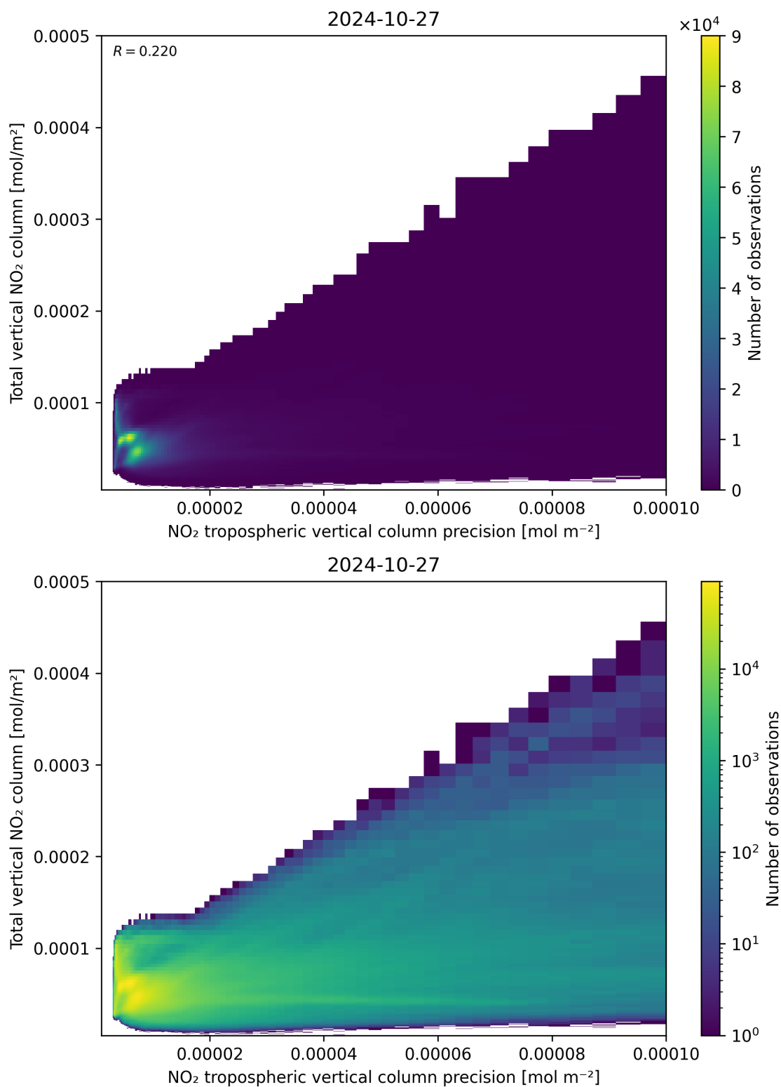
Figure 138: Scatter density plot of “NO 2 tropospheric vertical column precision” against “Total vertical NO 2 column” for 2024-10-26 to 2024-10-28.
