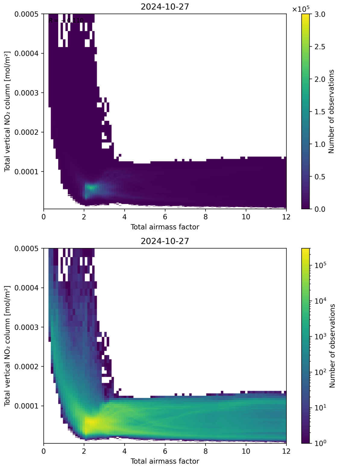
Figure 67: Scatter density plot of “Total airmass factor” against “Total vertical NO 2 column” for 2024-10-26 to 2024-10-28.
