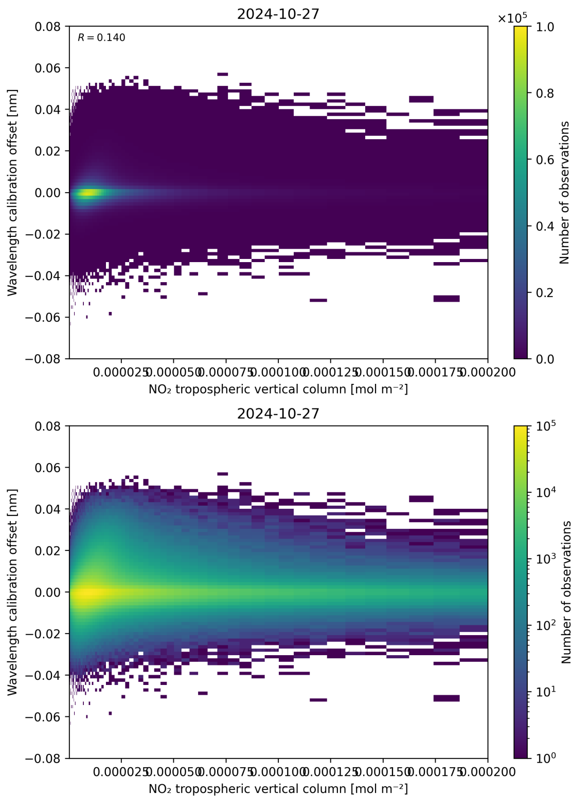
Figure 143: Scatter density plot of “NO 2 tropospheric vertical column” against “Wavelength calibration offset” for 2024-10-26 to 2024-10-28.
