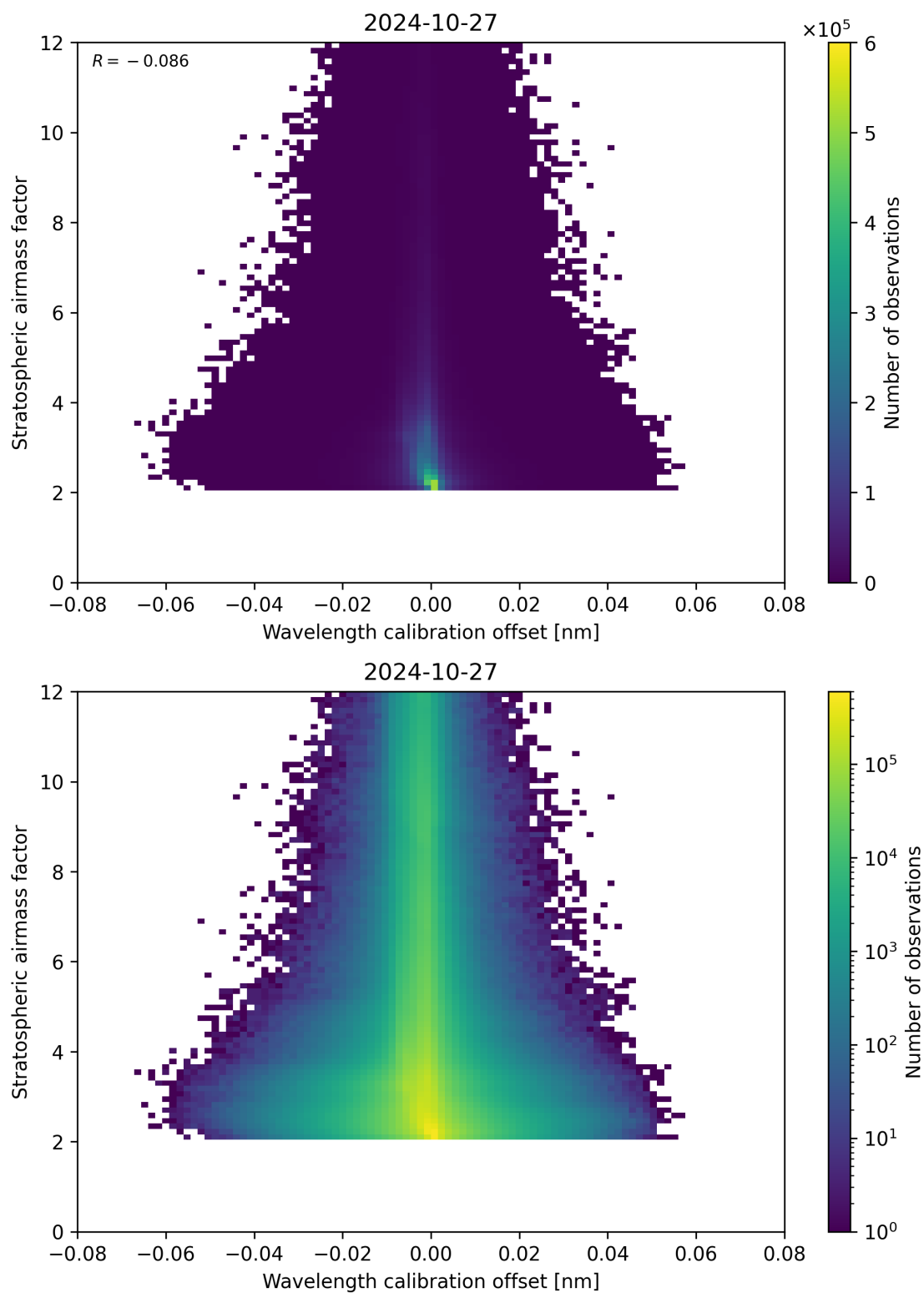
Figure 174: Scatter density plot of “Wavelength calibration offset” against “Stratospheric airmass factor” for 2024-10-26 to 2024-10-28.
