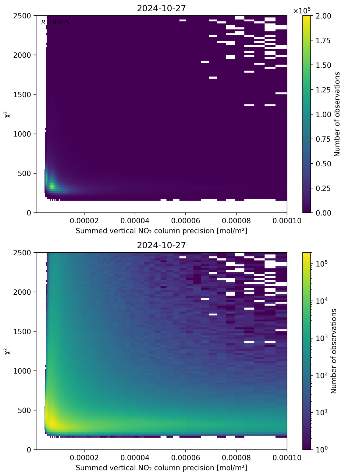
Figure 107: Scatter density plot of “Summed vertical NO 2 column precision” against “ \chi^2 ” for 2024-10-26 to 2024-10-28.
