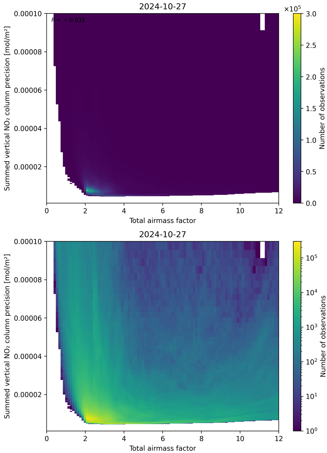
Figure 66: Scatter density plot of “Total airmass factor” against “Summed vertical NO 2 column precision” for 2024-10-26 to 2024-10-28.
