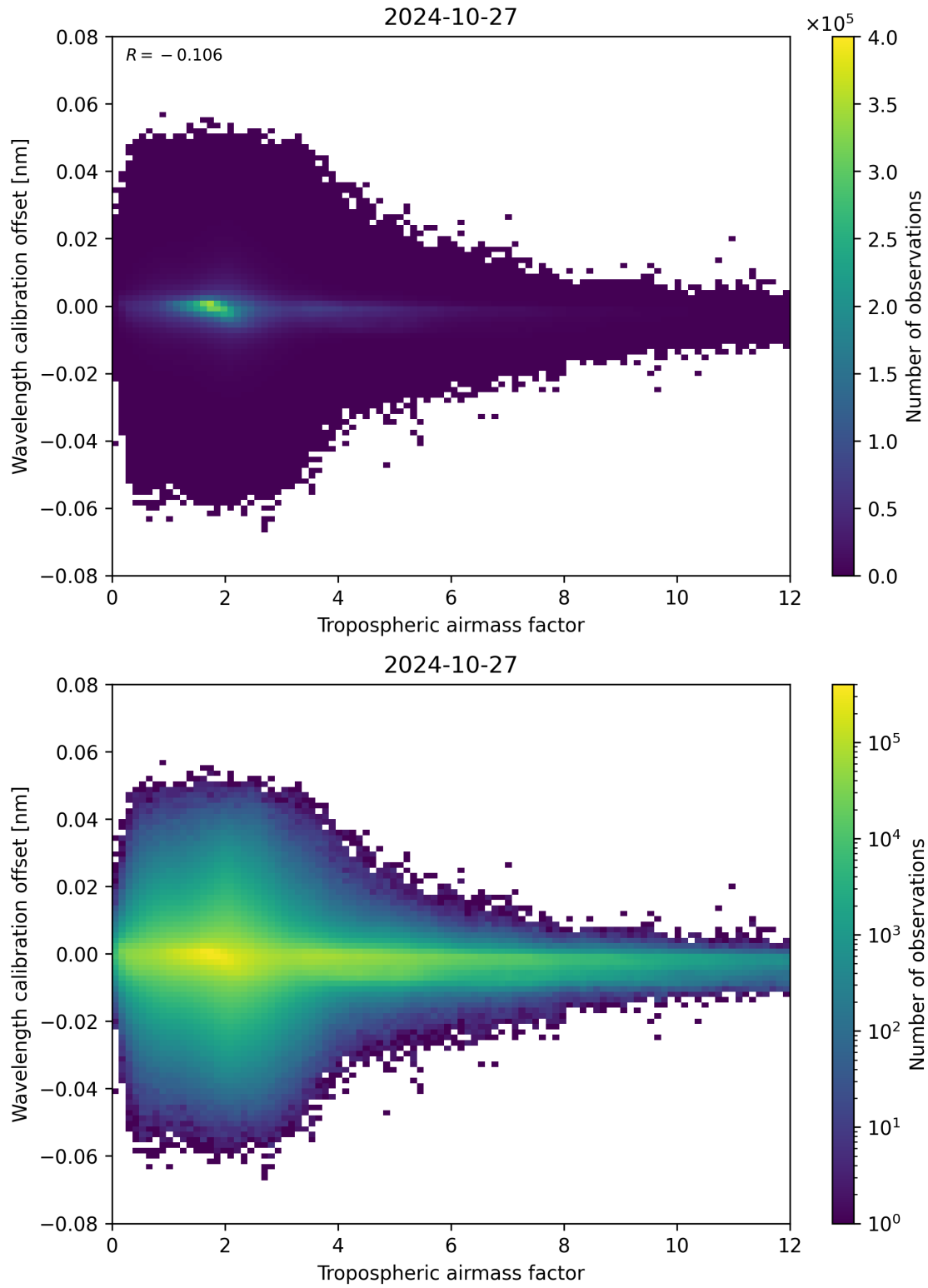
Figure 80: Scatter density plot of “Tropospheric airmass factor” against “Wavelength calibration offset” for 2024-10-26 to 2024-10-28.
