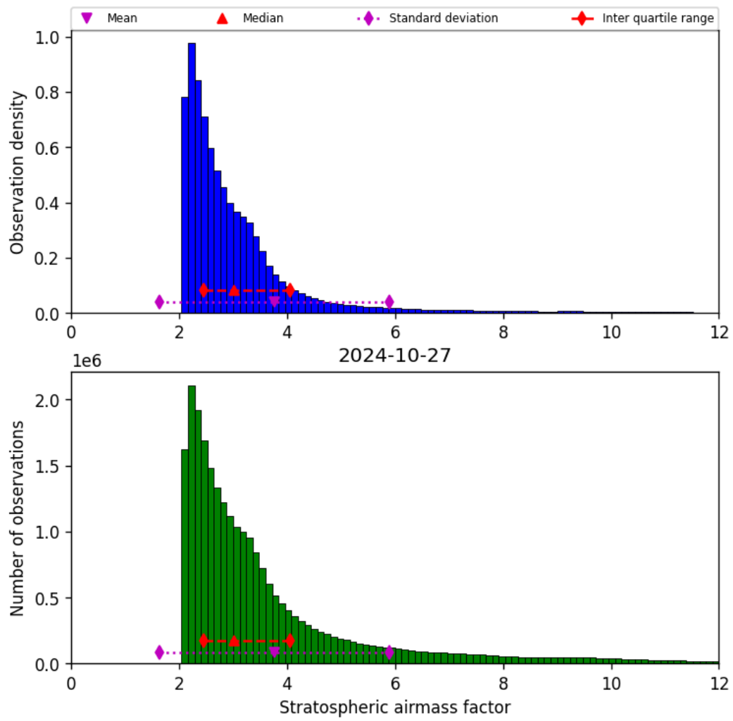
Figure 44: Histogram of “Stratospheric airmass factor” for 2024-10-26 to 2024-10-28
