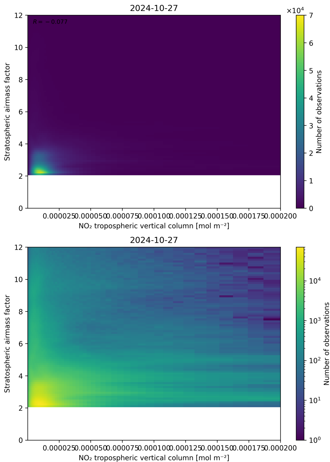
Figure 121: Scatter density plot of “NO 2 tropospheric vertical column” against “Stratospheric airmass factor” for 2024-10-26 to 2024-10-28.
