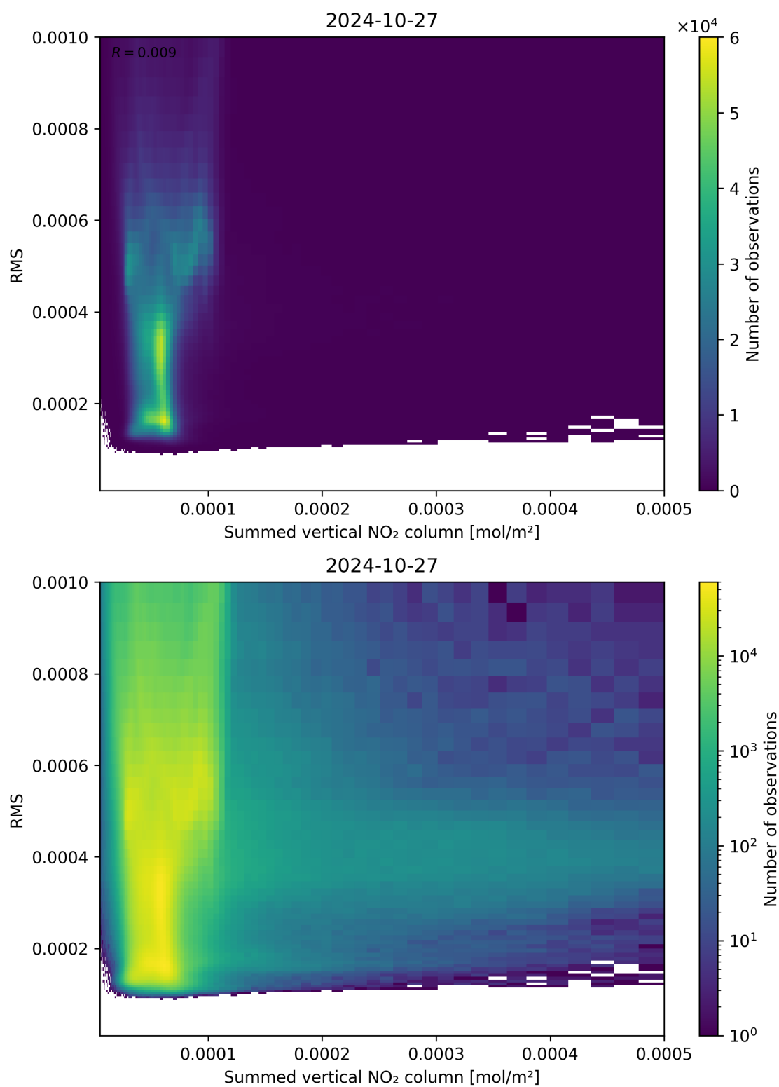
Figure 109: Scatter density plot of “Summed vertical NO 2 column” against “RMS” for 2024-10-26 to 2024-10-28.
