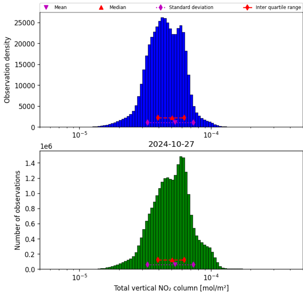
Figure 38: Histogram of “Total vertical NO 2 column” for 2024-10-26 to 2024-10-28
