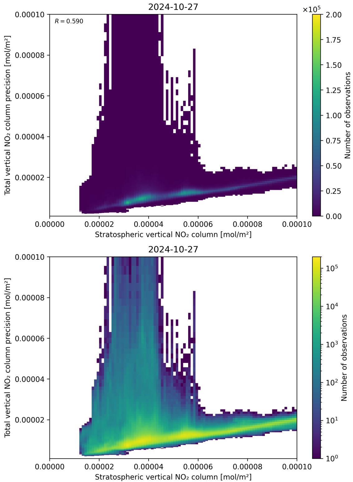
Figure 101: Scatter density plot of “Stratospheric vertical NO 2 column” against “Total vertical NO 2 column precision” for 2024-10-26 to 2024-10-28.
