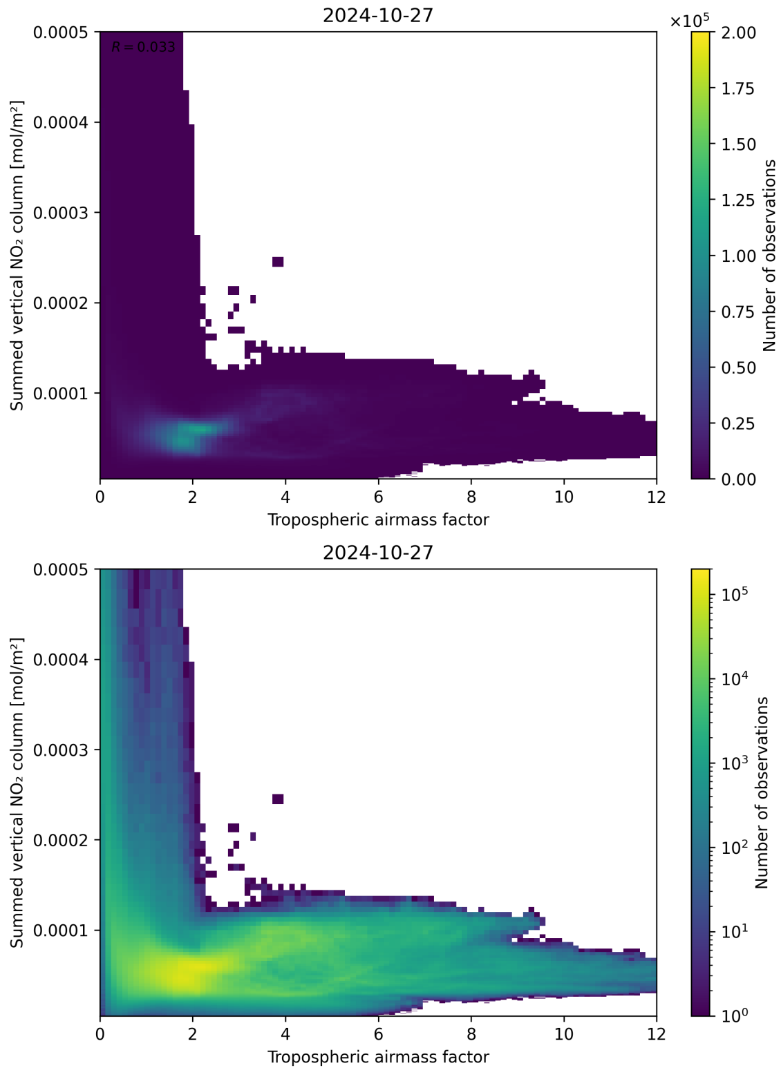
Figure 75: Scatter density plot of “Tropospheric airmass factor” against “Summed vertical NO 2 column” for 2024-10-26 to 2024-10-28.
