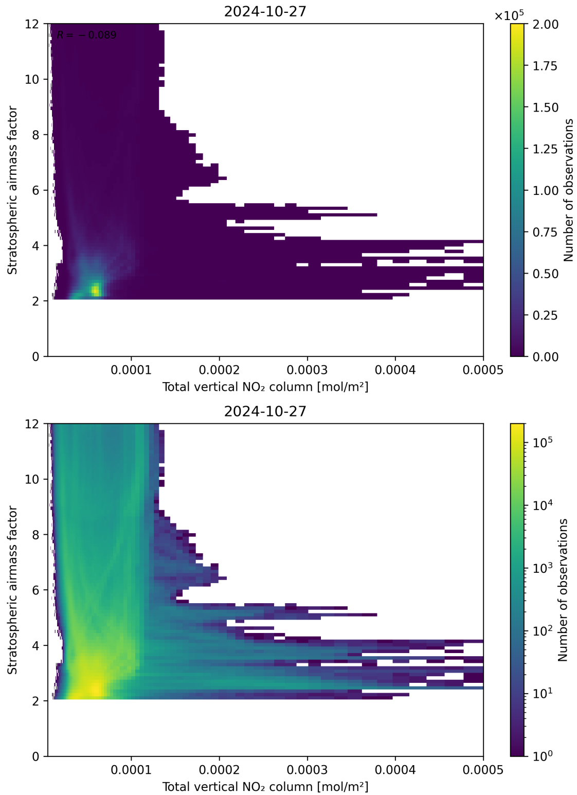
Figure 110: Scatter density plot of “Total vertical NO 2 column” against “Stratospheric air mass factor” for 2024-10-26 to 2024-10-28.
