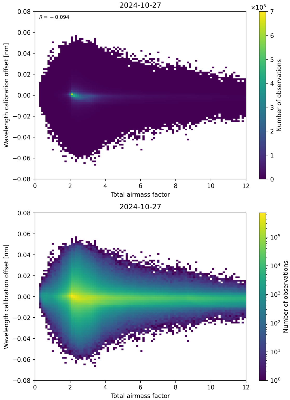
Figure 70: Scatter density plot of “Total airmass factor” against “Wavelength calibration offset” for 2024-10-26 to 2024-10-28.
