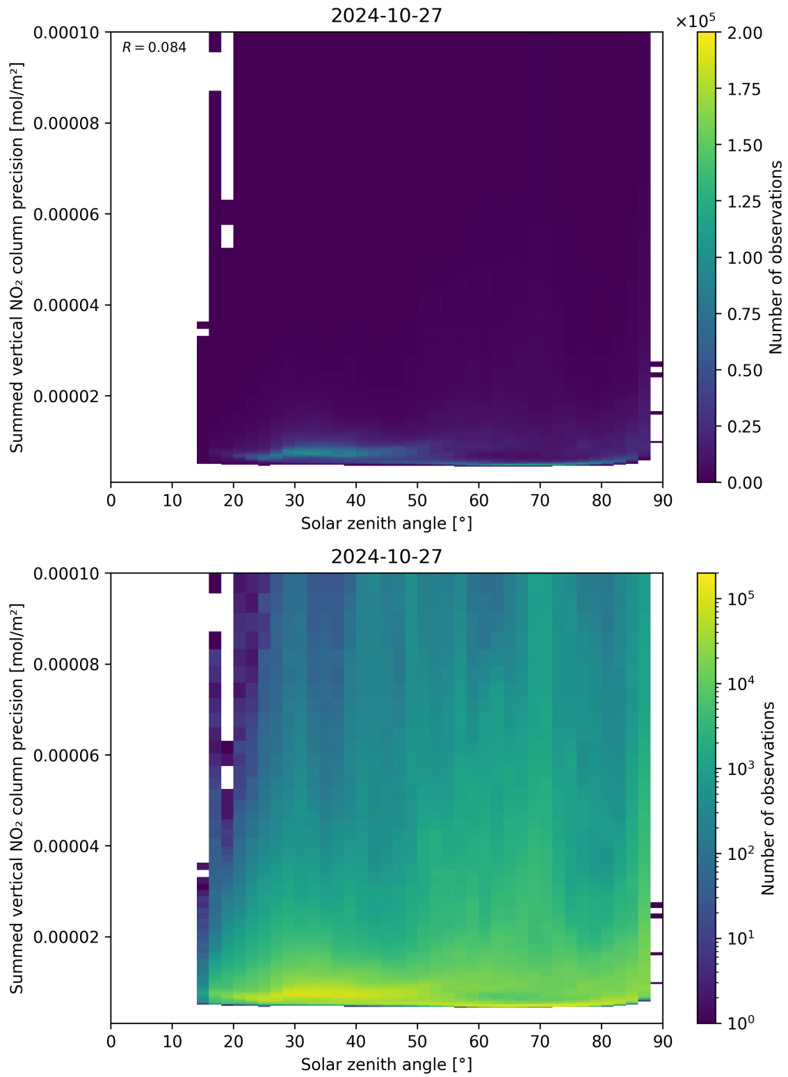
Figure 152: Scatter density plot of “Solar zenith angle” against “Summed vertical NO 2 column precision” for 2024-10-26 to 2024-10-28.
