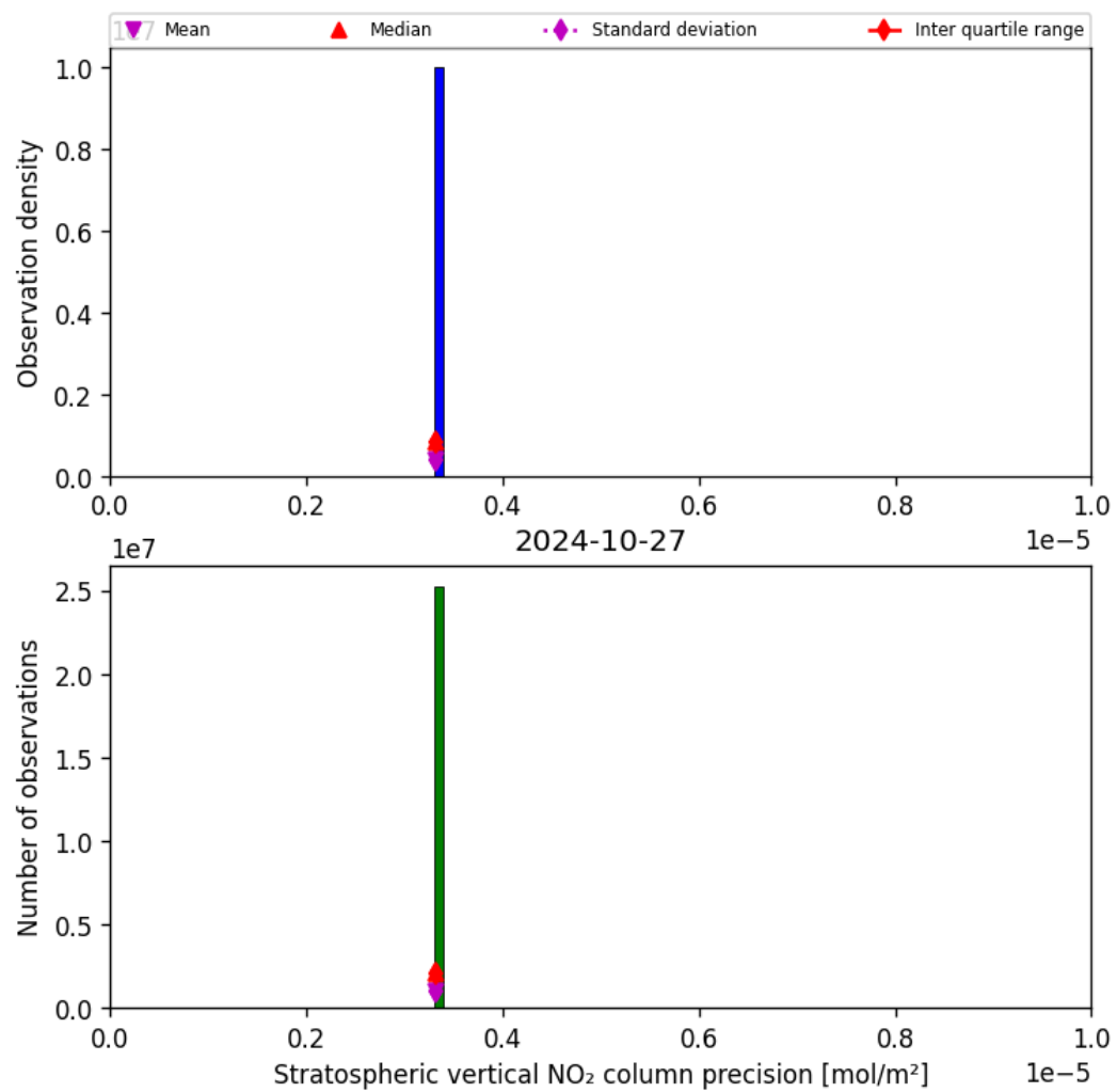
Figure 37: Histogram of “Stratospheric vertical NO 2 column precision” for 2024-10-26 to 2024-10-28
