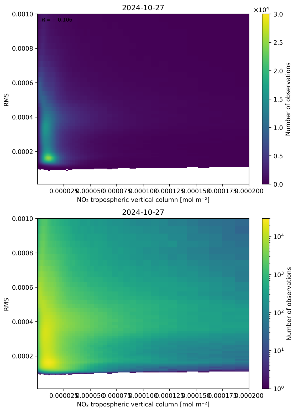
Figure 142: Scatter density plot of “NO 2 tropospheric vertical column” against “RMS” for 2024-10-26 to 2024-10-28.
