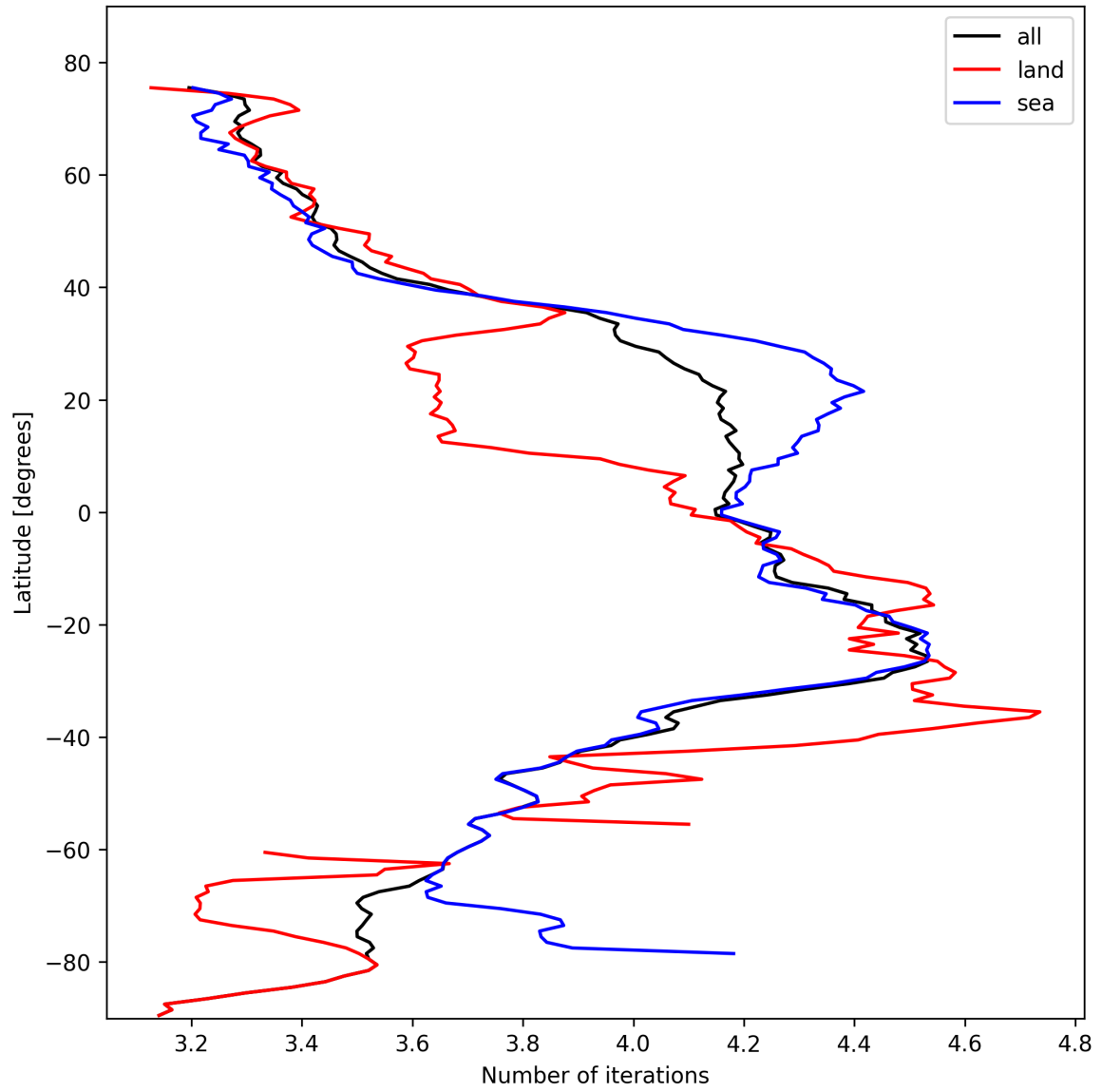
Figure 17: Zonal average of “Number of iterations” for 2024-10-26 to 2024-10-28.
