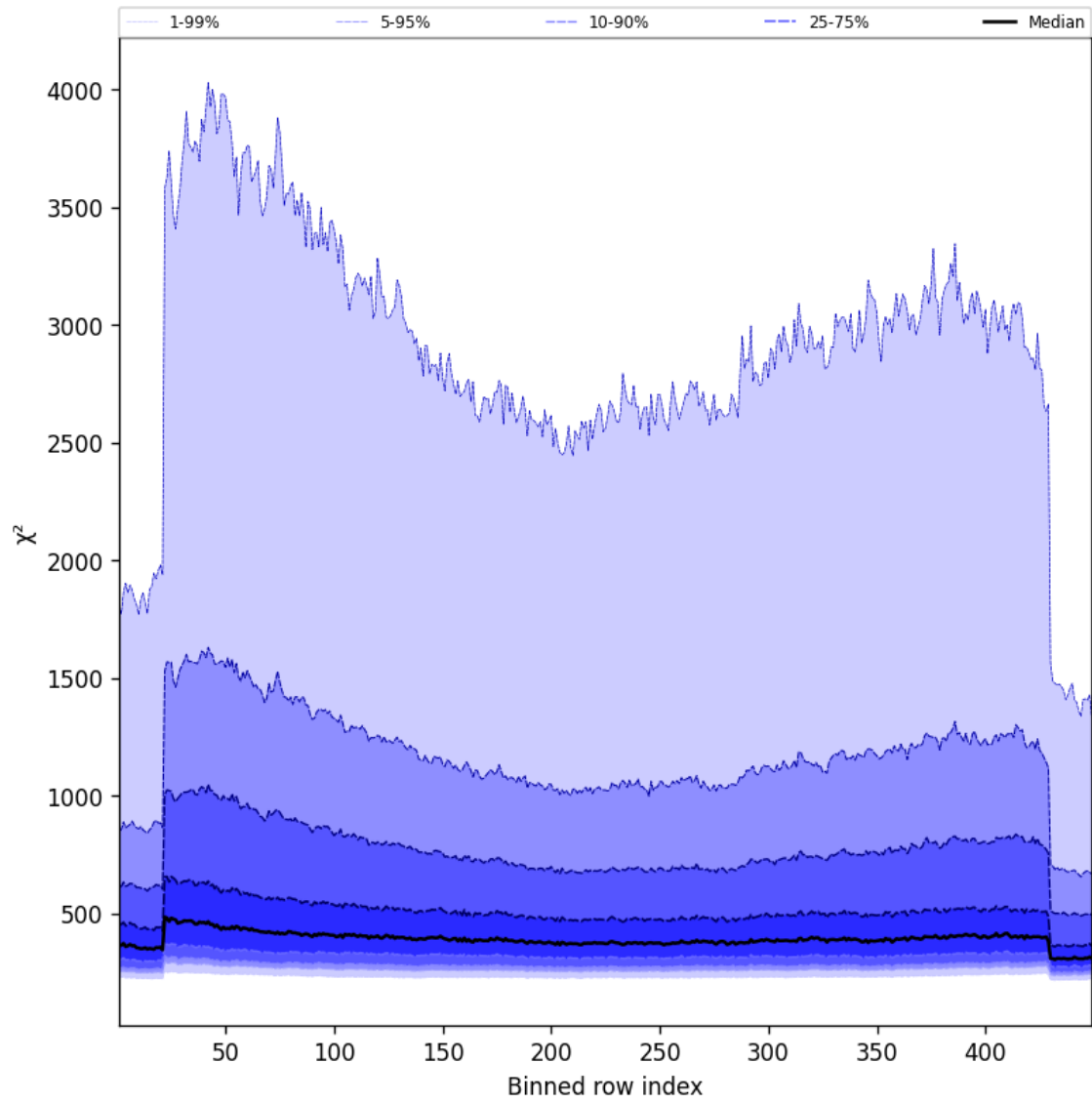
Figure 59: Along track statistics of “ \chi^2 ” for 2024-10-26 to 2024-10-28
