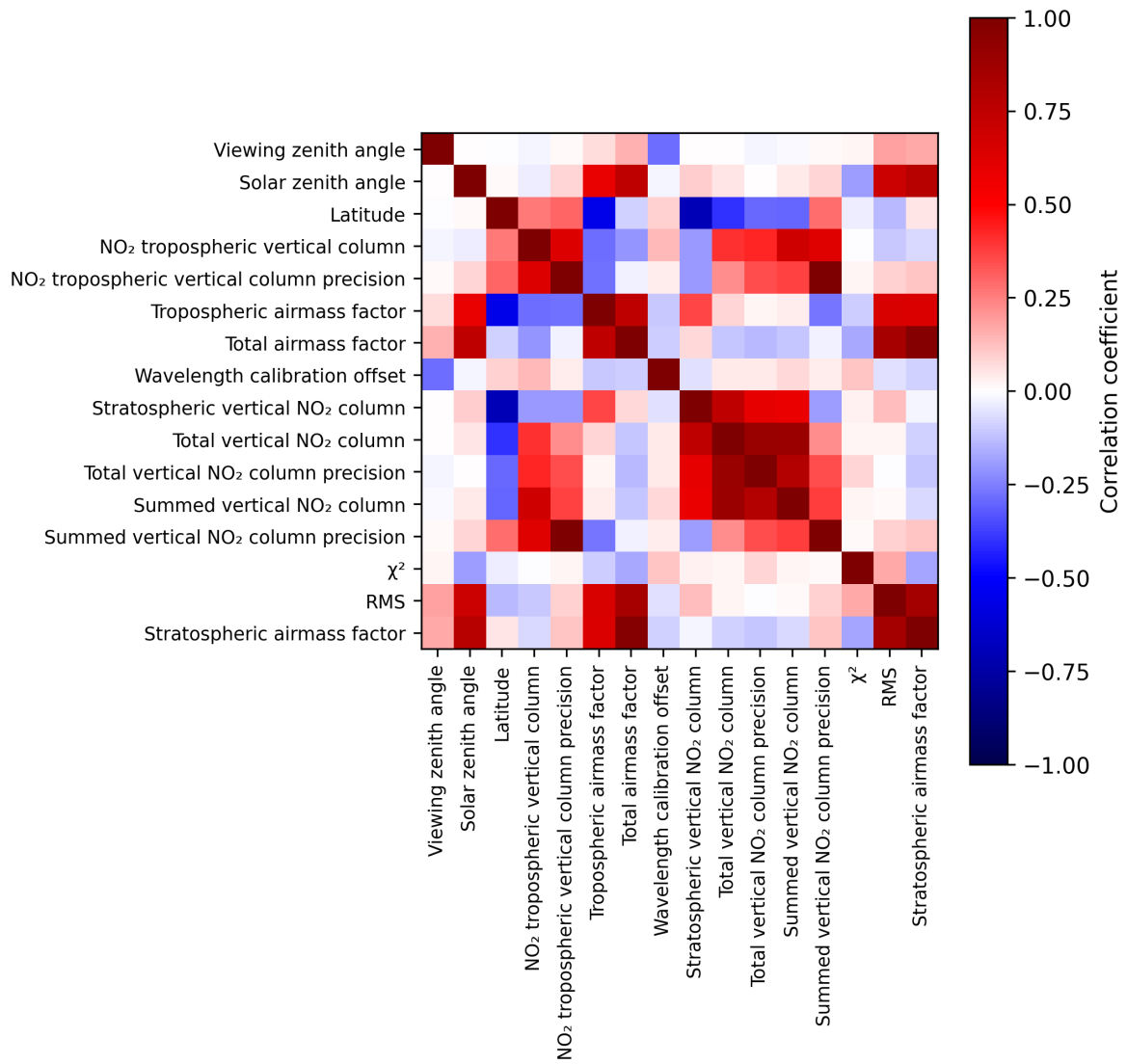
Figure 2: Map of correlation matrix for 2024-10-26 to 2024-10-28.
