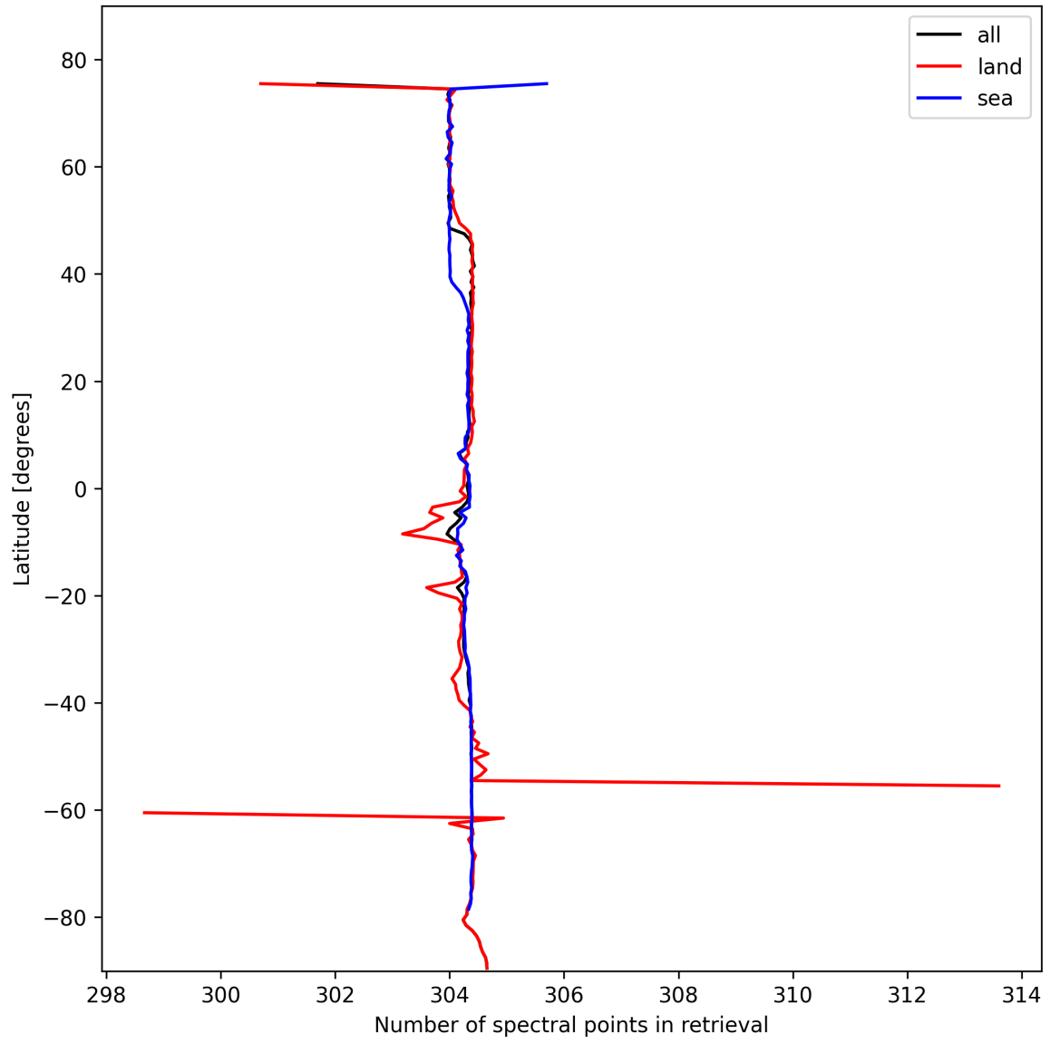
Figure 16: Zonal average of “Number of spectral points in retrieval” for 2024-10-26 to 2024-10-28.
