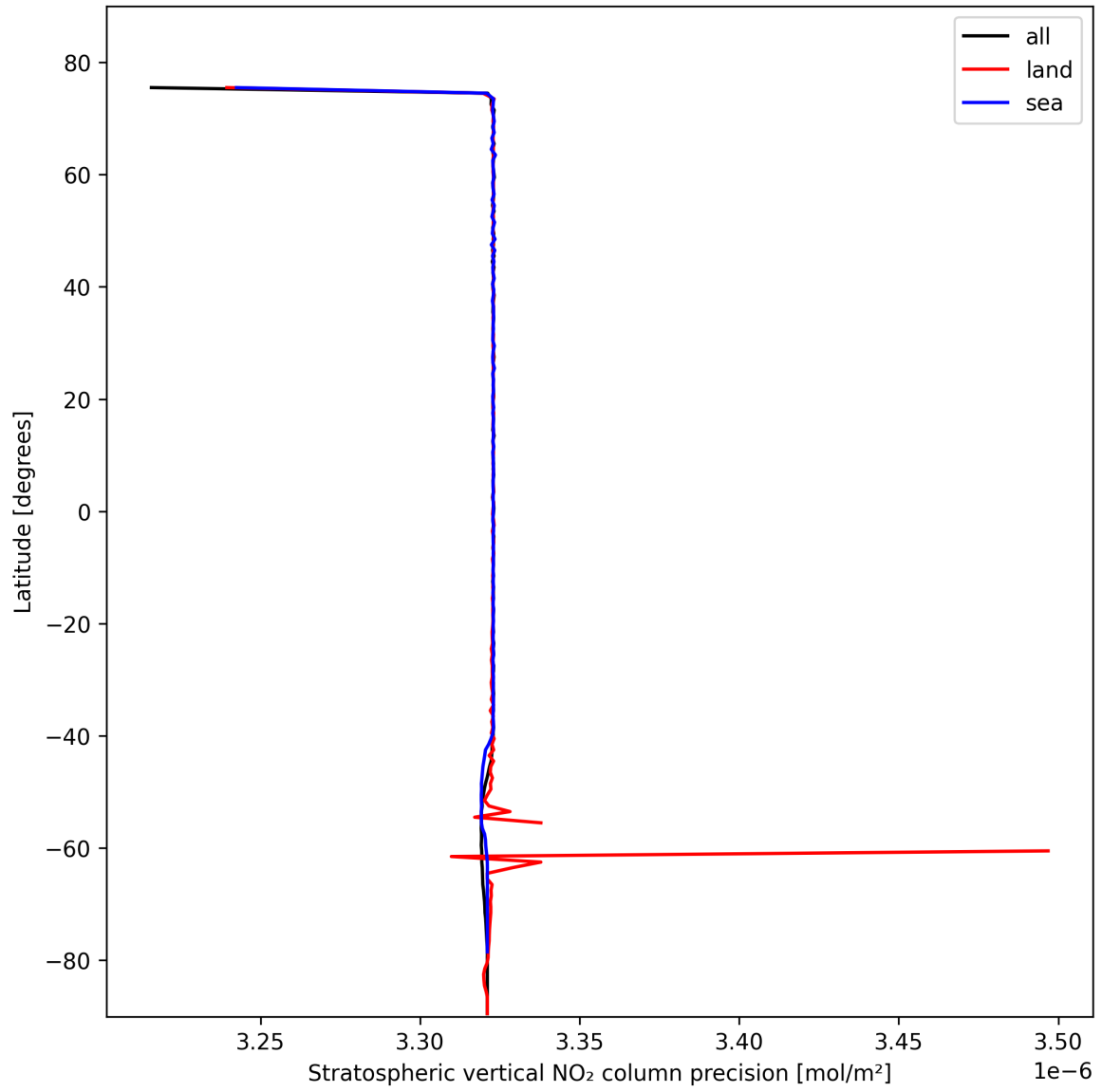
Figure 20: Zonal average of “Stratospheric vertical NO 2 column precision” for 2024-10-26 to 2024-10-28.
