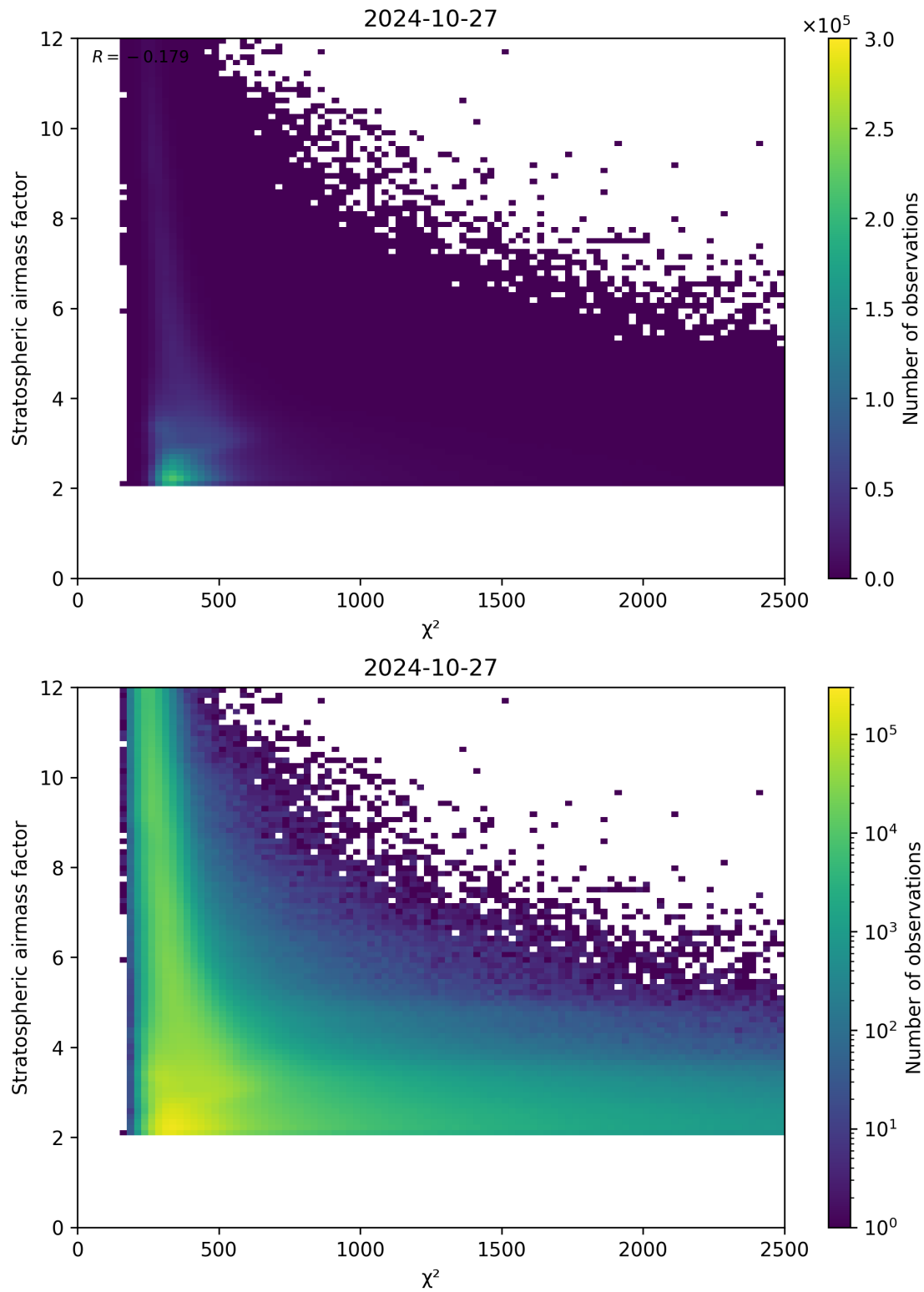
Figure 81: Scatter density plot of “ \chi^2 ” against “Stratospheric airmass factor” for 2024-10-26 to 2024-10-28.
