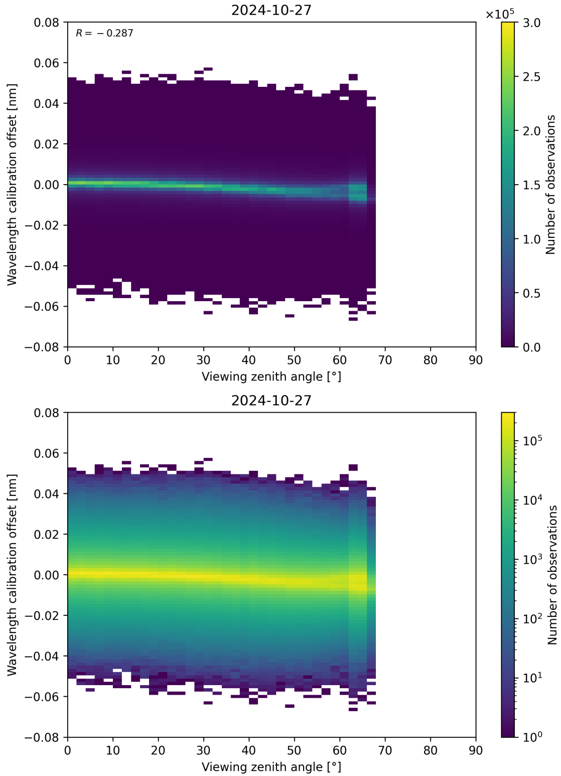
Figure 173: Scatter density plot of “Viewing zenith angle” against “Wavelength calibration offset” for 2024-10-26 to 2024-10-28.
