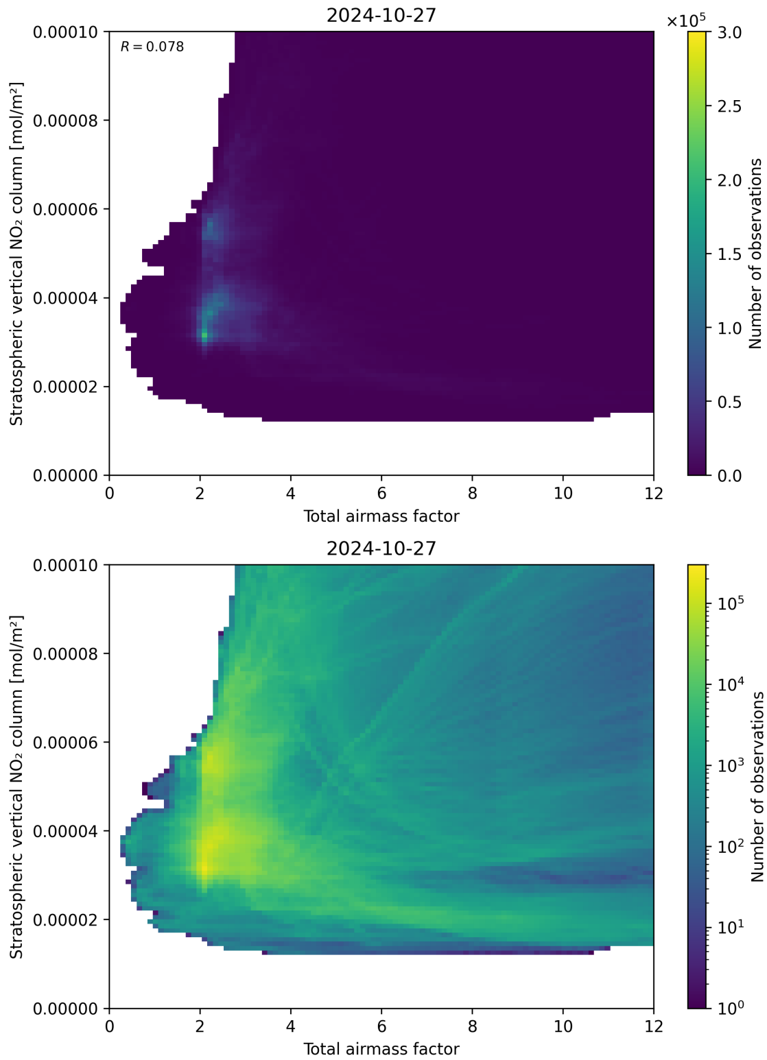
Figure 64: Scatter density plot of “Total airmass factor” against “Stratospheric vertical NO 2 column” for 2024-10-26 to 2024-10-28.
