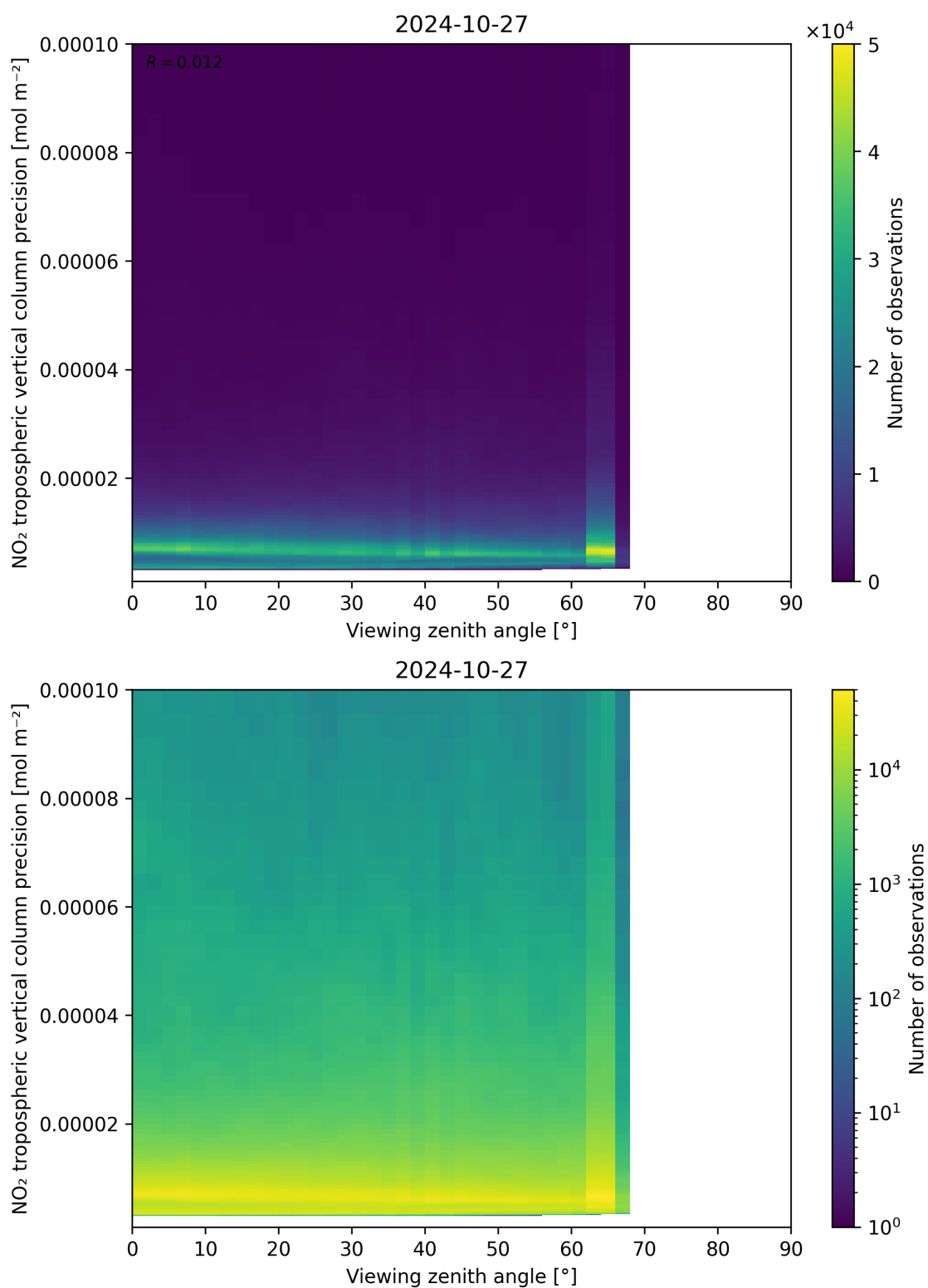
Figure 170: Scatter density plot of “Viewing zenith angle” against “NO 2 tropospheric vertical column precision” for 2024-10-26 to 2024-10-28.
