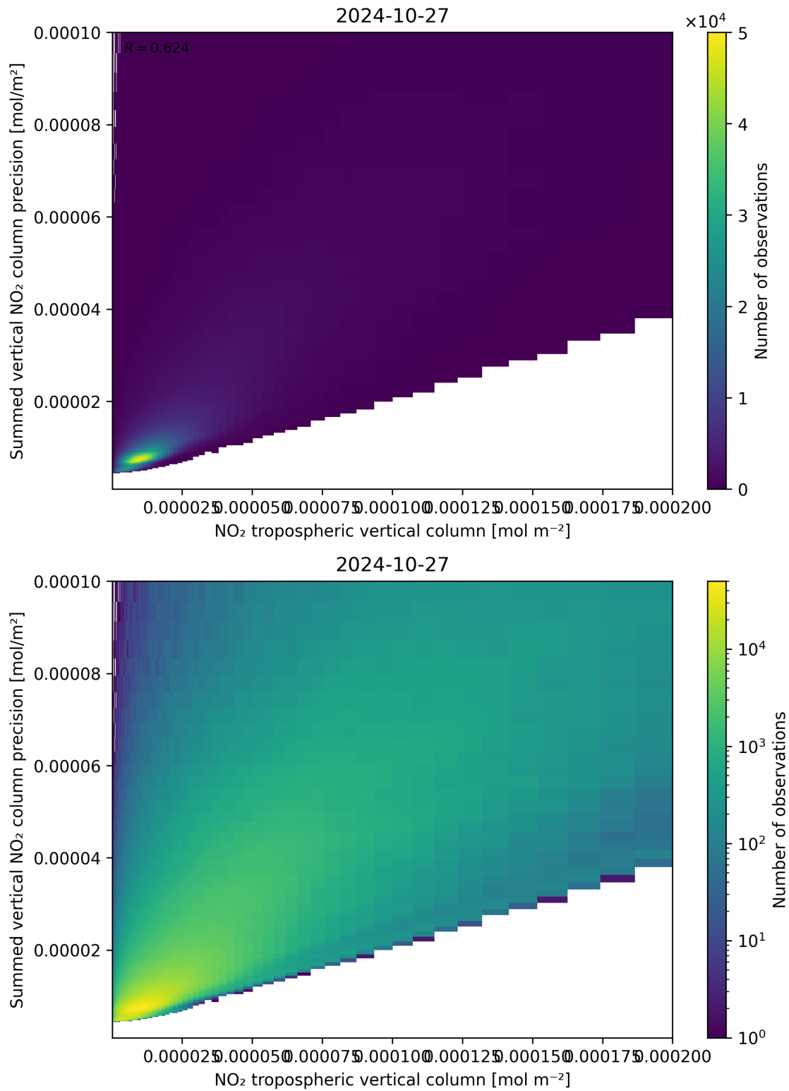
Figure 127: Scatter density plot of “NO 2 tropospheric vertical column” against “Summed vertical NO 2 column precision” for 2024-10-26 to 2024-10-28.
