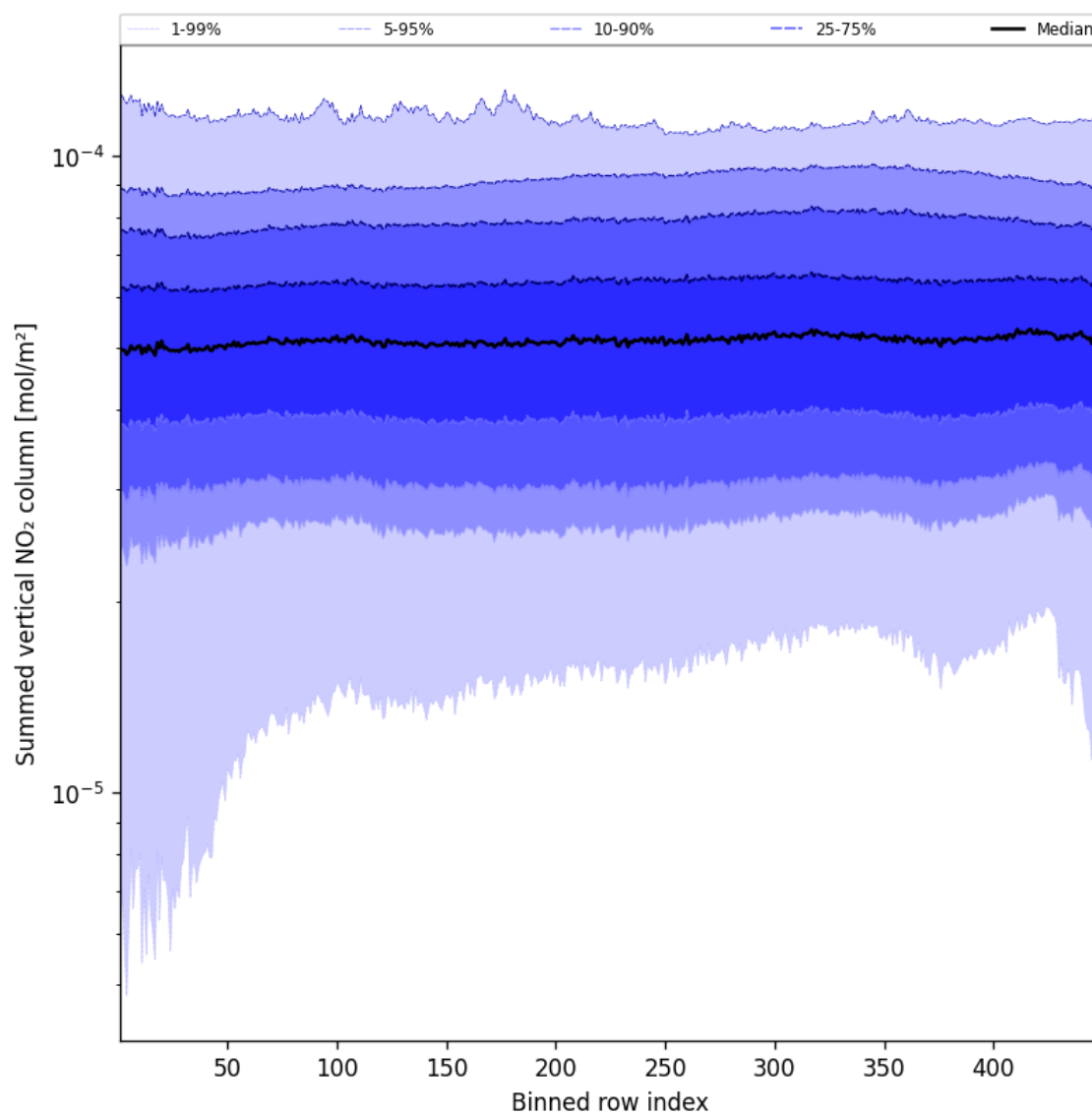
Figure 57: Along track statistics of “Summed vertical NO 2 column” for 2024-10-26 to 2024-10-28
