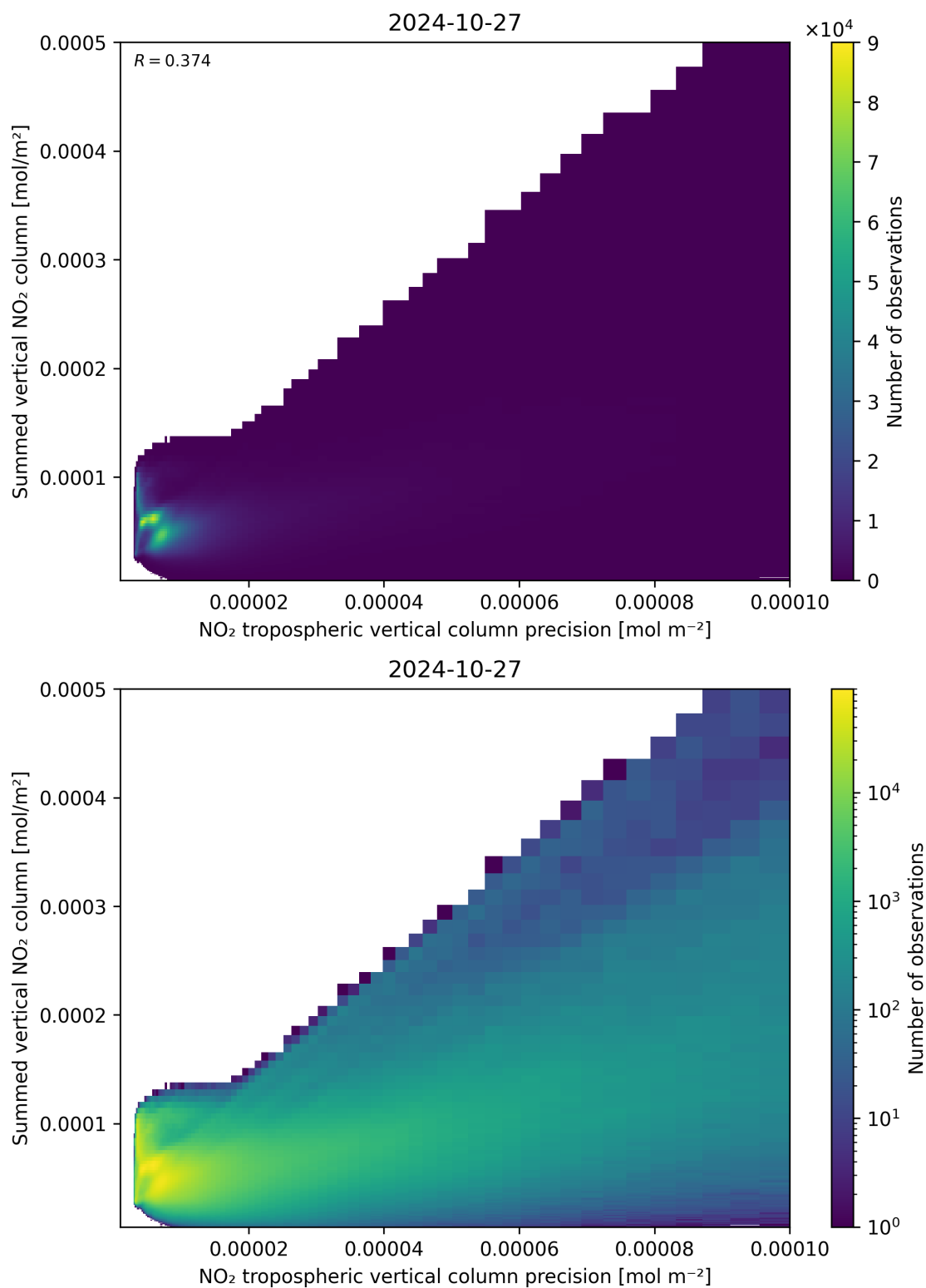
Figure 136: Scatter density plot of “NO 2 tropospheric vertical column precision” against “Summed vertical NO 2 column” for 2024-10-26 to 2024-10-28.
