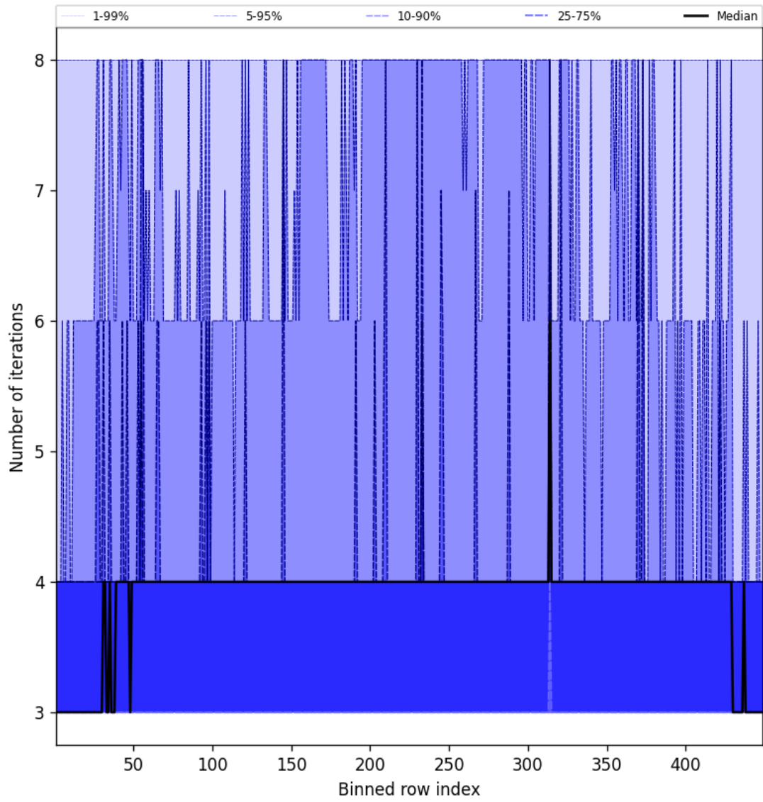
Figure 51: Along track statistics of “Number of iterations” for 2024-10-26 to 2024-10-28
