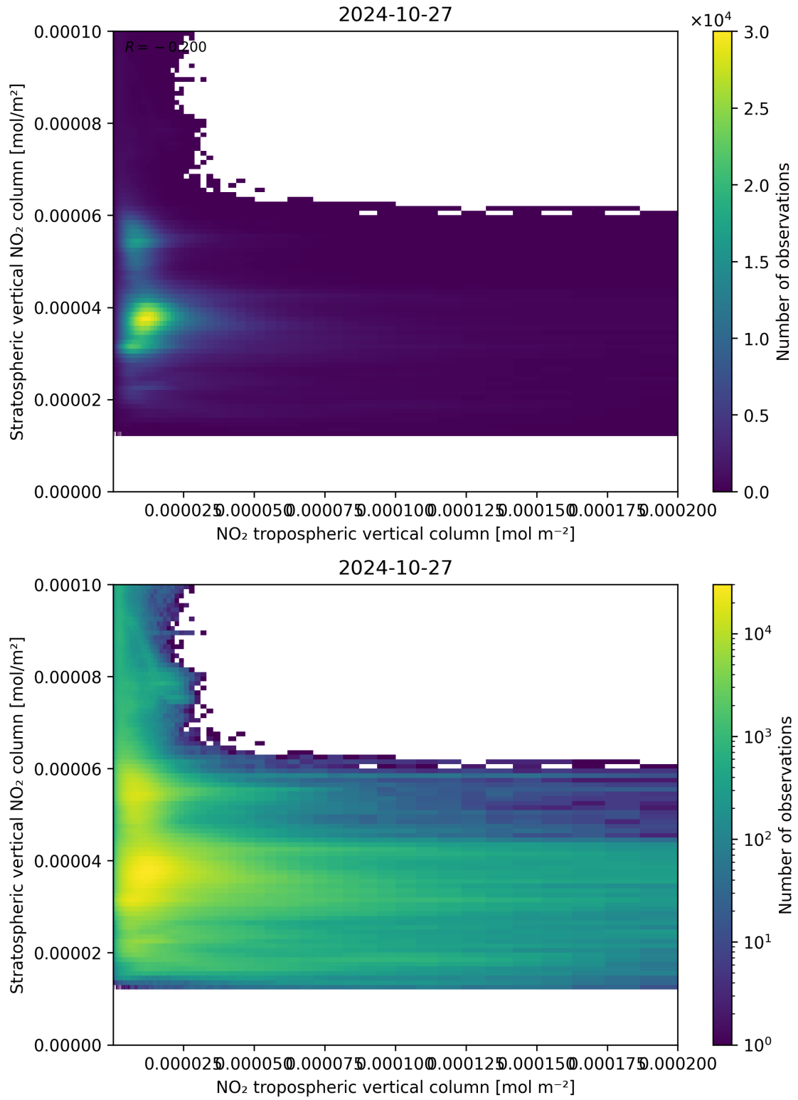
Figure 125: Scatter density plot of “NO 2 tropospheric vertical column” against “Stratospheric vertical NO 2 column” for 2024-10-26 to 2024-10-28.
