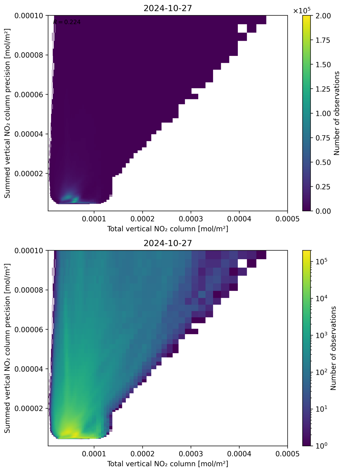
Figure 113: Scatter density plot of “Total vertical NO 2 column” against “Summed vertical NO 2 column precision” for 2024-10-26 to 2024-10-28.
