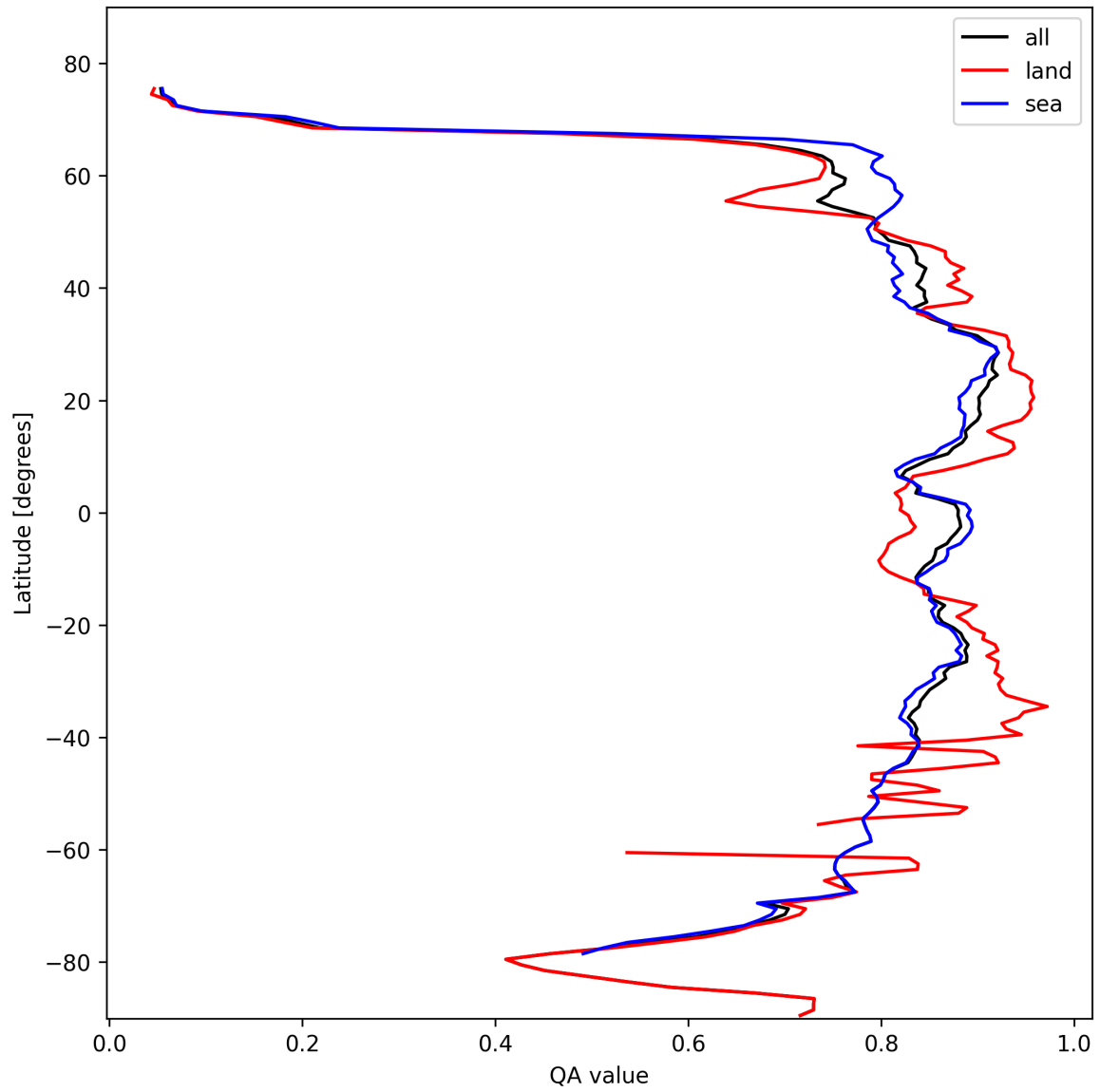
Figure 11: Zonal average of “QA value” for 2024-10-26 to 2024-10-28.
