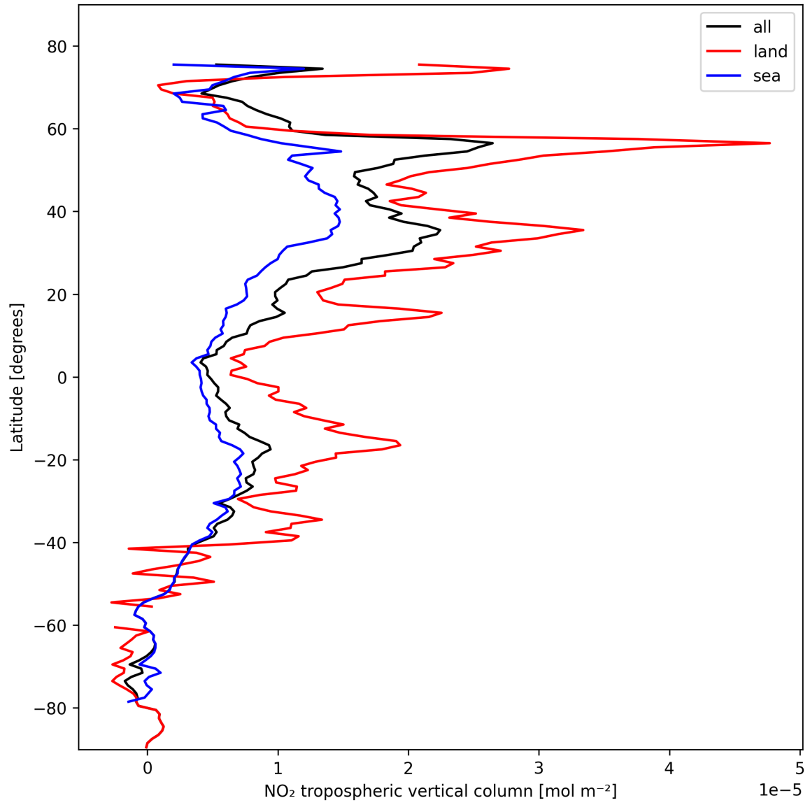
Figure 12: Zonal average of “NO 2 tropospheric vertical column” for 2024-10-26 to 2024-10-28.
