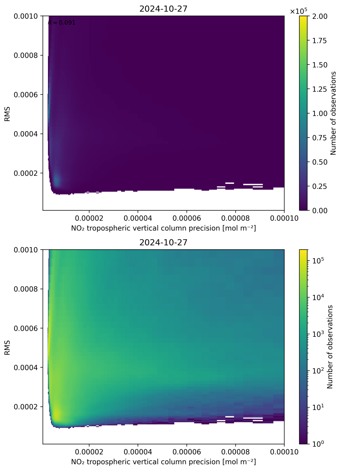
Figure 140: Scatter density plot of “NO 2 tropospheric vertical column precision” against “RMS” for 2024-10-26 to 2024-10-28.
