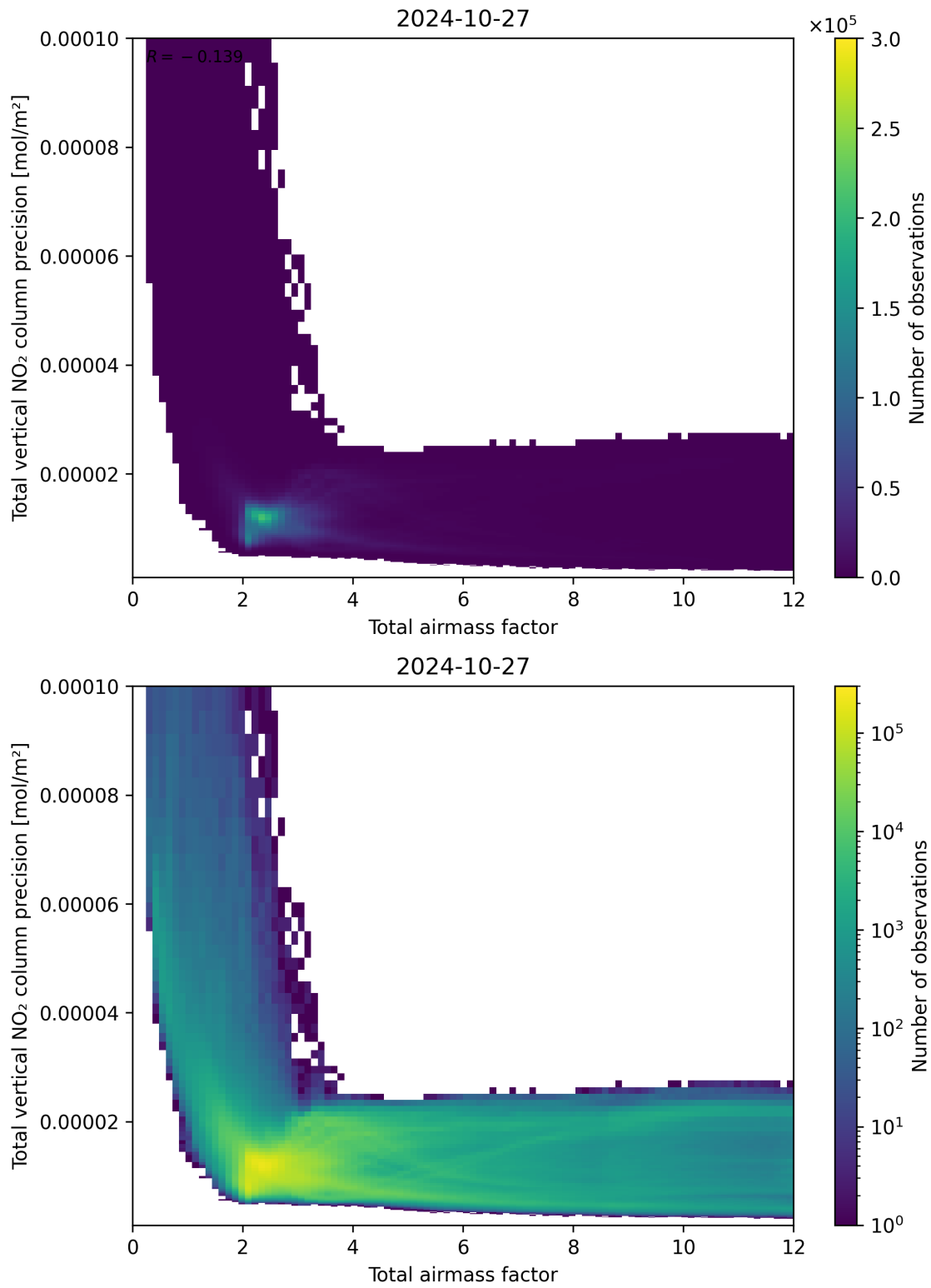
Figure 68: Scatter density plot of “Total airmass factor” against “Total vertical NO 2 column precision” for 2024-10-26 to 2024-10-28.
