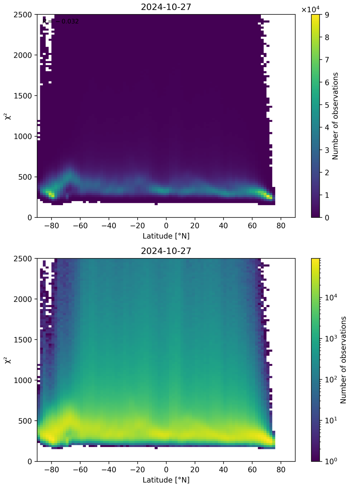
Figure 86: Scatter density plot of “Latitude” against “ \chi^2 ” for 2024-10-26 to 2024-10-28.
