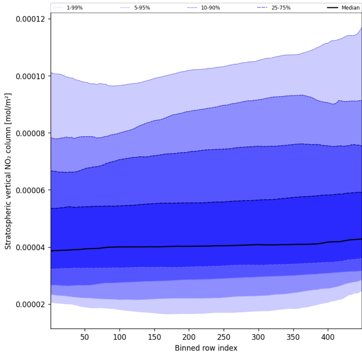
Figure 53: Along track statistics of “Stratospheric vertical NO 2 column” for 2024-10-26 to 2024-10-28
