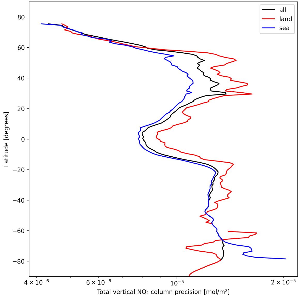
Figure 22: Zonal average of “Total vertical NO 2 column precision” for 2024-10-26 to 2024-10-28.
