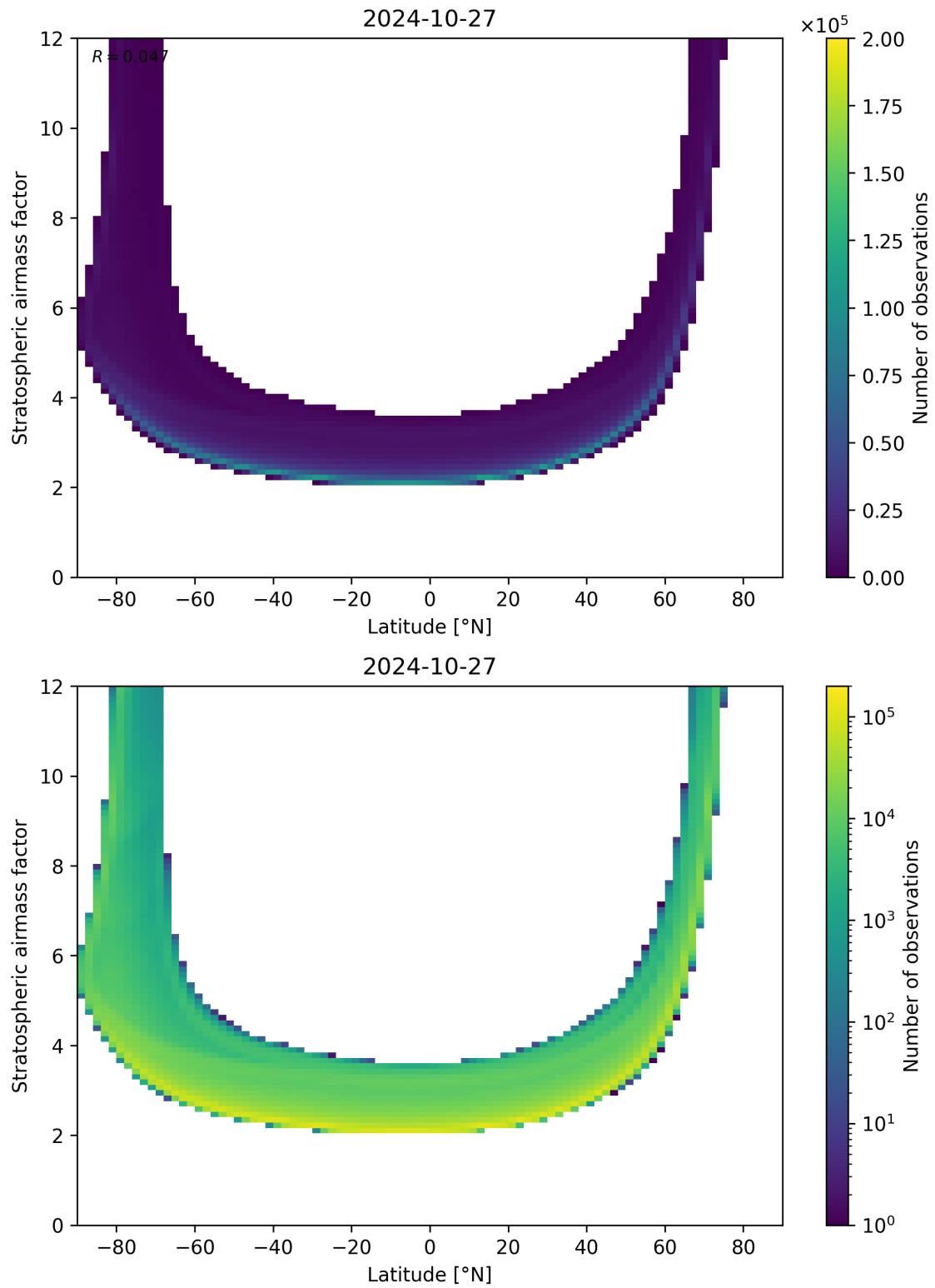
Figure 83: Scatter density plot of “Latitude” against “Stratospheric air mass factor” for 2024-10-26 to 2024-10-28.
