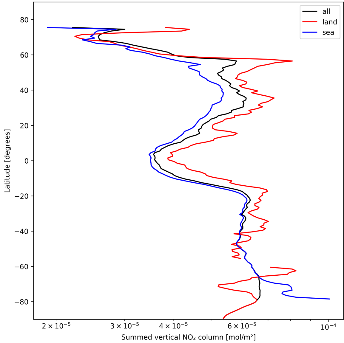
Figure 23: Zonal average of “Summed vertical NO 2 column” for 2024-10-26 to 2024-10-28.
