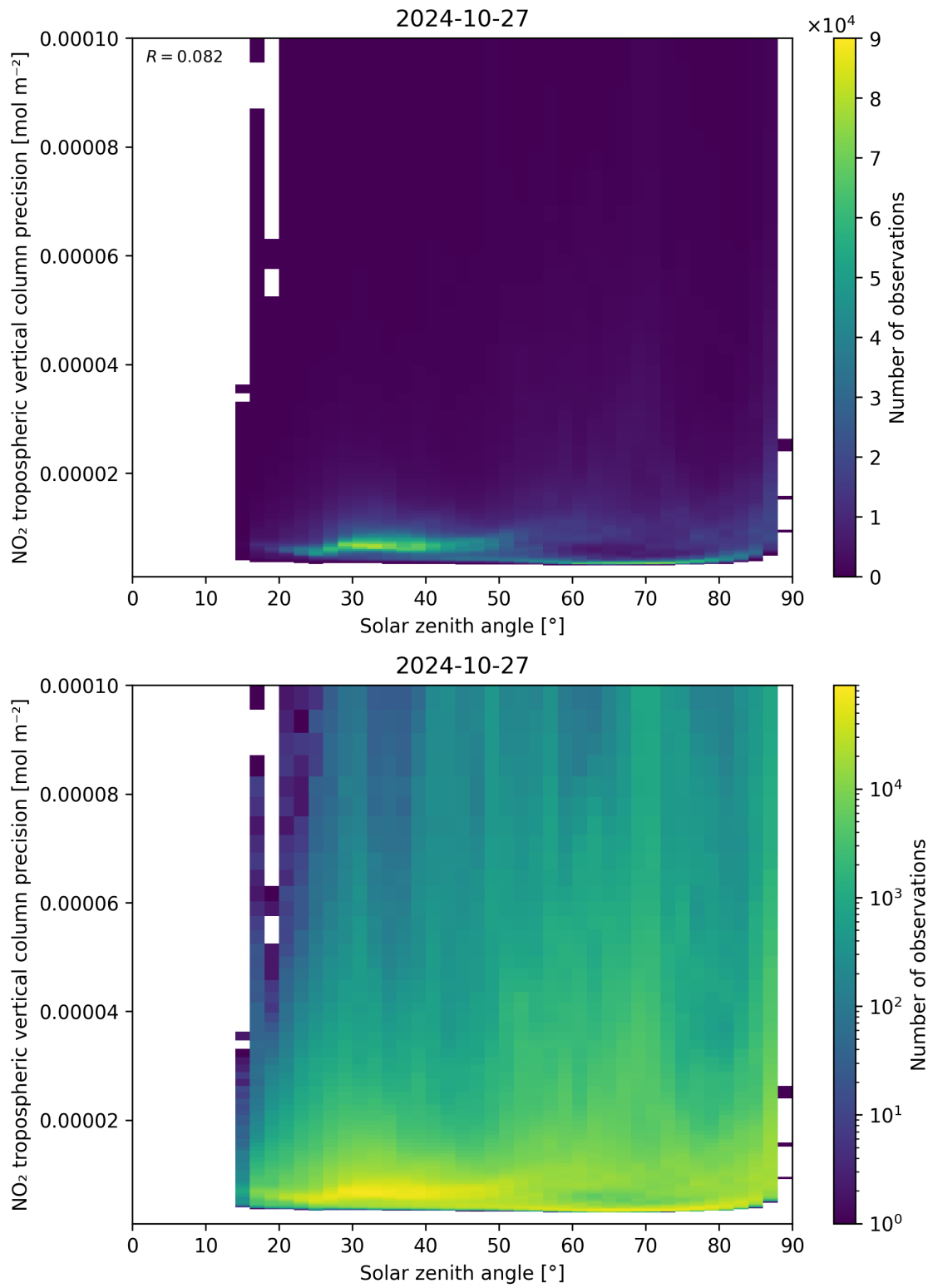
Figure 156: Scatter density plot of “Solar zenith angle” against “NO 2 tropospheric vertical column precision” for 2024-10-26 to 2024-10-28.
