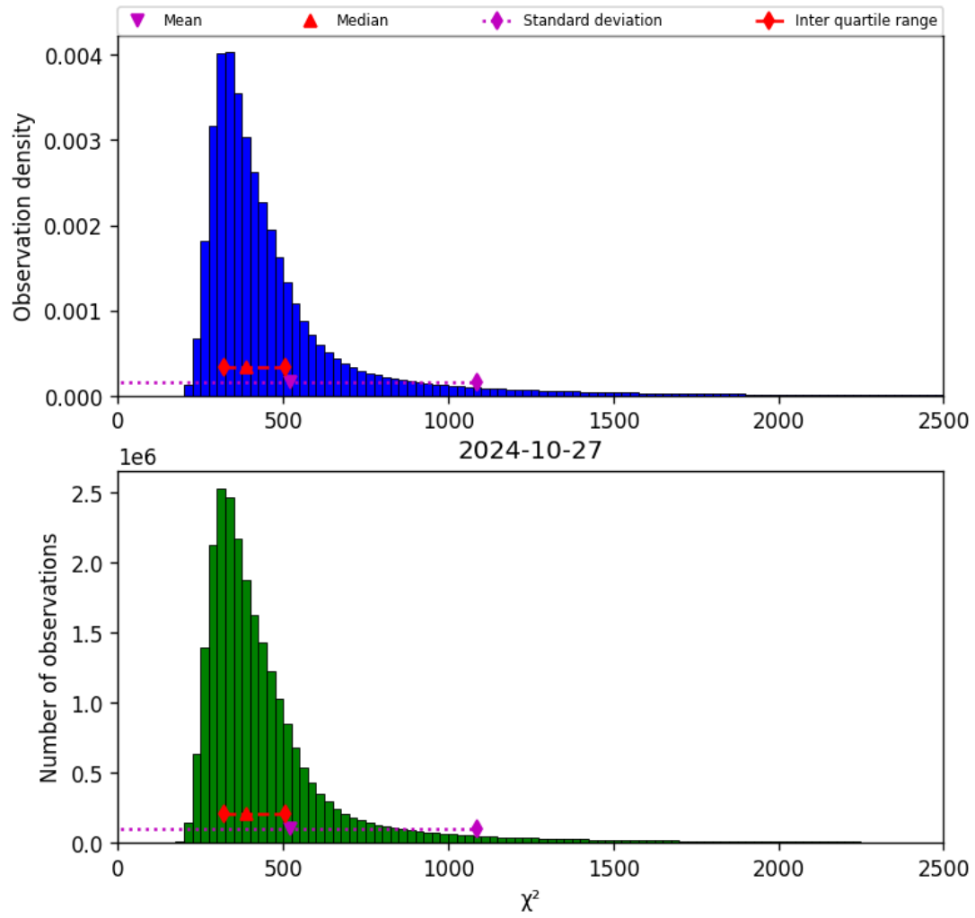
Figure 42: Histogram of “ \chi^2 ” for 2024-10-26 to 2024-10-28
