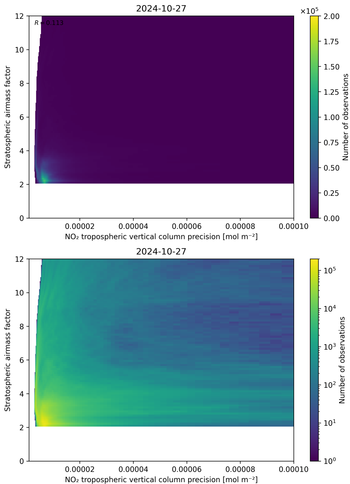
Figure 131: Scatter density plot of “NO 2 tropospheric vertical column precision” against “Stratospheric airmass factor” for 2024-10-26 to 2024-10-28.
