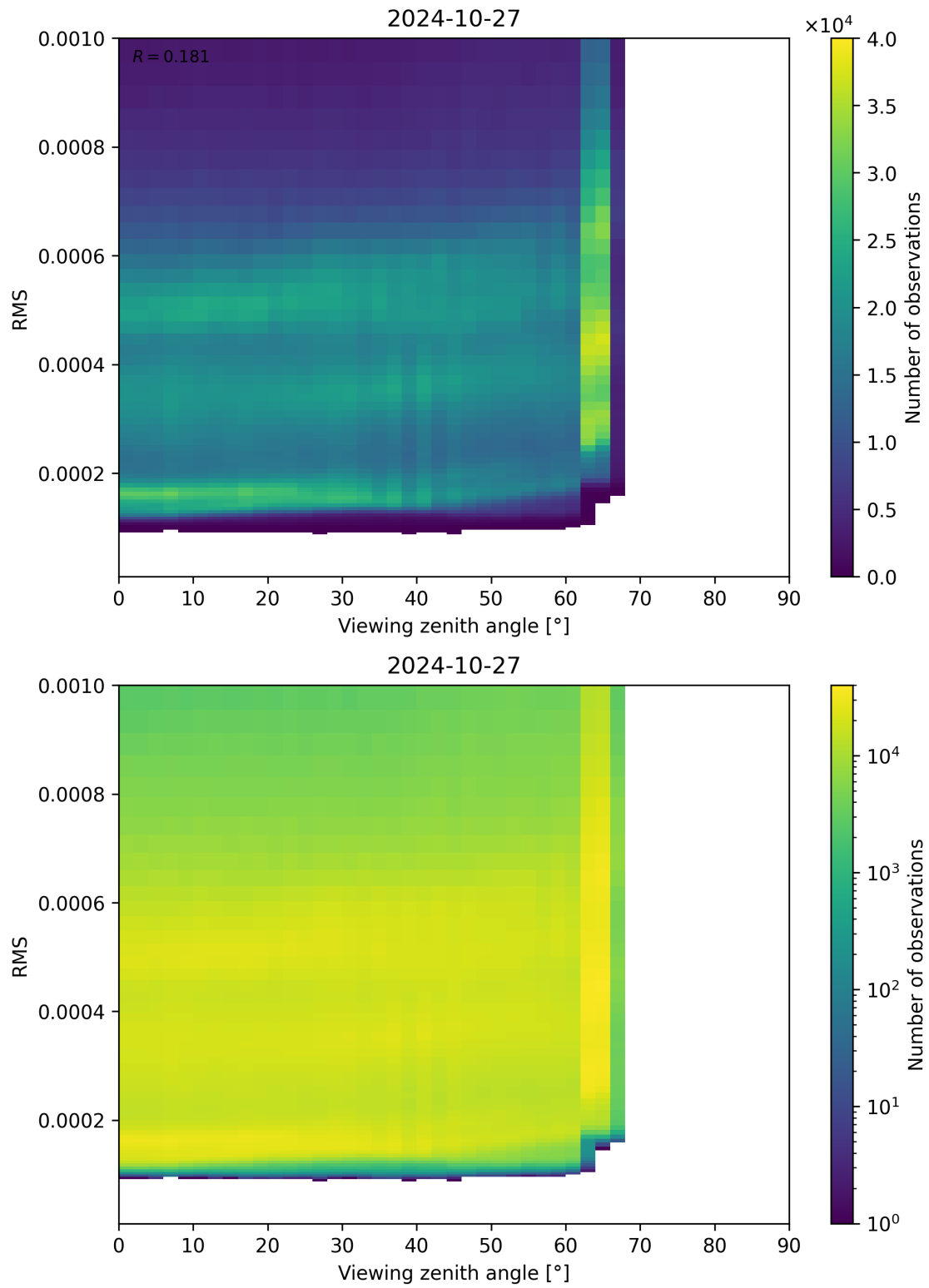
Figure 171: Scatter density plot of “Viewing zenith angle” against “RMS” for 2024-10-26 to 2024-10-28.
