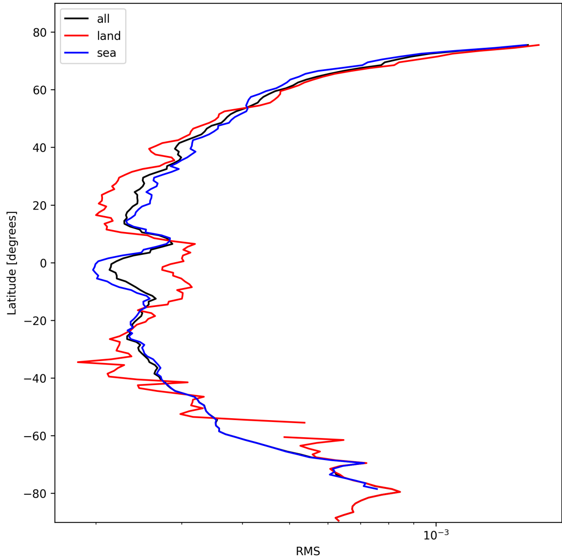
Figure 26: Zonal average of “RMS” for 2024-10-26 to 2024-10-28.
