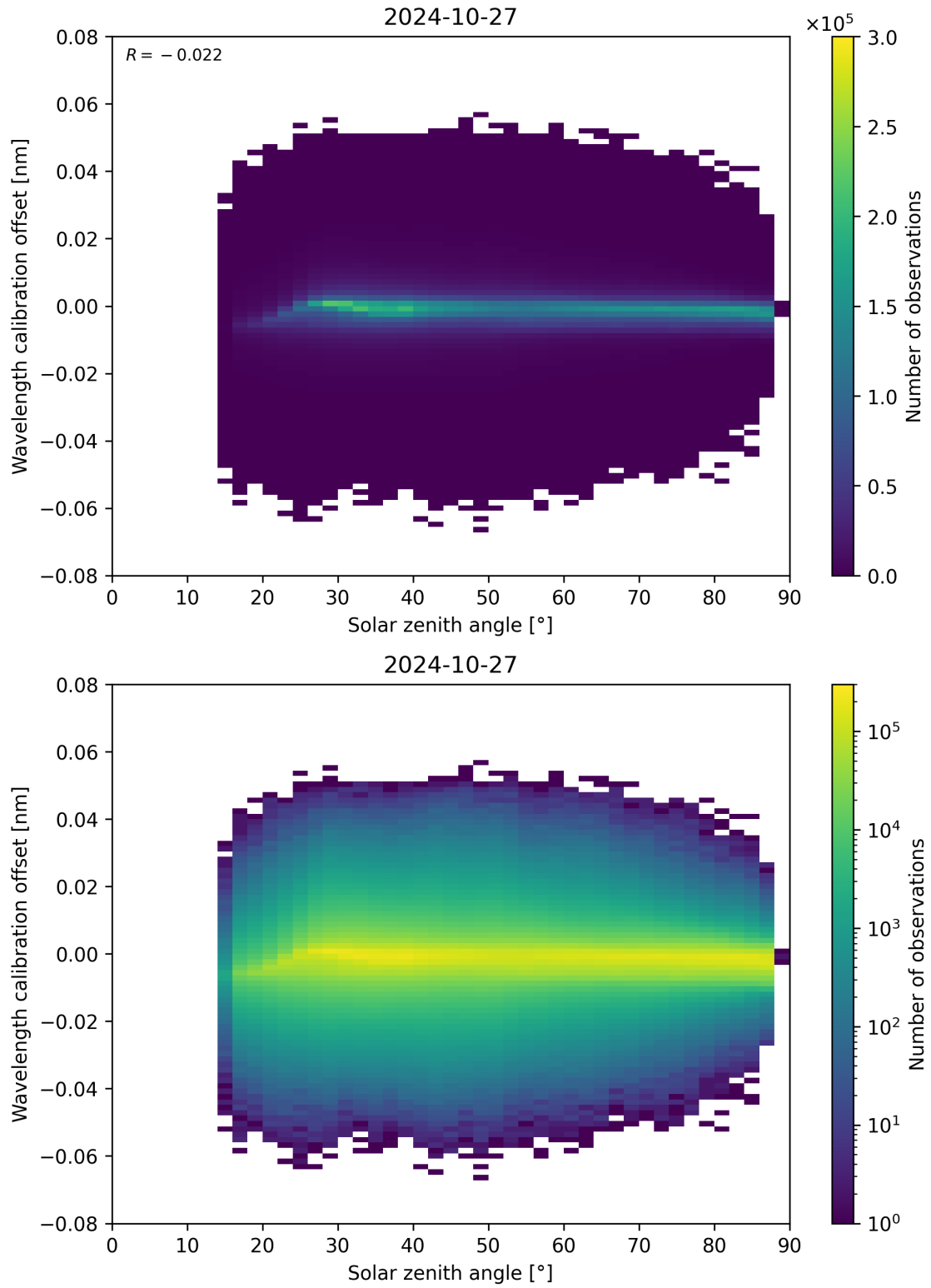
Figure 158: Scatter density plot of “Solar zenith angle” against “Wavelength calibration offset” for 2024-10-26 to 2024-10-28.
