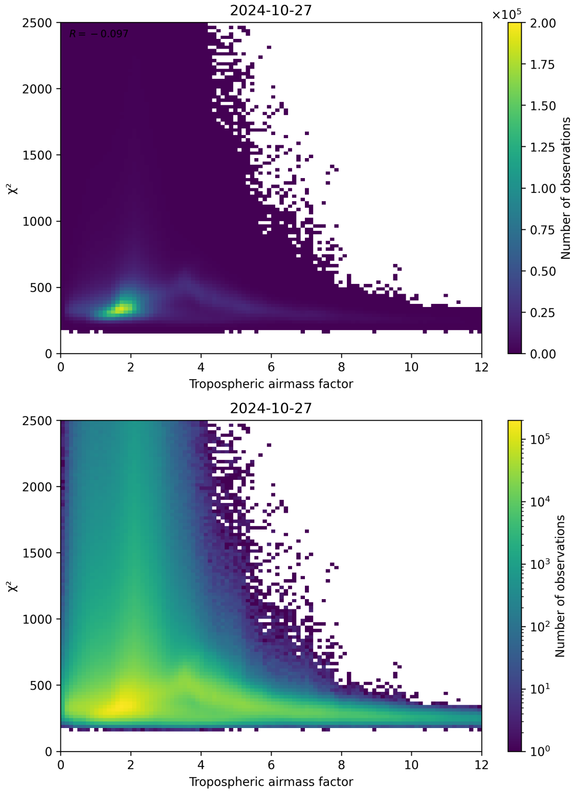
Figure 73: Scatter density plot of “Tropospheric airmass factor” against “ \chi^2 ” for 2024-10-26 to 2024-10-28.
