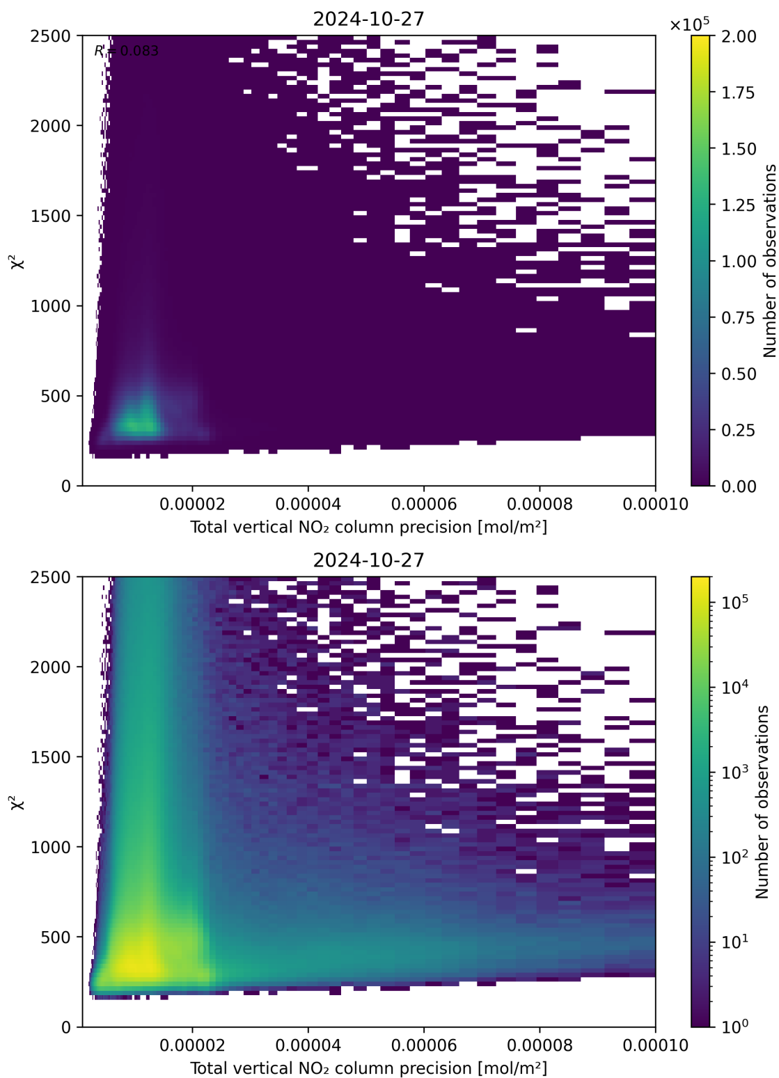
Figure 116: Scatter density plot of “Total vertical NO 2 column precision” against “ \chi^2 ” for 2024-10-26 to 2024-10-28.
