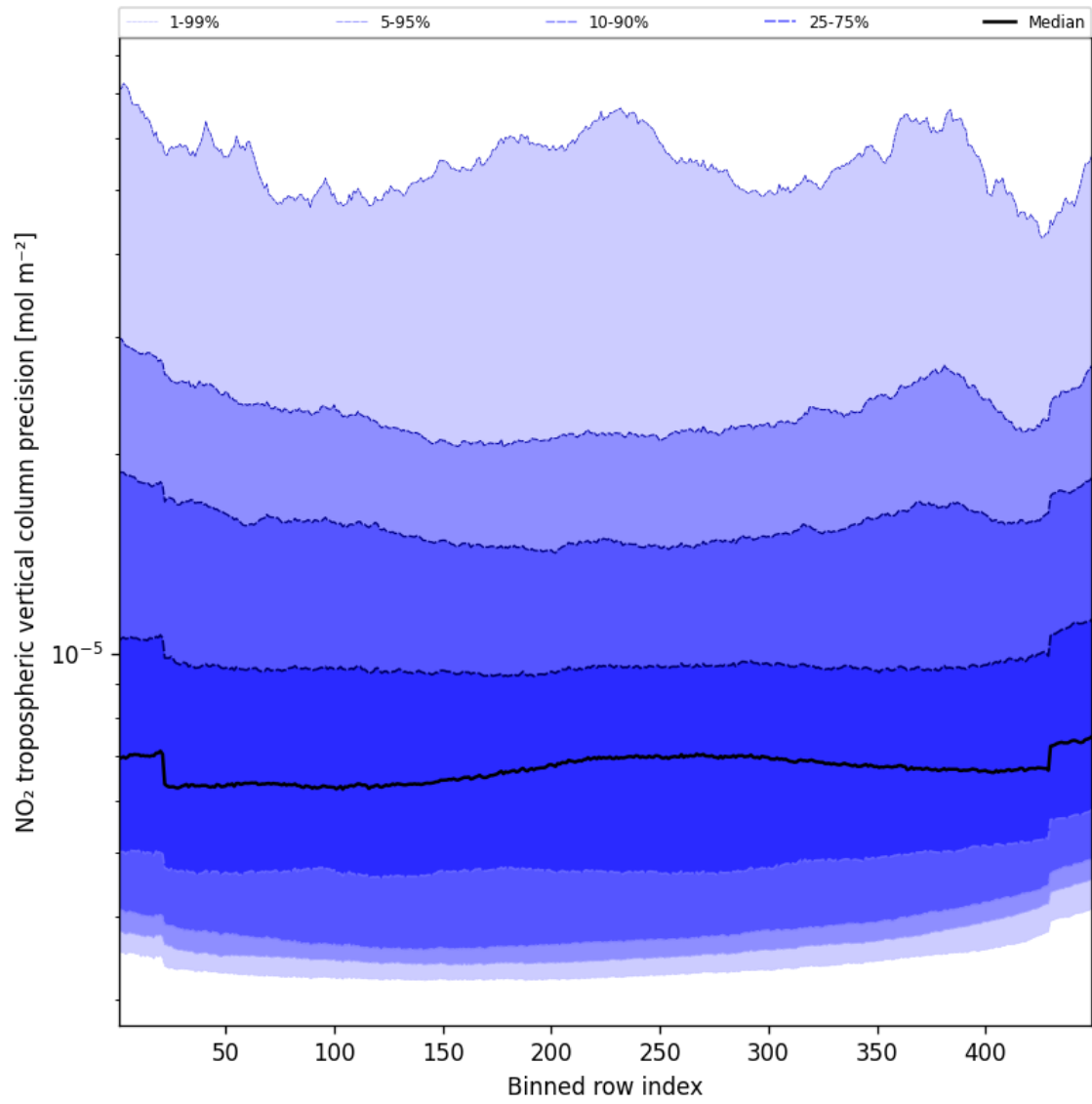
Figure 47: Along track statistics of “NO 2 tropospheric vertical column precision” for 2024-10-26 to 2024-10-28
