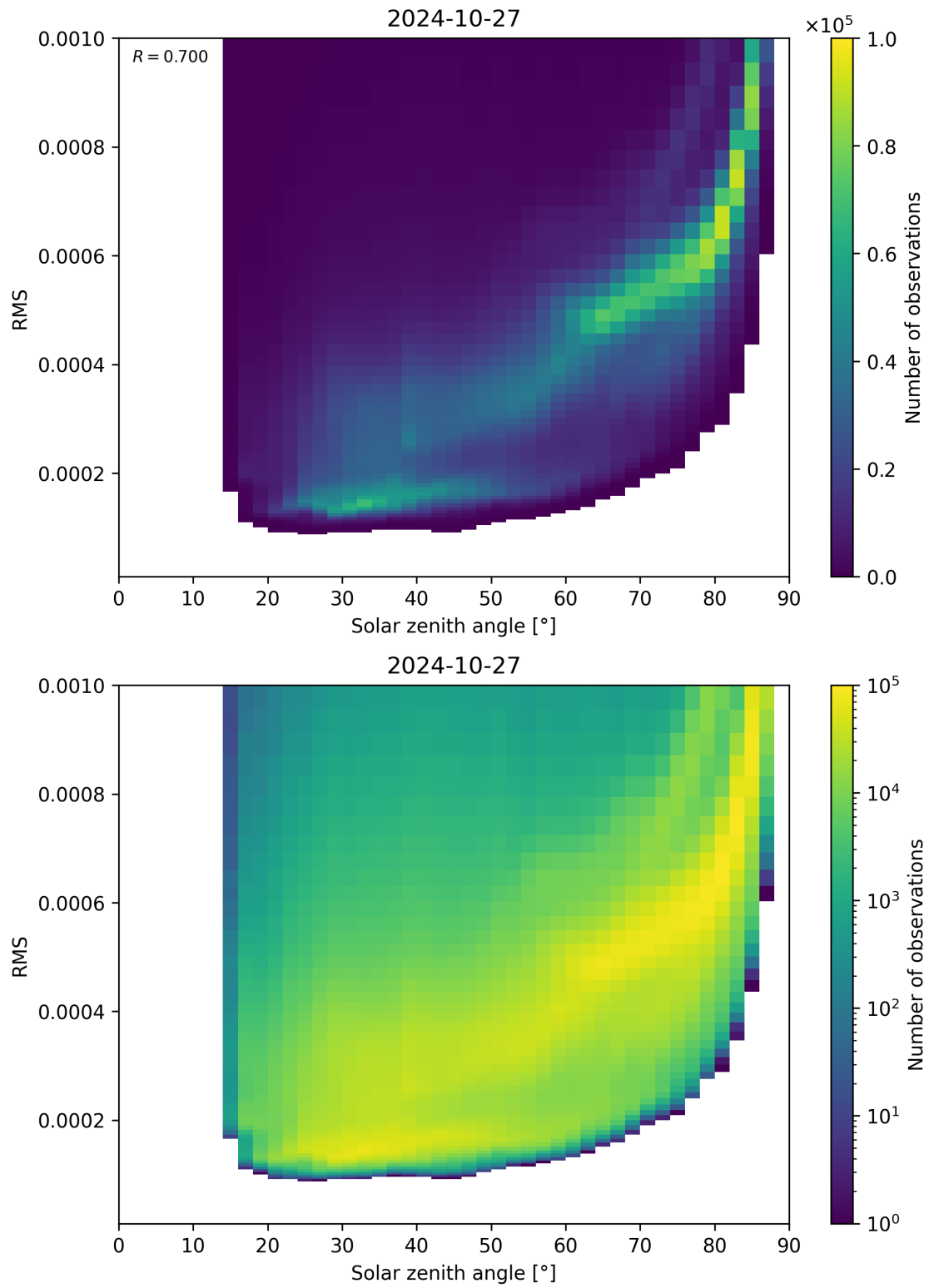
Figure 157: Scatter density plot of “Solar zenith angle” against “RMS” for 2024-10-26 to 2024-10-28.
