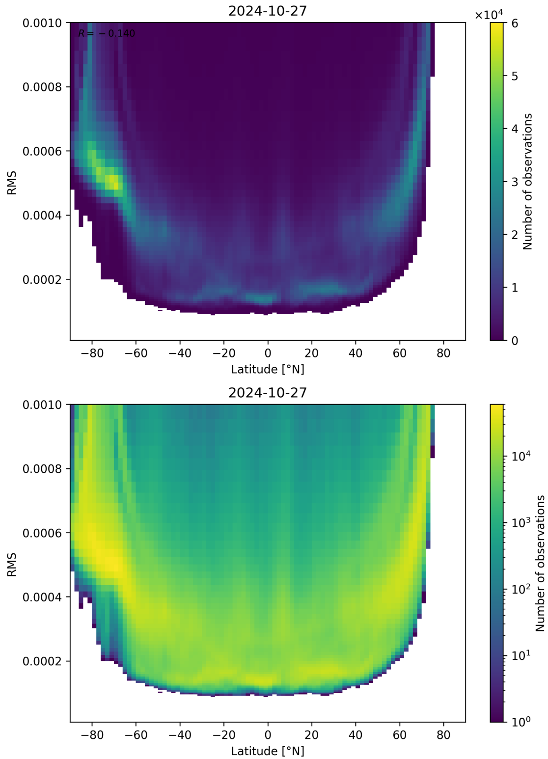
Figure 94: Scatter density plot of “Latitude” against “RMS” for 2024-10-26 to 2024-10-28.
