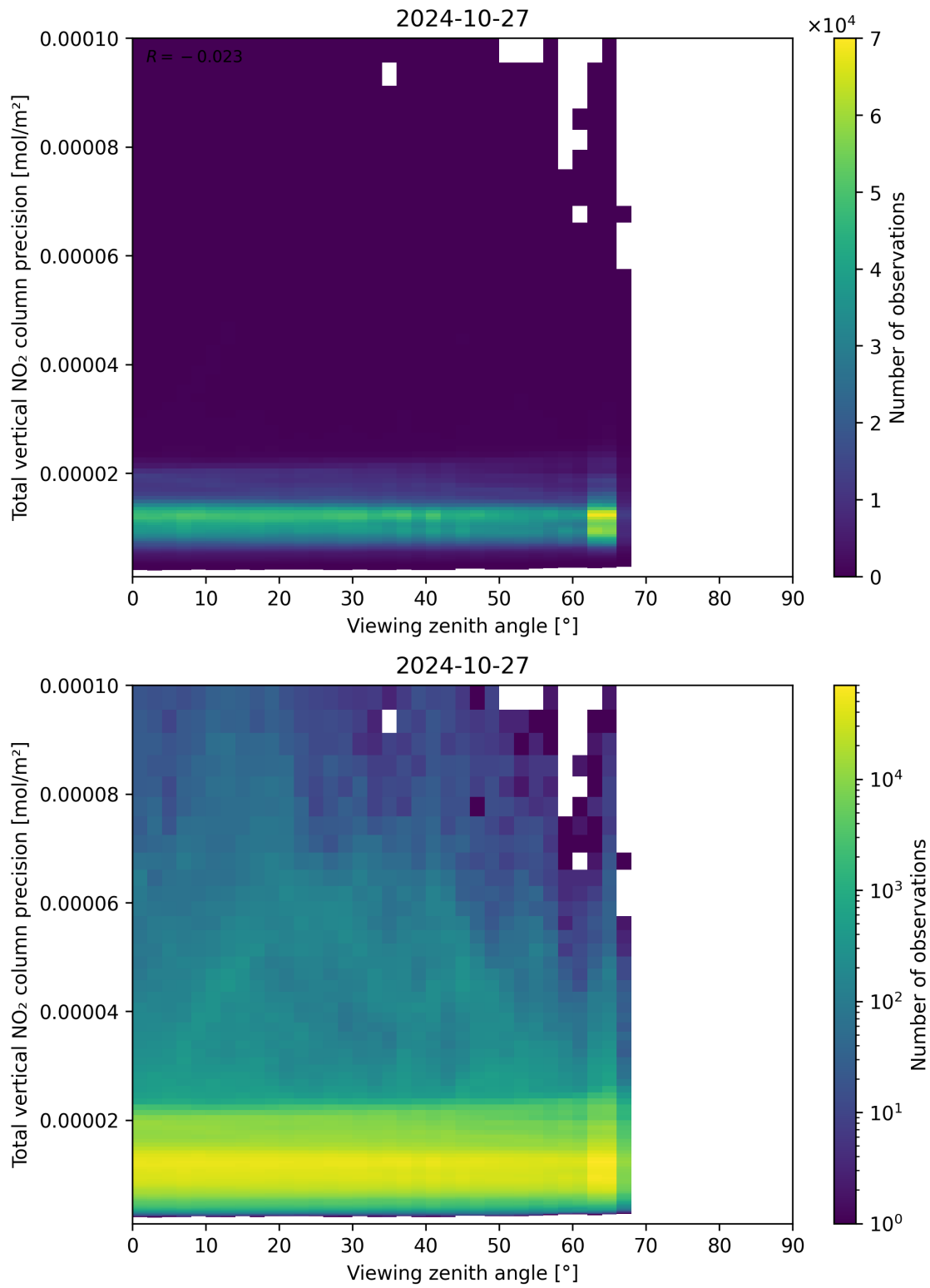
Figure 168: Scatter density plot of “Viewing zenith angle” against “Total vertical NO 2 column precision” for 2024-10-26 to 2024-10-28.
