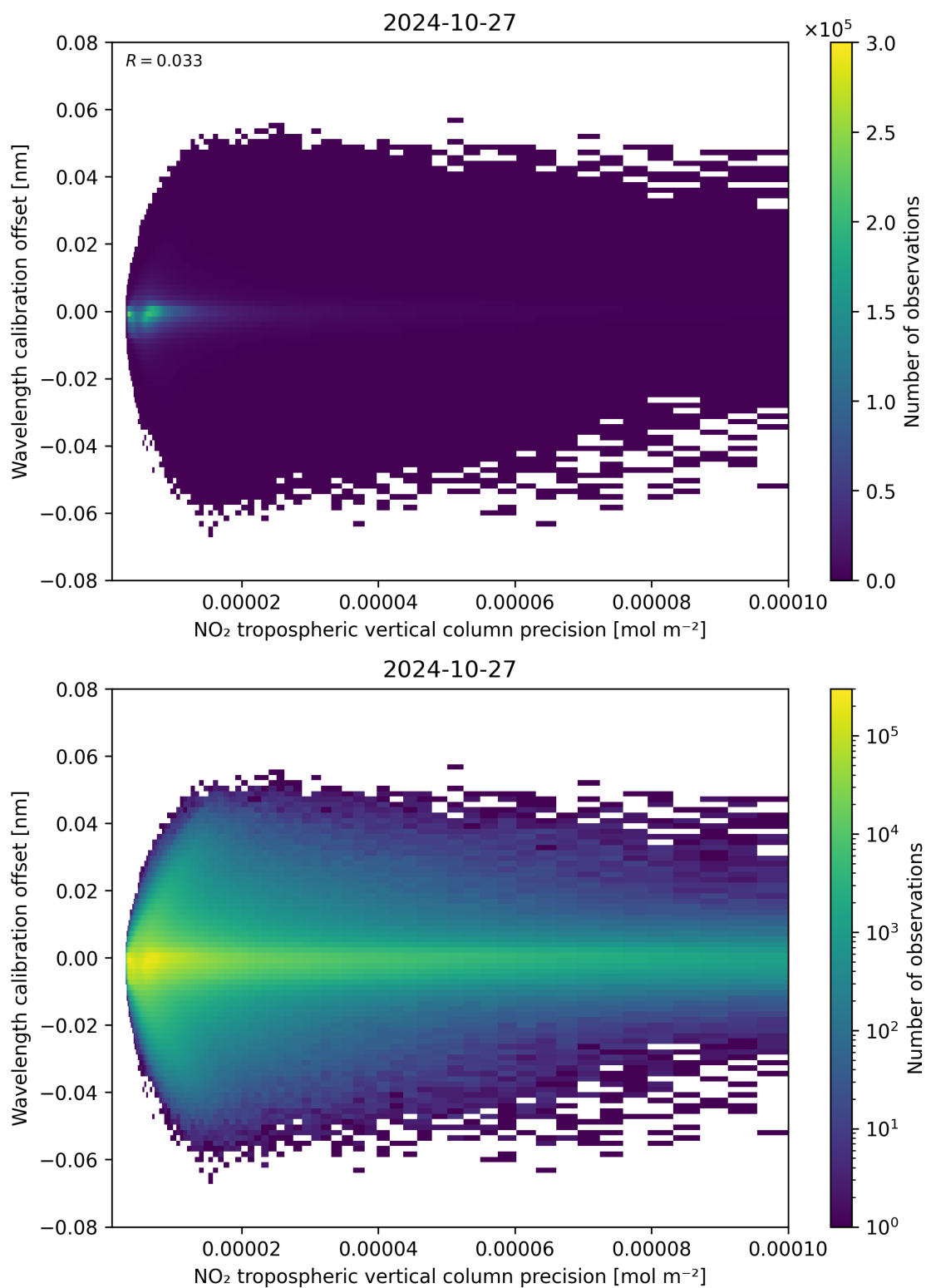
Figure 141: Scatter density plot of “NO 2 tropospheric vertical column precision” against “Wavelength calibration offset” for 2024-10-26 to 2024-10-28.
