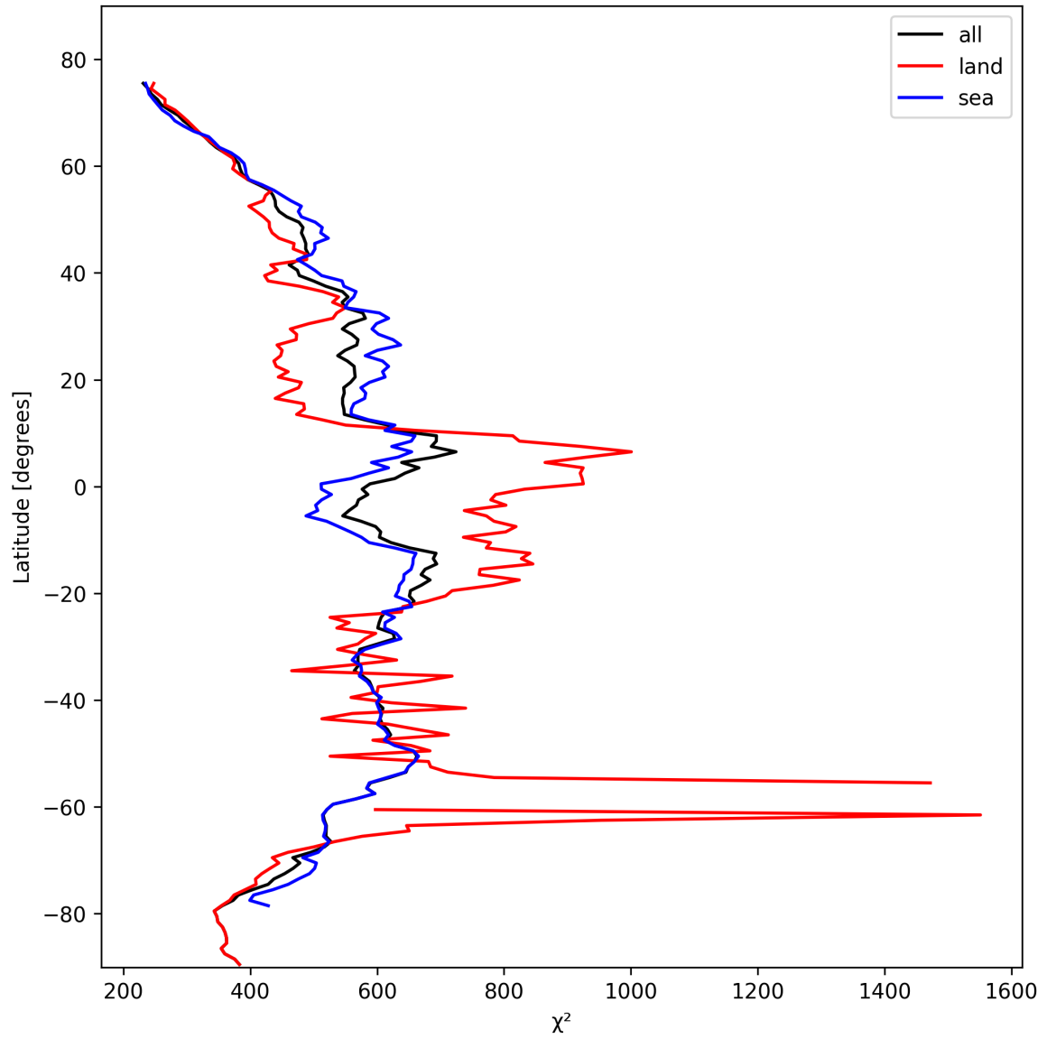
Figure 25: Zonal average of “ \chi^2 ” for 2024-10-26 to 2024-10-28.
