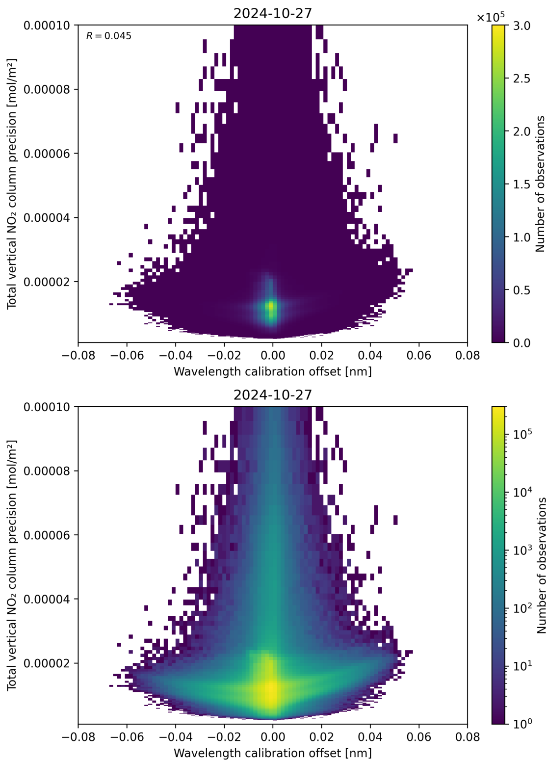
Figure 180: Scatter density plot of “Wavelength calibration offset” against “Total vertical NO 2 column precision” for 2024-10-26 to 2024-10-28.
