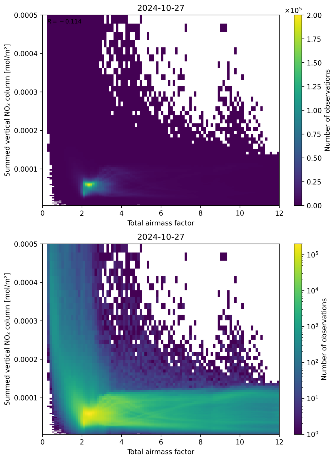
Figure 65: Scatter density plot of “Total airmass factor” against “Summed vertical NO 2 column” for 2024-10-26 to 2024-10-28.
