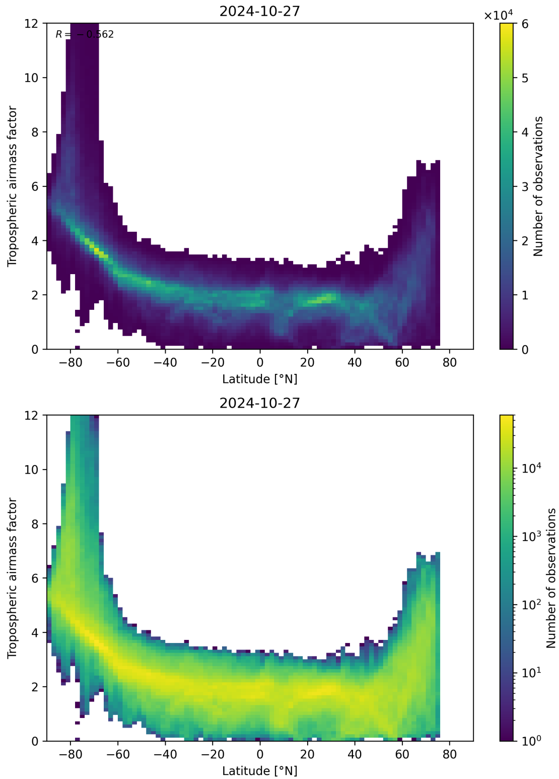
Figure 85: Scatter density plot of “Latitude” against “Tropospheric airmass factor” for 2024-10-26 to 2024-10-28.
