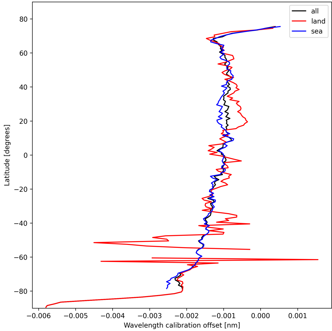
Figure 18: Zonal average of “Wavelength calibration offset” for 2024-10-26 to 2024-10-28.
