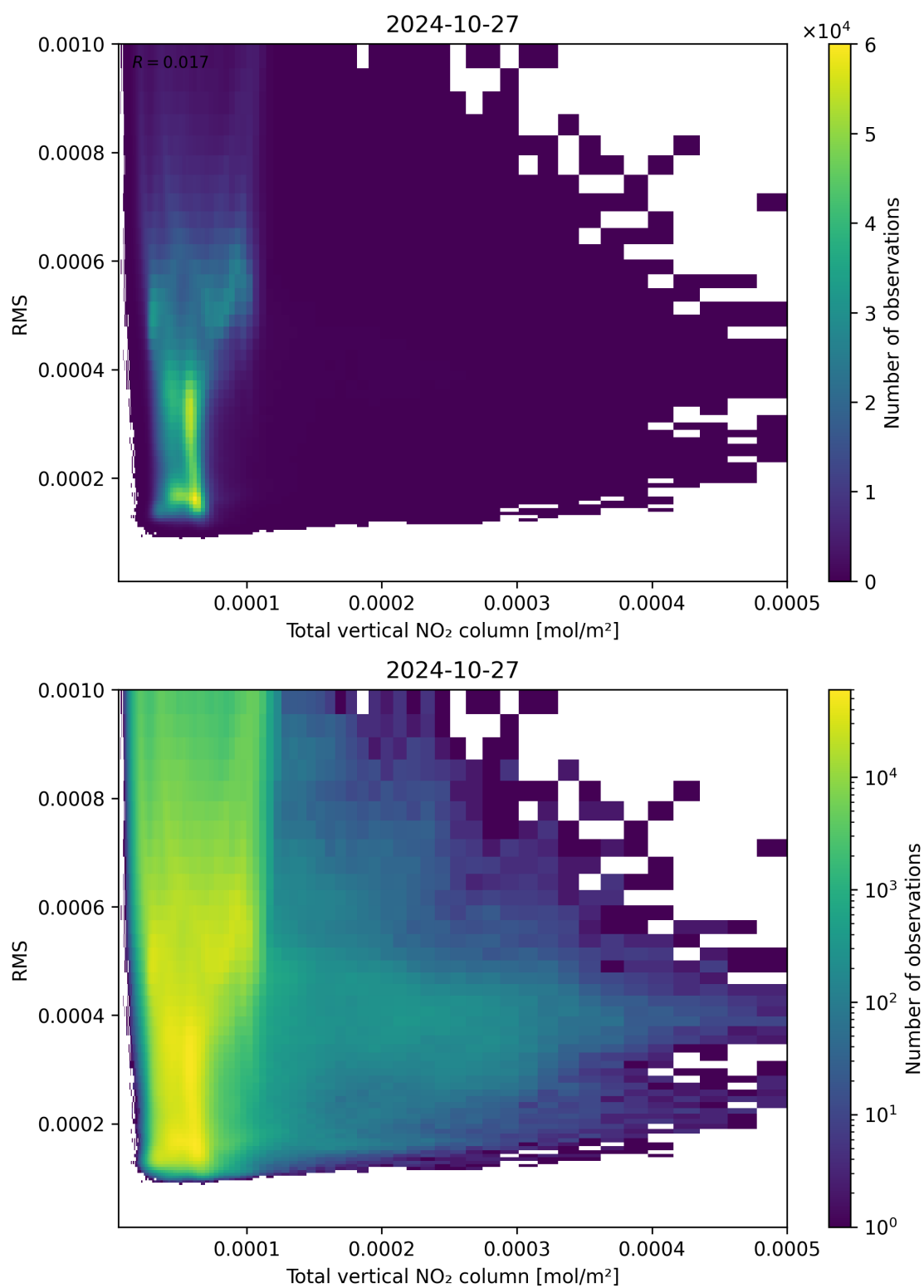
Figure 120: Scatter density plot of “Total vertical NO 2 column” against “RMS” for 2024-10-26 to 2024-10-28.
