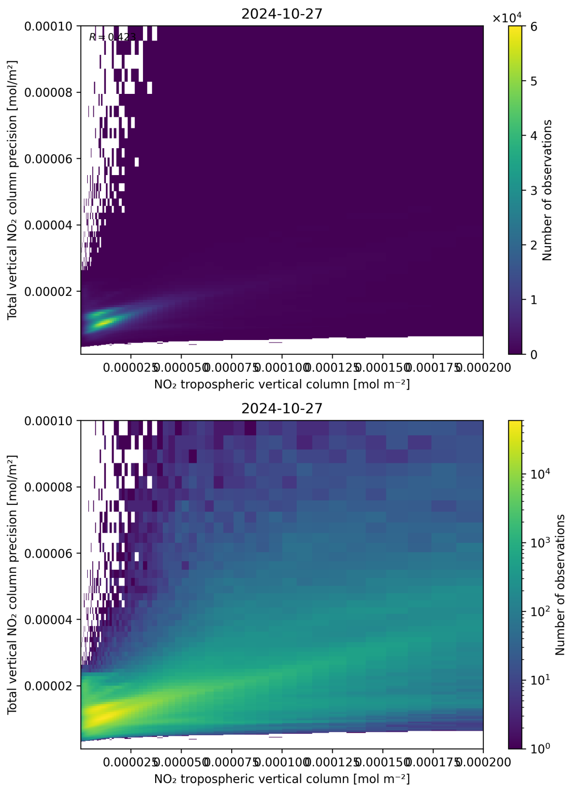
Figure 129: Scatter density plot of “NO 2 tropospheric vertical column” against “Total vertical NO 2 column precision” for 2024-10-26 to 2024-10-28.
