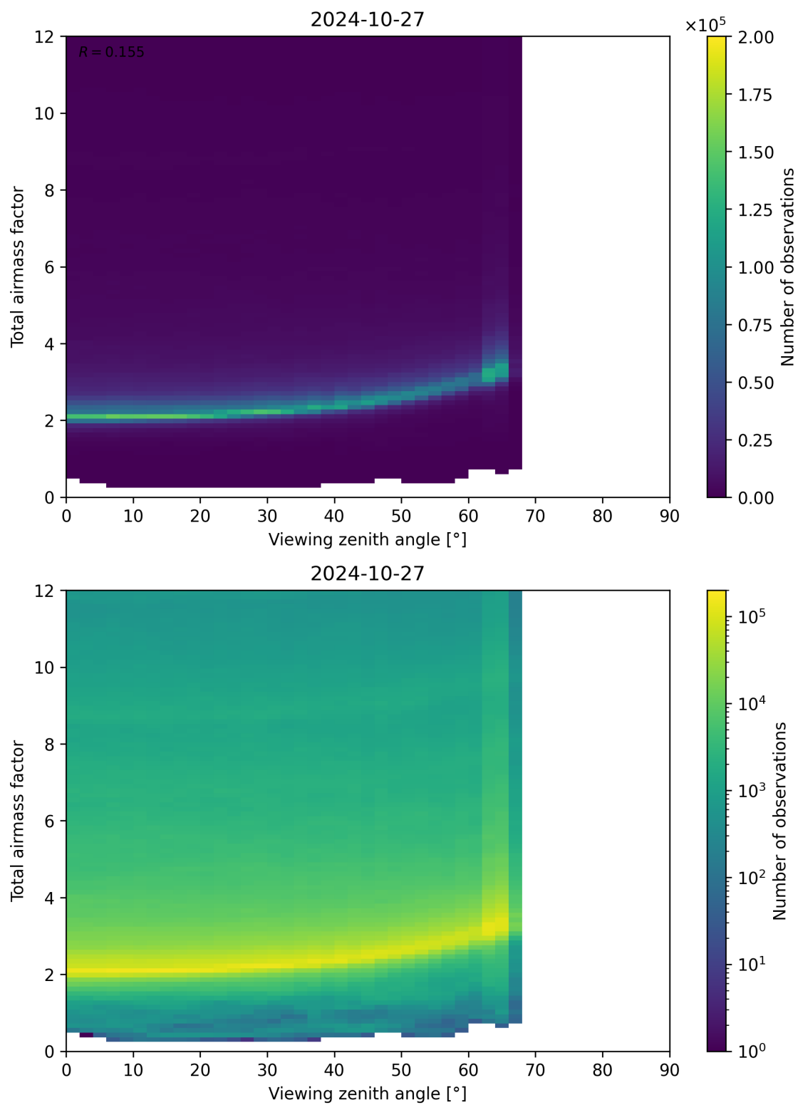
Figure 160: Scatter density plot of “Viewing zenith angle” against “Total airmass factor” for 2024-10-26 to 2024-10-28.
