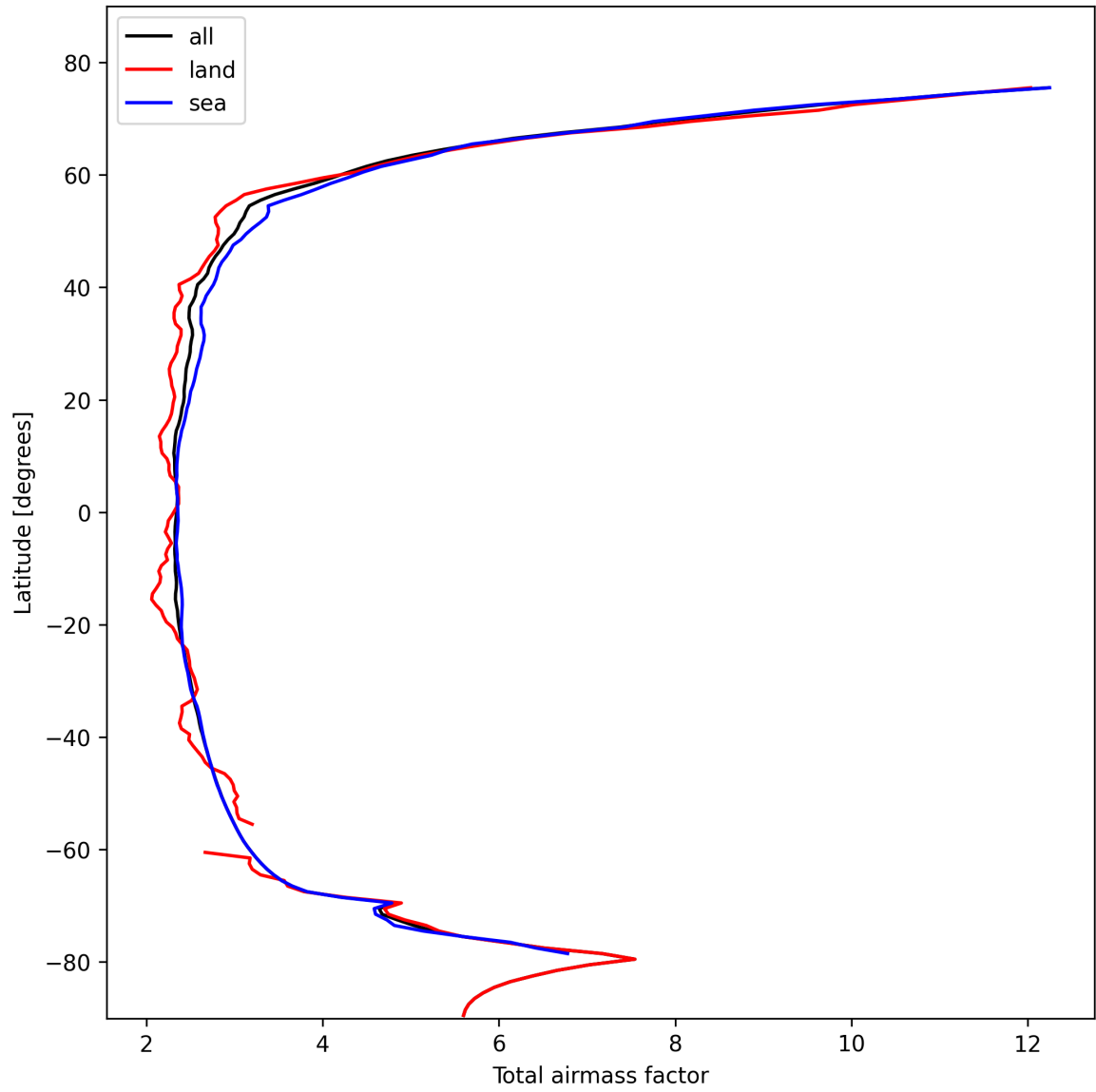
Figure 15: Zonal average of “Total airmass factor” for 2024-10-26 to 2024-10-28.
