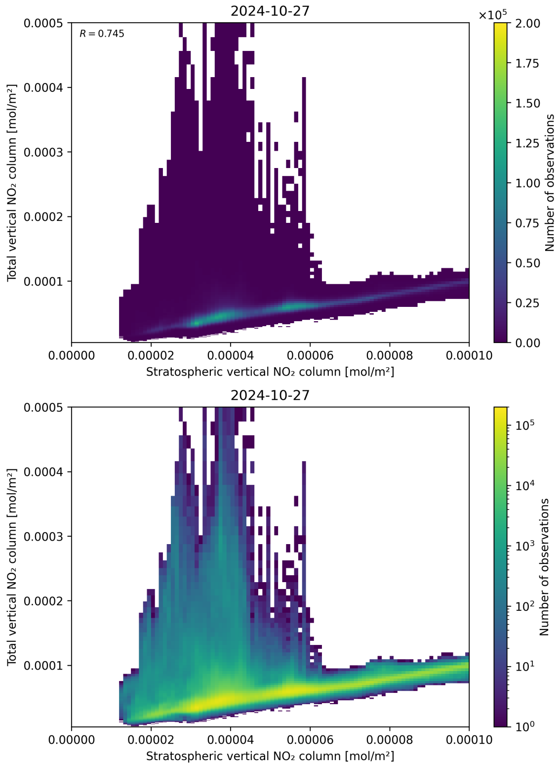
Figure 100: Scatter density plot of “Stratospheric vertical NO 2 column” against “Total vertical NO 2 column” for 2024-10-26 to 2024-10-28.
