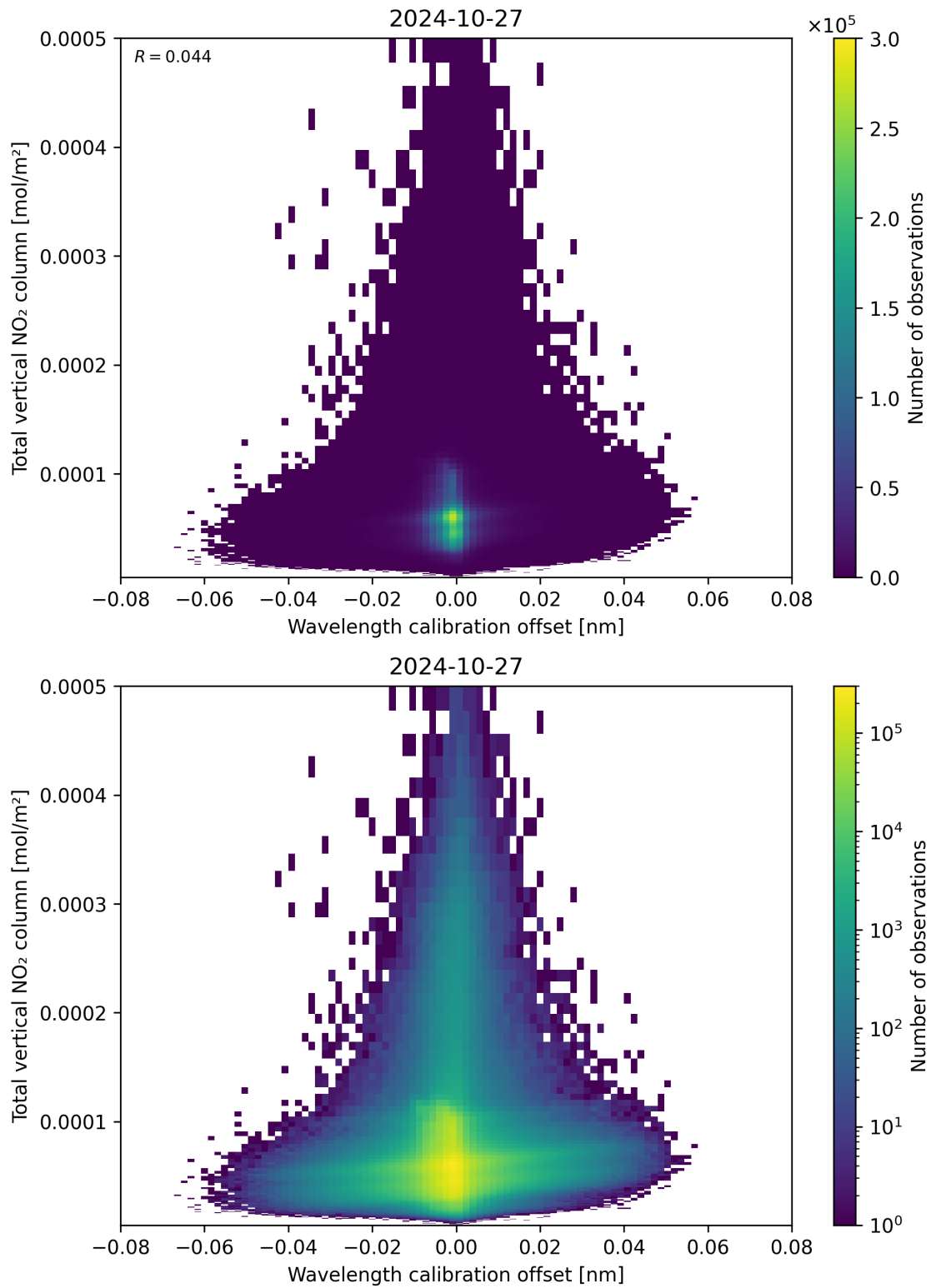
Figure 179: Scatter density plot of “Wavelength calibration offset” against “Total vertical NO 2 column” for 2024-10-26 to 2024-10-28.
