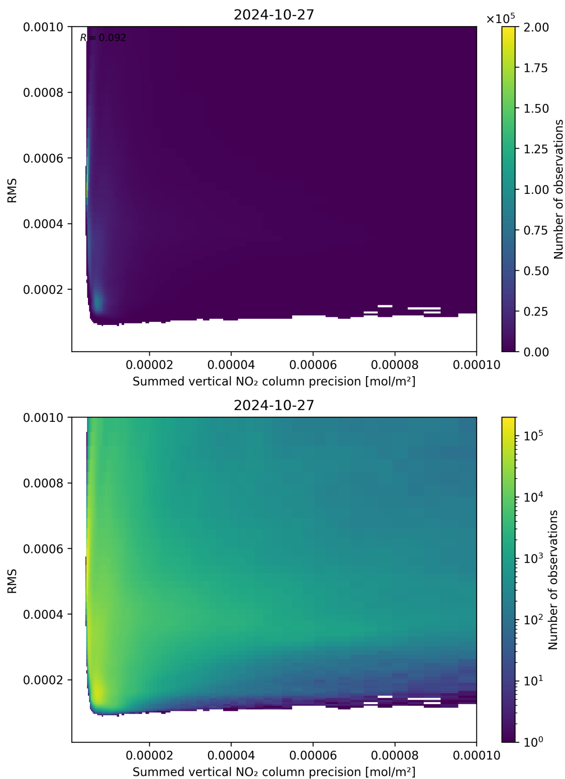
Figure 108: Scatter density plot of “Summed vertical NO 2 column precision” against “RMS” for 2024-10-26 to 2024-10-28.
