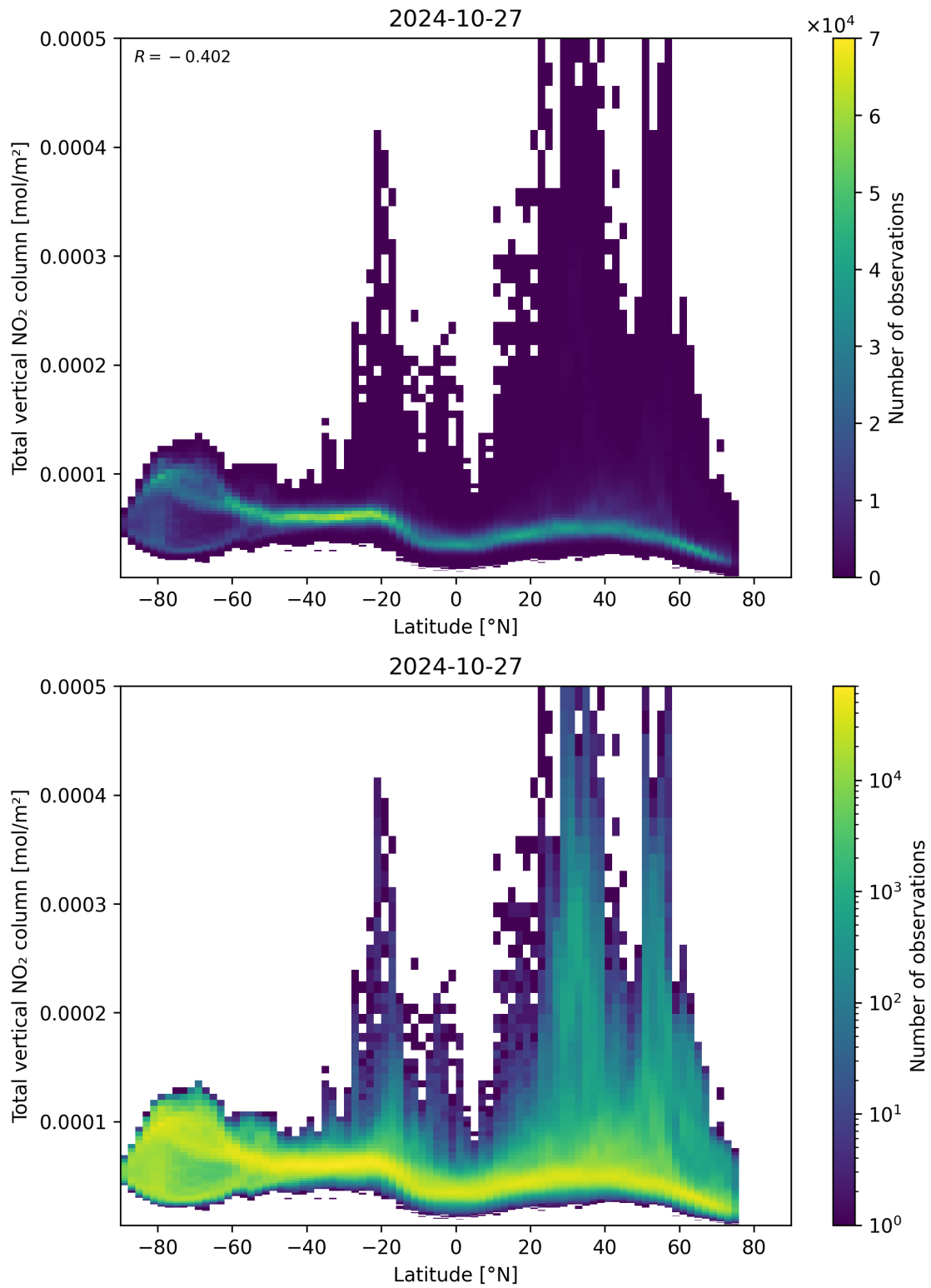
Figure 90: Scatter density plot of “Latitude” against “Total vertical NO 2 column” for 2024-10-26 to 2024-10-28.
