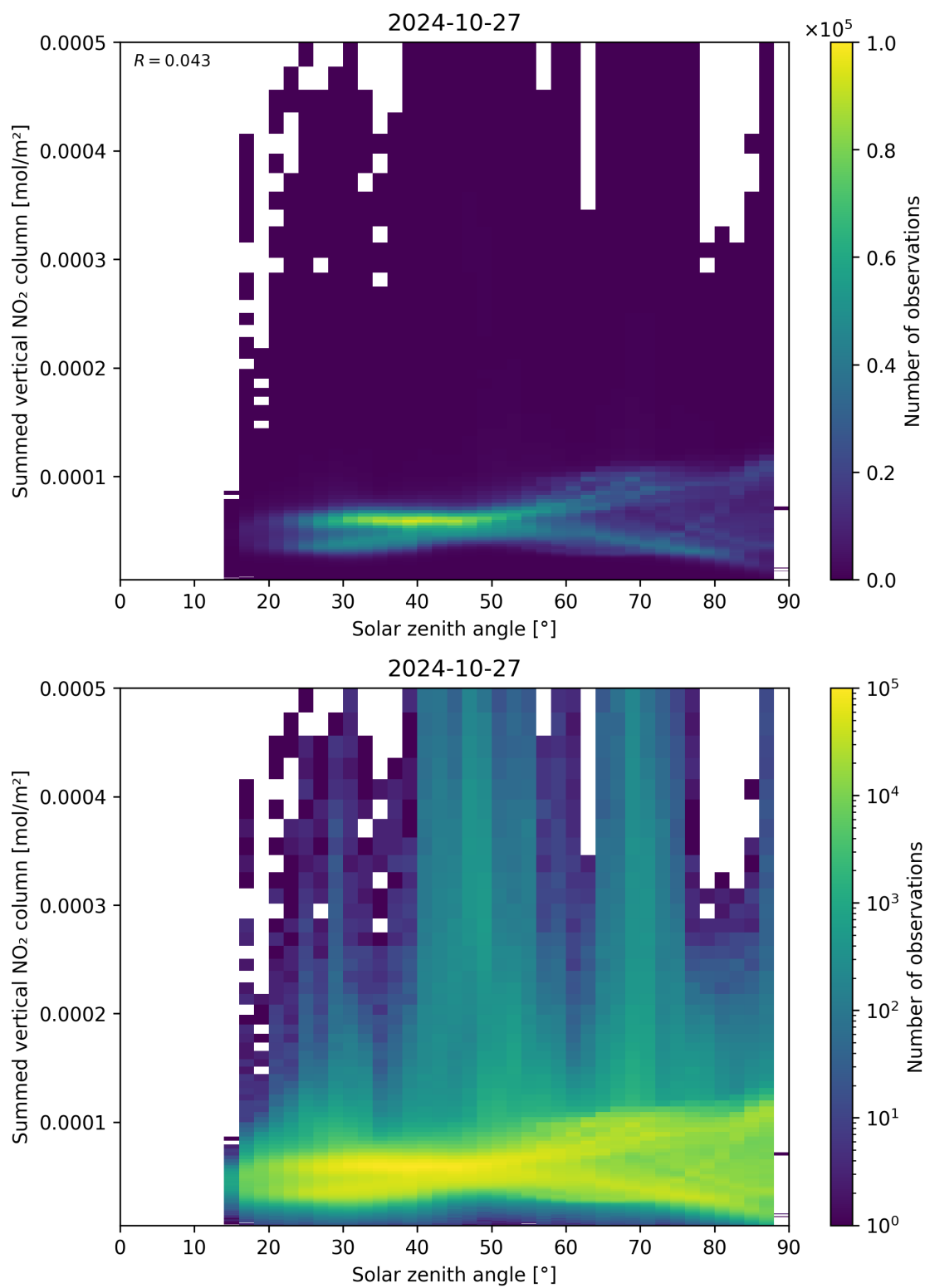
Figure 151: Scatter density plot of “Solar zenith angle” against “Summed vertical NO 2 column” for 2024-10-26 to 2024-10-28.
