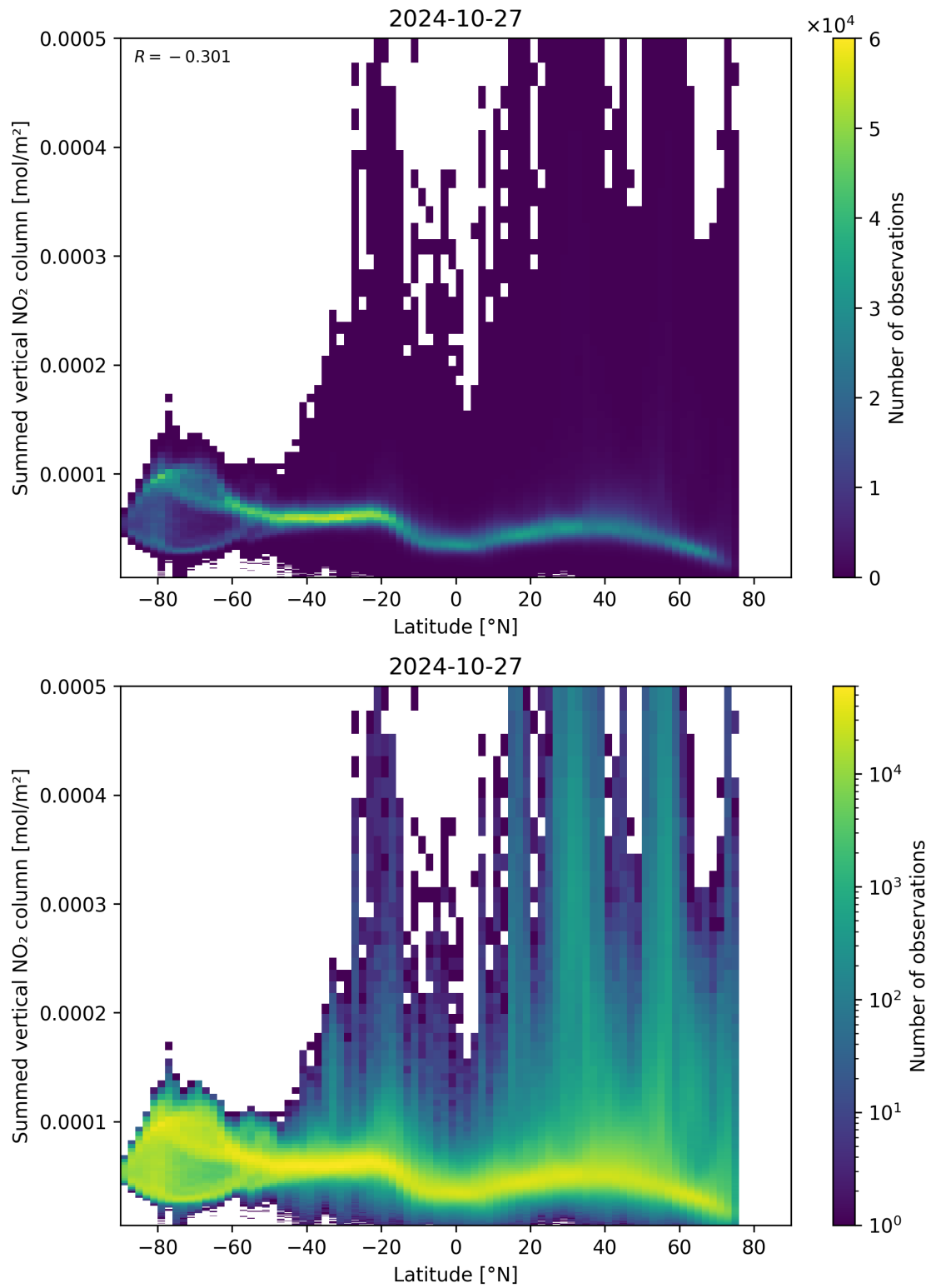
Figure 88: Scatter density plot of “Latitude” against “Summed vertical NO 2 column” for 2024-10-26 to 2024-10-28.
