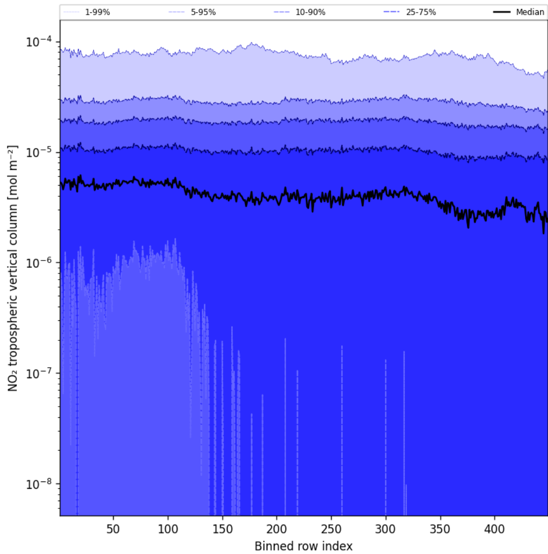
Figure 46: Along track statistics of “NO 2 tropospheric vertical column” for 2024-10-26 to 2024-10-28
