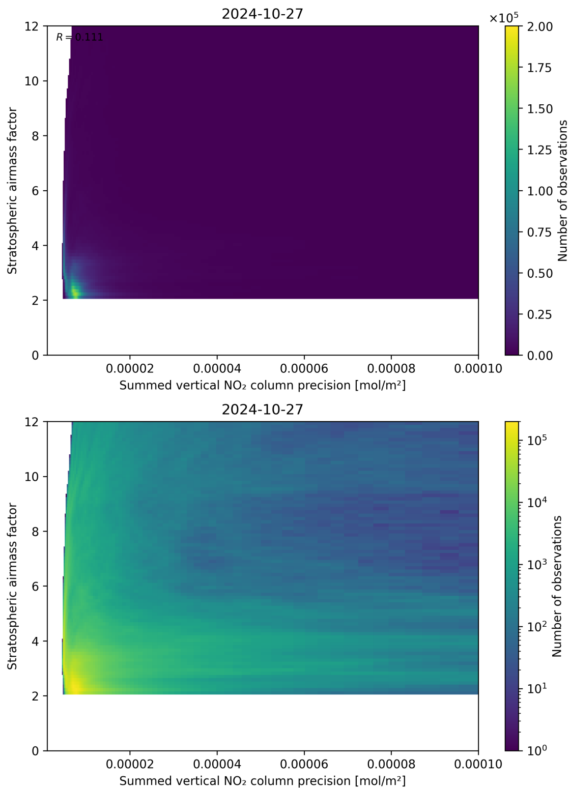
Figure 106: Scatter density plot of “Summed vertical NO 2 column precision” against “Stratospheric airmass factor” for 2024-10-26 to 2024-10-28.
