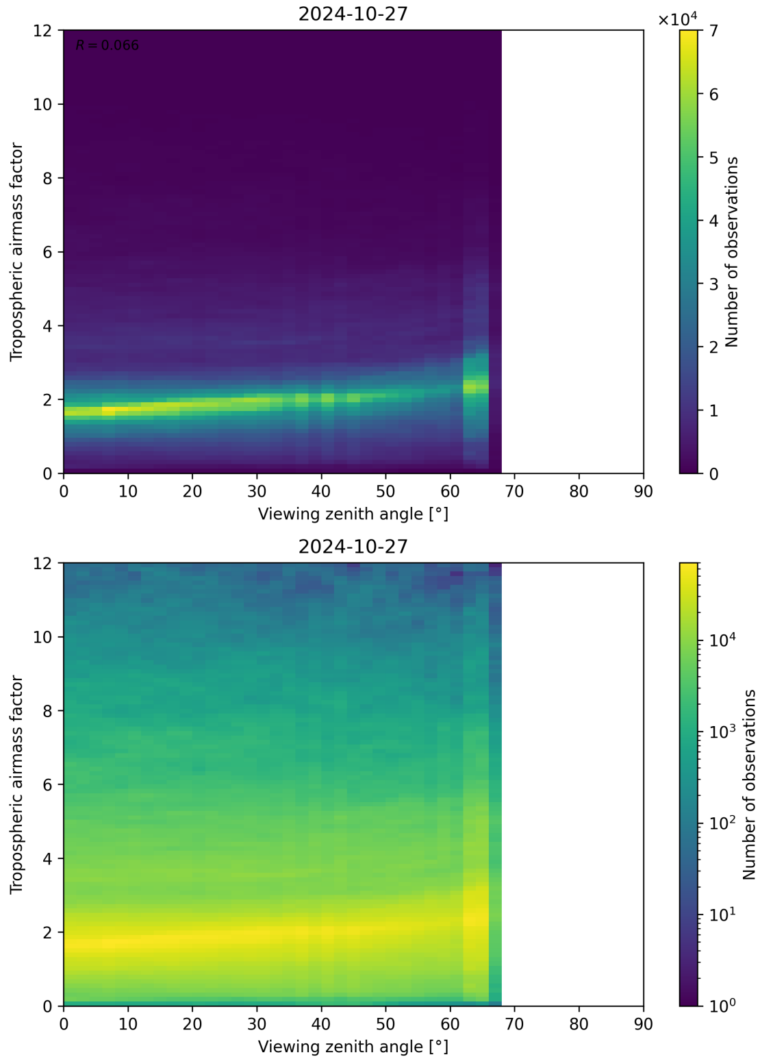
Figure 161: Scatter density plot of “Viewing zenith angle” against “Tropospheric airmass factor” for 2024-10-26 to 2024-10-28.
