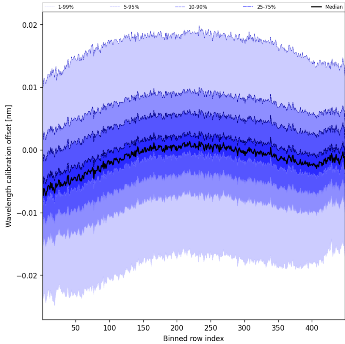
Figure 52: Along track statistics of “Wavelength calibration offset” for 2024-10-26 to 2024-10-28
