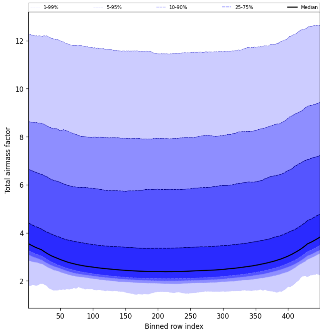
Figure 49: Along track statistics of “Total airmass factor” for 2024-10-26 to 2024-10-28
