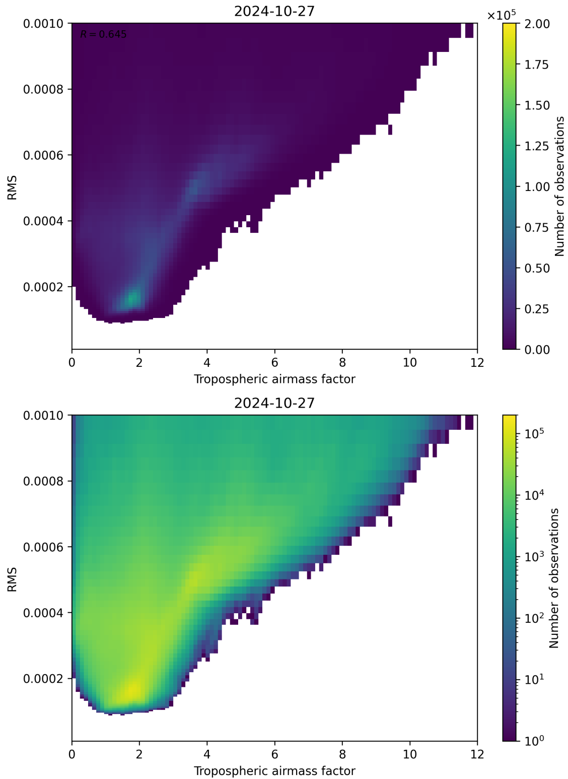
Figure 79: Scatter density plot of “Tropospheric airmass factor” against “RMS” for 2024-10-26 to 2024-10-28.
