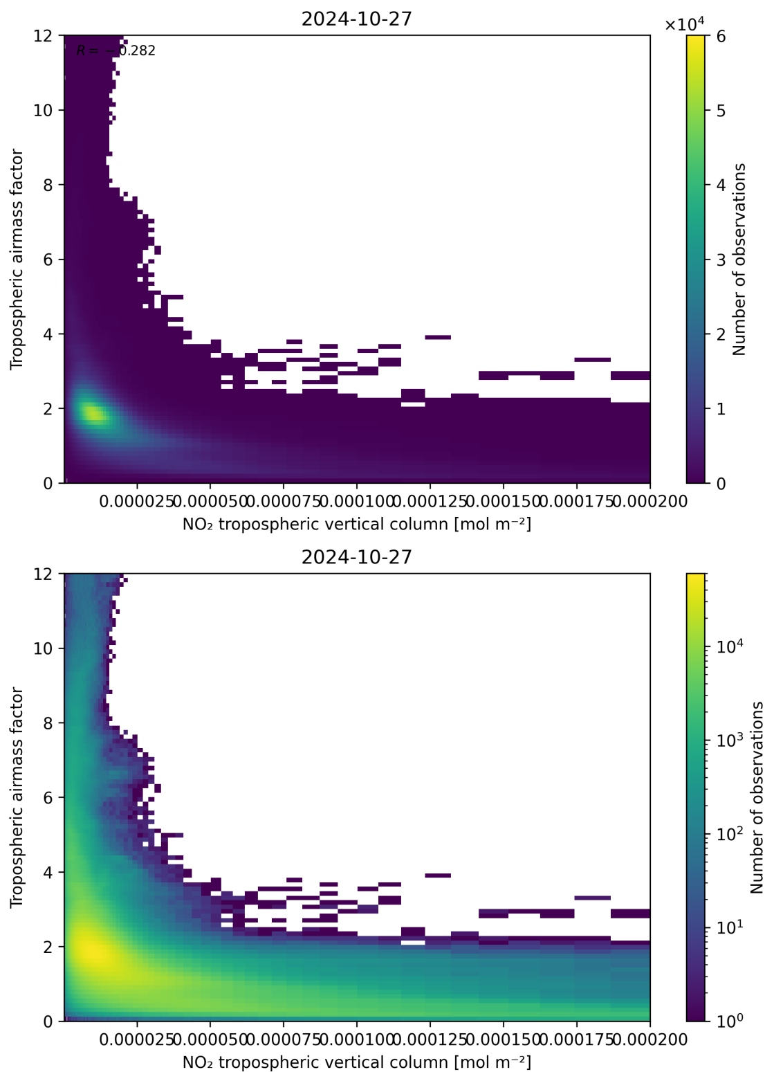
Figure 123: Scatter density plot of “NO 2 tropospheric vertical column” against “Tropospheric air mass factor” for 2024-10-26 to 2024-10-28.
