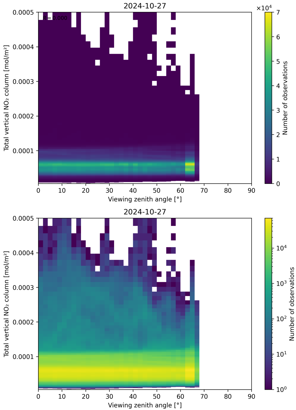
Figure 167: Scatter density plot of “Viewing zenith angle” against “Total vertical NO 2 column” for 2024-10-26 to 2024-10-28.
