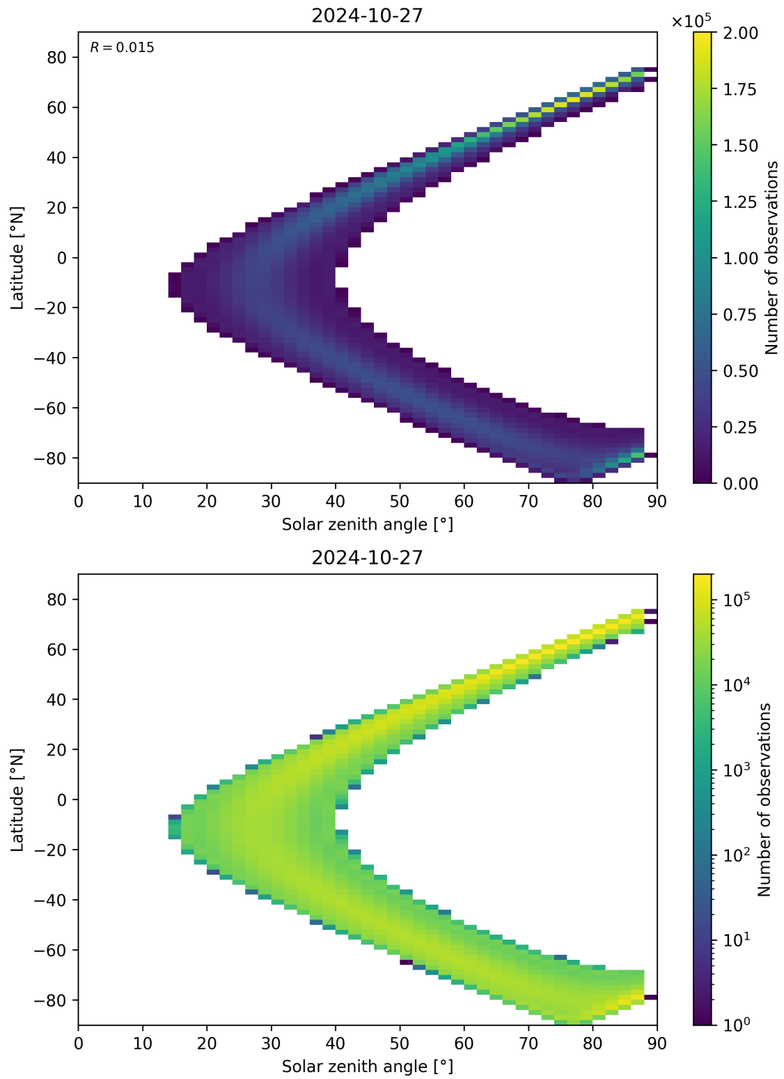
Figure 149: Scatter density plot of “Solar zenith angle” against “Latitude” for 2024-10-26 to 2024-10-28.
