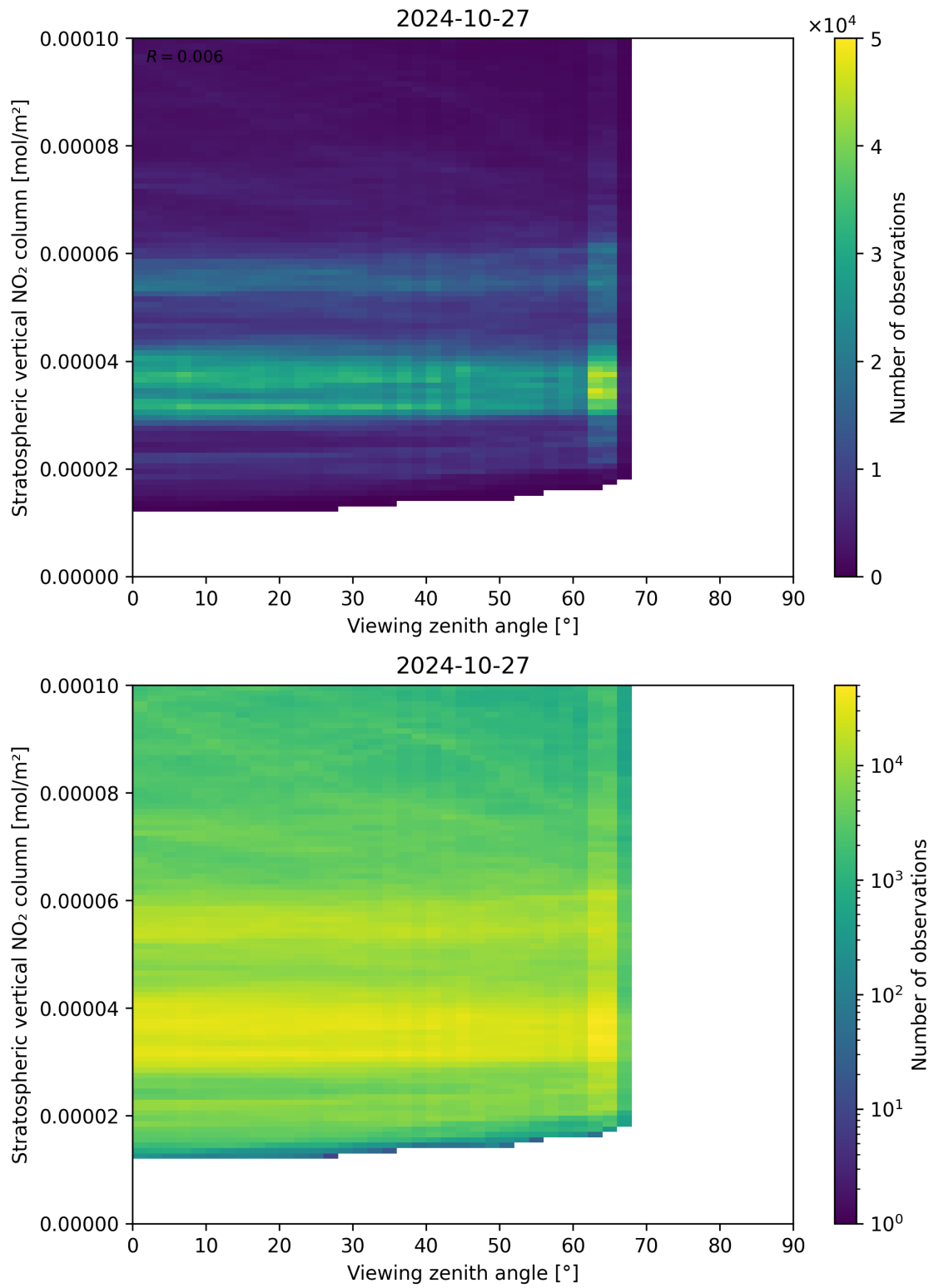
Figure 164: Scatter density plot of “Viewing zenith angle” against “Stratospheric vertical NO 2 column” for 2024-10-26 to 2024-10-28.
