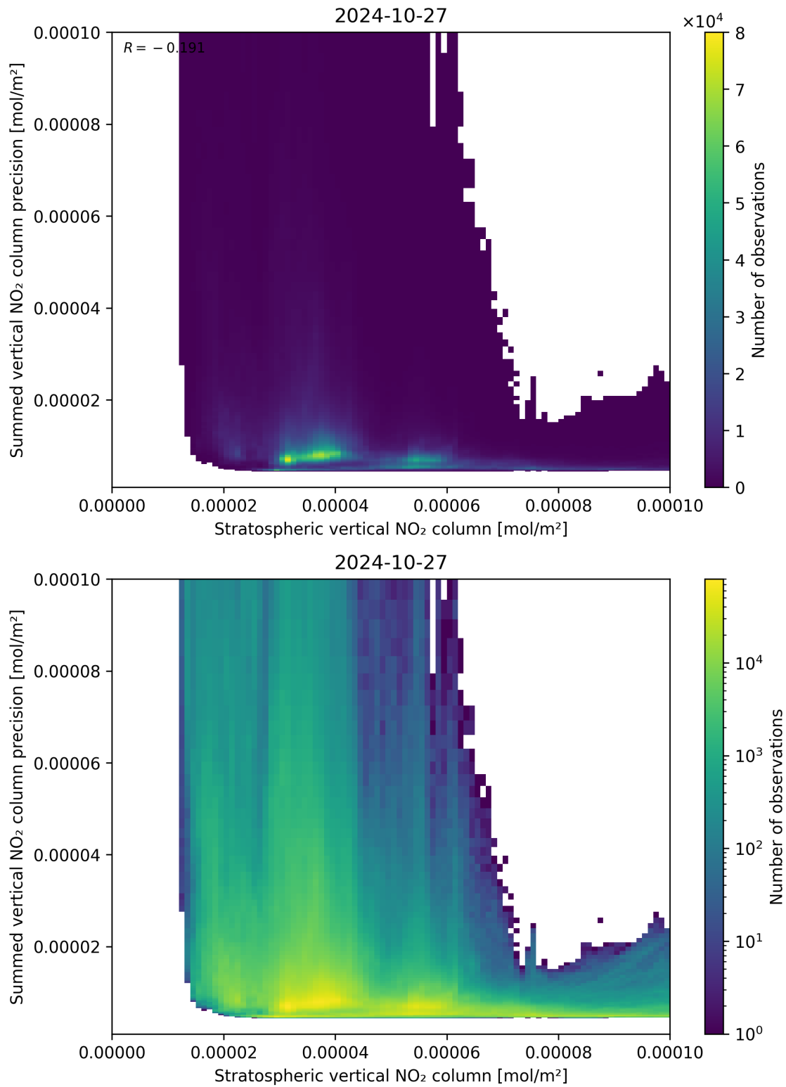
Figure 99: Scatter density plot of “Stratospheric vertical NO 2 column” against “Summed vertical NO 2 column precision” for 2024-10-26 to 2024-10-28.
