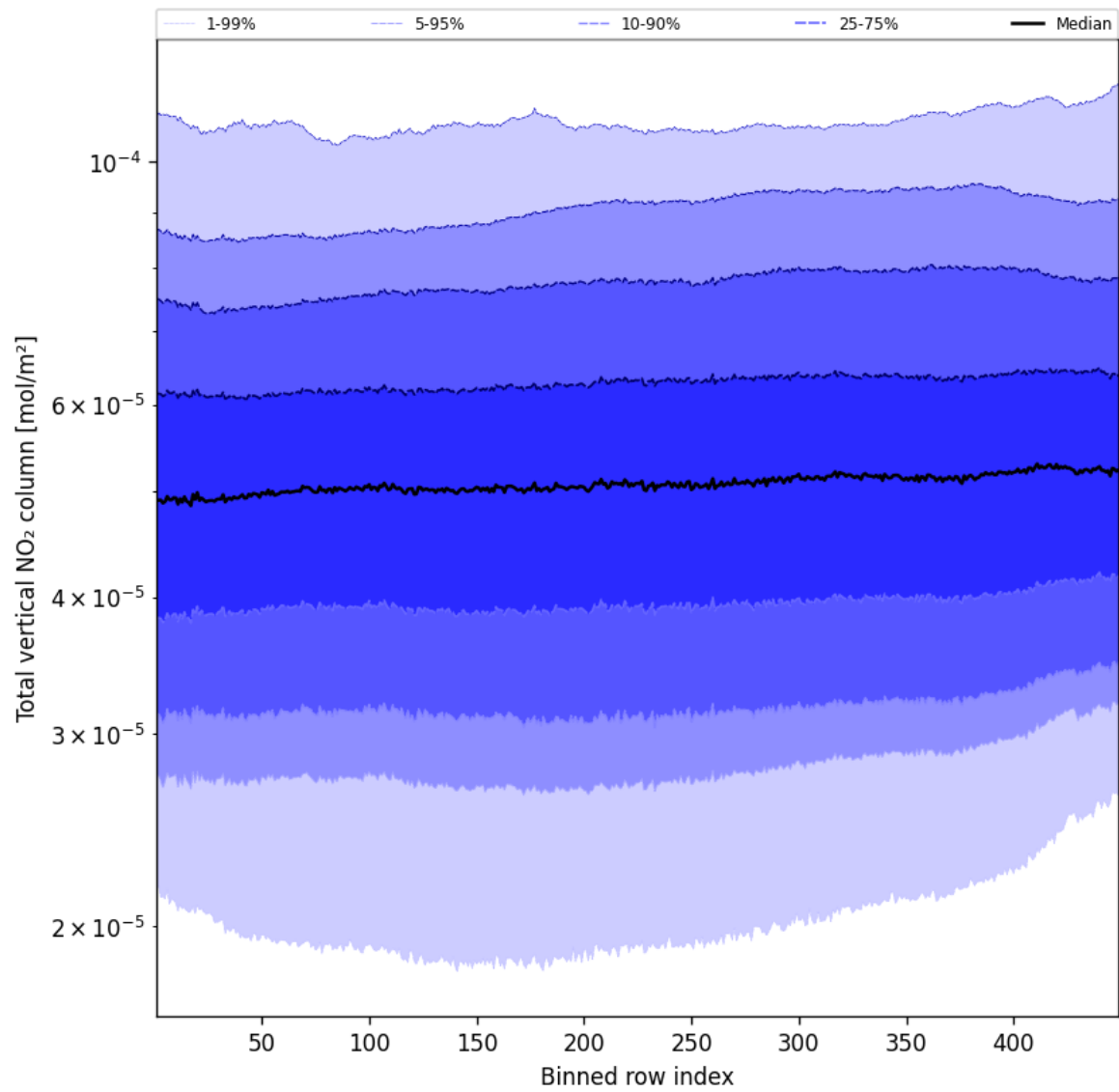
Figure 55: Along track statistics of “Total vertical NO 2 column” for 2024-10-26 to 2024-10-28
