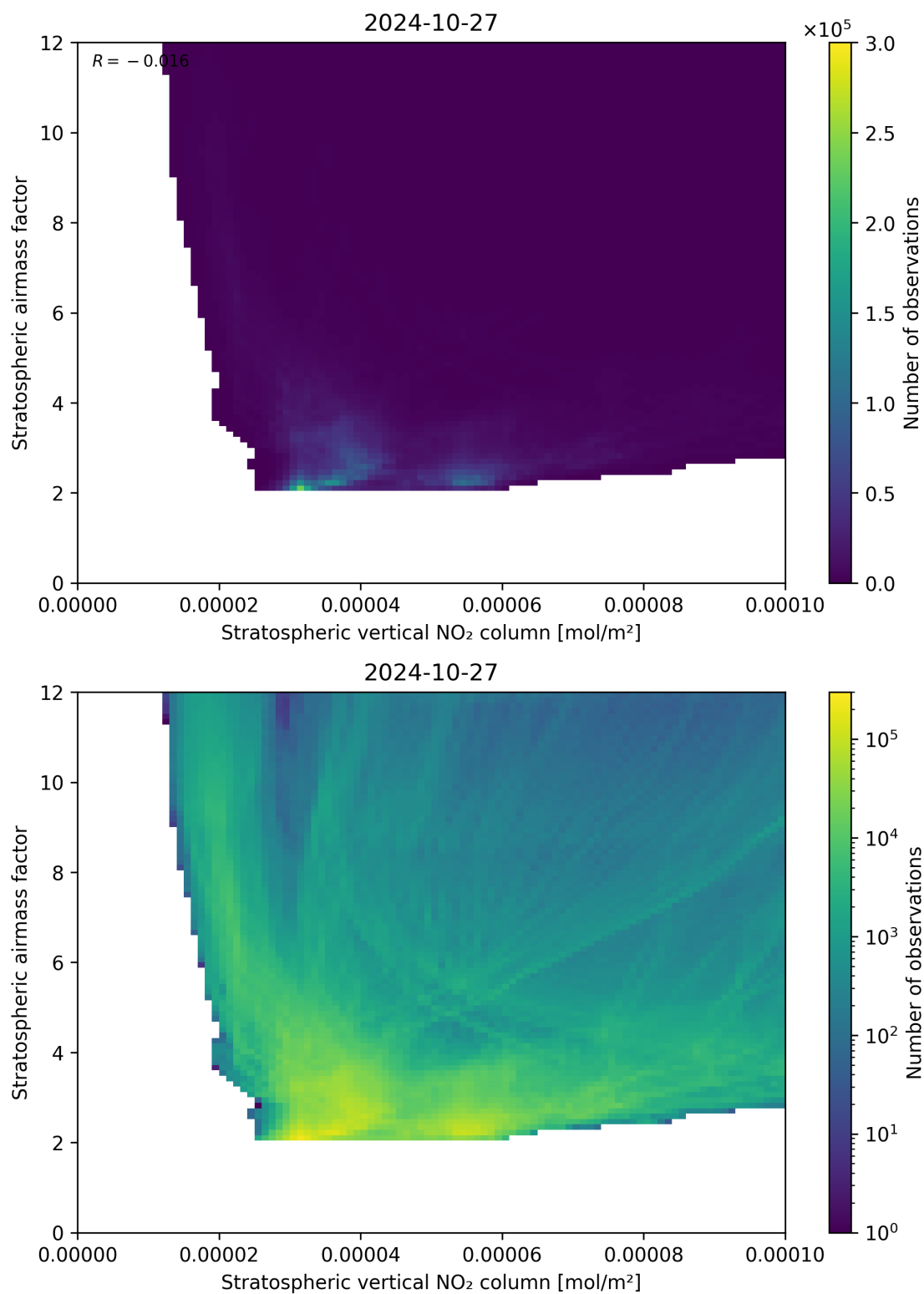
Figure 96: Scatter density plot of “Stratospheric vertical NO 2 column” against “Stratospheric airmass factor” for 2024-10-26 to 2024-10-28.
