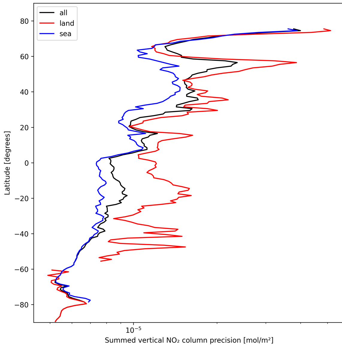
Figure 24: Zonal average of “Summed vertical NO 2 column precision” for 2024-10-26 to 2024-10-28.
