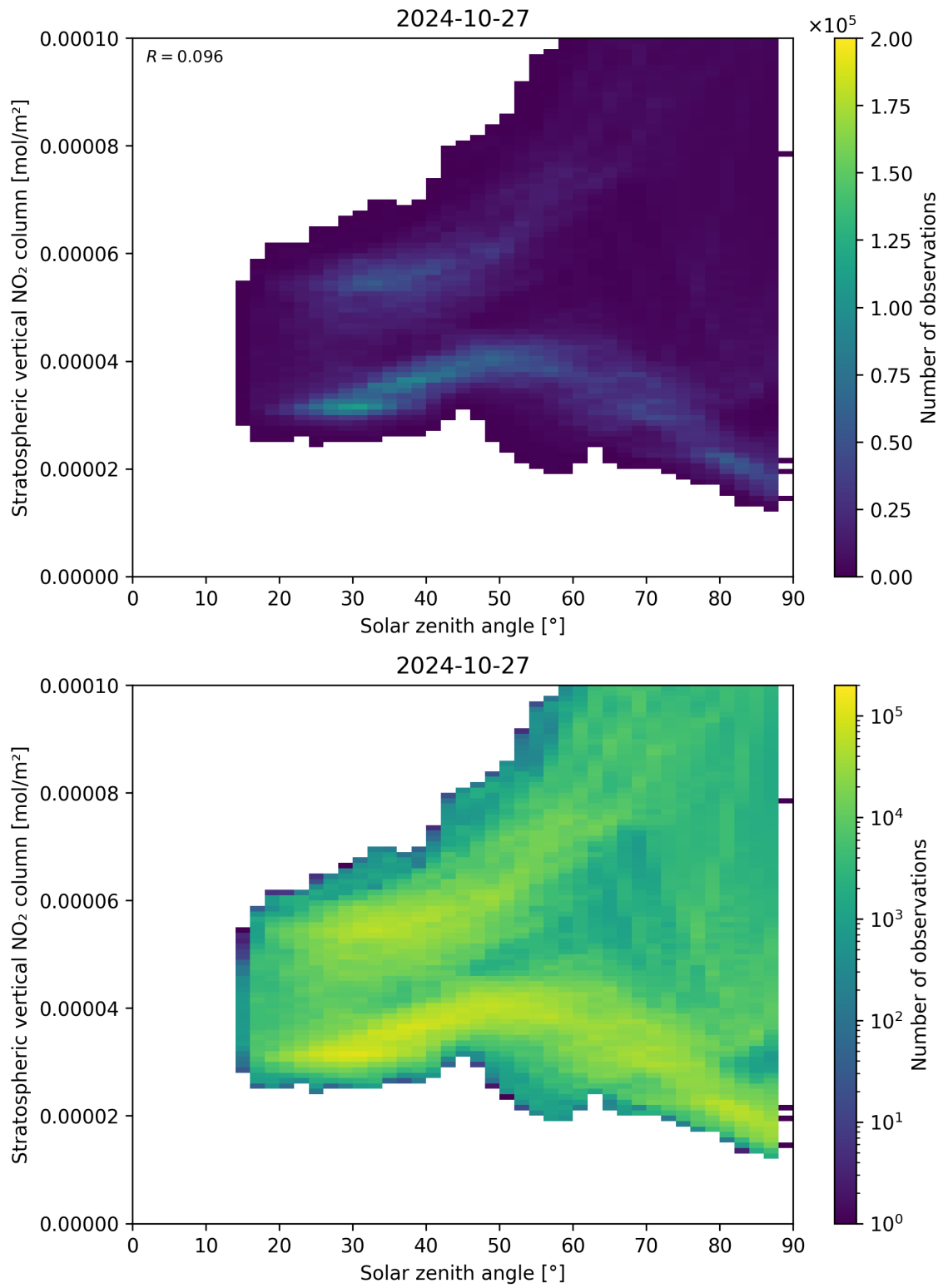
Figure 150: Scatter density plot of “Solar zenith angle” against “Stratospheric vertical NO 2 column” for 2024-10-26 to 2024-10-28.
