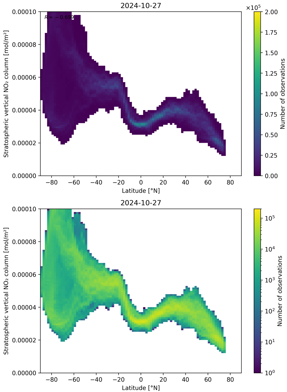
Figure 87: Scatter density plot of “Latitude” against “Stratospheric vertical NO 2 column” for 2024-10-26 to 2024-10-28.
