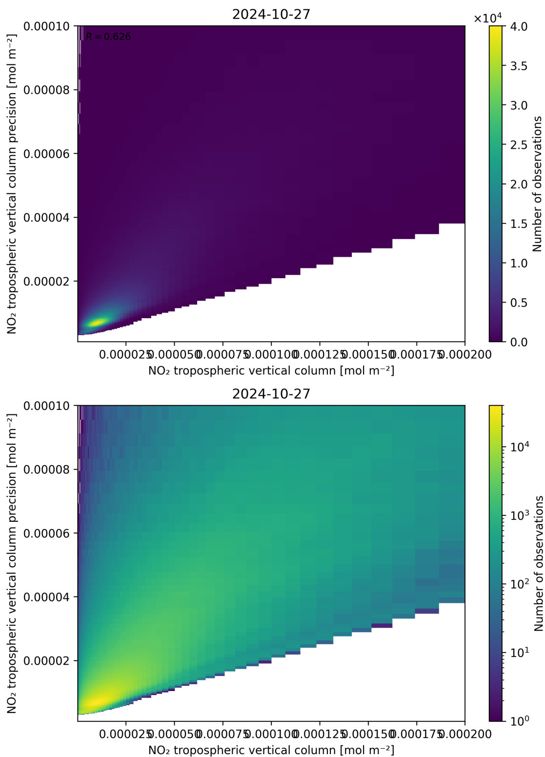
Figure 130: Scatter density plot of “NO 2 tropospheric vertical column” against “NO 2 tropospheric vertical column precision” for 2024-10-26 to 2024-10-28.
