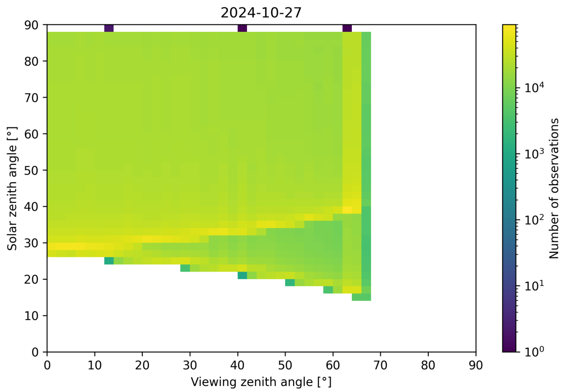
Figure 172: Scatter density plot of “Viewing zenith angle” against “Solar zenith angle” for 2024-10-26 to 2024-10-28.
