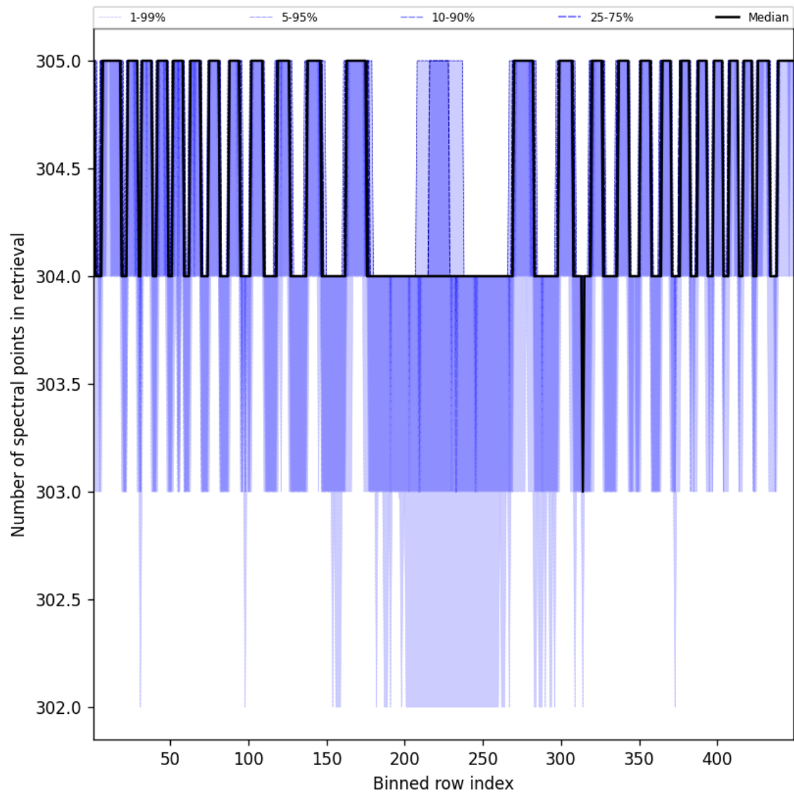
Figure 50: Along track statistics of “Number of spectral points in retrieval” for 2024-10-26 to 2024-10-28
