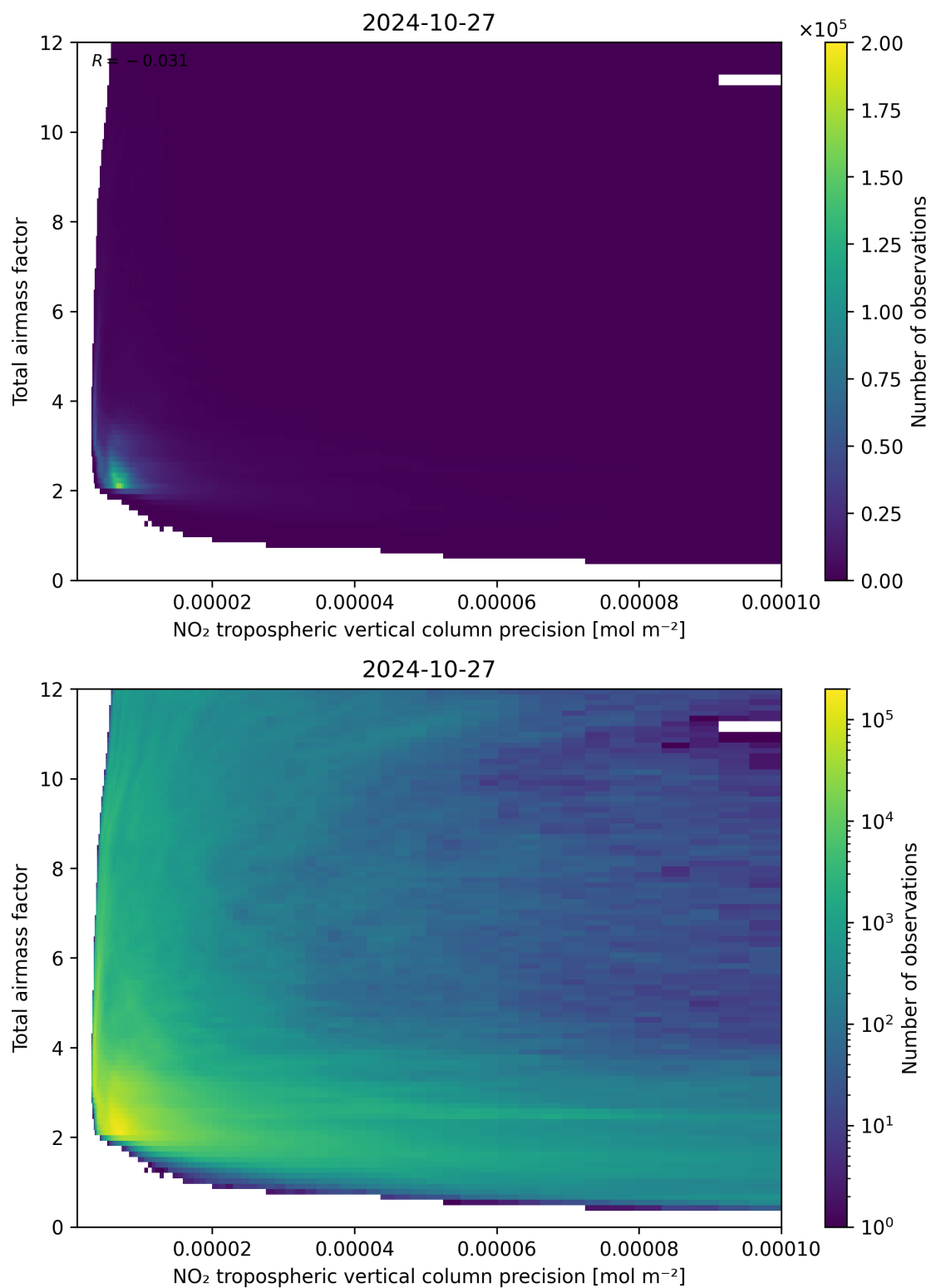
Figure 132: Scatter density plot of “NO 2 tropospheric vertical column precision” against “Total airmass factor” for 2024-10-26 to 2024-10-28.
