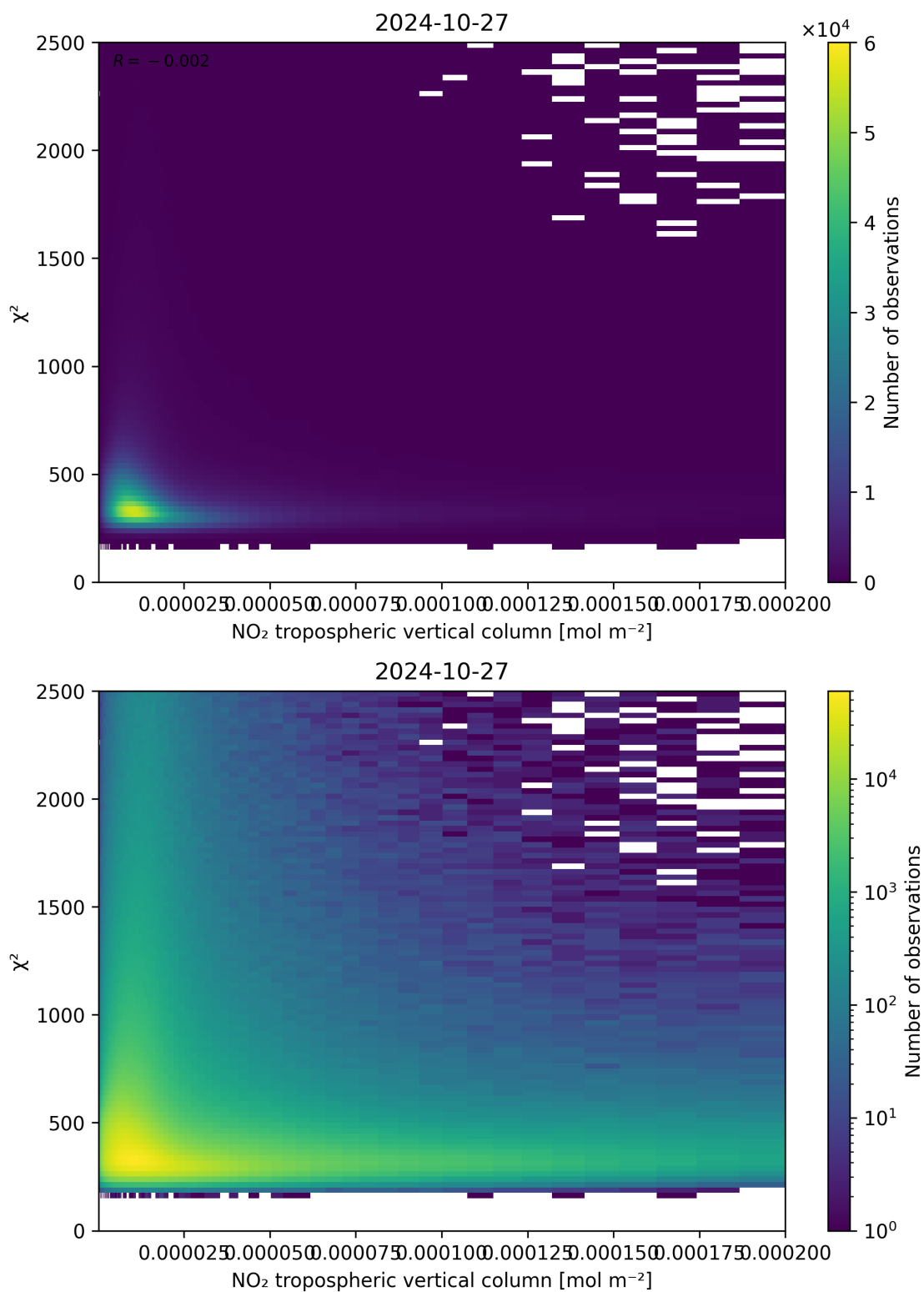
Figure 124: Scatter density plot of “NO 2 tropospheric vertical column” against “ \chi^2 ” for 2024-10-26 to 2024-10-28.
