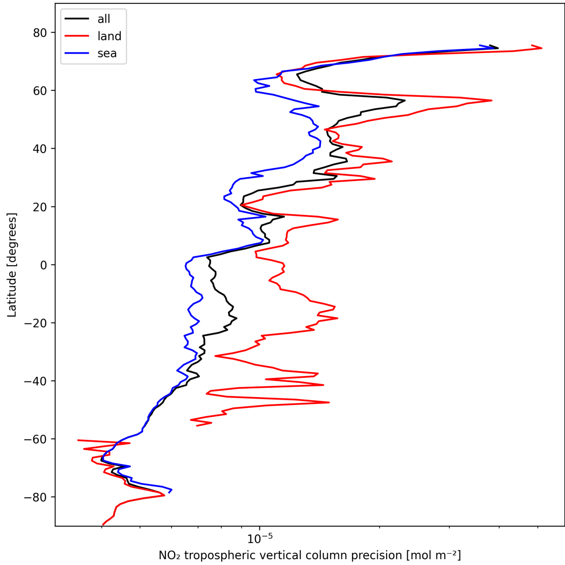
Figure 13: Zonal average of “NO 2 tropospheric vertical column precision” for 2024-10-26 to 2024-10-28.
