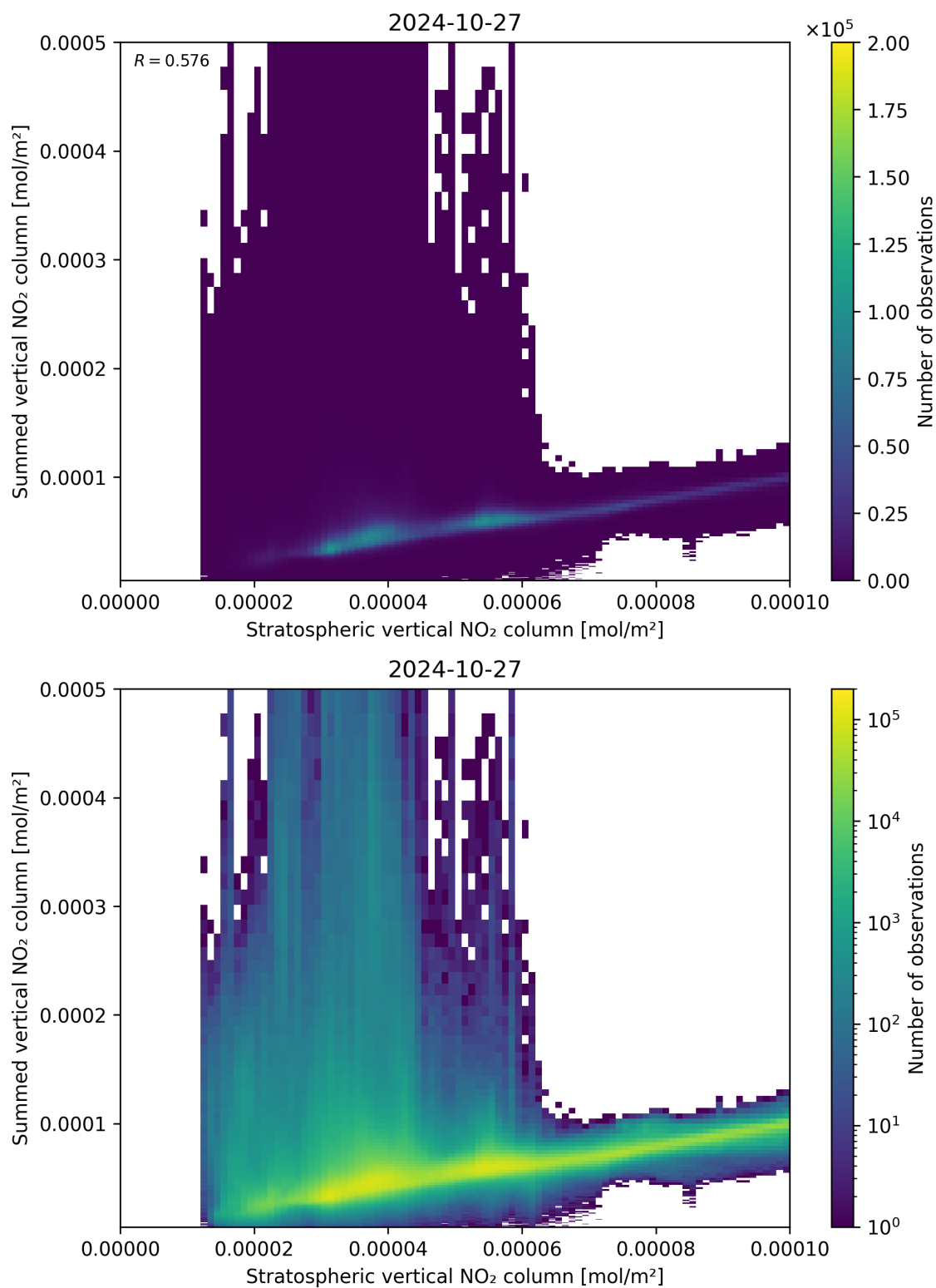
Figure 98: Scatter density plot of “Stratospheric vertical NO 2 column” against “Summed vertical NO 2 column” for 2024-10-26 to 2024-10-28.
