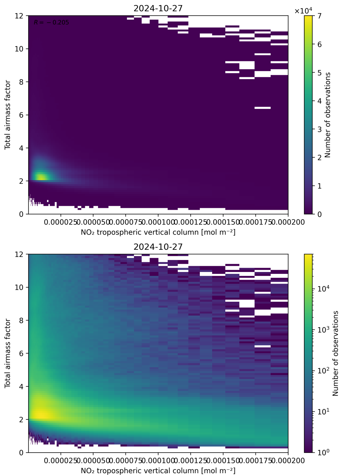
Figure 122: Scatter density plot of “NO 2 tropospheric vertical column” against “Total air mass factor” for 2024-10-26 to 2024-10-28.
