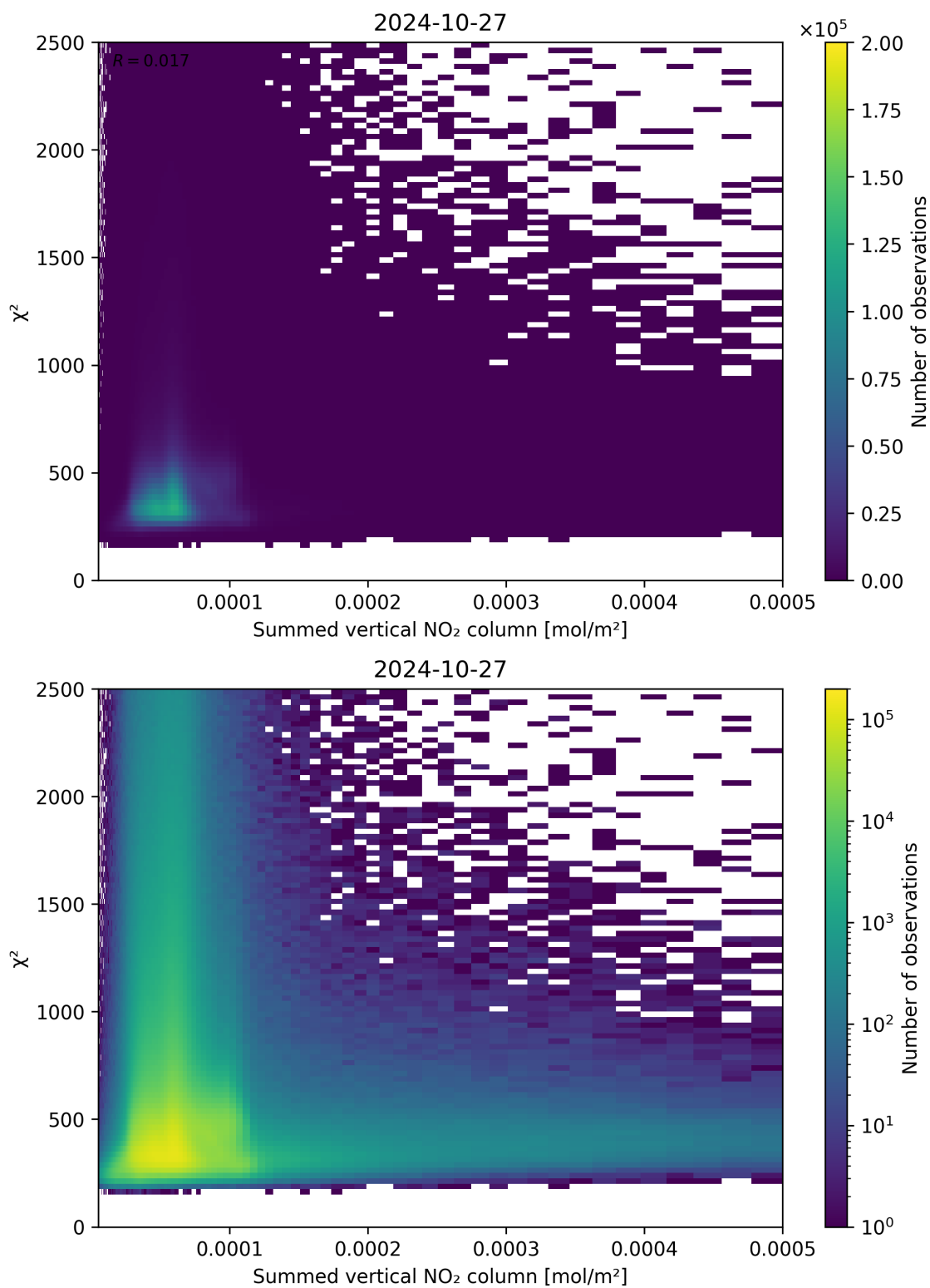
Figure 104: Scatter density plot of “Summed vertical NO 2 column” against “ \chi^2 ” for 2024-10-26 to 2024-10-28.
