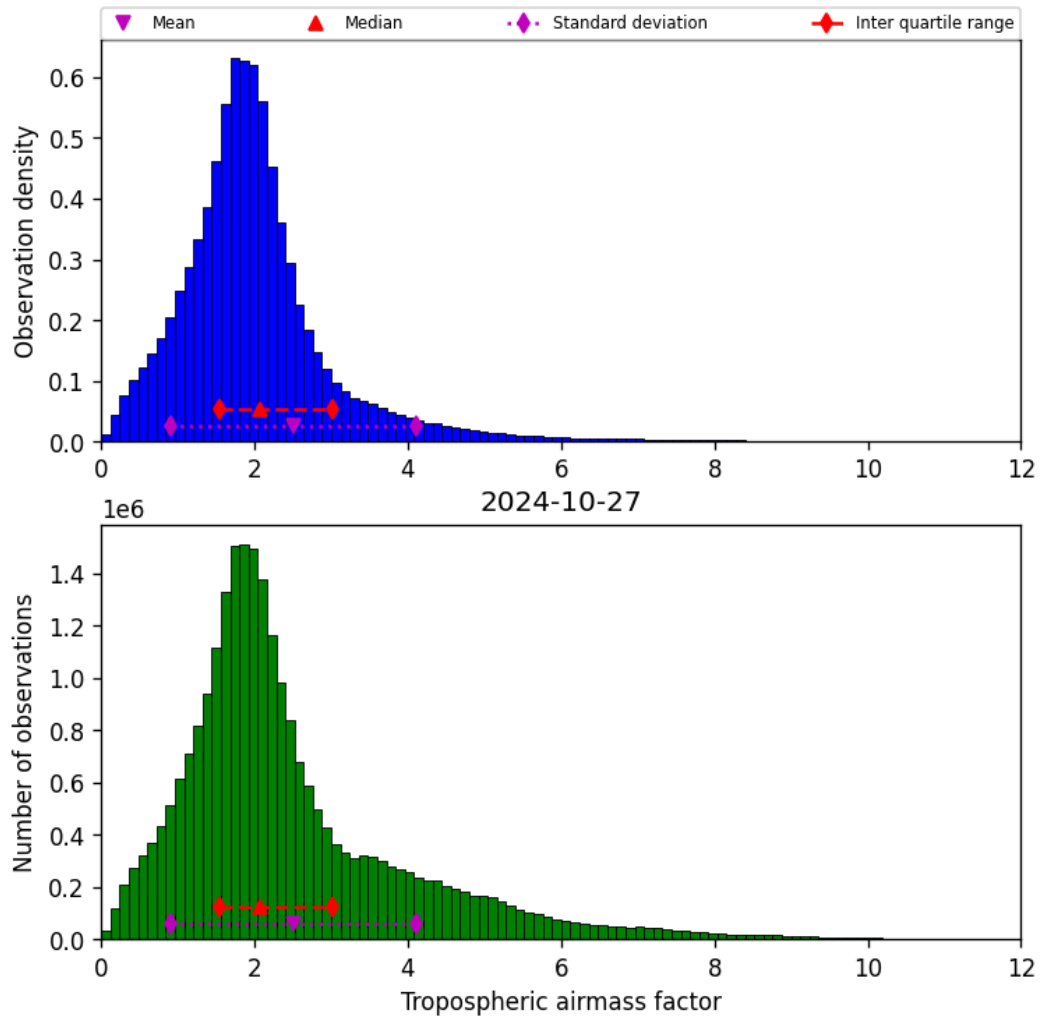
Figure 31: Histogram of “Tropospheric airmass factor” for 2024-10-26 to 2024-10-28
