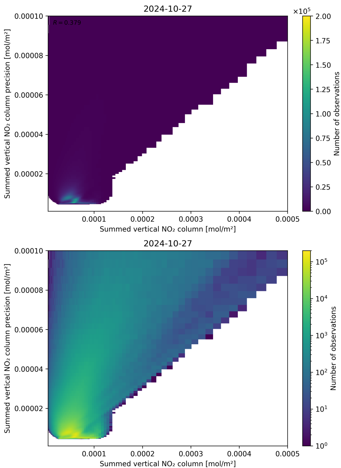
Figure 105: Scatter density plot of “Summed vertical NO 2 column” against “Summed vertical NO 2 column precision” for 2024-10-26 to 2024-10-28.
