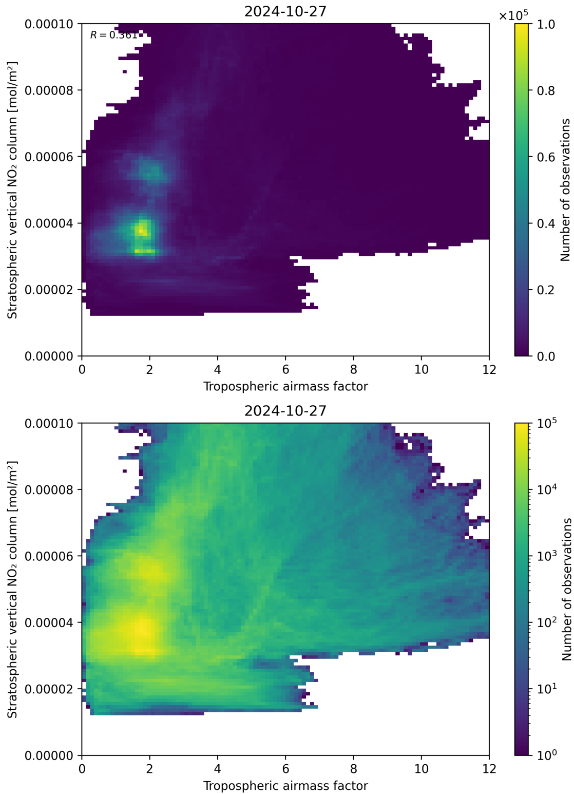
Figure 74: Scatter density plot of “Tropospheric air mass factor” against “Stratospheric vertical NO 2 column” for 2024-10-26 to 2024-10-28.
