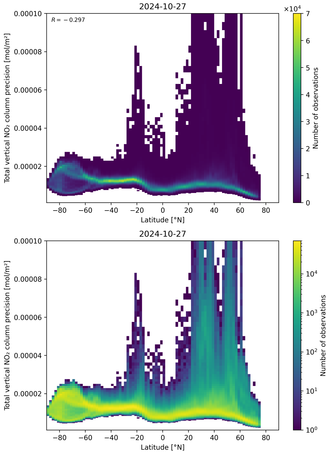
Figure 91: Scatter density plot of “Latitude” against “Total vertical NO 2 column precision” for 2024-10-26 to 2024-10-28.
