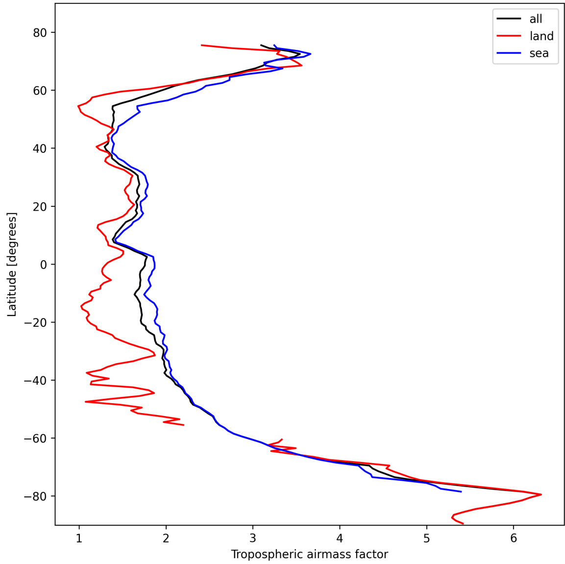
Figure 14: Zonal average of “Tropospheric airmass factor” for 2024-10-26 to 2024-10-28.
