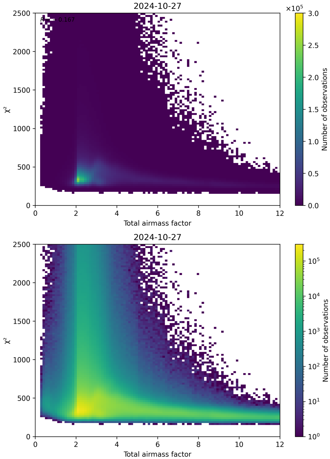
Figure 63: Scatter density plot of “Total airmass factor” against “ \chi^2 ” for 2024-10-26 to 2024-10-28.
