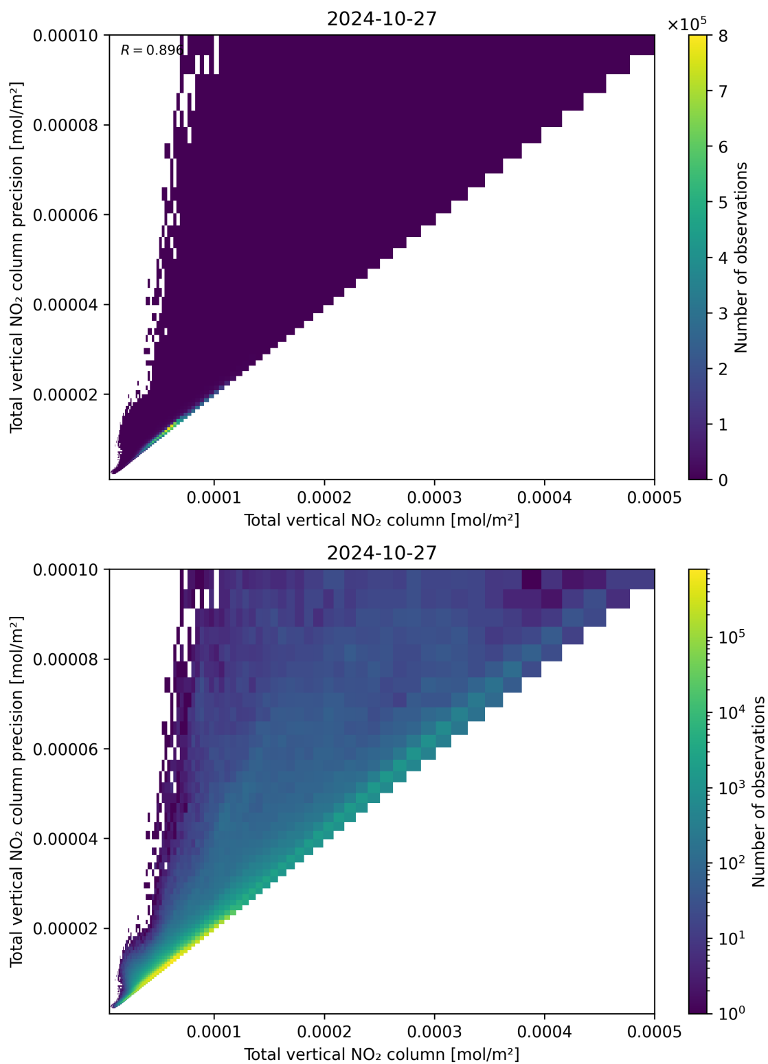
Figure 114: Scatter density plot of “Total vertical NO 2 column” against “Total vertical NO 2 column precision” for 2024-10-26 to 2024-10-28.
