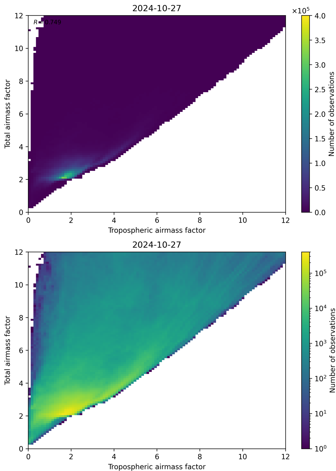
Figure 72: Scatter density plot of “Tropospheric airmass factor” against “Total airmass factor” for 2024-10-26 to 2024-10-28.
