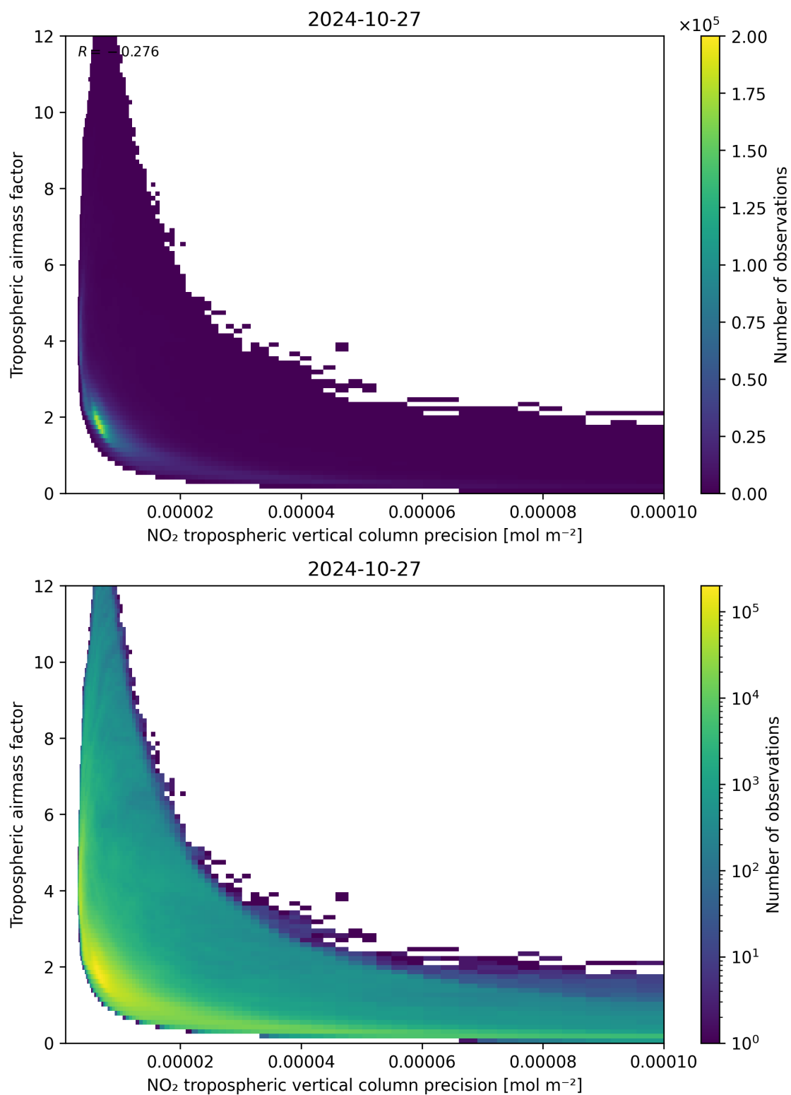
Figure 133: Scatter density plot of “NO 2 tropospheric vertical column precision” against “Tropospheric airmass factor” for 2024-10-26 to 2024-10-28.
