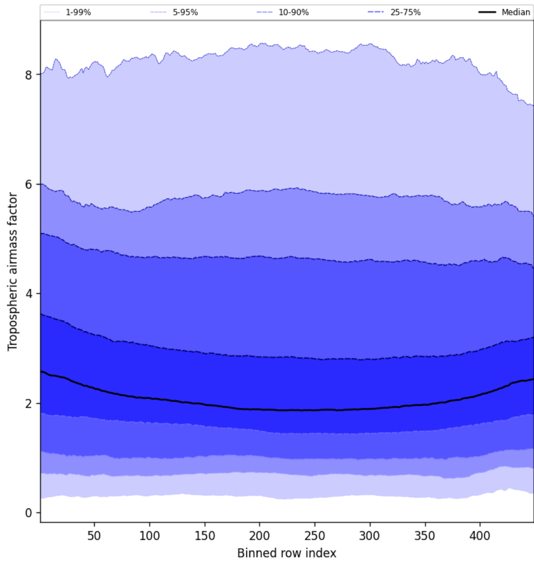
Figure 48: Along track statistics of “Tropospheric airmass factor” for 2024-10-26 to 2024-10-28
