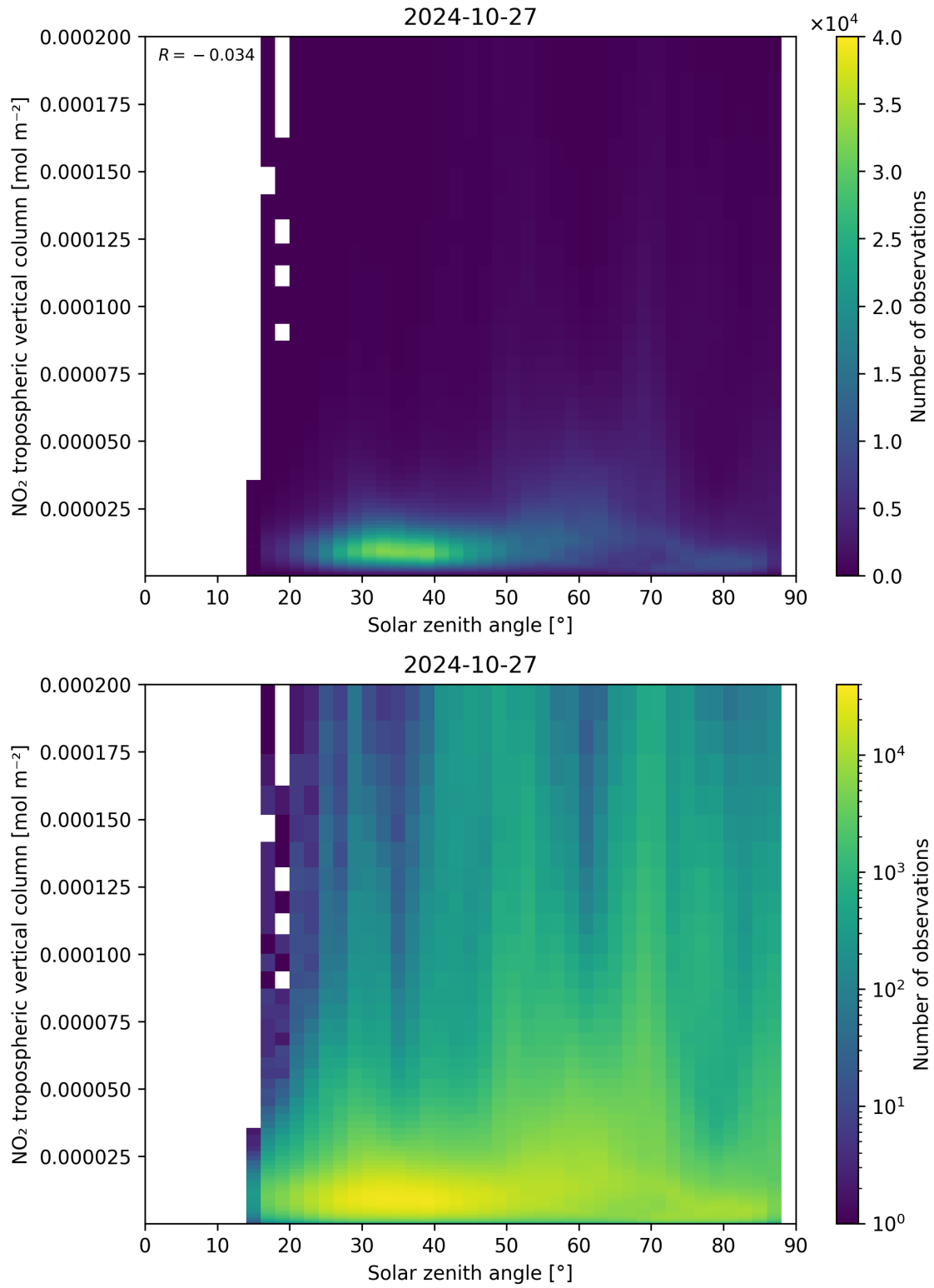
Figure 155: Scatter density plot of “Solar zenith angle” against “NO 2 tropospheric vertical column” for 2024-10-26 to 2024-10-28.
