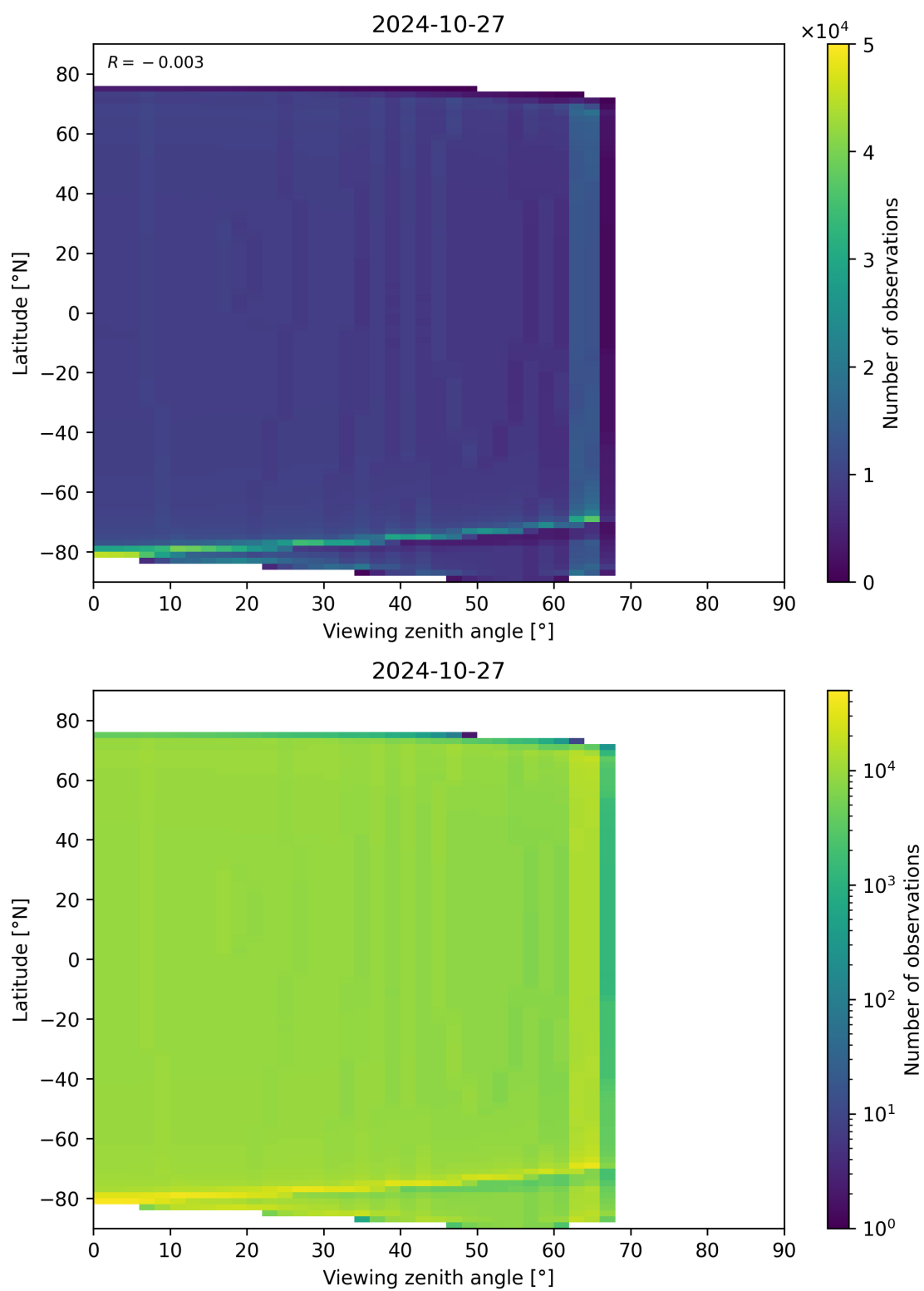
Figure 163: Scatter density plot of “Viewing zenith angle” against “Latitude” for 2024-10-26 to 2024-10-28.
