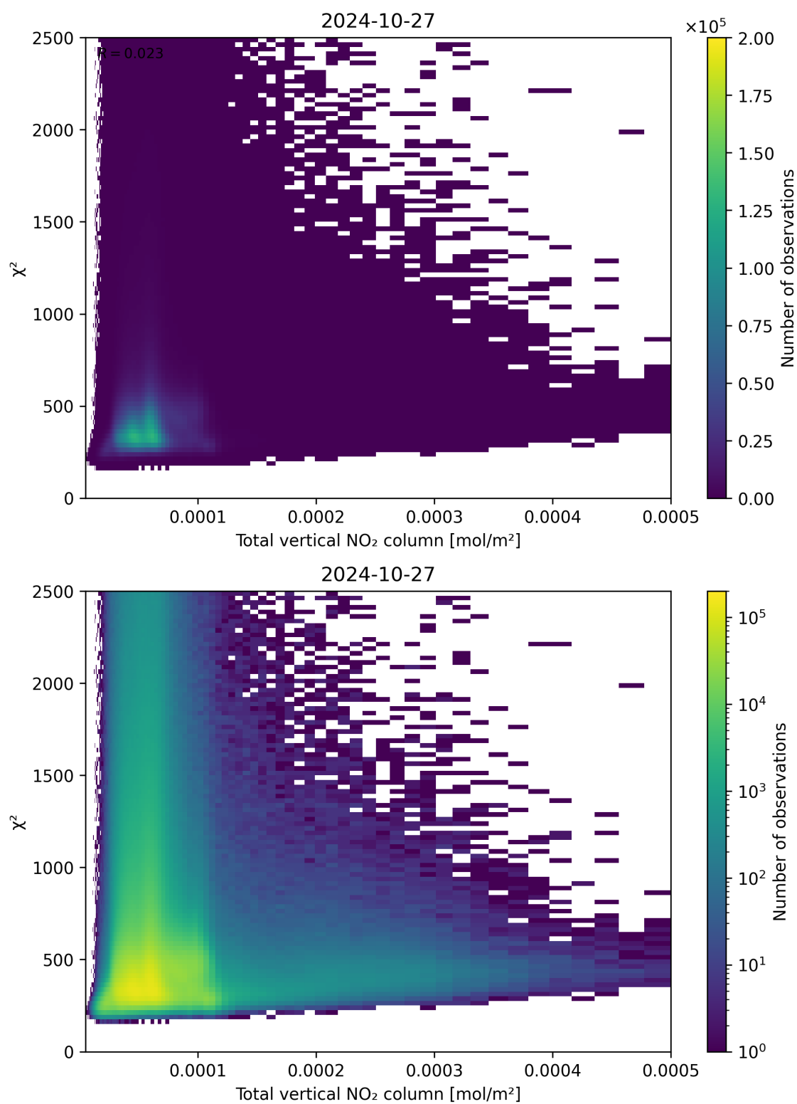
Figure 111: Scatter density plot of “Total vertical NO 2 column” against “ \chi^2 ” for 2024-10-26 to 2024-10-28.
