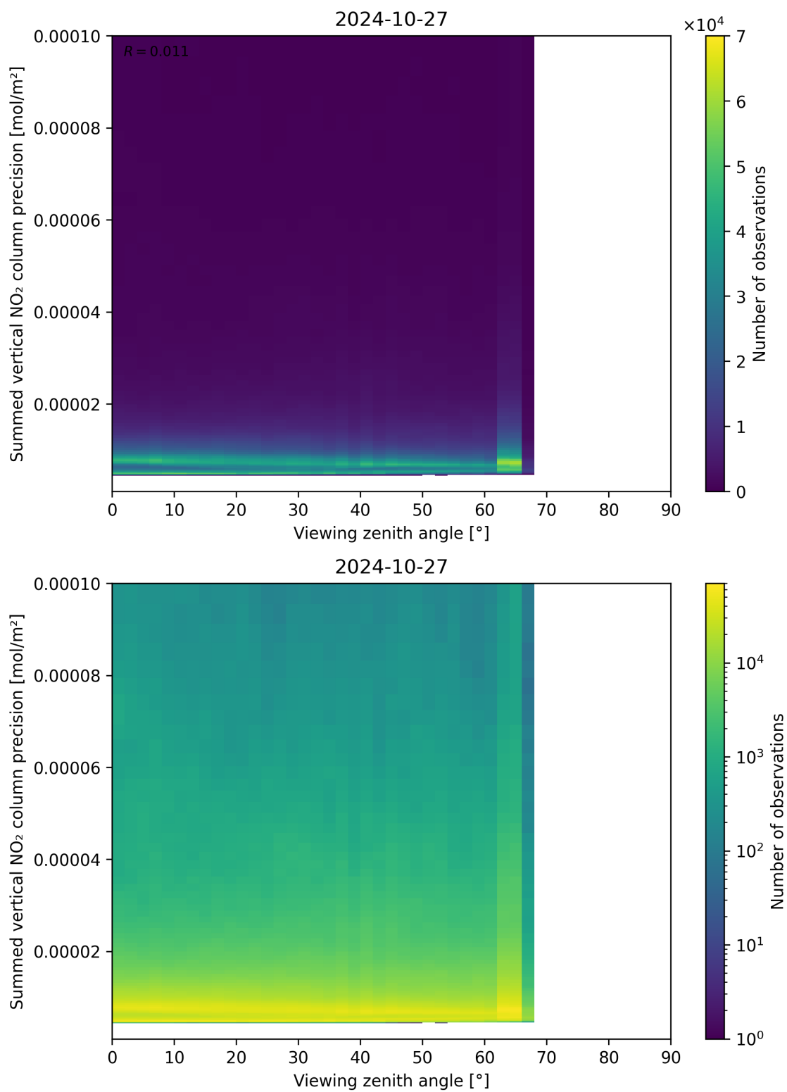
Figure 166: Scatter density plot of “Viewing zenith angle” against “Summed vertical NO 2 column precision” for 2024-10-26 to 2024-10-28.
