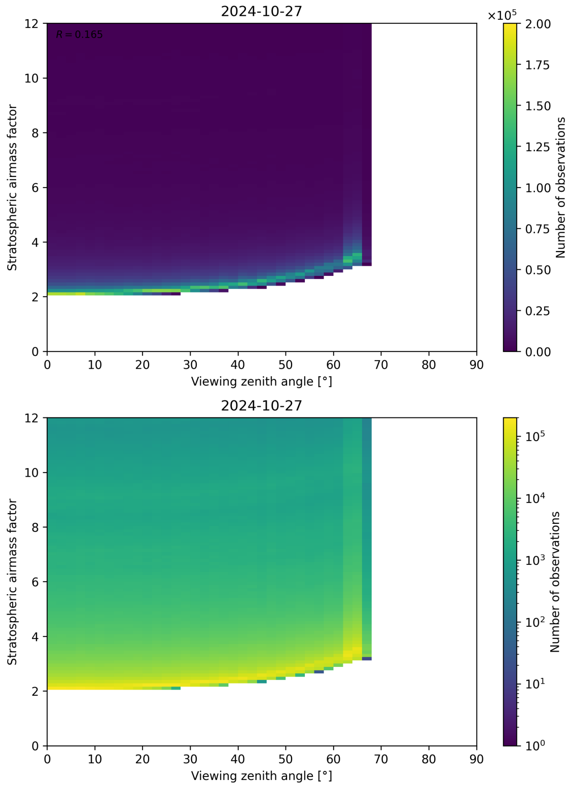
Figure 159: Scatter density plot of “Viewing zenith angle” against “Stratospheric airmass factor” for 2024-10-26 to 2024-10-28.
