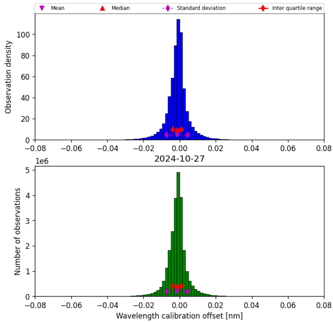
Figure 35: Histogram of “Wavelength calibration offset” for 2024-10-26 to 2024-10-28
