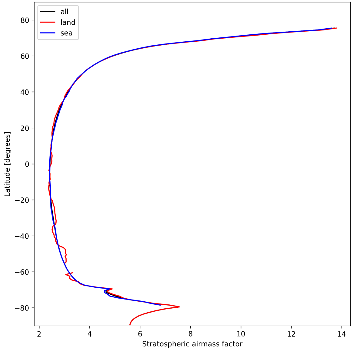
Figure 27: Zonal average of “Stratospheric air mass factor” for 2024-10-26 to 2024-10-28.
