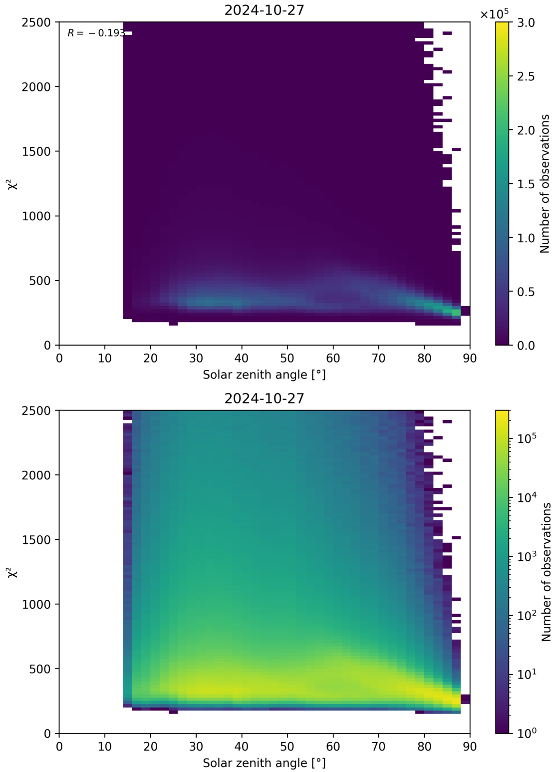
Figure 148: Scatter density plot of “Solar zenith angle” against “ \chi^2 ” for 2024-10-26 to 2024-10-28.
