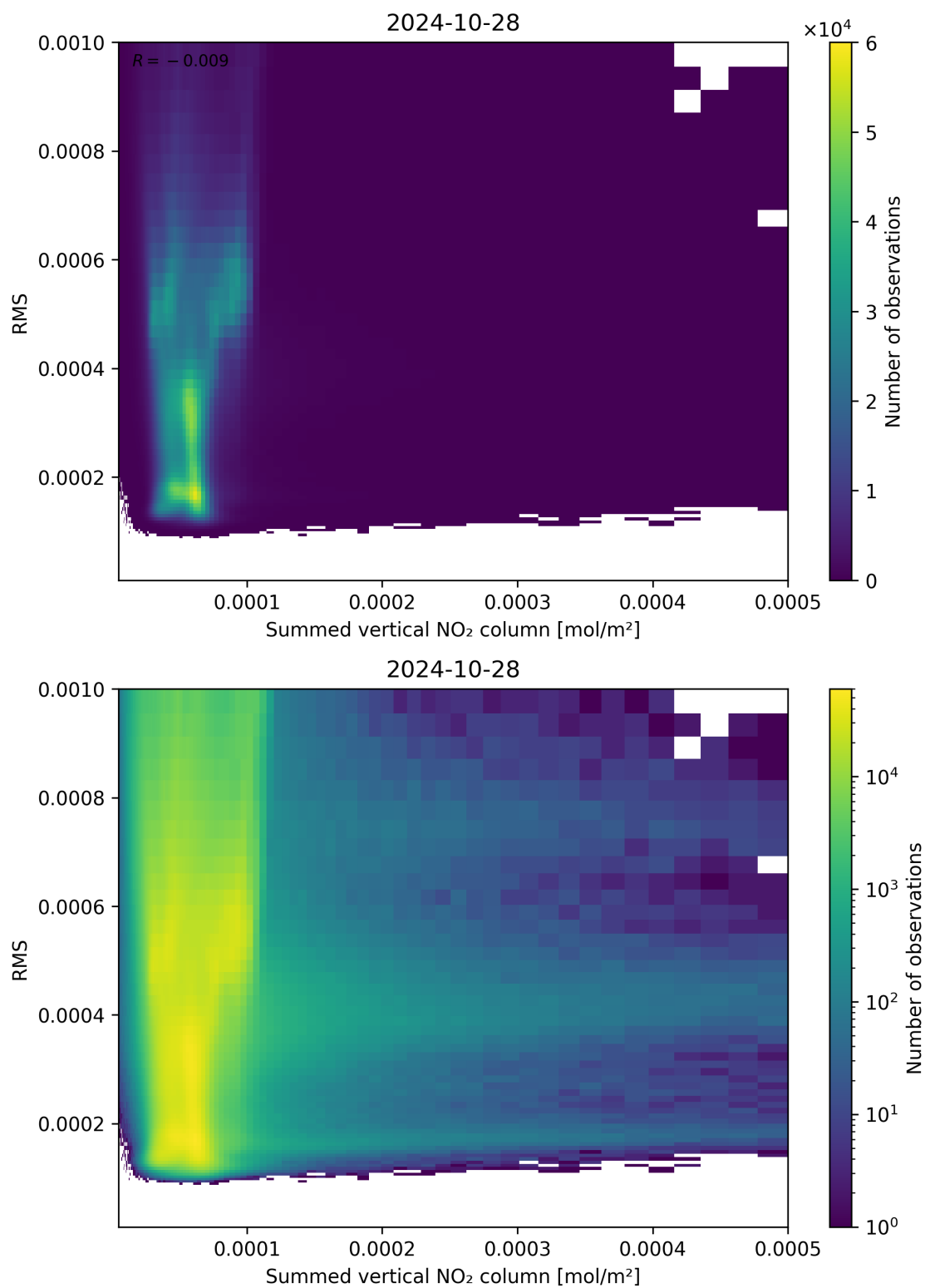
Figure 109: Scatter density plot of “Summed vertical NO 2 column” against “RMS” for 2024-10-27 to 2024-10-29.
