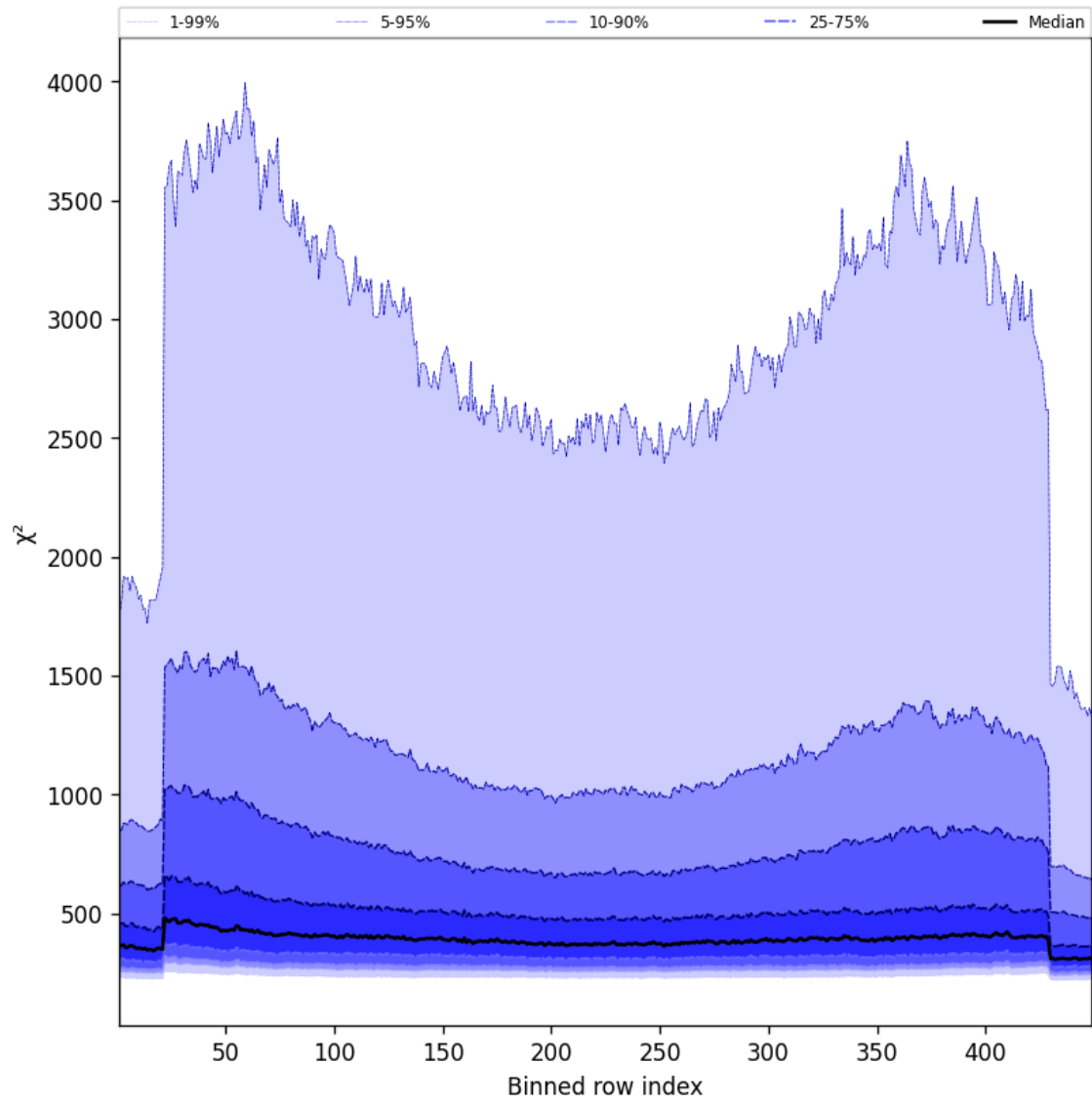
Figure 59: Along track statistics of “ \chi^2 ” for 2024-10-27 to 2024-10-29
