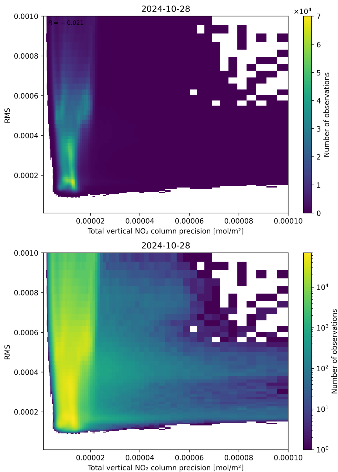
Figure 119: Scatter density plot of “Total vertical NO 2 column precision” against “RMS” for 2024-10-27 to 2024-10-29.
