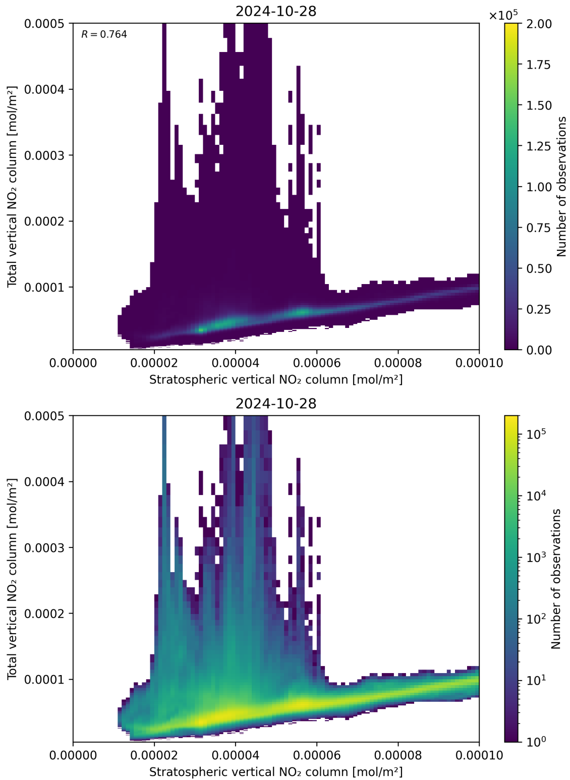
Figure 100: Scatter density plot of “Stratospheric vertical NO 2 column” against “Total vertical NO 2 column” for 2024-10-27 to 2024-10-29.
