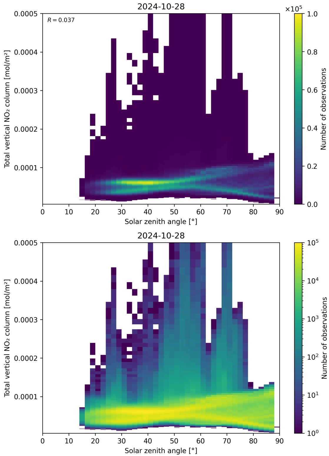
Figure 153: Scatter density plot of “Solar zenith angle” against “Total vertical NO 2 column” for 2024-10-27 to 2024-10-29.
