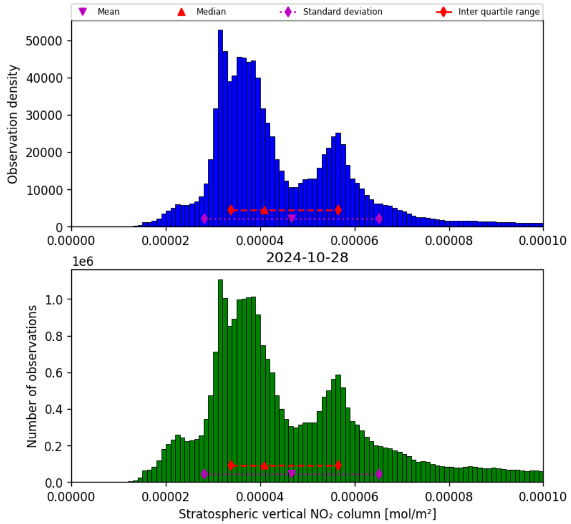
Figure 36: Histogram of “Stratospheric vertical NO 2 column” for 2024-10-27 to 2024-10-29
