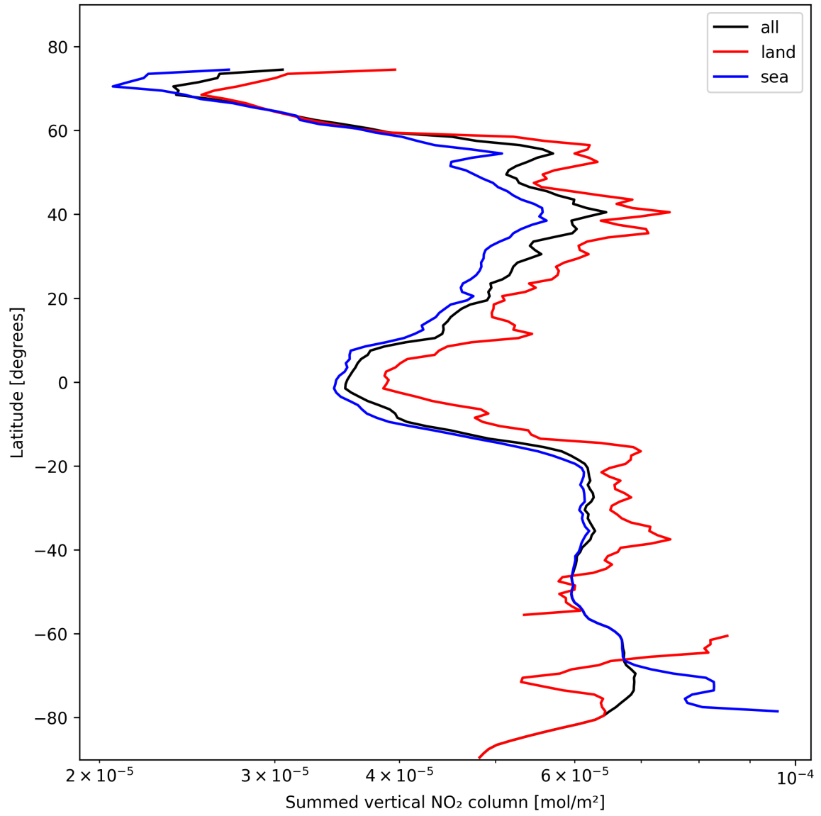
Figure 23: Zonal average of “Summed vertical NO 2 column” for 2024-10-27 to 2024-10-29.
