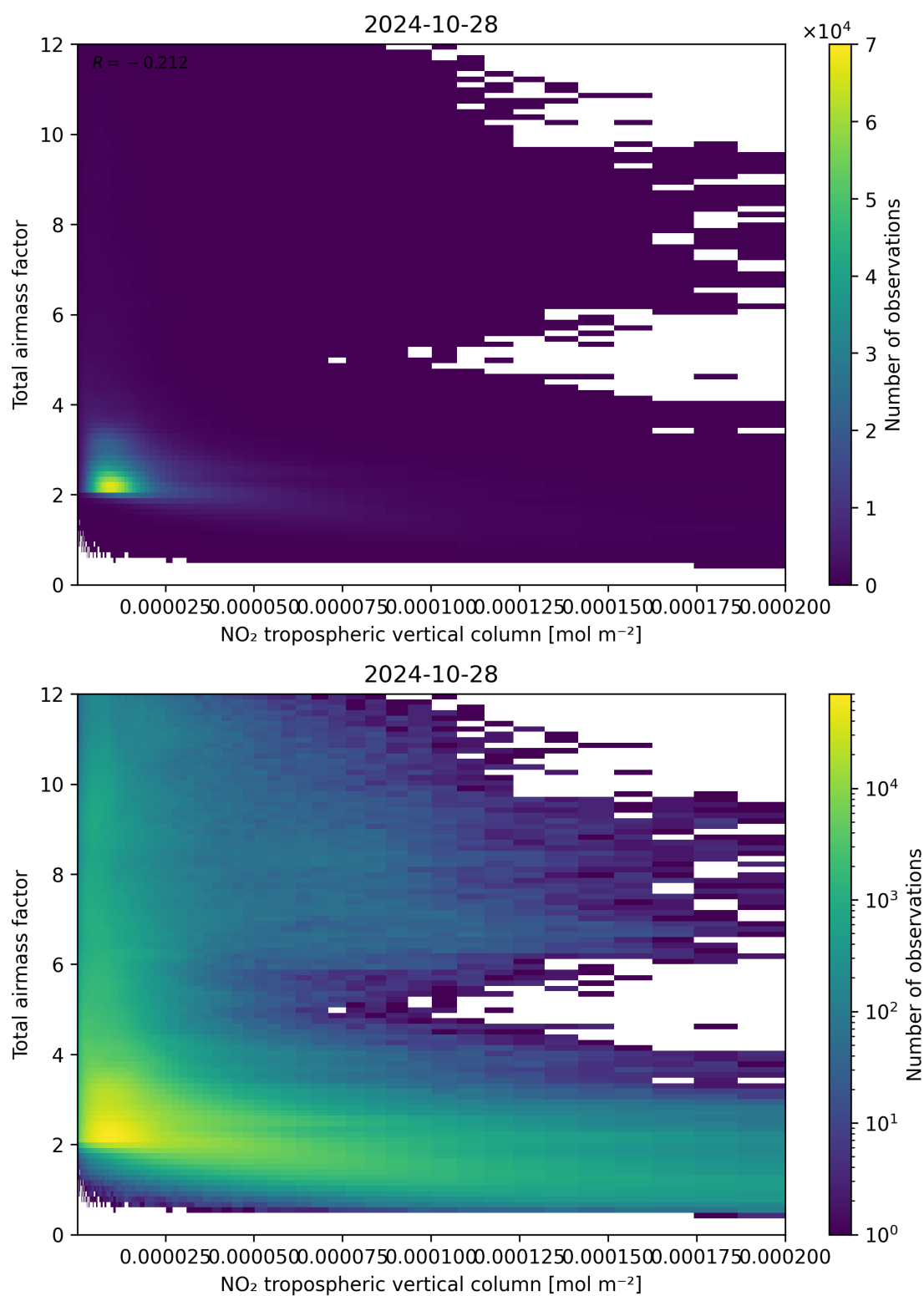
Figure 122: Scatter density plot of “NO 2 tropospheric vertical column” against “Total air mass factor” for 2024-10-27 to 2024-10-29.
