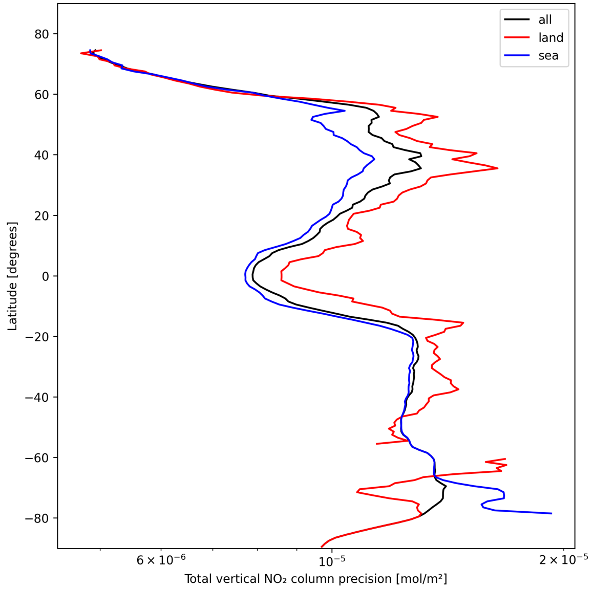
Figure 22: Zonal average of “Total vertical NO 2 column precision” for 2024-10-27 to 2024-10-29.
