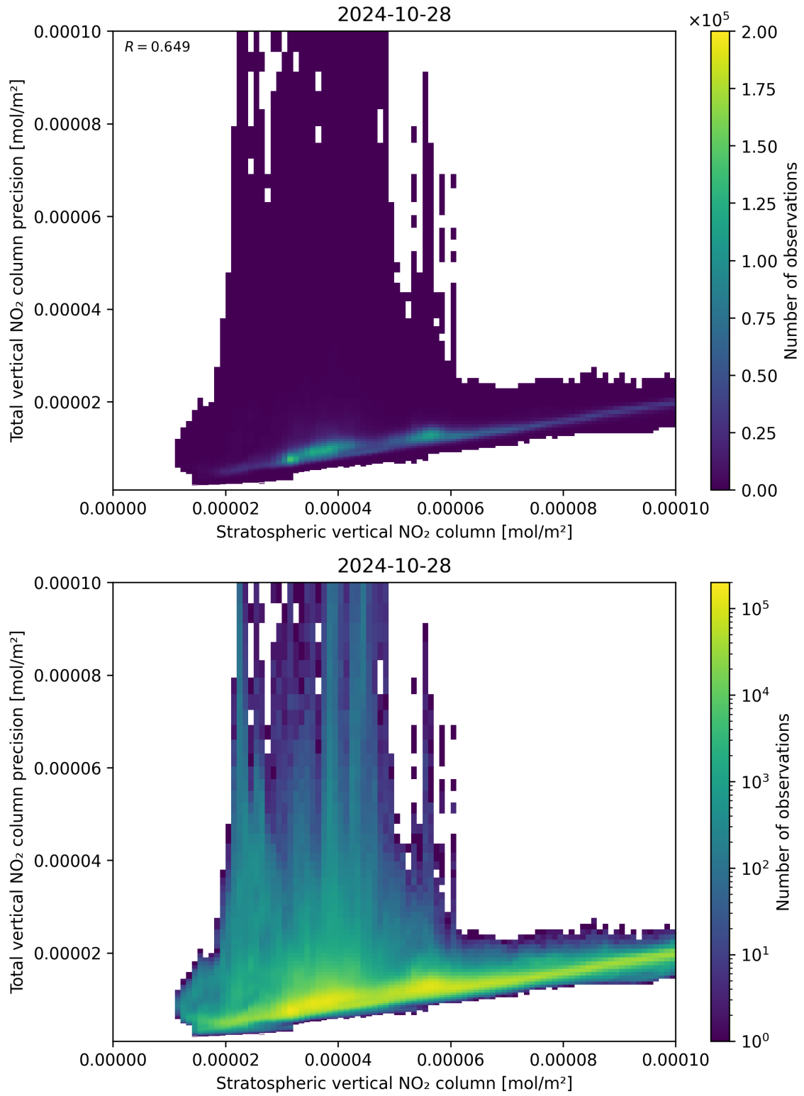
Figure 101: Scatter density plot of “Stratospheric vertical NO 2 column” against “Total vertical NO 2 column precision” for 2024-10-27 to 2024-10-29.
