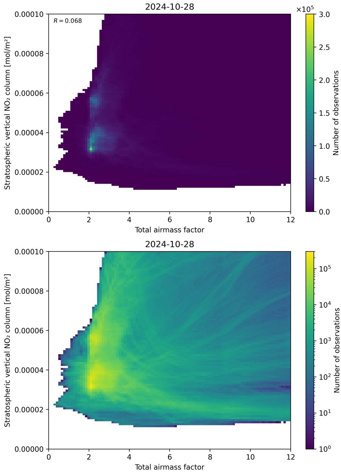
Figure 64: Scatter density plot of “Total airmass factor” against “Stratospheric vertical NO 2 column” for 2024-10-27 to 2024-10-29.
