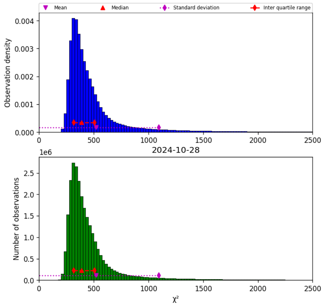
Figure 42: Histogram of “ \chi^2 ” for 2024-10-27 to 2024-10-29
