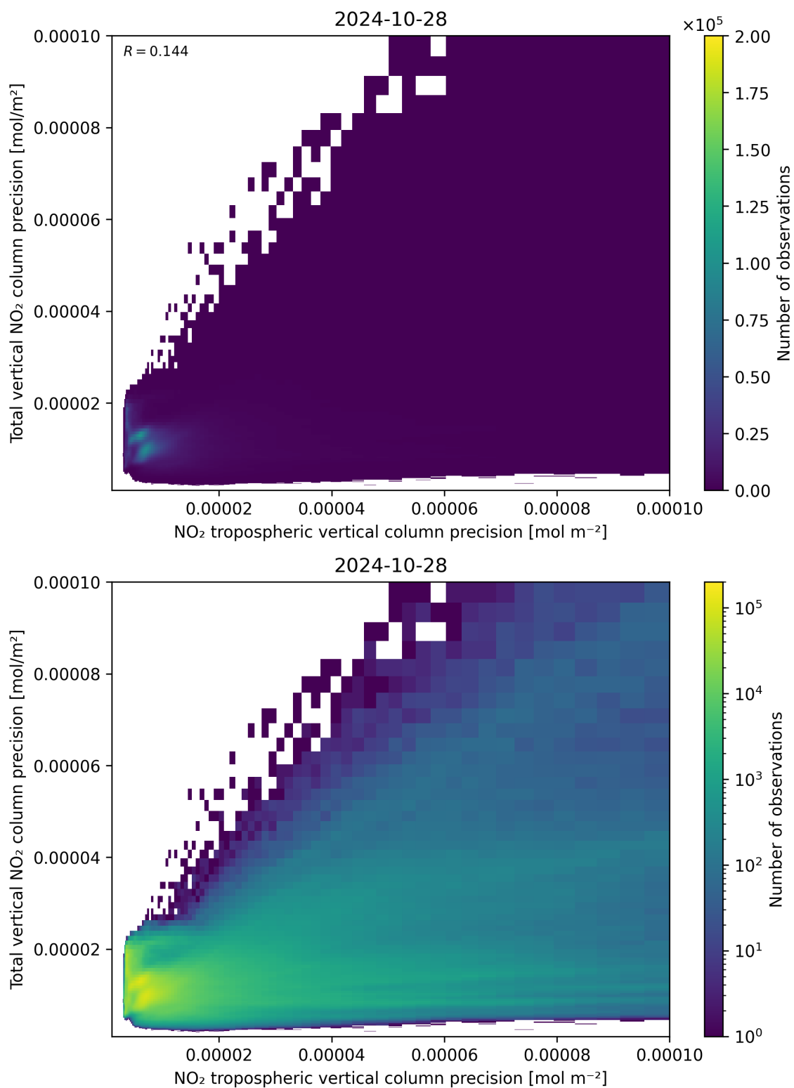
Figure 139: Scatter density plot of “NO 2 tropospheric vertical column precision” against “Total vertical NO 2 column precision” for 2024-10-27 to 2024-10-29.
