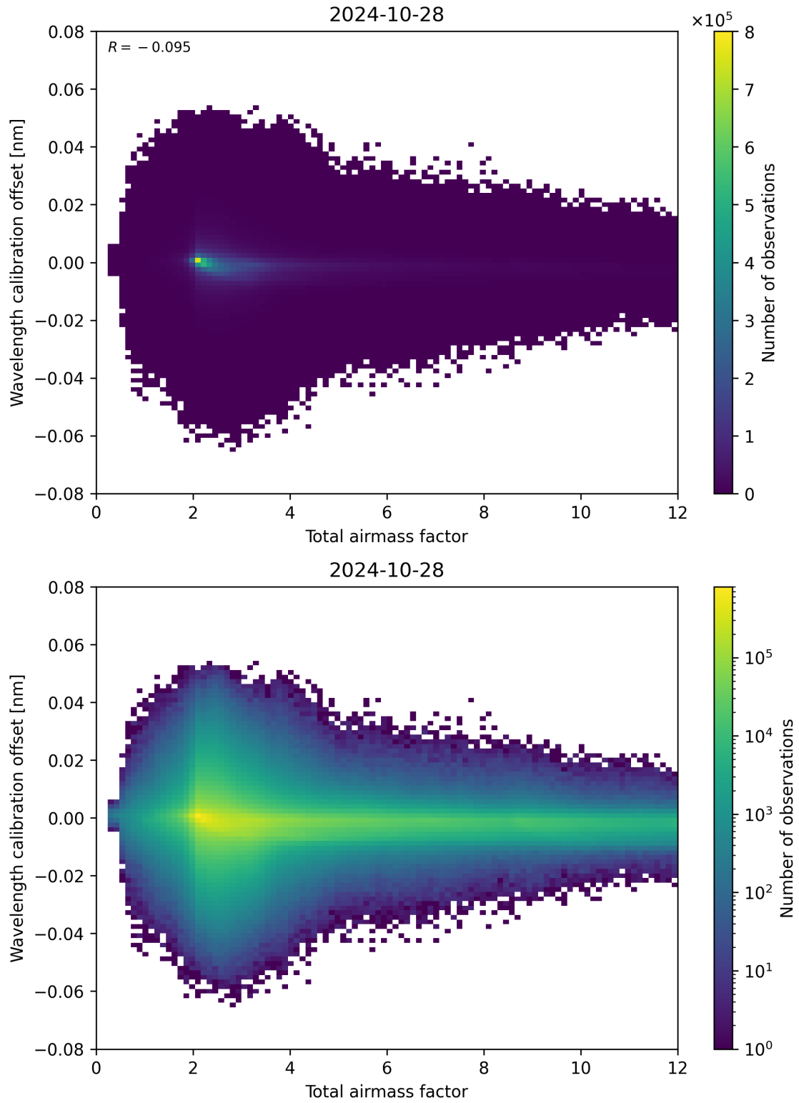
Figure 70: Scatter density plot of “Total airmass factor” against “Wavelength calibration offset” for 2024-10-27 to 2024-10-29.
