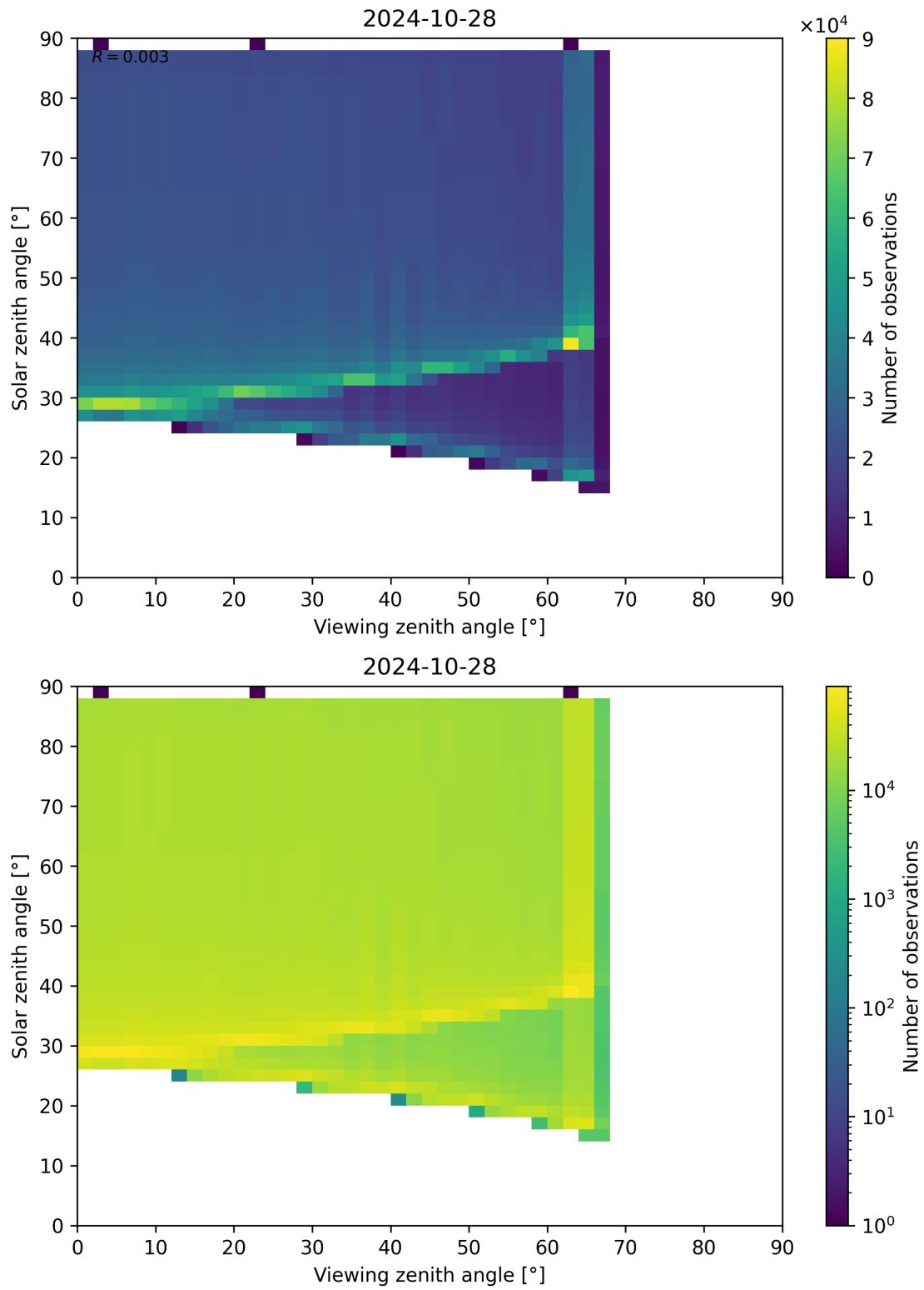
Figure 172: Scatter density plot of “Viewing zenith angle” against “Solar zenith angle” for 2024-10-27 to 2024-10-29.
