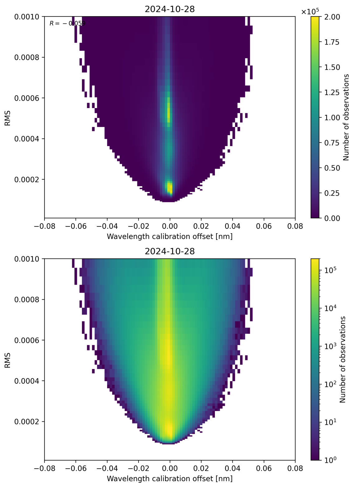
Figure 181: Scatter density plot of “Wavelength calibration offset” against “RMS” for 2024-10-27 to 2024-10-29.
