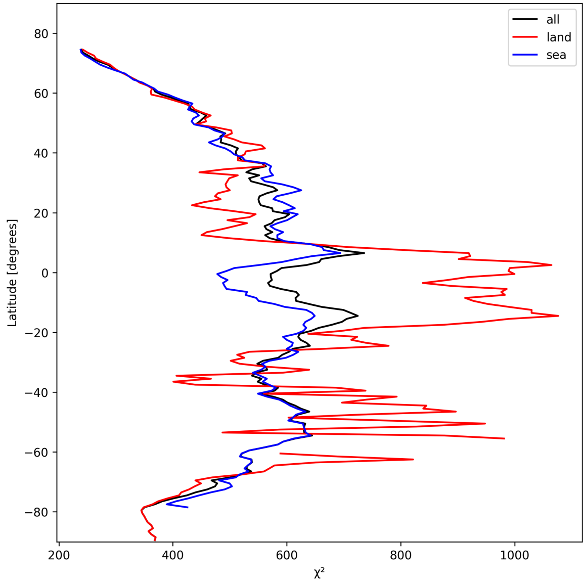
Figure 25: Zonal average of “ \chi^2 ” for 2024-10-27 to 2024-10-29.
