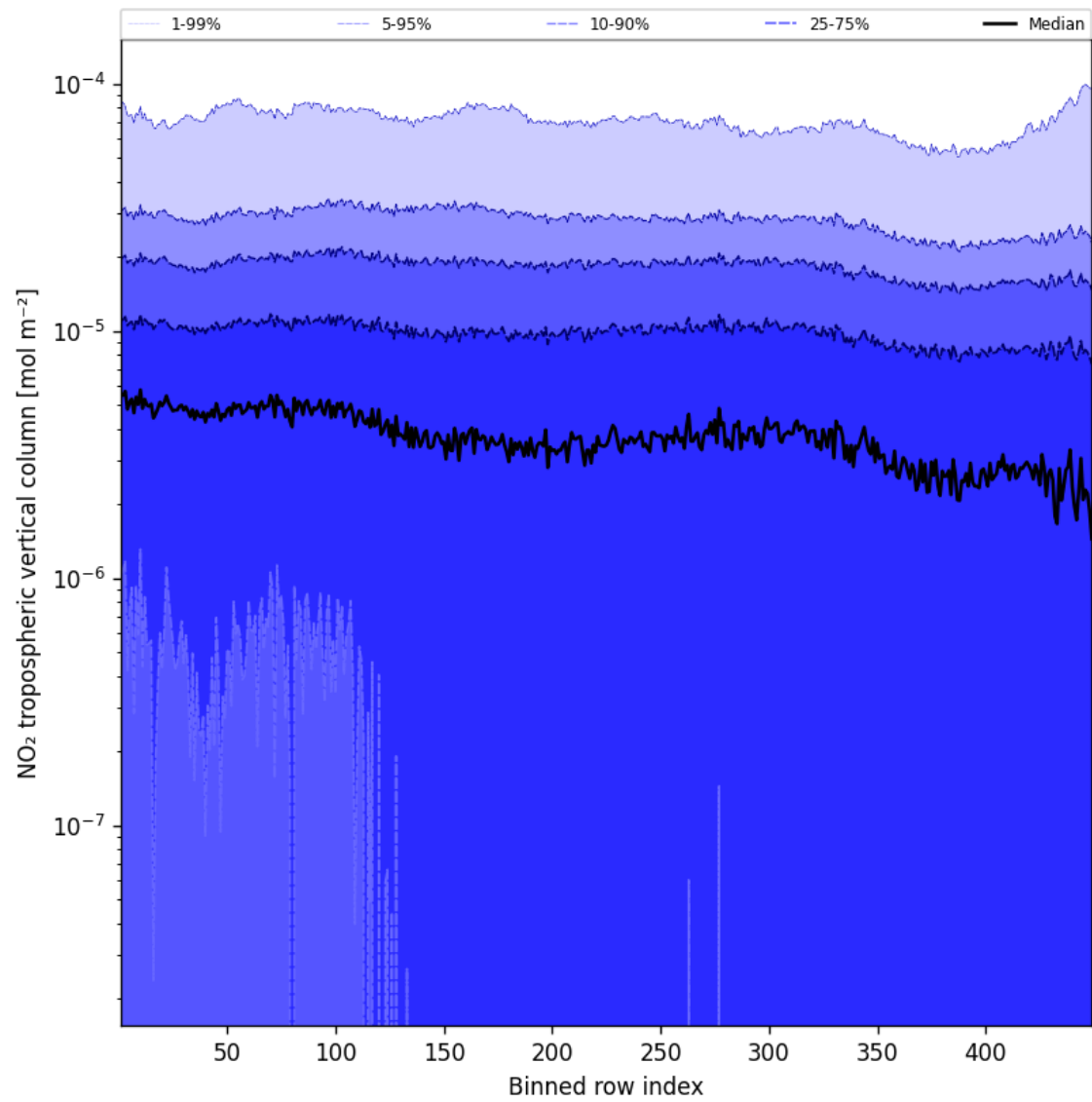
Figure 46: Along track statistics of “NO 2 tropospheric vertical column” for 2024-10-27 to 2024-10-29
