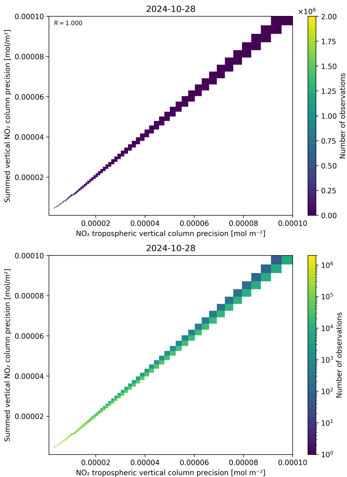
Figure 137: Scatter density plot of “NO 2 tropospheric vertical column precision” against “Summed vertical NO 2 column precision” for 2024-10-27 to 2024-10-29.
