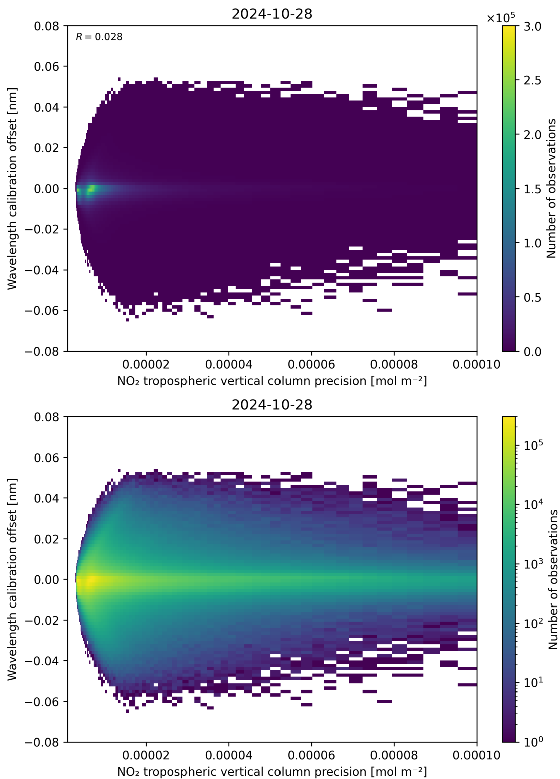
Figure 141: Scatter density plot of “NO 2 tropospheric vertical column precision” against “Wavelength calibration offset” for 2024-10-27 to 2024-10-29.
