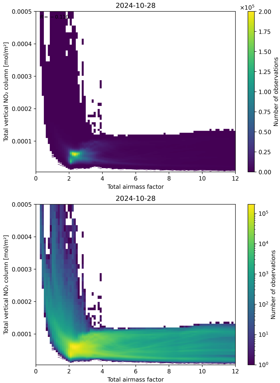
Figure 67: Scatter density plot of “Total airmass factor” against “Total vertical NO 2 column” for 2024-10-27 to 2024-10-29.
