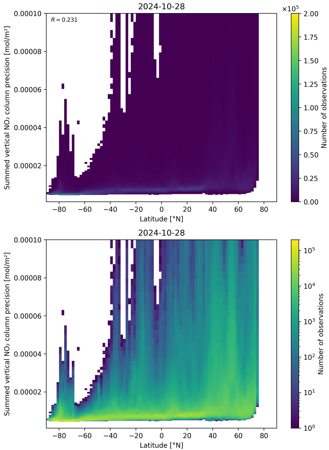
Figure 89: Scatter density plot of “Latitude” against “Summed vertical NO 2 column precision” for 2024-10-27 to 2024-10-29.
