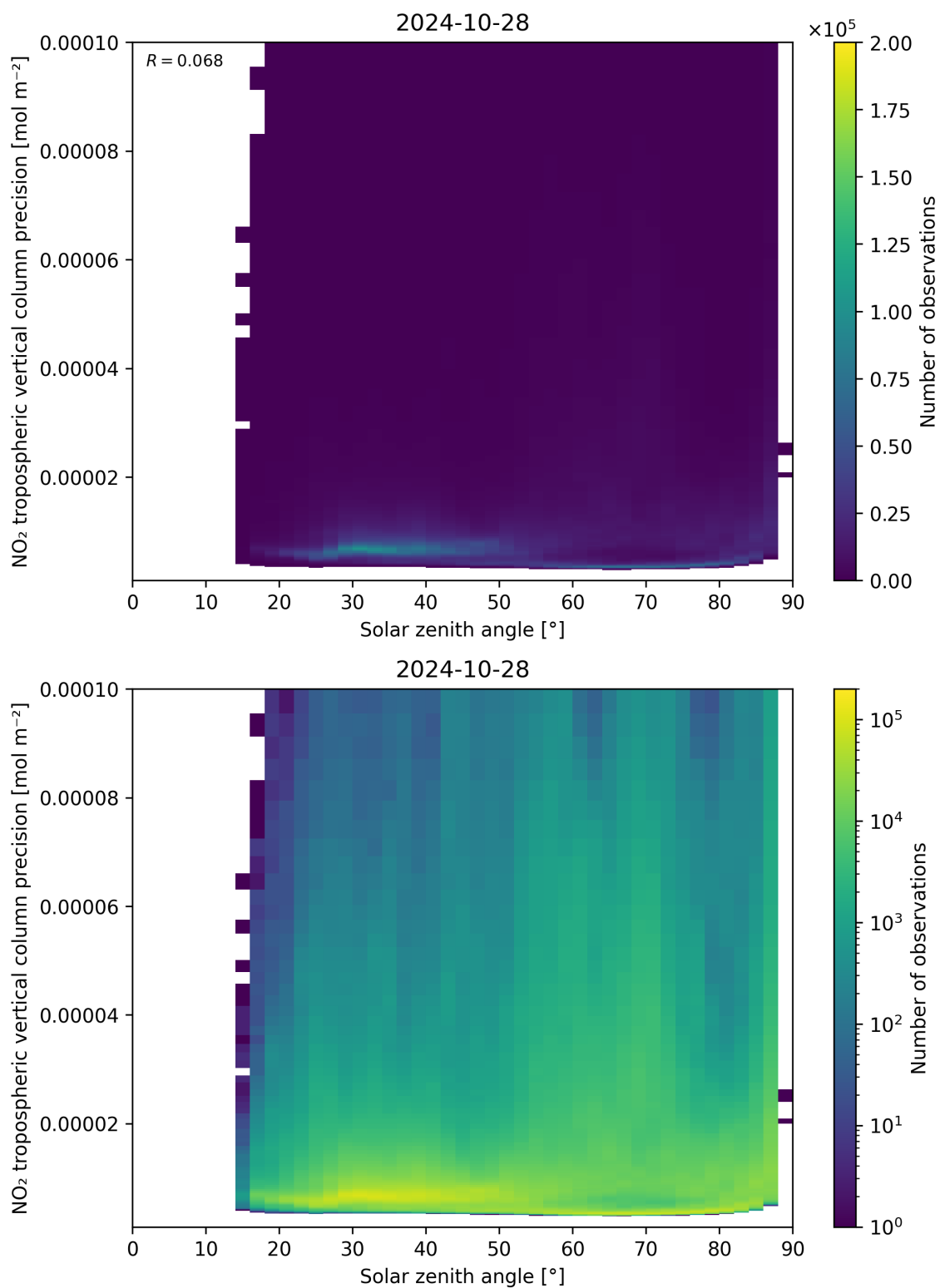
Figure 156: Scatter density plot of “Solar zenith angle” against “NO 2 tropospheric vertical column precision” for 2024-10-27 to 2024-10-29.
