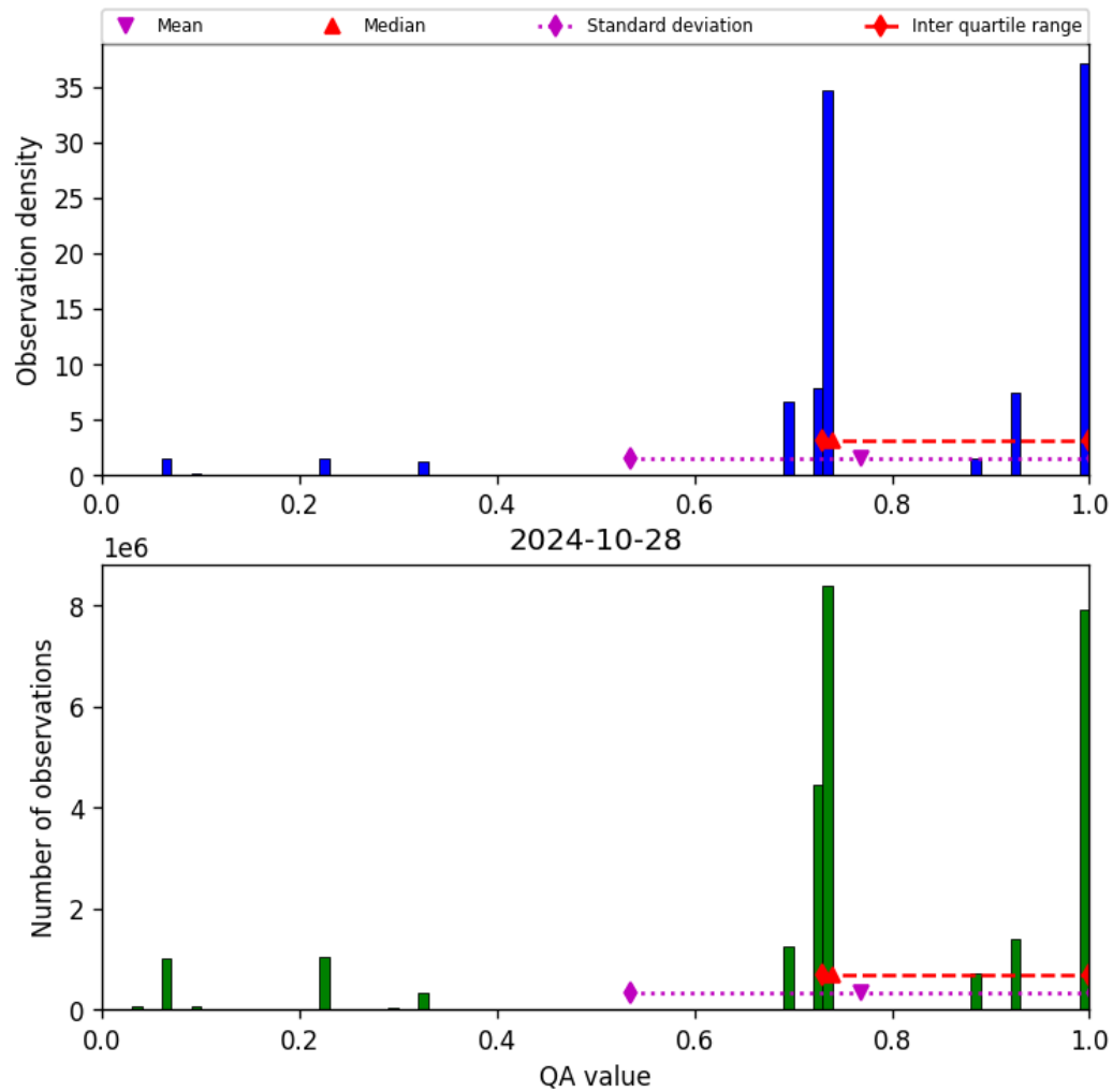
Figure 28: Histogram of “QA value” for 2024-10-27 to 2024-10-29
