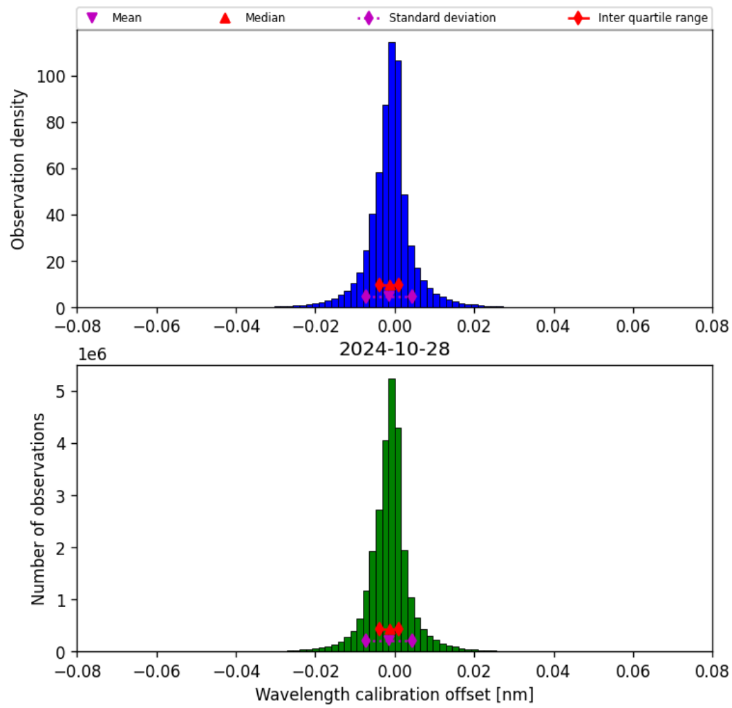
Figure 35: Histogram of “Wavelength calibration offset” for 2024-10-27 to 2024-10-29
