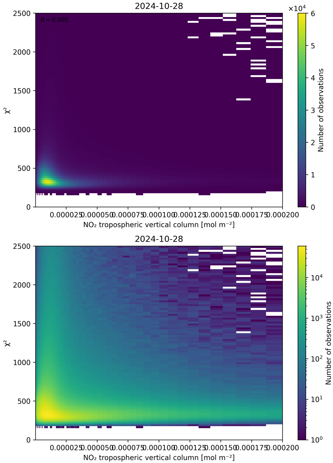
Figure 124: Scatter density plot of “NO 2 tropospheric vertical column” against “ \chi^2 ” for 2024-10-27 to 2024-10-29.
