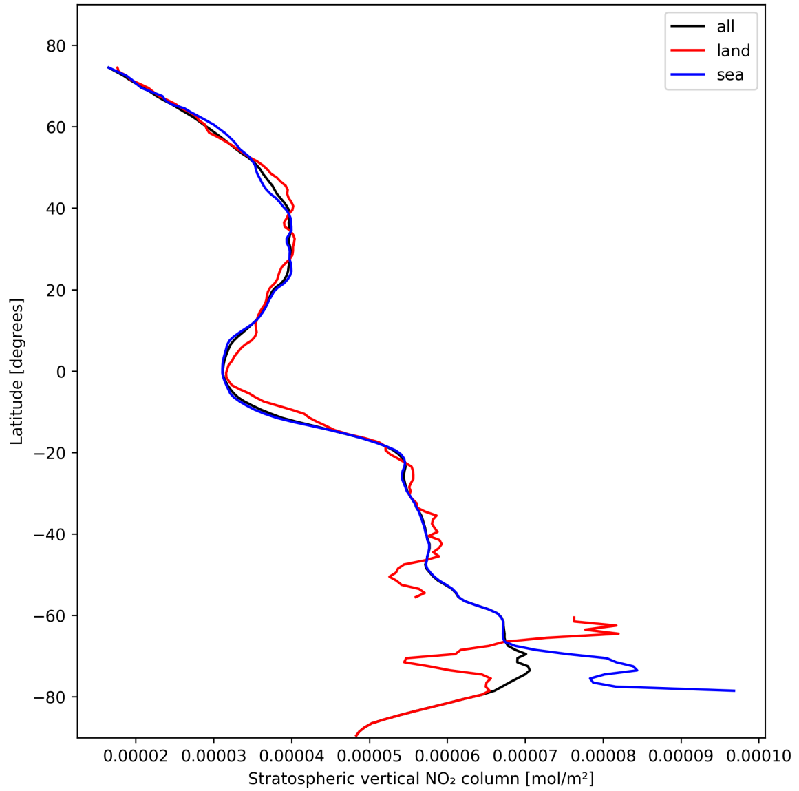
Figure 19: Zonal average of “Stratospheric vertical NO 2 column” for 2024-10-27 to 2024-10-29.
