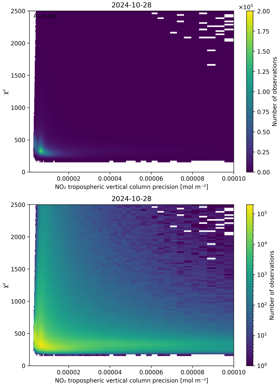
Figure 134: Scatter density plot of “NO 2 tropospheric vertical column precision” against “ \chi^2 ” for 2024-10-27 to 2024-10-29.
