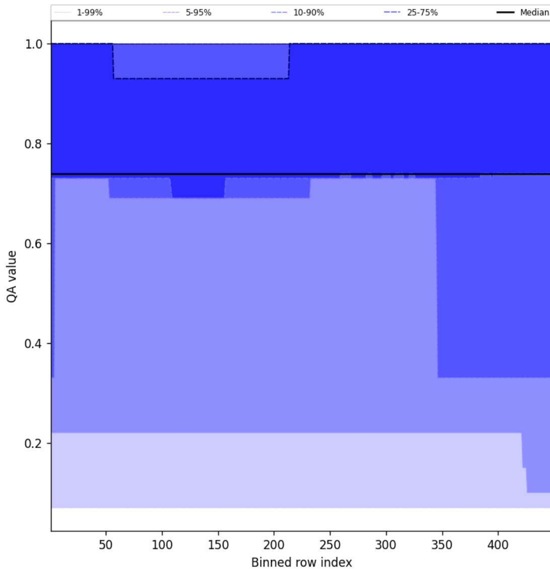
Figure 45: Along track statistics of “QA value” for 2024-10-27 to 2024-10-29
