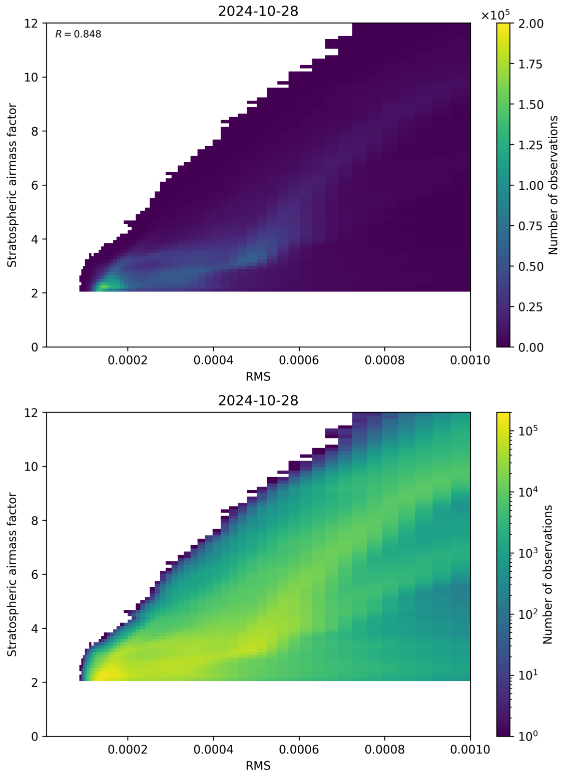
Figure 144: Scatter density plot of “RMS” against “Stratospheric airmass factor” for 2024-10-27 to 2024-10-29.
