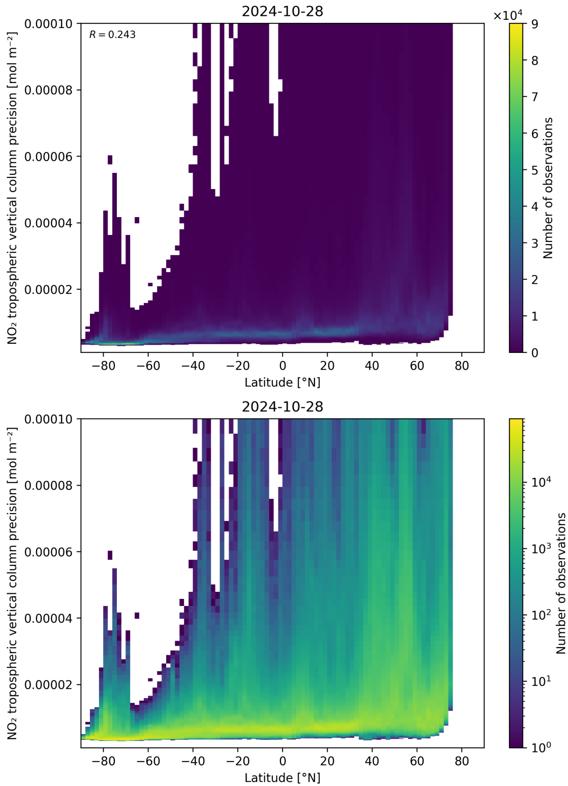
Figure 93: Scatter density plot of “Latitude” against “NO 2 tropospheric vertical column precision” for 2024-10-27 to 2024-10-29.
