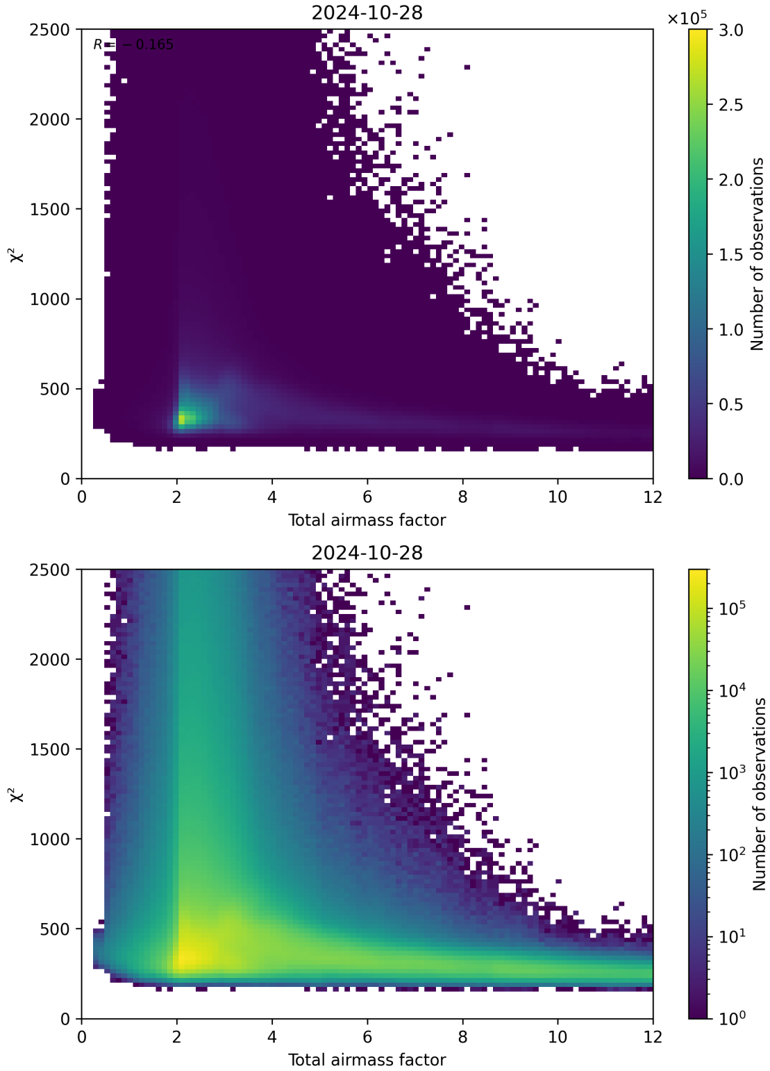
Figure 63: Scatter density plot of “Total airmass factor” against “ \chi^2 ” for 2024-10-27 to 2024-10-29.
