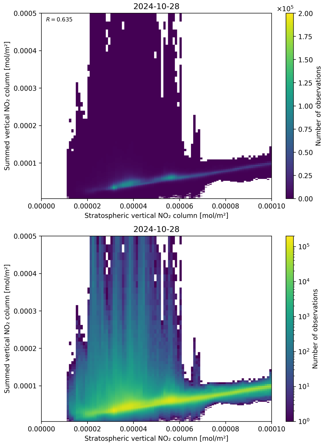
Figure 98: Scatter density plot of “Stratospheric vertical NO 2 column” against “Summed vertical NO 2 column” for 2024-10-27 to 2024-10-29.
