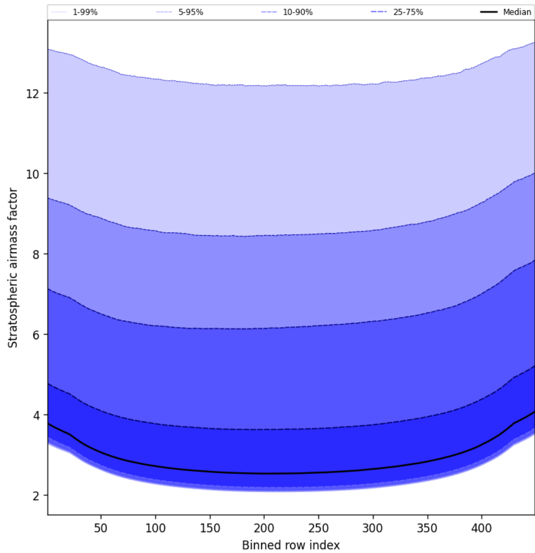
Figure 61: Along track statistics of “Stratospheric airmass factor” for 2024-10-27 to 2024-10-29
