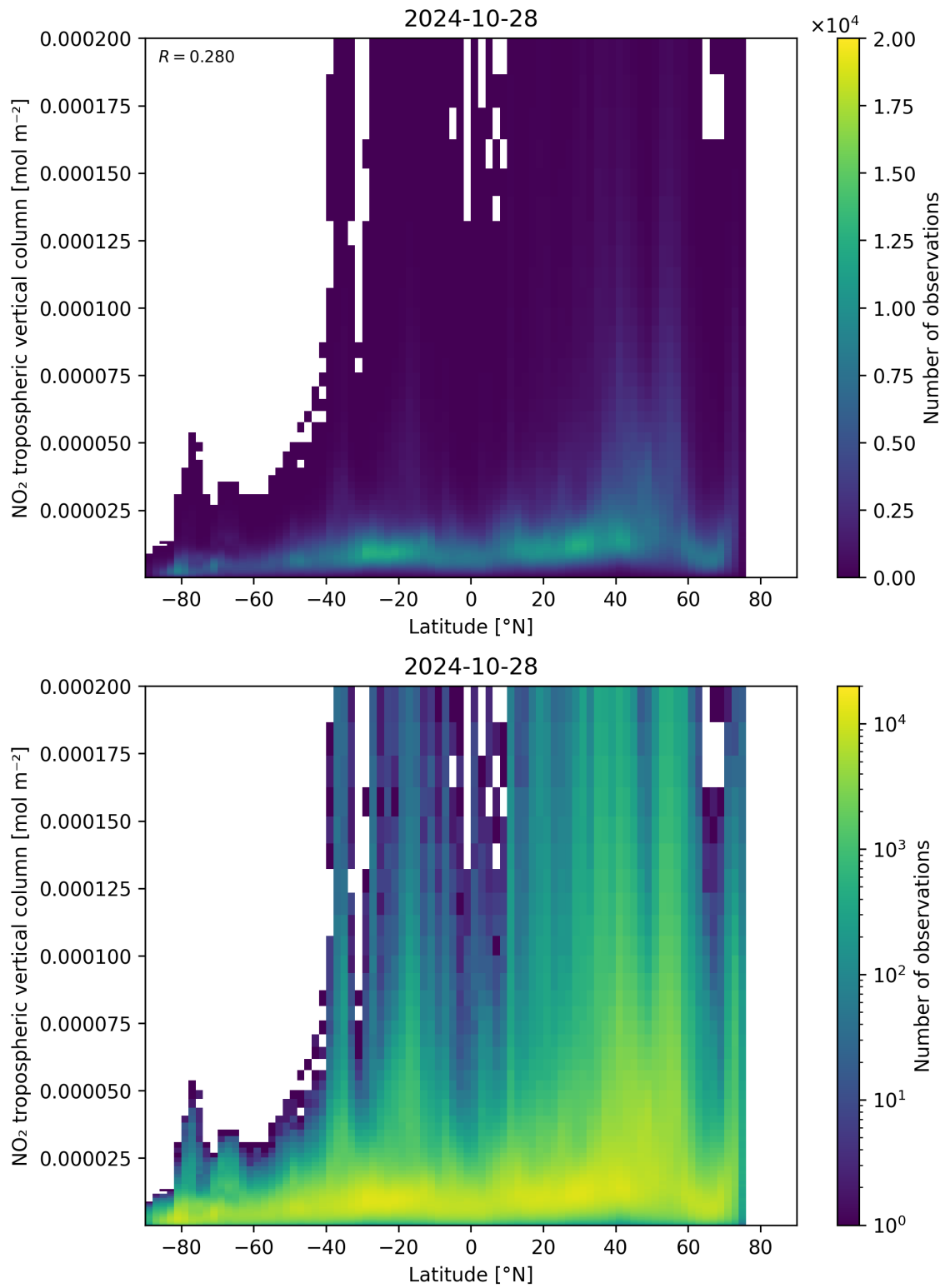
Figure 92: Scatter density plot of “Latitude” against “NO 2 tropospheric vertical column” for 2024-10-27 to 2024-10-29.
