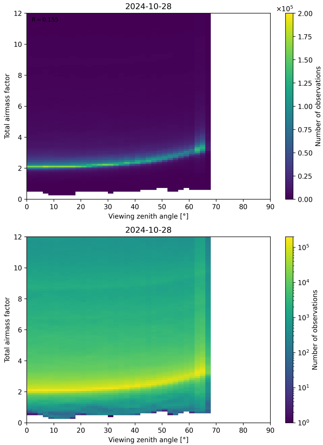
Figure 160: Scatter density plot of “Viewing zenith angle” against “Total airmass factor” for 2024-10-27 to 2024-10-29.
