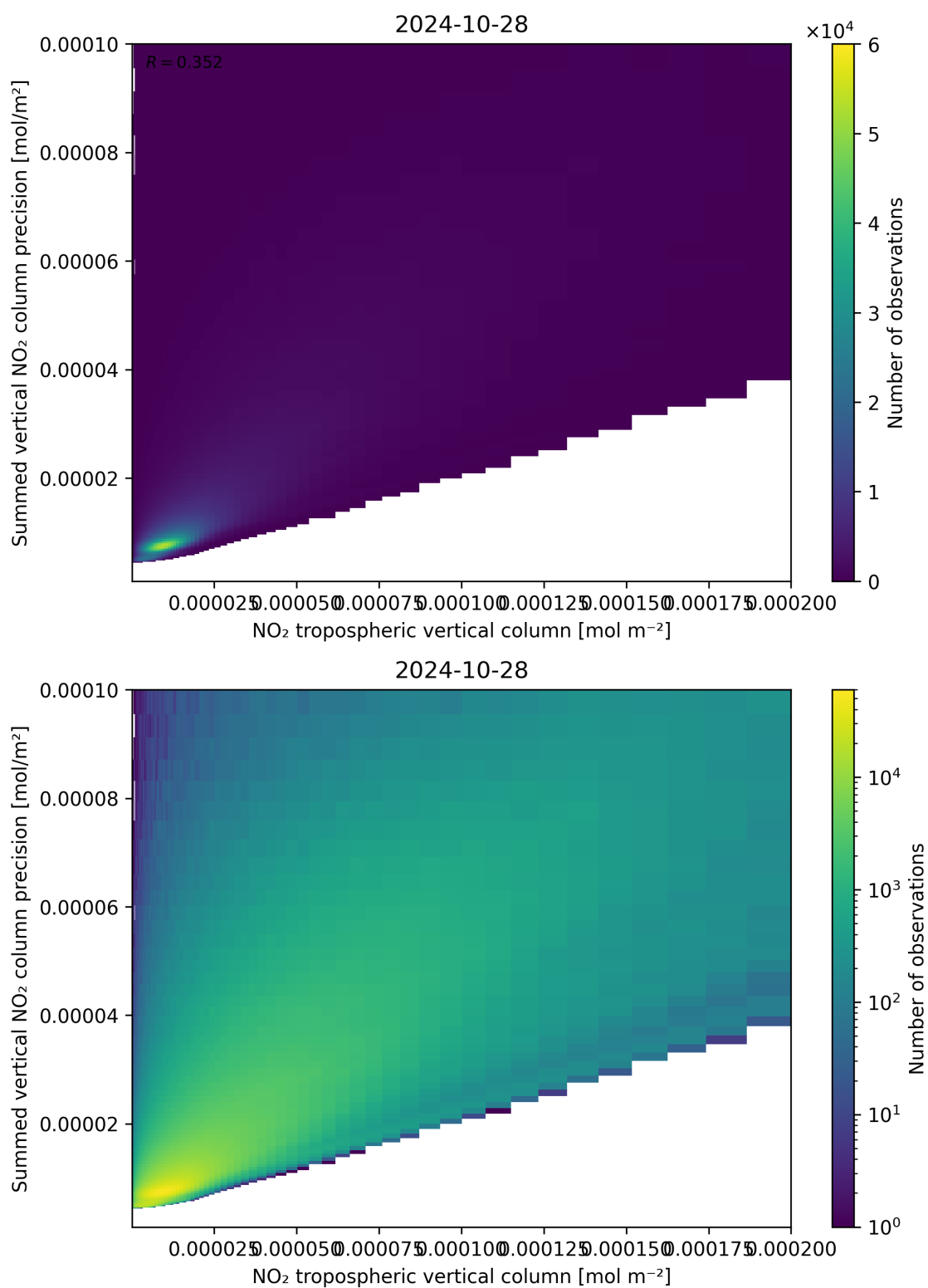
Figure 127: Scatter density plot of “NO 2 tropospheric vertical column” against “Summed vertical NO 2 column precision” for 2024-10-27 to 2024-10-29.
