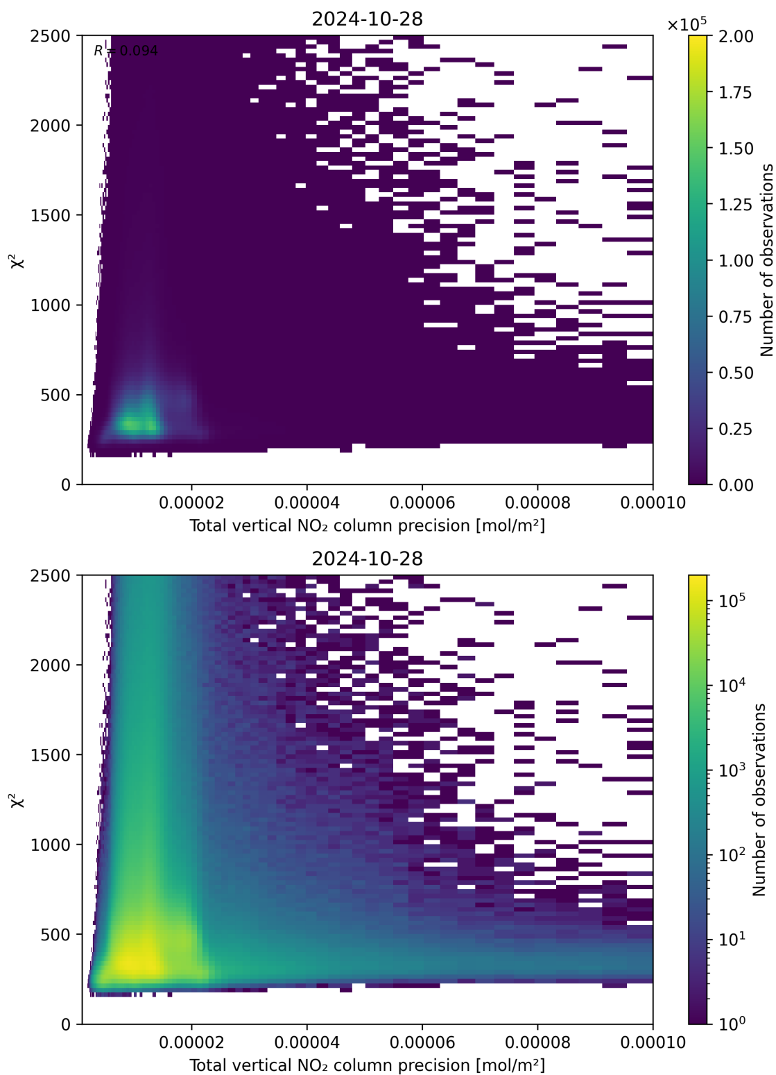
Figure 116: Scatter density plot of “Total vertical NO 2 column precision” against “ \chi^2 ” for 2024-10-27 to 2024-10-29.
