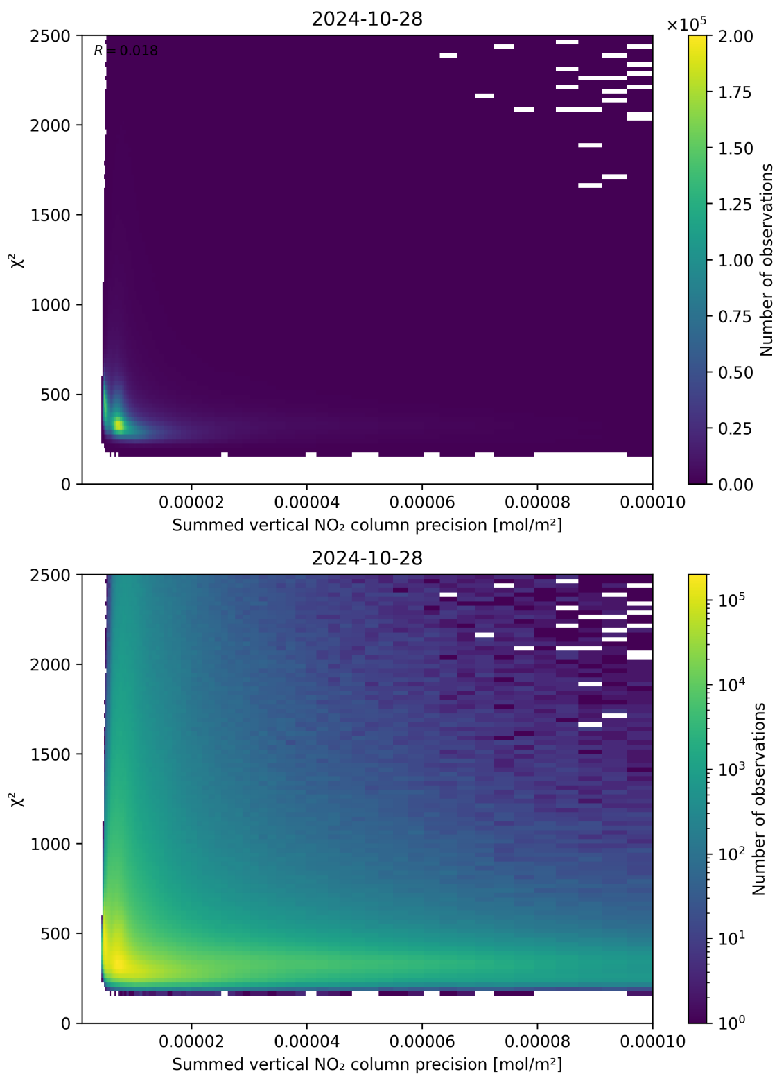
Figure 107: Scatter density plot of “Summed vertical NO 2 column precision” against “ \chi^2 ” for 2024-10-27 to 2024-10-29.
