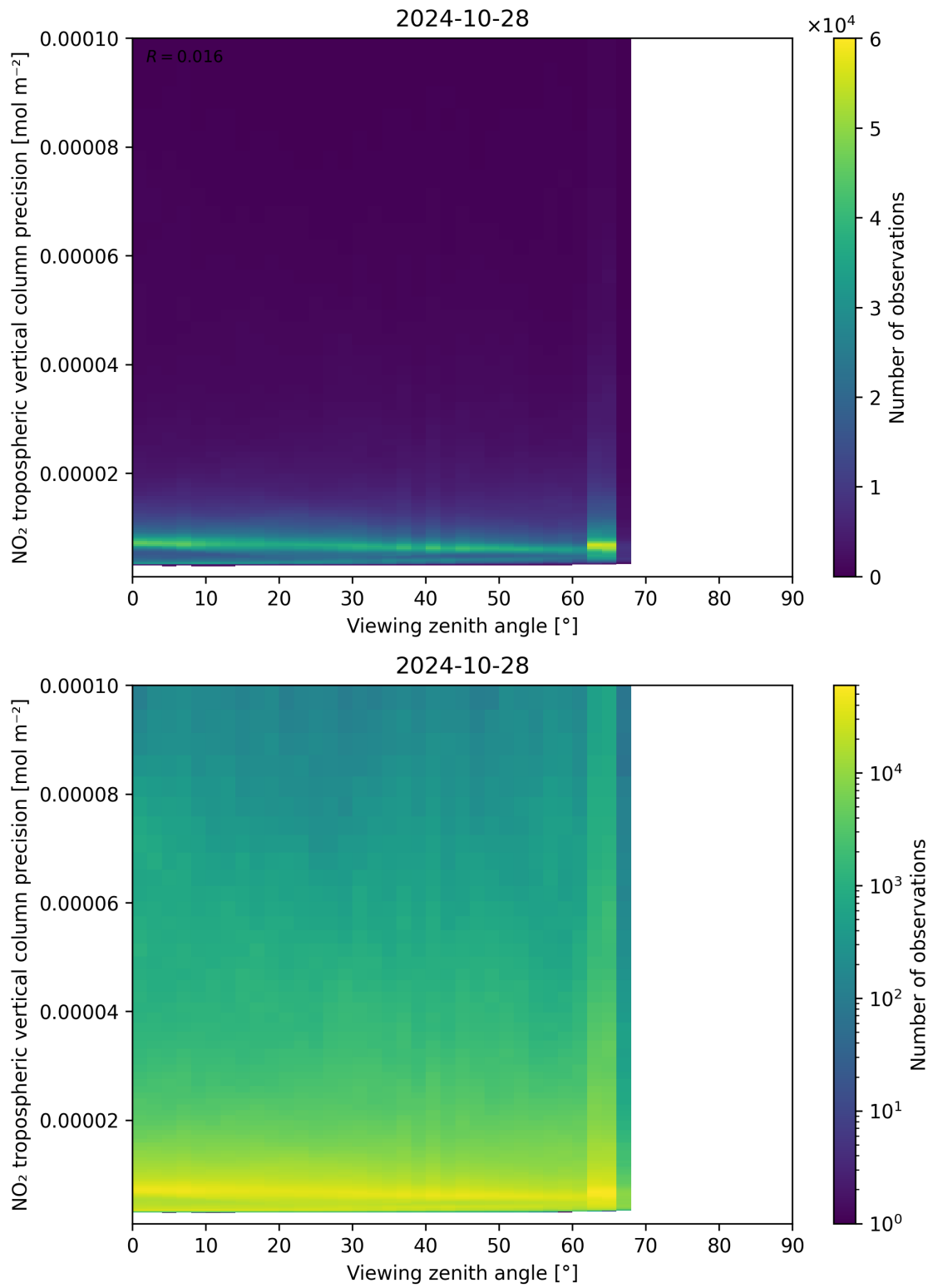
Figure 170: Scatter density plot of “Viewing zenith angle” against “NO 2 tropospheric vertical column precision” for 2024-10-27 to 2024-10-29.
