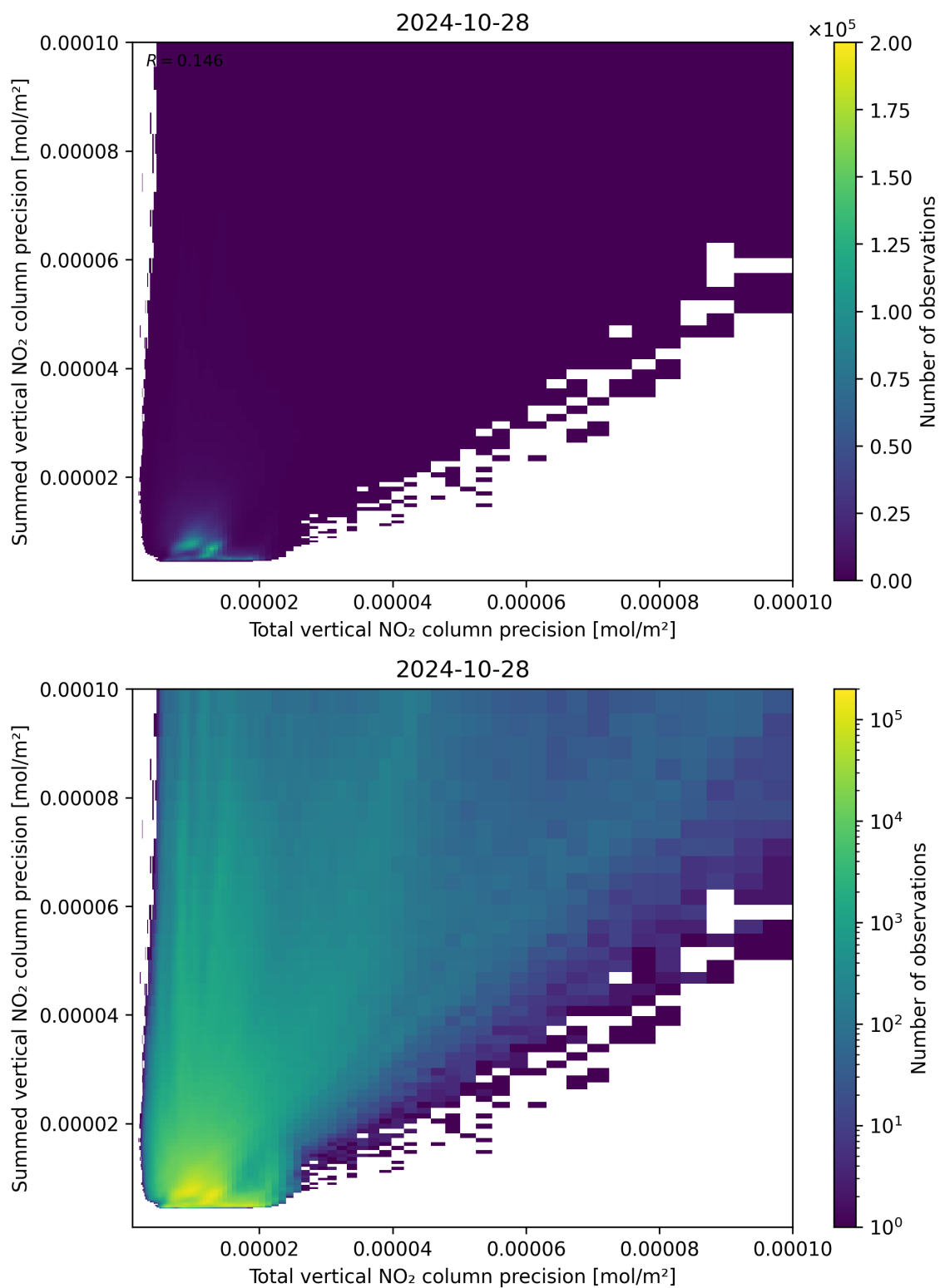
Figure 118: Scatter density plot of “Total vertical NO 2 column precision” against “Summed vertical NO 2 column precision” for 2024-10-27 to 2024-10-29.
