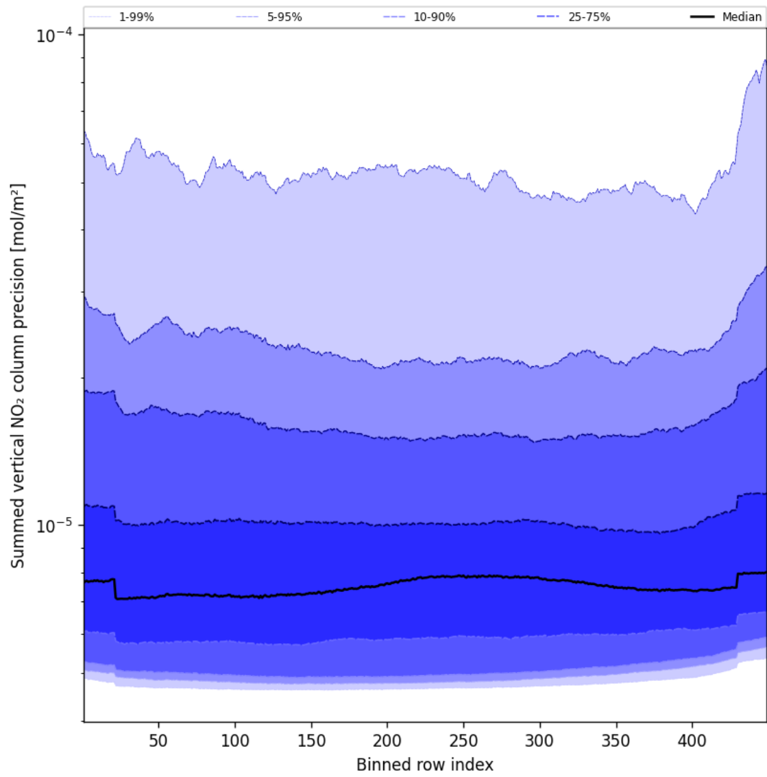
Figure 58: Along track statistics of “Summed vertical NO 2 column precision” for 2024-10-27 to 2024-10-29
