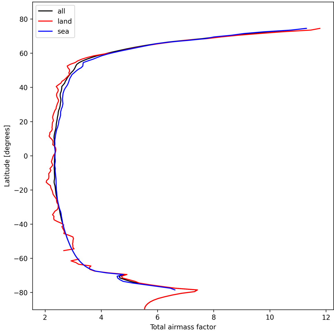
Figure 15: Zonal average of “Total airmass factor” for 2024-10-27 to 2024-10-29.
