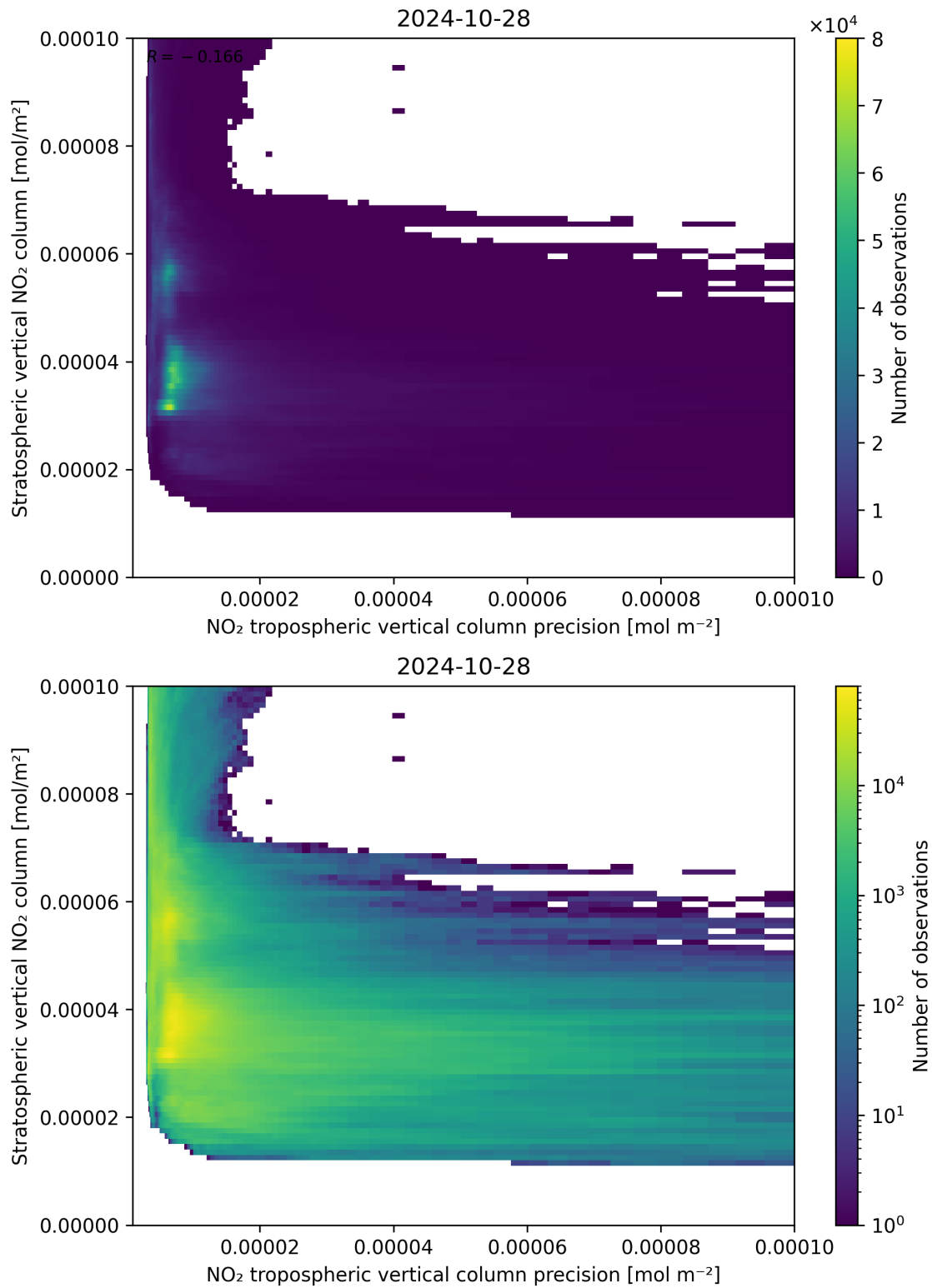
Figure 135: Scatter density plot of “NO 2 tropospheric vertical column precision” against “Stratospheric vertical NO 2 column” for 2024-10-27 to 2024-10-29.
