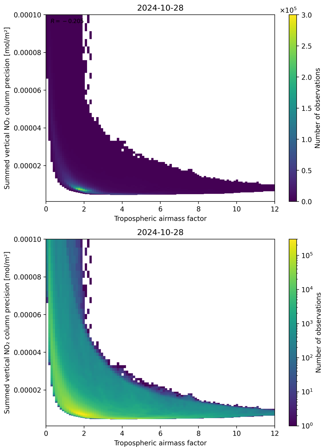
Figure 76: Scatter density plot of “Tropospheric airmass factor” against “Summed vertical NO 2 column precision” for 2024-10-27 to 2024-10-29.
