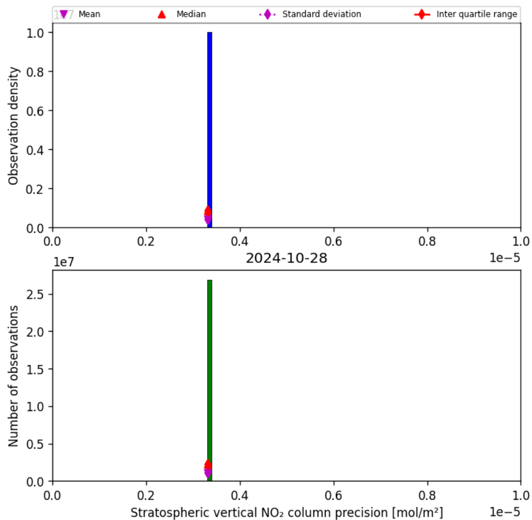
Figure 37: Histogram of “Stratospheric vertical NO 2 column precision” for 2024-10-27 to 2024-10-29
