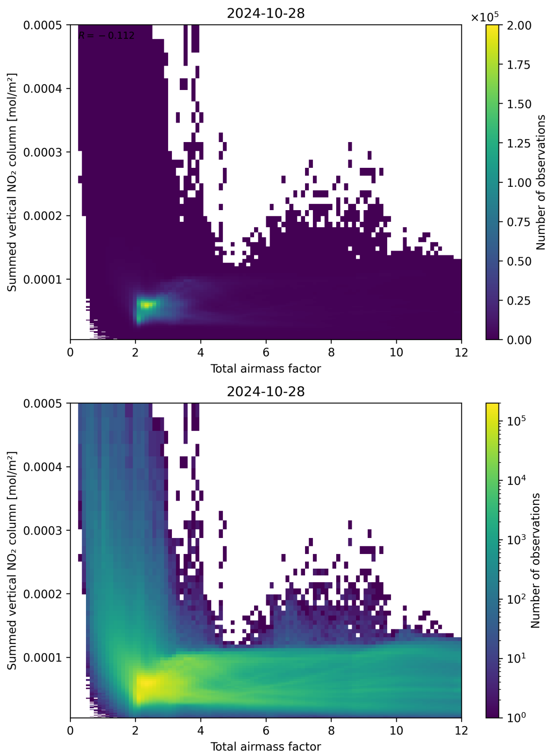
Figure 65: Scatter density plot of “Total airmass factor” against “Summed vertical NO 2 column” for 2024-10-27 to 2024-10-29.
