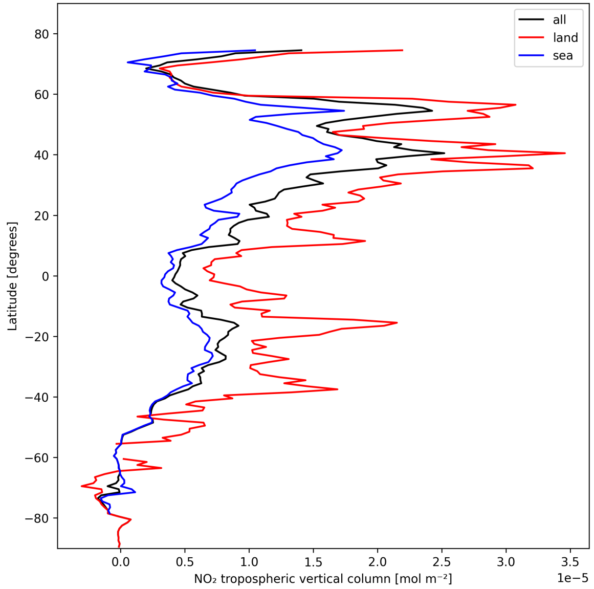
Figure 12: Zonal average of “NO 2 tropospheric vertical column” for 2024-10-27 to 2024-10-29.
