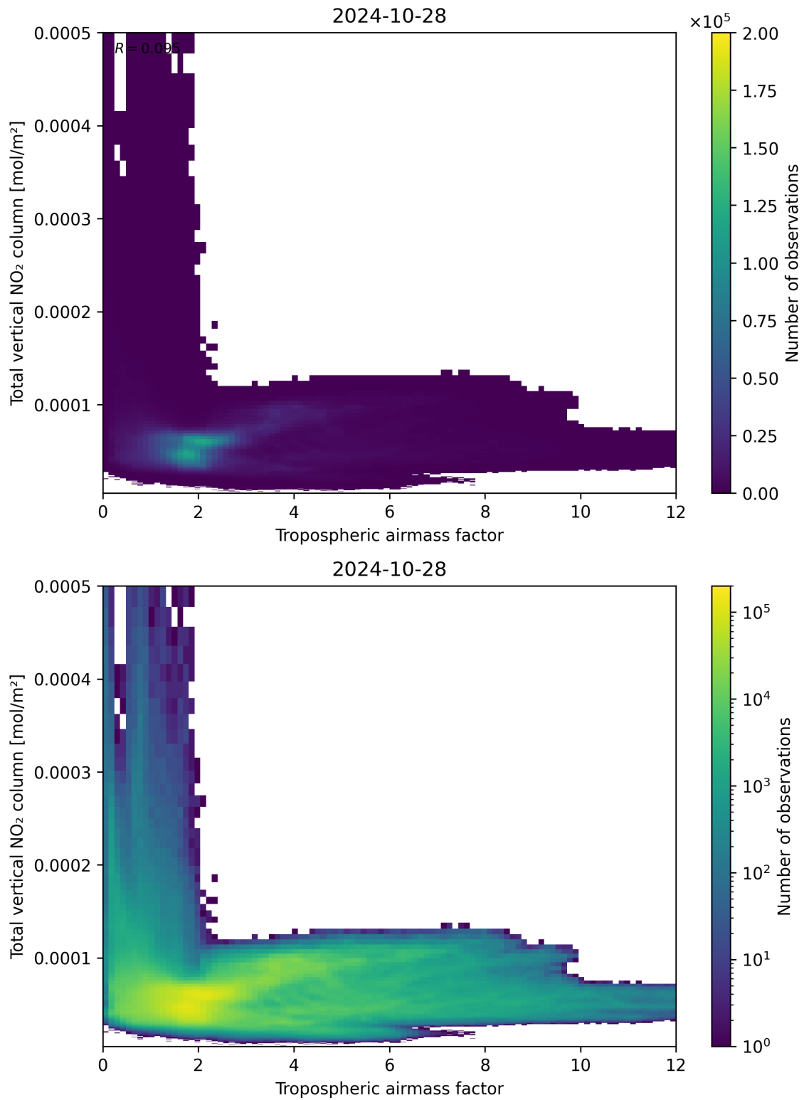
Figure 77: Scatter density plot of “Tropospheric airmass factor” against “Total vertical NO 2 column” for 2024-10-27 to 2024-10-29.
