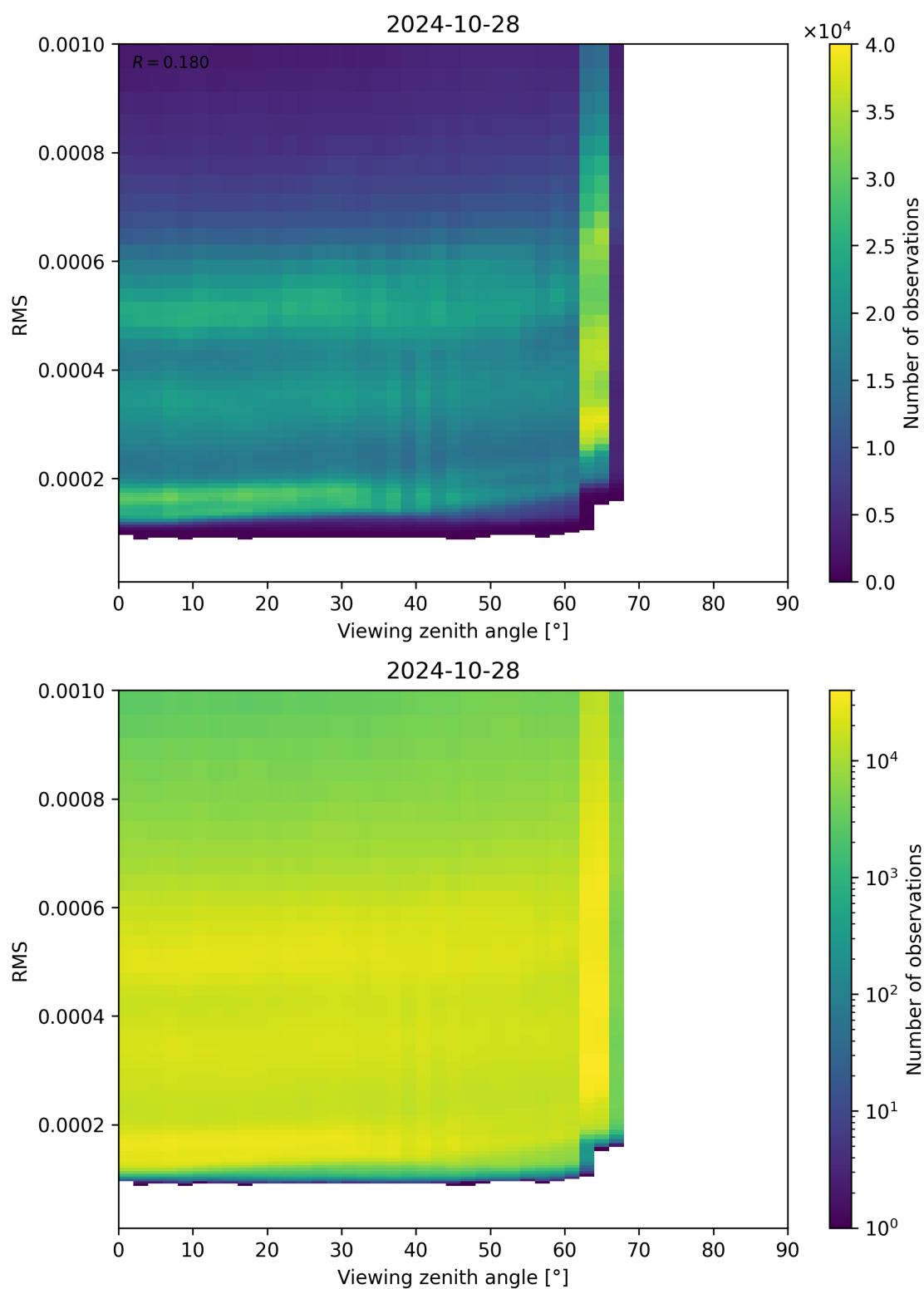
Figure 171: Scatter density plot of “Viewing zenith angle” against “RMS” for 2024-10-27 to 2024-10-29.
