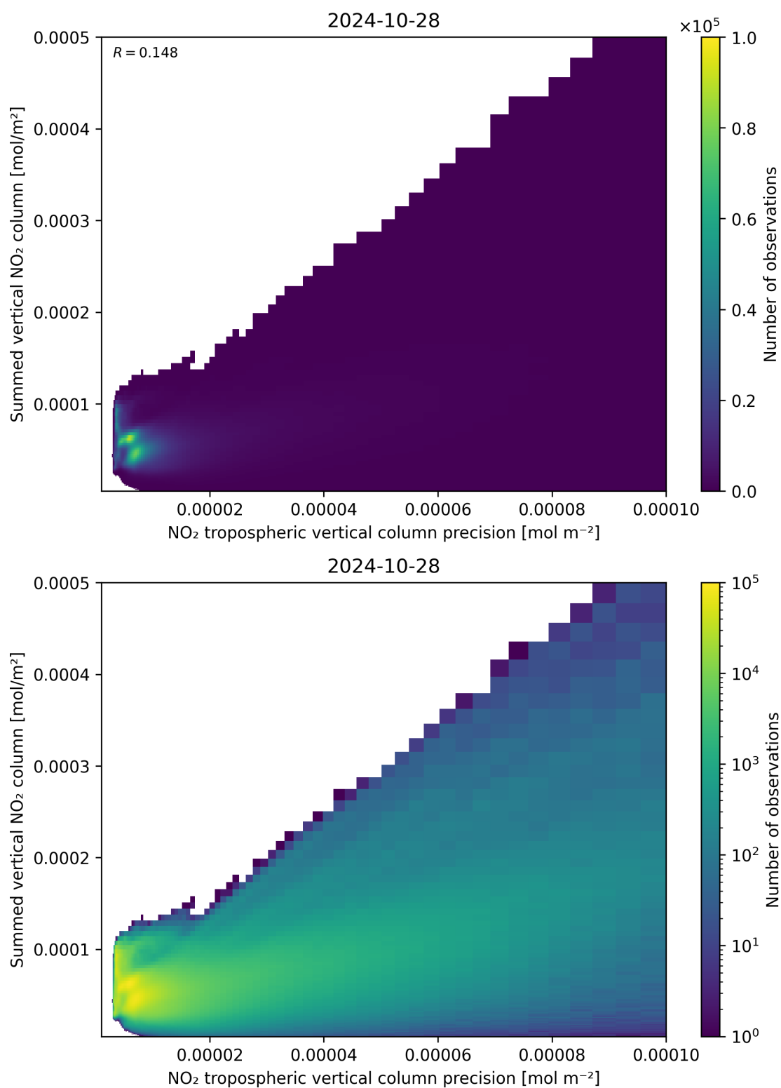
Figure 136: Scatter density plot of “NO 2 tropospheric vertical column precision” against “Summed vertical NO 2 column” for 2024-10-27 to 2024-10-29.
