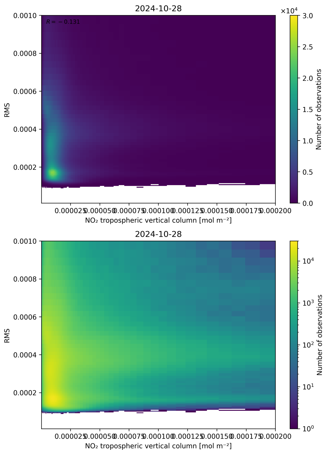
Figure 142: Scatter density plot of “NO 2 tropospheric vertical column” against “RMS” for 2024-10-27 to 2024-10-29.
