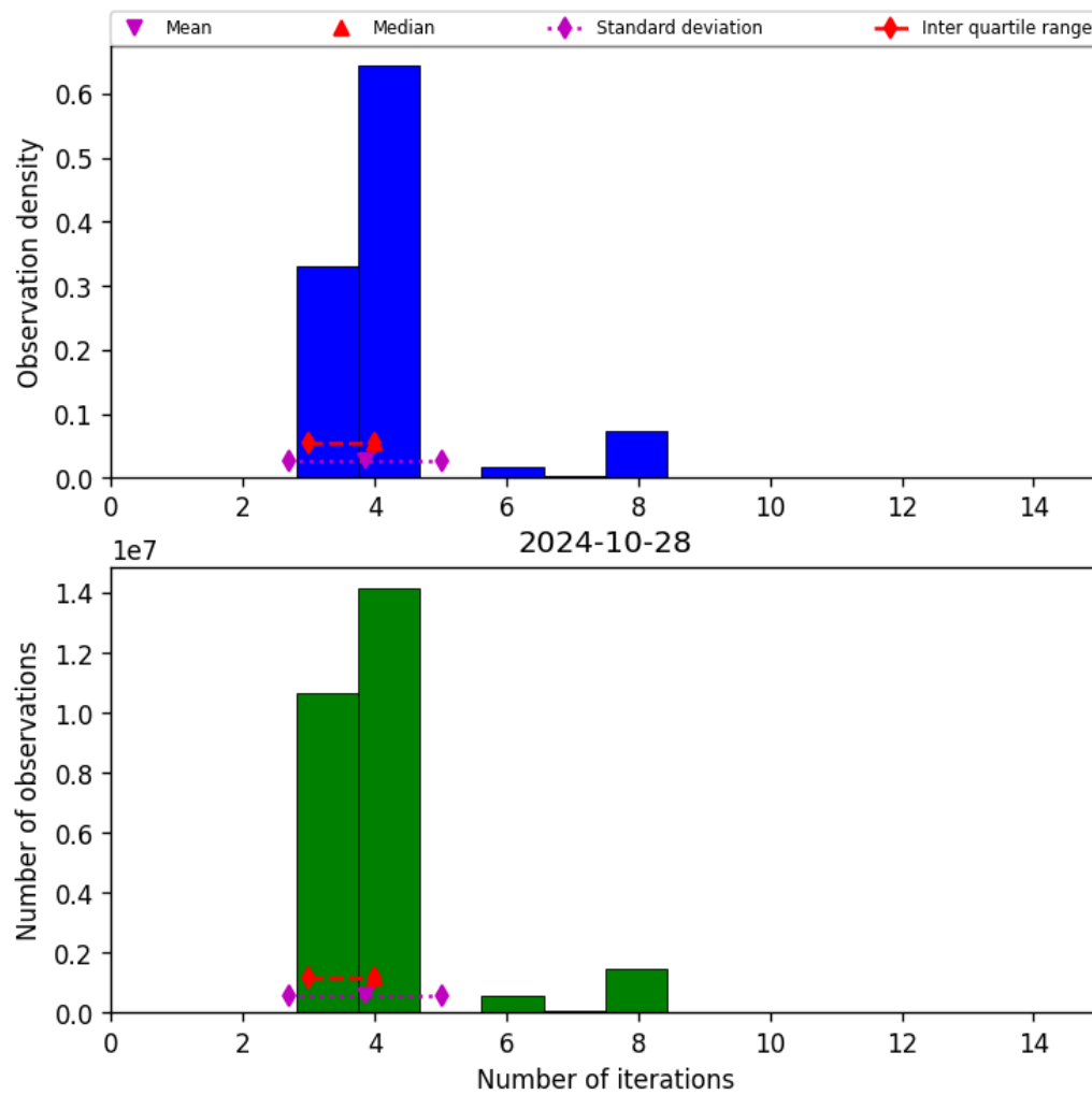
Figure 34: Histogram of “Number of iterations” for 2024-10-27 to 2024-10-29
