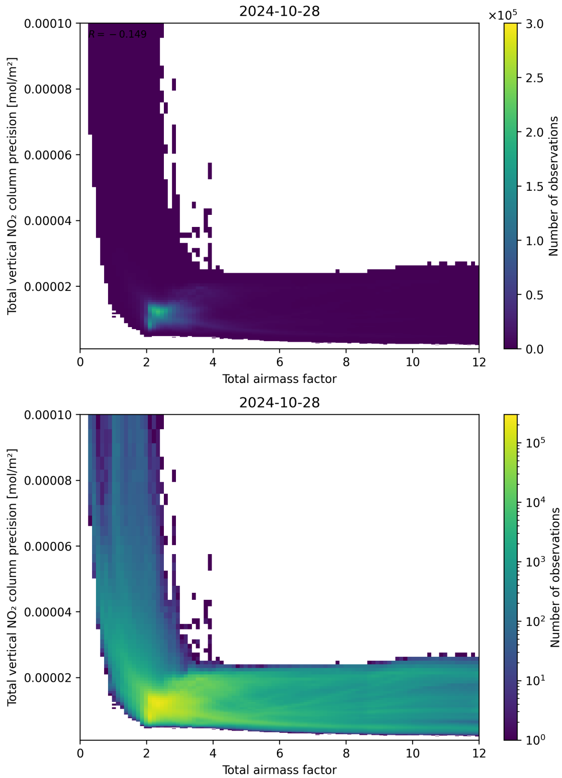
Figure 68: Scatter density plot of “Total airmass factor” against “Total vertical NO 2 column precision” for 2024-10-27 to 2024-10-29.
