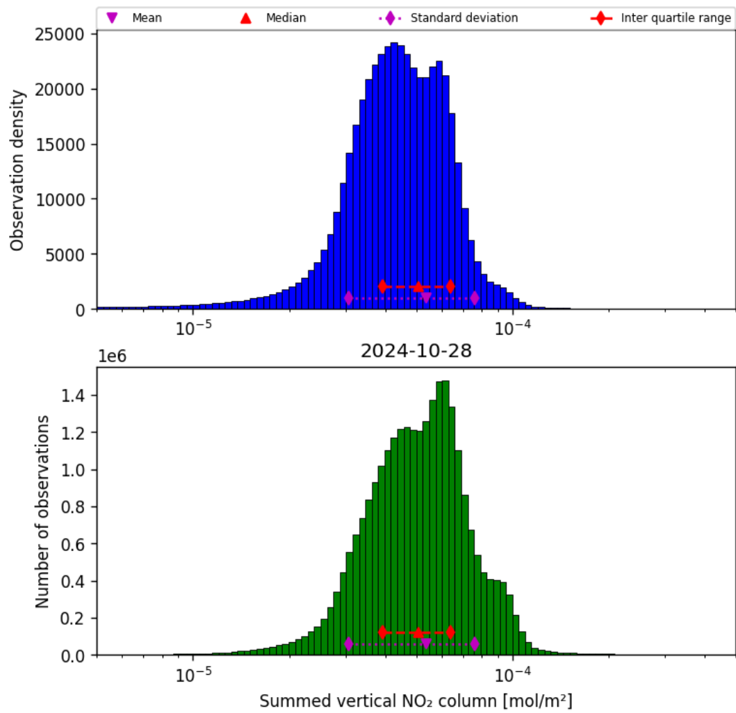
Figure 40: Histogram of “Summed vertical NO 2 column” for 2024-10-27 to 2024-10-29
