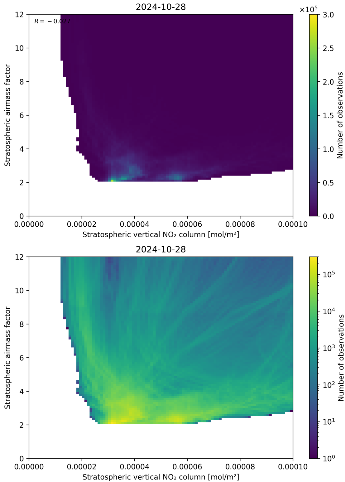
Figure 96: Scatter density plot of “Stratospheric vertical NO 2 column” against “Stratospheric airmass factor” for 2024-10-27 to 2024-10-29.
