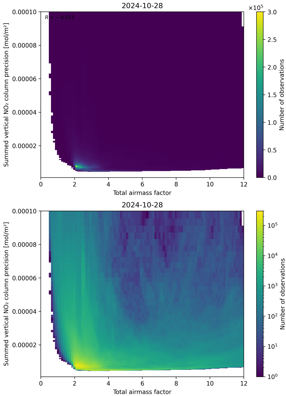
Figure 66: Scatter density plot of “Total airmass factor” against “Summed vertical NO 2 column precision” for 2024-10-27 to 2024-10-29.
