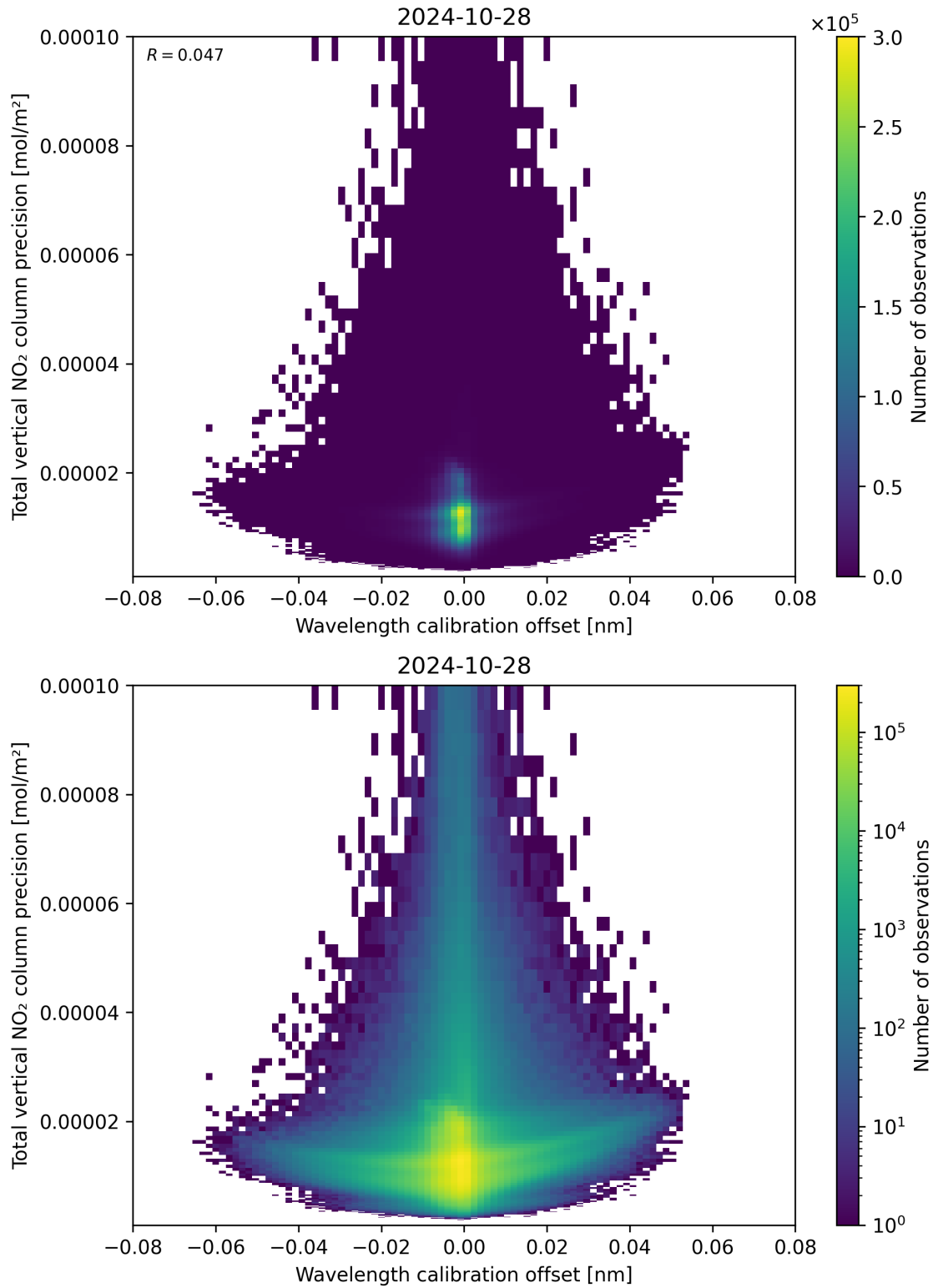
Figure 180: Scatter density plot of “Wavelength calibration offset” against “Total vertical NO 2 column precision” for 2024-10-27 to 2024-10-29.
