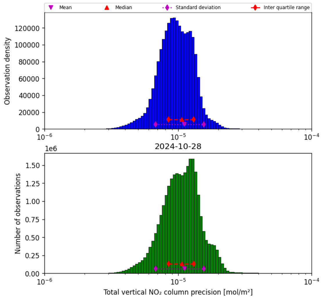
Figure 39: Histogram of “Total vertical NO 2 column precision” for 2024-10-27 to 2024-10-29
