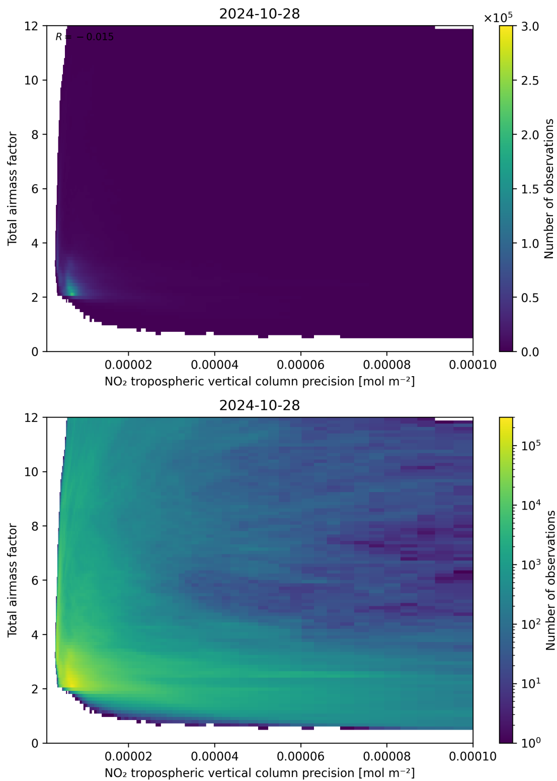
Figure 132: Scatter density plot of “NO 2 tropospheric vertical column precision” against “Total air mass factor” for 2024-10-27 to 2024-10-29.
