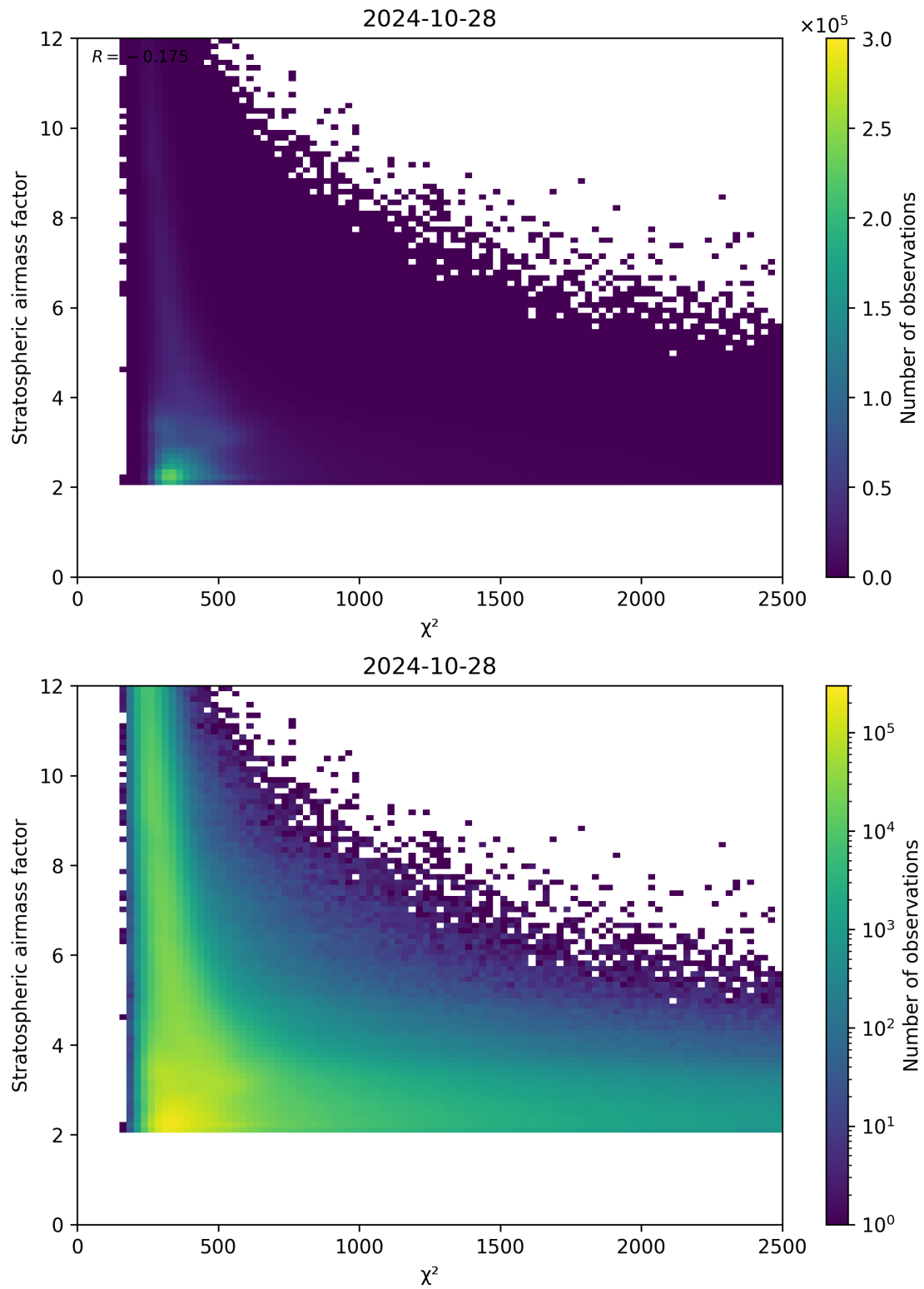
Figure 81: Scatter density plot of “ \chi^2 ” against “Stratospheric airmass factor” for 2024-10-27 to 2024-10-29.
