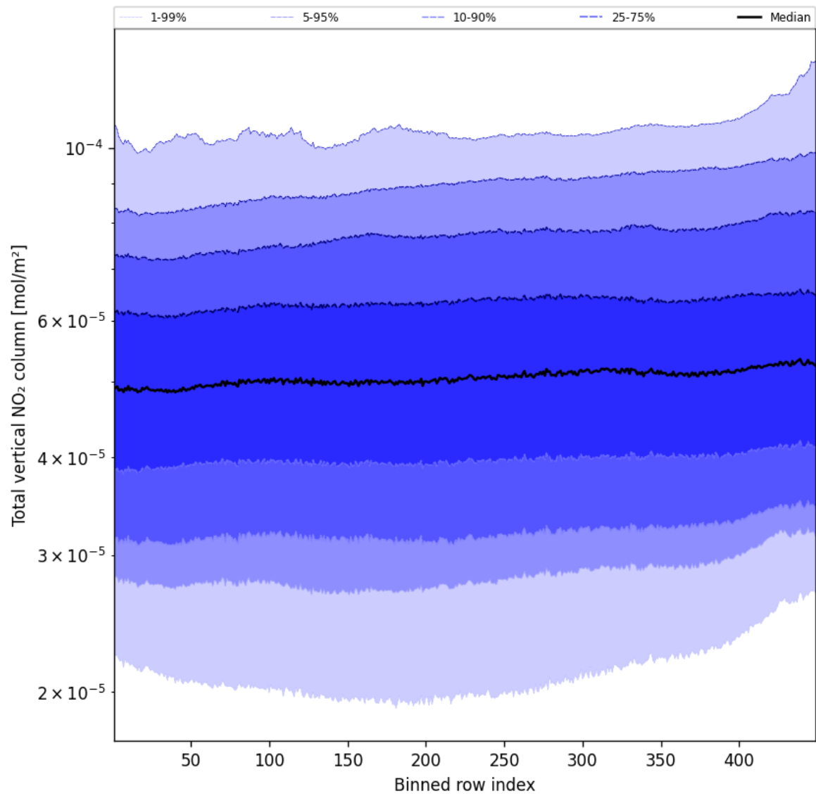
Figure 55: Along track statistics of “Total vertical NO 2 column” for 2024-10-27 to 2024-10-29
