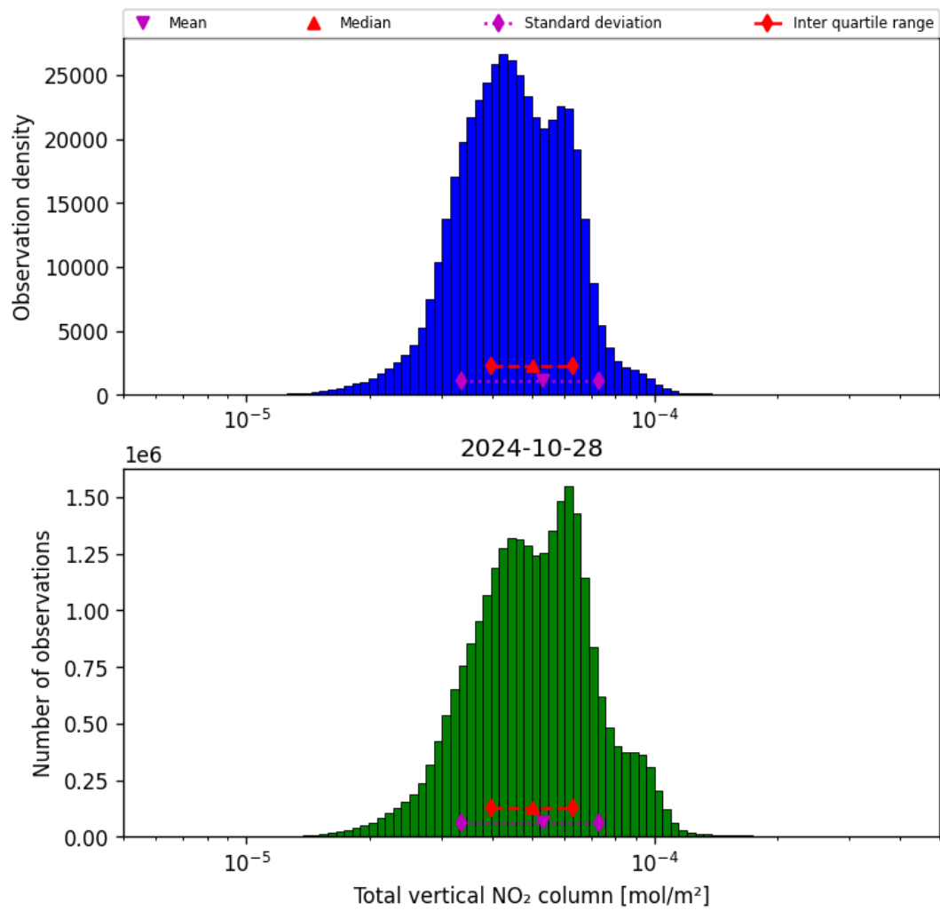
Figure 38: Histogram of “Total vertical NO 2 column” for 2024-10-27 to 2024-10-29
