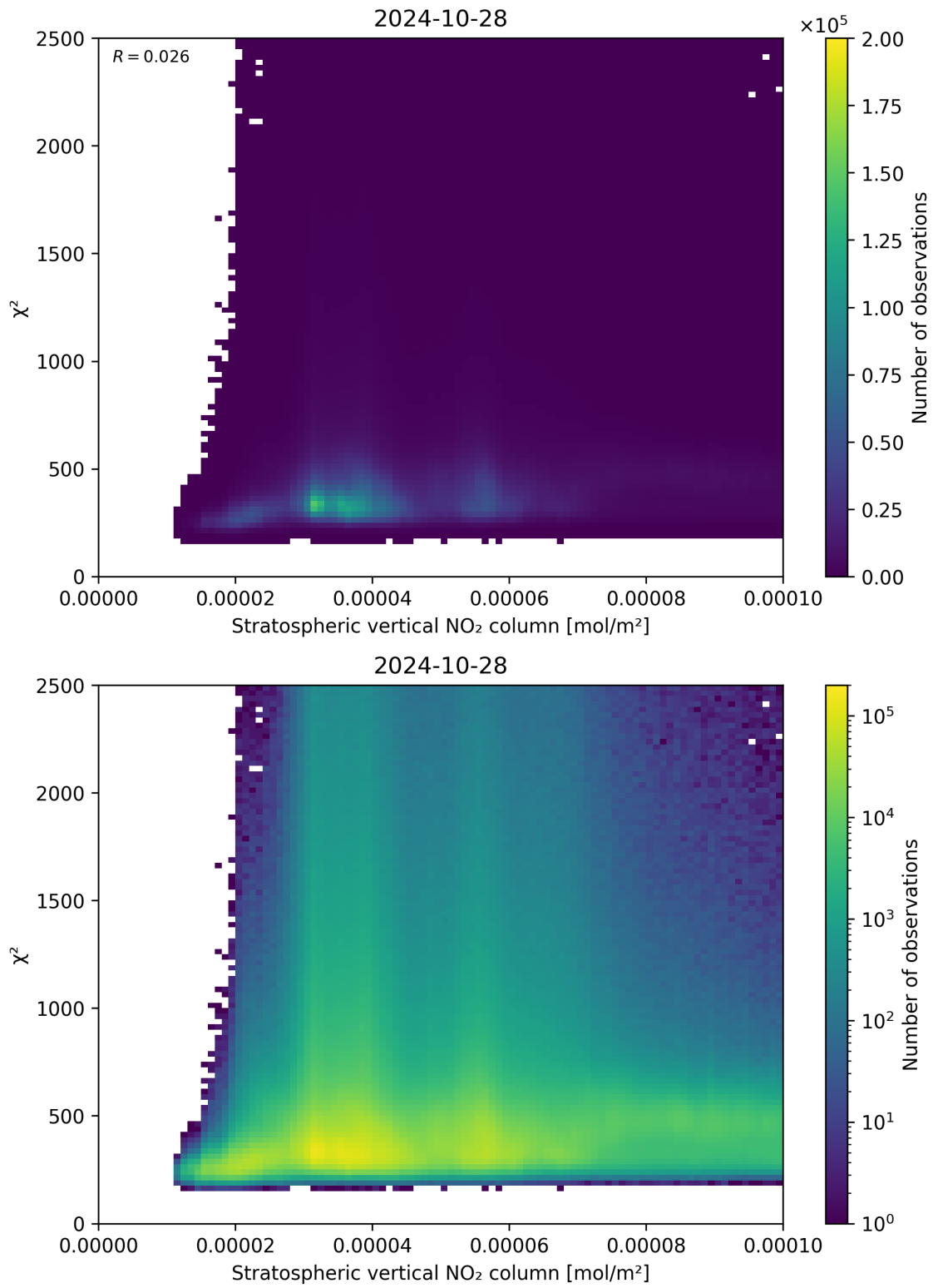
Figure 97: Scatter density plot of “Stratospheric vertical NO 2 column” against “ \chi^2 ” for 2024-10-27 to 2024-10-29.
