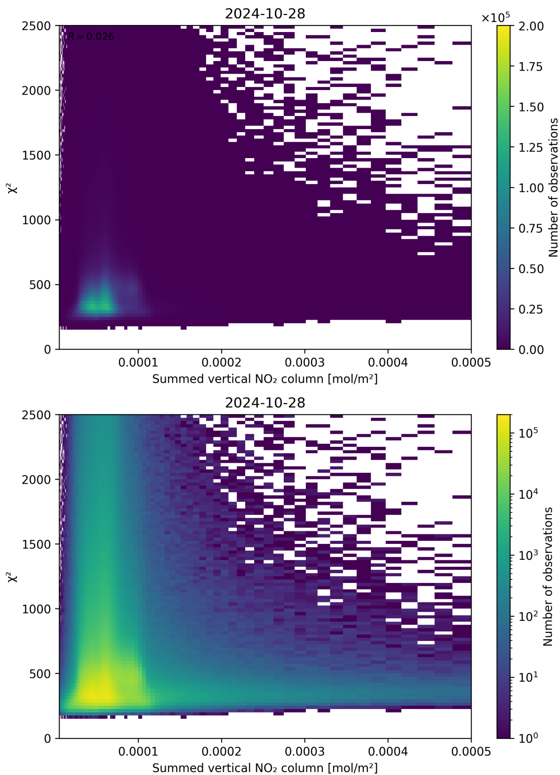
Figure 104: Scatter density plot of “Summed vertical NO 2 column” against “ \chi^2 ” for 2024-10-27 to 2024-10-29.
