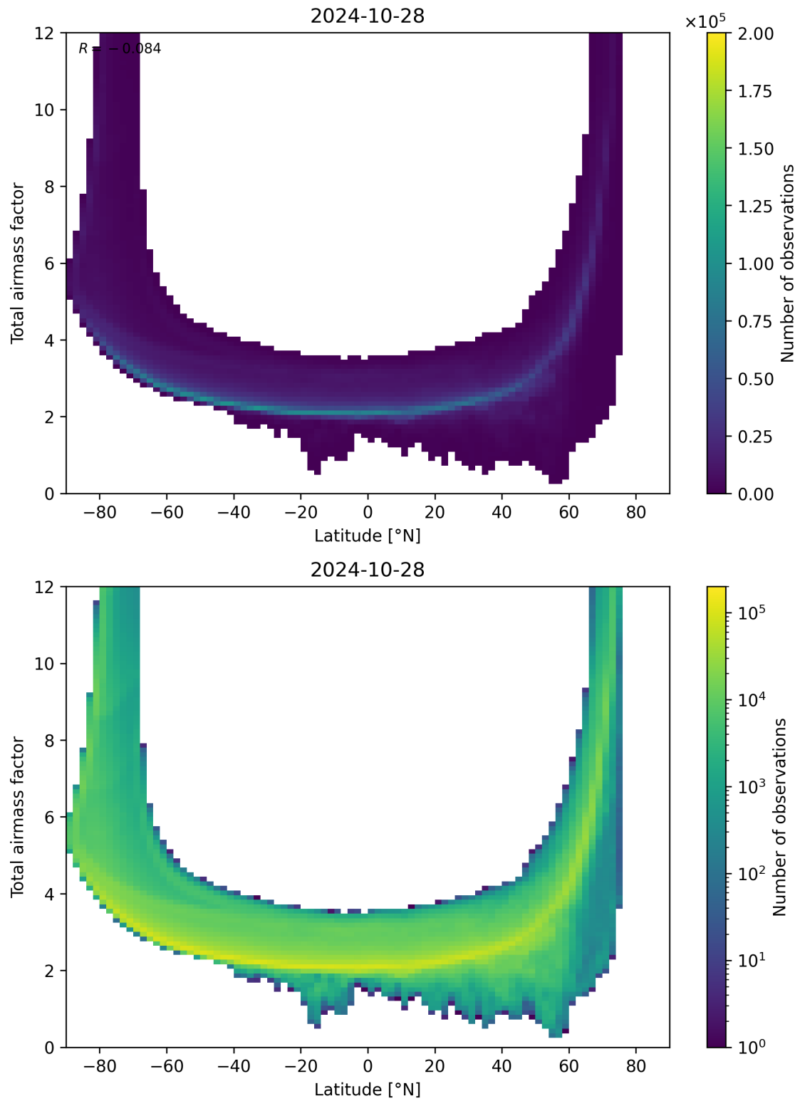
Figure 84: Scatter density plot of “Latitude” against “Total airmass factor” for 2024-10-27 to 2024-10-29.
