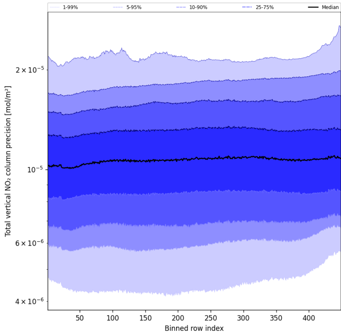
Figure 56: Along track statistics of “Total vertical NO 2 column precision” for 2024-10-27 to 2024-10-29
