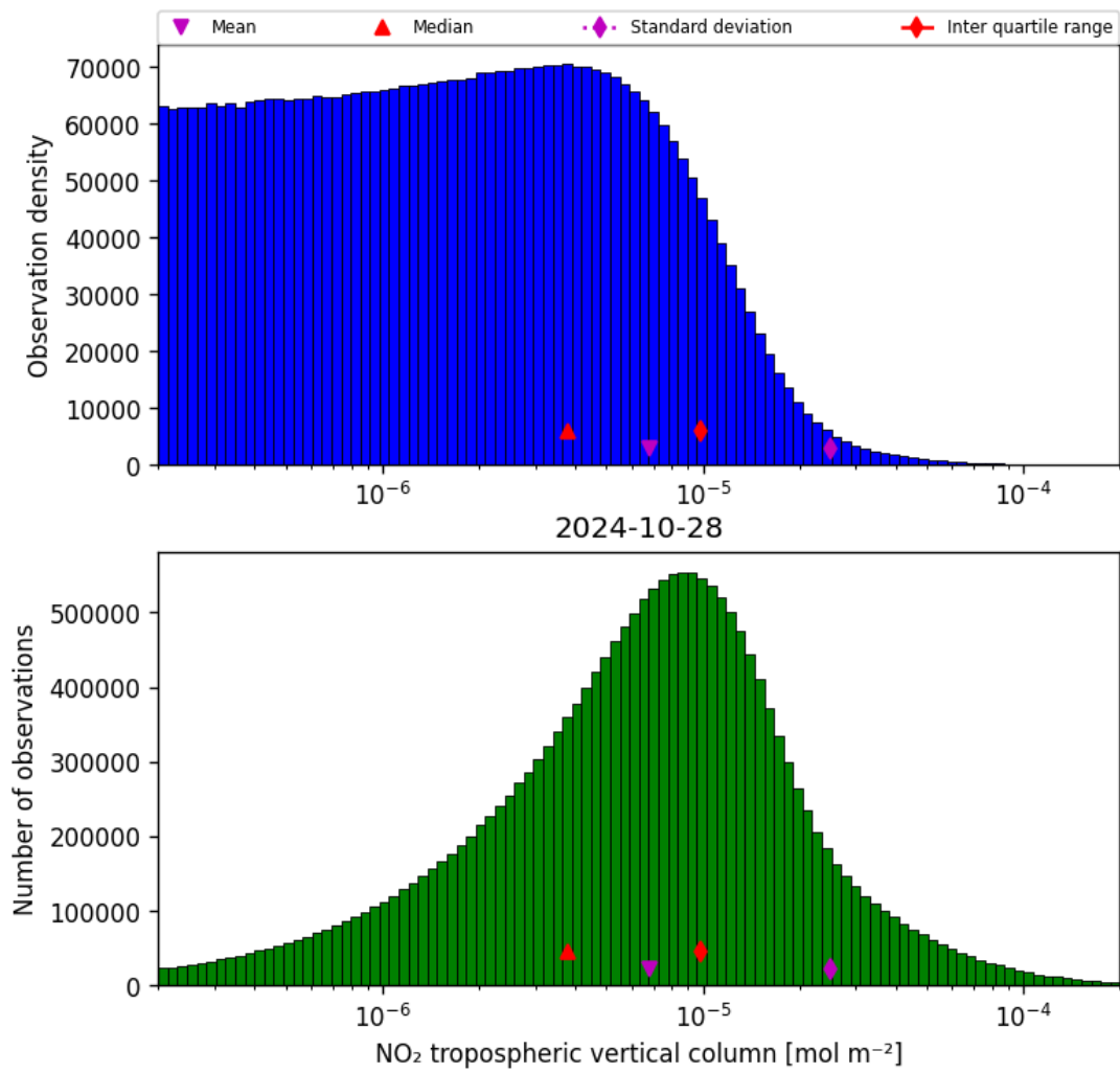
Figure 29: Histogram of “NO 2 tropospheric vertical column” for 2024-10-27 to 2024-10-29
