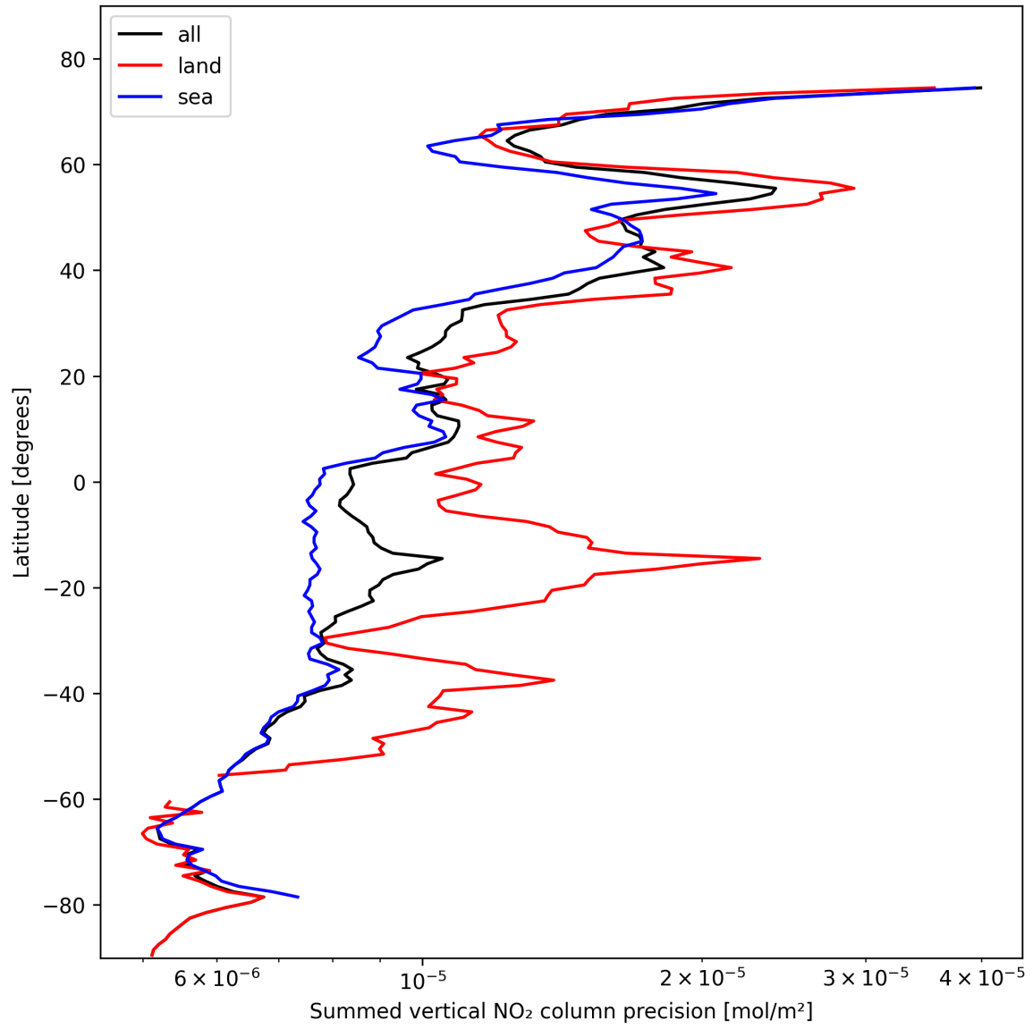
Figure 24: Zonal average of “Summed vertical NO 2 column precision” for 2024-10-27 to 2024-10-29.
