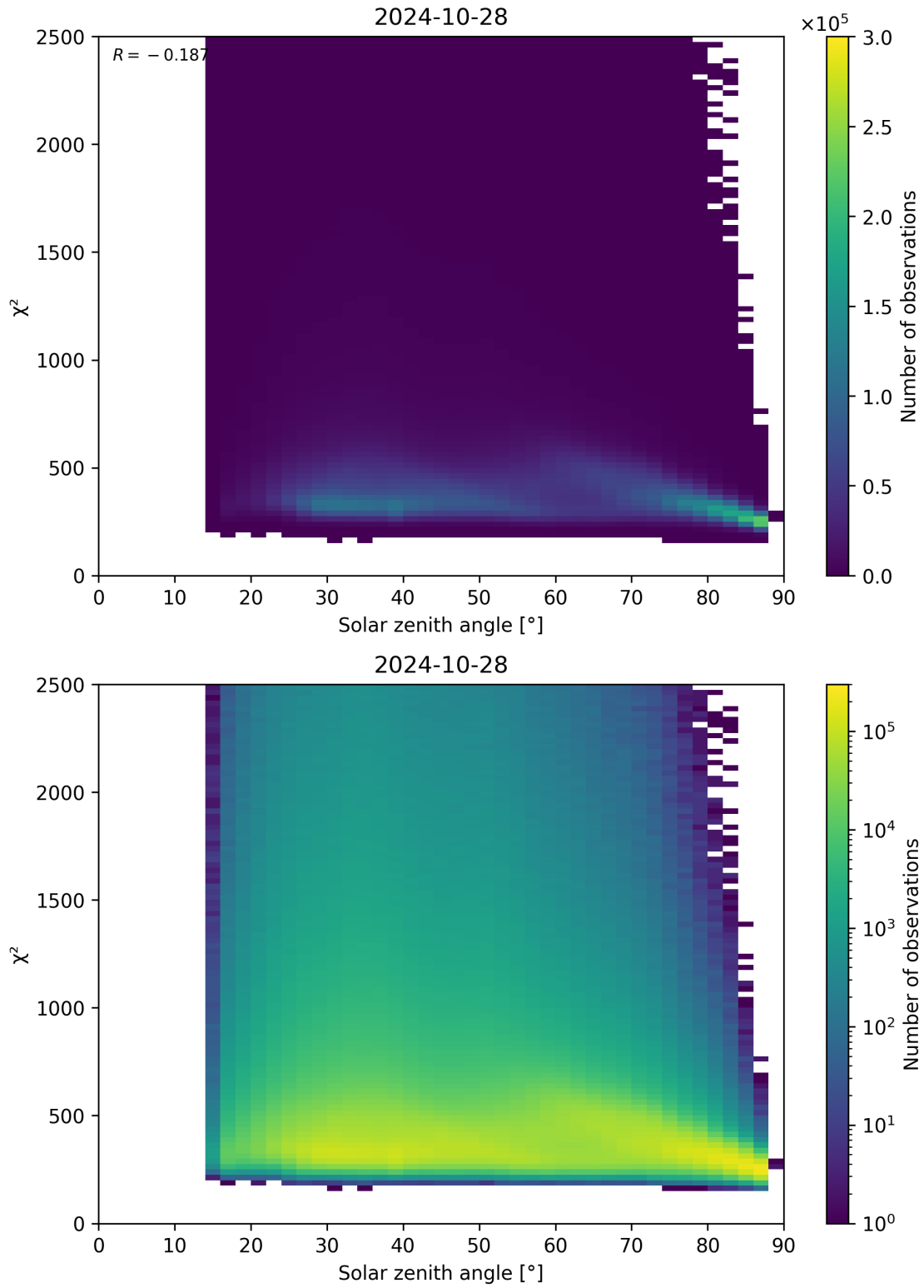
Figure 148: Scatter density plot of “Solar zenith angle” against “ \chi^2 ” for 2024-10-27 to 2024-10-29.
