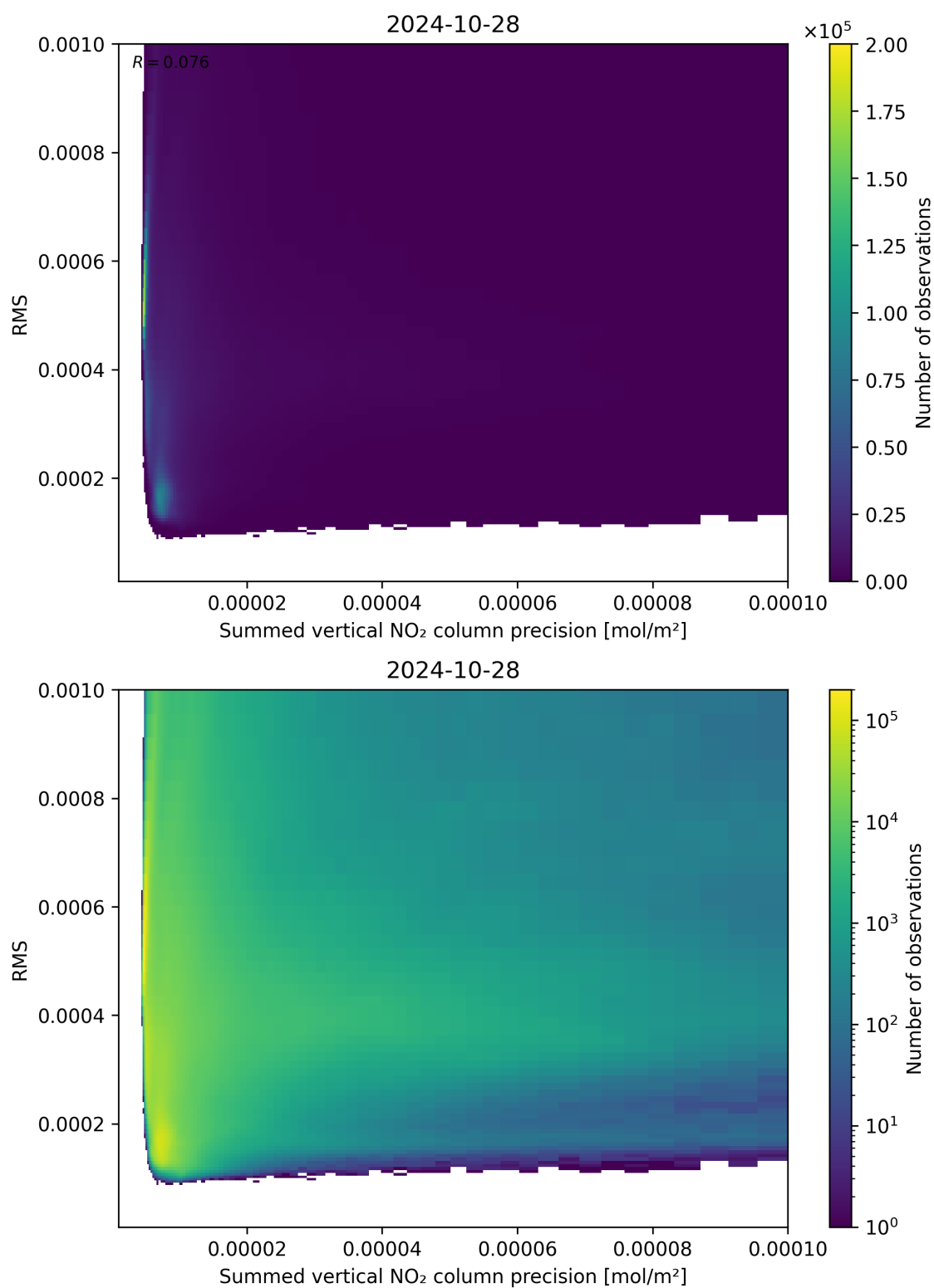
Figure 108: Scatter density plot of “Summed vertical NO 2 column precision” against “RMS” for 2024-10-27 to 2024-10-29.
