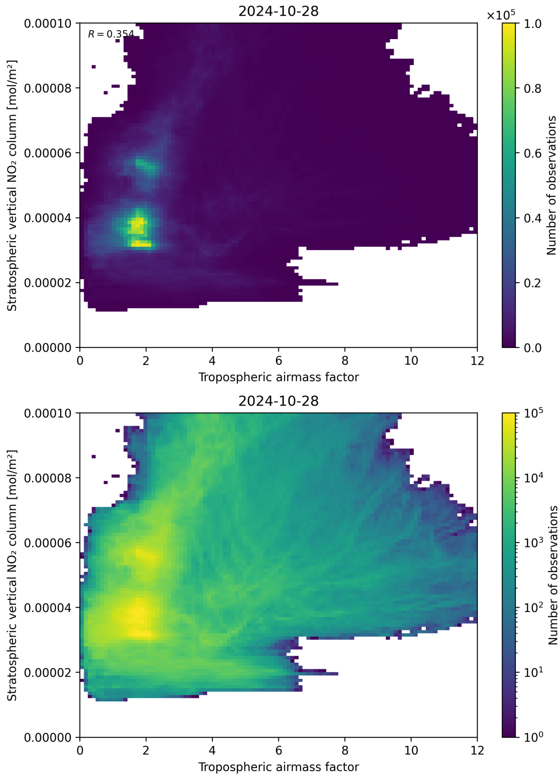
Figure 74: Scatter density plot of “Tropospheric air mass factor” against “Stratospheric vertical NO 2 column” for 2024-10-27 to 2024-10-29.
