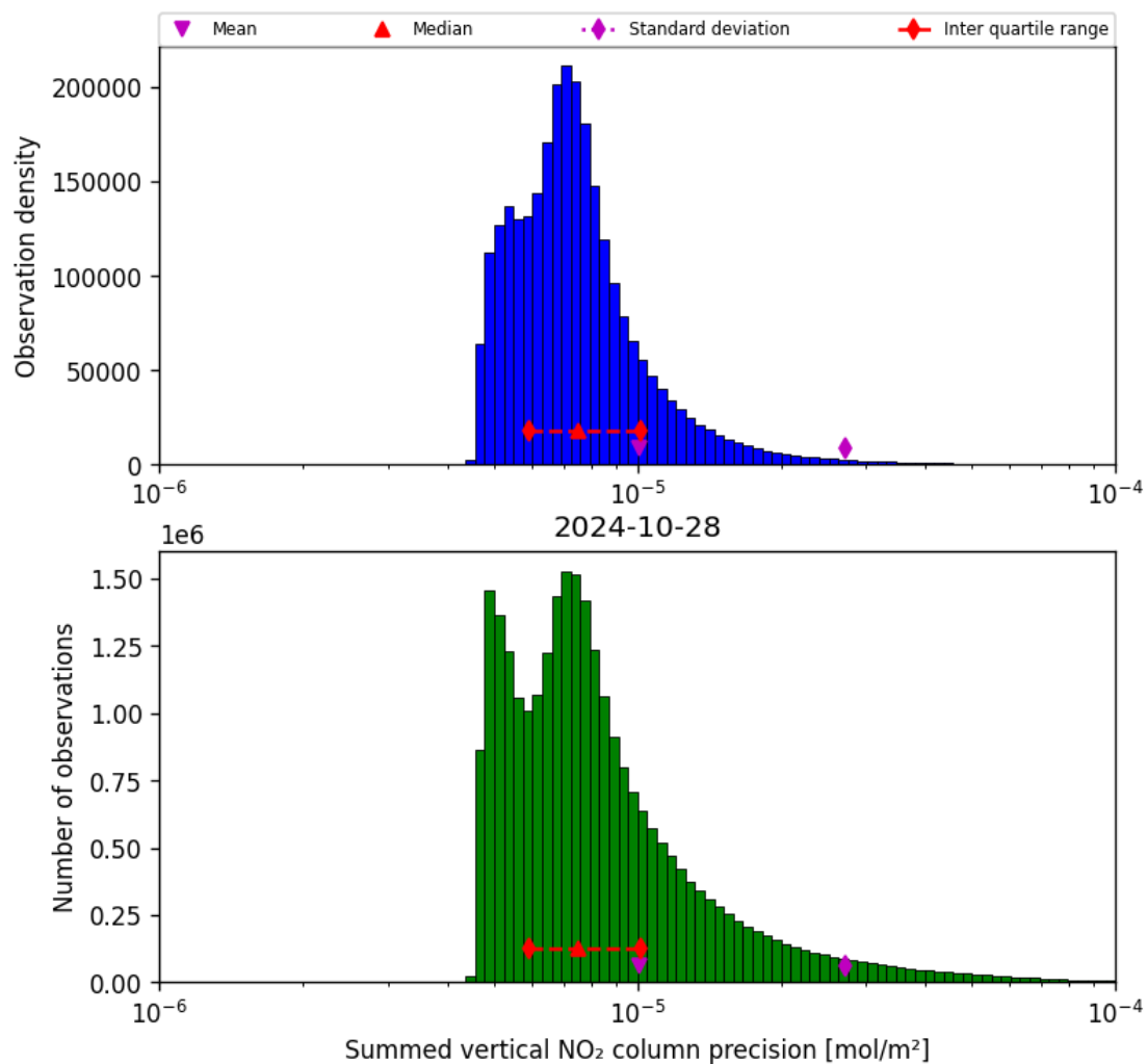
Figure 41: Histogram of "Summed vertical NO 2 column precision" for 2024-10-27 to 2024-10-29
