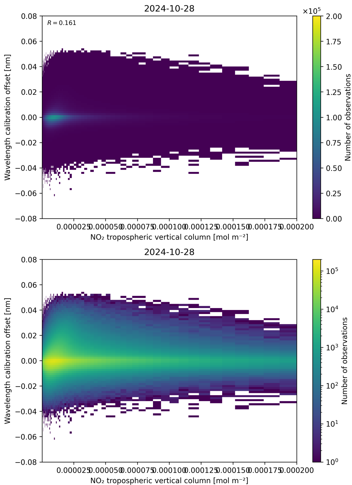
Figure 143: Scatter density plot of “NO 2 tropospheric vertical column” against “Wavelength calibration offset” for 2024-10-27 to 2024-10-29.
