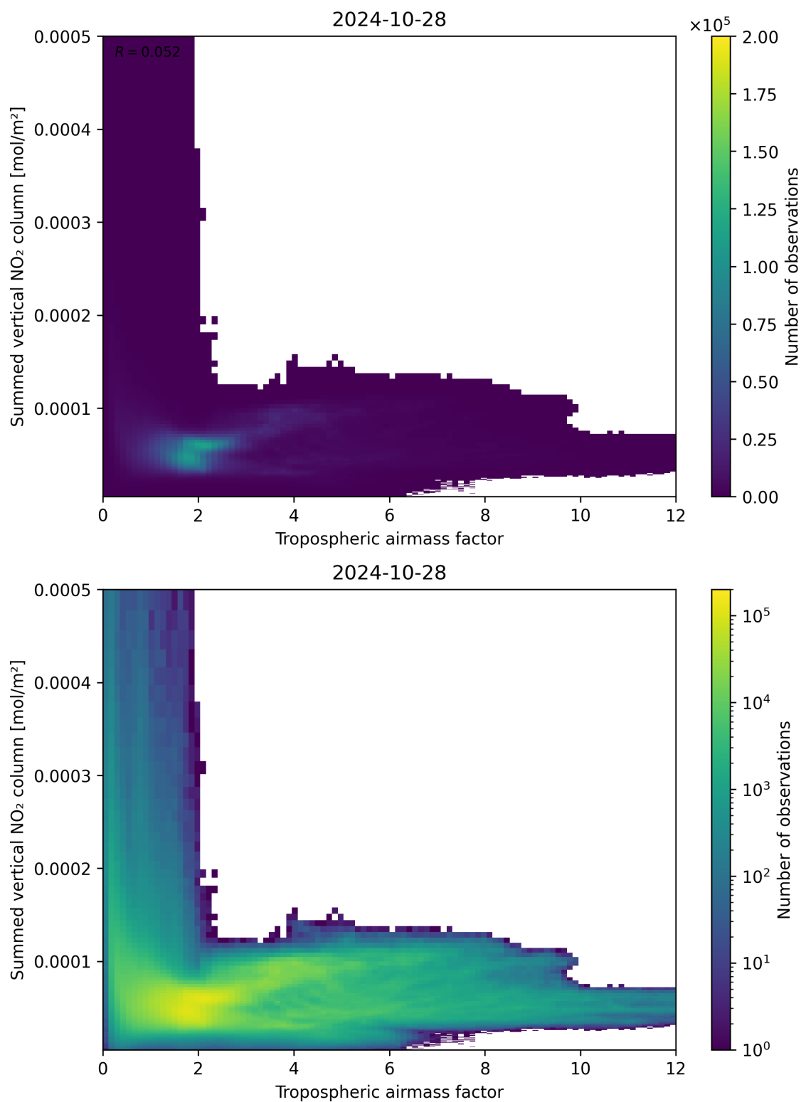
Figure 75: Scatter density plot of “Tropospheric air mass factor” against “Summed vertical NO 2 column” for 2024-10-27 to 2024-10-29.
