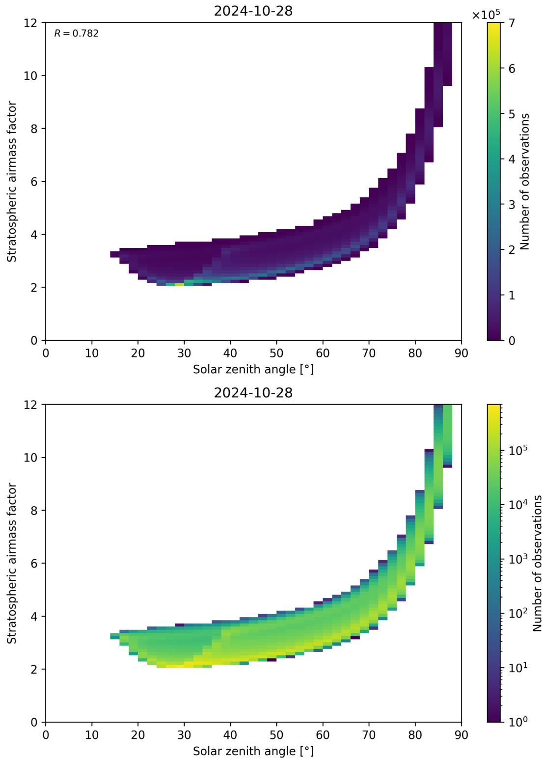
Figure 145: Scatter density plot of “Solar zenith angle” against “Stratospheric airmass factor” for 2024-10-27 to 2024-10-29.
