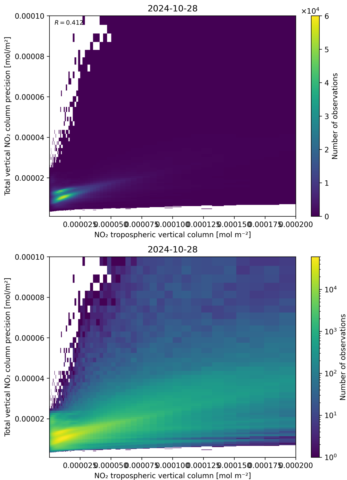
Figure 129: Scatter density plot of “NO 2 tropospheric vertical column” against “Total vertical NO 2 column precision” for 2024-10-27 to 2024-10-29.
