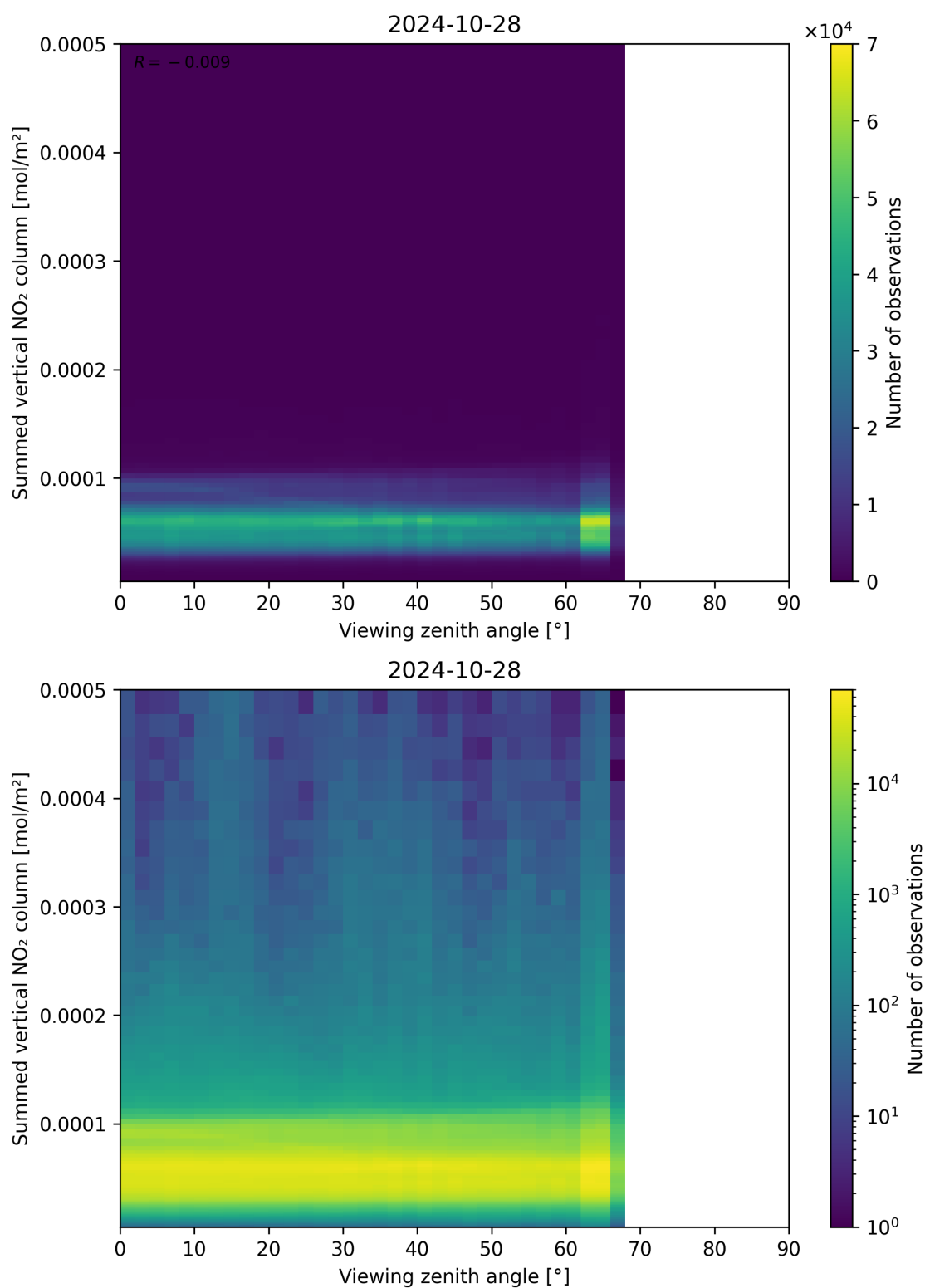
Figure 165: Scatter density plot of “Viewing zenith angle” against “Summed vertical NO 2 column” for 2024-10-27 to 2024-10-29.
