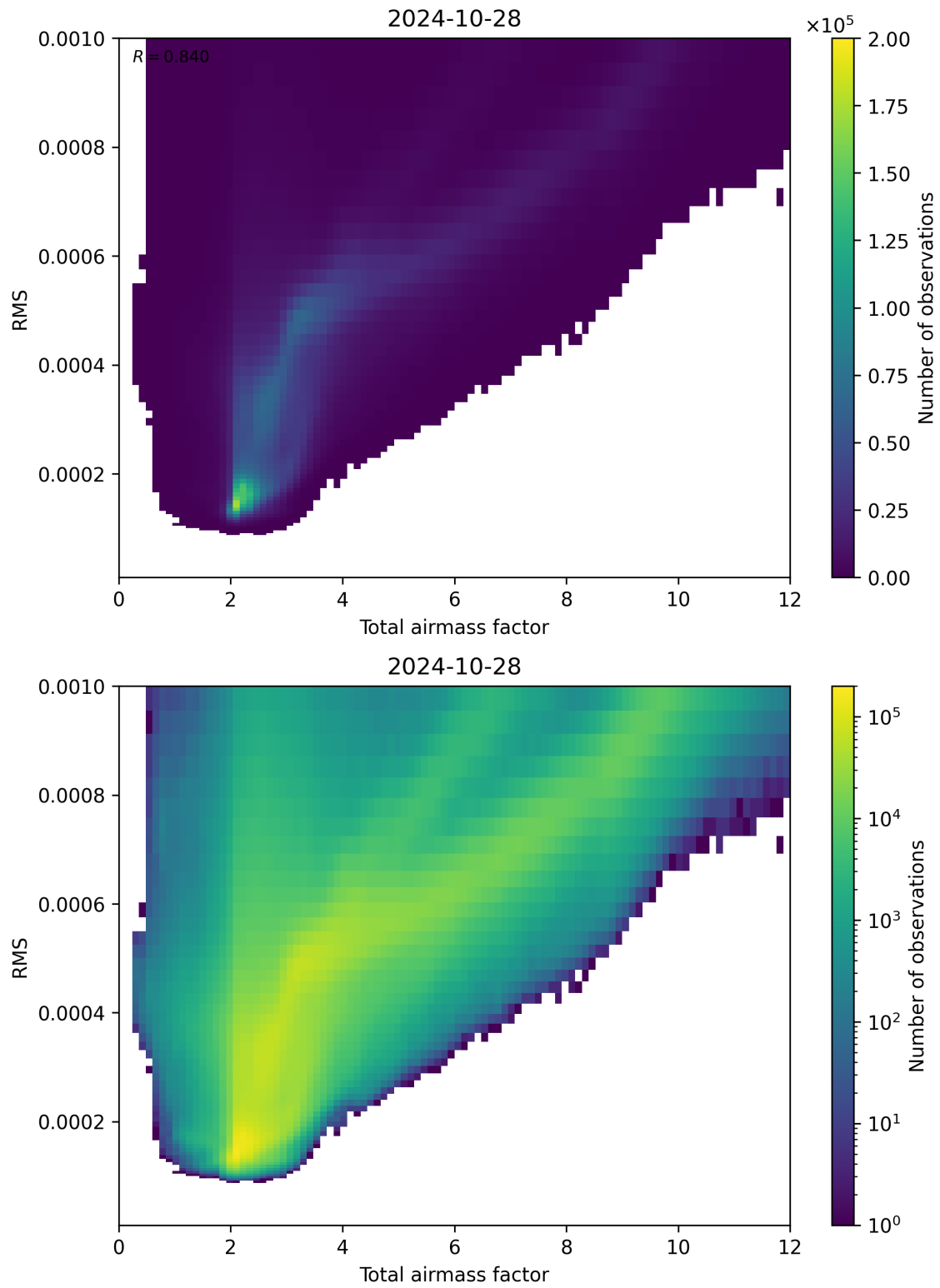
Figure 69: Scatter density plot of “Total airmass factor” against “RMS” for 2024-10-27 to 2024-10-29.
