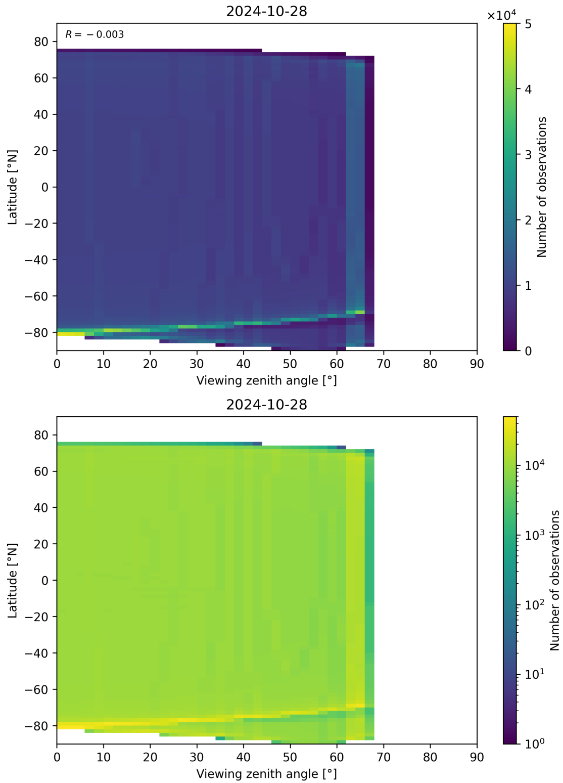
Figure 163: Scatter density plot of “Viewing zenith angle” against “Latitude” for 2024-10-27 to 2024-10-29.
