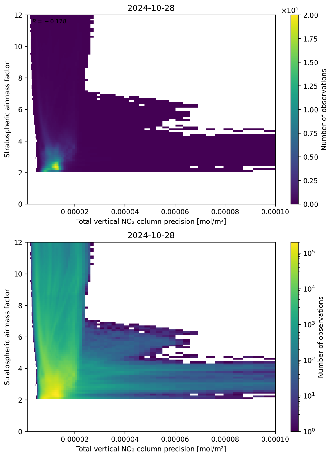
Figure 115: Scatter density plot of “Total vertical NO 2 column precision” against “Stratospheric air mass factor” for 2024-10-27 to 2024-10-29.
