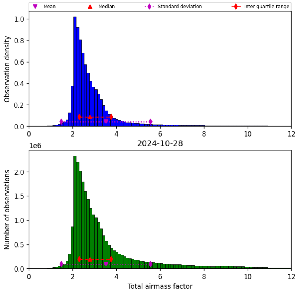
Figure 32: Histogram of “Total airmass factor” for 2024-10-27 to 2024-10-29
