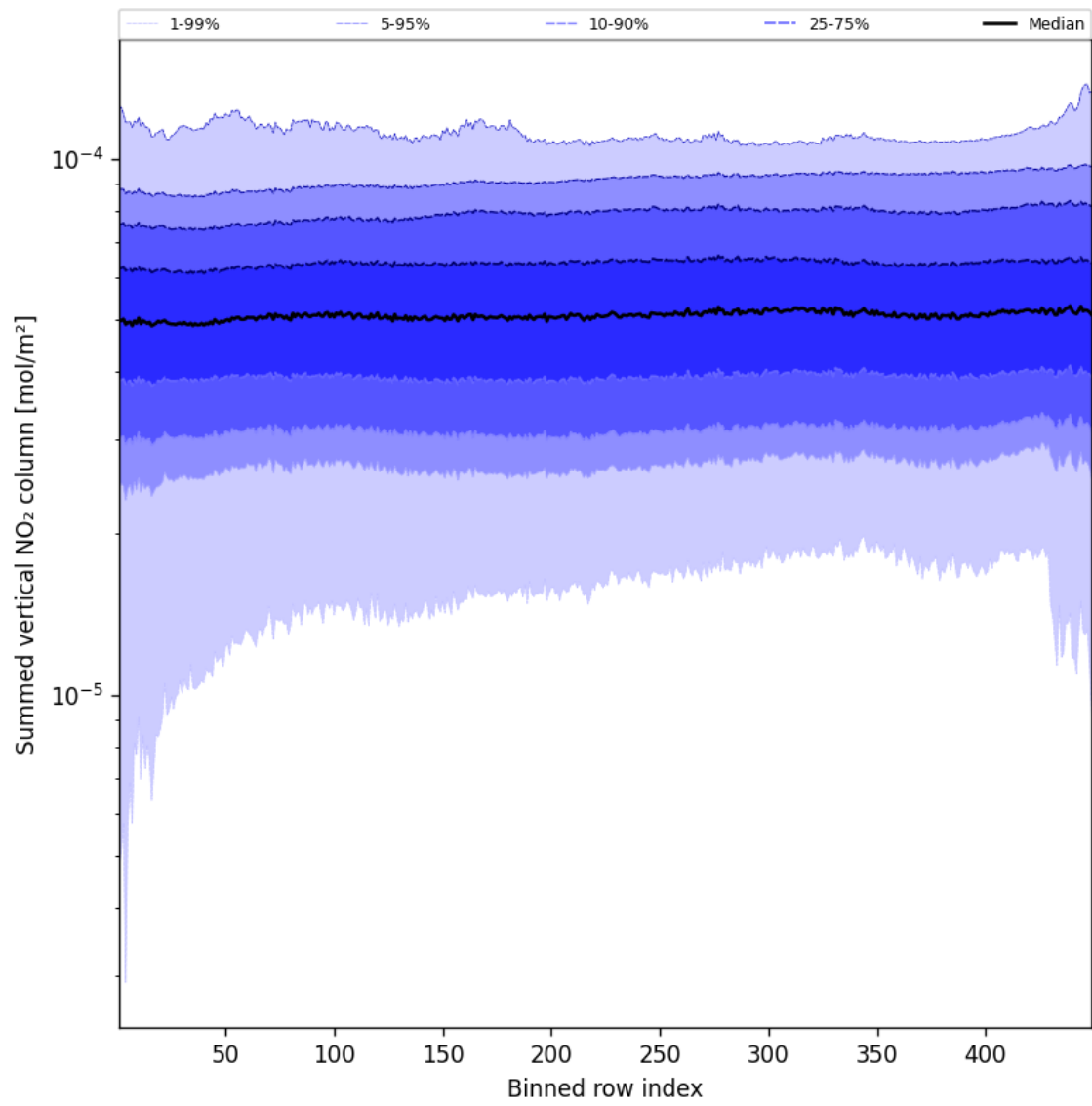
Figure 57: Along track statistics of “Summed vertical NO 2 column” for 2024-10-27 to 2024-10-29
