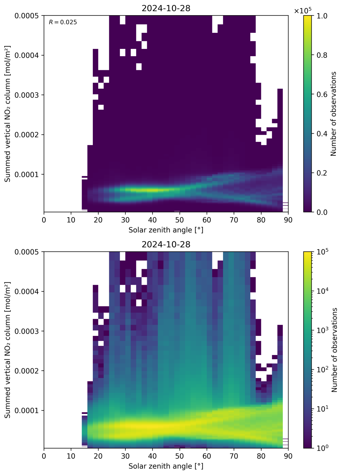
Figure 151: Scatter density plot of “Solar zenith angle” against “Summed vertical NO 2 column” for 2024-10-27 to 2024-10-29.
