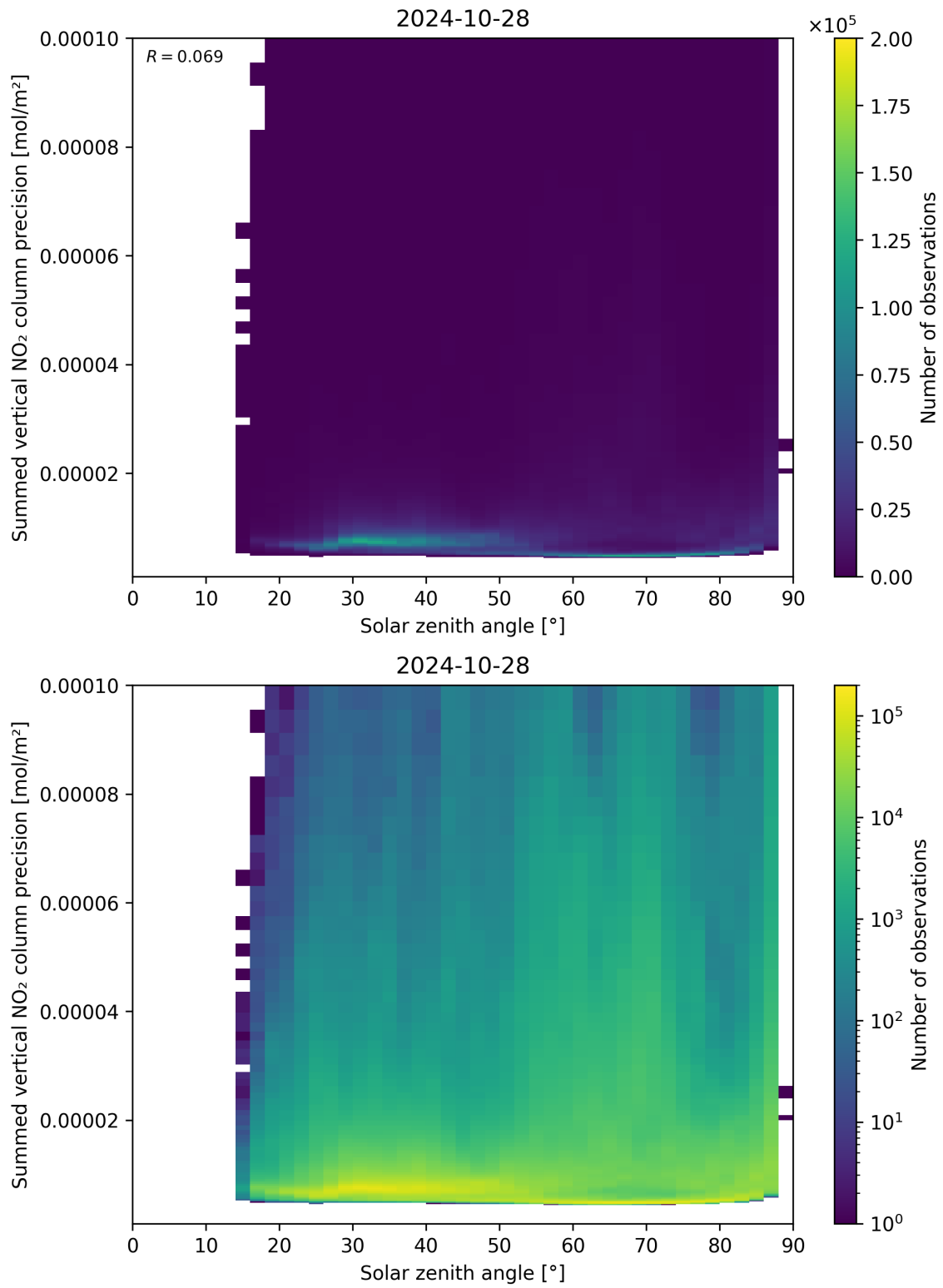
Figure 152: Scatter density plot of “Solar zenith angle” against “Summed vertical NO 2 column precision” for 2024-10-27 to 2024-10-29.
