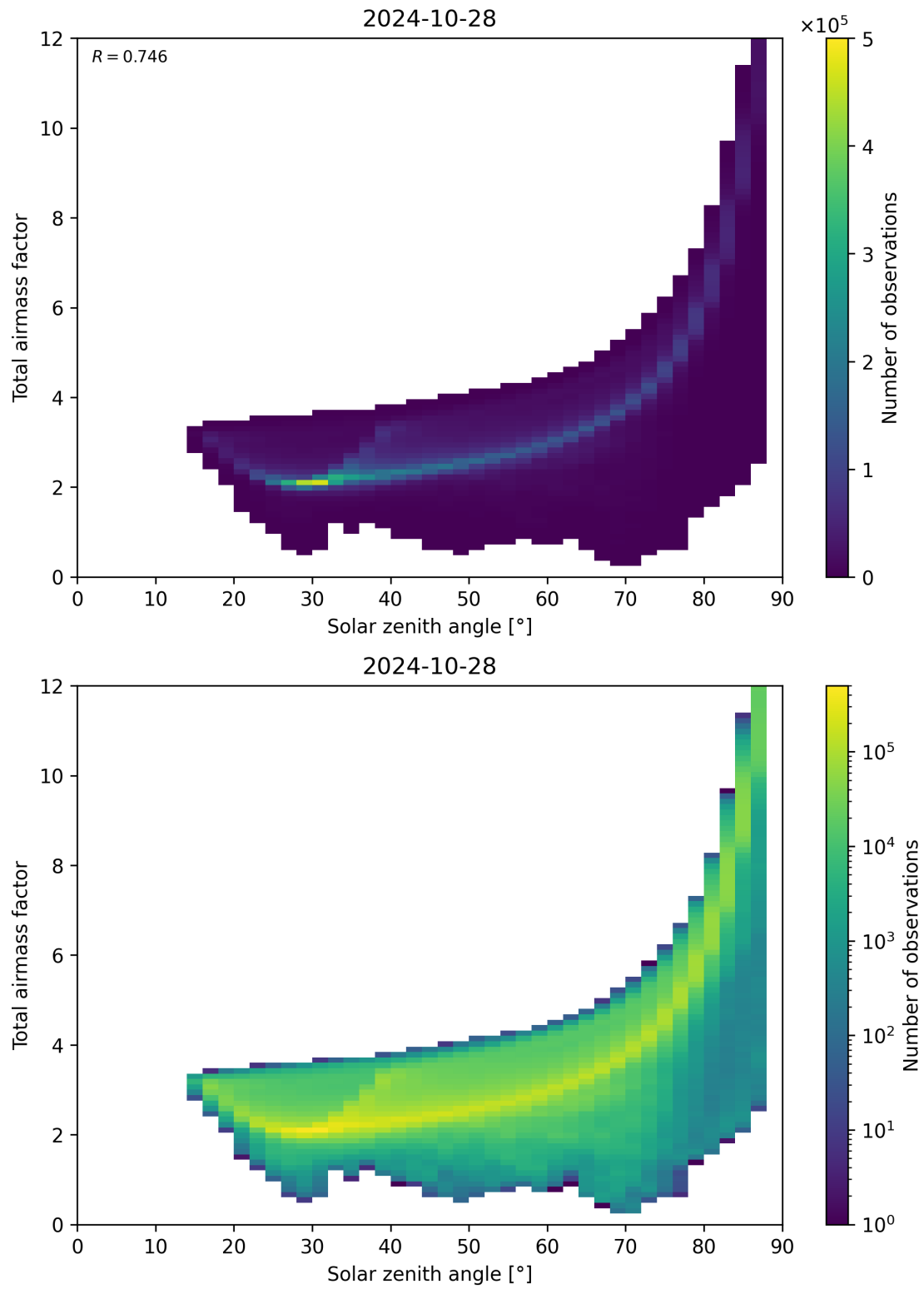
Figure 146: Scatter density plot of “Solar zenith angle” against “Total air mass factor” for 2024-10-27 to 2024-10-29.
