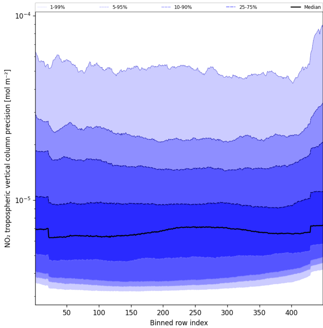
Figure 47: Along track statistics of “NO 2 tropospheric vertical column precision” for 2024-10-27 to 2024-10-29
