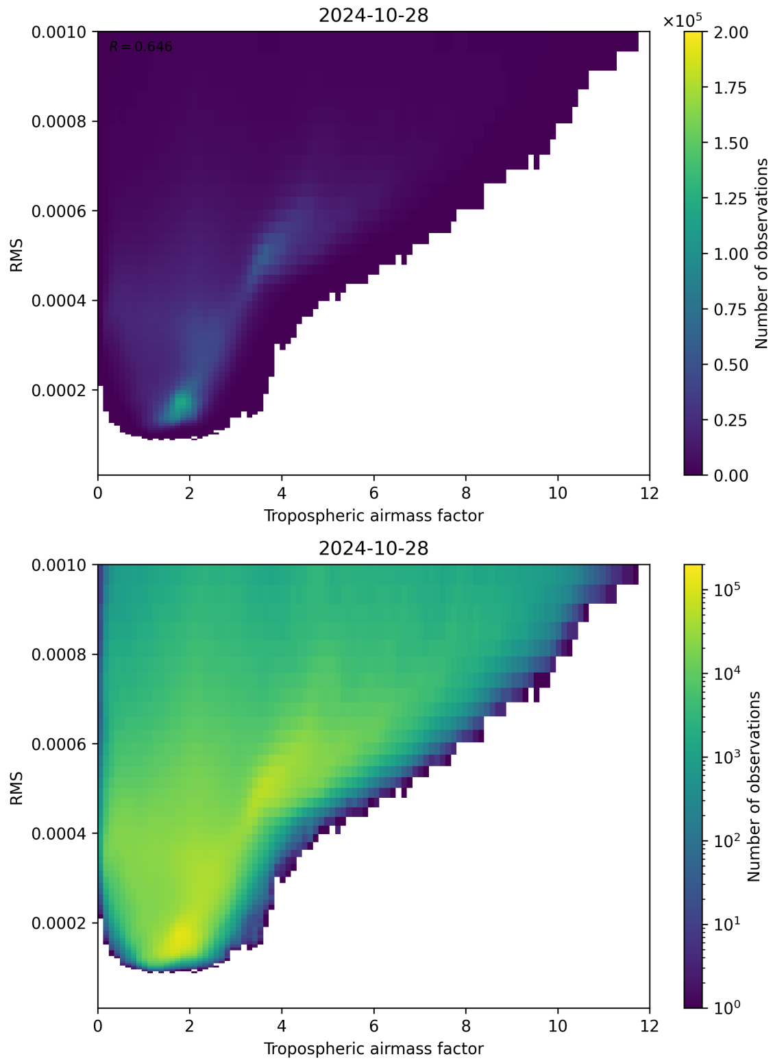
Figure 79: Scatter density plot of “Tropospheric airmass factor” against “RMS” for 2024-10-27 to 2024-10-29.
