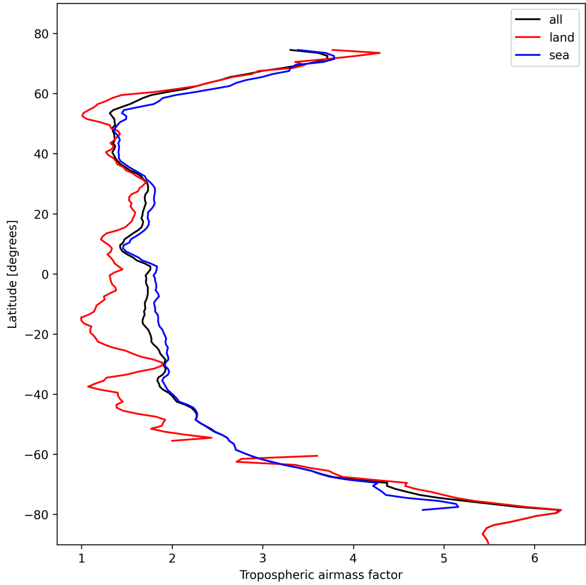
Figure 14: Zonal average of “Tropospheric airmass factor” for 2024-10-27 to 2024-10-29.
