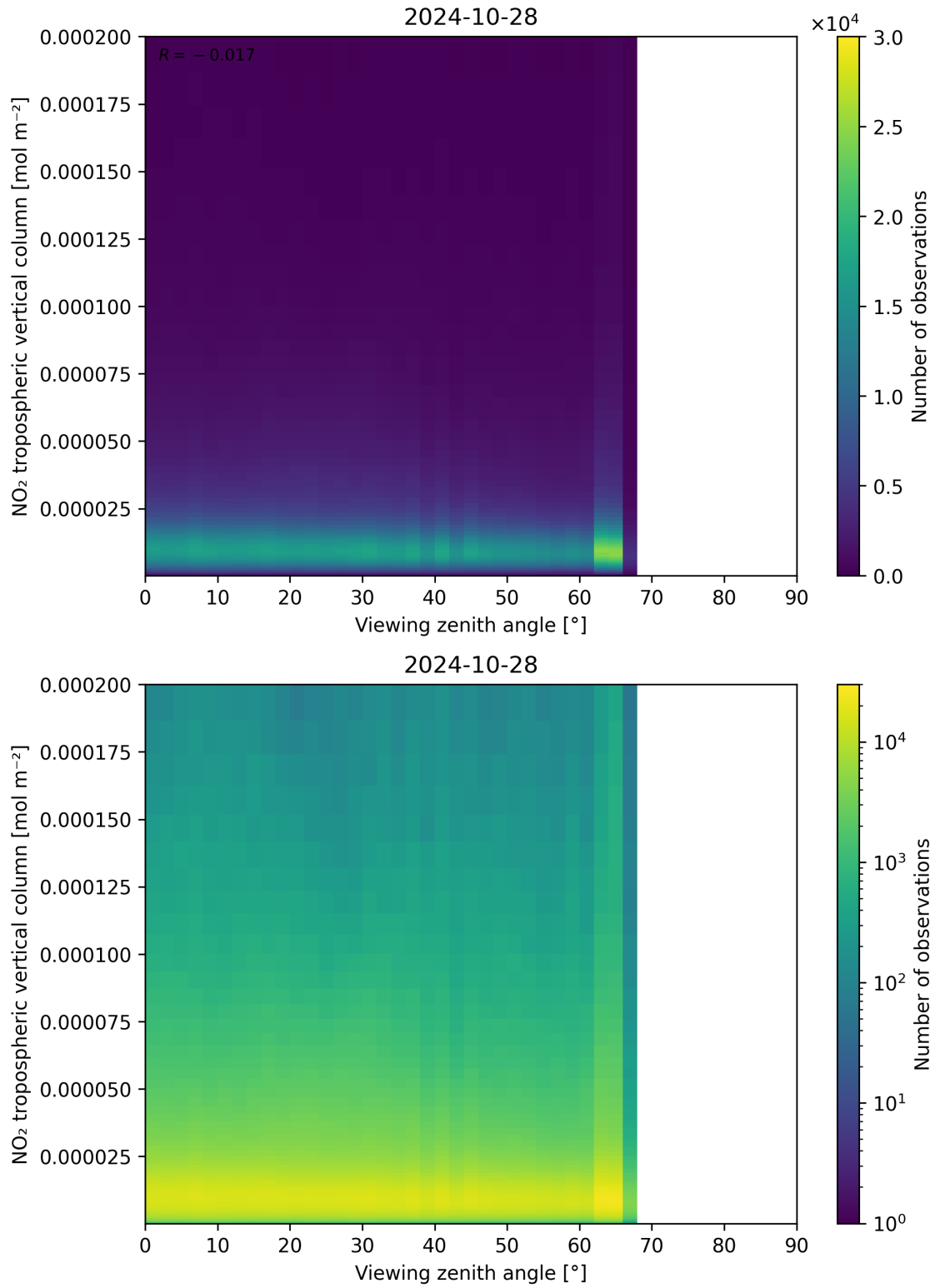
Figure 169: Scatter density plot of “Viewing zenith angle” against “NO 2 tropospheric vertical column” for 2024-10-27 to 2024-10-29.
