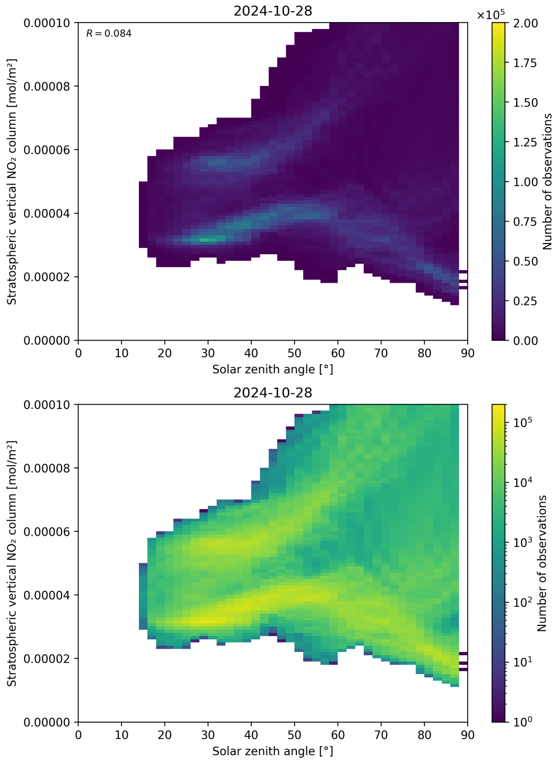
Figure 150: Scatter density plot of “Solar zenith angle” against “Stratospheric vertical NO 2 column” for 2024-10-27 to 2024-10-29.
