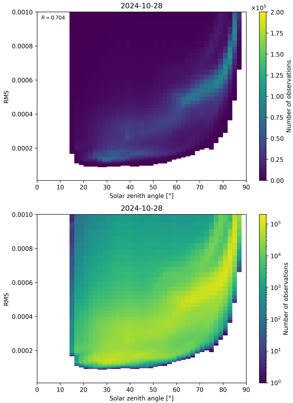
Figure 157: Scatter density plot of “Solar zenith angle” against “RMS” for 2024-10-27 to 2024-10-29.
