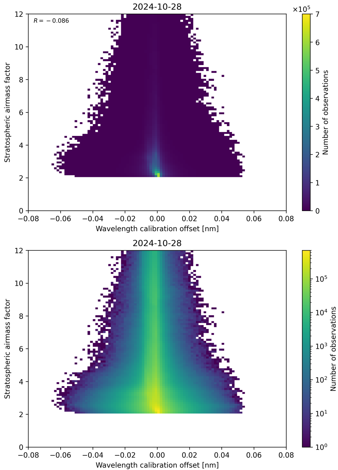
Figure 174: Scatter density plot of “Wavelength calibration offset” against “Stratospheric airmass factor” for 2024-10-27 to 2024-10-29.
