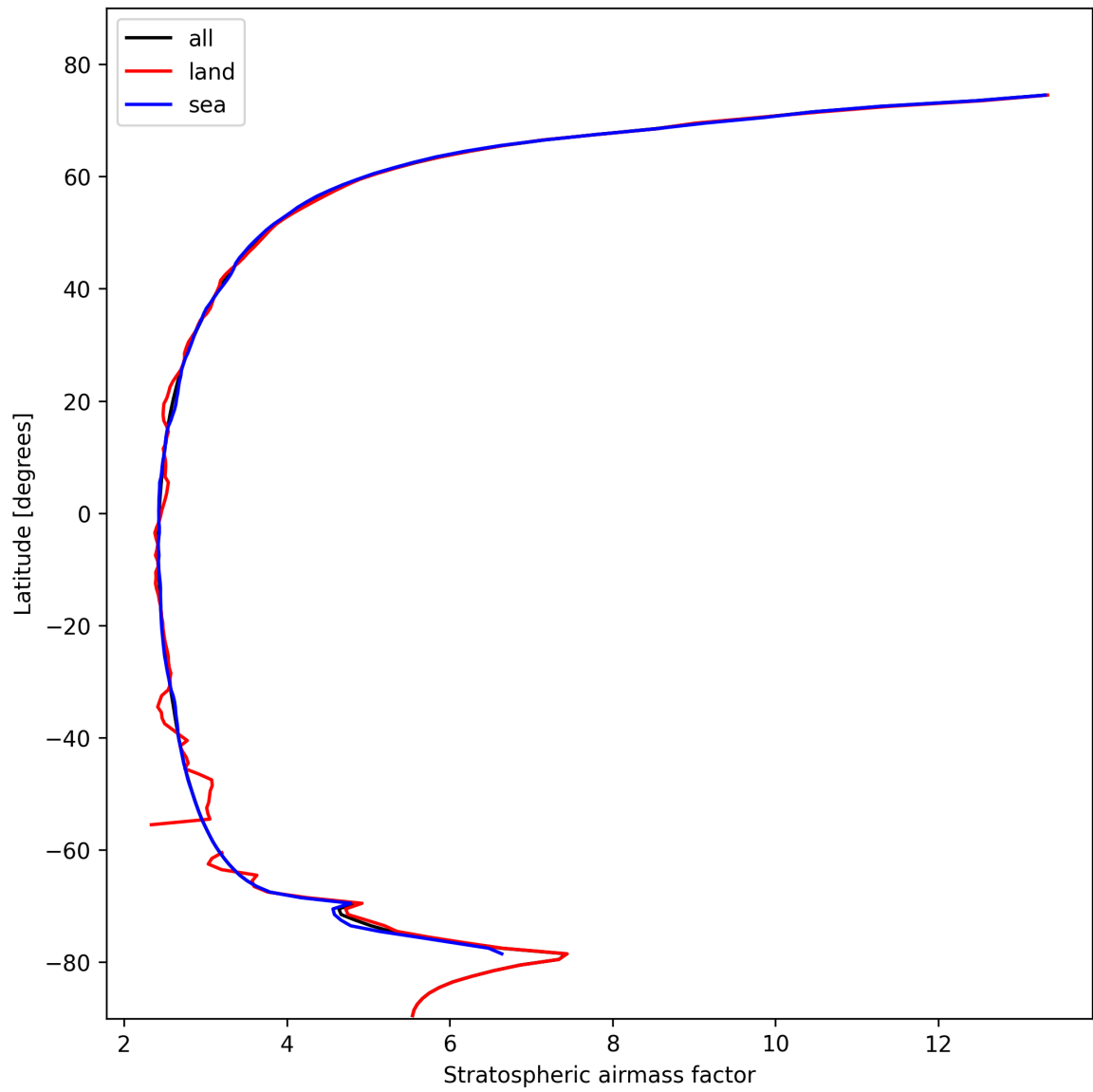
Figure 27: Zonal average of “Stratospheric airmass factor” for 2024-10-27 to 2024-10-29.
