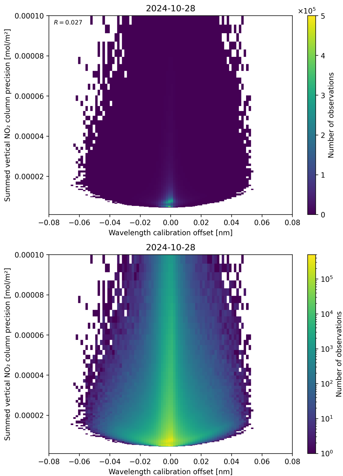
Figure 178: Scatter density plot of “Wavelength calibration offset” against “Summed vertical NO 2 column precision” for 2024-10-27 to 2024-10-29.
