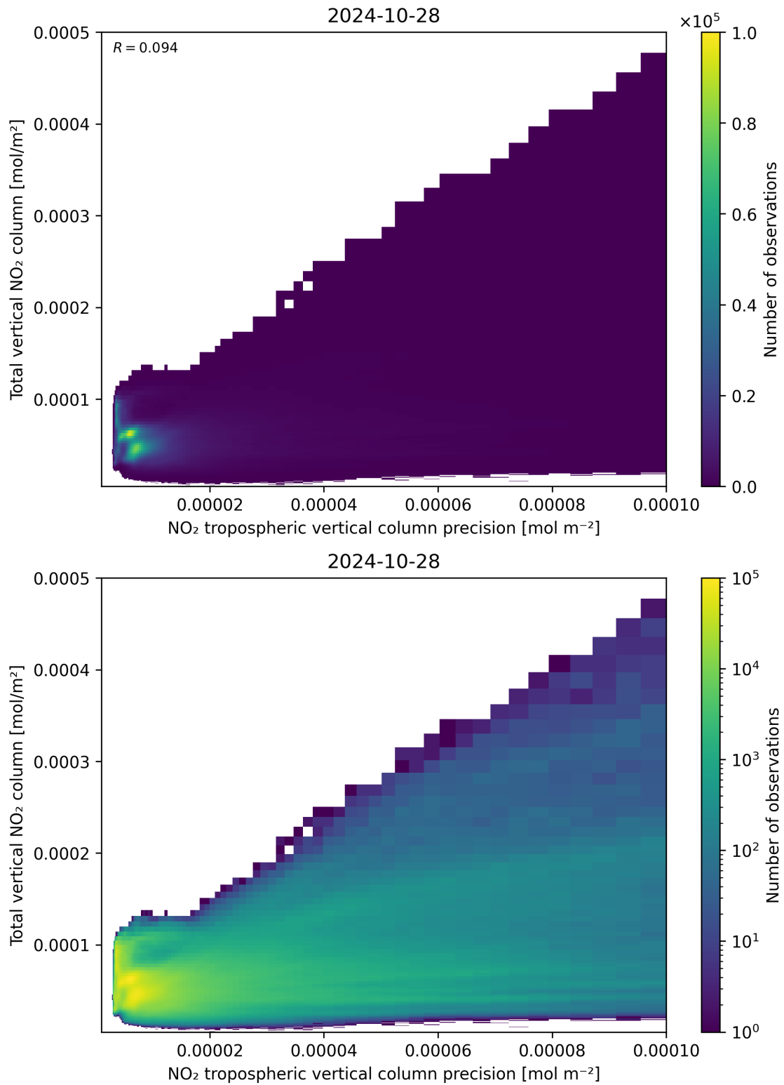
Figure 138: Scatter density plot of “NO 2 tropospheric vertical column precision” against “Total vertical NO 2 column” for 2024-10-27 to 2024-10-29.
