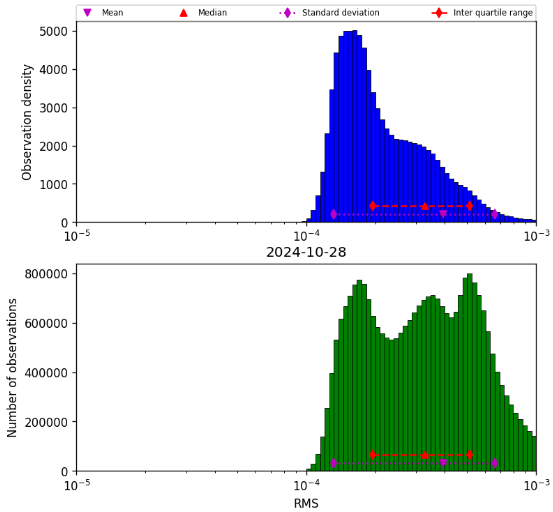
Figure 43: Histogram of “RMS” for 2024-10-27 to 2024-10-29
