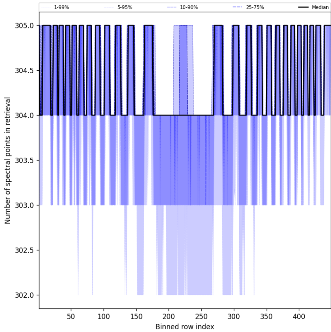
Figure 50: Along track statistics of “Number of spectral points in retrieval” for 2024-10-27 to 2024-10-29
