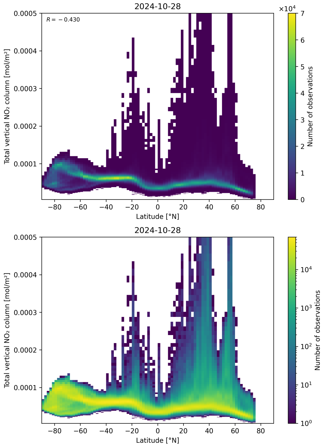
Figure 90: Scatter density plot of “Latitude” against “Total vertical NO 2 column” for 2024-10-27 to 2024-10-29.
