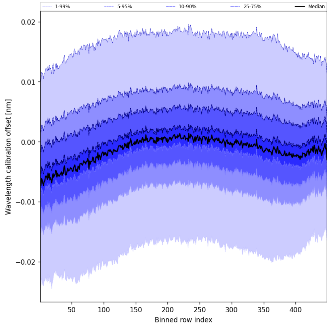
Figure 52: Along track statistics of “Wavelength calibration offset” for 2024-10-27 to 2024-10-29
