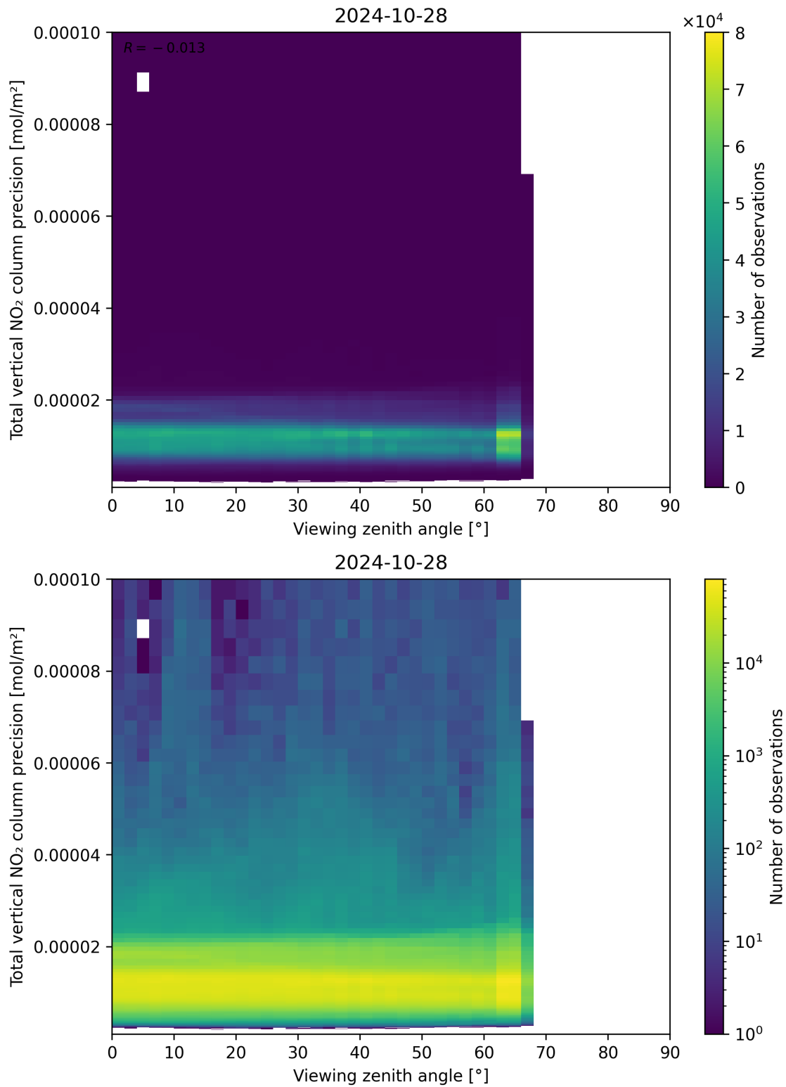
Figure 168: Scatter density plot of “Viewing zenith angle” against “Total vertical NO 2 column precision” for 2024-10-27 to 2024-10-29.
