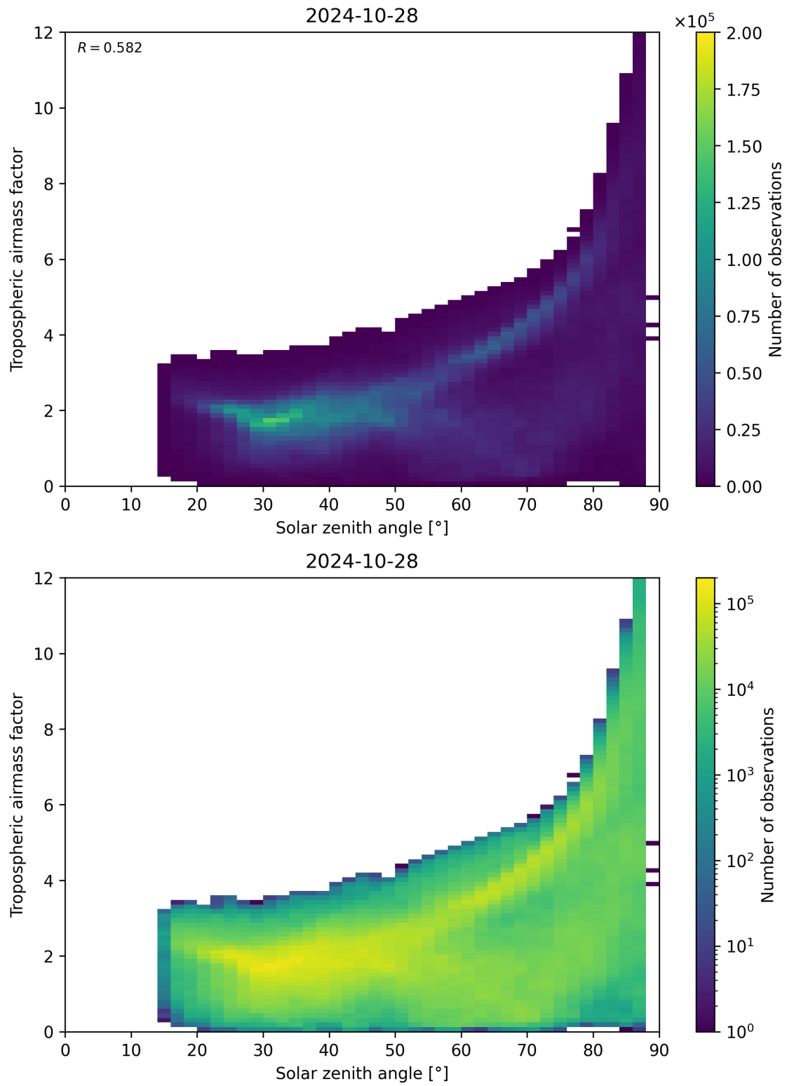
Figure 147: Scatter density plot of “Solar zenith angle” against “Tropospheric airmass factor” for 2024-10-27 to 2024-10-29.
