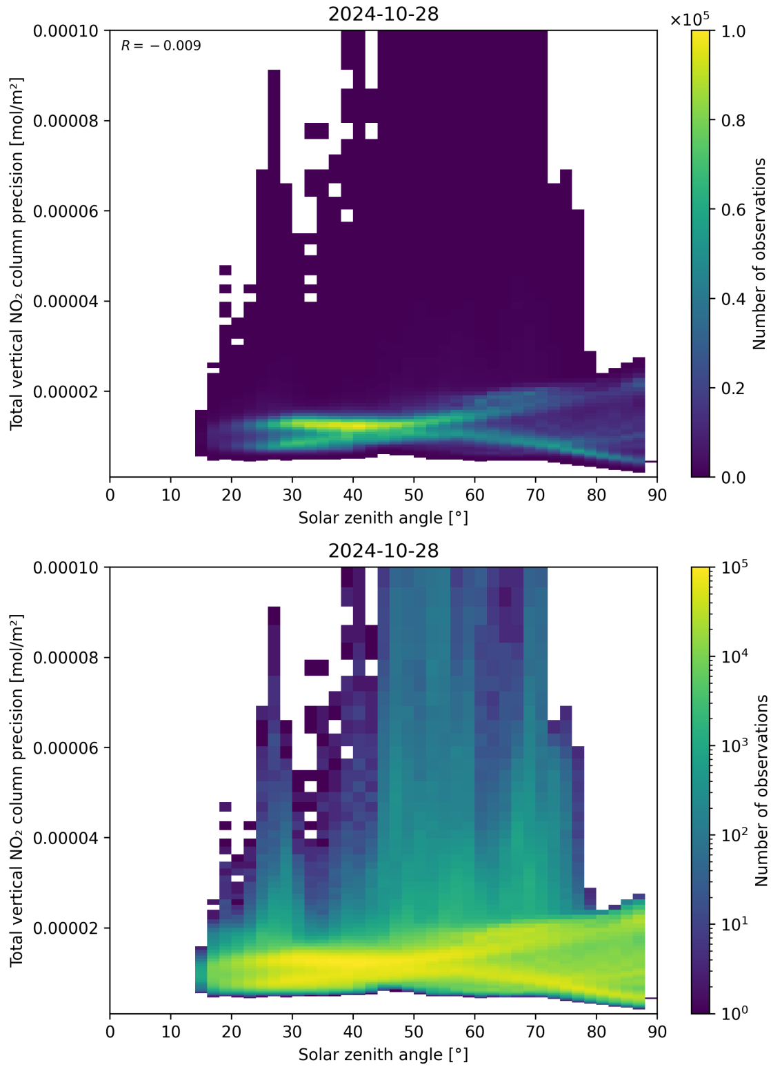
Figure 154: Scatter density plot of “Solar zenith angle” against “Total vertical NO 2 column precision” for 2024-10-27 to 2024-10-29.
