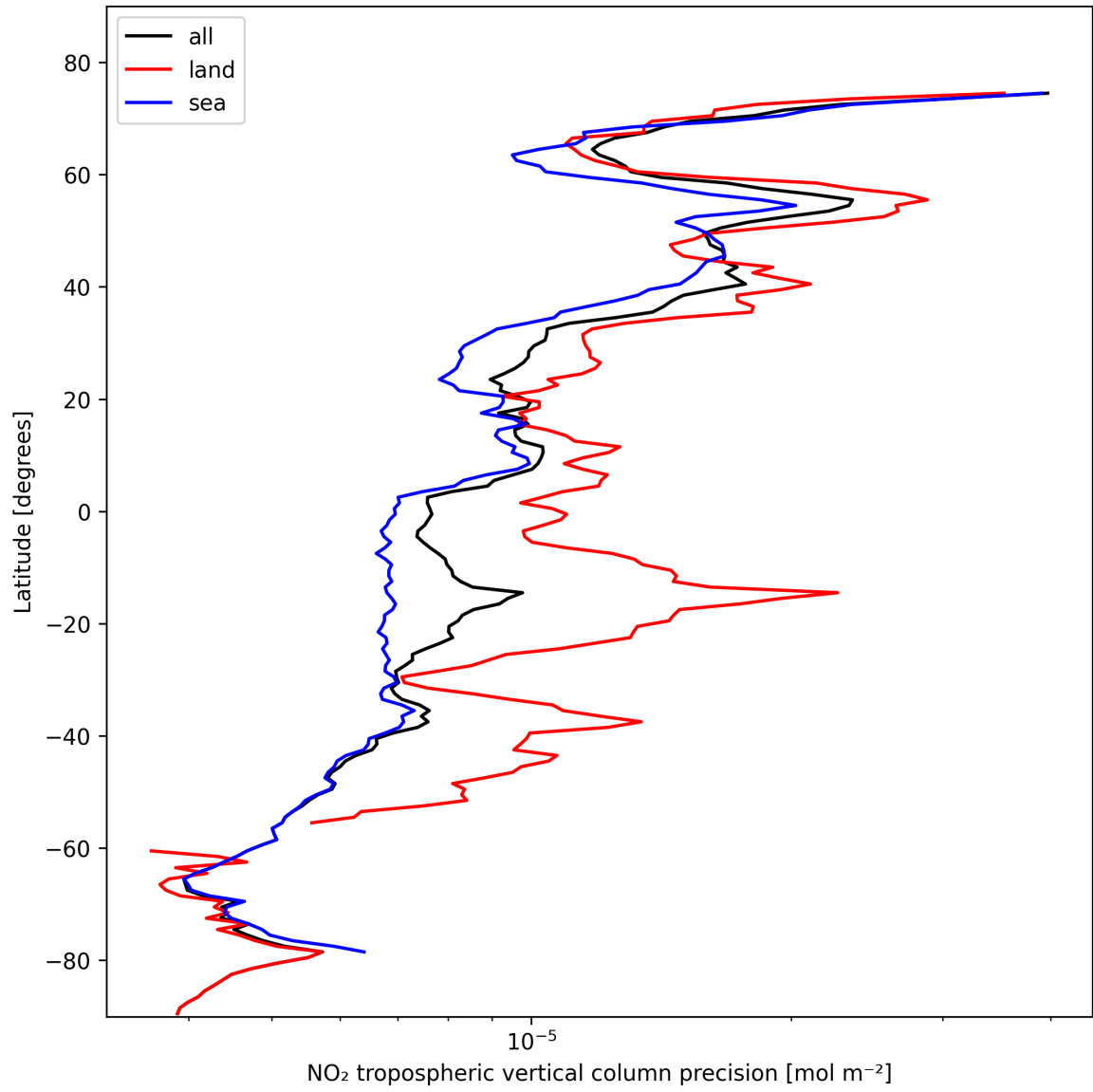
Figure 13: Zonal average of "NO 2 tropospheric vertical column precision" for 2024-10-27 to 2024-10-29.
