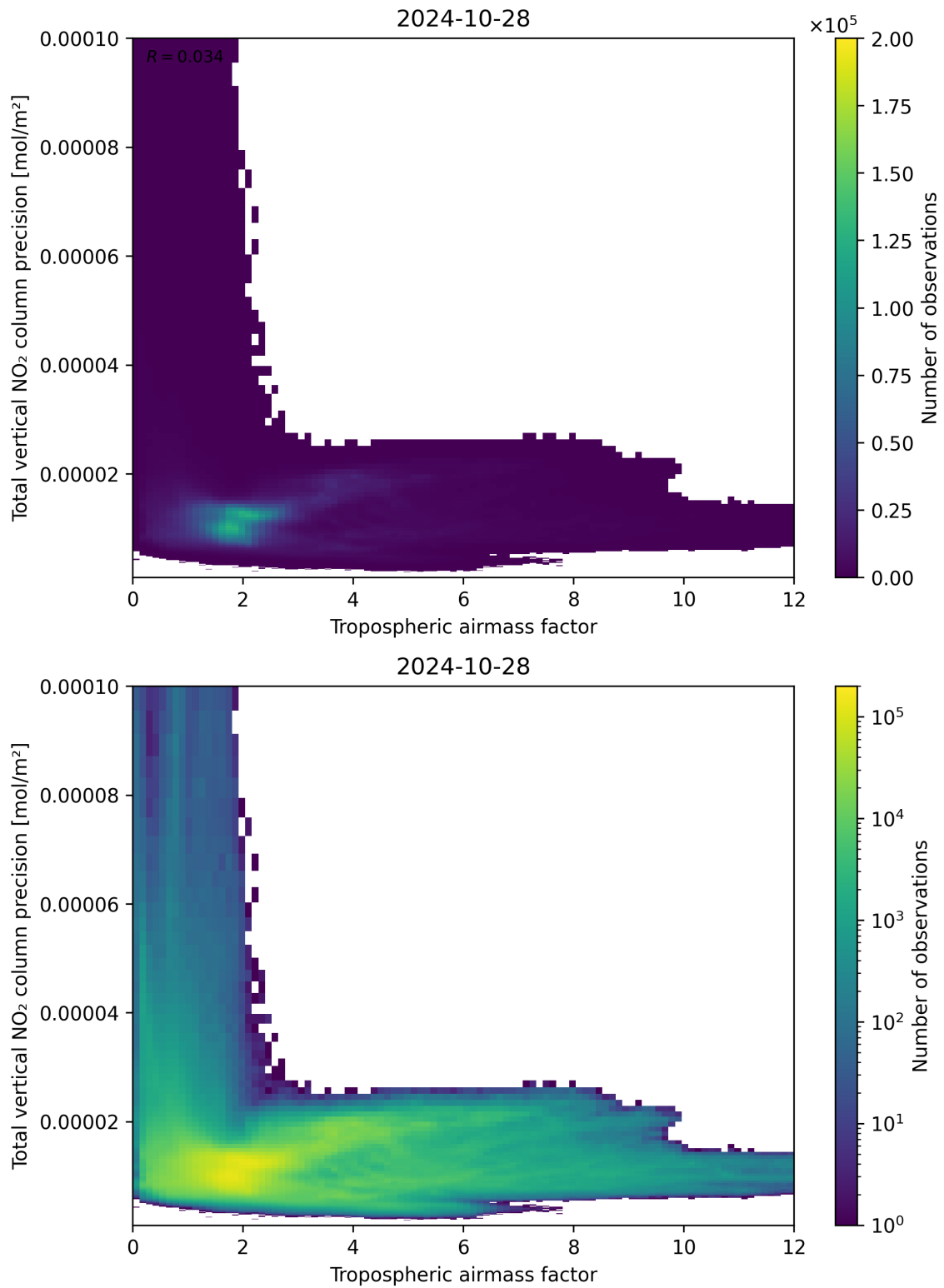
Figure 78: Scatter density plot of “Tropospheric air mass factor” against “Total vertical NO 2 column precision” for 2024-10-27 to 2024-10-29.
