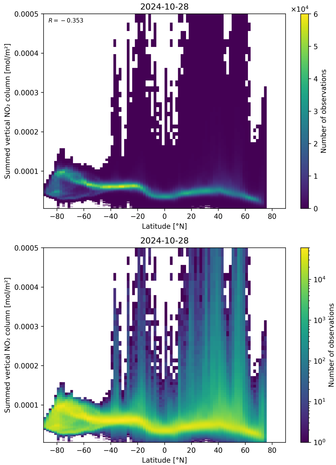
Figure 88: Scatter density plot of “Latitude” against “Summed vertical NO 2 column” for 2024-10-27 to 2024-10-29.
