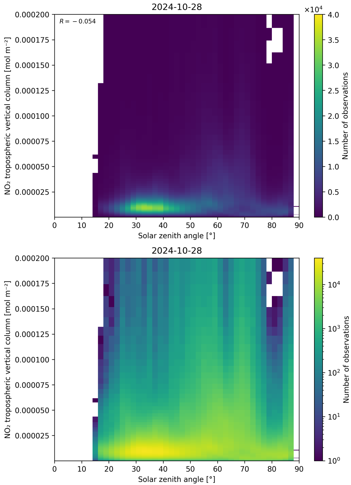
Figure 155: Scatter density plot of “Solar zenith angle” against “NO 2 tropospheric vertical column” for 2024-10-27 to 2024-10-29.
