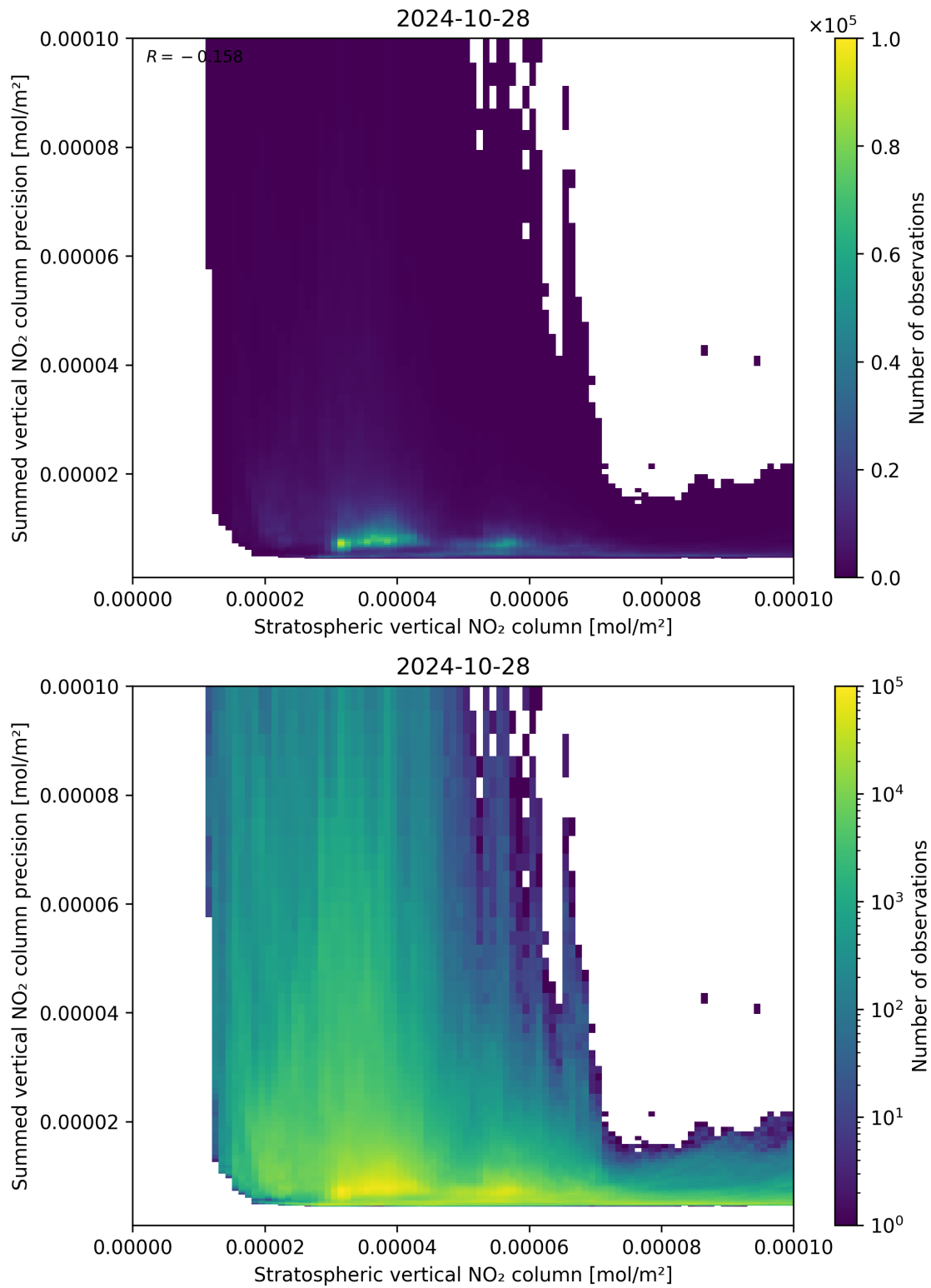
Figure 99: Scatter density plot of “Stratospheric vertical NO 2 column” against “Summed vertical NO 2 column precision” for 2024-10-27 to 2024-10-29.
