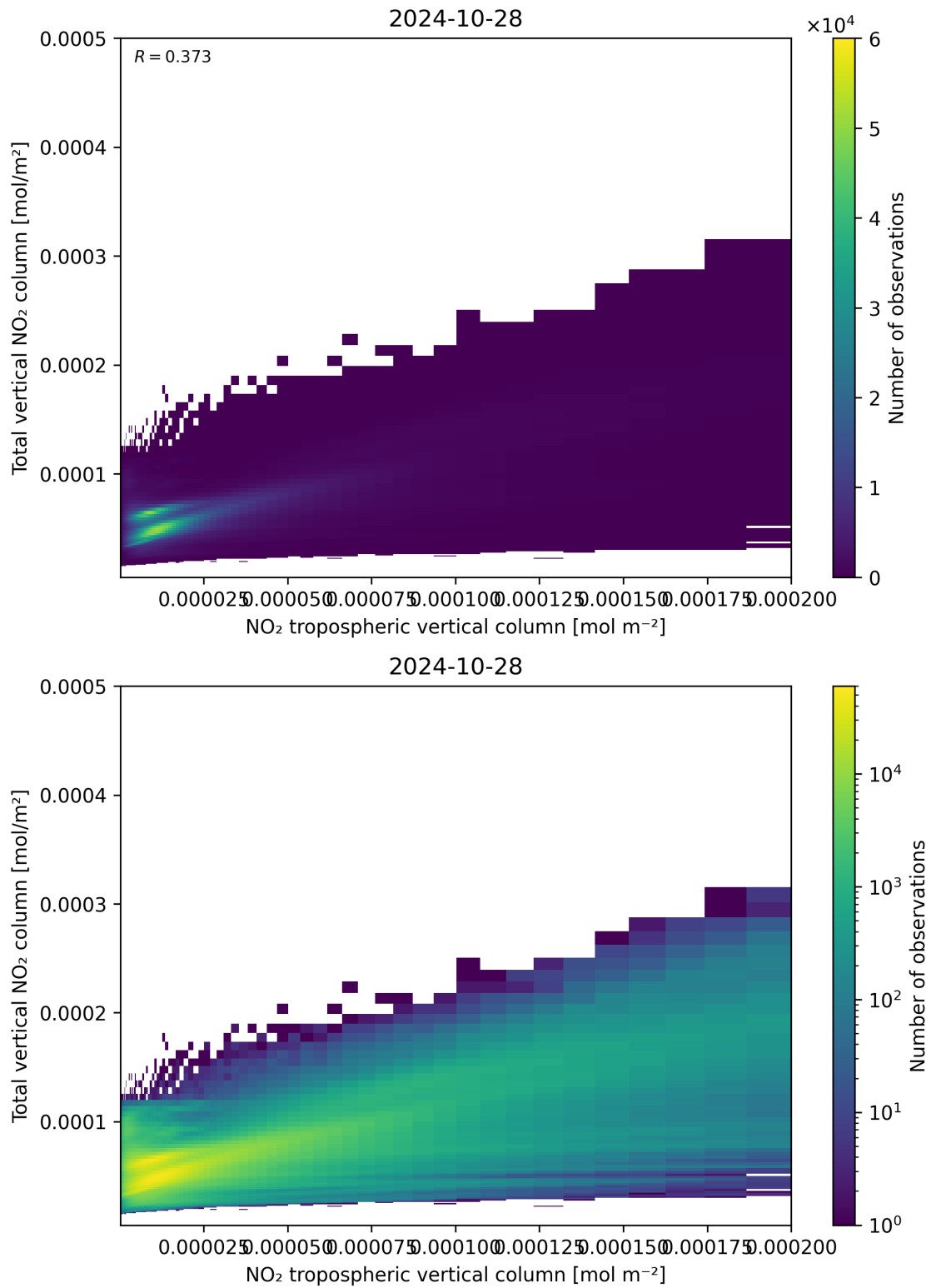
Figure 128: Scatter density plot of “NO 2 tropospheric vertical column” against “Total vertical NO 2 column” for 2024-10-27 to 2024-10-29.
