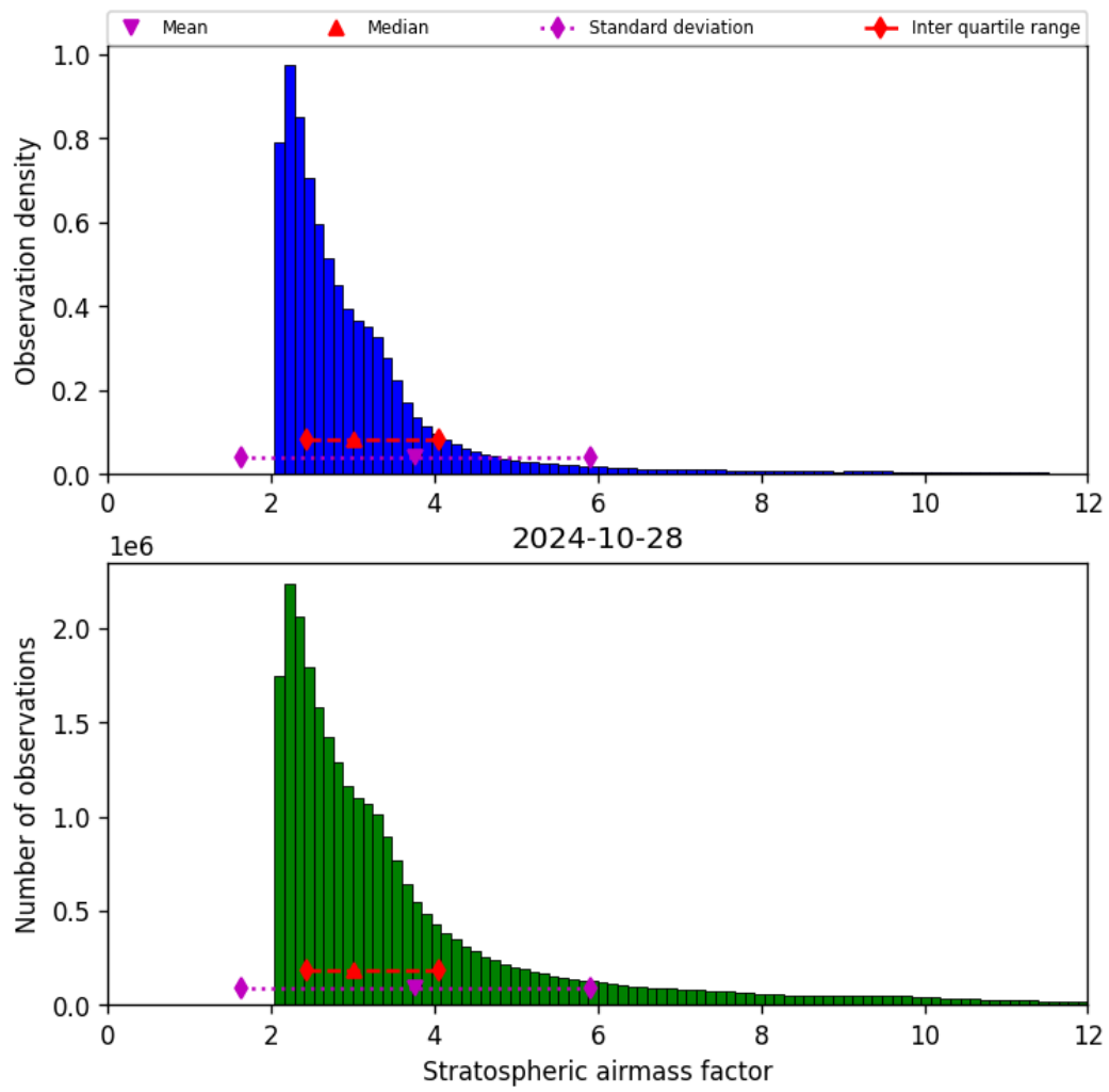
Figure 44: Histogram of “Stratospheric airmass factor” for 2024-10-27 to 2024-10-29
