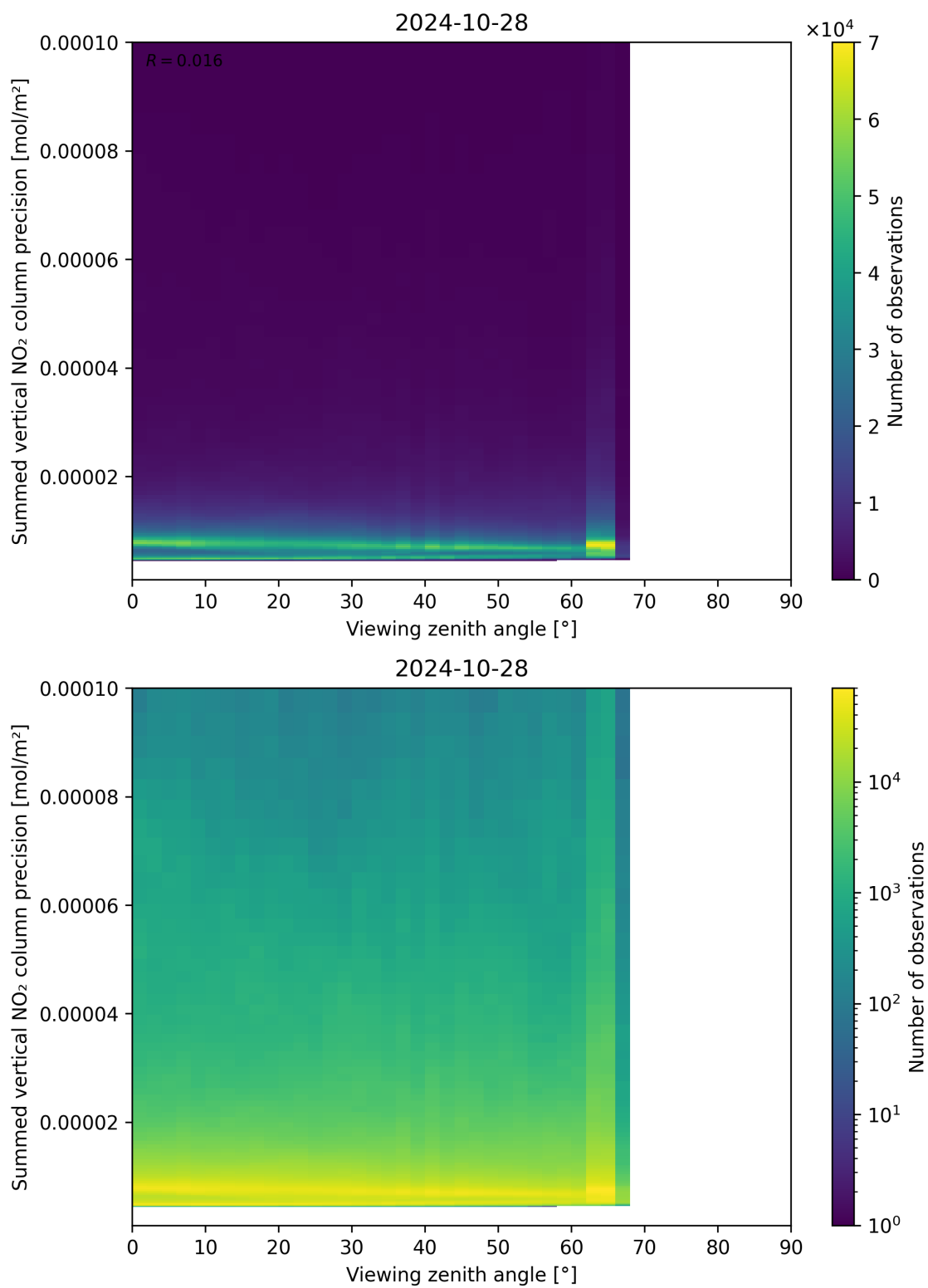
Figure 166: Scatter density plot of “Viewing zenith angle” against “Summed vertical NO 2 column precision” for 2024-10-27 to 2024-10-29.
