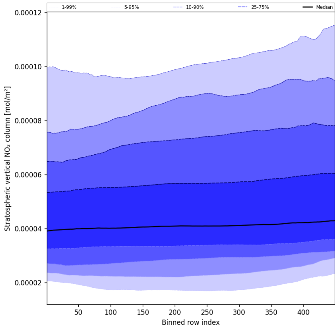
Figure 53: Along track statistics of “Stratospheric vertical NO 2 column” for 2024-10-27 to 2024-10-29
