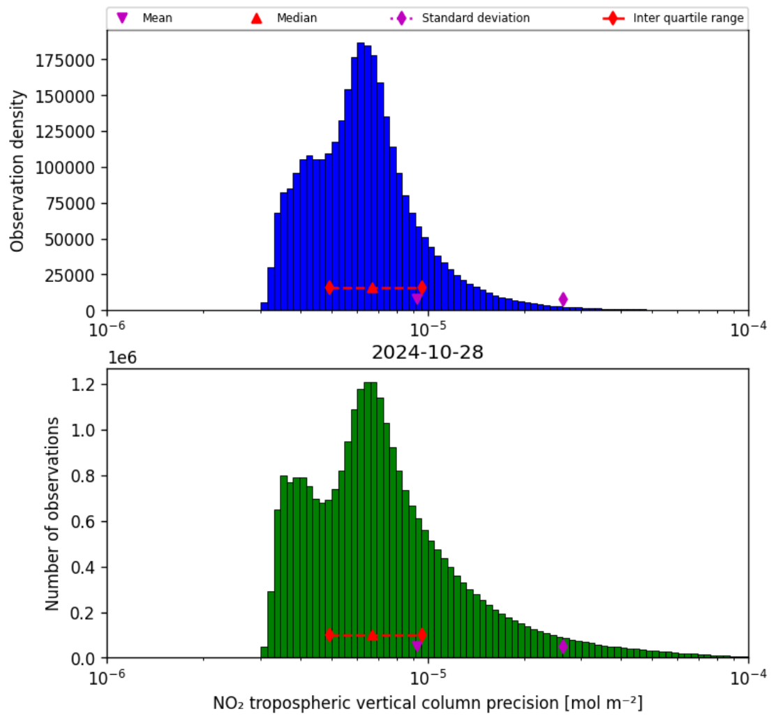
Figure 30: Histogram of “NO 2 tropospheric vertical column precision” for 2024-10-27 to 2024-10-29
