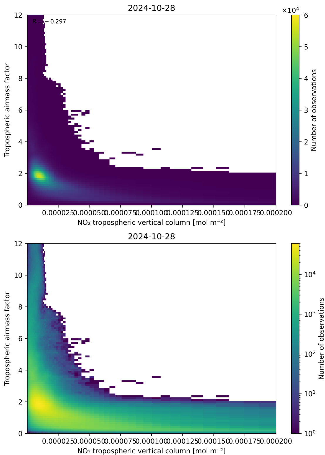
Figure 123: Scatter density plot of “NO 2 tropospheric vertical column” against “Tropospheric air mass factor” for 2024-10-27 to 2024-10-29.
