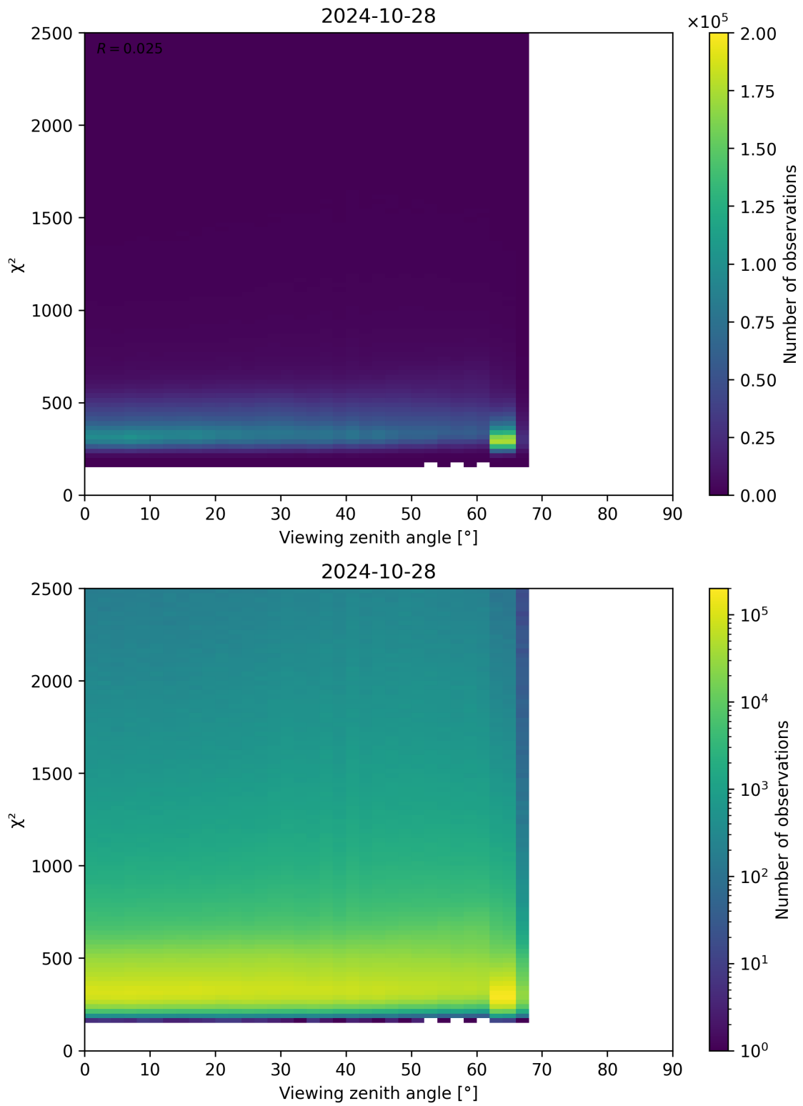
Figure 162: Scatter density plot of “Viewing zenith angle” against “ \chi^2 ” for 2024-10-27 to 2024-10-29.
