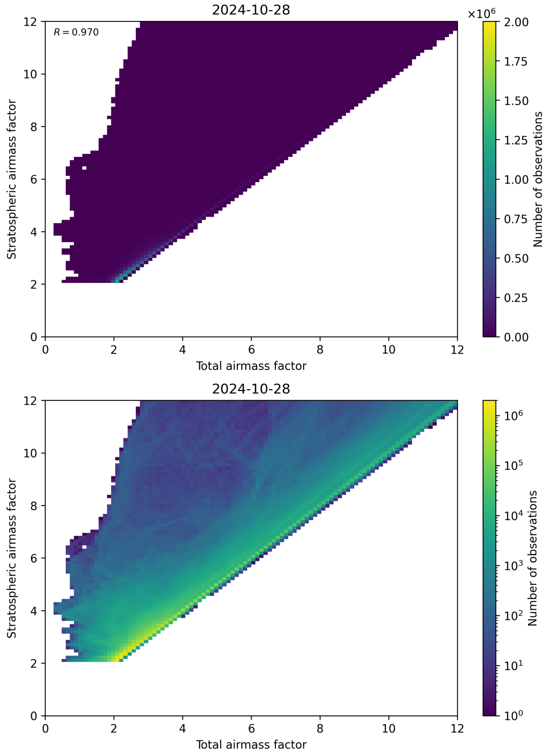
Figure 62: Scatter density plot of “Total airmass factor” against “Stratospheric airmass factor” for 2024-10-27 to 2024-10-29.
