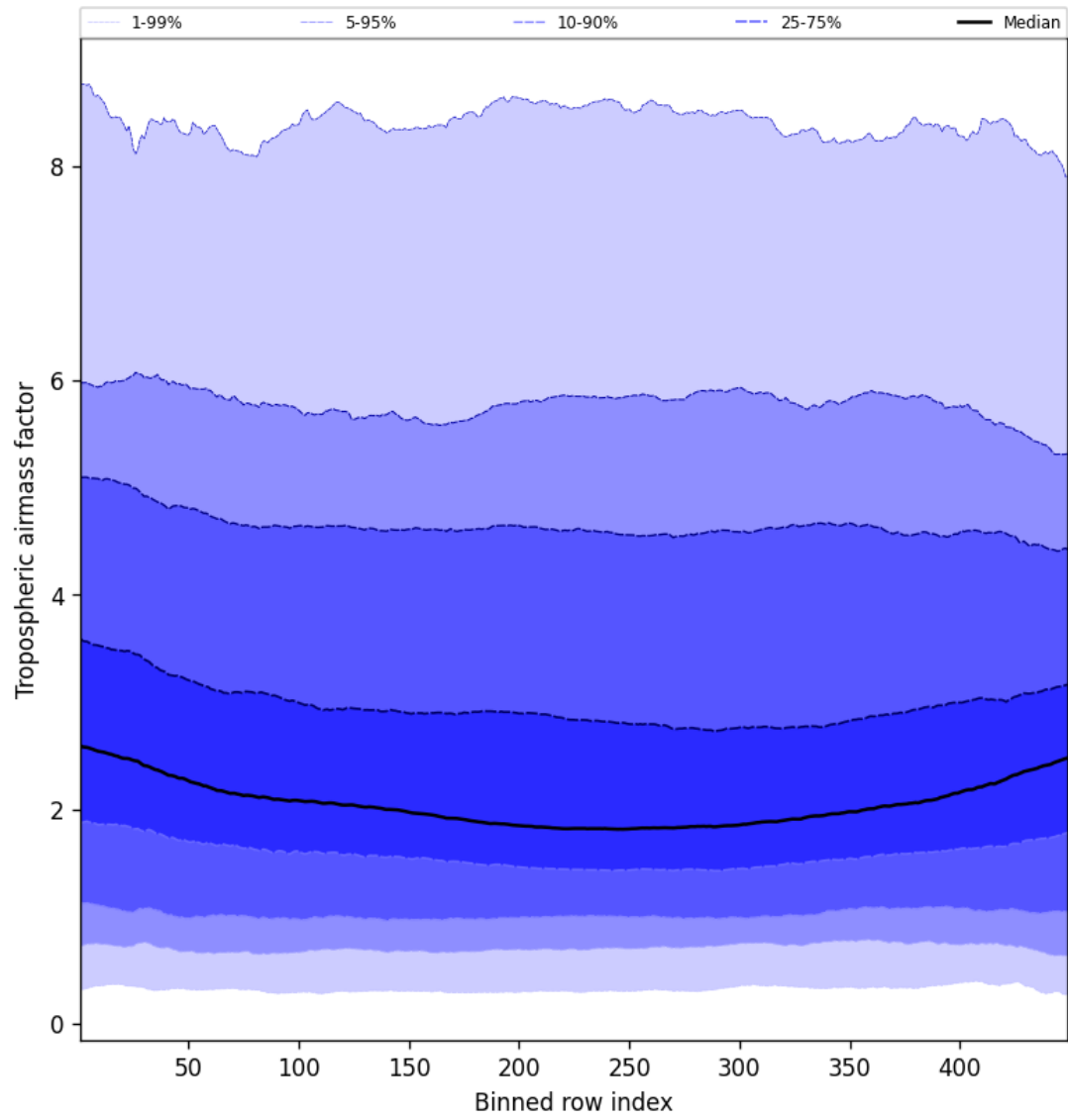
Figure 48: Along track statistics of “Tropospheric air mass factor” for 2024-10-27 to 2024-10-29
