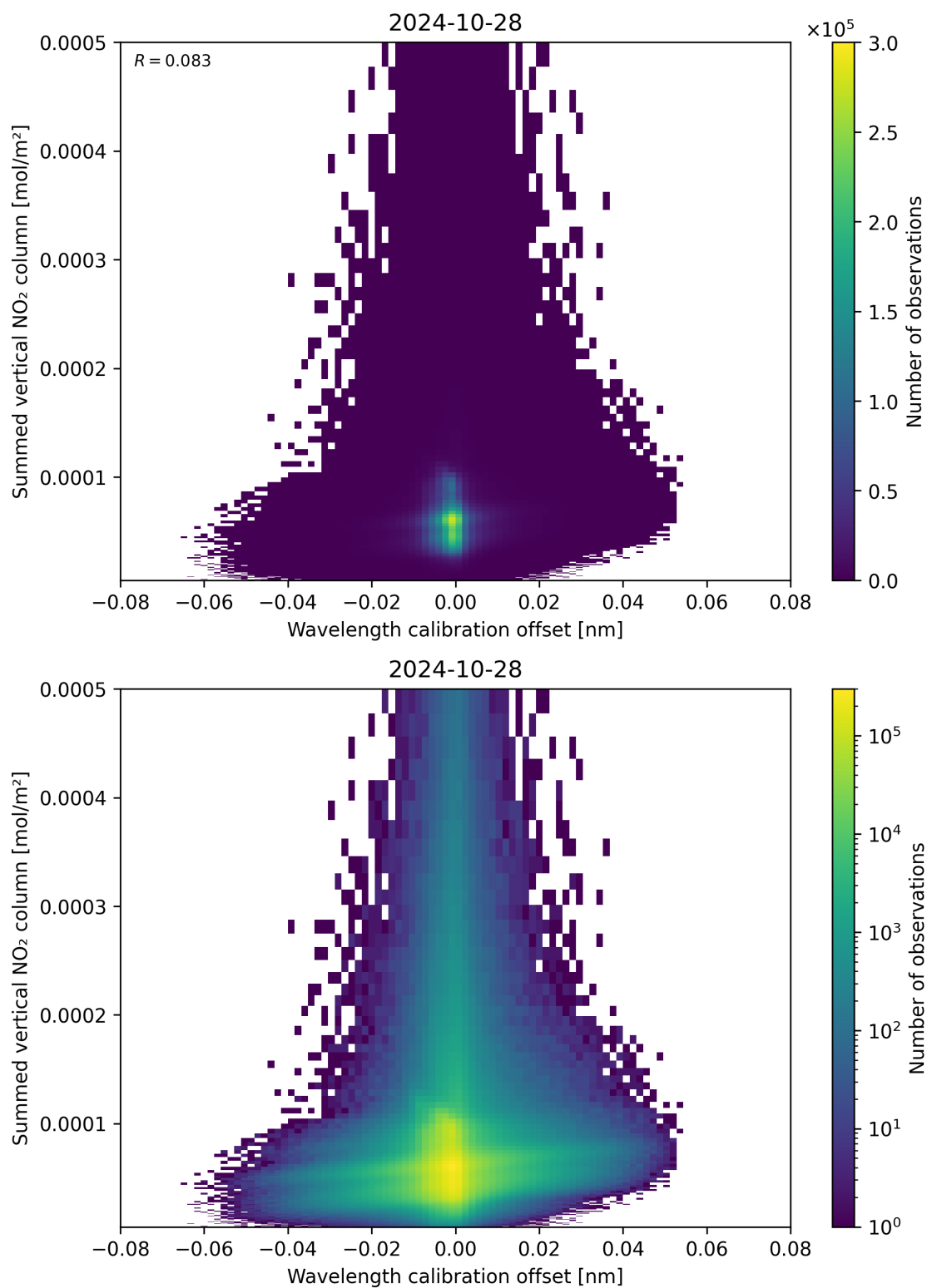
Figure 177: Scatter density plot of “Wavelength calibration offset” against “Summed vertical NO 2 column” for 2024-10-27 to 2024-10-29.
