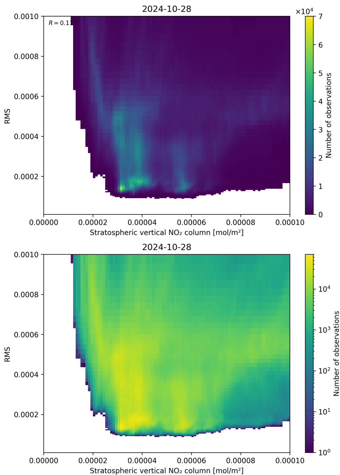
Figure 102: Scatter density plot of “Stratospheric vertical NO 2 column” against “RMS” for 2024-10-27 to 2024-10-29.
