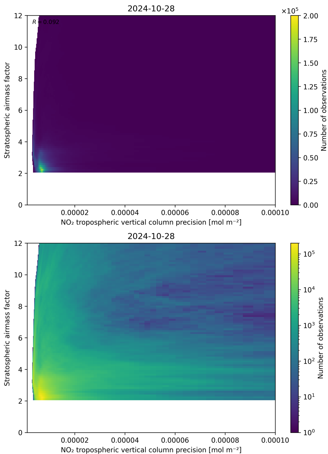
Figure 131: Scatter density plot of “NO 2 tropospheric vertical column precision” against “Stratospheric airmass factor” for 2024-10-27 to 2024-10-29.
