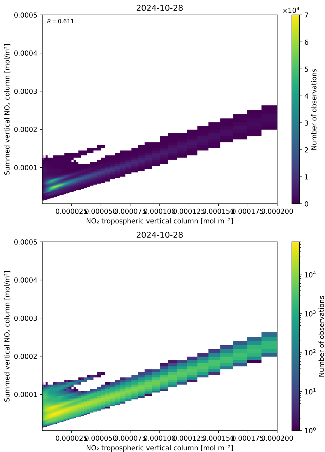
Figure 126: Scatter density plot of “NO 2 tropospheric vertical column” against “Summed vertical NO 2 column” for 2024-10-27 to 2024-10-29.
