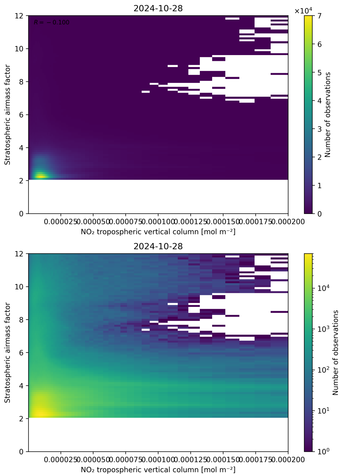
Figure 121: Scatter density plot of “NO 2 tropospheric vertical column” against “Stratospheric airmass factor” for 2024-10-27 to 2024-10-29.
