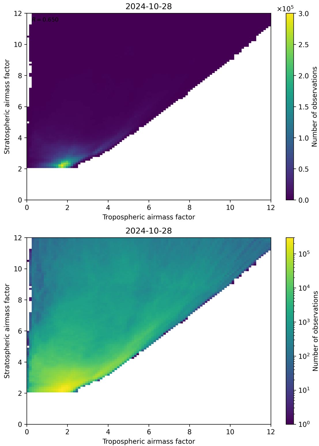
Figure 71: Scatter density plot of “Tropospheric airmass factor” against “Stratospheric airmass factor” for 2024-10-27 to 2024-10-29.
