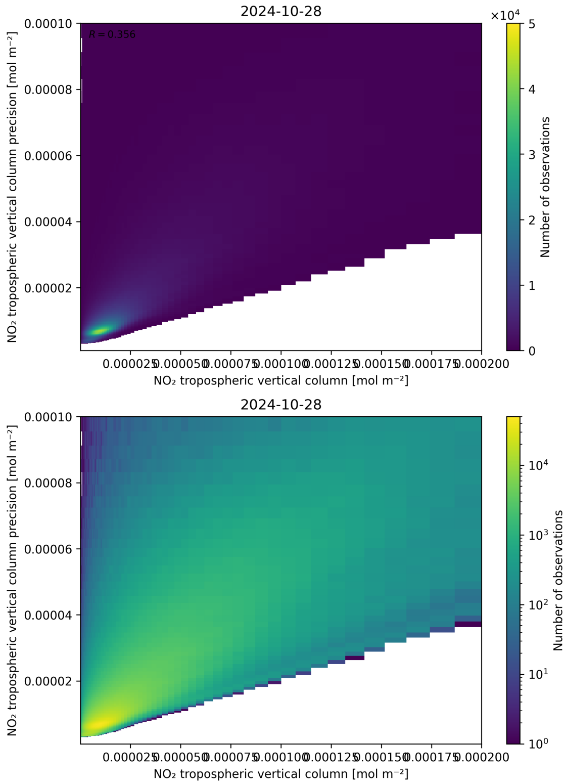
Figure 130: Scatter density plot of “NO 2 tropospheric vertical column” against “NO 2 tropospheric vertical column precision” for 2024-10-27 to 2024-10-29.
