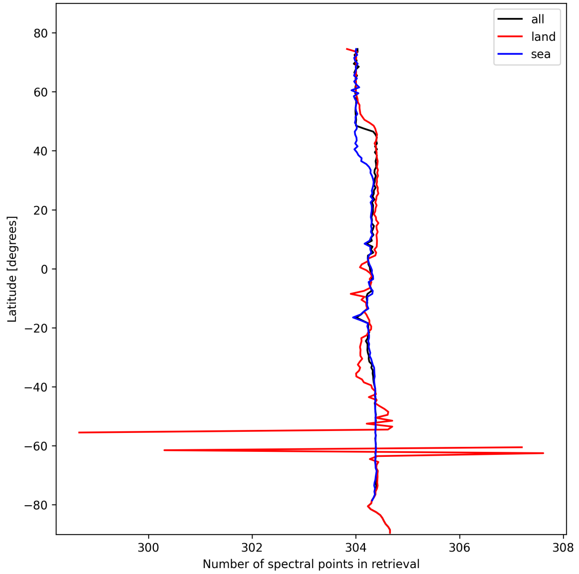
Figure 16: Zonal average of “Number of spectral points in retrieval” for 2024-10-27 to 2024-10-29.
