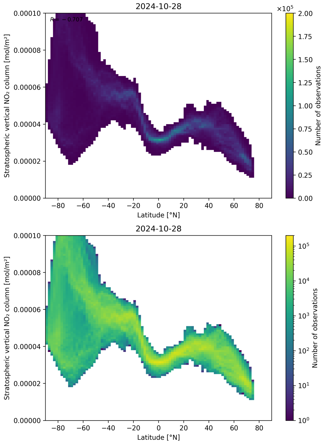
Figure 87: Scatter density plot of “Latitude” against “Stratospheric vertical NO 2 column” for 2024-10-27 to 2024-10-29.
