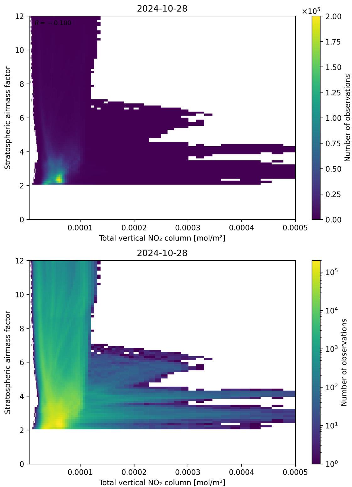
Figure 110: Scatter density plot of “Total vertical NO 2 column” against “Stratospheric airmass factor” for 2024-10-27 to 2024-10-29.
