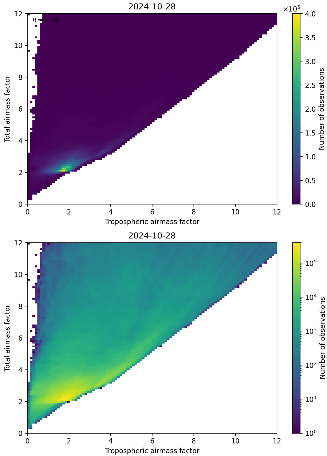
Figure 72: Scatter density plot of “Tropospheric airmass factor” against “Total airmass factor” for 2024-10-27 to 2024-10-29.
