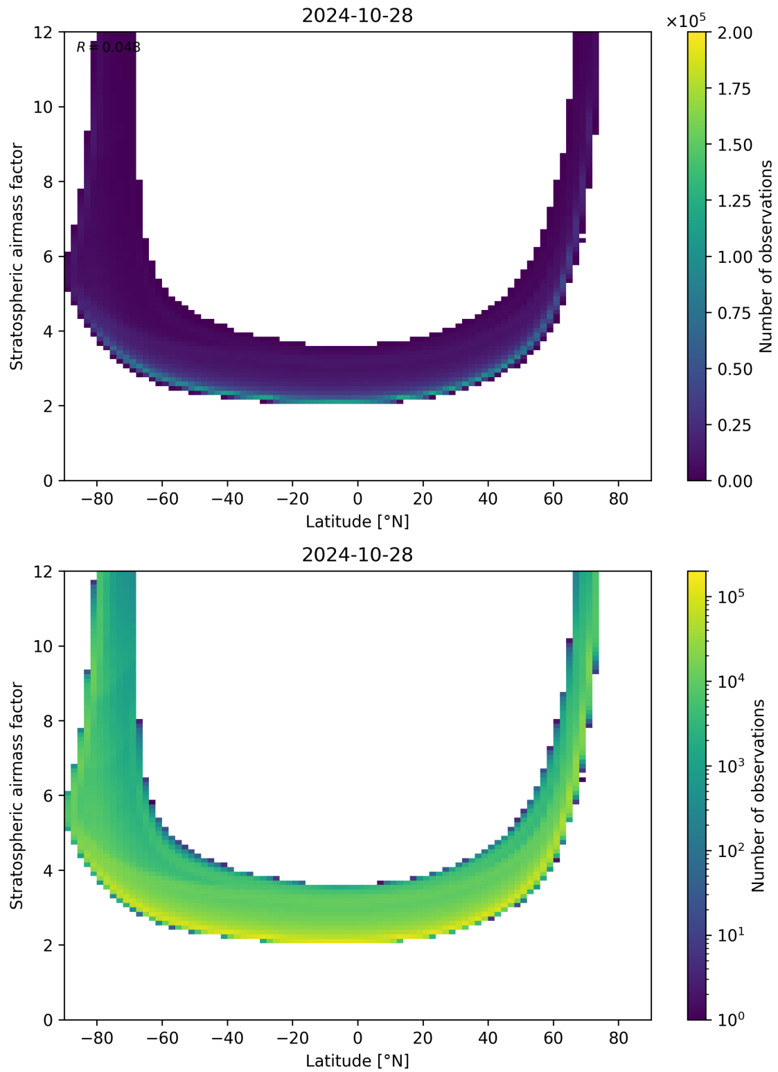
Figure 83: Scatter density plot of “Latitude” against “Stratospheric air mass factor” for 2024-10-27 to 2024-10-29.
