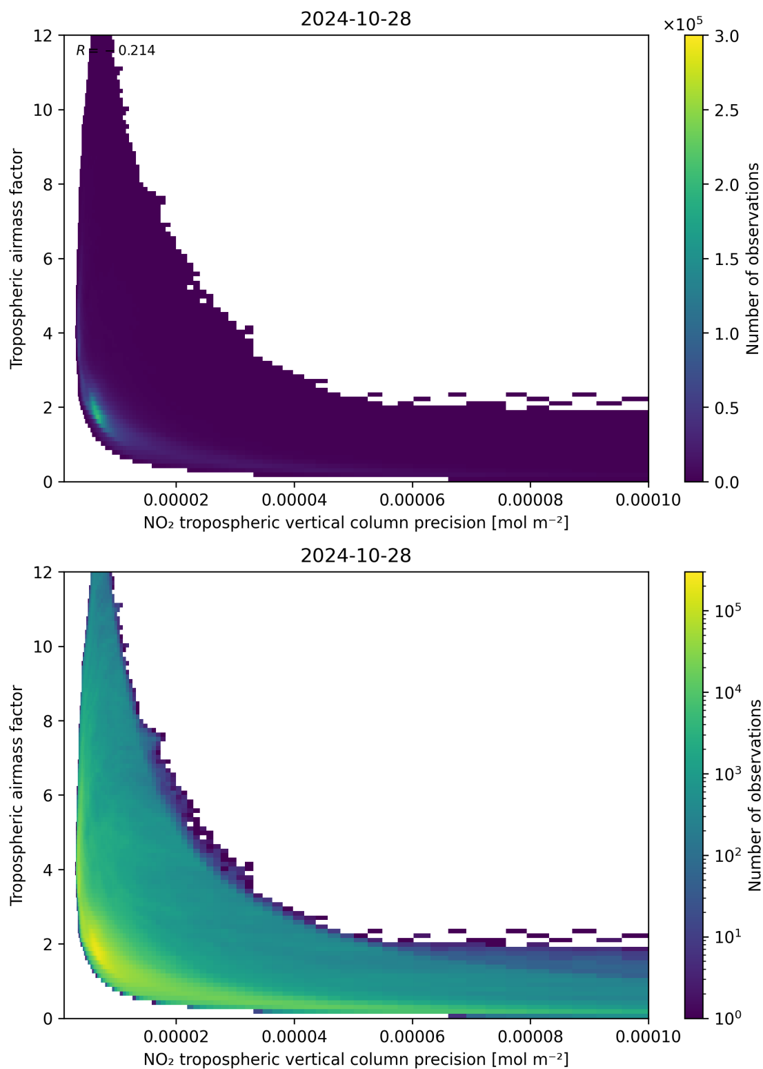
Figure 133: Scatter density plot of “NO 2 tropospheric vertical column precision” against “Tropospheric air mass factor” for 2024-10-27 to 2024-10-29.
