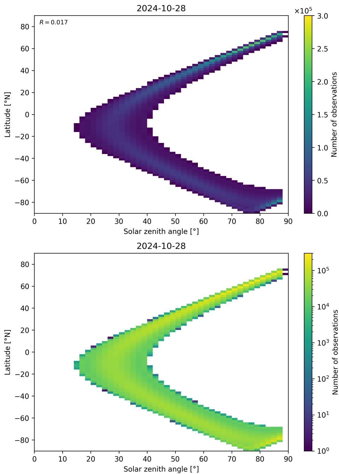
Figure 149: Scatter density plot of “Solar zenith angle” against “Latitude” for 2024-10-27 to 2024-10-29.
