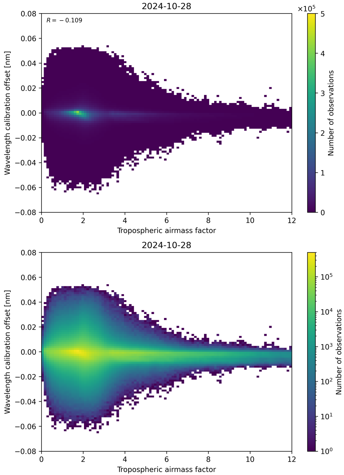
Figure 80: Scatter density plot of “Tropospheric airmass factor” against “Wavelength calibration offset” for 2024-10-27 to 2024-10-29.
