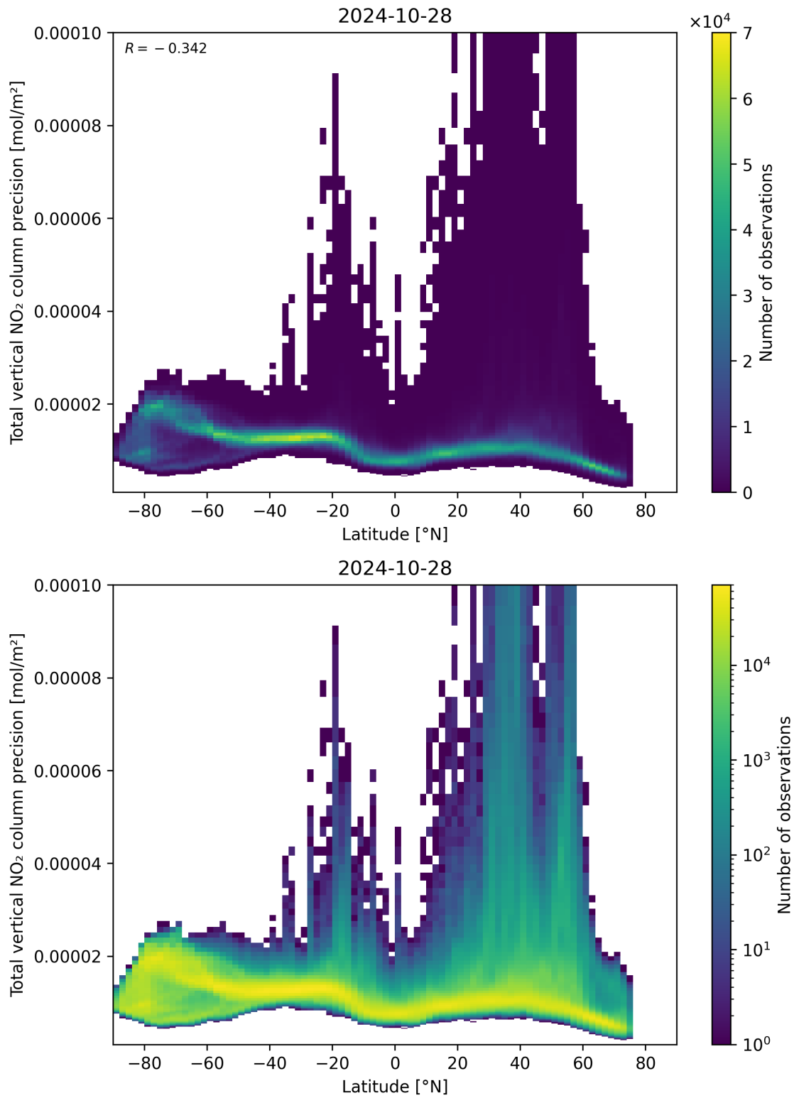
Figure 91: Scatter density plot of “Latitude” against “Total vertical NO 2 column precision” for 2024-10-27 to 2024-10-29.
