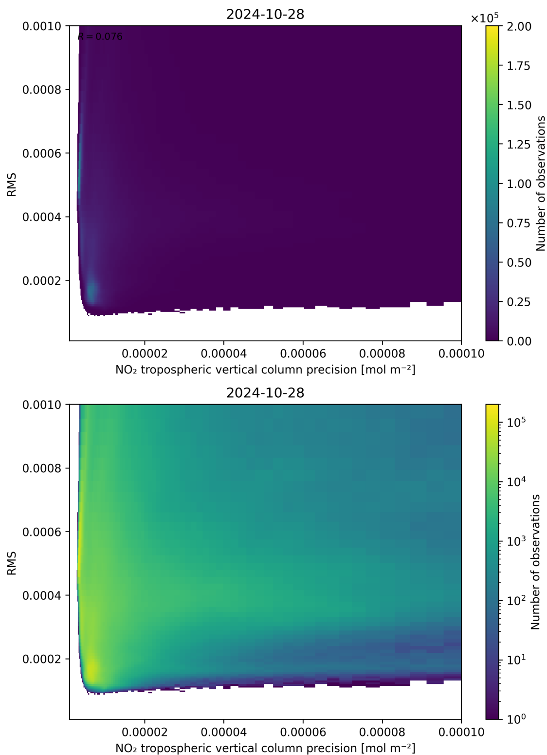
Figure 140: Scatter density plot of “NO 2 tropospheric vertical column precision” against “RMS” for 2024-10-27 to 2024-10-29.
