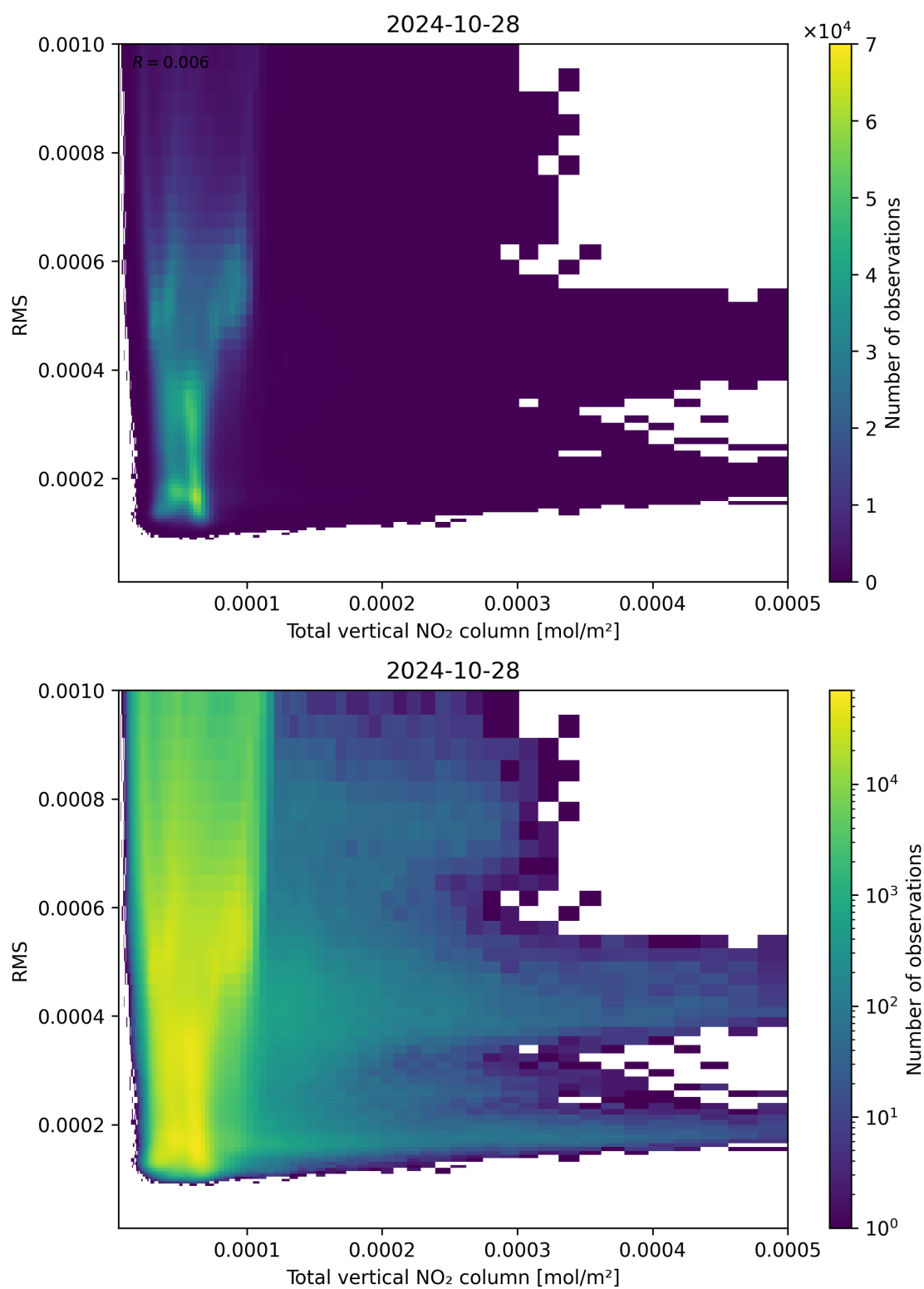
Figure 120: Scatter density plot of “Total vertical NO 2 column” against “RMS” for 2024-10-27 to 2024-10-29.
