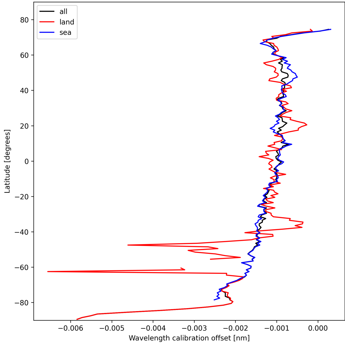
Figure 18: Zonal average of “Wavelength calibration offset” for 2024-10-27 to 2024-10-29.
