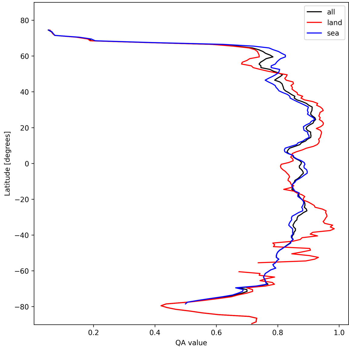
Figure 11: Zonal average of “QA value” for 2024-10-27 to 2024-10-29.
