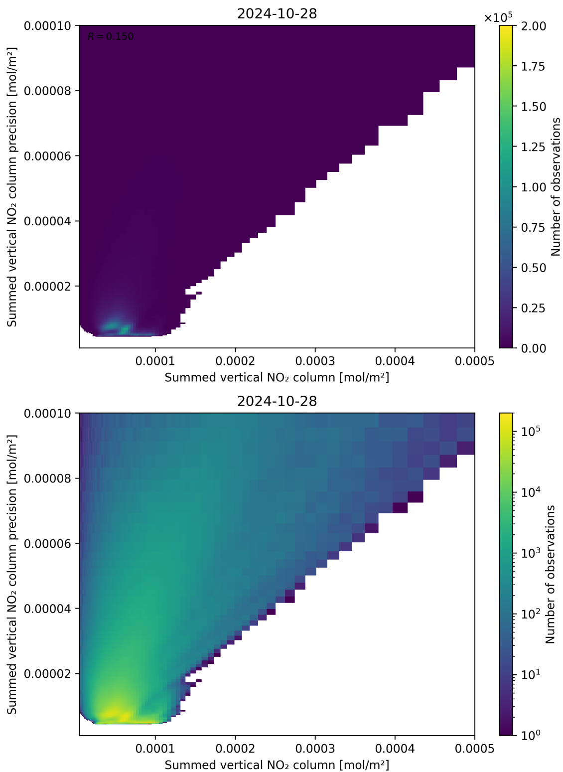
Figure 105: Scatter density plot of “Summed vertical NO 2 column” against “Summed vertical NO 2 column precision” for 2024-10-27 to 2024-10-29.
