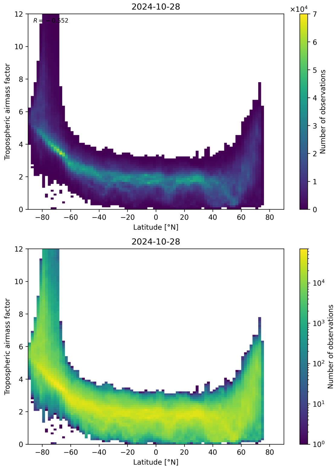
Figure 85: Scatter density plot of “Latitude” against “Tropospheric air mass factor” for 2024-10-27 to 2024-10-29.
