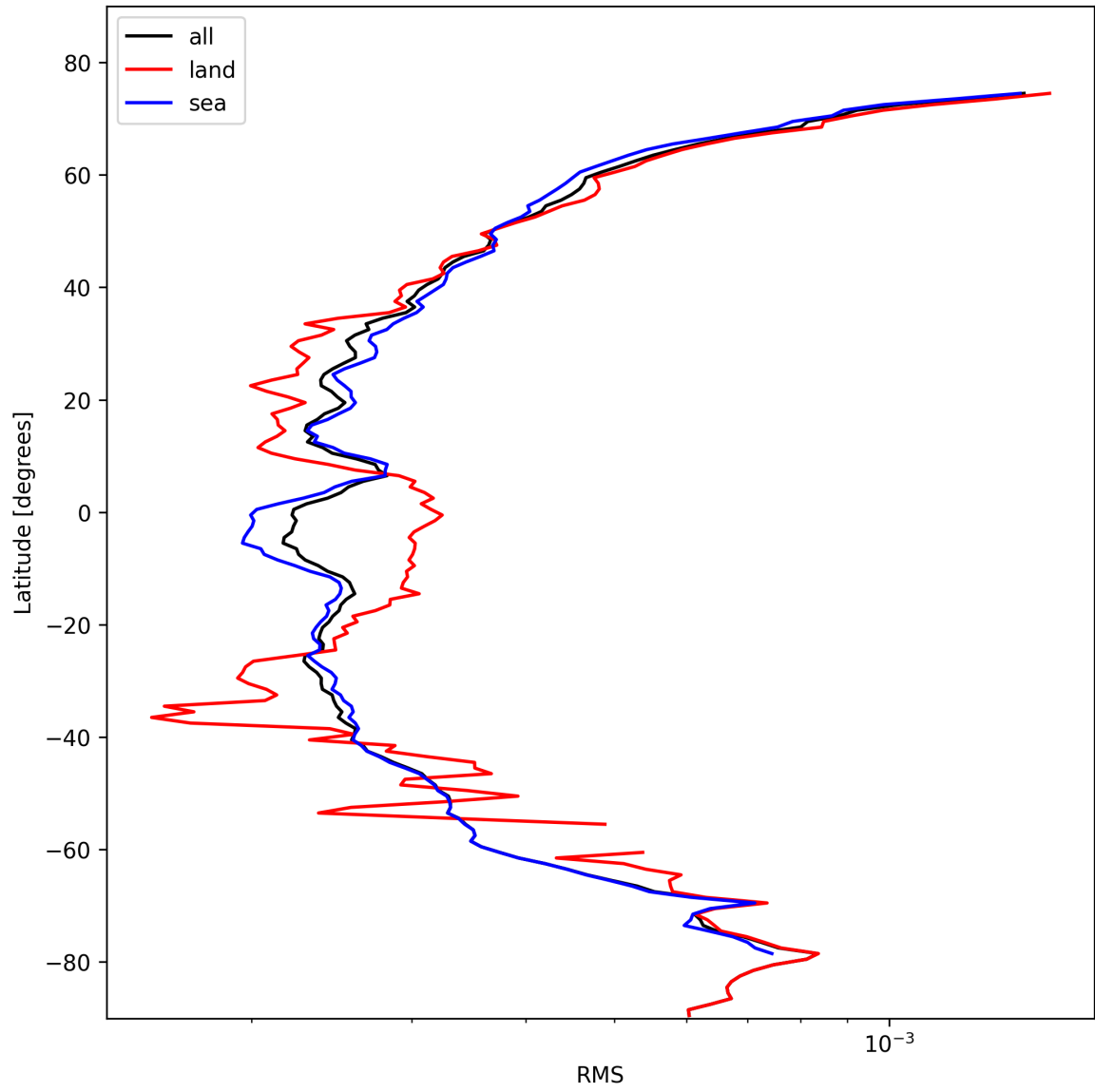
Figure 26: Zonal average of “RMS” for 2024-10-27 to 2024-10-29.
