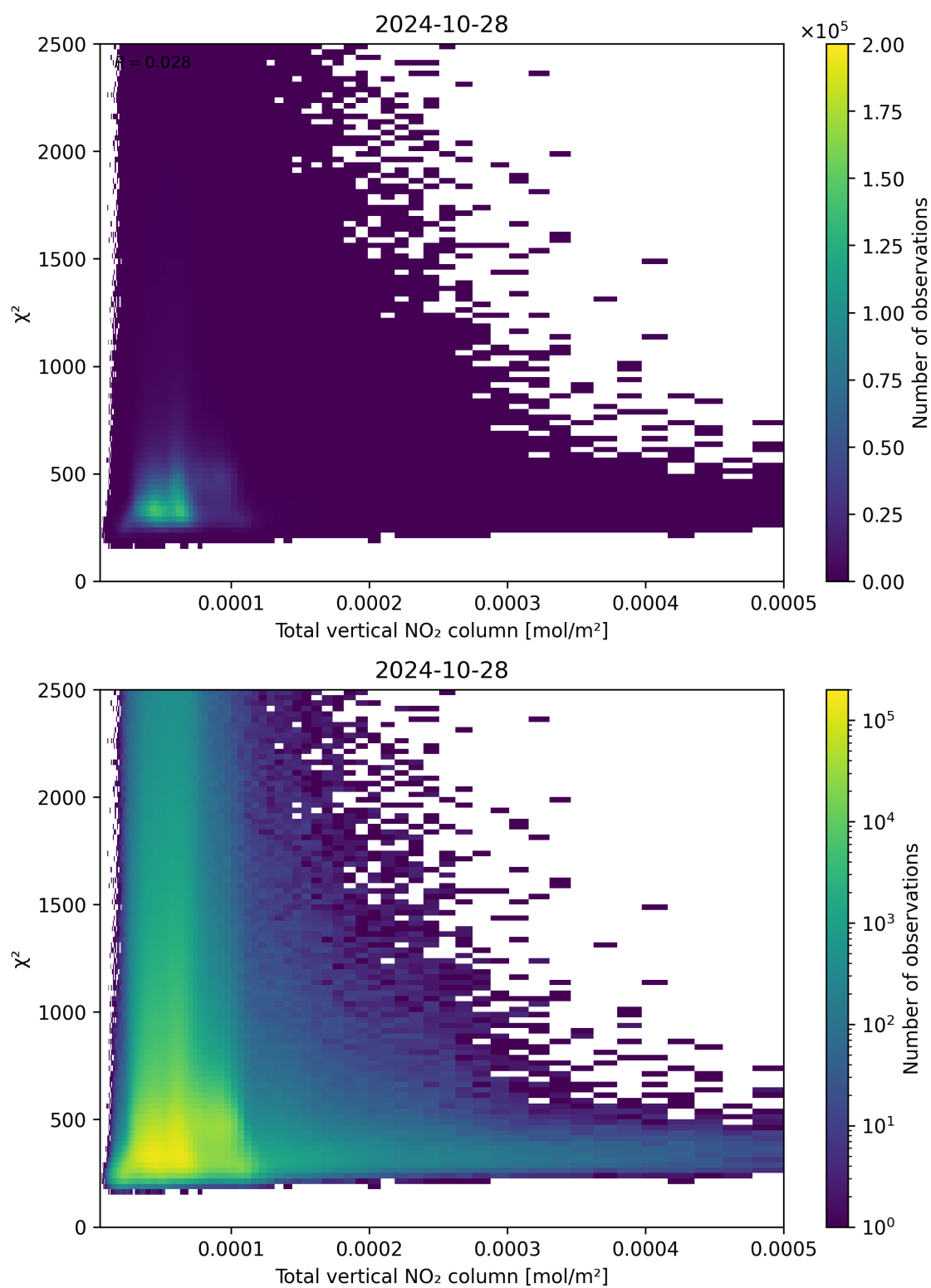
Figure 111: Scatter density plot of “Total vertical NO 2 column” against “ \chi^2 ” for 2024-10-27 to 2024-10-29.
