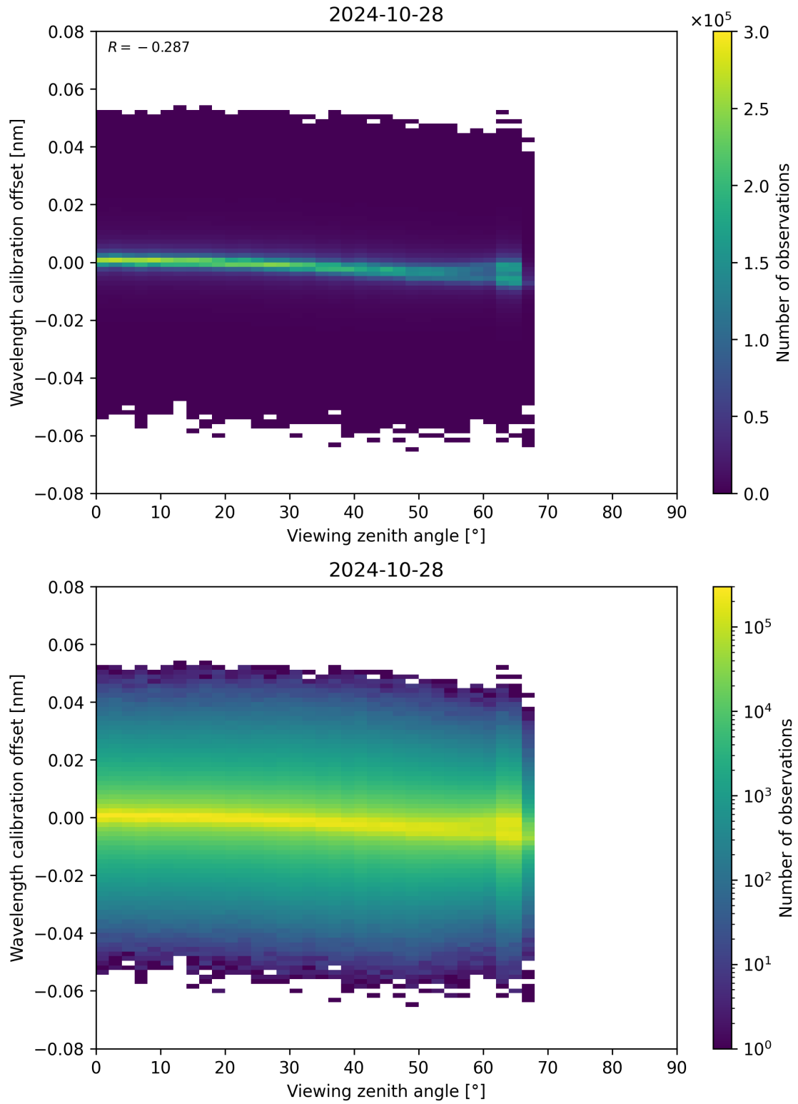
Figure 173: Scatter density plot of “Viewing zenith angle” against “Wavelength calibration offset” for 2024-10-27 to 2024-10-29.
