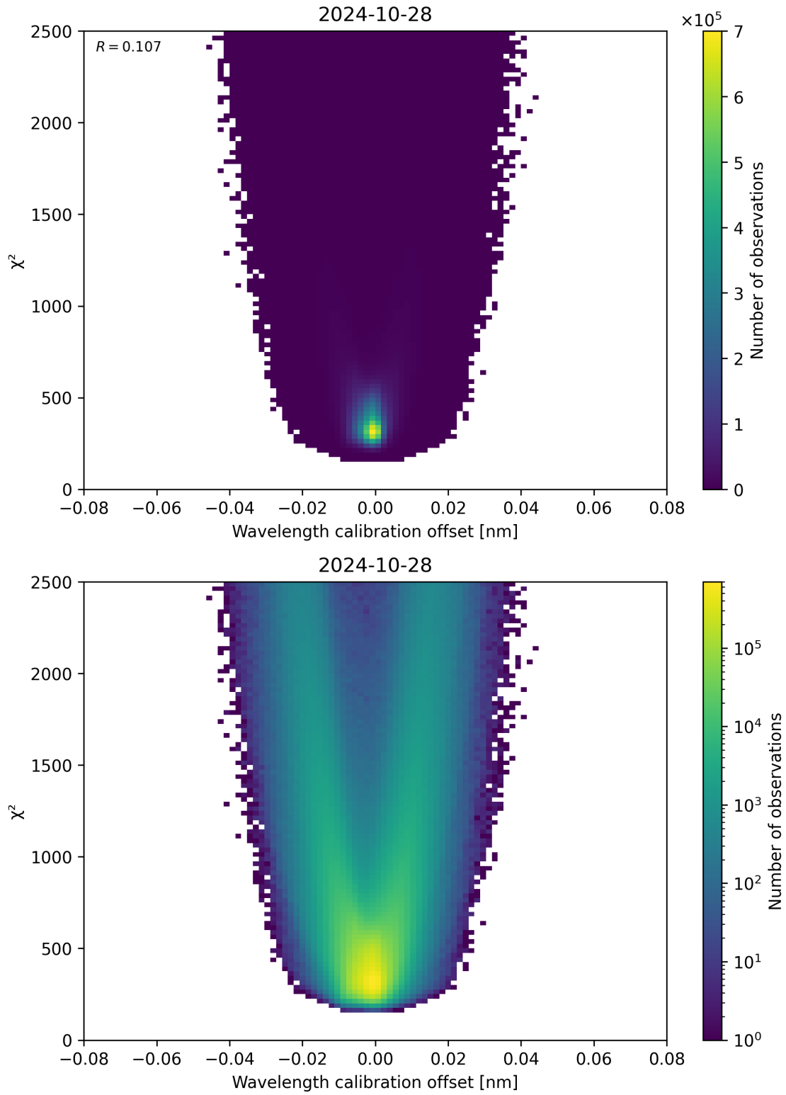
Figure 175: Scatter density plot of “Wavelength calibration offset” against “ \chi^2 ” for 2024-10-27 to 2024-10-29.
