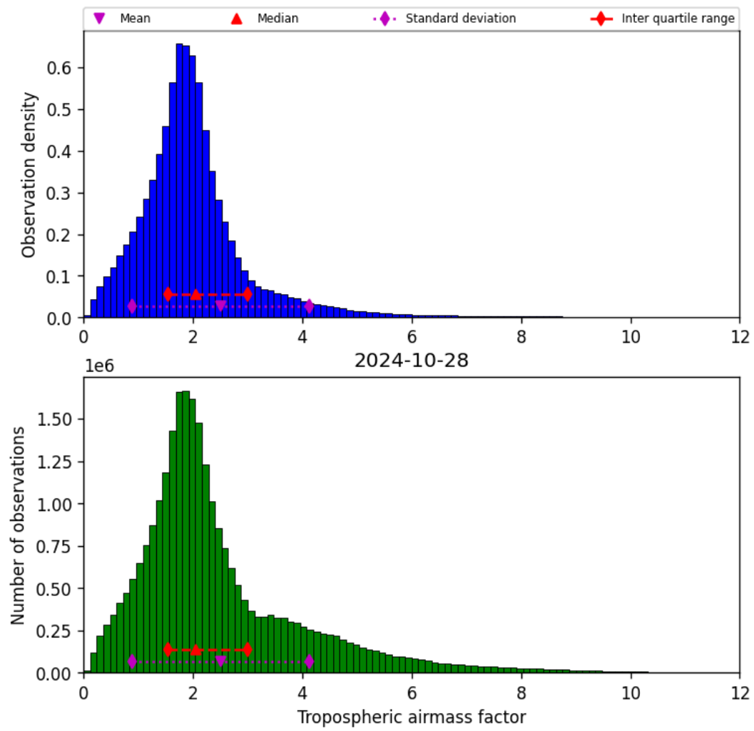
Figure 31: Histogram of “Tropospheric airmass factor” for 2024-10-27 to 2024-10-29
