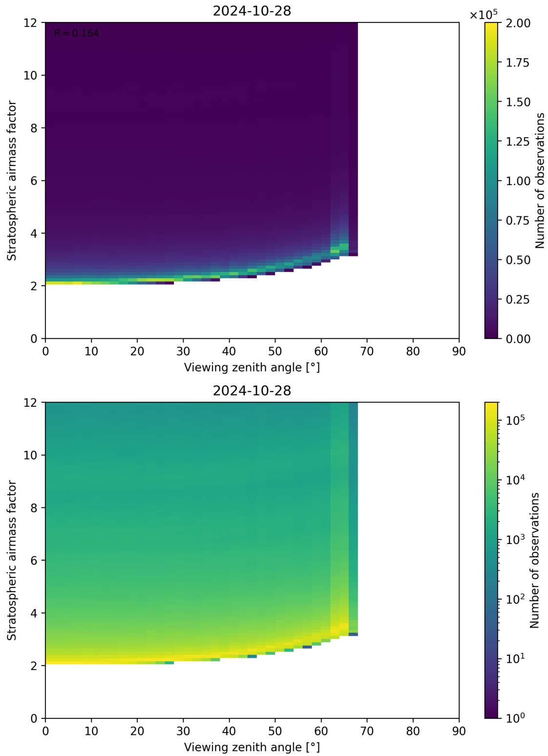
Figure 159: Scatter density plot of “Viewing zenith angle” against “Stratospheric airmass factor” for 2024-10-27 to 2024-10-29.
