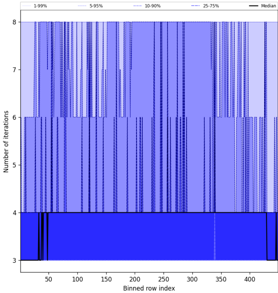
Figure 51: Along track statistics of “Number of iterations” for 2024-10-27 to 2024-10-29
