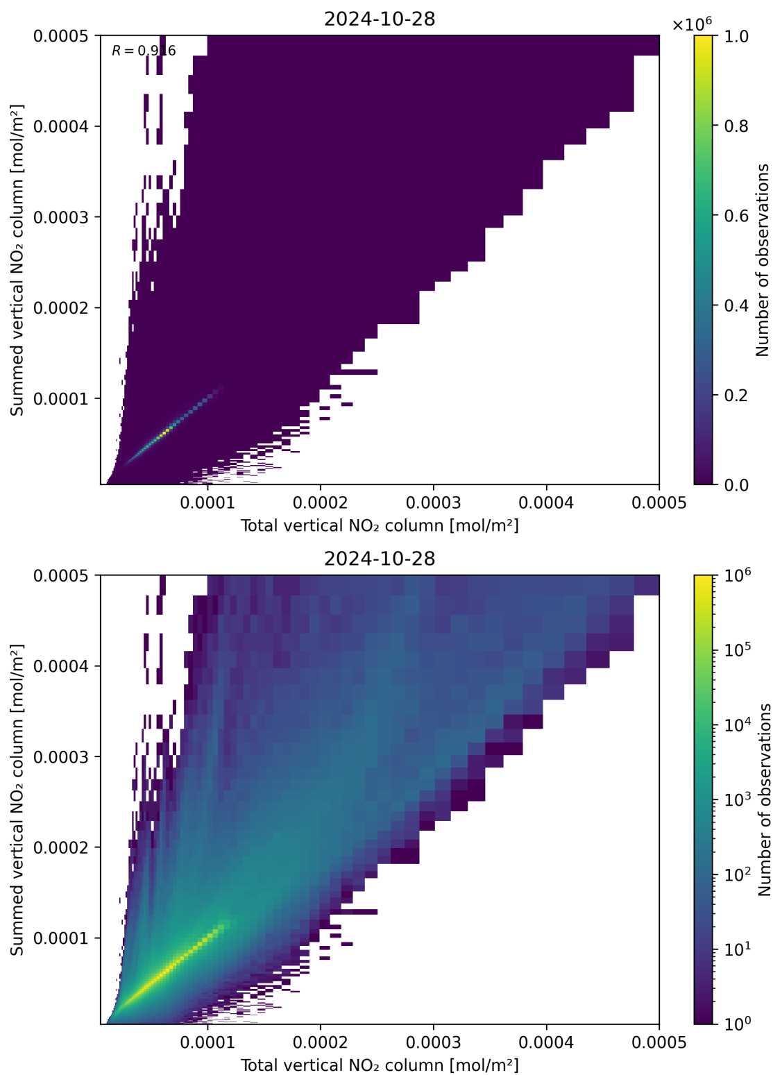
Figure 112: Scatter density plot of “Total vertical NO 2 column” against “Summed vertical NO 2 column” for 2024-10-27 to 2024-10-29.
