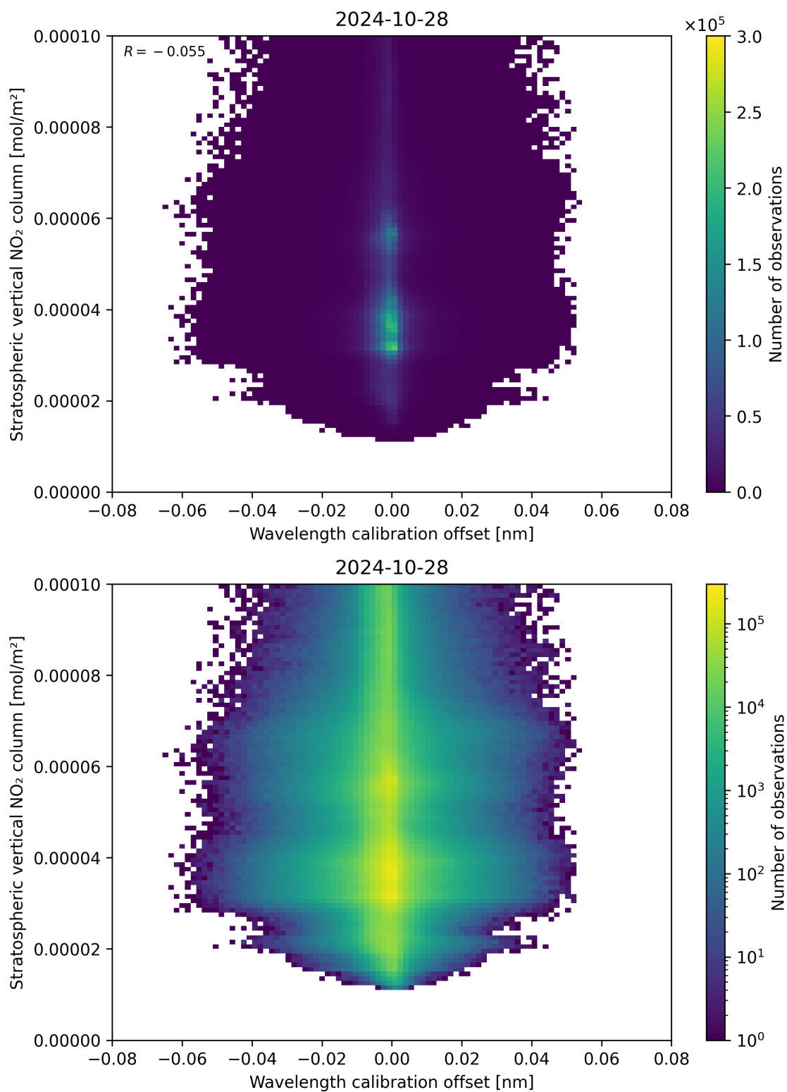
Figure 176: Scatter density plot of “Wavelength calibration offset” against “Stratospheric vertical NO 2 column” for 2024-10-27 to 2024-10-29.
