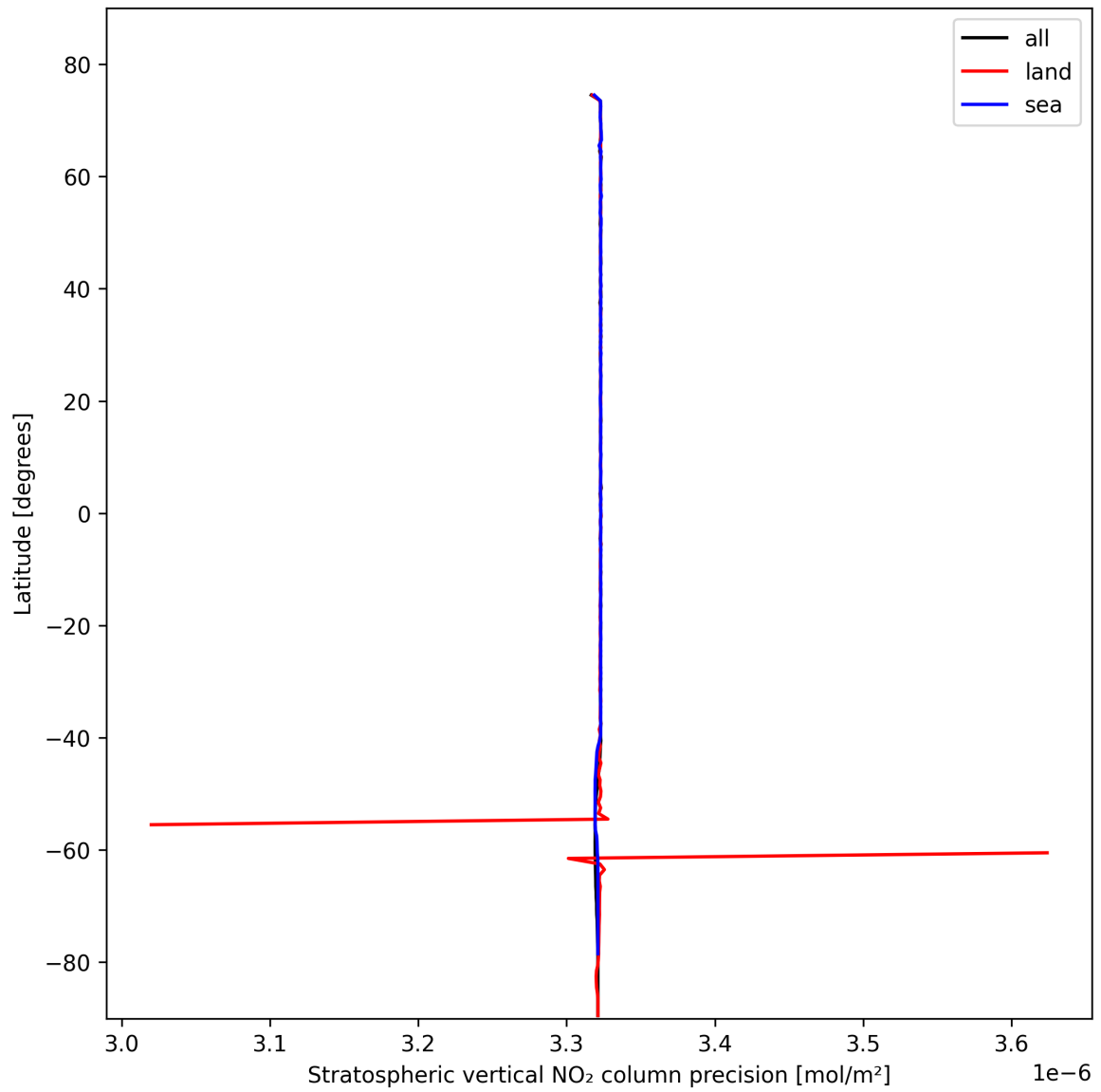
Figure 20: Zonal average of “Stratospheric vertical NO 2 column precision” for 2024-10-27 to 2024-10-29.
