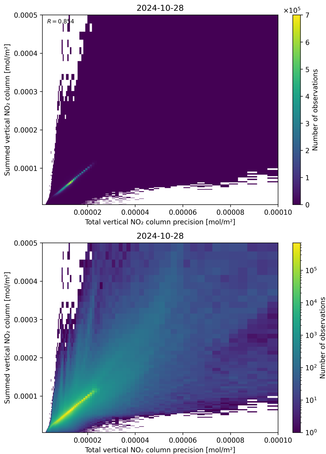
Figure 117: Scatter density plot of “Total vertical NO 2 column precision” against “Summed vertical NO 2 column” for 2024-10-27 to 2024-10-29.
