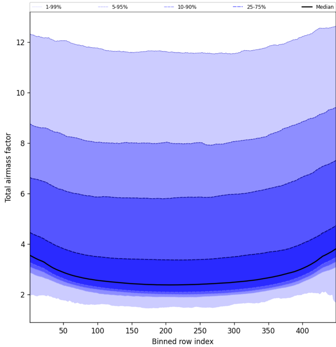
Figure 49: Along track statistics of “Total airmass factor” for 2024-10-27 to 2024-10-29
