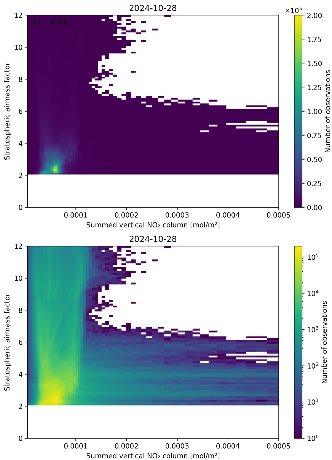
Figure 103: Scatter density plot of “Summed vertical NO 2 column” against “Stratospheric air mass factor” for 2024-10-27 to 2024-10-29.
