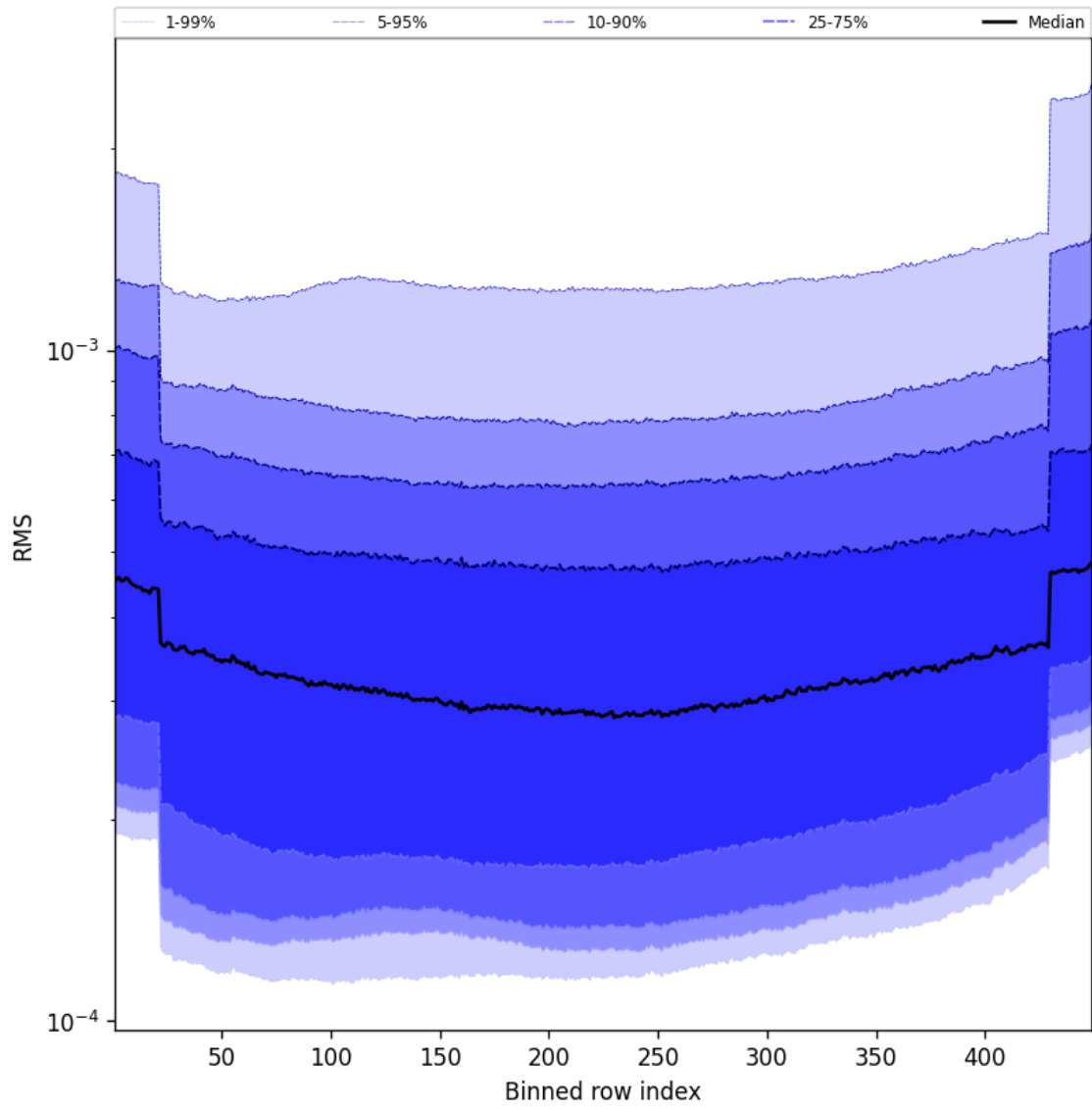
Figure 60: Along track statistics of “RMS” for 2024-10-27 to 2024-10-29
