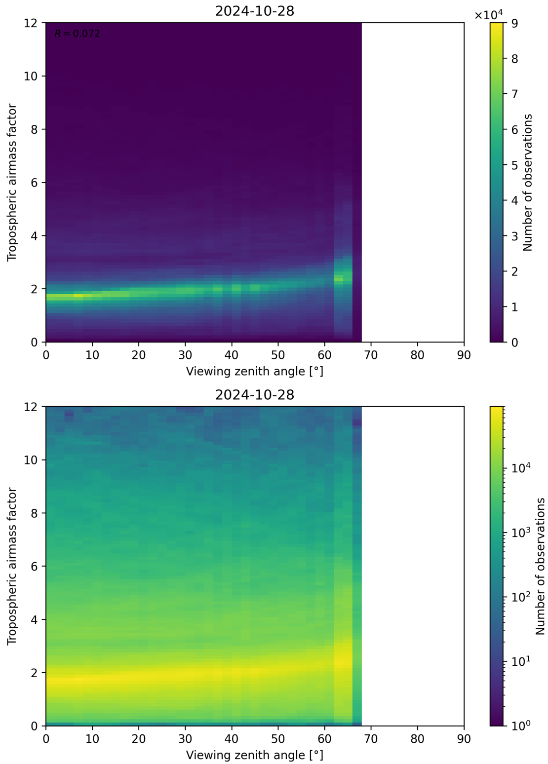
Figure 161: Scatter density plot of “Viewing zenith angle” against “Tropospheric airmass factor” for 2024-10-27 to 2024-10-29.
