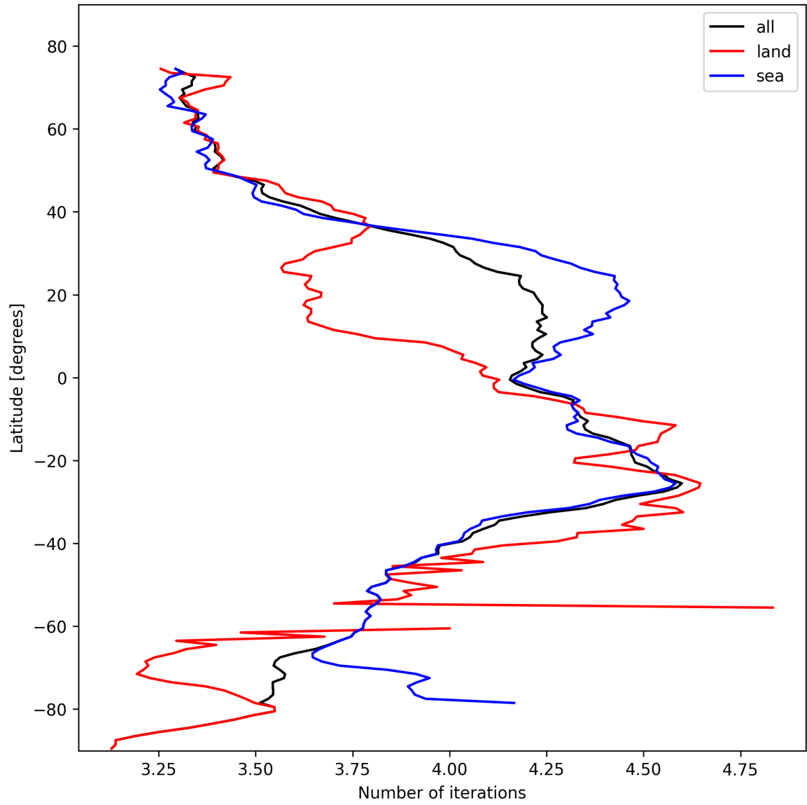
Figure 17: Zonal average of “Number of iterations” for 2024-10-27 to 2024-10-29.
