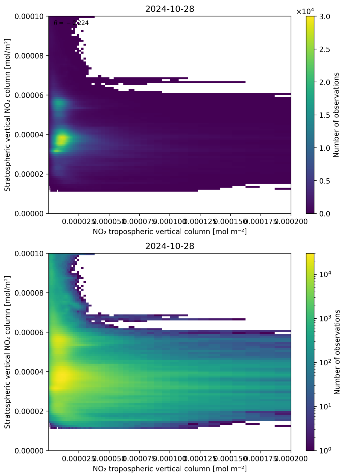
Figure 125: Scatter density plot of “NO 2 tropospheric vertical column” against “Stratospheric vertical NO 2 column” for 2024-10-27 to 2024-10-29.
