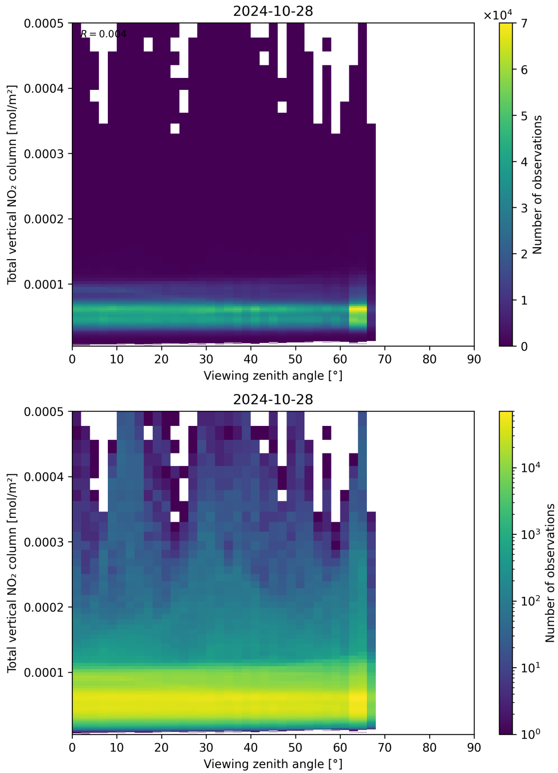
Figure 167: Scatter density plot of “Viewing zenith angle” against “Total vertical NO 2 column” for 2024-10-27 to 2024-10-29.
