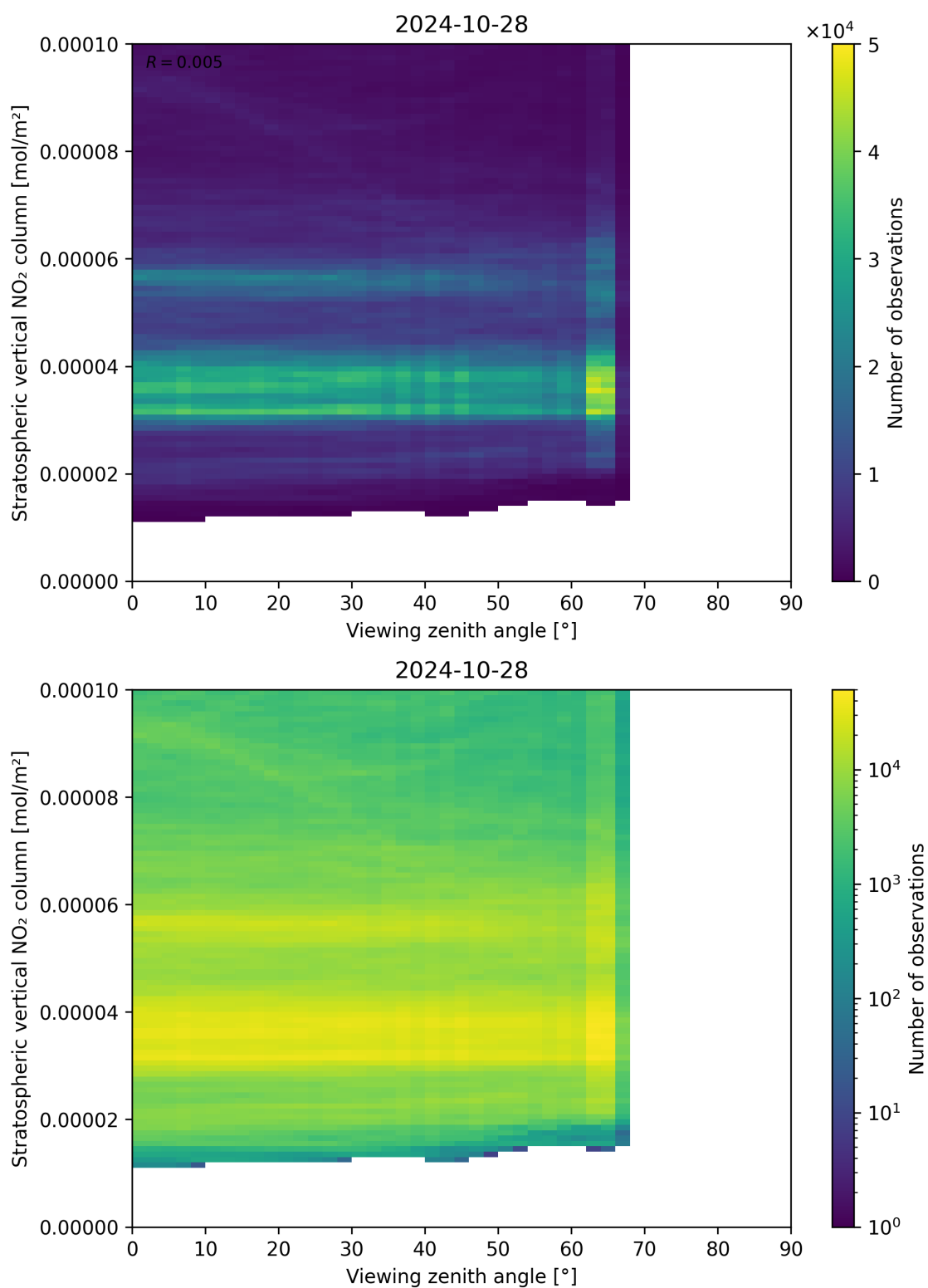
Figure 164: Scatter density plot of “Viewing zenith angle” against “Stratospheric vertical NO 2 column” for 2024-10-27 to 2024-10-29.
