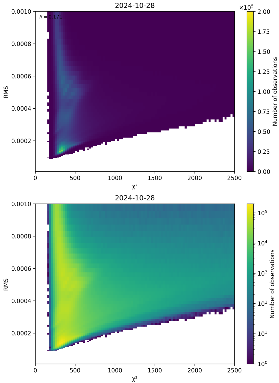
Figure 82: Scatter density plot of “ \chi^2 ” against “RMS” for 2024-10-27 to 2024-10-29.
