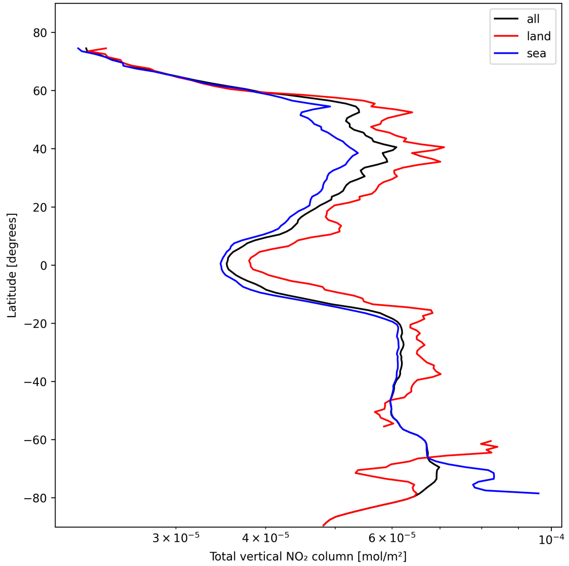
Figure 21: Zonal average of “Total vertical NO 2 column” for 2024-10-27 to 2024-10-29.
