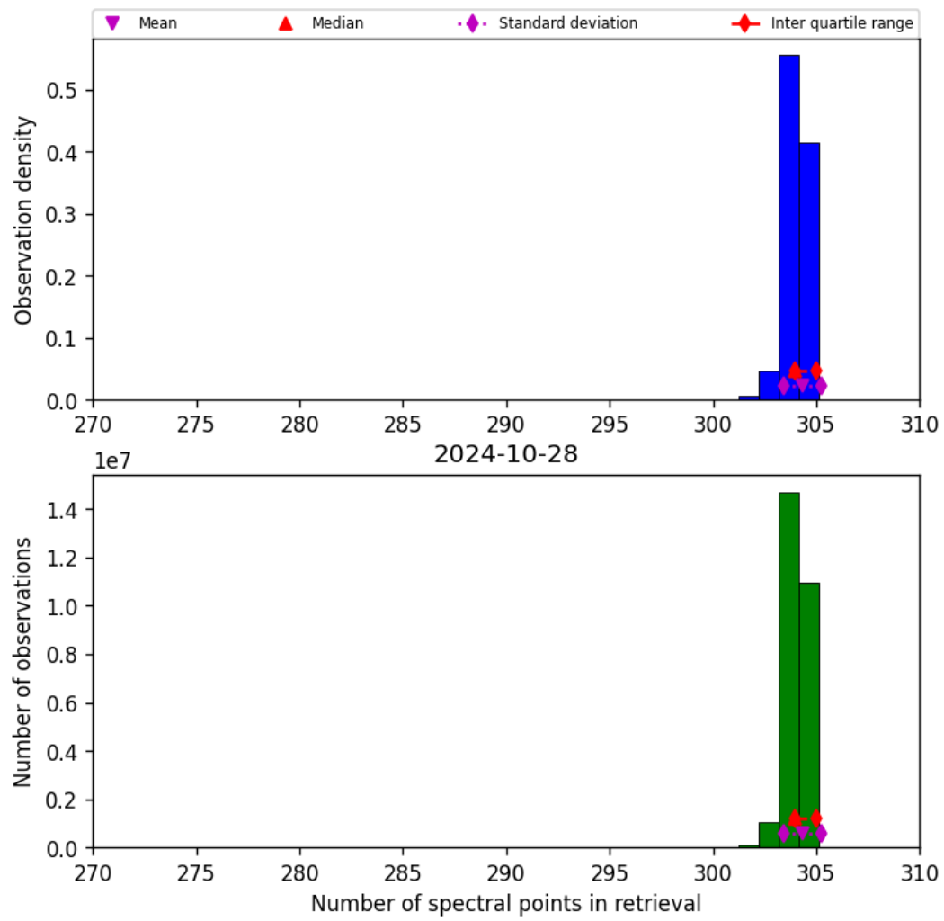
Figure 33: Histogram of “Number of spectral points in retrieval” for 2024-10-27 to 2024-10-29
