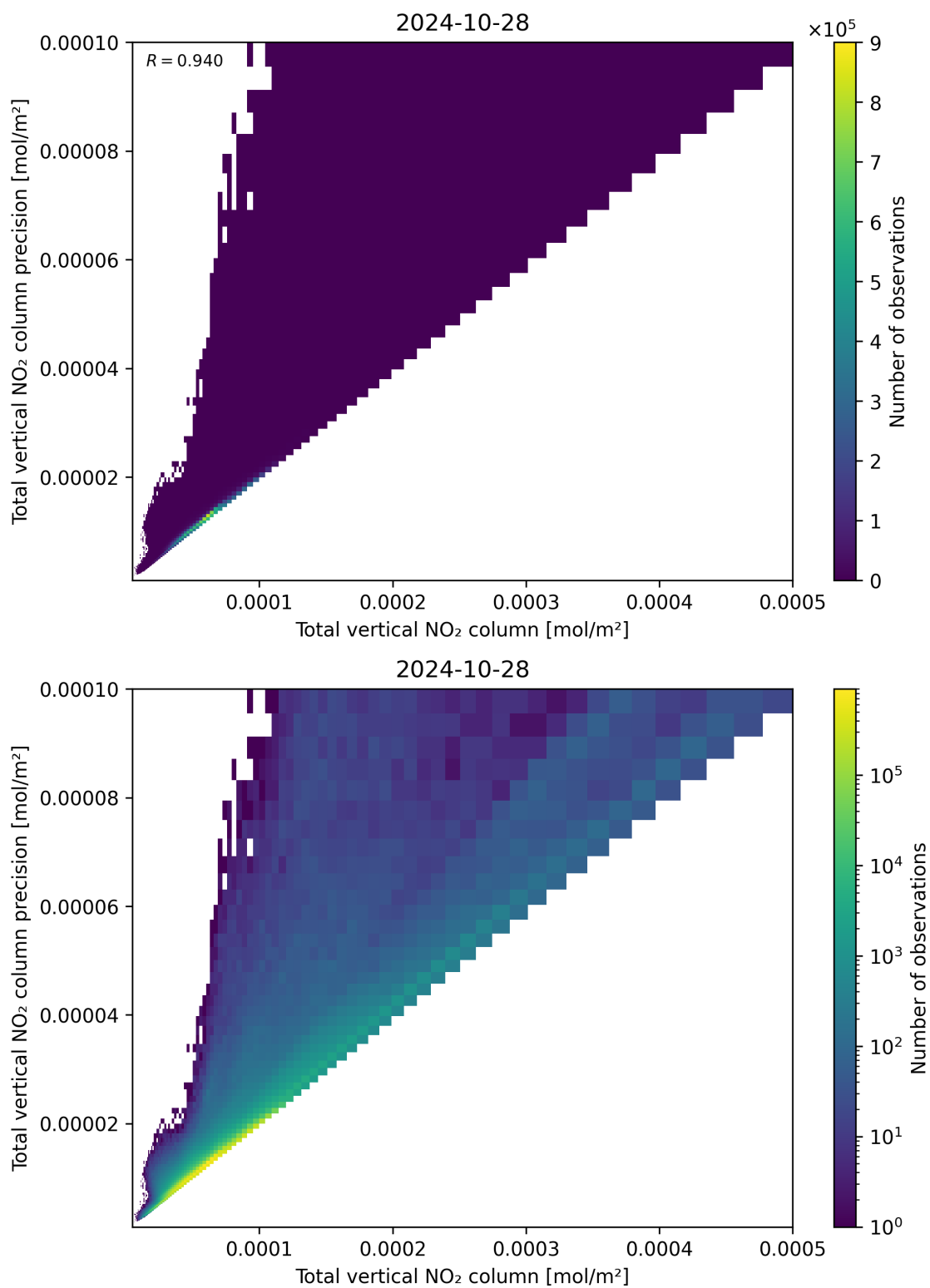
Figure 114: Scatter density plot of “Total vertical NO 2 column” against “Total vertical NO 2 column precision” for 2024-10-27 to 2024-10-29.
