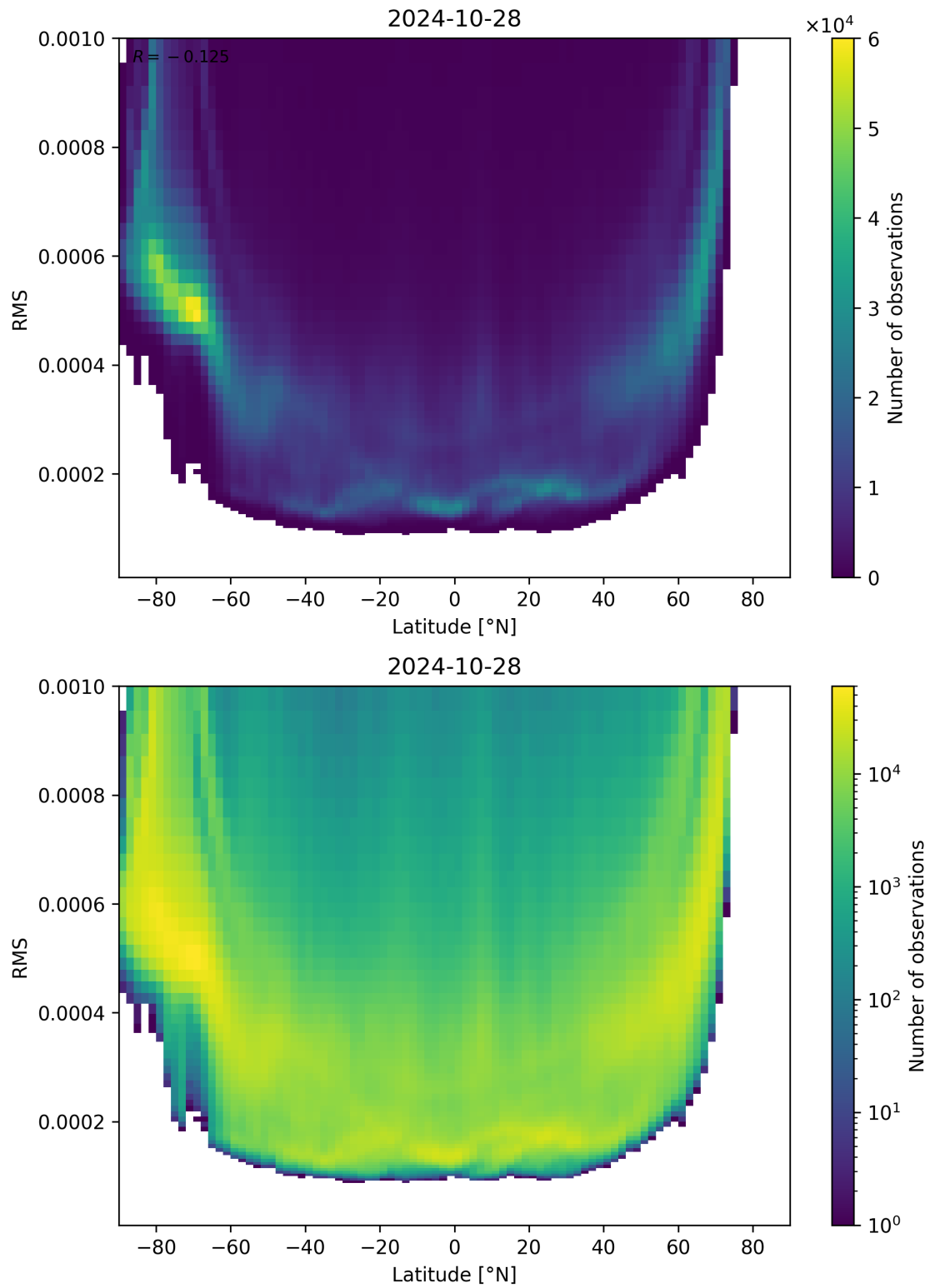
Figure 94: Scatter density plot of “Latitude” against “RMS” for 2024-10-27 to 2024-10-29.
