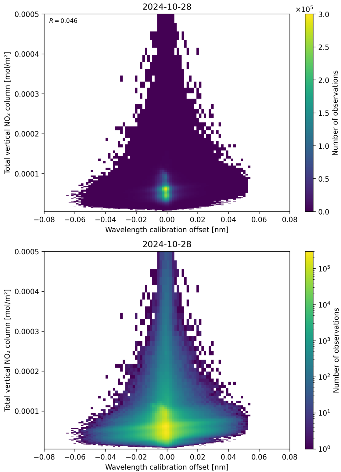
Figure 179: Scatter density plot of “Wavelength calibration offset” against “Total vertical NO 2 column” for 2024-10-27 to 2024-10-29.
