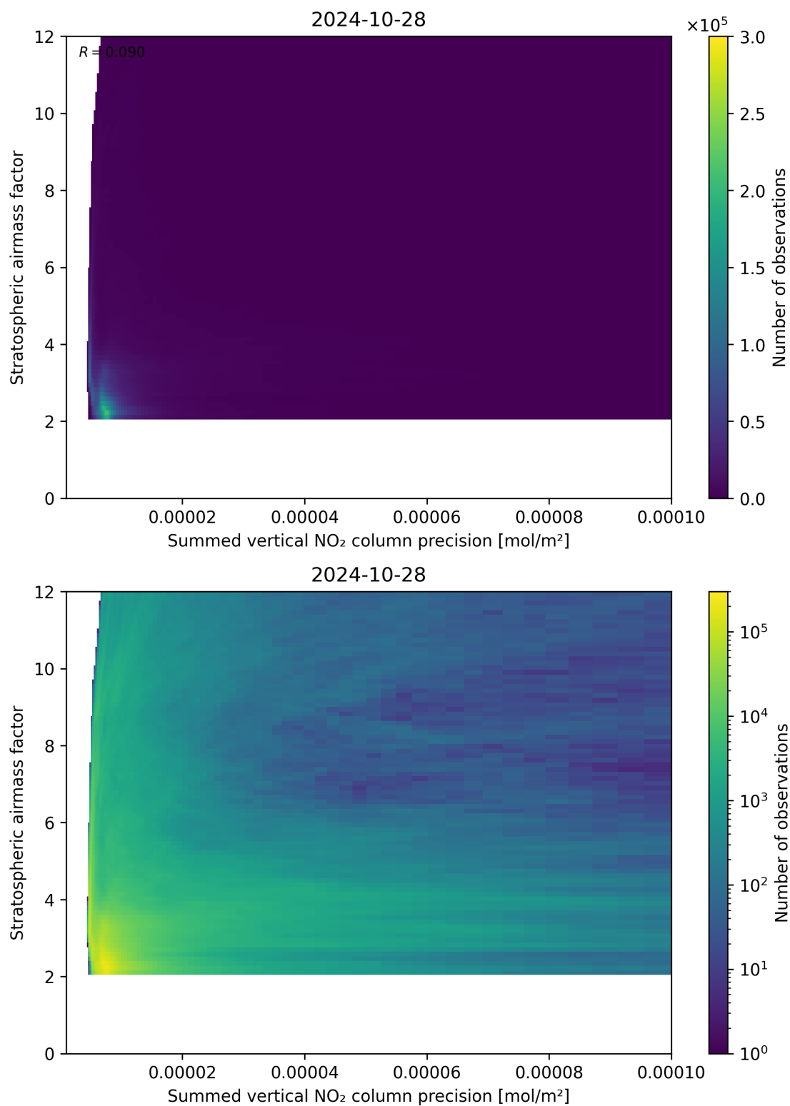
Figure 106: Scatter density plot of “Summed vertical NO 2 column precision” against “Stratospheric airmass factor” for 2024-10-27 to 2024-10-29.
