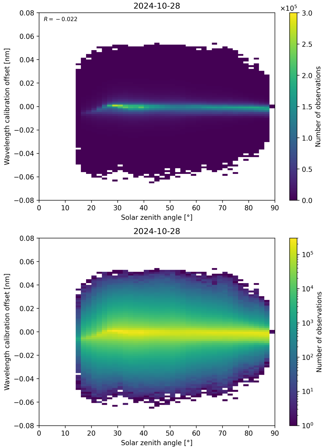
Figure 158: Scatter density plot of “Solar zenith angle” against “Wavelength calibration offset” for 2024-10-27 to 2024-10-29.
