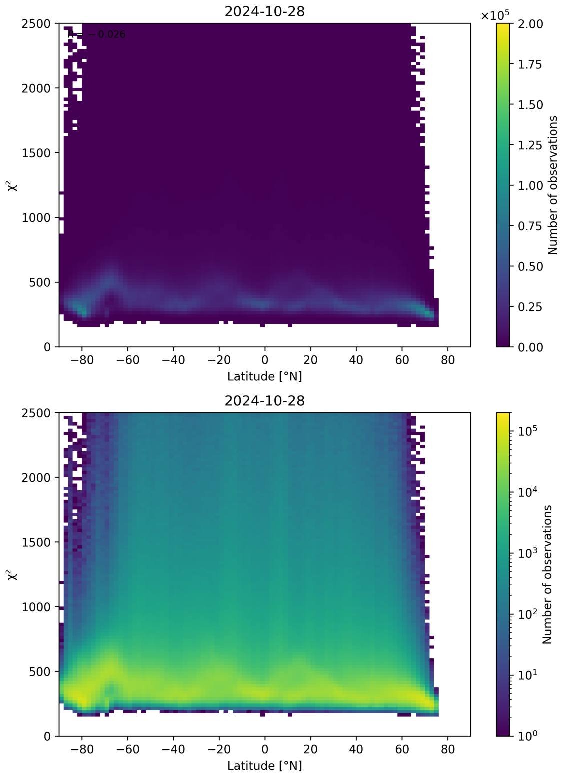
Figure 86: Scatter density plot of “Latitude” against “ \chi^2 ” for 2024-10-27 to 2024-10-29.
