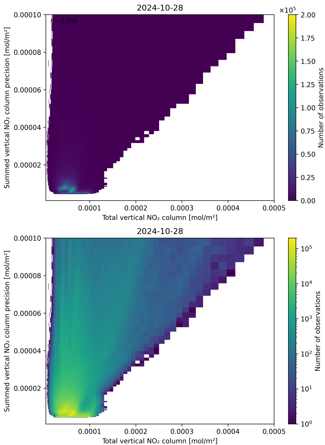
Figure 113: Scatter density plot of “Total vertical NO 2 column” against “Summed vertical NO 2 column precision” for 2024-10-27 to 2024-10-29.
