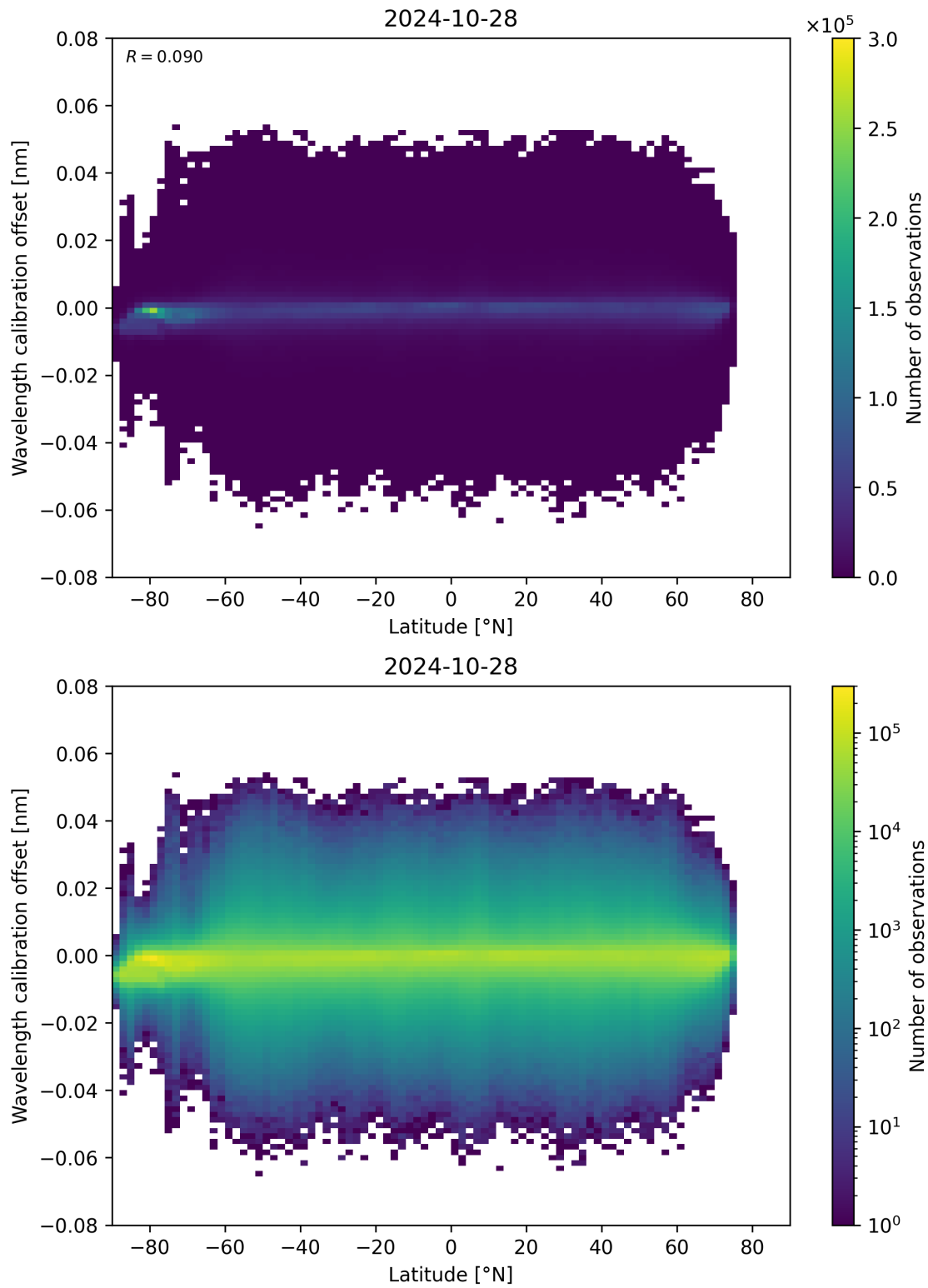
Figure 95: Scatter density plot of “Latitude” against “Wavelength calibration offset” for 2024-10-27 to 2024-10-29.
