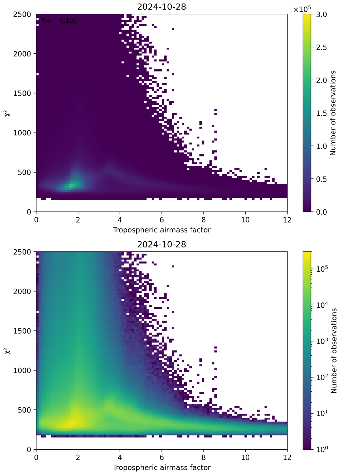
Figure 73: Scatter density plot of “Tropospheric airmass factor” against “ \chi^2 ” for 2024-10-27 to 2024-10-29.
