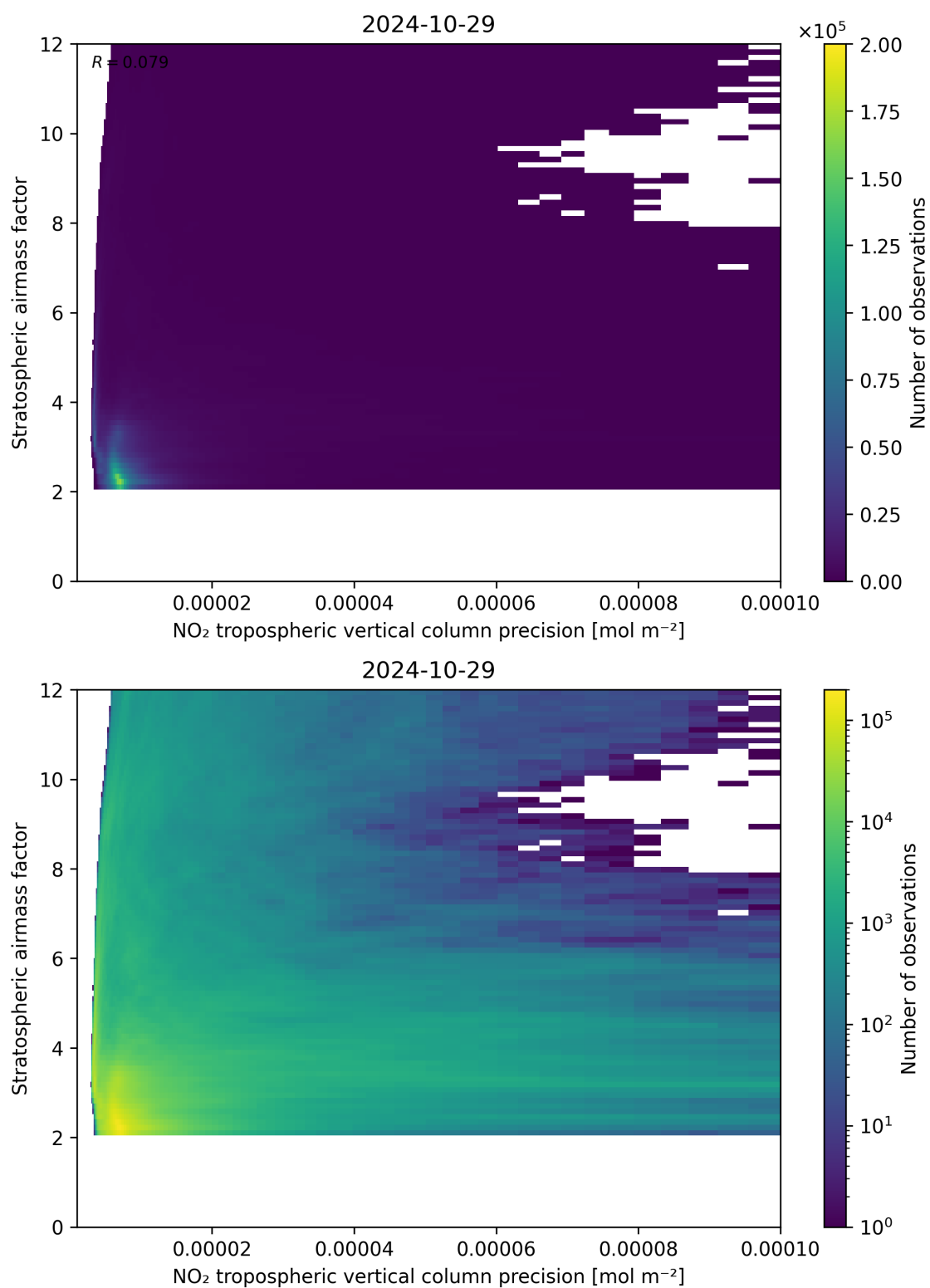
Figure 131: Scatter density plot of “NO 2 tropospheric vertical column precision” against “Stratospheric airmass factor” for 2024-10-29 to 2024-10-30.
