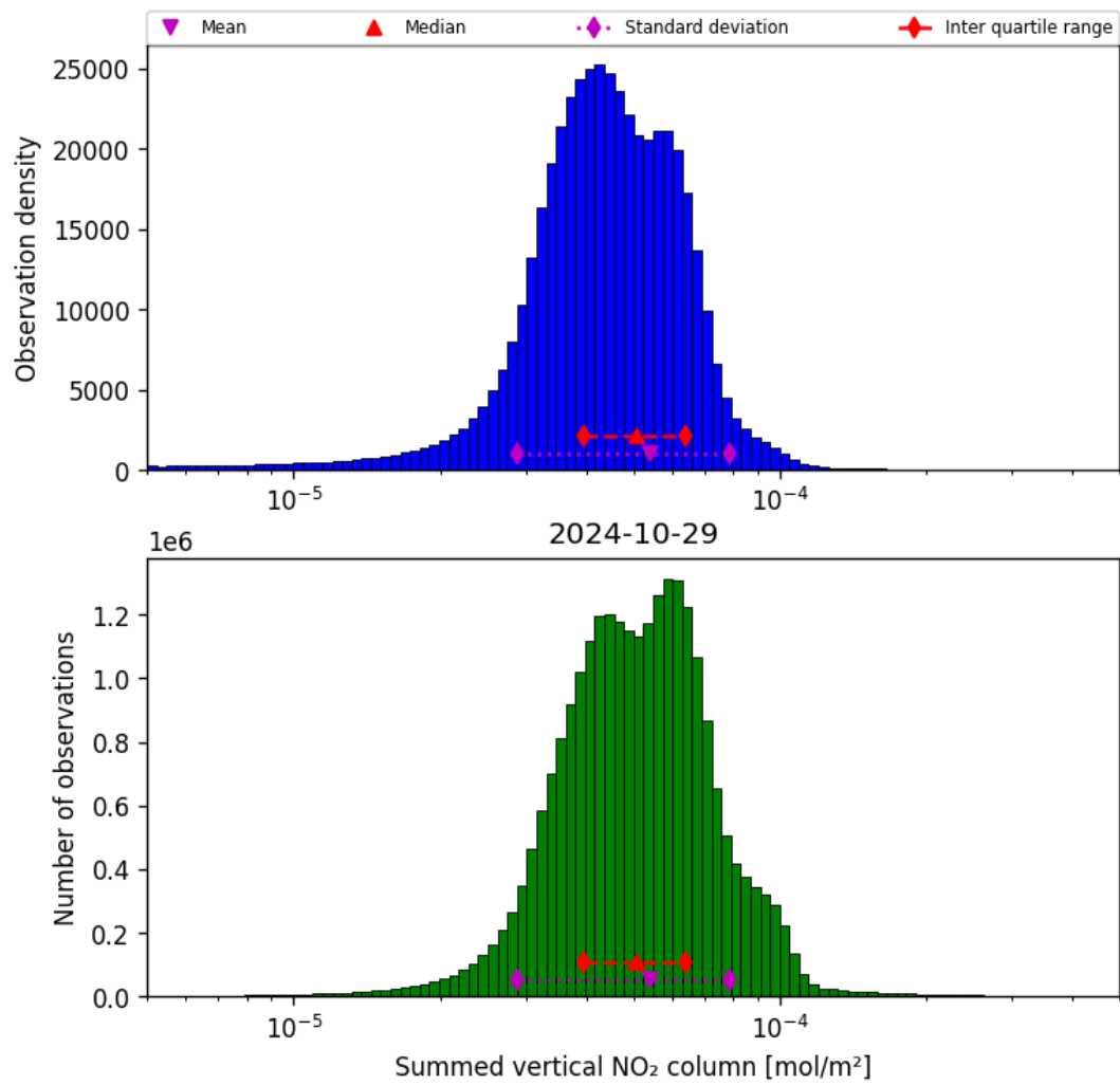
Figure 40: Histogram of “Summed vertical NO 2 column” for 2024-10-29 to 2024-10-30
