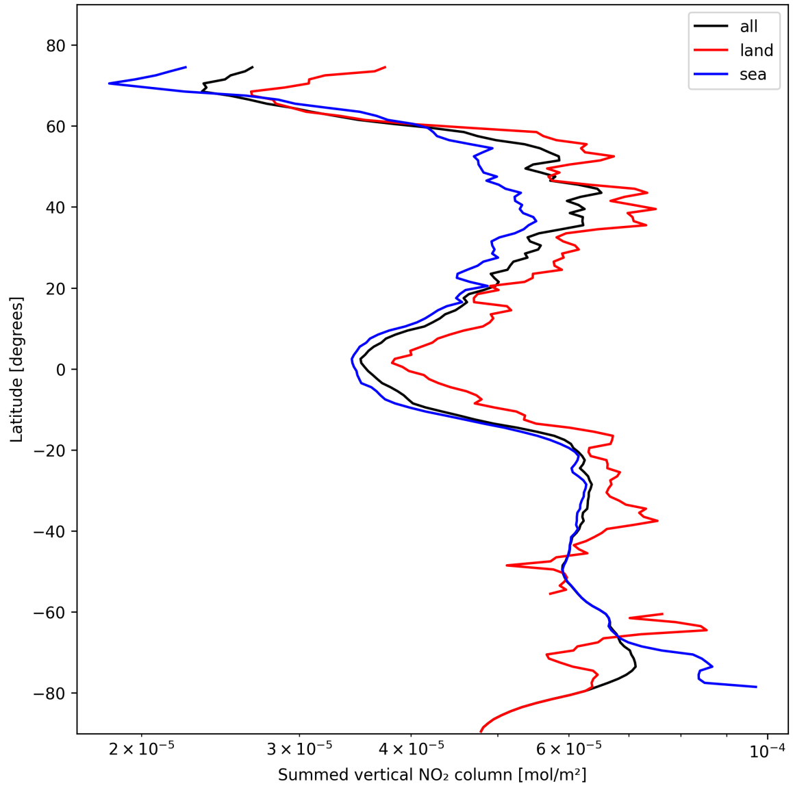
Figure 23: Zonal average of “Summed vertical NO 2 column” for 2024-10-29 to 2024-10-30.
