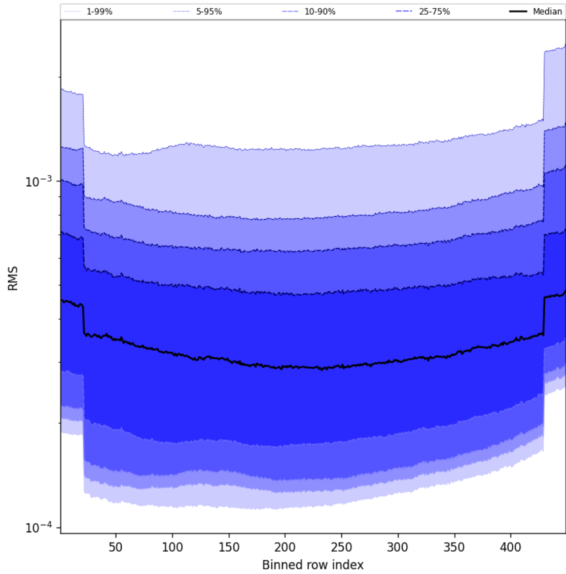
Figure 60: Along track statistics of “RMS” for 2024-10-29 to 2024-10-30
