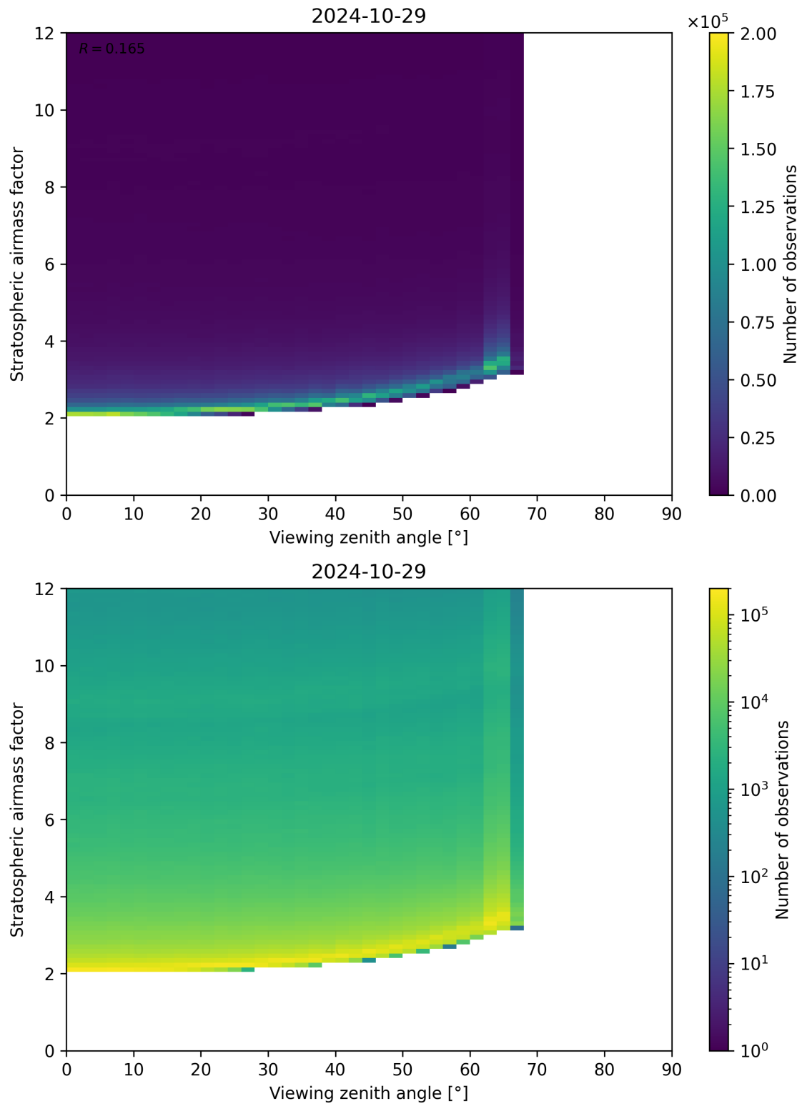
Figure 159: Scatter density plot of “Viewing zenith angle” against “Stratospheric airmass factor” for 2024-10-29 to 2024-10-30.
