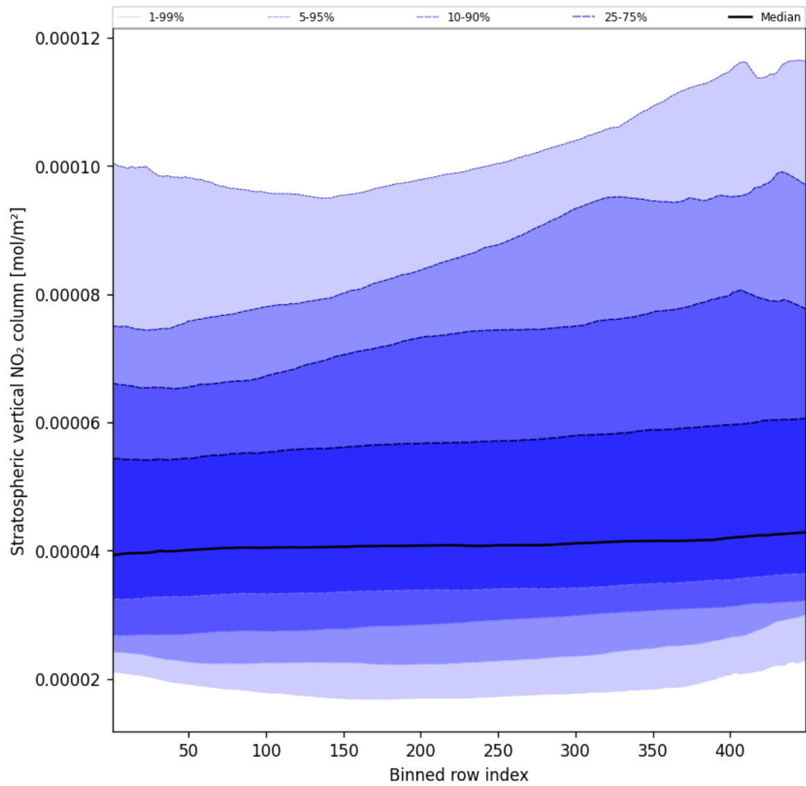
Figure 53: Along track statistics of “Stratospheric vertical NO 2 column” for 2024-10-29 to 2024-10-30
