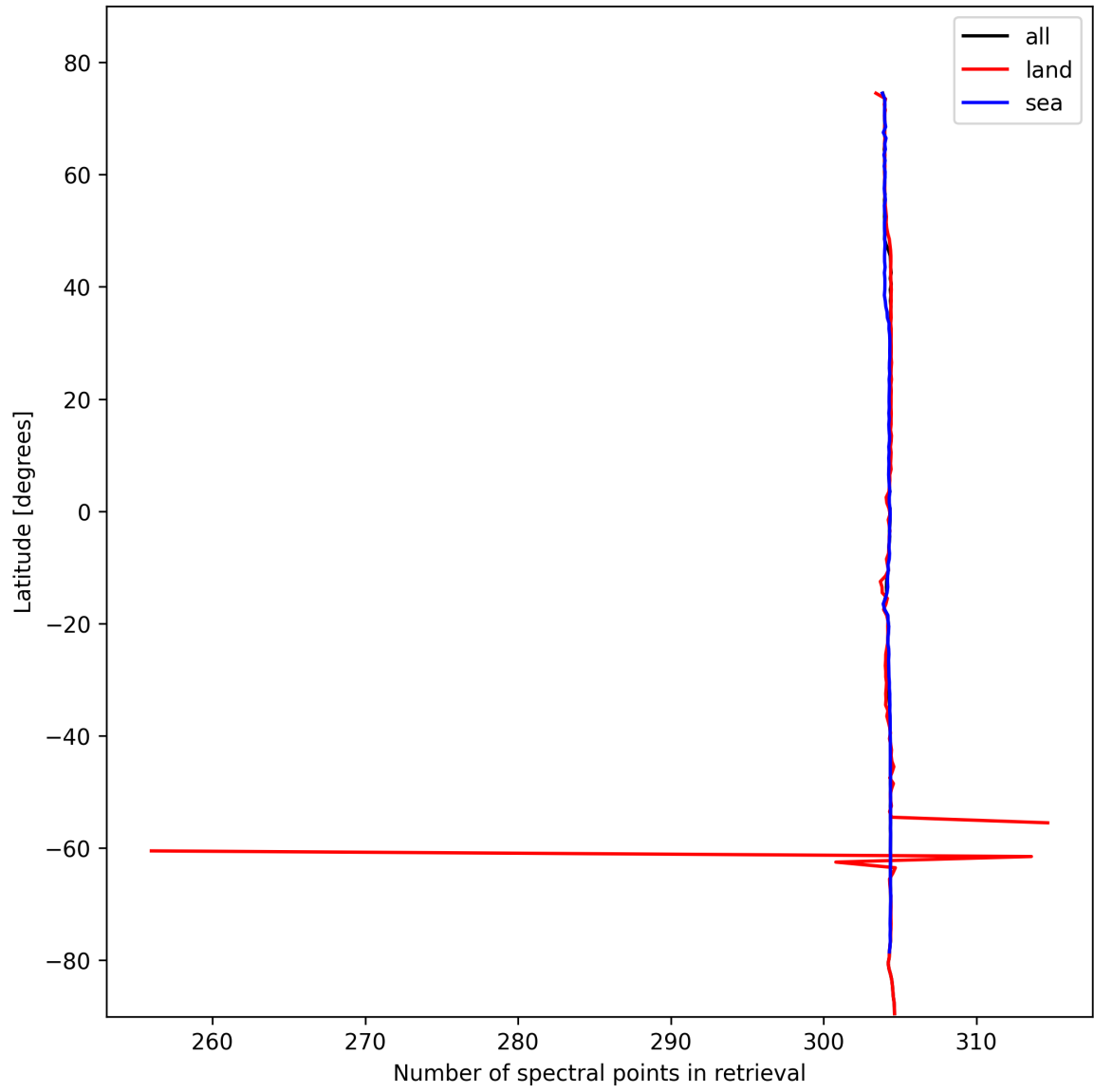
Figure 16: Zonal average of “Number of spectral points in retrieval” for 2024-10-29 to 2024-10-30.
