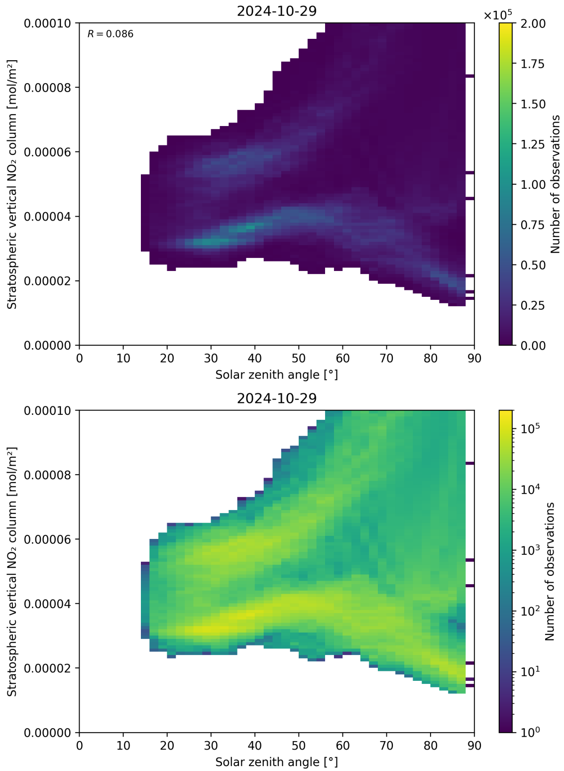
Figure 150: Scatter density plot of “Solar zenith angle” against “Stratospheric vertical NO 2 column” for 2024-10-29 to 2024-10-30.
