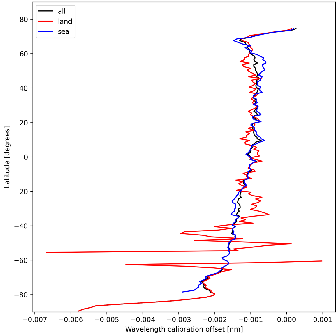
Figure 18: Zonal average of “Wavelength calibration offset” for 2024-10-29 to 2024-10-30.
