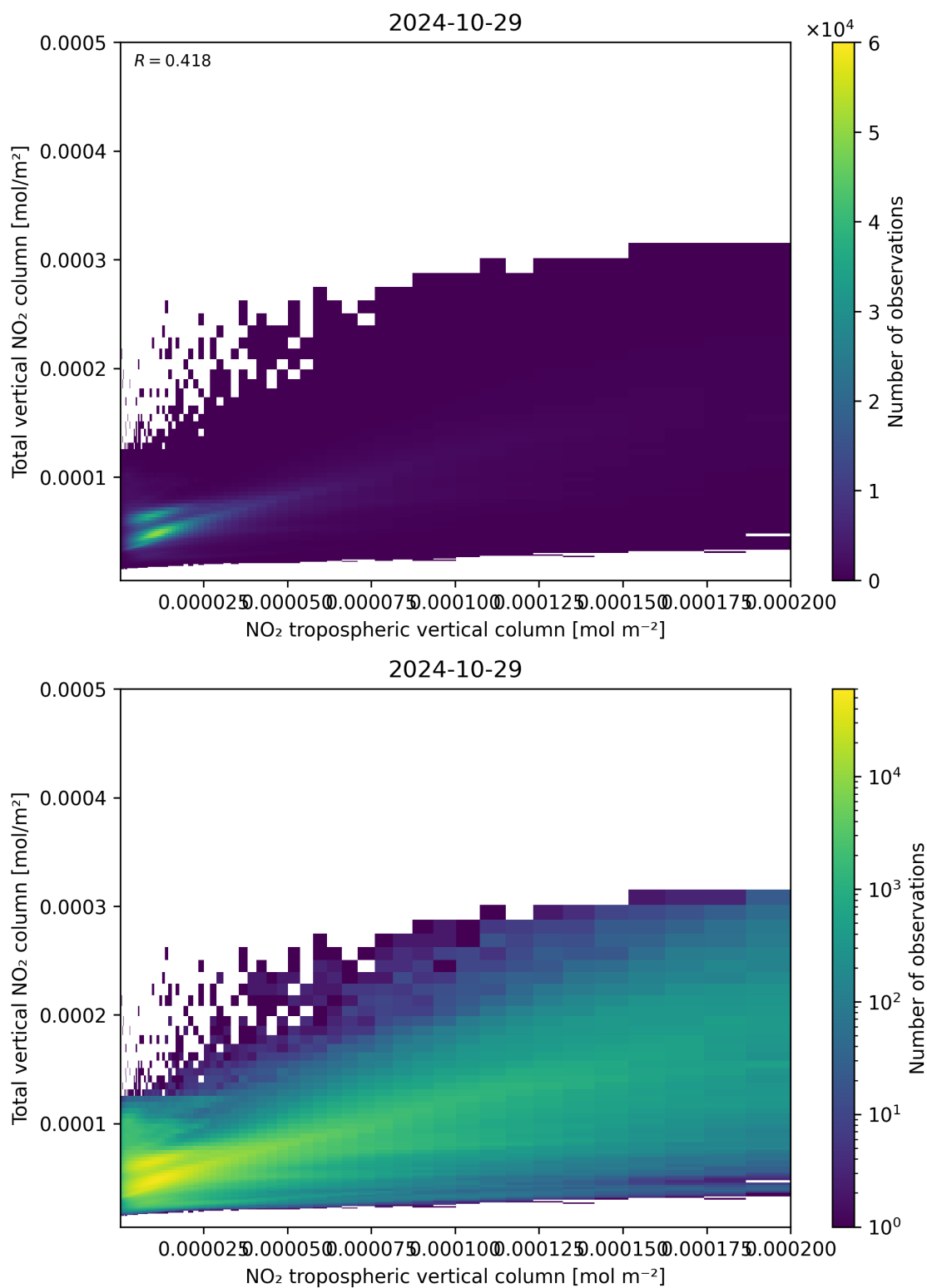
Figure 128: Scatter density plot of “NO 2 tropospheric vertical column” against “Total vertical NO 2 column” for 2024-10-29 to 2024-10-30.
