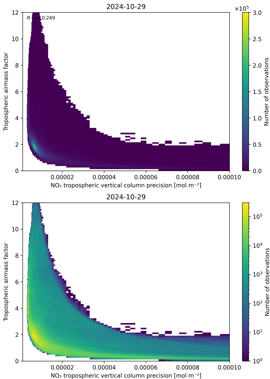
Figure 133: Scatter density plot of “NO 2 tropospheric vertical column precision” against “Tropospheric airmass factor” for 2024-10-29 to 2024-10-30.
