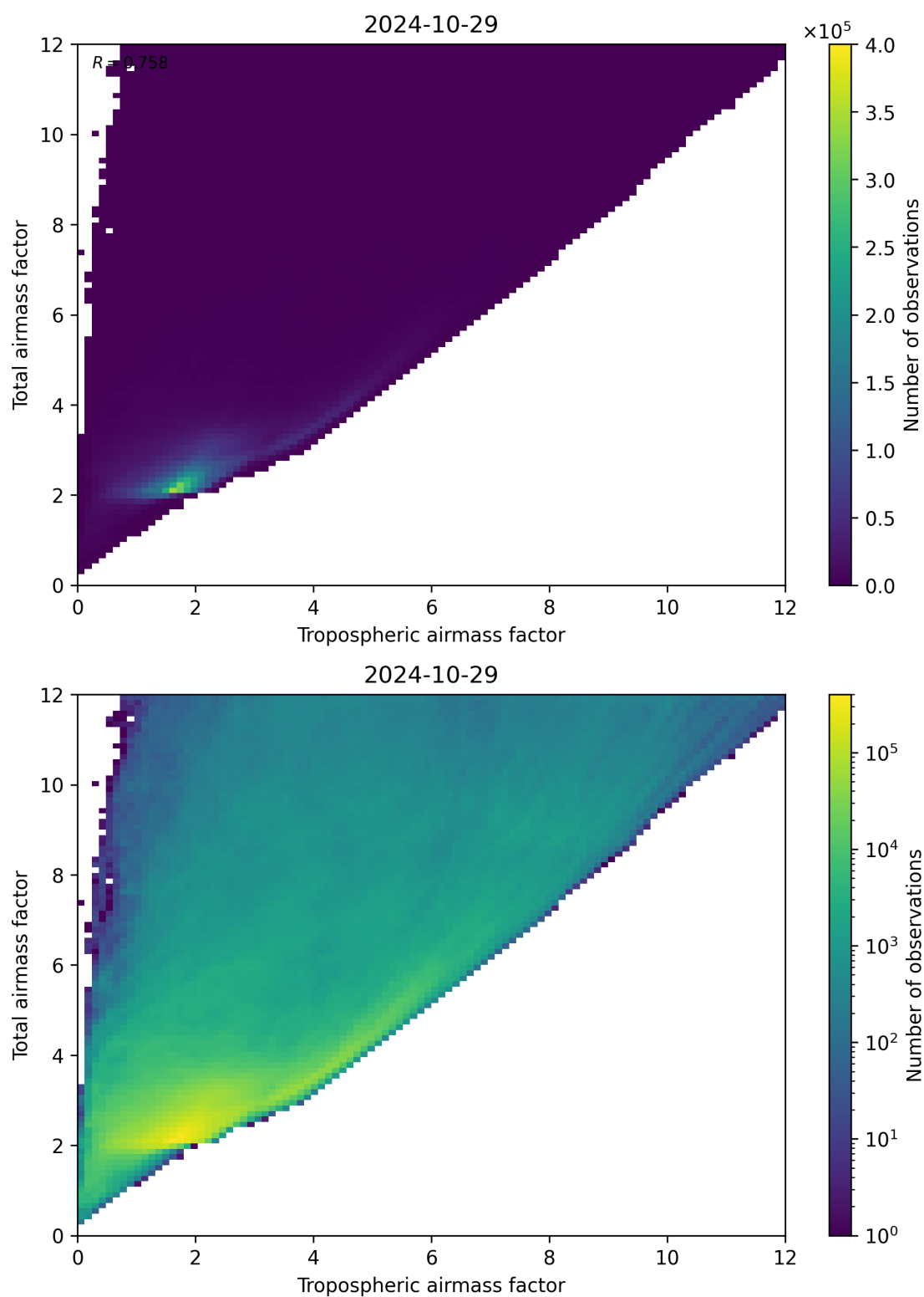
Figure 72: Scatter density plot of “Tropospheric airmass factor” against “Total airmass factor” for 2024-10-29 to 2024-10-30.
