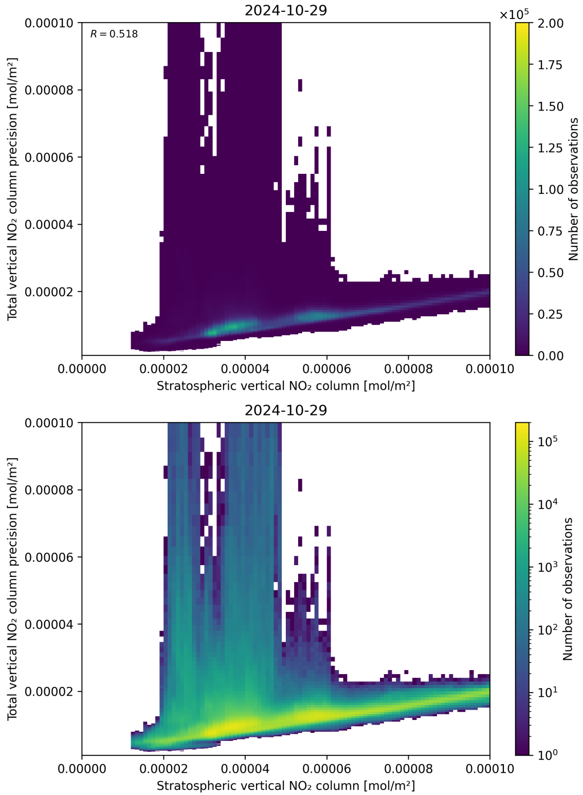
Figure 101: Scatter density plot of “Stratospheric vertical NO 2 column” against “Total vertical NO 2 column precision” for 2024-10-29 to 2024-10-30.
