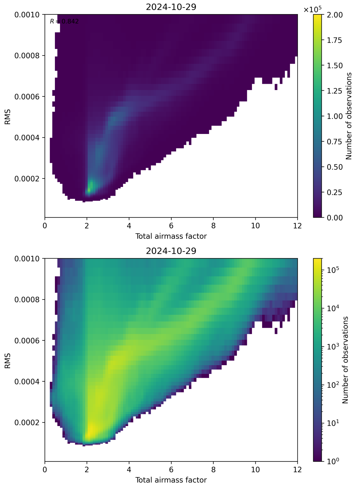
Figure 69: Scatter density plot of “Total airmass factor” against “RMS” for 2024-10-29 to 2024-10-30.
