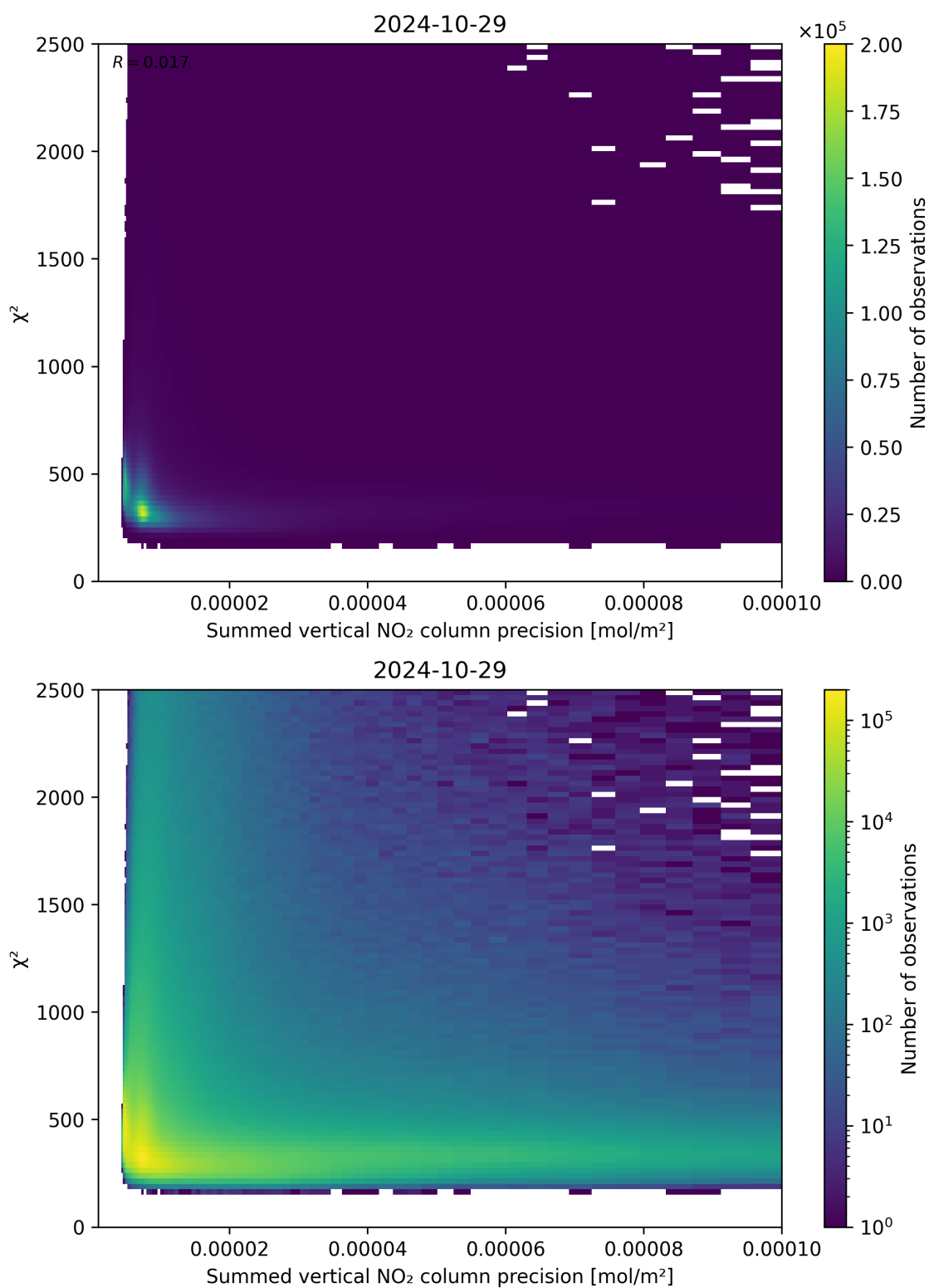
Figure 107: Scatter density plot of “Summed vertical NO 2 column precision” against “ \chi^2 ” for 2024-10-29 to 2024-10-30.
