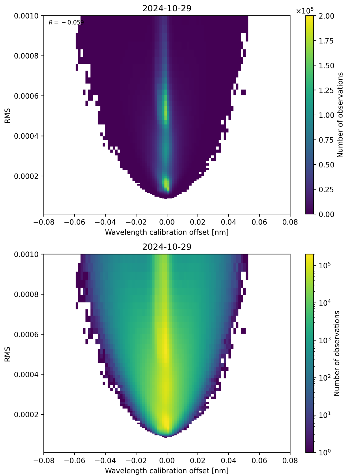
Figure 181: Scatter density plot of “Wavelength calibration offset” against “RMS” for 2024-10-29 to 2024-10-30.
