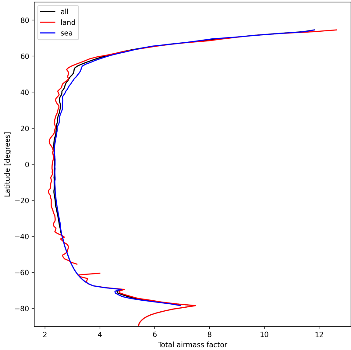
Figure 15: Zonal average of “Total airmass factor” for 2024-10-29 to 2024-10-30.
