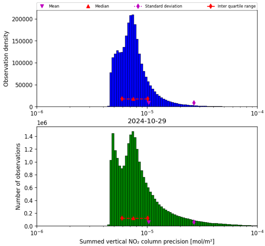
Figure 41: Histogram of "Summed vertical NO 2 column precision" for 2024-10-29 to 2024-10-30
