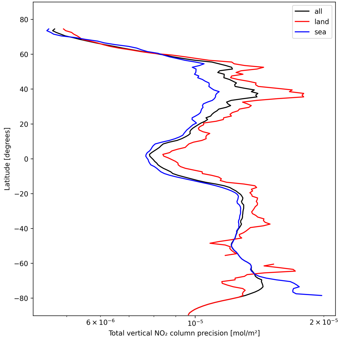
Figure 22: Zonal average of “Total vertical NO 2 column precision” for 2024-10-29 to 2024-10-30.
