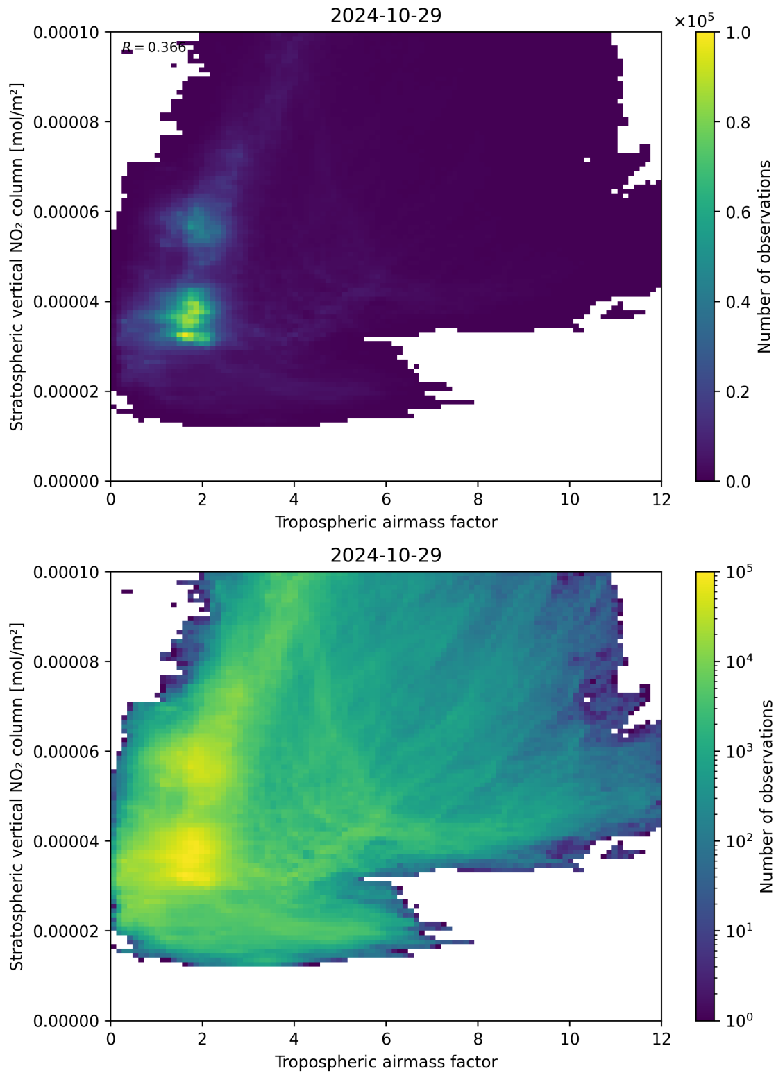
Figure 74: Scatter density plot of “Tropospheric air mass factor” against “Stratospheric vertical NO 2 column” for 2024-10-29 to 2024-10-30.
