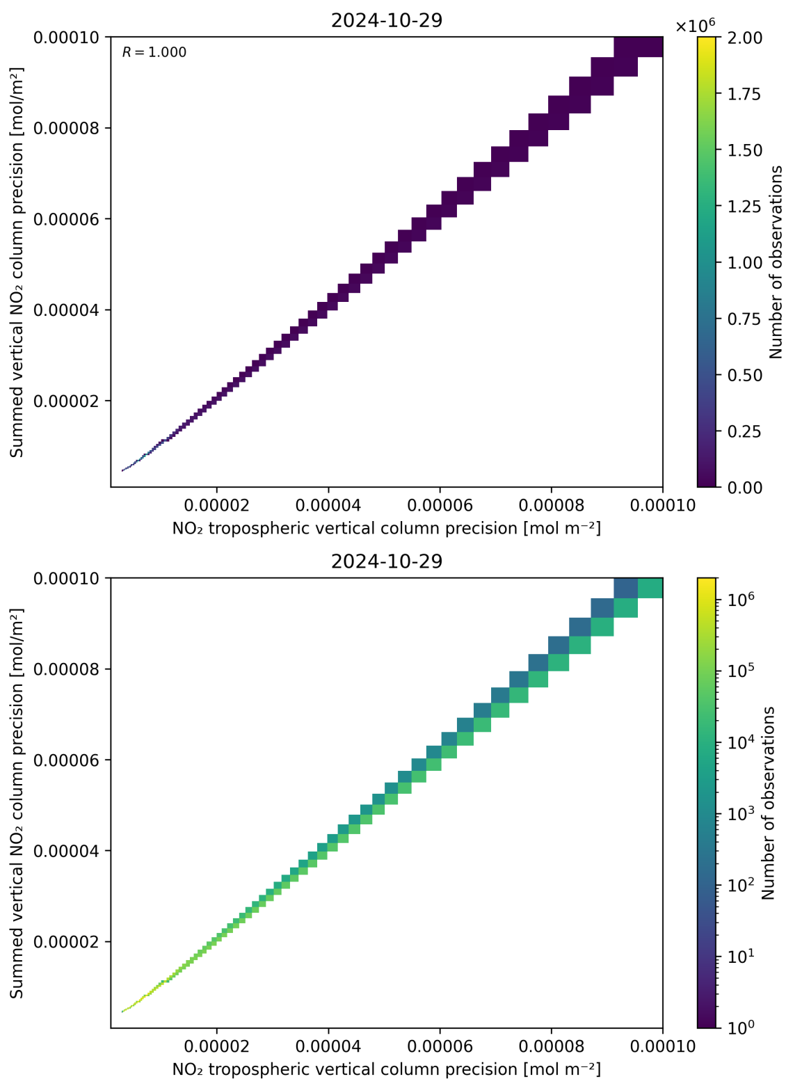
Figure 137: Scatter density plot of “NO 2 tropospheric vertical column precision” against “Summed vertical NO 2 column precision” for 2024-10-29 to 2024-10-30.
