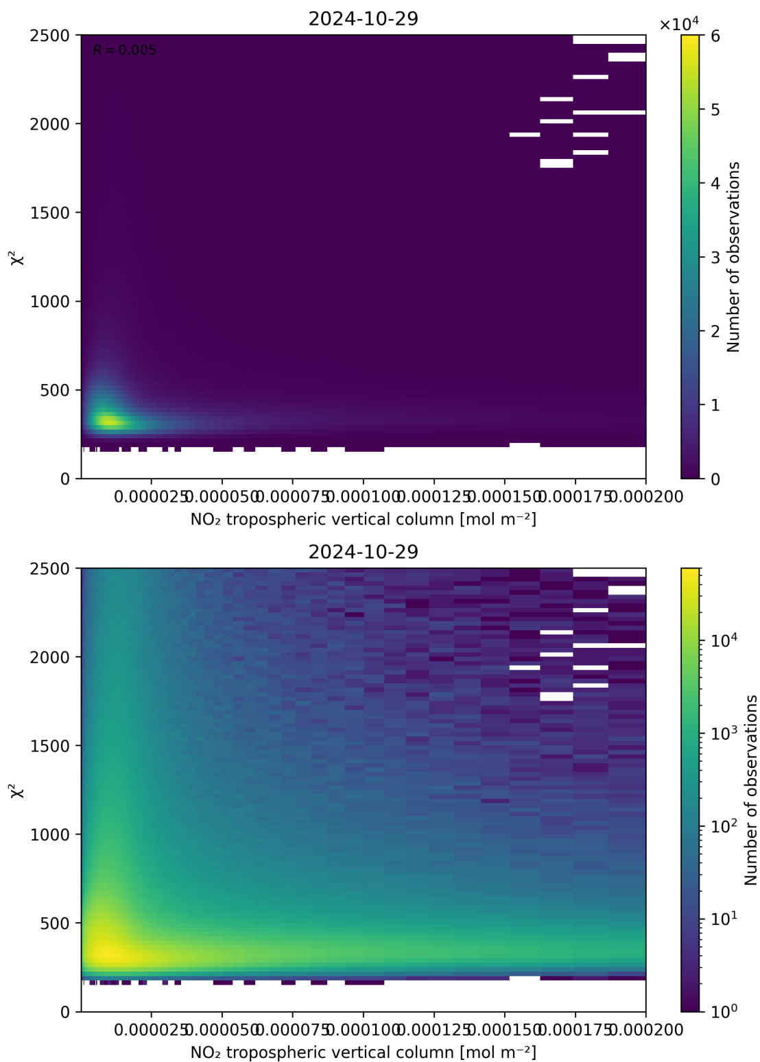
Figure 124: Scatter density plot of “NO 2 tropospheric vertical column” against “ \chi^2 ” for 2024-10-29 to 2024-10-30.
