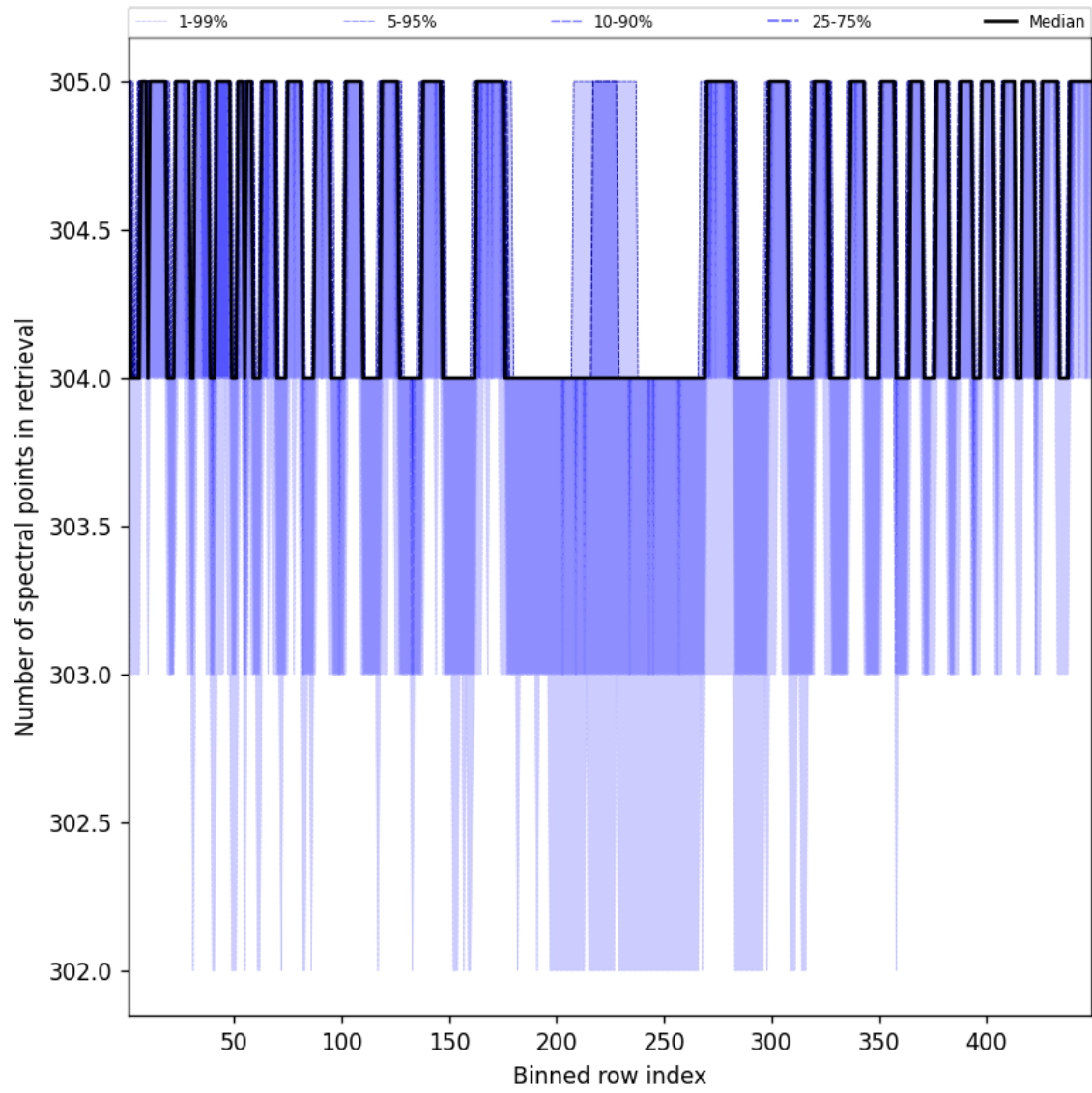
Figure 50: Along track statistics of “Number of spectral points in retrieval” for 2024-10-29 to 2024-10-30
