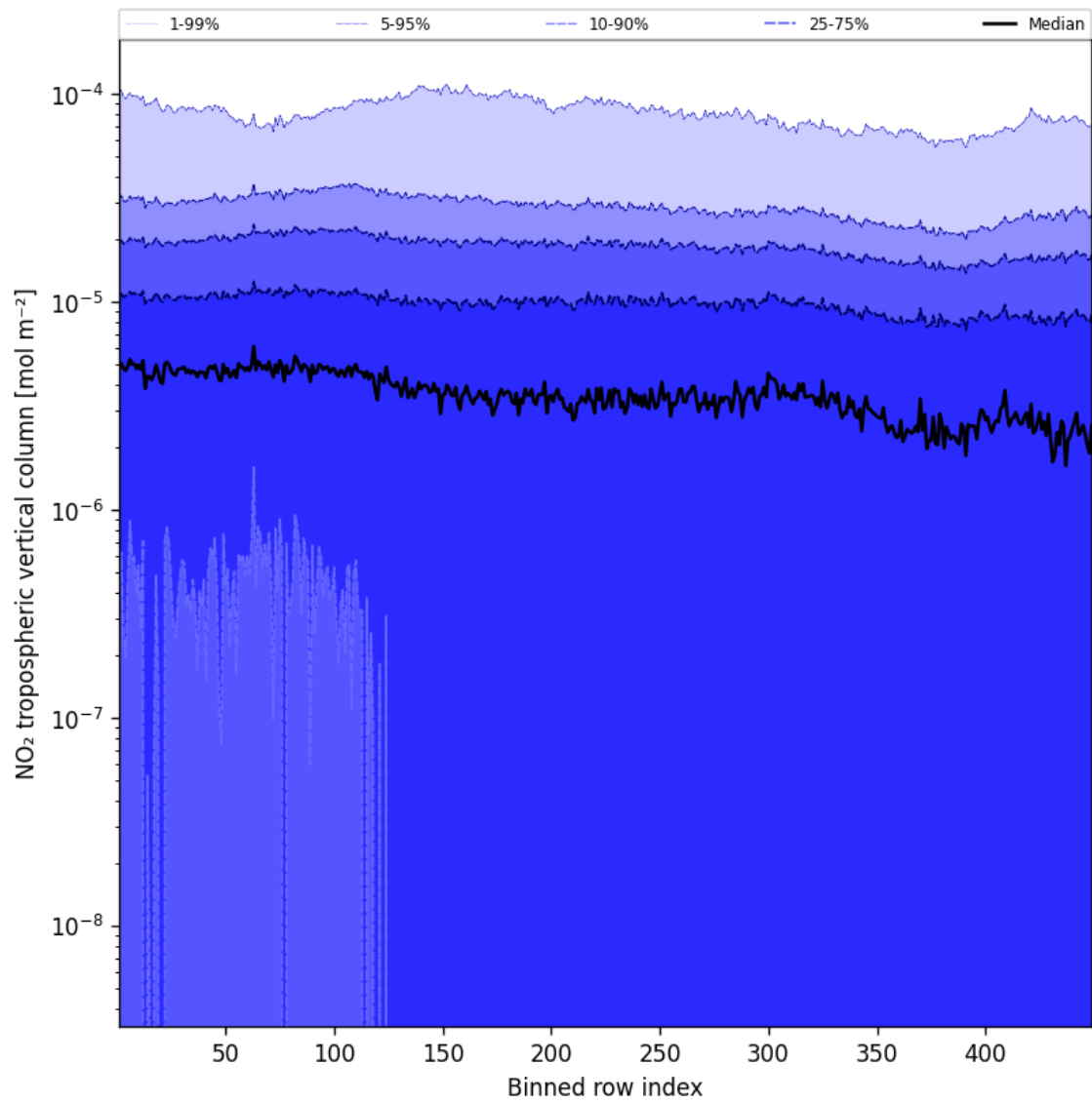
Figure 46: Along track statistics of “NO 2 tropospheric vertical column” for 2024-10-29 to 2024-10-30
