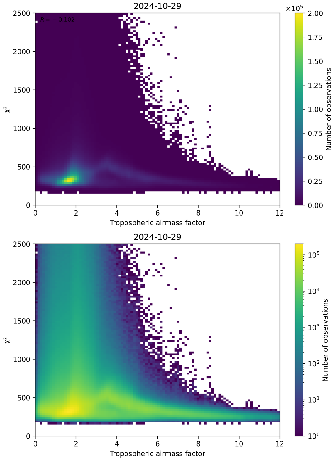
Figure 73: Scatter density plot of “Tropospheric airmass factor” against “ \chi^2 ” for 2024-10-29 to 2024-10-30.
