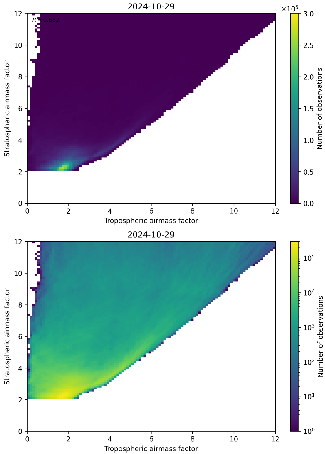
Figure 71: Scatter density plot of “Tropospheric airmass factor” against “Stratospheric airmass factor” for 2024-10-29 to 2024-10-30.
