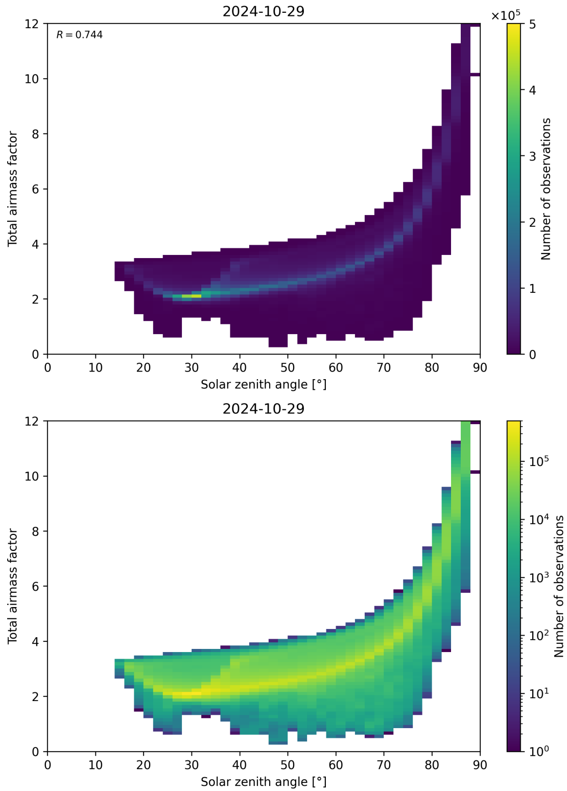
Figure 146: Scatter density plot of “Solar zenith angle” against “Total air mass factor” for 2024-10-29 to 2024-10-30.
