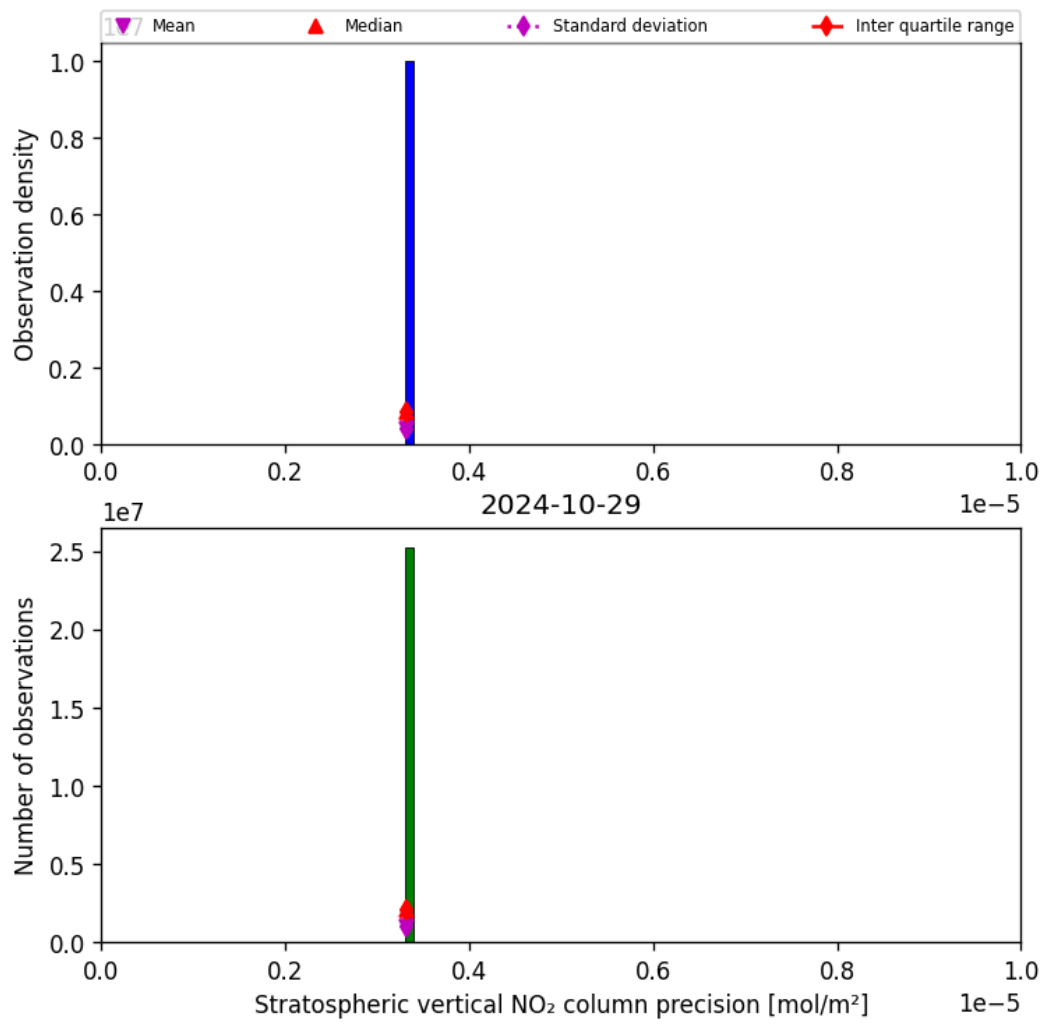
Figure 37: Histogram of “Stratospheric vertical NO 2 column precision” for 2024-10-29 to 2024-10-30
