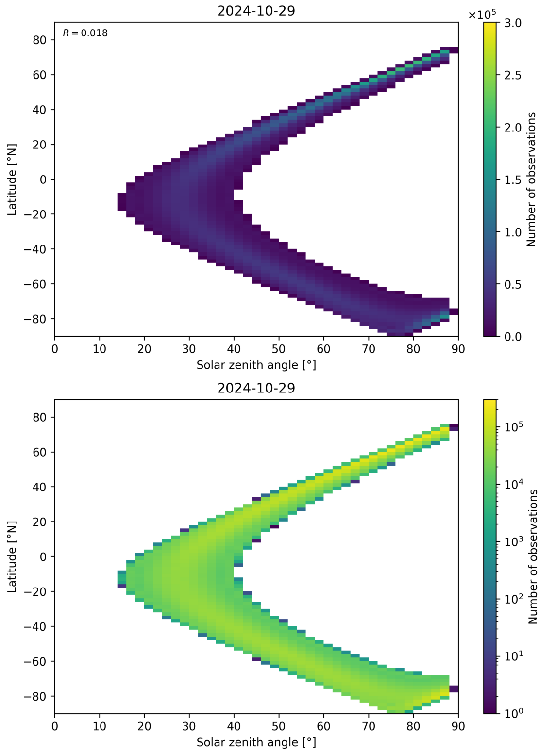
Figure 149: Scatter density plot of “Solar zenith angle” against “Latitude” for 2024-10-29 to 2024-10-30.
