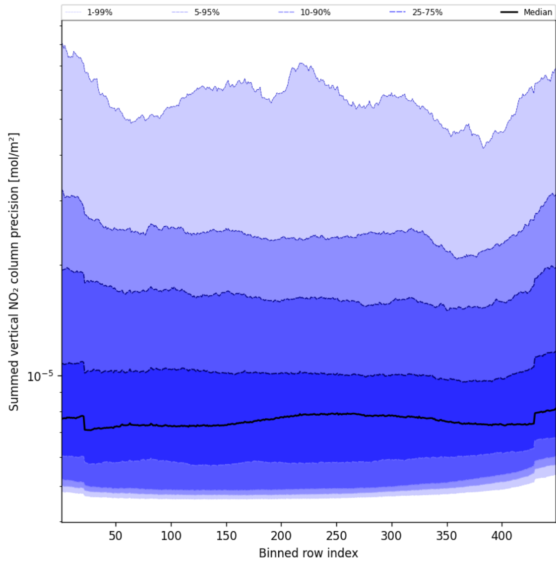
Figure 58: Along track statistics of “Summed vertical NO 2 column precision” for 2024-10-29 to 2024-10-30
