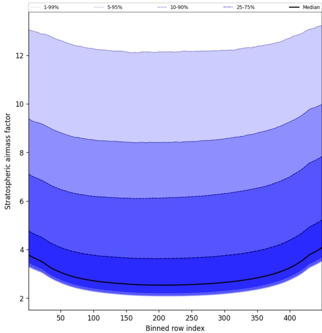
Figure 61: Along track statistics of “Stratospheric airmass factor” for 2024-10-29 to 2024-10-30
