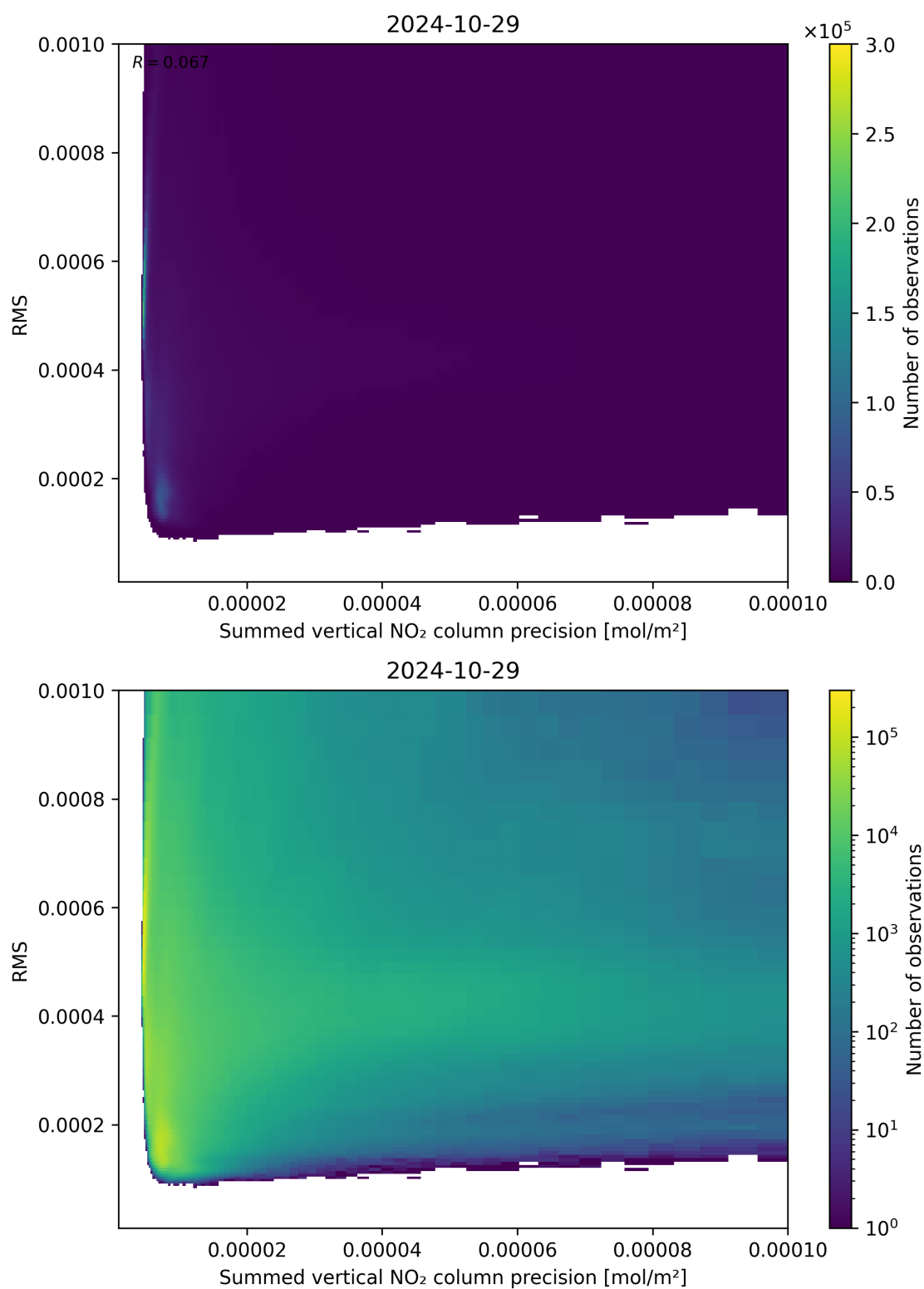
Figure 108: Scatter density plot of “Summed vertical NO 2 column precision” against “RMS” for 2024-10-29 to 2024-10-30.
