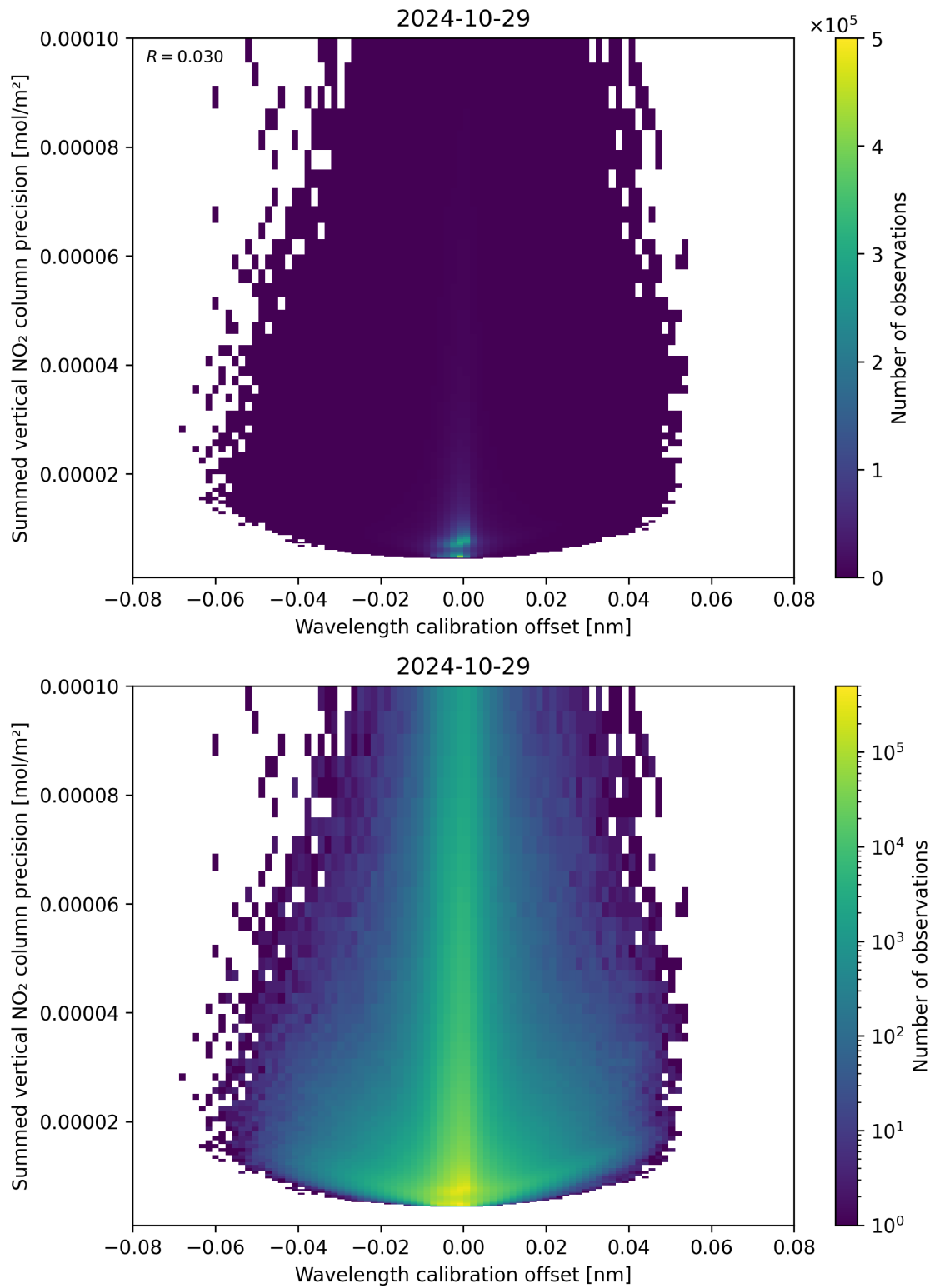
Figure 178: Scatter density plot of “Wavelength calibration offset” against “Summed vertical NO 2 column precision” for 2024-10-29 to 2024-10-30.
