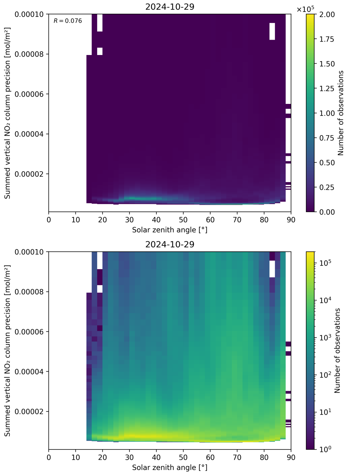
Figure 152: Scatter density plot of “Solar zenith angle” against “Summed vertical NO 2 column precision” for 2024-10-29 to 2024-10-30.
