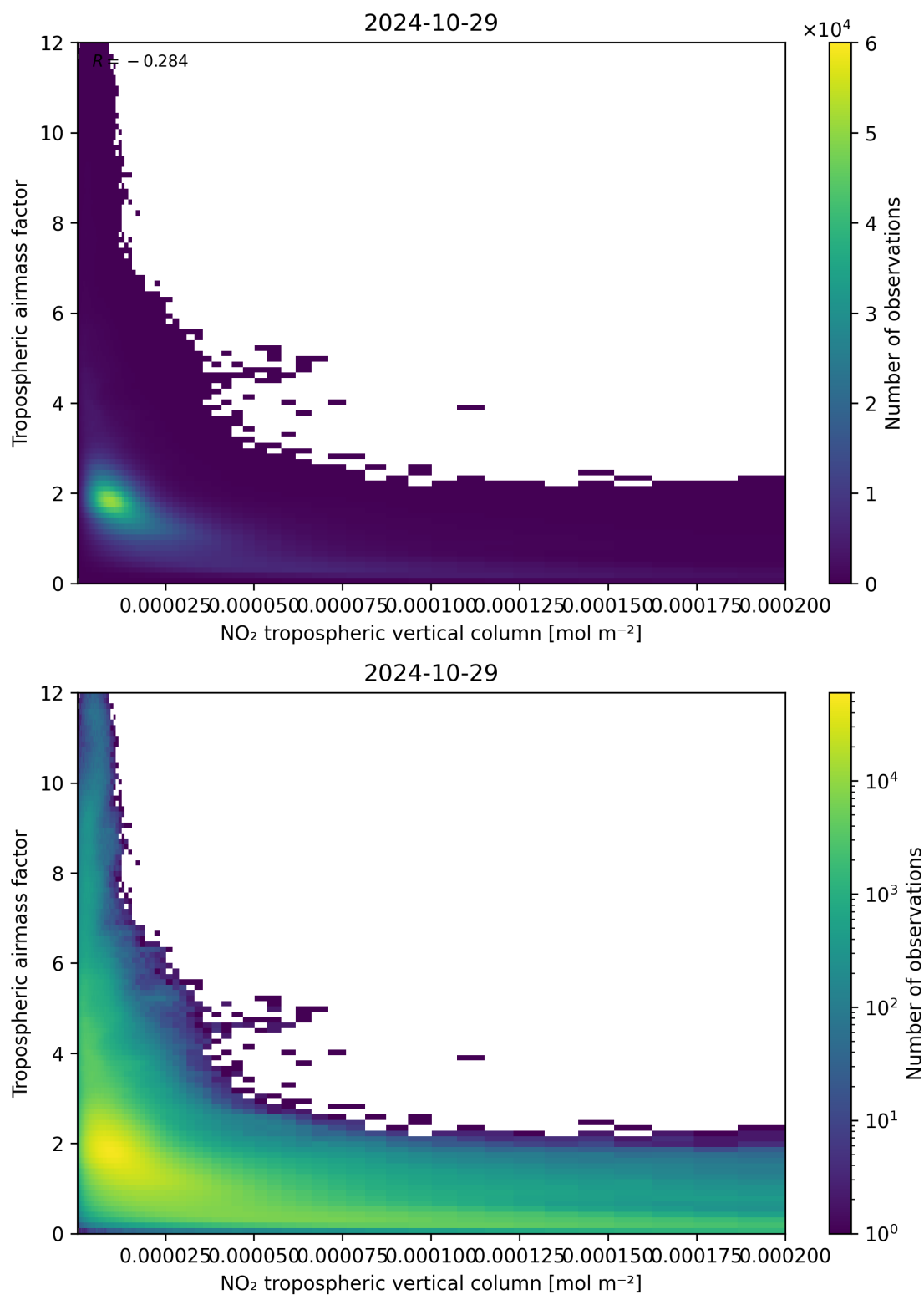
Figure 123: Scatter density plot of “NO 2 tropospheric vertical column” against “Tropospheric air mass factor” for 2024-10-29 to 2024-10-30.
