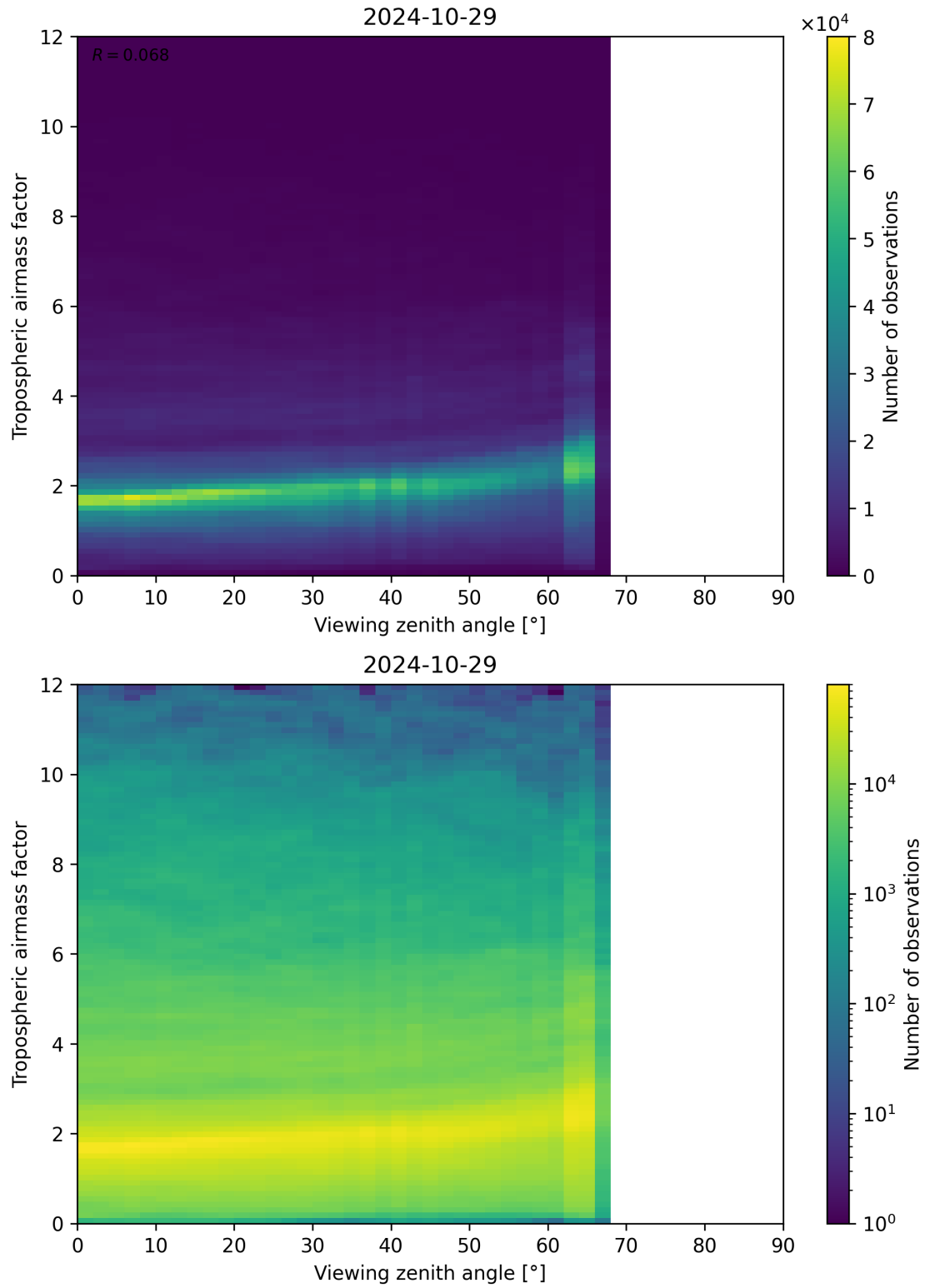
Figure 161: Scatter density plot of “Viewing zenith angle” against “Tropospheric airmass factor” for 2024-10-29 to 2024-10-30.
