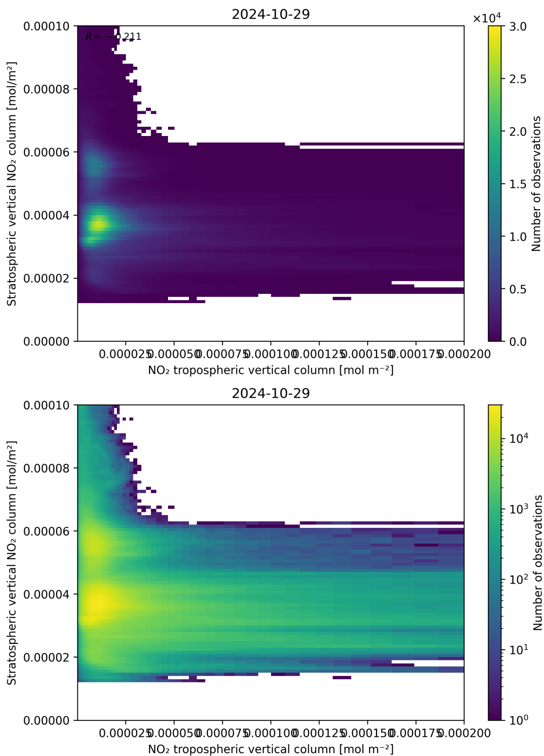
Figure 125: Scatter density plot of “NO 2 tropospheric vertical column” against “Stratospheric vertical NO 2 column” for 2024-10-29 to 2024-10-30.
