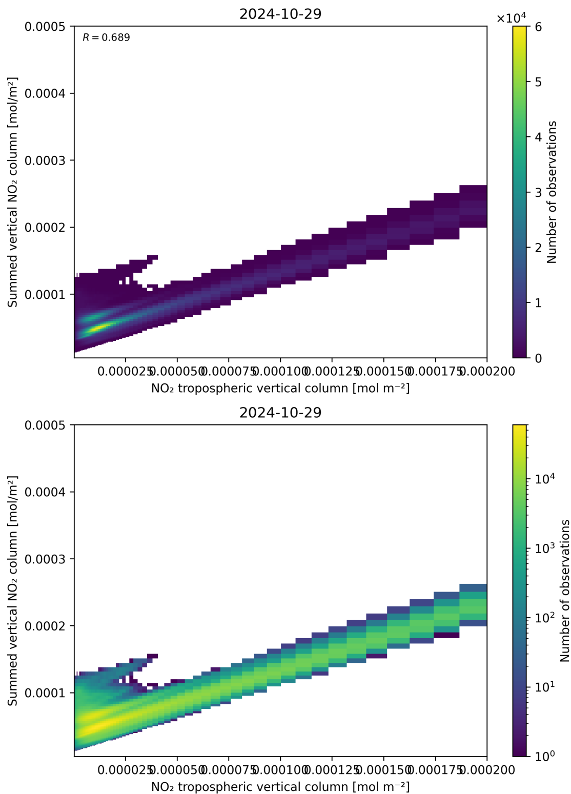
Figure 126: Scatter density plot of “NO 2 tropospheric vertical column” against “Summed vertical NO 2 column” for 2024-10-29 to 2024-10-30.
