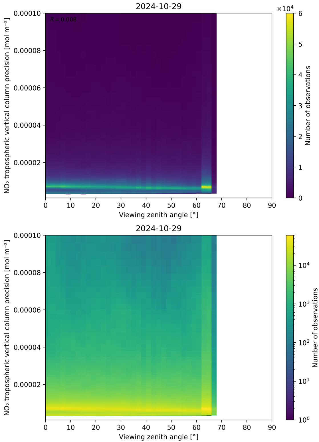
Figure 170: Scatter density plot of “Viewing zenith angle” against “NO 2 tropospheric vertical column precision” for 2024-10-29 to 2024-10-30.
