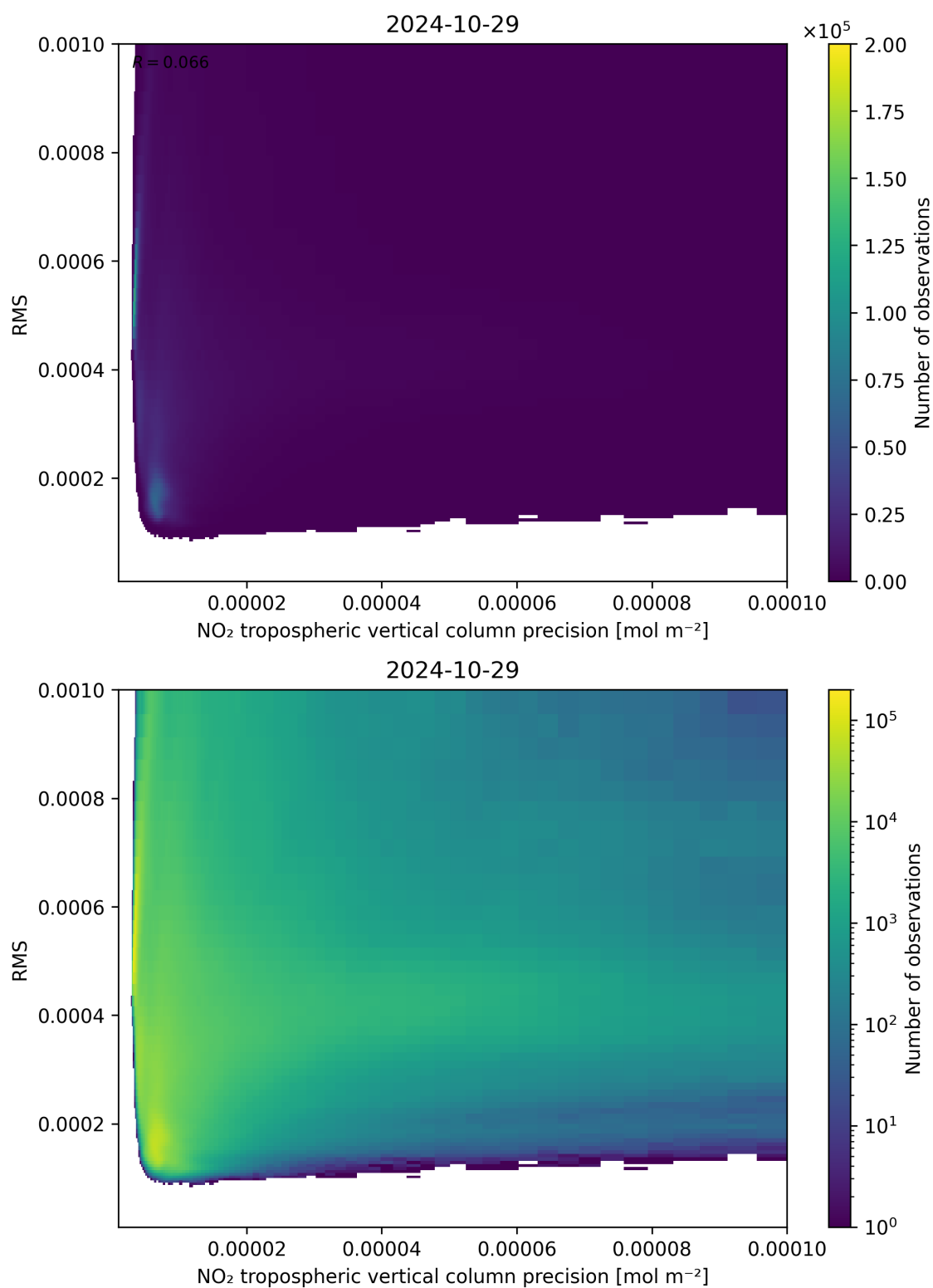
Figure 140: Scatter density plot of “NO 2 tropospheric vertical column precision” against “RMS” for 2024-10-29 to 2024-10-30.
