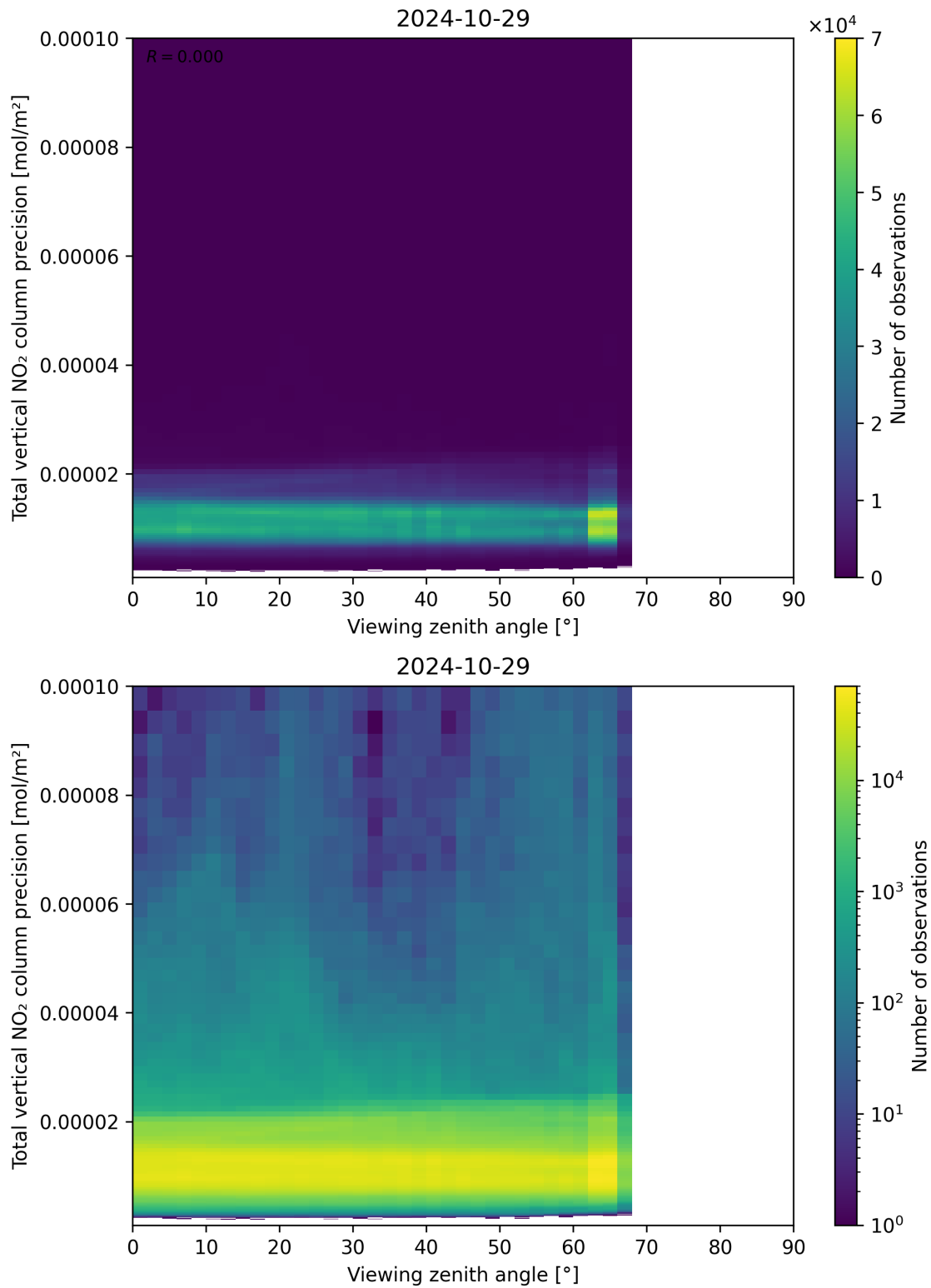
Figure 168: Scatter density plot of “Viewing zenith angle” against “Total vertical NO 2 column precision” for 2024-10-29 to 2024-10-30.
