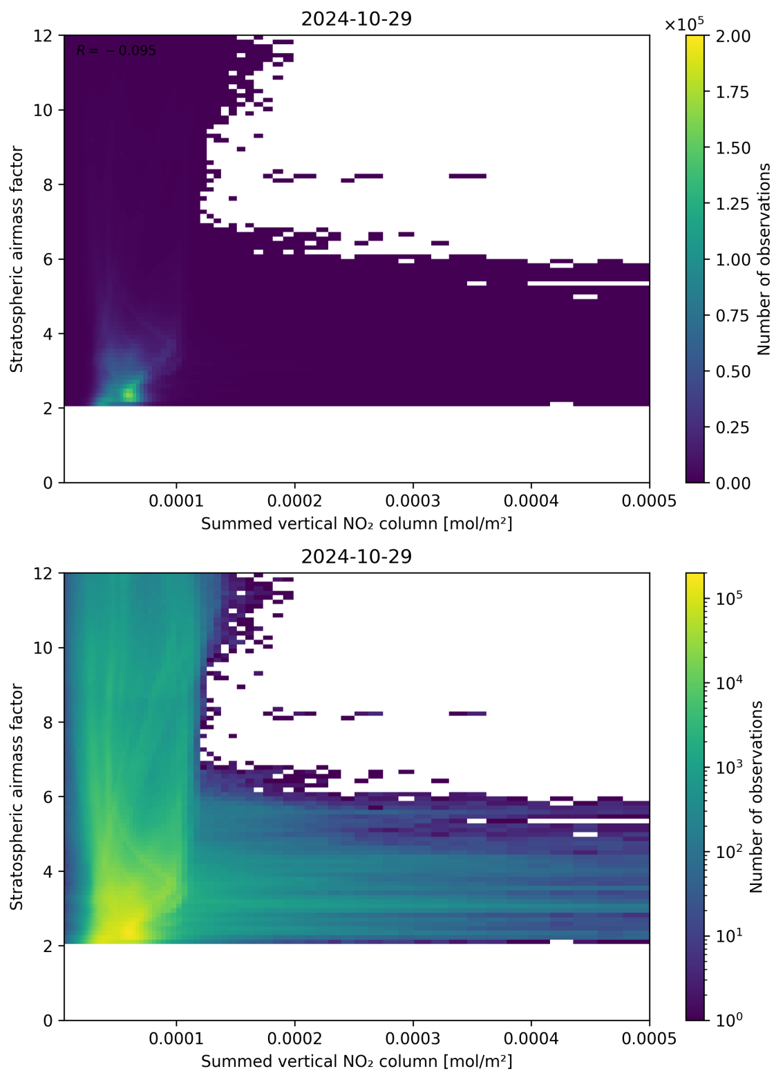
Figure 103: Scatter density plot of “Summed vertical NO 2 column” against “Stratospheric air mass factor” for 2024-10-29 to 2024-10-30.
