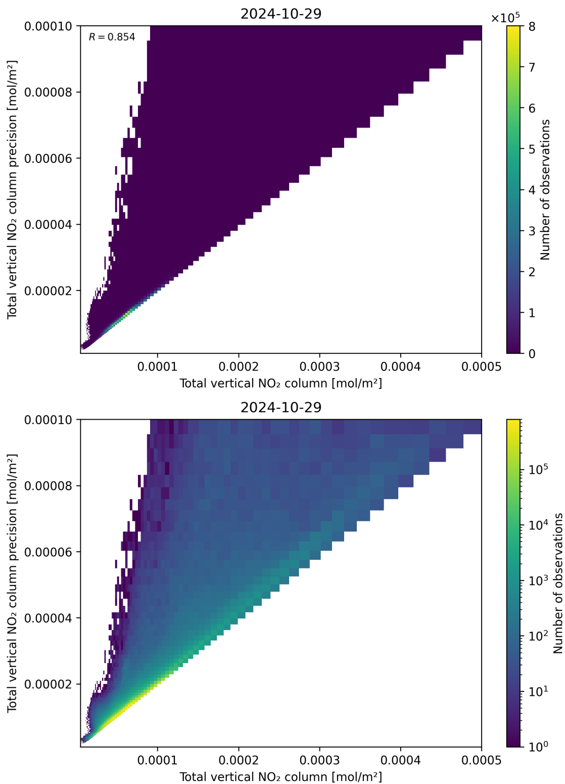
Figure 114: Scatter density plot of “Total vertical NO 2 column” against “Total vertical NO 2 column precision” for 2024-10-29 to 2024-10-30.
