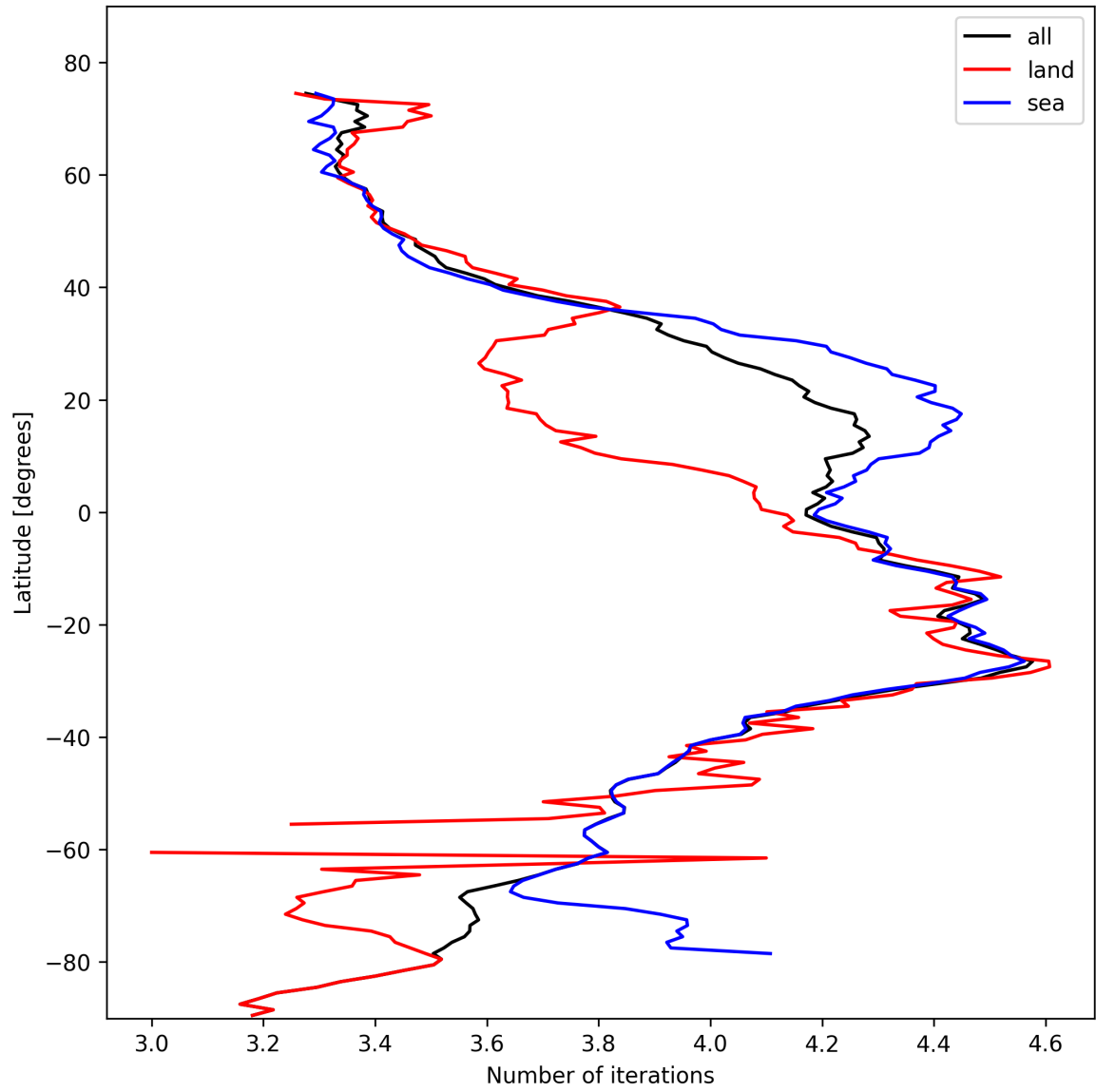
Figure 17: Zonal average of “Number of iterations” for 2024-10-29 to 2024-10-30.
