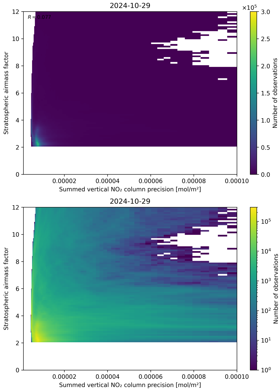
Figure 106: Scatter density plot of “Summed vertical NO 2 column precision” against “Stratospheric airmass factor” for 2024-10-29 to 2024-10-30.
