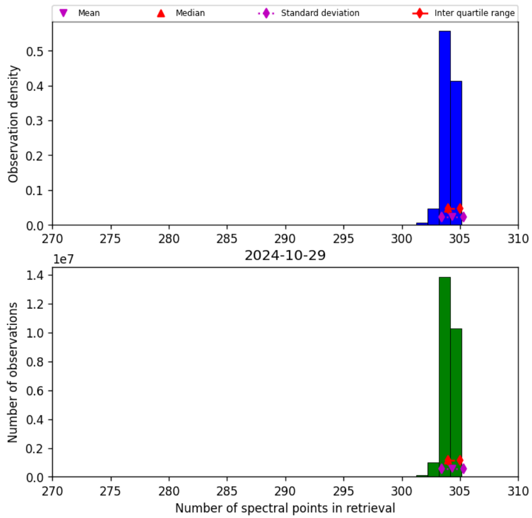
Figure 33: Histogram of “Number of spectral points in retrieval” for 2024-10-29 to 2024-10-30
