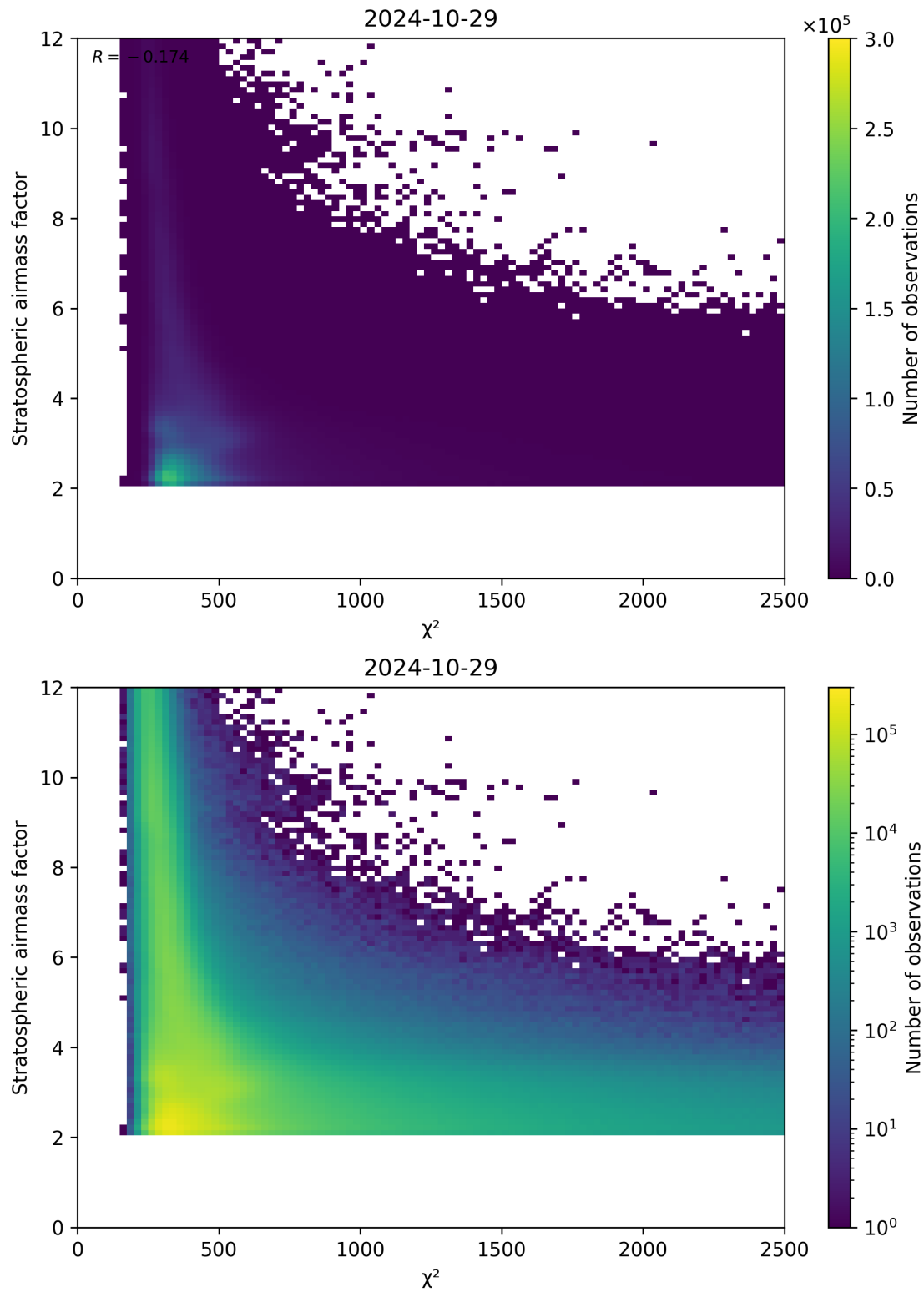
Figure 81: Scatter density plot of “ \chi^2 ” against “Stratospheric airmass factor” for 2024-10-29 to 2024-10-30.
