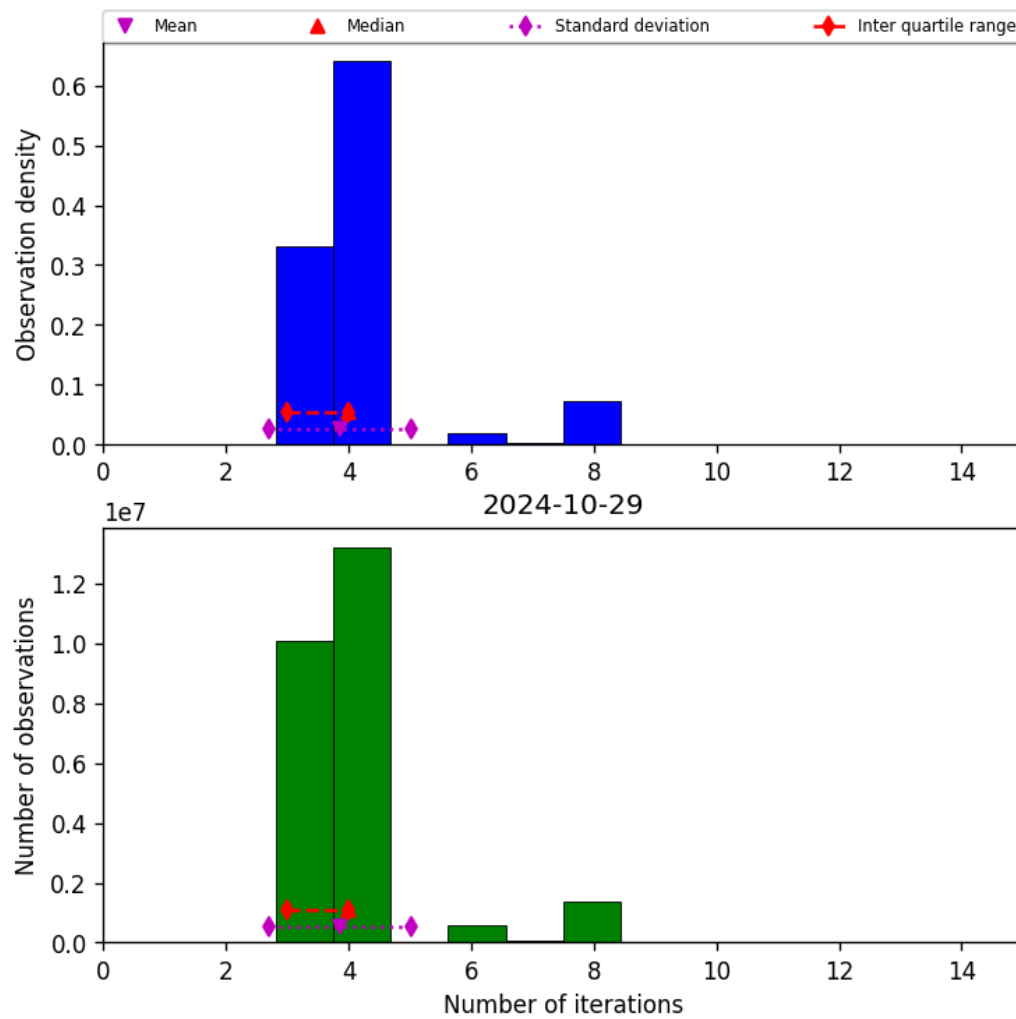
Figure 34: Histogram of “Number of iterations” for 2024-10-29 to 2024-10-30
