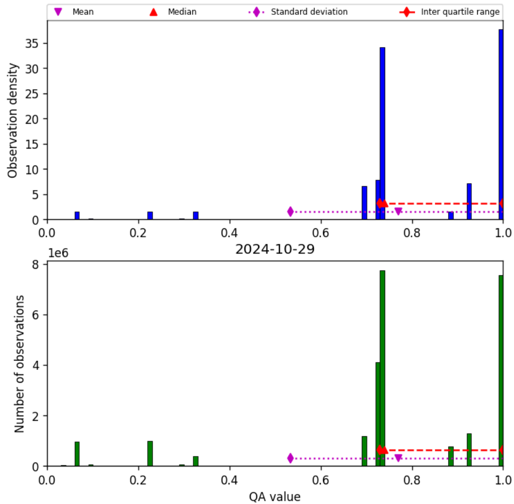
Figure 28: Histogram of “QA value” for 2024-10-29 to 2024-10-30
