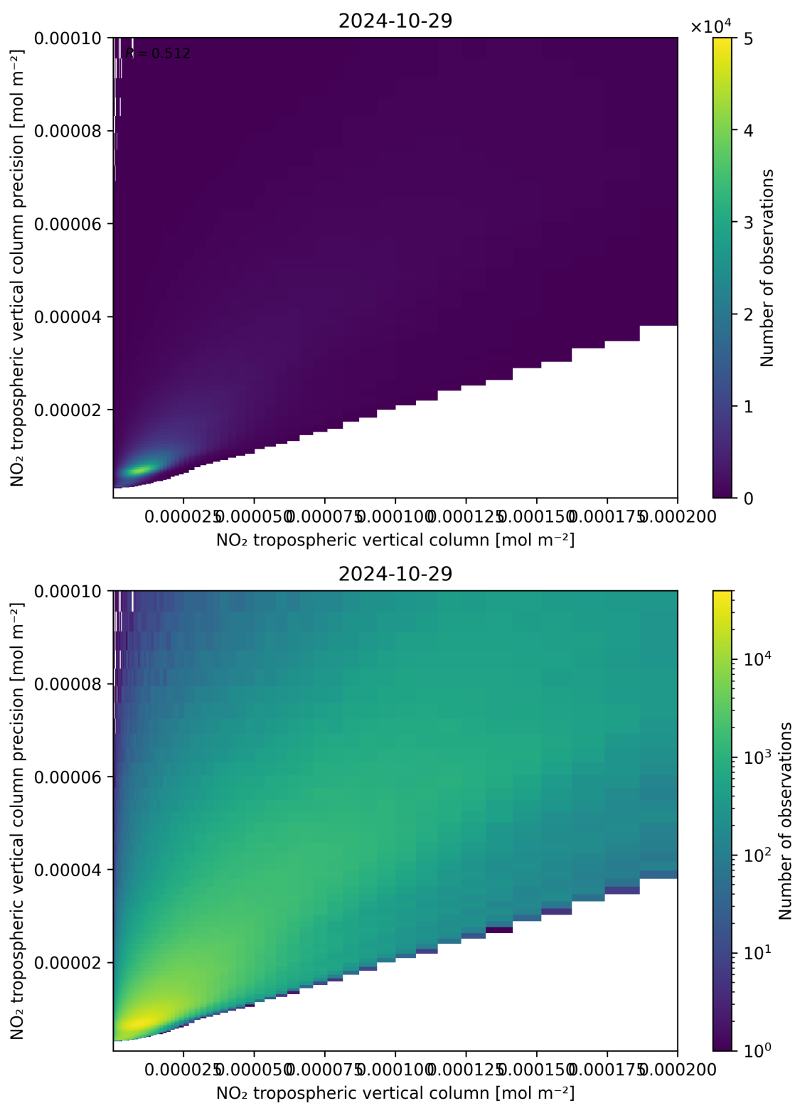
Figure 130: Scatter density plot of “NO 2 tropospheric vertical column” against “NO 2 tropospheric vertical column precision” for 2024-10-29 to 2024-10-30.
