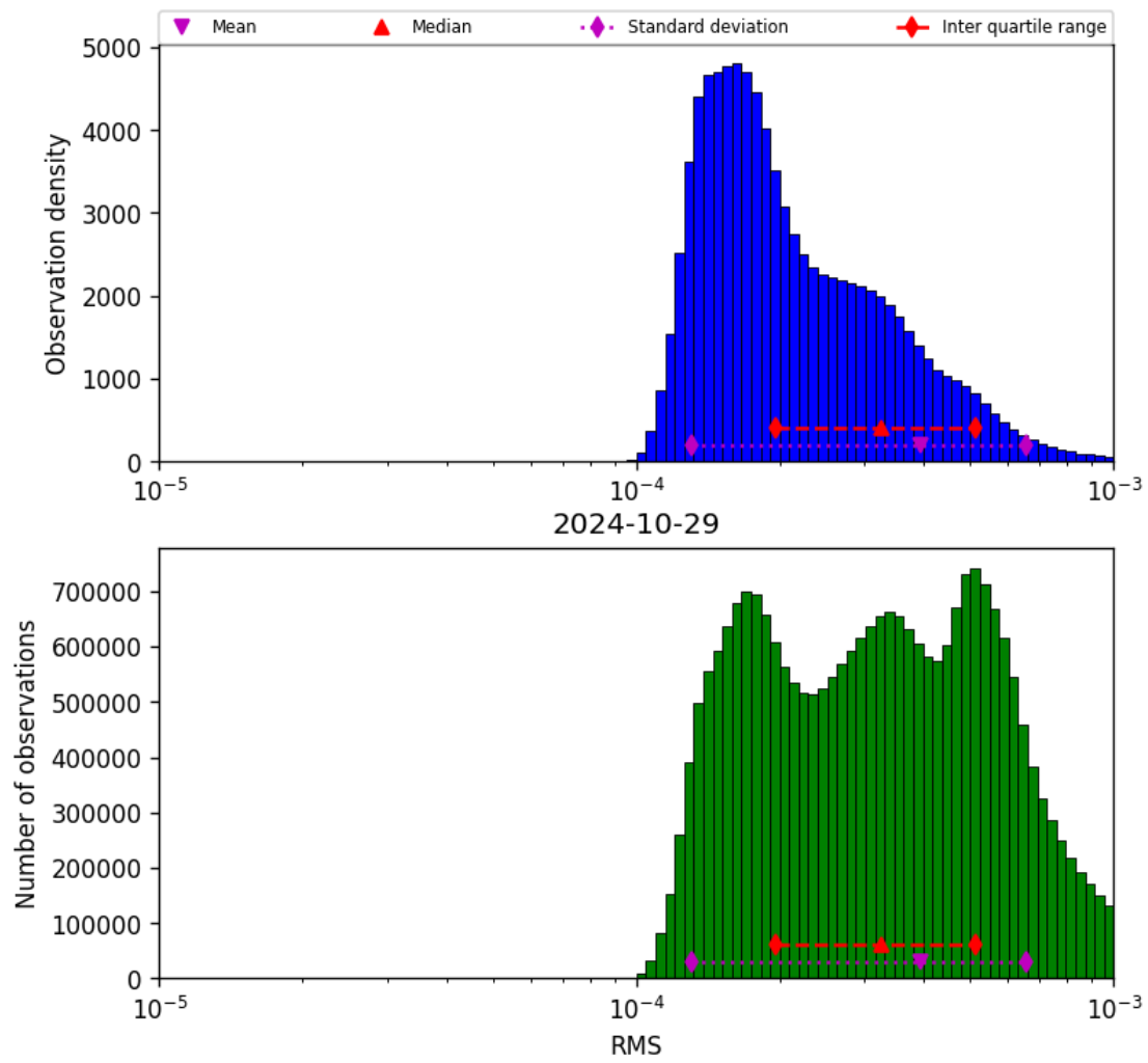
Figure 43: Histogram of “RMS” for 2024-10-29 to 2024-10-30
