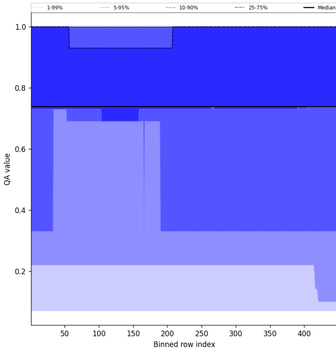
Figure 45: Along track statistics of “QA value” for 2024-10-29 to 2024-10-30
