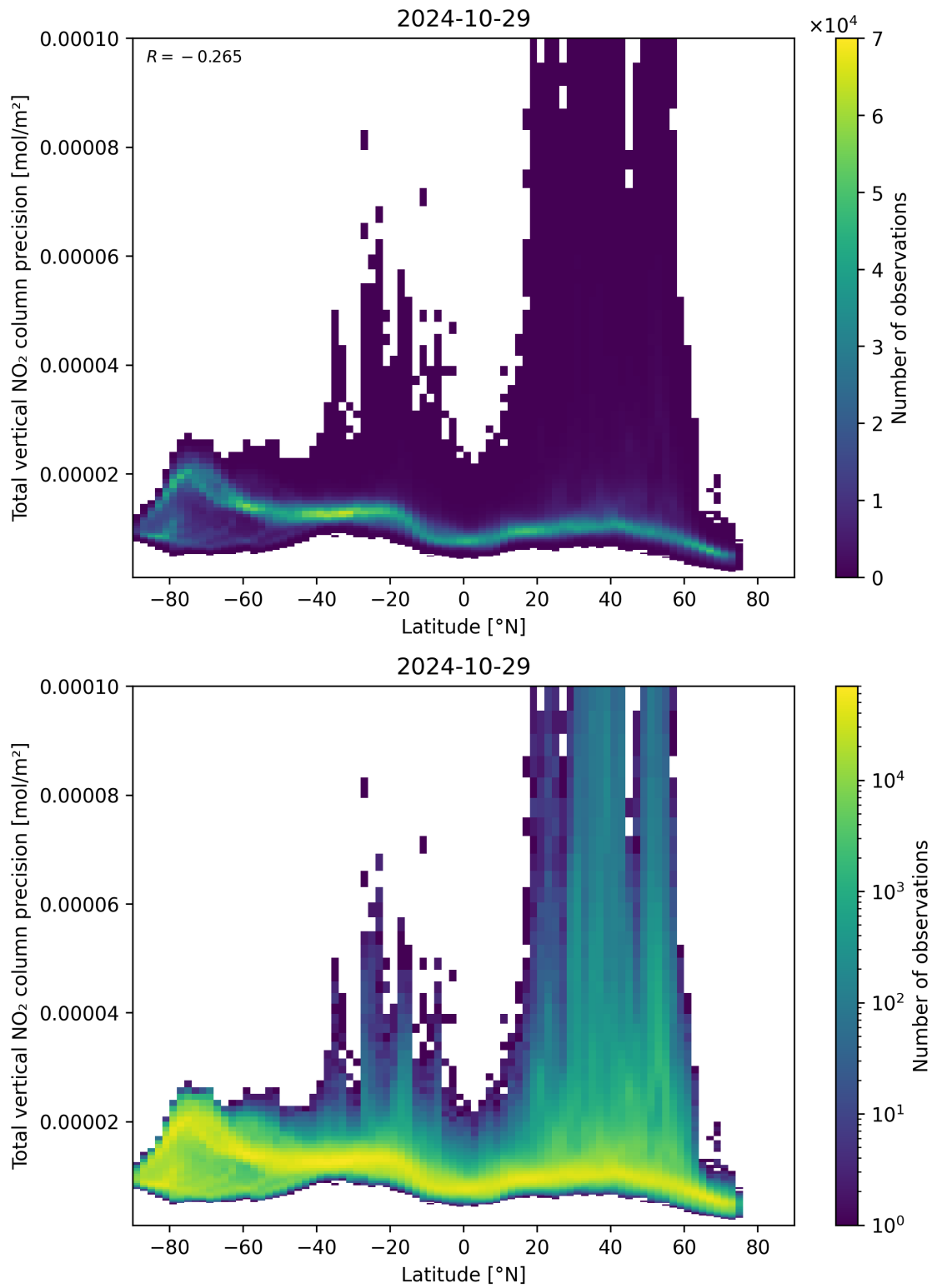
Figure 91: Scatter density plot of “Latitude” against “Total vertical NO 2 column precision” for 2024-10-29 to 2024-10-30.
