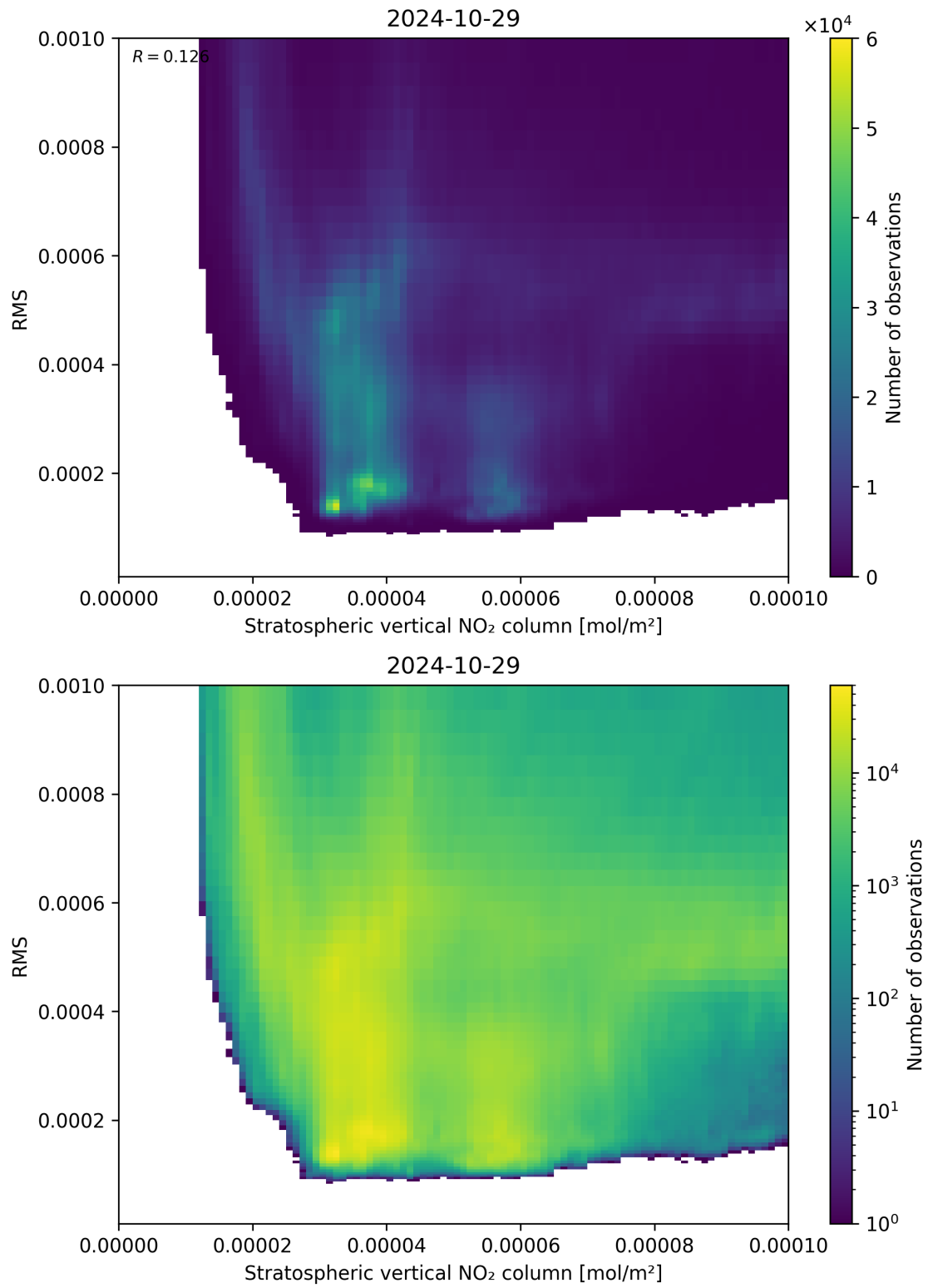
Figure 102: Scatter density plot of “Stratospheric vertical NO 2 column” against “RMS” for 2024-10-29 to 2024-10-30.
