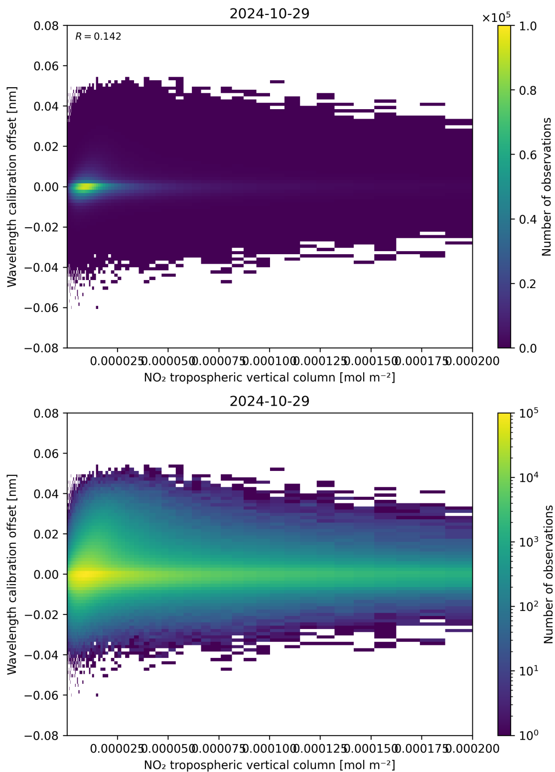
Figure 143: Scatter density plot of “NO 2 tropospheric vertical column” against “Wavelength calibration offset” for 2024-10-29 to 2024-10-30.
