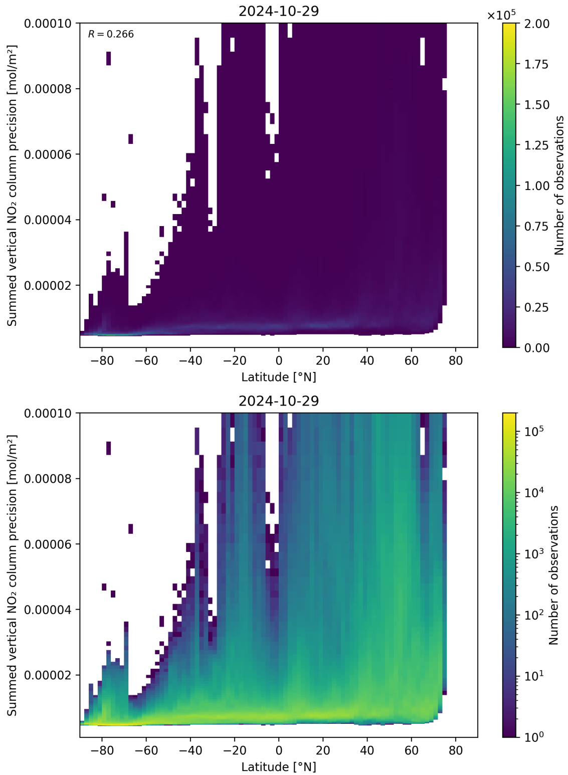
Figure 89: Scatter density plot of “Latitude” against “Summed vertical NO 2 column precision” for 2024-10-29 to 2024-10-30.
