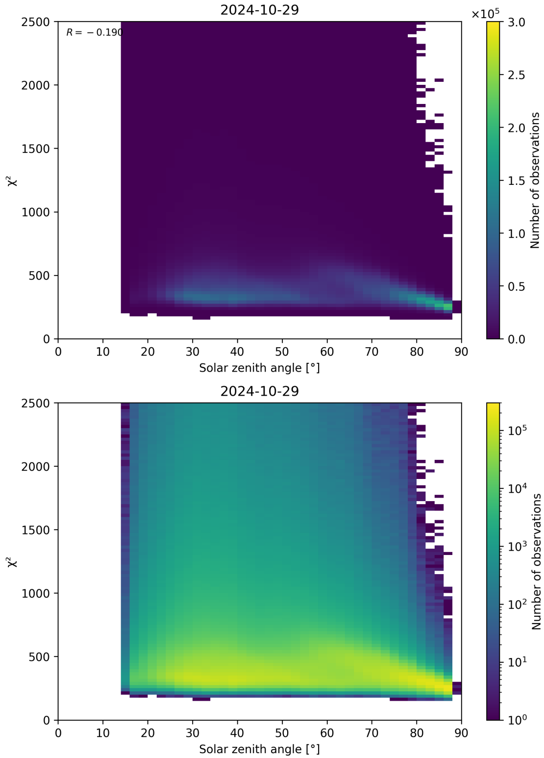
Figure 148: Scatter density plot of “Solar zenith angle” against “ \chi^2 ” for 2024-10-29 to 2024-10-30.
