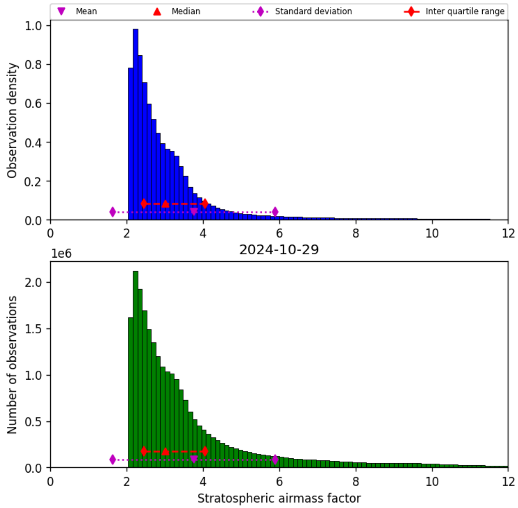
Figure 44: Histogram of “Stratospheric airmass factor” for 2024-10-29 to 2024-10-30
