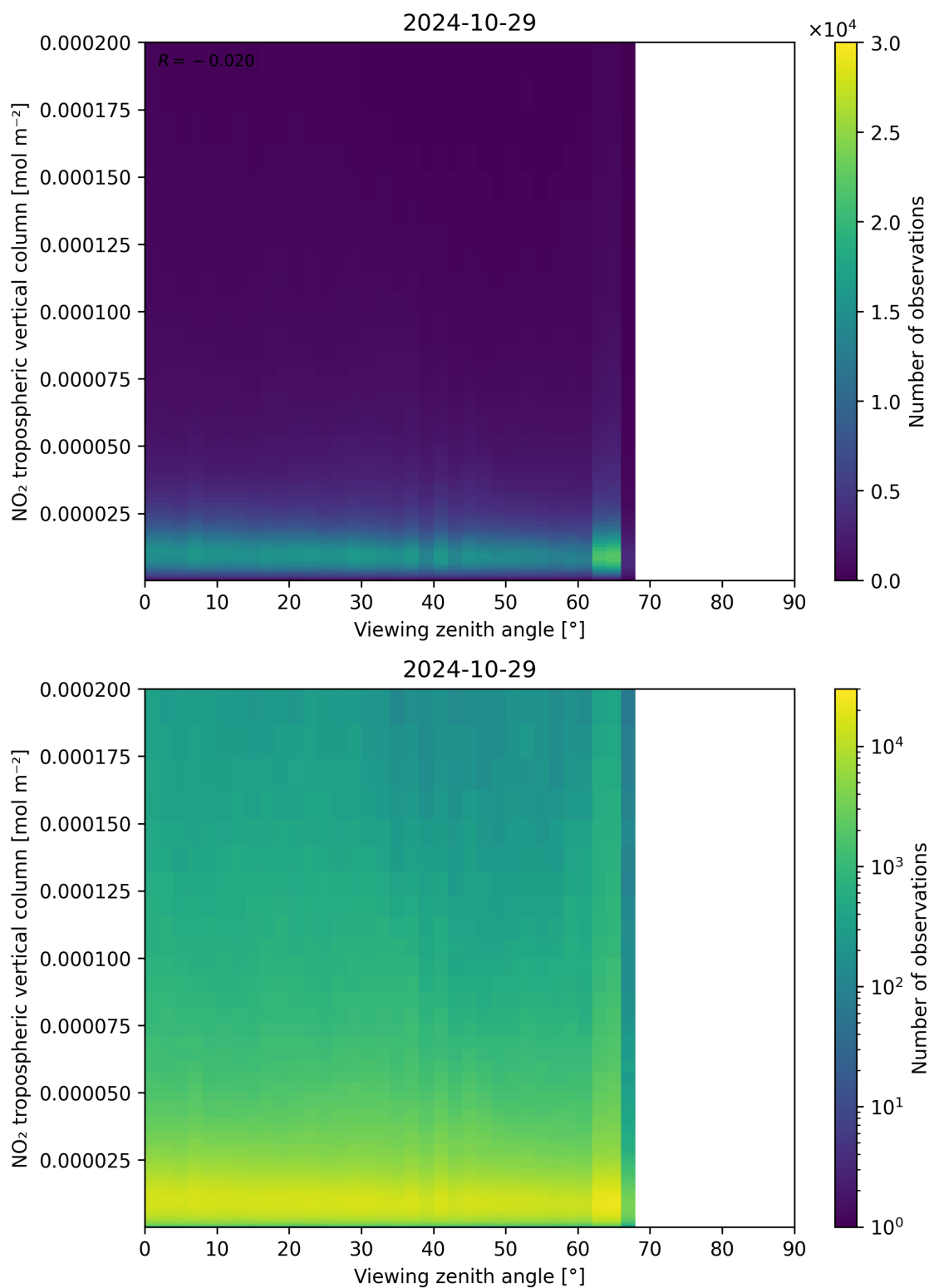
Figure 169: Scatter density plot of “Viewing zenith angle” against “NO 2 tropospheric vertical column” for 2024-10-29 to 2024-10-30.
