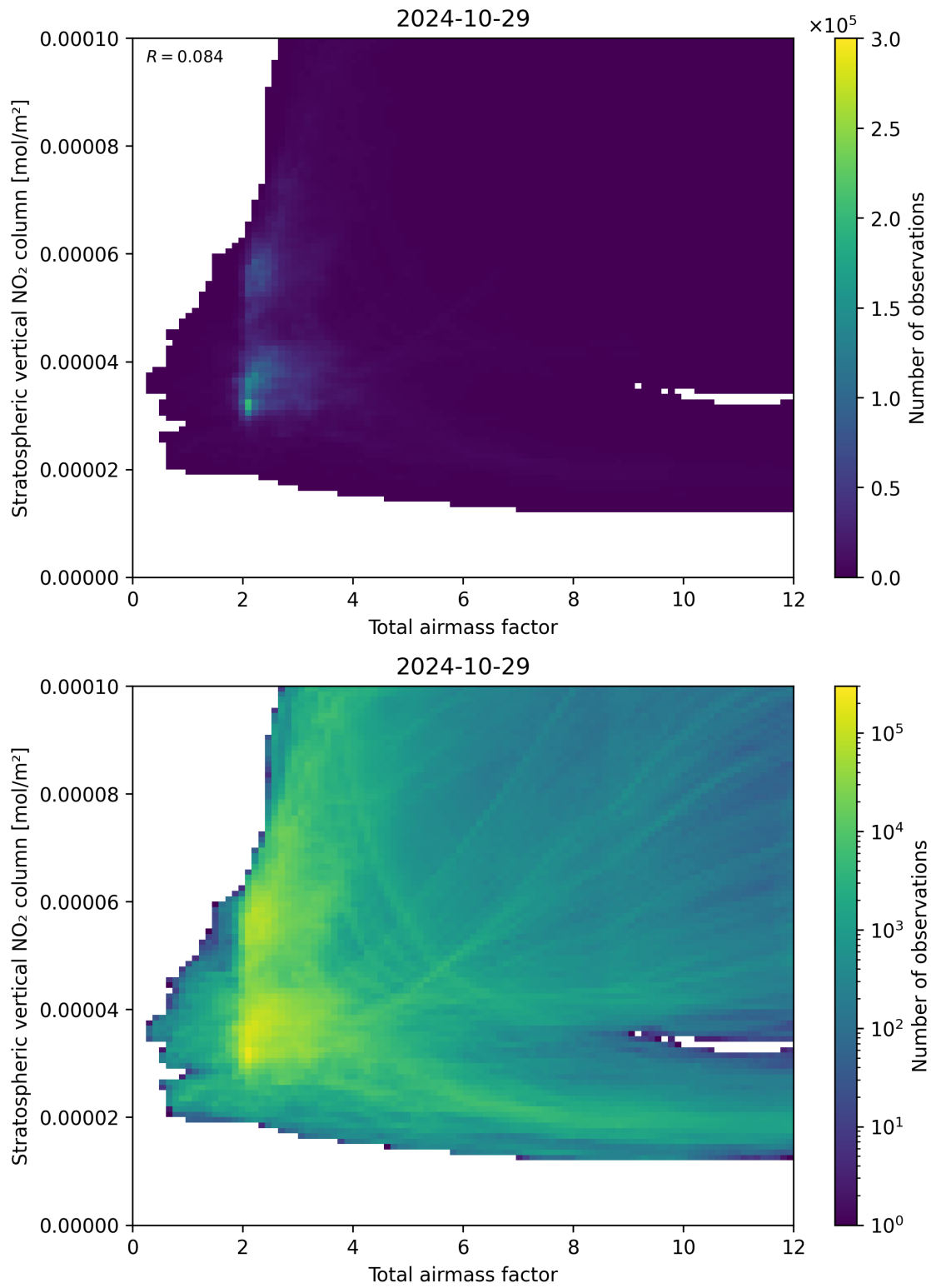
Figure 64: Scatter density plot of “Total airmass factor” against “Stratospheric vertical NO 2 column” for 2024-10-29 to 2024-10-30.
