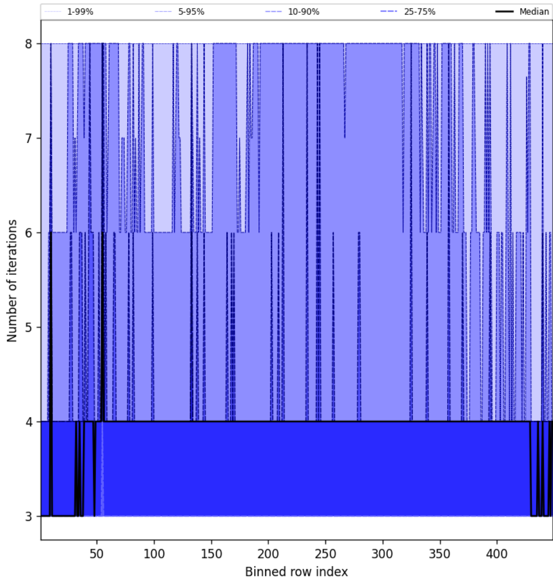
Figure 51: Along track statistics of “Number of iterations” for 2024-10-29 to 2024-10-30
