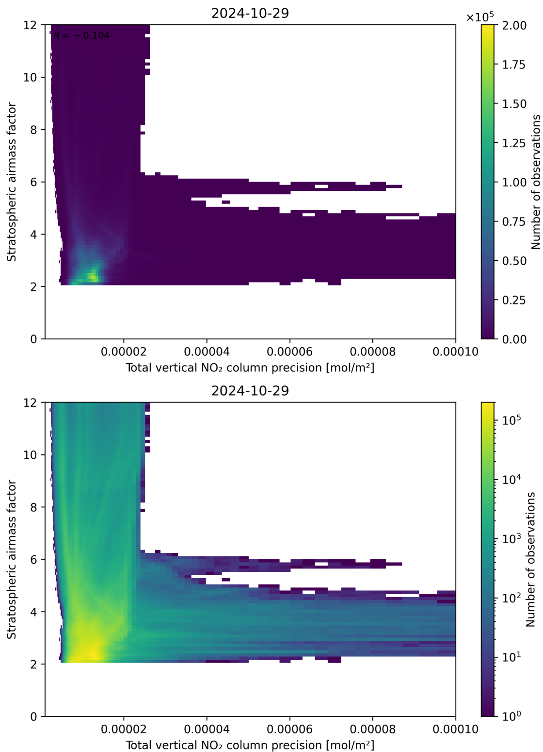
Figure 115: Scatter density plot of “Total vertical NO 2 column precision” against “Stratospheric air mass factor” for 2024-10-29 to 2024-10-30.
