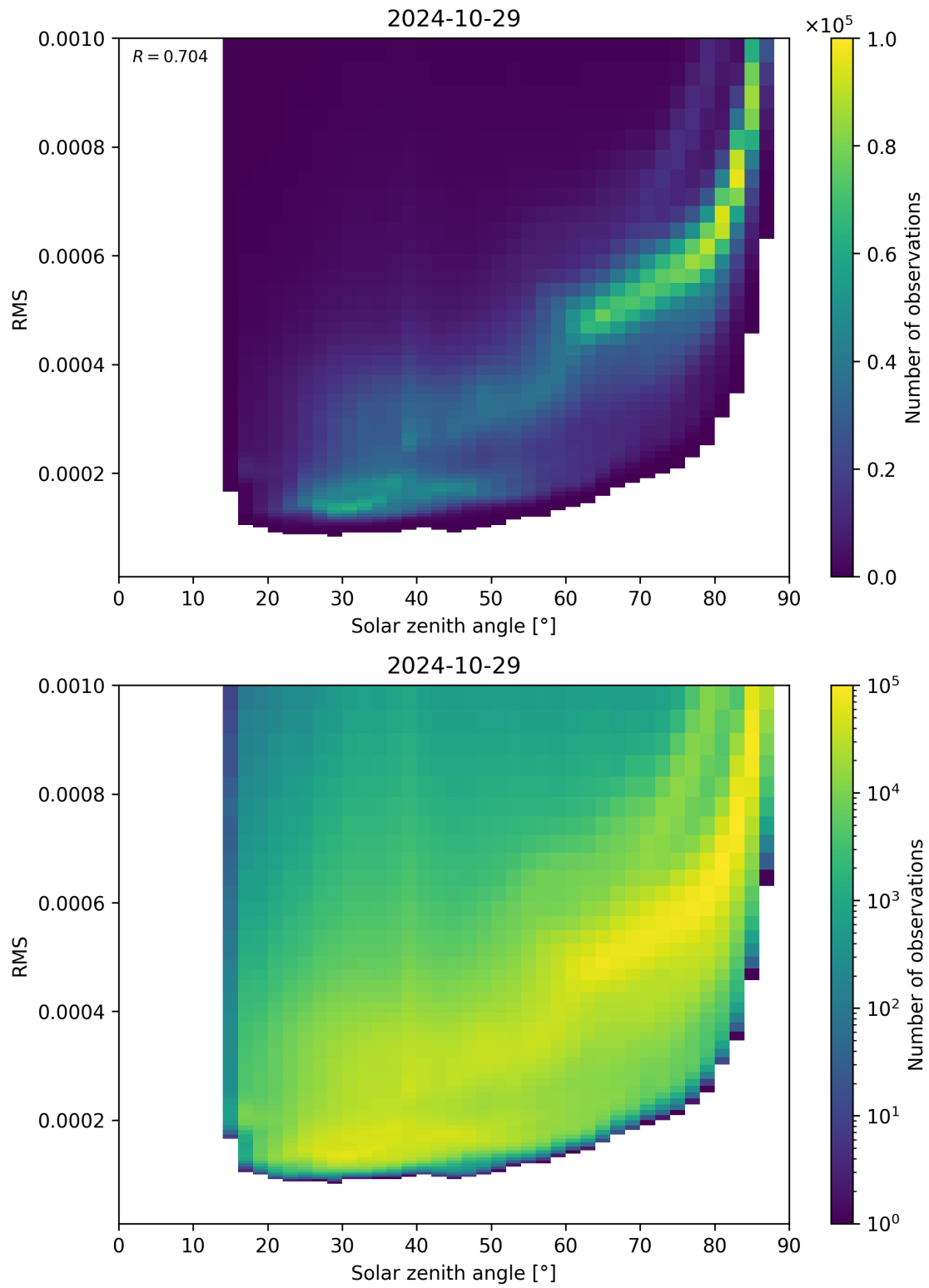
Figure 157: Scatter density plot of “Solar zenith angle” against “RMS” for 2024-10-29 to 2024-10-30.
