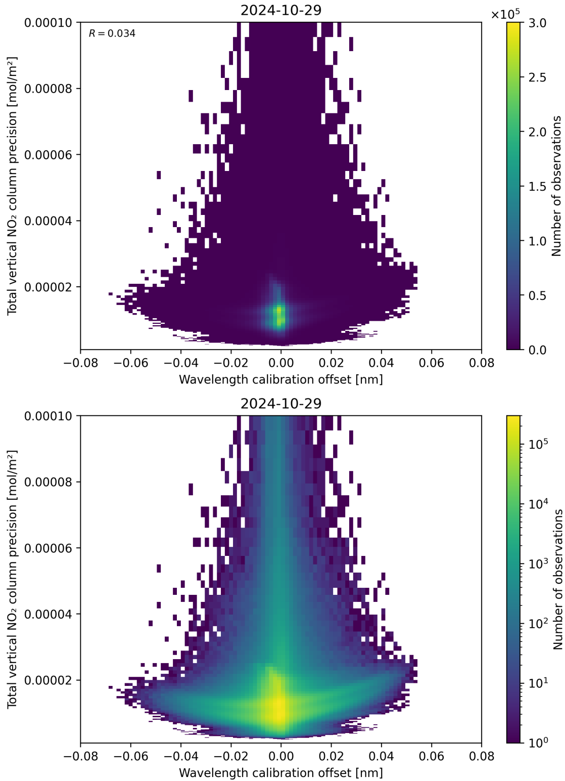
Figure 180: Scatter density plot of “Wavelength calibration offset” against “Total vertical NO 2 column precision” for 2024-10-29 to 2024-10-30.
