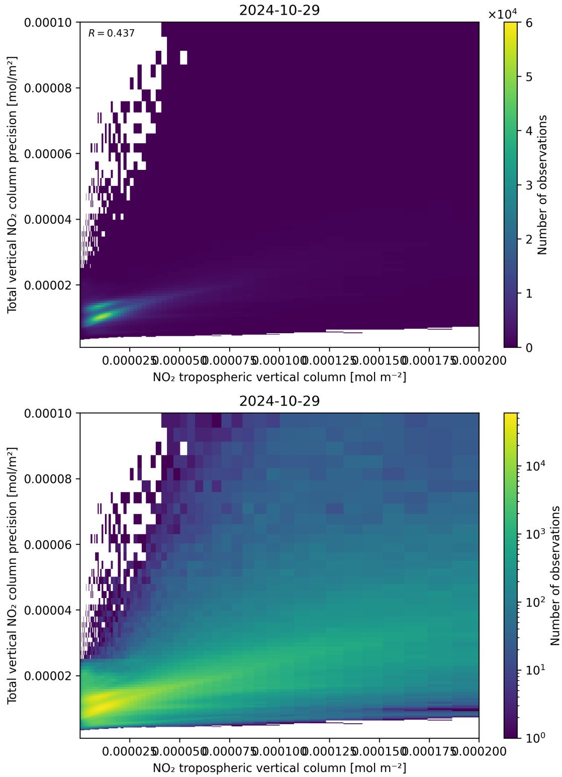
Figure 129: Scatter density plot of “NO 2 tropospheric vertical column” against “Total vertical NO 2 column precision” for 2024-10-29 to 2024-10-30.
