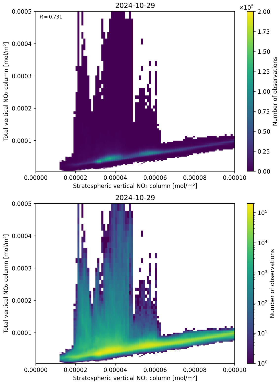
Figure 100: Scatter density plot of “Stratospheric vertical NO 2 column” against “Total vertical NO 2 column” for 2024-10-29 to 2024-10-30.
