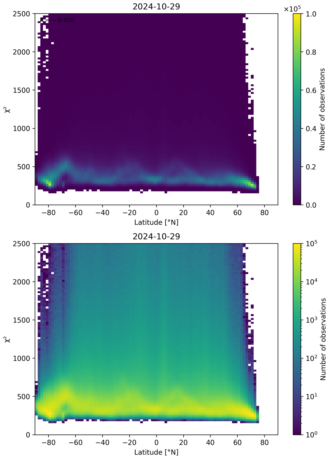
Figure 86: Scatter density plot of “Latitude” against “ \chi^2 ” for 2024-10-29 to 2024-10-30.
