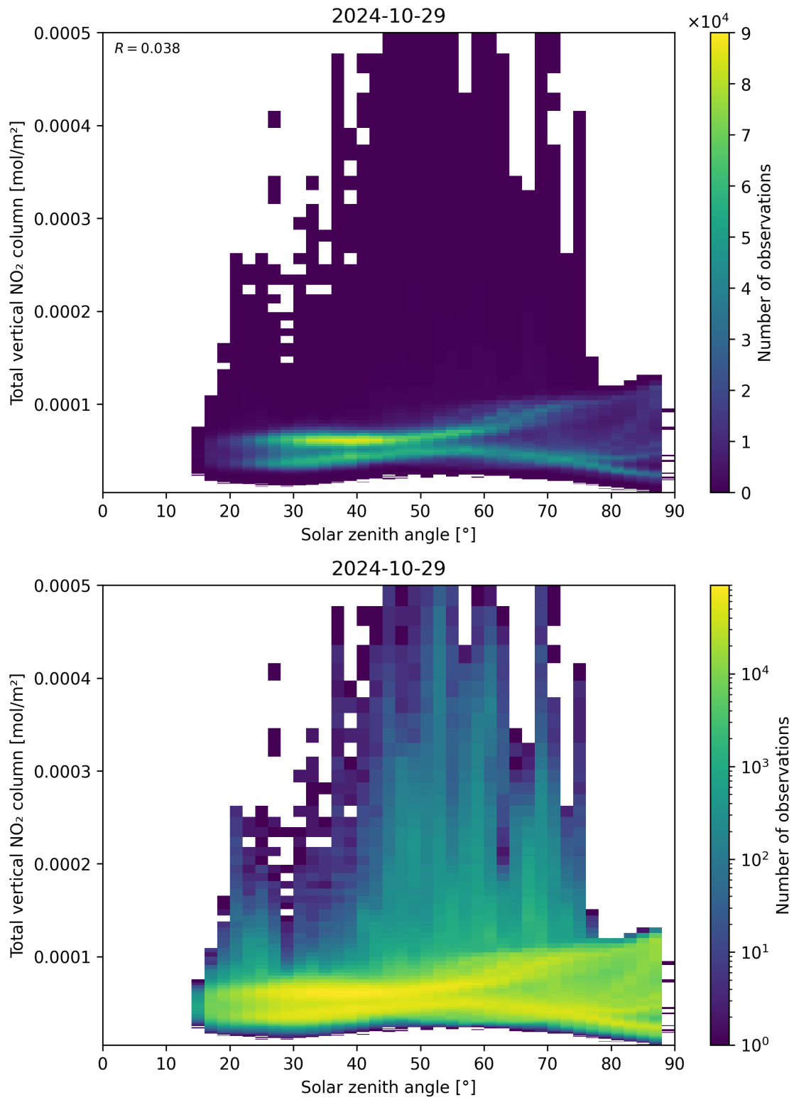
Figure 153: Scatter density plot of “Solar zenith angle” against “Total vertical NO 2 column” for 2024-10-29 to 2024-10-30.
