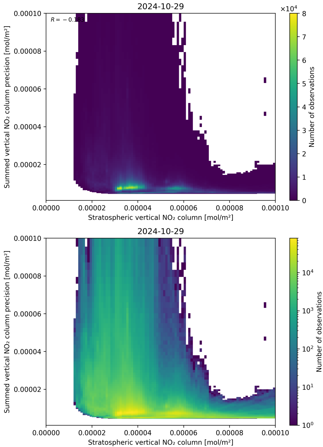
Figure 99: Scatter density plot of “Stratospheric vertical NO 2 column” against “Summed vertical NO 2 column precision” for 2024-10-29 to 2024-10-30.
