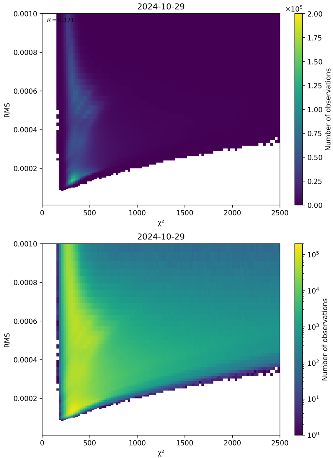
Figure 82: Scatter density plot of “ \chi^2 ” against “RMS” for 2024-10-29 to 2024-10-30.
