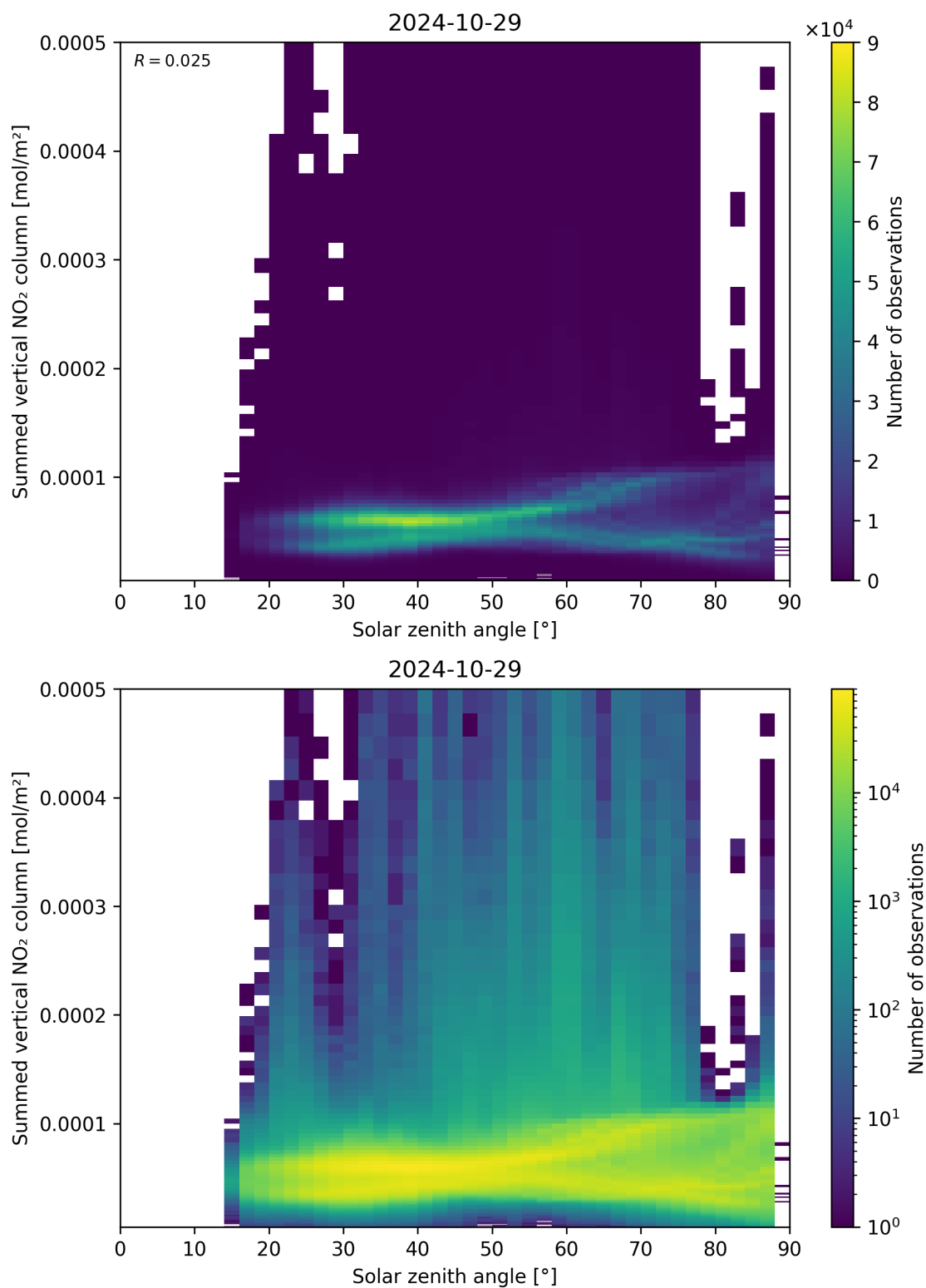
Figure 151: Scatter density plot of “Solar zenith angle” against “Summed vertical NO 2 column” for 2024-10-29 to 2024-10-30.
