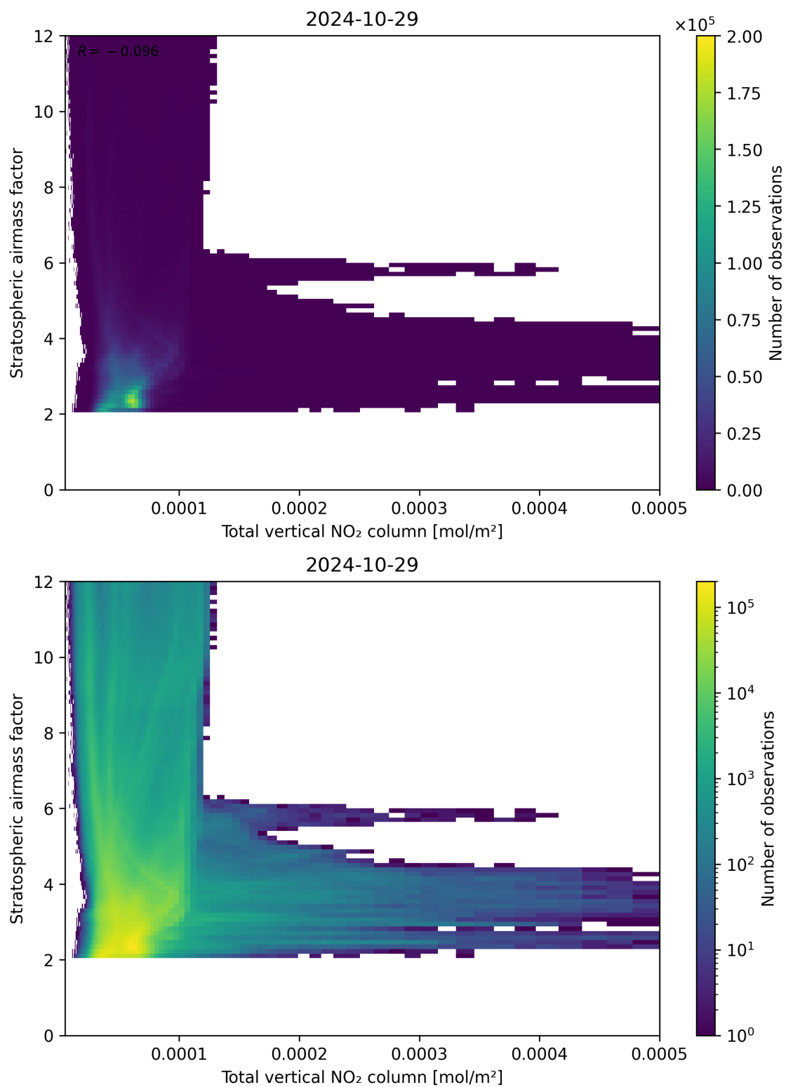
Figure 110: Scatter density plot of “Total vertical NO 2 column” against “Stratospheric airmass factor” for 2024-10-29 to 2024-10-30.
