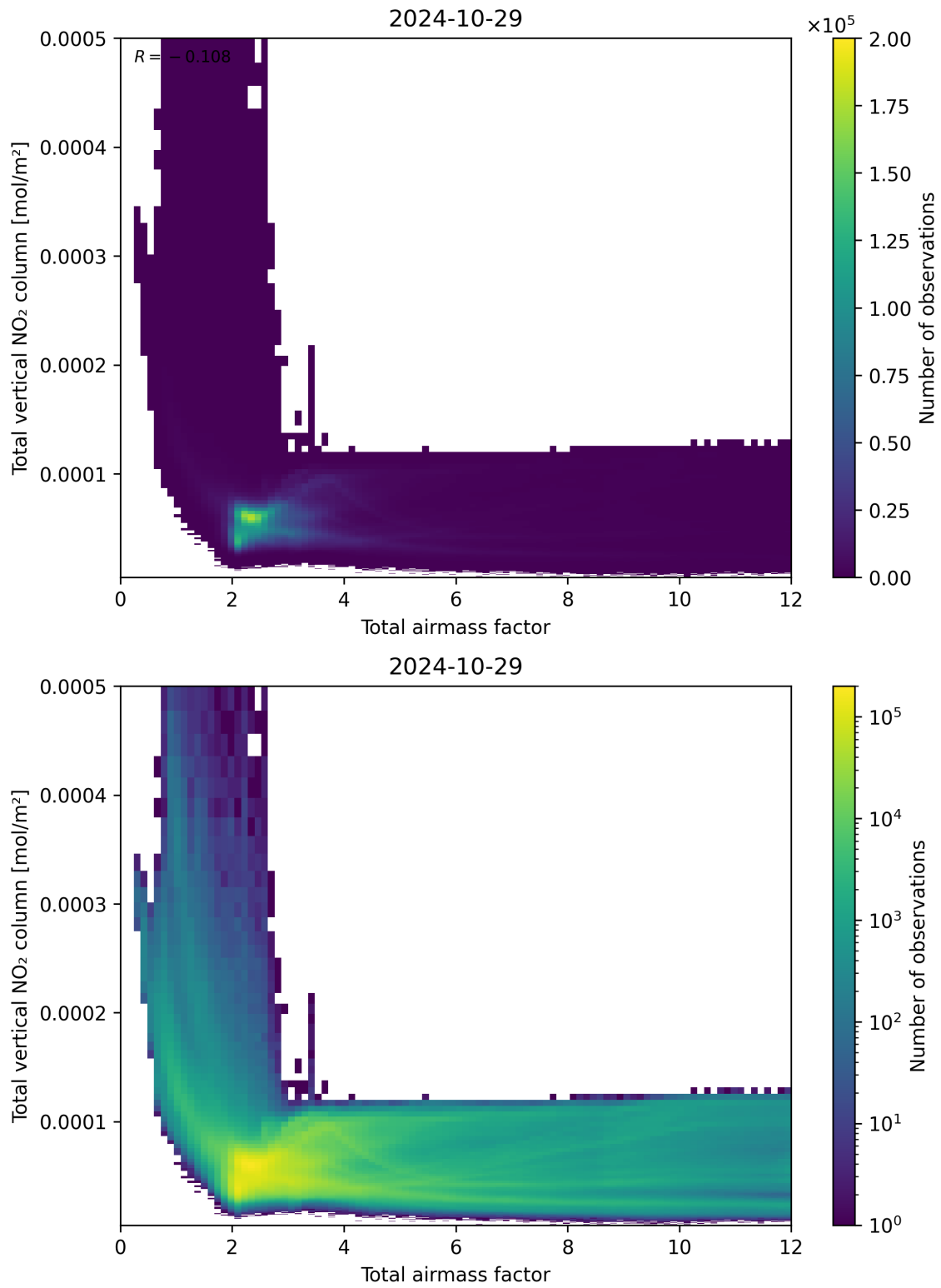
Figure 67: Scatter density plot of “Total air mass factor” against “Total vertical NO 2 column” for 2024-10-29 to 2024-10-30.
