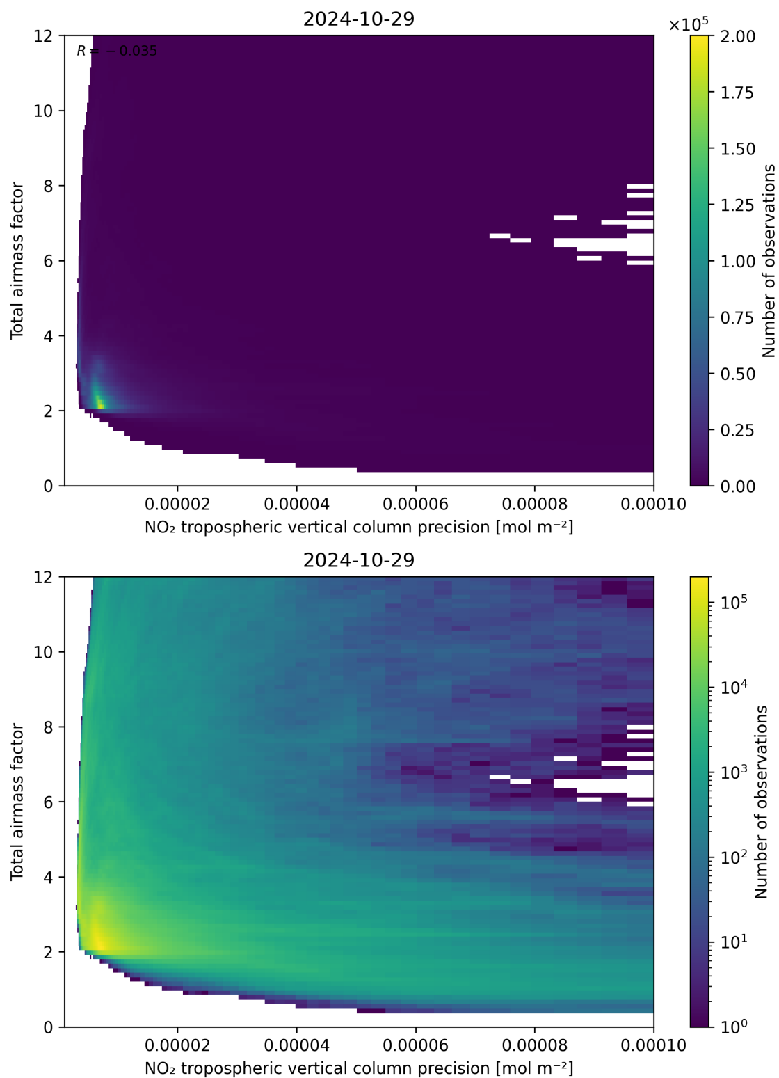
Figure 132: Scatter density plot of “NO 2 tropospheric vertical column precision” against “Total air mass factor” for 2024-10-29 to 2024-10-30.
