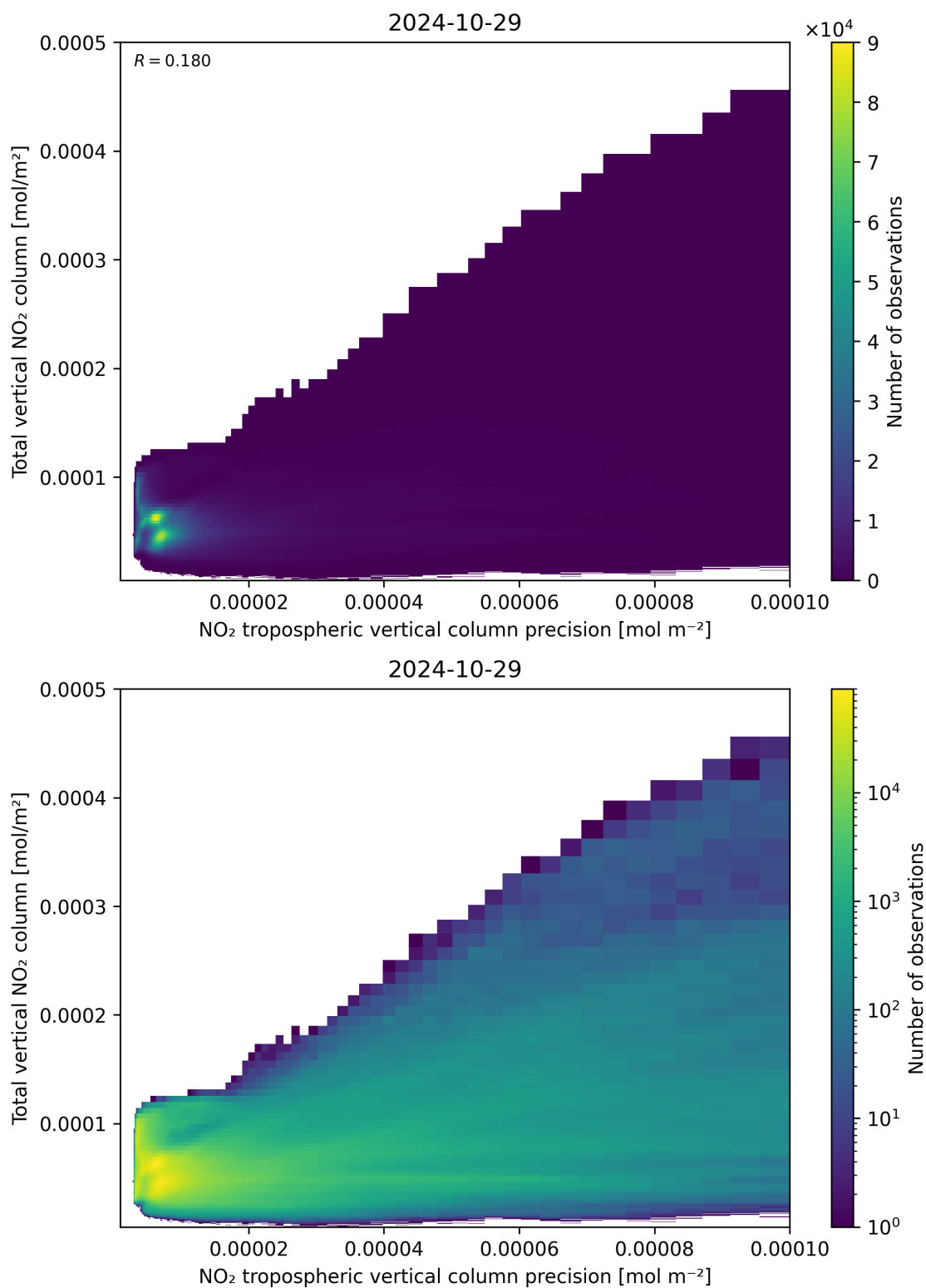
Figure 138: Scatter density plot of “NO 2 tropospheric vertical column precision” against “Total vertical NO 2 column” for 2024-10-29 to 2024-10-30.
