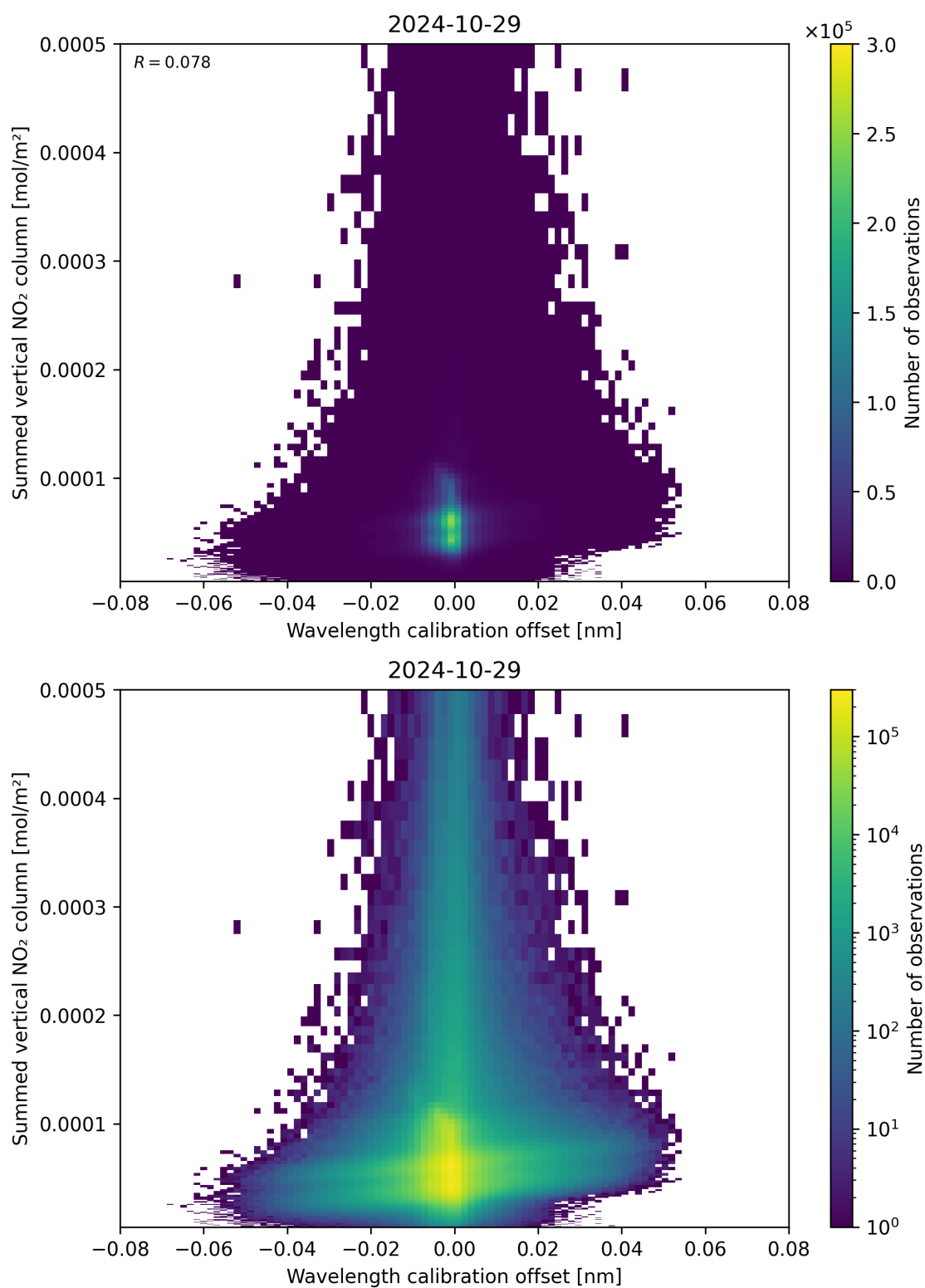
Figure 177: Scatter density plot of “Wavelength calibration offset” against “Summed vertical NO 2 column” for 2024-10-29 to 2024-10-30.
