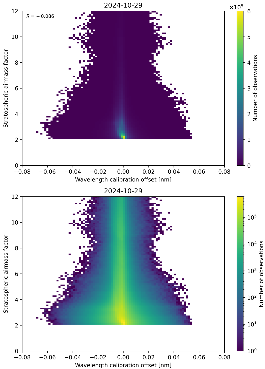
Figure 174: Scatter density plot of “Wavelength calibration offset” against “Stratospheric airmass factor” for 2024-10-29 to 2024-10-30.
