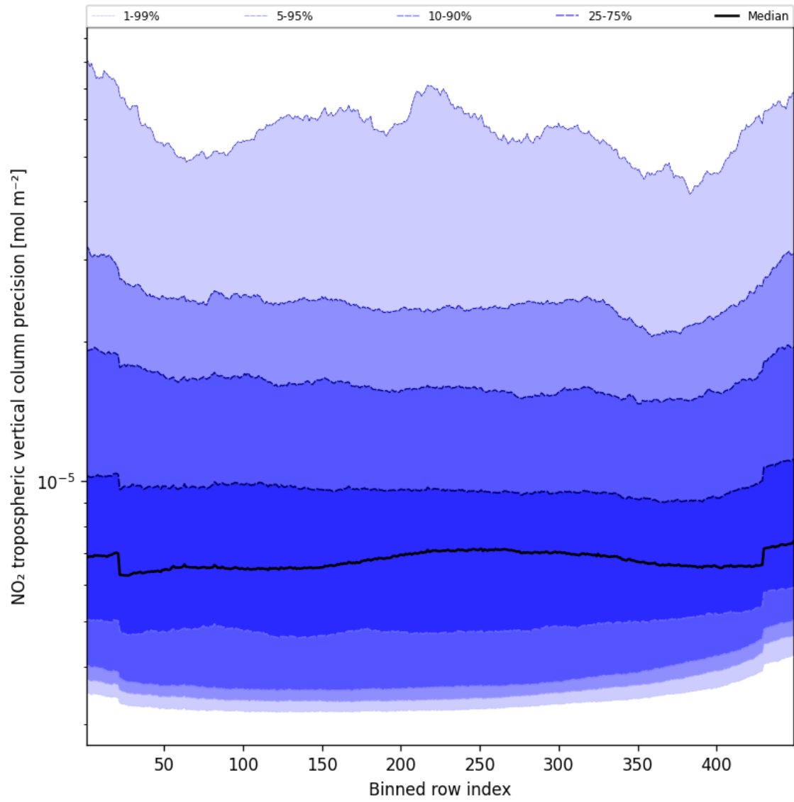
Figure 47: Along track statistics of “NO 2 tropospheric vertical column precision” for 2024-10-29 to 2024-10-30
