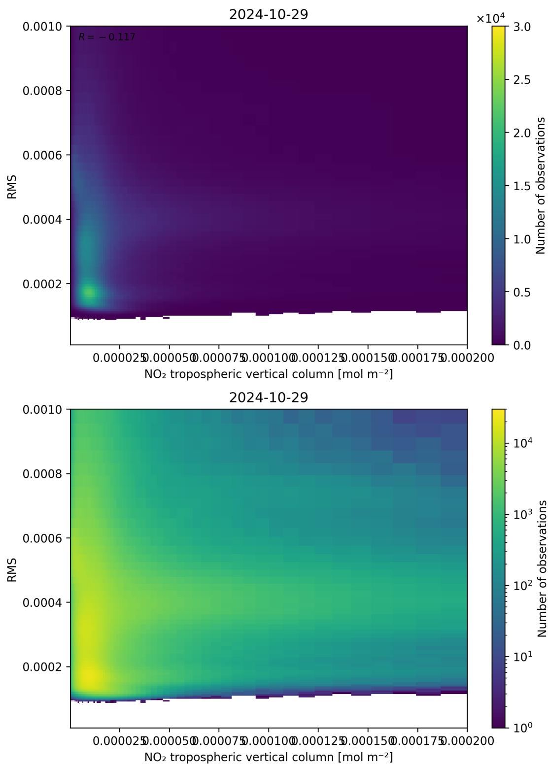
Figure 142: Scatter density plot of “NO 2 tropospheric vertical column” against “RMS” for 2024-10-29 to 2024-10-30.
