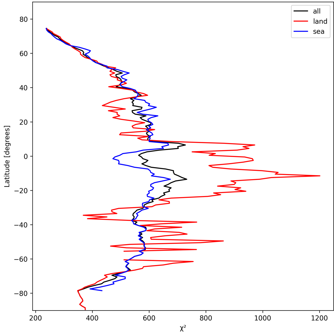
Figure 25: Zonal average of “ \chi^2 ” for 2024-10-29 to 2024-10-30.
