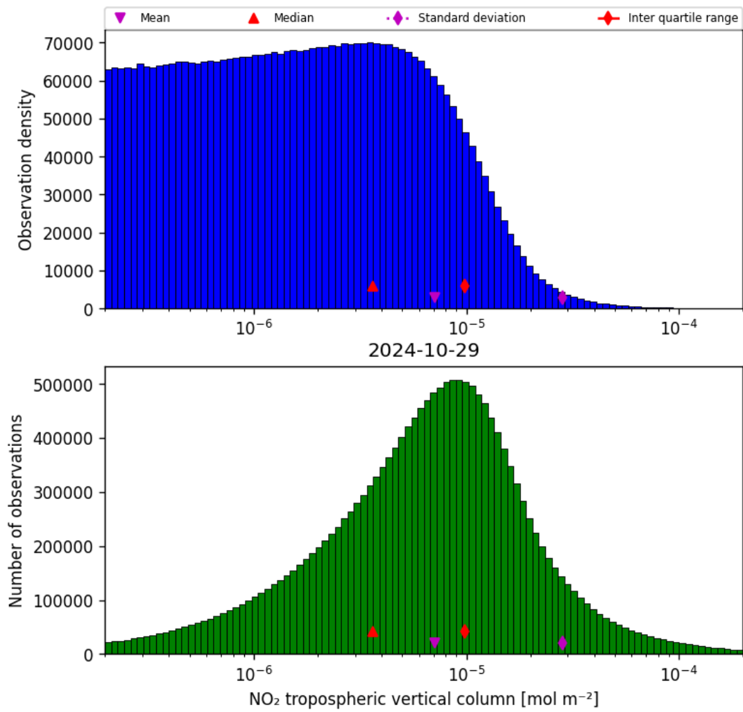
Figure 29: Histogram of “NO 2 tropospheric vertical column” for 2024-10-29 to 2024-10-30
