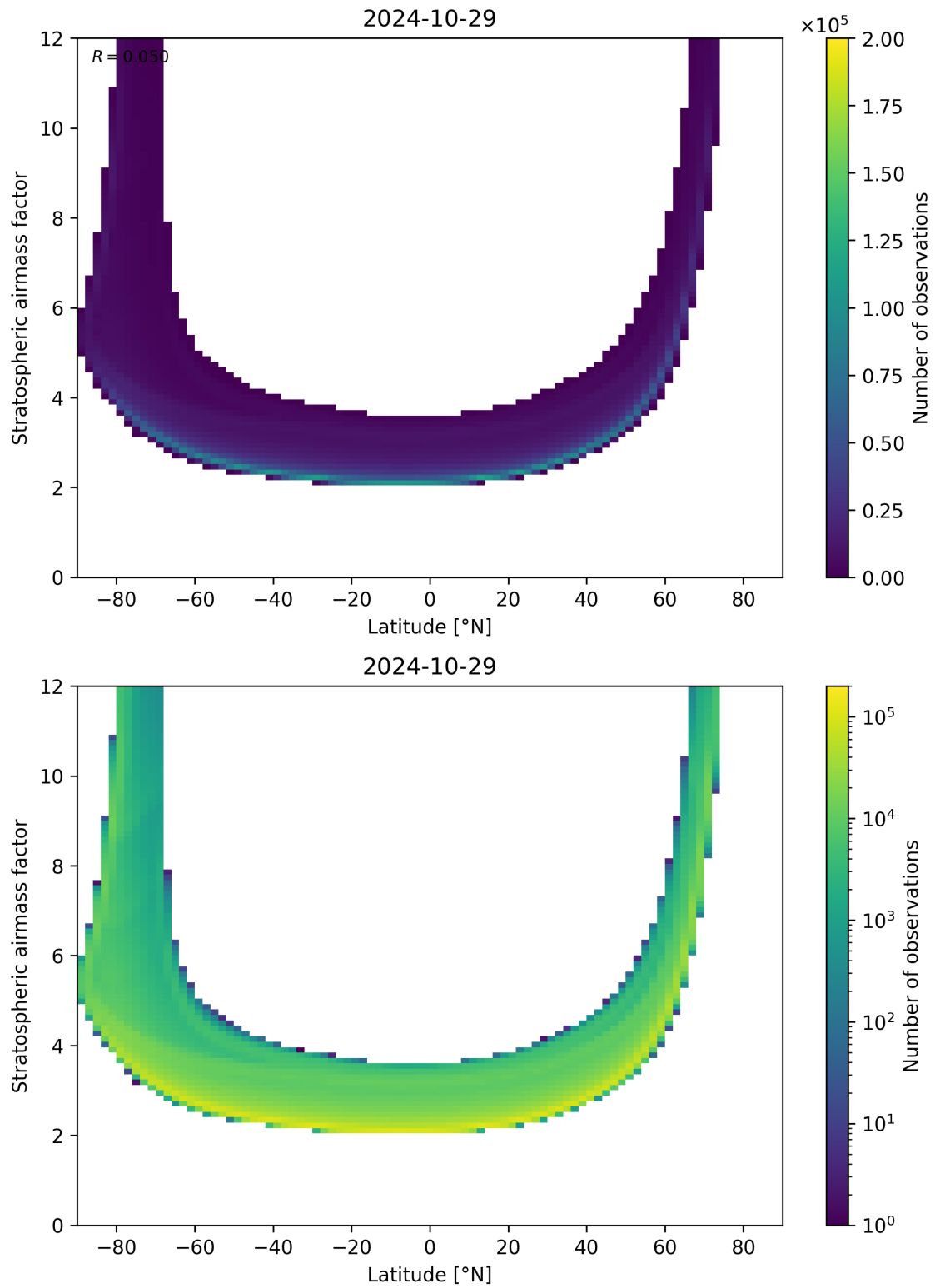
Figure 83: Scatter density plot of “Latitude” against “Stratospheric air mass factor” for 2024-10-29 to 2024-10-30.
