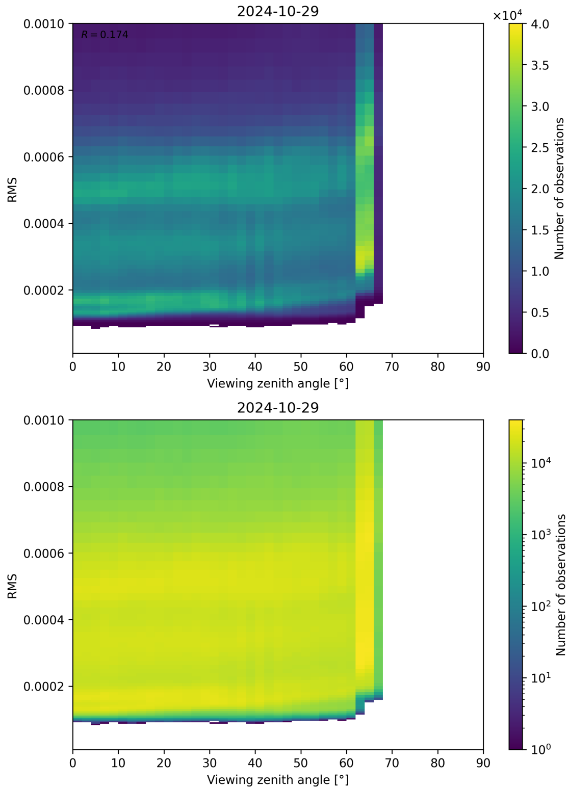
Figure 171: Scatter density plot of “Viewing zenith angle” against “RMS” for 2024-10-29 to 2024-10-30.
