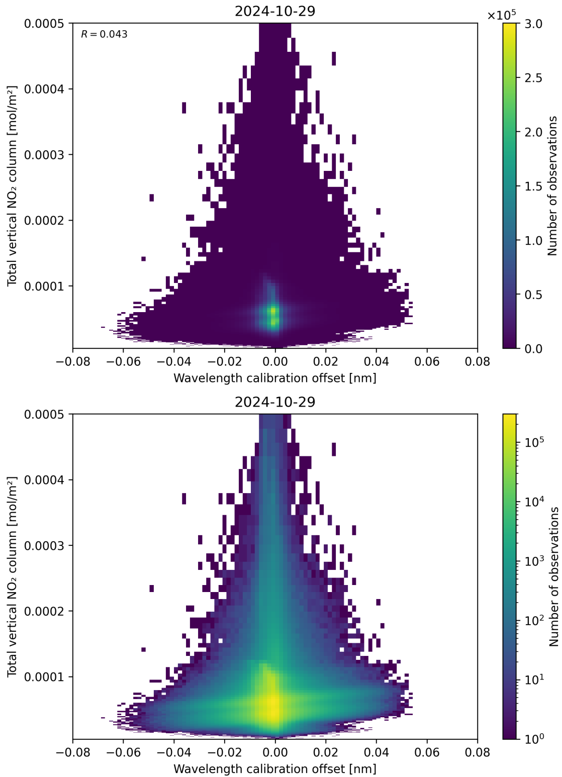
Figure 179: Scatter density plot of “Wavelength calibration offset” against “Total vertical NO 2 column” for 2024-10-29 to 2024-10-30.
