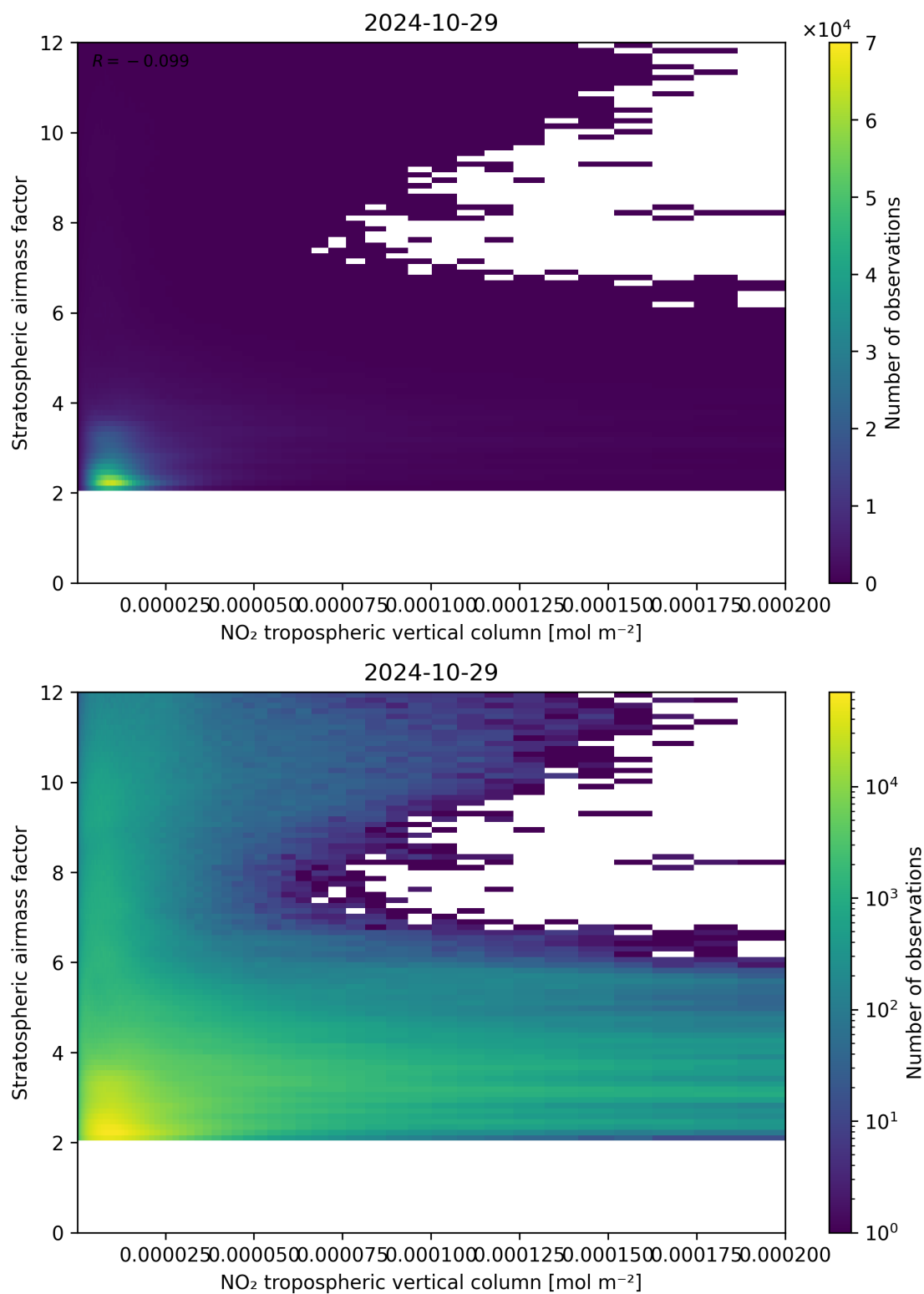
Figure 121: Scatter density plot of “NO 2 tropospheric vertical column” against “Stratospheric air mass factor” for 2024-10-29 to 2024-10-30.
