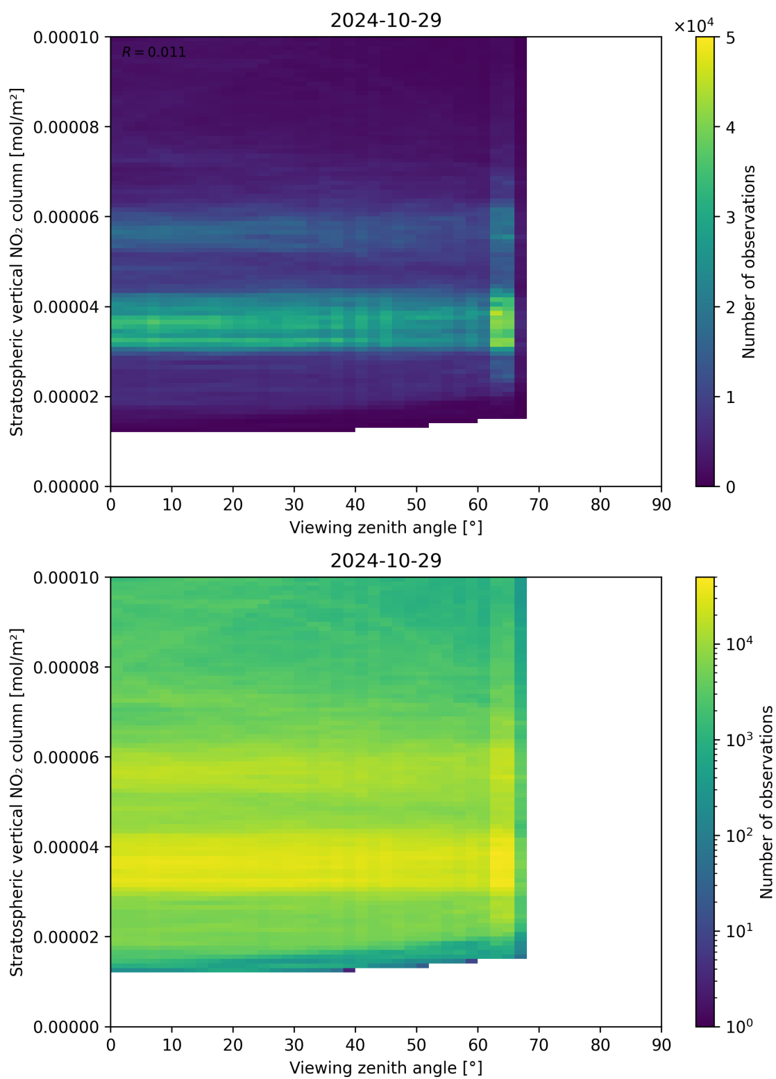
Figure 164: Scatter density plot of “Viewing zenith angle” against “Stratospheric vertical NO 2 column” for 2024-10-29 to 2024-10-30.
