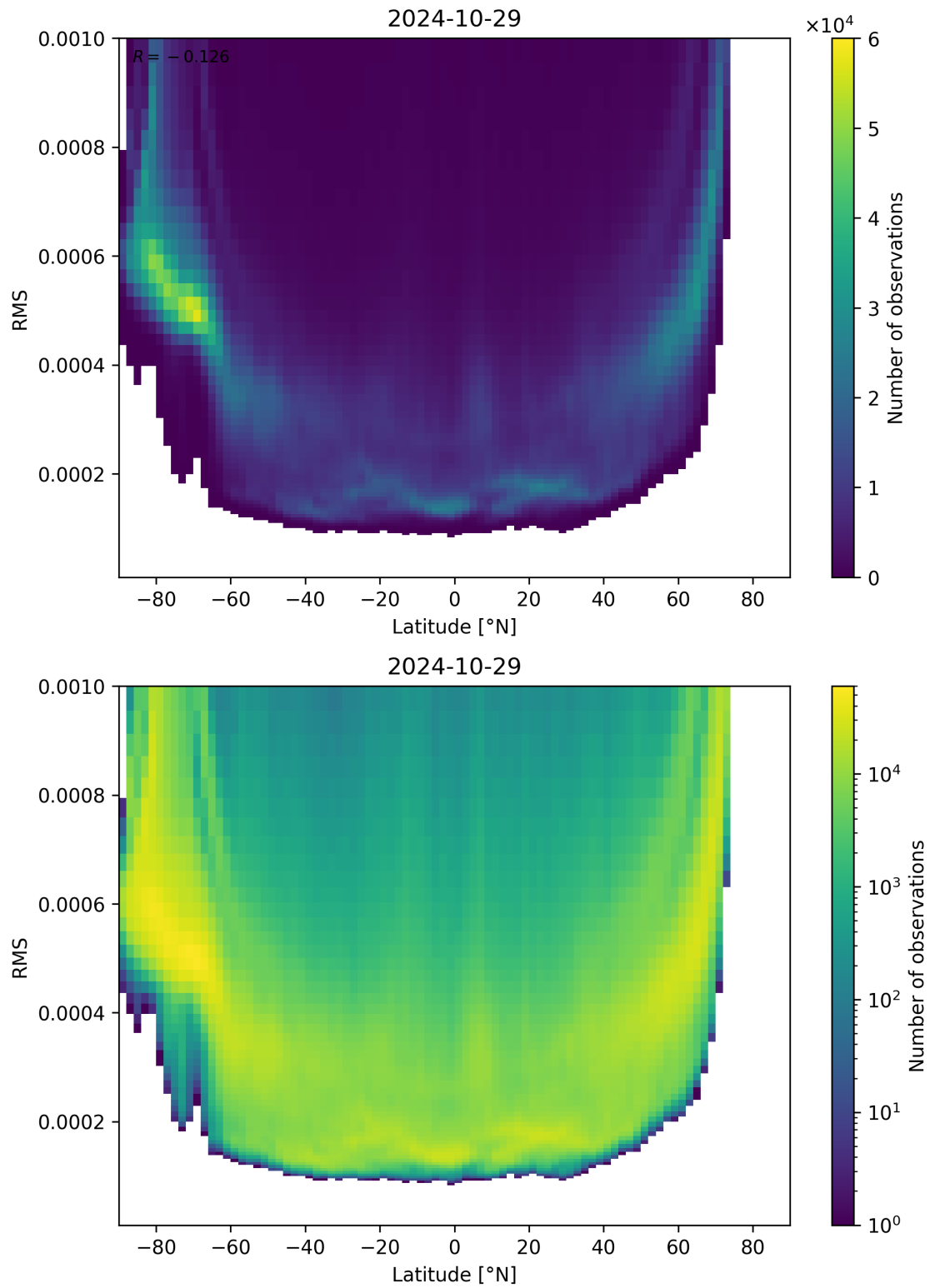
Figure 94: Scatter density plot of “Latitude” against “RMS” for 2024-10-29 to 2024-10-30.
