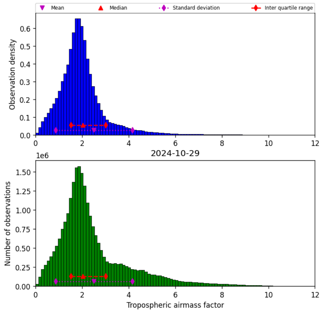
Figure 31: Histogram of “Tropospheric airmass factor” for 2024-10-29 to 2024-10-30
