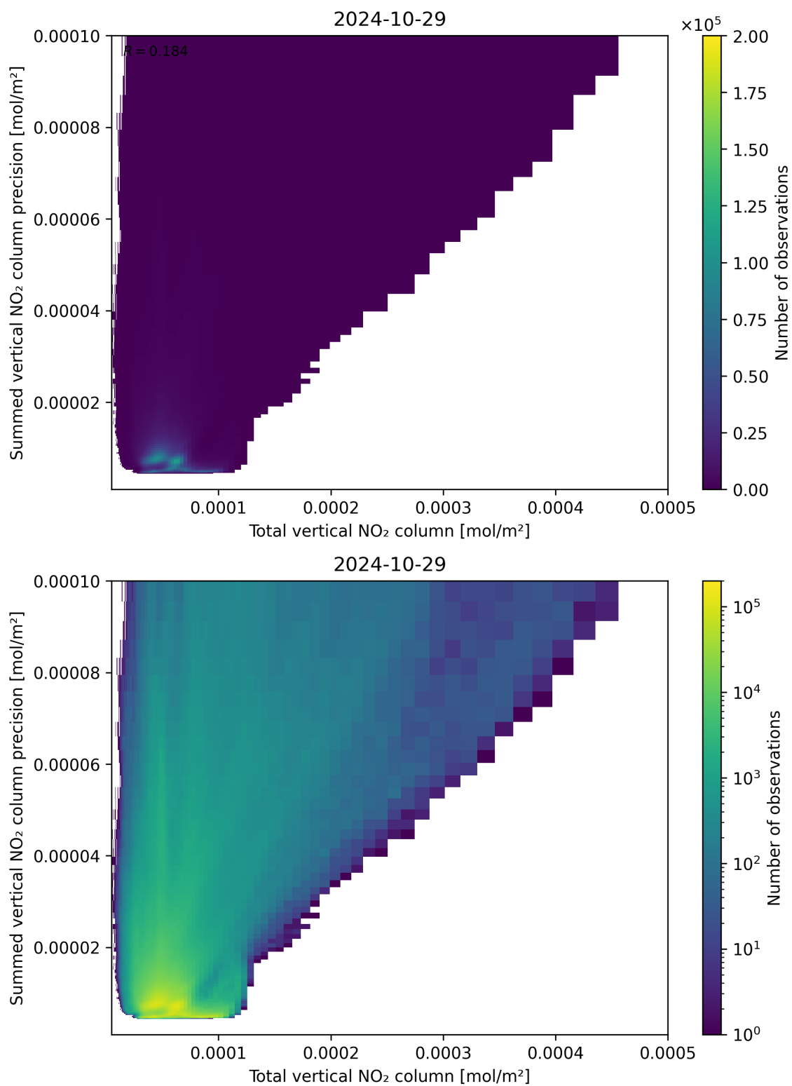
Figure 113: Scatter density plot of “Total vertical NO 2 column” against “Summed vertical NO 2 column precision” for 2024-10-29 to 2024-10-30.
