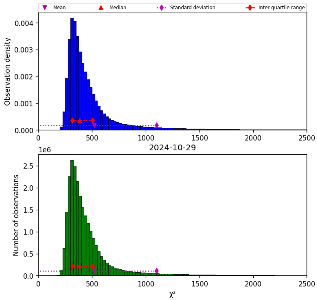
Figure 42: Histogram of “ \chi^2 ” for 2024-10-29 to 2024-10-30
