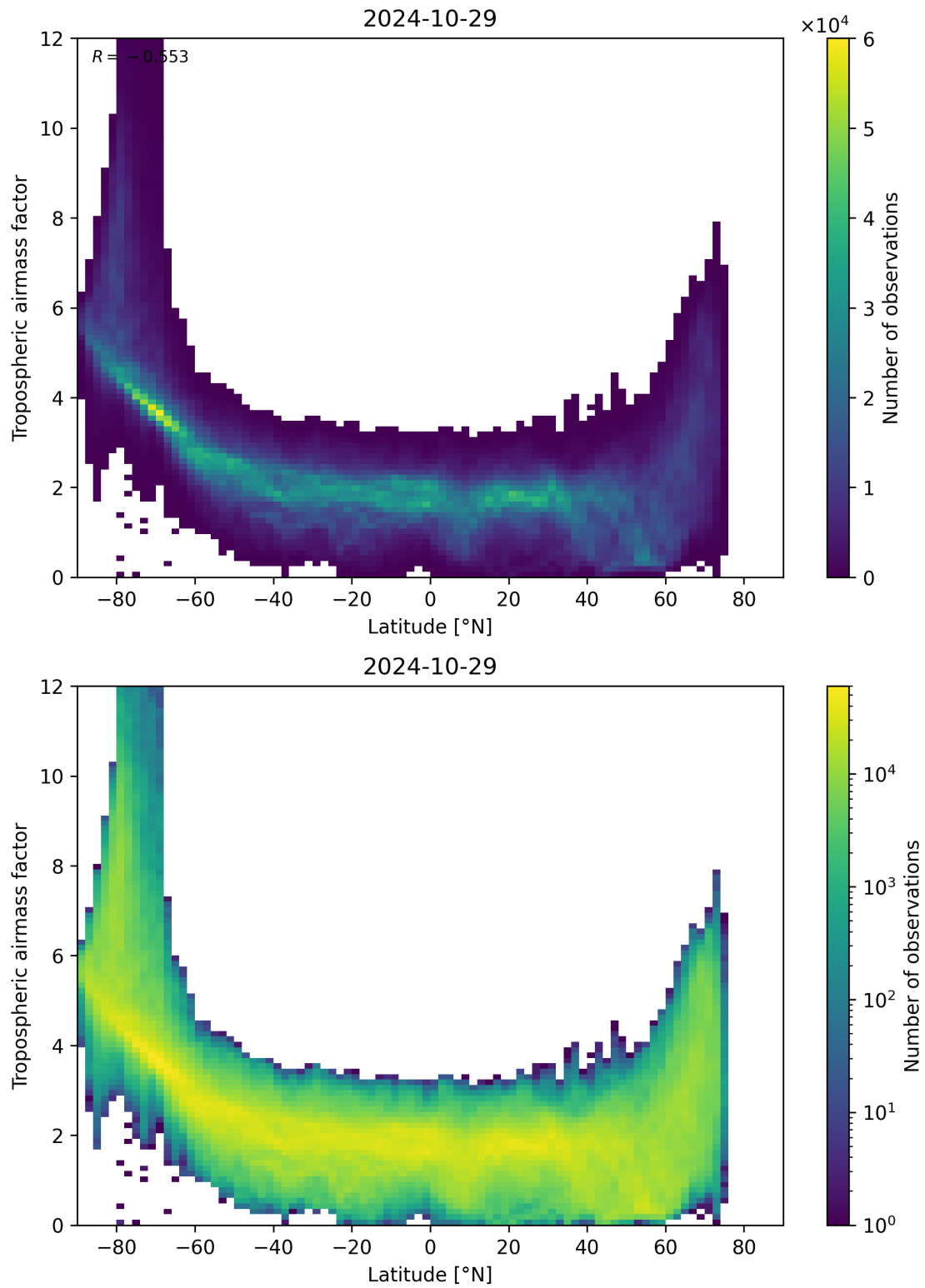
Figure 85: Scatter density plot of “Latitude” against “Tropospheric airmass factor” for 2024-10-29 to 2024-10-30.
