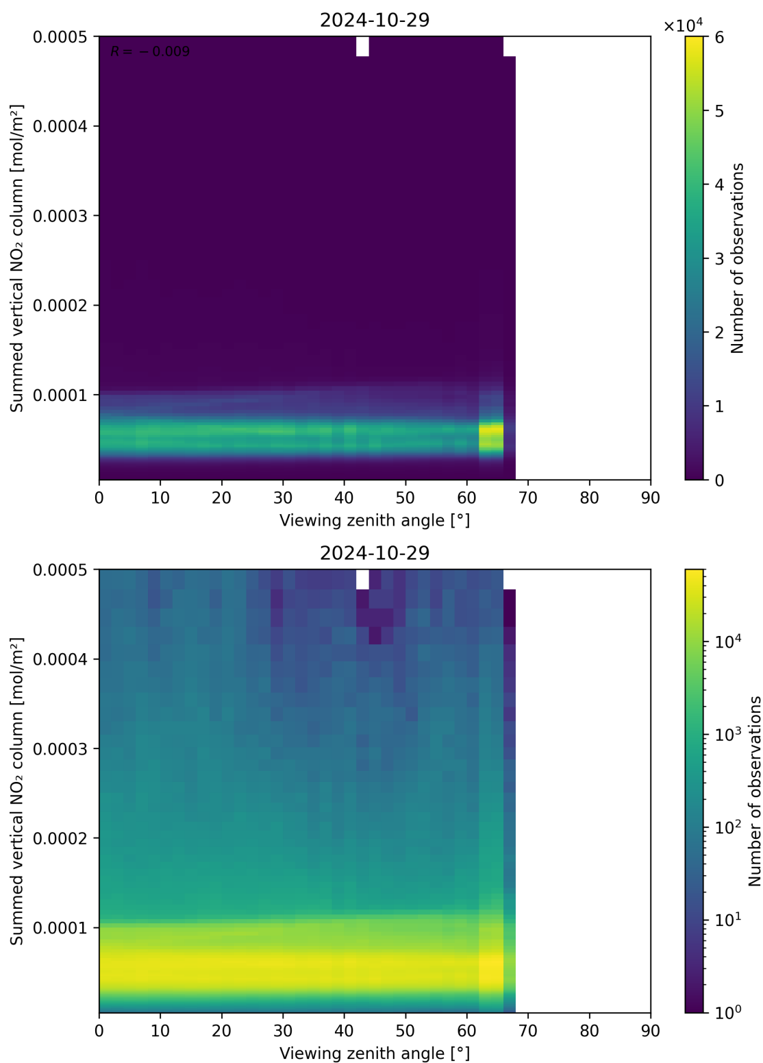
Figure 165: Scatter density plot of “Viewing zenith angle” against “Summed vertical NO 2 column” for 2024-10-29 to 2024-10-30.
