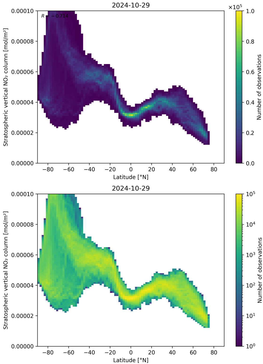
Figure 87: Scatter density plot of “Latitude” against “Stratospheric vertical NO 2 column” for 2024-10-29 to 2024-10-30.
