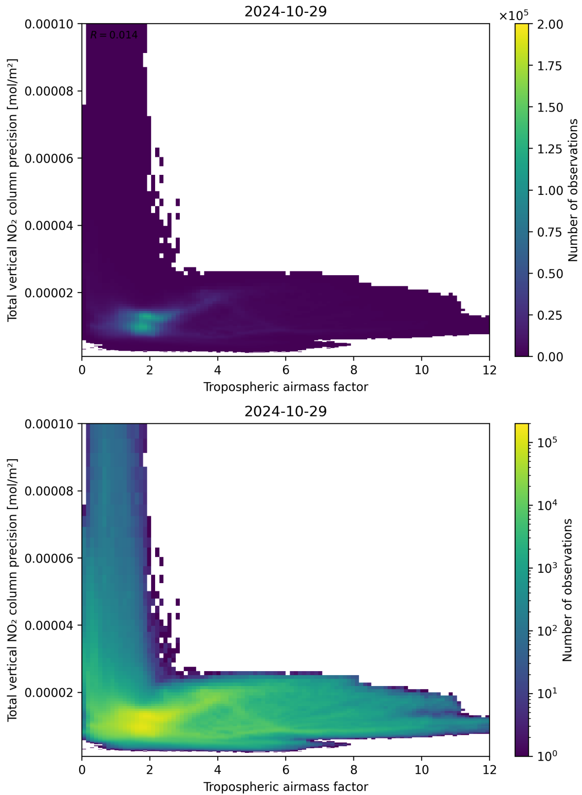
Figure 78: Scatter density plot of “Tropospheric airmass factor” against “Total vertical NO 2 column precision” for 2024-10-29 to 2024-10-30.
