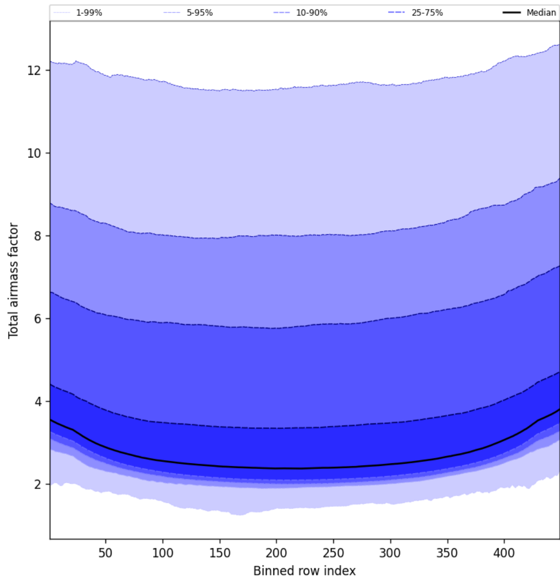
Figure 49: Along track statistics of “Total airmass factor” for 2024-10-29 to 2024-10-30
