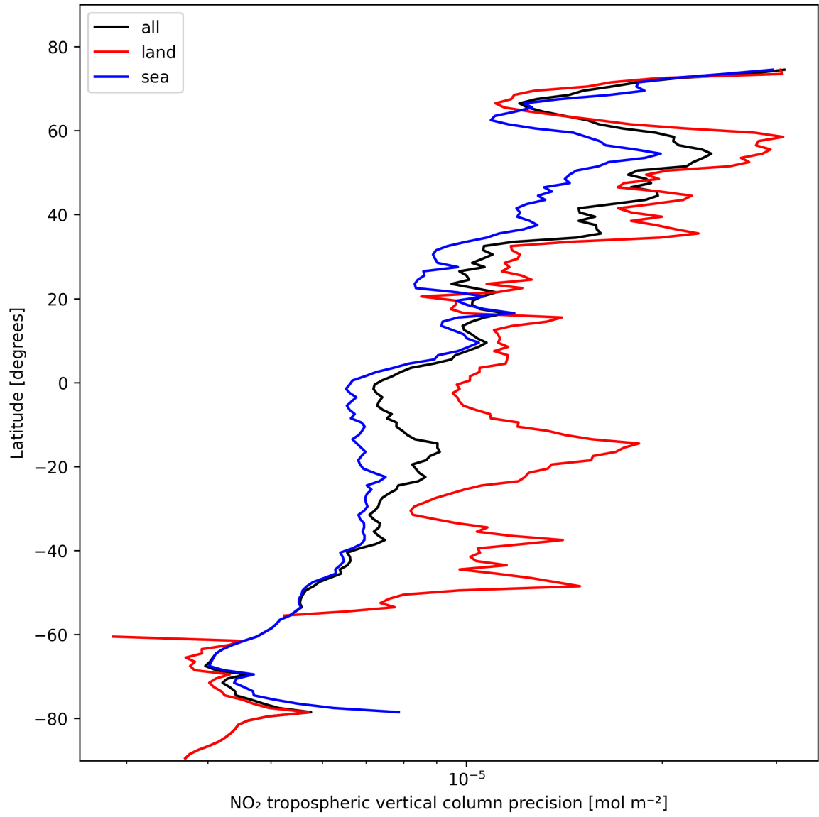
Figure 13: Zonal average of “NO 2 tropospheric vertical column precision” for 2024-10-29 to 2024-10-30.
