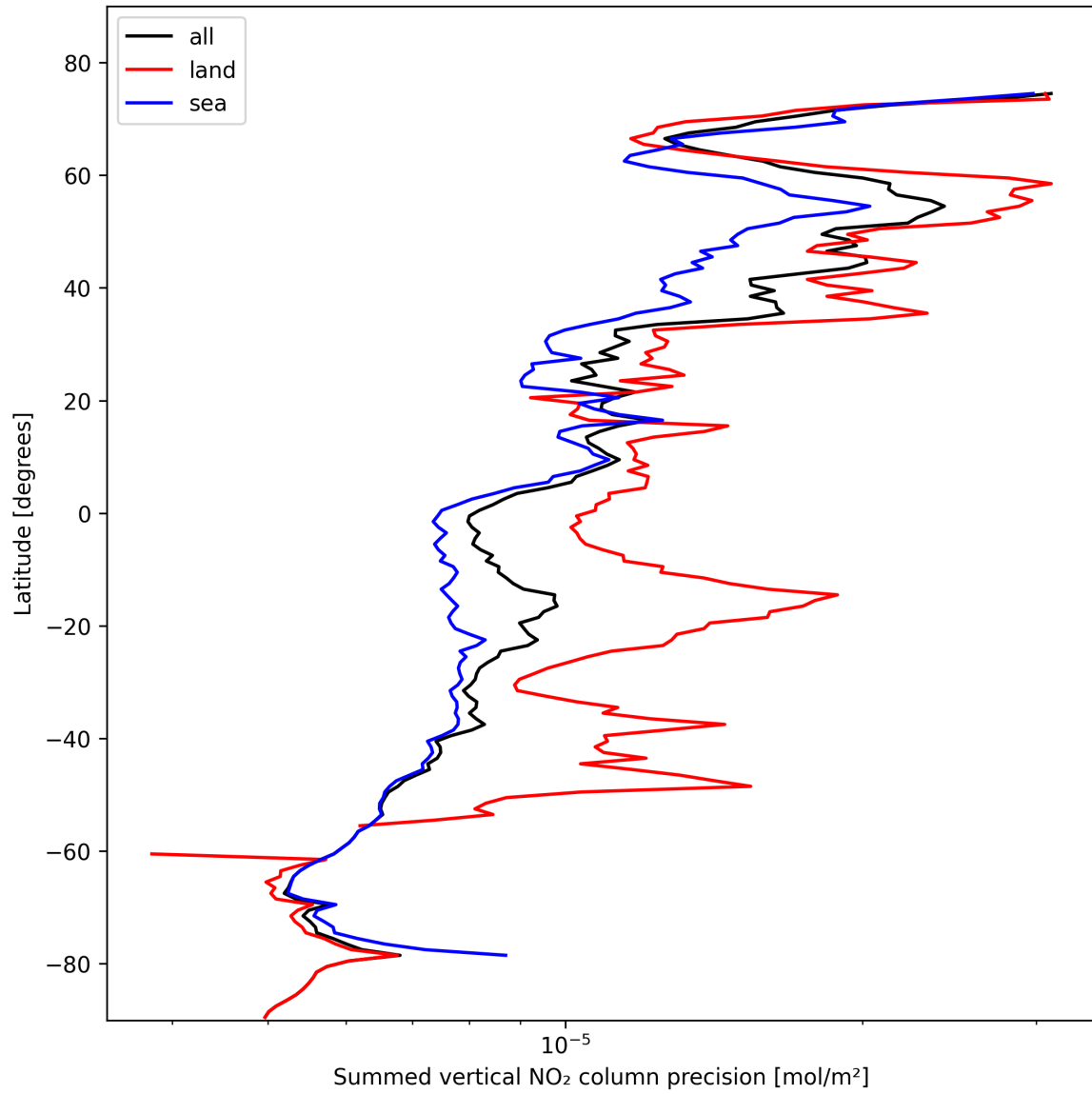
Figure 24: Zonal average of “Summed vertical NO 2 column precision” for 2024-10-29 to 2024-10-30.
