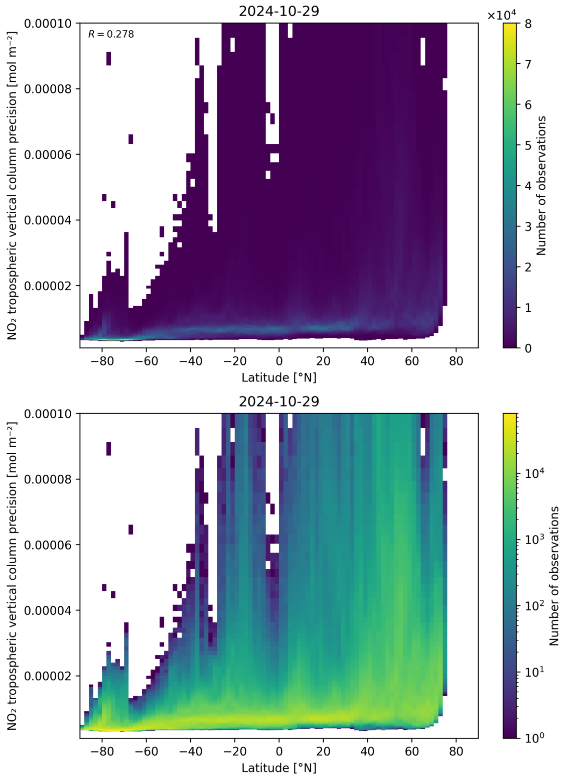
Figure 93: Scatter density plot of “Latitude” against “NO 2 tropospheric vertical column precision” for 2024-10-29 to 2024-10-30.
