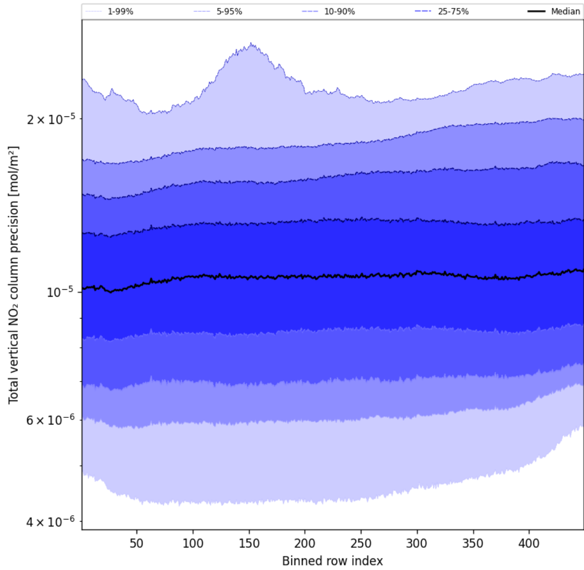
Figure 56: Along track statistics of "Total vertical NO 2 column precision" for 2024-10-29 to 2024-10-30
