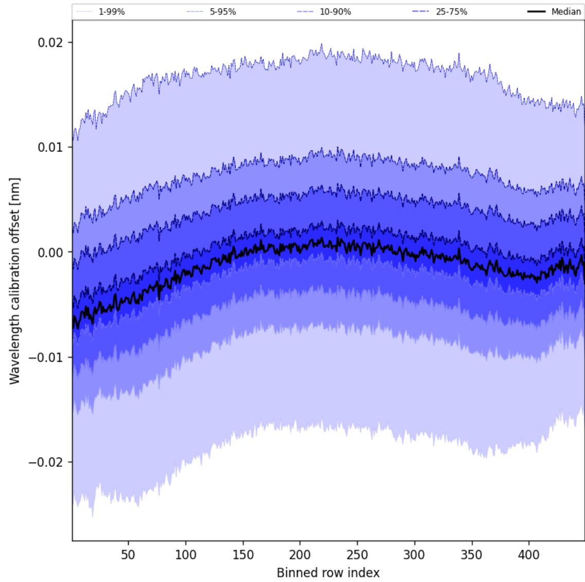
Figure 52: Along track statistics of “Wavelength calibration offset” for 2024-10-29 to 2024-10-30
