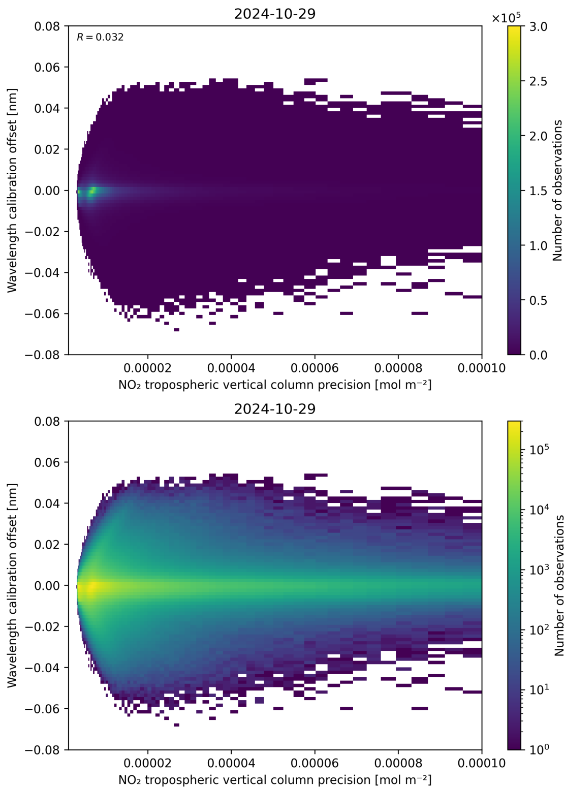
Figure 141: Scatter density plot of “NO 2 tropospheric vertical column precision” against “Wavelength calibration offset” for 2024-10-29 to 2024-10-30.
