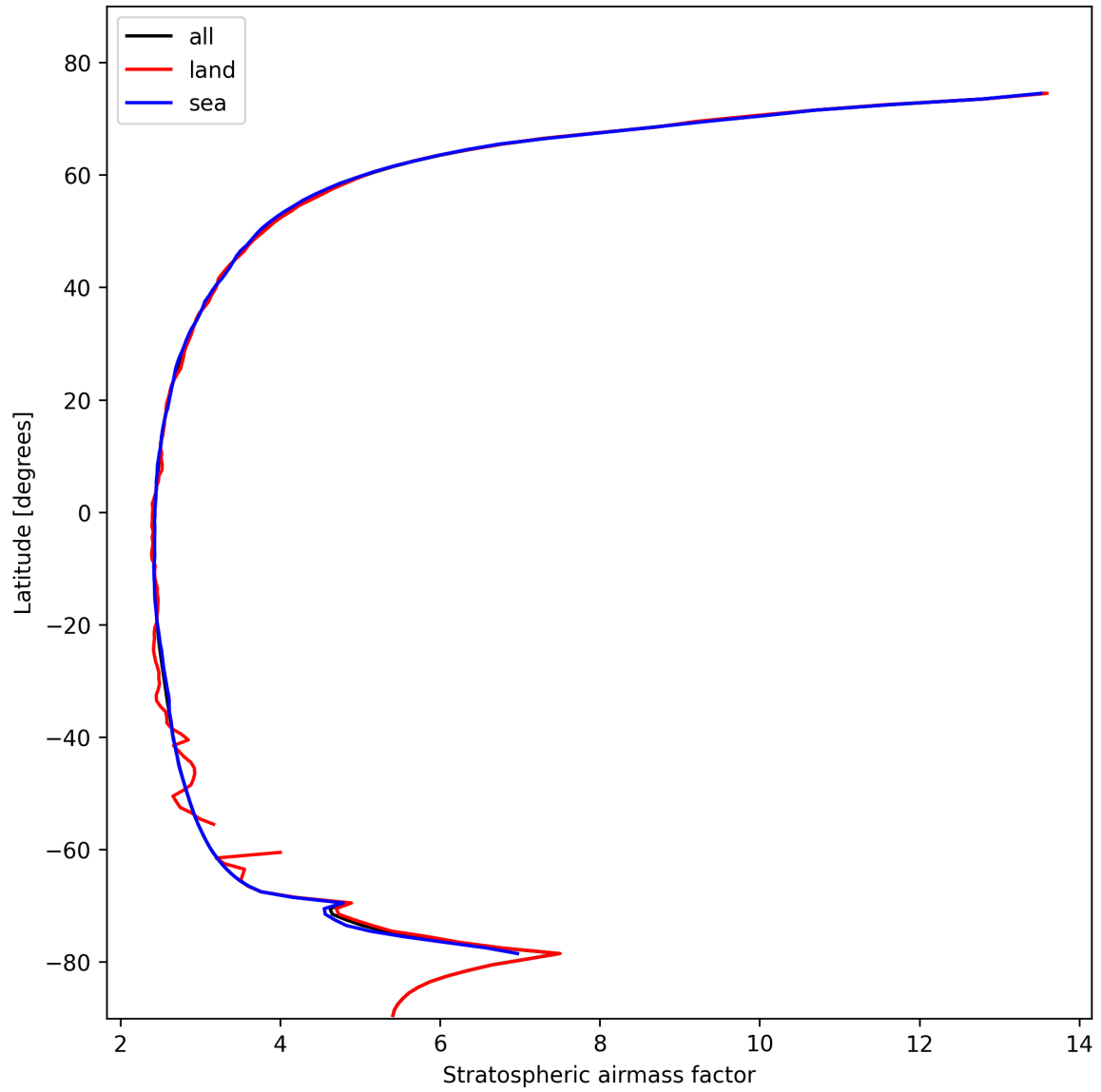
Figure 27: Zonal average of “Stratospheric air mass factor” for 2024-10-29 to 2024-10-30.
