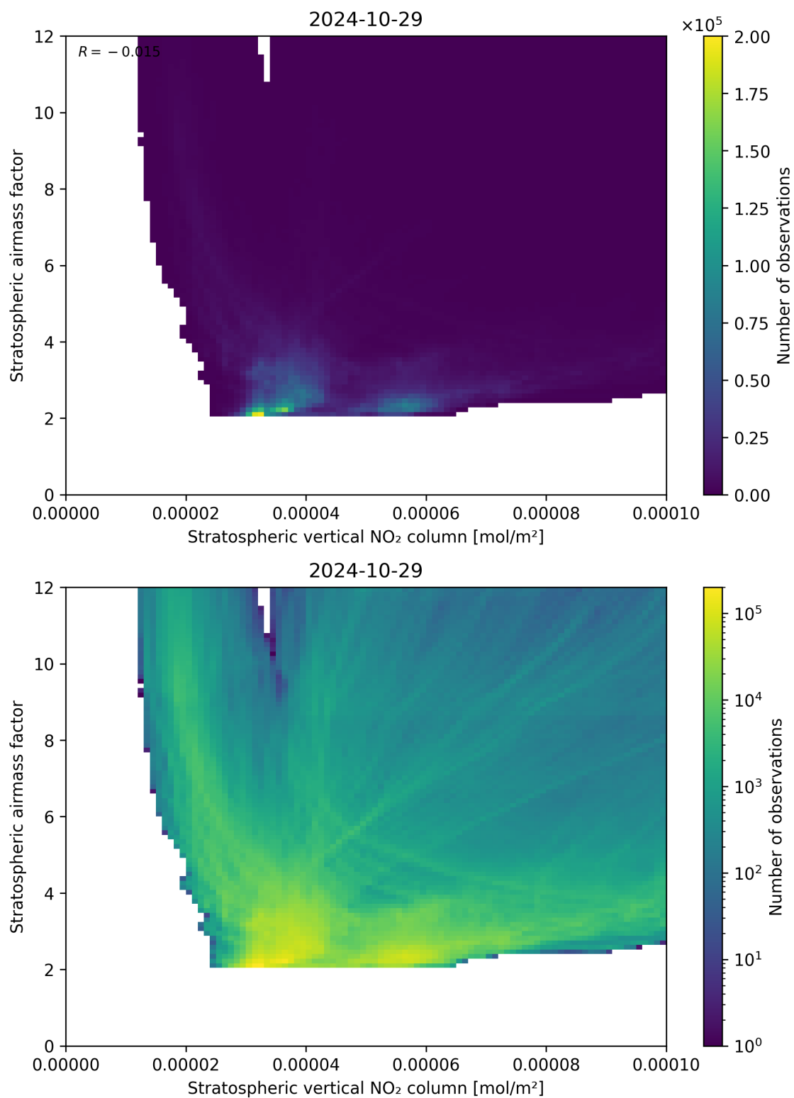
Figure 96: Scatter density plot of “Stratospheric vertical NO 2 column” against “Stratospheric airmass factor” for 2024-10-29 to 2024-10-30.
