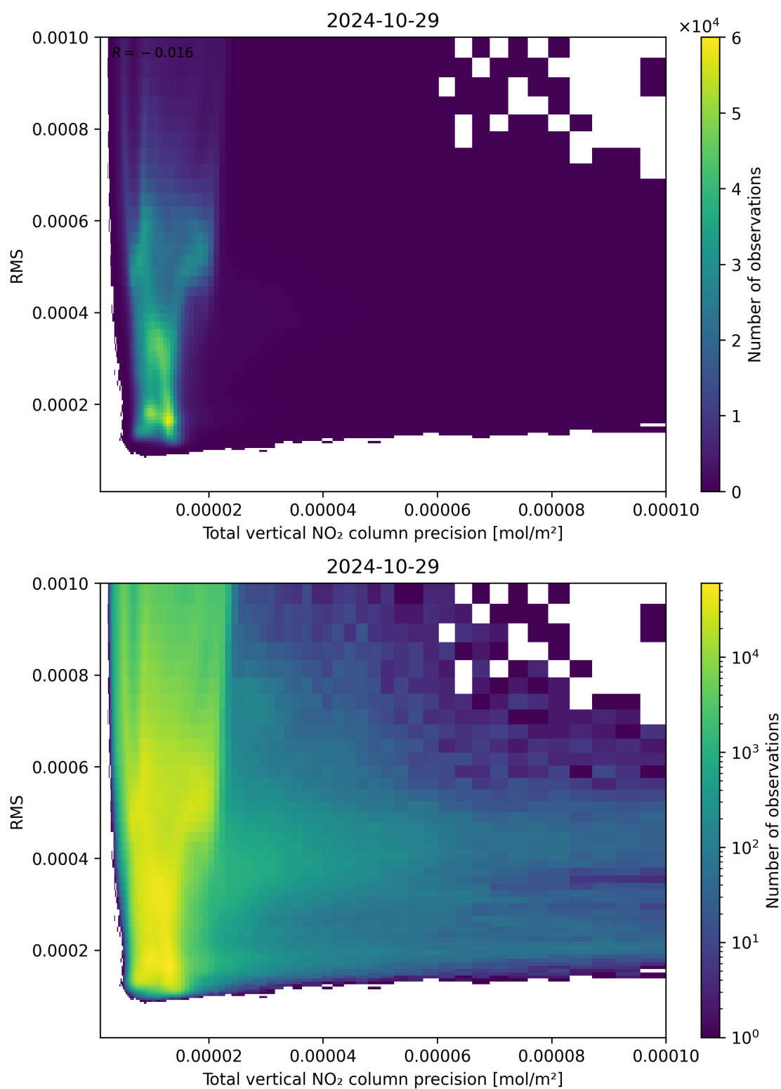
Figure 119: Scatter density plot of “Total vertical NO 2 column precision” against “RMS” for 2024-10-29 to 2024-10-30.
