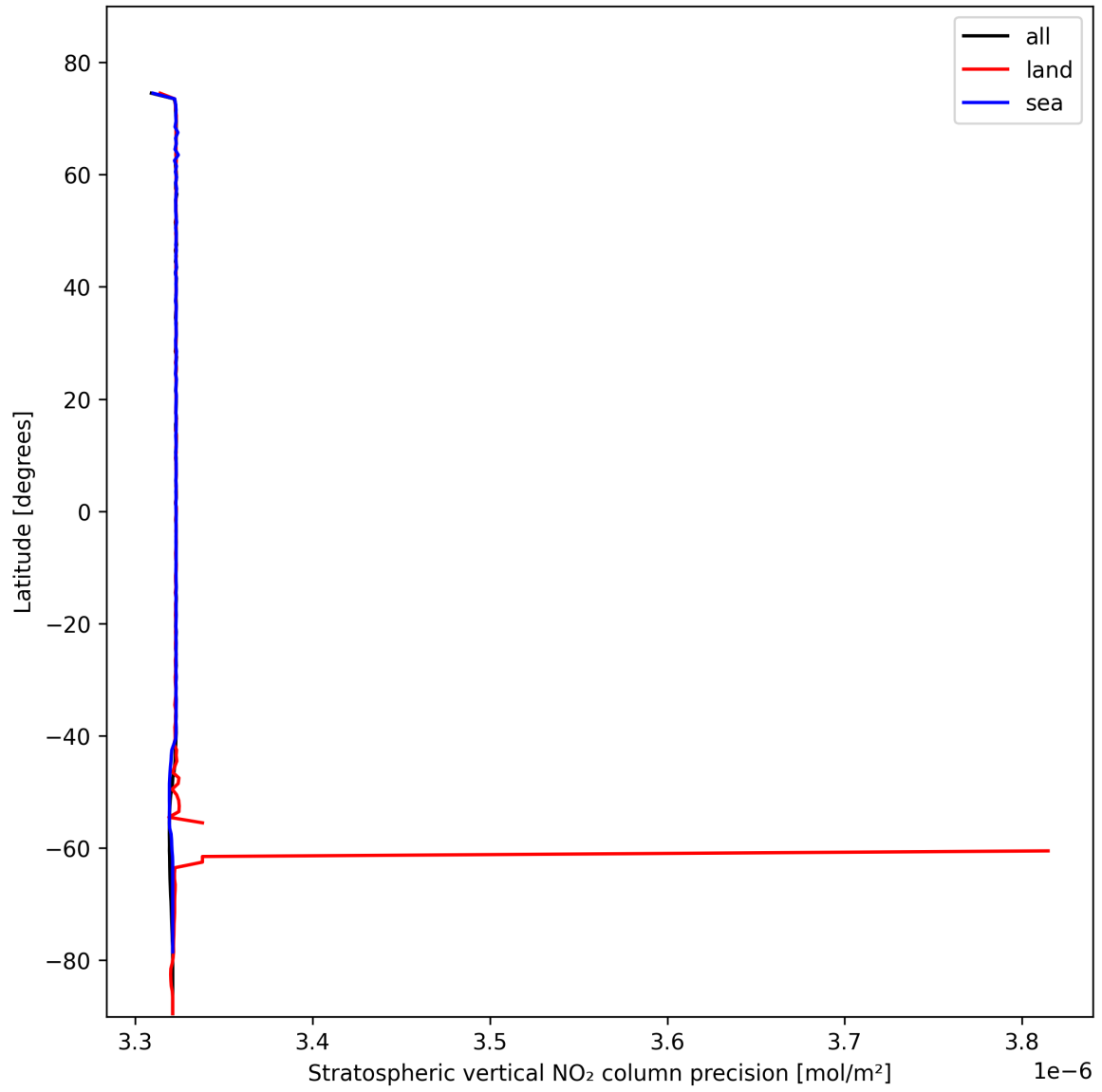
Figure 20: Zonal average of "Stratospheric vertical NO 2 column precision" for 2024-10-29 to 2024-10-30.
