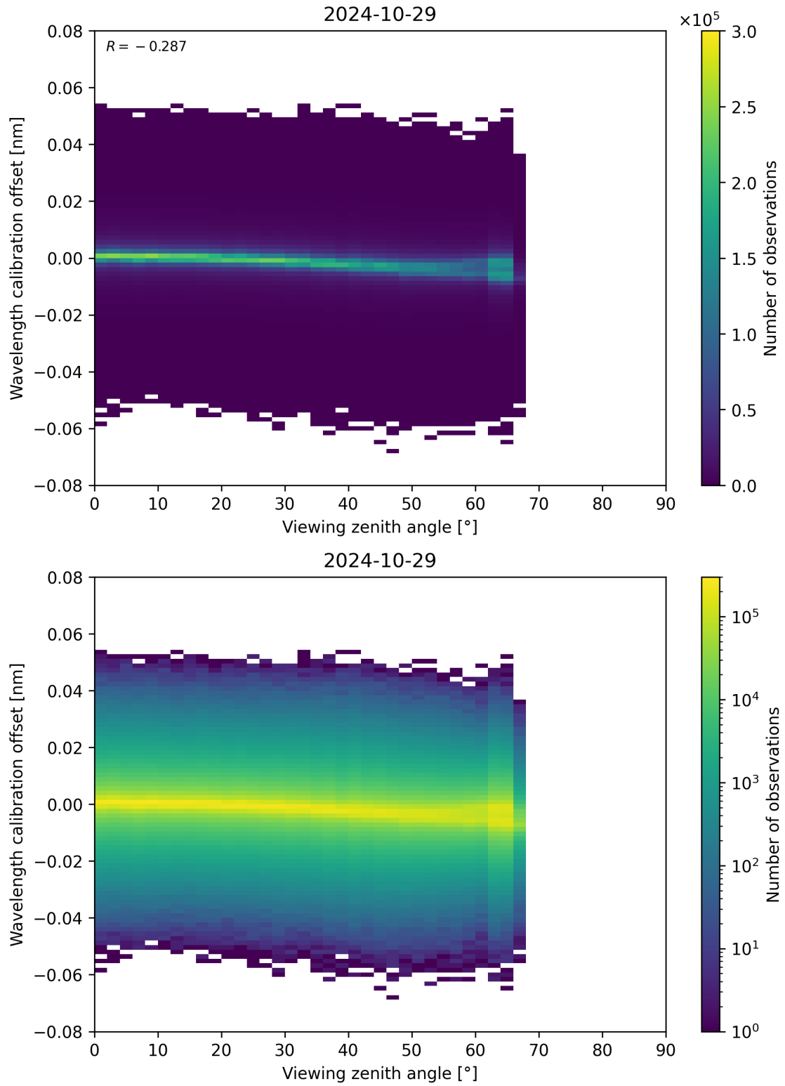
Figure 173: Scatter density plot of “Viewing zenith angle” against “Wavelength calibration offset” for 2024-10-29 to 2024-10-30.
