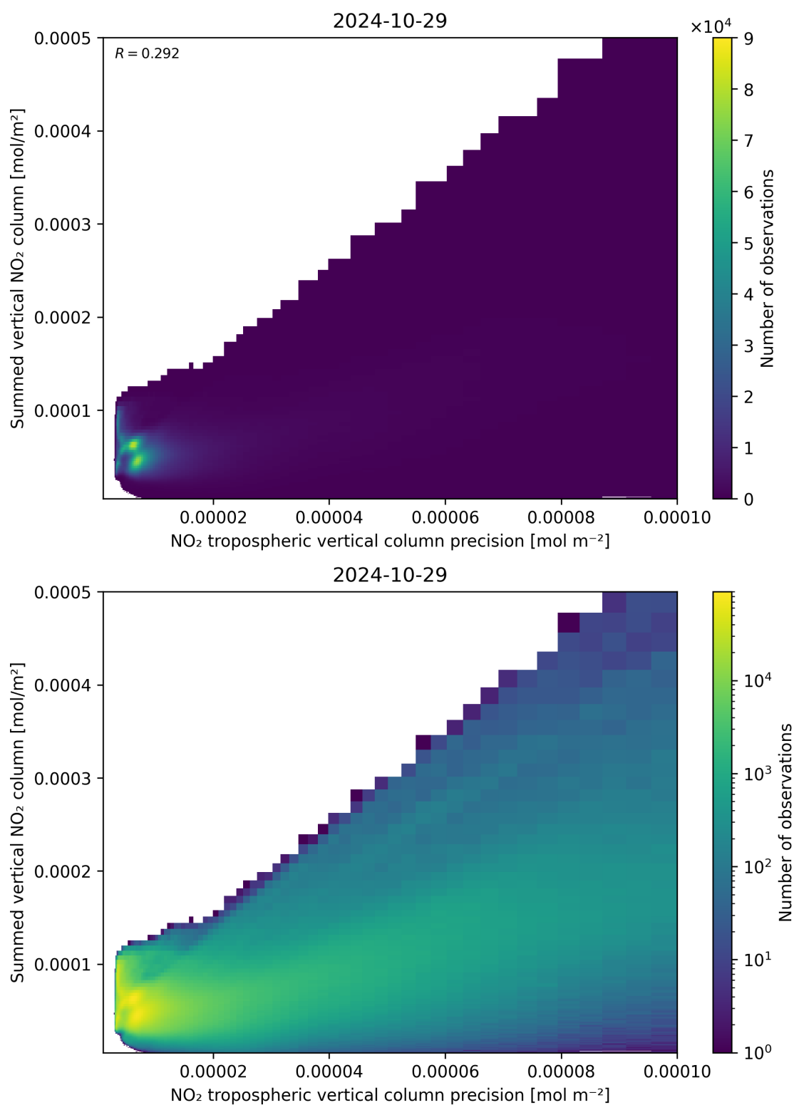
Figure 136: Scatter density plot of “NO 2 tropospheric vertical column precision” against “Summed vertical NO 2 column” for 2024-10-29 to 2024-10-30.
