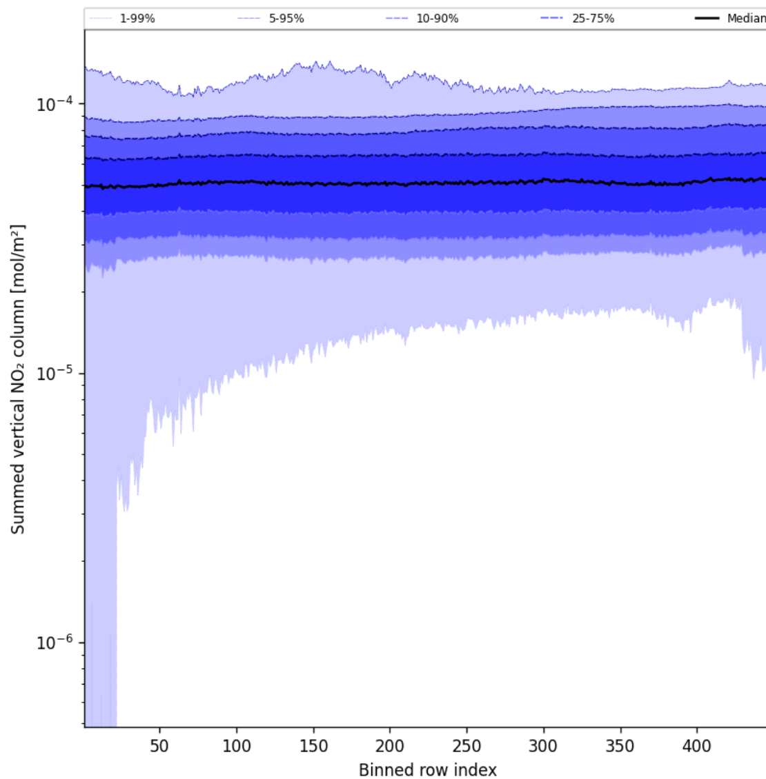
Figure 57: Along track statistics of “Summed vertical NO 2 column” for 2024-10-29 to 2024-10-30
