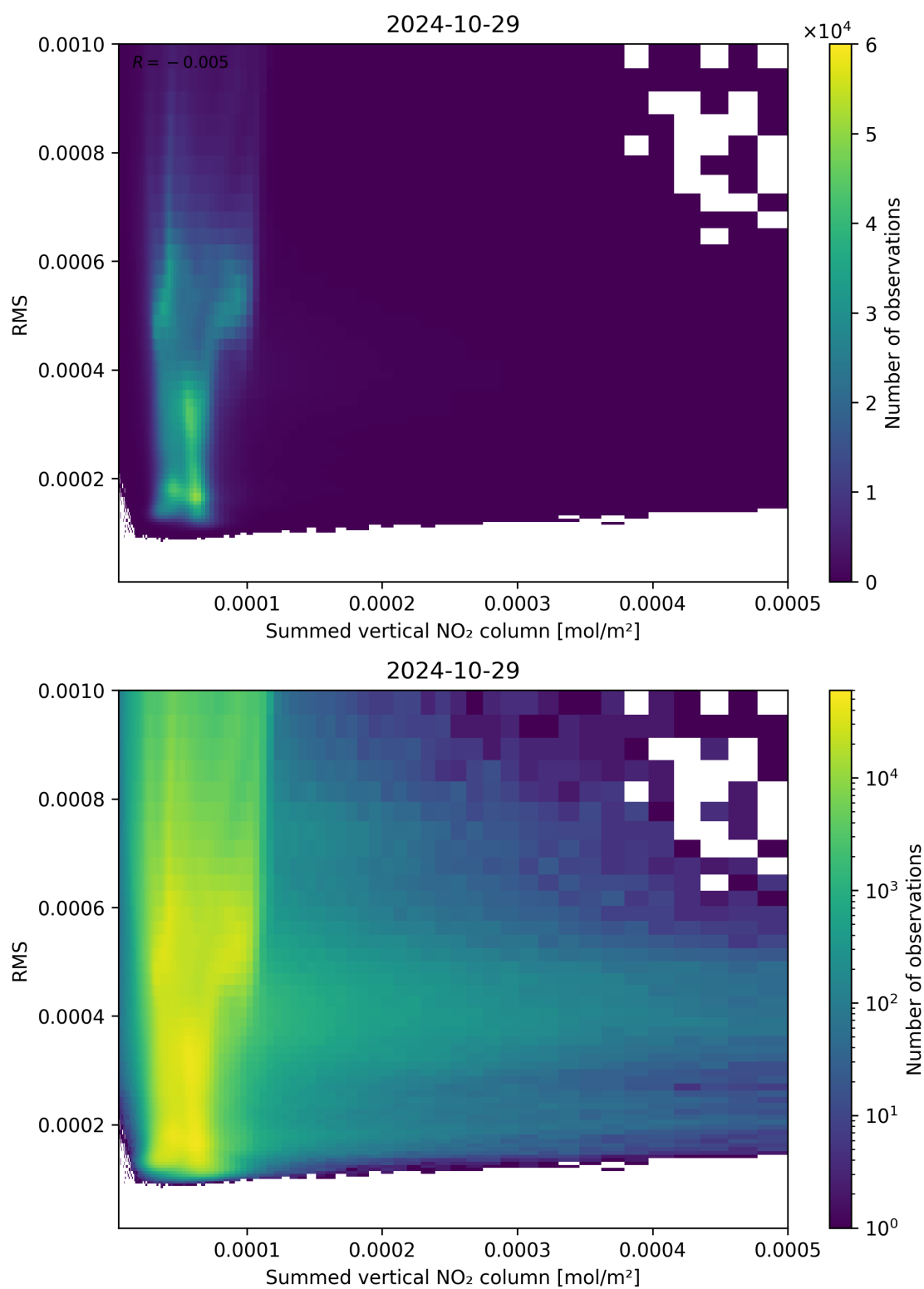
Figure 109: Scatter density plot of “Summed vertical NO 2 column” against “RMS” for 2024-10-29 to 2024-10-30.
