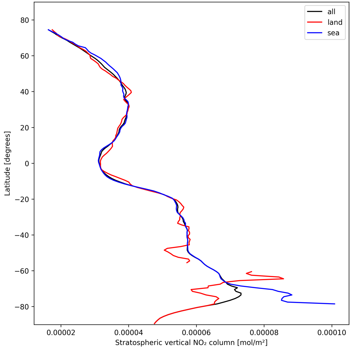
Figure 19: Zonal average of “Stratospheric vertical NO 2 column” for 2024-10-29 to 2024-10-30.
