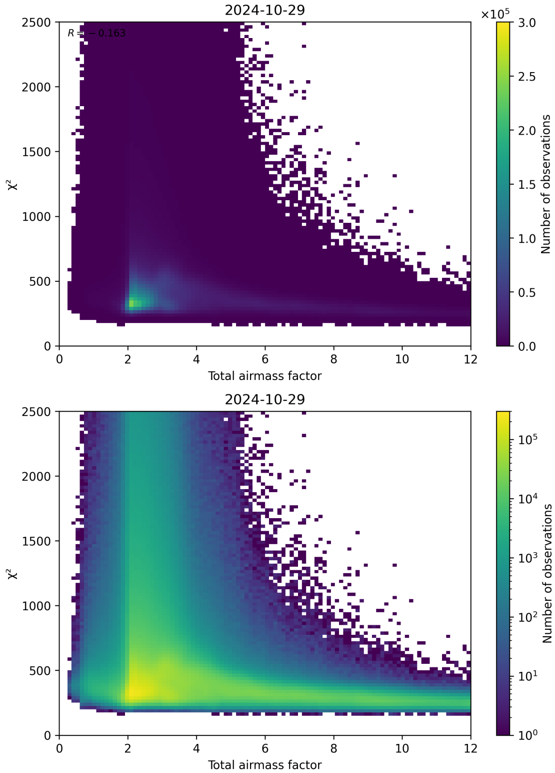
Figure 63: Scatter density plot of “Total airmass factor” against “ \chi^2 ” for 2024-10-29 to 2024-10-30.
