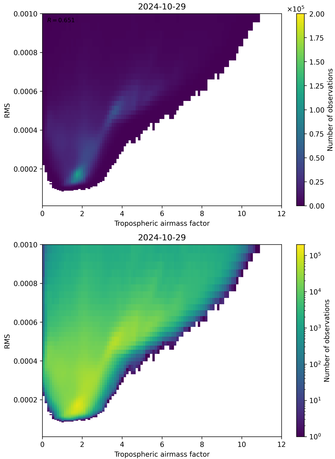
Figure 79: Scatter density plot of “Tropospheric airmass factor” against “RMS” for 2024-10-29 to 2024-10-30.
