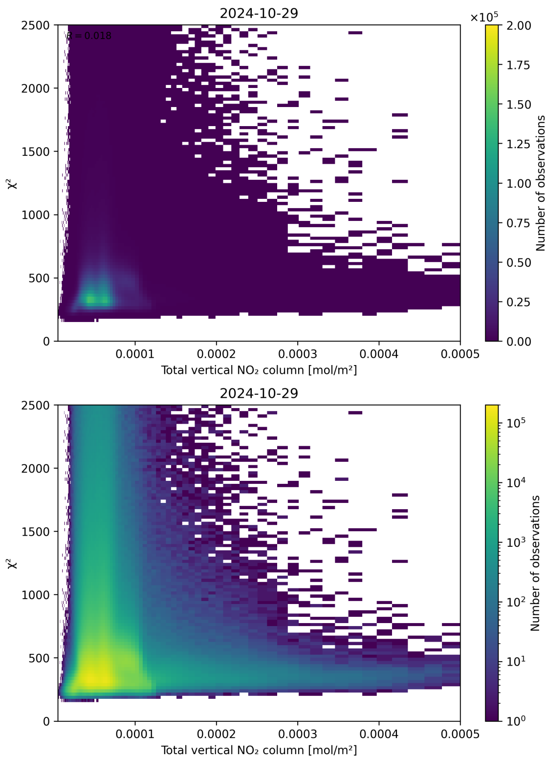
Figure 111: Scatter density plot of “Total vertical NO 2 column” against “ \chi^2 ” for 2024-10-29 to 2024-10-30.
