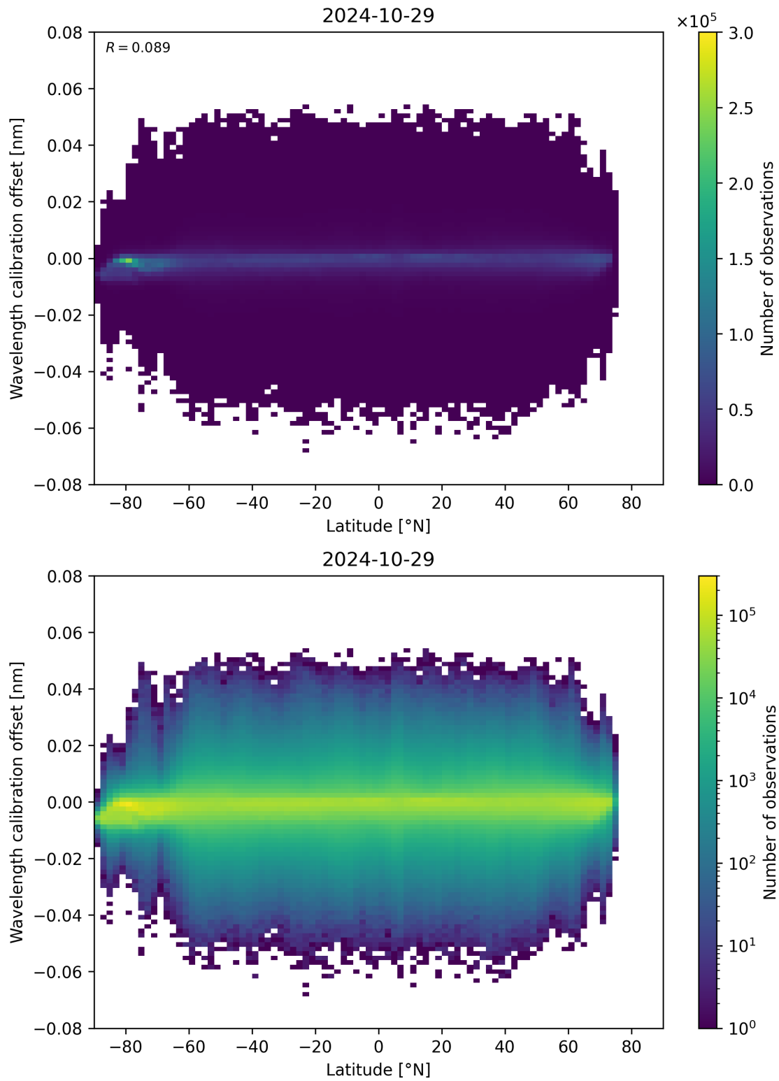
Figure 95: Scatter density plot of “Latitude” against “Wavelength calibration offset” for 2024-10-29 to 2024-10-30.
