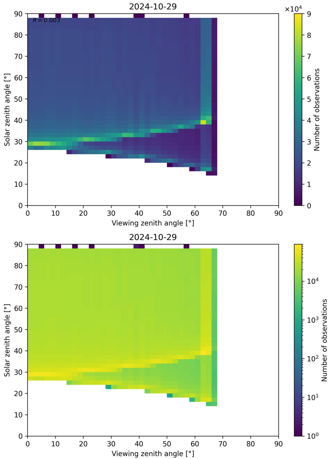
Figure 172: Scatter density plot of “Viewing zenith angle” against “Solar zenith angle” for 2024-10-29 to 2024-10-30.
