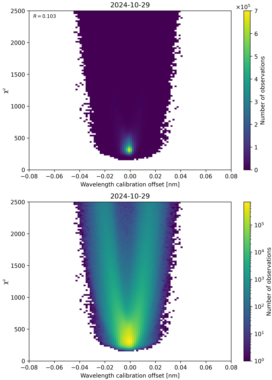
Figure 175: Scatter density plot of “Wavelength calibration offset” against “ \chi^2 ” for 2024-10-29 to 2024-10-30.
