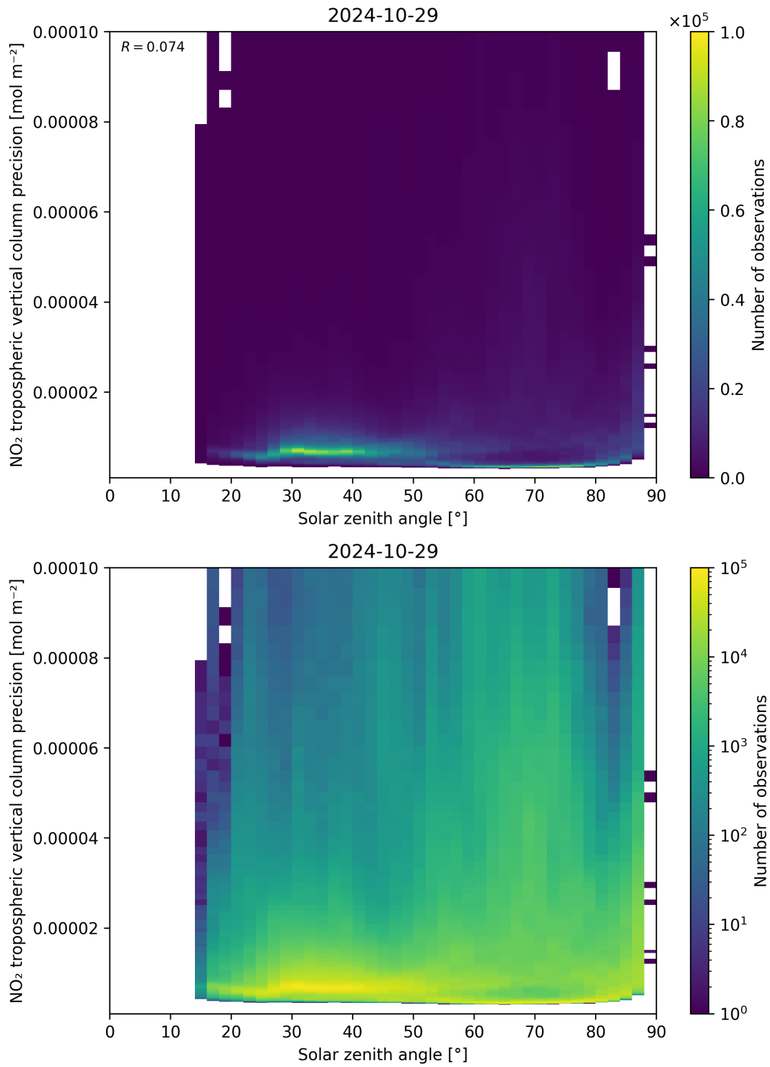
Figure 156: Scatter density plot of “Solar zenith angle” against “NO 2 tropospheric vertical column precision” for 2024-10-29 to 2024-10-30.
