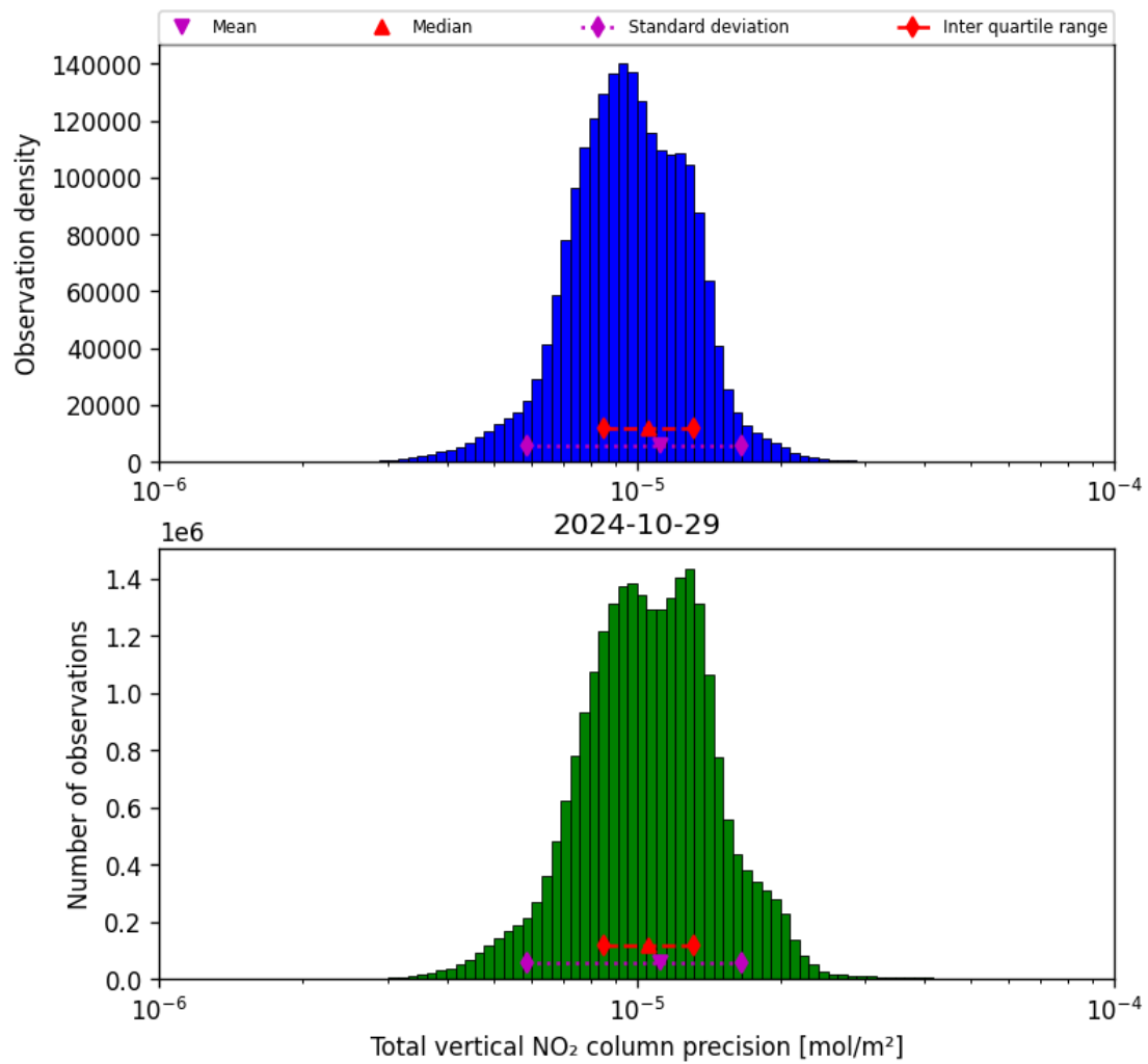
Figure 39: Histogram of "Total vertical NO 2 column precision" for 2024-10-29 to 2024-10-30
