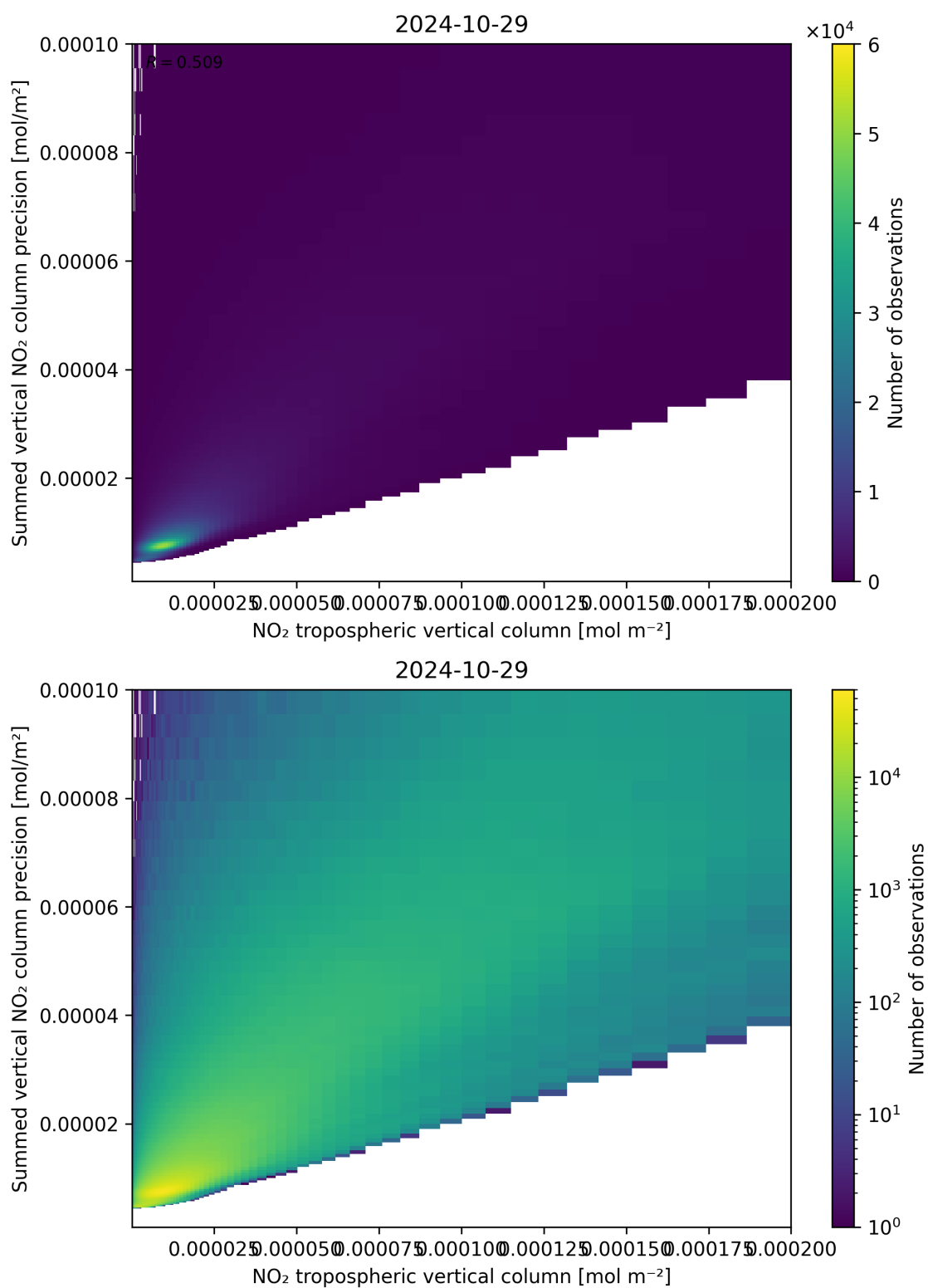
Figure 127: Scatter density plot of “NO 2 tropospheric vertical column” against “Summed vertical NO 2 column precision” for 2024-10-29 to 2024-10-30.
