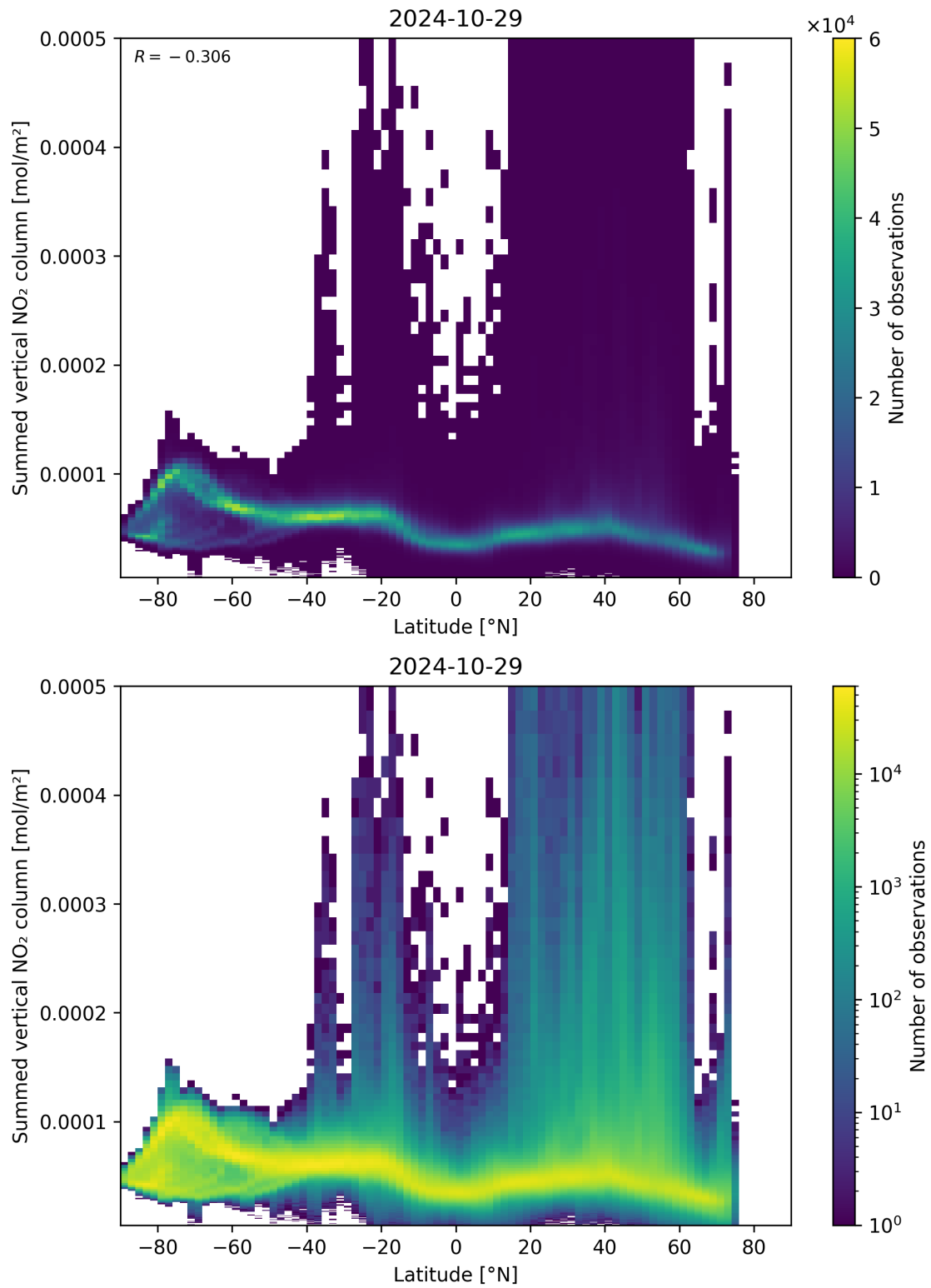
Figure 88: Scatter density plot of “Latitude” against “Summed vertical NO 2 column” for 2024-10-29 to 2024-10-30.
