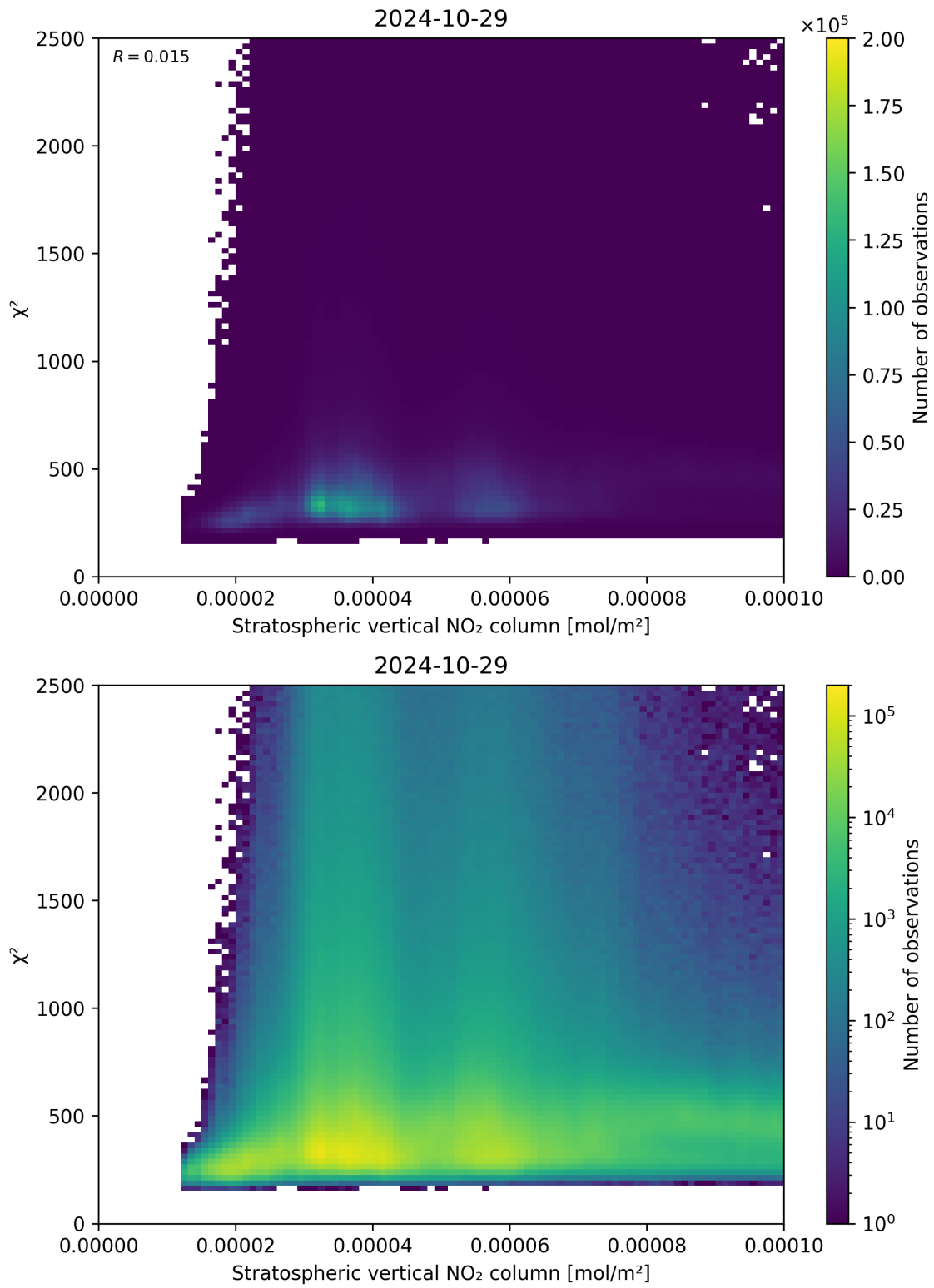
Figure 97: Scatter density plot of “Stratospheric vertical NO 2 column” against “ \chi^2 ” for 2024-10-29 to 2024-10-30.
