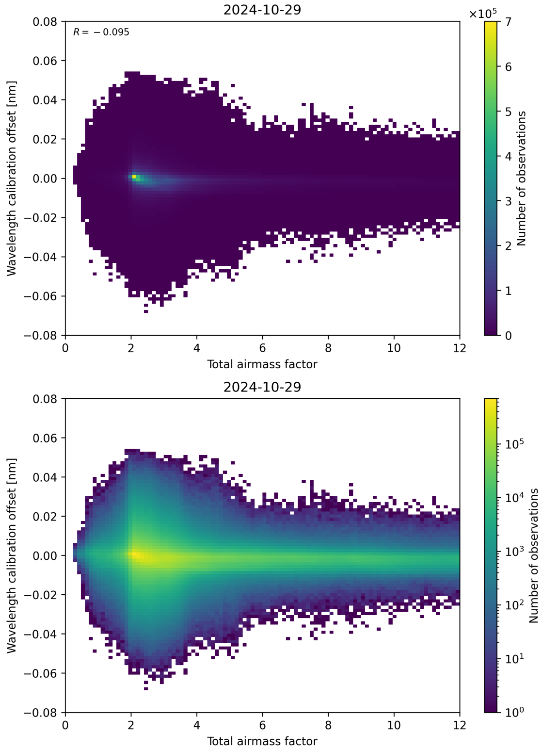
Figure 70: Scatter density plot of “Total airmass factor” against “Wavelength calibration offset” for 2024-10-29 to 2024-10-30.
