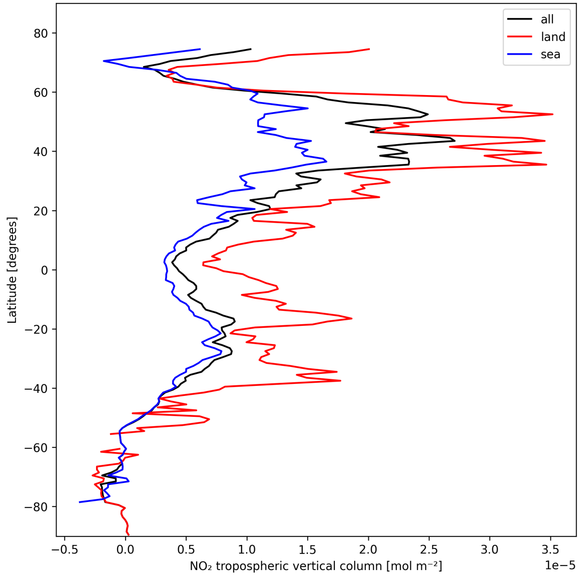
Figure 12: Zonal average of “NO 2 tropospheric vertical column” for 2024-10-29 to 2024-10-30.
