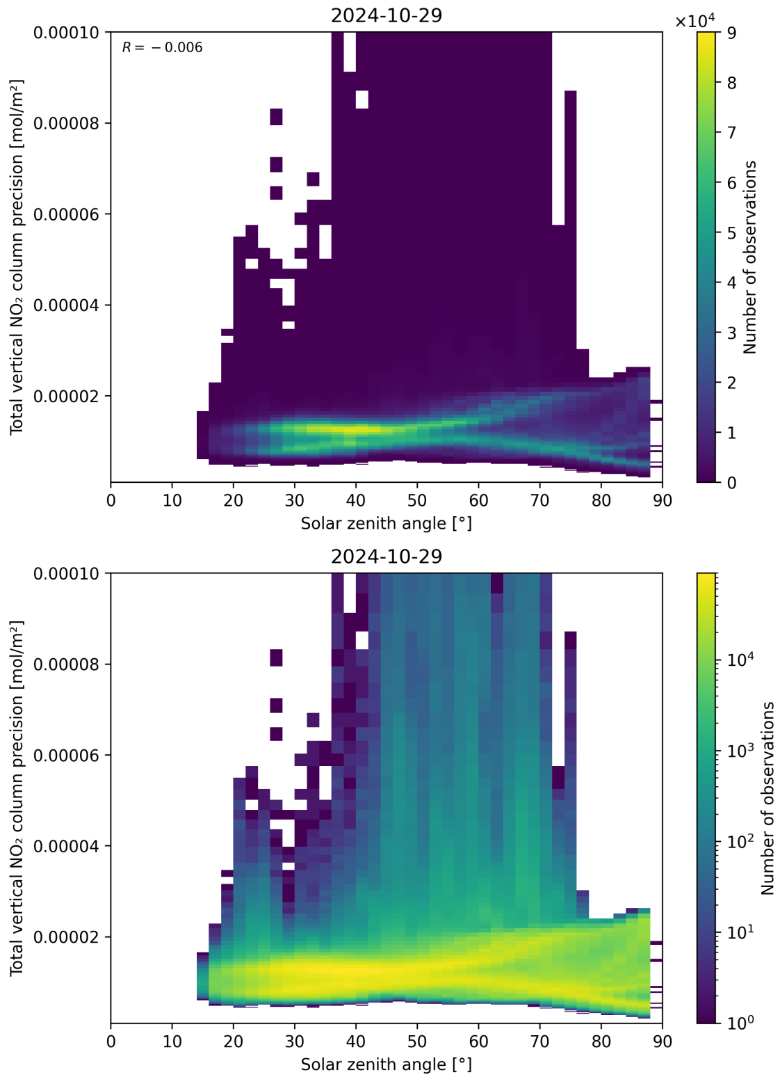
Figure 154: Scatter density plot of “Solar zenith angle” against “Total vertical NO 2 column precision” for 2024-10-29 to 2024-10-30.
