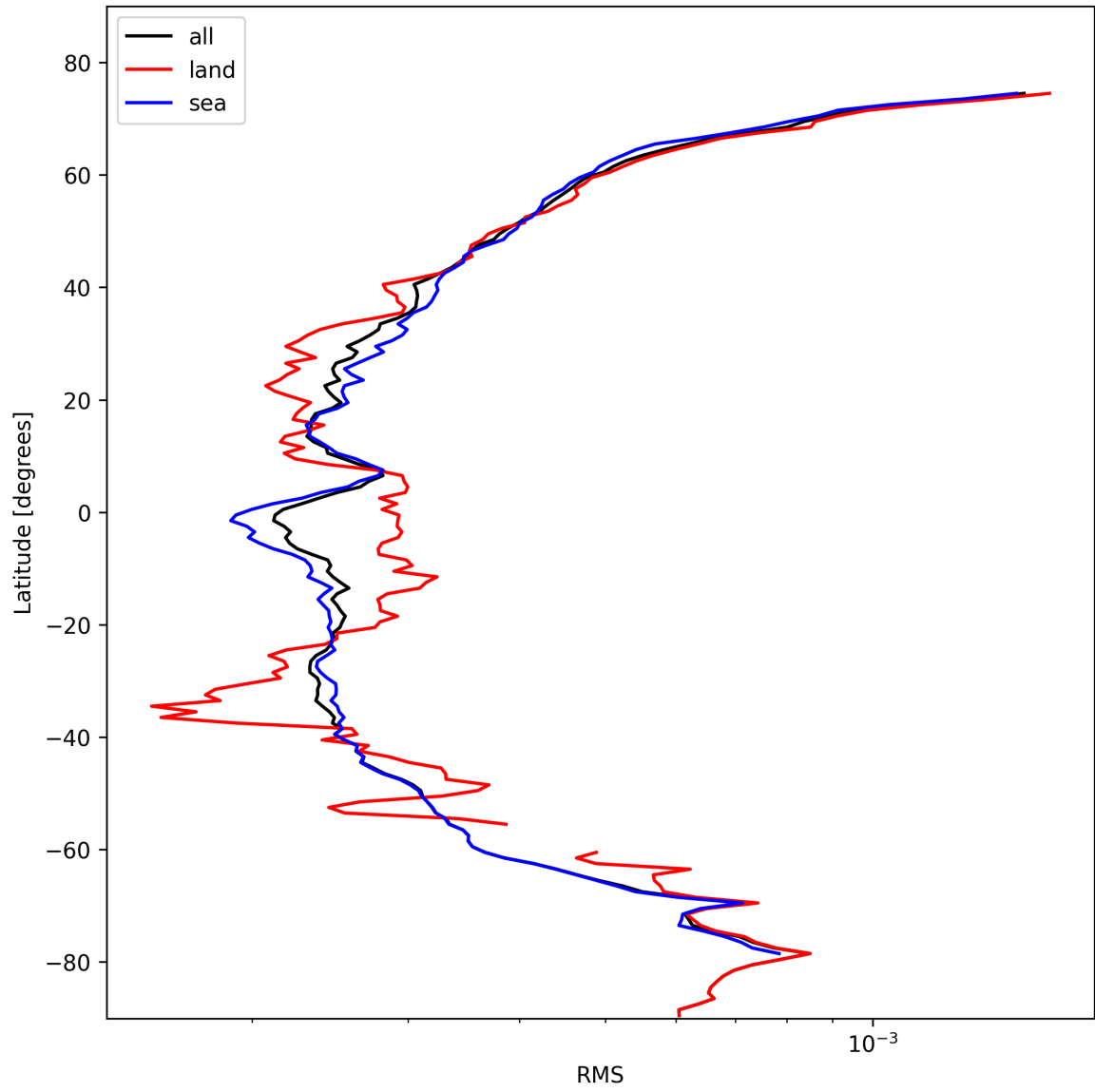
Figure 26: Zonal average of “RMS” for 2024-10-29 to 2024-10-30.
