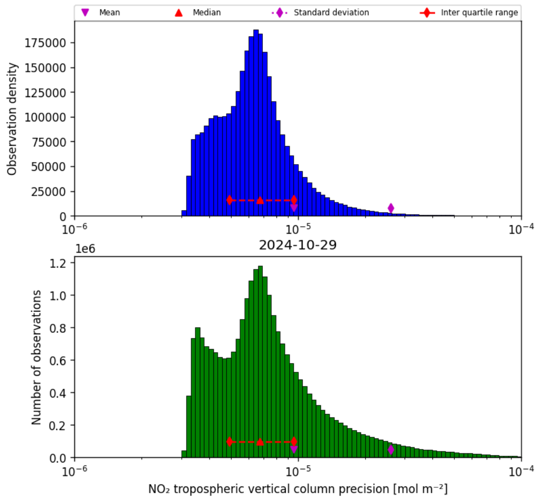
Figure 30: Histogram of “NO 2 tropospheric vertical column precision” for 2024-10-29 to 2024-10-30
