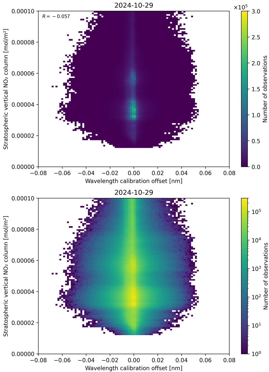
Figure 176: Scatter density plot of “Wavelength calibration offset” against “Stratospheric vertical NO 2 column” for 2024-10-29 to 2024-10-30.
