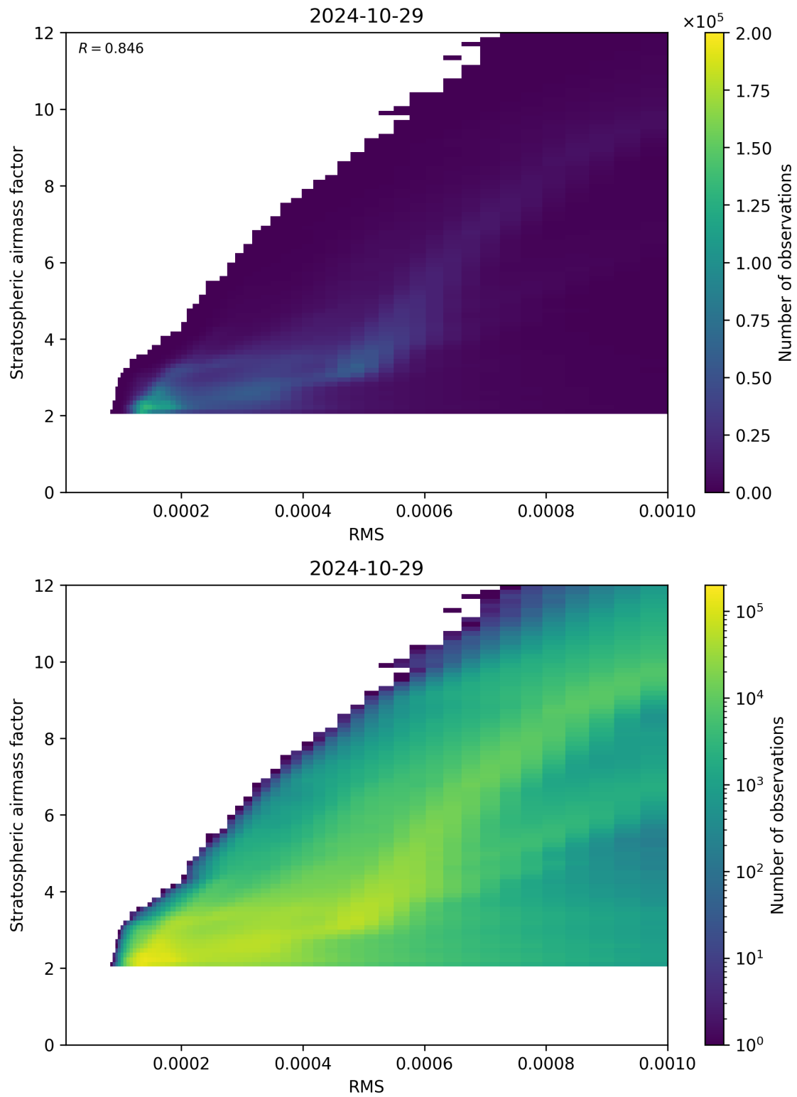
Figure 144: Scatter density plot of “RMS” against “Stratospheric airmass factor” for 2024-10-29 to 2024-10-30.
