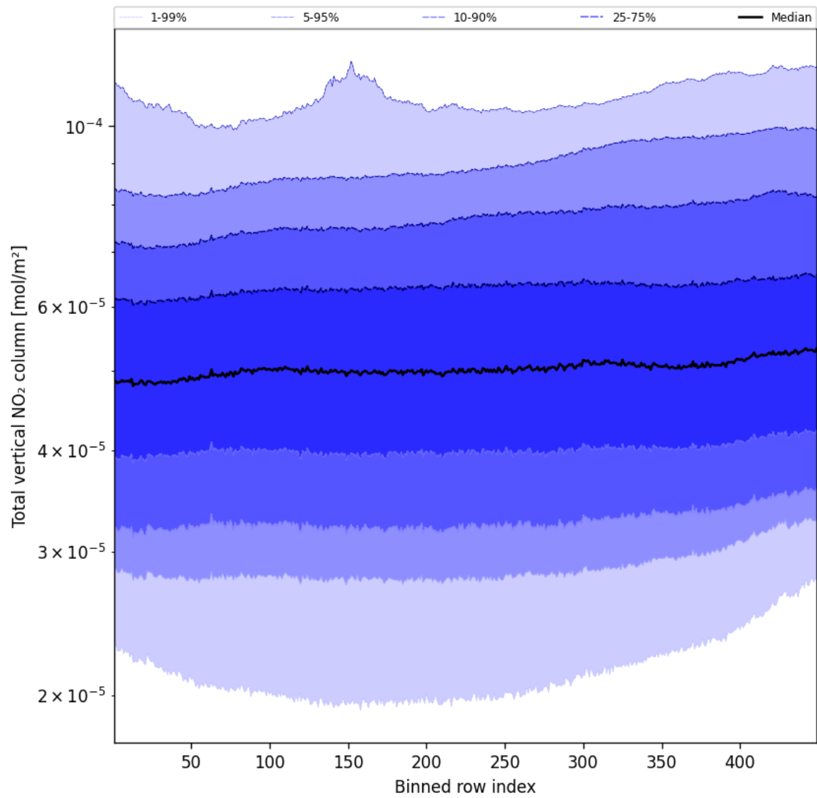
Figure 55: Along track statistics of “Total vertical NO 2 column” for 2024-10-29 to 2024-10-30
