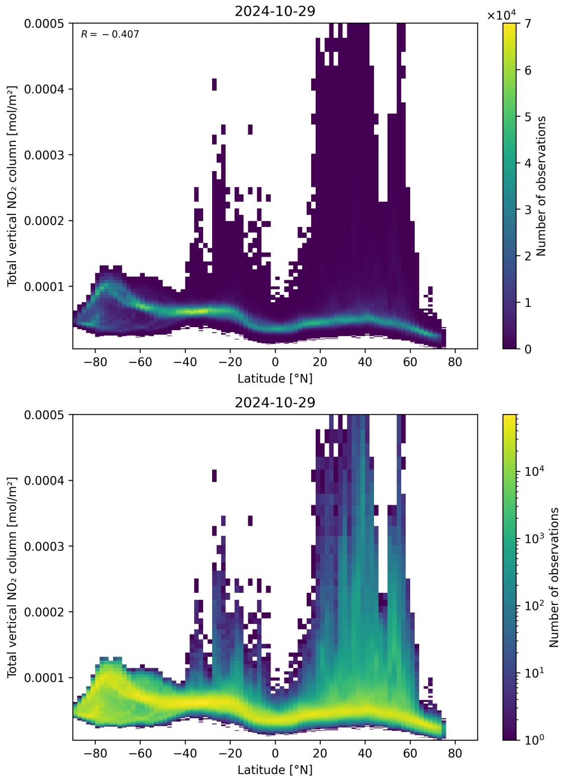
Figure 90: Scatter density plot of “Latitude” against “Total vertical NO 2 column” for 2024-10-29 to 2024-10-30.
