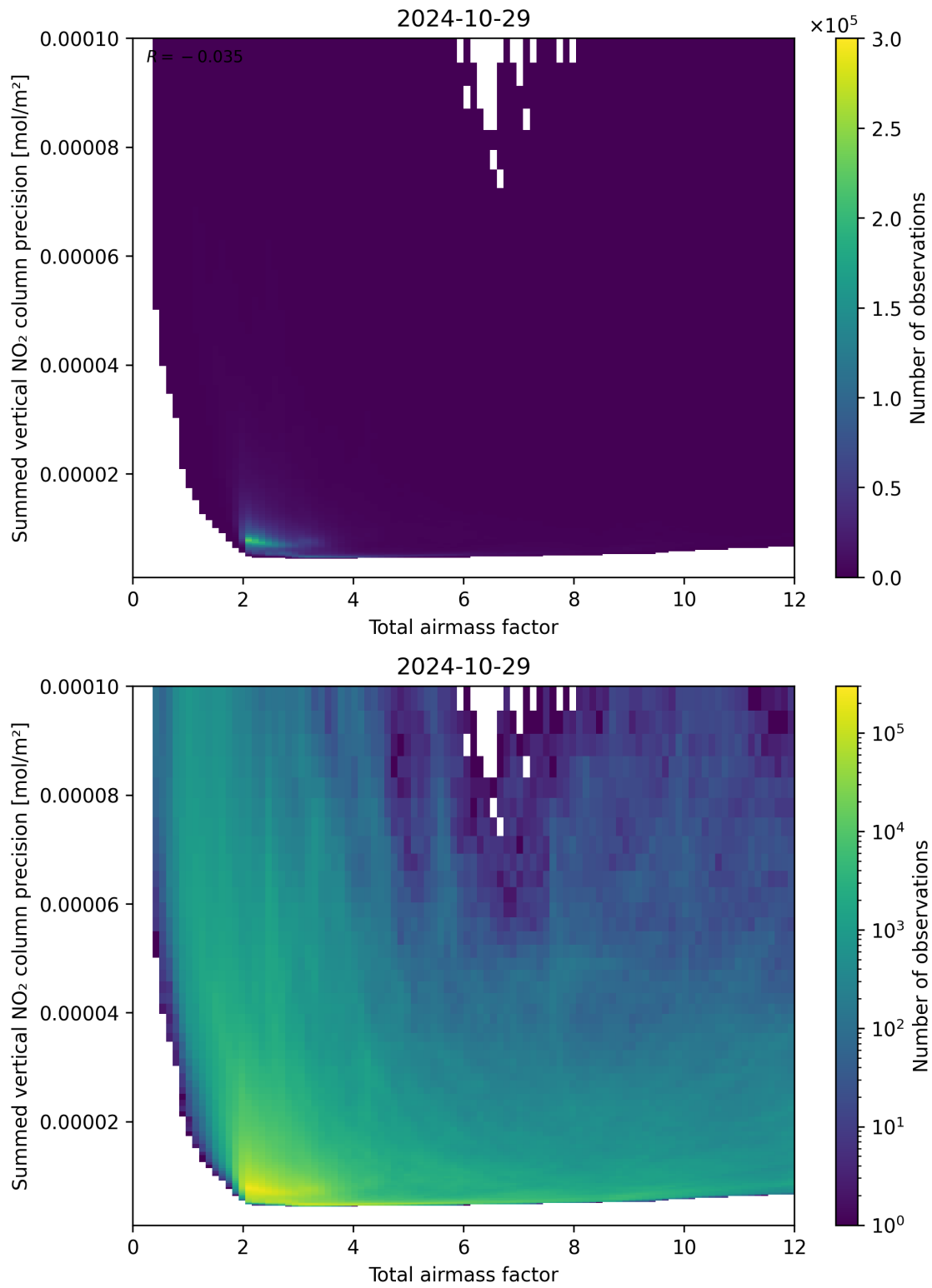
Figure 66: Scatter density plot of “Total airmass factor” against “Summed vertical NO 2 column precision” for 2024-10-29 to 2024-10-30.
