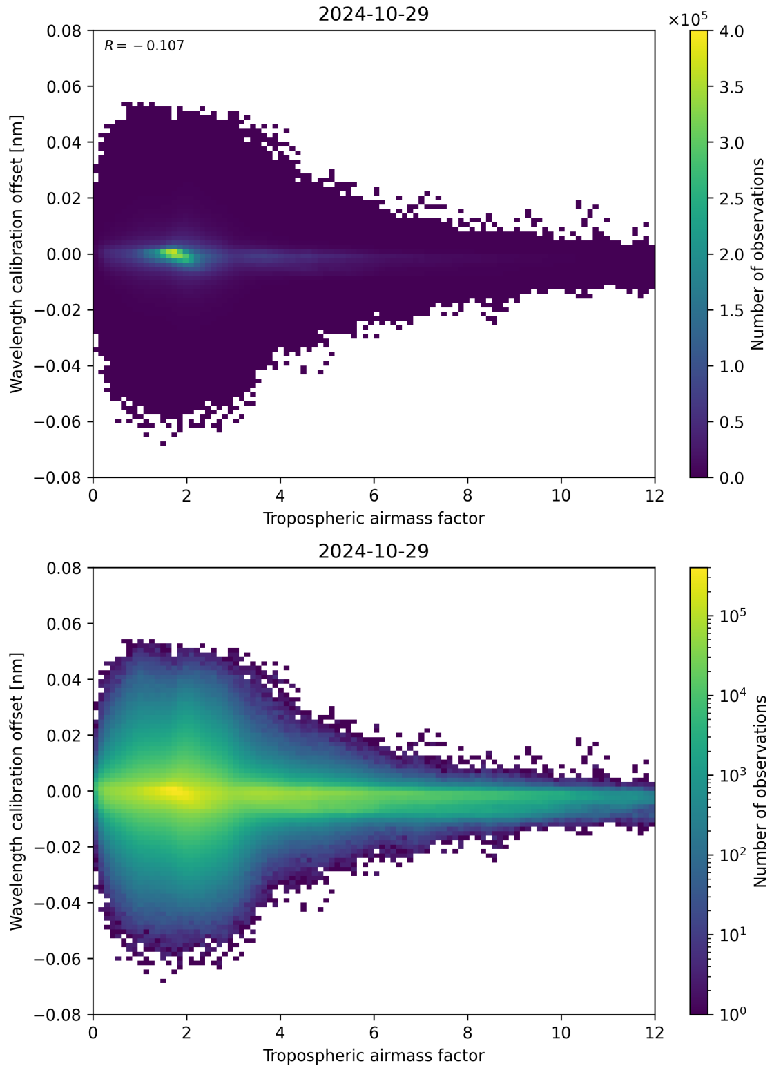
Figure 80: Scatter density plot of “Tropospheric airmass factor” against “Wavelength calibration offset” for 2024-10-29 to 2024-10-30.
