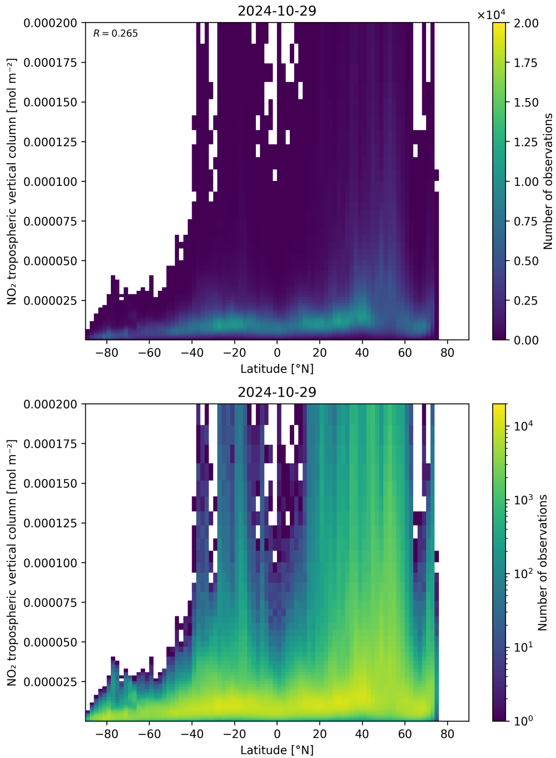
Figure 92: Scatter density plot of “Latitude” against “NO 2 tropospheric vertical column” for 2024-10-29 to 2024-10-30.
