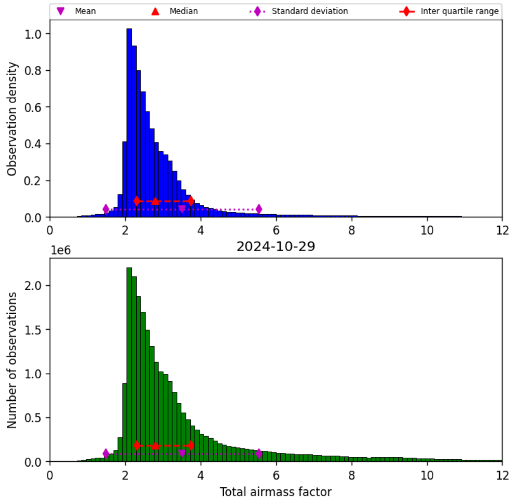
Figure 32: Histogram of “Total airmass factor” for 2024-10-29 to 2024-10-30
