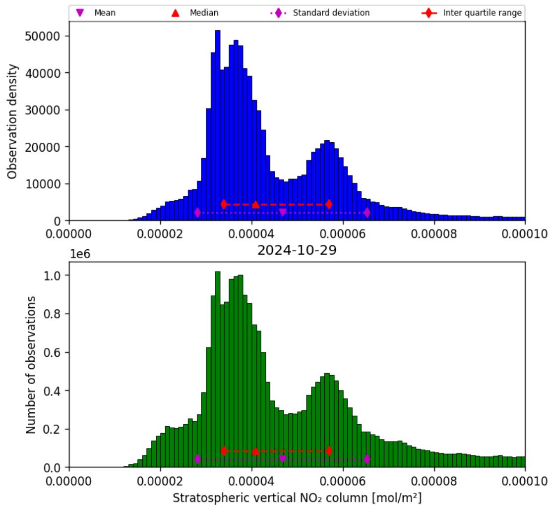
Figure 36: Histogram of “Stratospheric vertical NO 2 column” for 2024-10-29 to 2024-10-30
