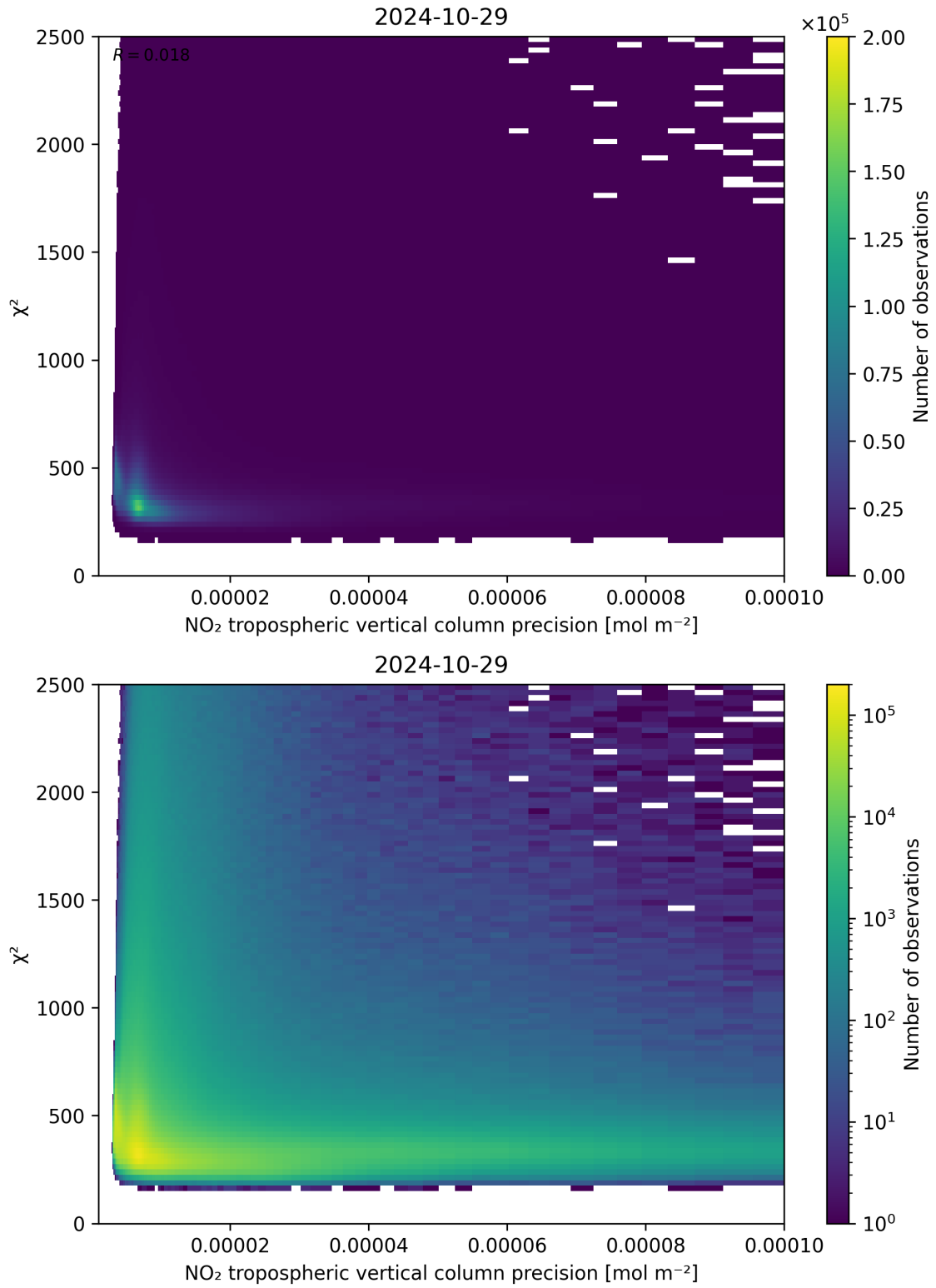
Figure 134: Scatter density plot of “NO 2 tropospheric vertical column precision” against “ \chi^2 ” for 2024-10-29 to 2024-10-30.
