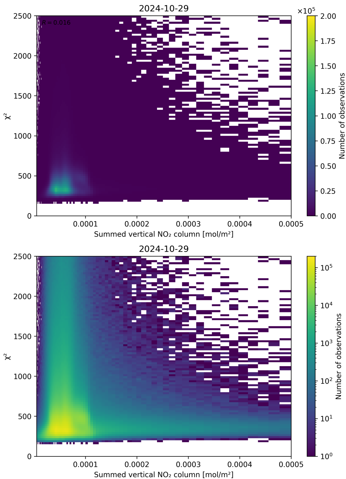
Figure 104: Scatter density plot of “Summed vertical NO 2 column” against “ \chi^2 ” for 2024-10-29 to 2024-10-30.
