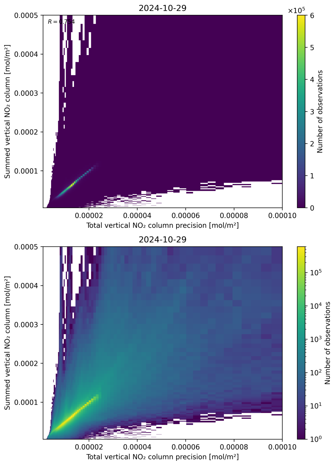
Figure 117: Scatter density plot of “Total vertical NO 2 column precision” against “Summed vertical NO 2 column” for 2024-10-29 to 2024-10-30.
