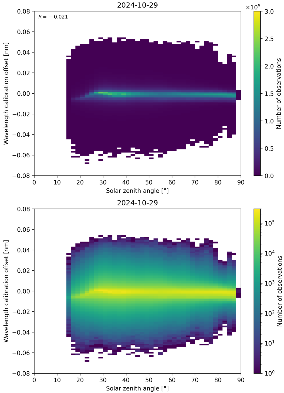
Figure 158: Scatter density plot of “Solar zenith angle” against “Wavelength calibration offset” for 2024-10-29 to 2024-10-30.
