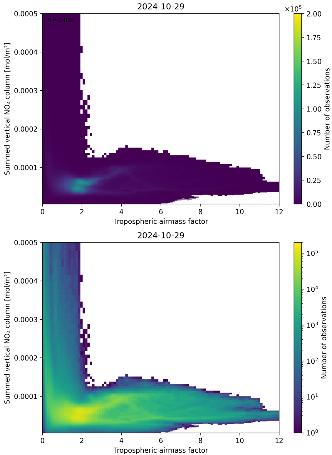
Figure 75: Scatter density plot of “Tropospheric air mass factor” against “Summed vertical NO 2 column” for 2024-10-29 to 2024-10-30.
