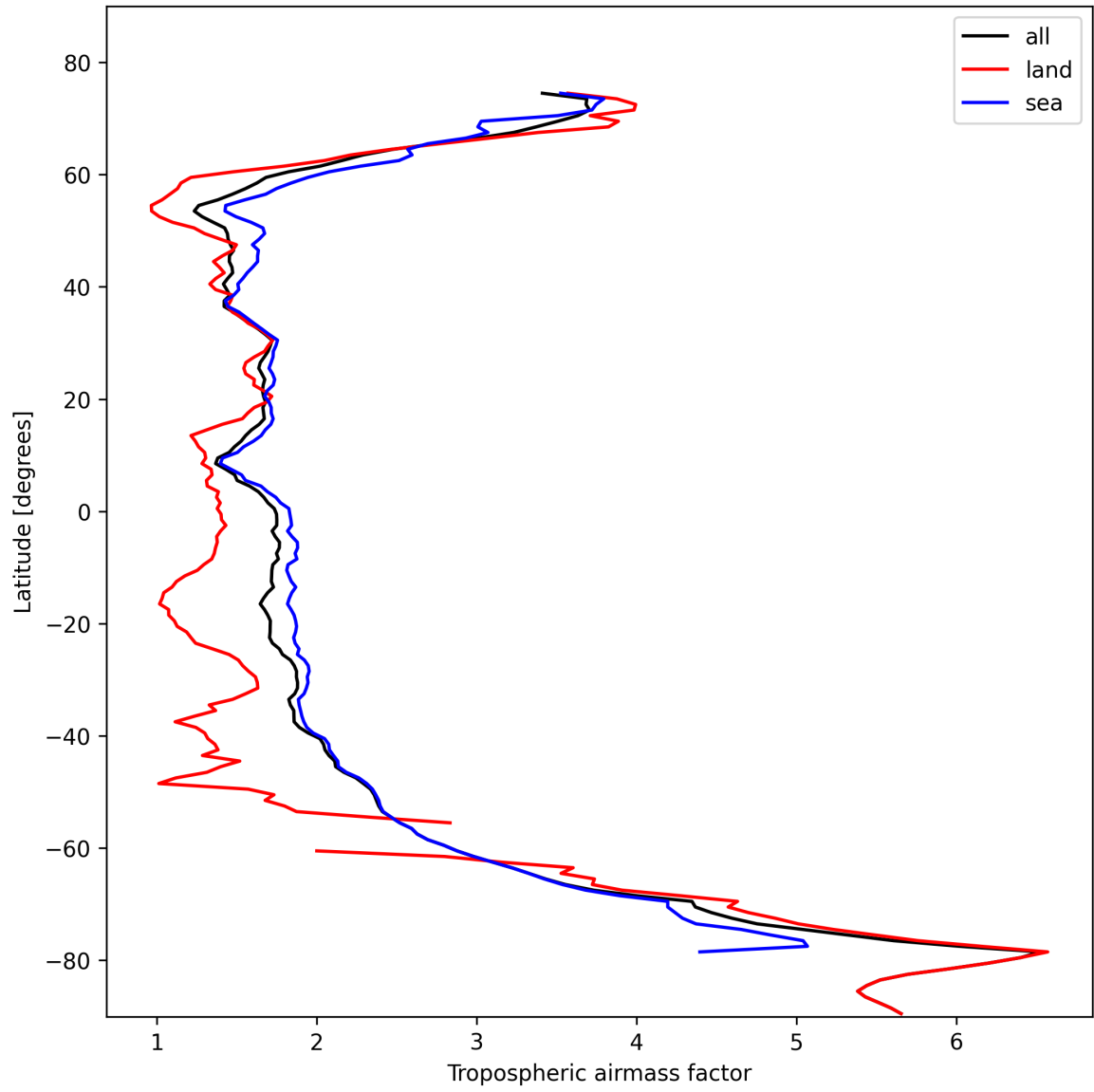
Figure 14: Zonal average of “Tropospheric airmass factor” for 2024-10-29 to 2024-10-30.
