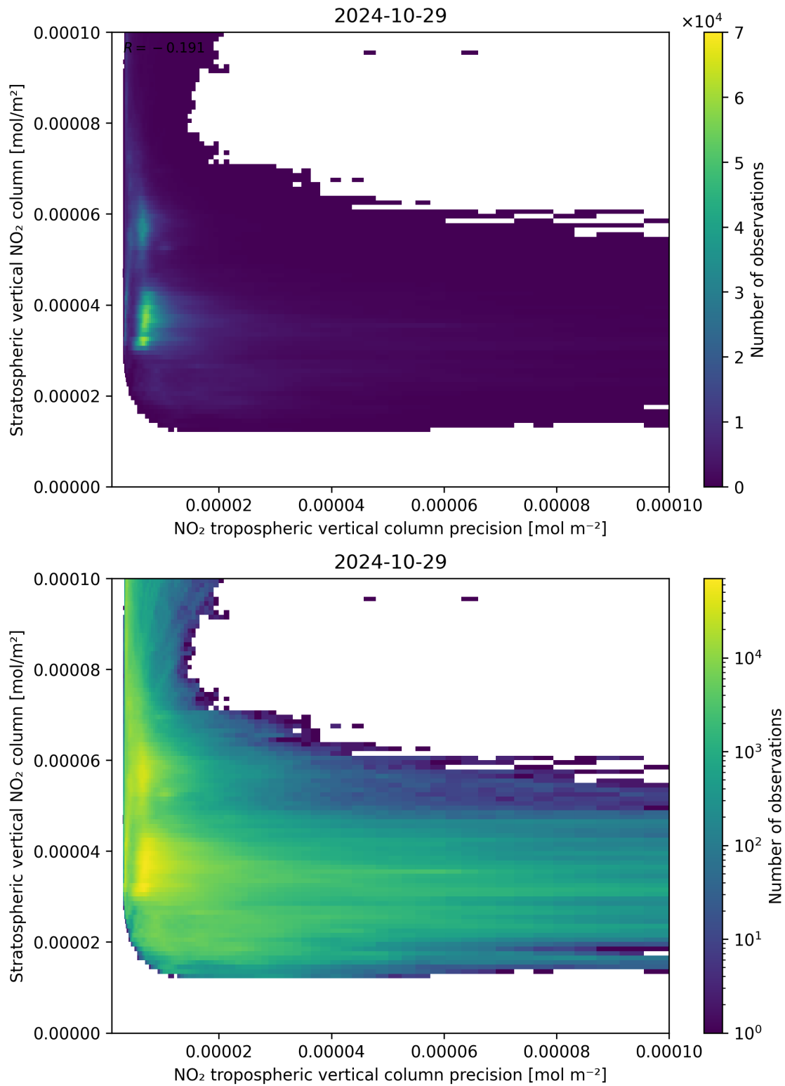
Figure 135: Scatter density plot of “NO 2 tropospheric vertical column precision” against “Stratospheric vertical NO 2 column” for 2024-10-29 to 2024-10-30.
