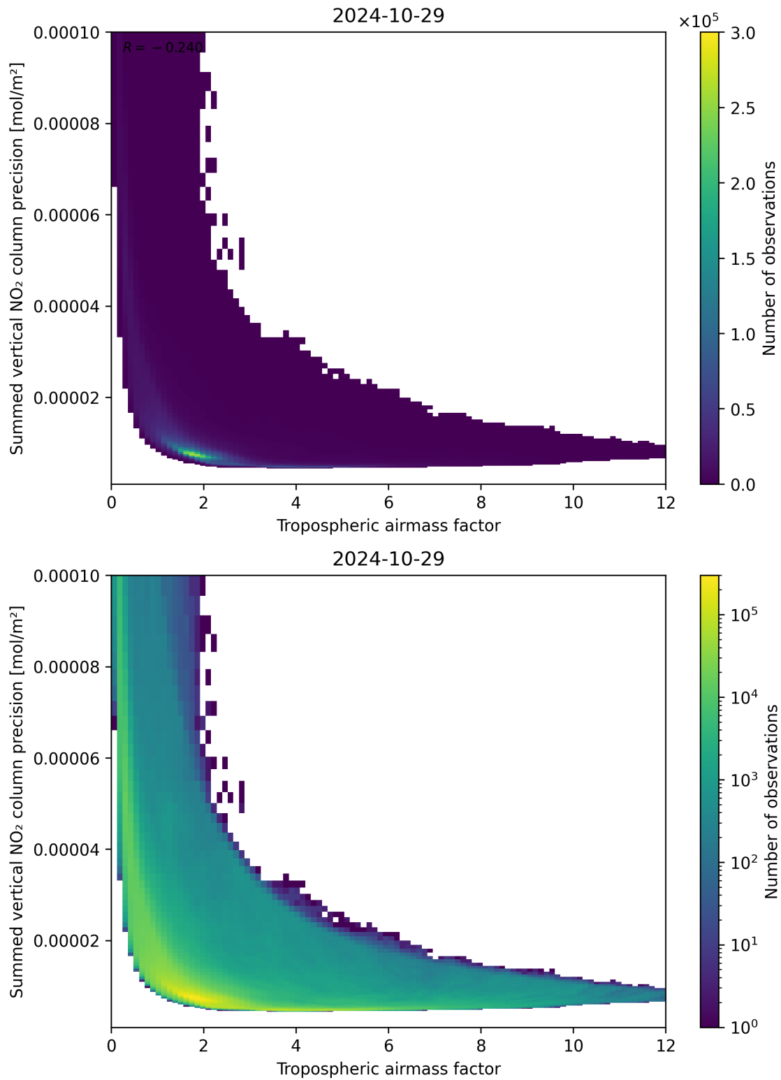
Figure 76: Scatter density plot of “Tropospheric air mass factor” against “Summed vertical NO 2 column precision” for 2024-10-29 to 2024-10-30.
