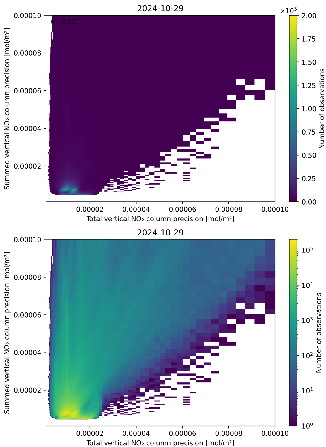
Figure 118: Scatter density plot of “Total vertical NO 2 column precision” against “Summed vertical NO 2 column precision” for 2024-10-29 to 2024-10-30.
