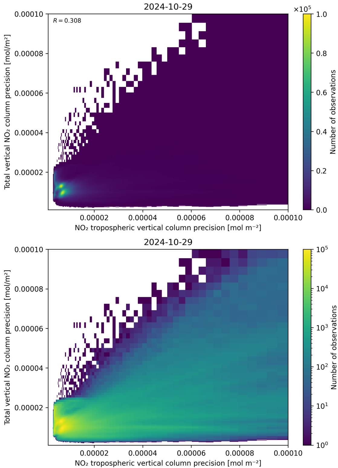
Figure 139: Scatter density plot of “NO 2 tropospheric vertical column precision” against “Total vertical NO 2 column precision” for 2024-10-29 to 2024-10-30.
