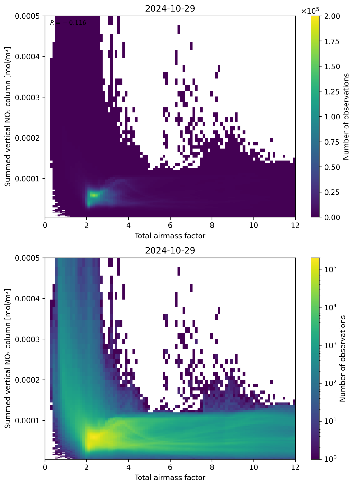
Figure 65: Scatter density plot of “Total airmass factor” against “Summed vertical NO 2 column” for 2024-10-29 to 2024-10-30.
