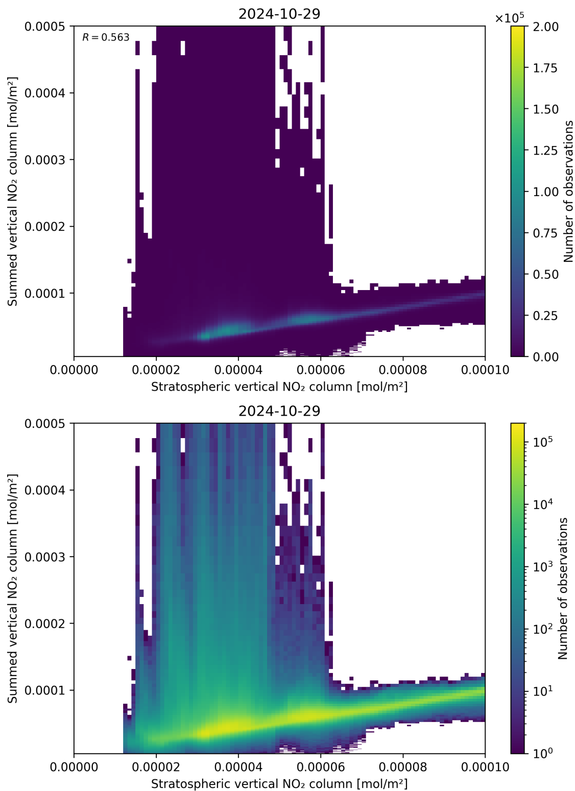
Figure 98: Scatter density plot of “Stratospheric vertical NO 2 column” against “Summed vertical NO 2 column” for 2024-10-29 to 2024-10-30.
