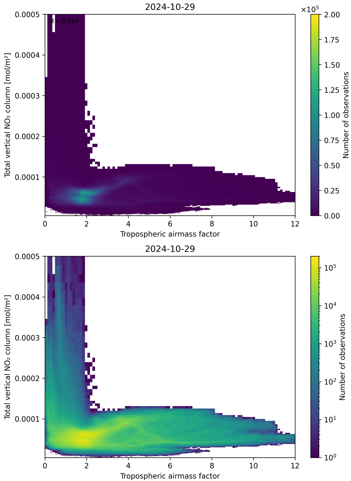
Figure 77: Scatter density plot of “Tropospheric airmass factor” against “Total vertical NO 2 column” for 2024-10-29 to 2024-10-30.
