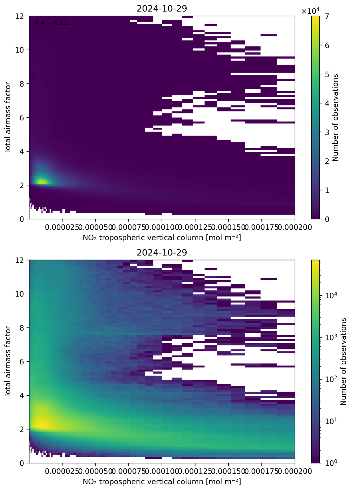
Figure 122: Scatter density plot of “NO 2 tropospheric vertical column” against “Total air mass factor” for 2024-10-29 to 2024-10-30.
