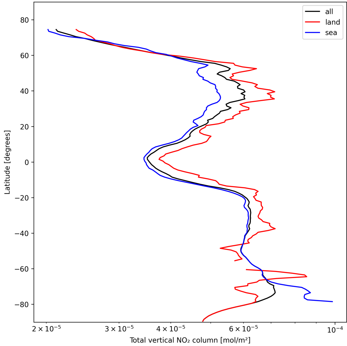
Figure 21: Zonal average of “Total vertical NO 2 column” for 2024-10-29 to 2024-10-30.
