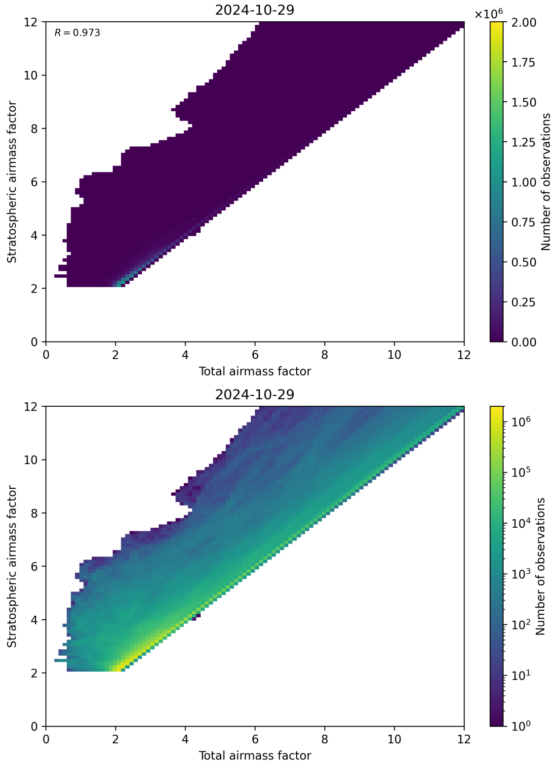
Figure 62: Scatter density plot of “Total airmass factor” against “Stratospheric airmass factor” for 2024-10-29 to 2024-10-30.
