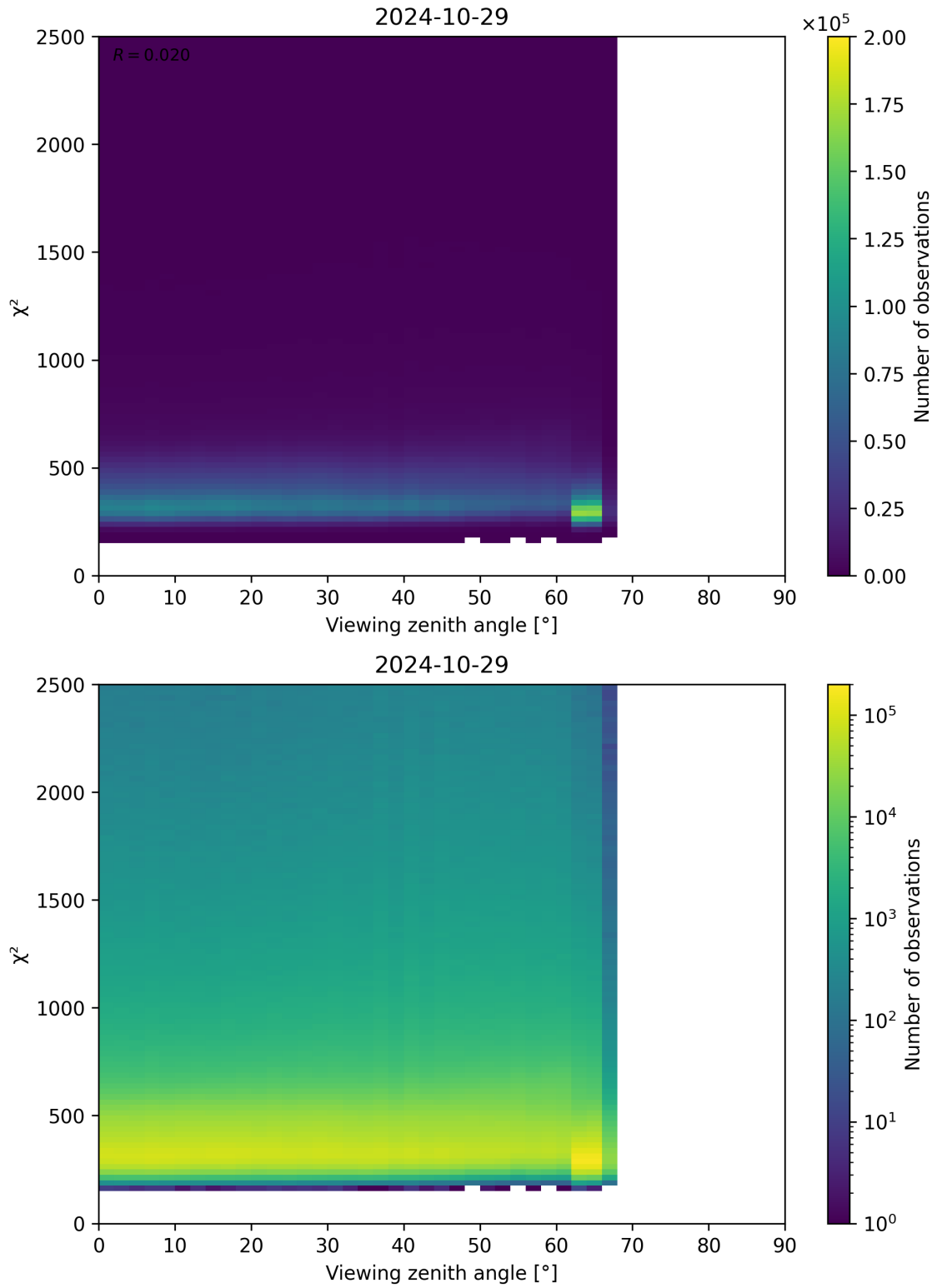
Figure 162: Scatter density plot of “Viewing zenith angle” against “ \chi^2 ” for 2024-10-29 to 2024-10-30.
