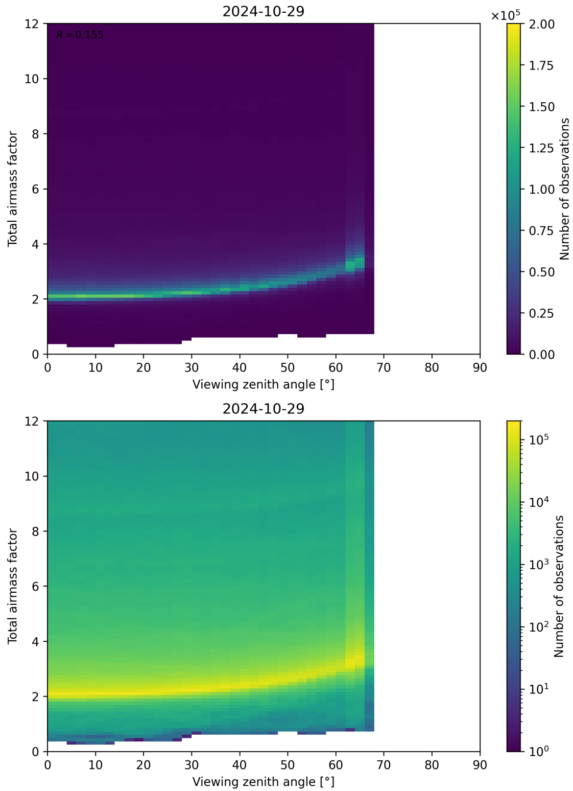
Figure 160: Scatter density plot of “Viewing zenith angle” against “Total airmass factor” for 2024-10-29 to 2024-10-30.
