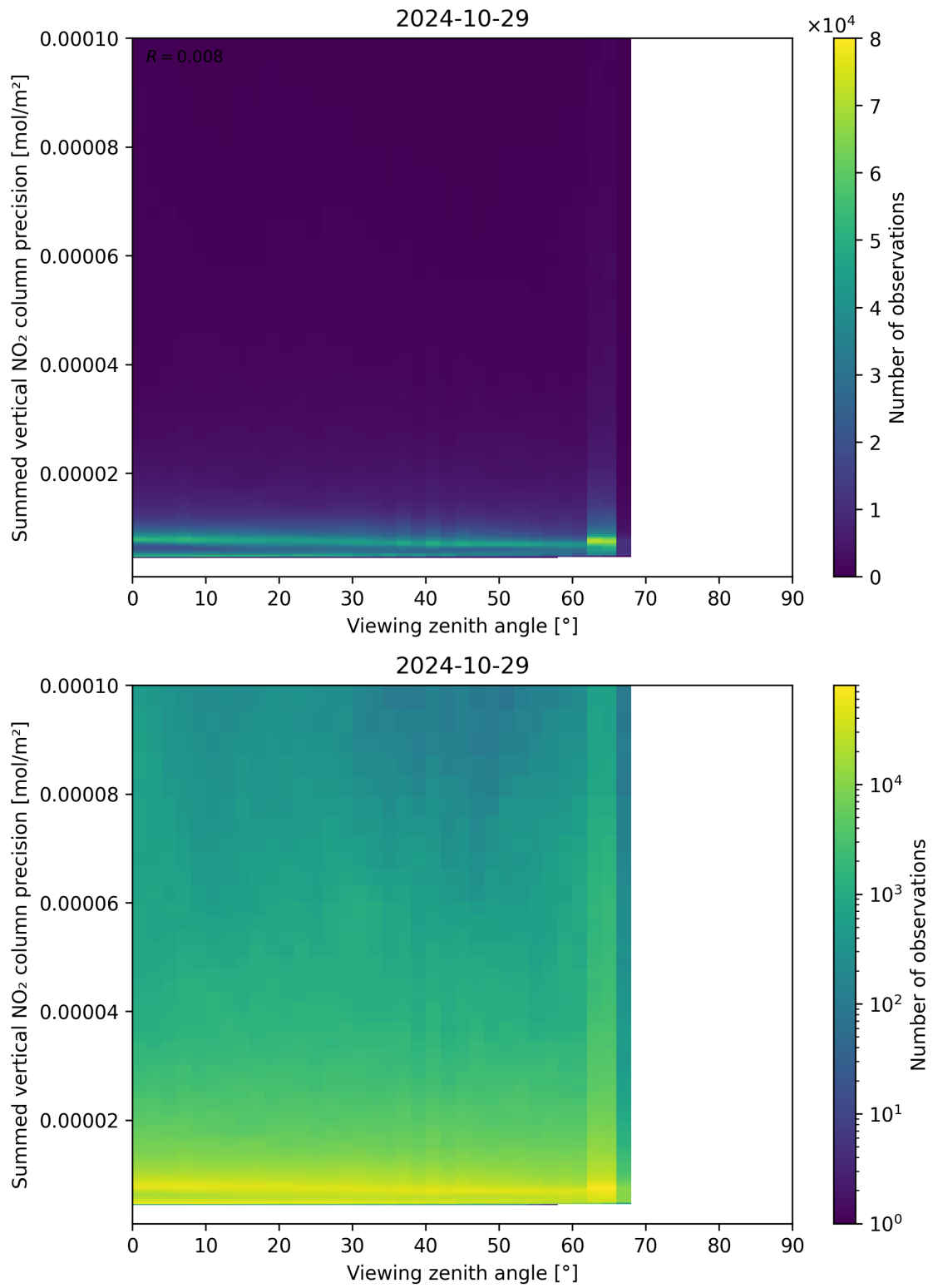
Figure 166: Scatter density plot of “Viewing zenith angle” against “Summed vertical NO 2 column precision” for 2024-10-29 to 2024-10-30.
