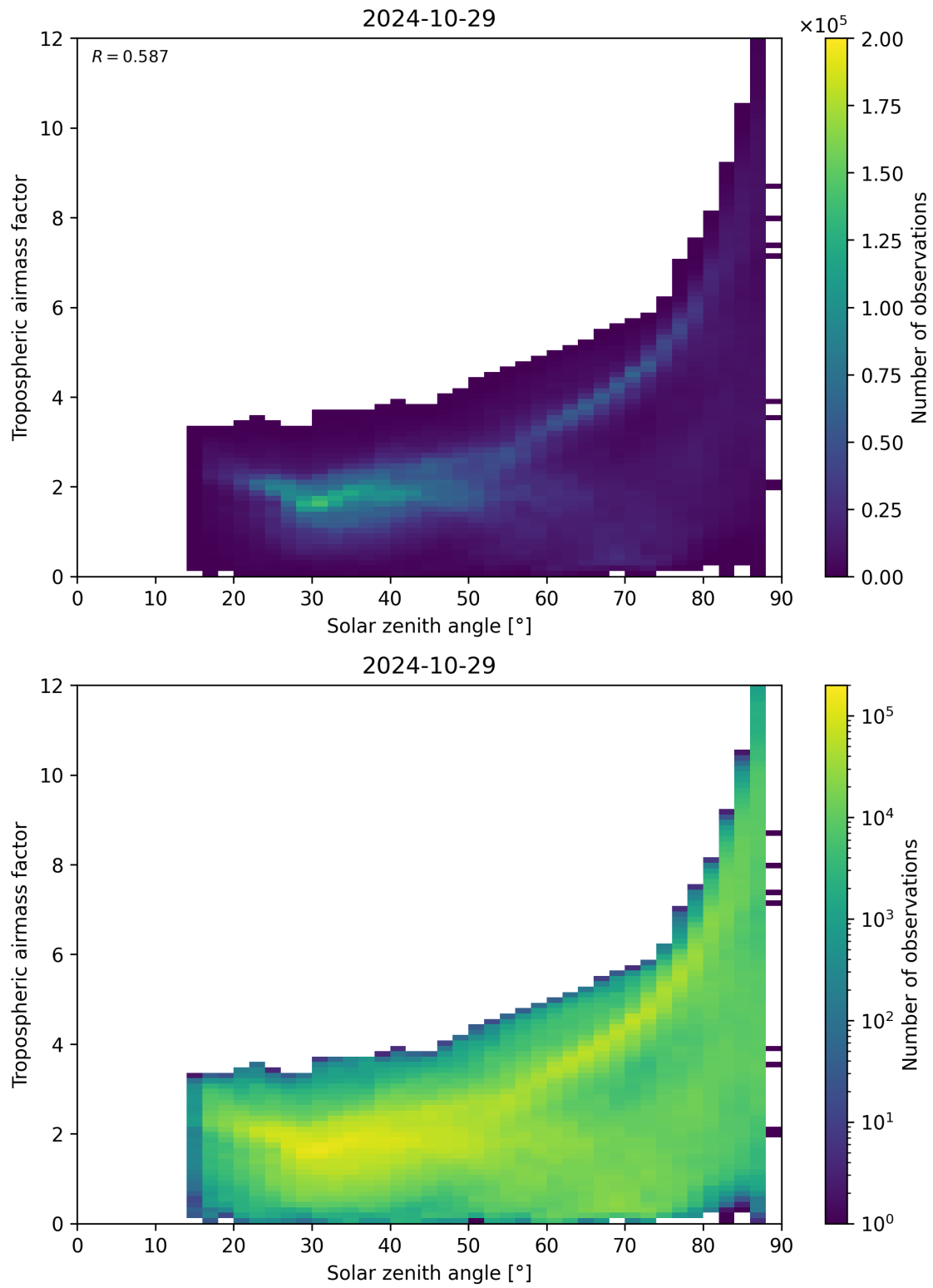
Figure 147: Scatter density plot of “Solar zenith angle” against “Tropospheric airmass factor” for 2024-10-29 to 2024-10-30.
