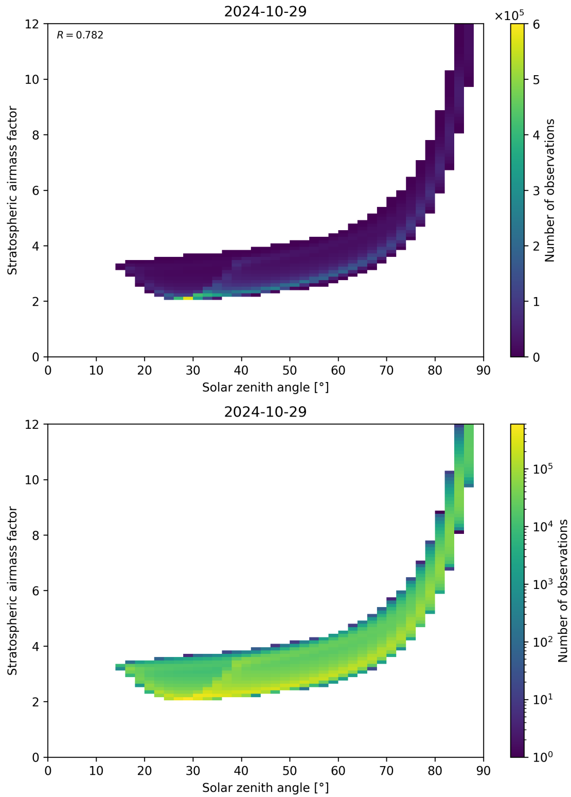
Figure 145: Scatter density plot of “Solar zenith angle” against “Stratospheric airmass factor” for 2024-10-29 to 2024-10-30.
