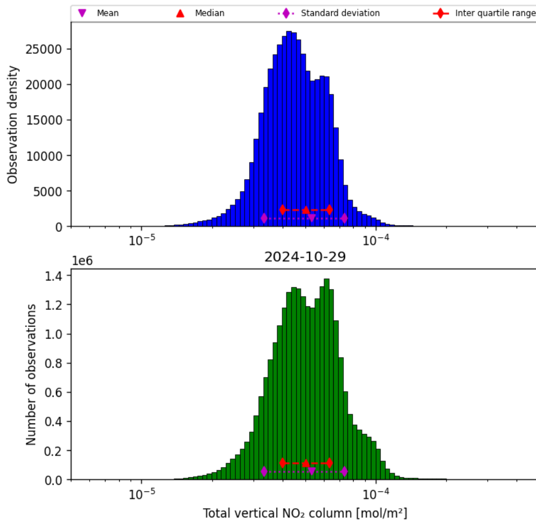
Figure 38: Histogram of “Total vertical NO 2 column” for 2024-10-29 to 2024-10-30
