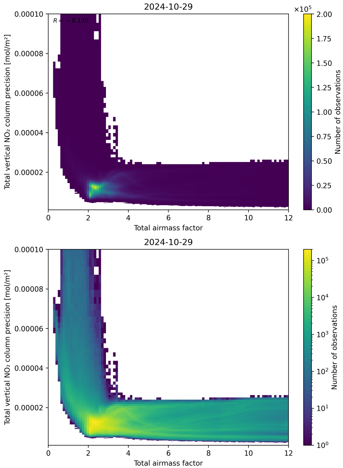
Figure 68: Scatter density plot of “Total airmass factor” against “Total vertical NO 2 column precision” for 2024-10-29 to 2024-10-30.
