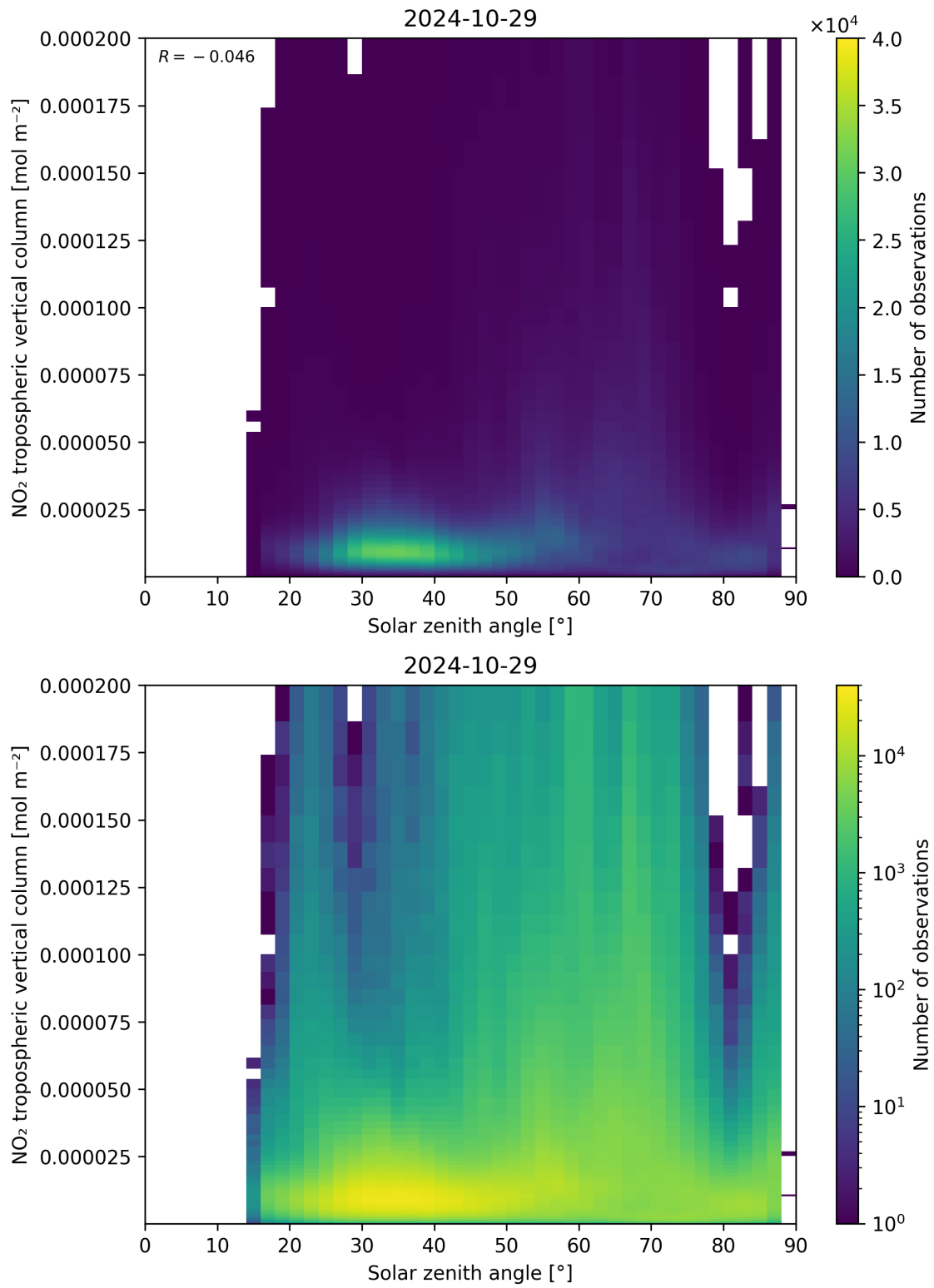
Figure 155: Scatter density plot of “Solar zenith angle” against “NO 2 tropospheric vertical column” for 2024-10-29 to 2024-10-30.
