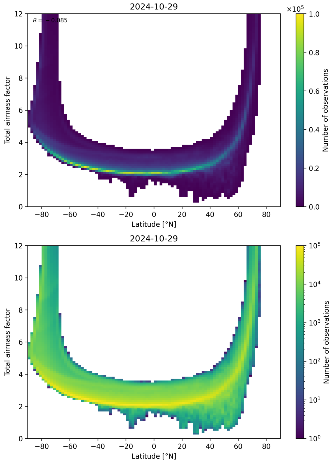
Figure 84: Scatter density plot of “Latitude” against “Total airmass factor” for 2024-10-29 to 2024-10-30.
