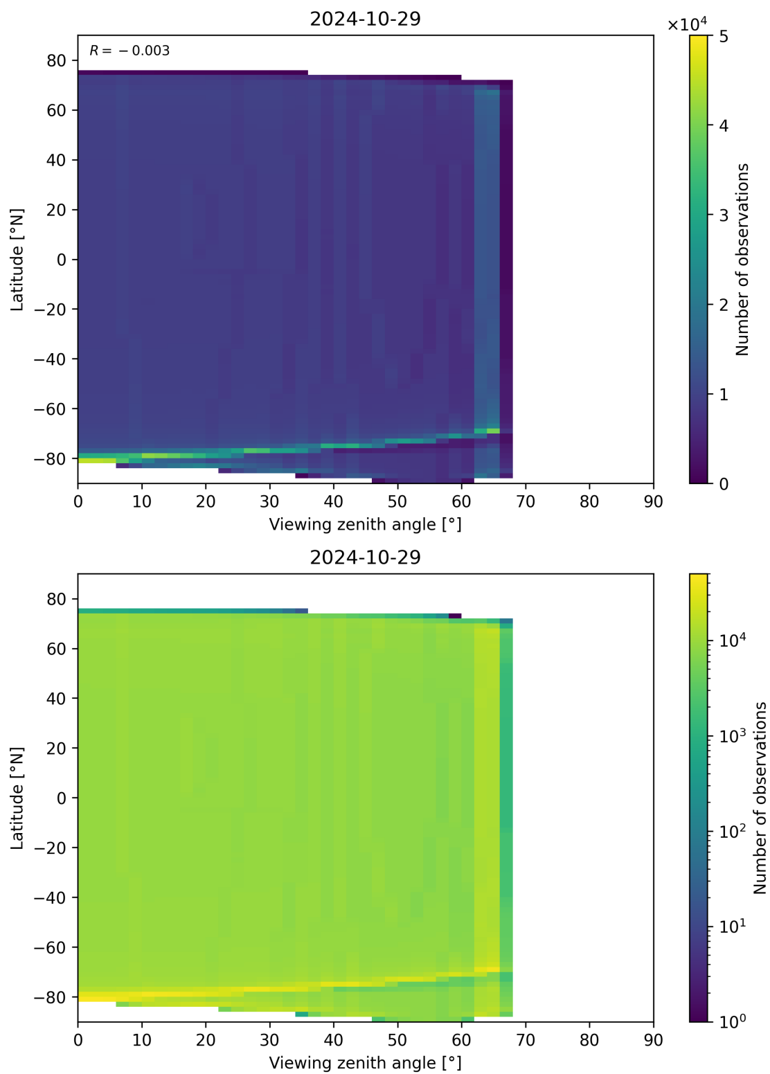
Figure 163: Scatter density plot of “Viewing zenith angle” against “Latitude” for 2024-10-29 to 2024-10-30.
