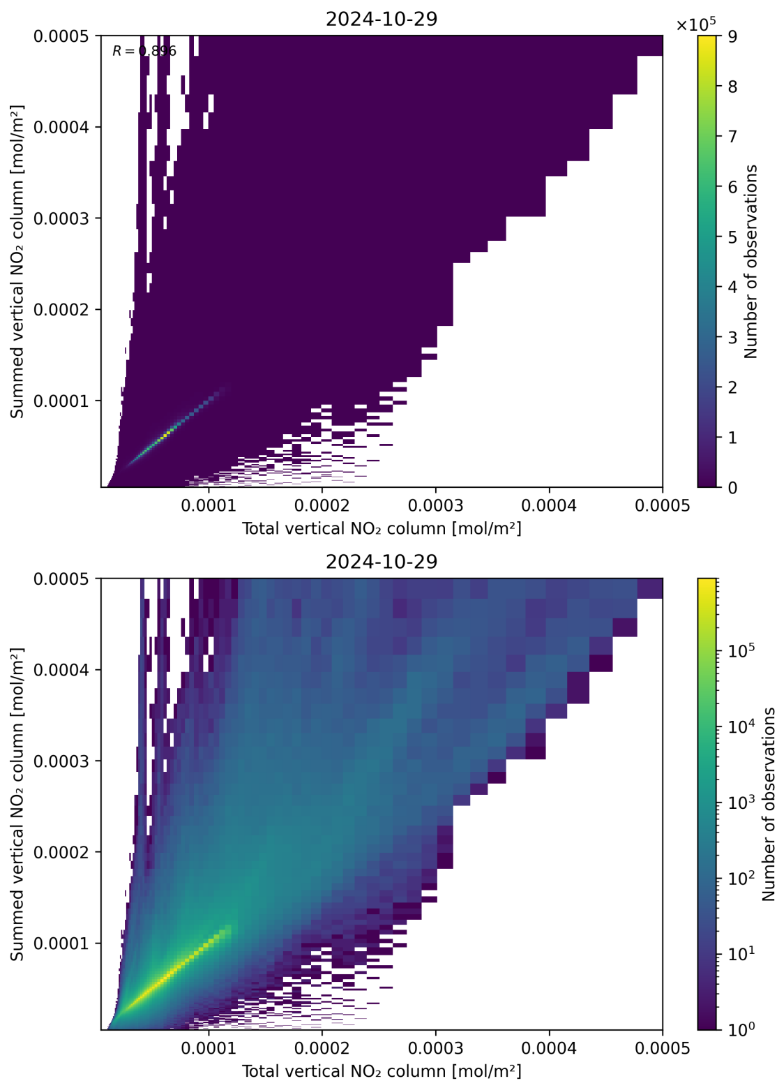
Figure 112: Scatter density plot of “Total vertical NO 2 column” against “Summed vertical NO 2 column” for 2024-10-29 to 2024-10-30.
