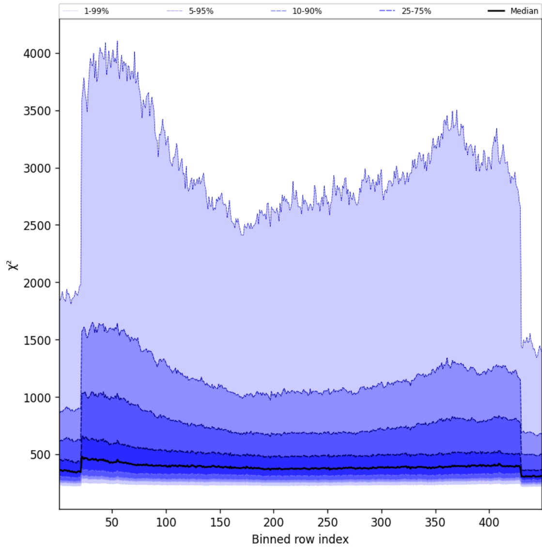
Figure 59: Along track statistics of “ \chi^2 ” for 2024-10-29 to 2024-10-30
