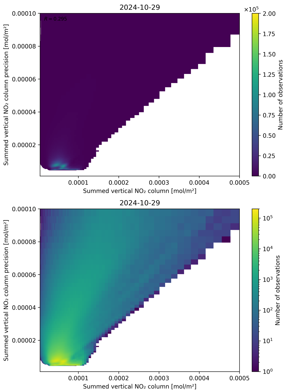
Figure 105: Scatter density plot of “Summed vertical NO 2 column” against “Summed vertical NO 2 column precision” for 2024-10-29 to 2024-10-30.
