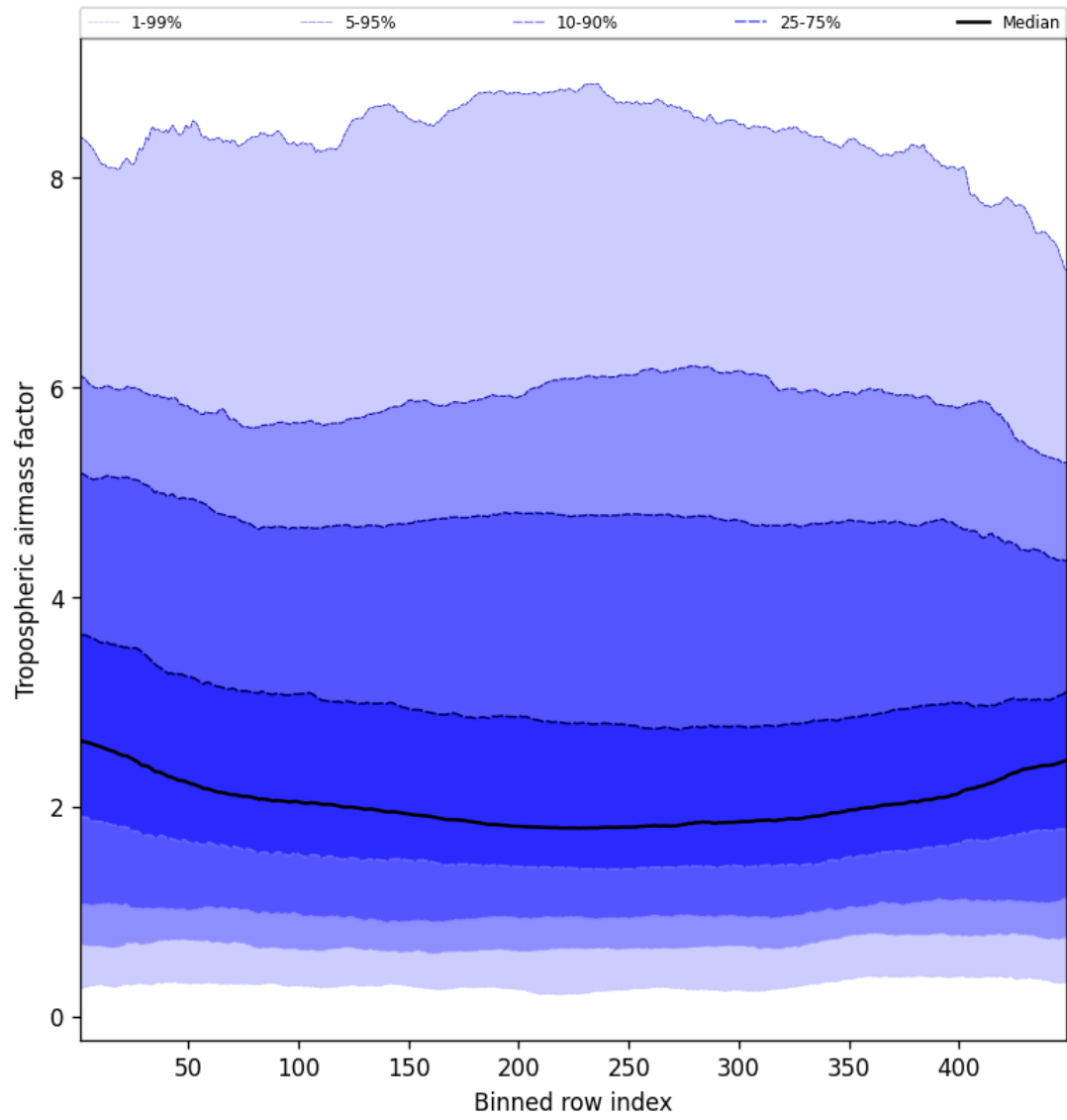
Figure 48: Along track statistics of “Tropospheric airmass factor” for 2024-10-29 to 2024-10-30
