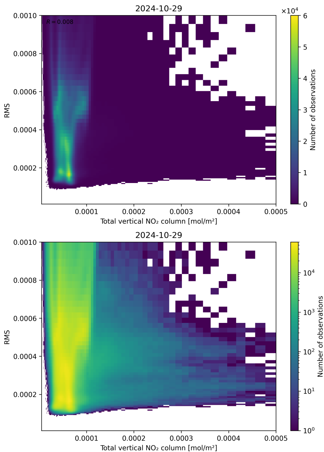
Figure 120: Scatter density plot of “Total vertical NO 2 column” against “RMS” for 2024-10-29 to 2024-10-30.
