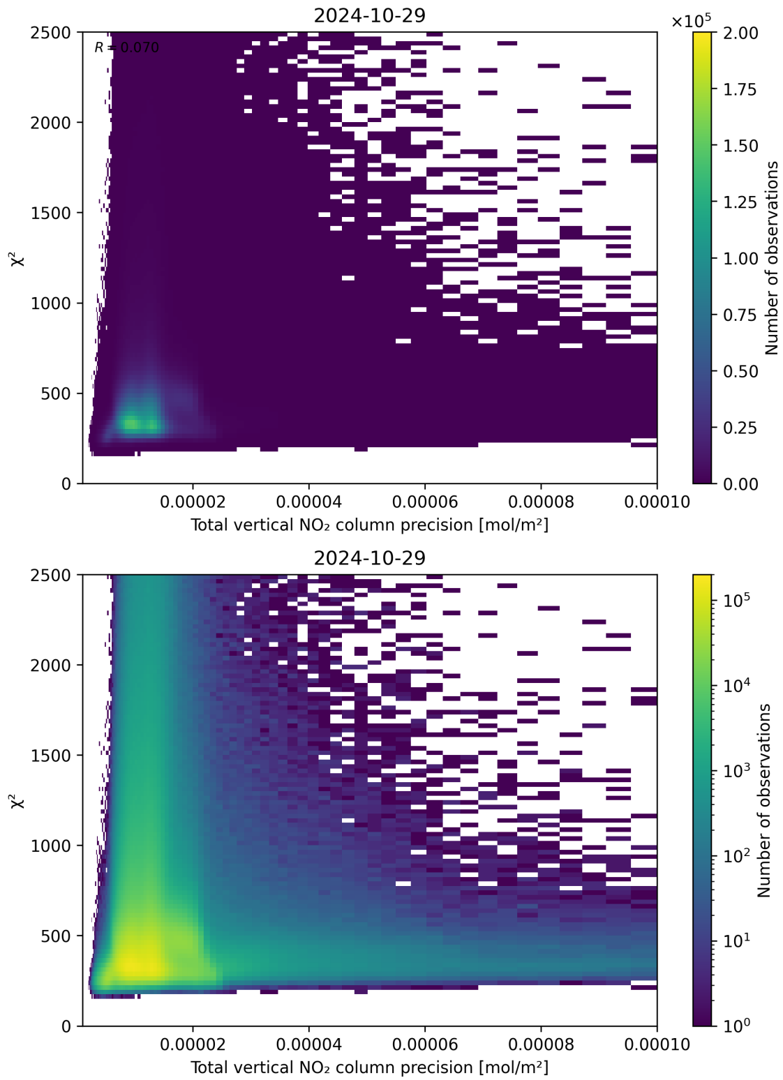
Figure 116: Scatter density plot of “Total vertical NO 2 column precision” against “ \chi^2 ” for 2024-10-29 to 2024-10-30.
