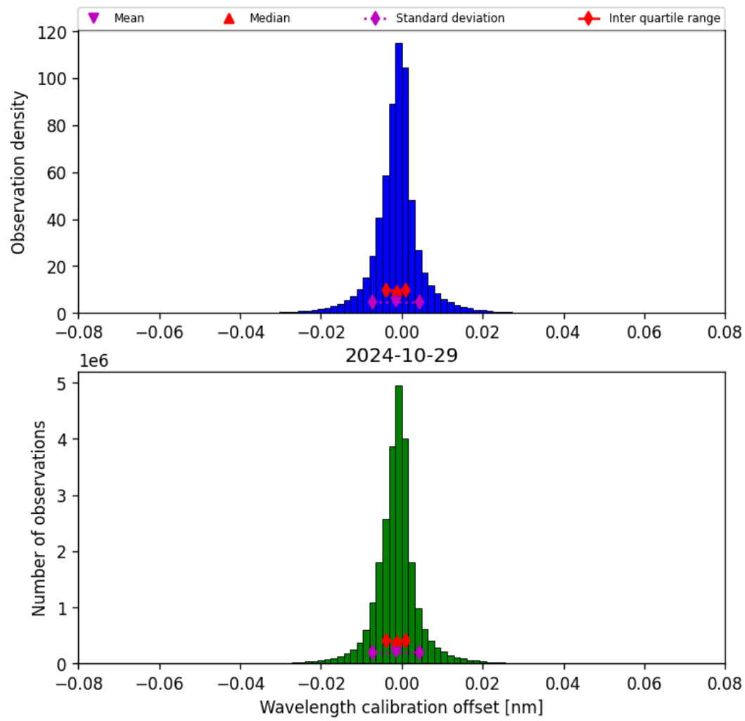
Figure 35: Histogram of “Wavelength calibration offset” for 2024-10-29 to 2024-10-30
