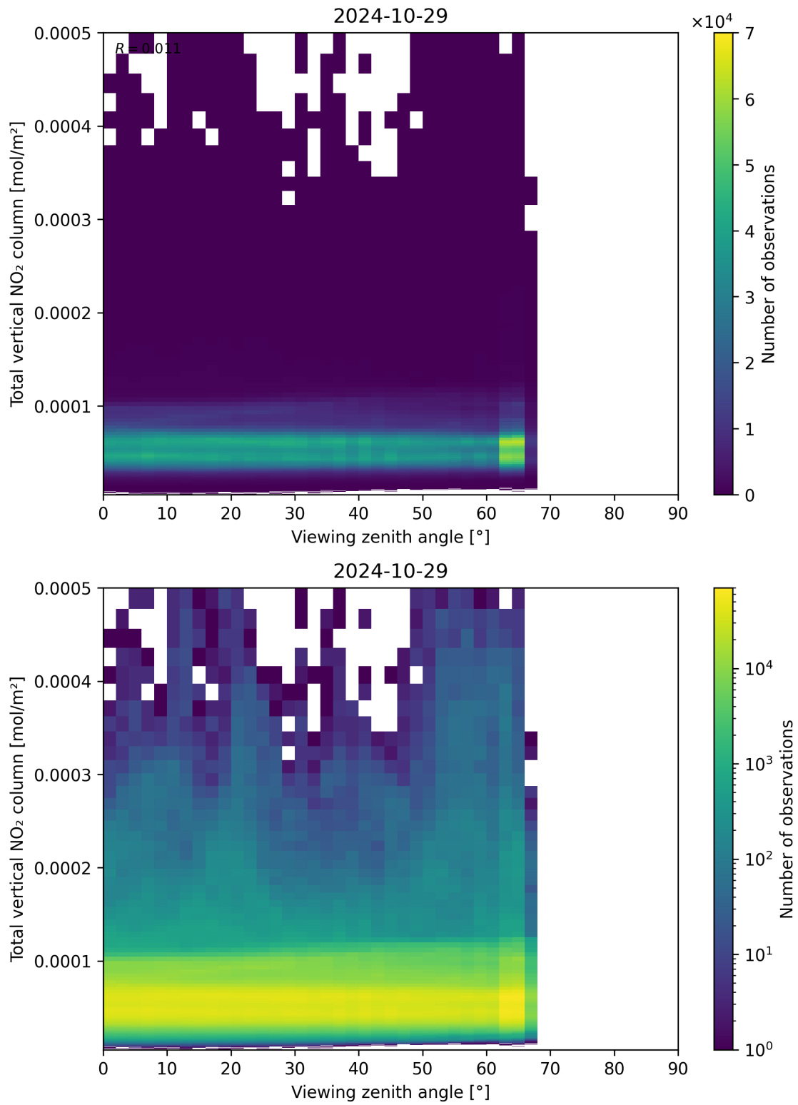
Figure 167: Scatter density plot of “Viewing zenith angle” against “Total vertical NO 2 column” for 2024-10-29 to 2024-10-30.
