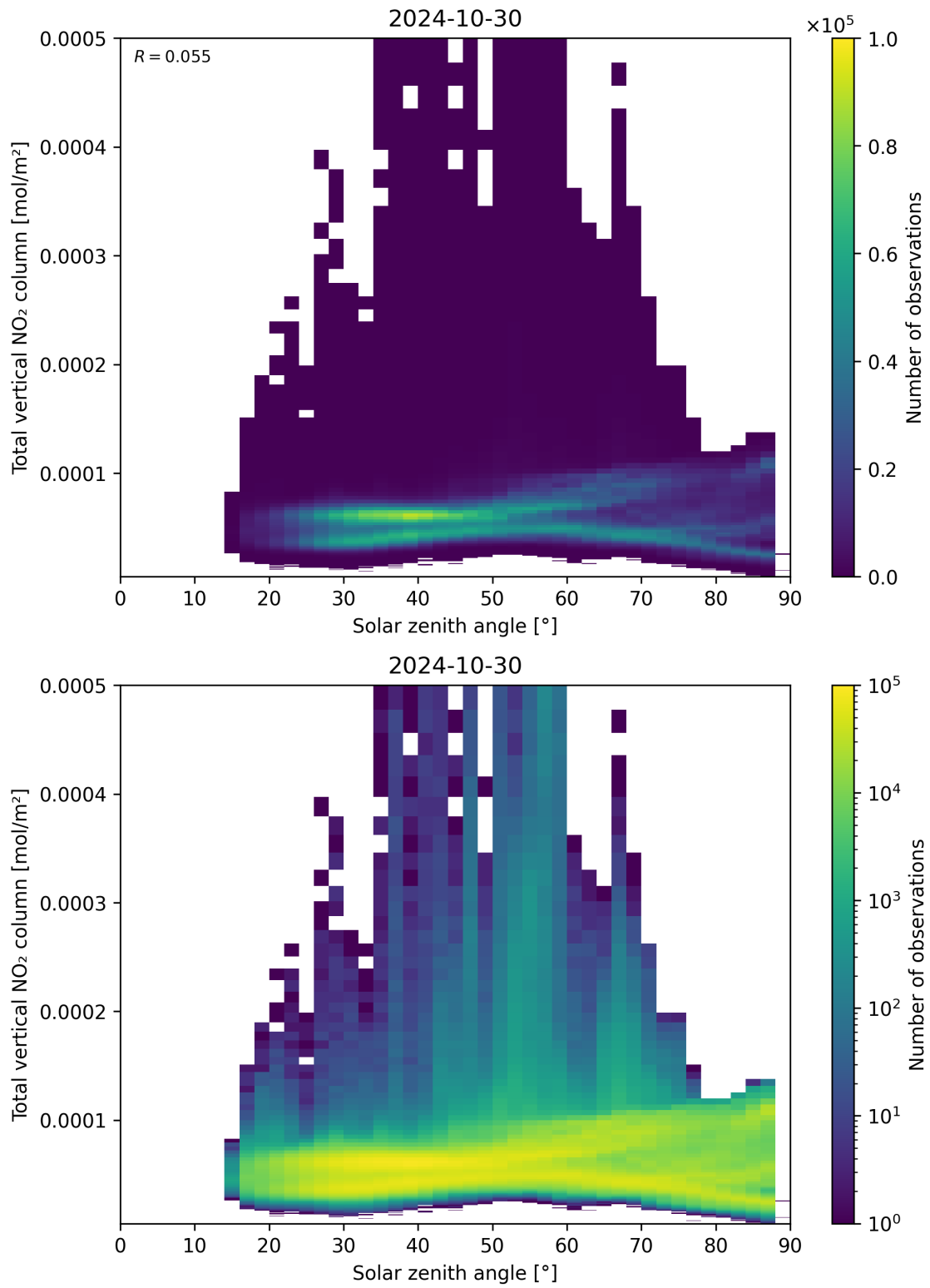
Figure 153: Scatter density plot of “Solar zenith angle” against “Total vertical NO 2 column” for 2024-10-30 to 2024-10-31.
