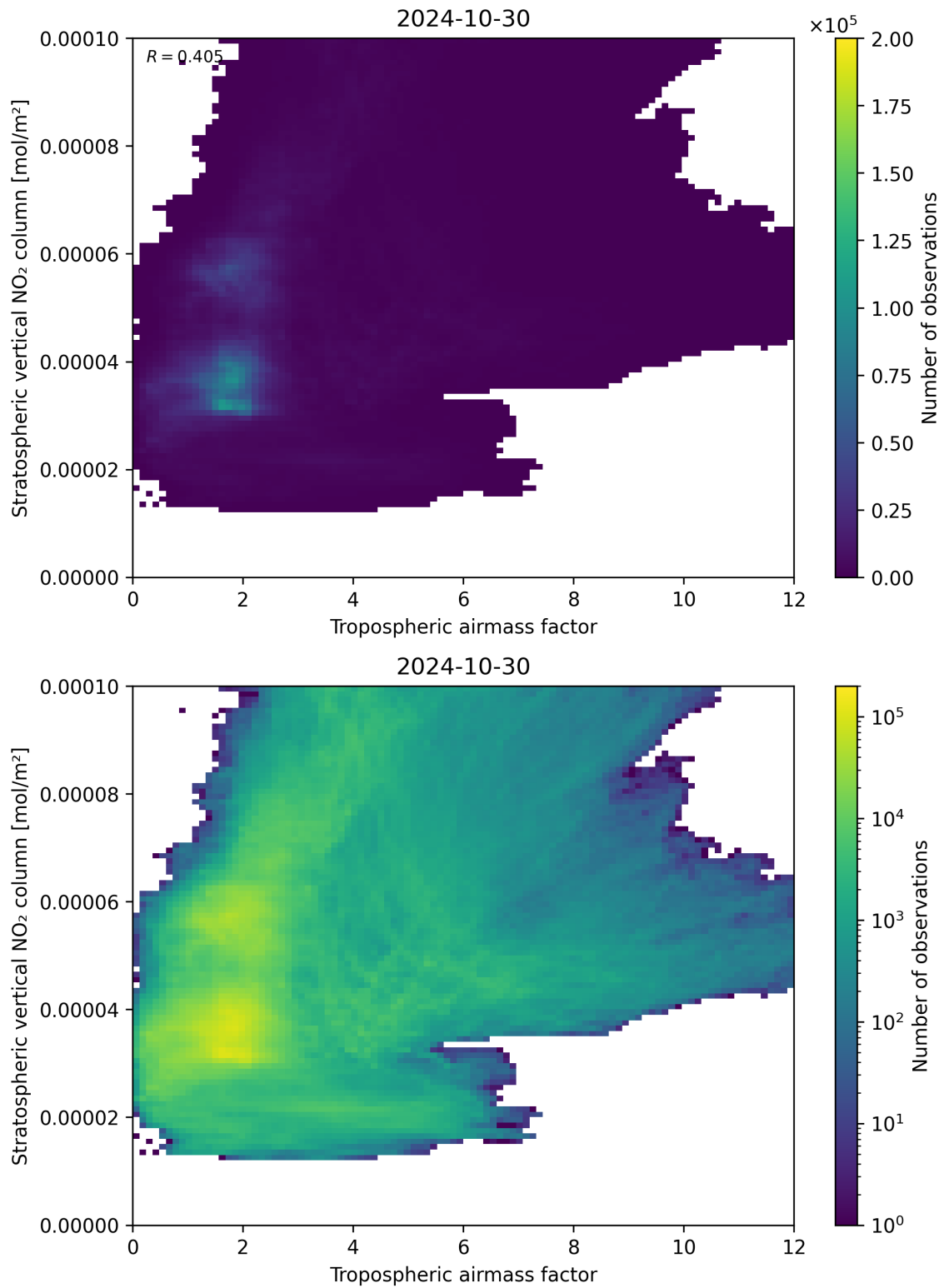
Figure 74: Scatter density plot of “Tropospheric airmass factor” against “Stratospheric vertical NO 2 column” for 2024-10-30 to 2024-10-31.
