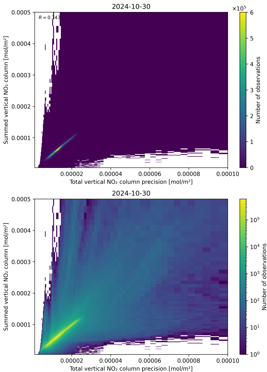
Figure 117: Scatter density plot of “Total vertical NO 2 column precision” against “Summed vertical NO 2 column” for 2024-10-30 to 2024-10-31.
