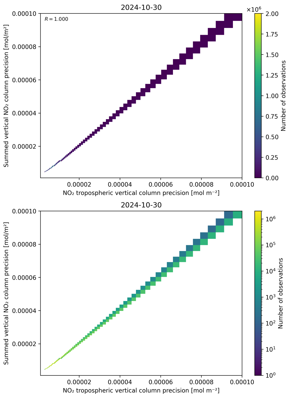
Figure 137: Scatter density plot of “NO 2 tropospheric vertical column precision” against “Summed vertical NO 2 column precision” for 2024-10-30 to 2024-10-31.
