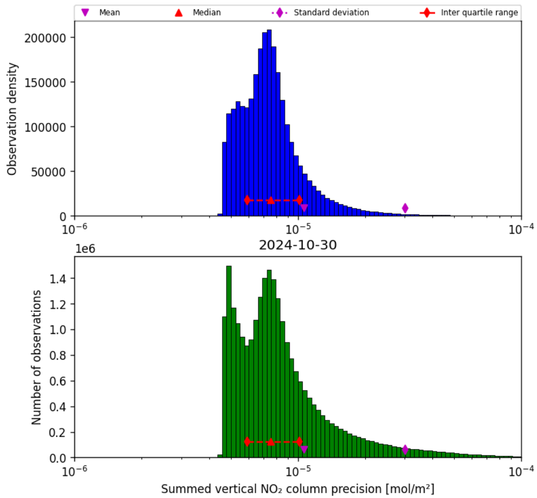
Figure 41: Histogram of “Summed vertical NO 2 column precision” for 2024-10-30 to 2024-10-31
