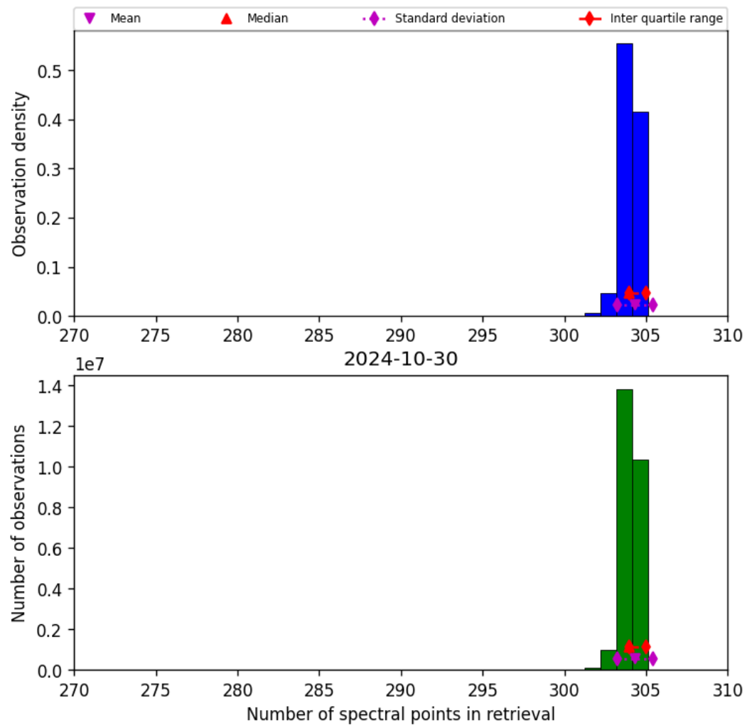
Figure 33: Histogram of “Number of spectral points in retrieval” for 2024-10-30 to 2024-10-31
