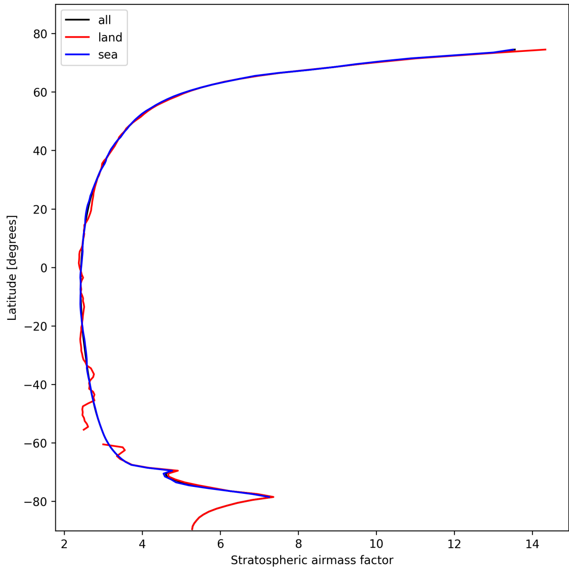
Figure 27: Zonal average of “Stratospheric air mass factor” for 2024-10-30 to 2024-10-31.
