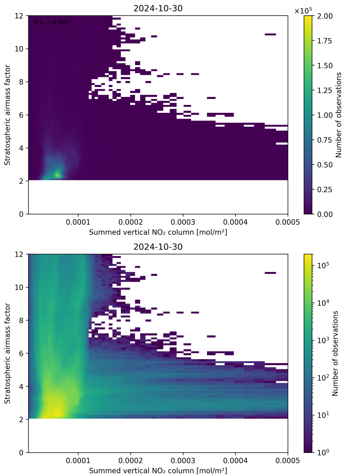
Figure 103: Scatter density plot of “Summed vertical NO 2 column” against “Stratospheric air mass factor” for 2024-10-30 to 2024-10-31.
