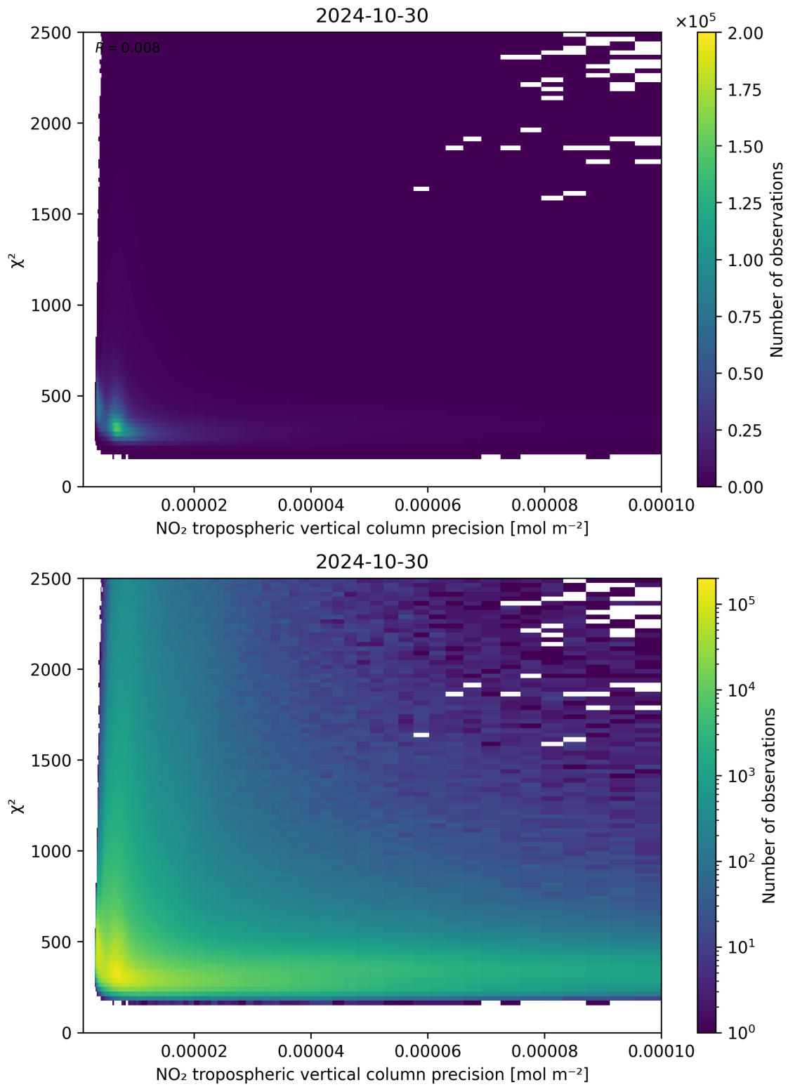
Figure 134: Scatter density plot of “NO 2 tropospheric vertical column precision” against “ \chi^2 ” for 2024-10-30 to 2024-10-31.
