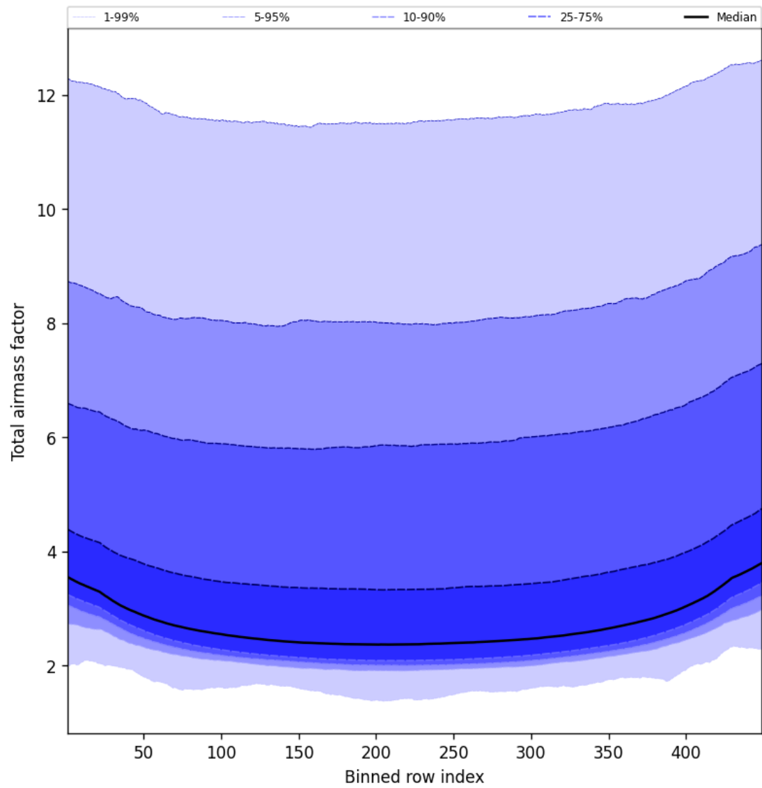
Figure 49: Along track statistics of “Total airmass factor” for 2024-10-30 to 2024-10-31
