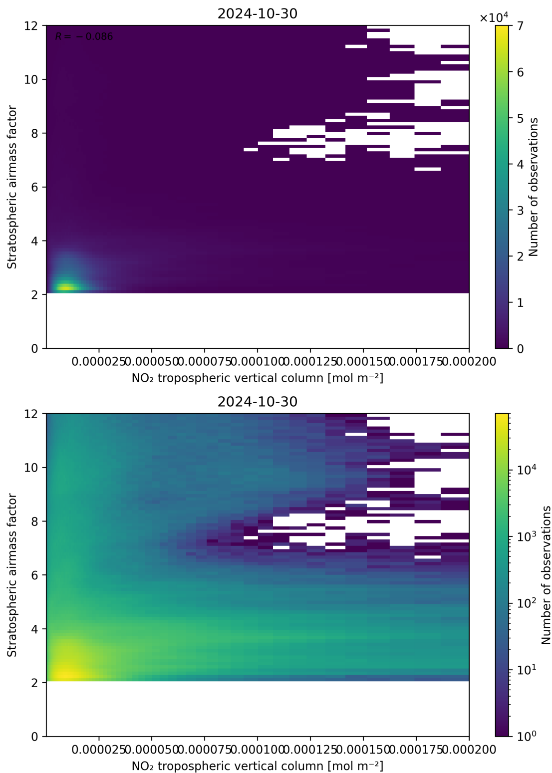
Figure 121: Scatter density plot of “NO 2 tropospheric vertical column” against “Stratospheric airmass factor” for 2024-10-30 to 2024-10-31.
