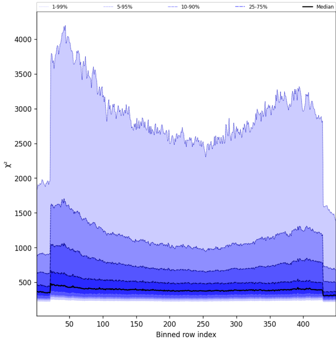
Figure 59: Along track statistics of “ \chi^2 ” for 2024-10-30 to 2024-10-31
