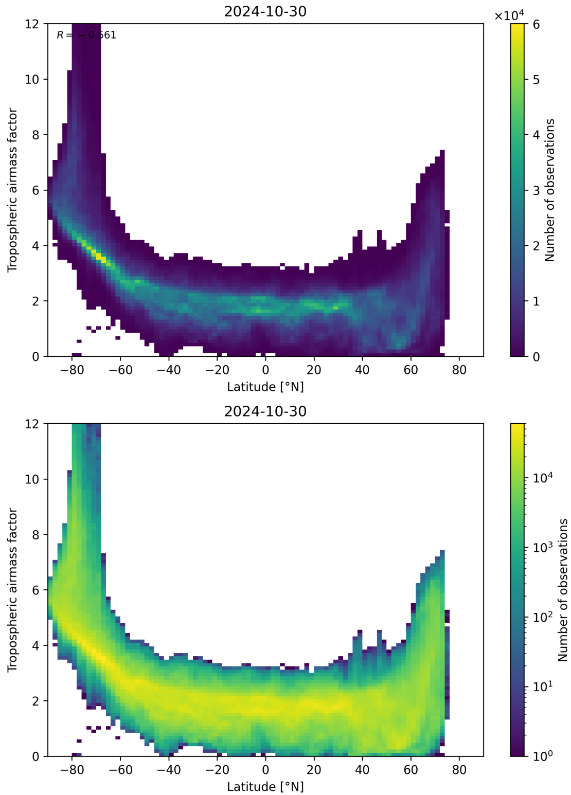
Figure 85: Scatter density plot of “Latitude” against “Tropospheric air mass factor” for 2024-10-30 to 2024-10-31.
