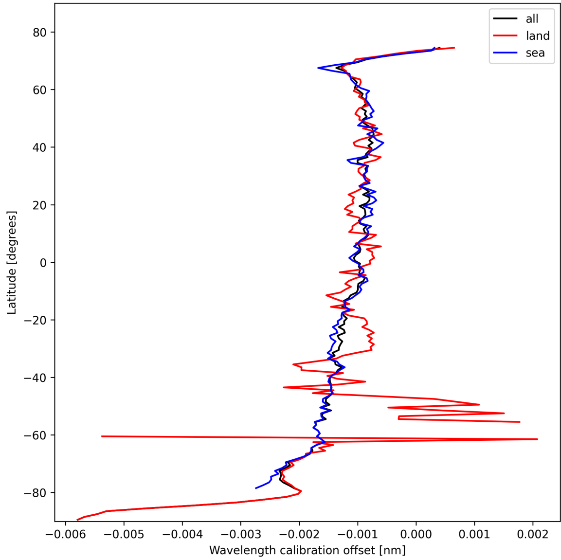
Figure 18: Zonal average of “Wavelength calibration offset” for 2024-10-30 to 2024-10-31.
