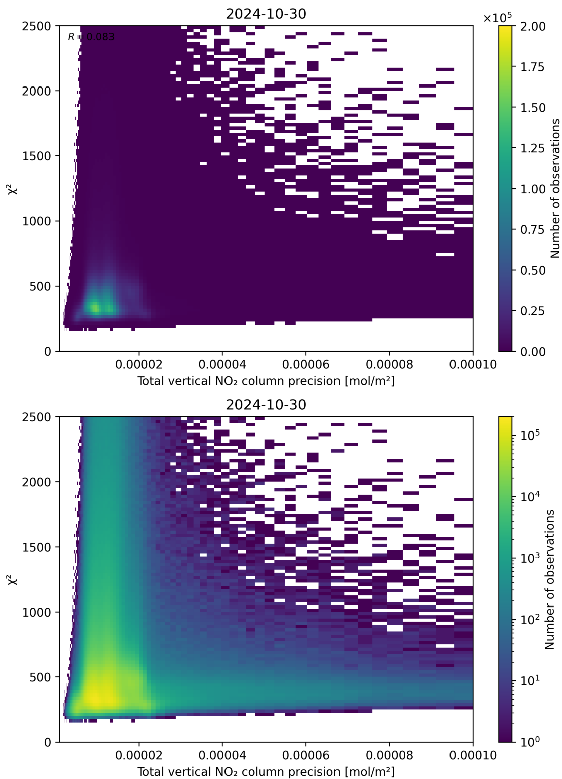
Figure 116: Scatter density plot of “Total vertical NO 2 column precision” against “ \chi^2 ” for 2024-10-30 to 2024-10-31.
