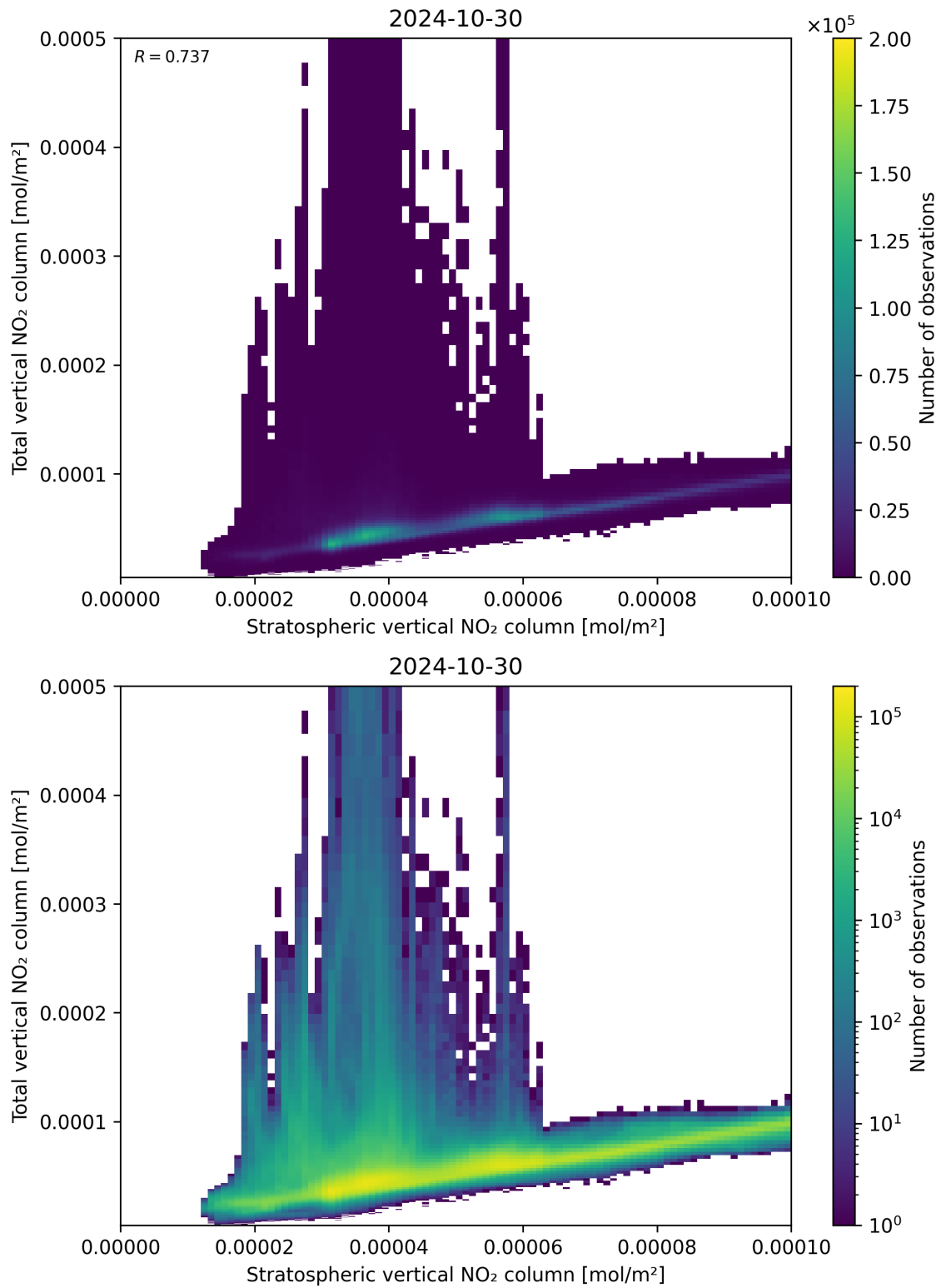
Figure 100: Scatter density plot of “Stratospheric vertical NO 2 column” against “Total vertical NO 2 column” for 2024-10-30 to 2024-10-31.
