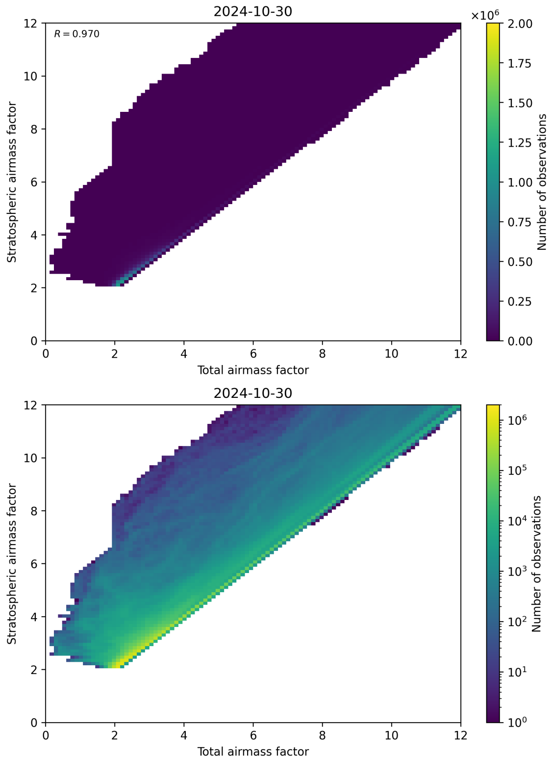
Figure 62: Scatter density plot of “Total airmass factor” against “Stratospheric airmass factor” for 2024-10-30 to 2024-10-31.
