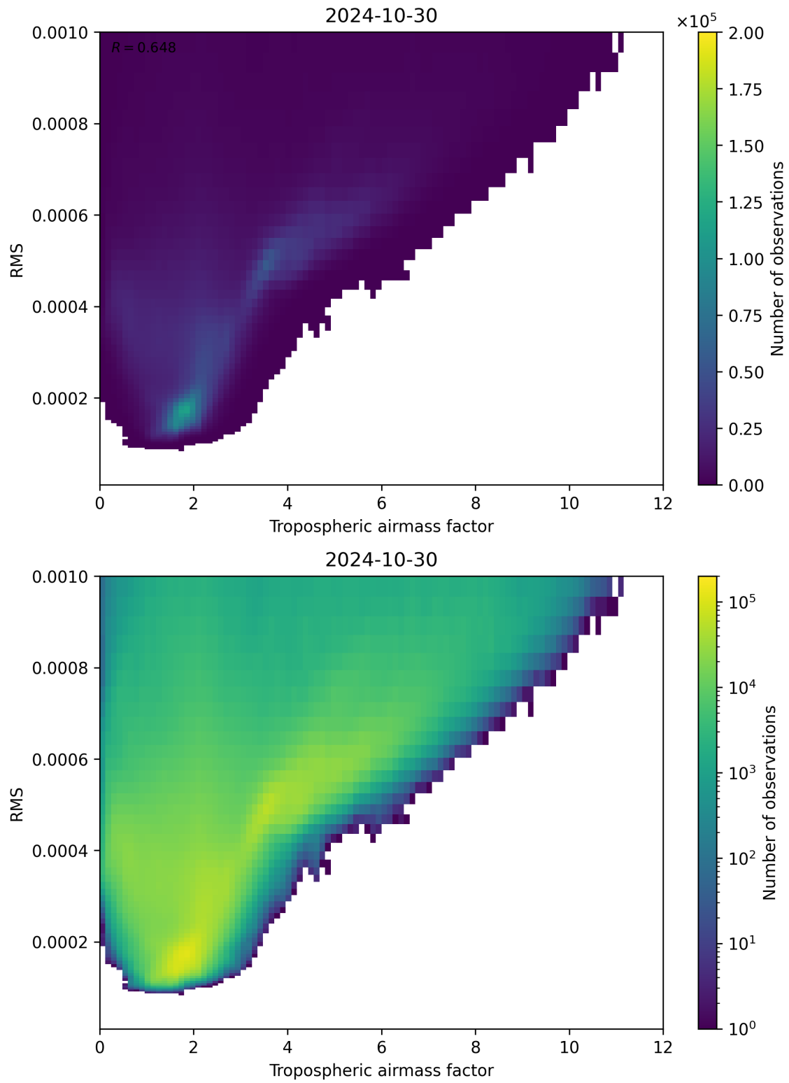
Figure 79: Scatter density plot of “Tropospheric airmass factor” against “RMS” for 2024-10-30 to 2024-10-31.
