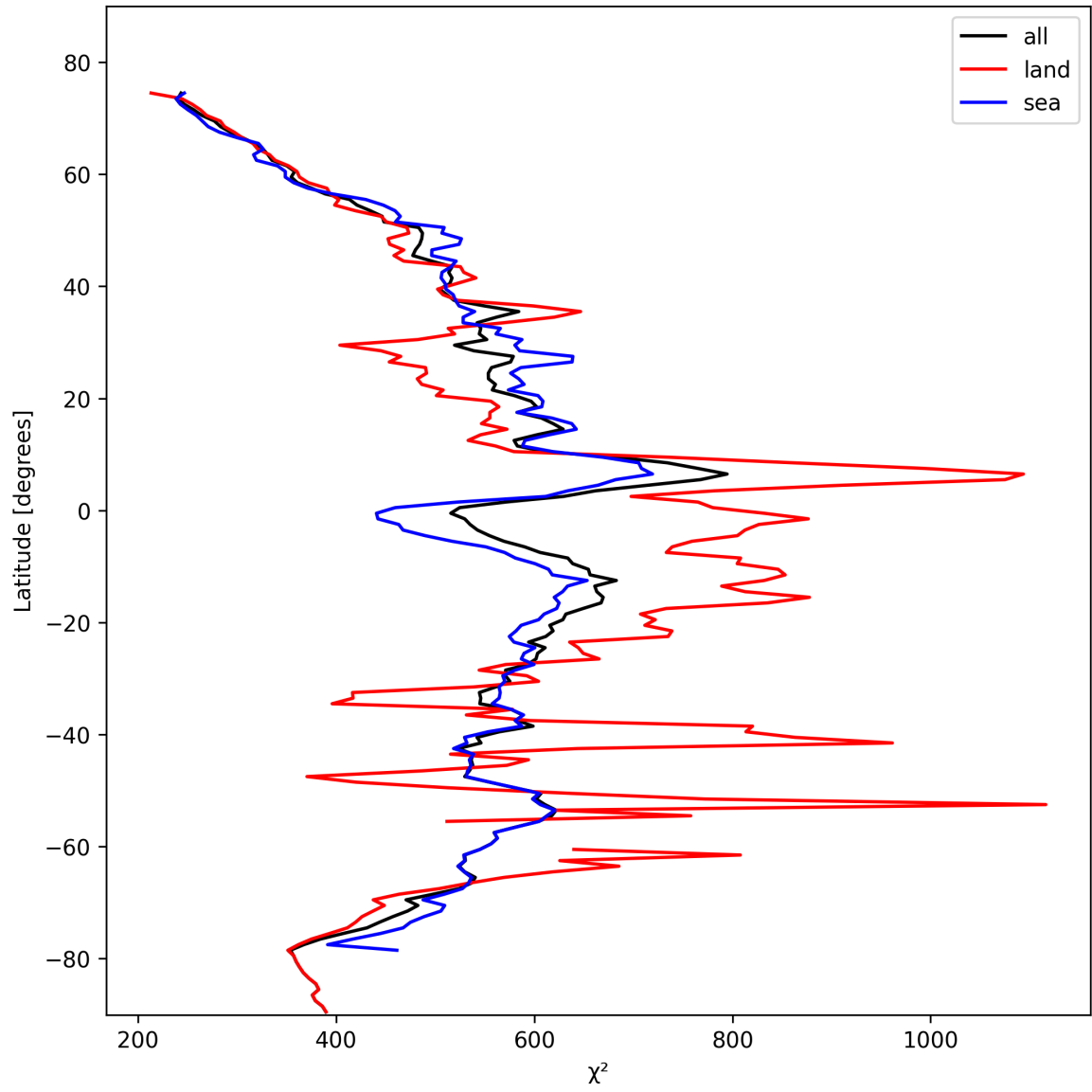
Figure 25: Zonal average of “ \chi^2 ” for 2024-10-30 to 2024-10-31.
