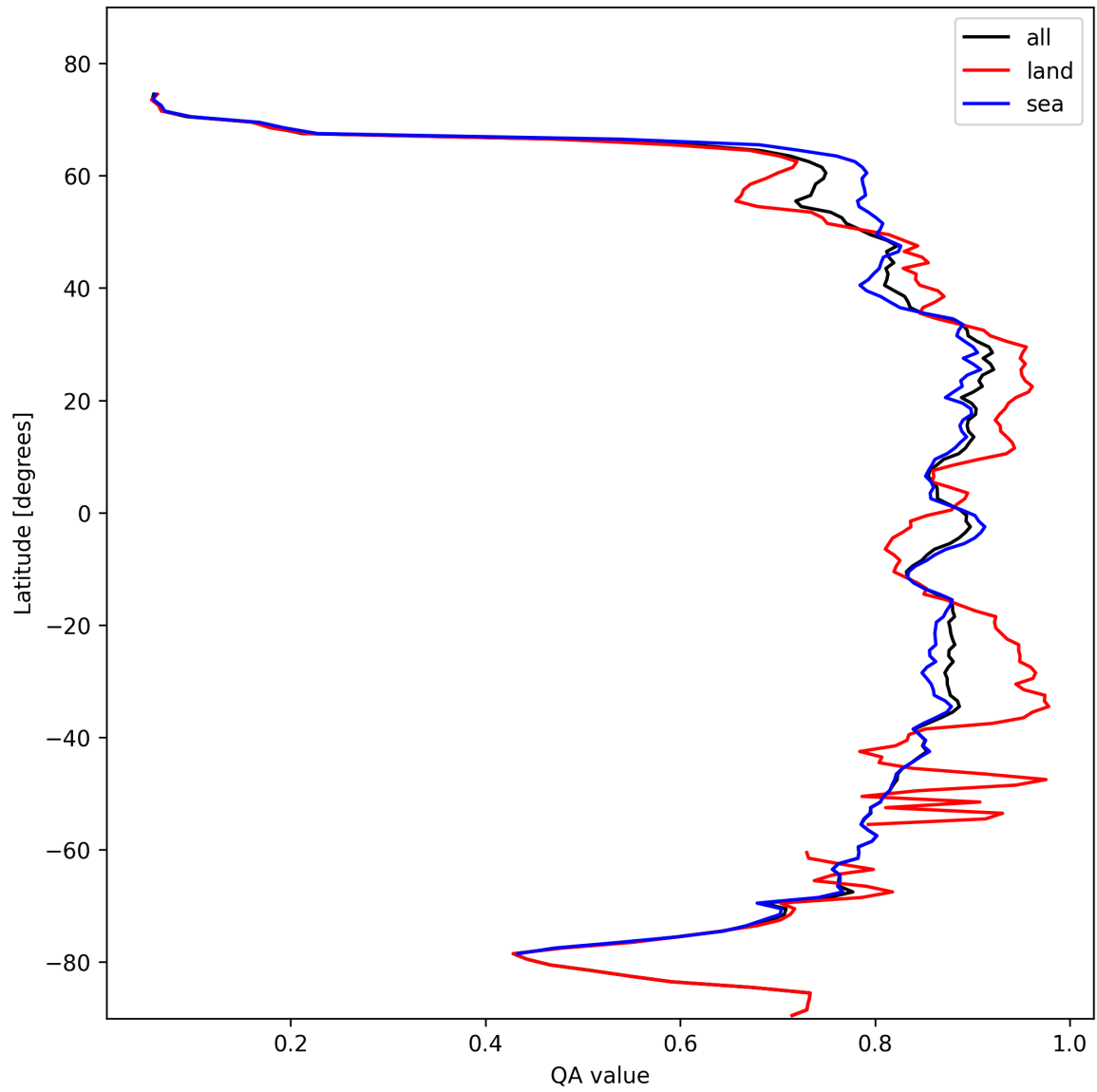
Figure 11: Zonal average of “QA value” for 2024-10-30 to 2024-10-31.
