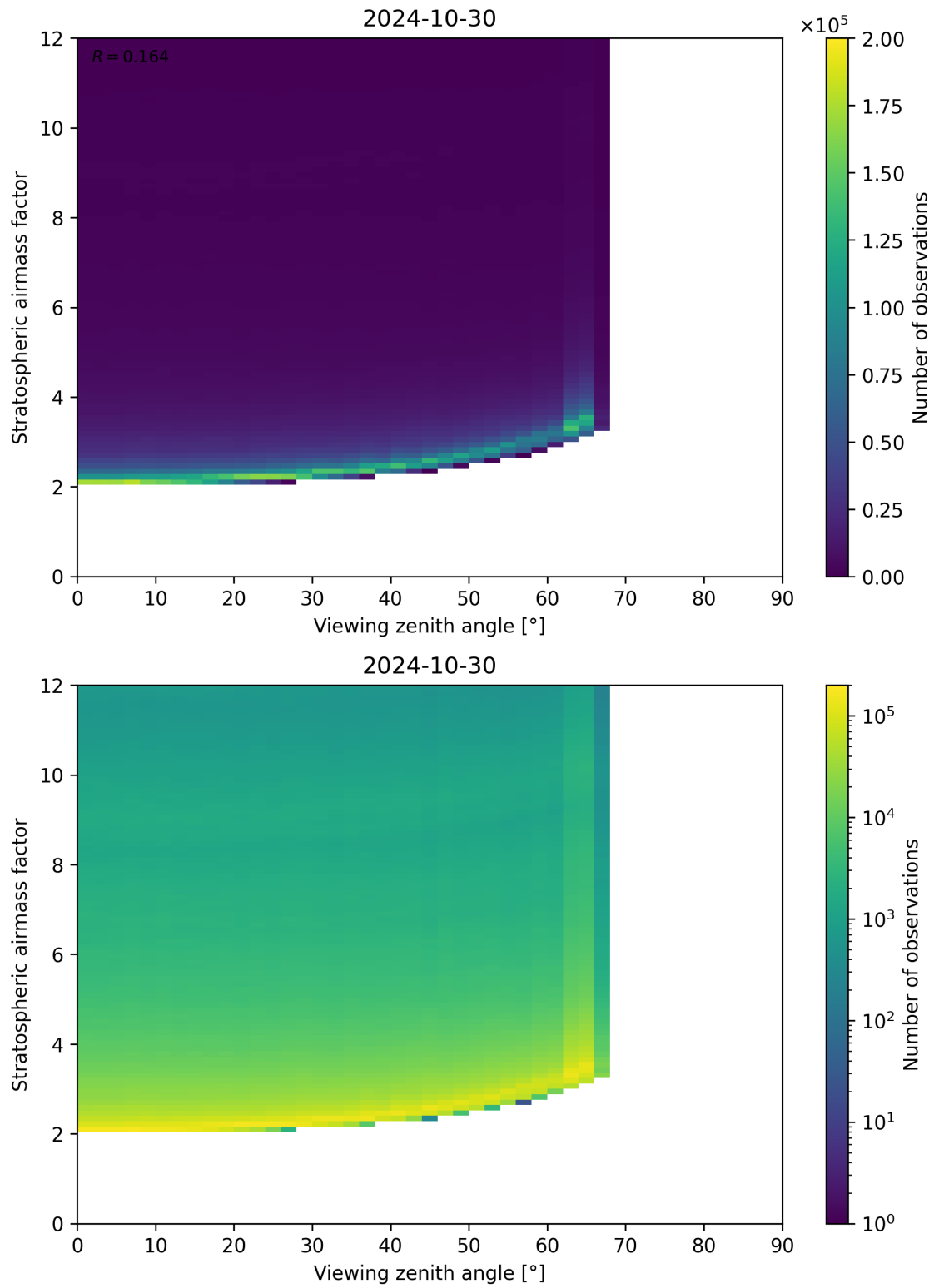
Figure 159: Scatter density plot of “Viewing zenith angle” against “Stratospheric airmass factor” for 2024-10-30 to 2024-10-31.
