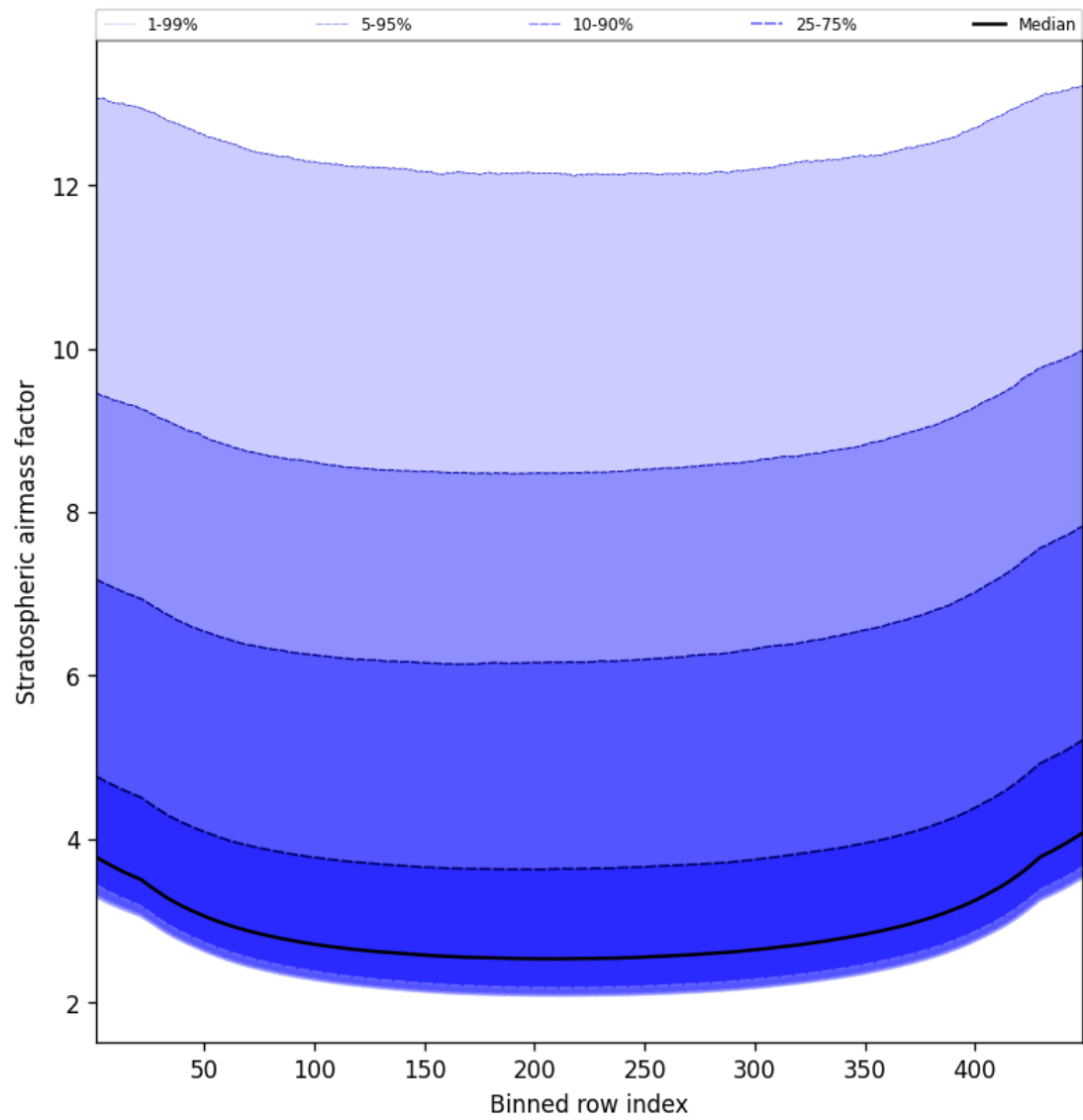
Figure 61: Along track statistics of “Stratospheric airmass factor” for 2024-10-30 to 2024-10-31
