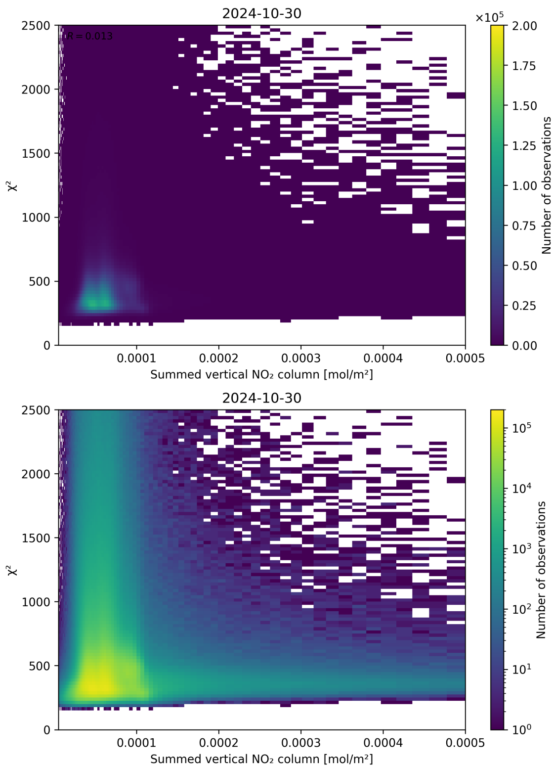
Figure 104: Scatter density plot of “Summed vertical NO 2 column” against “ \chi^2 ” for 2024-10-30 to 2024-10-31.
