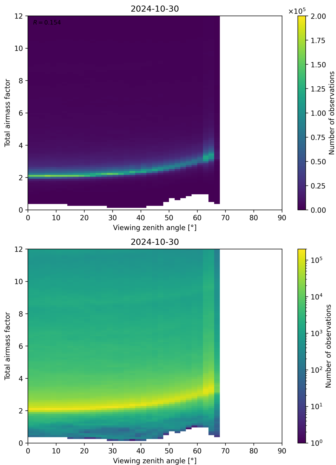
Figure 160: Scatter density plot of “Viewing zenith angle” against “Total airmass factor” for 2024-10-30 to 2024-10-31.
