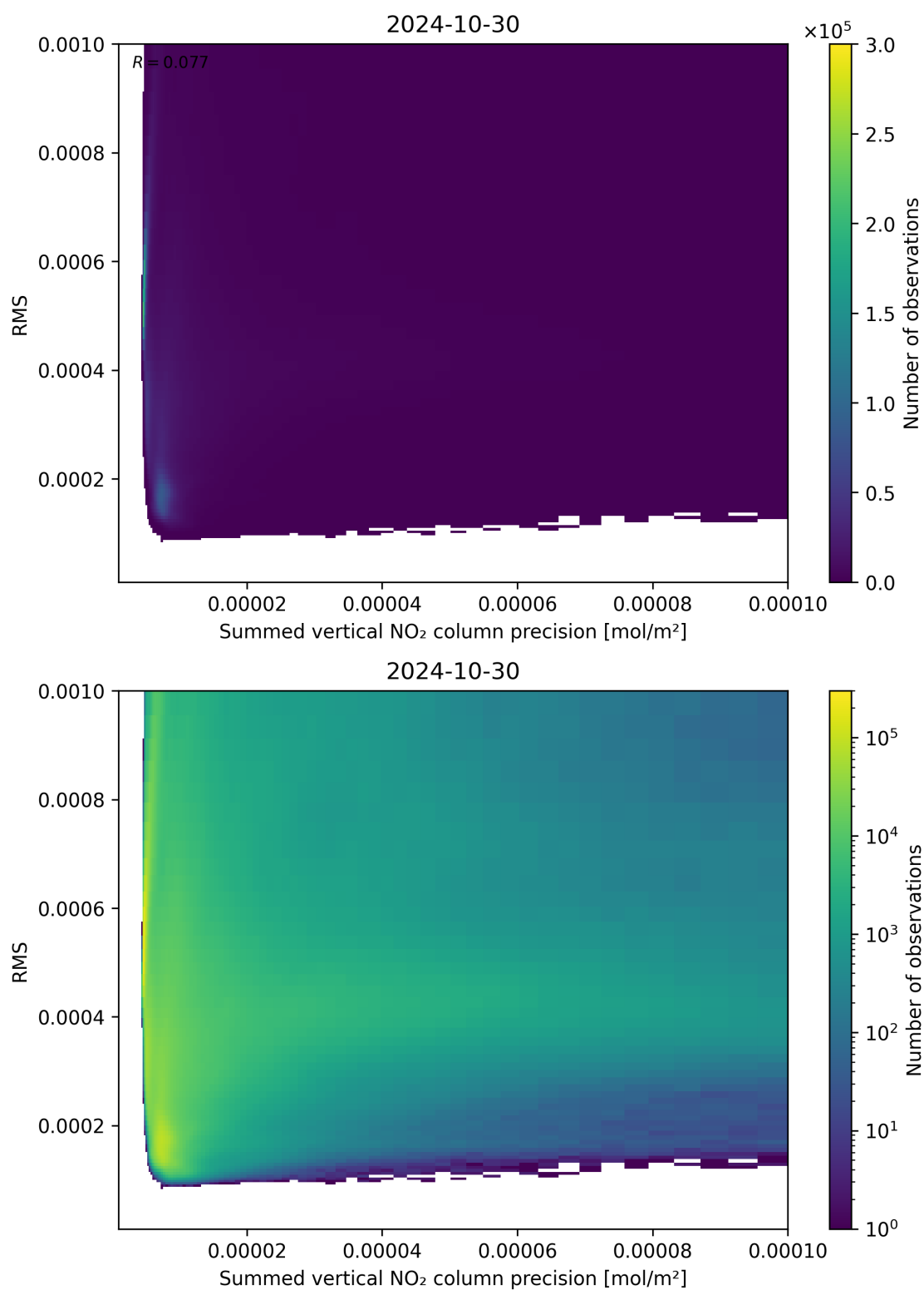
Figure 108: Scatter density plot of “Summed vertical NO 2 column precision” against “RMS” for 2024-10-30 to 2024-10-31.
