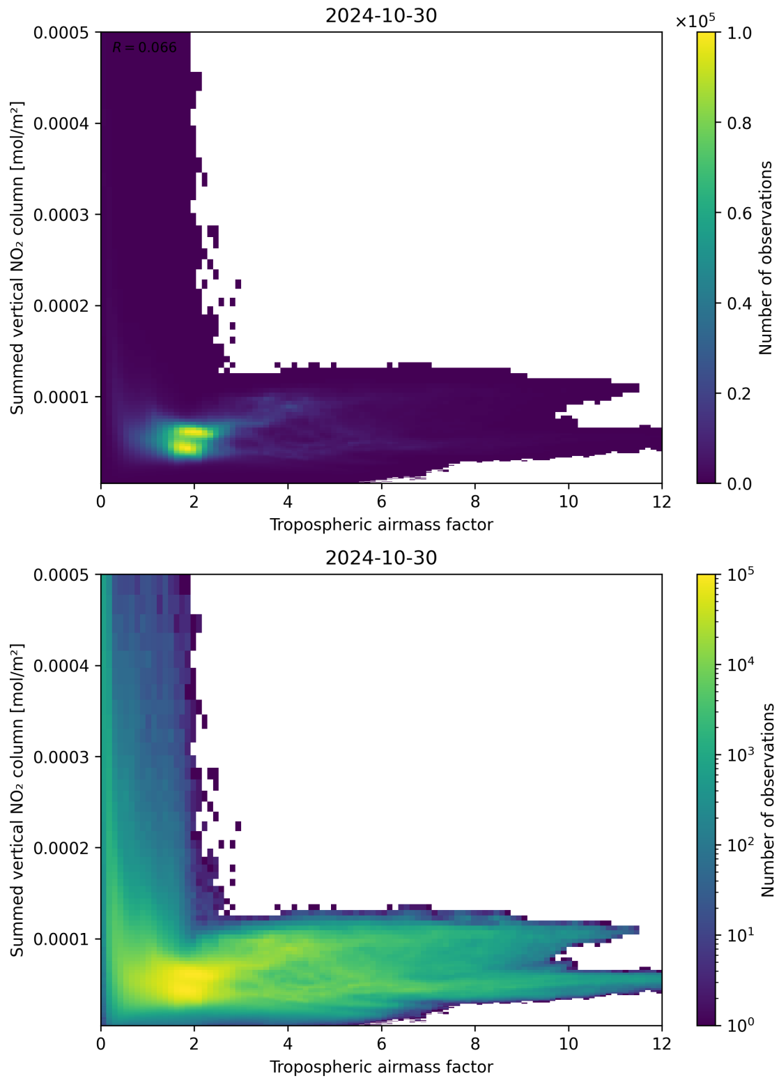
Figure 75: Scatter density plot of “Tropospheric air mass factor” against “Summed vertical NO 2 column” for 2024-10-30 to 2024-10-31.
