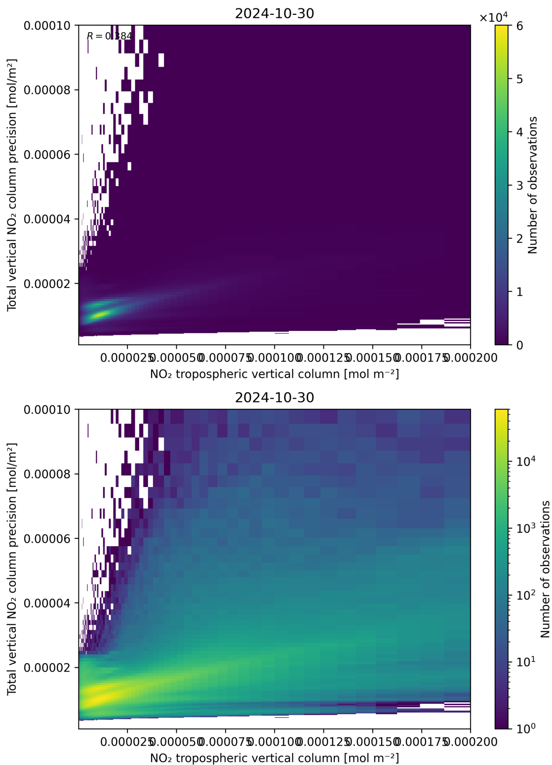
Figure 129: Scatter density plot of “NO 2 tropospheric vertical column” against “Total vertical NO 2 column precision” for 2024-10-30 to 2024-10-31.
