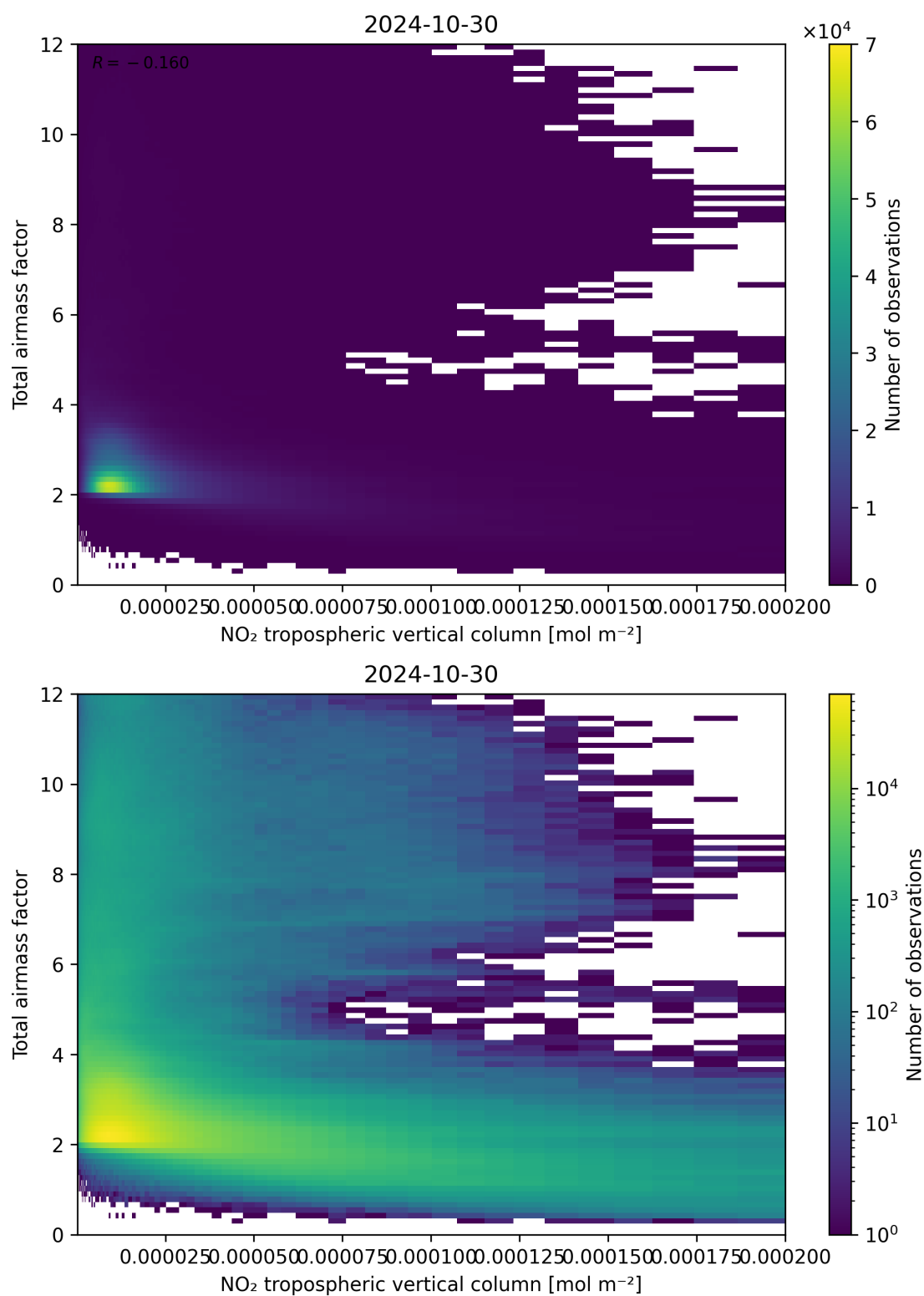
Figure 122: Scatter density plot of “NO 2 tropospheric vertical column” against “Total air mass factor” for 2024-10-30 to 2024-10-31.
