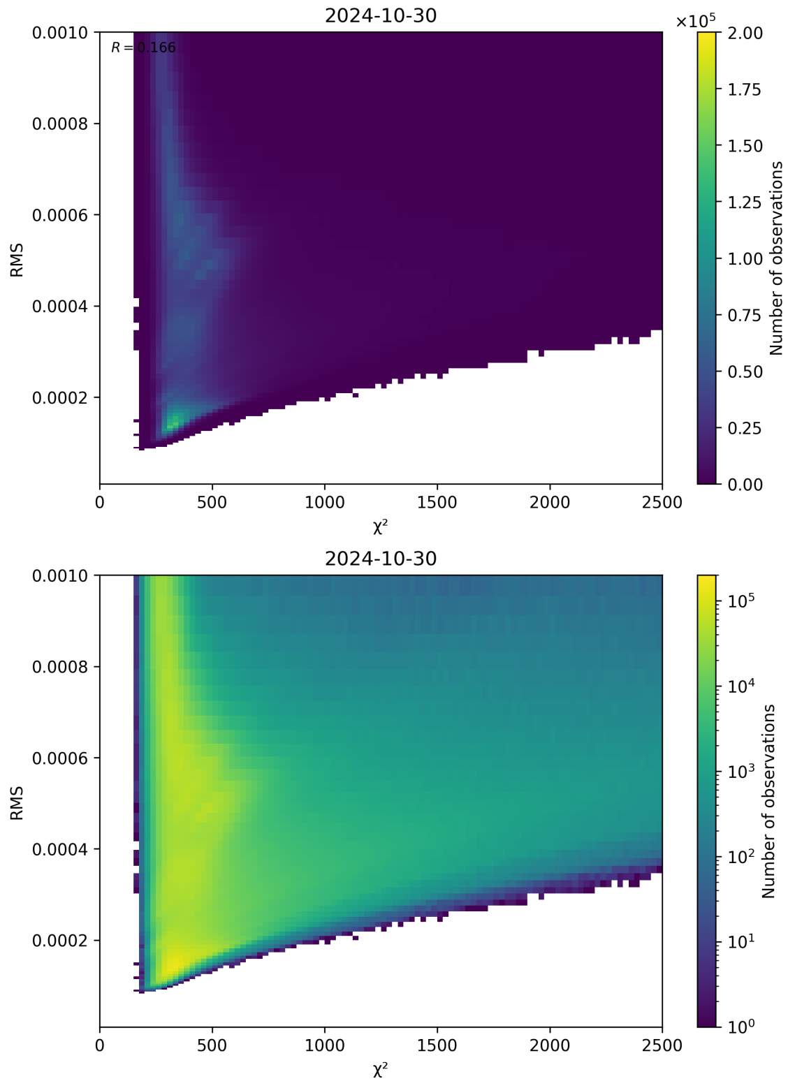
Figure 82: Scatter density plot of “ \chi^2 ” against “RMS” for 2024-10-30 to 2024-10-31.
