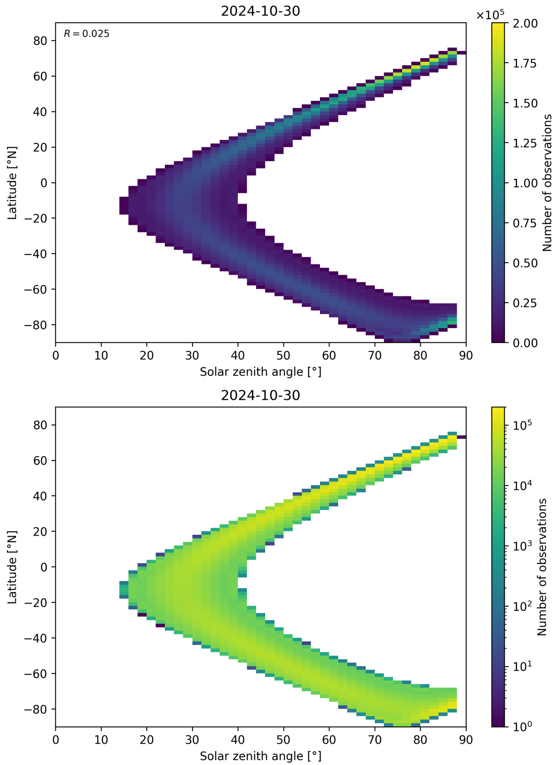
Figure 149: Scatter density plot of “Solar zenith angle” against “Latitude” for 2024-10-30 to 2024-10-31.
