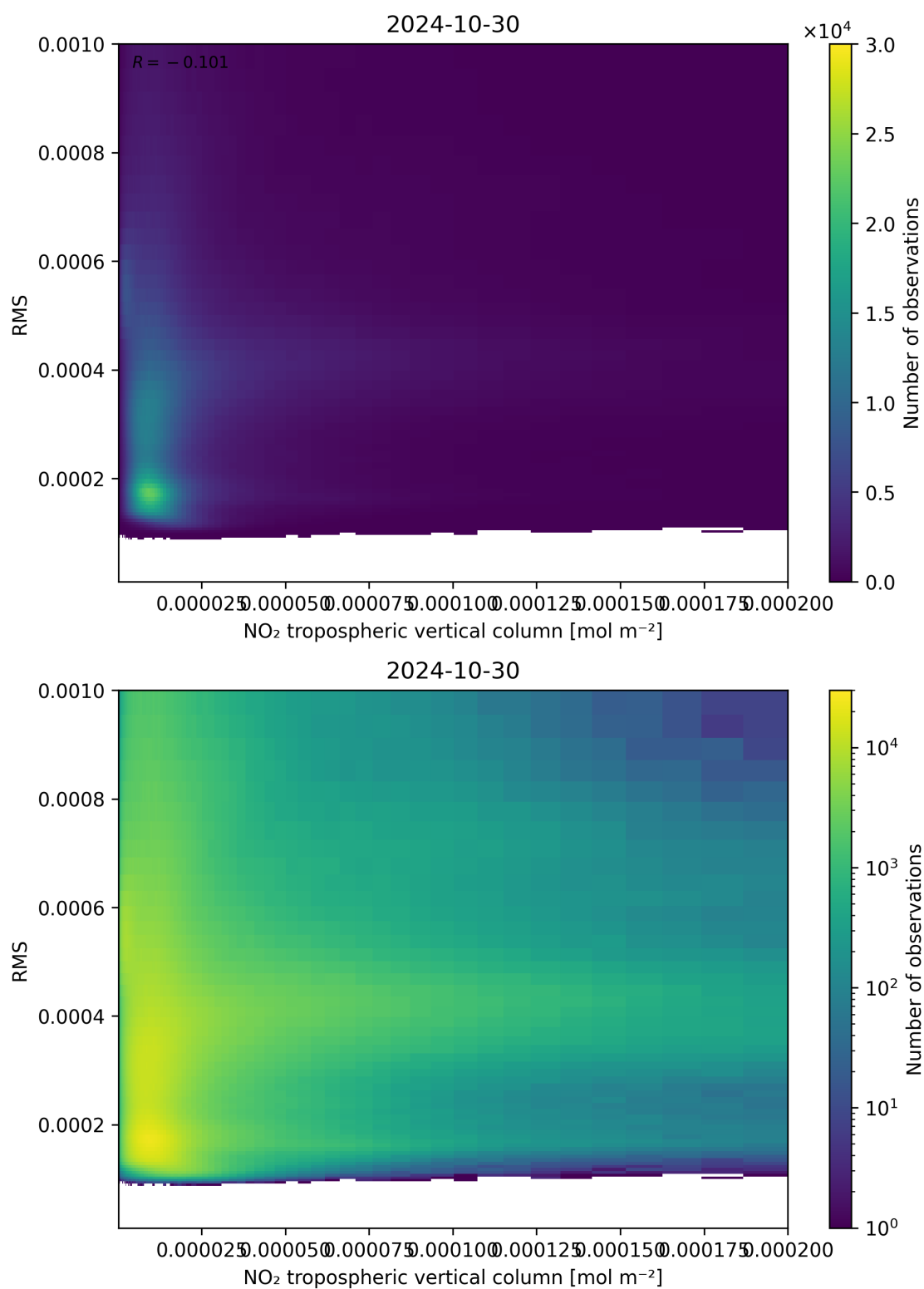
Figure 142: Scatter density plot of “NO 2 tropospheric vertical column” against “RMS” for 2024-10-30 to 2024-10-31.
