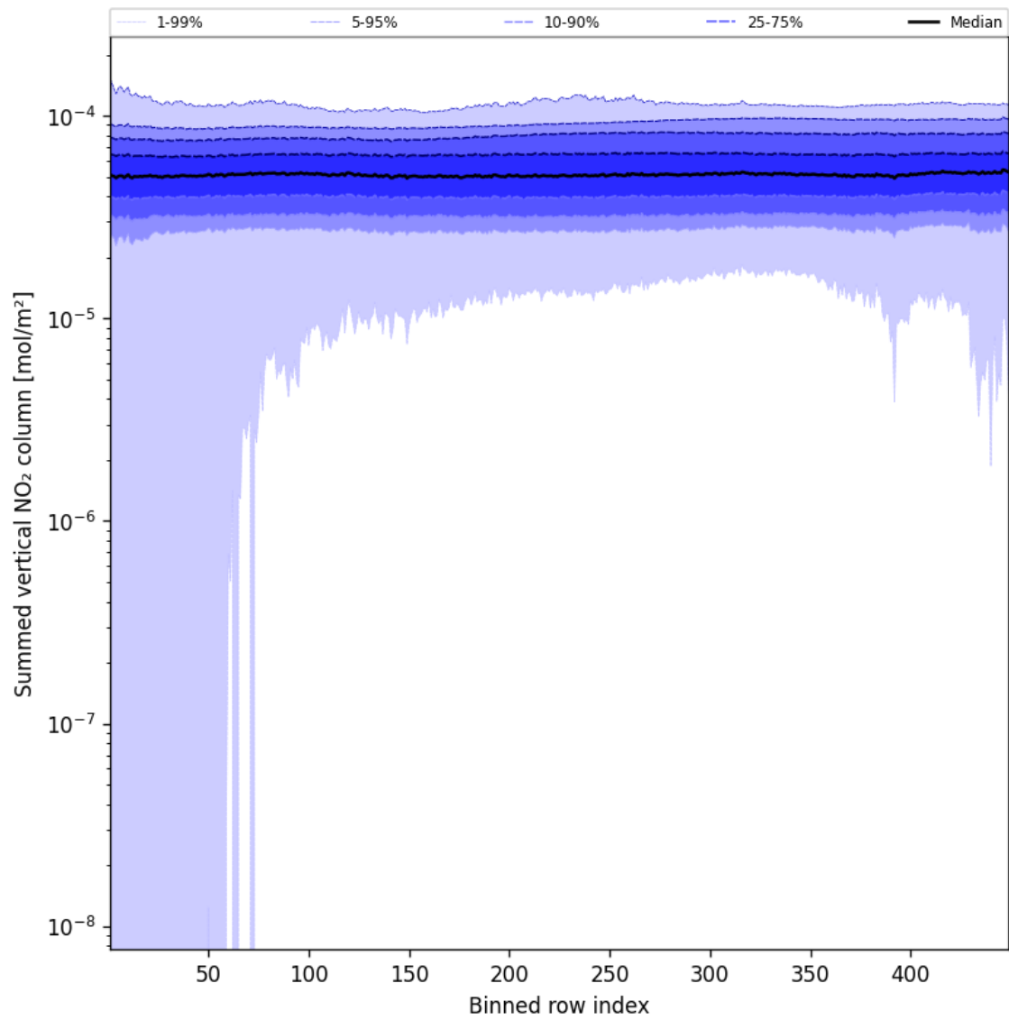
Figure 57: Along track statistics of “Summed vertical NO 2 column” for 2024-10-30 to 2024-10-31
