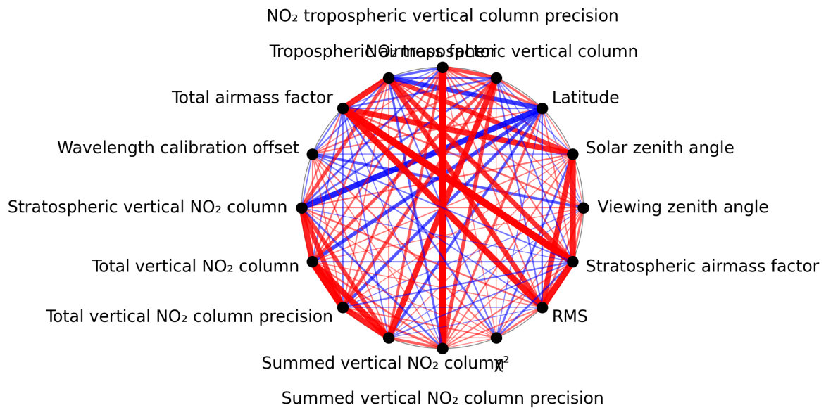
Figure 1: Map of correlation graph for 2024-10-30 to 2024-10-31.
