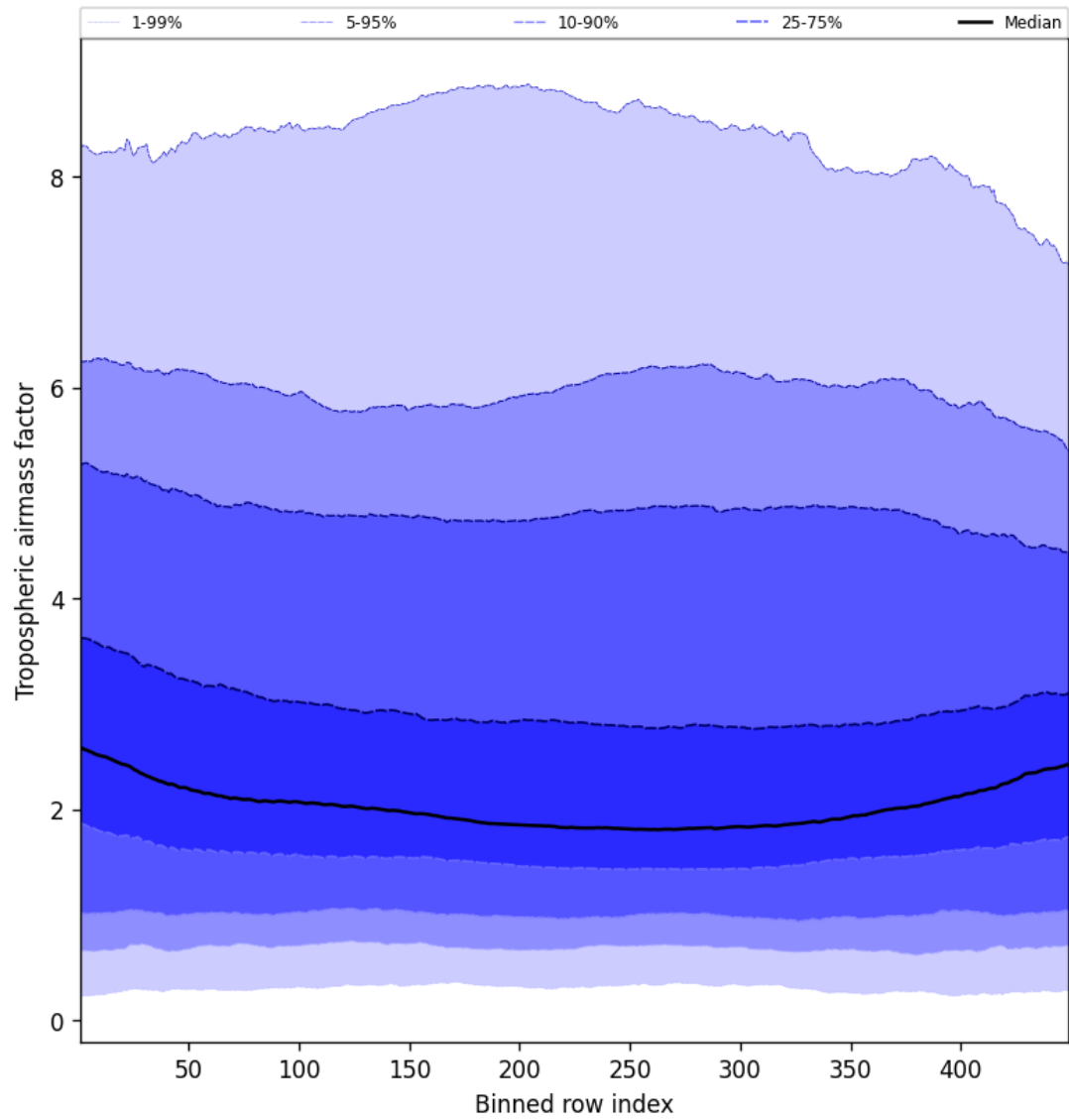
Figure 48: Along track statistics of “Tropospheric airmass factor” for 2024-10-30 to 2024-10-31
