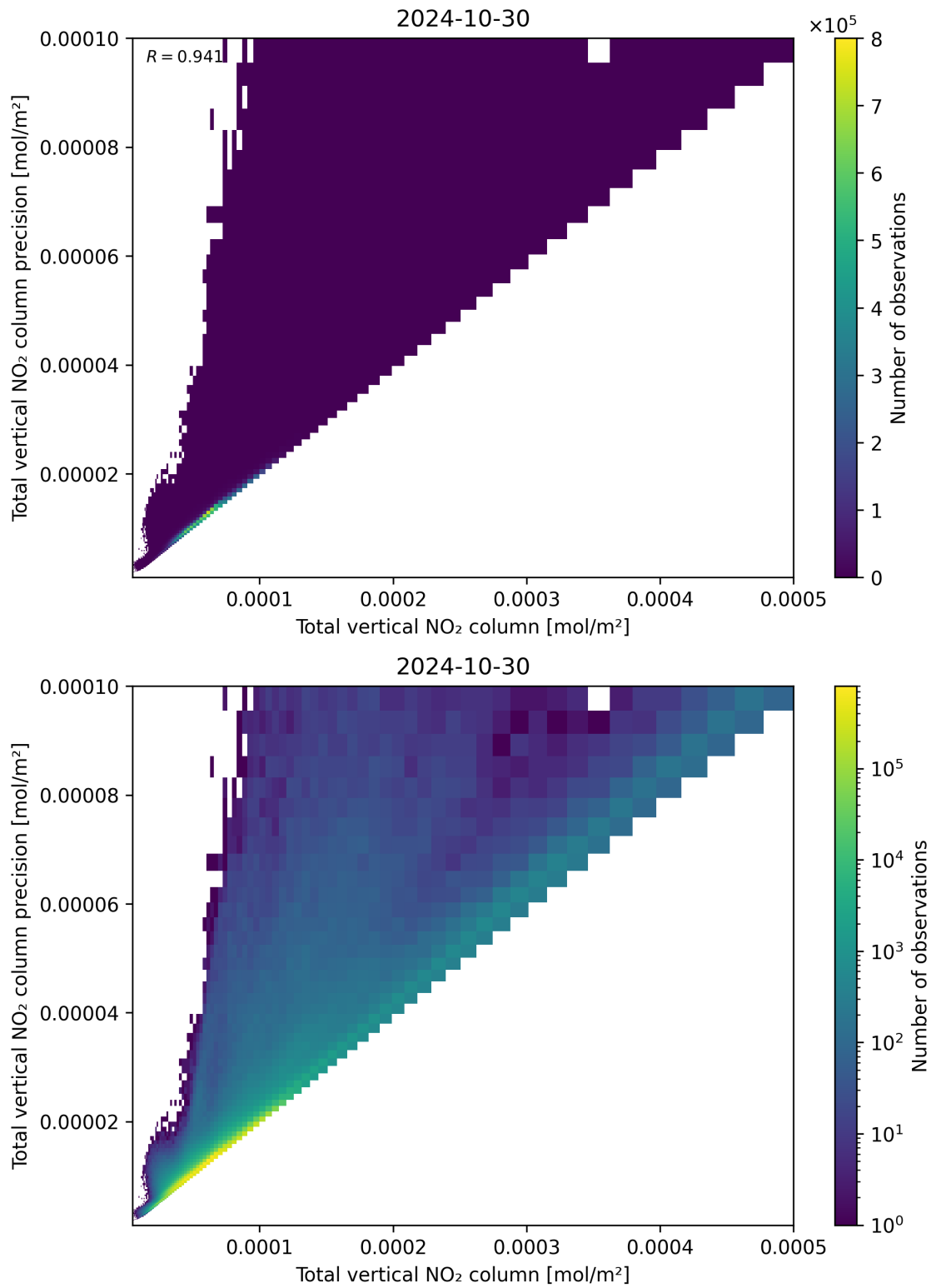
Figure 114: Scatter density plot of “Total vertical NO 2 column” against “Total vertical NO 2 column precision” for 2024-10-30 to 2024-10-31.
