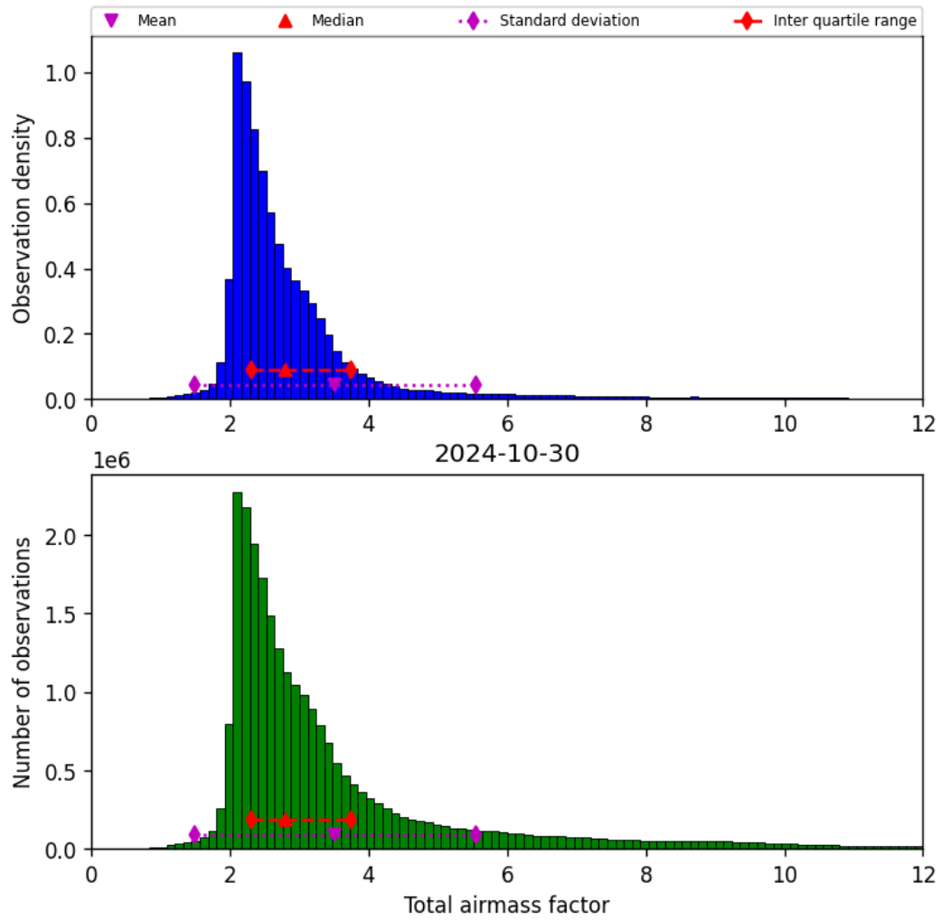
Figure 32: Histogram of “Total airmass factor” for 2024-10-30 to 2024-10-31
