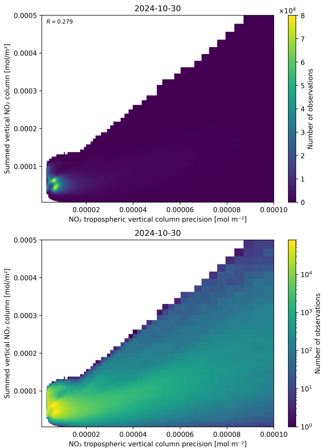
Figure 136: Scatter density plot of “NO 2 tropospheric vertical column precision” against “Summed vertical NO 2 column” for 2024-10-30 to 2024-10-31.
