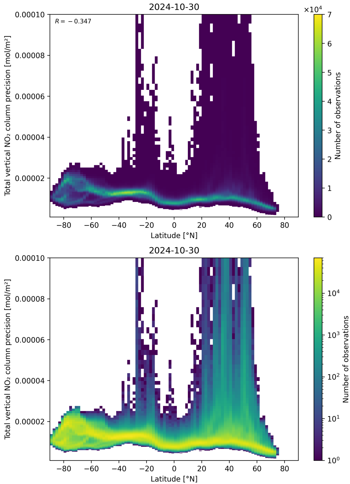
Figure 91: Scatter density plot of “Latitude” against “Total vertical NO 2 column precision” for 2024-10-30 to 2024-10-31.
