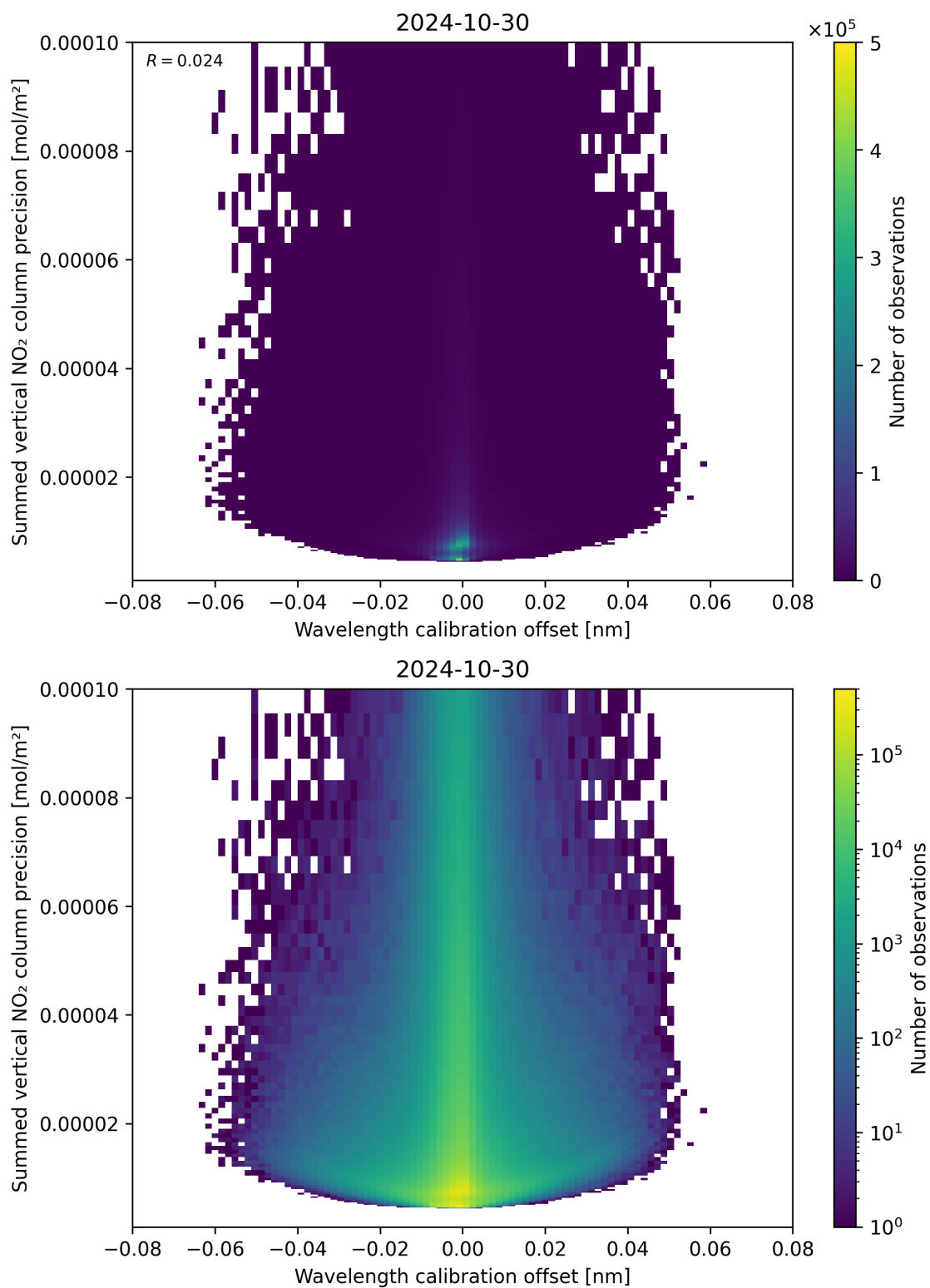
Figure 178: Scatter density plot of “Wavelength calibration offset” against “Summed vertical NO 2 column precision” for 2024-10-30 to 2024-10-31.
