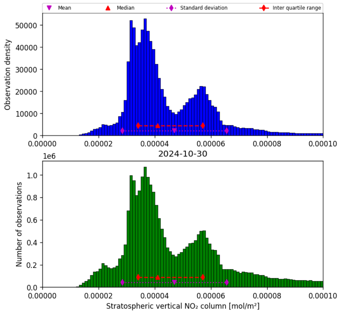
Figure 36: Histogram of “Stratospheric vertical NO 2 column” for 2024-10-30 to 2024-10-31
