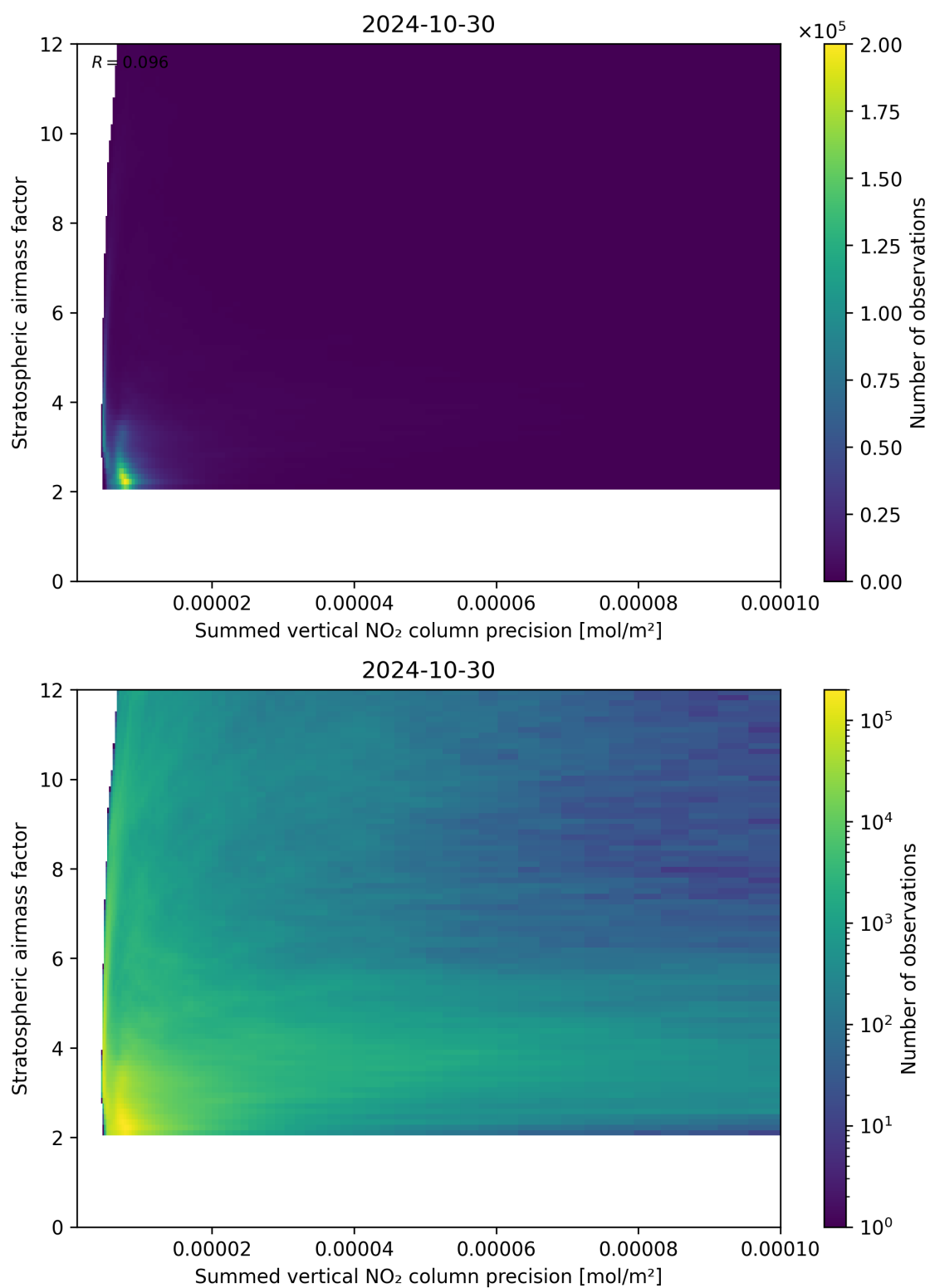
Figure 106: Scatter density plot of “Summed vertical NO 2 column precision” against “Stratospheric airmass factor” for 2024-10-30 to 2024-10-31.
