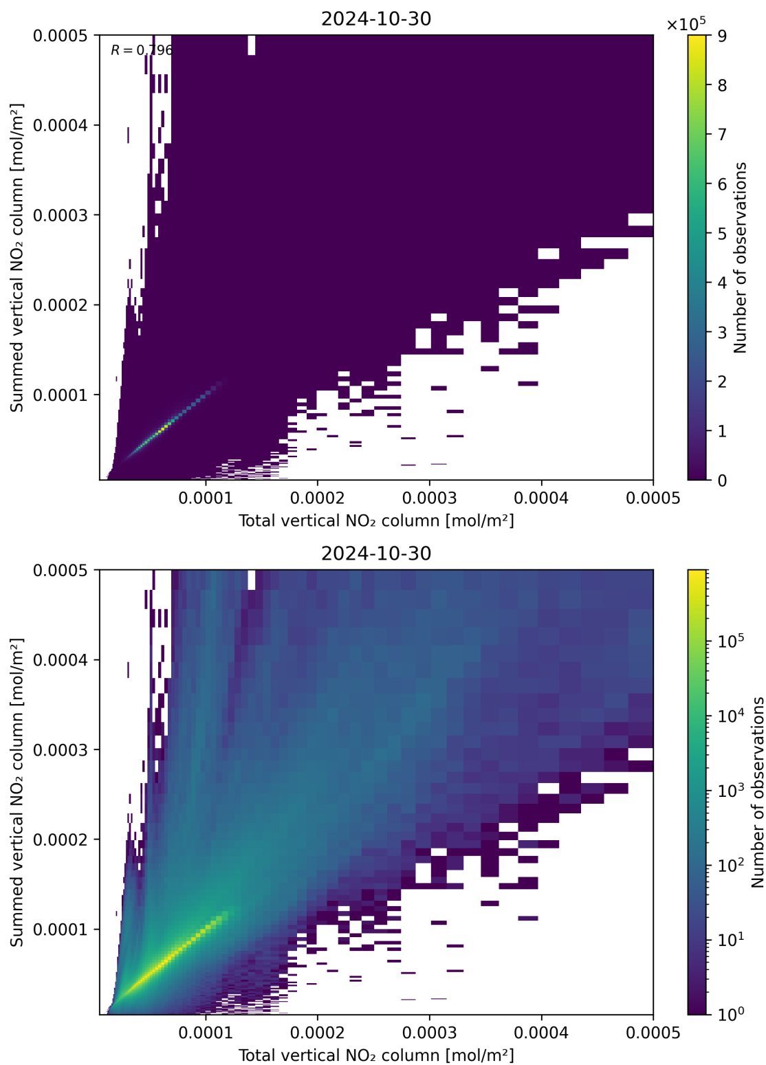
Figure 112: Scatter density plot of “Total vertical NO 2 column” against “Summed vertical NO 2 column” for 2024-10-30 to 2024-10-31.
