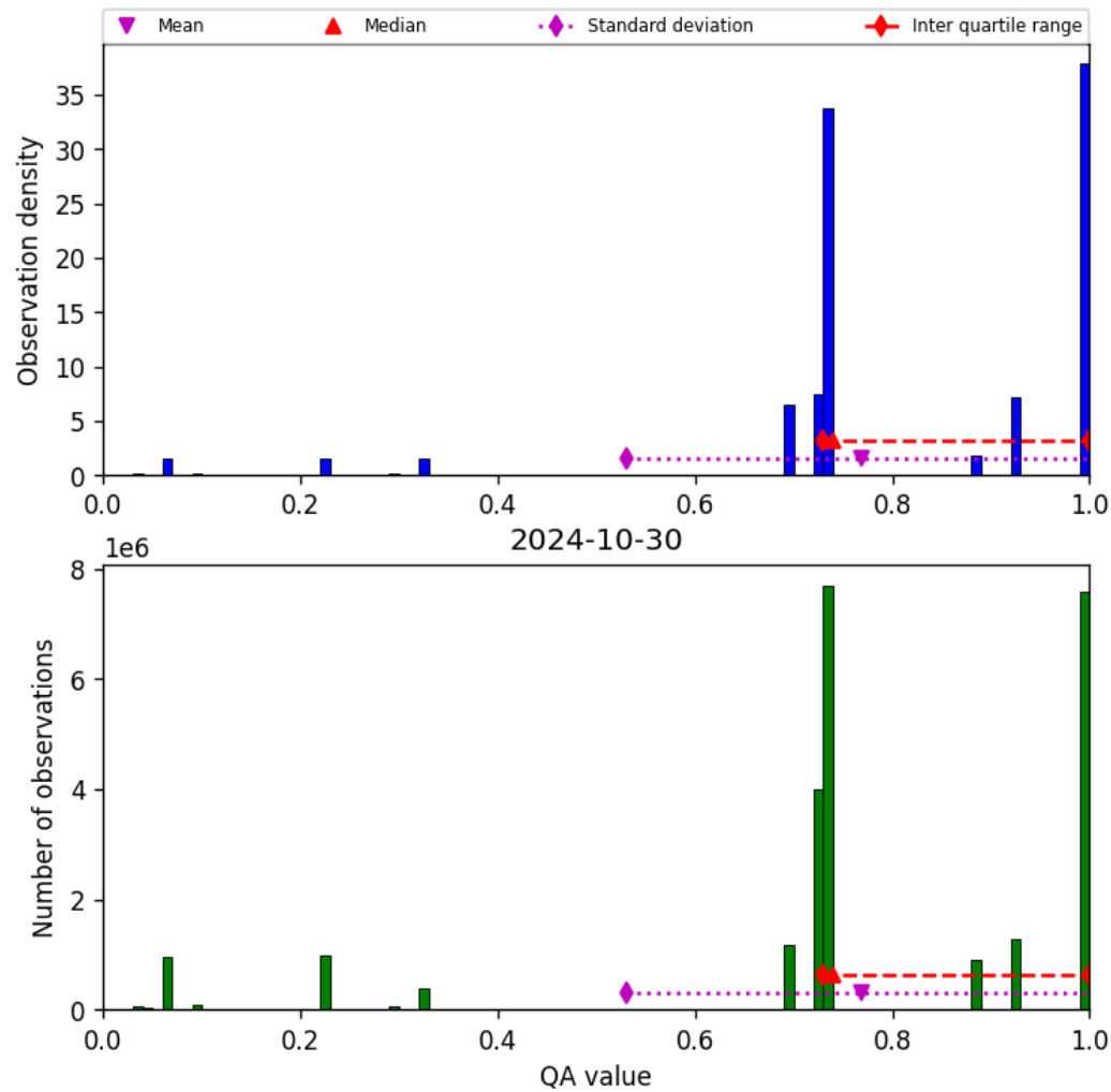
Figure 28: Histogram of “QA value” for 2024-10-30 to 2024-10-31
