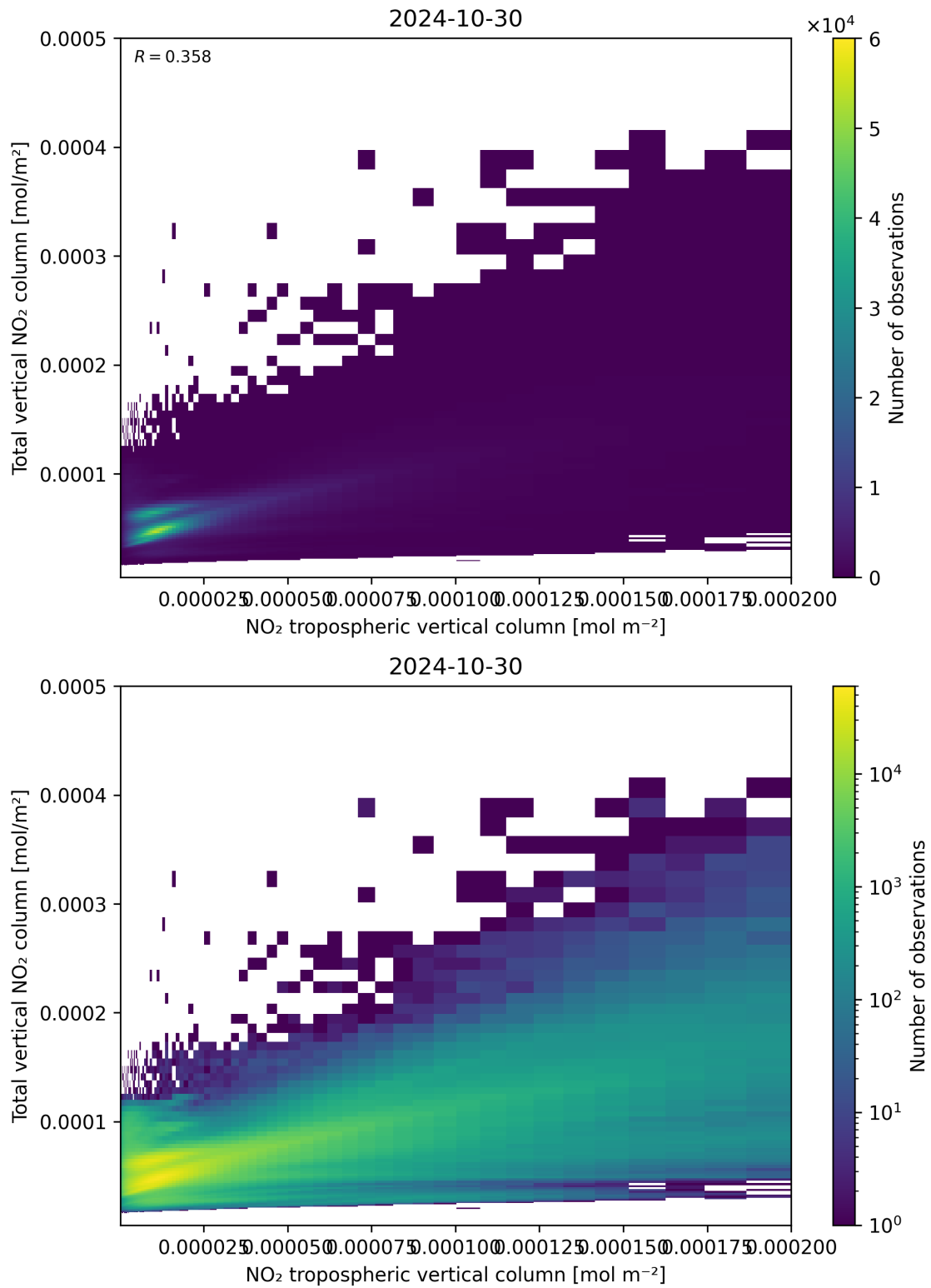
Figure 128: Scatter density plot of “NO 2 tropospheric vertical column” against “Total vertical NO 2 column” for 2024-10-30 to 2024-10-31.
