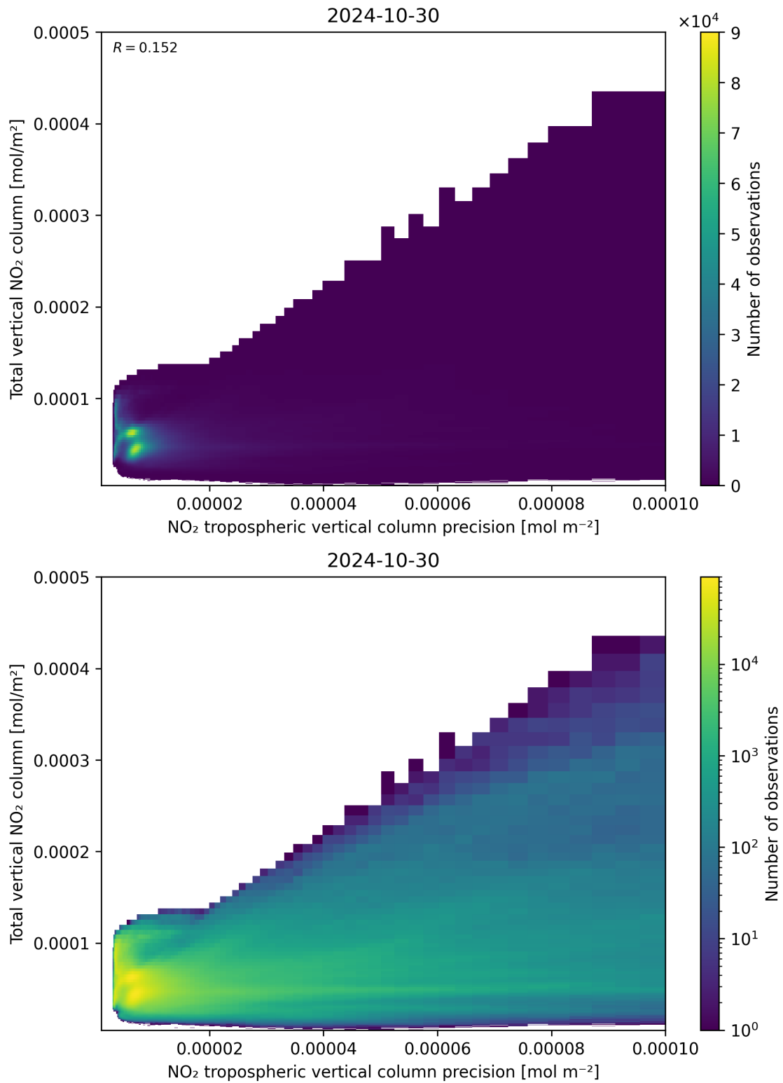
Figure 138: Scatter density plot of “NO 2 tropospheric vertical column precision” against “Total vertical NO 2 column” for 2024-10-30 to 2024-10-31.
