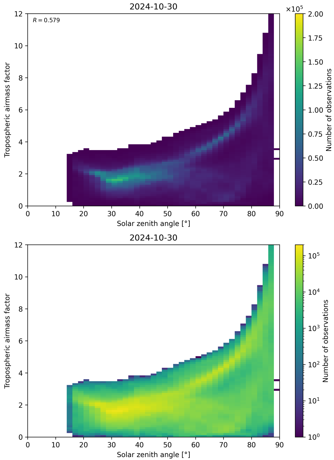
Figure 147: Scatter density plot of “Solar zenith angle” against “Tropospheric airmass factor” for 2024-10-30 to 2024-10-31.
