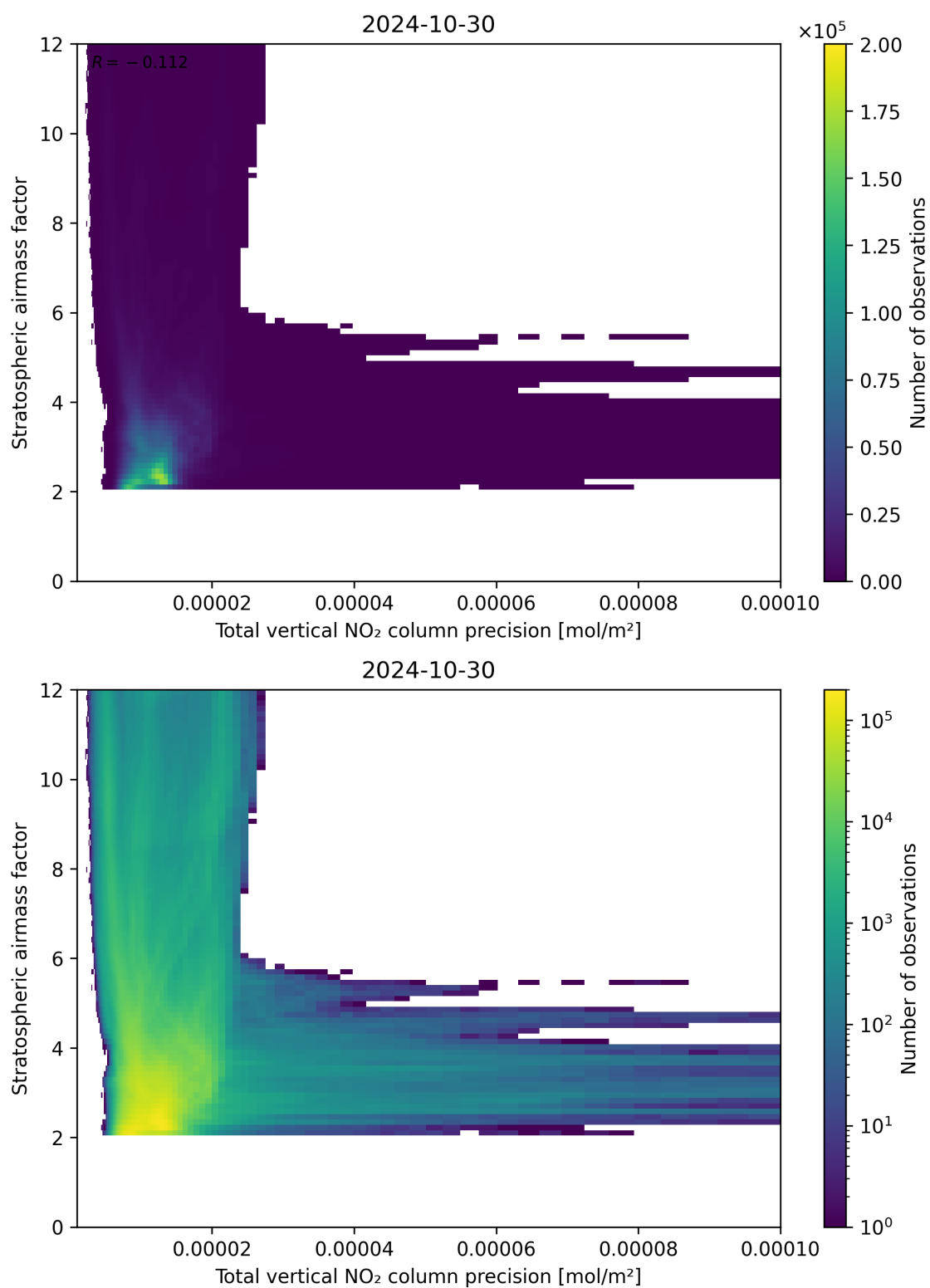
Figure 115: Scatter density plot of “Total vertical NO 2 column precision” against “Stratospheric air mass factor” for 2024-10-30 to 2024-10-31.
