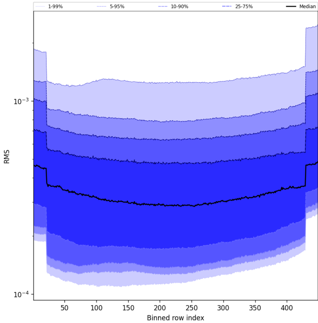
Figure 60: Along track statistics of “RMS” for 2024-10-30 to 2024-10-31
