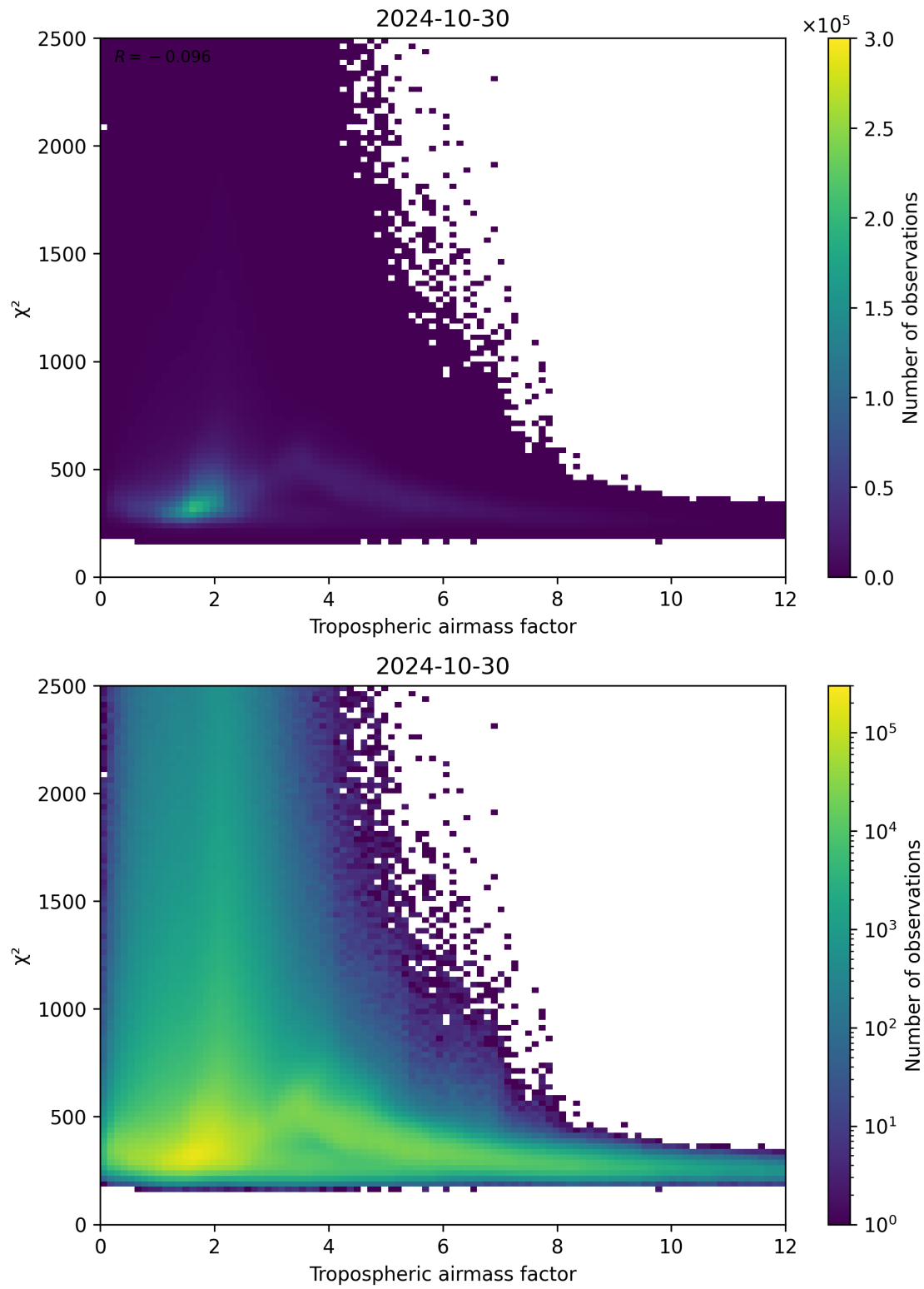
Figure 73: Scatter density plot of “Tropospheric airmass factor” against “ \chi^2 ” for 2024-10-30 to 2024-10-31.
