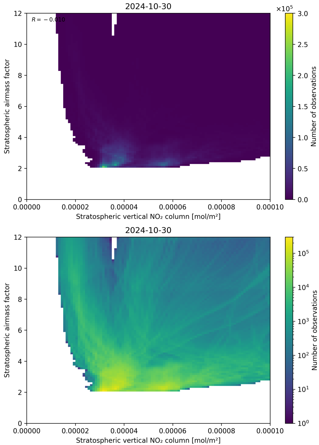
Figure 96: Scatter density plot of “Stratospheric vertical NO 2 column” against “Stratospheric airmass factor” for 2024-10-30 to 2024-10-31.
