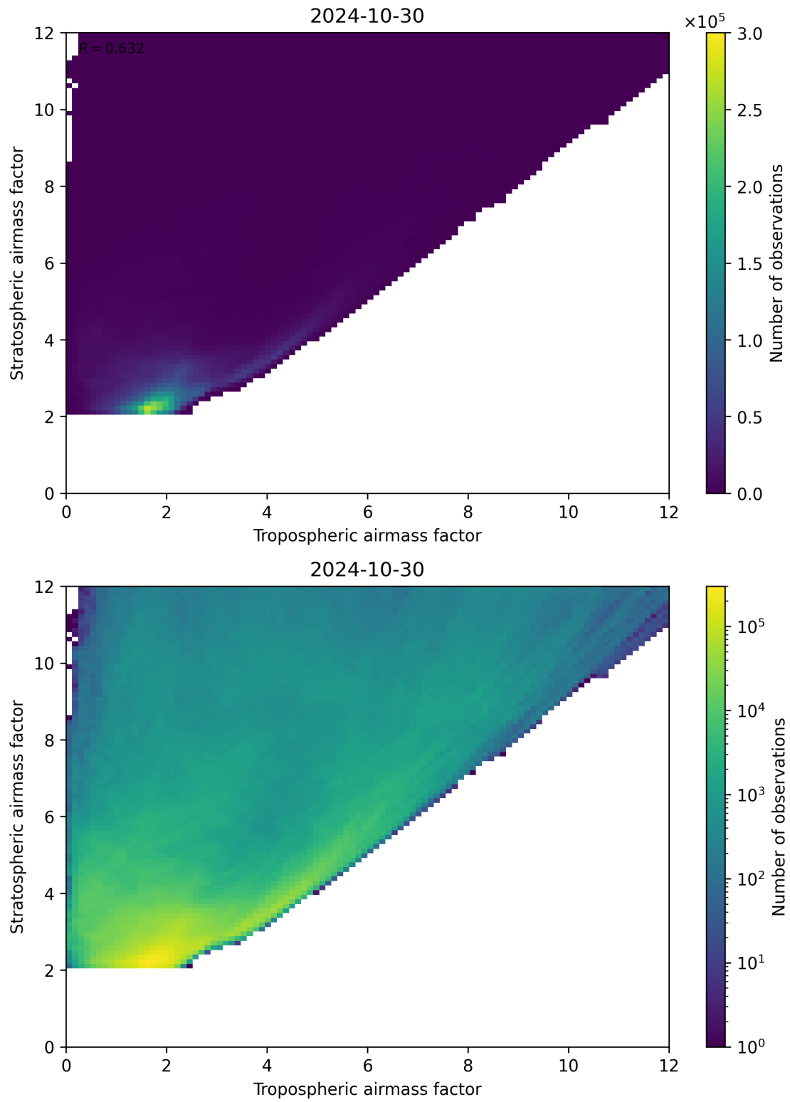
Figure 71: Scatter density plot of “Tropospheric airmass factor” against “Stratospheric airmass factor” for 2024-10-30 to 2024-10-31.
