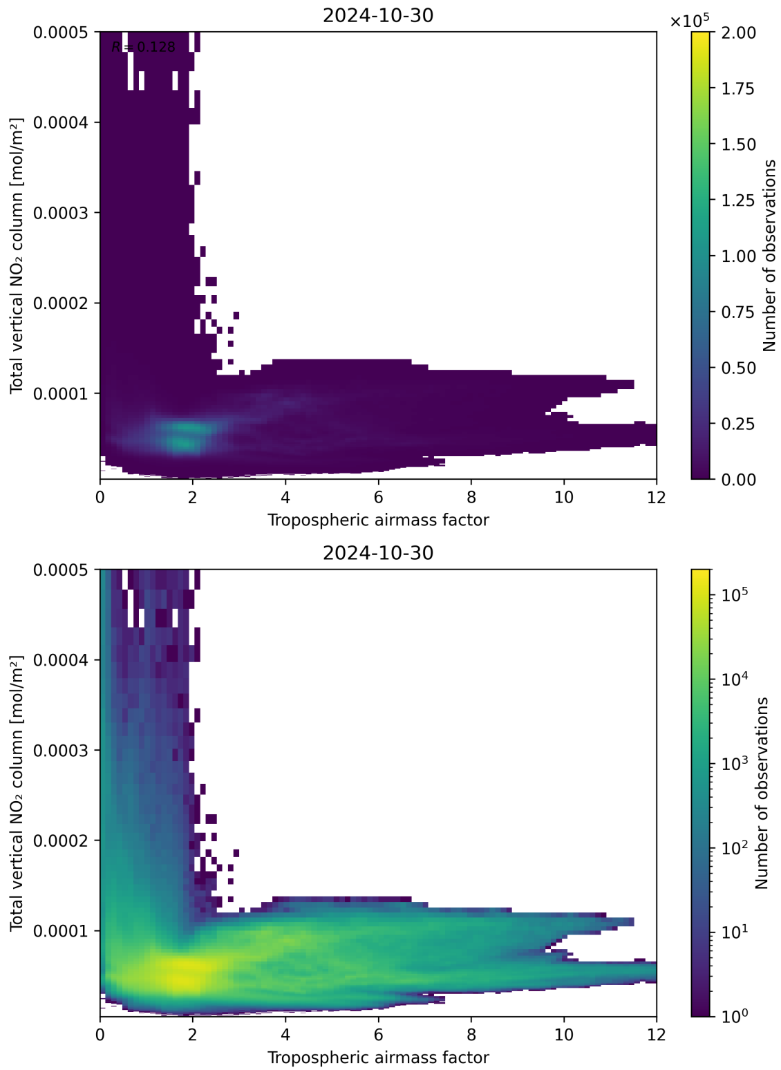
Figure 77: Scatter density plot of “Tropospheric airmass factor” against “Total vertical NO 2 column” for 2024-10-30 to 2024-10-31.
