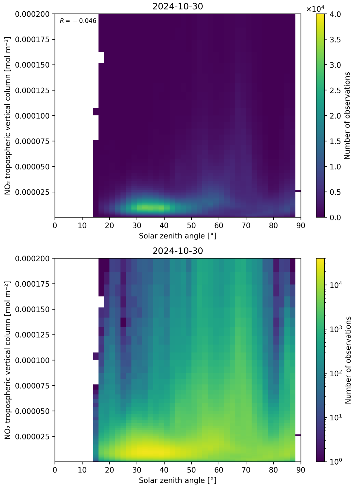
Figure 155: Scatter density plot of “Solar zenith angle” against “NO 2 tropospheric vertical column” for 2024-10-30 to 2024-10-31.
