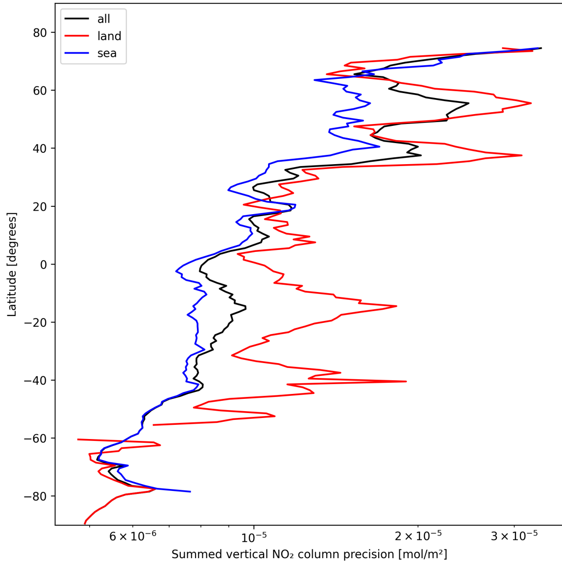
Figure 24: Zonal average of “Summed vertical NO 2 column precision” for 2024-10-30 to 2024-10-31.
