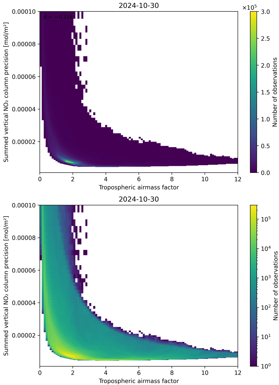
Figure 76: Scatter density plot of “Tropospheric air mass factor” against “Summed vertical NO 2 column precision” for 2024-10-30 to 2024-10-31.
