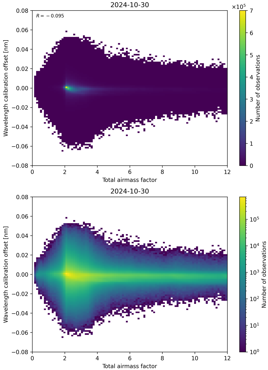
Figure 70: Scatter density plot of “Total airmass factor” against “Wavelength calibration offset” for 2024-10-30 to 2024-10-31.
