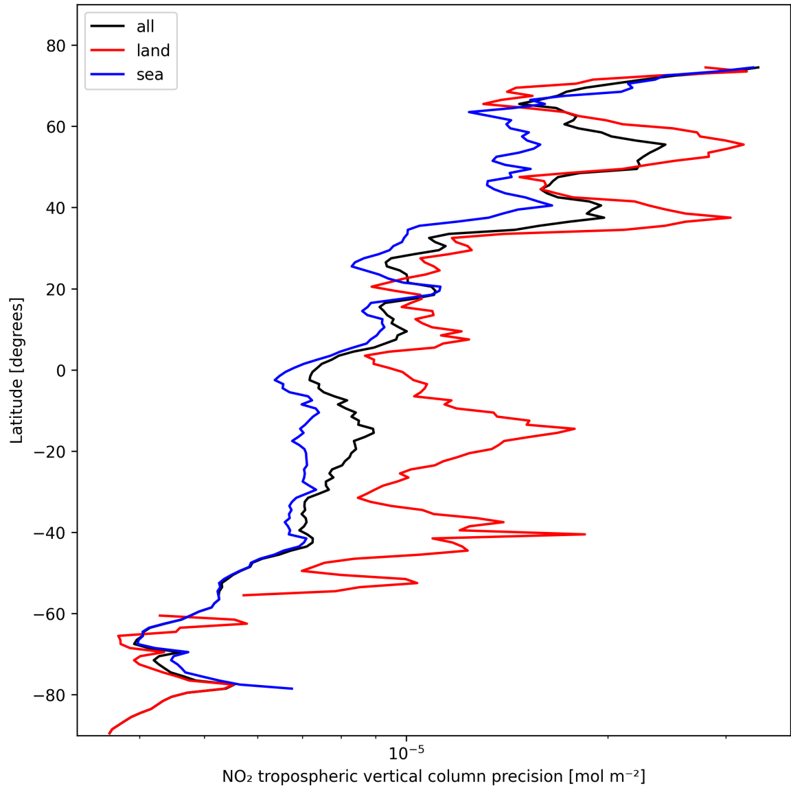
Figure 13: Zonal average of “NO 2 tropospheric vertical column precision” for 2024-10-30 to 2024-10-31.
