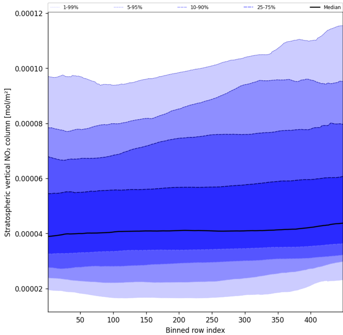
Figure 53: Along track statistics of “Stratospheric vertical NO 2 column” for 2024-10-30 to 2024-10-31
