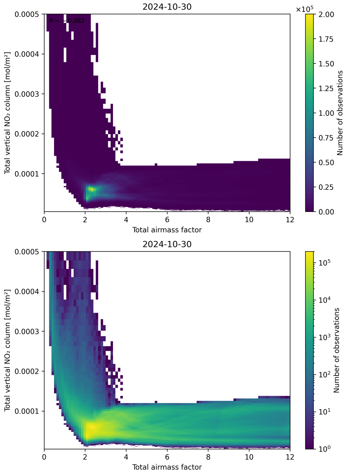
Figure 67: Scatter density plot of “Total airmass factor” against “Total vertical NO 2 column” for 2024-10-30 to 2024-10-31.
