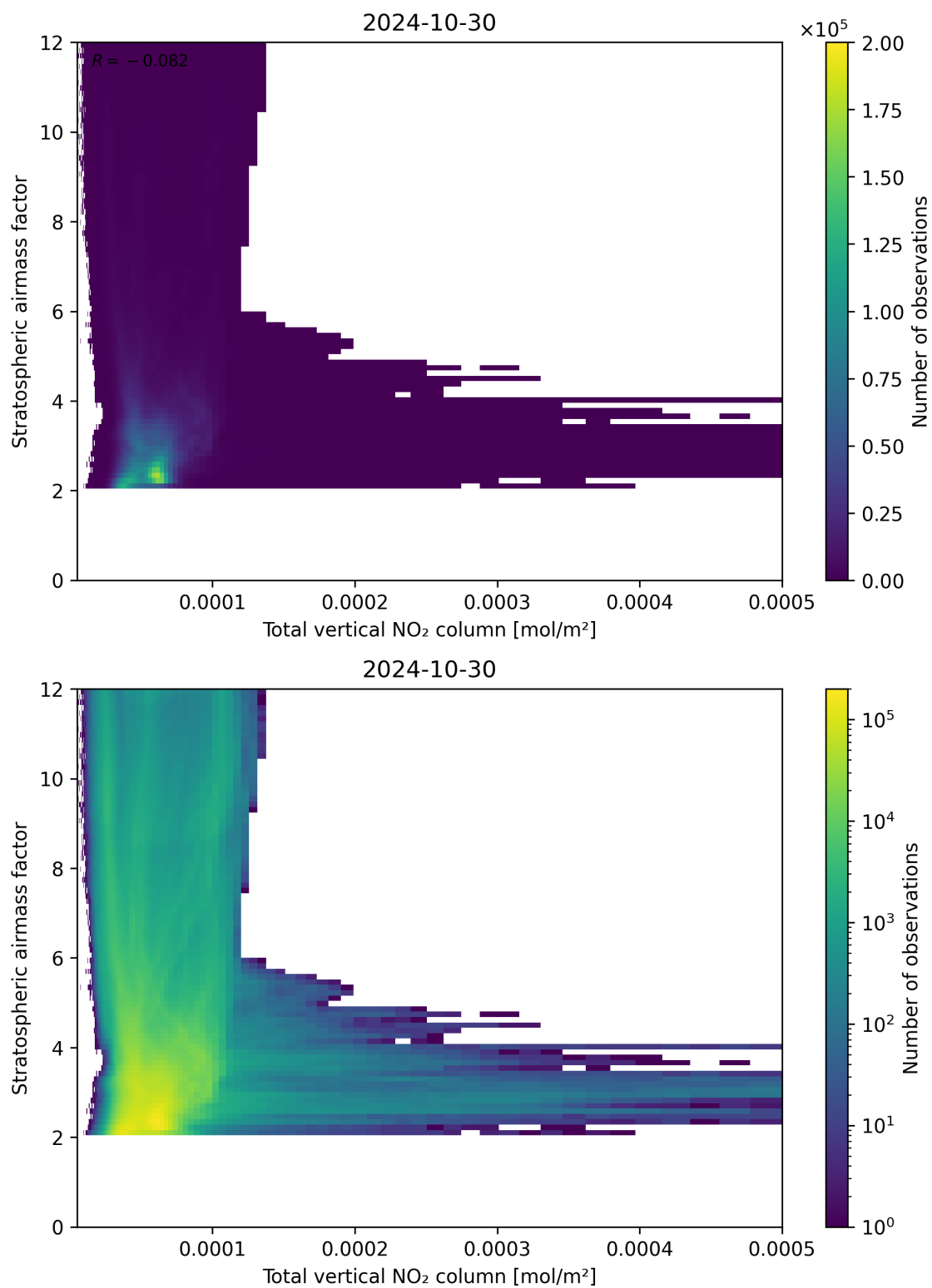
Figure 110: Scatter density plot of “Total vertical NO 2 column” against “Stratospheric airmass factor” for 2024-10-30 to 2024-10-31.
