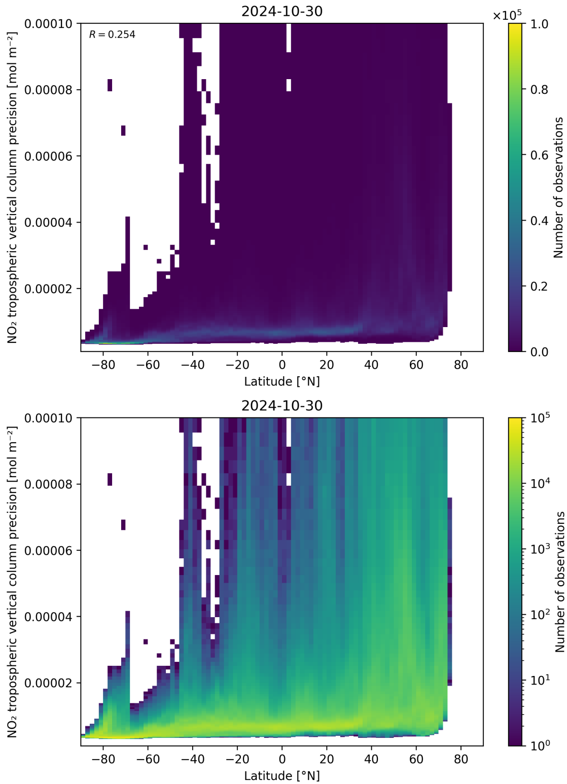
Figure 93: Scatter density plot of “Latitude” against “NO 2 tropospheric vertical column precision” for 2024-10-30 to 2024-10-31.
