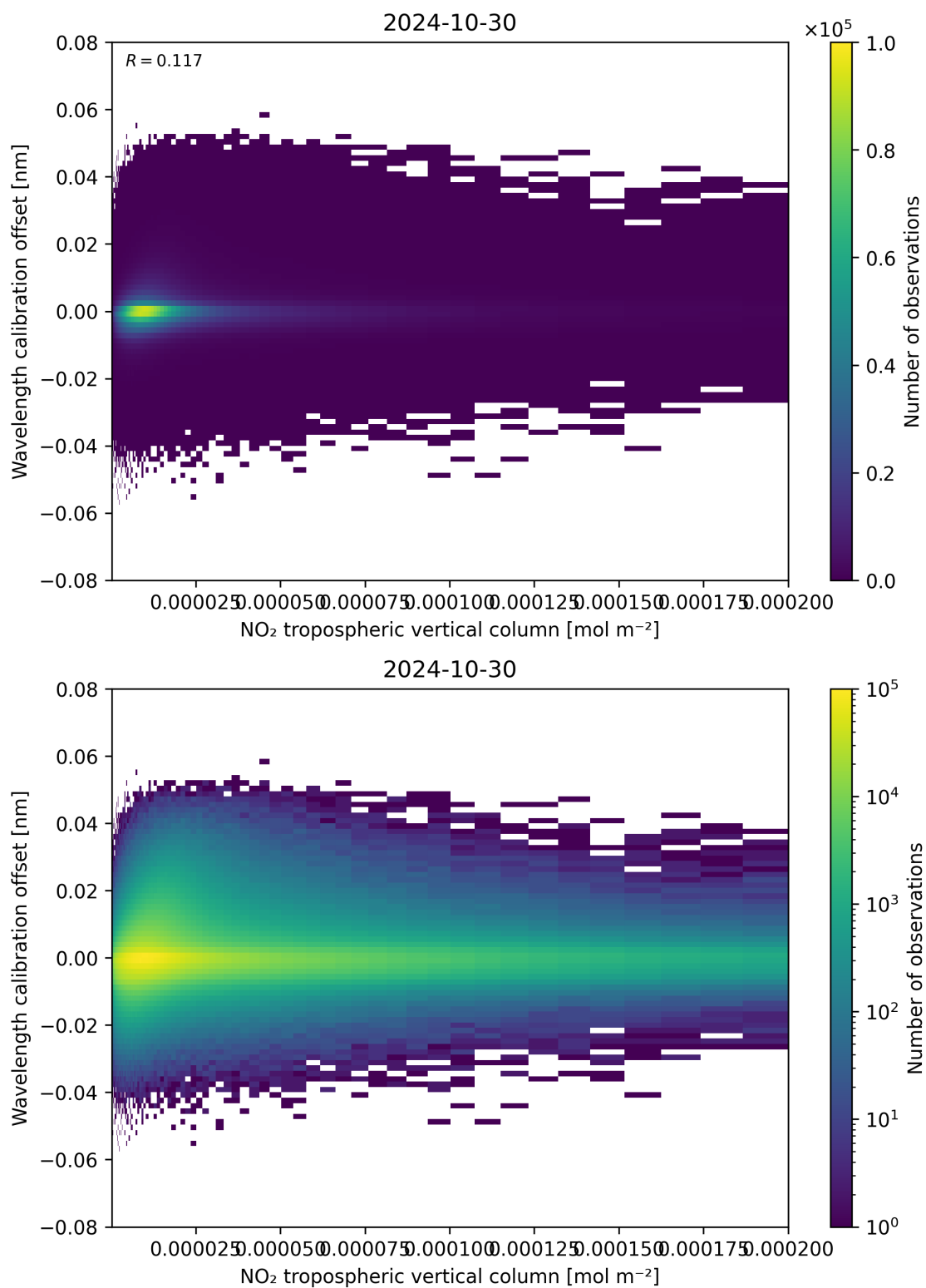
Figure 143: Scatter density plot of “NO 2 tropospheric vertical column” against “Wavelength calibration offset” for 2024-10-30 to 2024-10-31.
