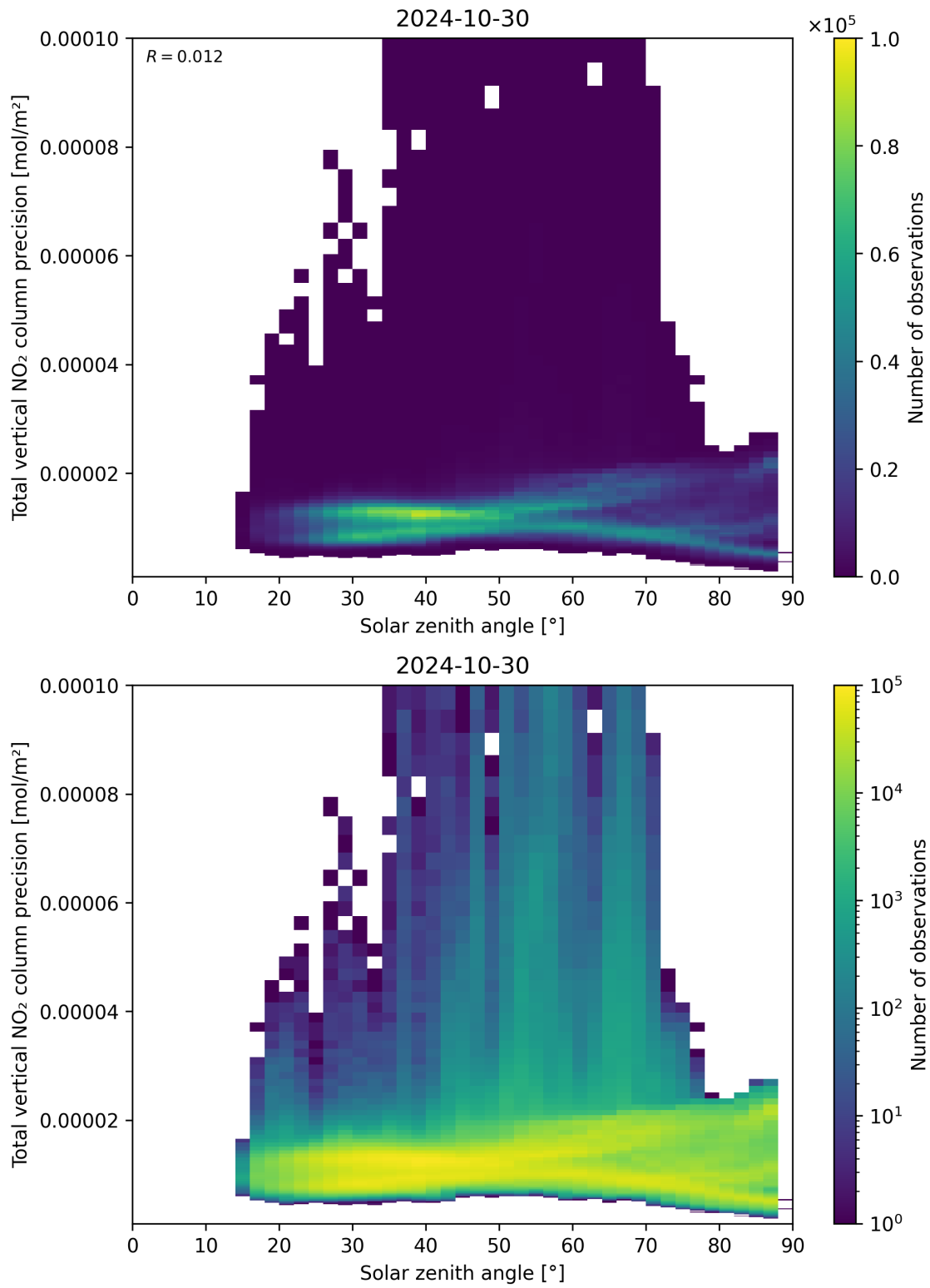
Figure 154: Scatter density plot of “Solar zenith angle” against “Total vertical NO 2 column precision” for 2024-10-30 to 2024-10-31.
