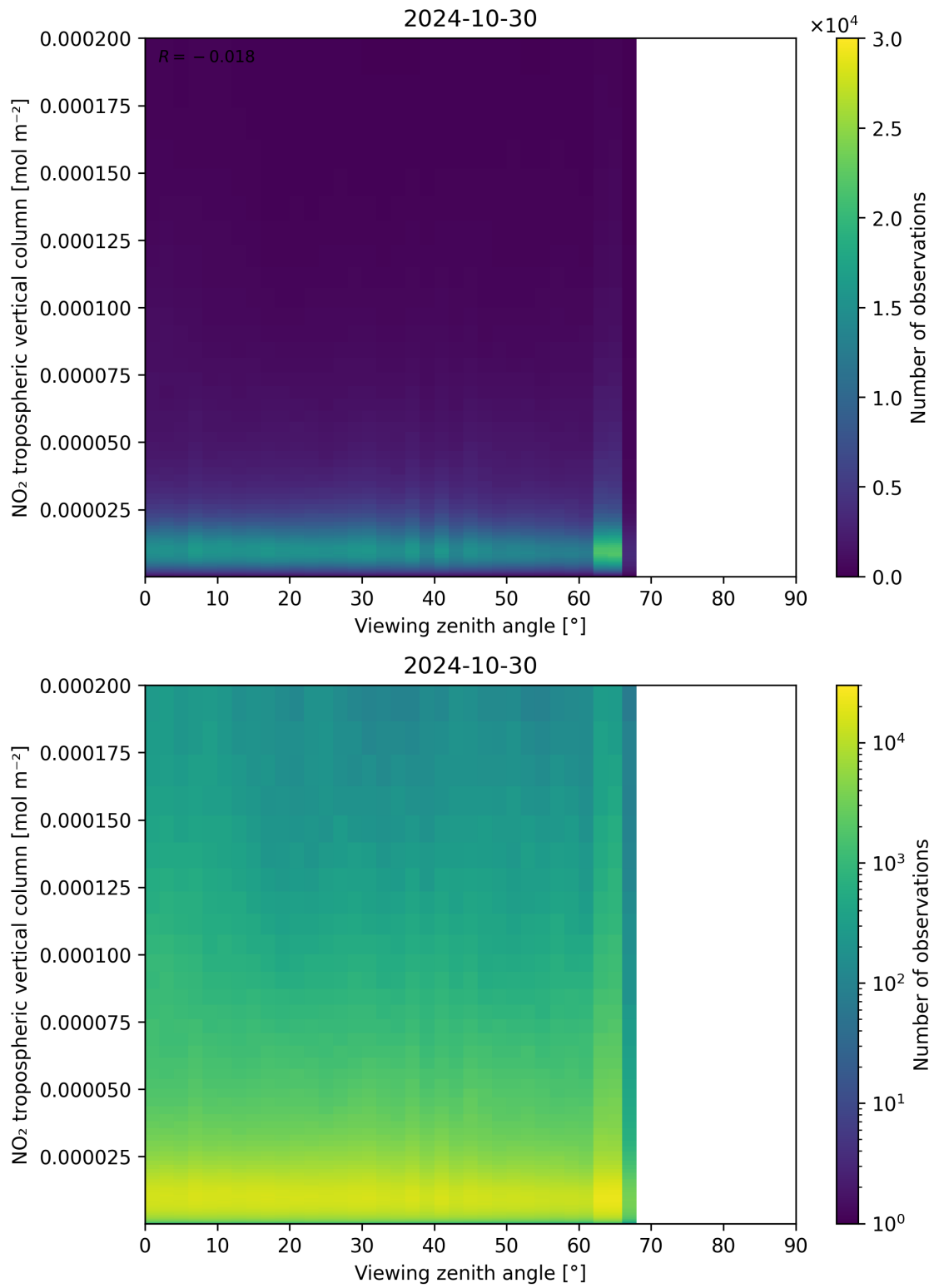
Figure 169: Scatter density plot of “Viewing zenith angle” against “NO 2 tropospheric vertical column” for 2024-10-30 to 2024-10-31.
