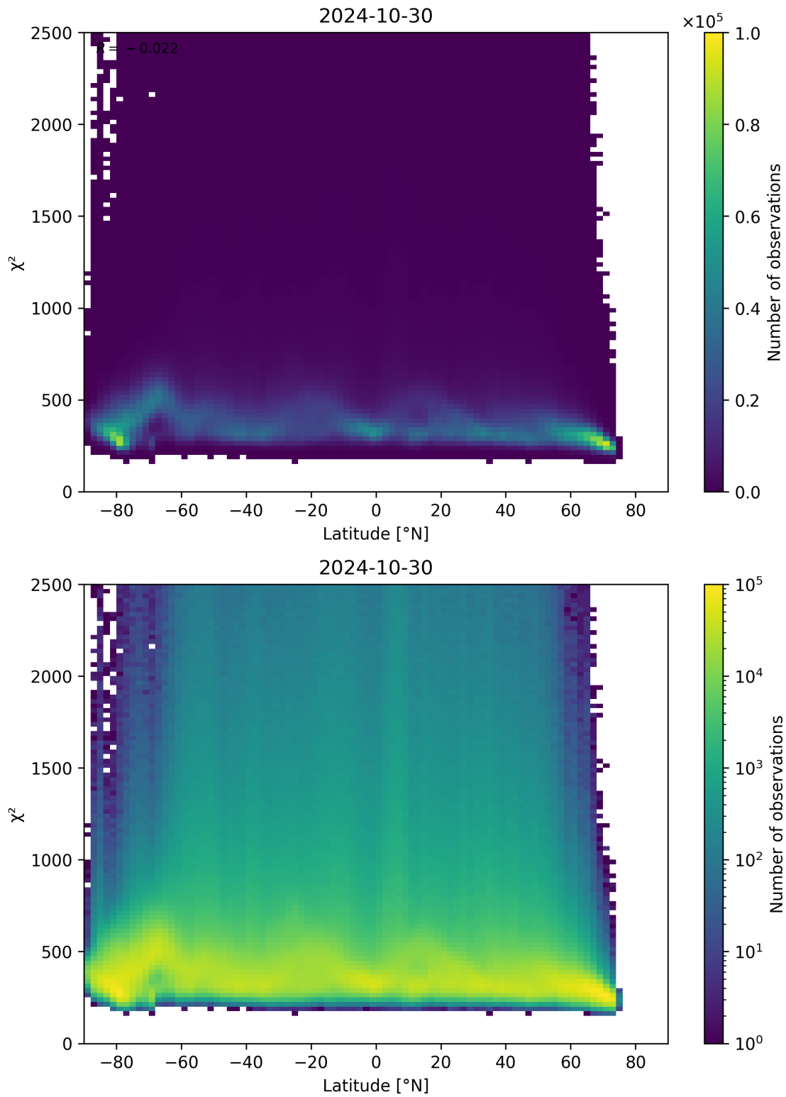
Figure 86: Scatter density plot of “Latitude” against “ \chi^2 ” for 2024-10-30 to 2024-10-31.
