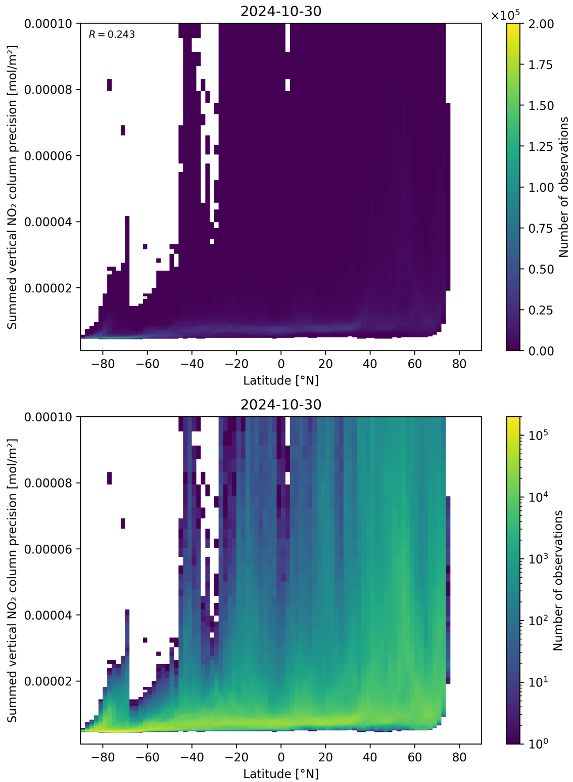
Figure 89: Scatter density plot of “Latitude” against “Summed vertical NO 2 column precision” for 2024-10-30 to 2024-10-31.
