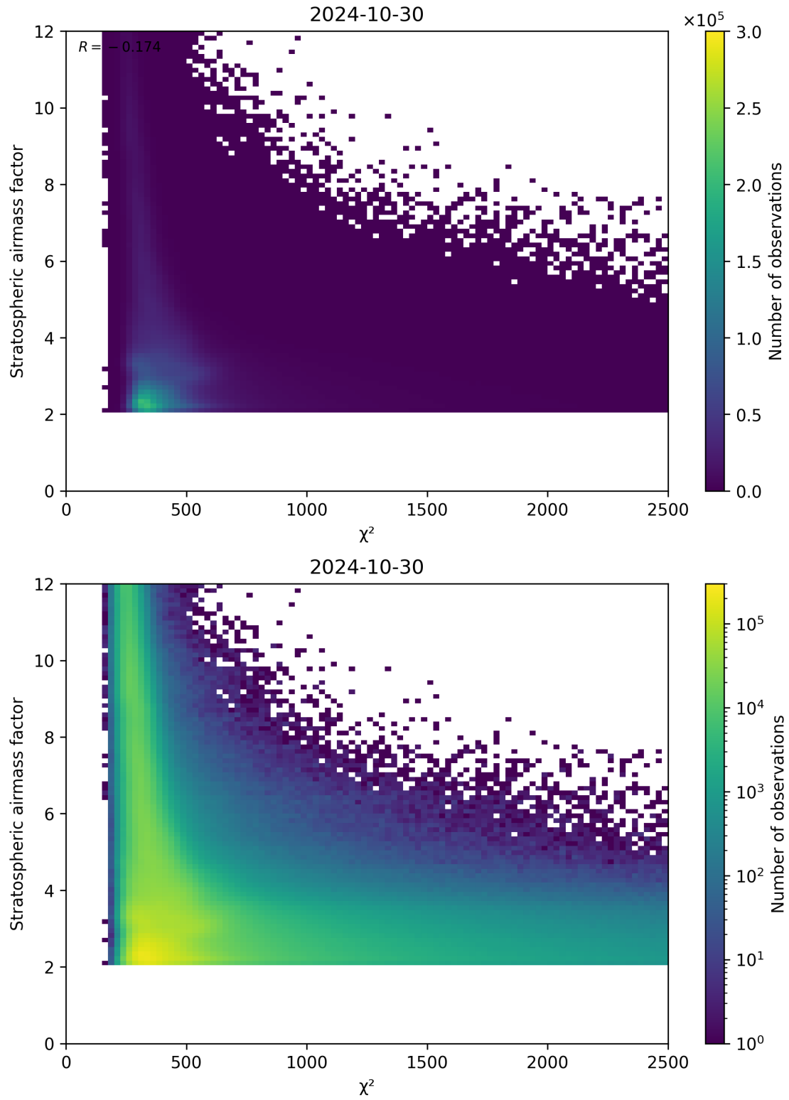
Figure 81: Scatter density plot of “ \chi^2 ” against “Stratospheric airmass factor” for 2024-10-30 to 2024-10-31.
