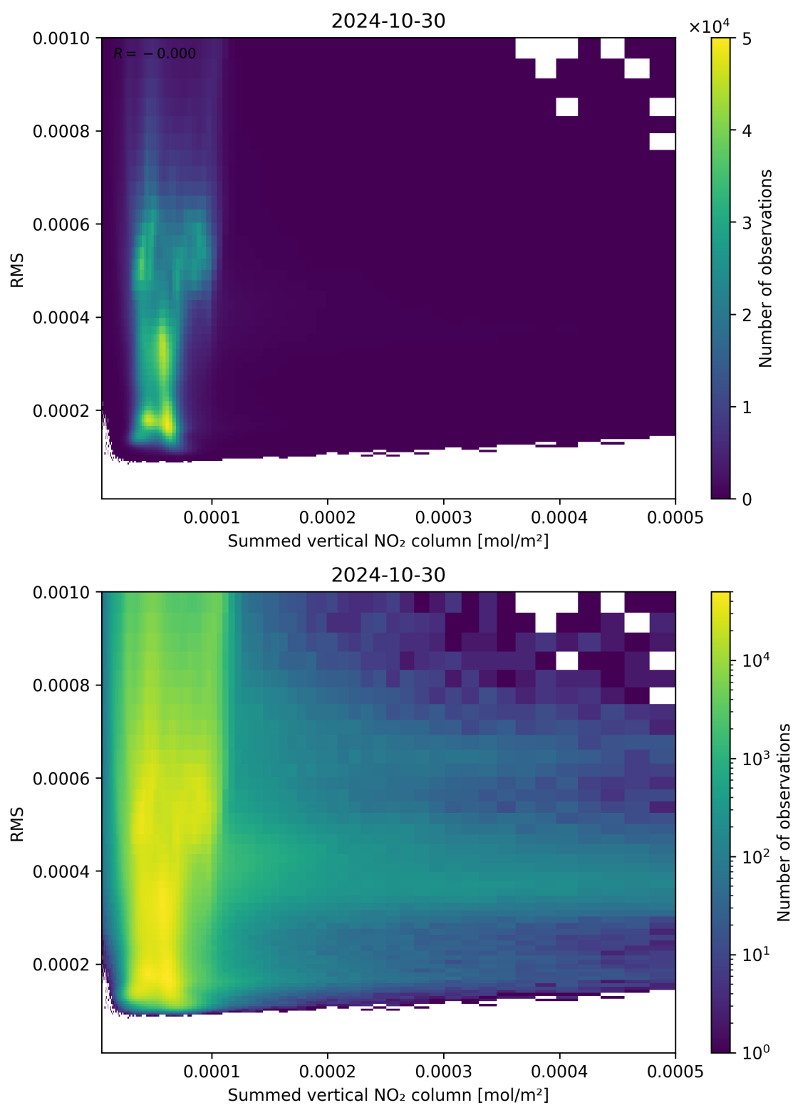
Figure 109: Scatter density plot of “Summed vertical NO 2 column” against “RMS” for 2024-10-30 to 2024-10-31.
