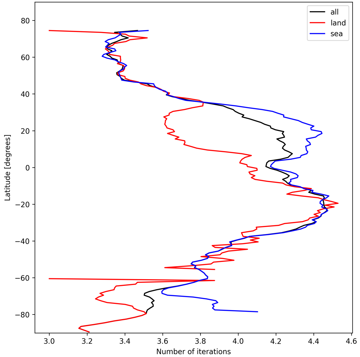
Figure 17: Zonal average of “Number of iterations” for 2024-10-30 to 2024-10-31.
