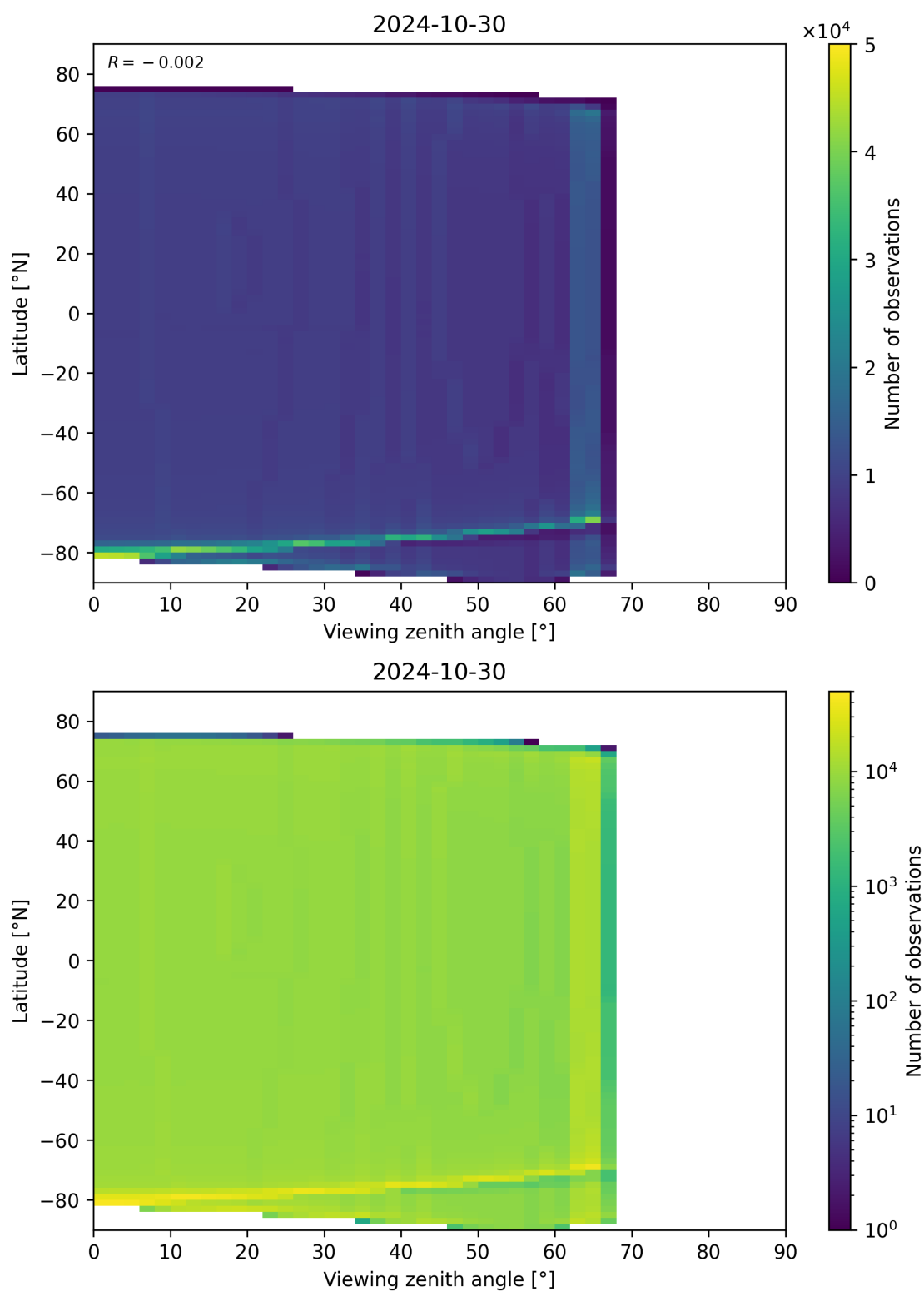
Figure 163: Scatter density plot of “Viewing zenith angle” against “Latitude” for 2024-10-30 to 2024-10-31.
