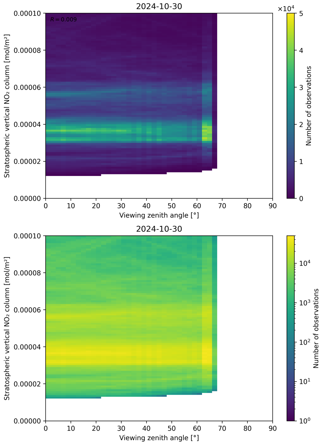
Figure 164: Scatter density plot of “Viewing zenith angle” against “Stratospheric vertical NO 2 column” for 2024-10-30 to 2024-10-31.
