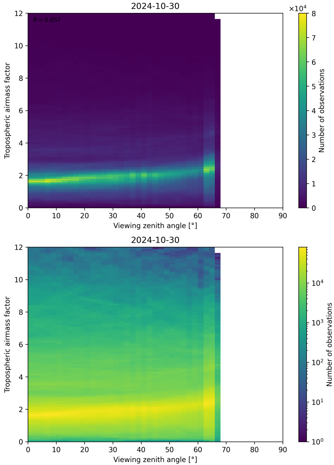
Figure 161: Scatter density plot of “Viewing zenith angle” against “Tropospheric airmass factor” for 2024-10-30 to 2024-10-31.
