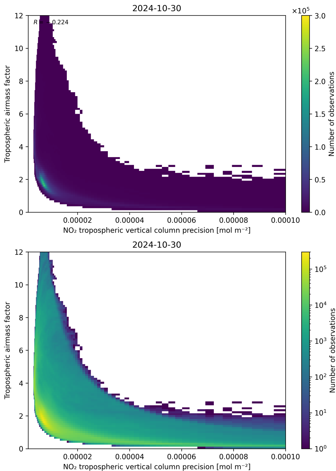
Figure 133: Scatter density plot of “NO 2 tropospheric vertical column precision” against “Tropospheric airmass factor” for 2024-10-30 to 2024-10-31.
