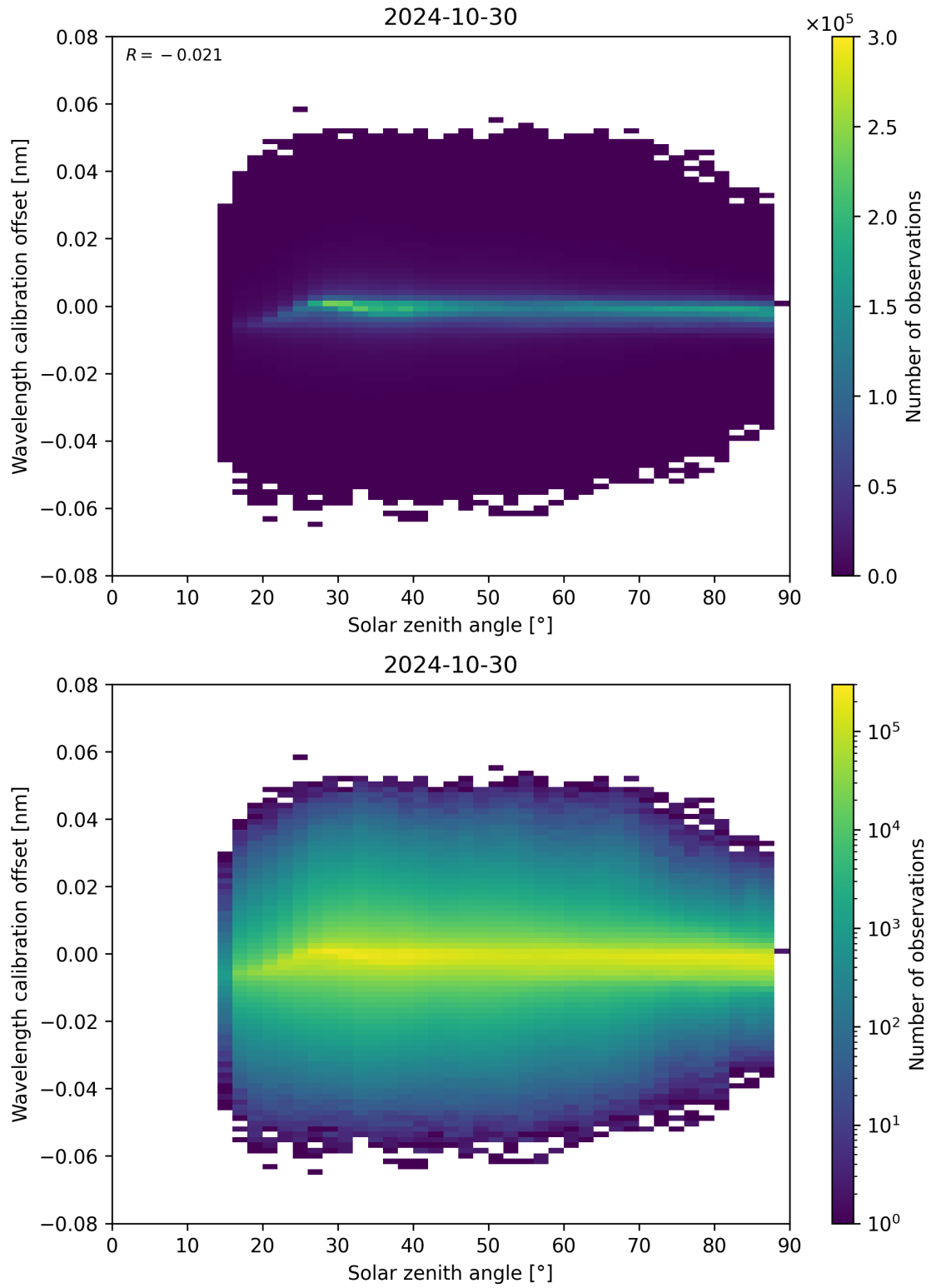
Figure 158: Scatter density plot of “Solar zenith angle” against “Wavelength calibration offset” for 2024-10-30 to 2024-10-31.
