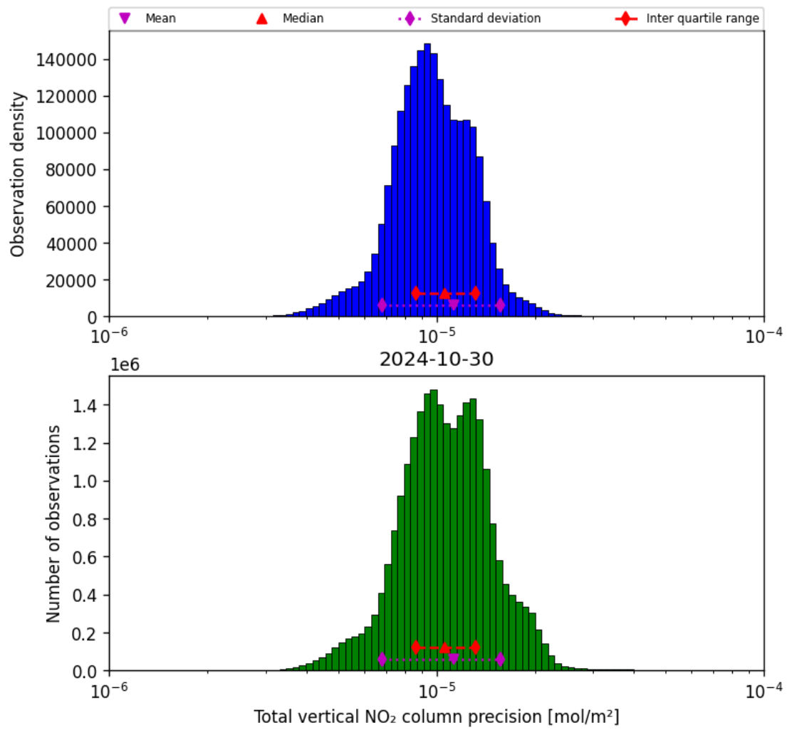
Figure 39: Histogram of “Total vertical NO 2 column precision” for 2024-10-30 to 2024-10-31
