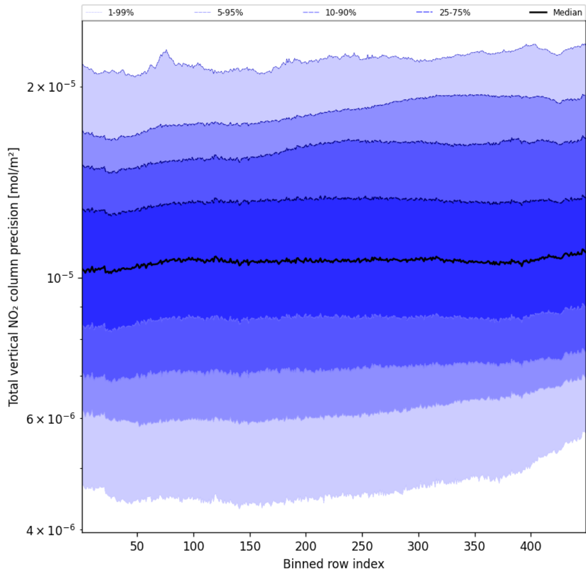
Figure 56: Along track statistics of “Total vertical NO 2 column precision” for 2024-10-30 to 2024-10-31
