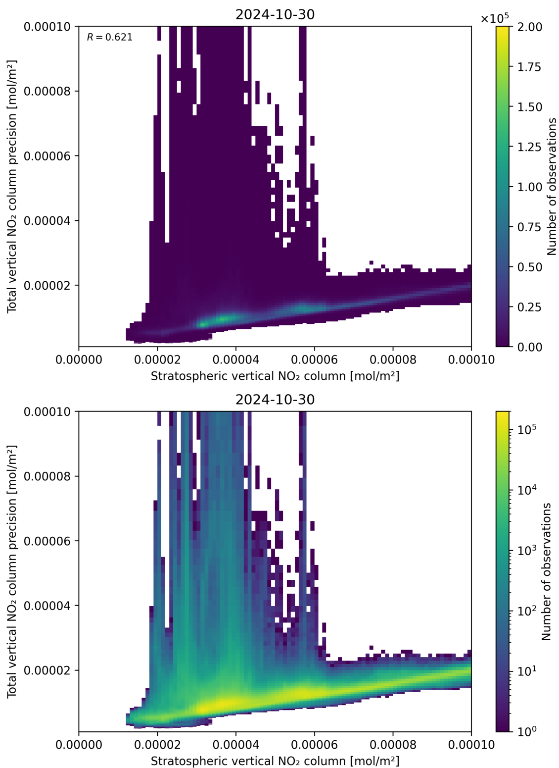
Figure 101: Scatter density plot of “Stratospheric vertical NO 2 column” against “Total vertical NO 2 column precision” for 2024-10-30 to 2024-10-31.
