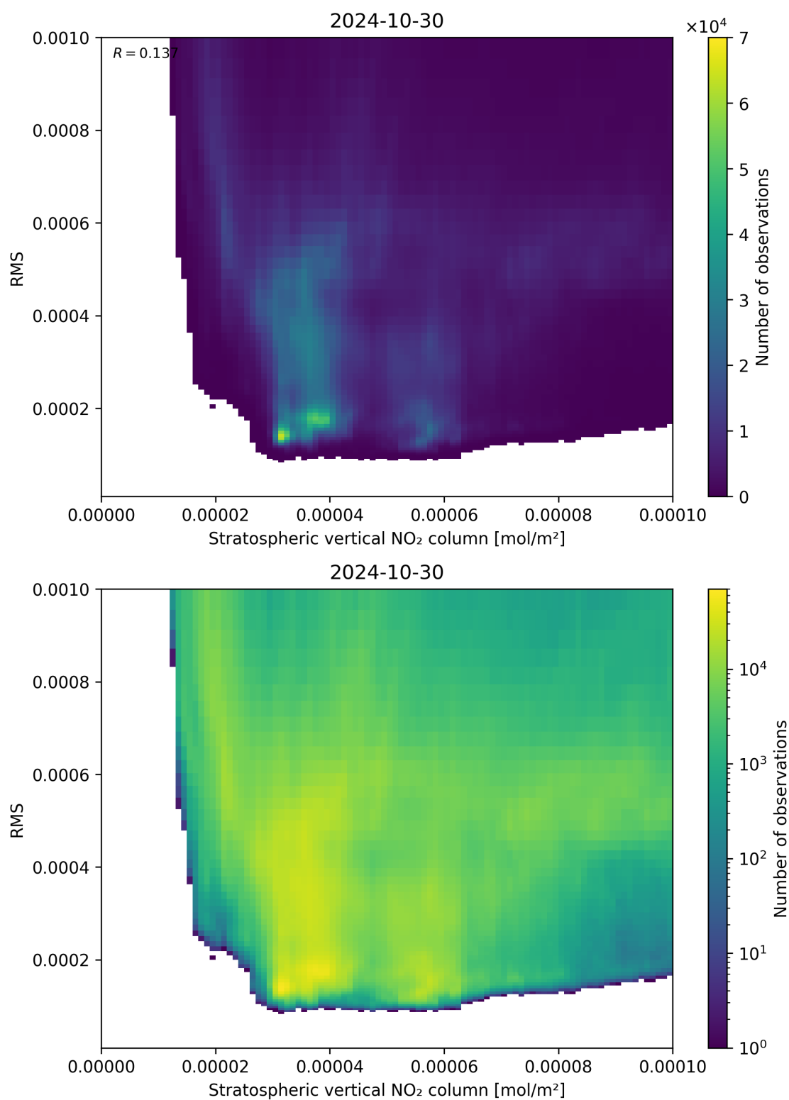
Figure 102: Scatter density plot of “Stratospheric vertical NO 2 column” against “RMS” for 2024-10-30 to 2024-10-31.
