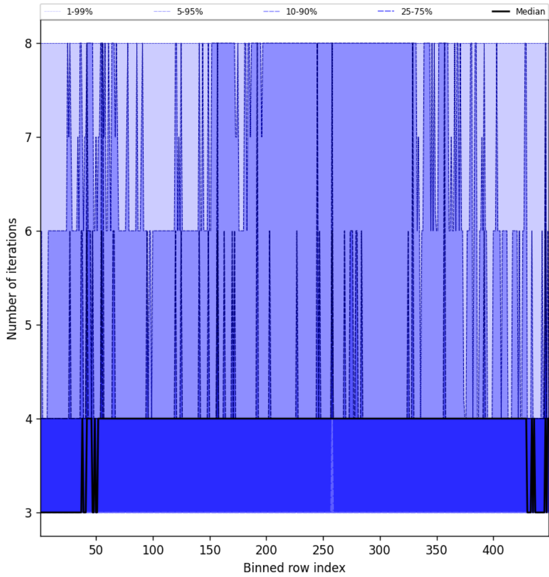
Figure 51: Along track statistics of “Number of iterations” for 2024-10-30 to 2024-10-31
