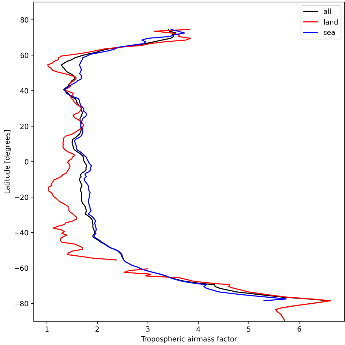
Figure 14: Zonal average of “Tropospheric airmass factor” for 2024-10-30 to 2024-10-31.
