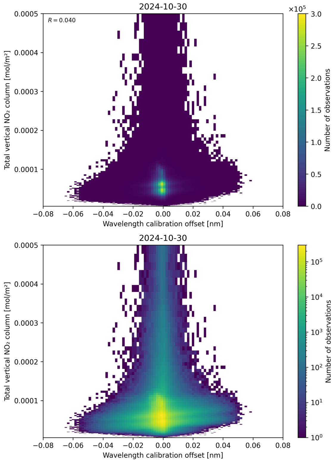
Figure 179: Scatter density plot of “Wavelength calibration offset” against “Total vertical NO 2 column” for 2024-10-30 to 2024-10-31.
