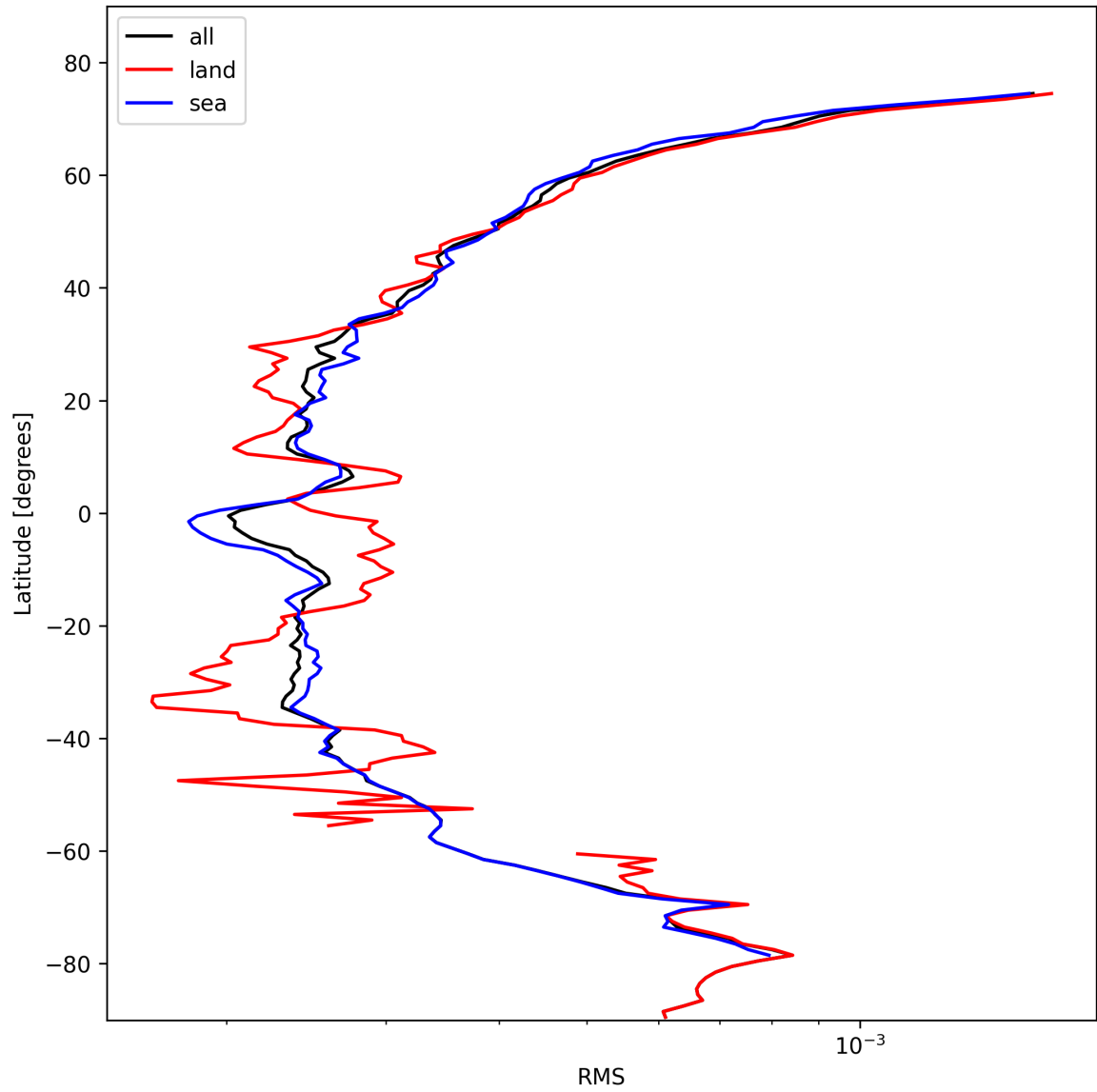
Figure 26: Zonal average of “RMS” for 2024-10-30 to 2024-10-31.
