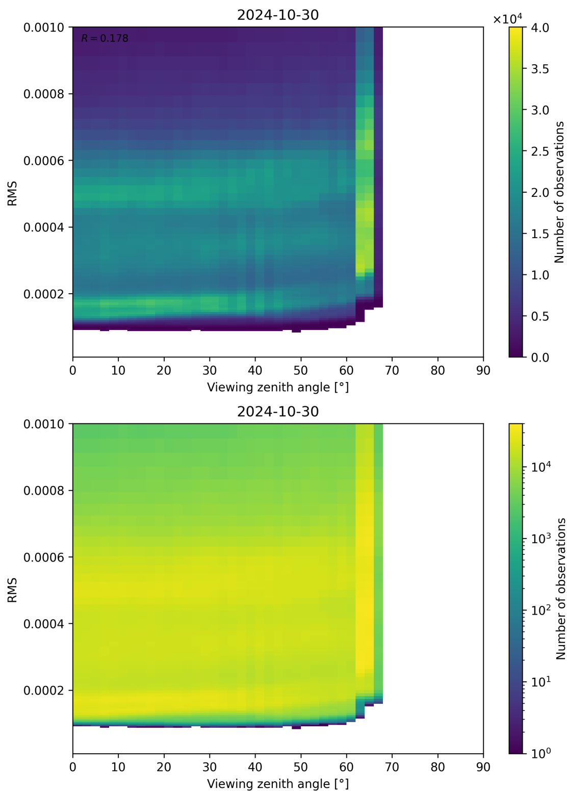
Figure 171: Scatter density plot of “Viewing zenith angle” against “RMS” for 2024-10-30 to 2024-10-31.
