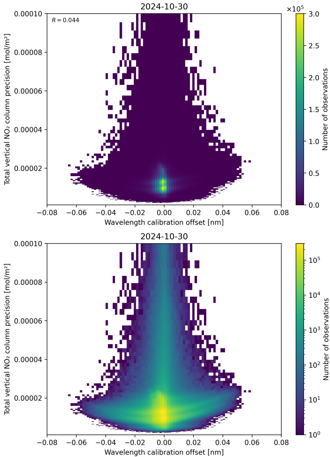
Figure 180: Scatter density plot of “Wavelength calibration offset” against “Total vertical NO 2 column precision” for 2024-10-30 to 2024-10-31.
