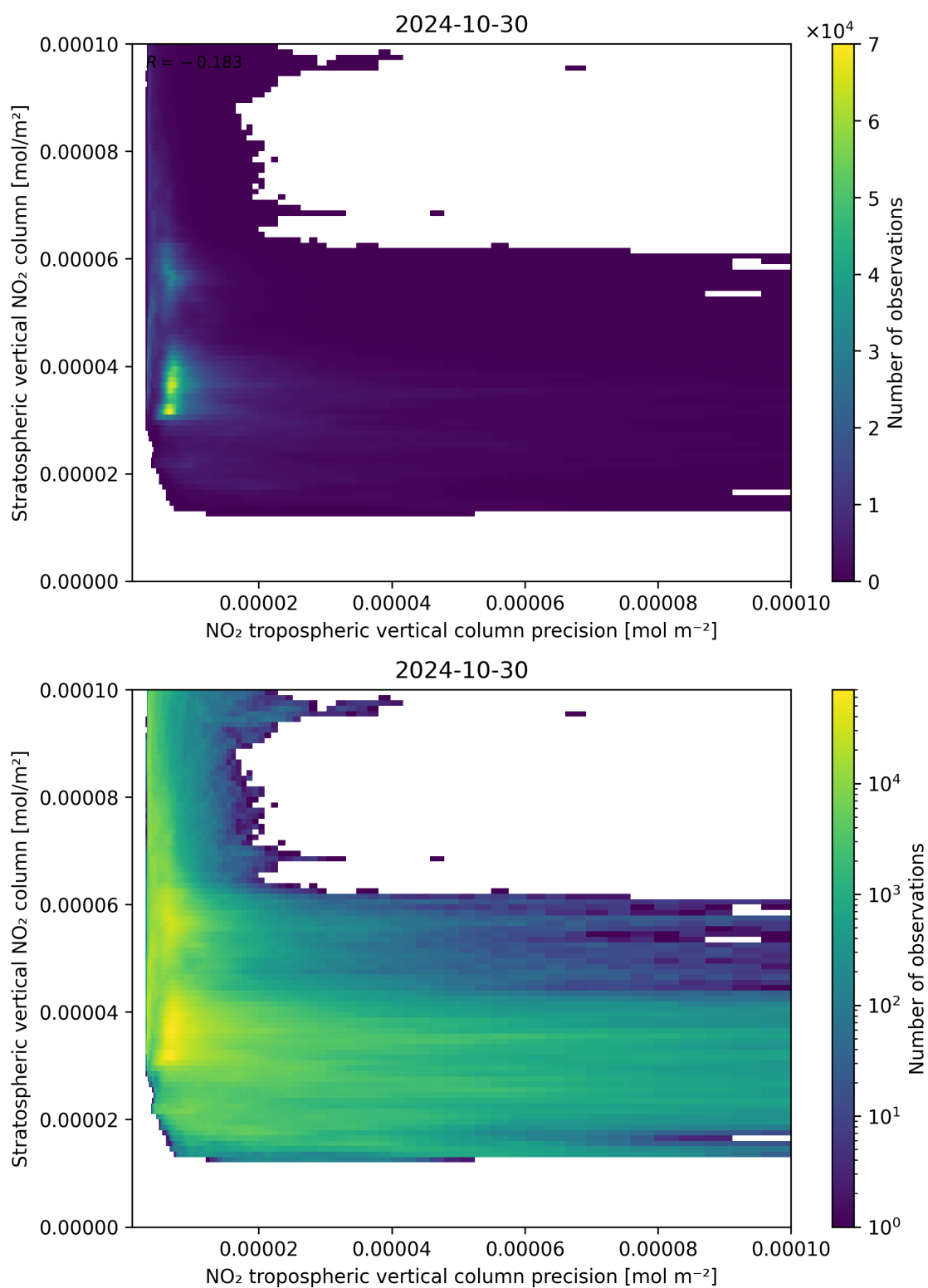
Figure 135: Scatter density plot of “NO 2 tropospheric vertical column precision” against “Stratospheric vertical NO 2 column” for 2024-10-30 to 2024-10-31.
