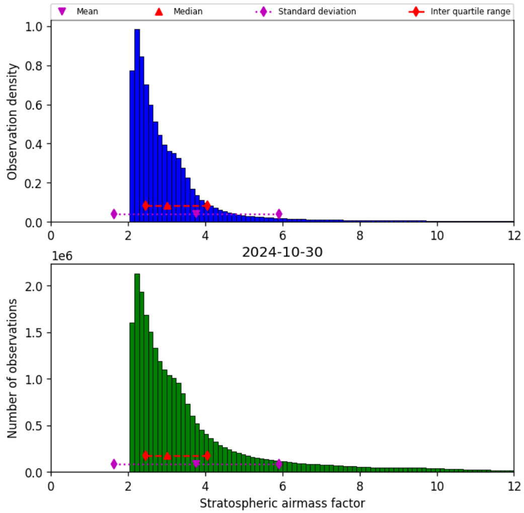
Figure 44: Histogram of “Stratospheric airmass factor” for 2024-10-30 to 2024-10-31
