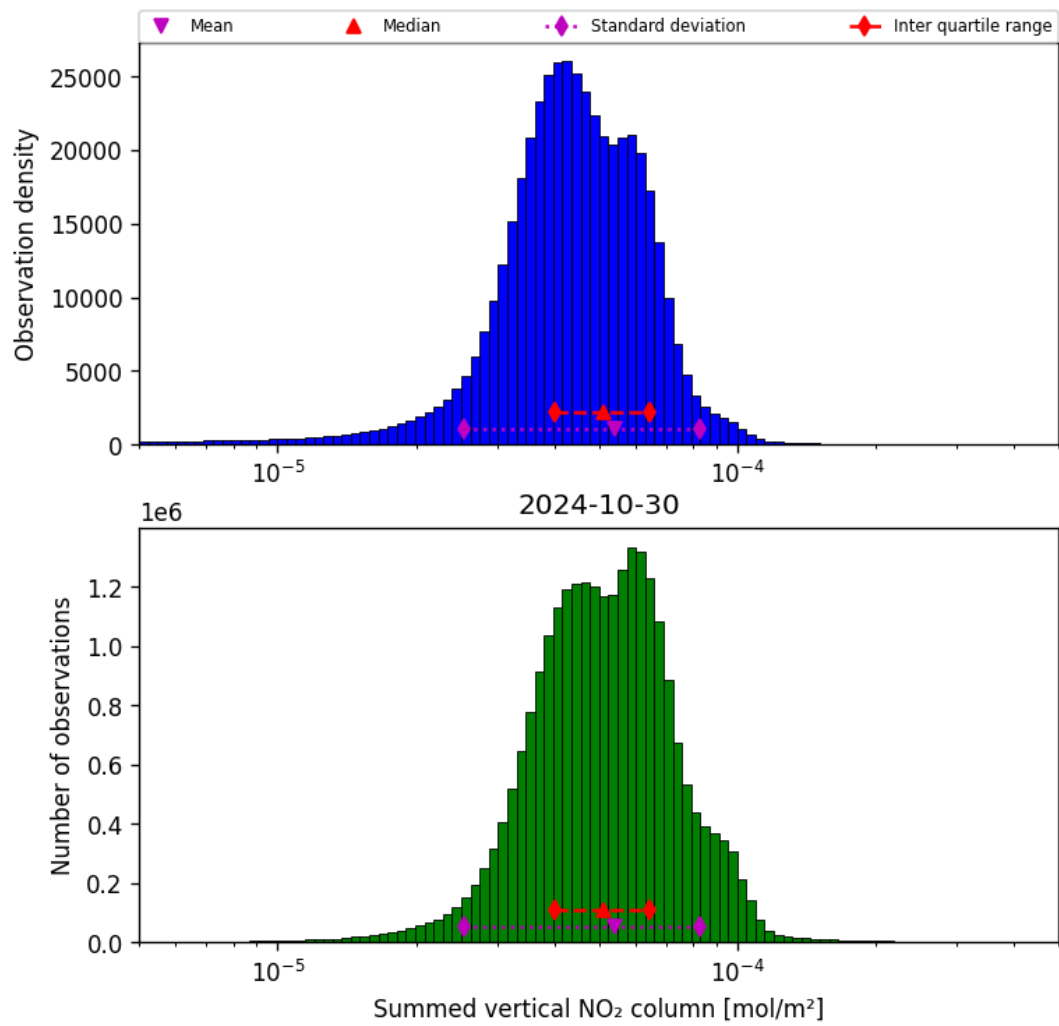
Figure 40: Histogram of “Summed vertical NO 2 column” for 2024-10-30 to 2024-10-31
