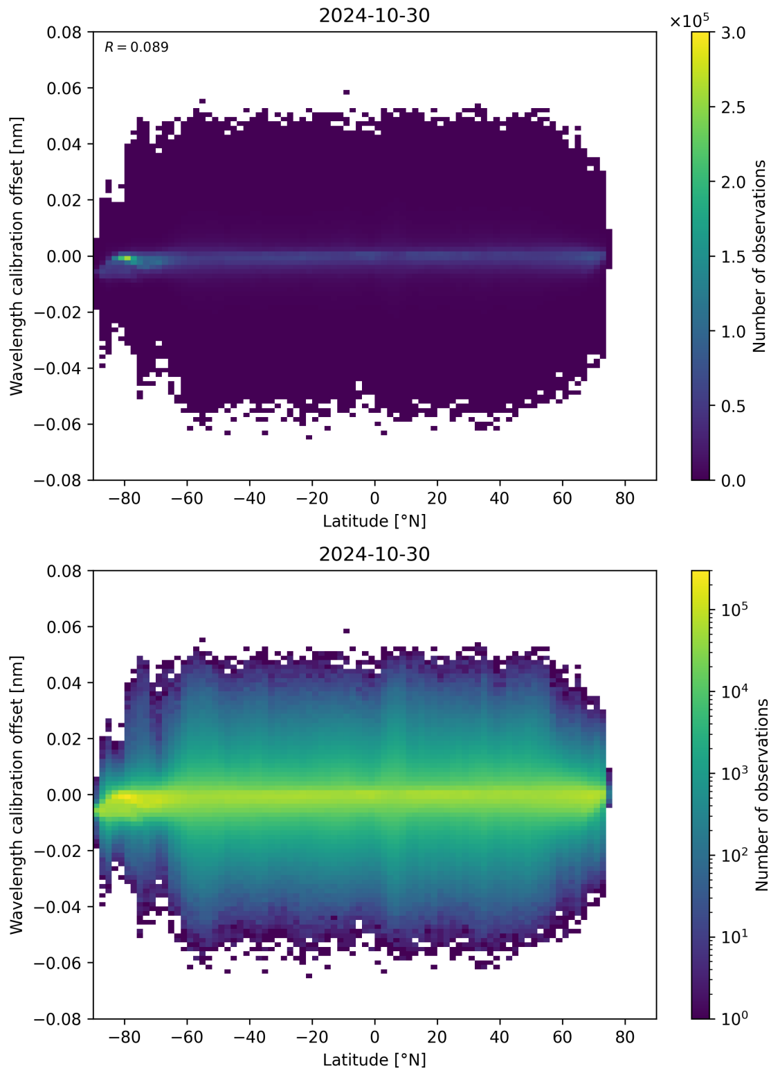
Figure 95: Scatter density plot of “Latitude” against “Wavelength calibration offset” for 2024-10-30 to 2024-10-31.
