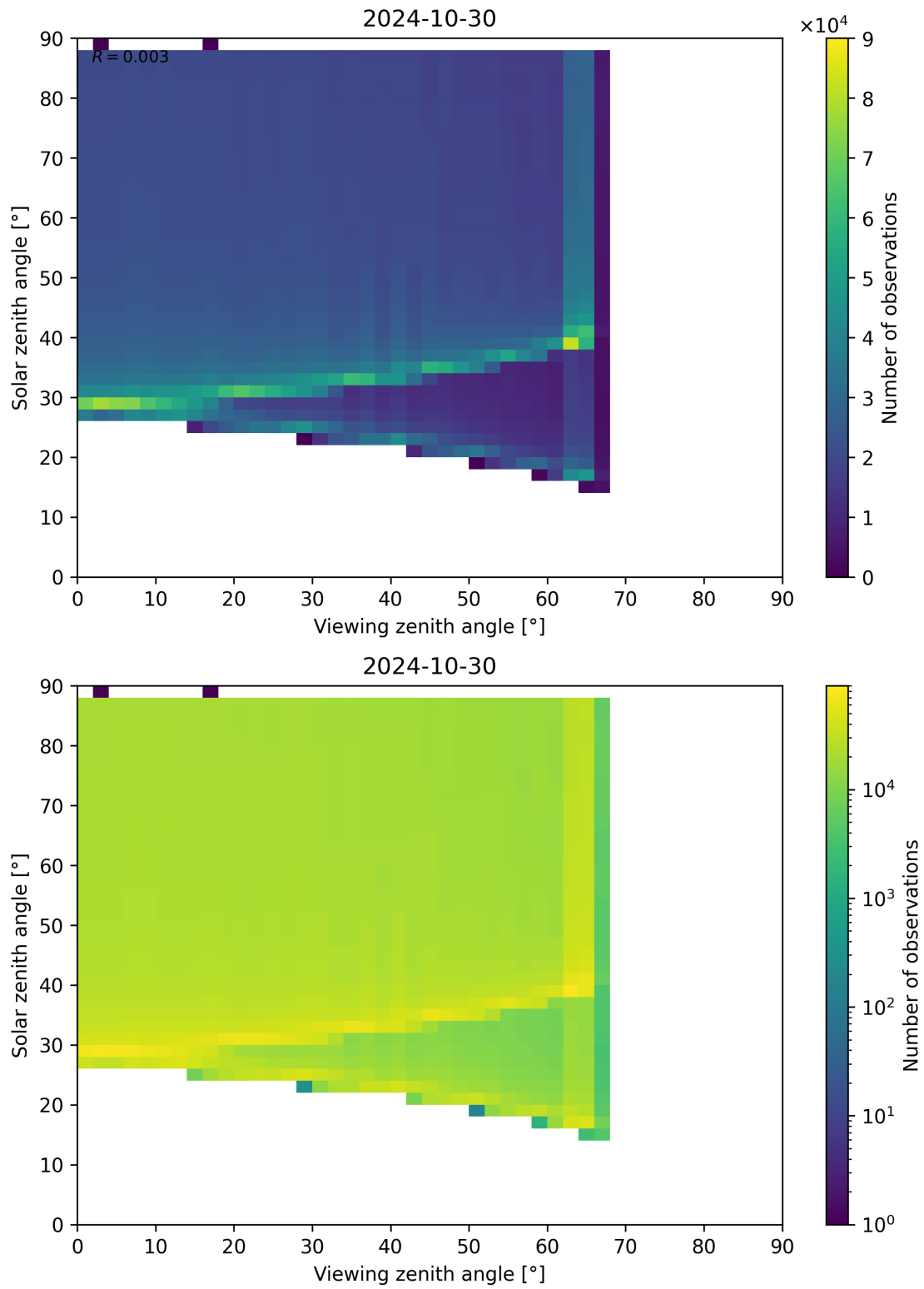
Figure 172: Scatter density plot of “Viewing zenith angle” against “Solar zenith angle” for 2024-10-30 to 2024-10-31.
