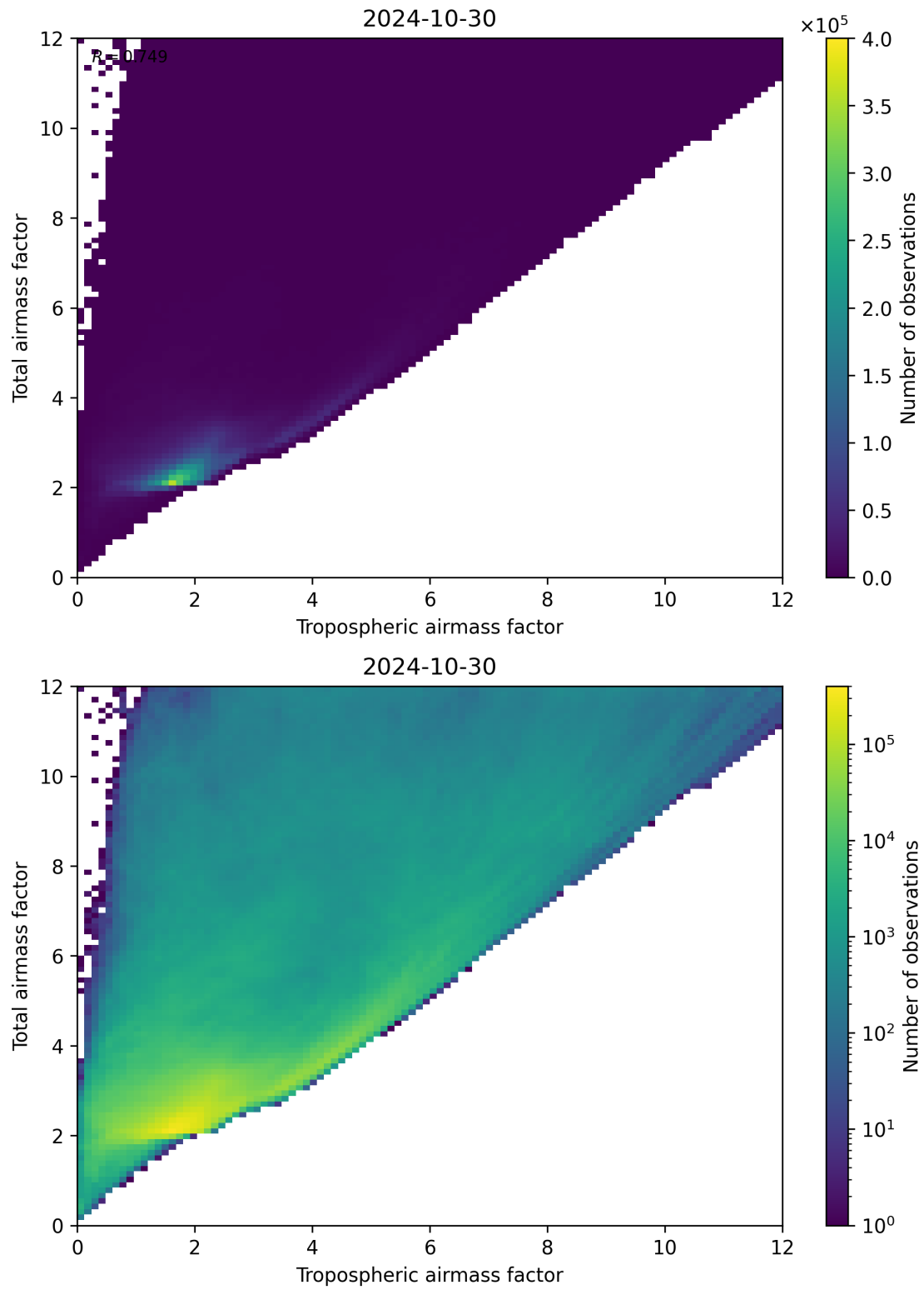
Figure 72: Scatter density plot of “Tropospheric airmass factor” against “Total airmass factor” for 2024-10-30 to 2024-10-31.
