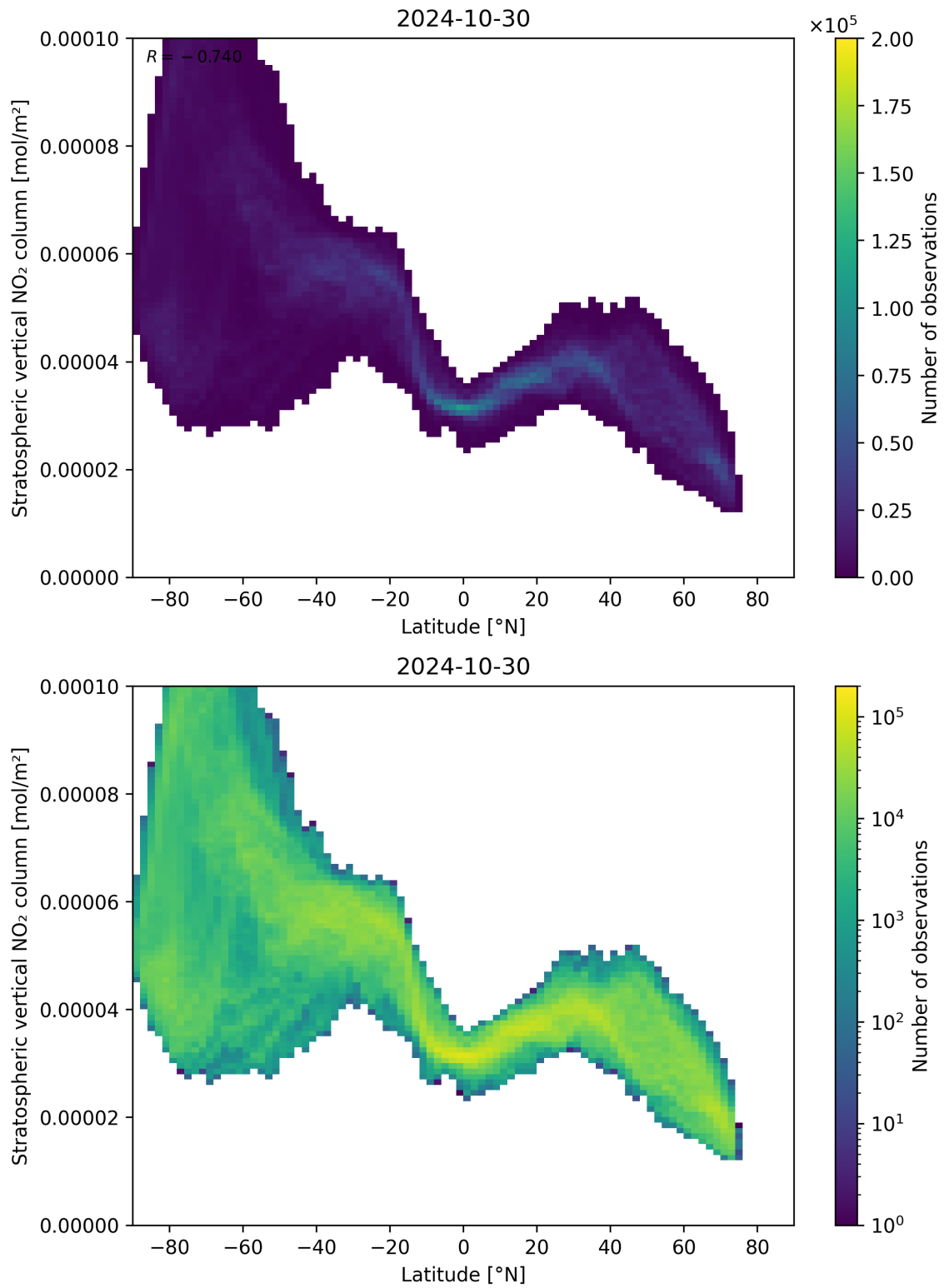
Figure 87: Scatter density plot of “Latitude” against “Stratospheric vertical NO 2 column” for 2024-10-30 to 2024-10-31.
