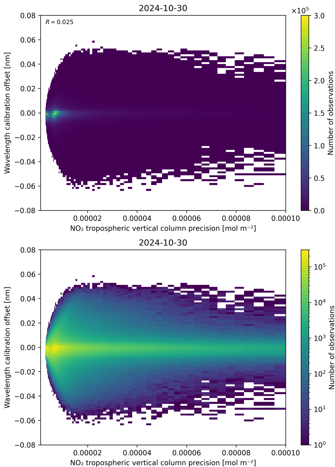
Figure 141: Scatter density plot of “NO 2 tropospheric vertical column precision” against “Wavelength calibration offset” for 2024-10-30 to 2024-10-31.
