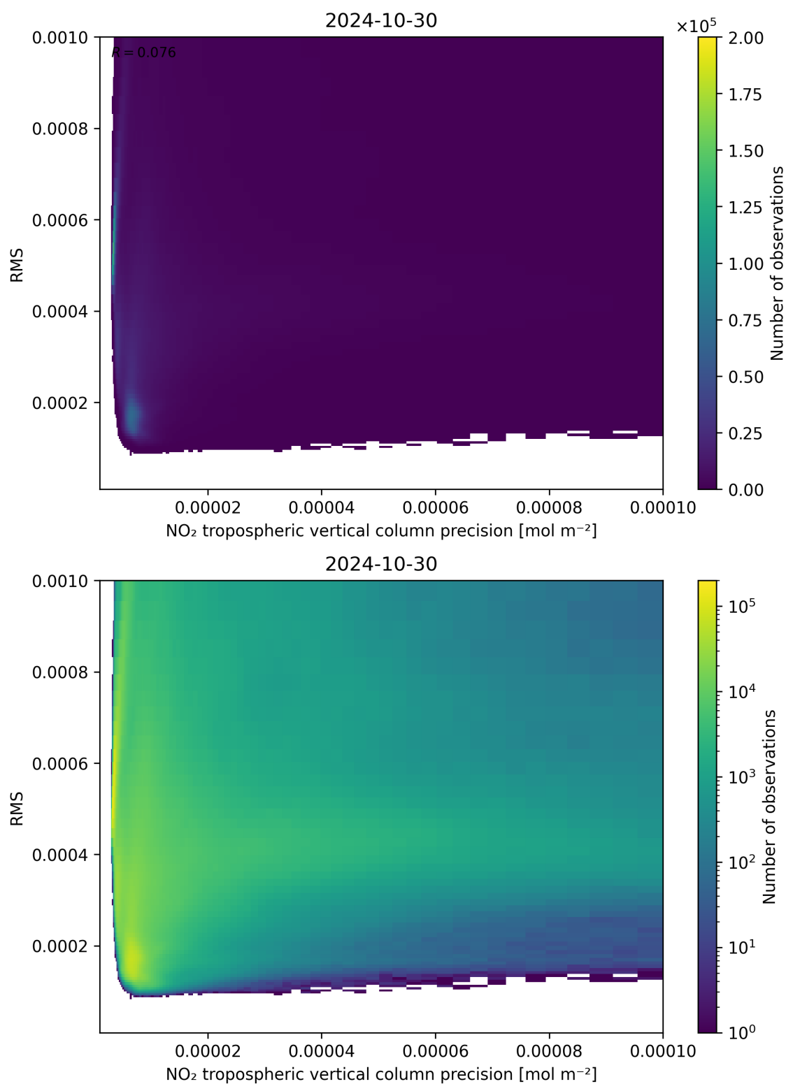
Figure 140: Scatter density plot of “NO 2 tropospheric vertical column precision” against “RMS” for 2024-10-30 to 2024-10-31.
