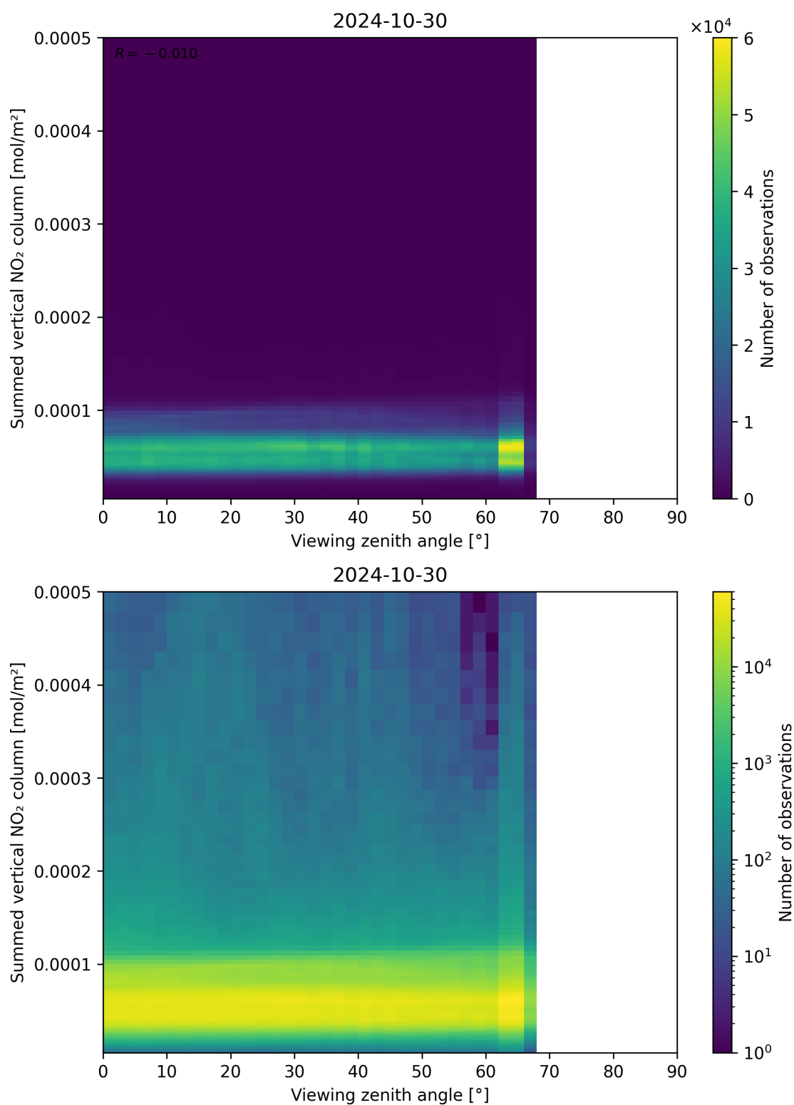
Figure 165: Scatter density plot of “Viewing zenith angle” against “Summed vertical NO 2 column” for 2024-10-30 to 2024-10-31.
