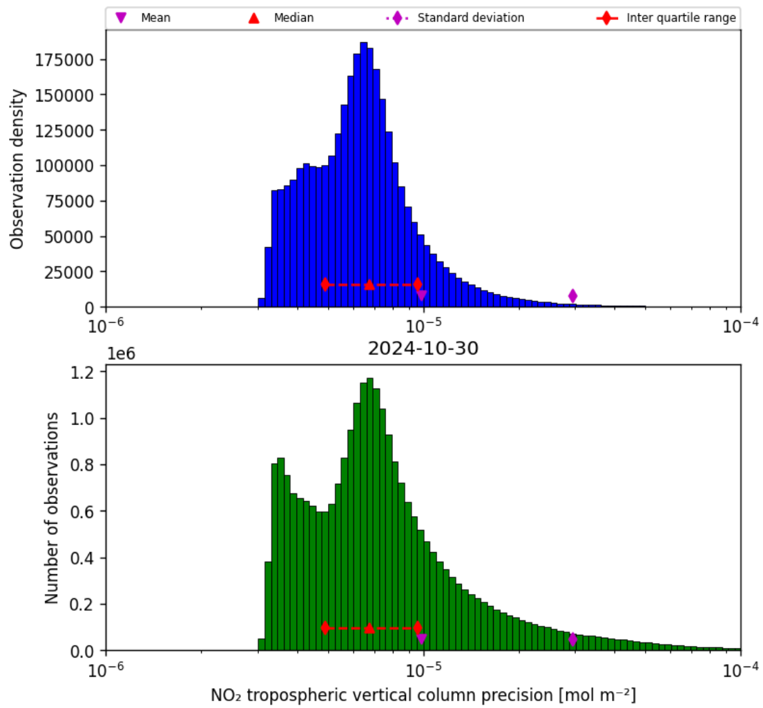
Figure 30: Histogram of “NO 2 tropospheric vertical column precision” for 2024-10-30 to 2024-10-31
