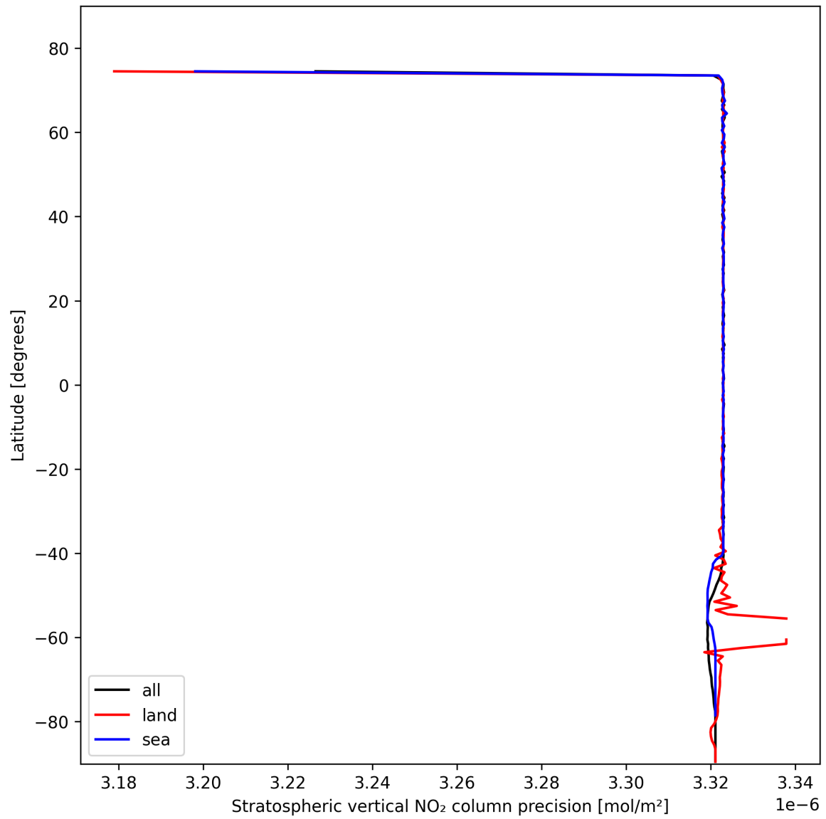
Figure 20: Zonal average of “Stratospheric vertical NO 2 column precision” for 2024-10-30 to 2024-10-31.
