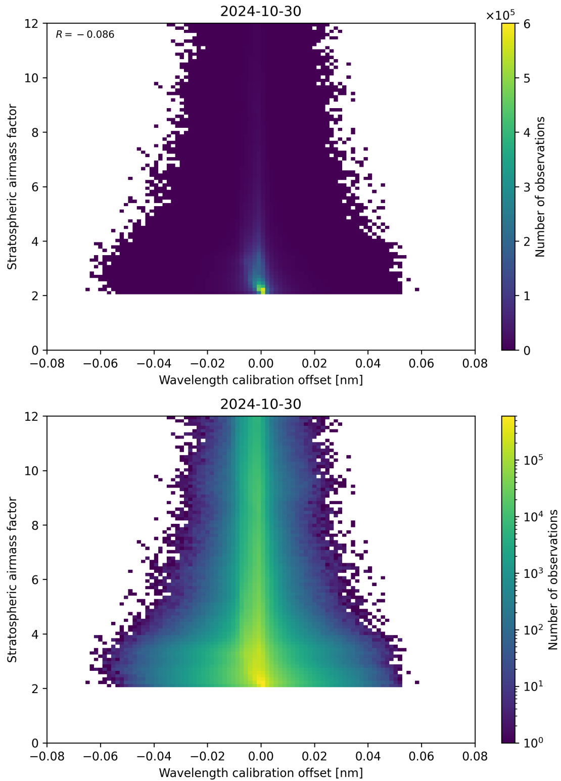
Figure 174: Scatter density plot of “Wavelength calibration offset” against “Stratospheric airmass factor” for 2024-10-30 to 2024-10-31.
