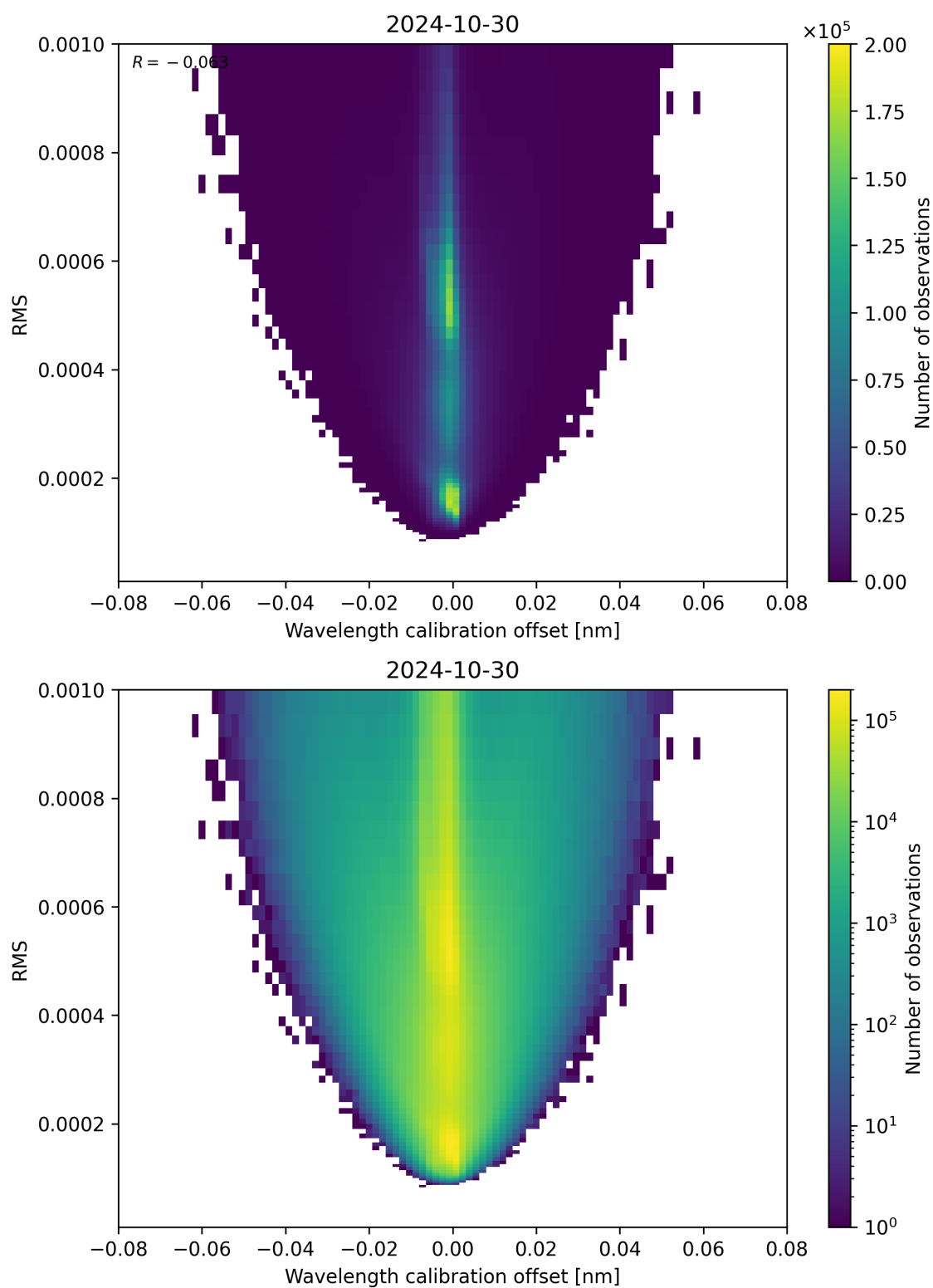
Figure 181: Scatter density plot of “Wavelength calibration offset” against “RMS” for 2024-10-30 to 2024-10-31.
