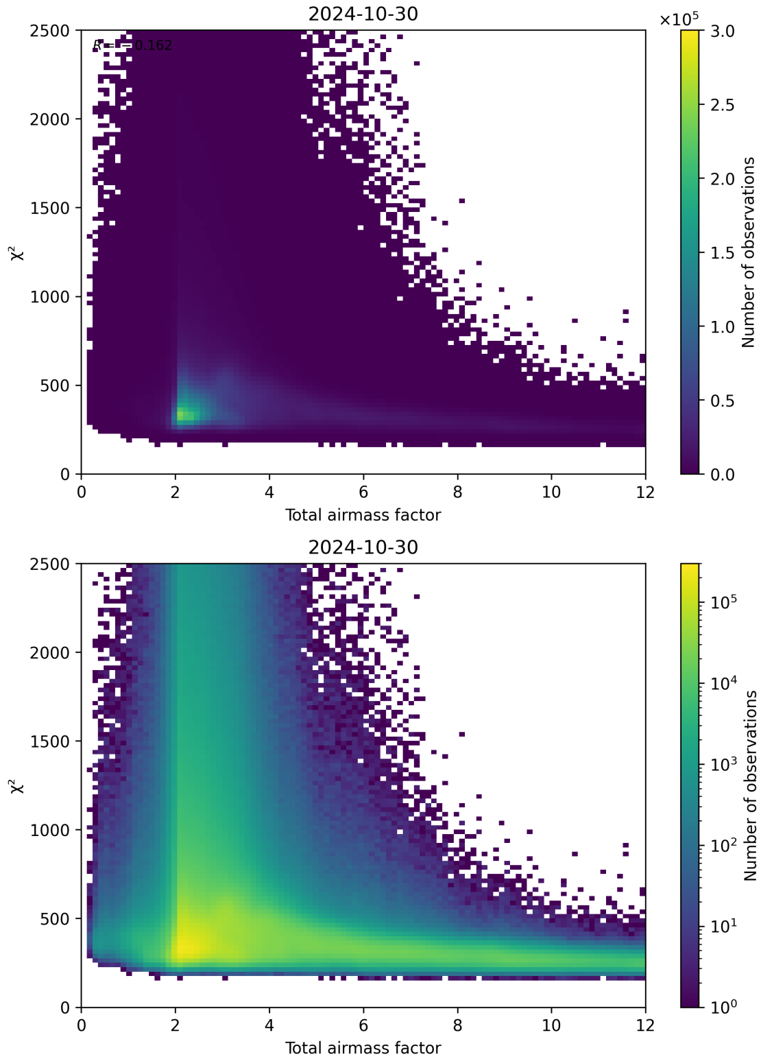
Figure 63: Scatter density plot of “Total airmass factor” against “ \chi^2 ” for 2024-10-30 to 2024-10-31.
