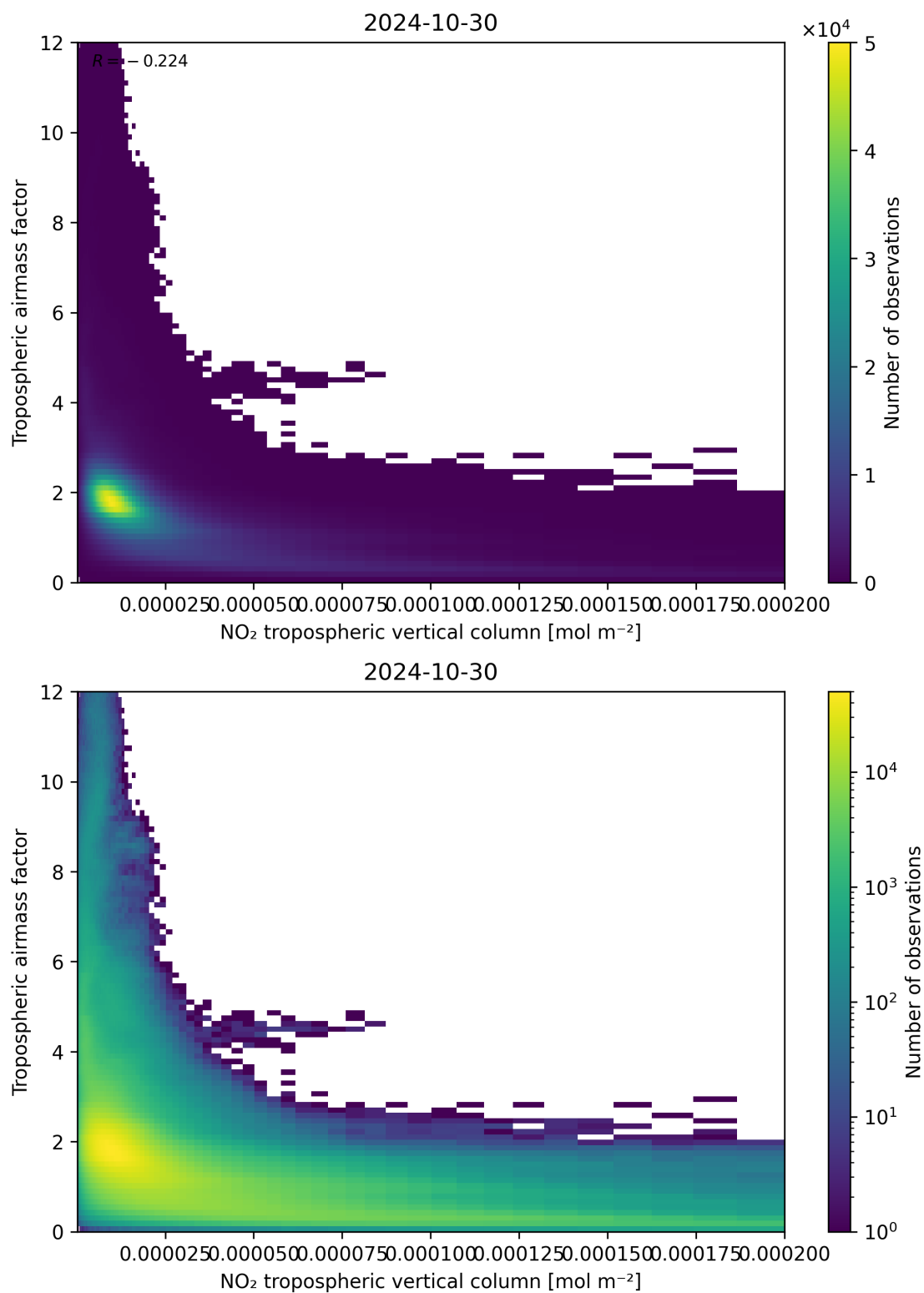
Figure 123: Scatter density plot of “NO 2 tropospheric vertical column” against “Tropospheric air mass factor” for 2024-10-30 to 2024-10-31.
