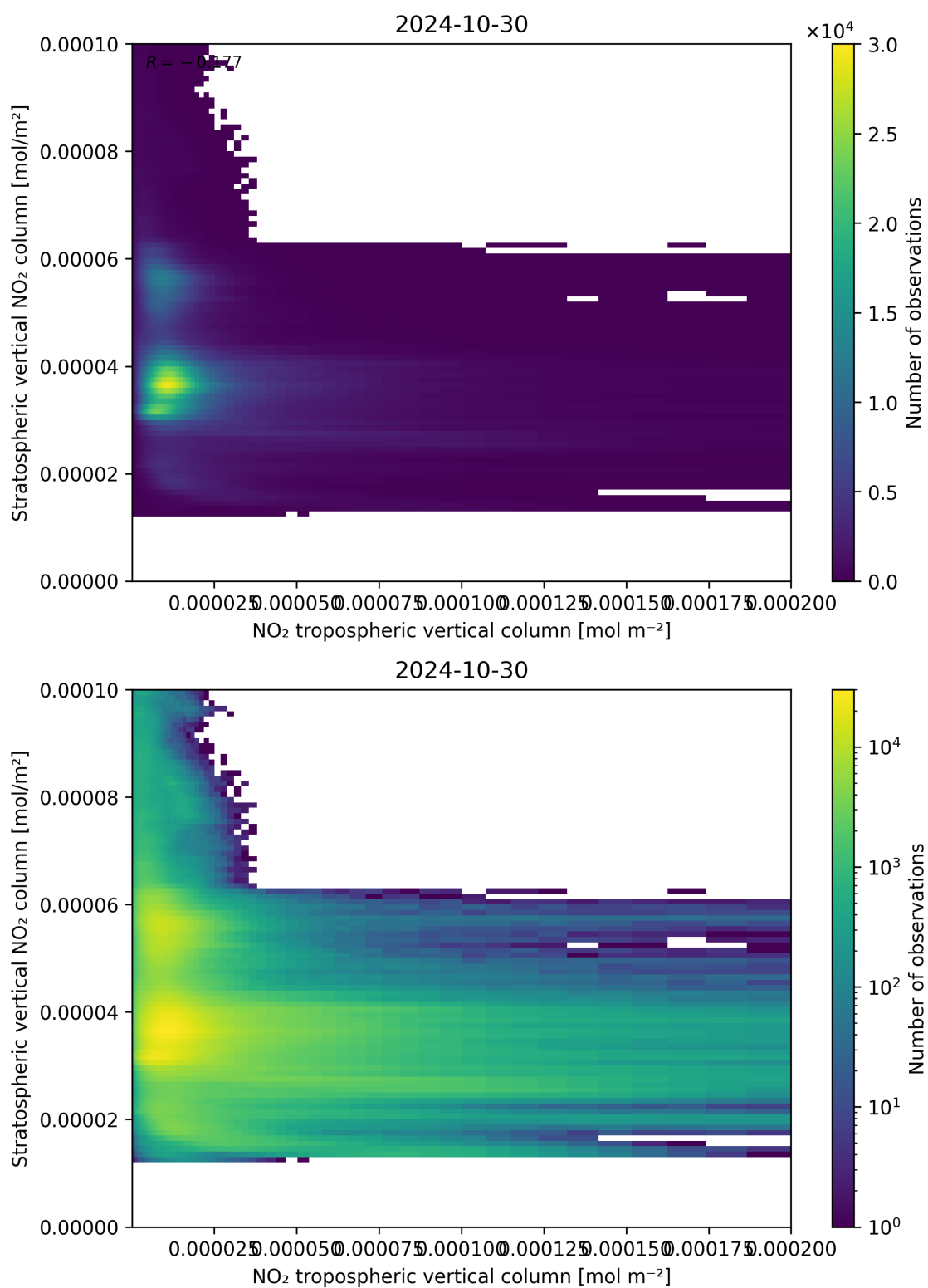
Figure 125: Scatter density plot of “NO 2 tropospheric vertical column” against “Stratospheric vertical NO 2 column” for 2024-10-30 to 2024-10-31.
