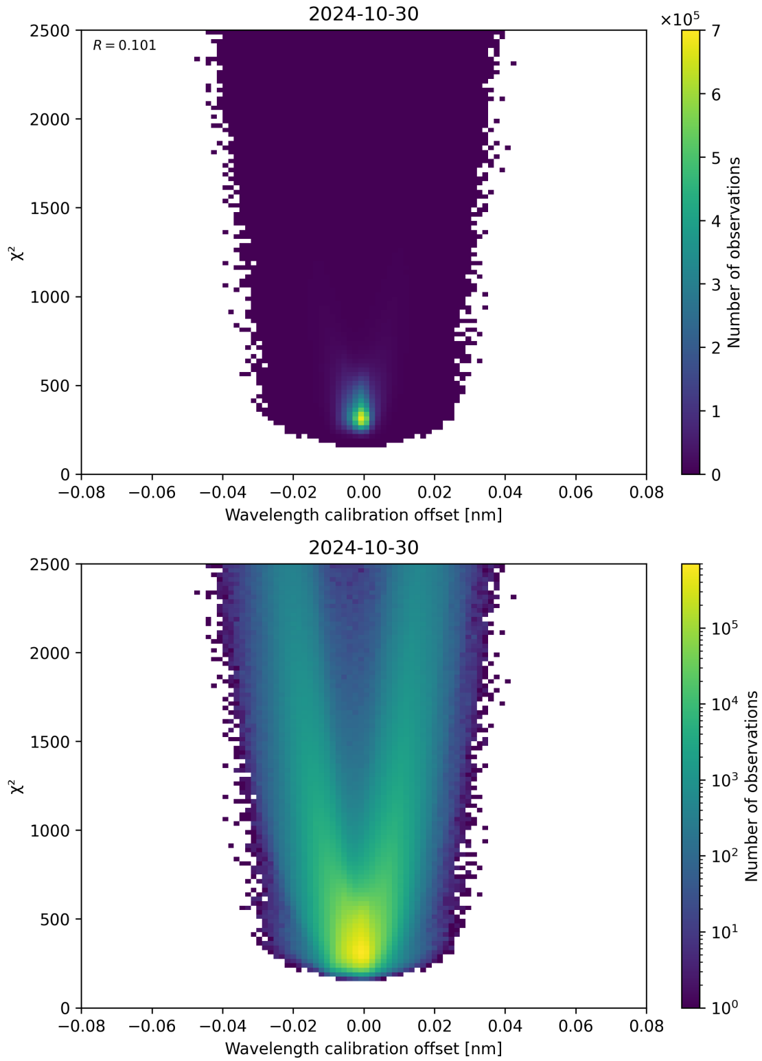
Figure 175: Scatter density plot of “Wavelength calibration offset” against “ \chi^2 ” for 2024-10-30 to 2024-10-31.
