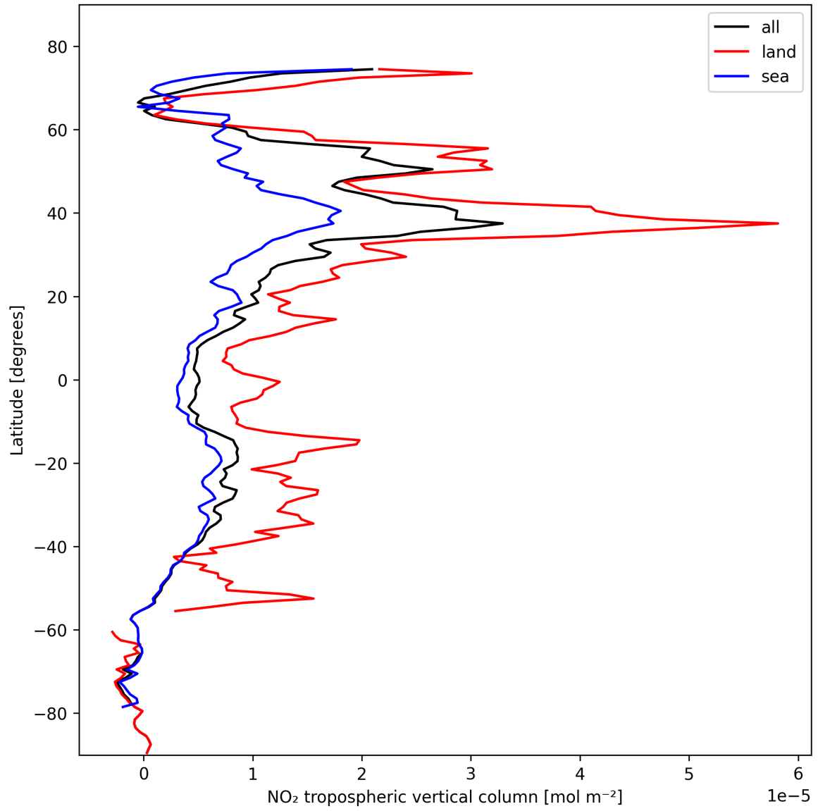
Figure 12: Zonal average of “NO 2 tropospheric vertical column” for 2024-10-30 to 2024-10-31.
