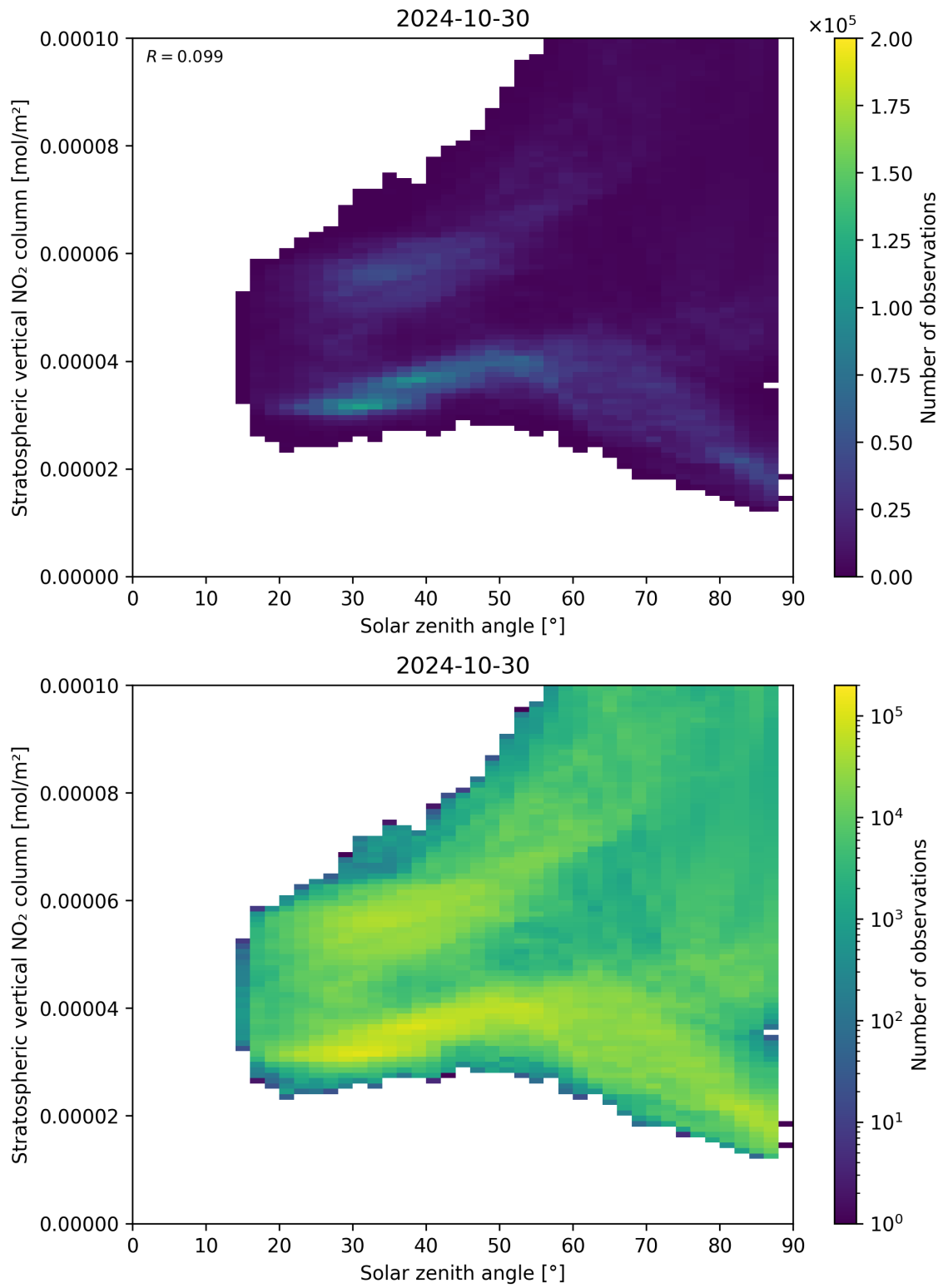
Figure 150: Scatter density plot of “Solar zenith angle” against “Stratospheric vertical NO 2 column” for 2024-10-30 to 2024-10-31.
