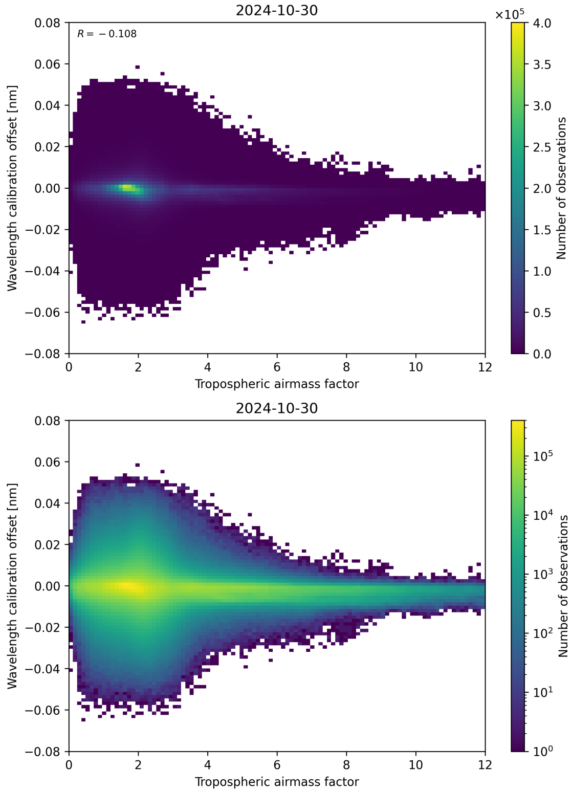
Figure 80: Scatter density plot of “Tropospheric airmass factor” against “Wavelength calibration offset” for 2024-10-30 to 2024-10-31.
