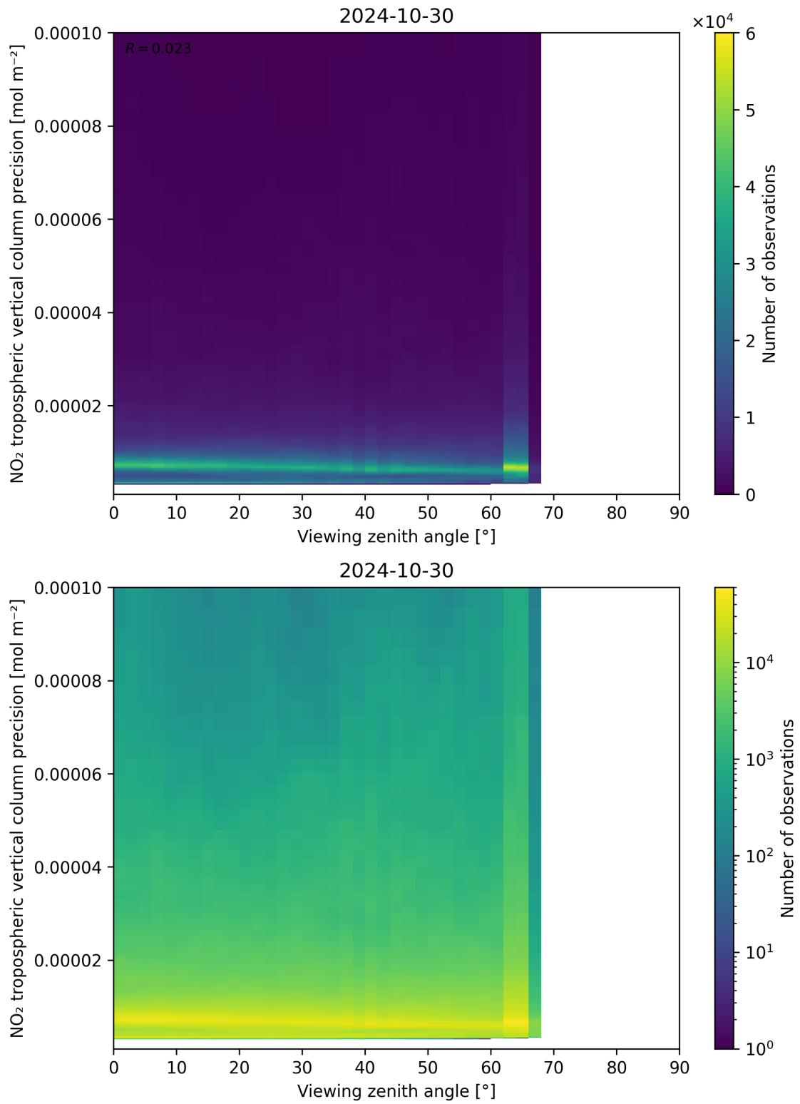
Figure 170: Scatter density plot of “Viewing zenith angle” against “NO 2 tropospheric vertical column precision” for 2024-10-30 to 2024-10-31.
