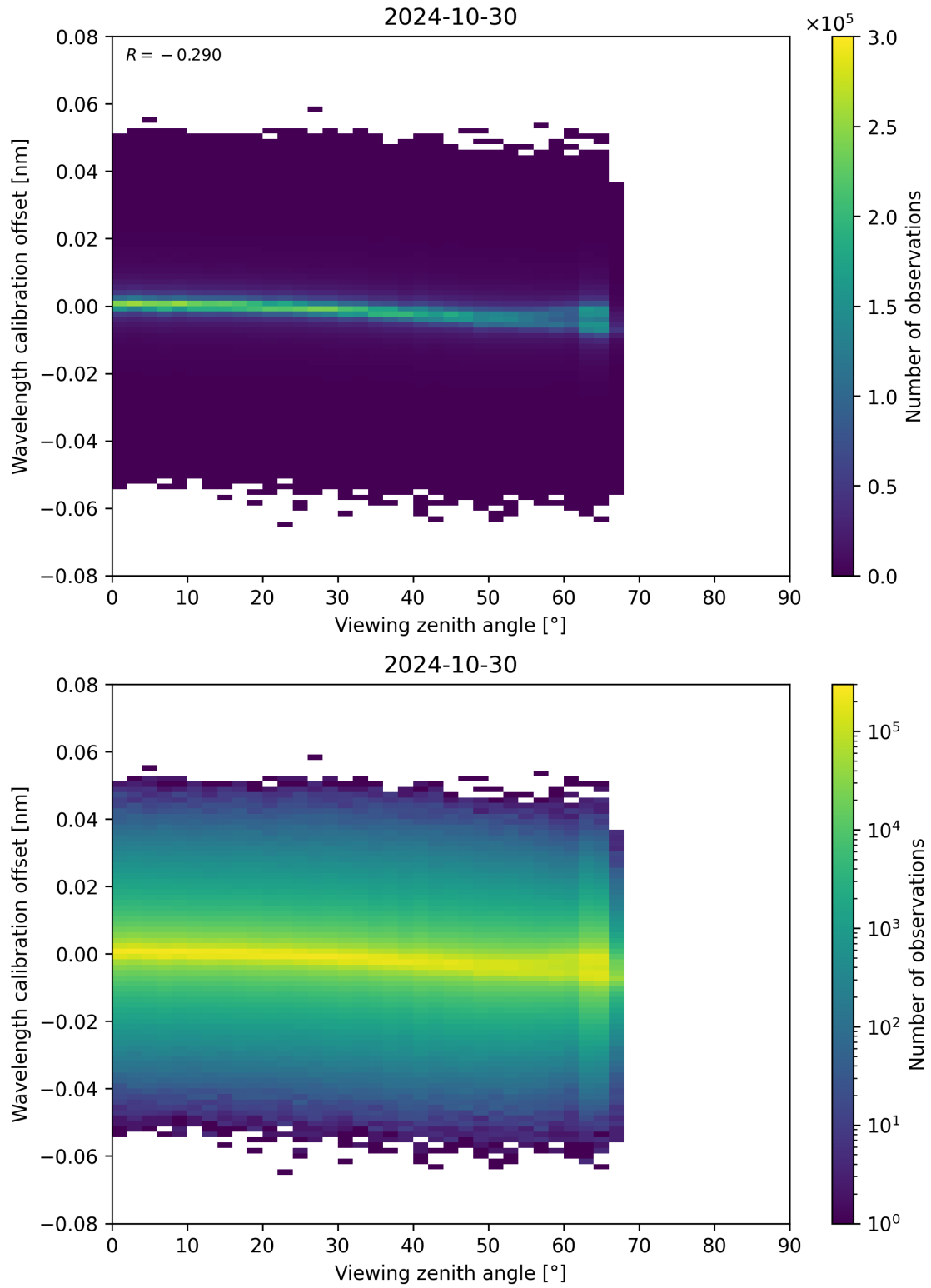
Figure 173: Scatter density plot of “Viewing zenith angle” against “Wavelength calibration offset” for 2024-10-30 to 2024-10-31.
