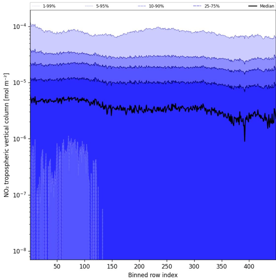
Figure 46: Along track statistics of “NO 2 tropospheric vertical column” for 2024-10-30 to 2024-10-31
