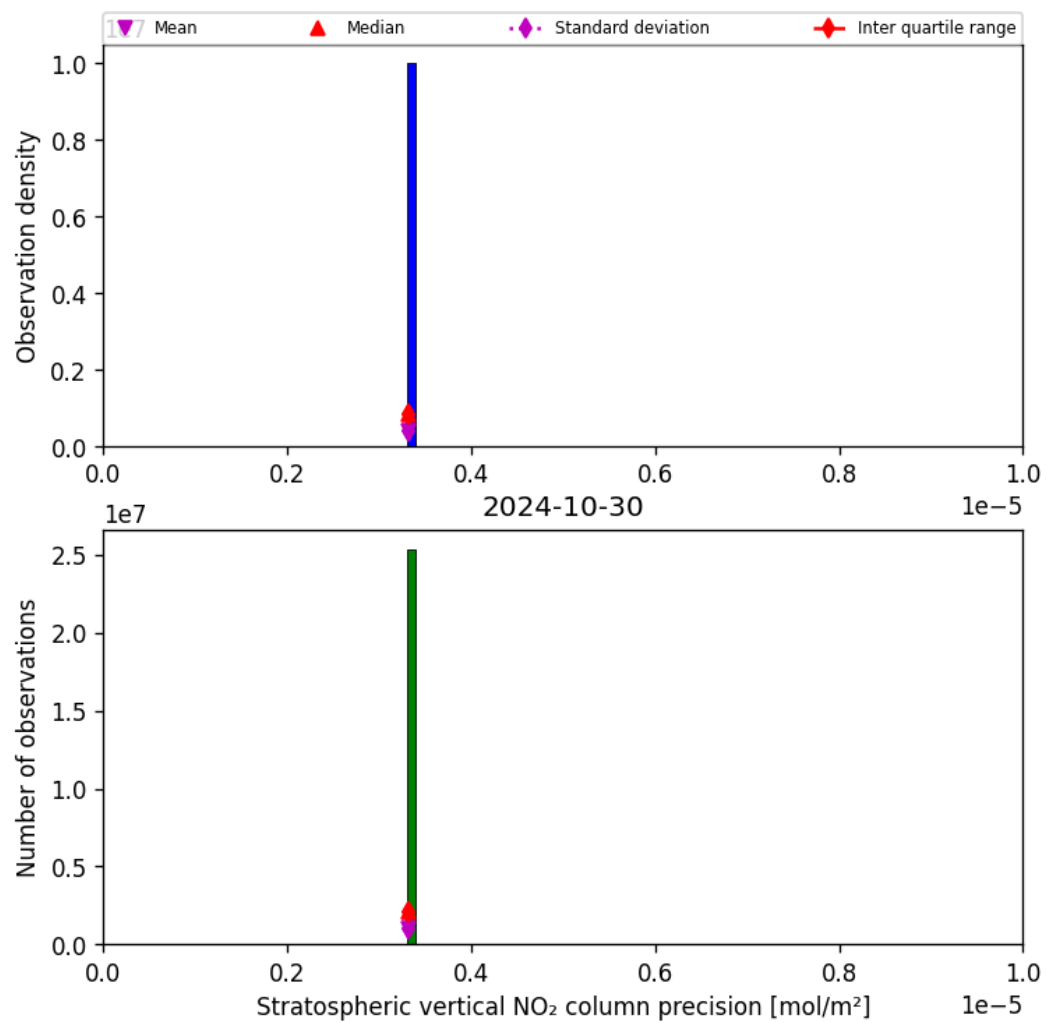
Figure 37: Histogram of “Stratospheric vertical NO 2 column precision” for 2024-10-30 to 2024-10-31
