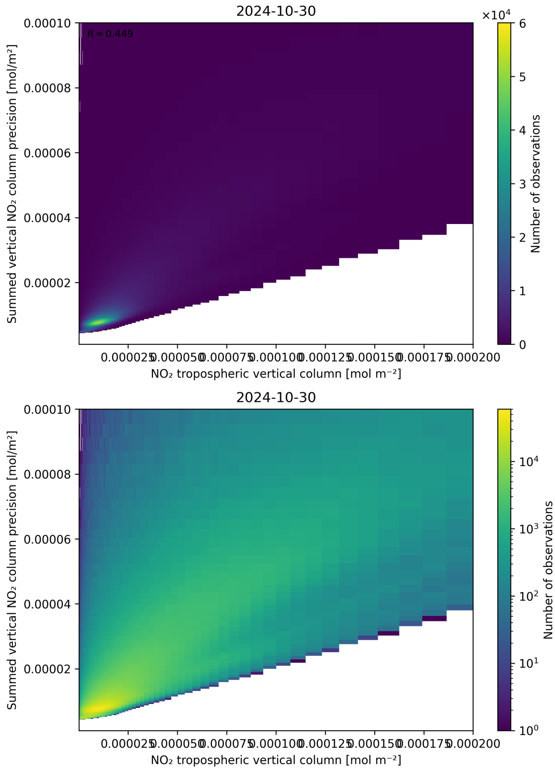
Figure 127: Scatter density plot of “NO 2 tropospheric vertical column” against “Summed vertical NO 2 column precision” for 2024-10-30 to 2024-10-31.
