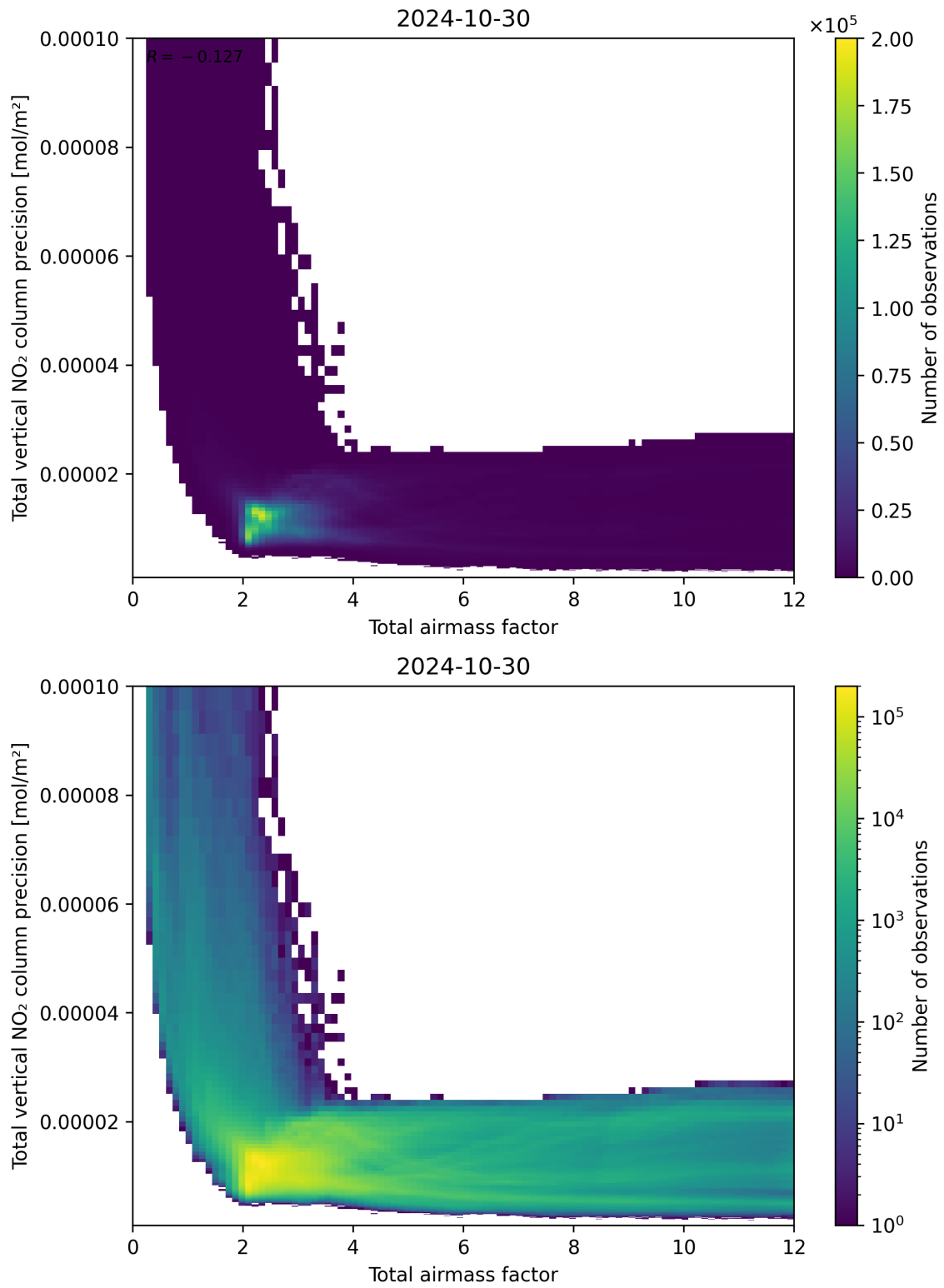
Figure 68: Scatter density plot of “Total airmass factor” against “Total vertical NO 2 column precision” for 2024-10-30 to 2024-10-31.
