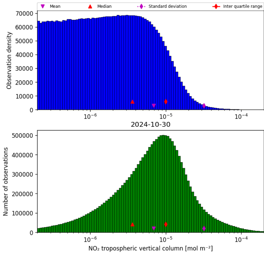
Figure 29: Histogram of “NO 2 tropospheric vertical column” for 2024-10-30 to 2024-10-31
