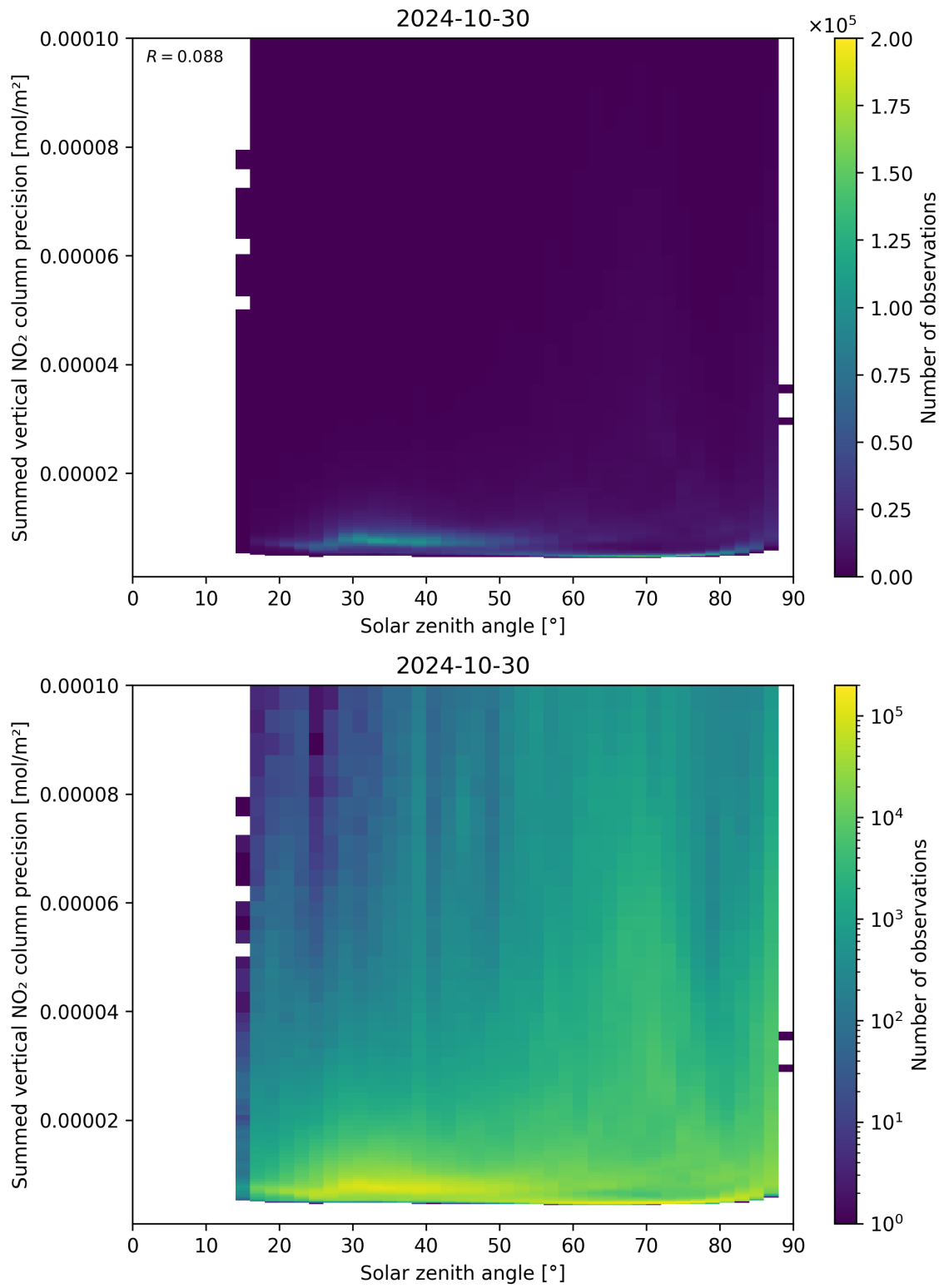
Figure 152: Scatter density plot of “Solar zenith angle” against “Summed vertical NO 2 column precision” for 2024-10-30 to 2024-10-31.
