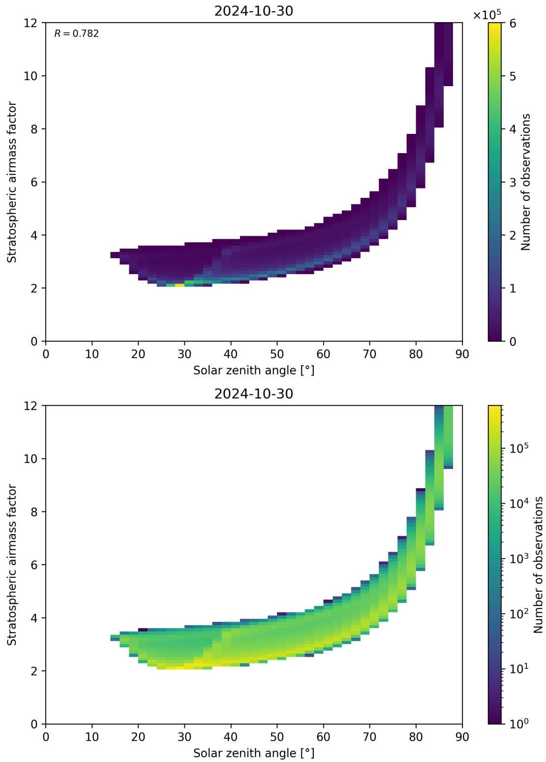
Figure 145: Scatter density plot of “Solar zenith angle” against “Stratospheric airmass factor” for 2024-10-30 to 2024-10-31.
