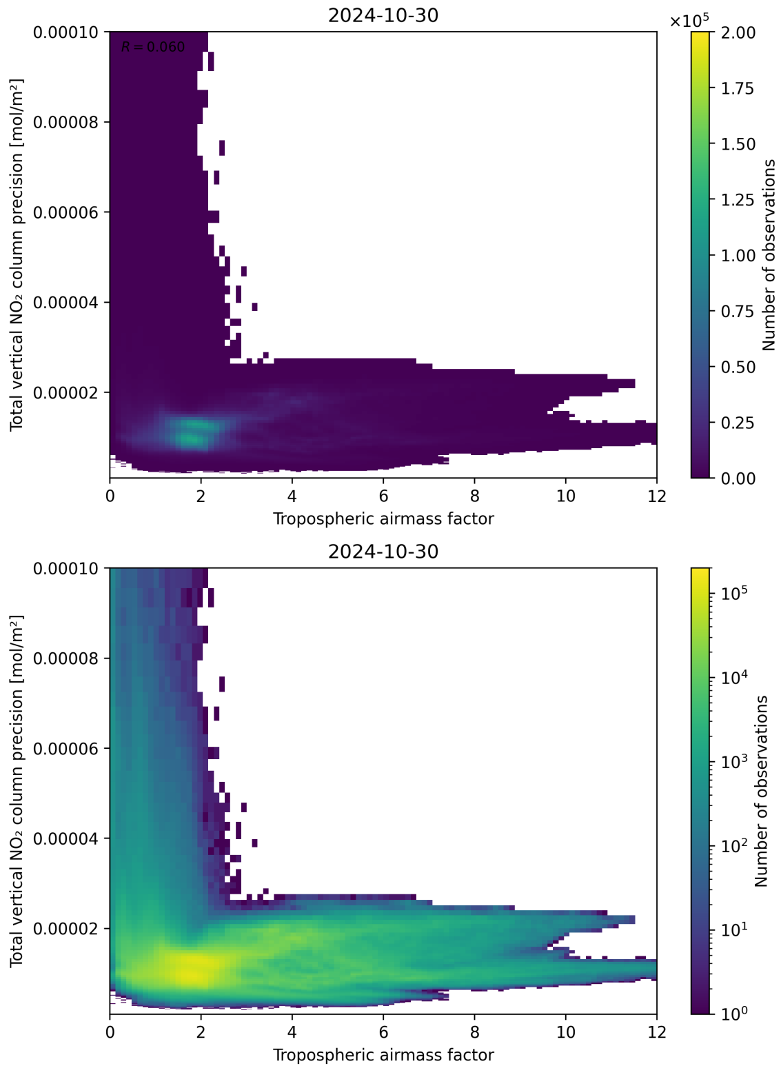
Figure 78: Scatter density plot of “Tropospheric airmass factor” against “Total vertical NO 2 column precision” for 2024-10-30 to 2024-10-31.
