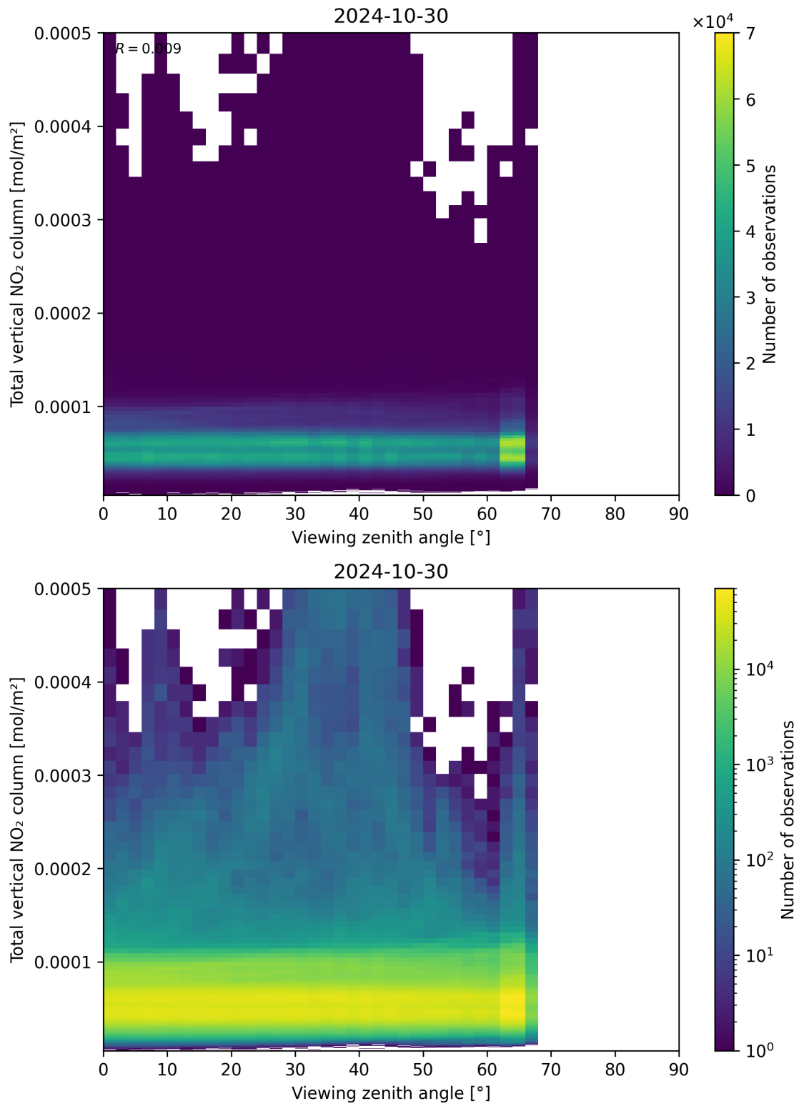
Figure 167: Scatter density plot of “Viewing zenith angle” against “Total vertical NO 2 column” for 2024-10-30 to 2024-10-31.
