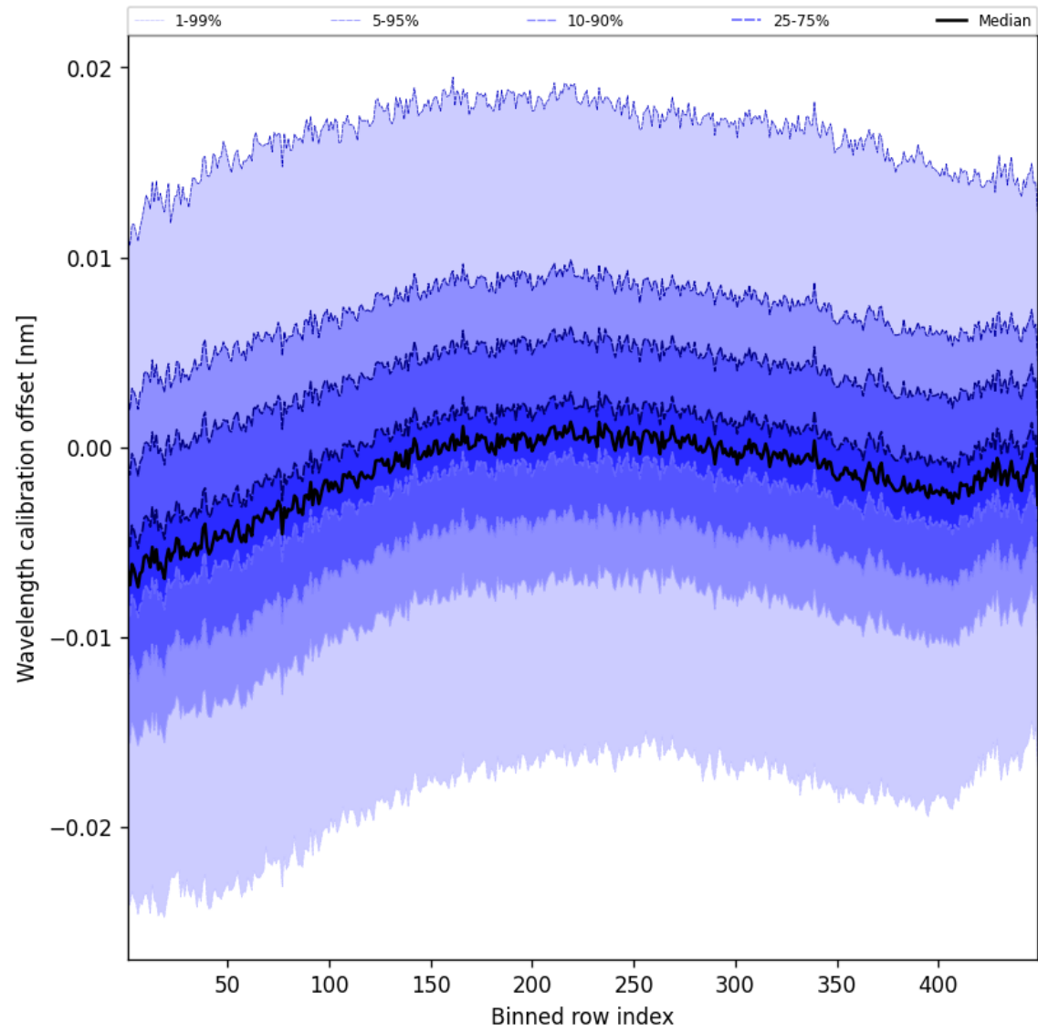
Figure 52: Along track statistics of “Wavelength calibration offset” for 2024-10-30 to 2024-10-31
