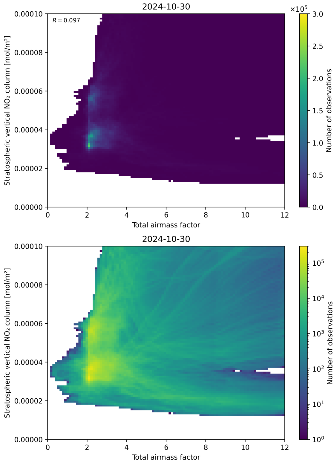
Figure 64: Scatter density plot of “Total airmass factor” against “Stratospheric vertical NO 2 column” for 2024-10-30 to 2024-10-31.
