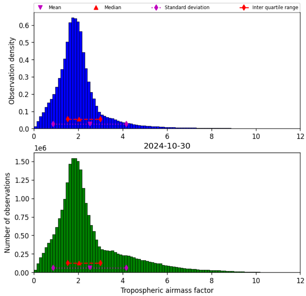
Figure 31: Histogram of “Tropospheric airmass factor” for 2024-10-30 to 2024-10-31
