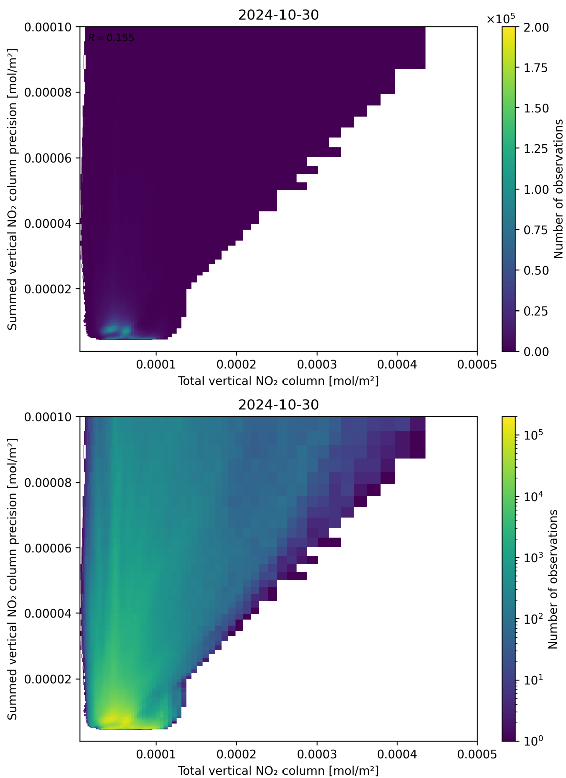
Figure 113: Scatter density plot of “Total vertical NO 2 column” against “Summed vertical NO 2 column precision” for 2024-10-30 to 2024-10-31.
