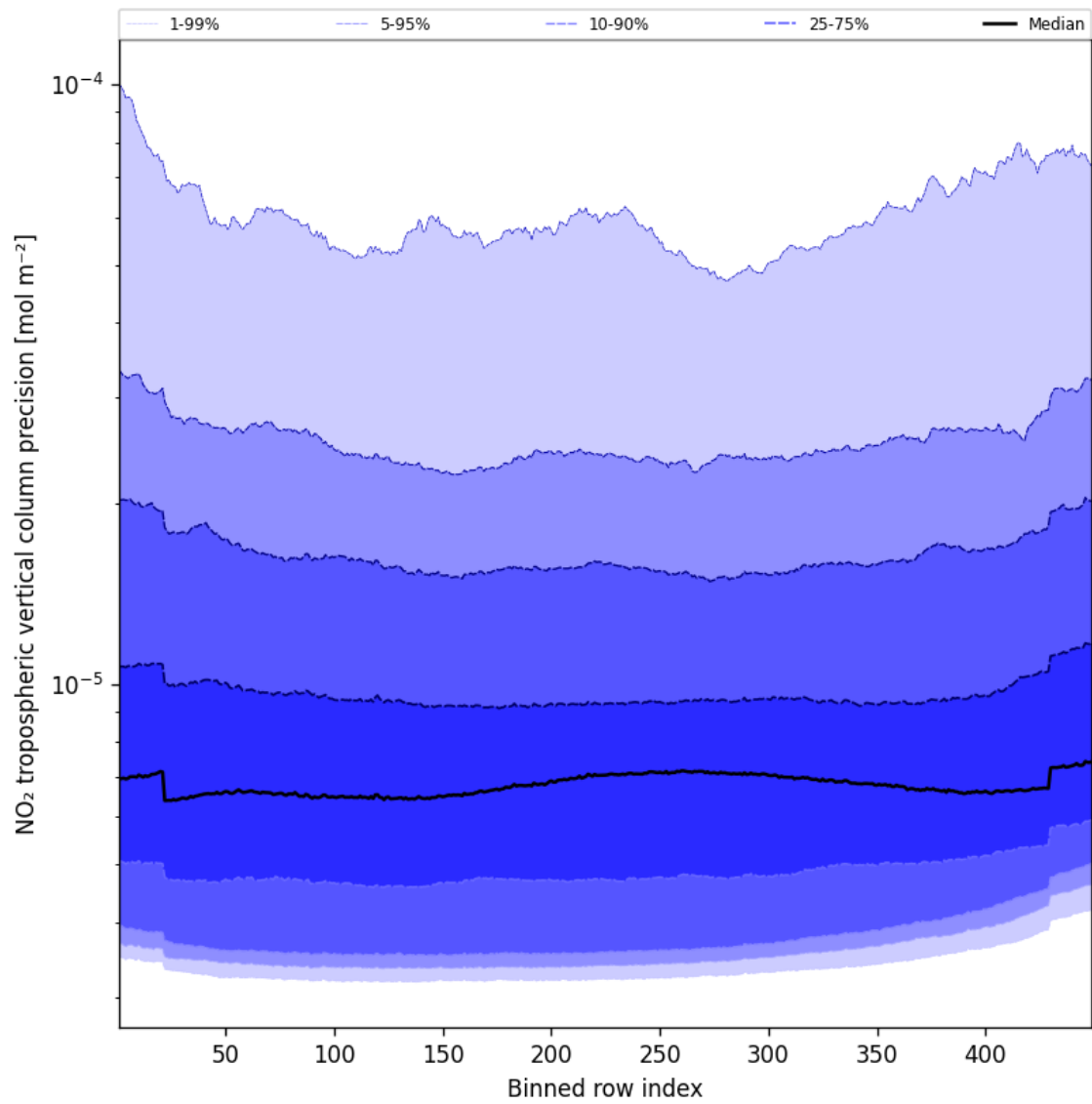
Figure 47: Along track statistics of “NO 2 tropospheric vertical column precision” for 2024-10-30 to 2024-10-31
