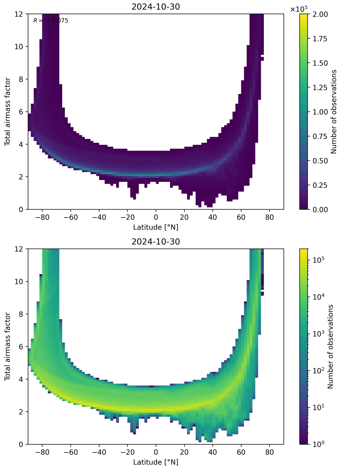
Figure 84: Scatter density plot of “Latitude” against “Total airmass factor” for 2024-10-30 to 2024-10-31.
