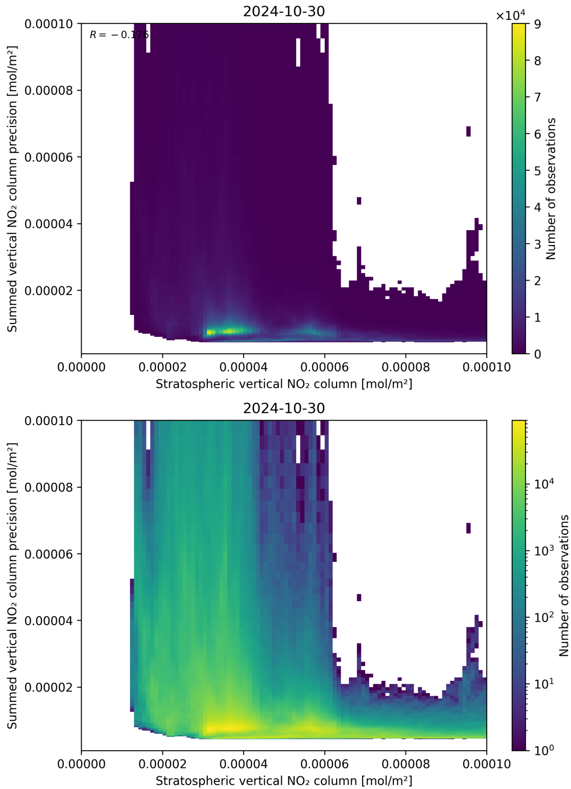
Figure 99: Scatter density plot of “Stratospheric vertical NO 2 column” against “Summed vertical NO 2 column precision” for 2024-10-30 to 2024-10-31.
