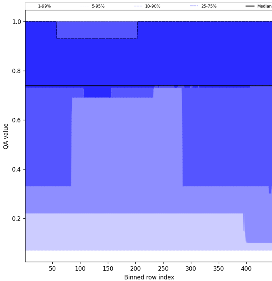
Figure 45: Along track statistics of “QA value” for 2024-10-30 to 2024-10-31
