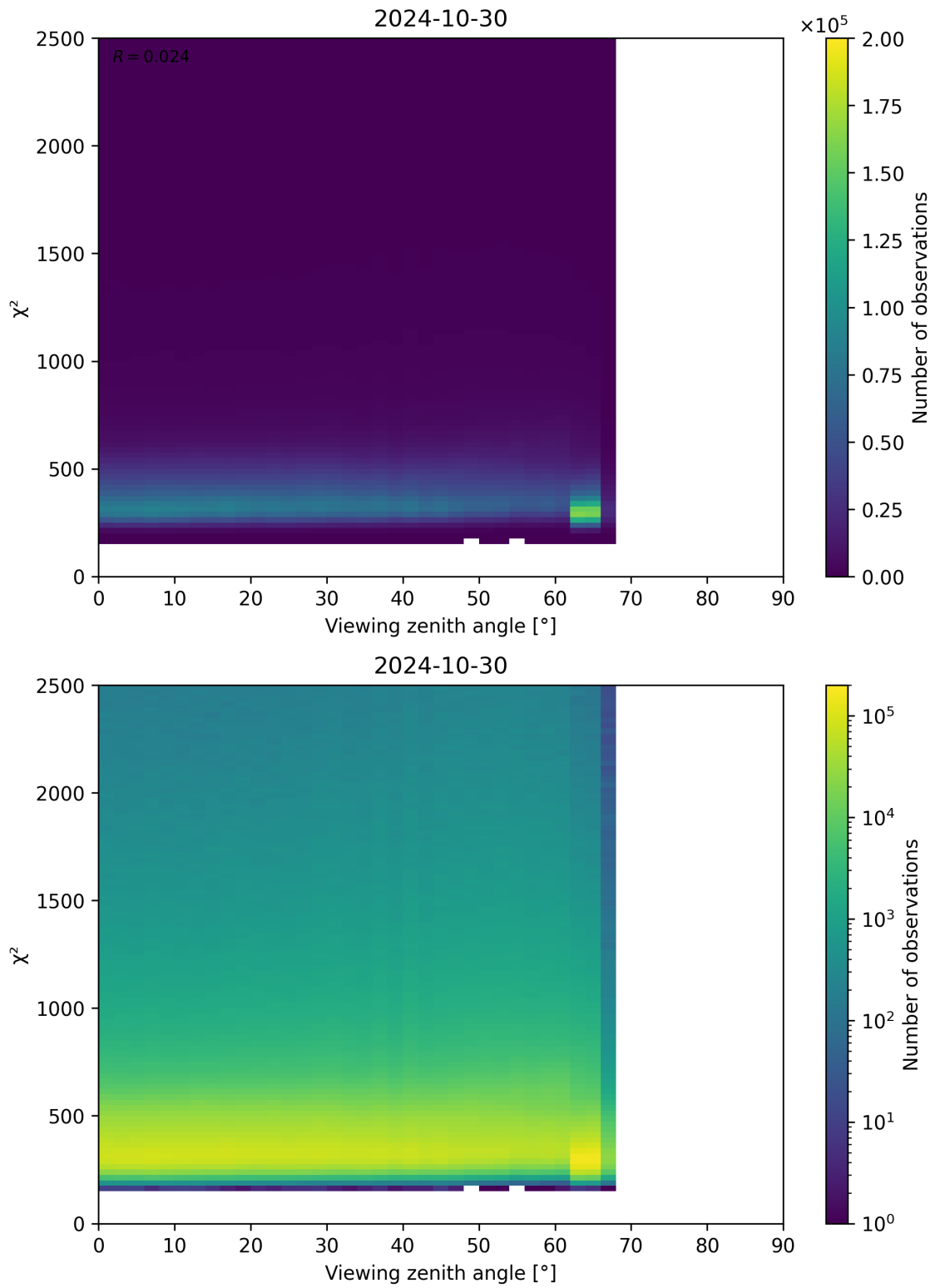
Figure 162: Scatter density plot of “Viewing zenith angle” against “ \chi^2 ” for 2024-10-30 to 2024-10-31.
