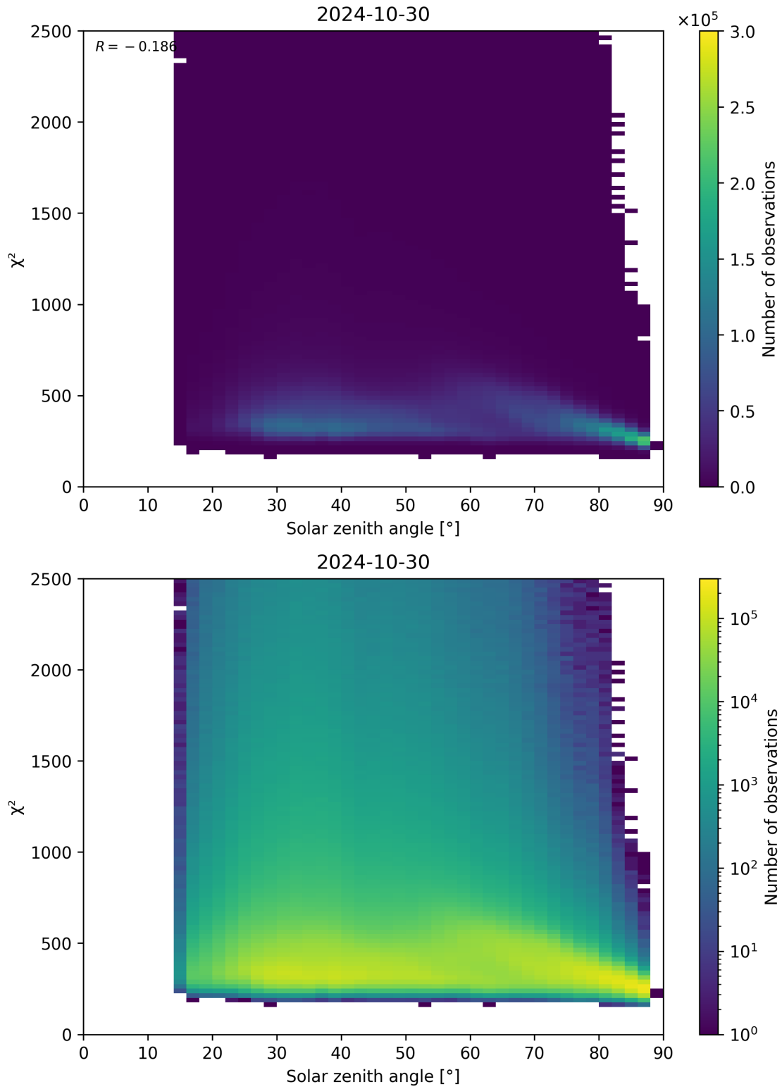
Figure 148: Scatter density plot of “Solar zenith angle” against “ \chi^2 ” for 2024-10-30 to 2024-10-31.
