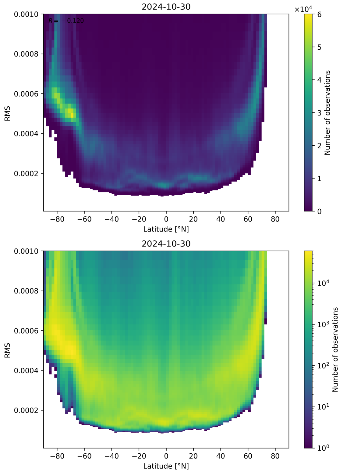
Figure 94: Scatter density plot of “Latitude” against “RMS” for 2024-10-30 to 2024-10-31.
