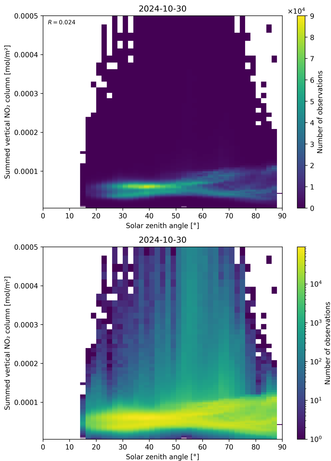
Figure 151: Scatter density plot of “Solar zenith angle” against “Summed vertical NO 2 column” for 2024-10-30 to 2024-10-31.
