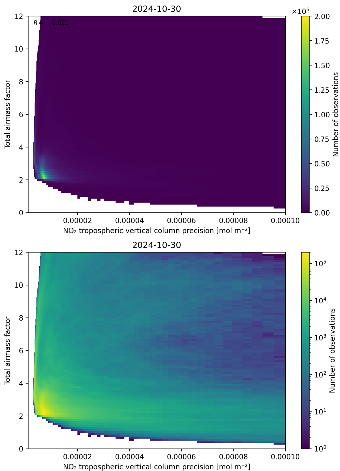
Figure 132: Scatter density plot of “NO 2 tropospheric vertical column precision” against “Total air mass factor” for 2024-10-30 to 2024-10-31.
