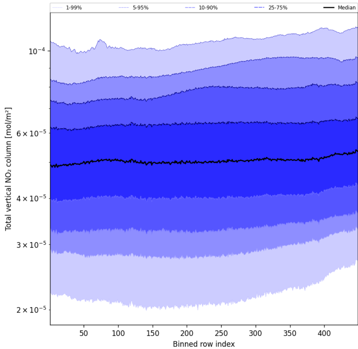
Figure 55: Along track statistics of “Total vertical NO 2 column” for 2024-10-30 to 2024-10-31
