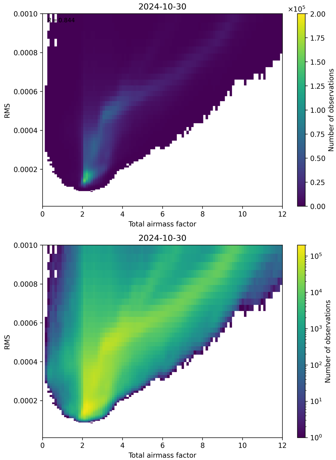
Figure 69: Scatter density plot of “Total airmass factor” against “RMS” for 2024-10-30 to 2024-10-31.
