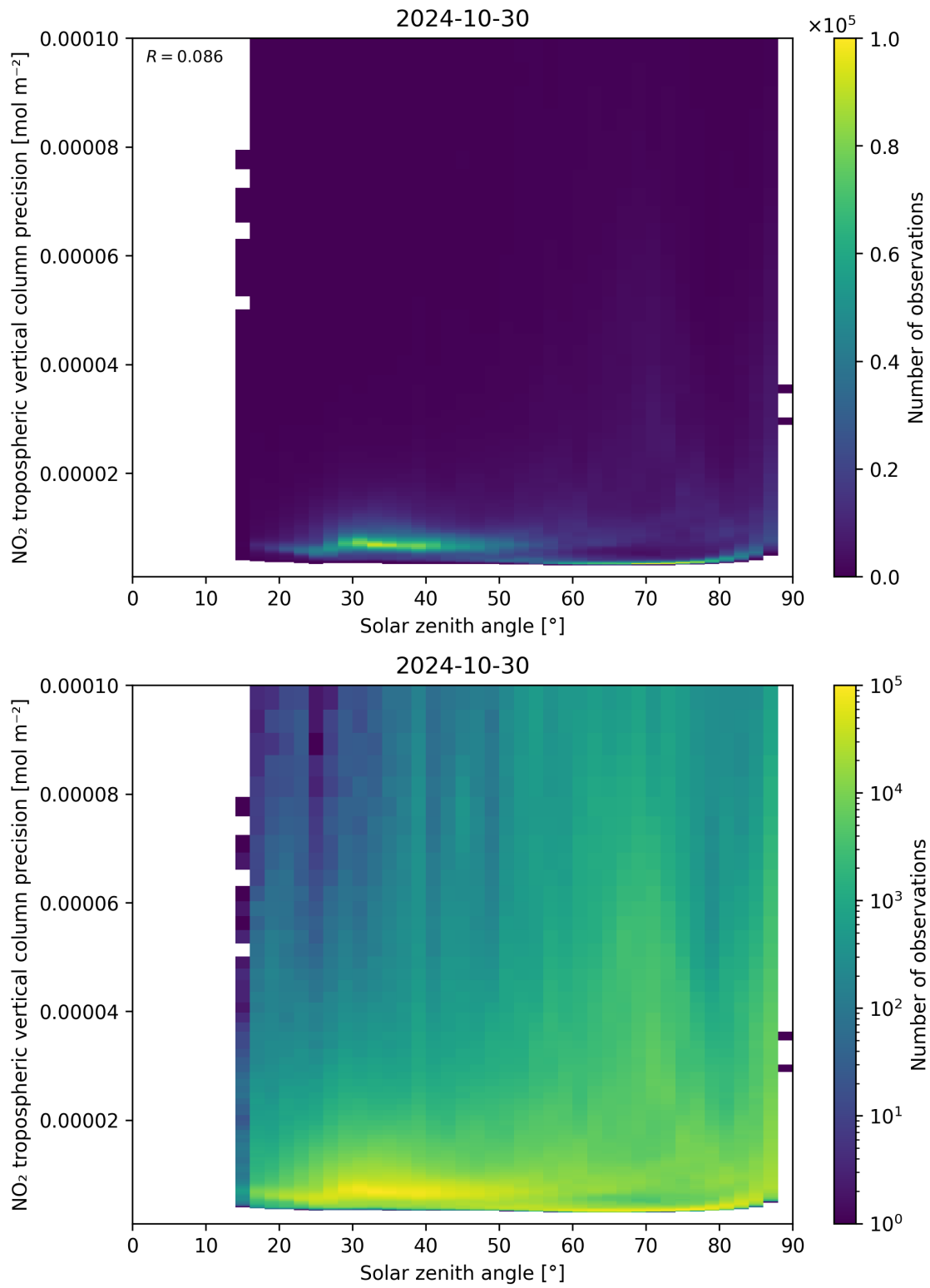
Figure 156: Scatter density plot of “Solar zenith angle” against “NO 2 tropospheric vertical column precision” for 2024-10-30 to 2024-10-31.
