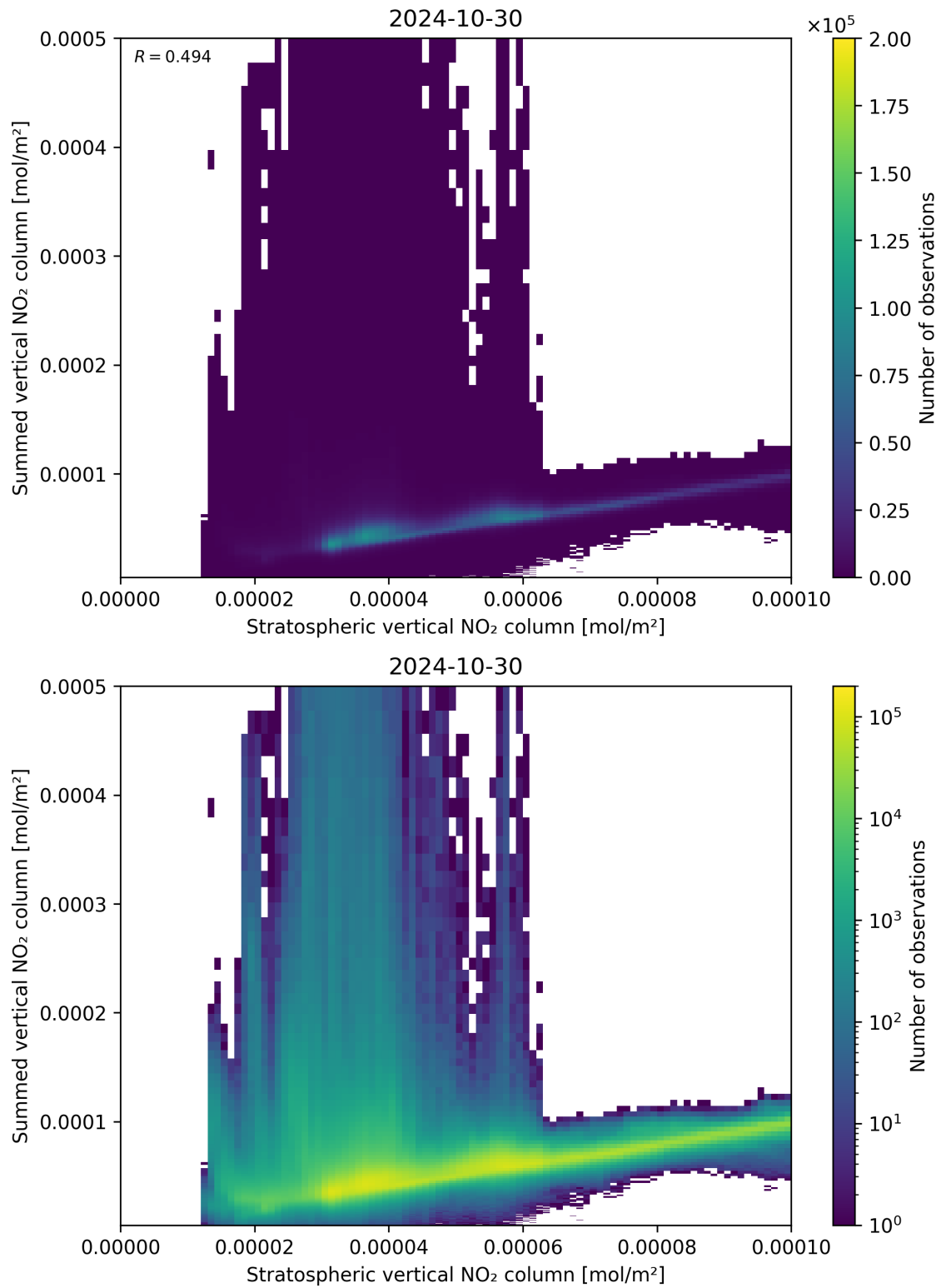
Figure 98: Scatter density plot of “Stratospheric vertical NO 2 column” against “Summed vertical NO 2 column” for 2024-10-30 to 2024-10-31.
