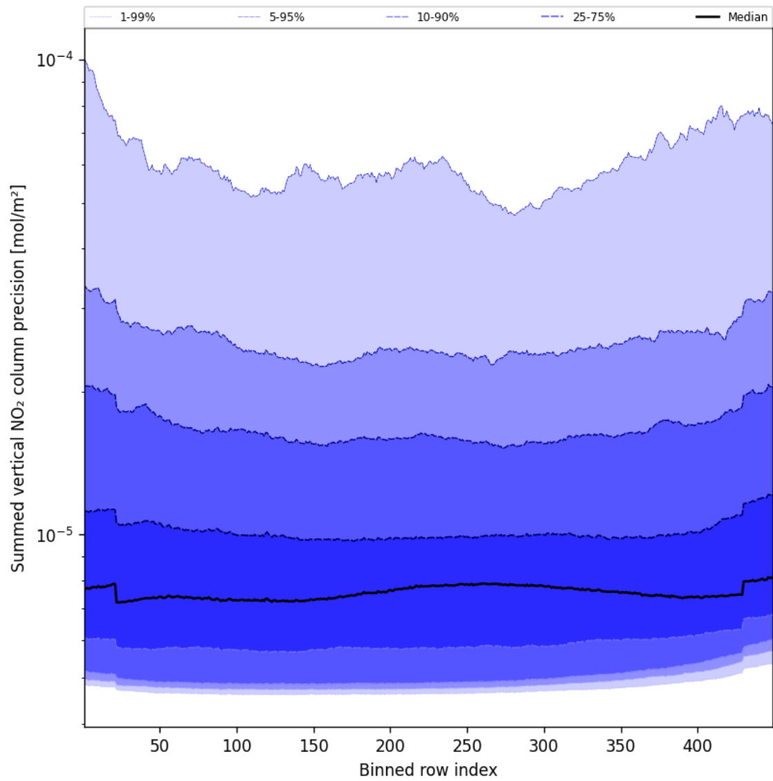
Figure 58: Along track statistics of “Summed vertical NO 2 column precision” for 2024-10-30 to 2024-10-31
