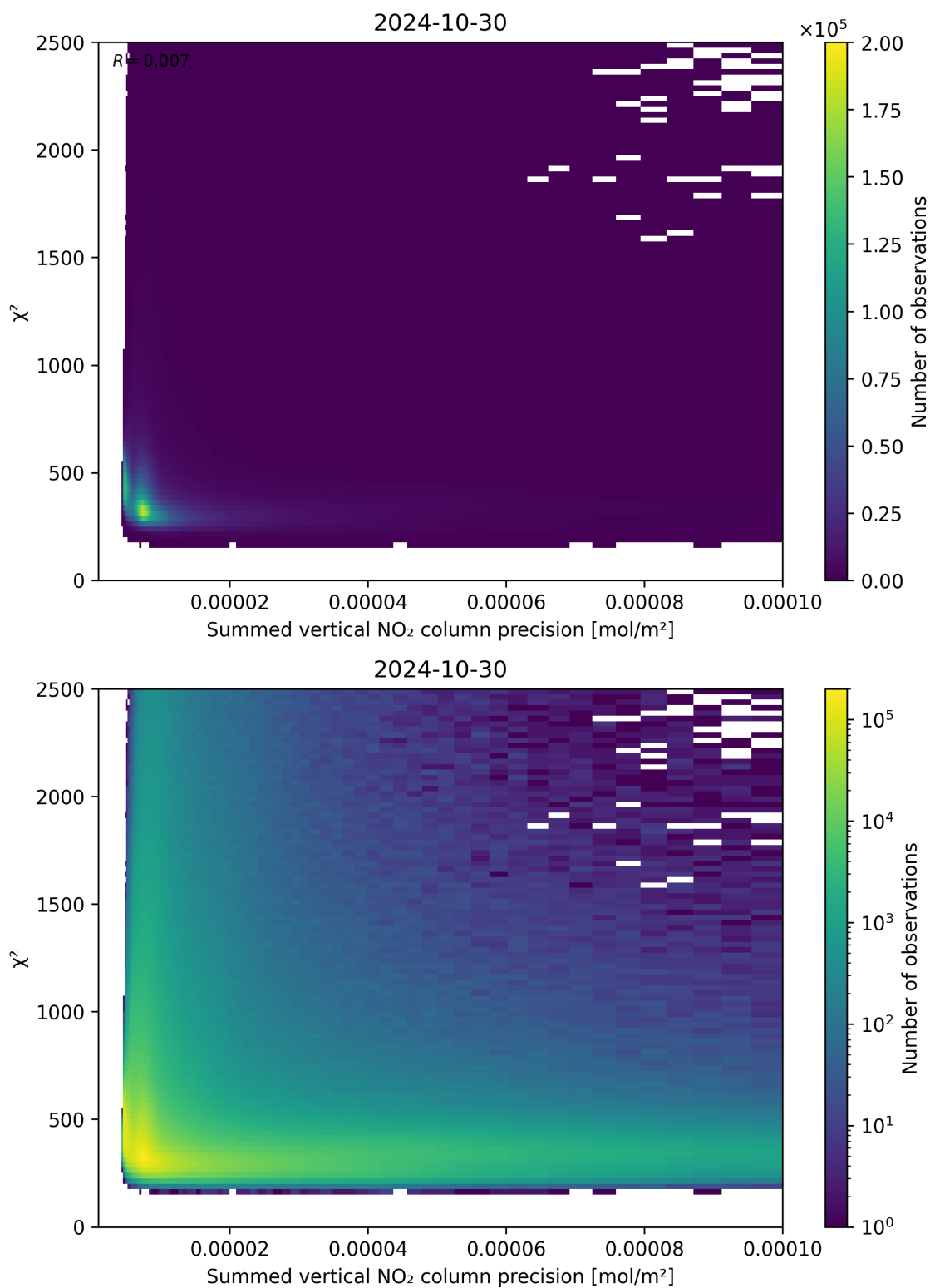
Figure 107: Scatter density plot of “Summed vertical NO 2 column precision” against “ \chi^2 ” for 2024-10-30 to 2024-10-31.
