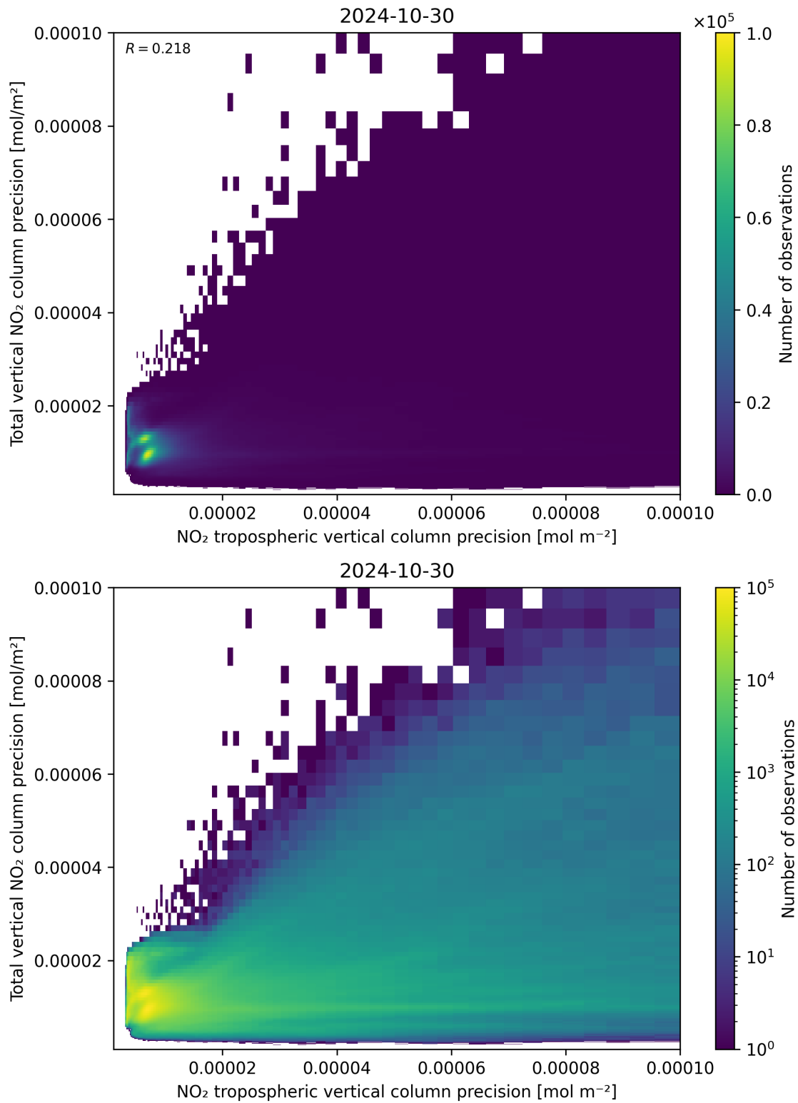
Figure 139: Scatter density plot of “NO 2 tropospheric vertical column precision” against “Total vertical NO 2 column precision” for 2024-10-30 to 2024-10-31.
