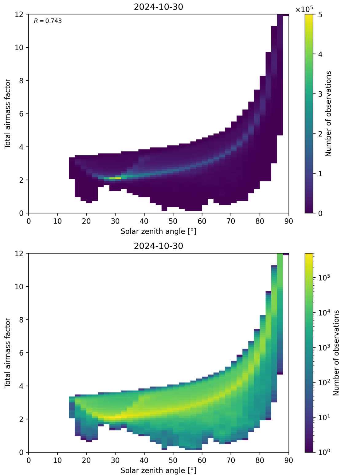
Figure 146: Scatter density plot of “Solar zenith angle” against “Total air mass factor” for 2024-10-30 to 2024-10-31.
