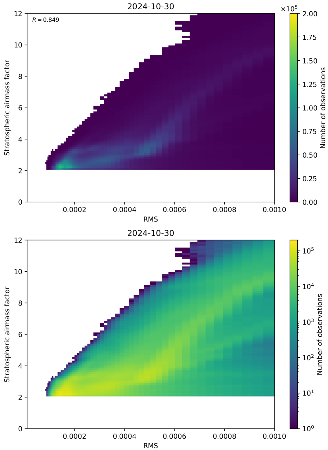
Figure 144: Scatter density plot of “RMS” against “Stratospheric airmass factor” for 2024-10-30 to 2024-10-31.
