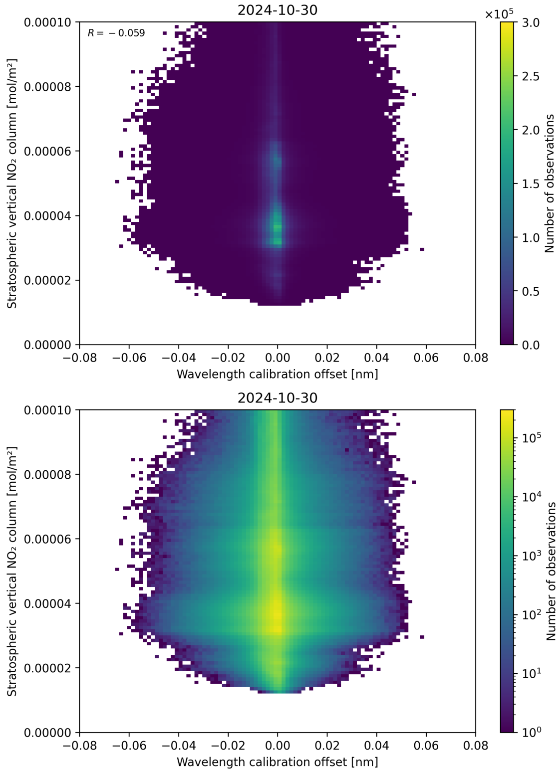
Figure 176: Scatter density plot of “Wavelength calibration offset” against “Stratospheric vertical NO 2 column” for 2024-10-30 to 2024-10-31.
