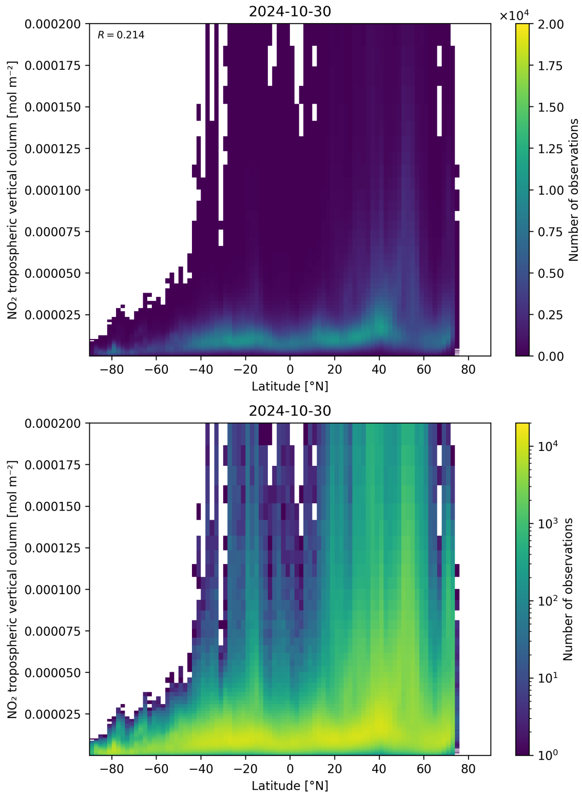
Figure 92: Scatter density plot of “Latitude” against “NO 2 tropospheric vertical column” for 2024-10-30 to 2024-10-31.
