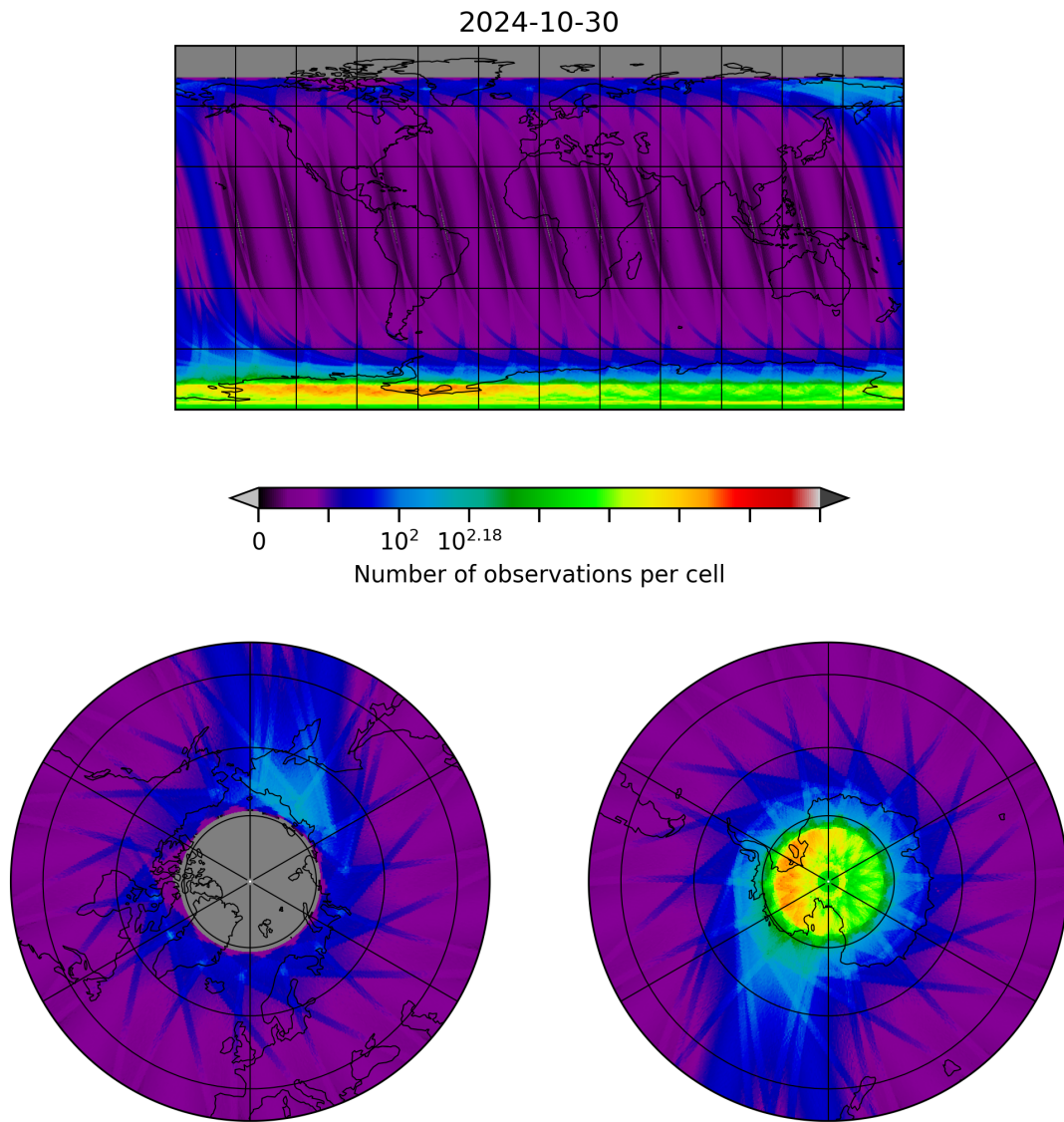
Figure 10: Map of the number of observations for 2024-10-30 to 2024-10-31
