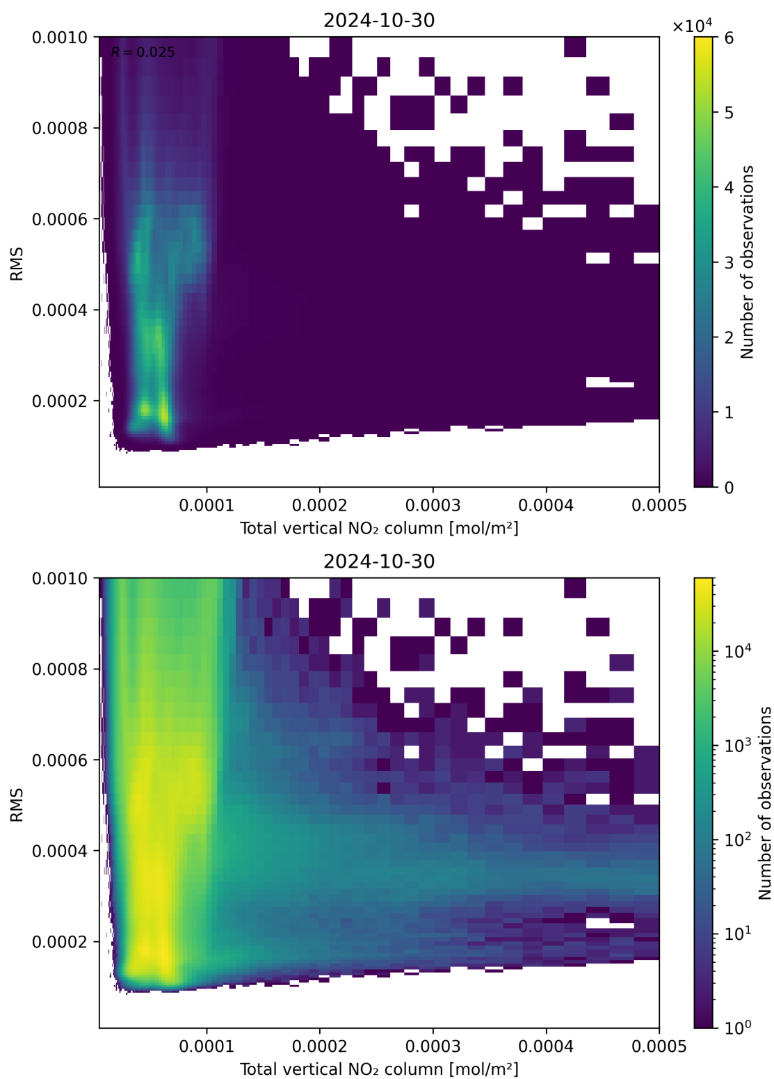
Figure 120: Scatter density plot of “Total vertical NO 2 column” against “RMS” for 2024-10-30 to 2024-10-31.
