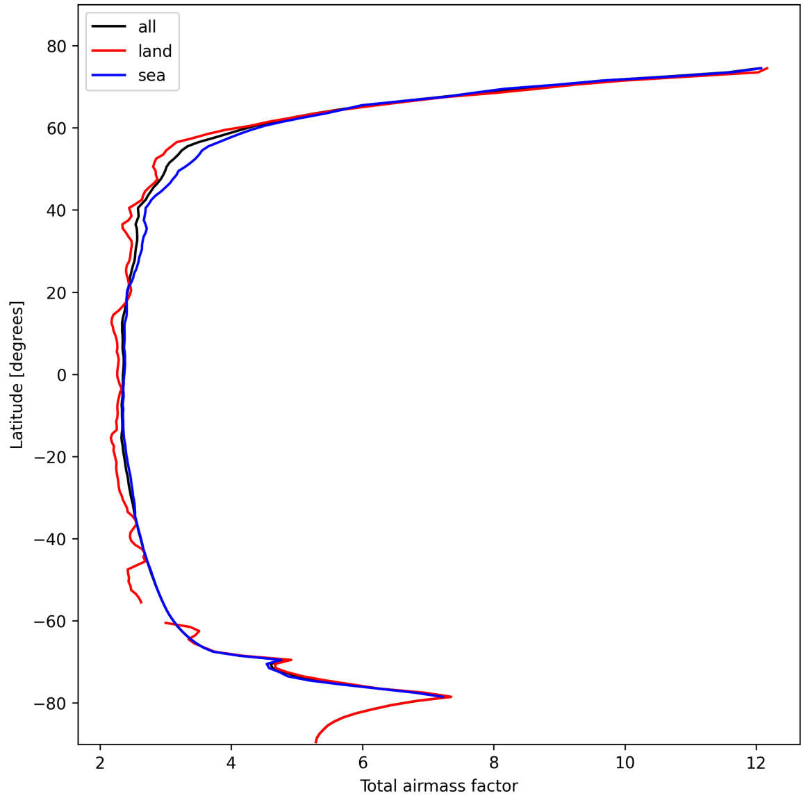
Figure 15: Zonal average of “Total airmass factor” for 2024-10-30 to 2024-10-31.
