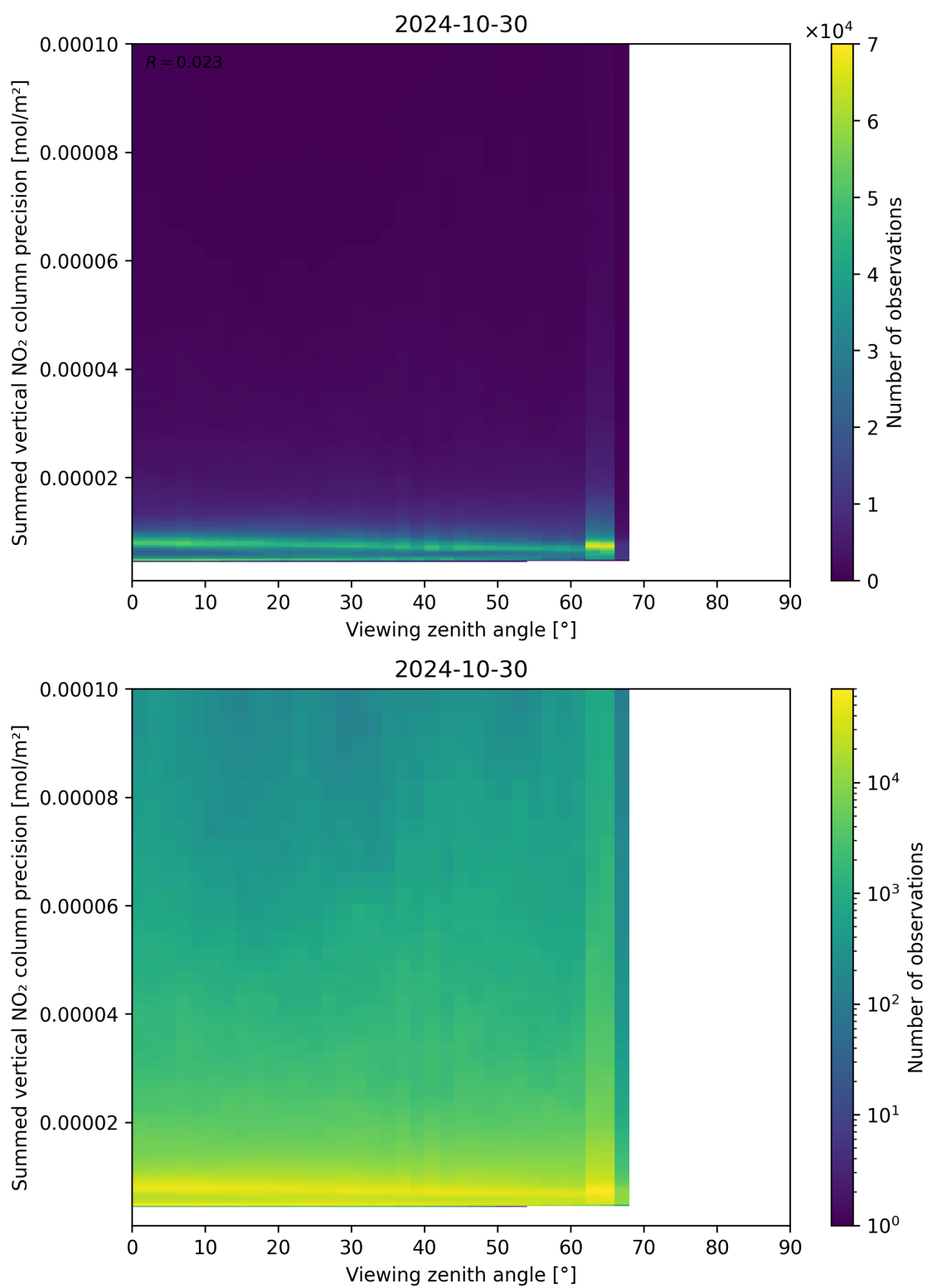
Figure 166: Scatter density plot of “Viewing zenith angle” against “Summed vertical NO 2 column precision” for 2024-10-30 to 2024-10-31.
