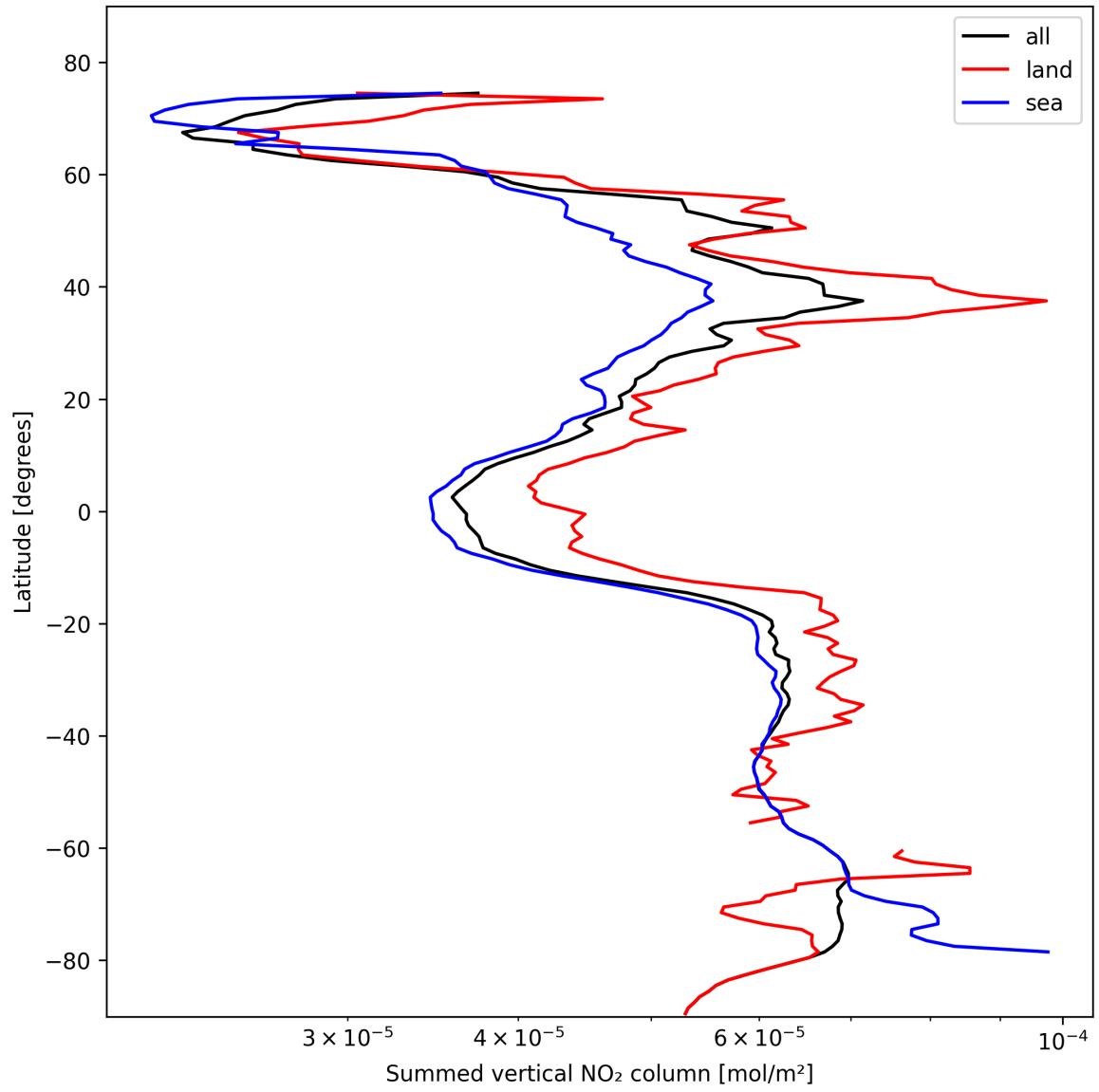
Figure 23: Zonal average of “Summed vertical NO 2 column” for 2024-10-30 to 2024-10-31.
