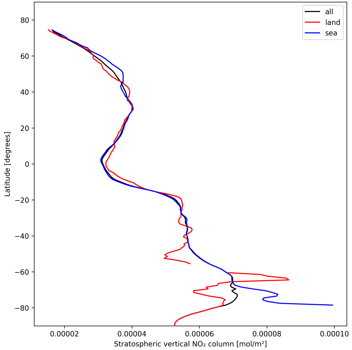
Figure 19: Zonal average of “Stratospheric vertical NO 2 column” for 2024-10-30 to 2024-10-31.
