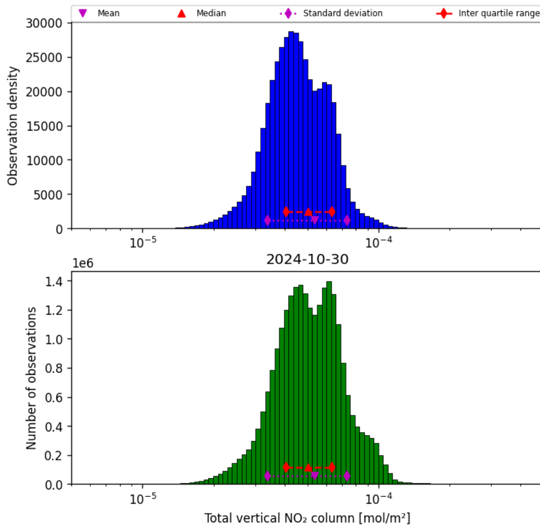
Figure 38: Histogram of “Total vertical NO 2 column” for 2024-10-30 to 2024-10-31
