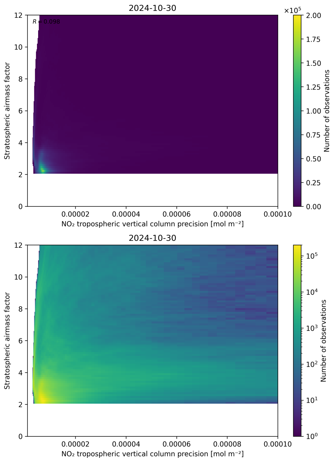
Figure 131: Scatter density plot of “NO 2 tropospheric vertical column precision” against “Stratospheric airmass factor” for 2024-10-30 to 2024-10-31.
