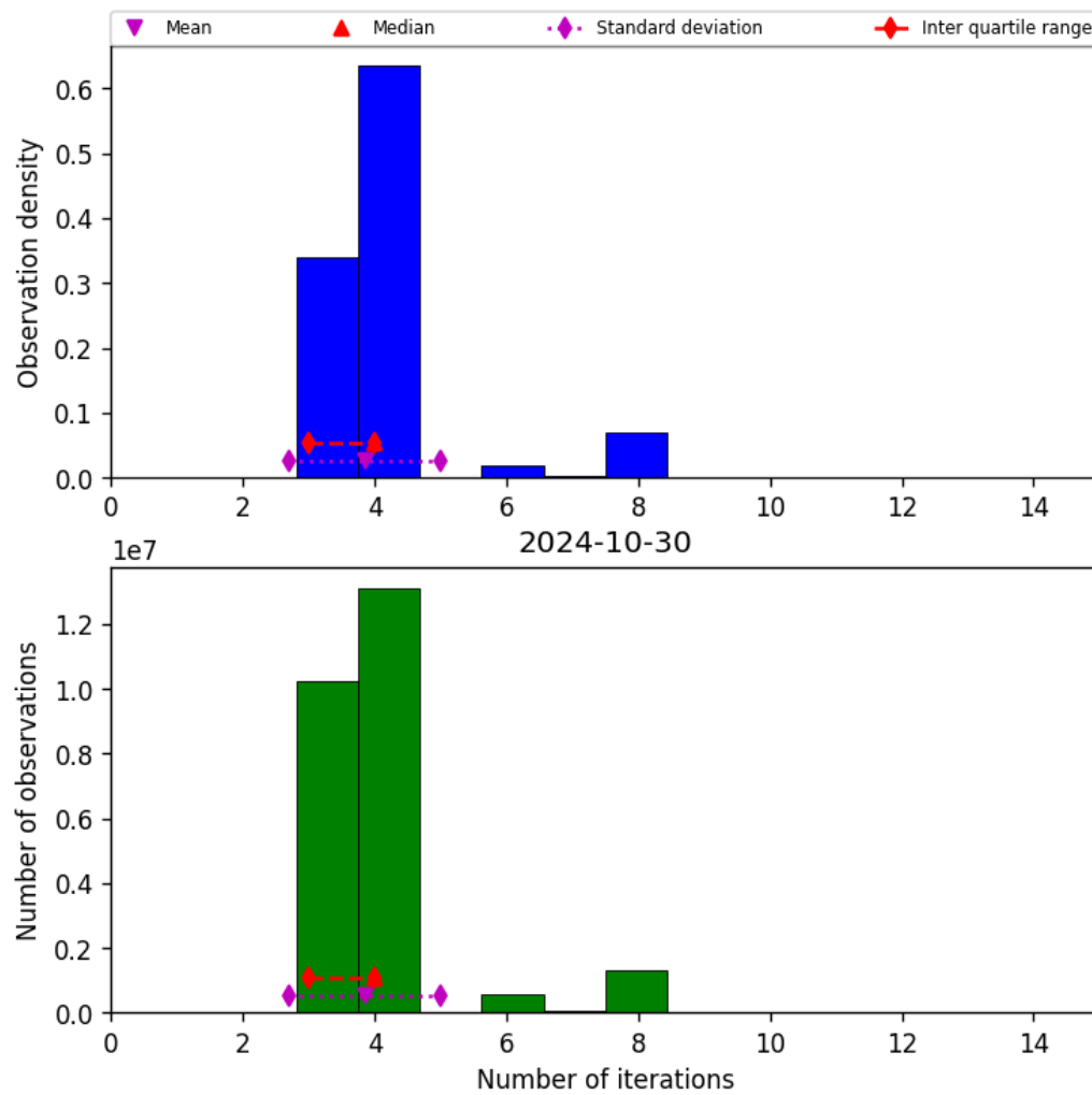
Figure 34: Histogram of “Number of iterations” for 2024-10-30 to 2024-10-31
