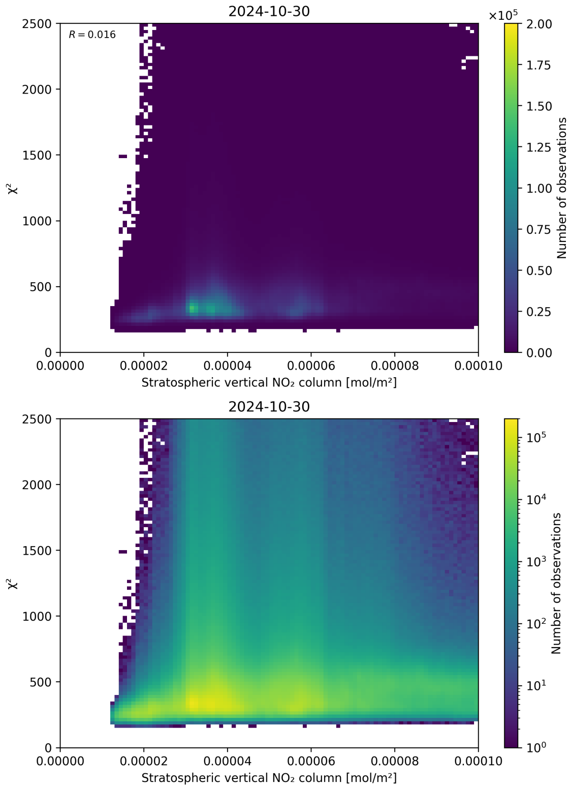
Figure 97: Scatter density plot of “Stratospheric vertical NO 2 column” against “ \chi^2 ” for 2024-10-30 to 2024-10-31.
