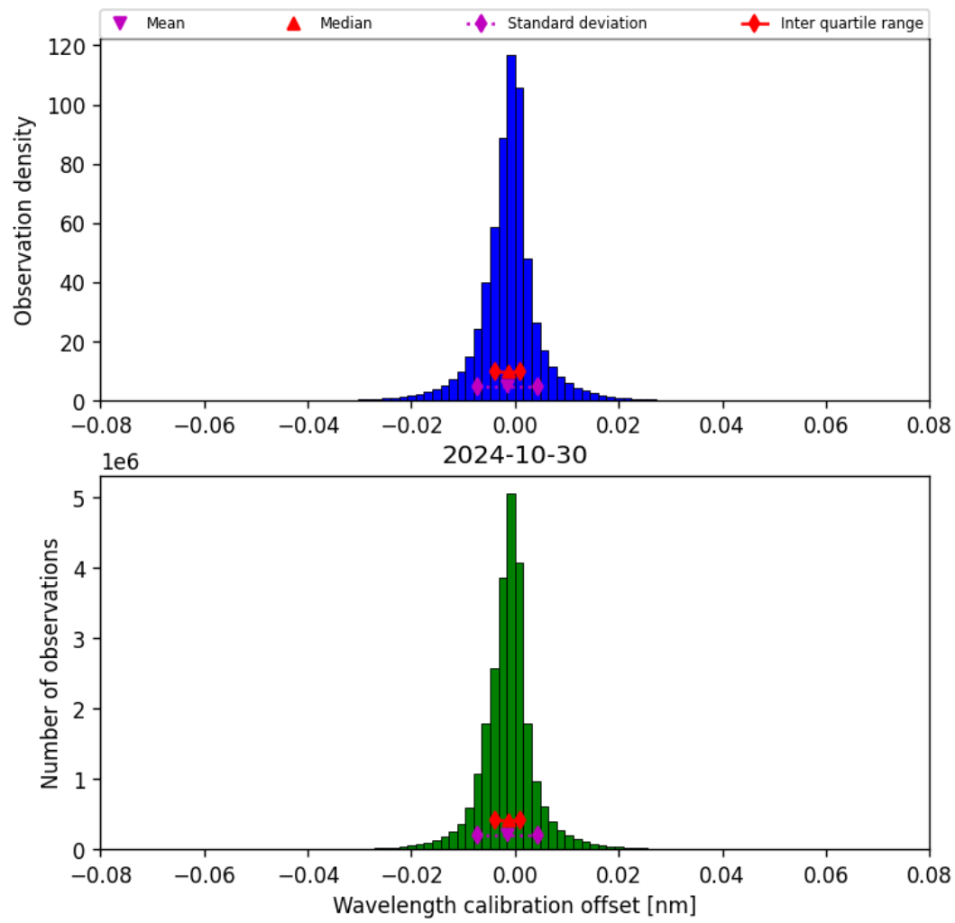
Figure 35: Histogram of “Wavelength calibration offset” for 2024-10-30 to 2024-10-31
