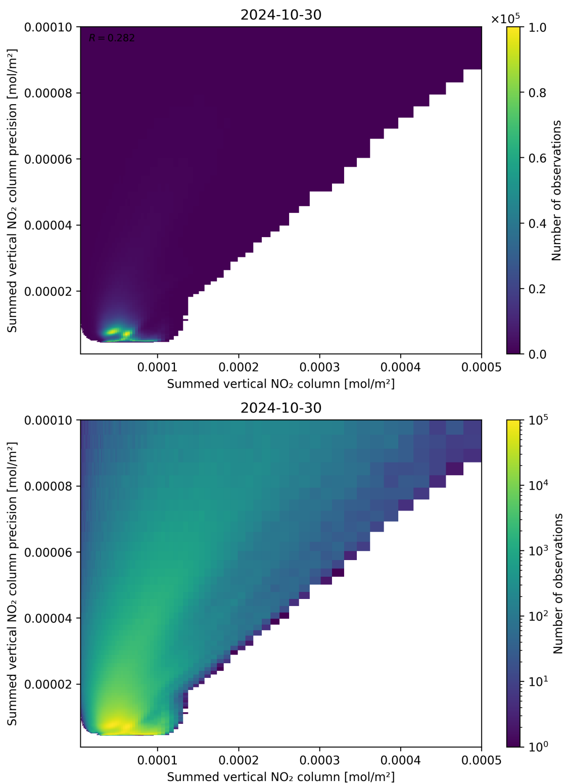
Figure 105: Scatter density plot of “Summed vertical NO 2 column” against “Summed vertical NO 2 column precision” for 2024-10-30 to 2024-10-31.
