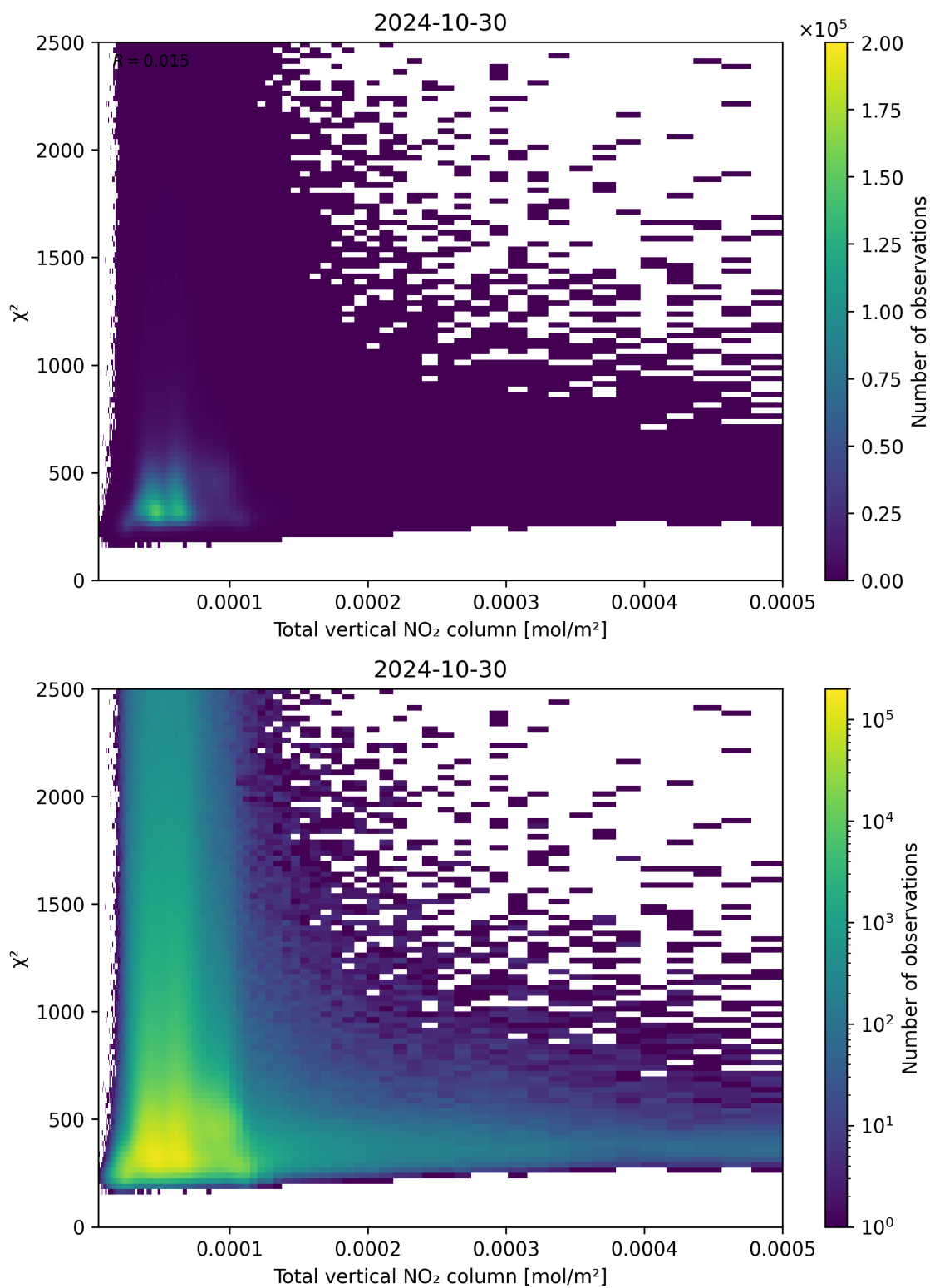
Figure 111: Scatter density plot of “Total vertical NO 2 column” against “ \chi^2 ” for 2024-10-30 to 2024-10-31.
