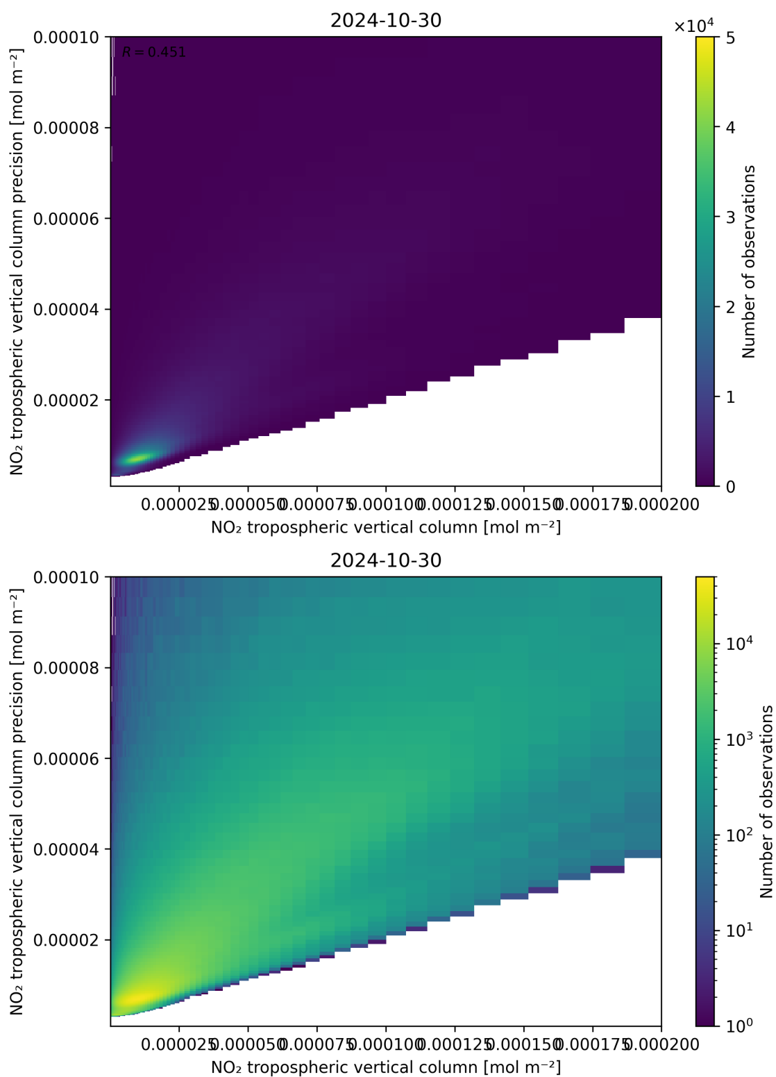
Figure 130: Scatter density plot of “NO 2 tropospheric vertical column” against “NO 2 tropospheric vertical column precision” for 2024-10-30 to 2024-10-31.
