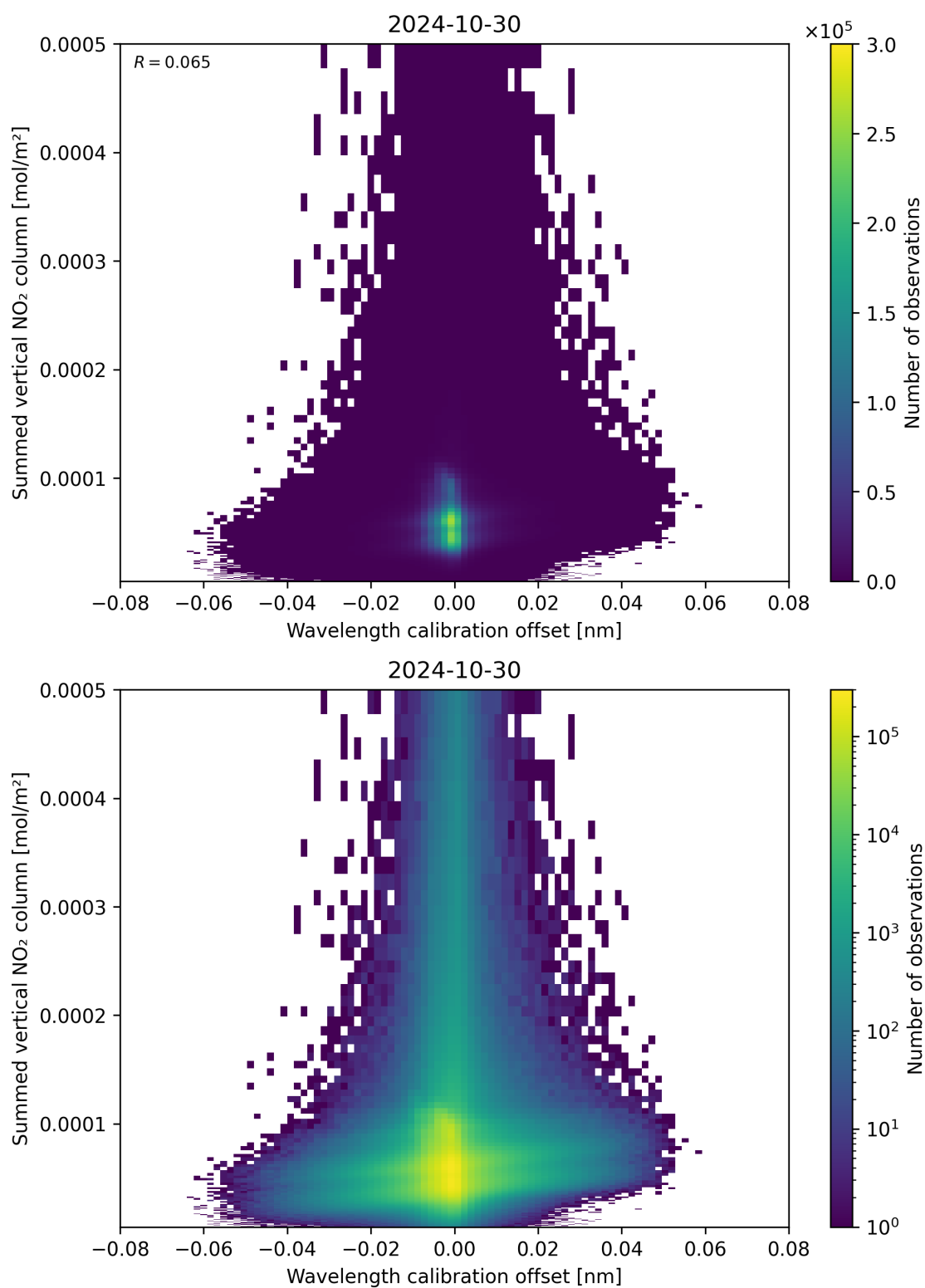
Figure 177: Scatter density plot of “Wavelength calibration offset” against “Summed vertical NO 2 column” for 2024-10-30 to 2024-10-31.
