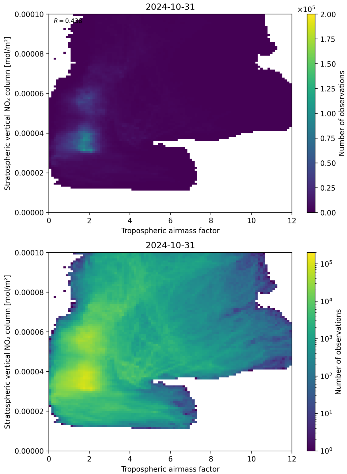
Figure 74: Scatter density plot of “Tropospheric air mass factor” against “Stratospheric vertical NO 2 column” for 2024-10-30 to 2024-11-01.
