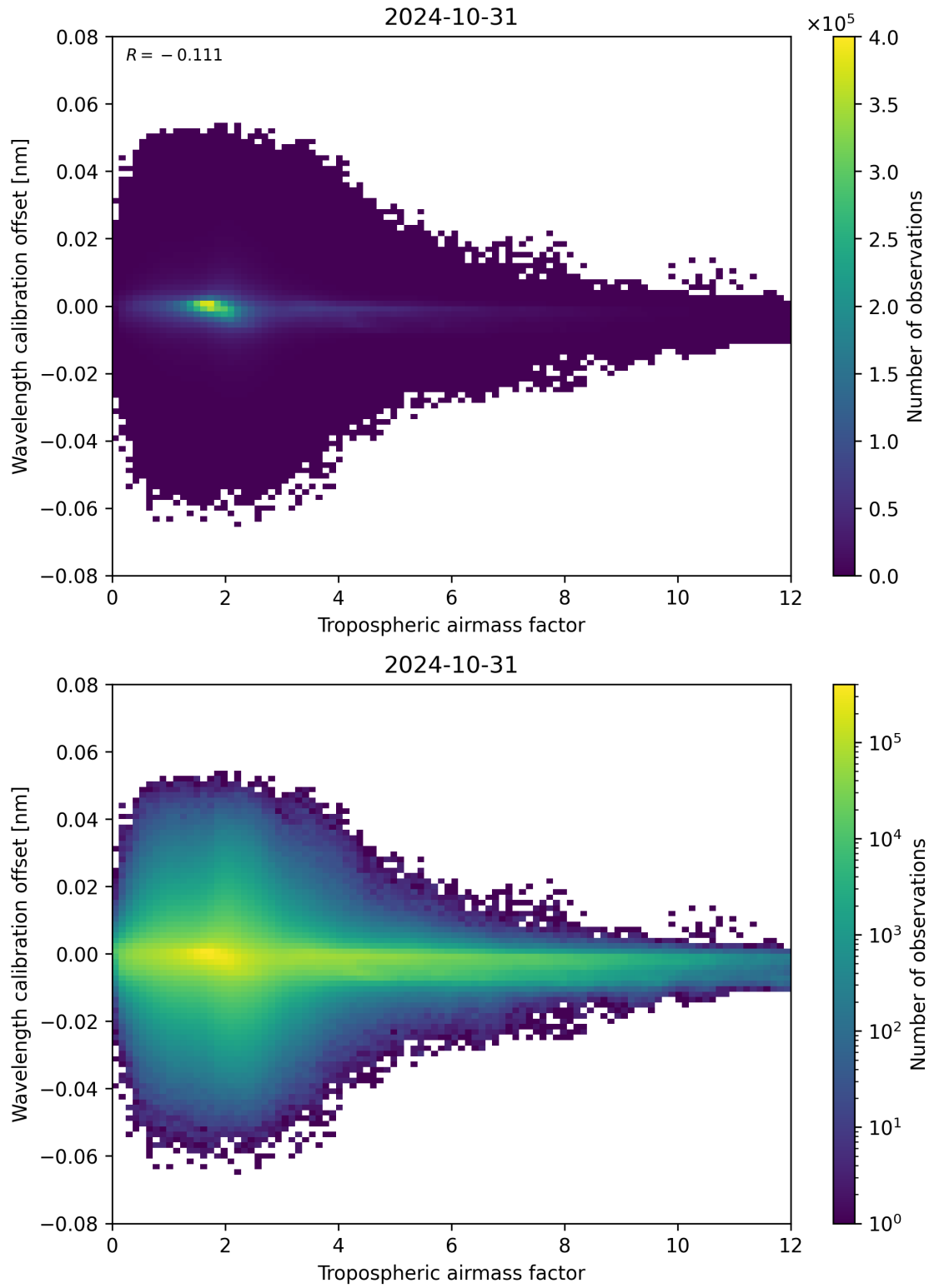
Figure 80: Scatter density plot of “Tropospheric airmass factor” against “Wavelength calibration offset” for 2024-10-30 to 2024-11-01.
