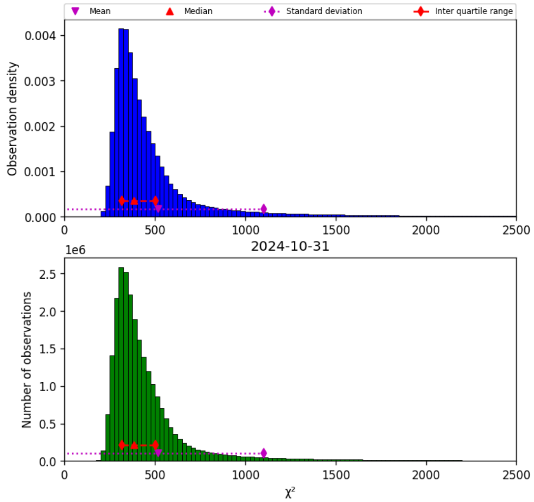
Figure 42: Histogram of “ \chi^2 ” for 2024-10-30 to 2024-11-01
