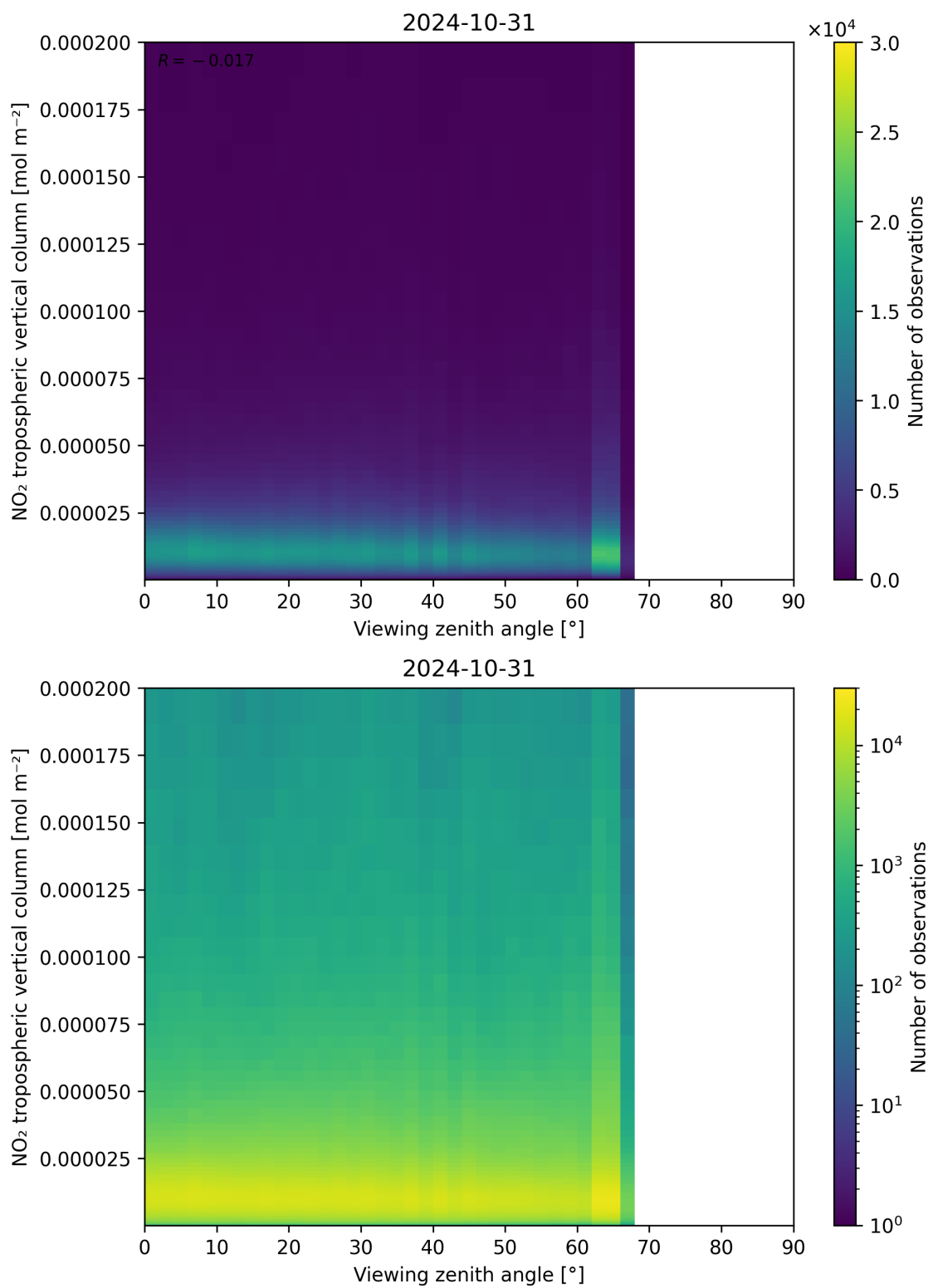
Figure 169: Scatter density plot of “Viewing zenith angle” against “NO 2 tropospheric vertical column” for 2024-10-30 to 2024-11-01.
