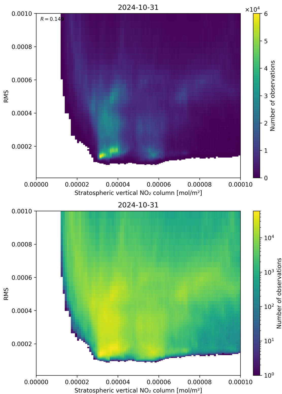
Figure 102: Scatter density plot of “Stratospheric vertical NO 2 column” against “RMS” for 2024-10-30 to 2024-11-01.
