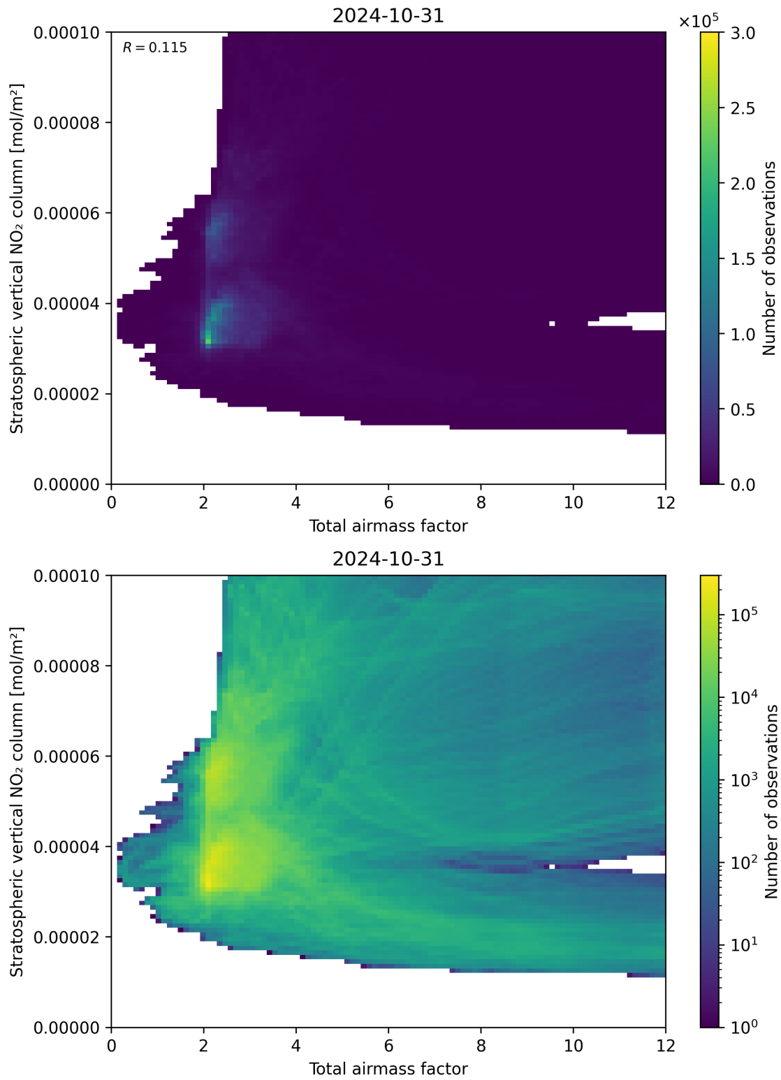
Figure 64: Scatter density plot of “Total airmass factor” against “Stratospheric vertical NO 2 column” for 2024-10-30 to 2024-11-01.
