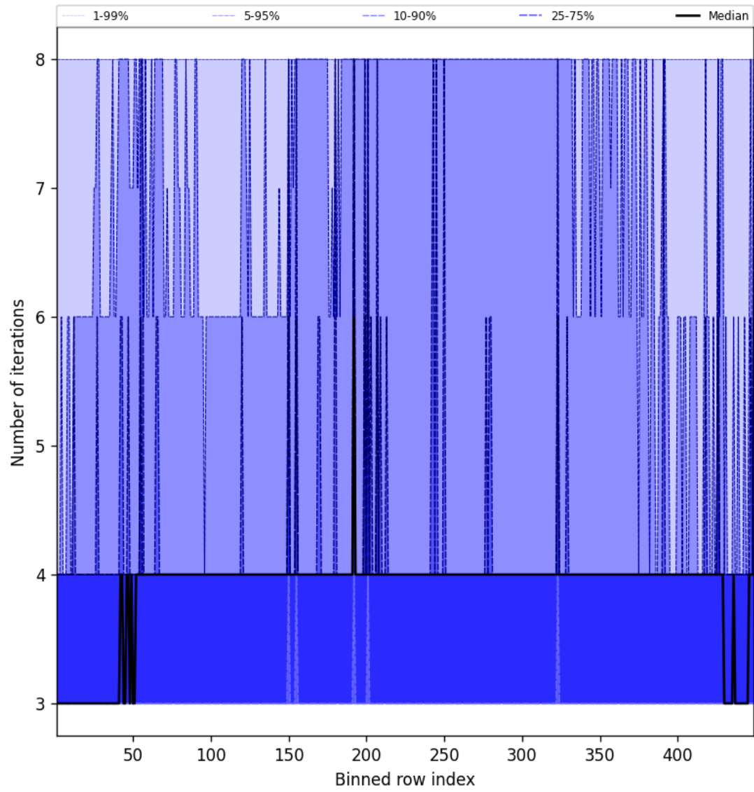
Figure 51: Along track statistics of “Number of iterations” for 2024-10-30 to 2024-11-01
