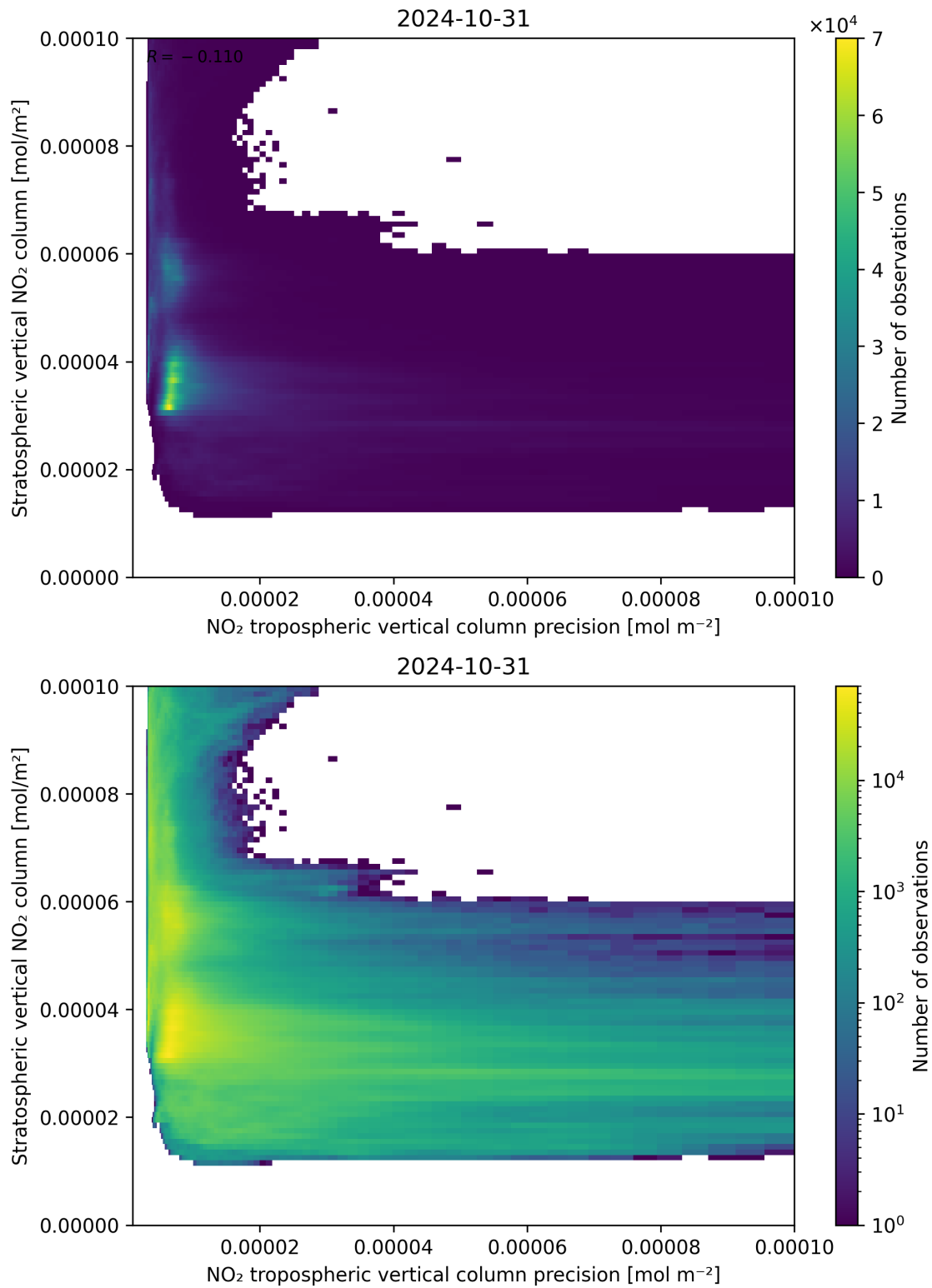
Figure 135: Scatter density plot of “NO 2 tropospheric vertical column precision” against “Stratospheric vertical NO 2 column” for 2024-10-30 to 2024-11-01.
