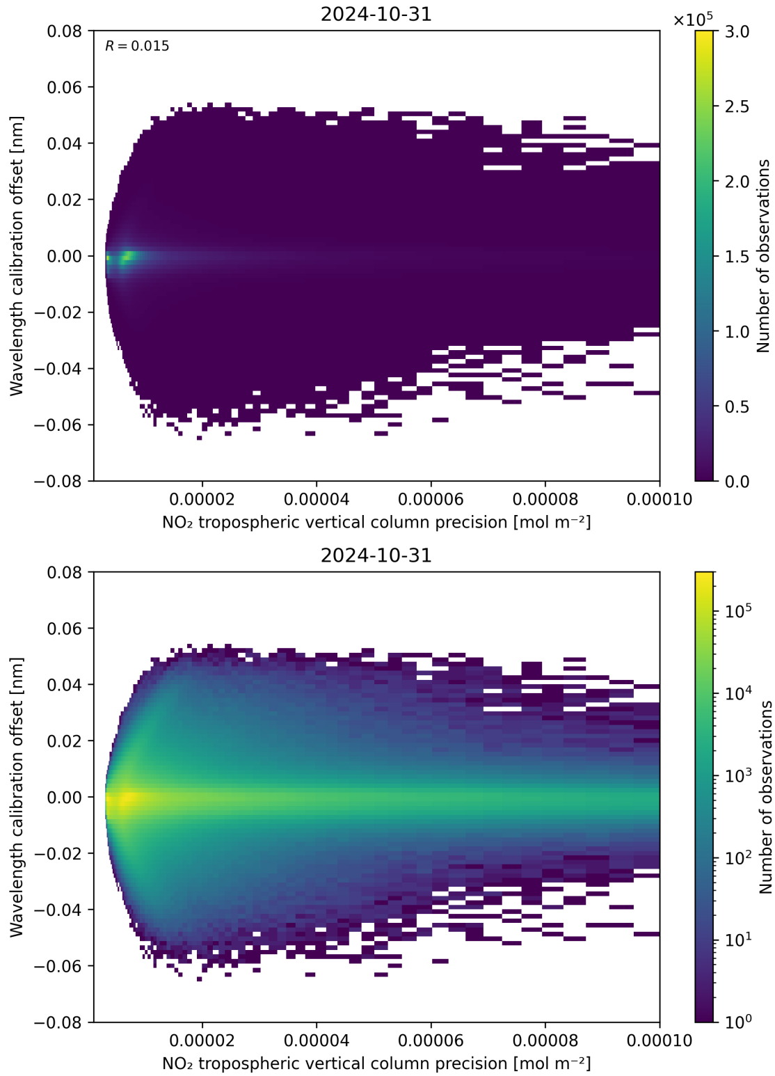
Figure 141: Scatter density plot of “NO 2 tropospheric vertical column precision” against “Wavelength calibration offset” for 2024-10-30 to 2024-11-01.
