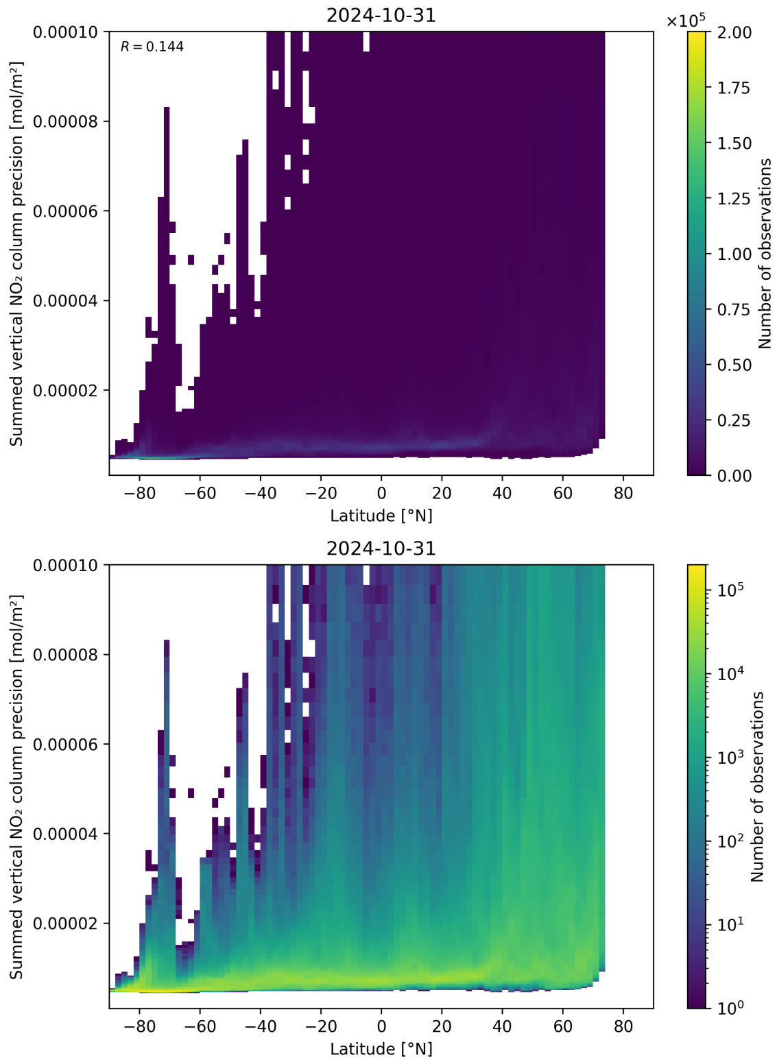
Figure 89: Scatter density plot of “Latitude” against “Summed vertical NO 2 column precision” for 2024-10-30 to 2024-11-01.
