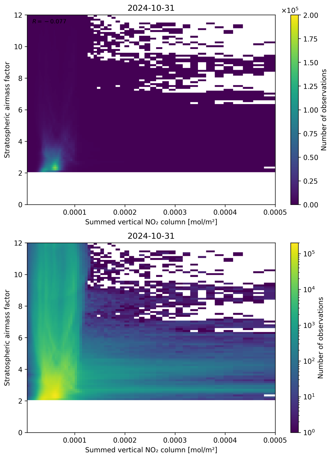
Figure 103: Scatter density plot of “Summed vertical NO 2 column” against “Stratospheric air mass factor” for 2024-10-30 to 2024-11-01.
