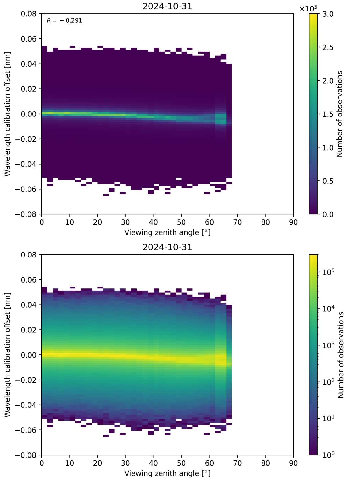
Figure 173: Scatter density plot of “Viewing zenith angle” against “Wavelength calibration offset” for 2024-10-30 to 2024-11-01.
