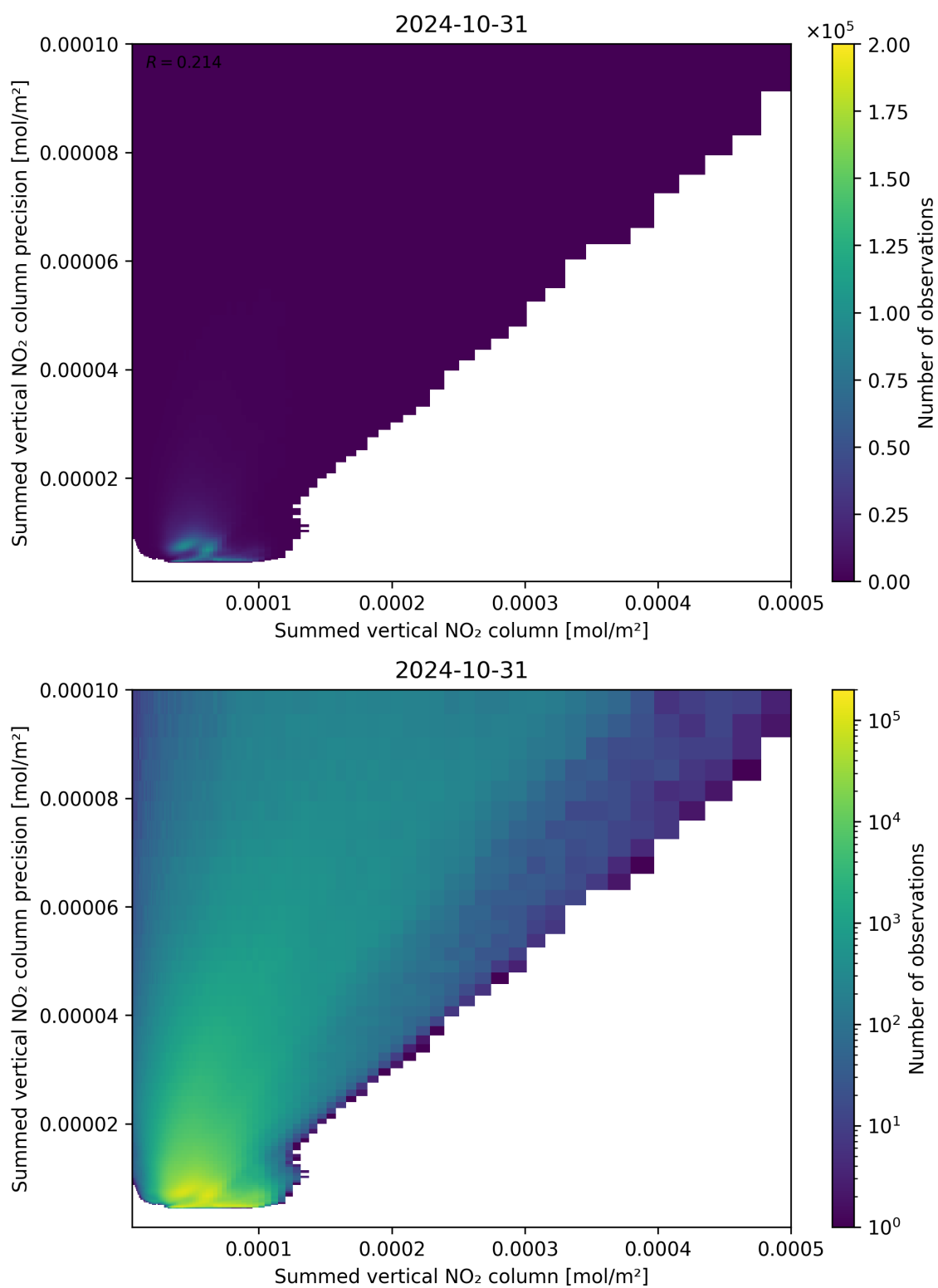
Figure 105: Scatter density plot of “Summed vertical NO 2 column” against “Summed vertical NO 2 column precision” for 2024-10-30 to 2024-11-01.
