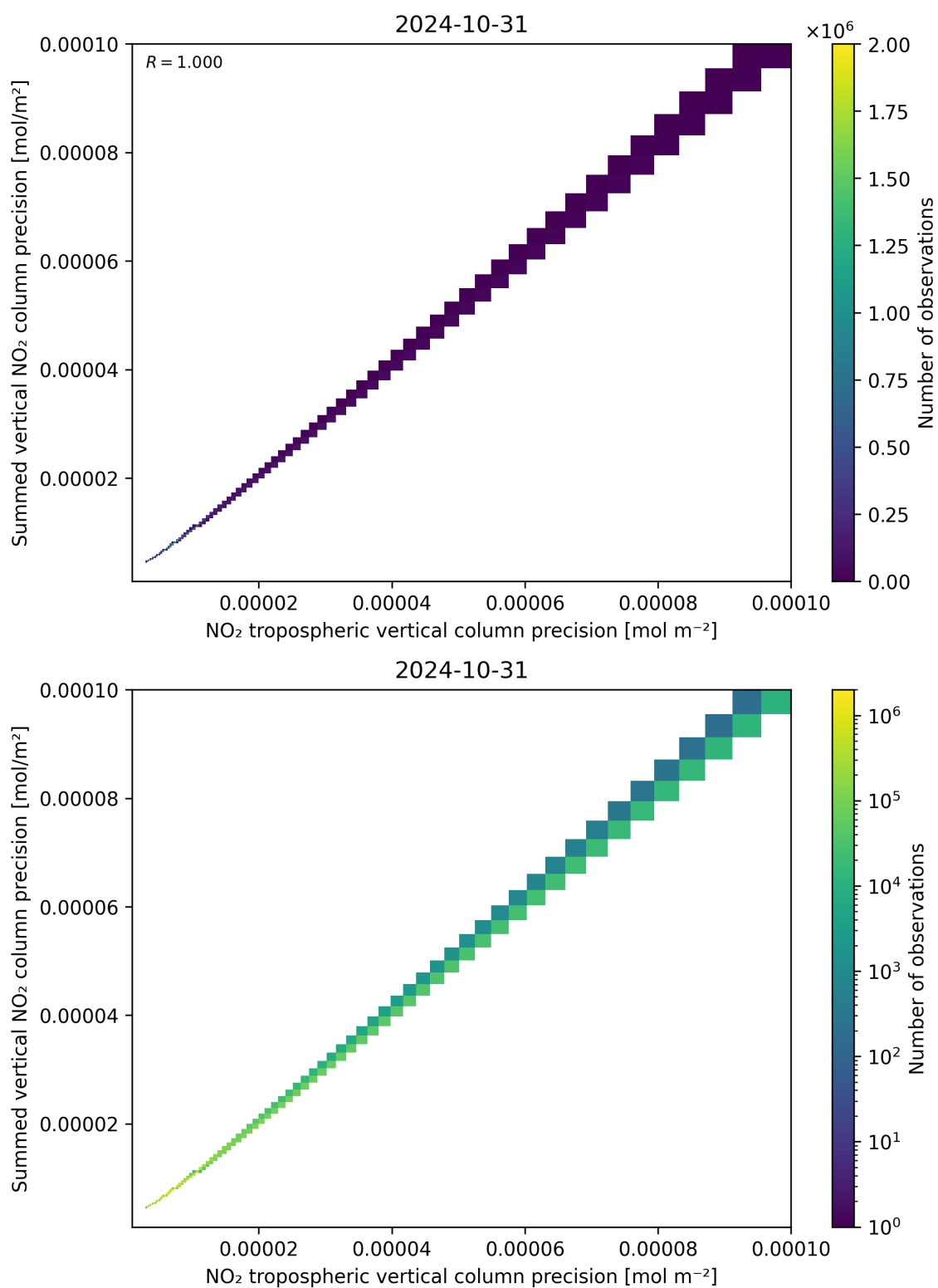
Figure 137: Scatter density plot of “NO 2 tropospheric vertical column precision” against “Summed vertical NO 2 column precision” for 2024-10-30 to 2024-11-01.
