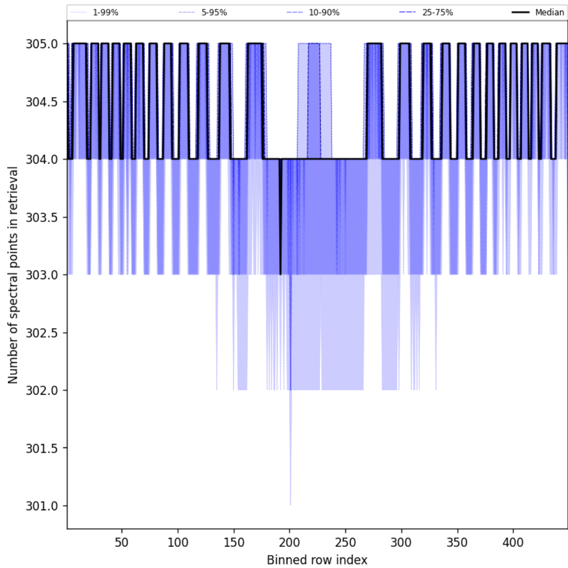
Figure 50: Along track statistics of “Number of spectral points in retrieval” for 2024-10-30 to 2024-11-01
