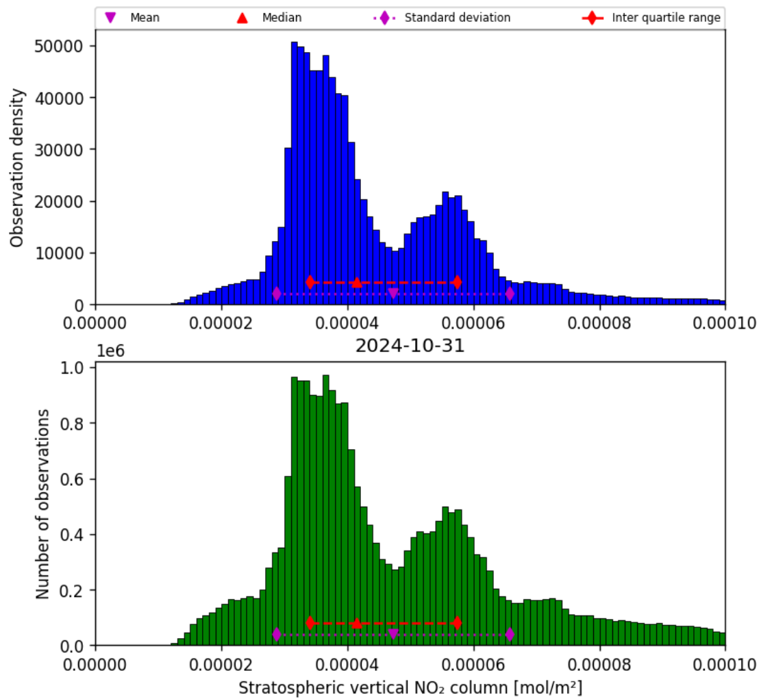
Figure 36: Histogram of “Stratospheric vertical NO 2 column” for 2024-10-30 to 2024-11-01
