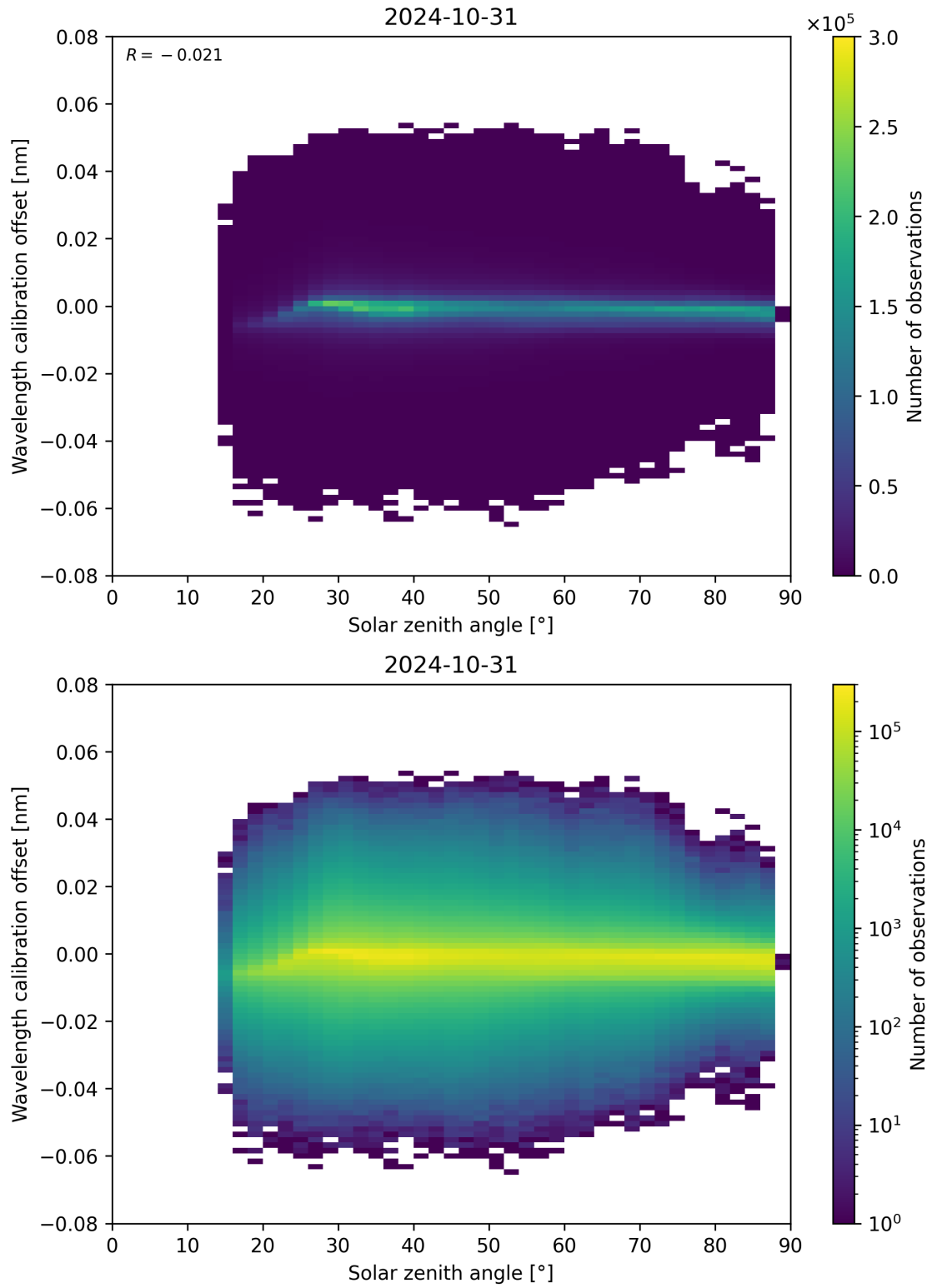
Figure 158: Scatter density plot of “Solar zenith angle” against “Wavelength calibration offset” for 2024-10-30 to 2024-11-01.
