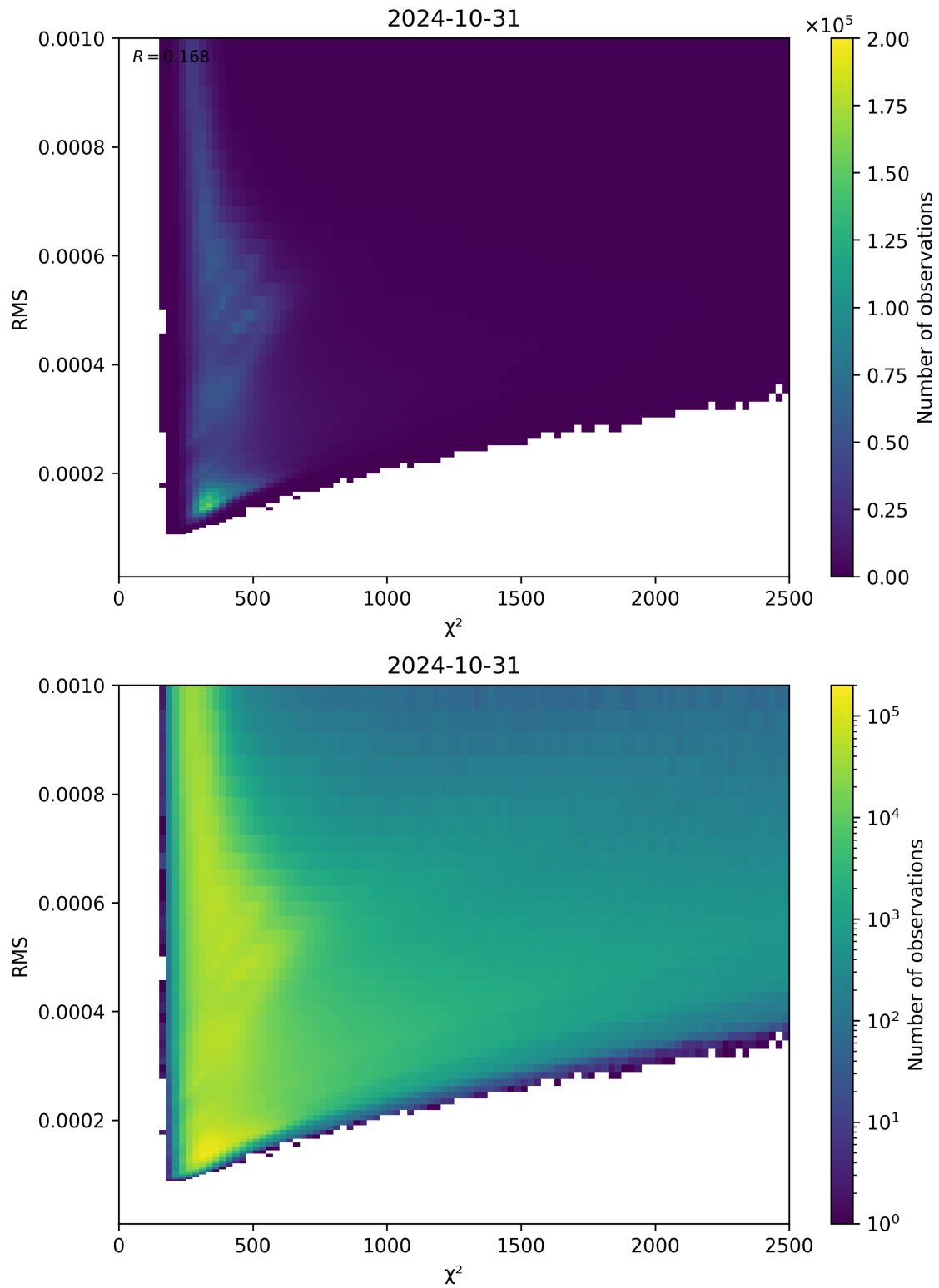
Figure 82: Scatter density plot of “ \chi^2 ” against “RMS” for 2024-10-30 to 2024-11-01.
