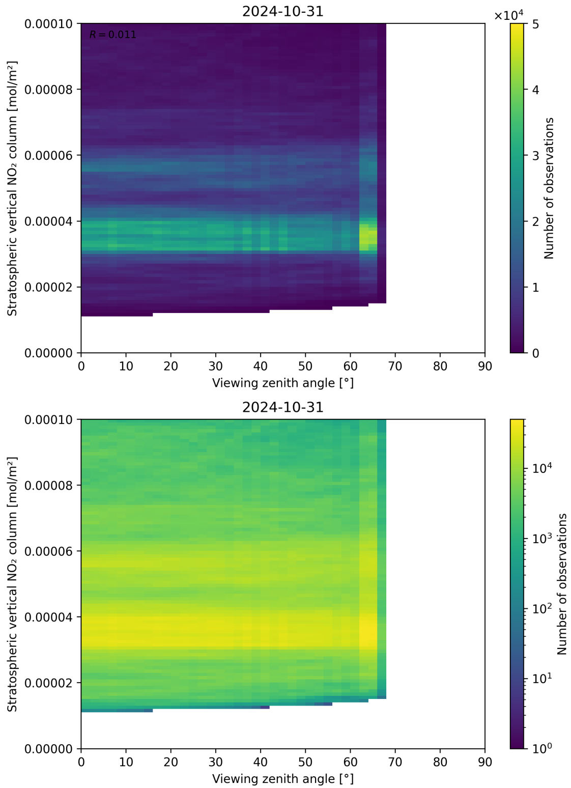
Figure 164: Scatter density plot of “Viewing zenith angle” against “Stratospheric vertical NO 2 column” for 2024-10-30 to 2024-11-01.
