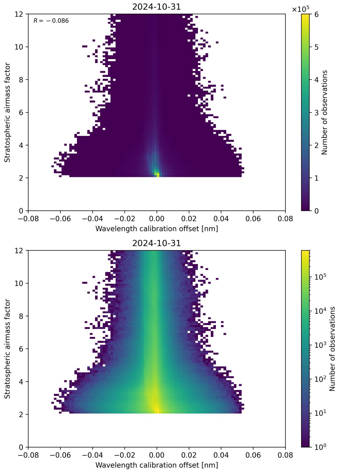
Figure 174: Scatter density plot of “Wavelength calibration offset” against “Stratospheric air mass factor” for 2024-10-30 to 2024-11-01.
