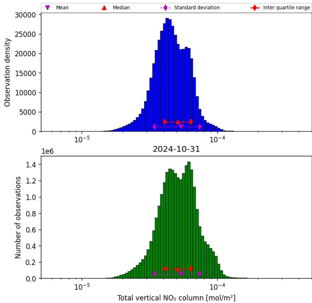
Figure 38: Histogram of “Total vertical NO 2 column” for 2024-10-30 to 2024-11-01
