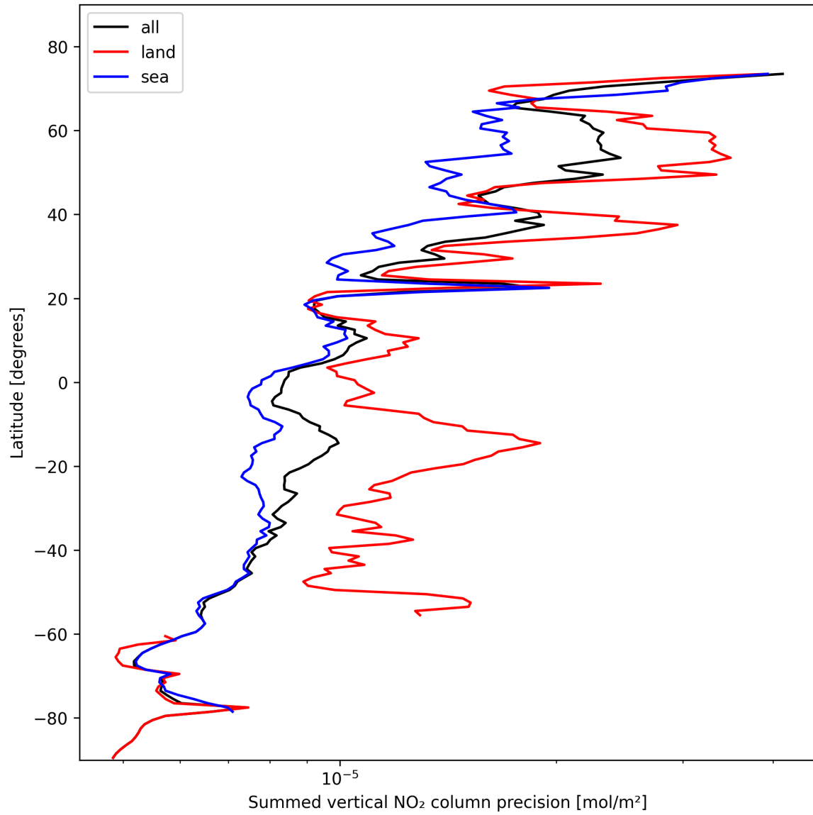
Figure 24: Zonal average of “Summed vertical NO 2 column precision” for 2024-10-30 to 2024-11-01.
