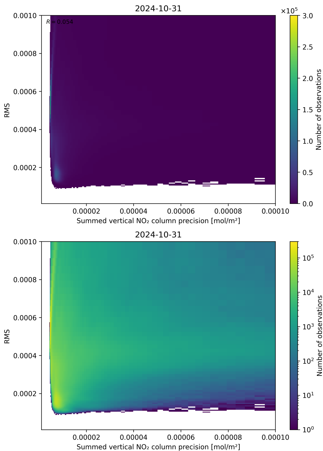
Figure 108: Scatter density plot of “Summed vertical NO 2 column precision” against “RMS” for 2024-10-30 to 2024-11-01.
