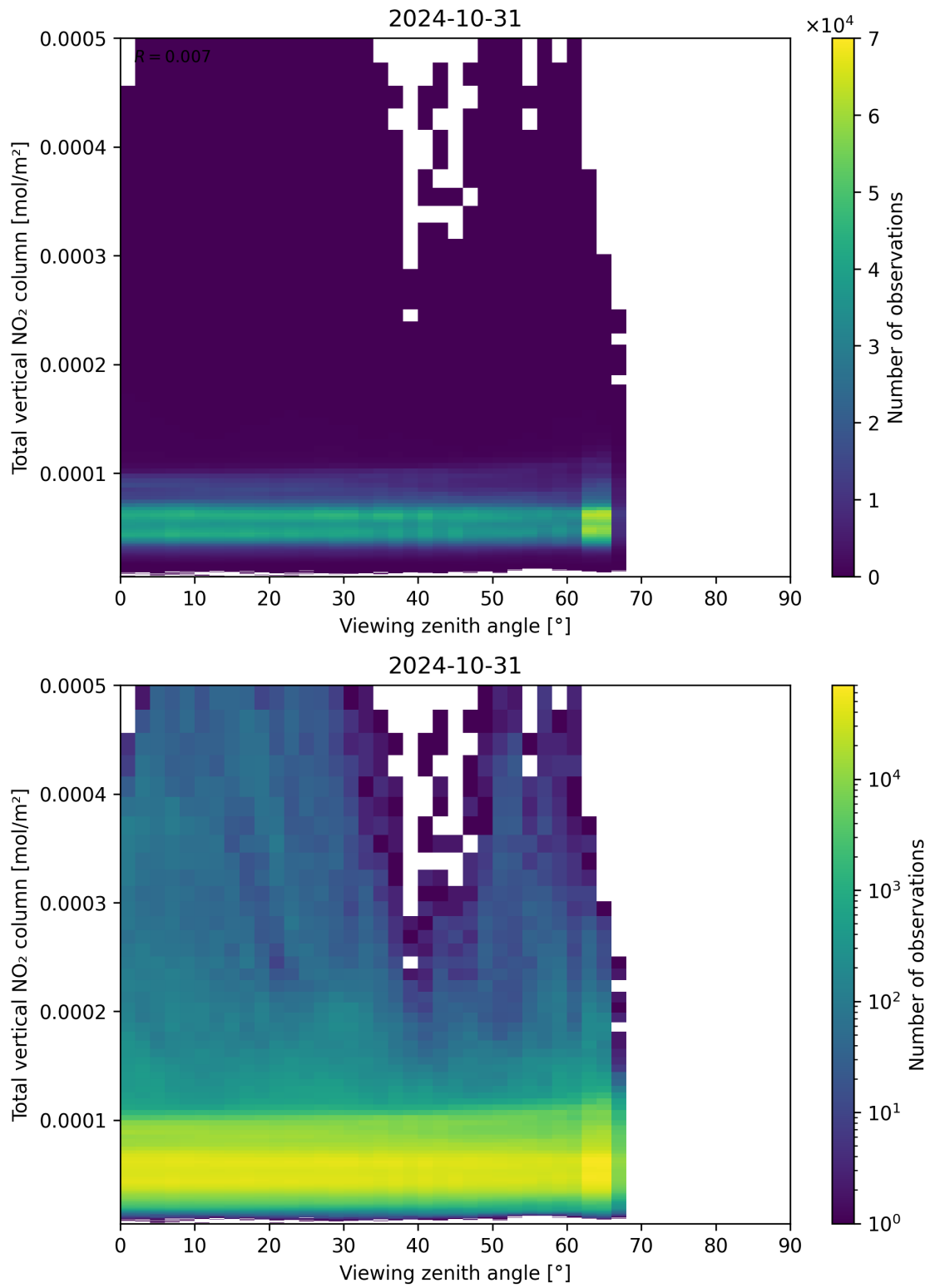
Figure 167: Scatter density plot of “Viewing zenith angle” against “Total vertical NO 2 column” for 2024-10-30 to 2024-11-01.
