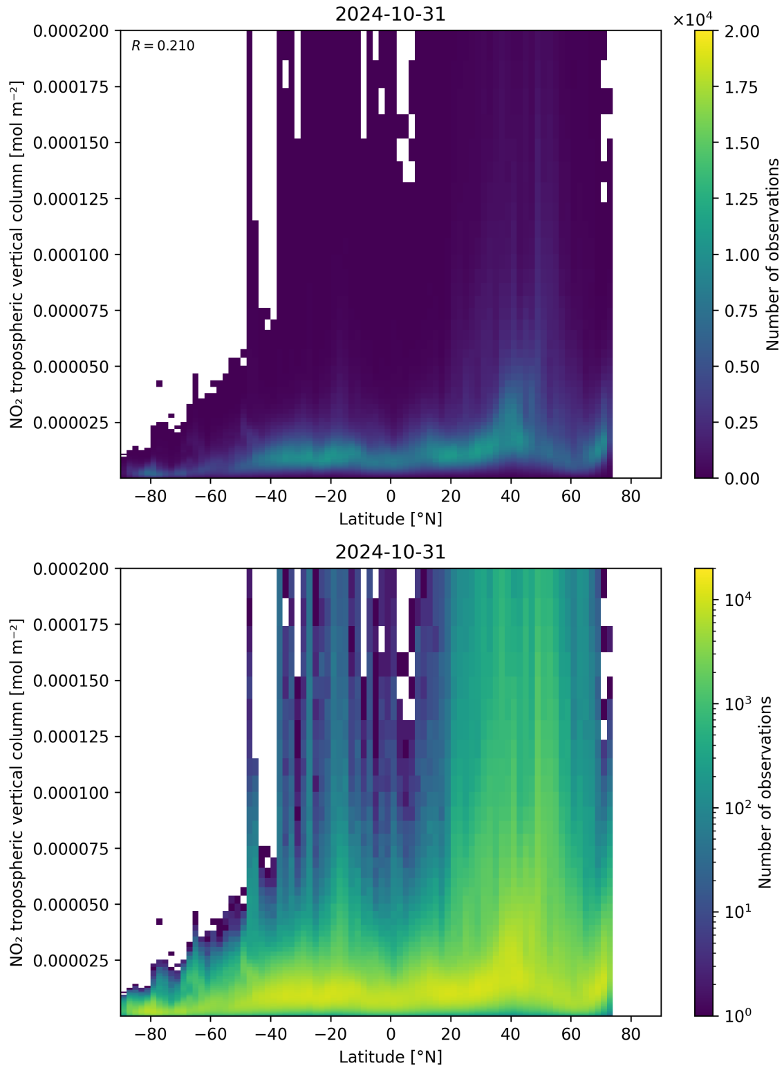
Figure 92: Scatter density plot of “Latitude” against “NO 2 tropospheric vertical column” for 2024-10-30 to 2024-11-01.
