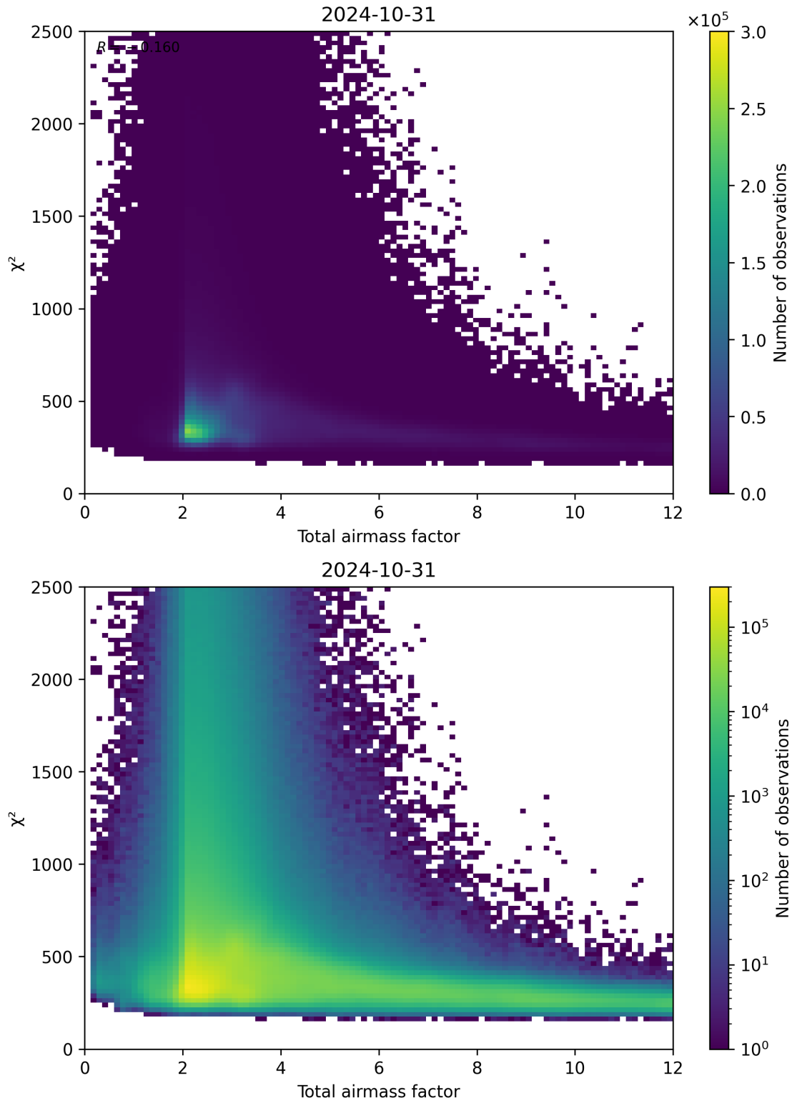
Figure 63: Scatter density plot of “Total airmass factor” against “ \chi^2 ” for 2024-10-30 to 2024-11-01.
