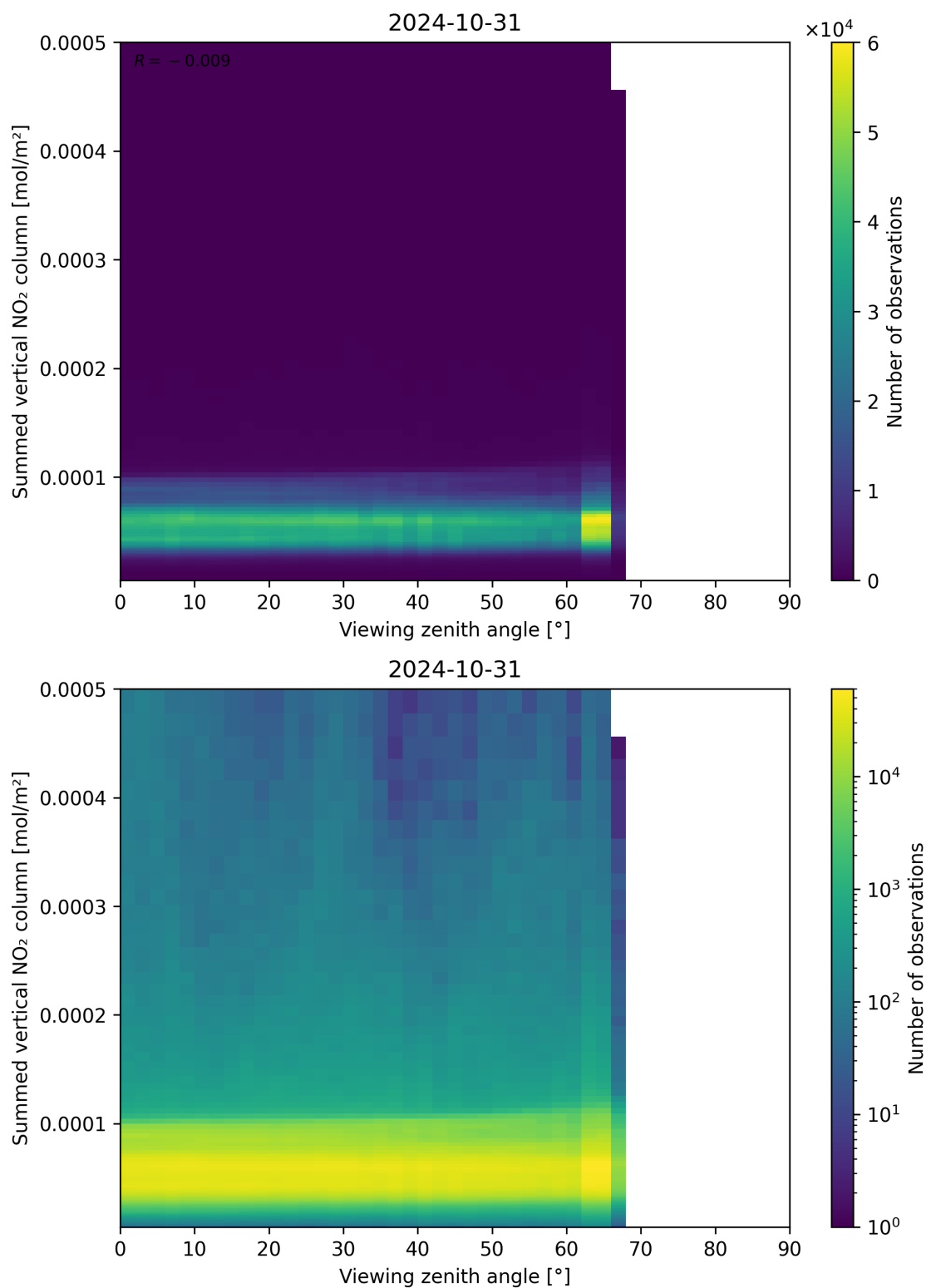
Figure 165: Scatter density plot of “Viewing zenith angle” against “Summed vertical NO 2 column” for 2024-10-30 to 2024-11-01.
