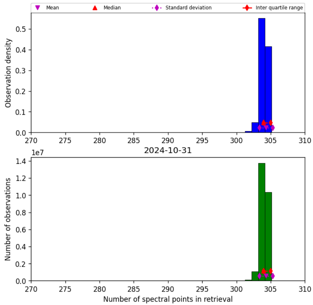
Figure 33: Histogram of “Number of spectral points in retrieval” for 2024-10-30 to 2024-11-01
