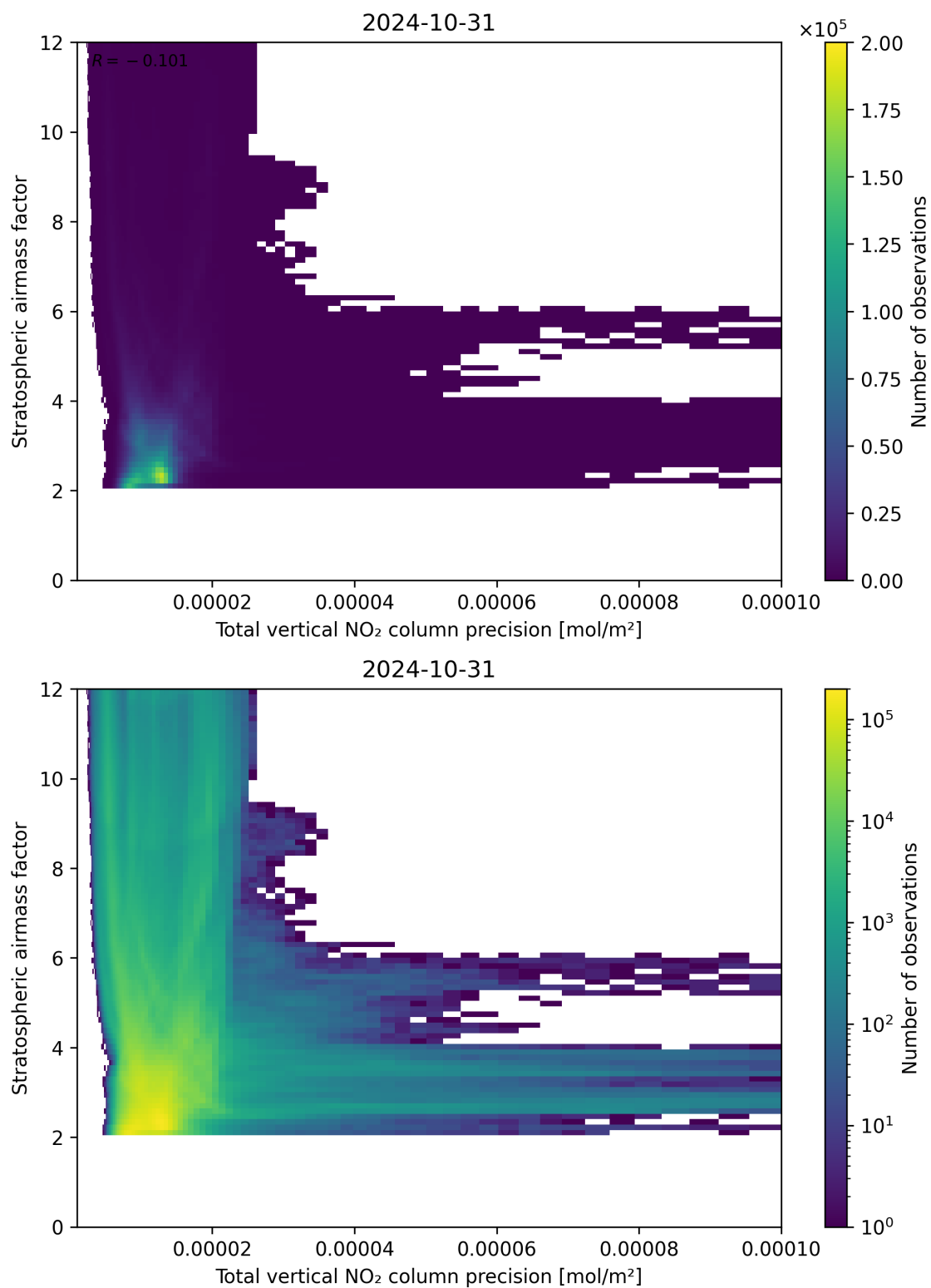
Figure 115: Scatter density plot of “Total vertical NO 2 column precision” against “Stratospheric air mass factor” for 2024-10-30 to 2024-11-01.
