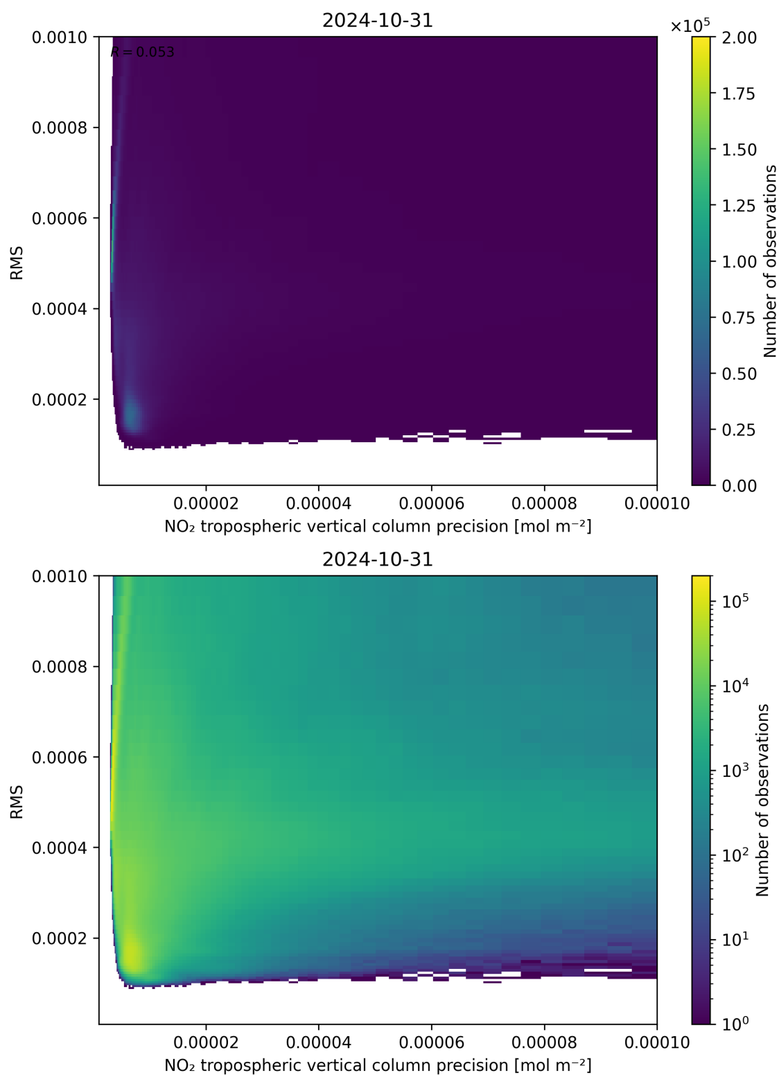
Figure 140: Scatter density plot of “NO 2 tropospheric vertical column precision” against “RMS” for 2024-10-30 to 2024-11-01.
