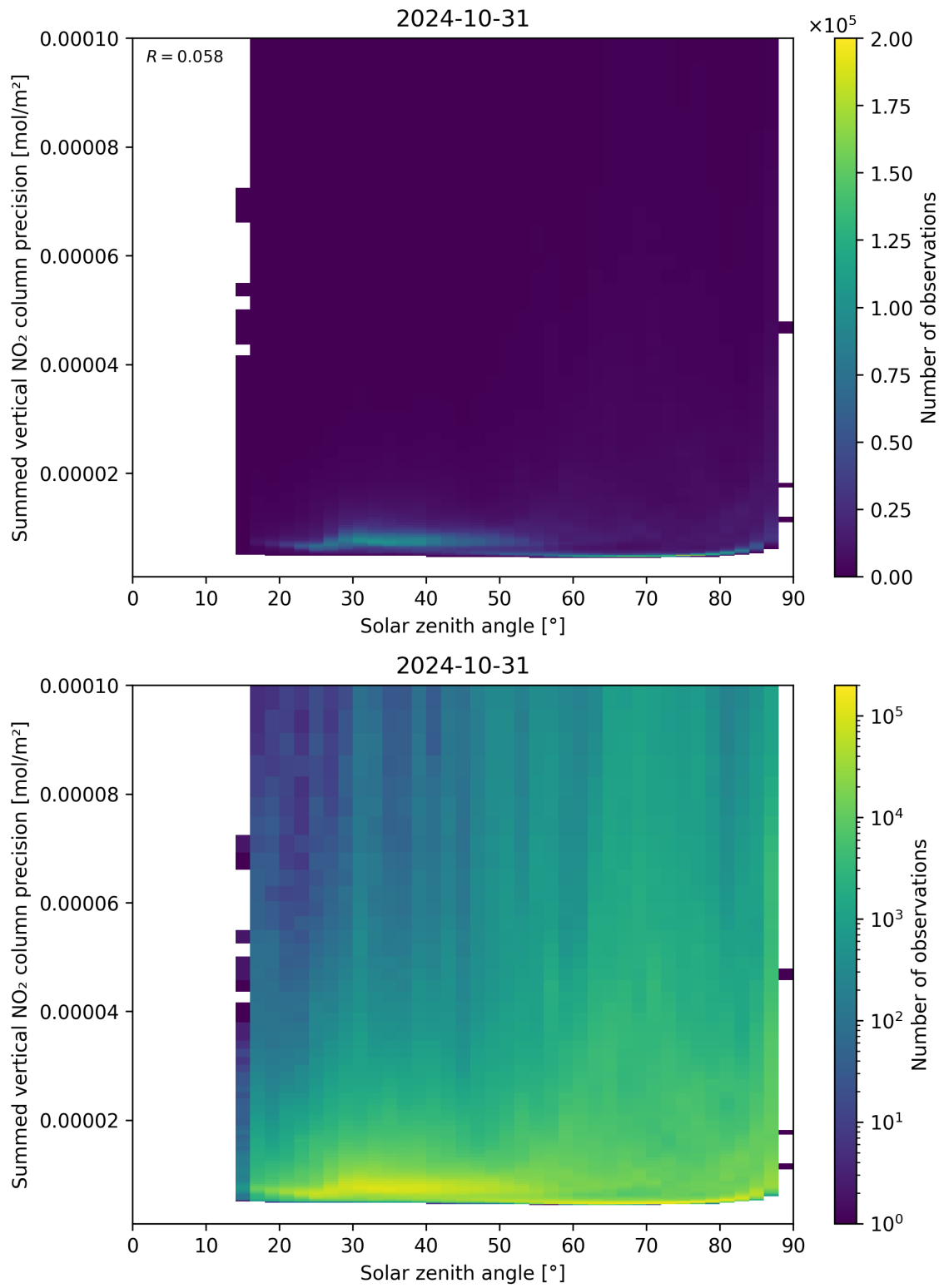
Figure 152: Scatter density plot of “Solar zenith angle” against “Summed vertical NO 2 column precision” for 2024-10-30 to 2024-11-01.
