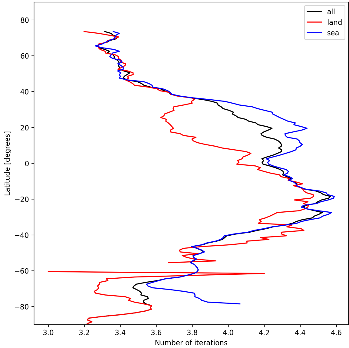
Figure 17: Zonal average of “Number of iterations” for 2024-10-30 to 2024-11-01.
