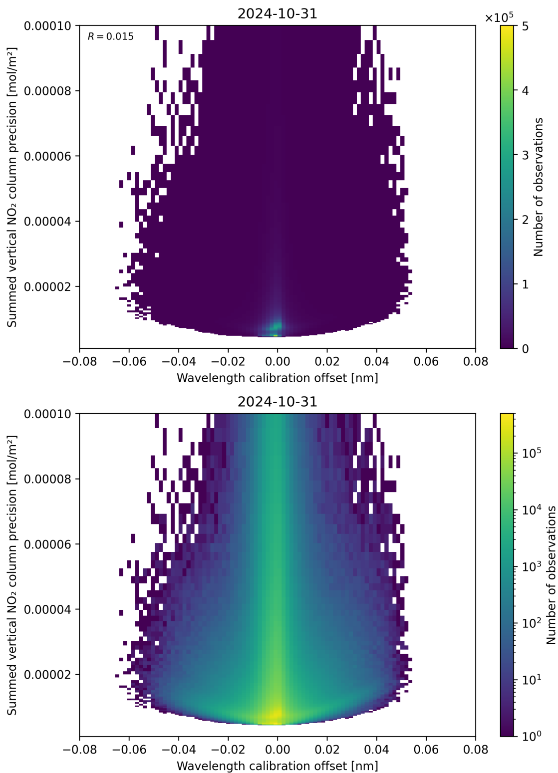
Figure 178: Scatter density plot of “Wavelength calibration offset” against “Summed vertical NO 2 column precision” for 2024-10-30 to 2024-11-01.
