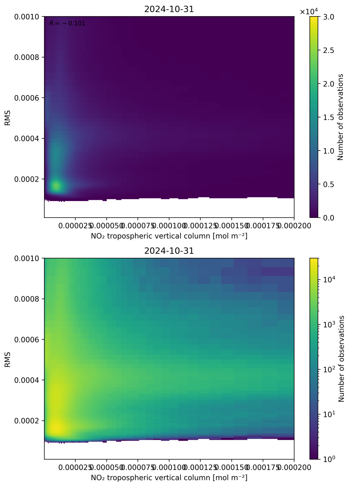
Figure 142: Scatter density plot of “NO 2 tropospheric vertical column” against “RMS” for 2024-10-30 to 2024-11-01.
