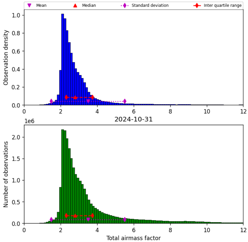
Figure 32: Histogram of “Total airmass factor” for 2024-10-30 to 2024-11-01
