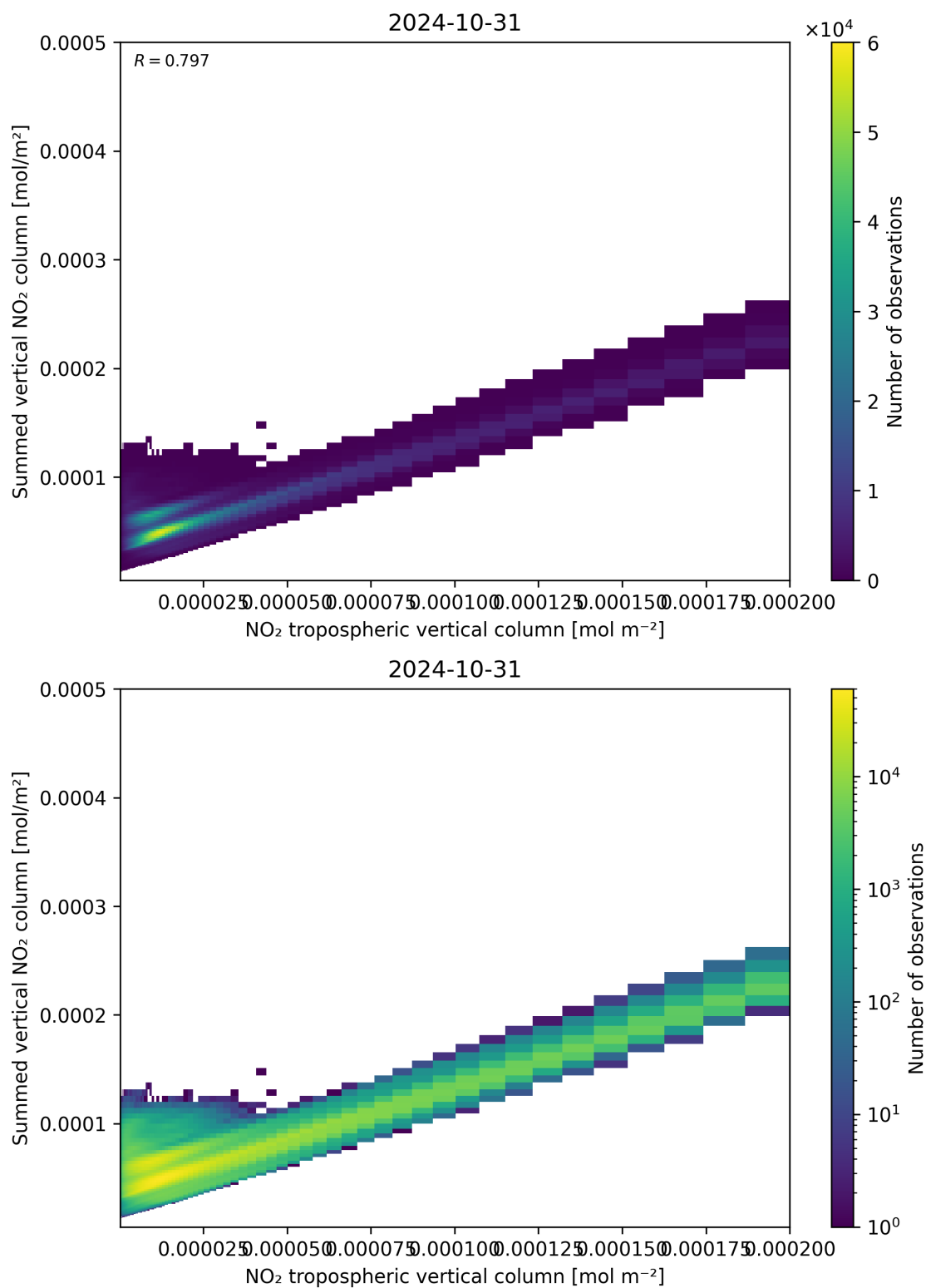
Figure 126: Scatter density plot of “NO 2 tropospheric vertical column” against “Summed vertical NO 2 column” for 2024-10-30 to 2024-11-01.
