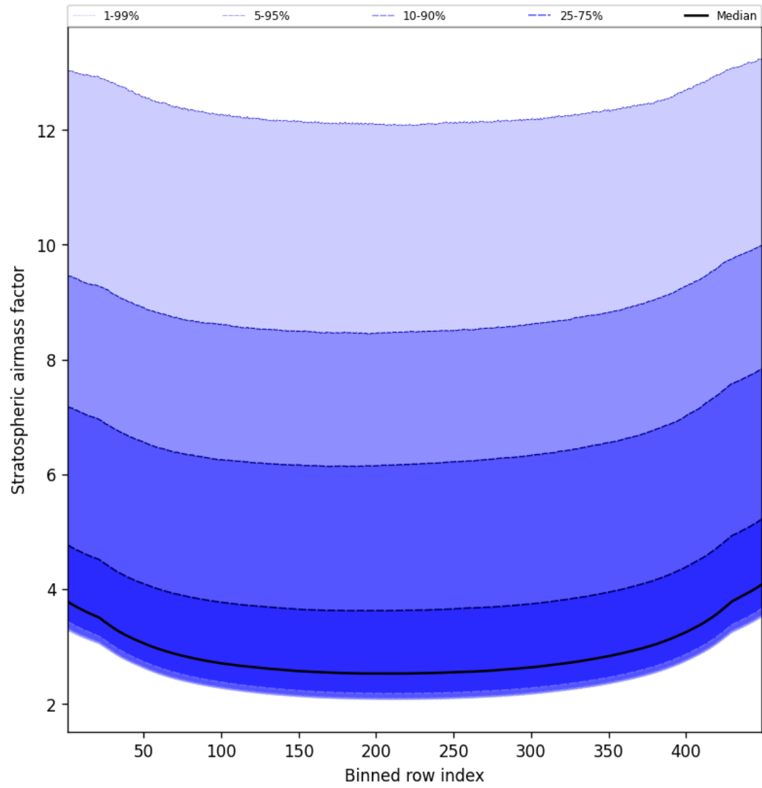
Figure 61: Along track statistics of “Stratospheric airmass factor” for 2024-10-30 to 2024-11-01
