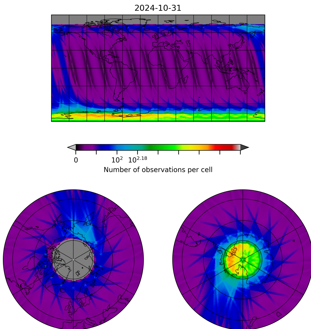
Figure 10: Map of the number of observations for 2024-10-30 to 2024-11-01
