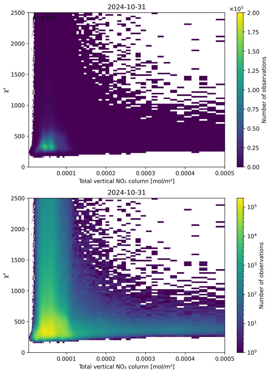
Figure 111: Scatter density plot of “Total vertical NO 2 column” against “ \chi^2 ” for 2024-10-30 to 2024-11-01.
