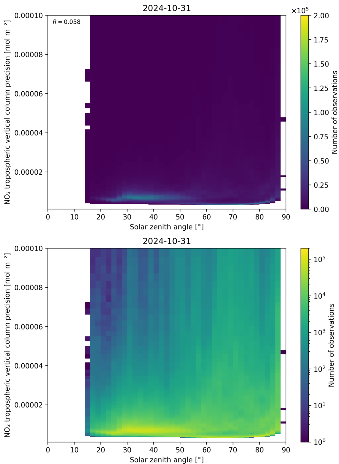
Figure 156: Scatter density plot of “Solar zenith angle” against “NO 2 tropospheric vertical column precision” for 2024-10-30 to 2024-11-01.
