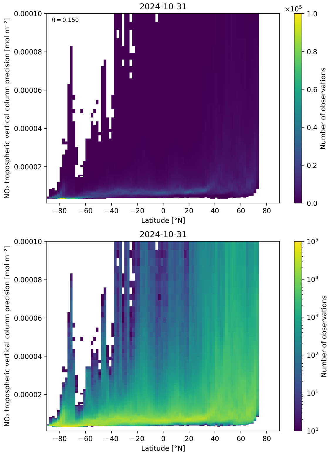
Figure 93: Scatter density plot of “Latitude” against “NO 2 tropospheric vertical column precision” for 2024-10-30 to 2024-11-01.
