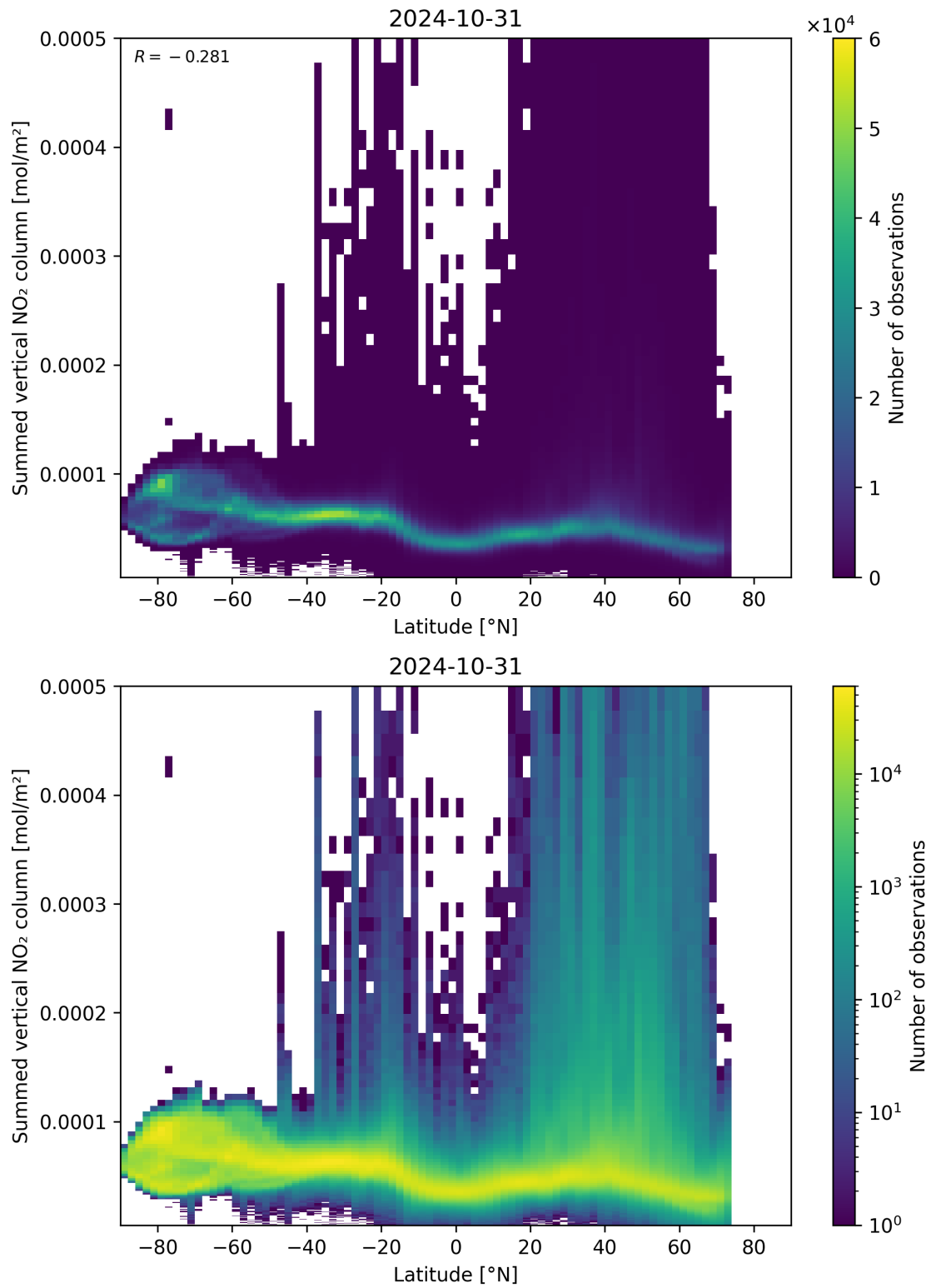
Figure 88: Scatter density plot of “Latitude” against “Summed vertical NO 2 column” for 2024-10-30 to 2024-11-01.
