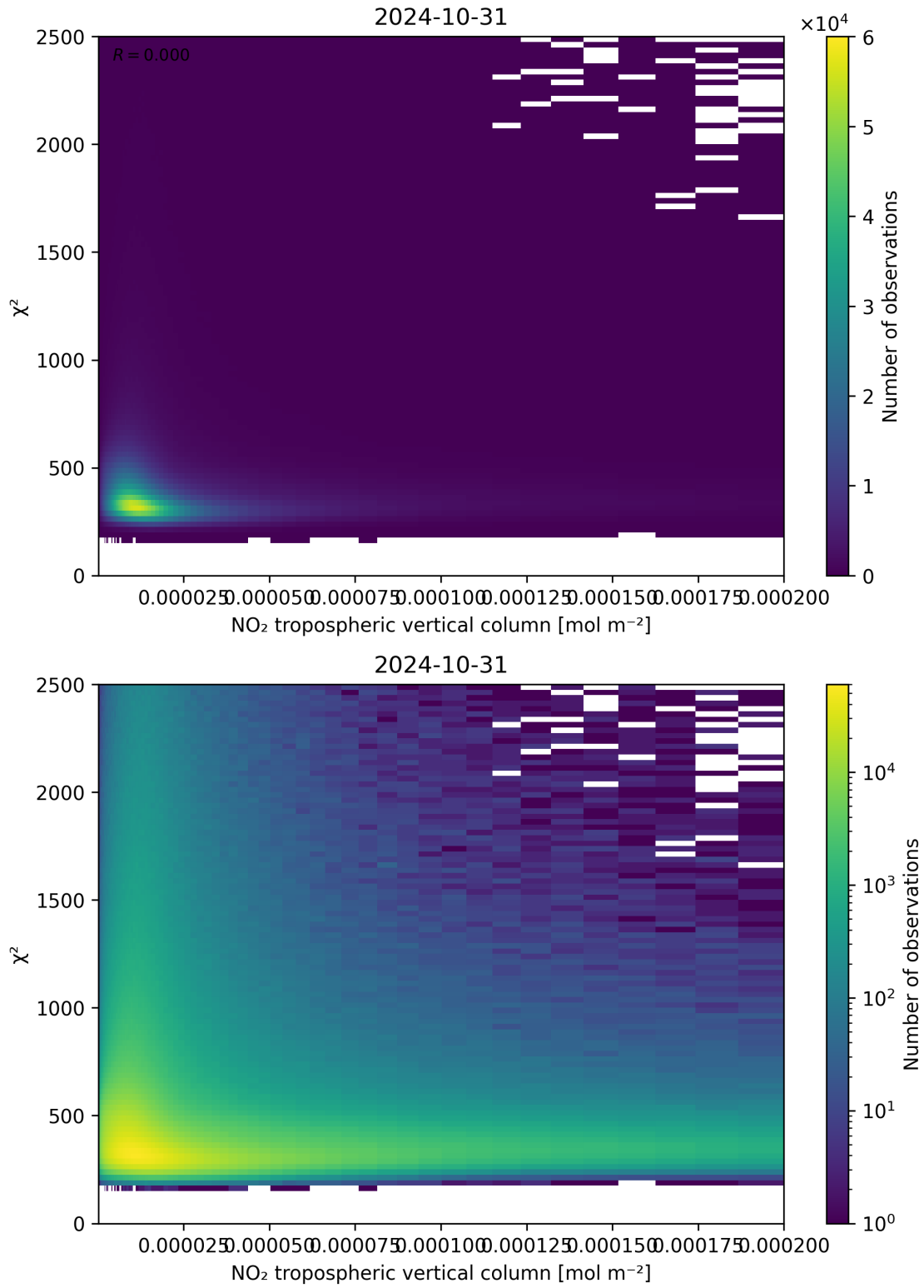
Figure 124: Scatter density plot of “NO 2 tropospheric vertical column” against “ \chi^2 ” for 2024-10-30 to 2024-11-01.
