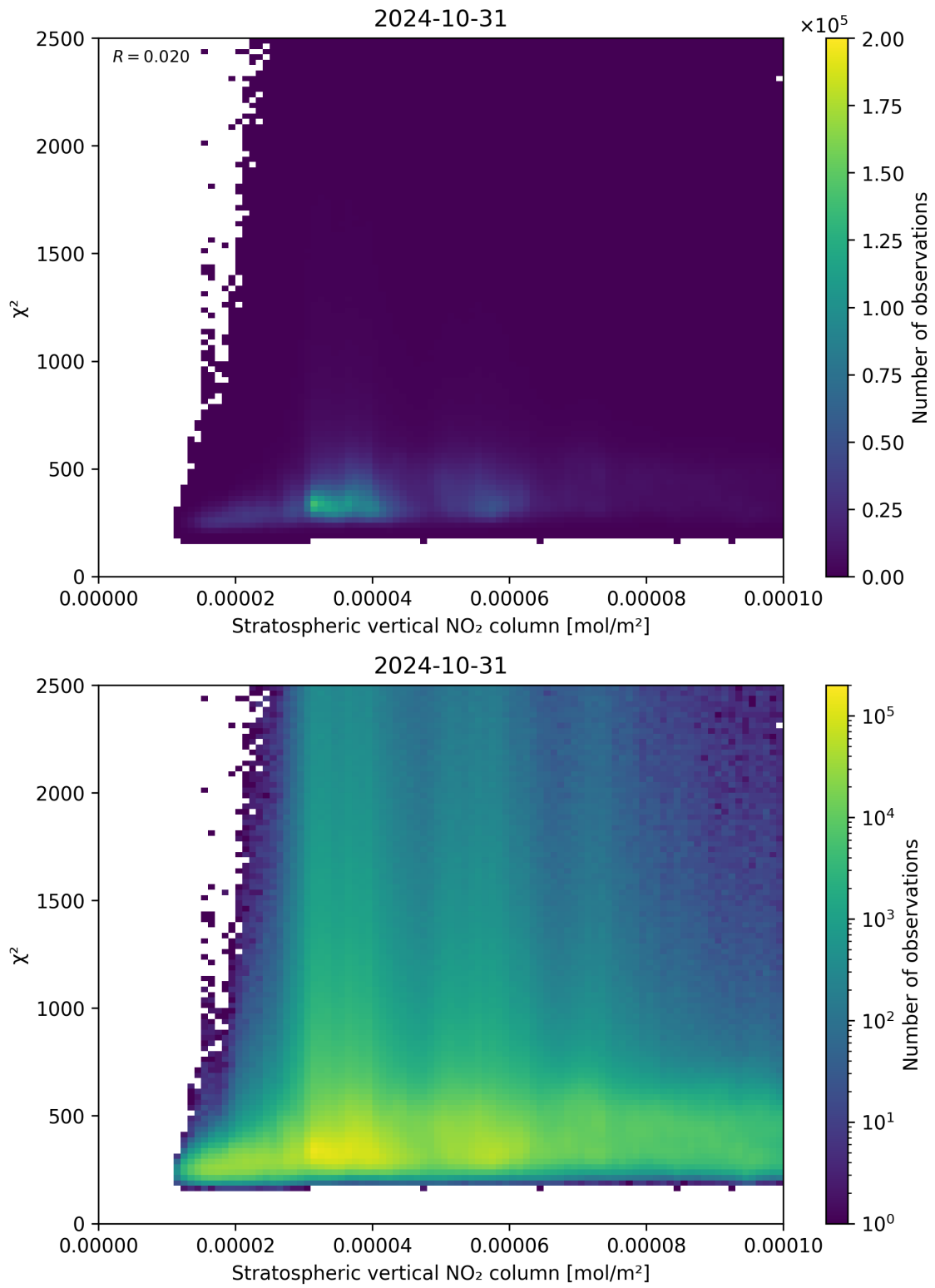
Figure 97: Scatter density plot of “Stratospheric vertical NO 2 column” against “ \chi^2 ” for 2024-10-30 to 2024-11-01.
