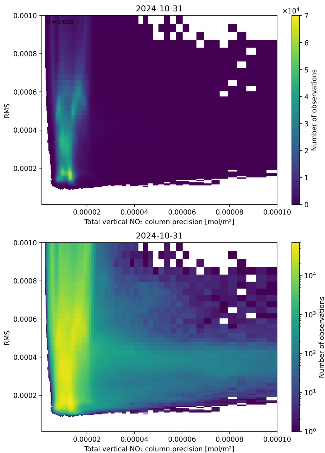
Figure 119: Scatter density plot of “Total vertical NO 2 column precision” against “RMS” for 2024-10-30 to 2024-11-01.
