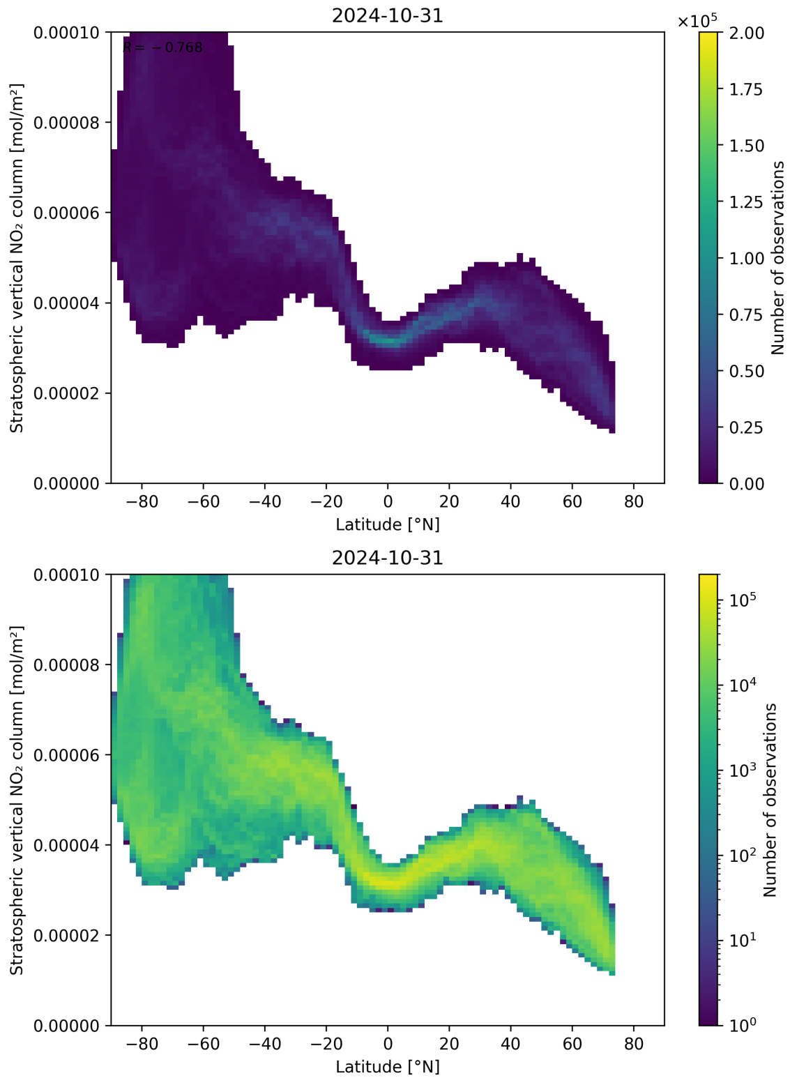
Figure 87: Scatter density plot of “Latitude” against “Stratospheric vertical NO 2 column” for 2024-10-30 to 2024-11-01.
