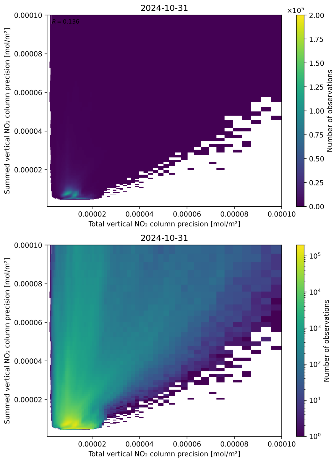
Figure 118: Scatter density plot of “Total vertical NO 2 column precision” against “Summed vertical NO 2 column precision” for 2024-10-30 to 2024-11-01.
