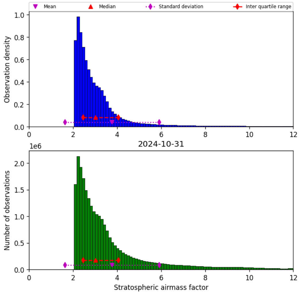
Figure 44: Histogram of “Stratospheric airmass factor” for 2024-10-30 to 2024-11-01
