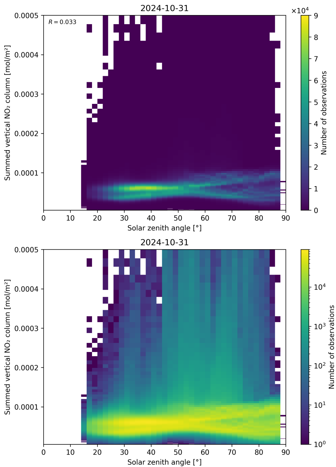
Figure 151: Scatter density plot of “Solar zenith angle” against “Summed vertical NO 2 column” for 2024-10-30 to 2024-11-01.
