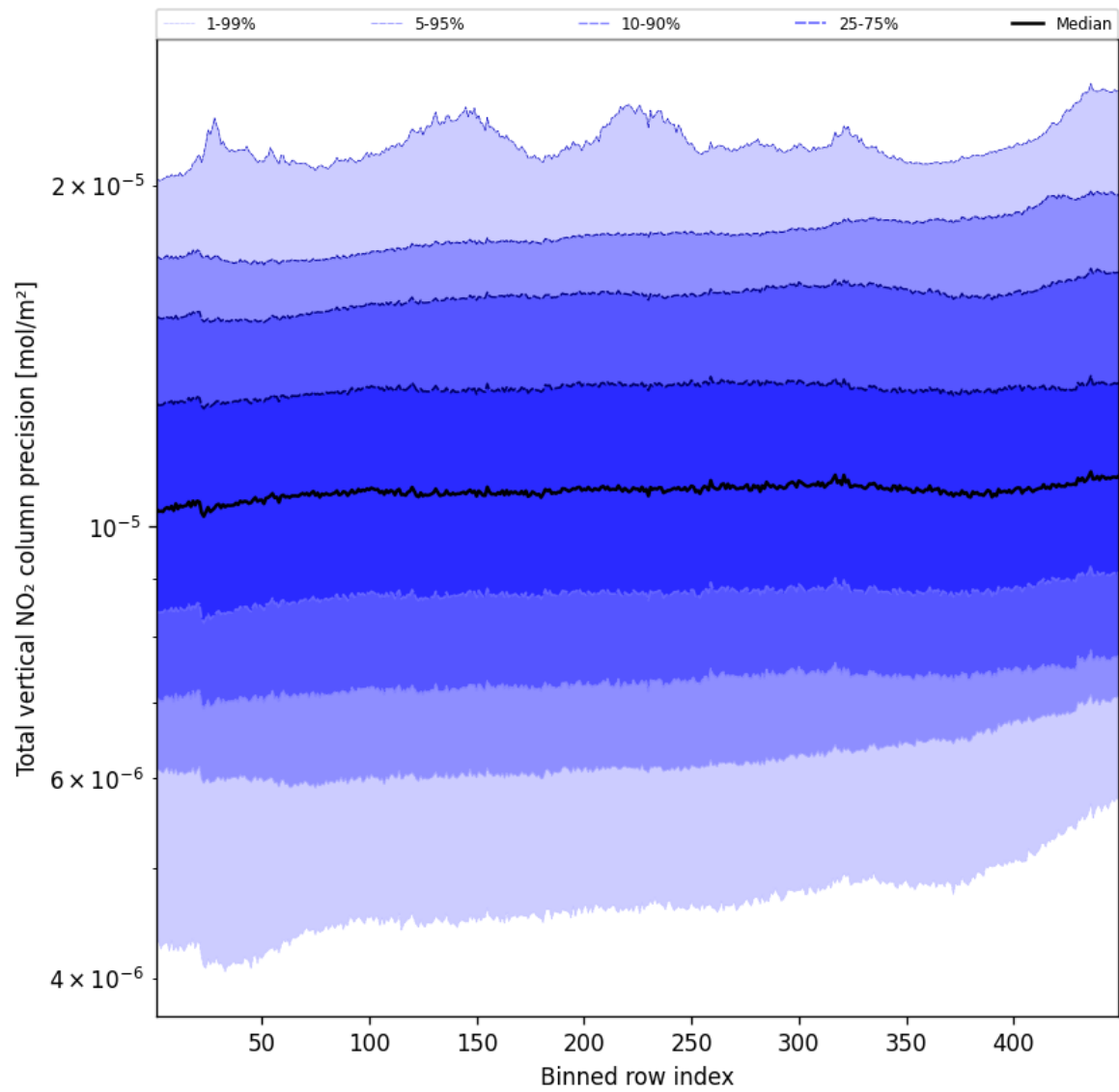
Figure 56: Along track statistics of “Total vertical NO 2 column precision” for 2024-10-30 to 2024-11-01
