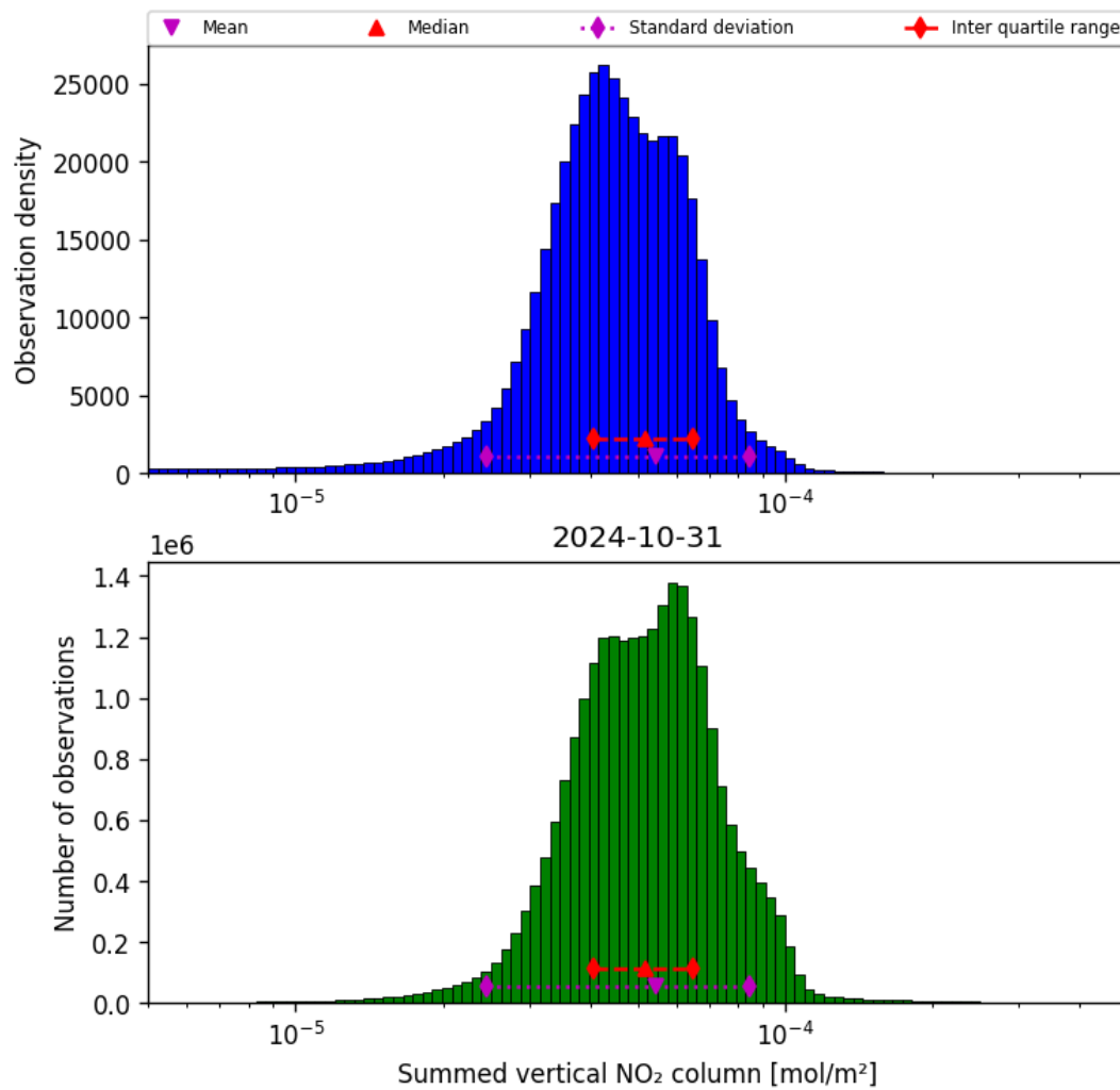
Figure 40: Histogram of “Summed vertical NO 2 column” for 2024-10-30 to 2024-11-01
