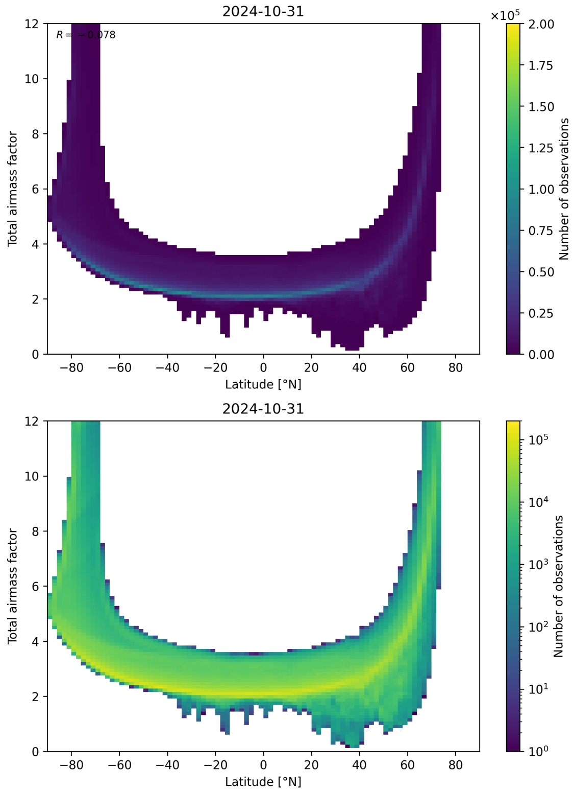
Figure 84: Scatter density plot of “Latitude” against “Total airmass factor” for 2024-10-30 to 2024-11-01.
