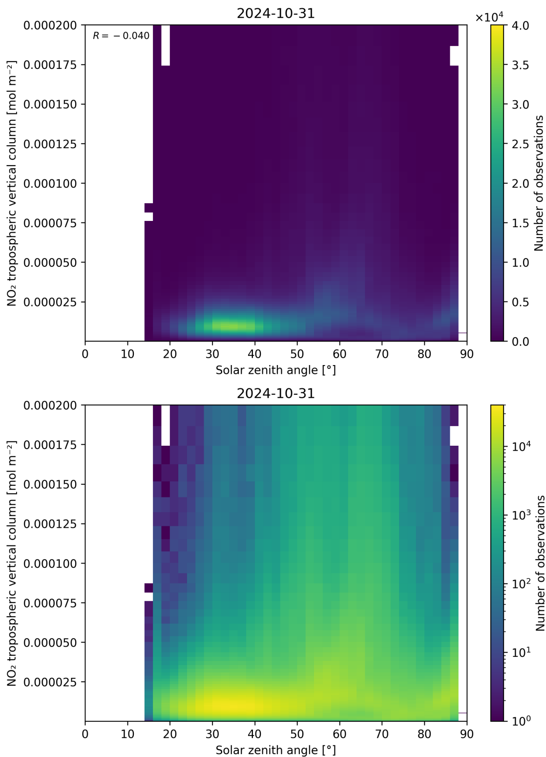
Figure 155: Scatter density plot of “Solar zenith angle” against “NO 2 tropospheric vertical column” for 2024-10-30 to 2024-11-01.
