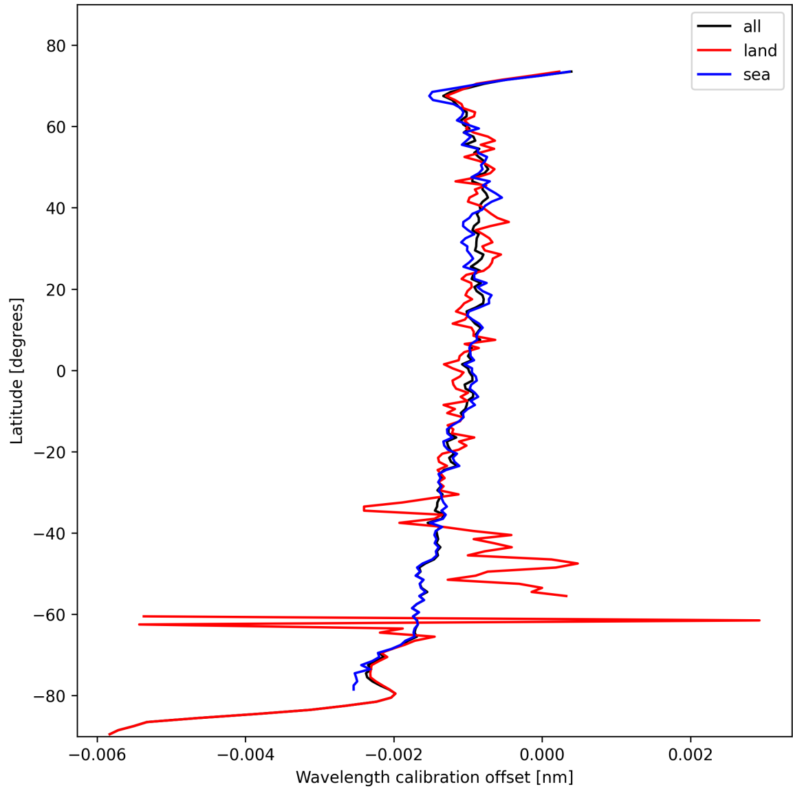
Figure 18: Zonal average of “Wavelength calibration offset” for 2024-10-30 to 2024-11-01.
