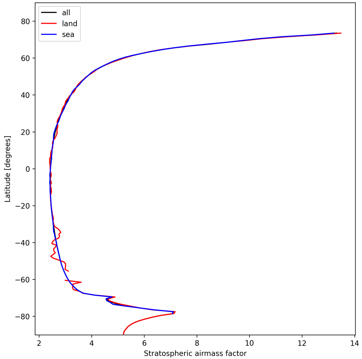
Figure 27: Zonal average of “Stratospheric air mass factor” for 2024-10-30 to 2024-11-01.
