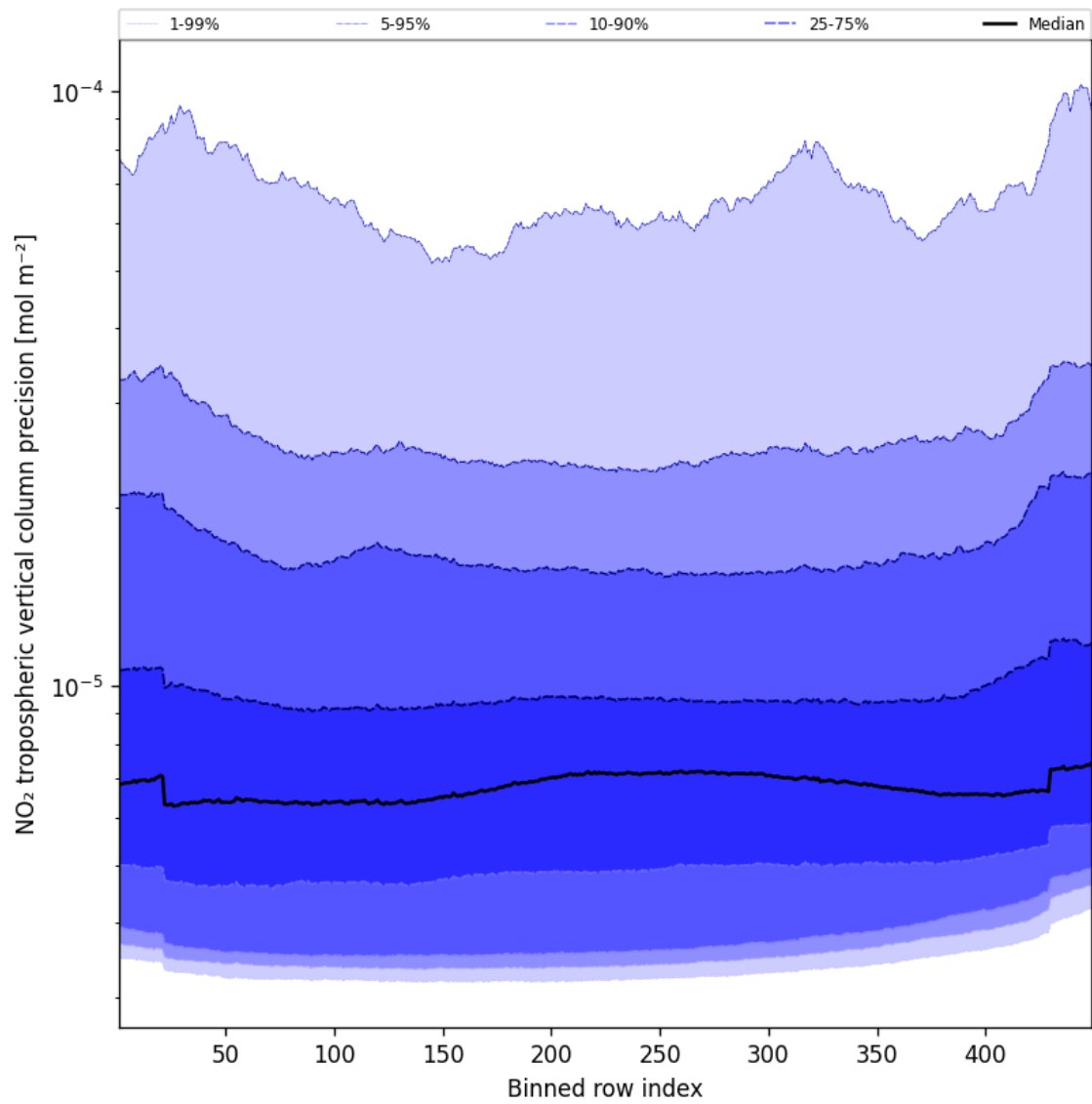
Figure 47: Along track statistics of “NO 2 tropospheric vertical column precision” for 2024-10-30 to 2024-11-01
