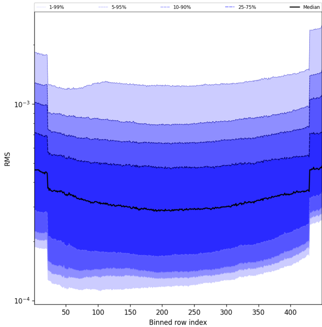
Figure 60: Along track statistics of “RMS” for 2024-10-30 to 2024-11-01
