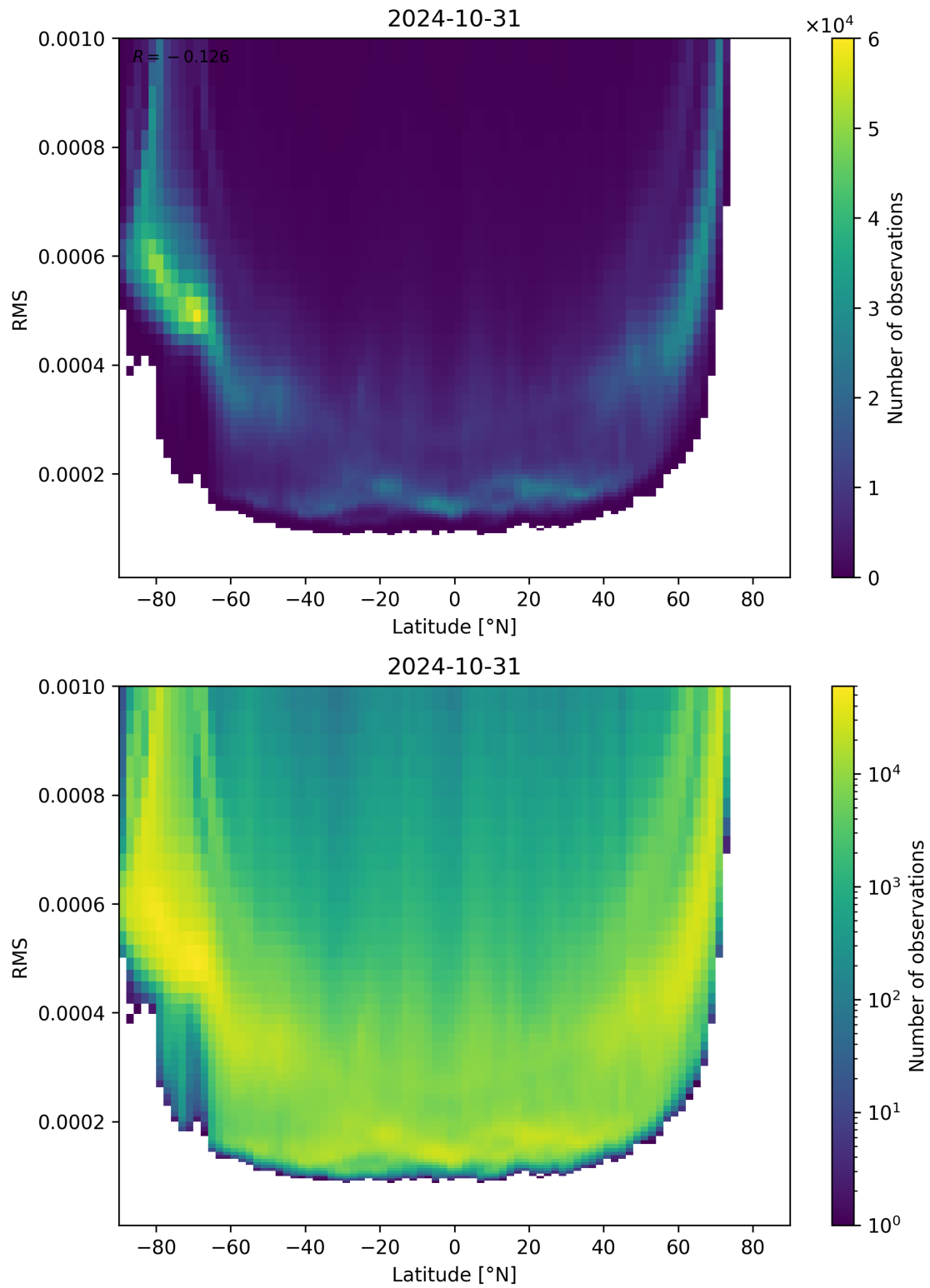
Figure 94: Scatter density plot of “Latitude” against “RMS” for 2024-10-30 to 2024-11-01.
