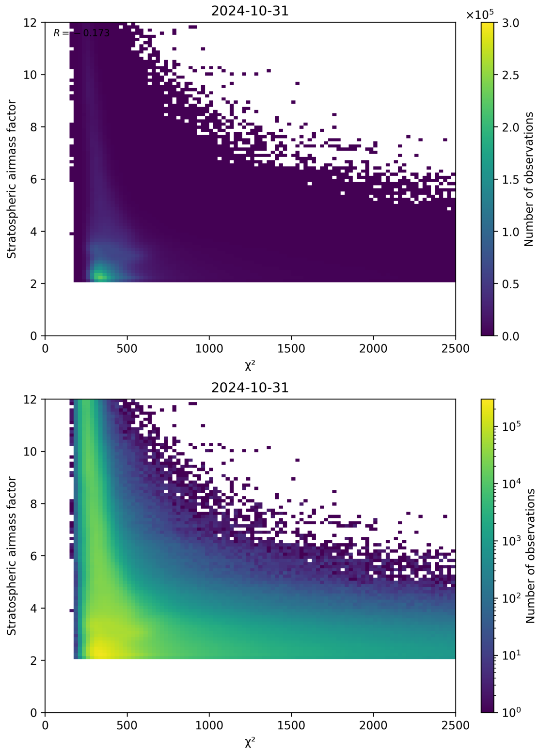
Figure 81: Scatter density plot of “ \chi^2 ” against “Stratospheric airmass factor” for 2024-10-30 to 2024-11-01.
