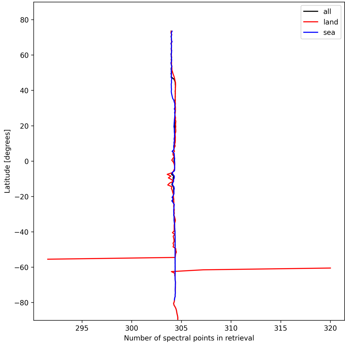
Figure 16: Zonal average of “Number of spectral points in retrieval” for 2024-10-30 to 2024-11-01.
