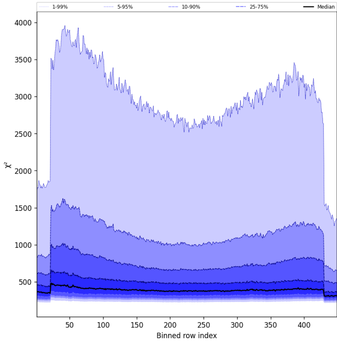
Figure 59: Along track statistics of “ \chi^2 ” for 2024-10-30 to 2024-11-01
