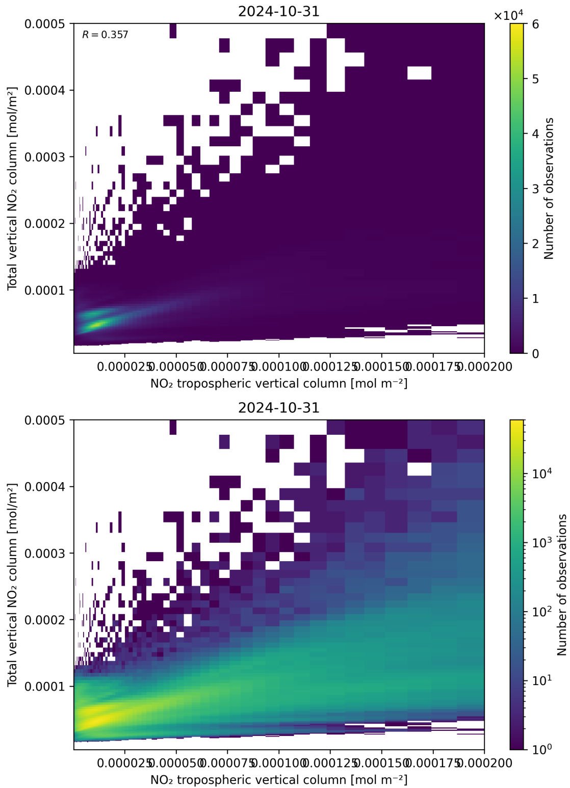
Figure 128: Scatter density plot of “NO 2 tropospheric vertical column” against “Total vertical NO 2 column” for 2024-10-30 to 2024-11-01.
