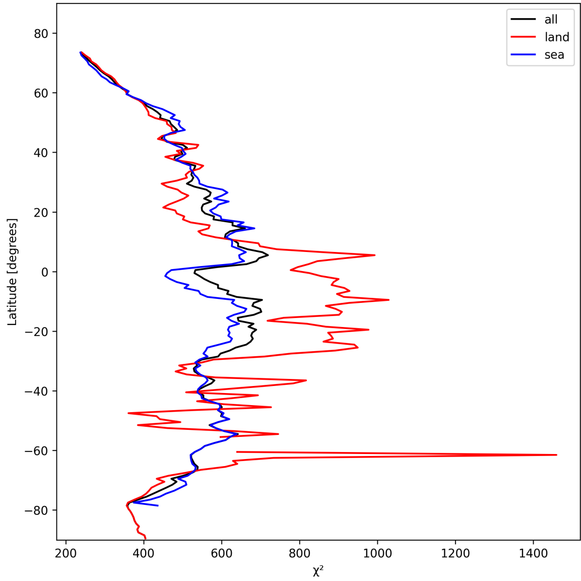
Figure 25: Zonal average of “ \chi^2 ” for 2024-10-30 to 2024-11-01.
