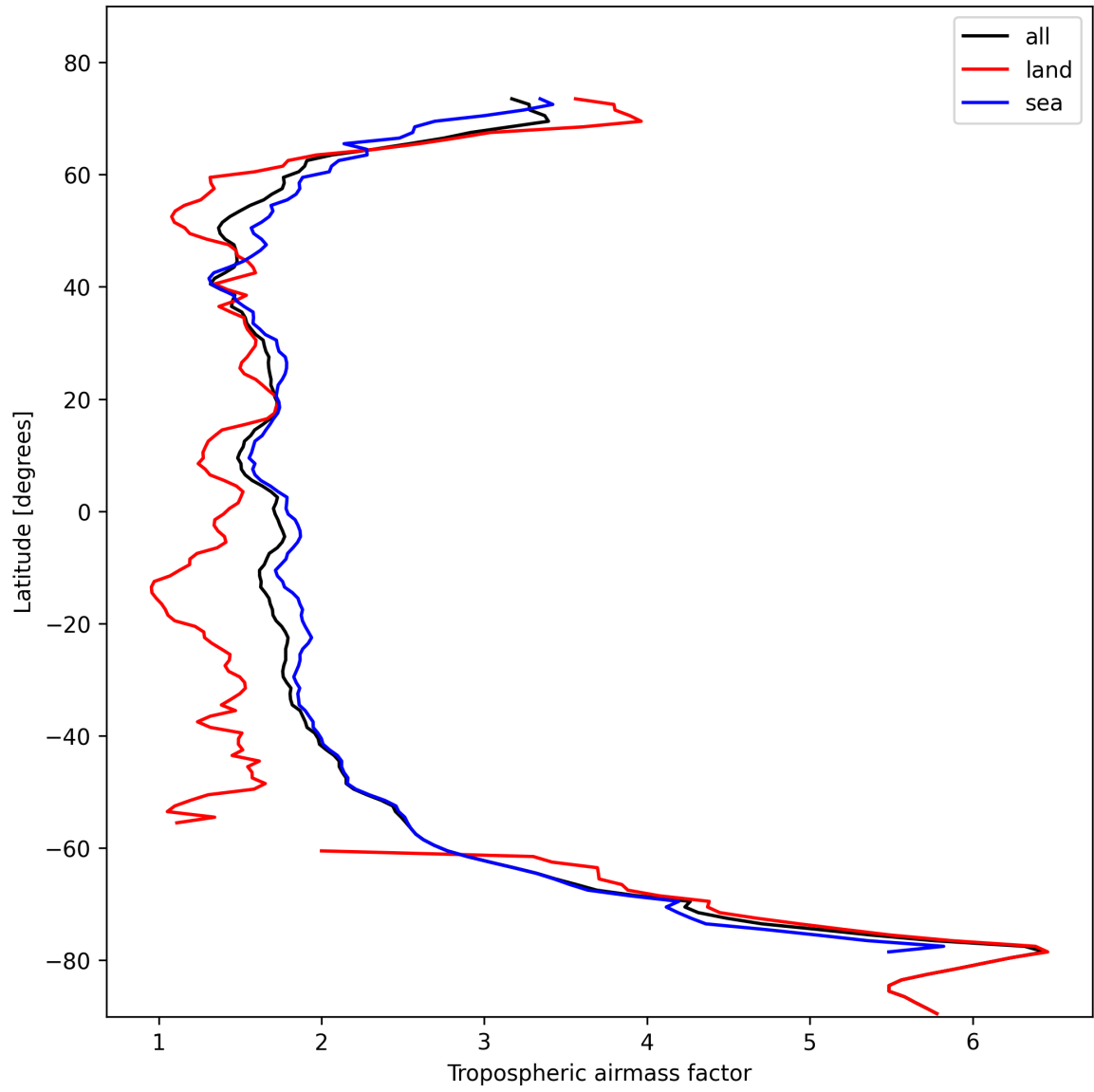
Figure 14: Zonal average of “Tropospheric airmass factor” for 2024-10-30 to 2024-11-01.
