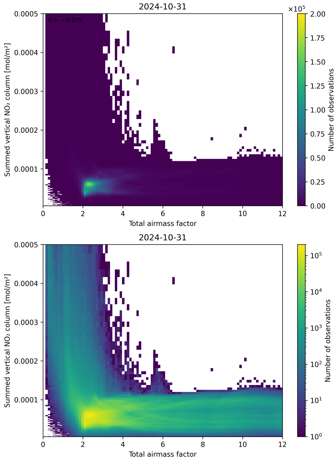
Figure 65: Scatter density plot of “Total airmass factor” against “Summed vertical NO 2 column” for 2024-10-30 to 2024-11-01.
