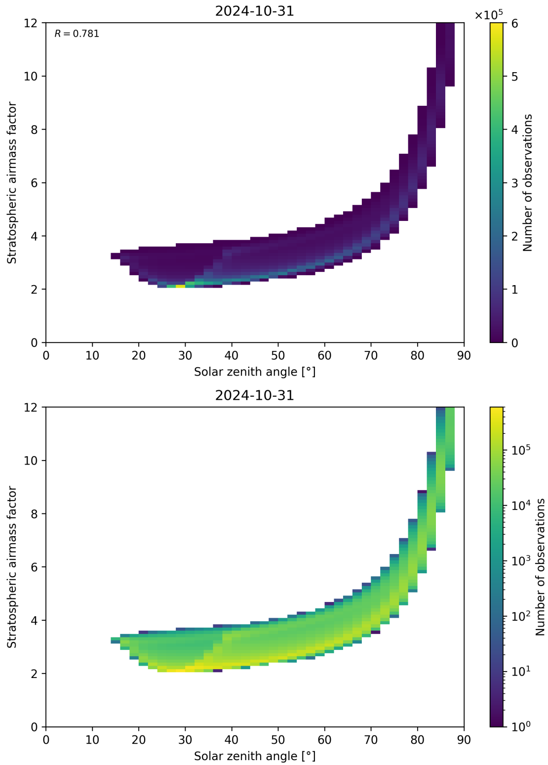
Figure 145: Scatter density plot of “Solar zenith angle” against “Stratospheric airmass factor” for 2024-10-30 to 2024-11-01.
