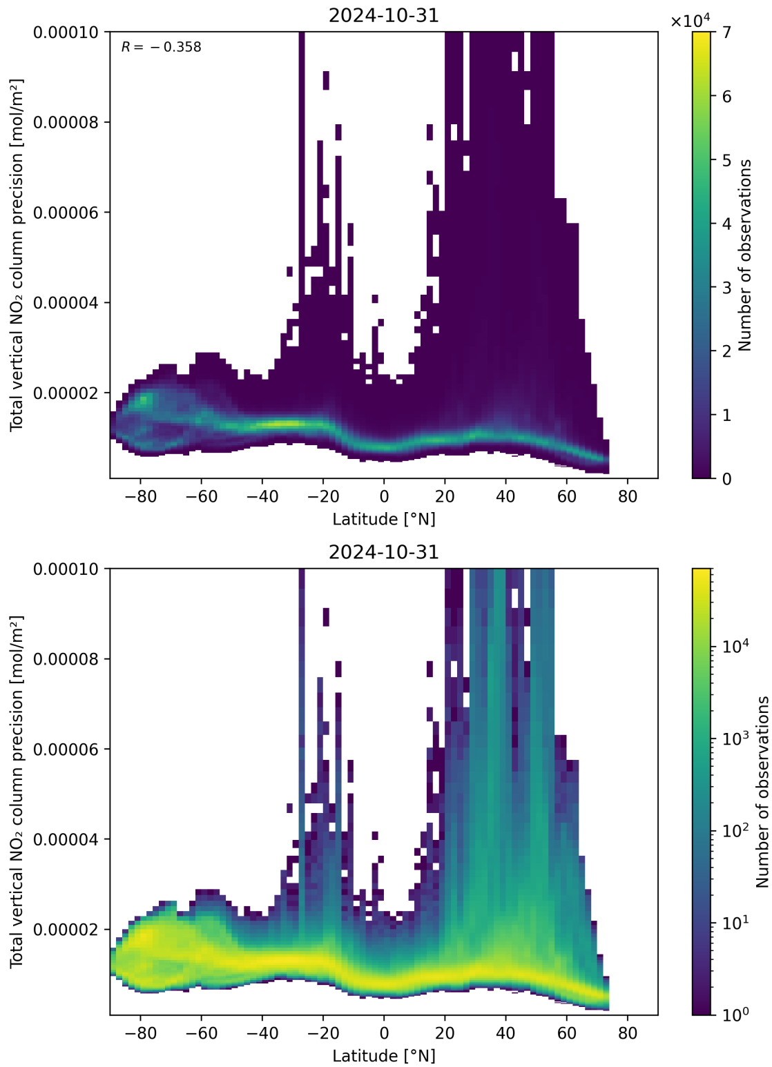
Figure 91: Scatter density plot of “Latitude” against “Total vertical NO 2 column precision” for 2024-10-30 to 2024-11-01.
