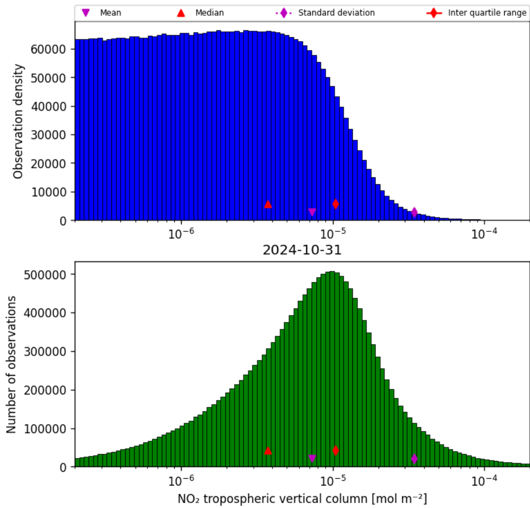
Figure 29: Histogram of “NO 2 tropospheric vertical column” for 2024-10-30 to 2024-11-01
