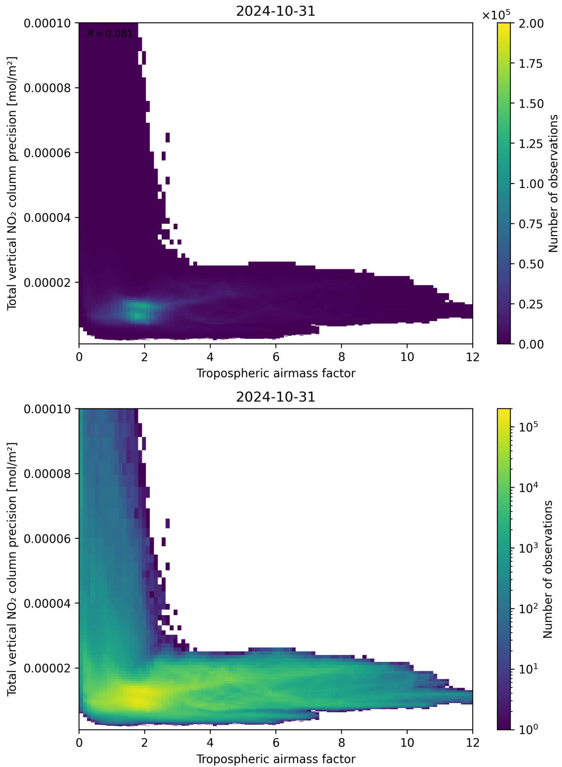
Figure 78: Scatter density plot of “Tropospheric air mass factor” against “Total vertical NO 2 column precision” for 2024-10-30 to 2024-11-01.
