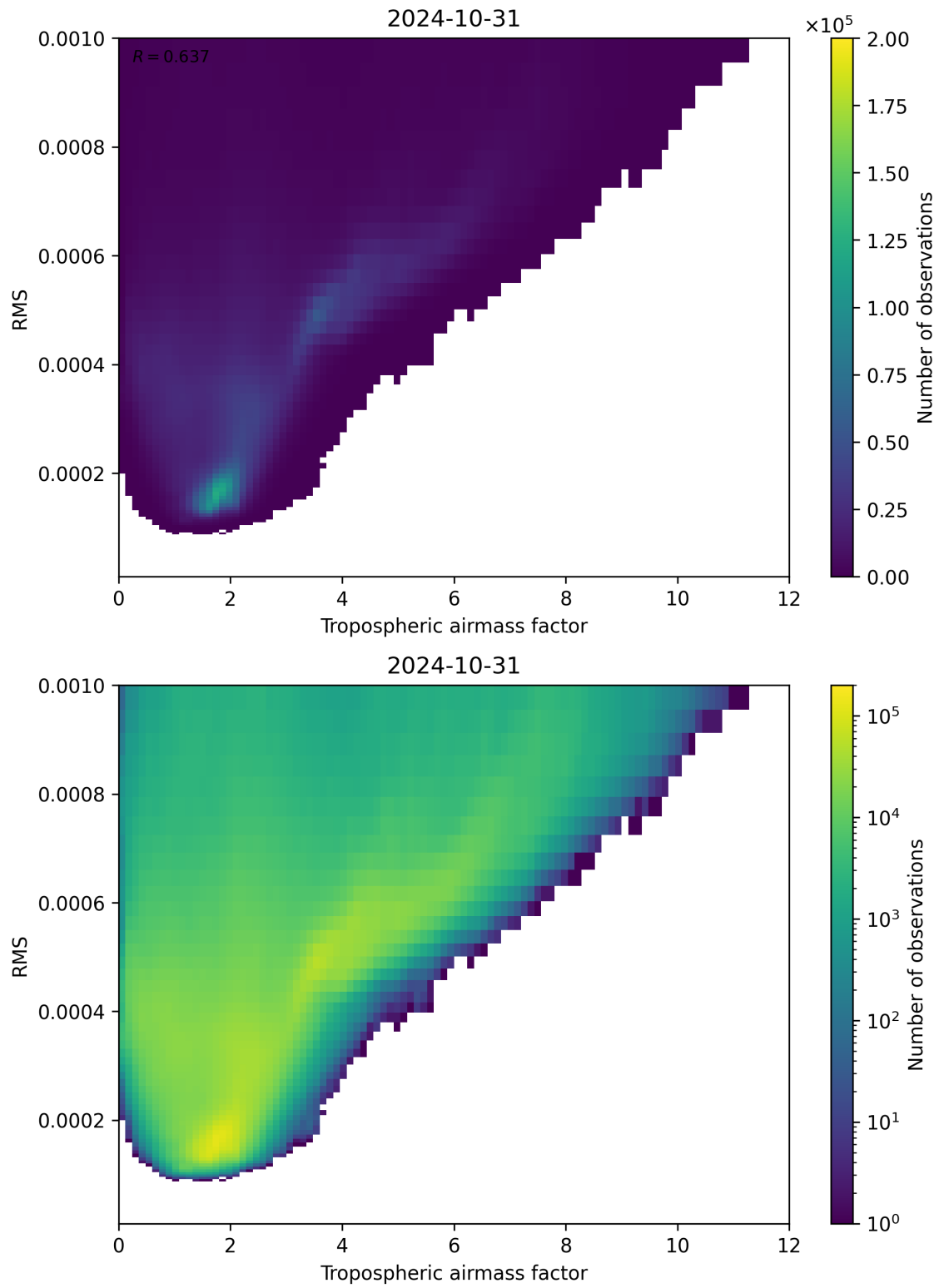
Figure 79: Scatter density plot of “Tropospheric airmass factor” against “RMS” for 2024-10-30 to 2024-11-01.
