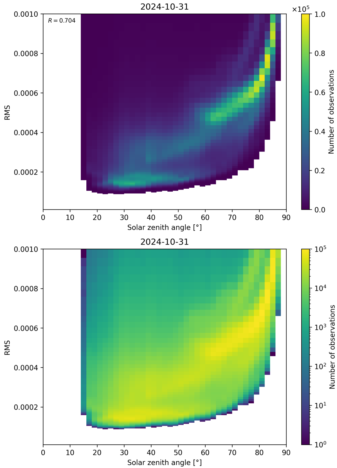
Figure 157: Scatter density plot of “Solar zenith angle” against “RMS” for 2024-10-30 to 2024-11-01.
