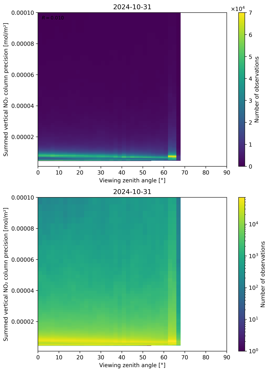
Figure 166: Scatter density plot of “Viewing zenith angle” against “Summed vertical NO 2 column precision” for 2024-10-30 to 2024-11-01.
