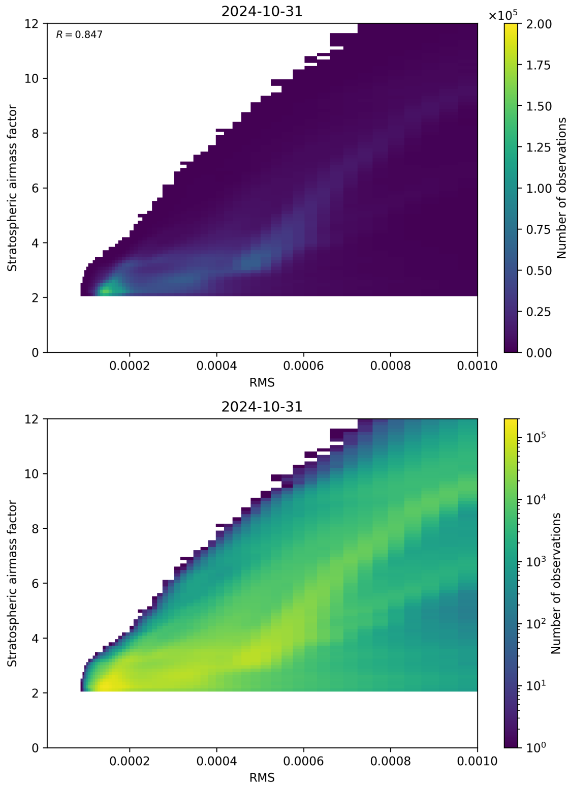
Figure 144: Scatter density plot of “RMS” against “Stratospheric airmass factor” for 2024-10-30 to 2024-11-01.
