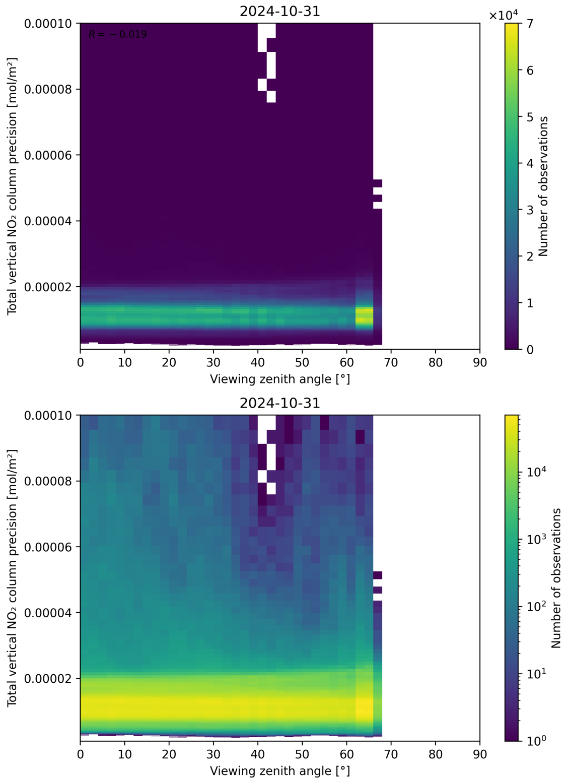
Figure 168: Scatter density plot of “Viewing zenith angle” against “Total vertical NO 2 column precision” for 2024-10-30 to 2024-11-01.
