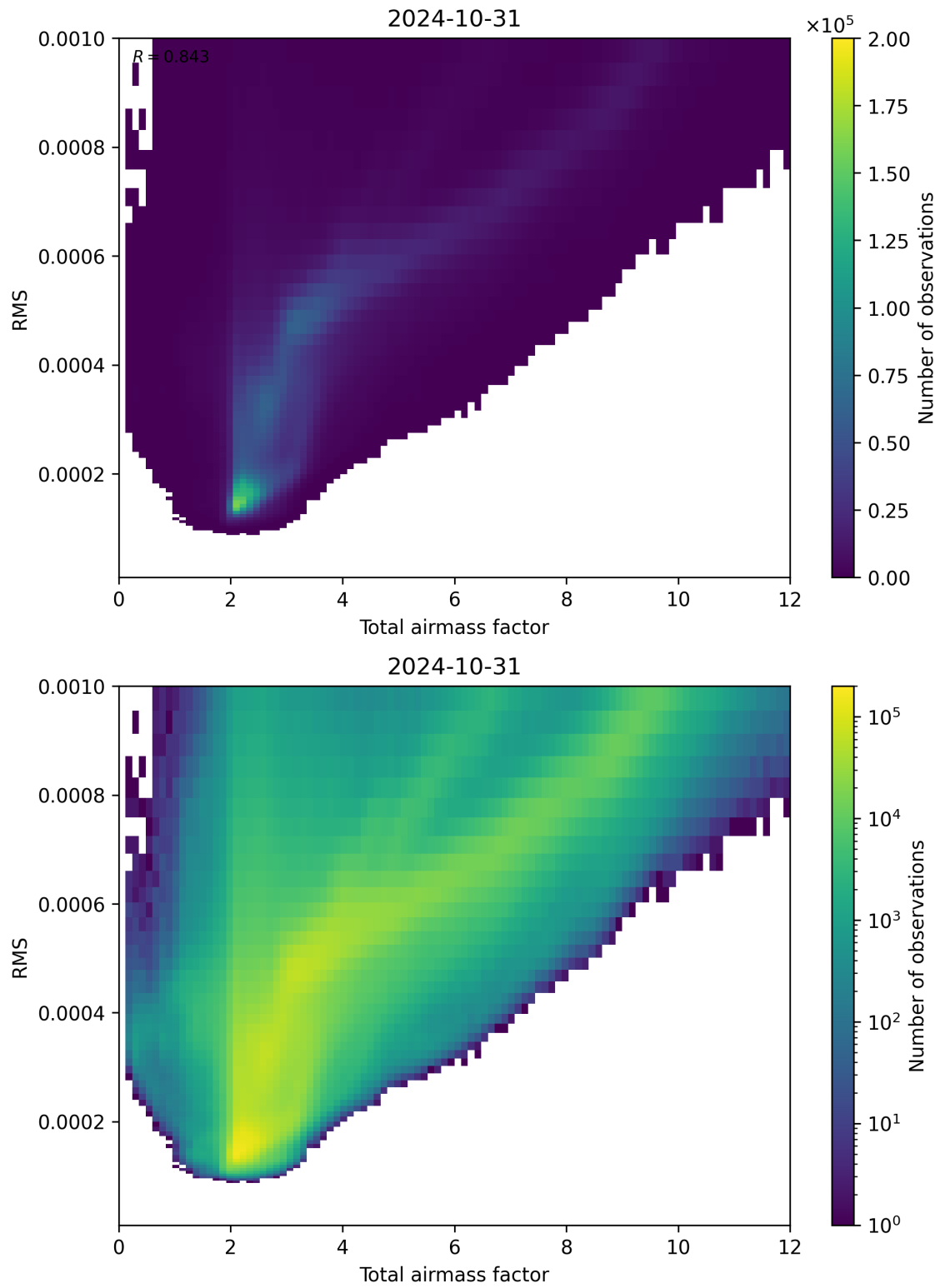
Figure 69: Scatter density plot of “Total airmass factor” against “RMS” for 2024-10-30 to 2024-11-01.
