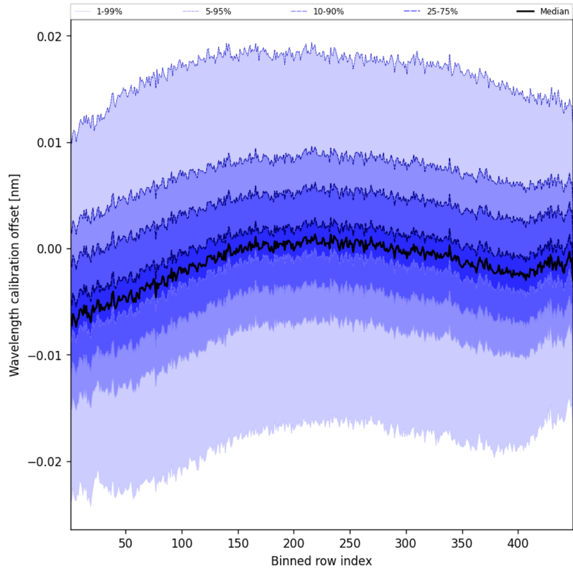
Figure 52: Along track statistics of “Wavelength calibration offset” for 2024-10-30 to 2024-11-01
