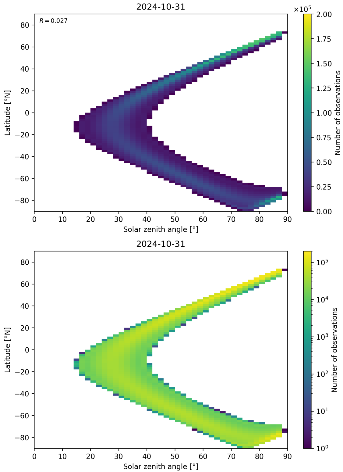
Figure 149: Scatter density plot of “Solar zenith angle” against “Latitude” for 2024-10-30 to 2024-11-01.
