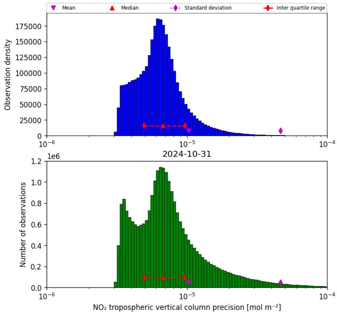
Figure 30: Histogram of “NO 2 tropospheric vertical column precision” for 2024-10-30 to 2024-11-01
