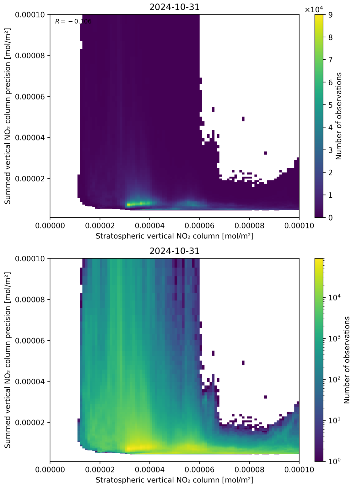
Figure 99: Scatter density plot of “Stratospheric vertical NO 2 column” against “Summed vertical NO 2 column precision” for 2024-10-30 to 2024-11-01.
