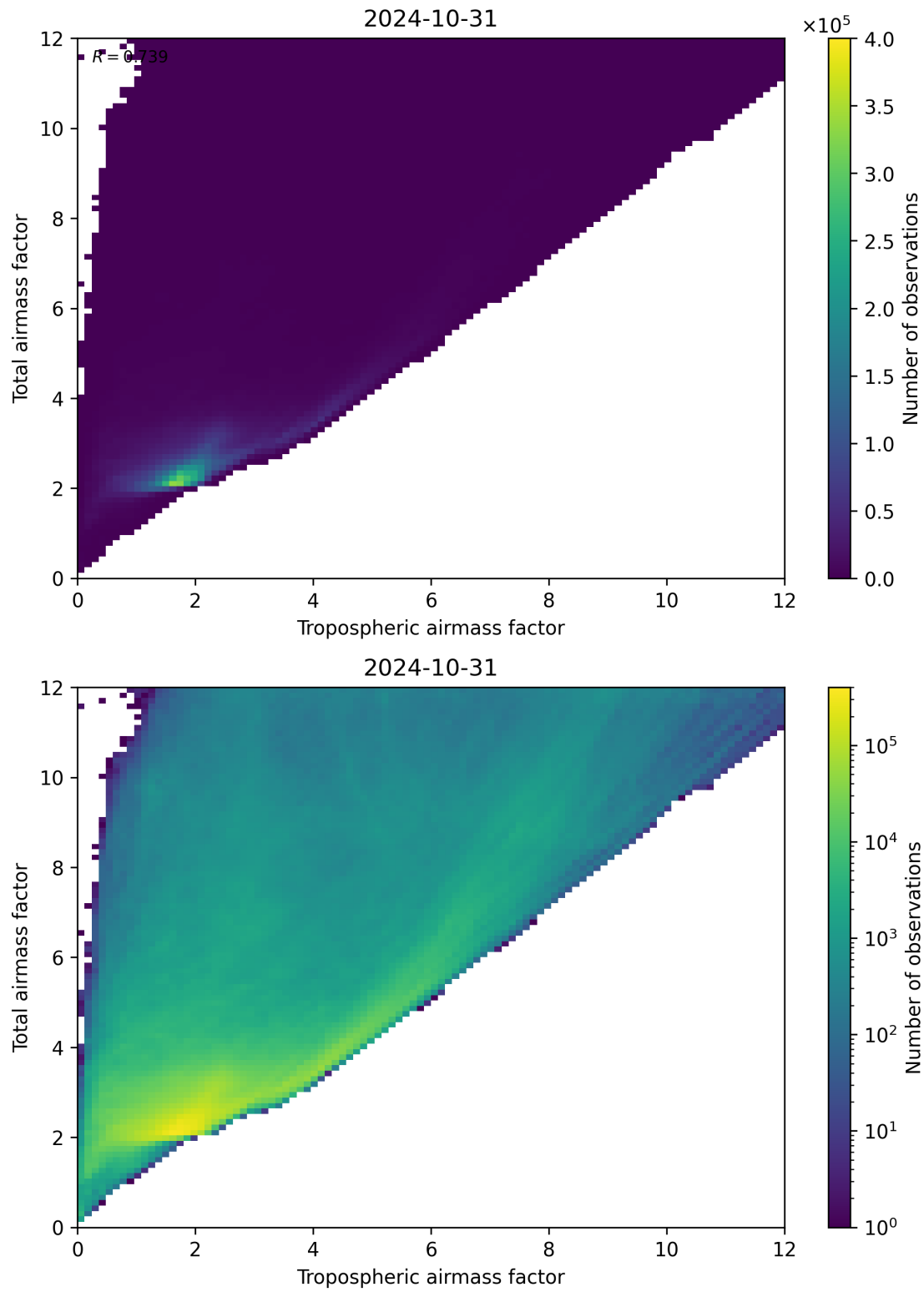
Figure 72: Scatter density plot of “Tropospheric airmass factor” against “Total airmass factor” for 2024-10-30 to 2024-11-01.
