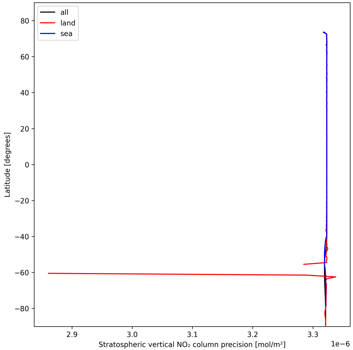
Figure 20: Zonal average of “Stratospheric vertical NO 2 column precision” for 2024-10-30 to 2024-11-01.
