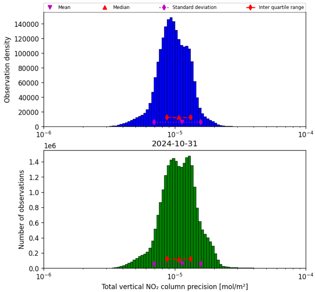
Figure 39: Histogram of “Total vertical NO 2 column precision” for 2024-10-30 to 2024-11-01
