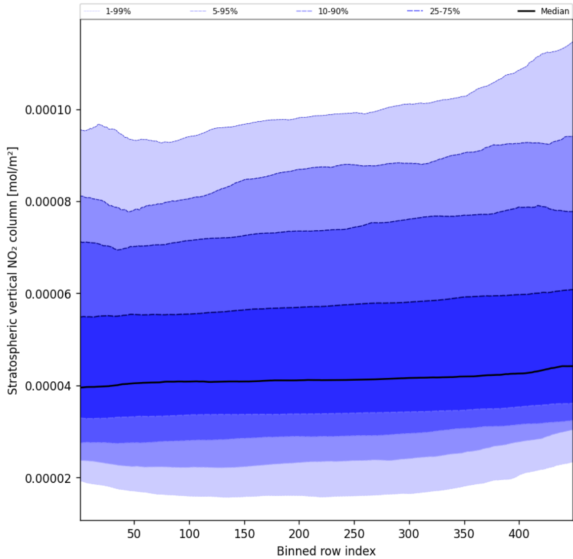
Figure 53: Along track statistics of “Stratospheric vertical NO 2 column” for 2024-10-30 to 2024-11-01
