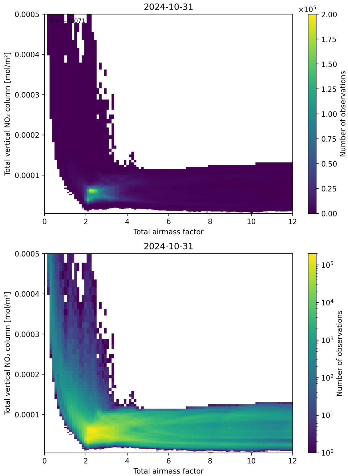
Figure 67: Scatter density plot of “Total airmass factor” against “Total vertical NO 2 column” for 2024-10-30 to 2024-11-01.
