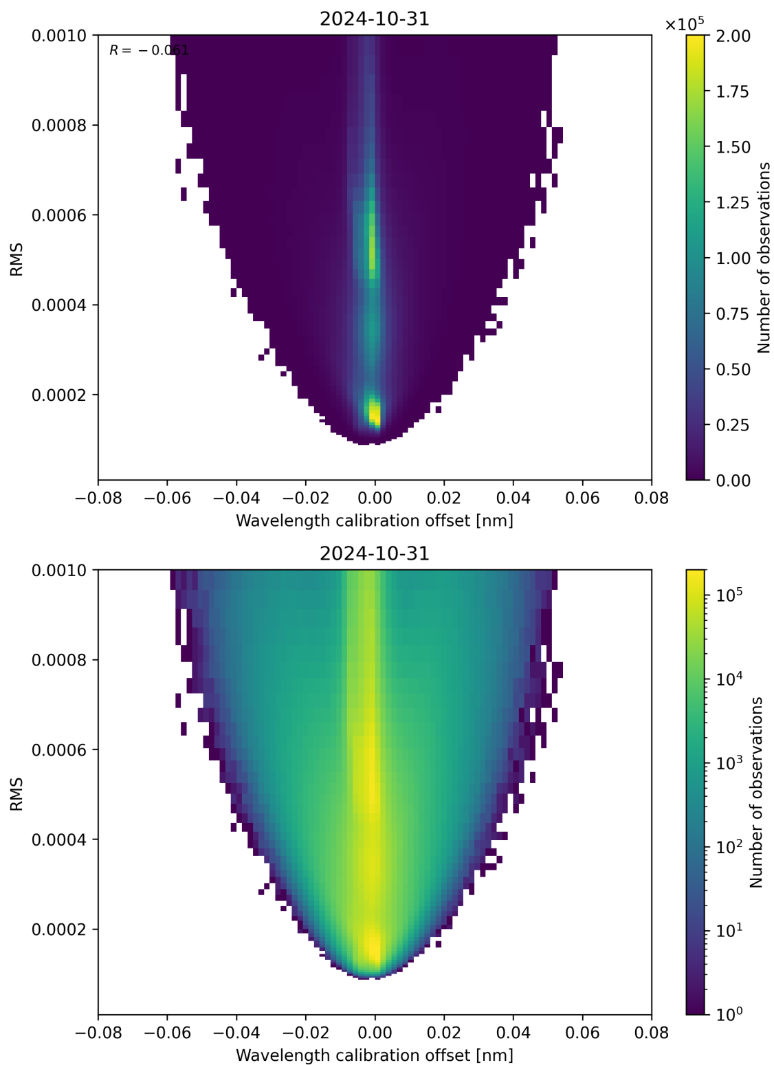
Figure 181: Scatter density plot of “Wavelength calibration offset” against “RMS” for 2024-10-30 to 2024-11-01.
