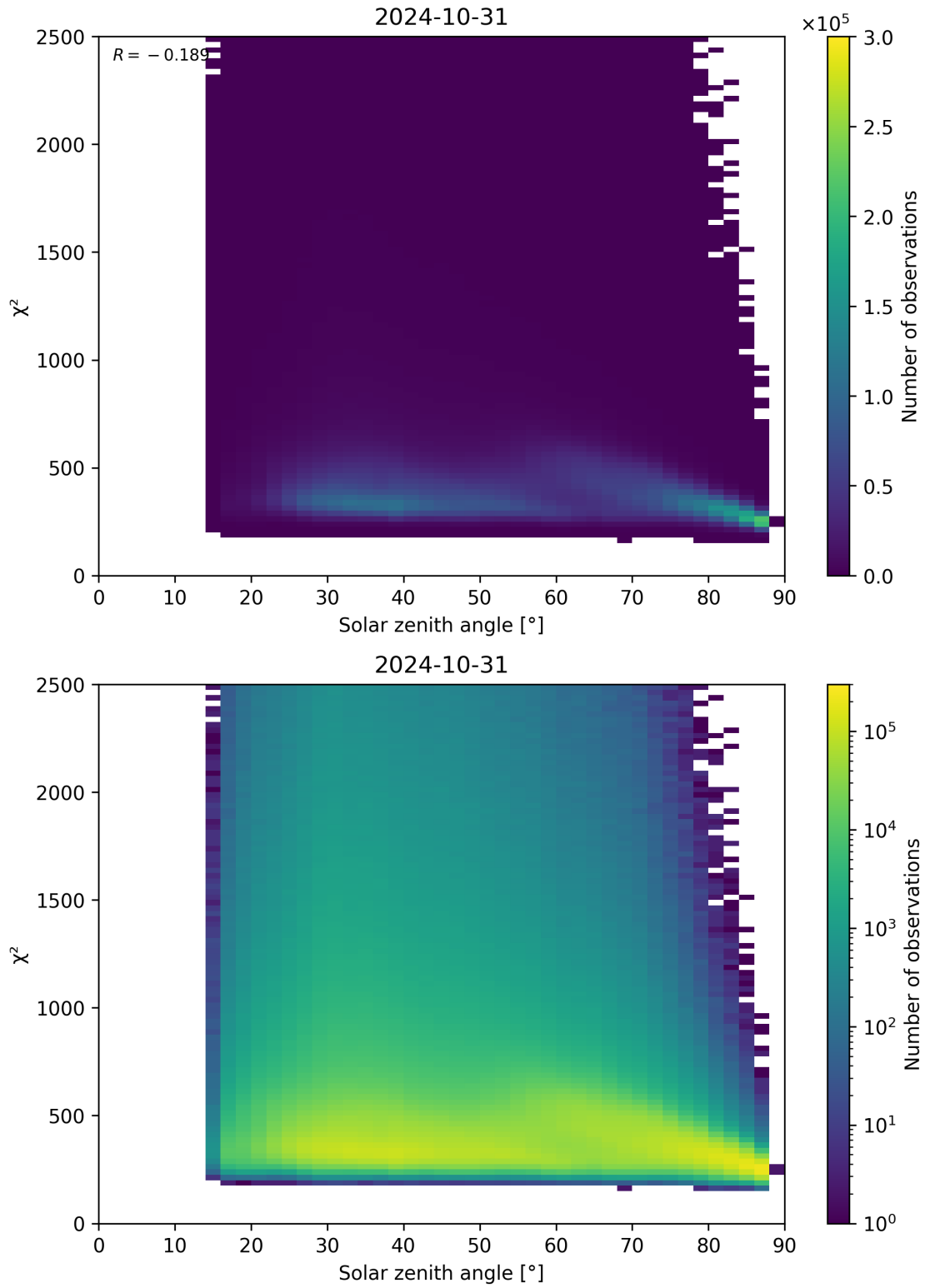
Figure 148: Scatter density plot of “Solar zenith angle” against “ \chi^2 ” for 2024-10-30 to 2024-11-01.
