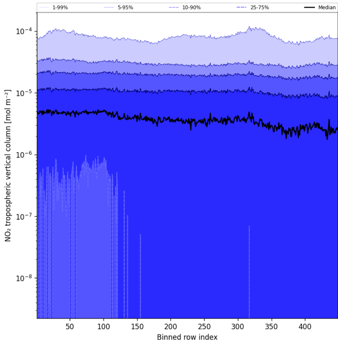
Figure 46: Along track statistics of “NO 2 tropospheric vertical column” for 2024-10-30 to 2024-11-01
