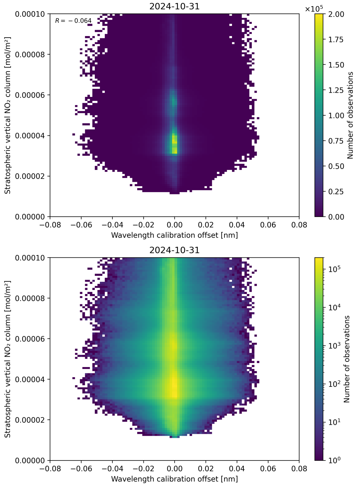
Figure 176: Scatter density plot of “Wavelength calibration offset” against “Stratospheric vertical NO 2 column” for 2024-10-30 to 2024-11-01.
