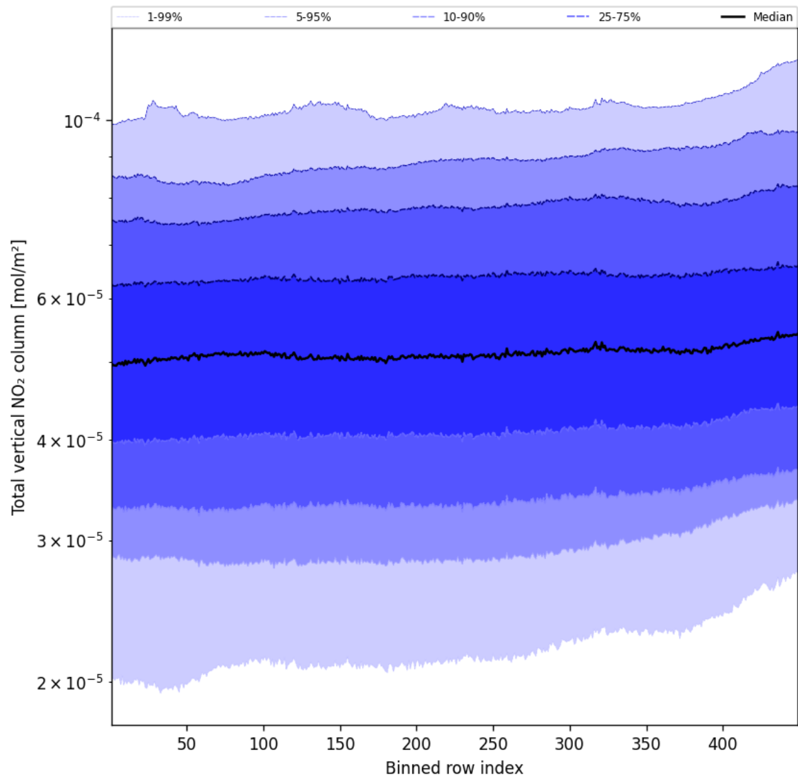
Figure 55: Along track statistics of “Total vertical NO 2 column” for 2024-10-30 to 2024-11-01
