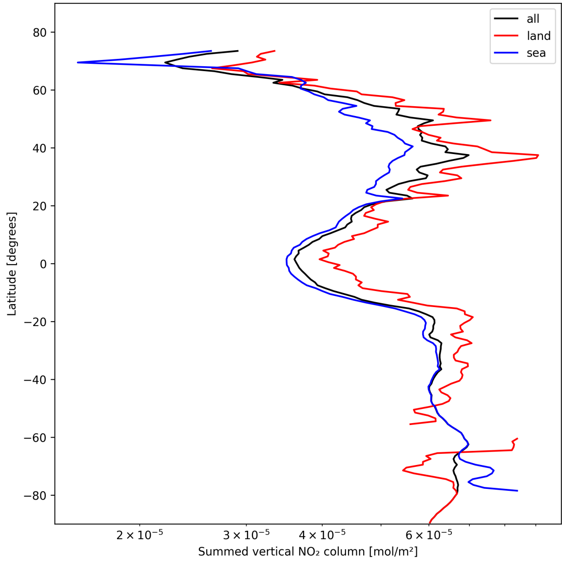
Figure 23: Zonal average of “Summed vertical NO 2 column” for 2024-10-30 to 2024-11-01.
