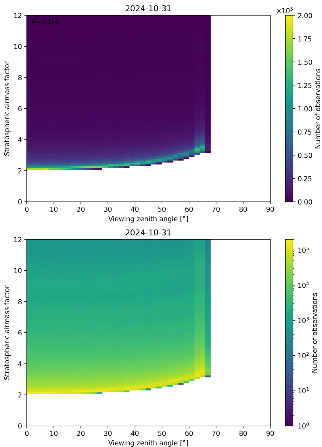
Figure 159: Scatter density plot of “Viewing zenith angle” against “Stratospheric airmass factor” for 2024-10-30 to 2024-11-01.
