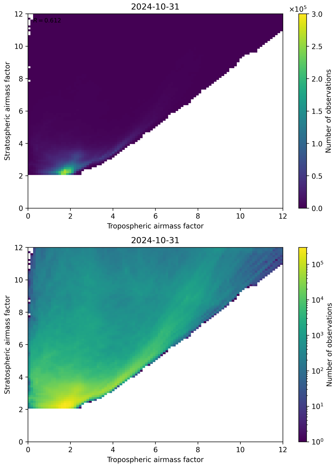
Figure 71: Scatter density plot of “Tropospheric airmass factor” against “Stratospheric airmass factor” for 2024-10-30 to 2024-11-01.
