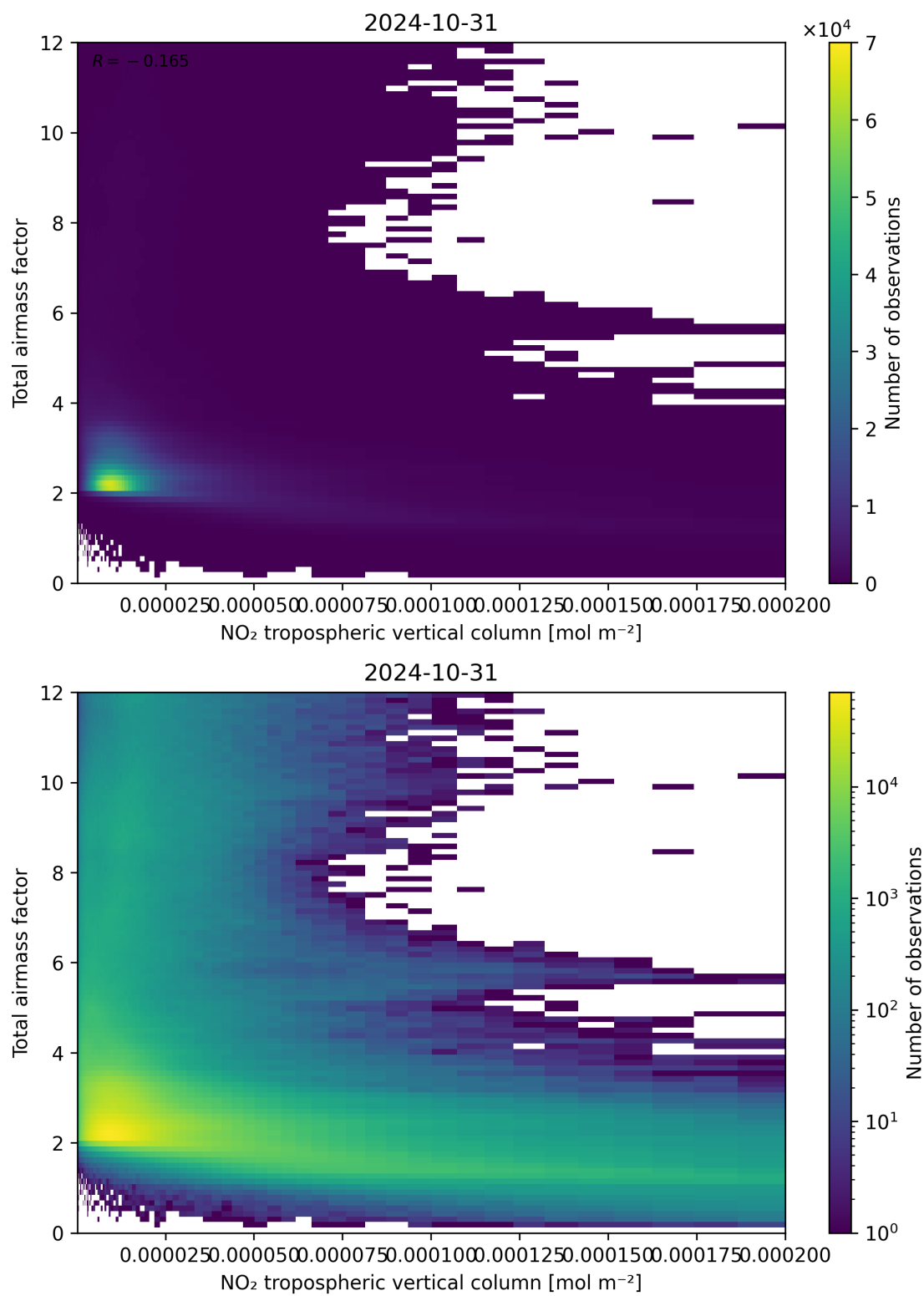
Figure 122: Scatter density plot of “NO 2 tropospheric vertical column” against “Total air mass factor” for 2024-10-30 to 2024-11-01.
