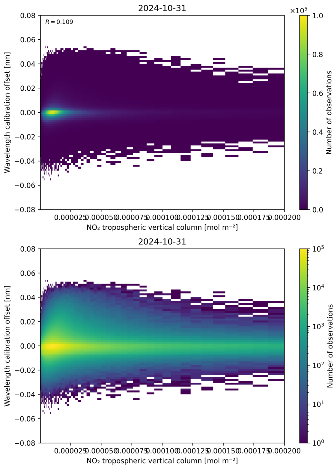
Figure 143: Scatter density plot of “NO 2 tropospheric vertical column” against “Wavelength calibration offset” for 2024-10-30 to 2024-11-01.
