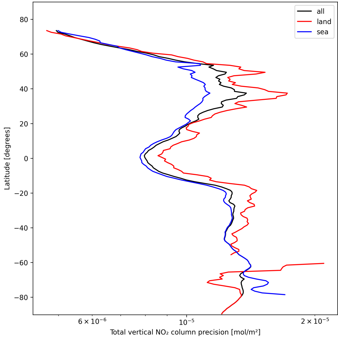
Figure 22: Zonal average of “Total vertical NO 2 column precision” for 2024-10-30 to 2024-11-01.
