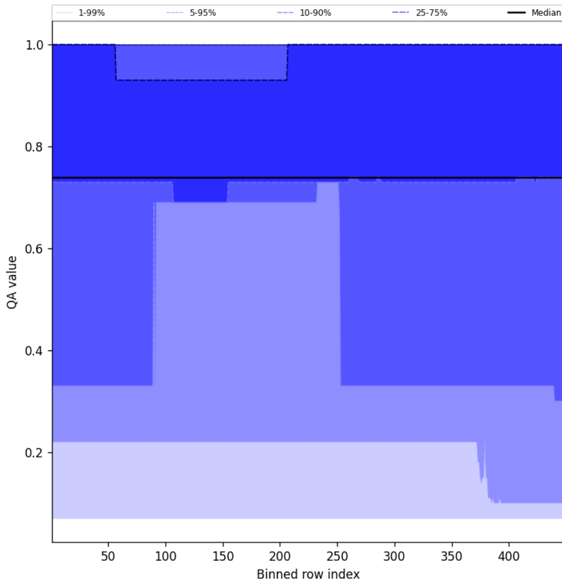
Figure 45: Along track statistics of “QA value” for 2024-10-30 to 2024-11-01
