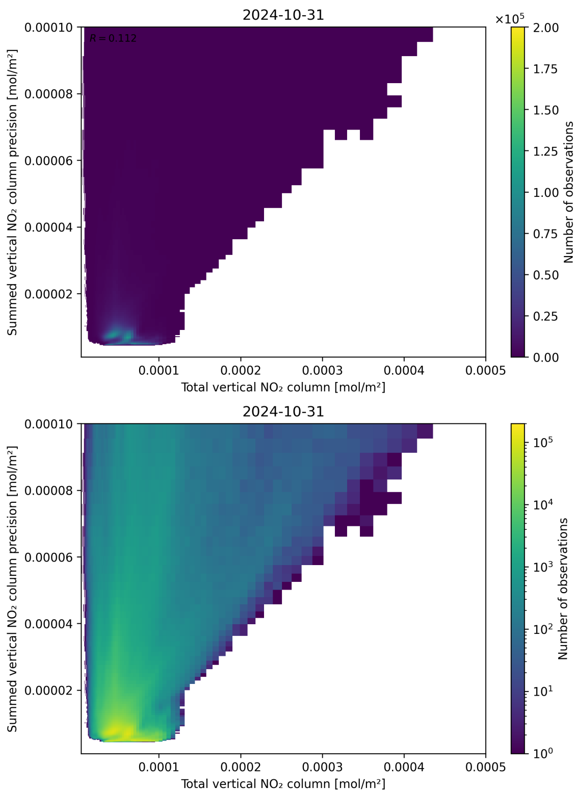
Figure 113: Scatter density plot of “Total vertical NO 2 column” against “Summed vertical NO 2 column precision” for 2024-10-30 to 2024-11-01.
