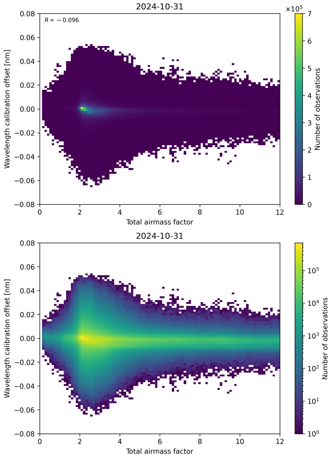
Figure 70: Scatter density plot of “Total airmass factor” against “Wavelength calibration offset” for 2024-10-30 to 2024-11-01.
