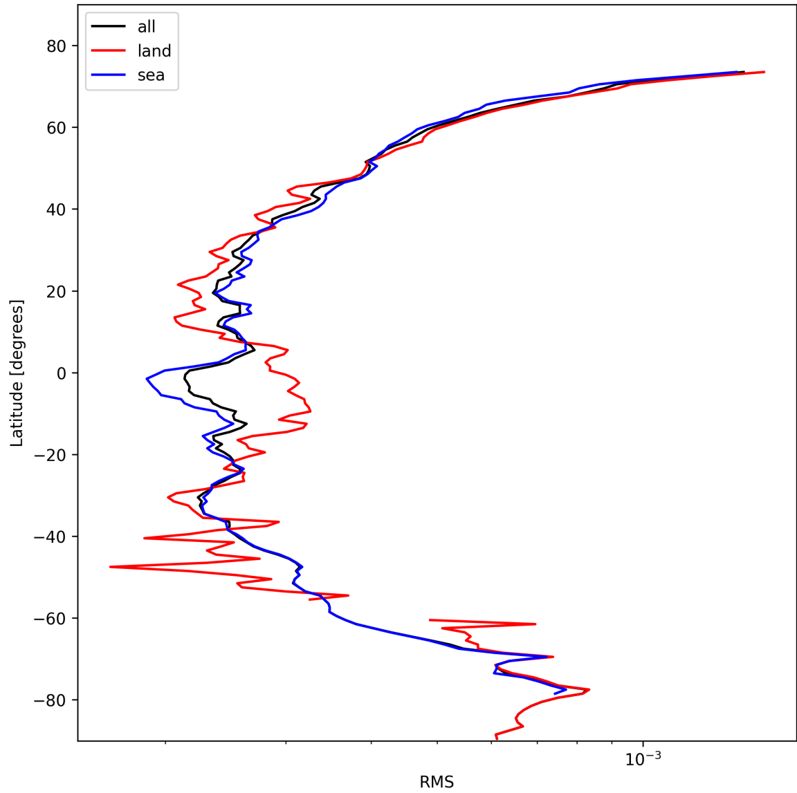
Figure 26: Zonal average of “RMS” for 2024-10-30 to 2024-11-01.
