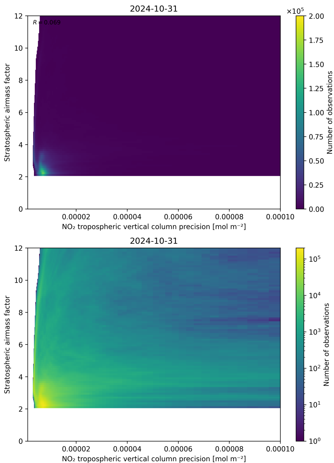
Figure 131: Scatter density plot of “NO 2 tropospheric vertical column precision” against “Stratospheric airmass factor” for 2024-10-30 to 2024-11-01.
