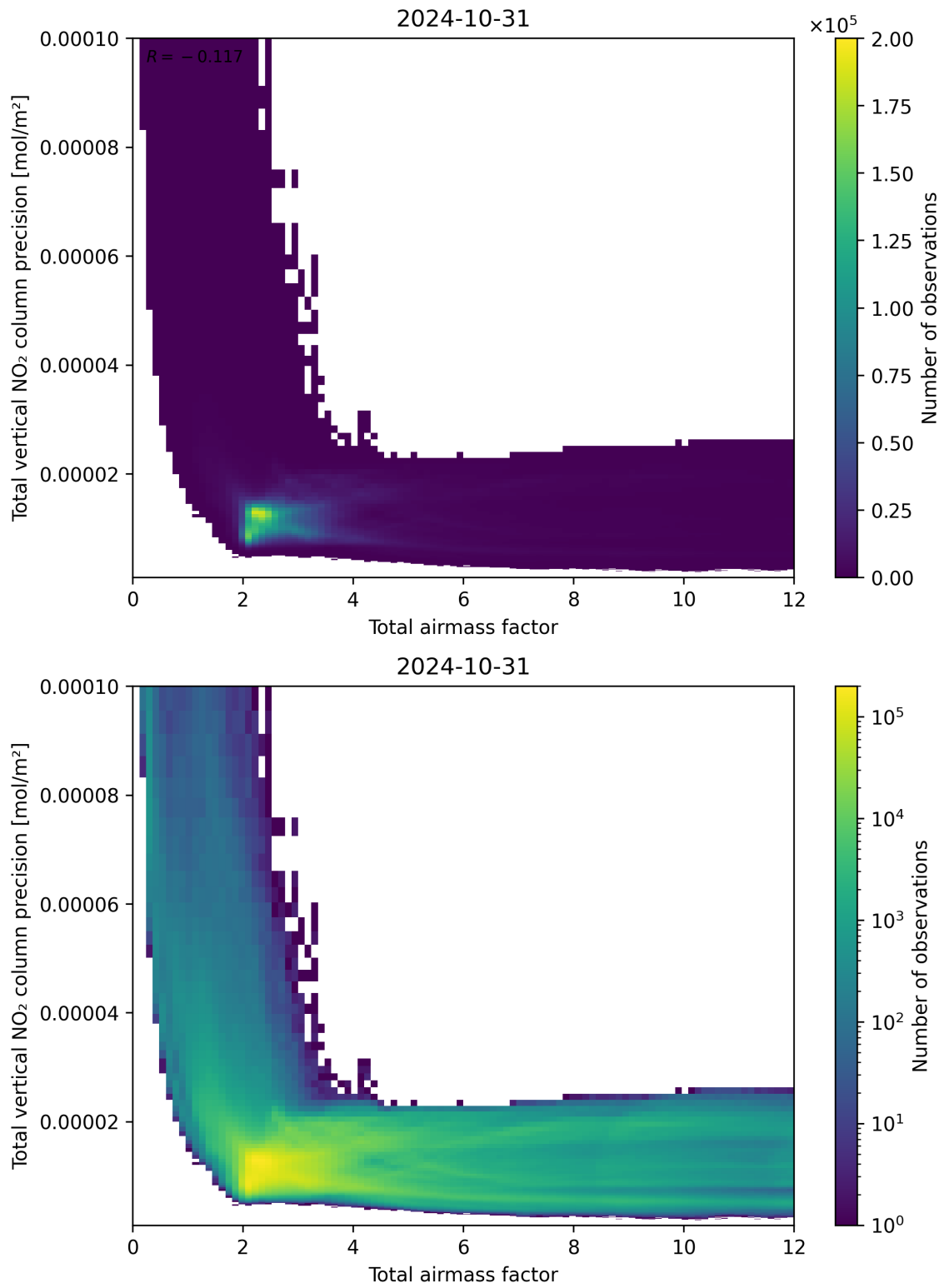
Figure 68: Scatter density plot of “Total airmass factor” against “Total vertical NO 2 column precision” for 2024-10-30 to 2024-11-01.
