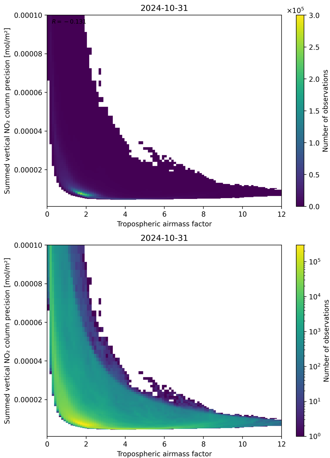
Figure 76: Scatter density plot of “Tropospheric air mass factor” against “Summed vertical NO 2 column precision” for 2024-10-30 to 2024-11-01.
