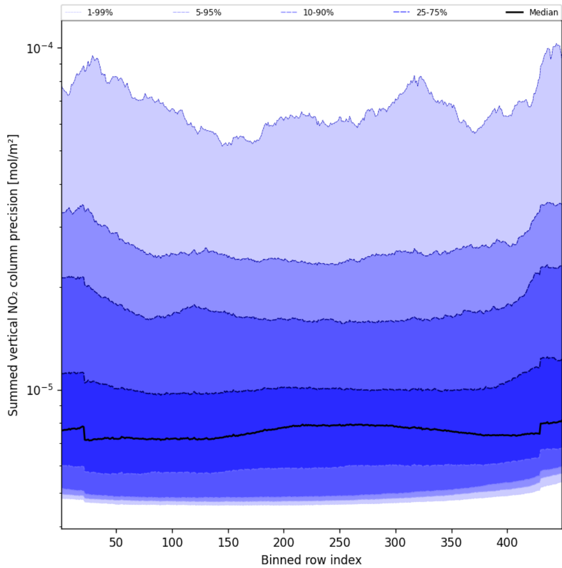
Figure 58: Along track statistics of “Summed vertical NO 2 column precision” for 2024-10-30 to 2024-11-01
