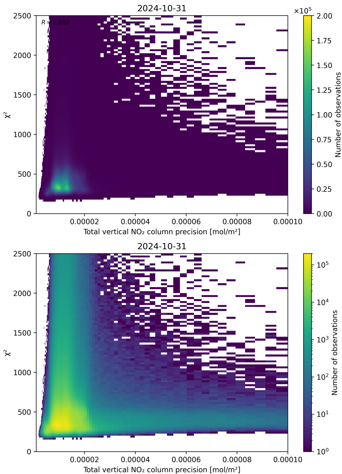
Figure 116: Scatter density plot of “Total vertical NO 2 column precision” against “ \chi^2 ” for 2024-10-30 to 2024-11-01.
