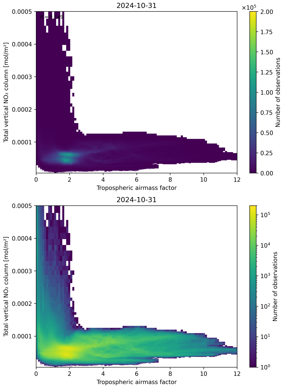
Figure 77: Scatter density plot of “Tropospheric airmass factor” against “Total vertical NO 2 column” for 2024-10-30 to 2024-11-01.
