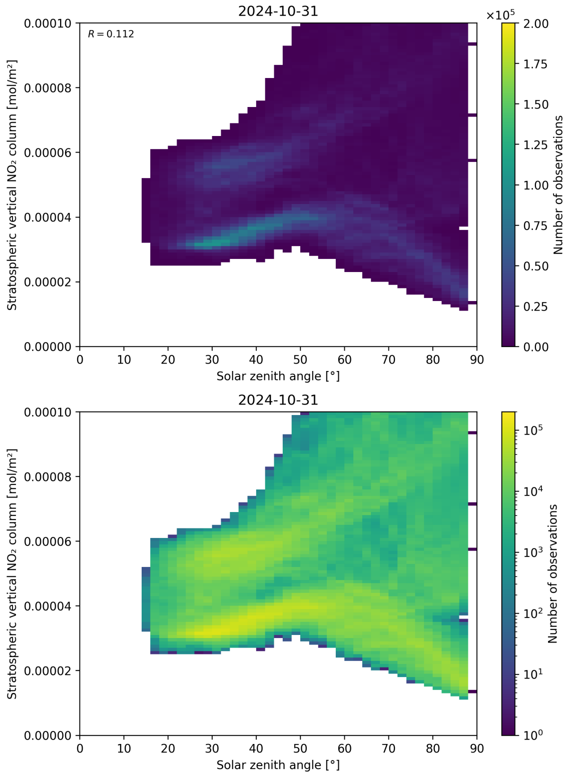
Figure 150: Scatter density plot of “Solar zenith angle” against “Stratospheric vertical NO 2 column” for 2024-10-30 to 2024-11-01.
