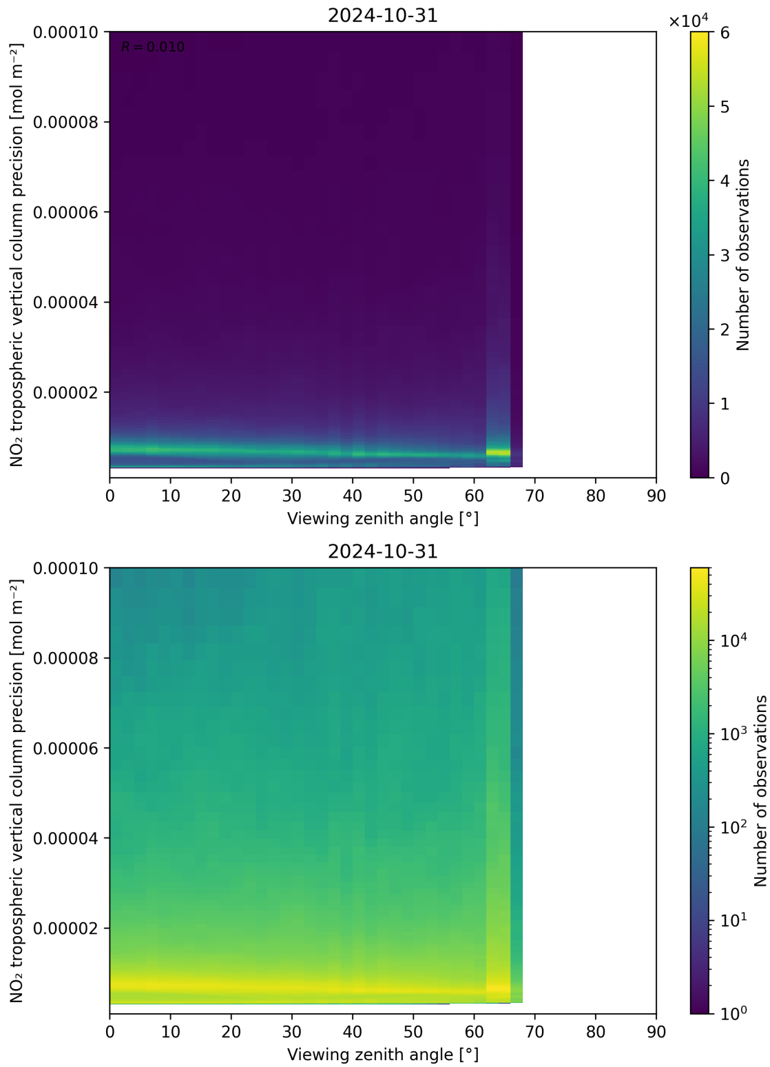
Figure 170: Scatter density plot of “Viewing zenith angle” against “NO 2 tropospheric vertical column precision” for 2024-10-30 to 2024-11-01.
