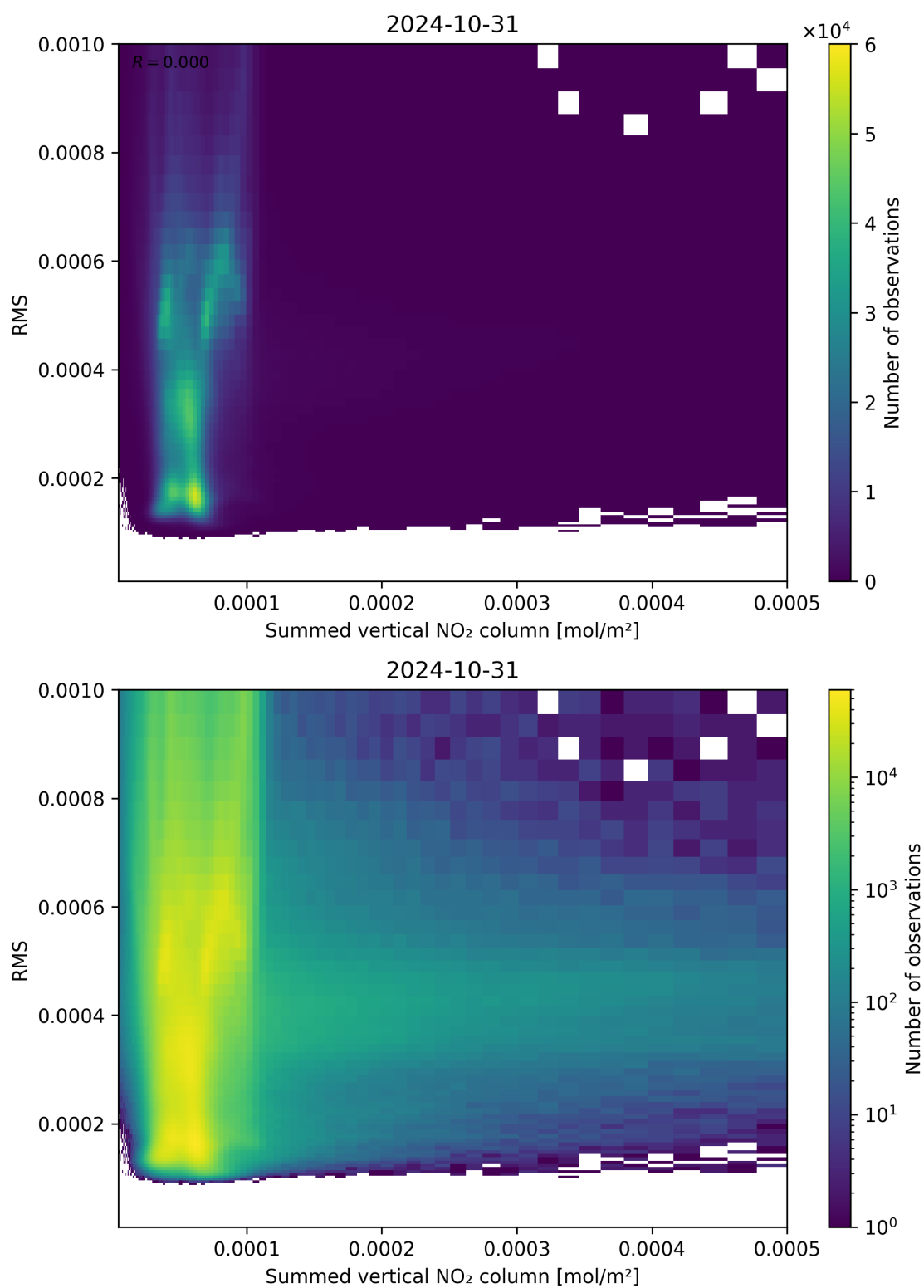
Figure 109: Scatter density plot of “Summed vertical NO 2 column” against “RMS” for 2024-10-30 to 2024-11-01.
