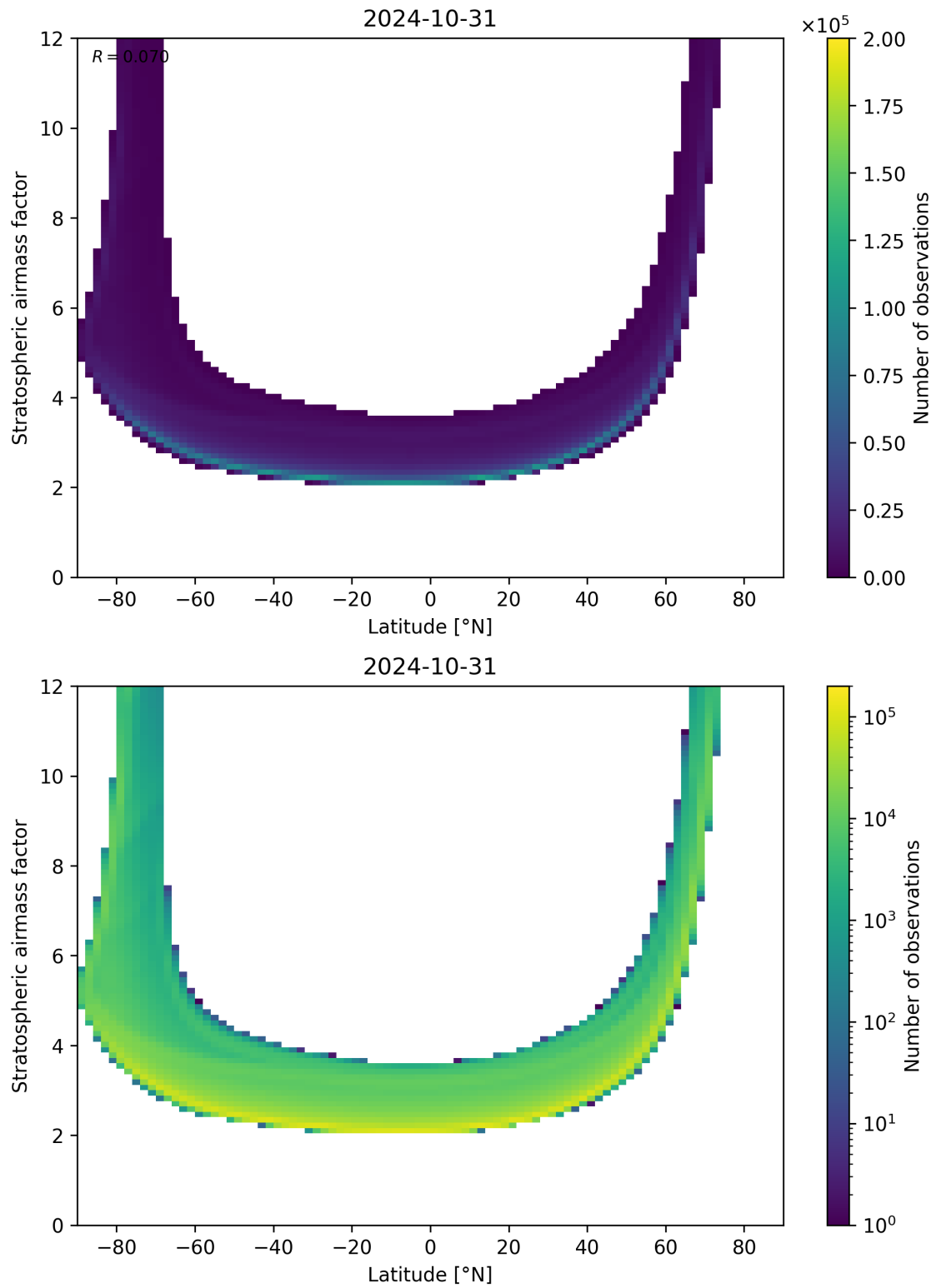
Figure 83: Scatter density plot of “Latitude” against “Stratospheric air mass factor” for 2024-10-30 to 2024-11-01.
