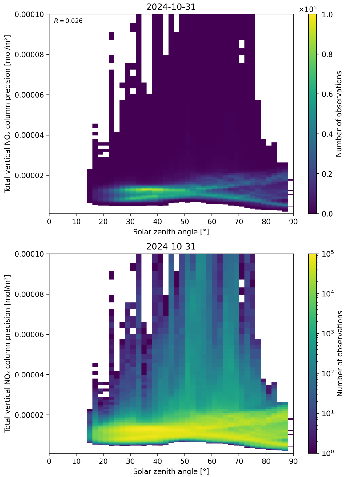
Figure 154: Scatter density plot of “Solar zenith angle” against “Total vertical NO 2 column precision” for 2024-10-30 to 2024-11-01.
