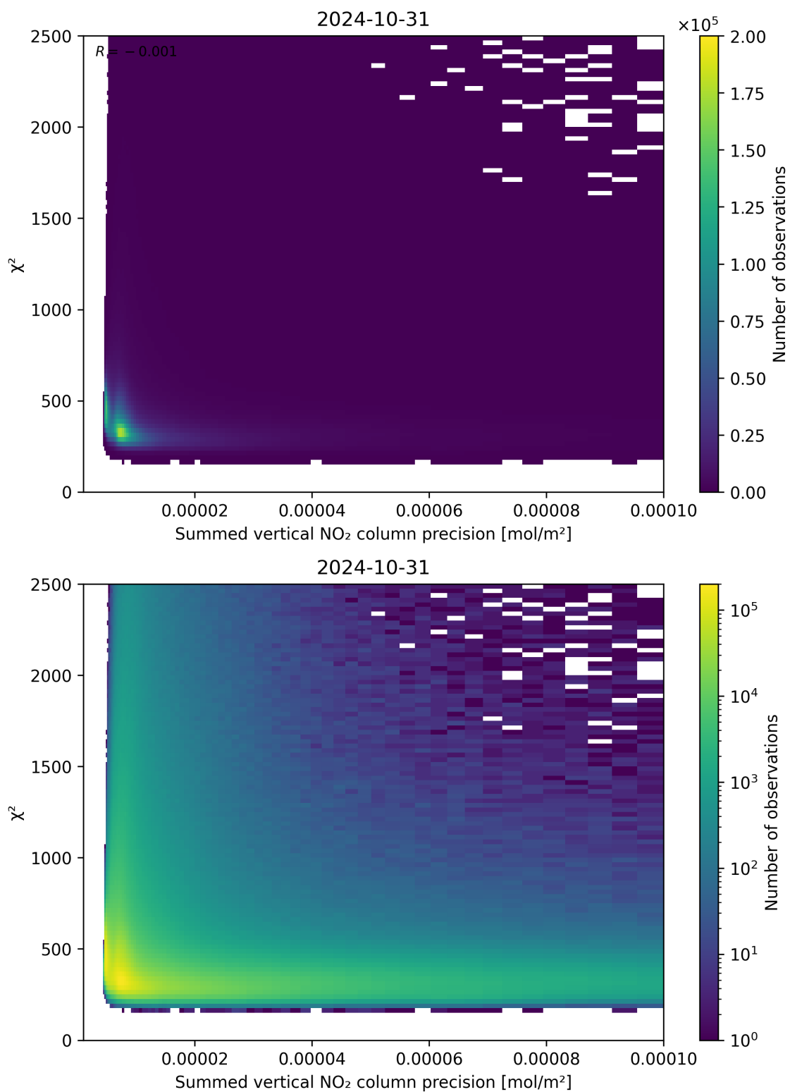
Figure 107: Scatter density plot of “Summed vertical NO 2 column precision” against “ \chi^2 ” for 2024-10-30 to 2024-11-01.
