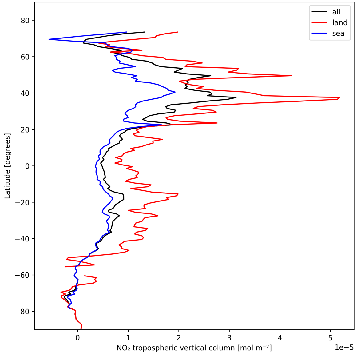
Figure 12: Zonal average of “NO 2 tropospheric vertical column” for 2024-10-30 to 2024-11-01.
