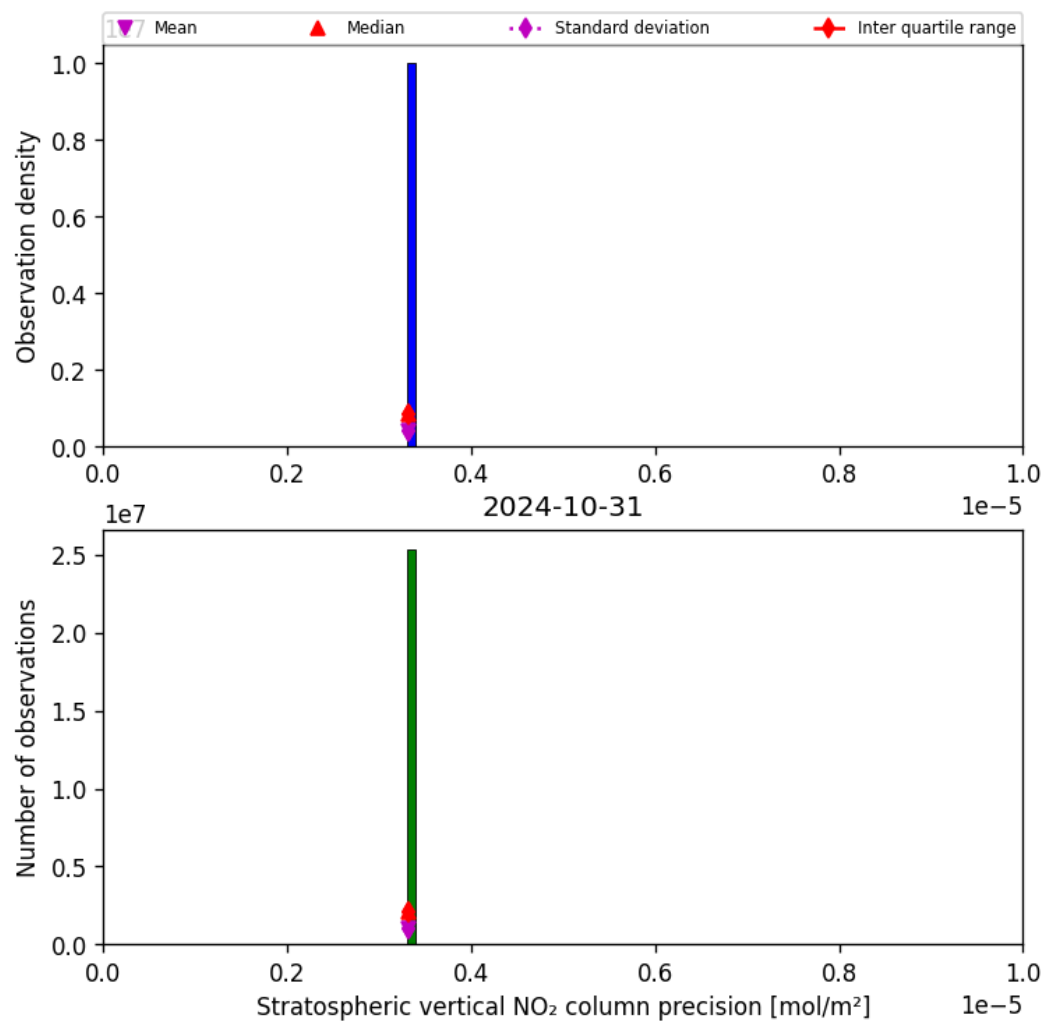
Figure 37: Histogram of “Stratospheric vertical NO 2 column precision” for 2024-10-30 to 2024-11-01
