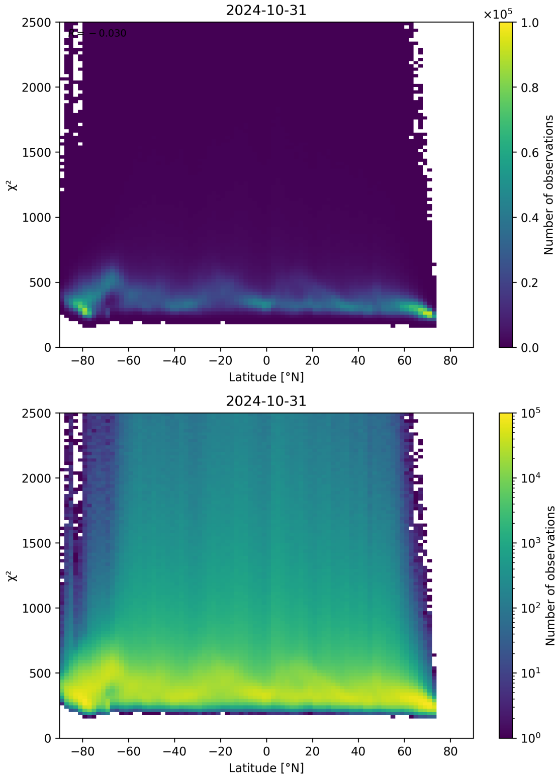
Figure 86: Scatter density plot of “Latitude” against “ \chi^2 ” for 2024-10-30 to 2024-11-01.
