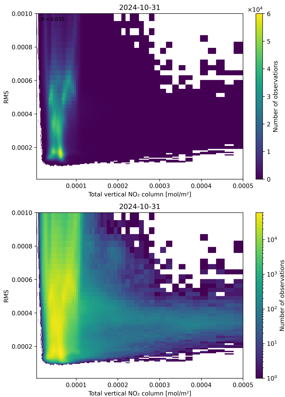
Figure 120: Scatter density plot of “Total vertical NO 2 column” against “RMS” for 2024-10-30 to 2024-11-01.
