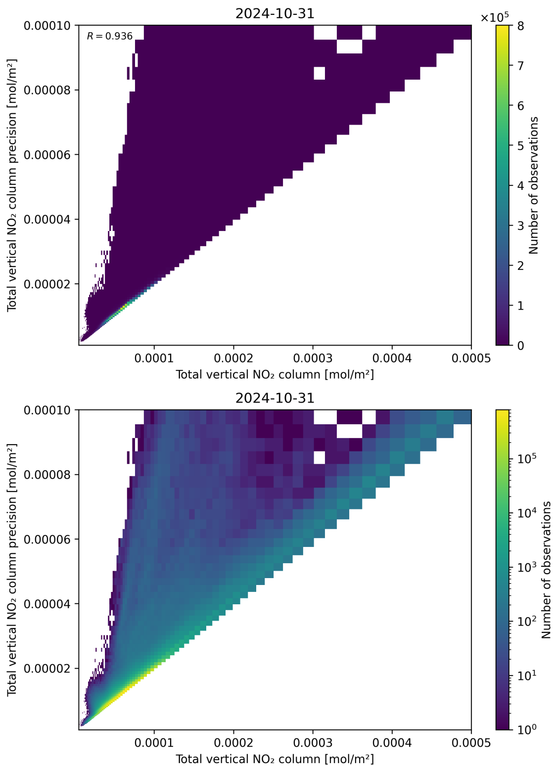
Figure 114: Scatter density plot of “Total vertical NO 2 column” against “Total vertical NO 2 column precision” for 2024-10-30 to 2024-11-01.
