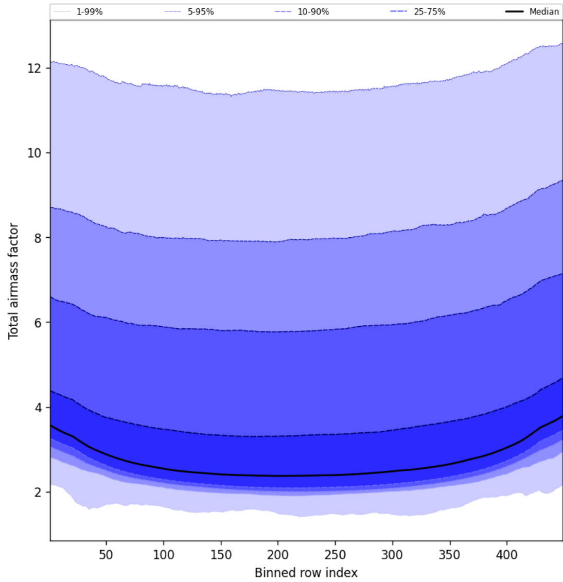
Figure 49: Along track statistics of “Total airmass factor” for 2024-10-30 to 2024-11-01
