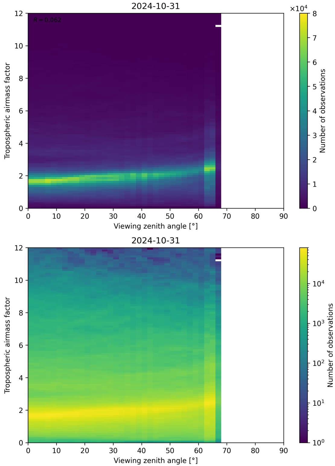
Figure 161: Scatter density plot of “Viewing zenith angle” against “Tropospheric airmass factor” for 2024-10-30 to 2024-11-01.
