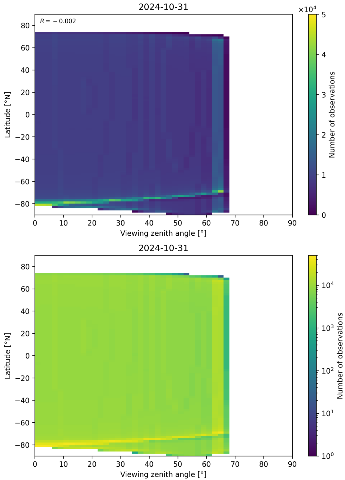
Figure 163: Scatter density plot of “Viewing zenith angle” against “Latitude” for 2024-10-30 to 2024-11-01.
