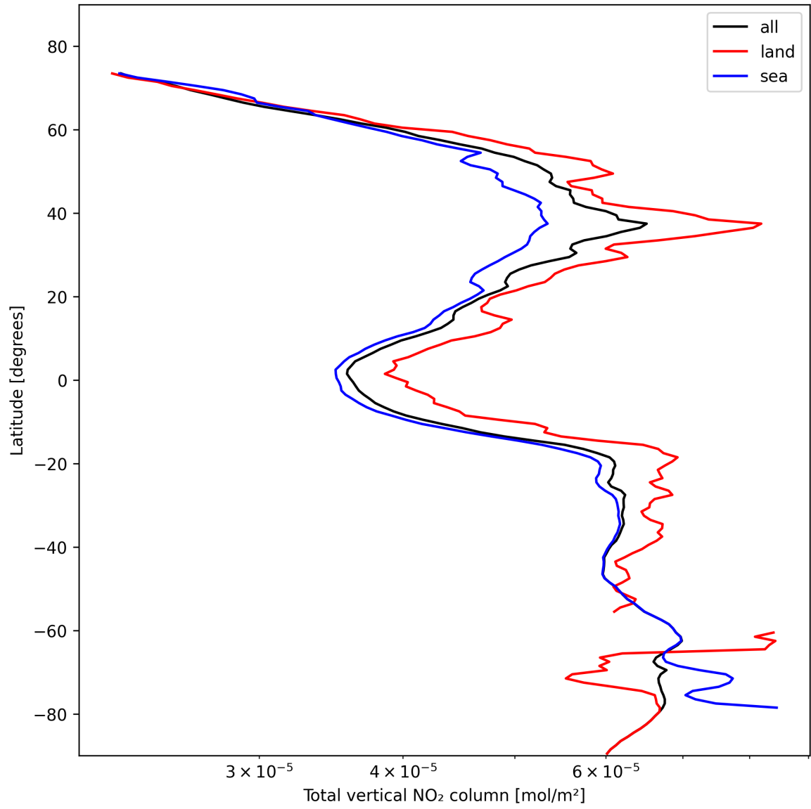
Figure 21: Zonal average of “Total vertical NO 2 column” for 2024-10-30 to 2024-11-01.
