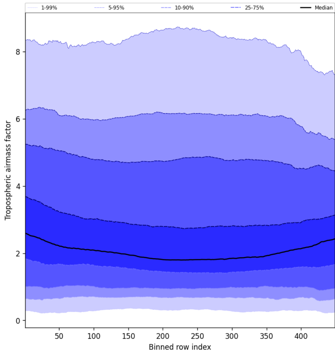
Figure 48: Along track statistics of “Tropospheric air mass factor” for 2024-10-30 to 2024-11-01
