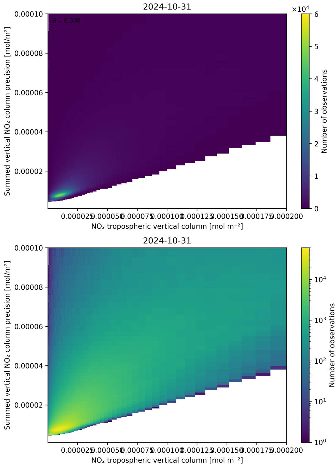
Figure 127: Scatter density plot of “NO 2 tropospheric vertical column” against “Summed vertical NO 2 column precision” for 2024-10-30 to 2024-11-01.
