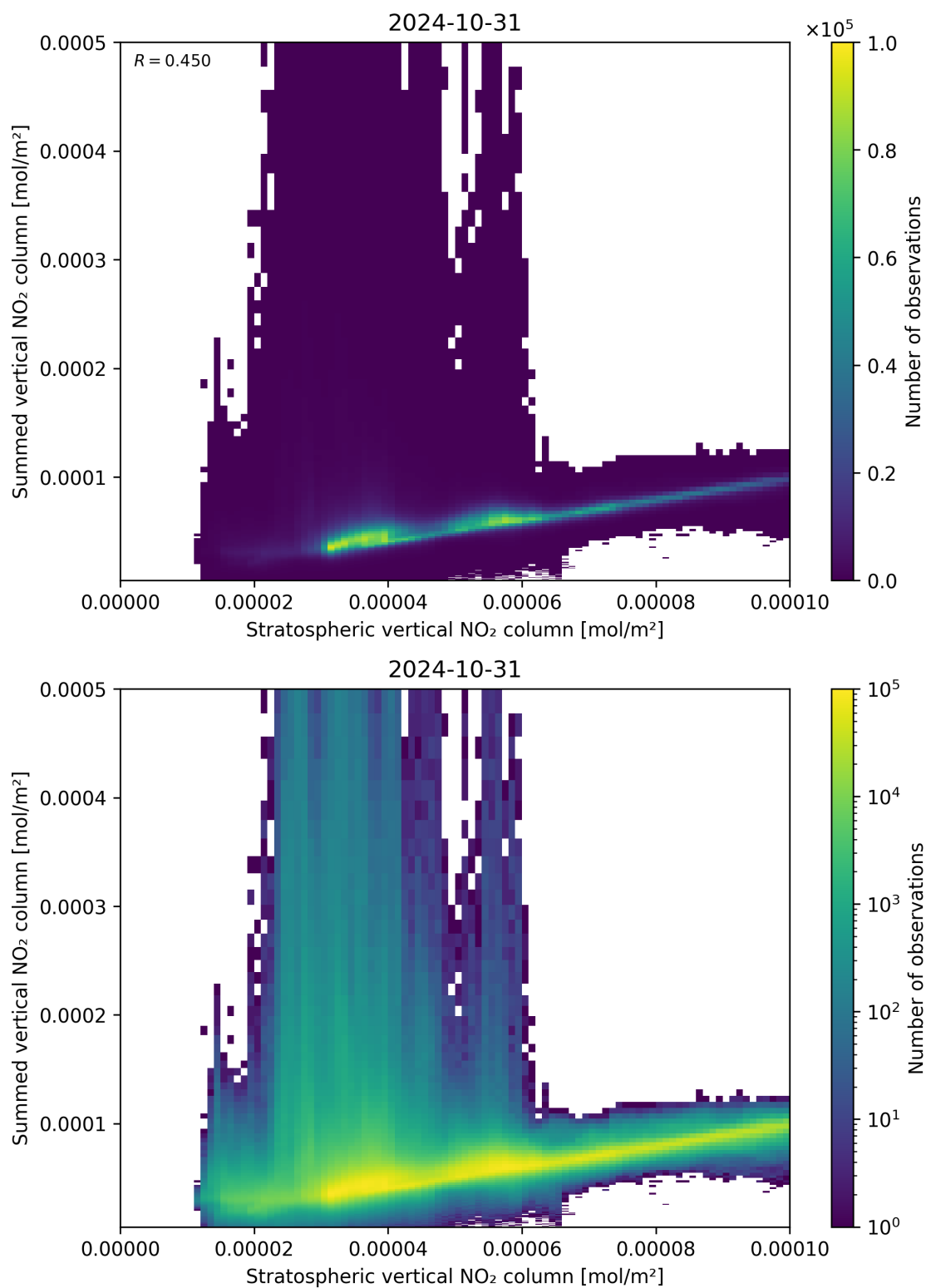
Figure 98: Scatter density plot of “Stratospheric vertical NO 2 column” against “Summed vertical NO 2 column” for 2024-10-30 to 2024-11-01.
