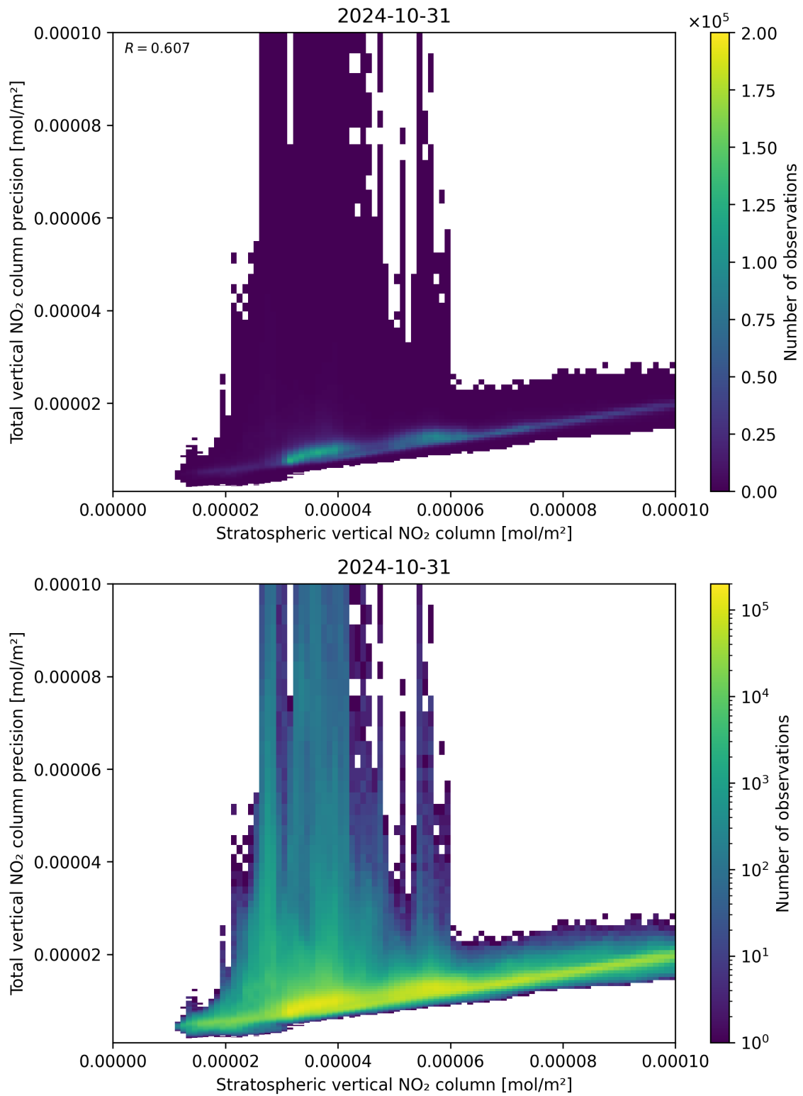
Figure 101: Scatter density plot of “Stratospheric vertical NO 2 column” against “Total vertical NO 2 column precision” for 2024-10-30 to 2024-11-01.
