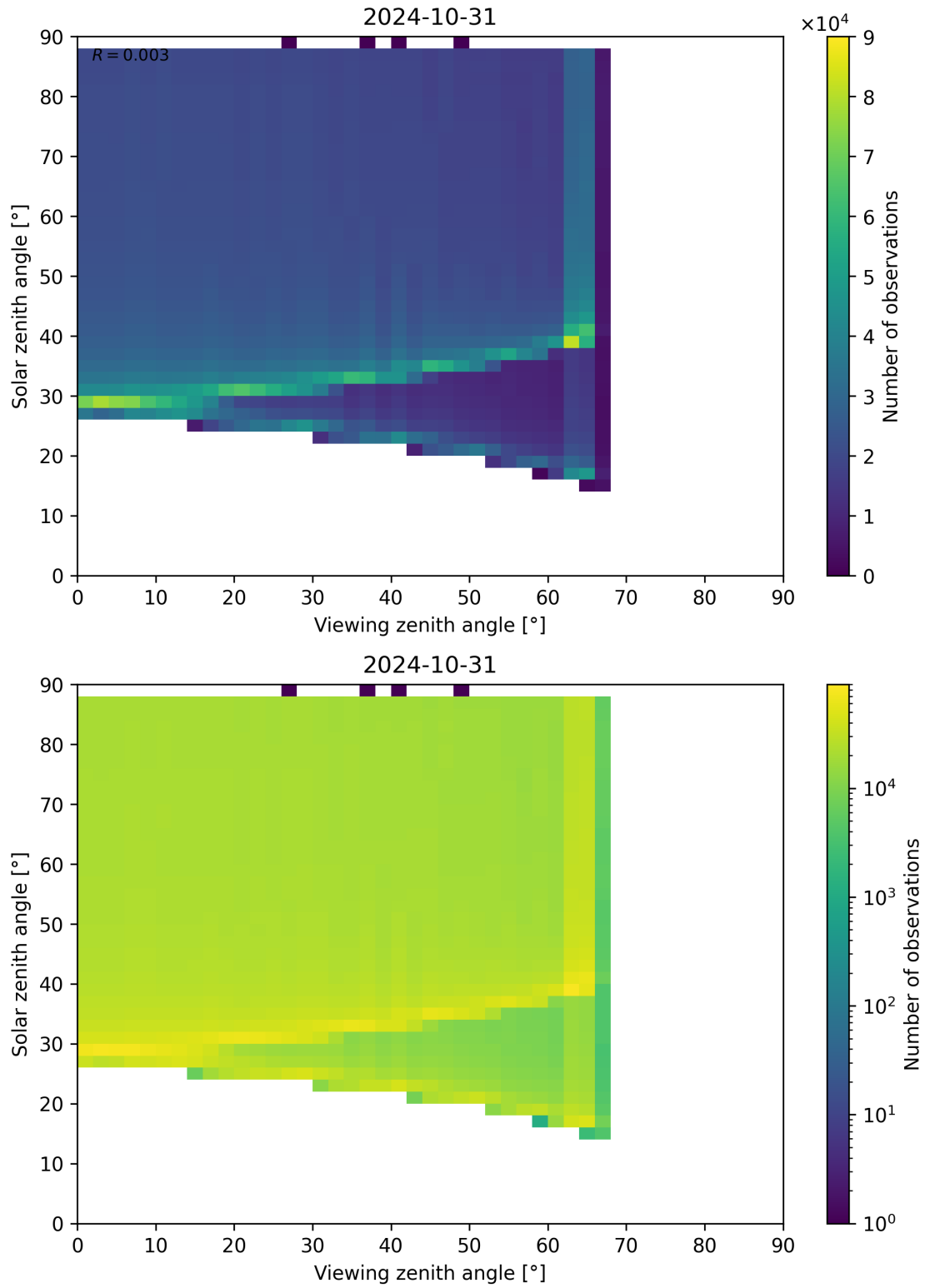
Figure 172: Scatter density plot of “Viewing zenith angle” against “Solar zenith angle” for 2024-10-30 to 2024-11-01.
