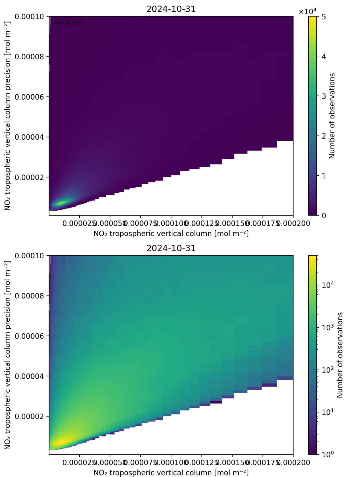
Figure 130: Scatter density plot of “NO 2 tropospheric vertical column” against “NO 2 tropospheric vertical column precision” for 2024-10-30 to 2024-11-01.
