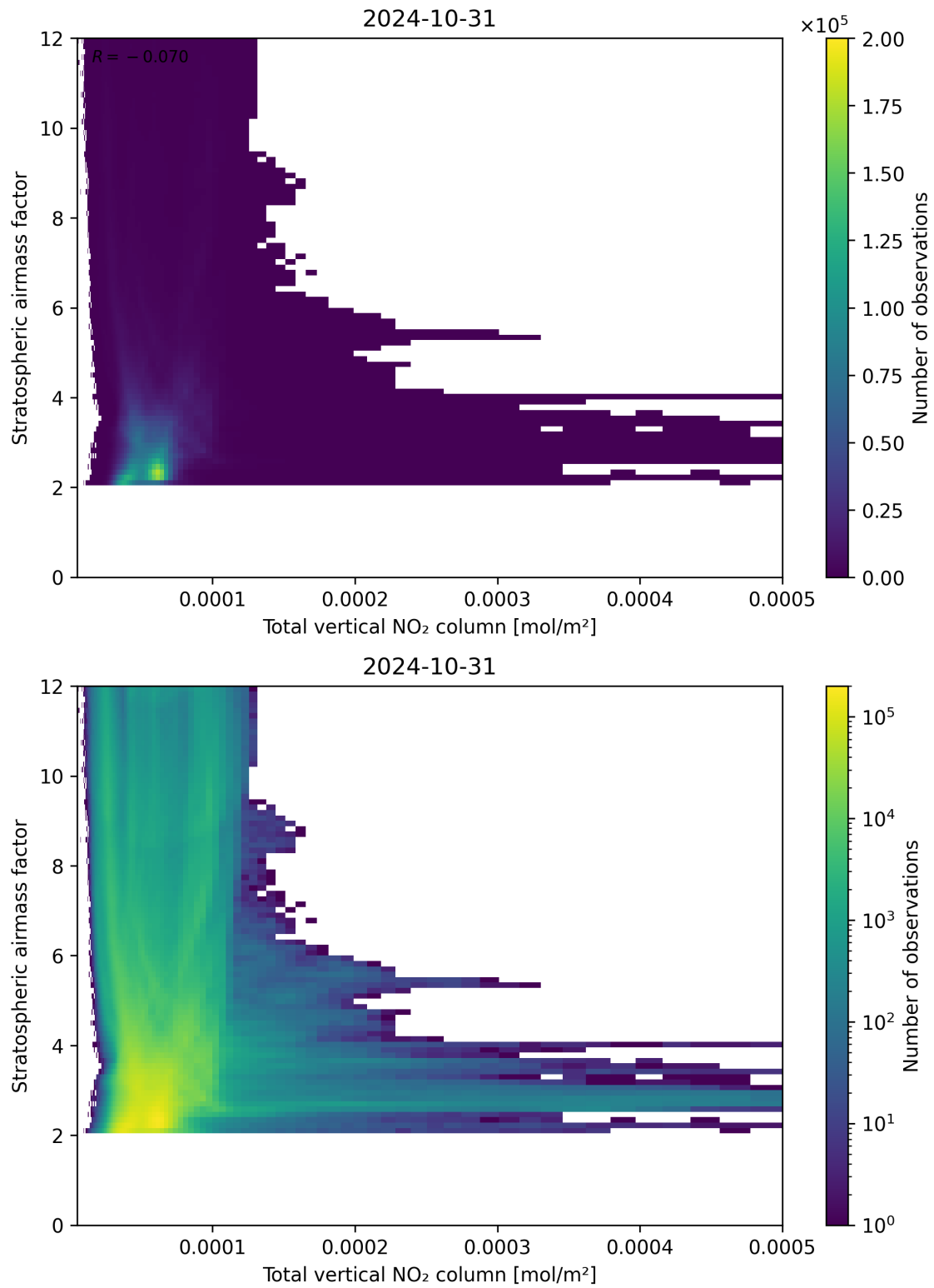
Figure 110: Scatter density plot of “Total vertical NO 2 column” against “Stratospheric air mass factor” for 2024-10-30 to 2024-11-01.
