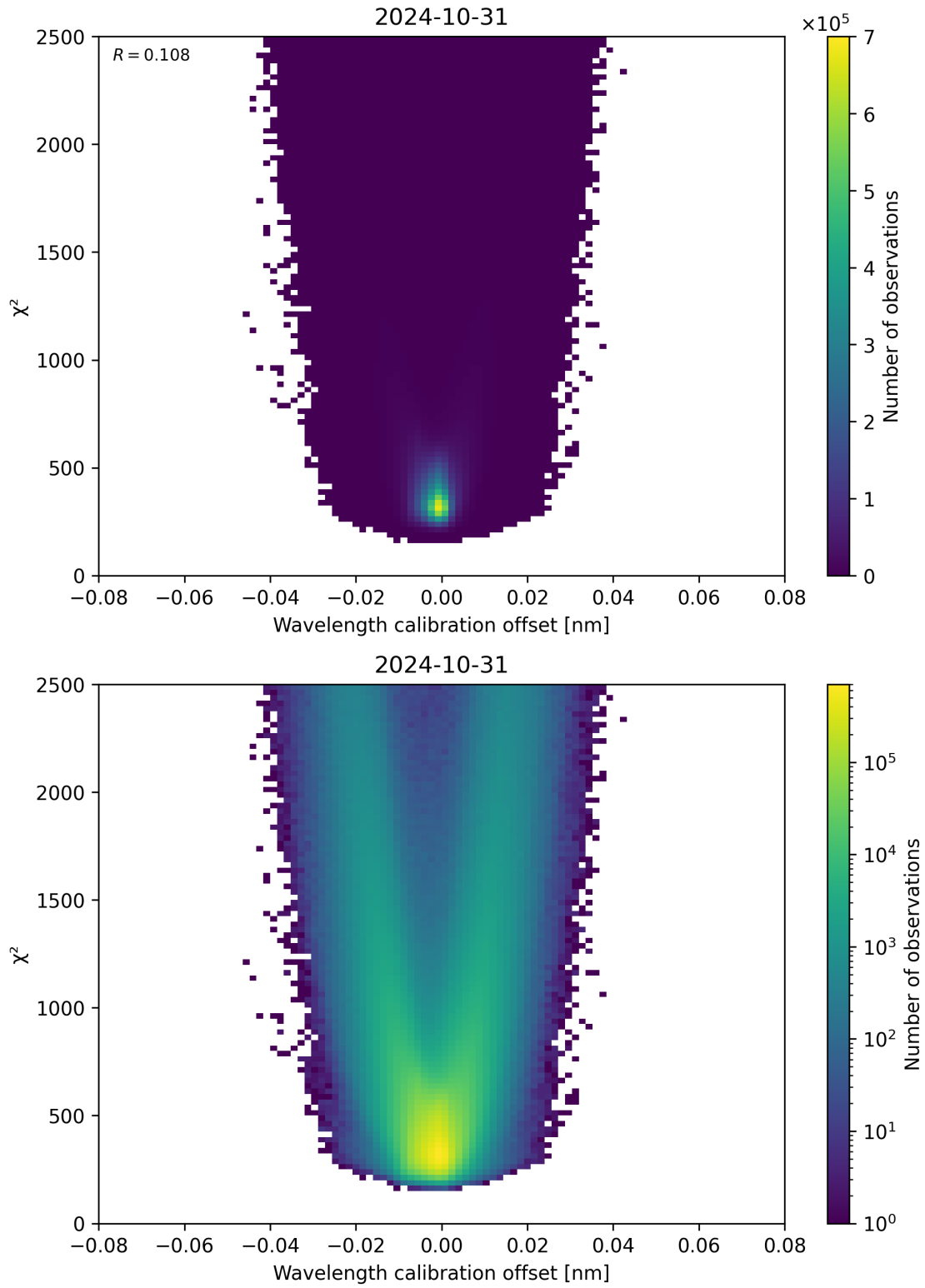
Figure 175: Scatter density plot of “Wavelength calibration offset” against “ \chi^2 ” for 2024-10-30 to 2024-11-01.
