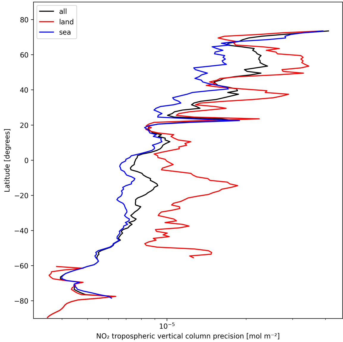
Figure 13: Zonal average of “NO 2 tropospheric vertical column precision” for 2024-10-30 to 2024-11-01.
