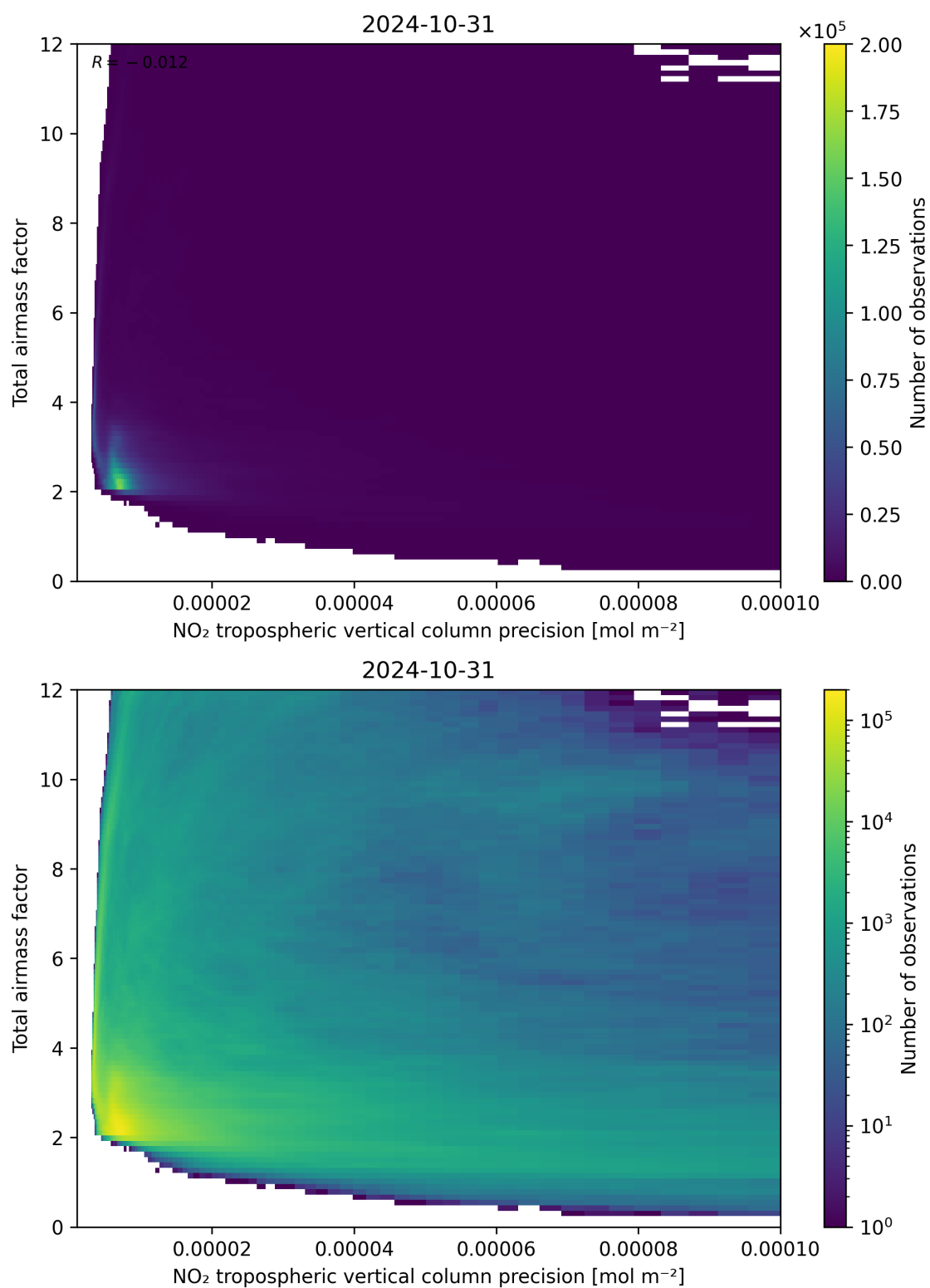
Figure 132: Scatter density plot of “NO 2 tropospheric vertical column precision” against “Total airmass factor” for 2024-10-30 to 2024-11-01.
