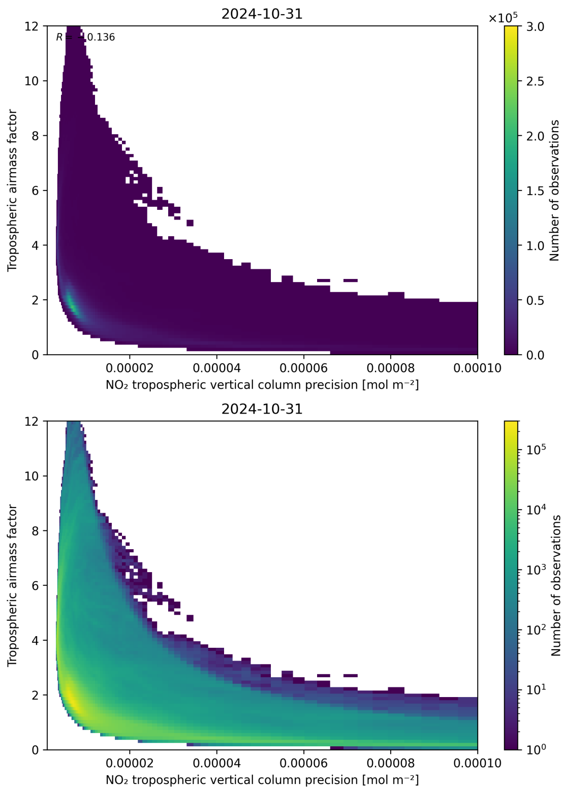
Figure 133: Scatter density plot of “NO 2 tropospheric vertical column precision” against “Tropospheric airmass factor” for 2024-10-30 to 2024-11-01.
