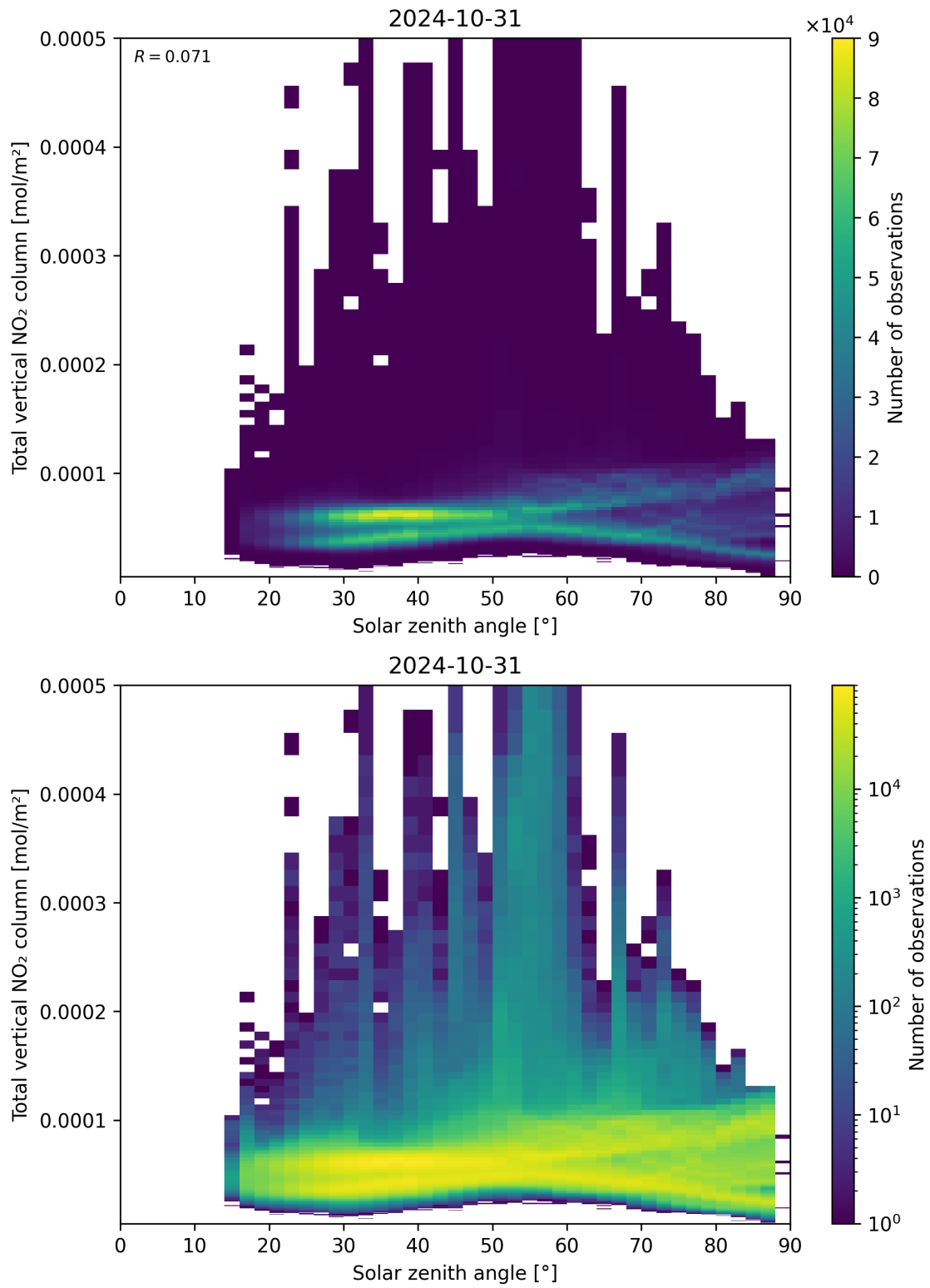
Figure 153: Scatter density plot of “Solar zenith angle” against “Total vertical NO 2 column” for 2024-10-30 to 2024-11-01.
