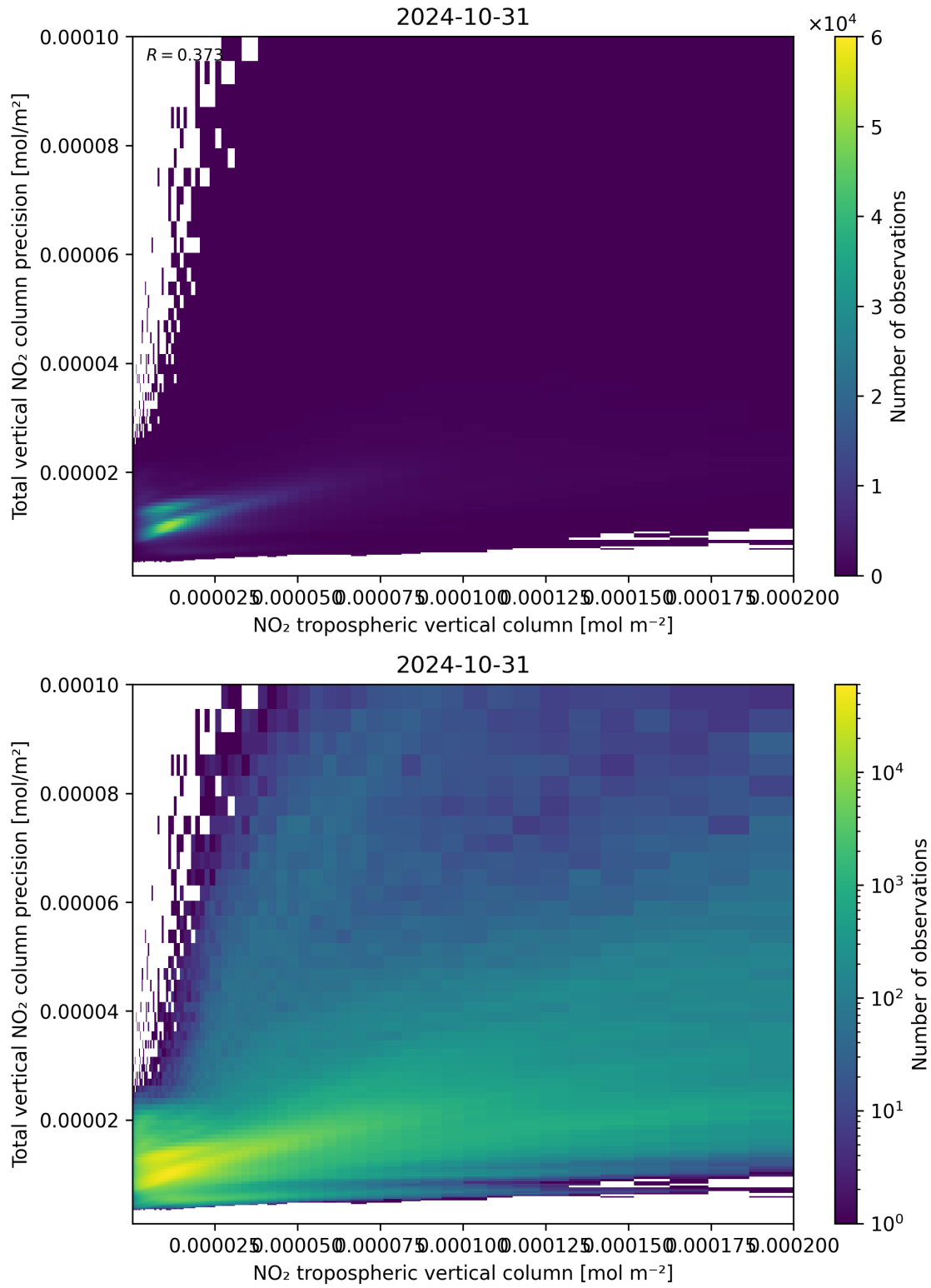
Figure 129: Scatter density plot of “NO 2 tropospheric vertical column” against “Total vertical NO 2 column precision” for 2024-10-30 to 2024-11-01.
