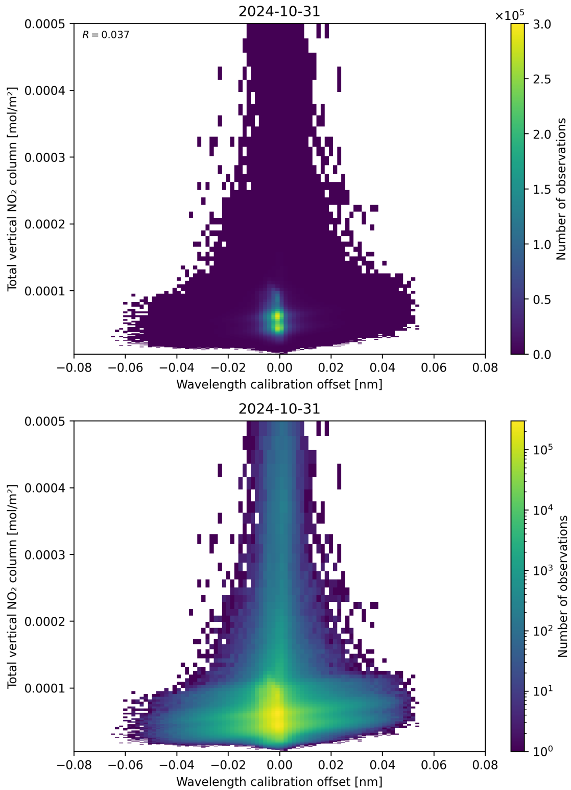
Figure 179: Scatter density plot of “Wavelength calibration offset” against “Total vertical NO 2 column” for 2024-10-30 to 2024-11-01.
