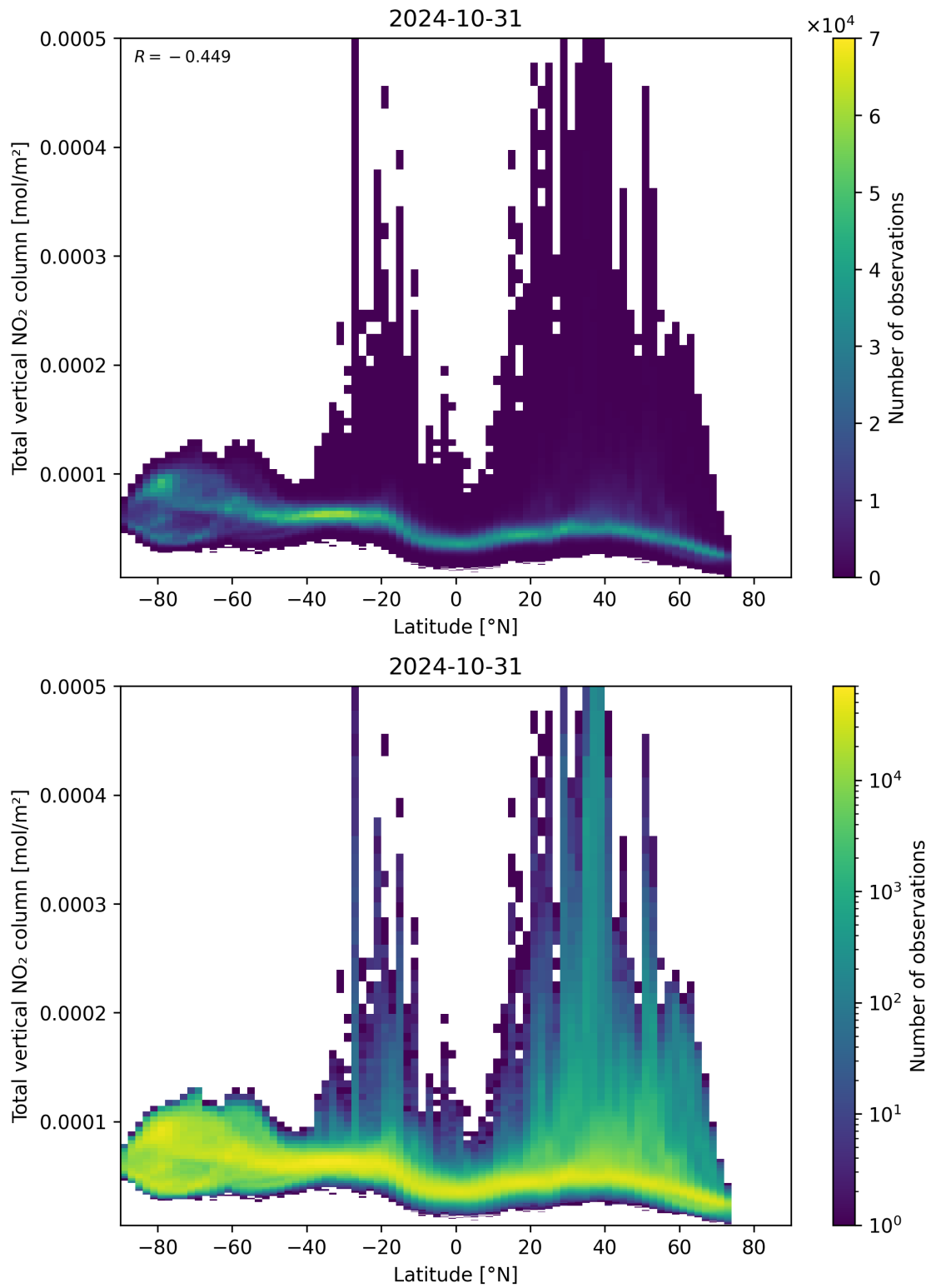
Figure 90: Scatter density plot of “Latitude” against “Total vertical NO 2 column” for 2024-10-30 to 2024-11-01.
