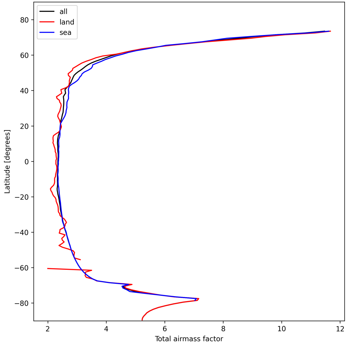
Figure 15: Zonal average of “Total airmass factor” for 2024-10-30 to 2024-11-01.
