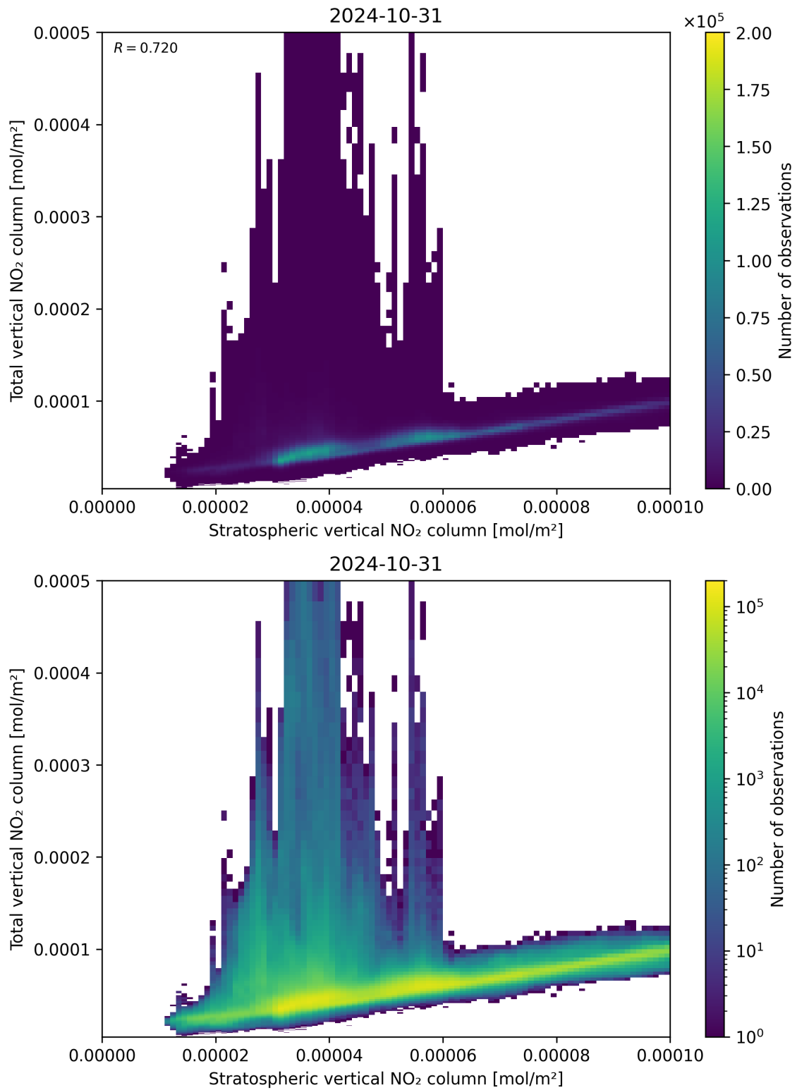
Figure 100: Scatter density plot of “Stratospheric vertical NO 2 column” against “Total vertical NO 2 column” for 2024-10-30 to 2024-11-01.
