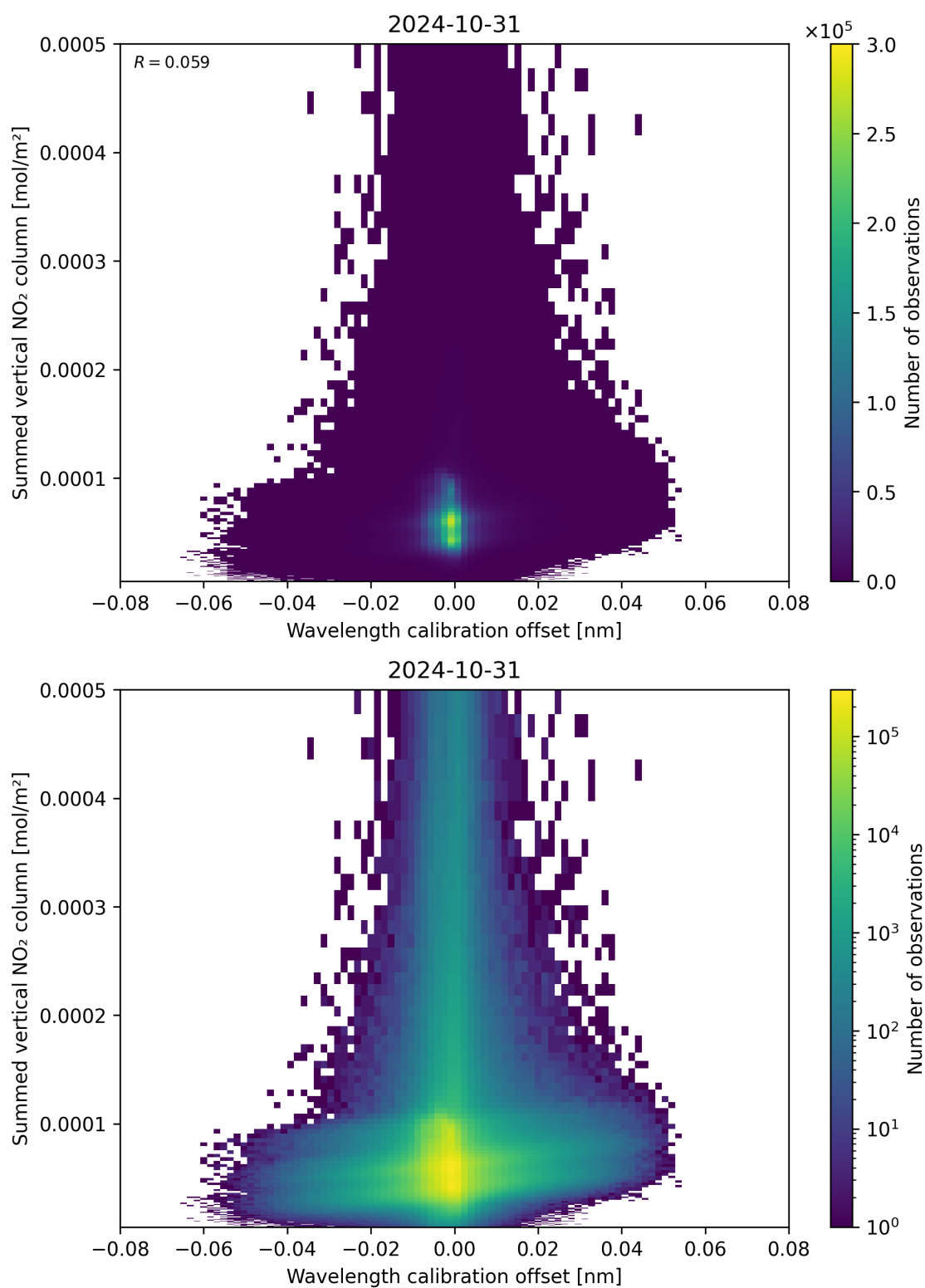
Figure 177: Scatter density plot of “Wavelength calibration offset” against “Summed vertical NO 2 column” for 2024-10-30 to 2024-11-01.
