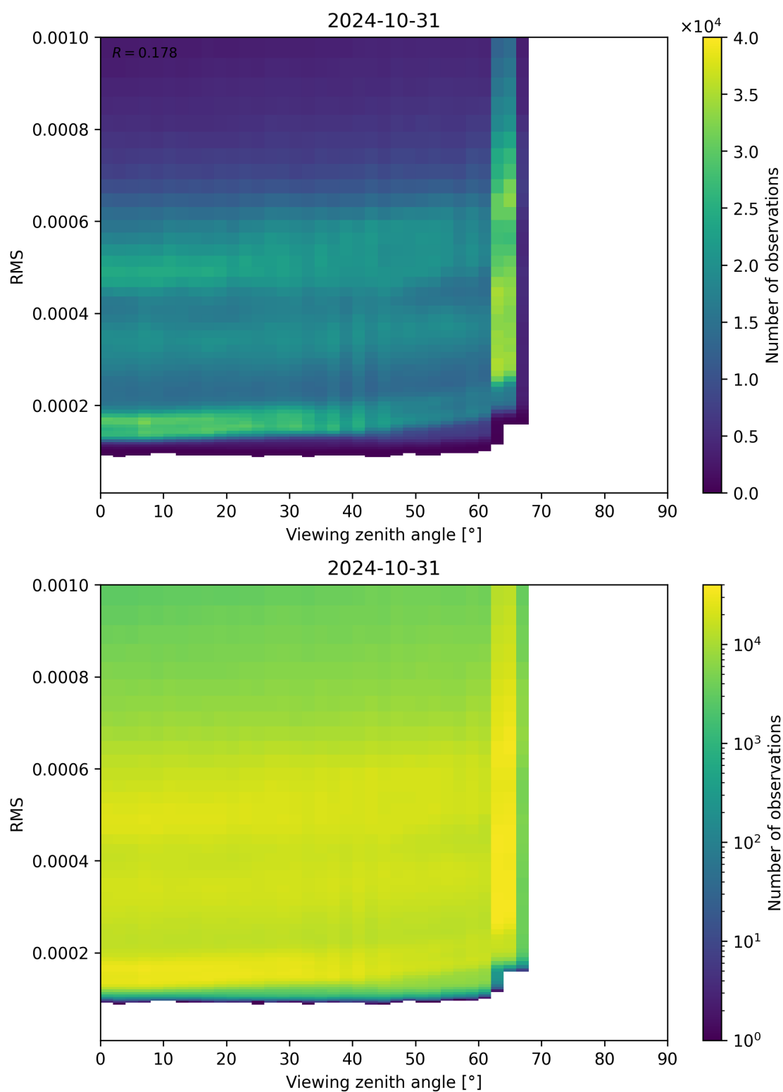
Figure 171: Scatter density plot of “Viewing zenith angle” against “RMS” for 2024-10-30 to 2024-11-01.
