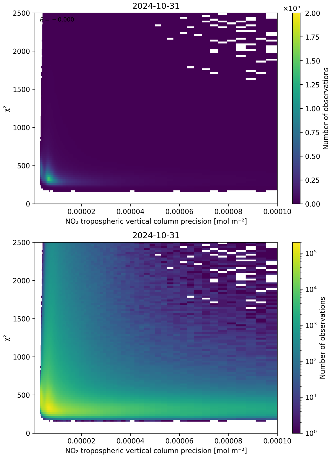
Figure 134: Scatter density plot of “NO 2 tropospheric vertical column precision” against “ \chi^2 ” for 2024-10-30 to 2024-11-01.
