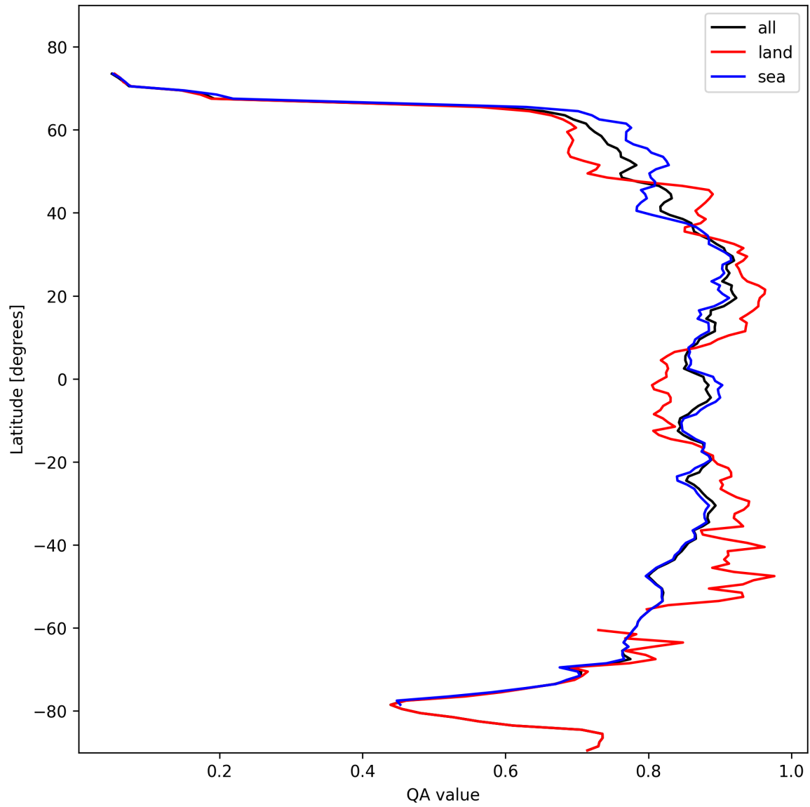
Figure 11: Zonal average of “QA value” for 2024-10-30 to 2024-11-01.
