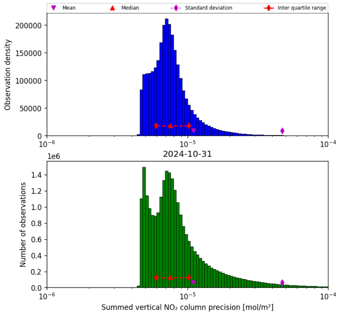
Figure 41: Histogram of "Summed vertical NO 2 column precision" for 2024-10-30 to 2024-11-01
