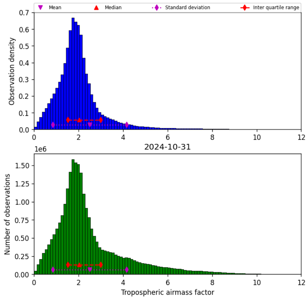
Figure 31: Histogram of “Tropospheric airmass factor” for 2024-10-30 to 2024-11-01
