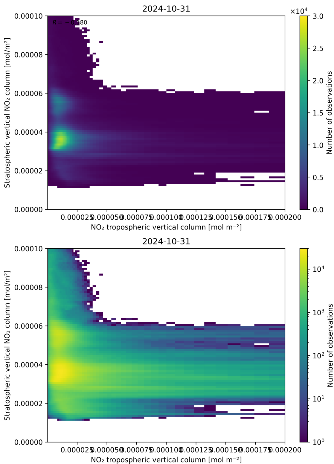
Figure 125: Scatter density plot of “NO 2 tropospheric vertical column” against “Stratospheric vertical NO 2 column” for 2024-10-30 to 2024-11-01.
