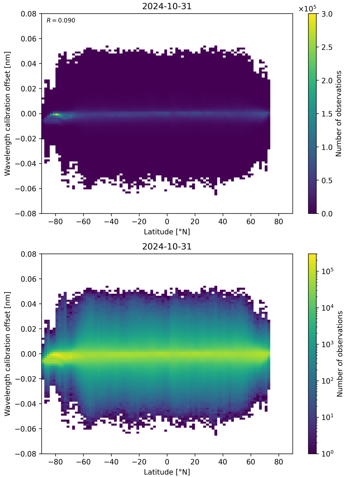
Figure 95: Scatter density plot of “Latitude” against “Wavelength calibration offset” for 2024-10-30 to 2024-11-01.
