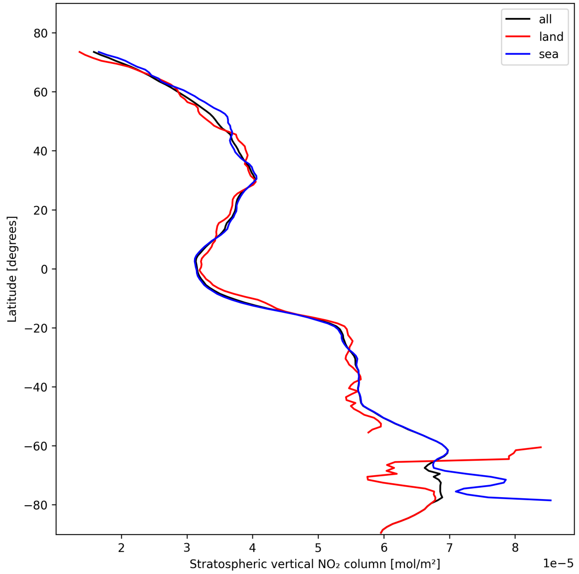
Figure 19: Zonal average of “Stratospheric vertical NO 2 column” for 2024-10-30 to 2024-11-01.
