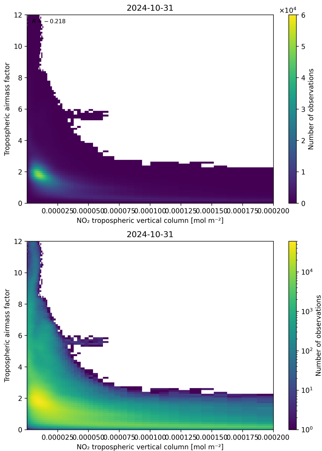
Figure 123: Scatter density plot of “NO 2 tropospheric vertical column” against “Tropospheric air mass factor” for 2024-10-30 to 2024-11-01.
