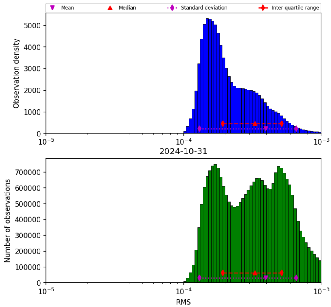
Figure 43: Histogram of “RMS” for 2024-10-30 to 2024-11-01
