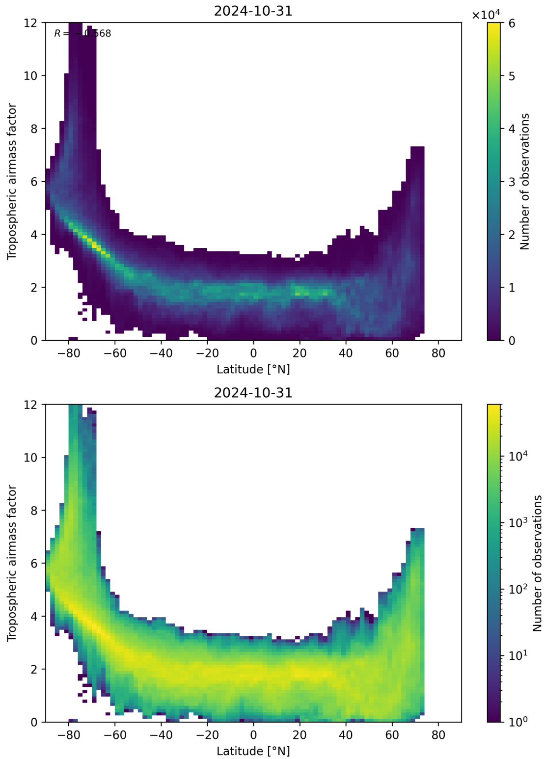
Figure 85: Scatter density plot of “Latitude” against “Tropospheric air mass factor” for 2024-10-30 to 2024-11-01.
