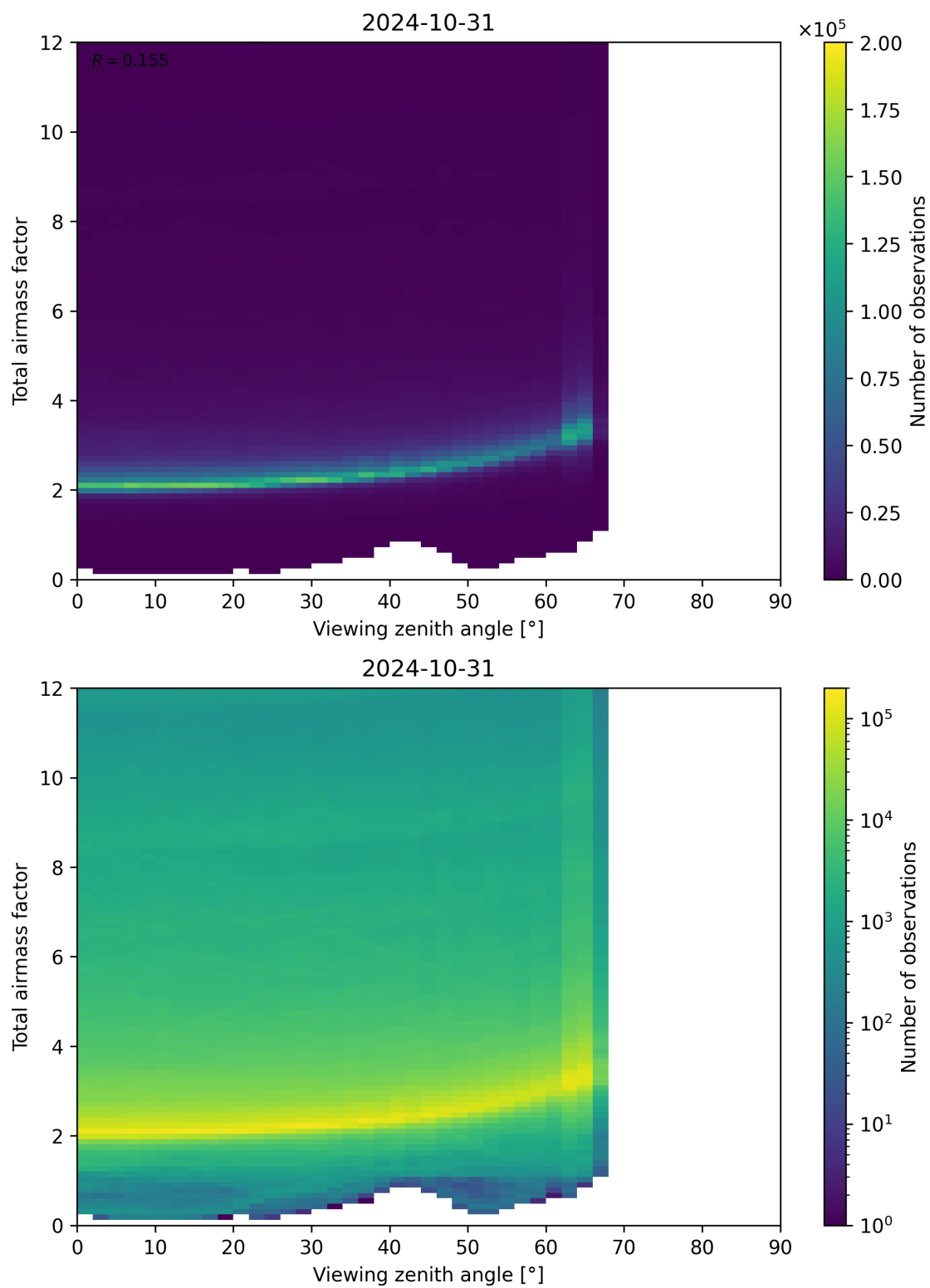
Figure 160: Scatter density plot of “Viewing zenith angle” against “Total airmass factor” for 2024-10-30 to 2024-11-01.
