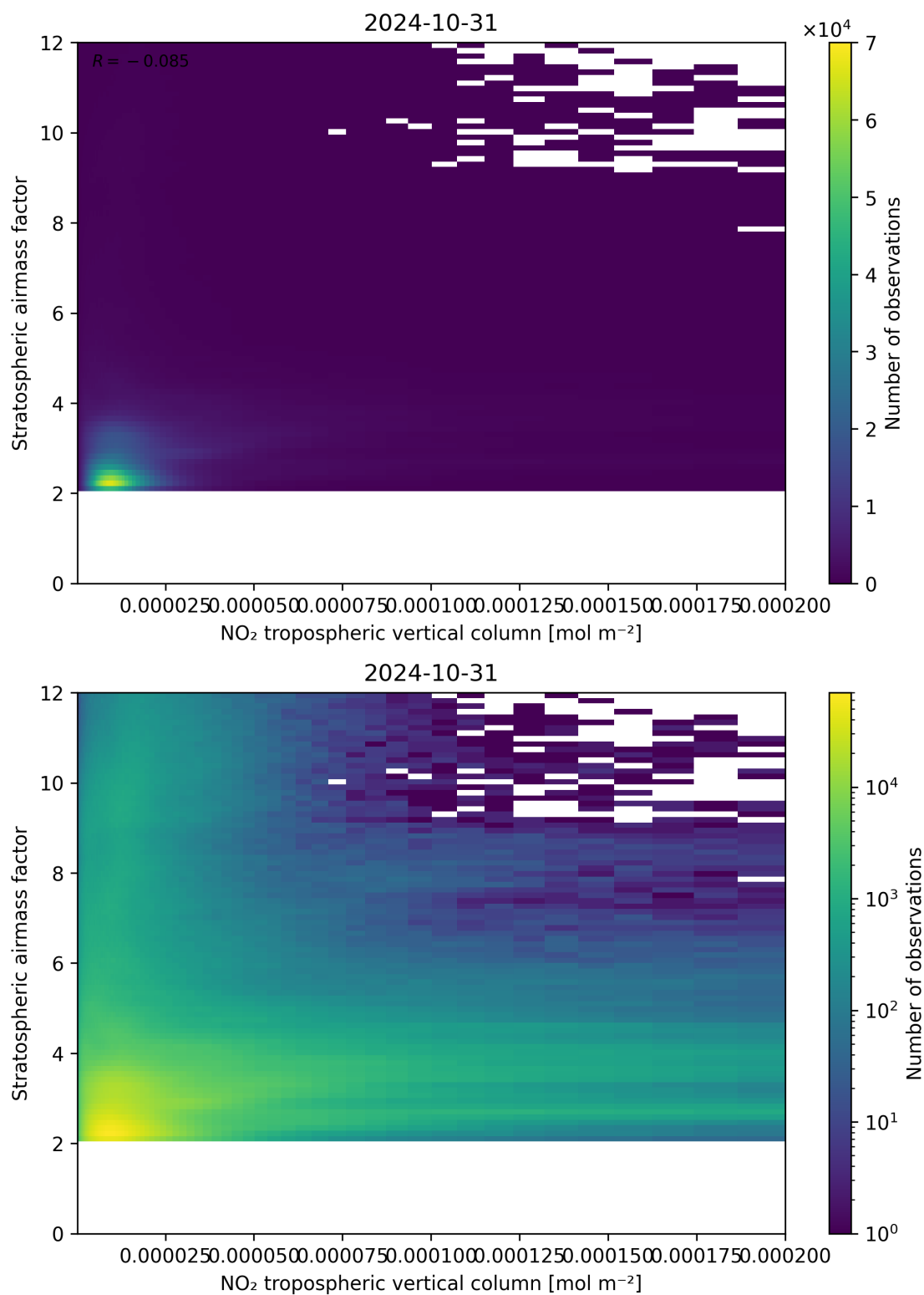
Figure 121: Scatter density plot of “NO 2 tropospheric vertical column” against “Stratospheric air mass factor” for 2024-10-30 to 2024-11-01.
