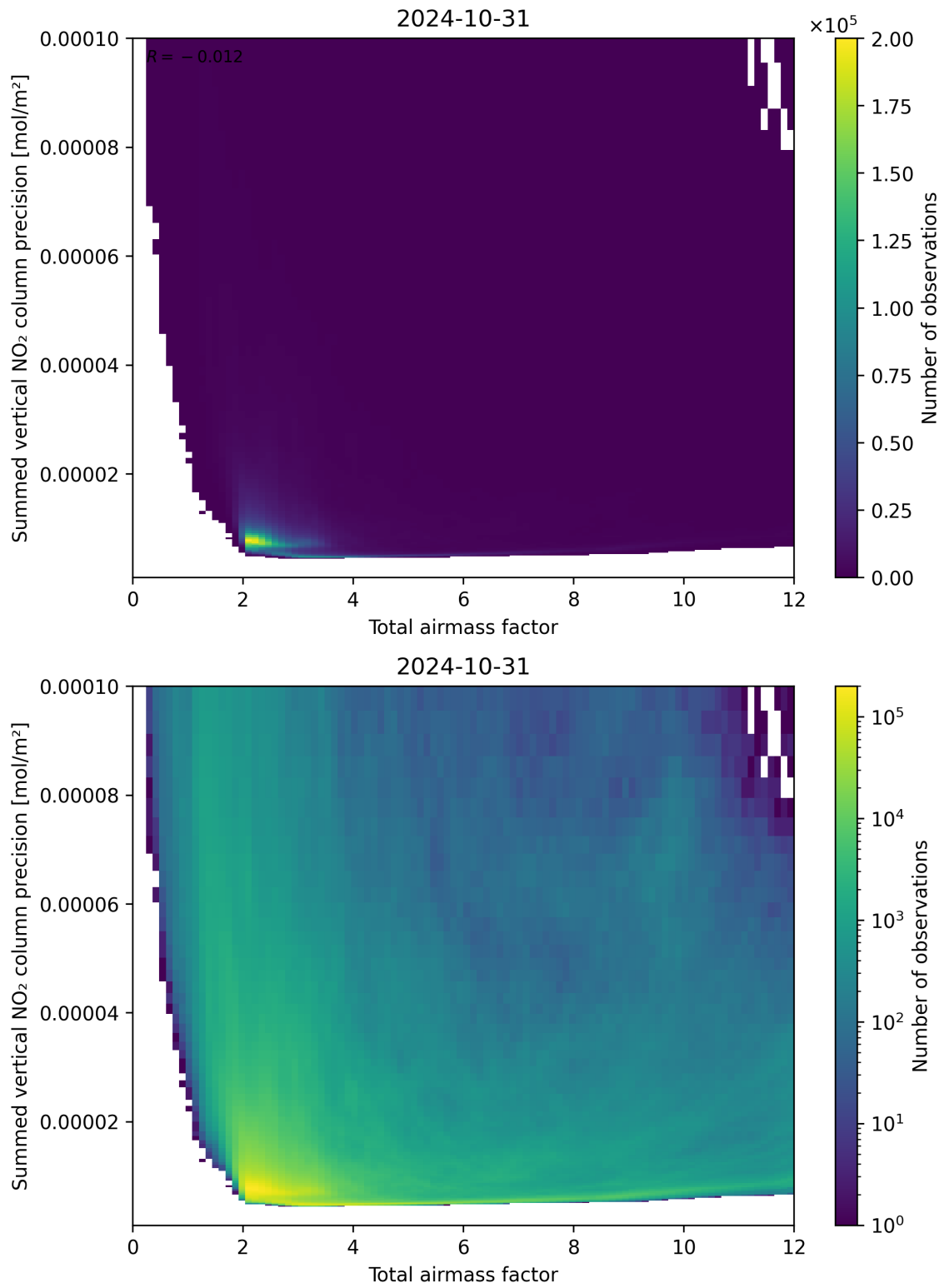
Figure 66: Scatter density plot of “Total airmass factor” against “Summed vertical NO 2 column precision” for 2024-10-30 to 2024-11-01.
