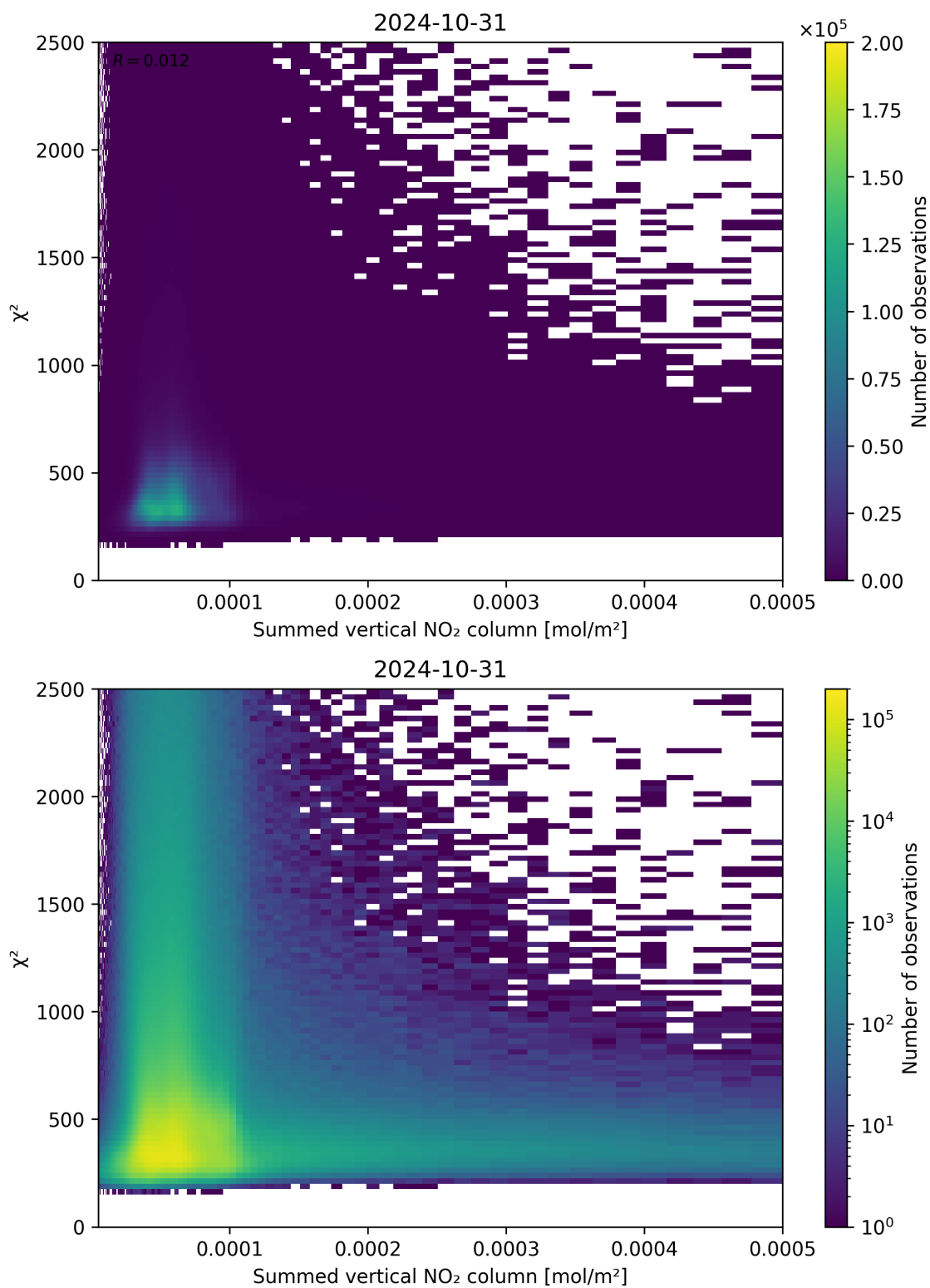
Figure 104: Scatter density plot of “Summed vertical NO 2 column” against “ \chi^2 ” for 2024-10-30 to 2024-11-01.
