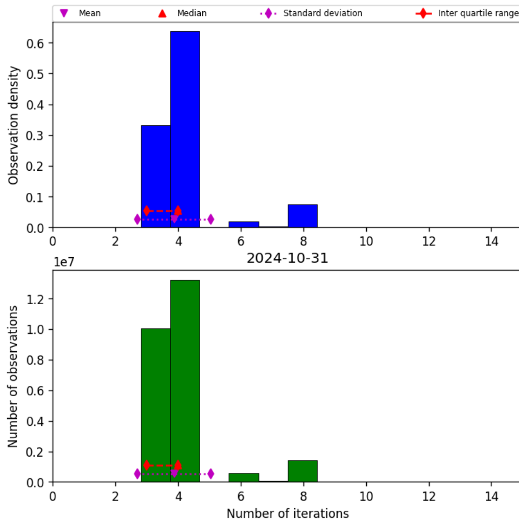
Figure 34: Histogram of “Number of iterations” for 2024-10-30 to 2024-11-01
