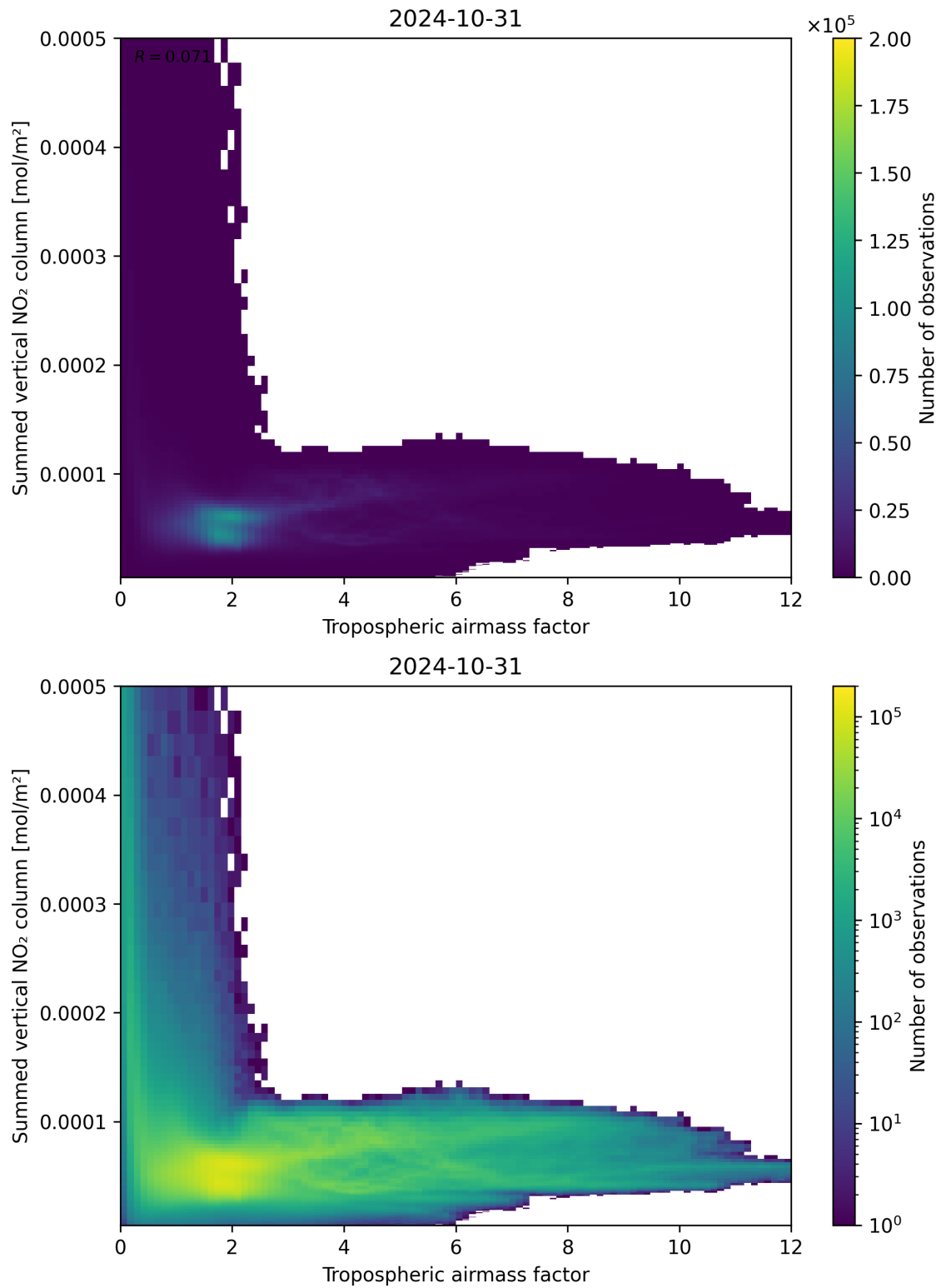
Figure 75: Scatter density plot of “Tropospheric airmass factor” against “Summed vertical NO 2 column” for 2024-10-30 to 2024-11-01.
