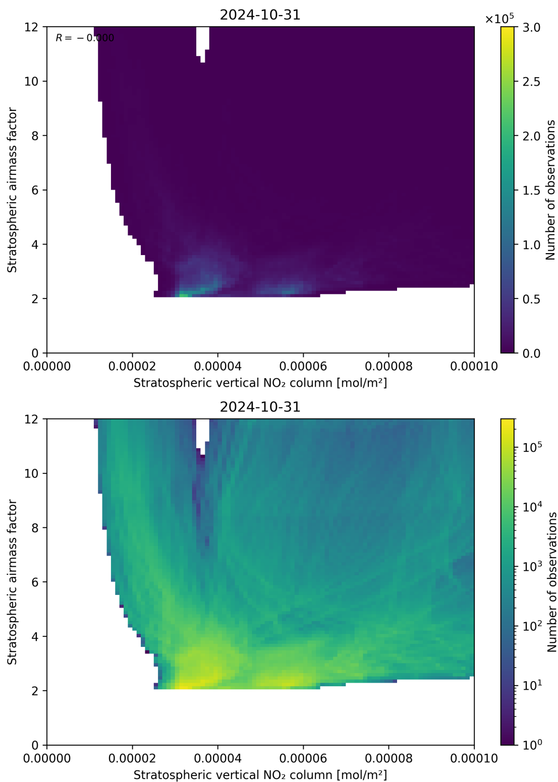
Figure 96: Scatter density plot of “Stratospheric vertical NO 2 column” against “Stratospheric airmass factor” for 2024-10-30 to 2024-11-01.
