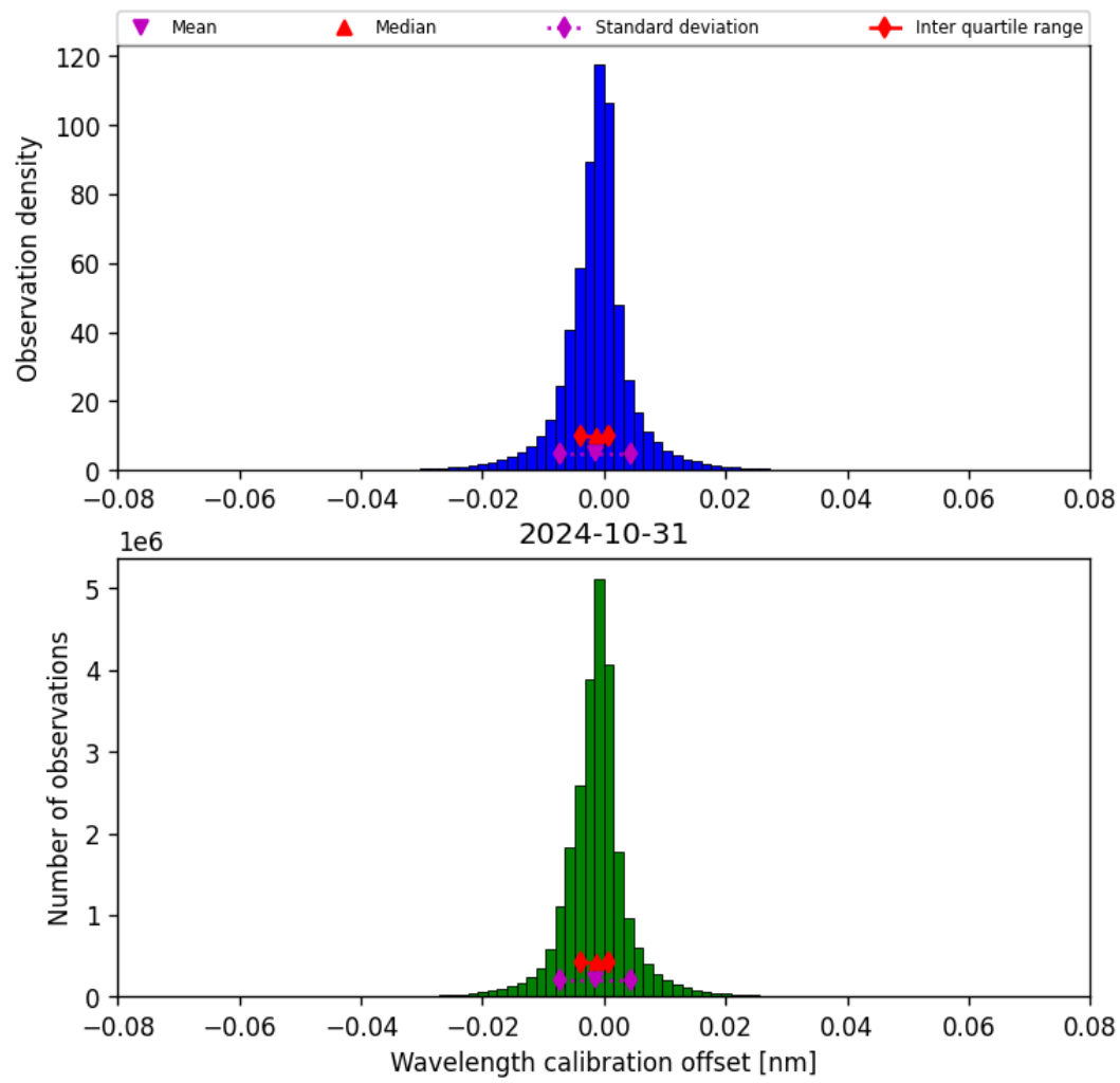
Figure 35: Histogram of “Wavelength calibration offset” for 2024-10-30 to 2024-11-01
