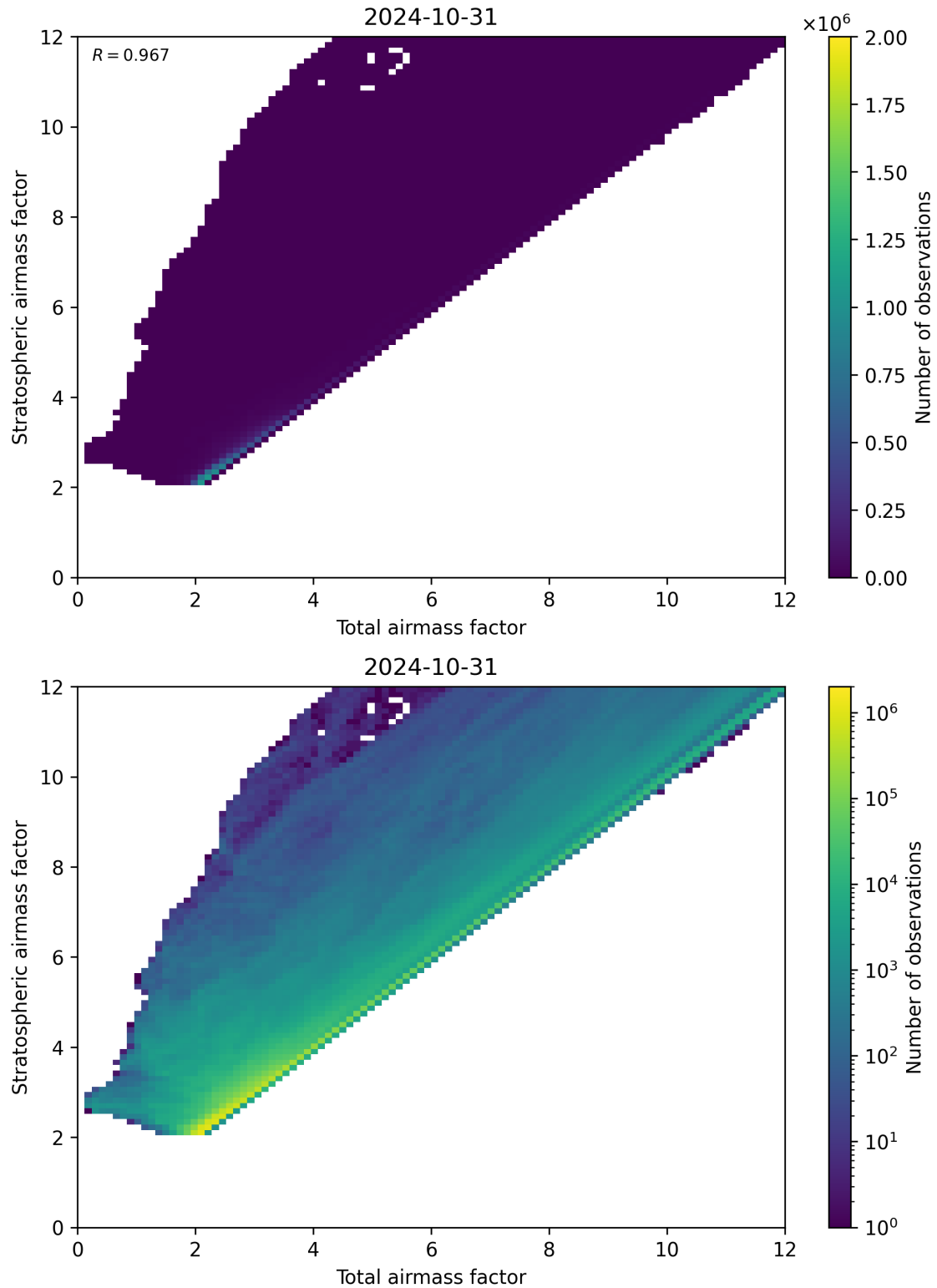
Figure 62: Scatter density plot of “Total airmass factor” against “Stratospheric airmass factor” for 2024-10-30 to 2024-11-01.
