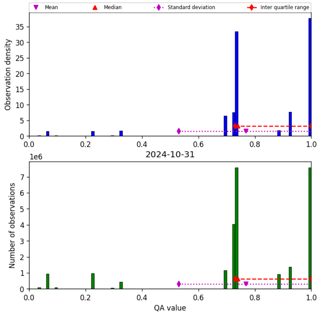
Figure 28: Histogram of “QA value” for 2024-10-30 to 2024-11-01
