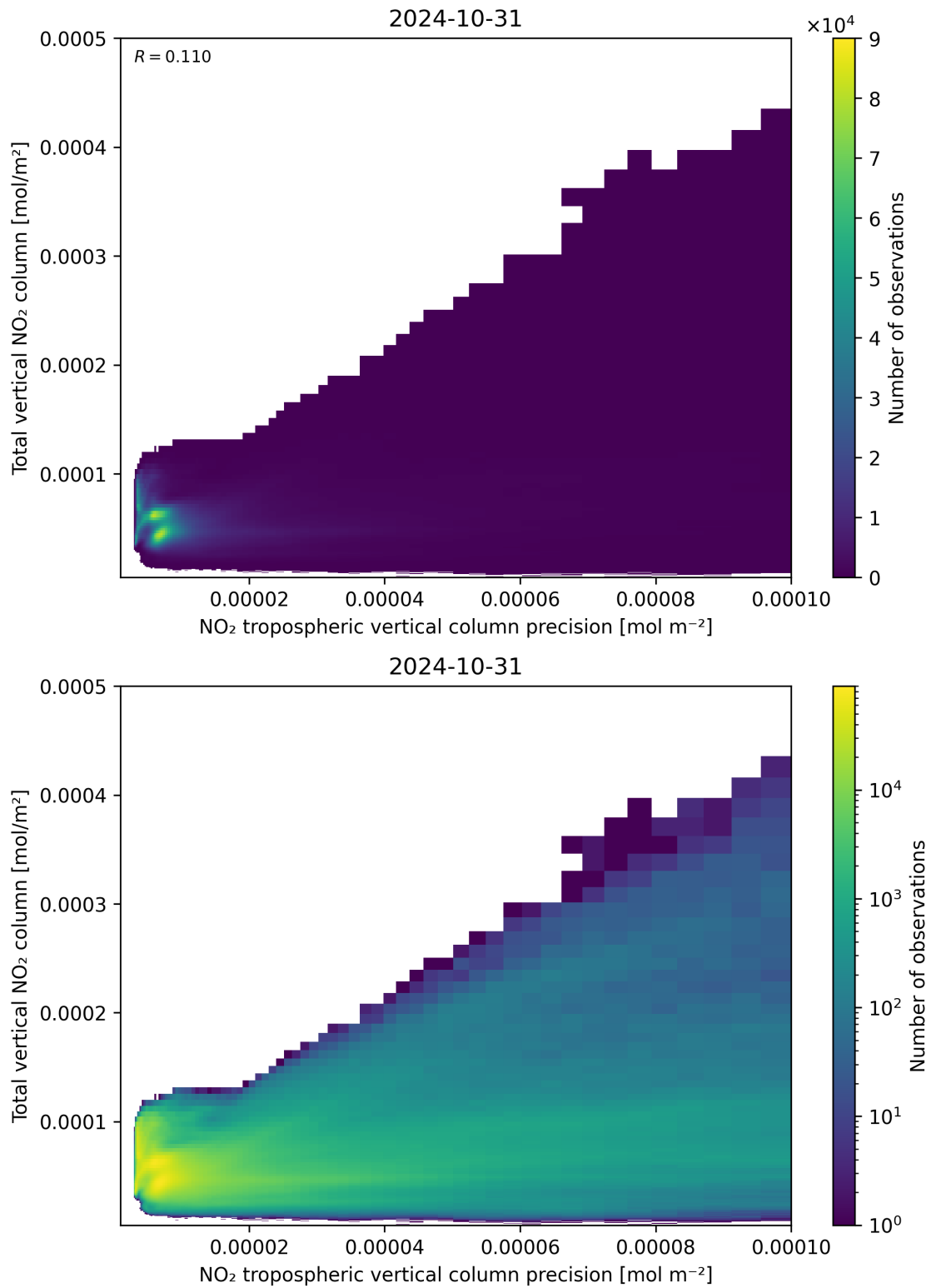
Figure 138: Scatter density plot of “NO 2 tropospheric vertical column precision” against “Total vertical NO 2 column” for 2024-10-30 to 2024-11-01.
