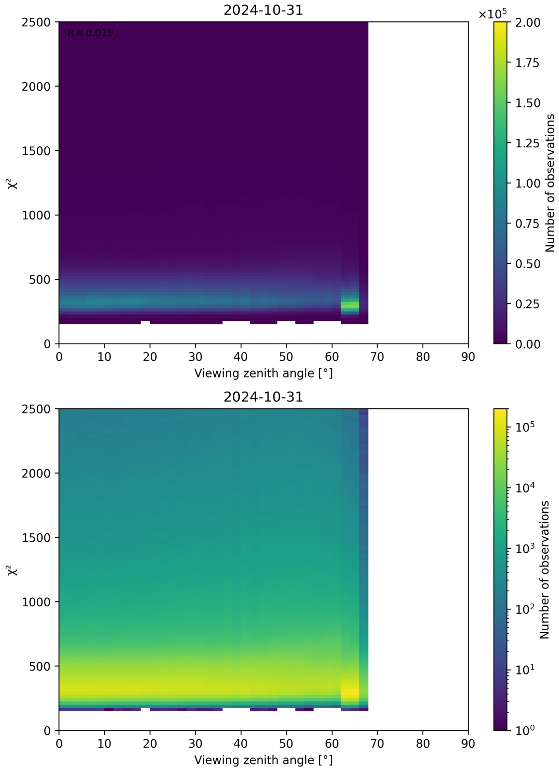
Figure 162: Scatter density plot of “Viewing zenith angle” against “ \chi^2 ” for 2024-10-30 to 2024-11-01.
