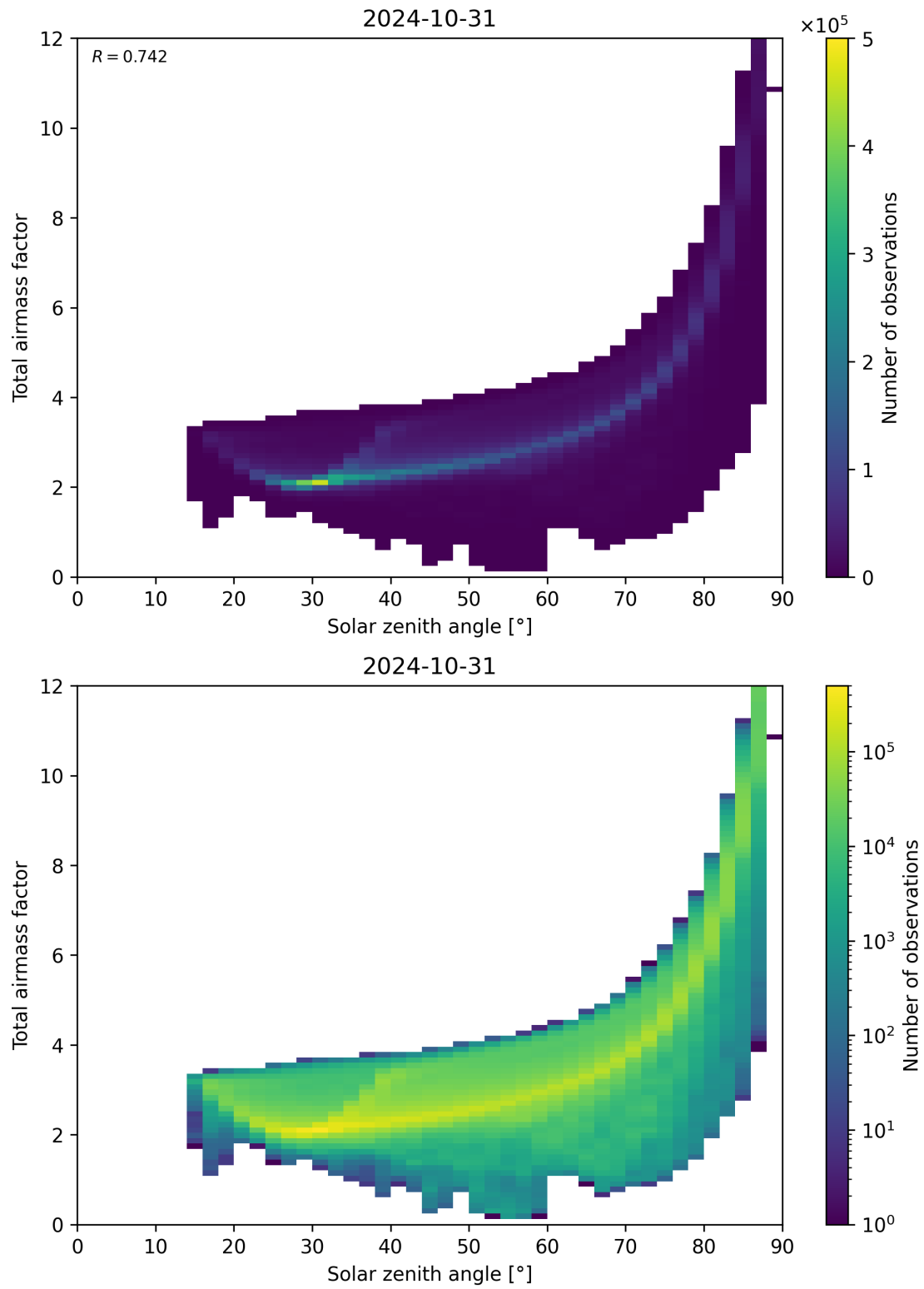
Figure 146: Scatter density plot of “Solar zenith angle” against “Total air mass factor” for 2024-10-30 to 2024-11-01.
