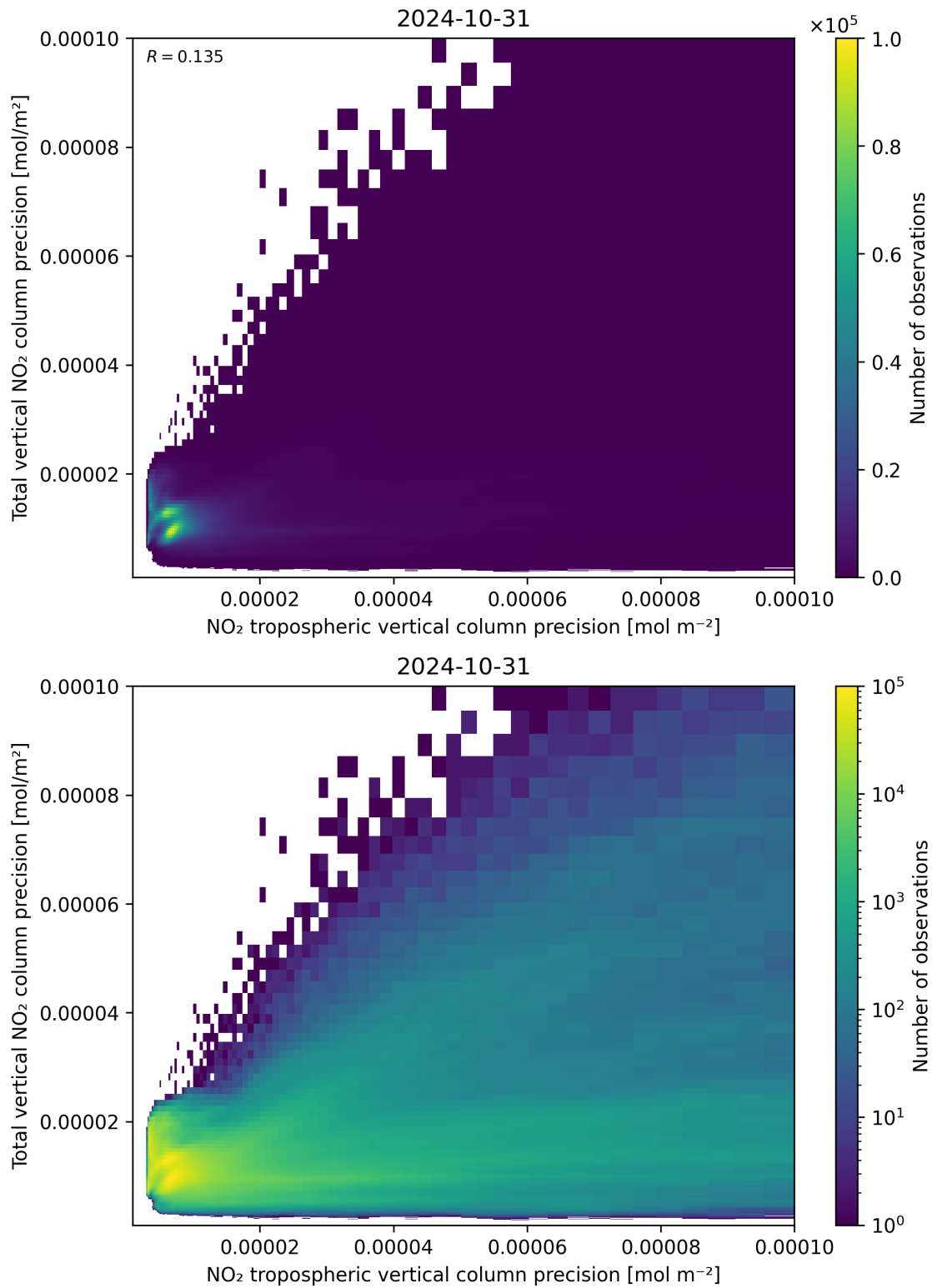
Figure 139: Scatter density plot of “NO 2 tropospheric vertical column precision” against “Total vertical NO 2 column precision” for 2024-10-30 to 2024-11-01.
