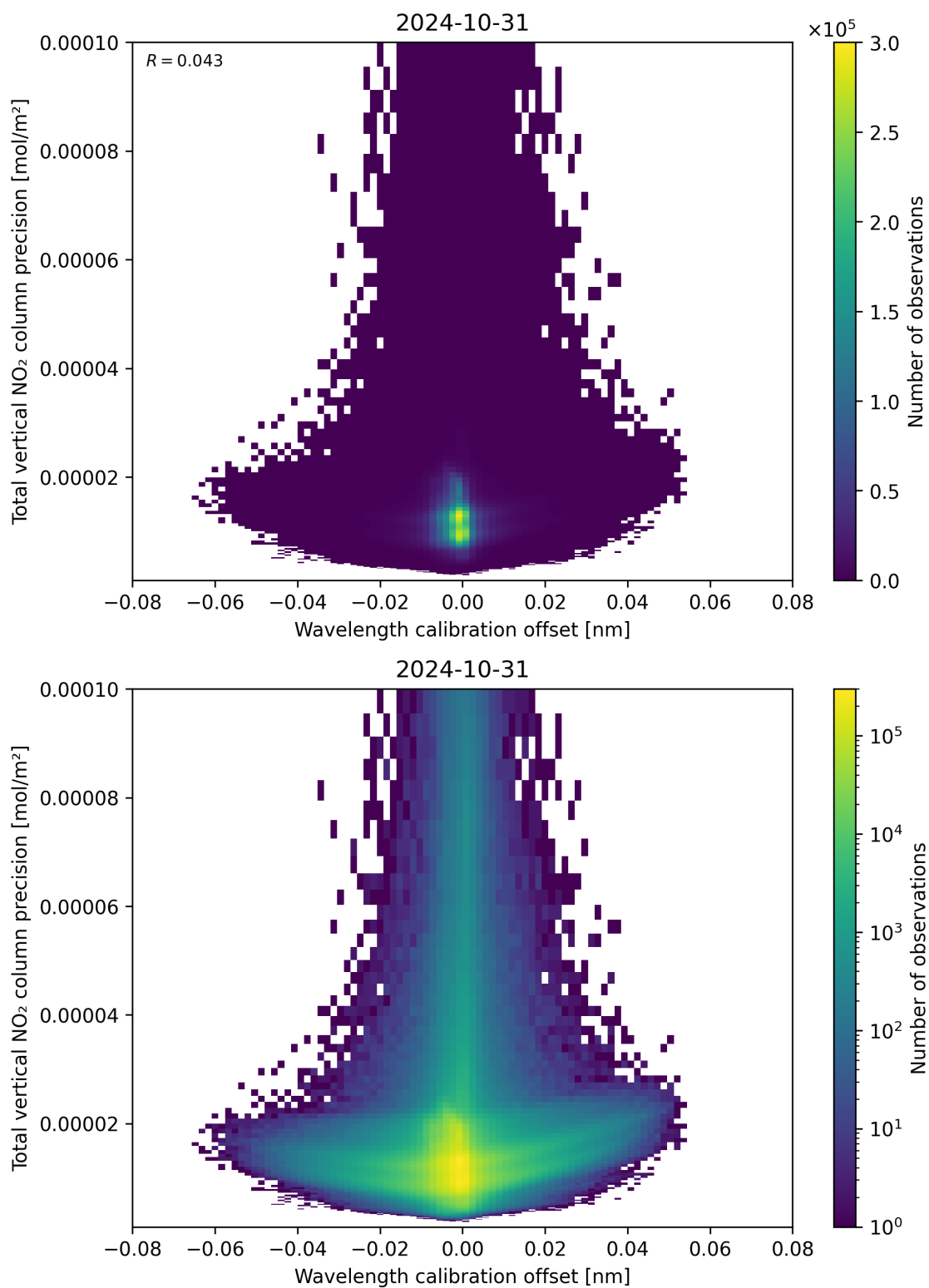
Figure 180: Scatter density plot of “Wavelength calibration offset” against “Total vertical NO 2 column precision” for 2024-10-30 to 2024-11-01.
