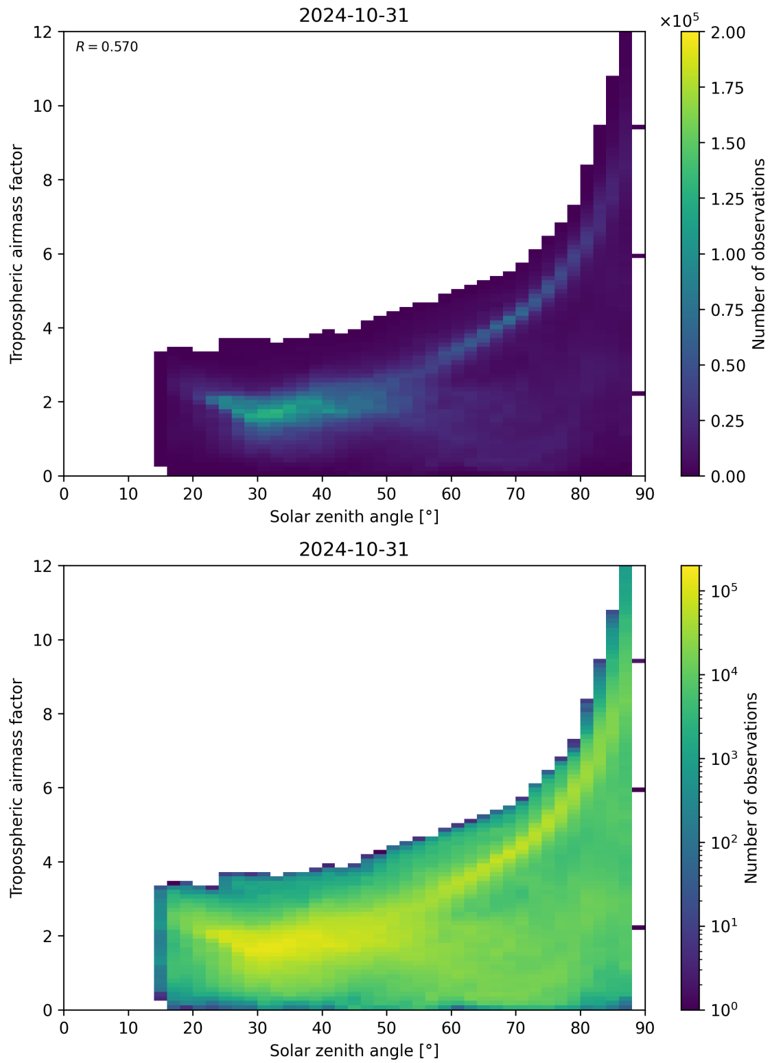
Figure 147: Scatter density plot of “Solar zenith angle” against “Tropospheric airmass factor” for 2024-10-30 to 2024-11-01.
