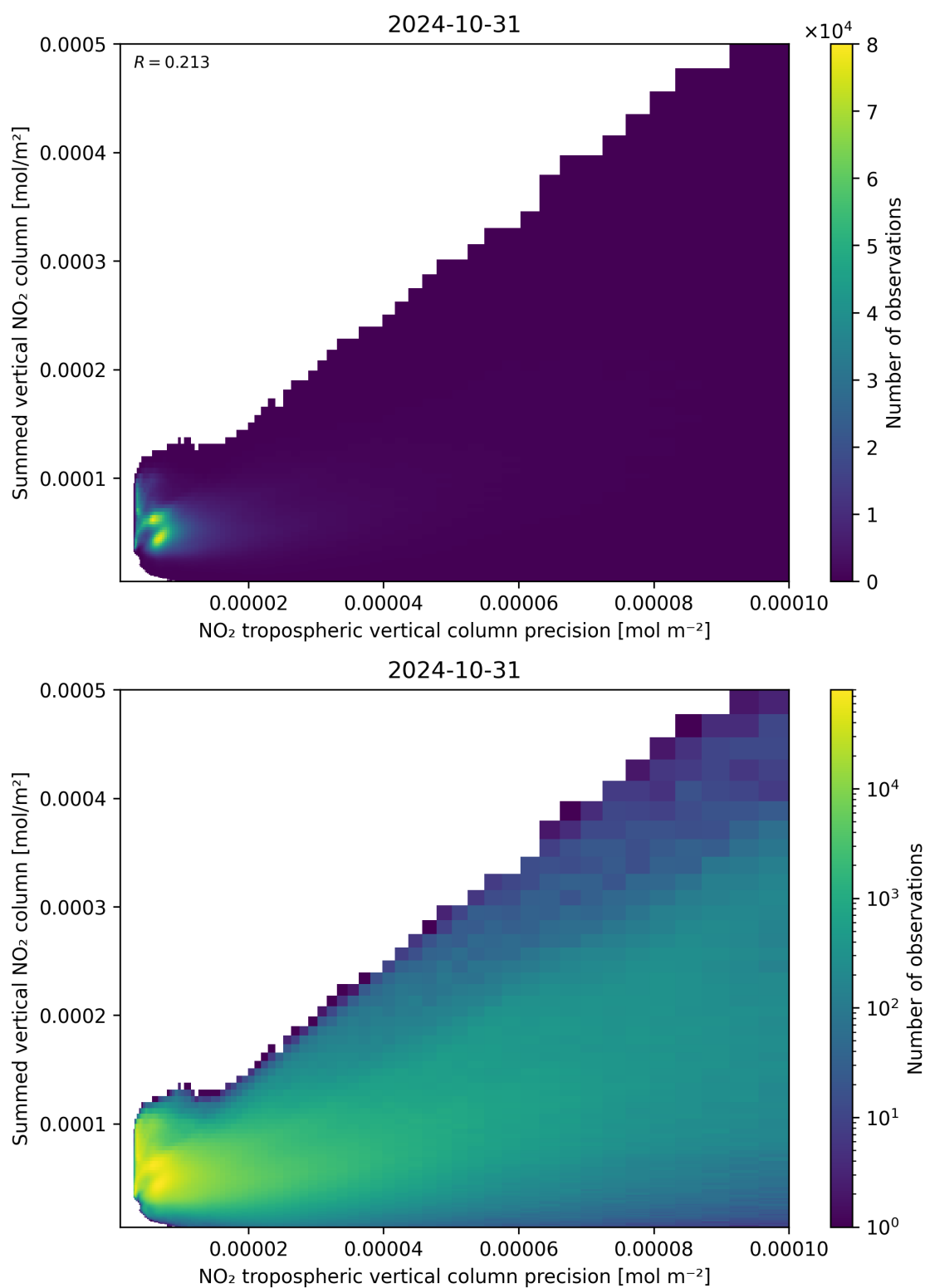
Figure 136: Scatter density plot of “NO 2 tropospheric vertical column precision” against “Summed vertical NO 2 column” for 2024-10-30 to 2024-11-01.
