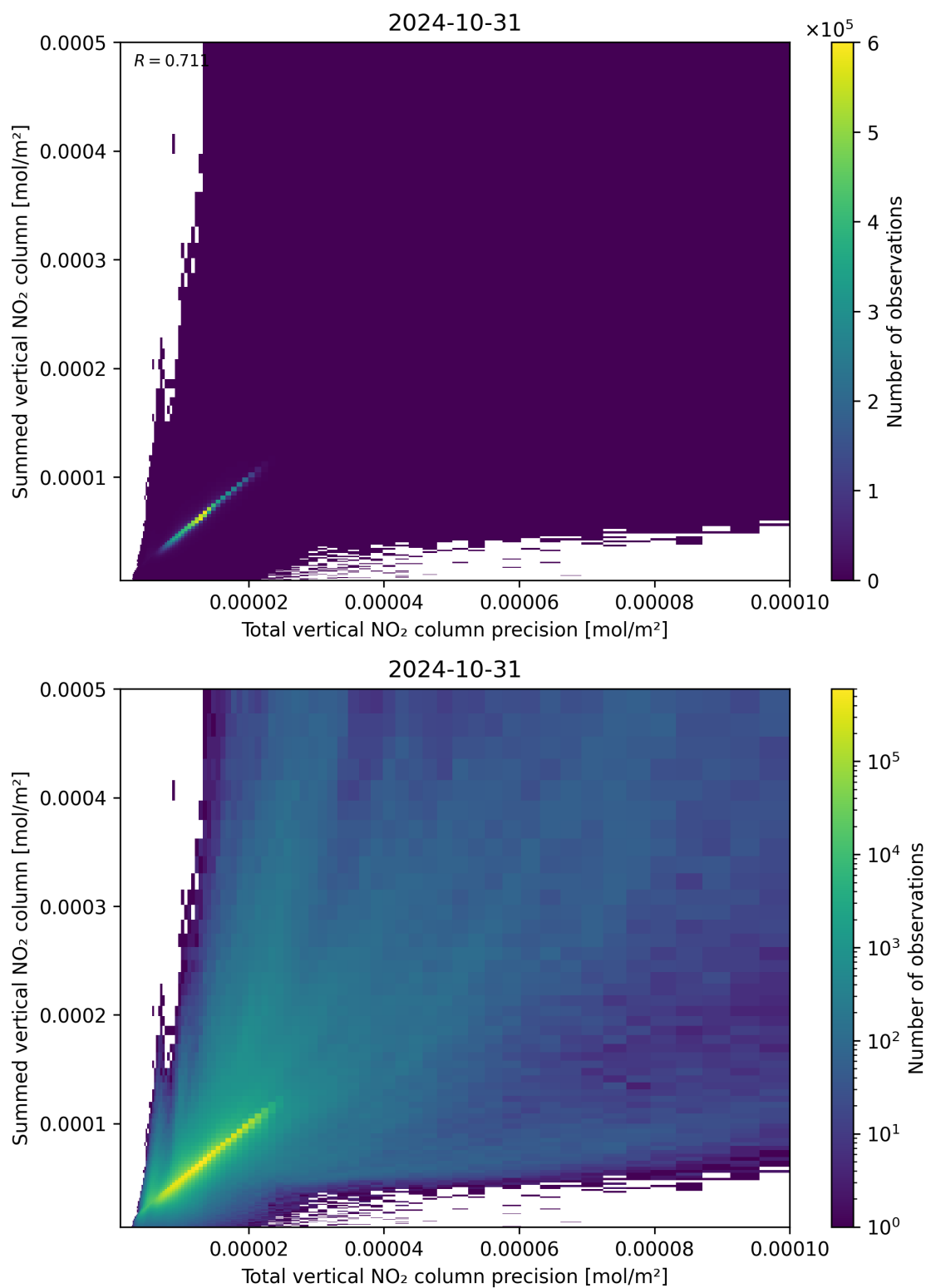
Figure 117: Scatter density plot of “Total vertical NO 2 column precision” against “Summed vertical NO 2 column” for 2024-10-30 to 2024-11-01.
