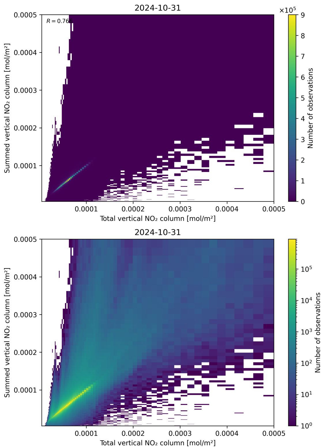
Figure 112: Scatter density plot of “Total vertical NO 2 column” against “Summed vertical NO 2 column” for 2024-10-30 to 2024-11-01.
