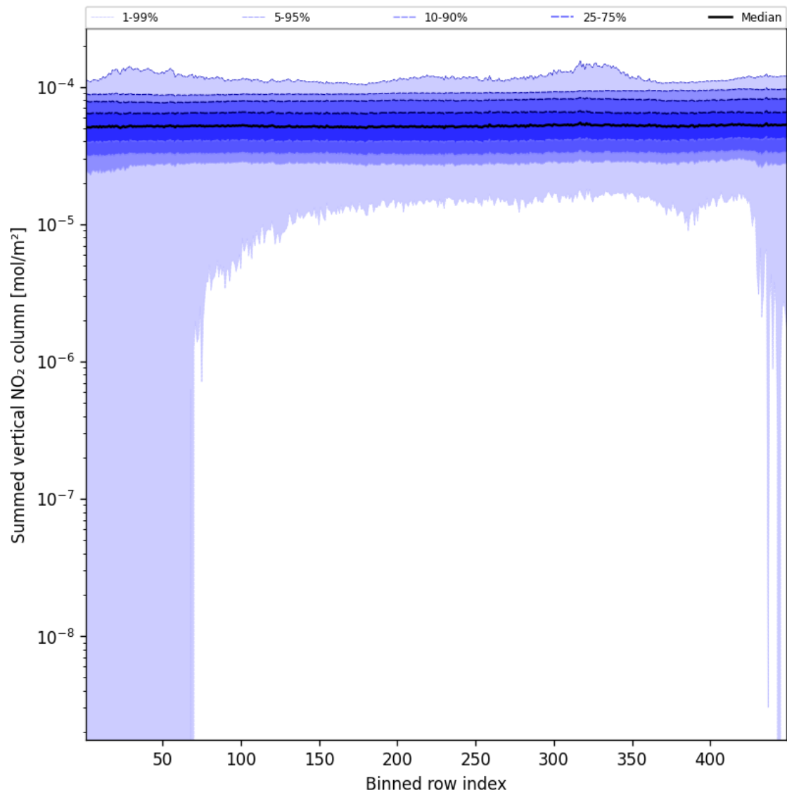
Figure 57: Along track statistics of “Summed vertical NO 2 column” for 2024-10-30 to 2024-11-01
