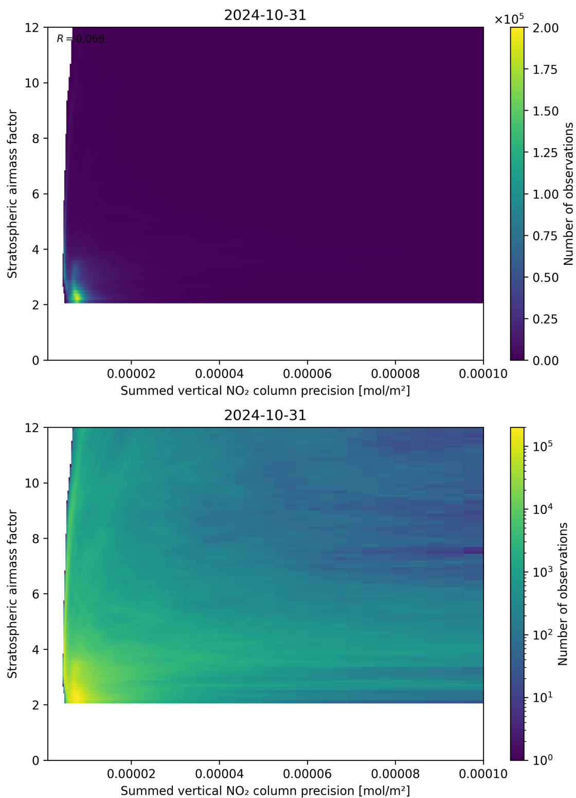
Figure 106: Scatter density plot of “Summed vertical NO 2 column precision” against “Stratospheric airmass factor” for 2024-10-30 to 2024-11-01.
