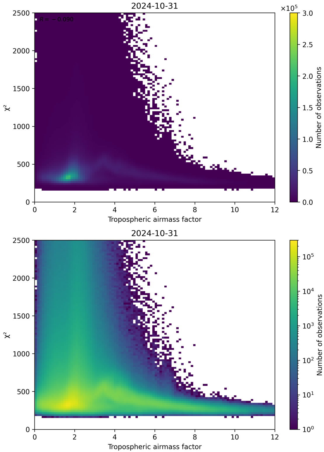
Figure 73: Scatter density plot of “Tropospheric airmass factor” against “ \chi^2 ” for 2024-10-30 to 2024-11-01.
