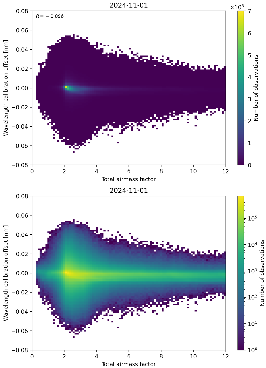
Figure 70: Scatter density plot of “Total airmass factor” against “Wavelength calibration offset” for 2024-10-31 to 2024-11-02.
