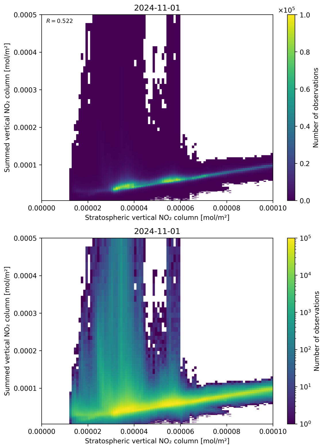
Figure 98: Scatter density plot of “Stratospheric vertical NO 2 column” against “Summed vertical NO 2 column” for 2024-10-31 to 2024-11-02.
