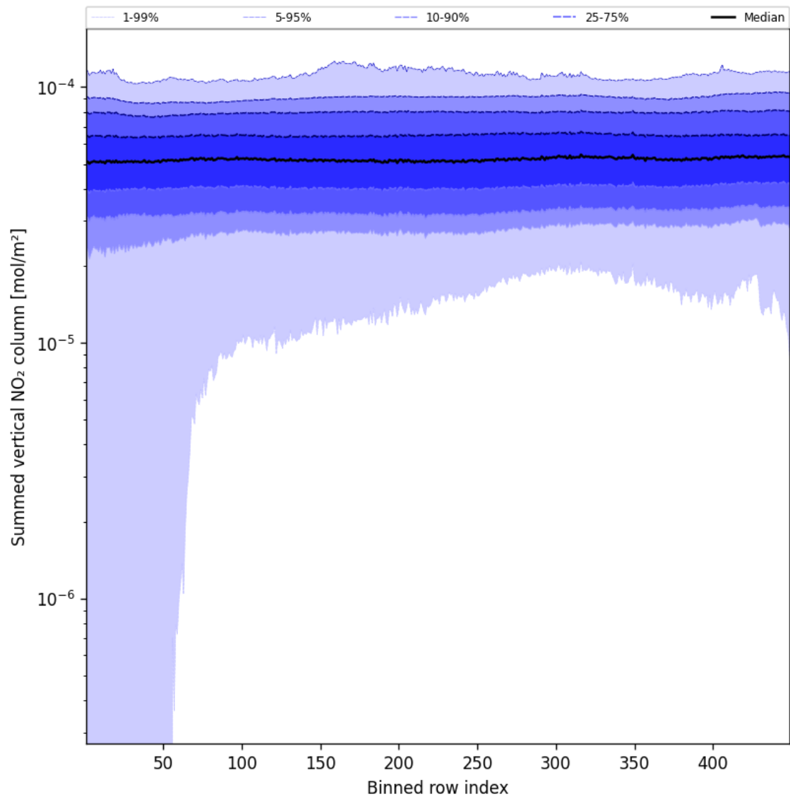
Figure 57: Along track statistics of “Summed vertical NO 2 column” for 2024-10-31 to 2024-11-02
