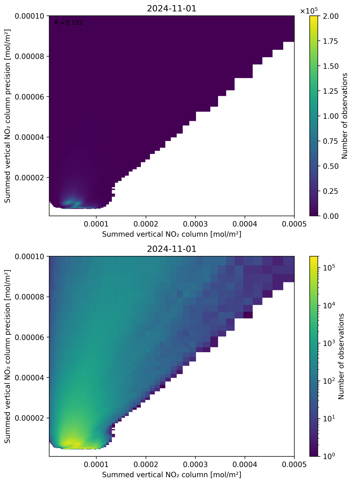
Figure 105: Scatter density plot of “Summed vertical NO 2 column” against “Summed vertical NO 2 column precision” for 2024-10-31 to 2024-11-02.
