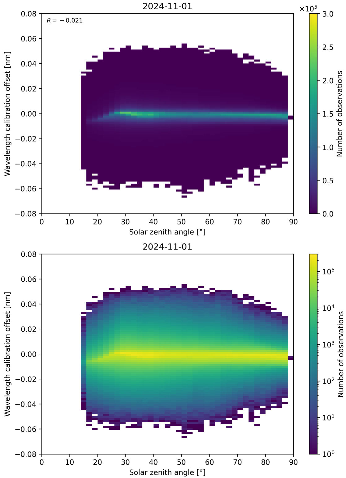
Figure 158: Scatter density plot of “Solar zenith angle” against “Wavelength calibration offset” for 2024-10-31 to 2024-11-02.
