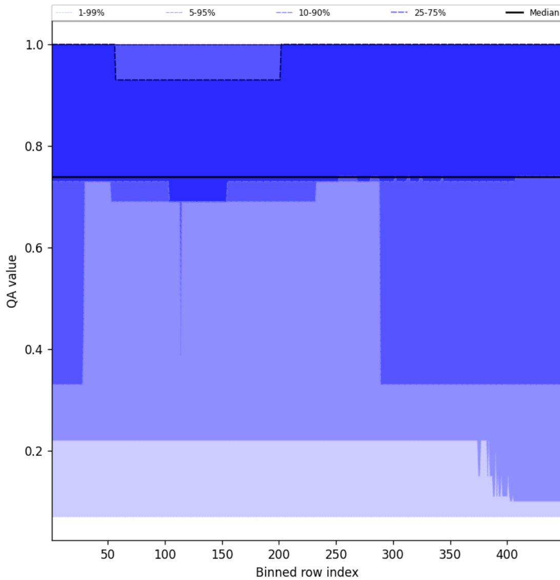
Figure 45: Along track statistics of “QA value” for 2024-10-31 to 2024-11-02
