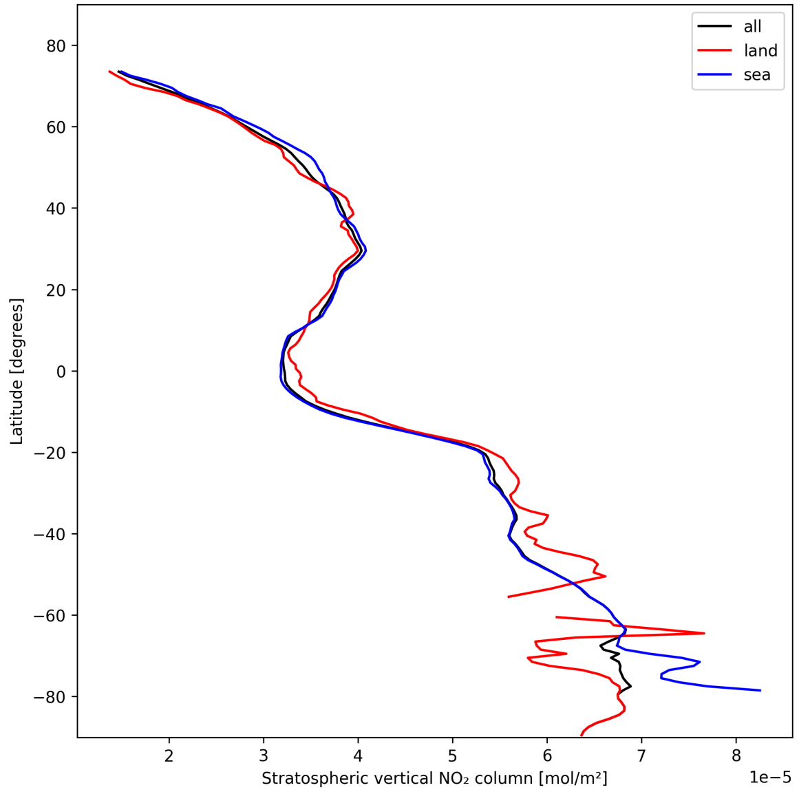
Figure 19: Zonal average of “Stratospheric vertical NO 2 column” for 2024-10-31 to 2024-11-02.
