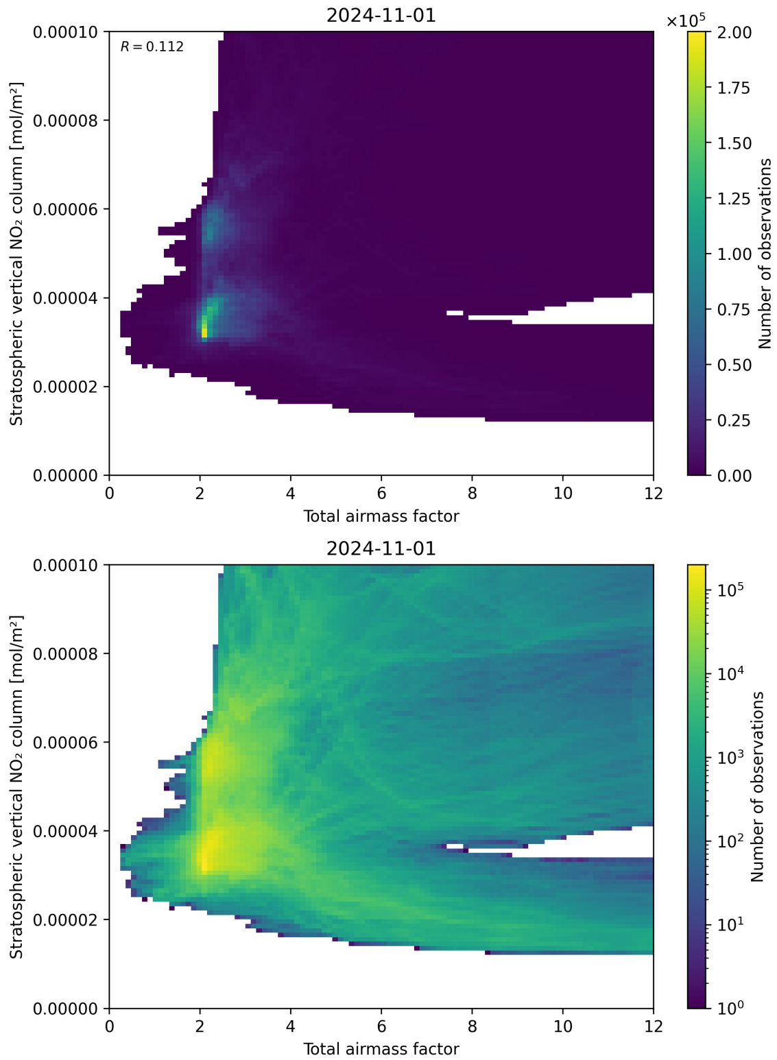
Figure 64: Scatter density plot of “Total airmass factor” against “Stratospheric vertical NO 2 column” for 2024-10-31 to 2024-11-02.
