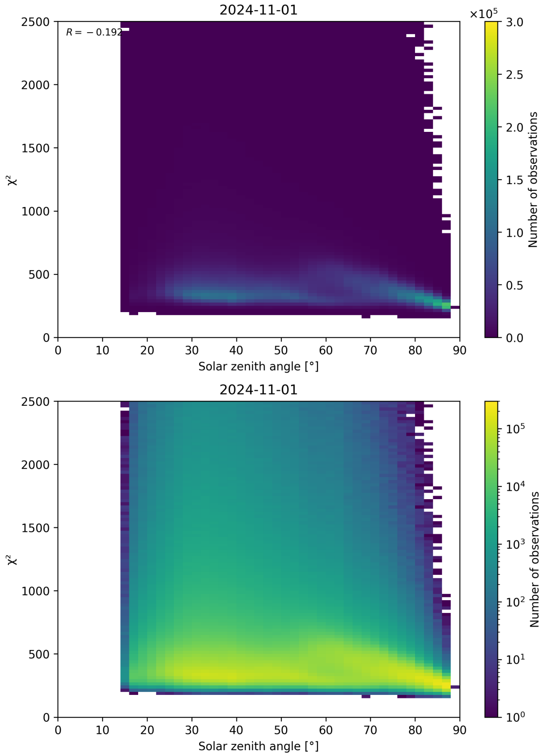
Figure 148: Scatter density plot of “Solar zenith angle” against “ \chi^2 ” for 2024-10-31 to 2024-11-02.
