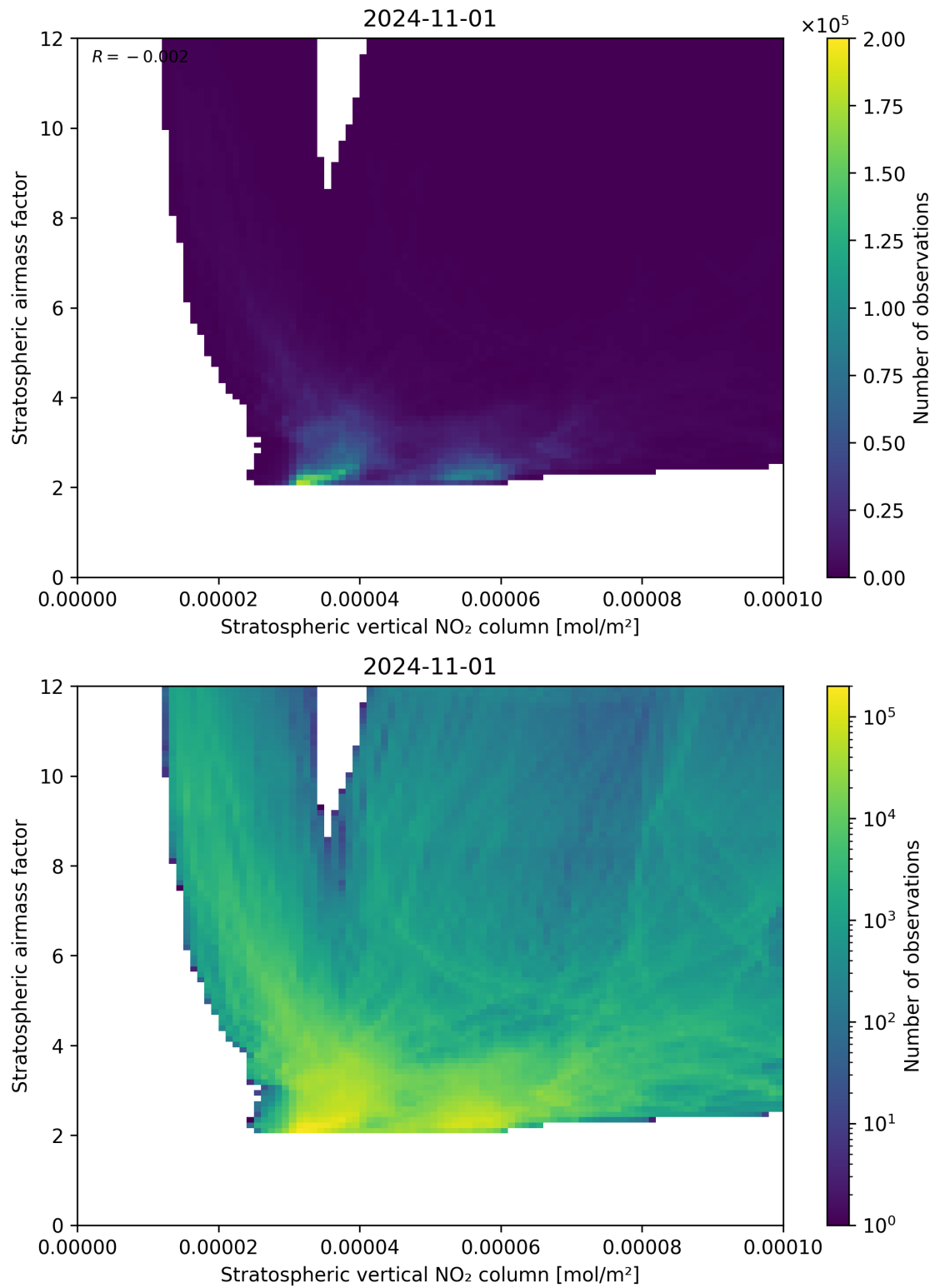
Figure 96: Scatter density plot of “Stratospheric vertical NO 2 column” against “Stratospheric airmass factor” for 2024-10-31 to 2024-11-02.
