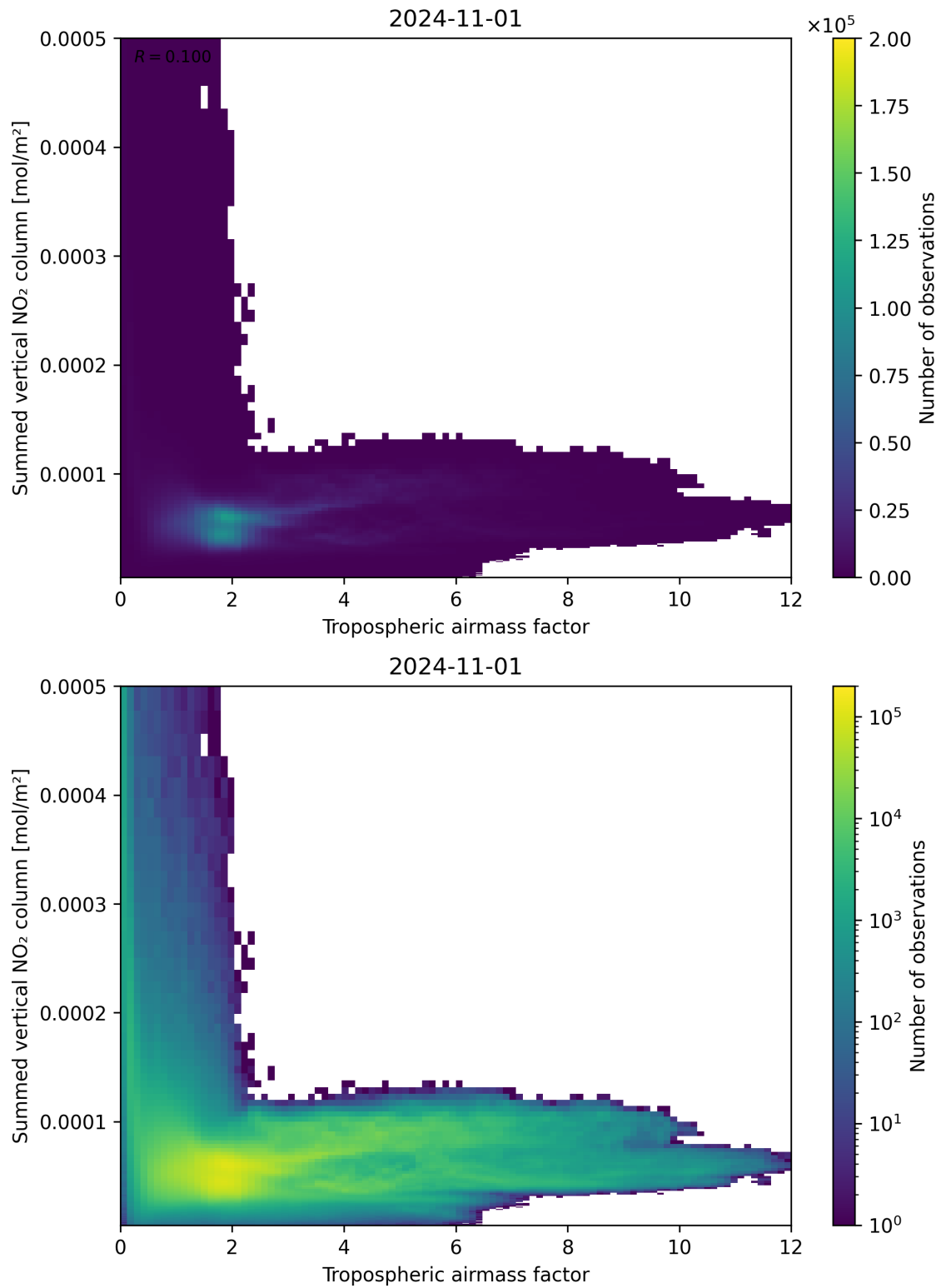
Figure 75: Scatter density plot of “Tropospheric airmass factor” against “Summed vertical NO 2 column” for 2024-10-31 to 2024-11-02.
