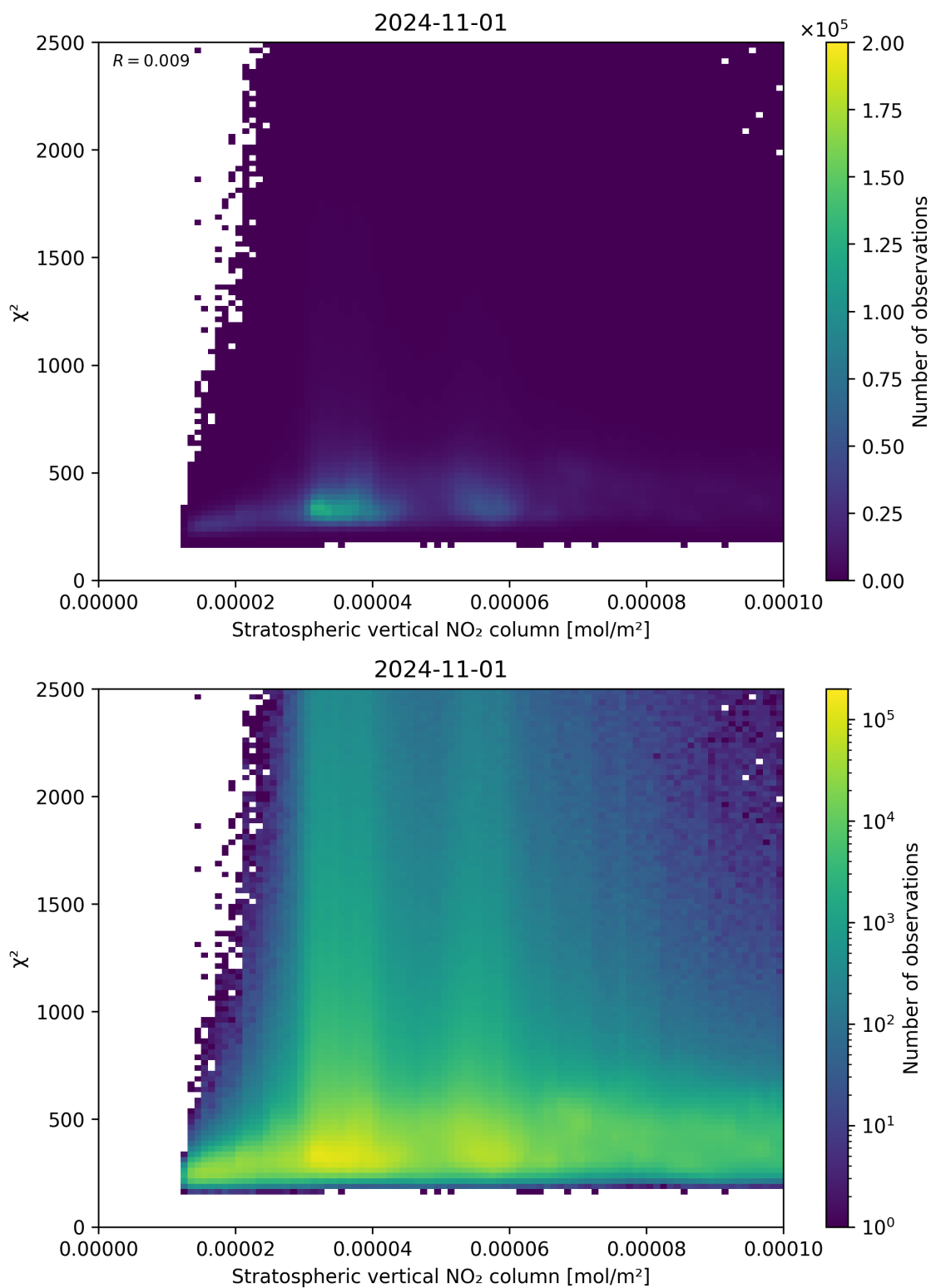
Figure 97: Scatter density plot of “Stratospheric vertical NO 2 column” against “ \chi^2 ” for 2024-10-31 to 2024-11-02.
