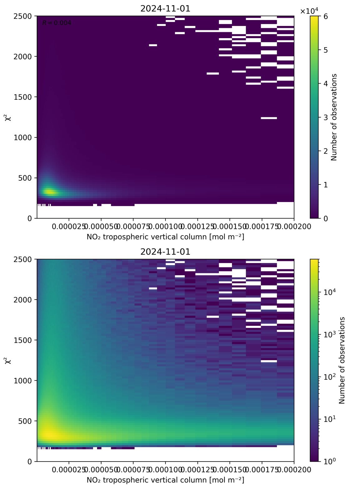
Figure 124: Scatter density plot of “NO 2 tropospheric vertical column” against “ \chi^2 ” for 2024-10-31 to 2024-11-02.
