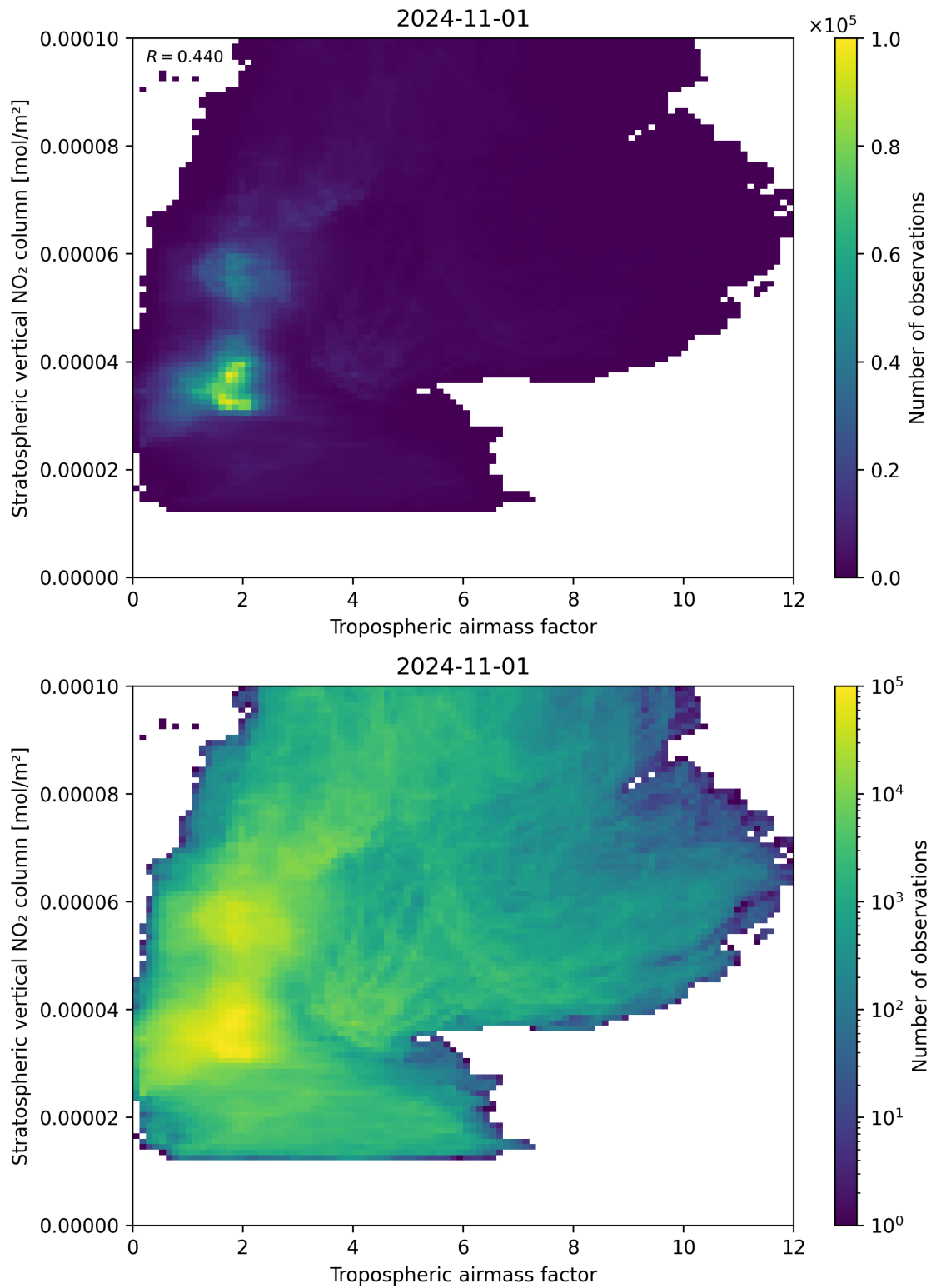
Figure 74: Scatter density plot of “Tropospheric air mass factor” against “Stratospheric vertical NO 2 column” for 2024-10-31 to 2024-11-02.
