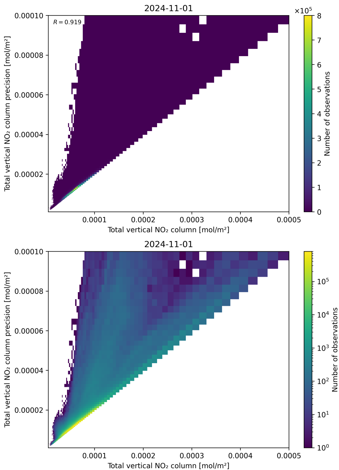
Figure 114: Scatter density plot of “Total vertical NO 2 column” against “Total vertical NO 2 column precision” for 2024-10-31 to 2024-11-02.
