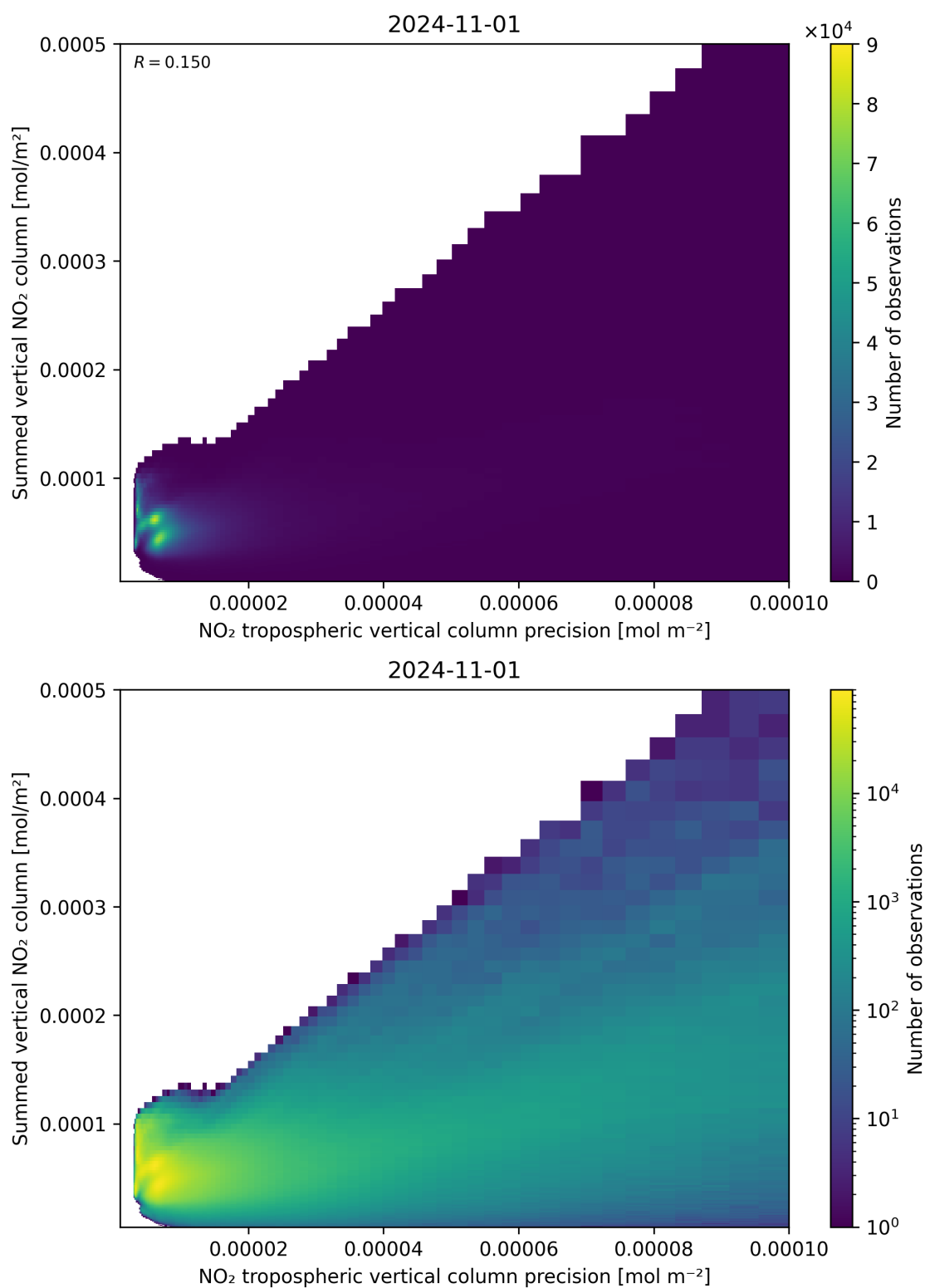
Figure 136: Scatter density plot of “NO 2 tropospheric vertical column precision” against “Summed vertical NO 2 column” for 2024-10-31 to 2024-11-02.
