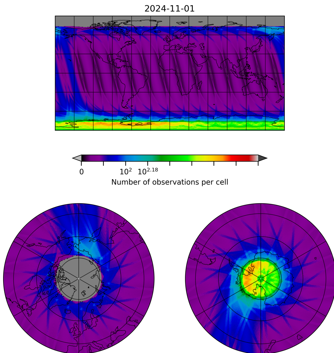
Figure 10: Map of the number of observations for 2024-10-31 to 2024-11-02
