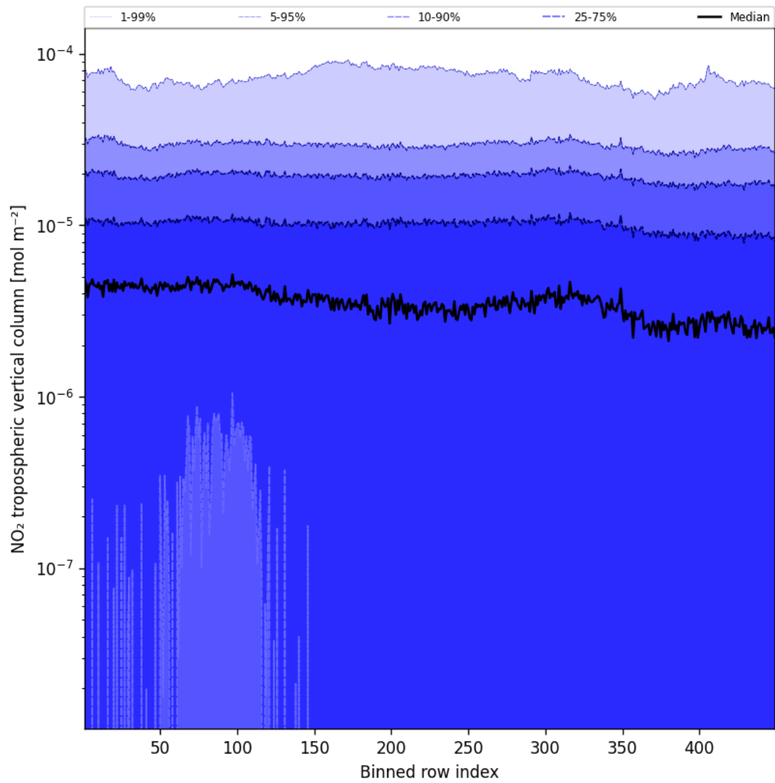
Figure 46: Along track statistics of “NO 2 tropospheric vertical column” for 2024-10-31 to 2024-11-02
