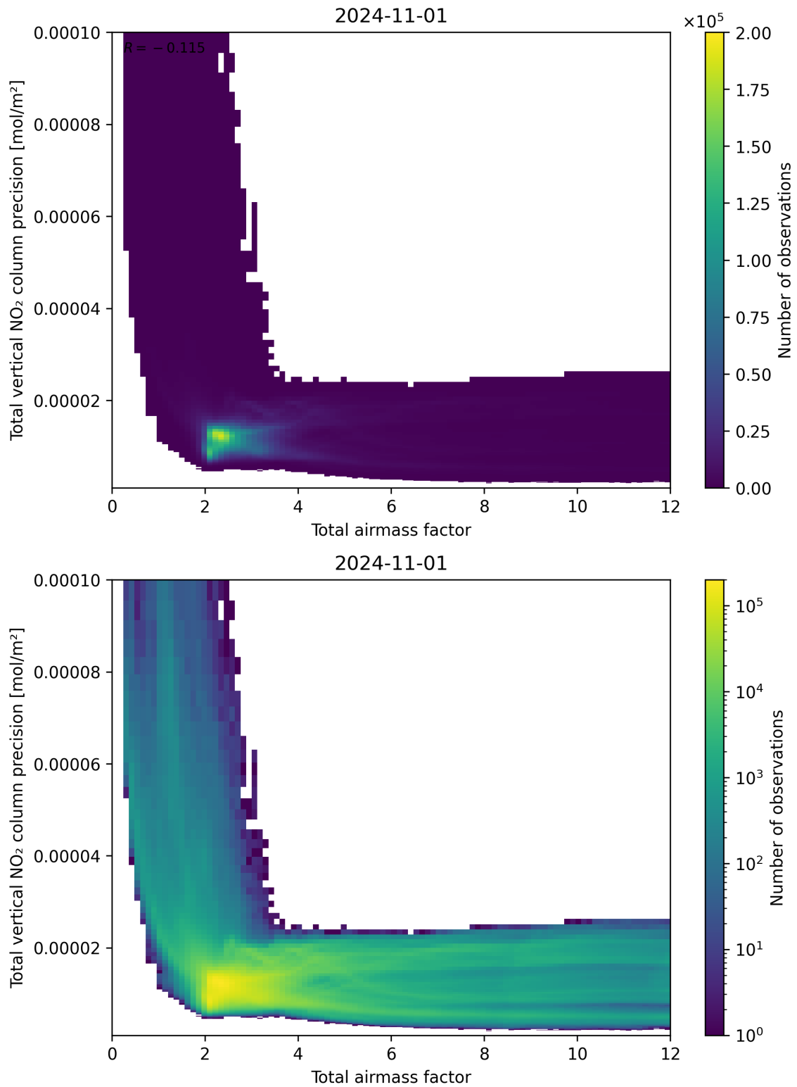
Figure 68: Scatter density plot of “Total airmass factor” against “Total vertical NO 2 column precision” for 2024-10-31 to 2024-11-02.
