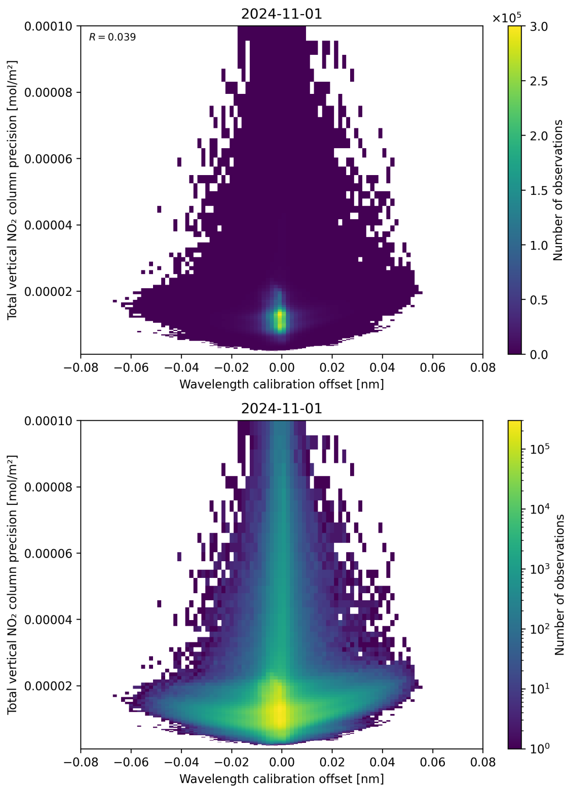
Figure 180: Scatter density plot of “Wavelength calibration offset” against “Total vertical NO 2 column precision” for 2024-10-31 to 2024-11-02.
