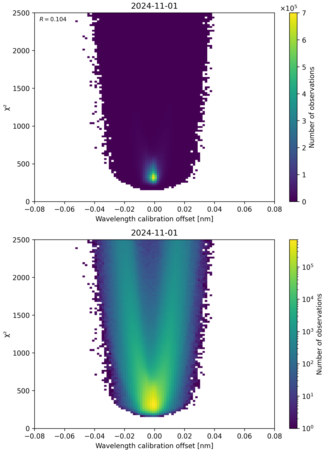
Figure 175: Scatter density plot of “Wavelength calibration offset” against “ \chi^2 ” for 2024-10-31 to 2024-11-02.
