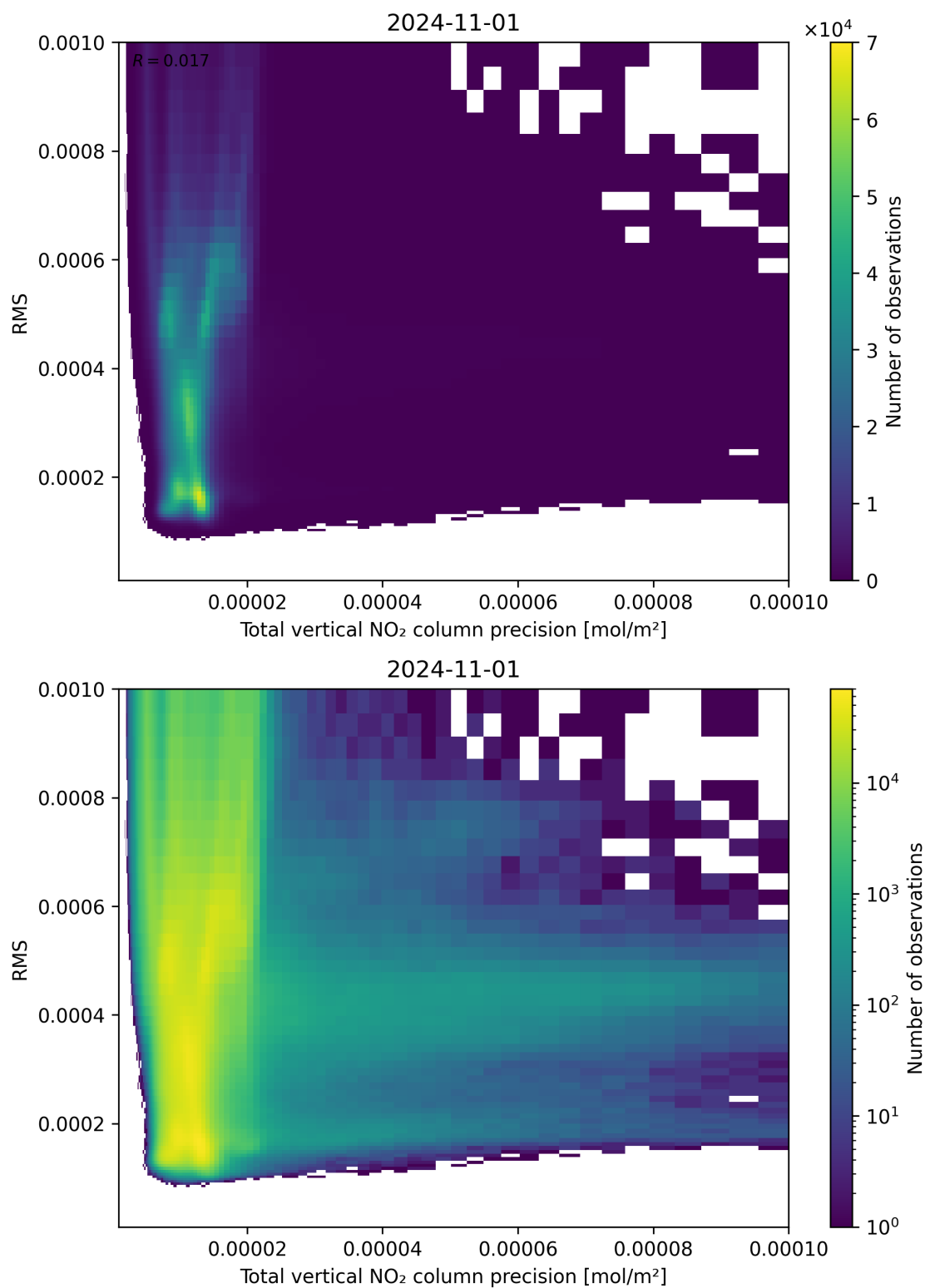
Figure 119: Scatter density plot of “Total vertical NO 2 column precision” against “RMS” for 2024-10-31 to 2024-11-02.
