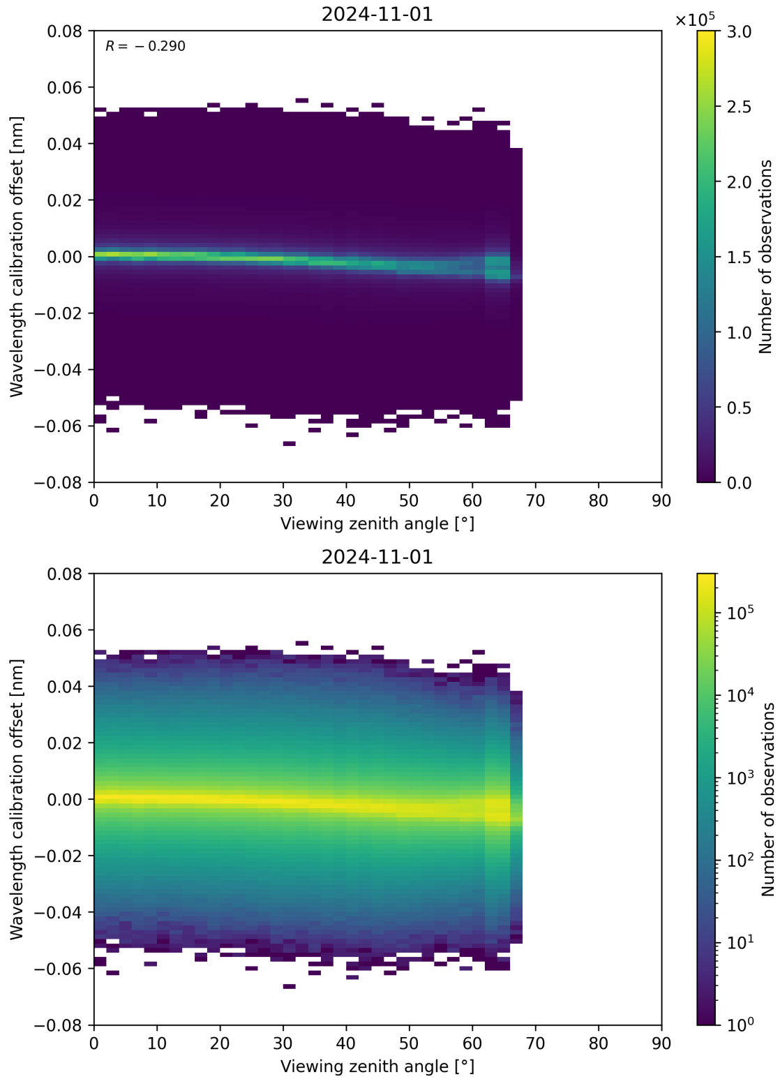
Figure 173: Scatter density plot of “Viewing zenith angle” against “Wavelength calibration offset” for 2024-10-31 to 2024-11-02.
