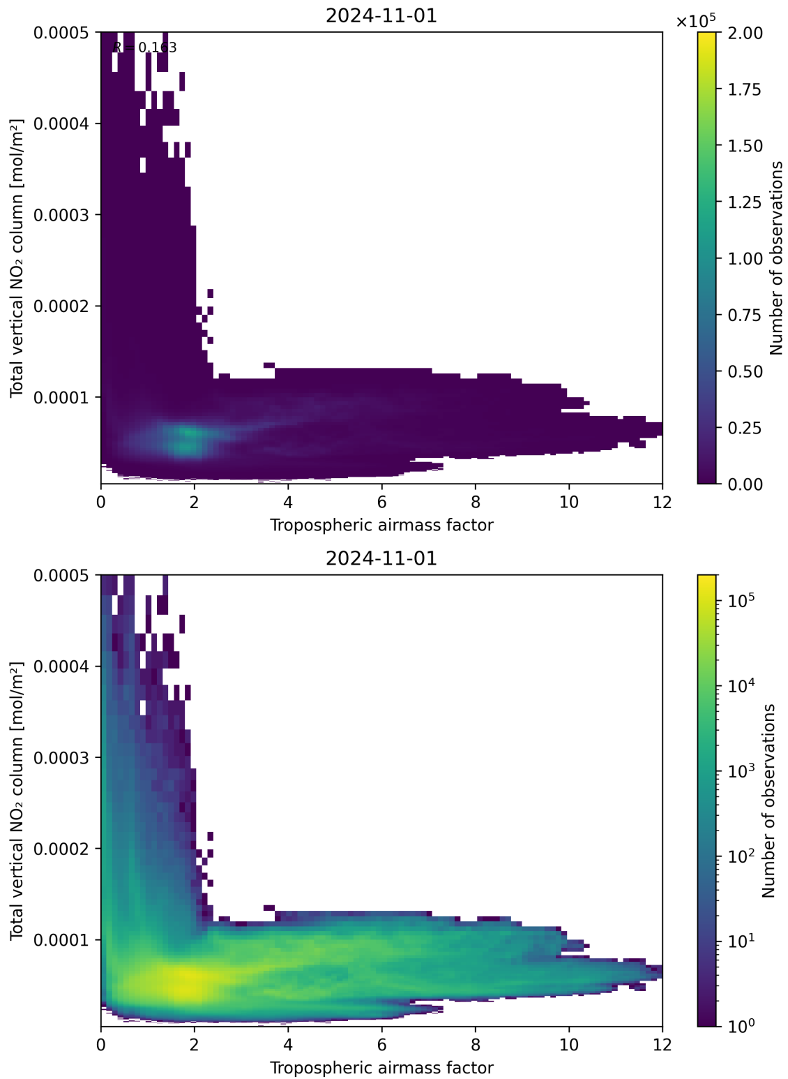
Figure 77: Scatter density plot of “Tropospheric airmass factor” against “Total vertical NO 2 column” for 2024-10-31 to 2024-11-02.
