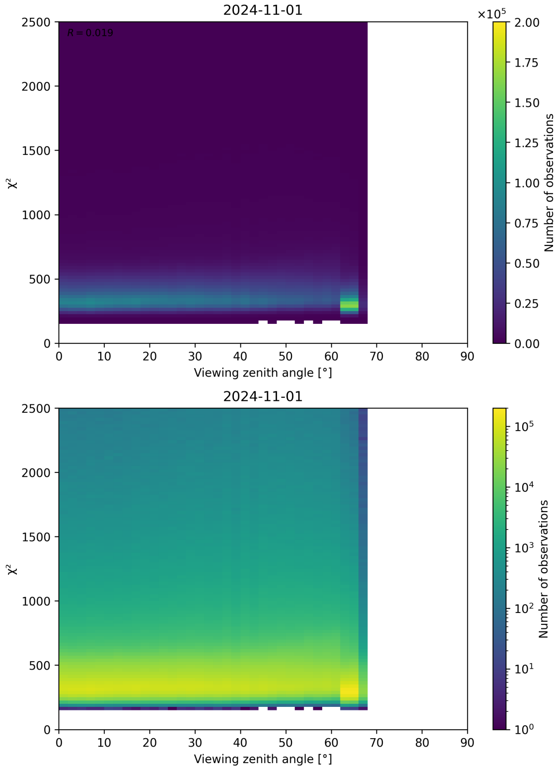
Figure 162: Scatter density plot of “Viewing zenith angle” against “ \chi^2 ” for 2024-10-31 to 2024-11-02.
