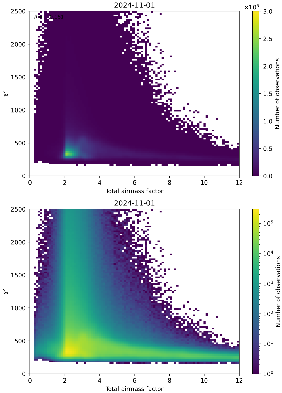
Figure 63: Scatter density plot of “Total airmass factor” against “ \chi^2 ” for 2024-10-31 to 2024-11-02.
