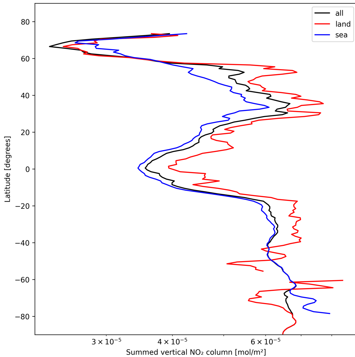
Figure 23: Zonal average of “Summed vertical NO 2 column” for 2024-10-31 to 2024-11-02.
