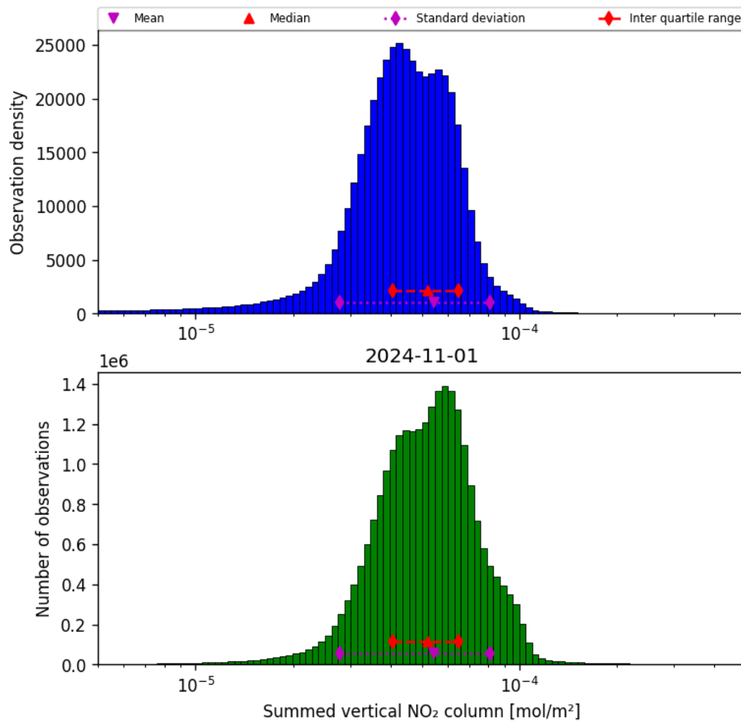
Figure 40: Histogram of “Summed vertical NO 2 column” for 2024-10-31 to 2024-11-02
