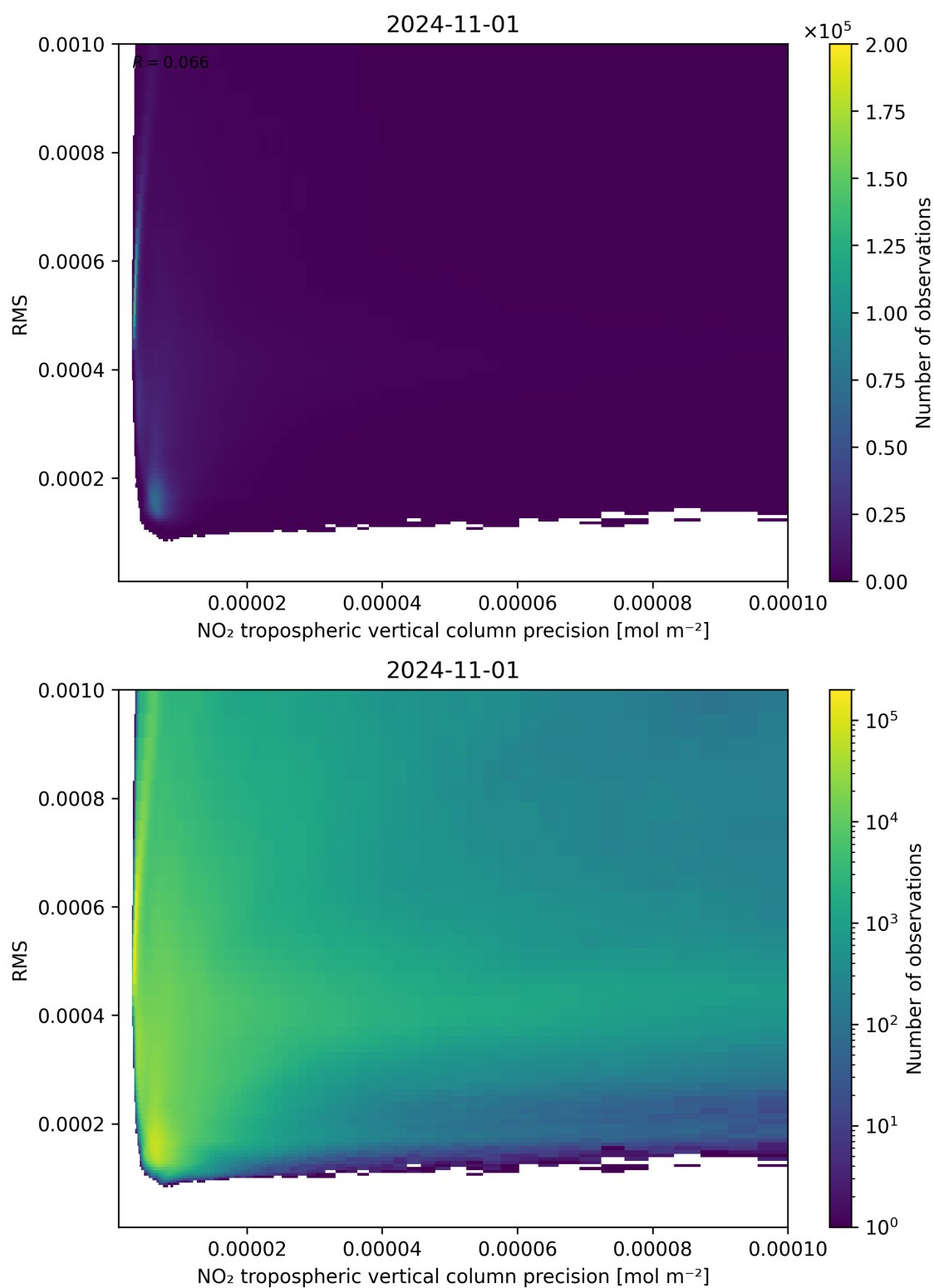
Figure 140: Scatter density plot of “NO 2 tropospheric vertical column precision” against “RMS” for 2024-10-31 to 2024-11-02.
