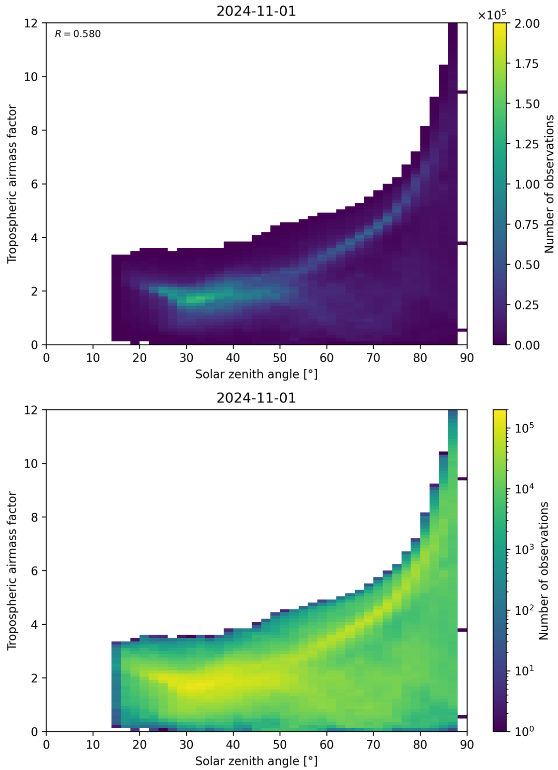
Figure 147: Scatter density plot of “Solar zenith angle” against “Tropospheric airmass factor” for 2024-10-31 to 2024-11-02.
