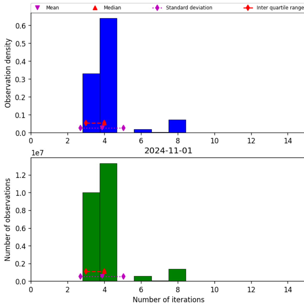
Figure 34: Histogram of “Number of iterations” for 2024-10-31 to 2024-11-02
