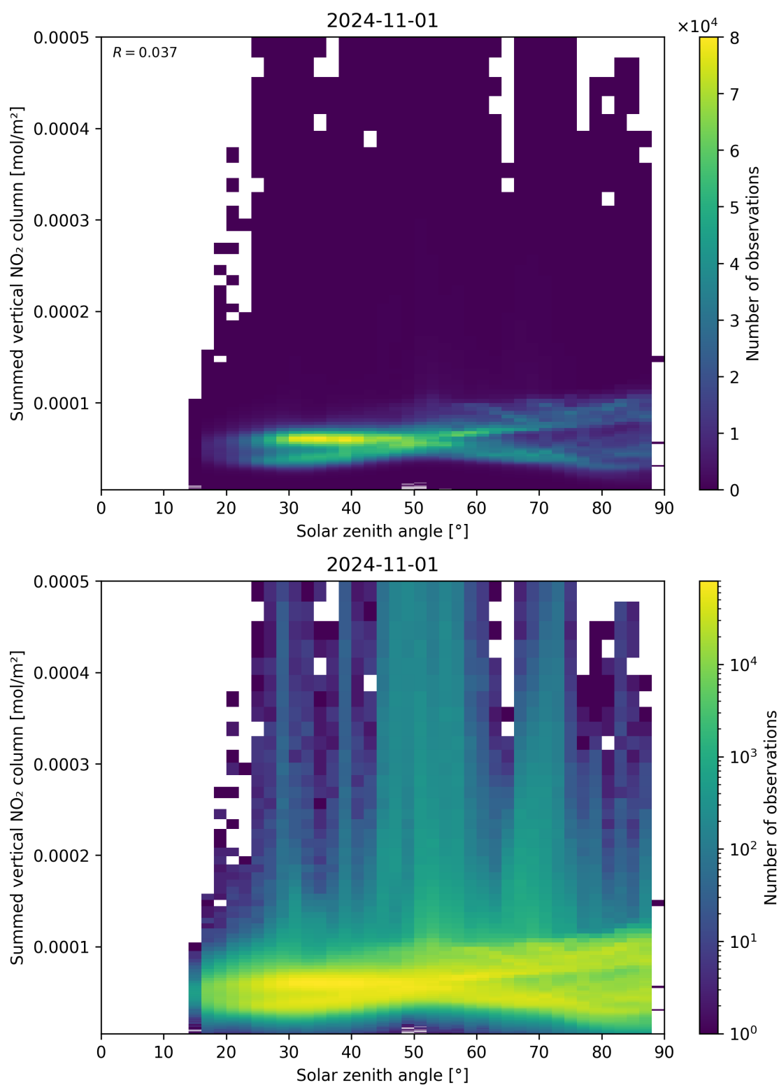
Figure 151: Scatter density plot of “Solar zenith angle” against “Summed vertical NO 2 column” for 2024-10-31 to 2024-11-02.
