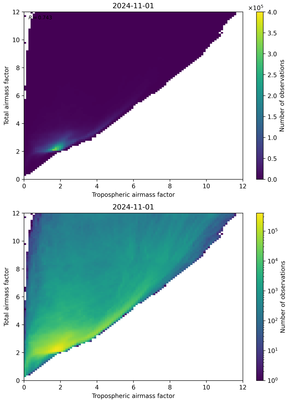
Figure 72: Scatter density plot of “Tropospheric airmass factor” against “Total airmass factor” for 2024-10-31 to 2024-11-02.
