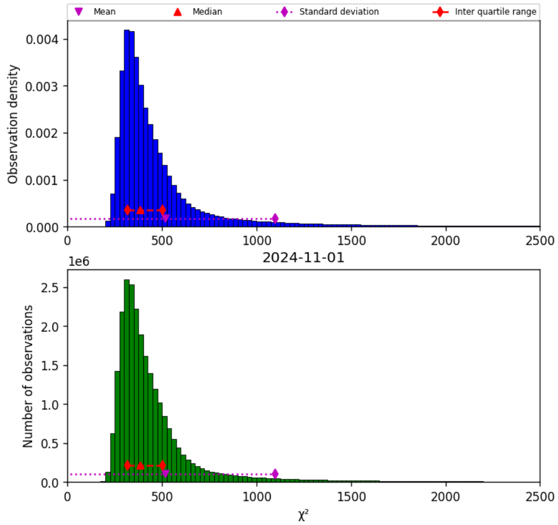
Figure 42: Histogram of “ \chi^2 ” for 2024-10-31 to 2024-11-02
