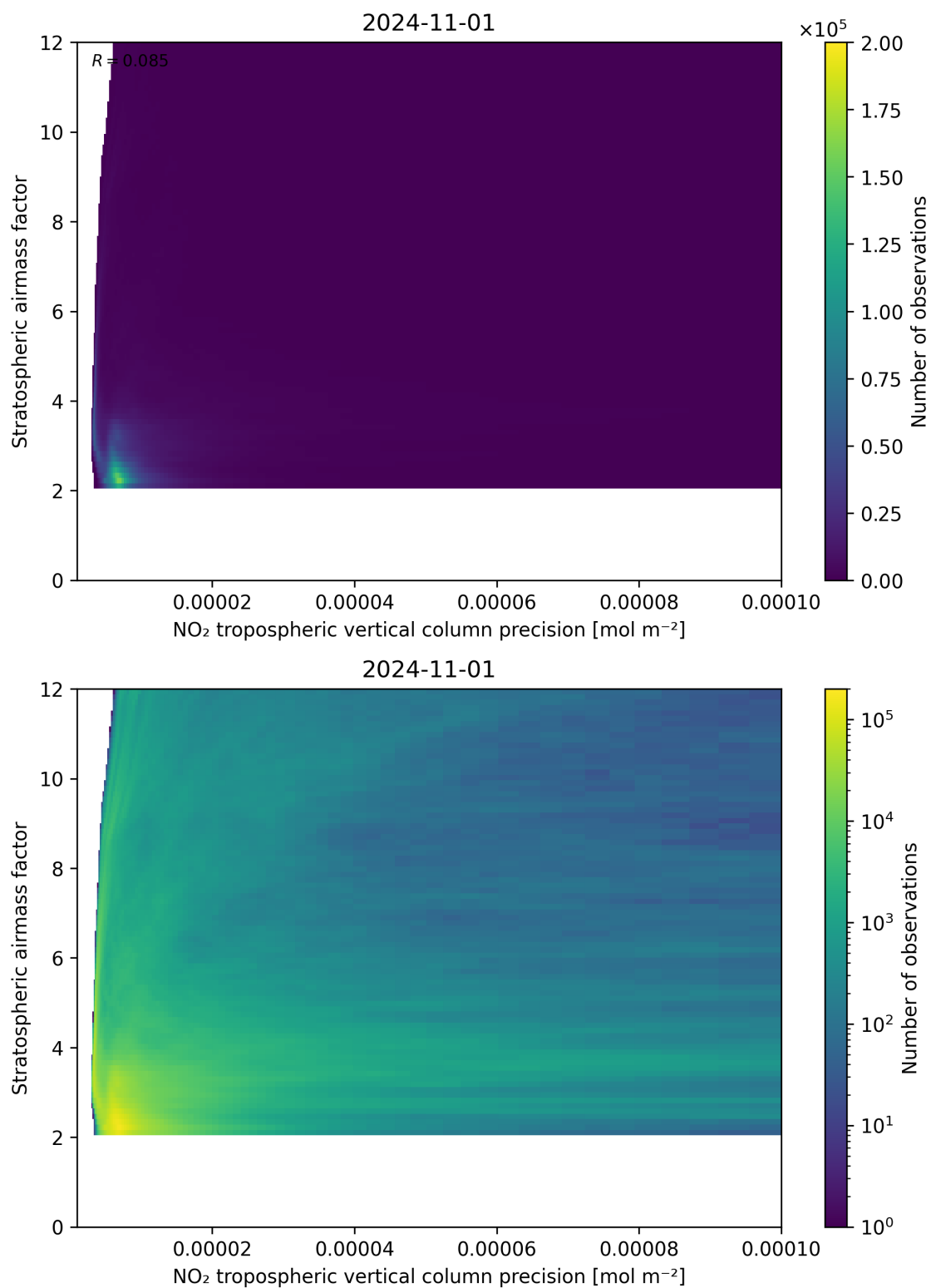
Figure 131: Scatter density plot of “NO 2 tropospheric vertical column precision” against “Stratospheric airmass factor” for 2024-10-31 to 2024-11-02.
