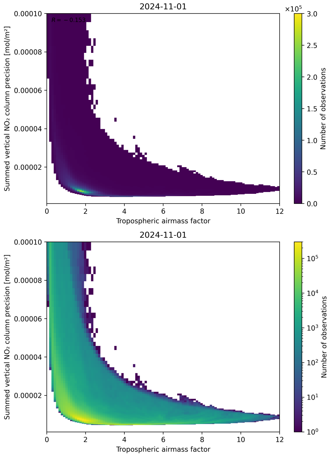
Figure 76: Scatter density plot of “Tropospheric air mass factor” against “Summed vertical NO 2 column precision” for 2024-10-31 to 2024-11-02.
