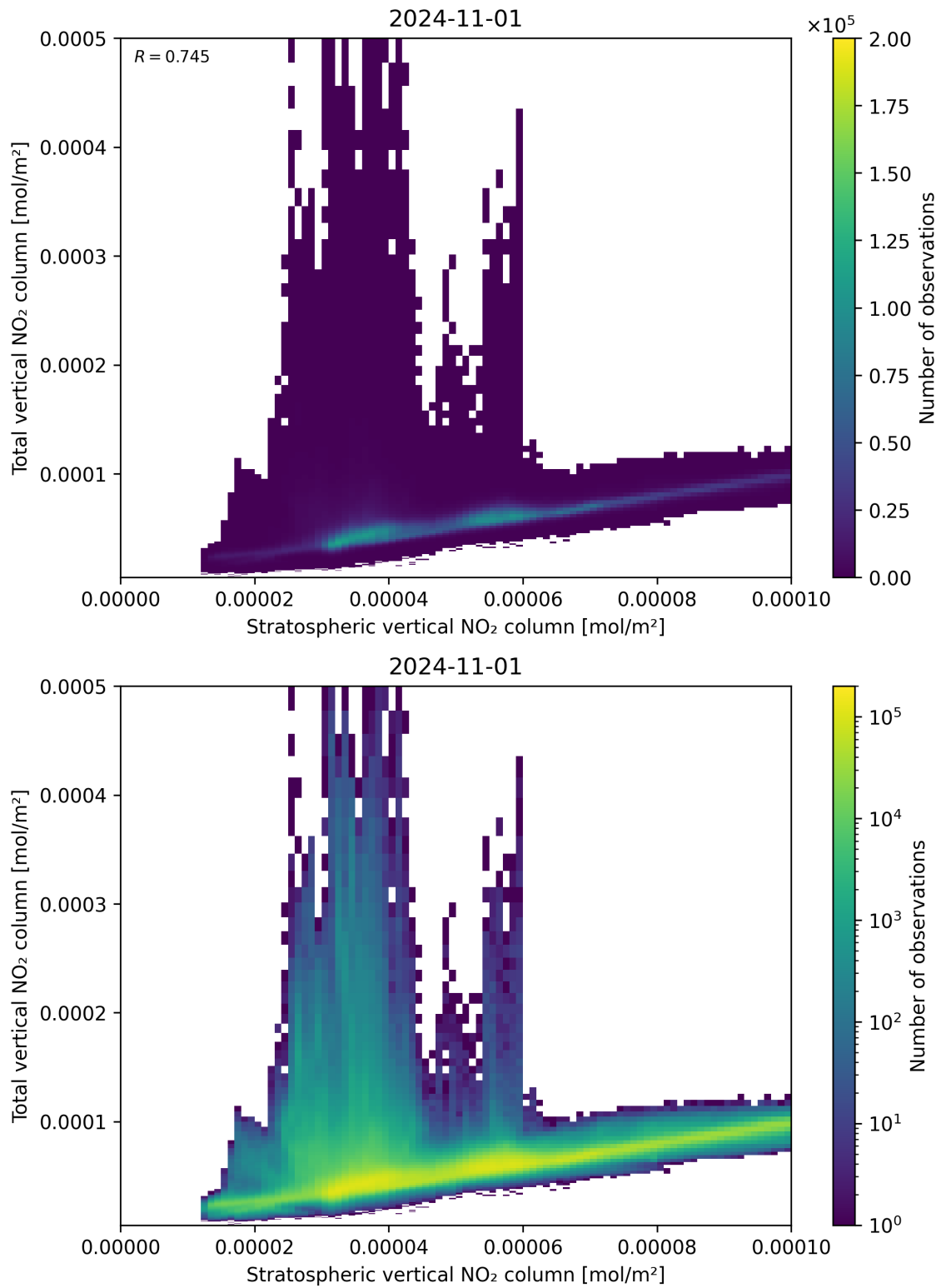
Figure 100: Scatter density plot of “Stratospheric vertical NO 2 column” against “Total vertical NO 2 column” for 2024-10-31 to 2024-11-02.
