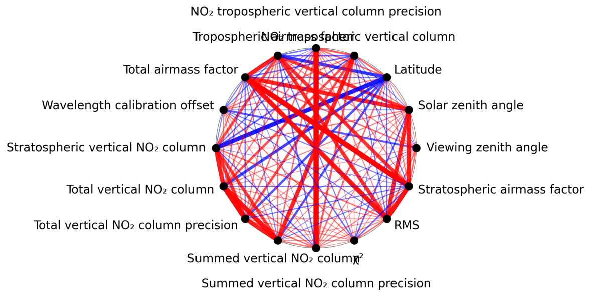
Figure 1: Map of correlation graph for 2024-10-31 to 2024-11-02.
