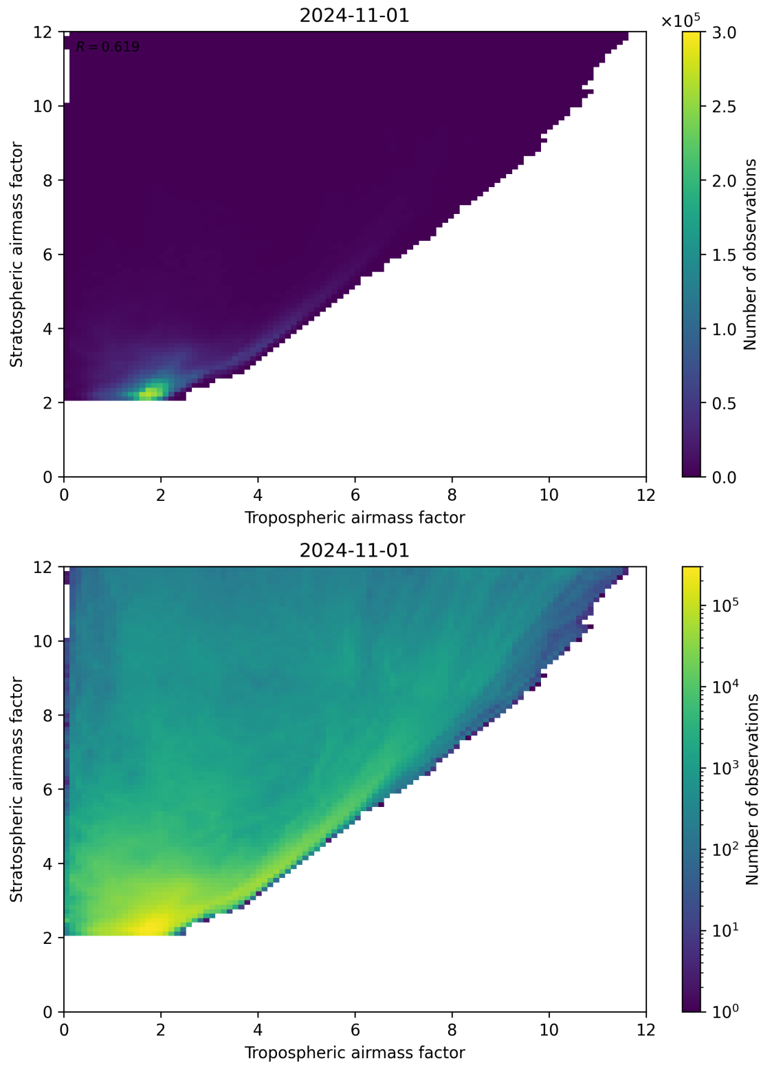
Figure 71: Scatter density plot of “Tropospheric airmass factor” against “Stratospheric airmass factor” for 2024-10-31 to 2024-11-02.
