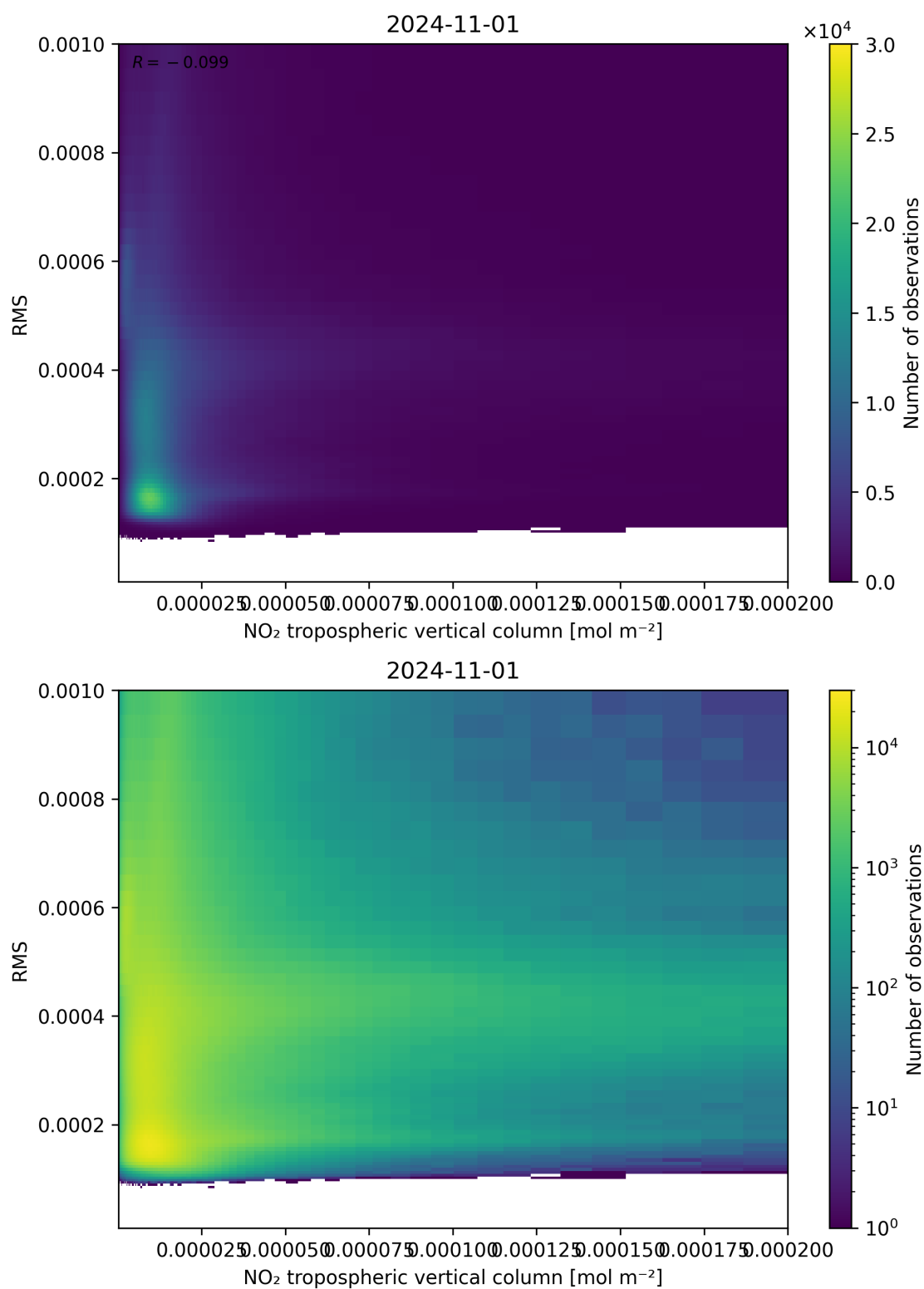
Figure 142: Scatter density plot of “NO 2 tropospheric vertical column” against “RMS” for 2024-10-31 to 2024-11-02.
