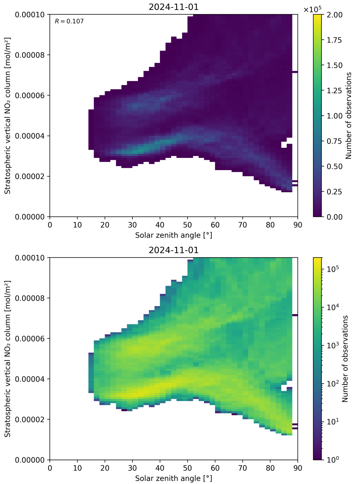
Figure 150: Scatter density plot of “Solar zenith angle” against “Stratospheric vertical NO 2 column” for 2024-10-31 to 2024-11-02.
