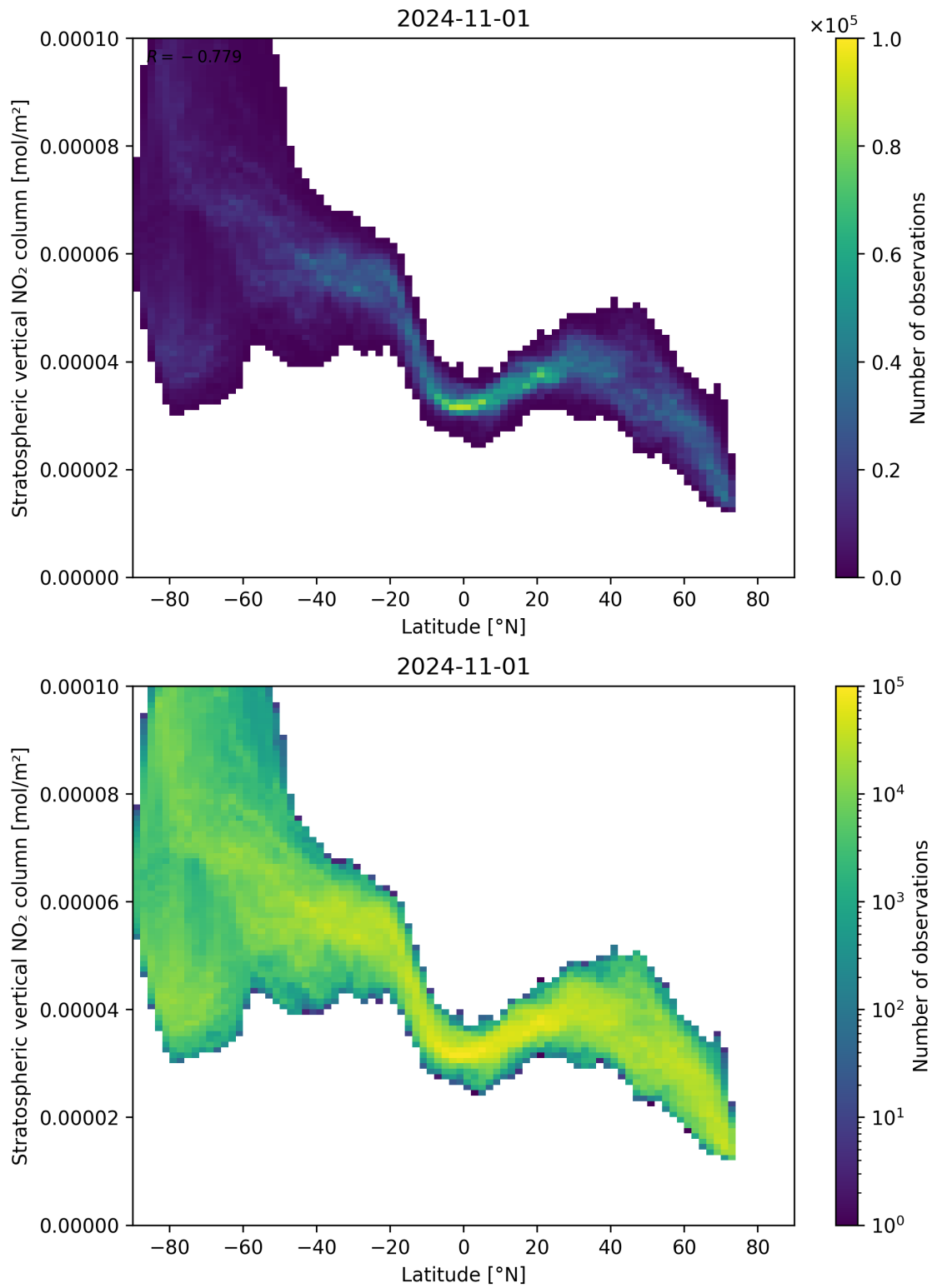
Figure 87: Scatter density plot of “Latitude” against “Stratospheric vertical NO 2 column” for 2024-10-31 to 2024-11-02.
