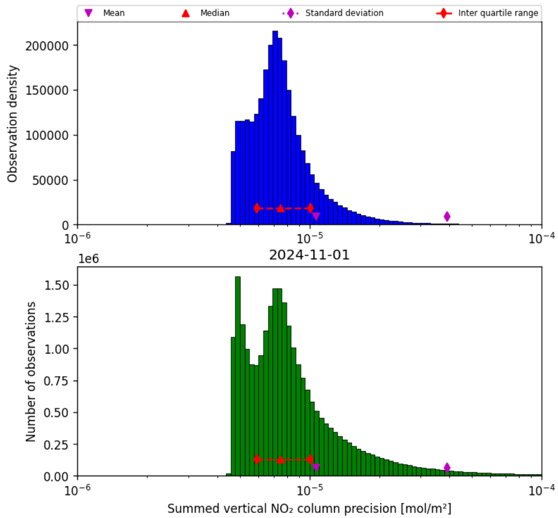
Figure 41: Histogram of "Summed vertical NO 2 column precision" for 2024-10-31 to 2024-11-02
