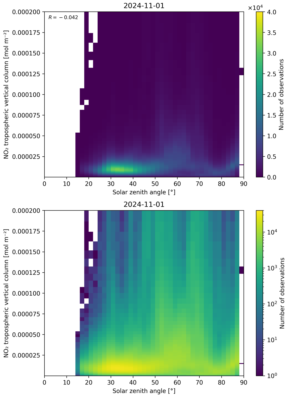
Figure 155: Scatter density plot of “Solar zenith angle” against “NO 2 tropospheric vertical column” for 2024-10-31 to 2024-11-02.
