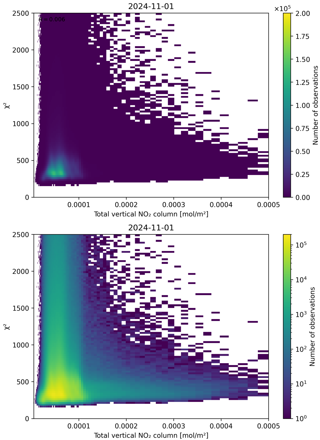
Figure 111: Scatter density plot of “Total vertical NO 2 column” against “ \chi^2 ” for 2024-10-31 to 2024-11-02.
