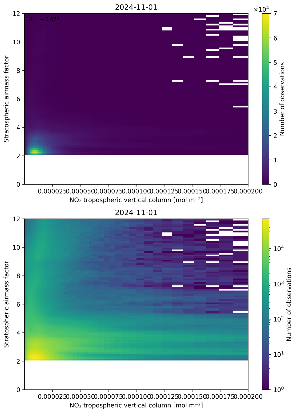
Figure 121: Scatter density plot of “NO 2 tropospheric vertical column” against “Stratospheric airmass factor” for 2024-10-31 to 2024-11-02.
