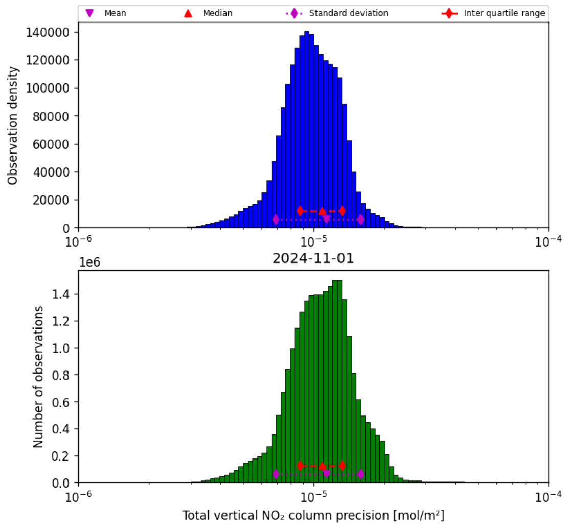
Figure 39: Histogram of “Total vertical NO 2 column precision” for 2024-10-31 to 2024-11-02
