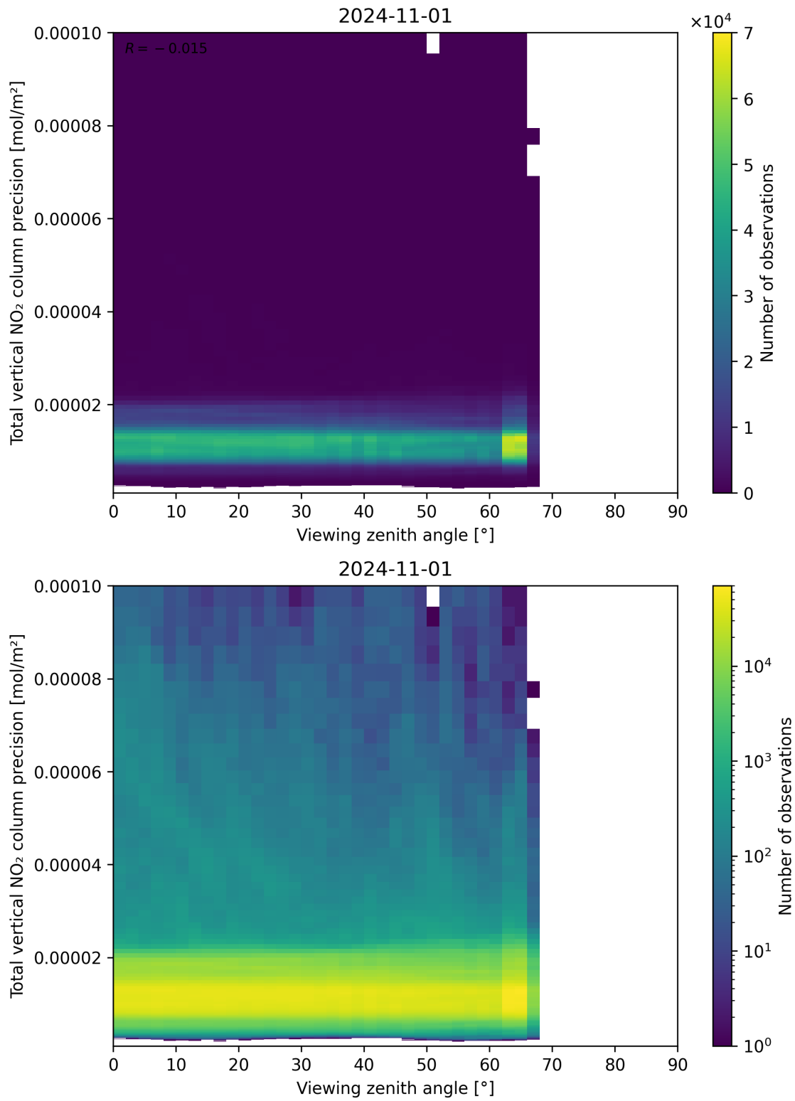
Figure 168: Scatter density plot of “Viewing zenith angle” against “Total vertical NO 2 column precision” for 2024-10-31 to 2024-11-02.
