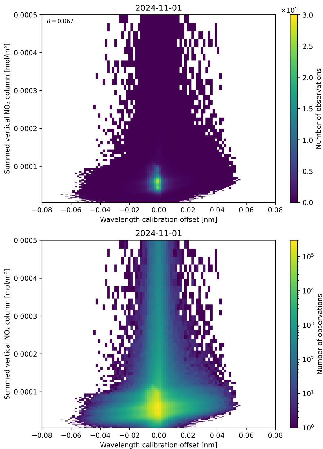
Figure 177: Scatter density plot of “Wavelength calibration offset” against “Summed vertical NO 2 column” for 2024-10-31 to 2024-11-02.
