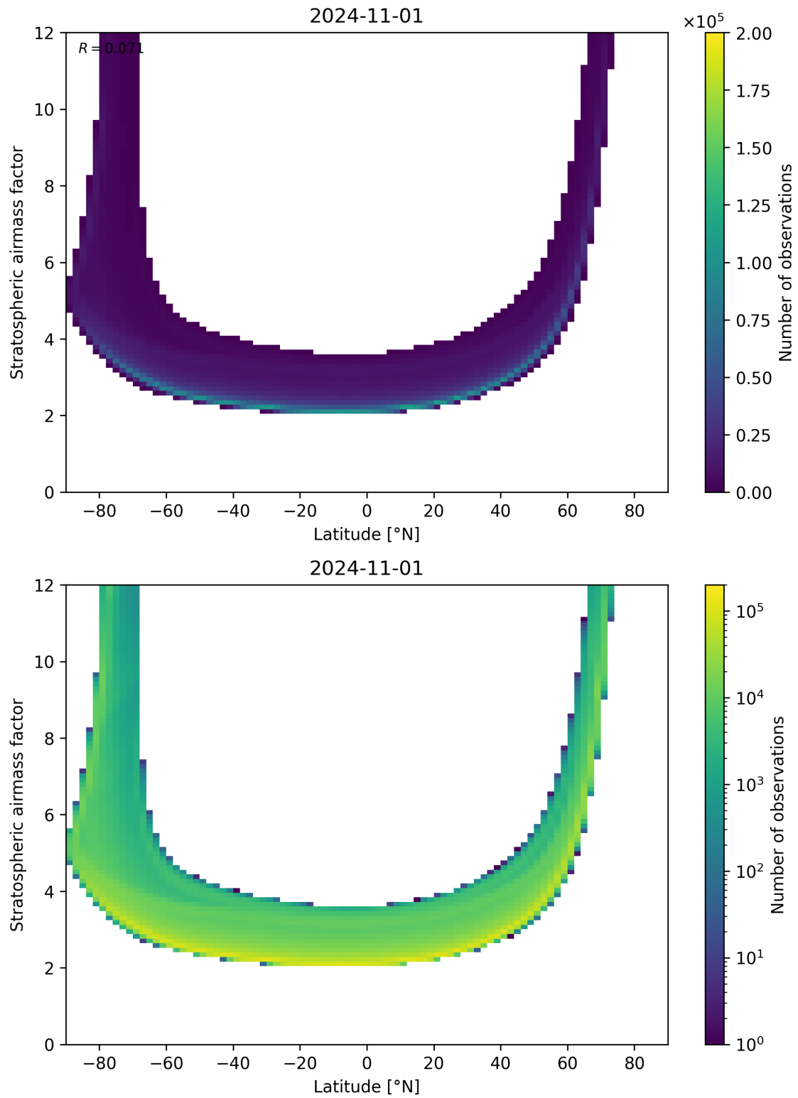
Figure 83: Scatter density plot of “Latitude” against “Stratospheric airmass factor” for 2024-10-31 to 2024-11-02.
