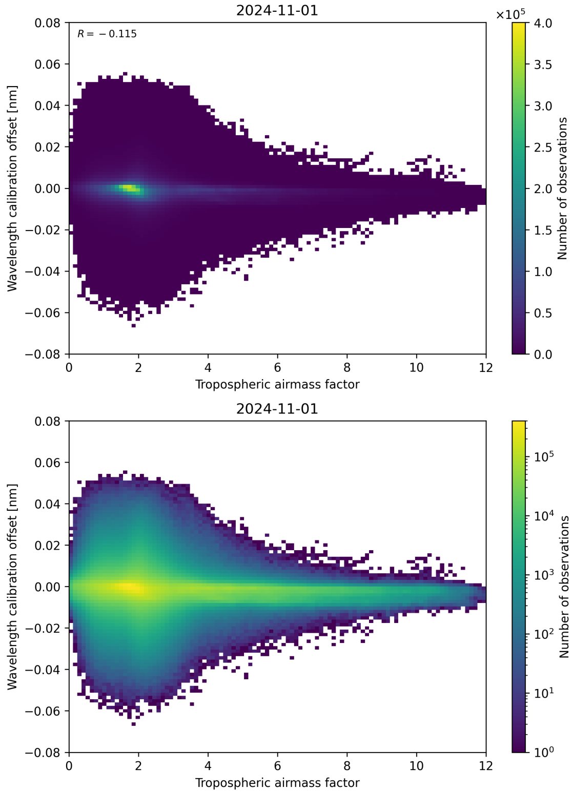
Figure 80: Scatter density plot of “Tropospheric air mass factor” against “Wavelength calibration offset” for 2024-10-31 to 2024-11-02.
