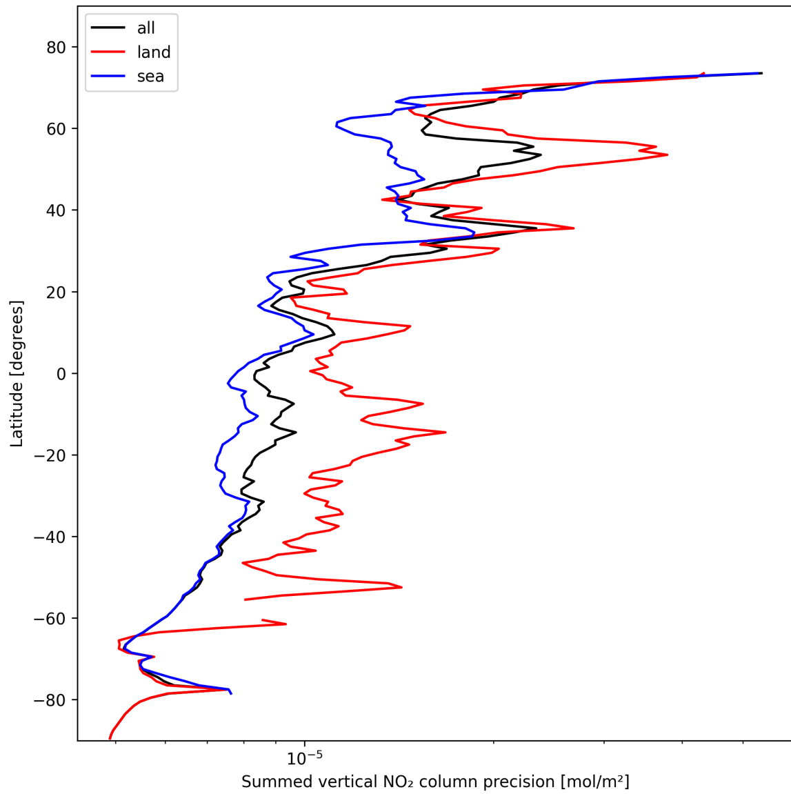
Figure 24: Zonal average of “Summed vertical NO 2 column precision” for 2024-10-31 to 2024-11-02.
