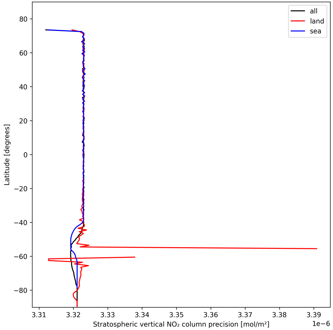
Figure 20: Zonal average of “Stratospheric vertical NO 2 column precision” for 2024-10-31 to 2024-11-02.
