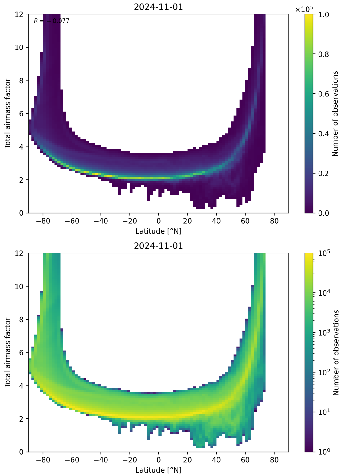
Figure 84: Scatter density plot of “Latitude” against “Total airmass factor” for 2024-10-31 to 2024-11-02.
