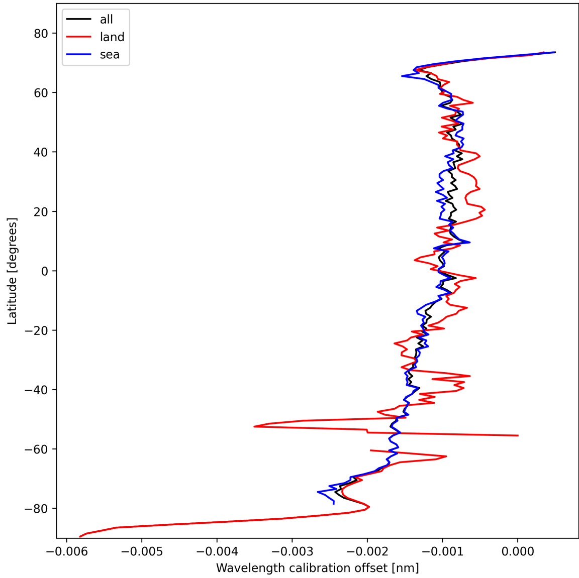
Figure 18: Zonal average of “Wavelength calibration offset” for 2024-10-31 to 2024-11-02.
