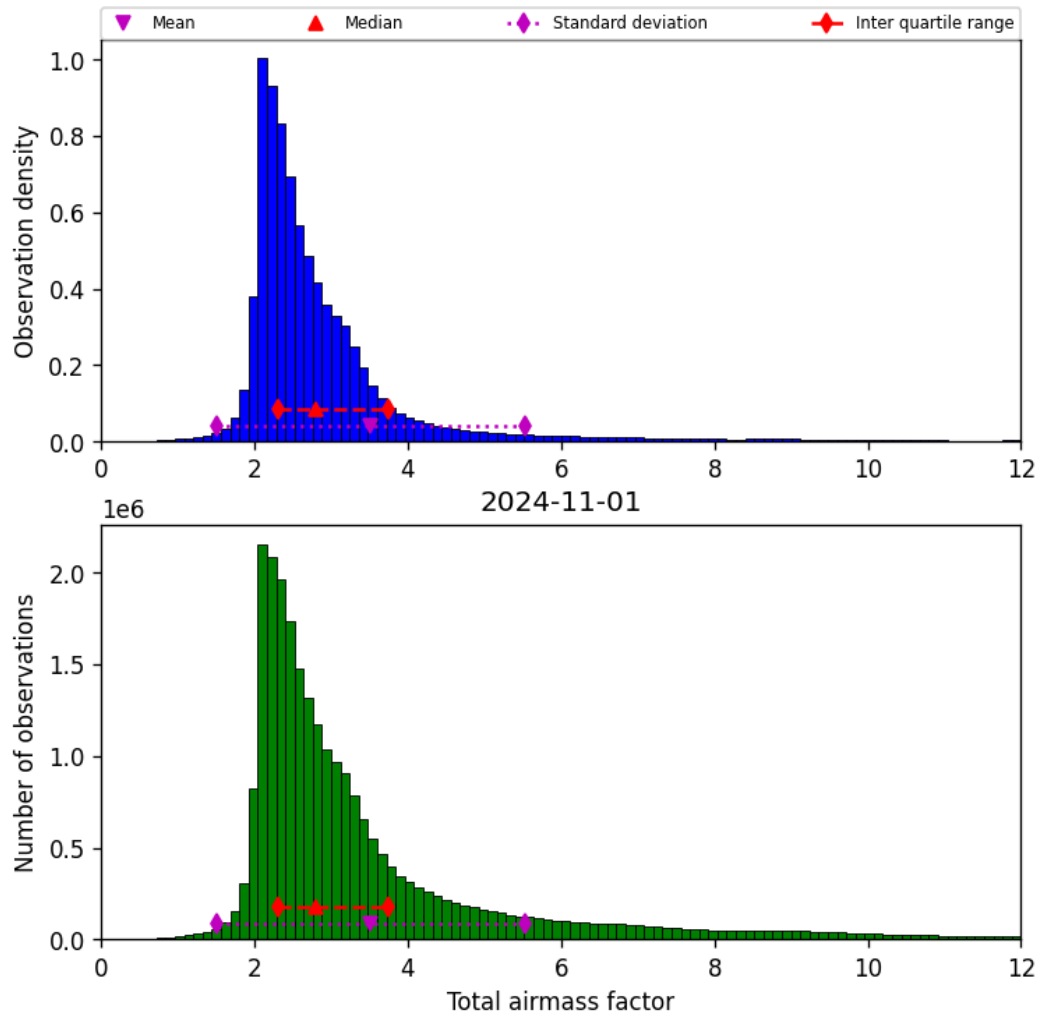
Figure 32: Histogram of “Total airmass factor” for 2024-10-31 to 2024-11-02
