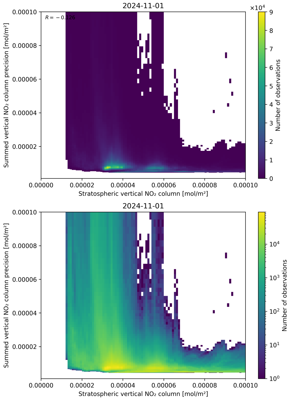
Figure 99: Scatter density plot of “Stratospheric vertical NO 2 column” against “Summed vertical NO 2 column precision” for 2024-10-31 to 2024-11-02.
