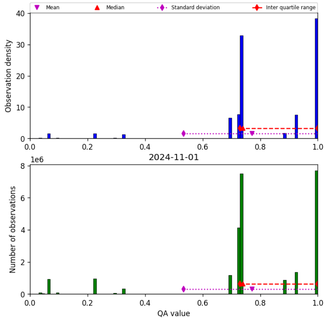
Figure 28: Histogram of “QA value” for 2024-10-31 to 2024-11-02
