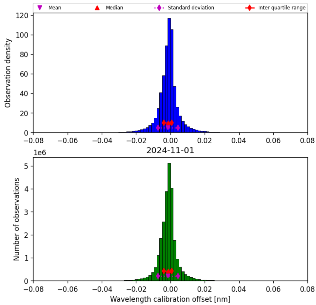
Figure 35: Histogram of “Wavelength calibration offset” for 2024-10-31 to 2024-11-02
