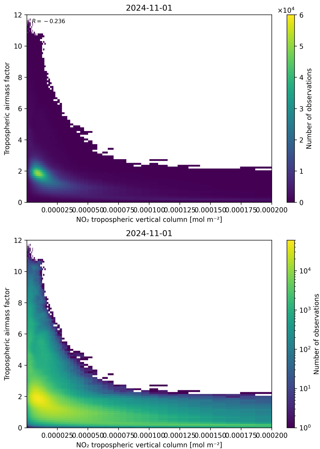
Figure 123: Scatter density plot of “NO 2 tropospheric vertical column” against “Tropospheric air mass factor” for 2024-10-31 to 2024-11-02.
