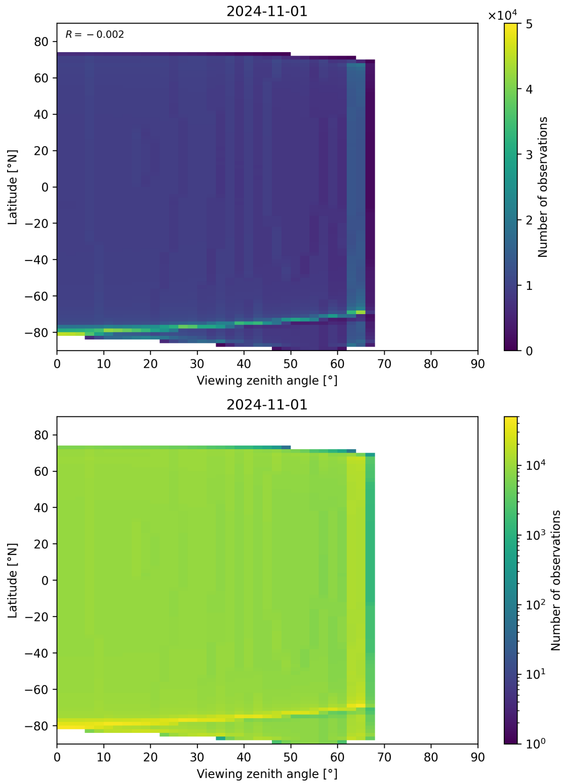
Figure 163: Scatter density plot of “Viewing zenith angle” against “Latitude” for 2024-10-31 to 2024-11-02.
