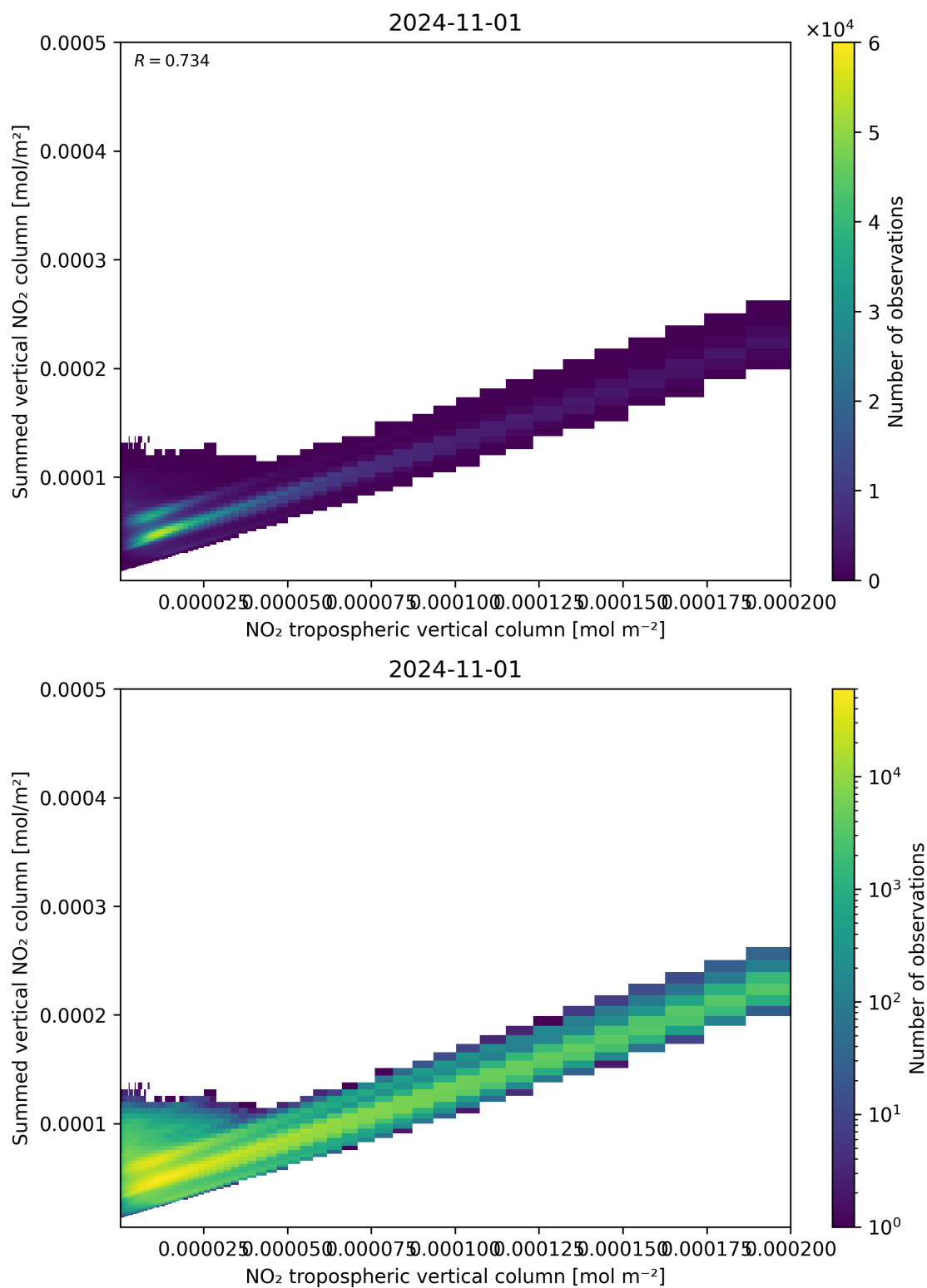
Figure 126: Scatter density plot of “NO 2 tropospheric vertical column” against “Summed vertical NO 2 column” for 2024-10-31 to 2024-11-02.
