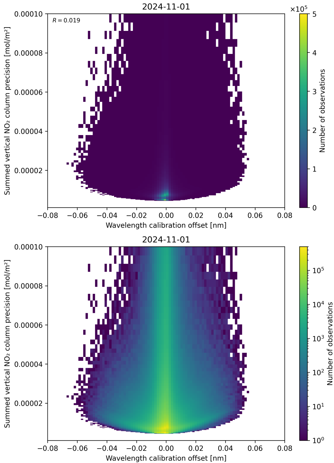
Figure 178: Scatter density plot of “Wavelength calibration offset” against “Summed vertical NO 2 column precision” for 2024-10-31 to 2024-11-02.
