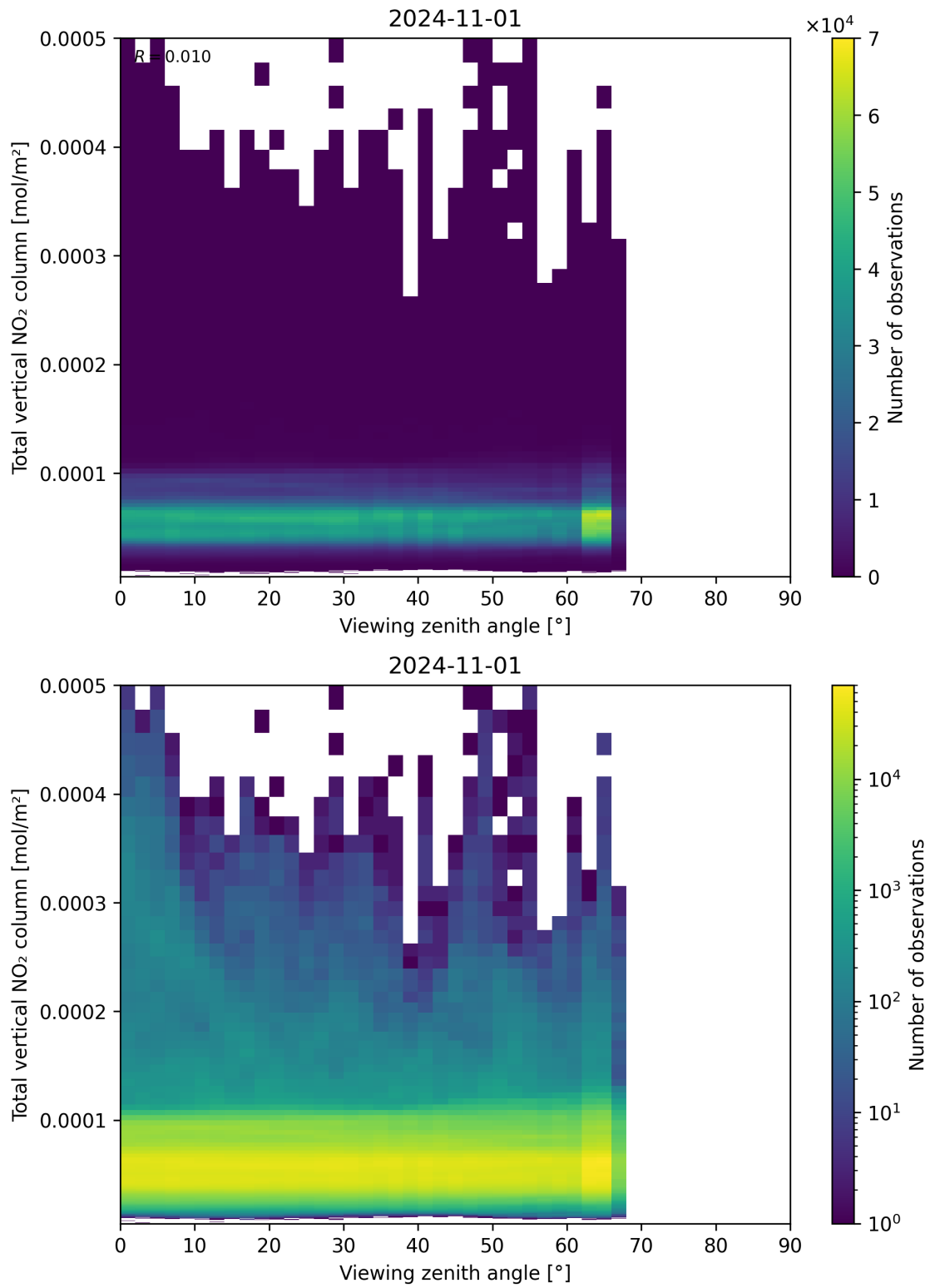
Figure 167: Scatter density plot of “Viewing zenith angle” against “Total vertical NO 2 column” for 2024-10-31 to 2024-11-02.
