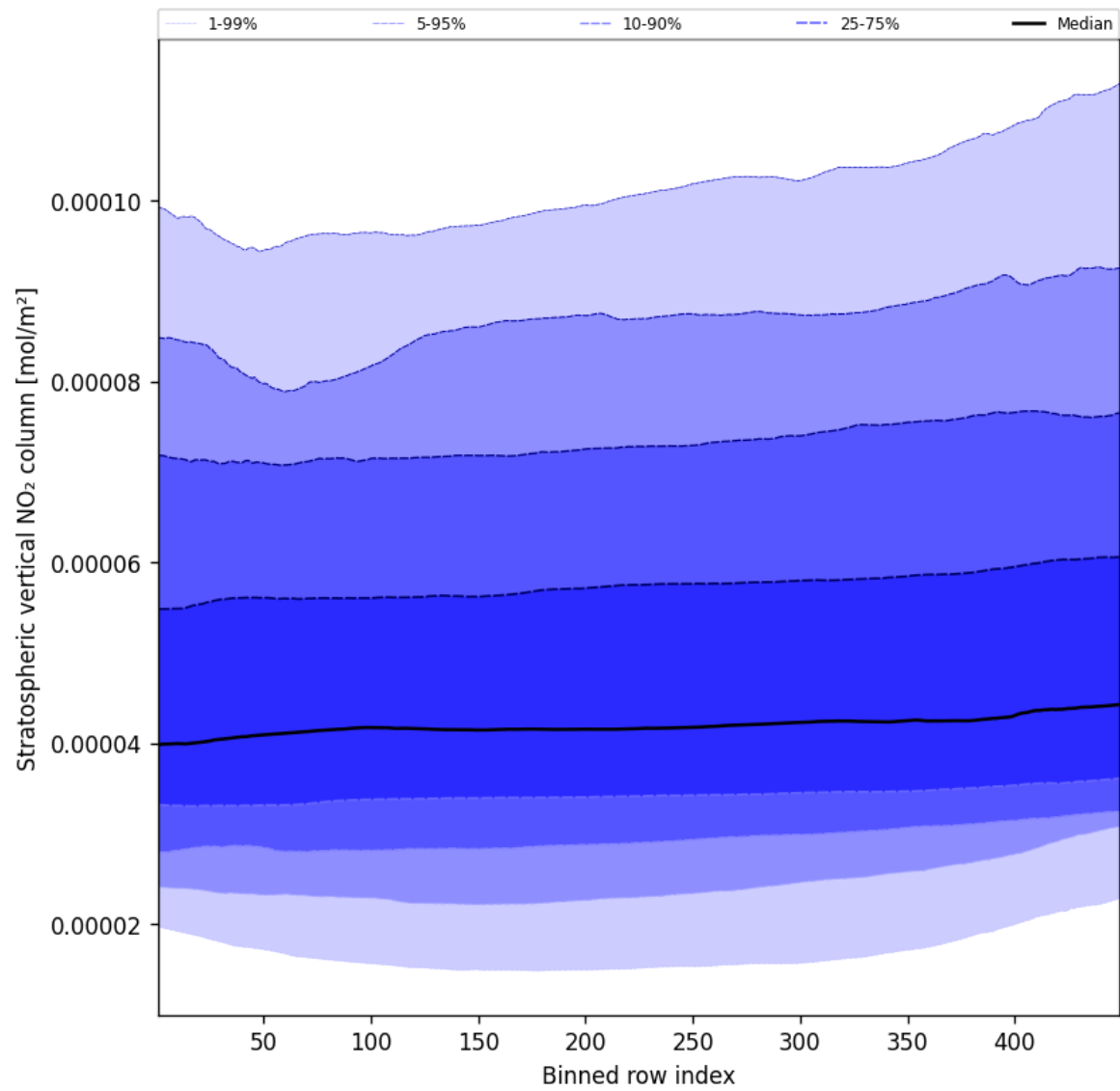
Figure 53: Along track statistics of “Stratospheric vertical NO 2 column” for 2024-10-31 to 2024-11-02
