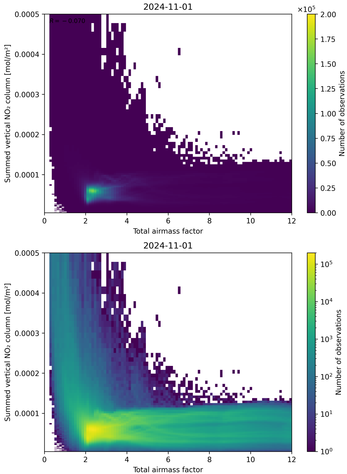
Figure 65: Scatter density plot of “Total airmass factor” against “Summed vertical NO 2 column” for 2024-10-31 to 2024-11-02.
