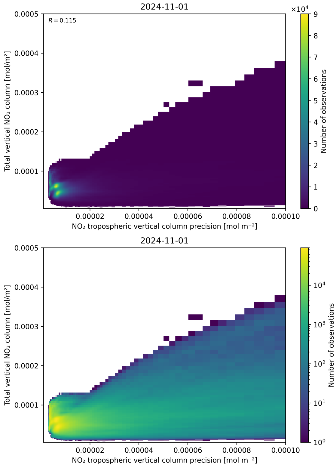
Figure 138: Scatter density plot of “NO 2 tropospheric vertical column precision” against “Total vertical NO 2 column” for 2024-10-31 to 2024-11-02.
