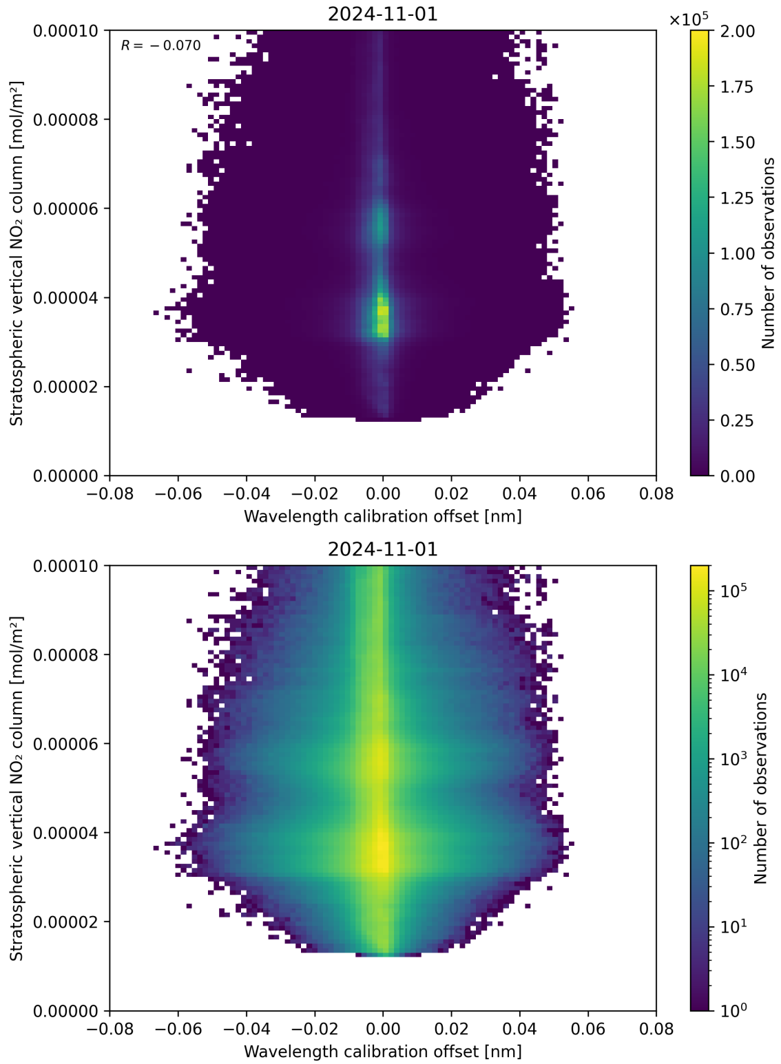
Figure 176: Scatter density plot of “Wavelength calibration offset” against “Stratospheric vertical NO 2 column” for 2024-10-31 to 2024-11-02.
