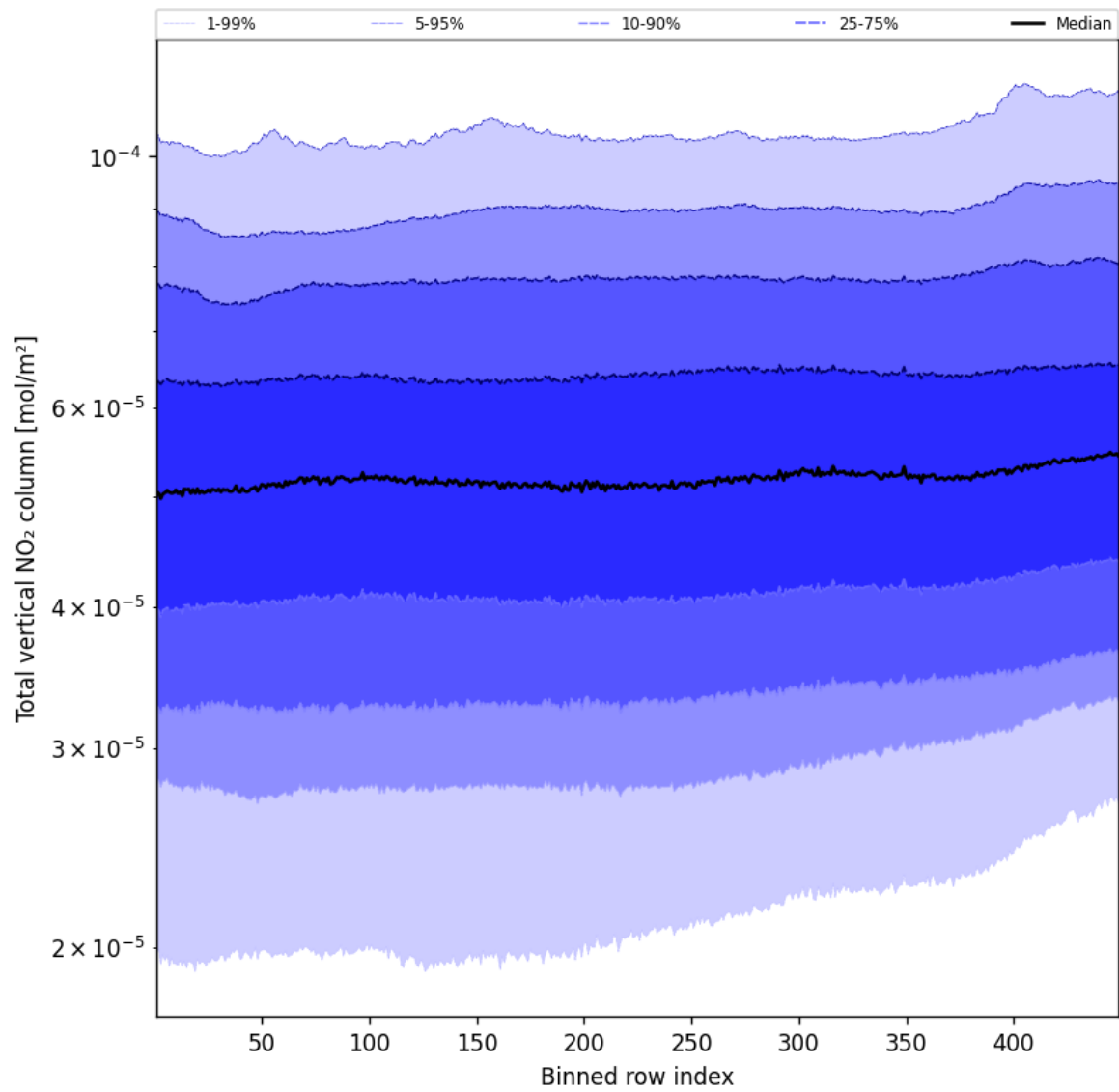
Figure 55: Along track statistics of “Total vertical NO 2 column” for 2024-10-31 to 2024-11-02
