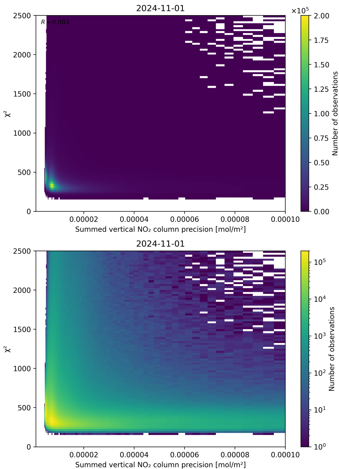
Figure 107: Scatter density plot of “Summed vertical NO 2 column precision” against “ \chi^2 ” for 2024-10-31 to 2024-11-02.
