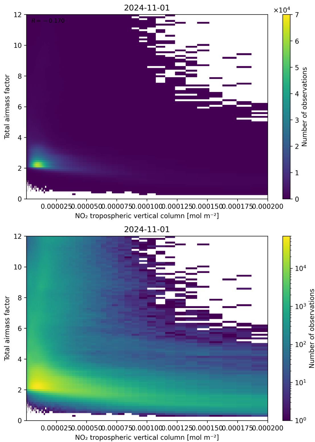
Figure 122: Scatter density plot of “NO 2 tropospheric vertical column” against “Total air mass factor” for 2024-10-31 to 2024-11-02.
