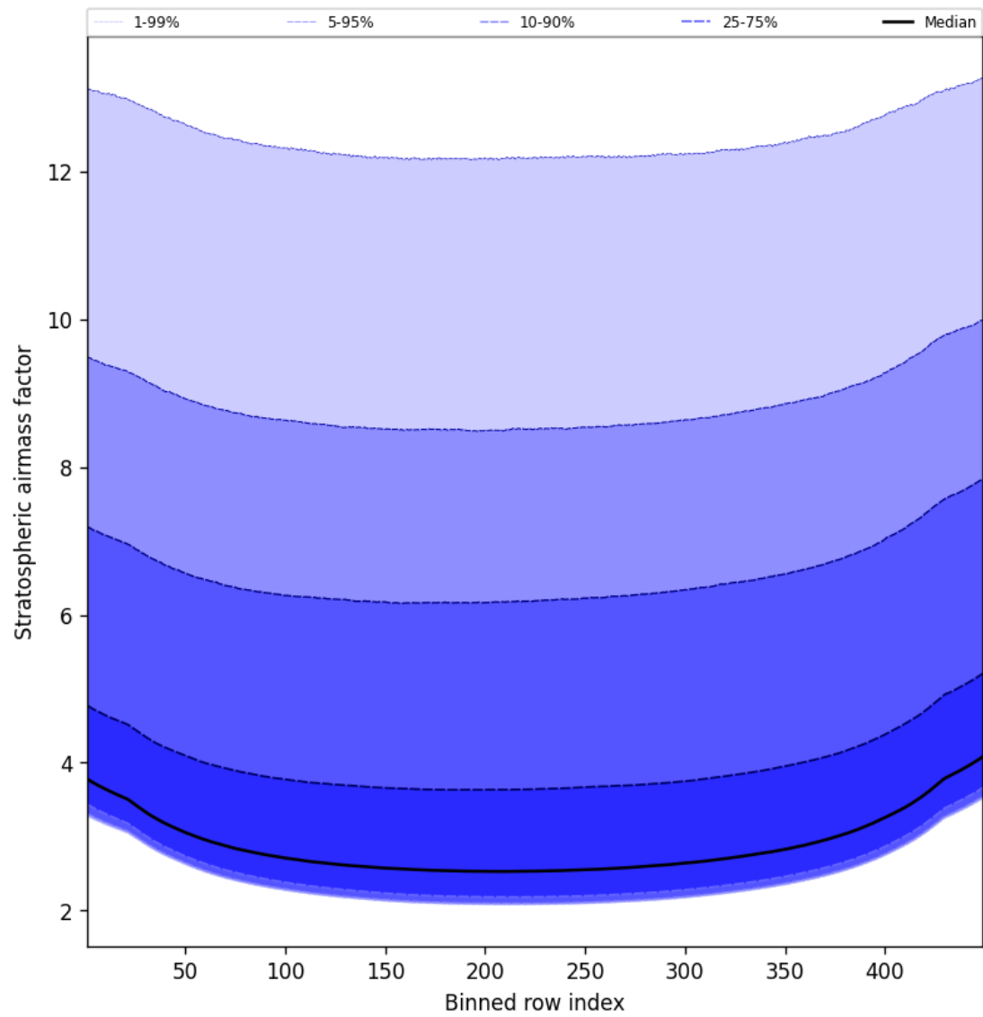
Figure 61: Along track statistics of “Stratospheric airmass factor” for 2024-10-31 to 2024-11-02
