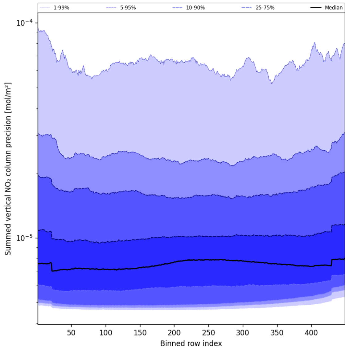
Figure 58: Along track statistics of “Summed vertical NO 2 column precision” for 2024-10-31 to 2024-11-02
