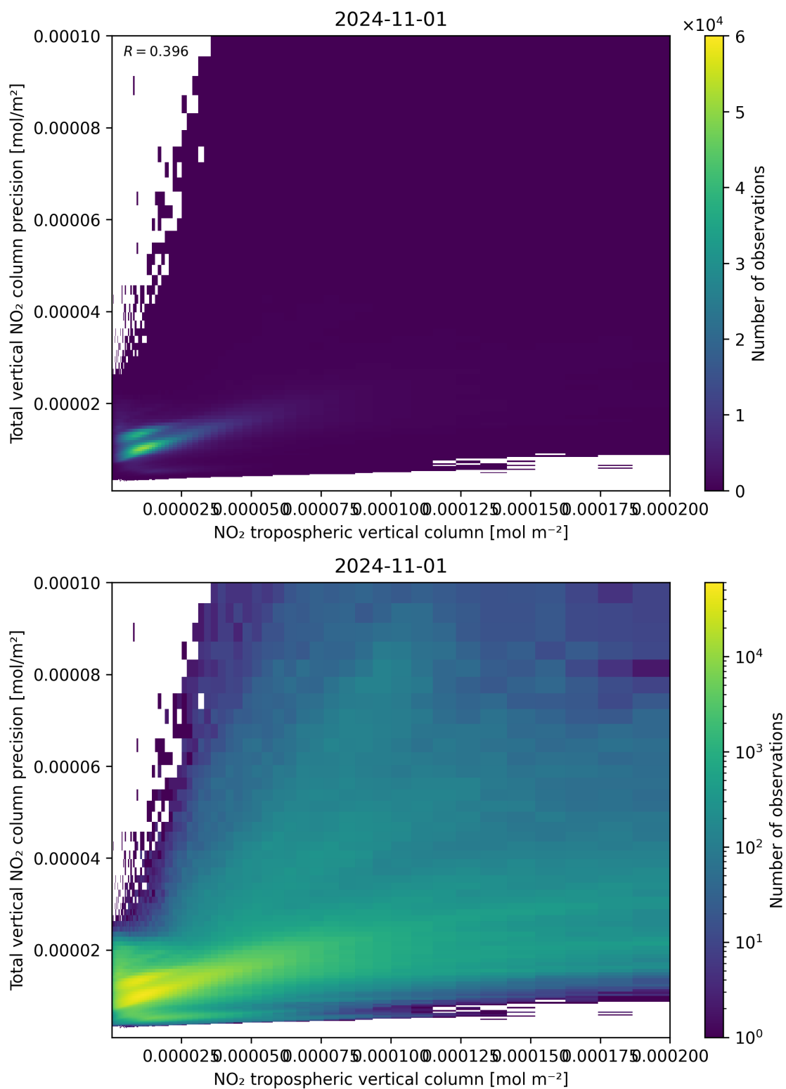
Figure 129: Scatter density plot of “NO 2 tropospheric vertical column” against “Total vertical NO 2 column precision” for 2024-10-31 to 2024-11-02.
