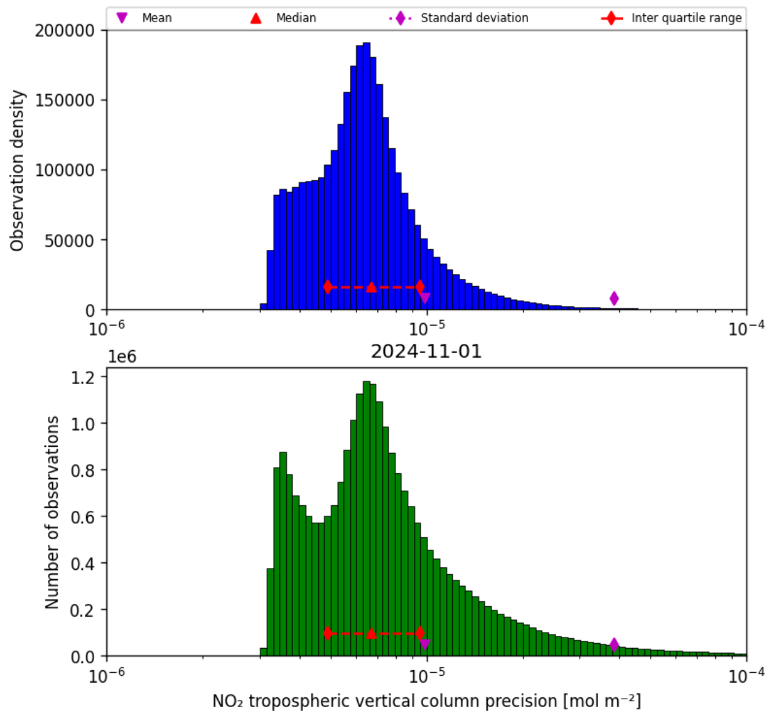
Figure 30: Histogram of “NO 2 tropospheric vertical column precision” for 2024-10-31 to 2024-11-02
