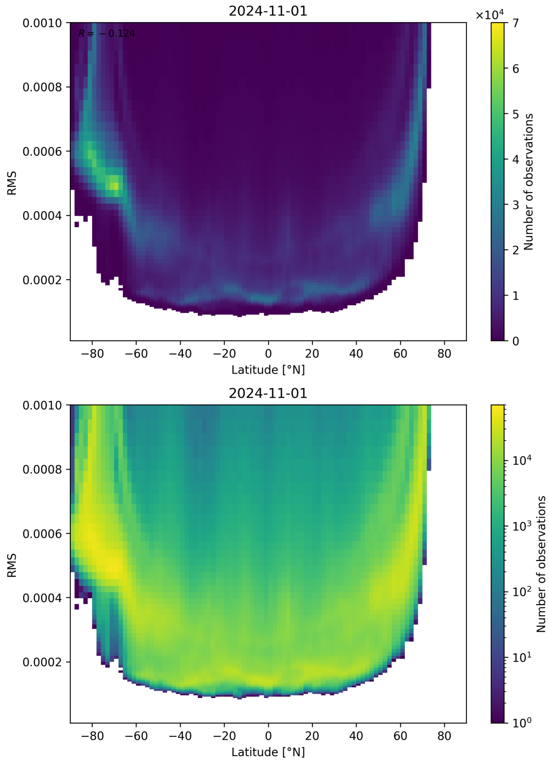
Figure 94: Scatter density plot of “Latitude” against “RMS” for 2024-10-31 to 2024-11-02.
