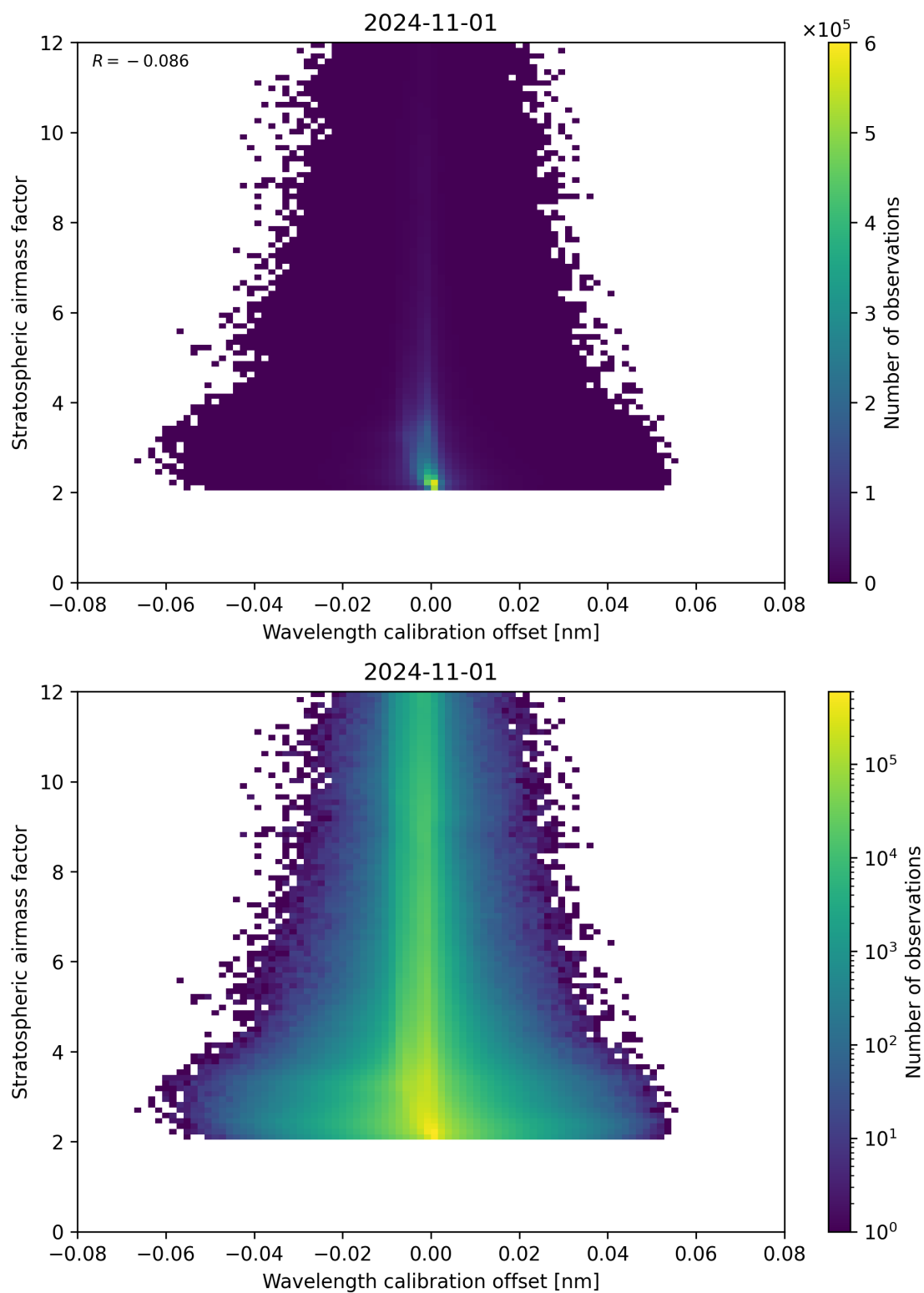
Figure 174: Scatter density plot of “Wavelength calibration offset” against “Stratospheric air mass factor” for 2024-10-31 to 2024-11-02.
