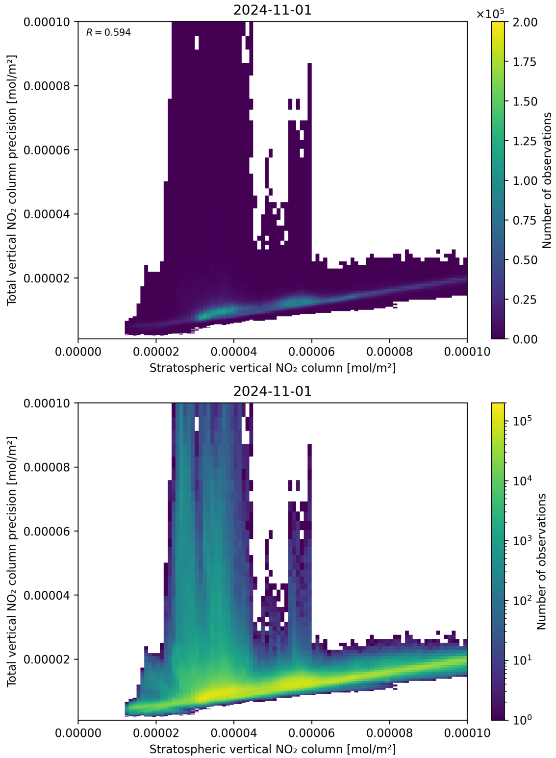
Figure 101: Scatter density plot of “Stratospheric vertical NO 2 column” against “Total vertical NO 2 column precision” for 2024-10-31 to 2024-11-02.
