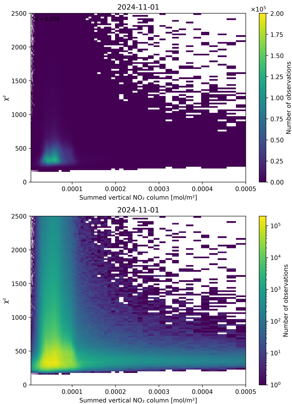
Figure 104: Scatter density plot of “Summed vertical NO 2 column” against “ \chi^2 ” for 2024-10-31 to 2024-11-02.
