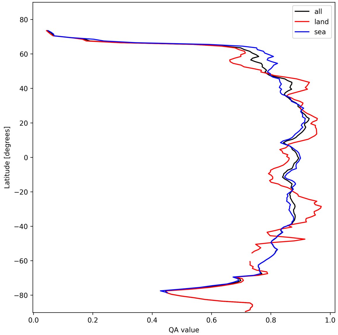
Figure 11: Zonal average of “QA value” for 2024-10-31 to 2024-11-02.
