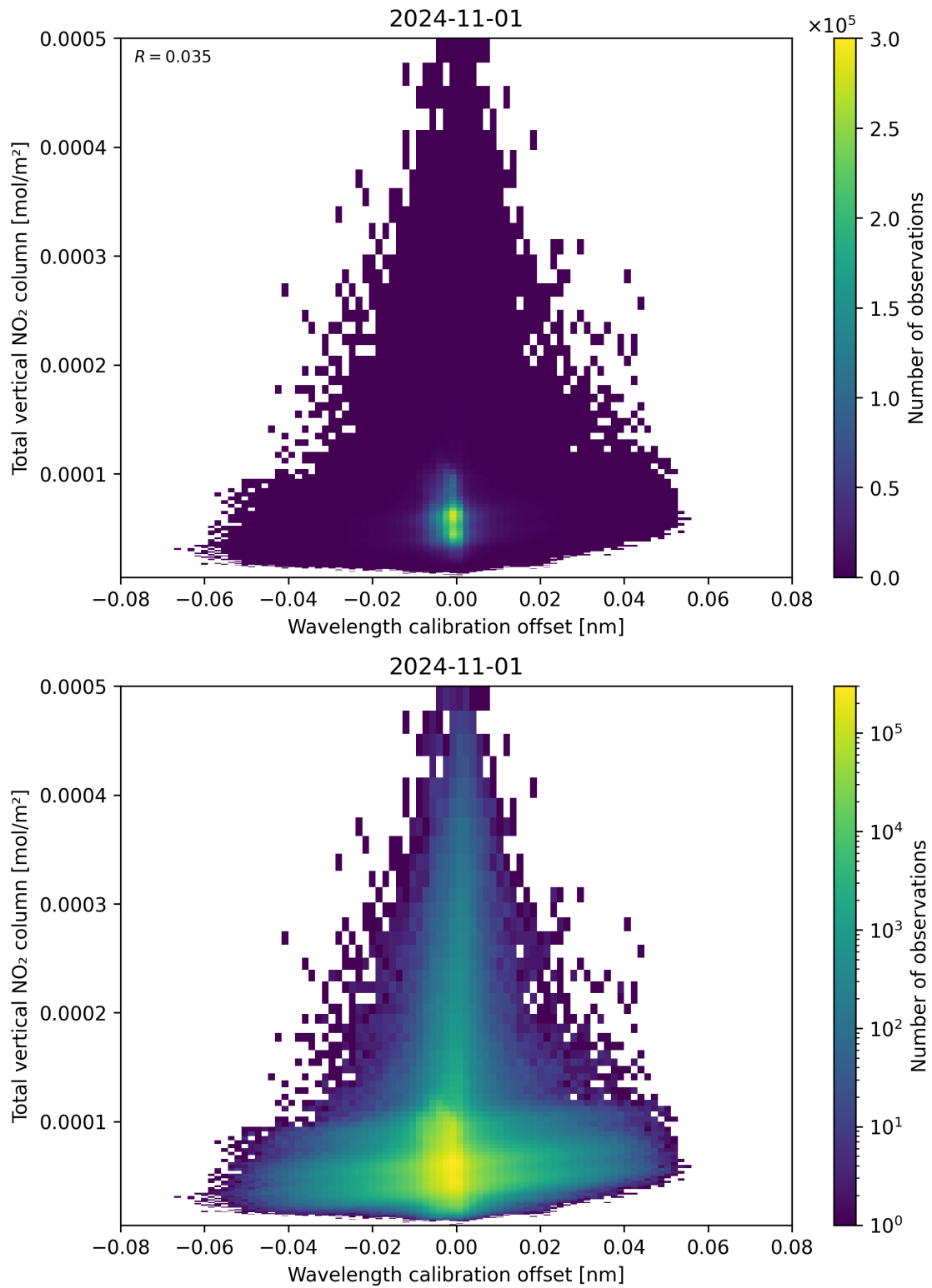
Figure 179: Scatter density plot of “Wavelength calibration offset” against “Total vertical NO 2 column” for 2024-10-31 to 2024-11-02.
