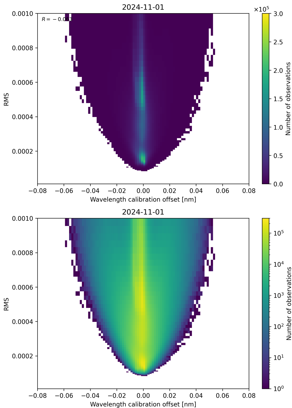
Figure 181: Scatter density plot of “Wavelength calibration offset” against “RMS” for 2024-10-31 to 2024-11-02.
