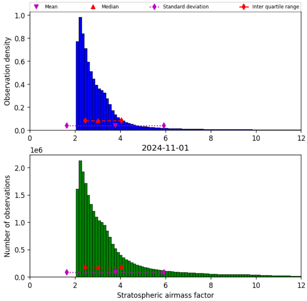
Figure 44: Histogram of “Stratospheric airmass factor” for 2024-10-31 to 2024-11-02
