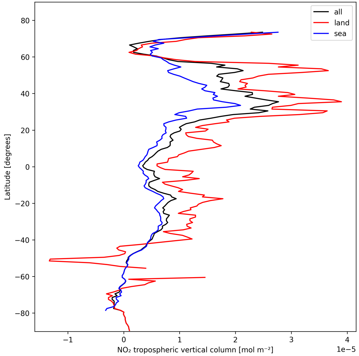
Figure 12: Zonal average of “NO 2 tropospheric vertical column” for 2024-10-31 to 2024-11-02.
