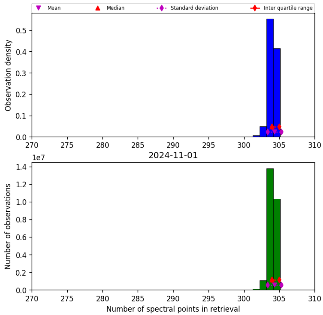
Figure 33: Histogram of “Number of spectral points in retrieval” for 2024-10-31 to 2024-11-02
