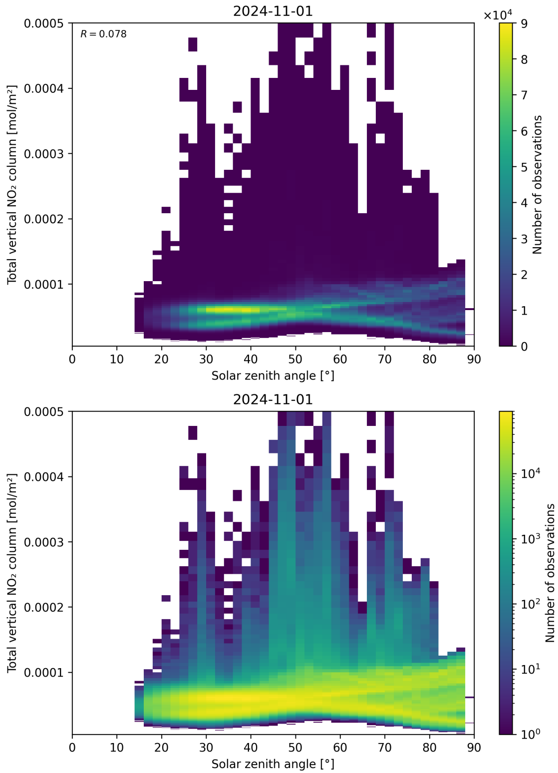
Figure 153: Scatter density plot of “Solar zenith angle” against “Total vertical NO 2 column” for 2024-10-31 to 2024-11-02.
