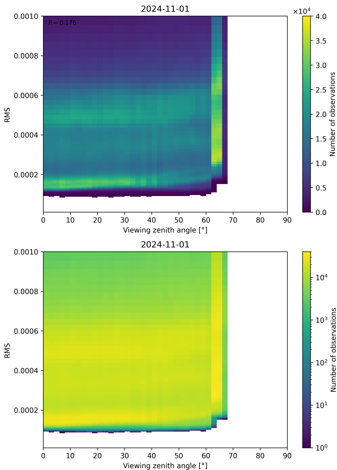
Figure 171: Scatter density plot of “Viewing zenith angle” against “RMS” for 2024-10-31 to 2024-11-02.
