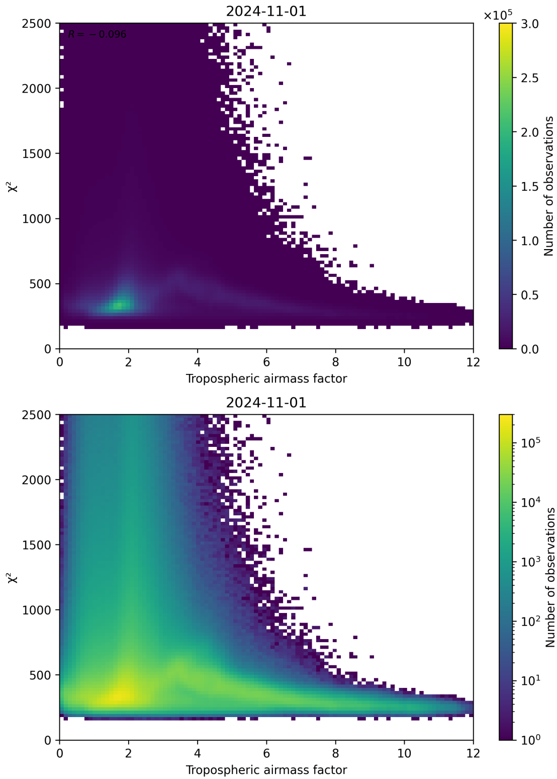
Figure 73: Scatter density plot of “Tropospheric airmass factor” against “ \chi^2 ” for 2024-10-31 to 2024-11-02.
