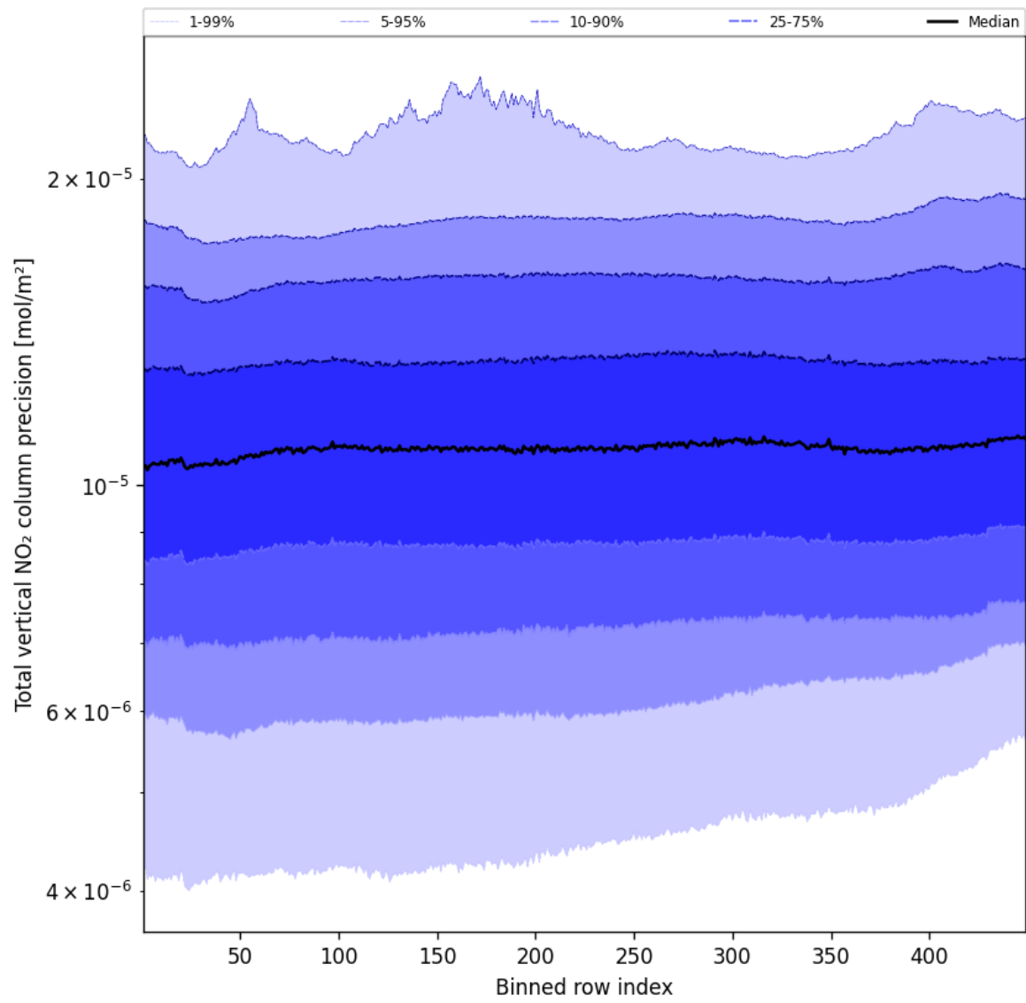
Figure 56: Along track statistics of “Total vertical NO 2 column precision” for 2024-10-31 to 2024-11-02
