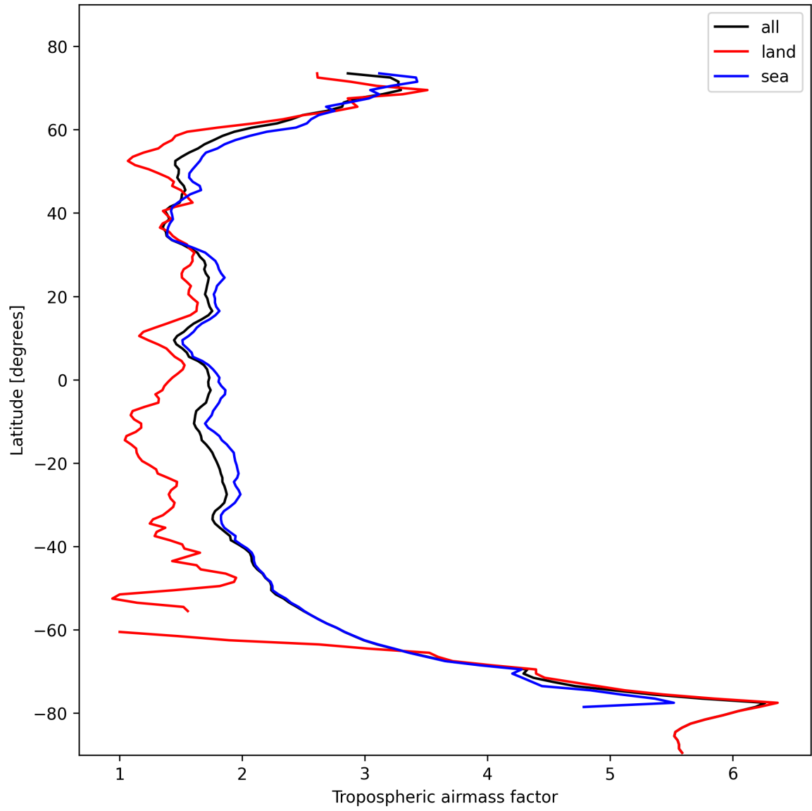
Figure 14: Zonal average of “Tropospheric airmass factor” for 2024-10-31 to 2024-11-02.
