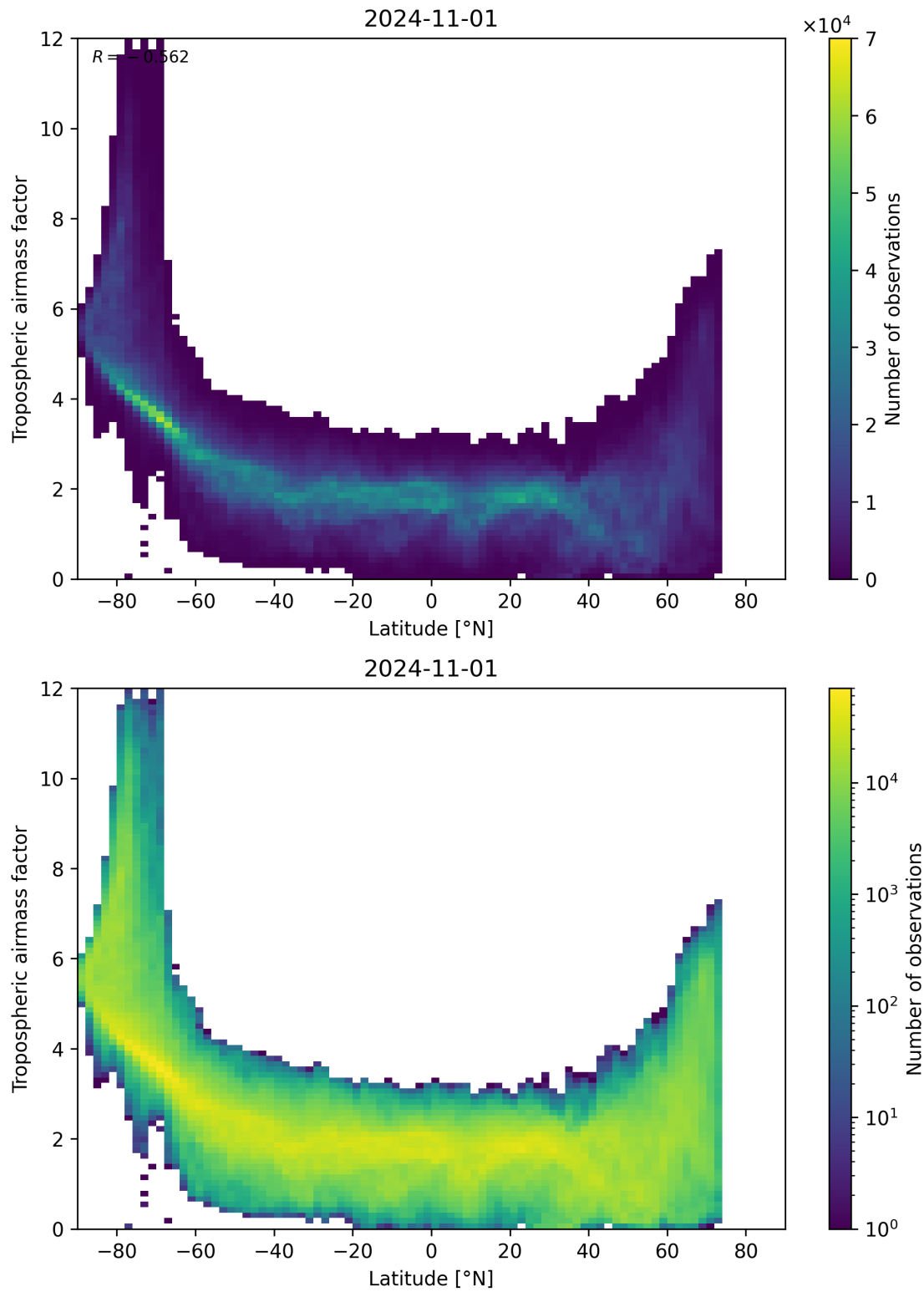
Figure 85: Scatter density plot of “Latitude” against “Tropospheric air mass factor” for 2024-10-31 to 2024-11-02.
