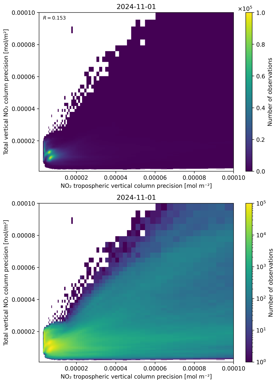
Figure 139: Scatter density plot of “NO 2 tropospheric vertical column precision” against “Total vertical NO 2 column precision” for 2024-10-31 to 2024-11-02.
