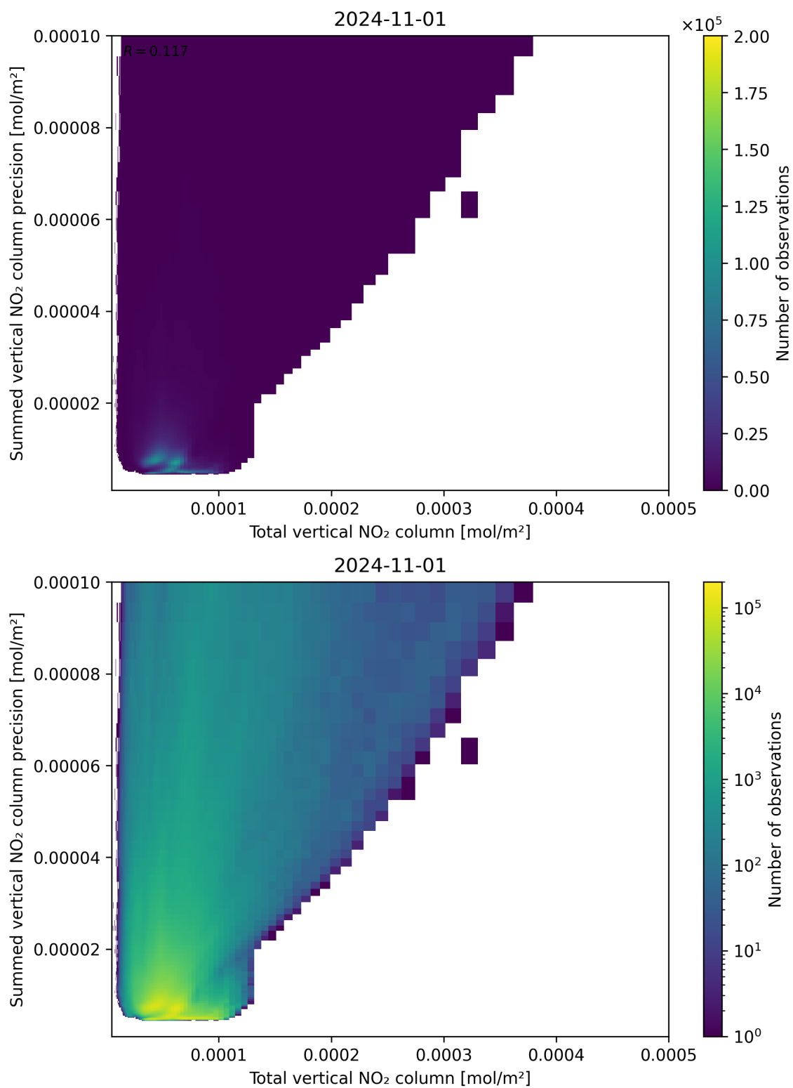
Figure 113: Scatter density plot of “Total vertical NO 2 column” against “Summed vertical NO 2 column precision” for 2024-10-31 to 2024-11-02.
