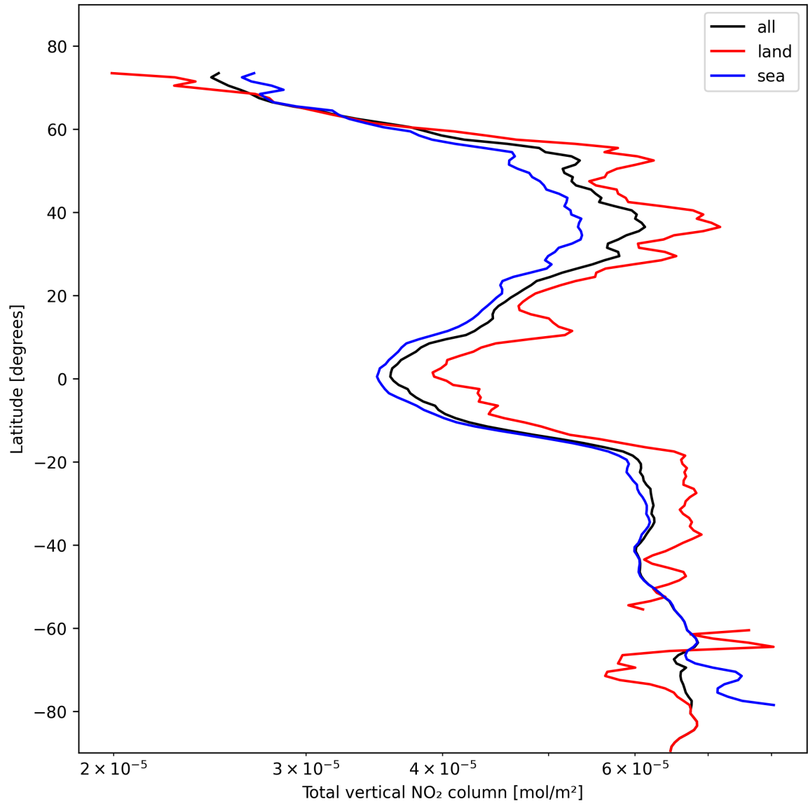
Figure 21: Zonal average of “Total vertical NO 2 column” for 2024-10-31 to 2024-11-02.
