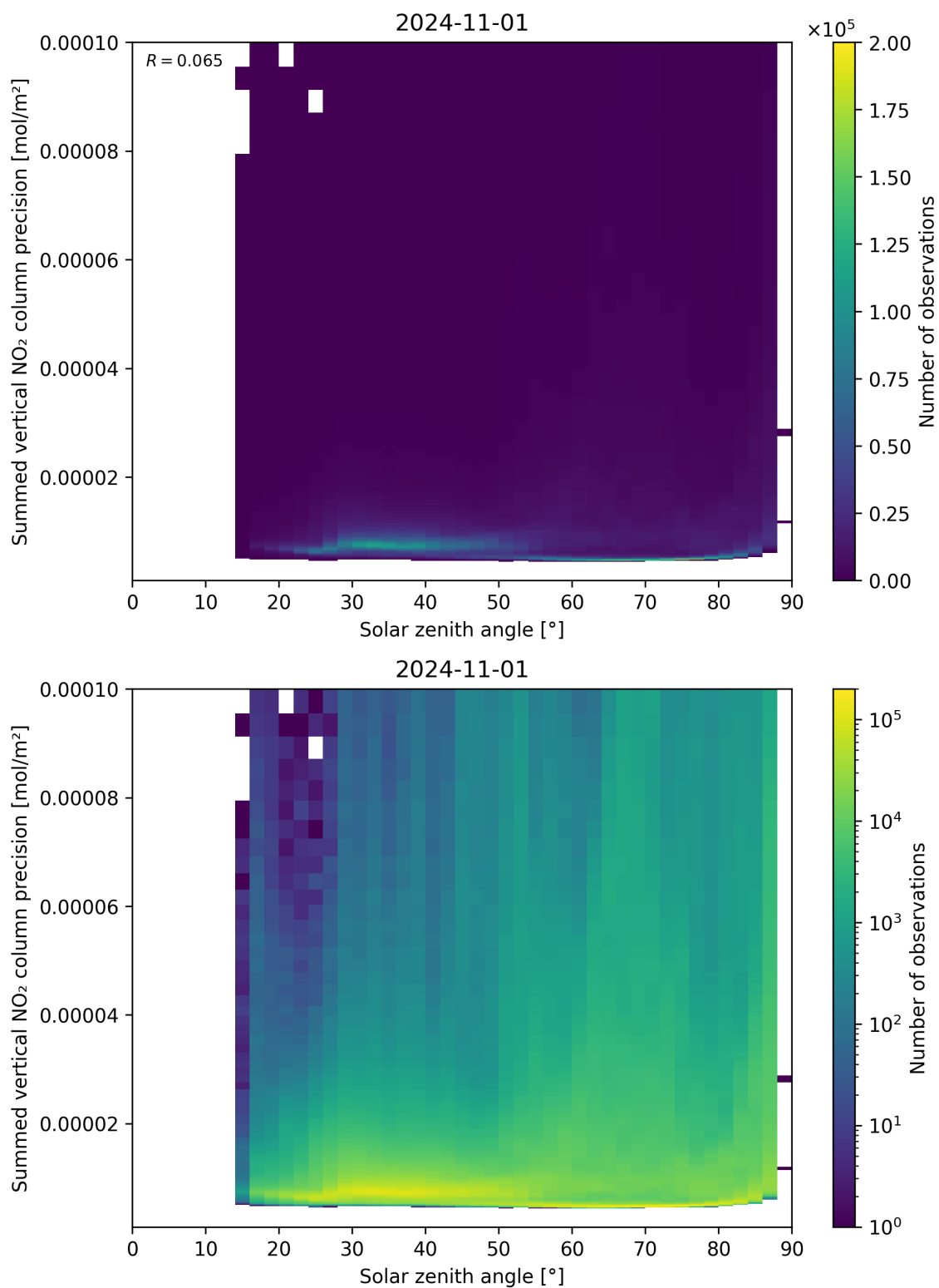
Figure 152: Scatter density plot of “Solar zenith angle” against “Summed vertical NO 2 column precision” for 2024-10-31 to 2024-11-02.
