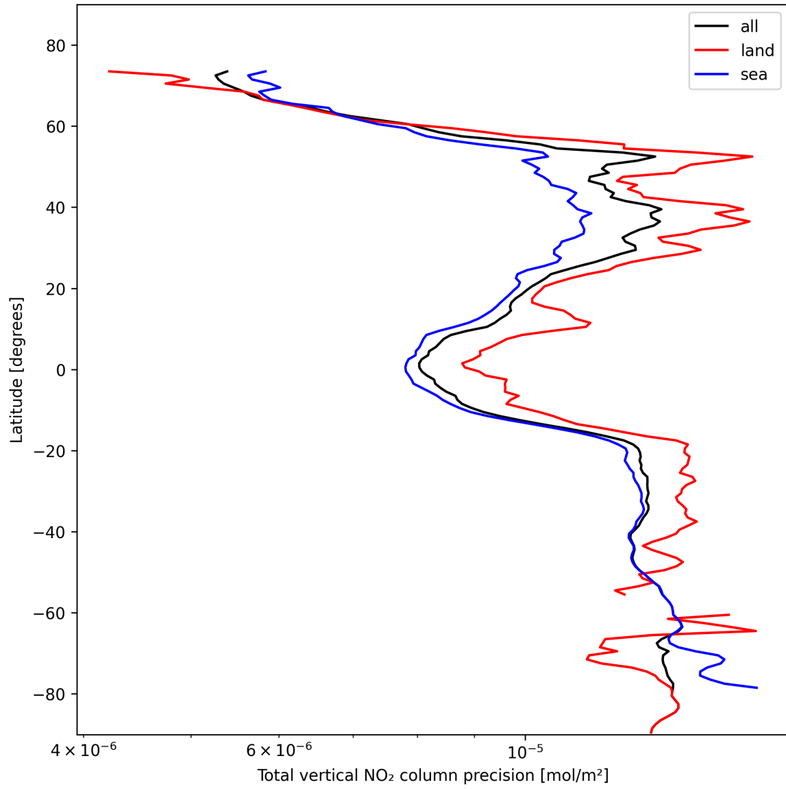
Figure 22: Zonal average of “Total vertical NO 2 column precision” for 2024-10-31 to 2024-11-02.
