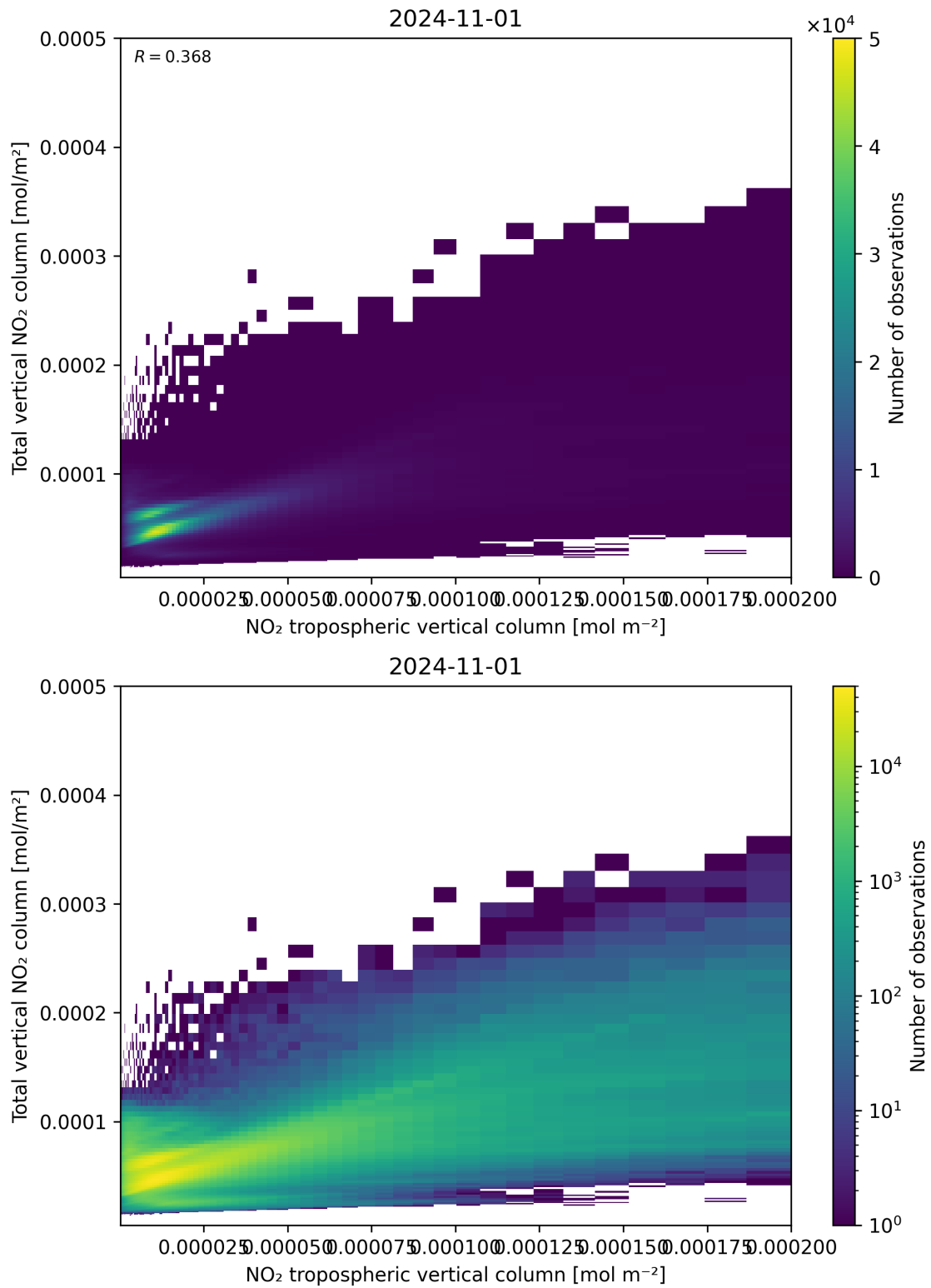
Figure 128: Scatter density plot of “NO 2 tropospheric vertical column” against “Total vertical NO 2 column” for 2024-10-31 to 2024-11-02.
