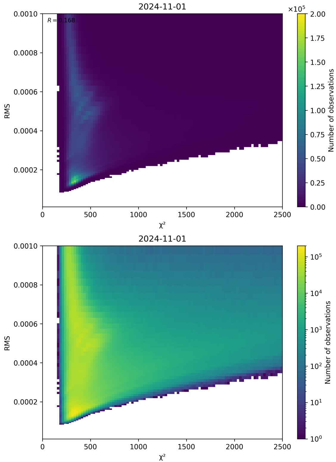
Figure 82: Scatter density plot of “ \chi^2 ” against “RMS” for 2024-10-31 to 2024-11-02.
