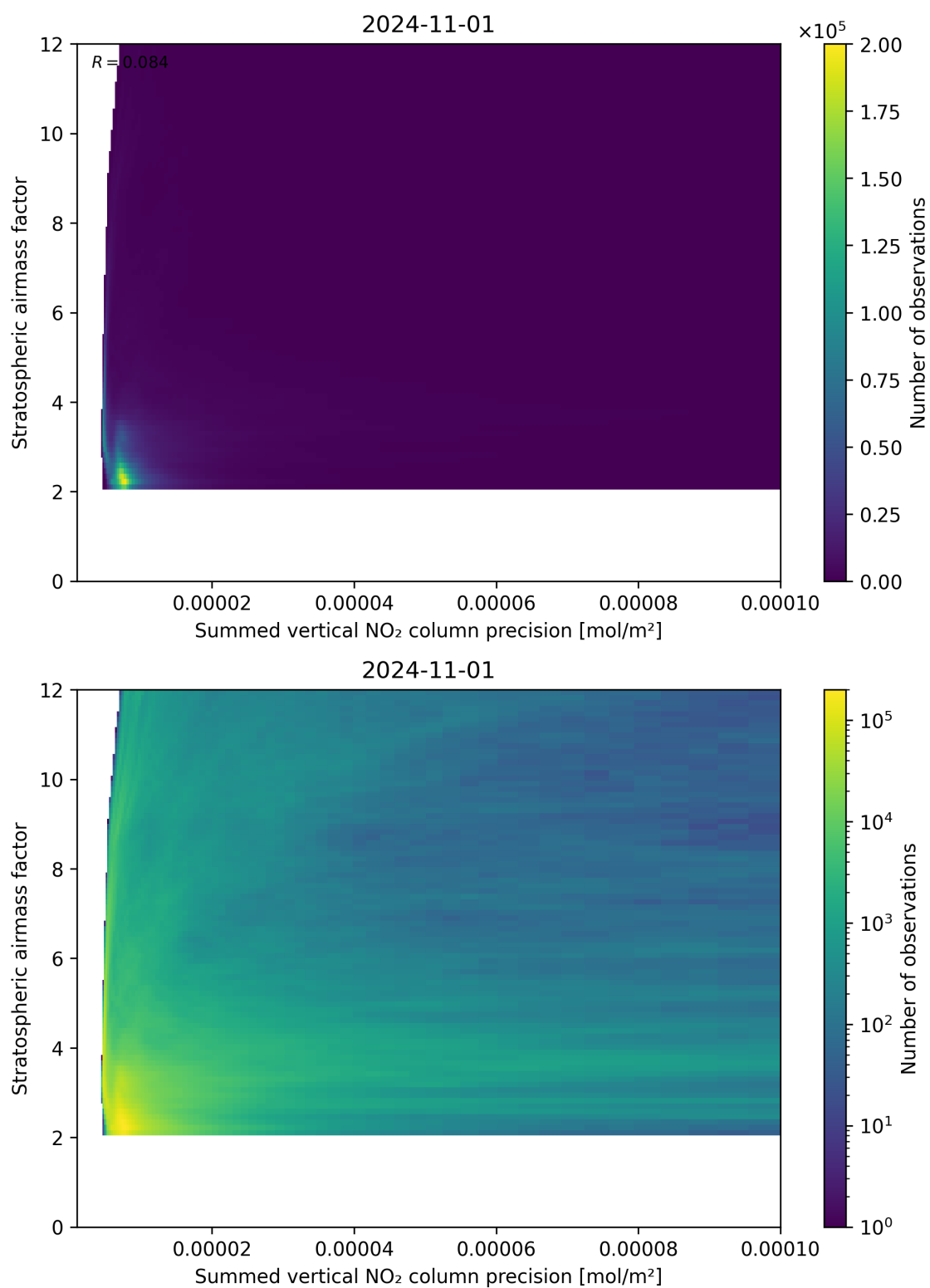
Figure 106: Scatter density plot of “Summed vertical NO 2 column precision” against “Stratospheric airmass factor” for 2024-10-31 to 2024-11-02.
