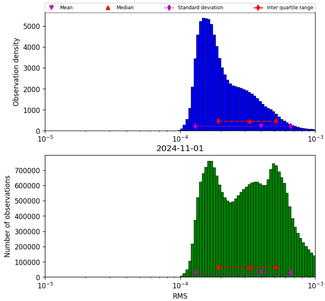
Figure 43: Histogram of “RMS” for 2024-10-31 to 2024-11-02
