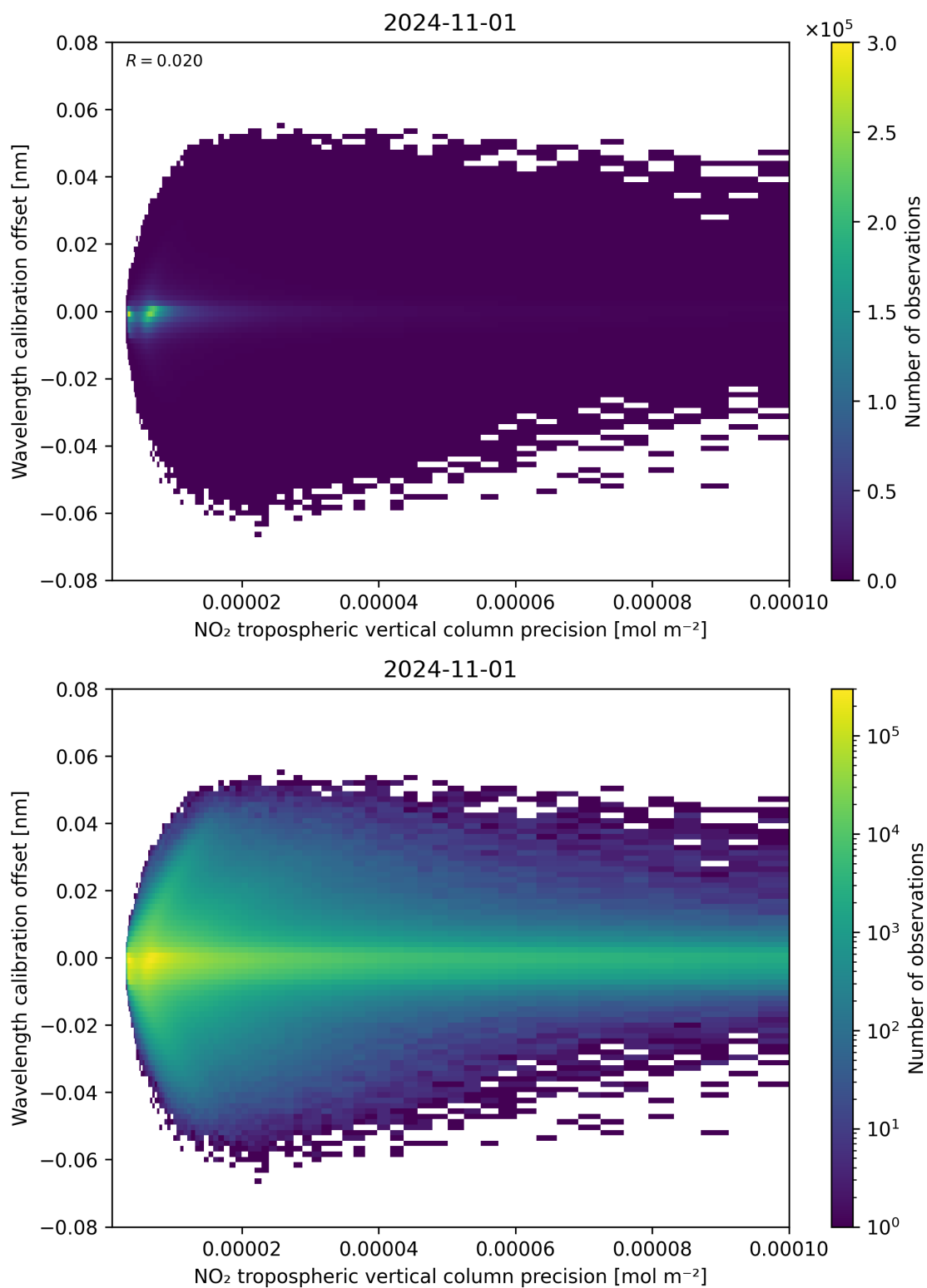
Figure 141: Scatter density plot of “NO 2 tropospheric vertical column precision” against “Wavelength calibration offset” for 2024-10-31 to 2024-11-02.
