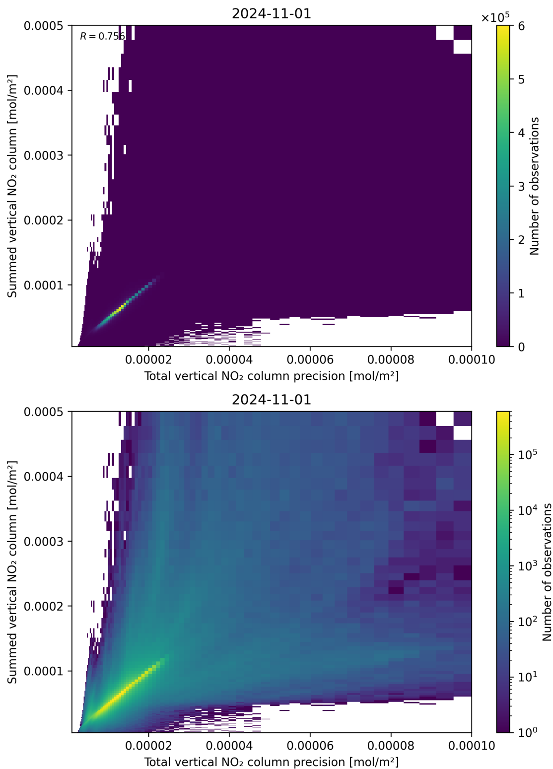
Figure 117: Scatter density plot of “Total vertical NO 2 column precision” against “Summed vertical NO 2 column” for 2024-10-31 to 2024-11-02.
