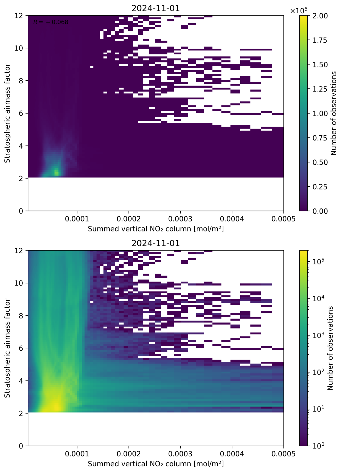
Figure 103: Scatter density plot of “Summed vertical NO 2 column” against “Stratospheric air mass factor” for 2024-10-31 to 2024-11-02.
