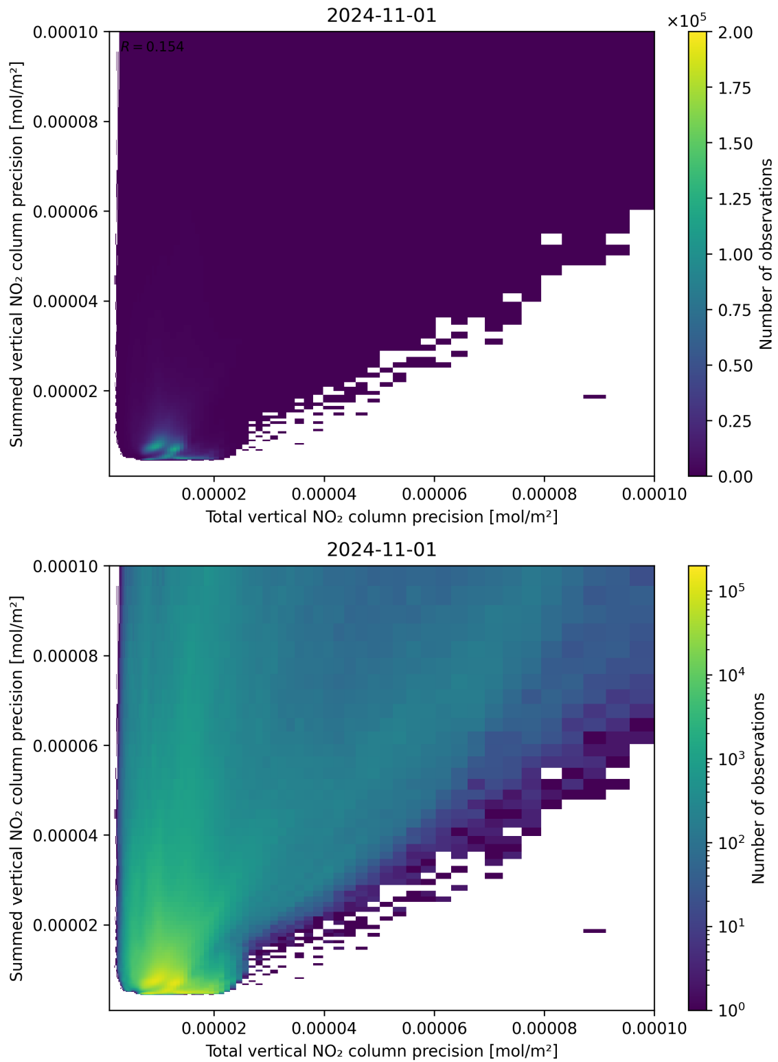
Figure 118: Scatter density plot of “Total vertical NO 2 column precision” against “Summed vertical NO 2 column precision” for 2024-10-31 to 2024-11-02.
