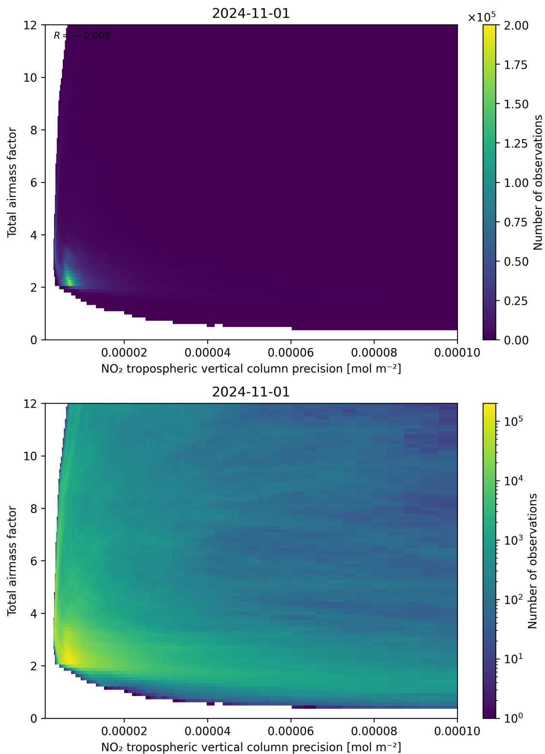
Figure 132: Scatter density plot of “NO 2 tropospheric vertical column precision” against “Total air mass factor” for 2024-10-31 to 2024-11-02.
