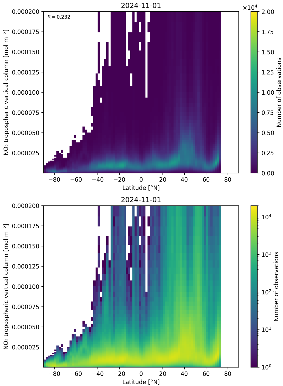
Figure 92: Scatter density plot of “Latitude” against “NO 2 tropospheric vertical column” for 2024-10-31 to 2024-11-02.
