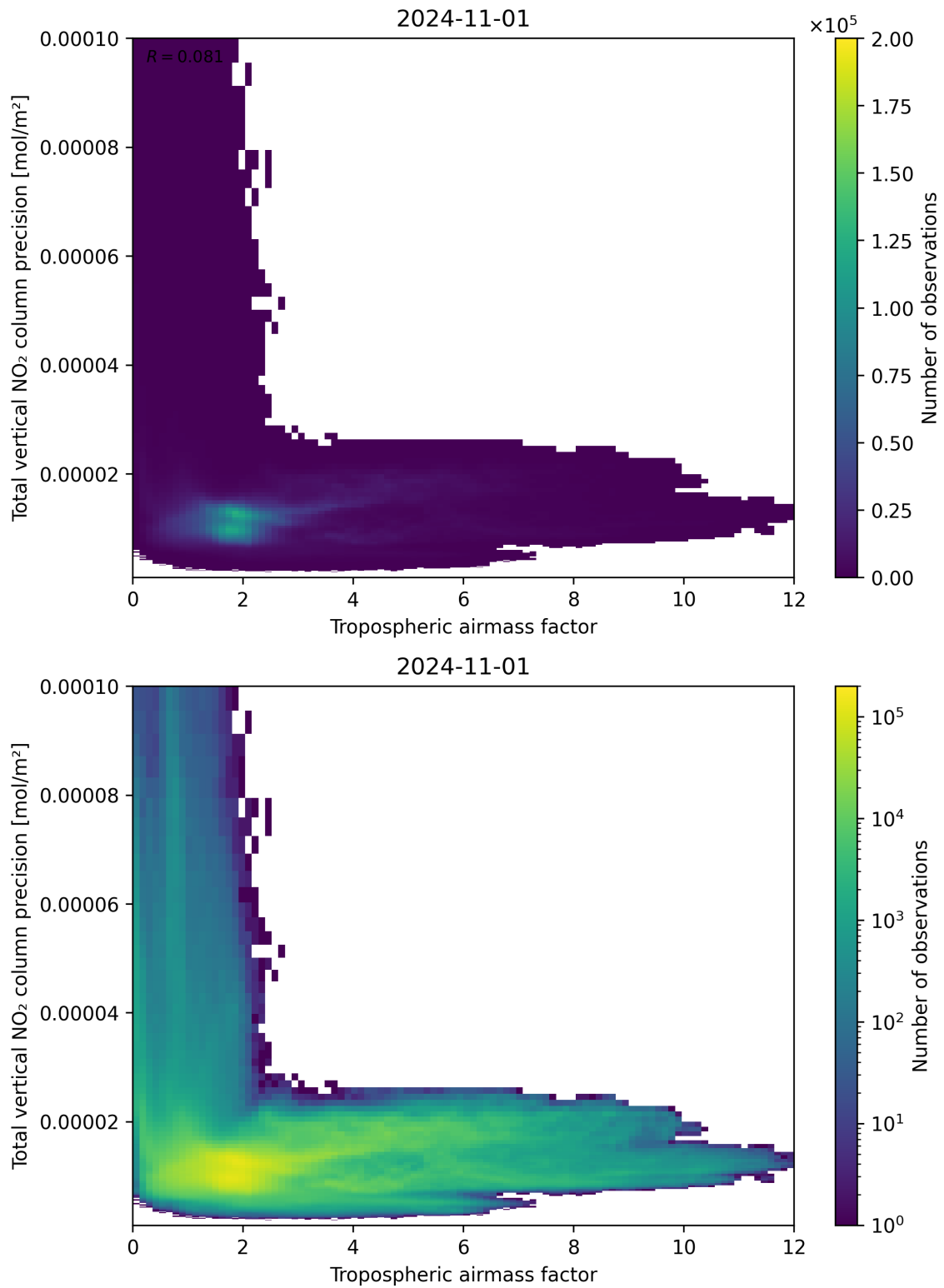
Figure 78: Scatter density plot of “Tropospheric airmass factor” against “Total vertical NO 2 column precision” for 2024-10-31 to 2024-11-02.
