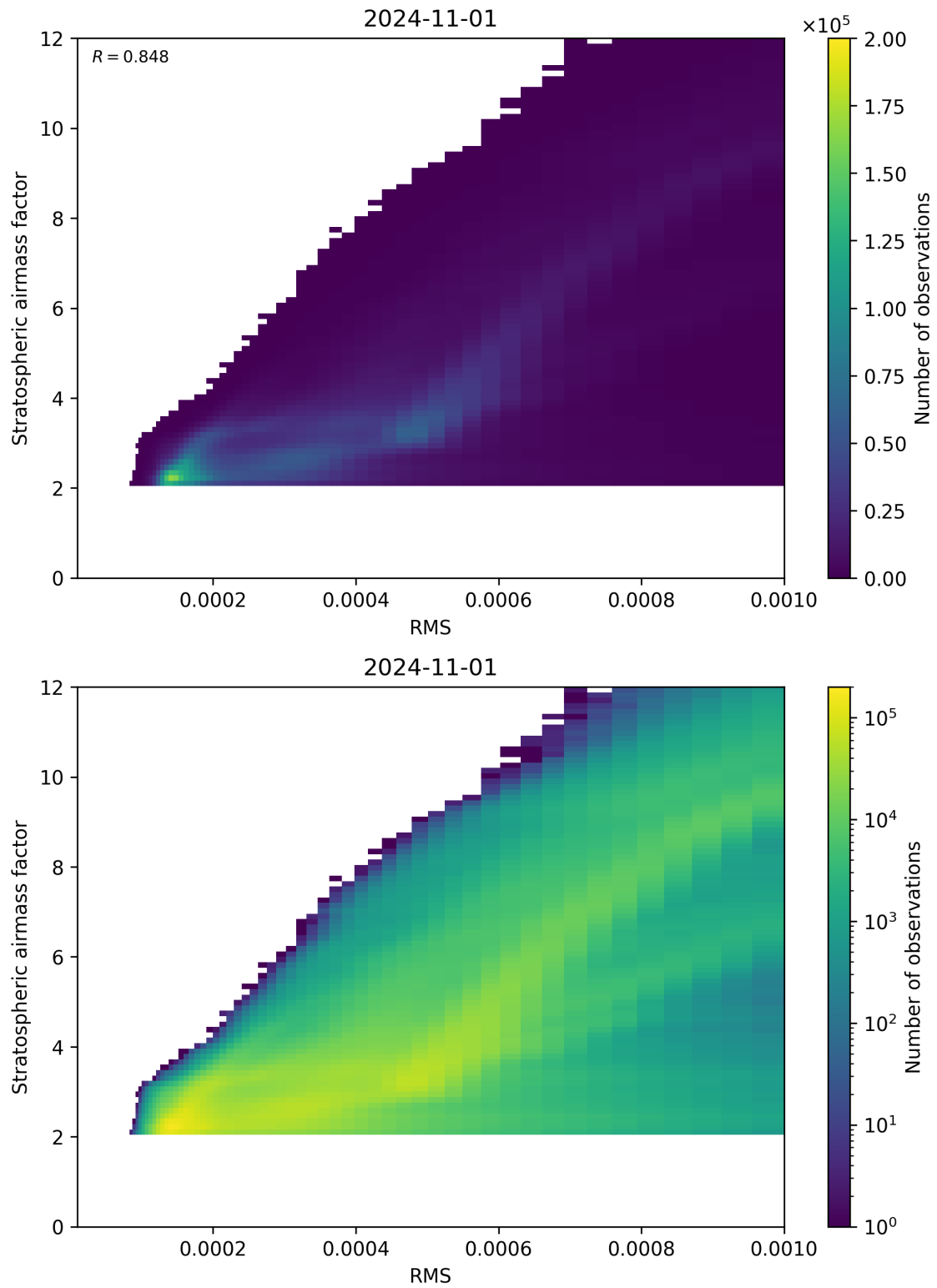
Figure 144: Scatter density plot of “RMS” against “Stratospheric airmass factor” for 2024-10-31 to 2024-11-02.
