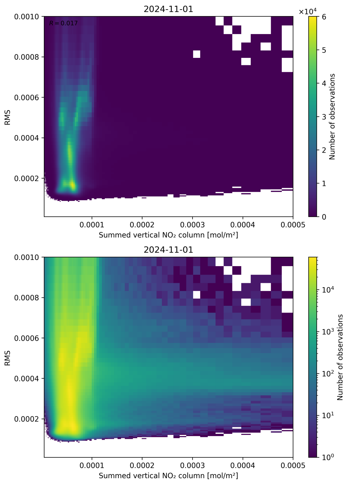
Figure 109: Scatter density plot of “Summed vertical NO 2 column” against “RMS” for 2024-10-31 to 2024-11-02.
