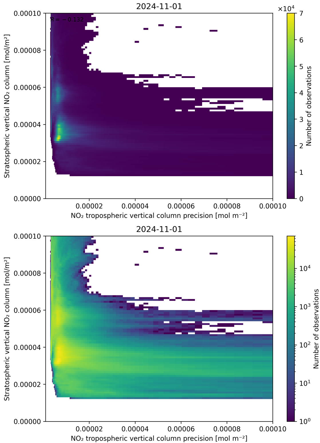
Figure 135: Scatter density plot of “NO 2 tropospheric vertical column precision” against “Stratospheric vertical NO 2 column” for 2024-10-31 to 2024-11-02.
