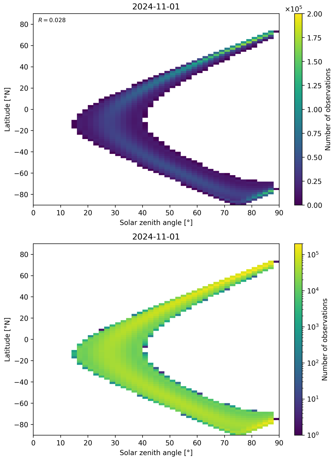
Figure 149: Scatter density plot of “Solar zenith angle” against “Latitude” for 2024-10-31 to 2024-11-02.
