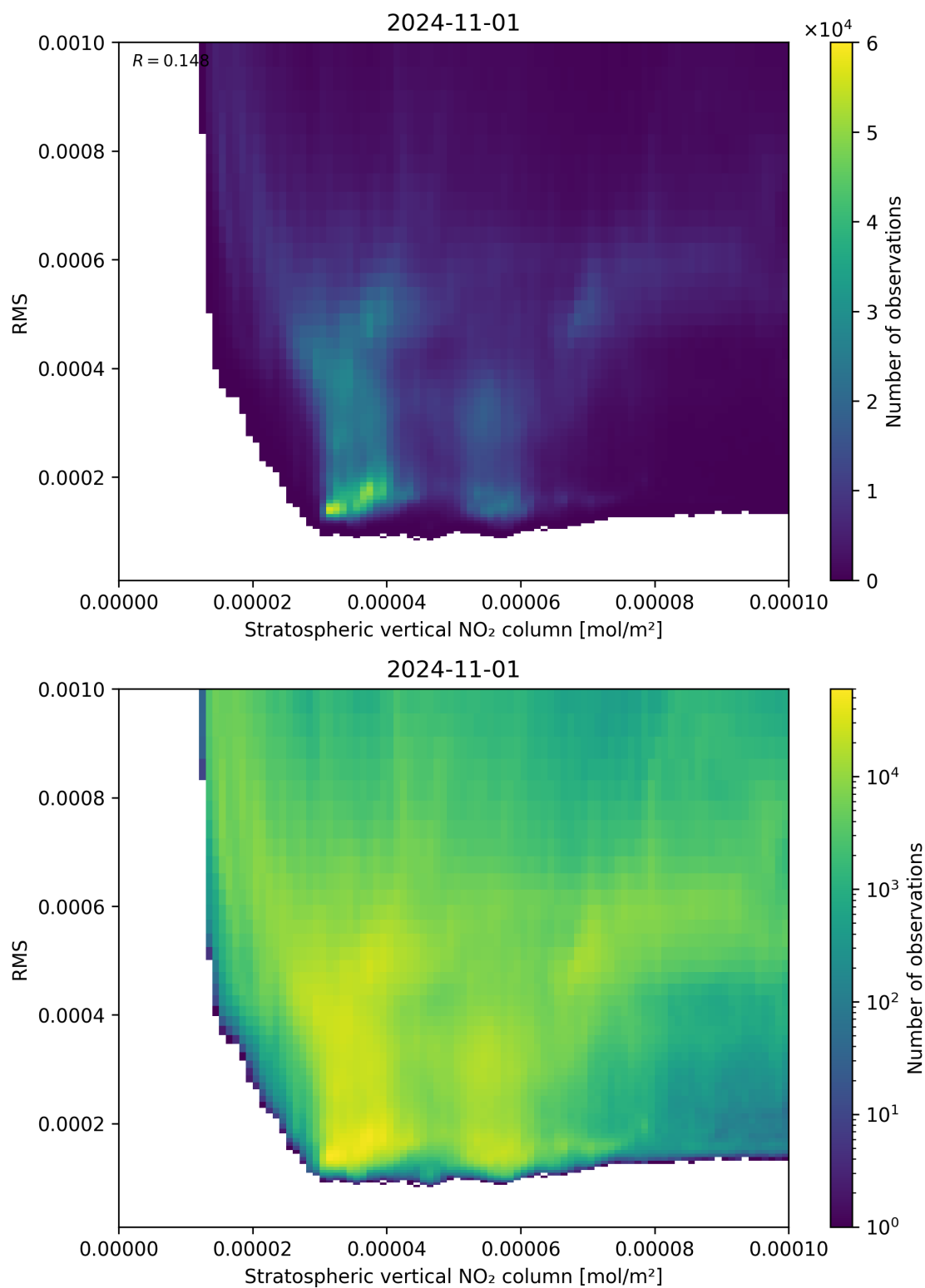
Figure 102: Scatter density plot of “Stratospheric vertical NO 2 column” against “RMS” for 2024-10-31 to 2024-11-02.
