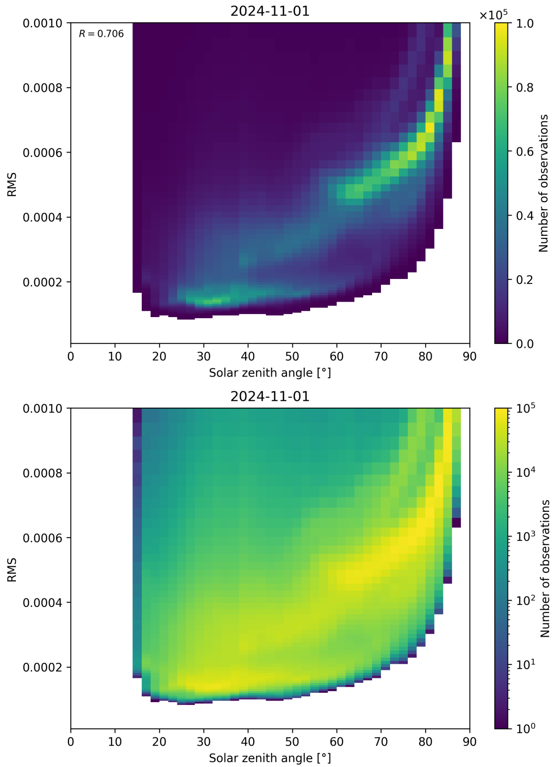
Figure 157: Scatter density plot of “Solar zenith angle” against “RMS” for 2024-10-31 to 2024-11-02.
