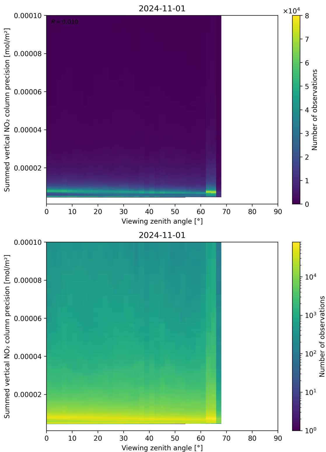
Figure 166: Scatter density plot of “Viewing zenith angle” against “Summed vertical NO 2 column precision” for 2024-10-31 to 2024-11-02.
