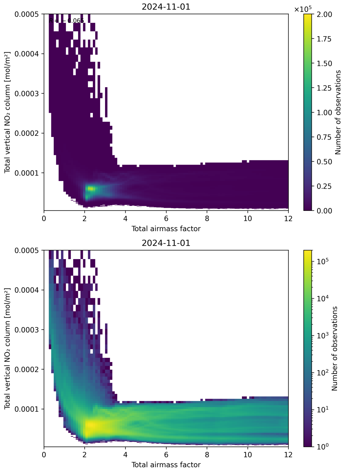
Figure 67: Scatter density plot of “Total airmass factor” against “Total vertical NO 2 column” for 2024-10-31 to 2024-11-02.
