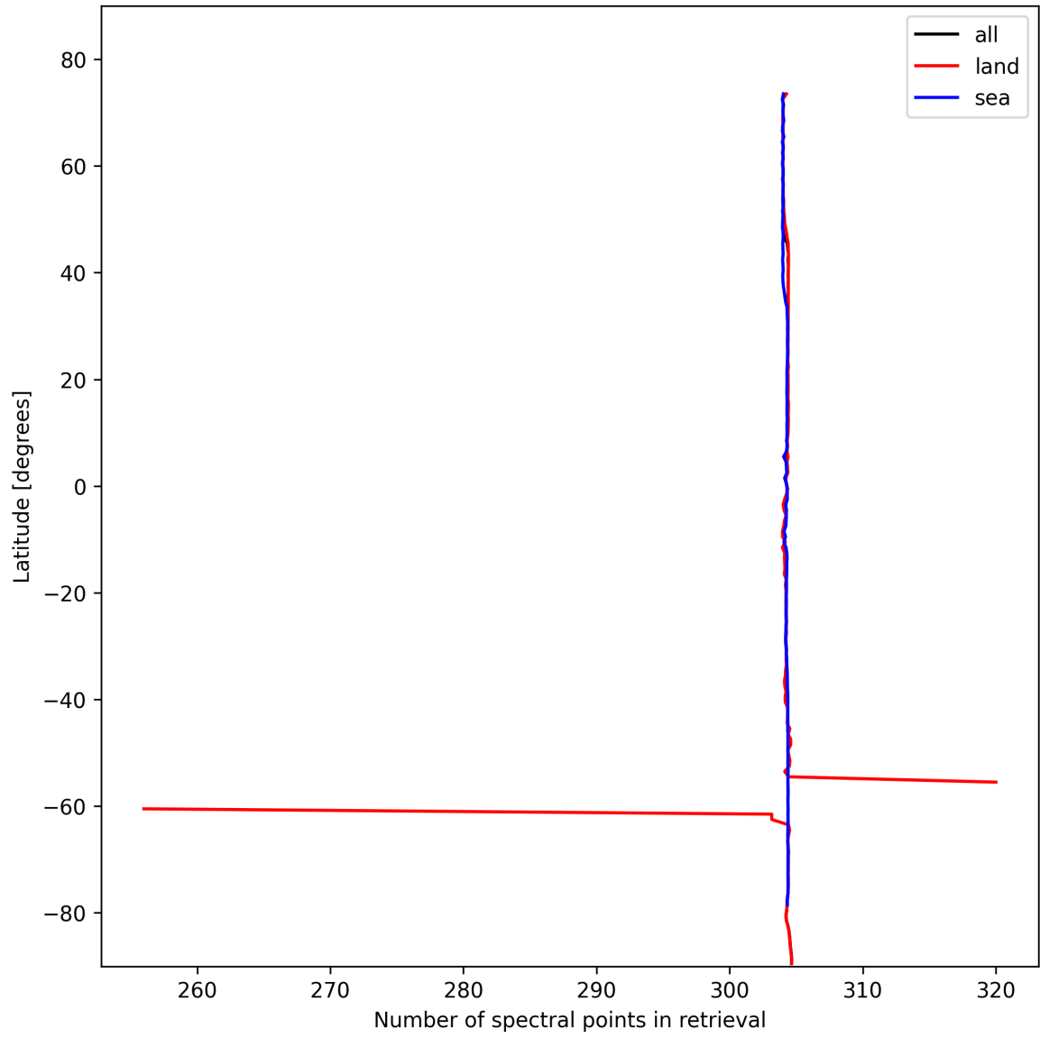
Figure 16: Zonal average of “Number of spectral points in retrieval” for 2024-10-31 to 2024-11-02.
