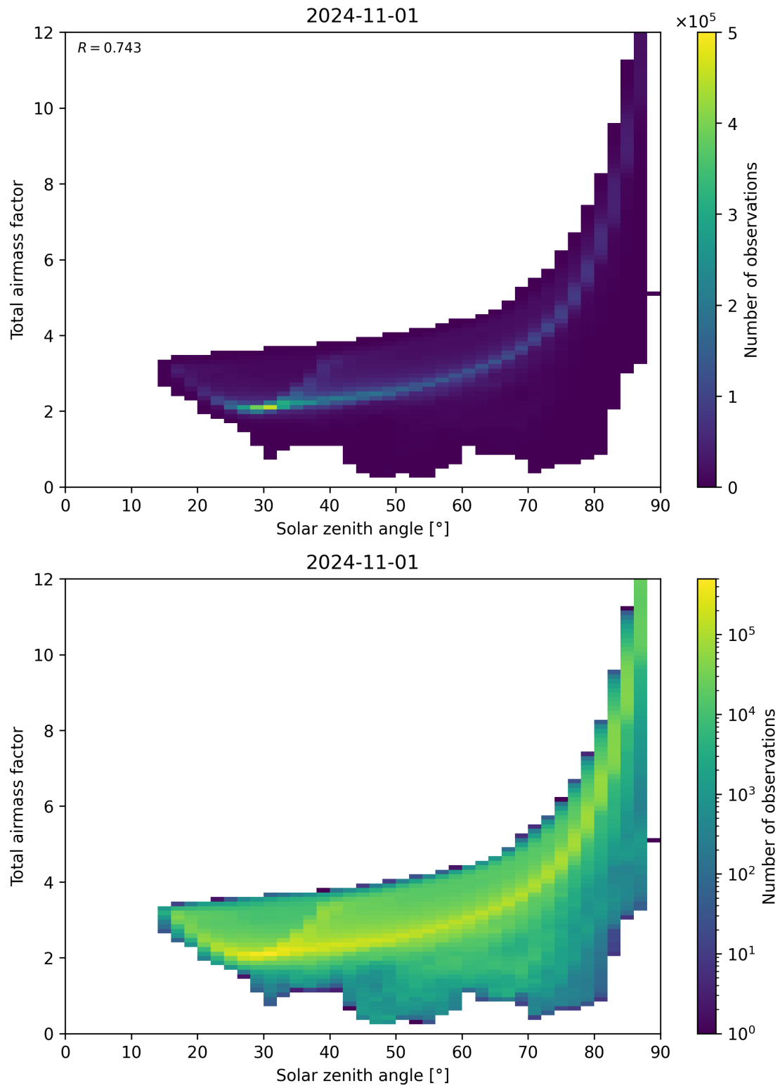
Figure 146: Scatter density plot of “Solar zenith angle” against “Total airmass factor” for 2024-10-31 to 2024-11-02.
