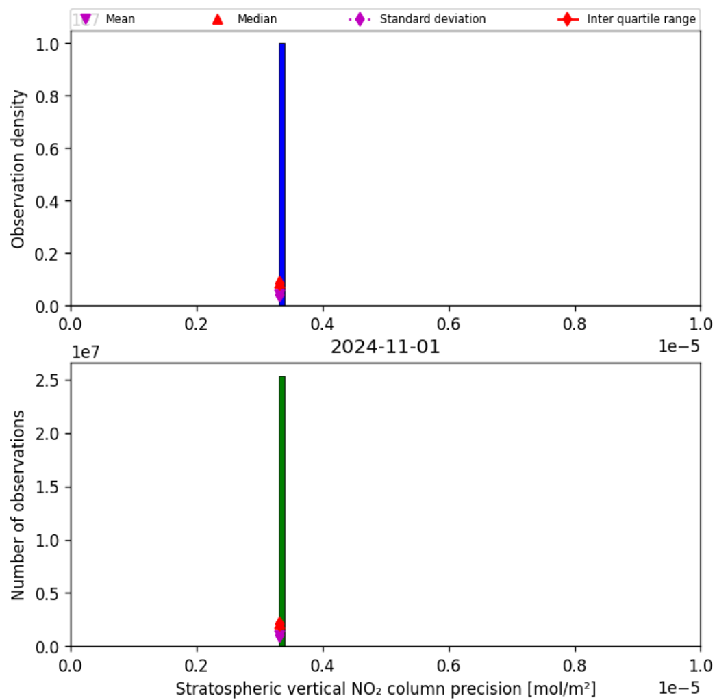
Figure 37: Histogram of “Stratospheric vertical NO 2 column precision” for 2024-10-31 to 2024-11-02
