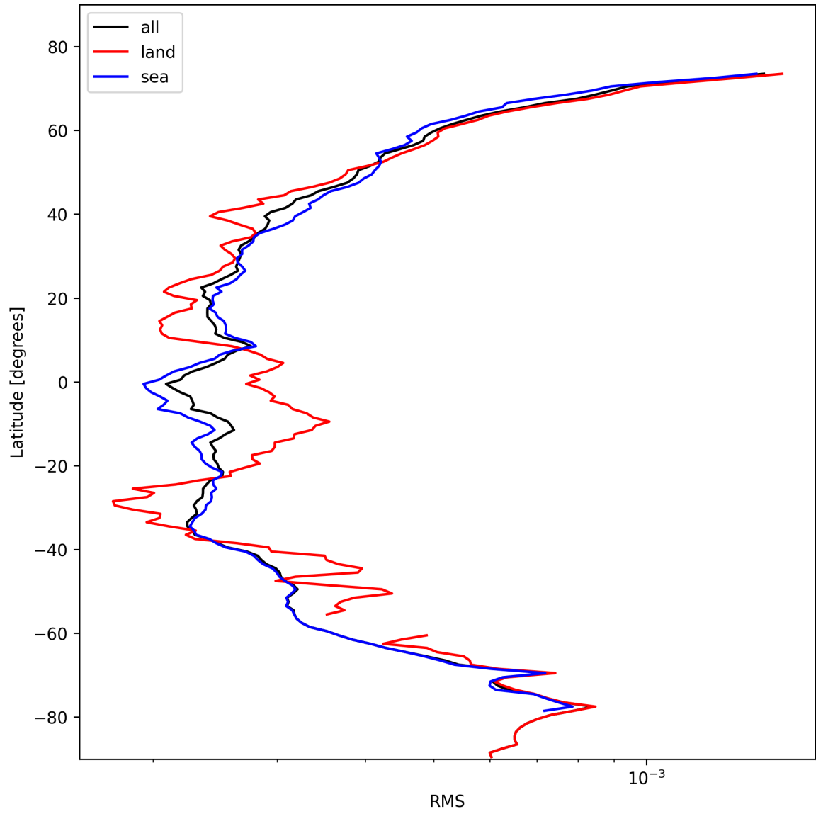
Figure 26: Zonal average of “RMS” for 2024-10-31 to 2024-11-02.
