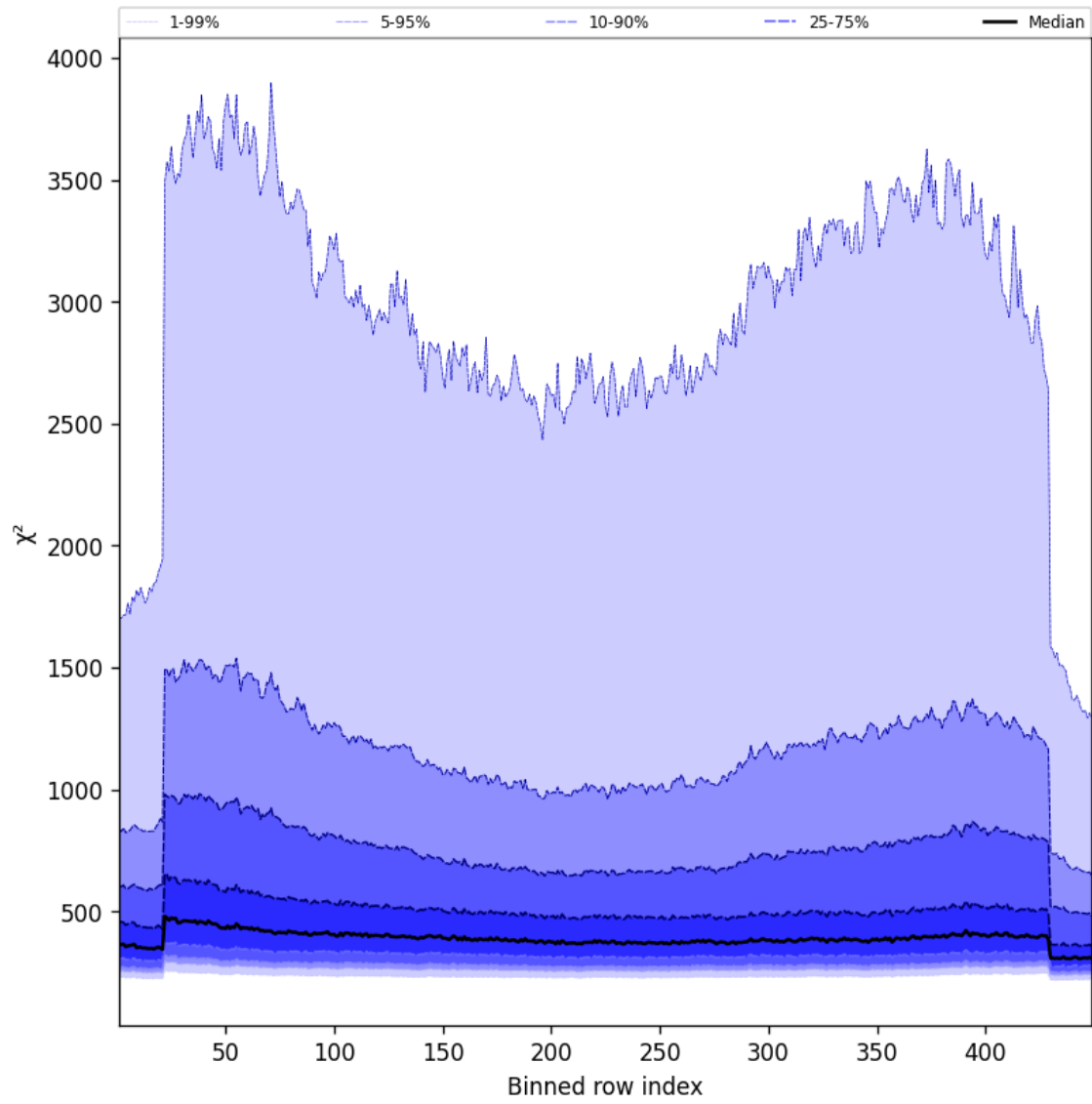
Figure 59: Along track statistics of “ \chi^2 ” for 2024-10-31 to 2024-11-02
