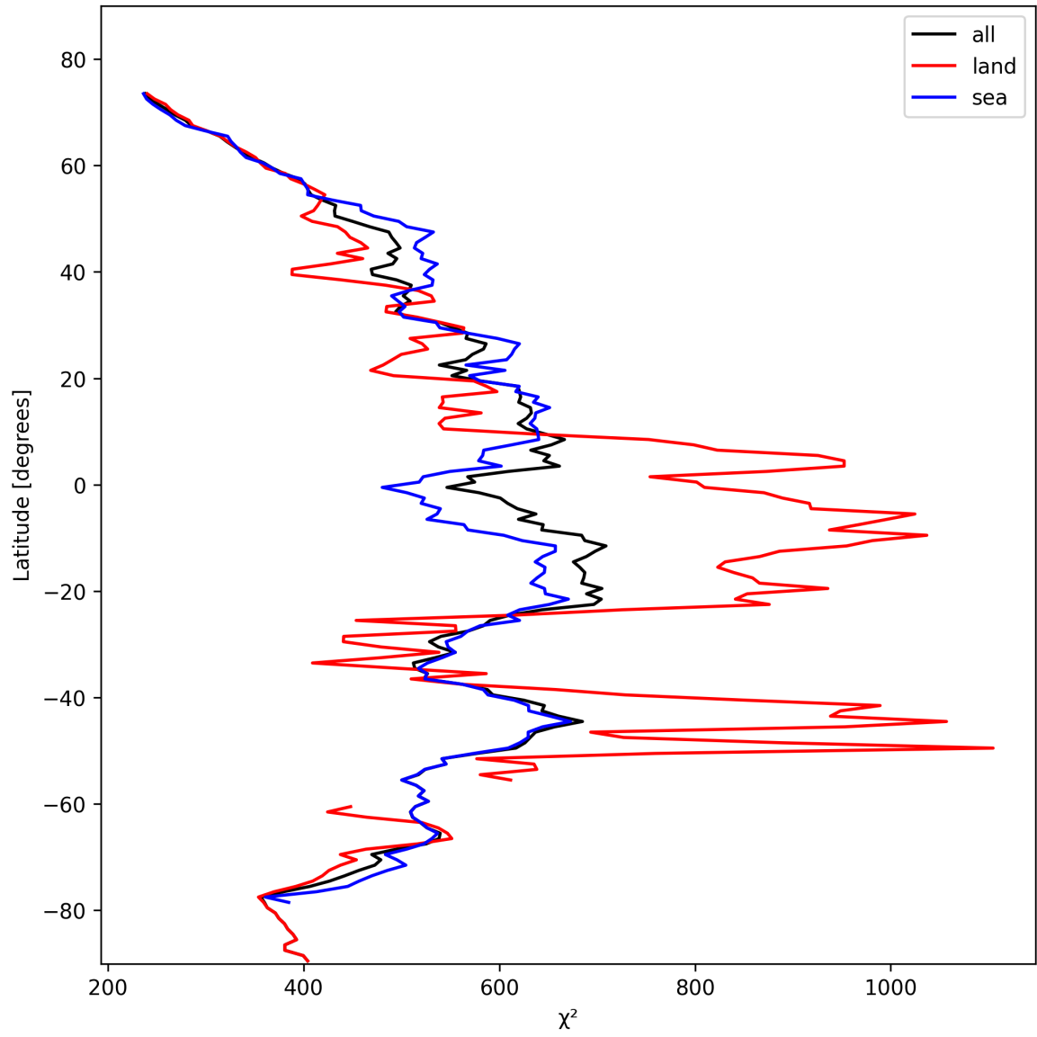
Figure 25: Zonal average of “ \chi^2 ” for 2024-10-31 to 2024-11-02.
