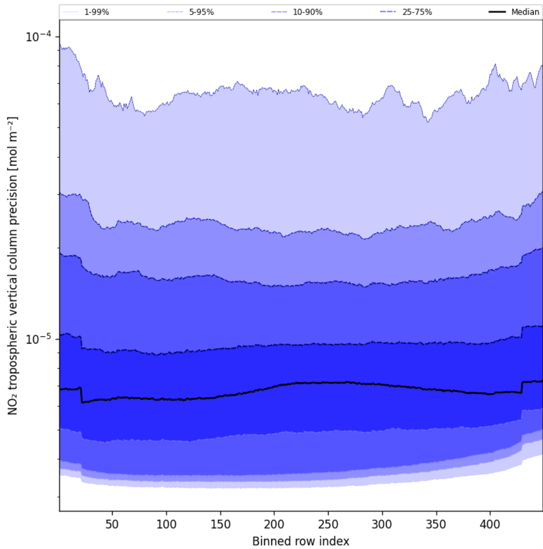
Figure 47: Along track statistics of “NO 2 tropospheric vertical column precision” for 2024-10-31 to 2024-11-02
