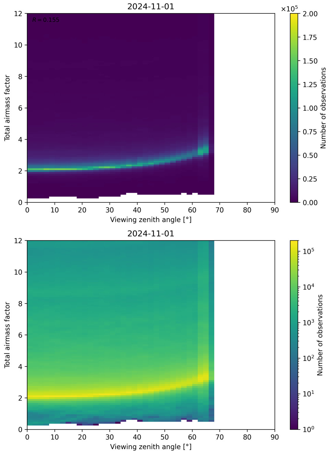
Figure 160: Scatter density plot of “Viewing zenith angle” against “Total airmass factor” for 2024-10-31 to 2024-11-02.
