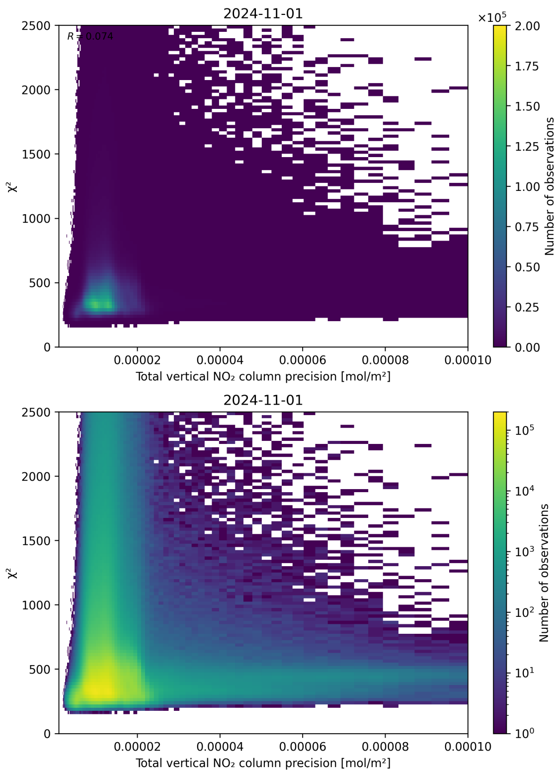
Figure 116: Scatter density plot of “Total vertical NO 2 column precision” against “ \chi^2 ” for 2024-10-31 to 2024-11-02.
