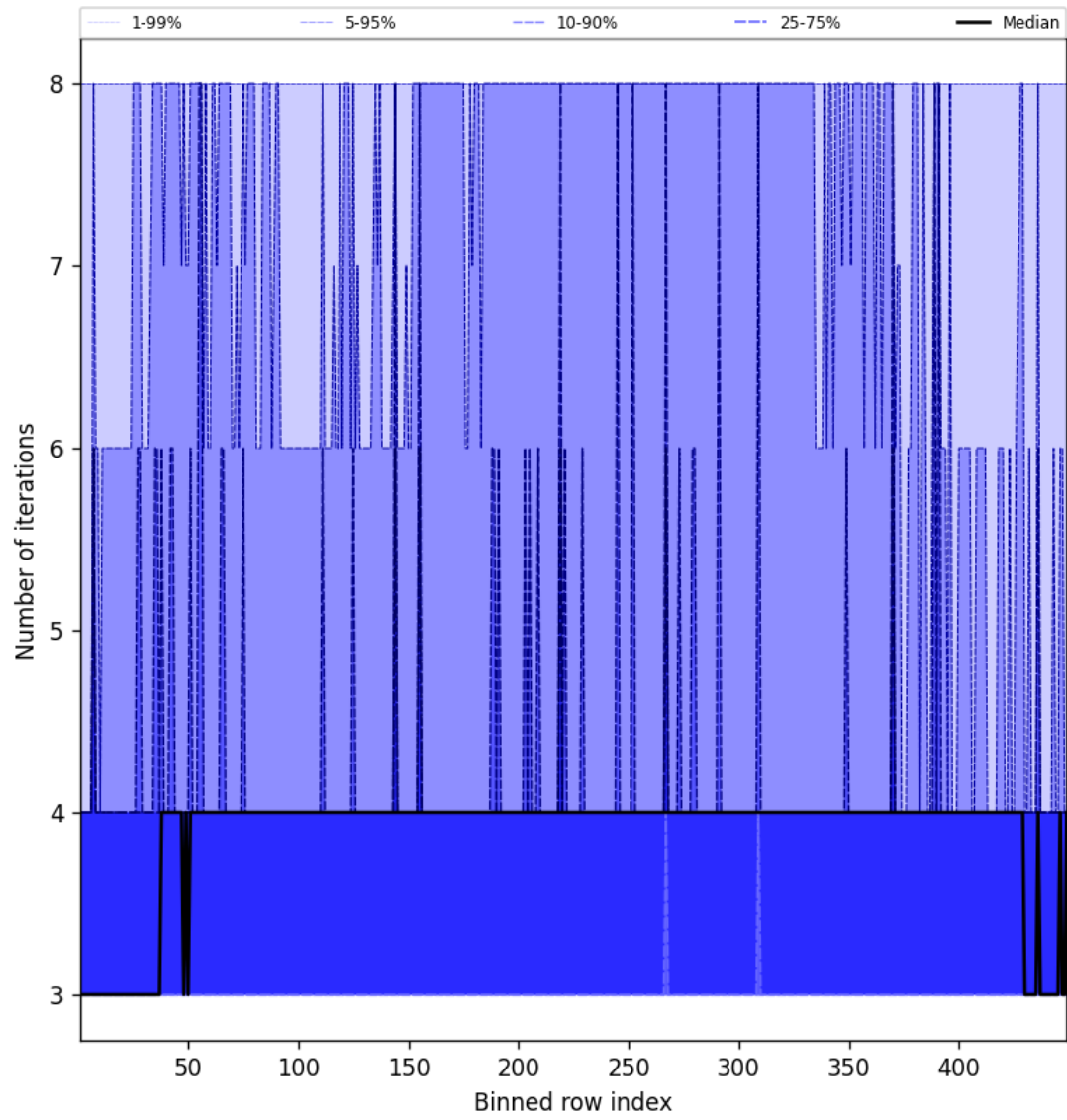
Figure 51: Along track statistics of “Number of iterations” for 2024-10-31 to 2024-11-02
