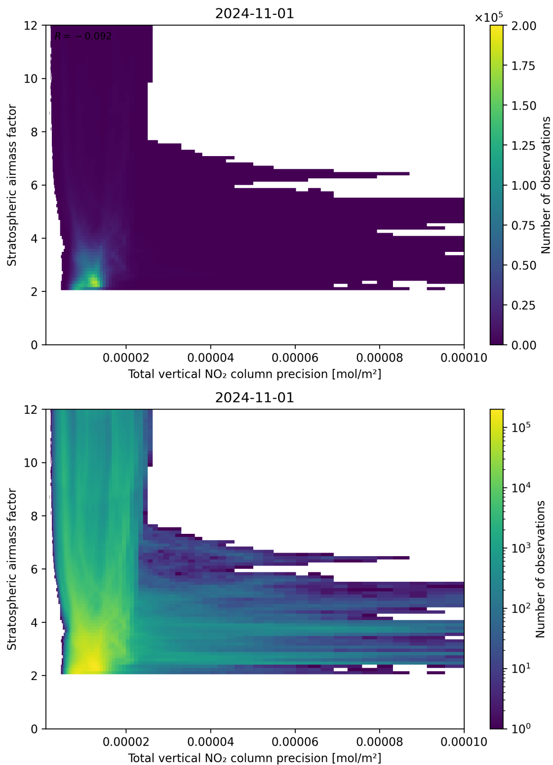
Figure 115: Scatter density plot of “Total vertical NO 2 column precision” against “Stratospheric air mass factor” for 2024-10-31 to 2024-11-02.
