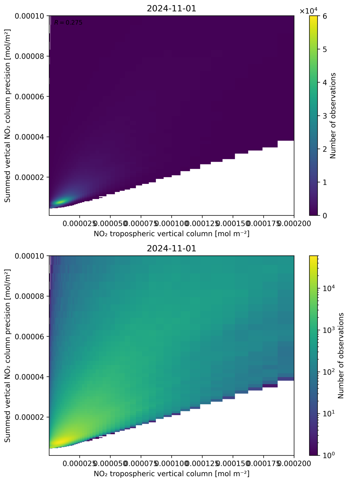
Figure 127: Scatter density plot of “NO 2 tropospheric vertical column” against “Summed vertical NO 2 column precision” for 2024-10-31 to 2024-11-02.
