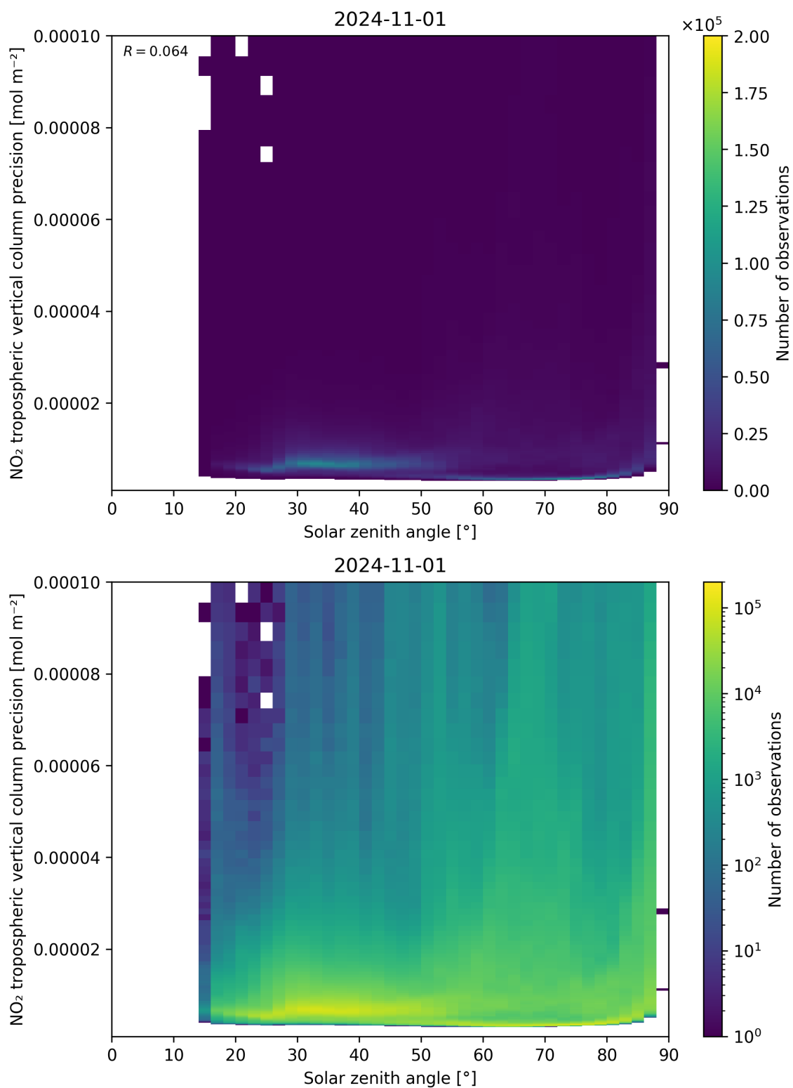
Figure 156: Scatter density plot of “Solar zenith angle” against “NO 2 tropospheric vertical column precision” for 2024-10-31 to 2024-11-02.
