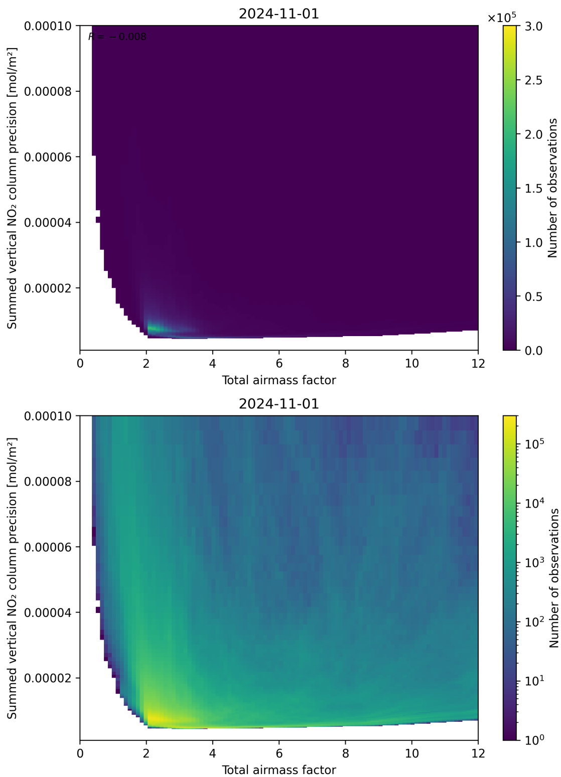
Figure 66: Scatter density plot of “Total airmass factor” against “Summed vertical NO 2 column precision” for 2024-10-31 to 2024-11-02.
