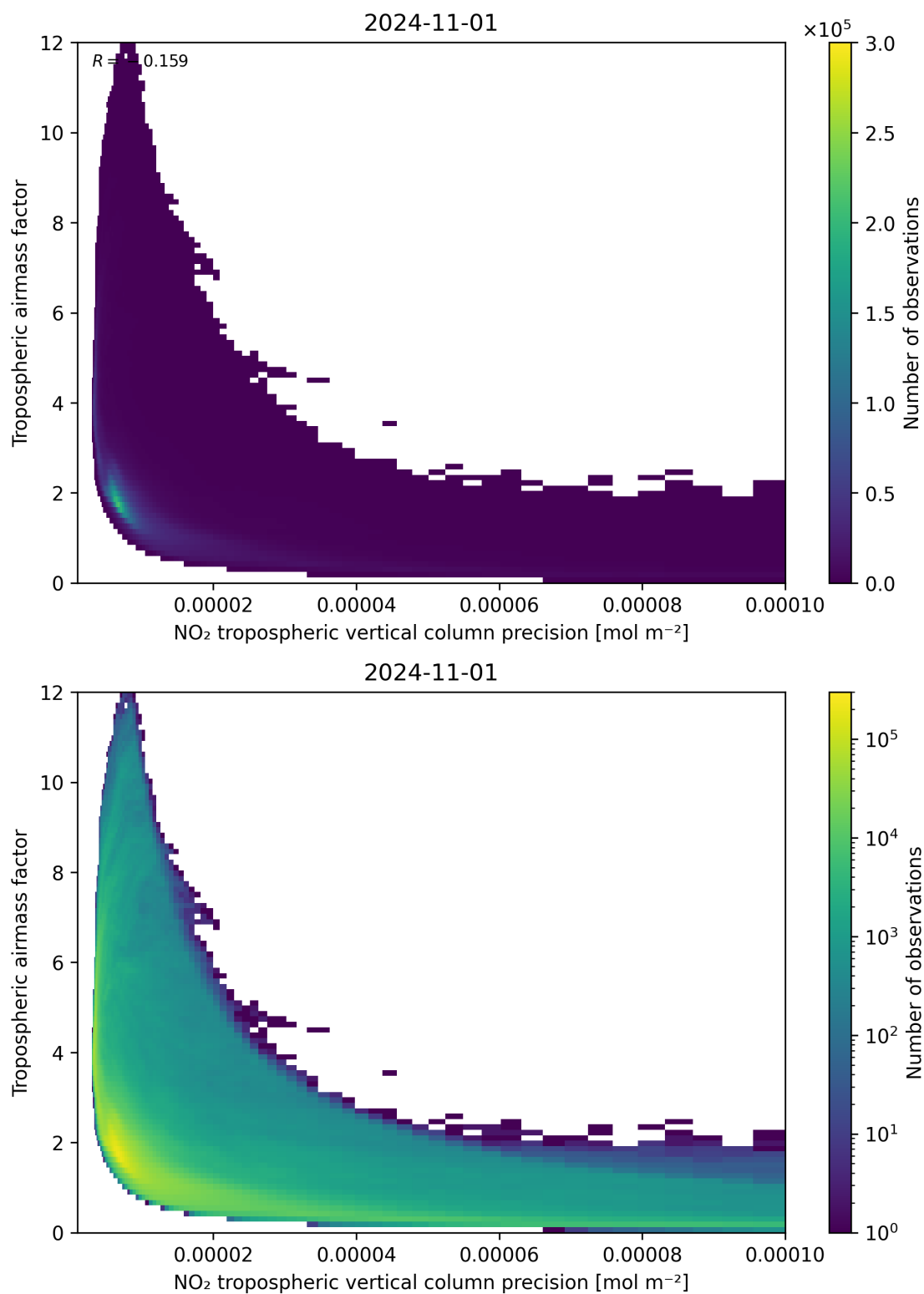
Figure 133: Scatter density plot of “NO 2 tropospheric vertical column precision” against “Tropospheric airmass factor” for 2024-10-31 to 2024-11-02.
