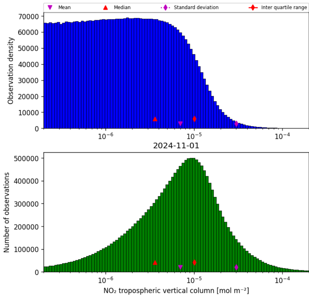
Figure 29: Histogram of “NO 2 tropospheric vertical column” for 2024-10-31 to 2024-11-02
