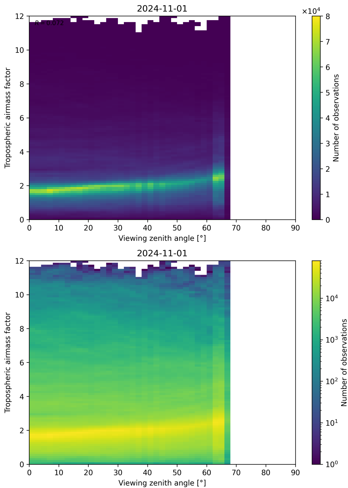
Figure 161: Scatter density plot of “Viewing zenith angle” against “Tropospheric airmass factor” for 2024-10-31 to 2024-11-02.
