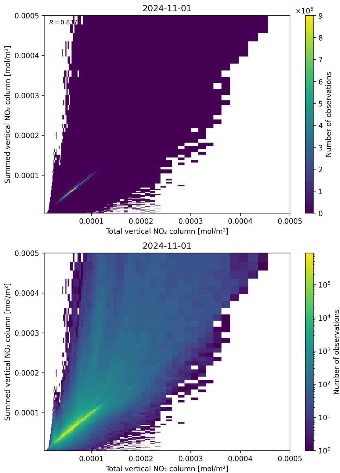
Figure 112: Scatter density plot of “Total vertical NO 2 column” against “Summed vertical NO 2 column” for 2024-10-31 to 2024-11-02.
