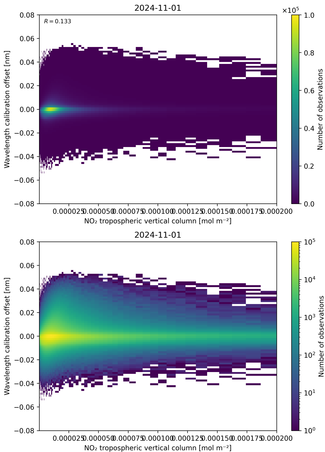
Figure 143: Scatter density plot of “NO 2 tropospheric vertical column” against “Wavelength calibration offset” for 2024-10-31 to 2024-11-02.
