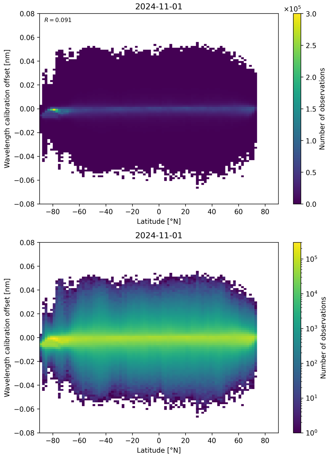
Figure 95: Scatter density plot of “Latitude” against “Wavelength calibration offset” for 2024-10-31 to 2024-11-02.
