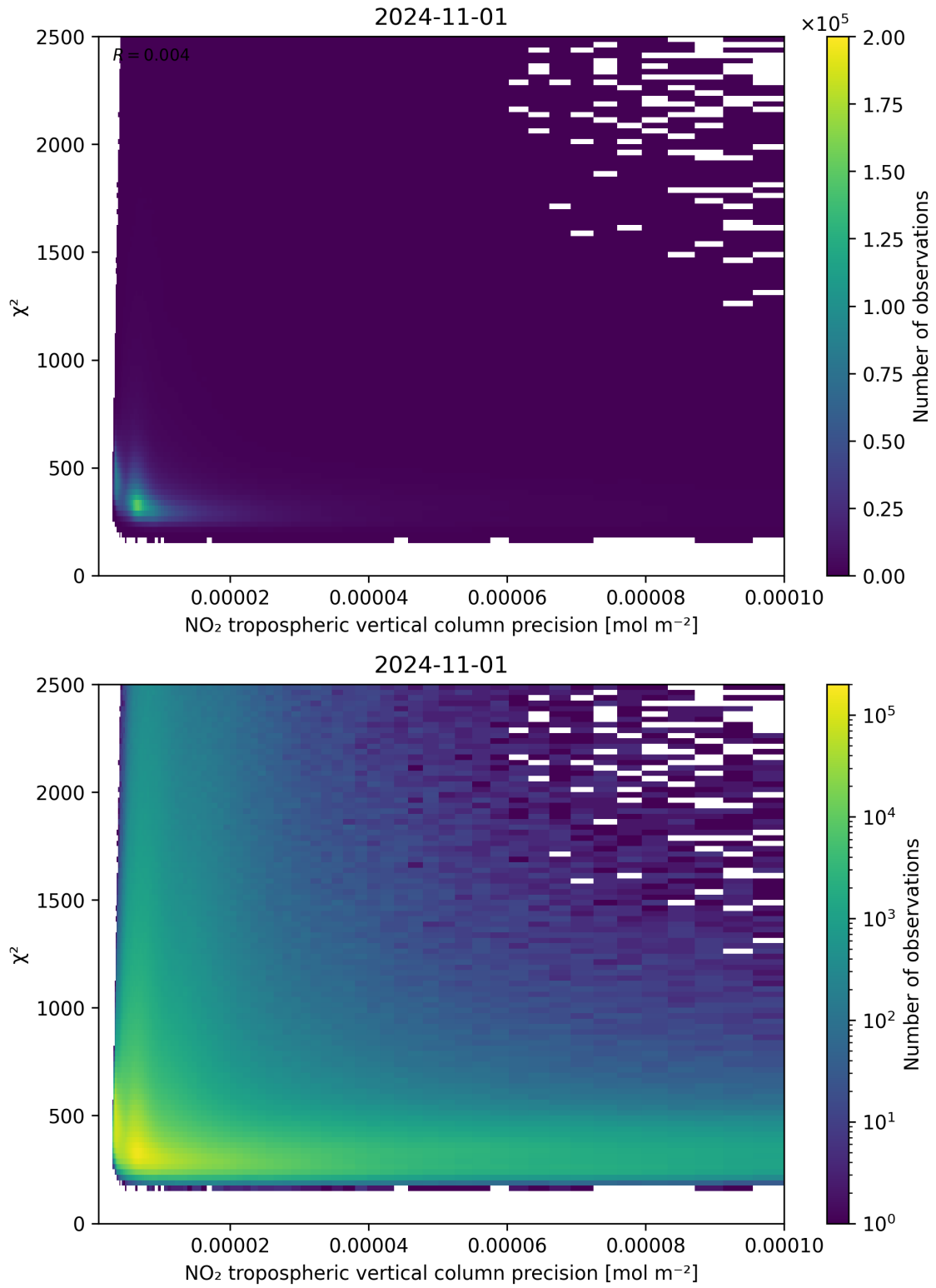
Figure 134: Scatter density plot of “NO 2 tropospheric vertical column precision” against “ \chi^2 ” for 2024-10-31 to 2024-11-02.
