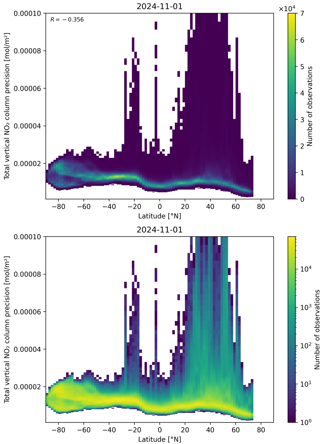
Figure 91: Scatter density plot of “Latitude” against “Total vertical NO 2 column precision” for 2024-10-31 to 2024-11-02.
