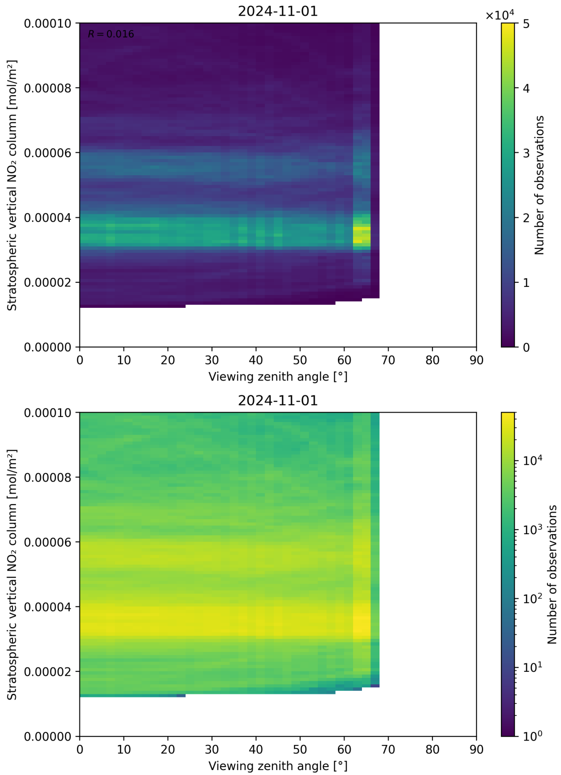
Figure 164: Scatter density plot of “Viewing zenith angle” against “Stratospheric vertical NO 2 column” for 2024-10-31 to 2024-11-02.
