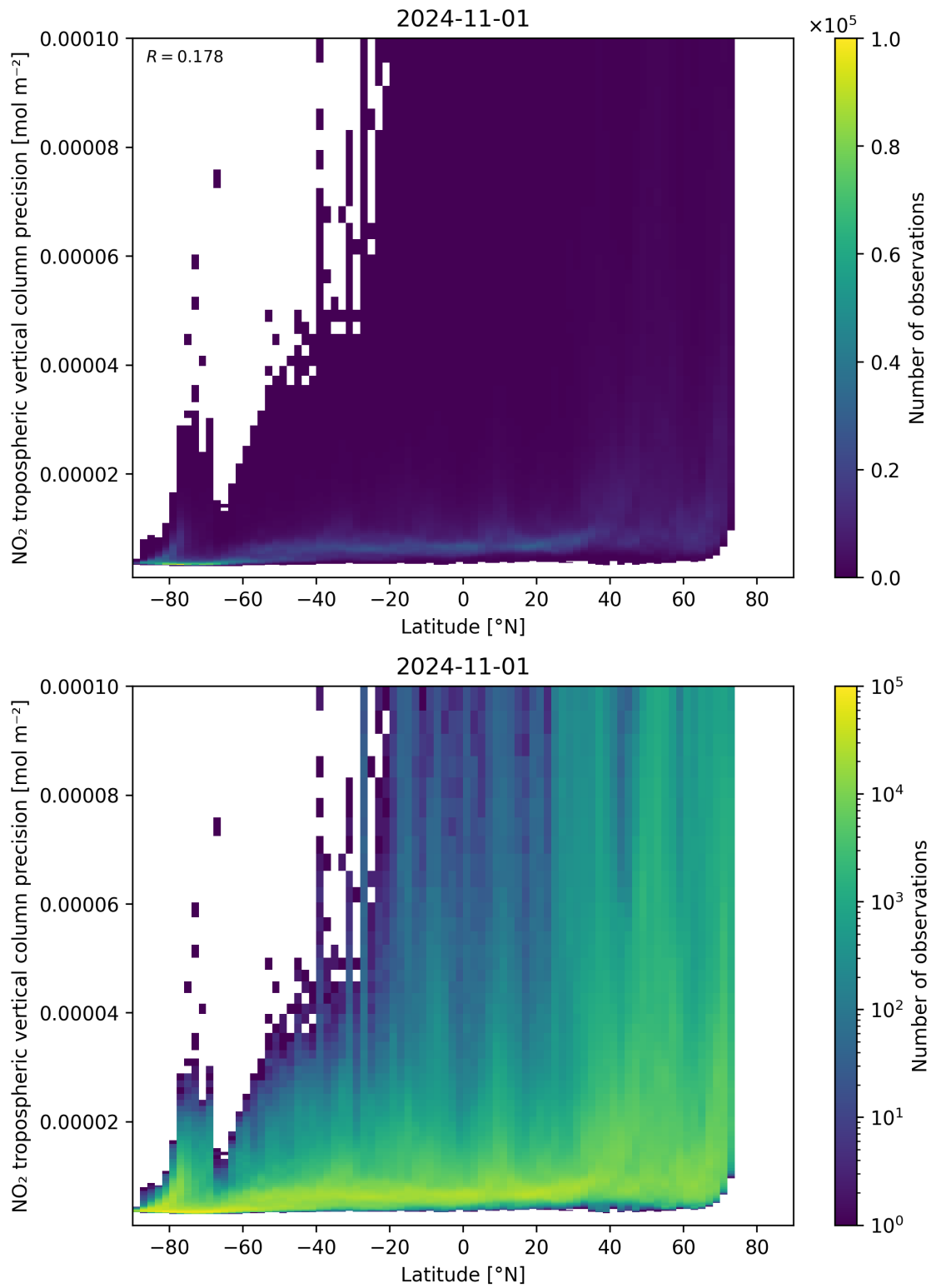
Figure 93: Scatter density plot of “Latitude” against “NO 2 tropospheric vertical column precision” for 2024-10-31 to 2024-11-02.
