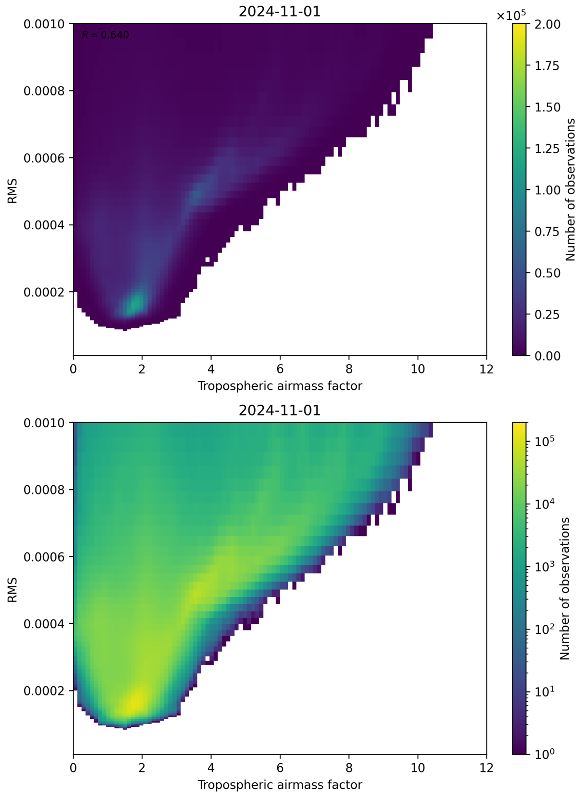
Figure 79: Scatter density plot of “Tropospheric airmass factor” against “RMS” for 2024-10-31 to 2024-11-02.
