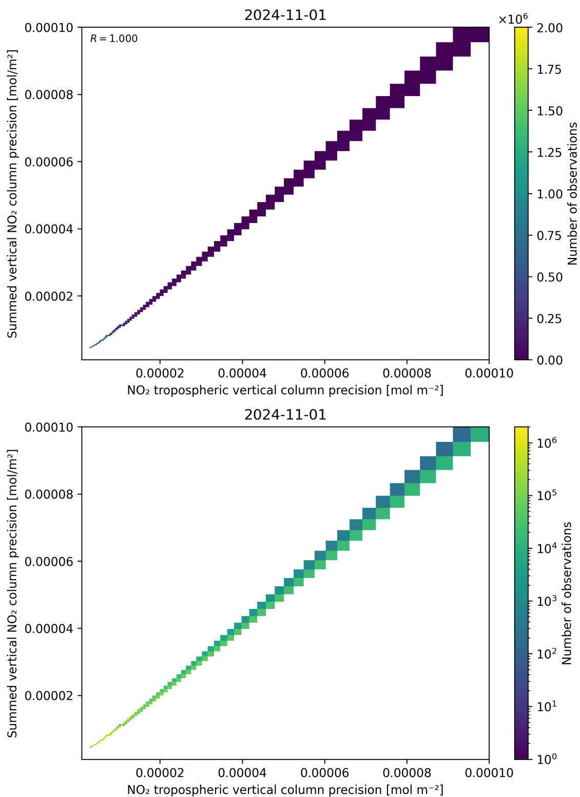
Figure 137: Scatter density plot of “NO 2 tropospheric vertical column precision” against “Summed vertical NO 2 column precision” for 2024-10-31 to 2024-11-02.
