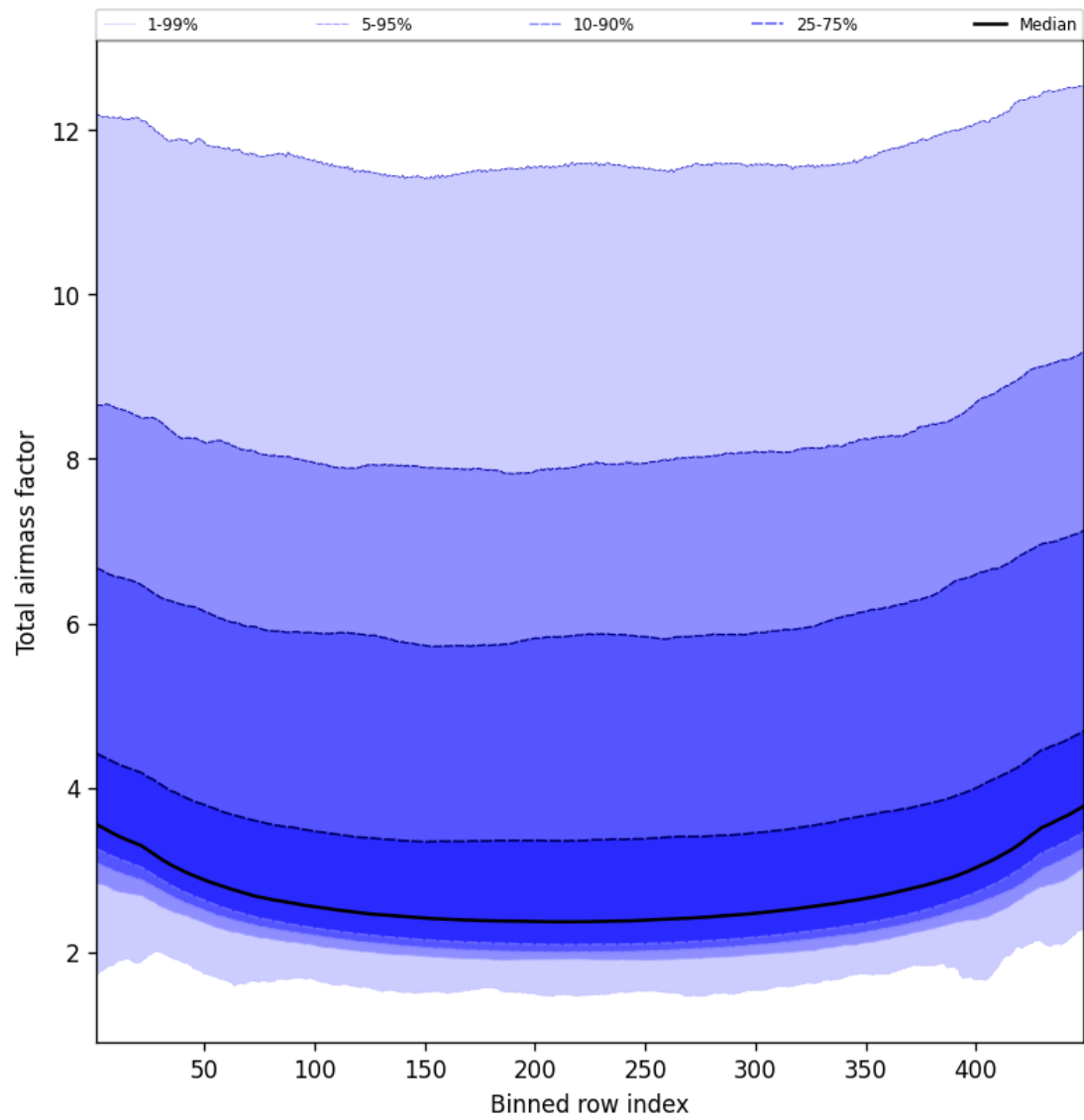
Figure 49: Along track statistics of “Total airmass factor” for 2024-10-31 to 2024-11-02
