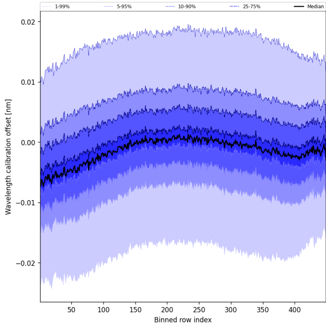
Figure 52: Along track statistics of “Wavelength calibration offset” for 2024-10-31 to 2024-11-02
