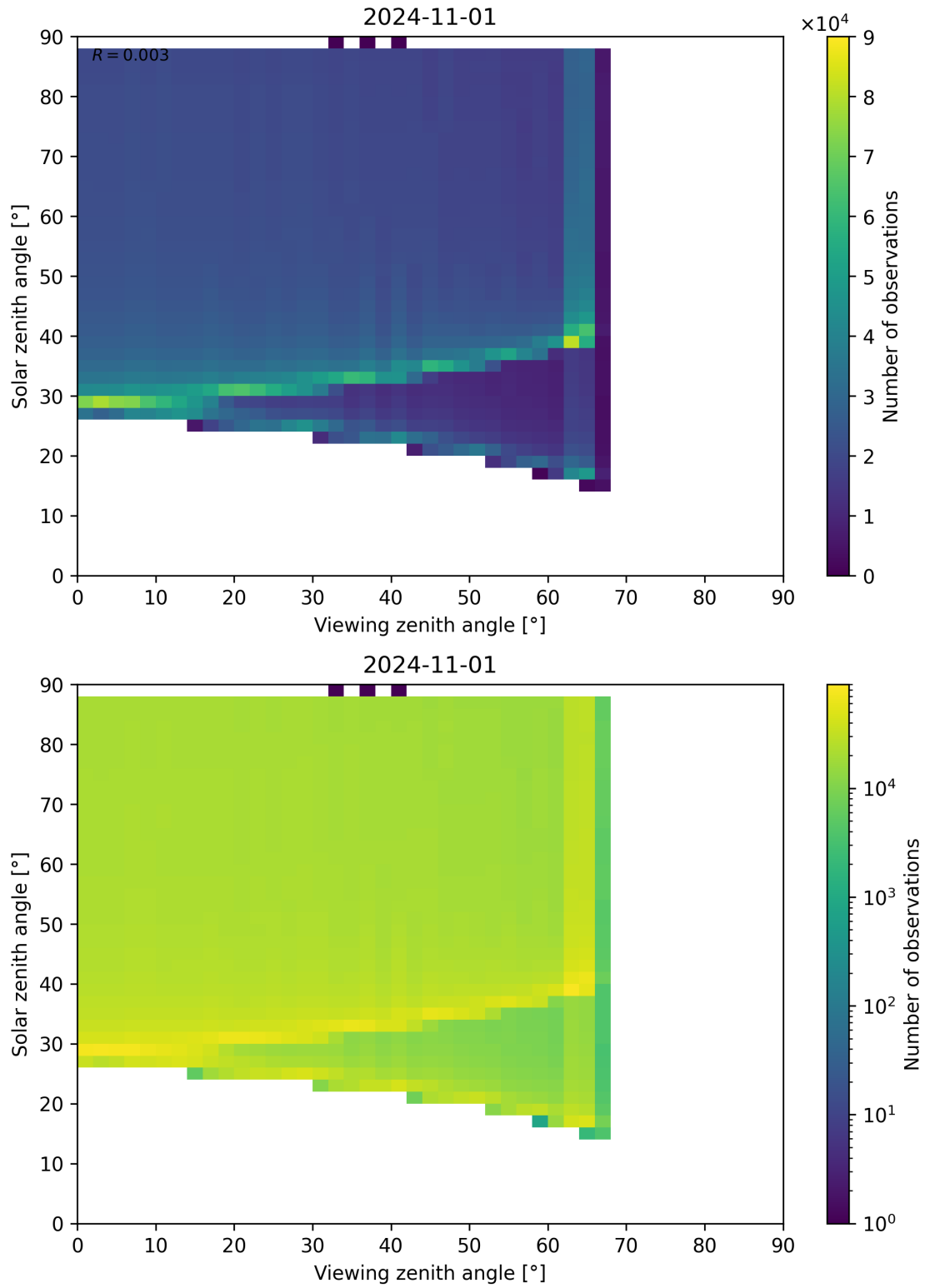
Figure 172: Scatter density plot of “Viewing zenith angle” against “Solar zenith angle” for 2024-10-31 to 2024-11-02.
