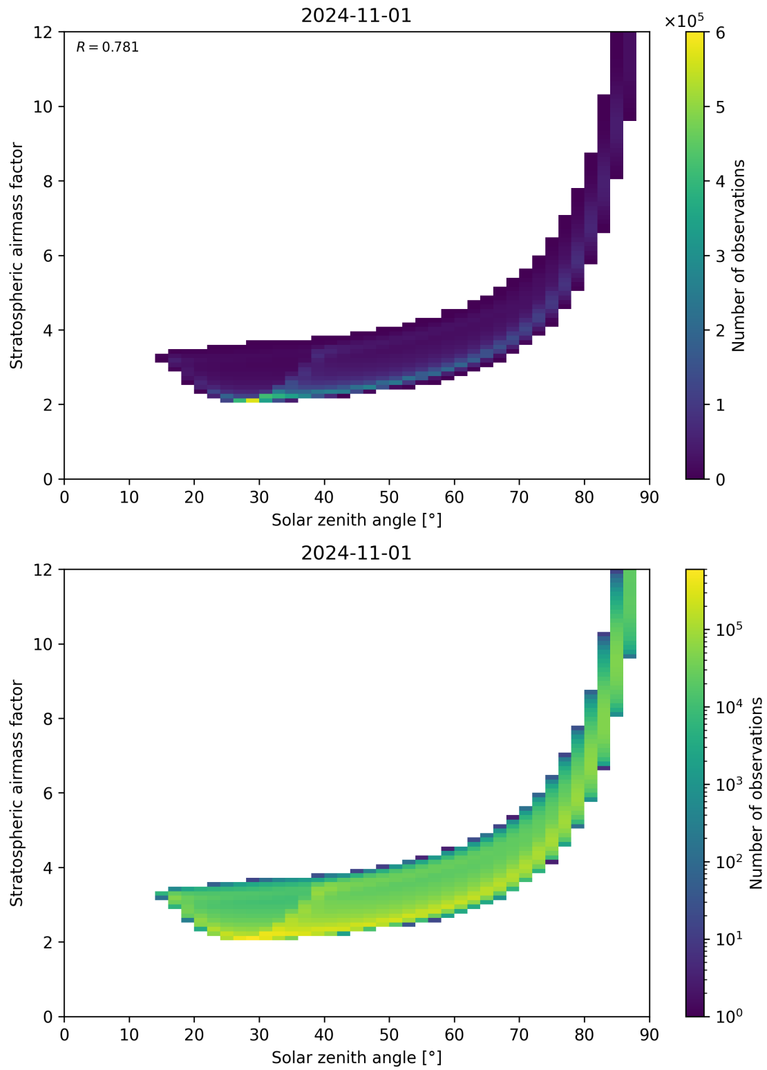
Figure 145: Scatter density plot of “Solar zenith angle” against “Stratospheric airmass factor” for 2024-10-31 to 2024-11-02.
