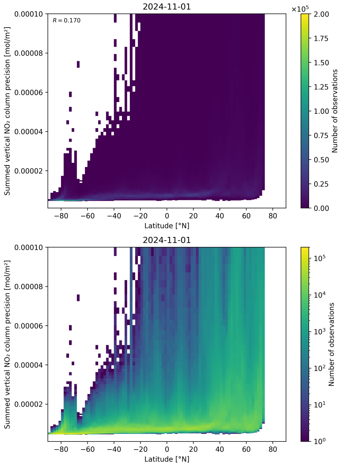
Figure 89: Scatter density plot of “Latitude” against “Summed vertical NO 2 column precision” for 2024-10-31 to 2024-11-02.
