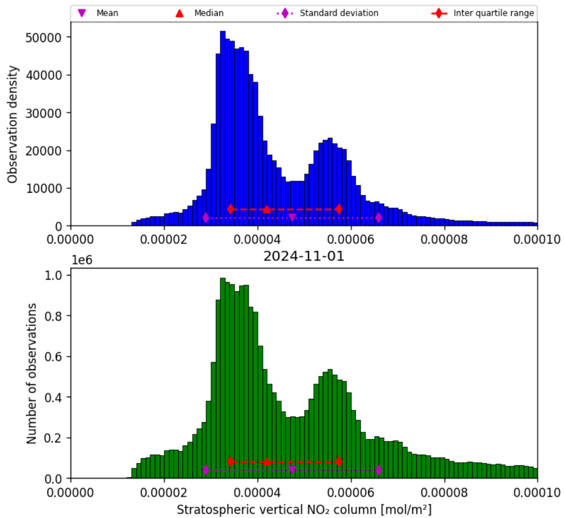
Figure 36: Histogram of “Stratospheric vertical NO 2 column” for 2024-10-31 to 2024-11-02
