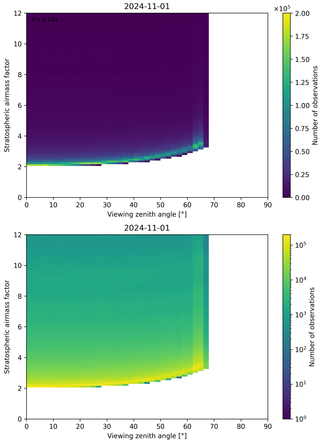
Figure 159: Scatter density plot of “Viewing zenith angle” against “Stratospheric airmass factor” for 2024-10-31 to 2024-11-02.
