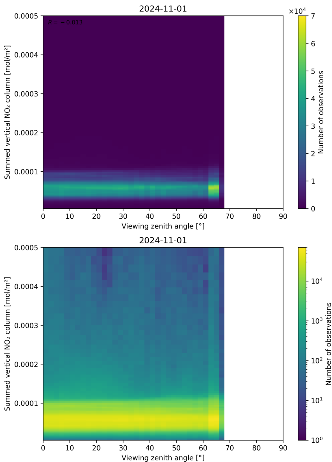
Figure 165: Scatter density plot of “Viewing zenith angle” against “Summed vertical NO 2 column” for 2024-10-31 to 2024-11-02.
