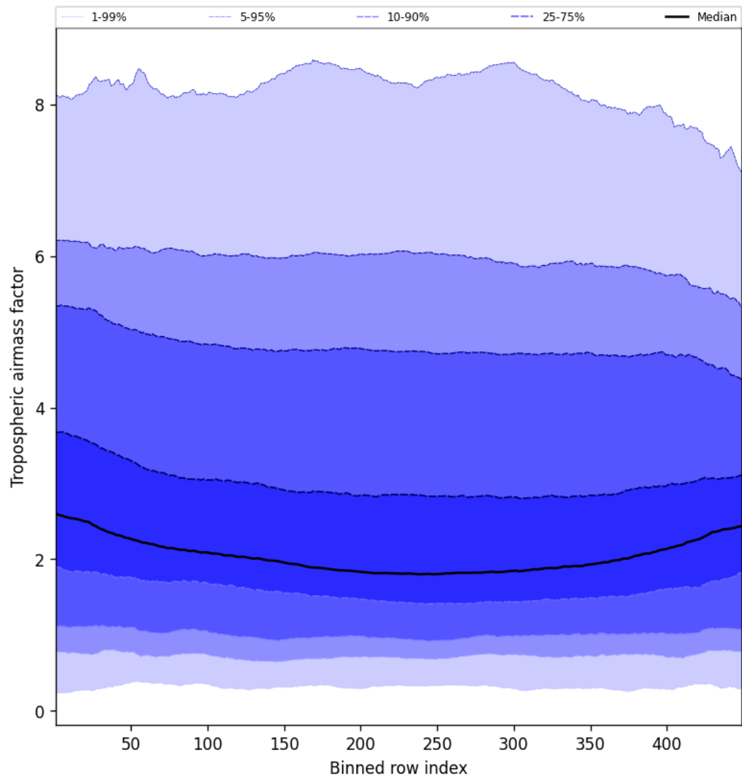
Figure 48: Along track statistics of “Tropospheric air mass factor” for 2024-10-31 to 2024-11-02
