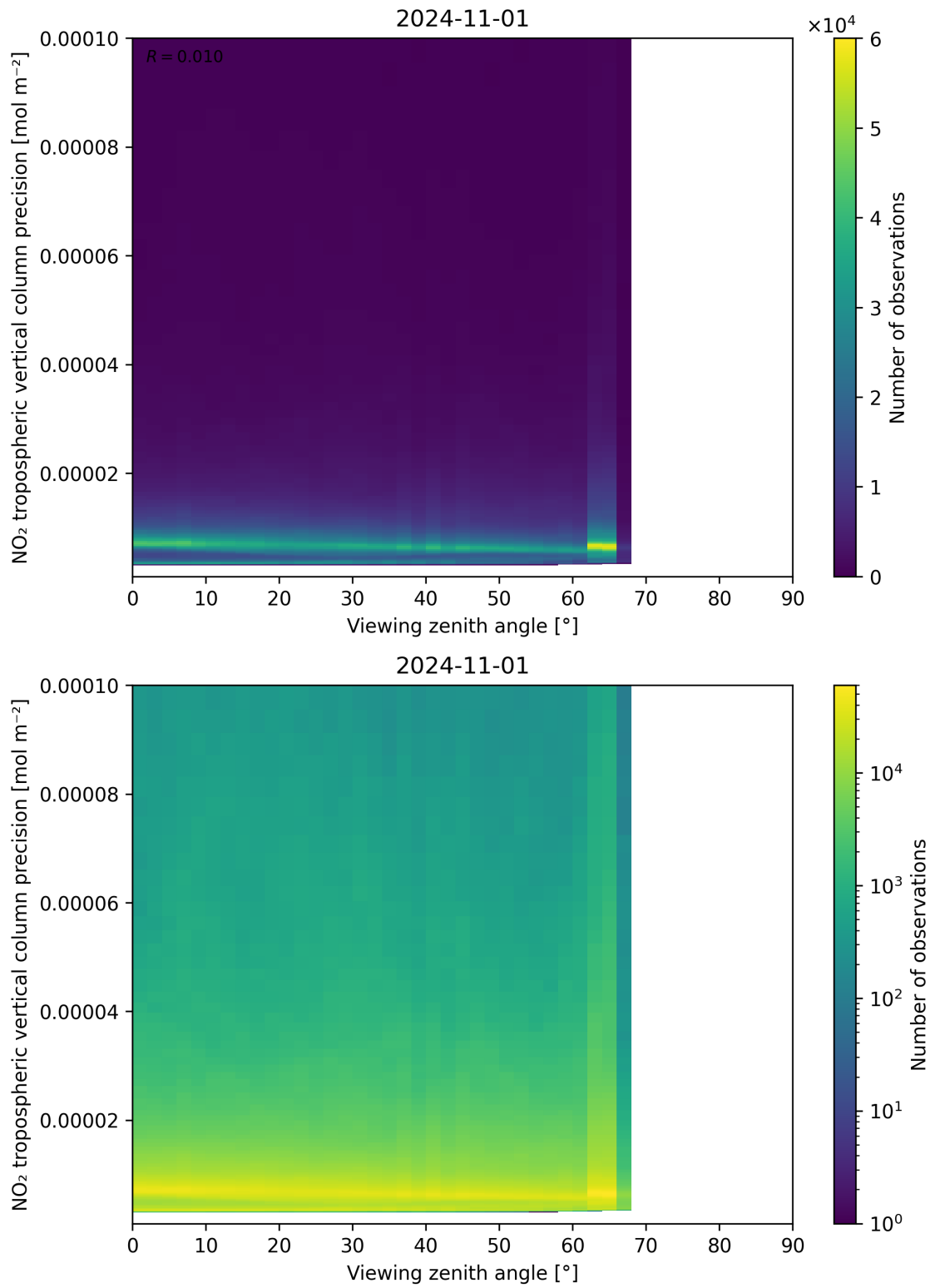
Figure 170: Scatter density plot of “Viewing zenith angle” against “NO 2 tropospheric vertical column precision” for 2024-10-31 to 2024-11-02.
