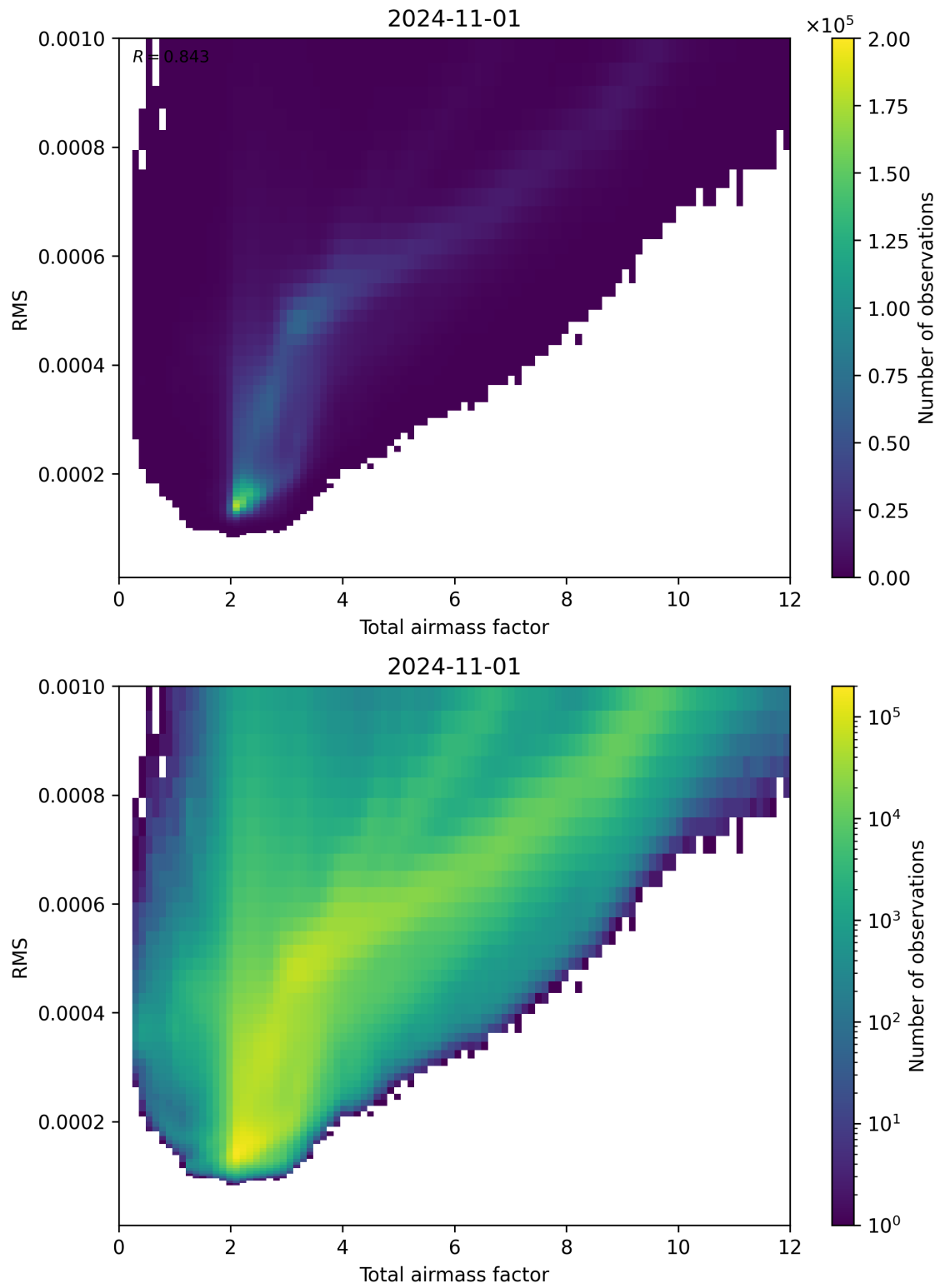
Figure 69: Scatter density plot of “Total airmass factor” against “RMS” for 2024-10-31 to 2024-11-02.
