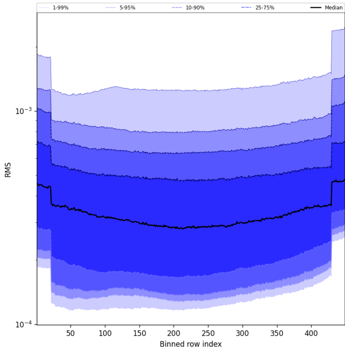
Figure 60: Along track statistics of “RMS” for 2024-10-31 to 2024-11-02
