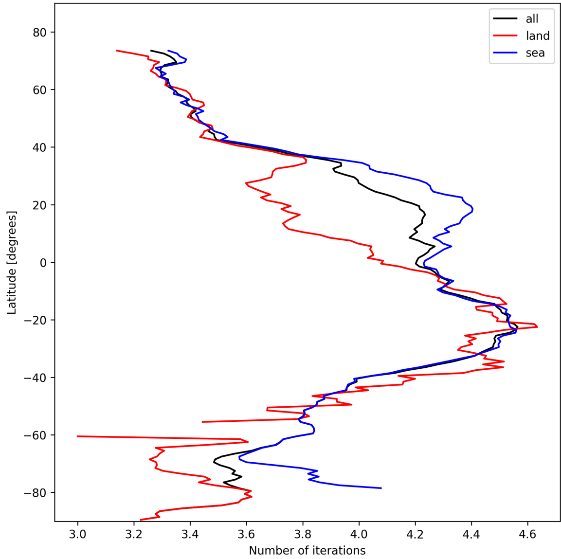
Figure 17: Zonal average of “Number of iterations” for 2024-10-31 to 2024-11-02.
