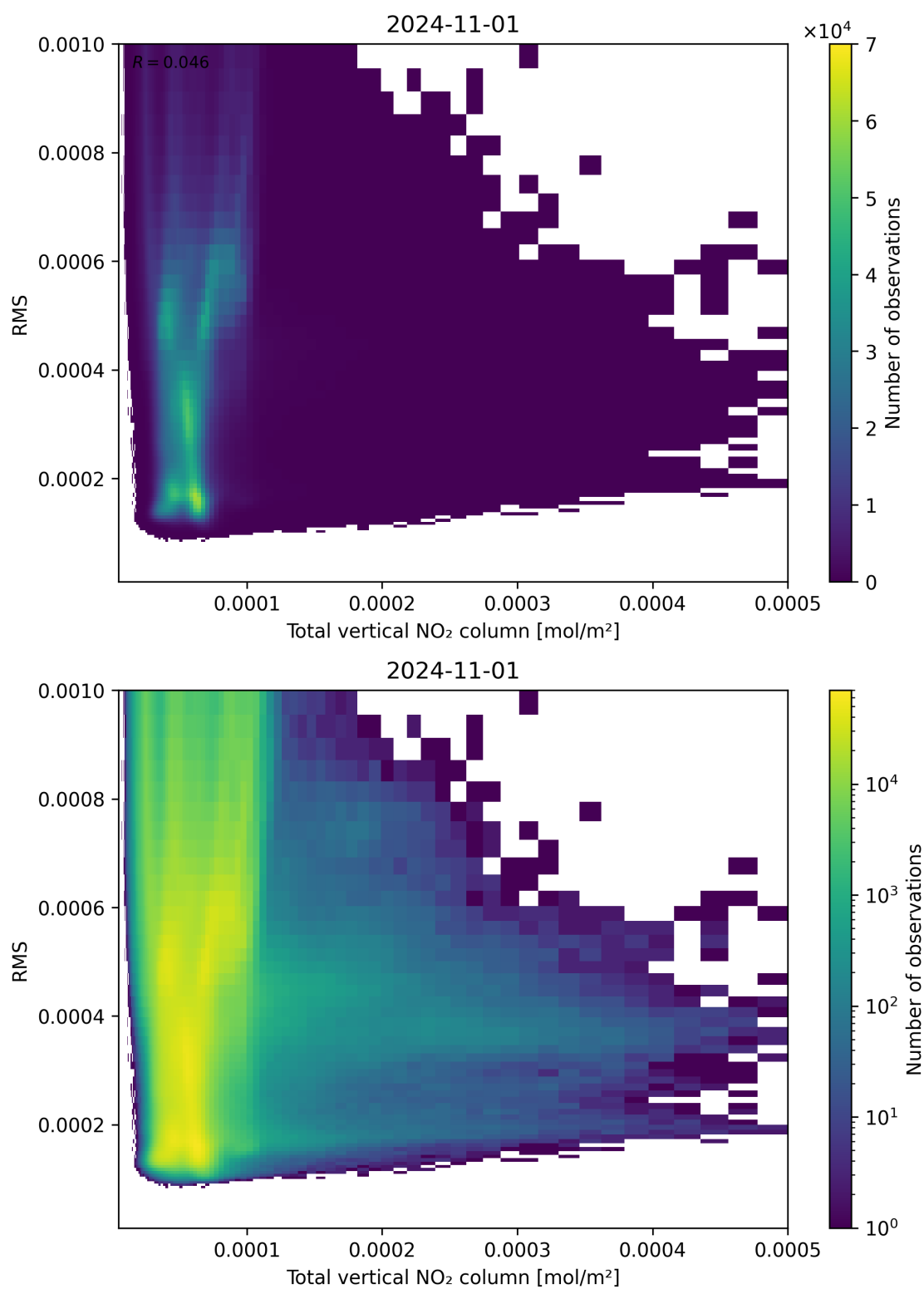
Figure 120: Scatter density plot of “Total vertical NO 2 column” against “RMS” for 2024-10-31 to 2024-11-02.
