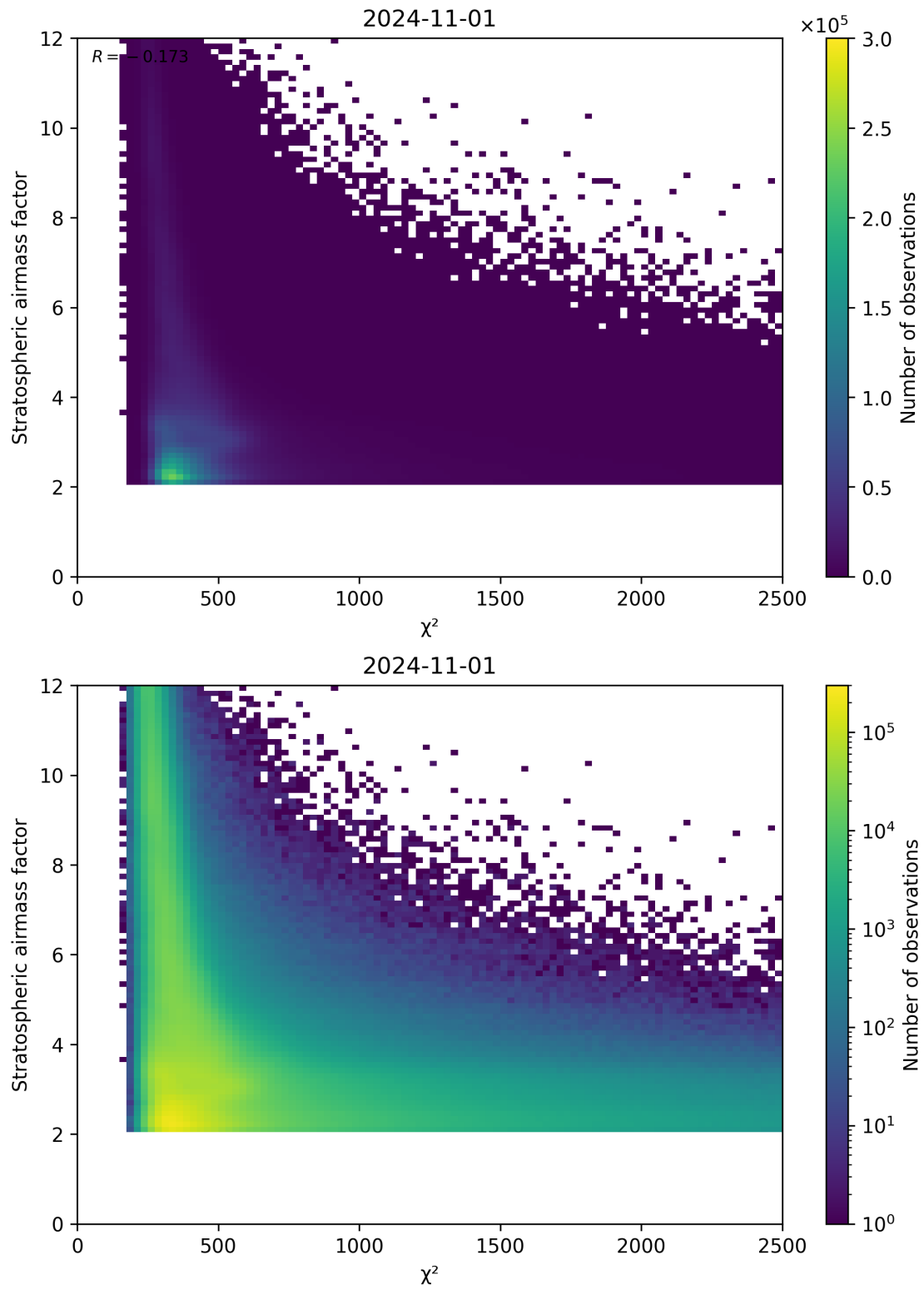
Figure 81: Scatter density plot of “ \chi^2 ” against “Stratospheric airmass factor” for 2024-10-31 to 2024-11-02.
