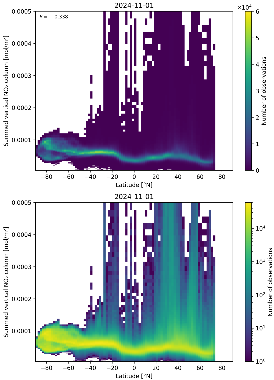
Figure 88: Scatter density plot of “Latitude” against “Summed vertical NO 2 column” for 2024-10-31 to 2024-11-02.
