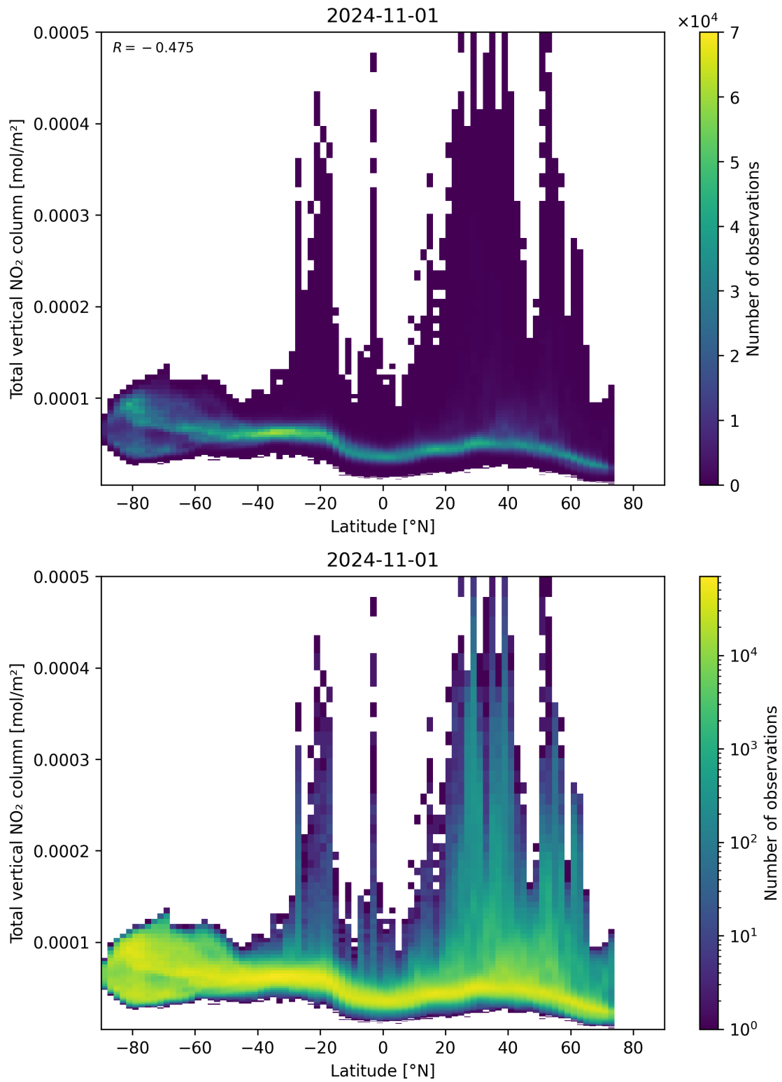
Figure 90: Scatter density plot of “Latitude” against “Total vertical NO 2 column” for 2024-10-31 to 2024-11-02.
