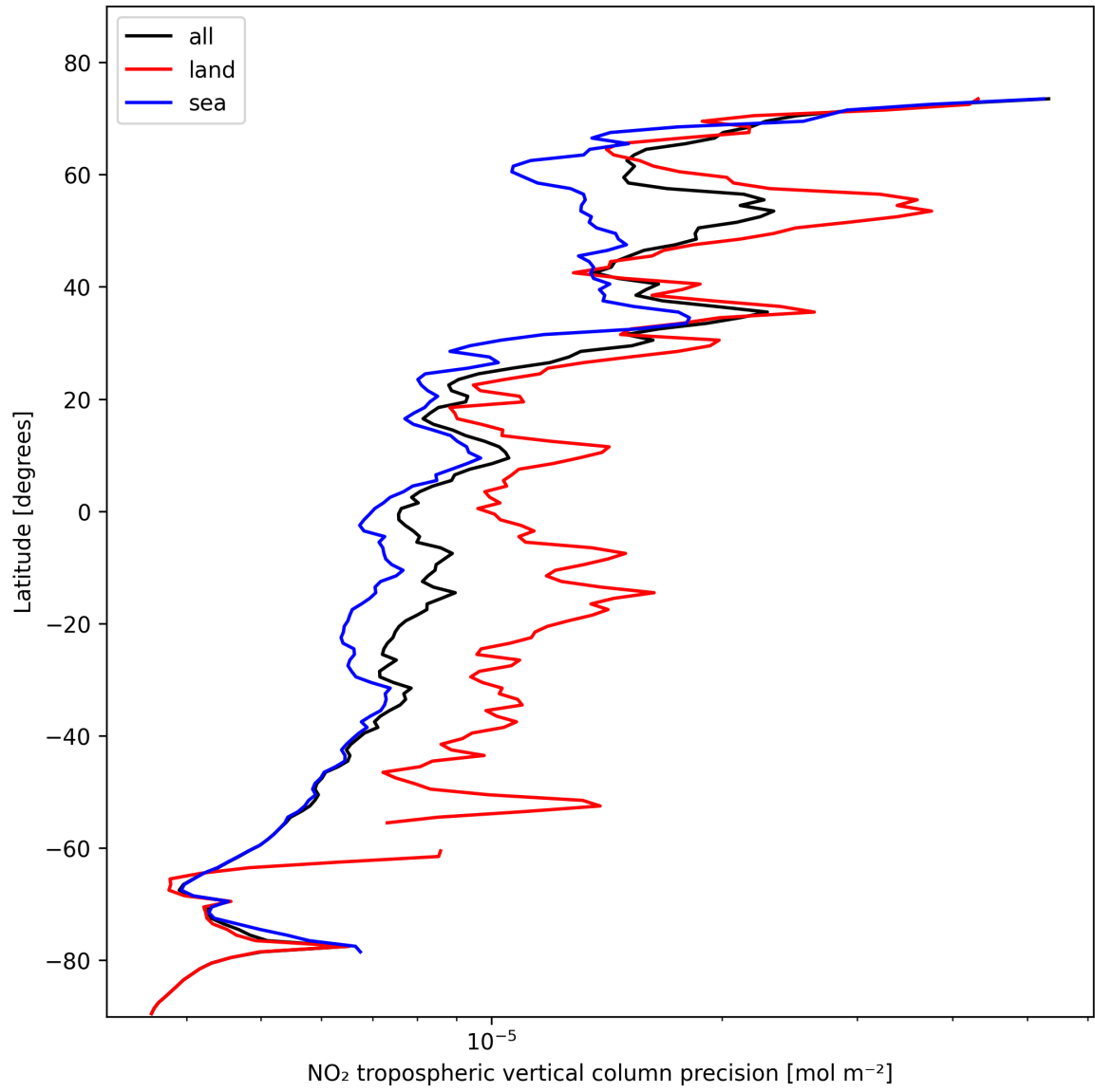
Figure 13: Zonal average of “NO 2 tropospheric vertical column precision” for 2024-10-31 to 2024-11-02.
