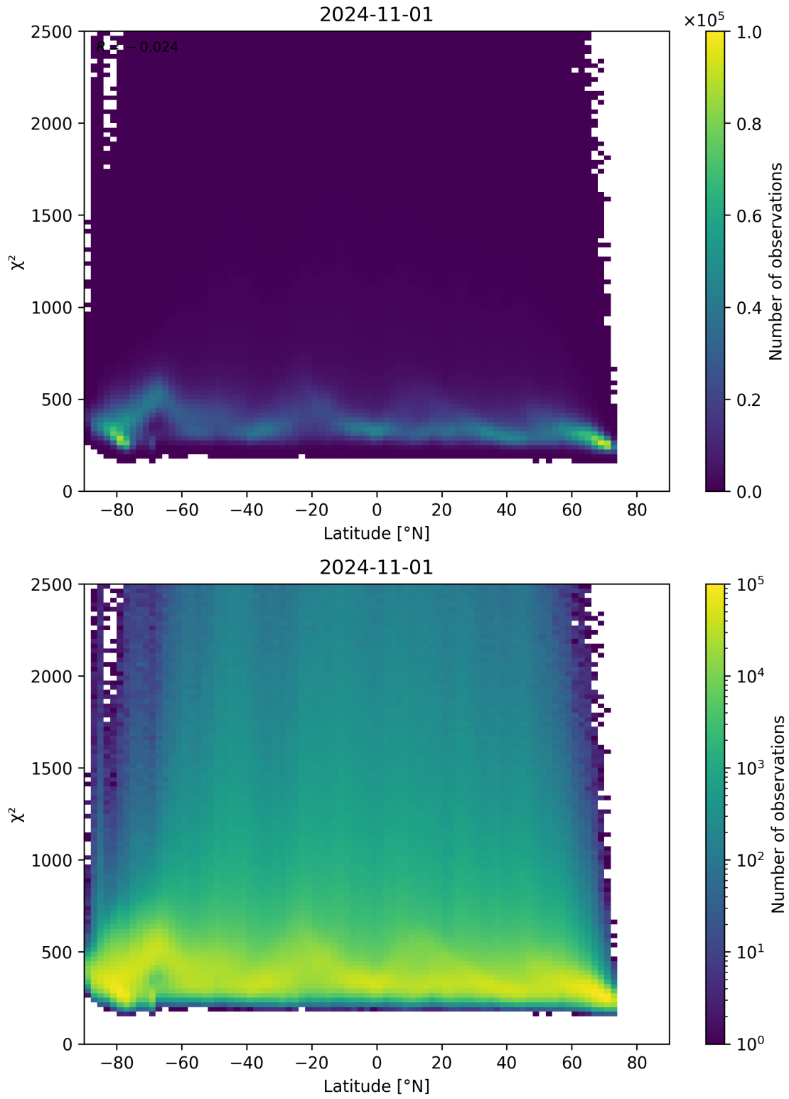
Figure 86: Scatter density plot of “Latitude” against “ \chi^2 ” for 2024-10-31 to 2024-11-02.
