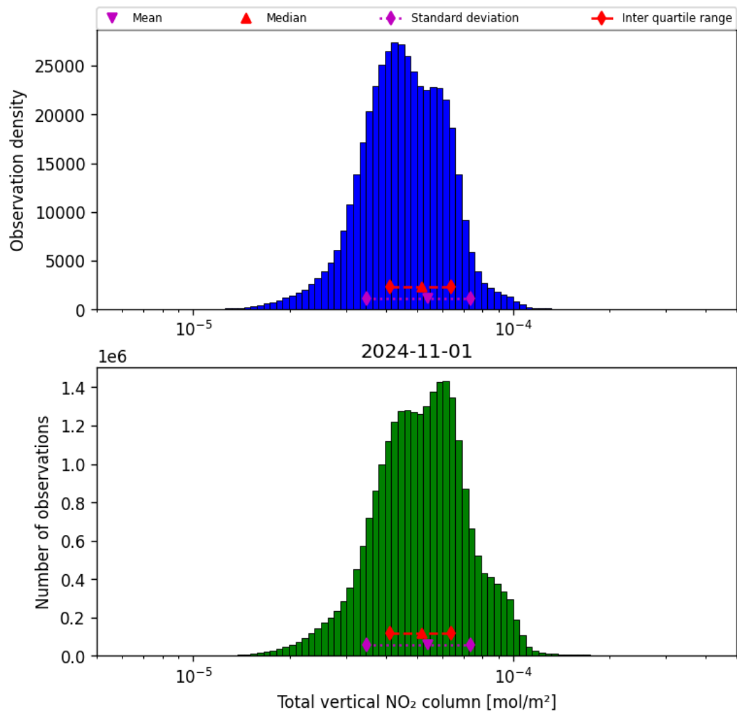
Figure 38: Histogram of “Total vertical NO 2 column” for 2024-10-31 to 2024-11-02
