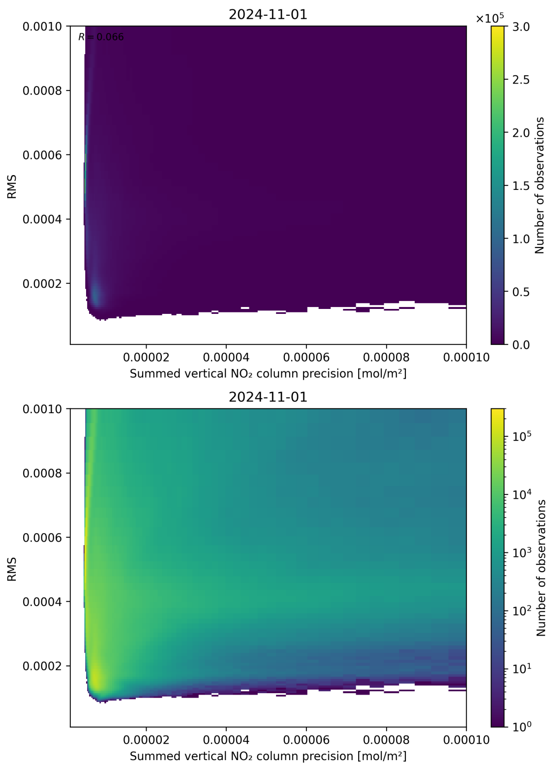
Figure 108: Scatter density plot of “Summed vertical NO 2 column precision” against “RMS” for 2024-10-31 to 2024-11-02.
