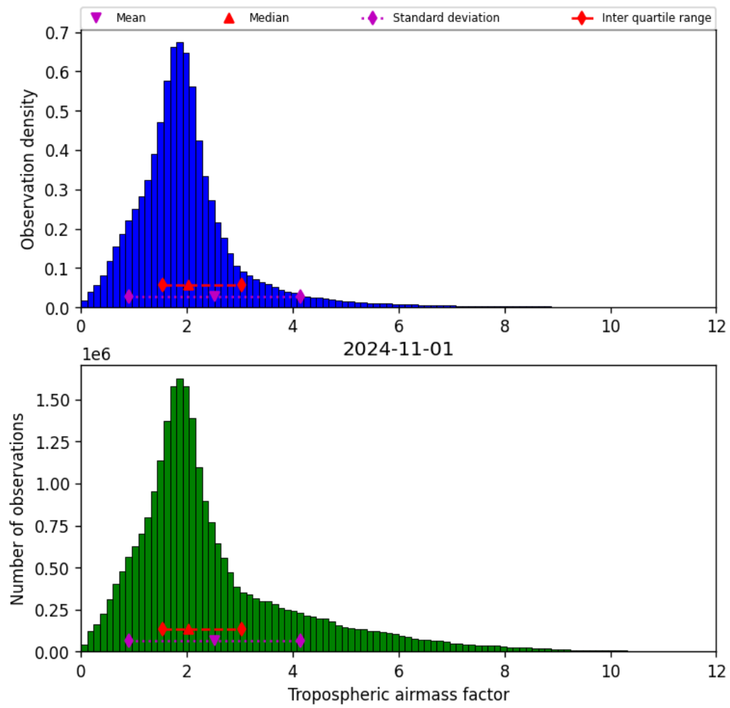
Figure 31: Histogram of “Tropospheric airmass factor” for 2024-10-31 to 2024-11-02
