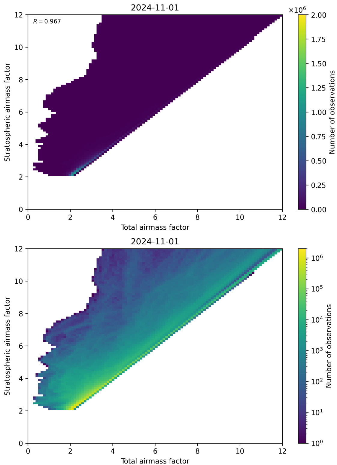
Figure 62: Scatter density plot of “Total airmass factor” against “Stratospheric airmass factor” for 2024-10-31 to 2024-11-02.
