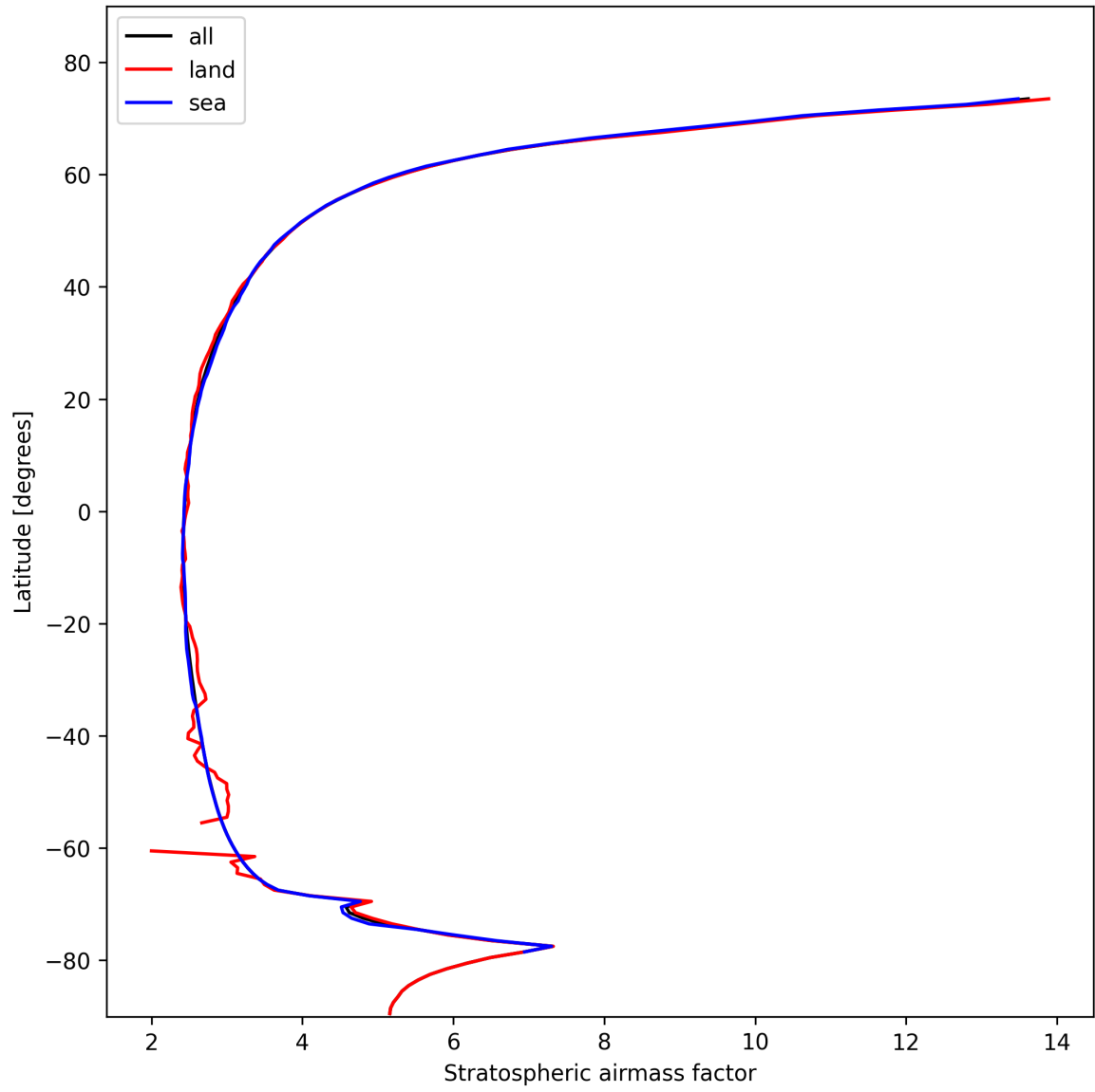
Figure 27: Zonal average of “Stratospheric air mass factor” for 2024-10-31 to 2024-11-02.
