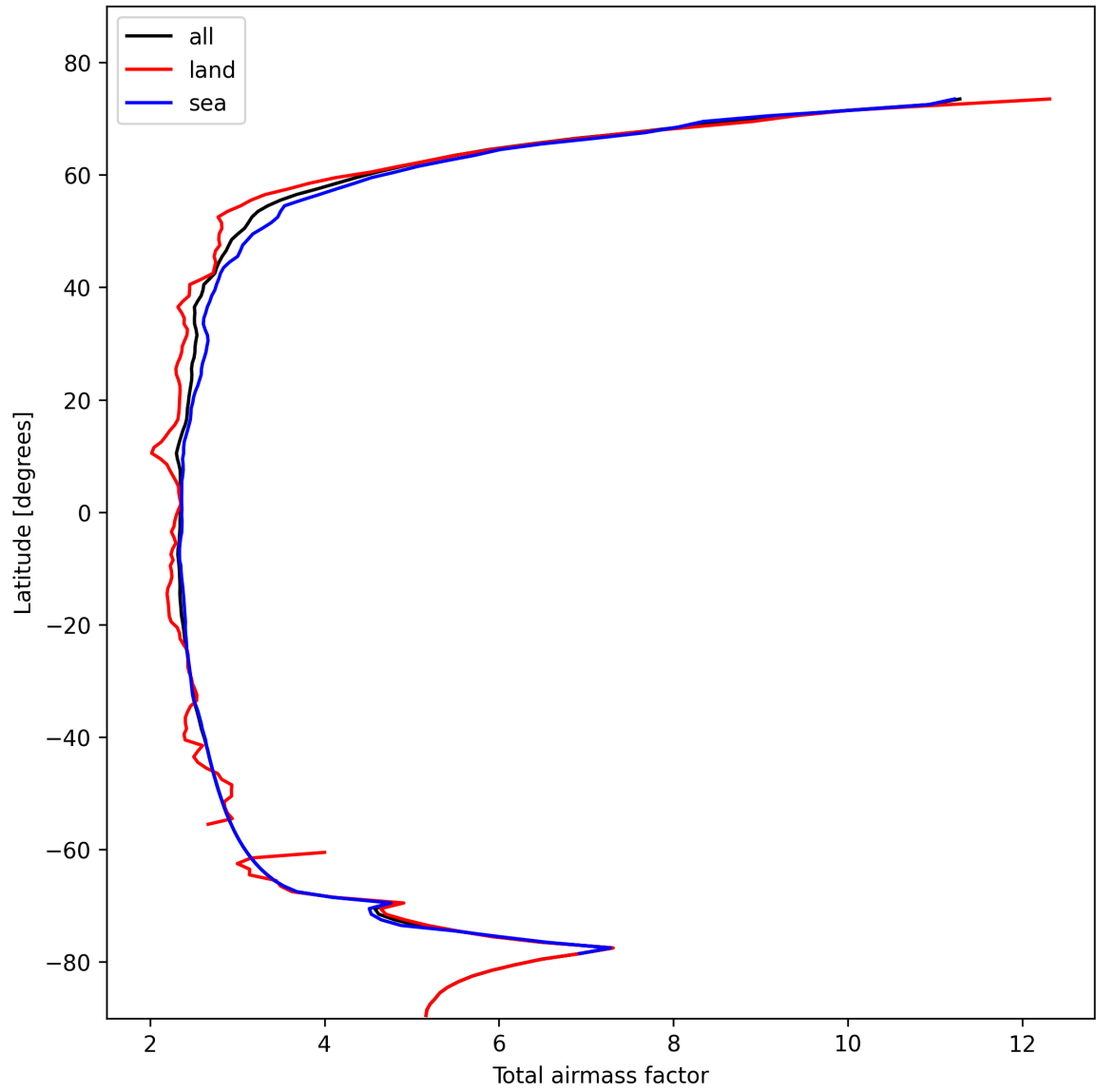
Figure 15: Zonal average of “Total airmass factor” for 2024-10-31 to 2024-11-02.
