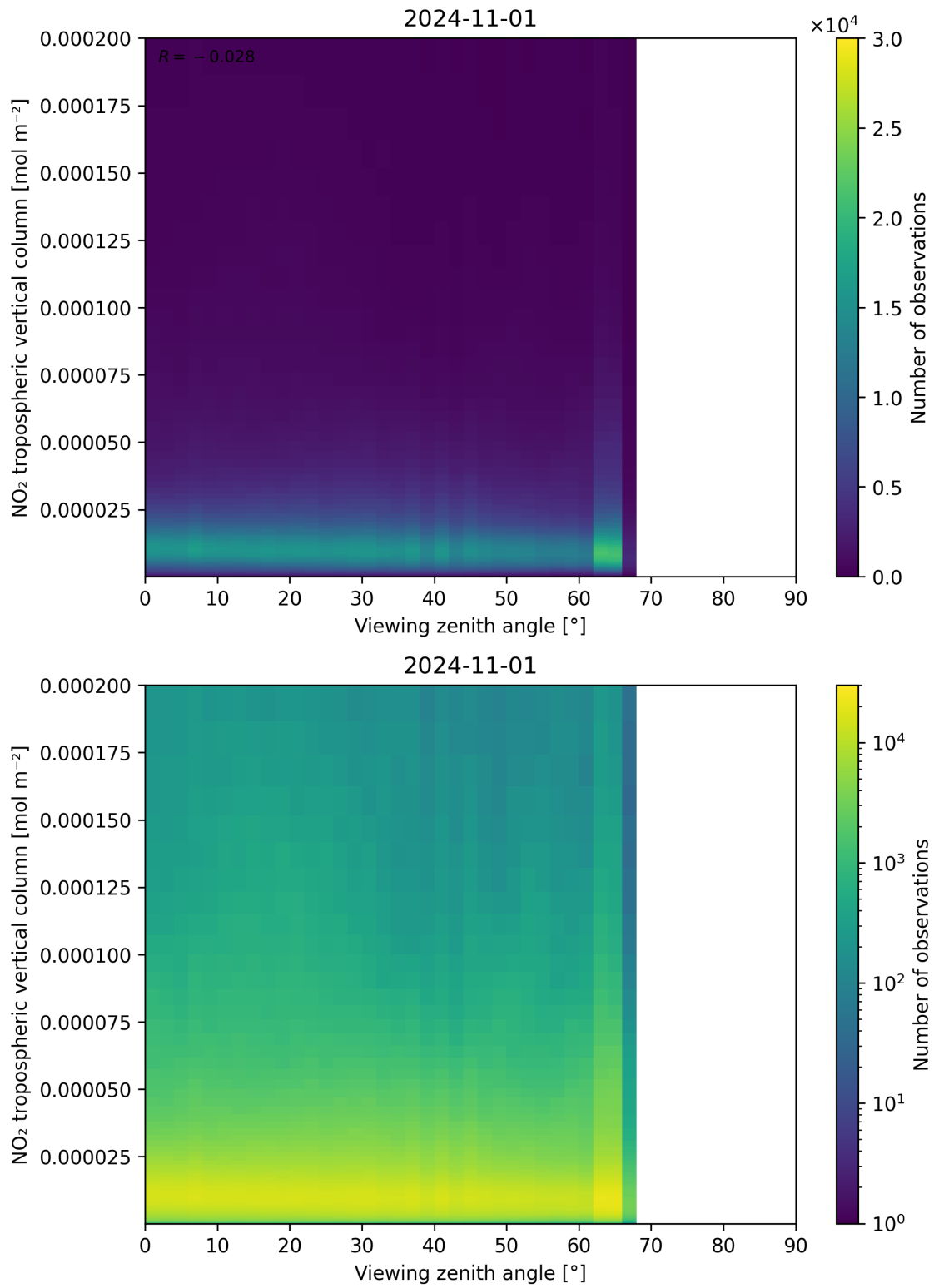
Figure 169: Scatter density plot of “Viewing zenith angle” against “NO 2 tropospheric vertical column” for 2024-10-31 to 2024-11-02.
