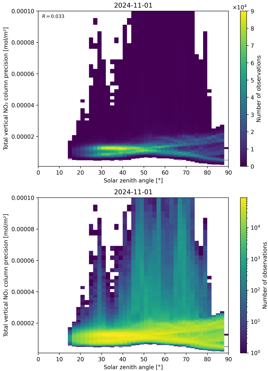
Figure 154: Scatter density plot of “Solar zenith angle” against “Total vertical NO 2 column precision” for 2024-10-31 to 2024-11-02.
