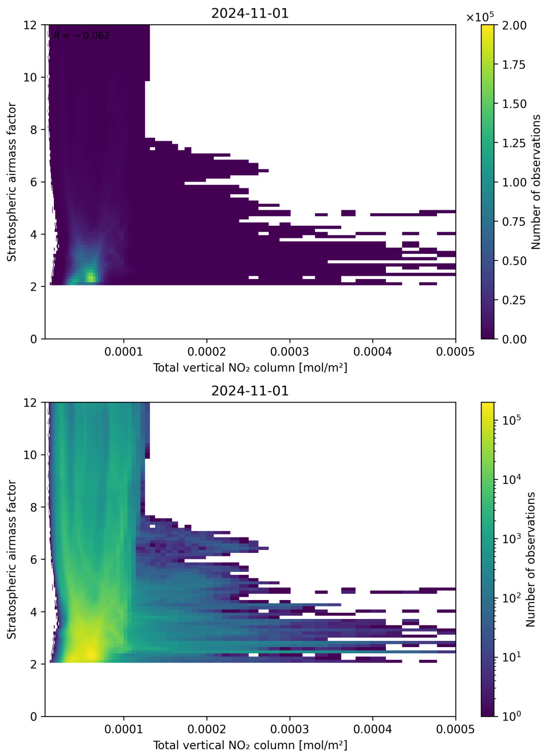
Figure 110: Scatter density plot of “Total vertical NO 2 column” against “Stratospheric airmass factor” for 2024-10-31 to 2024-11-02.
