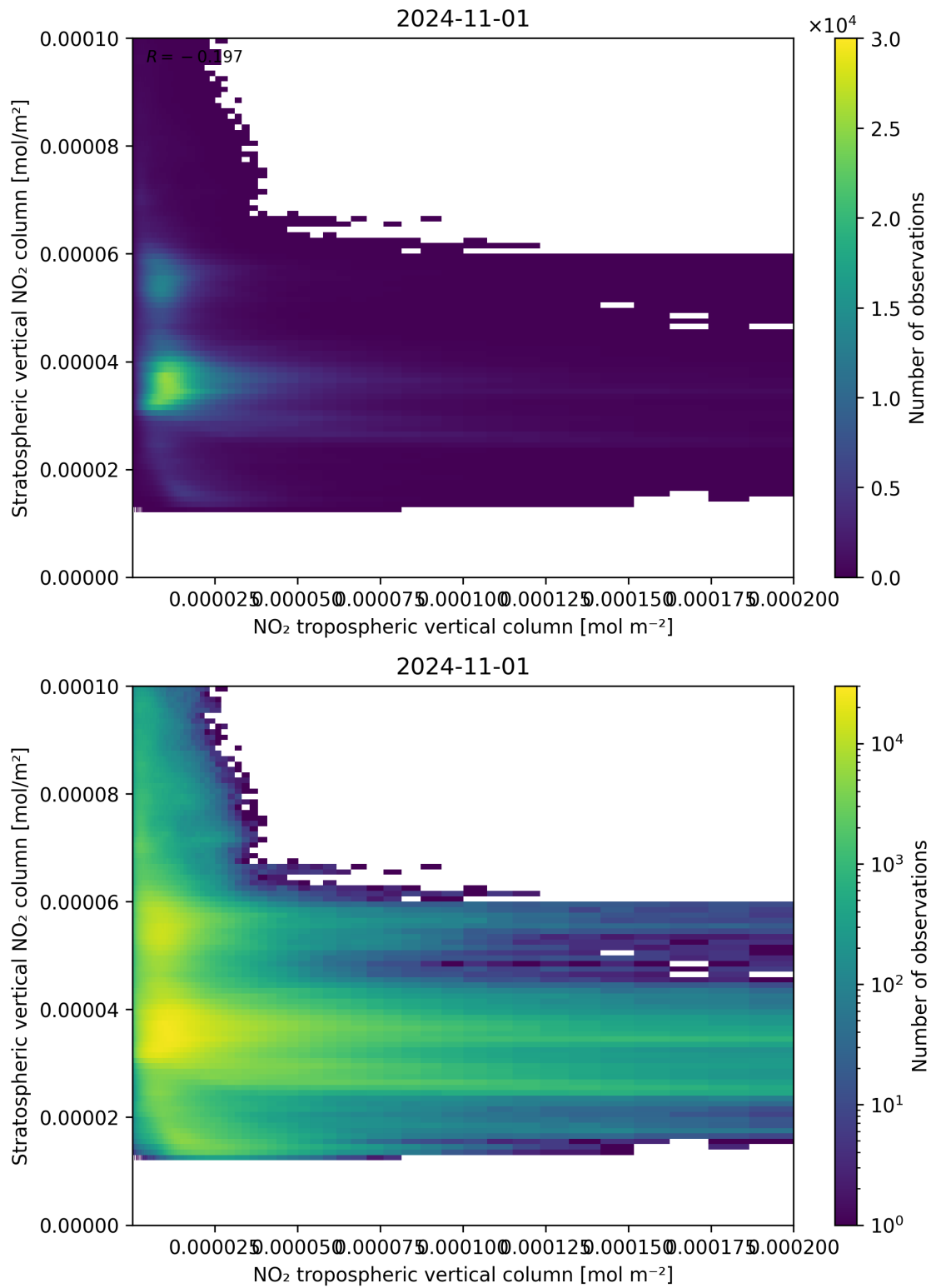
Figure 125: Scatter density plot of “NO 2 tropospheric vertical column” against “Stratospheric vertical NO 2 column” for 2024-10-31 to 2024-11-02.
