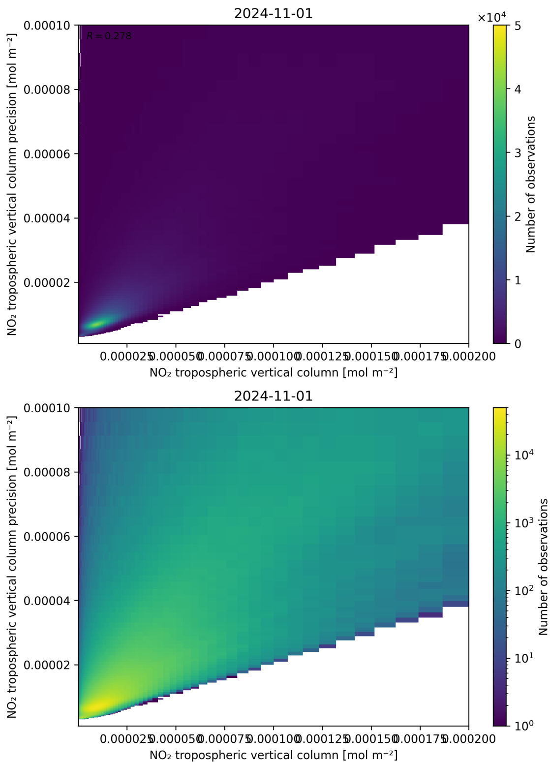
Figure 130: Scatter density plot of “NO 2 tropospheric vertical column” against “NO 2 tropospheric vertical column precision” for 2024-10-31 to 2024-11-02.
