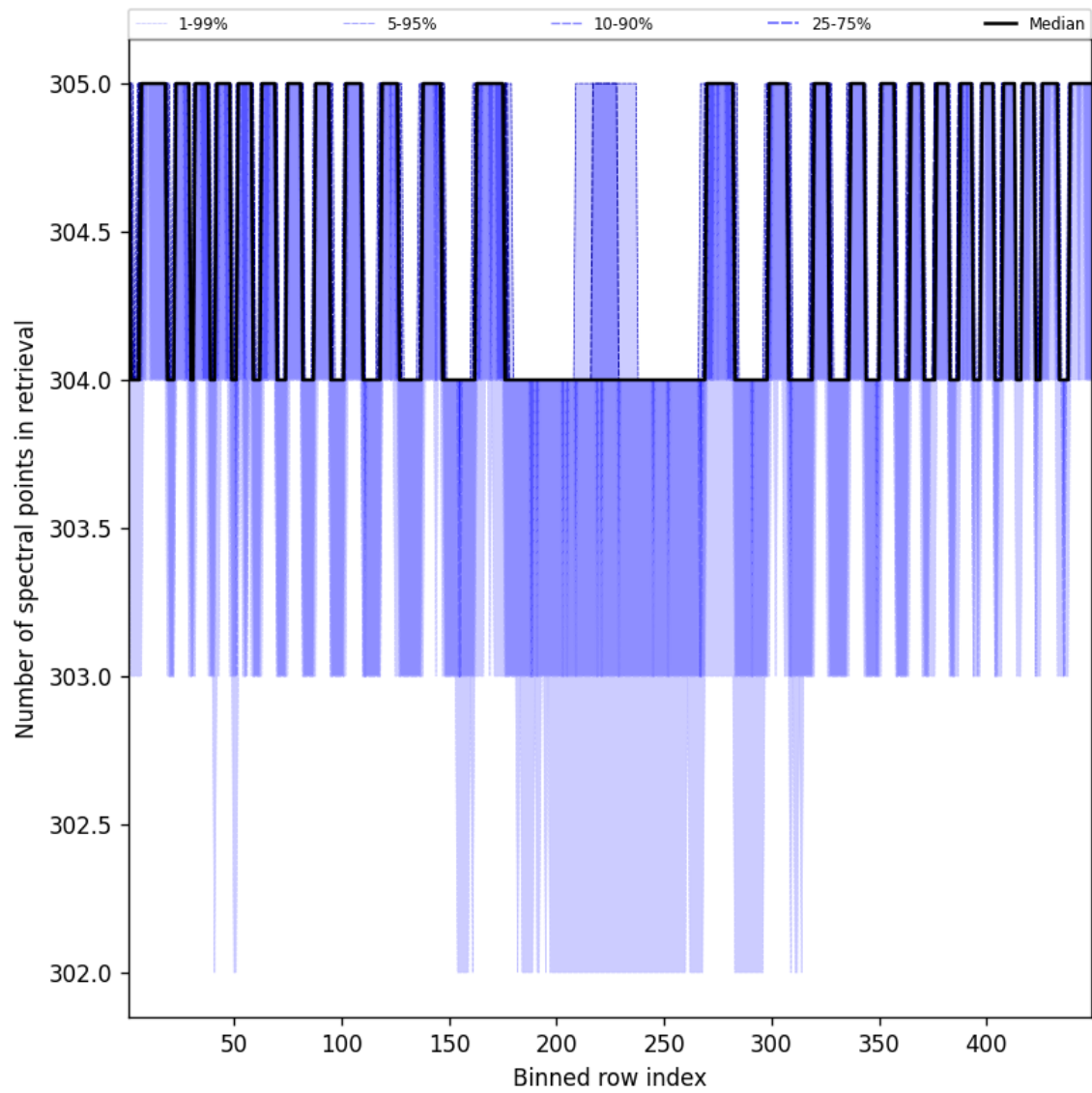
Figure 50: Along track statistics of “Number of spectral points in retrieval” for 2024-10-31 to 2024-11-02
