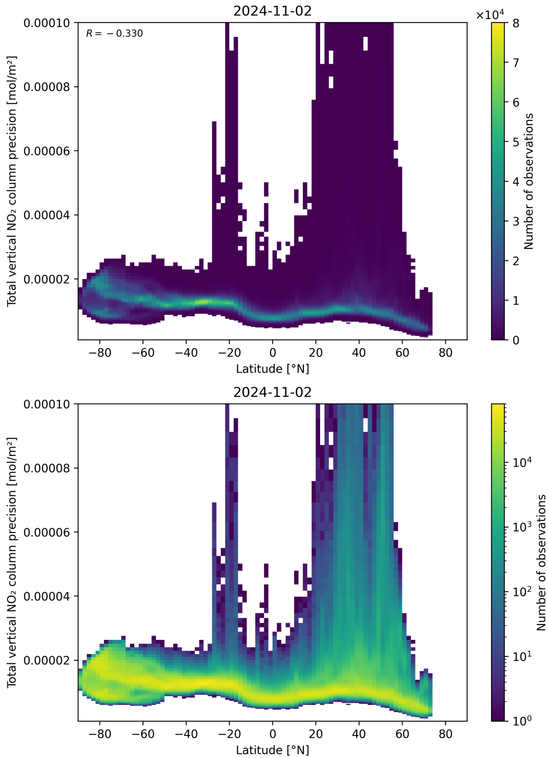
Figure 91: Scatter density plot of “Latitude” against “Total vertical NO 2 column precision” for 2024-11-01 to 2024-11-03.
