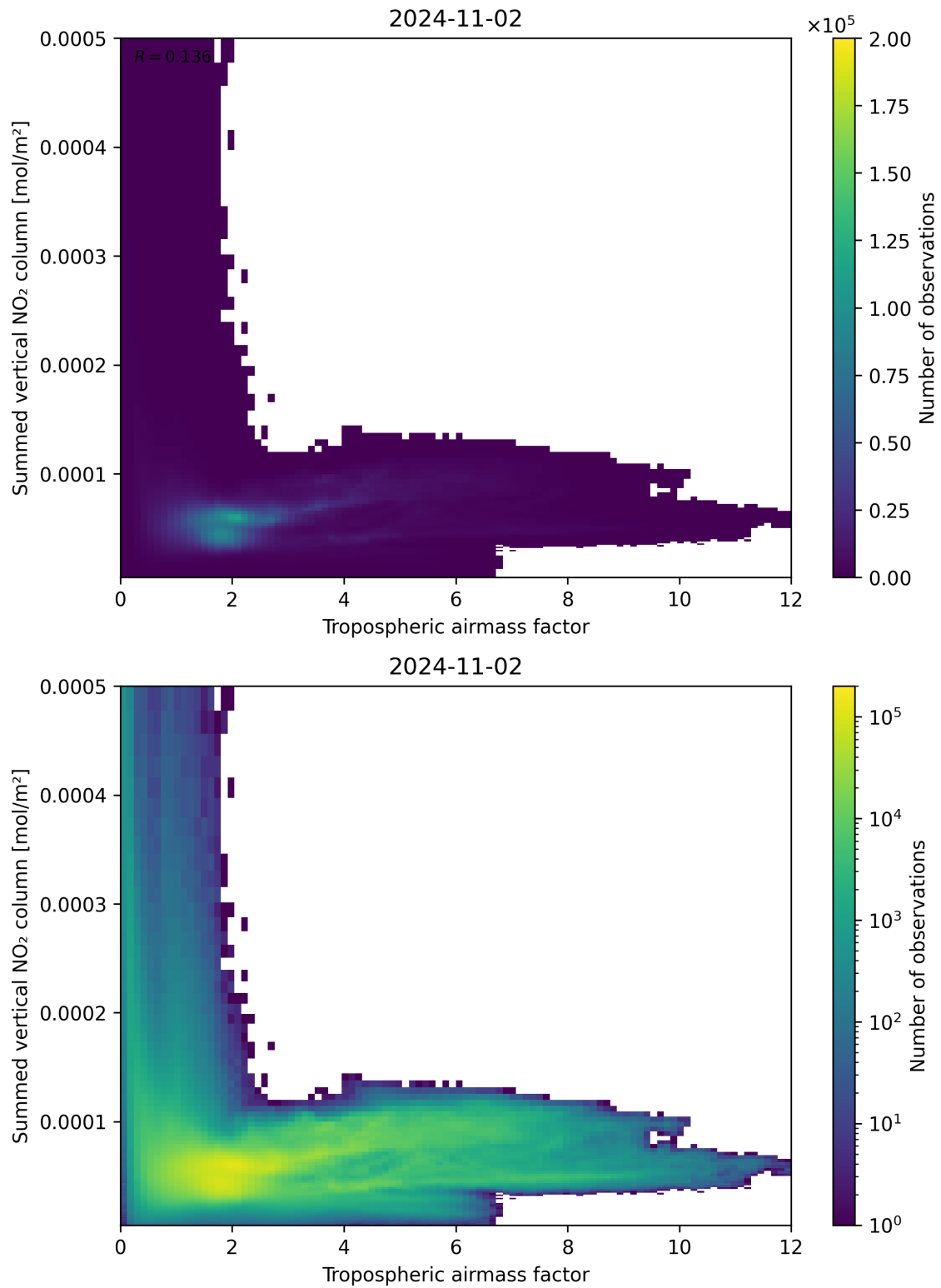
Figure 75: Scatter density plot of “Tropospheric air mass factor” against “Summed vertical NO 2 column” for 2024-11-01 to 2024-11-03.
