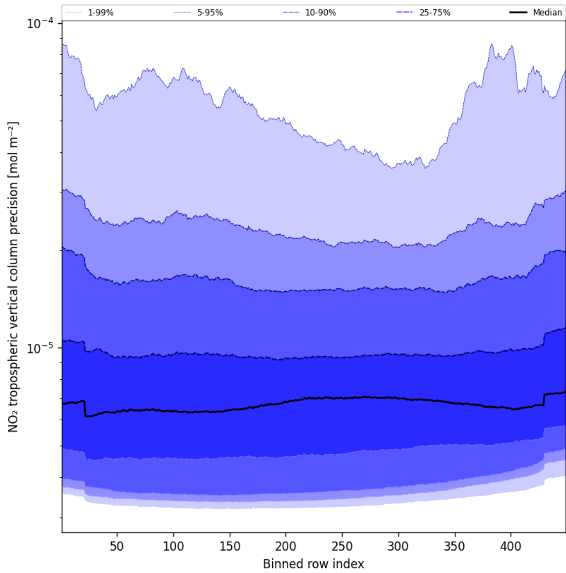
Figure 47: Along track statistics of “NO 2 tropospheric vertical column precision” for 2024-11-01 to 2024-11-03
