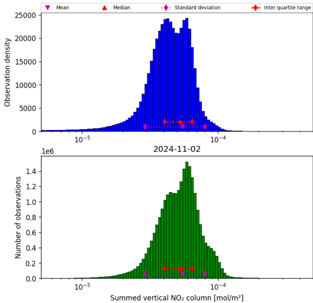
Figure 40: Histogram of “Summed vertical NO 2 column” for 2024-11-01 to 2024-11-03
