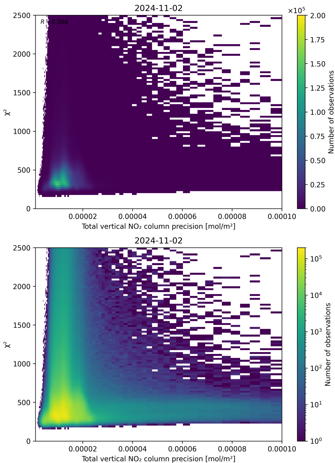
Figure 116: Scatter density plot of “Total vertical NO 2 column precision” against “ \chi^2 ” for 2024-11-01 to 2024-11-03.
