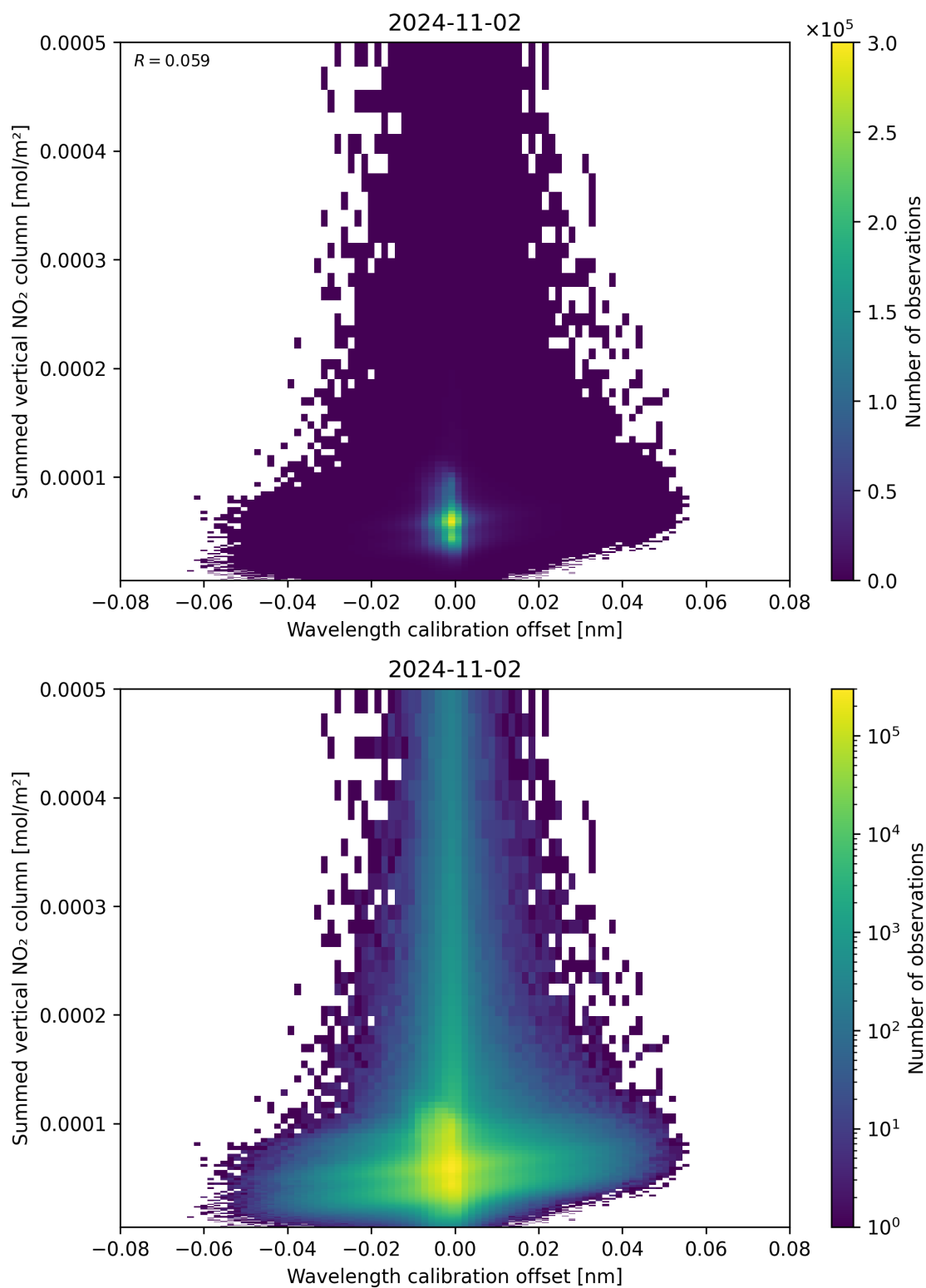
Figure 177: Scatter density plot of “Wavelength calibration offset” against “Summed vertical NO 2 column” for 2024-11-01 to 2024-11-03.
