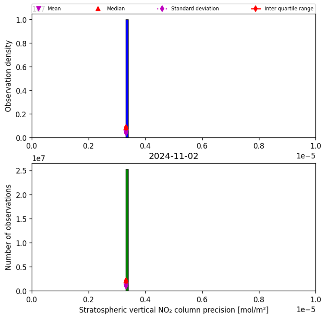
Figure 37: Histogram of “Stratospheric vertical NO 2 column precision” for 2024-11-01 to 2024-11-03
