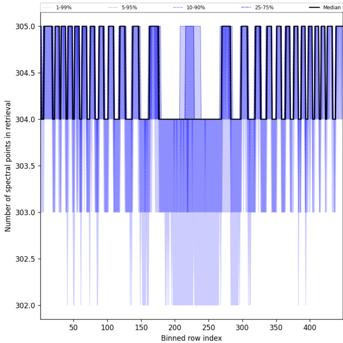
Figure 50: Along track statistics of “Number of spectral points in retrieval” for 2024-11-01 to 2024-11-03
