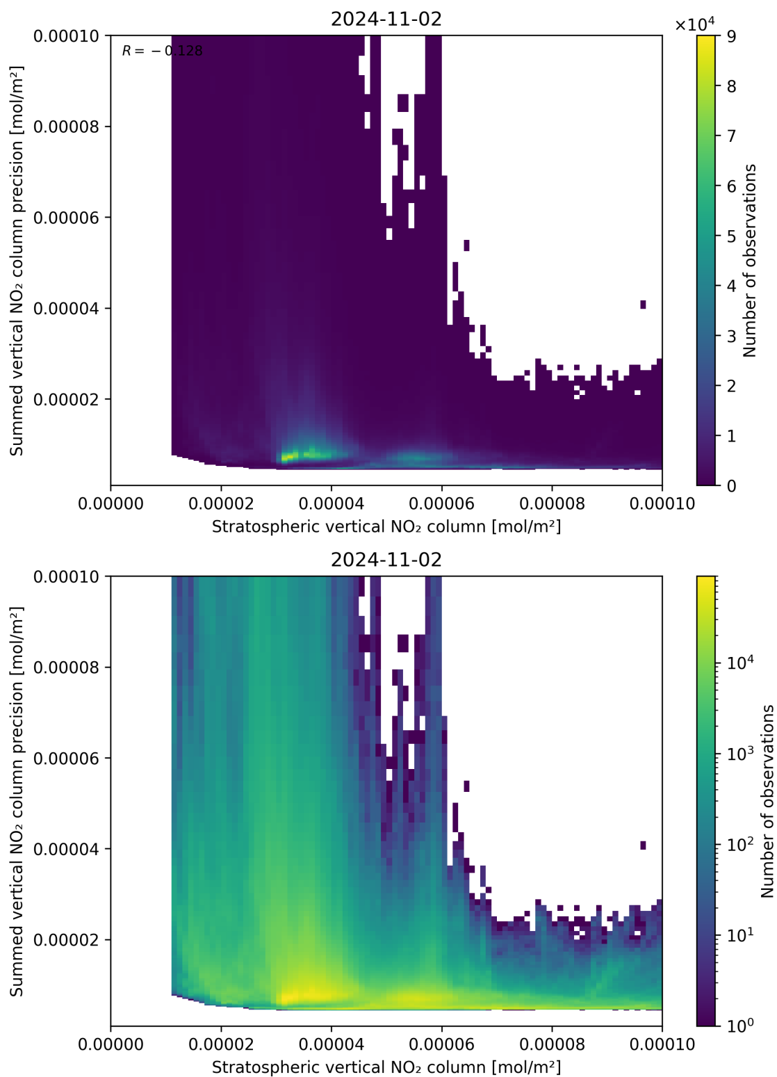
Figure 99: Scatter density plot of “Stratospheric vertical NO 2 column” against “Summed vertical NO 2 column precision” for 2024-11-01 to 2024-11-03.
