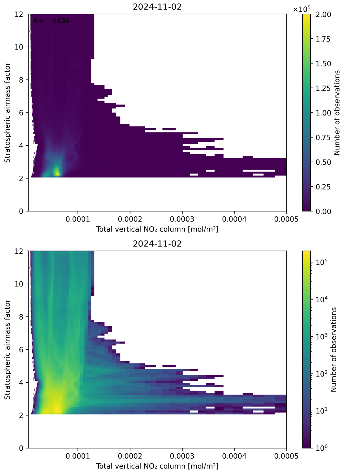
Figure 110: Scatter density plot of “Total vertical NO 2 column” against “Stratospheric airmass factor” for 2024-11-01 to 2024-11-03.
