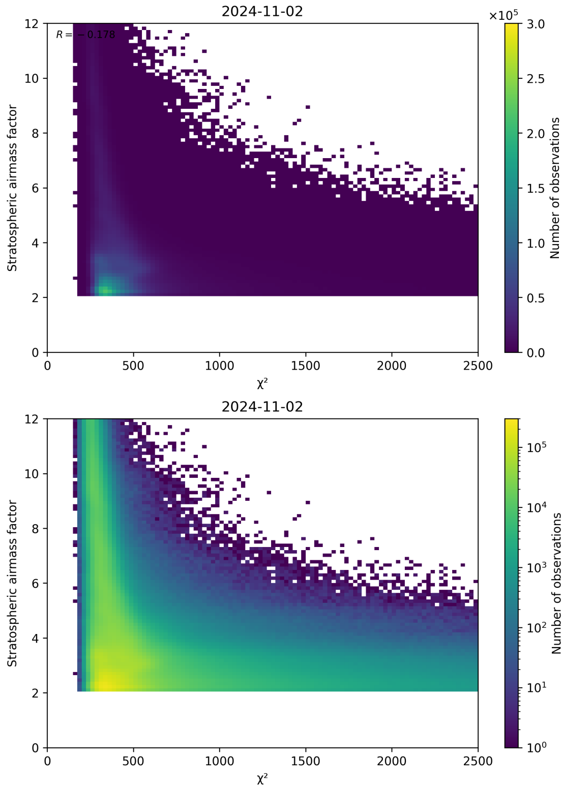
Figure 81: Scatter density plot of “ \chi^2 ” against “Stratospheric airmass factor” for 2024-11-01 to 2024-11-03.
