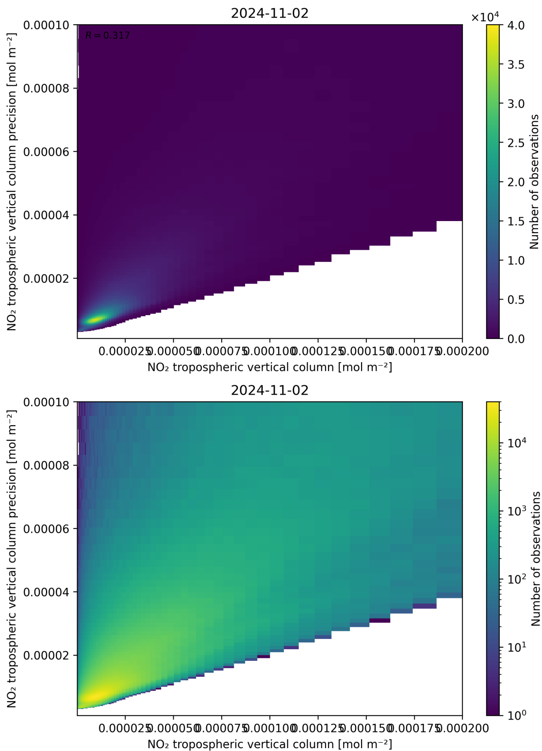
Figure 130: Scatter density plot of “NO 2 tropospheric vertical column” against “NO 2 tropospheric vertical column precision” for 2024-11-01 to 2024-11-03.
