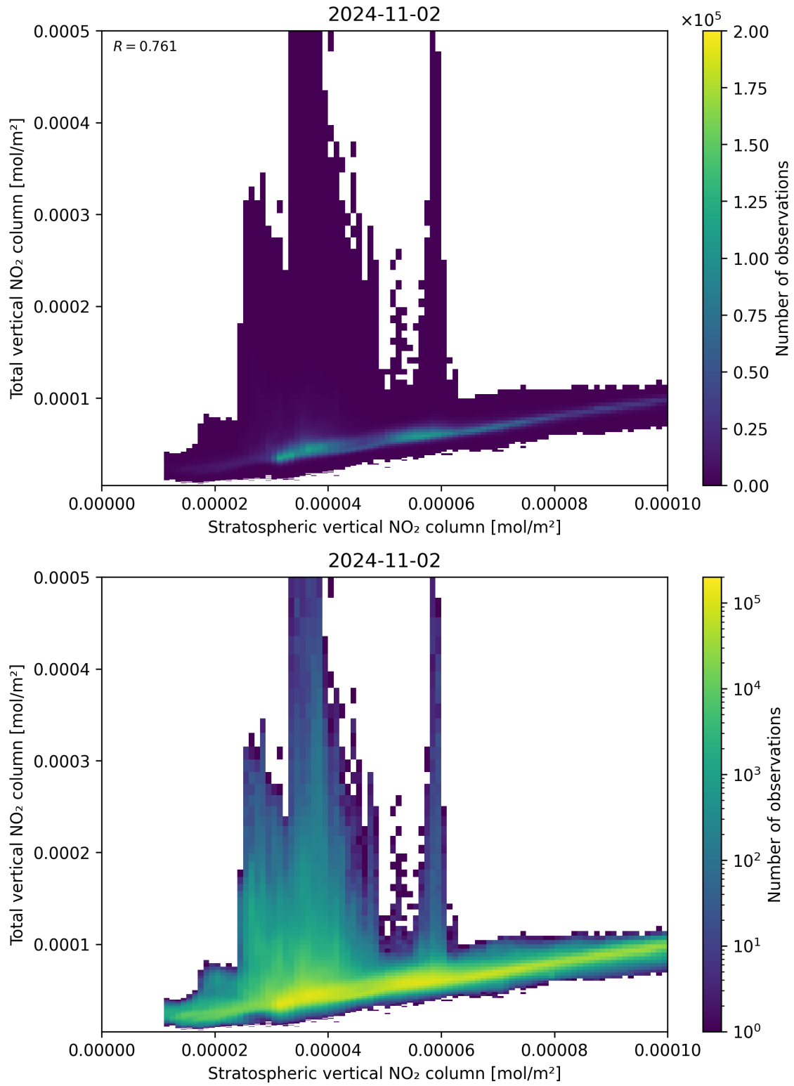
Figure 100: Scatter density plot of “Stratospheric vertical NO 2 column” against “Total vertical NO 2 column” for 2024-11-01 to 2024-11-03.
