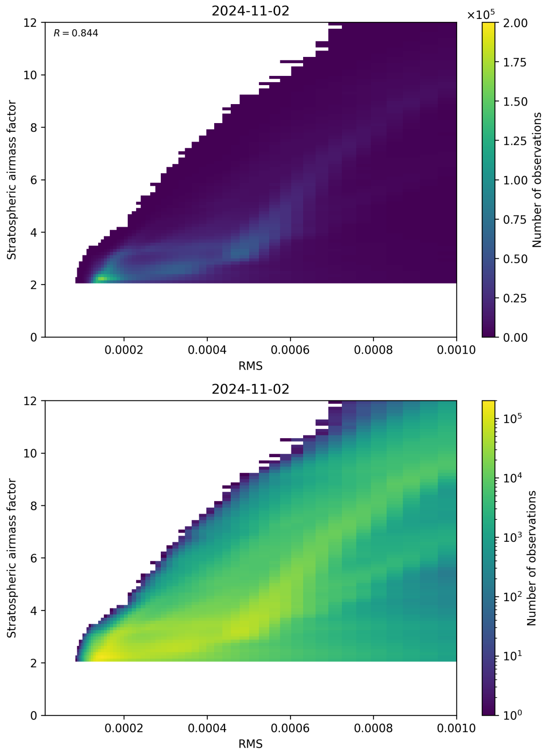
Figure 144: Scatter density plot of “RMS” against “Stratospheric airmass factor” for 2024-11-01 to 2024-11-03.
