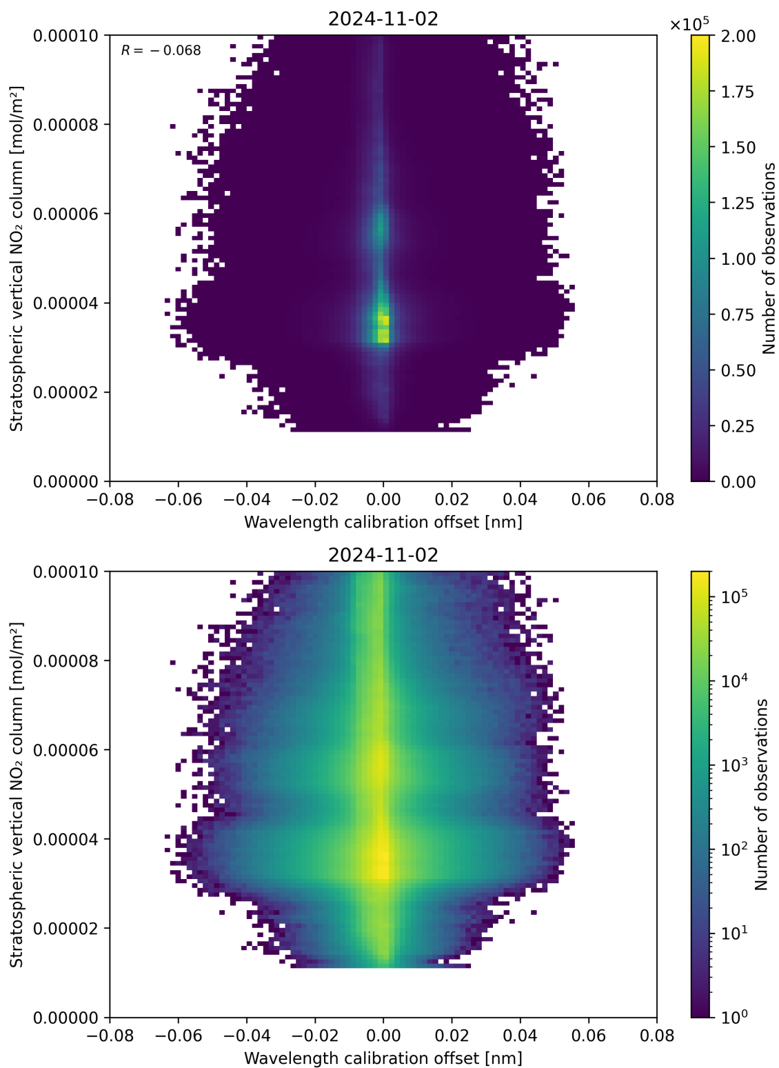
Figure 176: Scatter density plot of “Wavelength calibration offset” against “Stratospheric vertical NO 2 column” for 2024-11-01 to 2024-11-03.
