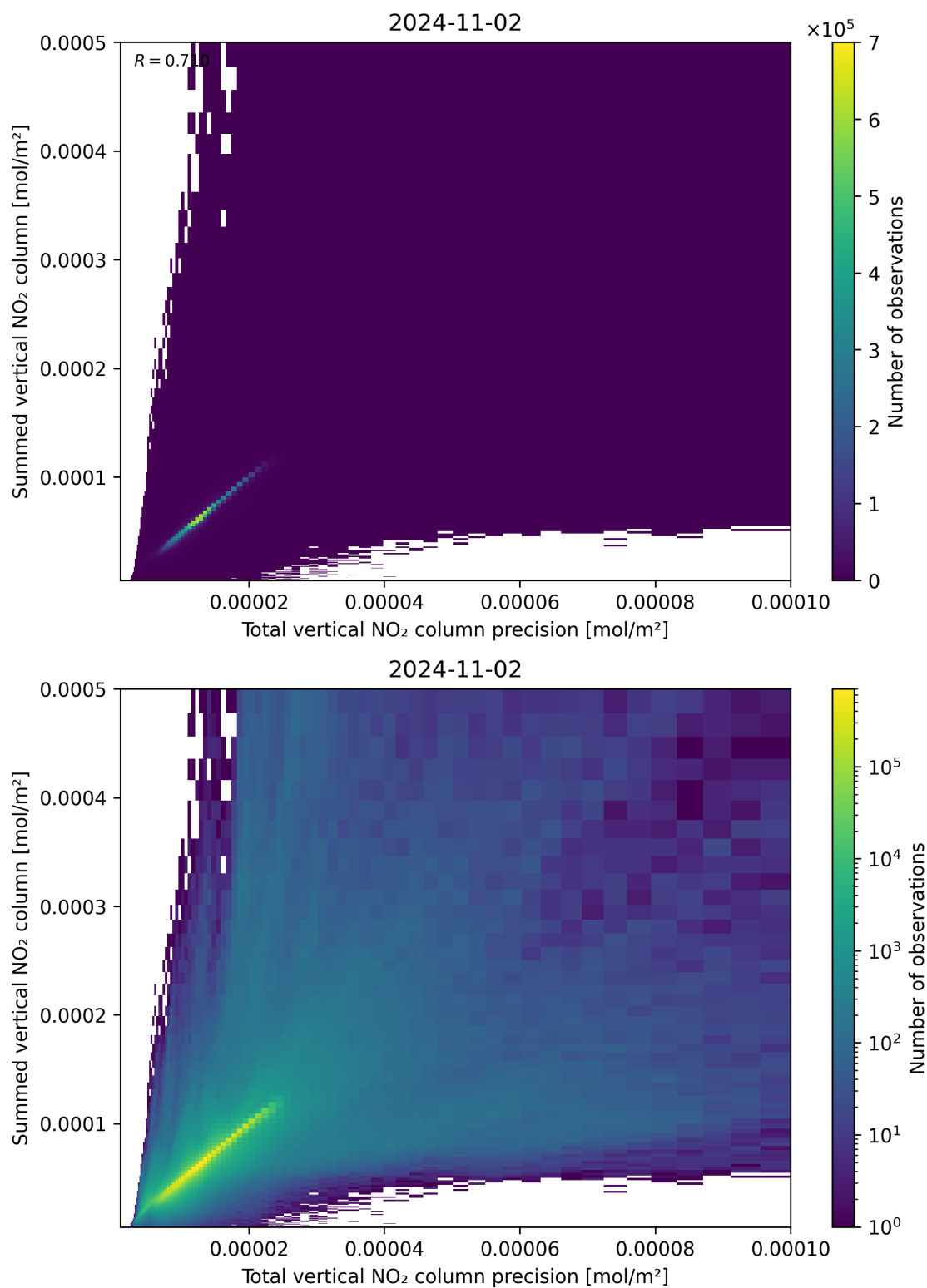
Figure 117: Scatter density plot of “Total vertical NO 2 column precision” against “Summed vertical NO 2 column” for 2024-11-01 to 2024-11-03.
