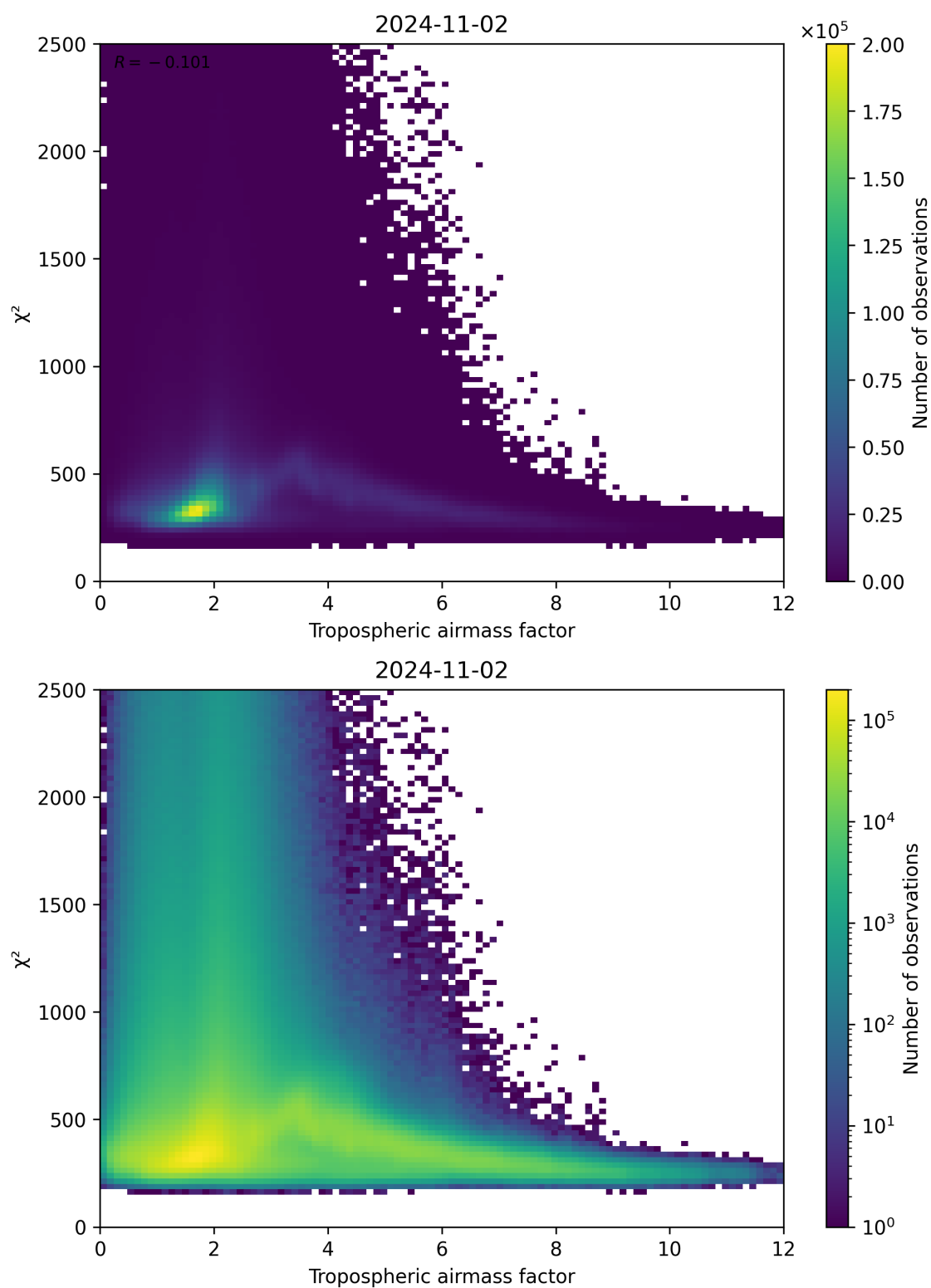
Figure 73: Scatter density plot of “Tropospheric airmass factor” against “ \chi^2 ” for 2024-11-01 to 2024-11-03.
