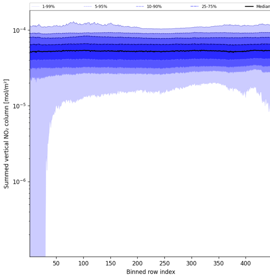
Figure 57: Along track statistics of “Summed vertical NO 2 column” for 2024-11-01 to 2024-11-03
