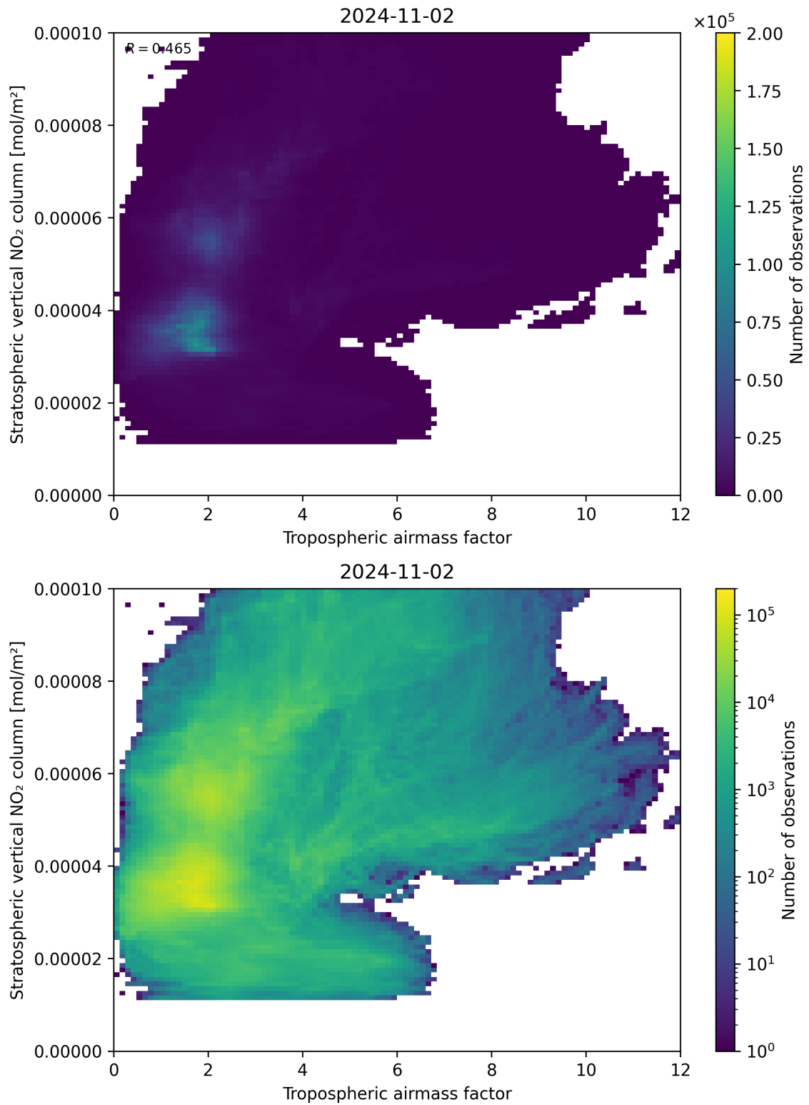
Figure 74: Scatter density plot of “Tropospheric airmass factor” against “Stratospheric vertical NO 2 column” for 2024-11-01 to 2024-11-03.
