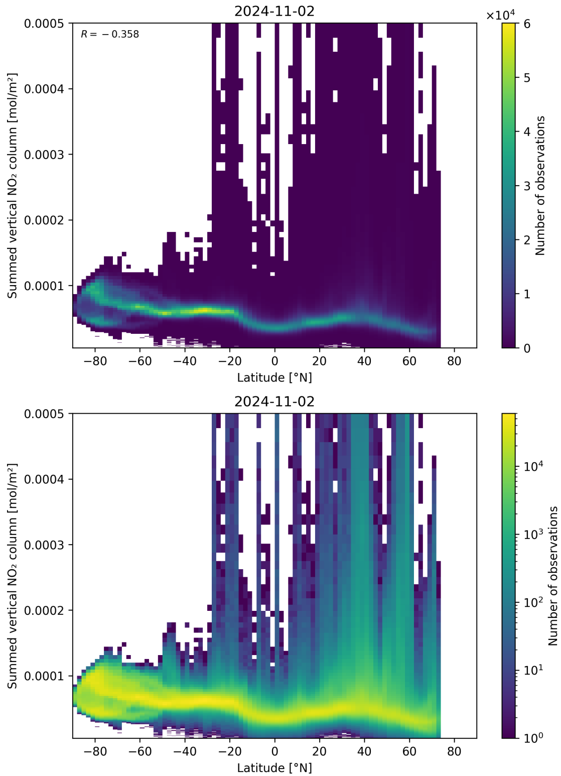
Figure 88: Scatter density plot of “Latitude” against “Summed vertical NO 2 column” for 2024-11-01 to 2024-11-03.
