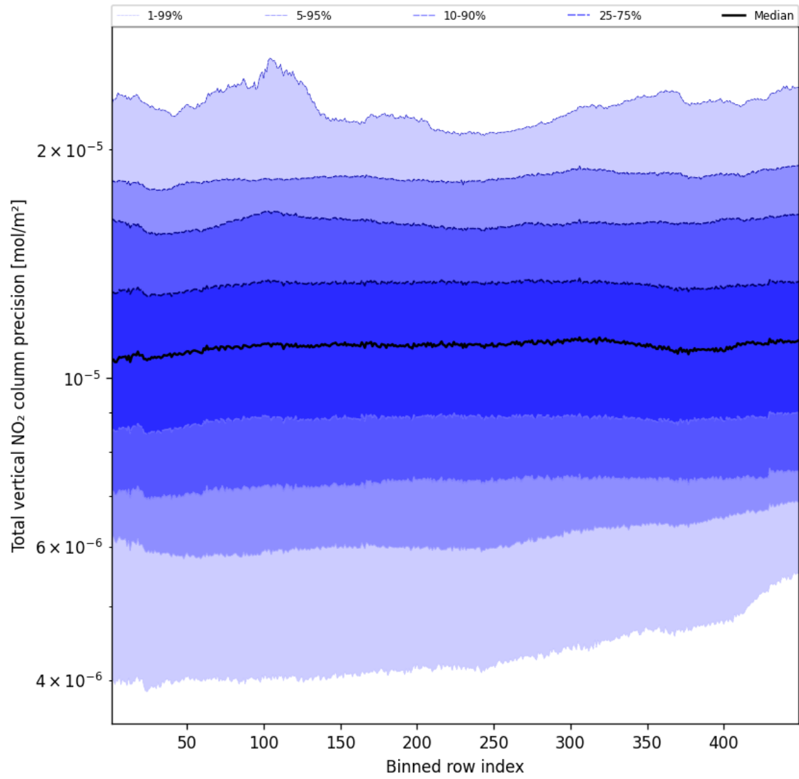
Figure 56: Along track statistics of “Total vertical NO 2 column precision” for 2024-11-01 to 2024-11-03
