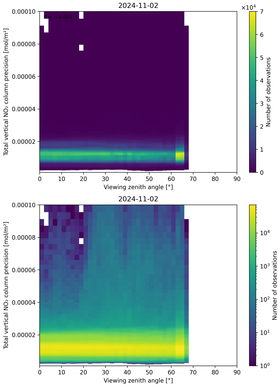
Figure 168: Scatter density plot of “Viewing zenith angle” against “Total vertical NO 2 column precision” for 2024-11-01 to 2024-11-03.
