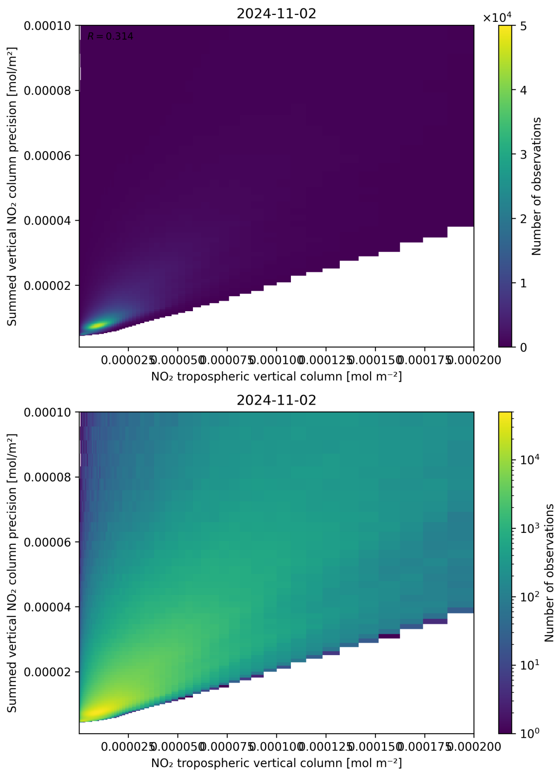
Figure 127: Scatter density plot of “NO 2 tropospheric vertical column” against “Summed vertical NO 2 column precision” for 2024-11-01 to 2024-11-03.
