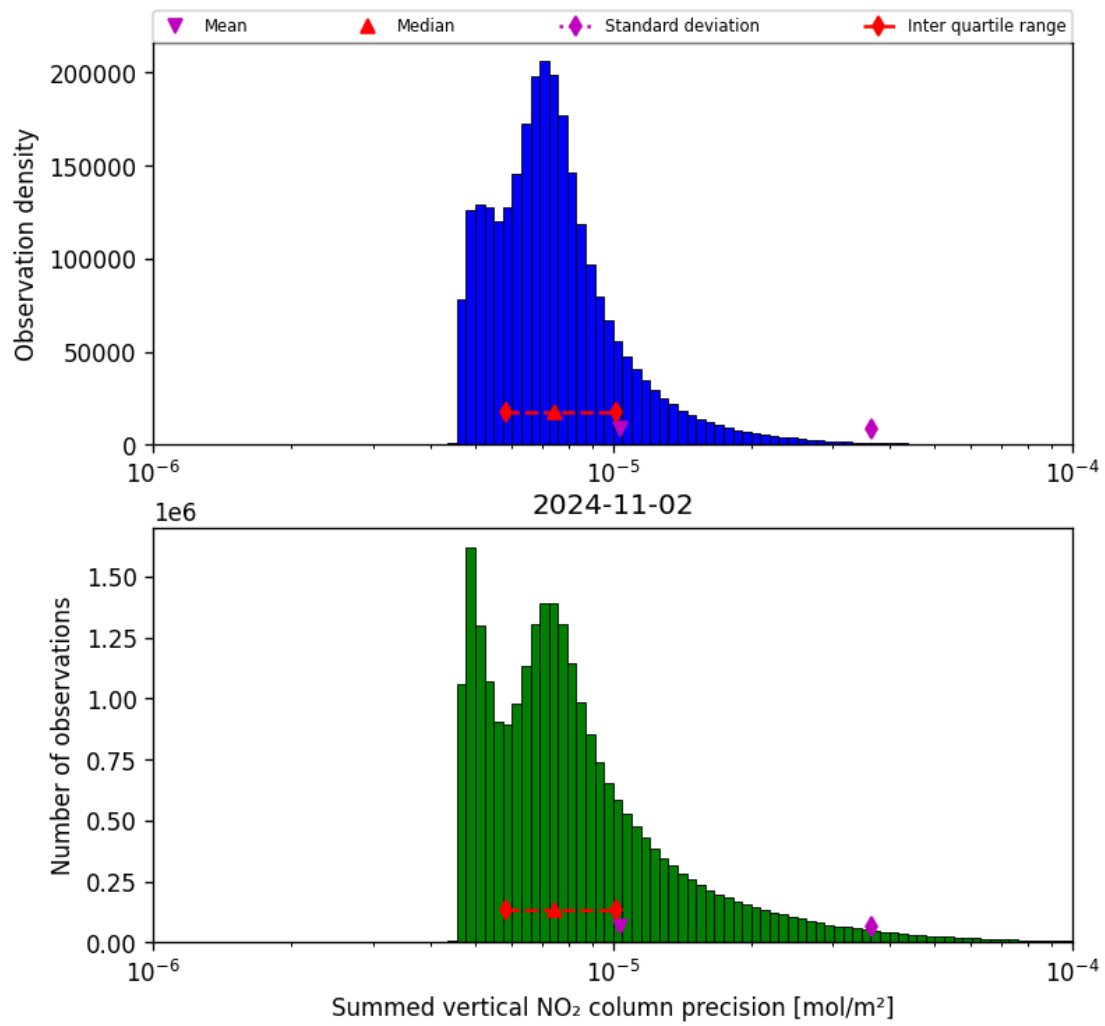
Figure 41: Histogram of "Summed vertical NO 2 column precision" for 2024-11-01 to 2024-11-03
