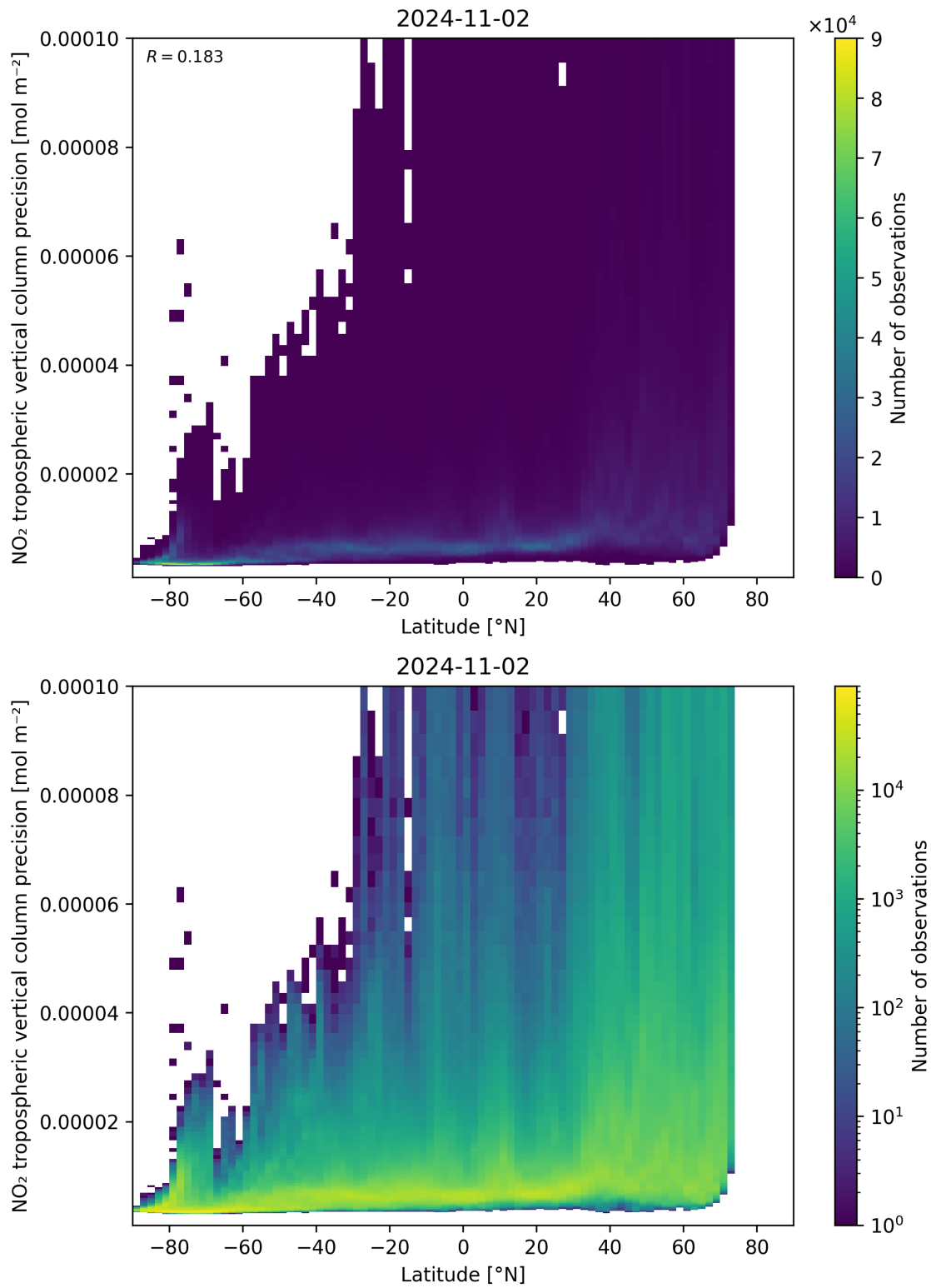
Figure 93: Scatter density plot of “Latitude” against “NO 2 tropospheric vertical column precision” for 2024-11-01 to 2024-11-03.
