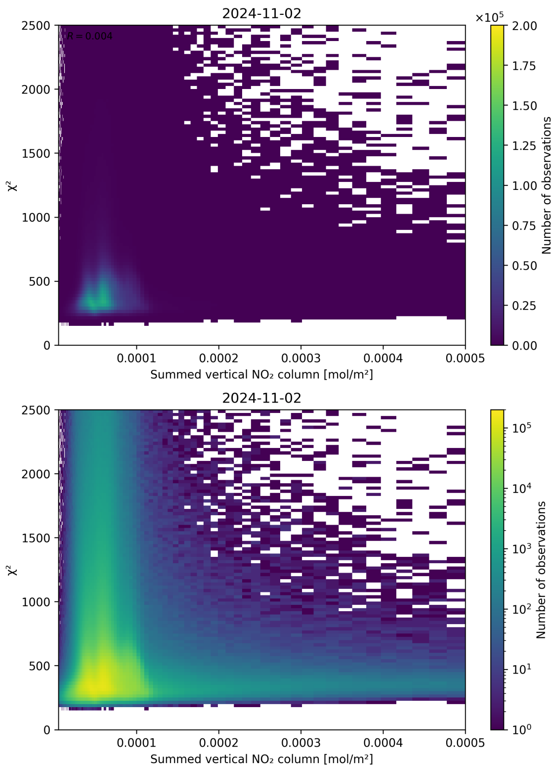
Figure 104: Scatter density plot of “Summed vertical NO 2 column” against “ \chi^2 ” for 2024-11-01 to 2024-11-03.
