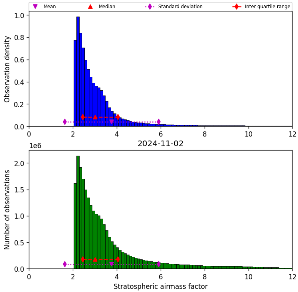
Figure 44: Histogram of “Stratospheric airmass factor” for 2024-11-01 to 2024-11-03
