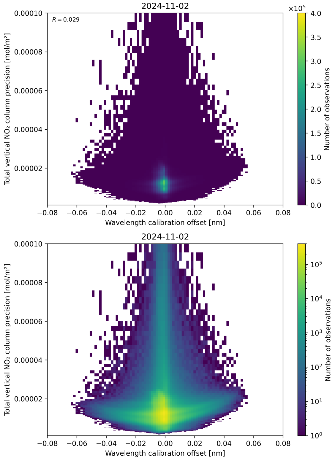
Figure 180: Scatter density plot of “Wavelength calibration offset” against “Total vertical NO 2 column precision” for 2024-11-01 to 2024-11-03.
