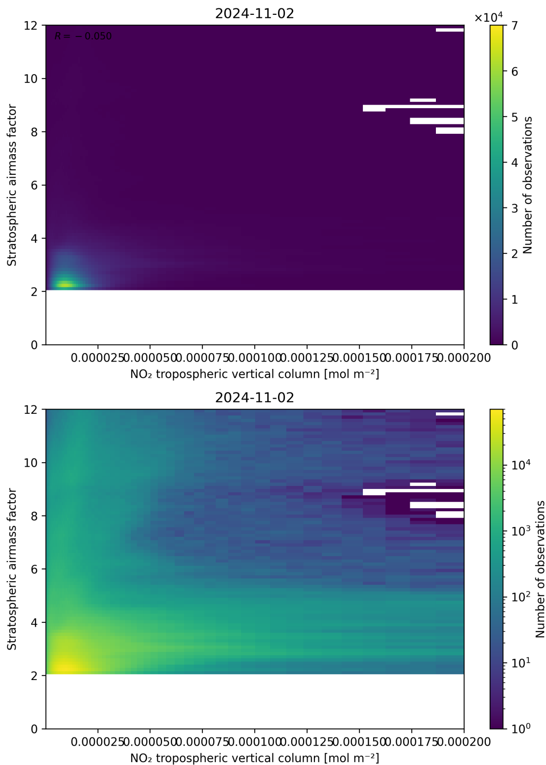
Figure 121: Scatter density plot of “NO 2 tropospheric vertical column” against “Stratospheric airmass factor” for 2024-11-01 to 2024-11-03.
