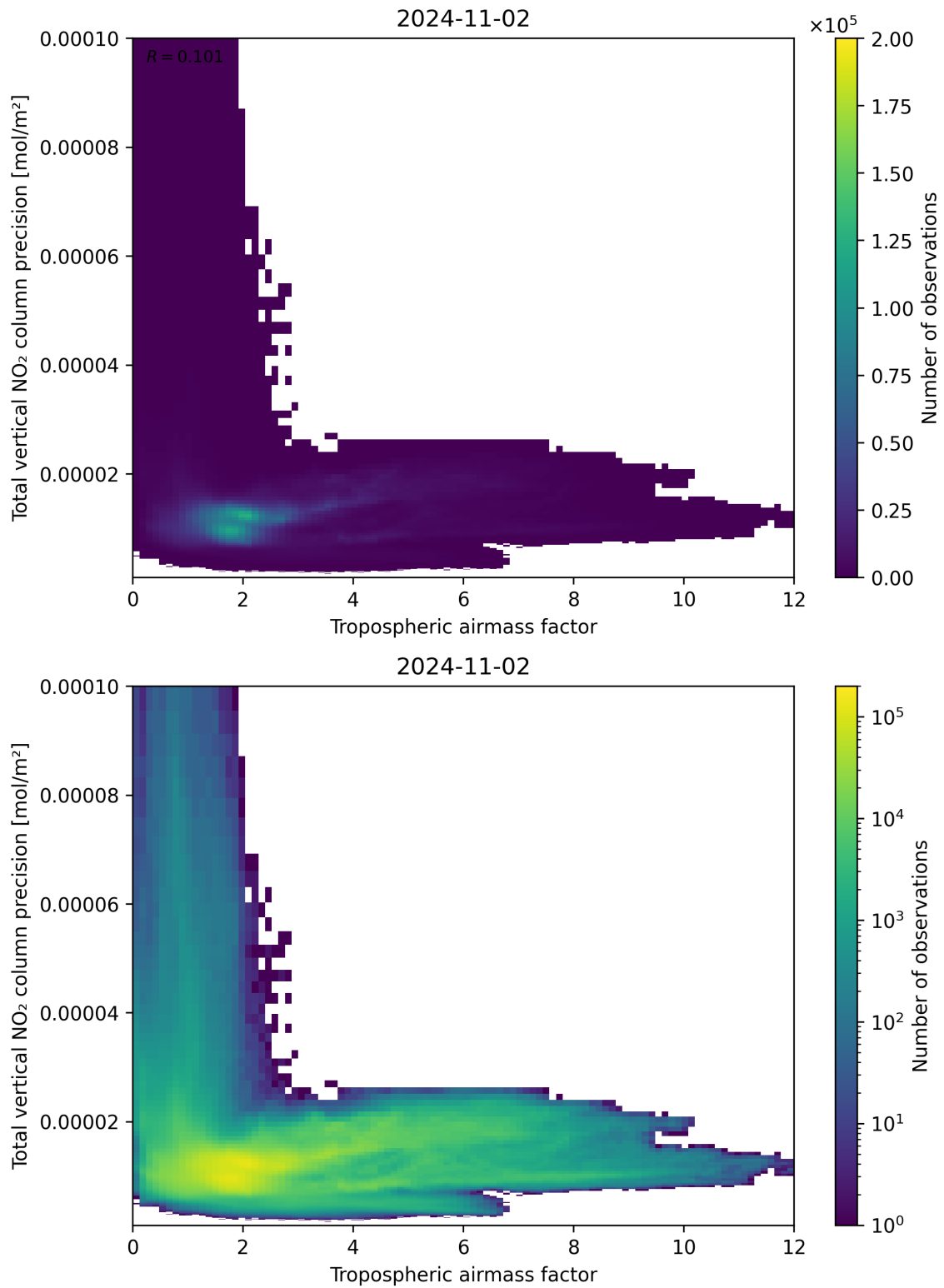
Figure 78: Scatter density plot of “Tropospheric air mass factor” against “Total vertical NO 2 column precision” for 2024-11-01 to 2024-11-03.
