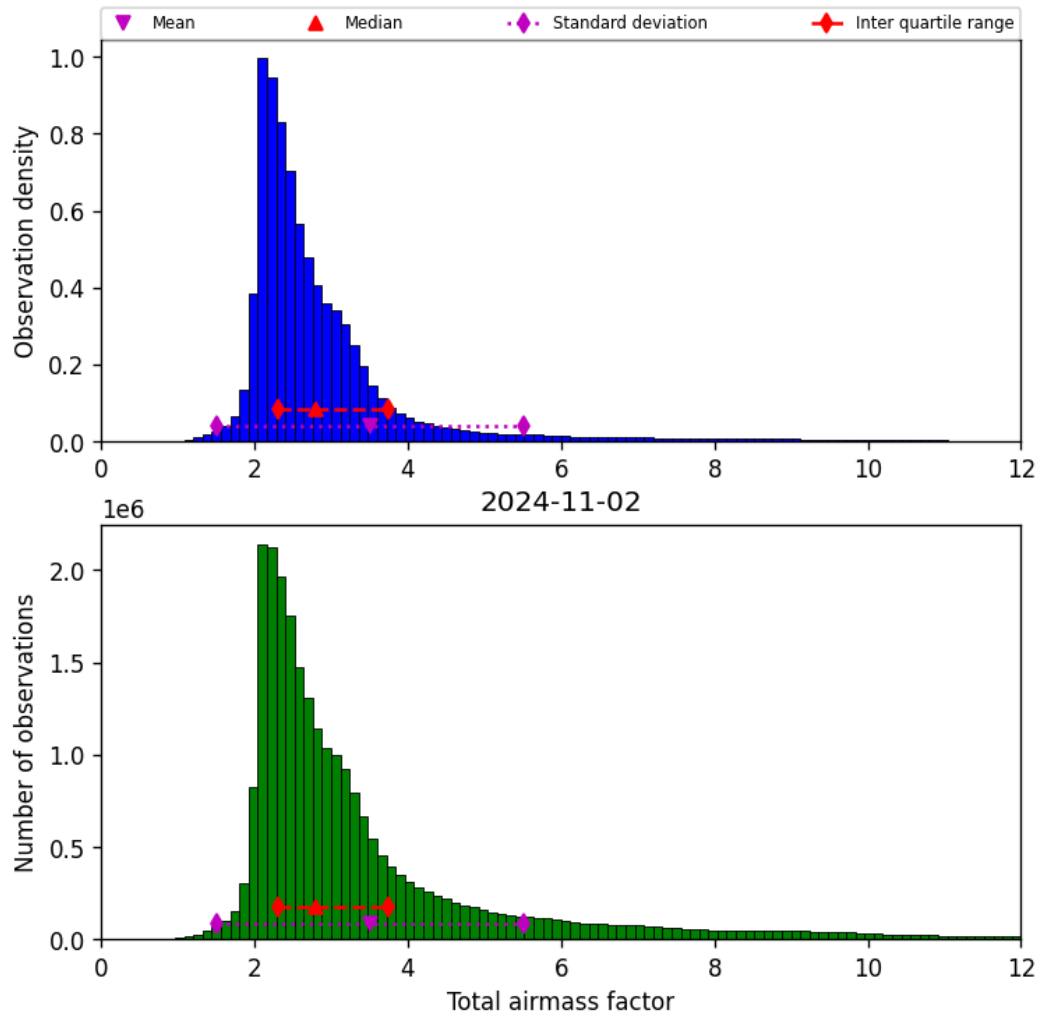
Figure 32: Histogram of “Total airmass factor” for 2024-11-01 to 2024-11-03
