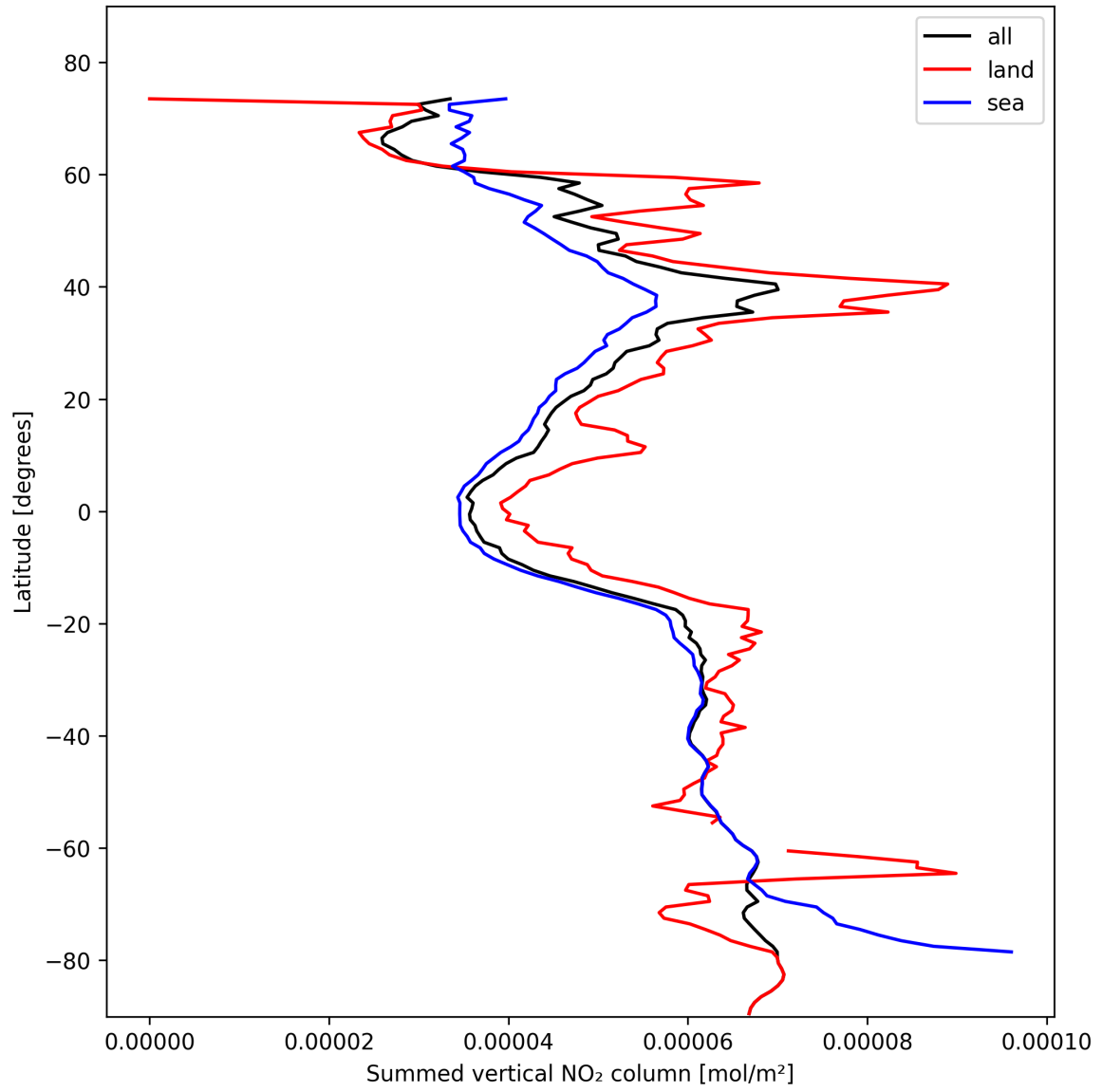
Figure 23: Zonal average of “Summed vertical NO 2 column” for 2024-11-01 to 2024-11-03.
