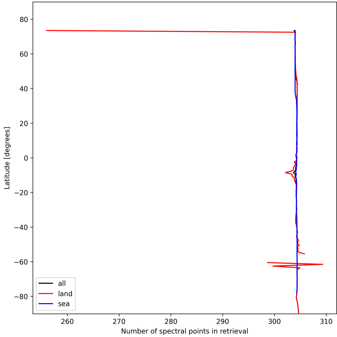
Figure 16: Zonal average of “Number of spectral points in retrieval” for 2024-11-01 to 2024-11-03.
