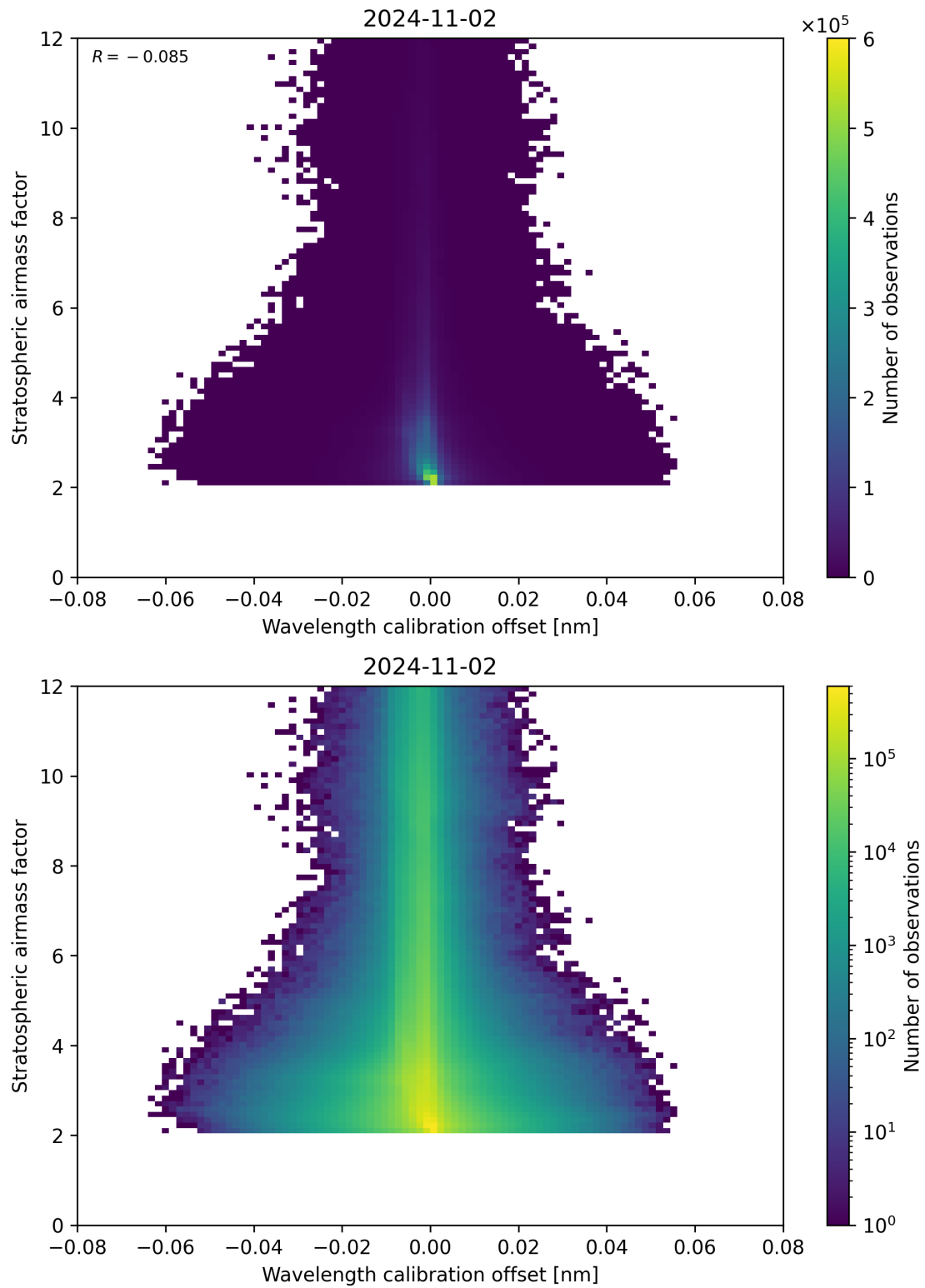
Figure 174: Scatter density plot of “Wavelength calibration offset” against “Stratospheric airmass factor” for 2024-11-01 to 2024-11-03.
