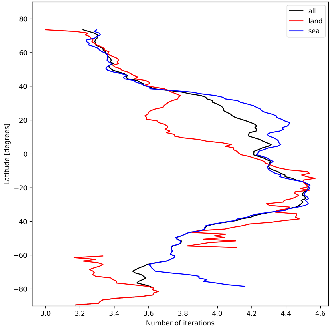
Figure 17: Zonal average of “Number of iterations” for 2024-11-01 to 2024-11-03.
