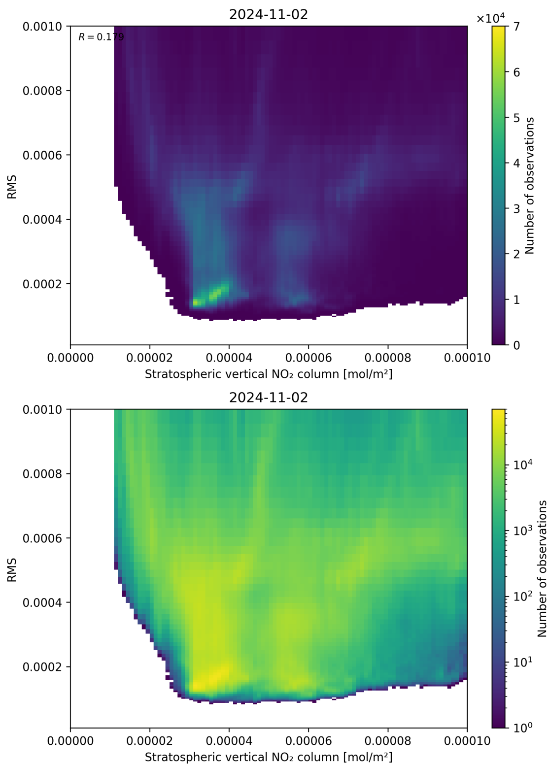
Figure 102: Scatter density plot of “Stratospheric vertical NO 2 column” against “RMS” for 2024-11-01 to 2024-11-03.
