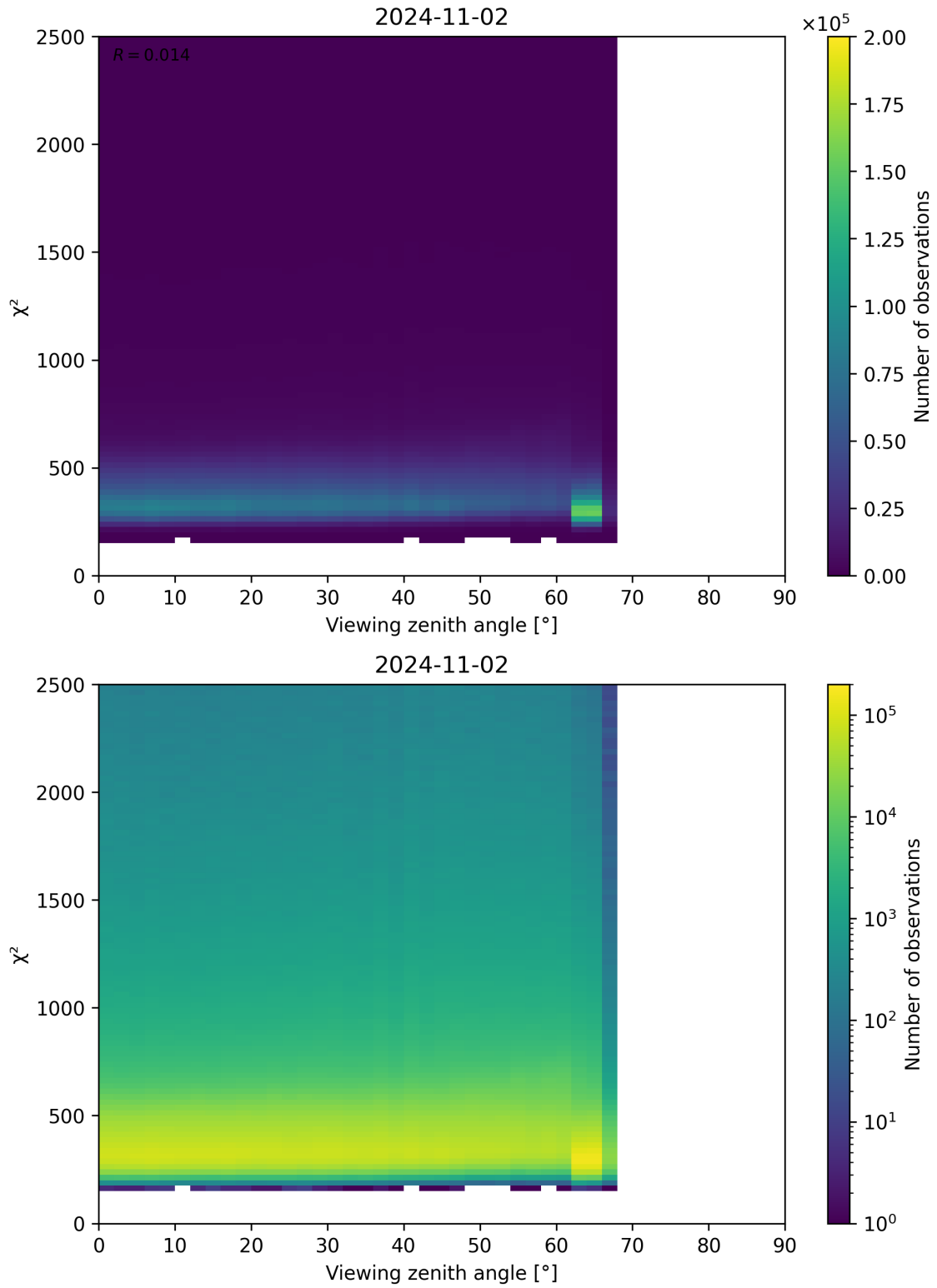
Figure 162: Scatter density plot of “Viewing zenith angle” against “ \chi^2 ” for 2024-11-01 to 2024-11-03.
