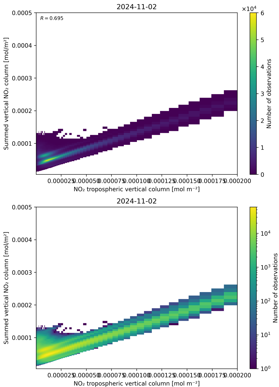
Figure 126: Scatter density plot of “NO 2 tropospheric vertical column” against “Summed vertical NO 2 column” for 2024-11-01 to 2024-11-03.
