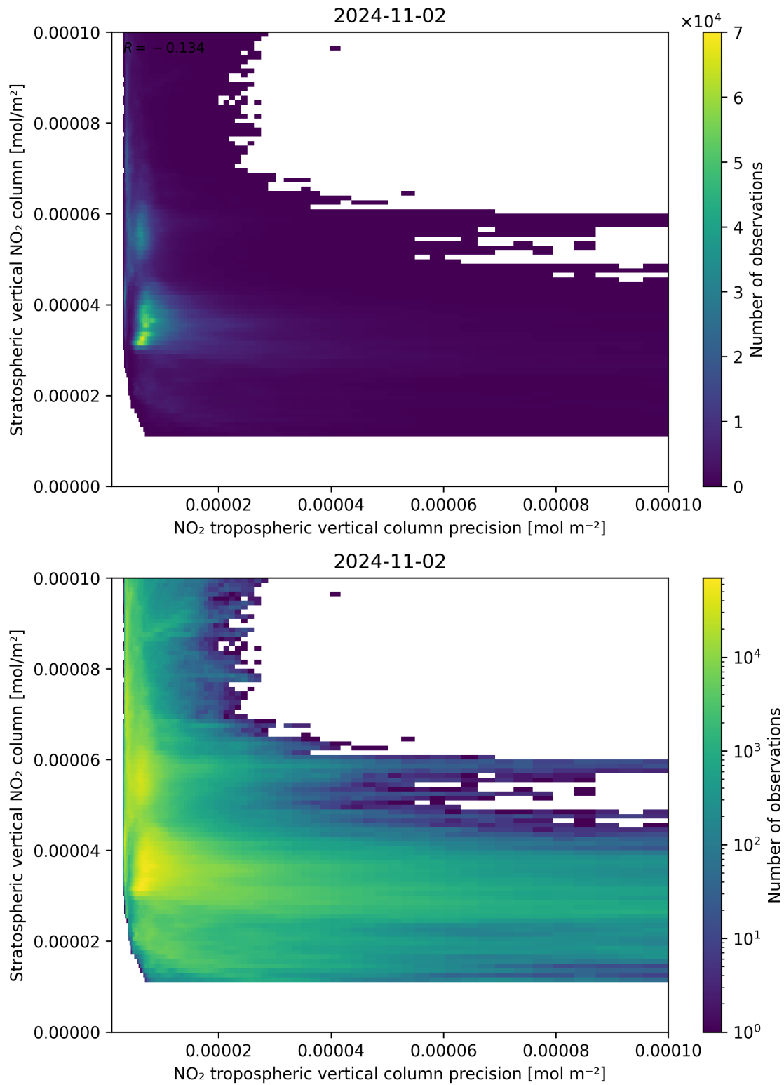
Figure 135: Scatter density plot of “NO 2 tropospheric vertical column precision” against “Stratospheric vertical NO 2 column” for 2024-11-01 to 2024-11-03.
