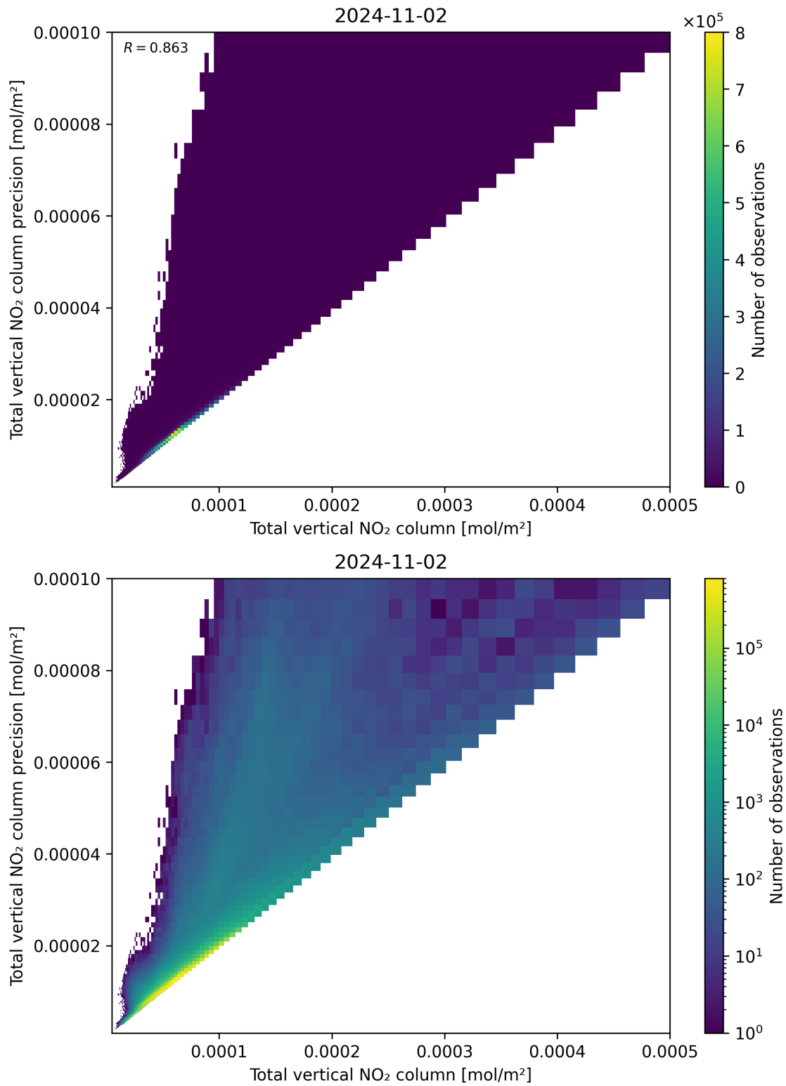
Figure 114: Scatter density plot of “Total vertical NO 2 column” against “Total vertical NO 2 column precision” for 2024-11-01 to 2024-11-03.
