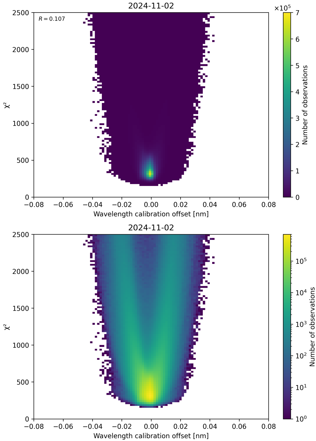
Figure 175: Scatter density plot of “Wavelength calibration offset” against “ \chi^2 ” for 2024-11-01 to 2024-11-03.
