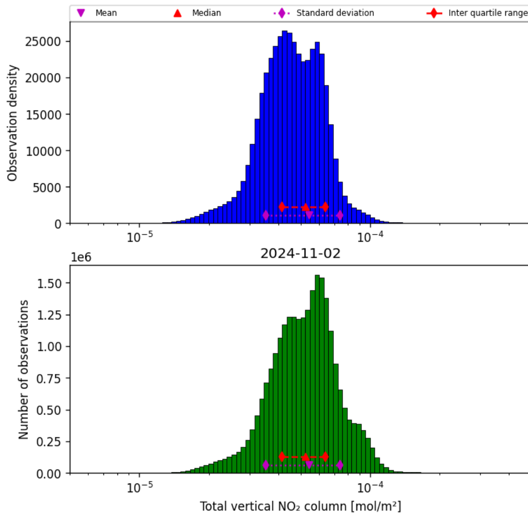
Figure 38: Histogram of “Total vertical NO 2 column” for 2024-11-01 to 2024-11-03
