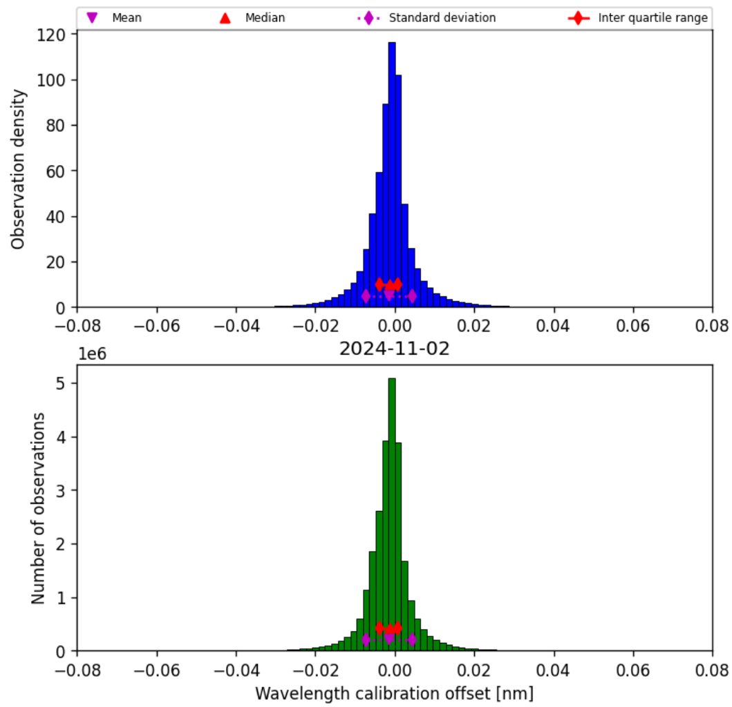
Figure 35: Histogram of “Wavelength calibration offset” for 2024-11-01 to 2024-11-03
