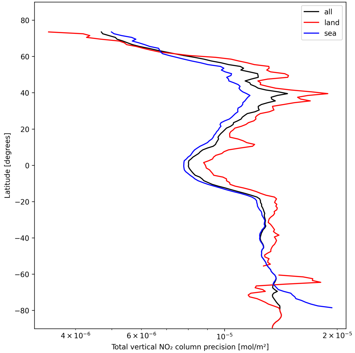
Figure 22: Zonal average of “Total vertical NO 2 column precision” for 2024-11-01 to 2024-11-03.
