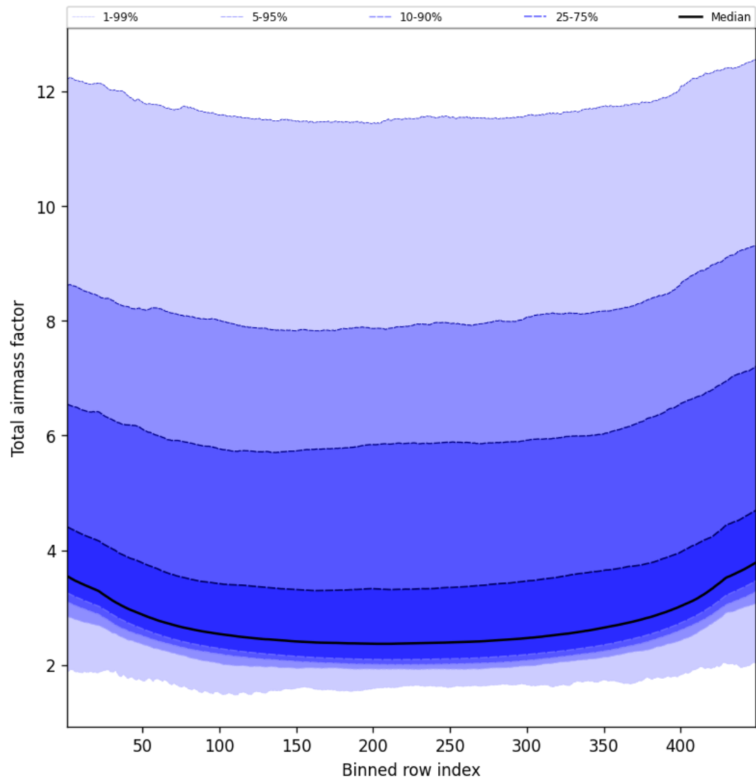
Figure 49: Along track statistics of “Total airmass factor” for 2024-11-01 to 2024-11-03
