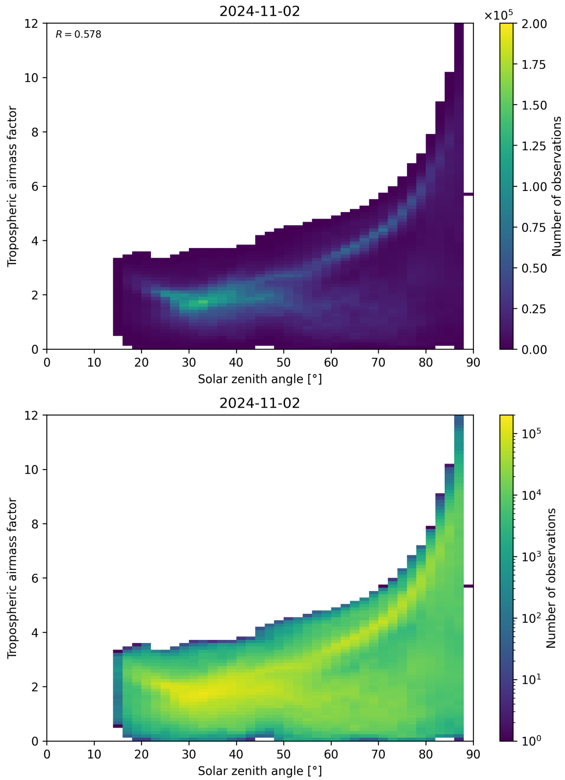
Figure 147: Scatter density plot of “Solar zenith angle” against “Tropospheric airmass factor” for 2024-11-01 to 2024-11-03.
