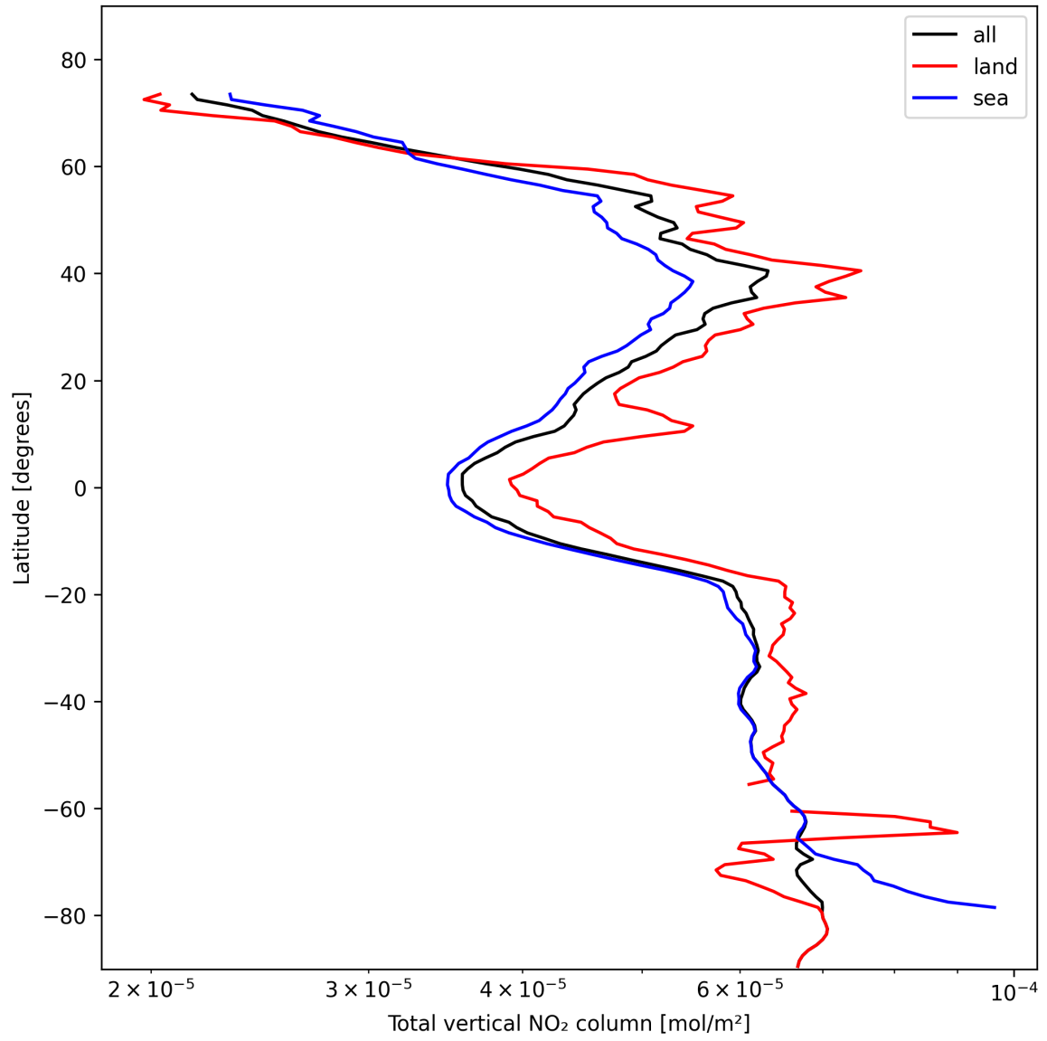
Figure 21: Zonal average of “Total vertical NO 2 column” for 2024-11-01 to 2024-11-03.
