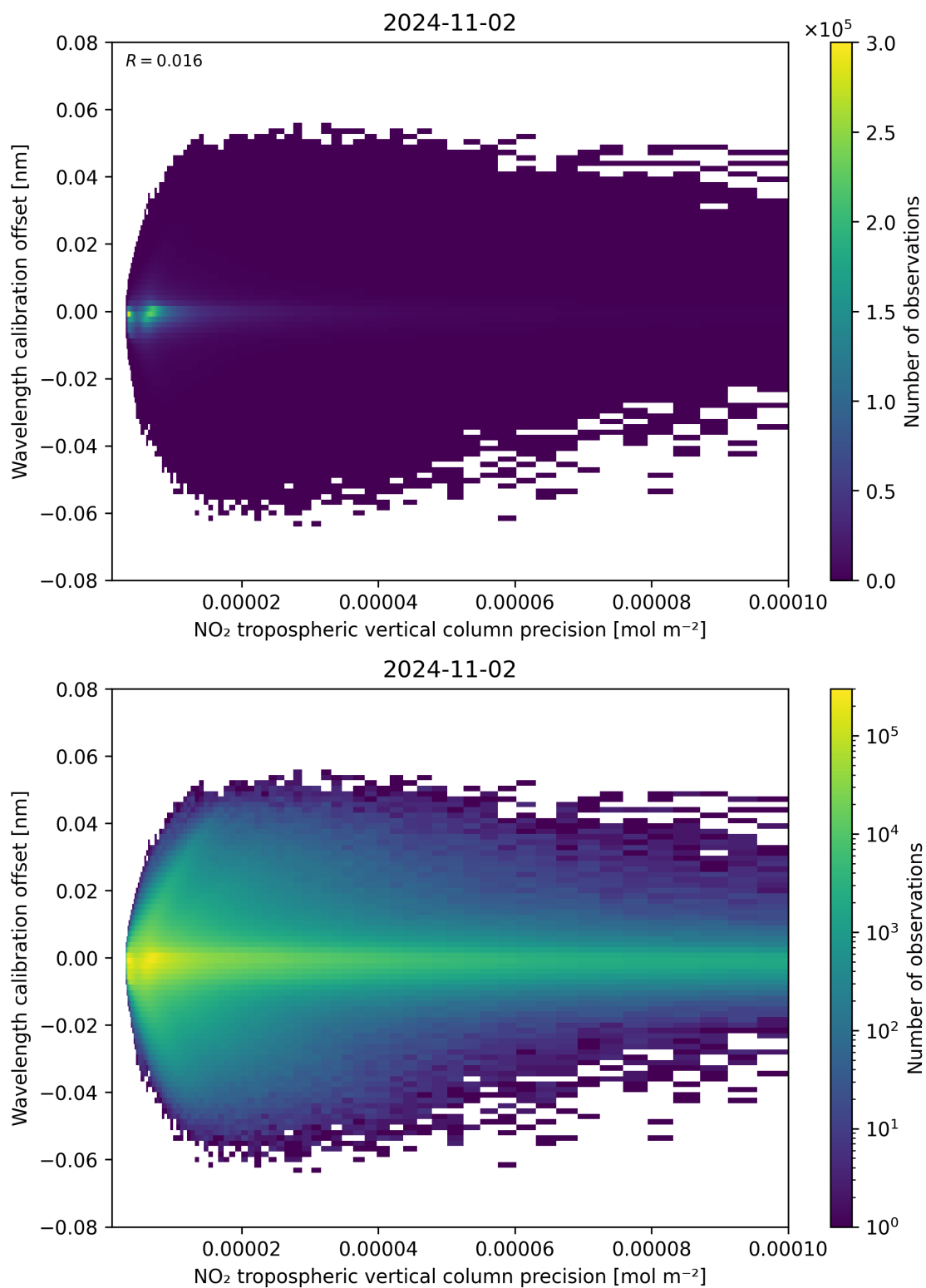
Figure 141: Scatter density plot of “NO 2 tropospheric vertical column precision” against “Wavelength calibration offset” for 2024-11-01 to 2024-11-03.
