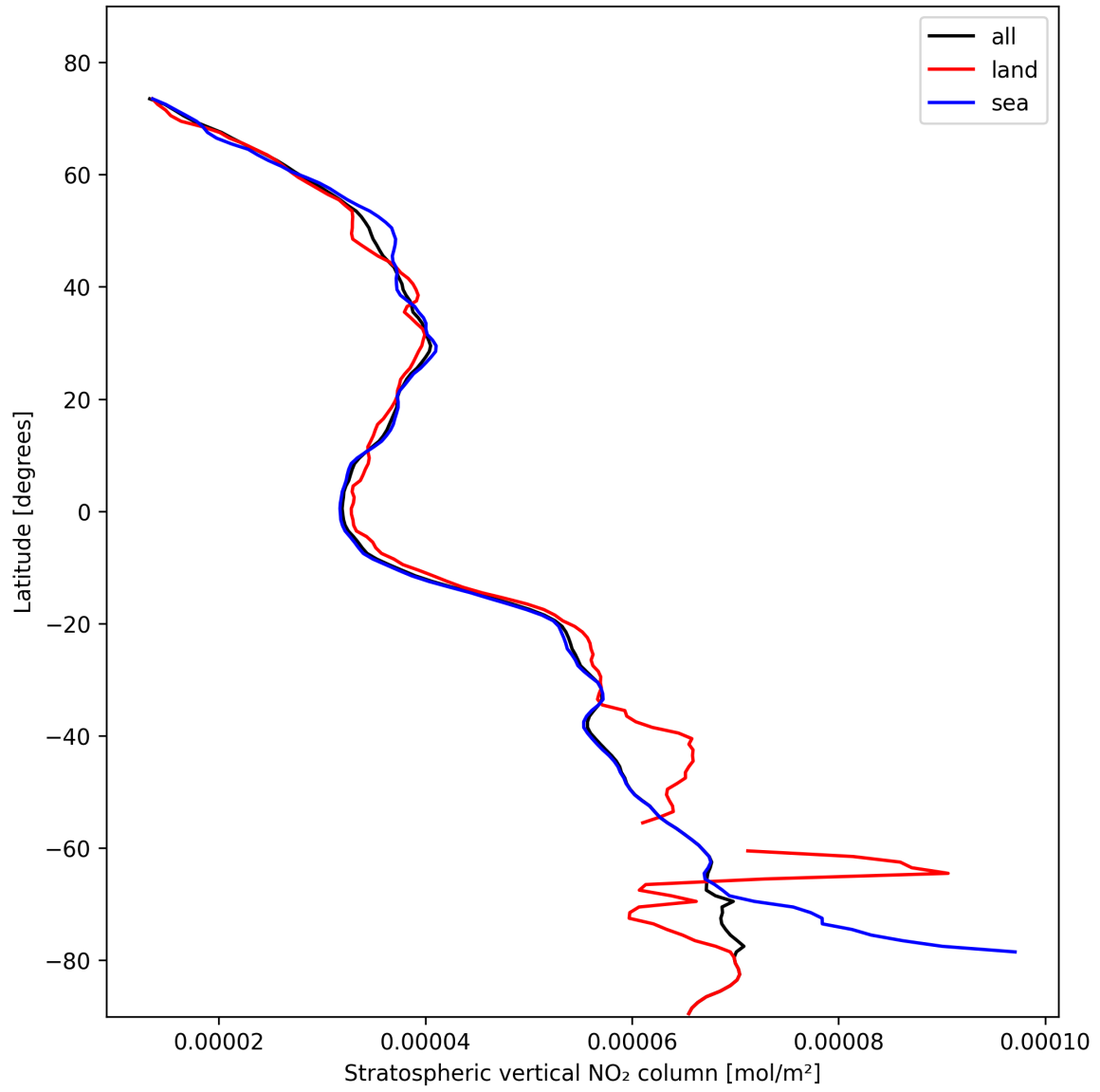
Figure 19: Zonal average of “Stratospheric vertical NO 2 column” for 2024-11-01 to 2024-11-03.
