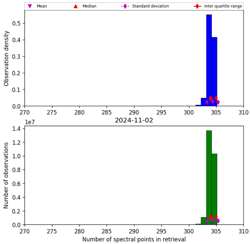
Figure 33: Histogram of “Number of spectral points in retrieval” for 2024-11-01 to 2024-11-03
