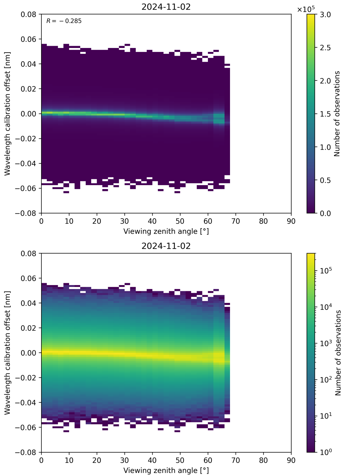
Figure 173: Scatter density plot of “Viewing zenith angle” against “Wavelength calibration offset” for 2024-11-01 to 2024-11-03.
