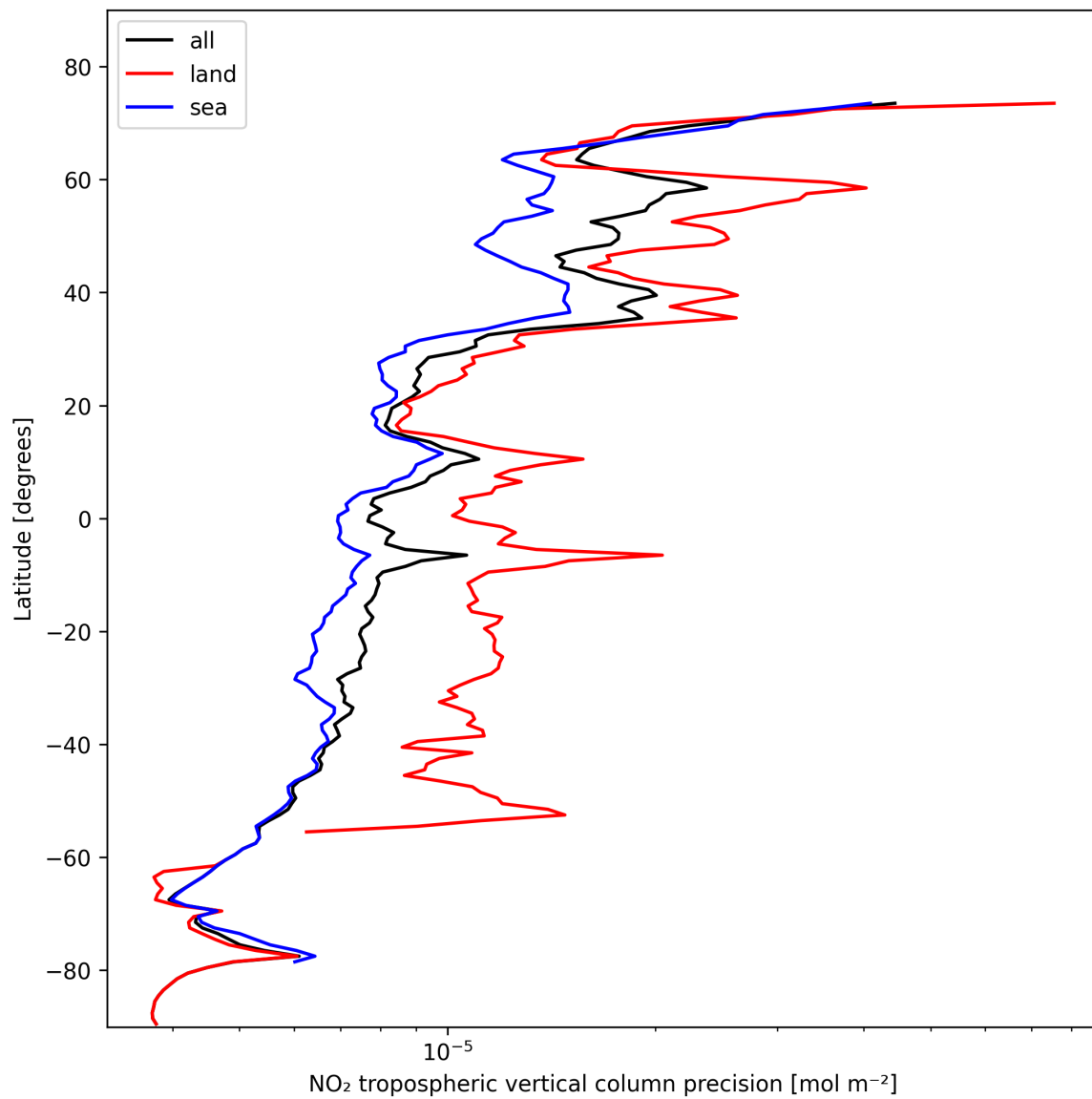
Figure 13: Zonal average of “NO 2 tropospheric vertical column precision” for 2024-11-01 to 2024-11-03.
