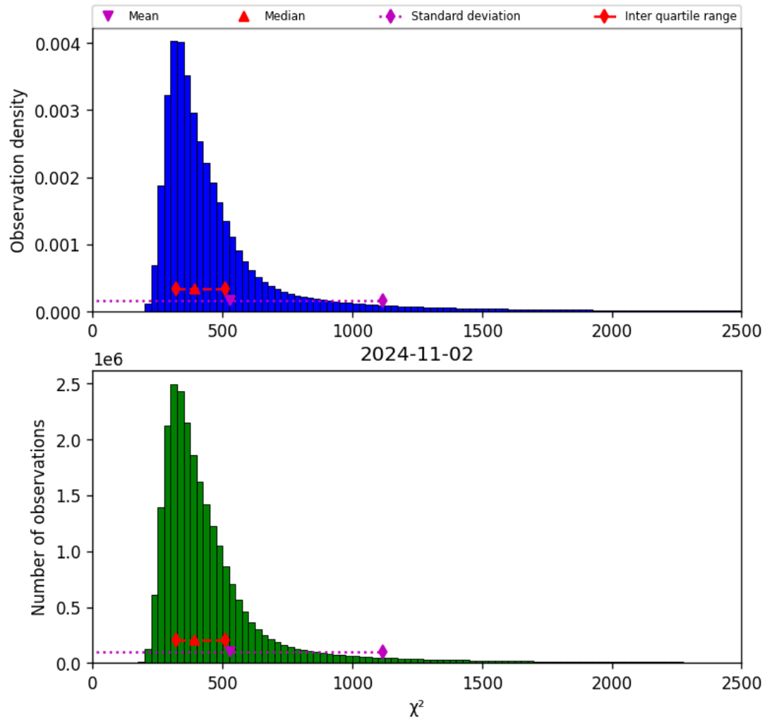
Figure 42: Histogram of “ \chi^2 ” for 2024-11-01 to 2024-11-03
