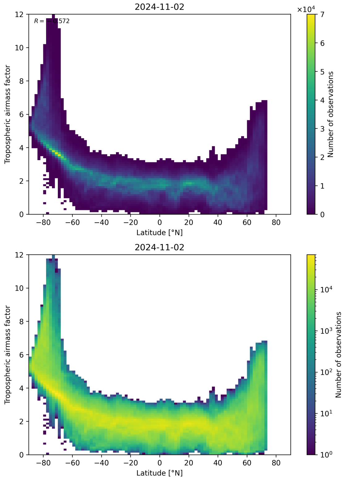
Figure 85: Scatter density plot of “Latitude” against “Tropospheric air mass factor” for 2024-11-01 to 2024-11-03.
