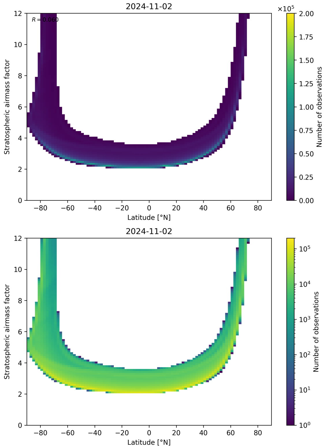
Figure 83: Scatter density plot of “Latitude” against “Stratospheric air mass factor” for 2024-11-01 to 2024-11-03.
