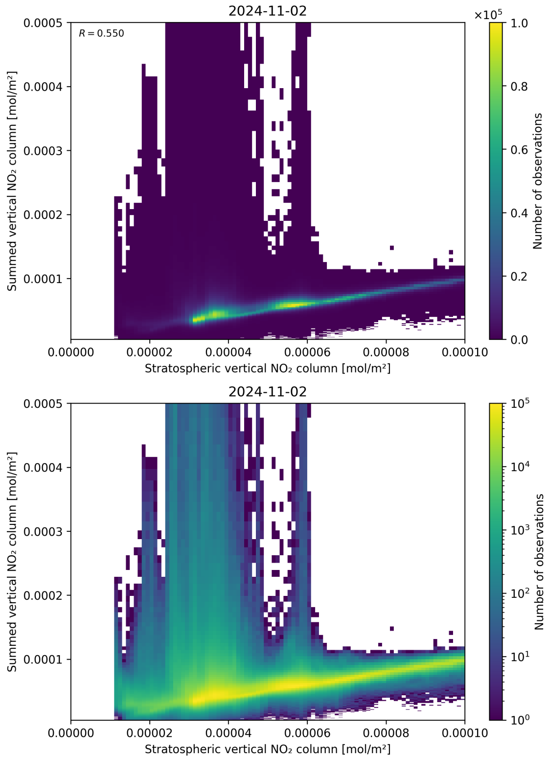
Figure 98: Scatter density plot of “Stratospheric vertical NO 2 column” against “Summed vertical NO 2 column” for 2024-11-01 to 2024-11-03.
