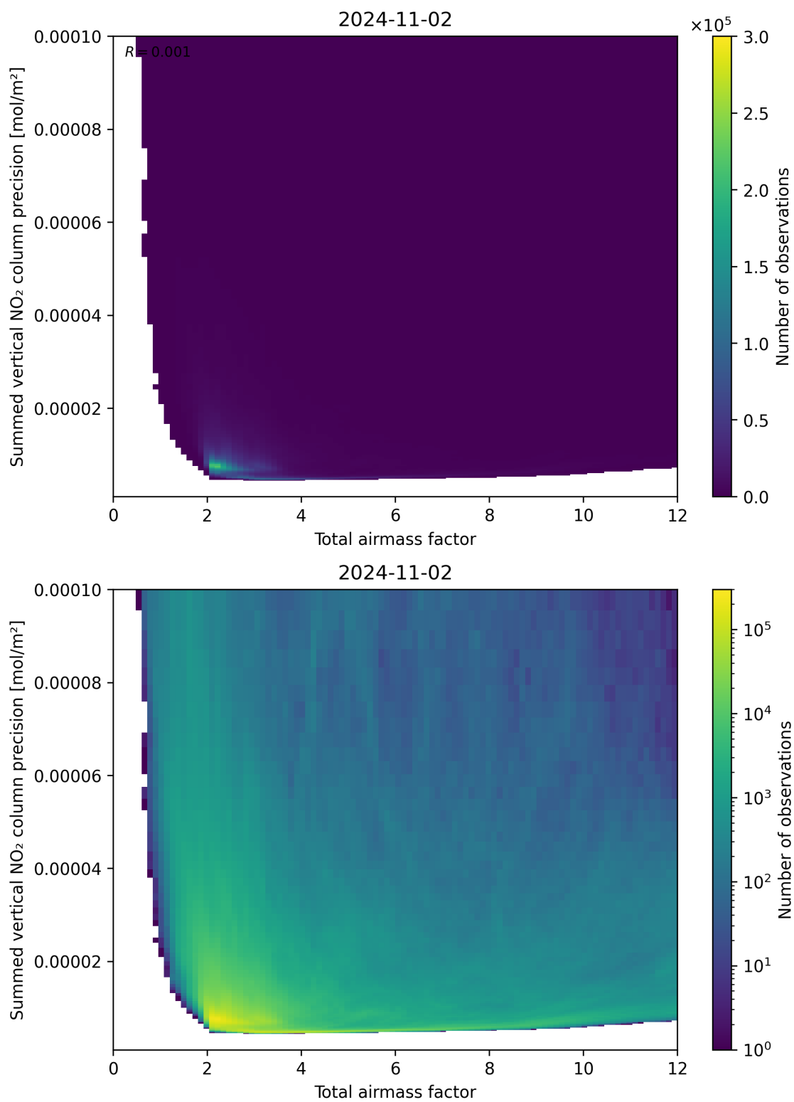
Figure 66: Scatter density plot of “Total airmass factor” against “Summed vertical NO 2 column precision” for 2024-11-01 to 2024-11-03.
