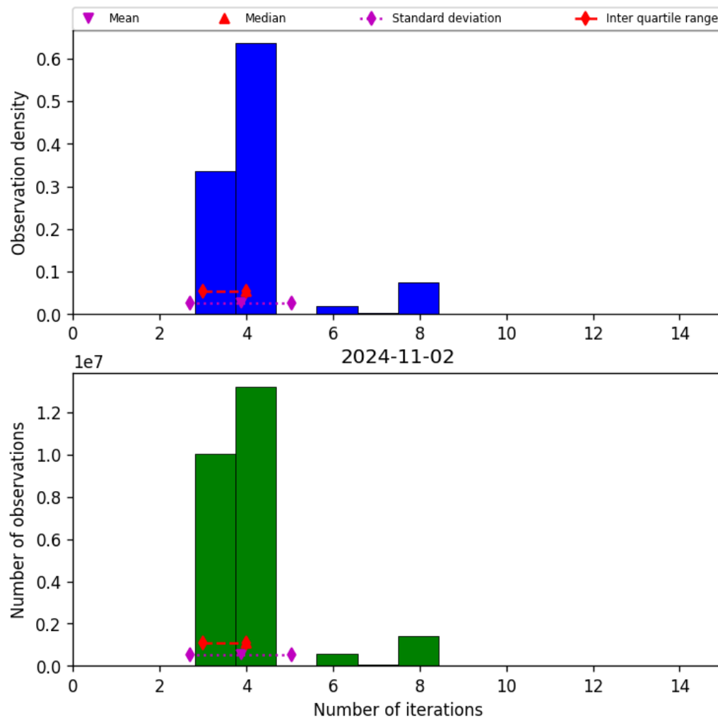
Figure 34: Histogram of “Number of iterations” for 2024-11-01 to 2024-11-03
