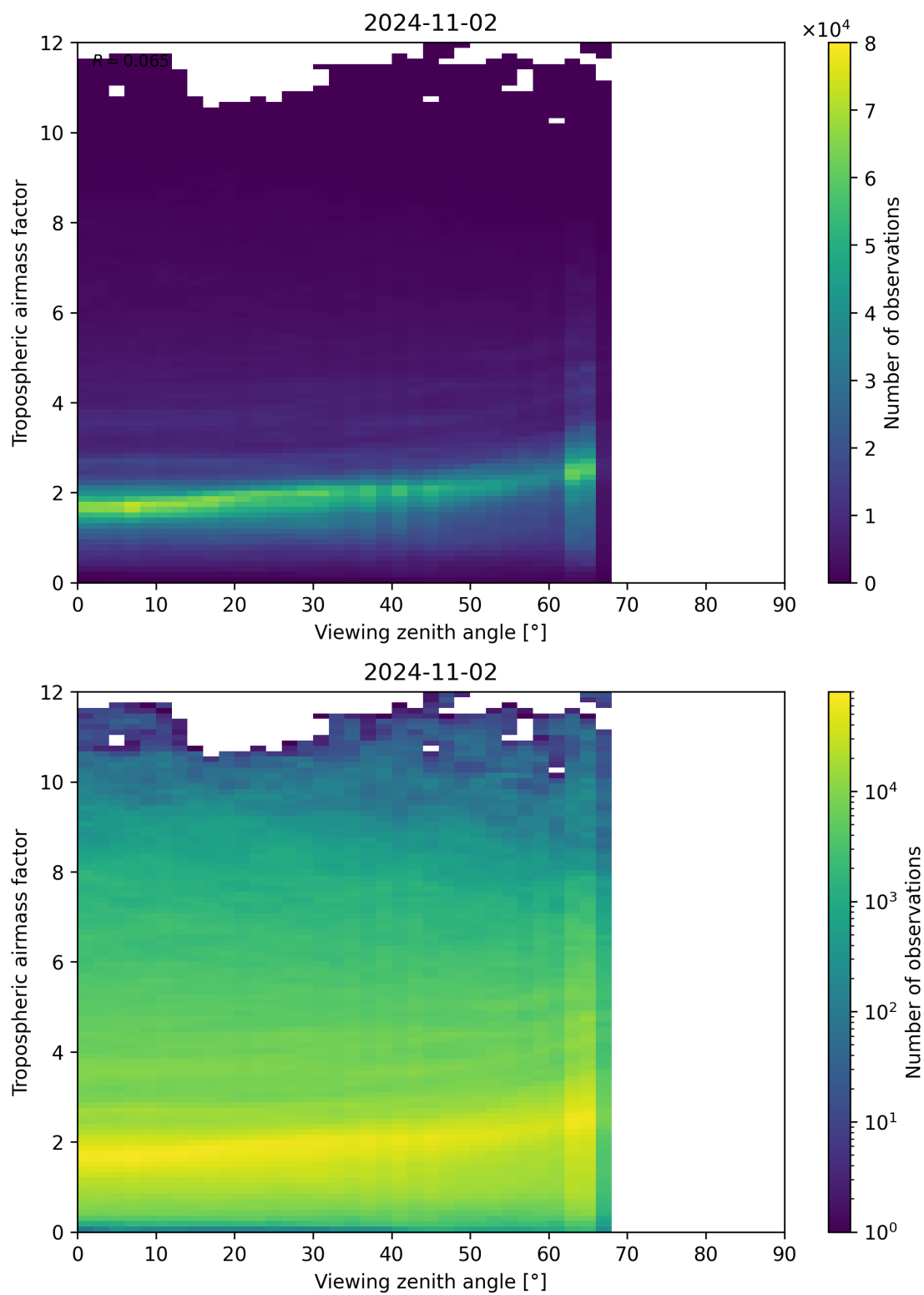
Figure 161: Scatter density plot of “Viewing zenith angle” against “Tropospheric airmass factor” for 2024-11-01 to 2024-11-03.
