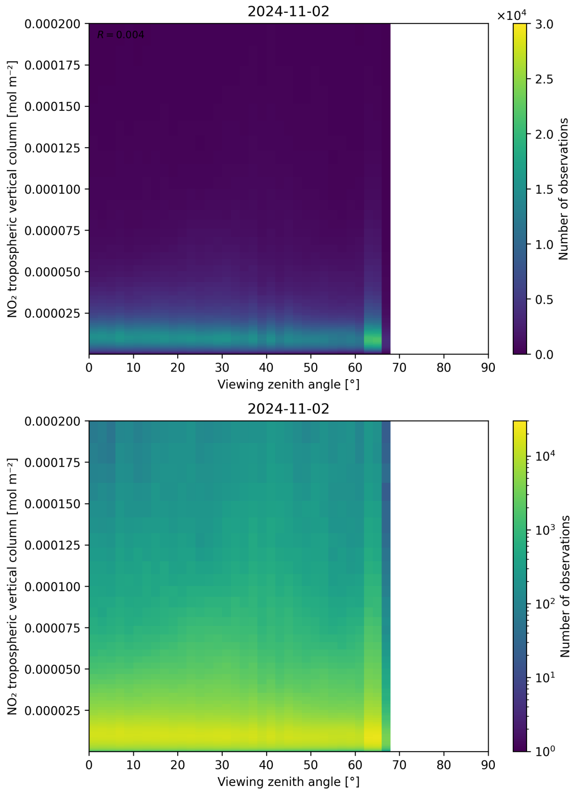
Figure 169: Scatter density plot of “Viewing zenith angle” against “NO 2 tropospheric vertical column” for 2024-11-01 to 2024-11-03.
