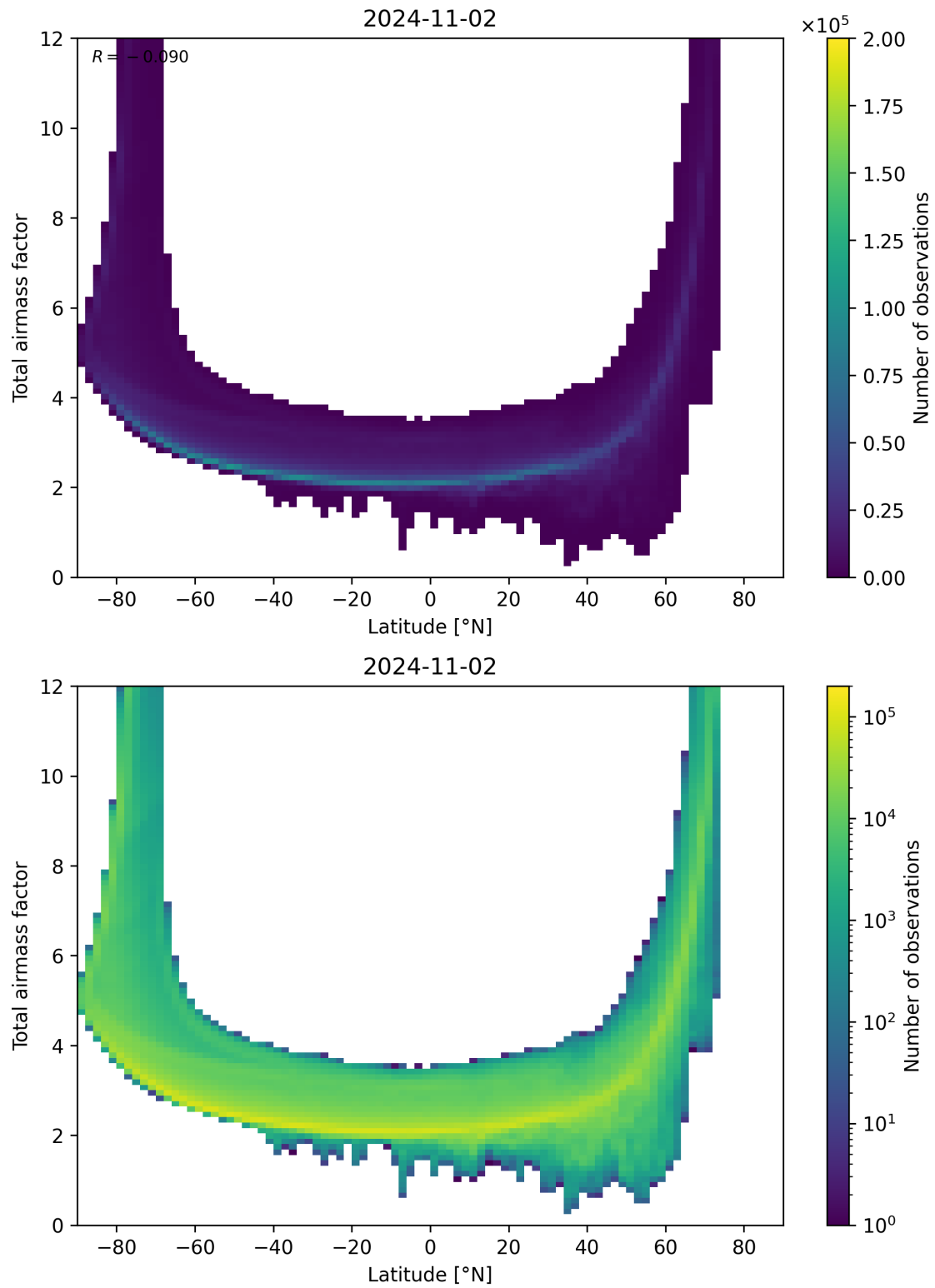
Figure 84: Scatter density plot of “Latitude” against “Total airmass factor” for 2024-11-01 to 2024-11-03.
