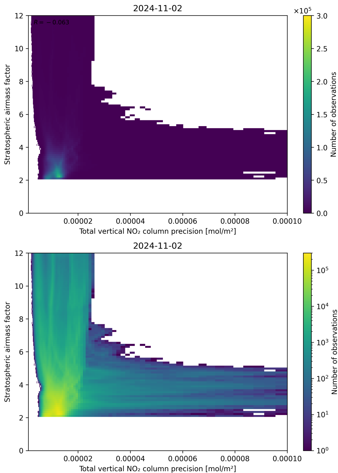
Figure 115: Scatter density plot of “Total vertical NO 2 column precision” against “Stratospheric airmass factor” for 2024-11-01 to 2024-11-03.
