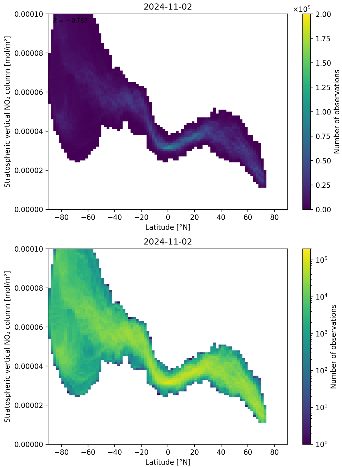
Figure 87: Scatter density plot of “Latitude” against “Stratospheric vertical NO 2 column” for 2024-11-01 to 2024-11-03.
