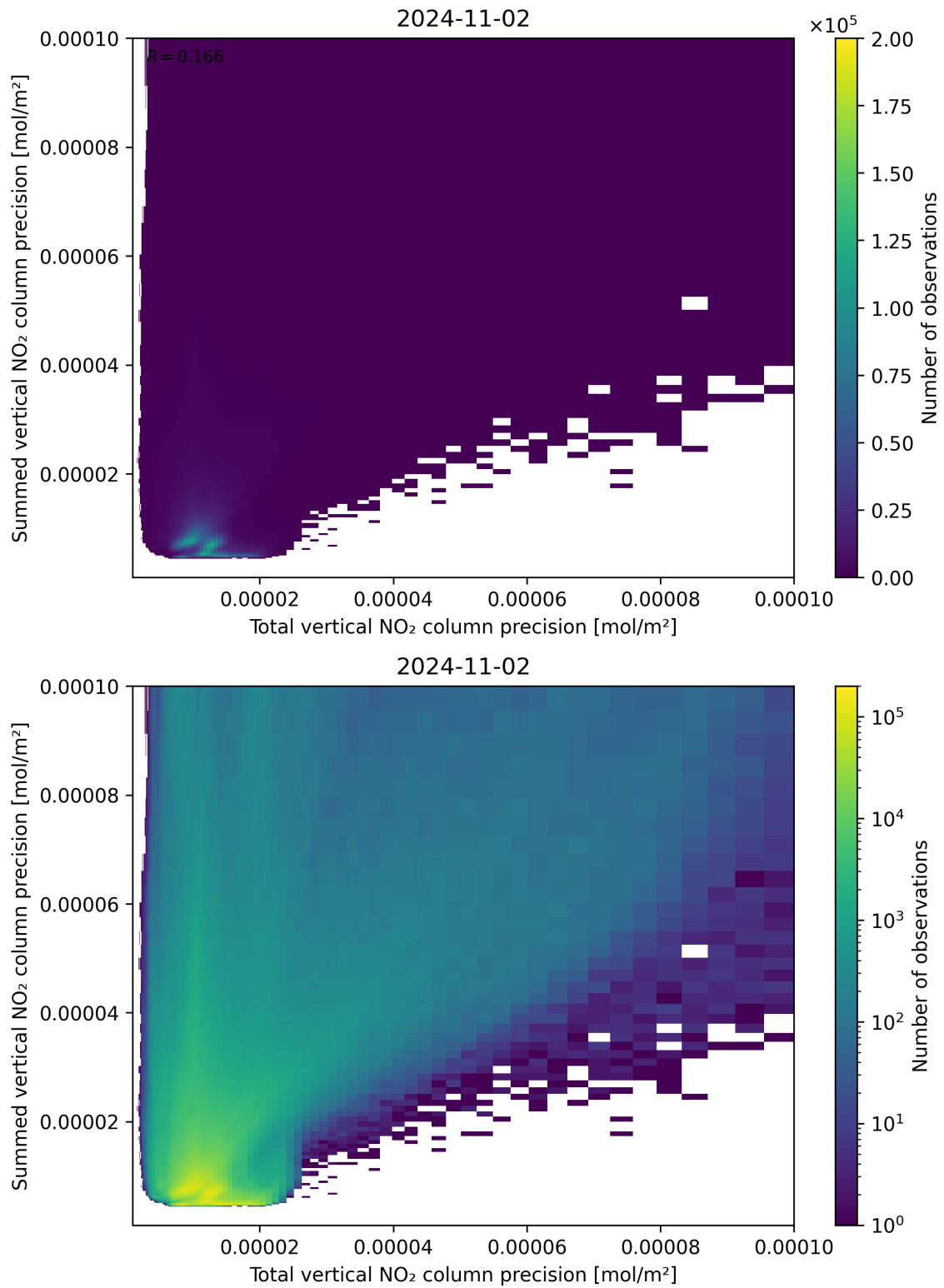
Figure 118: Scatter density plot of “Total vertical NO 2 column precision” against “Summed vertical NO 2 column precision” for 2024-11-01 to 2024-11-03.
