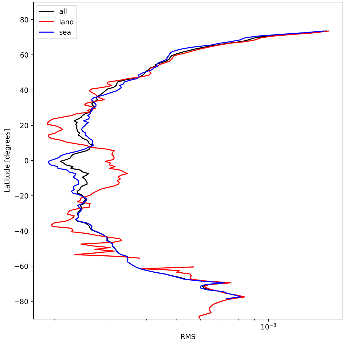
Figure 26: Zonal average of “RMS” for 2024-11-01 to 2024-11-03.
