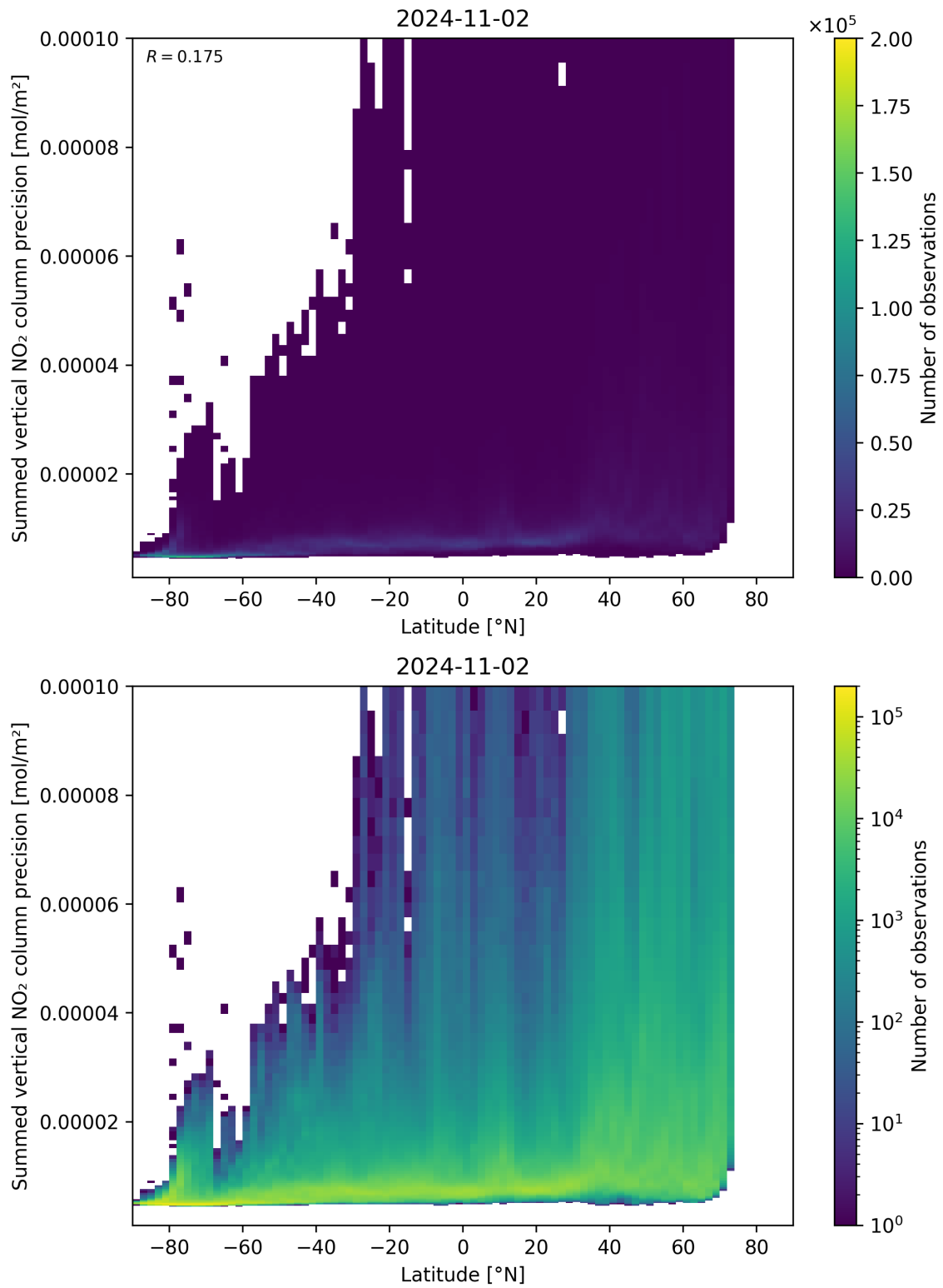
Figure 89: Scatter density plot of “Latitude” against “Summed vertical NO 2 column precision” for 2024-11-01 to 2024-11-03.
