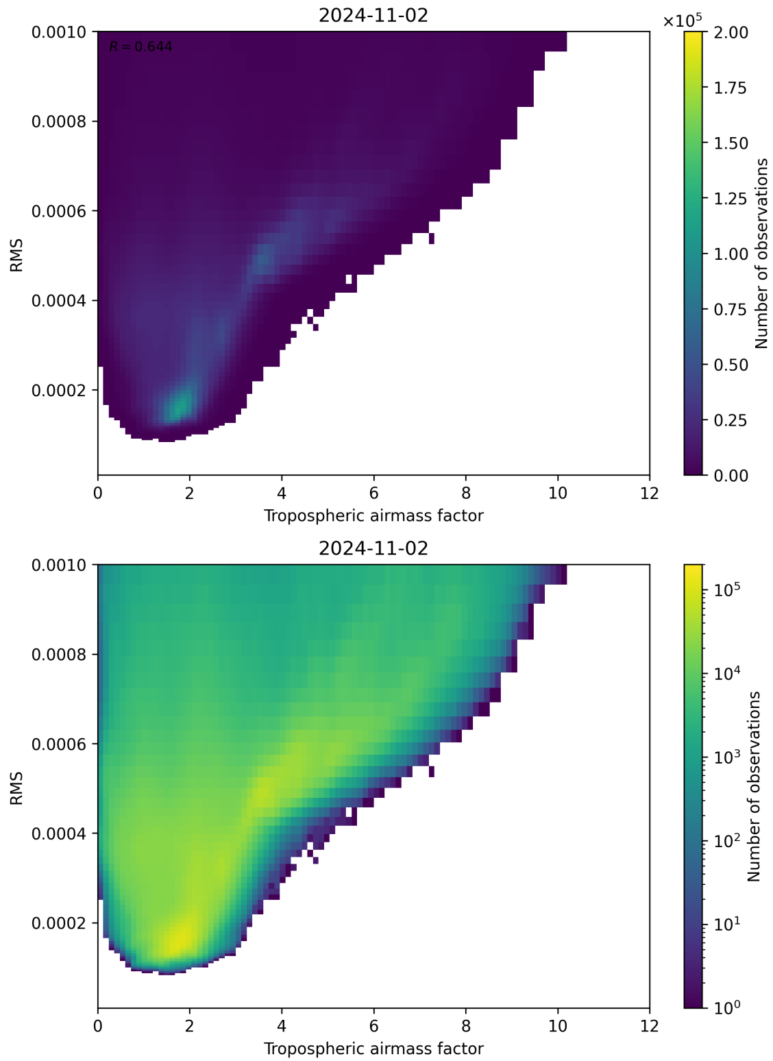
Figure 79: Scatter density plot of “Tropospheric airmass factor” against “RMS” for 2024-11-01 to 2024-11-03.
