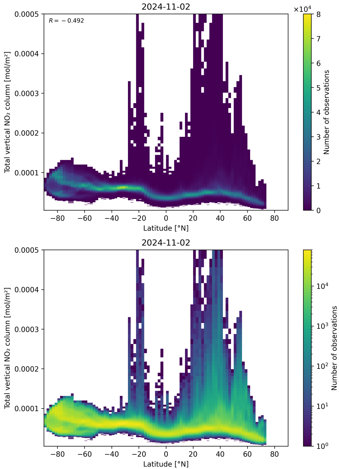
Figure 90: Scatter density plot of “Latitude” against “Total vertical NO 2 column” for 2024-11-01 to 2024-11-03.
