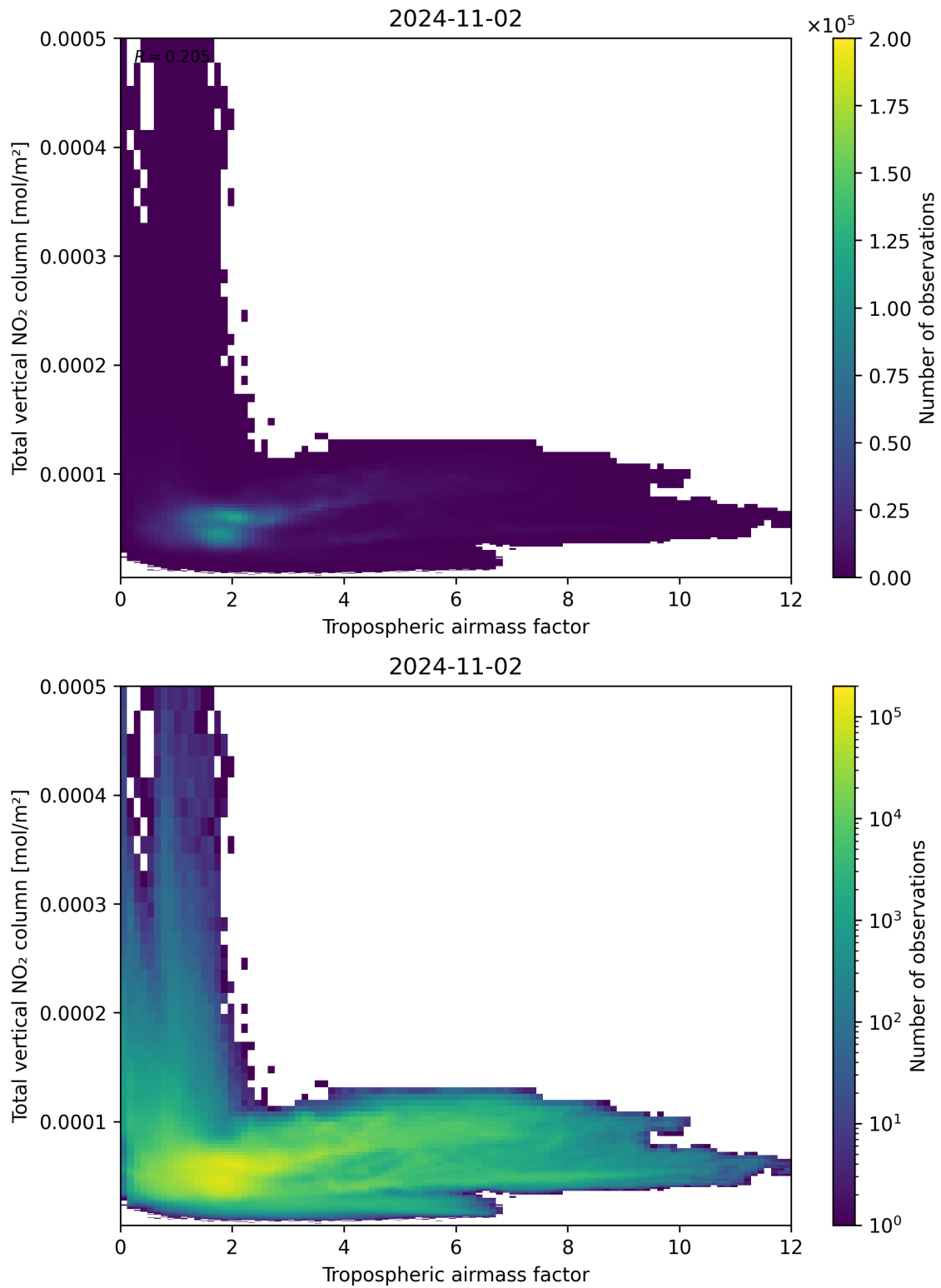
Figure 77: Scatter density plot of “Tropospheric airmass factor” against “Total vertical NO 2 column” for 2024-11-01 to 2024-11-03.
