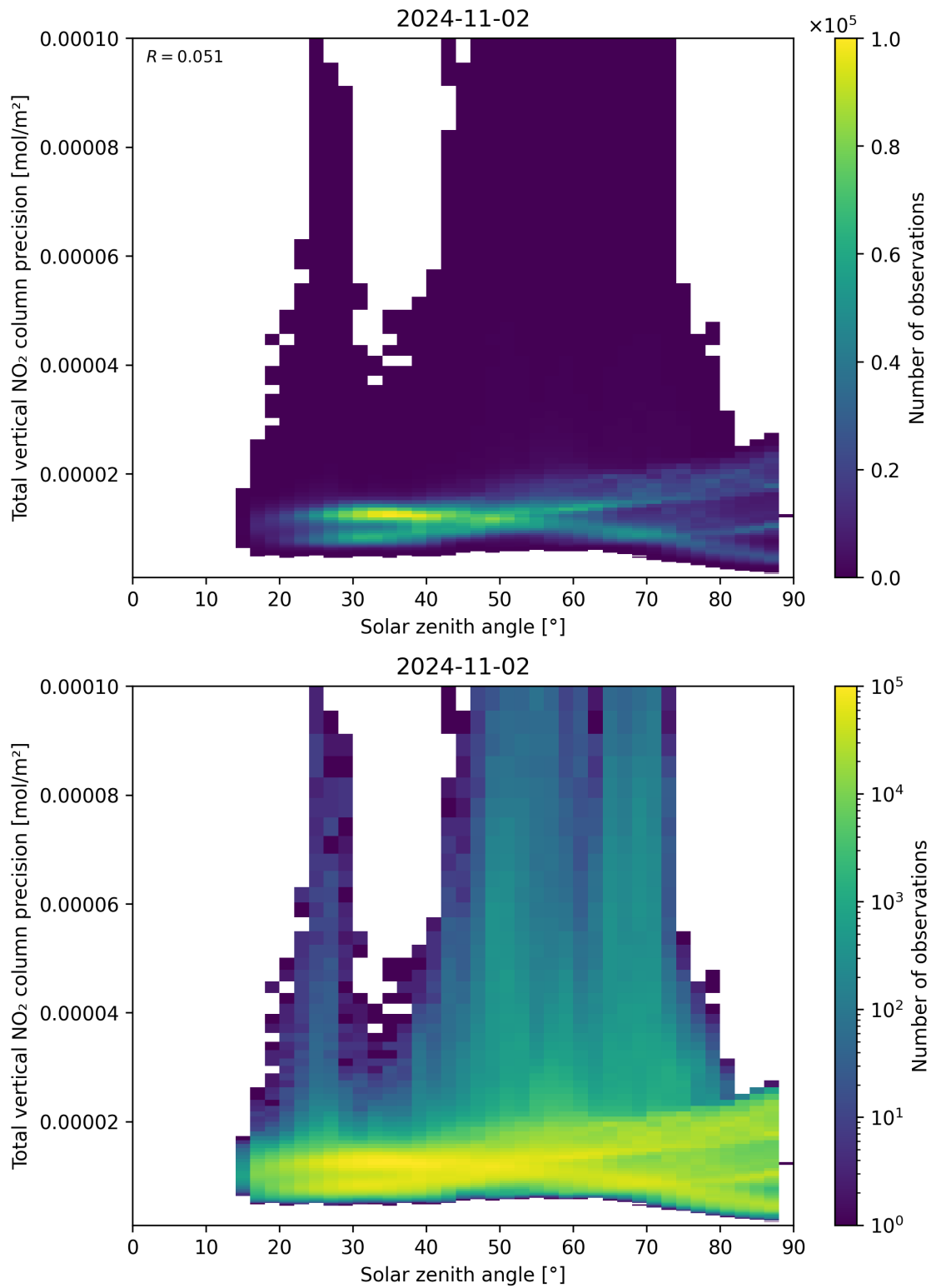
Figure 154: Scatter density plot of “Solar zenith angle” against “Total vertical NO 2 column precision” for 2024-11-01 to 2024-11-03.
