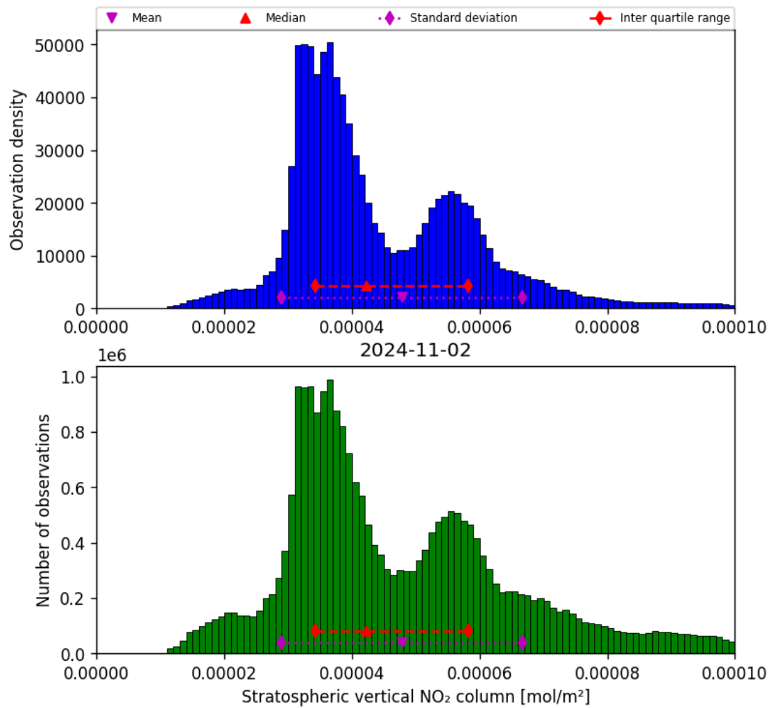
Figure 36: Histogram of “Stratospheric vertical NO 2 column” for 2024-11-01 to 2024-11-03
