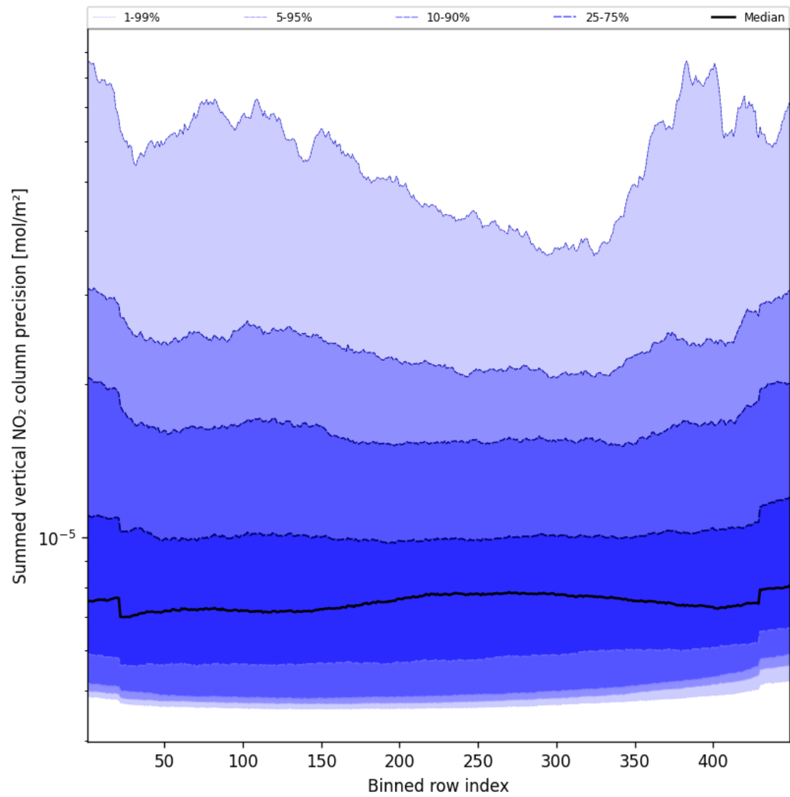
Figure 58: Along track statistics of “Summed vertical NO 2 column precision” for 2024-11-01 to 2024-11-03
