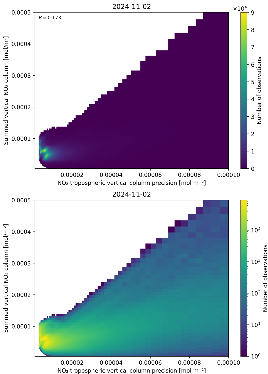
Figure 136: Scatter density plot of “NO 2 tropospheric vertical column precision” against “Summed vertical NO 2 column” for 2024-11-01 to 2024-11-03.
