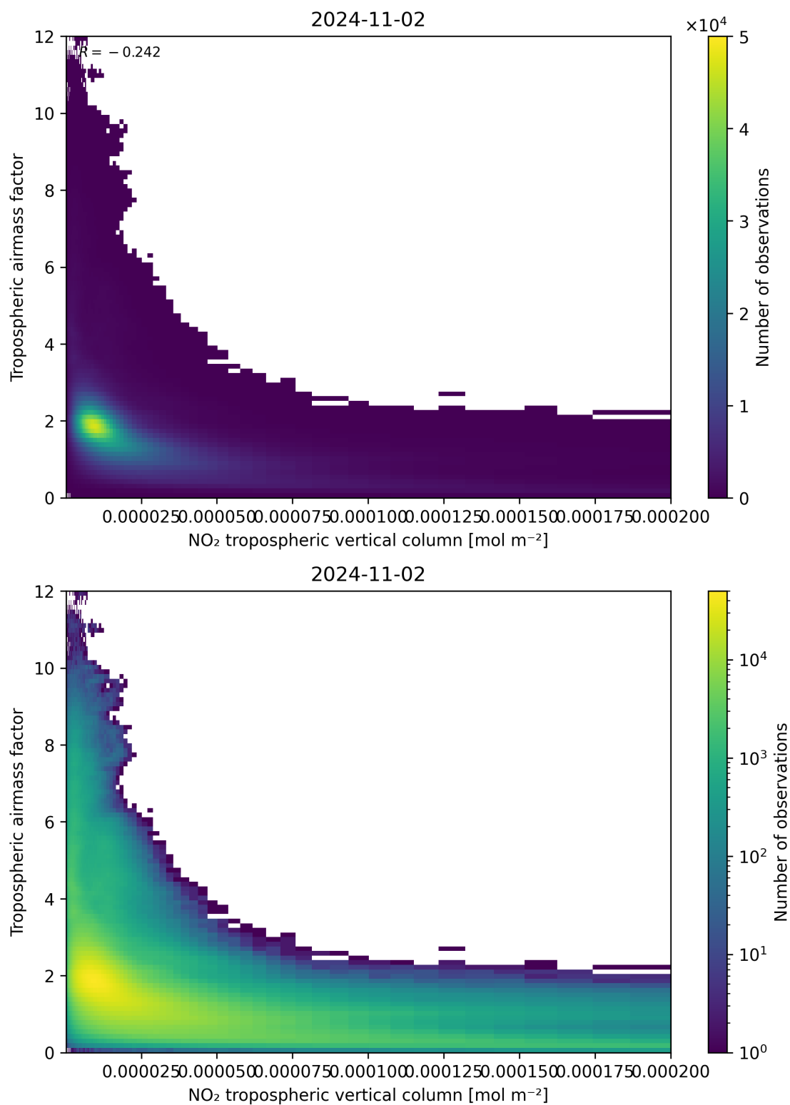
Figure 123: Scatter density plot of “NO 2 tropospheric vertical column” against “Tropospheric air mass factor” for 2024-11-01 to 2024-11-03.
