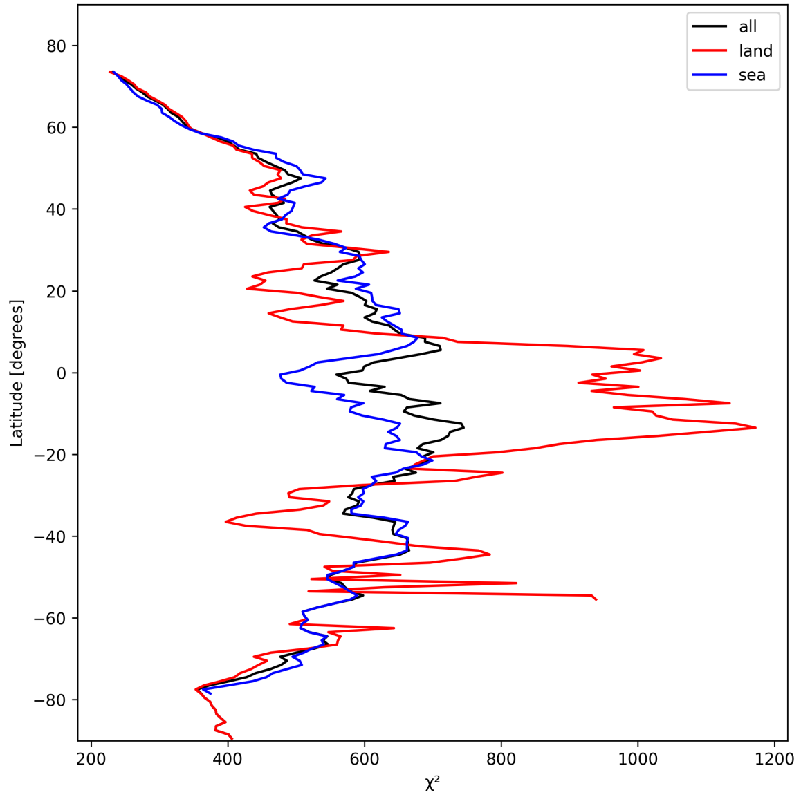
Figure 25: Zonal average of “ \chi^2 ” for 2024-11-01 to 2024-11-03.
