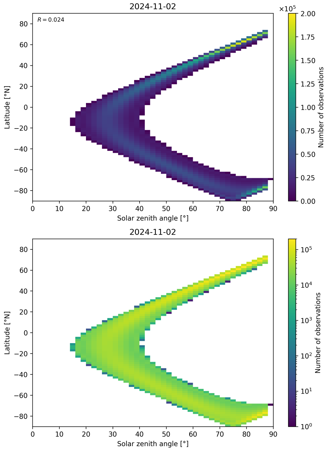
Figure 149: Scatter density plot of “Solar zenith angle” against “Latitude” for 2024-11-01 to 2024-11-03.
