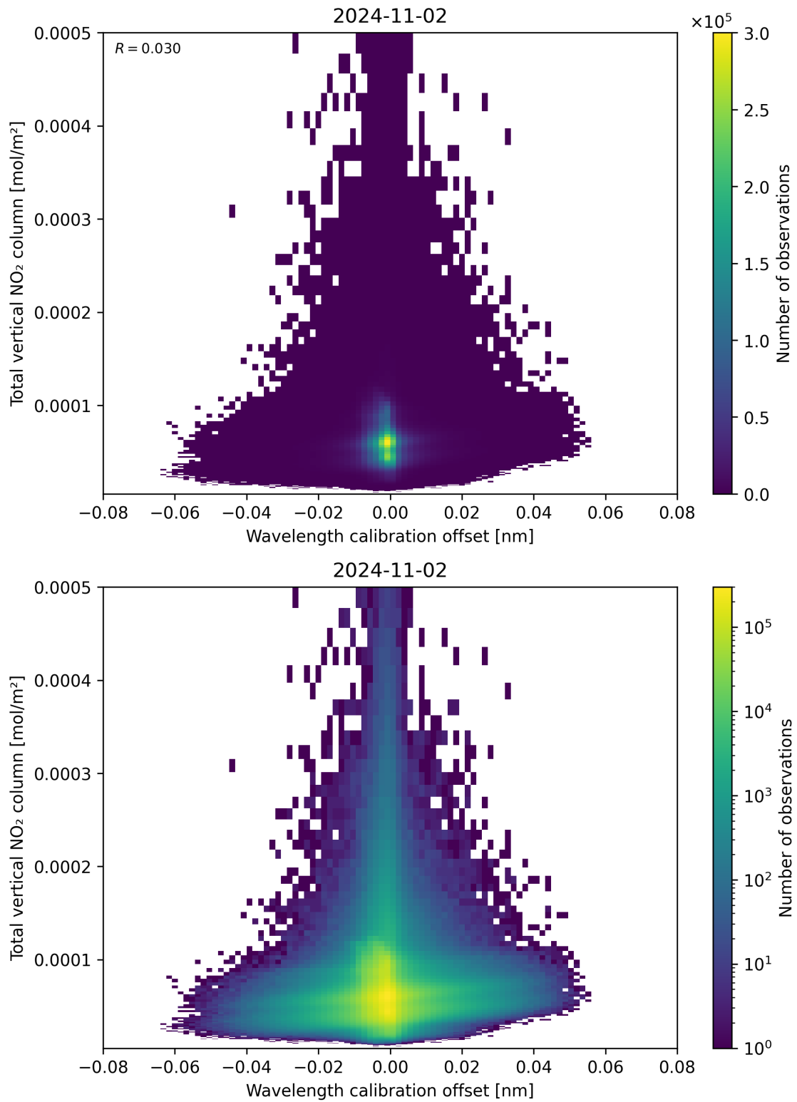
Figure 179: Scatter density plot of “Wavelength calibration offset” against “Total vertical NO 2 column” for 2024-11-01 to 2024-11-03.
