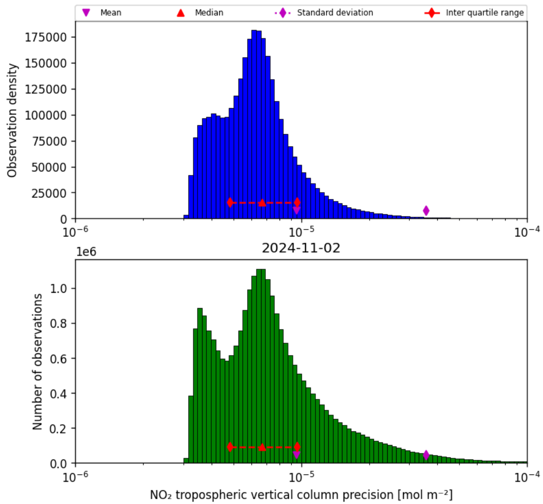
Figure 30: Histogram of “NO 2 tropospheric vertical column precision” for 2024-11-01 to 2024-11-03
