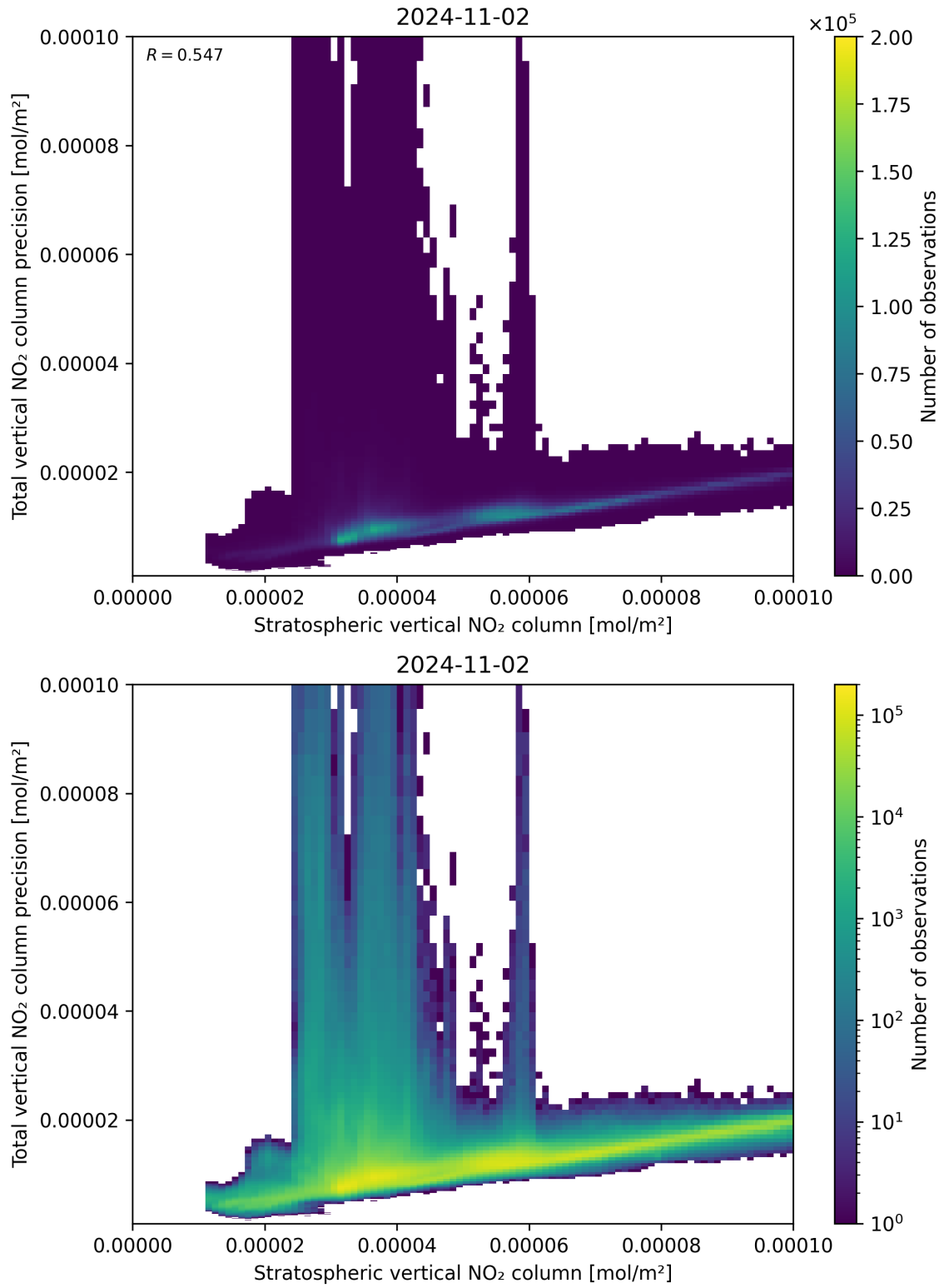
Figure 101: Scatter density plot of “Stratospheric vertical NO 2 column” against “Total vertical NO 2 column precision” for 2024-11-01 to 2024-11-03.
