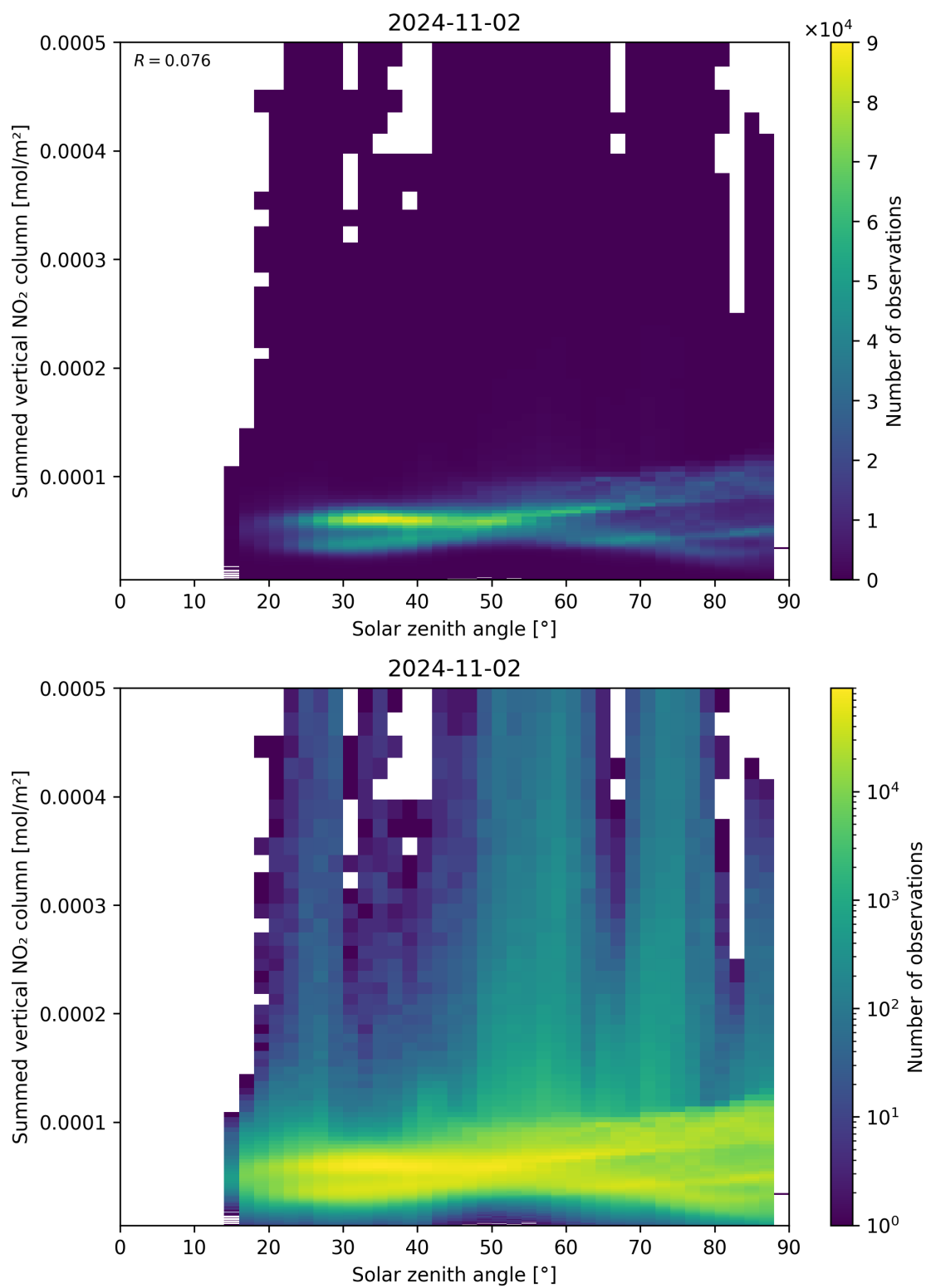
Figure 151: Scatter density plot of “Solar zenith angle” against “Summed vertical NO 2 column” for 2024-11-01 to 2024-11-03.
