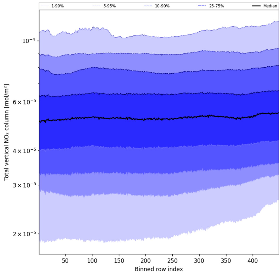
Figure 55: Along track statistics of “Total vertical NO 2 column” for 2024-11-01 to 2024-11-03
