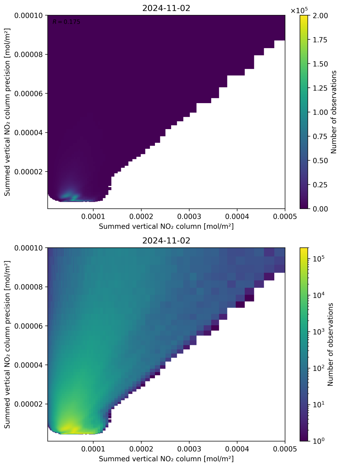
Figure 105: Scatter density plot of “Summed vertical NO 2 column” against “Summed vertical NO 2 column precision” for 2024-11-01 to 2024-11-03.
