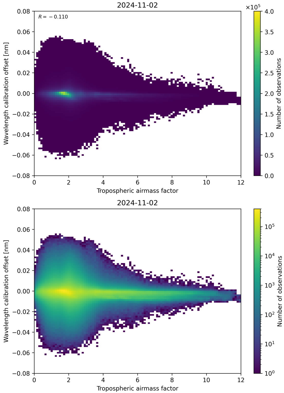
Figure 80: Scatter density plot of “Tropospheric airmass factor” against “Wavelength calibration offset” for 2024-11-01 to 2024-11-03.
