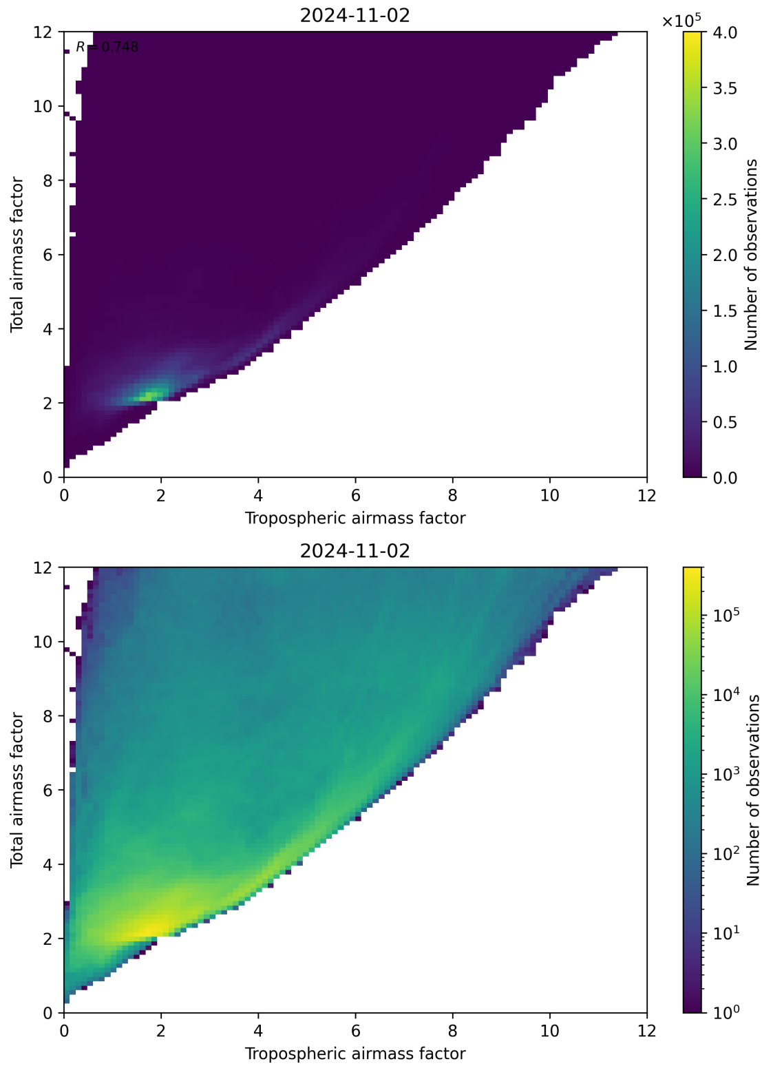
Figure 72: Scatter density plot of “Tropospheric airmass factor” against “Total airmass factor” for 2024-11-01 to 2024-11-03.
