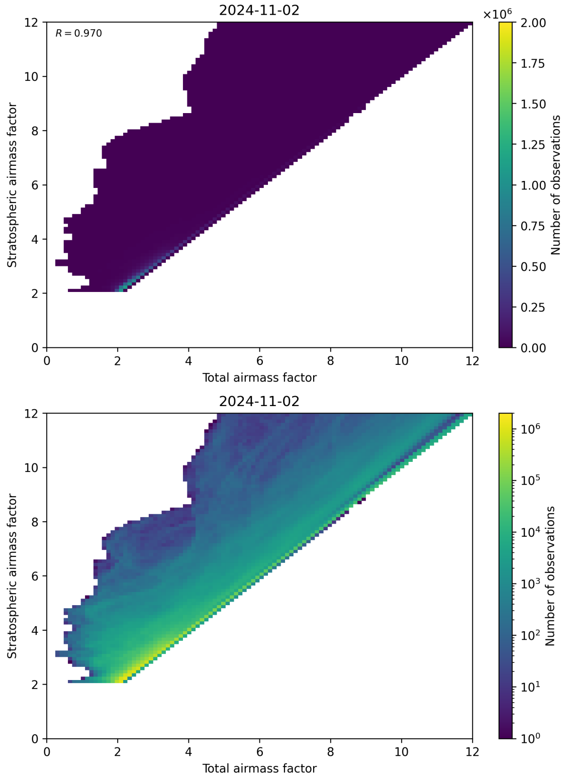
Figure 62: Scatter density plot of “Total airmass factor” against “Stratospheric airmass factor” for 2024-11-01 to 2024-11-03.
