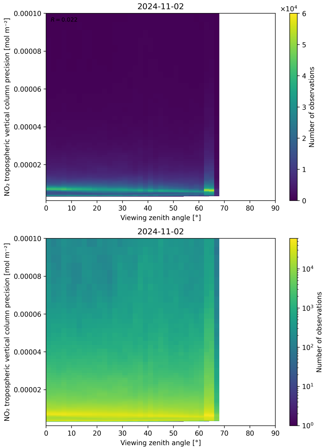
Figure 170: Scatter density plot of “Viewing zenith angle” against “NO 2 tropospheric vertical column precision” for 2024-11-01 to 2024-11-03.
