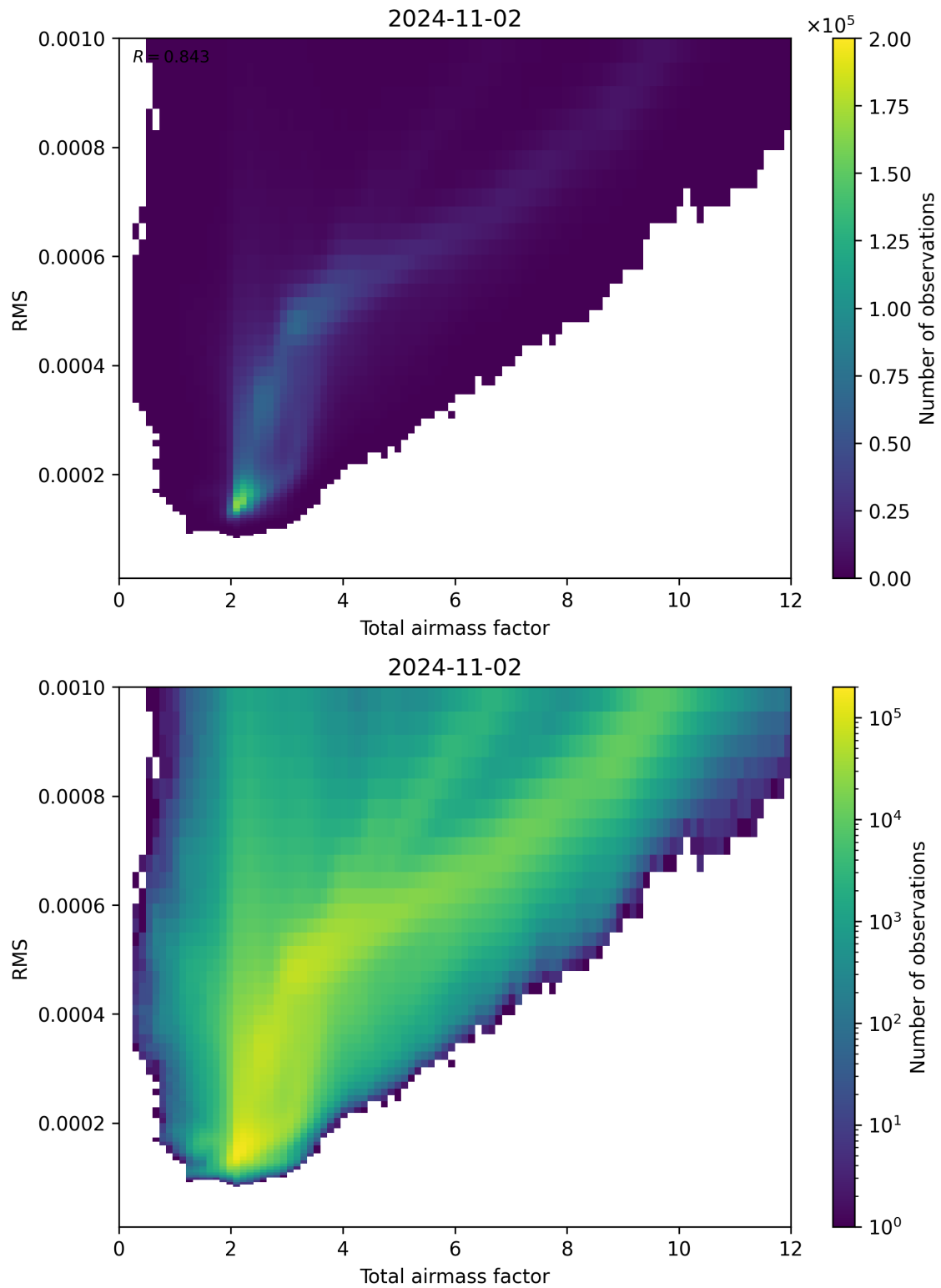
Figure 69: Scatter density plot of “Total airmass factor” against “RMS” for 2024-11-01 to 2024-11-03.
