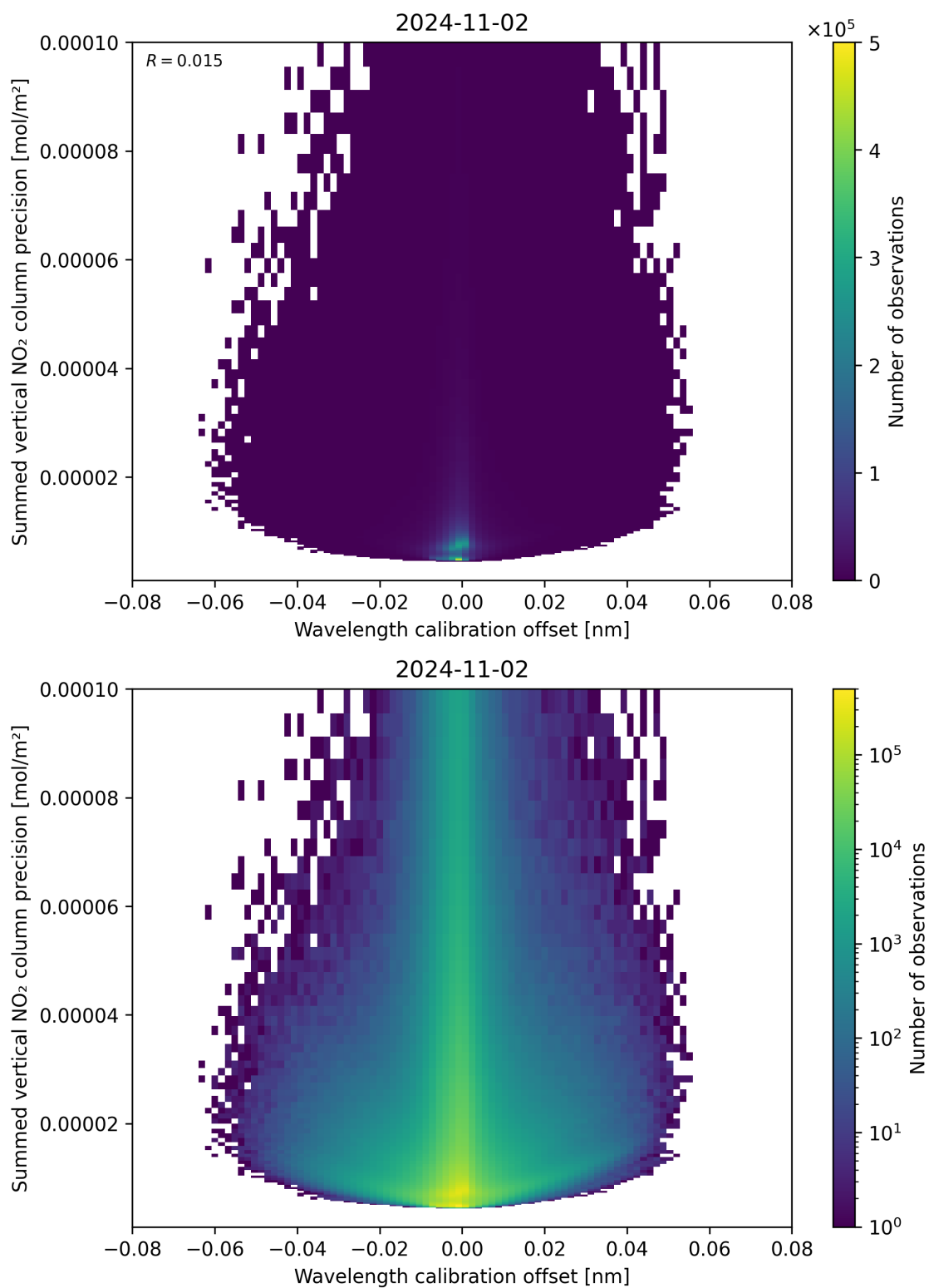
Figure 178: Scatter density plot of “Wavelength calibration offset” against “Summed vertical NO 2 column precision” for 2024-11-01 to 2024-11-03.
