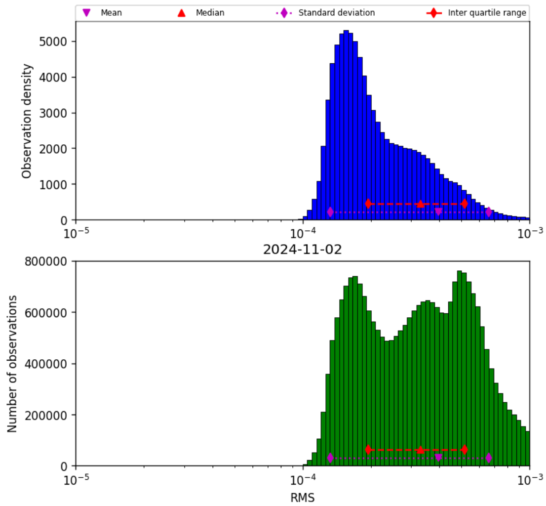
Figure 43: Histogram of “RMS” for 2024-11-01 to 2024-11-03
