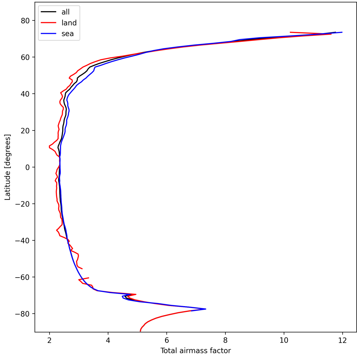
Figure 15: Zonal average of “Total airmass factor” for 2024-11-01 to 2024-11-03.
