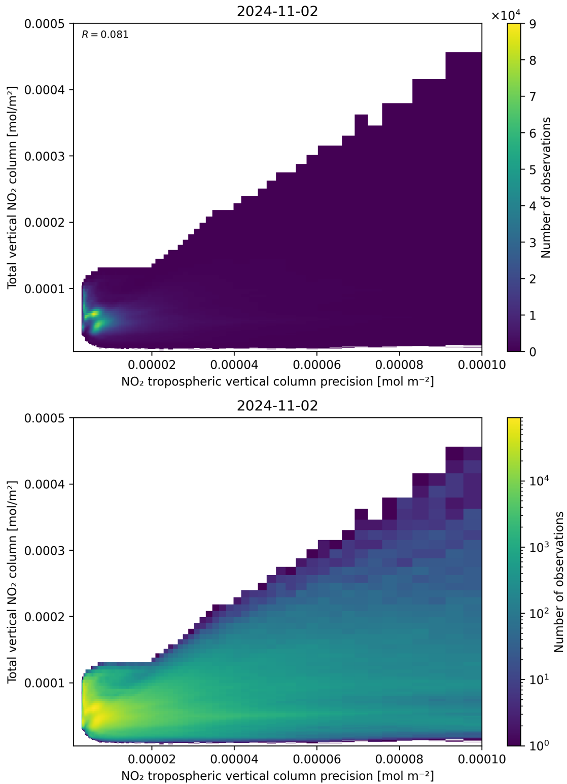
Figure 138: Scatter density plot of “NO 2 tropospheric vertical column precision” against “Total vertical NO 2 column” for 2024-11-01 to 2024-11-03.
