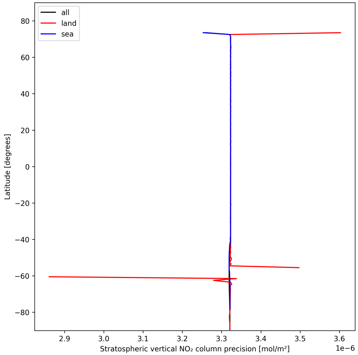
Figure 20: Zonal average of “Stratospheric vertical NO 2 column precision” for 2024-11-01 to 2024-11-03.
