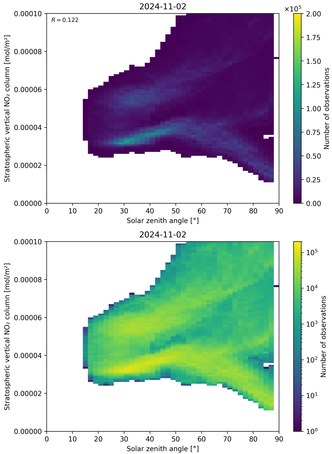
Figure 150: Scatter density plot of “Solar zenith angle” against “Stratospheric vertical NO 2 column” for 2024-11-01 to 2024-11-03.
