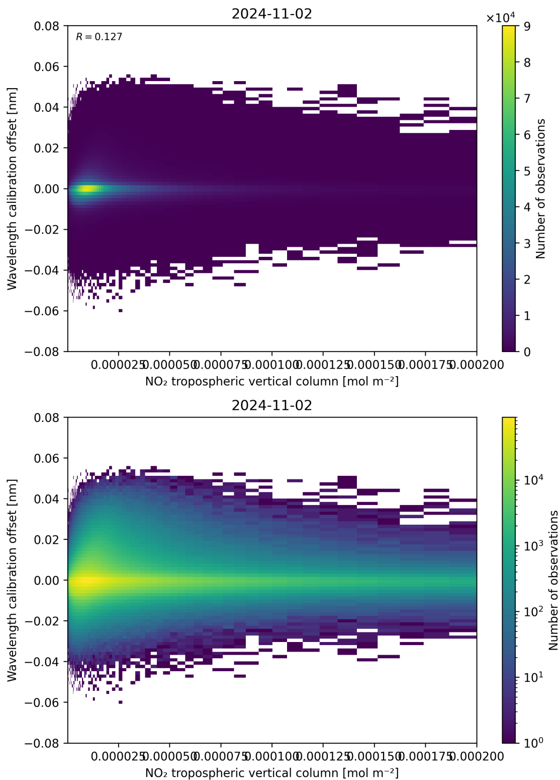
Figure 143: Scatter density plot of “NO 2 tropospheric vertical column” against “Wavelength calibration offset” for 2024-11-01 to 2024-11-03.
