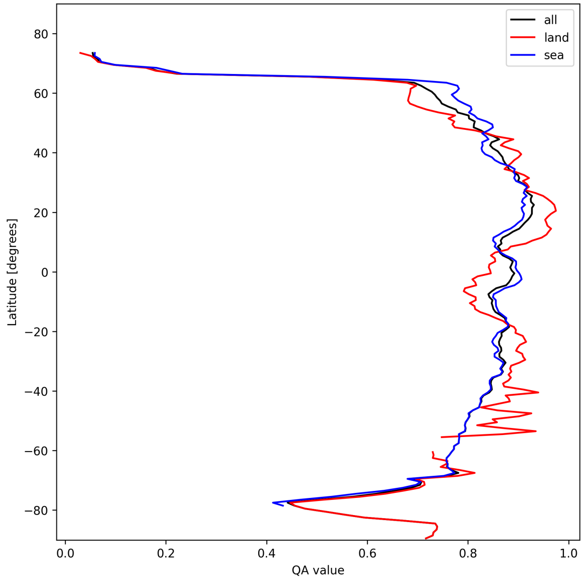
Figure 11: Zonal average of “QA value” for 2024-11-01 to 2024-11-03.
