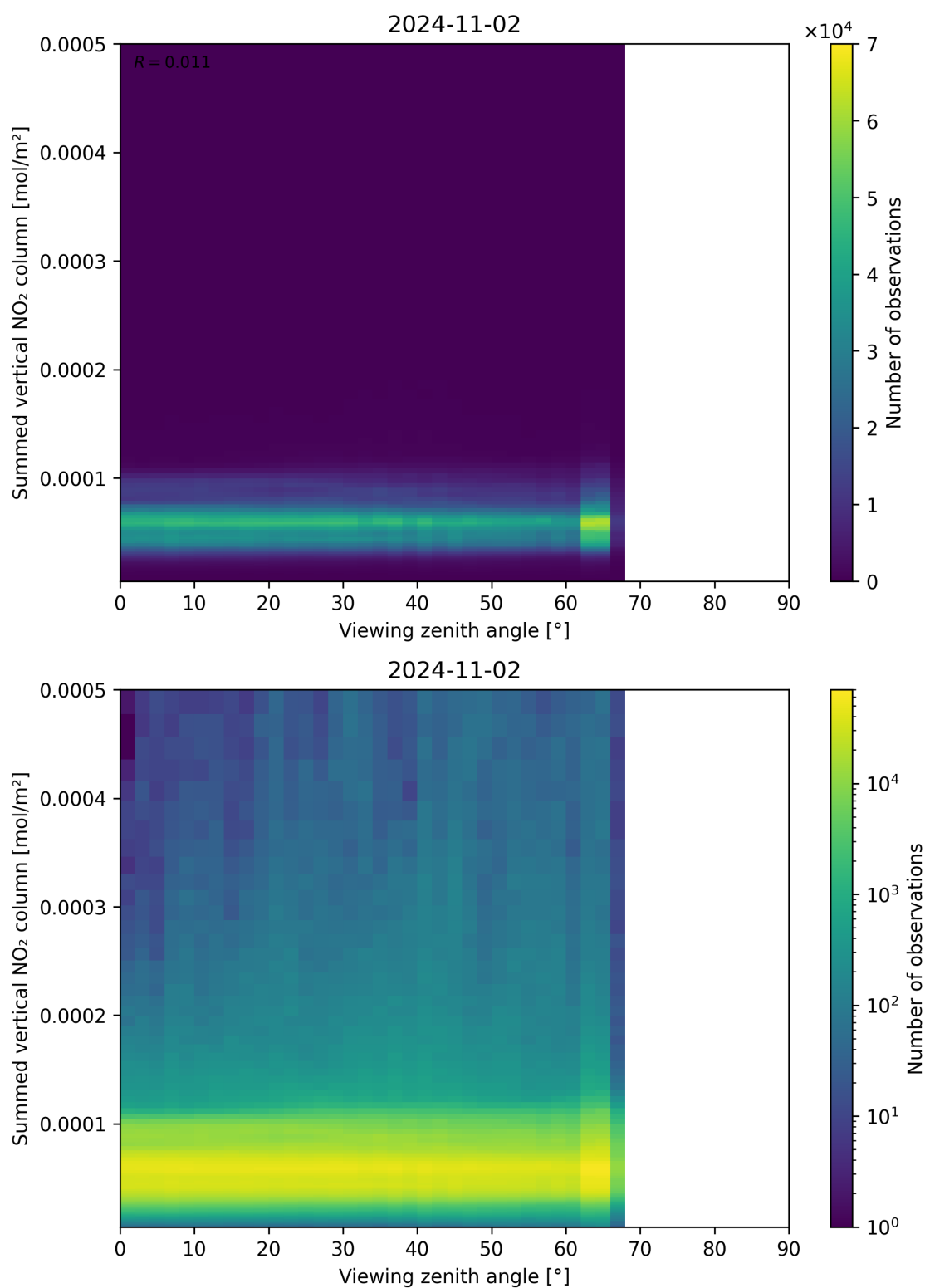
Figure 165: Scatter density plot of “Viewing zenith angle” against “Summed vertical NO 2 column” for 2024-11-01 to 2024-11-03.
