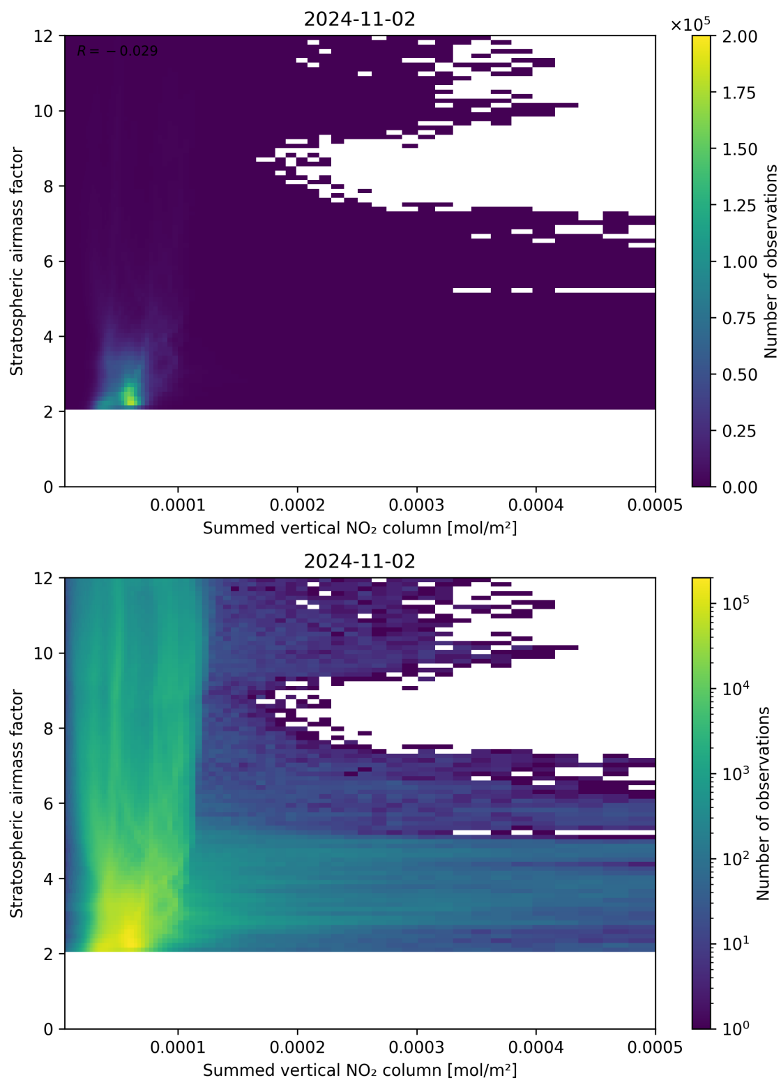
Figure 103: Scatter density plot of “Summed vertical NO 2 column” against “Stratospheric airmass factor” for 2024-11-01 to 2024-11-03.
