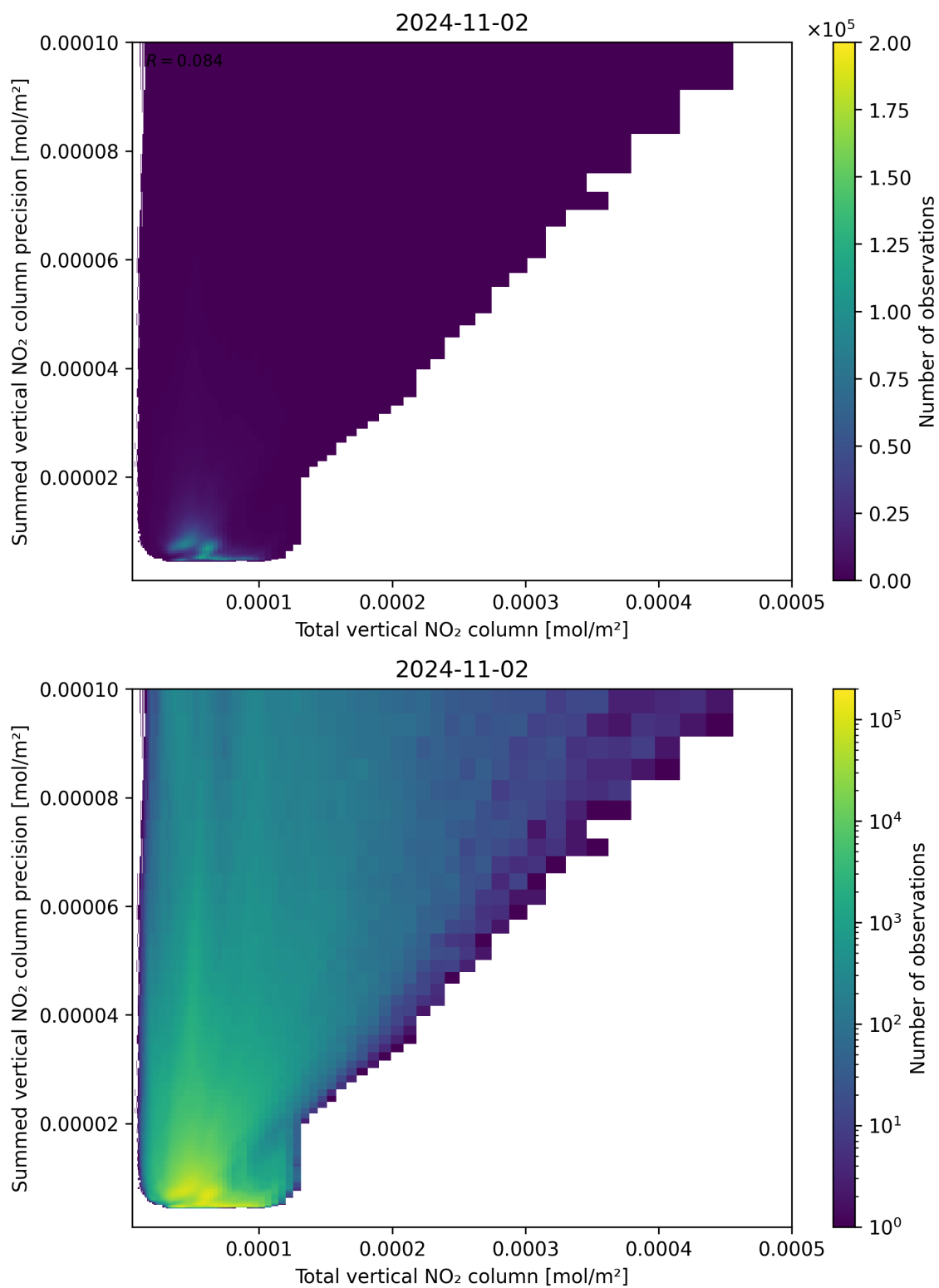
Figure 113: Scatter density plot of “Total vertical NO 2 column” against “Summed vertical NO 2 column precision” for 2024-11-01 to 2024-11-03.
