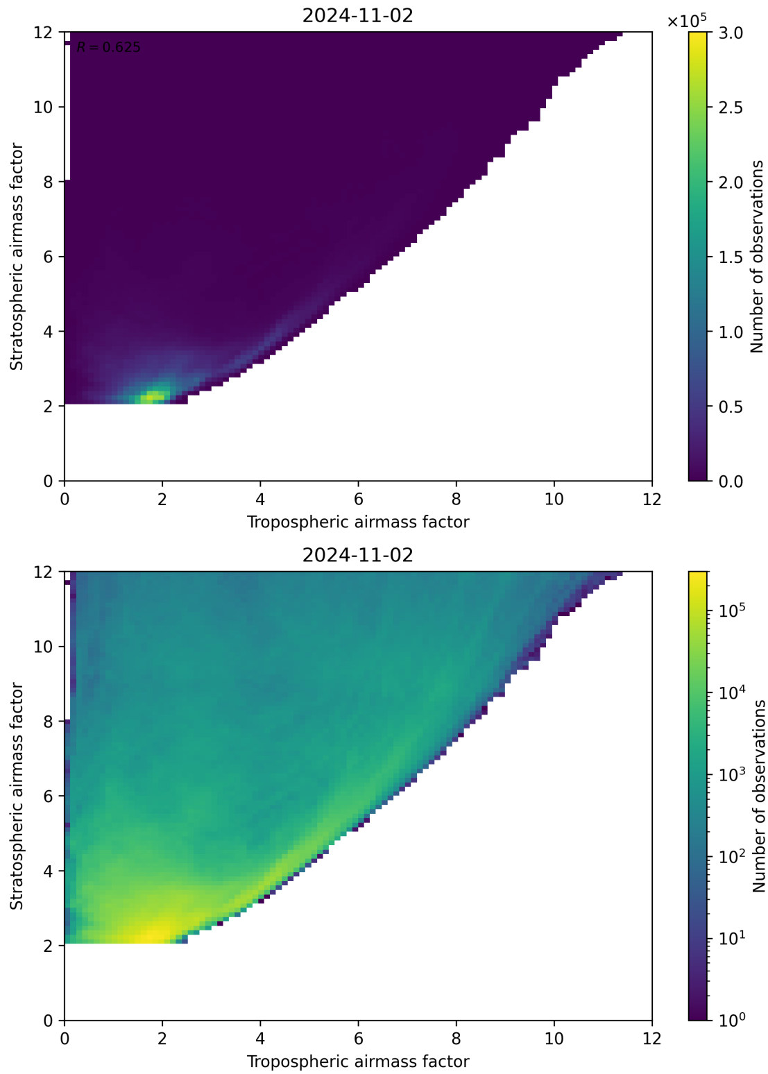
Figure 71: Scatter density plot of “Tropospheric airmass factor” against “Stratospheric airmass factor” for 2024-11-01 to 2024-11-03.
