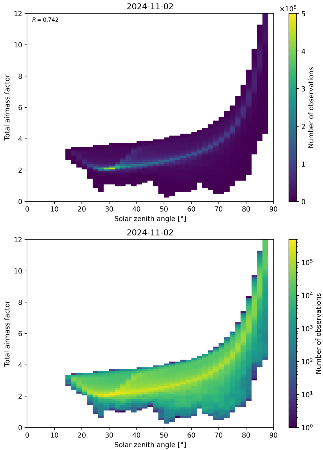
Figure 146: Scatter density plot of “Solar zenith angle” against “Total airmass factor” for 2024-11-01 to 2024-11-03.
