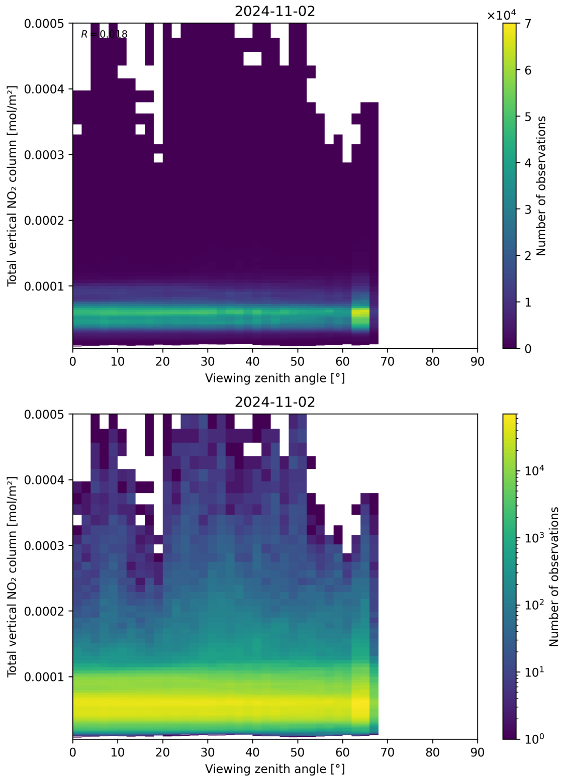
Figure 167: Scatter density plot of “Viewing zenith angle” against “Total vertical NO 2 column” for 2024-11-01 to 2024-11-03.
