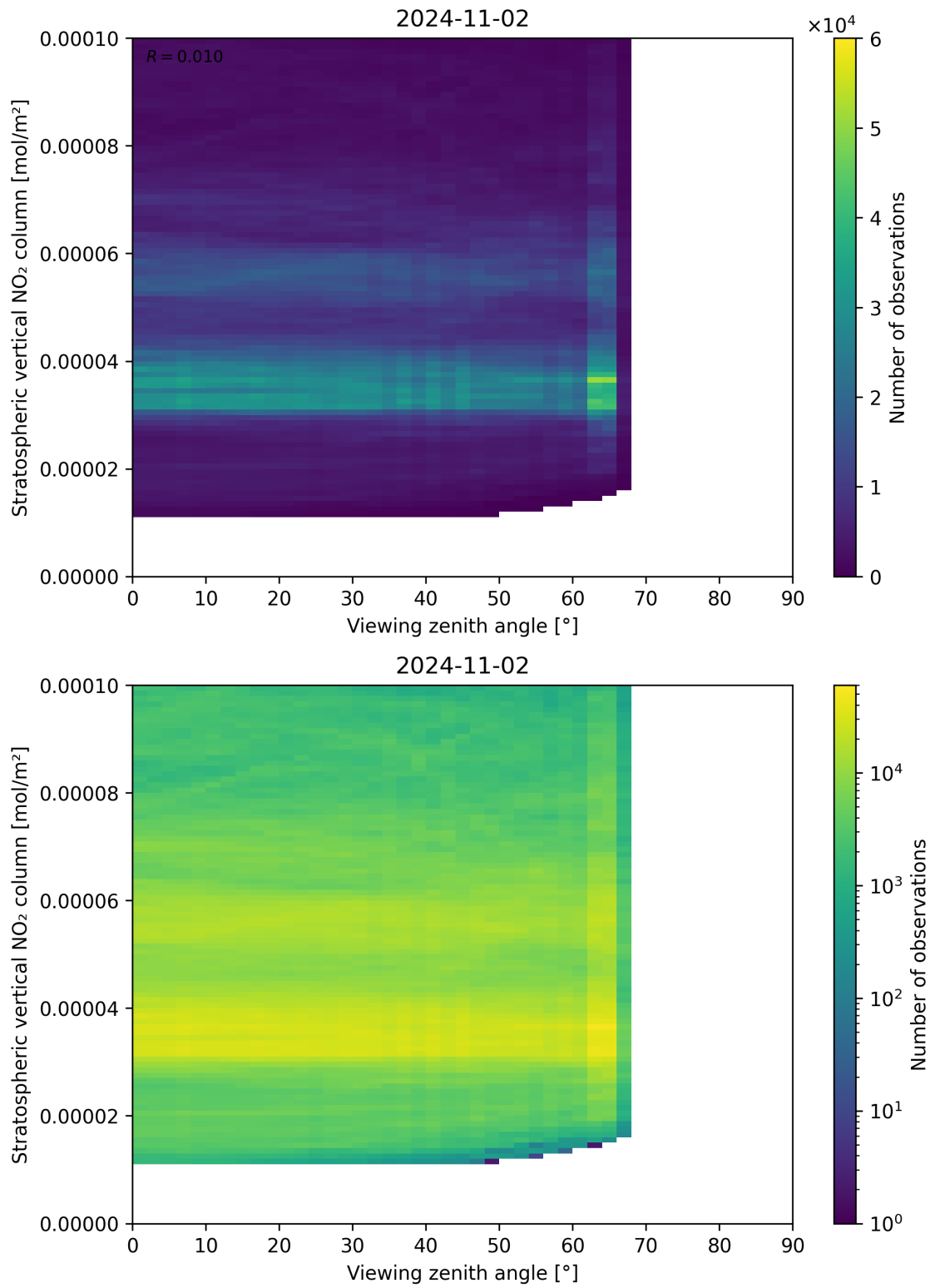
Figure 164: Scatter density plot of “Viewing zenith angle” against “Stratospheric vertical NO 2 column” for 2024-11-01 to 2024-11-03.
