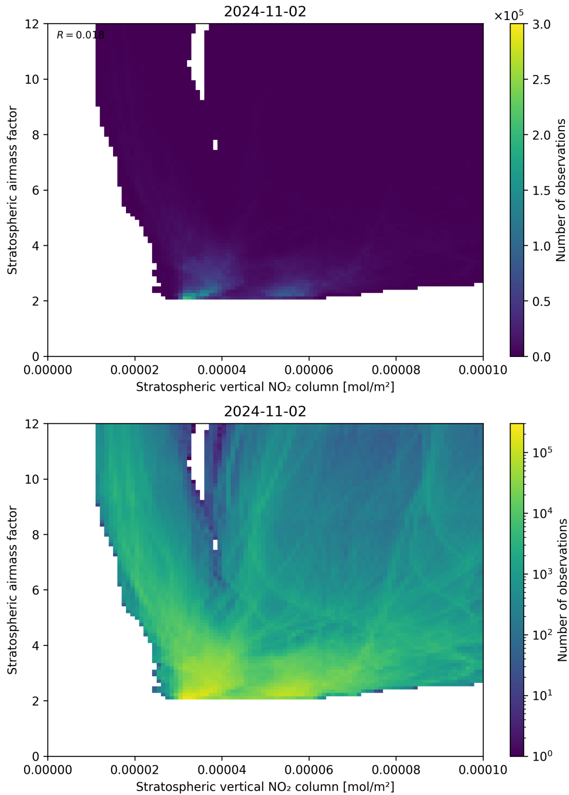
Figure 96: Scatter density plot of “Stratospheric vertical NO 2 column” against “Stratospheric airmass factor” for 2024-11-01 to 2024-11-03.
