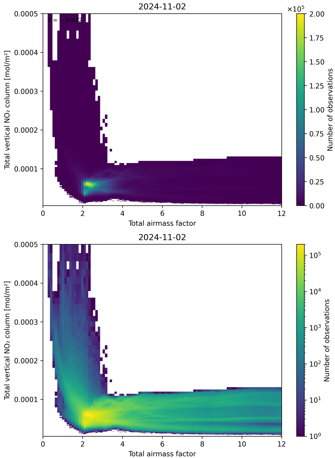
Figure 67: Scatter density plot of “Total airmass factor” against “Total vertical NO 2 column” for 2024-11-01 to 2024-11-03.
