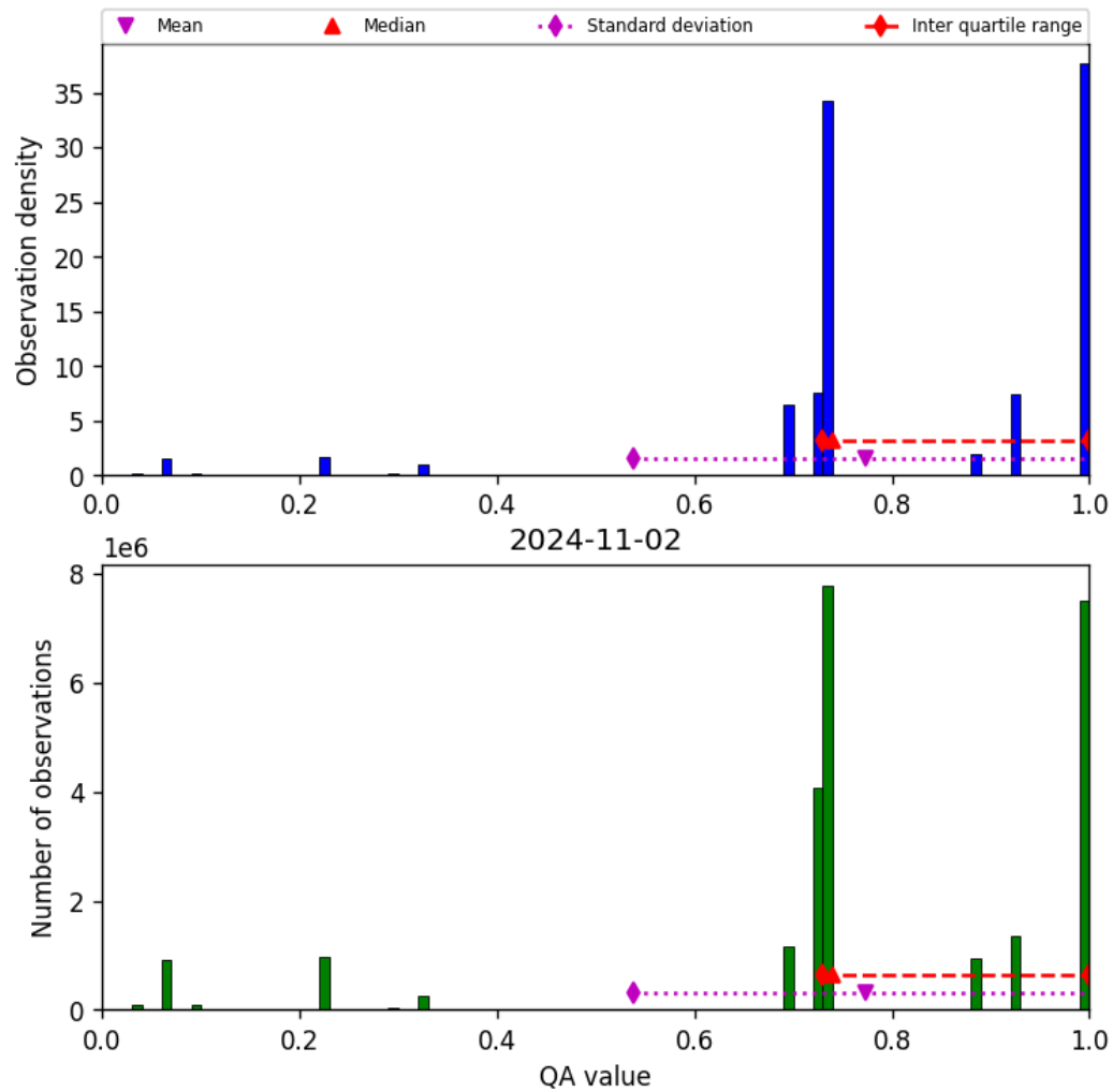
Figure 28: Histogram of “QA value” for 2024-11-01 to 2024-11-03
