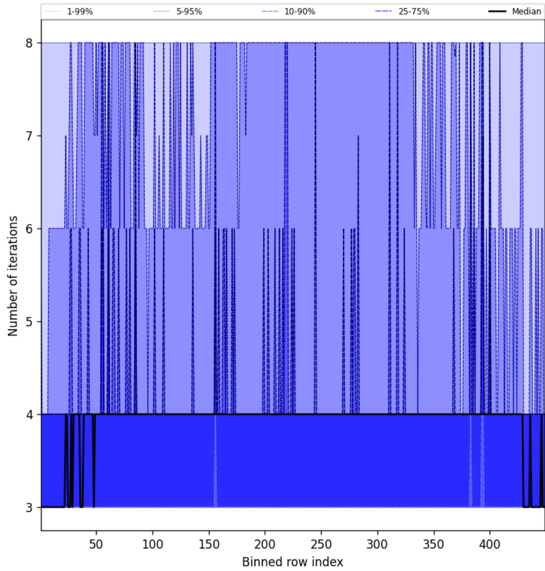
Figure 51: Along track statistics of “Number of iterations” for 2024-11-01 to 2024-11-03
