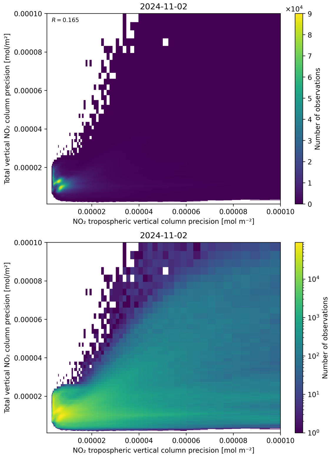
Figure 139: Scatter density plot of “NO 2 tropospheric vertical column precision” against “Total vertical NO 2 column precision” for 2024-11-01 to 2024-11-03.
