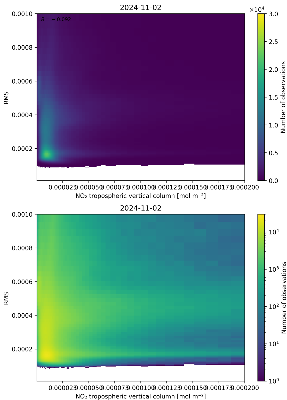
Figure 142: Scatter density plot of “NO 2 tropospheric vertical column” against “RMS” for 2024-11-01 to 2024-11-03.
