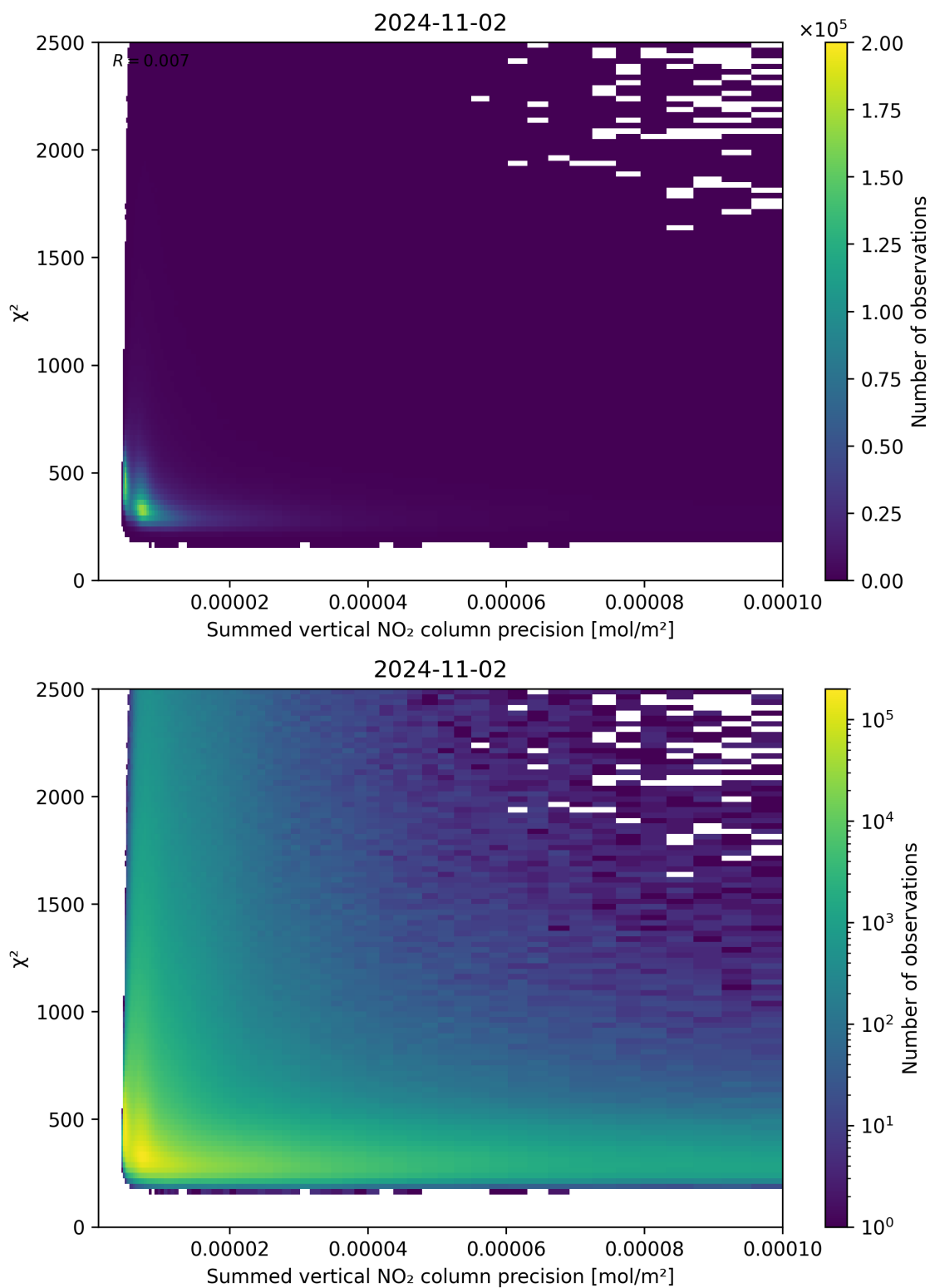
Figure 107: Scatter density plot of “Summed vertical NO 2 column precision” against “ \chi^2 ” for 2024-11-01 to 2024-11-03.
