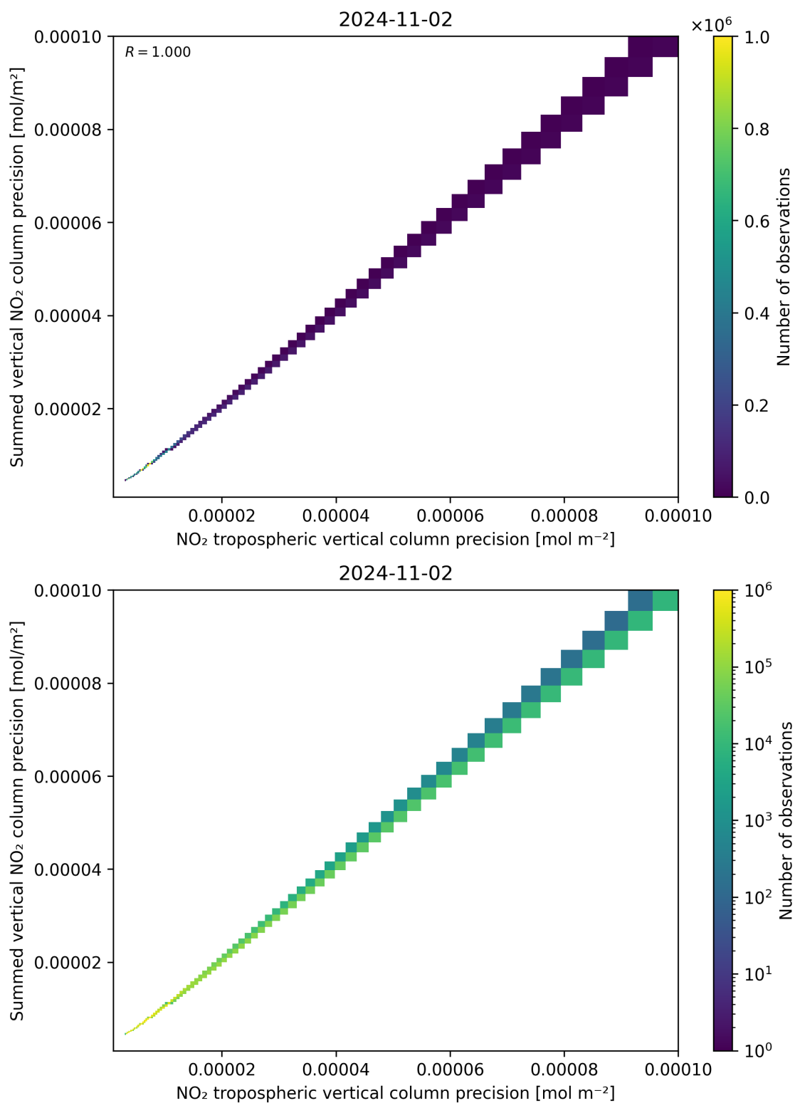
Figure 137: Scatter density plot of “NO 2 tropospheric vertical column precision” against “Summed vertical NO 2 column precision” for 2024-11-01 to 2024-11-03.
