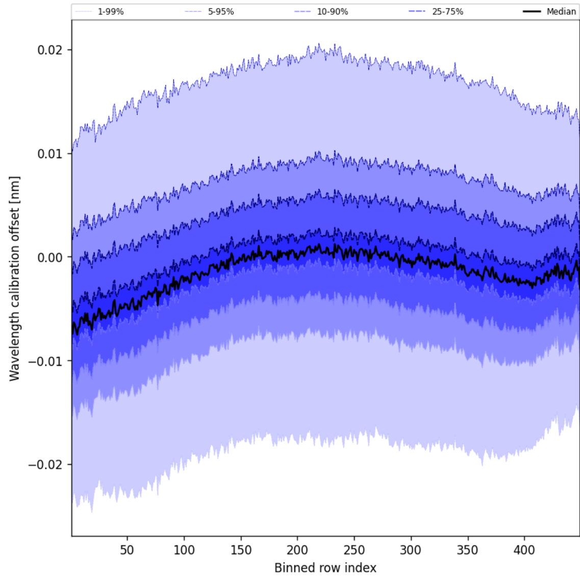
Figure 52: Along track statistics of “Wavelength calibration offset” for 2024-11-01 to 2024-11-03
