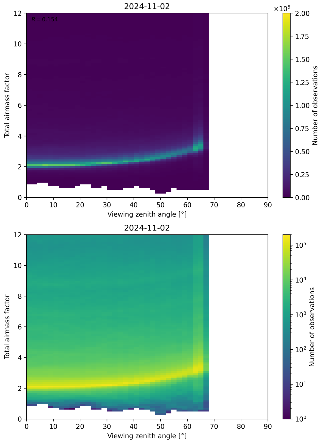
Figure 160: Scatter density plot of “Viewing zenith angle” against “Total airmass factor” for 2024-11-01 to 2024-11-03.
