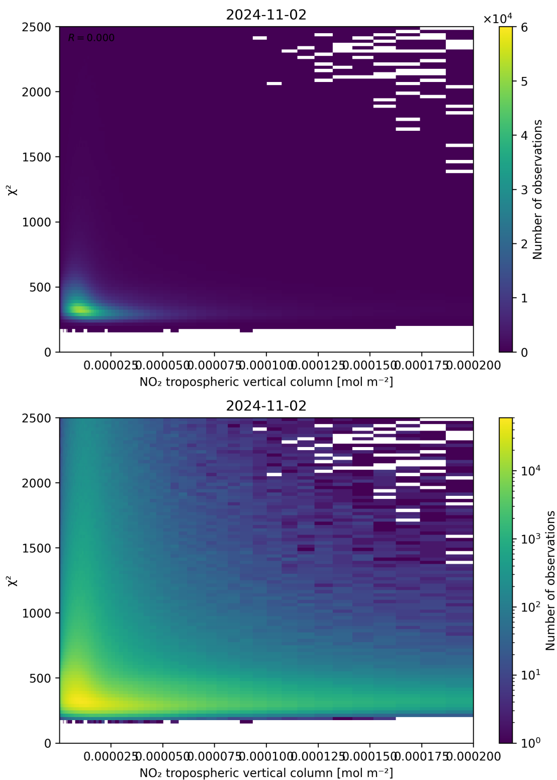
Figure 124: Scatter density plot of “NO 2 tropospheric vertical column” against “ \chi^2 ” for 2024-11-01 to 2024-11-03.
