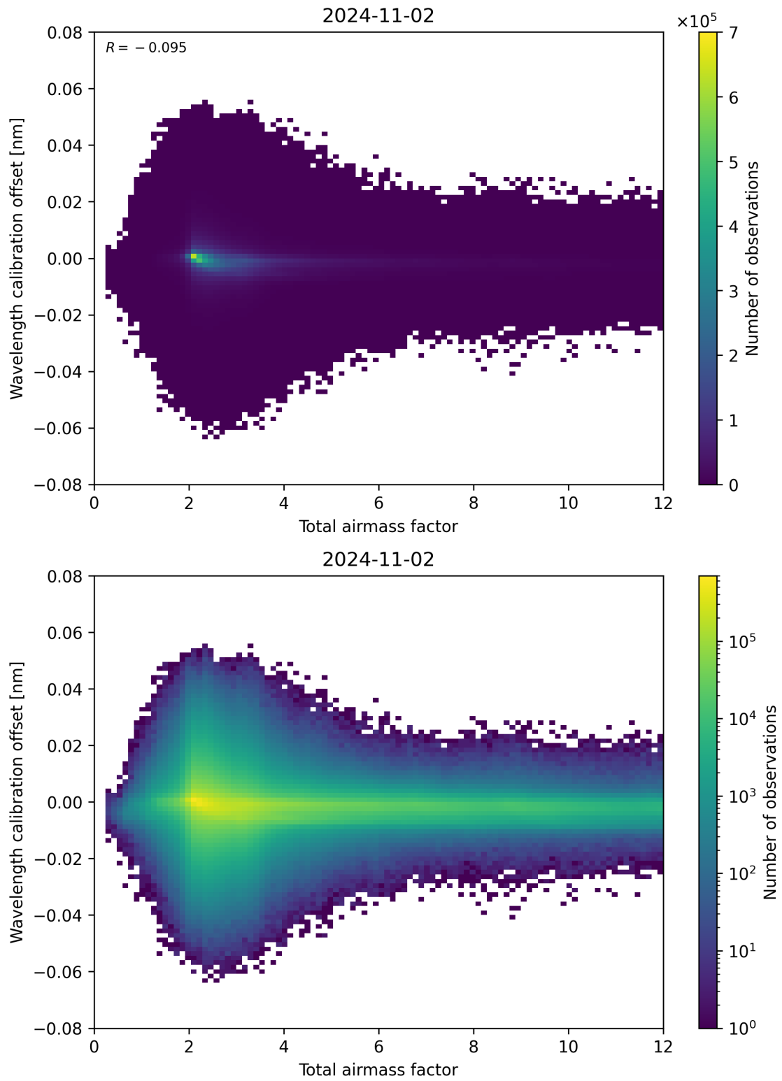
Figure 70: Scatter density plot of “Total airmass factor” against “Wavelength calibration offset” for 2024-11-01 to 2024-11-03.
