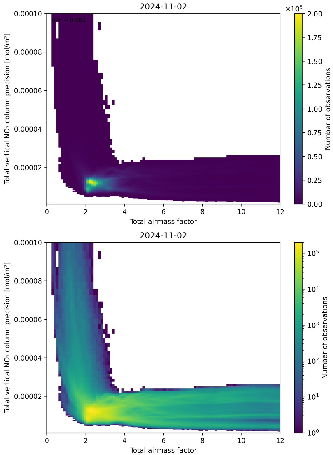
Figure 68: Scatter density plot of “Total airmass factor” against “Total vertical NO 2 column precision” for 2024-11-01 to 2024-11-03.
