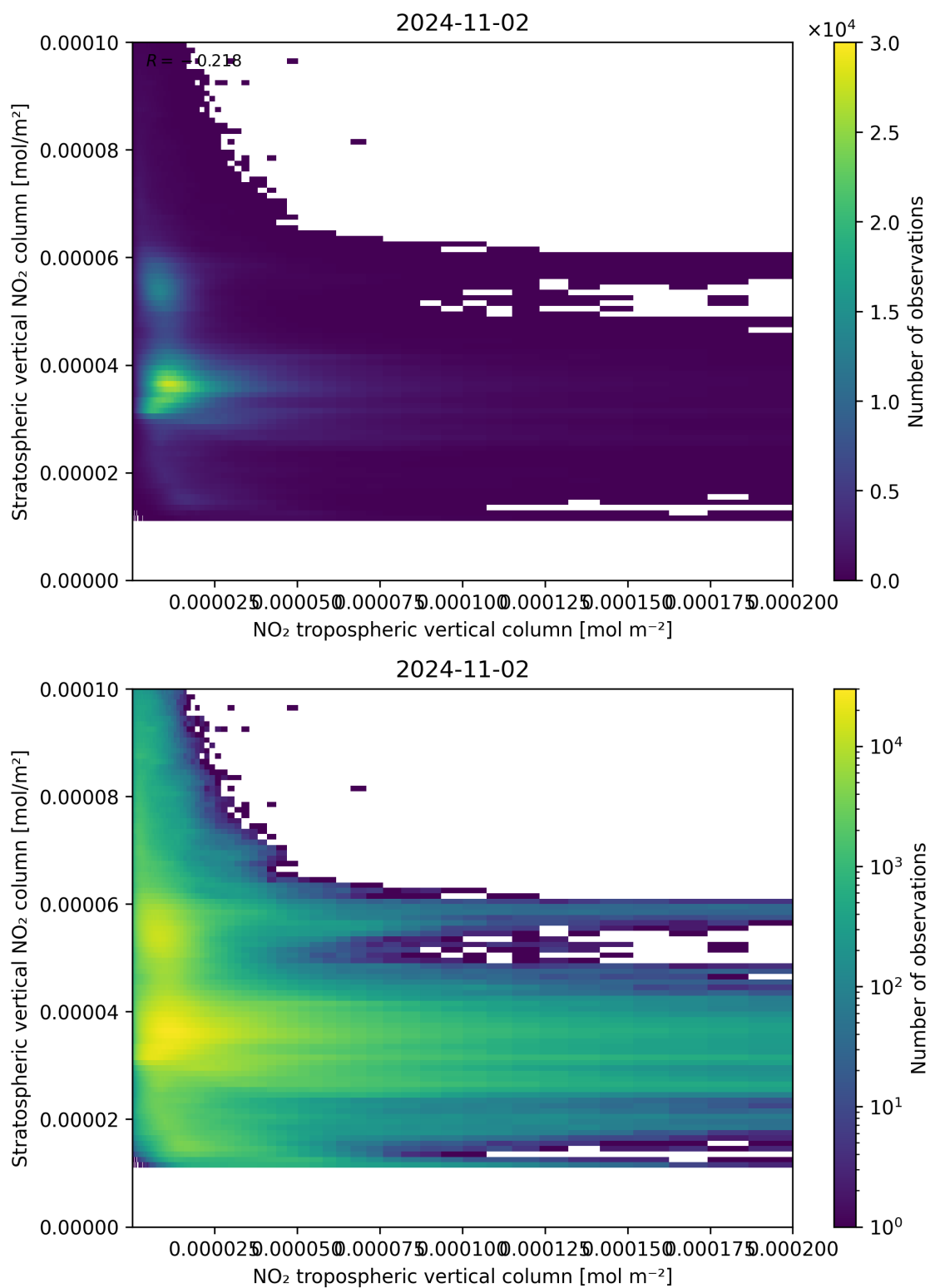
Figure 125: Scatter density plot of “NO 2 tropospheric vertical column” against “Stratospheric vertical NO 2 column” for 2024-11-01 to 2024-11-03.
