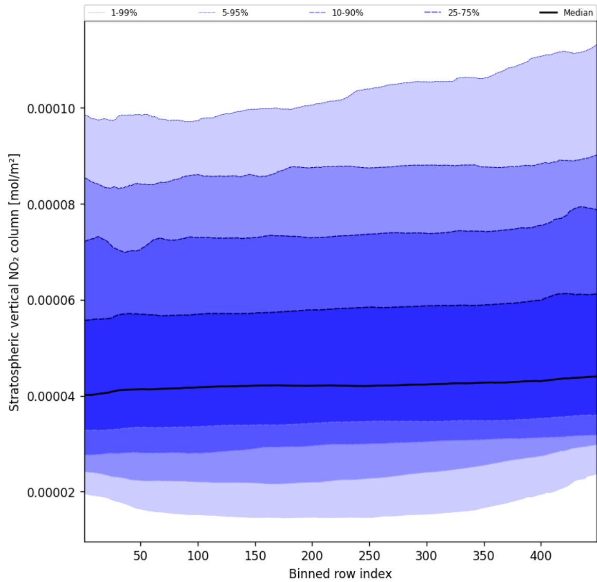
Figure 53: Along track statistics of “Stratospheric vertical NO 2 column” for 2024-11-01 to 2024-11-03
