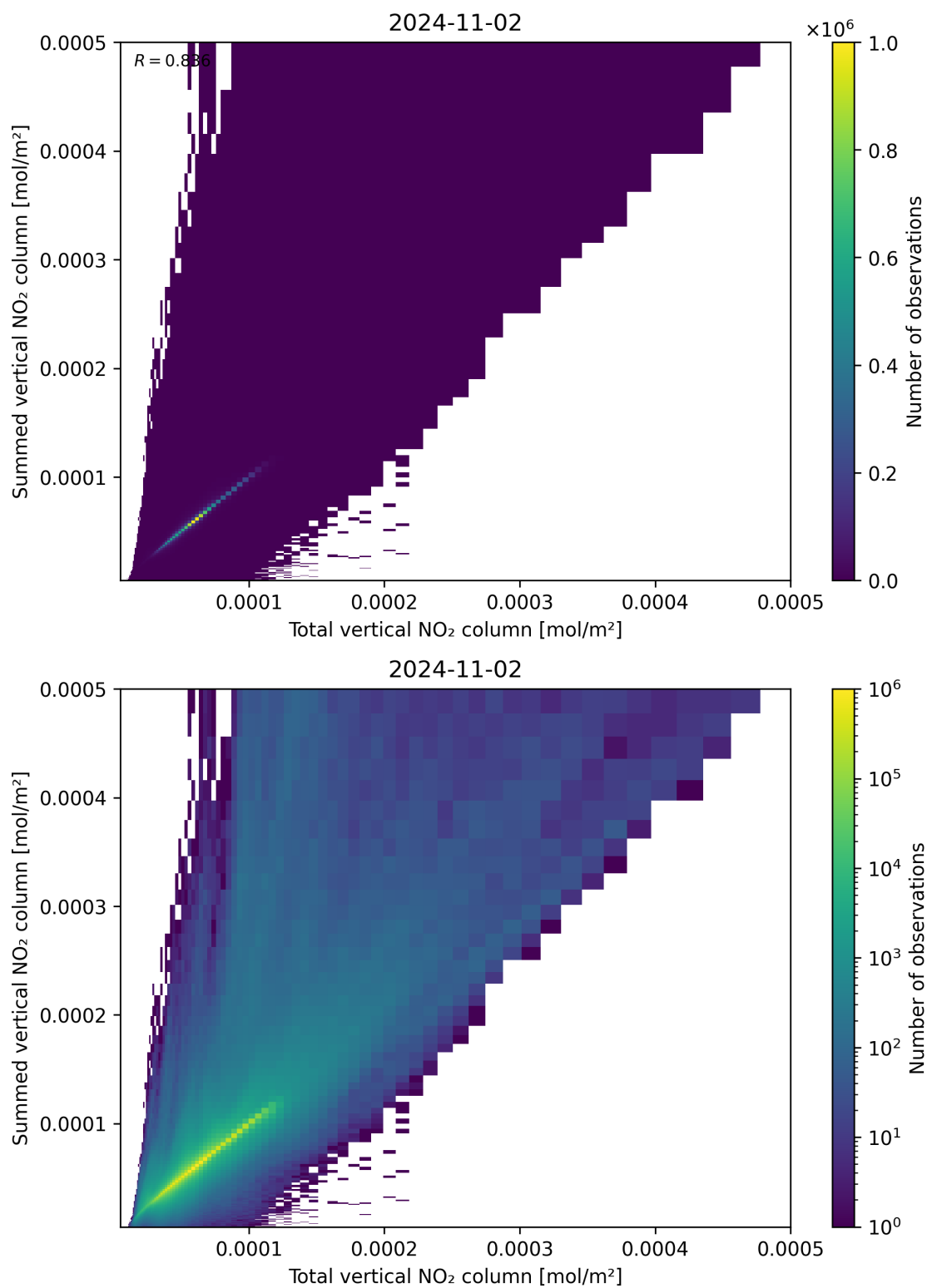
Figure 112: Scatter density plot of “Total vertical NO 2 column” against “Summed vertical NO 2 column” for 2024-11-01 to 2024-11-03.
