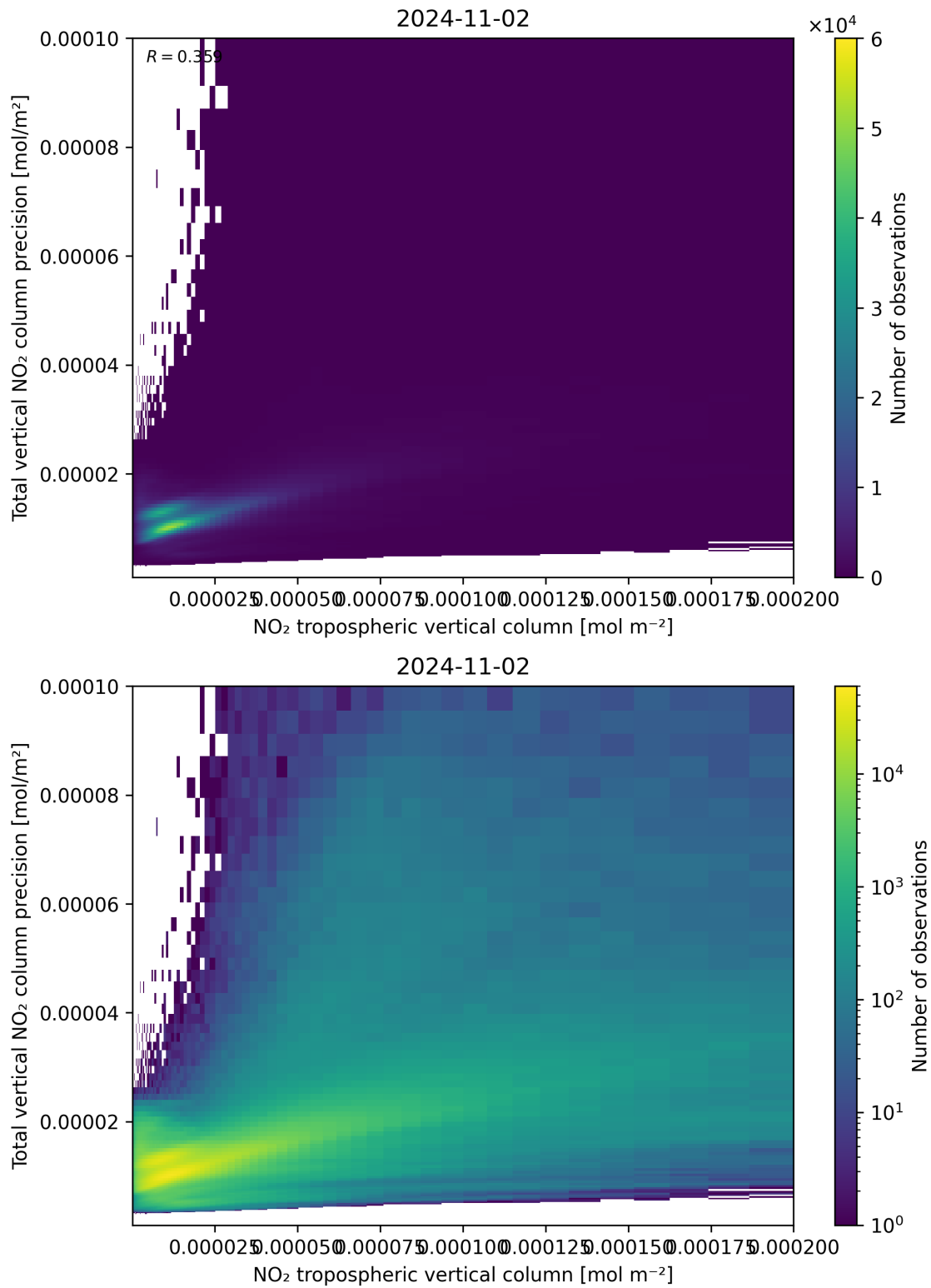
Figure 129: Scatter density plot of “NO 2 tropospheric vertical column” against “Total vertical NO 2 column precision” for 2024-11-01 to 2024-11-03.
