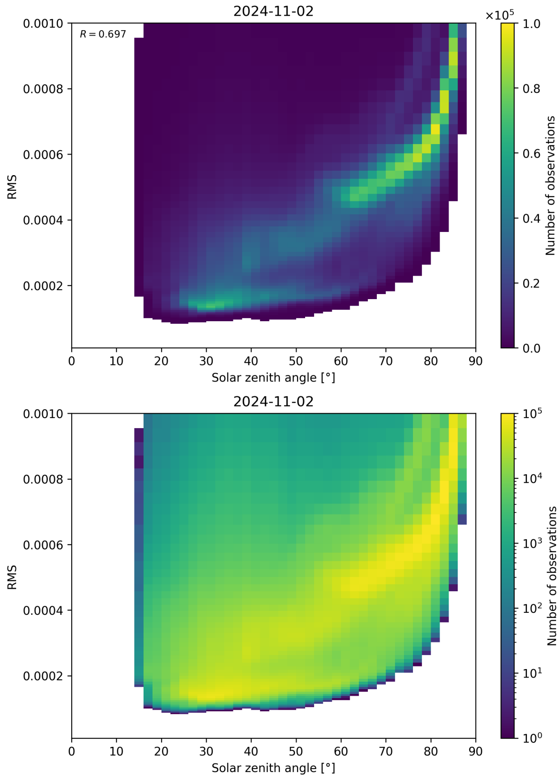
Figure 157: Scatter density plot of “Solar zenith angle” against “RMS” for 2024-11-01 to 2024-11-03.
