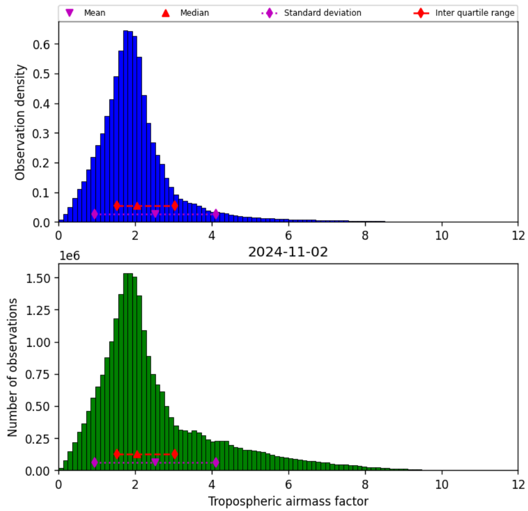
Figure 31: Histogram of “Tropospheric airmass factor” for 2024-11-01 to 2024-11-03
