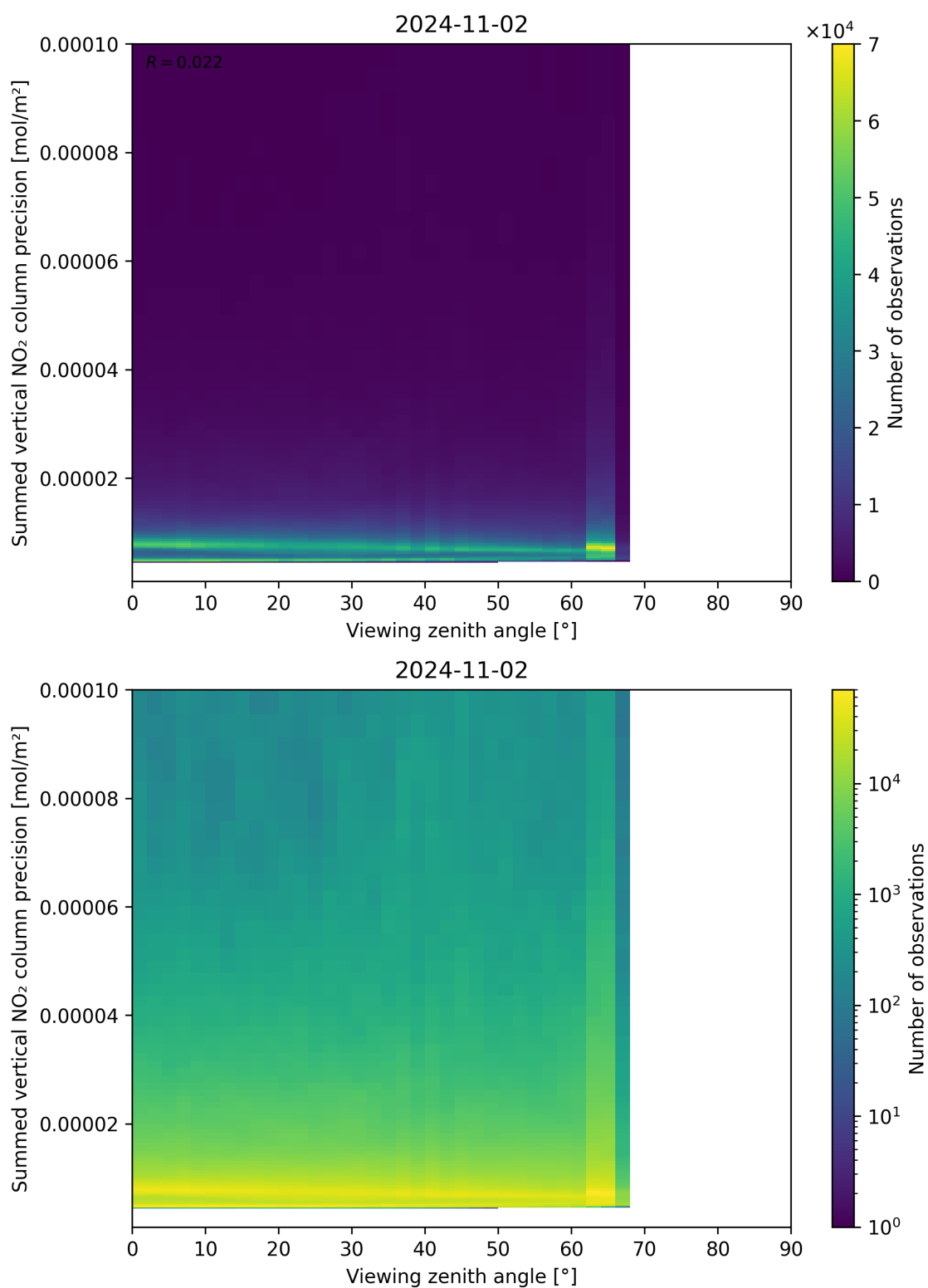
Figure 166: Scatter density plot of “Viewing zenith angle” against “Summed vertical NO 2 column precision” for 2024-11-01 to 2024-11-03.
