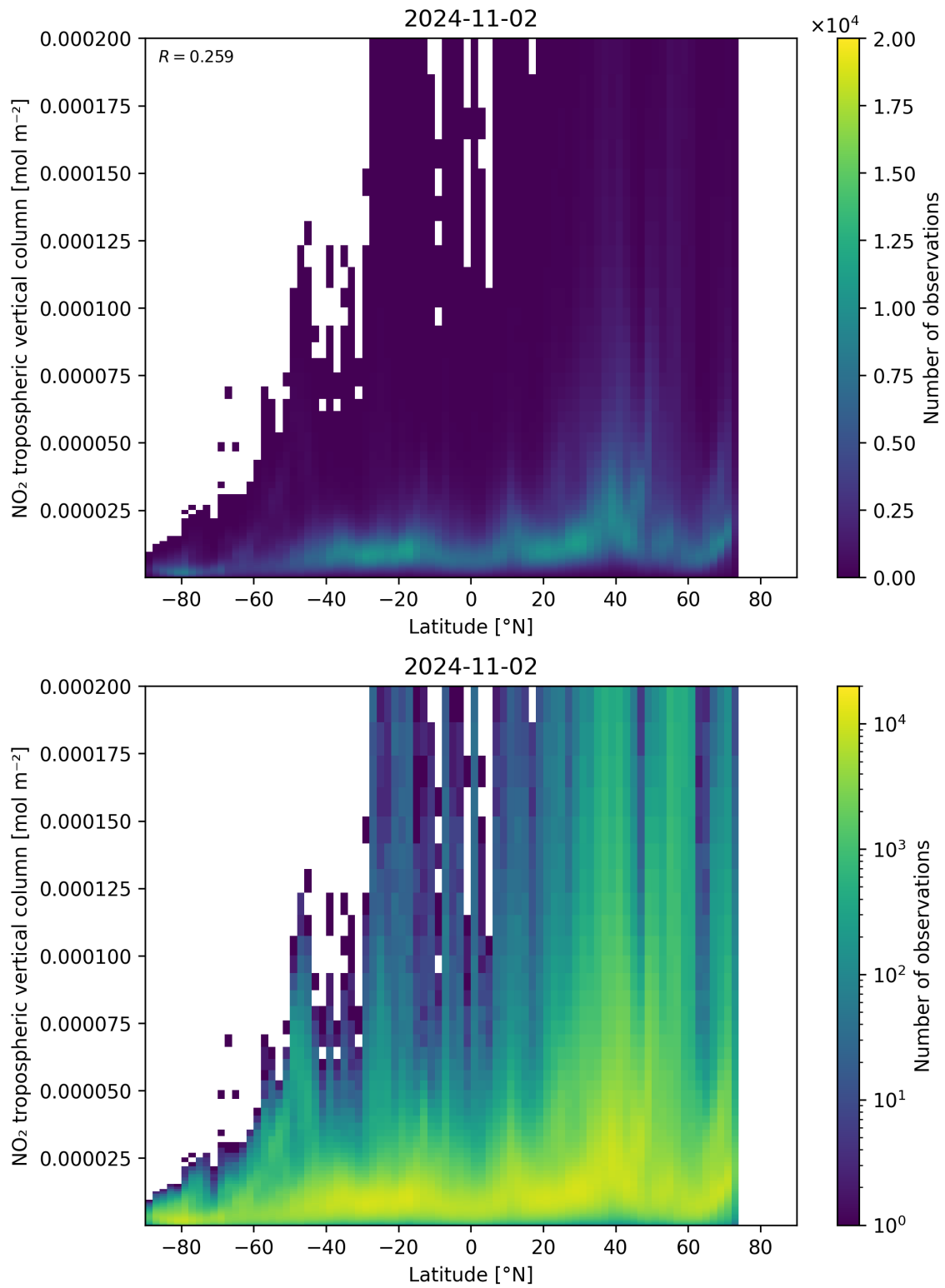
Figure 92: Scatter density plot of “Latitude” against “NO 2 tropospheric vertical column” for 2024-11-01 to 2024-11-03.
