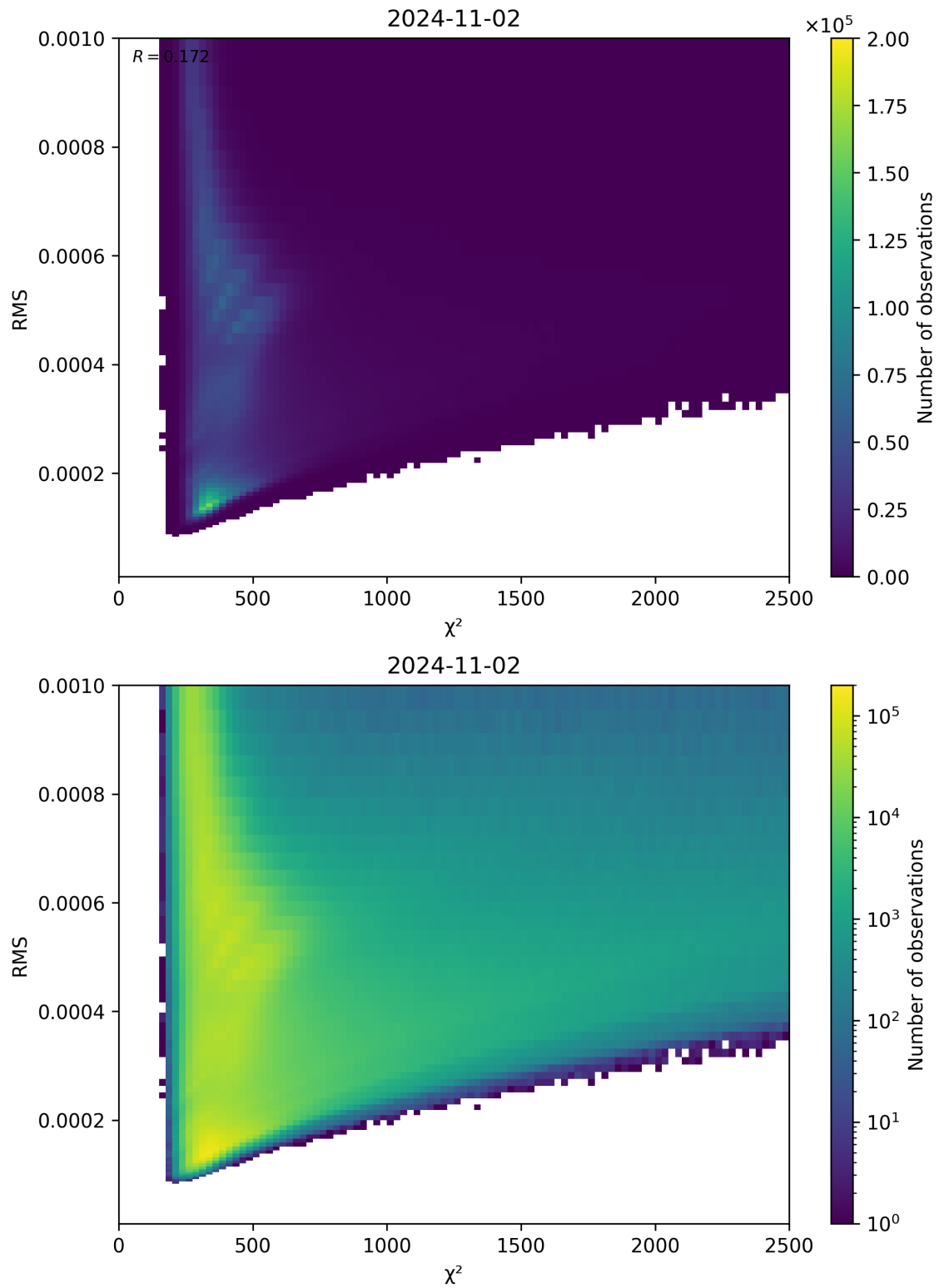
Figure 82: Scatter density plot of “ \chi^2 ” against “RMS” for 2024-11-01 to 2024-11-03.
