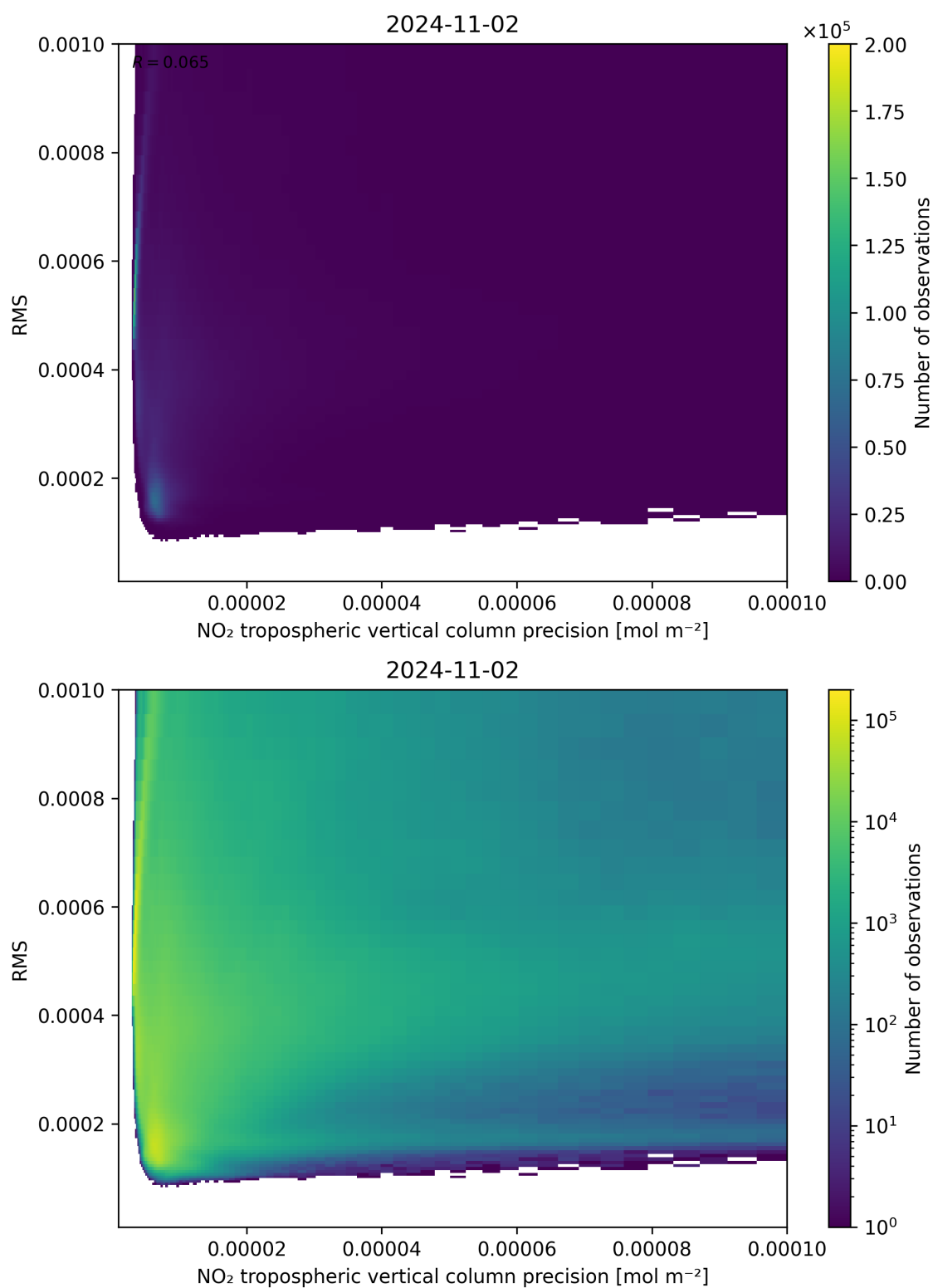
Figure 140: Scatter density plot of “NO 2 tropospheric vertical column precision” against “RMS” for 2024-11-01 to 2024-11-03.
