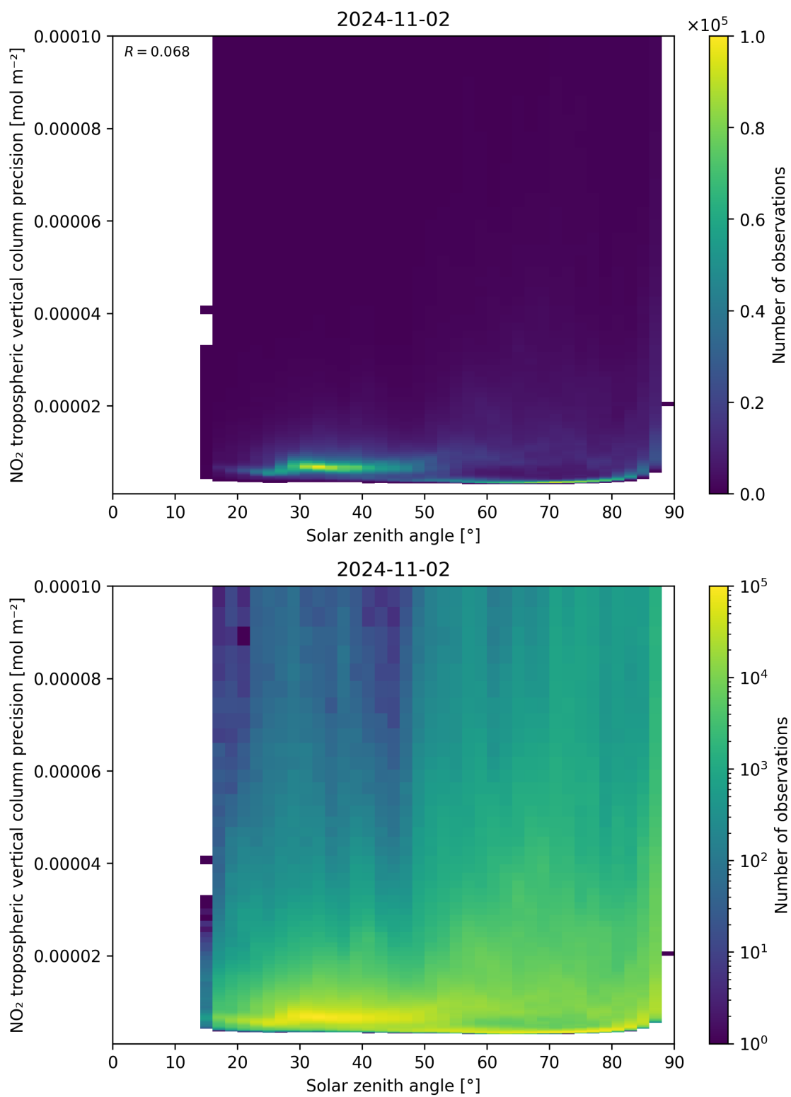
Figure 156: Scatter density plot of “Solar zenith angle” against “NO 2 tropospheric vertical column precision” for 2024-11-01 to 2024-11-03.
