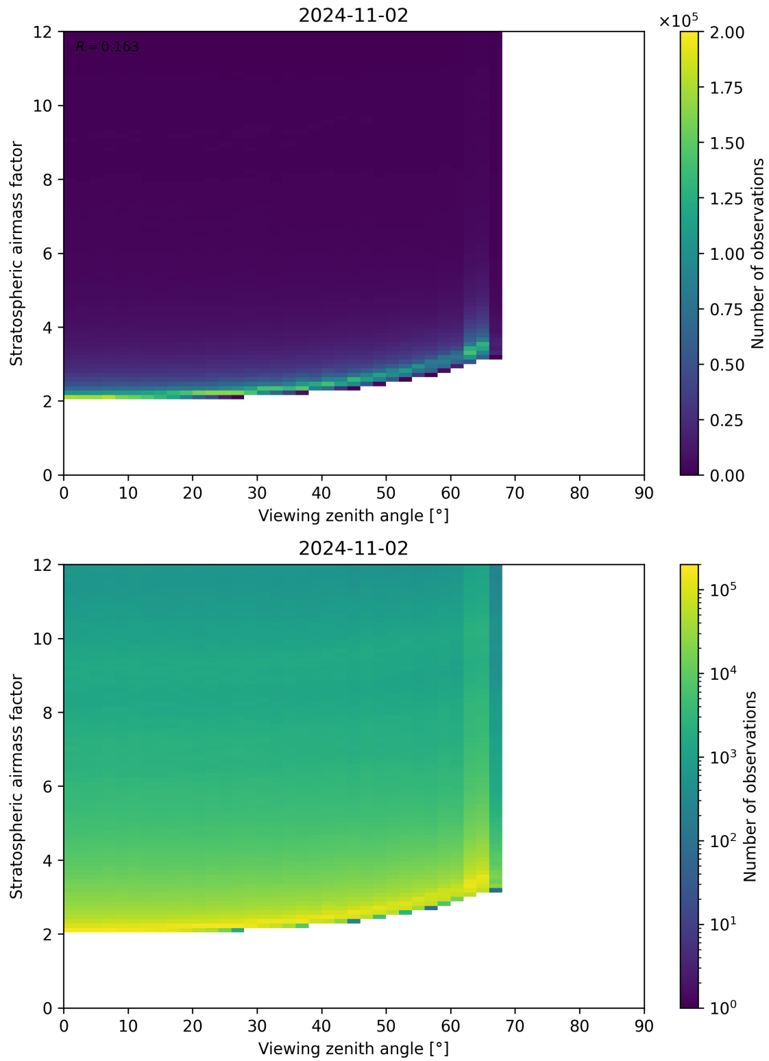
Figure 159: Scatter density plot of “Viewing zenith angle” against “Stratospheric airmass factor” for 2024-11-01 to 2024-11-03.
