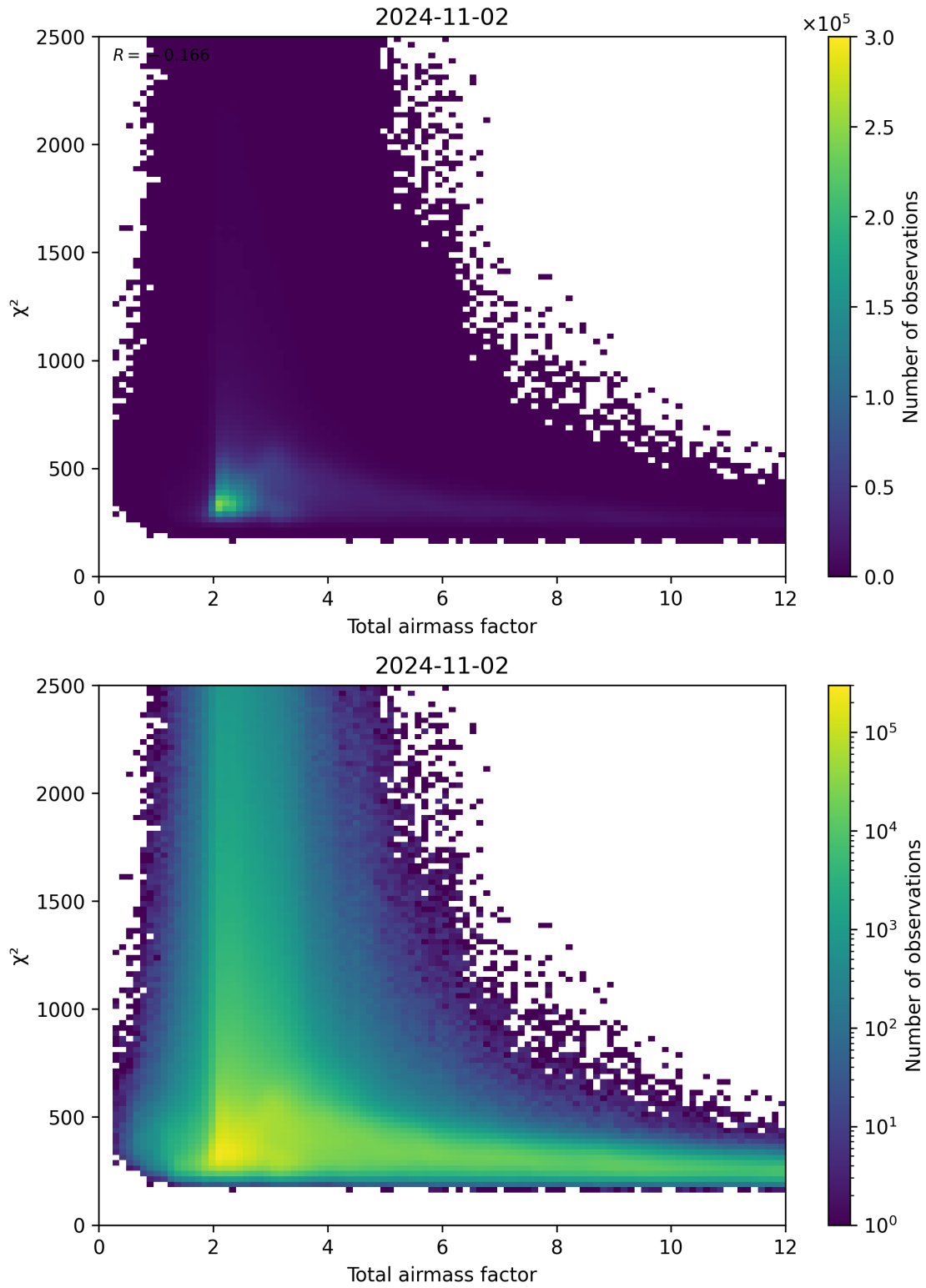
Figure 63: Scatter density plot of “Total airmass factor” against “ \chi^2 ” for 2024-11-01 to 2024-11-03.
