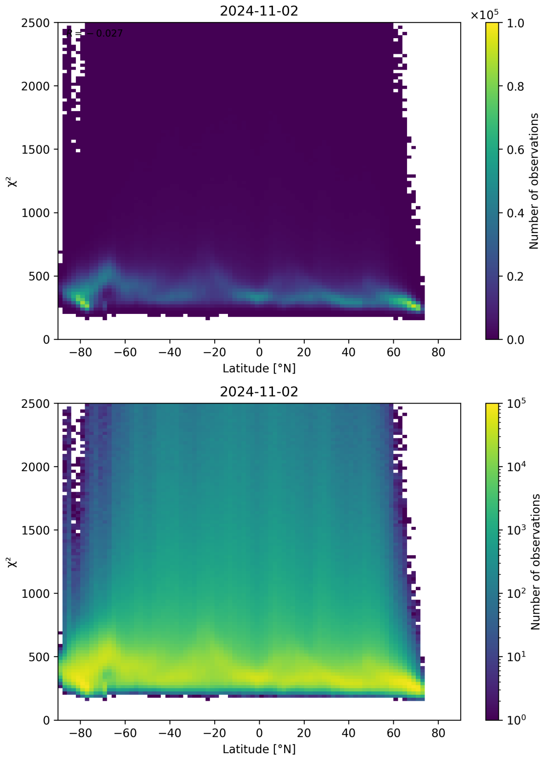
Figure 86: Scatter density plot of “Latitude” against “ \chi^2 ” for 2024-11-01 to 2024-11-03.
