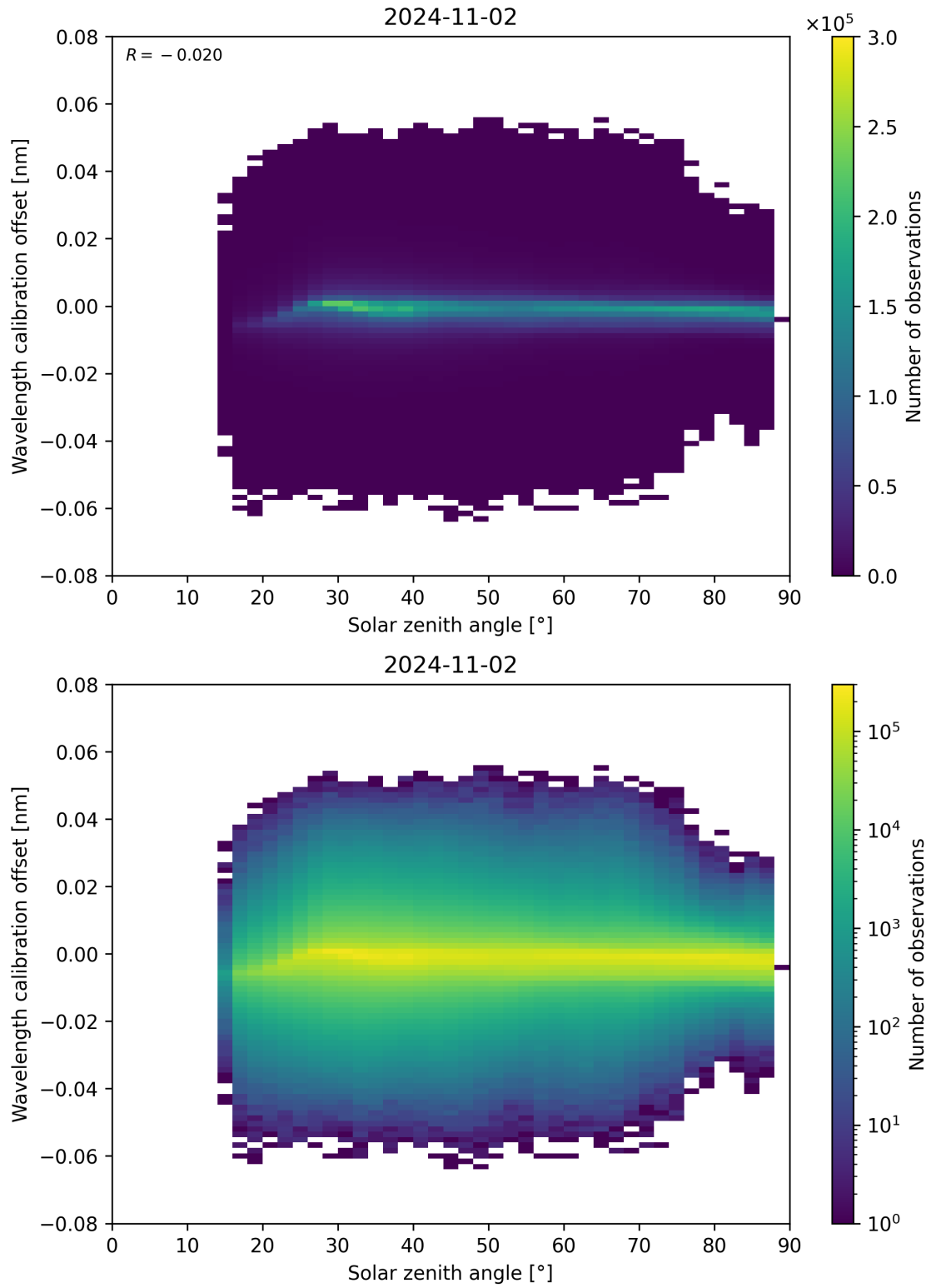
Figure 158: Scatter density plot of “Solar zenith angle” against “Wavelength calibration offset” for 2024-11-01 to 2024-11-03.
