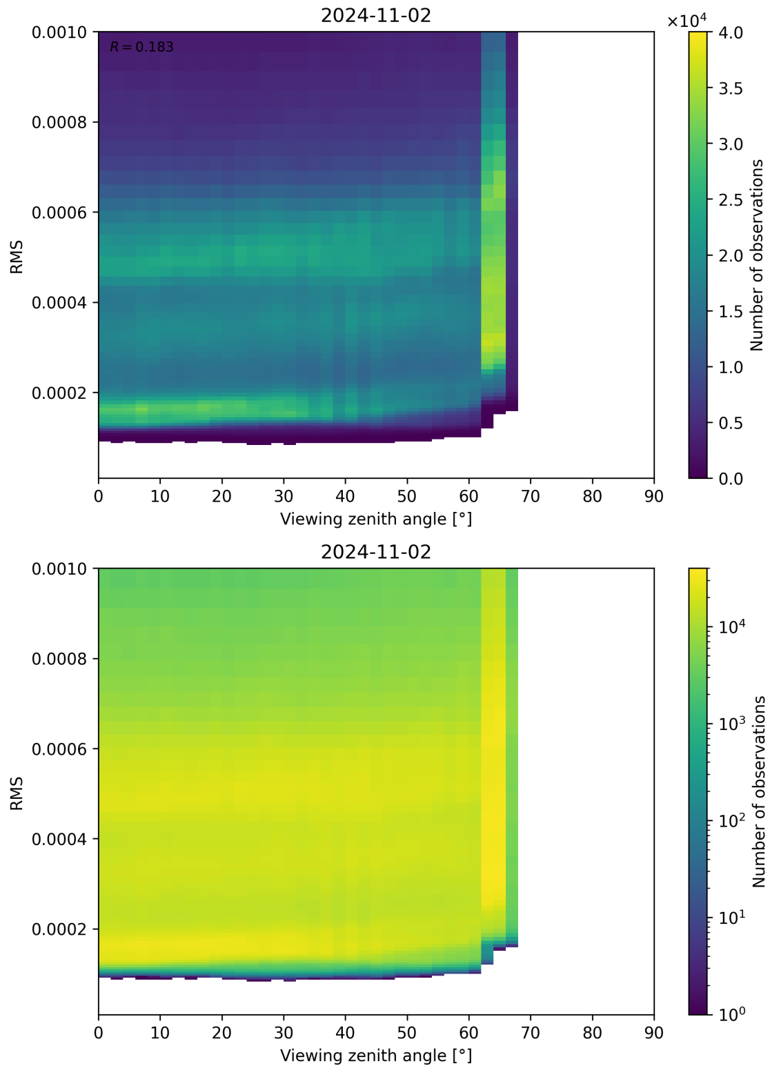
Figure 171: Scatter density plot of “Viewing zenith angle” against “RMS” for 2024-11-01 to 2024-11-03.
