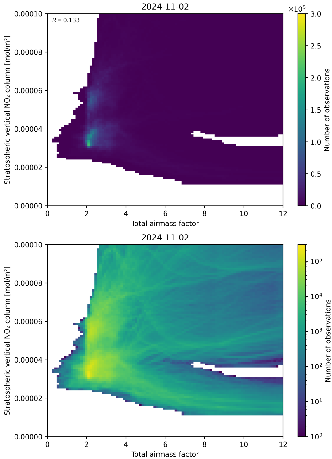
Figure 64: Scatter density plot of “Total airmass factor” against “Stratospheric vertical \text{NO}_2 column” for 2024-11-01 to 2024-11-03.
