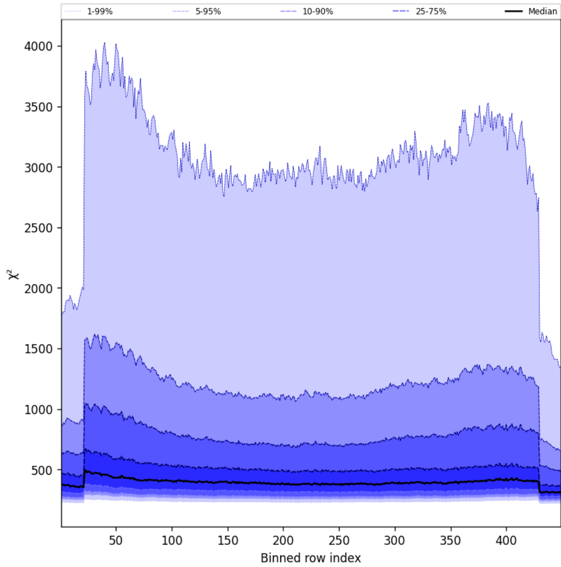
Figure 59: Along track statistics of “ \chi^2 ” for 2024-11-01 to 2024-11-03
