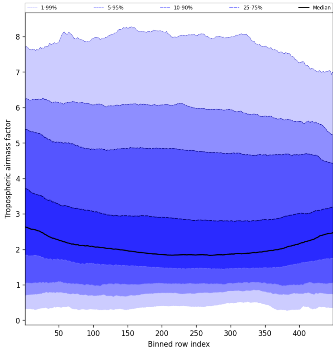
Figure 48: Along track statistics of “Tropospheric air mass factor” for 2024-11-01 to 2024-11-03
