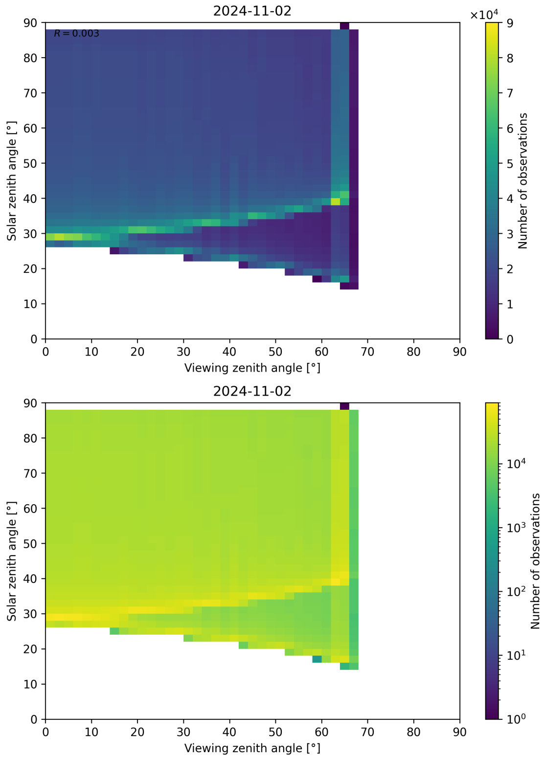
Figure 172: Scatter density plot of “Viewing zenith angle” against “Solar zenith angle” for 2024-11-01 to 2024-11-03.
