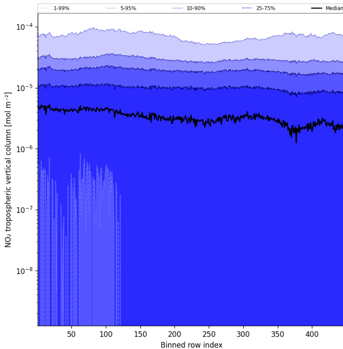
Figure 46: Along track statistics of “NO 2 tropospheric vertical column” for 2024-11-01 to 2024-11-03
