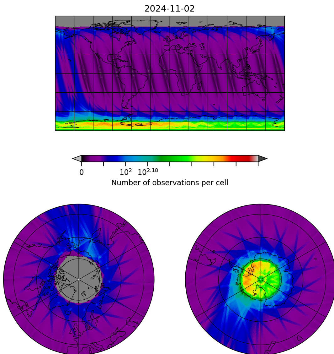
Figure 10: Map of the number of observations for 2024-11-01 to 2024-11-03
