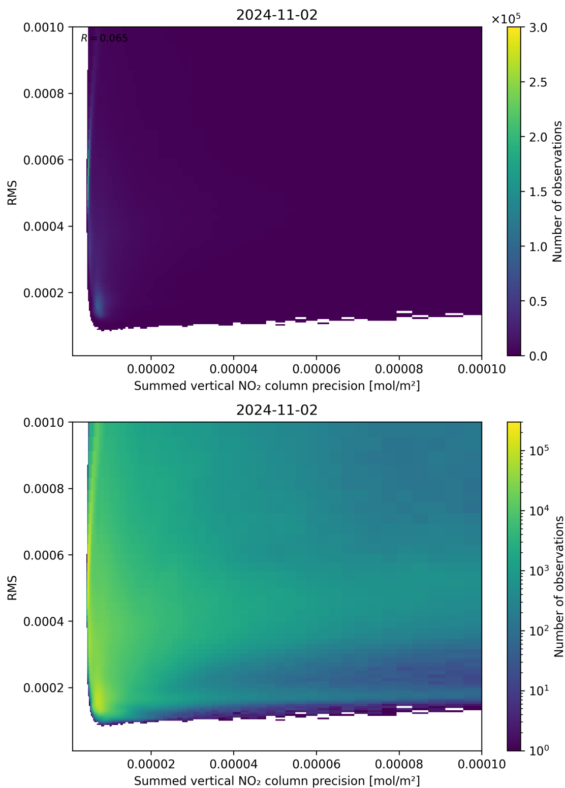
Figure 108: Scatter density plot of “Summed vertical NO 2 column precision” against “RMS” for 2024-11-01 to 2024-11-03.
