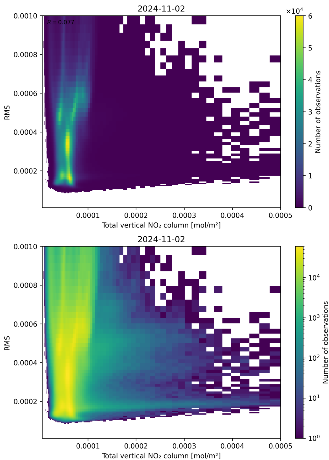
Figure 120: Scatter density plot of “Total vertical NO 2 column” against “RMS” for 2024-11-01 to 2024-11-03.
