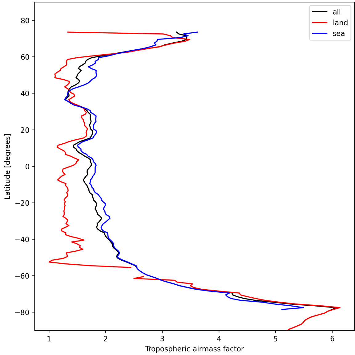
Figure 14: Zonal average of “Tropospheric airmass factor” for 2024-11-01 to 2024-11-03.
