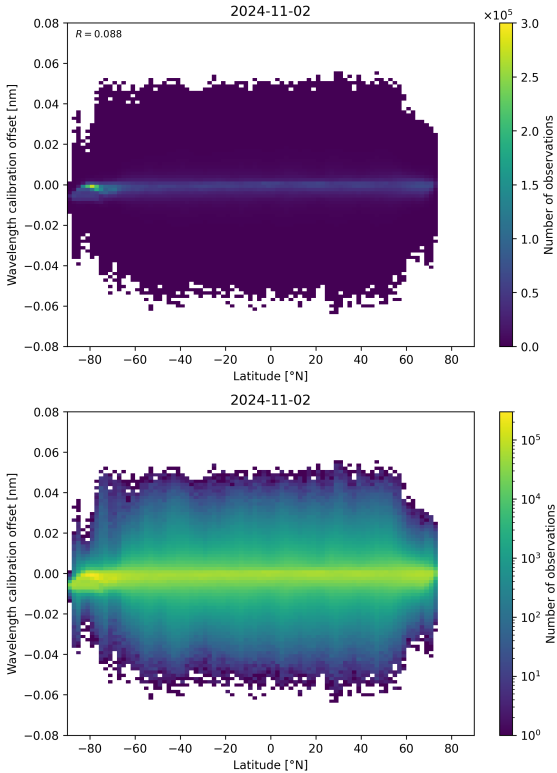
Figure 95: Scatter density plot of “Latitude” against “Wavelength calibration offset” for 2024-11-01 to 2024-11-03.
