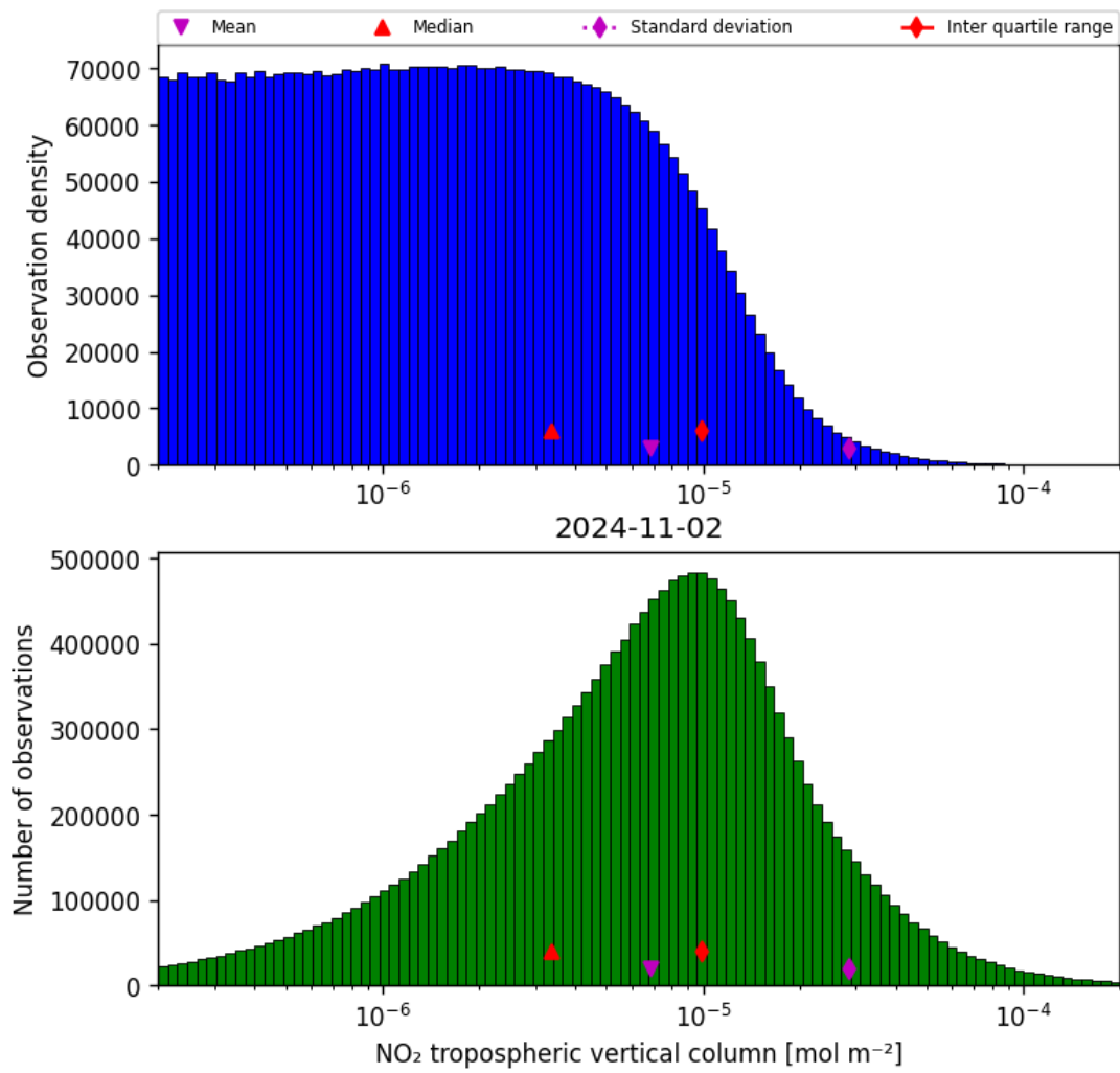
Figure 29: Histogram of “NO 2 tropospheric vertical column” for 2024-11-01 to 2024-11-03
