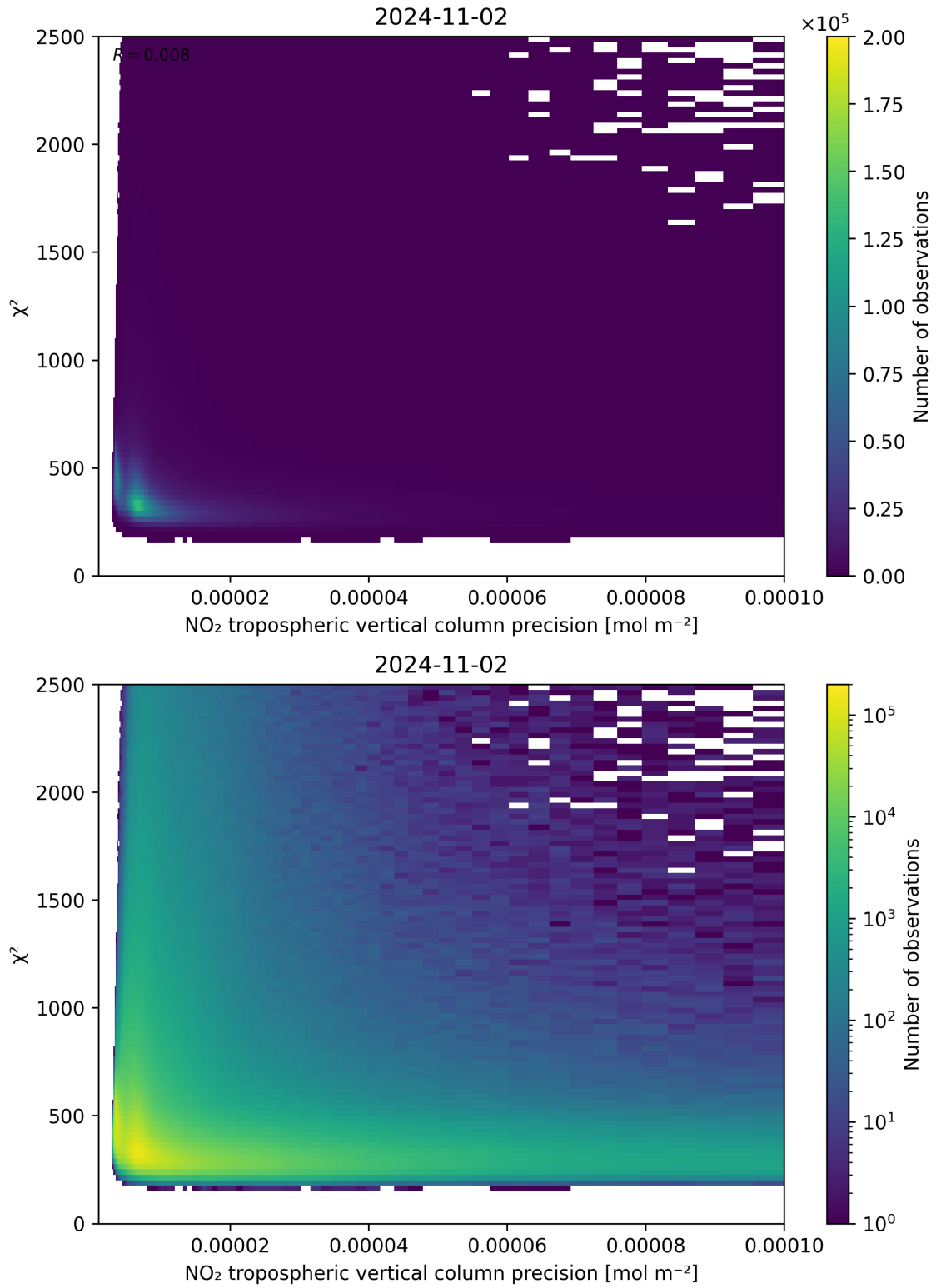
Figure 134: Scatter density plot of “NO 2 tropospheric vertical column precision” against “ \chi^2 ” for 2024-11-01 to 2024-11-03.
