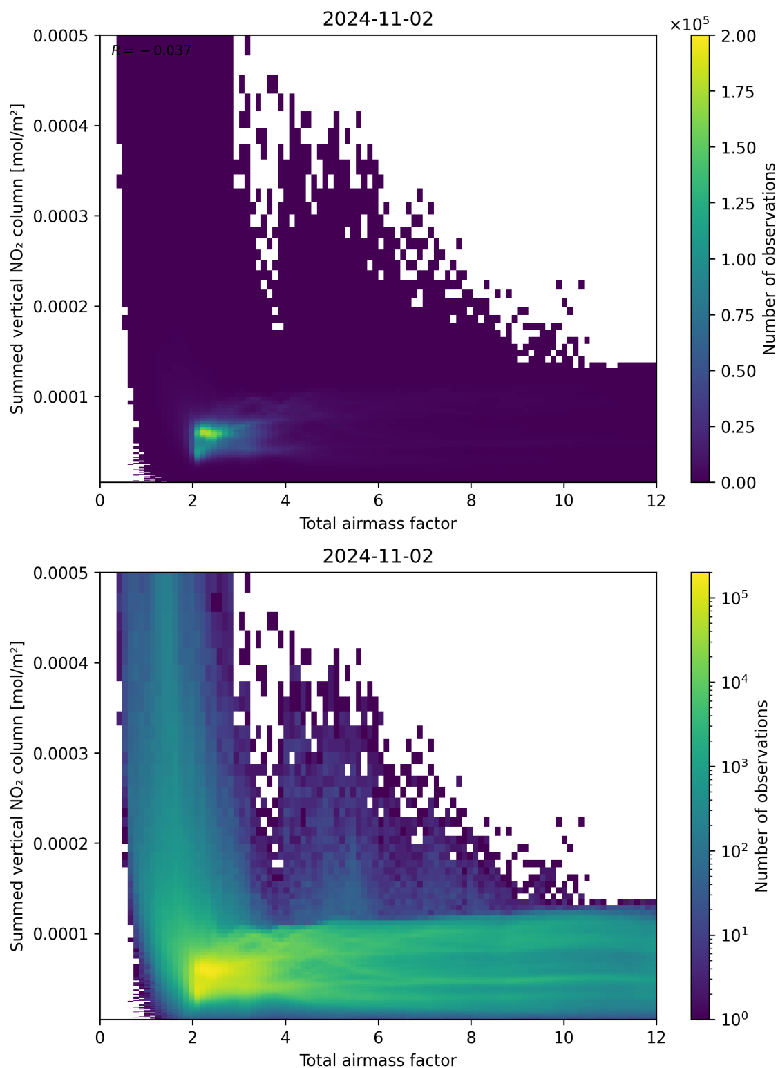
Figure 65: Scatter density plot of “Total airmass factor” against “Summed vertical NO 2 column” for 2024-11-01 to 2024-11-03.
