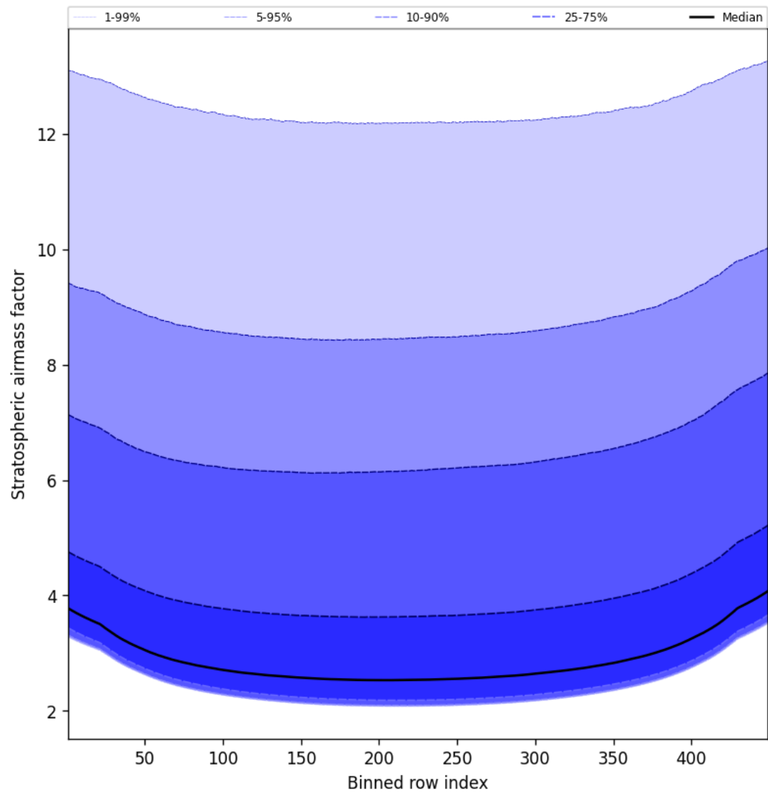
Figure 61: Along track statistics of “Stratospheric airmass factor” for 2024-11-01 to 2024-11-03
