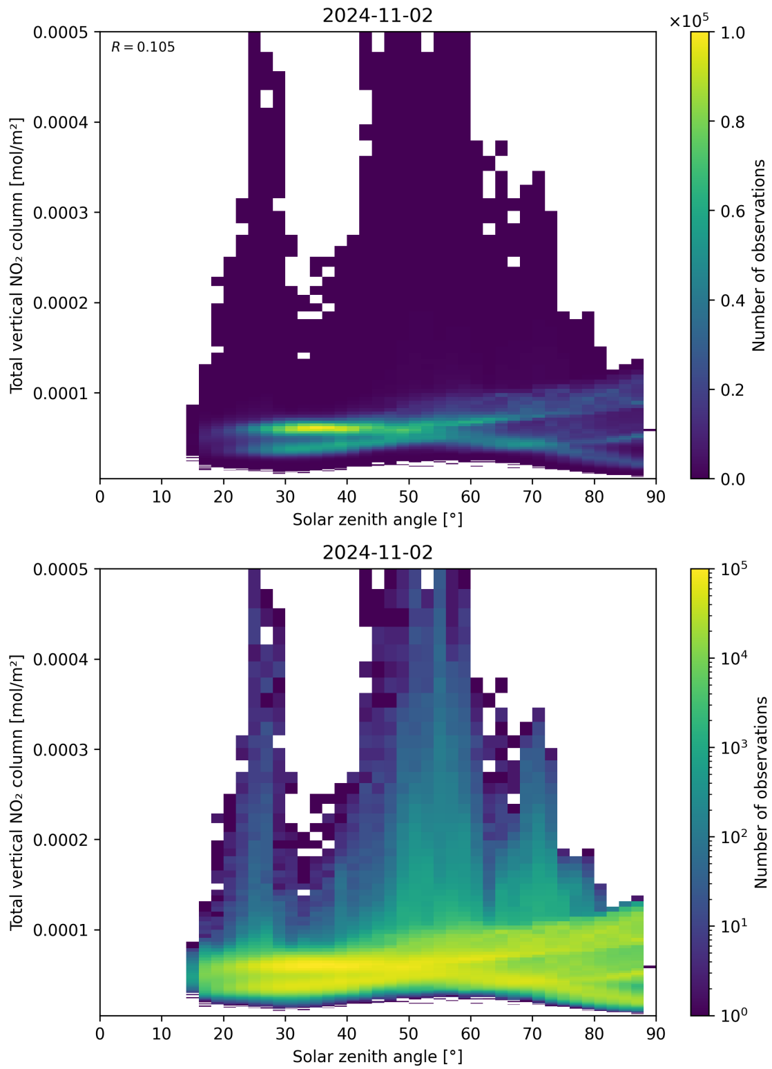
Figure 153: Scatter density plot of “Solar zenith angle” against “Total vertical NO 2 column” for 2024-11-01 to 2024-11-03.
