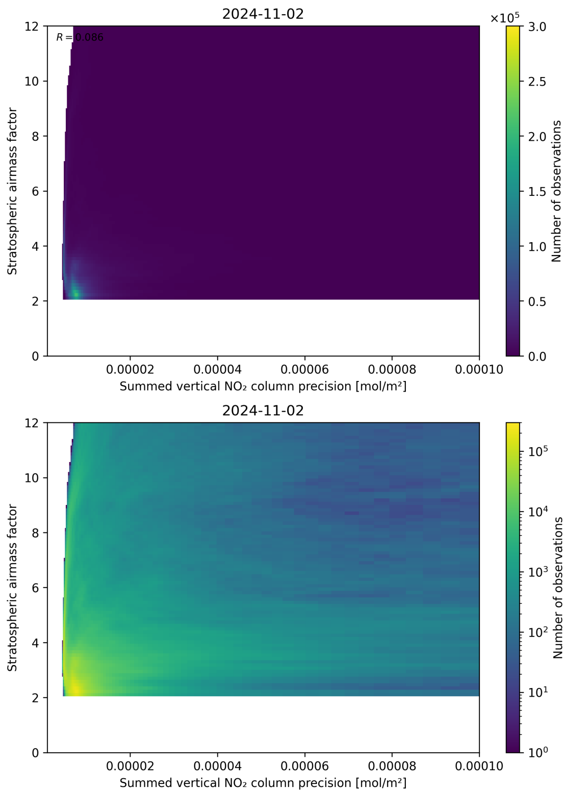
Figure 106: Scatter density plot of “Summed vertical NO 2 column precision” against “Stratospheric airmass factor” for 2024-11-01 to 2024-11-03.
