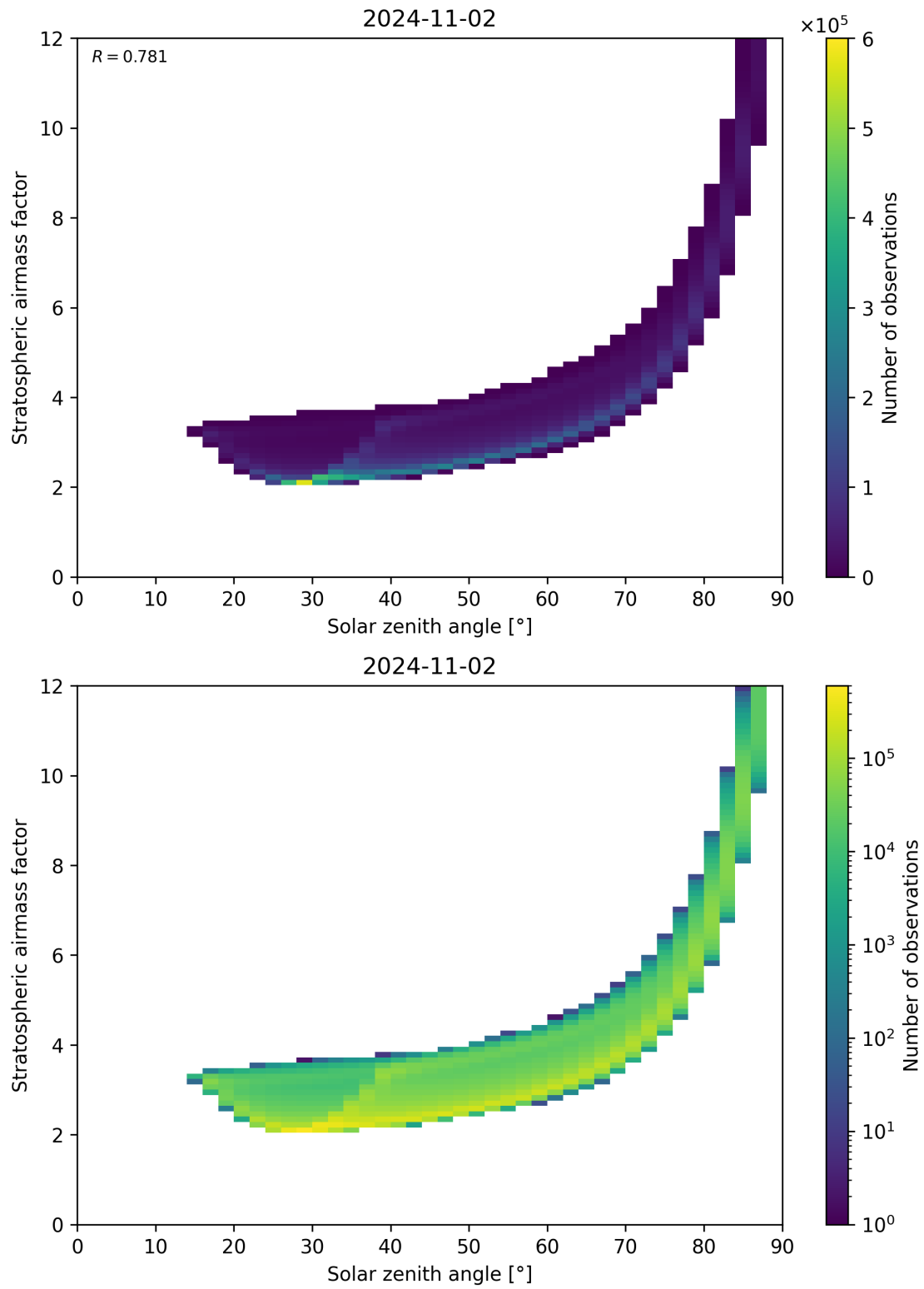
Figure 145: Scatter density plot of “Solar zenith angle” against “Stratospheric airmass factor” for 2024-11-01 to 2024-11-03.
