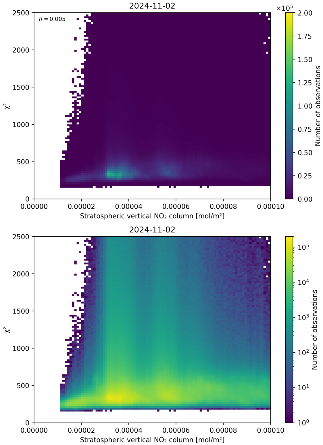
Figure 97: Scatter density plot of “Stratospheric vertical NO 2 column” against “ \chi^2 ” for 2024-11-01 to 2024-11-03.
