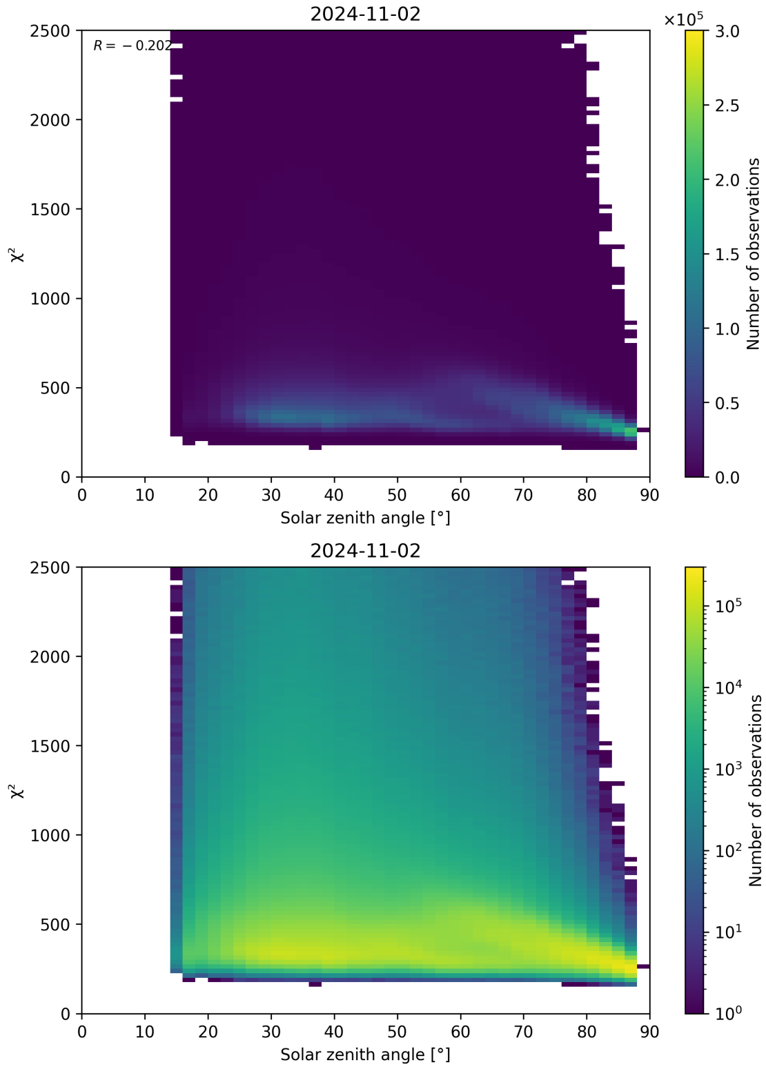
Figure 148: Scatter density plot of “Solar zenith angle” against “ \chi^2 ” for 2024-11-01 to 2024-11-03.
