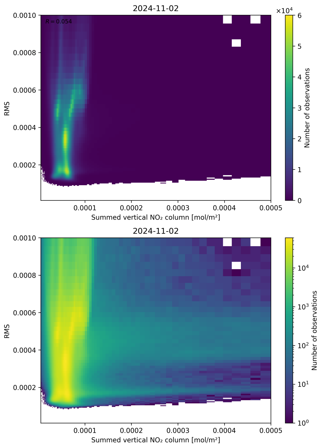
Figure 109: Scatter density plot of “Summed vertical NO 2 column” against “RMS” for 2024-11-01 to 2024-11-03.
