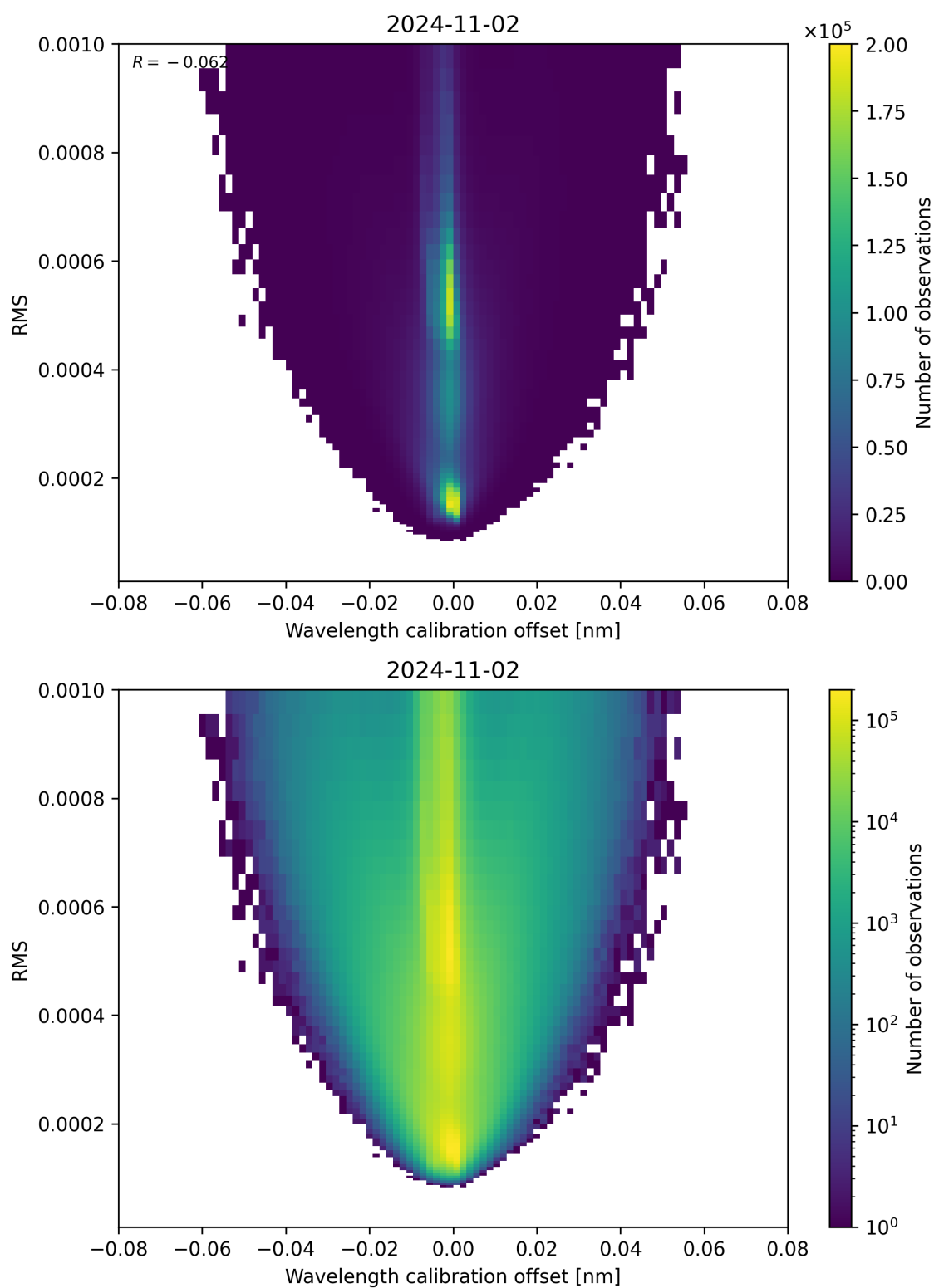
Figure 181: Scatter density plot of “Wavelength calibration offset” against “RMS” for 2024-11-01 to 2024-11-03.
