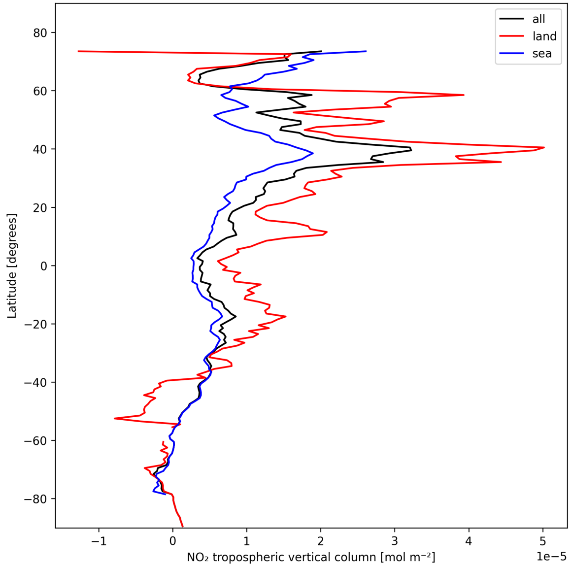
Figure 12: Zonal average of “NO 2 tropospheric vertical column” for 2024-11-01 to 2024-11-03.
