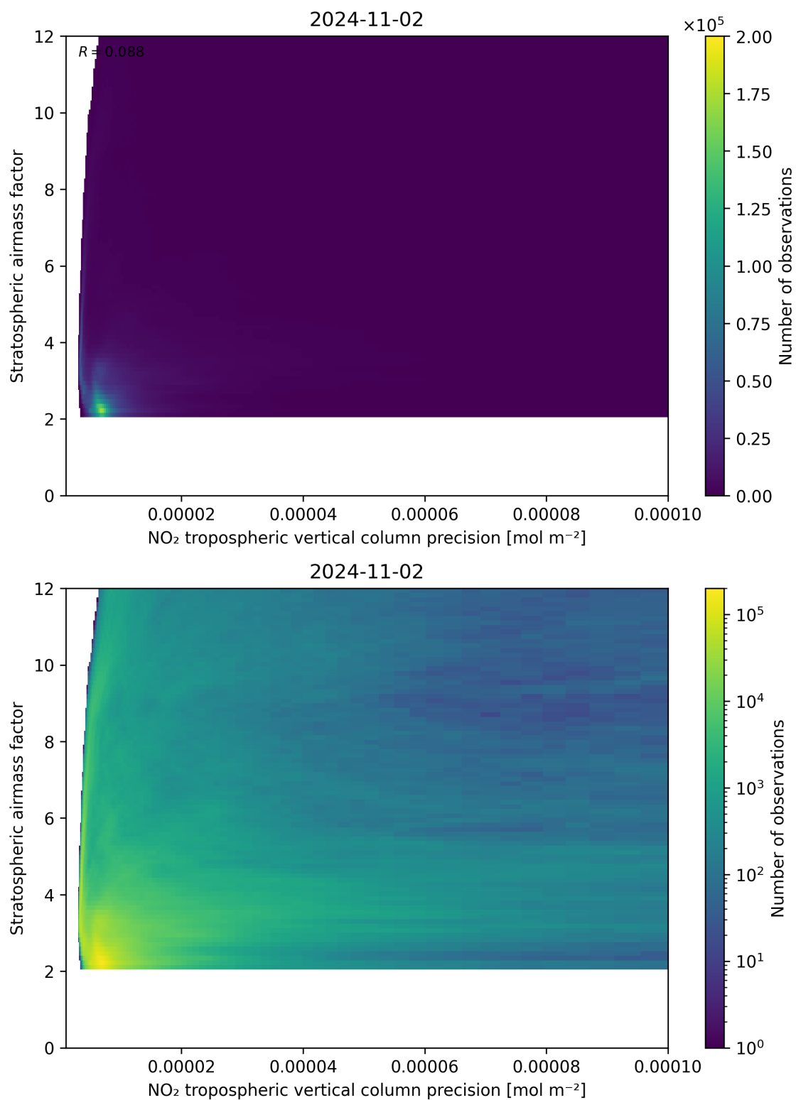
Figure 131: Scatter density plot of “NO 2 tropospheric vertical column precision” against “Stratospheric airmass factor” for 2024-11-01 to 2024-11-03.
