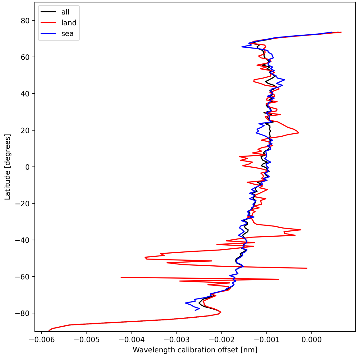
Figure 18: Zonal average of “Wavelength calibration offset” for 2024-11-01 to 2024-11-03.
