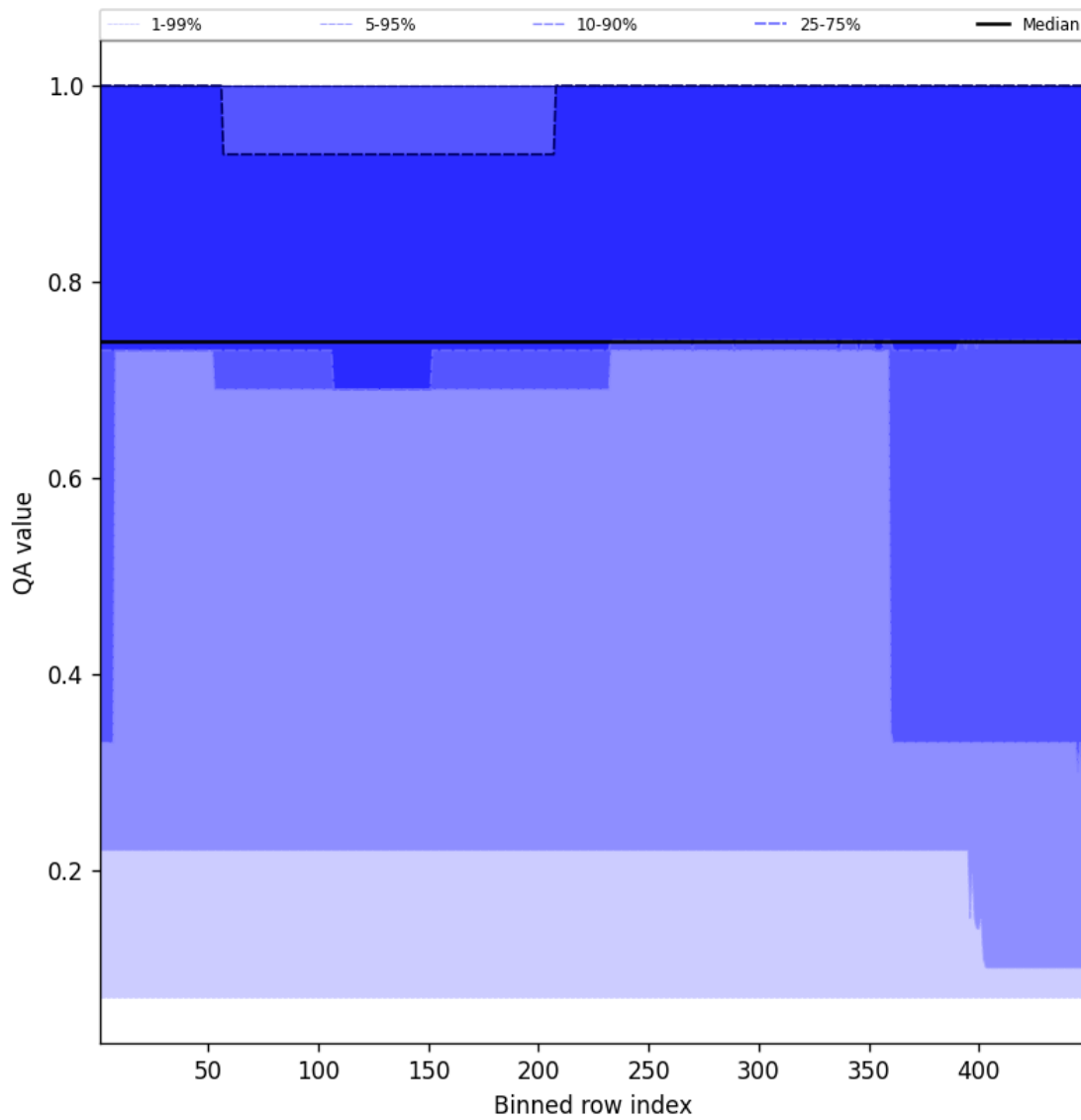
Figure 45: Along track statistics of “QA value” for 2024-11-01 to 2024-11-03
