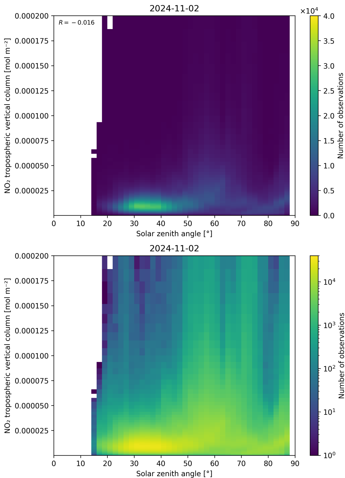
Figure 155: Scatter density plot of “Solar zenith angle” against “NO 2 tropospheric vertical column” for 2024-11-01 to 2024-11-03.
