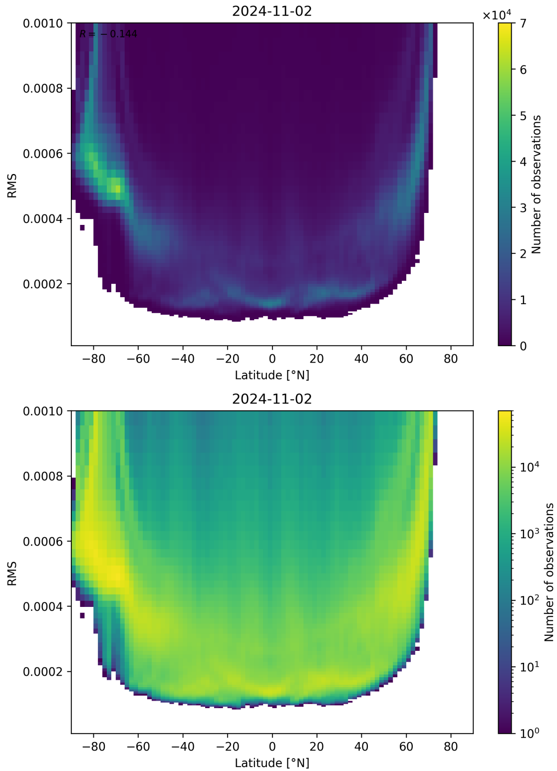
Figure 94: Scatter density plot of “Latitude” against “RMS” for 2024-11-01 to 2024-11-03.
