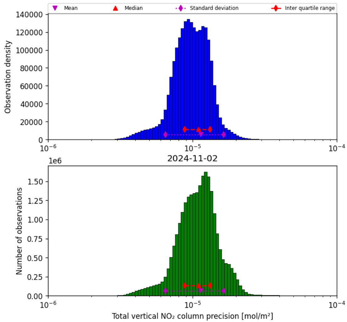
Figure 39: Histogram of “Total vertical NO 2 column precision” for 2024-11-01 to 2024-11-03
