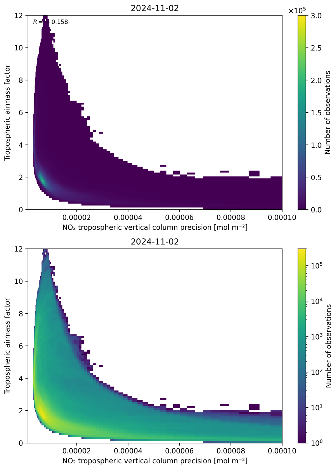
Figure 133: Scatter density plot of “NO 2 tropospheric vertical column precision” against “Tropospheric airmass factor” for 2024-11-01 to 2024-11-03.
