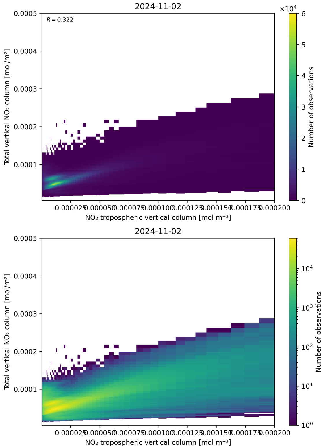
Figure 128: Scatter density plot of “NO 2 tropospheric vertical column” against “Total vertical NO 2 column” for 2024-11-01 to 2024-11-03.
