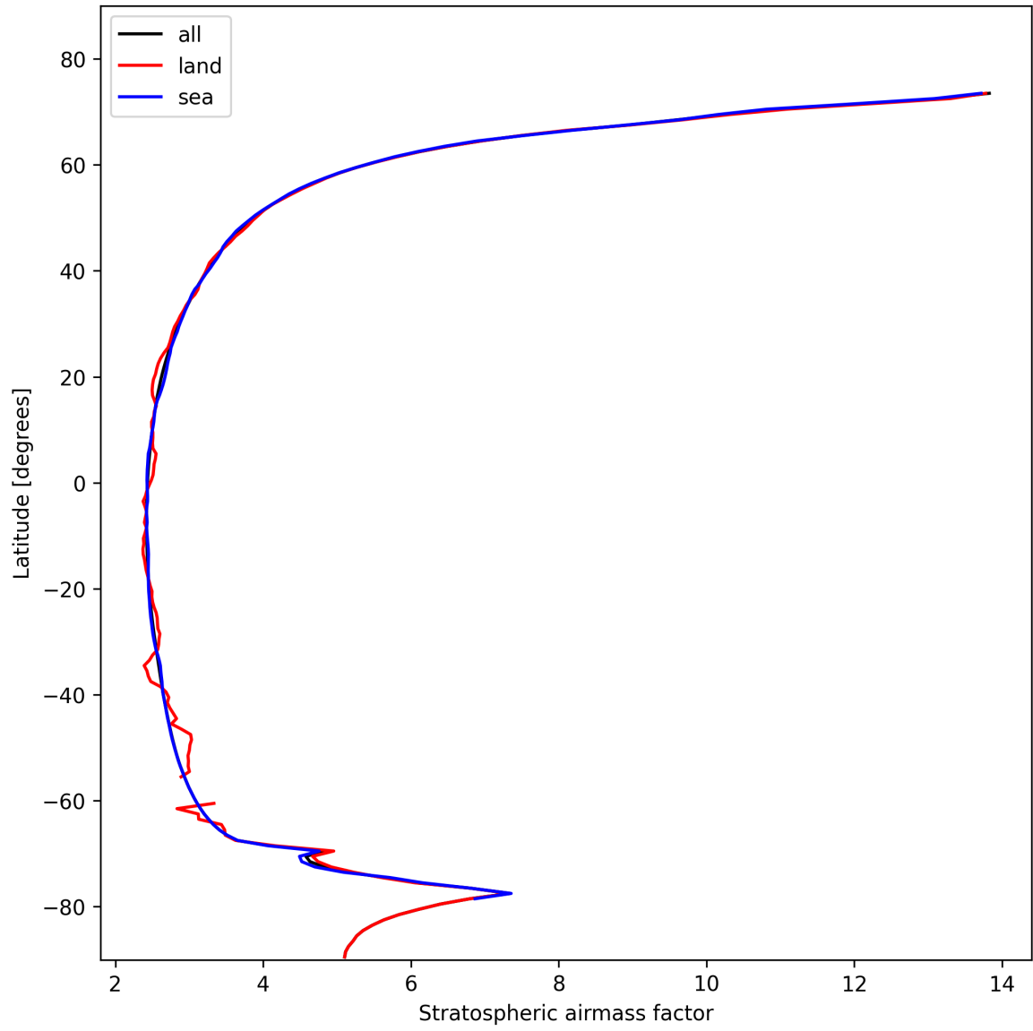
Figure 27: Zonal average of “Stratospheric air mass factor” for 2024-11-01 to 2024-11-03.
