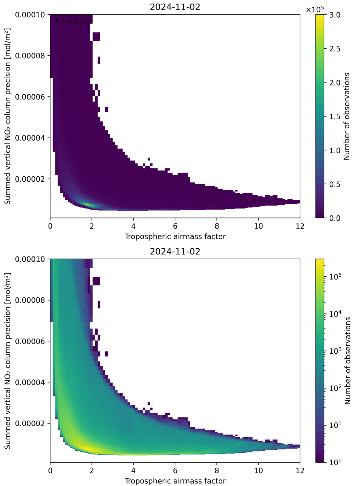
Figure 76: Scatter density plot of “Tropospheric air mass factor” against “Summed vertical NO 2 column precision” for 2024-11-01 to 2024-11-03.
