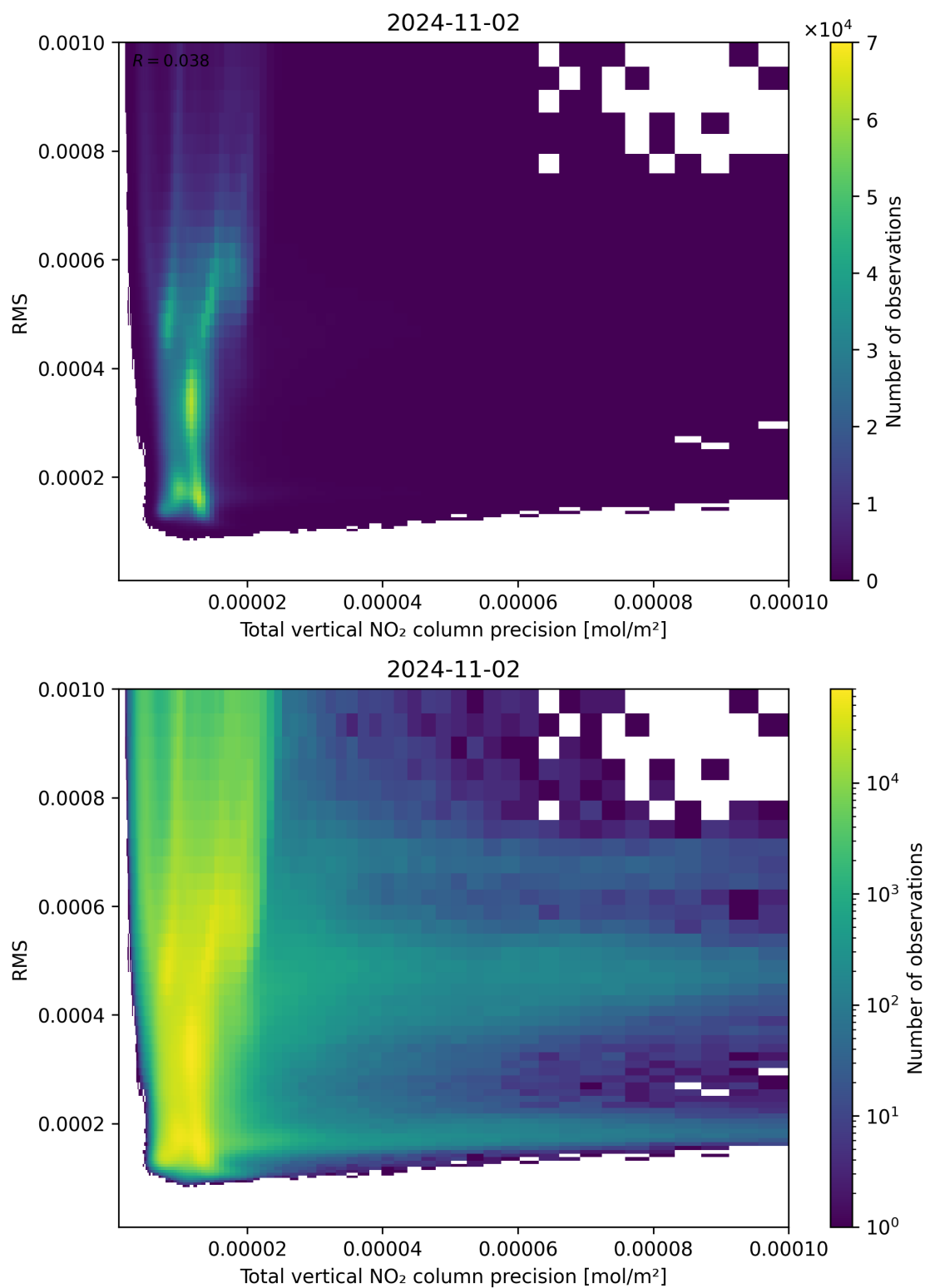
Figure 119: Scatter density plot of “Total vertical NO 2 column precision” against “RMS” for 2024-11-01 to 2024-11-03.
