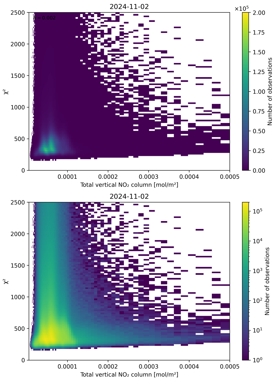
Figure 111: Scatter density plot of “Total vertical NO 2 column” against “ \chi^2 ” for 2024-11-01 to 2024-11-03.
