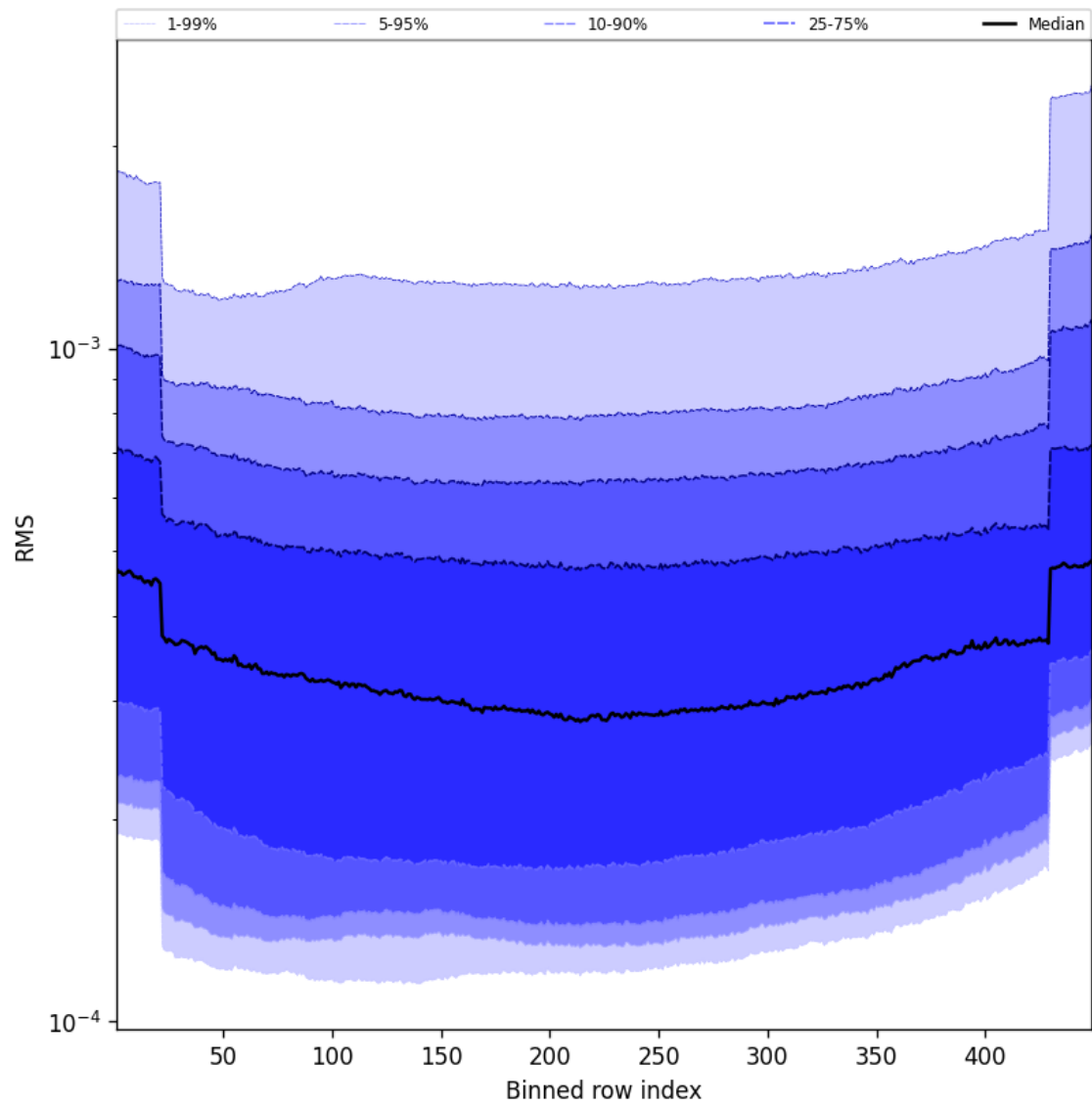
Figure 60: Along track statistics of “RMS” for 2024-11-01 to 2024-11-03
