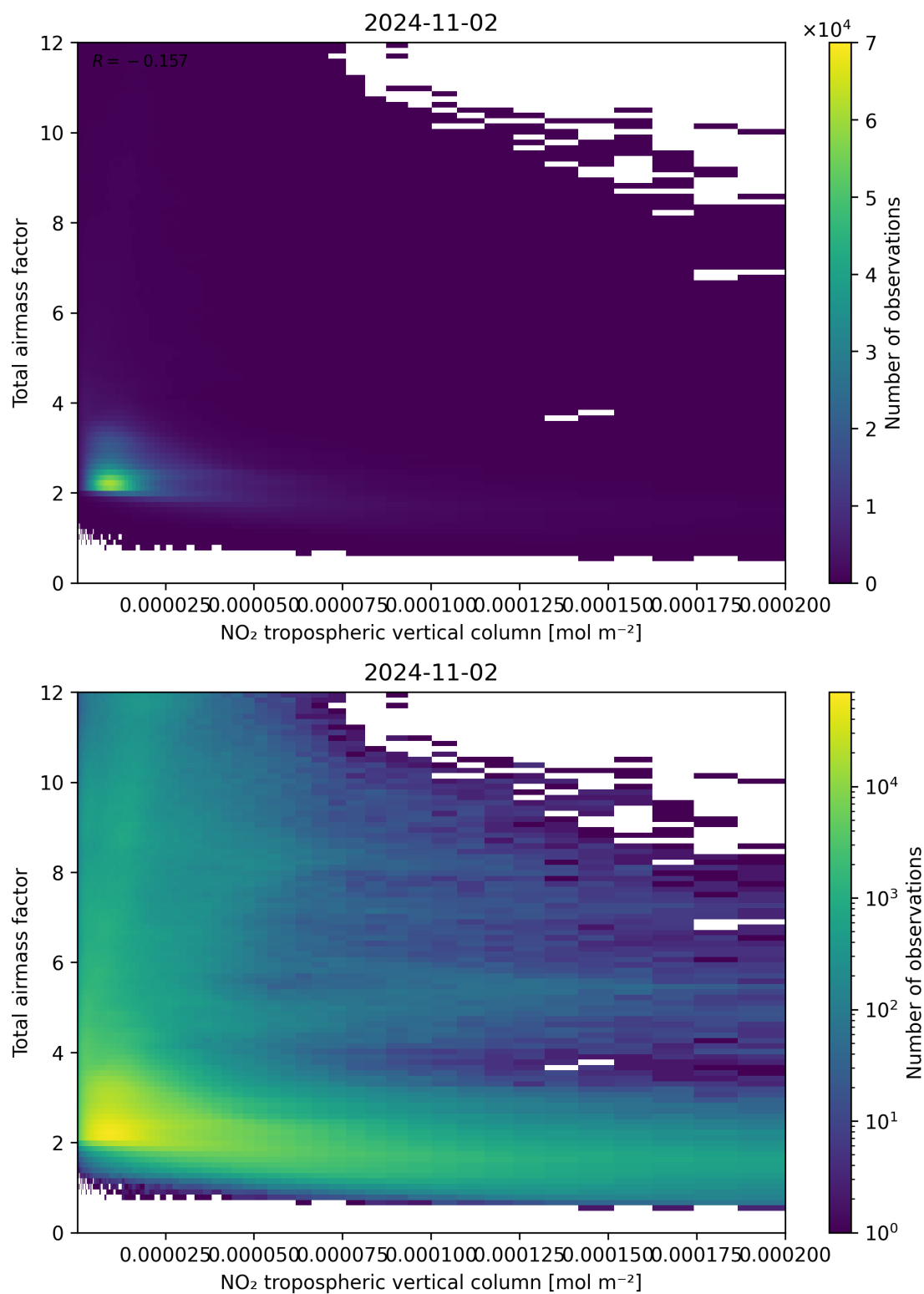
Figure 122: Scatter density plot of “NO 2 tropospheric vertical column” against “Total airmass factor” for 2024-11-01 to 2024-11-03.
