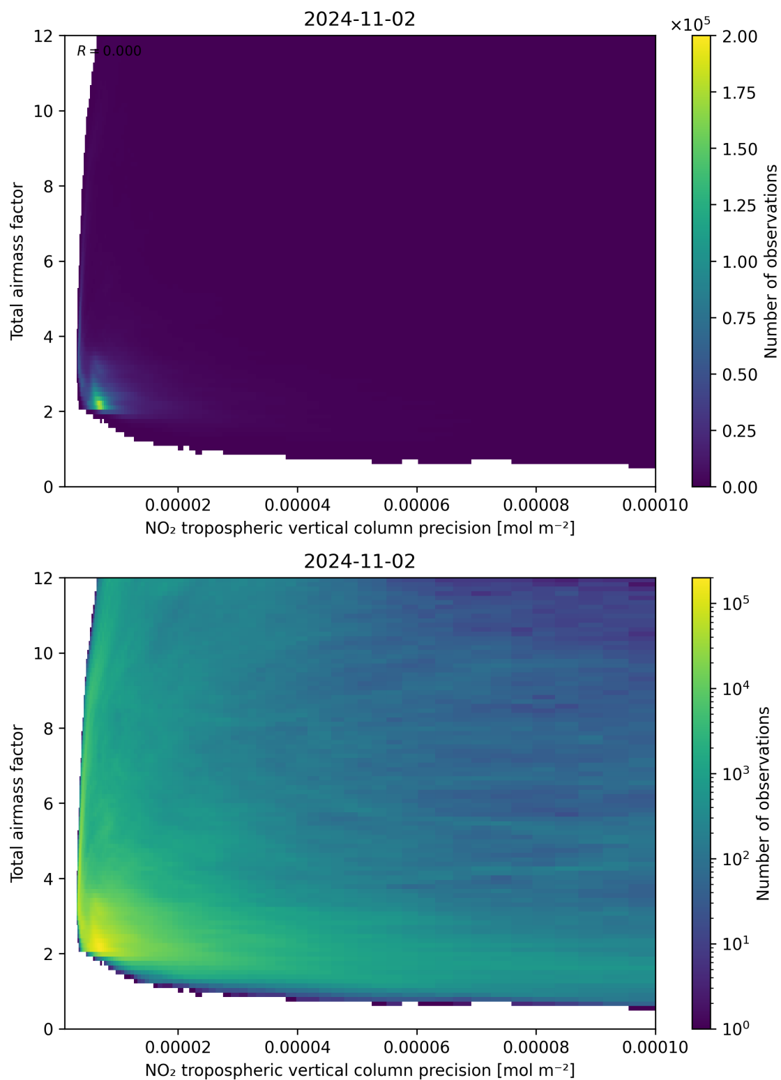
Figure 132: Scatter density plot of “NO 2 tropospheric vertical column precision” against “Total air mass factor” for 2024-11-01 to 2024-11-03.
