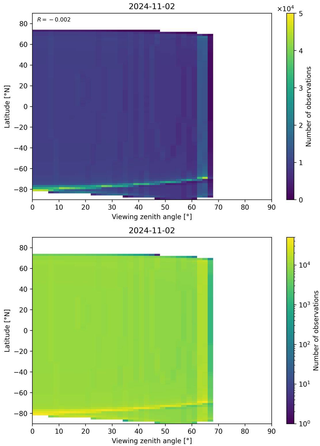
Figure 163: Scatter density plot of “Viewing zenith angle” against “Latitude” for 2024-11-01 to 2024-11-03.
