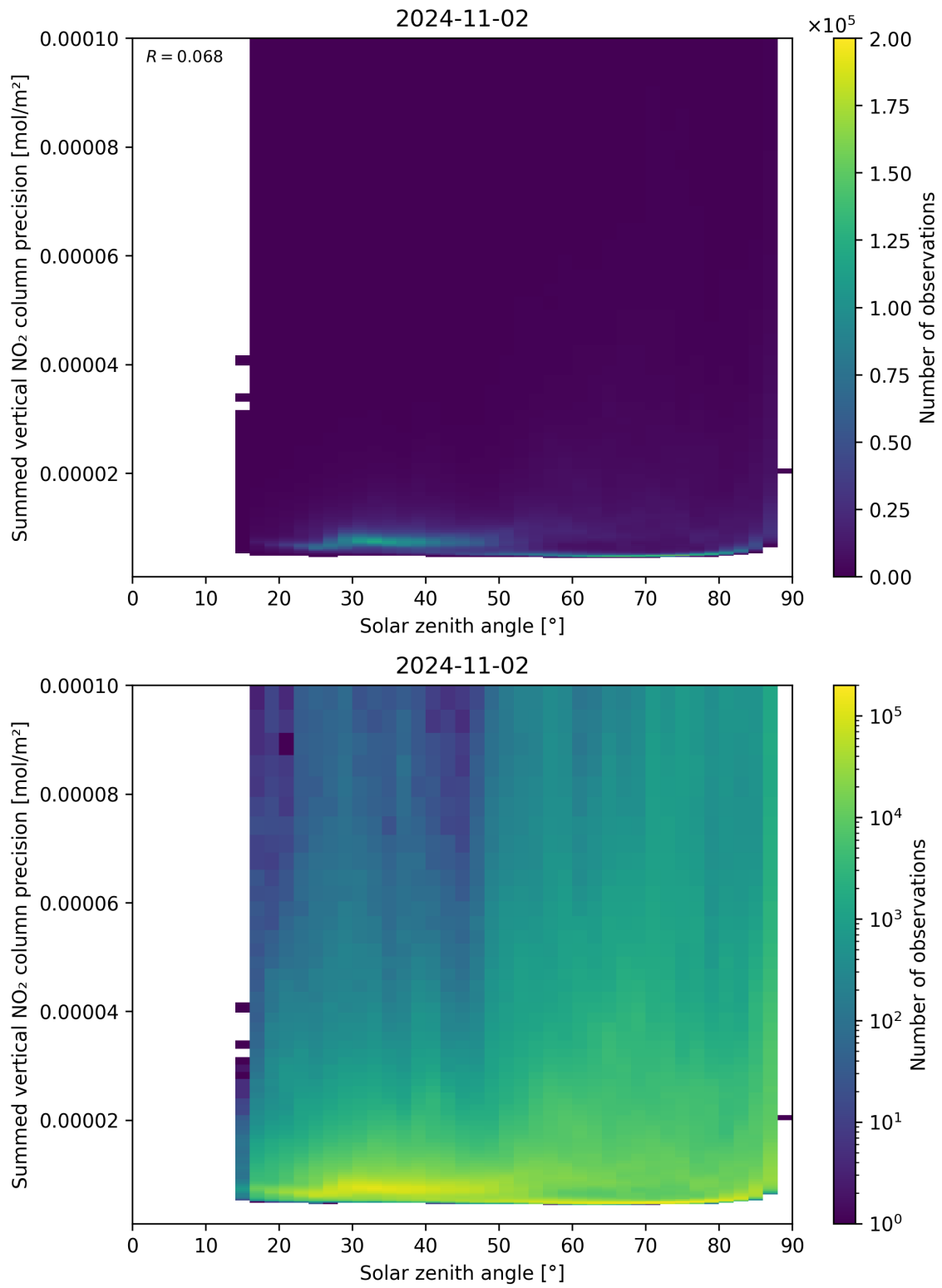
Figure 152: Scatter density plot of “Solar zenith angle” against “Summed vertical NO 2 column precision” for 2024-11-01 to 2024-11-03.
