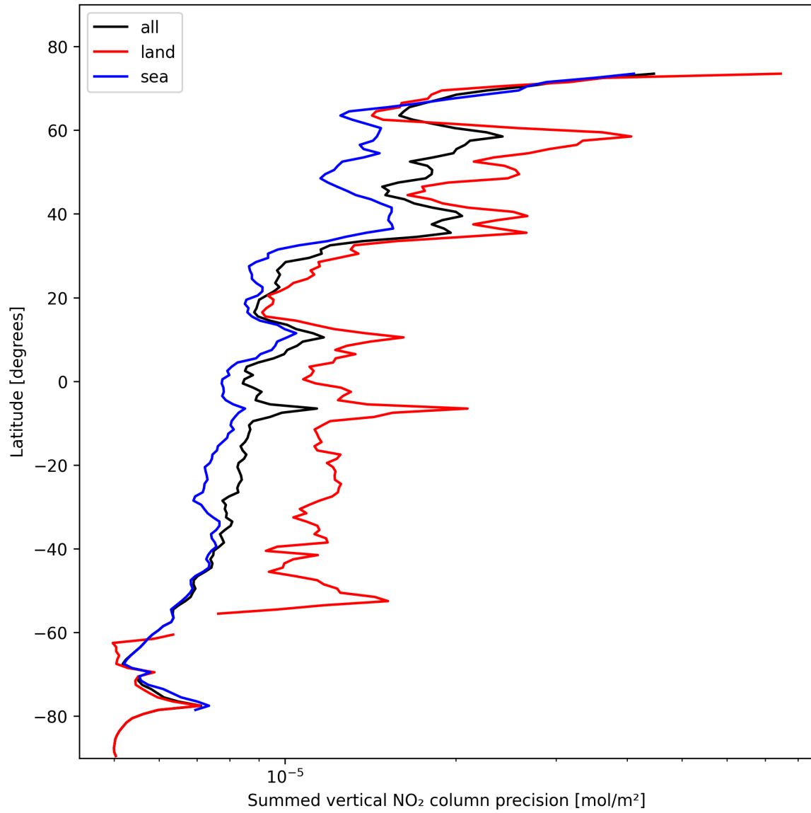
Figure 24: Zonal average of “Summed vertical NO 2 column precision” for 2024-11-01 to 2024-11-03.
