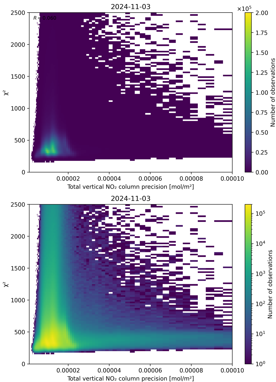
Figure 116: Scatter density plot of “Total vertical NO 2 column precision” against “ \chi^2 ” for 2024-11-02 to 2024-11-04.
