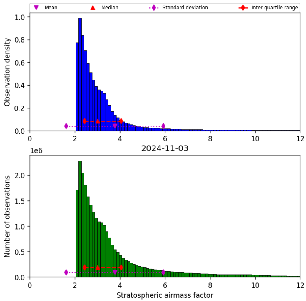
Figure 44: Histogram of “Stratospheric airmass factor” for 2024-11-02 to 2024-11-04
