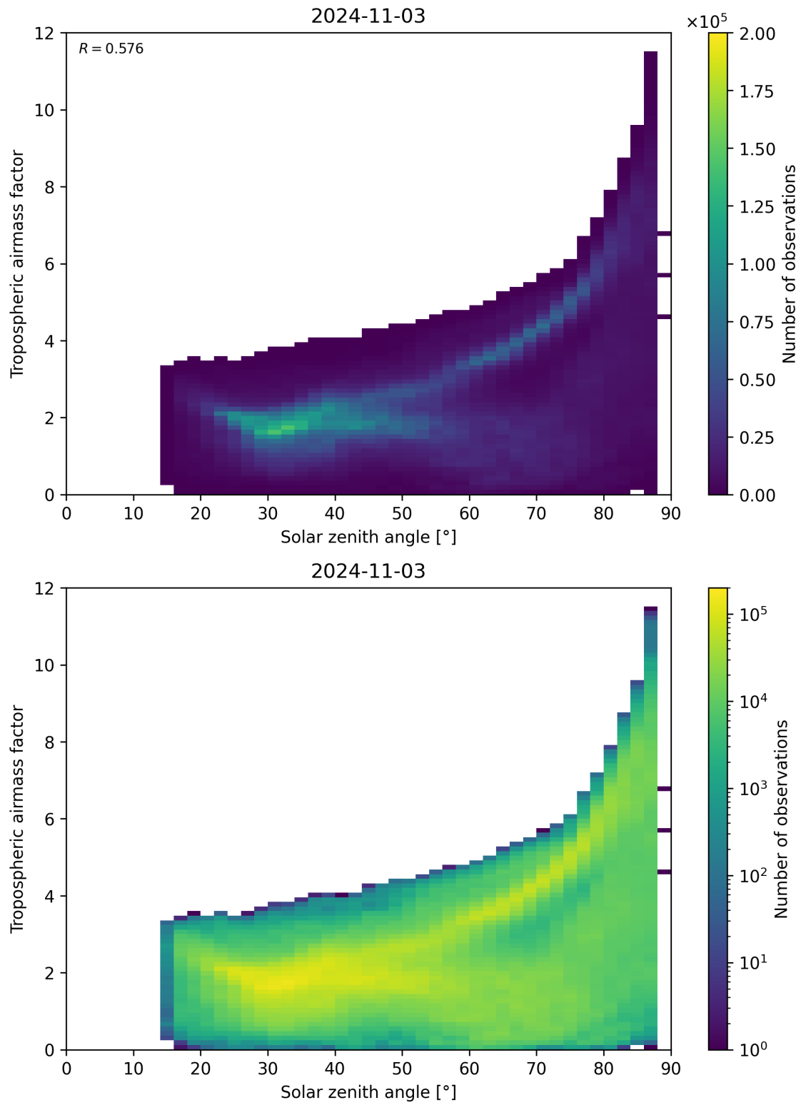
Figure 147: Scatter density plot of “Solar zenith angle” against “Tropospheric airmass factor” for 2024-11-02 to 2024-11-04.
