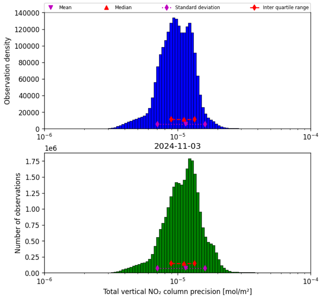
Figure 39: Histogram of “Total vertical NO 2 column precision” for 2024-11-02 to 2024-11-04
