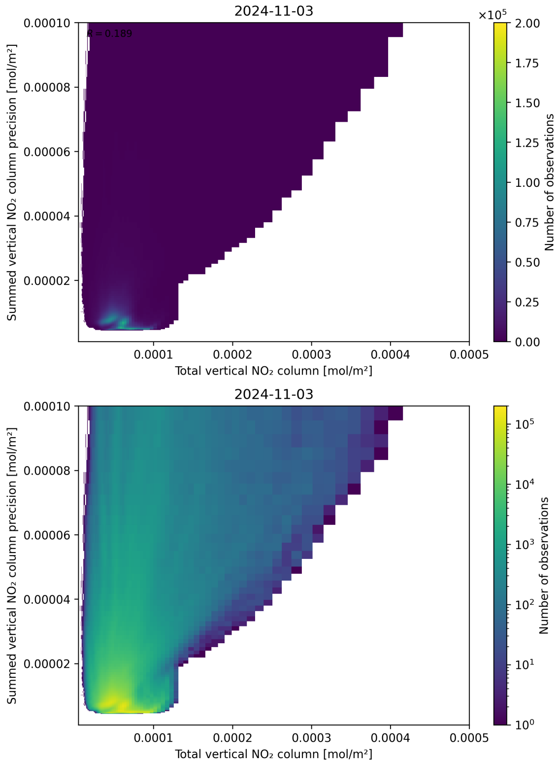
Figure 113: Scatter density plot of “Total vertical NO 2 column” against “Summed vertical NO 2 column precision” for 2024-11-02 to 2024-11-04.
