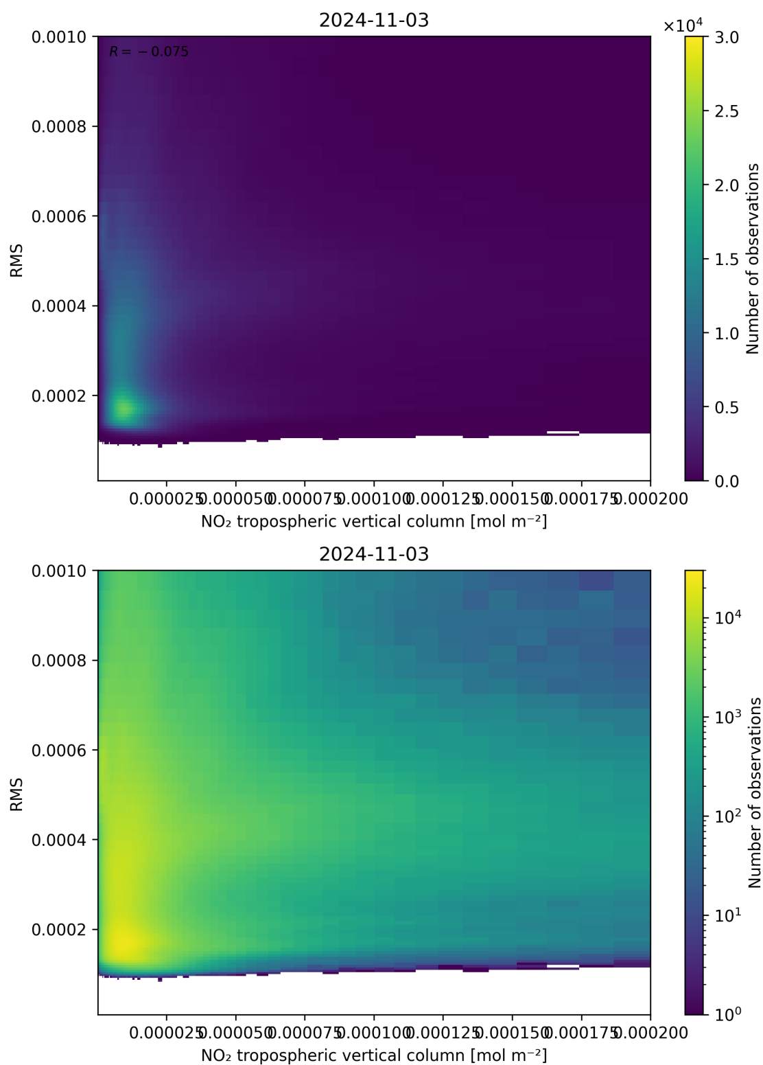
Figure 142: Scatter density plot of “NO 2 tropospheric vertical column” against “RMS” for 2024-11-02 to 2024-11-04.
