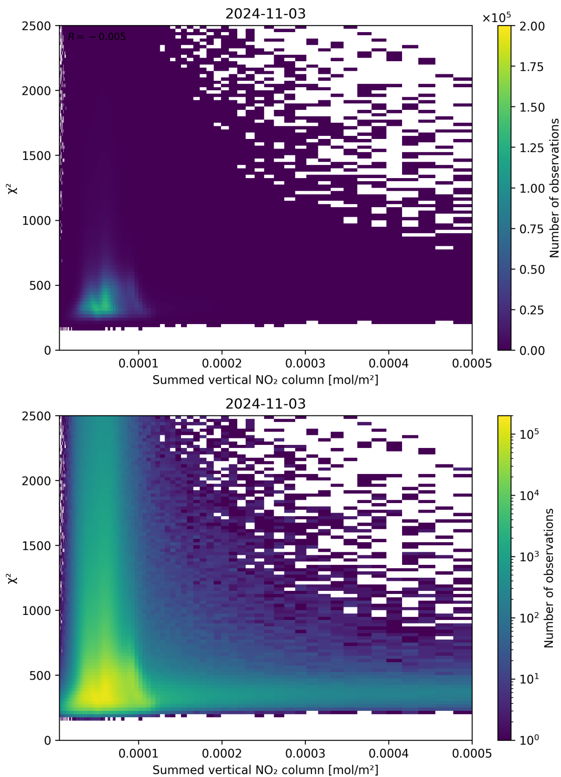
Figure 104: Scatter density plot of “Summed vertical NO 2 column” against “ \chi^2 ” for 2024-11-02 to 2024-11-04.
