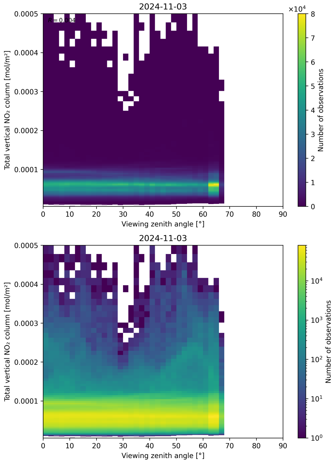
Figure 167: Scatter density plot of “Viewing zenith angle” against “Total vertical NO 2 column” for 2024-11-02 to 2024-11-04.
