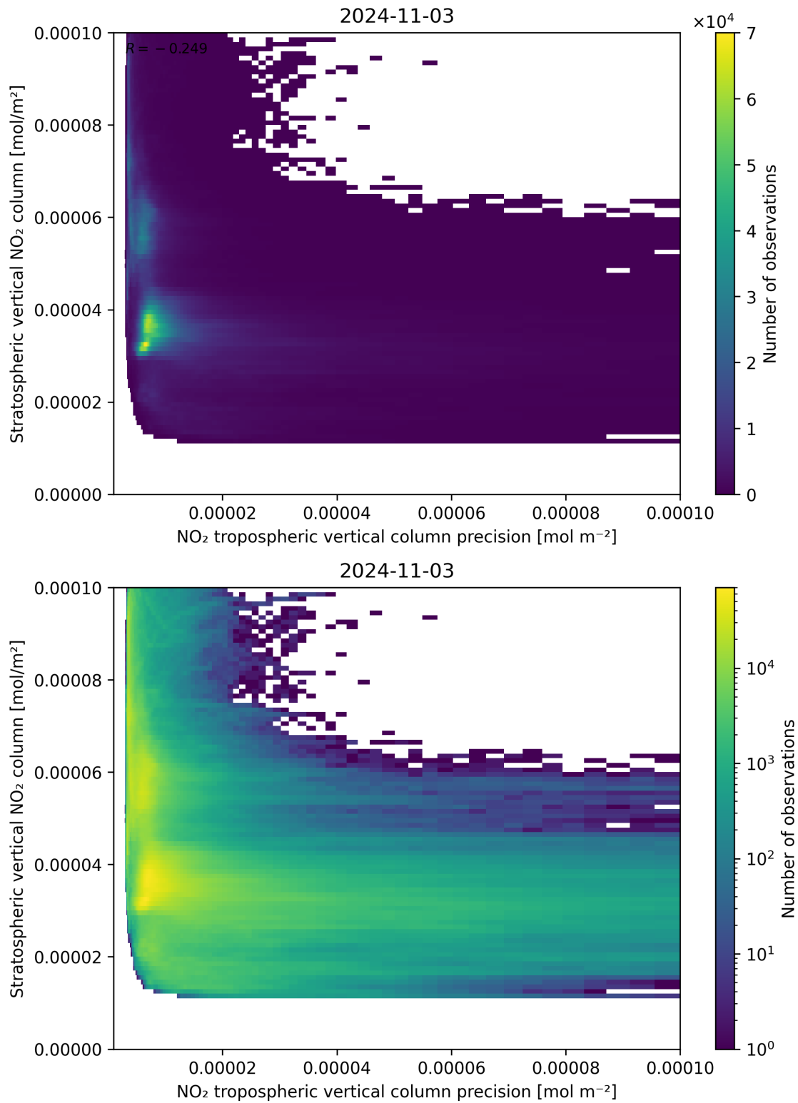
Figure 135: Scatter density plot of “NO 2 tropospheric vertical column precision” against “Stratospheric vertical NO 2 column” for 2024-11-02 to 2024-11-04.
