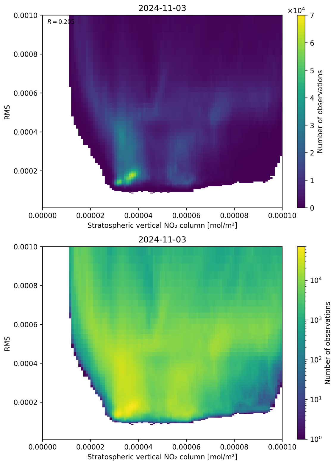
Figure 102: Scatter density plot of “Stratospheric vertical NO 2 column” against “RMS” for 2024-11-02 to 2024-11-04.
