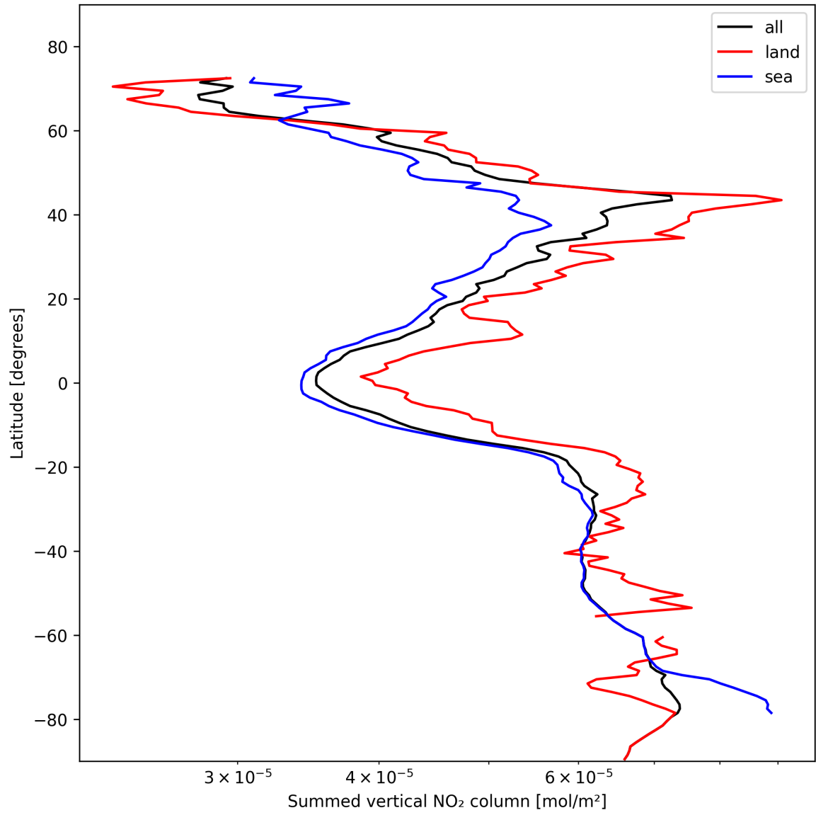
Figure 23: Zonal average of “Summed vertical NO 2 column” for 2024-11-02 to 2024-11-04.
