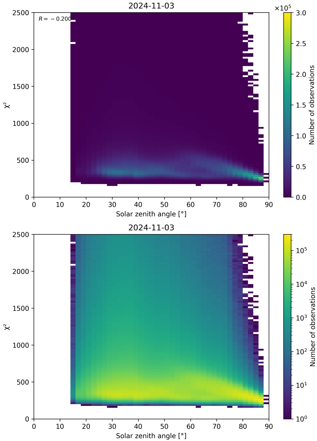
Figure 148: Scatter density plot of “Solar zenith angle” against “ \chi^2 ” for 2024-11-02 to 2024-11-04.
