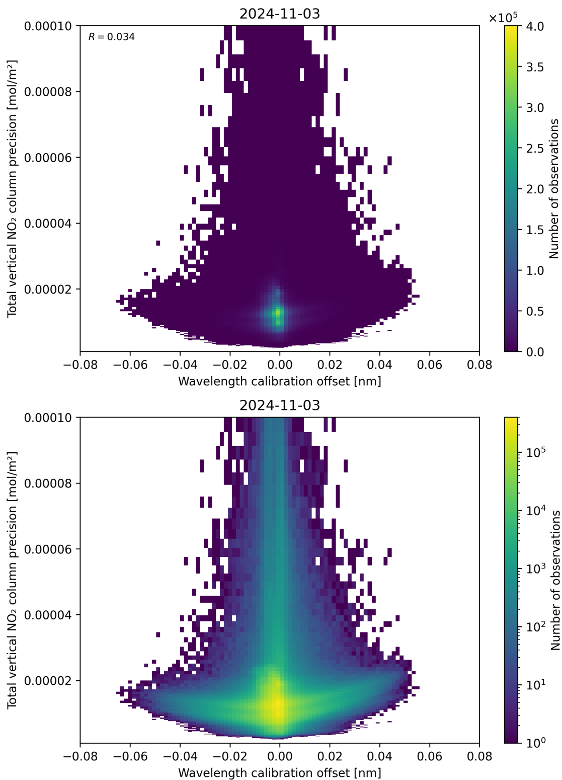
Figure 180: Scatter density plot of “Wavelength calibration offset” against “Total vertical NO 2 column precision” for 2024-11-02 to 2024-11-04.
