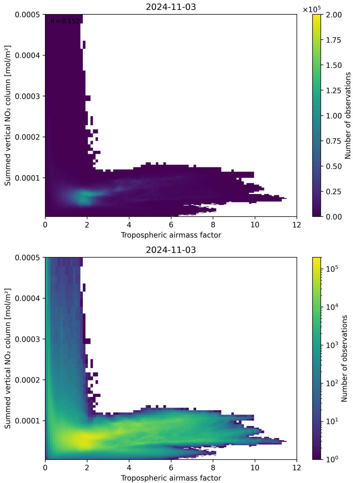
Figure 75: Scatter density plot of “Tropospheric air mass factor” against “Summed vertical NO 2 column” for 2024-11-02 to 2024-11-04.
