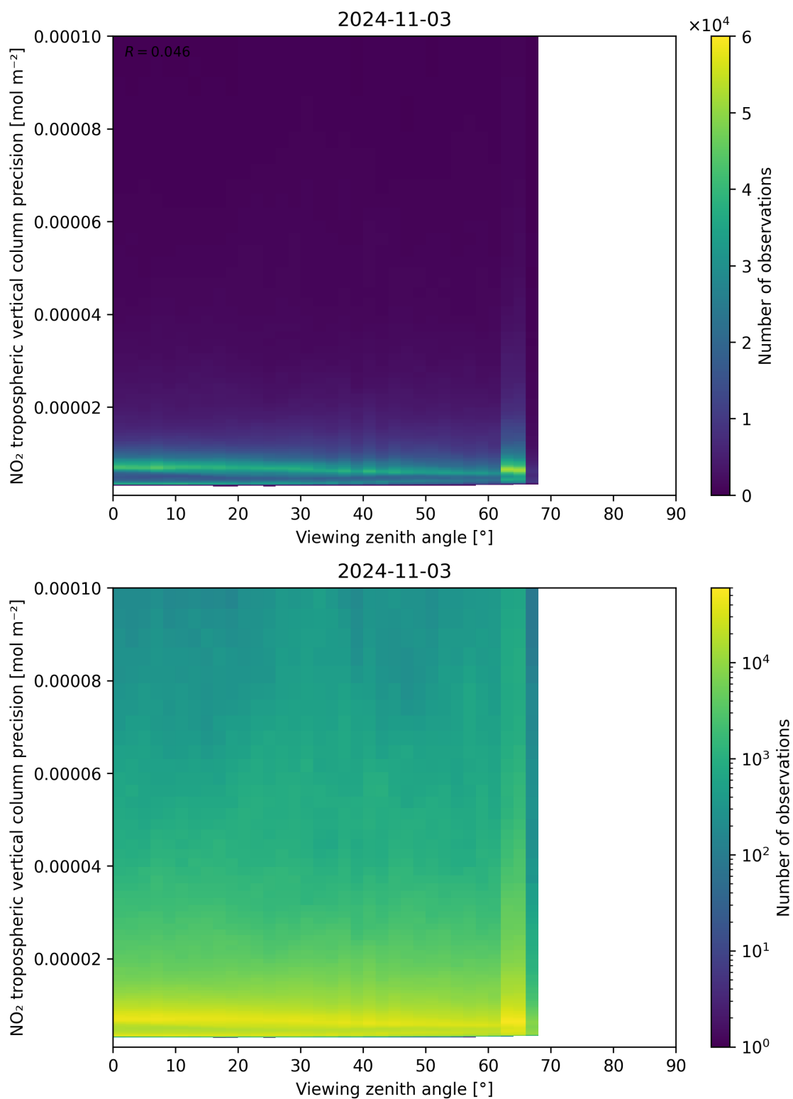
Figure 170: Scatter density plot of “Viewing zenith angle” against “NO 2 tropospheric vertical column precision” for 2024-11-02 to 2024-11-04.
