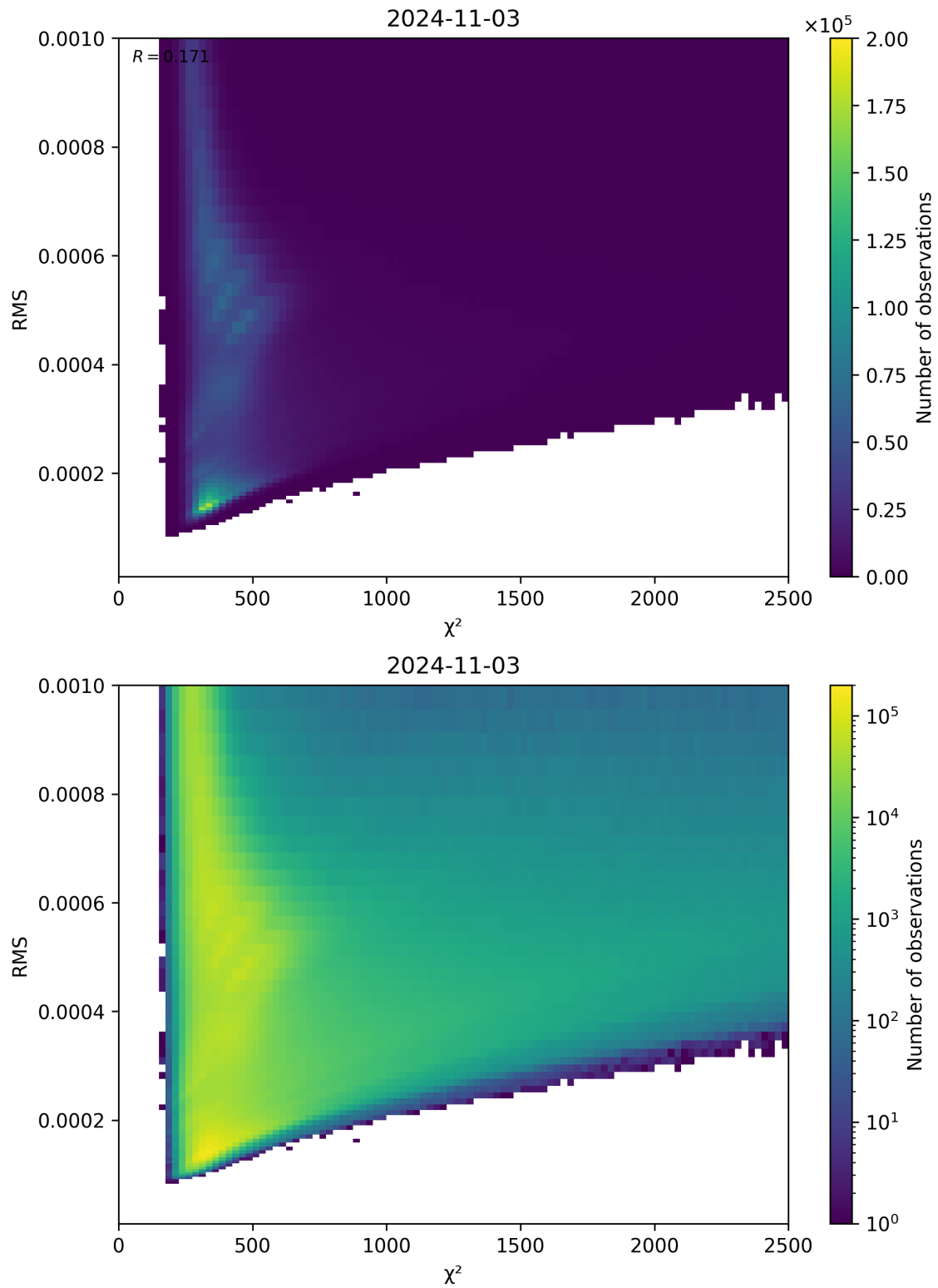
Figure 82: Scatter density plot of “ \chi^2 ” against “RMS” for 2024-11-02 to 2024-11-04.
