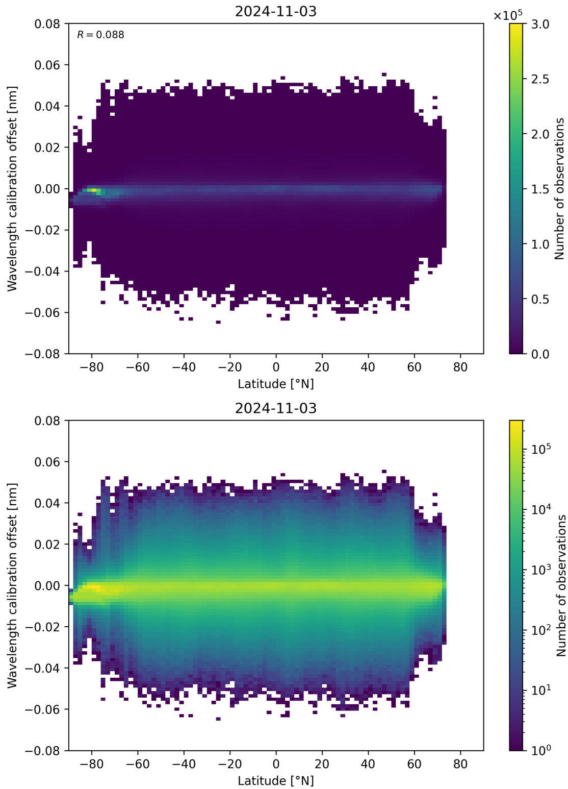
Figure 95: Scatter density plot of “Latitude” against “Wavelength calibration offset” for 2024-11-02 to 2024-11-04.
