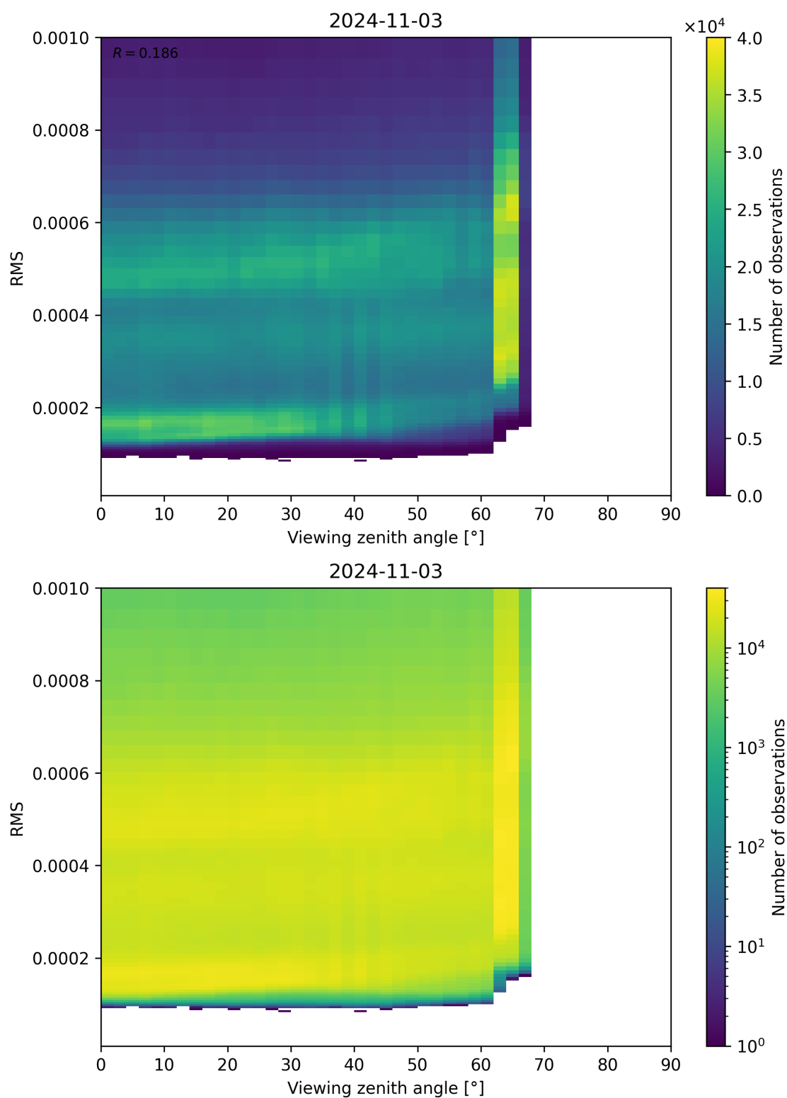
Figure 171: Scatter density plot of “Viewing zenith angle” against “RMS” for 2024-11-02 to 2024-11-04.
