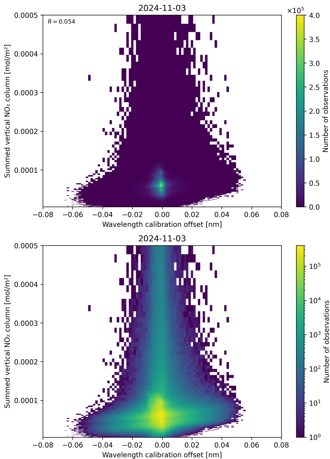
Figure 177: Scatter density plot of “Wavelength calibration offset” against “Summed vertical NO 2 column” for 2024-11-02 to 2024-11-04.
