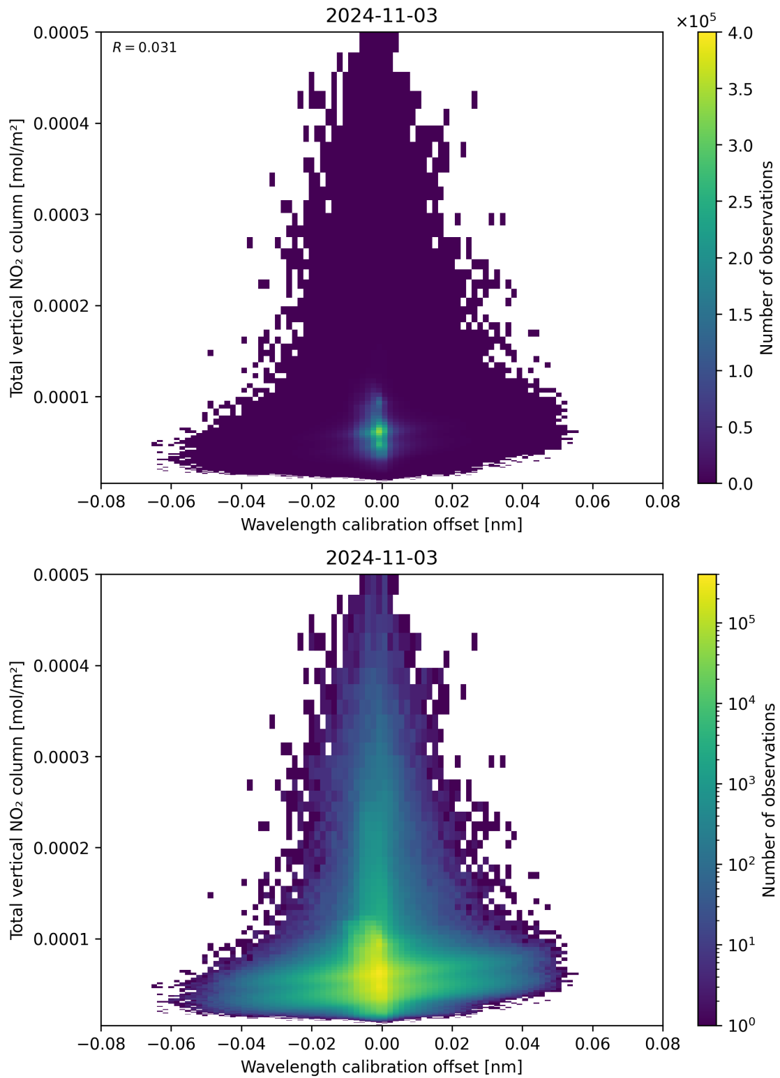
Figure 179: Scatter density plot of “Wavelength calibration offset” against “Total vertical NO 2 column” for 2024-11-02 to 2024-11-04.
