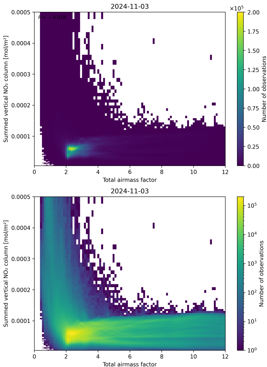
Figure 65: Scatter density plot of “Total airmass factor” against “Summed vertical NO 2 column” for 2024-11-02 to 2024-11-04.
