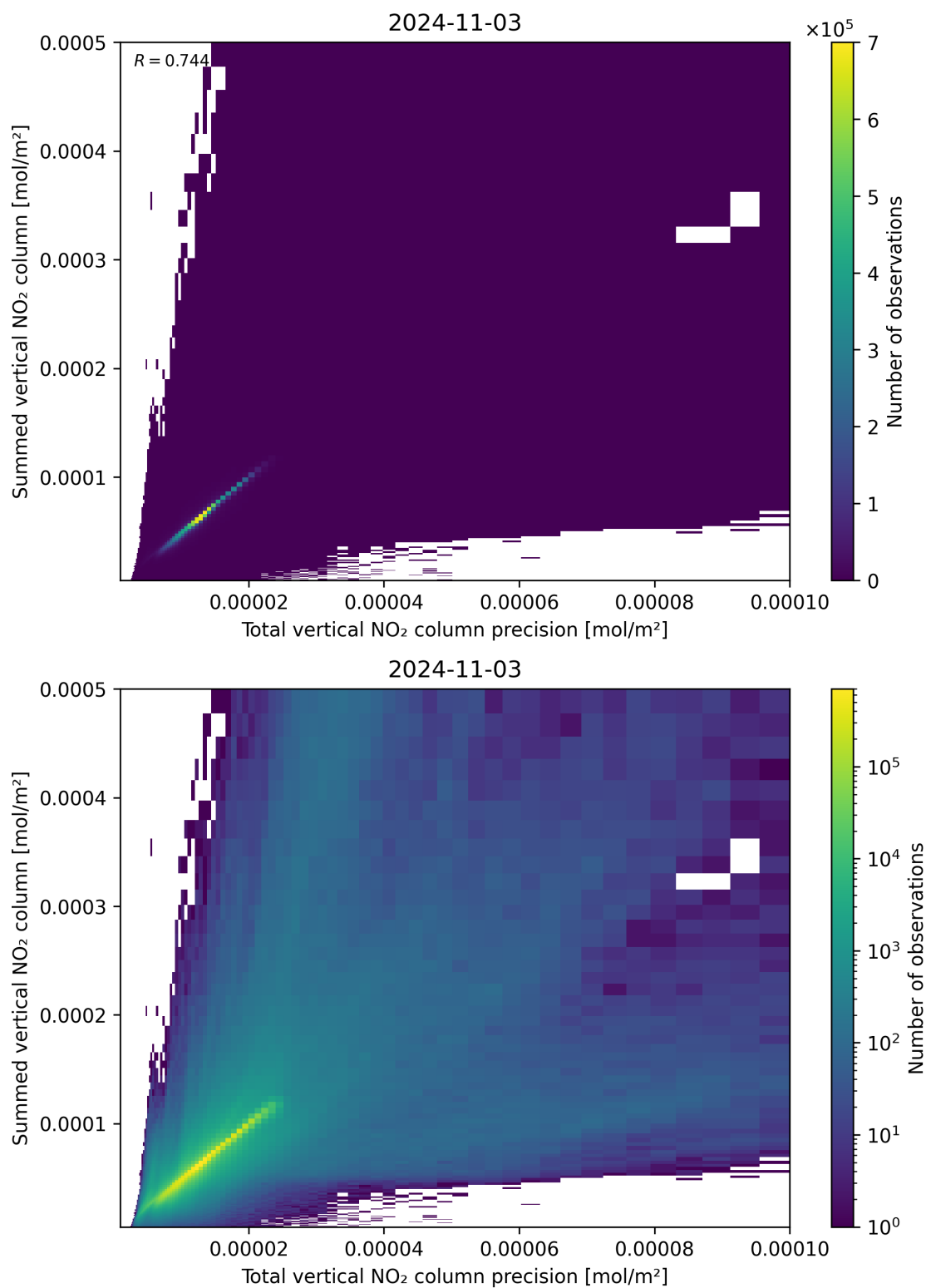
Figure 117: Scatter density plot of “Total vertical NO 2 column precision” against “Summed vertical NO 2 column” for 2024-11-02 to 2024-11-04.
