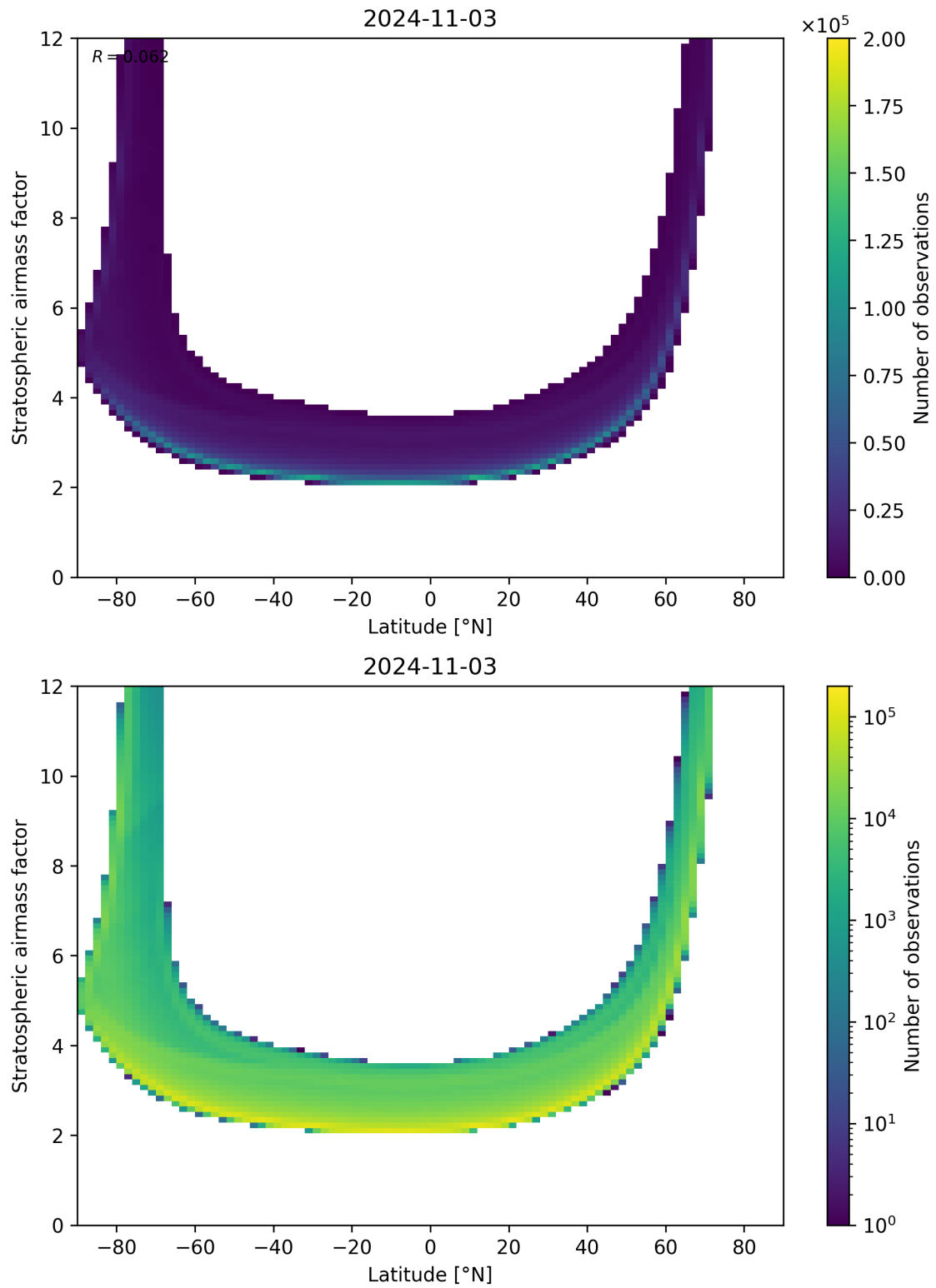
Figure 83: Scatter density plot of “Latitude” against “Stratospheric air mass factor” for 2024-11-02 to 2024-11-04.
