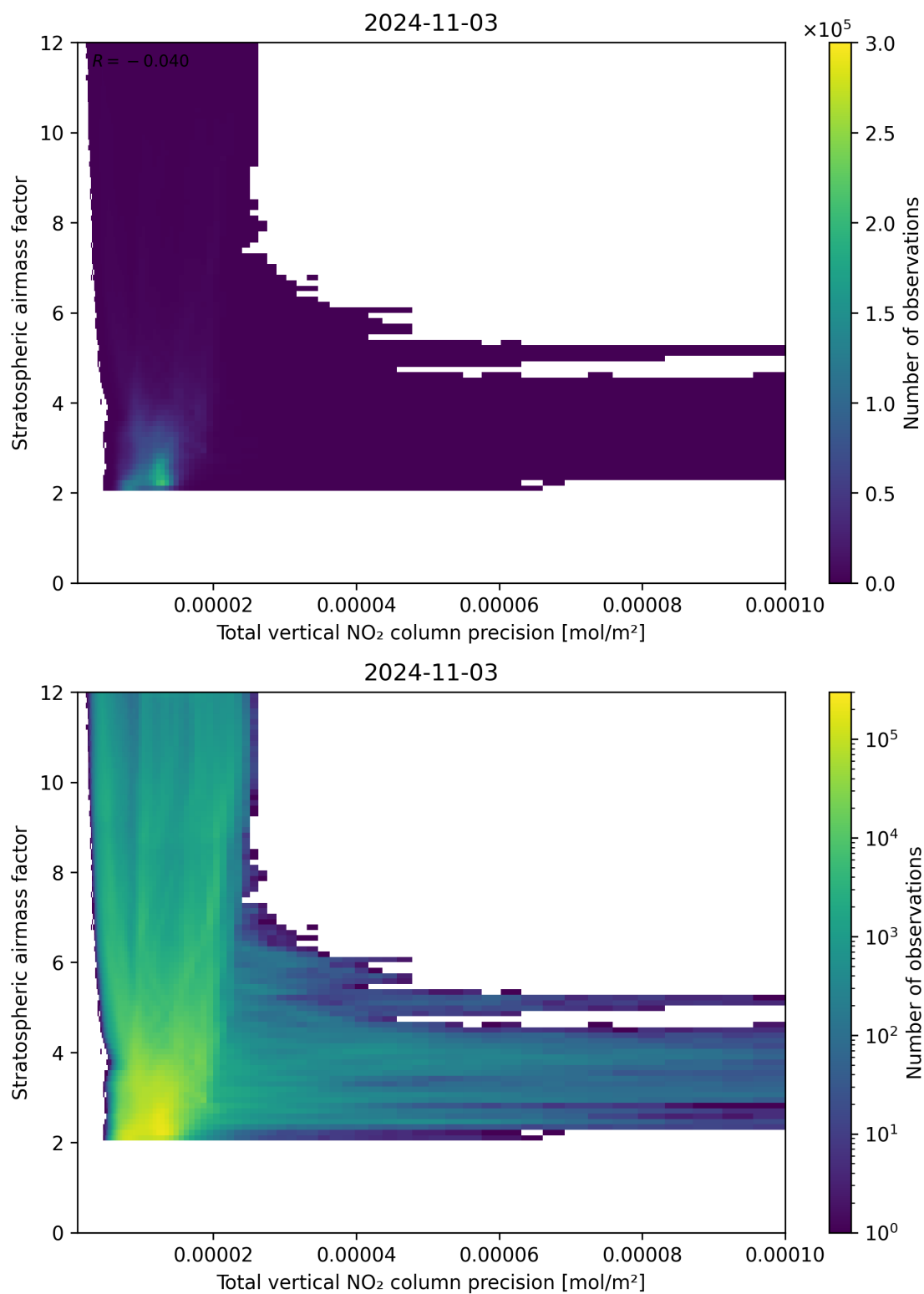
Figure 115: Scatter density plot of “Total vertical NO 2 column precision” against “Stratospheric air mass factor” for 2024-11-02 to 2024-11-04.
