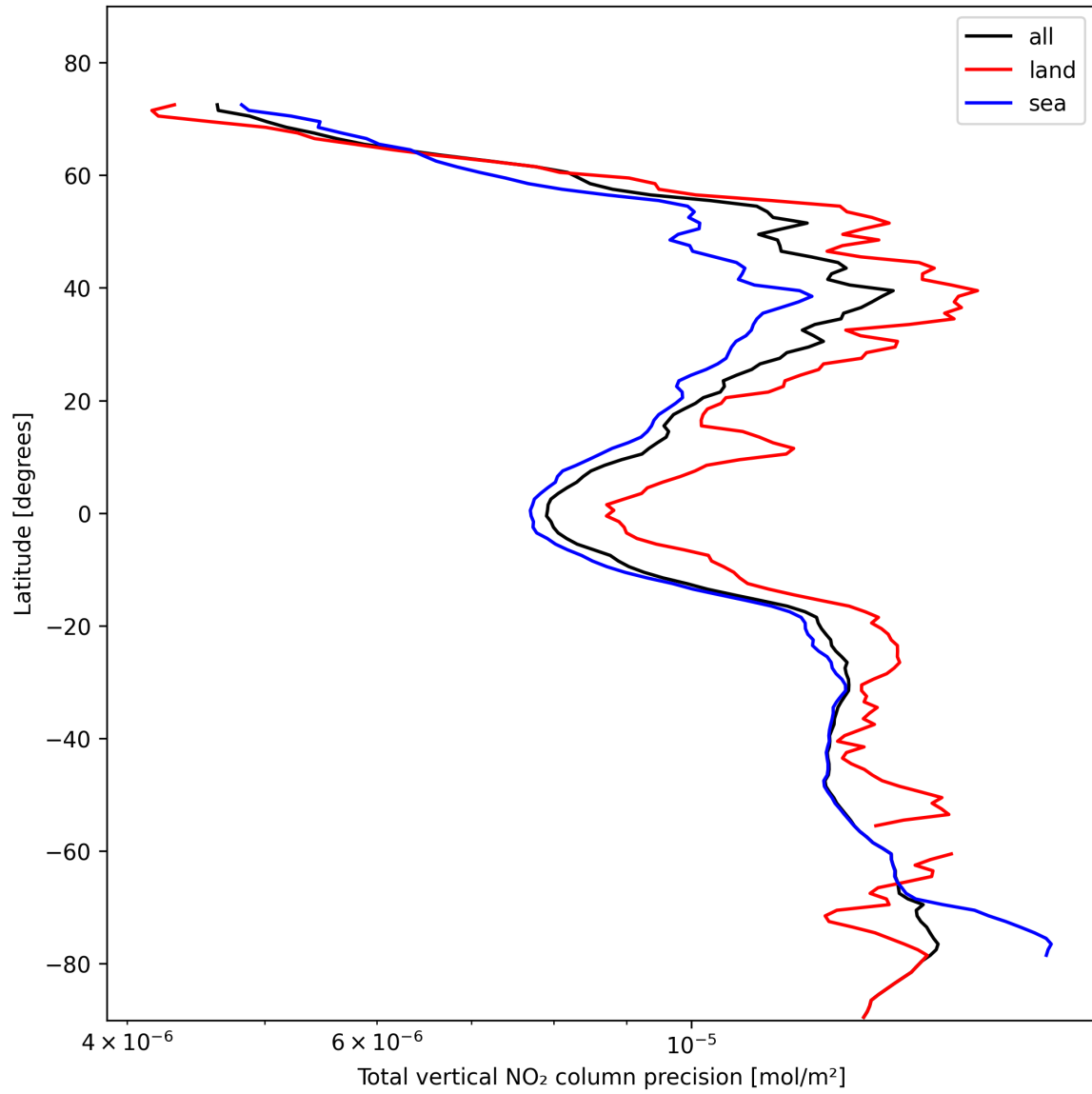
Figure 22: Zonal average of “Total vertical NO 2 column precision” for 2024-11-02 to 2024-11-04.
