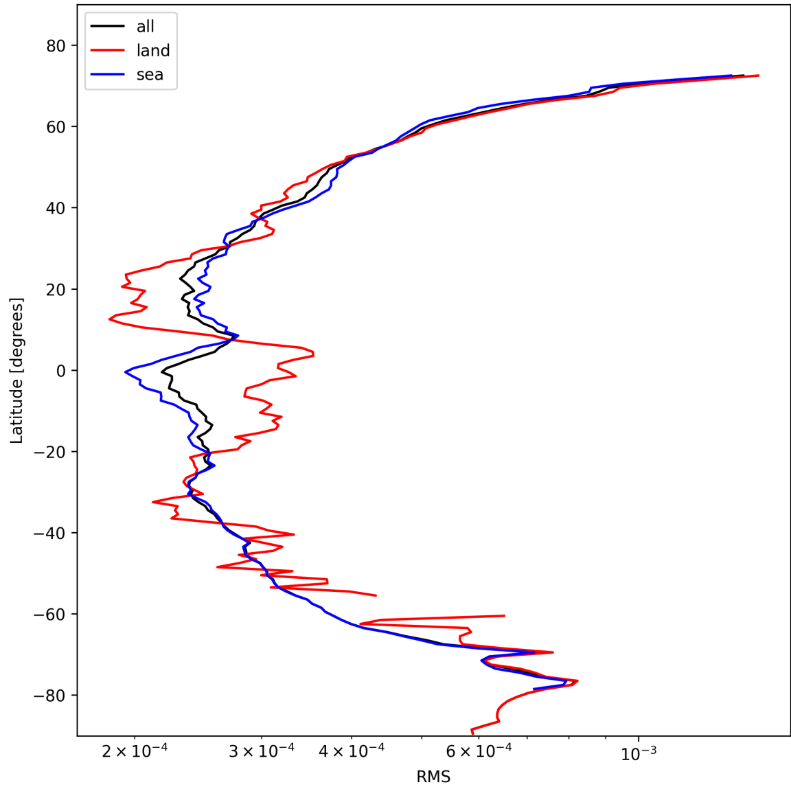
Figure 26: Zonal average of “RMS” for 2024-11-02 to 2024-11-04.
