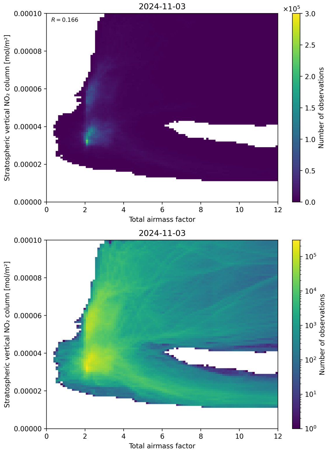
Figure 64: Scatter density plot of “Total airmass factor” against “Stratospheric vertical NO 2 column” for 2024-11-02 to 2024-11-04.
