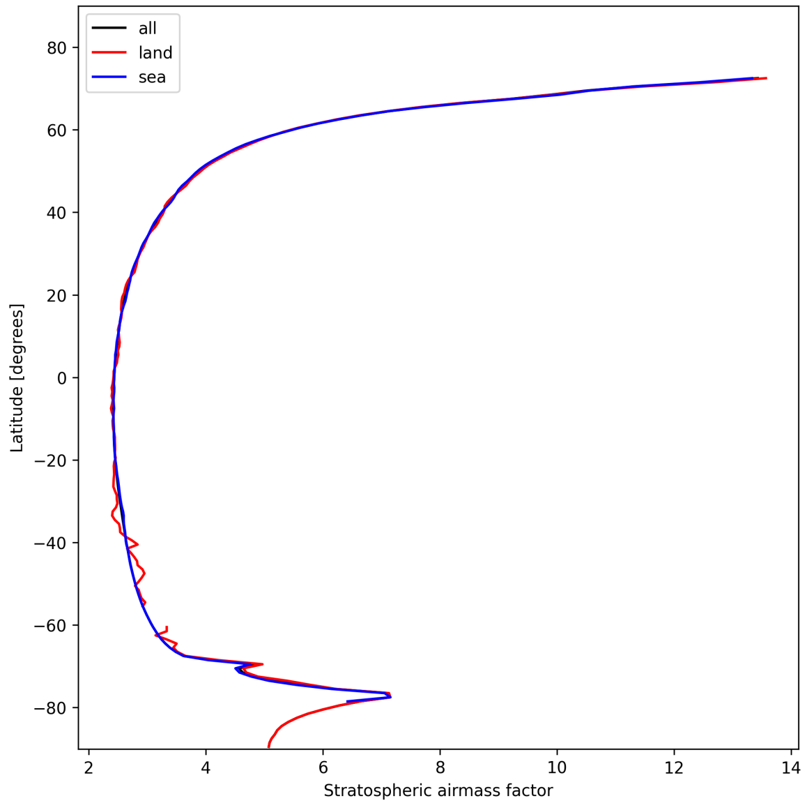
Figure 27: Zonal average of “Stratospheric air mass factor” for 2024-11-02 to 2024-11-04.
