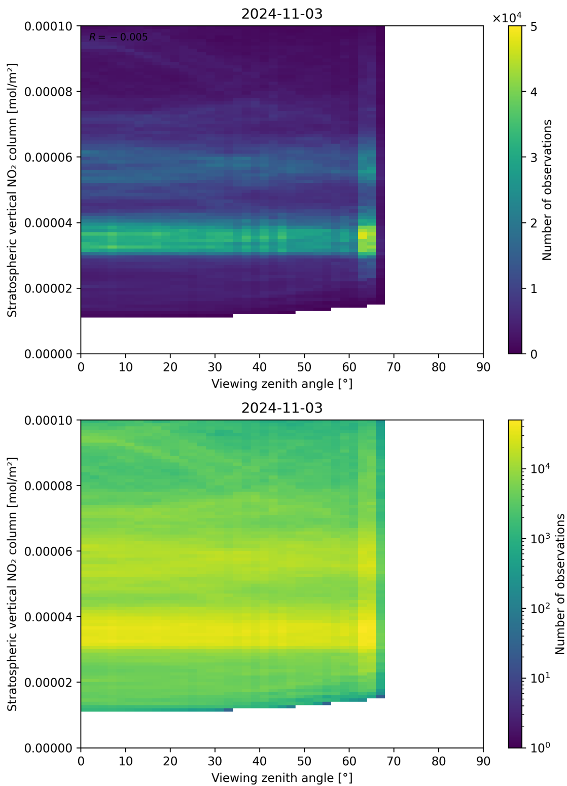
Figure 164: Scatter density plot of “Viewing zenith angle” against “Stratospheric vertical NO 2 column” for 2024-11-02 to 2024-11-04.
