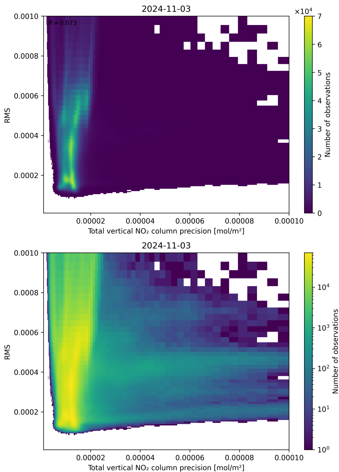
Figure 119: Scatter density plot of “Total vertical NO 2 column precision” against “RMS” for 2024-11-02 to 2024-11-04.
