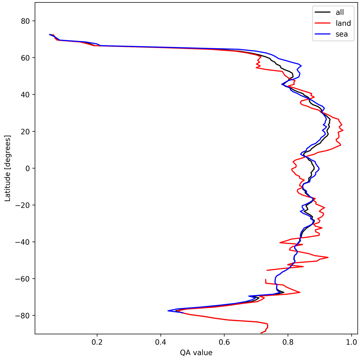
Figure 11: Zonal average of “QA value” for 2024-11-02 to 2024-11-04.
