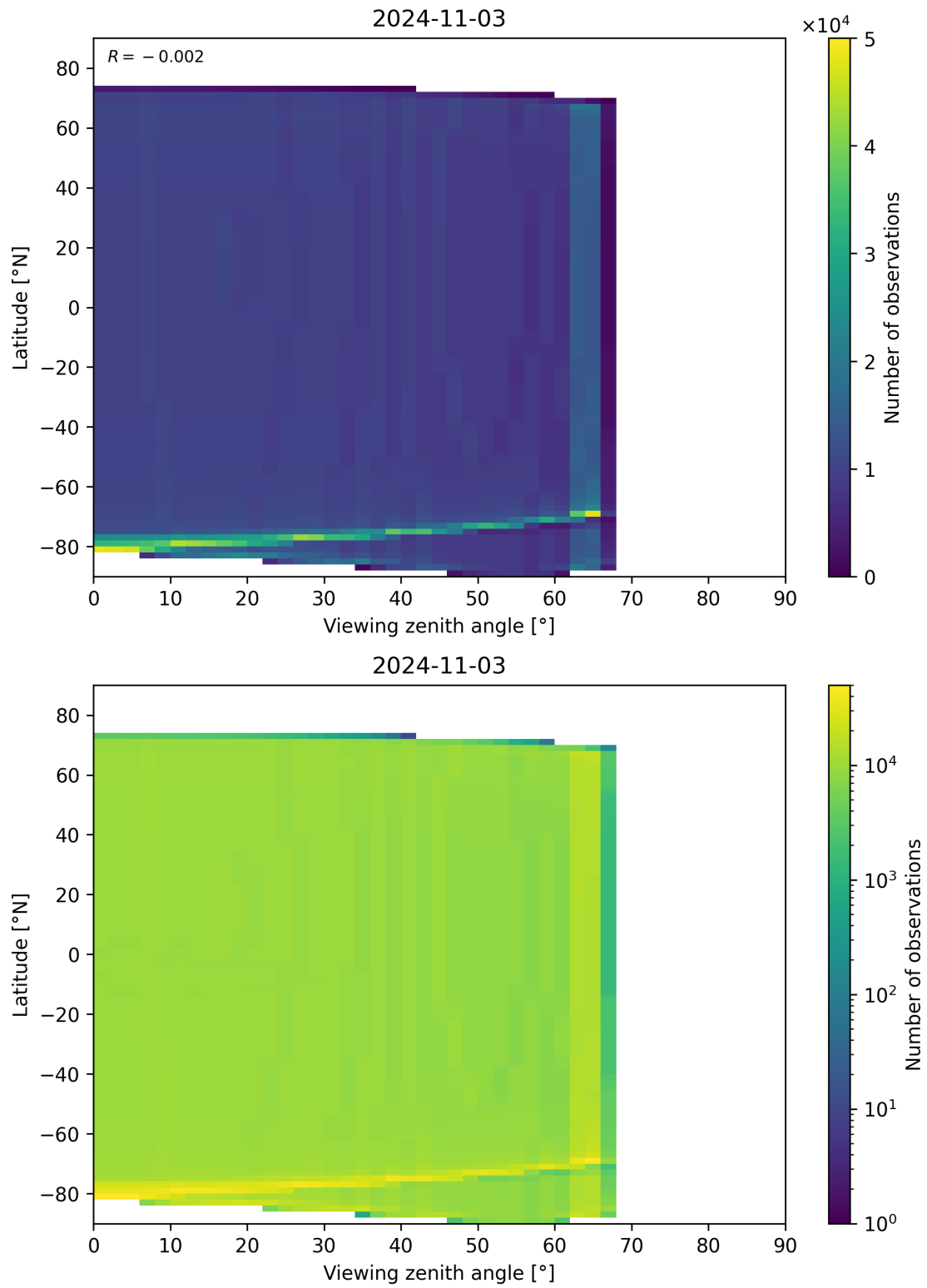
Figure 163: Scatter density plot of “Viewing zenith angle” against “Latitude” for 2024-11-02 to 2024-11-04.
