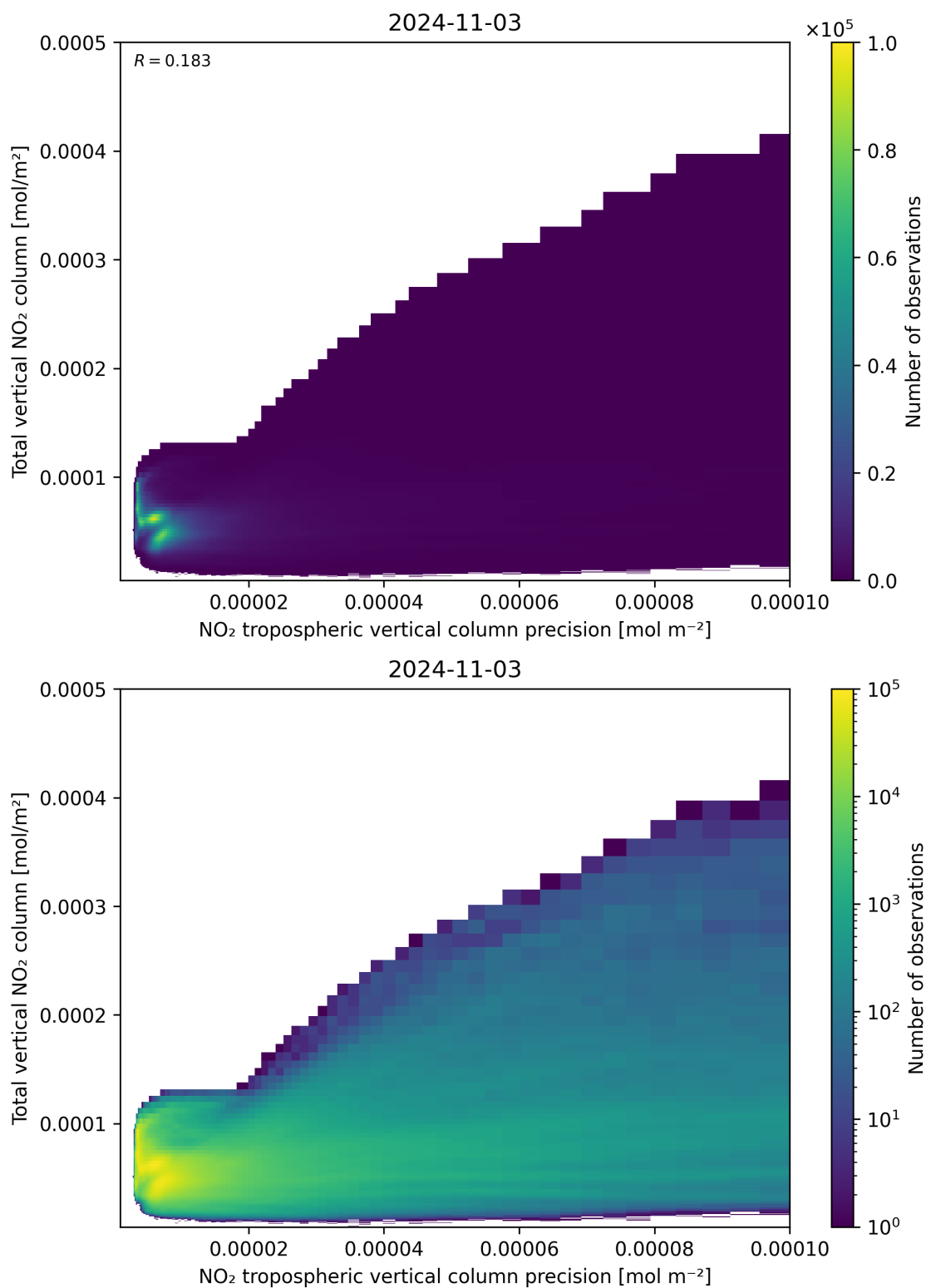
Figure 138: Scatter density plot of “NO 2 tropospheric vertical column precision” against “Total vertical NO 2 column” for 2024-11-02 to 2024-11-04.
