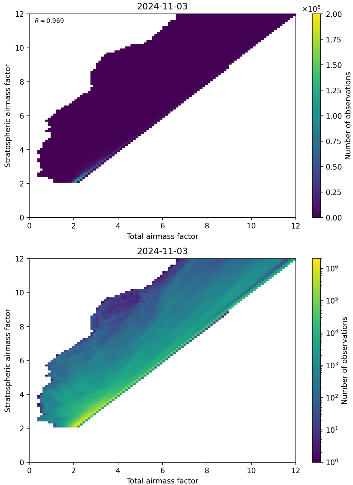
Figure 62: Scatter density plot of “Total air mass factor” against “Stratospheric air mass factor” for 2024-11-02 to 2024-11-04.
