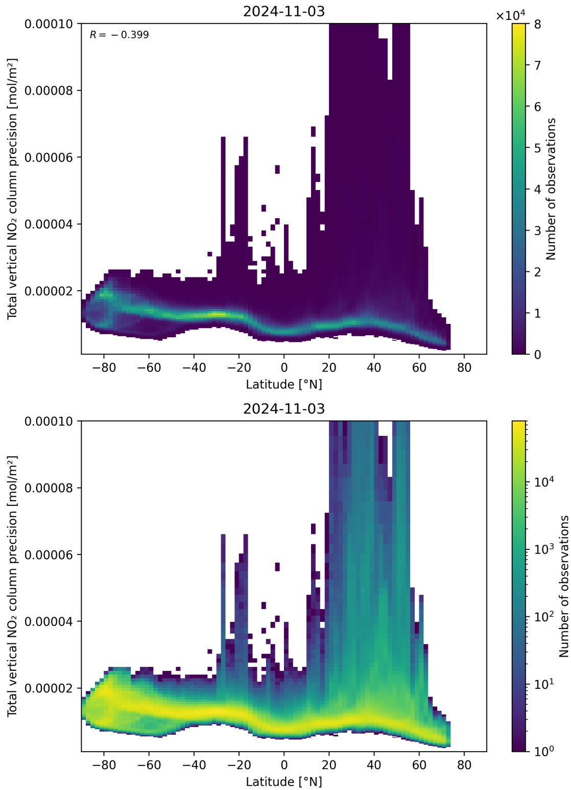
Figure 91: Scatter density plot of “Latitude” against “Total vertical NO 2 column precision” for 2024-11-02 to 2024-11-04.
