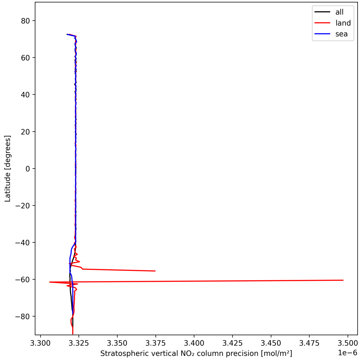
Figure 20: Zonal average of “Stratospheric vertical NO 2 column precision” for 2024-11-02 to 2024-11-04.
