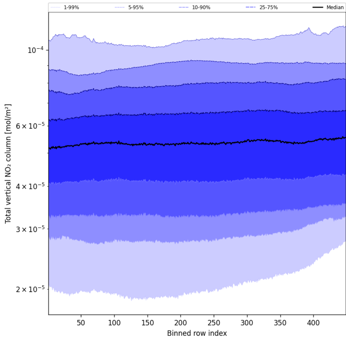
Figure 55: Along track statistics of “Total vertical NO 2 column” for 2024-11-02 to 2024-11-04
