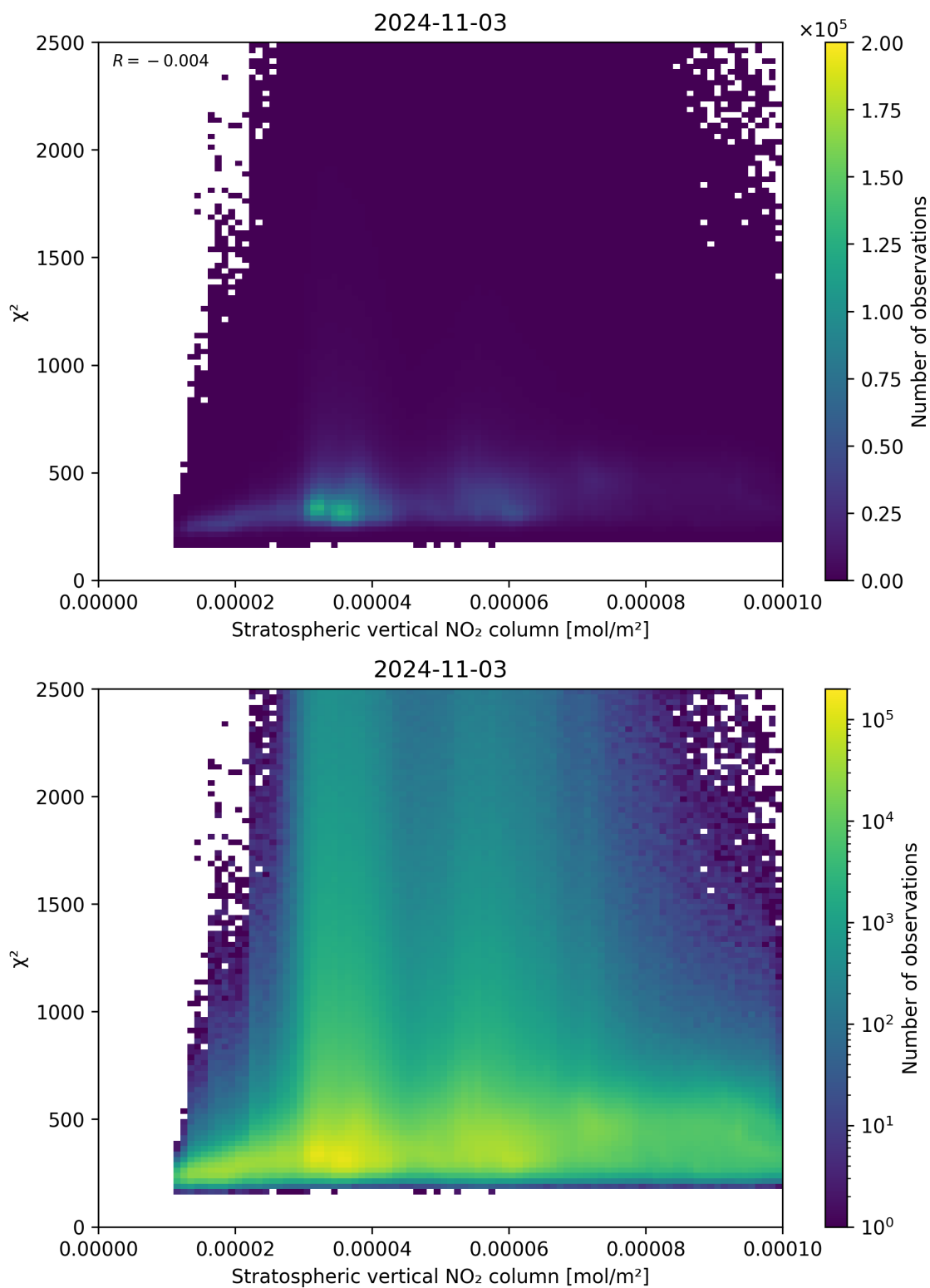
Figure 97: Scatter density plot of “Stratospheric vertical NO 2 column” against “ \chi^2 ” for 2024-11-02 to 2024-11-04.
