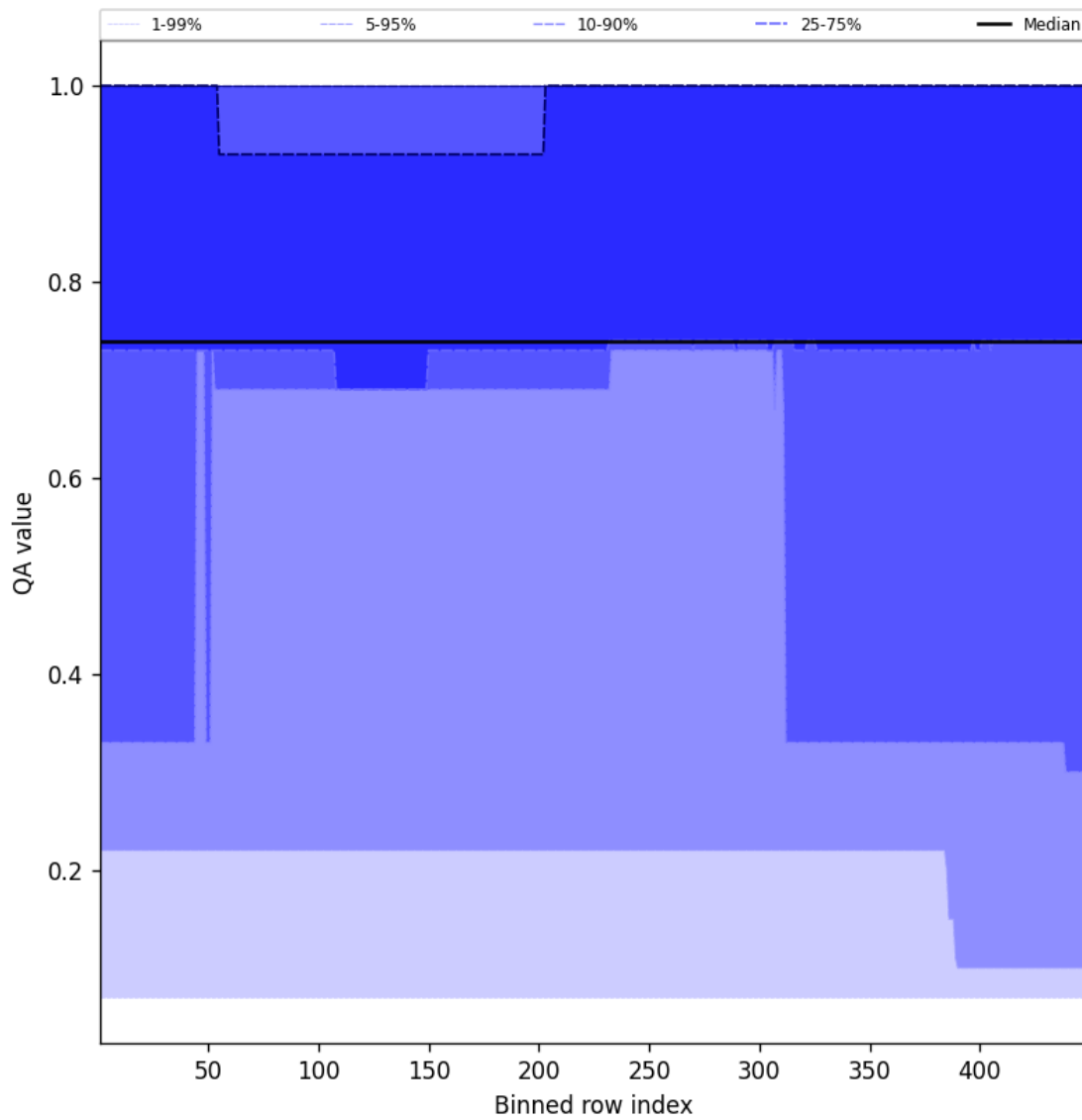
Figure 45: Along track statistics of “QA value” for 2024-11-02 to 2024-11-04
