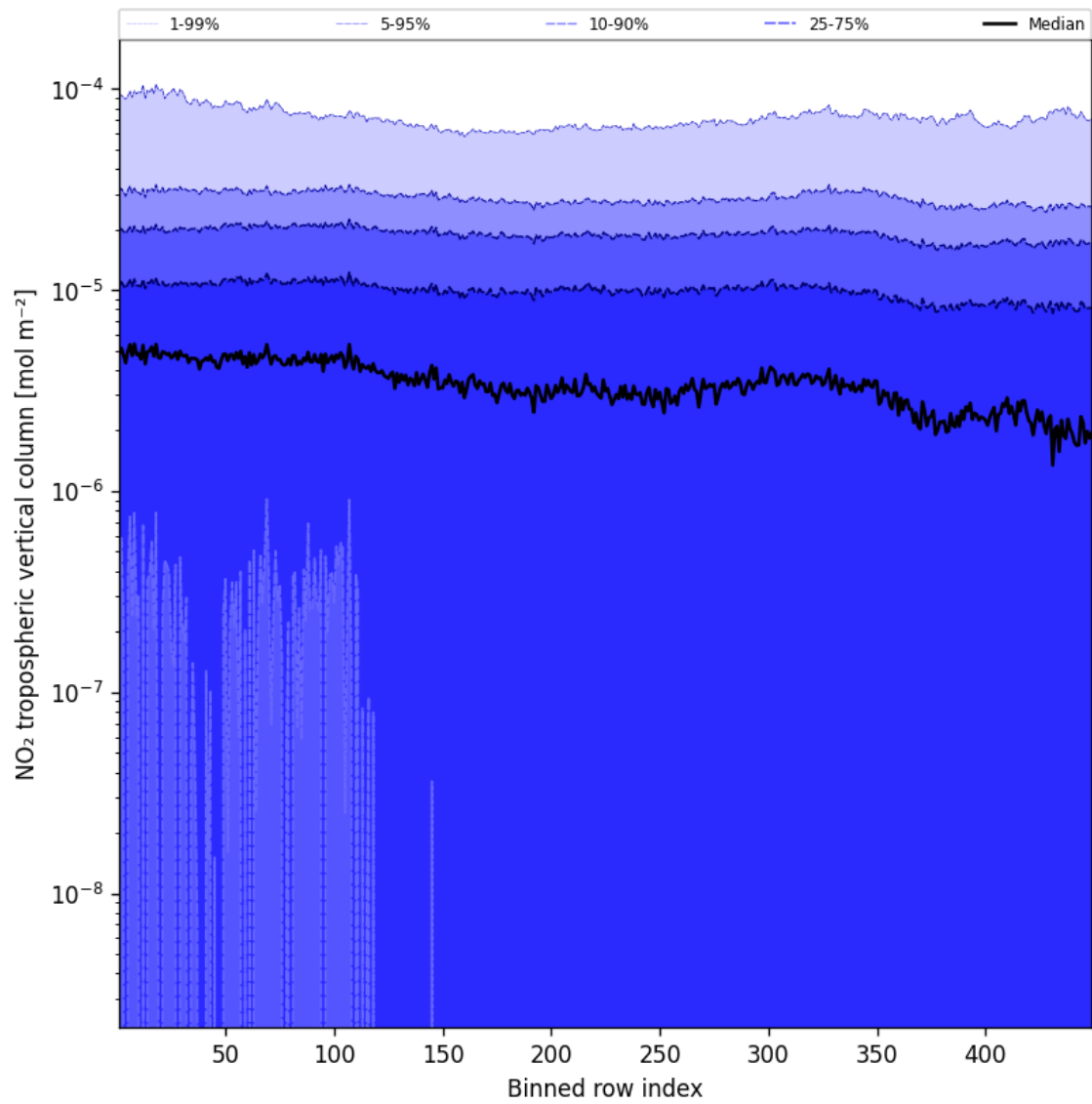
Figure 46: Along track statistics of “NO 2 tropospheric vertical column” for 2024-11-02 to 2024-11-04
