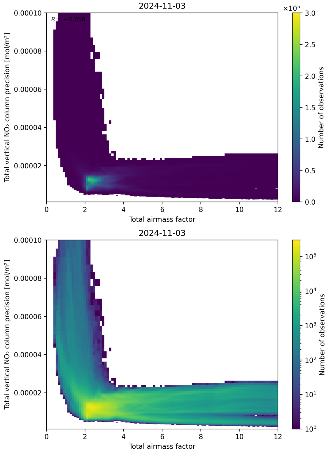
Figure 68: Scatter density plot of “Total airmass factor” against “Total vertical NO 2 column precision” for 2024-11-02 to 2024-11-04.
