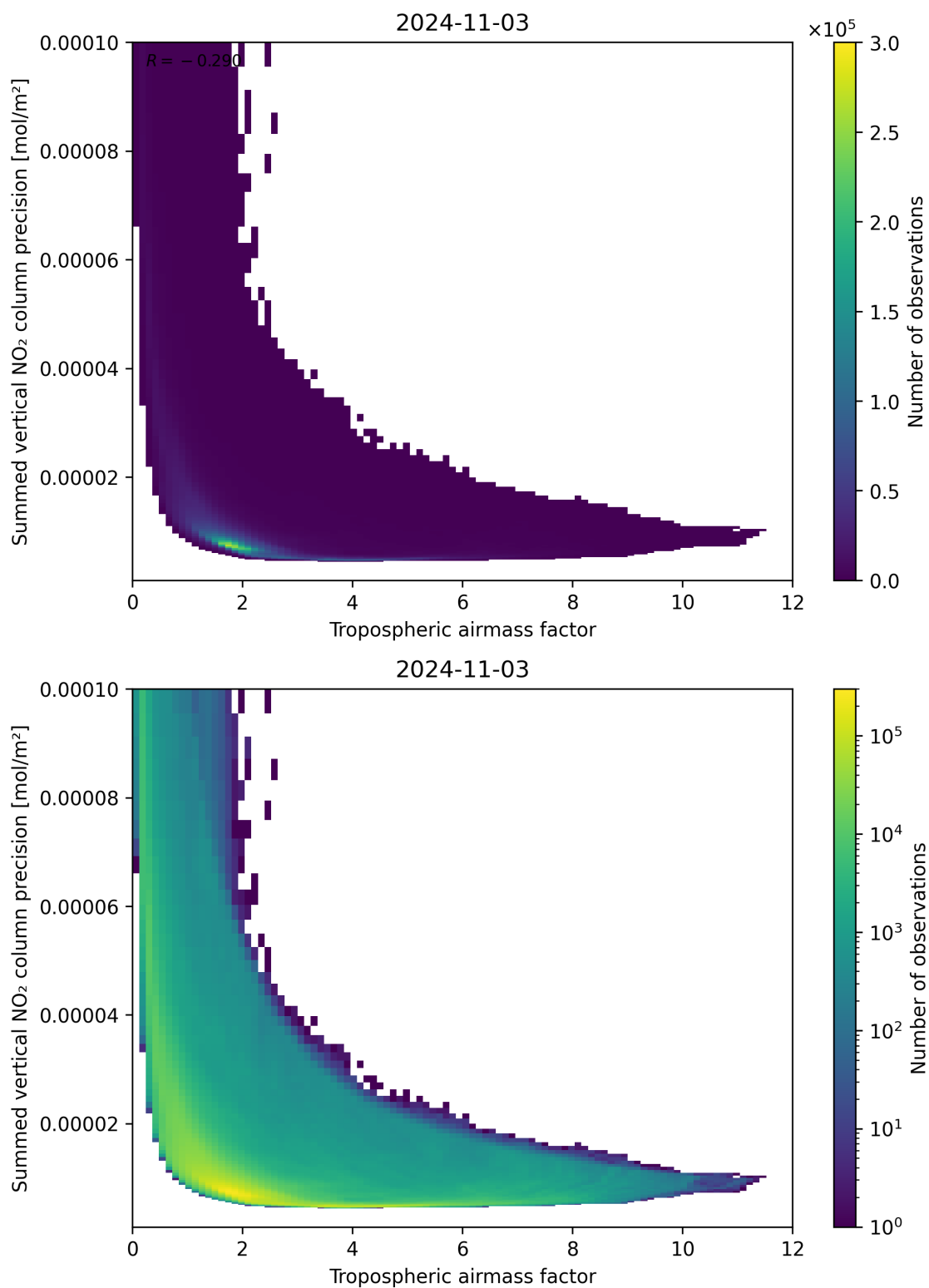
Figure 76: Scatter density plot of “Tropospheric air mass factor” against “Summed vertical NO 2 column precision” for 2024-11-02 to 2024-11-04.
