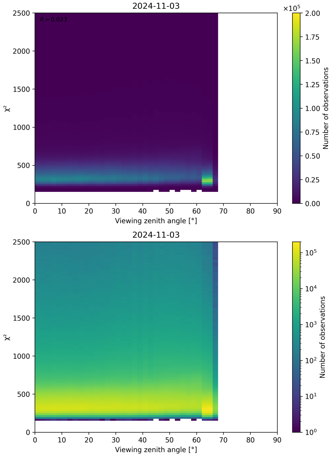
Figure 162: Scatter density plot of “Viewing zenith angle” against “ \chi^2 ” for 2024-11-02 to 2024-11-04.
