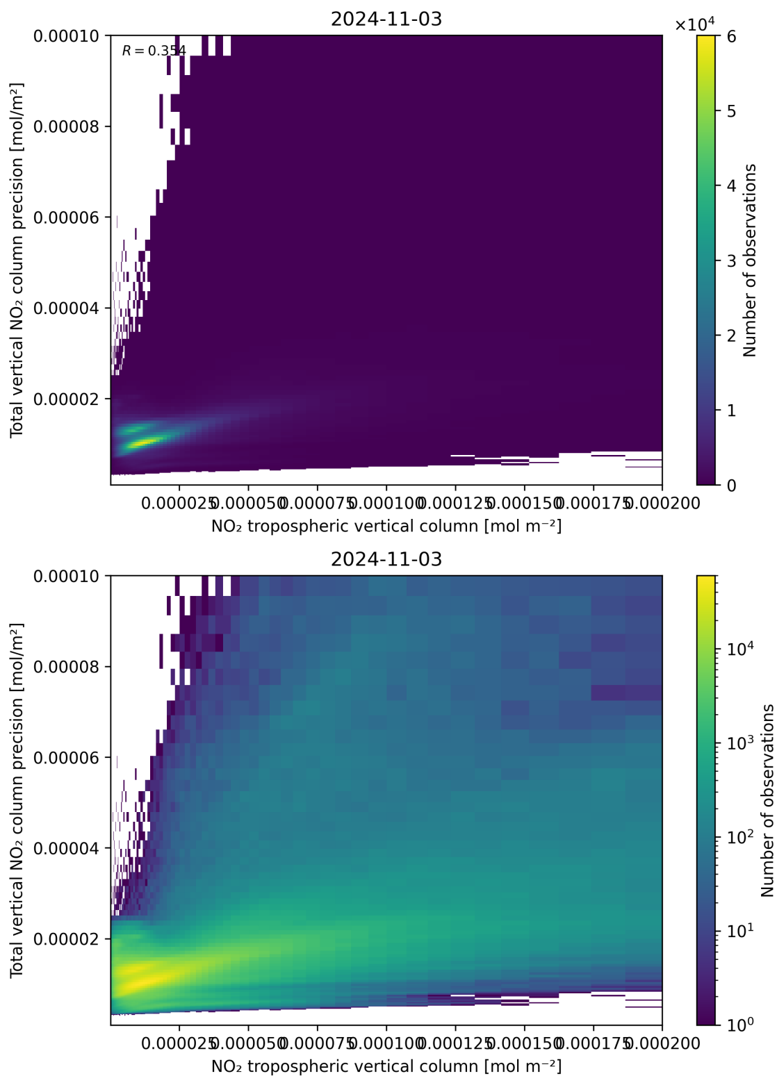
Figure 129: Scatter density plot of “NO 2 tropospheric vertical column” against “Total vertical NO 2 column precision” for 2024-11-02 to 2024-11-04.
