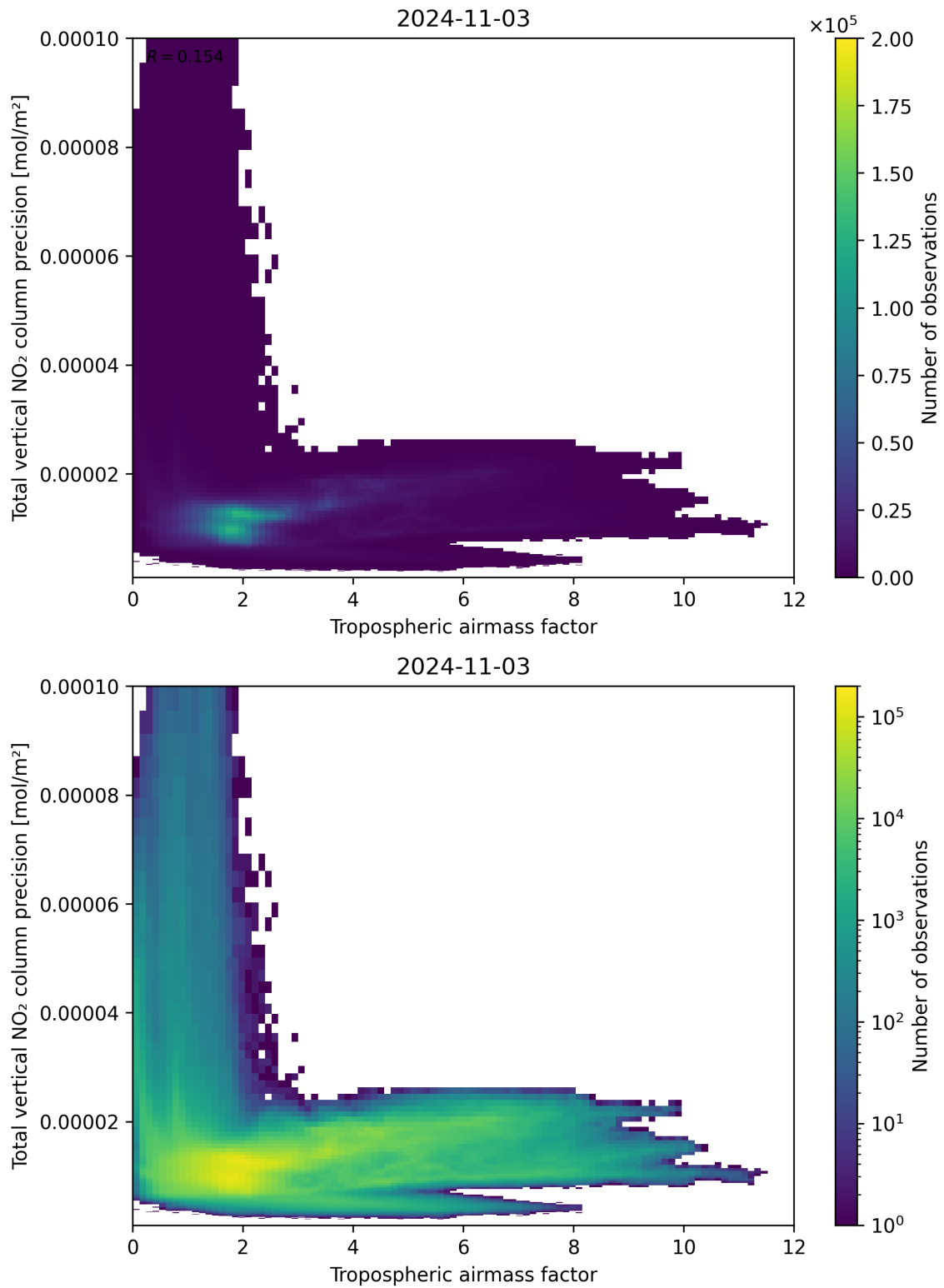
Figure 78: Scatter density plot of “Tropospheric air mass factor” against “Total vertical NO 2 column precision” for 2024-11-02 to 2024-11-04.
