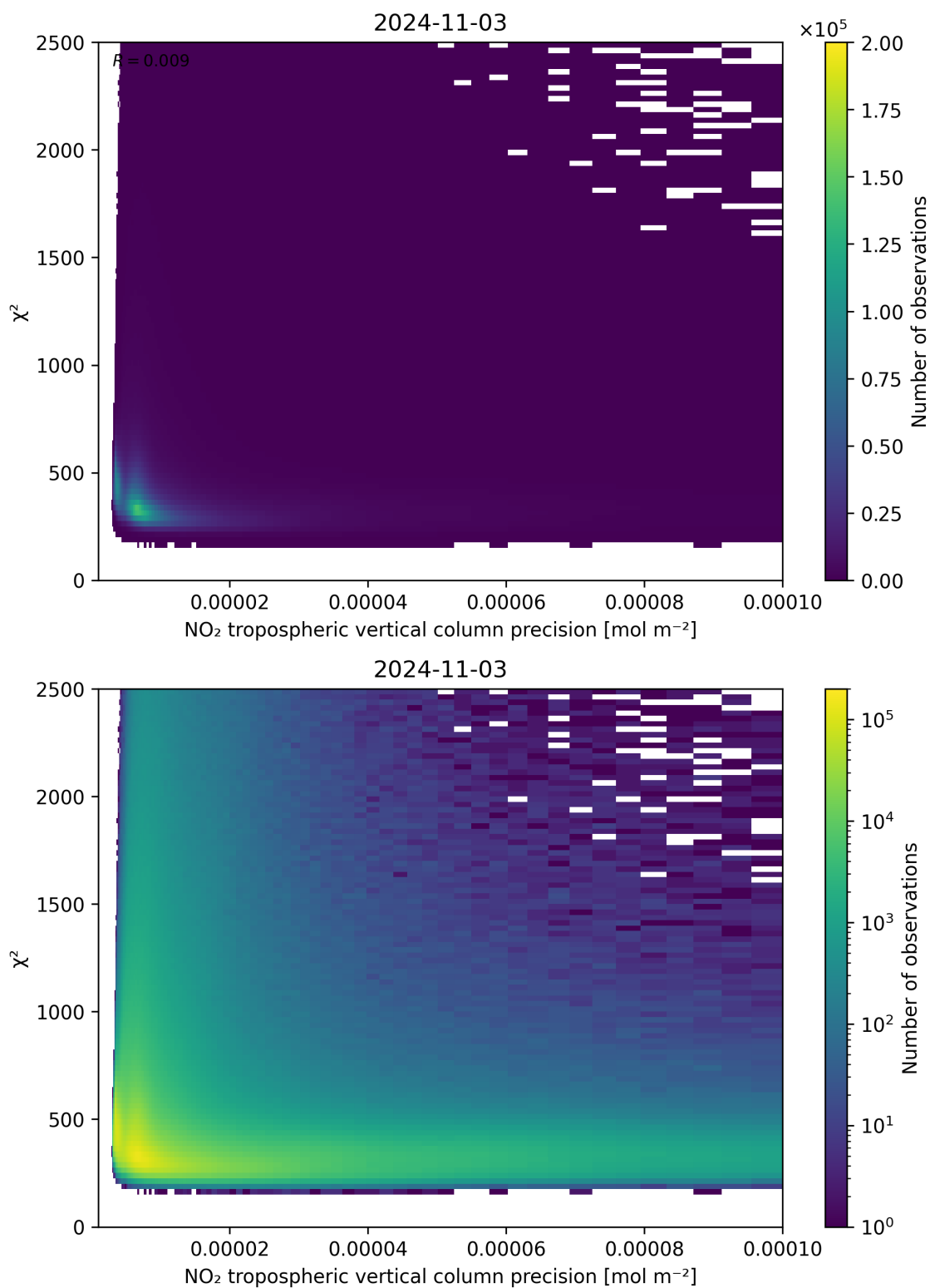
Figure 134: Scatter density plot of “NO 2 tropospheric vertical column precision” against “ \chi^2 ” for 2024-11-02 to 2024-11-04.
