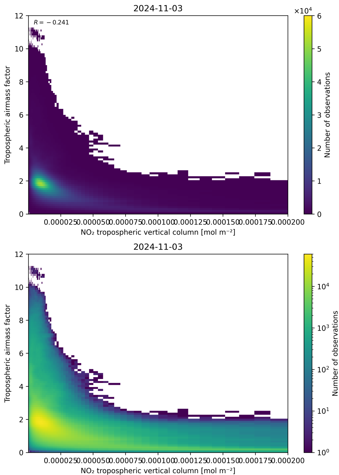
Figure 123: Scatter density plot of “NO 2 tropospheric vertical column” against “Tropospheric air mass factor” for 2024-11-02 to 2024-11-04.
