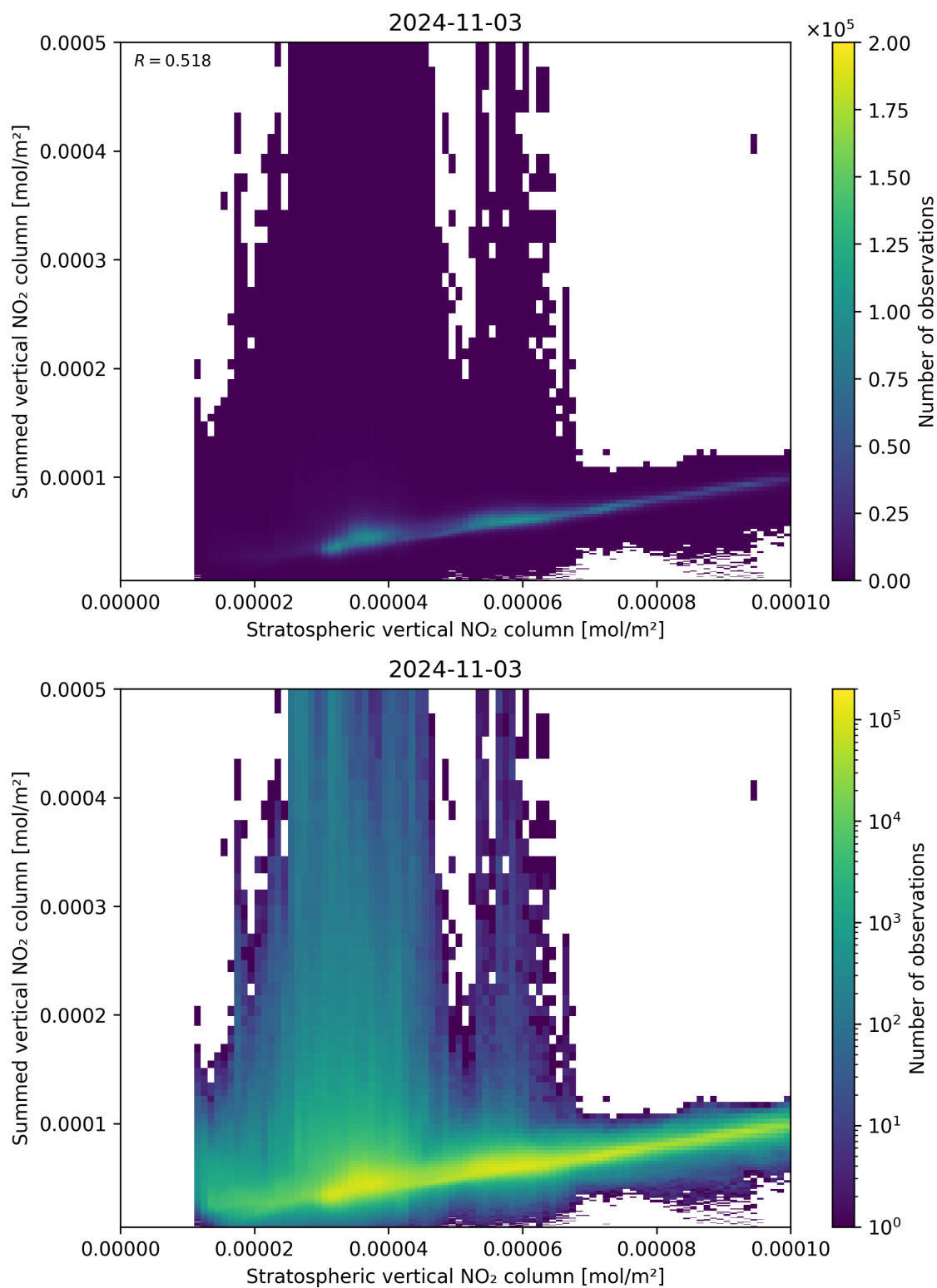
Figure 98: Scatter density plot of “Stratospheric vertical NO 2 column” against “Summed vertical NO 2 column” for 2024-11-02 to 2024-11-04.
