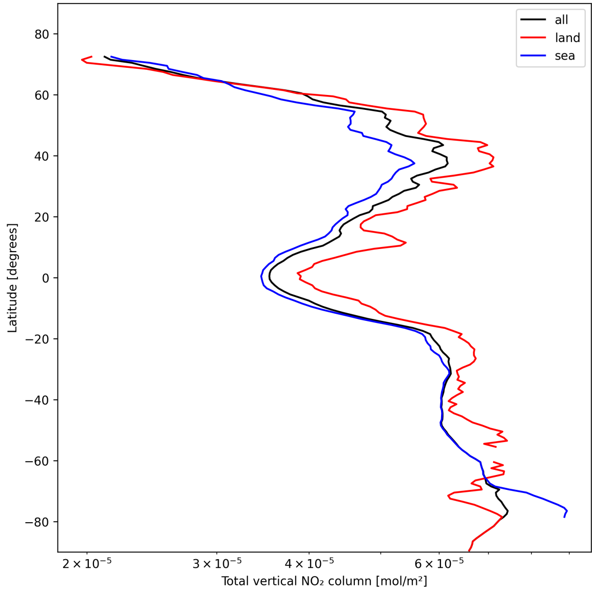
Figure 21: Zonal average of “Total vertical NO 2 column” for 2024-11-02 to 2024-11-04.
