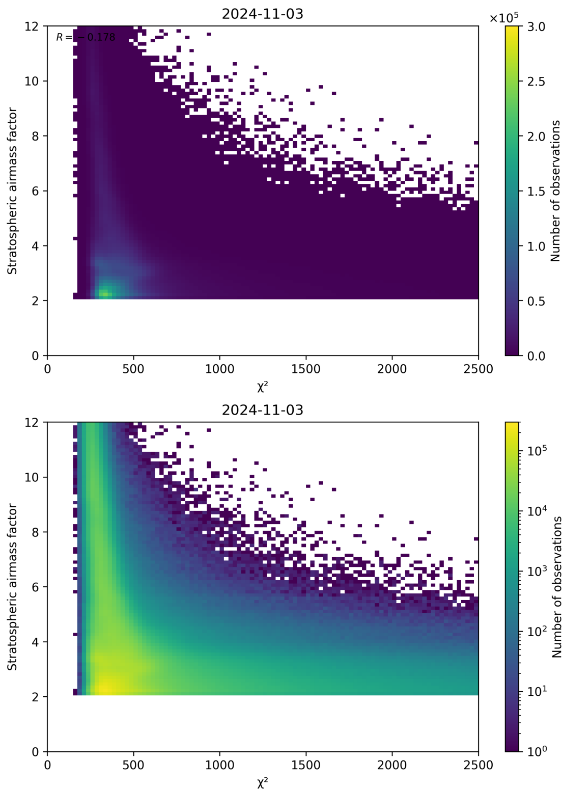
Figure 81: Scatter density plot of “ \chi^2 ” against “Stratospheric airmass factor” for 2024-11-02 to 2024-11-04.
