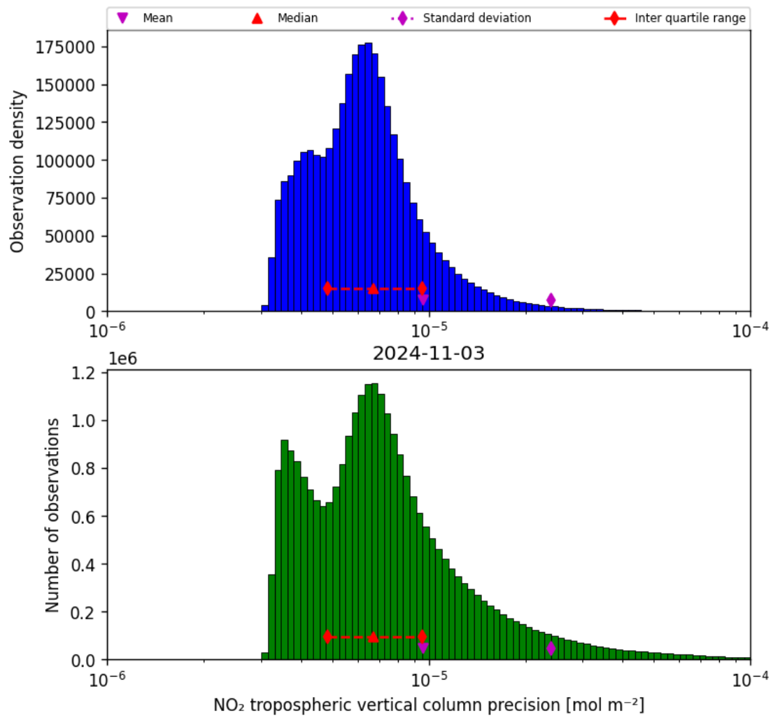
Figure 30: Histogram of “NO 2 tropospheric vertical column precision” for 2024-11-02 to 2024-11-04
