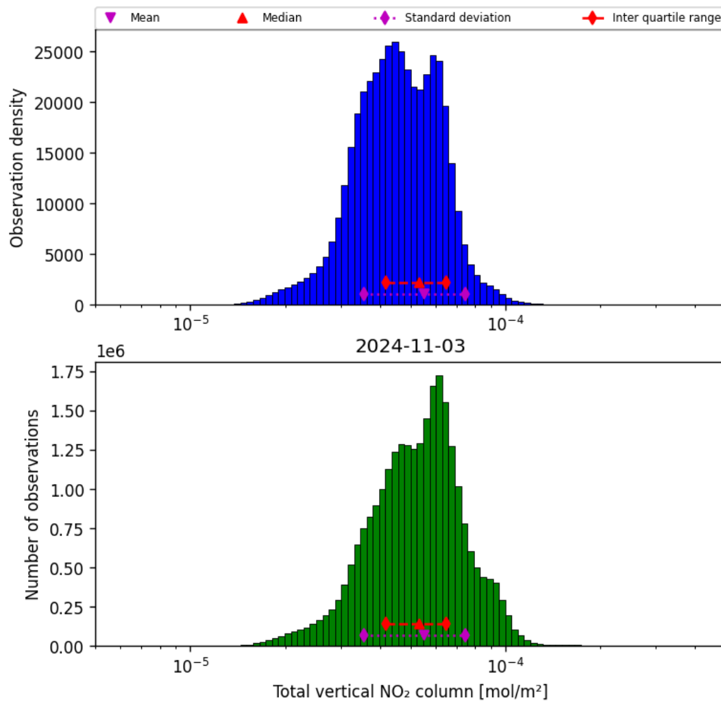
Figure 38: Histogram of “Total vertical NO 2 column” for 2024-11-02 to 2024-11-04
