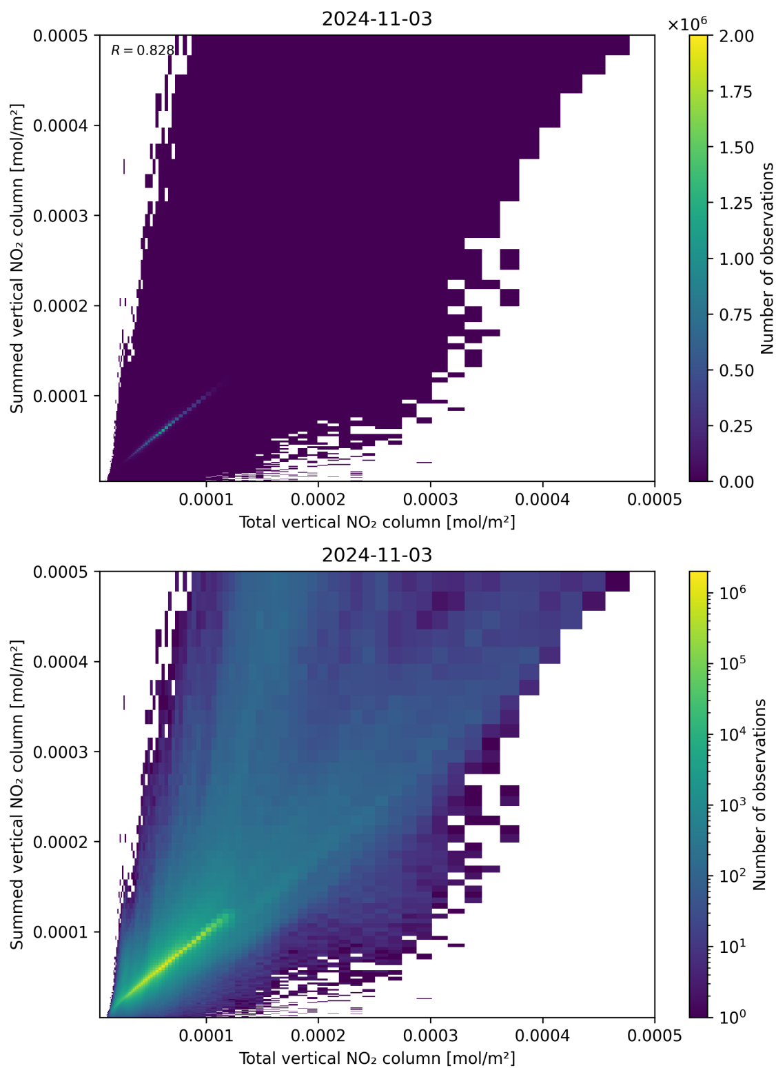
Figure 112: Scatter density plot of “Total vertical NO 2 column” against “Summed vertical NO 2 column” for 2024-11-02 to 2024-11-04.
