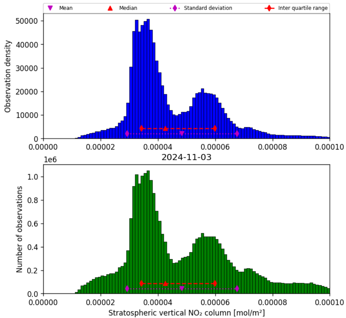
Figure 36: Histogram of “Stratospheric vertical NO 2 column” for 2024-11-02 to 2024-11-04
