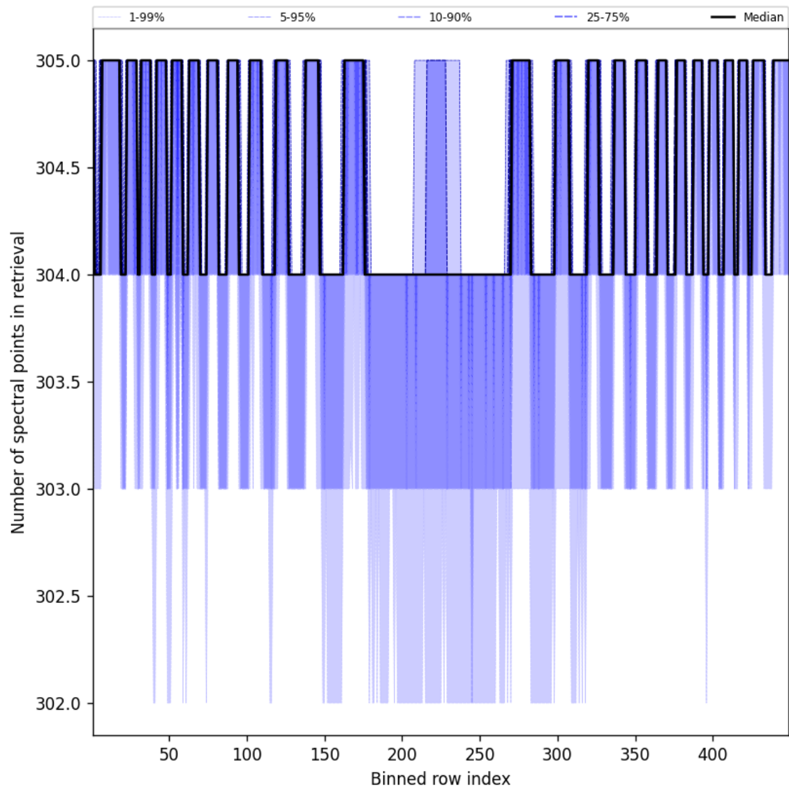
Figure 50: Along track statistics of “Number of spectral points in retrieval” for 2024-11-02 to 2024-11-04
