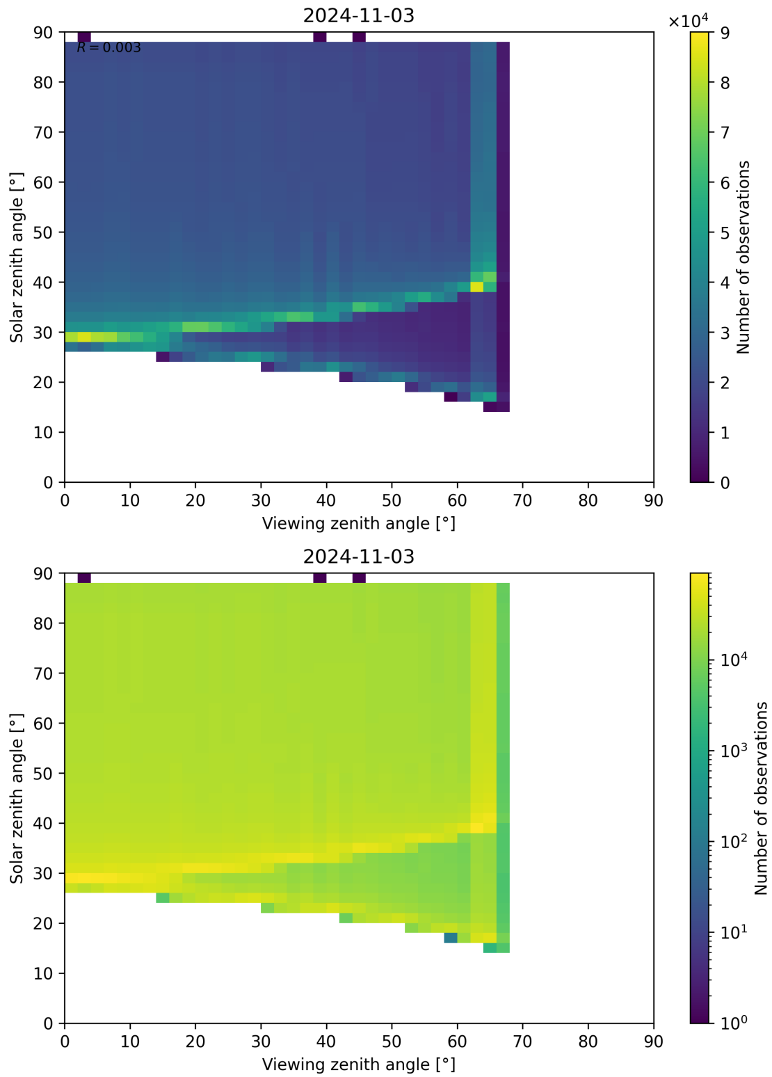
Figure 172: Scatter density plot of “Viewing zenith angle” against “Solar zenith angle” for 2024-11-02 to 2024-11-04.
