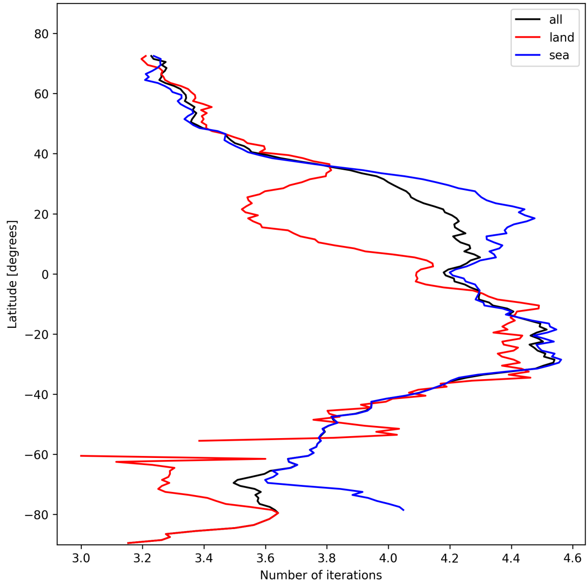
Figure 17: Zonal average of “Number of iterations” for 2024-11-02 to 2024-11-04.
