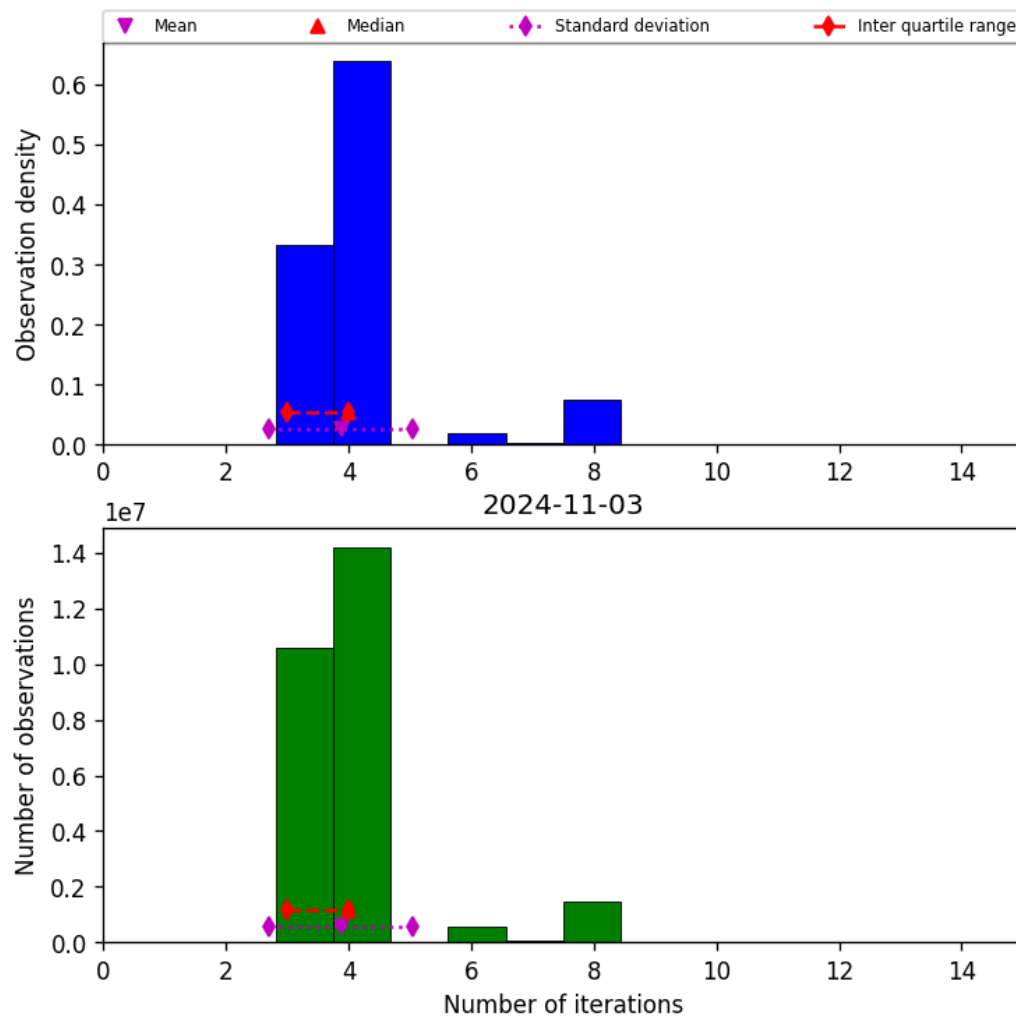
Figure 34: Histogram of “Number of iterations” for 2024-11-02 to 2024-11-04
