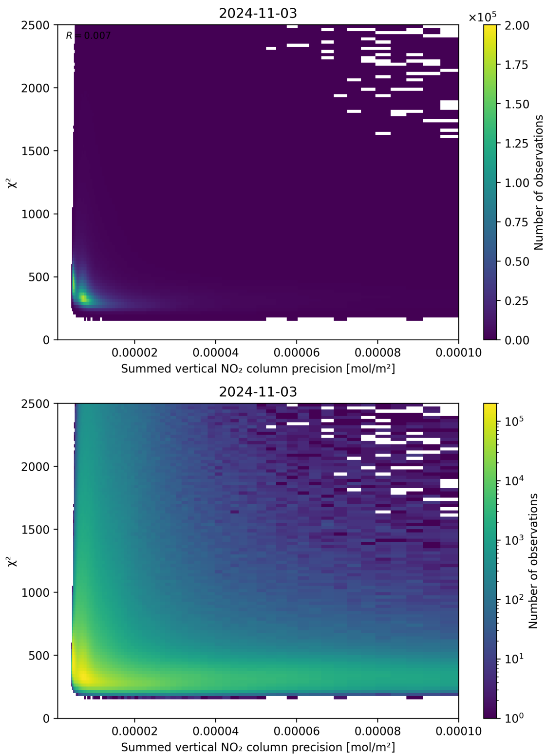
Figure 107: Scatter density plot of “Summed vertical NO 2 column precision” against “ \chi^2 ” for 2024-11-02 to 2024-11-04.
