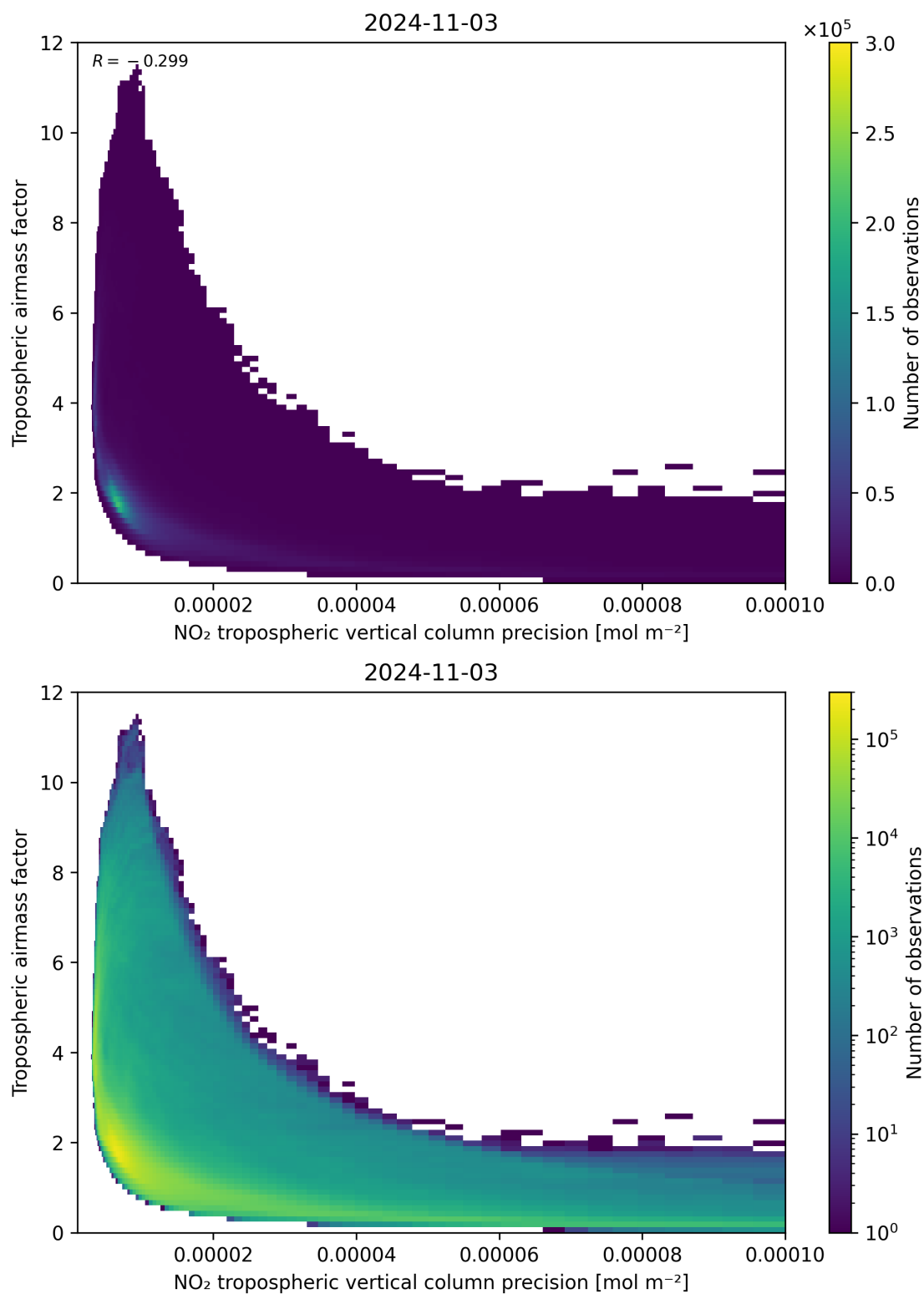
Figure 133: Scatter density plot of “NO 2 tropospheric vertical column precision” against “Tropospheric airmass factor” for 2024-11-02 to 2024-11-04.
