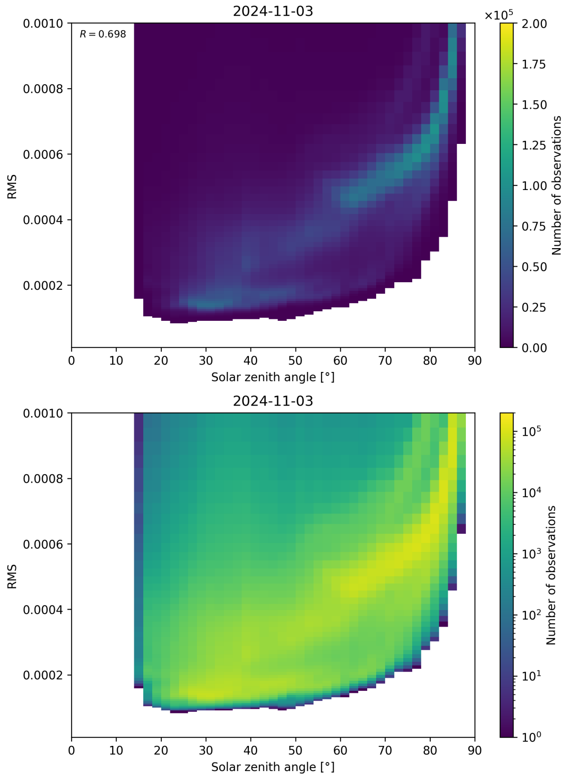
Figure 157: Scatter density plot of “Solar zenith angle” against “RMS” for 2024-11-02 to 2024-11-04.
