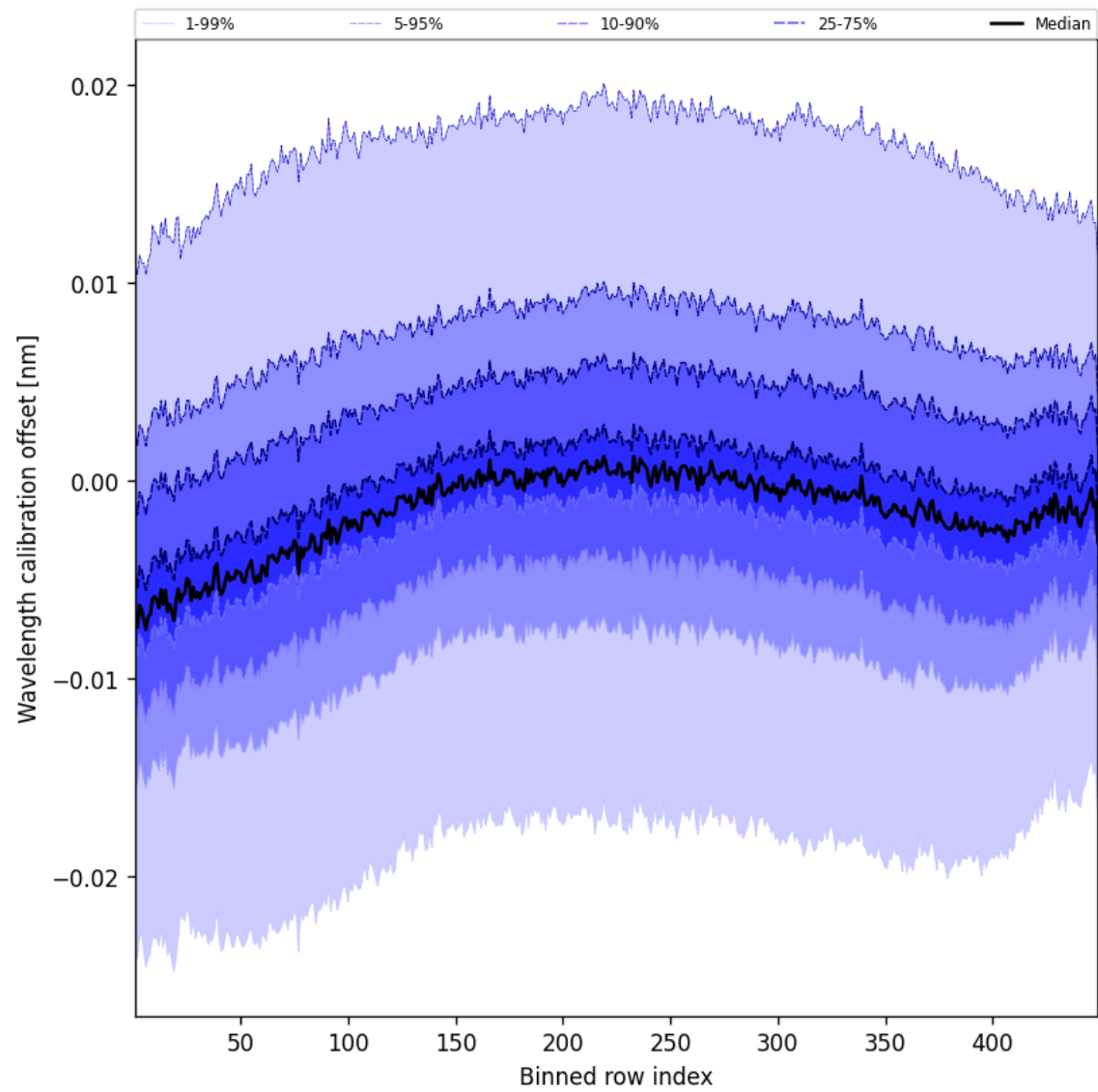
Figure 52: Along track statistics of “Wavelength calibration offset” for 2024-11-02 to 2024-11-04
