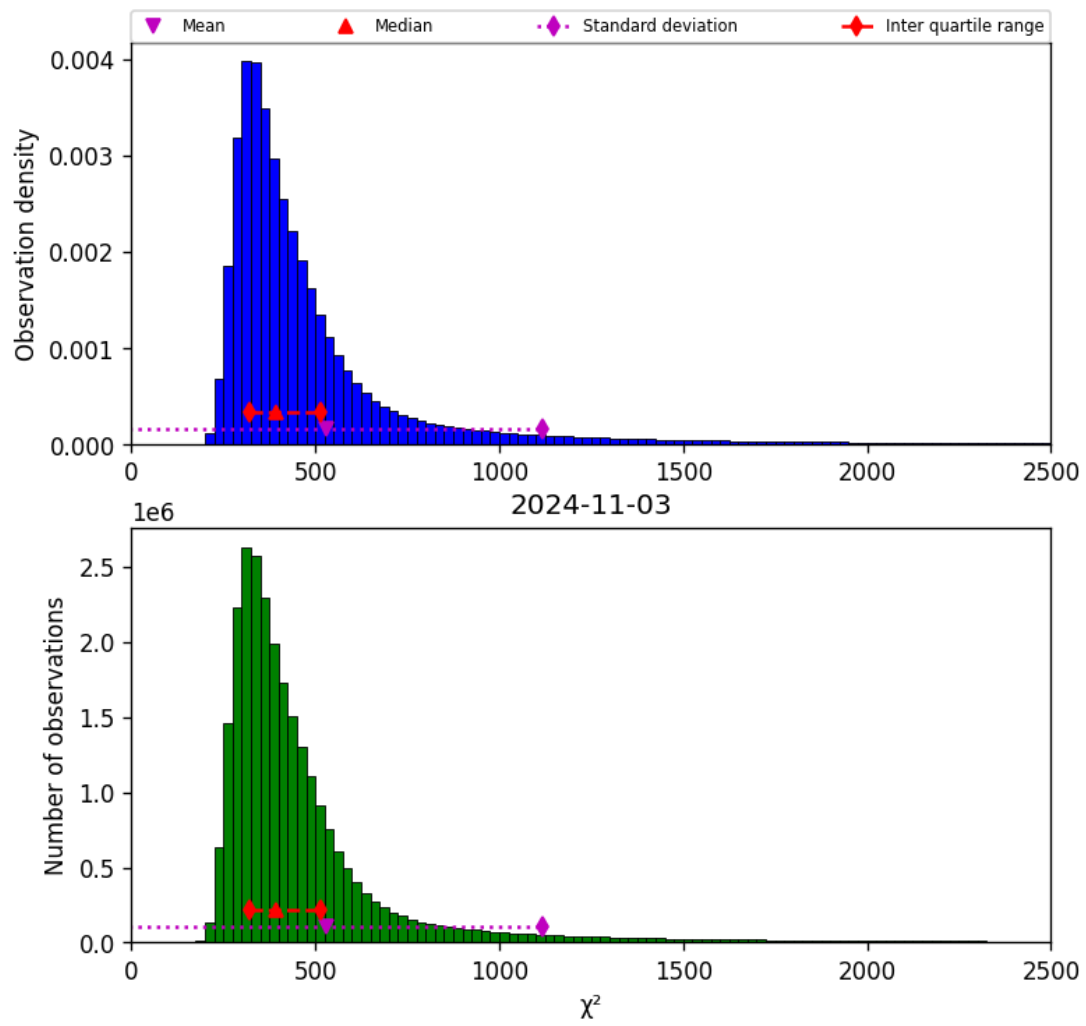
Figure 42: Histogram of “ \chi^2 ” for 2024-11-02 to 2024-11-04
