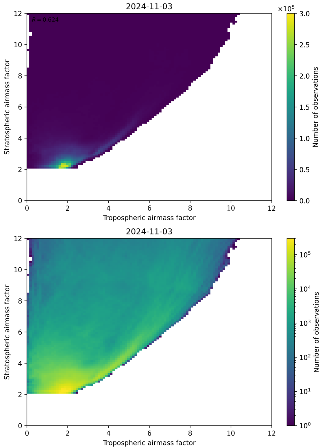
Figure 71: Scatter density plot of “Tropospheric airmass factor” against “Stratospheric airmass factor” for 2024-11-02 to 2024-11-04.
