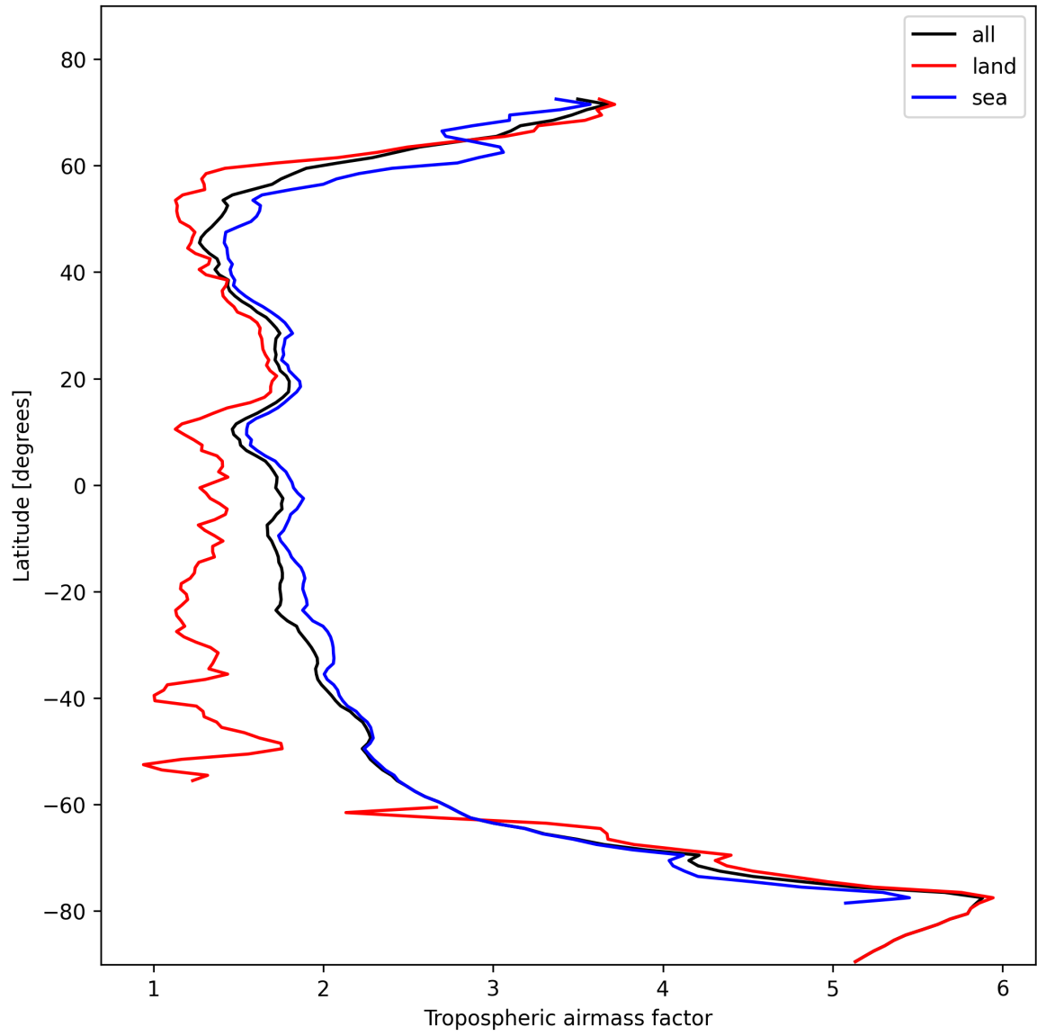
Figure 14: Zonal average of “Tropospheric airmass factor” for 2024-11-02 to 2024-11-04.
