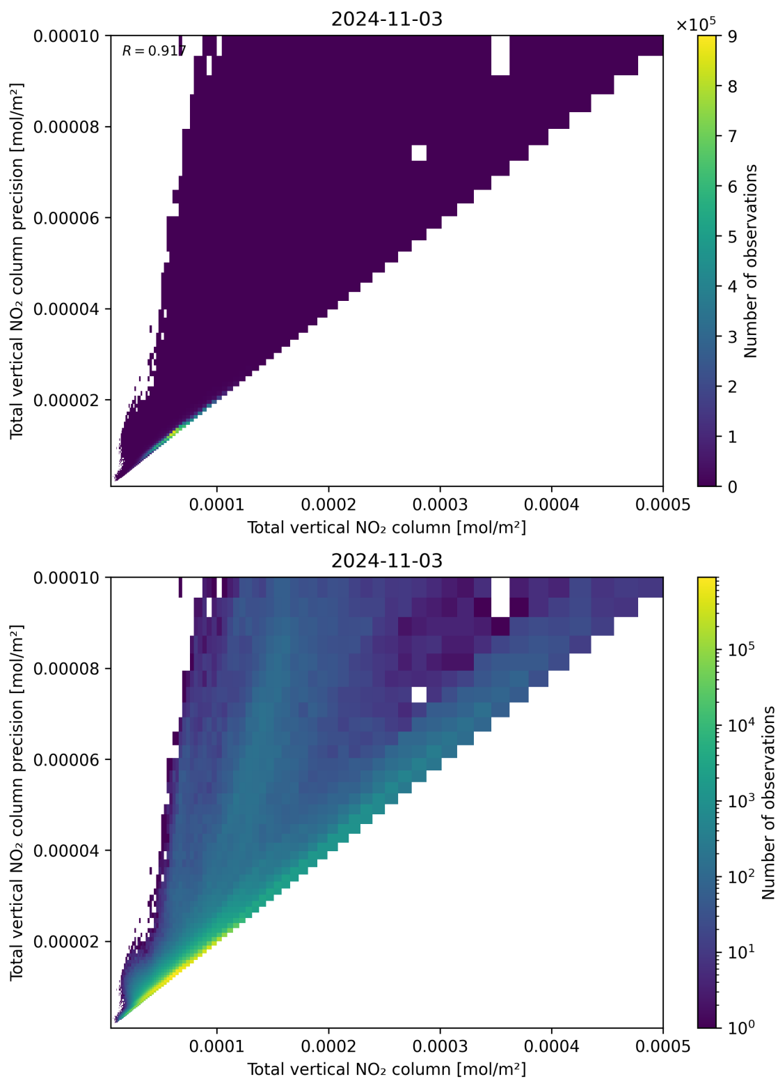
Figure 114: Scatter density plot of “Total vertical NO 2 column” against “Total vertical NO 2 column precision” for 2024-11-02 to 2024-11-04.
