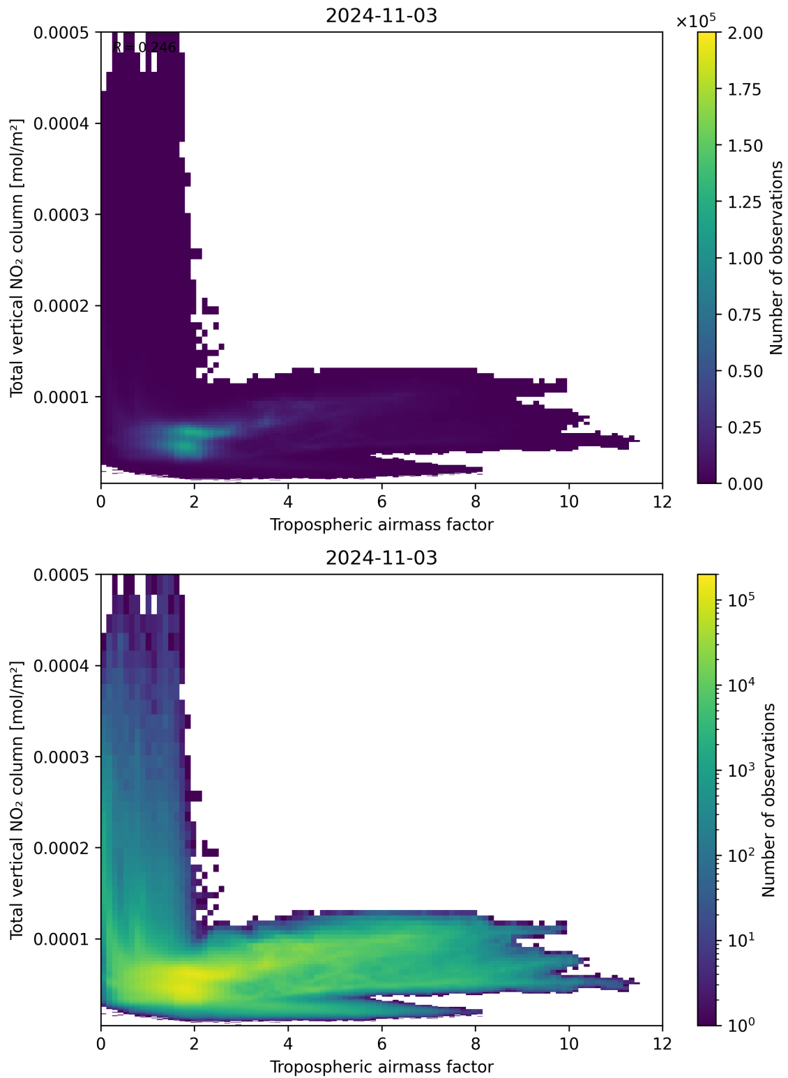
Figure 77: Scatter density plot of “Tropospheric airmass factor” against “Total vertical NO 2 column” for 2024-11-02 to 2024-11-04.
