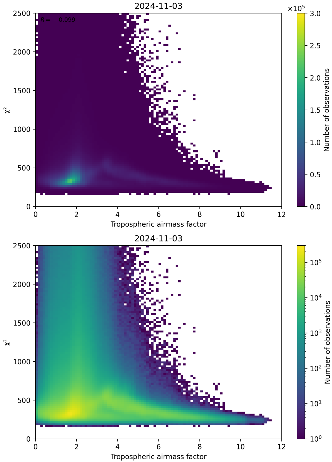
Figure 73: Scatter density plot of “Tropospheric airmass factor” against “ \chi^2 ” for 2024-11-02 to 2024-11-04.
