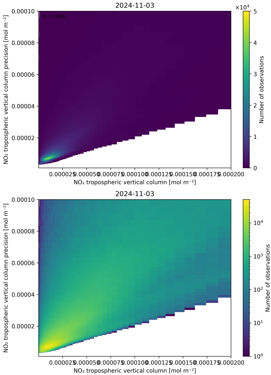
Figure 130: Scatter density plot of “NO 2 tropospheric vertical column” against “NO 2 tropospheric vertical column precision” for 2024-11-02 to 2024-11-04.
