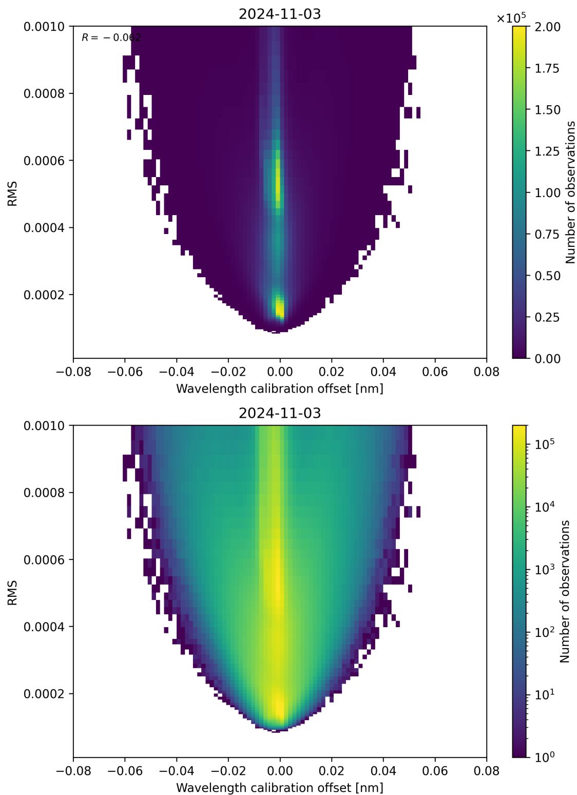
Figure 181: Scatter density plot of “Wavelength calibration offset” against “RMS” for 2024-11-02 to 2024-11-04.
