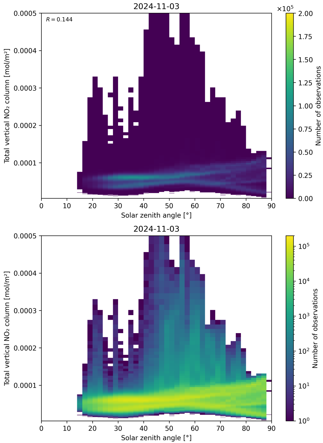
Figure 153: Scatter density plot of “Solar zenith angle” against “Total vertical NO 2 column” for 2024-11-02 to 2024-11-04.
