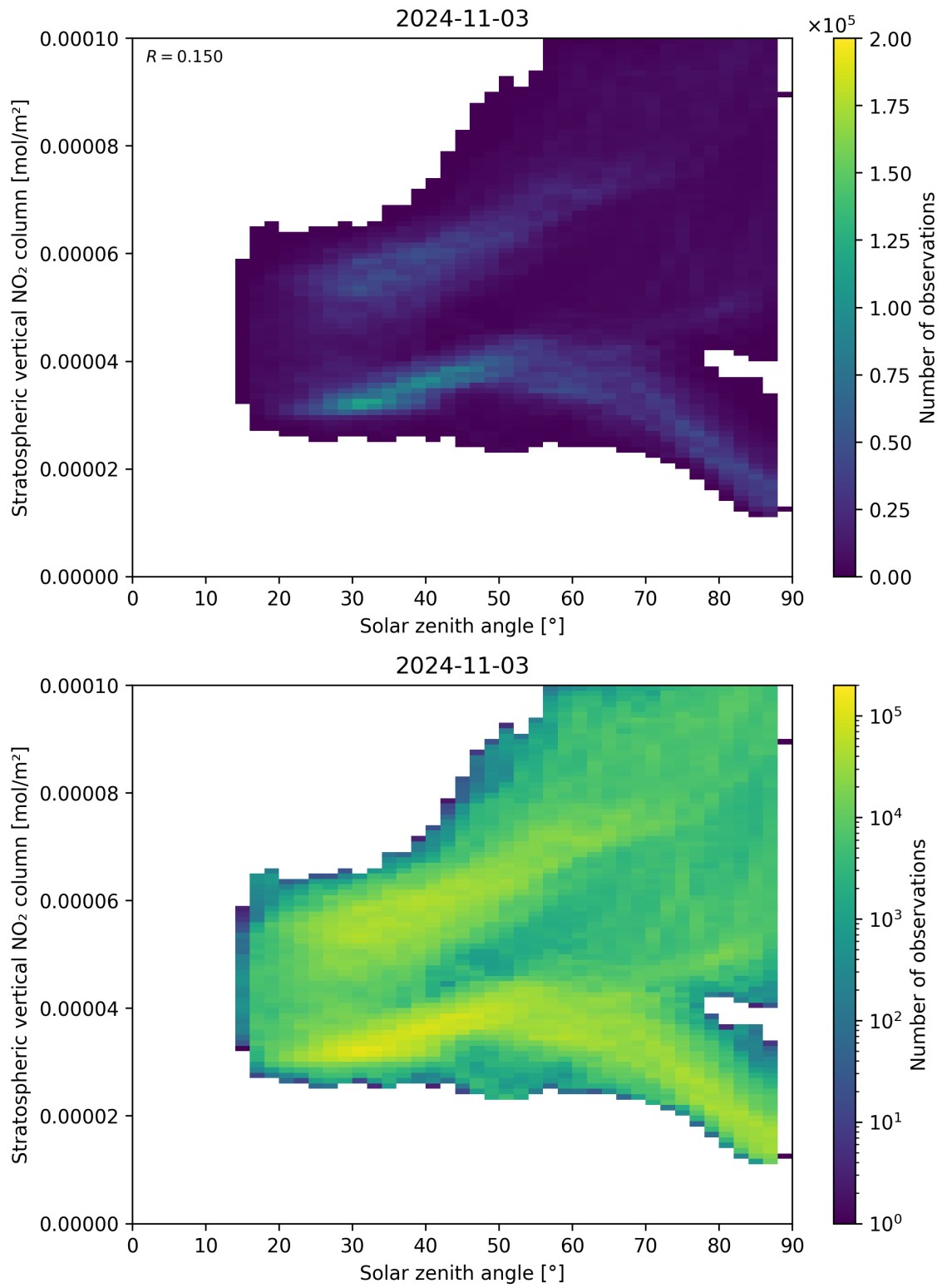
Figure 150: Scatter density plot of “Solar zenith angle” against “Stratospheric vertical NO 2 column” for 2024-11-02 to 2024-11-04.
