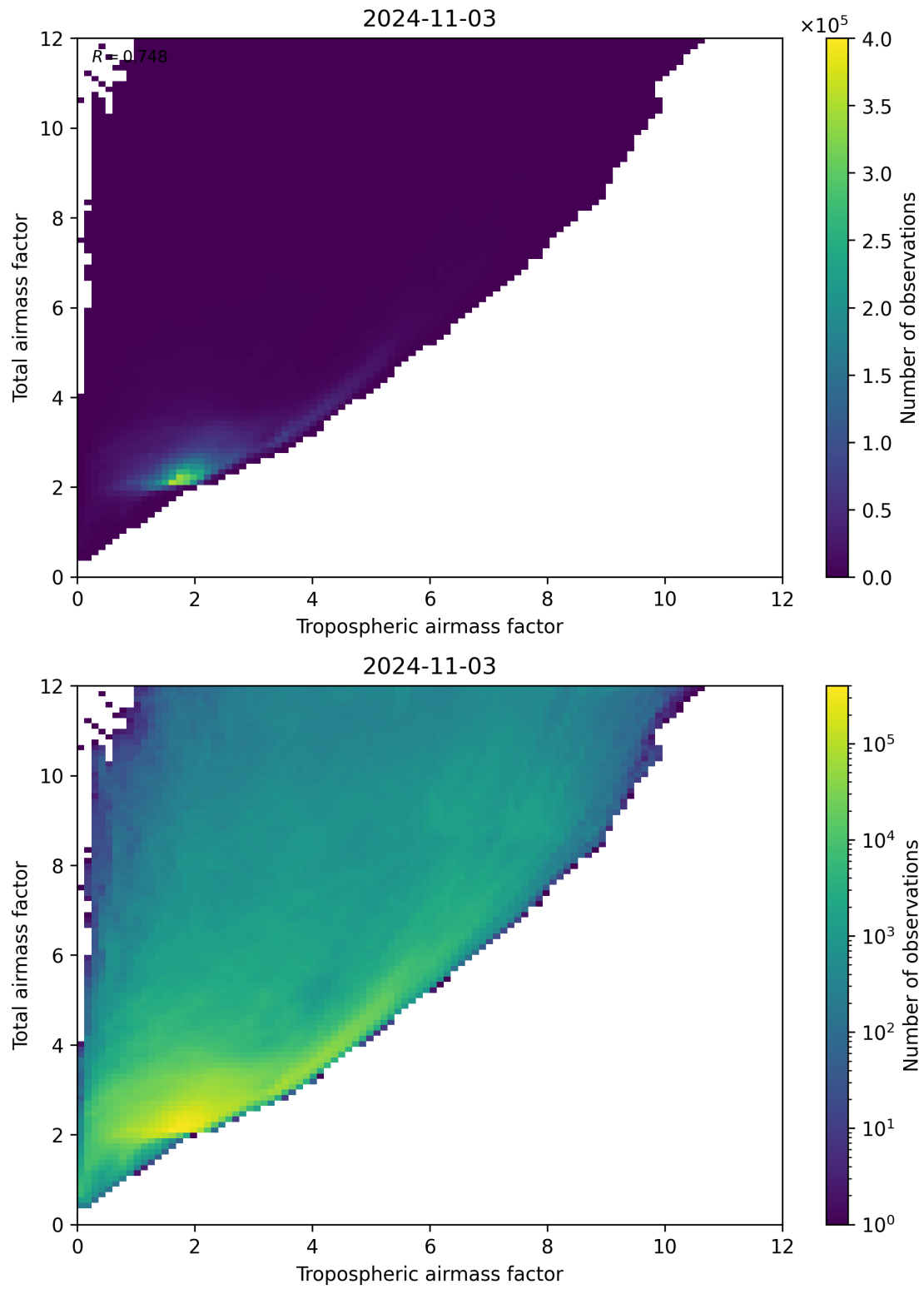
Figure 72: Scatter density plot of “Tropospheric airmass factor” against “Total airmass factor” for 2024-11-02 to 2024-11-04.
