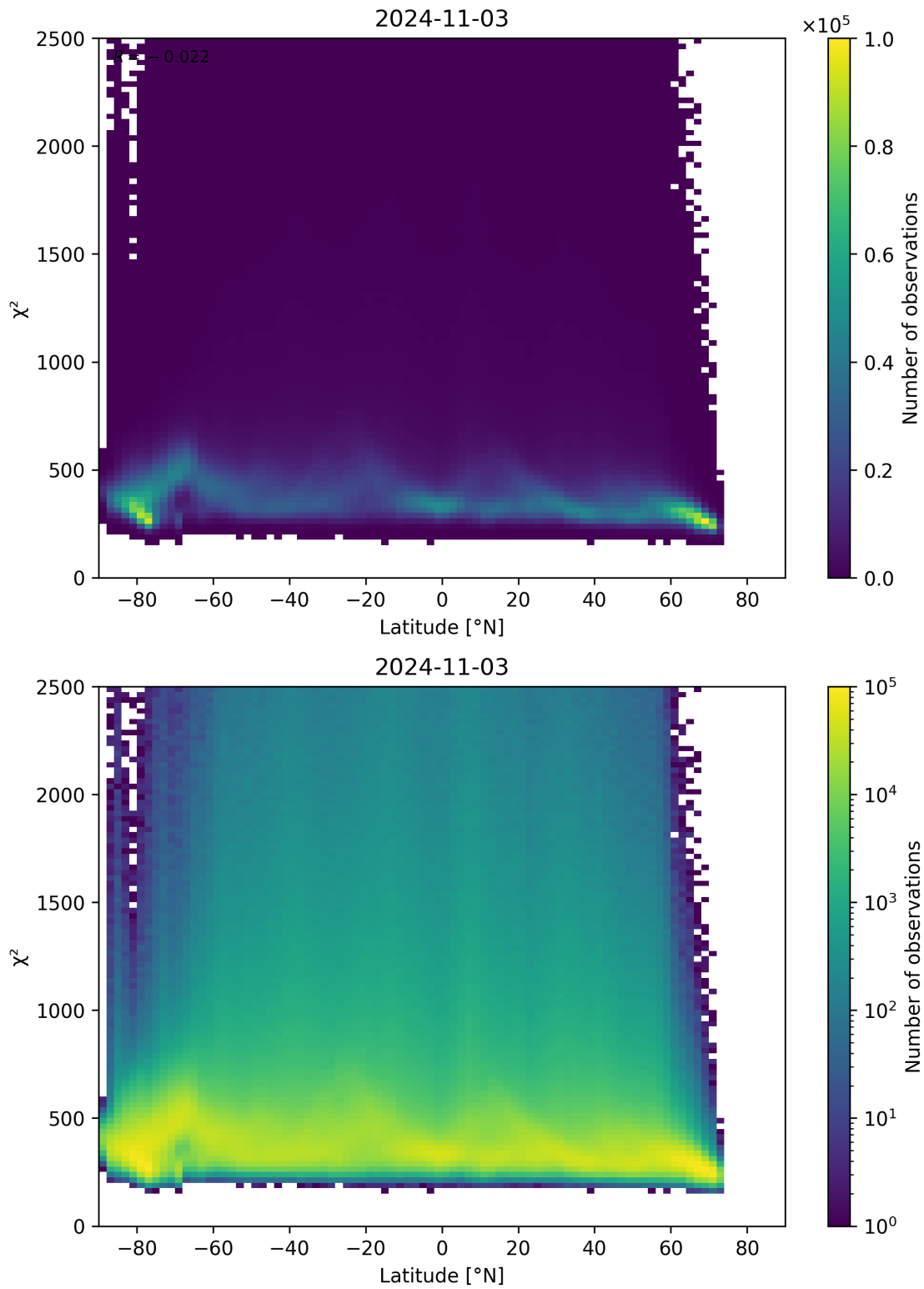
Figure 86: Scatter density plot of “Latitude” against “ \chi^2 ” for 2024-11-02 to 2024-11-04.
