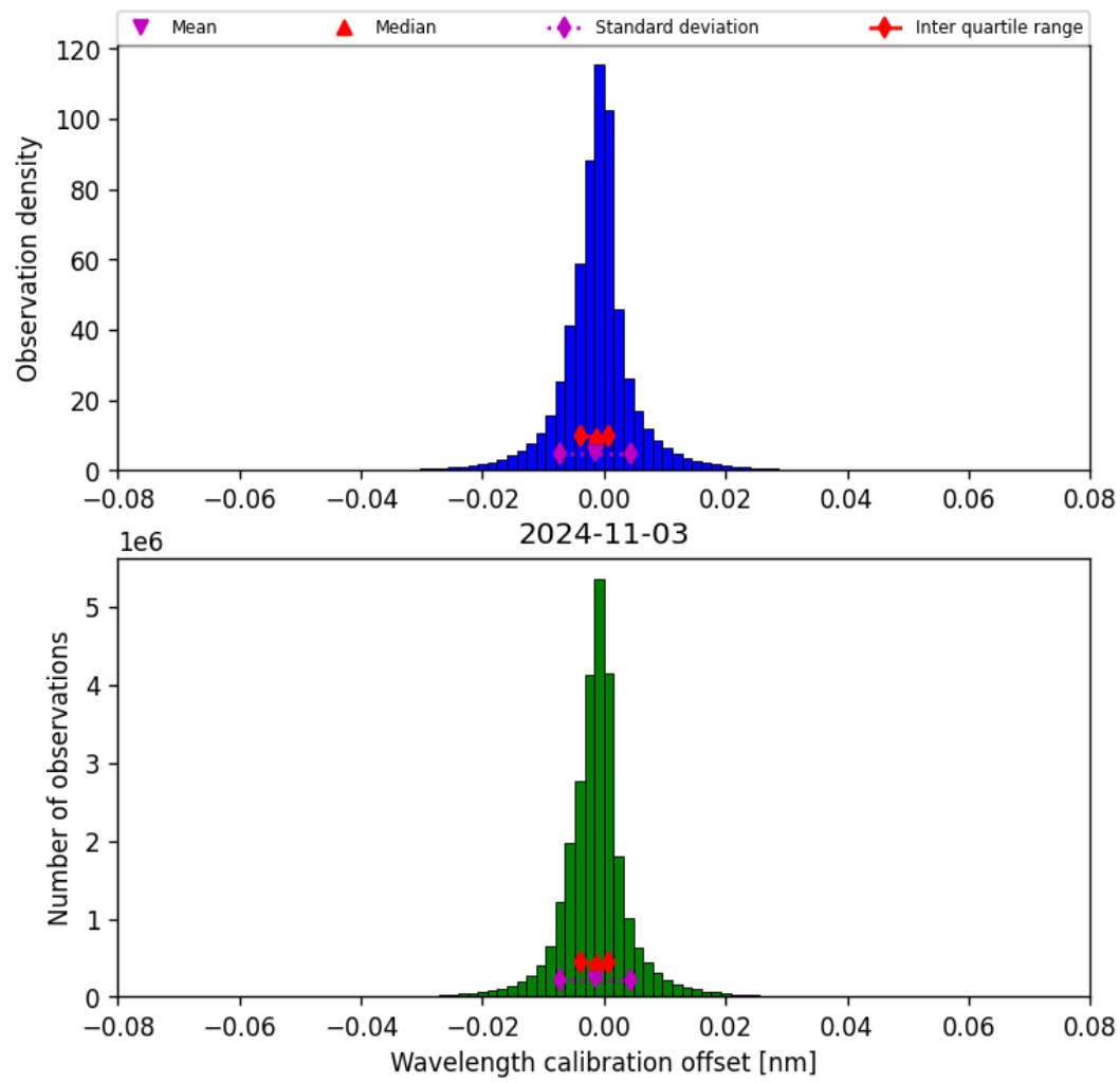
Figure 35: Histogram of “Wavelength calibration offset” for 2024-11-02 to 2024-11-04
