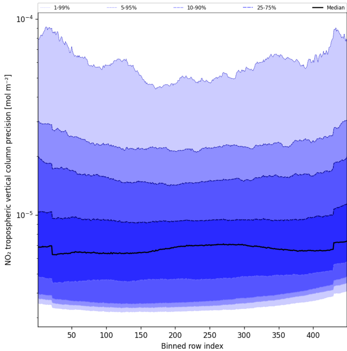
Figure 47: Along track statistics of “NO 2 tropospheric vertical column precision” for 2024-11-02 to 2024-11-04
