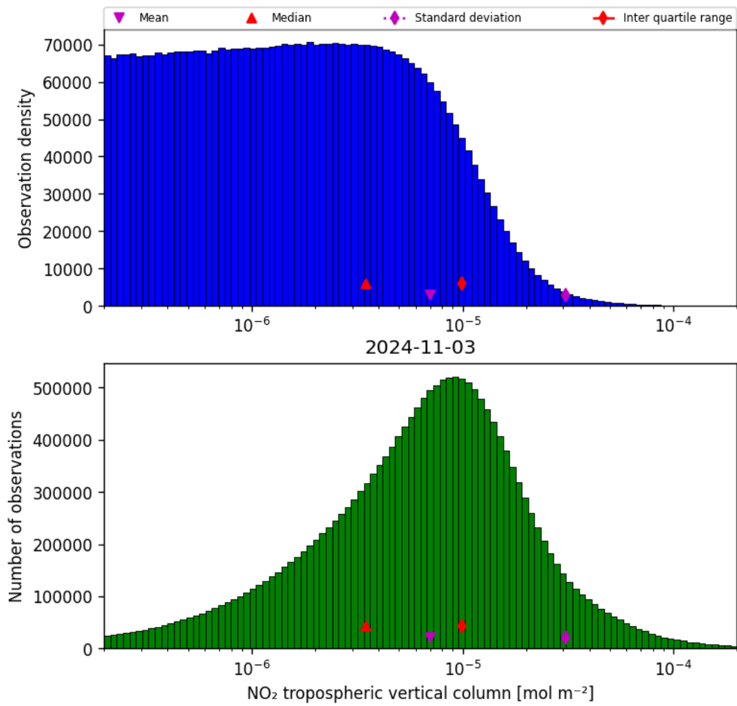
Figure 29: Histogram of “NO 2 tropospheric vertical column” for 2024-11-02 to 2024-11-04
