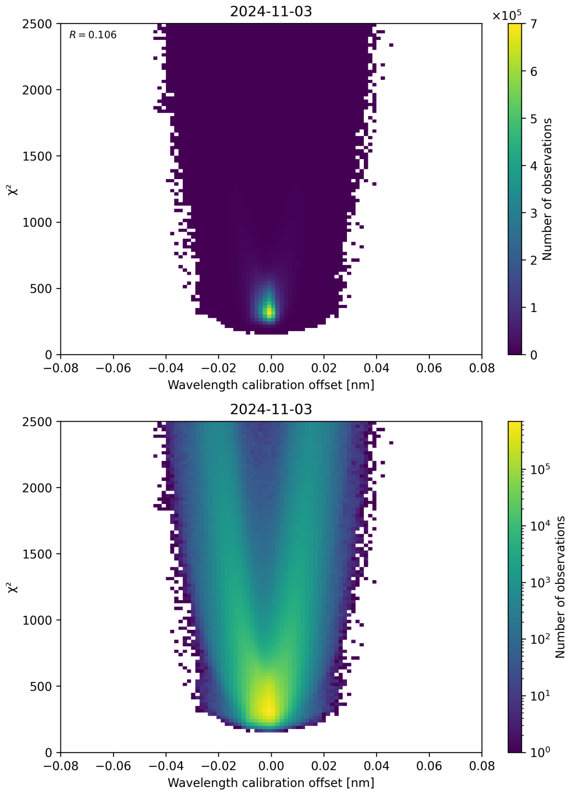
Figure 175: Scatter density plot of “Wavelength calibration offset” against “ \chi^2 ” for 2024-11-02 to 2024-11-04.
