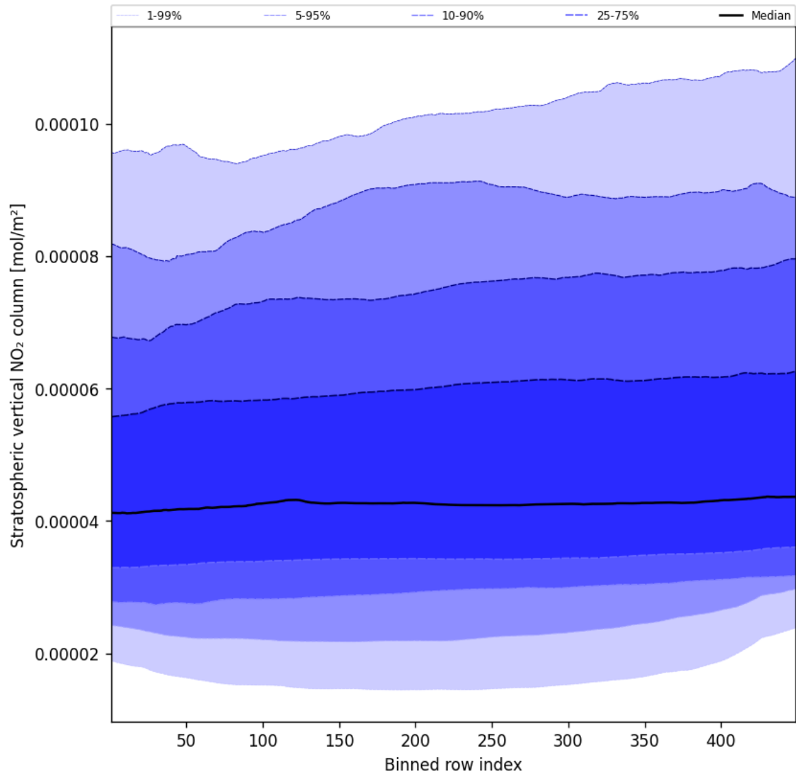
Figure 53: Along track statistics of “Stratospheric vertical NO 2 column” for 2024-11-02 to 2024-11-04
