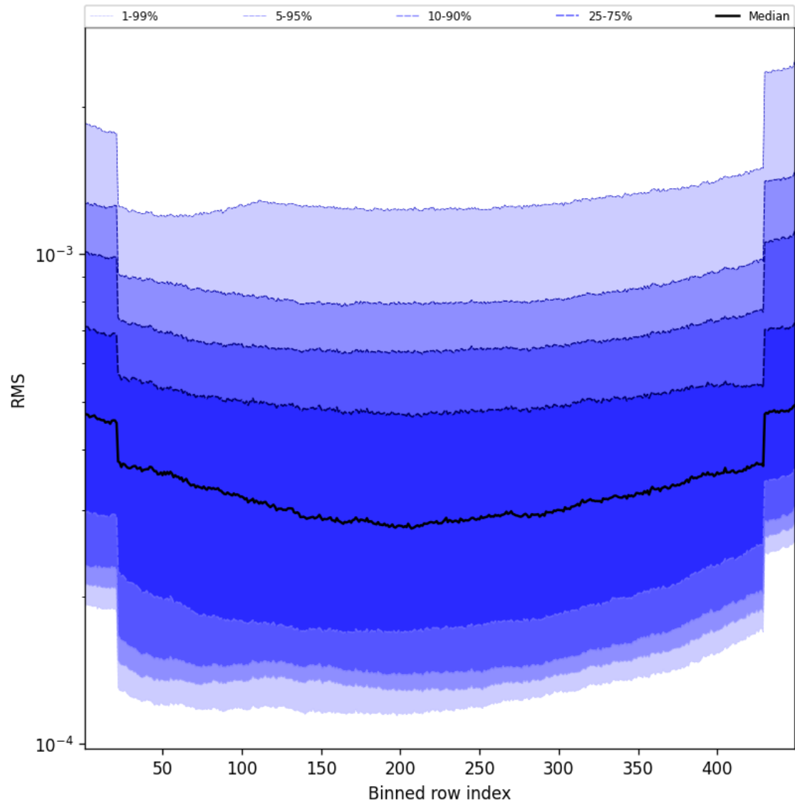
Figure 60: Along track statistics of “RMS” for 2024-11-02 to 2024-11-04
