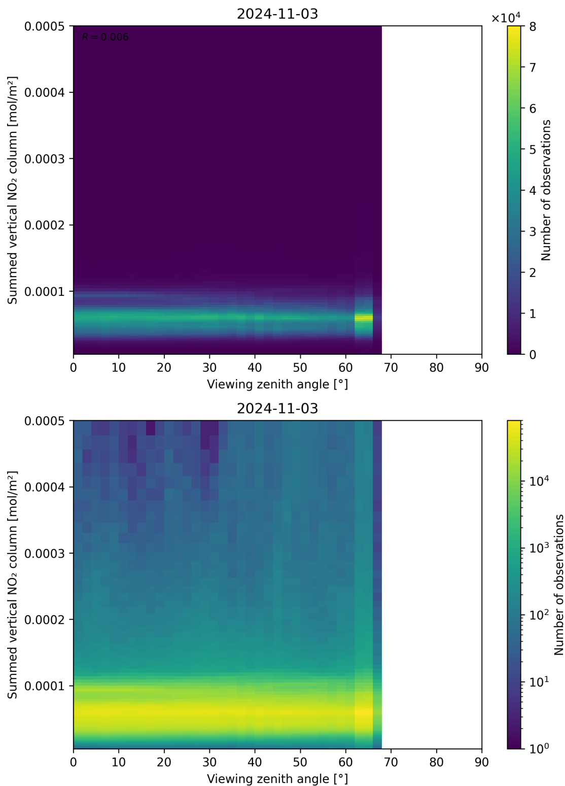
Figure 165: Scatter density plot of “Viewing zenith angle” against “Summed vertical NO 2 column” for 2024-11-02 to 2024-11-04.
