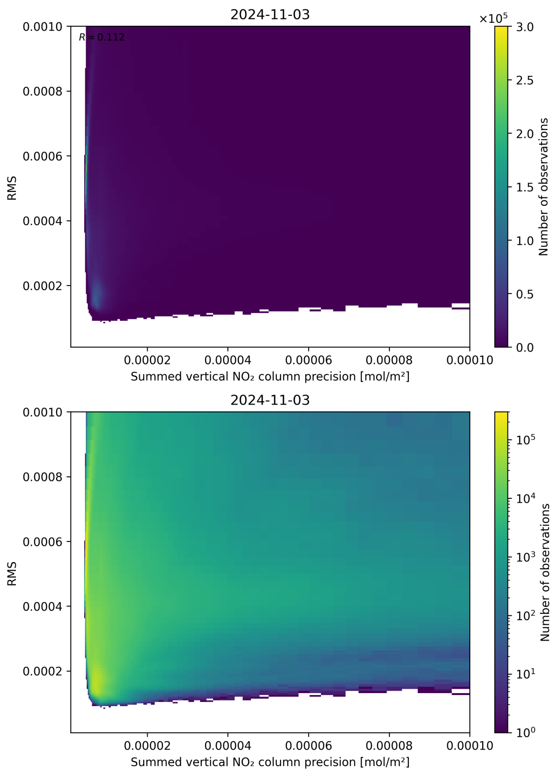
Figure 108: Scatter density plot of “Summed vertical NO 2 column precision” against “RMS” for 2024-11-02 to 2024-11-04.
