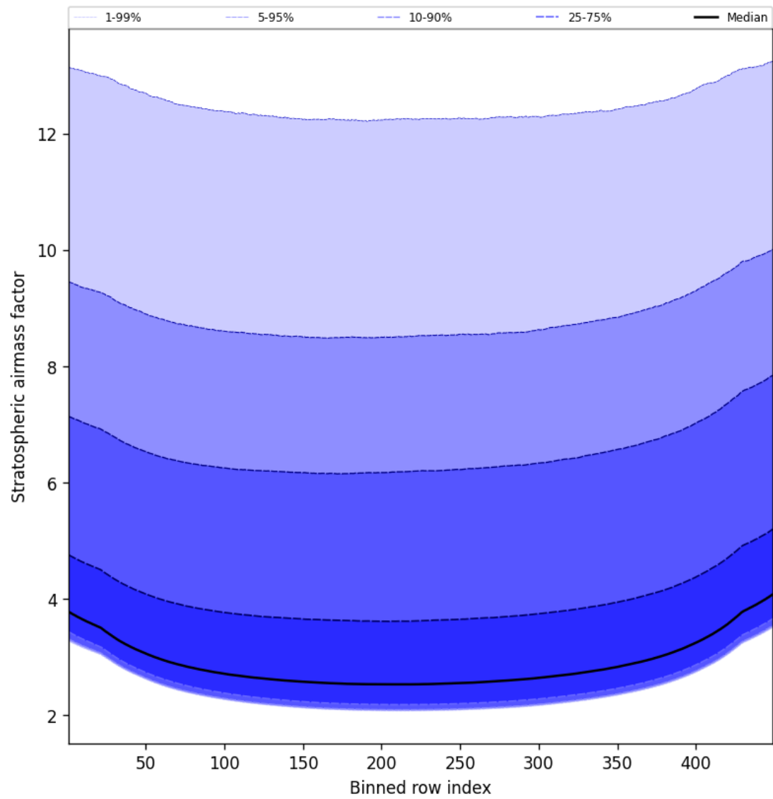
Figure 61: Along track statistics of “Stratospheric airmass factor” for 2024-11-02 to 2024-11-04
