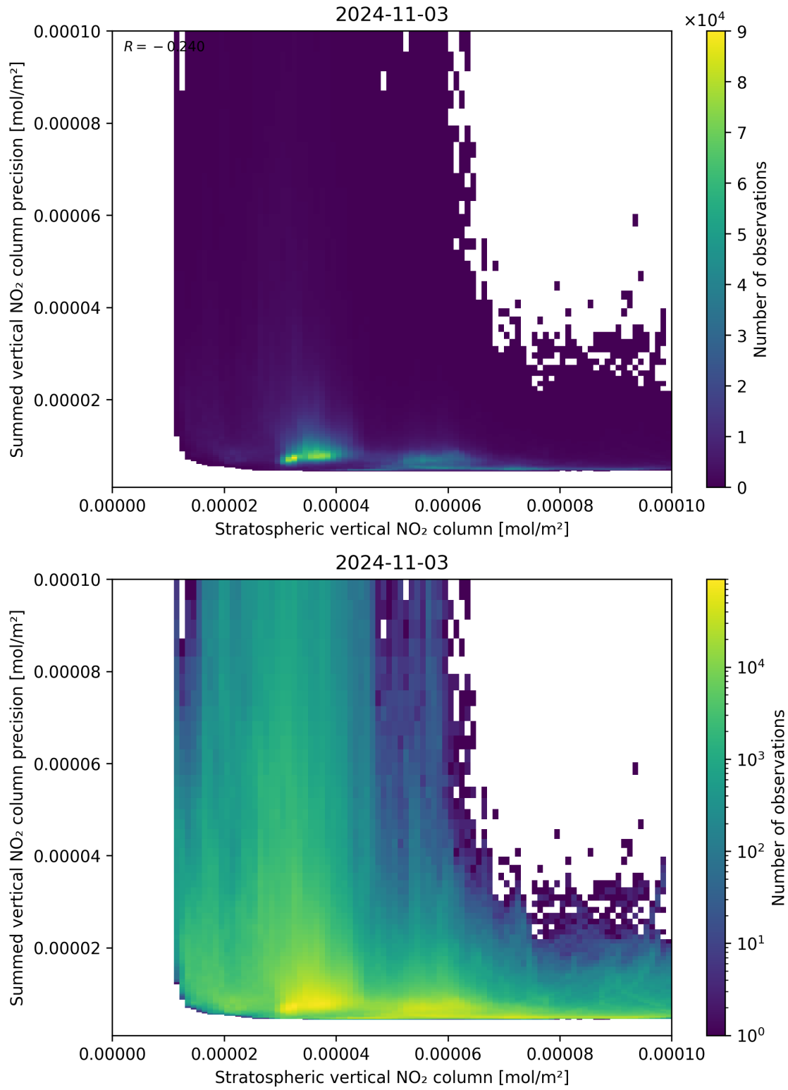
Figure 99: Scatter density plot of “Stratospheric vertical NO 2 column” against “Summed vertical NO 2 column precision” for 2024-11-02 to 2024-11-04.
