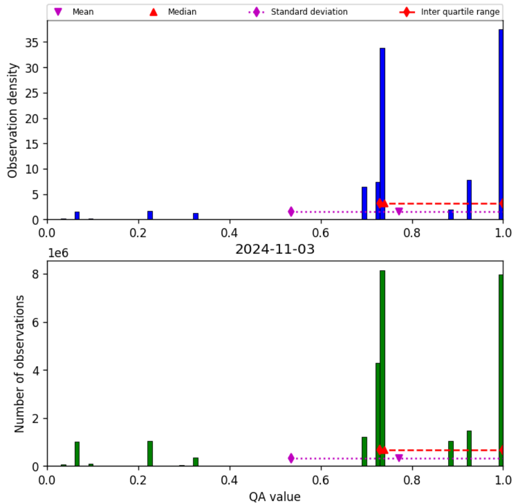
Figure 28: Histogram of “QA value” for 2024-11-02 to 2024-11-04
