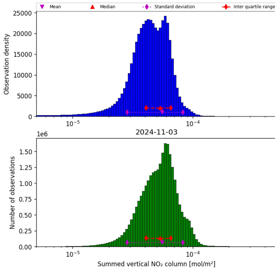
Figure 40: Histogram of “Summed vertical NO 2 column” for 2024-11-02 to 2024-11-04
