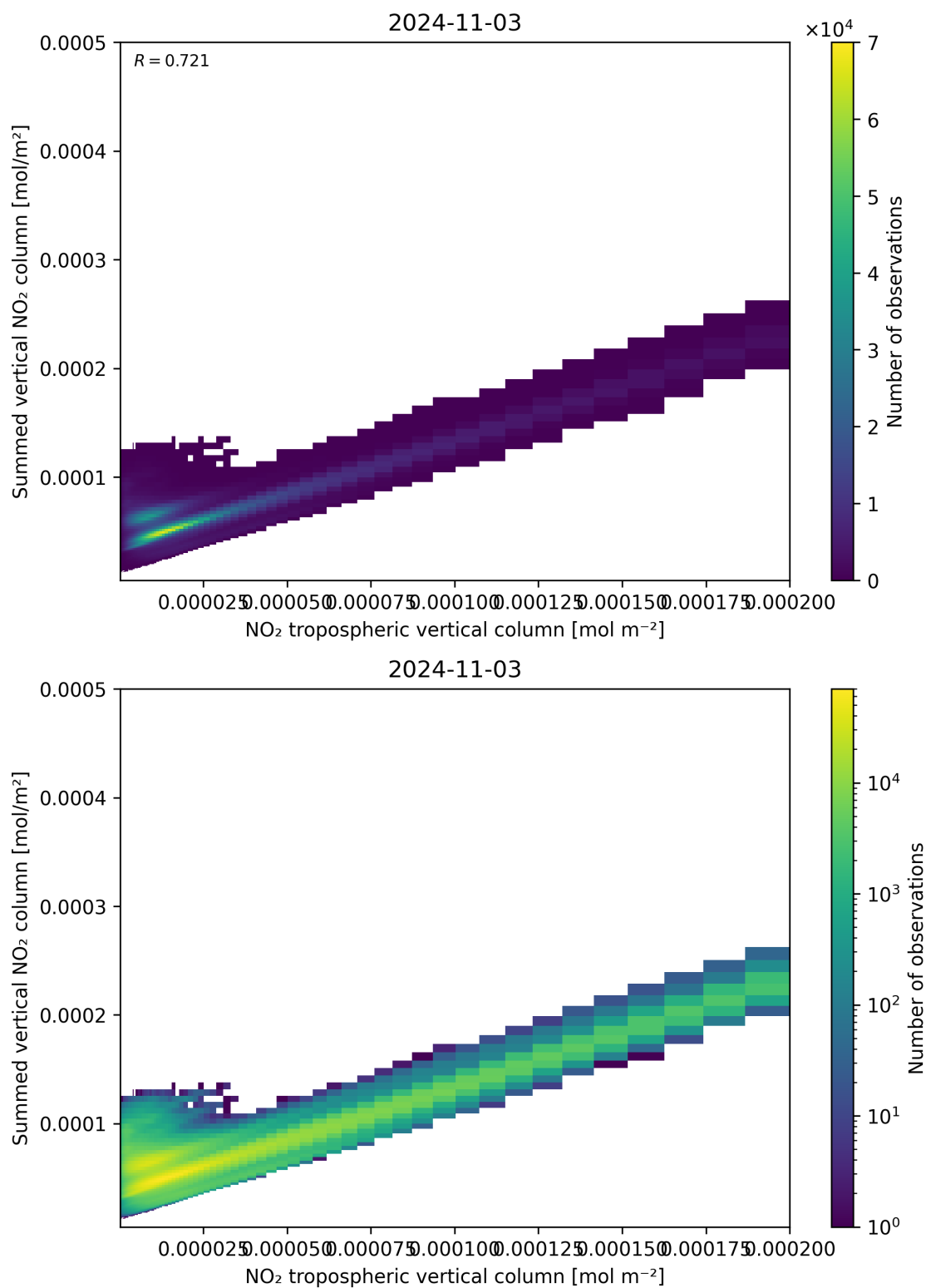
Figure 126: Scatter density plot of “NO 2 tropospheric vertical column” against “Summed vertical NO 2 column” for 2024-11-02 to 2024-11-04.
