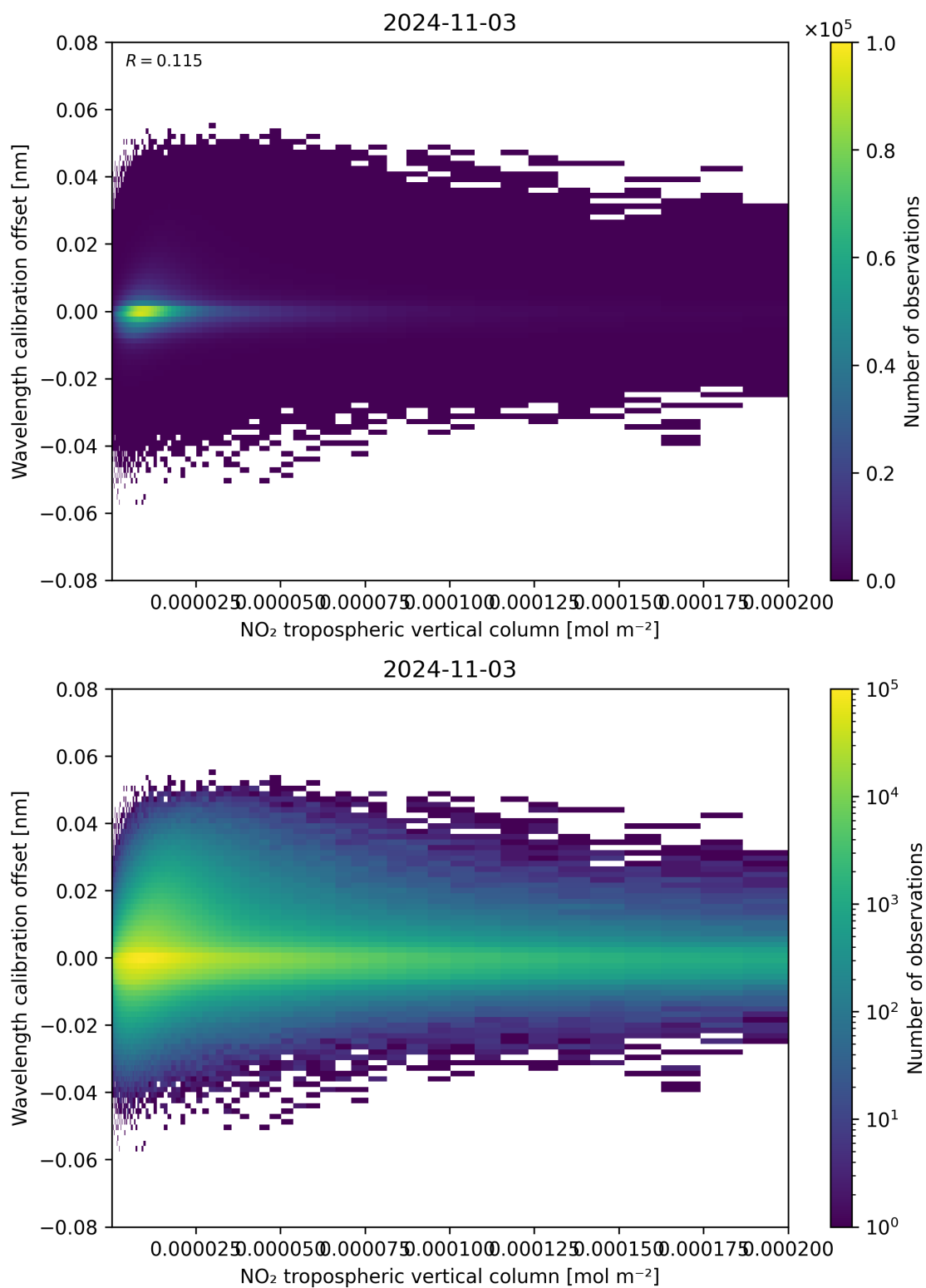
Figure 143: Scatter density plot of “NO 2 tropospheric vertical column” against “Wavelength calibration offset” for 2024-11-02 to 2024-11-04.
