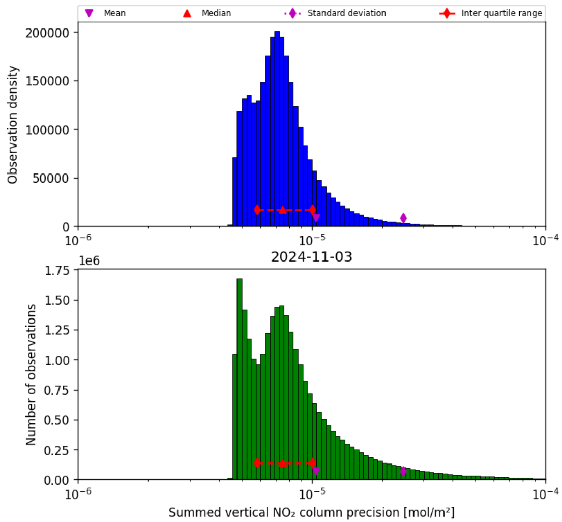
Figure 41: Histogram of "Summed vertical NO 2 column precision" for 2024-11-02 to 2024-11-04
