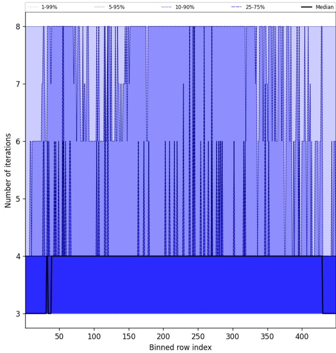
Figure 51: Along track statistics of “Number of iterations” for 2024-11-02 to 2024-11-04
