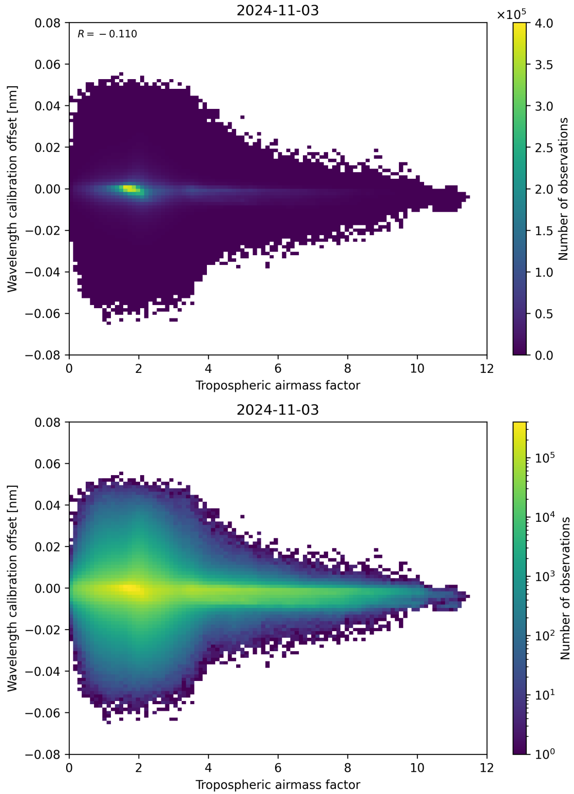
Figure 80: Scatter density plot of “Tropospheric airmass factor” against “Wavelength calibration offset” for 2024-11-02 to 2024-11-04.
