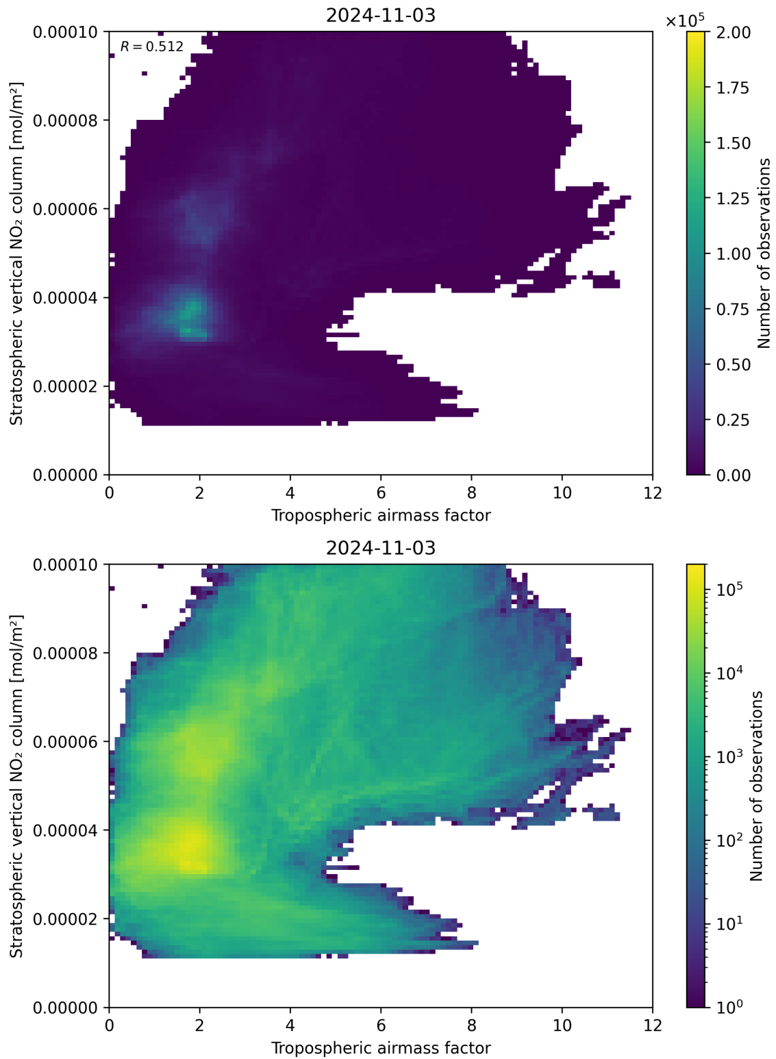
Figure 74: Scatter density plot of “Tropospheric air mass factor” against “Stratospheric vertical NO 2 column” for 2024-11-02 to 2024-11-04.
