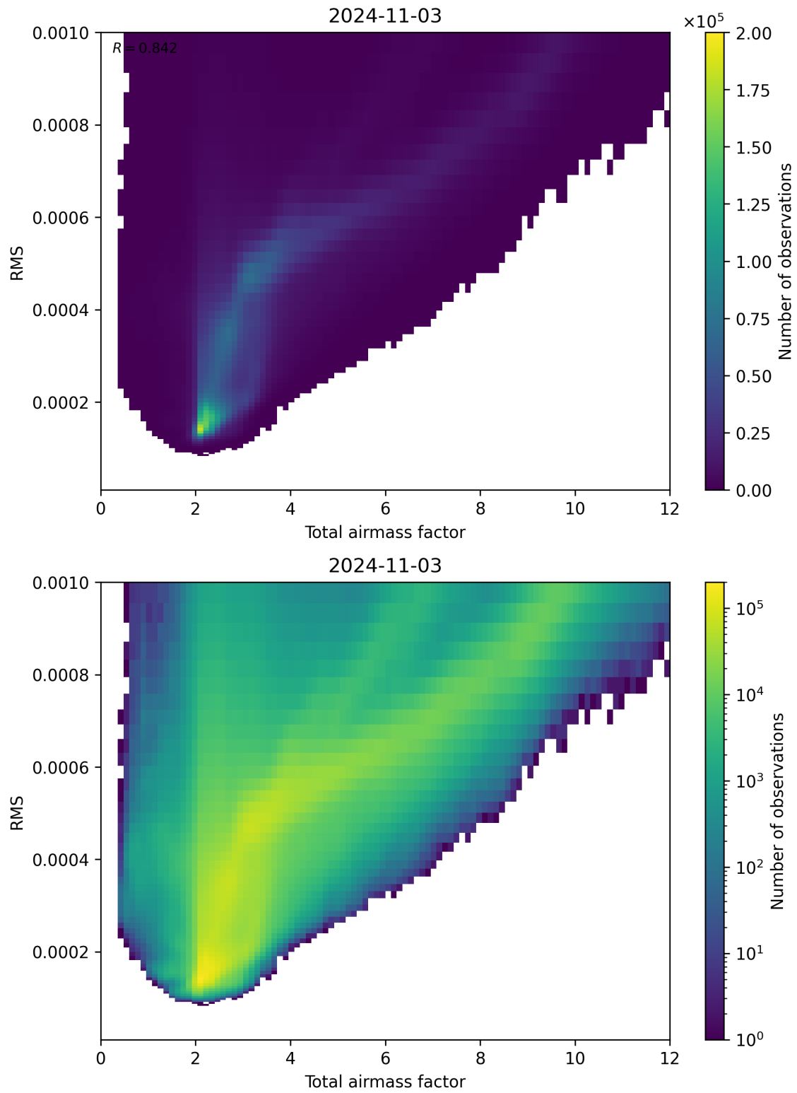
Figure 69: Scatter density plot of “Total airmass factor” against “RMS” for 2024-11-02 to 2024-11-04.
