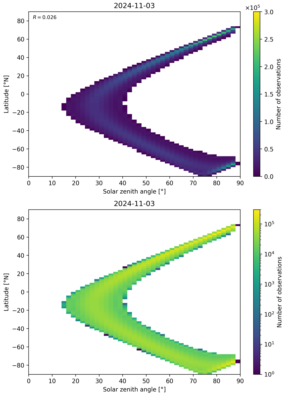
Figure 149: Scatter density plot of “Solar zenith angle” against “Latitude” for 2024-11-02 to 2024-11-04.
