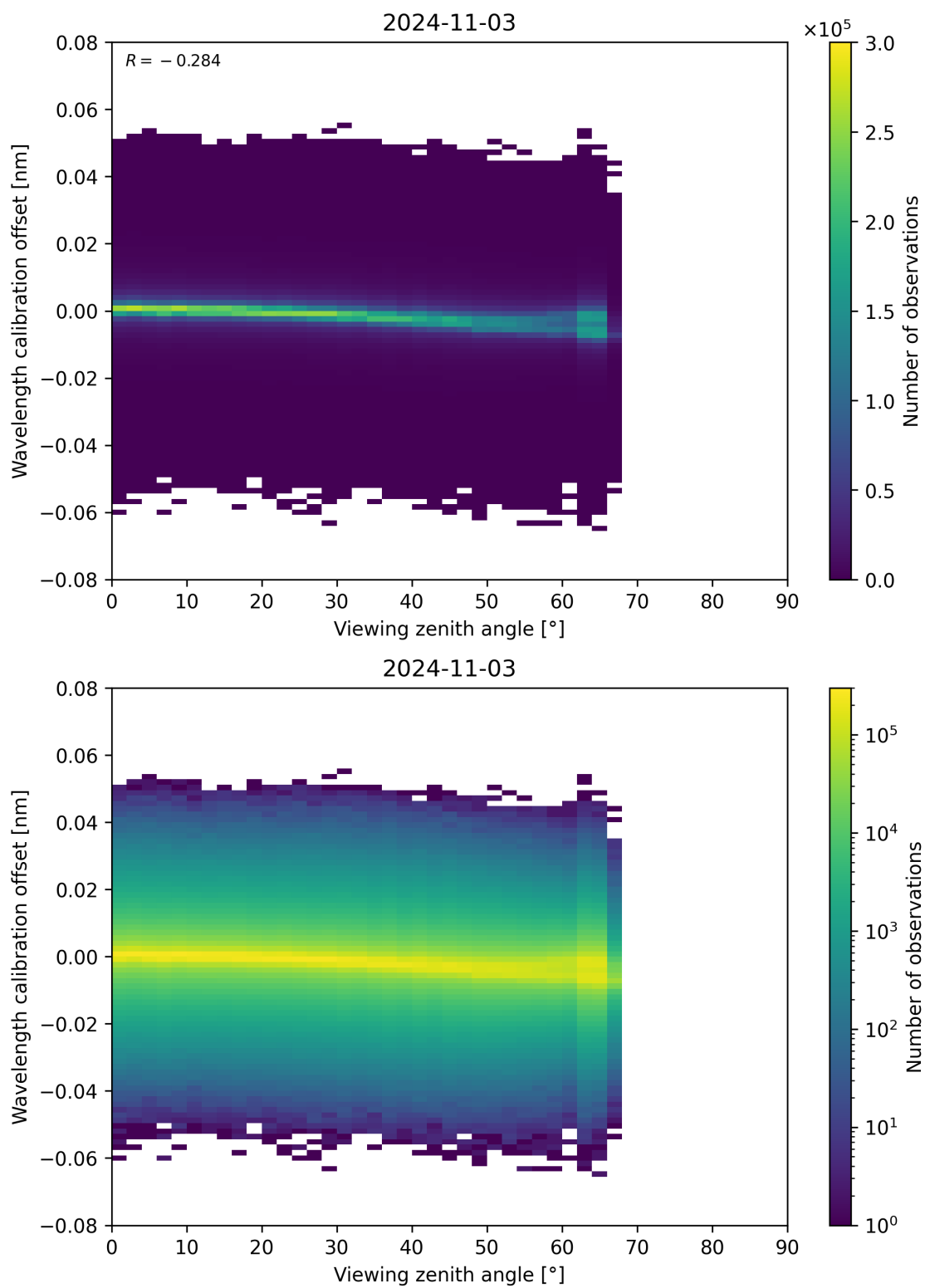
Figure 173: Scatter density plot of “Viewing zenith angle” against “Wavelength calibration offset” for 2024-11-02 to 2024-11-04.
