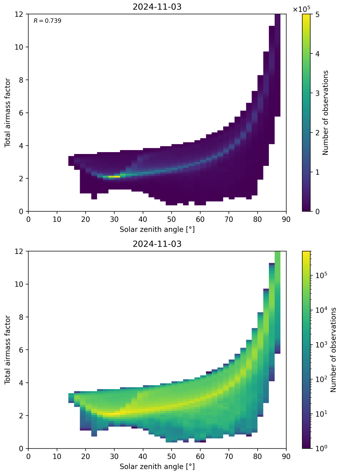
Figure 146: Scatter density plot of “Solar zenith angle” against “Total airmass factor” for 2024-11-02 to 2024-11-04.
