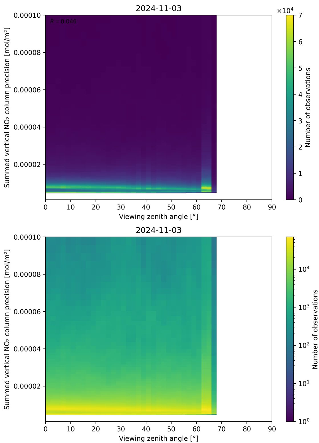
Figure 166: Scatter density plot of “Viewing zenith angle” against “Summed vertical NO 2 column precision” for 2024-11-02 to 2024-11-04.
