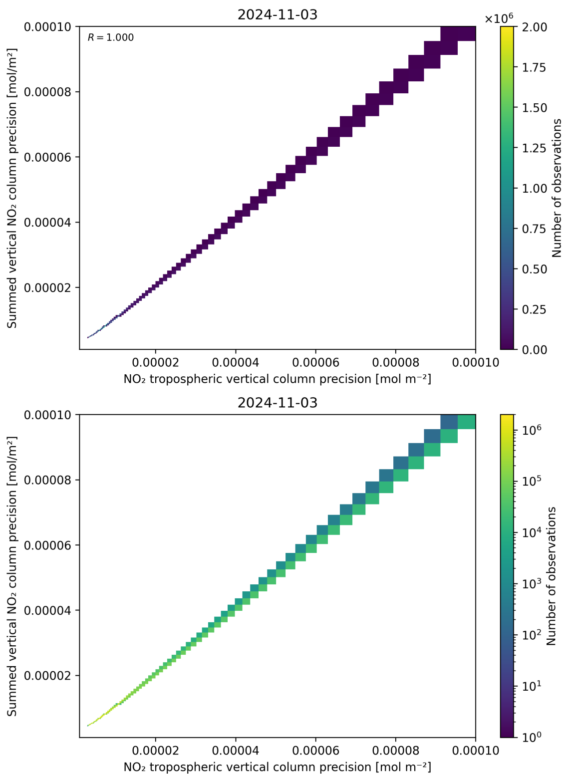
Figure 137: Scatter density plot of “NO 2 tropospheric vertical column precision” against “Summed vertical NO 2 column precision” for 2024-11-02 to 2024-11-04.
