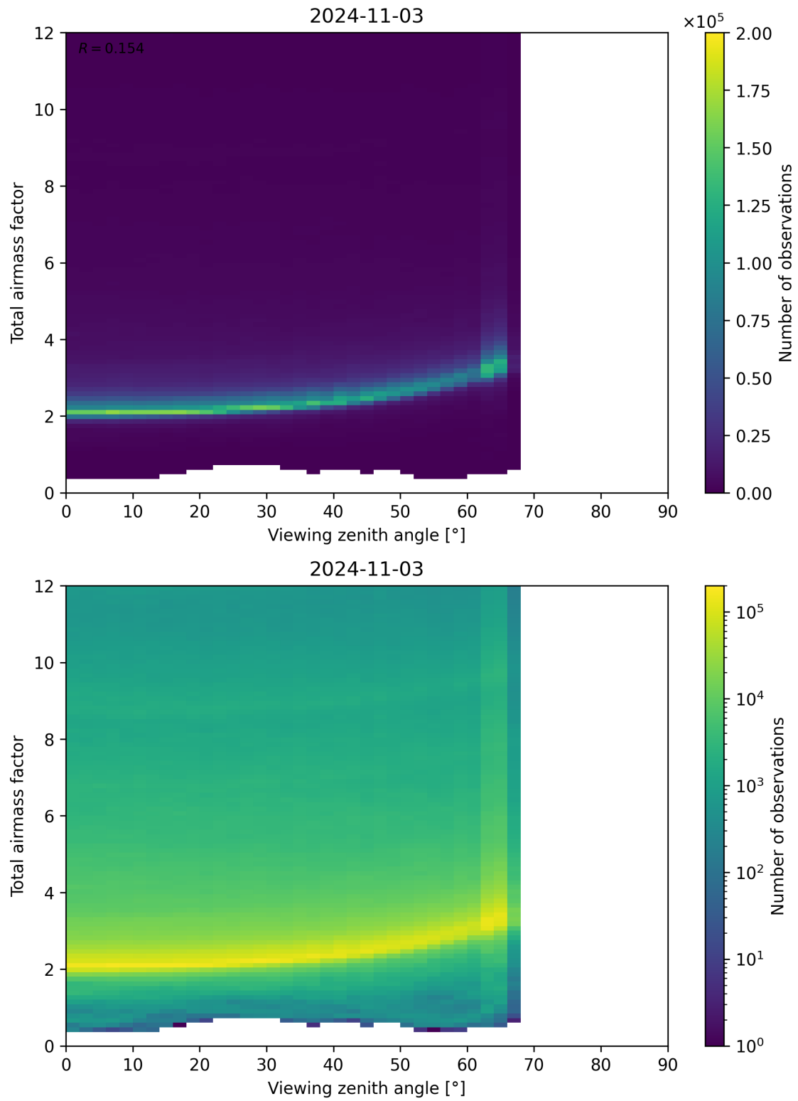
Figure 160: Scatter density plot of “Viewing zenith angle” against “Total airmass factor” for 2024-11-02 to 2024-11-04.
