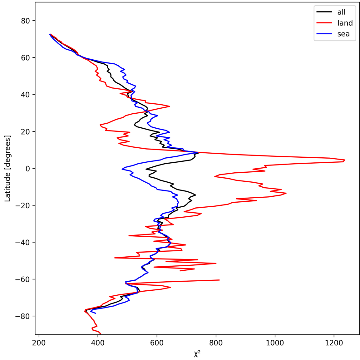
Figure 25: Zonal average of “ \chi^2 ” for 2024-11-02 to 2024-11-04.
