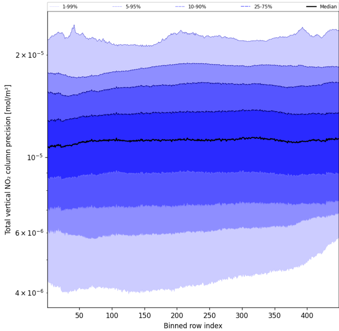
Figure 56: Along track statistics of “Total vertical NO 2 column precision” for 2024-11-02 to 2024-11-04
