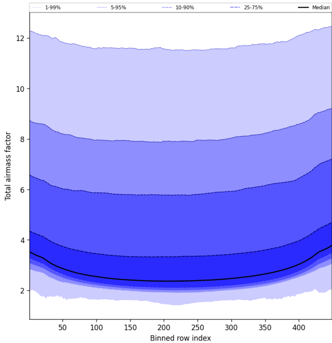
Figure 49: Along track statistics of “Total airmass factor” for 2024-11-02 to 2024-11-04
