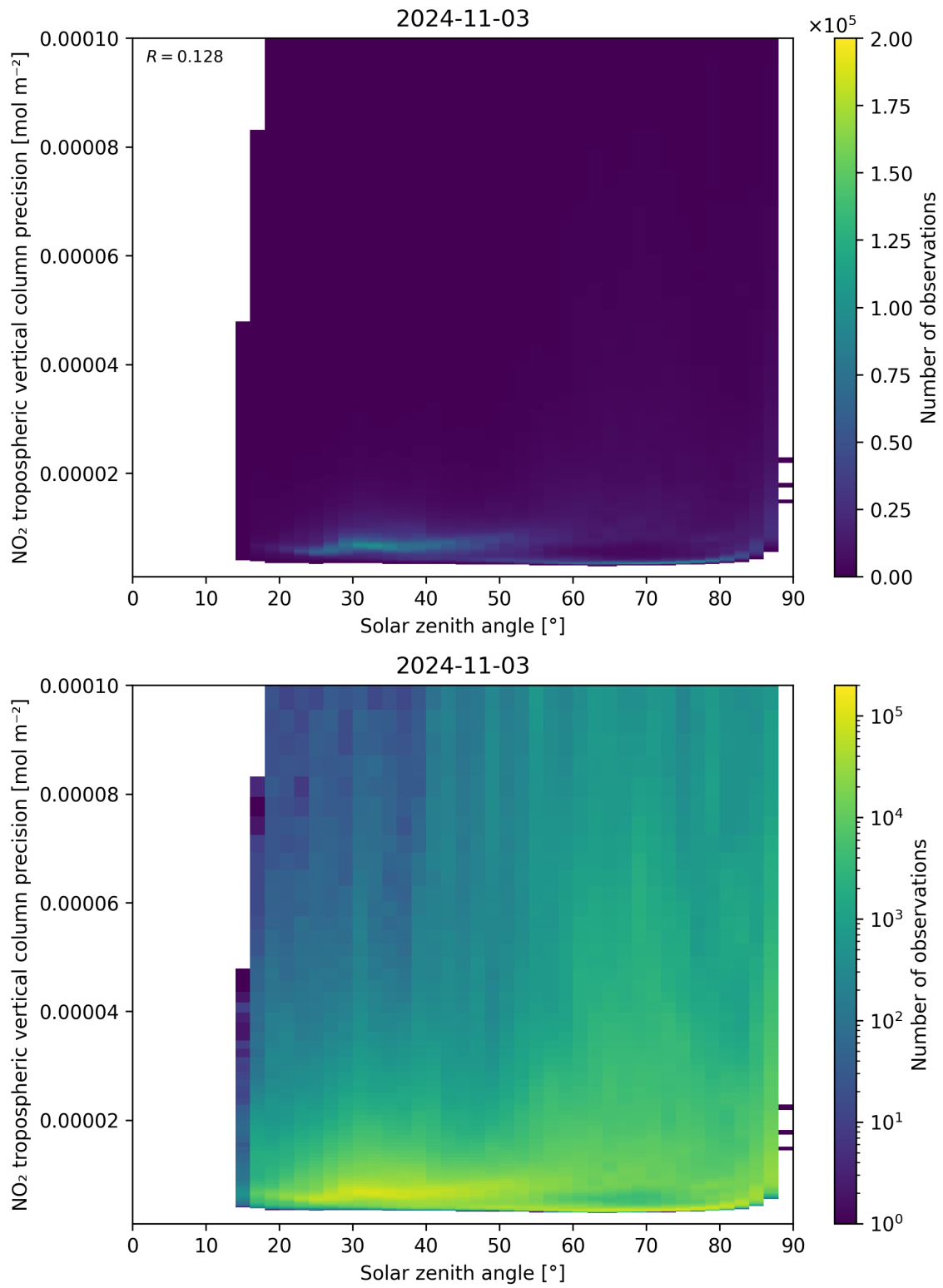
Figure 156: Scatter density plot of “Solar zenith angle” against “NO 2 tropospheric vertical column precision” for 2024-11-02 to 2024-11-04.
