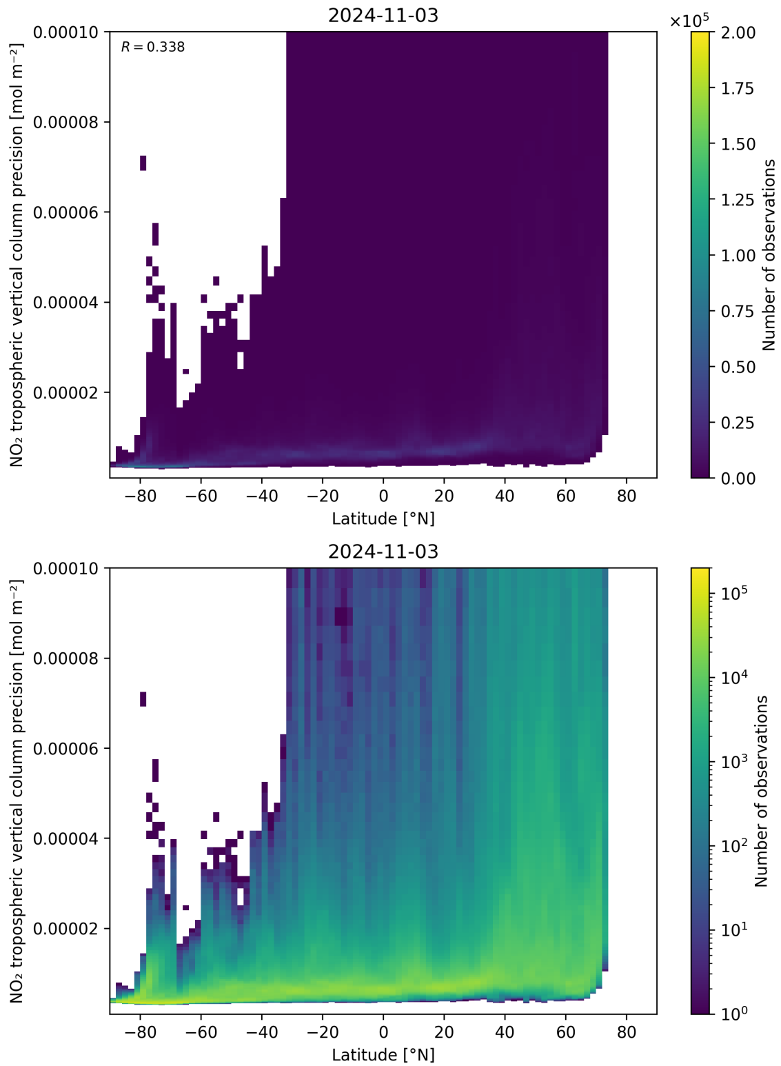
Figure 93: Scatter density plot of “Latitude” against “NO 2 tropospheric vertical column precision” for 2024-11-02 to 2024-11-04.
