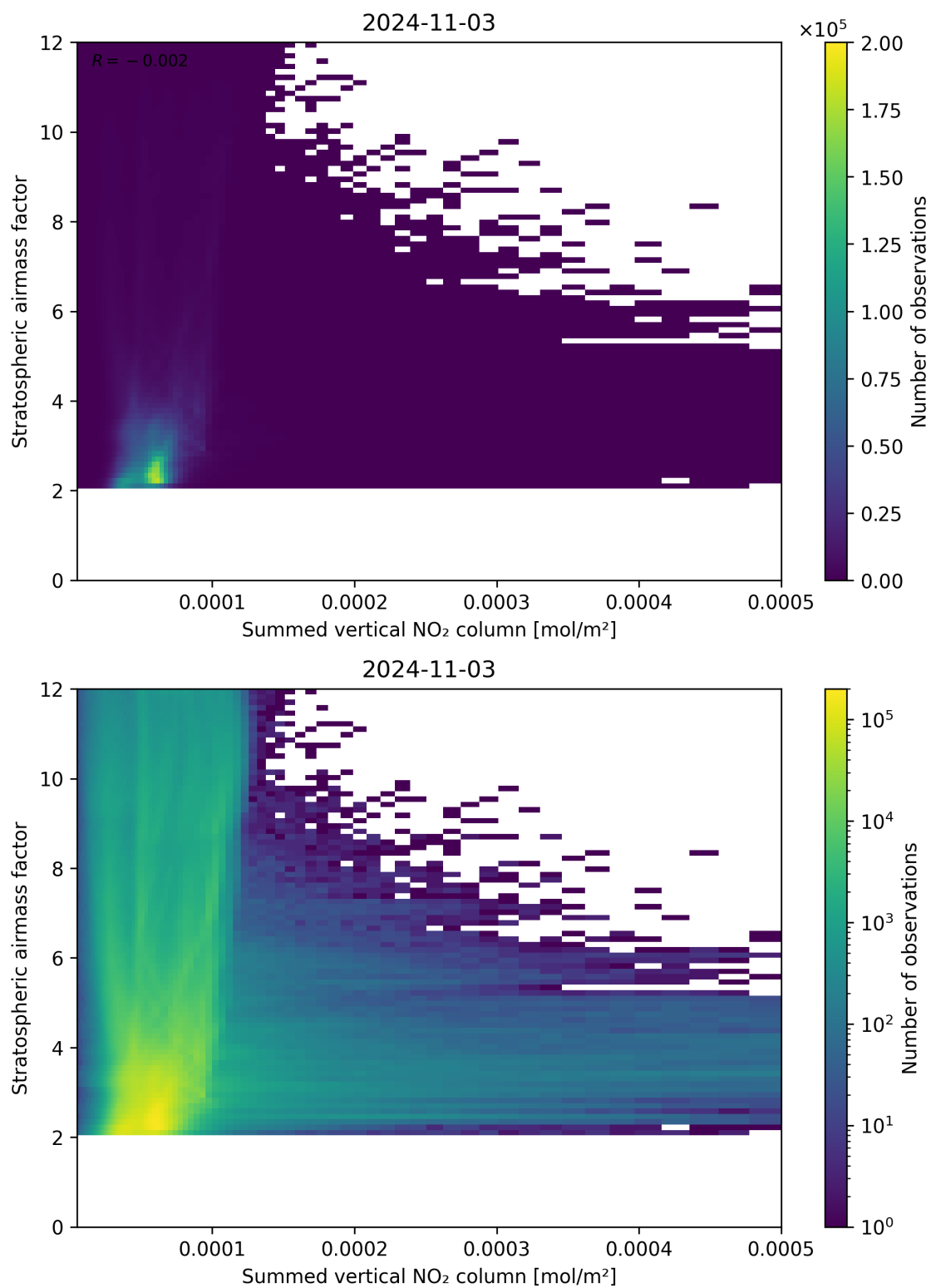
Figure 103: Scatter density plot of “Summed vertical NO 2 column” against “Stratospheric airmass factor” for 2024-11-02 to 2024-11-04.
