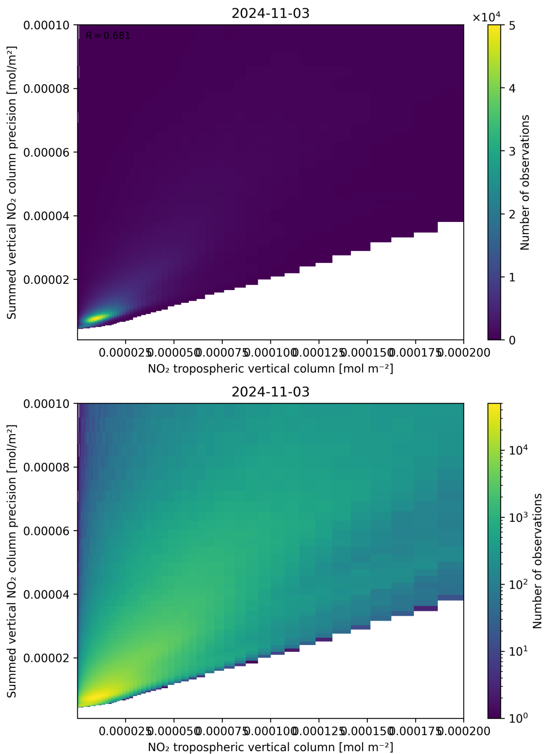
Figure 127: Scatter density plot of “NO 2 tropospheric vertical column” against “Summed vertical NO 2 column precision” for 2024-11-02 to 2024-11-04.
