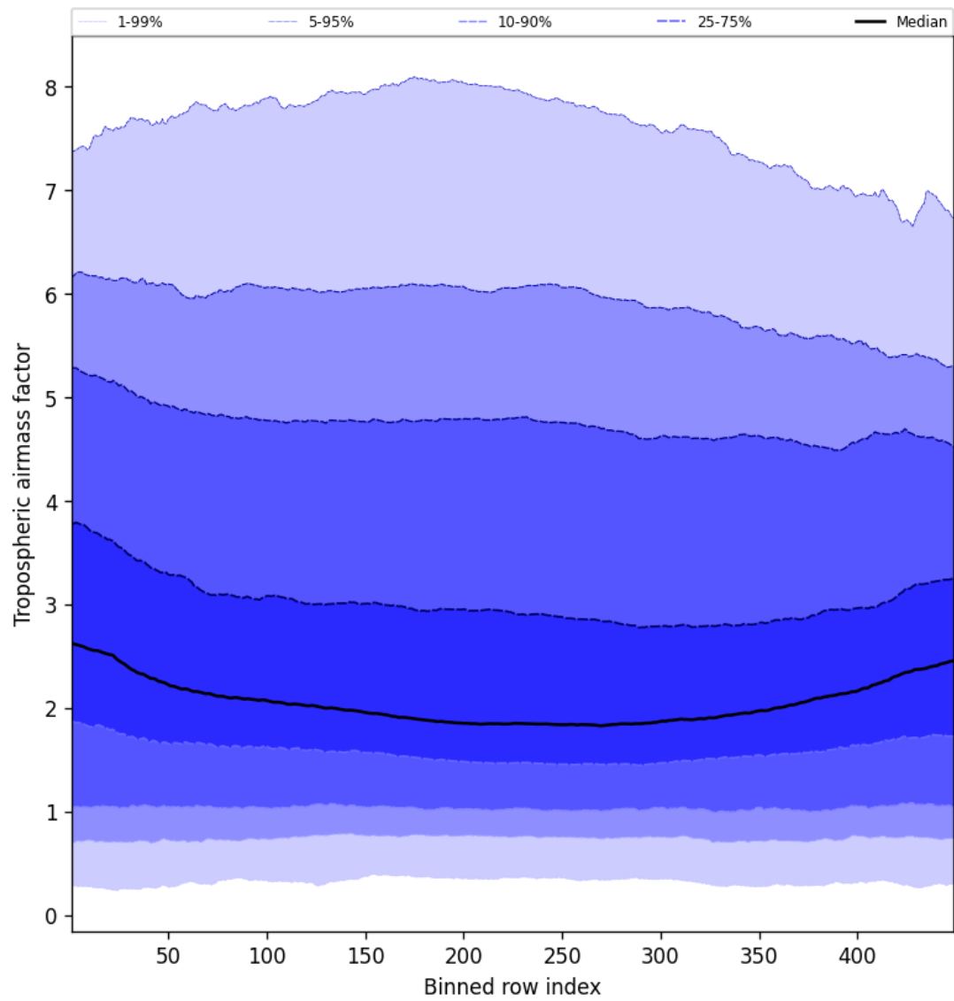
Figure 48: Along track statistics of “Tropospheric air mass factor” for 2024-11-02 to 2024-11-04
