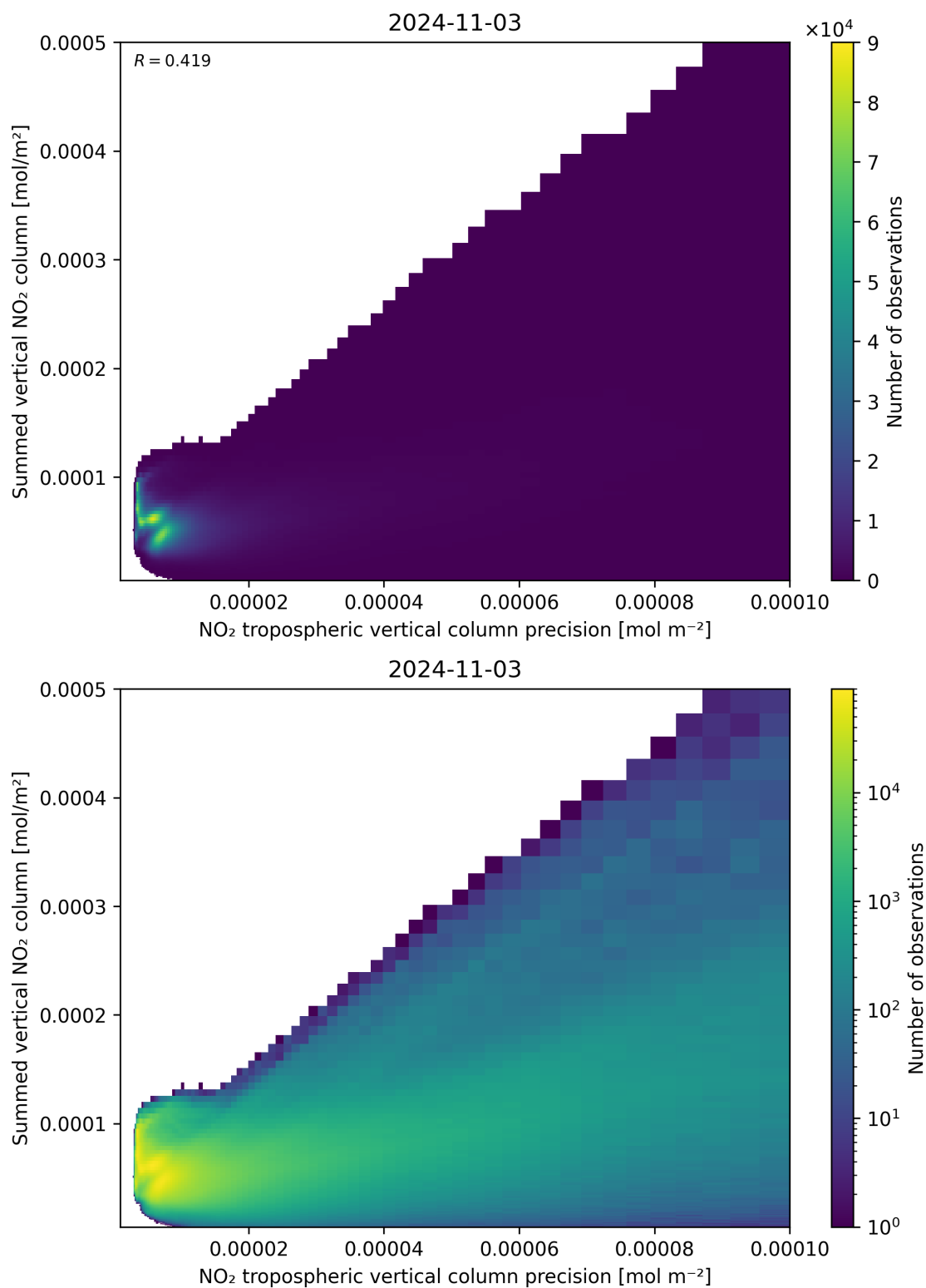
Figure 136: Scatter density plot of “NO 2 tropospheric vertical column precision” against “Summed vertical NO 2 column” for 2024-11-02 to 2024-11-04.
