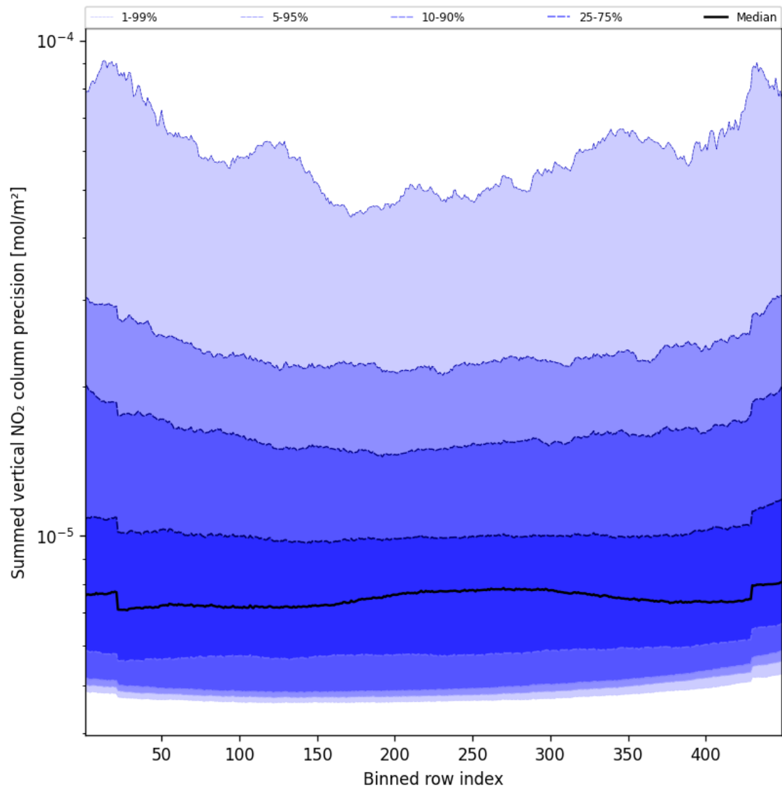
Figure 58: Along track statistics of “Summed vertical NO 2 column precision” for 2024-11-02 to 2024-11-04
