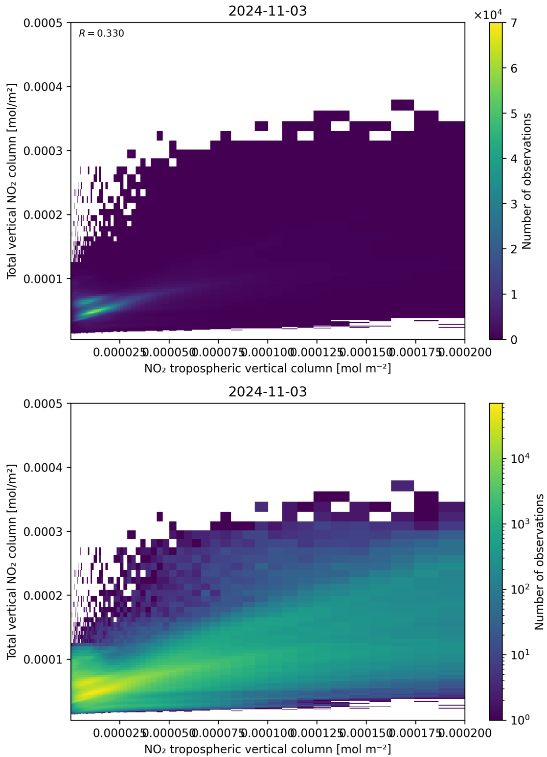
Figure 128: Scatter density plot of “NO 2 tropospheric vertical column” against “Total vertical NO 2 column” for 2024-11-02 to 2024-11-04.
