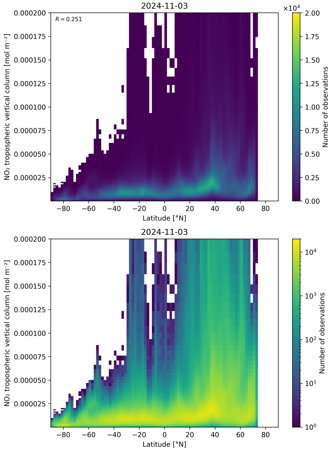
Figure 92: Scatter density plot of “Latitude” against “NO 2 tropospheric vertical column” for 2024-11-02 to 2024-11-04.
