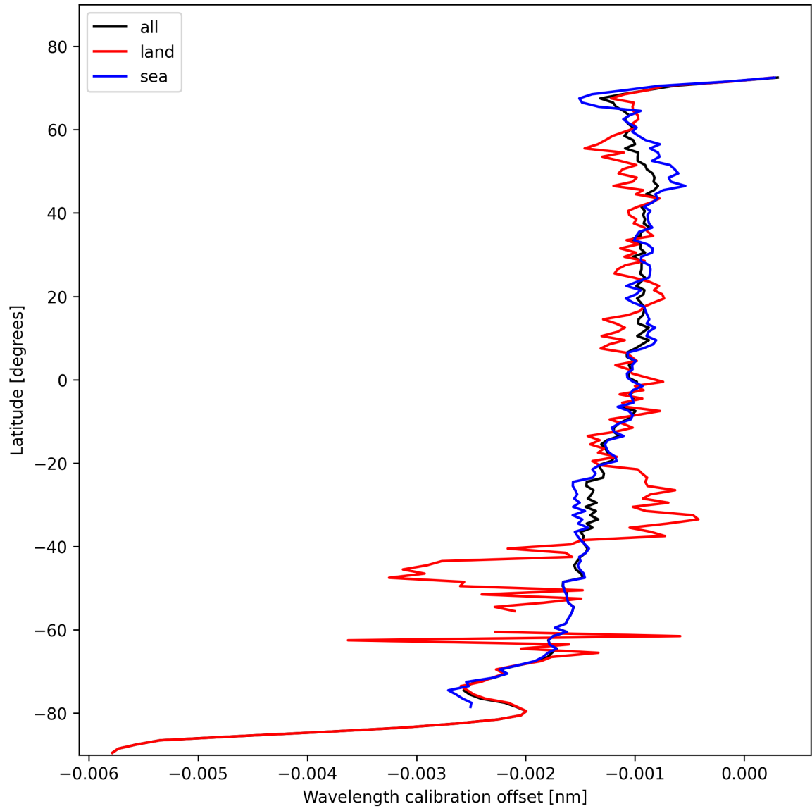
Figure 18: Zonal average of “Wavelength calibration offset” for 2024-11-02 to 2024-11-04.
