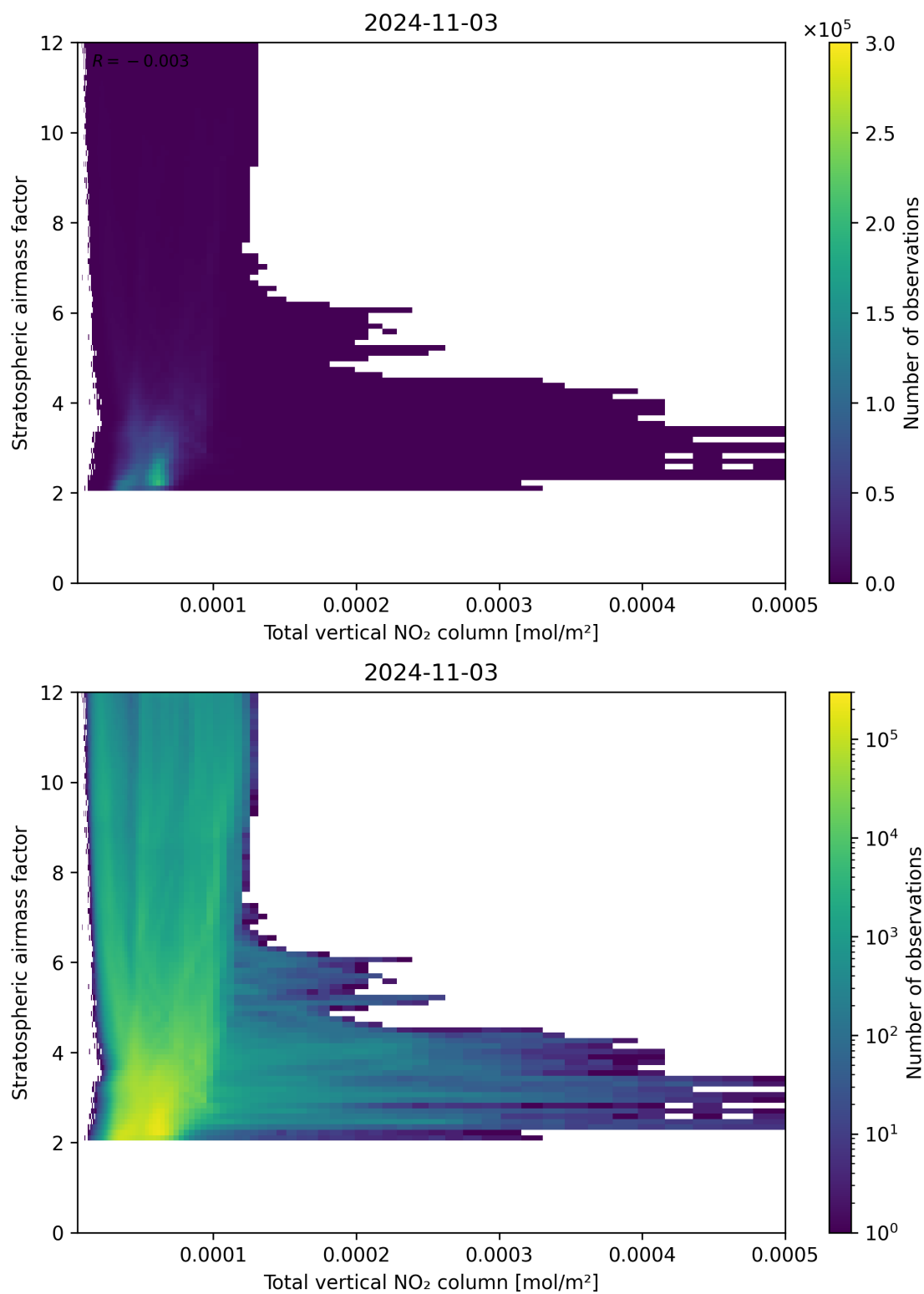
Figure 110: Scatter density plot of “Total vertical NO 2 column” against “Stratospheric airmass factor” for 2024-11-02 to 2024-11-04.
