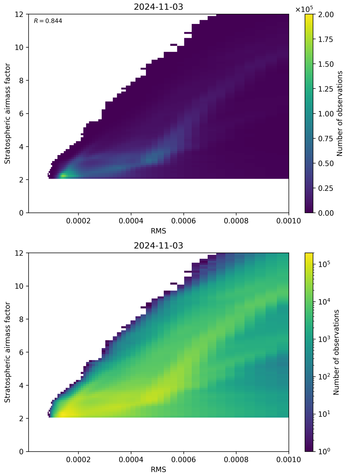
Figure 144: Scatter density plot of “RMS” against “Stratospheric airmass factor” for 2024-11-02 to 2024-11-04.
