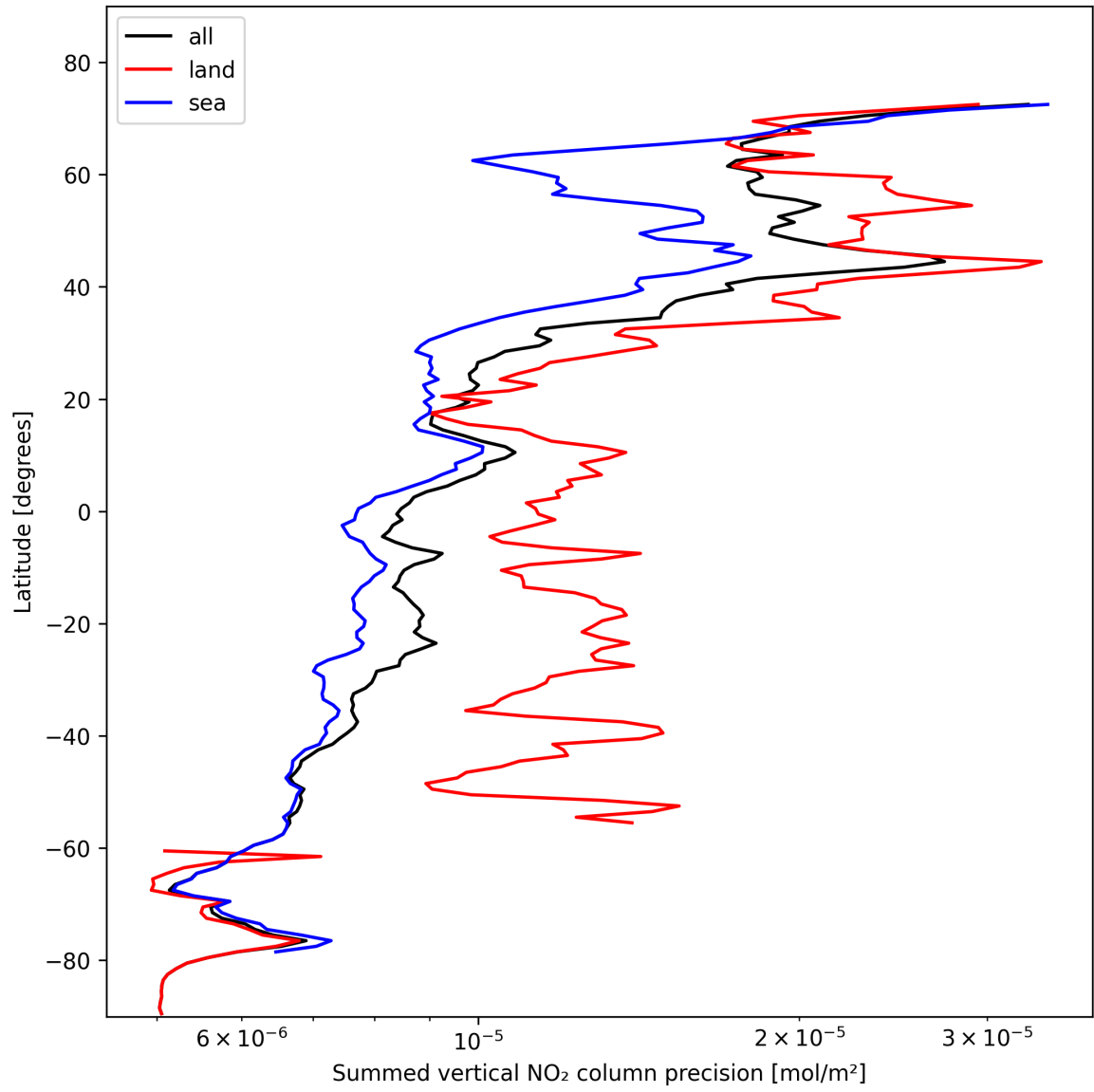
Figure 24: Zonal average of “Summed vertical NO 2 column precision” for 2024-11-02 to 2024-11-04.
