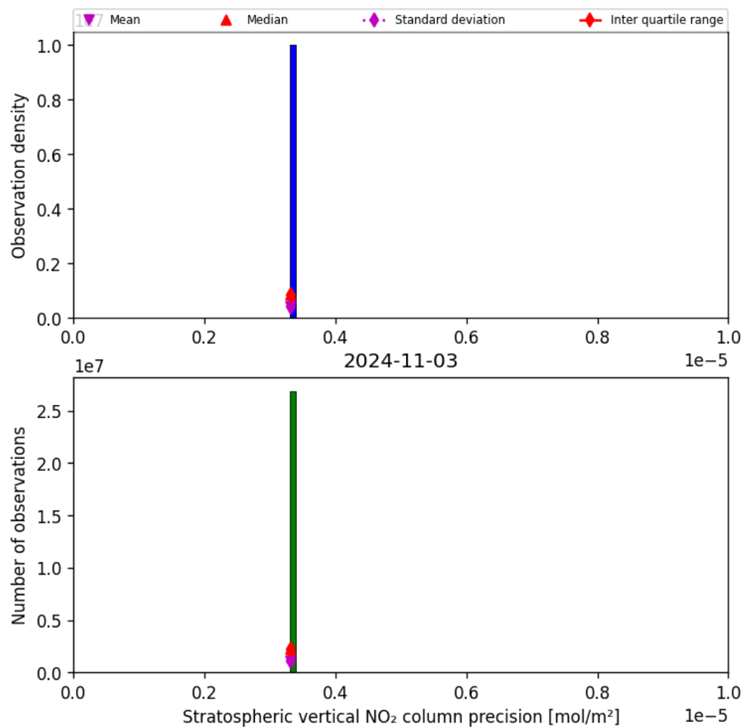
Figure 37: Histogram of “Stratospheric vertical NO 2 column precision” for 2024-11-02 to 2024-11-04
