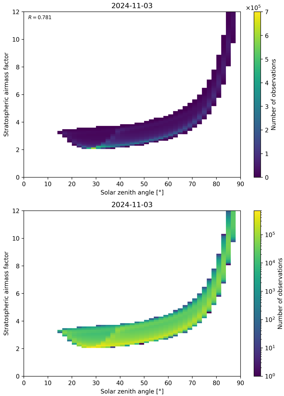
Figure 145: Scatter density plot of “Solar zenith angle” against “Stratospheric airmass factor” for 2024-11-02 to 2024-11-04.
