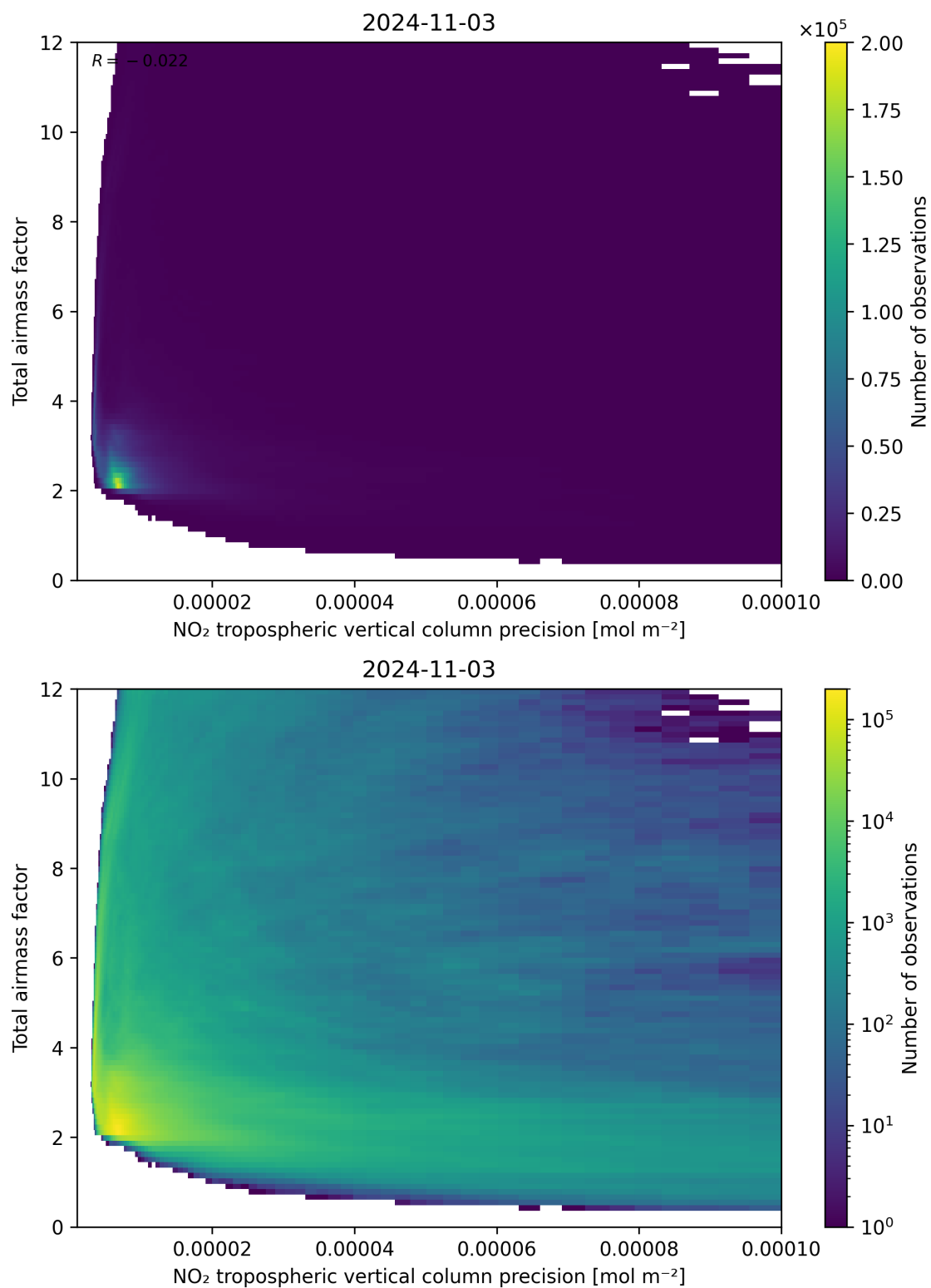
Figure 132: Scatter density plot of “NO 2 tropospheric vertical column precision” against “Total air mass factor” for 2024-11-02 to 2024-11-04.
