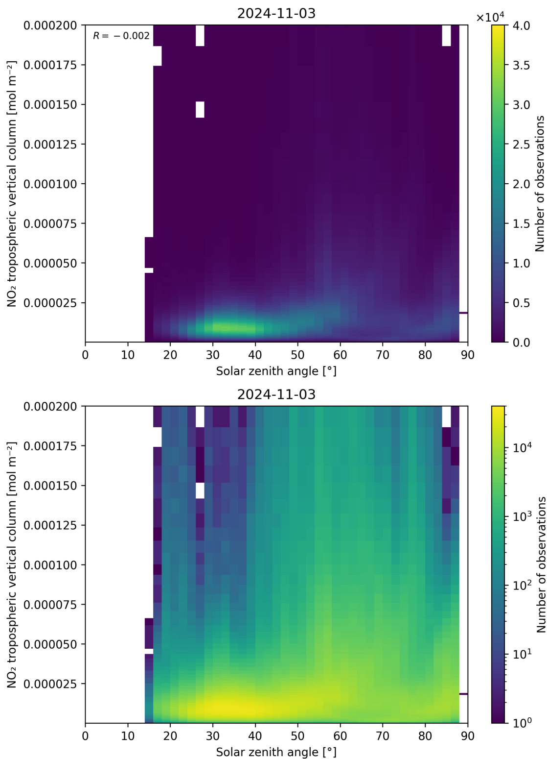
Figure 155: Scatter density plot of “Solar zenith angle” against “NO 2 tropospheric vertical column” for 2024-11-02 to 2024-11-04.
