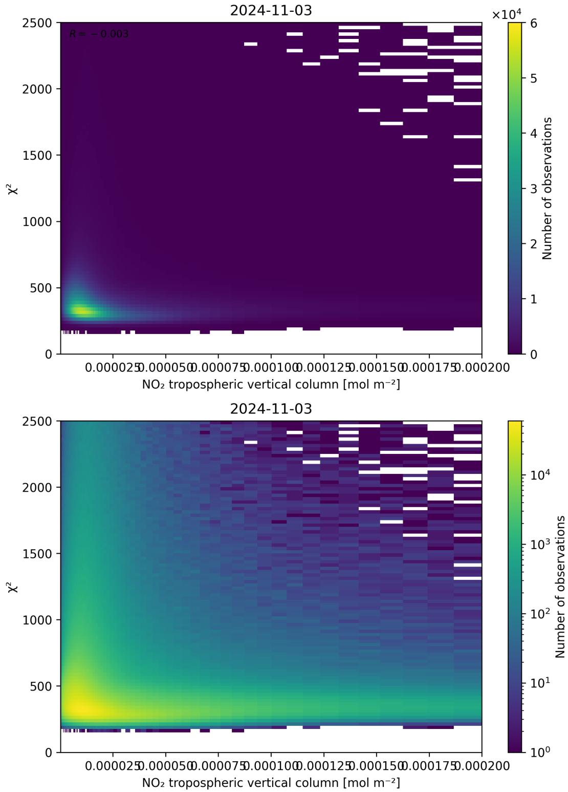
Figure 124: Scatter density plot of “NO 2 tropospheric vertical column” against “ \chi^2 ” for 2024-11-02 to 2024-11-04.
