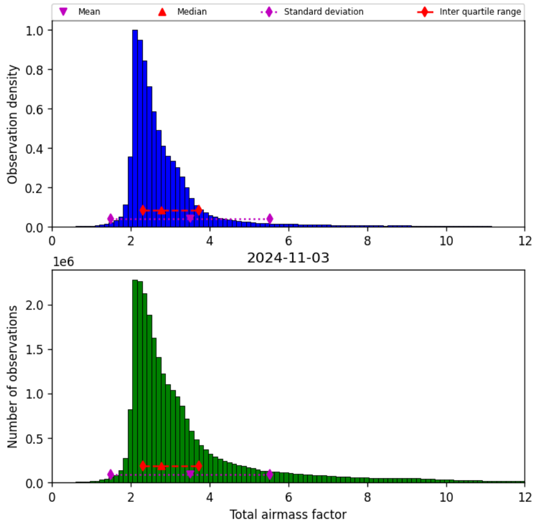
Figure 32: Histogram of “Total airmass factor” for 2024-11-02 to 2024-11-04
