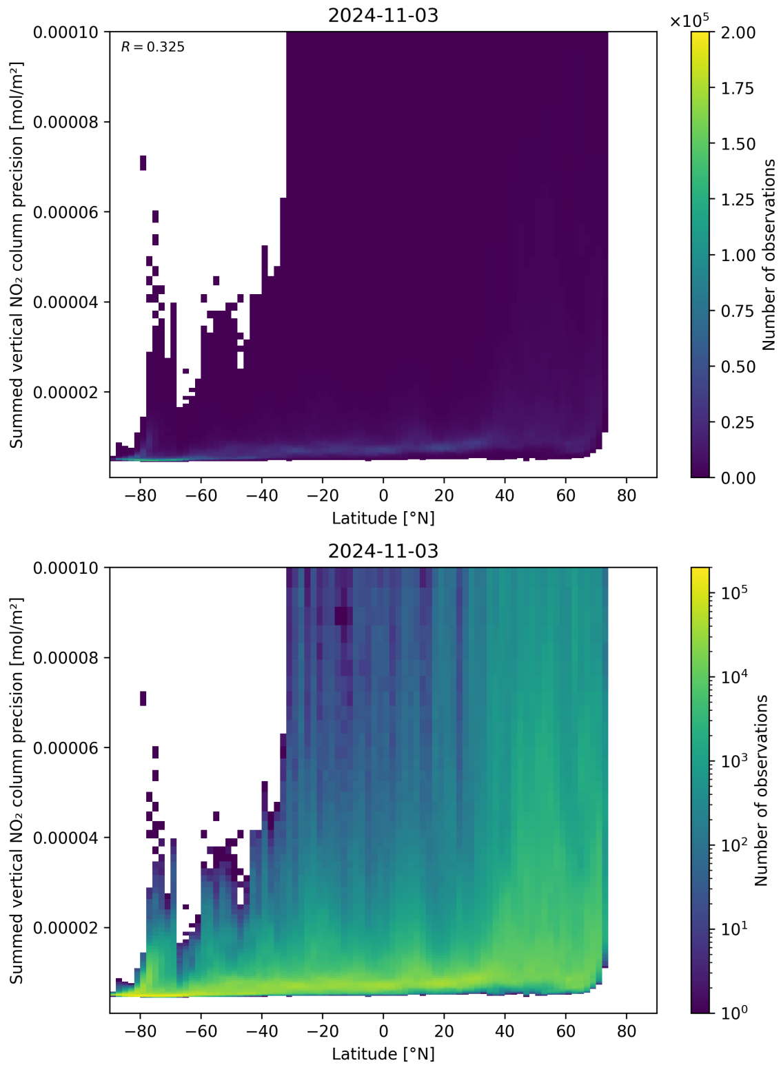
Figure 89: Scatter density plot of “Latitude” against “Summed vertical NO 2 column precision” for 2024-11-02 to 2024-11-04.
