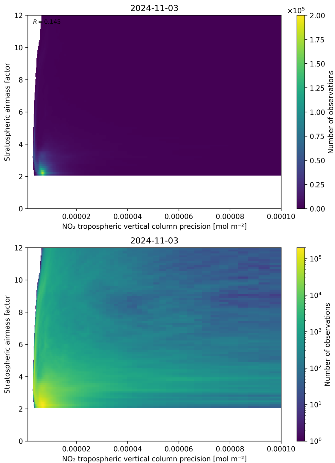
Figure 131: Scatter density plot of “NO 2 tropospheric vertical column precision” against “Stratospheric airmass factor” for 2024-11-02 to 2024-11-04.
