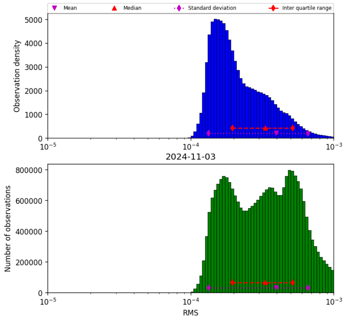
Figure 43: Histogram of “RMS” for 2024-11-02 to 2024-11-04
