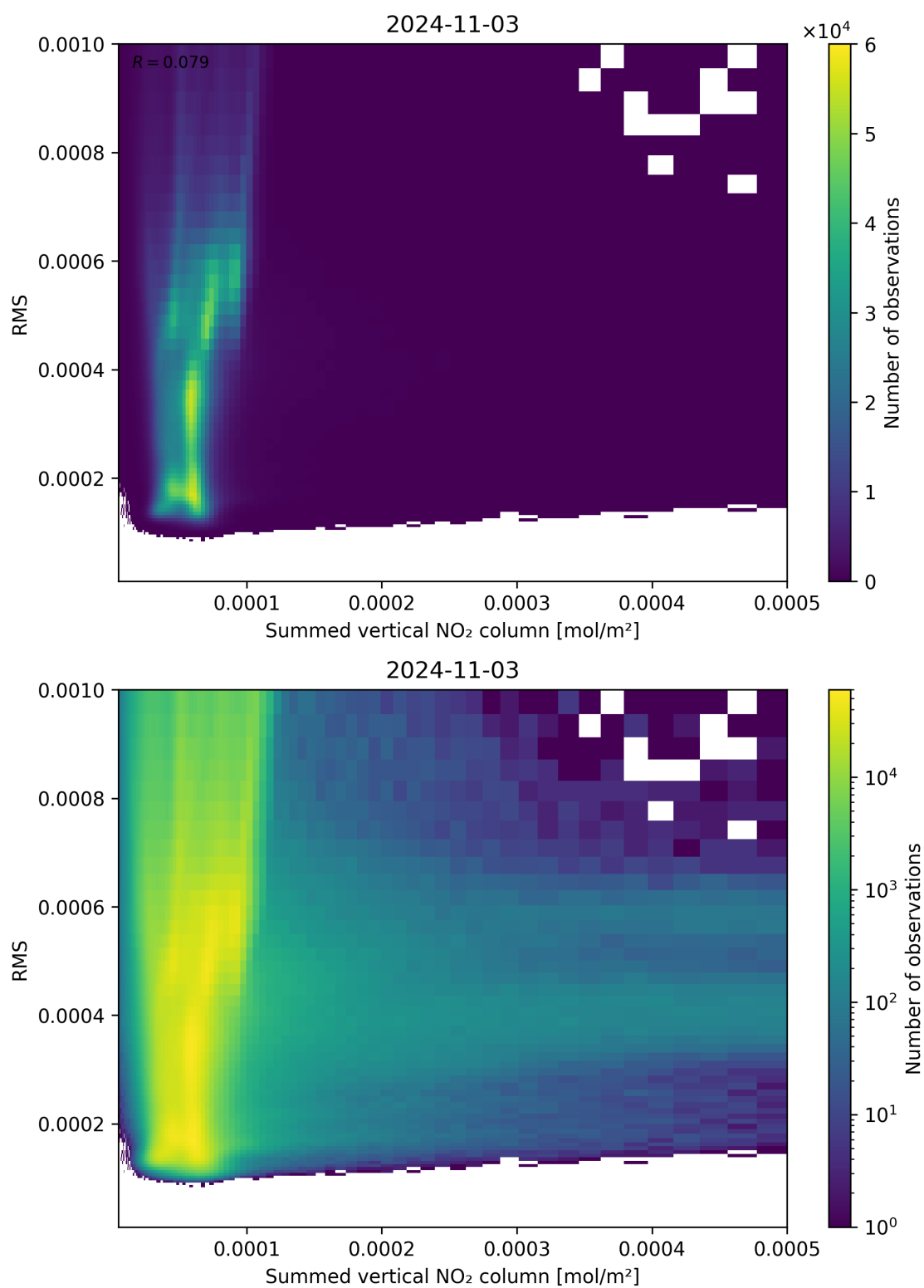
Figure 109: Scatter density plot of “Summed vertical NO 2 column” against “RMS” for 2024-11-02 to 2024-11-04.
