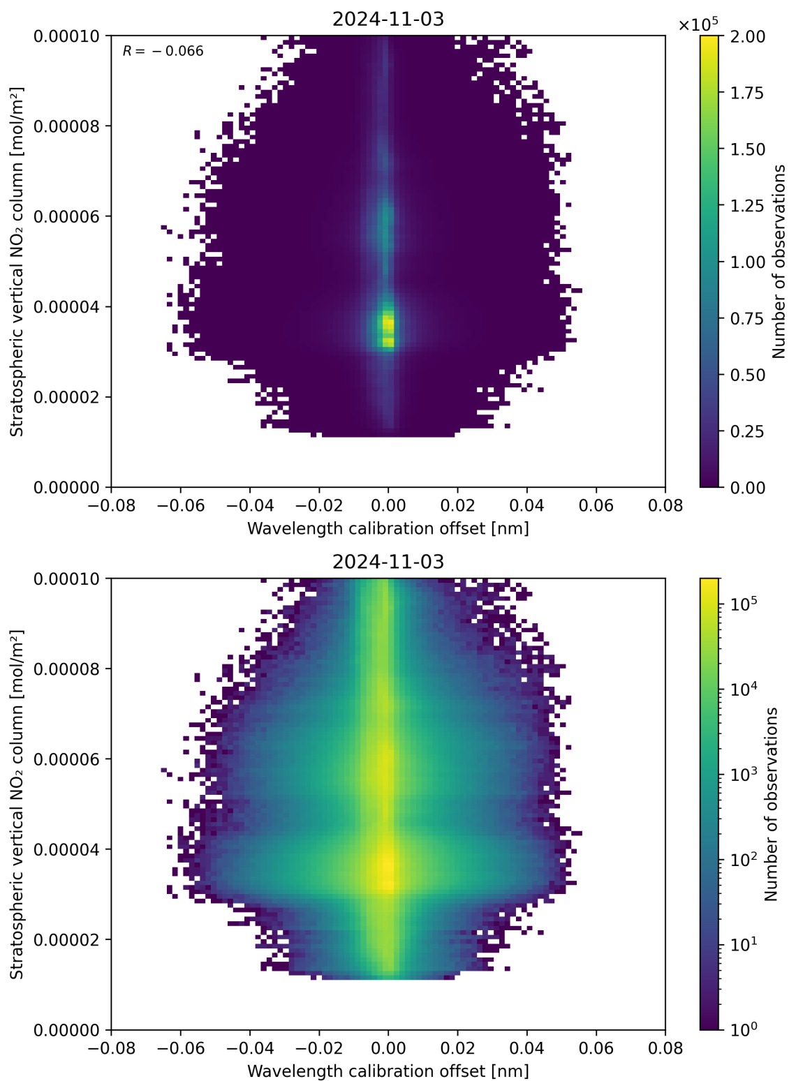
Figure 176: Scatter density plot of “Wavelength calibration offset” against “Stratospheric vertical NO 2 column” for 2024-11-02 to 2024-11-04.
