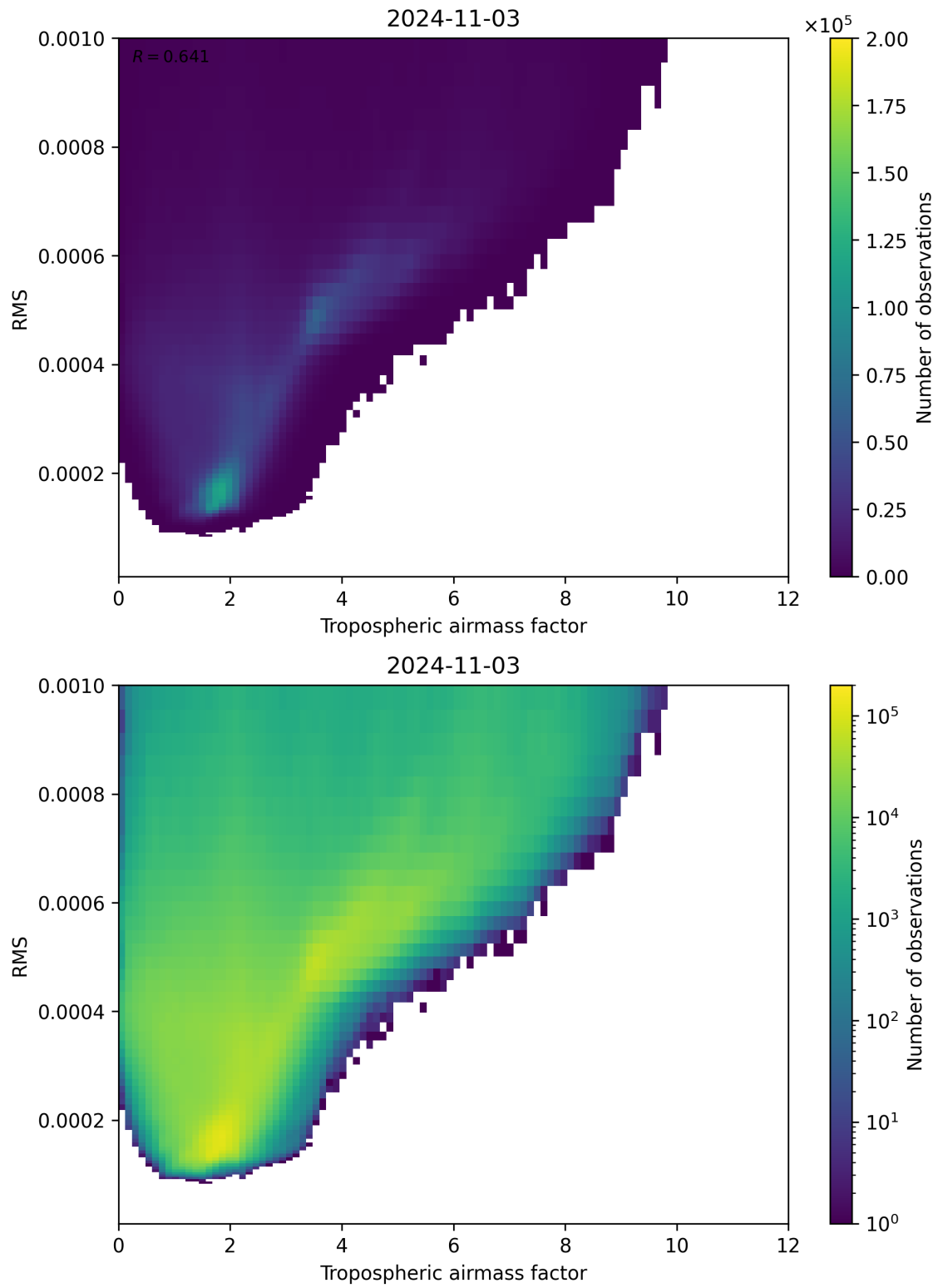
Figure 79: Scatter density plot of “Tropospheric airmass factor” against “RMS” for 2024-11-02 to 2024-11-04.
