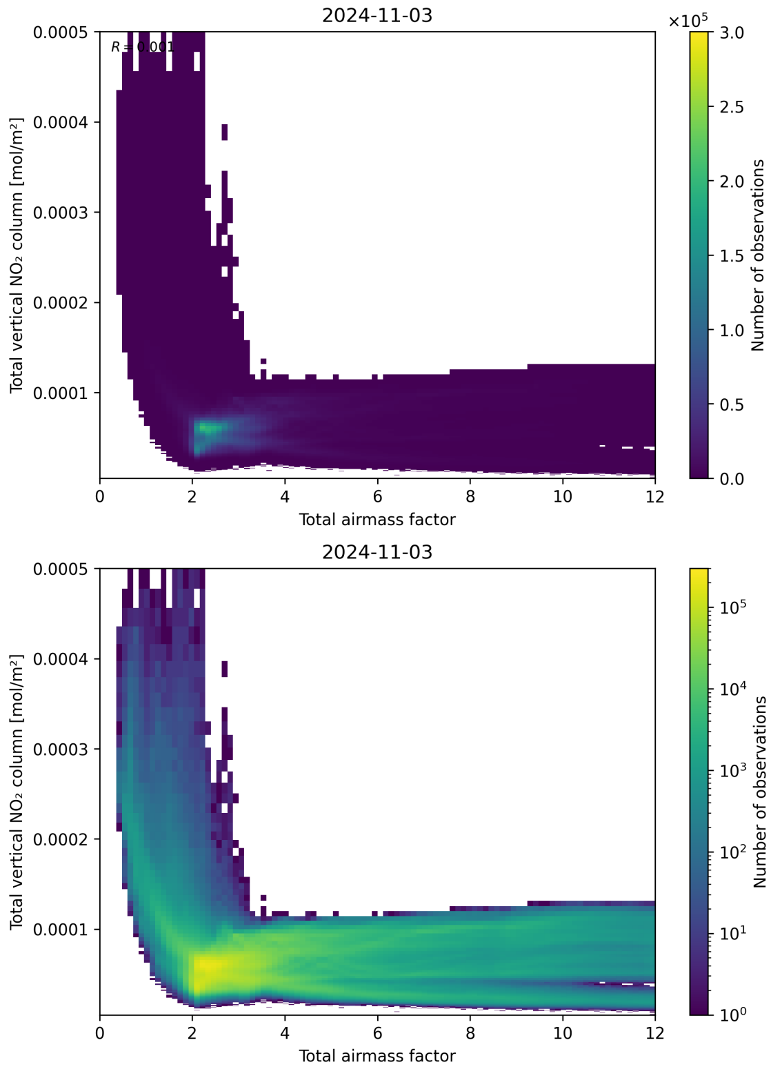
Figure 67: Scatter density plot of “Total airmass factor” against “Total vertical NO 2 column” for 2024-11-02 to 2024-11-04.
