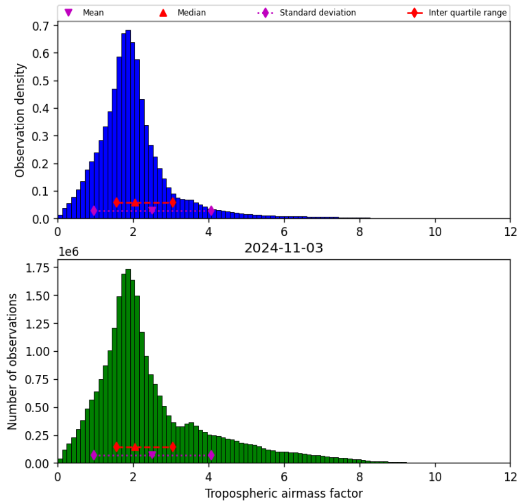
Figure 31: Histogram of “Tropospheric airmass factor” for 2024-11-02 to 2024-11-04
