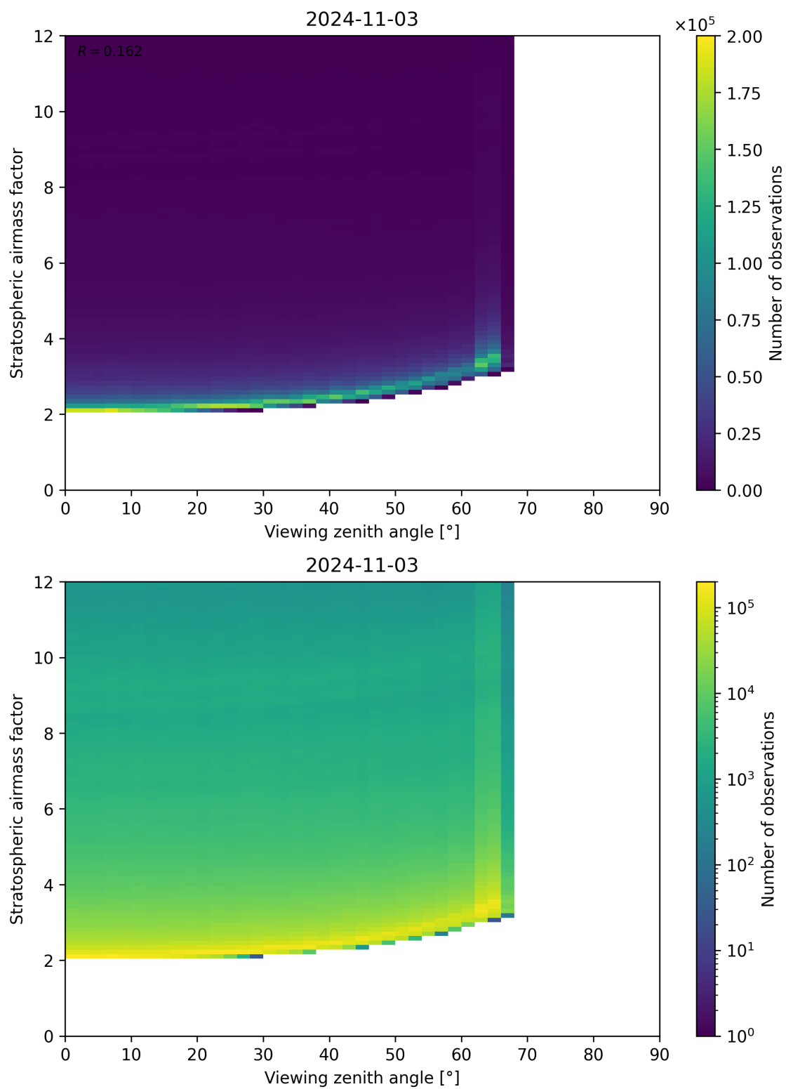
Figure 159: Scatter density plot of “Viewing zenith angle” against “Stratospheric airmass factor” for 2024-11-02 to 2024-11-04.
