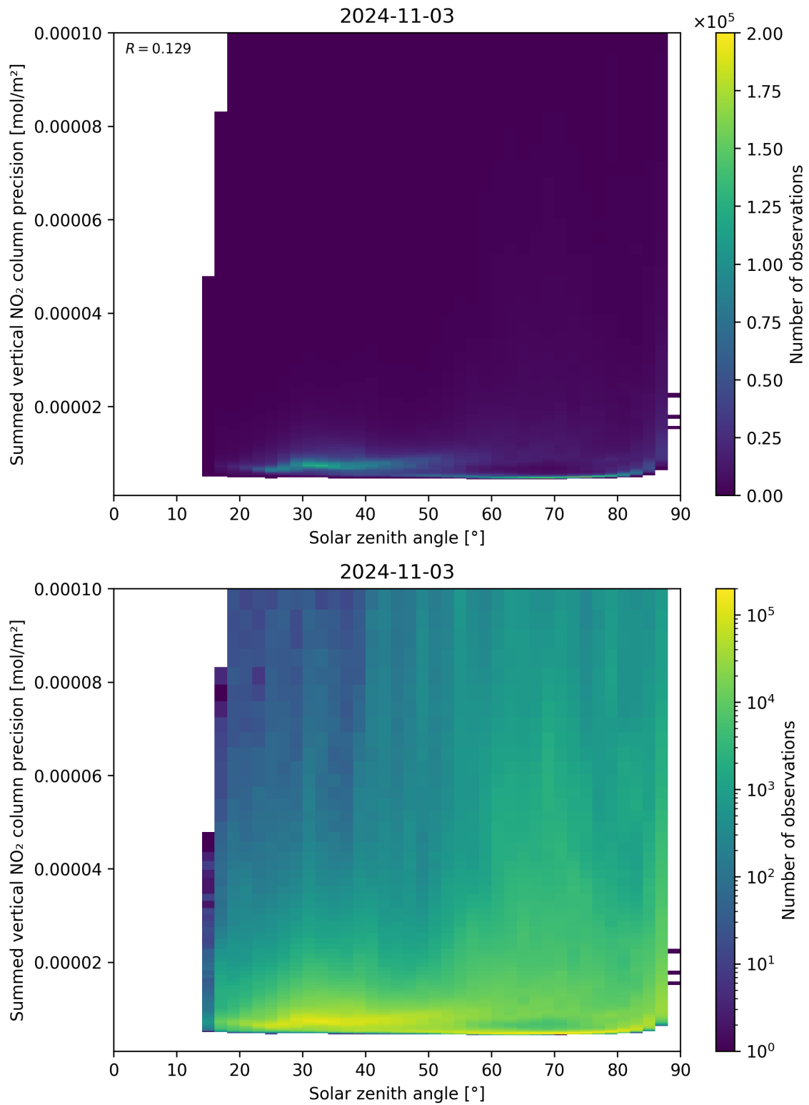
Figure 152: Scatter density plot of “Solar zenith angle” against “Summed vertical NO 2 column precision” for 2024-11-02 to 2024-11-04.
