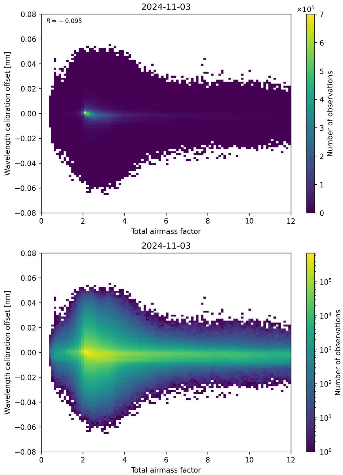
Figure 70: Scatter density plot of “Total airmass factor” against “Wavelength calibration offset” for 2024-11-02 to 2024-11-04.
