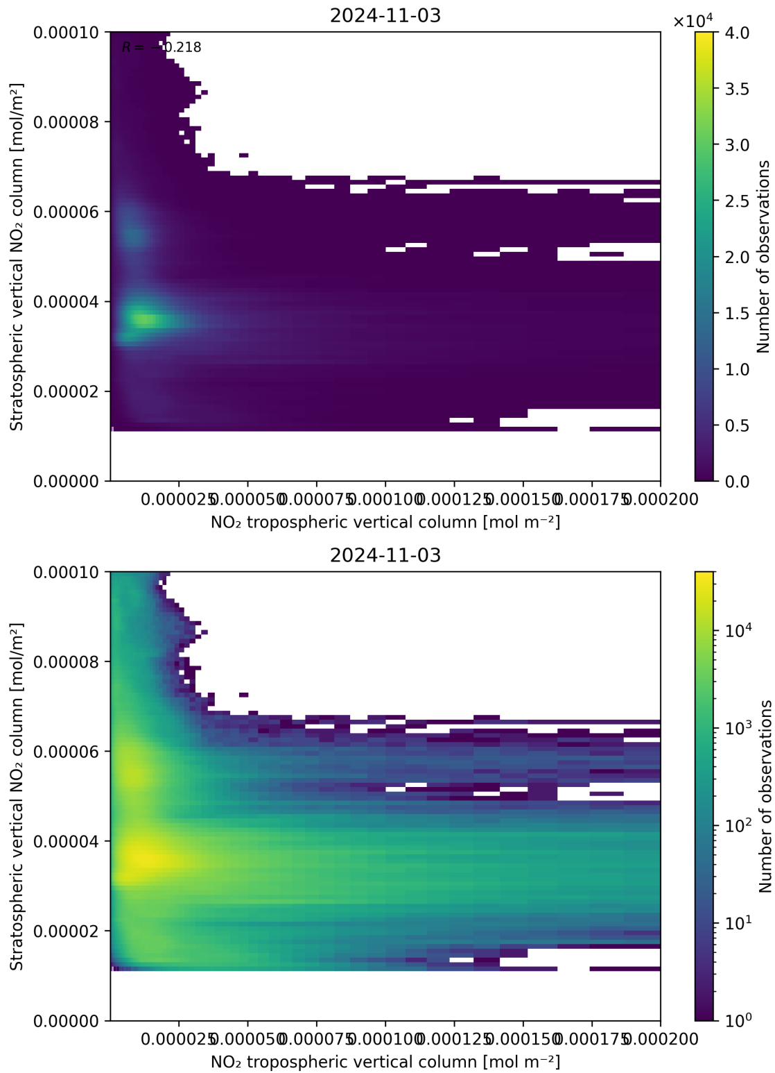
Figure 125: Scatter density plot of “NO 2 tropospheric vertical column” against “Stratospheric vertical NO 2 column” for 2024-11-02 to 2024-11-04.
