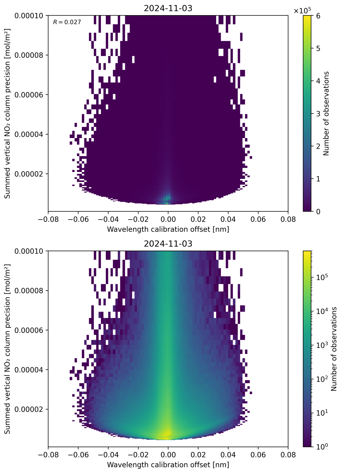
Figure 178: Scatter density plot of “Wavelength calibration offset” against “Summed vertical NO 2 column precision” for 2024-11-02 to 2024-11-04.
