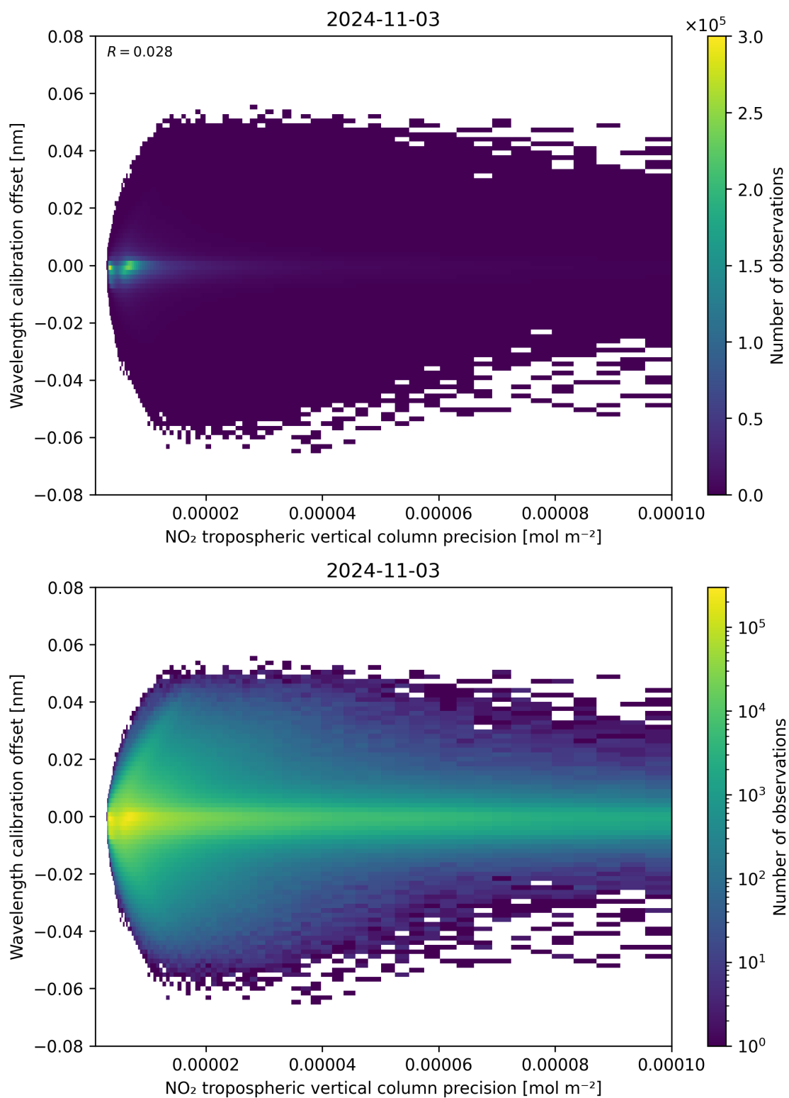
Figure 141: Scatter density plot of “NO 2 tropospheric vertical column precision” against “Wavelength calibration offset” for 2024-11-02 to 2024-11-04.
