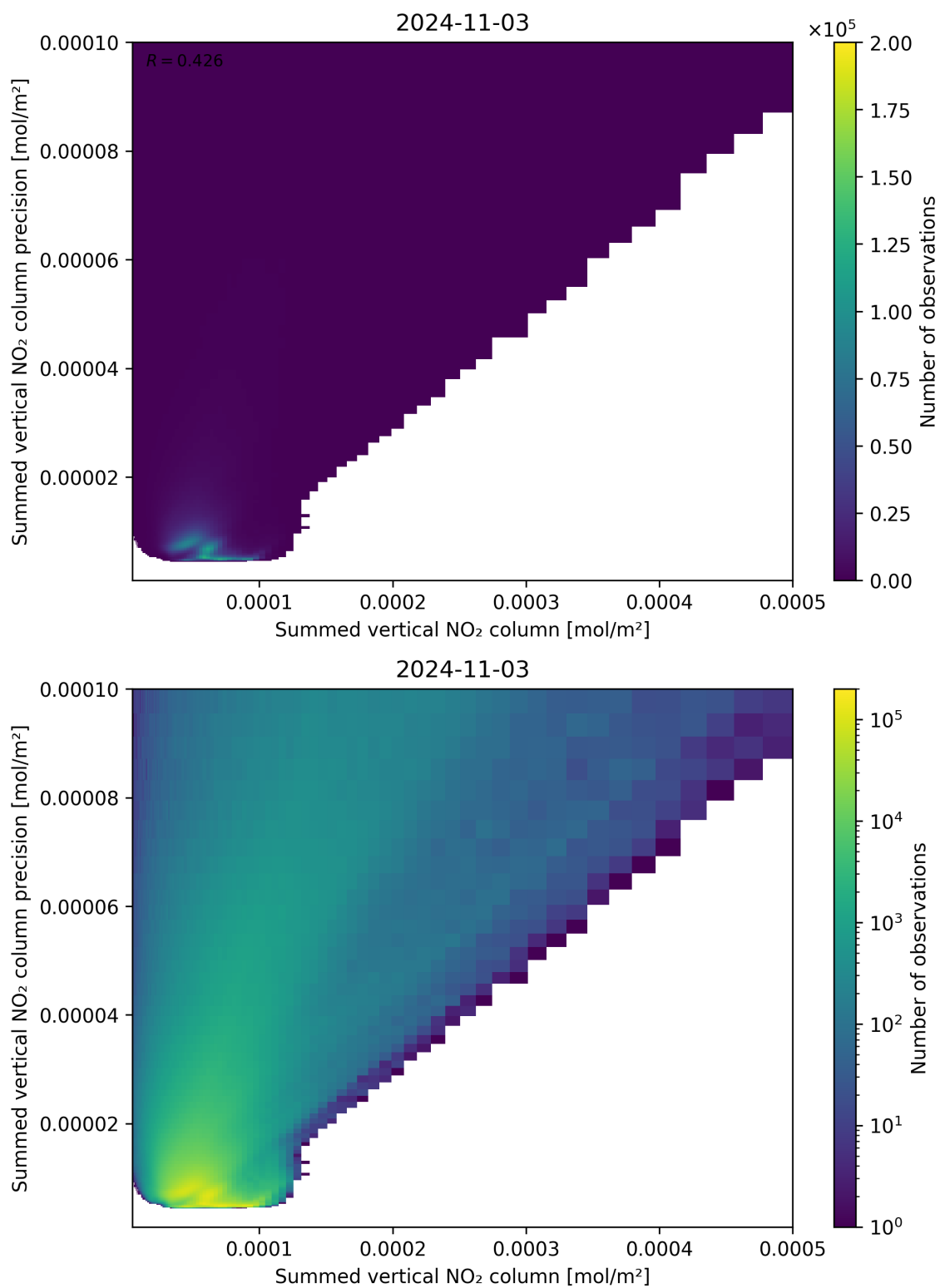
Figure 105: Scatter density plot of “Summed vertical NO 2 column” against “Summed vertical NO 2 column precision” for 2024-11-02 to 2024-11-04.
