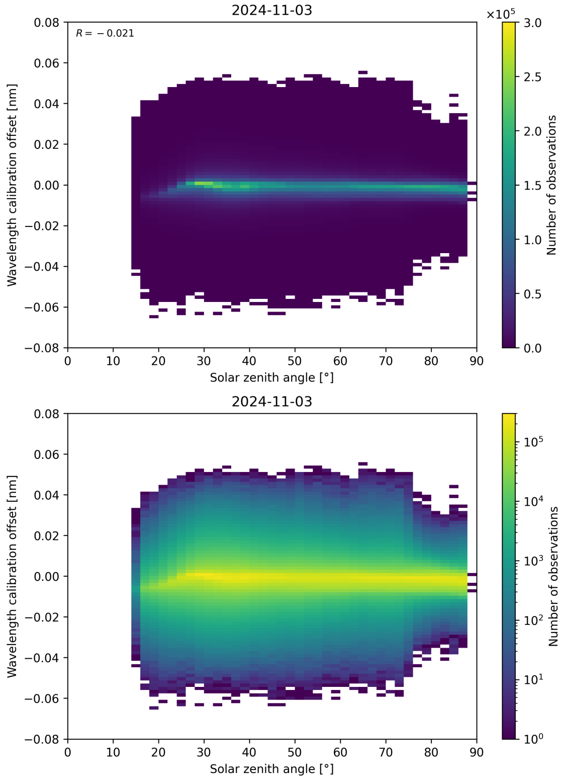
Figure 158: Scatter density plot of “Solar zenith angle” against “Wavelength calibration offset” for 2024-11-02 to 2024-11-04.
