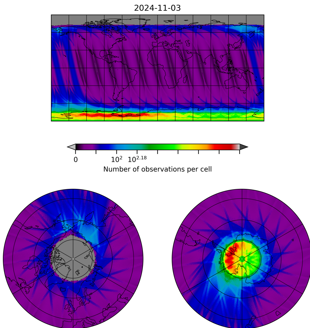
Figure 10: Map of the number of observations for 2024-11-02 to 2024-11-04
