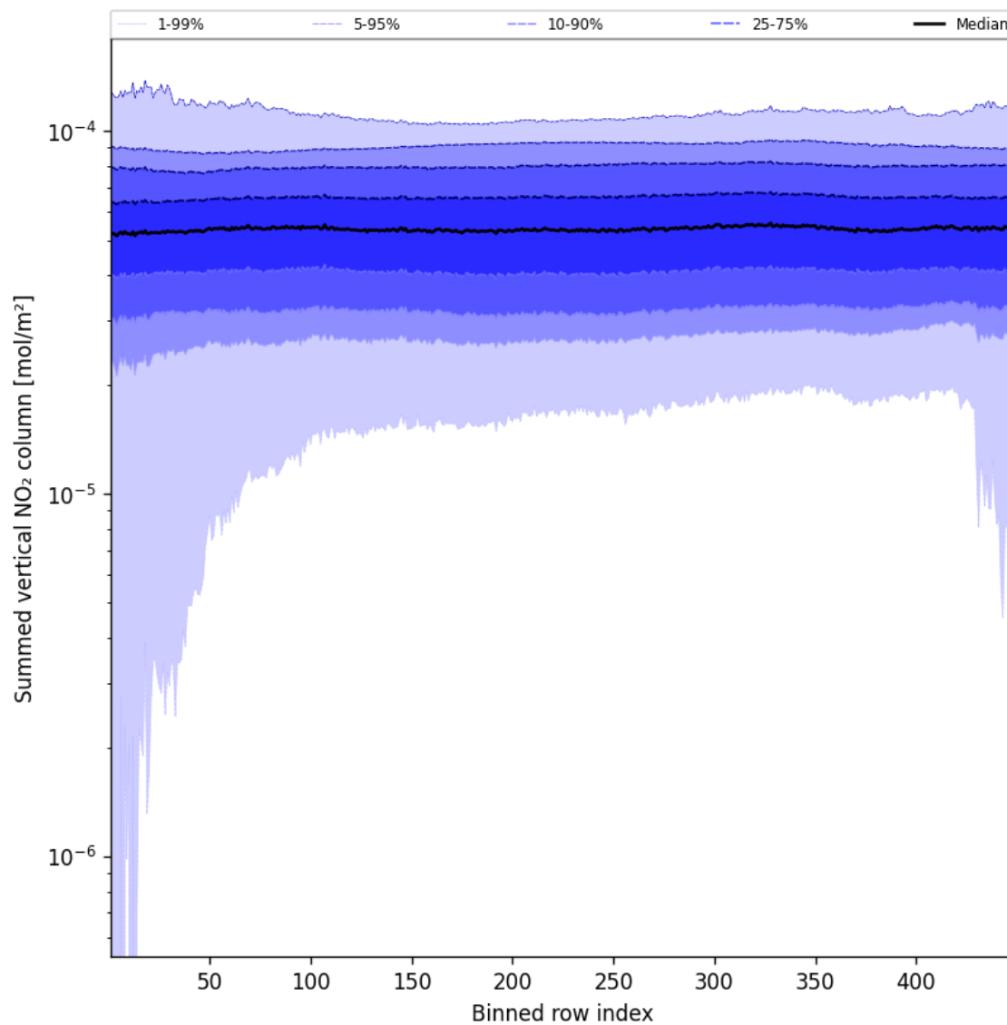
Figure 57: Along track statistics of “Summed vertical NO 2 column” for 2024-11-02 to 2024-11-04
