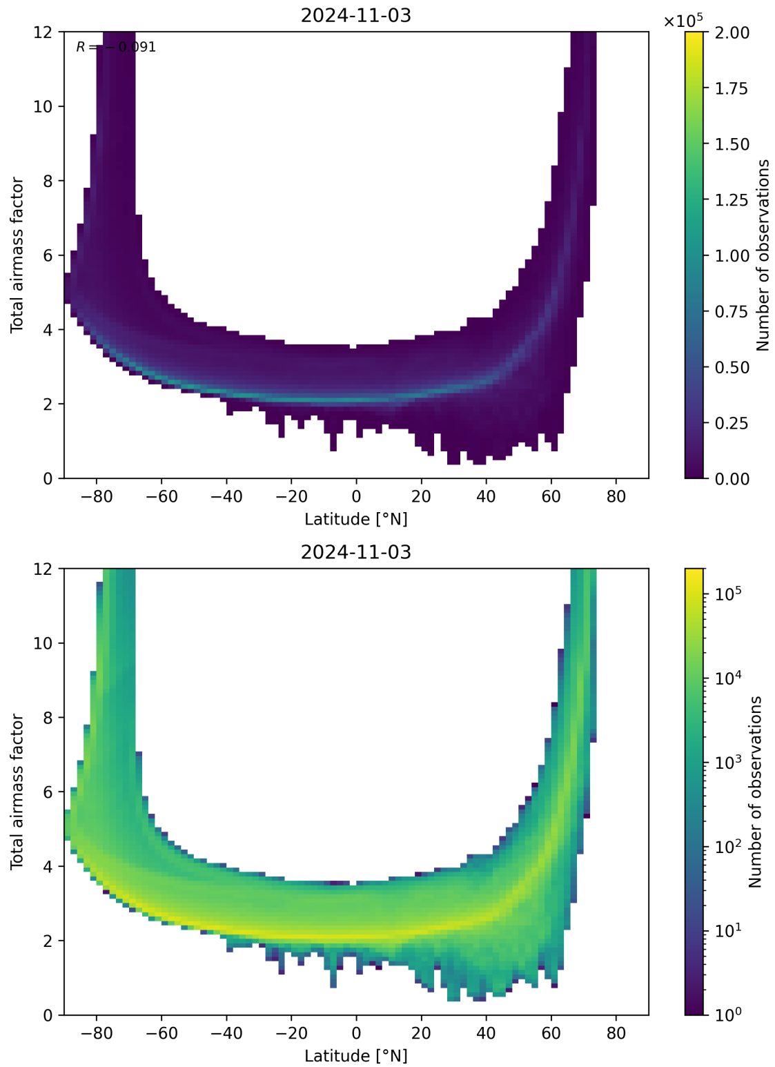
Figure 84: Scatter density plot of “Latitude” against “Total airmass factor” for 2024-11-02 to 2024-11-04.
