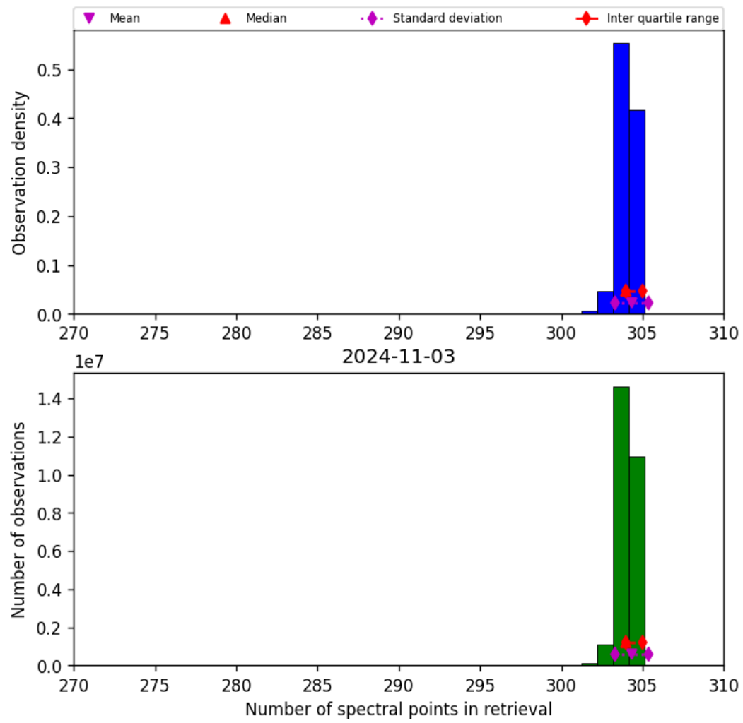
Figure 33: Histogram of “Number of spectral points in retrieval” for 2024-11-02 to 2024-11-04
