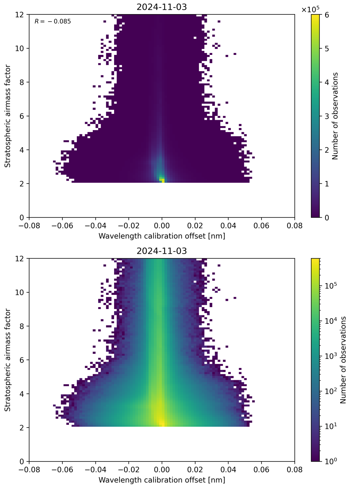
Figure 174: Scatter density plot of “Wavelength calibration offset” against “Stratospheric air mass factor” for 2024-11-02 to 2024-11-04.
