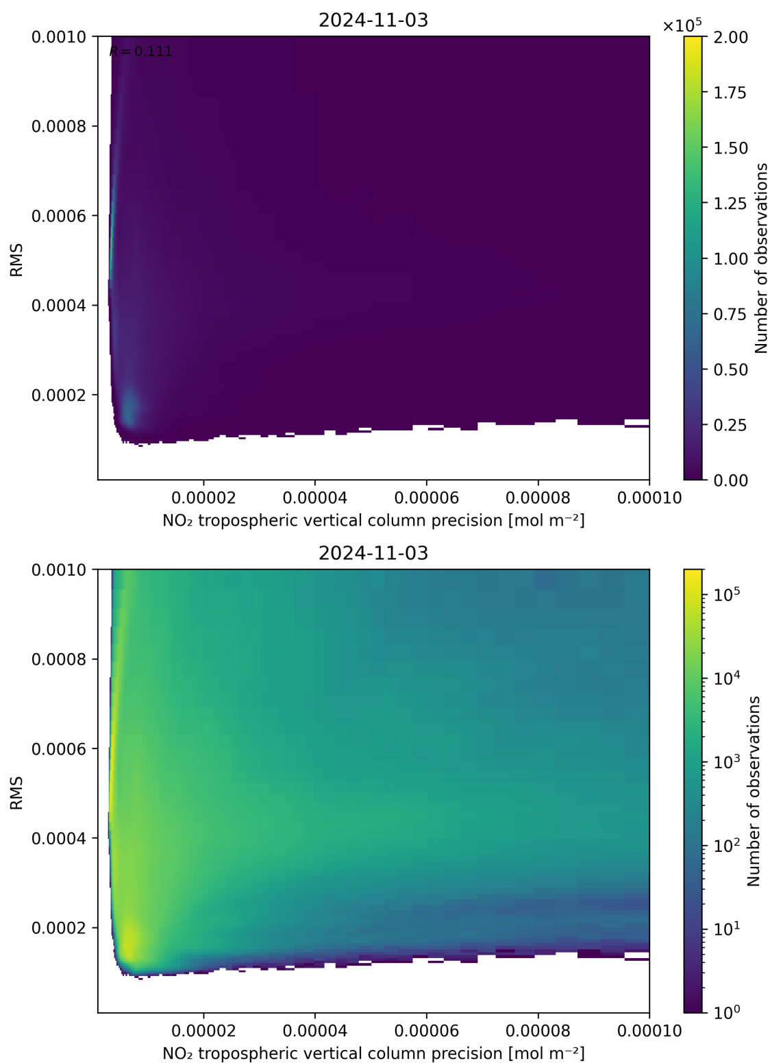
Figure 140: Scatter density plot of “NO 2 tropospheric vertical column precision” against “RMS” for 2024-11-02 to 2024-11-04.
