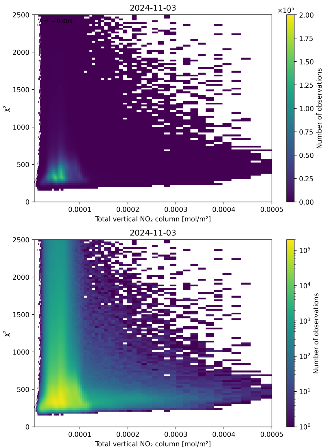
Figure 111: Scatter density plot of “Total vertical NO 2 column” against “ \chi^2 ” for 2024-11-02 to 2024-11-04.
