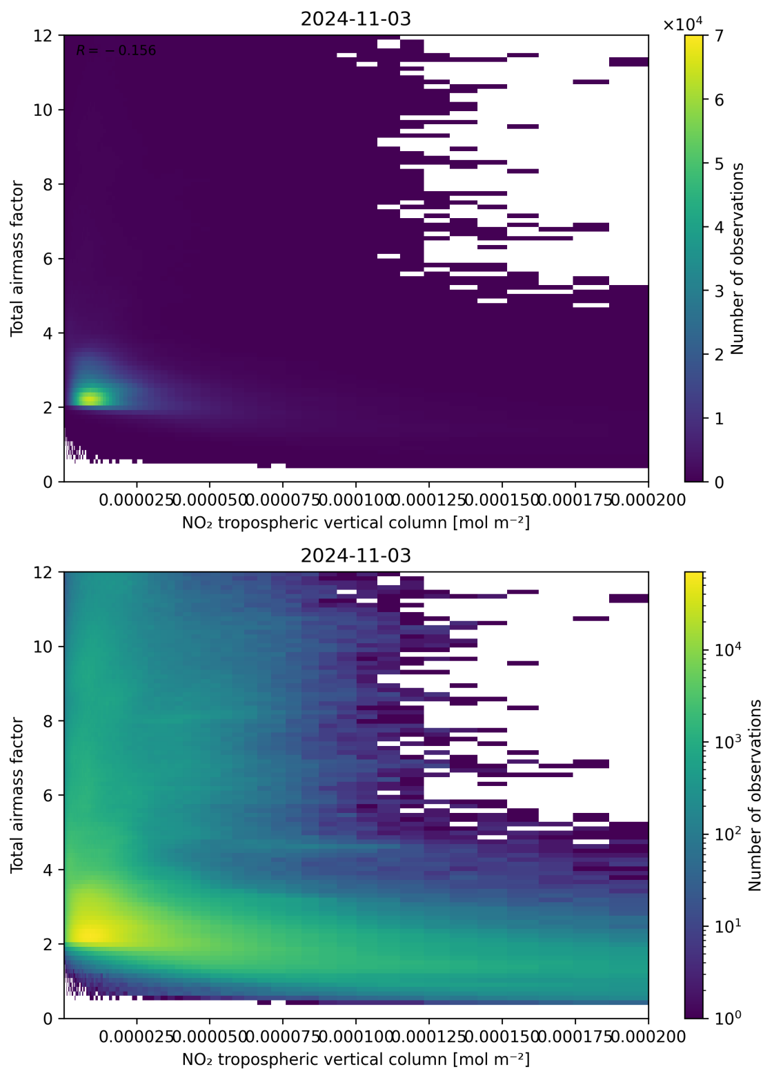
Figure 122: Scatter density plot of “NO 2 tropospheric vertical column” against “Total air mass factor” for 2024-11-02 to 2024-11-04.
