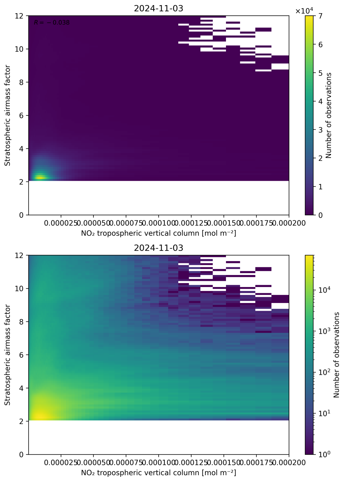
Figure 121: Scatter density plot of “NO 2 tropospheric vertical column” against “Stratospheric airmass factor” for 2024-11-02 to 2024-11-04.
