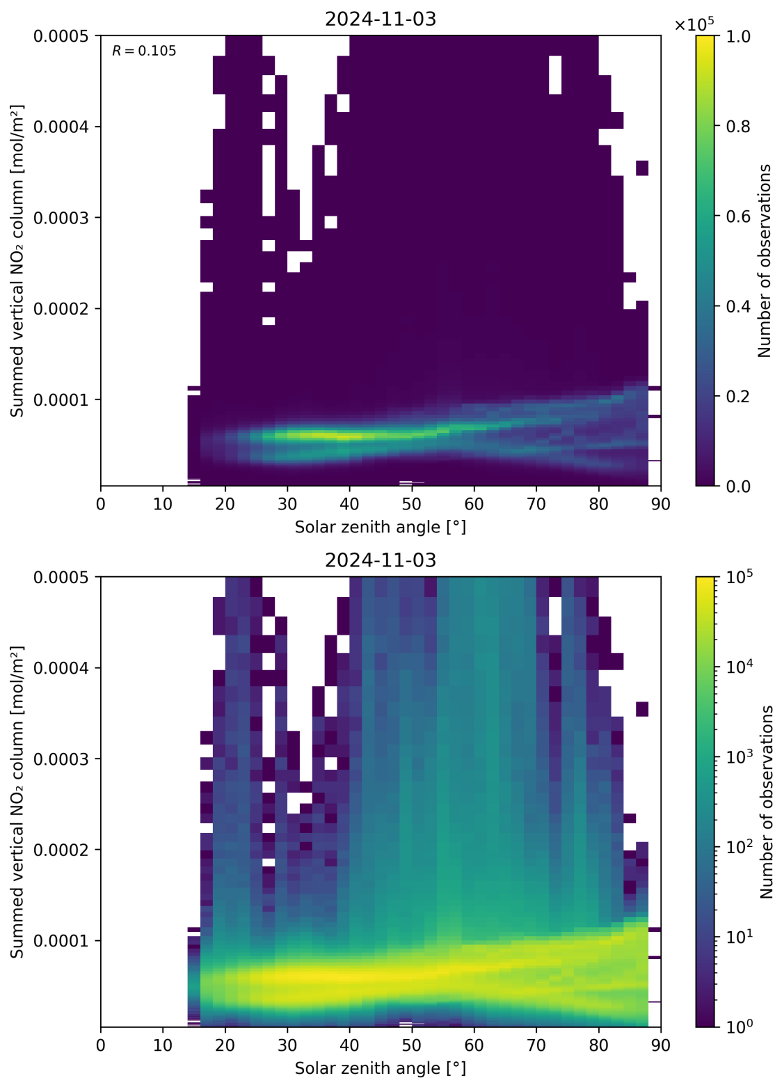
Figure 151: Scatter density plot of “Solar zenith angle” against “Summed vertical NO 2 column” for 2024-11-02 to 2024-11-04.
