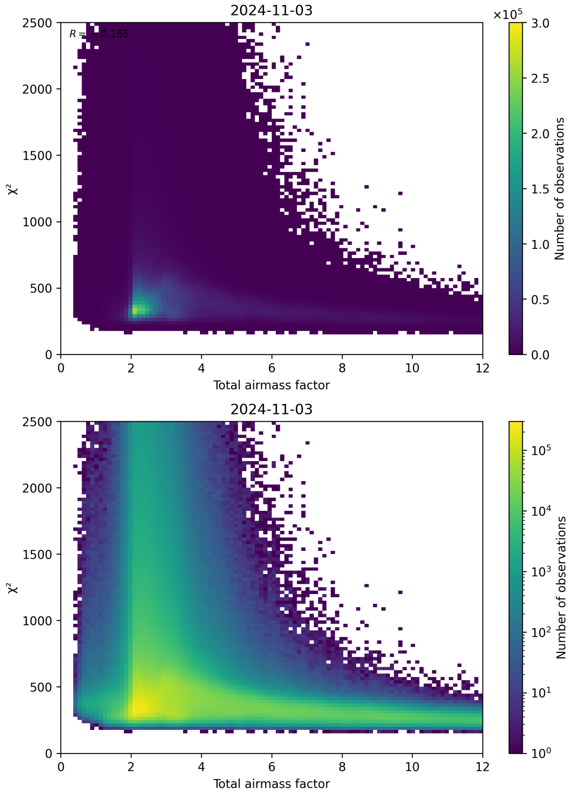
Figure 63: Scatter density plot of “Total airmass factor” against “ \chi^2 ” for 2024-11-02 to 2024-11-04.
