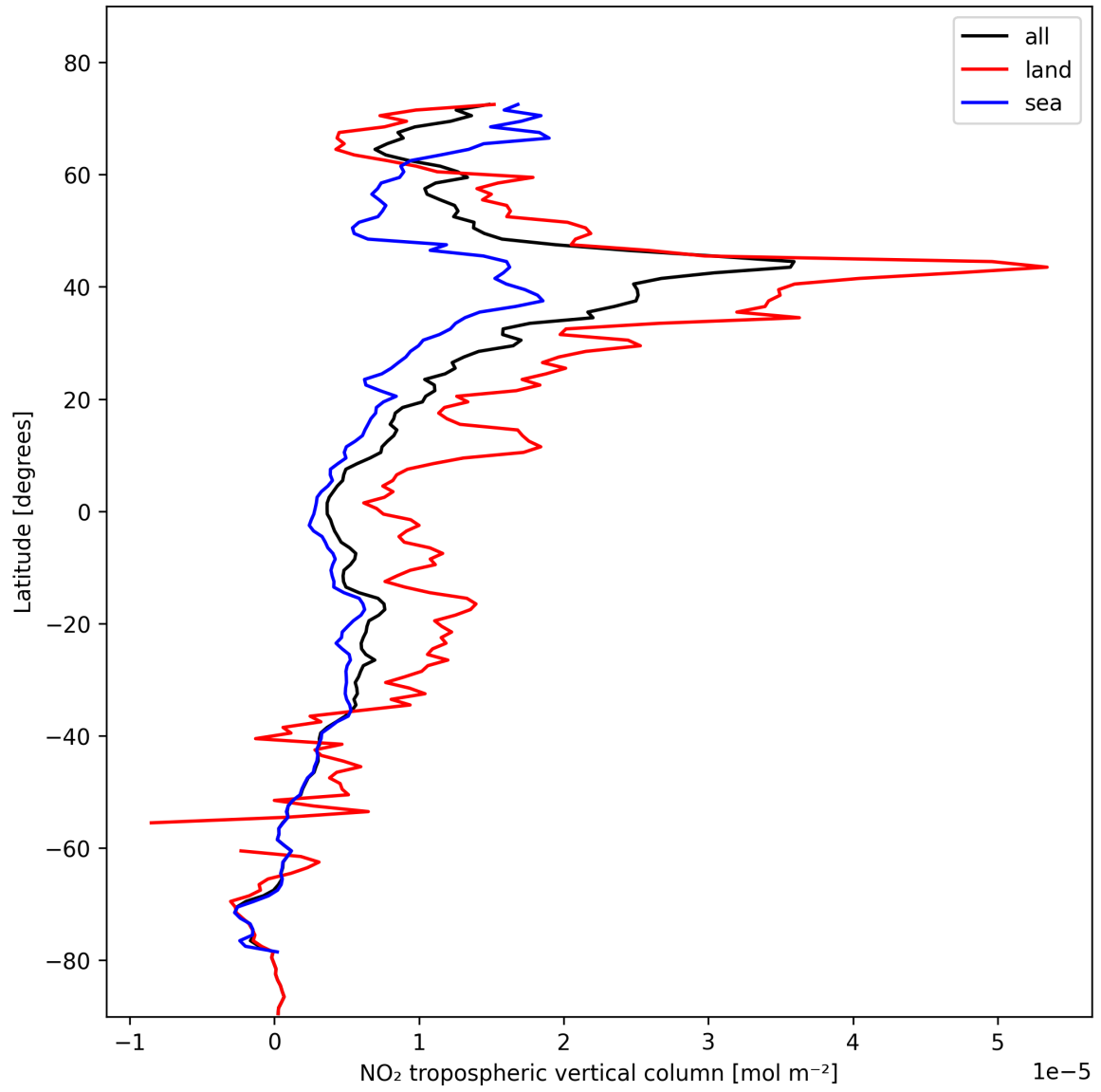
Figure 12: Zonal average of “NO 2 tropospheric vertical column” for 2024-11-02 to 2024-11-04.
