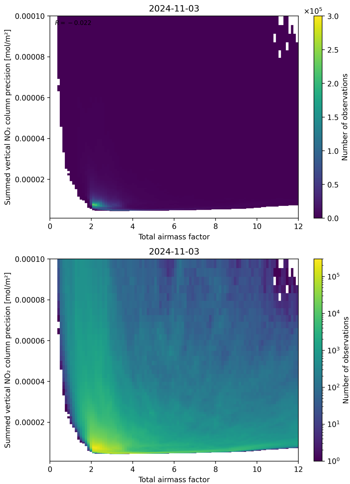
Figure 66: Scatter density plot of “Total airmass factor” against “Summed vertical NO 2 column precision” for 2024-11-02 to 2024-11-04.
