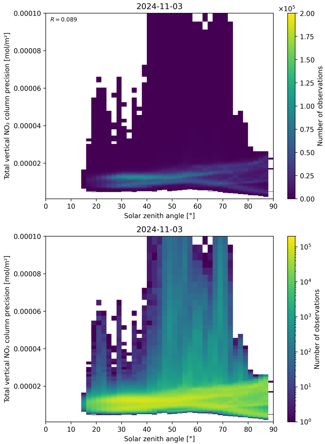
Figure 154: Scatter density plot of “Solar zenith angle” against “Total vertical NO 2 column precision” for 2024-11-02 to 2024-11-04.
