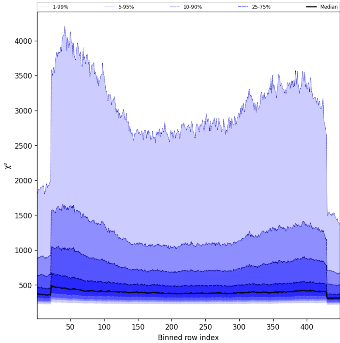
Figure 59: Along track statistics of “ \chi^2 ” for 2024-11-02 to 2024-11-04
