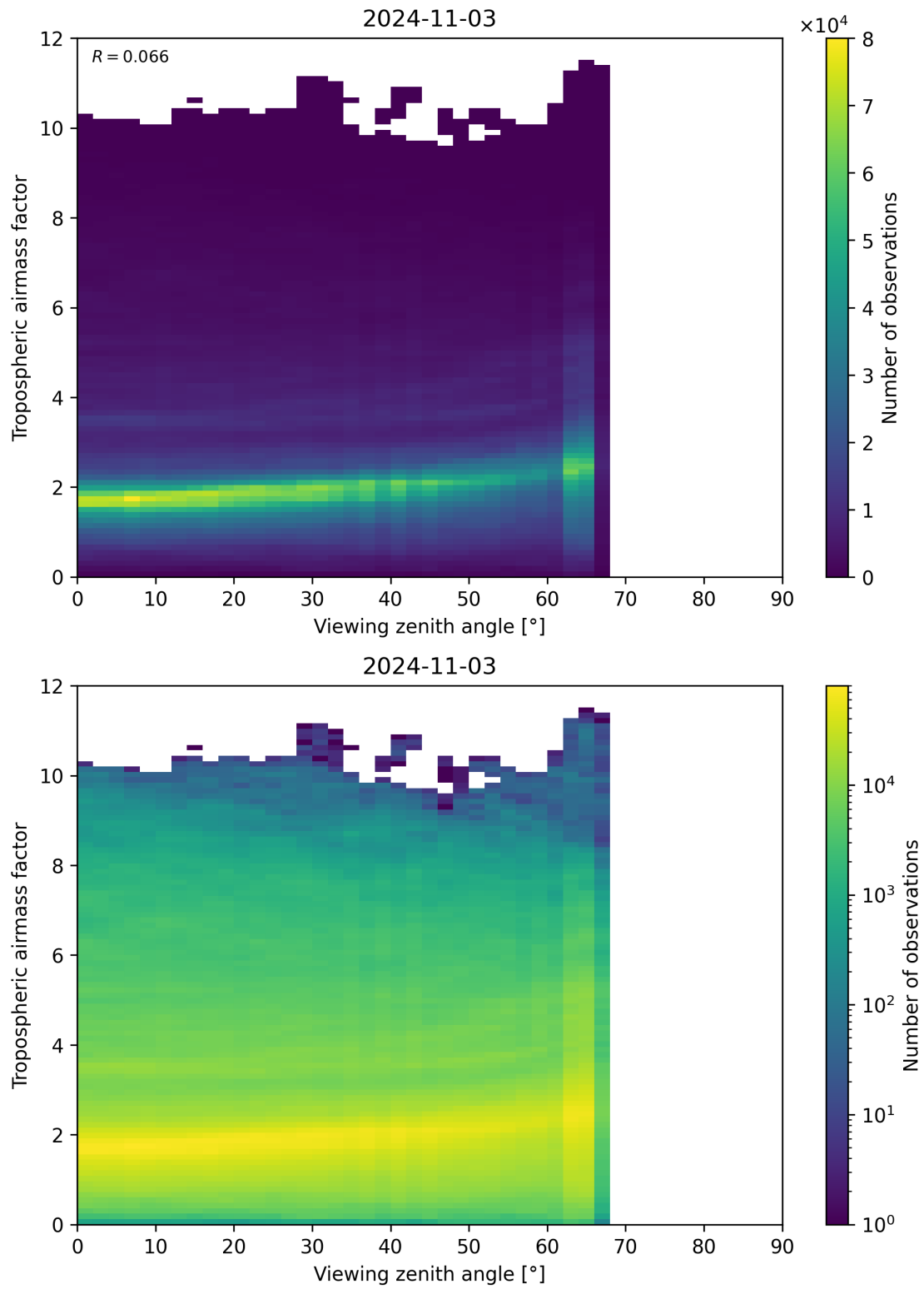
Figure 161: Scatter density plot of “Viewing zenith angle” against “Tropospheric airmass factor” for 2024-11-02 to 2024-11-04.
