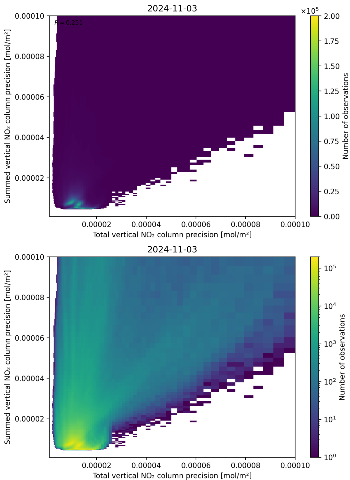
Figure 118: Scatter density plot of “Total vertical NO 2 column precision” against “Summed vertical NO 2 column precision” for 2024-11-02 to 2024-11-04.
