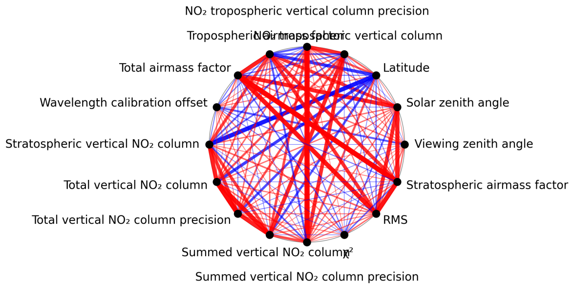
Figure 1: Map of correlation graph for 2024-11-02 to 2024-11-04.
