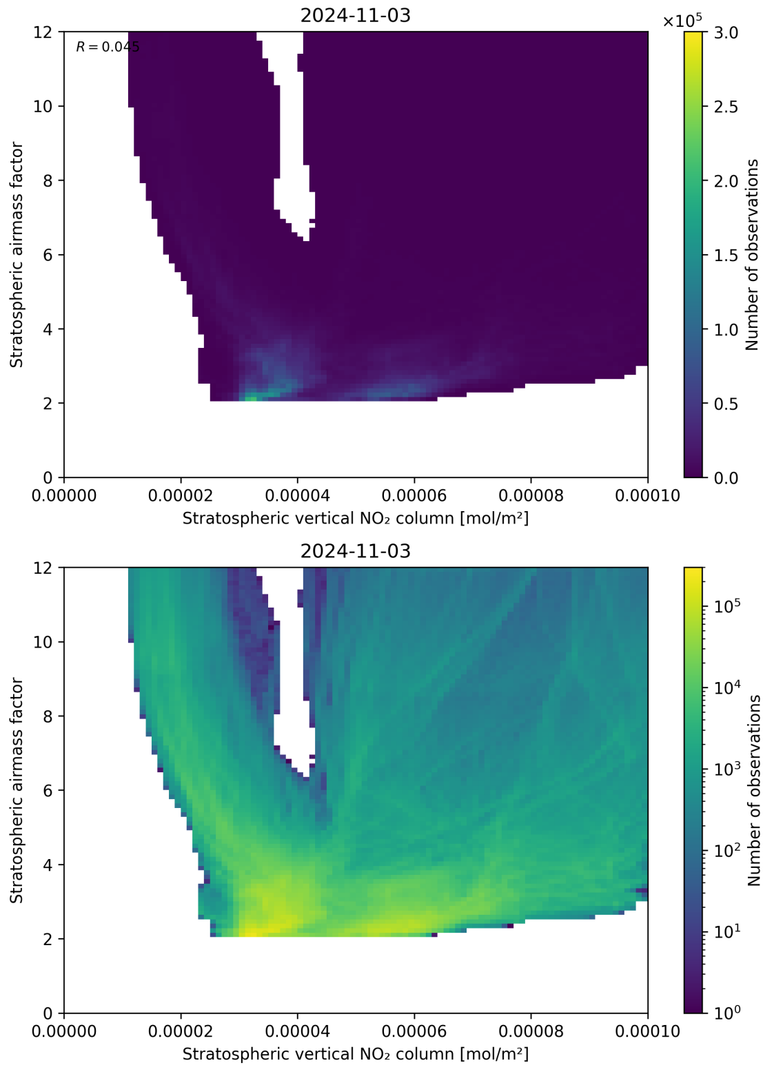
Figure 96: Scatter density plot of “Stratospheric vertical NO 2 column” against “Stratospheric airmass factor” for 2024-11-02 to 2024-11-04.
