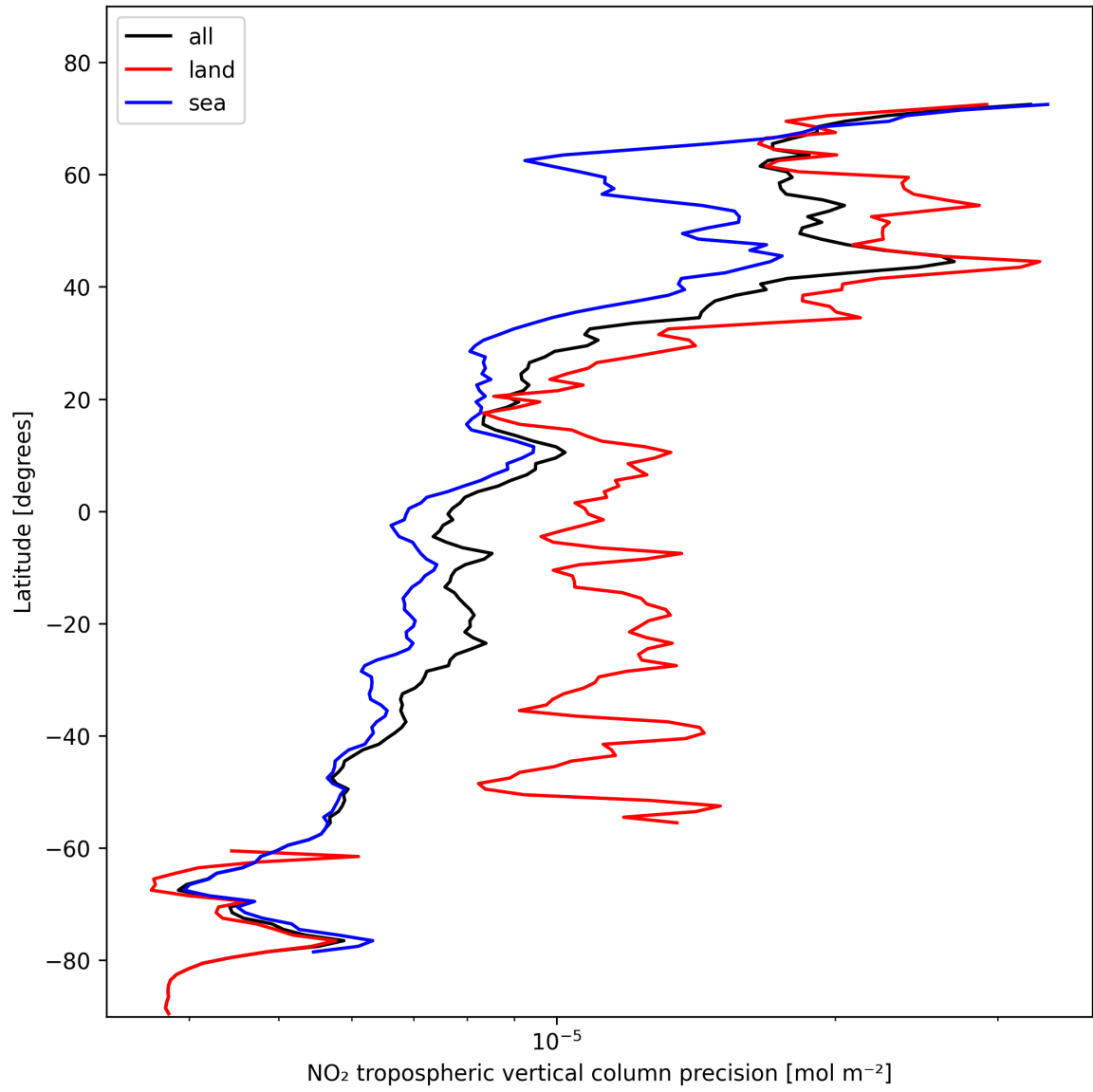
Figure 13: Zonal average of “NO 2 tropospheric vertical column precision” for 2024-11-02 to 2024-11-04.
