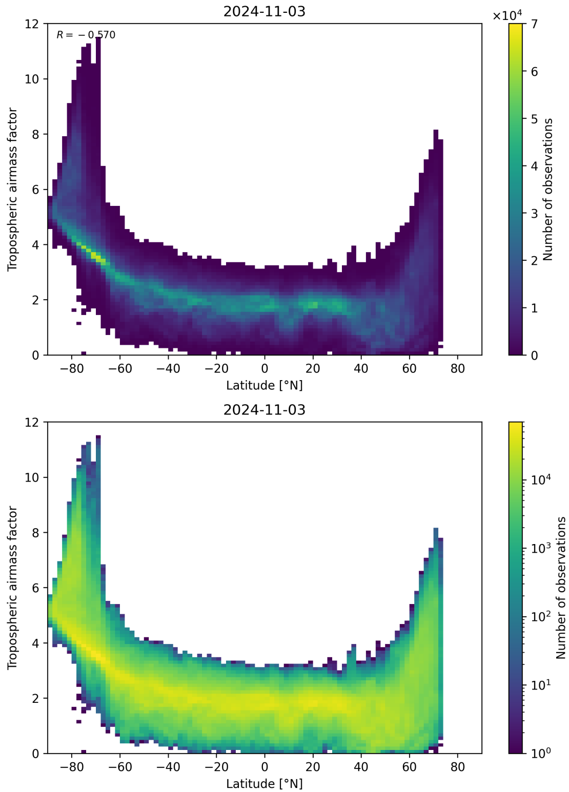
Figure 85: Scatter density plot of “Latitude” against “Tropospheric airmass factor” for 2024-11-02 to 2024-11-04.
