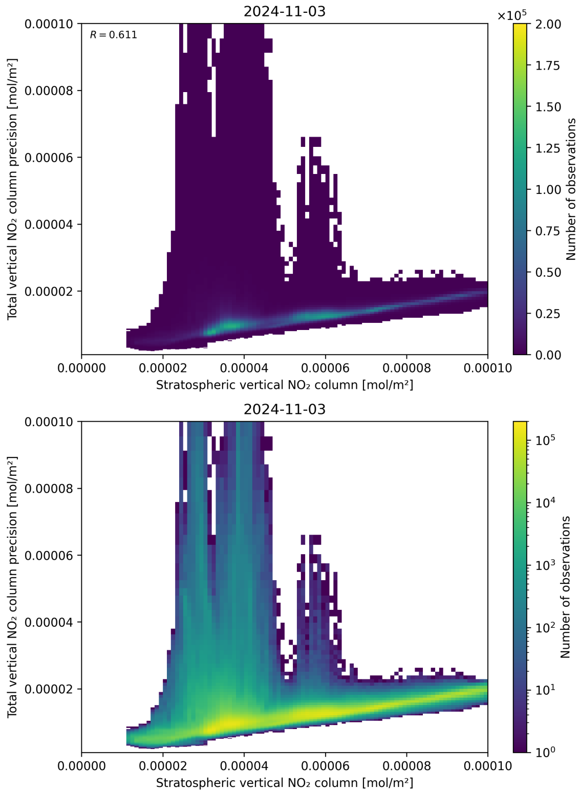
Figure 101: Scatter density plot of “Stratospheric vertical NO 2 column” against “Total vertical NO 2 column precision” for 2024-11-02 to 2024-11-04.
