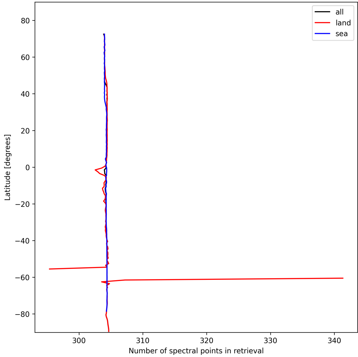
Figure 16: Zonal average of “Number of spectral points in retrieval” for 2024-11-02 to 2024-11-04.
