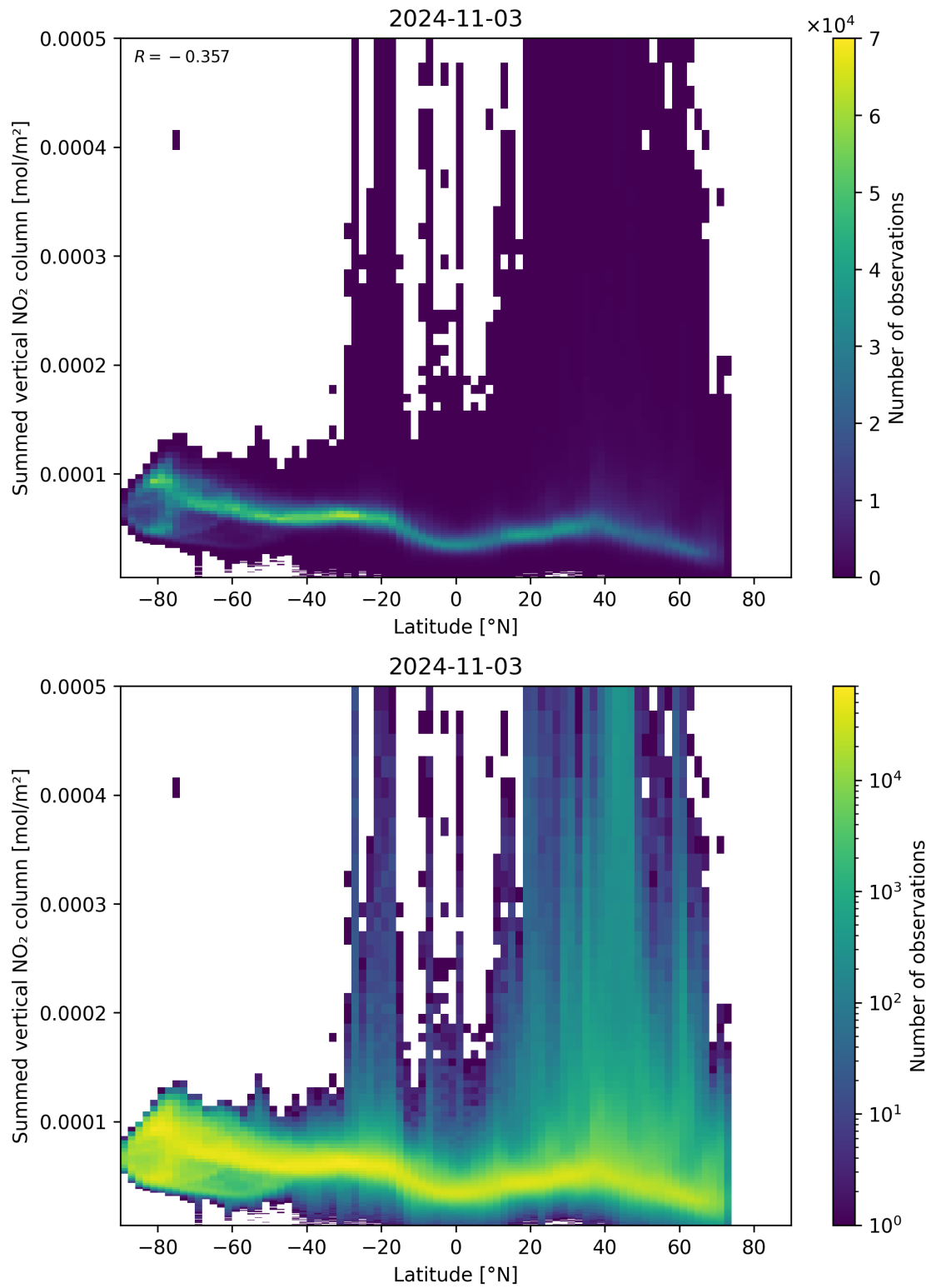
Figure 88: Scatter density plot of “Latitude” against “Summed vertical NO 2 column” for 2024-11-02 to 2024-11-04.
