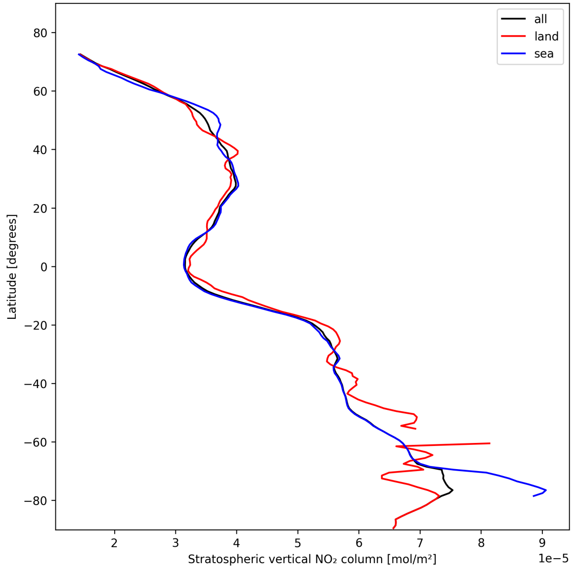
Figure 19: Zonal average of “Stratospheric vertical NO 2 column” for 2024-11-02 to 2024-11-04.
