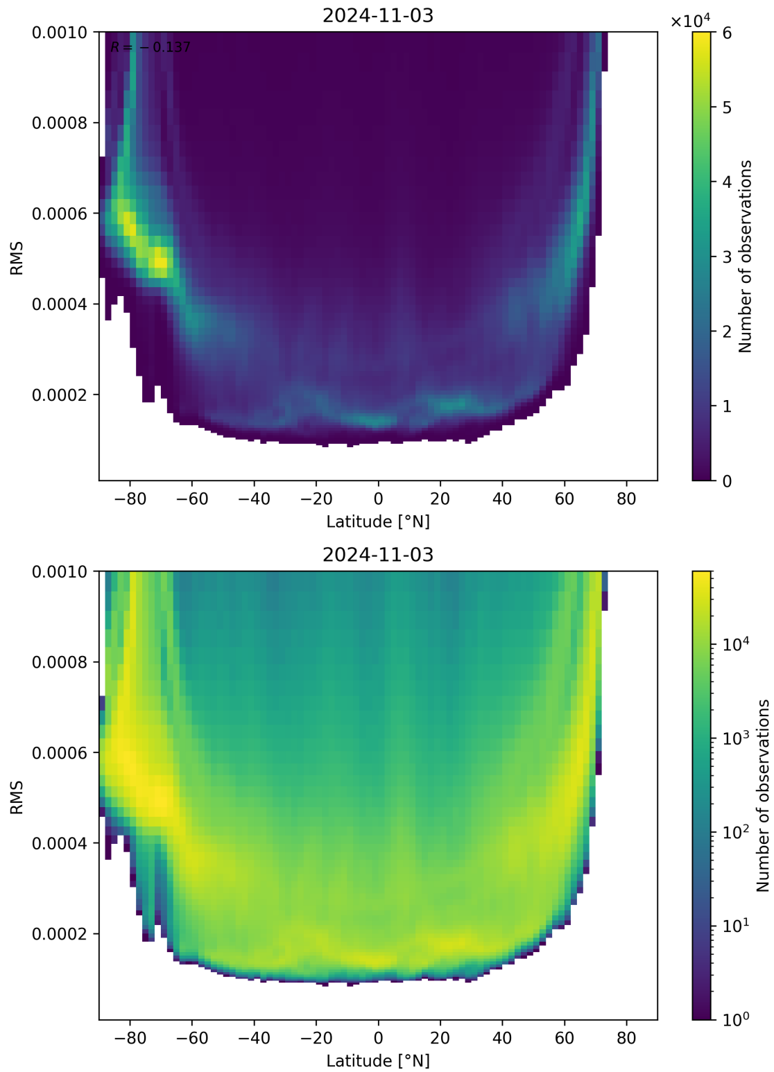
Figure 94: Scatter density plot of “Latitude” against “RMS” for 2024-11-02 to 2024-11-04.
