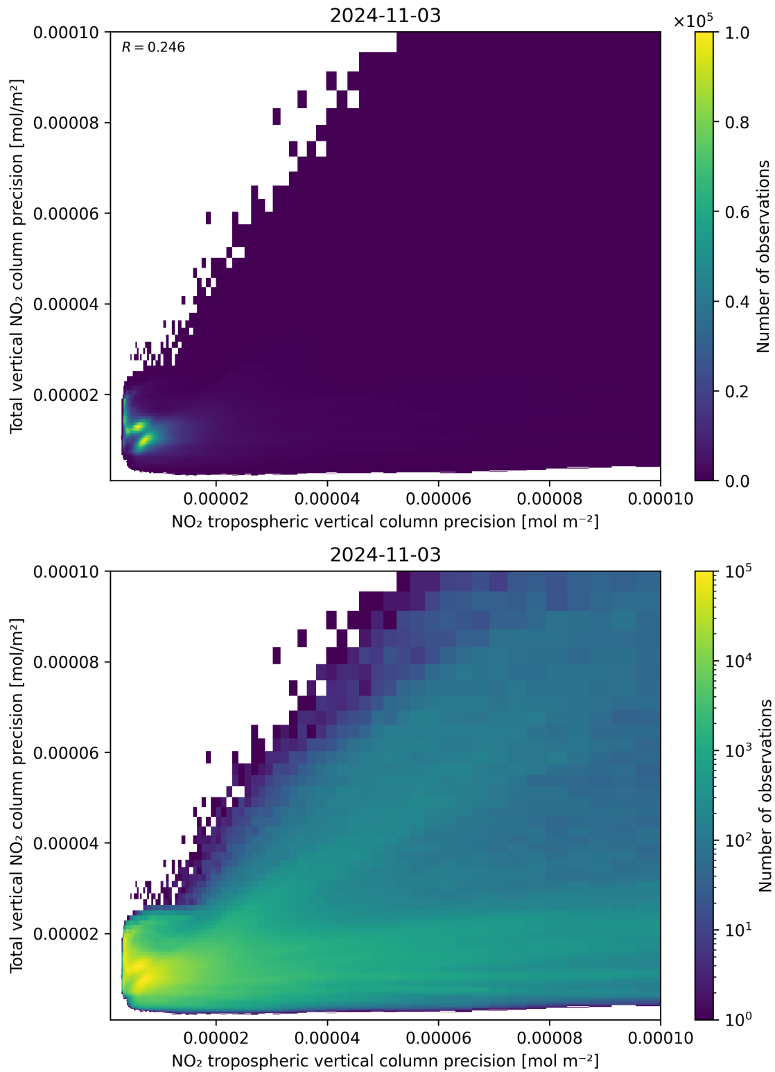
Figure 139: Scatter density plot of “NO 2 tropospheric vertical column precision” against “Total vertical NO 2 column precision” for 2024-11-02 to 2024-11-04.
