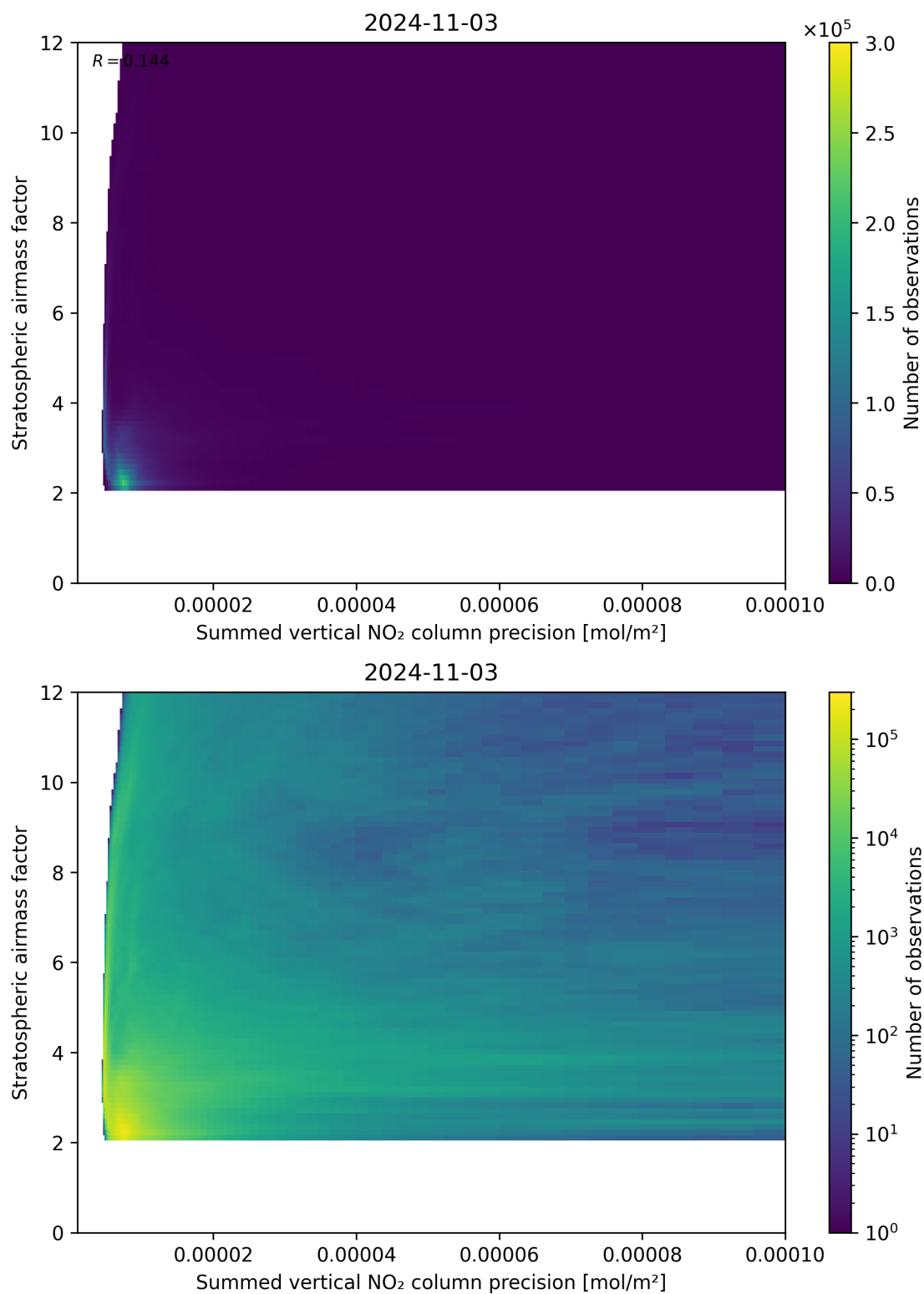
Figure 106: Scatter density plot of “Summed vertical NO 2 column precision” against “Stratospheric airmass factor” for 2024-11-02 to 2024-11-04.
