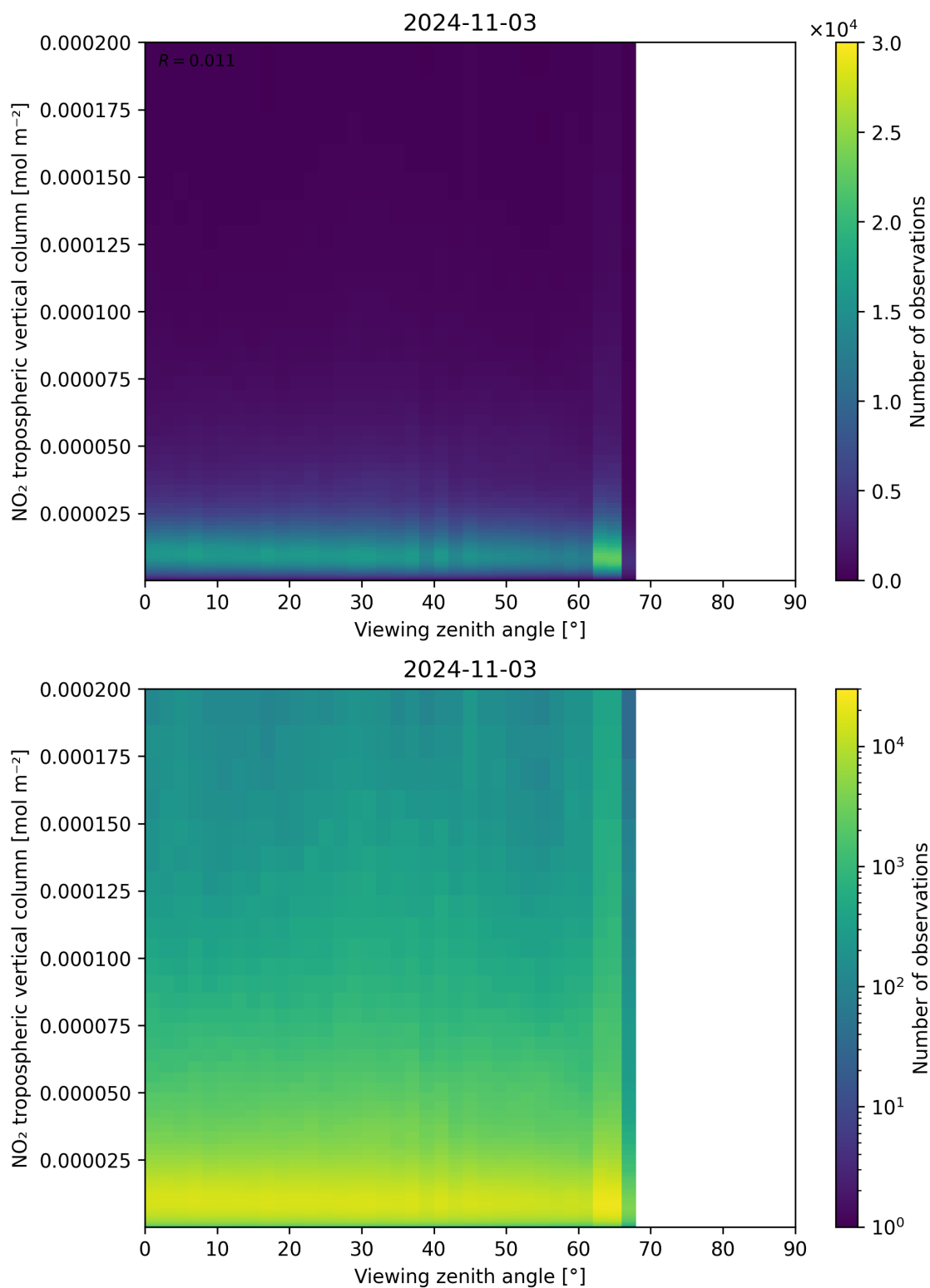
Figure 169: Scatter density plot of “Viewing zenith angle” against “NO 2 tropospheric vertical column” for 2024-11-02 to 2024-11-04.
