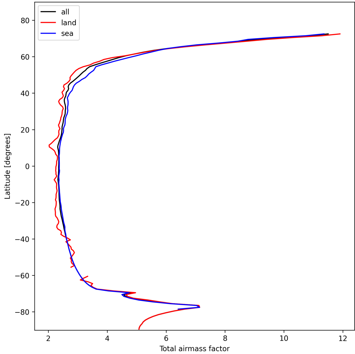
Figure 15: Zonal average of “Total airmass factor” for 2024-11-02 to 2024-11-04.
