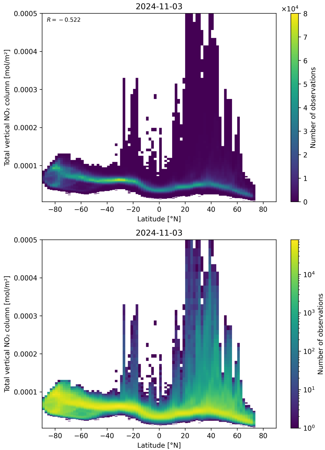
Figure 90: Scatter density plot of “Latitude” against “Total vertical NO 2 column” for 2024-11-02 to 2024-11-04.
