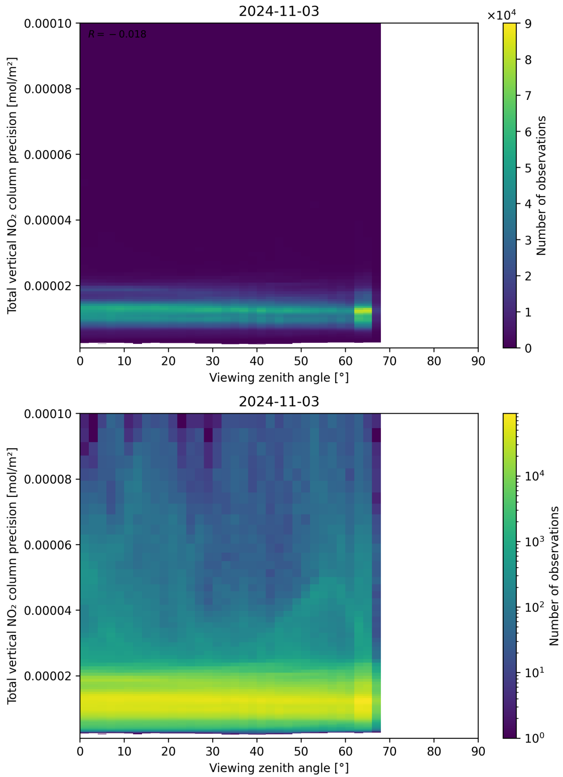
Figure 168: Scatter density plot of “Viewing zenith angle” against “Total vertical NO 2 column precision” for 2024-11-02 to 2024-11-04.
