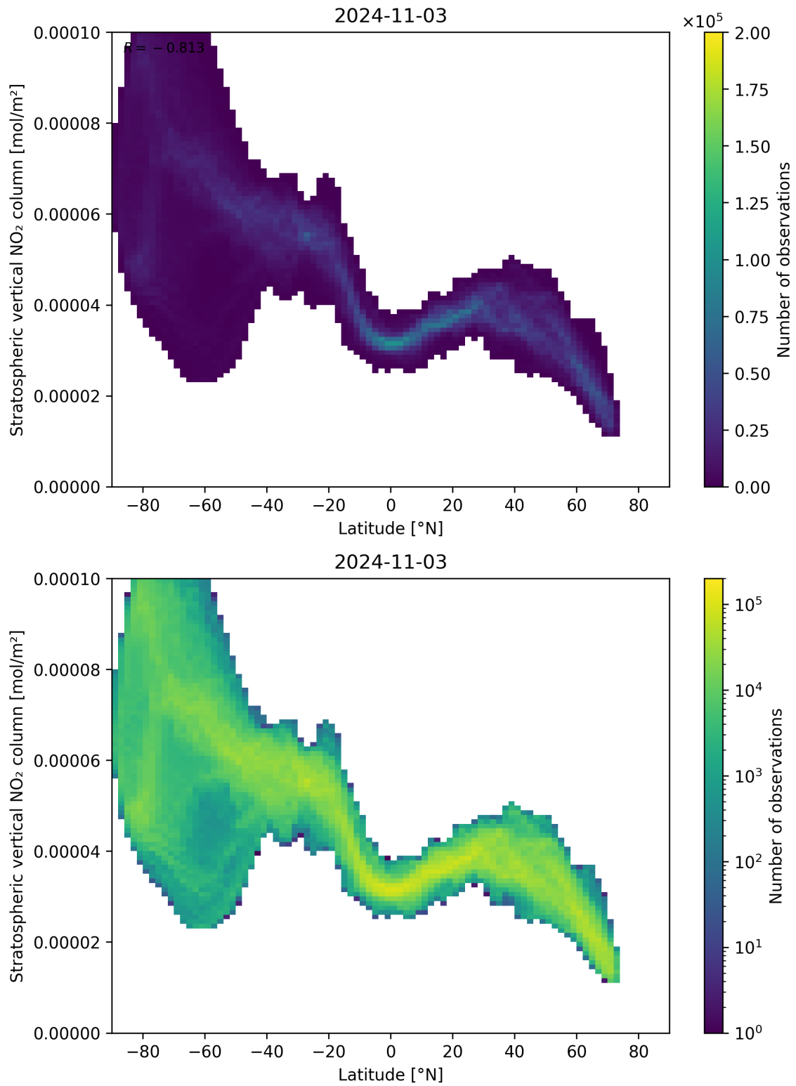
Figure 87: Scatter density plot of “Latitude” against “Stratospheric vertical NO 2 column” for 2024-11-02 to 2024-11-04.
