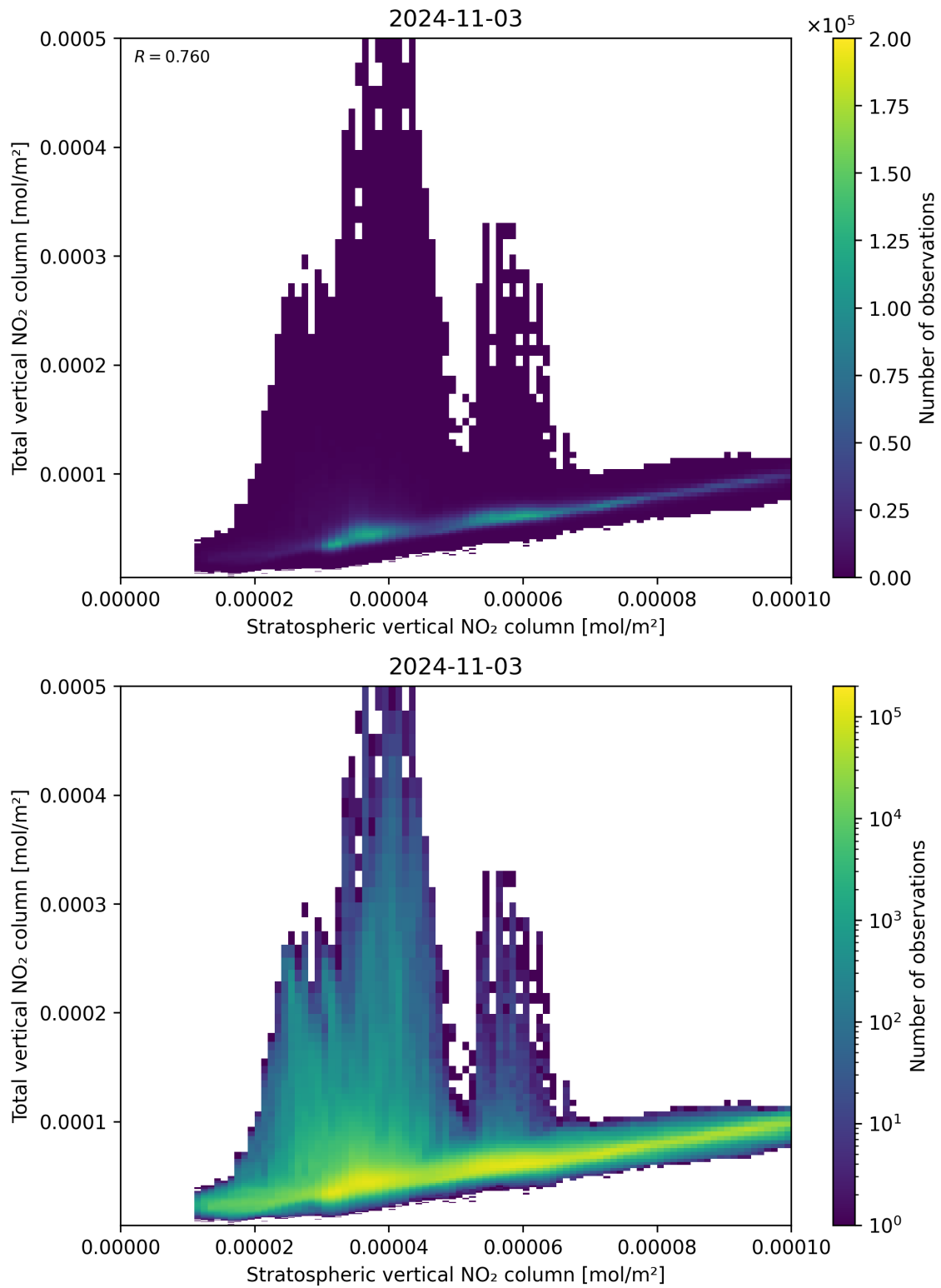
Figure 100: Scatter density plot of “Stratospheric vertical NO 2 column” against “Total vertical NO 2 column” for 2024-11-02 to 2024-11-04.
