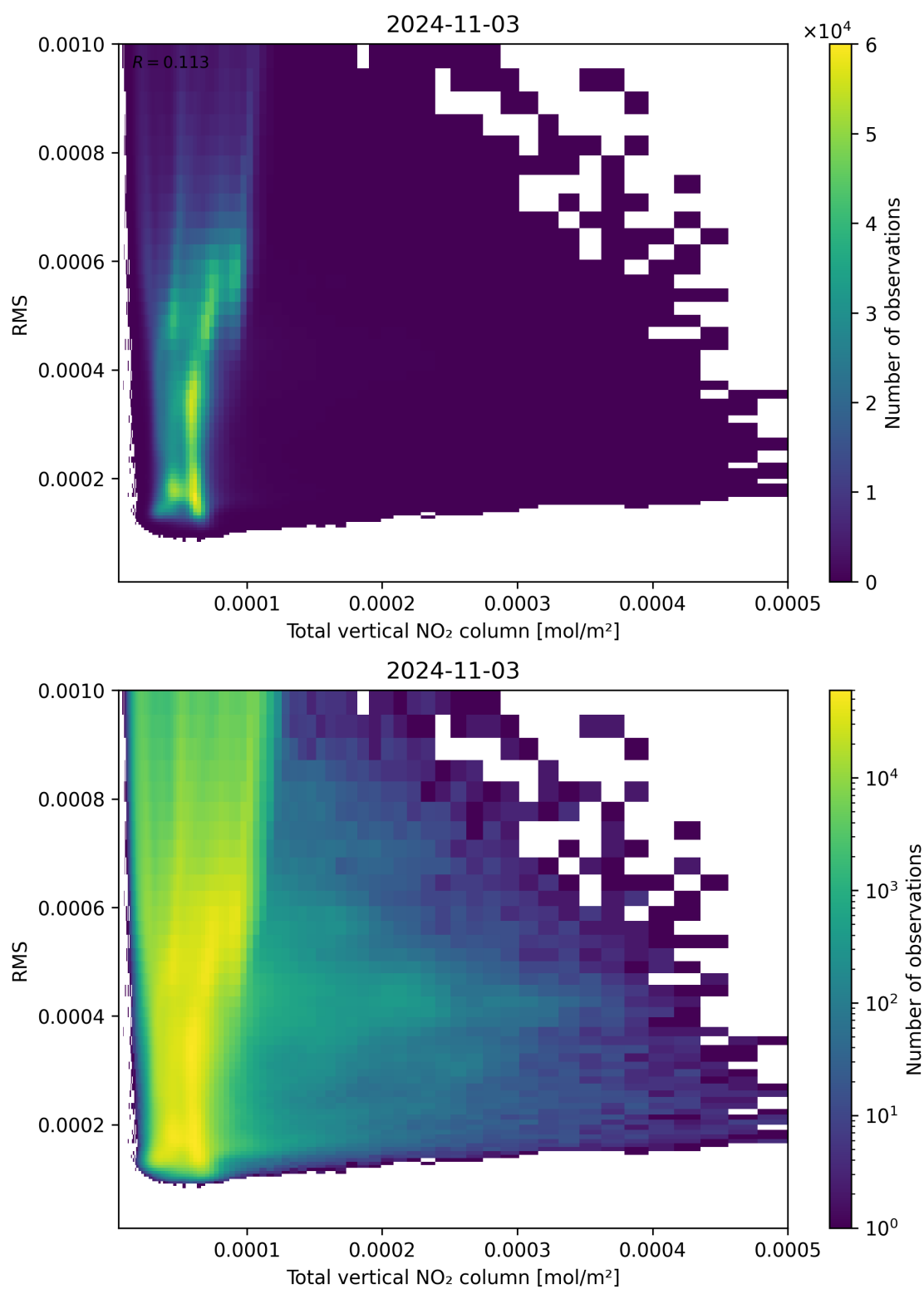
Figure 120: Scatter density plot of “Total vertical NO 2 column” against “RMS” for 2024-11-02 to 2024-11-04.
