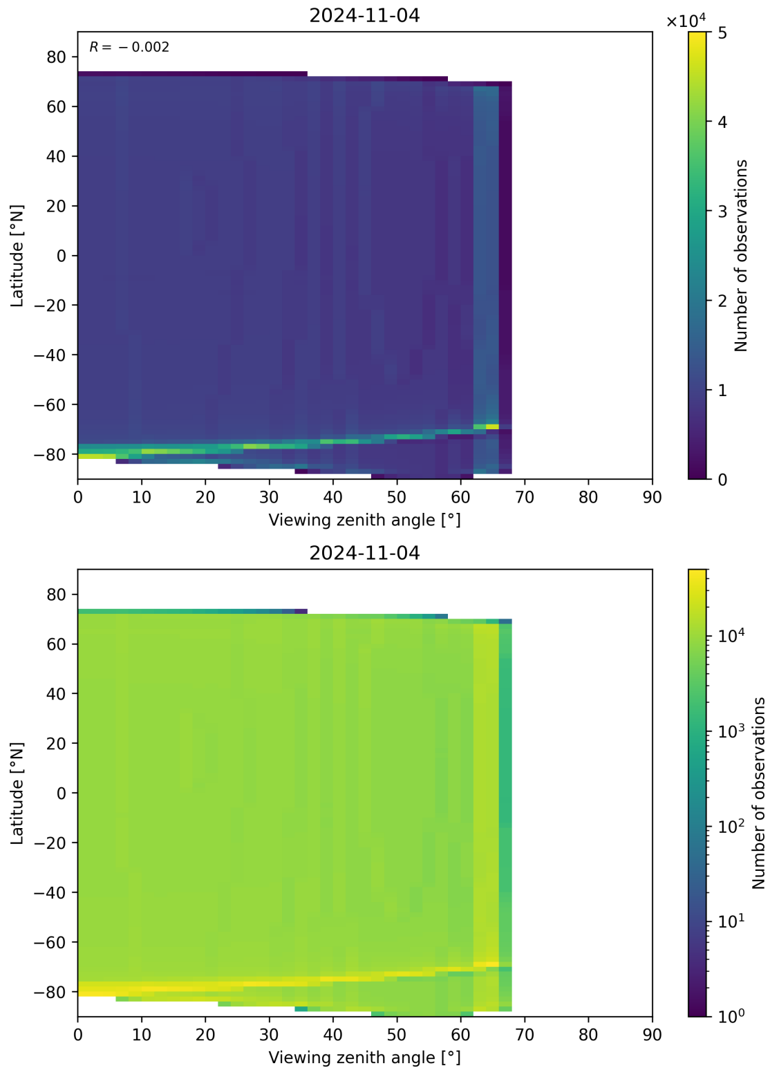
Figure 163: Scatter density plot of “Viewing zenith angle” against “Latitude” for 2024-11-04 to 2024-11-05.
