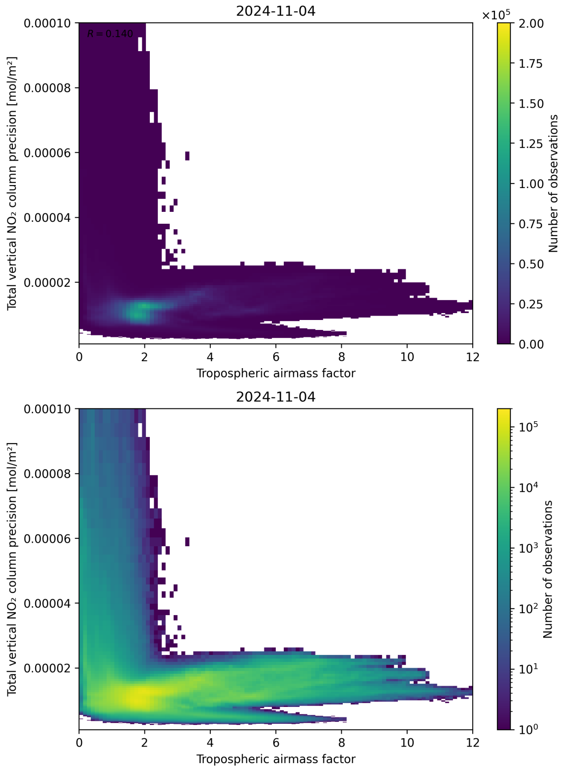
Figure 78: Scatter density plot of “Tropospheric air mass factor” against “Total vertical NO 2 column precision” for 2024-11-04 to 2024-11-05.
