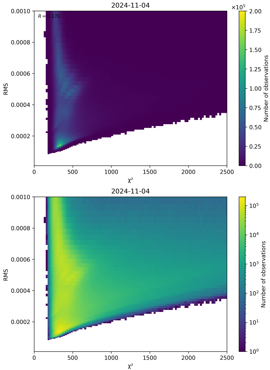
Figure 82: Scatter density plot of “ \chi^2 ” against “RMS” for 2024-11-04 to 2024-11-05.
