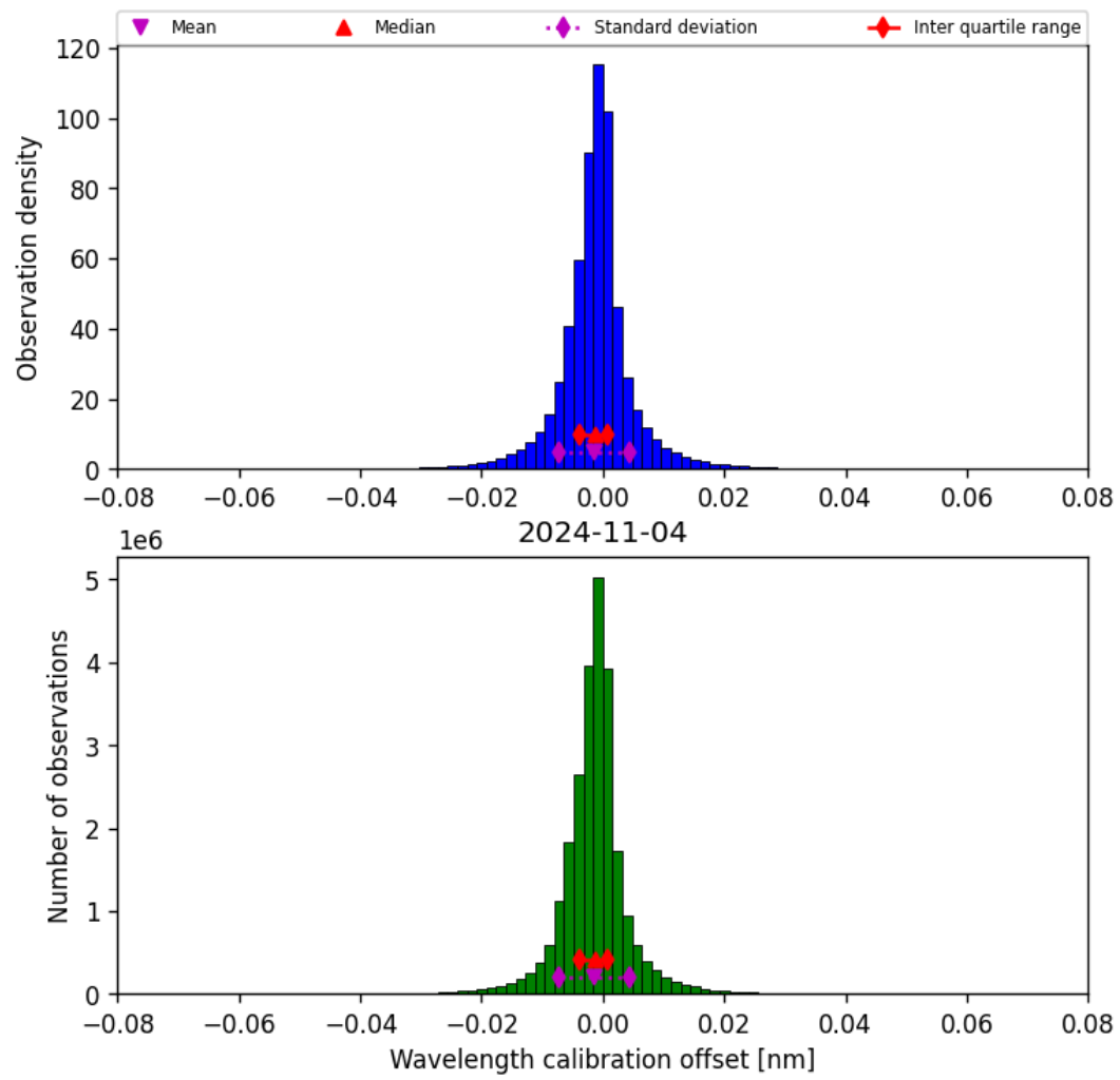
Figure 35: Histogram of “Wavelength calibration offset” for 2024-11-04 to 2024-11-05
