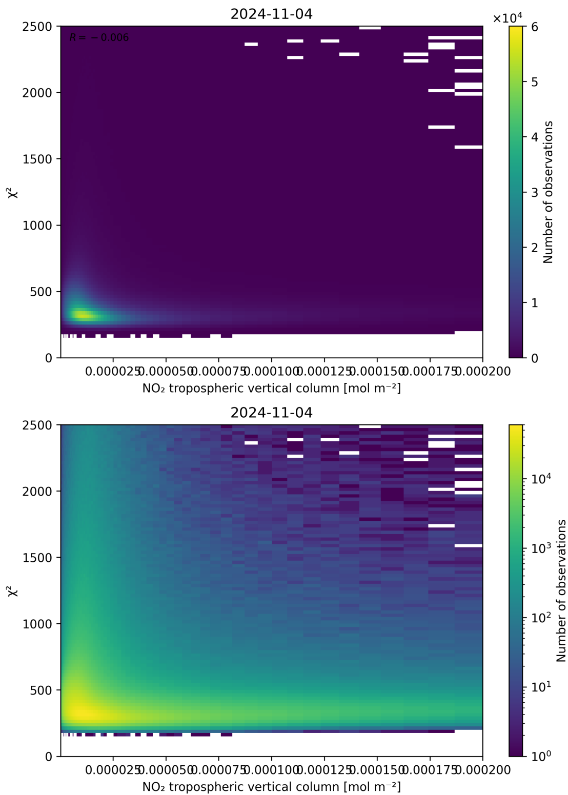
Figure 124: Scatter density plot of “NO 2 tropospheric vertical column” against “ \chi^2 ” for 2024-11-04 to 2024-11-05.
