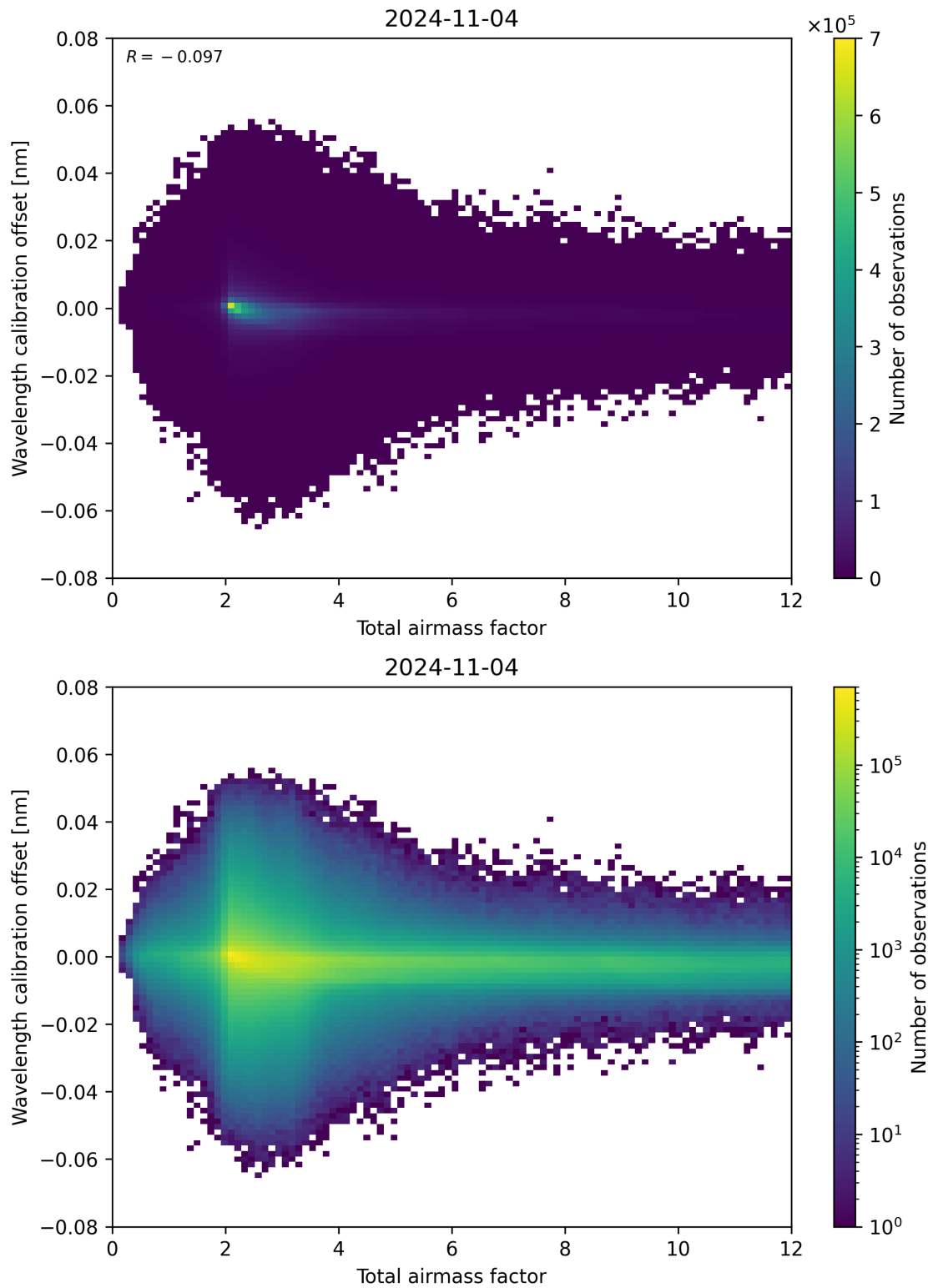
Figure 70: Scatter density plot of “Total airmass factor” against “Wavelength calibration offset” for 2024-11-04 to 2024-11-05.
