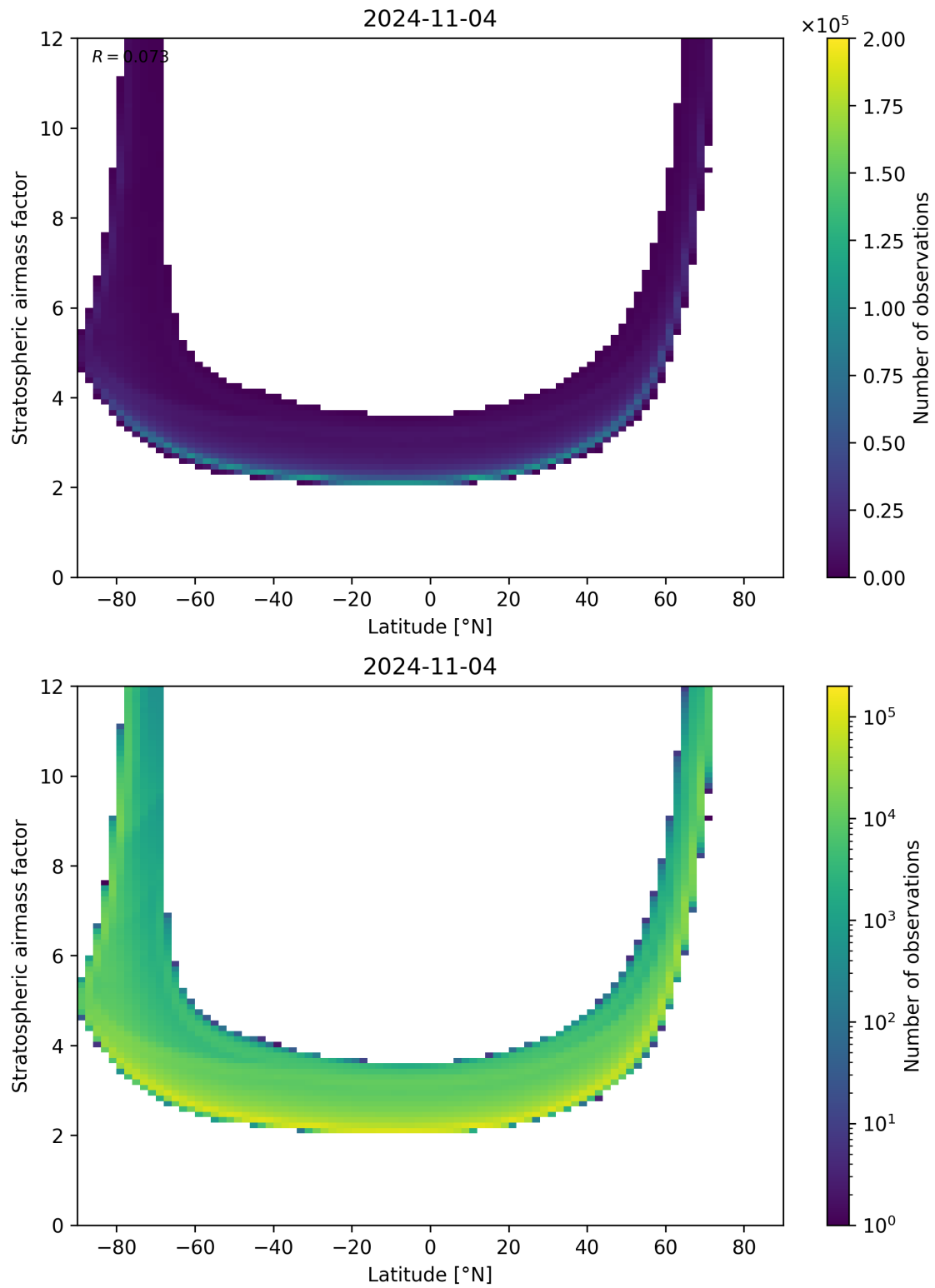
Figure 83: Scatter density plot of “Latitude” against “Stratospheric air mass factor” for 2024-11-04 to 2024-11-05.
