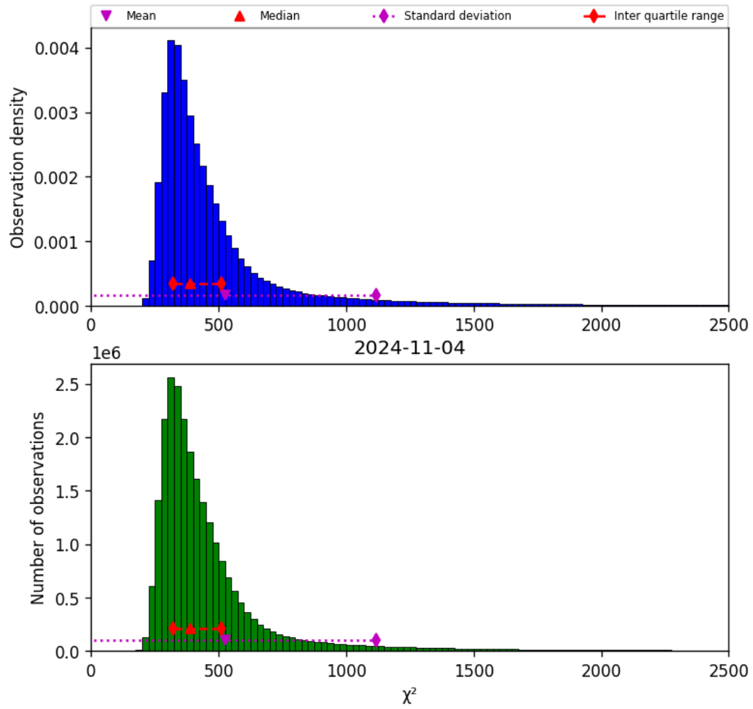
Figure 42: Histogram of “ \chi^2 ” for 2024-11-04 to 2024-11-05
