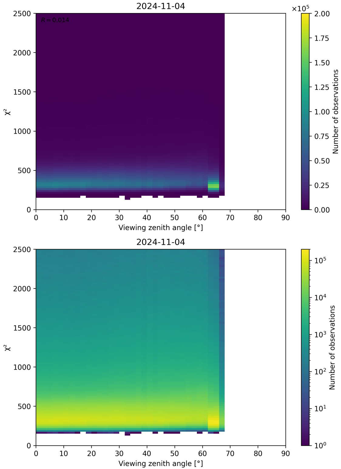
Figure 162: Scatter density plot of “Viewing zenith angle” against “ \chi^2 ” for 2024-11-04 to 2024-11-05.
