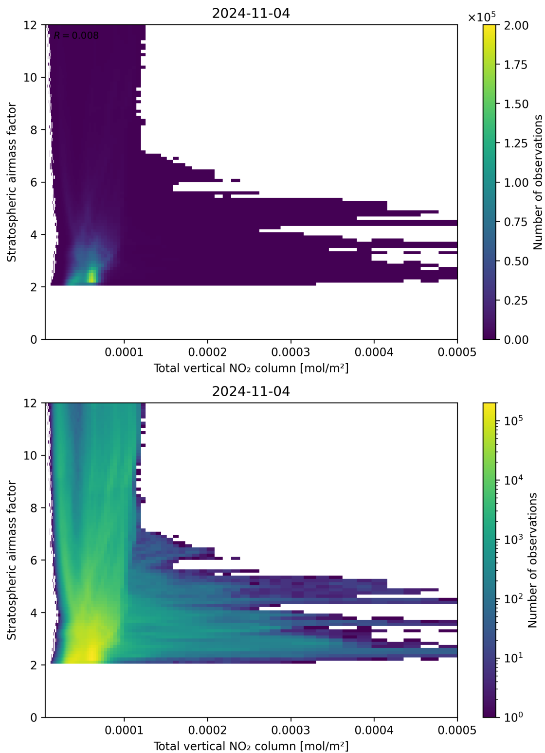
Figure 110: Scatter density plot of “Total vertical NO 2 column” against “Stratospheric airmass factor” for 2024-11-04 to 2024-11-05.
