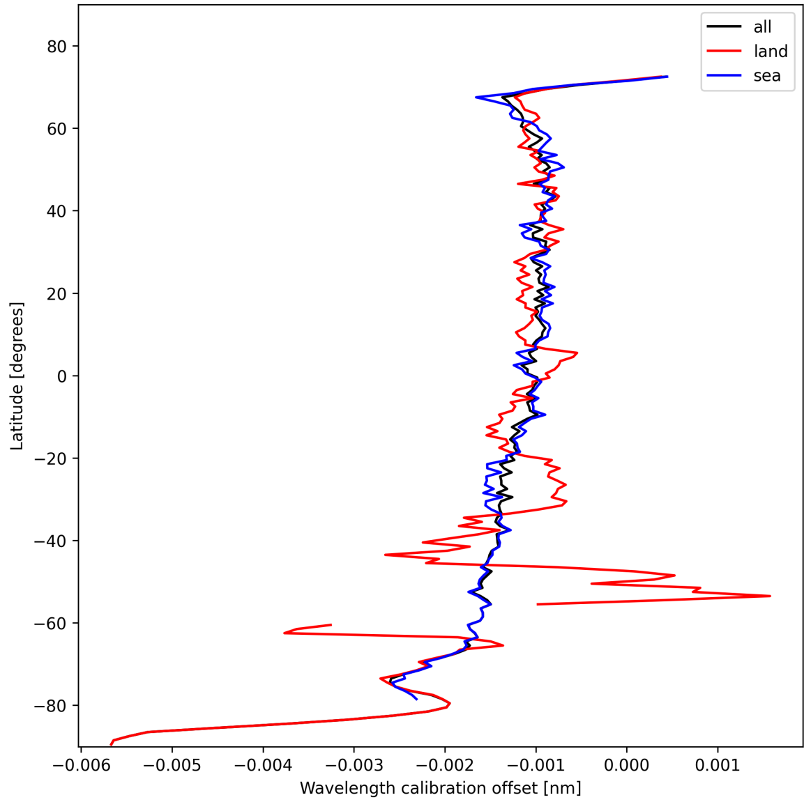
Figure 18: Zonal average of “Wavelength calibration offset” for 2024-11-04 to 2024-11-05.
