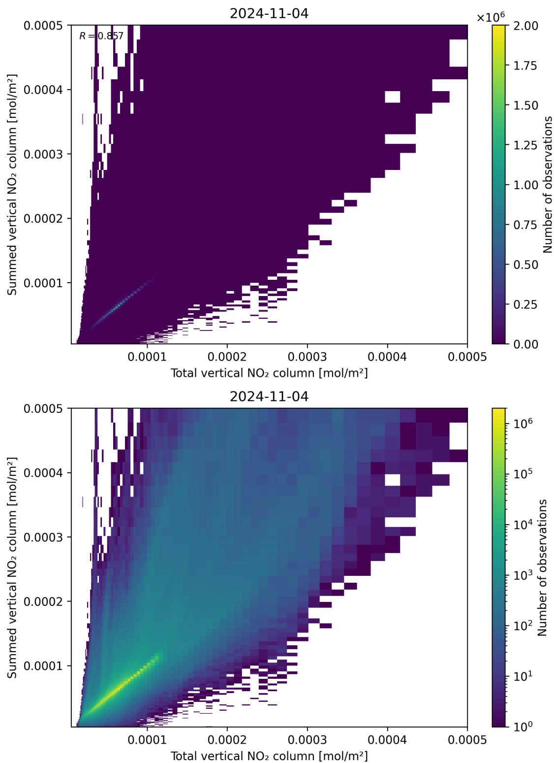
Figure 112: Scatter density plot of “Total vertical NO 2 column” against “Summed vertical NO 2 column” for 2024-11-04 to 2024-11-05.
