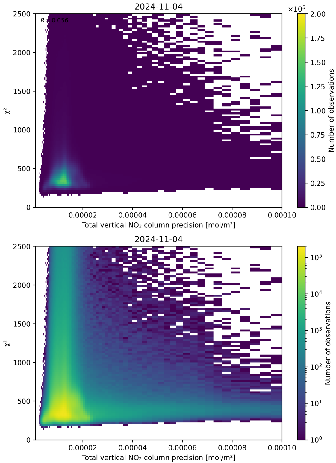
Figure 116: Scatter density plot of “Total vertical NO 2 column precision” against “ \chi^2 ” for 2024-11-04 to 2024-11-05.
