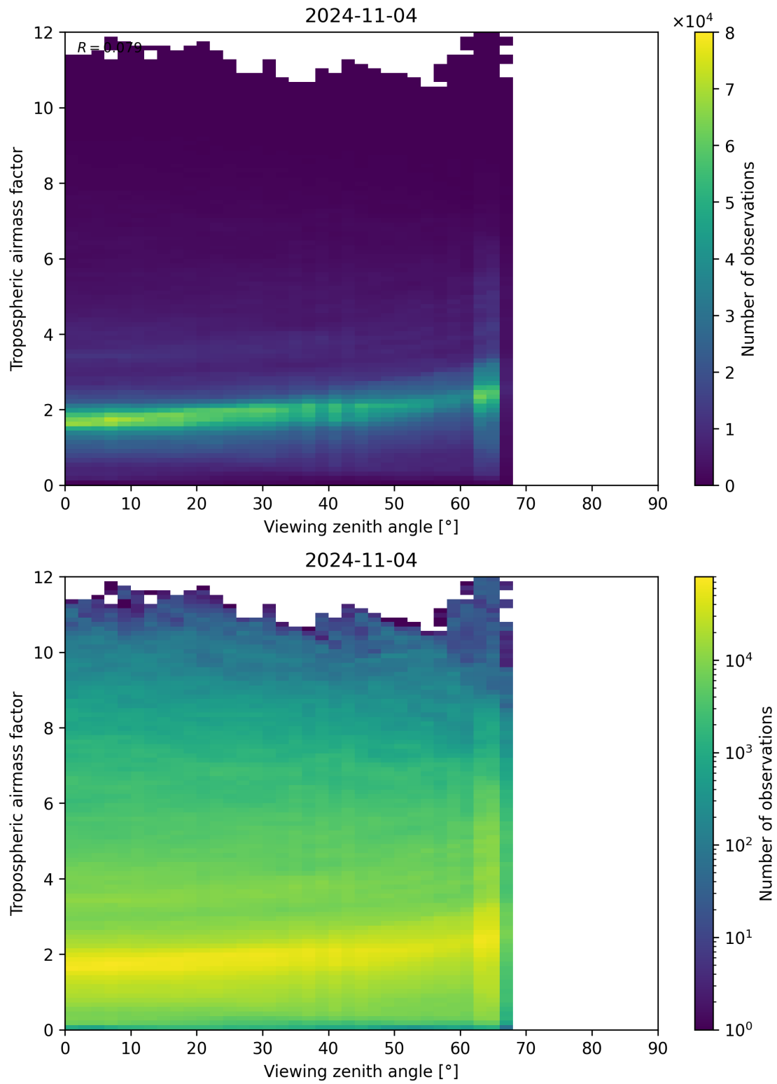
Figure 161: Scatter density plot of “Viewing zenith angle” against “Tropospheric airmass factor” for 2024-11-04 to 2024-11-05.
