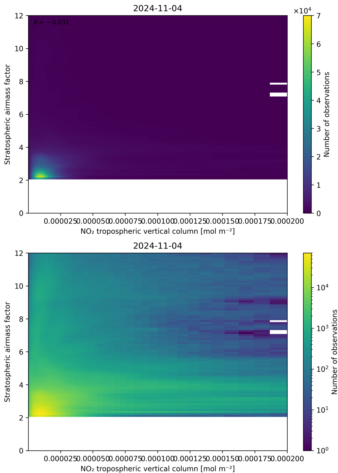
Figure 121: Scatter density plot of “NO 2 tropospheric vertical column” against “Stratospheric airmass factor” for 2024-11-04 to 2024-11-05.
