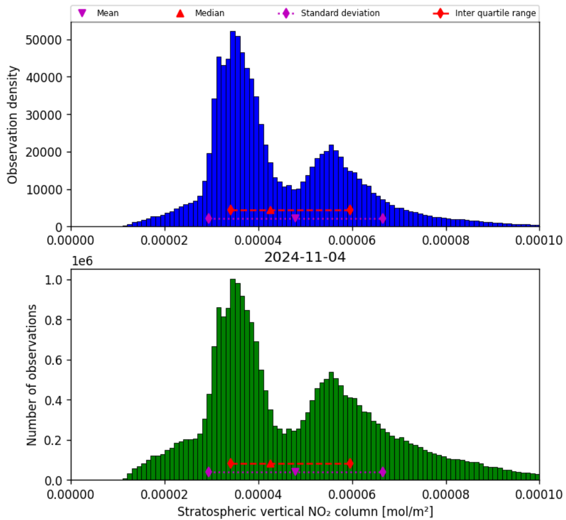
Figure 36: Histogram of “Stratospheric vertical NO 2 column” for 2024-11-04 to 2024-11-05
