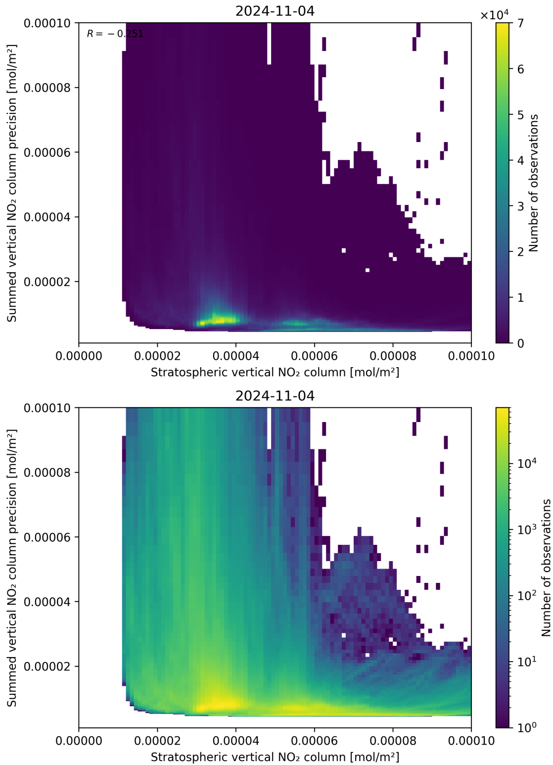
Figure 99: Scatter density plot of “Stratospheric vertical NO 2 column” against “Summed vertical NO 2 column precision” for 2024-11-04 to 2024-11-05.
