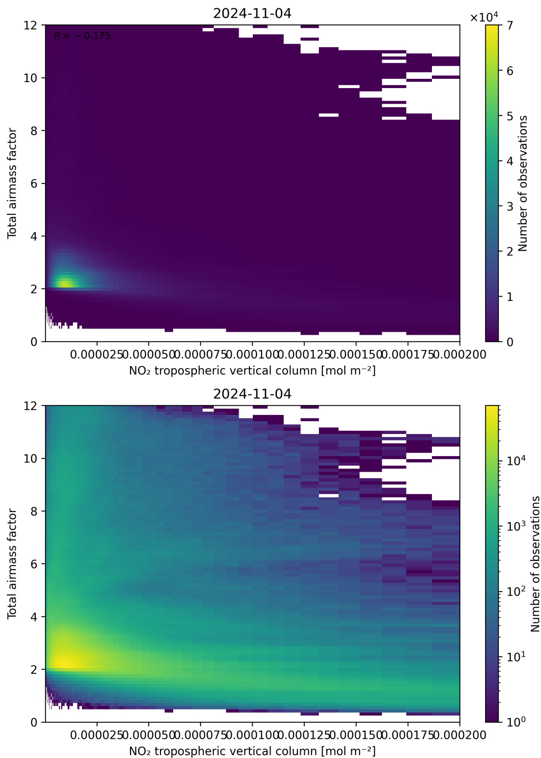
Figure 122: Scatter density plot of “NO 2 tropospheric vertical column” against “Total air mass factor” for 2024-11-04 to 2024-11-05.
