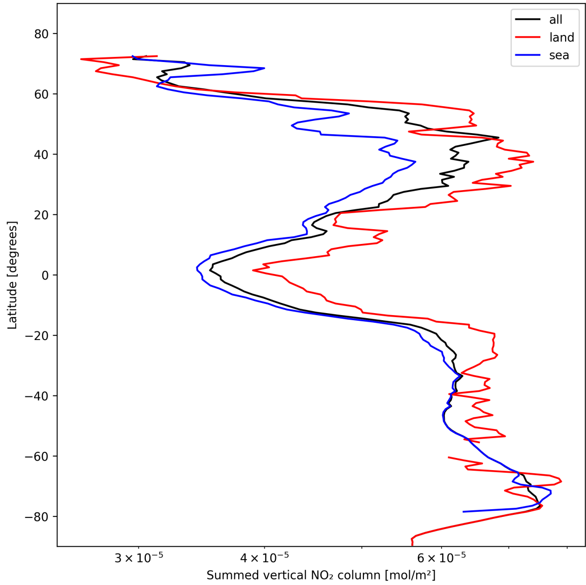
Figure 23: Zonal average of “Summed vertical NO 2 column” for 2024-11-04 to 2024-11-05.
