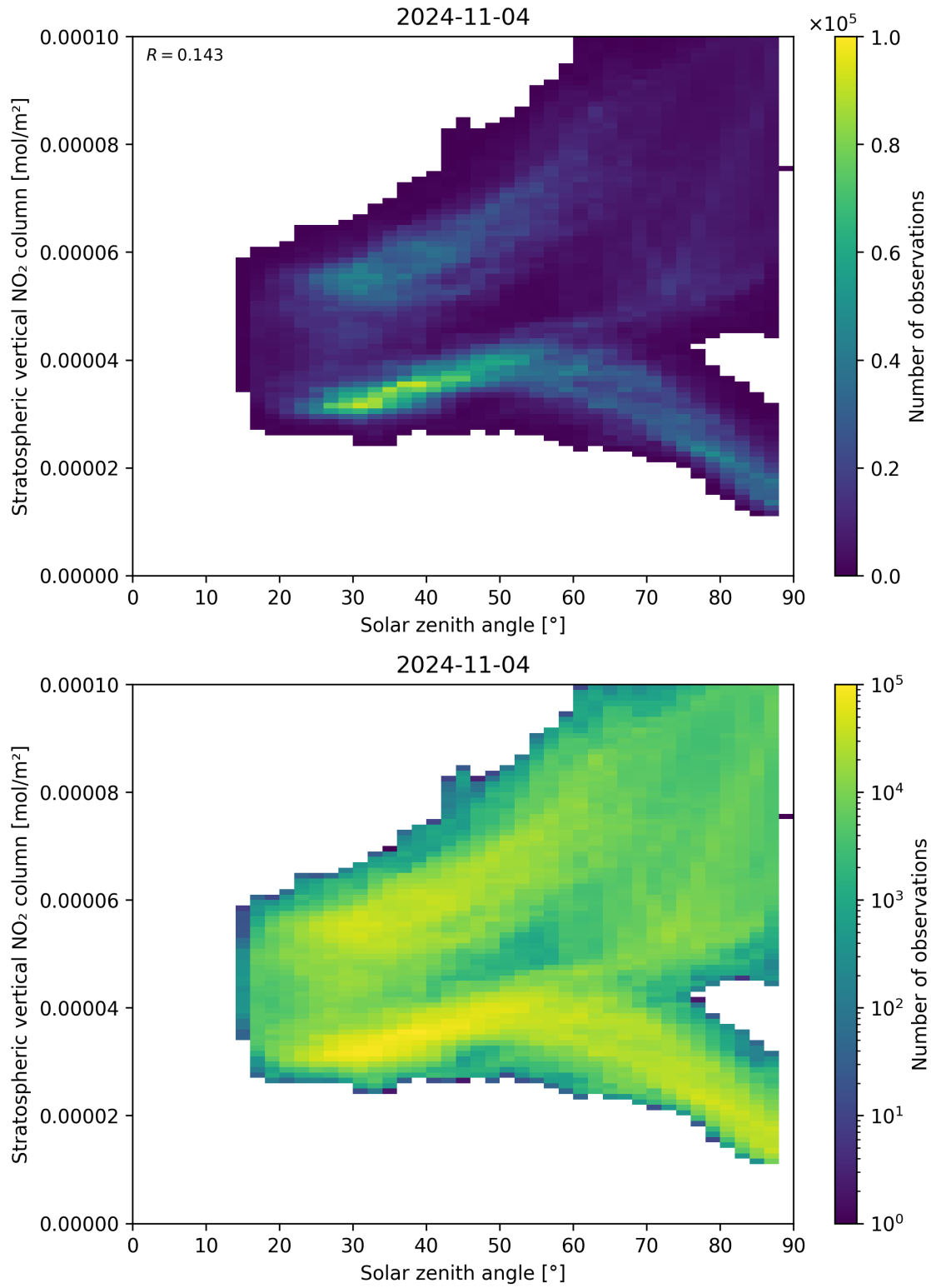
Figure 150: Scatter density plot of “Solar zenith angle” against “Stratospheric vertical NO 2 column” for 2024-11-04 to 2024-11-05.
