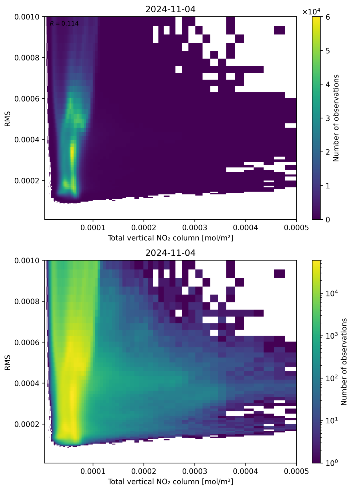
Figure 120: Scatter density plot of “Total vertical NO 2 column” against “RMS” for 2024-11-04 to 2024-11-05.
