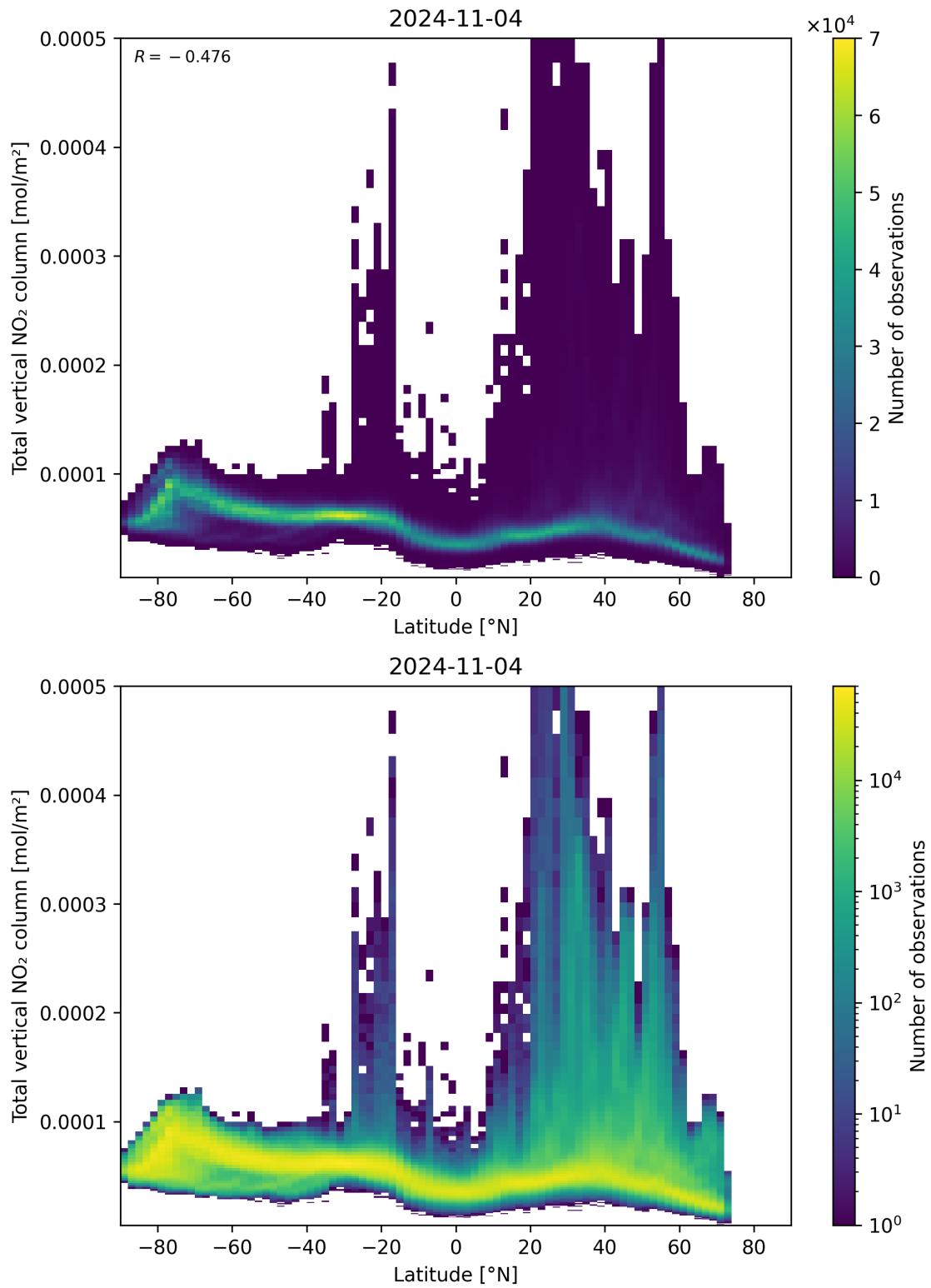
Figure 90: Scatter density plot of “Latitude” against “Total vertical NO 2 column” for 2024-11-04 to 2024-11-05.
