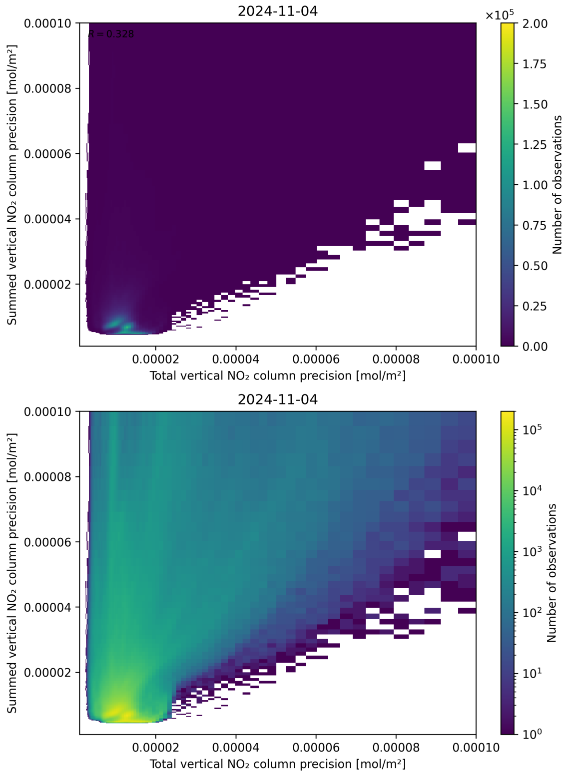
Figure 118: Scatter density plot of “Total vertical NO 2 column precision” against “Summed vertical NO 2 column precision” for 2024-11-04 to 2024-11-05.
