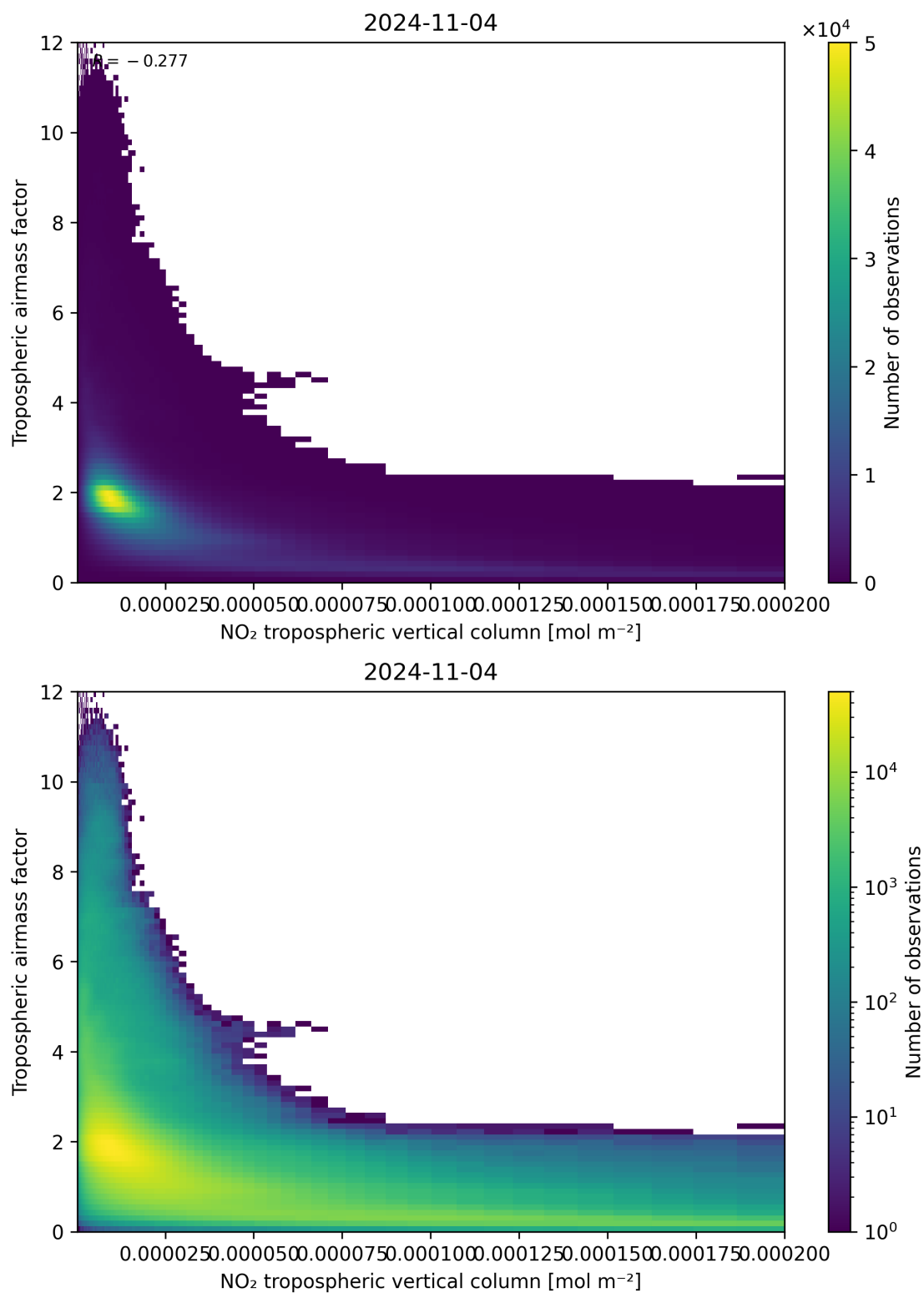
Figure 123: Scatter density plot of “NO 2 tropospheric vertical column” against “Tropospheric air mass factor” for 2024-11-04 to 2024-11-05.
