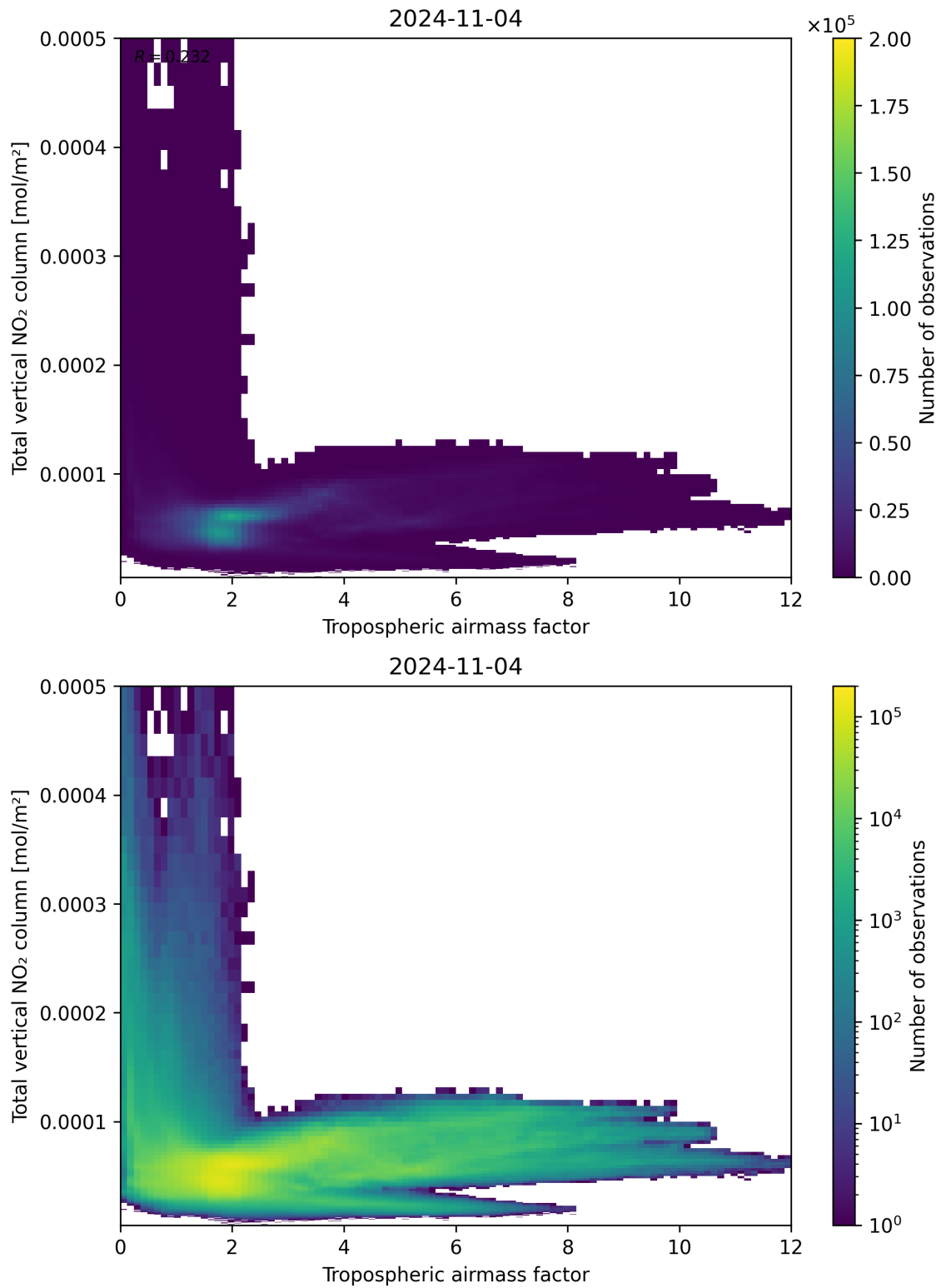
Figure 77: Scatter density plot of “Tropospheric airmass factor” against “Total vertical NO 2 column” for 2024-11-04 to 2024-11-05.
