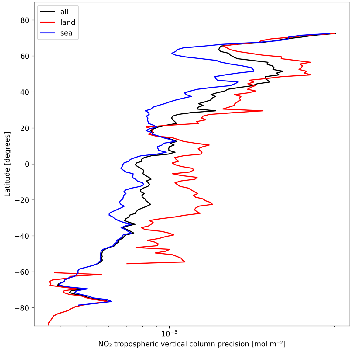
Figure 13: Zonal average of “NO 2 tropospheric vertical column precision” for 2024-11-04 to 2024-11-05.
