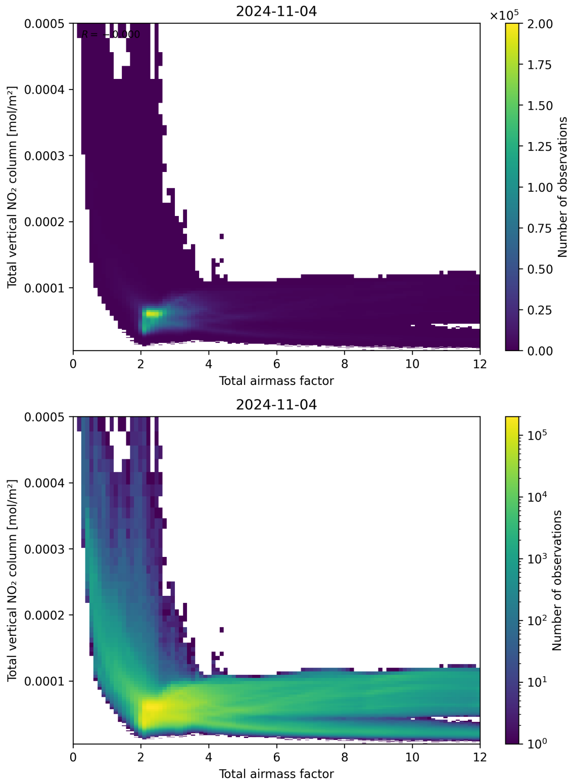
Figure 67: Scatter density plot of “Total airmass factor” against “Total vertical NO 2 column” for 2024-11-04 to 2024-11-05.
