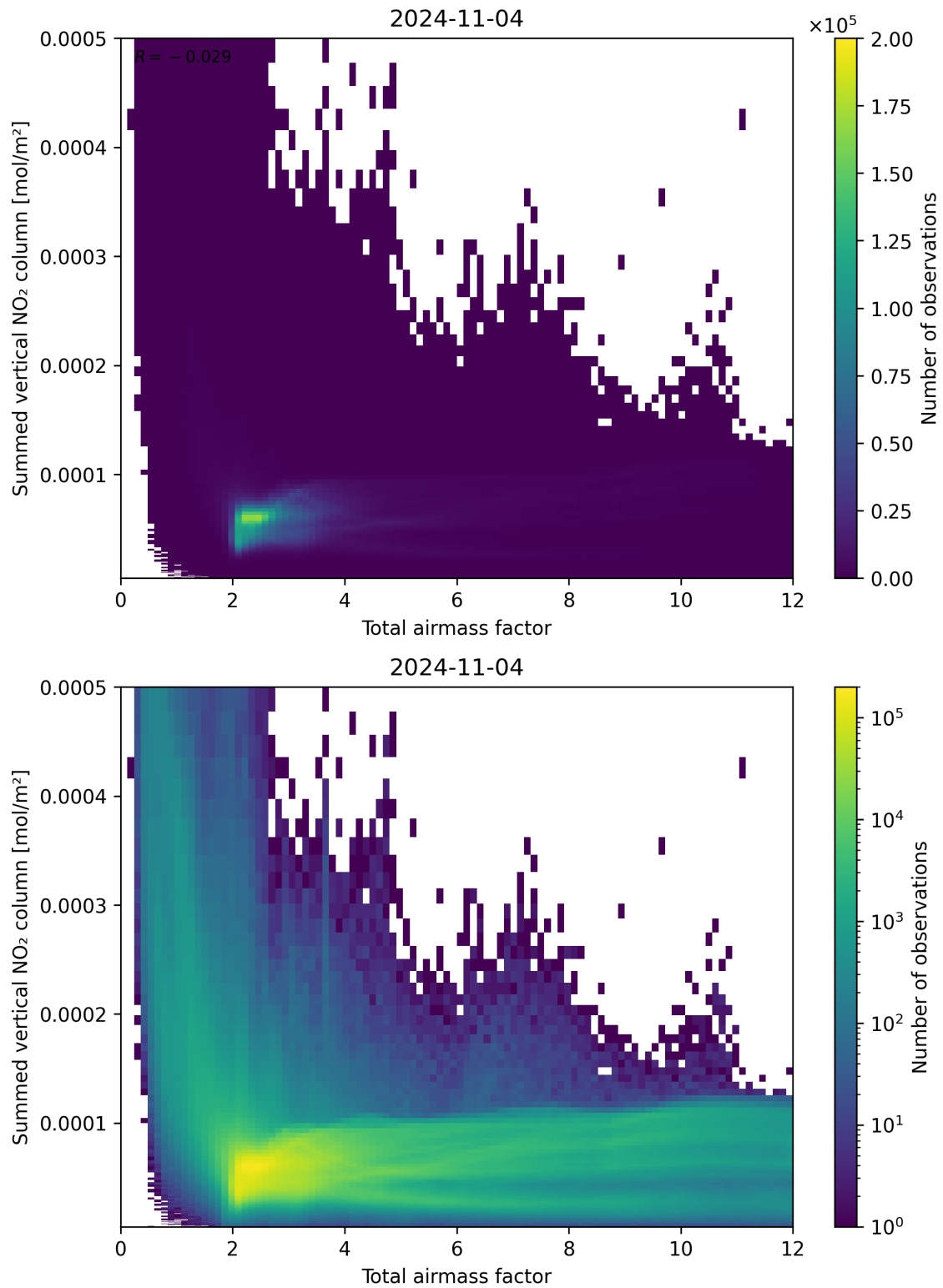
Figure 65: Scatter density plot of “Total airmass factor” against “Summed vertical NO 2 column” for 2024-11-04 to 2024-11-05.
