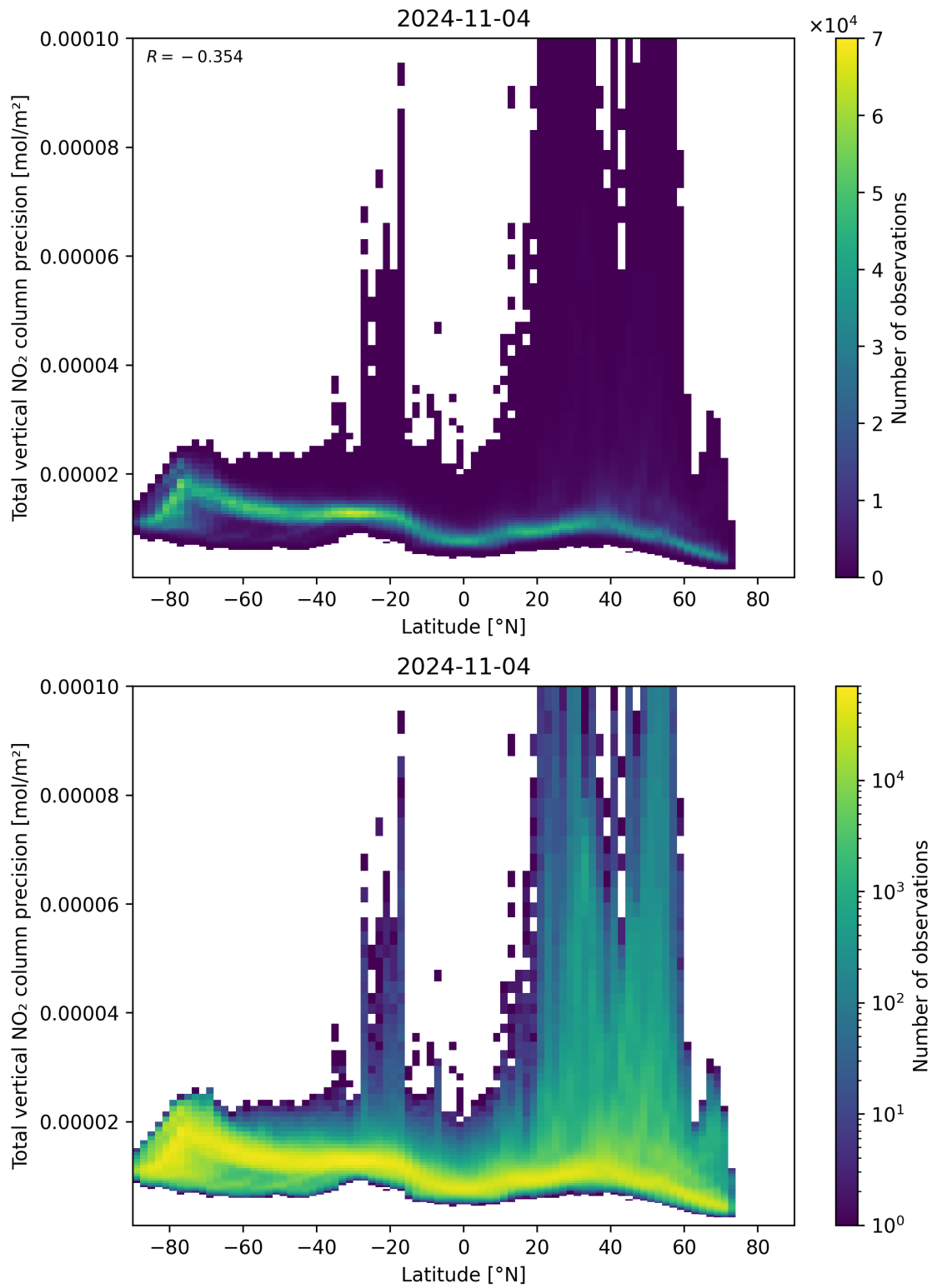
Figure 91: Scatter density plot of “Latitude” against “Total vertical NO 2 column precision” for 2024-11-04 to 2024-11-05.
