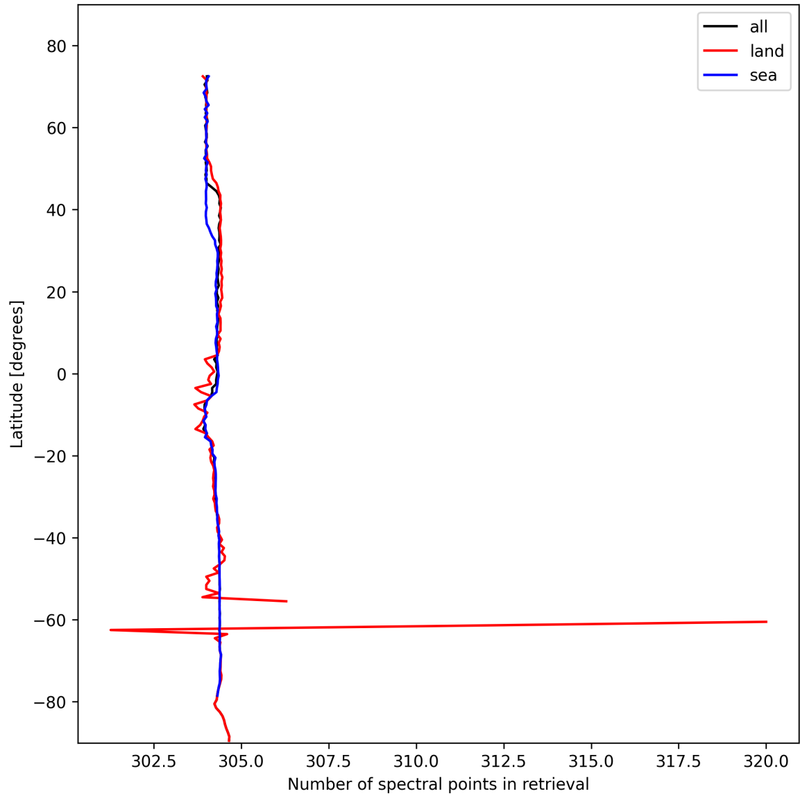
Figure 16: Zonal average of “Number of spectral points in retrieval” for 2024-11-04 to 2024-11-05.
