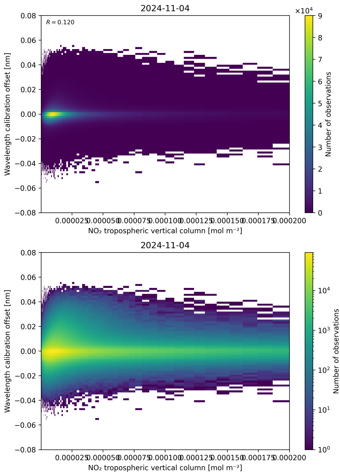
Figure 143: Scatter density plot of “NO 2 tropospheric vertical column” against “Wavelength calibration offset” for 2024-11-04 to 2024-11-05.
