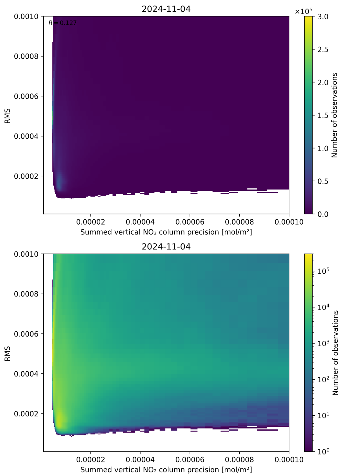
Figure 108: Scatter density plot of “Summed vertical NO 2 column precision” against “RMS” for 2024-11-04 to 2024-11-05.
