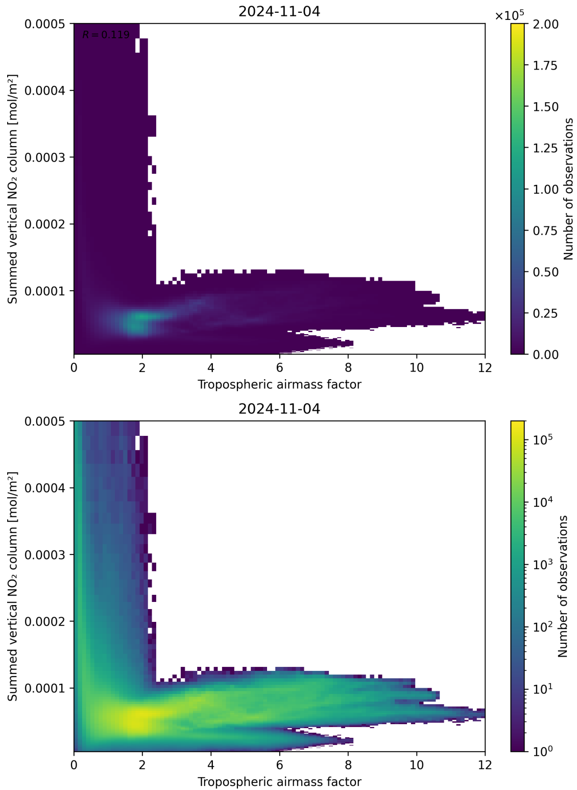
Figure 75: Scatter density plot of “Tropospheric airmass factor” against “Summed vertical NO 2 column” for 2024-11-04 to 2024-11-05.
