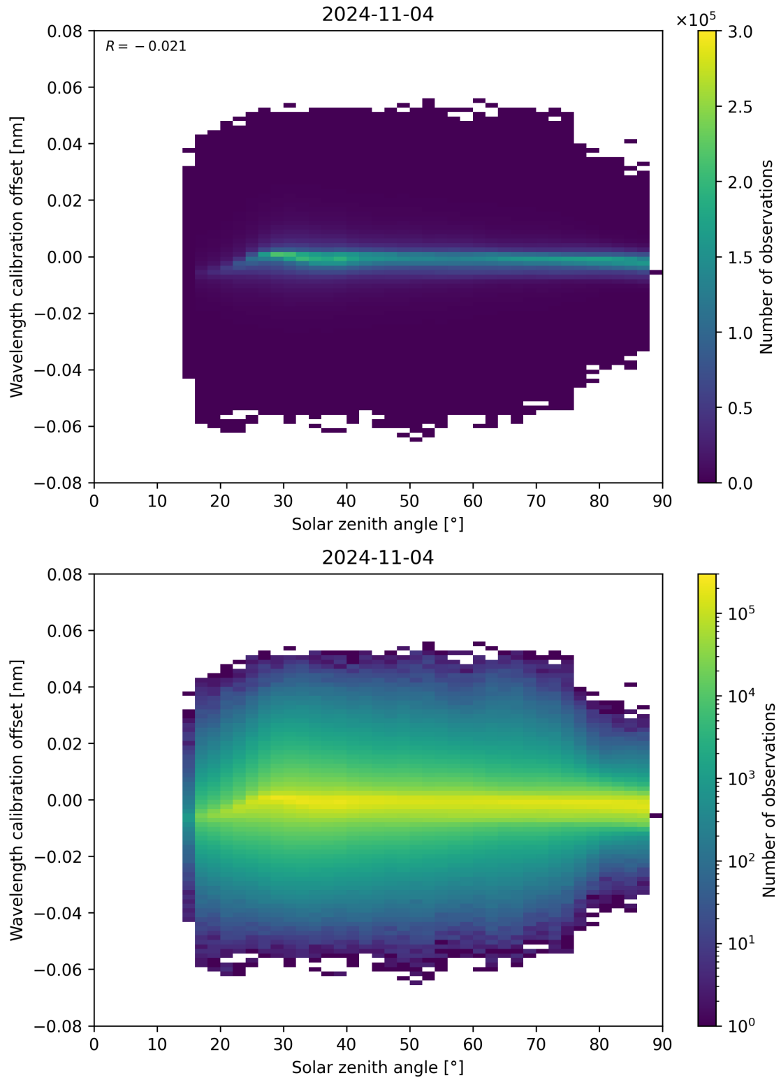
Figure 158: Scatter density plot of “Solar zenith angle” against “Wavelength calibration offset” for 2024-11-04 to 2024-11-05.
