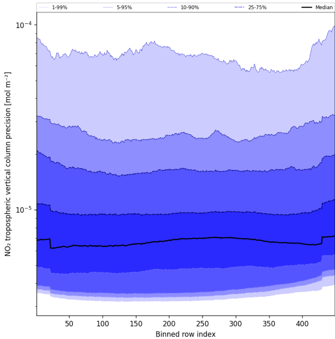
Figure 47: Along track statistics of “NO 2 tropospheric vertical column precision” for 2024-11-04 to 2024-11-05
