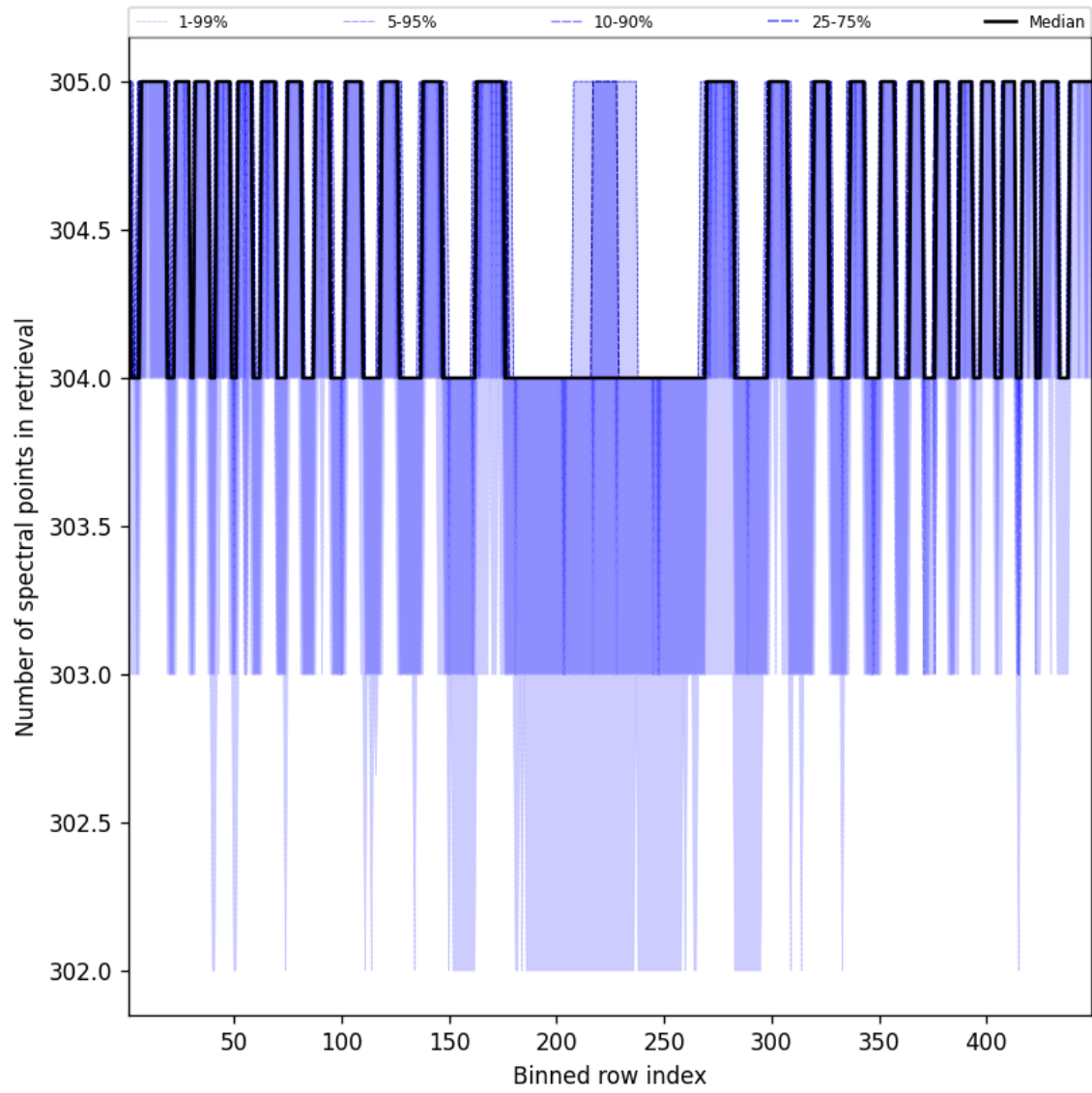
Figure 50: Along track statistics of “Number of spectral points in retrieval” for 2024-11-04 to 2024-11-05
