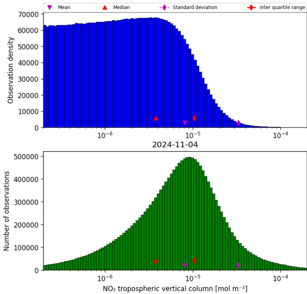
Figure 29: Histogram of “NO 2 tropospheric vertical column” for 2024-11-04 to 2024-11-05
