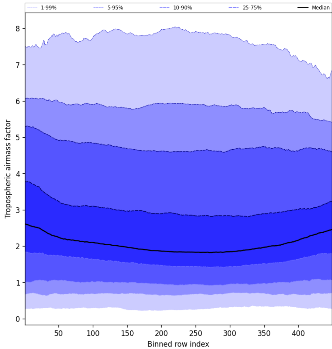
Figure 48: Along track statistics of “Tropospheric airmass factor” for 2024-11-04 to 2024-11-05
