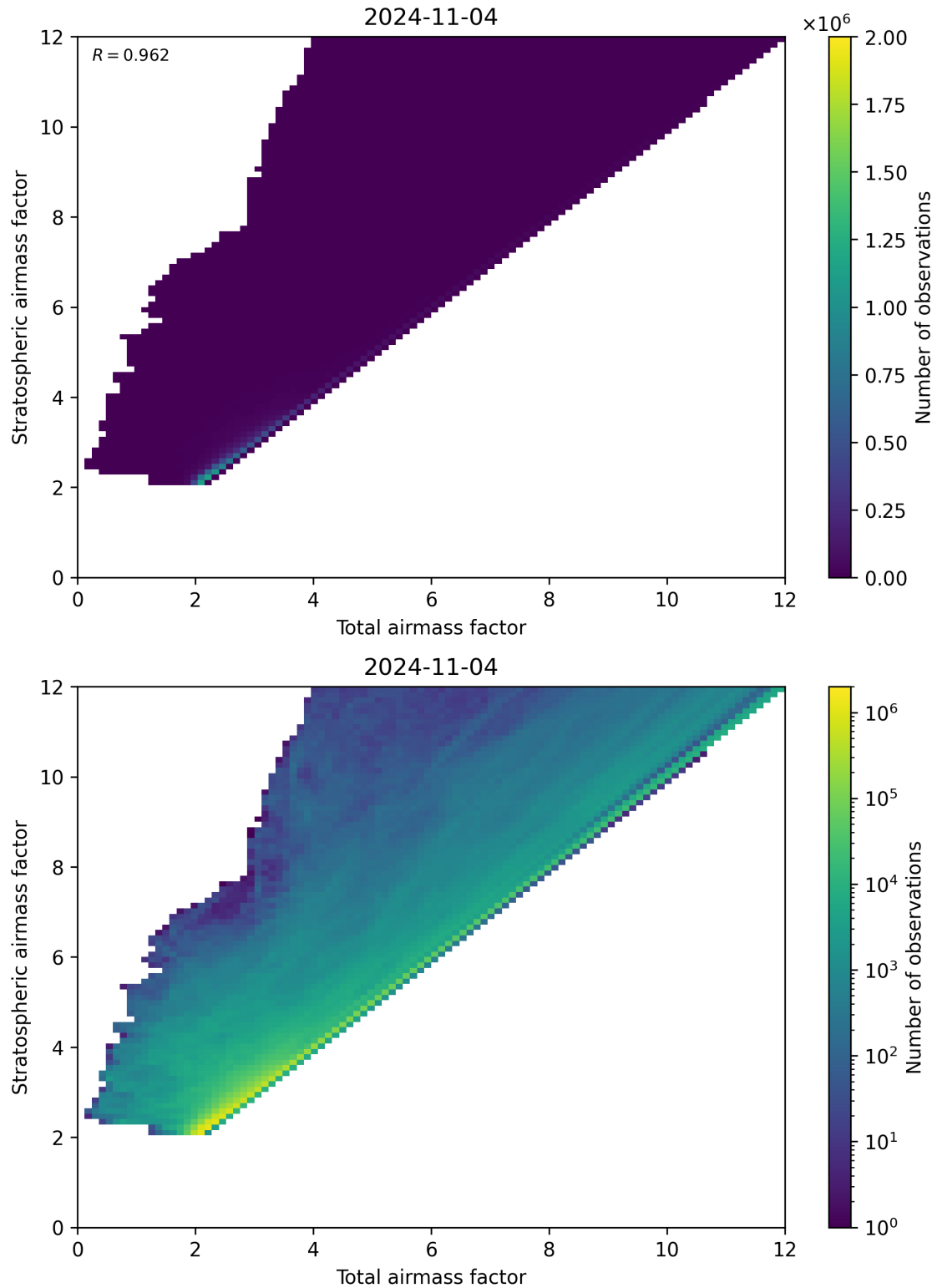
Figure 62: Scatter density plot of “Total airmass factor” against “Stratospheric airmass factor” for 2024-11-04 to 2024-11-05.
