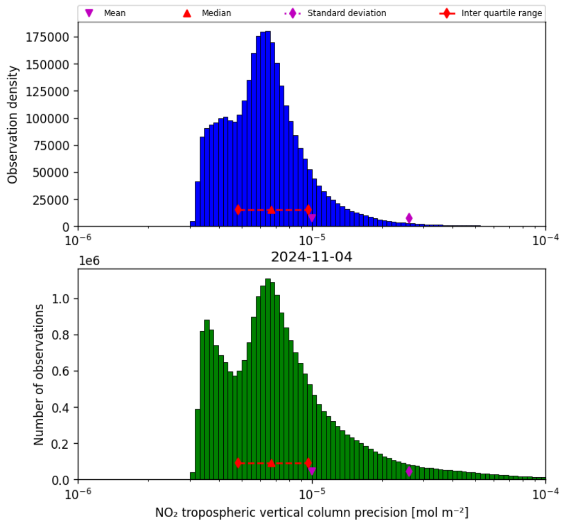
Figure 30: Histogram of “NO 2 tropospheric vertical column precision” for 2024-11-04 to 2024-11-05
