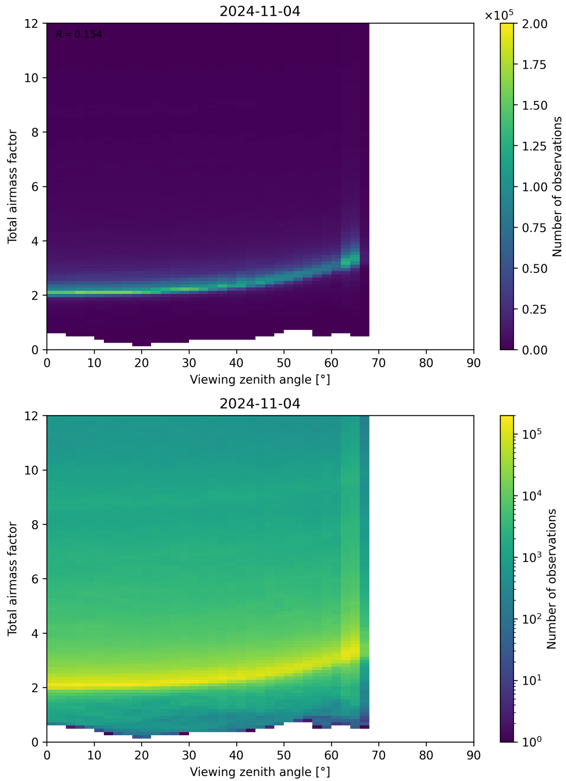
Figure 160: Scatter density plot of “Viewing zenith angle” against “Total airmass factor” for 2024-11-04 to 2024-11-05.
