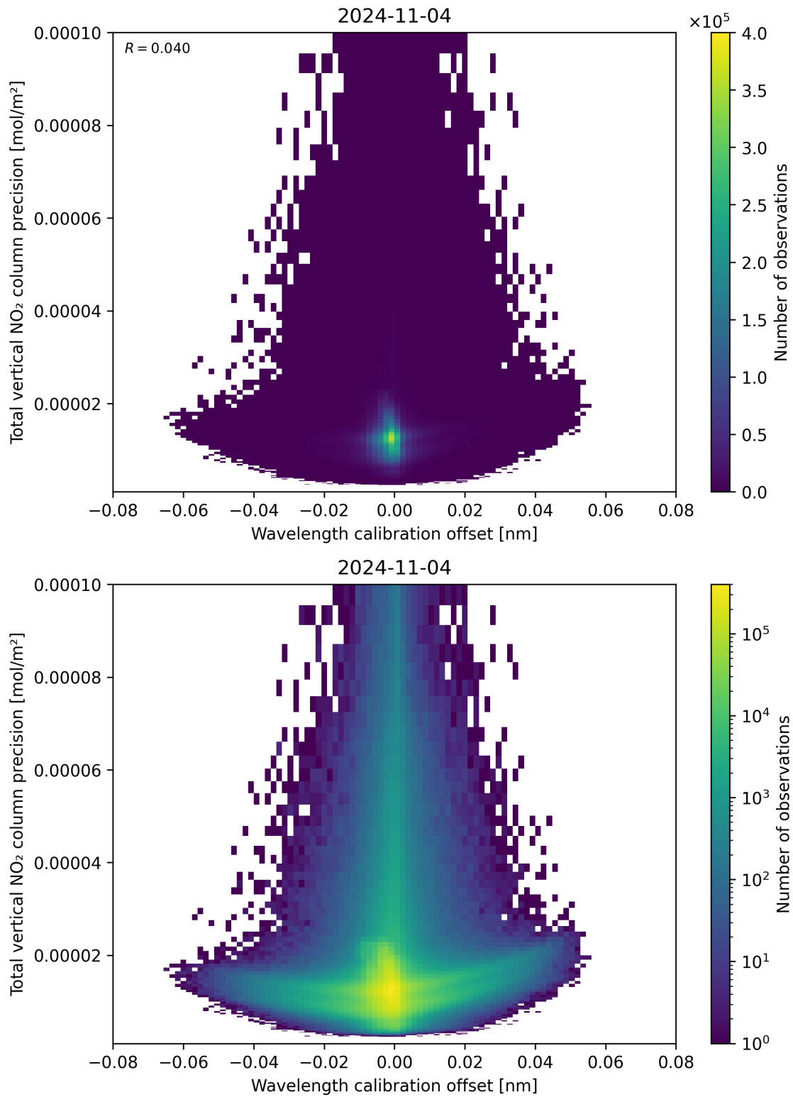
Figure 180: Scatter density plot of “Wavelength calibration offset” against “Total vertical NO 2 column precision” for 2024-11-04 to 2024-11-05.
