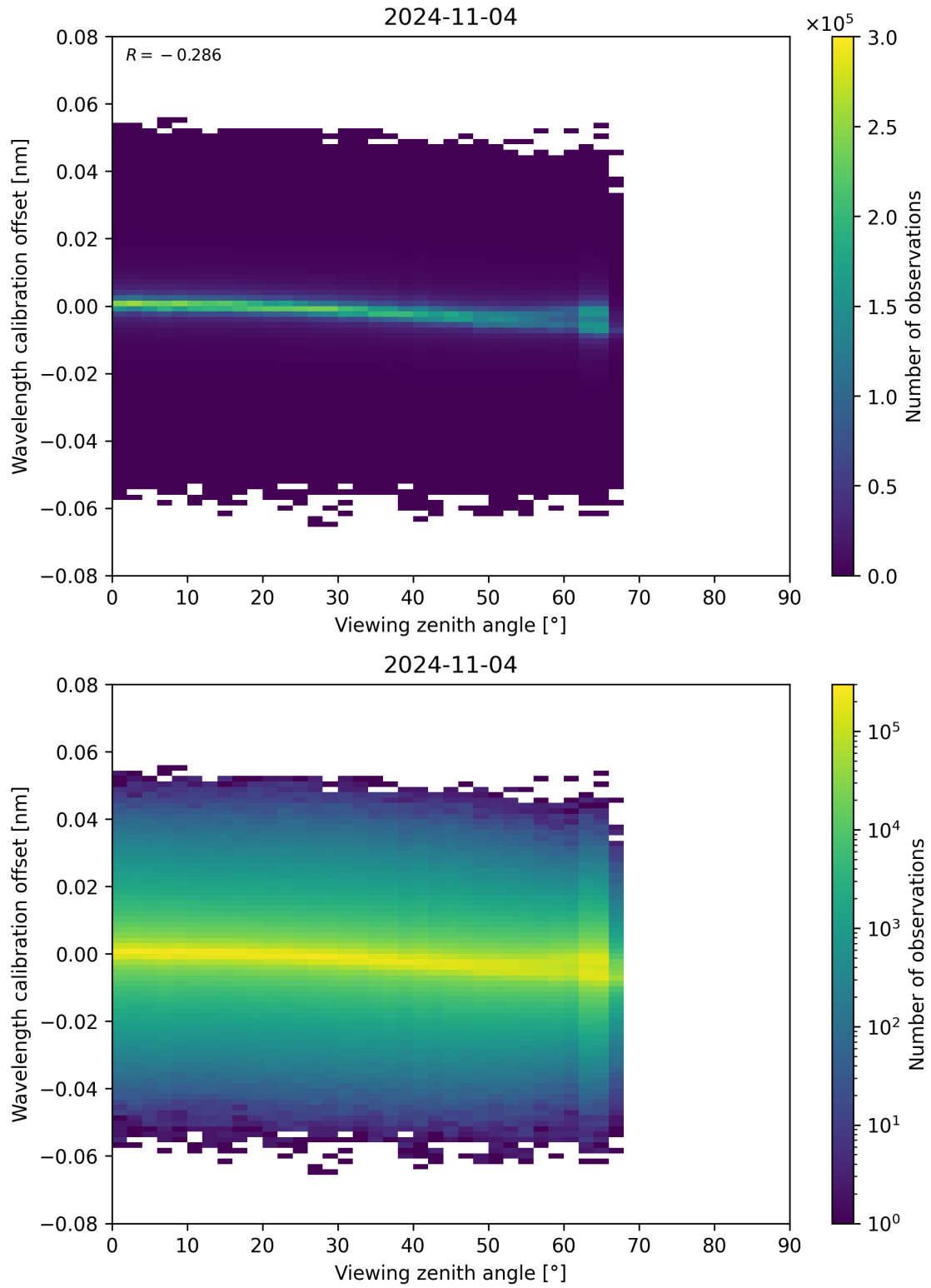
Figure 173: Scatter density plot of “Viewing zenith angle” against “Wavelength calibration offset” for 2024-11-04 to 2024-11-05.
