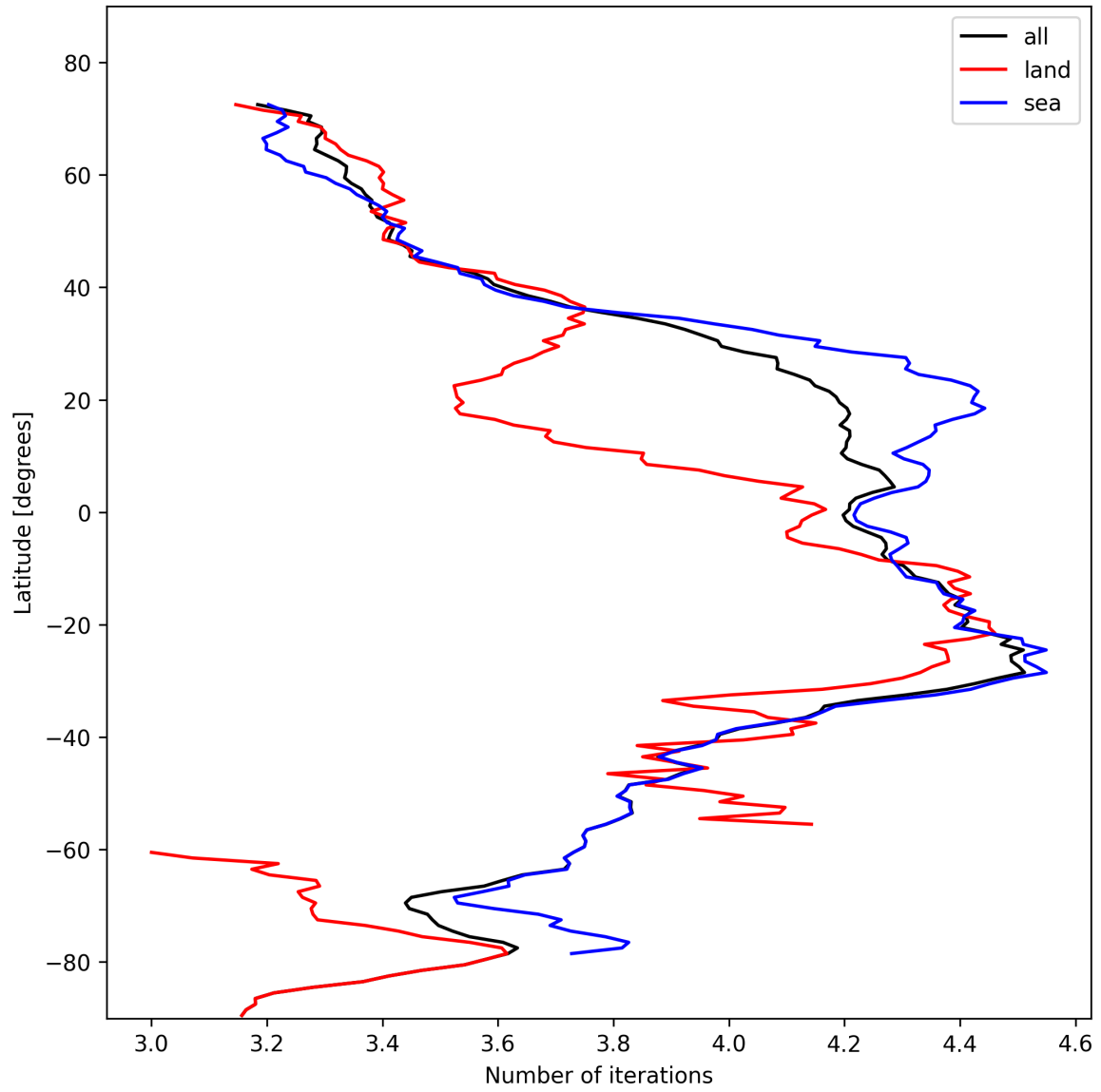
Figure 17: Zonal average of “Number of iterations” for 2024-11-04 to 2024-11-05.
