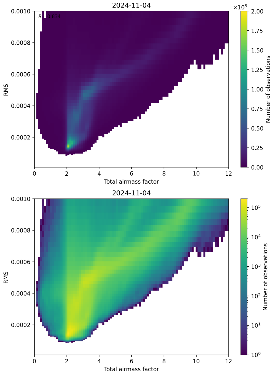
Figure 69: Scatter density plot of “Total airmass factor” against “RMS” for 2024-11-04 to 2024-11-05.
