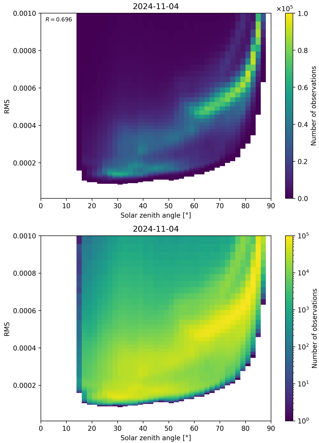
Figure 157: Scatter density plot of “Solar zenith angle” against “RMS” for 2024-11-04 to 2024-11-05.
