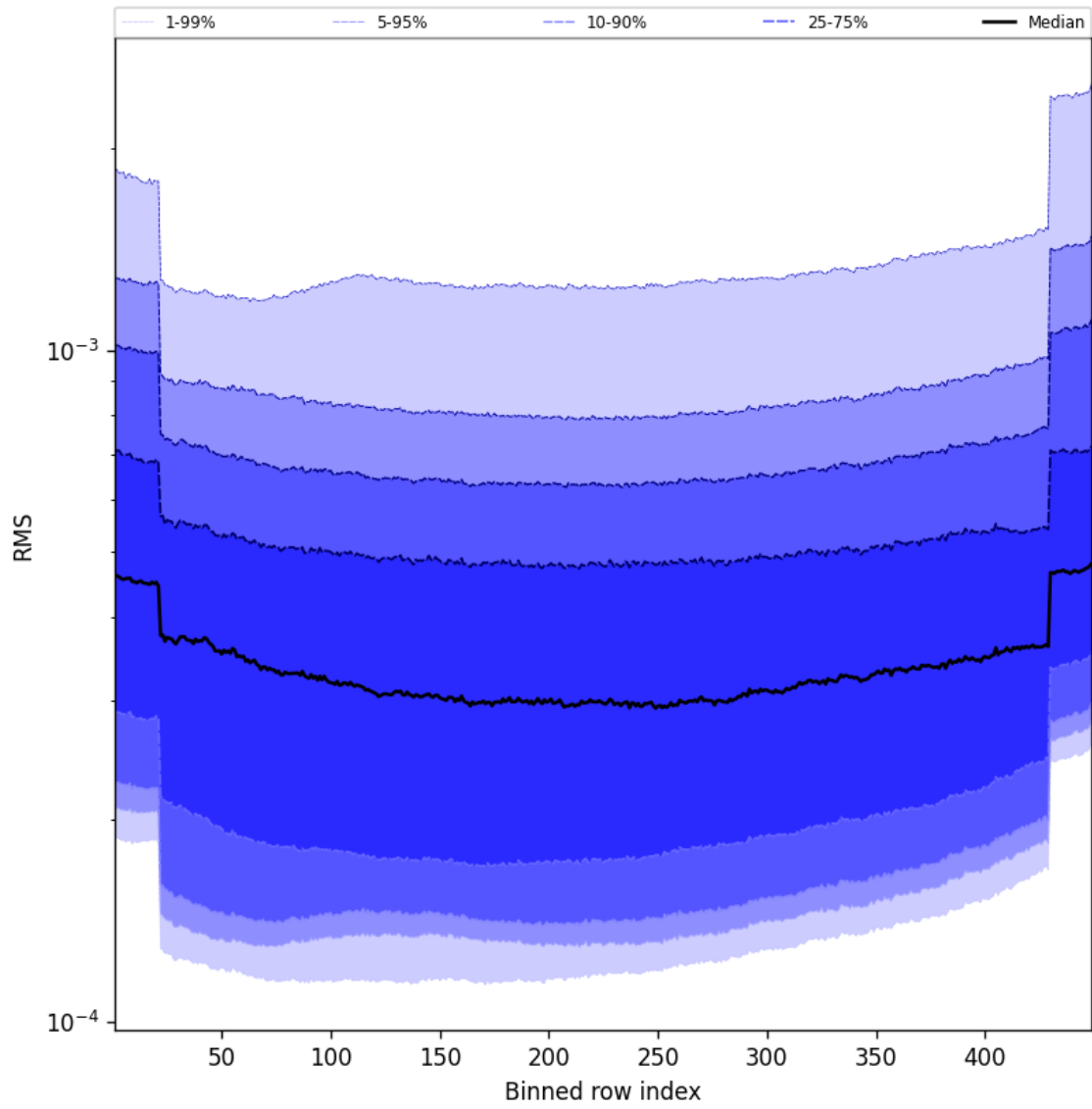
Figure 60: Along track statistics of “RMS” for 2024-11-04 to 2024-11-05
