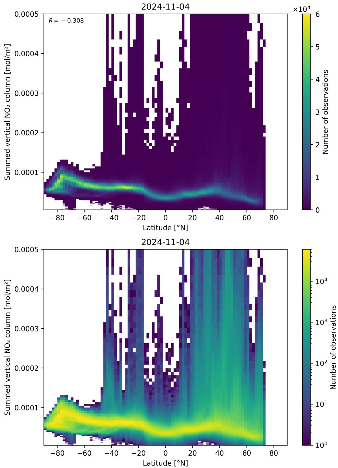
Figure 88: Scatter density plot of “Latitude” against “Summed vertical NO 2 column” for 2024-11-04 to 2024-11-05.
