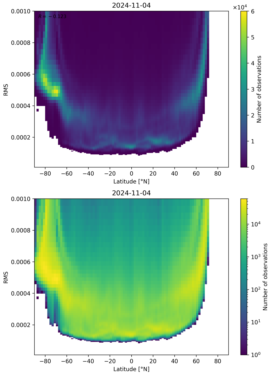
Figure 94: Scatter density plot of “Latitude” against “RMS” for 2024-11-04 to 2024-11-05.
