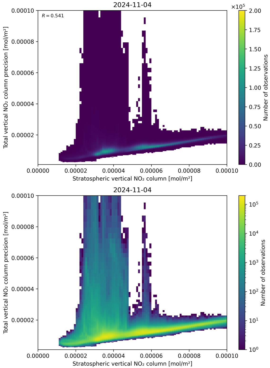
Figure 101: Scatter density plot of “Stratospheric vertical NO 2 column” against “Total vertical NO 2 column precision” for 2024-11-04 to 2024-11-05.
