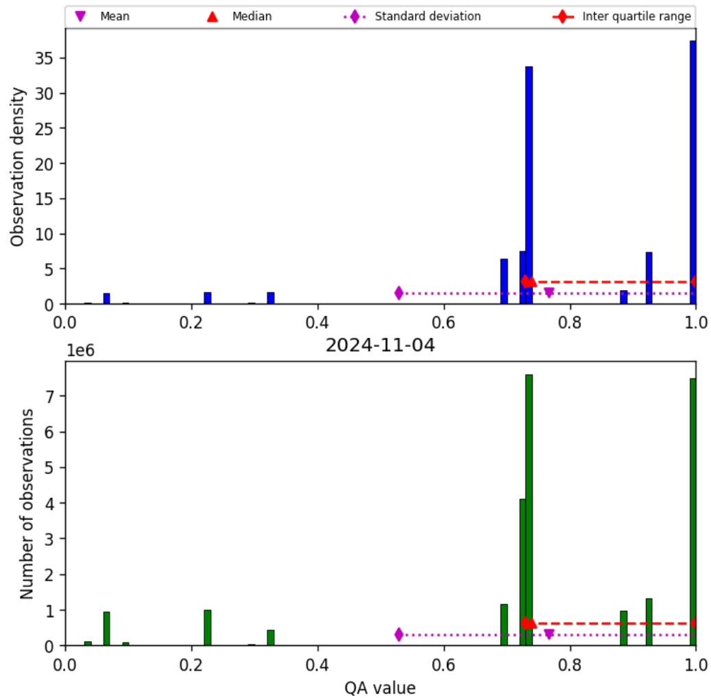
Figure 28: Histogram of “QA value” for 2024-11-04 to 2024-11-05
