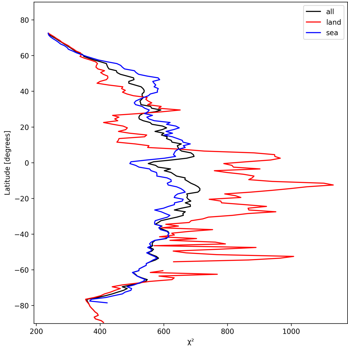
Figure 25: Zonal average of “ \chi^2 ” for 2024-11-04 to 2024-11-05.
