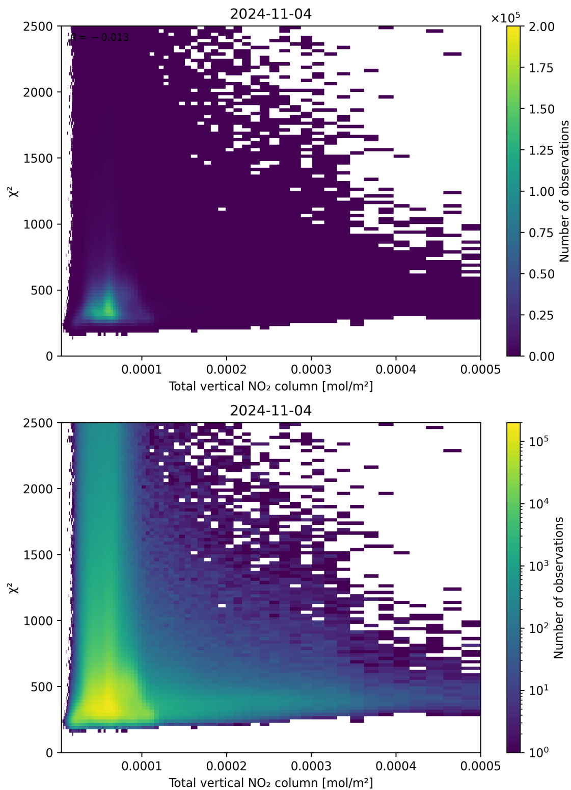
Figure 111: Scatter density plot of “Total vertical NO 2 column” against “ \chi^2 ” for 2024-11-04 to 2024-11-05.
