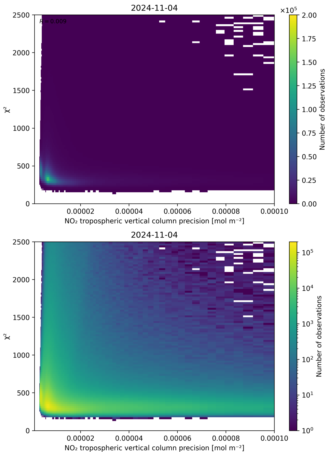
Figure 134: Scatter density plot of “NO 2 tropospheric vertical column precision” against “ \chi^2 ” for 2024-11-04 to 2024-11-05.
