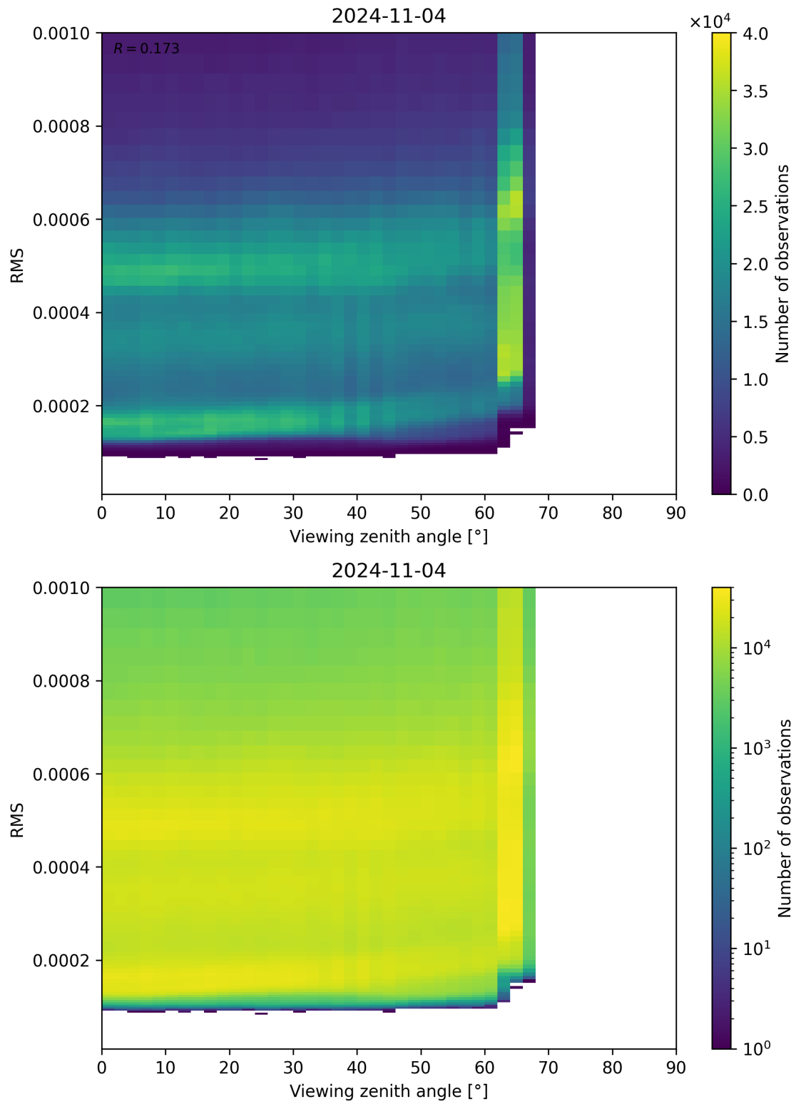
Figure 171: Scatter density plot of “Viewing zenith angle” against “RMS” for 2024-11-04 to 2024-11-05.
