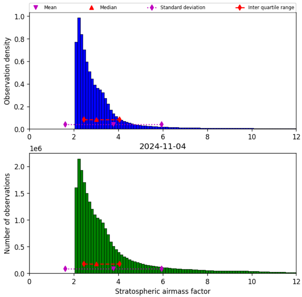
Figure 44: Histogram of “Stratospheric airmass factor” for 2024-11-04 to 2024-11-05
