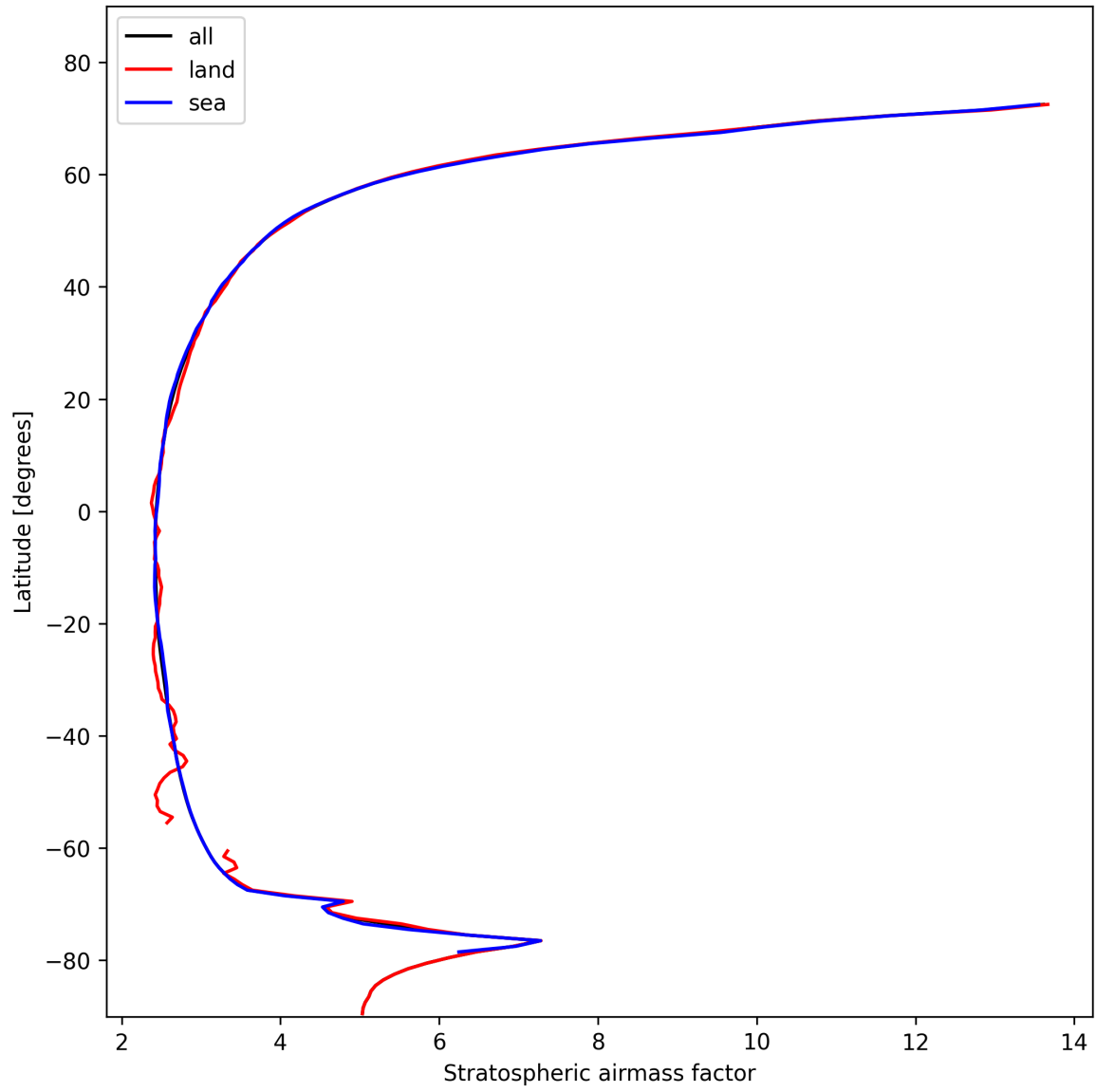
Figure 27: Zonal average of “Stratospheric air mass factor” for 2024-11-04 to 2024-11-05.
