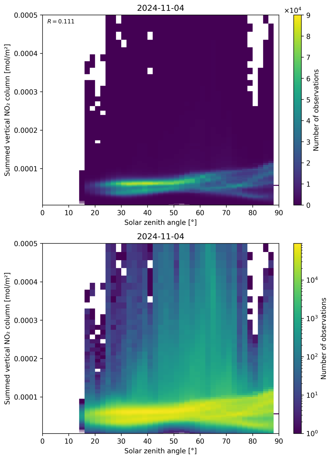
Figure 151: Scatter density plot of “Solar zenith angle” against “Summed vertical NO 2 column” for 2024-11-04 to 2024-11-05.
