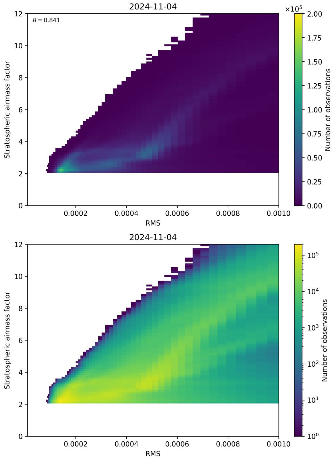
Figure 144: Scatter density plot of “RMS” against “Stratospheric airmass factor” for 2024-11-04 to 2024-11-05.
