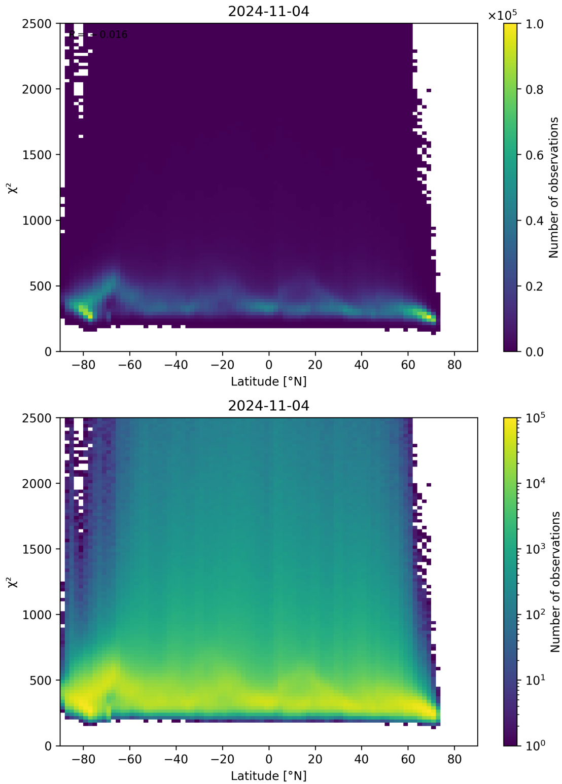
Figure 86: Scatter density plot of “Latitude” against “ \chi^2 ” for 2024-11-04 to 2024-11-05.
