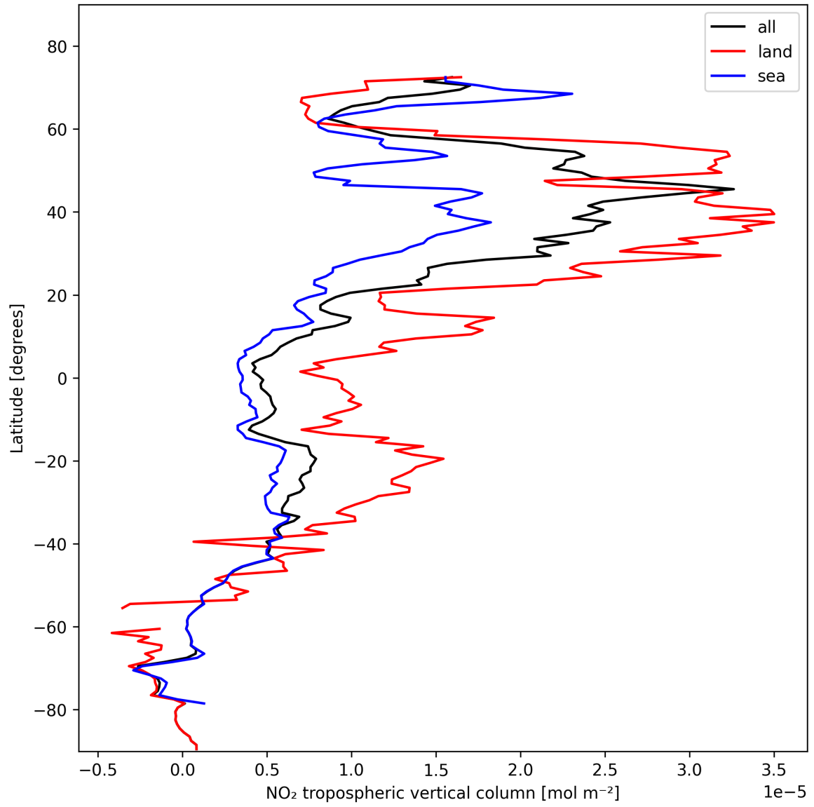
Figure 12: Zonal average of “NO 2 tropospheric vertical column” for 2024-11-04 to 2024-11-05.
