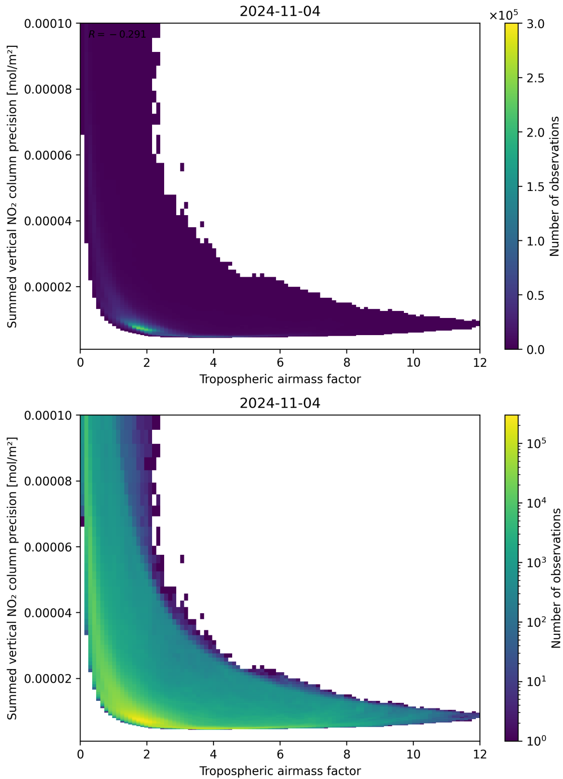
Figure 76: Scatter density plot of “Tropospheric air mass factor” against “Summed vertical NO 2 column precision” for 2024-11-04 to 2024-11-05.
