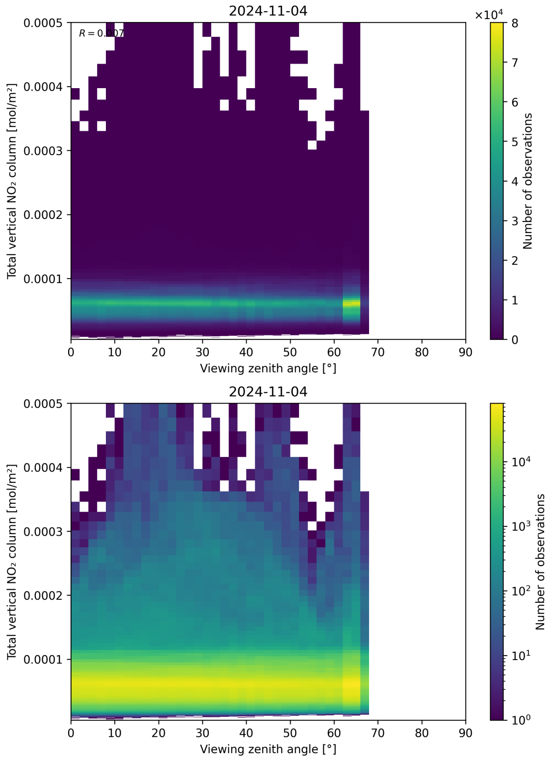
Figure 167: Scatter density plot of “Viewing zenith angle” against “Total vertical NO 2 column” for 2024-11-04 to 2024-11-05.
