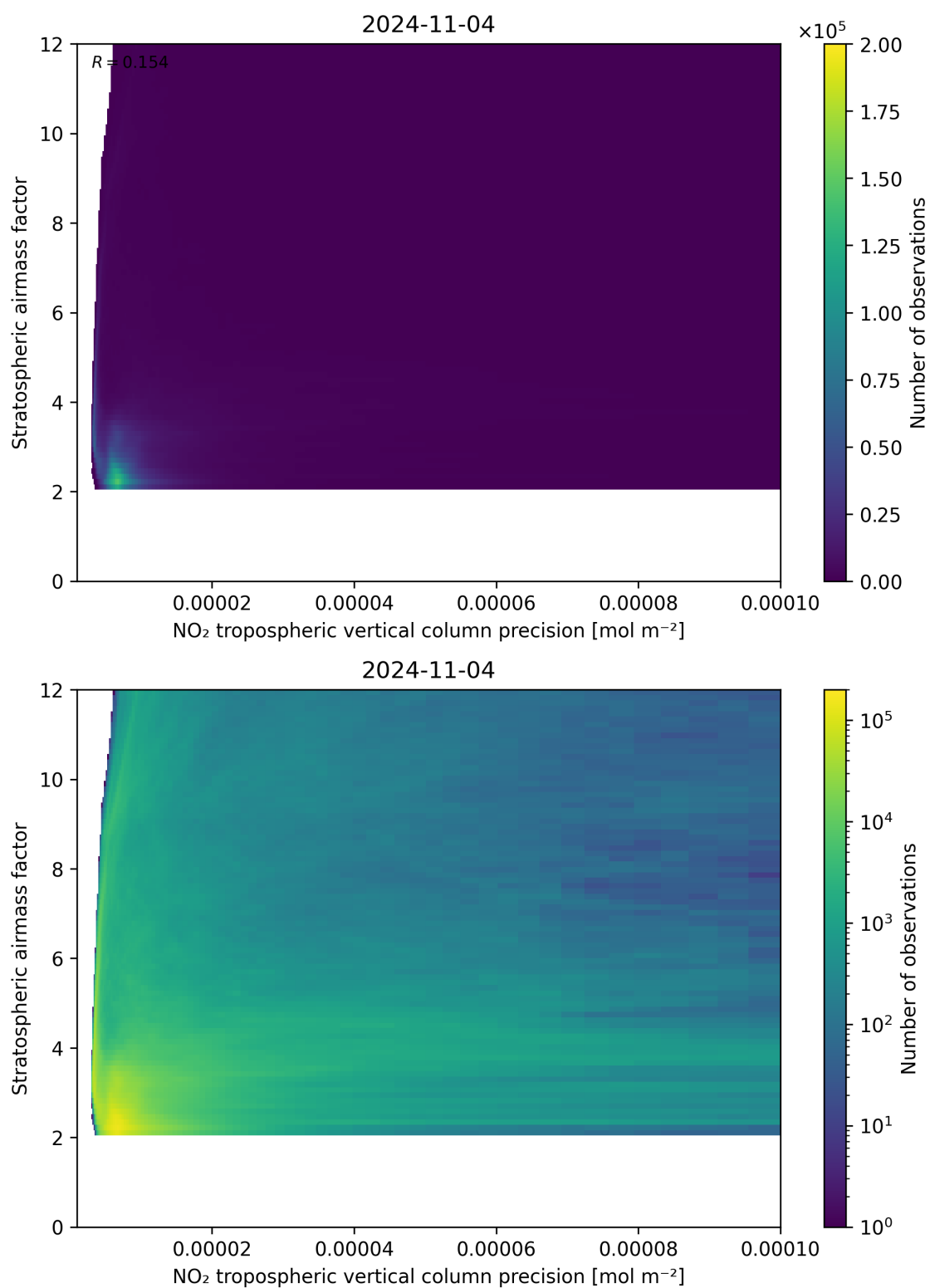
Figure 131: Scatter density plot of “NO 2 tropospheric vertical column precision” against “Stratospheric airmass factor” for 2024-11-04 to 2024-11-05.
