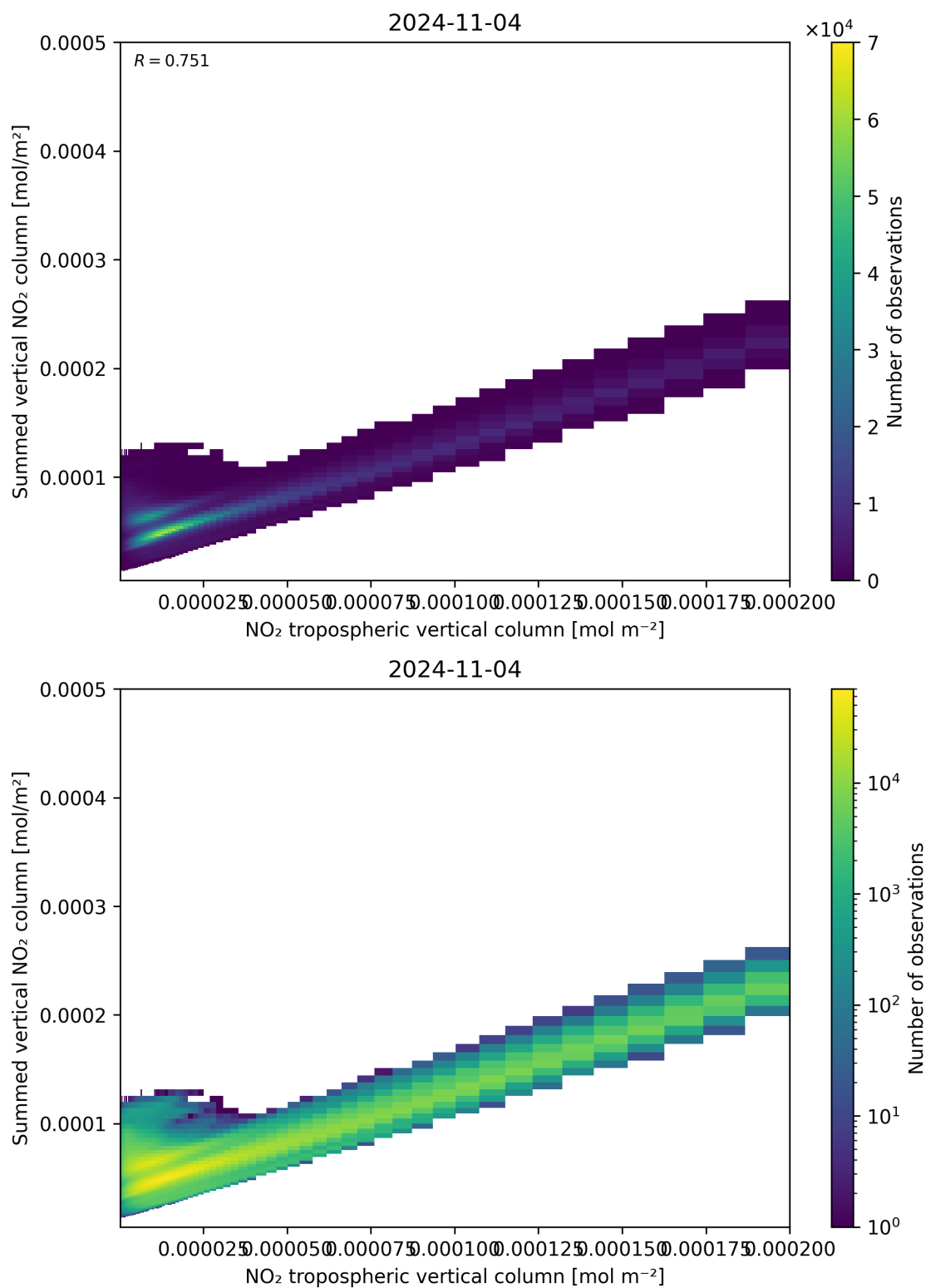
Figure 126: Scatter density plot of “NO 2 tropospheric vertical column” against “Summed vertical NO 2 column” for 2024-11-04 to 2024-11-05.
