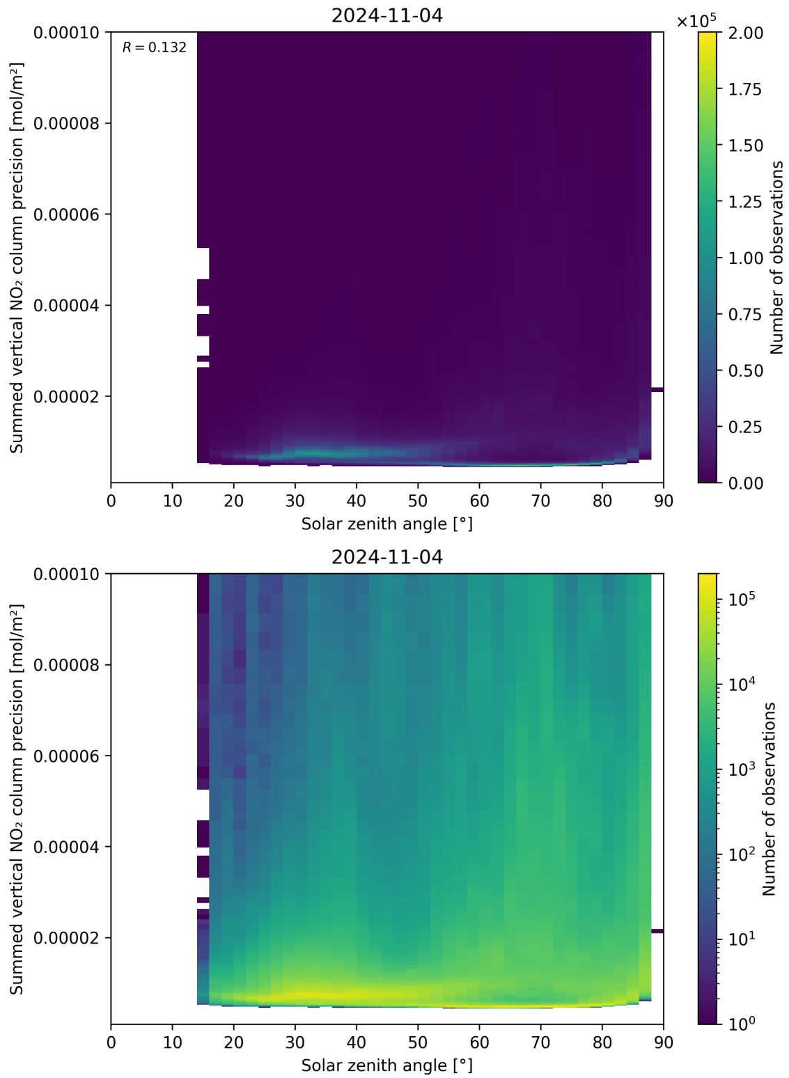
Figure 152: Scatter density plot of “Solar zenith angle” against “Summed vertical NO 2 column precision” for 2024-11-04 to 2024-11-05.
