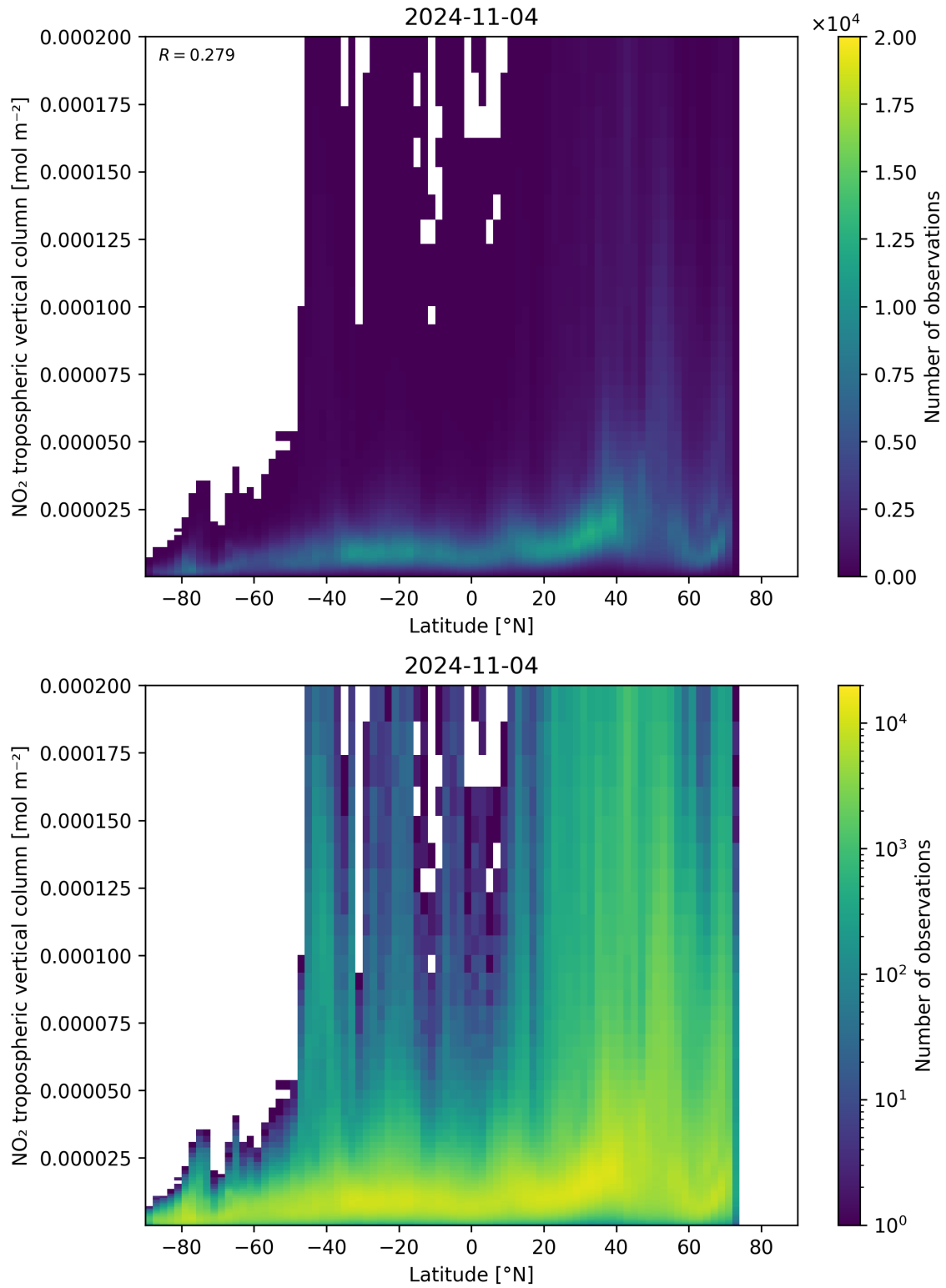
Figure 92: Scatter density plot of “Latitude” against “NO 2 tropospheric vertical column” for 2024-11-04 to 2024-11-05.
