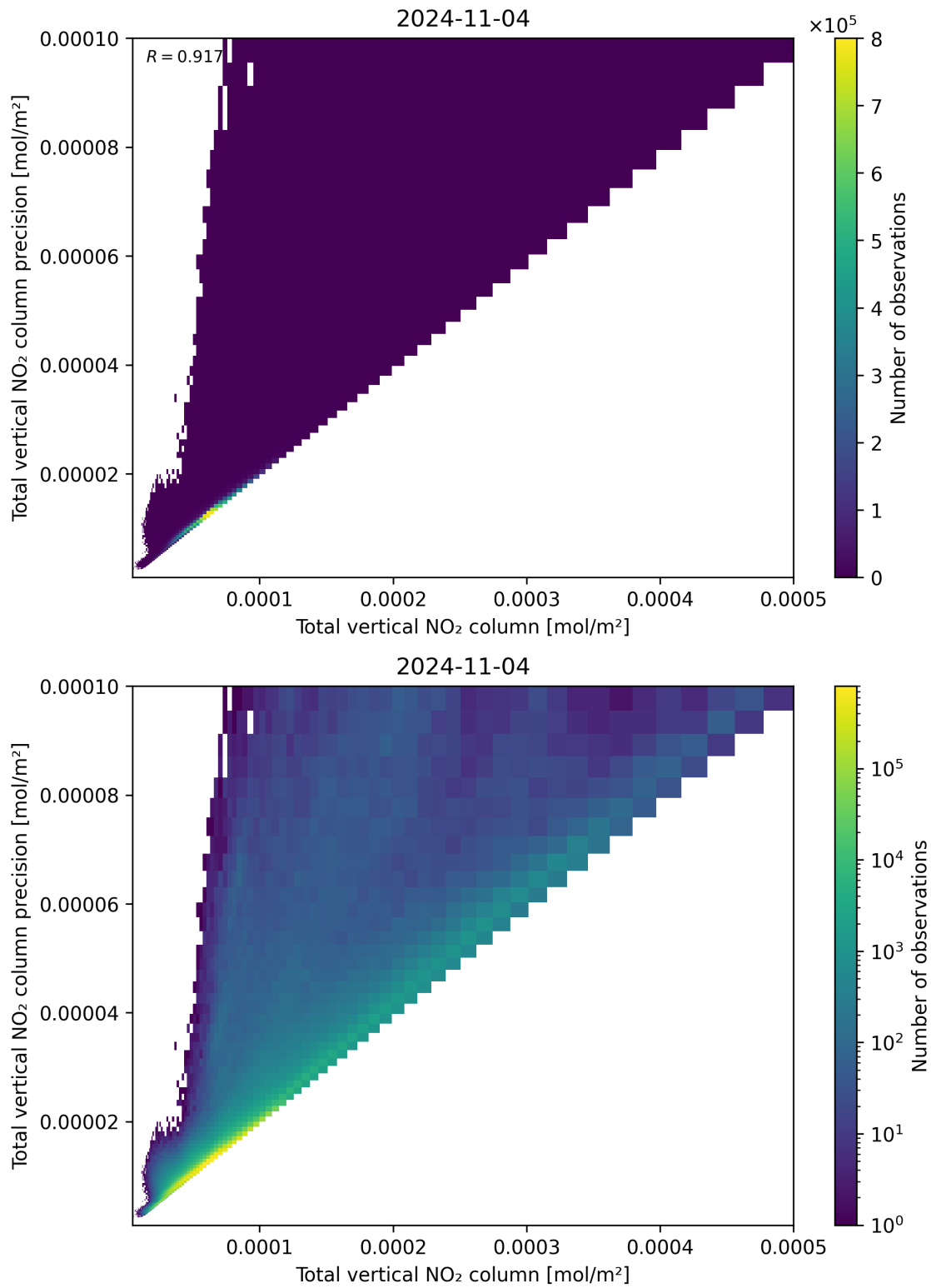
Figure 114: Scatter density plot of “Total vertical NO 2 column” against “Total vertical NO 2 column precision” for 2024-11-04 to 2024-11-05.
