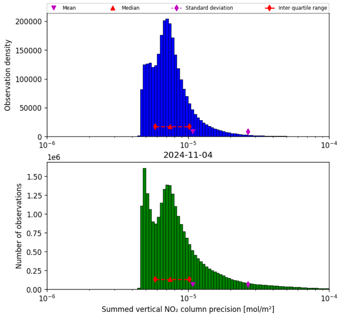
Figure 41: Histogram of "Summed vertical NO 2 column precision" for 2024-11-04 to 2024-11-05
