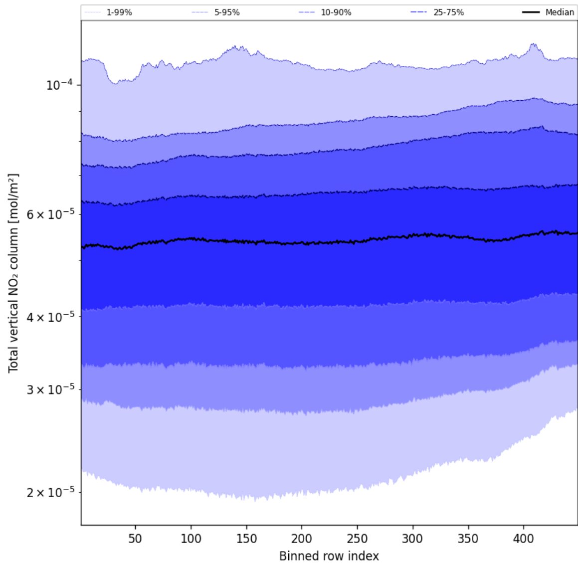
Figure 55: Along track statistics of “Total vertical NO 2 column” for 2024-11-04 to 2024-11-05
