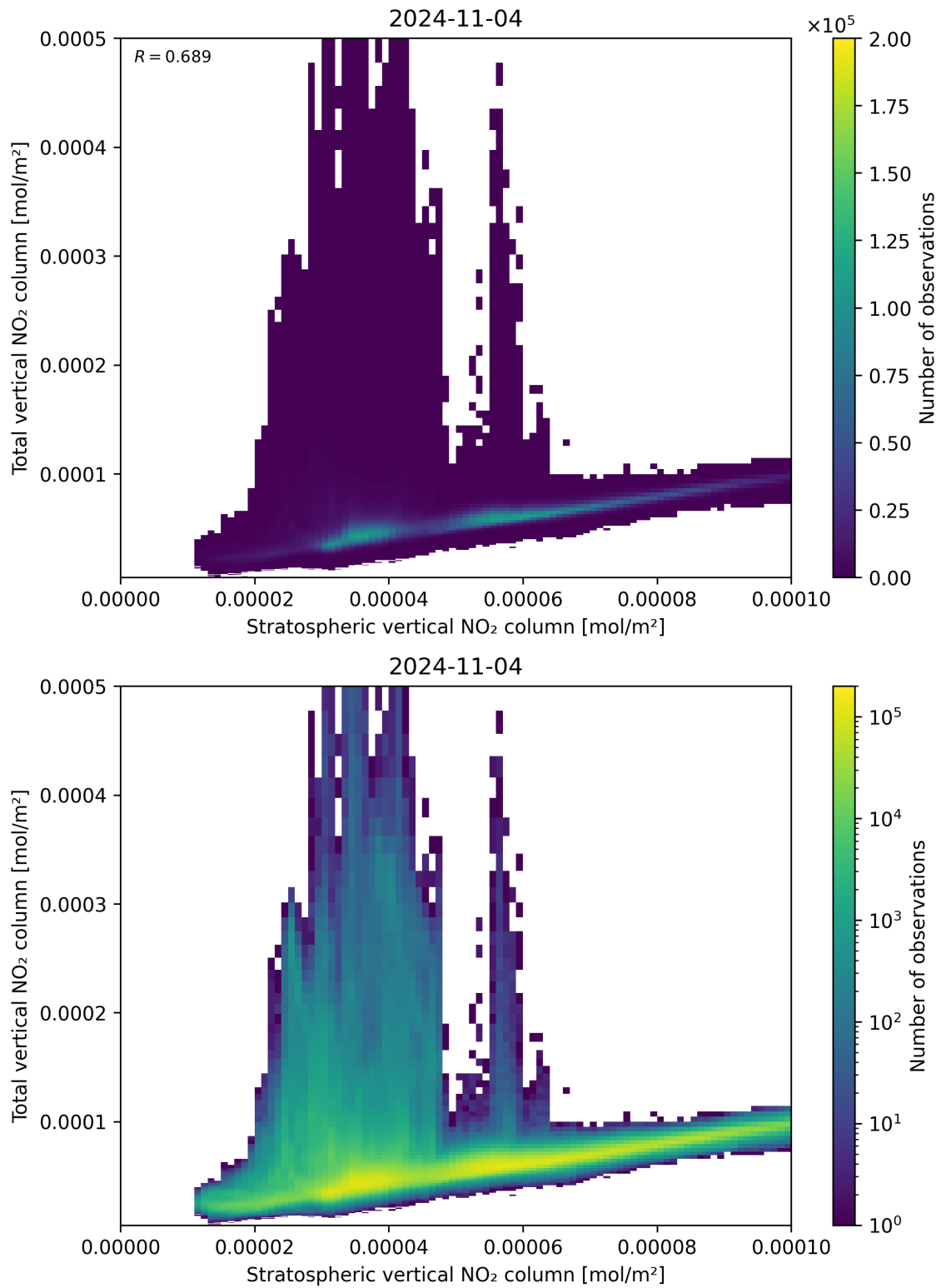
Figure 100: Scatter density plot of “Stratospheric vertical NO 2 column” against “Total vertical NO 2 column” for 2024-11-04 to 2024-11-05.
