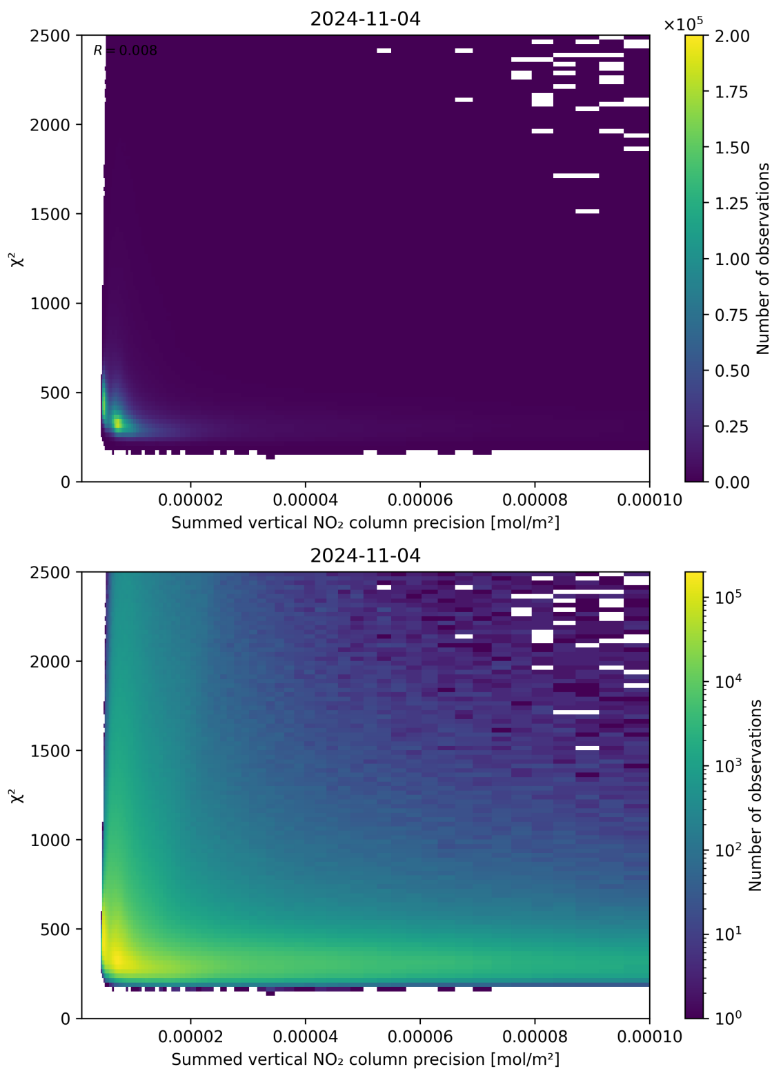
Figure 107: Scatter density plot of “Summed vertical NO 2 column precision” against “ \chi^2 ” for 2024-11-04 to 2024-11-05.
