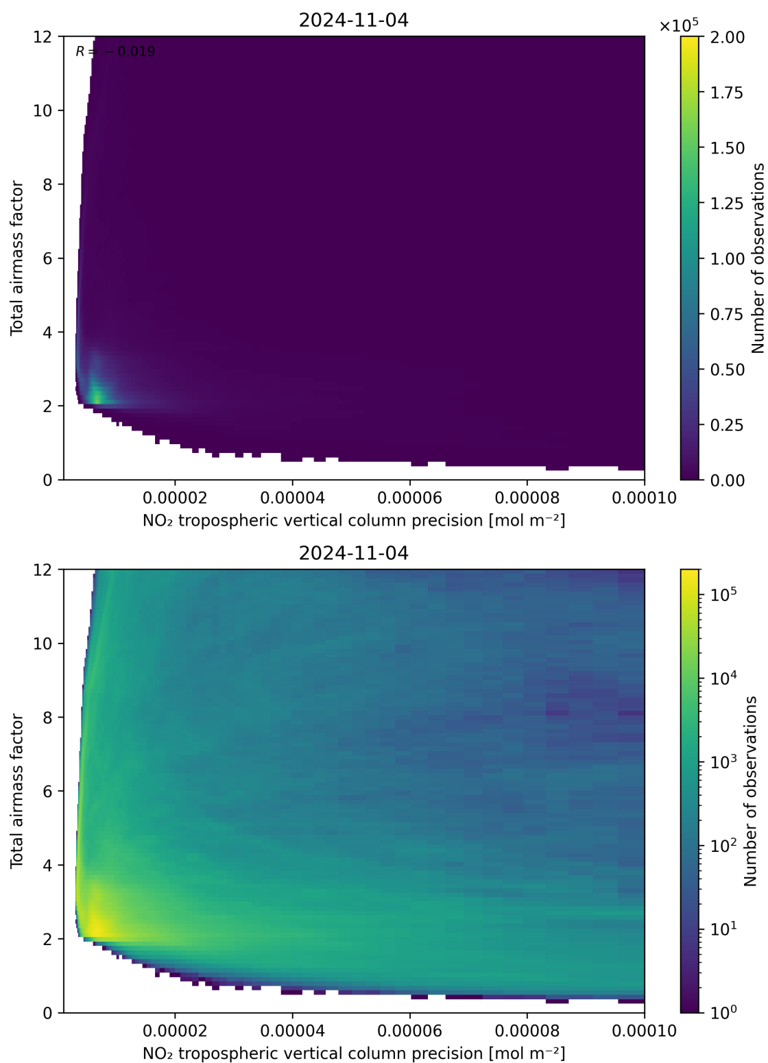
Figure 132: Scatter density plot of “NO 2 tropospheric vertical column precision” against “Total air mass factor” for 2024-11-04 to 2024-11-05.
