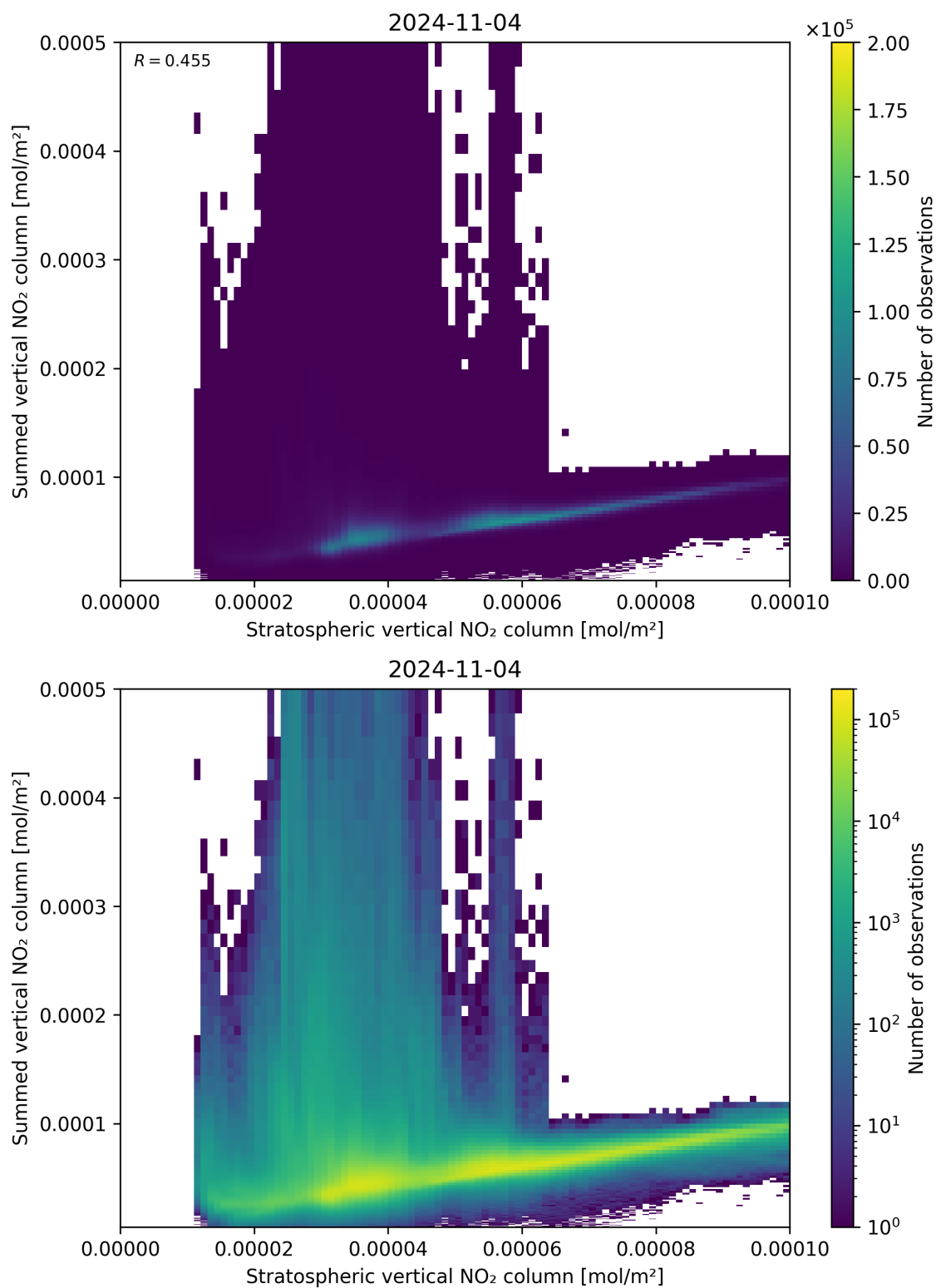
Figure 98: Scatter density plot of “Stratospheric vertical NO 2 column” against “Summed vertical NO 2 column” for 2024-11-04 to 2024-11-05.
