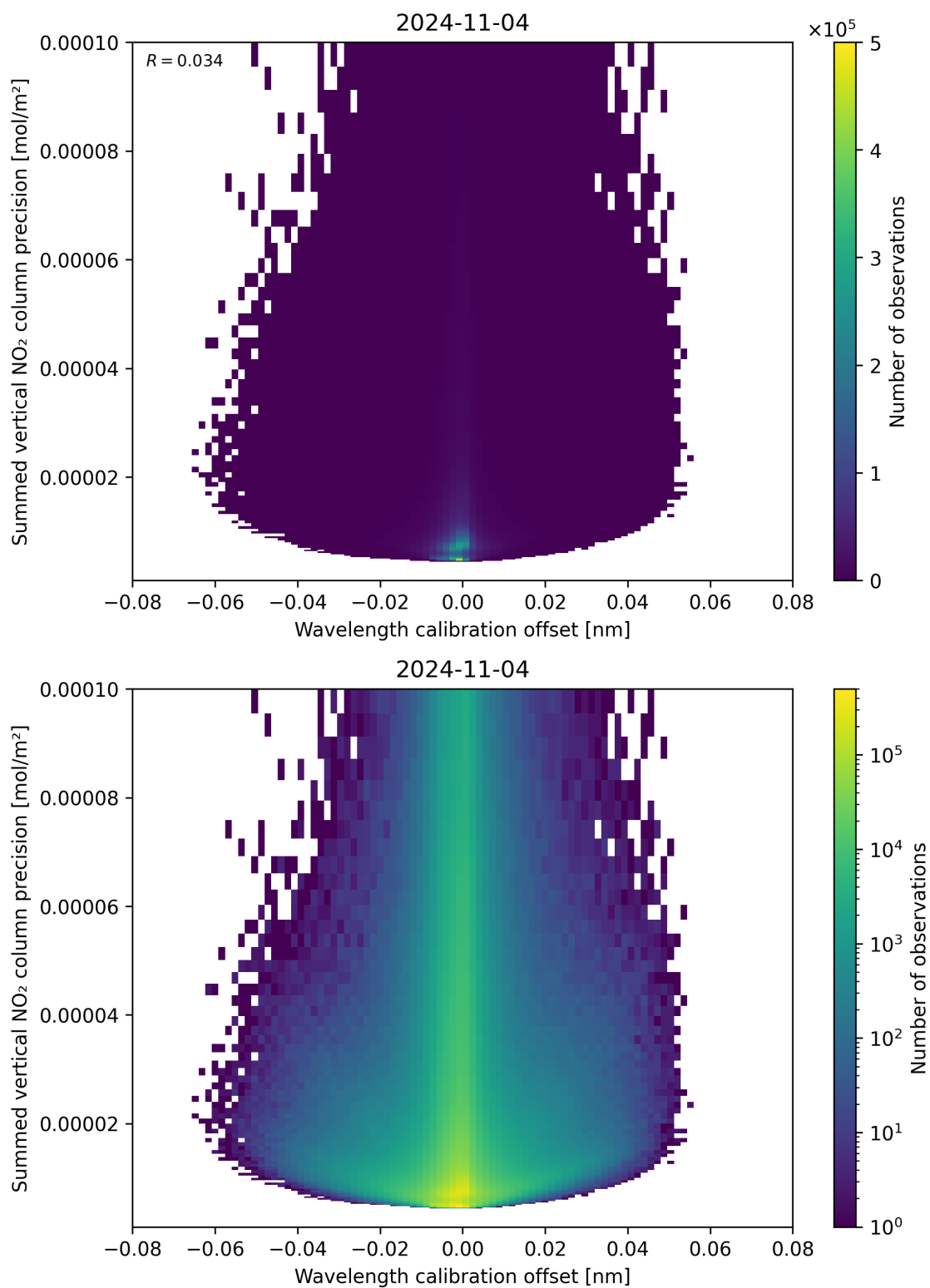
Figure 178: Scatter density plot of “Wavelength calibration offset” against “Summed vertical NO 2 column precision” for 2024-11-04 to 2024-11-05.
