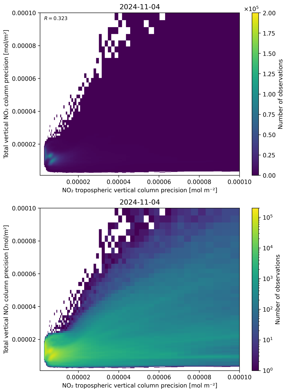
Figure 139: Scatter density plot of “NO 2 tropospheric vertical column precision” against “Total vertical NO 2 column precision” for 2024-11-04 to 2024-11-05.
