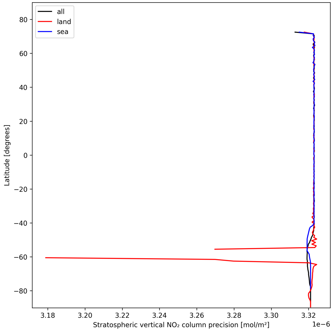
Figure 20: Zonal average of “Stratospheric vertical NO 2 column precision” for 2024-11-04 to 2024-11-05.
