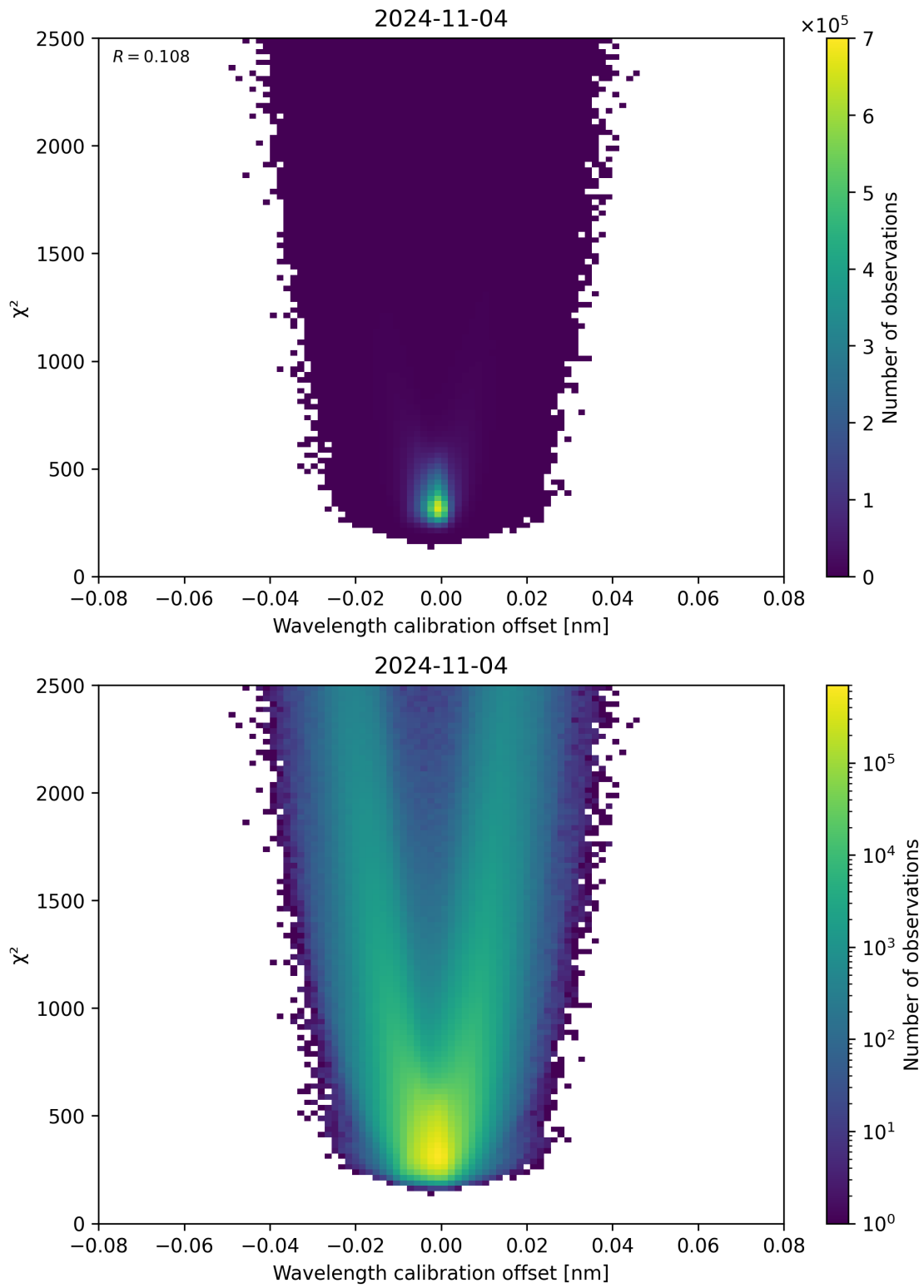
Figure 175: Scatter density plot of “Wavelength calibration offset” against “ \chi^2 ” for 2024-11-04 to 2024-11-05.
