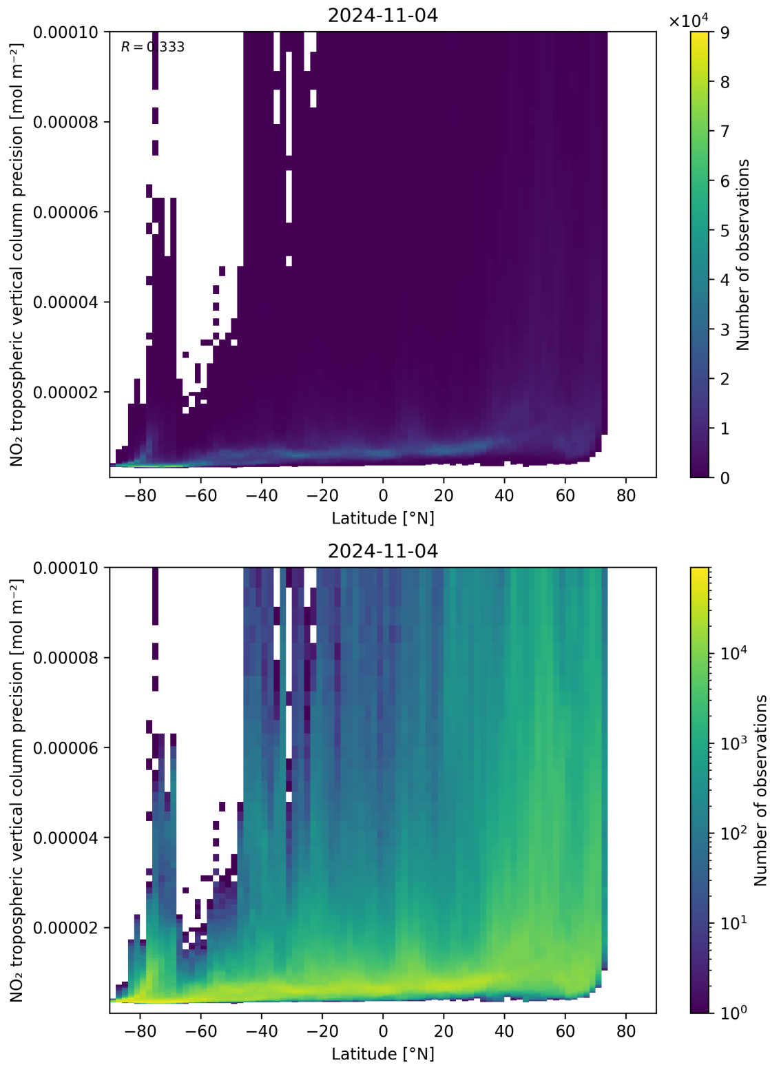
Figure 93: Scatter density plot of “Latitude” against “NO 2 tropospheric vertical column precision” for 2024-11-04 to 2024-11-05.
