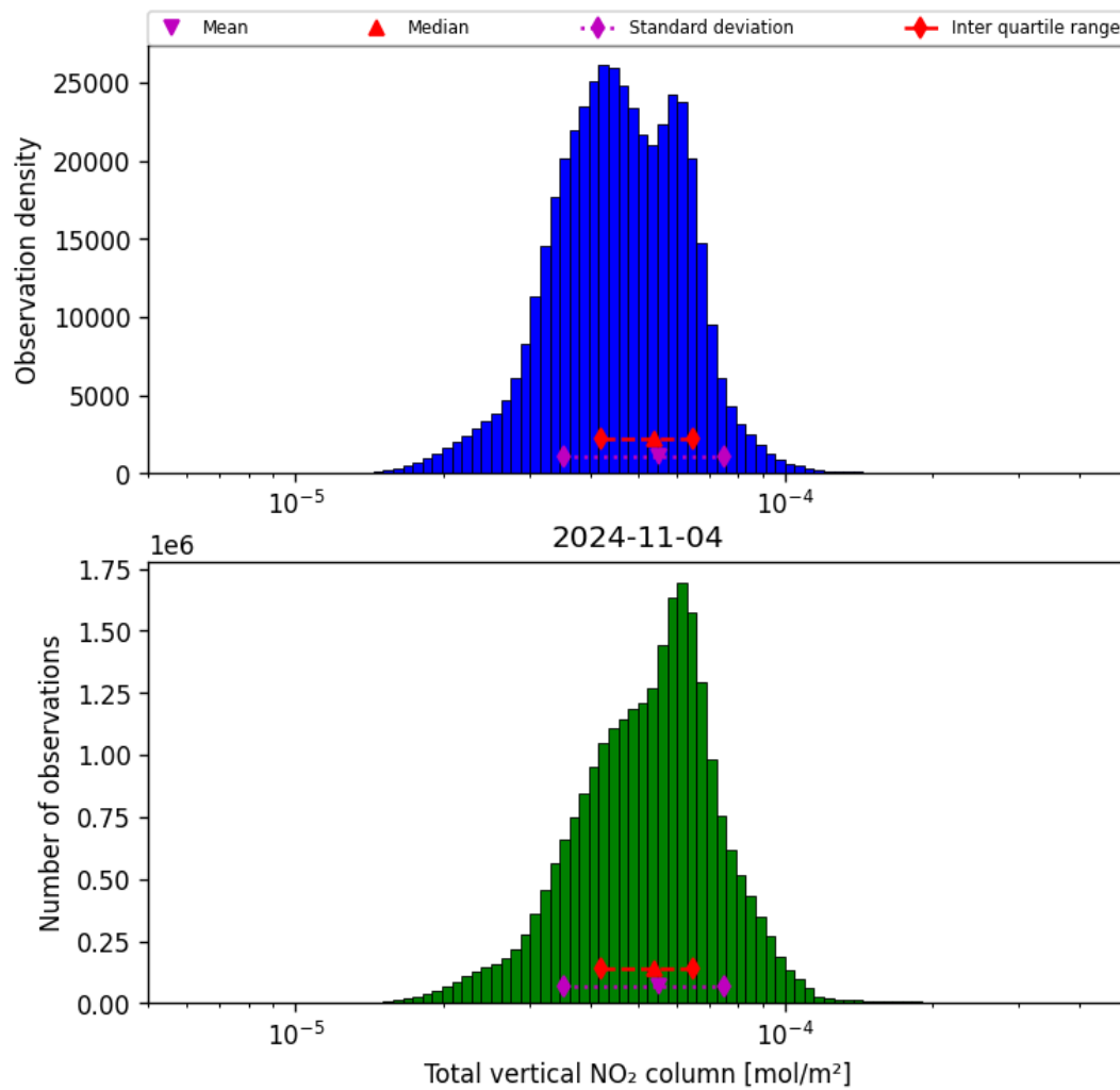
Figure 38: Histogram of “Total vertical NO 2 column” for 2024-11-04 to 2024-11-05
