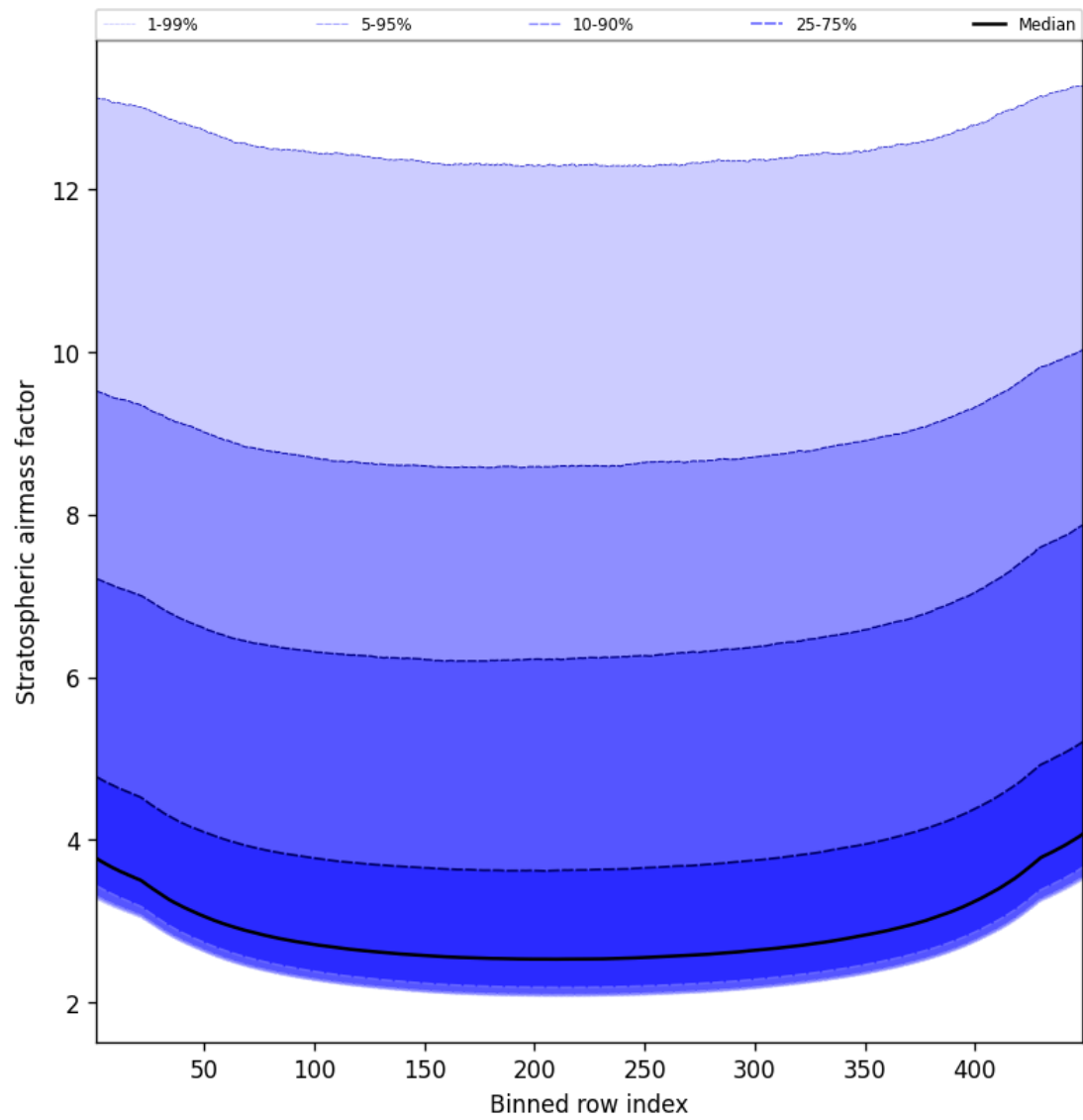
Figure 61: Along track statistics of “Stratospheric airmass factor” for 2024-11-04 to 2024-11-05
