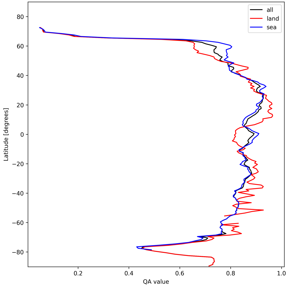
Figure 11: Zonal average of “QA value” for 2024-11-04 to 2024-11-05.
