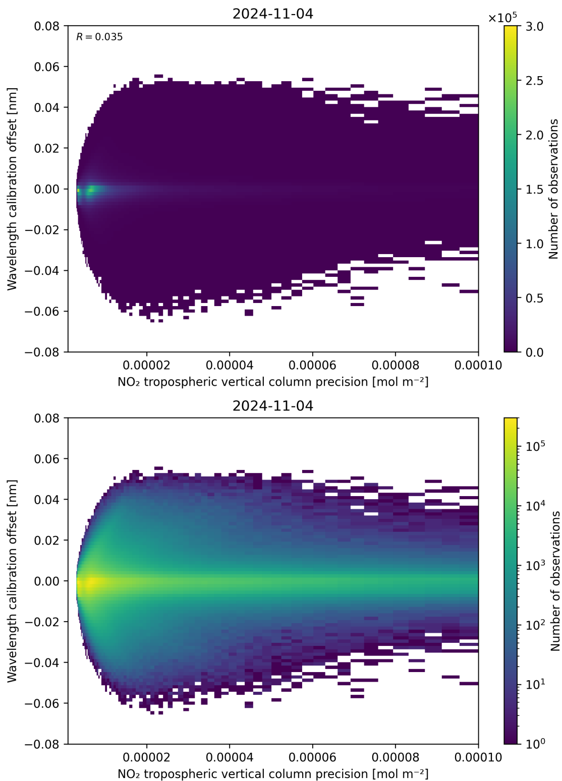
Figure 141: Scatter density plot of “NO 2 tropospheric vertical column precision” against “Wavelength calibration offset” for 2024-11-04 to 2024-11-05.
