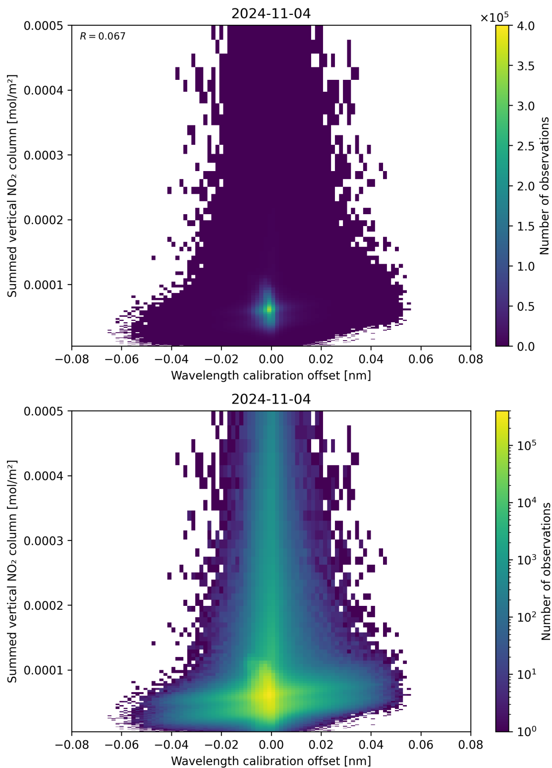
Figure 177: Scatter density plot of “Wavelength calibration offset” against “Summed vertical NO 2 column” for 2024-11-04 to 2024-11-05.
