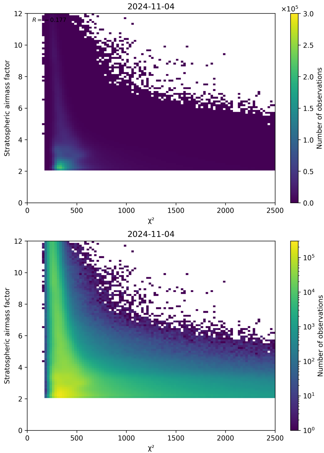
Figure 81: Scatter density plot of “ \chi^2 ” against “Stratospheric airmass factor” for 2024-11-04 to 2024-11-05.
