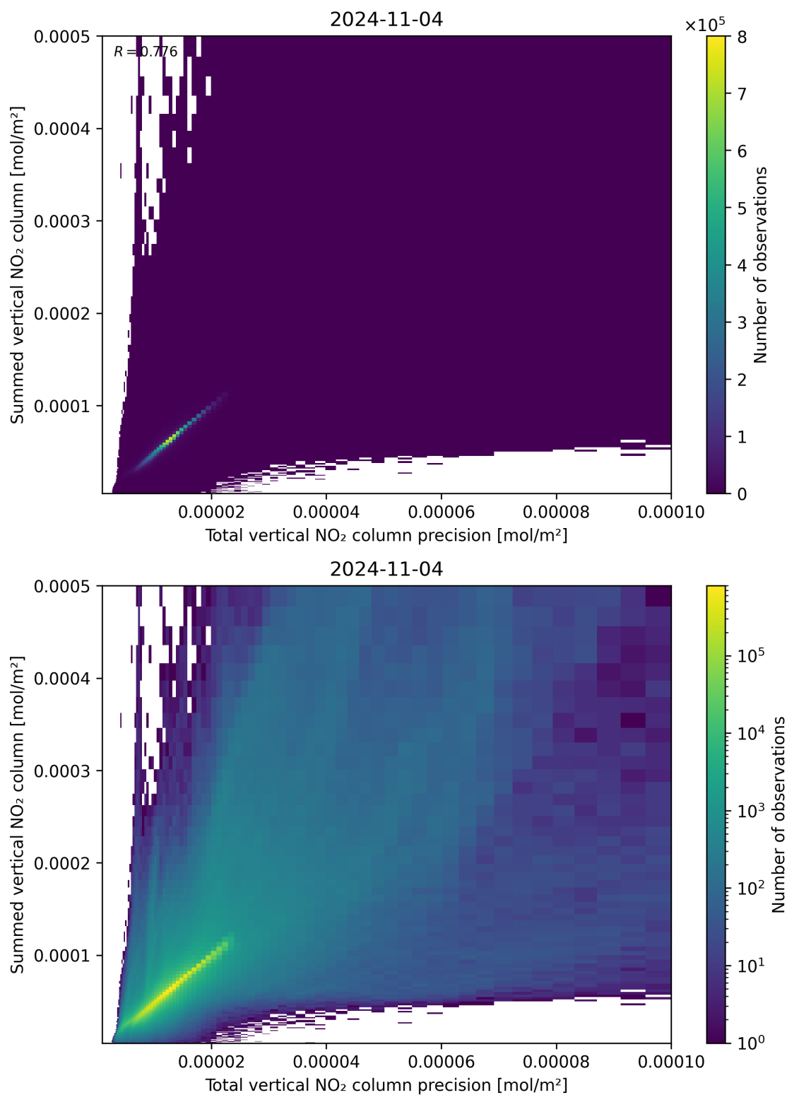
Figure 117: Scatter density plot of “Total vertical NO 2 column precision” against “Summed vertical NO 2 column” for 2024-11-04 to 2024-11-05.
