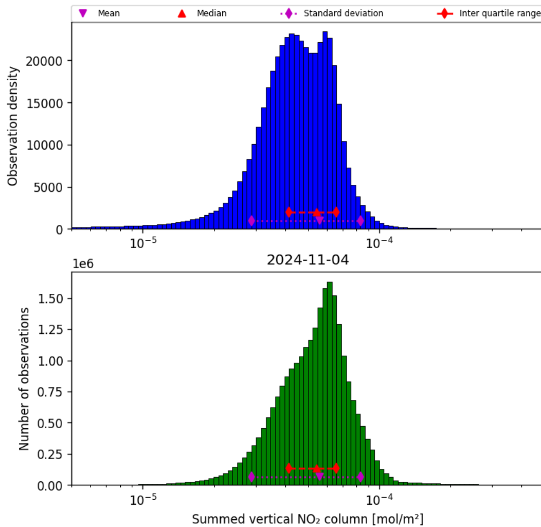
Figure 40: Histogram of “Summed vertical NO 2 column” for 2024-11-04 to 2024-11-05
