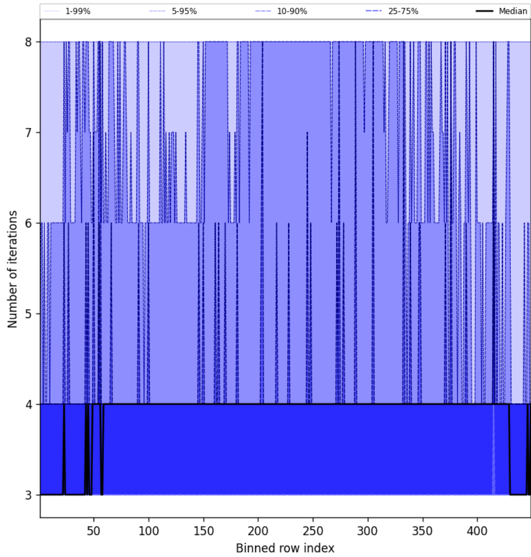
Figure 51: Along track statistics of “Number of iterations” for 2024-11-04 to 2024-11-05
