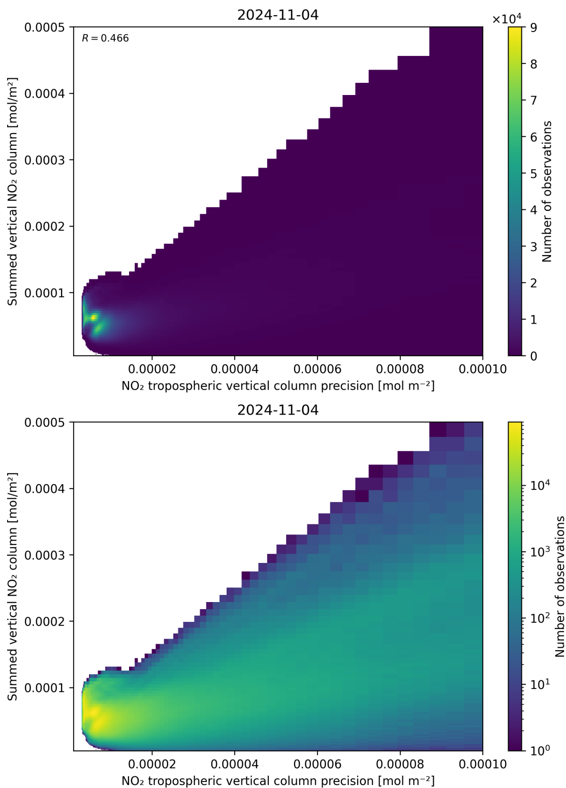
Figure 136: Scatter density plot of “NO 2 tropospheric vertical column precision” against “Summed vertical NO 2 column” for 2024-11-04 to 2024-11-05.
