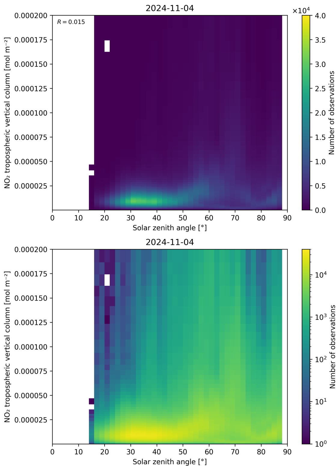
Figure 155: Scatter density plot of “Solar zenith angle” against “NO 2 tropospheric vertical column” for 2024-11-04 to 2024-11-05.
