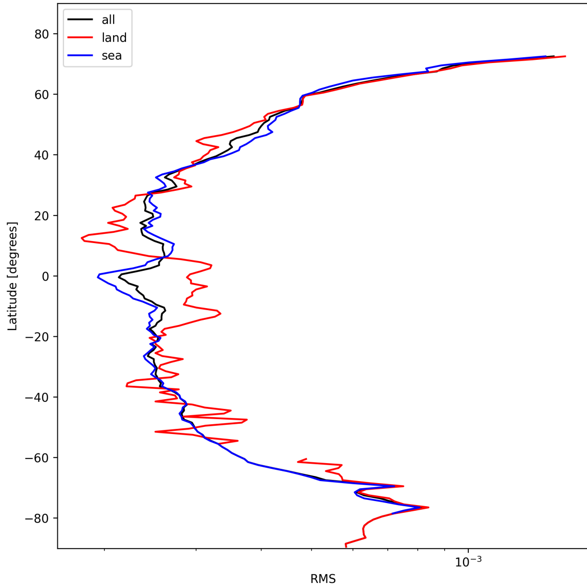
Figure 26: Zonal average of “RMS” for 2024-11-04 to 2024-11-05.
