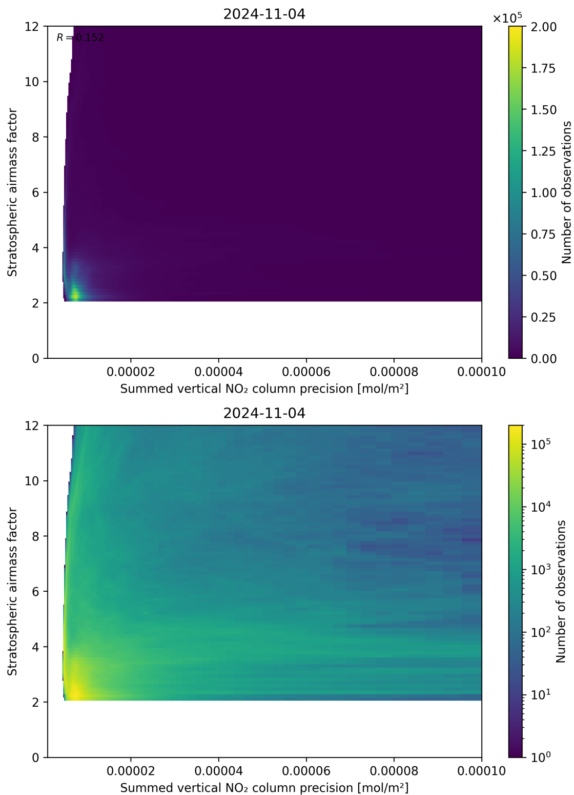
Figure 106: Scatter density plot of “Summed vertical NO 2 column precision” against “Stratospheric airmass factor” for 2024-11-04 to 2024-11-05.
