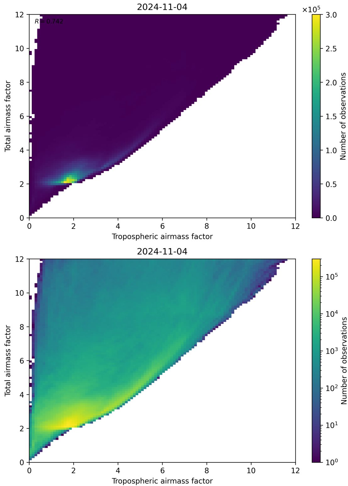
Figure 72: Scatter density plot of “Tropospheric airmass factor” against “Total airmass factor” for 2024-11-04 to 2024-11-05.
