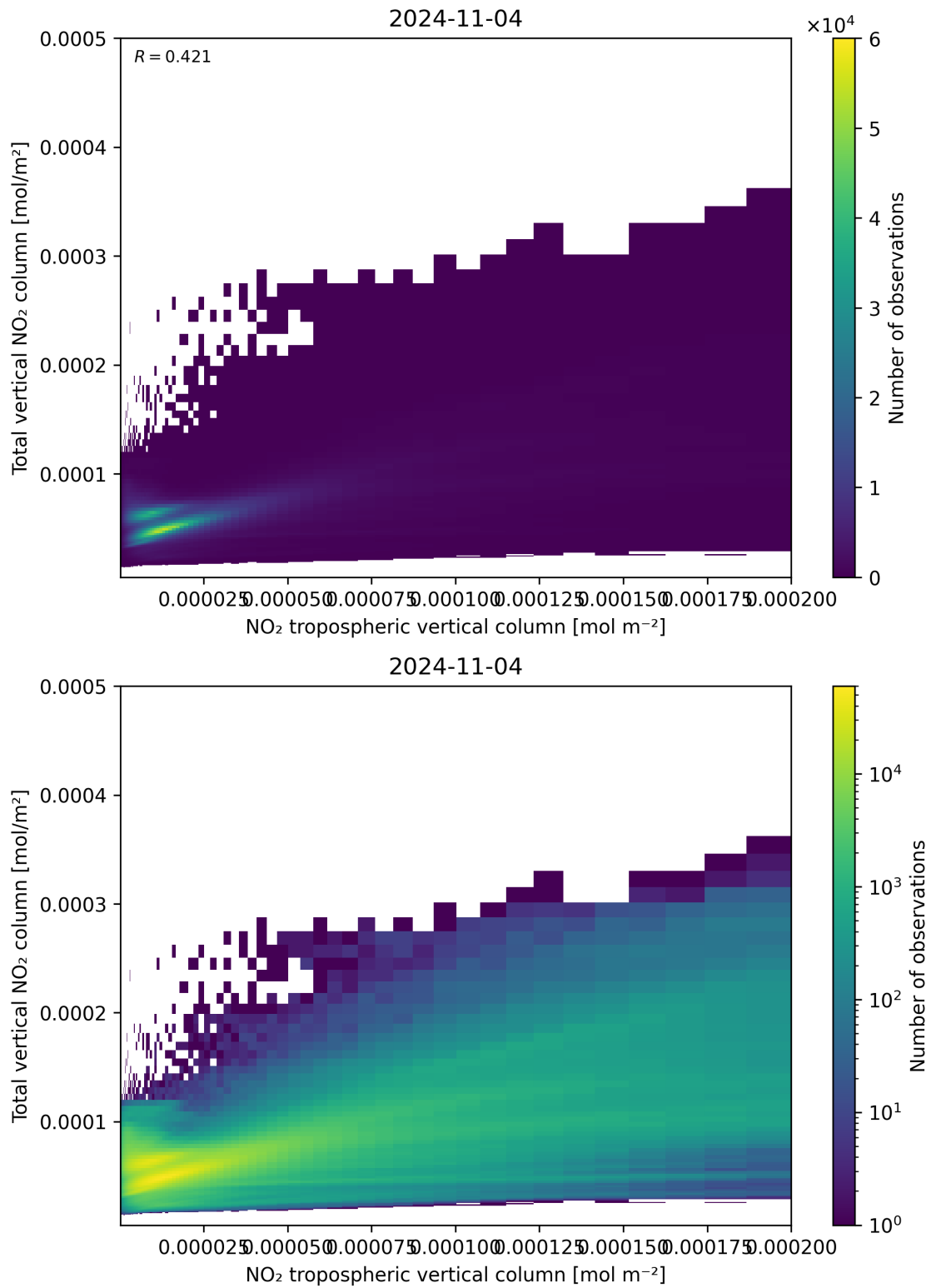
Figure 128: Scatter density plot of “NO 2 tropospheric vertical column” against “Total vertical NO 2 column” for 2024-11-04 to 2024-11-05.
