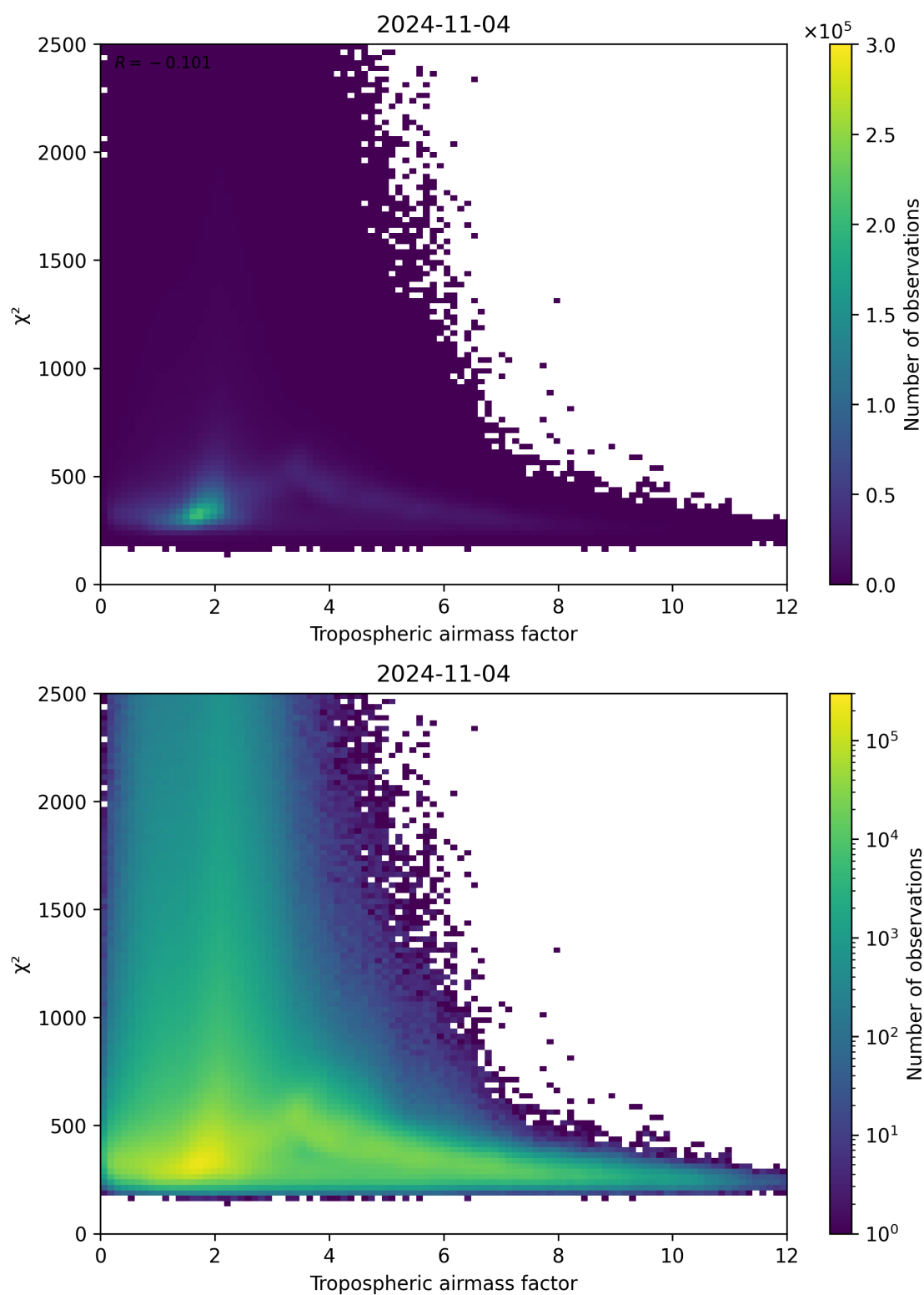
Figure 73: Scatter density plot of “Tropospheric airmass factor” against “ \chi^2 ” for 2024-11-04 to 2024-11-05.
