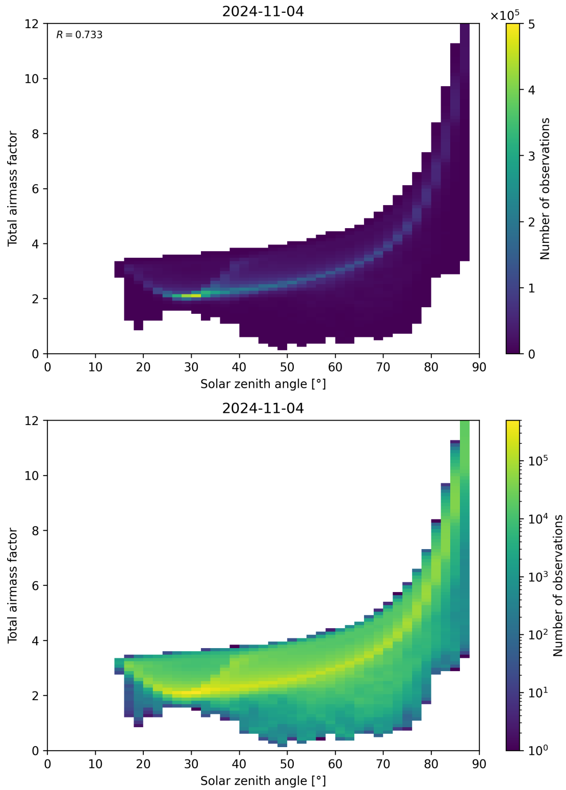
Figure 146: Scatter density plot of “Solar zenith angle” against “Total air mass factor” for 2024-11-04 to 2024-11-05.
