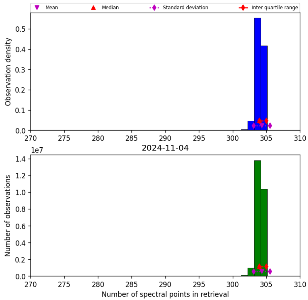
Figure 33: Histogram of “Number of spectral points in retrieval” for 2024-11-04 to 2024-11-05
