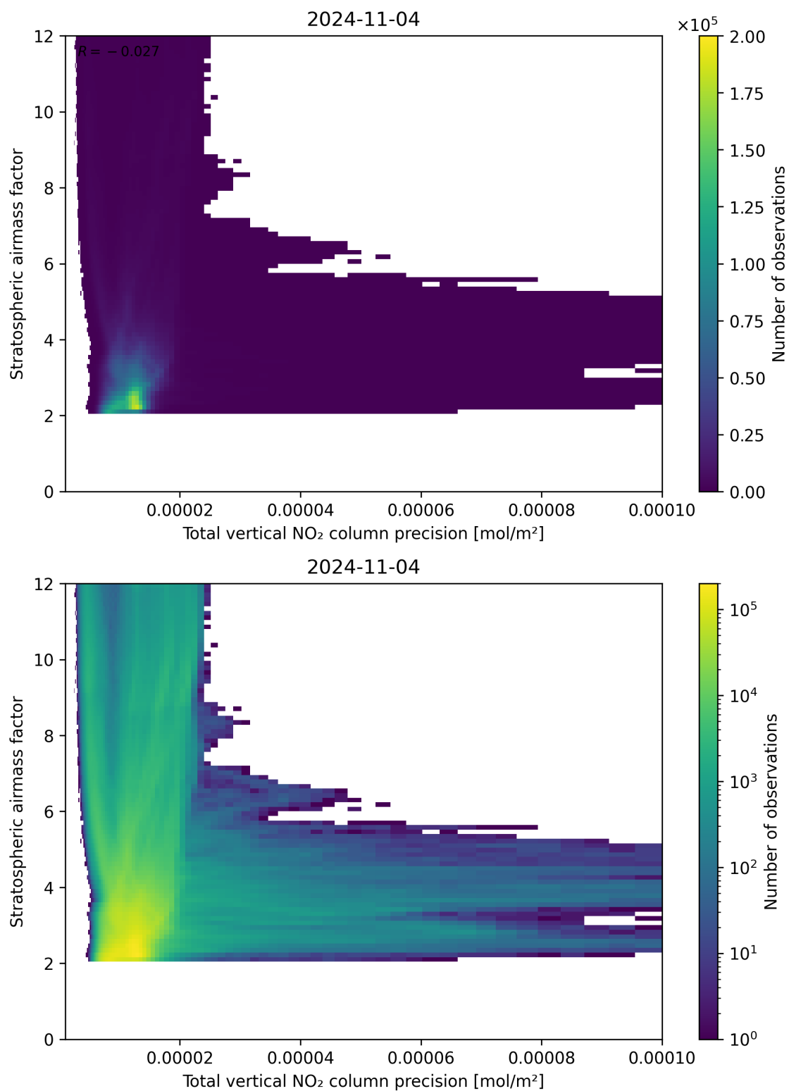
Figure 115: Scatter density plot of “Total vertical NO 2 column precision” against “Stratospheric air mass factor” for 2024-11-04 to 2024-11-05.
