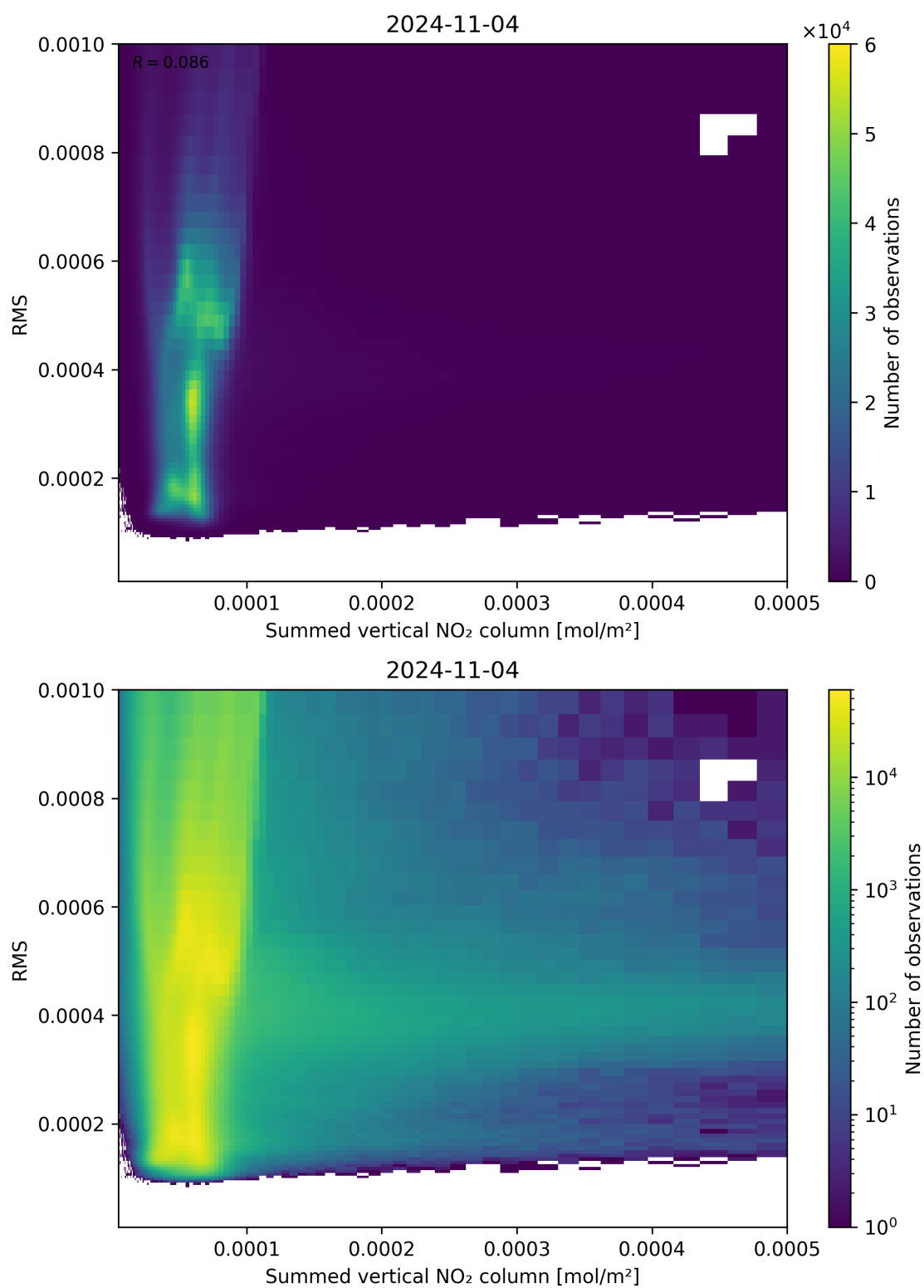
Figure 109: Scatter density plot of “Summed vertical NO 2 column” against “RMS” for 2024-11-04 to 2024-11-05.
