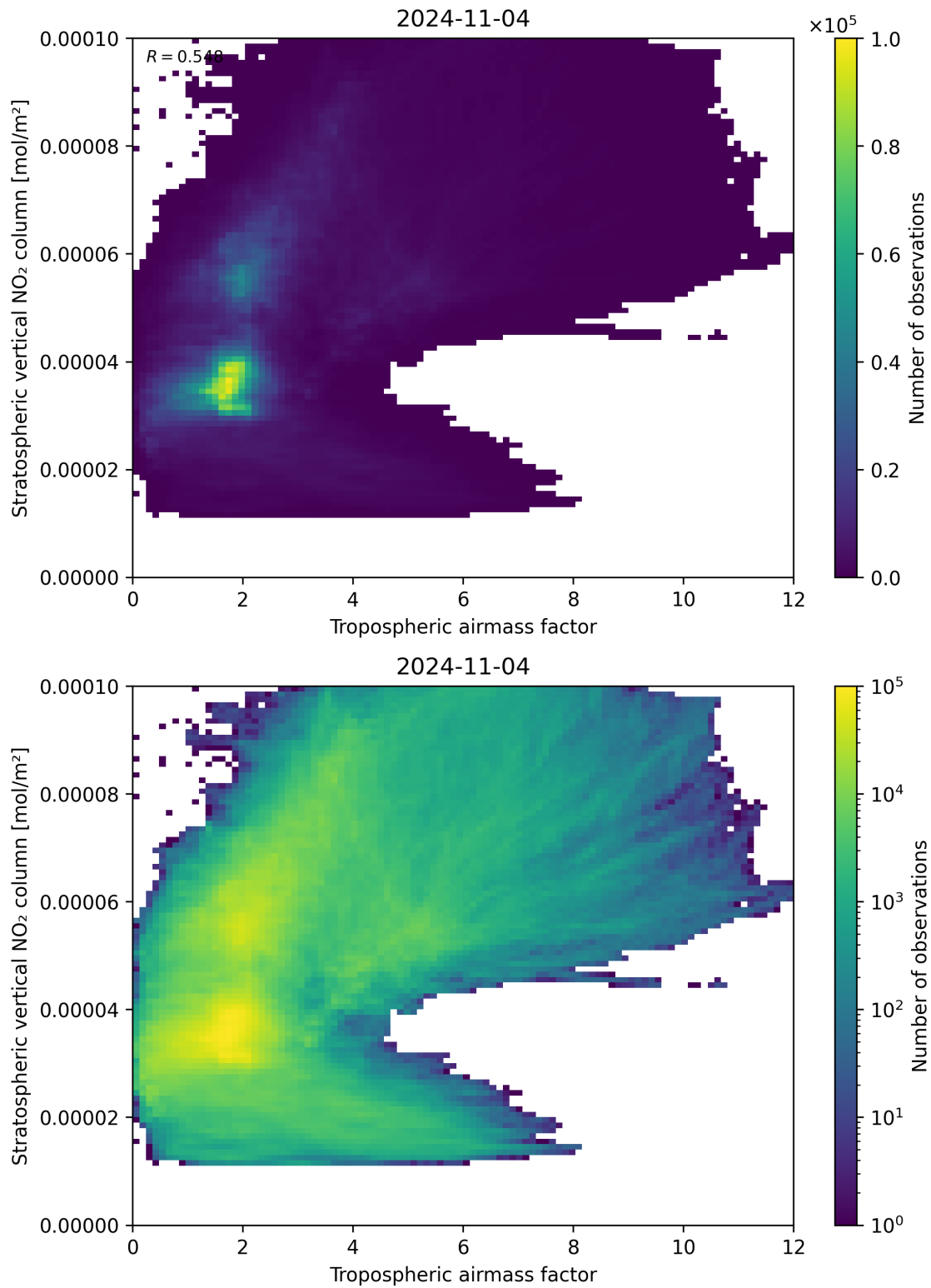
Figure 74: Scatter density plot of “Tropospheric air mass factor” against “Stratospheric vertical NO 2 column” for 2024-11-04 to 2024-11-05.
