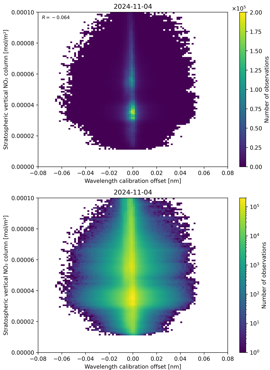
Figure 176: Scatter density plot of “Wavelength calibration offset” against “Stratospheric vertical NO 2 column” for 2024-11-04 to 2024-11-05.
