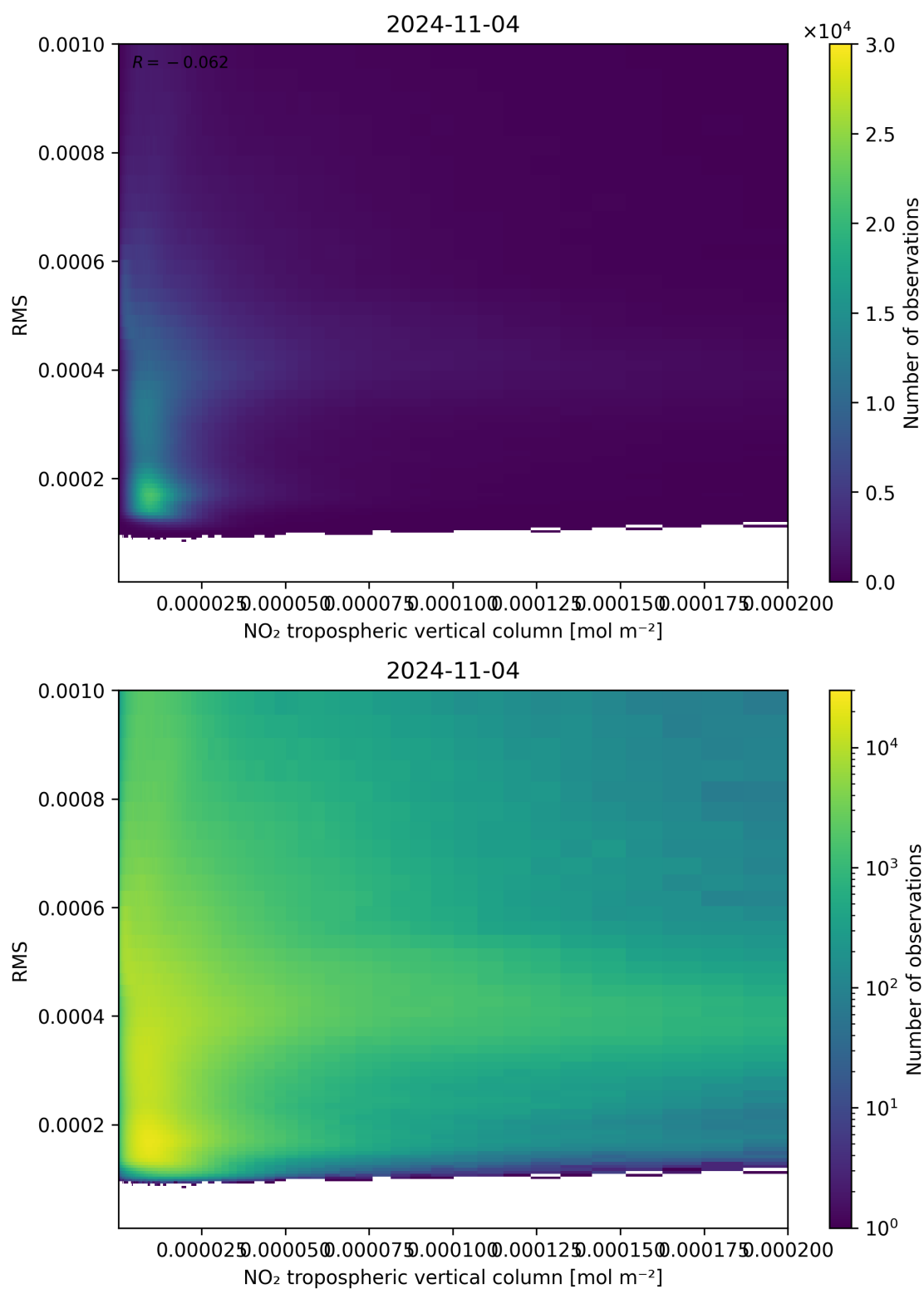
Figure 142: Scatter density plot of “NO 2 tropospheric vertical column” against “RMS” for 2024-11-04 to 2024-11-05.
