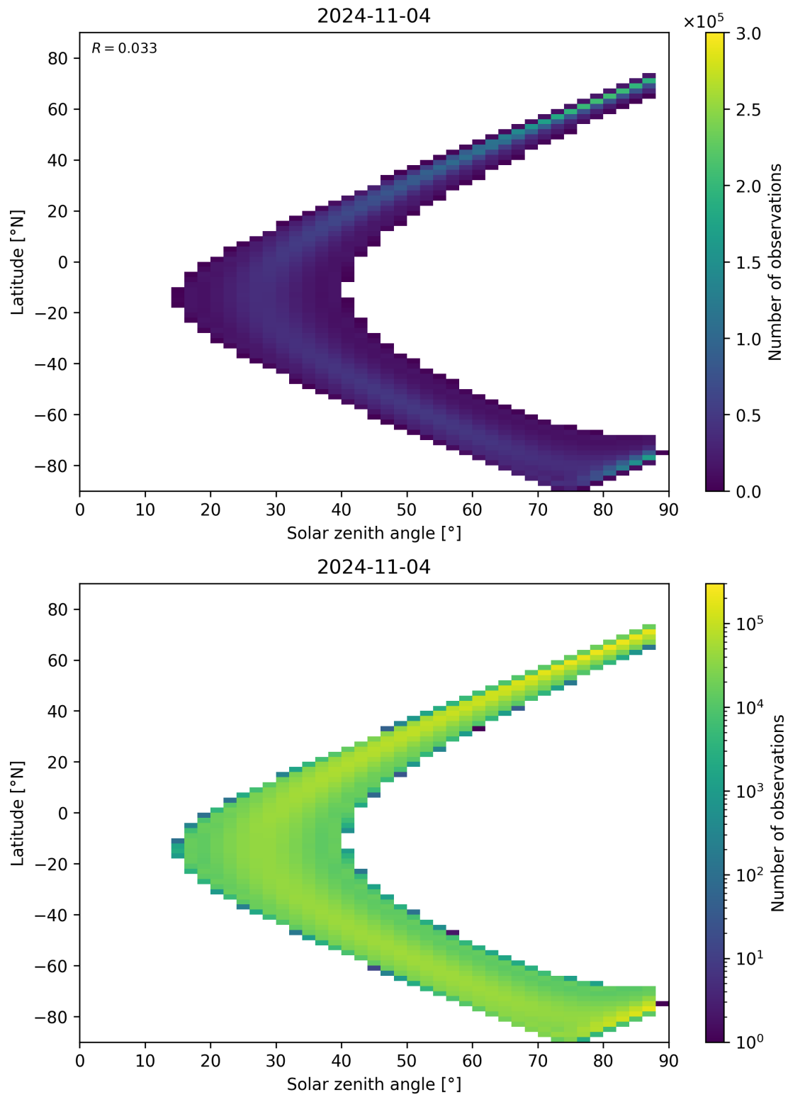
Figure 149: Scatter density plot of “Solar zenith angle” against “Latitude” for 2024-11-04 to 2024-11-05.
