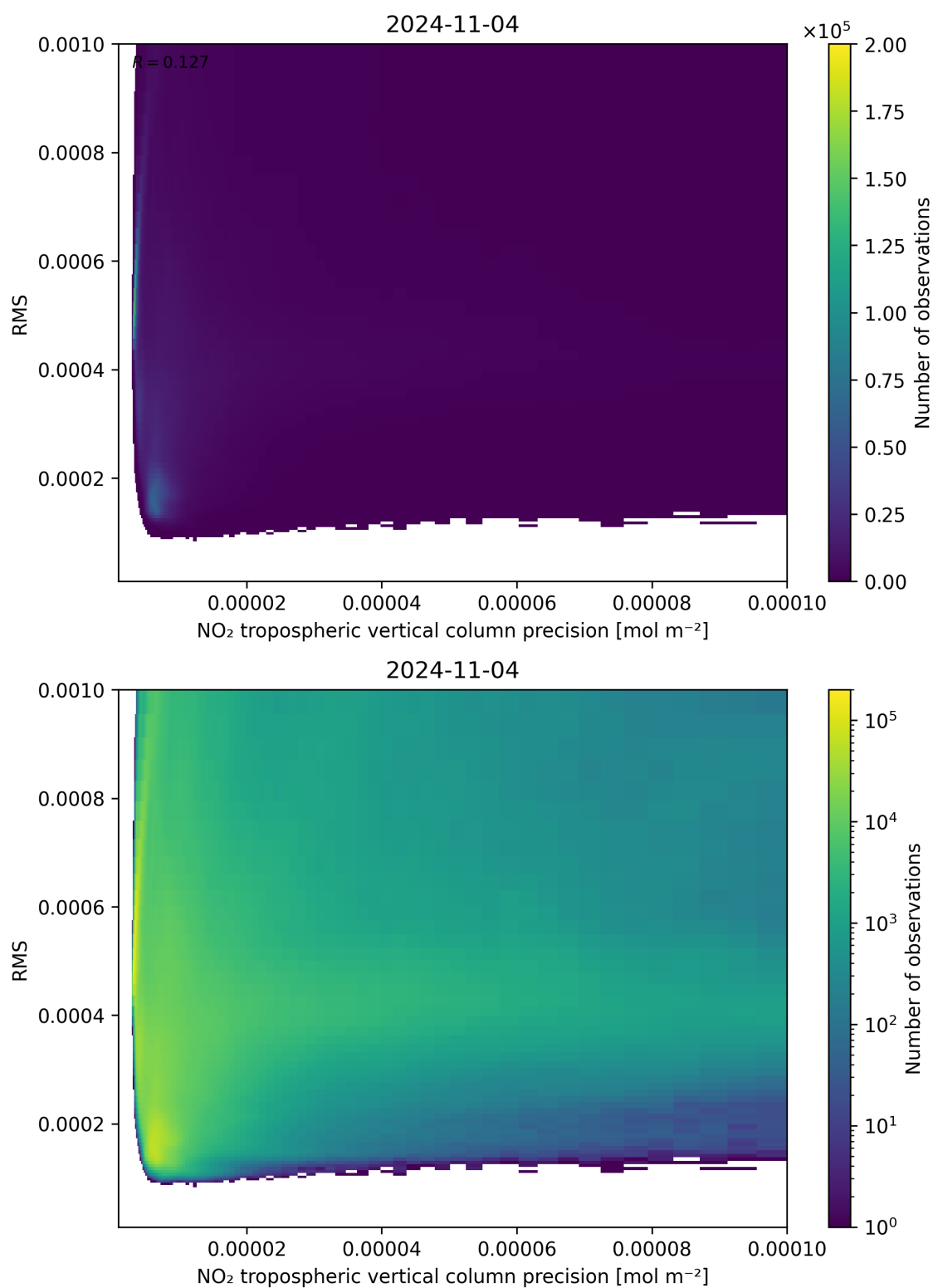
Figure 140: Scatter density plot of “NO 2 tropospheric vertical column precision” against “RMS” for 2024-11-04 to 2024-11-05.
