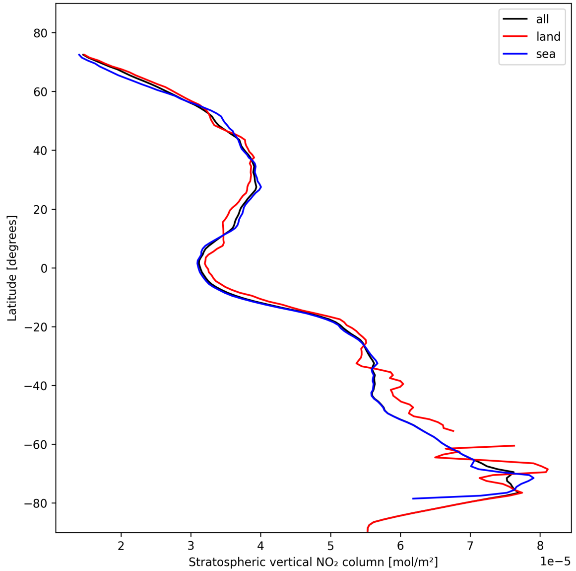
Figure 19: Zonal average of “Stratospheric vertical NO 2 column” for 2024-11-04 to 2024-11-05.
