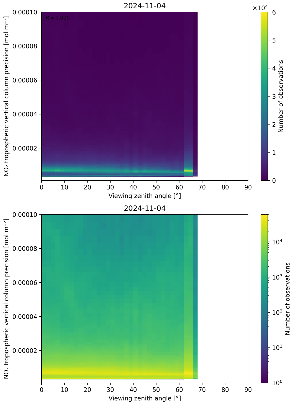
Figure 170: Scatter density plot of “Viewing zenith angle” against “NO 2 tropospheric vertical column precision” for 2024-11-04 to 2024-11-05.
