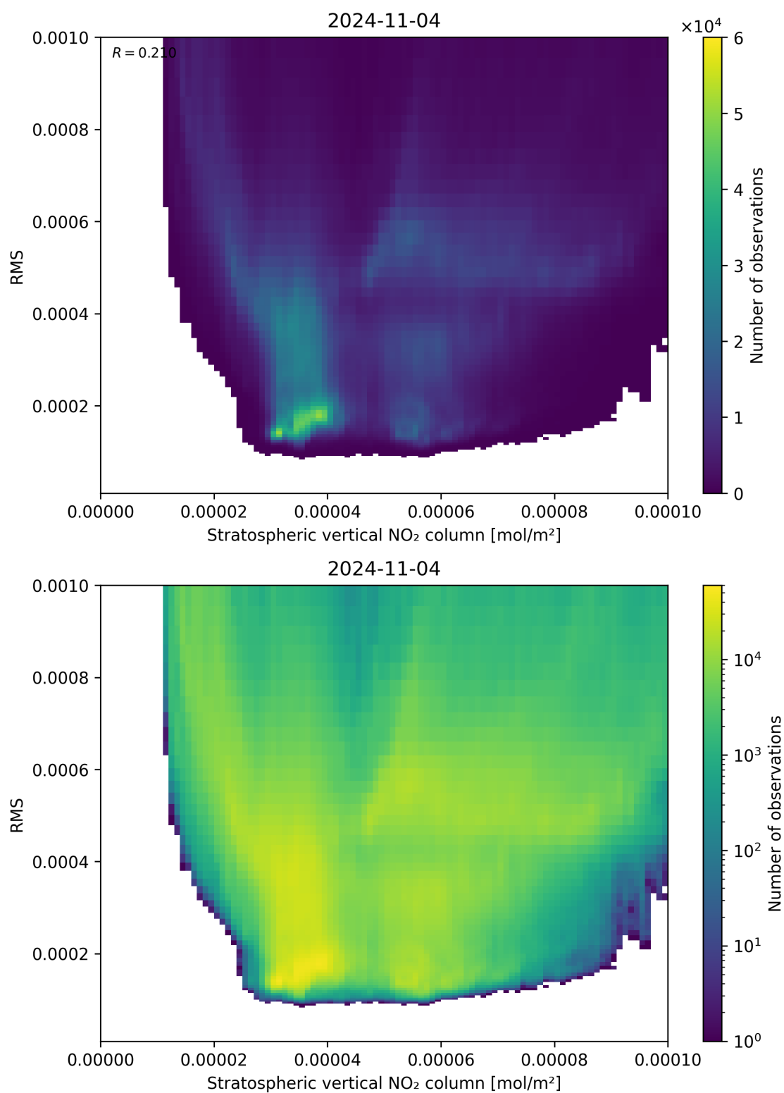
Figure 102: Scatter density plot of “Stratospheric vertical NO 2 column” against “RMS” for 2024-11-04 to 2024-11-05.
