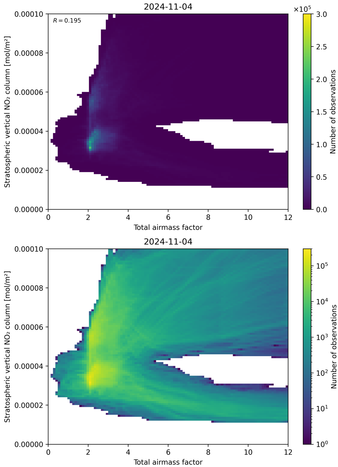
Figure 64: Scatter density plot of “Total airmass factor” against “Stratospheric vertical NO 2 column” for 2024-11-04 to 2024-11-05.
