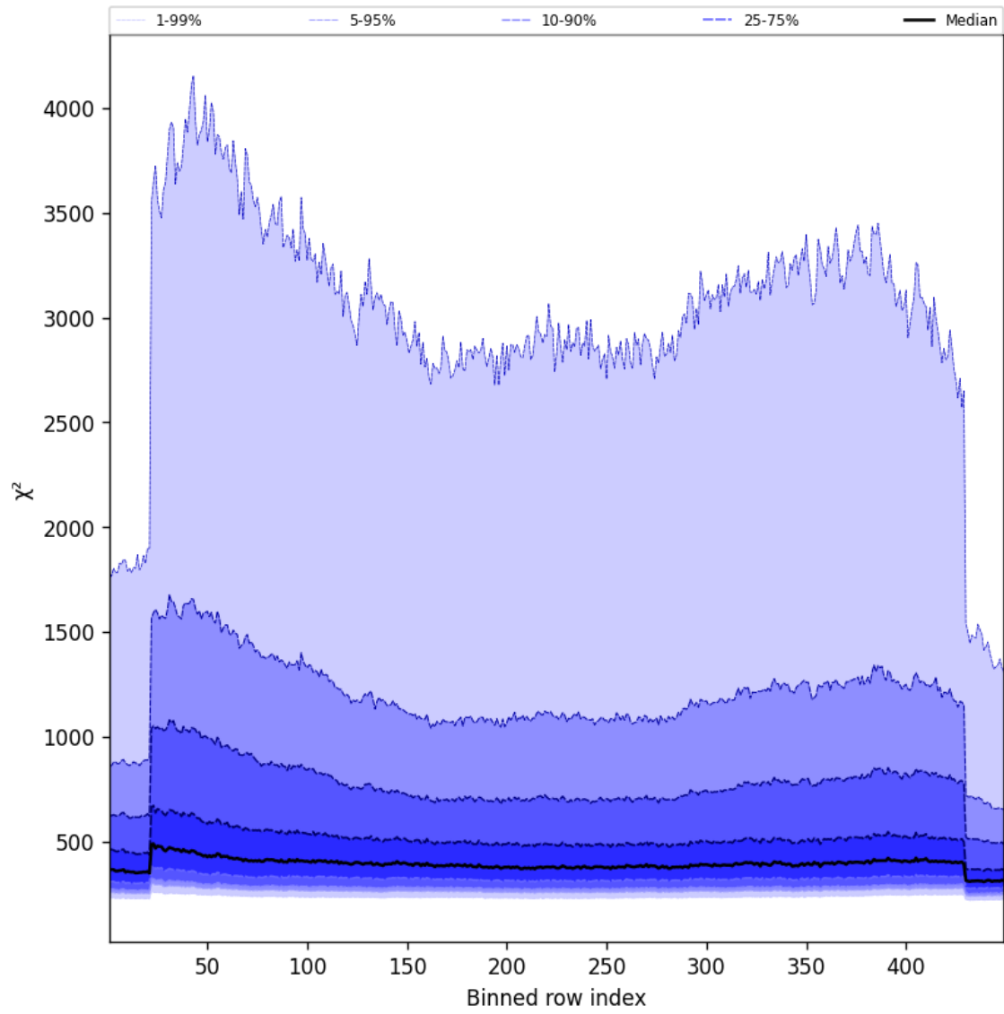
Figure 59: Along track statistics of “ \chi^2 ” for 2024-11-04 to 2024-11-05
