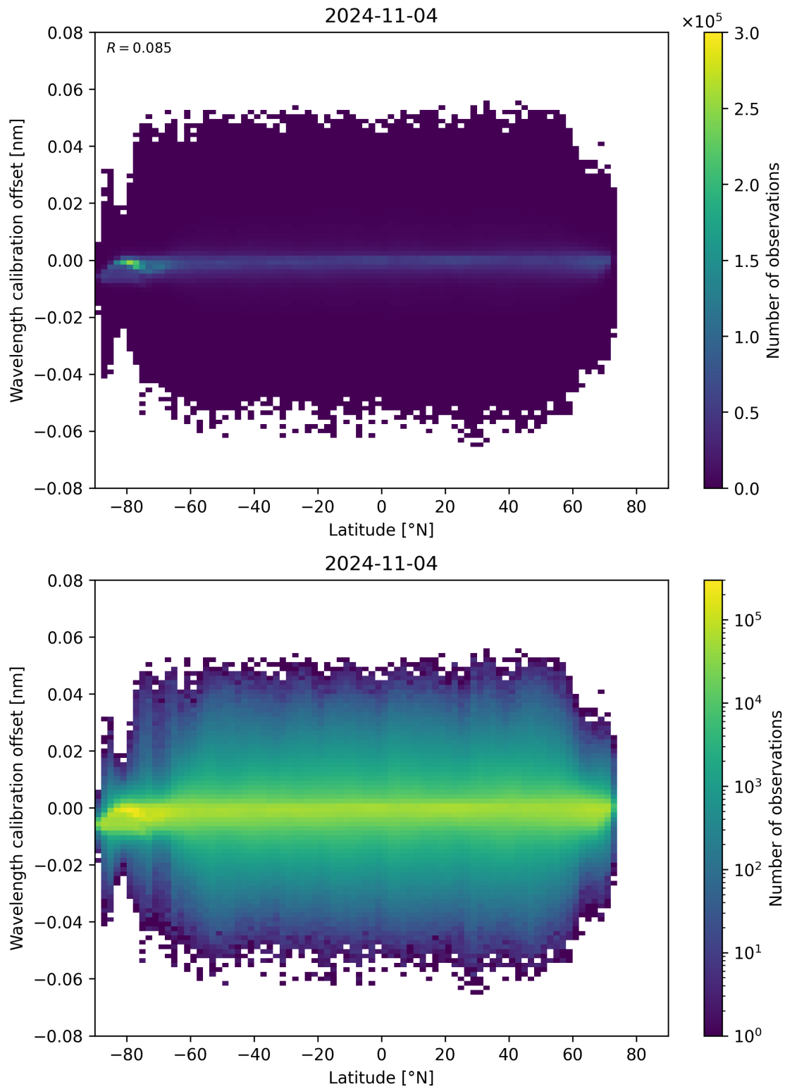
Figure 95: Scatter density plot of “Latitude” against “Wavelength calibration offset” for 2024-11-04 to 2024-11-05.
