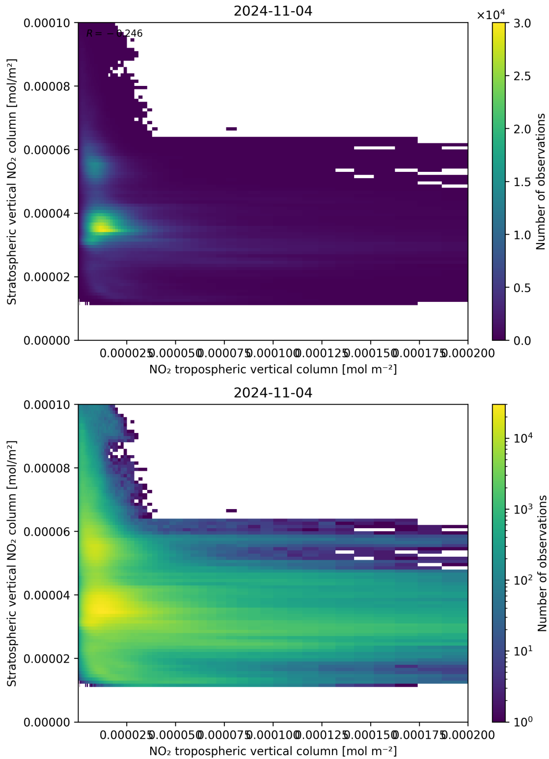
Figure 125: Scatter density plot of “NO 2 tropospheric vertical column” against “Stratospheric vertical NO 2 column” for 2024-11-04 to 2024-11-05.
