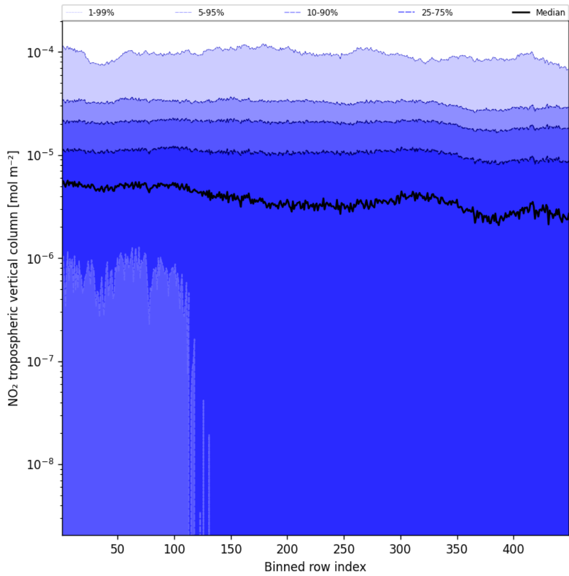
Figure 46: Along track statistics of “NO 2 tropospheric vertical column” for 2024-11-04 to 2024-11-05
