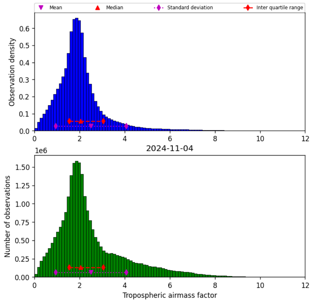
Figure 31: Histogram of “Tropospheric airmass factor” for 2024-11-04 to 2024-11-05
