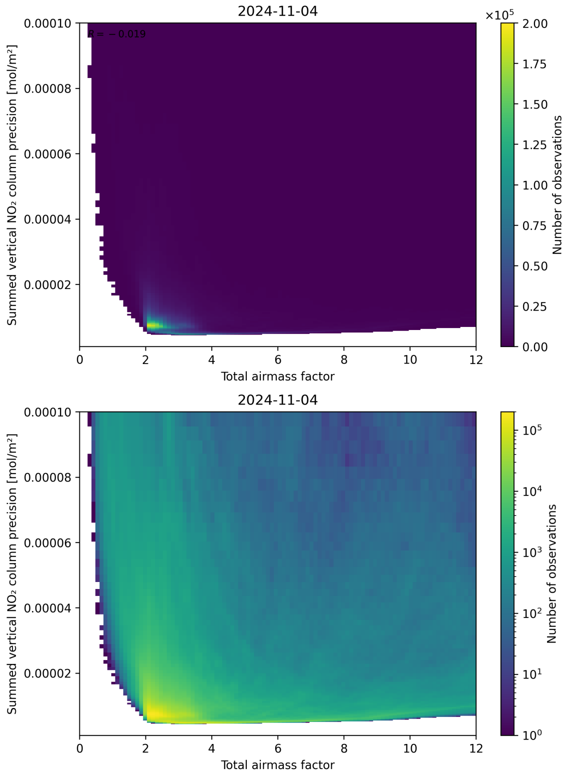
Figure 66: Scatter density plot of “Total airmass factor” against “Summed vertical NO 2 column precision” for 2024-11-04 to 2024-11-05.
