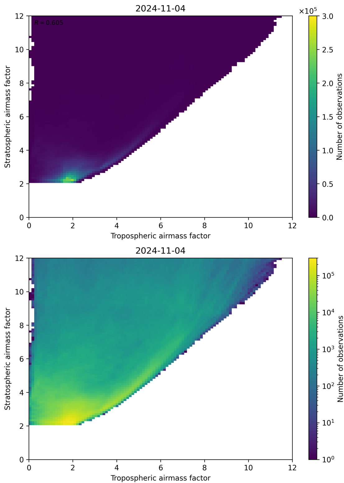
Figure 71: Scatter density plot of “Tropospheric airmass factor” against “Stratospheric airmass factor” for 2024-11-04 to 2024-11-05.
