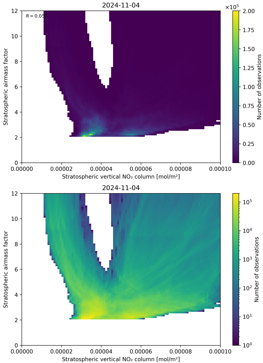
Figure 96: Scatter density plot of “Stratospheric vertical NO 2 column” against “Stratospheric airmass factor” for 2024-11-04 to 2024-11-05.
