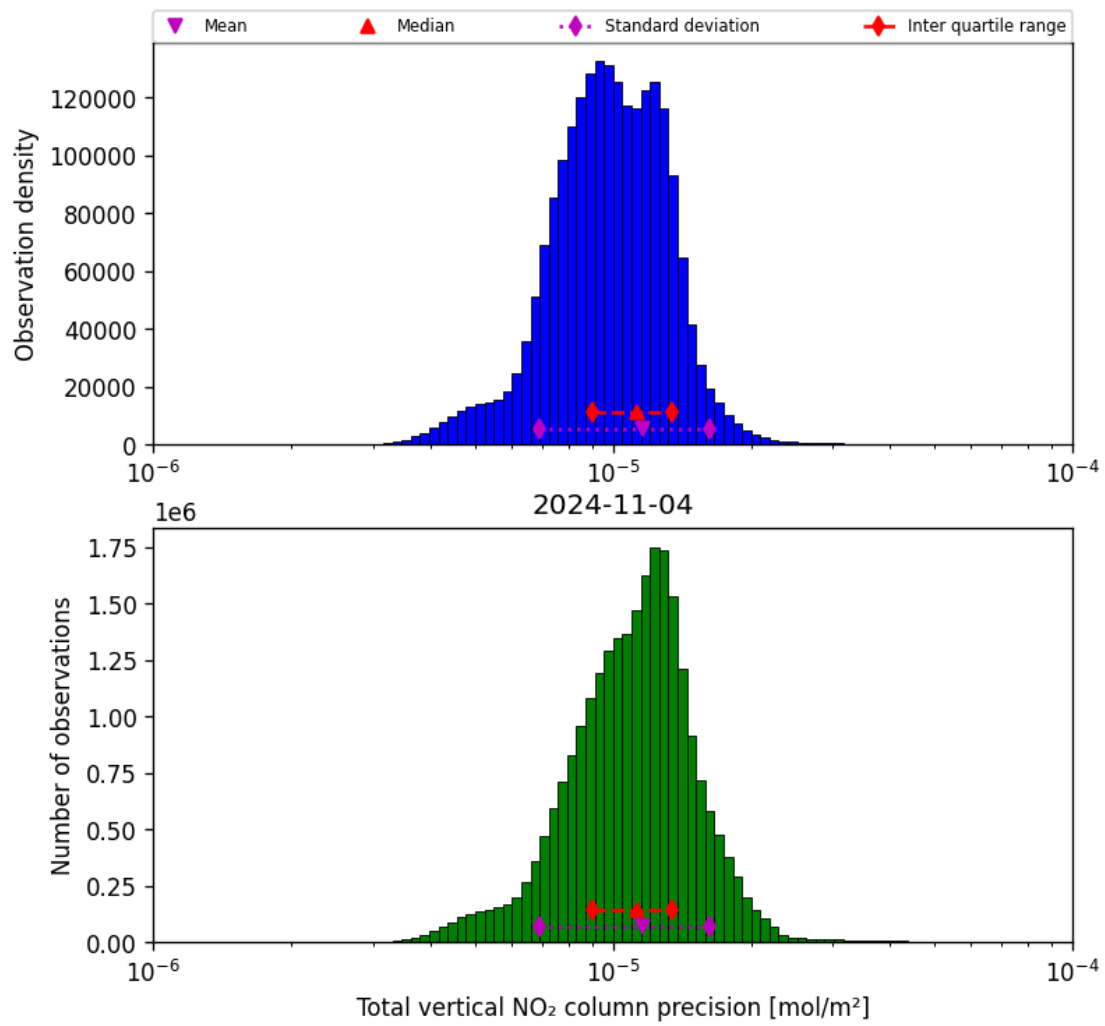
Figure 39: Histogram of “Total vertical NO 2 column precision” for 2024-11-04 to 2024-11-05
