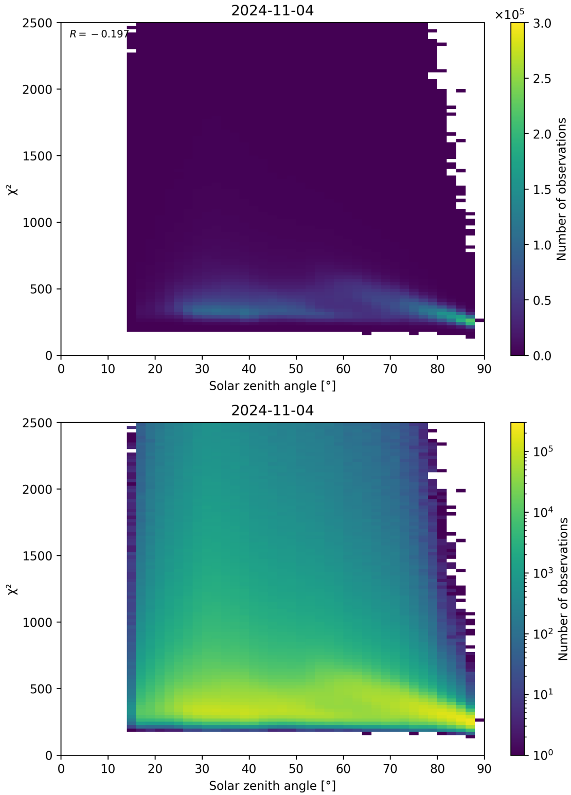
Figure 148: Scatter density plot of “Solar zenith angle” against “ \chi^2 ” for 2024-11-04 to 2024-11-05.
