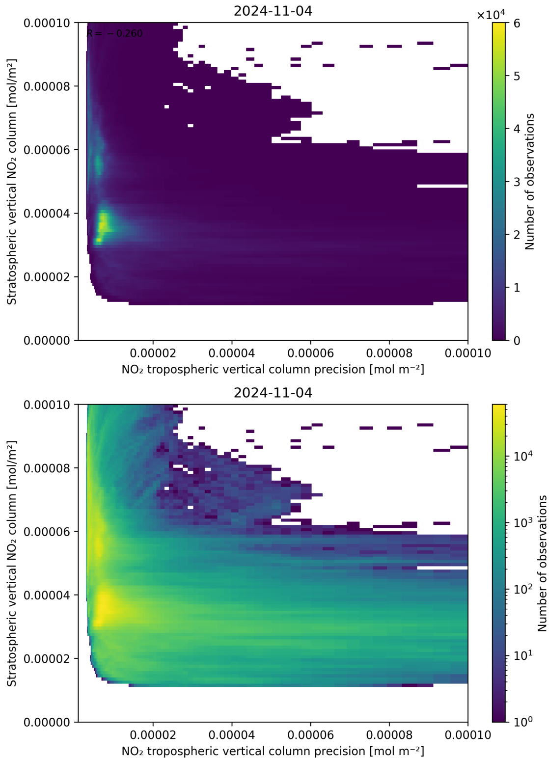
Figure 135: Scatter density plot of “NO 2 tropospheric vertical column precision” against “Stratospheric vertical NO 2 column” for 2024-11-04 to 2024-11-05.
