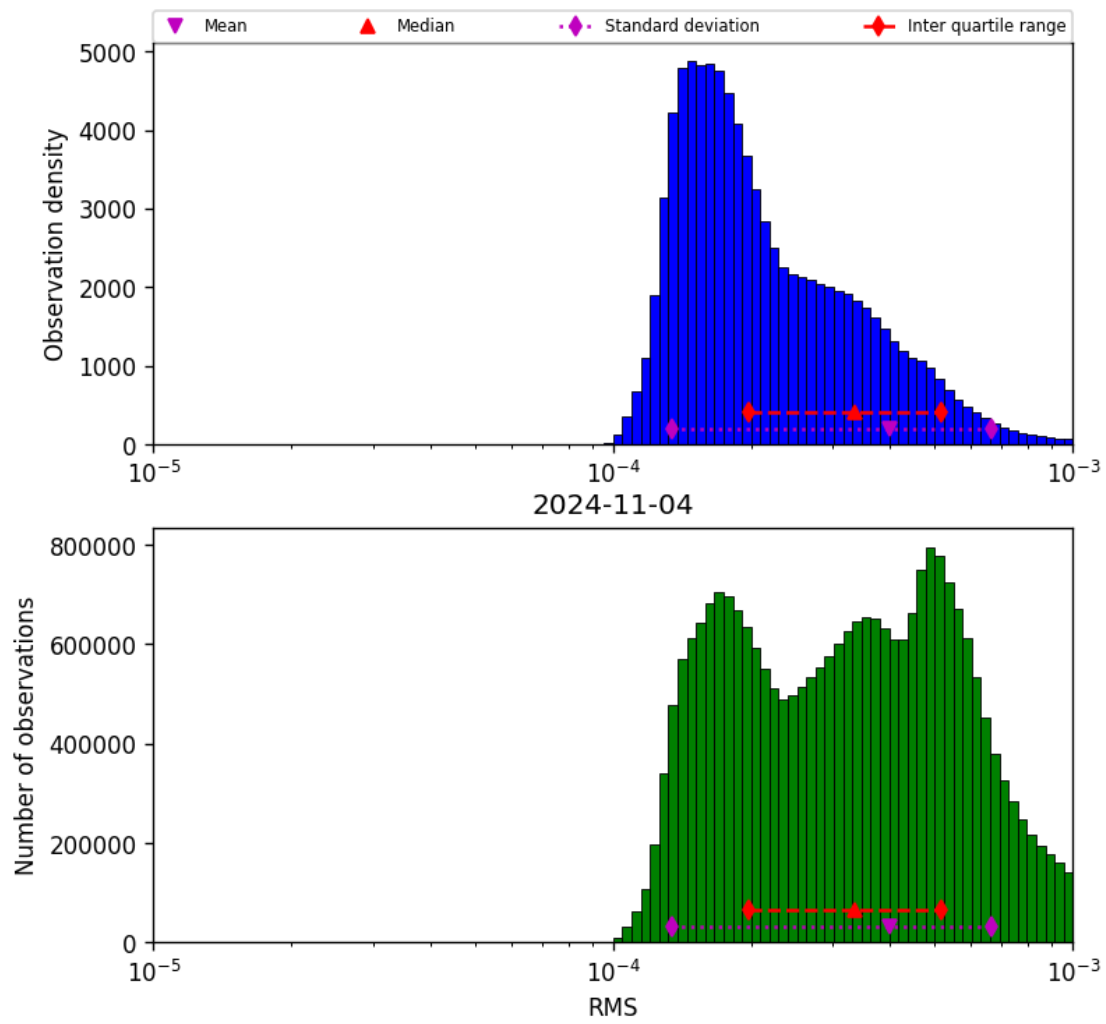
Figure 43: Histogram of “RMS” for 2024-11-04 to 2024-11-05
