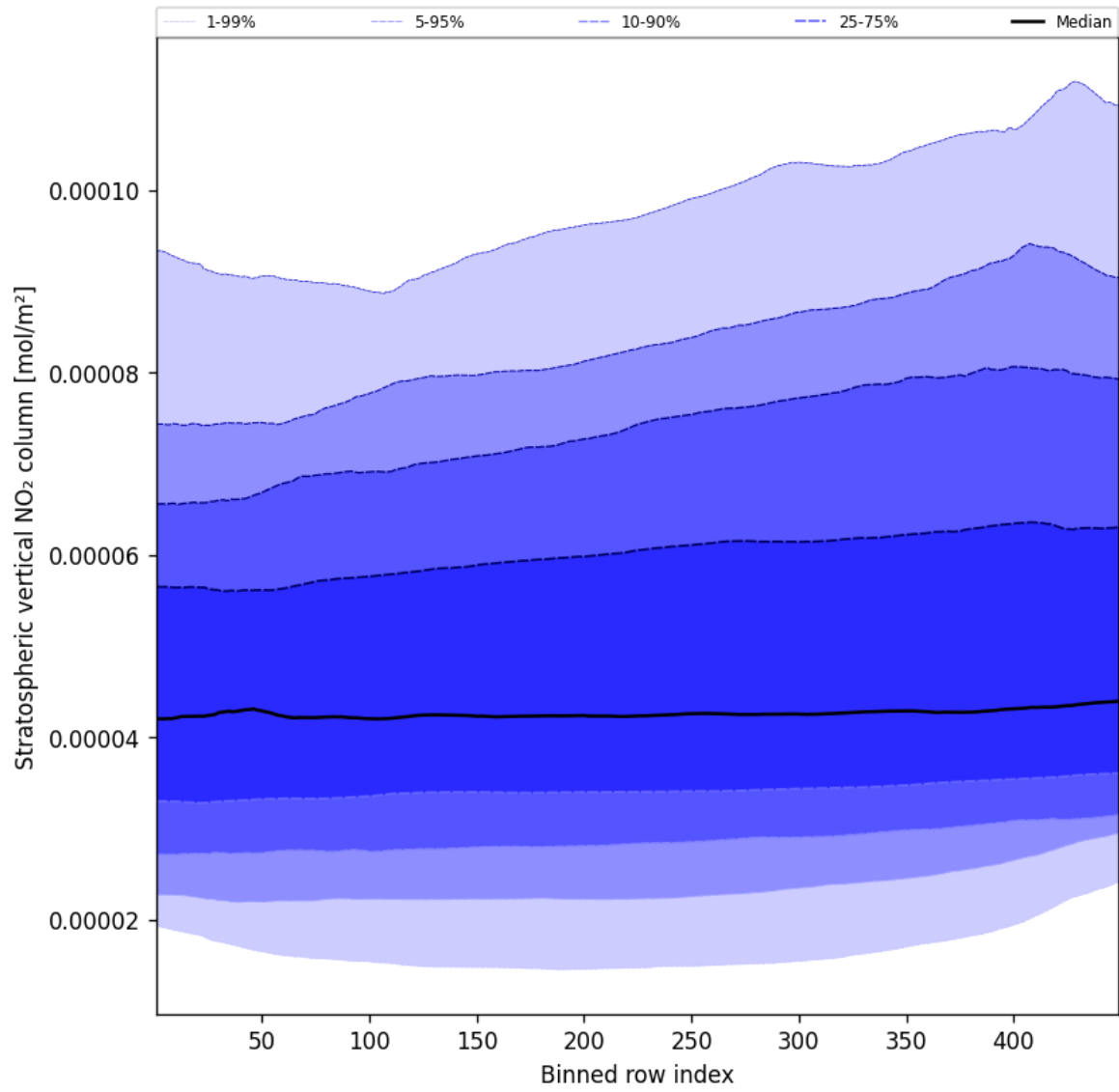
Figure 53: Along track statistics of “Stratospheric vertical NO 2 column” for 2024-11-04 to 2024-11-05
