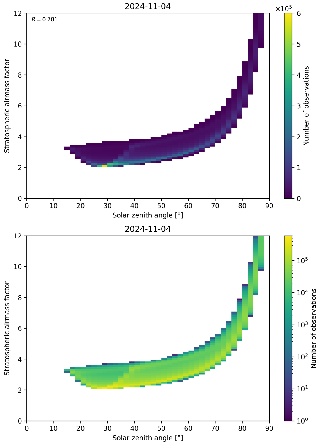
Figure 145: Scatter density plot of “Solar zenith angle” against “Stratospheric airmass factor” for 2024-11-04 to 2024-11-05.
