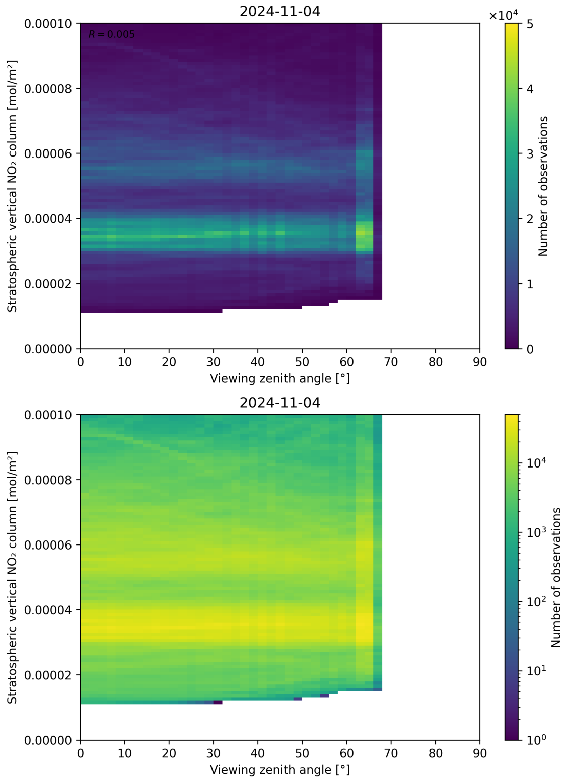
Figure 164: Scatter density plot of “Viewing zenith angle” against “Stratospheric vertical NO 2 column” for 2024-11-04 to 2024-11-05.
