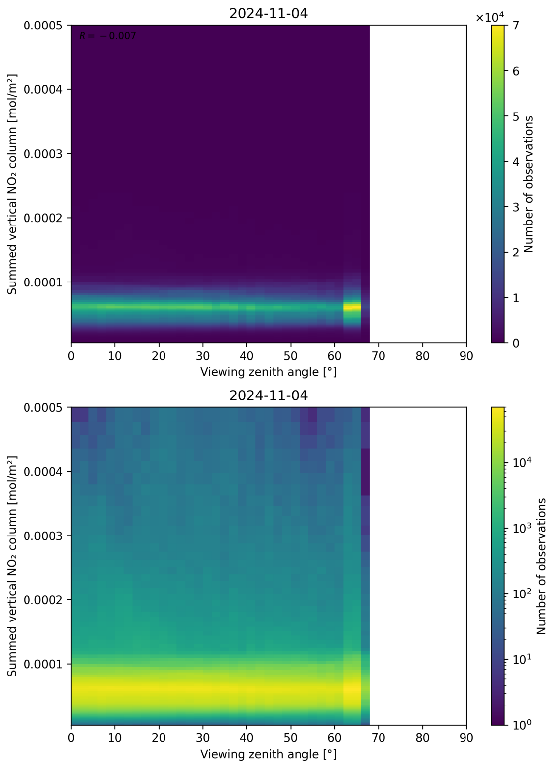
Figure 165: Scatter density plot of “Viewing zenith angle” against “Summed vertical NO 2 column” for 2024-11-04 to 2024-11-05.
