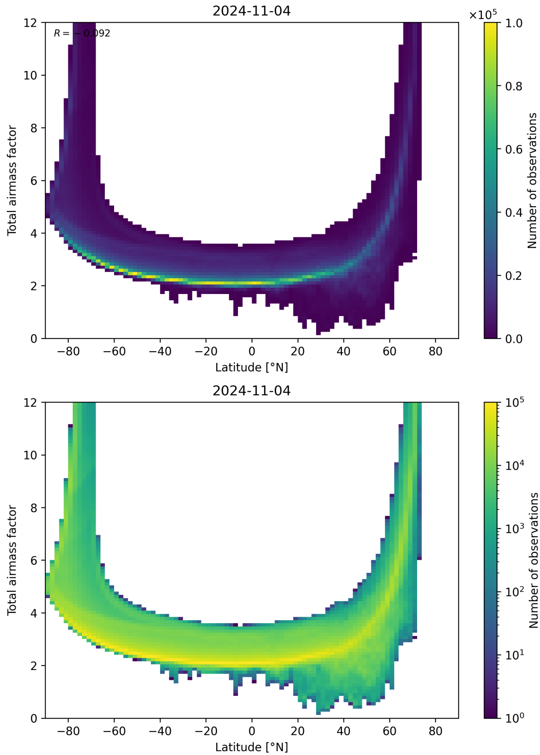
Figure 84: Scatter density plot of “Latitude” against “Total airmass factor” for 2024-11-04 to 2024-11-05.
