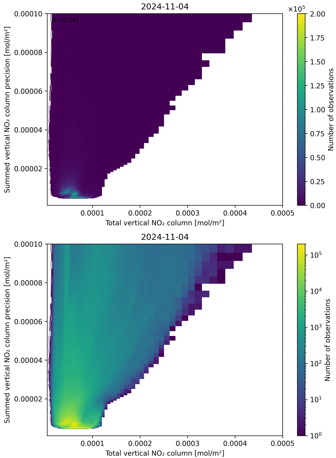
Figure 113: Scatter density plot of “Total vertical NO 2 column” against “Summed vertical NO 2 column precision” for 2024-11-04 to 2024-11-05.
