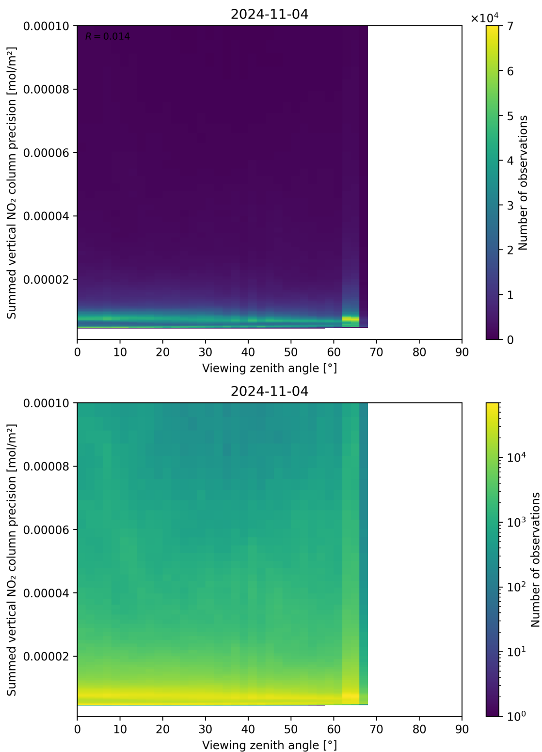
Figure 166: Scatter density plot of “Viewing zenith angle” against “Summed vertical NO 2 column precision” for 2024-11-04 to 2024-11-05.
