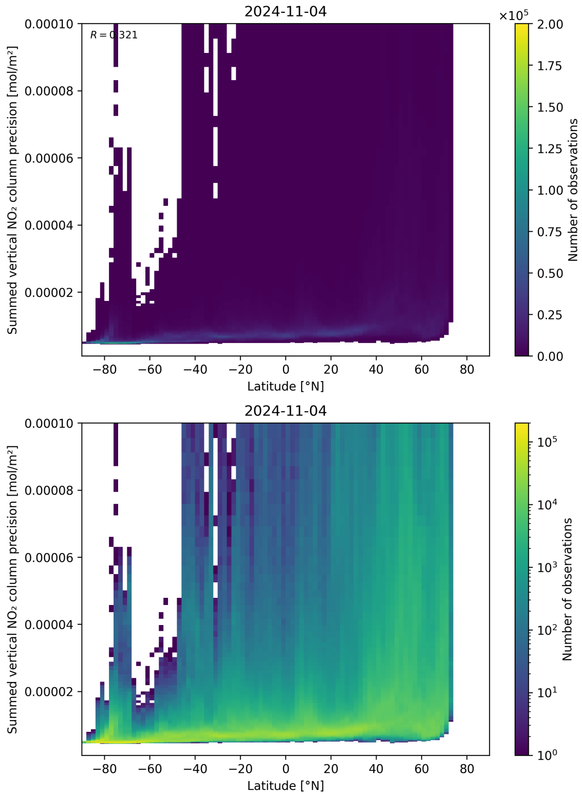
Figure 89: Scatter density plot of “Latitude” against “Summed vertical NO 2 column precision” for 2024-11-04 to 2024-11-05.
