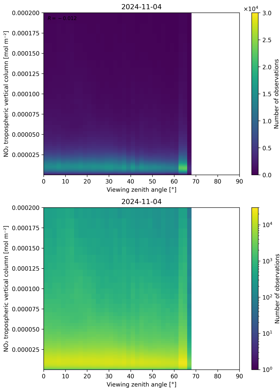
Figure 169: Scatter density plot of “Viewing zenith angle” against “NO 2 tropospheric vertical column” for 2024-11-04 to 2024-11-05.
