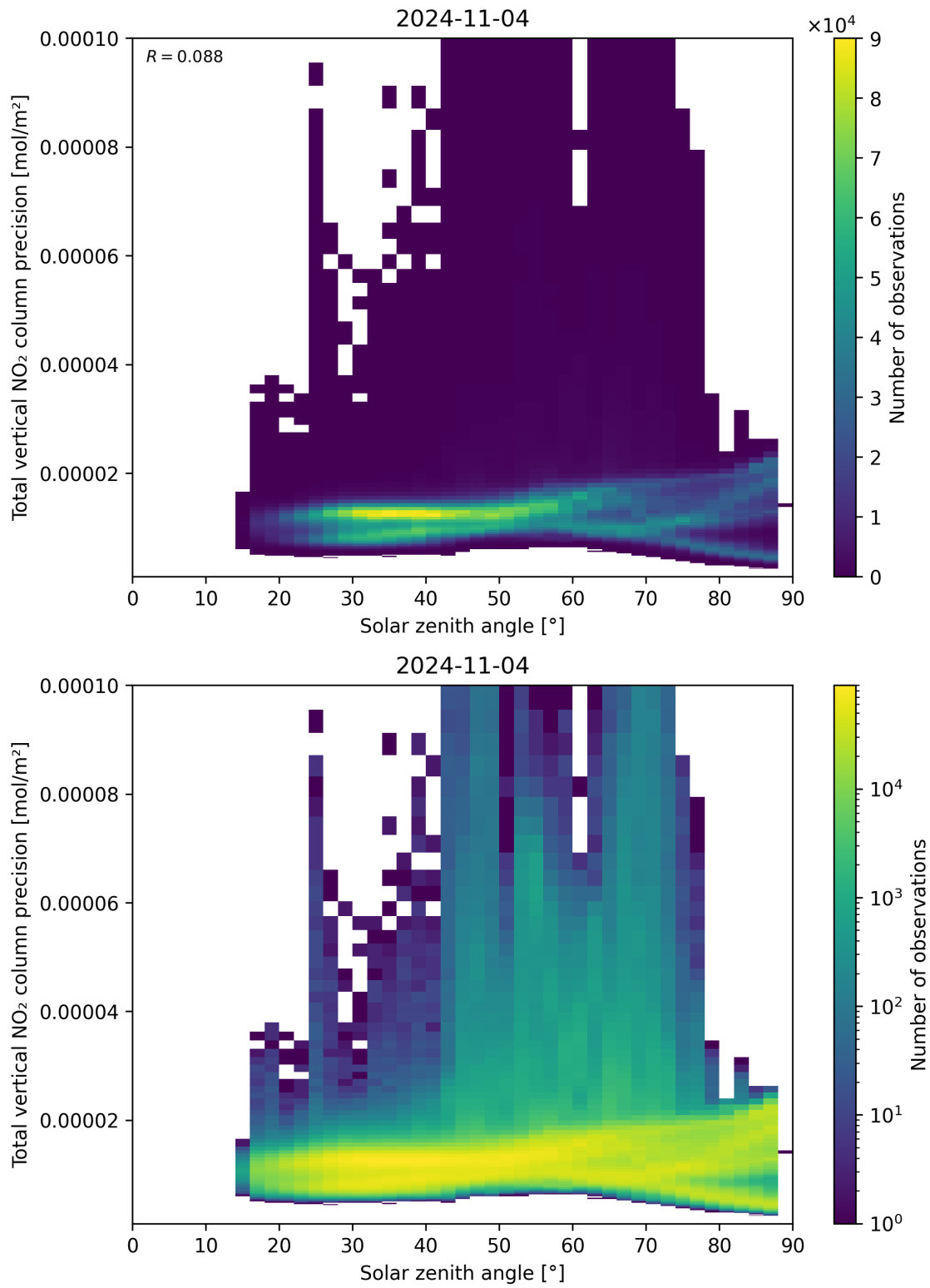
Figure 154: Scatter density plot of “Solar zenith angle” against “Total vertical NO 2 column precision” for 2024-11-04 to 2024-11-05.
