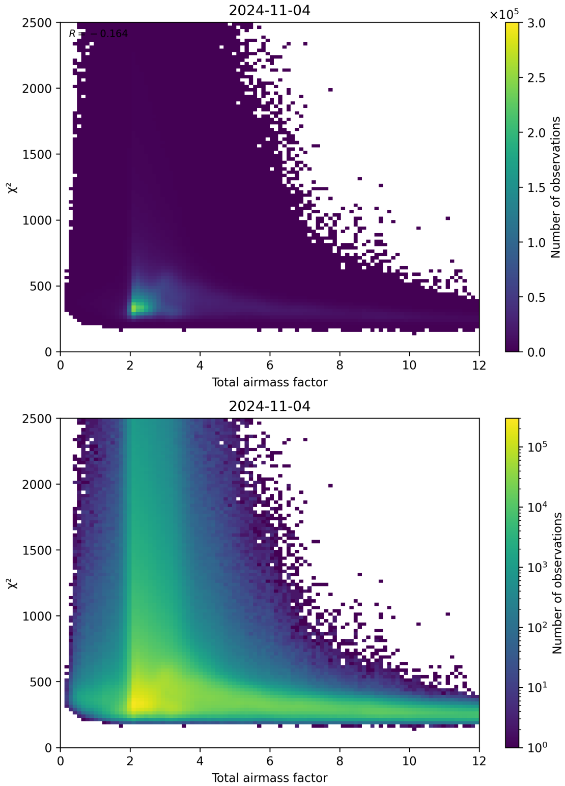
Figure 63: Scatter density plot of “Total airmass factor” against “ \chi^2 ” for 2024-11-04 to 2024-11-05.
