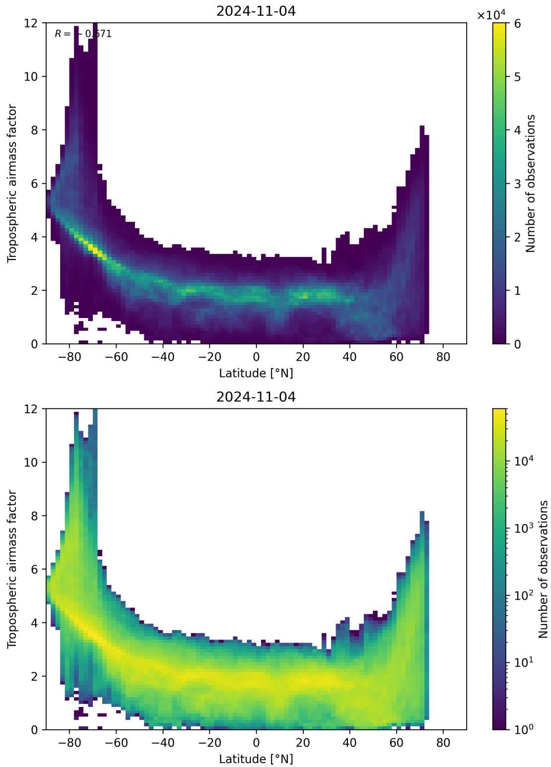
Figure 85: Scatter density plot of “Latitude” against “Tropospheric air mass factor” for 2024-11-04 to 2024-11-05.
