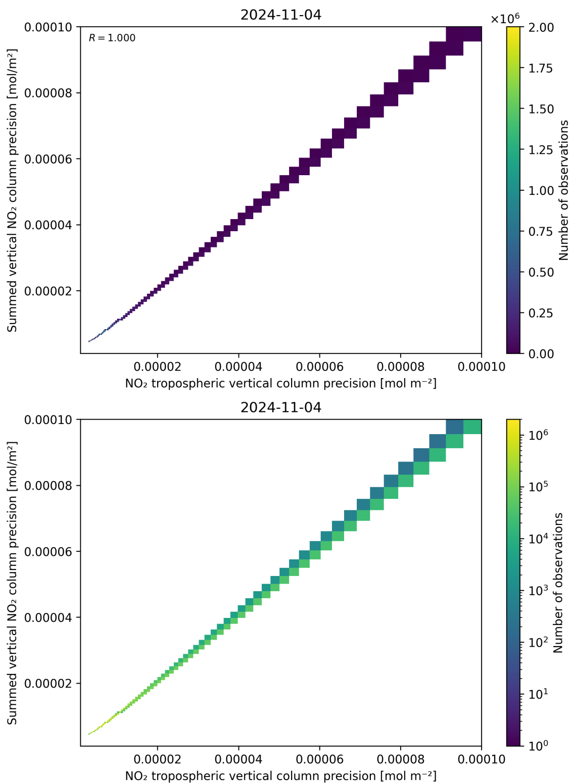
Figure 137: Scatter density plot of “NO 2 tropospheric vertical column precision” against “Summed vertical NO 2 column precision” for 2024-11-04 to 2024-11-05.
