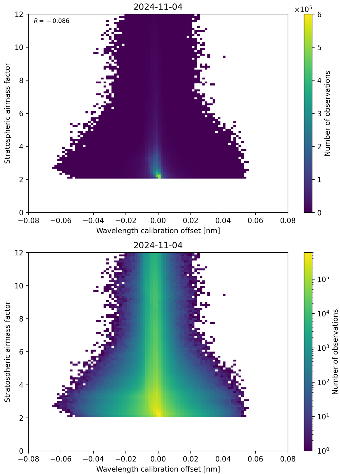
Figure 174: Scatter density plot of “Wavelength calibration offset” against “Stratospheric air mass factor” for 2024-11-04 to 2024-11-05.
