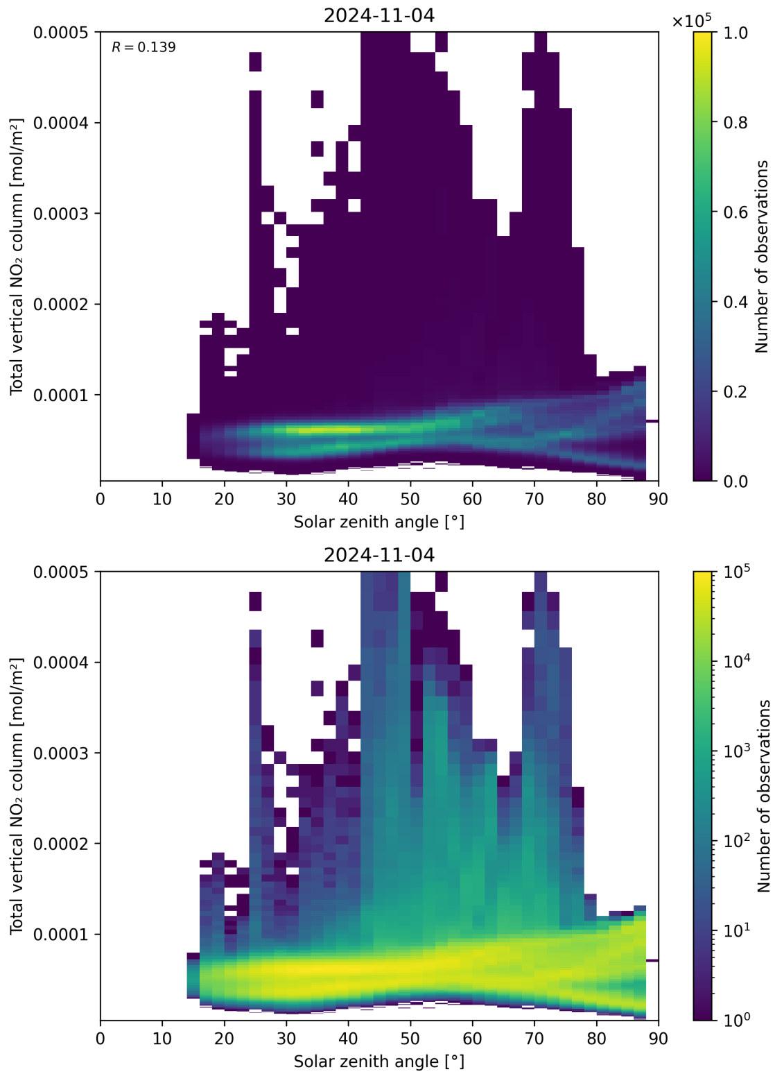
Figure 153: Scatter density plot of “Solar zenith angle” against “Total vertical NO 2 column” for 2024-11-04 to 2024-11-05.
