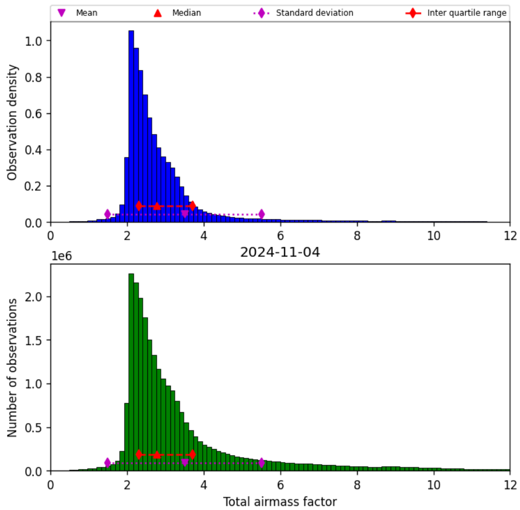
Figure 32: Histogram of “Total airmass factor” for 2024-11-04 to 2024-11-05
