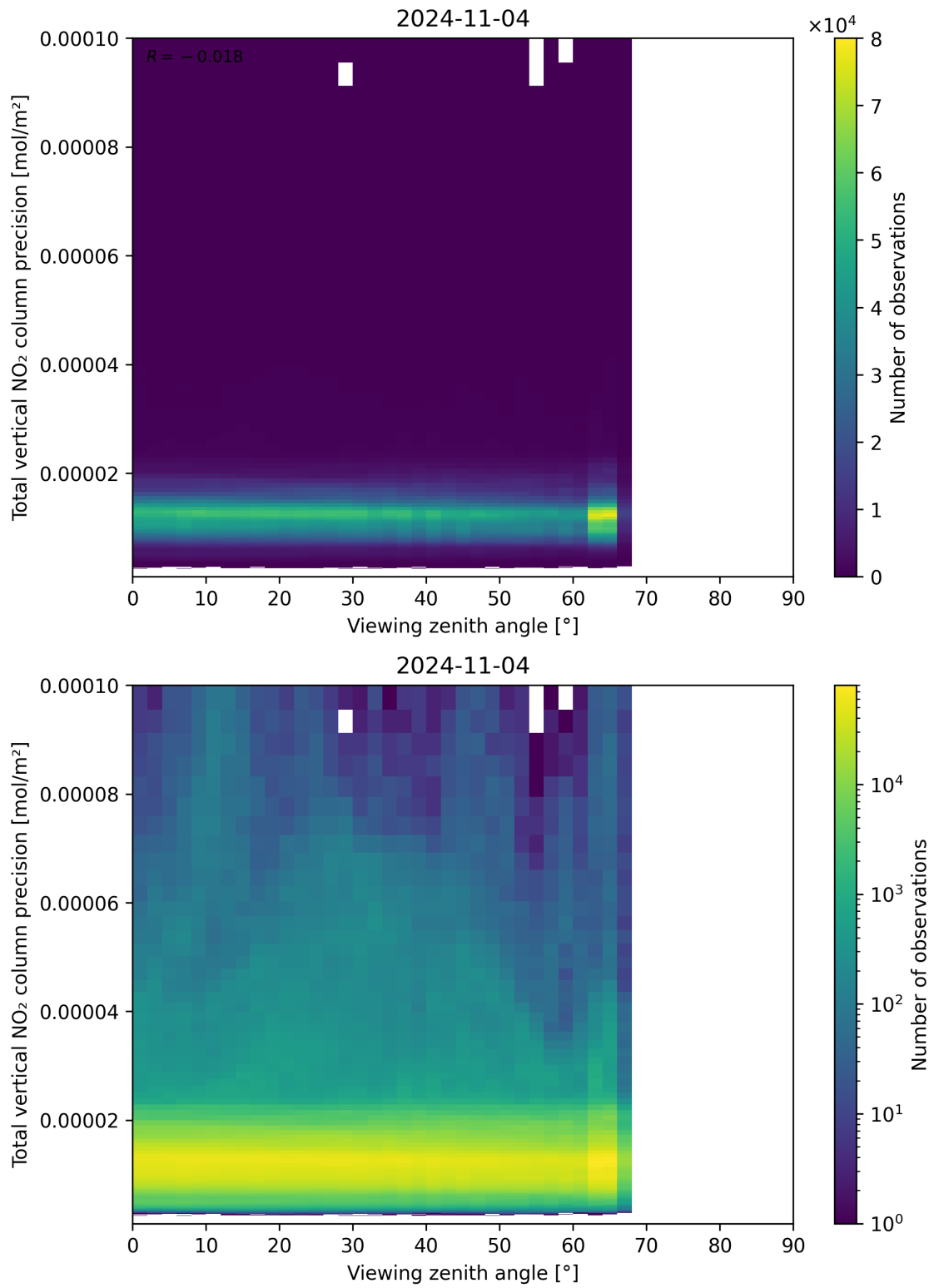
Figure 168: Scatter density plot of “Viewing zenith angle” against “Total vertical NO 2 column precision” for 2024-11-04 to 2024-11-05.
