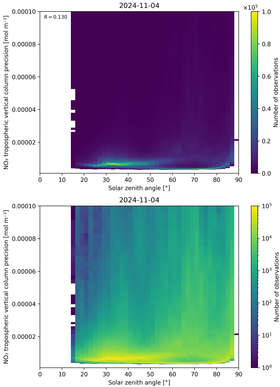
Figure 156: Scatter density plot of “Solar zenith angle” against “NO 2 tropospheric vertical column precision” for 2024-11-04 to 2024-11-05.
