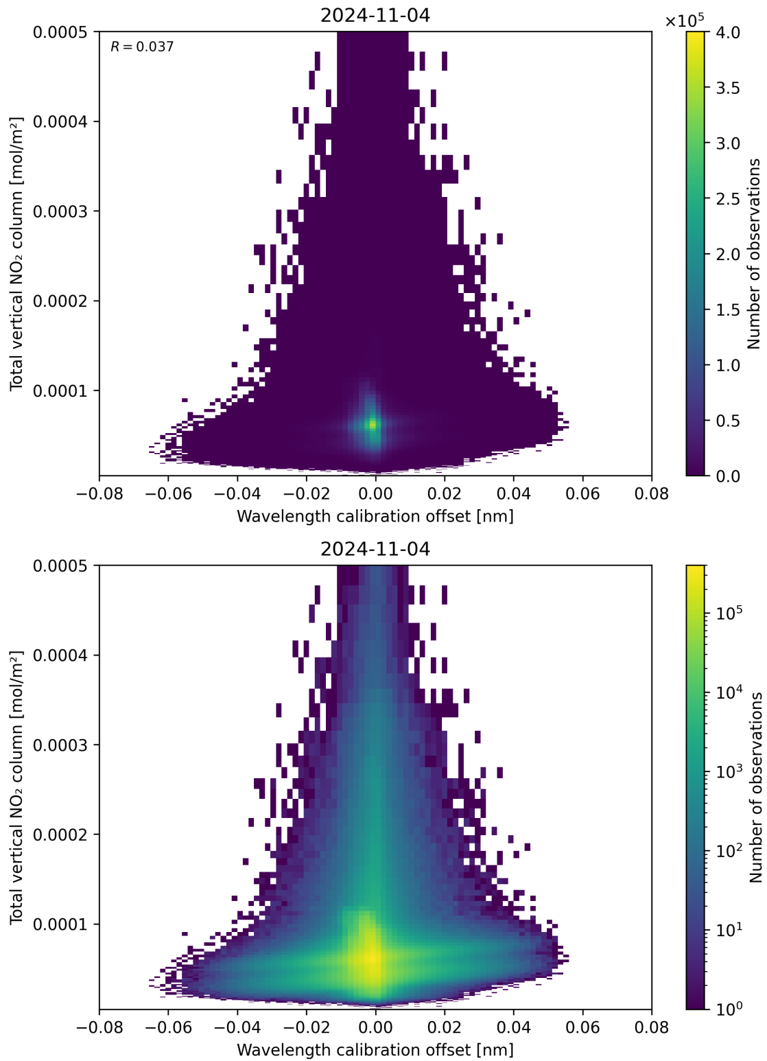
Figure 179: Scatter density plot of “Wavelength calibration offset” against “Total vertical NO 2 column” for 2024-11-04 to 2024-11-05.
