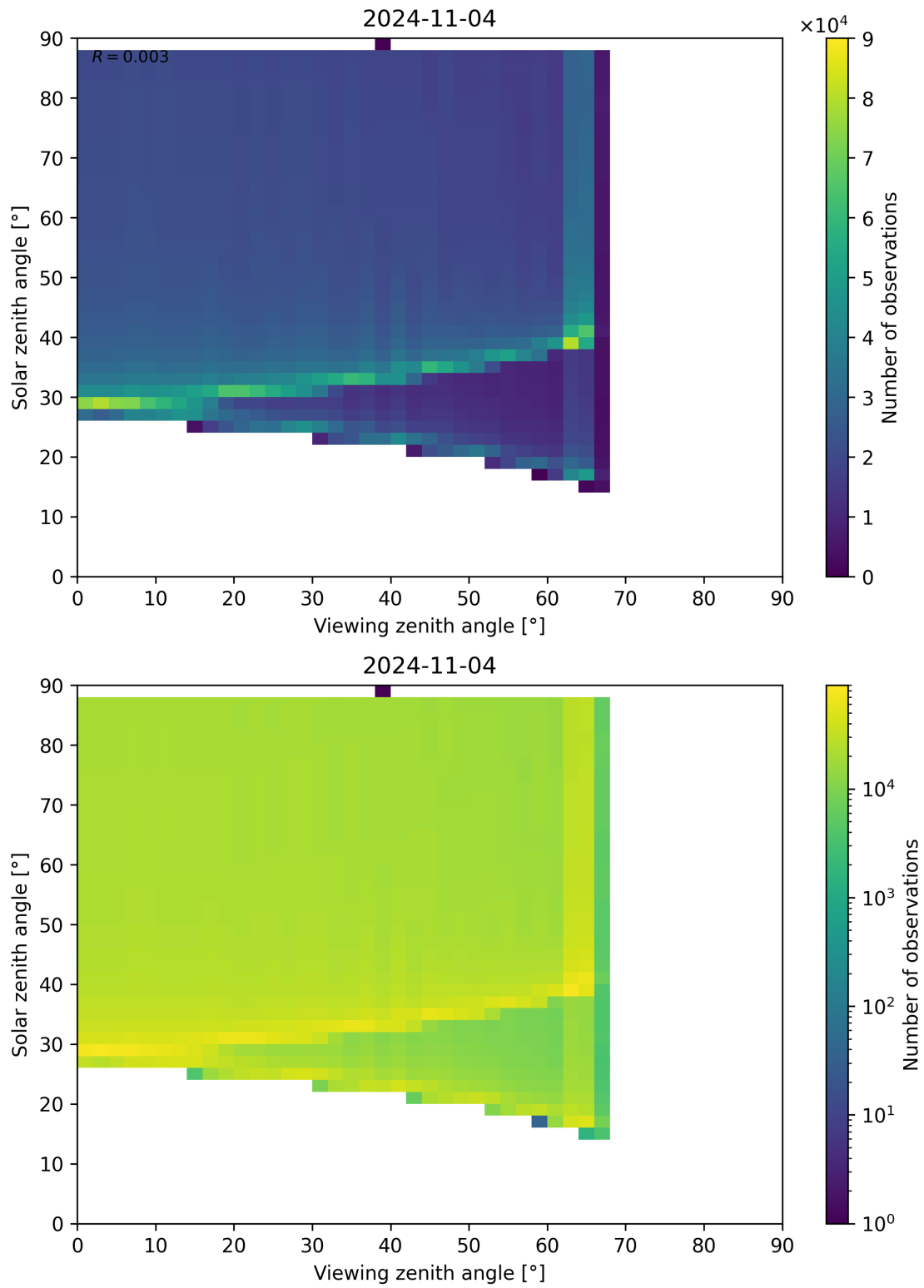
Figure 172: Scatter density plot of “Viewing zenith angle” against “Solar zenith angle” for 2024-11-04 to 2024-11-05.
