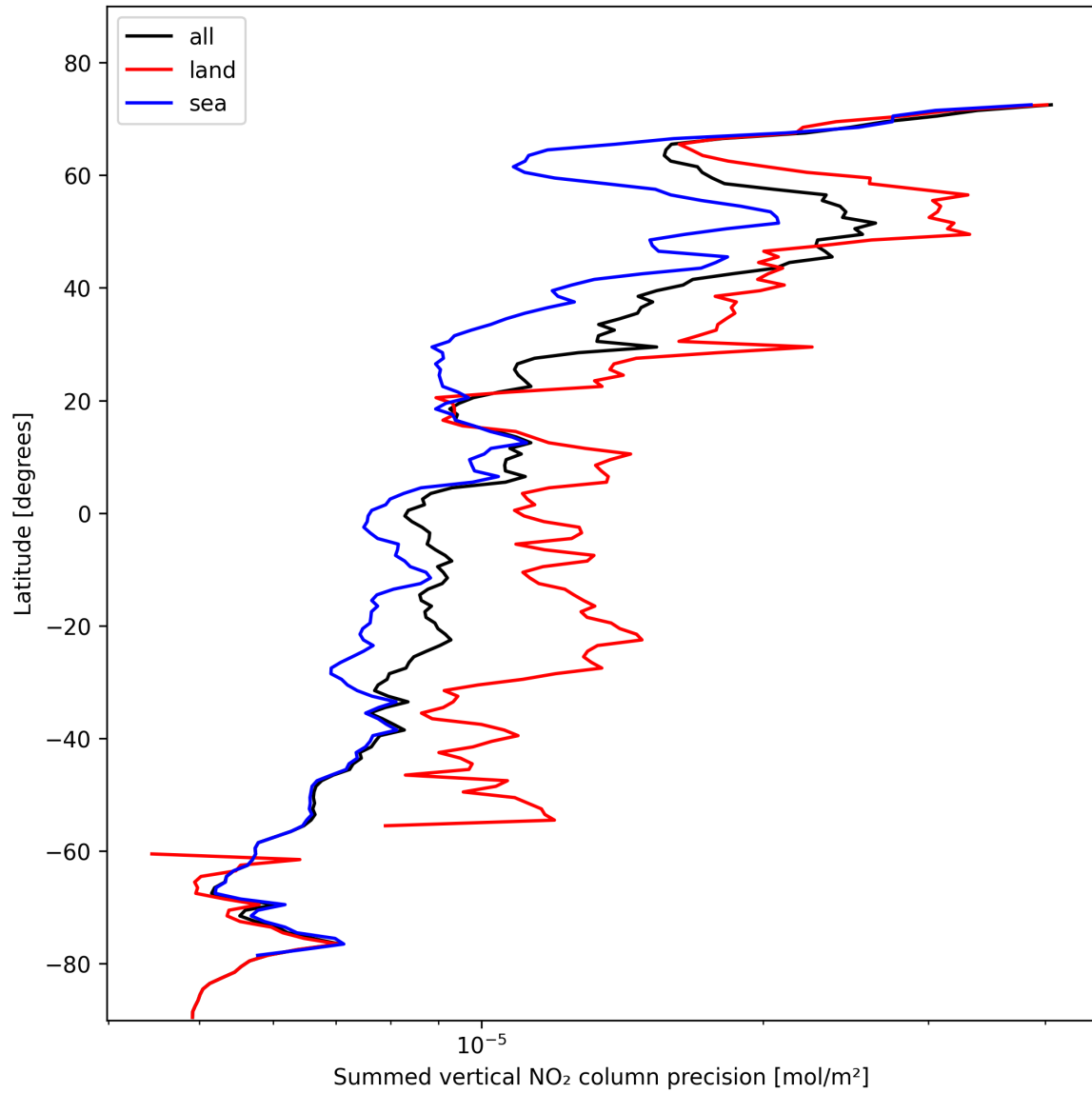
Figure 24: Zonal average of “Summed vertical NO 2 column precision” for 2024-11-04 to 2024-11-05.
