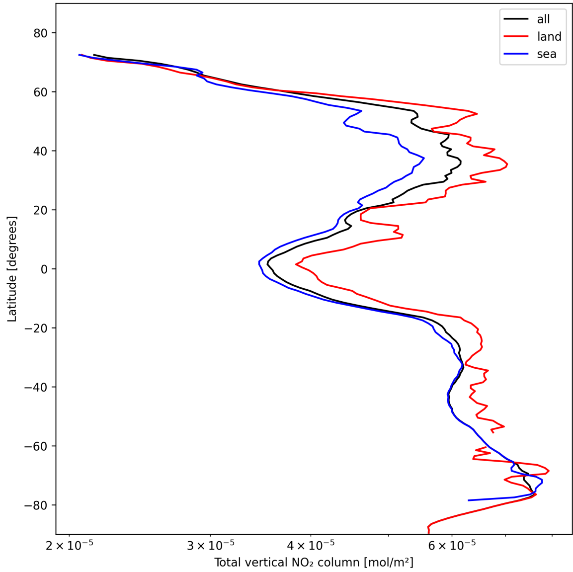
Figure 21: Zonal average of “Total vertical NO 2 column” for 2024-11-04 to 2024-11-05.
