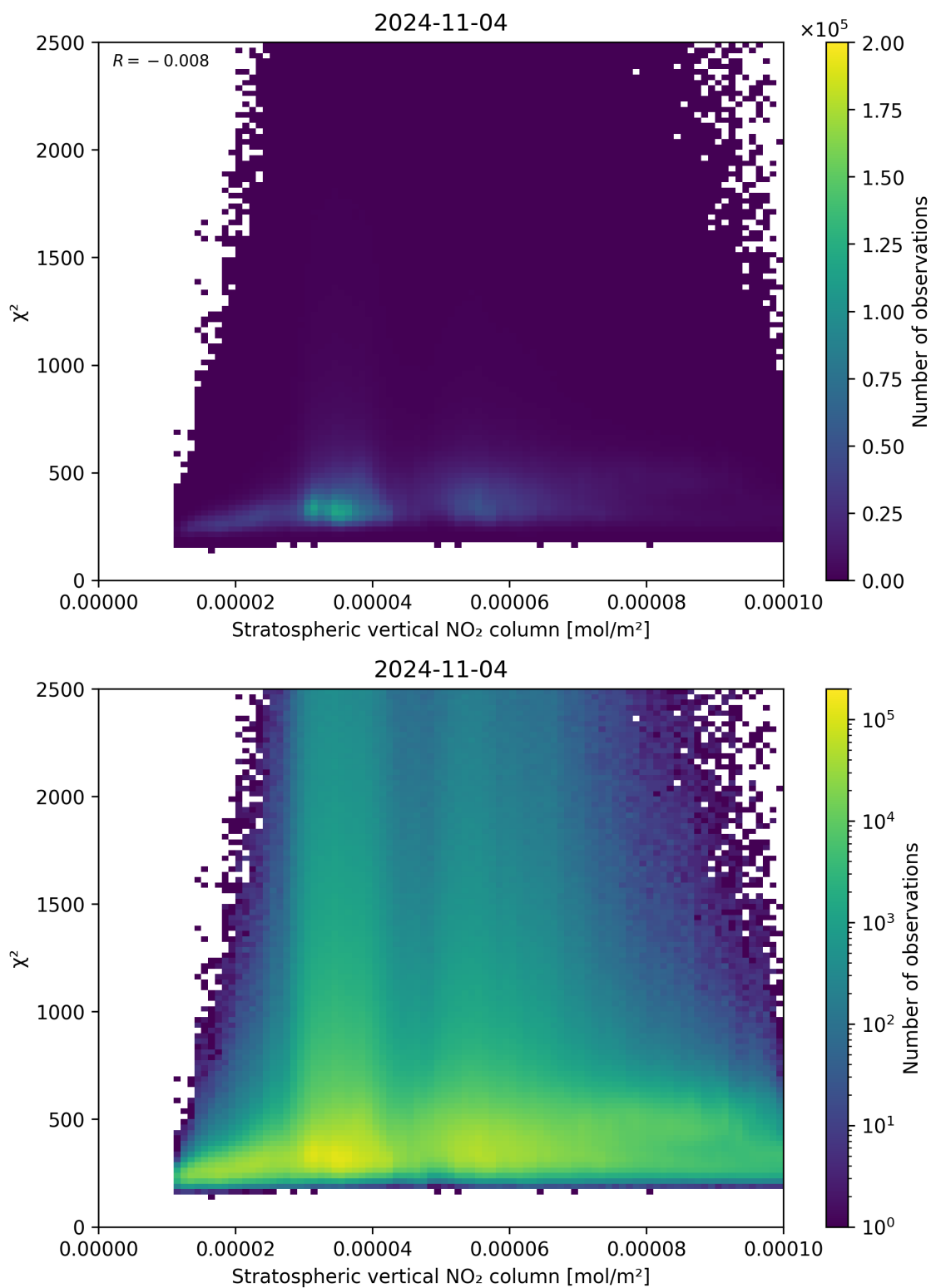
Figure 97: Scatter density plot of “Stratospheric vertical NO 2 column” against “ \chi^2 ” for 2024-11-04 to 2024-11-05.
