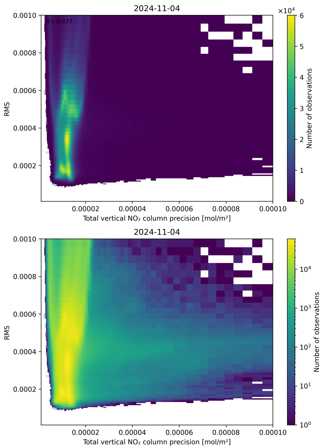
Figure 119: Scatter density plot of “Total vertical NO 2 column precision” against “RMS” for 2024-11-04 to 2024-11-05.
