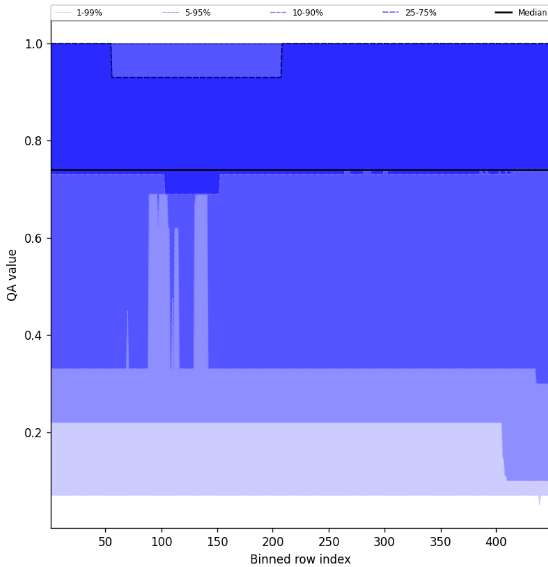
Figure 45: Along track statistics of “QA value” for 2024-11-04 to 2024-11-05
