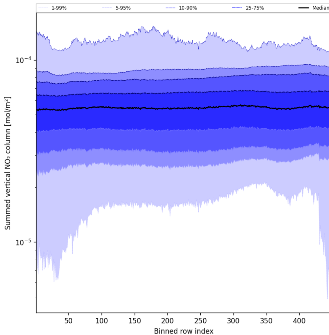
Figure 57: Along track statistics of “Summed vertical NO 2 column” for 2024-11-04 to 2024-11-05
