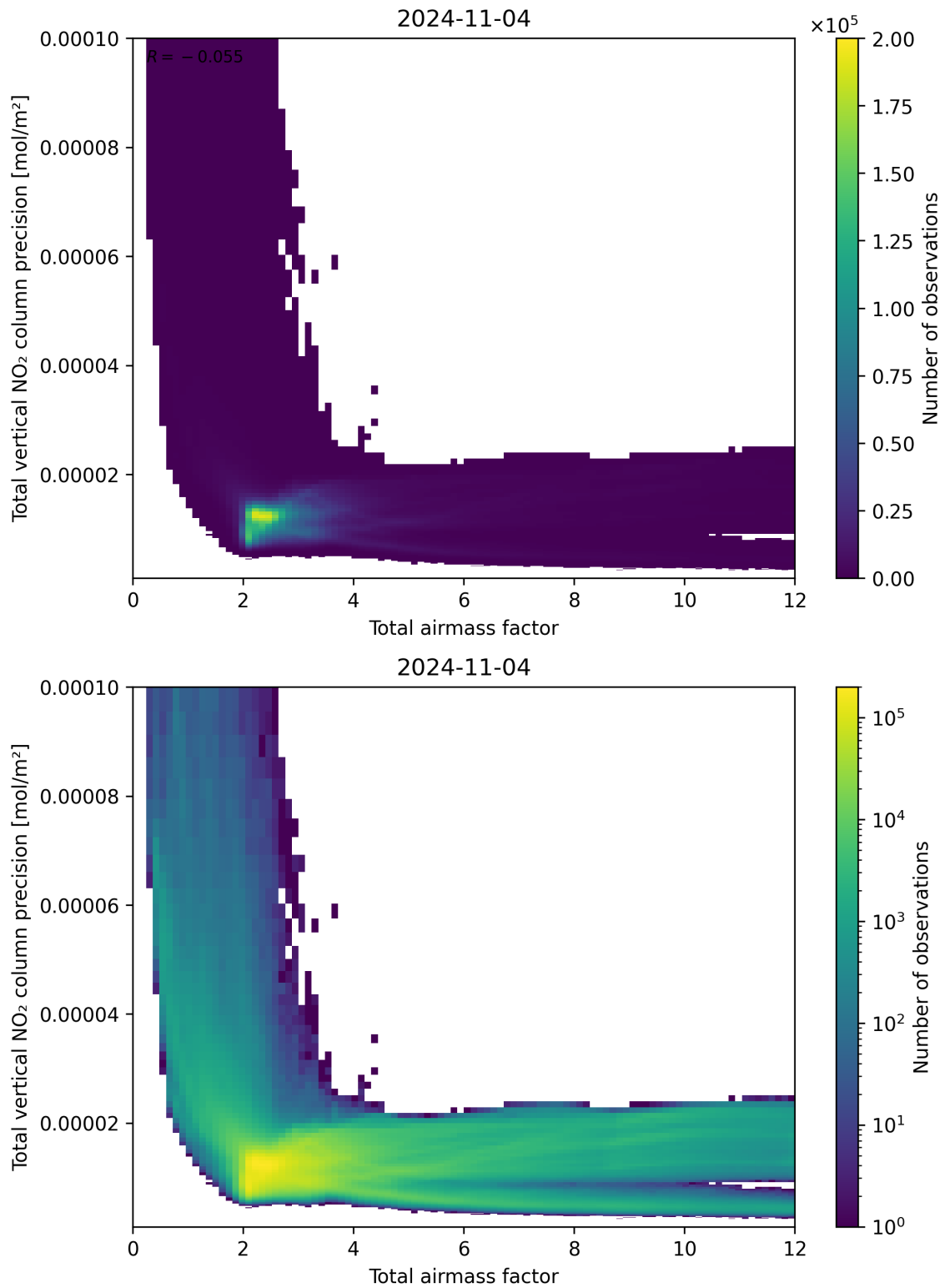
Figure 68: Scatter density plot of “Total airmass factor” against “Total vertical NO 2 column precision” for 2024-11-04 to 2024-11-05.
