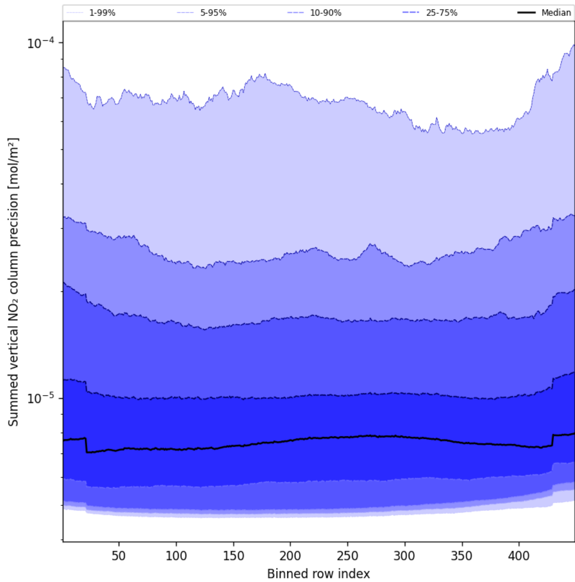
Figure 58: Along track statistics of “Summed vertical NO 2 column precision” for 2024-11-04 to 2024-11-05
