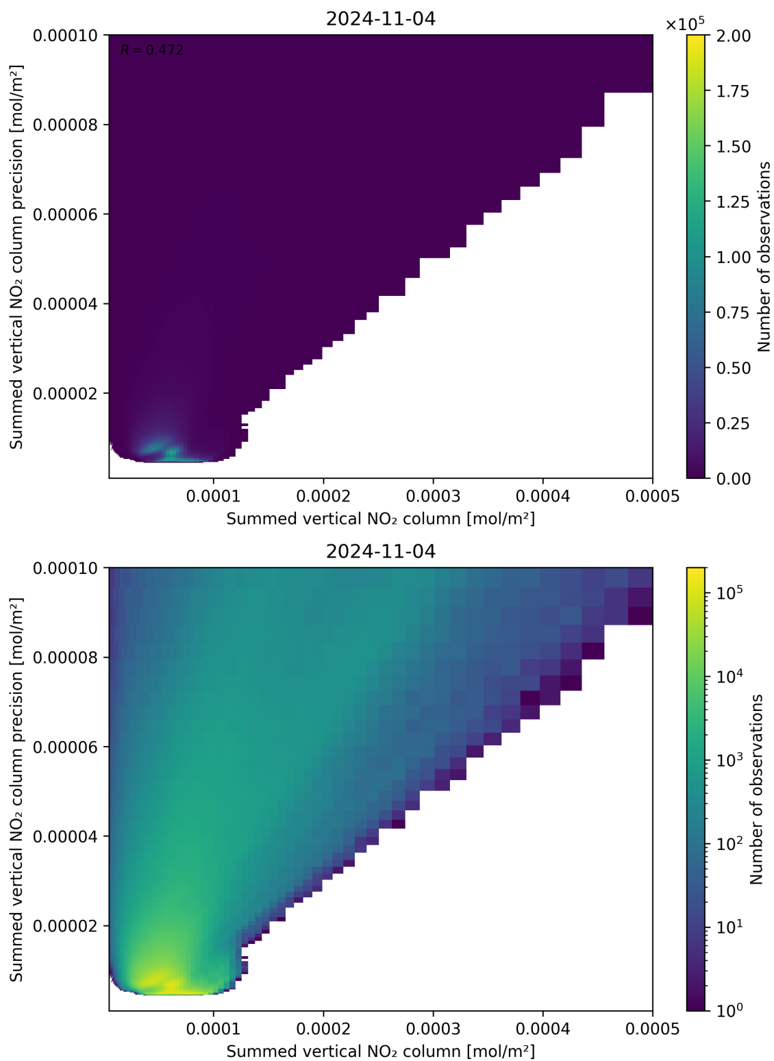
Figure 105: Scatter density plot of “Summed vertical NO 2 column” against “Summed vertical NO 2 column precision” for 2024-11-04 to 2024-11-05.
