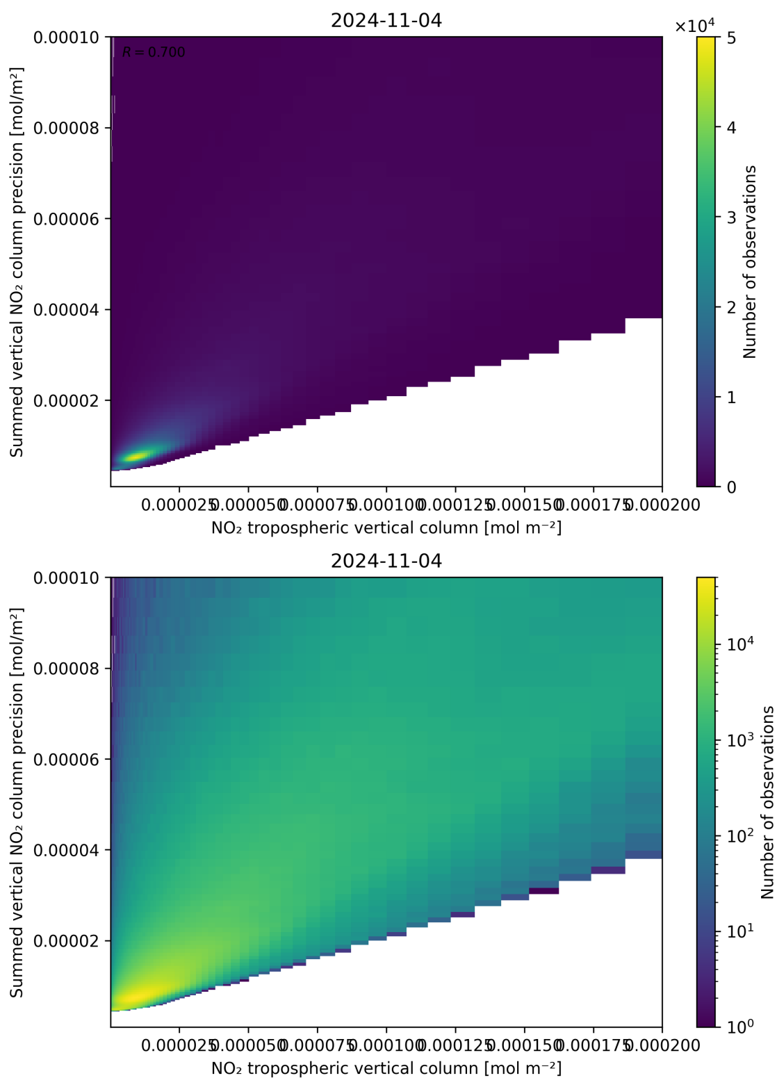
Figure 127: Scatter density plot of “NO 2 tropospheric vertical column” against “Summed vertical NO 2 column precision” for 2024-11-04 to 2024-11-05.
