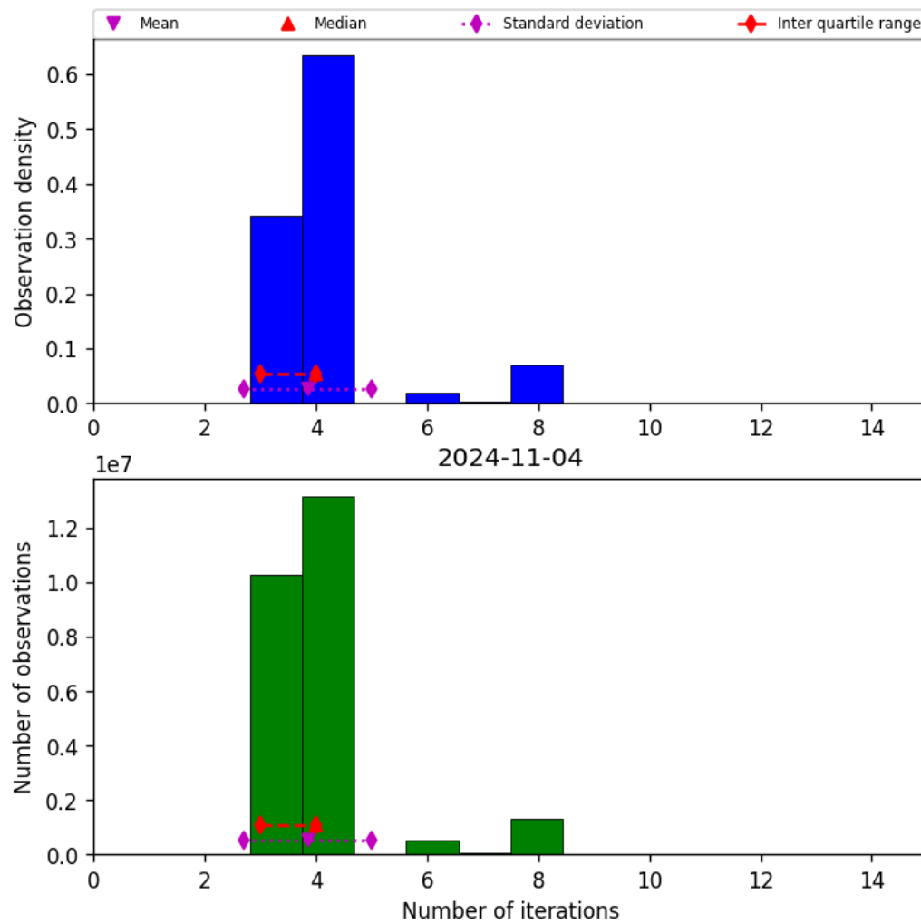
Figure 34: Histogram of “Number of iterations” for 2024-11-04 to 2024-11-05
