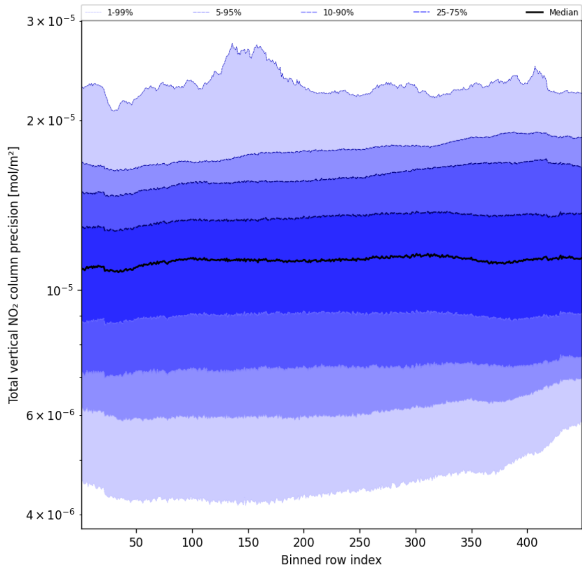
Figure 56: Along track statistics of “Total vertical NO 2 column precision” for 2024-11-04 to 2024-11-05
