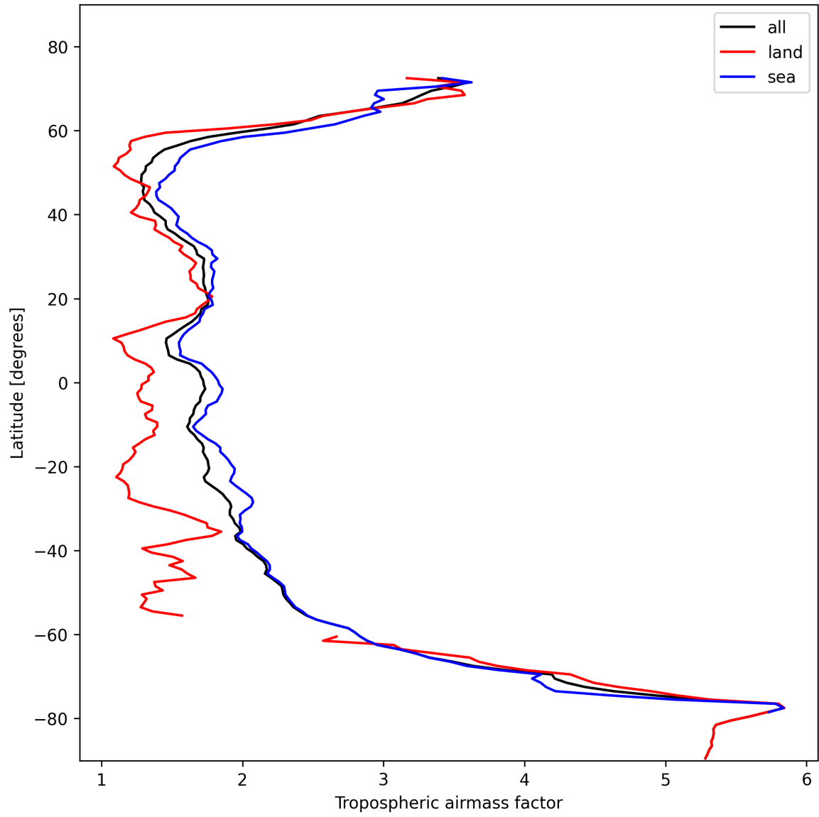
Figure 14: Zonal average of “Tropospheric airmass factor” for 2024-11-04 to 2024-11-05.
