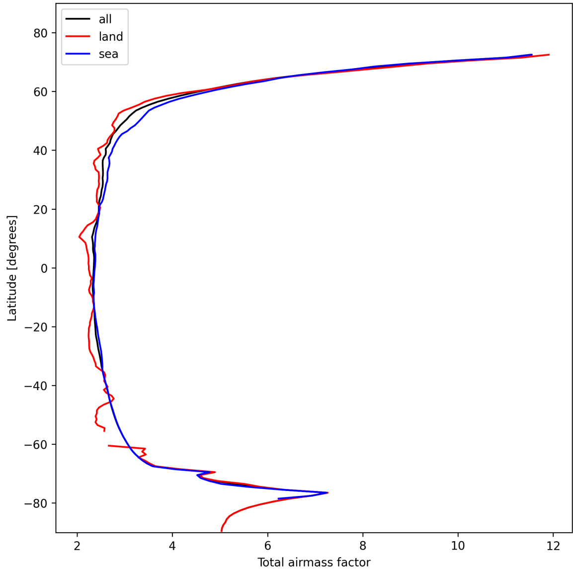
Figure 15: Zonal average of “Total airmass factor” for 2024-11-04 to 2024-11-05.
