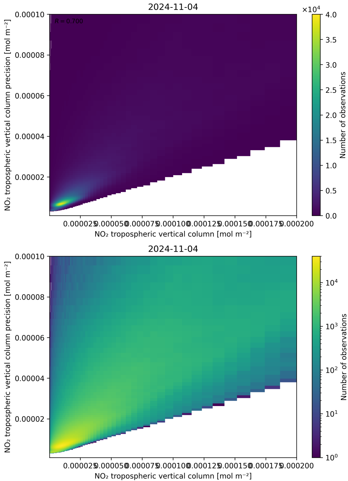
Figure 130: Scatter density plot of “NO 2 tropospheric vertical column” against “NO 2 tropospheric vertical column precision” for 2024-11-04 to 2024-11-05.
