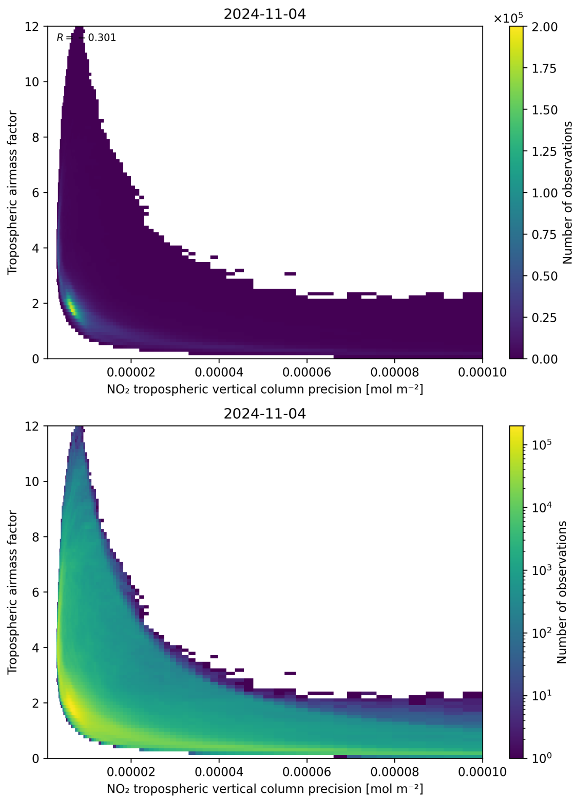
Figure 133: Scatter density plot of “NO 2 tropospheric vertical column precision” against “Tropospheric air mass factor” for 2024-11-04 to 2024-11-05.
