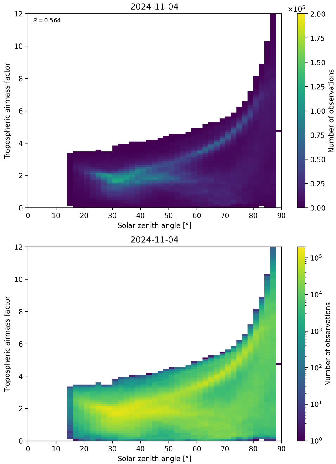
Figure 147: Scatter density plot of “Solar zenith angle” against “Tropospheric airmass factor” for 2024-11-04 to 2024-11-05.
