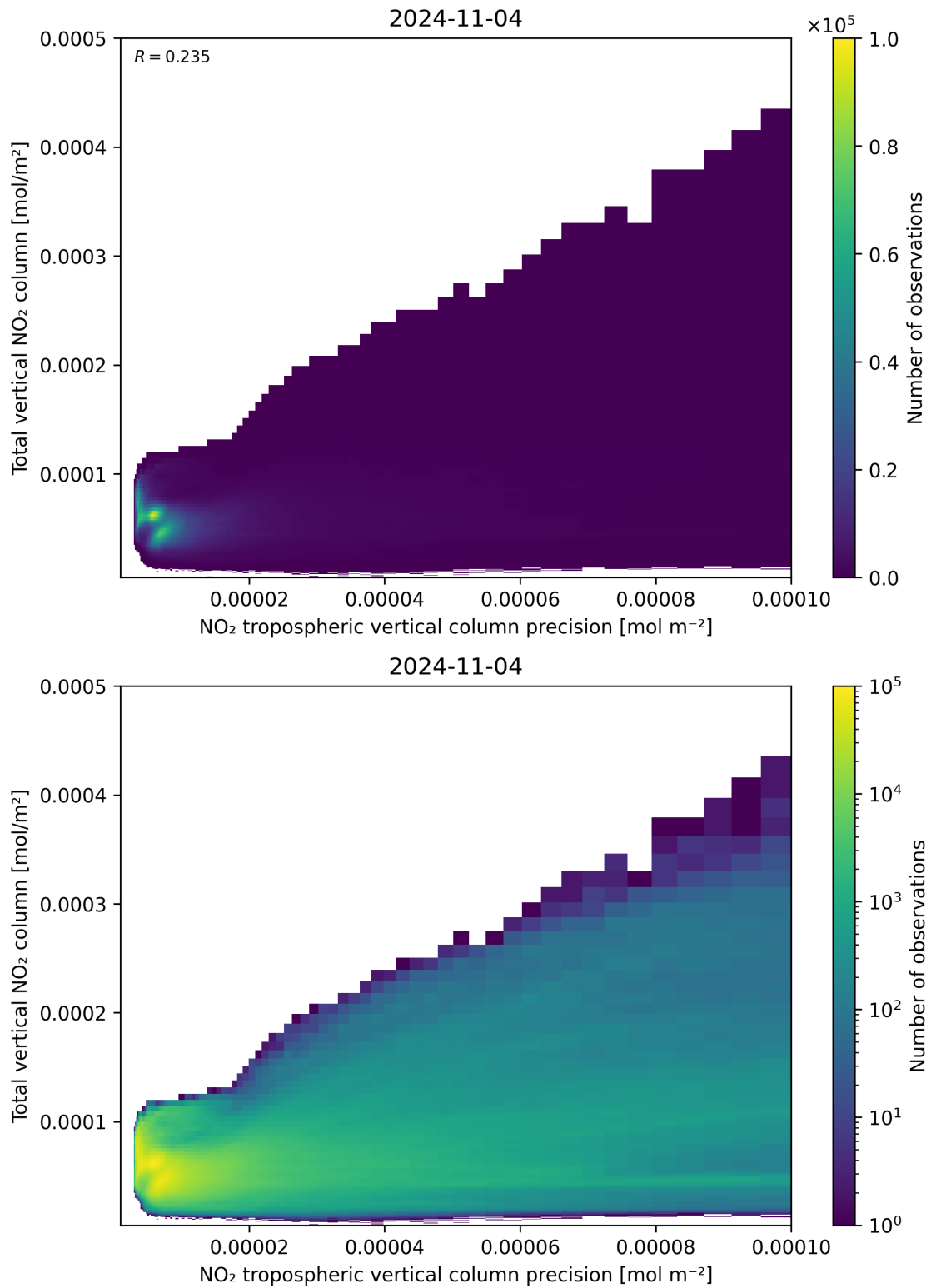
Figure 138: Scatter density plot of “NO 2 tropospheric vertical column precision” against “Total vertical NO 2 column” for 2024-11-04 to 2024-11-05.
