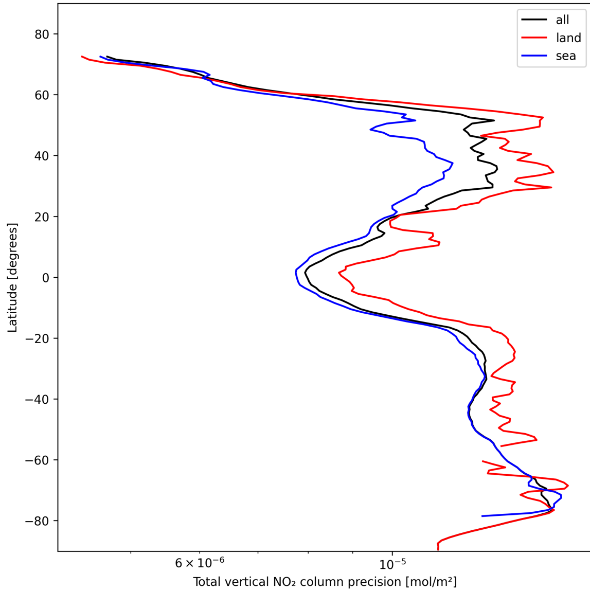
Figure 22: Zonal average of “Total vertical NO 2 column precision” for 2024-11-04 to 2024-11-05.
