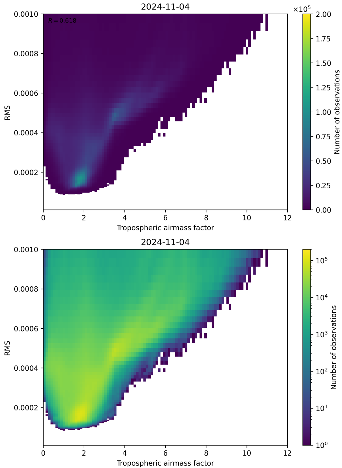
Figure 79: Scatter density plot of “Tropospheric airmass factor” against “RMS” for 2024-11-04 to 2024-11-05.
