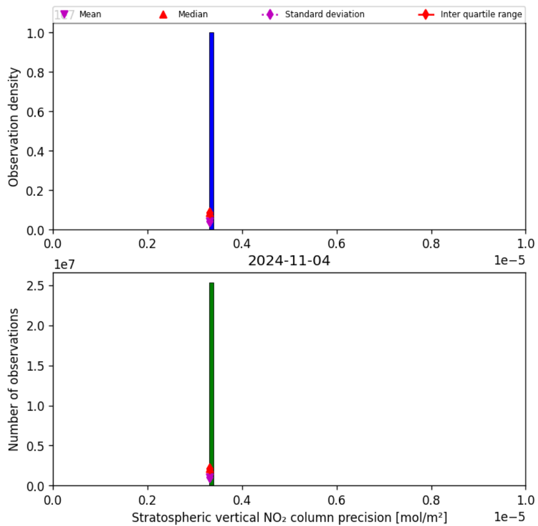
Figure 37: Histogram of “Stratospheric vertical NO 2 column precision” for 2024-11-04 to 2024-11-05
