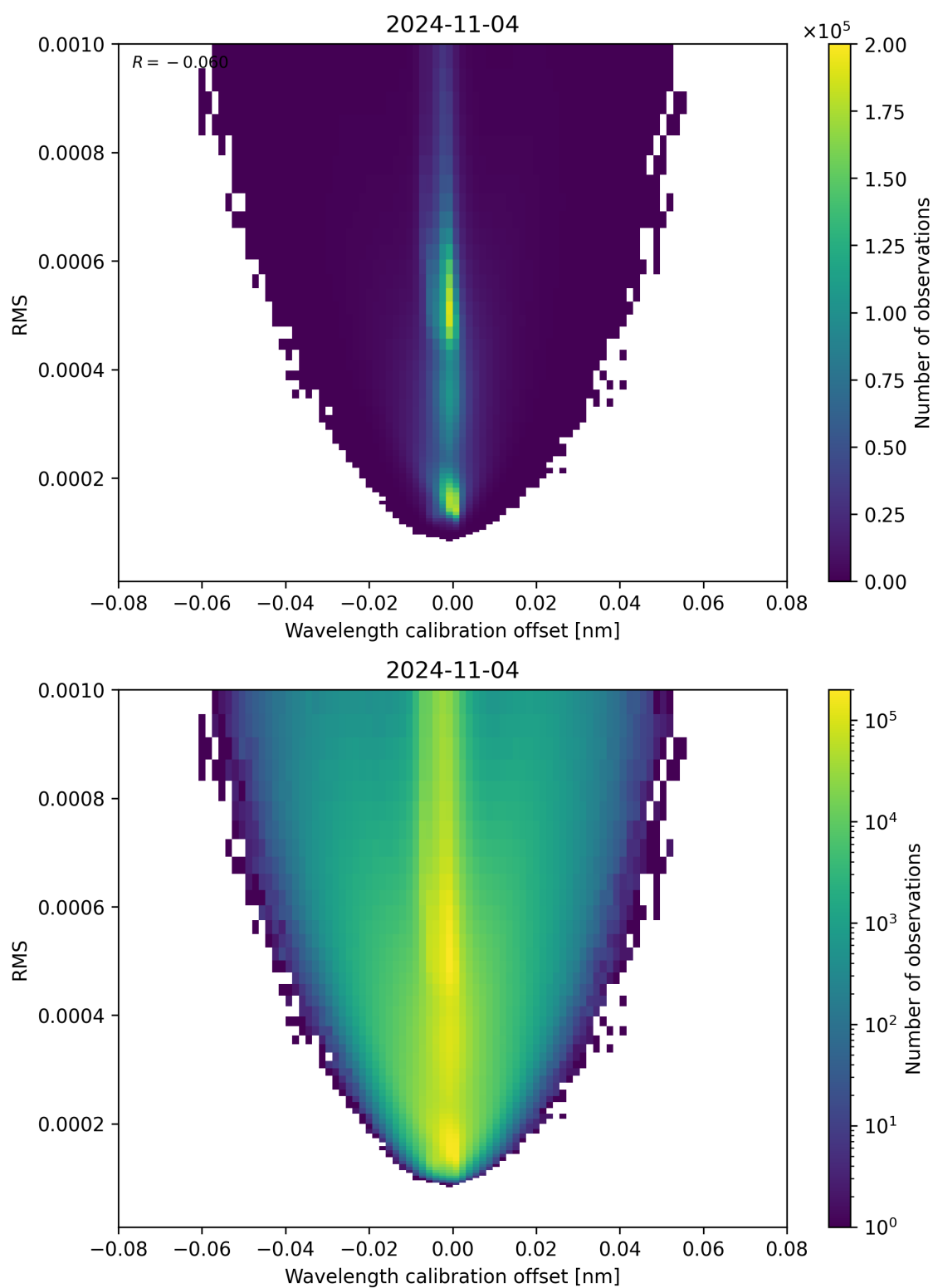
Figure 181: Scatter density plot of “Wavelength calibration offset” against “RMS” for 2024-11-04 to 2024-11-05.
