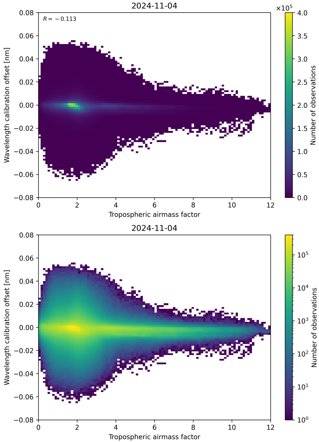
Figure 80: Scatter density plot of “Tropospheric airmass factor” against “Wavelength calibration offset” for 2024-11-04 to 2024-11-05.
