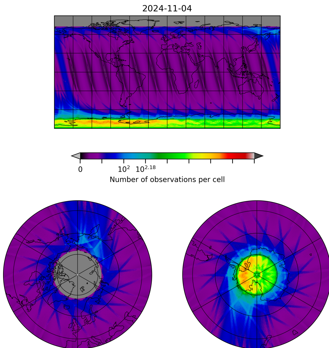
Figure 10: Map of the number of observations for 2024-11-04 to 2024-11-05
