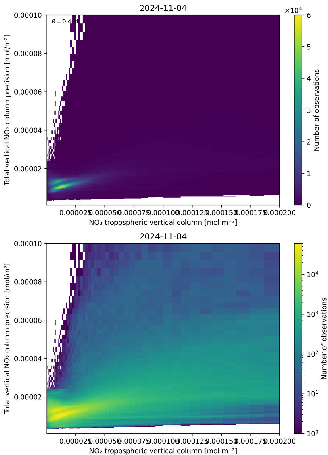
Figure 129: Scatter density plot of “NO 2 tropospheric vertical column” against “Total vertical NO 2 column precision” for 2024-11-04 to 2024-11-05.
