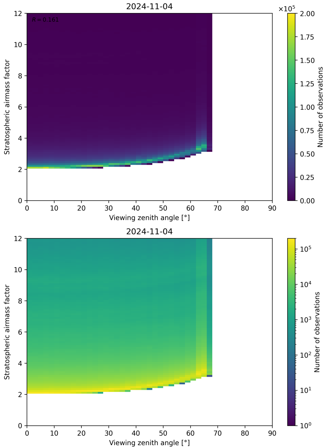
Figure 159: Scatter density plot of “Viewing zenith angle” against “Stratospheric airmass factor” for 2024-11-04 to 2024-11-05.
