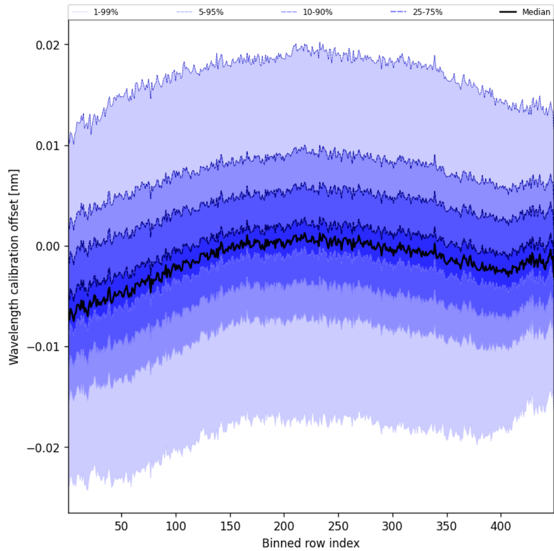
Figure 52: Along track statistics of “Wavelength calibration offset” for 2024-11-04 to 2024-11-05
