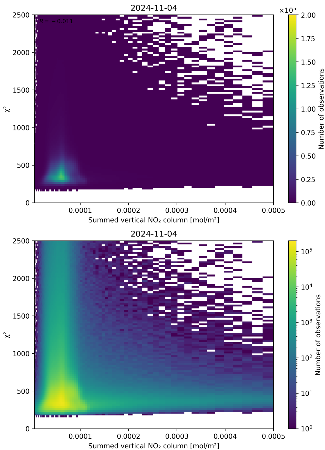
Figure 104: Scatter density plot of “Summed vertical NO 2 column” against “ \chi^2 ” for 2024-11-04 to 2024-11-05.
