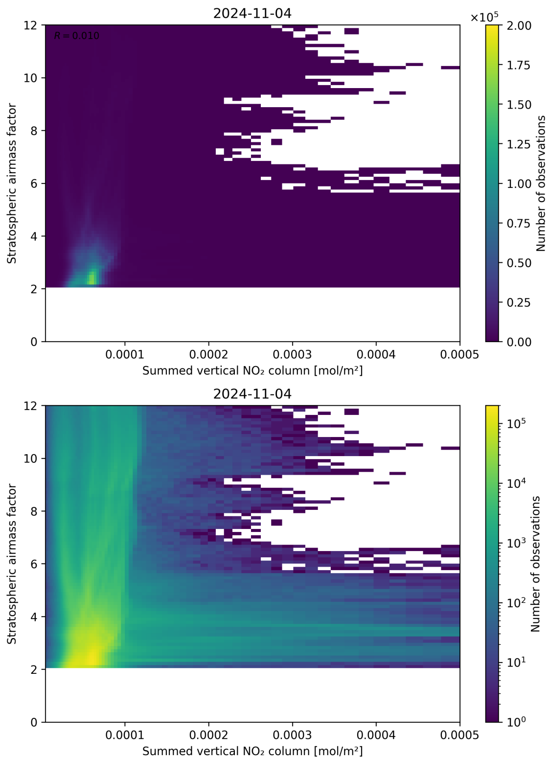
Figure 103: Scatter density plot of “Summed vertical NO 2 column” against “Stratospheric airmass factor” for 2024-11-04 to 2024-11-05.
