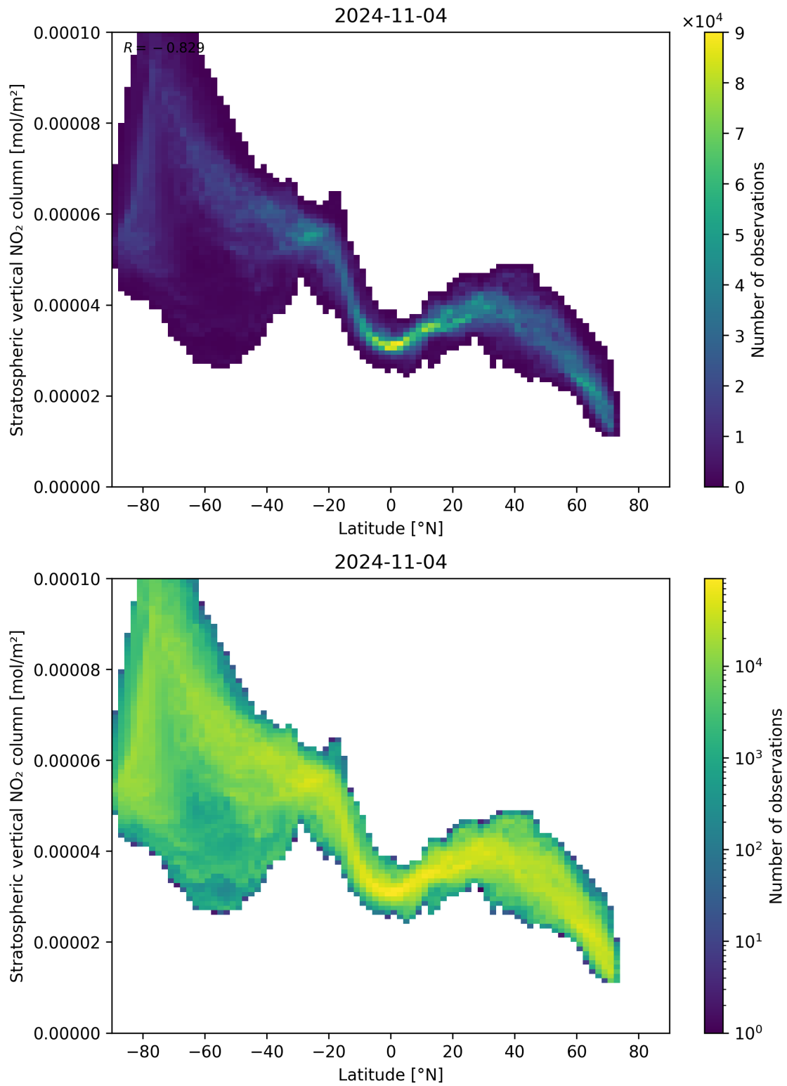
Figure 87: Scatter density plot of “Latitude” against “Stratospheric vertical NO 2 column” for 2024-11-04 to 2024-11-05.
