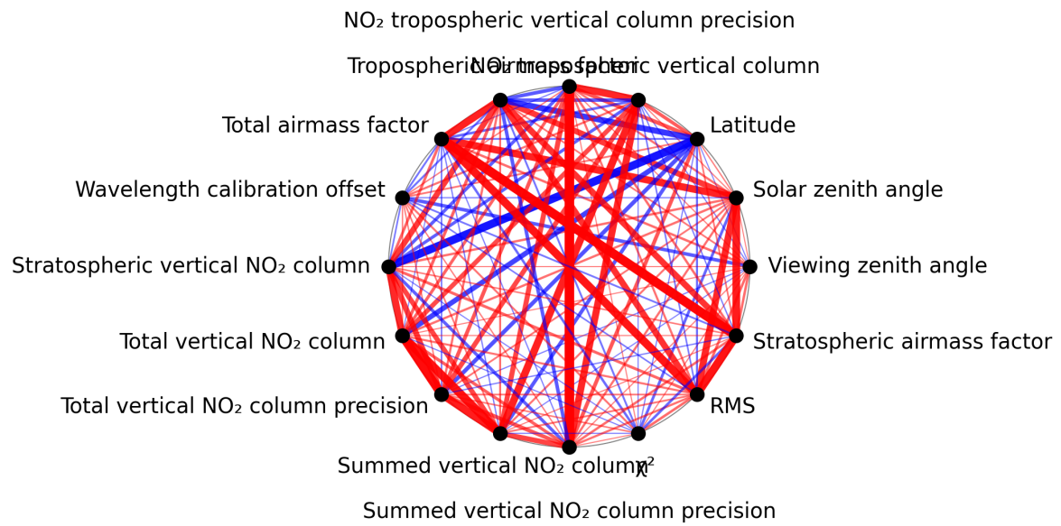
Figure 1: Map of correlation graph for 2024-11-04 to 2024-11-05.
