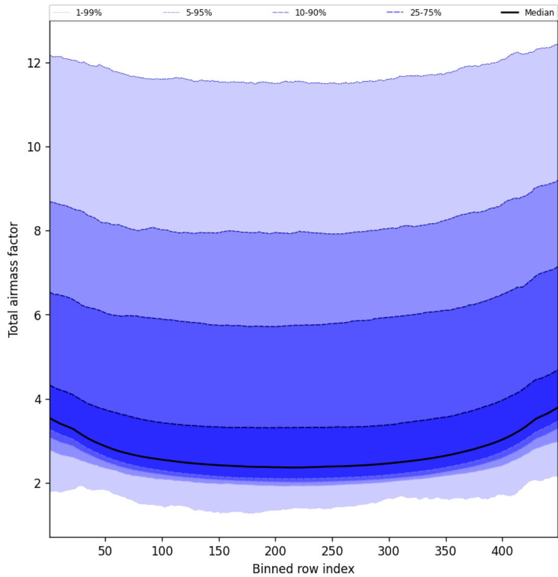
Figure 49: Along track statistics of “Total airmass factor” for 2024-11-04 to 2024-11-05
