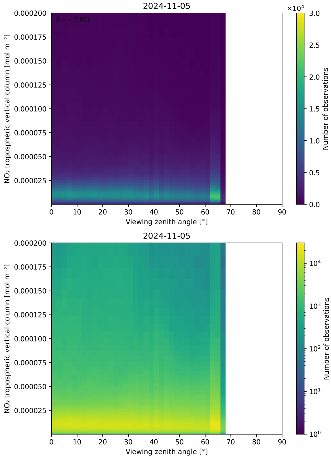
Figure 169: Scatter density plot of “Viewing zenith angle” against “NO 2 tropospheric vertical column” for 2024-11-04 to 2024-11-06.
