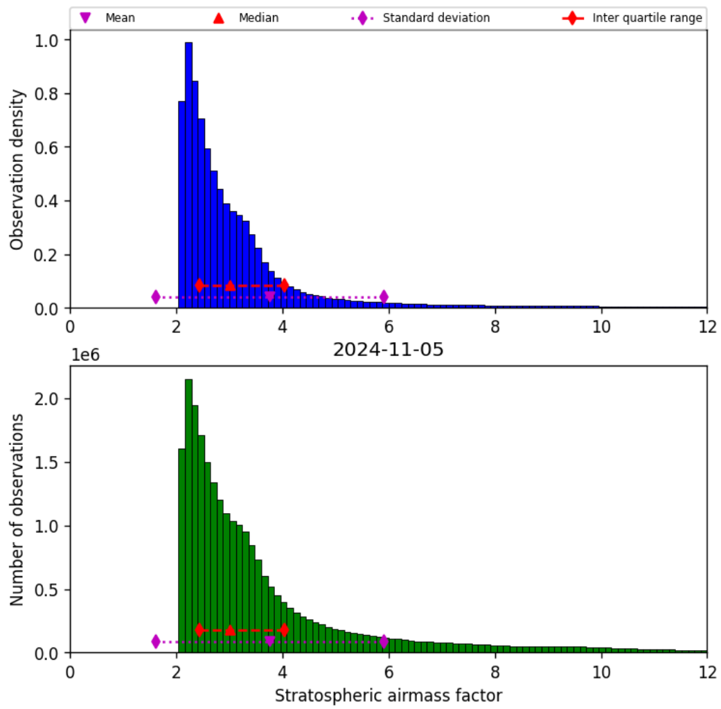
Figure 44: Histogram of “Stratospheric airmass factor” for 2024-11-04 to 2024-11-06
