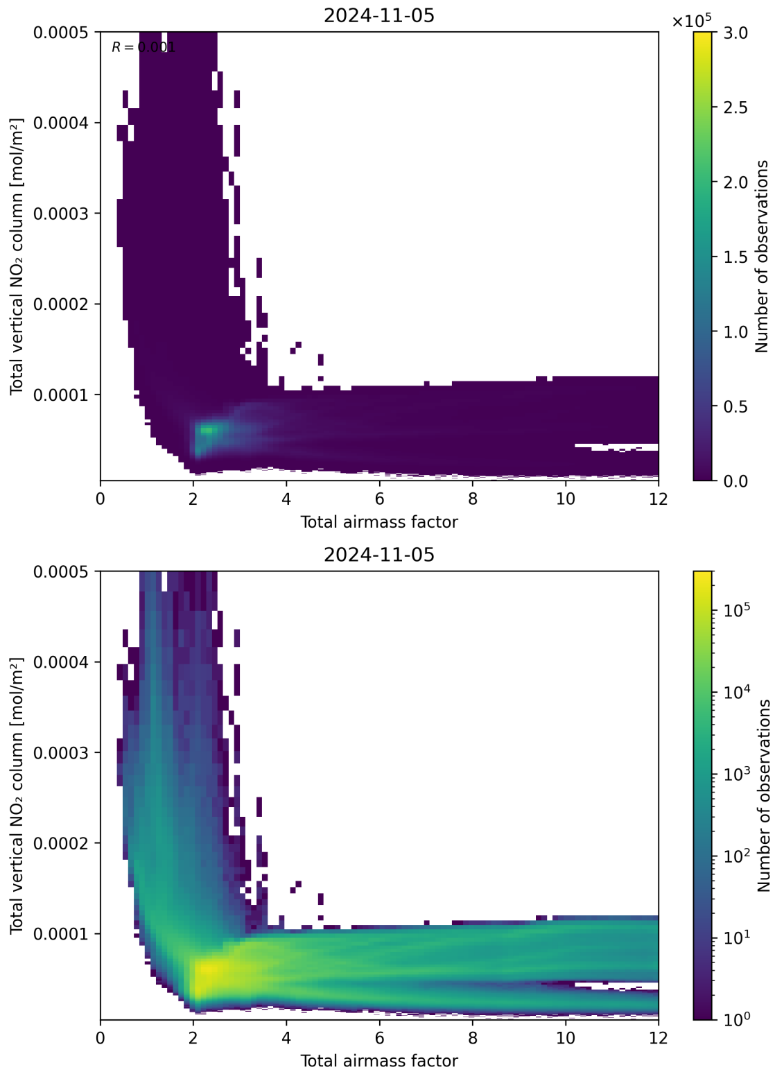
Figure 67: Scatter density plot of “Total airmass factor” against “Total vertical NO 2 column” for 2024-11-04 to 2024-11-06.
