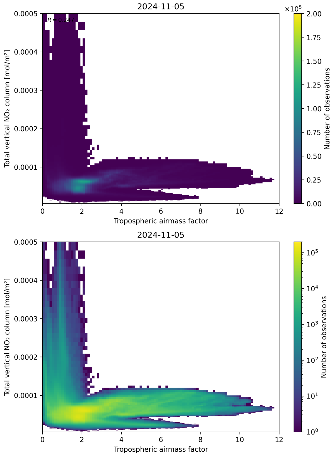
Figure 77: Scatter density plot of “Tropospheric airmass factor” against “Total vertical NO 2 column” for 2024-11-04 to 2024-11-06.
