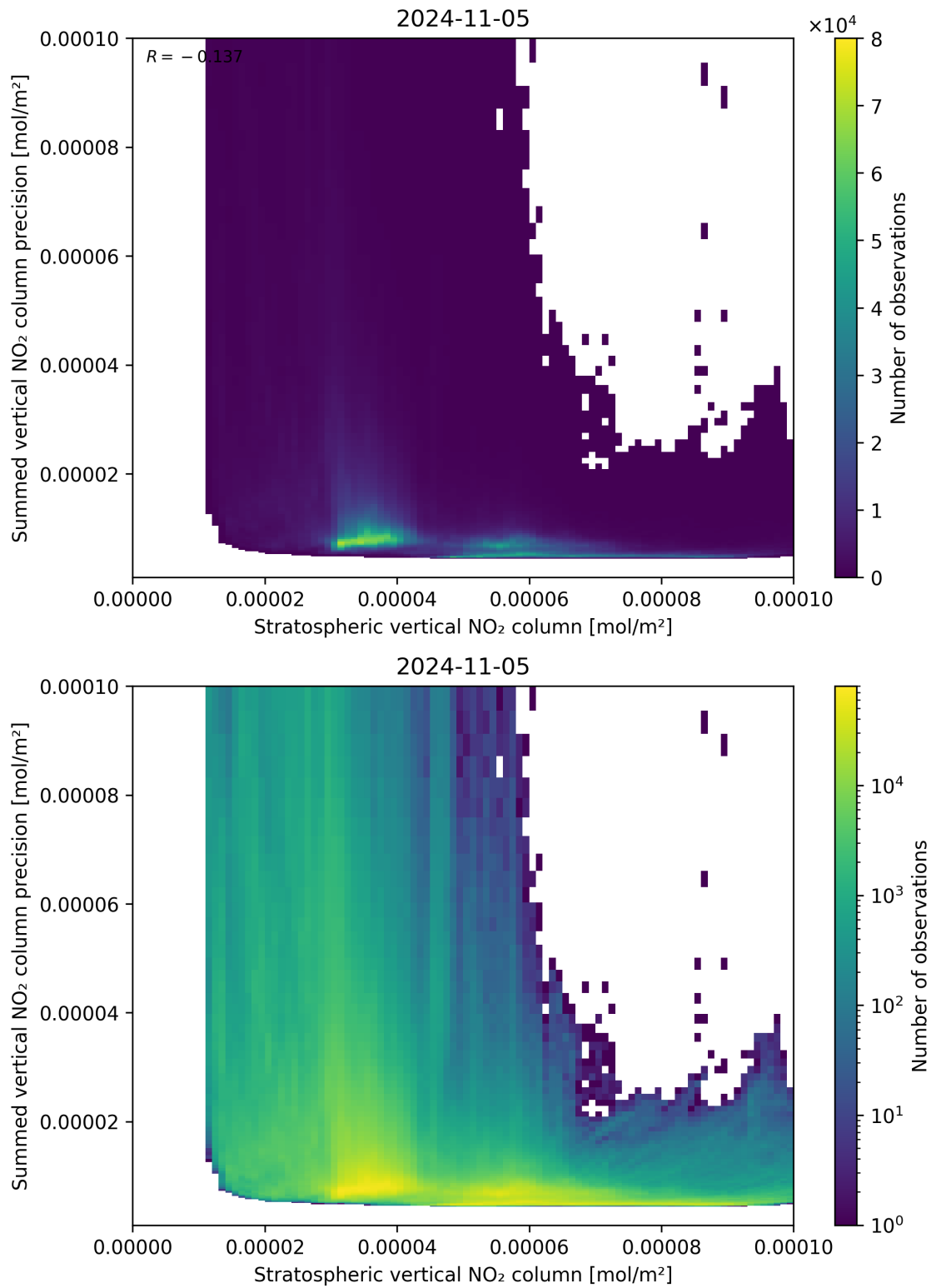
Figure 99: Scatter density plot of “Stratospheric vertical NO 2 column” against “Summed vertical NO 2 column precision” for 2024-11-04 to 2024-11-06.
