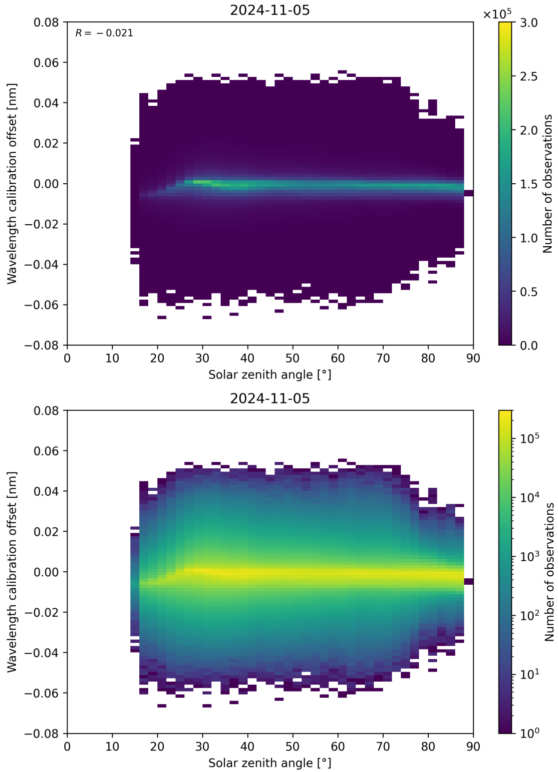
Figure 158: Scatter density plot of “Solar zenith angle” against “Wavelength calibration offset” for 2024-11-04 to 2024-11-06.
