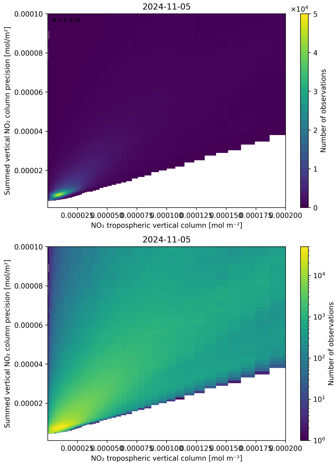
Figure 127: Scatter density plot of “NO 2 tropospheric vertical column” against “Summed vertical NO 2 column precision” for 2024-11-04 to 2024-11-06.
