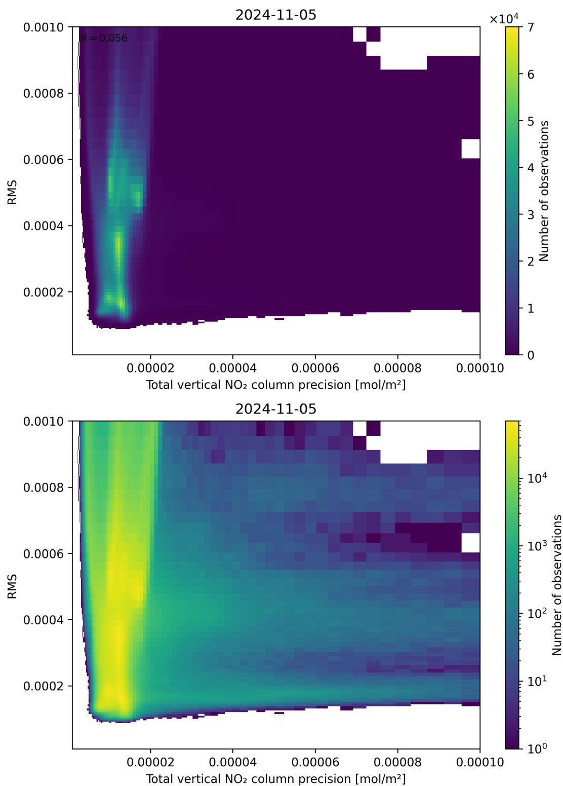
Figure 119: Scatter density plot of “Total vertical NO 2 column precision” against “RMS” for 2024-11-04 to 2024-11-06.
