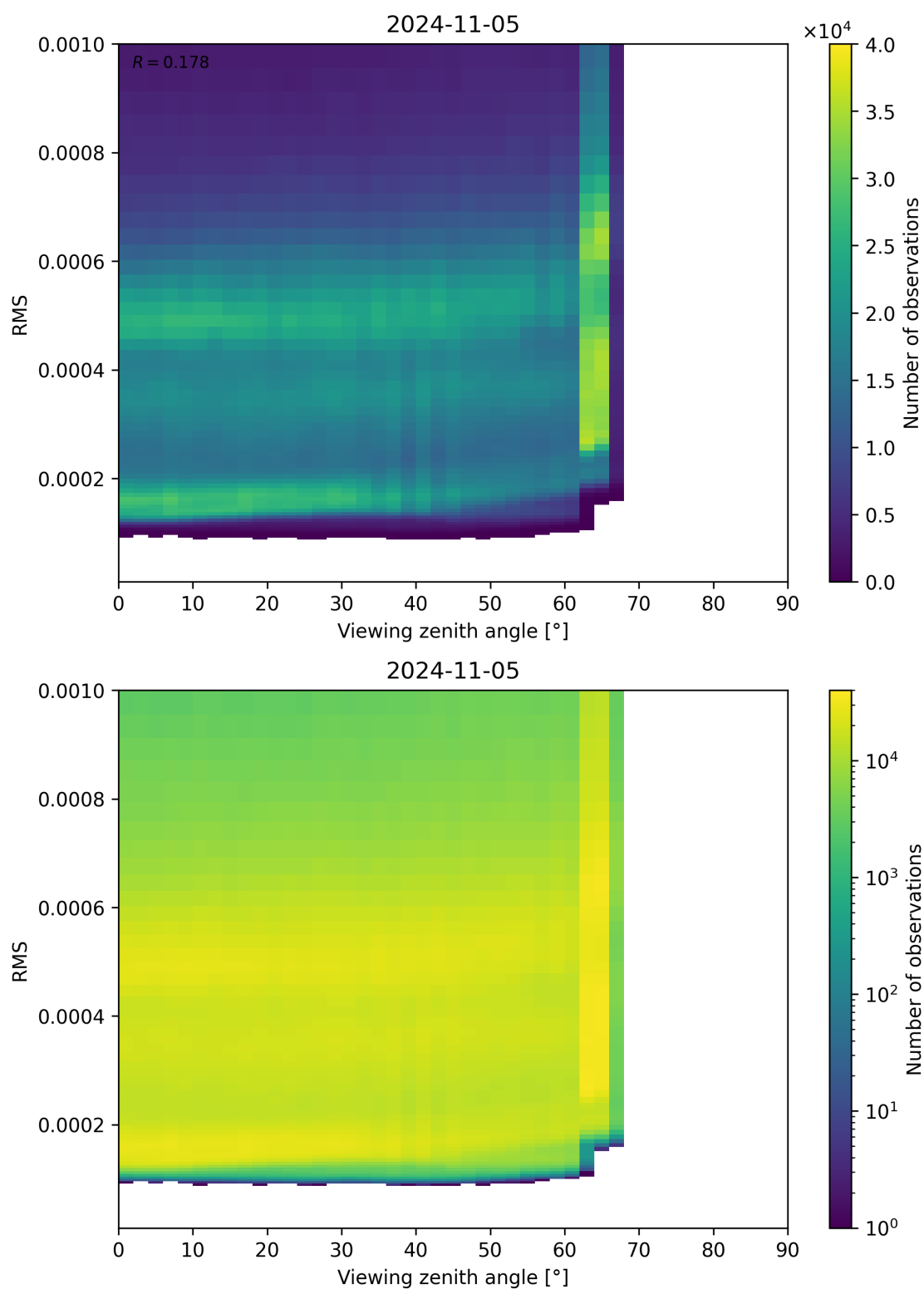
Figure 171: Scatter density plot of “Viewing zenith angle” against “RMS” for 2024-11-04 to 2024-11-06.
