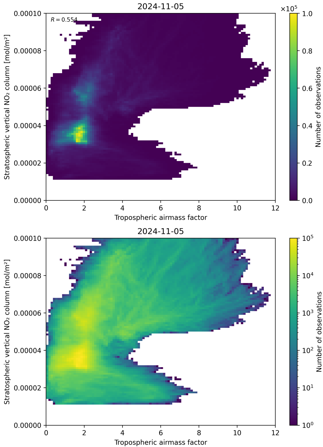
Figure 74: Scatter density plot of “Tropospheric air mass factor” against “Stratospheric vertical \text{NO}_2 column” for 2024-11-04 to 2024-11-06.
