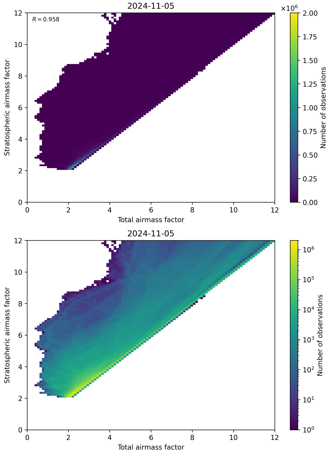
Figure 62: Scatter density plot of “Total airmass factor” against “Stratospheric airmass factor” for 2024-11-04 to 2024-11-06.
