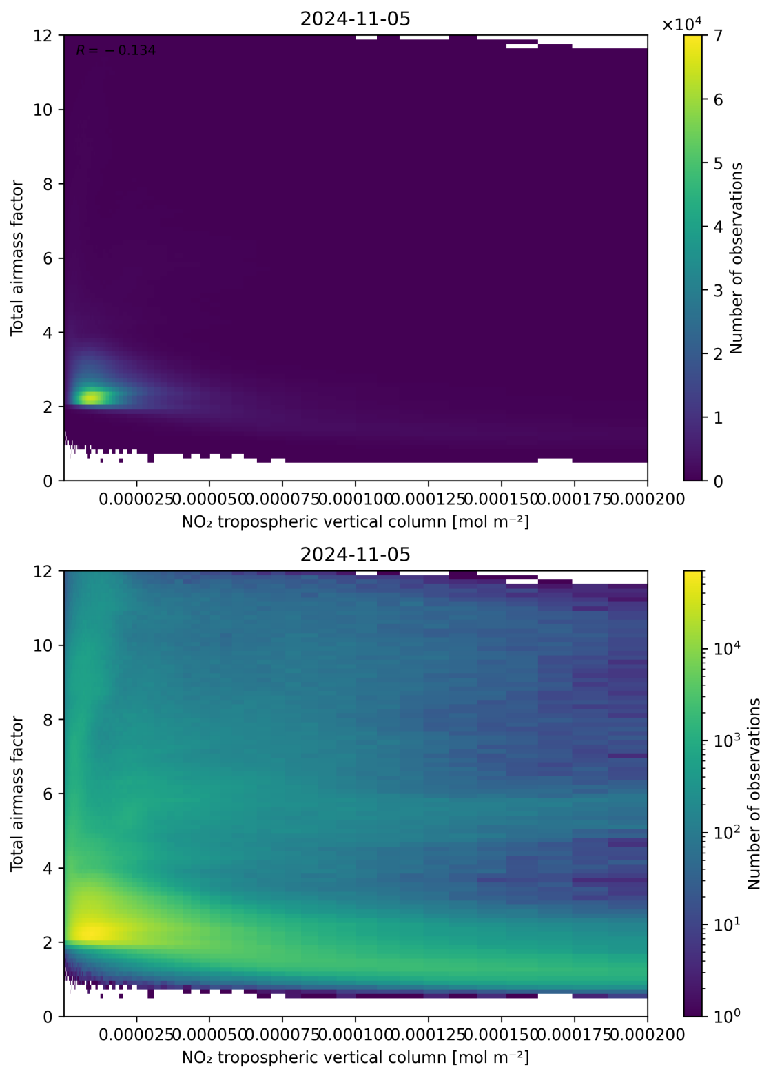
Figure 122: Scatter density plot of “NO 2 tropospheric vertical column” against “Total air mass factor” for 2024-11-04 to 2024-11-06.
