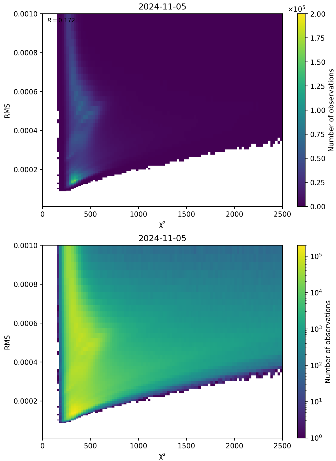
Figure 82: Scatter density plot of “ \chi^2 ” against “RMS” for 2024-11-04 to 2024-11-06.
