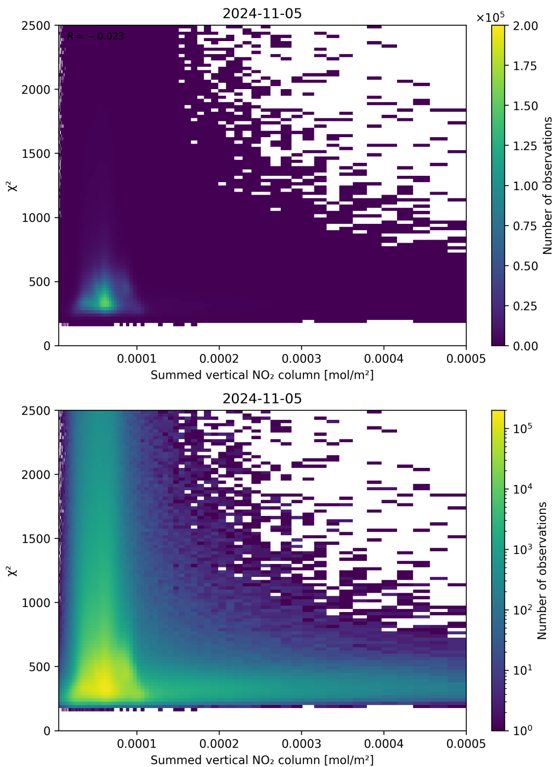
Figure 104: Scatter density plot of “Summed vertical NO 2 column” against “ \chi^2 ” for 2024-11-04 to 2024-11-06.
