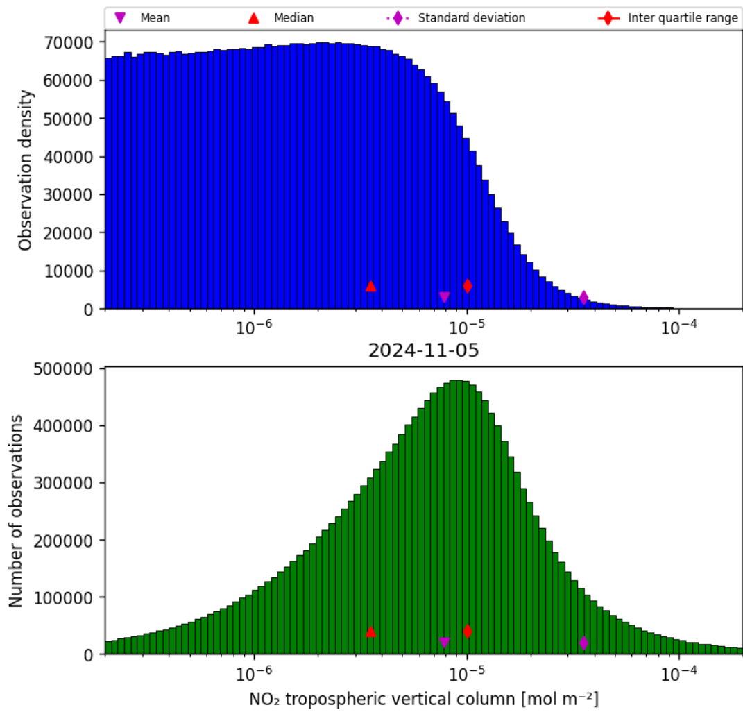
Figure 29: Histogram of “NO 2 tropospheric vertical column” for 2024-11-04 to 2024-11-06
