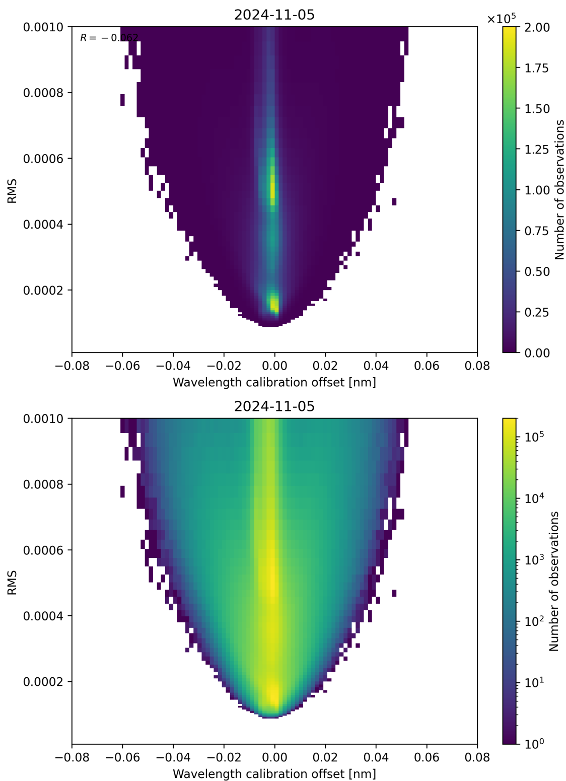
Figure 181: Scatter density plot of “Wavelength calibration offset” against “RMS” for 2024-11-04 to 2024-11-06.
