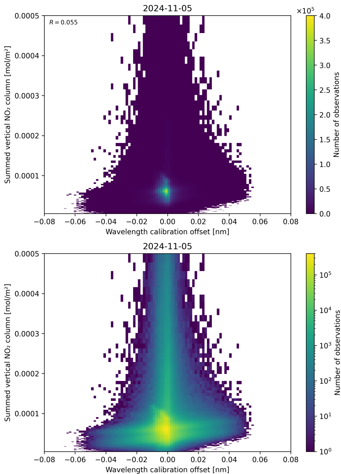
Figure 177: Scatter density plot of “Wavelength calibration offset” against “Summed vertical NO 2 column” for 2024-11-04 to 2024-11-06.
