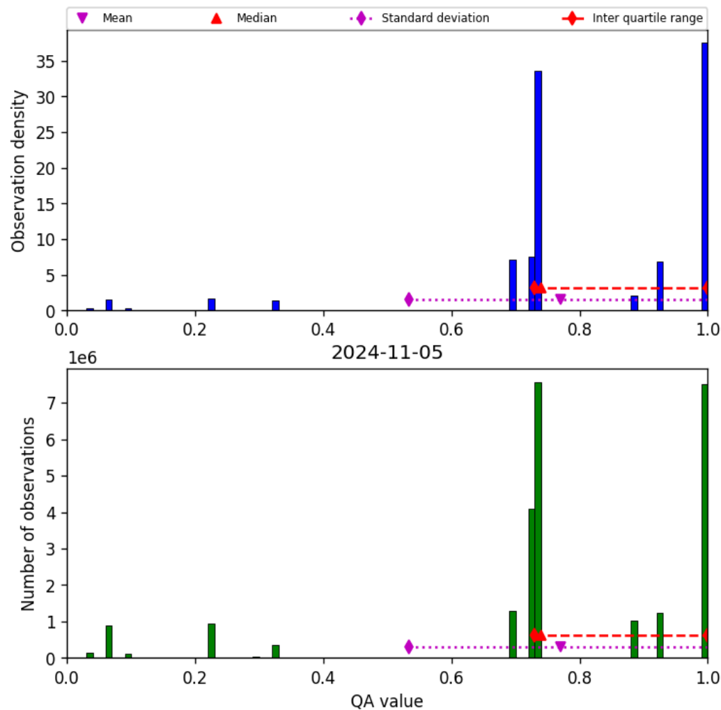
Figure 28: Histogram of “QA value” for 2024-11-04 to 2024-11-06
