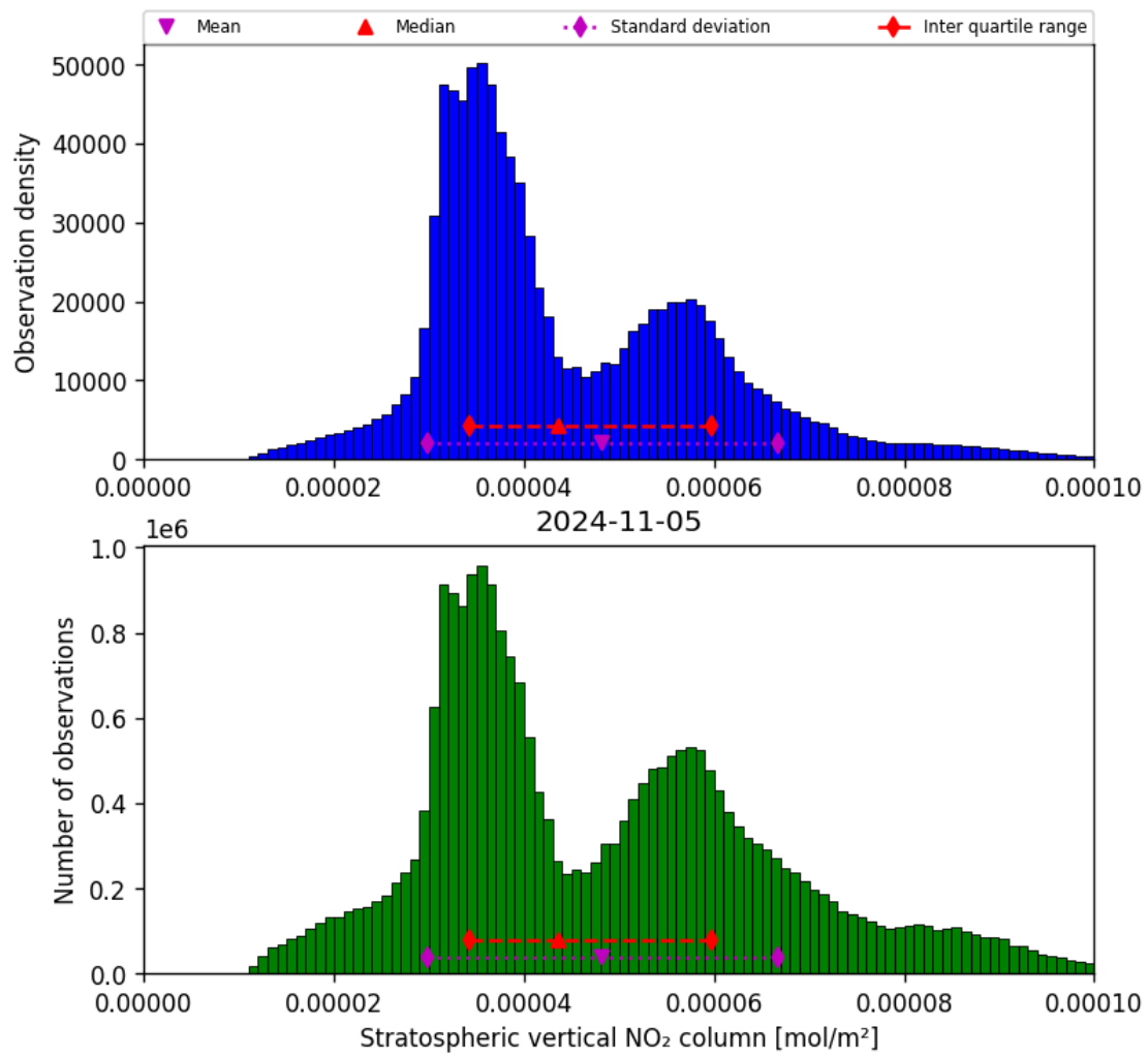
Figure 36: Histogram of “Stratospheric vertical NO 2 column” for 2024-11-04 to 2024-11-06
