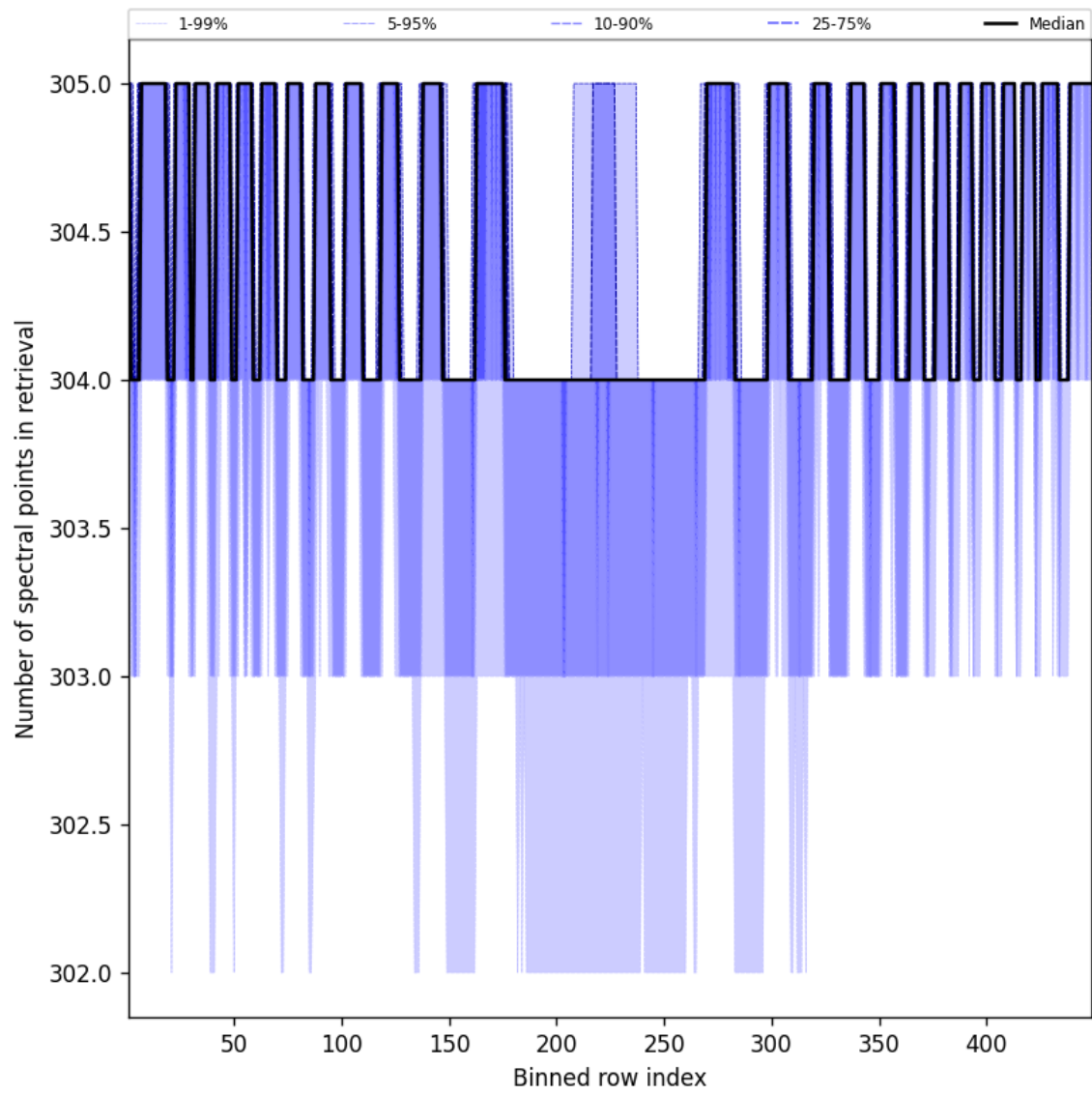
Figure 50: Along track statistics of “Number of spectral points in retrieval” for 2024-11-04 to 2024-11-06
