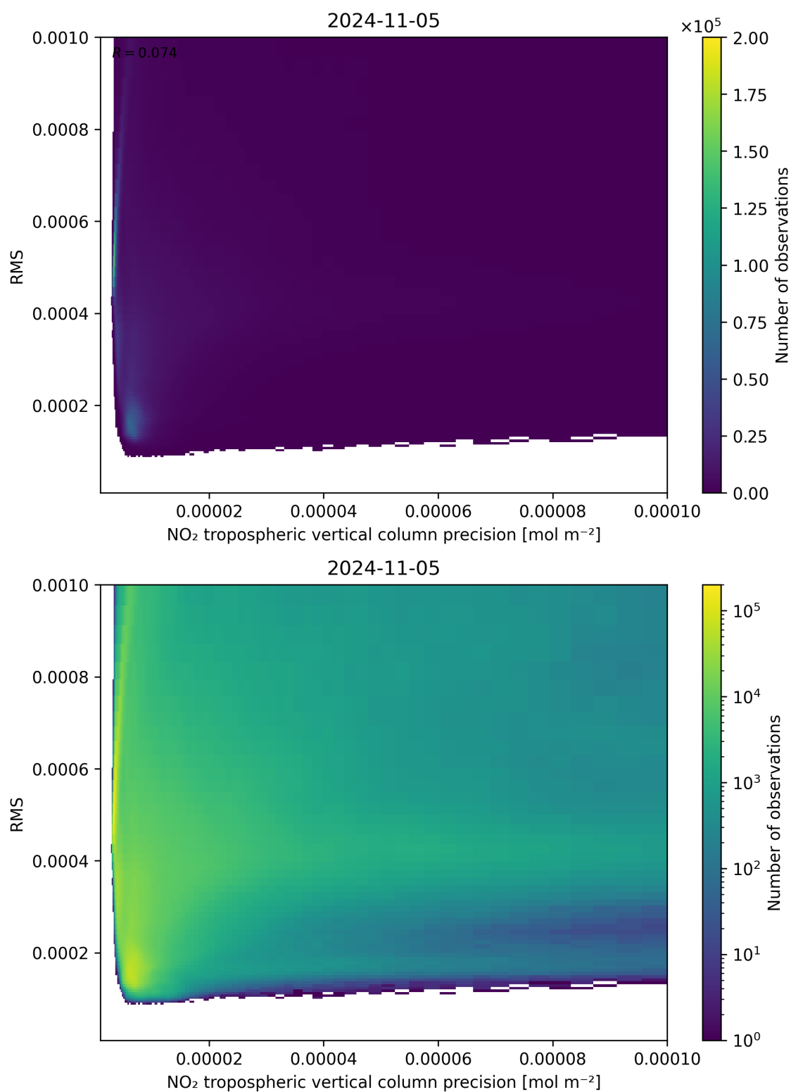
Figure 140: Scatter density plot of “NO 2 tropospheric vertical column precision” against “RMS” for 2024-11-04 to 2024-11-06.
