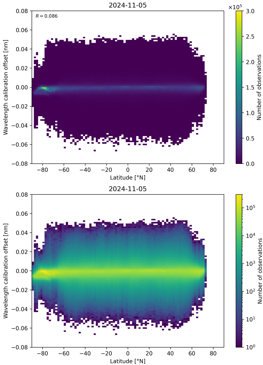
Figure 95: Scatter density plot of “Latitude” against “Wavelength calibration offset” for 2024-11-04 to 2024-11-06.
