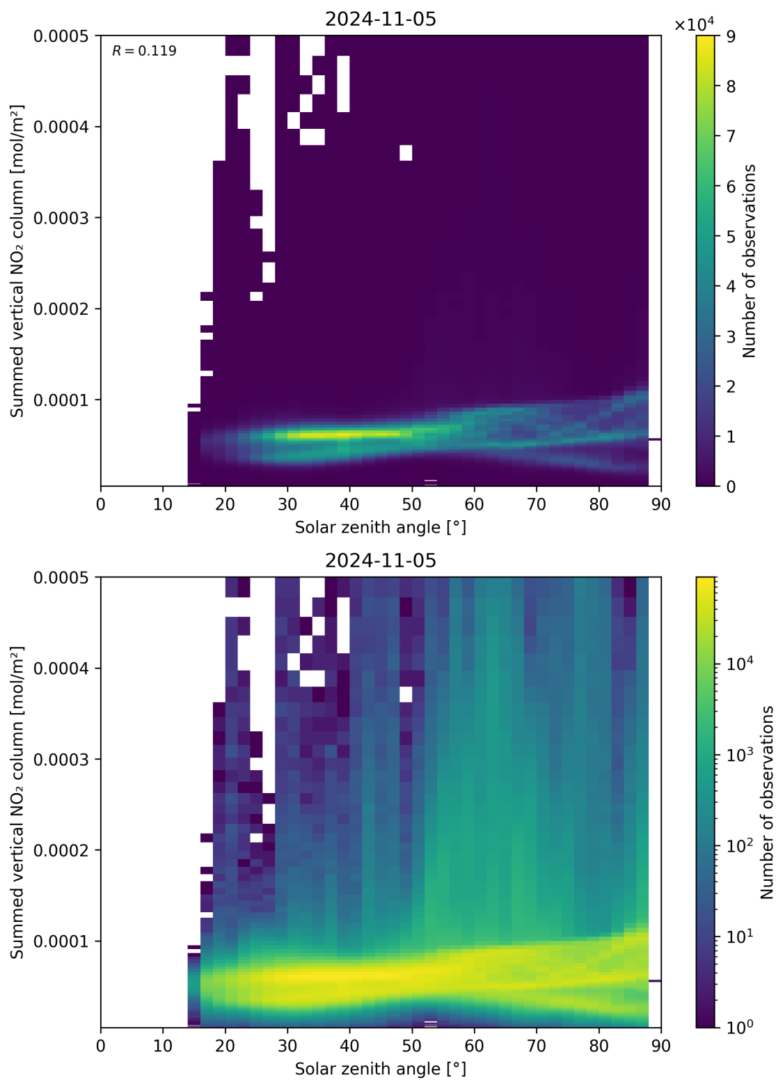
Figure 151: Scatter density plot of “Solar zenith angle” against “Summed vertical NO 2 column” for 2024-11-04 to 2024-11-06.
