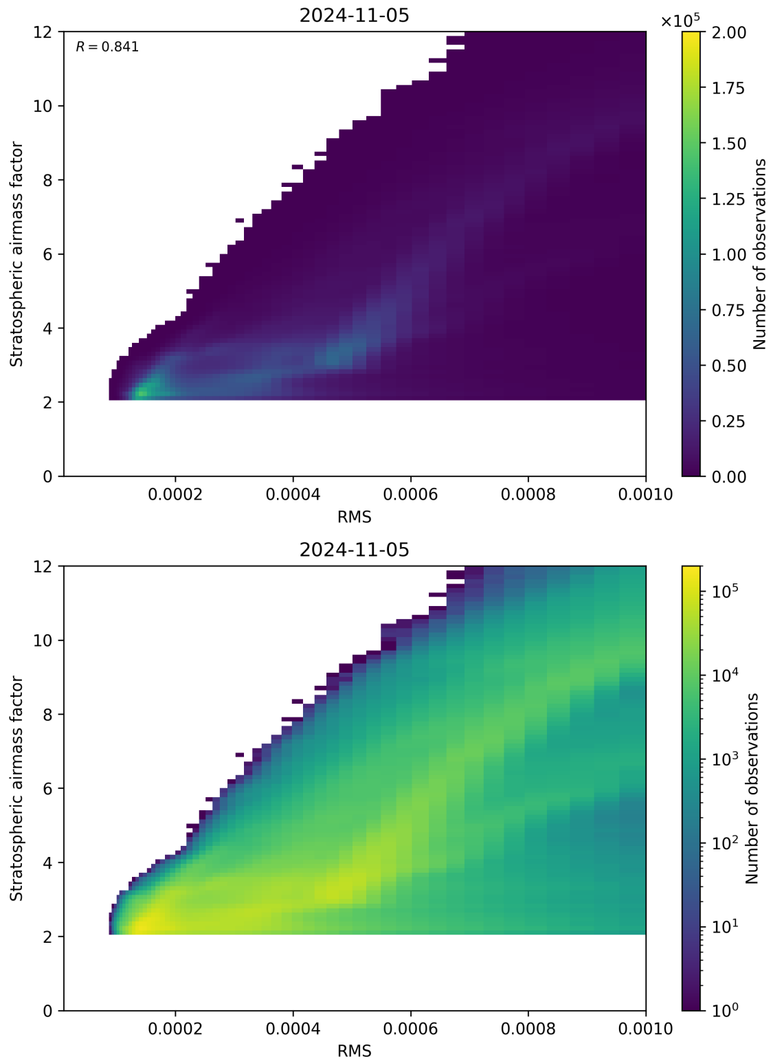
Figure 144: Scatter density plot of “RMS” against “Stratospheric airmass factor” for 2024-11-04 to 2024-11-06.
