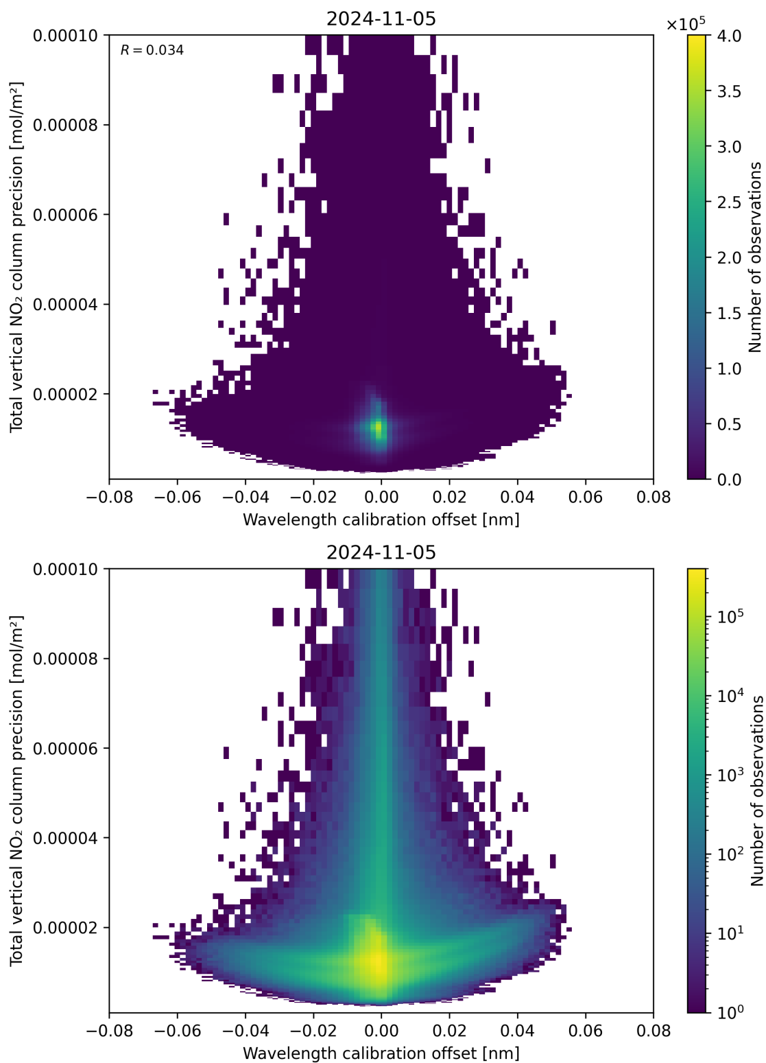
Figure 180: Scatter density plot of “Wavelength calibration offset” against “Total vertical NO 2 column precision” for 2024-11-04 to 2024-11-06.
