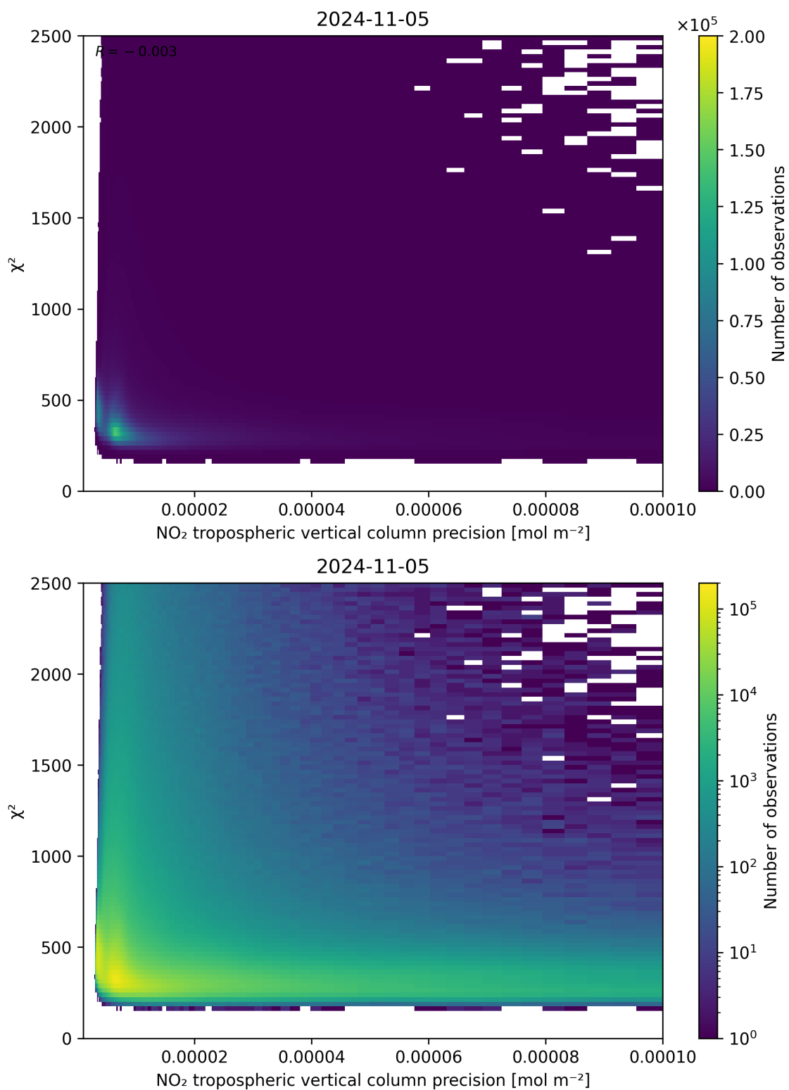
Figure 134: Scatter density plot of “NO 2 tropospheric vertical column precision” against “ \chi^2 ” for 2024-11-04 to 2024-11-06.
