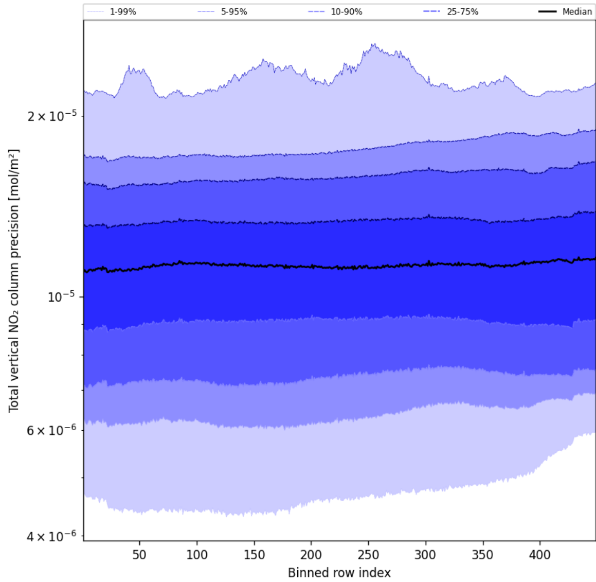
Figure 56: Along track statistics of "Total vertical NO 2 column precision" for 2024-11-04 to 2024-11-06
