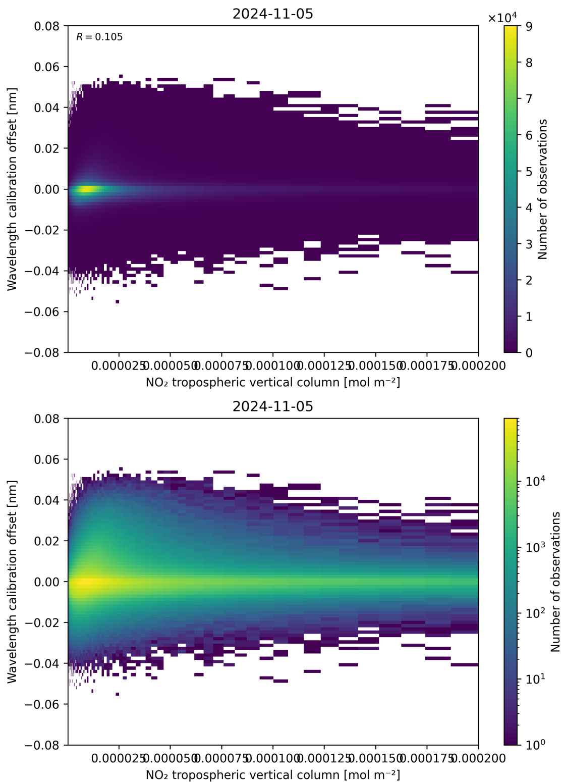
Figure 143: Scatter density plot of “NO 2 tropospheric vertical column” against “Wavelength calibration offset” for 2024-11-04 to 2024-11-06.
