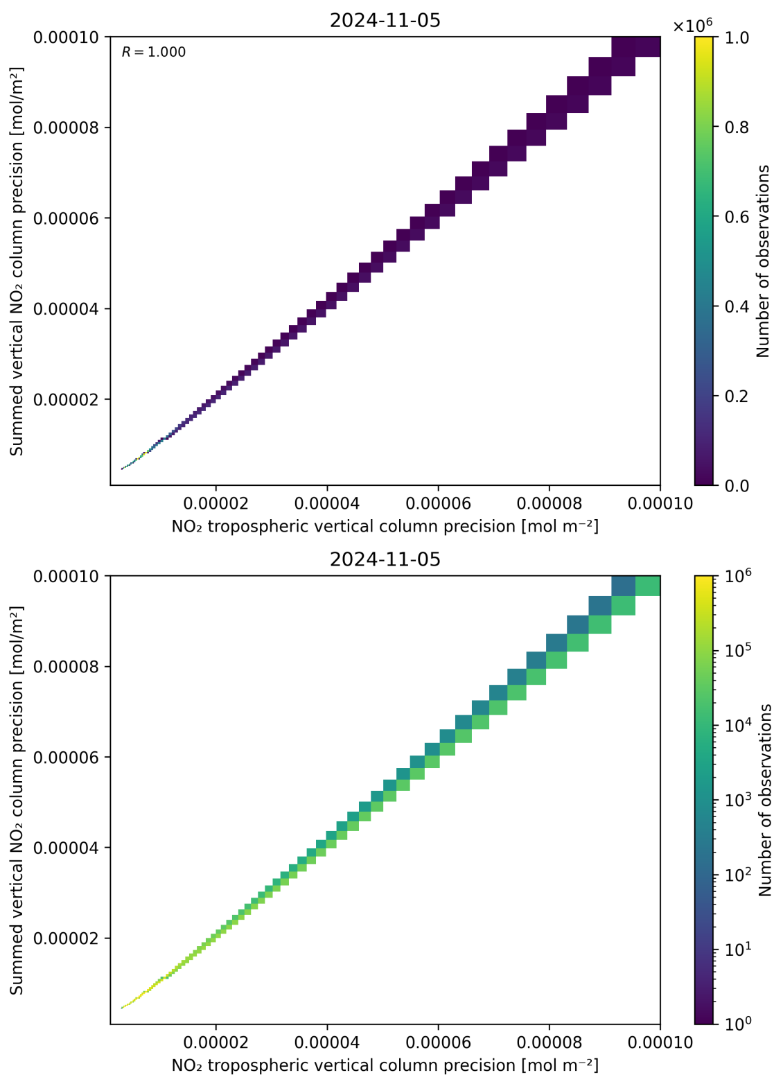
Figure 137: Scatter density plot of “NO 2 tropospheric vertical column precision” against “Summed vertical NO 2 column precision” for 2024-11-04 to 2024-11-06.
