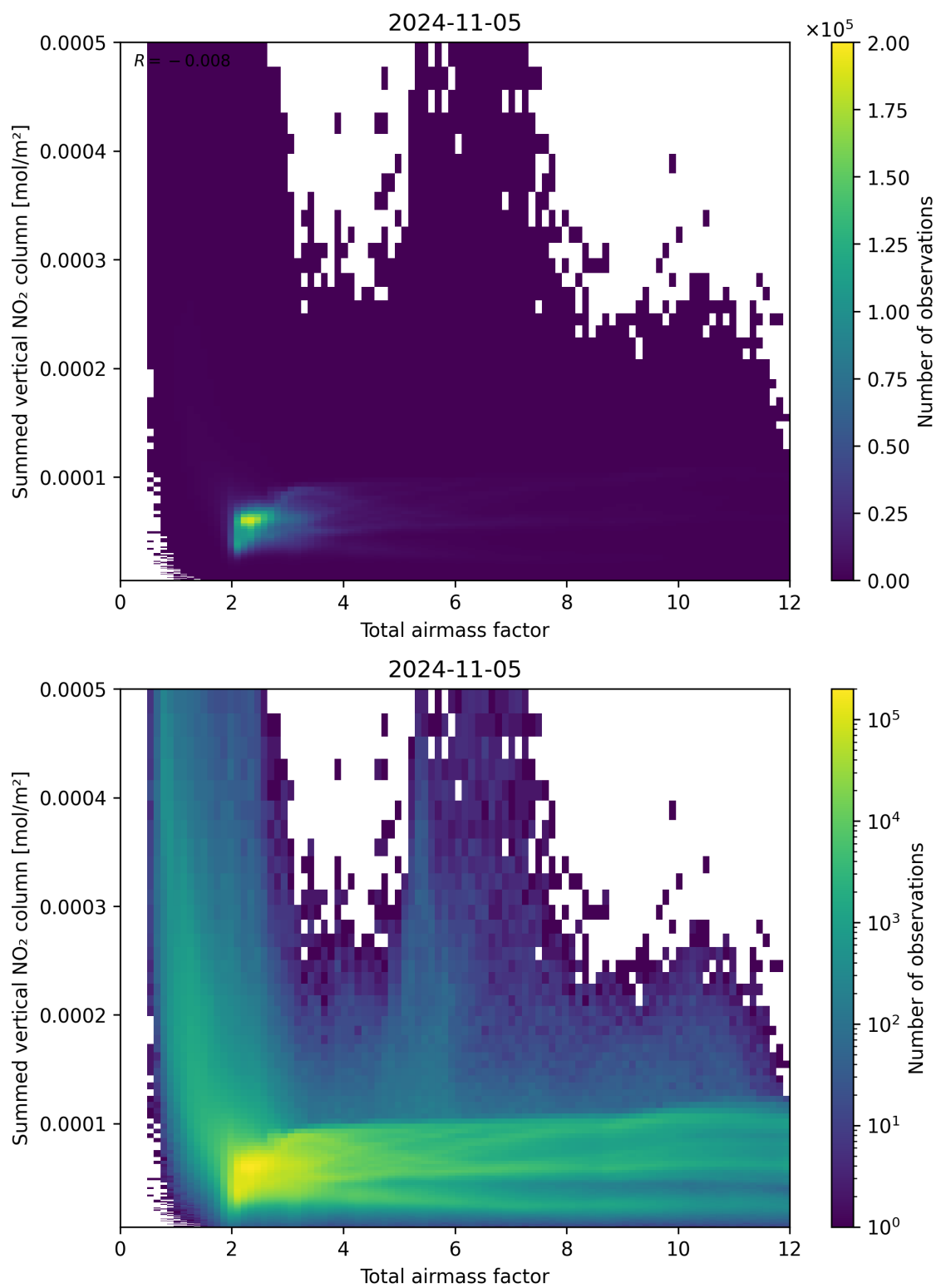
Figure 65: Scatter density plot of “Total airmass factor” against “Summed vertical NO 2 column” for 2024-11-04 to 2024-11-06.
