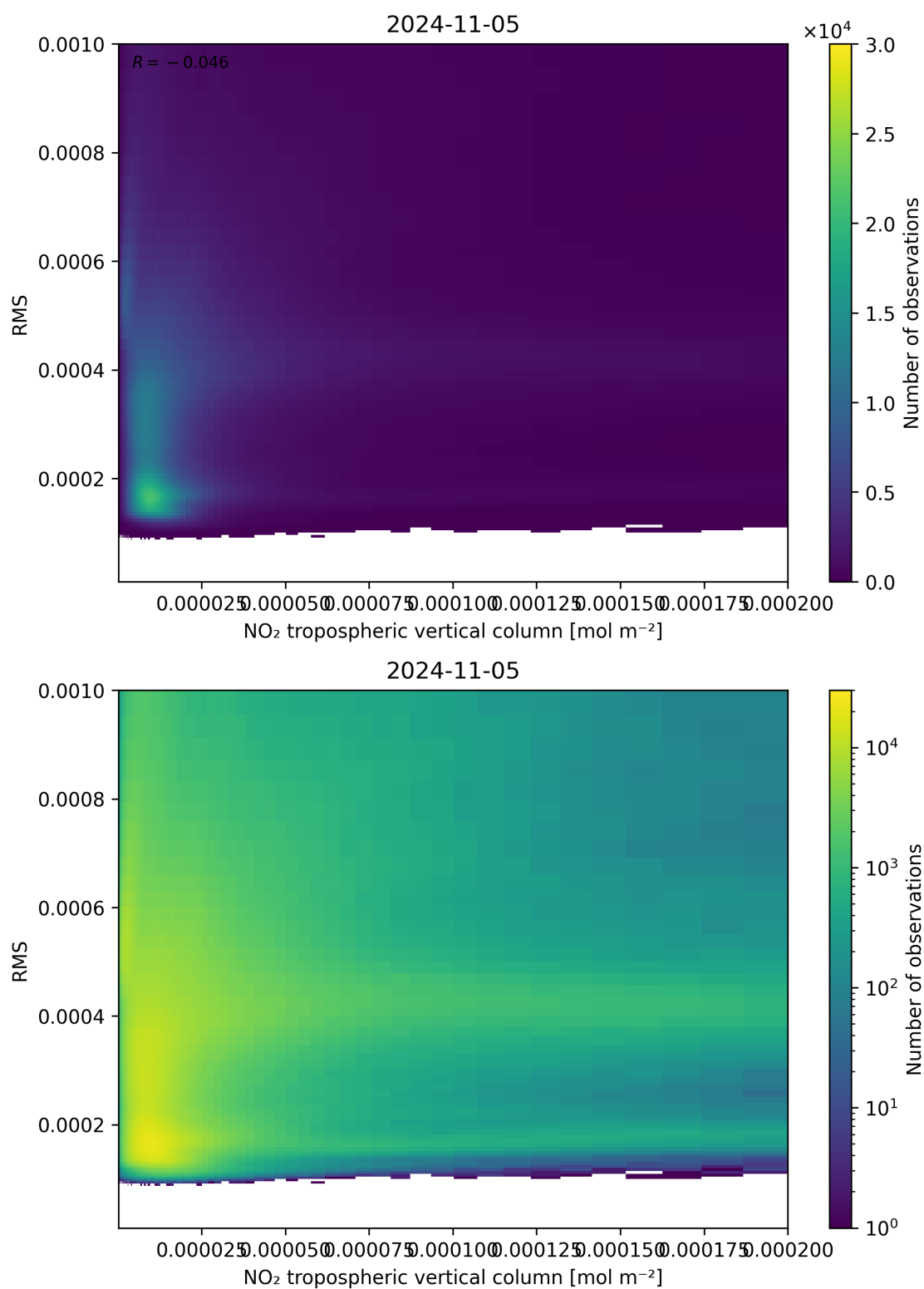
Figure 142: Scatter density plot of “NO 2 tropospheric vertical column” against “RMS” for 2024-11-04 to 2024-11-06.
