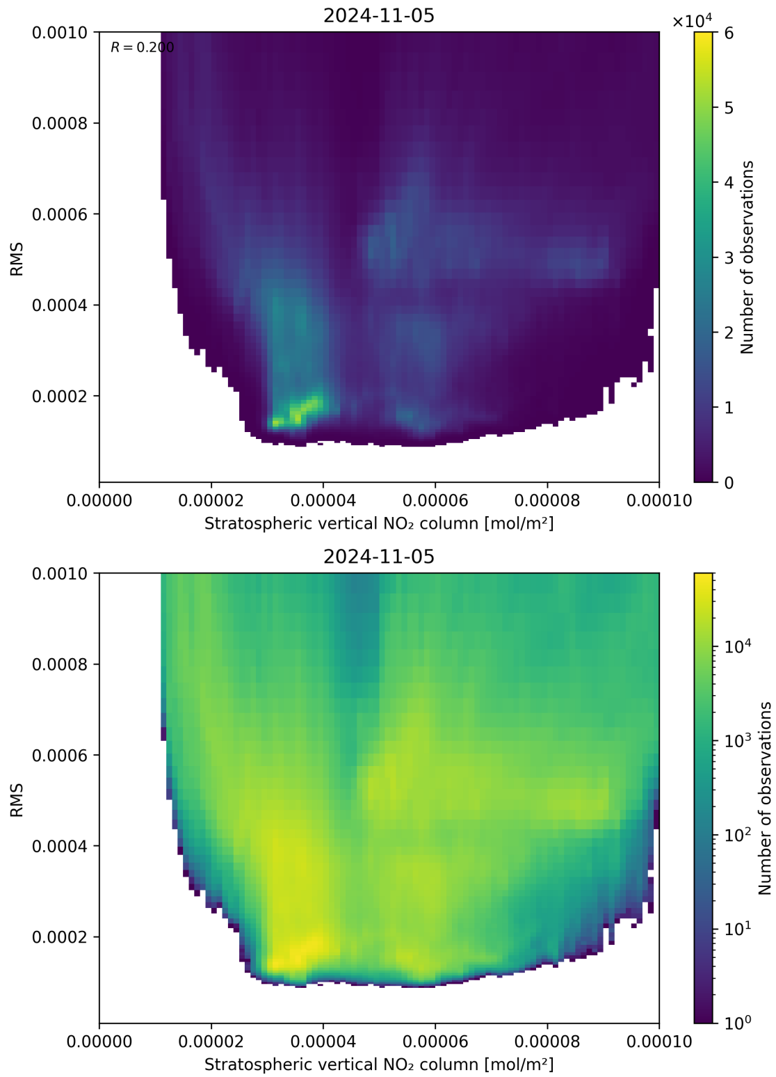
Figure 102: Scatter density plot of “Stratospheric vertical NO 2 column” against “RMS” for 2024-11-04 to 2024-11-06.
