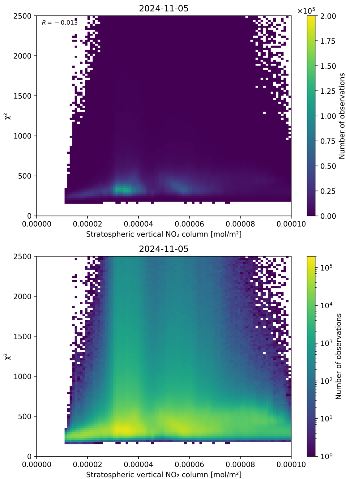
Figure 97: Scatter density plot of “Stratospheric vertical NO 2 column” against “ \chi^2 ” for 2024-11-04 to 2024-11-06.
