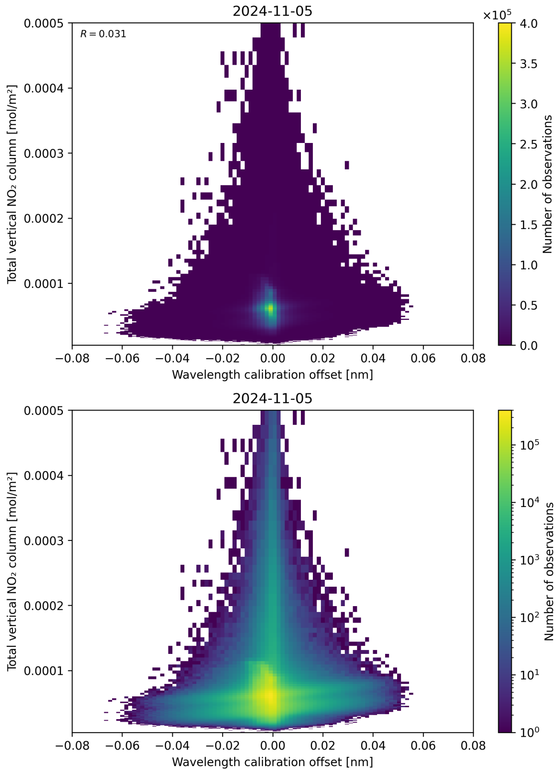
Figure 179: Scatter density plot of “Wavelength calibration offset” against “Total vertical NO 2 column” for 2024-11-04 to 2024-11-06.
