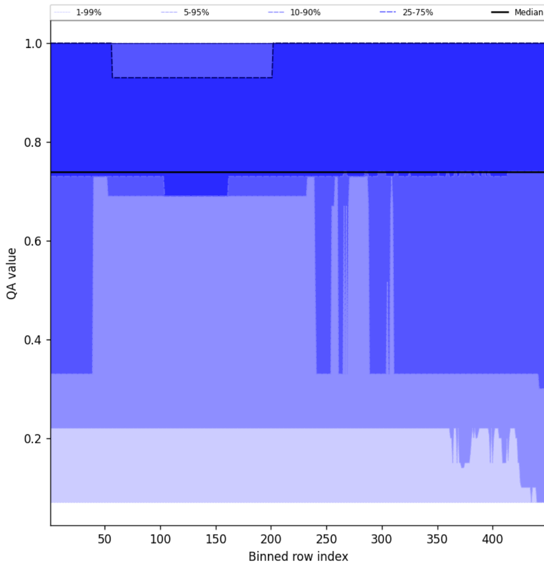
Figure 45: Along track statistics of “QA value” for 2024-11-04 to 2024-11-06
