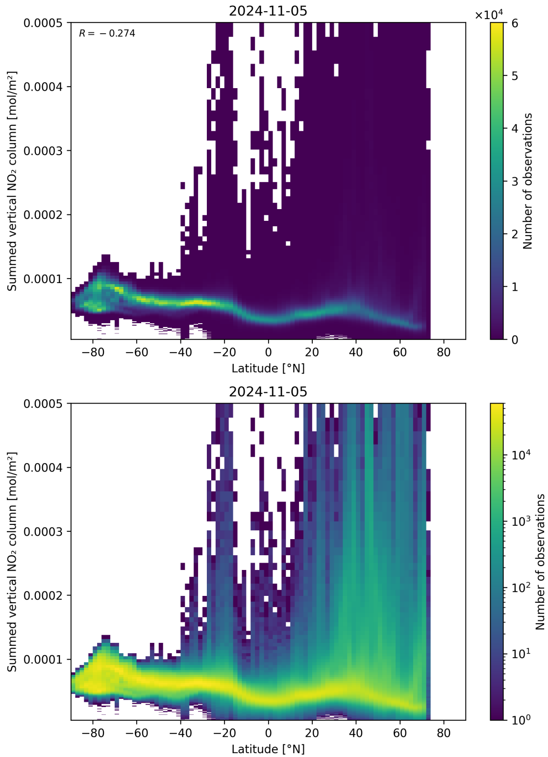
Figure 88: Scatter density plot of “Latitude” against “Summed vertical NO 2 column” for 2024-11-04 to 2024-11-06.
