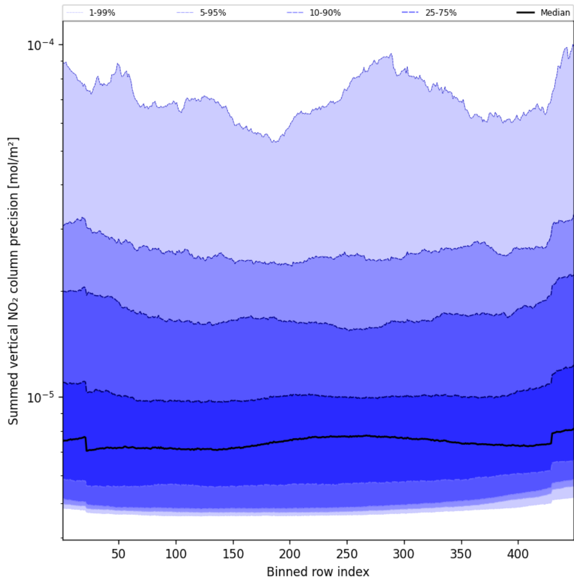
Figure 58: Along track statistics of “Summed vertical NO 2 column precision” for 2024-11-04 to 2024-11-06
