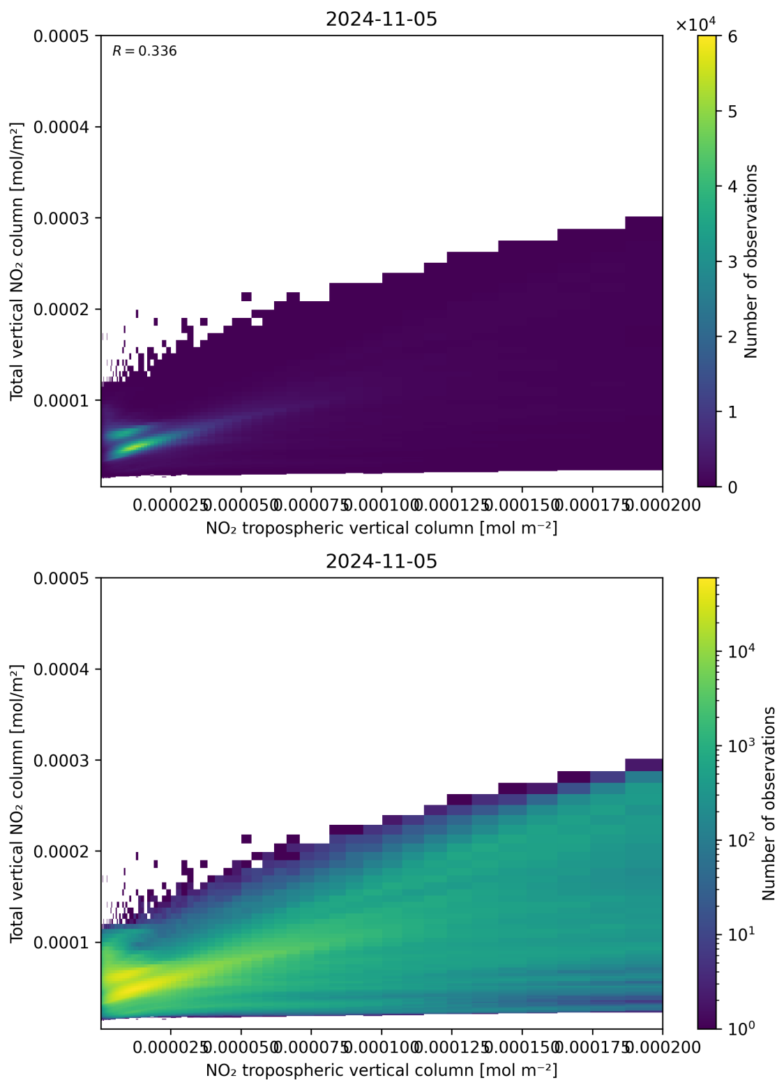
Figure 128: Scatter density plot of “NO 2 tropospheric vertical column” against “Total vertical NO 2 column” for 2024-11-04 to 2024-11-06.
