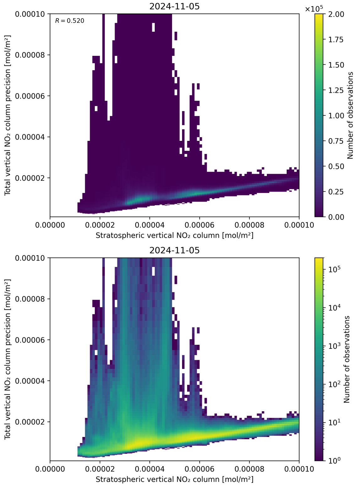
Figure 101: Scatter density plot of “Stratospheric vertical NO 2 column” against “Total vertical NO 2 column precision” for 2024-11-04 to 2024-11-06.
