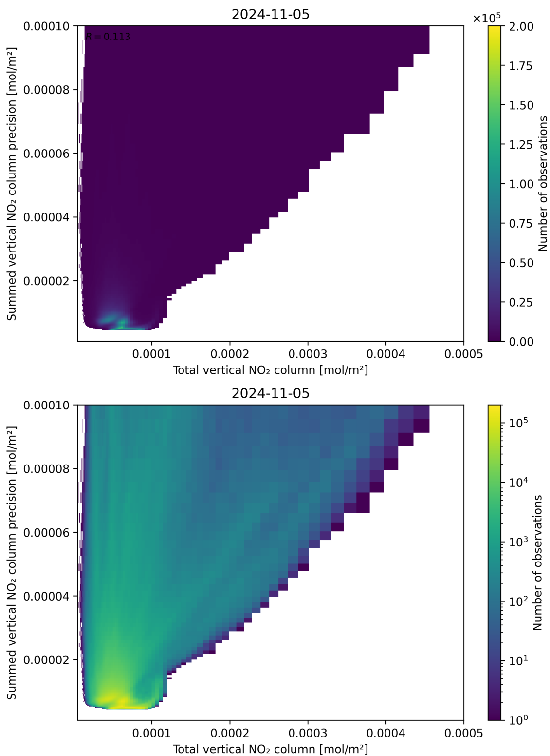
Figure 113: Scatter density plot of “Total vertical NO 2 column” against “Summed vertical NO 2 column precision” for 2024-11-04 to 2024-11-06.
