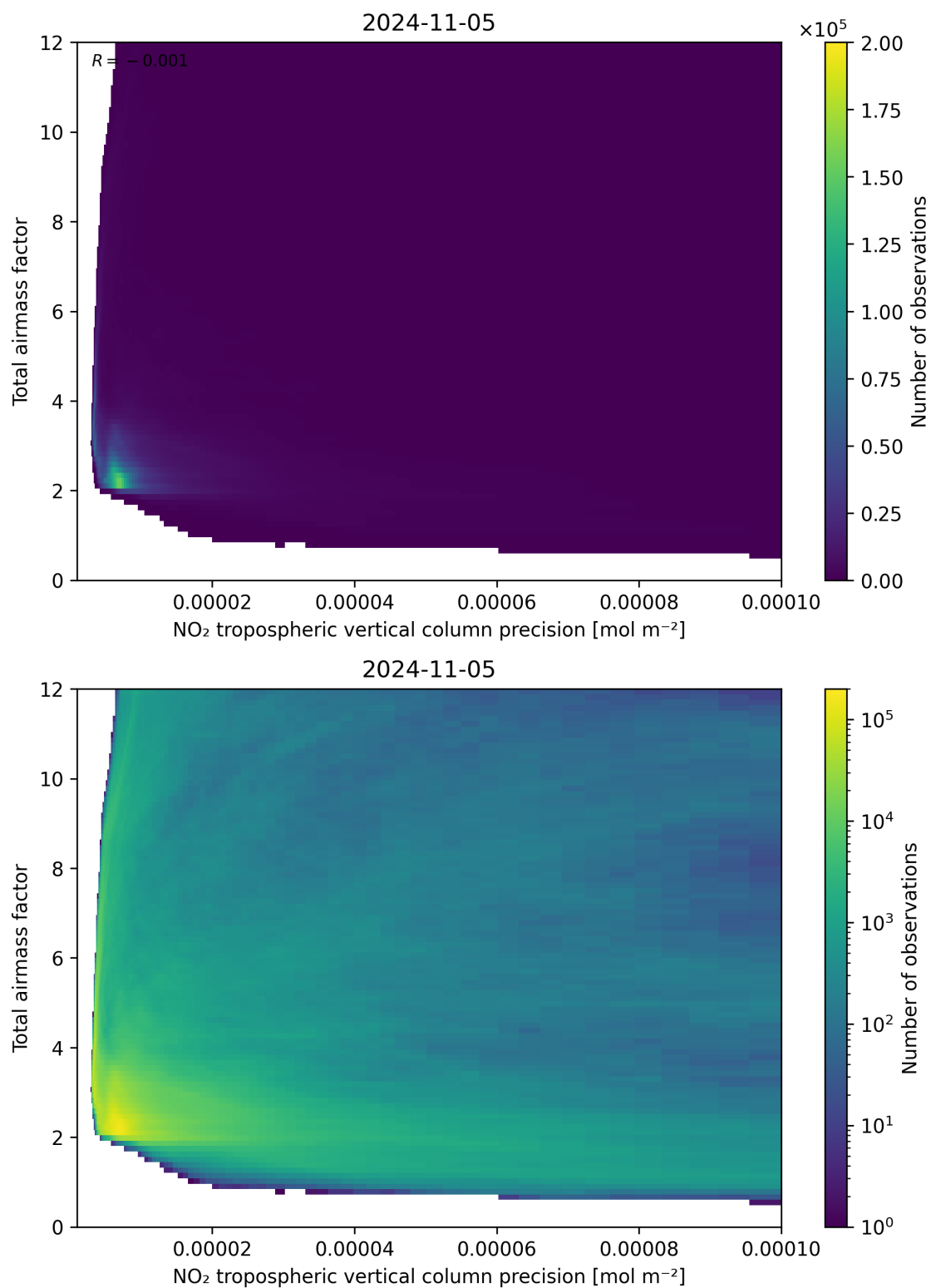
Figure 132: Scatter density plot of “NO 2 tropospheric vertical column precision” against “Total air mass factor” for 2024-11-04 to 2024-11-06.
