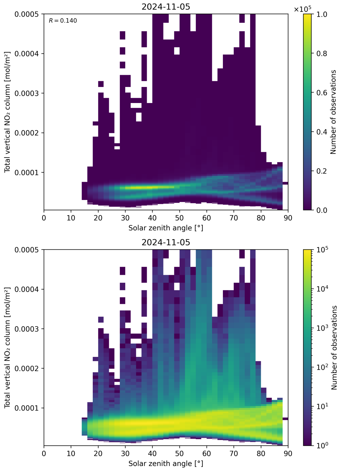
Figure 153: Scatter density plot of “Solar zenith angle” against “Total vertical NO 2 column” for 2024-11-04 to 2024-11-06.
