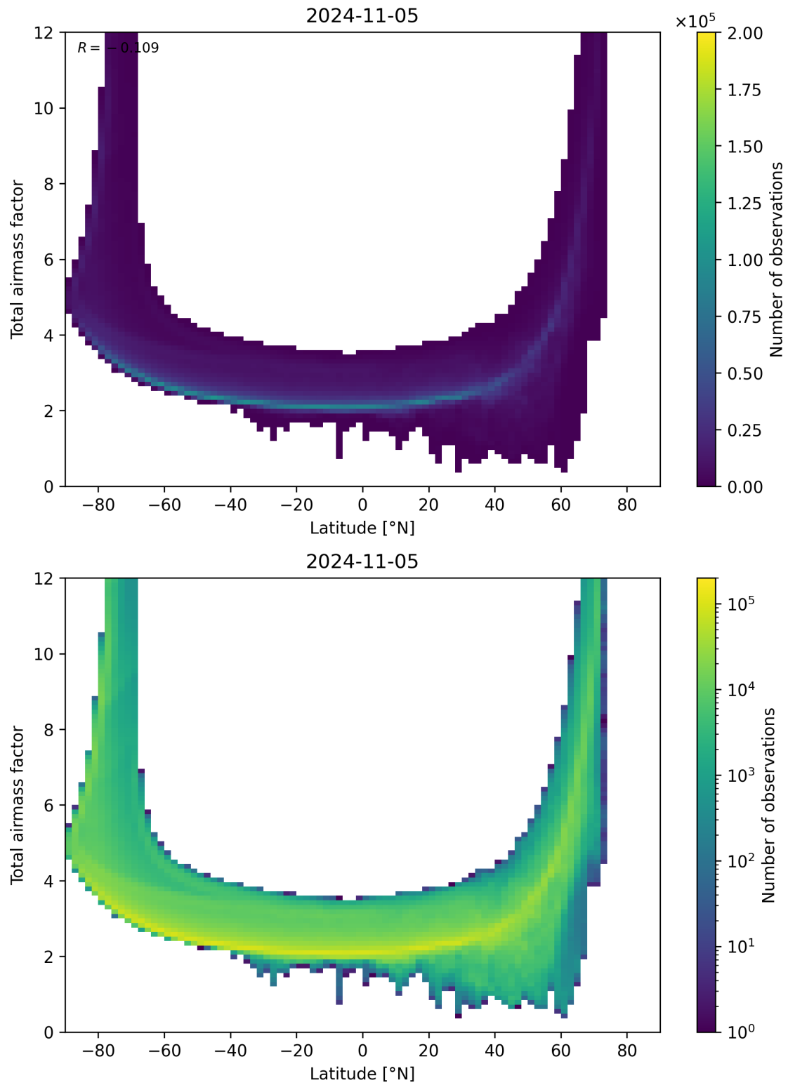
Figure 84: Scatter density plot of “Latitude” against “Total airmass factor” for 2024-11-04 to 2024-11-06.
