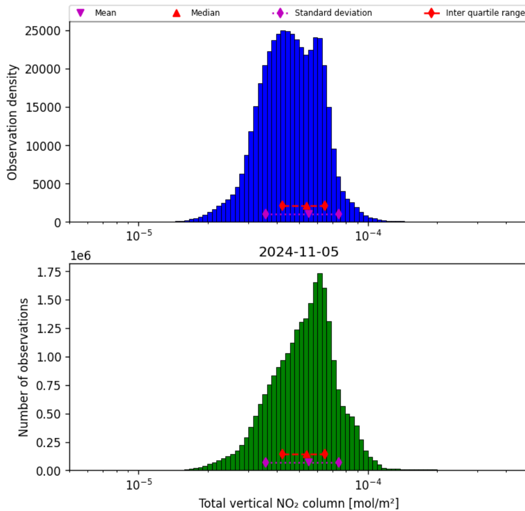
Figure 38: Histogram of “Total vertical NO 2 column” for 2024-11-04 to 2024-11-06
