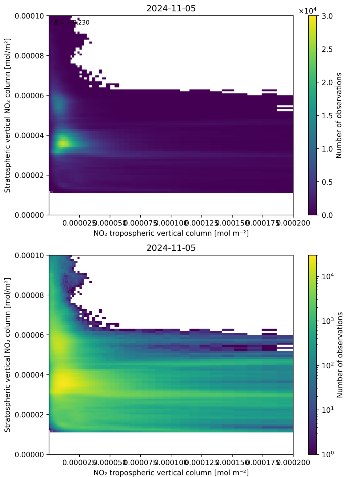
Figure 125: Scatter density plot of “NO 2 tropospheric vertical column” against “Stratospheric vertical NO 2 column” for 2024-11-04 to 2024-11-06.
