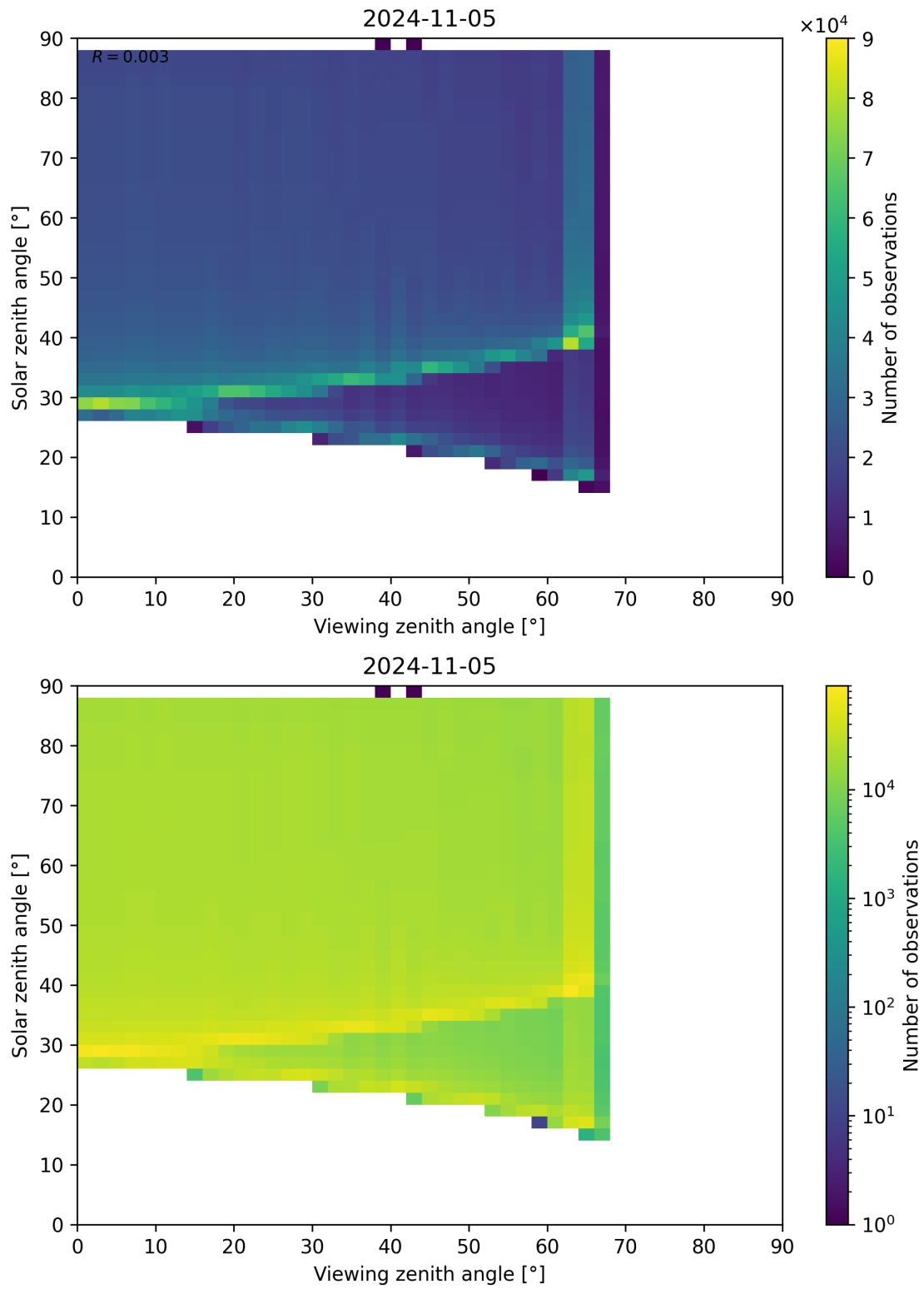
Figure 172: Scatter density plot of “Viewing zenith angle” against “Solar zenith angle” for 2024-11-04 to 2024-11-06.
