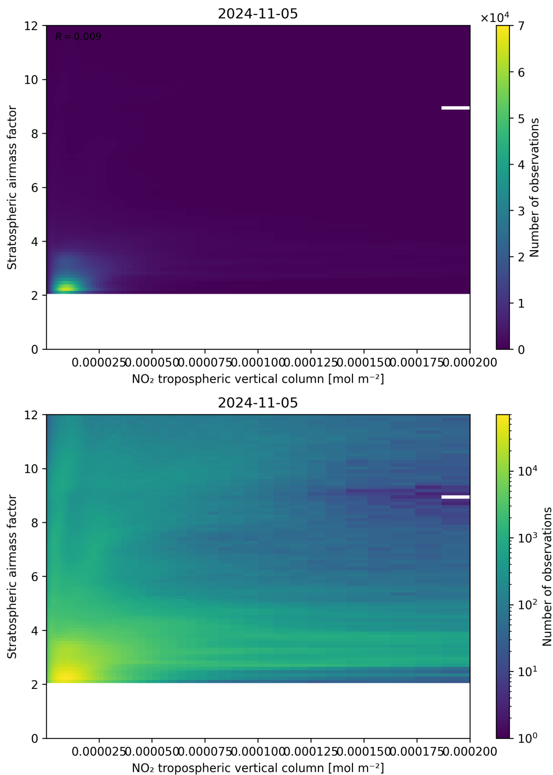
Figure 121: Scatter density plot of “NO 2 tropospheric vertical column” against “Stratospheric airmass factor” for 2024-11-04 to 2024-11-06.
