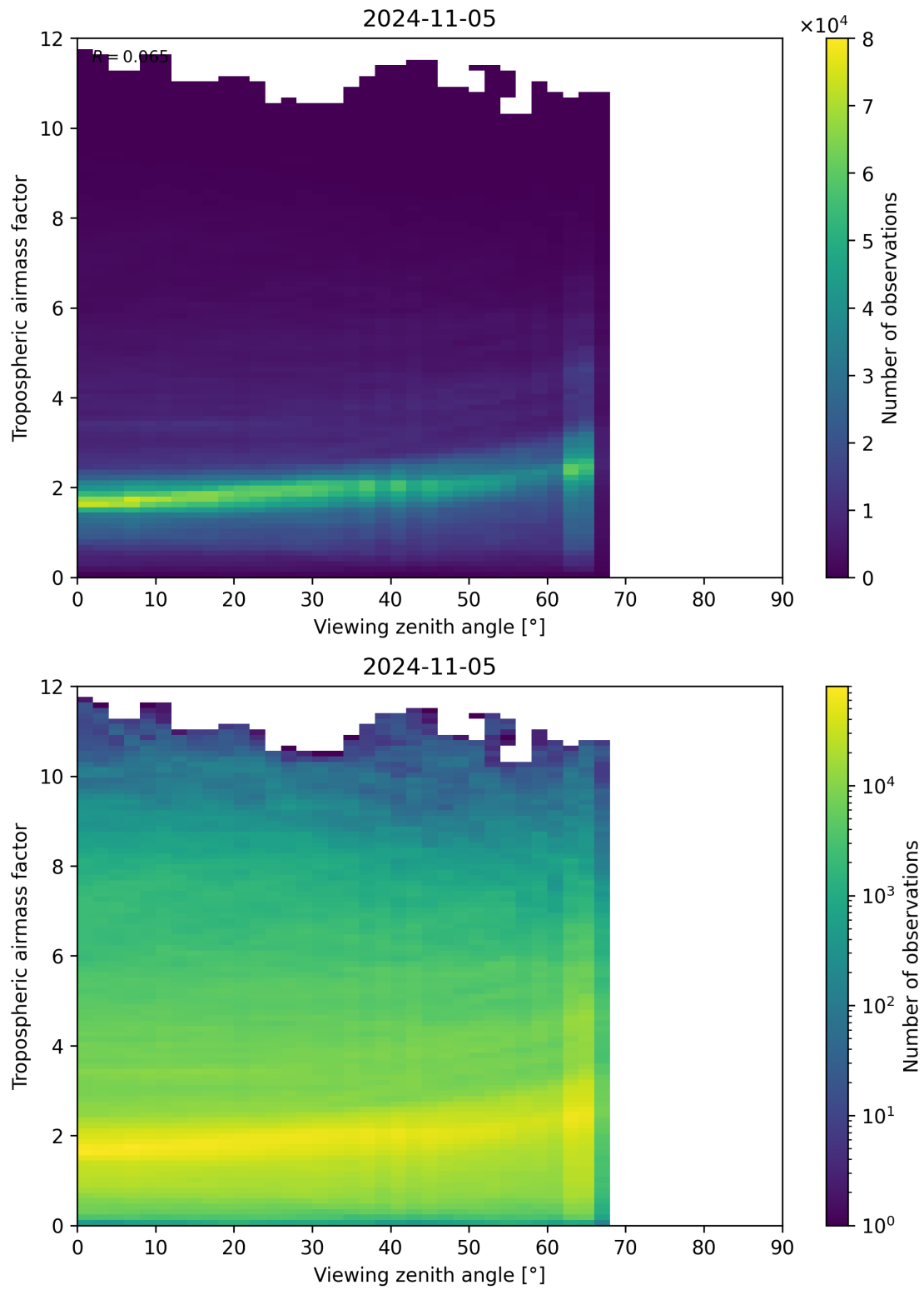
Figure 161: Scatter density plot of “Viewing zenith angle” against “Tropospheric airmass factor” for 2024-11-04 to 2024-11-06.
