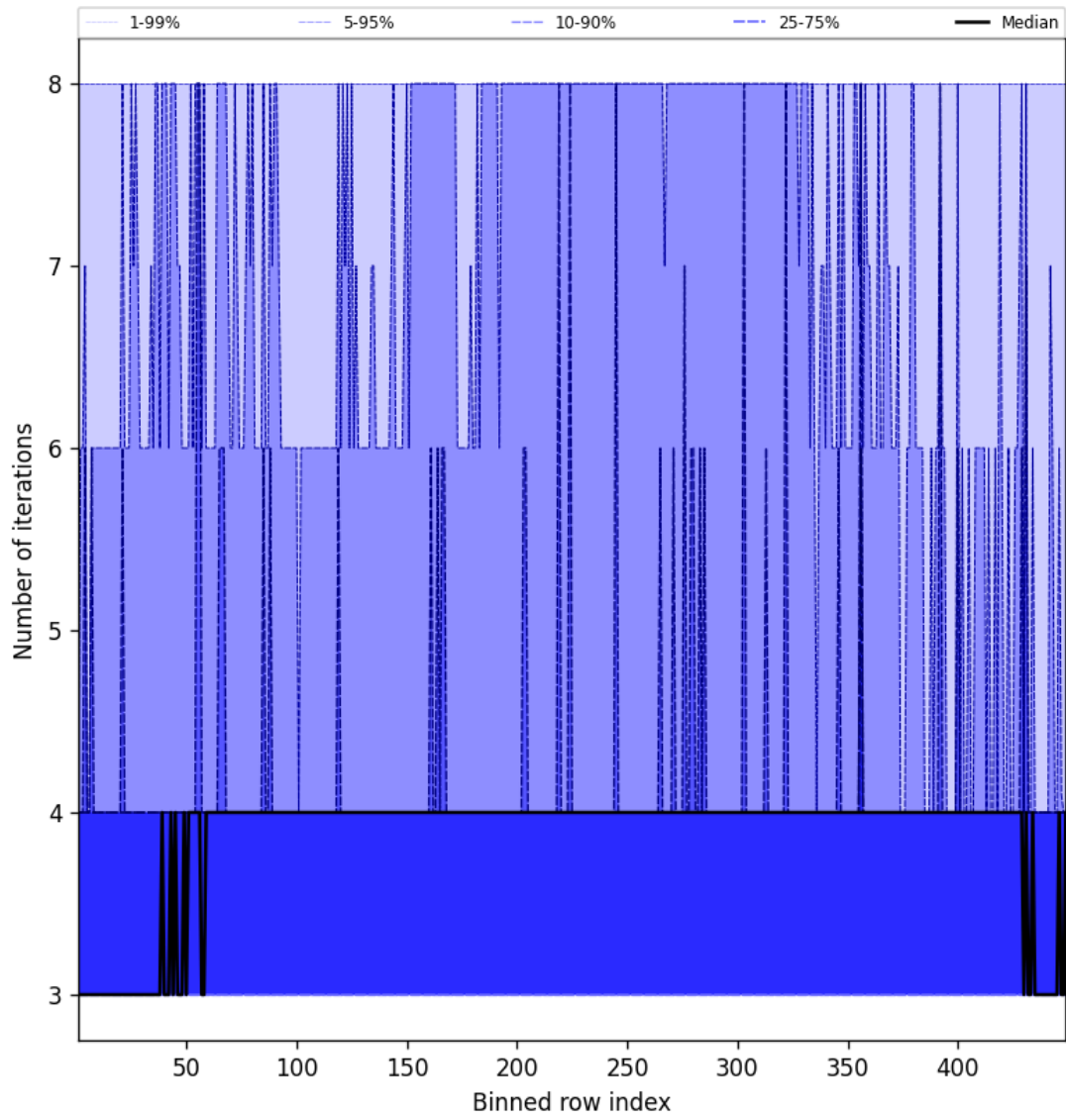
Figure 51: Along track statistics of “Number of iterations” for 2024-11-04 to 2024-11-06
