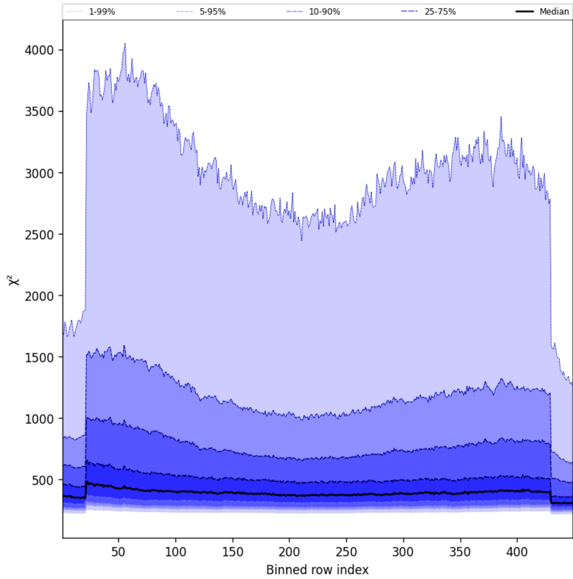
Figure 59: Along track statistics of “ \chi^2 ” for 2024-11-04 to 2024-11-06
