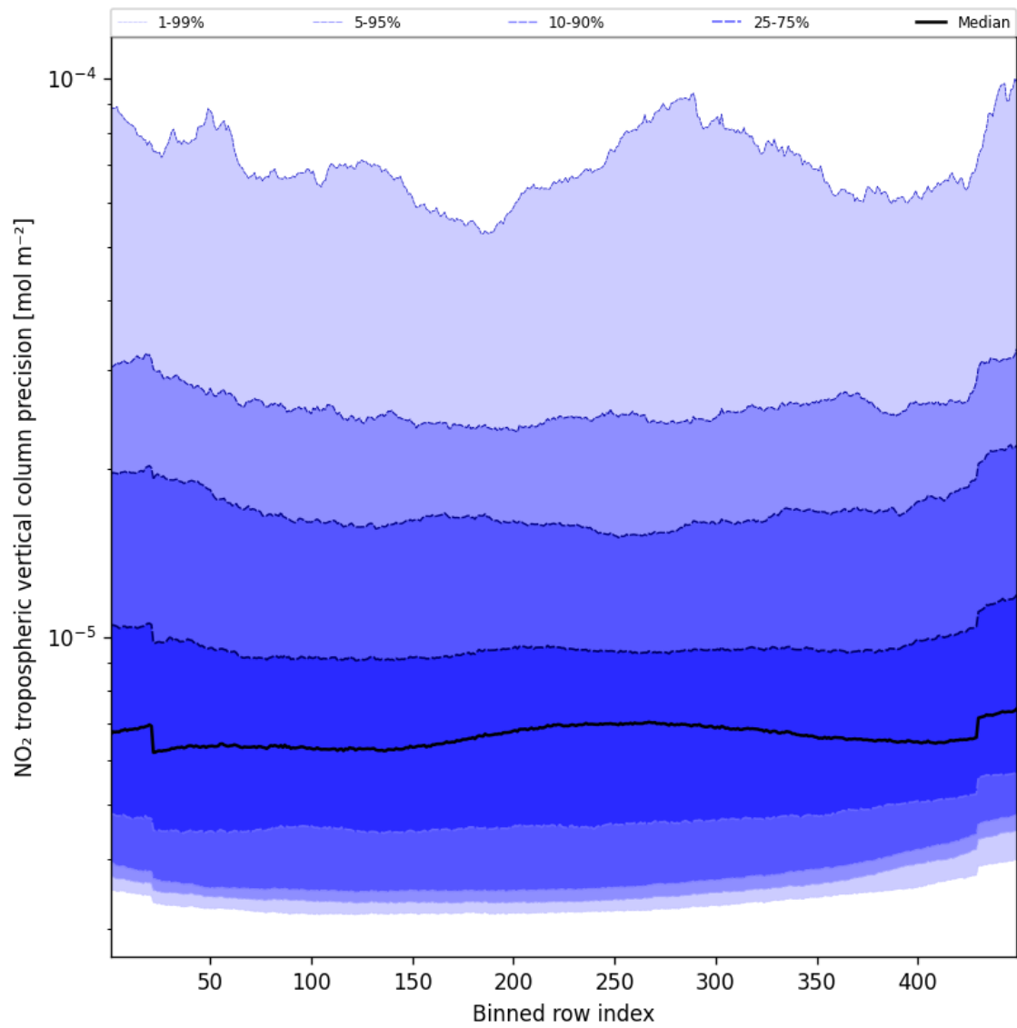
Figure 47: Along track statistics of “NO 2 tropospheric vertical column precision” for 2024-11-04 to 2024-11-06
