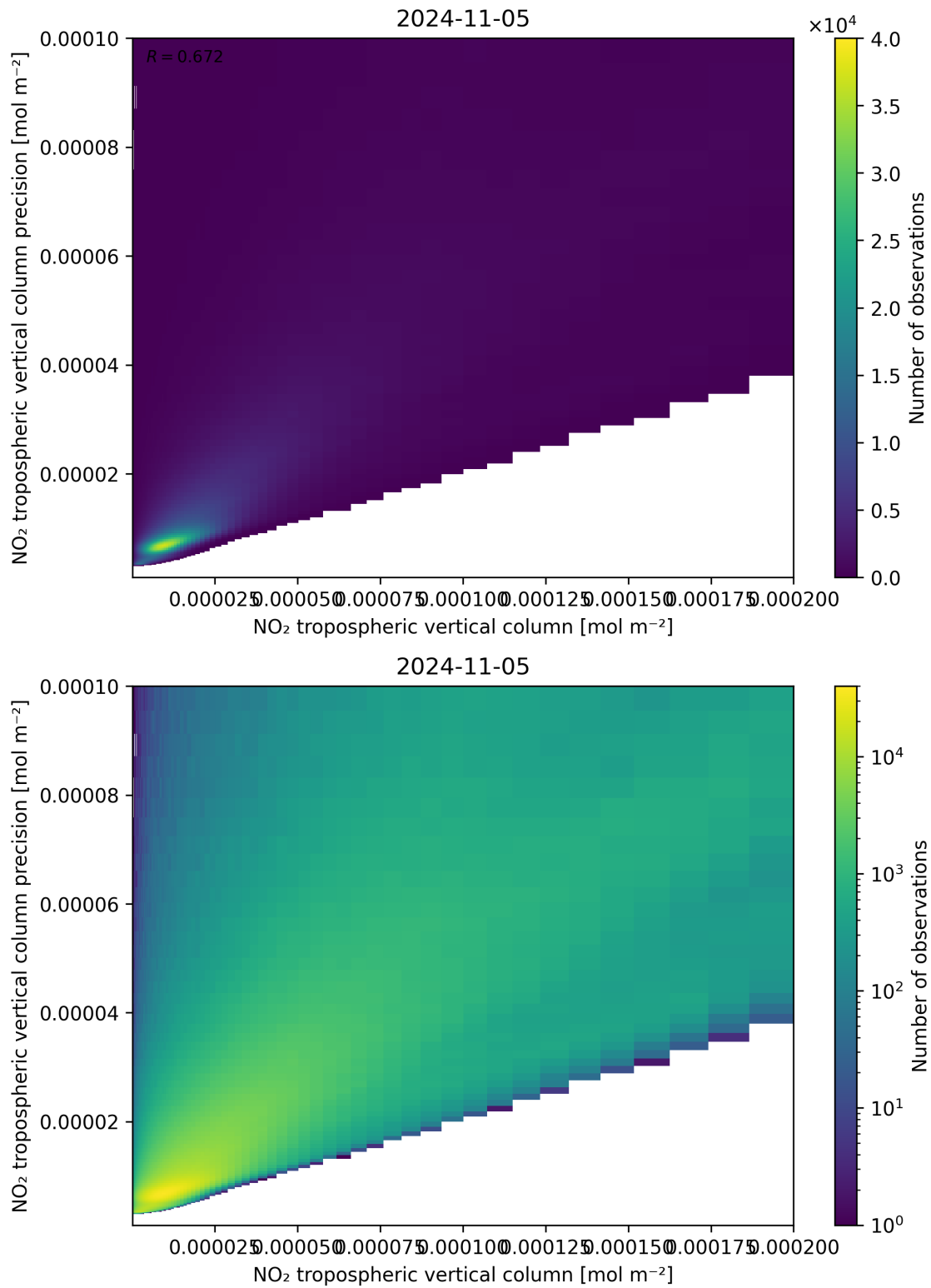
Figure 130: Scatter density plot of “NO 2 tropospheric vertical column” against “NO 2 tropospheric vertical column precision” for 2024-11-04 to 2024-11-06.
