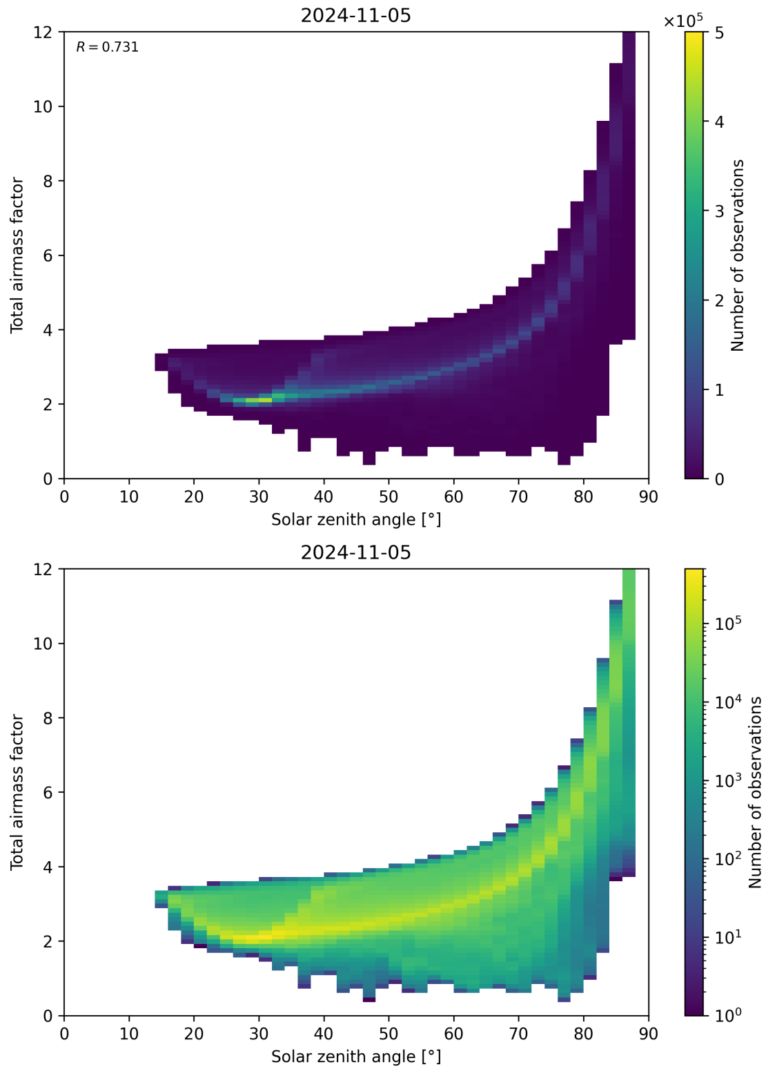
Figure 146: Scatter density plot of “Solar zenith angle” against “Total airmass factor” for 2024-11-04 to 2024-11-06.
