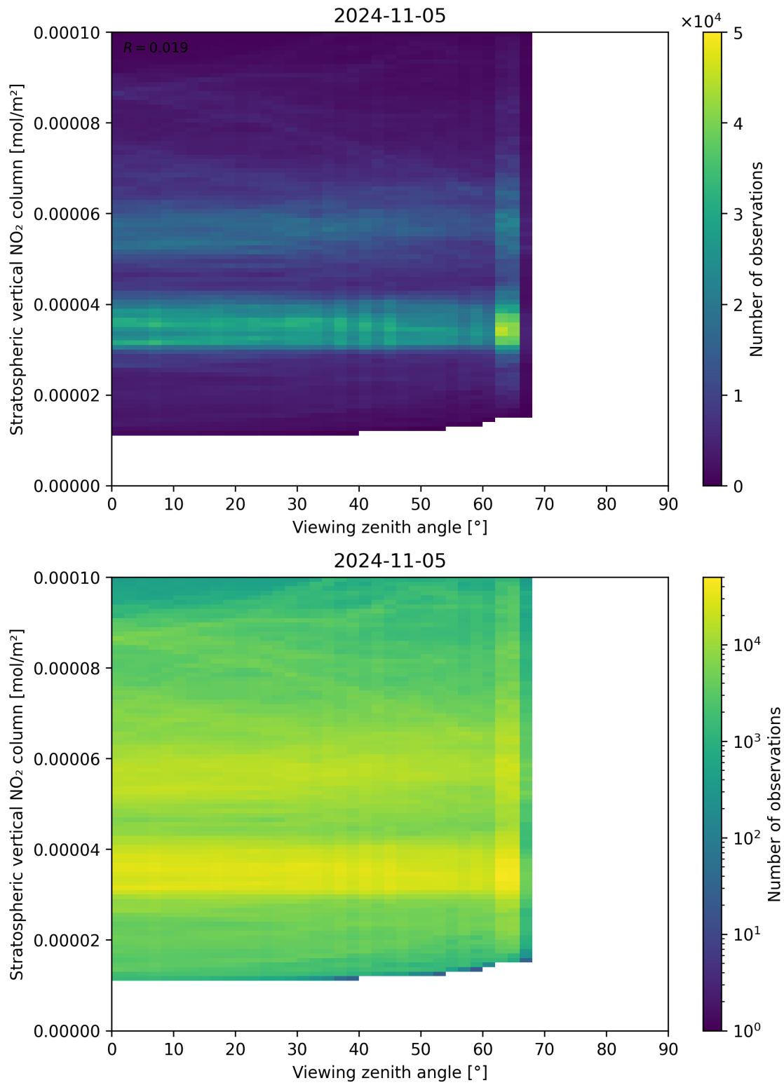
Figure 164: Scatter density plot of “Viewing zenith angle” against “Stratospheric vertical NO 2 column” for 2024-11-04 to 2024-11-06.
