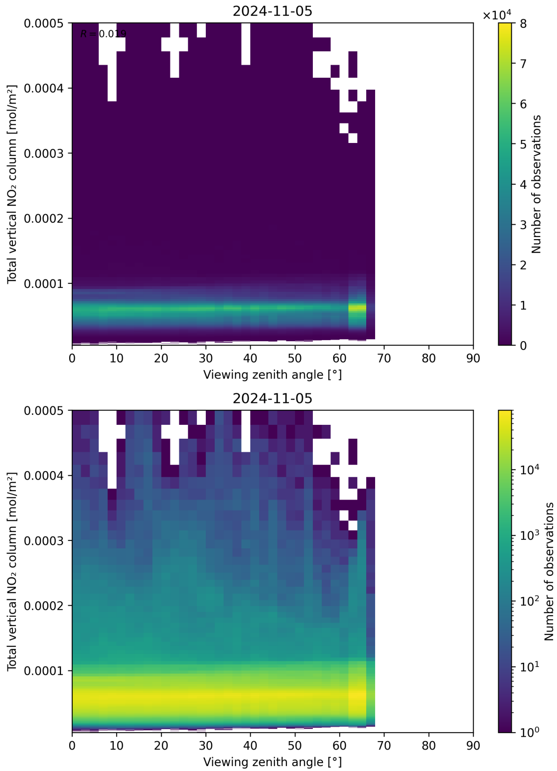
Figure 167: Scatter density plot of “Viewing zenith angle” against “Total vertical NO 2 column” for 2024-11-04 to 2024-11-06.
