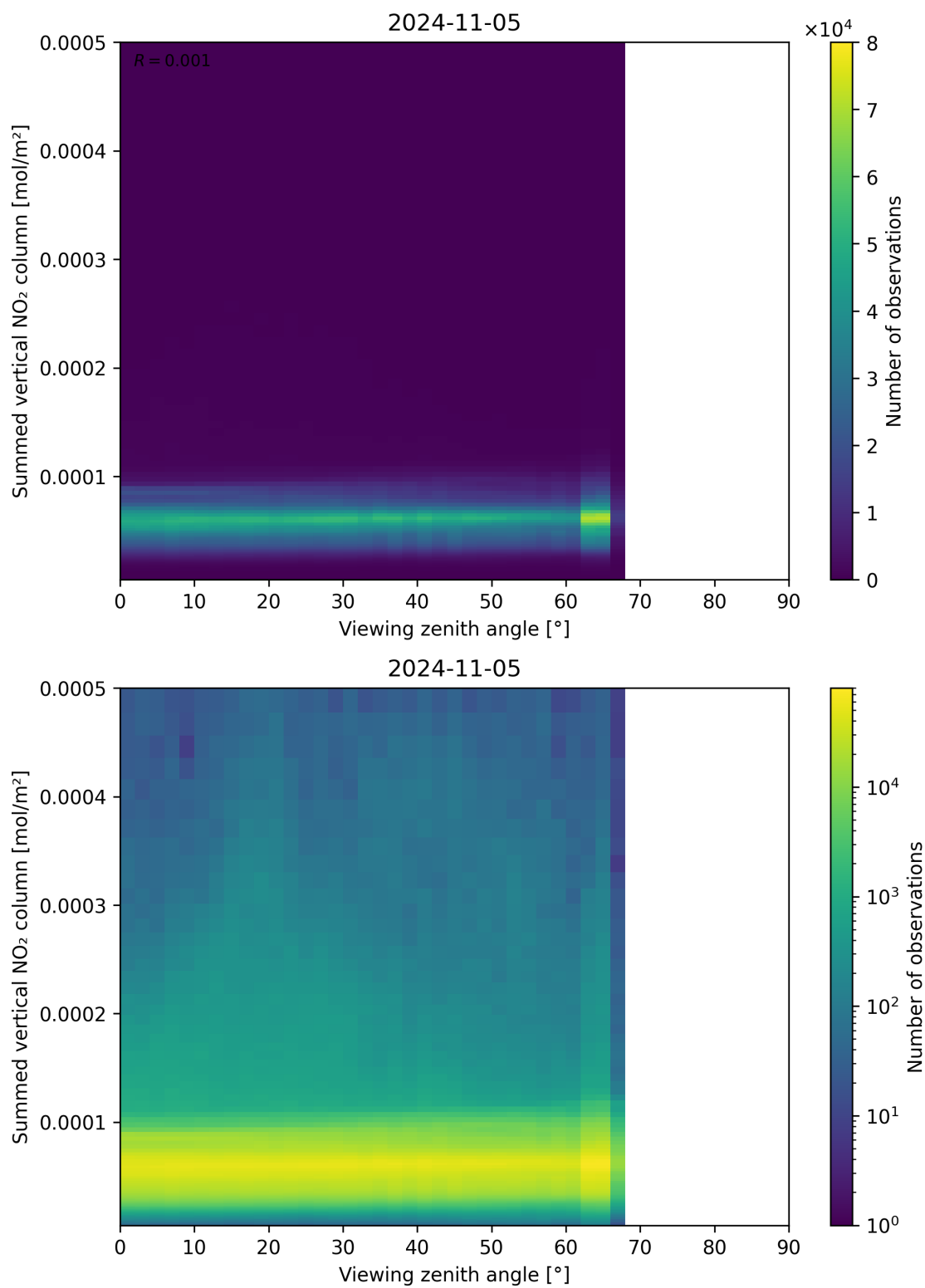
Figure 165: Scatter density plot of “Viewing zenith angle” against “Summed vertical NO 2 column” for 2024-11-04 to 2024-11-06.
