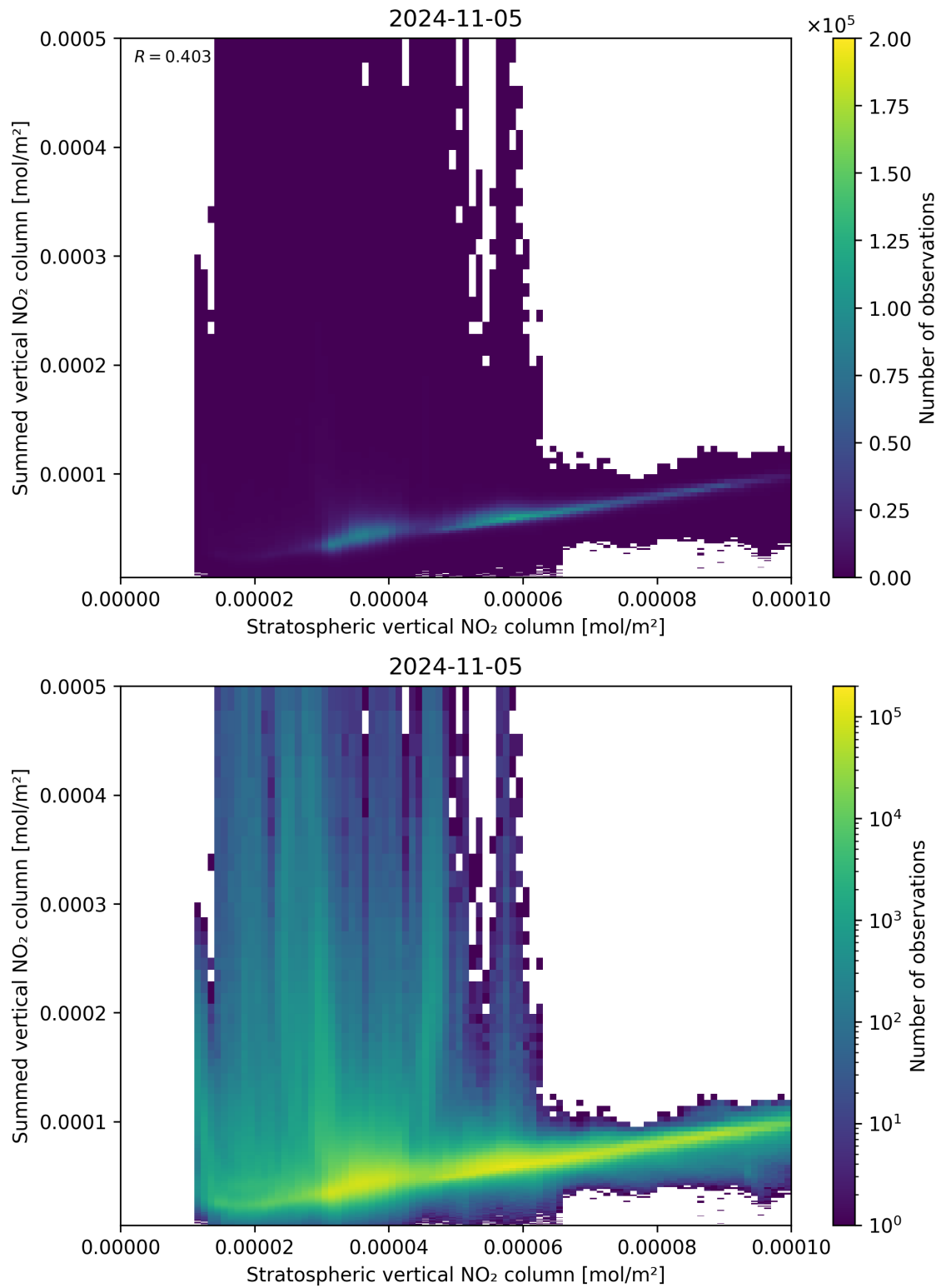
Figure 98: Scatter density plot of “Stratospheric vertical NO 2 column” against “Summed vertical NO 2 column” for 2024-11-04 to 2024-11-06.
