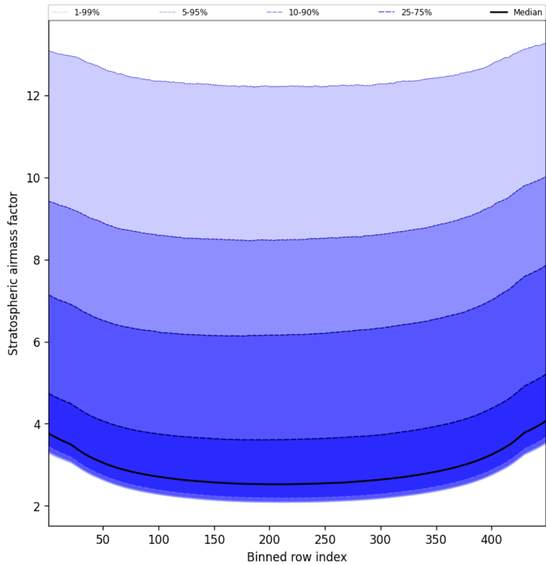
Figure 61: Along track statistics of “Stratospheric airmass factor” for 2024-11-04 to 2024-11-06
