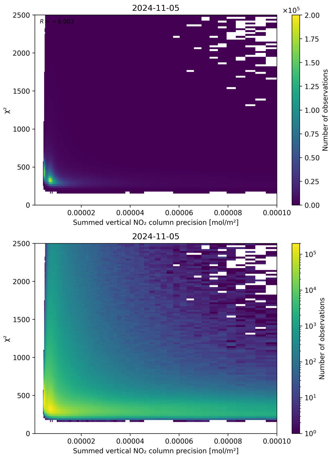
Figure 107: Scatter density plot of “Summed vertical NO 2 column precision” against “ \chi^2 ” for 2024-11-04 to 2024-11-06.
