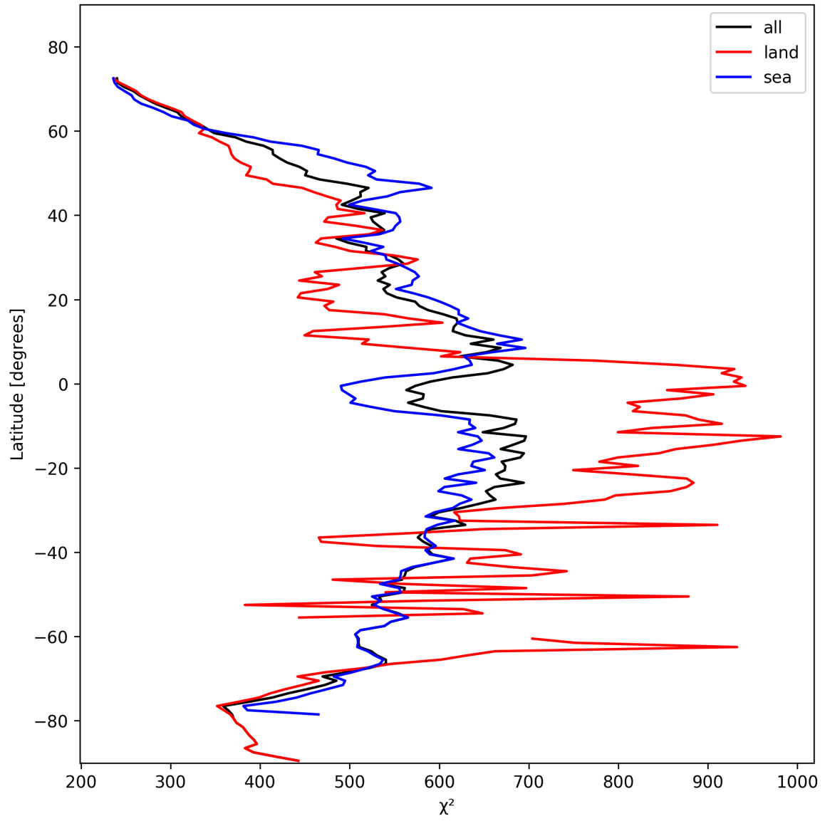
Figure 25: Zonal average of “ \chi^2 ” for 2024-11-04 to 2024-11-06.
