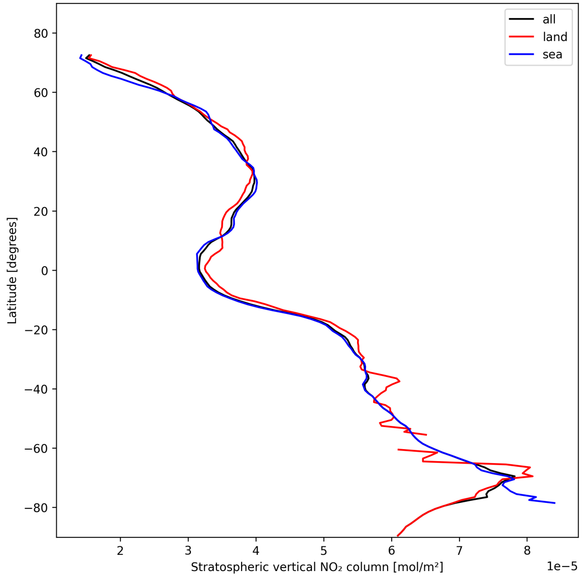
Figure 19: Zonal average of “Stratospheric vertical NO 2 column” for 2024-11-04 to 2024-11-06.
