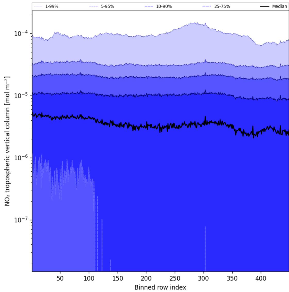
Figure 46: Along track statistics of “NO 2 tropospheric vertical column” for 2024-11-04 to 2024-11-06
