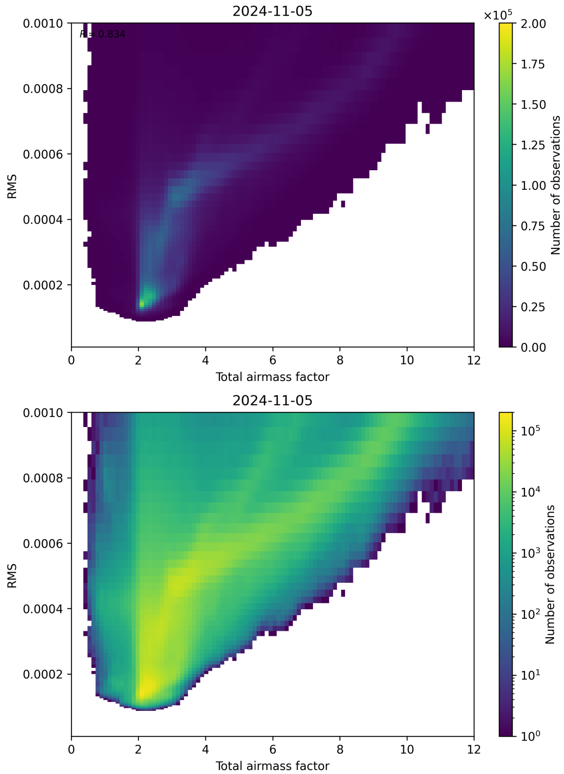
Figure 69: Scatter density plot of “Total airmass factor” against “RMS” for 2024-11-04 to 2024-11-06.
