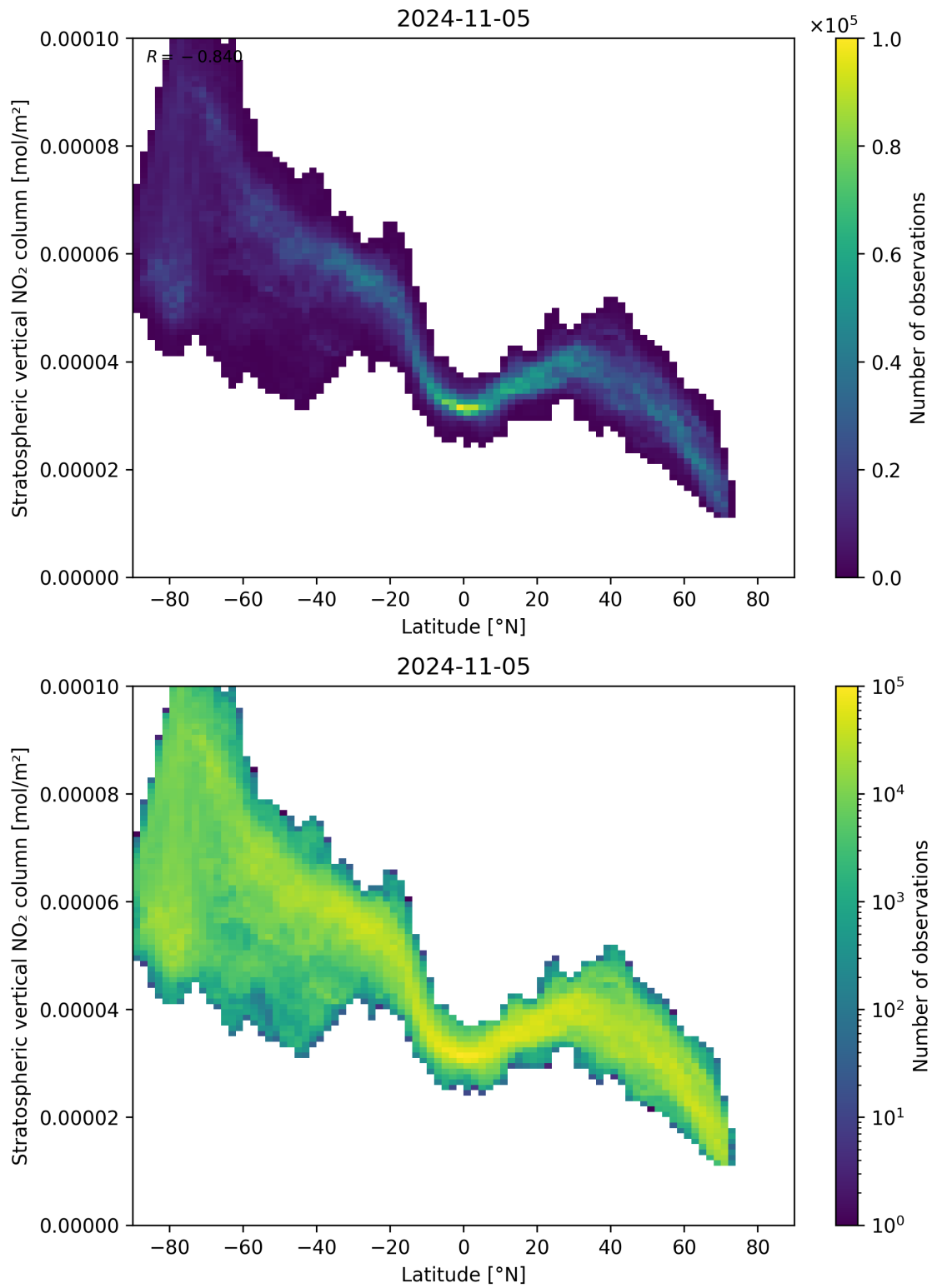
Figure 87: Scatter density plot of “Latitude” against “Stratospheric vertical NO 2 column” for 2024-11-04 to 2024-11-06.
