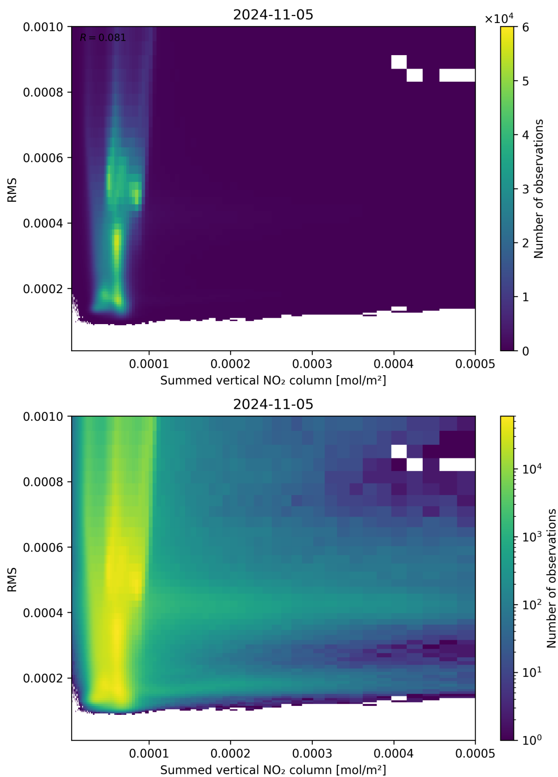
Figure 109: Scatter density plot of “Summed vertical NO 2 column” against “RMS” for 2024-11-04 to 2024-11-06.
