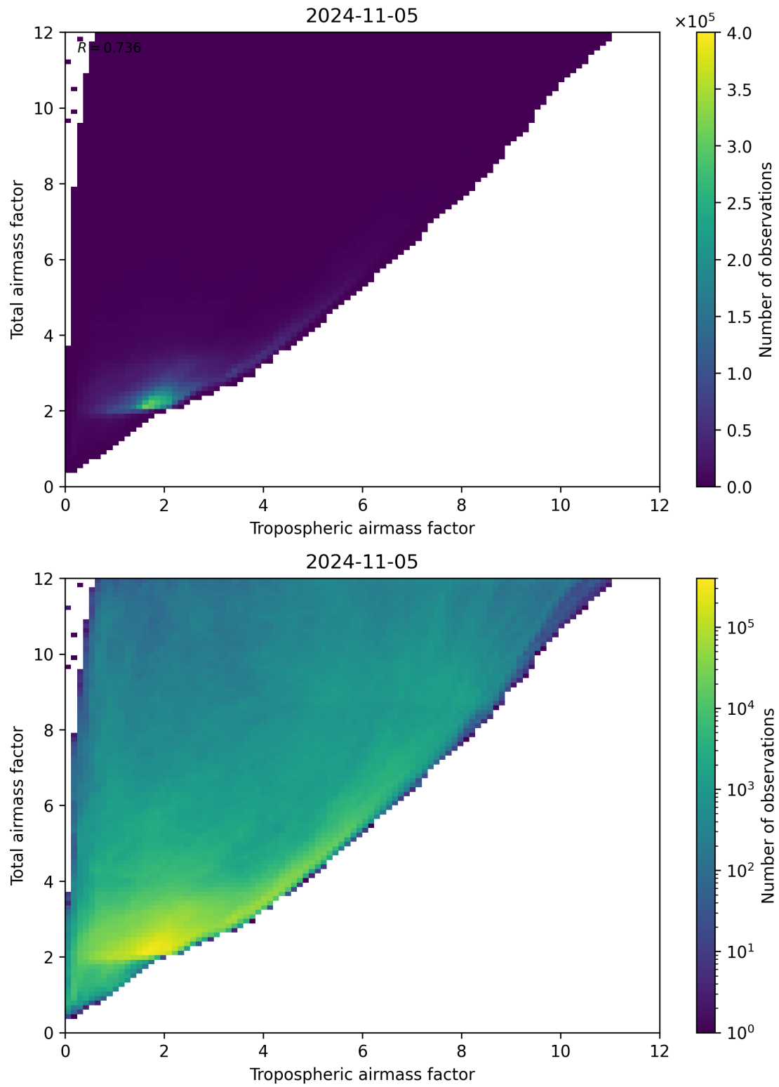
Figure 72: Scatter density plot of “Tropospheric airmass factor” against “Total airmass factor” for 2024-11-04 to 2024-11-06.
