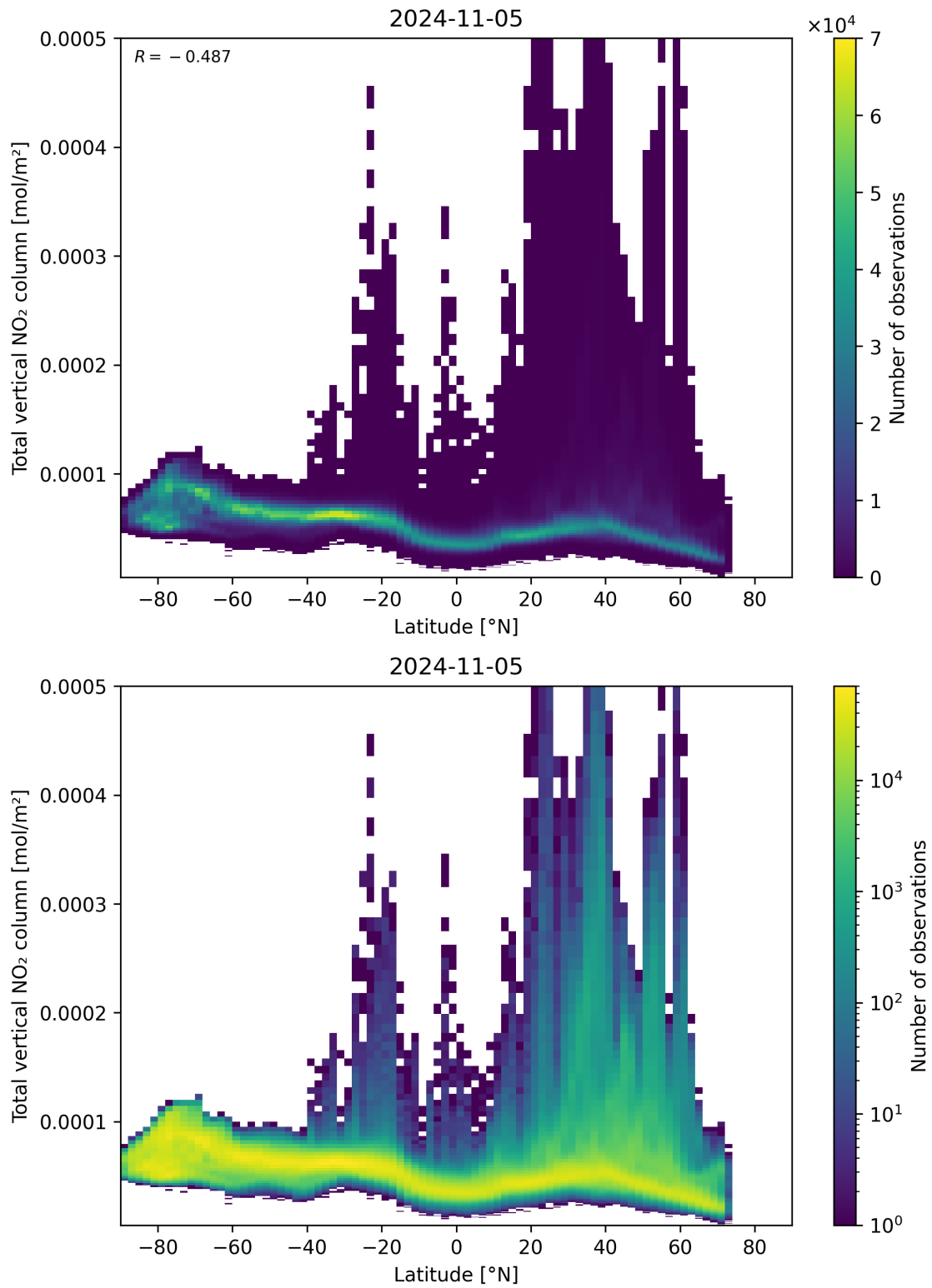
Figure 90: Scatter density plot of “Latitude” against “Total vertical NO 2 column” for 2024-11-04 to 2024-11-06.
