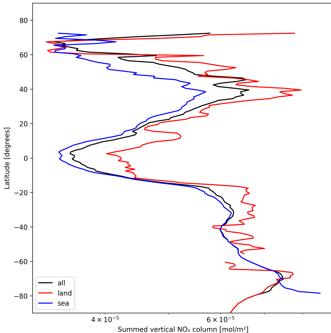
Figure 23: Zonal average of “Summed vertical NO 2 column” for 2024-11-04 to 2024-11-06.
