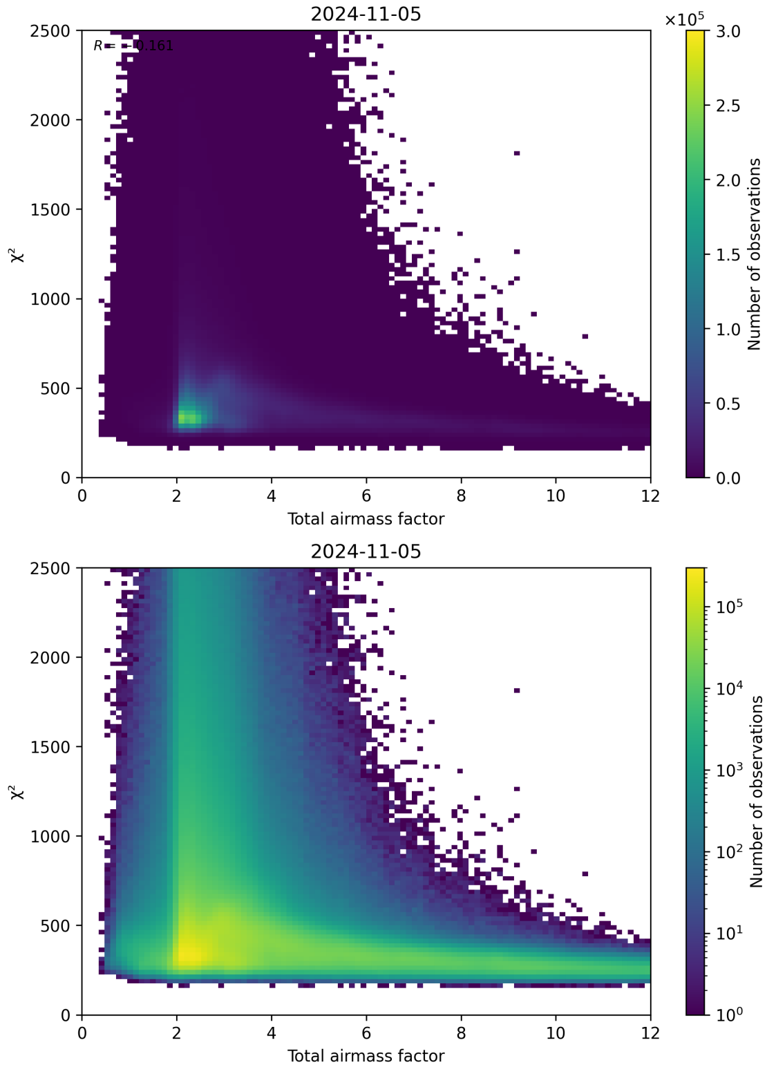
Figure 63: Scatter density plot of “Total airmass factor” against “ \chi^2 ” for 2024-11-04 to 2024-11-06.
