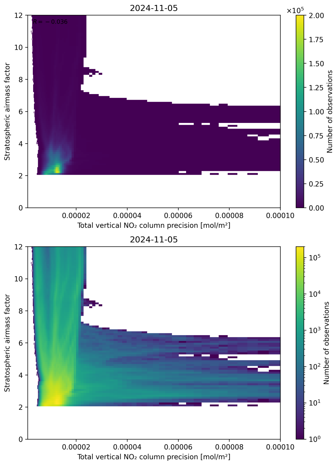
Figure 115: Scatter density plot of “Total vertical NO 2 column precision” against “Stratospheric air mass factor” for 2024-11-04 to 2024-11-06.
