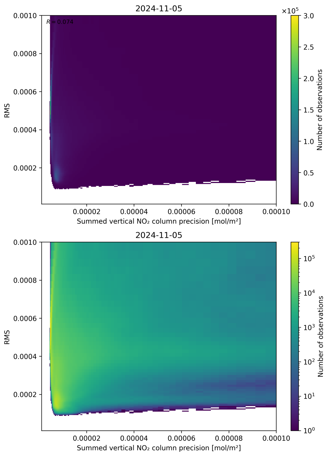
Figure 108: Scatter density plot of “Summed vertical NO 2 column precision” against “RMS” for 2024-11-04 to 2024-11-06.
