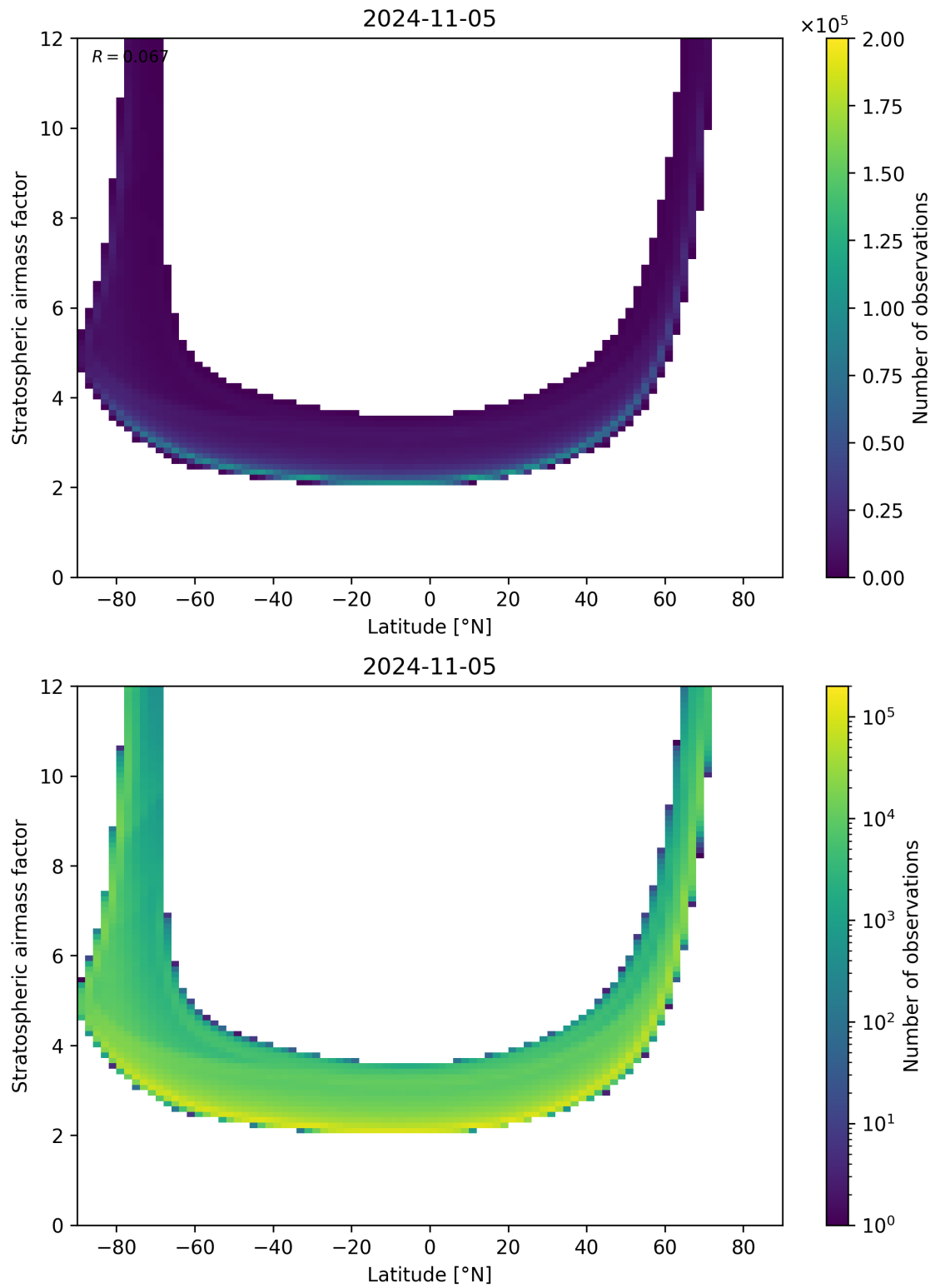
Figure 83: Scatter density plot of “Latitude” against “Stratospheric airmass factor” for 2024-11-04 to 2024-11-06.
