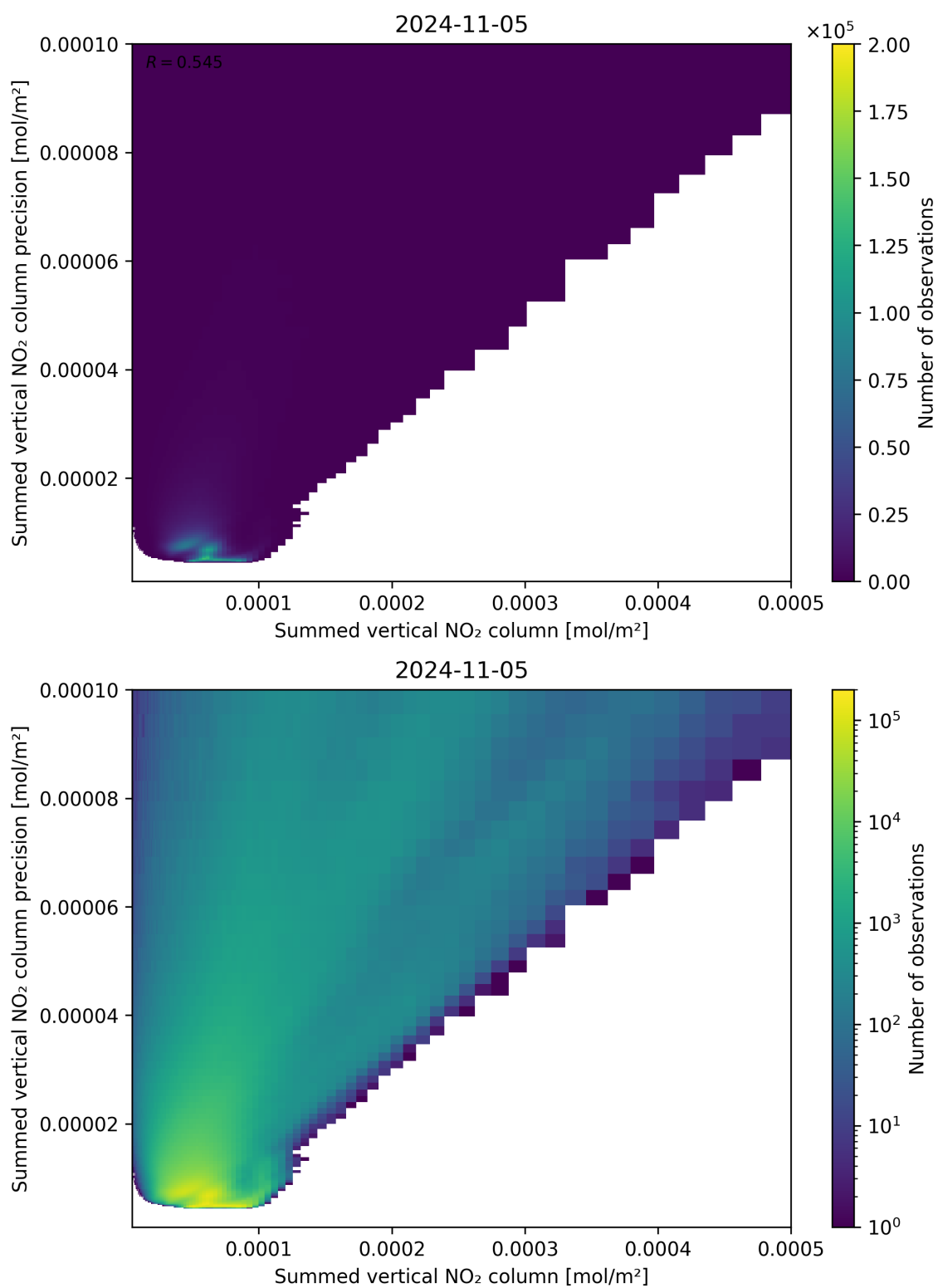
Figure 105: Scatter density plot of “Summed vertical NO 2 column” against “Summed vertical NO 2 column precision” for 2024-11-04 to 2024-11-06.
