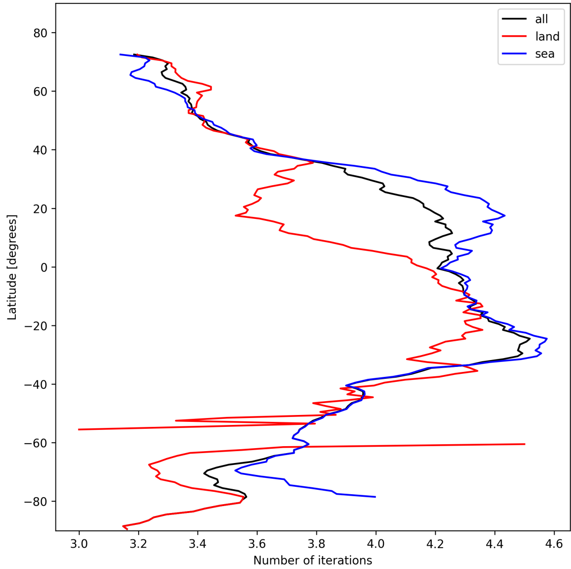
Figure 17: Zonal average of “Number of iterations” for 2024-11-04 to 2024-11-06.
