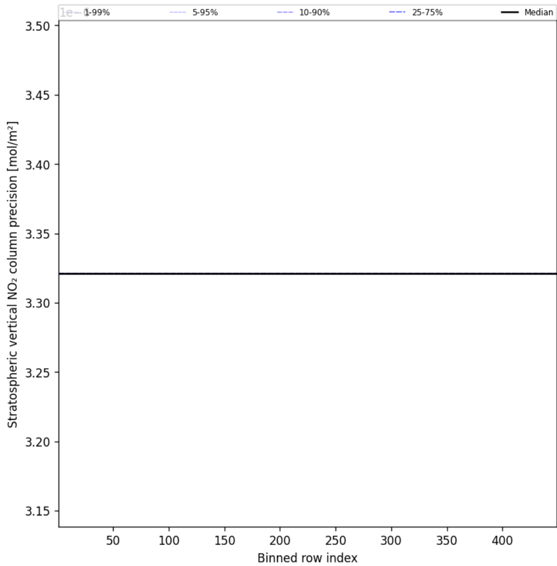
Figure 54: Along track statistics of “Stratospheric vertical NO 2 column precision” for 2024-11-04 to 2024-11-06
