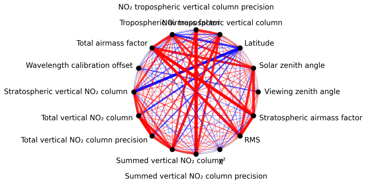
Figure 1: Map of correlation graph for 2024-11-04 to 2024-11-06.
