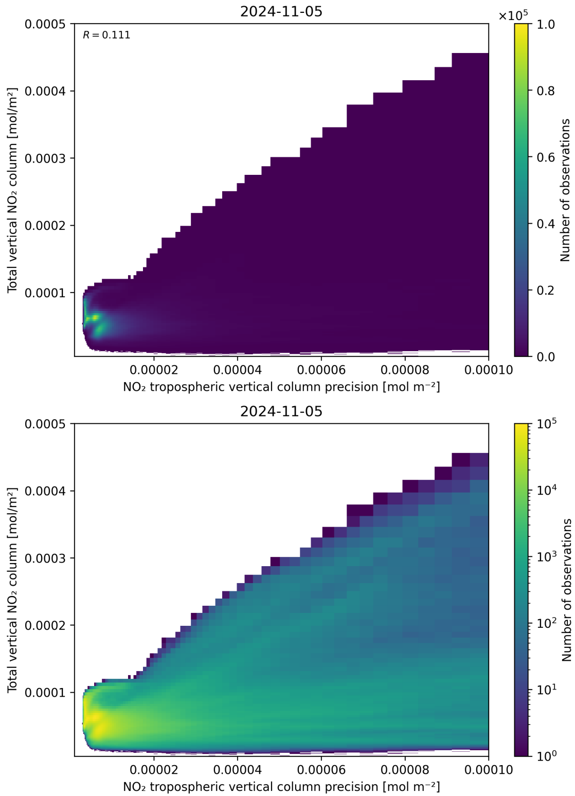
Figure 138: Scatter density plot of “NO 2 tropospheric vertical column precision” against “Total vertical NO 2 column” for 2024-11-04 to 2024-11-06.
