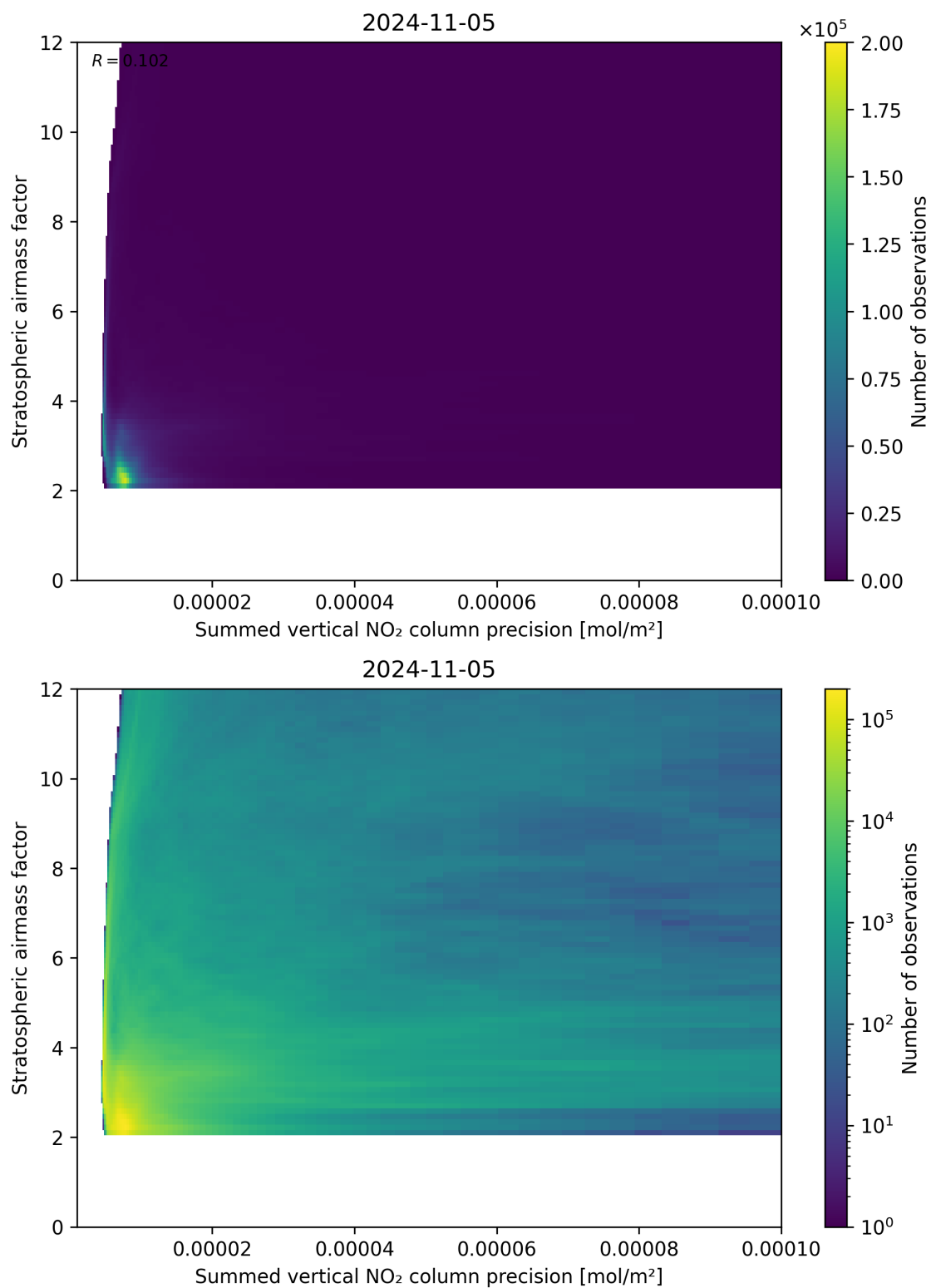
Figure 106: Scatter density plot of “Summed vertical NO 2 column precision” against “Stratospheric airmass factor” for 2024-11-04 to 2024-11-06.
