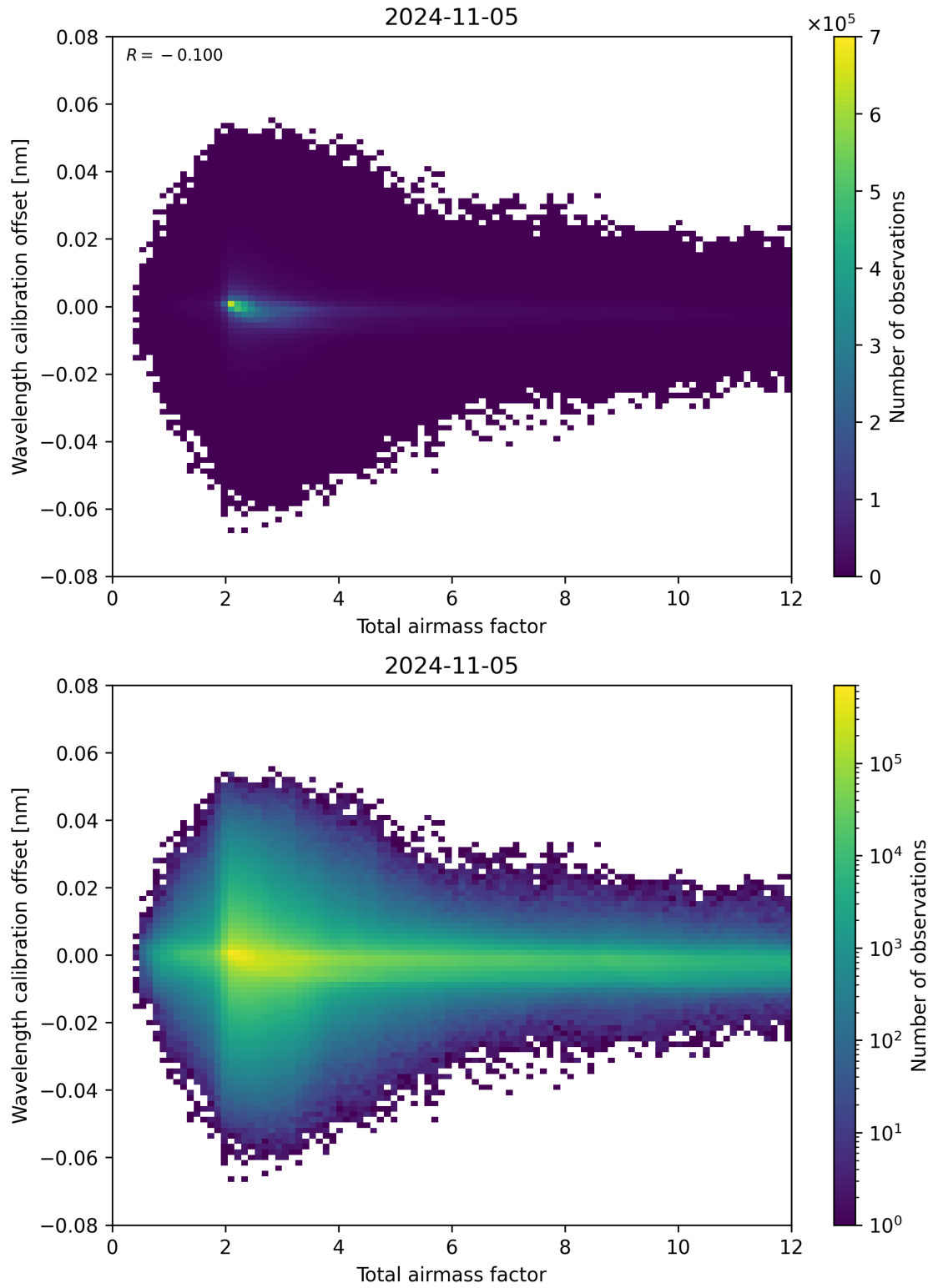
Figure 70: Scatter density plot of “Total airmass factor” against “Wavelength calibration offset” for 2024-11-04 to 2024-11-06.
