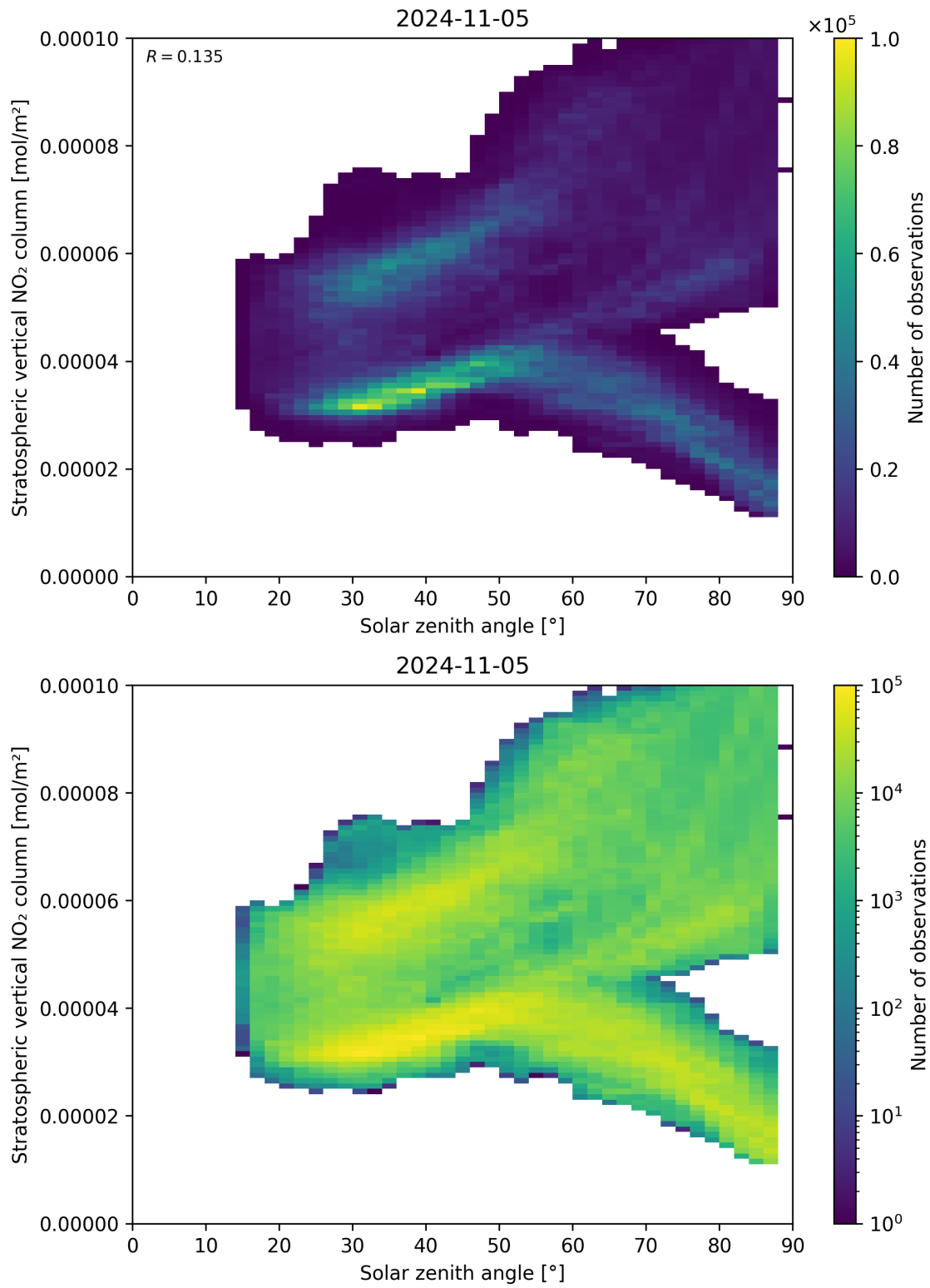
Figure 150: Scatter density plot of “Solar zenith angle” against “Stratospheric vertical NO 2 column” for 2024-11-04 to 2024-11-06.
