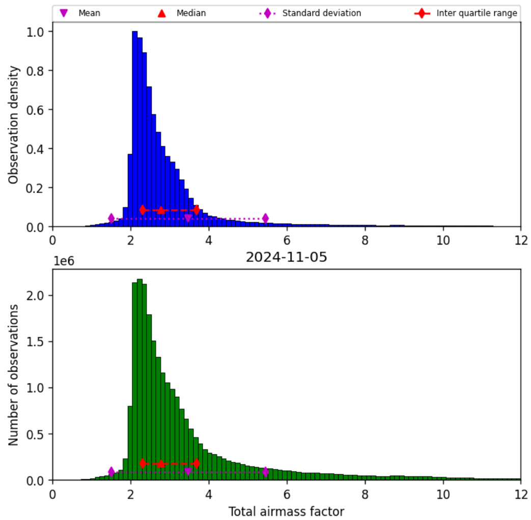
Figure 32: Histogram of “Total airmass factor” for 2024-11-04 to 2024-11-06
