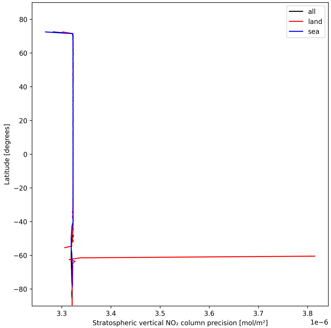
Figure 20: Zonal average of “Stratospheric vertical NO 2 column precision” for 2024-11-04 to 2024-11-06.
