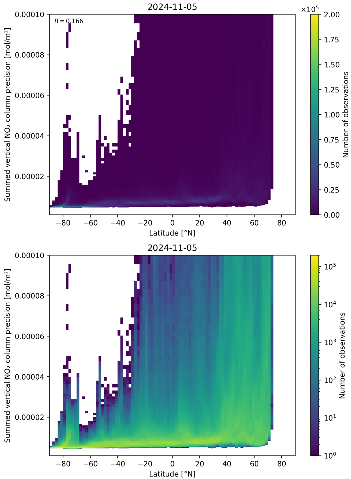
Figure 89: Scatter density plot of “Latitude” against “Summed vertical NO 2 column precision” for 2024-11-04 to 2024-11-06.
