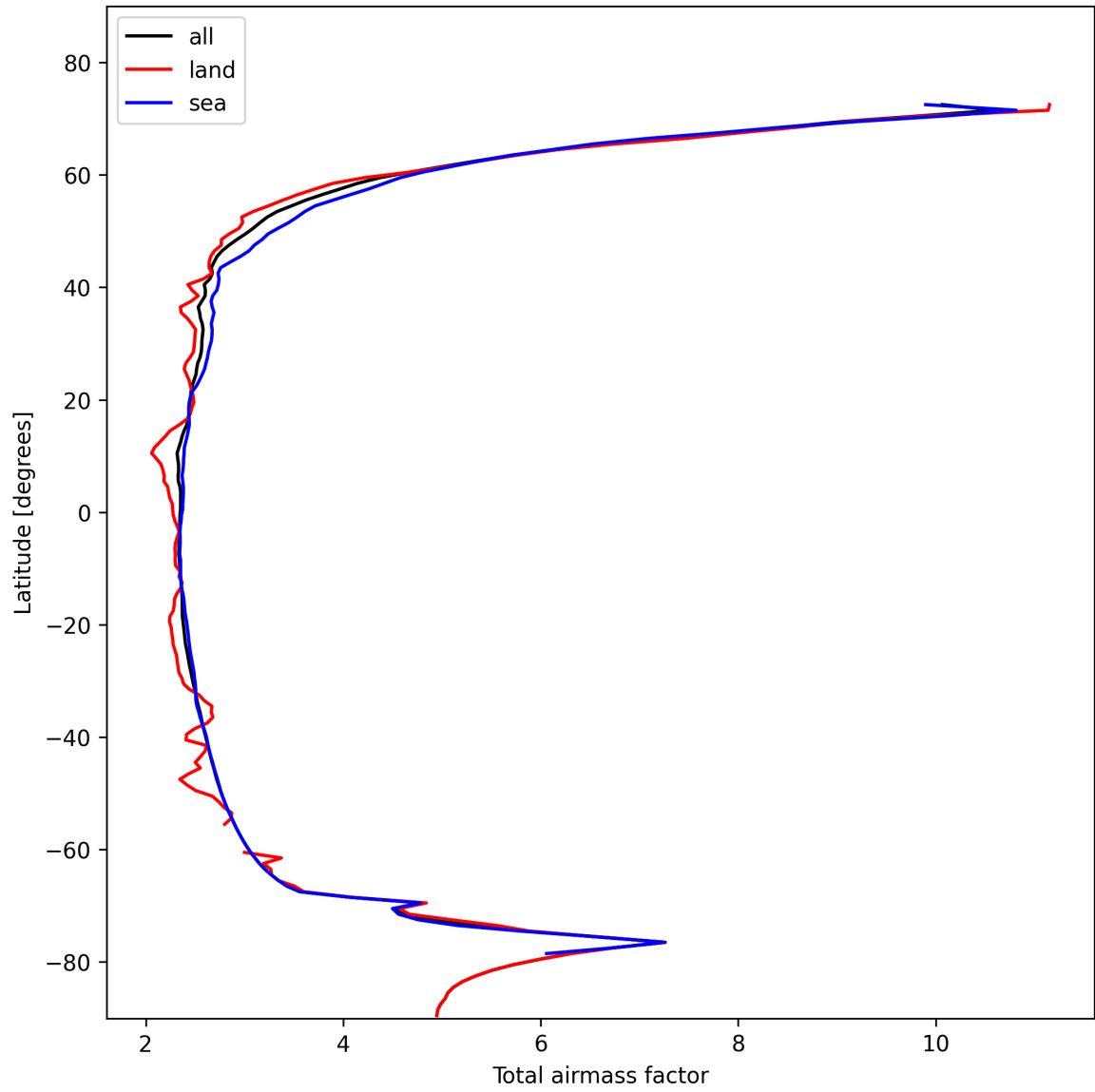
Figure 15: Zonal average of “Total airmass factor” for 2024-11-04 to 2024-11-06.
