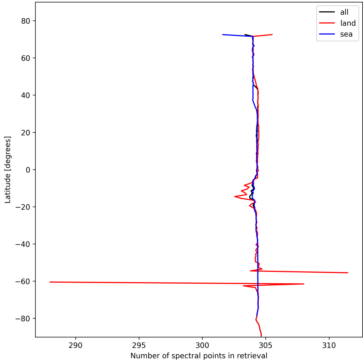
Figure 16: Zonal average of “Number of spectral points in retrieval” for 2024-11-04 to 2024-11-06.
