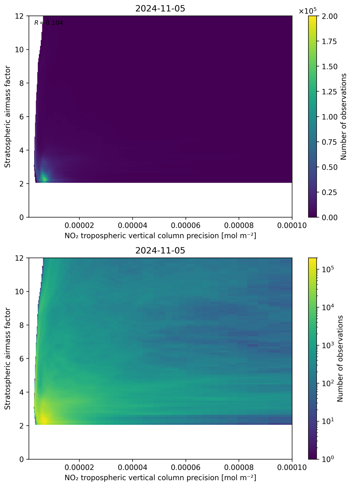
Figure 131: Scatter density plot of “NO 2 tropospheric vertical column precision” against “Stratospheric airmass factor” for 2024-11-04 to 2024-11-06.
