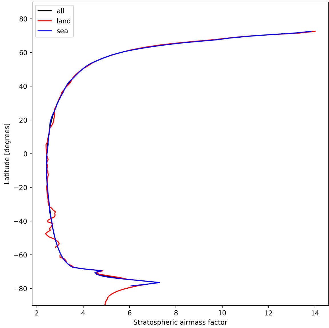
Figure 27: Zonal average of “Stratospheric air mass factor” for 2024-11-04 to 2024-11-06.
