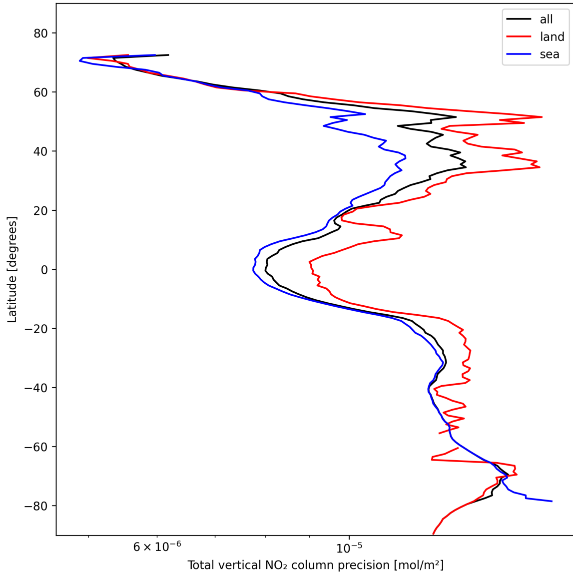
Figure 22: Zonal average of “Total vertical NO 2 column precision” for 2024-11-04 to 2024-11-06.
