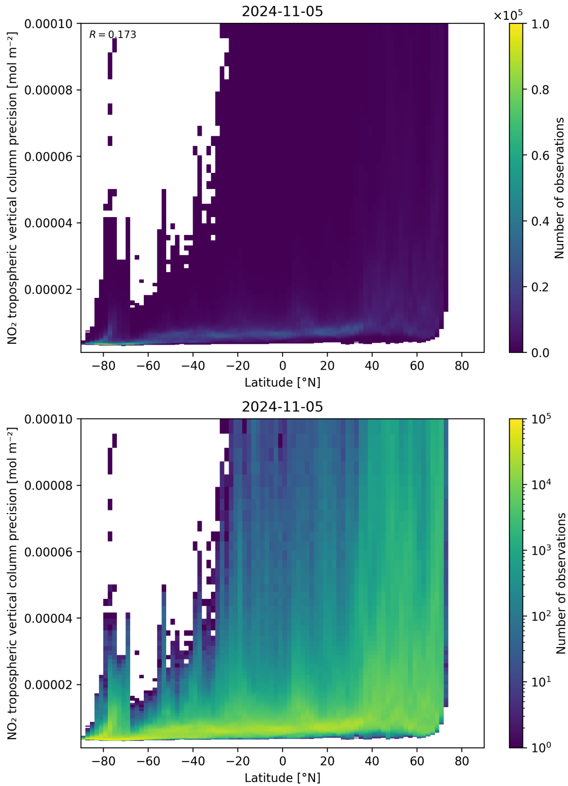
Figure 93: Scatter density plot of “Latitude” against “NO 2 tropospheric vertical column precision” for 2024-11-04 to 2024-11-06.
