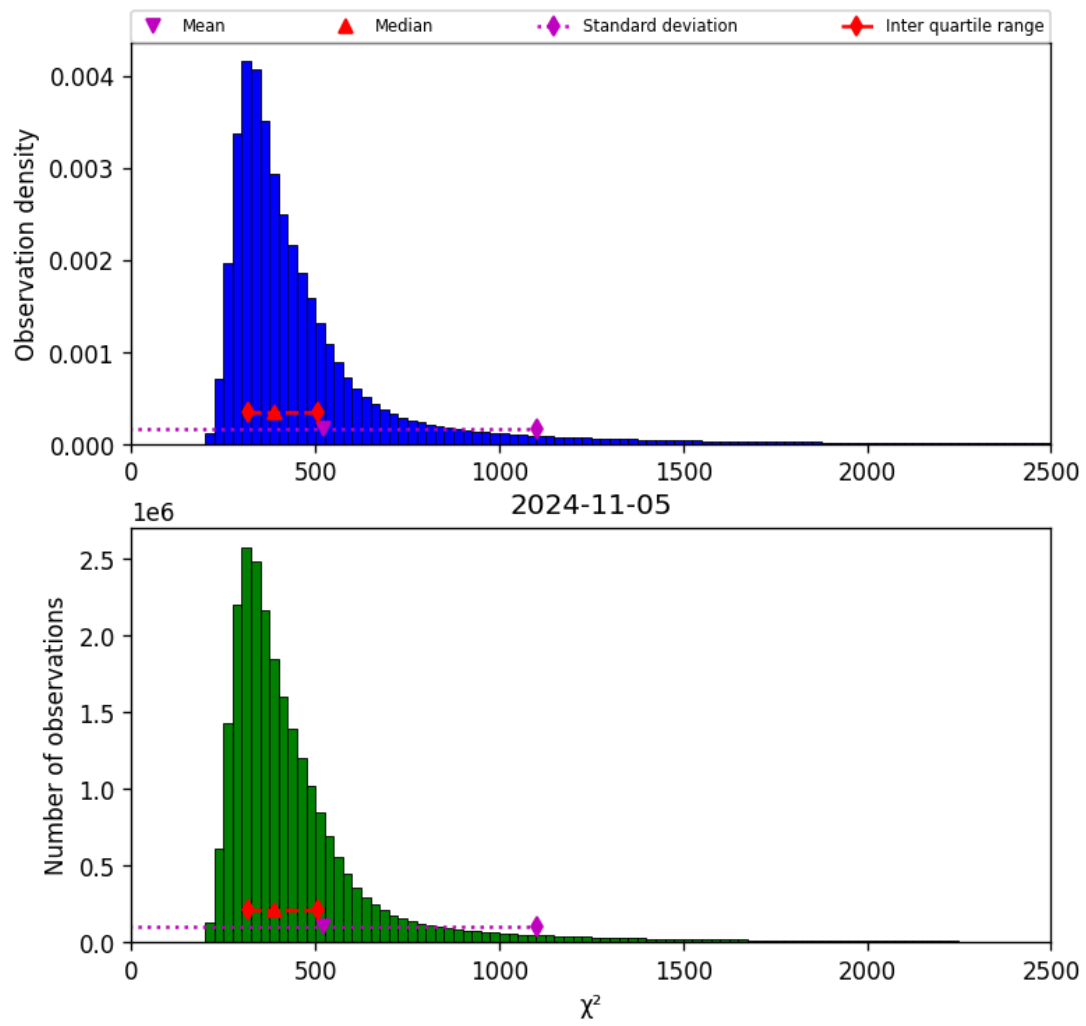
Figure 42: Histogram of “ \chi^2 ” for 2024-11-04 to 2024-11-06
