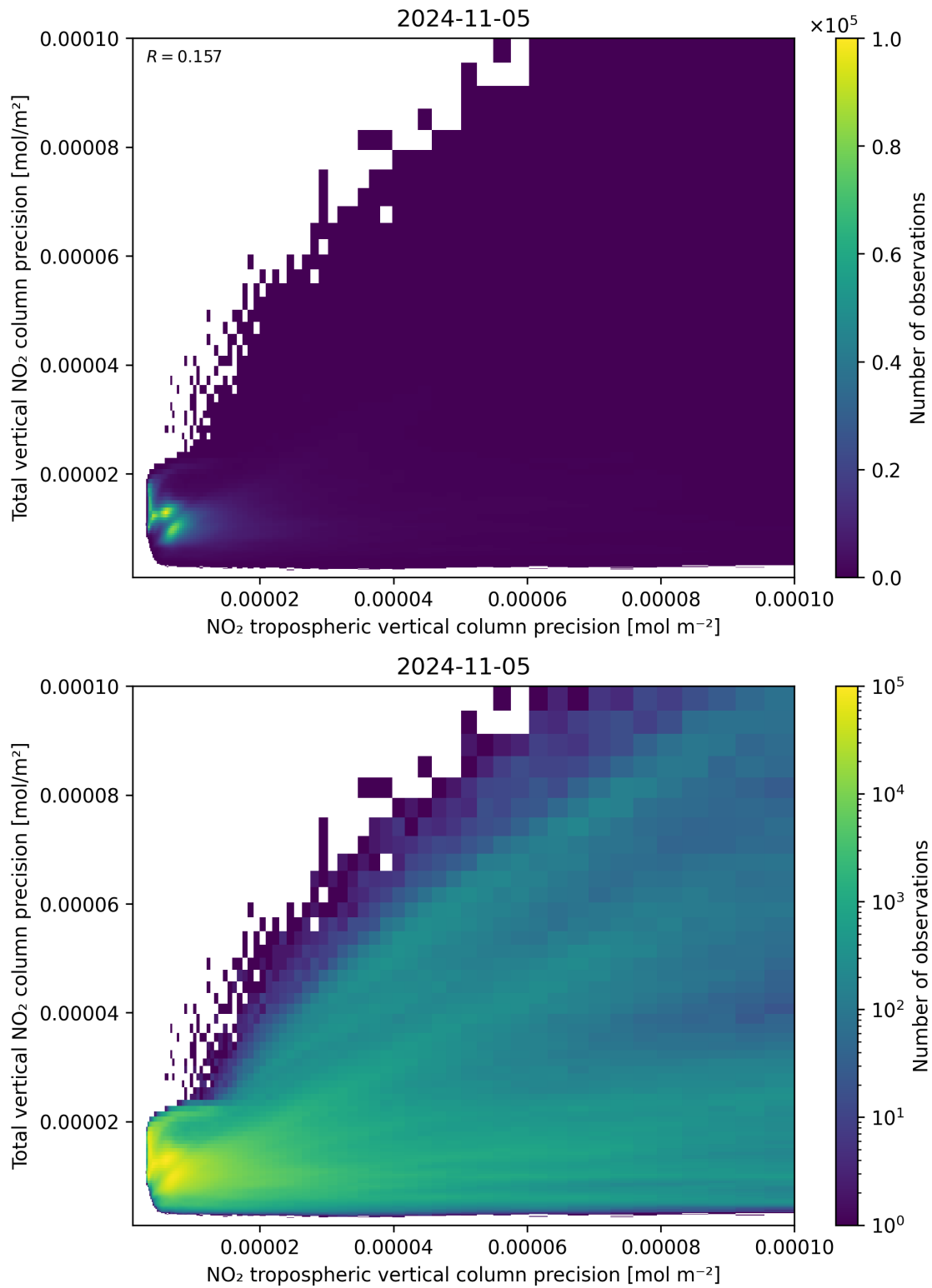
Figure 139: Scatter density plot of “NO 2 tropospheric vertical column precision” against “Total vertical NO 2 column precision” for 2024-11-04 to 2024-11-06.
