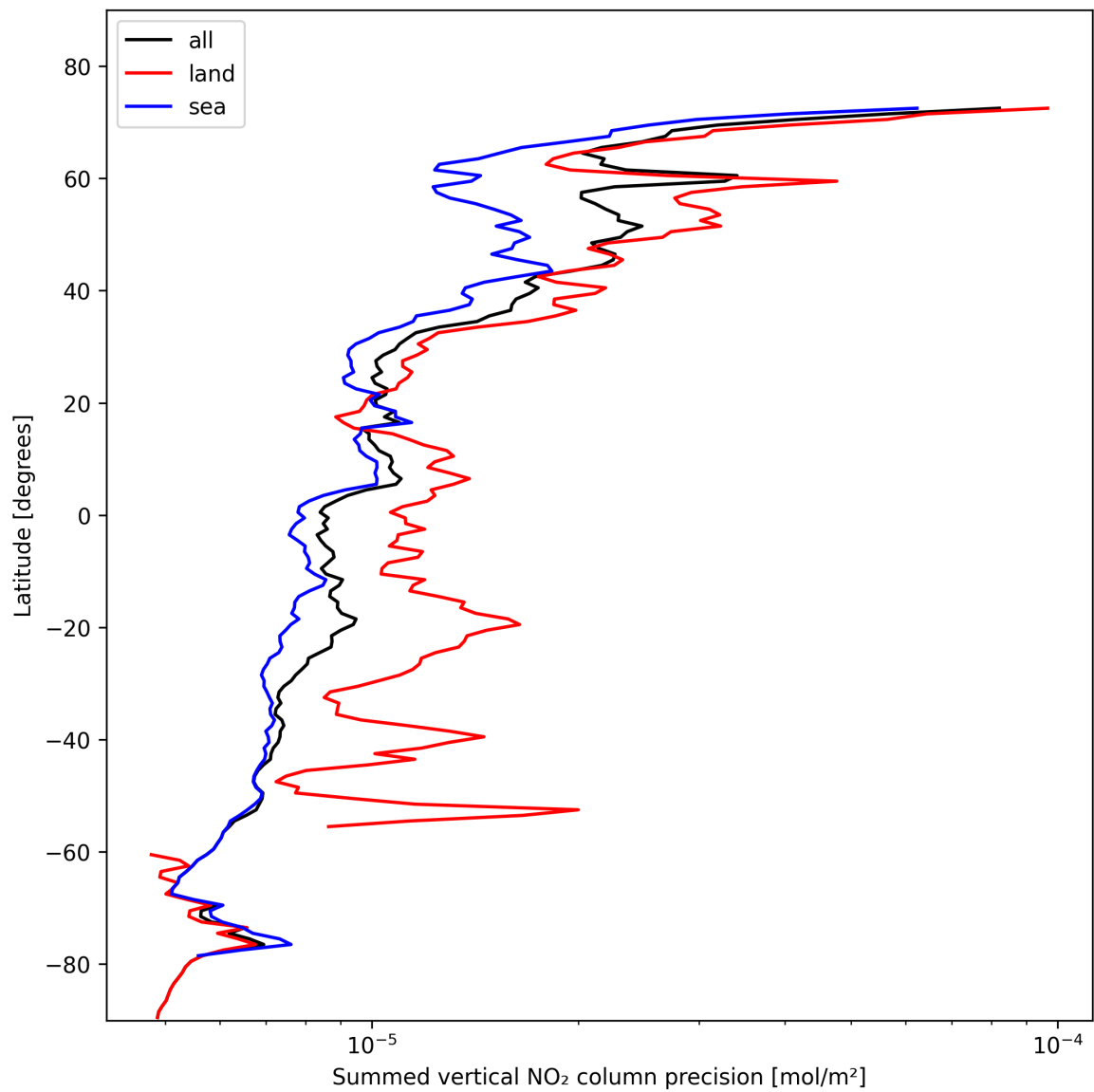
Figure 24: Zonal average of “Summed vertical NO 2 column precision” for 2024-11-04 to 2024-11-06.
