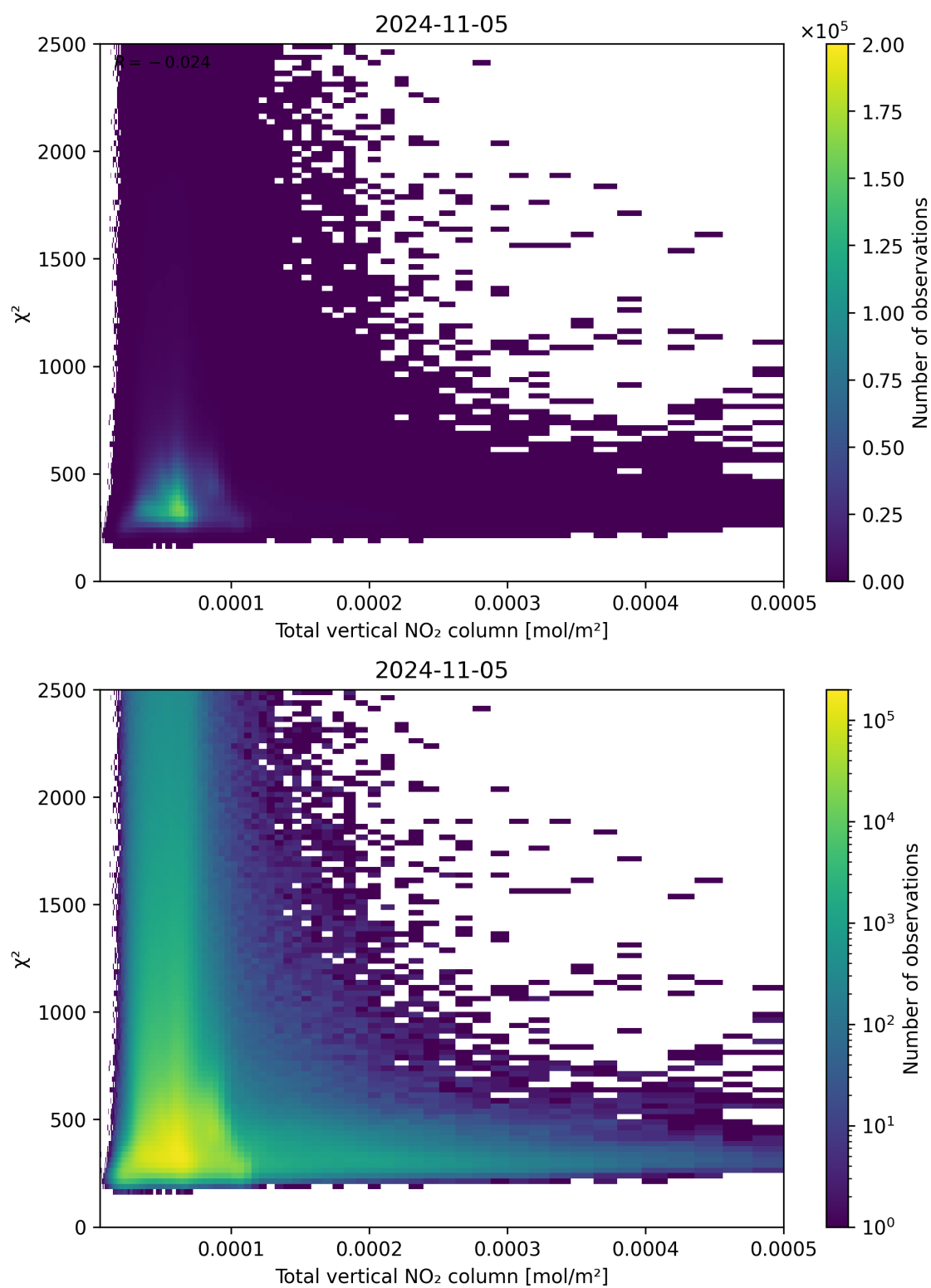
Figure 111: Scatter density plot of “Total vertical NO 2 column” against “ \chi^2 ” for 2024-11-04 to 2024-11-06.
