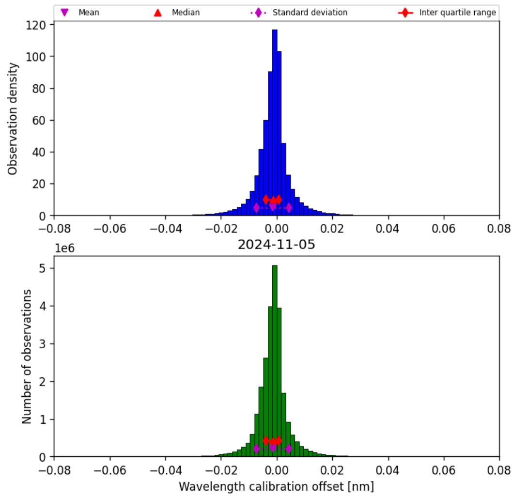
Figure 35: Histogram of “Wavelength calibration offset” for 2024-11-04 to 2024-11-06
