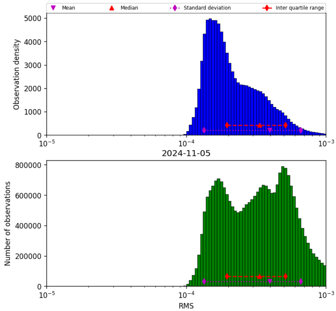
Figure 43: Histogram of “RMS” for 2024-11-04 to 2024-11-06
