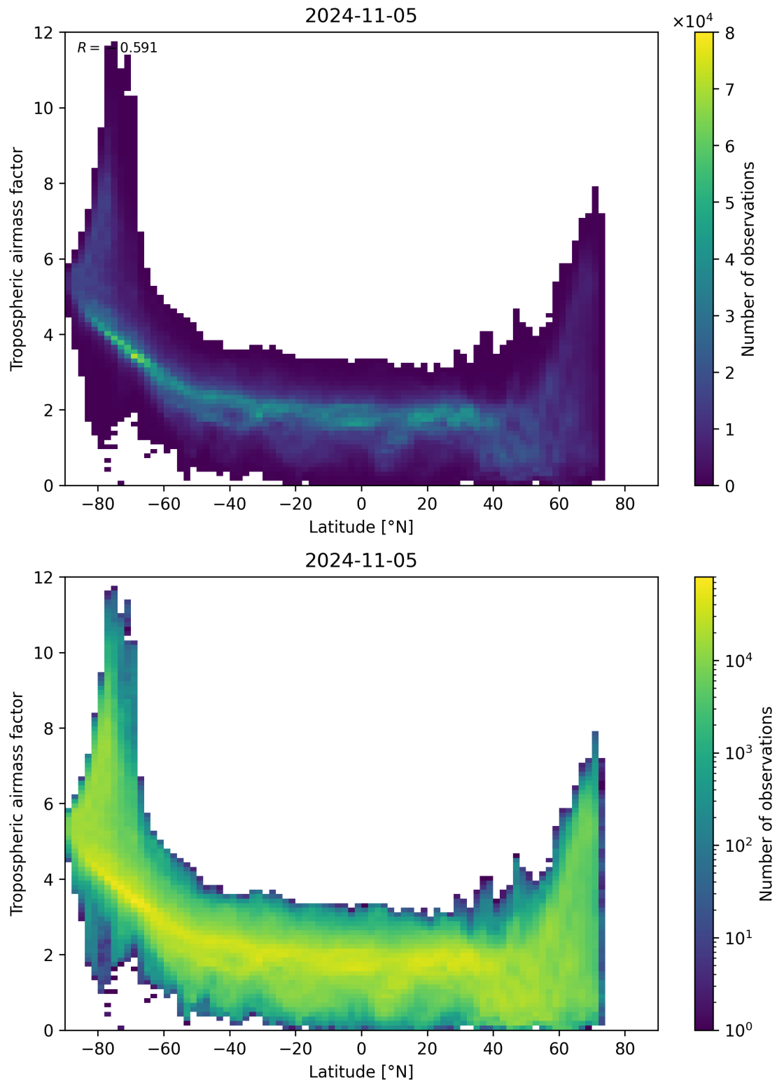
Figure 85: Scatter density plot of “Latitude” against “Tropospheric air mass factor” for 2024-11-04 to 2024-11-06.
