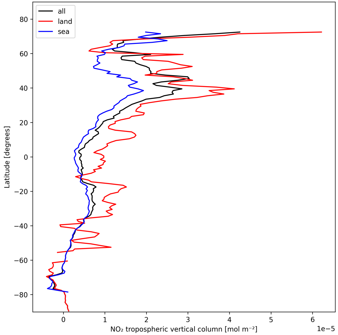
Figure 12: Zonal average of “NO 2 tropospheric vertical column” for 2024-11-04 to 2024-11-06.
