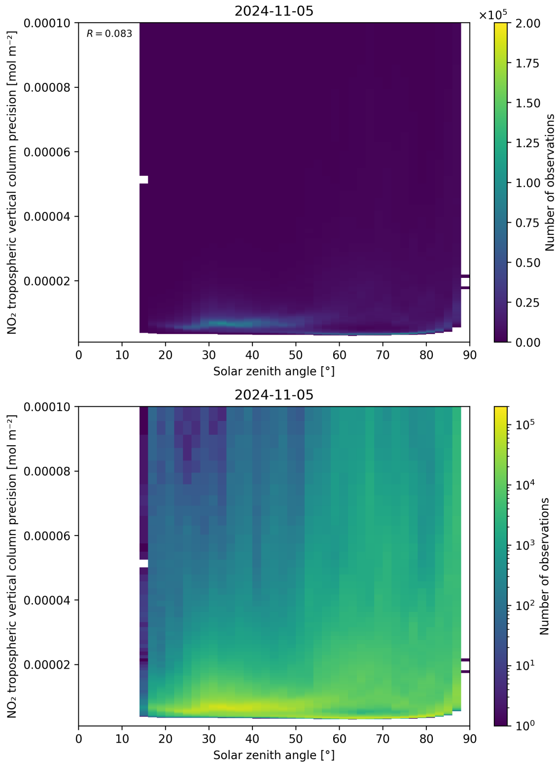
Figure 156: Scatter density plot of “Solar zenith angle” against “NO 2 tropospheric vertical column precision” for 2024-11-04 to 2024-11-06.
