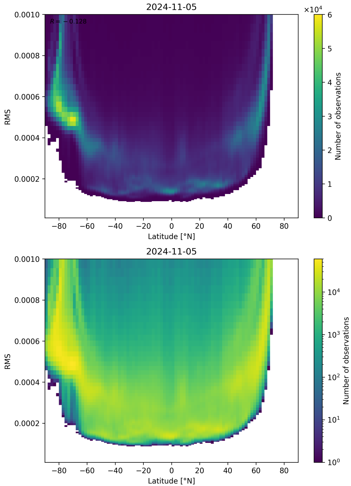
Figure 94: Scatter density plot of “Latitude” against “RMS” for 2024-11-04 to 2024-11-06.
