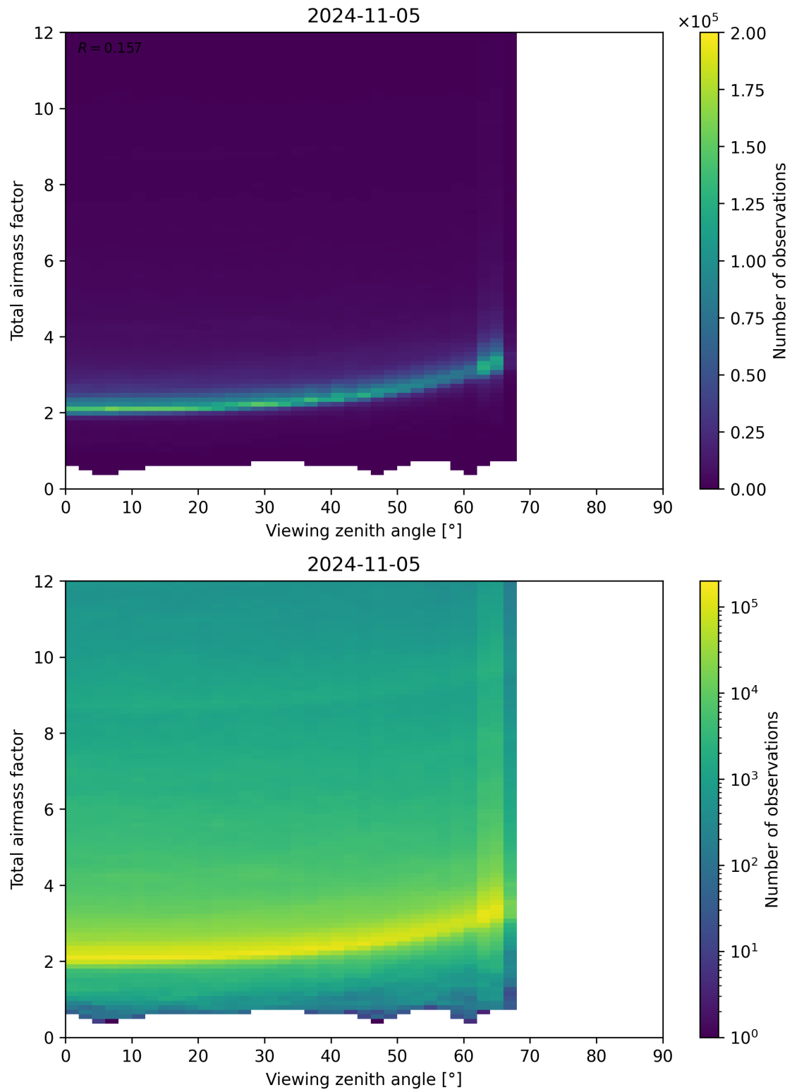
Figure 160: Scatter density plot of “Viewing zenith angle” against “Total airmass factor” for 2024-11-04 to 2024-11-06.
