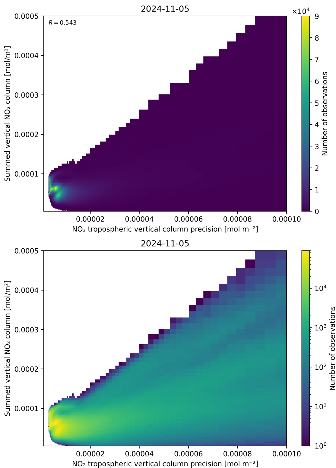
Figure 136: Scatter density plot of “NO 2 tropospheric vertical column precision” against “Summed vertical NO 2 column” for 2024-11-04 to 2024-11-06.
