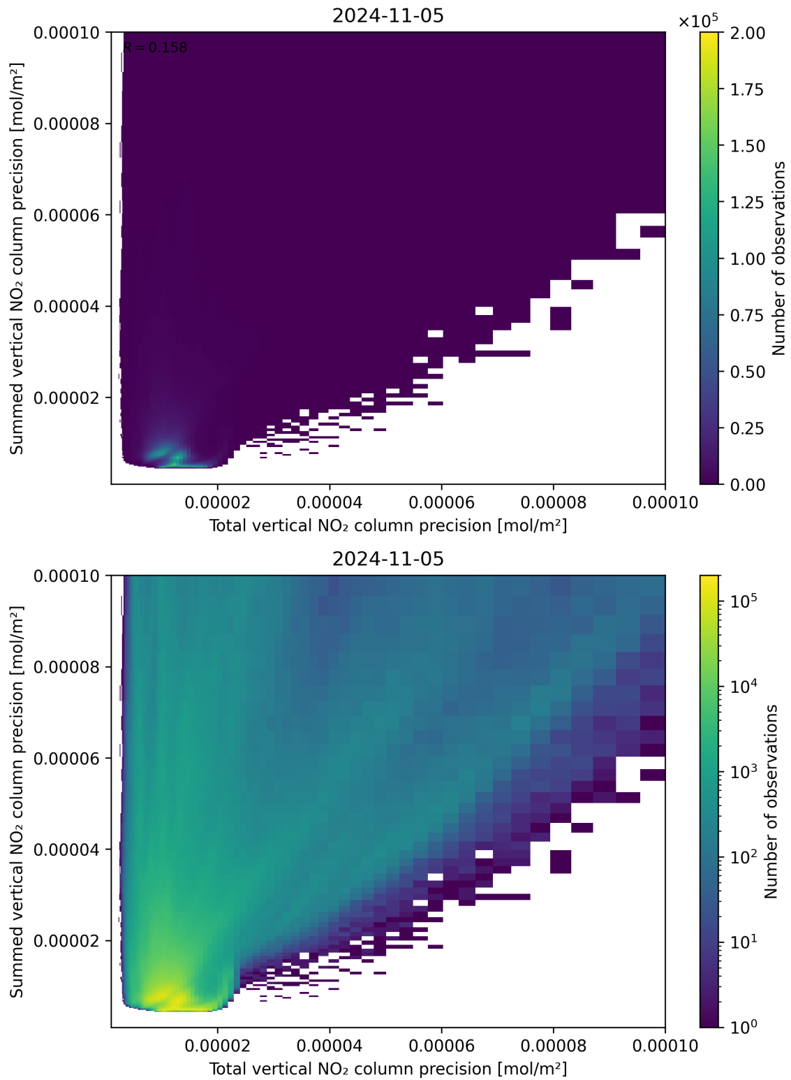
Figure 118: Scatter density plot of “Total vertical NO 2 column precision” against “Summed vertical NO 2 column precision” for 2024-11-04 to 2024-11-06.
