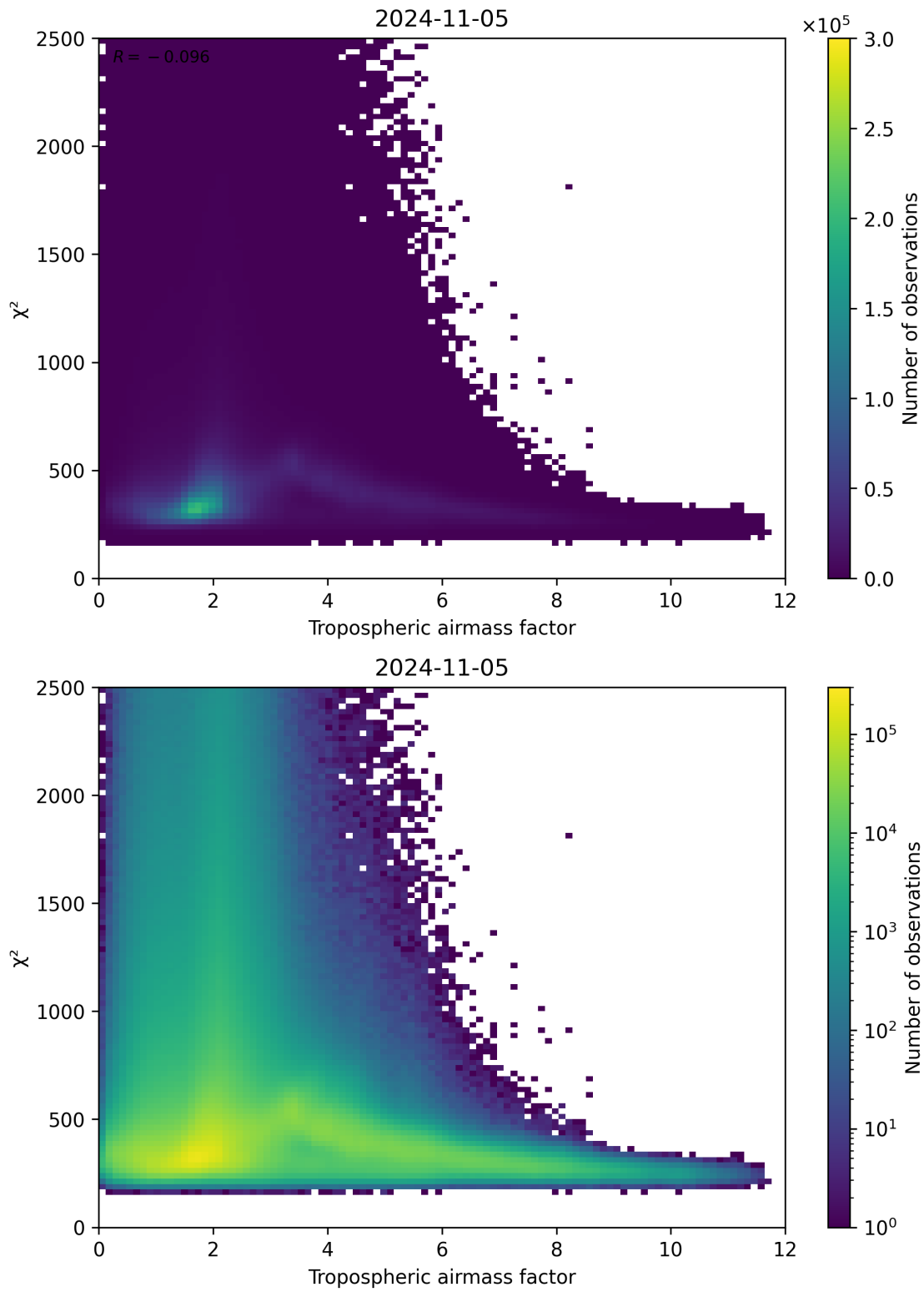
Figure 73: Scatter density plot of “Tropospheric airmass factor” against “ \chi^2 ” for 2024-11-04 to 2024-11-06.
