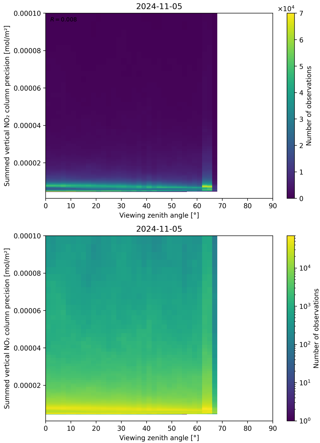
Figure 166: Scatter density plot of “Viewing zenith angle” against “Summed vertical NO 2 column precision” for 2024-11-04 to 2024-11-06.
