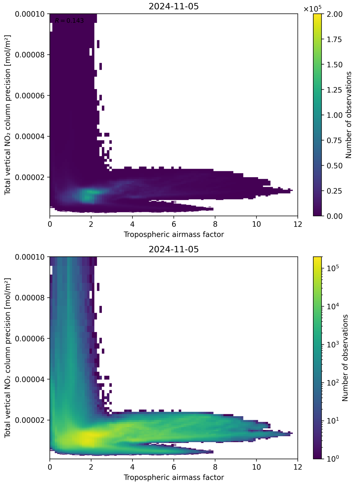
Figure 78: Scatter density plot of “Tropospheric airmass factor” against “Total vertical NO 2 column precision” for 2024-11-04 to 2024-11-06.
