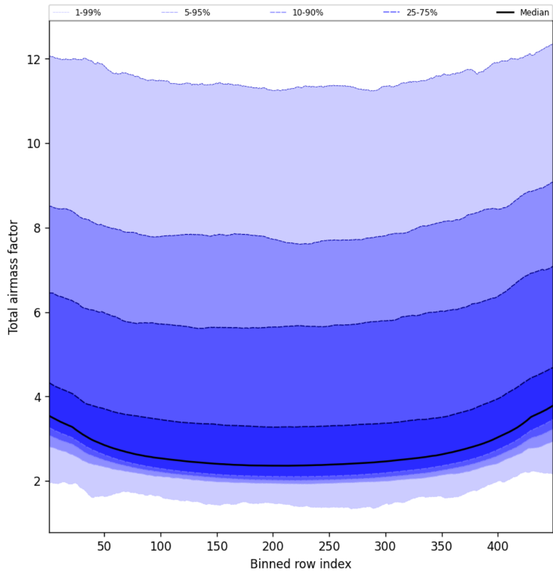
Figure 49: Along track statistics of “Total airmass factor” for 2024-11-04 to 2024-11-06
