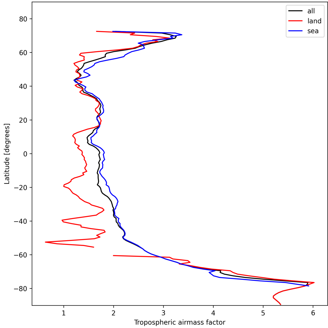
Figure 14: Zonal average of “Tropospheric airmass factor” for 2024-11-04 to 2024-11-06.
