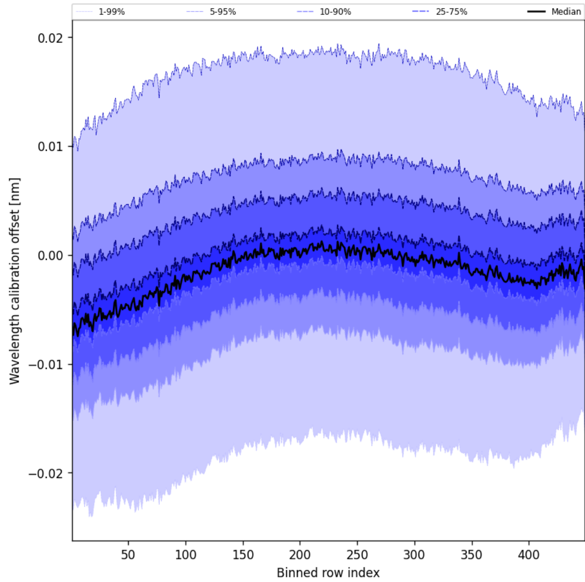
Figure 52: Along track statistics of “Wavelength calibration offset” for 2024-11-04 to 2024-11-06
