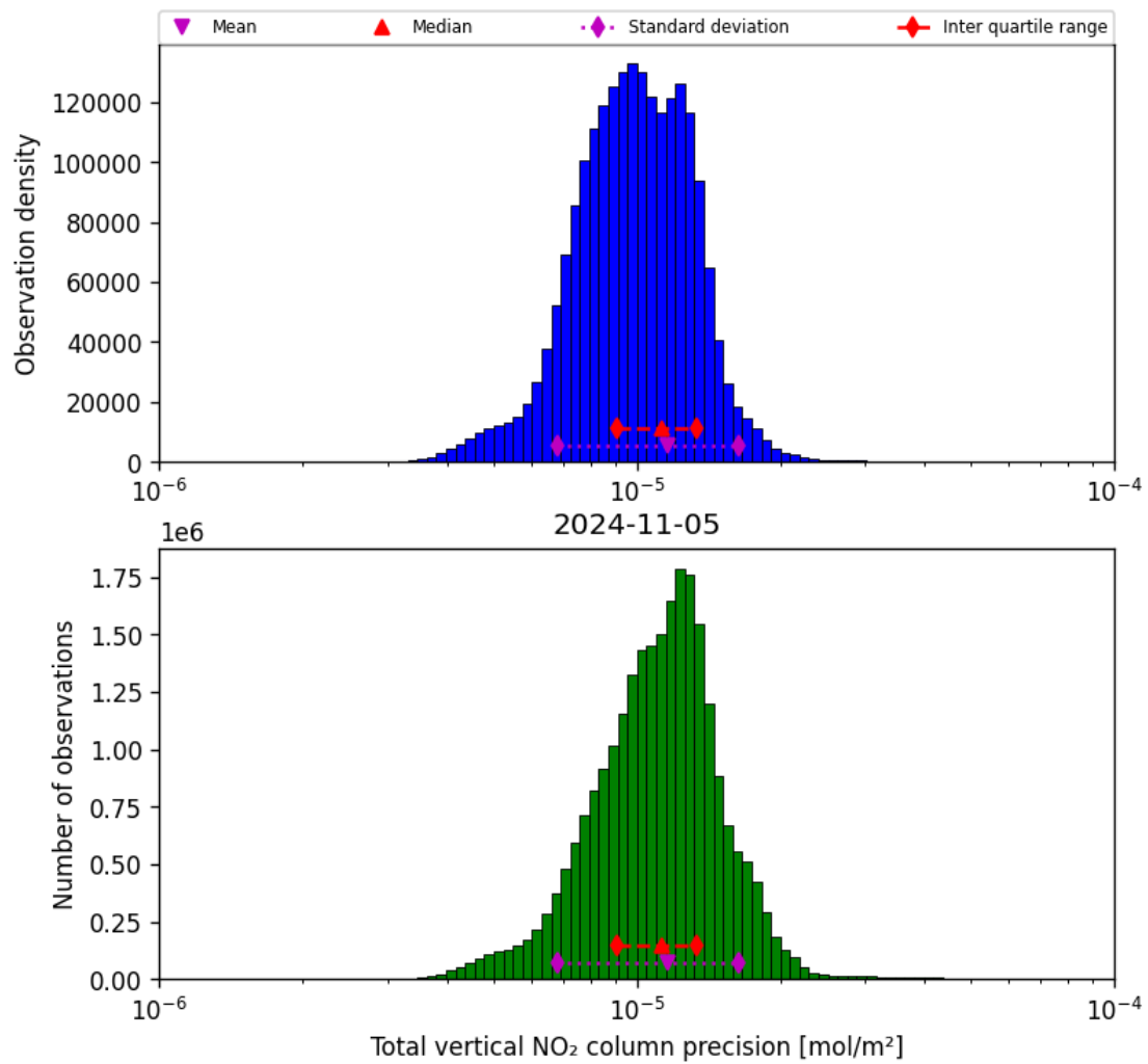
Figure 39: Histogram of “Total vertical NO 2 column precision” for 2024-11-04 to 2024-11-06
