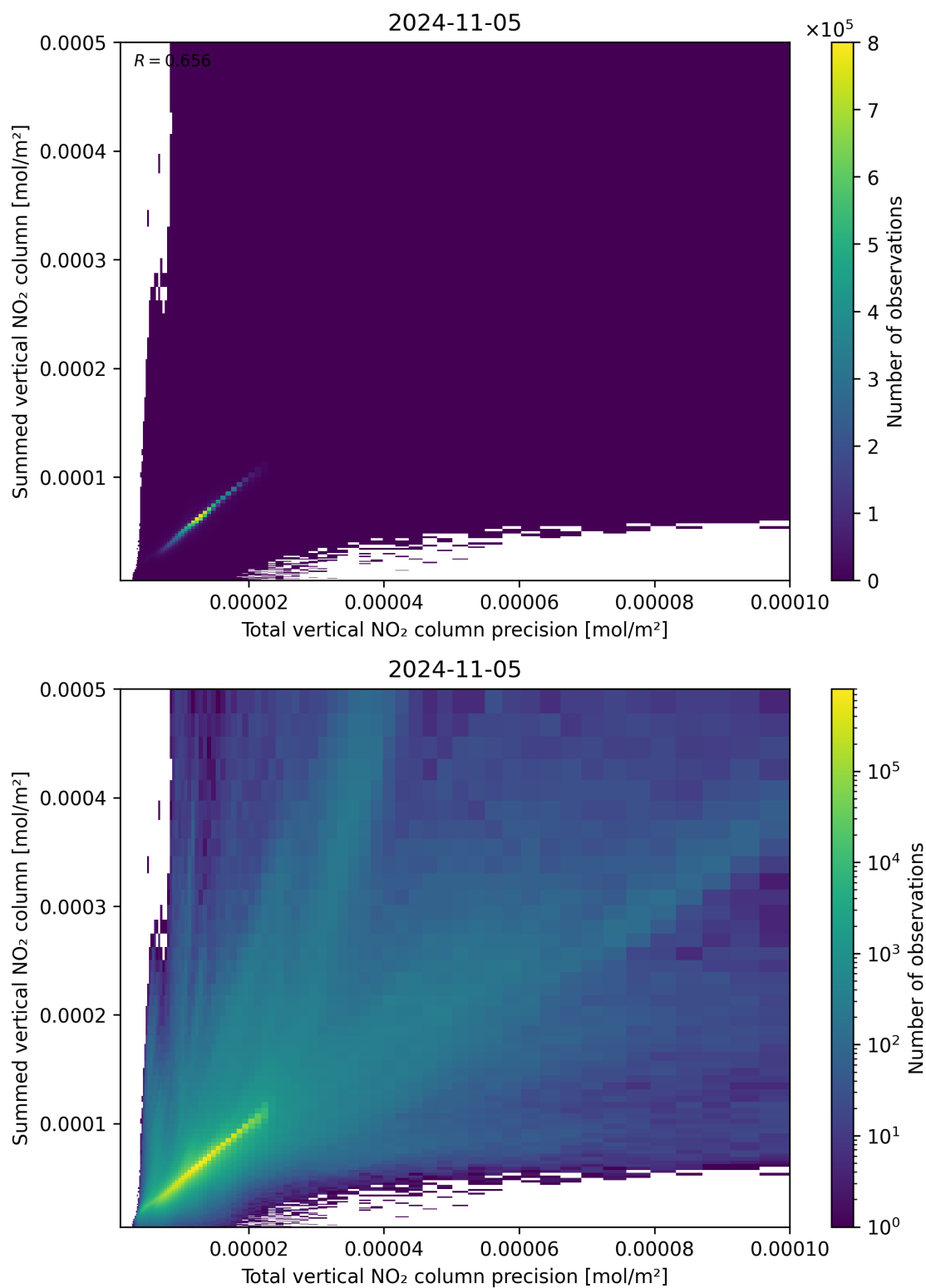
Figure 117: Scatter density plot of “Total vertical NO 2 column precision” against “Summed vertical NO 2 column” for 2024-11-04 to 2024-11-06.
