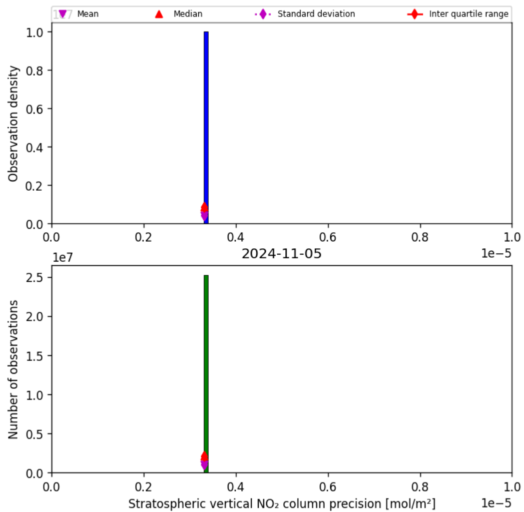
Figure 37: Histogram of “Stratospheric vertical NO 2 column precision” for 2024-11-04 to 2024-11-06
