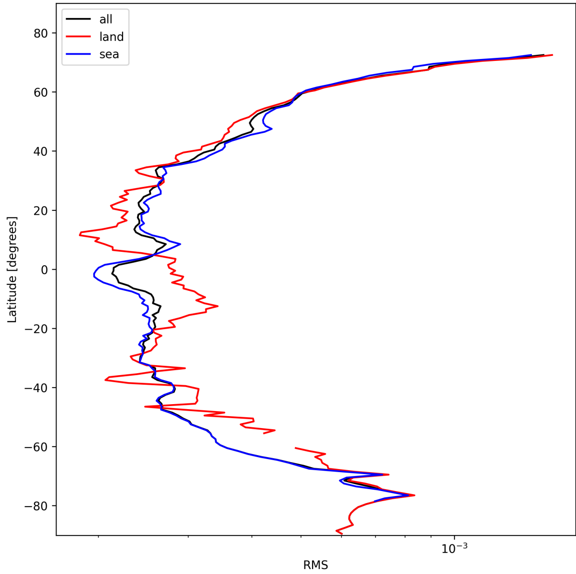
Figure 26: Zonal average of “RMS” for 2024-11-04 to 2024-11-06.
