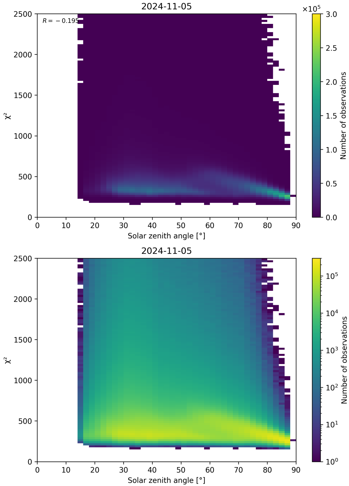
Figure 148: Scatter density plot of “Solar zenith angle” against “ \chi^2 ” for 2024-11-04 to 2024-11-06.
