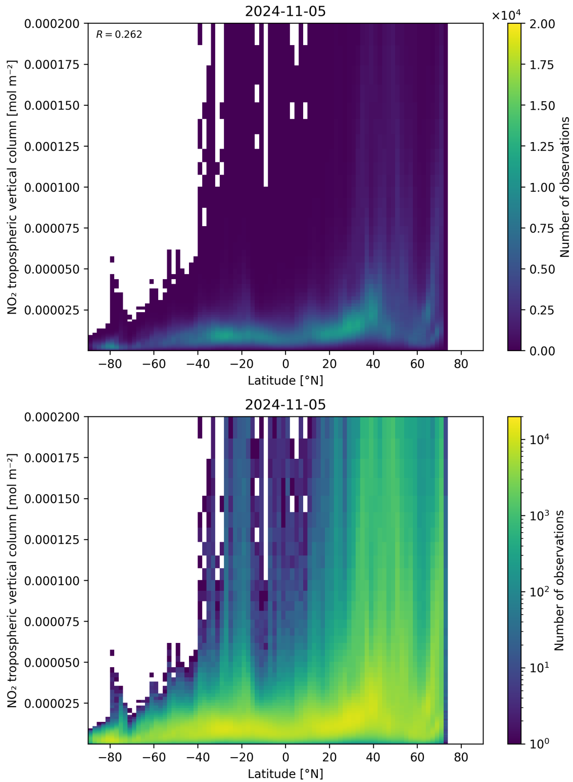
Figure 92: Scatter density plot of “Latitude” against “NO 2 tropospheric vertical column” for 2024-11-04 to 2024-11-06.
