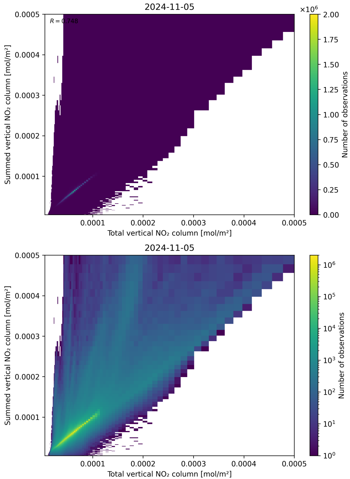
Figure 112: Scatter density plot of “Total vertical NO 2 column” against “Summed vertical NO 2 column” for 2024-11-04 to 2024-11-06.
