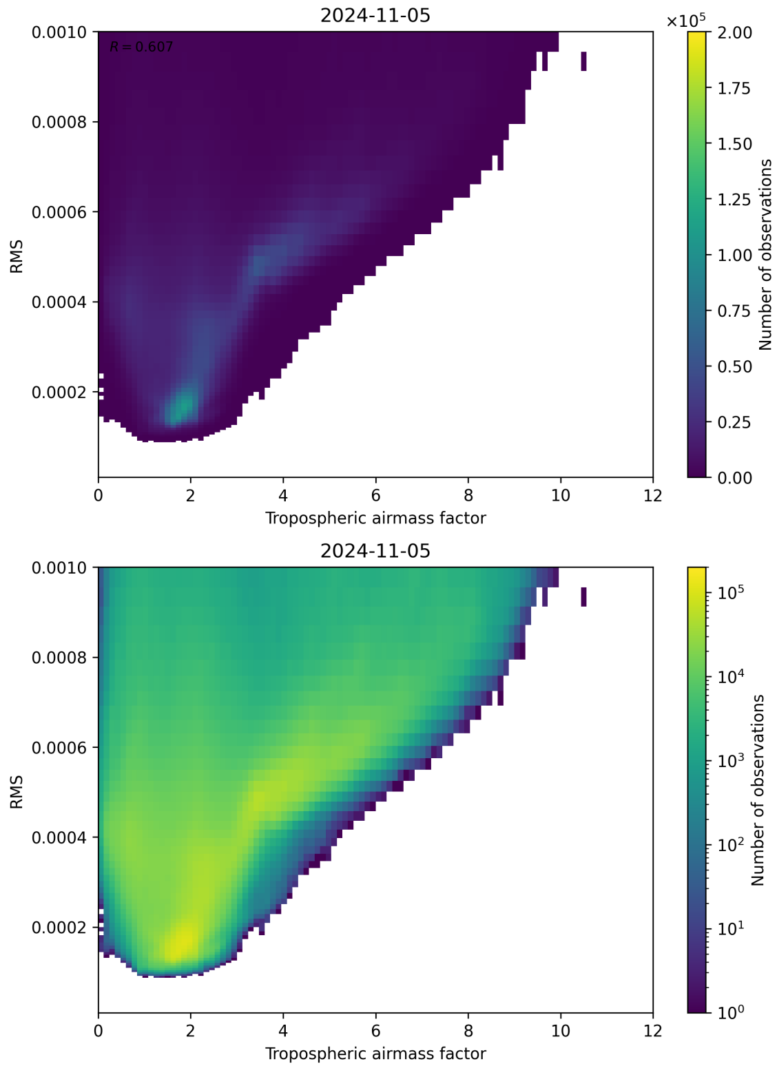
Figure 79: Scatter density plot of “Tropospheric airmass factor” against “RMS” for 2024-11-04 to 2024-11-06.
