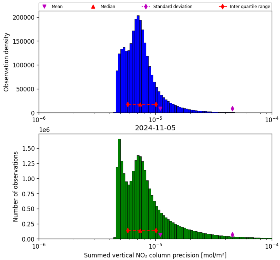
Figure 41: Histogram of "Summed vertical NO 2 column precision" for 2024-11-04 to 2024-11-06
