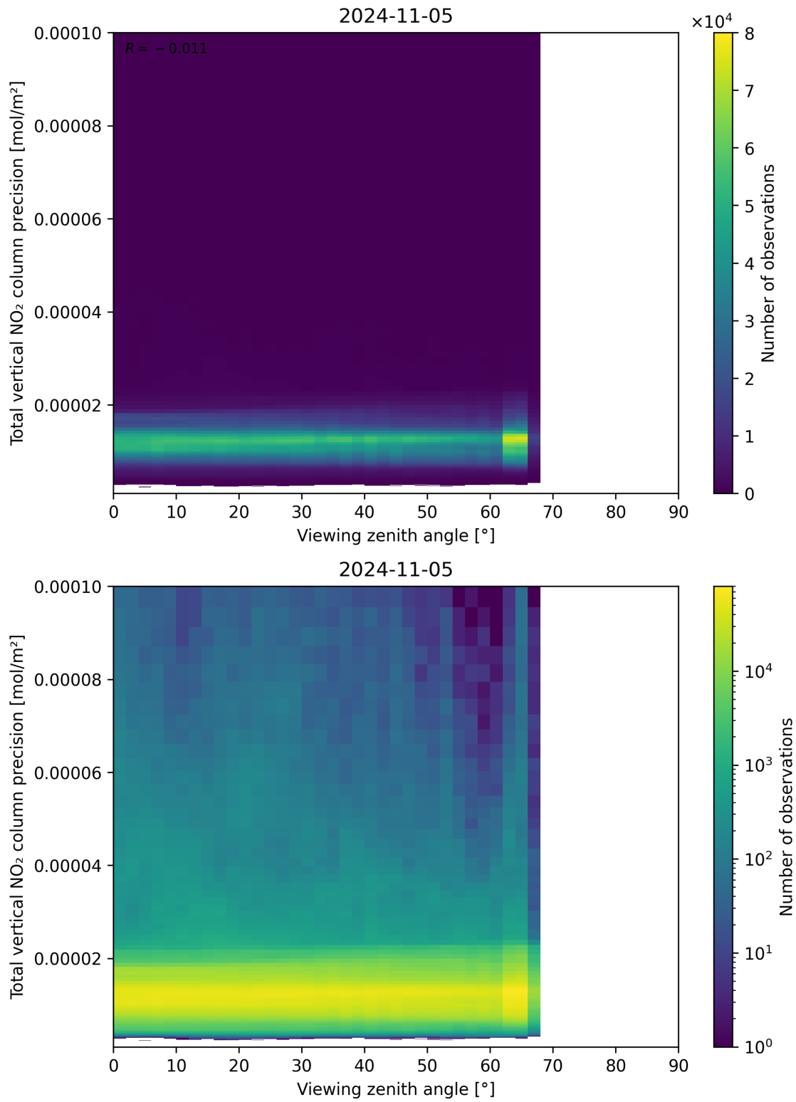
Figure 168: Scatter density plot of “Viewing zenith angle” against “Total vertical NO 2 column precision” for 2024-11-04 to 2024-11-06.
