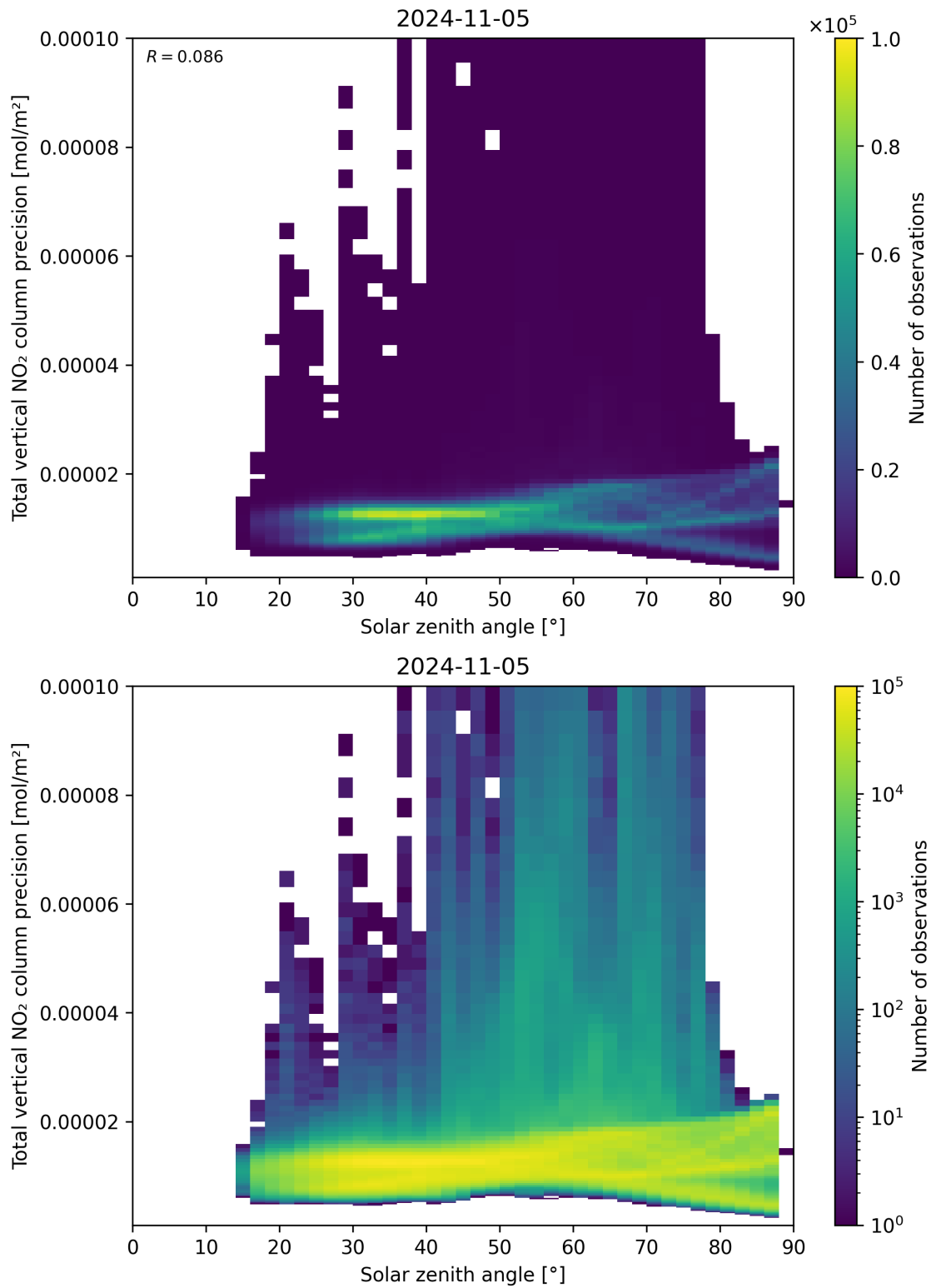
Figure 154: Scatter density plot of “Solar zenith angle” against “Total vertical NO 2 column precision” for 2024-11-04 to 2024-11-06.
