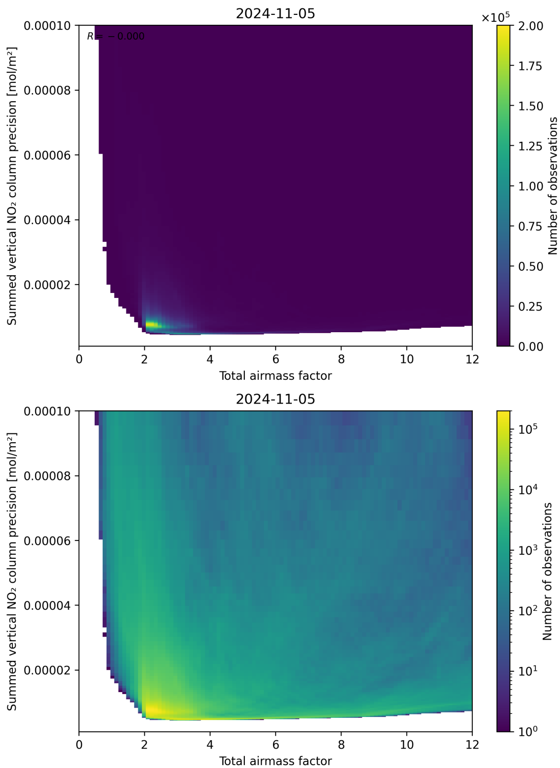
Figure 66: Scatter density plot of “Total airmass factor” against “Summed vertical NO 2 column precision” for 2024-11-04 to 2024-11-06.
