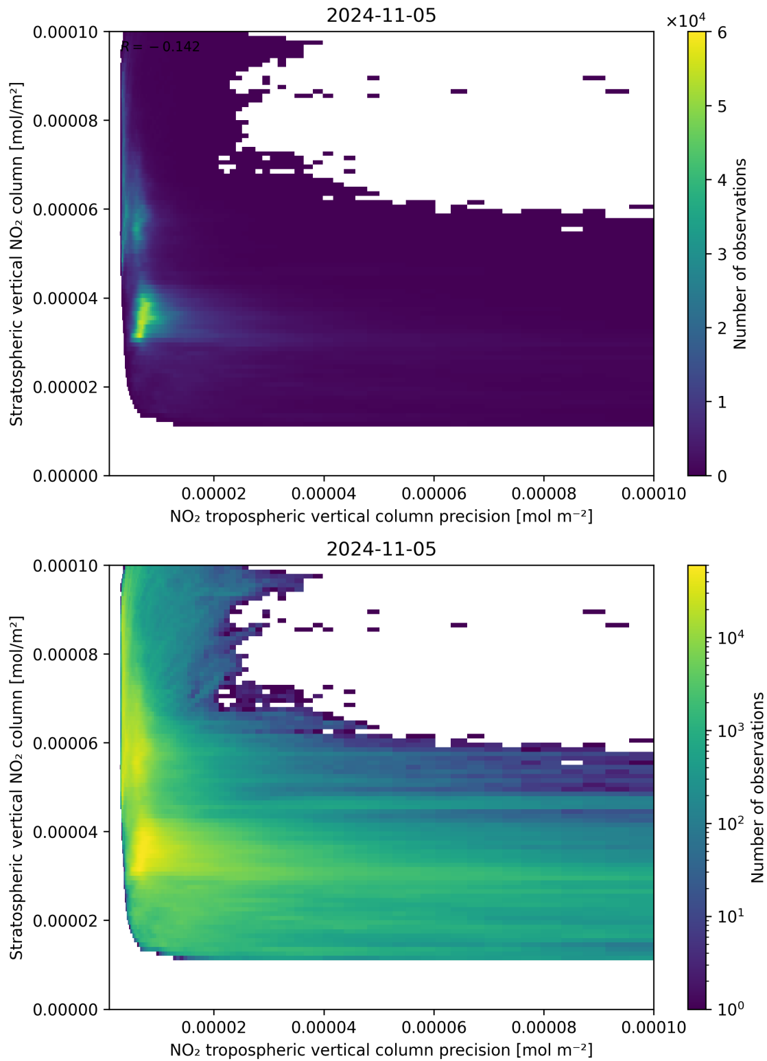
Figure 135: Scatter density plot of “NO 2 tropospheric vertical column precision” against “Stratospheric vertical NO 2 column” for 2024-11-04 to 2024-11-06.
