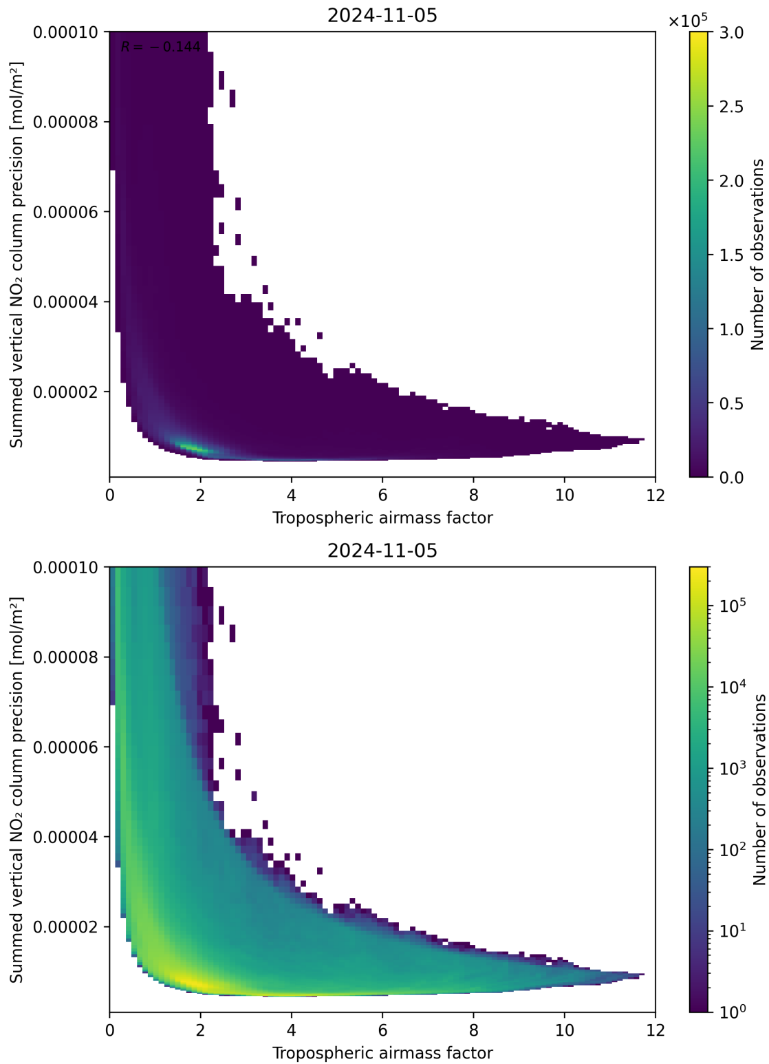
Figure 76: Scatter density plot of “Tropospheric airmass factor” against “Summed vertical NO 2 column precision” for 2024-11-04 to 2024-11-06.
