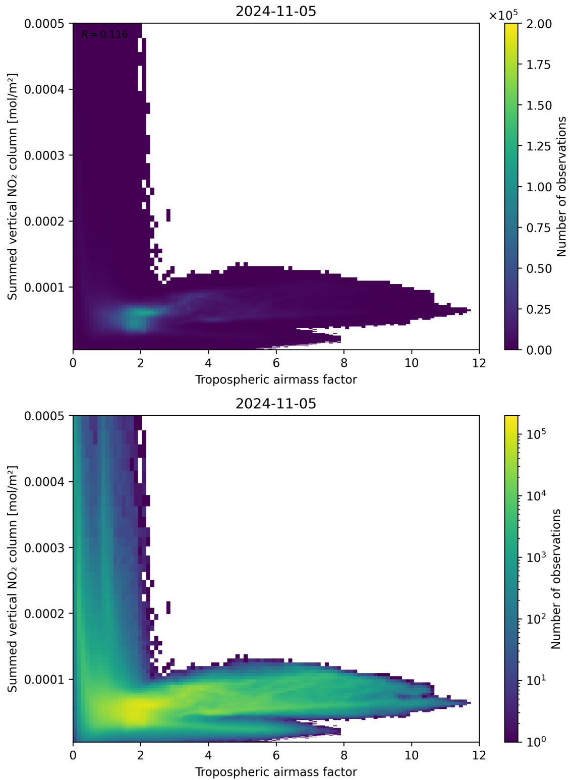
Figure 75: Scatter density plot of “Tropospheric airmass factor” against “Summed vertical NO 2 column” for 2024-11-04 to 2024-11-06.
