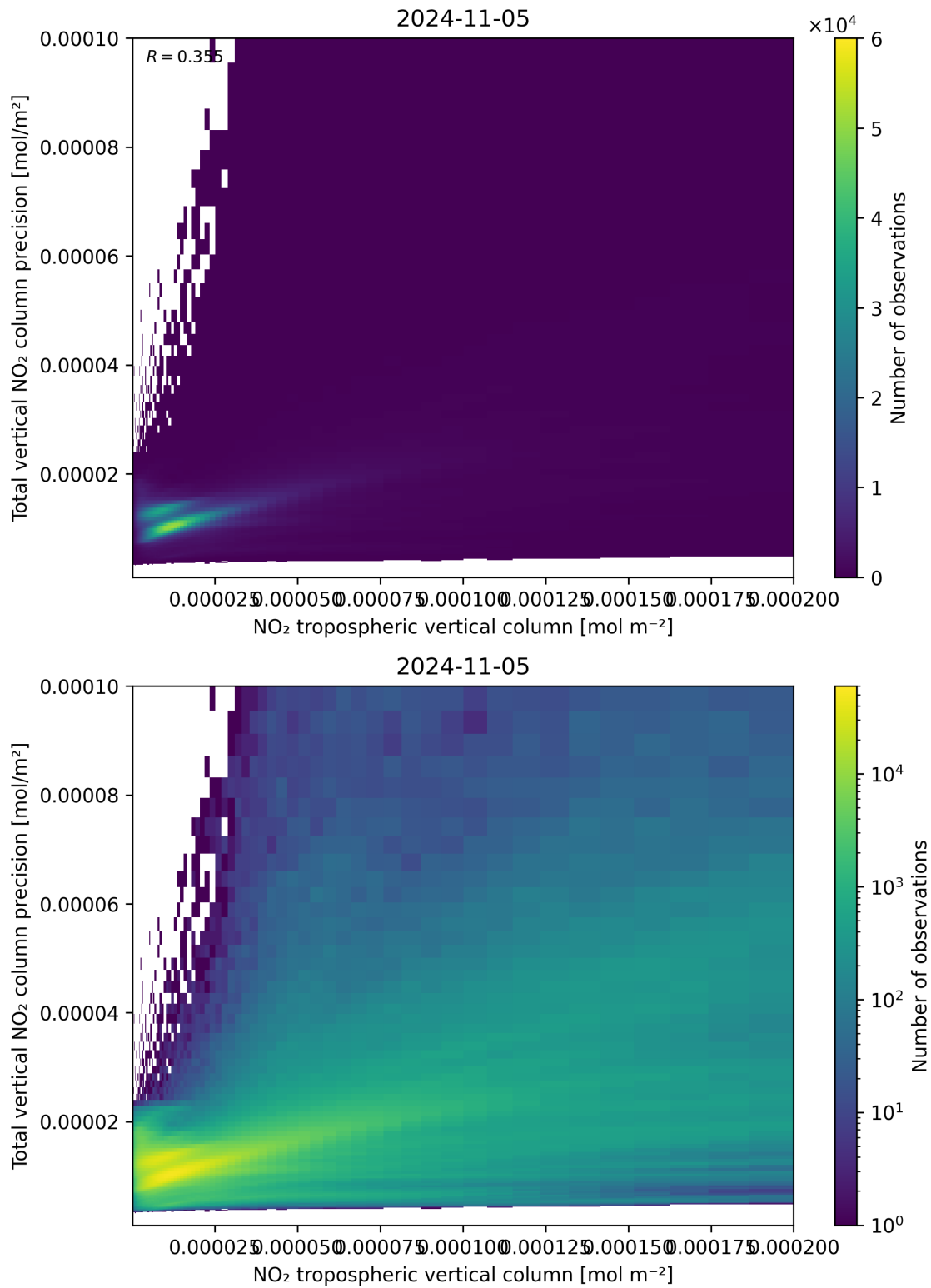
Figure 129: Scatter density plot of “NO 2 tropospheric vertical column” against “Total vertical NO 2 column precision” for 2024-11-04 to 2024-11-06.
