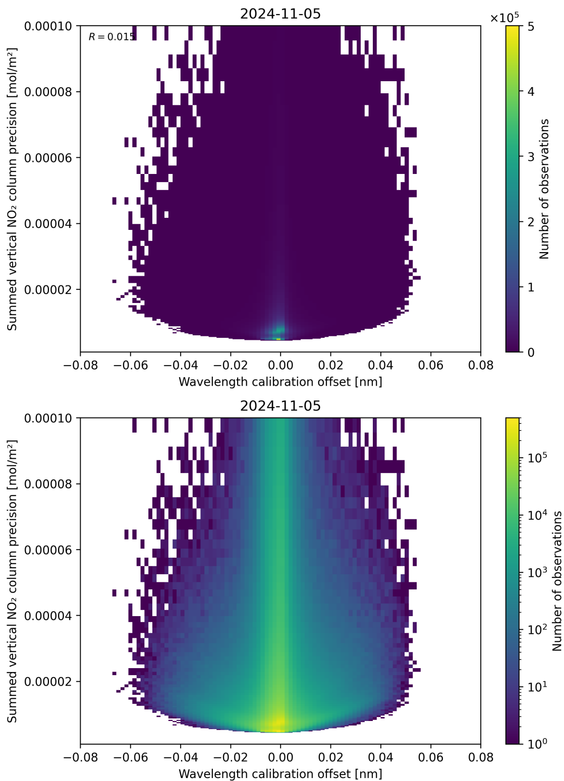
Figure 178: Scatter density plot of “Wavelength calibration offset” against “Summed vertical NO 2 column precision” for 2024-11-04 to 2024-11-06.
