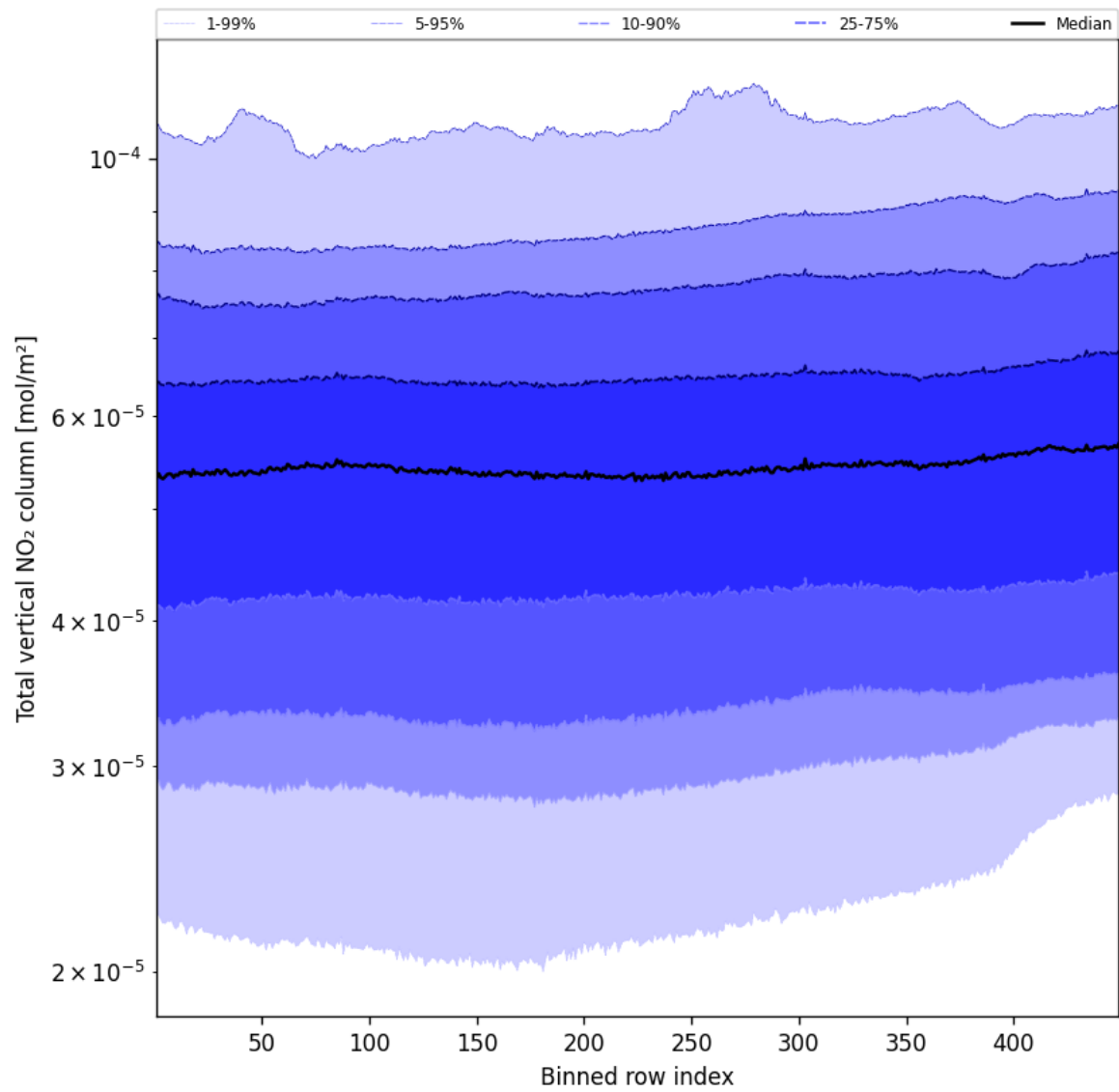
Figure 55: Along track statistics of “Total vertical NO 2 column” for 2024-11-04 to 2024-11-06
