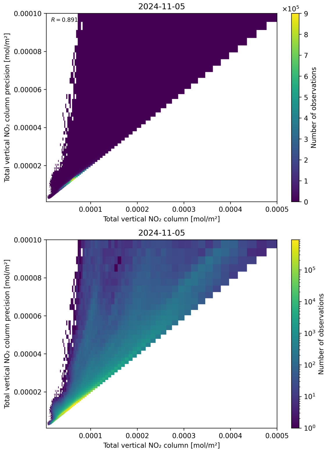
Figure 114: Scatter density plot of “Total vertical NO 2 column” against “Total vertical NO 2 column precision” for 2024-11-04 to 2024-11-06.
