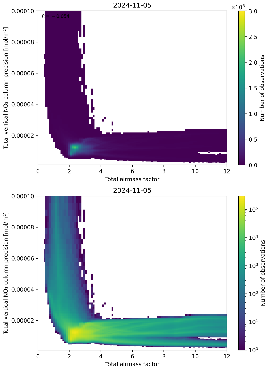
Figure 68: Scatter density plot of “Total airmass factor” against “Total vertical NO 2 column precision” for 2024-11-04 to 2024-11-06.
