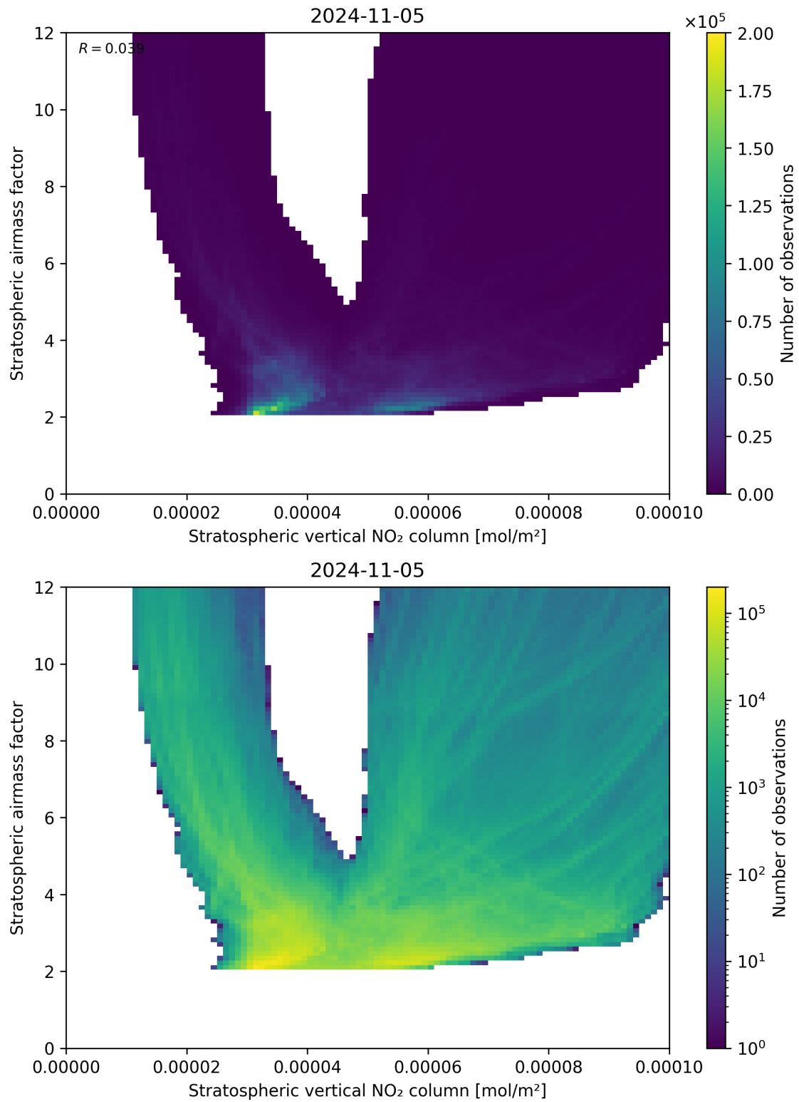
Figure 96: Scatter density plot of “Stratospheric vertical NO 2 column” against “Stratospheric airmass factor” for 2024-11-04 to 2024-11-06.
