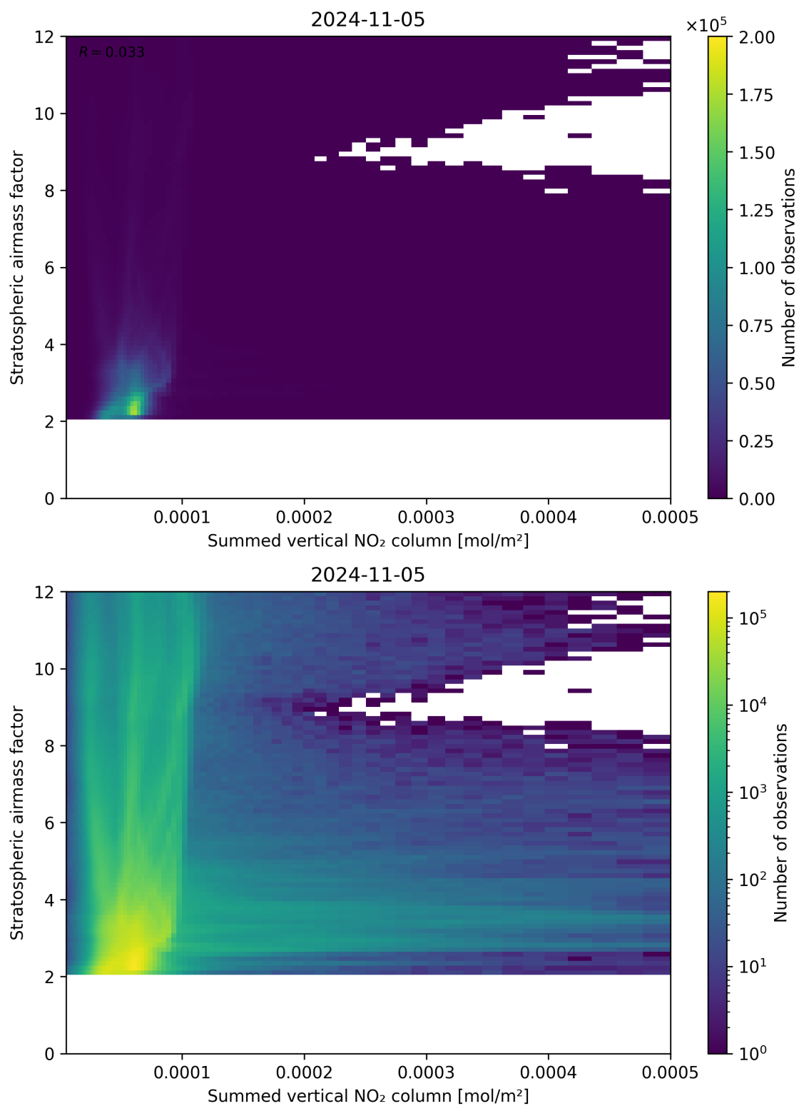
Figure 103: Scatter density plot of “Summed vertical NO 2 column” against “Stratospheric airmass factor” for 2024-11-04 to 2024-11-06.
