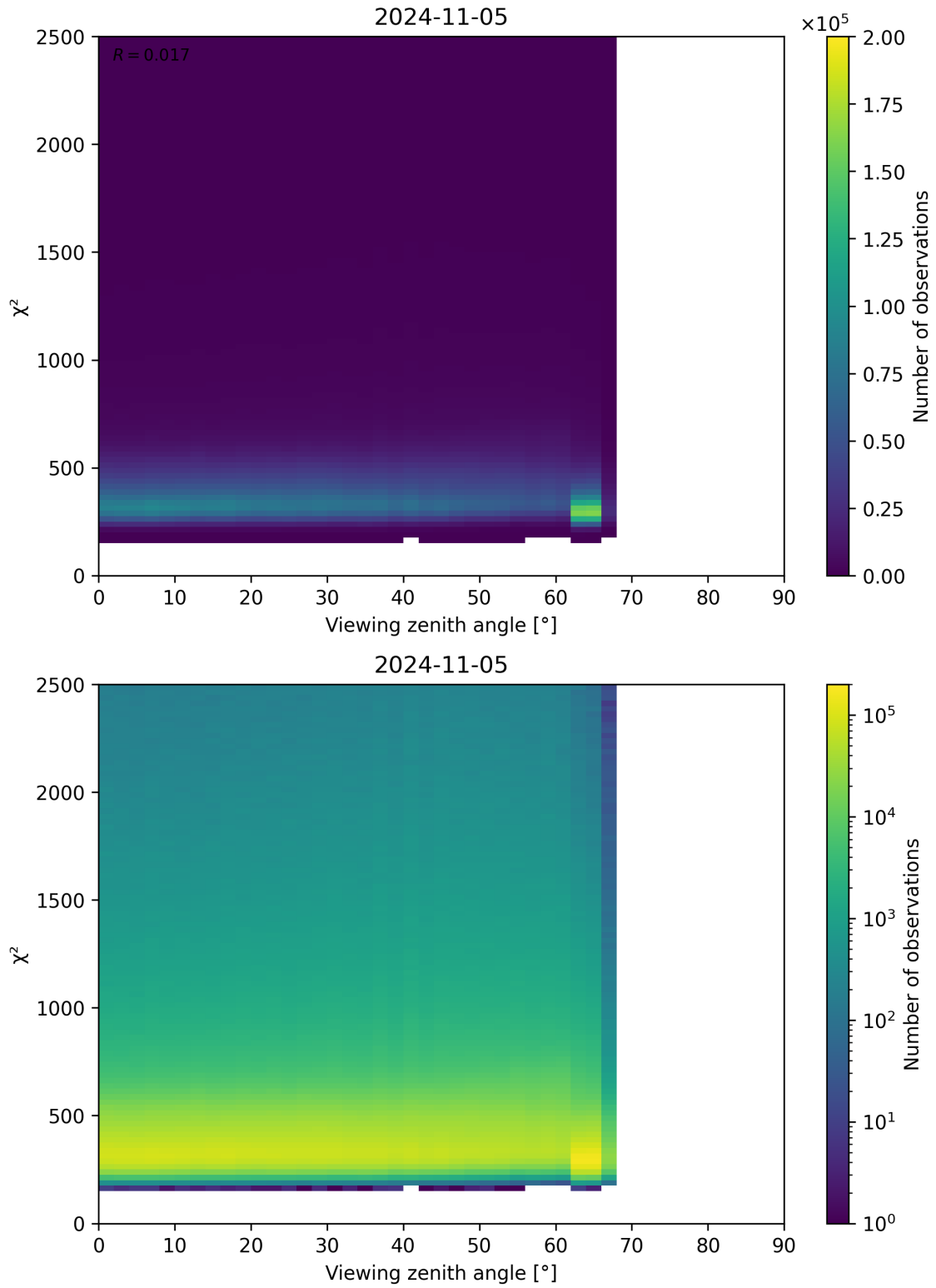
Figure 162: Scatter density plot of “Viewing zenith angle” against “ \chi^2 ” for 2024-11-04 to 2024-11-06.
