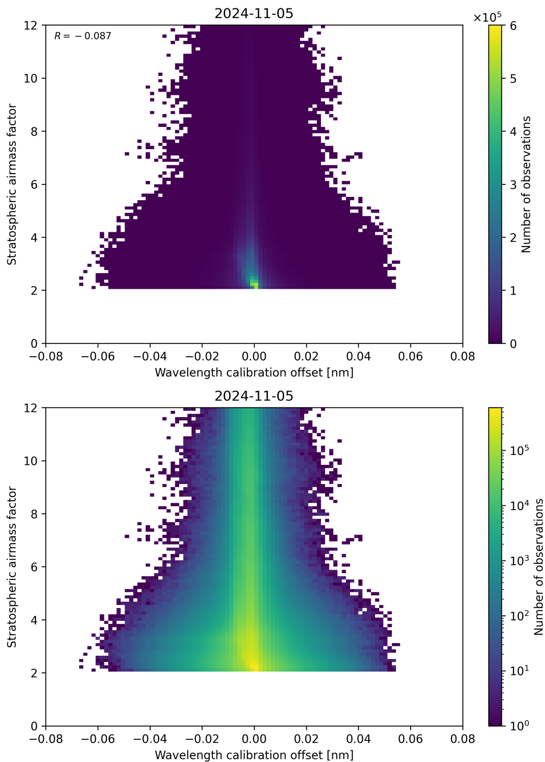
Figure 174: Scatter density plot of “Wavelength calibration offset” against “Stratospheric air mass factor” for 2024-11-04 to 2024-11-06.
