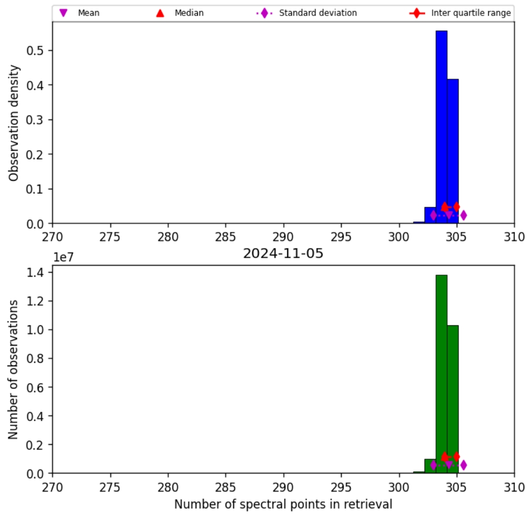
Figure 33: Histogram of “Number of spectral points in retrieval” for 2024-11-04 to 2024-11-06
