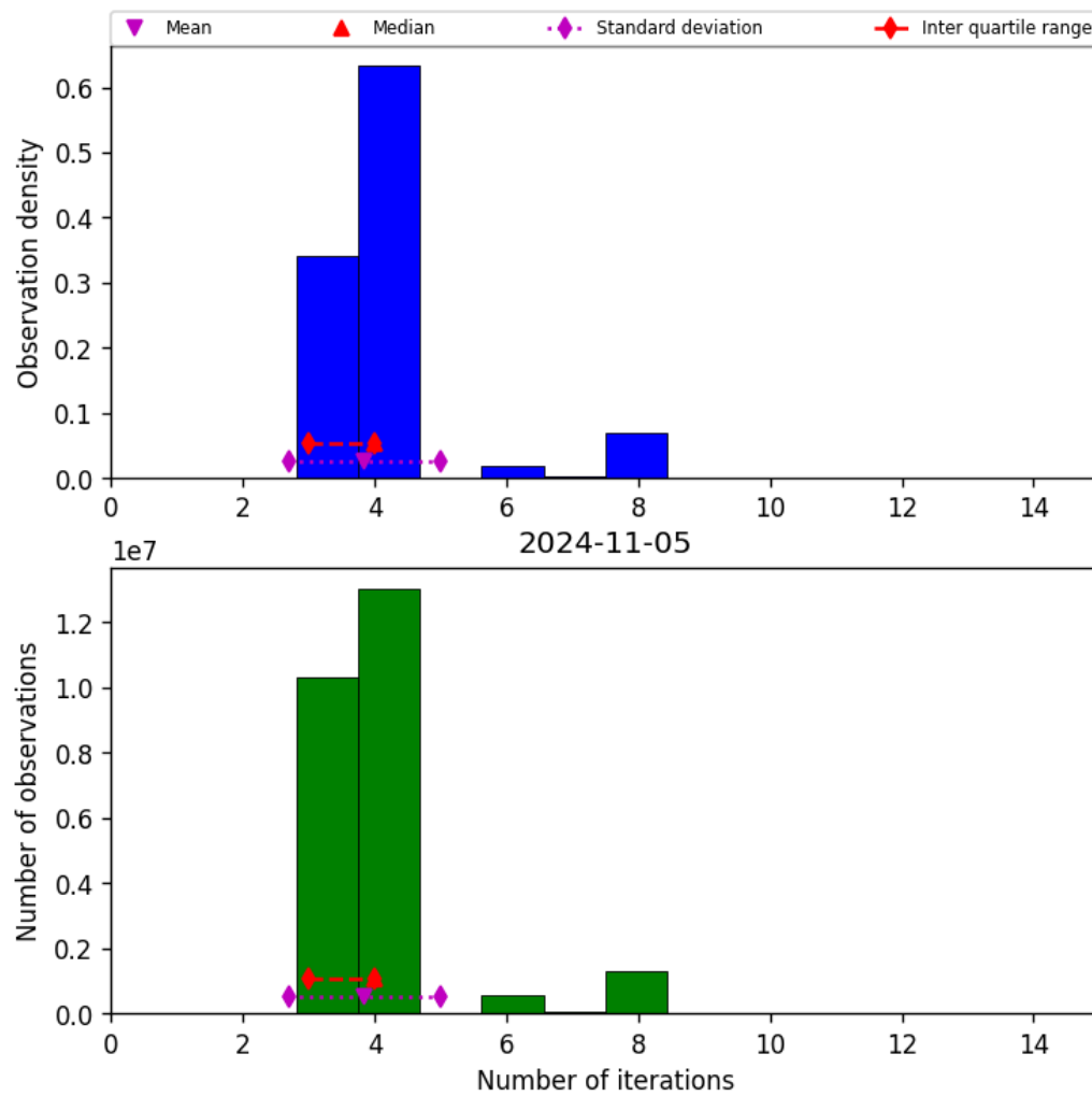
Figure 34: Histogram of “Number of iterations” for 2024-11-04 to 2024-11-06
