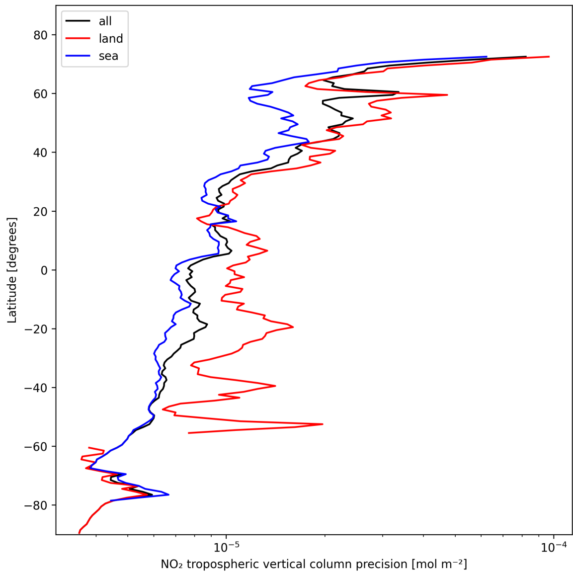
Figure 13: Zonal average of “NO 2 tropospheric vertical column precision” for 2024-11-04 to 2024-11-06.
