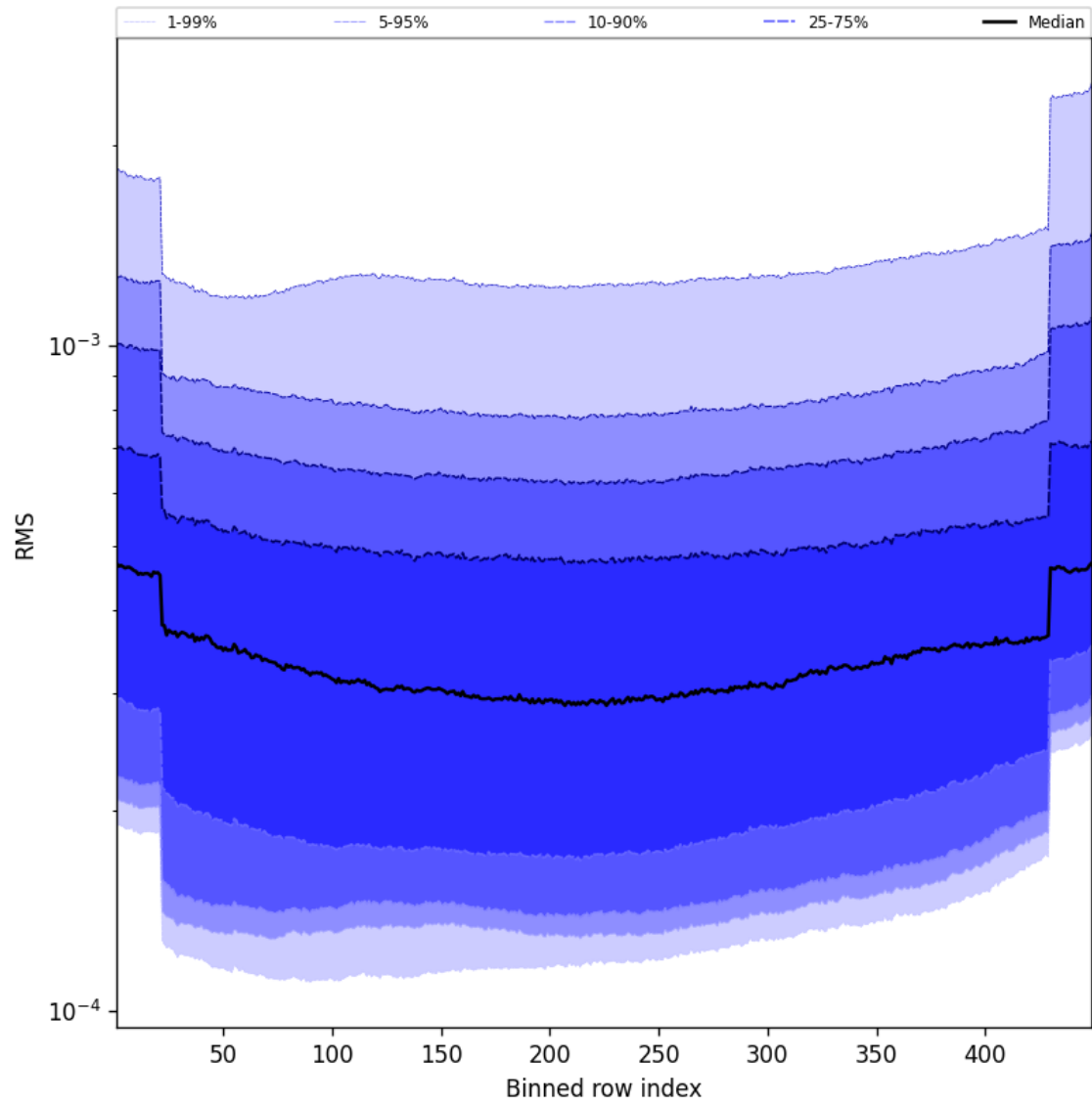
Figure 60: Along track statistics of “RMS” for 2024-11-04 to 2024-11-06
