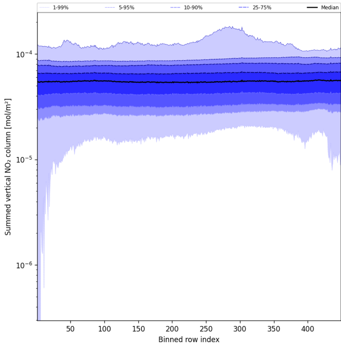
Figure 57: Along track statistics of “Summed vertical NO 2 column” for 2024-11-04 to 2024-11-06
