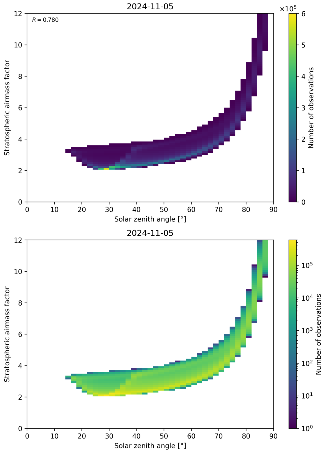
Figure 145: Scatter density plot of “Solar zenith angle” against “Stratospheric airmass factor” for 2024-11-04 to 2024-11-06.
