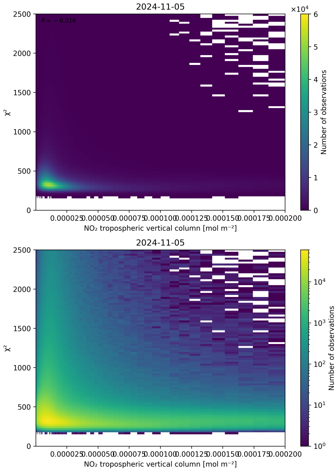
Figure 124: Scatter density plot of “NO 2 tropospheric vertical column” against “ \chi^2 ” for 2024-11-04 to 2024-11-06.
