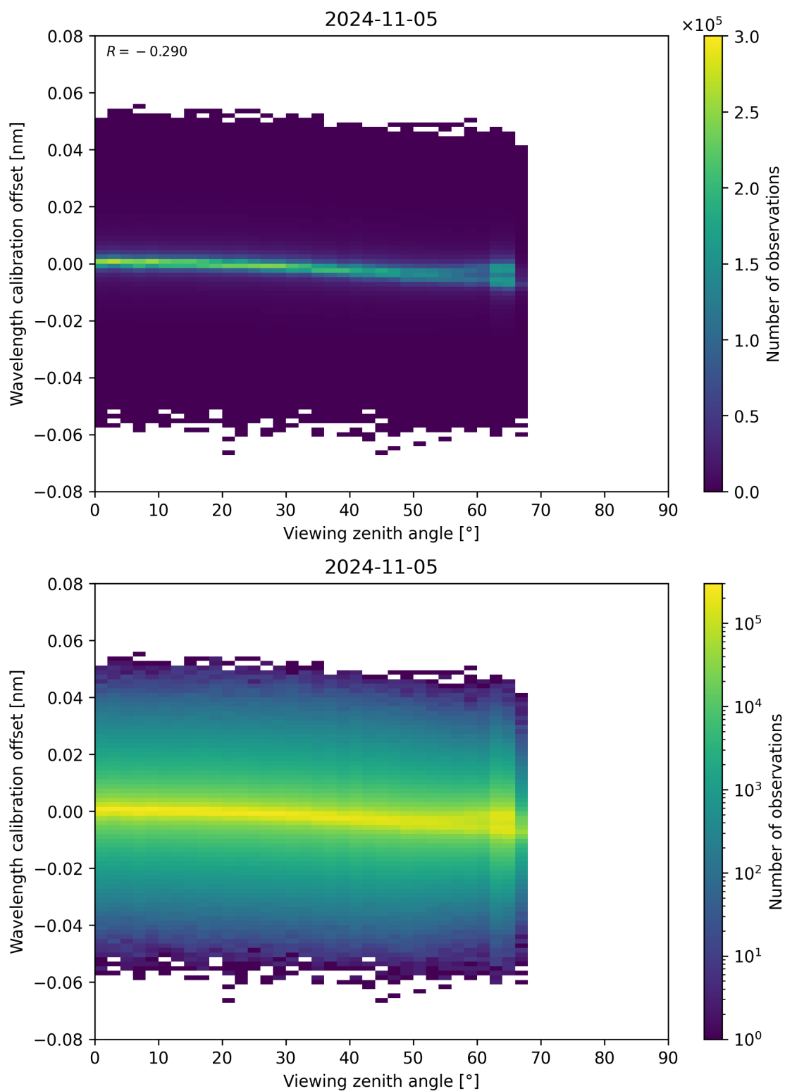
Figure 173: Scatter density plot of “Viewing zenith angle” against “Wavelength calibration offset” for 2024-11-04 to 2024-11-06.
