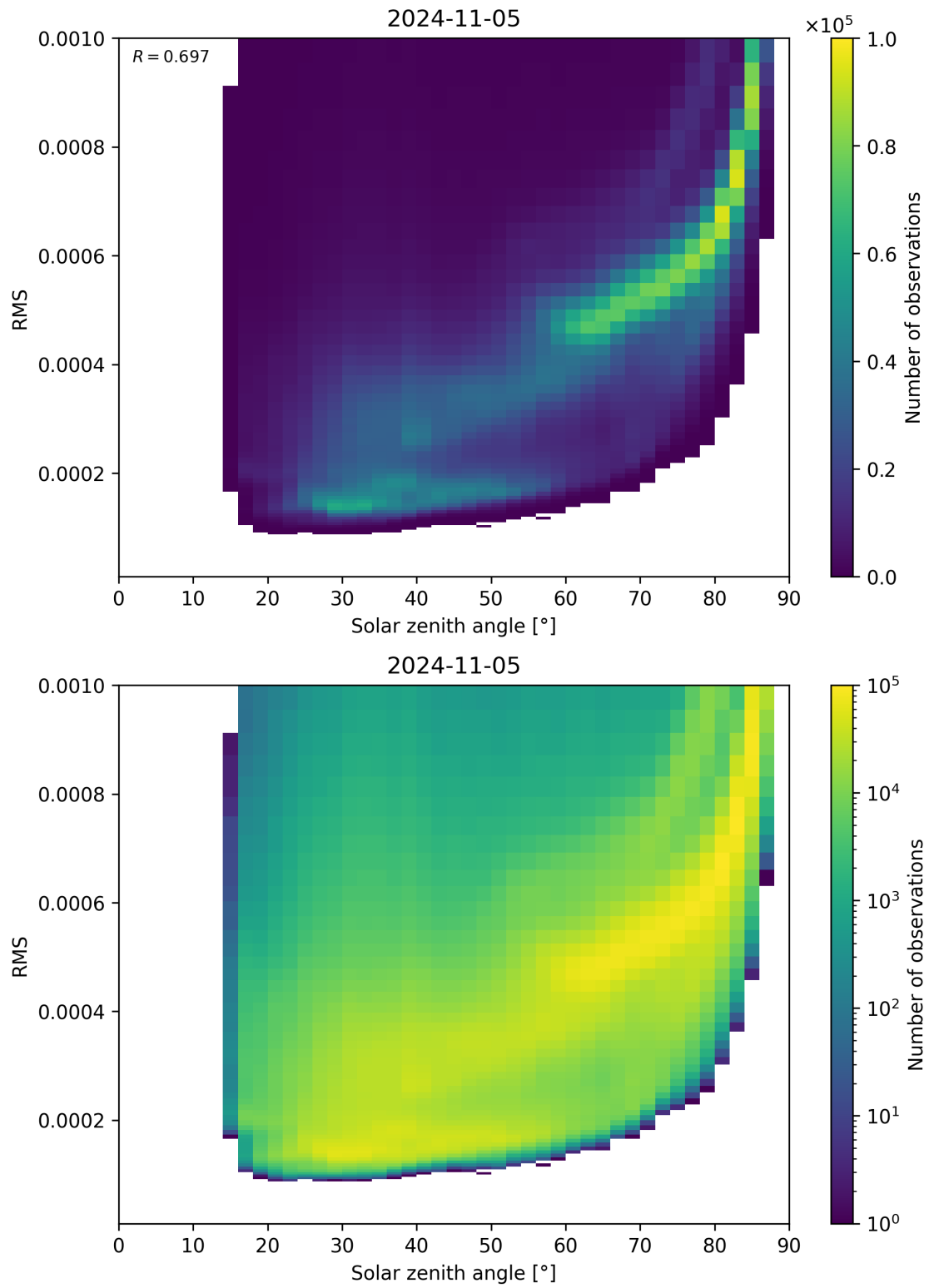
Figure 157: Scatter density plot of “Solar zenith angle” against “RMS” for 2024-11-04 to 2024-11-06.
