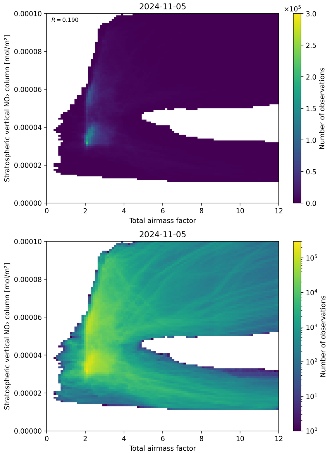
Figure 64: Scatter density plot of “Total airmass factor” against “Stratospheric vertical \text{NO}_2 column” for 2024-11-04 to 2024-11-06.
