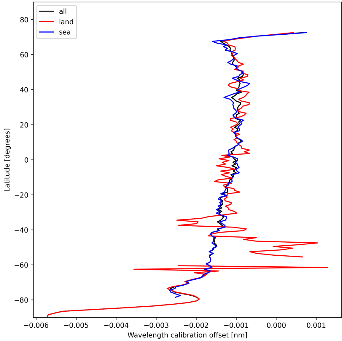
Figure 18: Zonal average of “Wavelength calibration offset” for 2024-11-04 to 2024-11-06.
