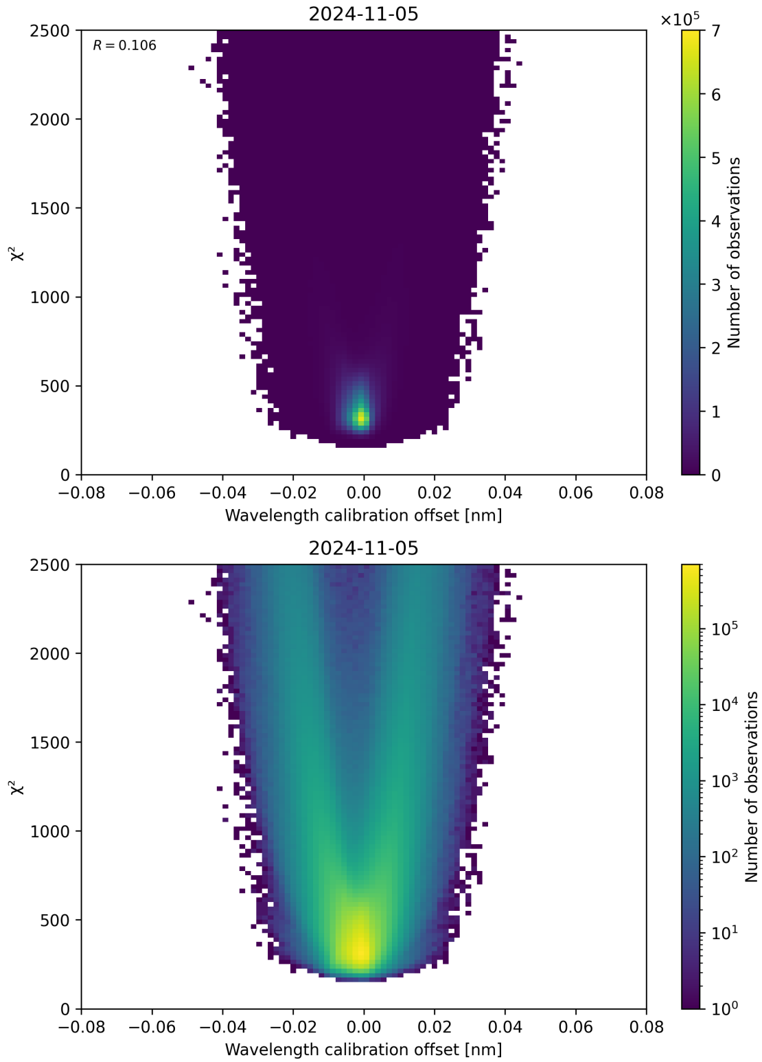
Figure 175: Scatter density plot of “Wavelength calibration offset” against “ \chi^2 ” for 2024-11-04 to 2024-11-06.
