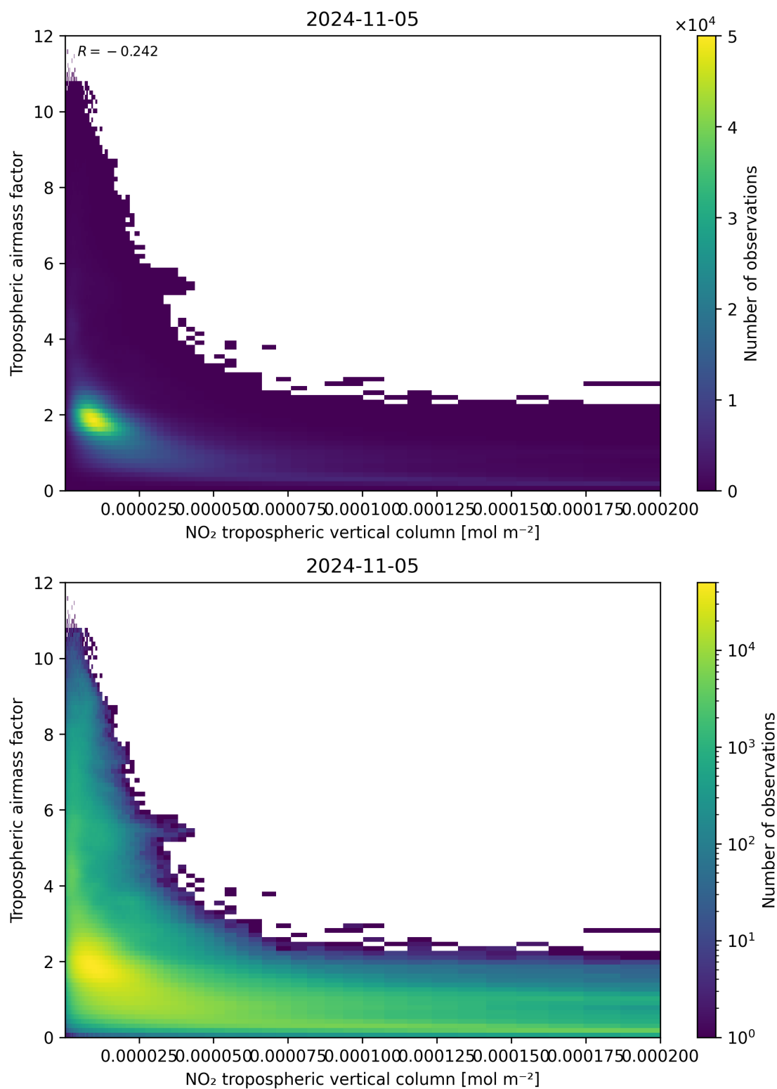
Figure 123: Scatter density plot of “NO 2 tropospheric vertical column” against “Tropospheric airmass factor” for 2024-11-04 to 2024-11-06.
