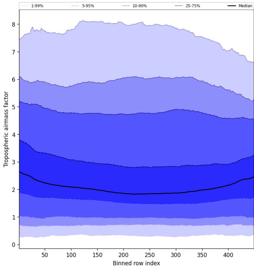
Figure 48: Along track statistics of “Tropospheric air mass factor” for 2024-11-04 to 2024-11-06
