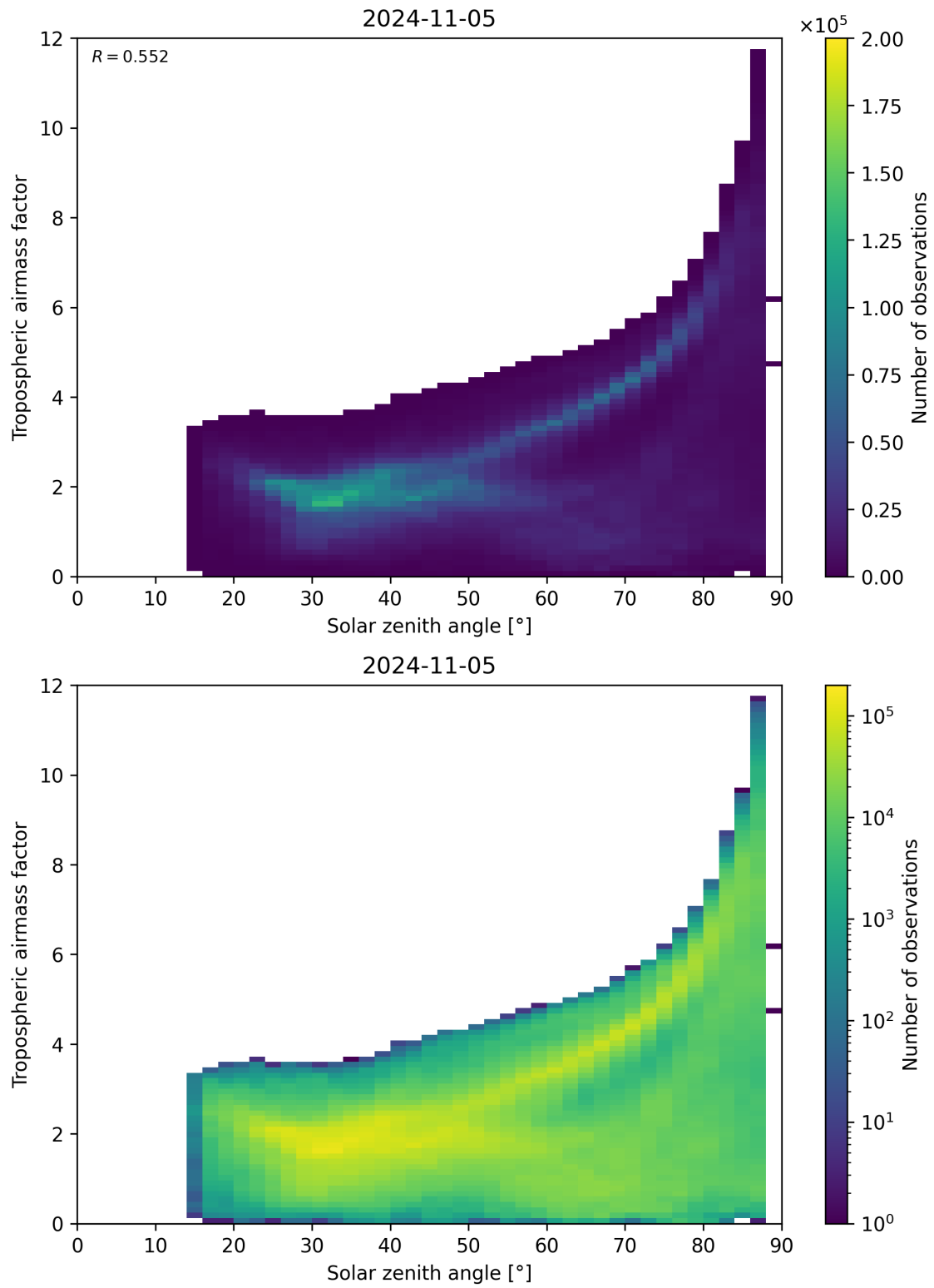
Figure 147: Scatter density plot of “Solar zenith angle” against “Tropospheric airmass factor” for 2024-11-04 to 2024-11-06.
