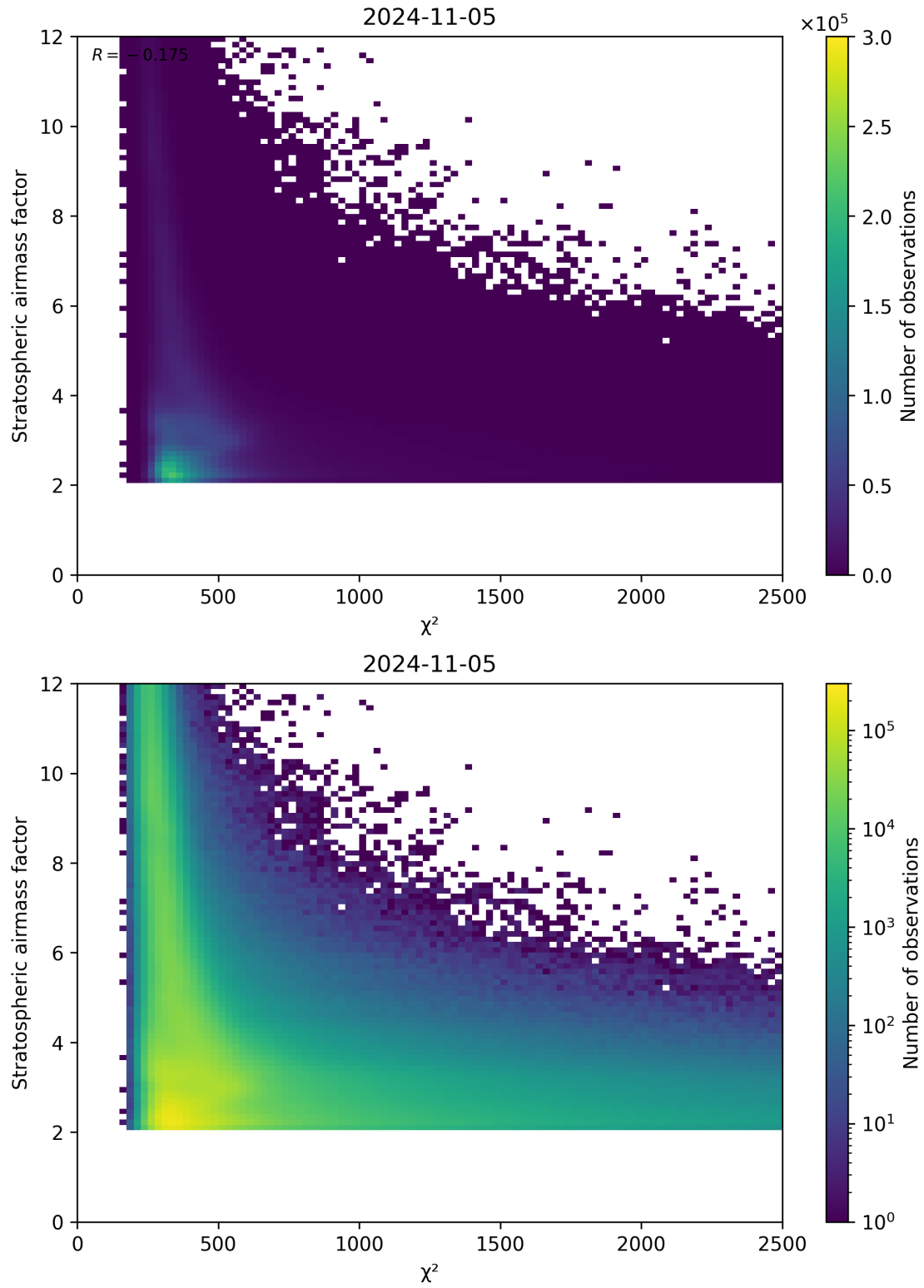
Figure 81: Scatter density plot of “ \chi^2 ” against “Stratospheric airmass factor” for 2024-11-04 to 2024-11-06.
