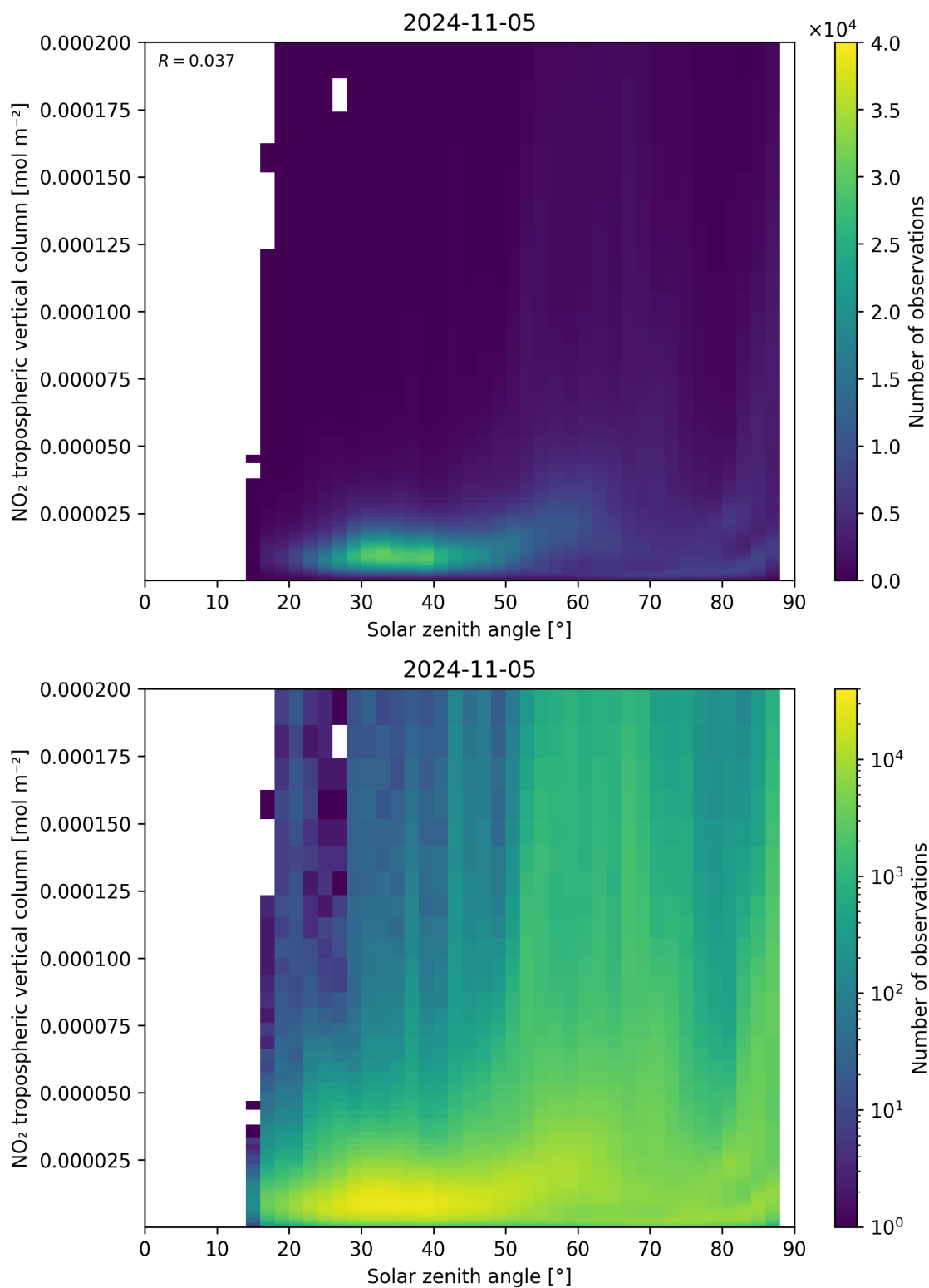
Figure 155: Scatter density plot of “Solar zenith angle” against “NO 2 tropospheric vertical column” for 2024-11-04 to 2024-11-06.
