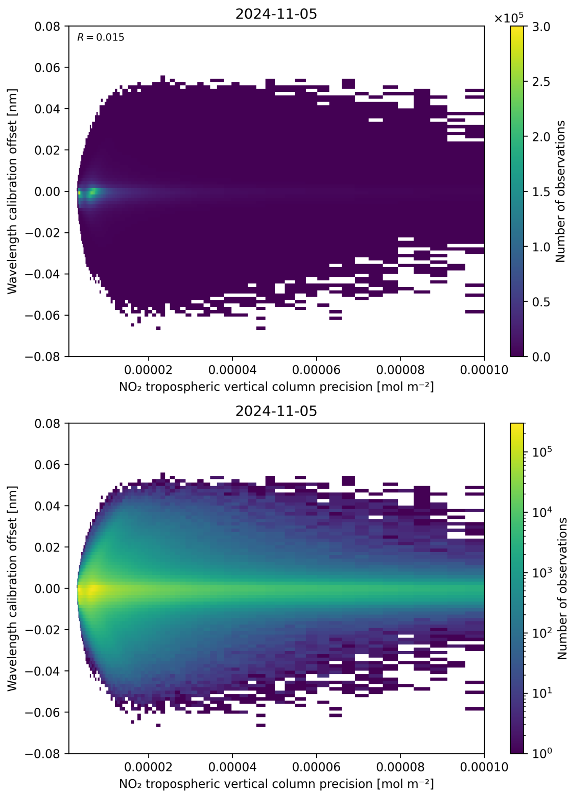
Figure 141: Scatter density plot of “NO 2 tropospheric vertical column precision” against “Wavelength calibration offset” for 2024-11-04 to 2024-11-06.
