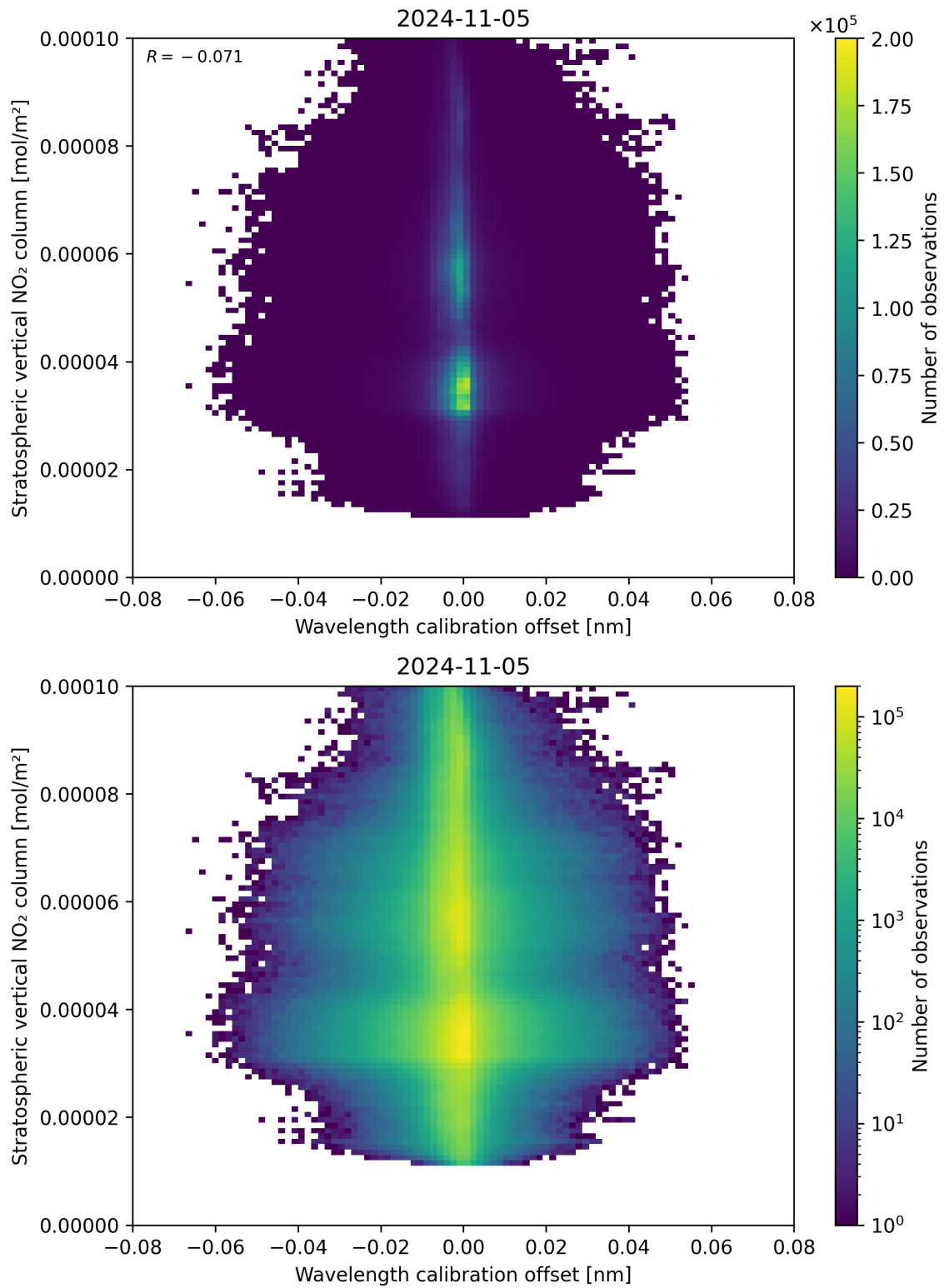
Figure 176: Scatter density plot of “Wavelength calibration offset” against “Stratospheric vertical NO 2 column” for 2024-11-04 to 2024-11-06.
