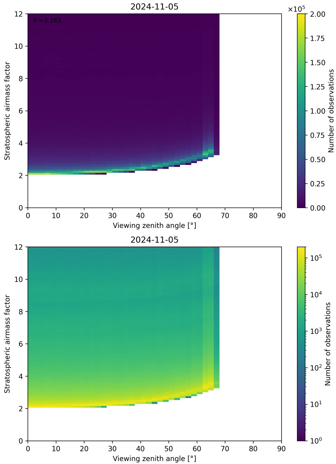
Figure 159: Scatter density plot of “Viewing zenith angle” against “Stratospheric airmass factor” for 2024-11-04 to 2024-11-06.
