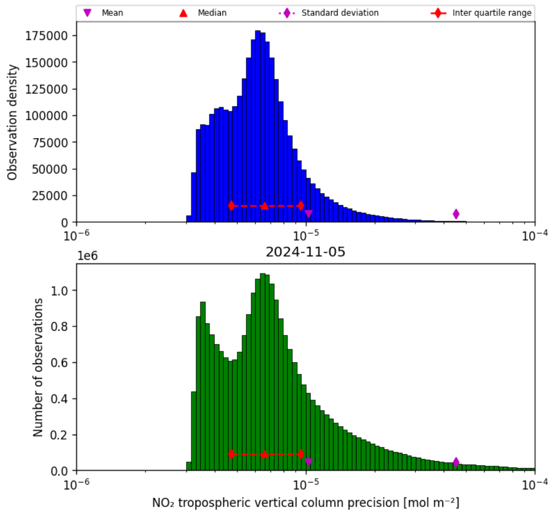
Figure 30: Histogram of “NO 2 tropospheric vertical column precision” for 2024-11-04 to 2024-11-06
