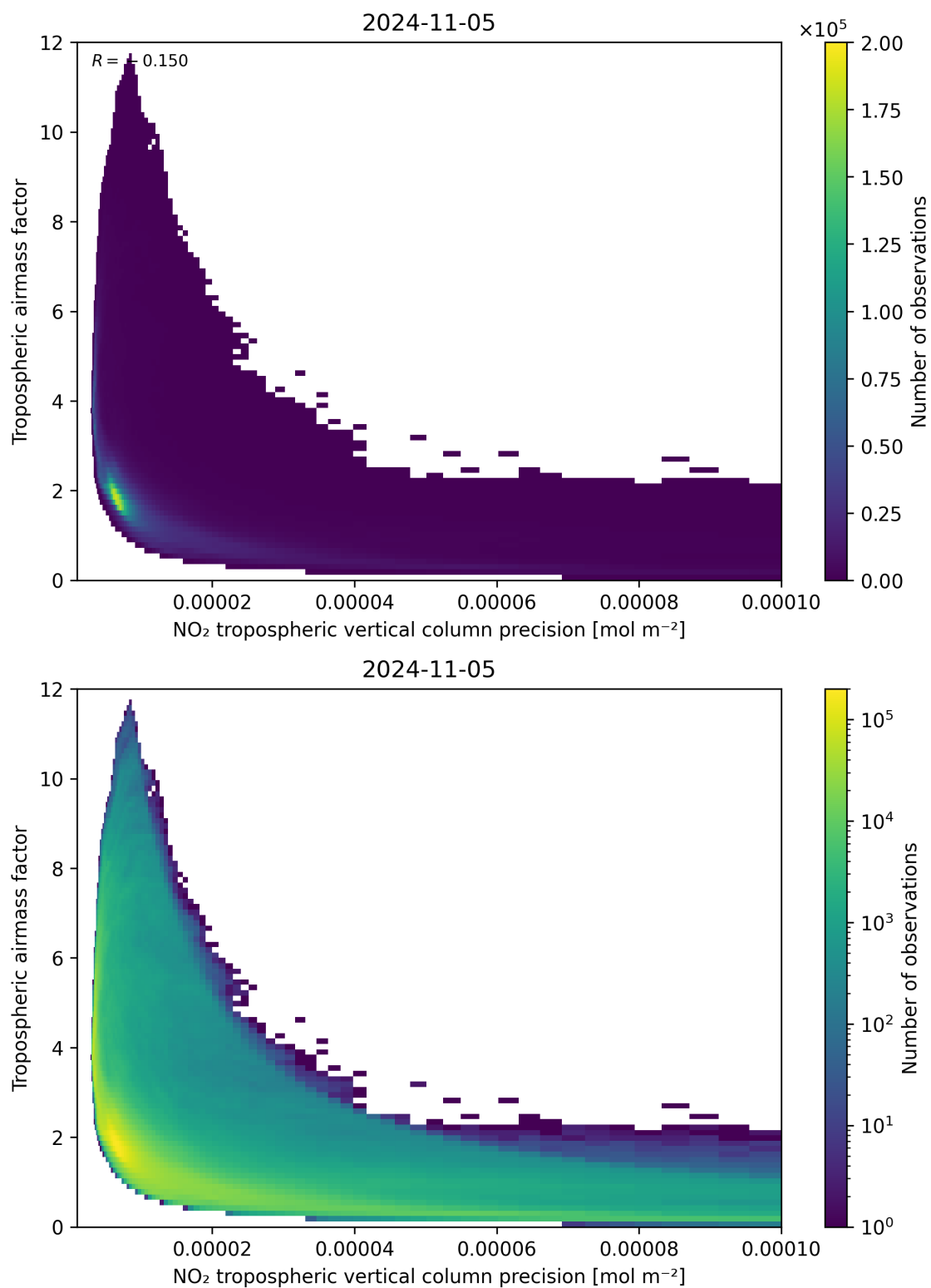
Figure 133: Scatter density plot of “NO 2 tropospheric vertical column precision” against “Tropospheric airmass factor” for 2024-11-04 to 2024-11-06.
