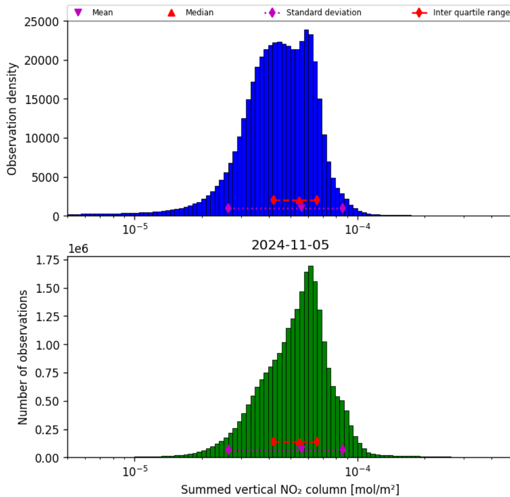
Figure 40: Histogram of “Summed vertical NO 2 column” for 2024-11-04 to 2024-11-06
