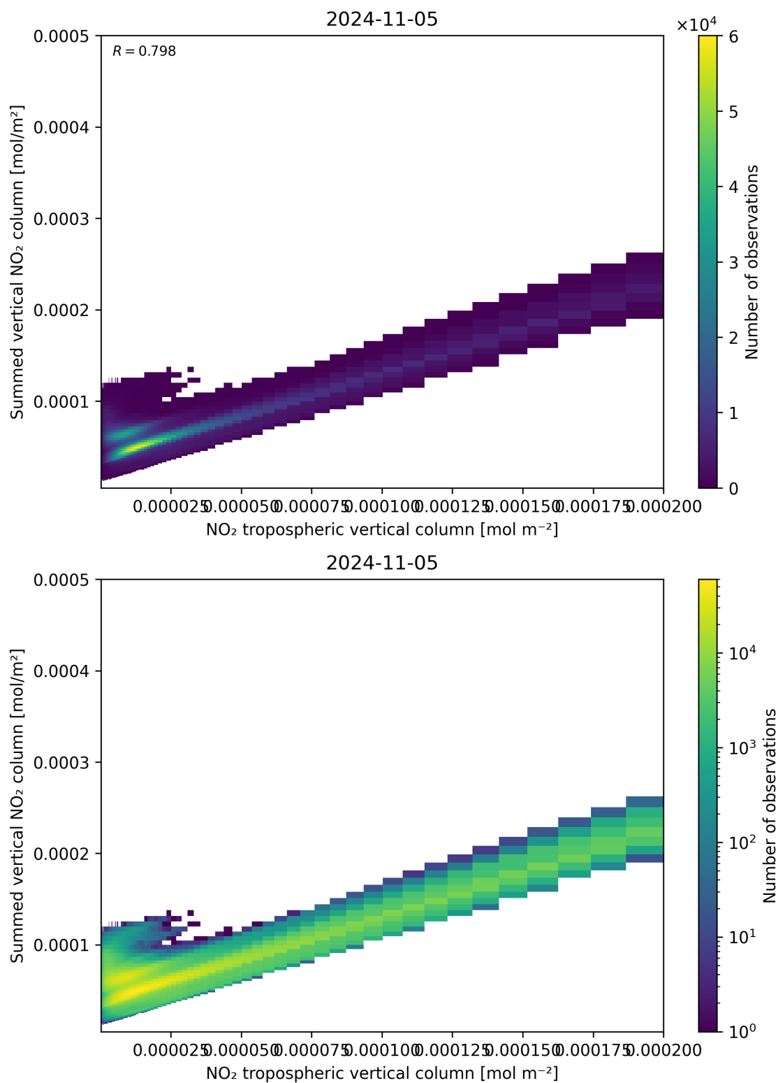
Figure 126: Scatter density plot of “NO 2 tropospheric vertical column” against “Summed vertical NO 2 column” for 2024-11-04 to 2024-11-06.
