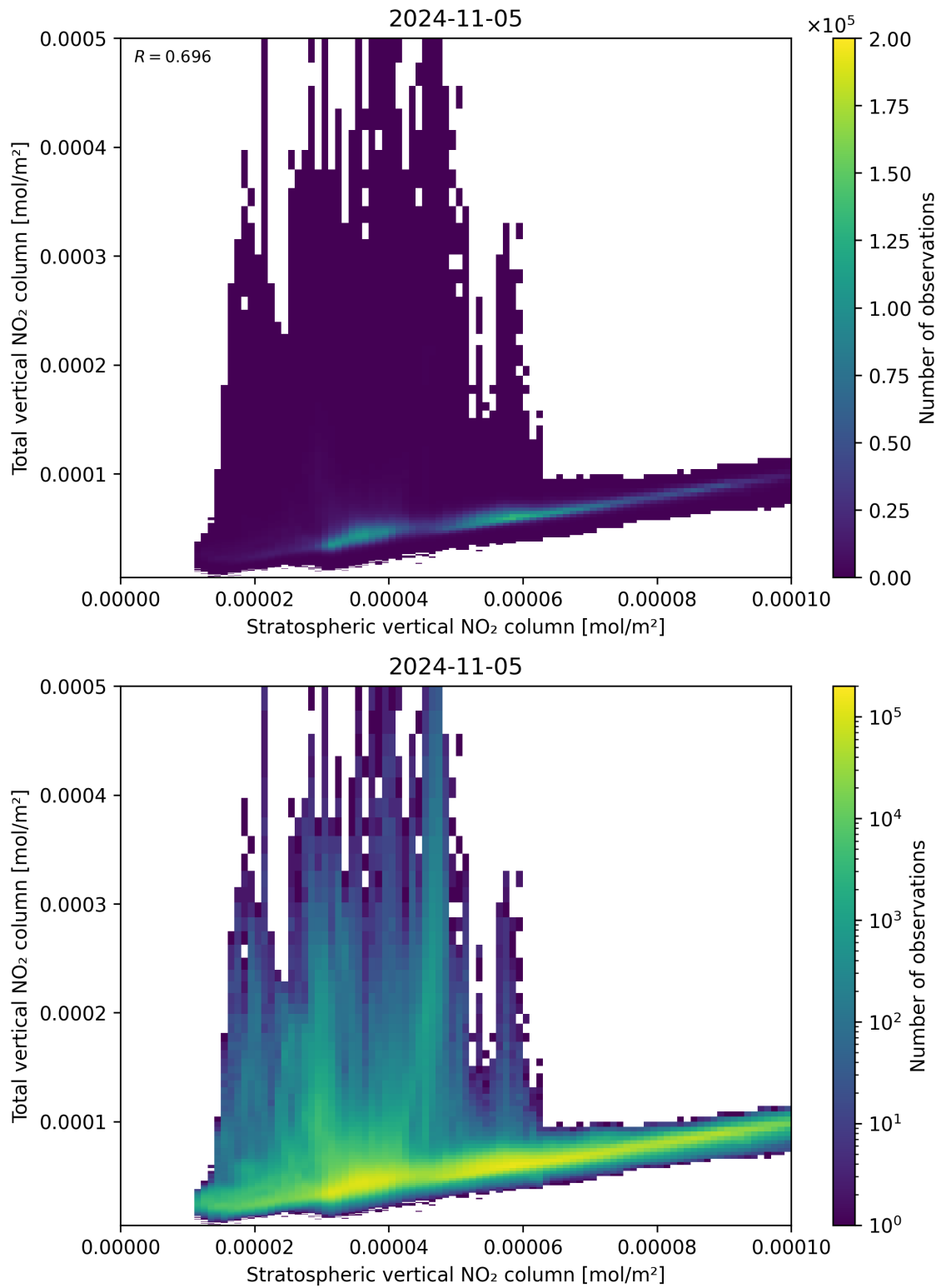
Figure 100: Scatter density plot of “Stratospheric vertical NO 2 column” against “Total vertical NO 2 column” for 2024-11-04 to 2024-11-06.
