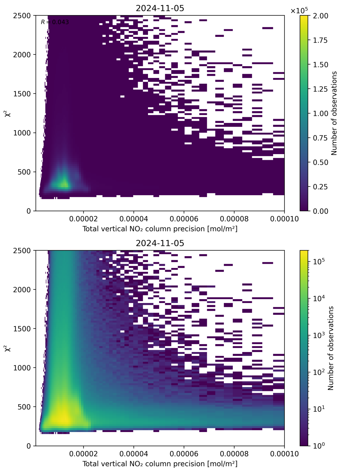
Figure 116: Scatter density plot of “Total vertical NO 2 column precision” against “ \chi^2 ” for 2024-11-04 to 2024-11-06.
