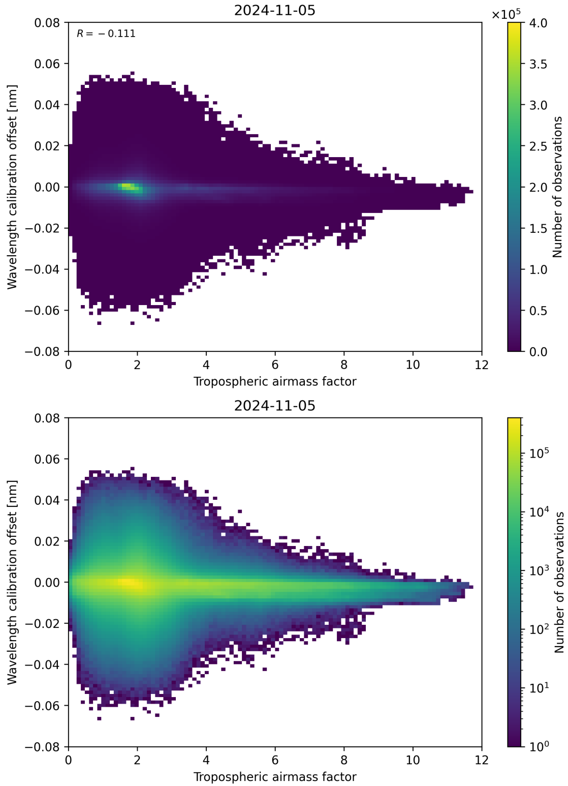
Figure 80: Scatter density plot of “Tropospheric airmass factor” against “Wavelength calibration offset” for 2024-11-04 to 2024-11-06.
