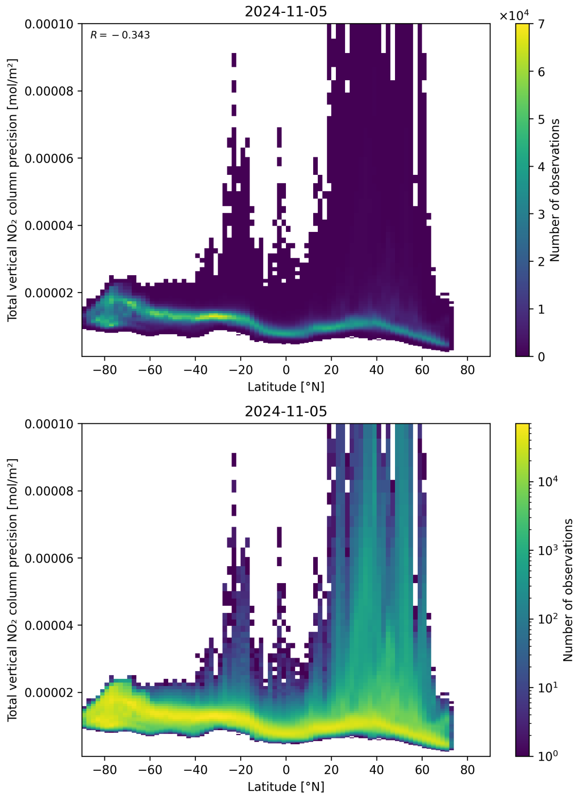
Figure 91: Scatter density plot of “Latitude” against “Total vertical NO 2 column precision” for 2024-11-04 to 2024-11-06.
