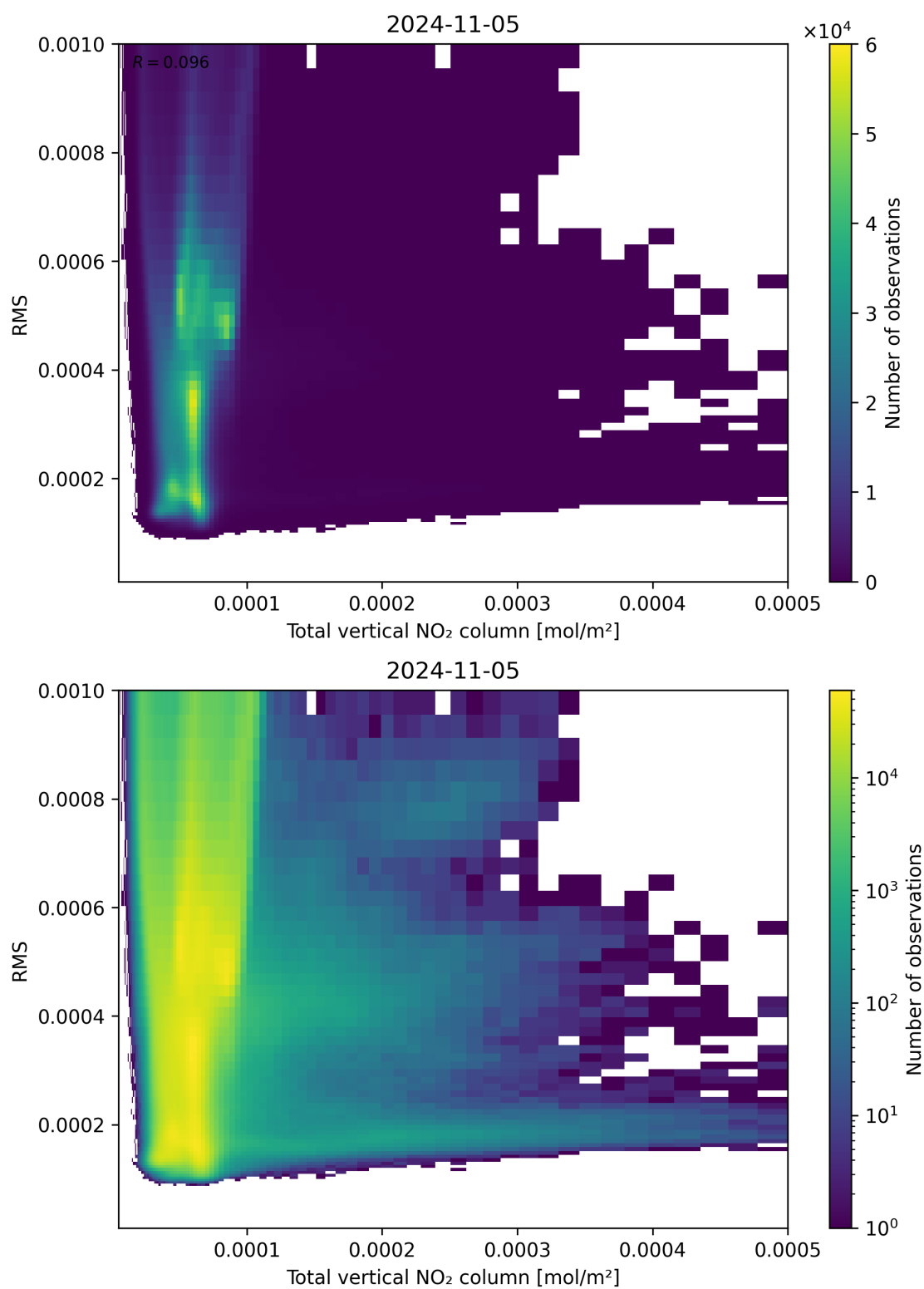
Figure 120: Scatter density plot of “Total vertical NO 2 column” against “RMS” for 2024-11-04 to 2024-11-06.
