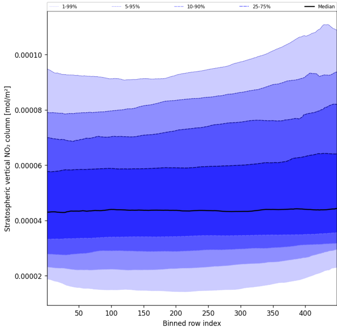
Figure 53: Along track statistics of “Stratospheric vertical NO 2 column” for 2024-11-04 to 2024-11-06
