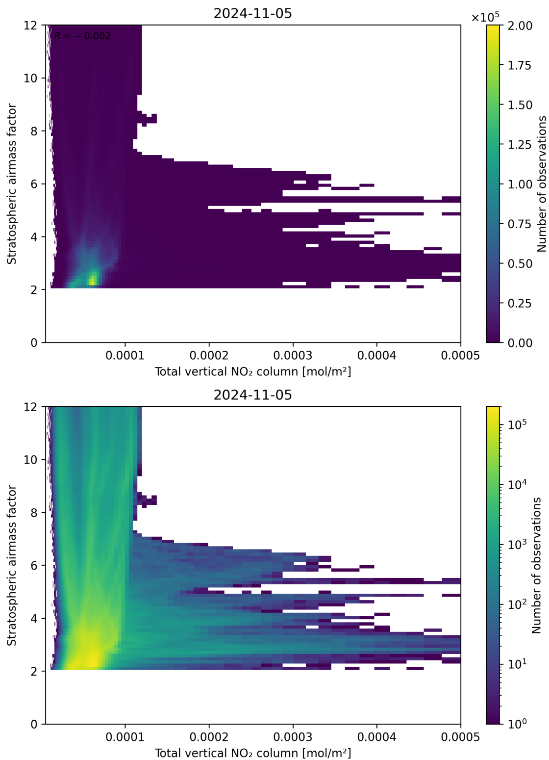
Figure 110: Scatter density plot of “Total vertical NO 2 column” against “Stratospheric airmass factor” for 2024-11-04 to 2024-11-06.
