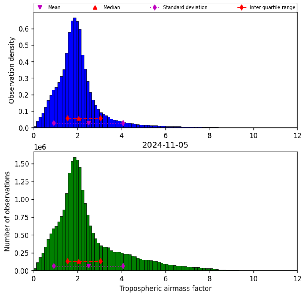
Figure 31: Histogram of “Tropospheric airmass factor” for 2024-11-04 to 2024-11-06
