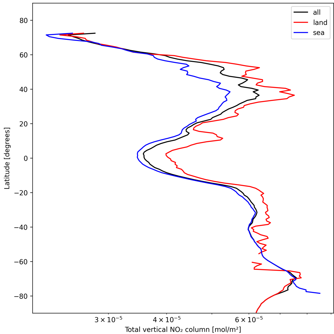
Figure 21: Zonal average of “Total vertical NO 2 column” for 2024-11-04 to 2024-11-06.
