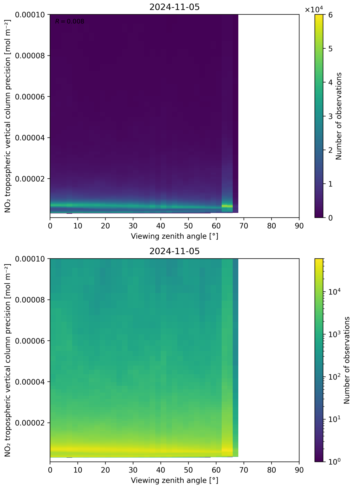
Figure 170: Scatter density plot of “Viewing zenith angle” against “NO 2 tropospheric vertical column precision” for 2024-11-04 to 2024-11-06.
