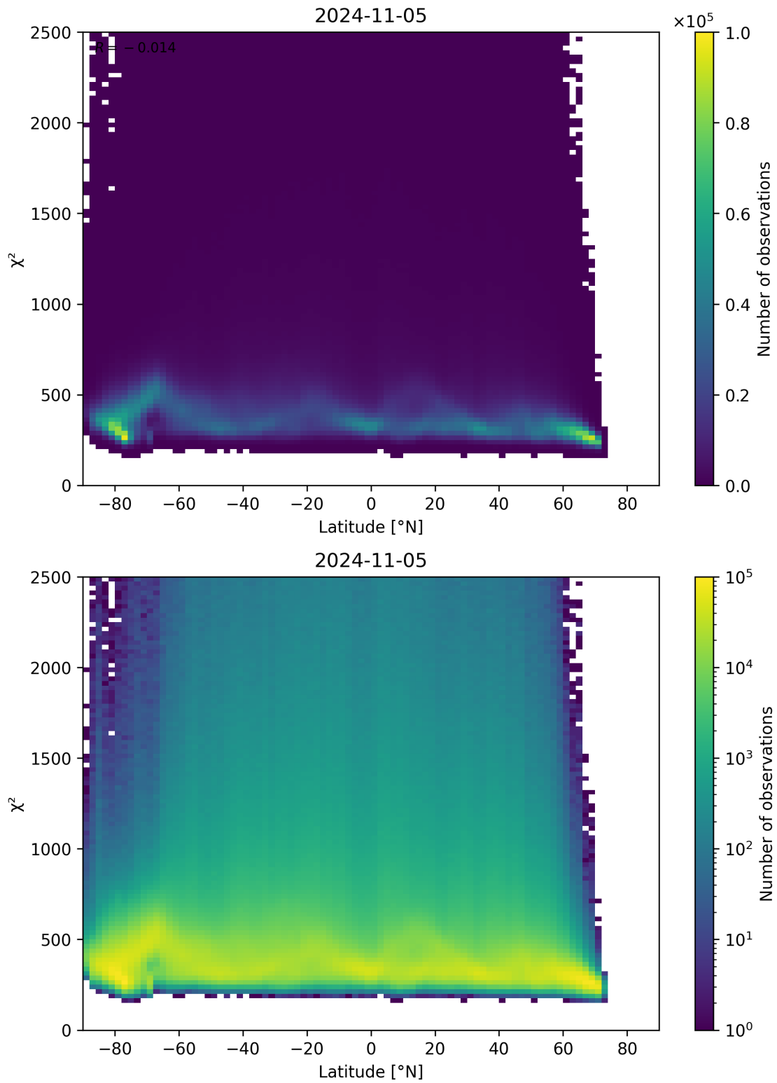
Figure 86: Scatter density plot of “Latitude” against “ \chi^2 ” for 2024-11-04 to 2024-11-06.
