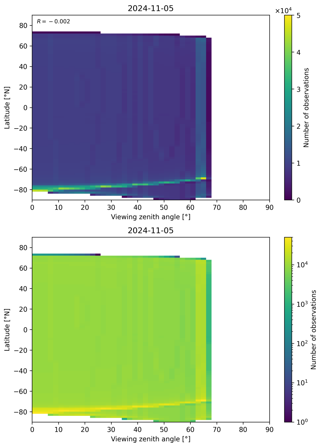
Figure 163: Scatter density plot of “Viewing zenith angle” against “Latitude” for 2024-11-04 to 2024-11-06.
