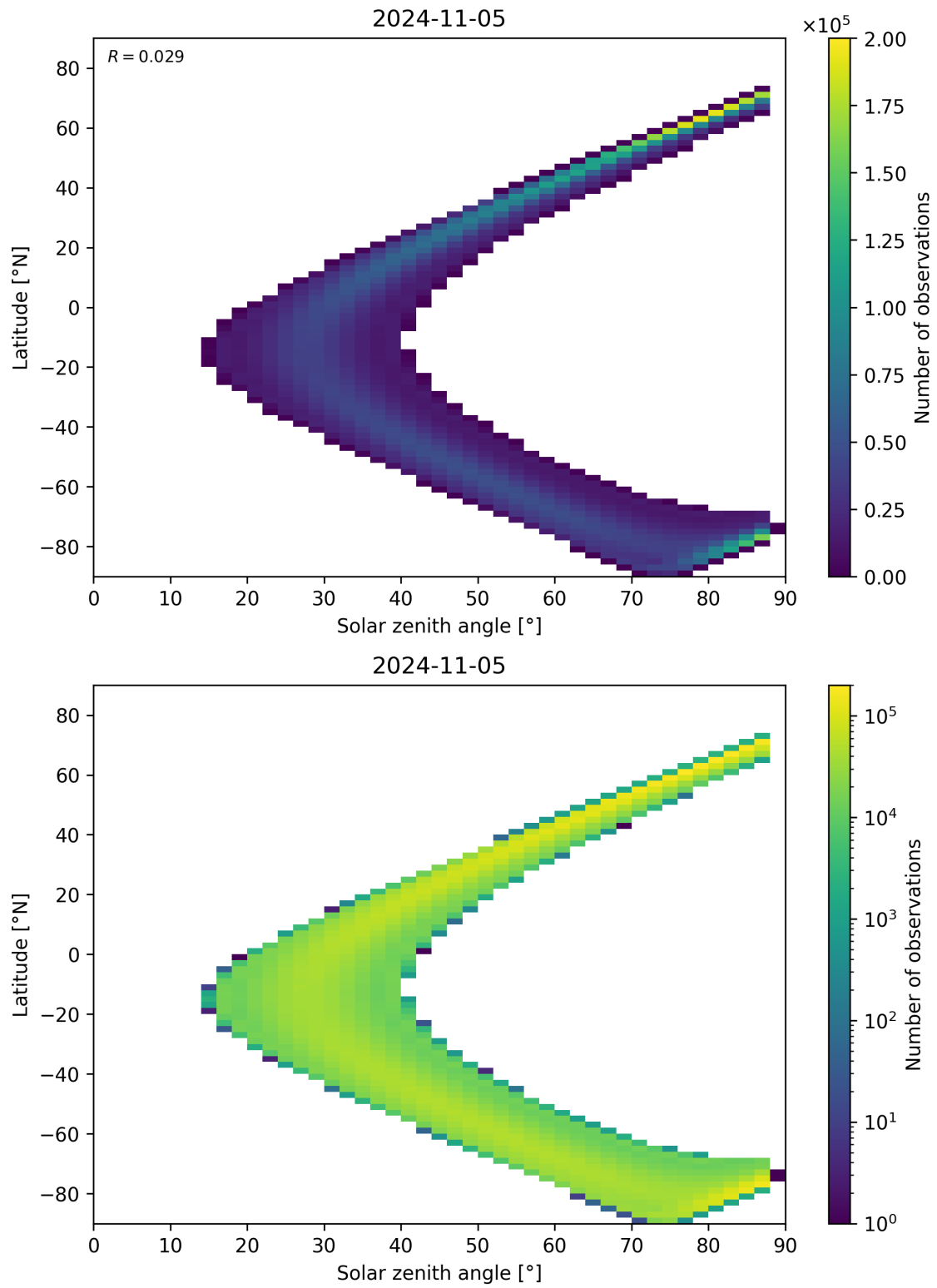
Figure 149: Scatter density plot of “Solar zenith angle” against “Latitude” for 2024-11-04 to 2024-11-06.
