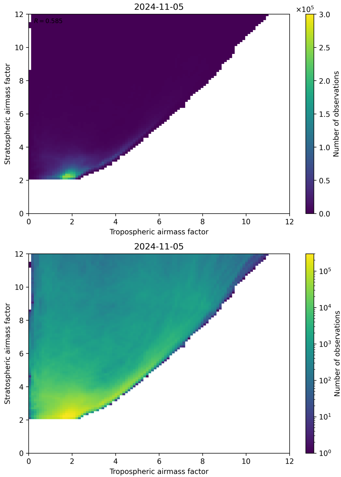
Figure 71: Scatter density plot of “Tropospheric airmass factor” against “Stratospheric airmass factor” for 2024-11-04 to 2024-11-06.
