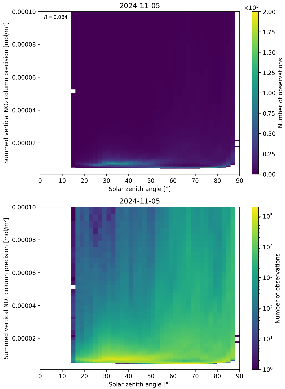
Figure 152: Scatter density plot of “Solar zenith angle” against “Summed vertical NO 2 column precision” for 2024-11-04 to 2024-11-06.
