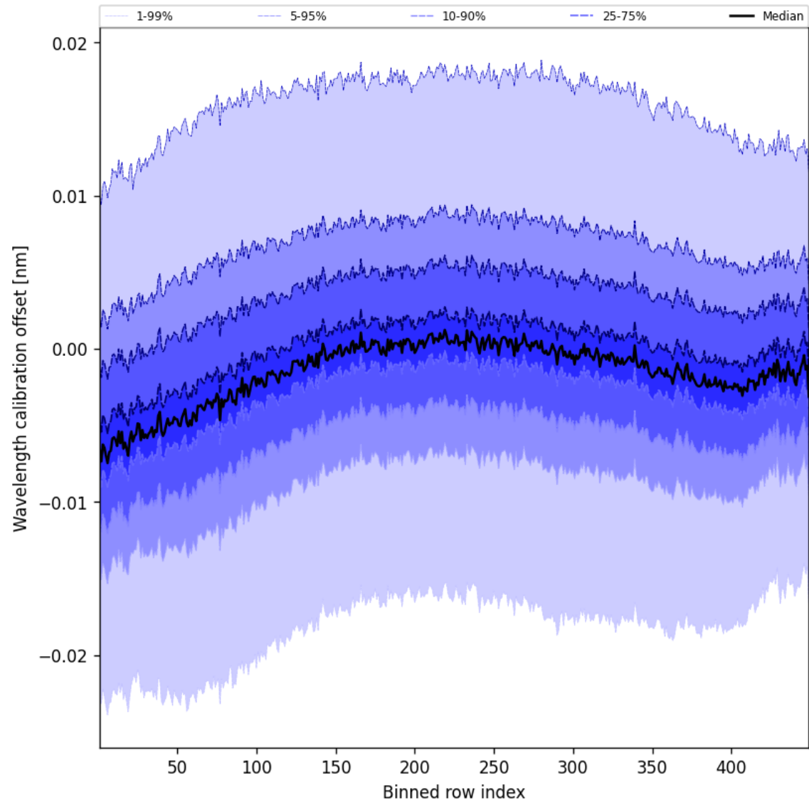
Figure 52: Along track statistics of “Wavelength calibration offset” for 2024-11-05 to 2024-11-07
