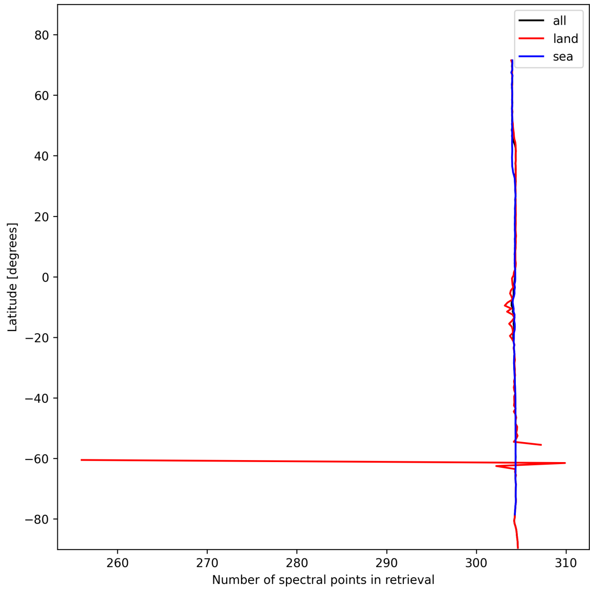
Figure 16: Zonal average of “Number of spectral points in retrieval” for 2024-11-05 to 2024-11-07.
