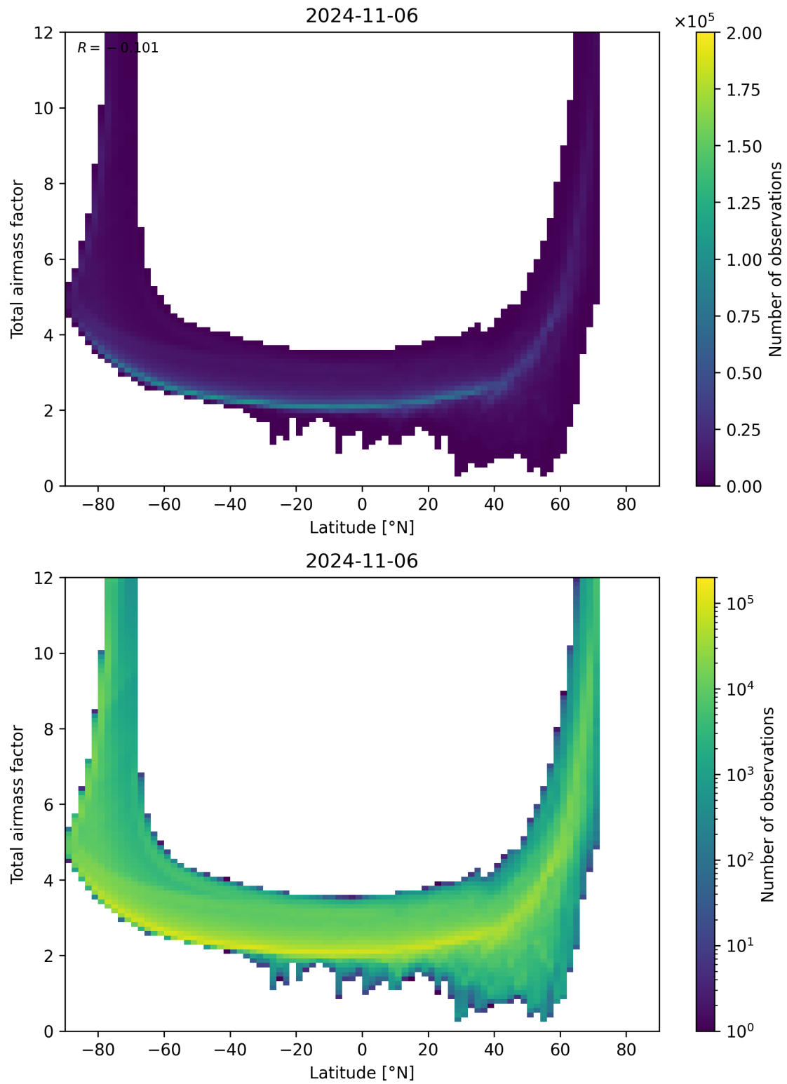
Figure 84: Scatter density plot of “Latitude” against “Total airmass factor” for 2024-11-05 to 2024-11-07.
