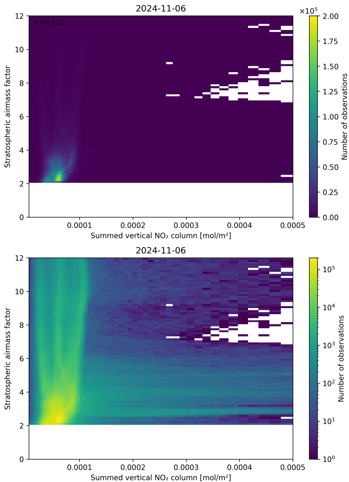
Figure 103: Scatter density plot of “Summed vertical NO 2 column” against “Stratospheric air mass factor” for 2024-11-05 to 2024-11-07.
