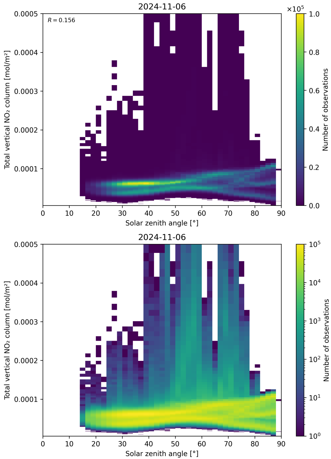
Figure 153: Scatter density plot of “Solar zenith angle” against “Total vertical NO 2 column” for 2024-11-05 to 2024-11-07.
