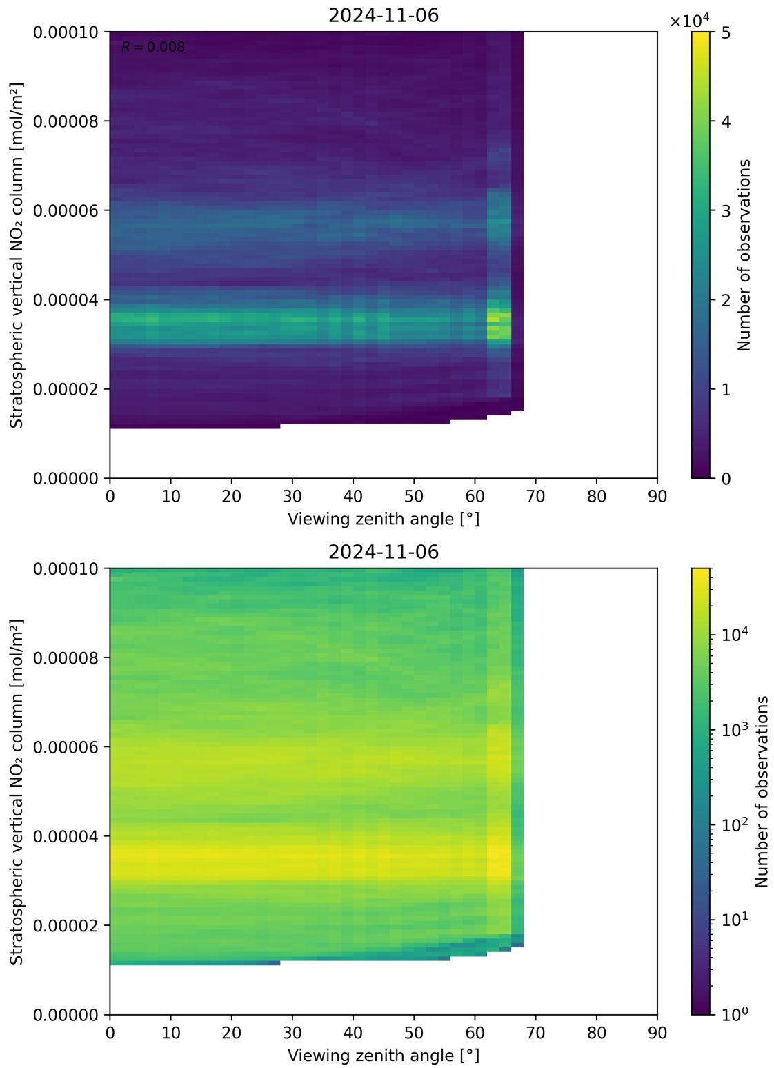
Figure 164: Scatter density plot of “Viewing zenith angle” against “Stratospheric vertical NO 2 column” for 2024-11-05 to 2024-11-07.
