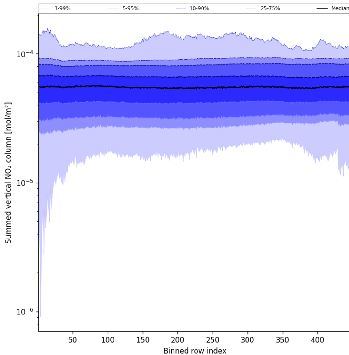
Figure 57: Along track statistics of “Summed vertical NO 2 column” for 2024-11-05 to 2024-11-07
