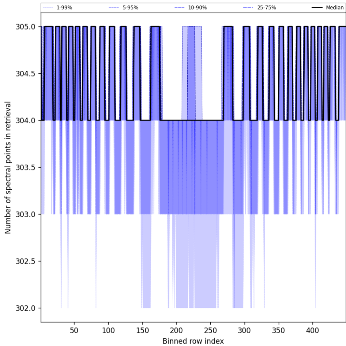
Figure 50: Along track statistics of “Number of spectral points in retrieval” for 2024-11-05 to 2024-11-07
