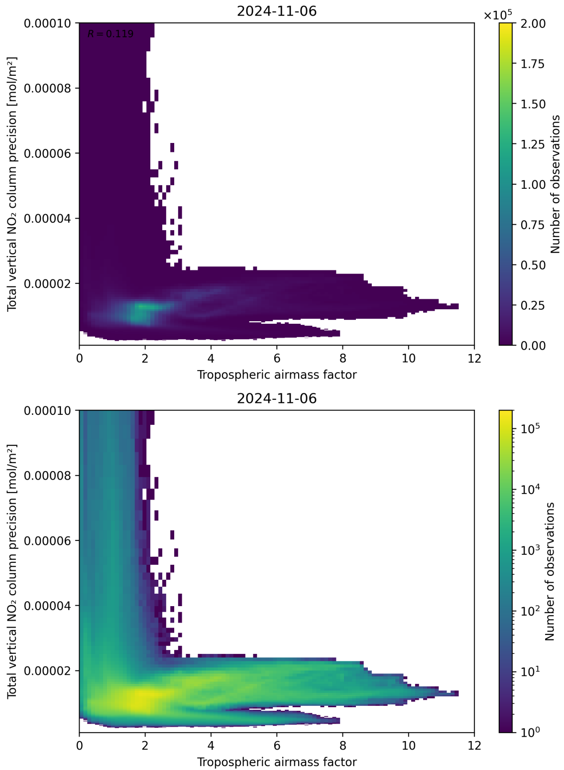
Figure 78: Scatter density plot of “Tropospheric air mass factor” against “Total vertical NO 2 column precision” for 2024-11-05 to 2024-11-07.
