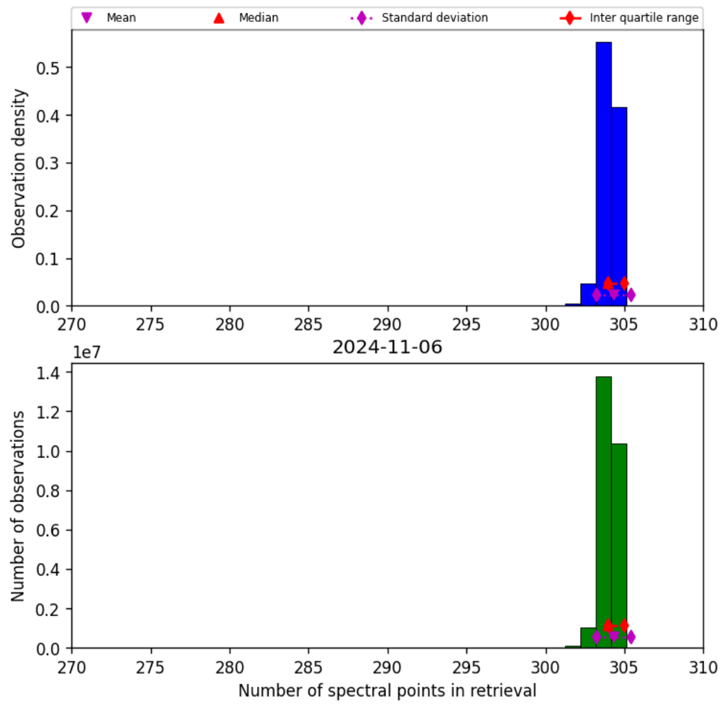
Figure 33: Histogram of “Number of spectral points in retrieval” for 2024-11-05 to 2024-11-07
