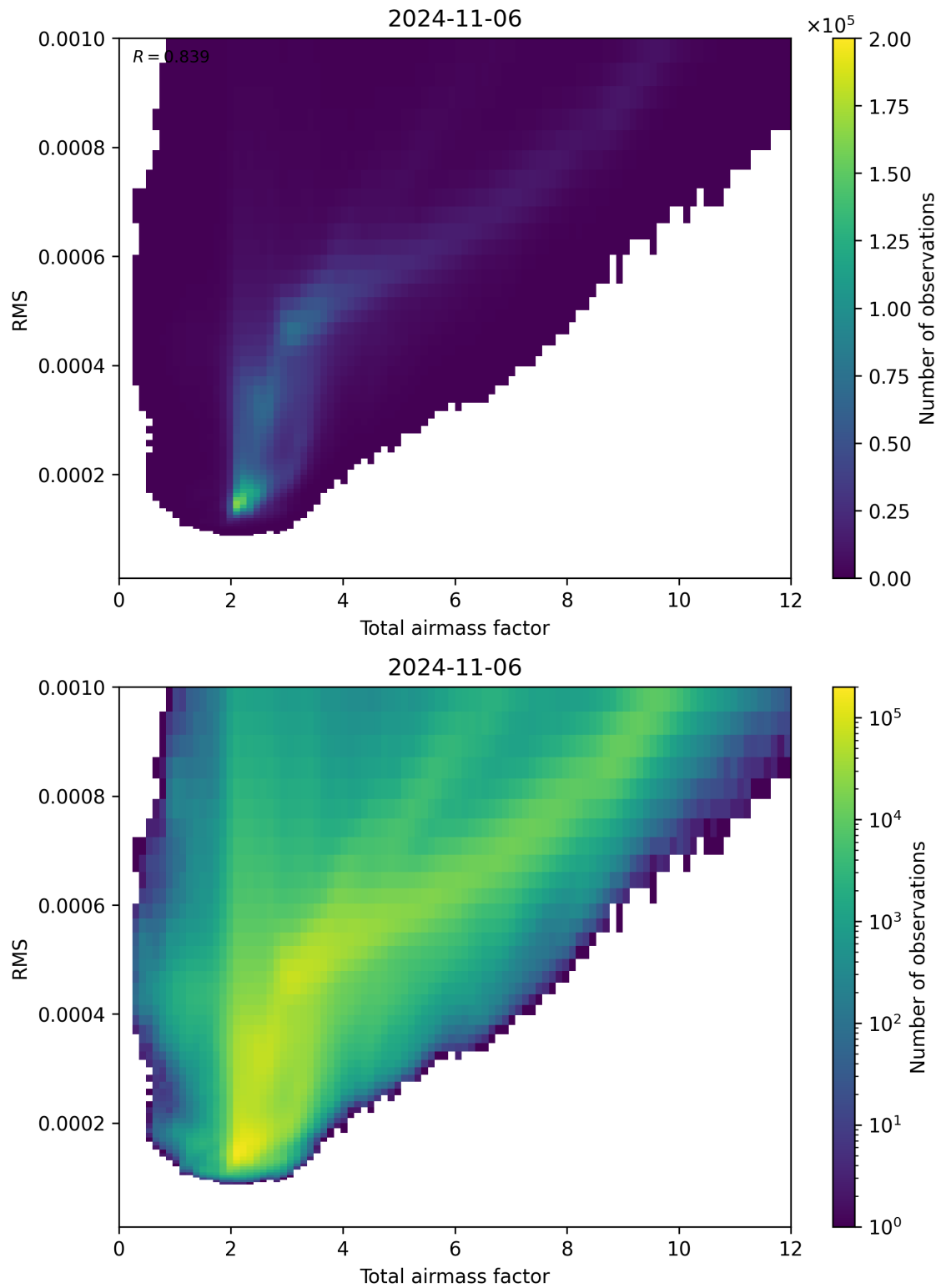
Figure 69: Scatter density plot of “Total airmass factor” against “RMS” for 2024-11-05 to 2024-11-07.
