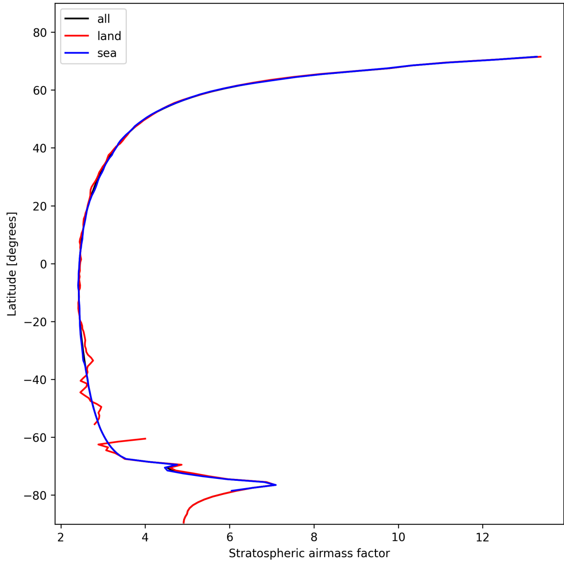
Figure 27: Zonal average of “Stratospheric air mass factor” for 2024-11-05 to 2024-11-07.
