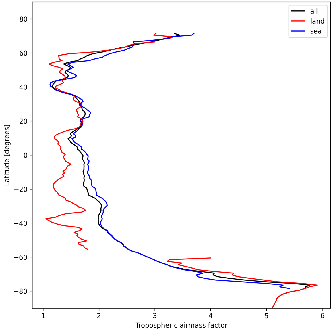
Figure 14: Zonal average of “Tropospheric airmass factor” for 2024-11-05 to 2024-11-07.
