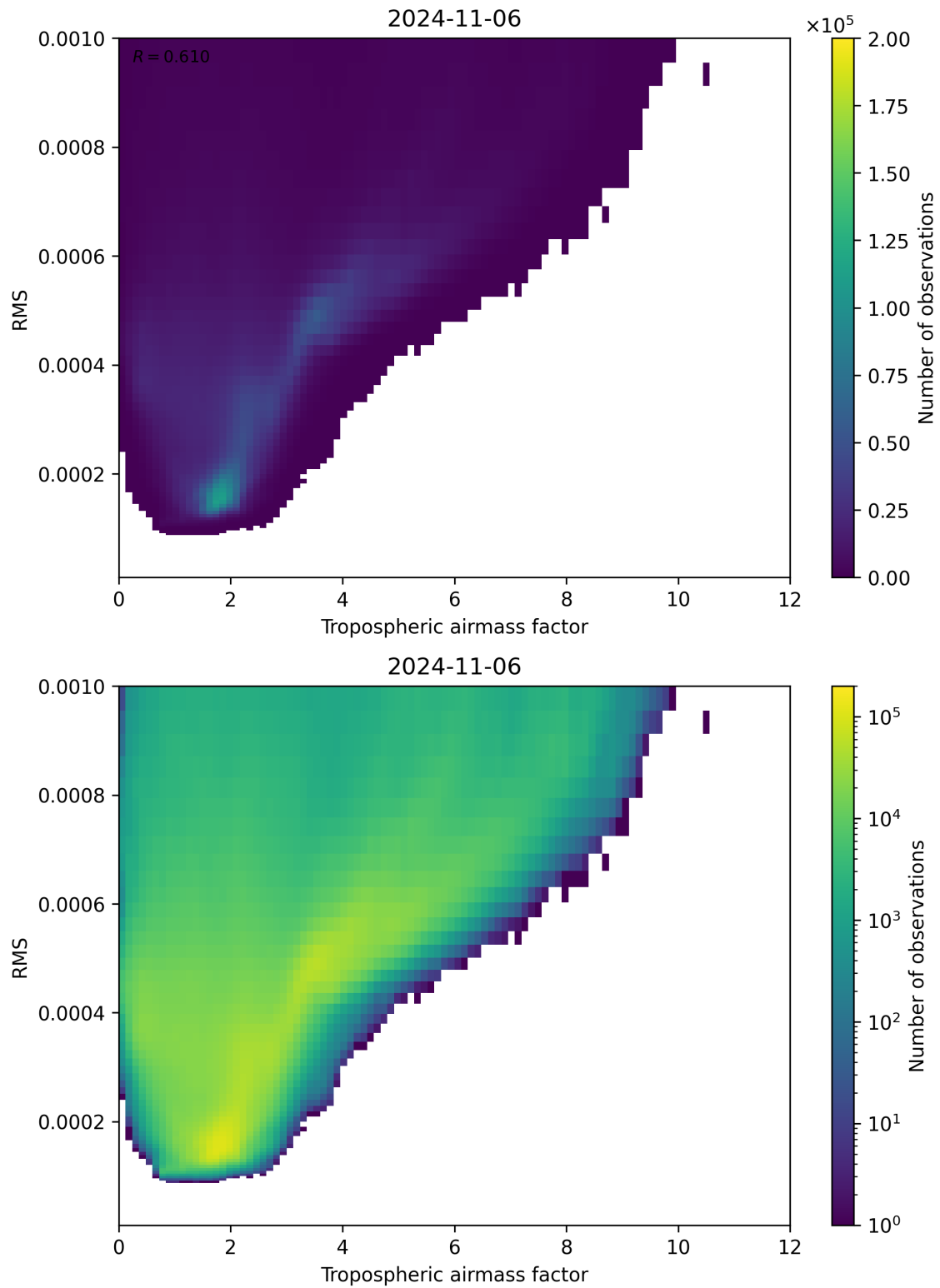
Figure 79: Scatter density plot of “Tropospheric airmass factor” against “RMS” for 2024-11-05 to 2024-11-07.
