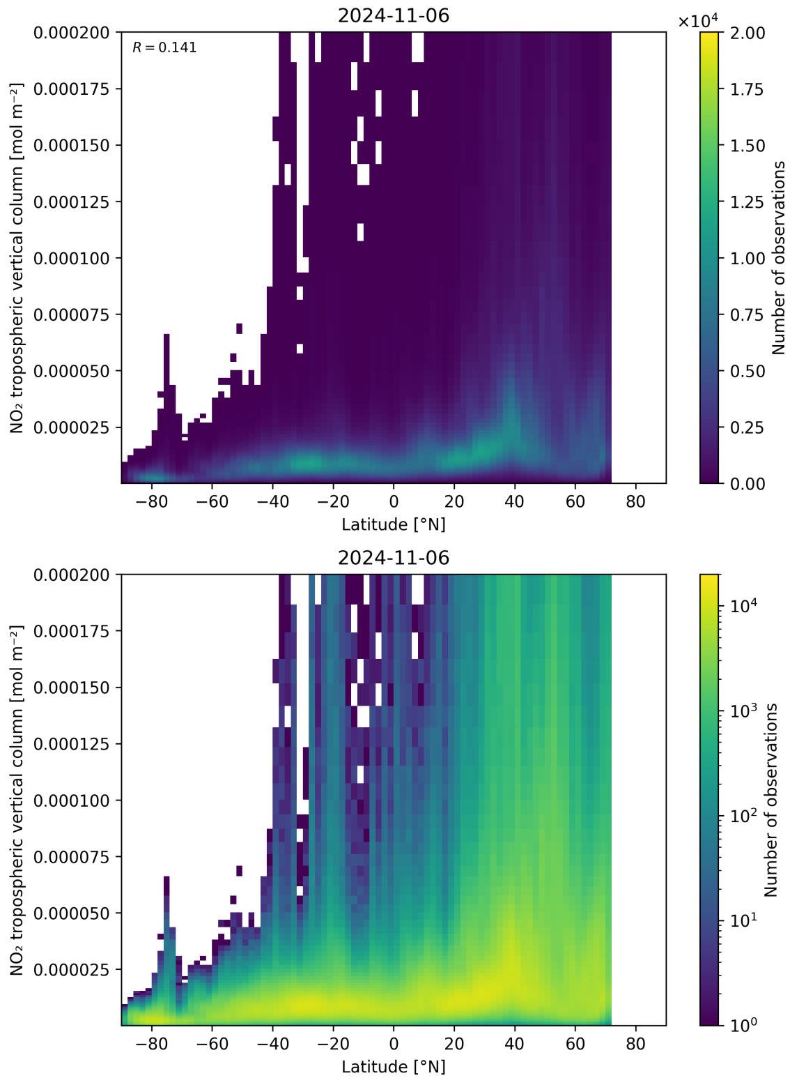
Figure 92: Scatter density plot of “Latitude” against “NO 2 tropospheric vertical column” for 2024-11-05 to 2024-11-07.
