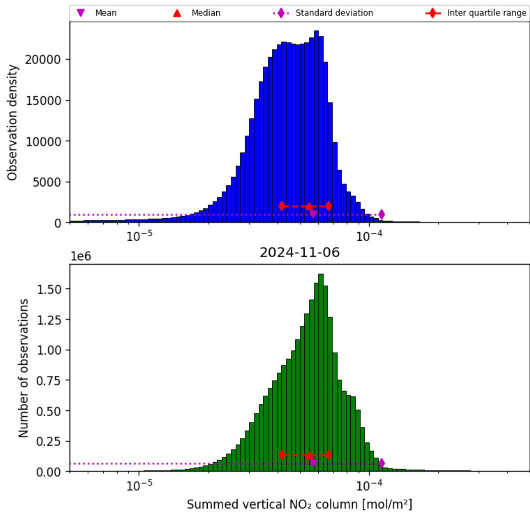
Figure 40: Histogram of "Summed vertical NO 2 column" for 2024-11-05 to 2024-11-07
