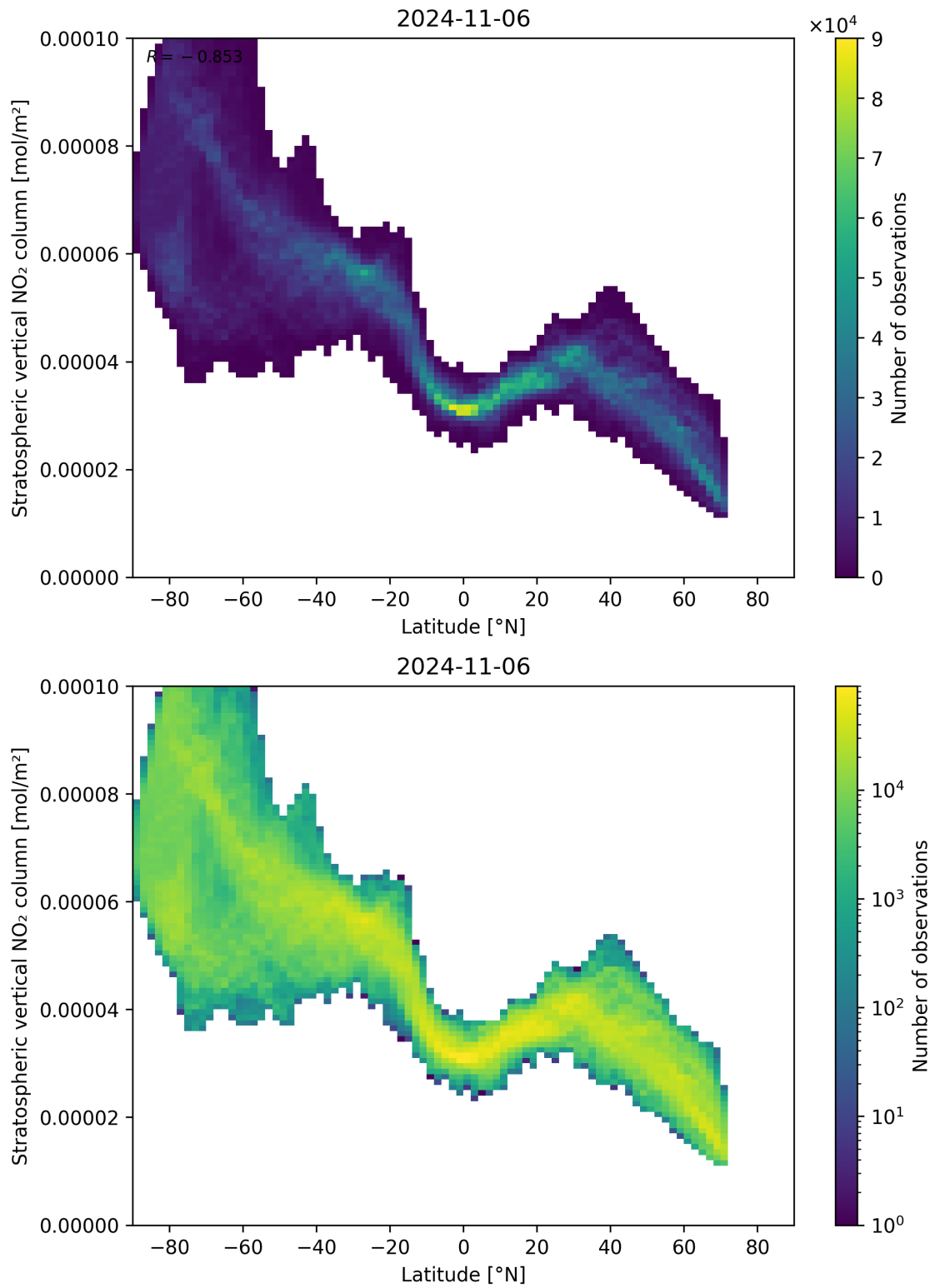
Figure 87: Scatter density plot of “Latitude” against “Stratospheric vertical NO 2 column” for 2024-11-05 to 2024-11-07.
