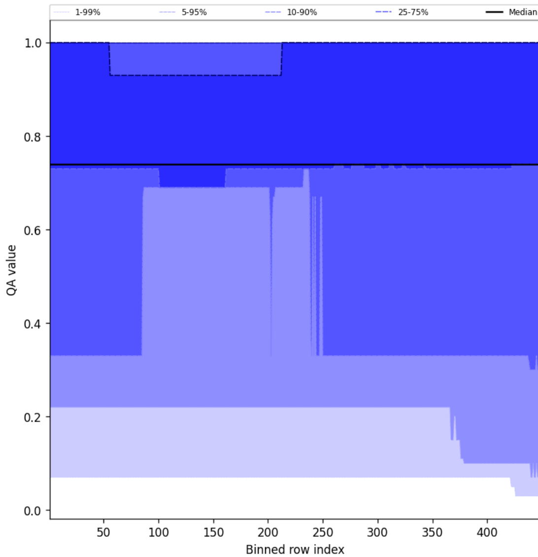
Figure 45: Along track statistics of “QA value” for 2024-11-05 to 2024-11-07
