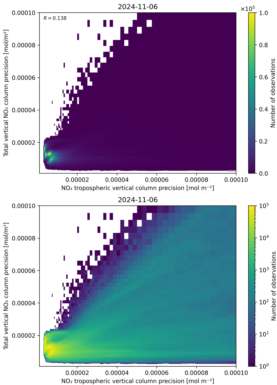
Figure 139: Scatter density plot of “NO 2 tropospheric vertical column precision” against “Total vertical NO 2 column precision” for 2024-11-05 to 2024-11-07.
