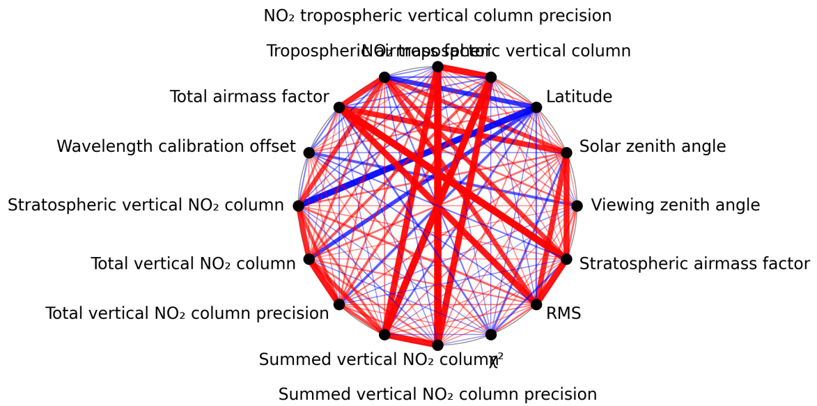
Figure 1: Map of correlation graph for 2024-11-05 to 2024-11-07.
