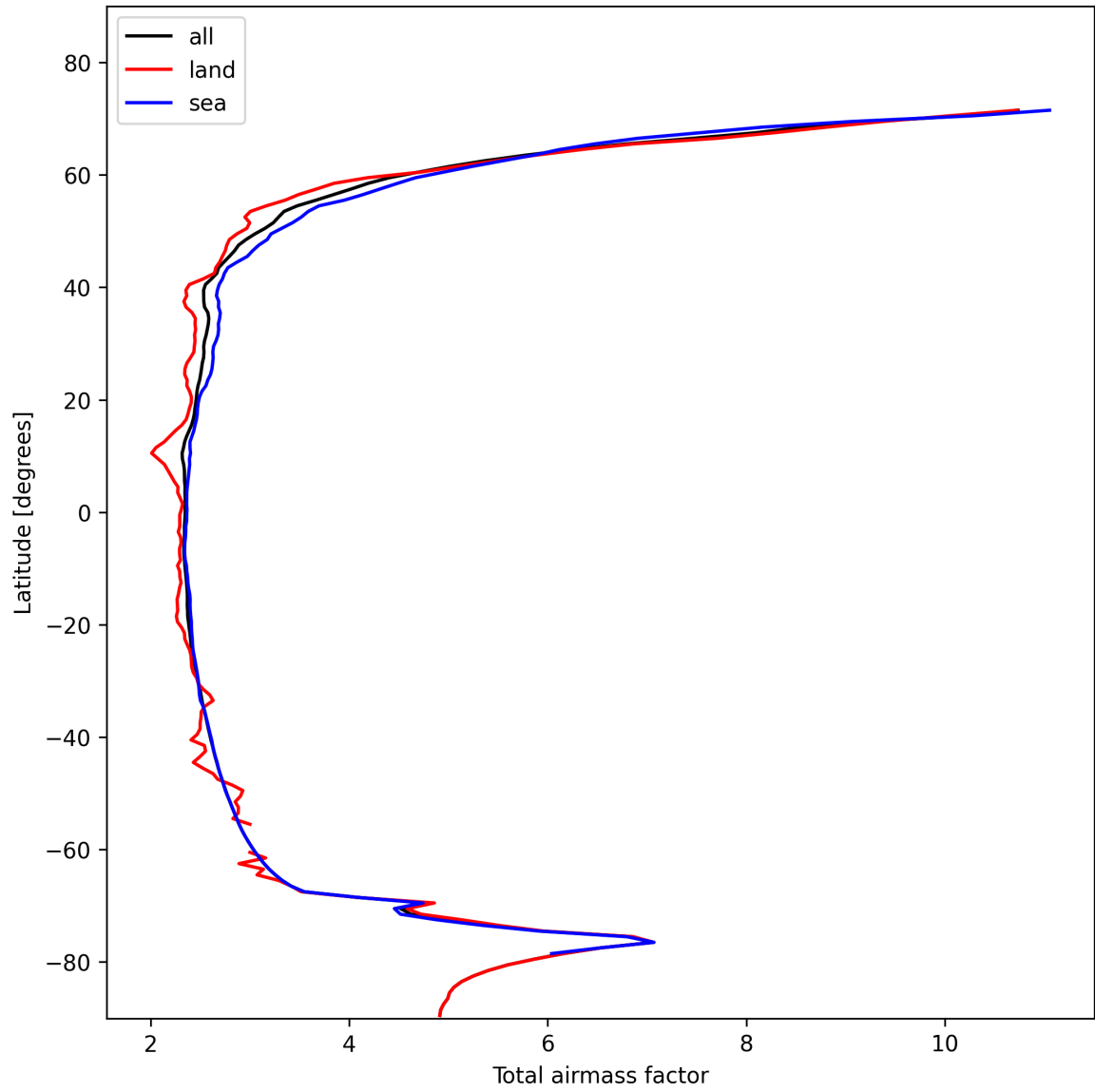
Figure 15: Zonal average of “Total airmass factor” for 2024-11-05 to 2024-11-07.
