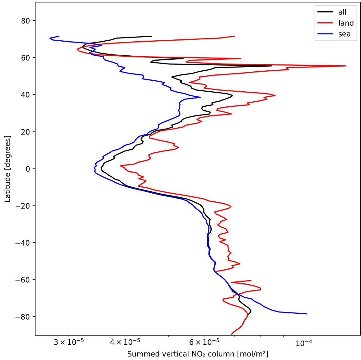
Figure 23: Zonal average of “Summed vertical NO 2 column” for 2024-11-05 to 2024-11-07.
