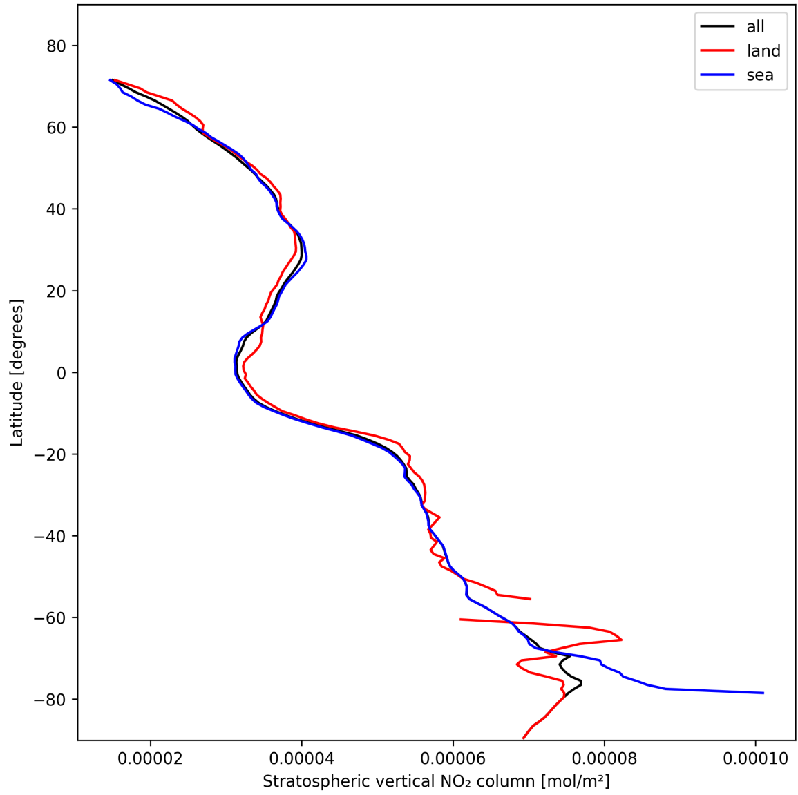
Figure 19: Zonal average of “Stratospheric vertical NO 2 column” for 2024-11-05 to 2024-11-07.
