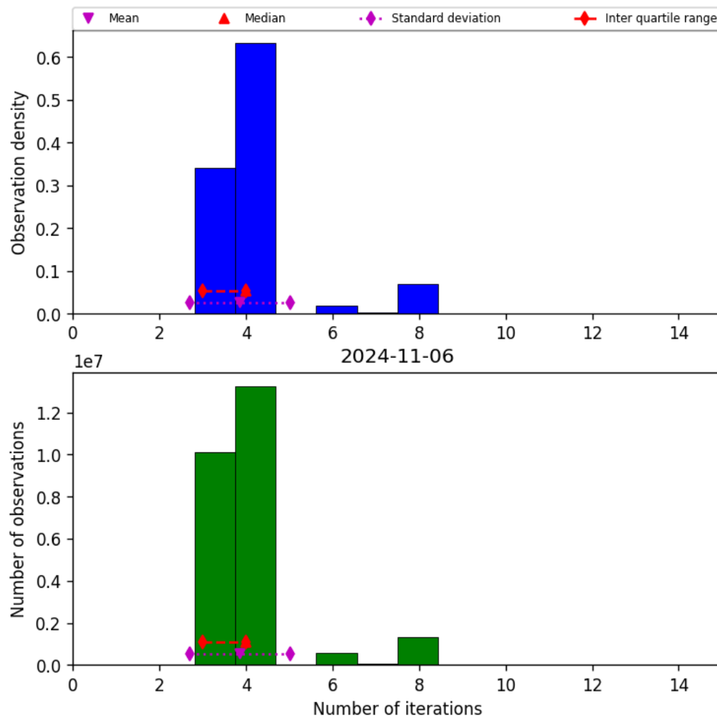
Figure 34: Histogram of “Number of iterations” for 2024-11-05 to 2024-11-07
