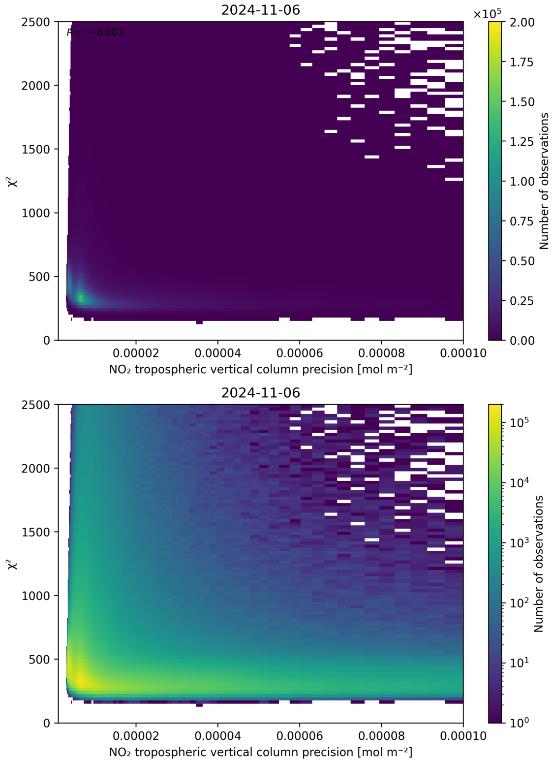
Figure 134: Scatter density plot of “NO 2 tropospheric vertical column precision” against “ \chi^2 ” for 2024-11-05 to 2024-11-07.
