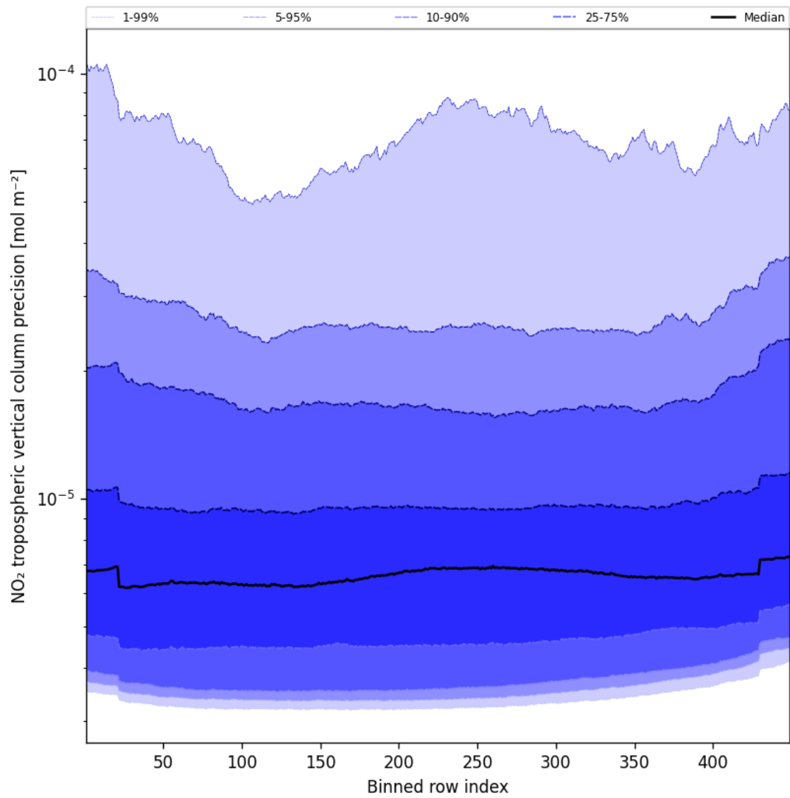
Figure 47: Along track statistics of “NO 2 tropospheric vertical column precision” for 2024-11-05 to 2024-11-07
