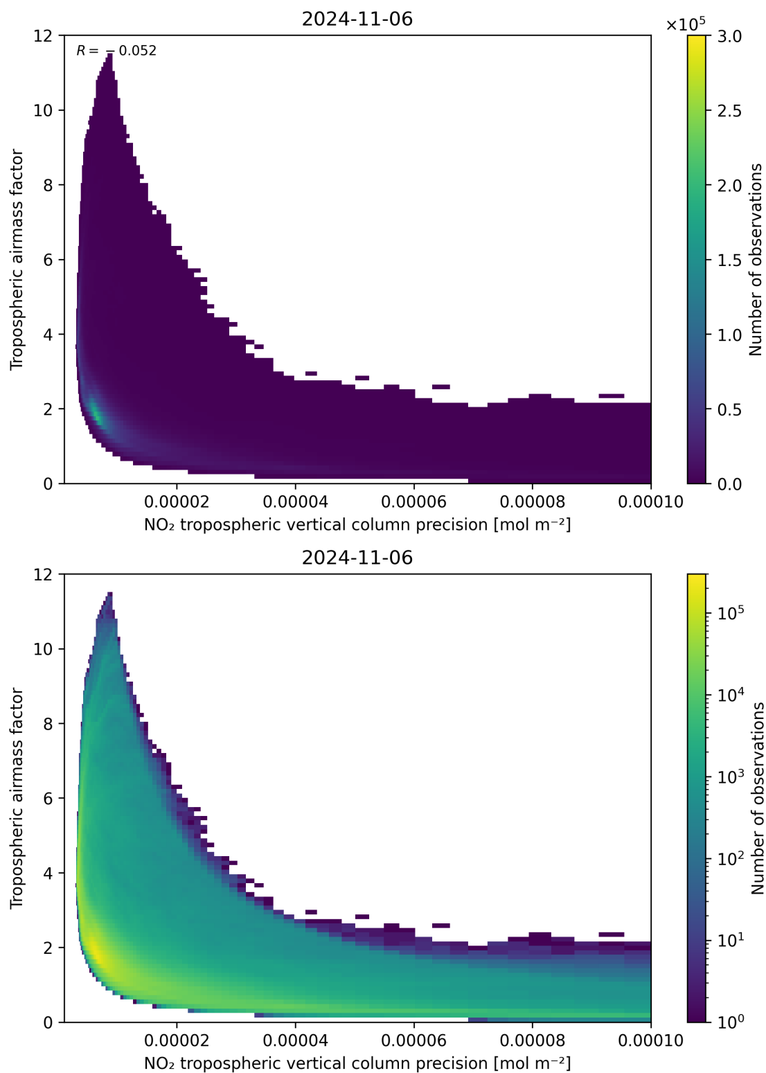
Figure 133: Scatter density plot of “NO 2 tropospheric vertical column precision” against “Tropospheric air mass factor” for 2024-11-05 to 2024-11-07.
