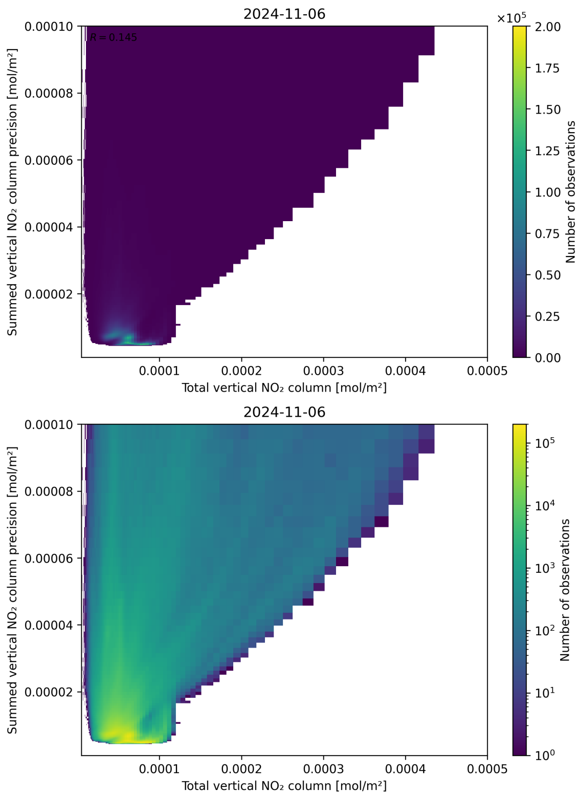
Figure 113: Scatter density plot of “Total vertical NO 2 column” against “Summed vertical NO 2 column precision” for 2024-11-05 to 2024-11-07.
