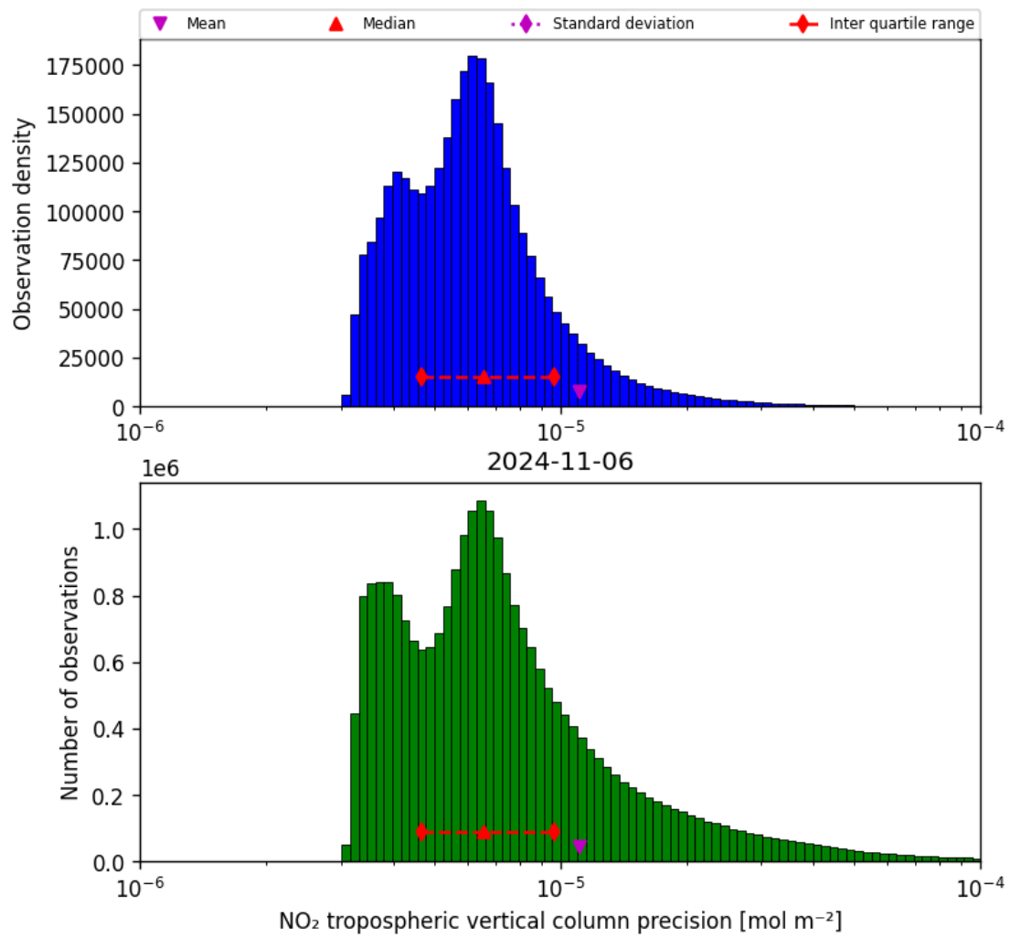
Figure 30: Histogram of “NO 2 tropospheric vertical column precision” for 2024-11-05 to 2024-11-07
