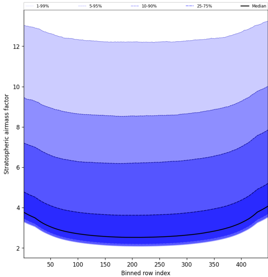
Figure 61: Along track statistics of “Stratospheric airmass factor” for 2024-11-05 to 2024-11-07
