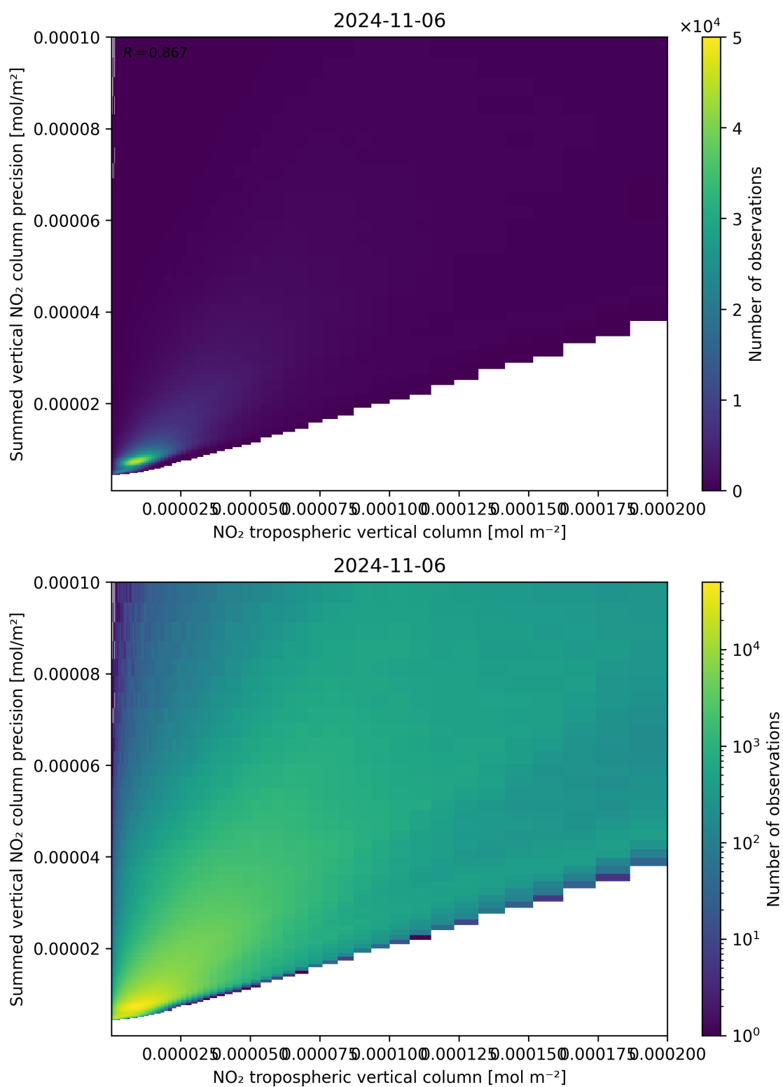
Figure 127: Scatter density plot of “NO 2 tropospheric vertical column” against “Summed vertical NO 2 column precision” for 2024-11-05 to 2024-11-07.
