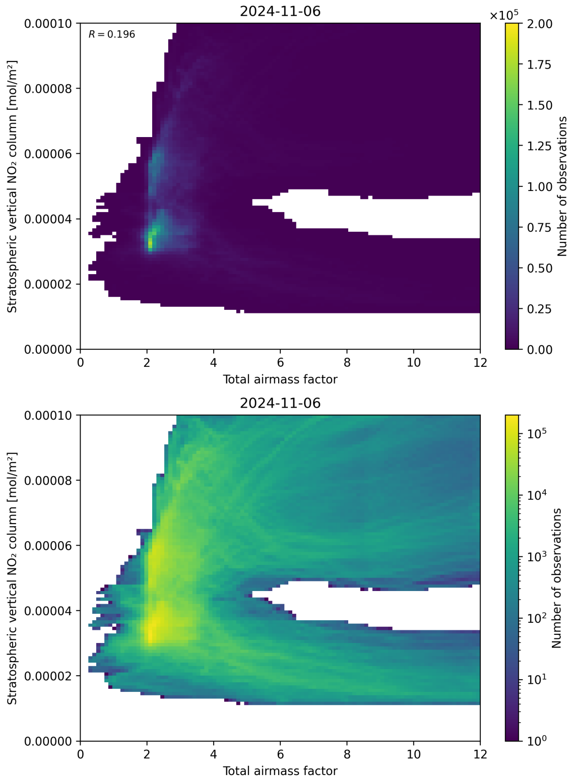
Figure 64: Scatter density plot of “Total airmass factor” against “Stratospheric vertical NO 2 column” for 2024-11-05 to 2024-11-07.
