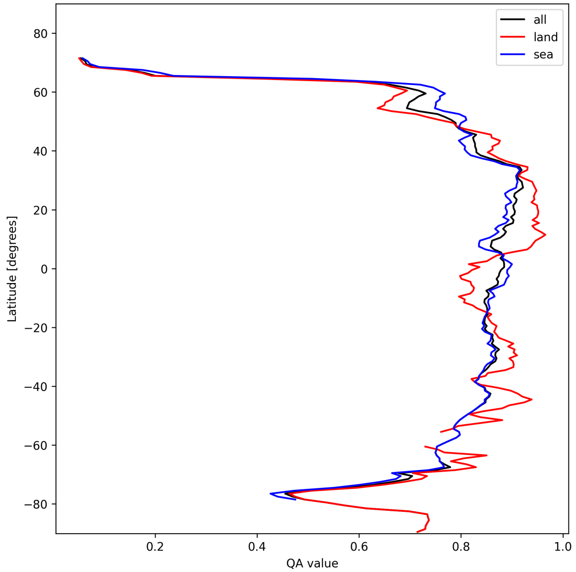
Figure 11: Zonal average of “QA value” for 2024-11-05 to 2024-11-07.
