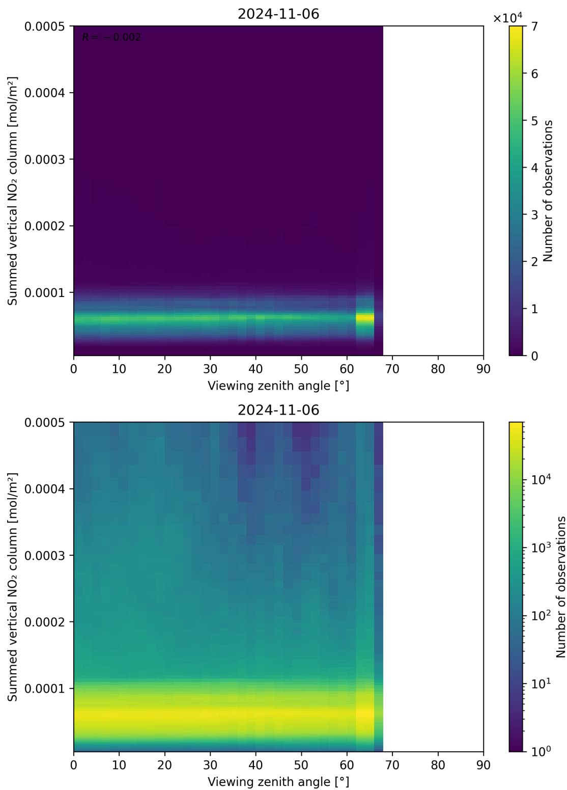
Figure 165: Scatter density plot of “Viewing zenith angle” against “Summed vertical NO 2 column” for 2024-11-05 to 2024-11-07.
