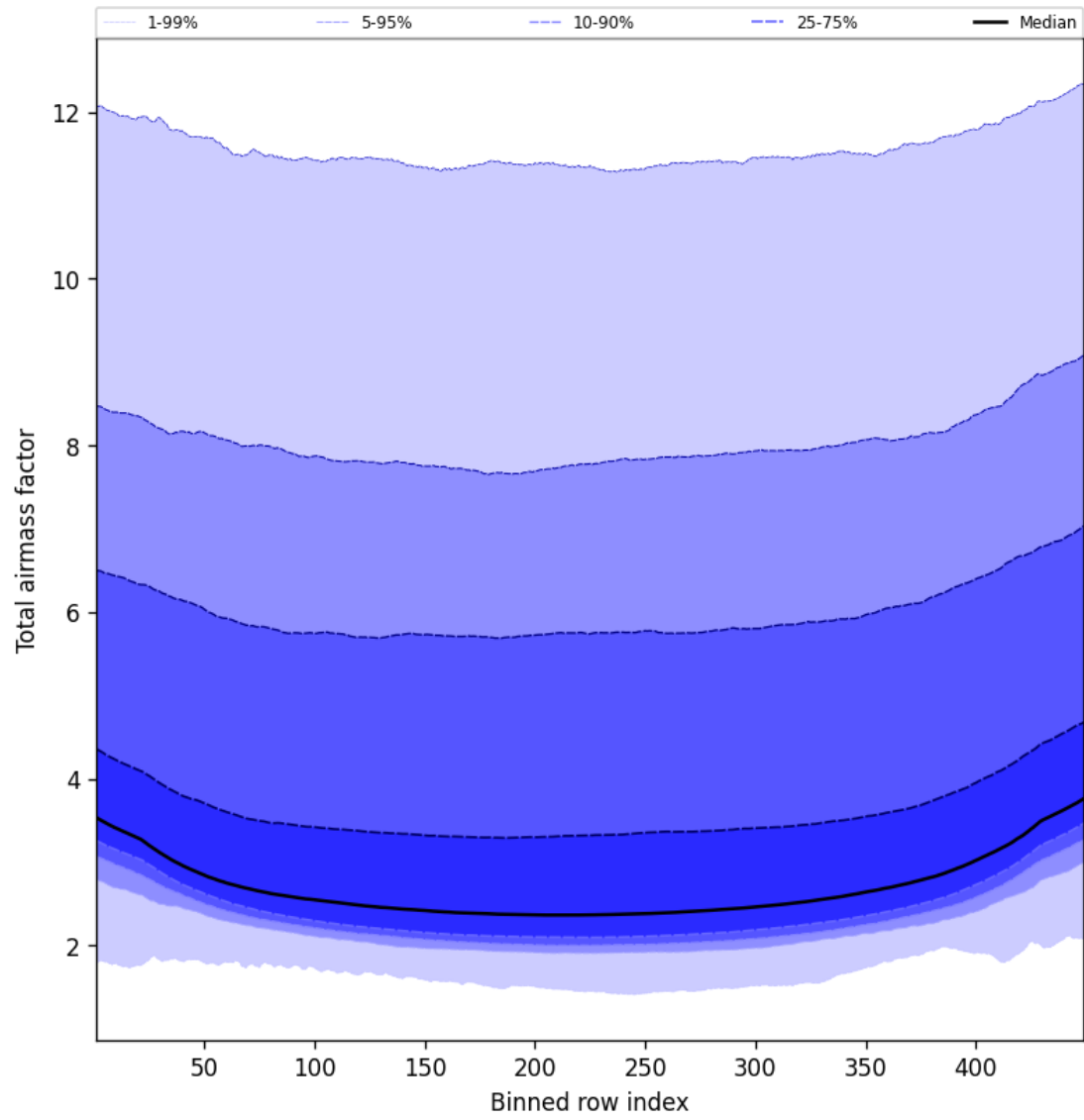
Figure 49: Along track statistics of “Total airmass factor” for 2024-11-05 to 2024-11-07
