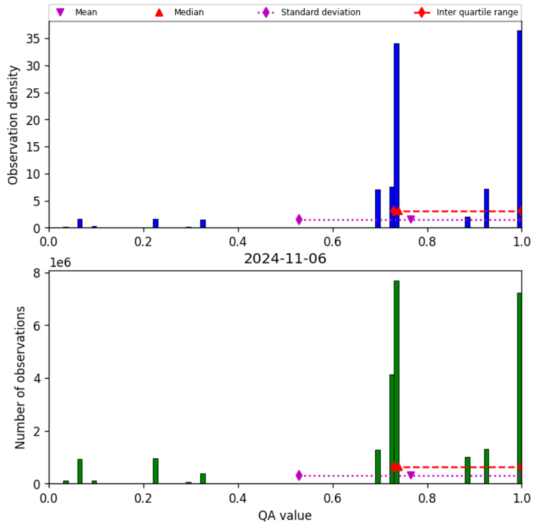
Figure 28: Histogram of “QA value” for 2024-11-05 to 2024-11-07
