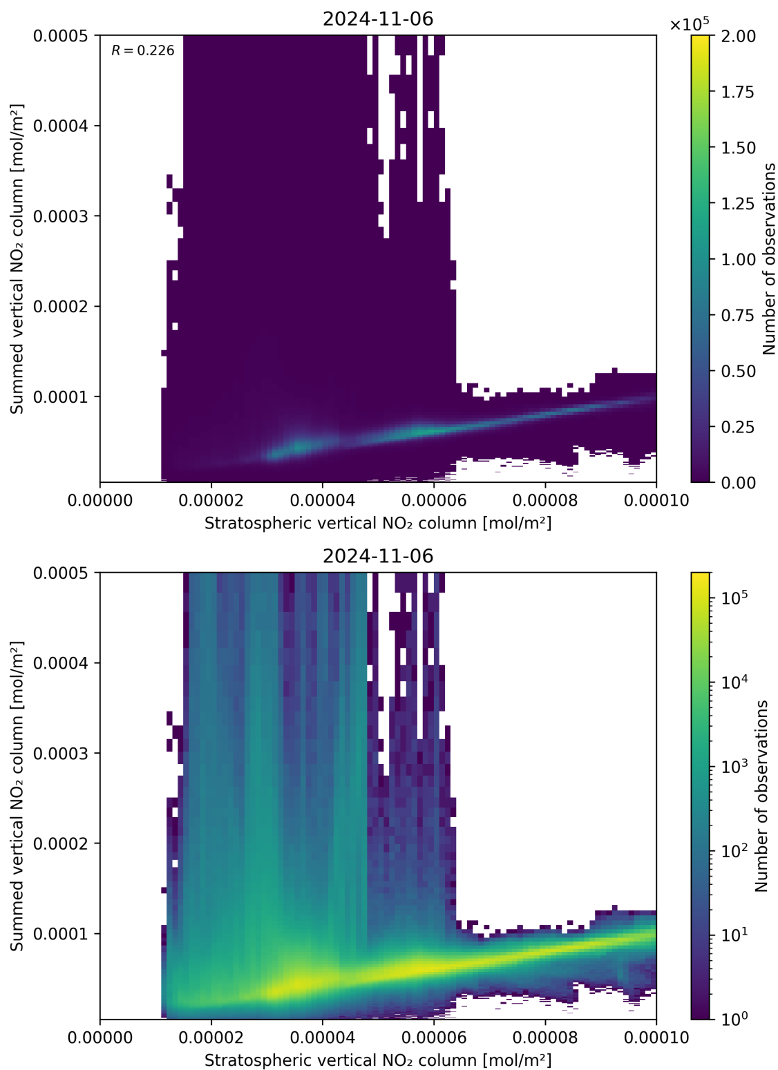
Figure 98: Scatter density plot of “Stratospheric vertical NO 2 column” against “Summed vertical NO 2 column” for 2024-11-05 to 2024-11-07.
