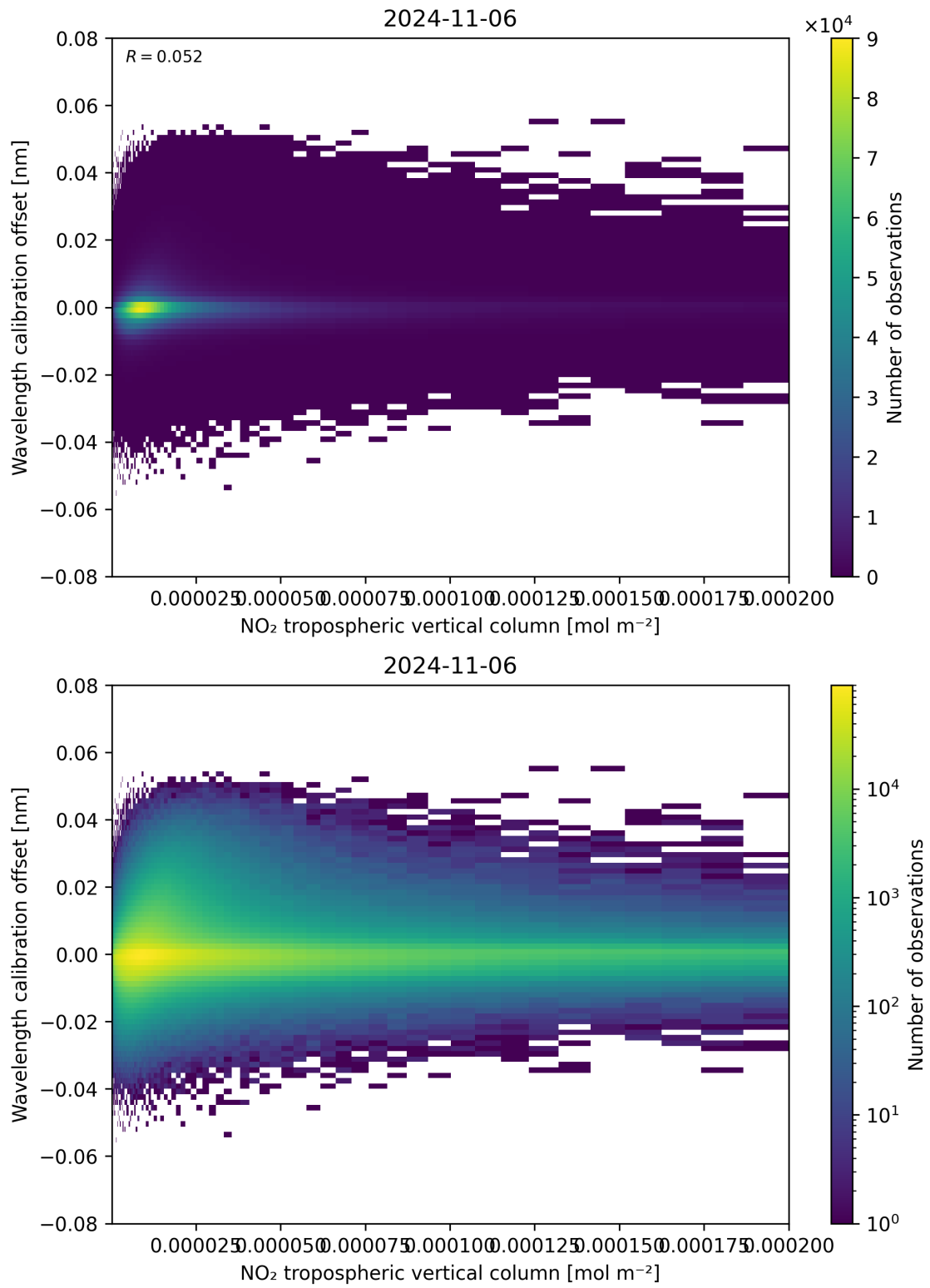
Figure 143: Scatter density plot of “NO 2 tropospheric vertical column” against “Wavelength calibration offset” for 2024-11-05 to 2024-11-07.
