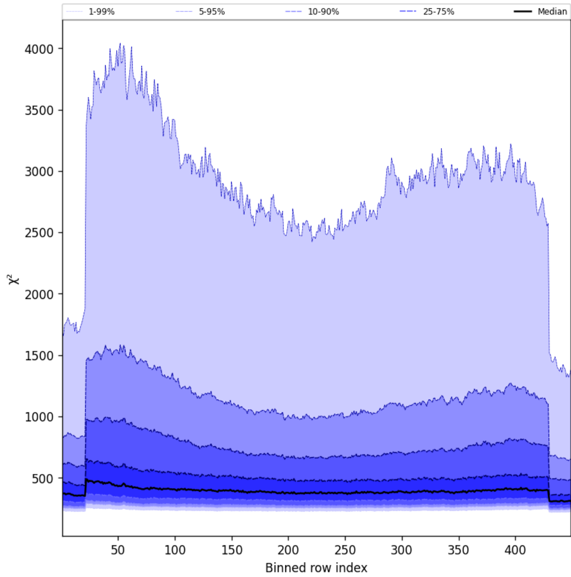
Figure 59: Along track statistics of “ \chi^2 ” for 2024-11-05 to 2024-11-07
