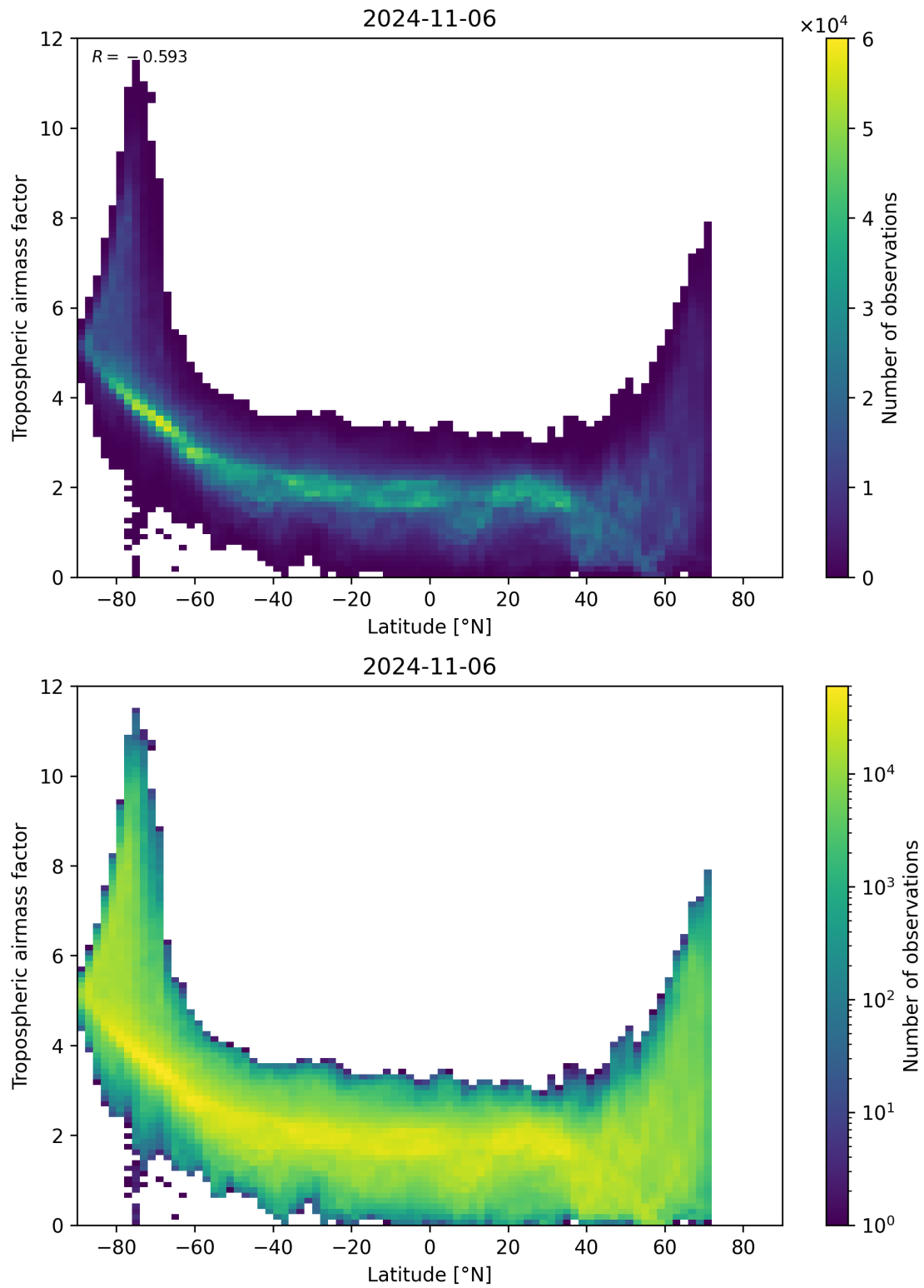
Figure 85: Scatter density plot of “Latitude” against “Tropospheric airmass factor” for 2024-11-05 to 2024-11-07.
