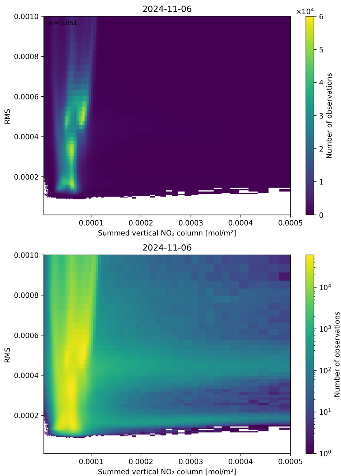
Figure 109: Scatter density plot of “Summed vertical NO 2 column” against “RMS” for 2024-11-05 to 2024-11-07.
