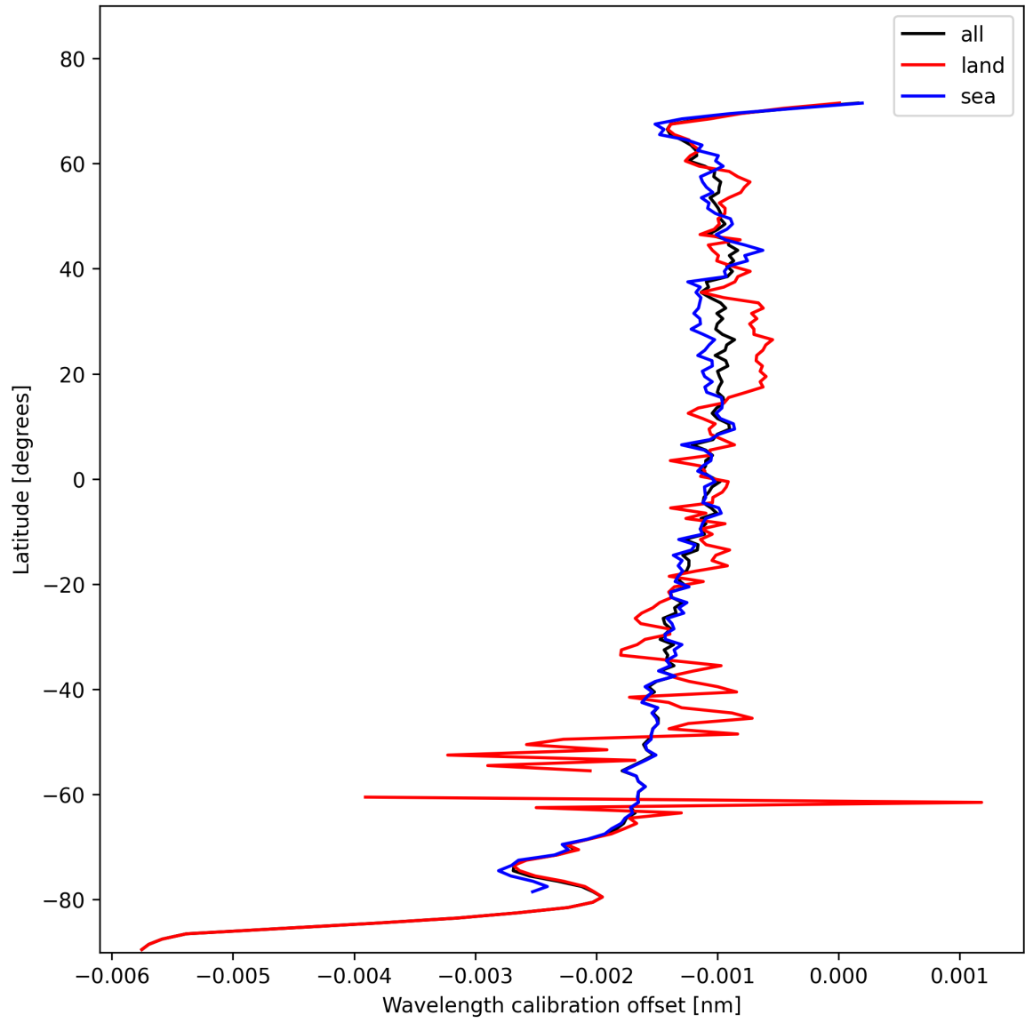
Figure 18: Zonal average of “Wavelength calibration offset” for 2024-11-05 to 2024-11-07.
