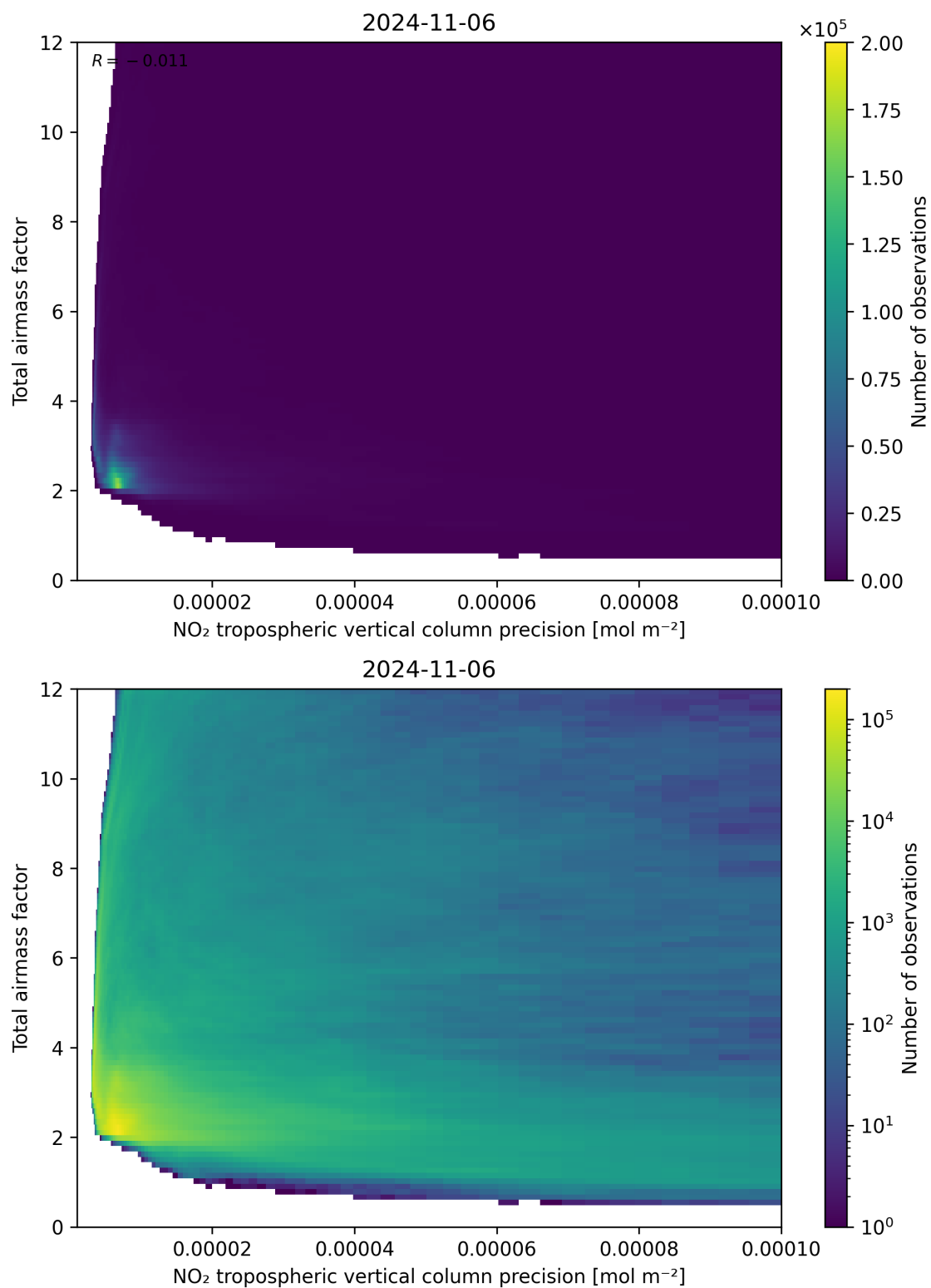
Figure 132: Scatter density plot of “NO 2 tropospheric vertical column precision” against “Total air mass factor” for 2024-11-05 to 2024-11-07.
