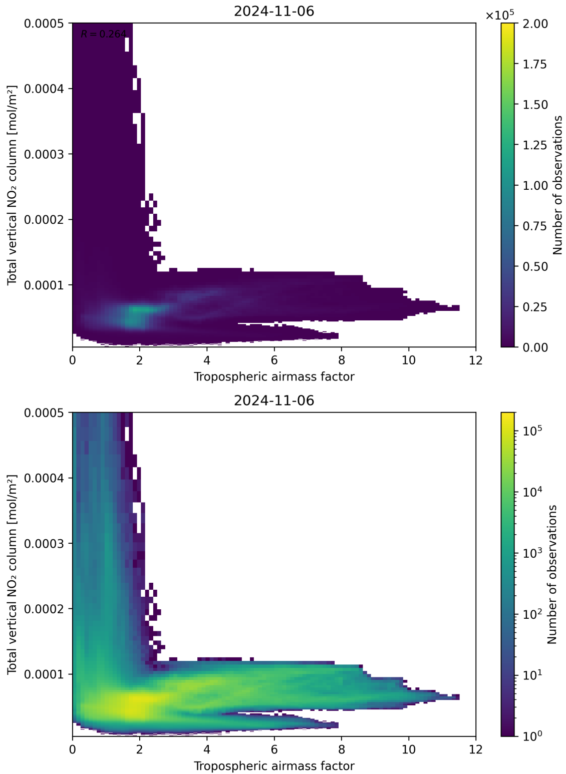
Figure 77: Scatter density plot of “Tropospheric airmass factor” against “Total vertical NO 2 column” for 2024-11-05 to 2024-11-07.
