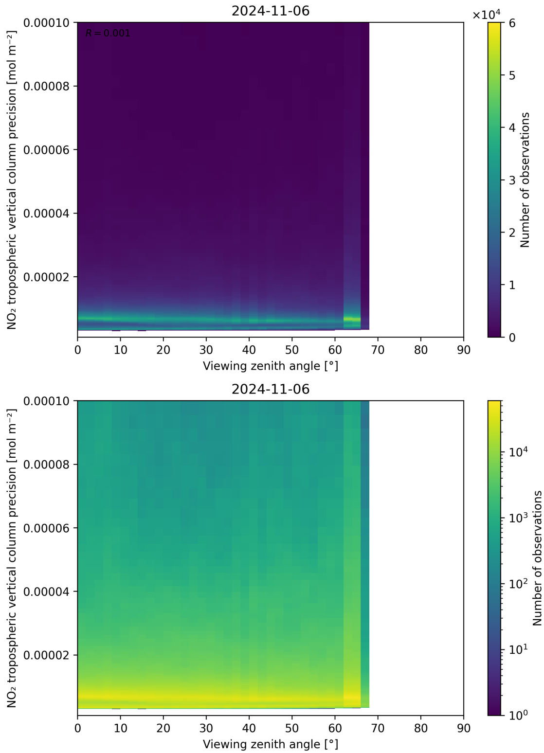
Figure 170: Scatter density plot of “Viewing zenith angle” against “NO 2 tropospheric vertical column precision” for 2024-11-05 to 2024-11-07.
