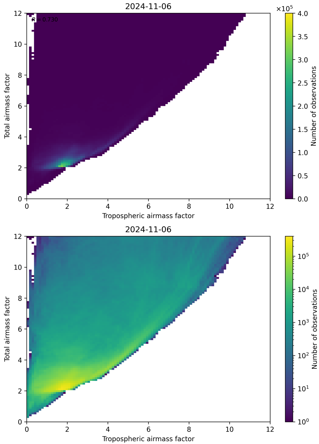
Figure 72: Scatter density plot of “Tropospheric airmass factor” against “Total airmass factor” for 2024-11-05 to 2024-11-07.
