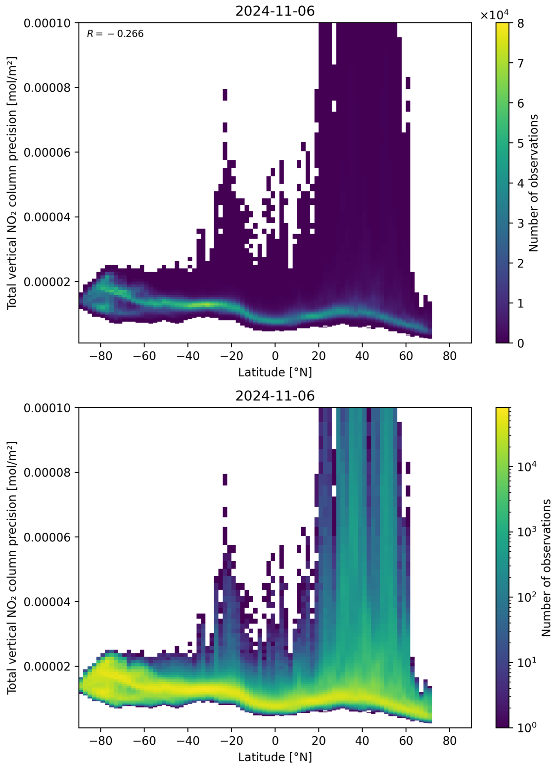
Figure 91: Scatter density plot of “Latitude” against “Total vertical NO 2 column precision” for 2024-11-05 to 2024-11-07.
