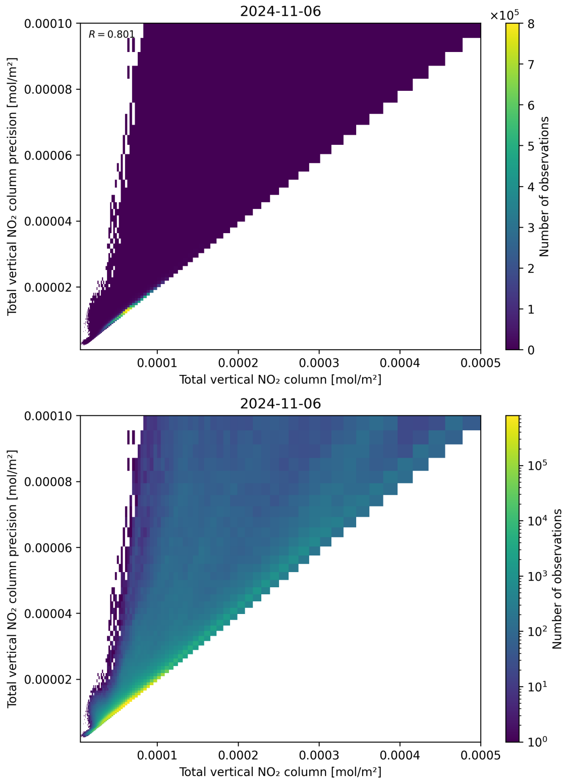
Figure 114: Scatter density plot of “Total vertical NO 2 column” against “Total vertical NO 2 column precision” for 2024-11-05 to 2024-11-07.
