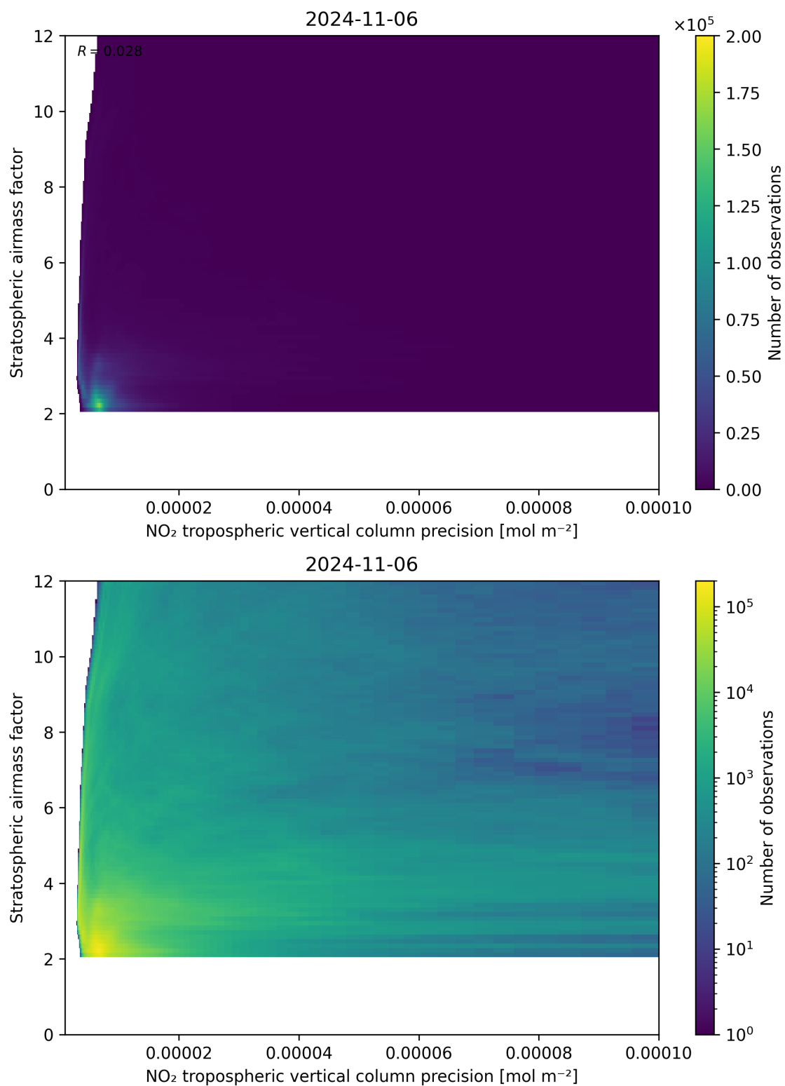
Figure 131: Scatter density plot of “NO 2 tropospheric vertical column precision” against “Stratospheric airmass factor” for 2024-11-05 to 2024-11-07.
