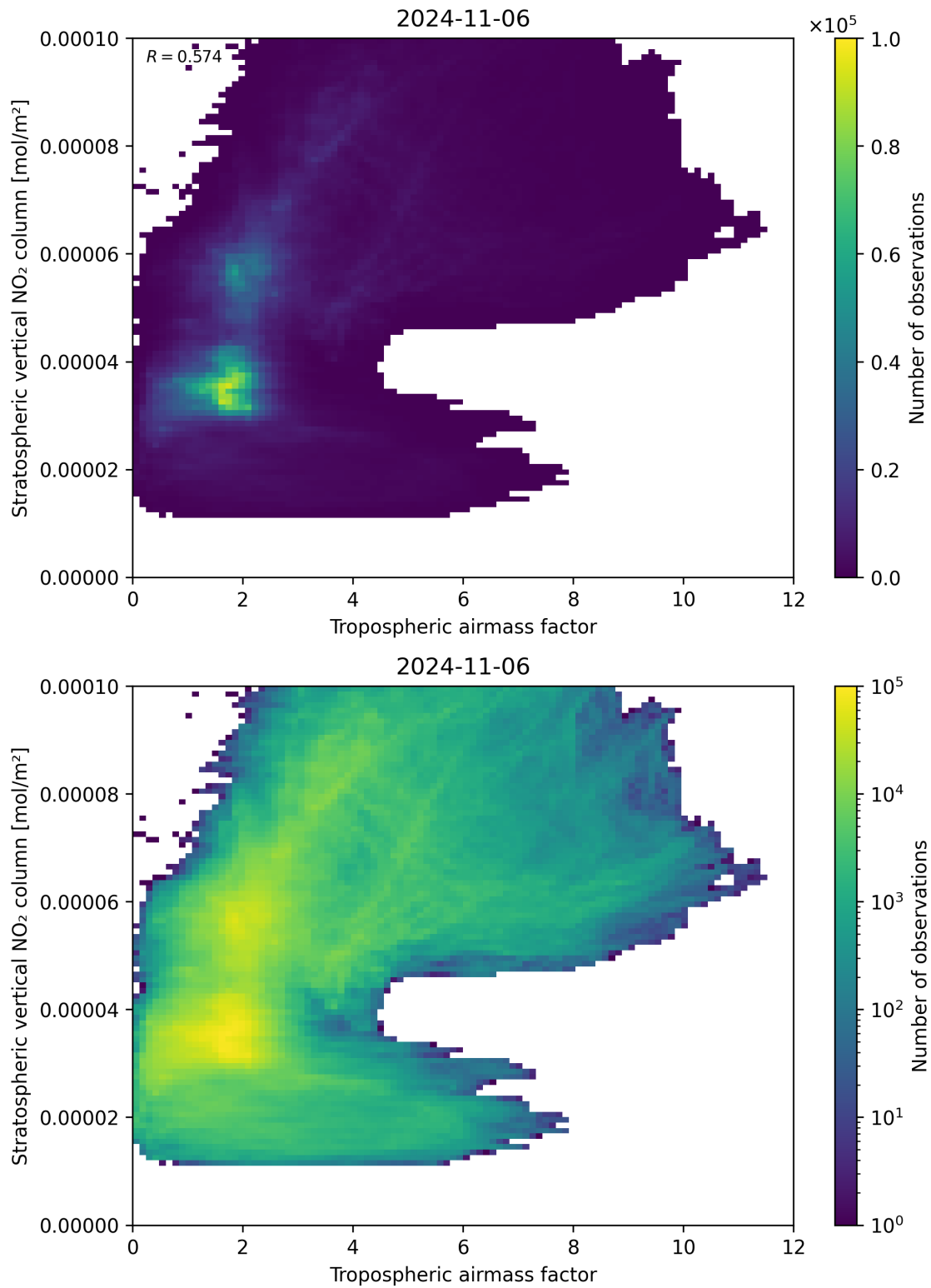
Figure 74: Scatter density plot of “Tropospheric air mass factor” against “Stratospheric vertical NO 2 column” for 2024-11-05 to 2024-11-07.
