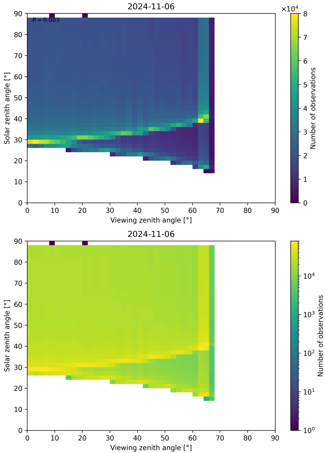
Figure 172: Scatter density plot of “Viewing zenith angle” against “Solar zenith angle” for 2024-11-05 to 2024-11-07.
