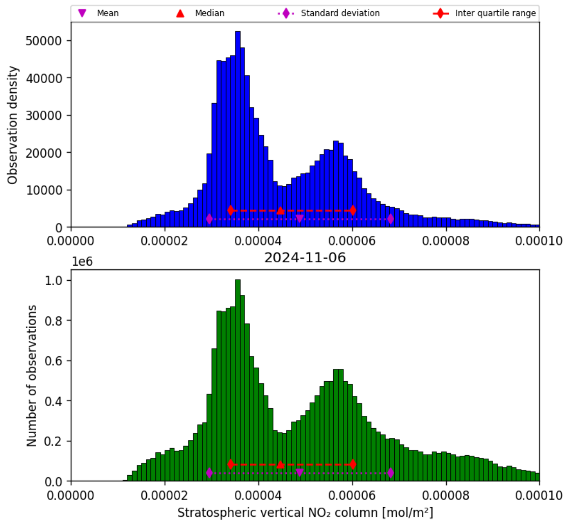
Figure 36: Histogram of “Stratospheric vertical NO 2 column” for 2024-11-05 to 2024-11-07
