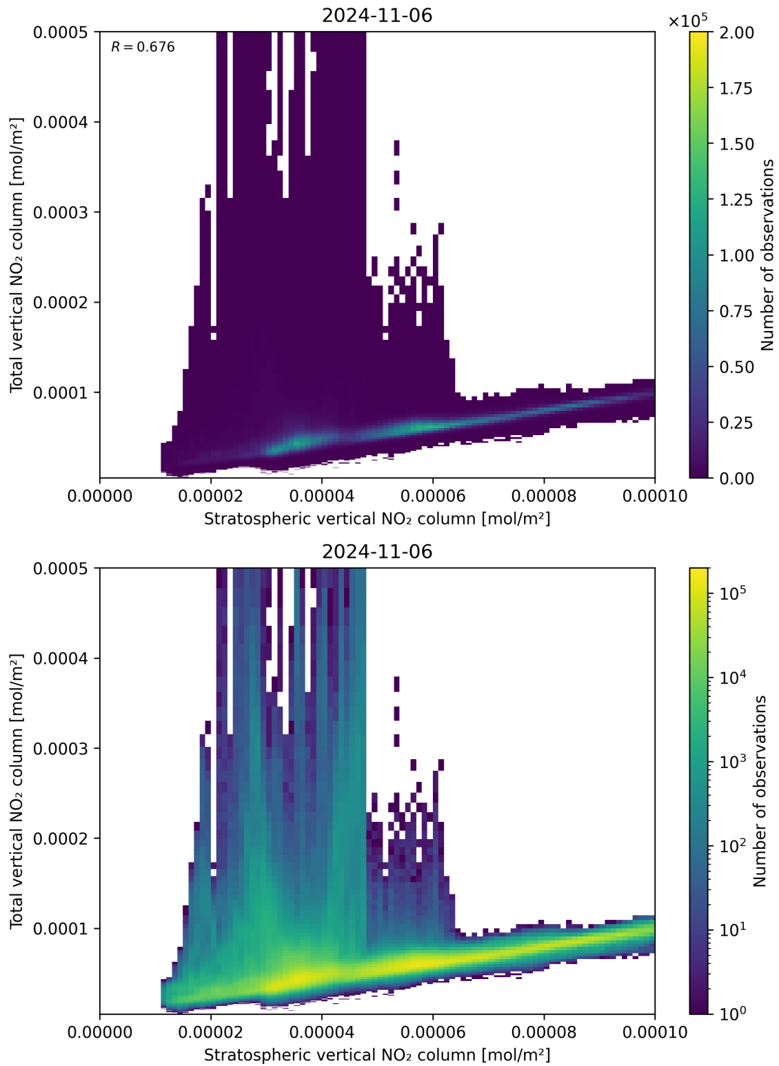
Figure 100: Scatter density plot of “Stratospheric vertical NO 2 column” against “Total vertical NO 2 column” for 2024-11-05 to 2024-11-07.
