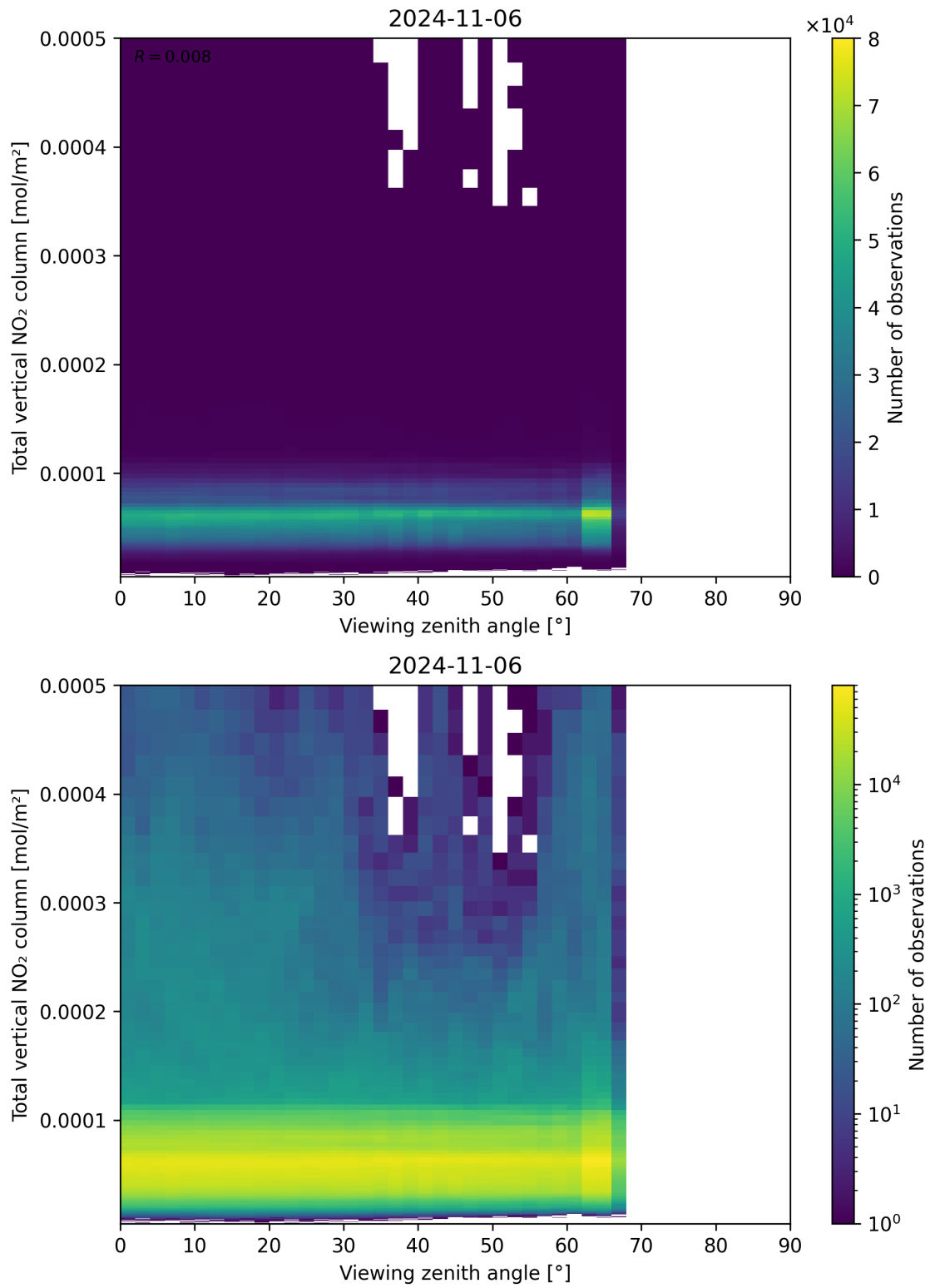
Figure 167: Scatter density plot of “Viewing zenith angle” against “Total vertical NO 2 column” for 2024-11-05 to 2024-11-07.
