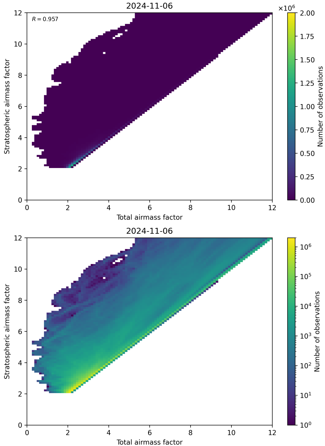
Figure 62: Scatter density plot of “Total airmass factor” against “Stratospheric airmass factor” for 2024-11-05 to 2024-11-07.
