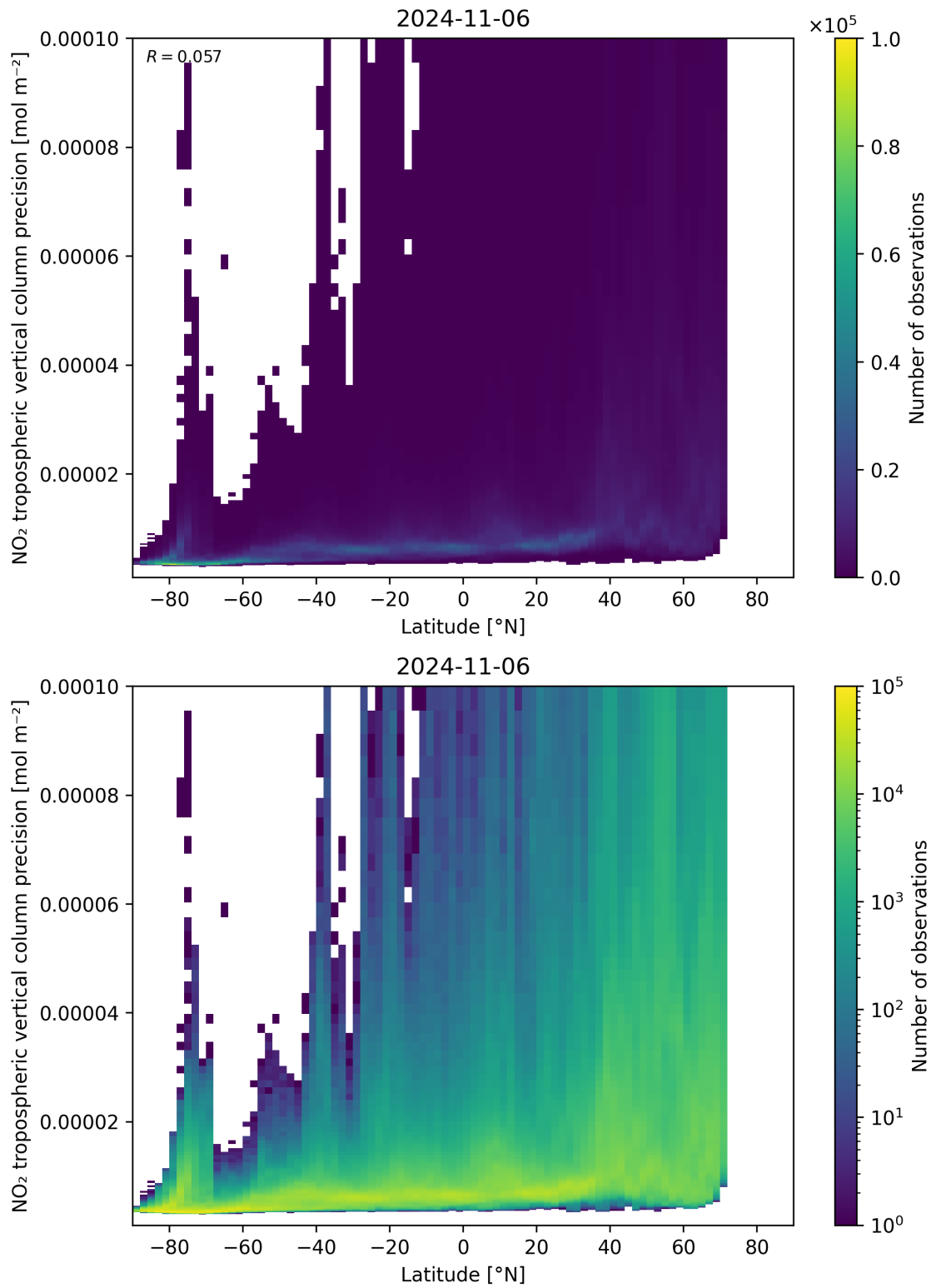
Figure 93: Scatter density plot of “Latitude” against “NO 2 tropospheric vertical column precision” for 2024-11-05 to 2024-11-07.
