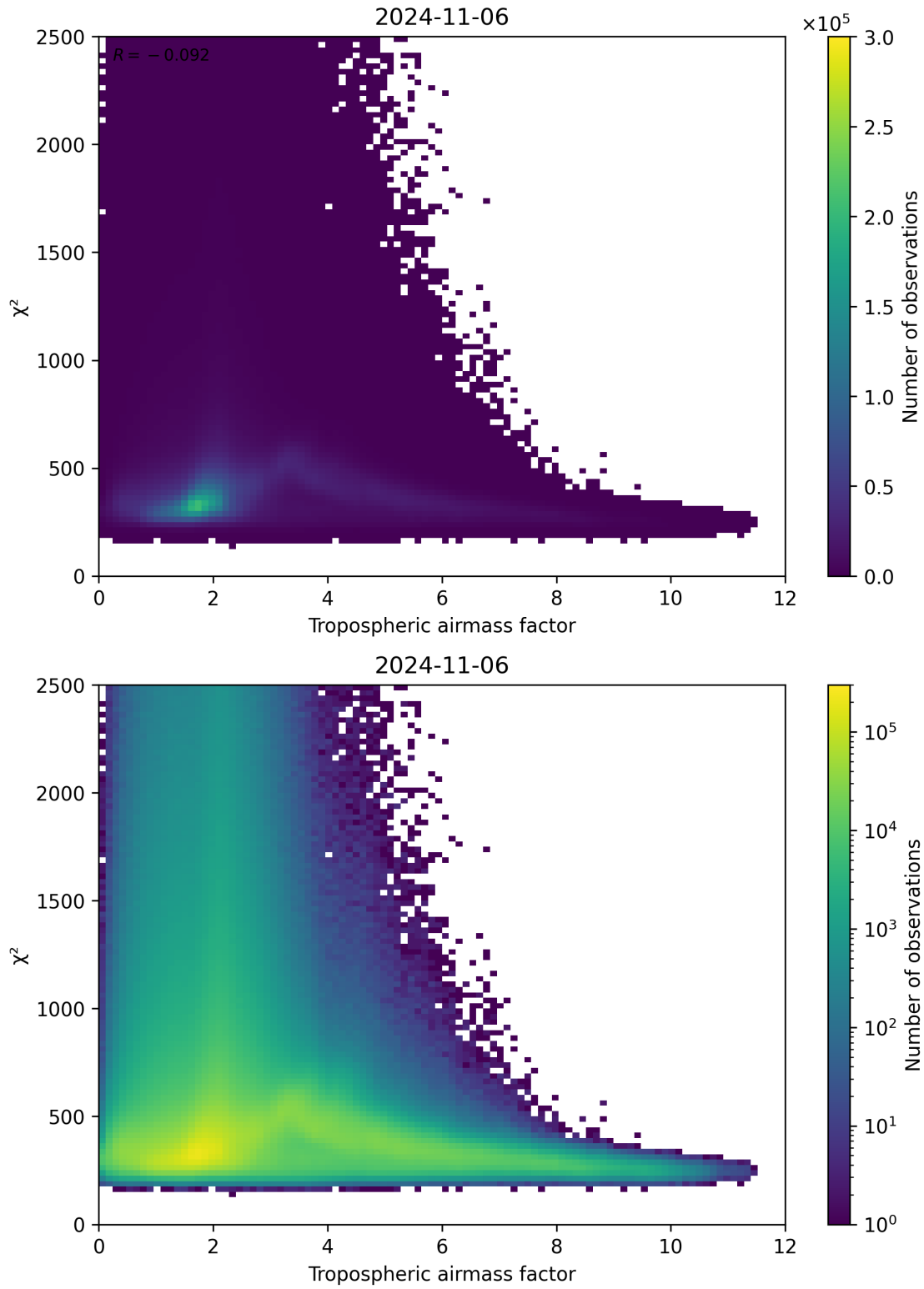
Figure 73: Scatter density plot of “Tropospheric airmass factor” against “ \chi^2 ” for 2024-11-05 to 2024-11-07.
