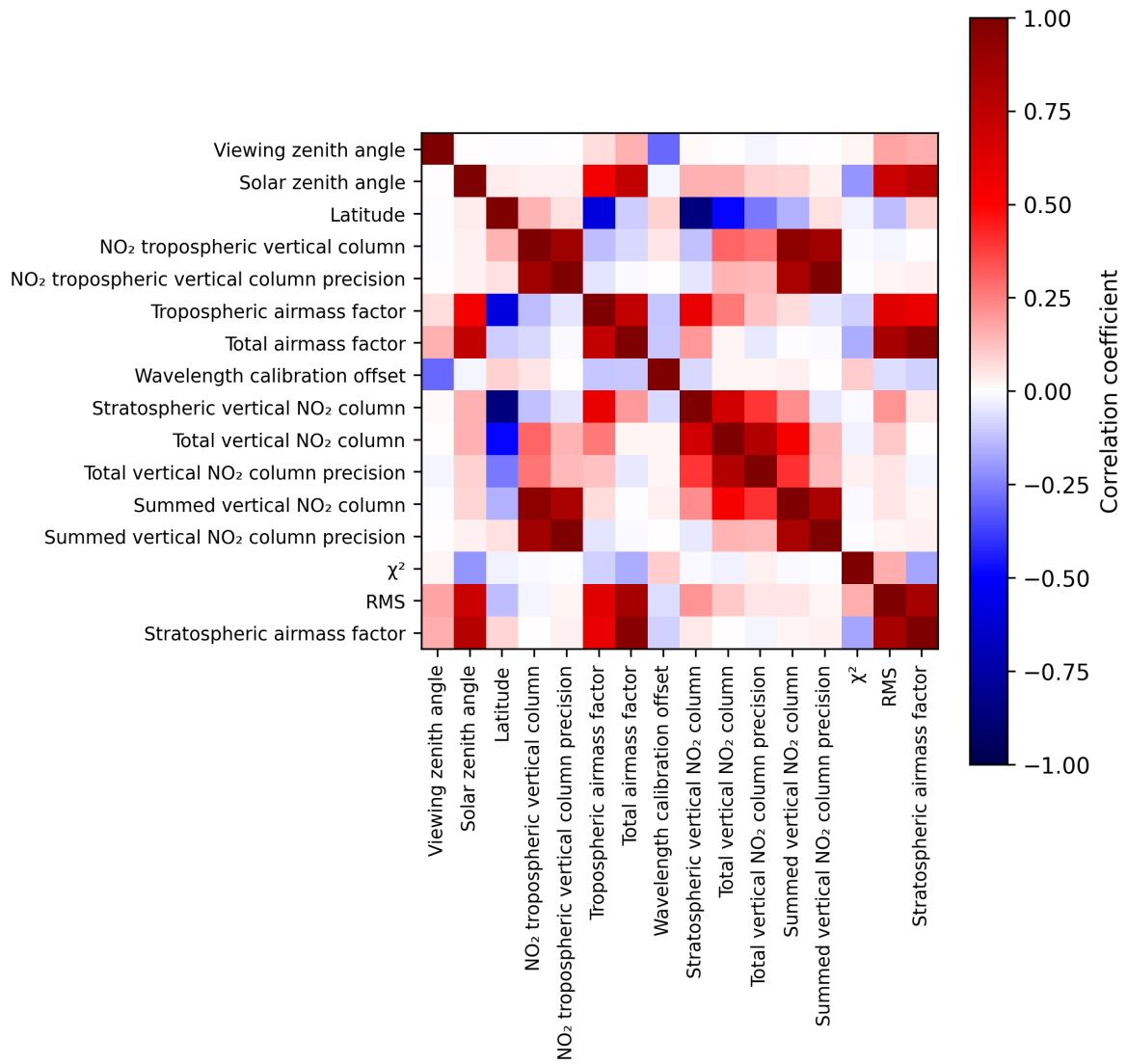
Figure 2: Map of correlation matrix for 2024-11-05 to 2024-11-07.
