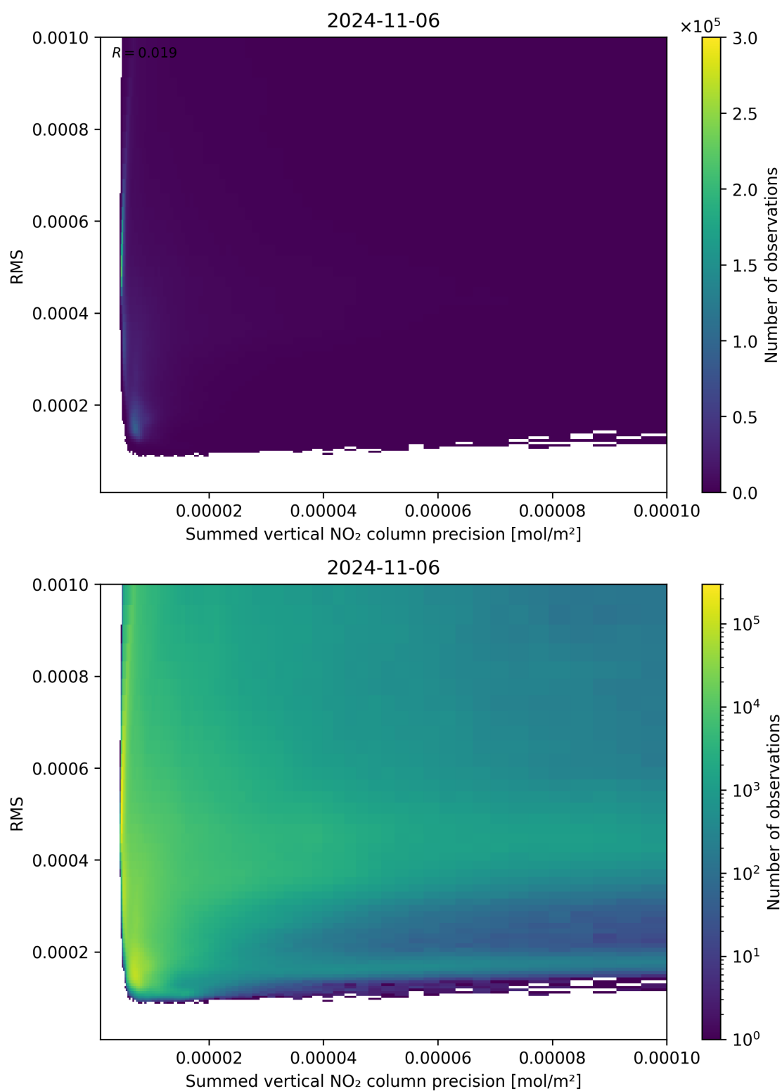
Figure 108: Scatter density plot of “Summed vertical NO 2 column precision” against “RMS” for 2024-11-05 to 2024-11-07.
