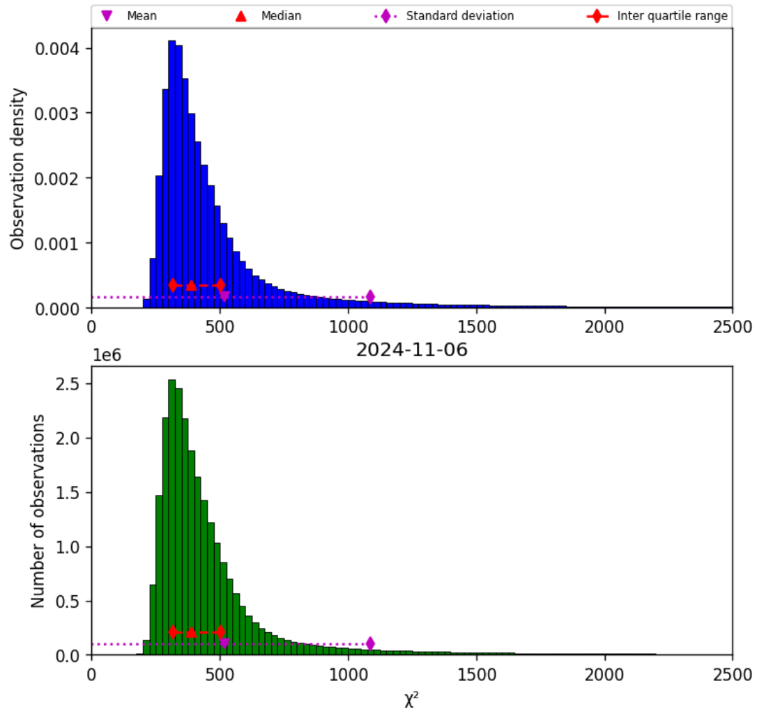
Figure 42: Histogram of “ \chi^2 ” for 2024-11-05 to 2024-11-07
