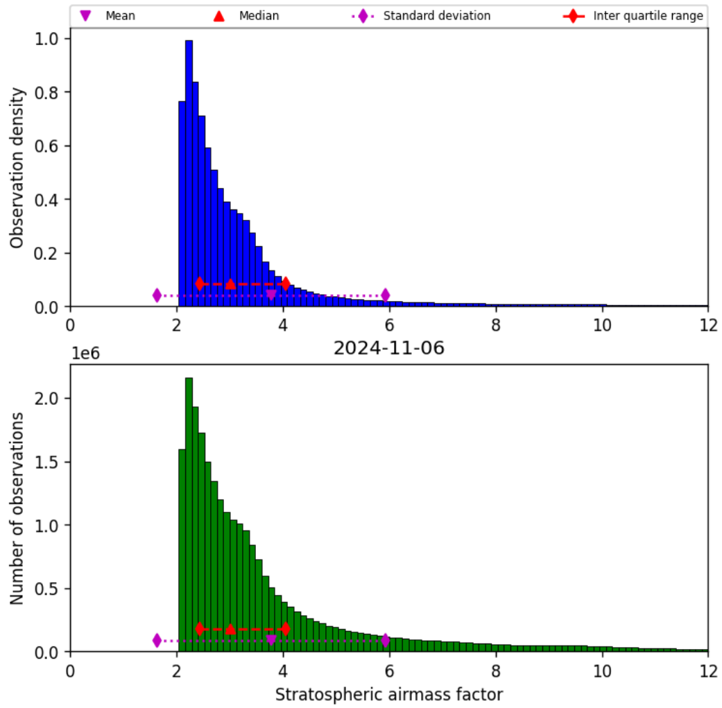
Figure 44: Histogram of “Stratospheric airmass factor” for 2024-11-05 to 2024-11-07
