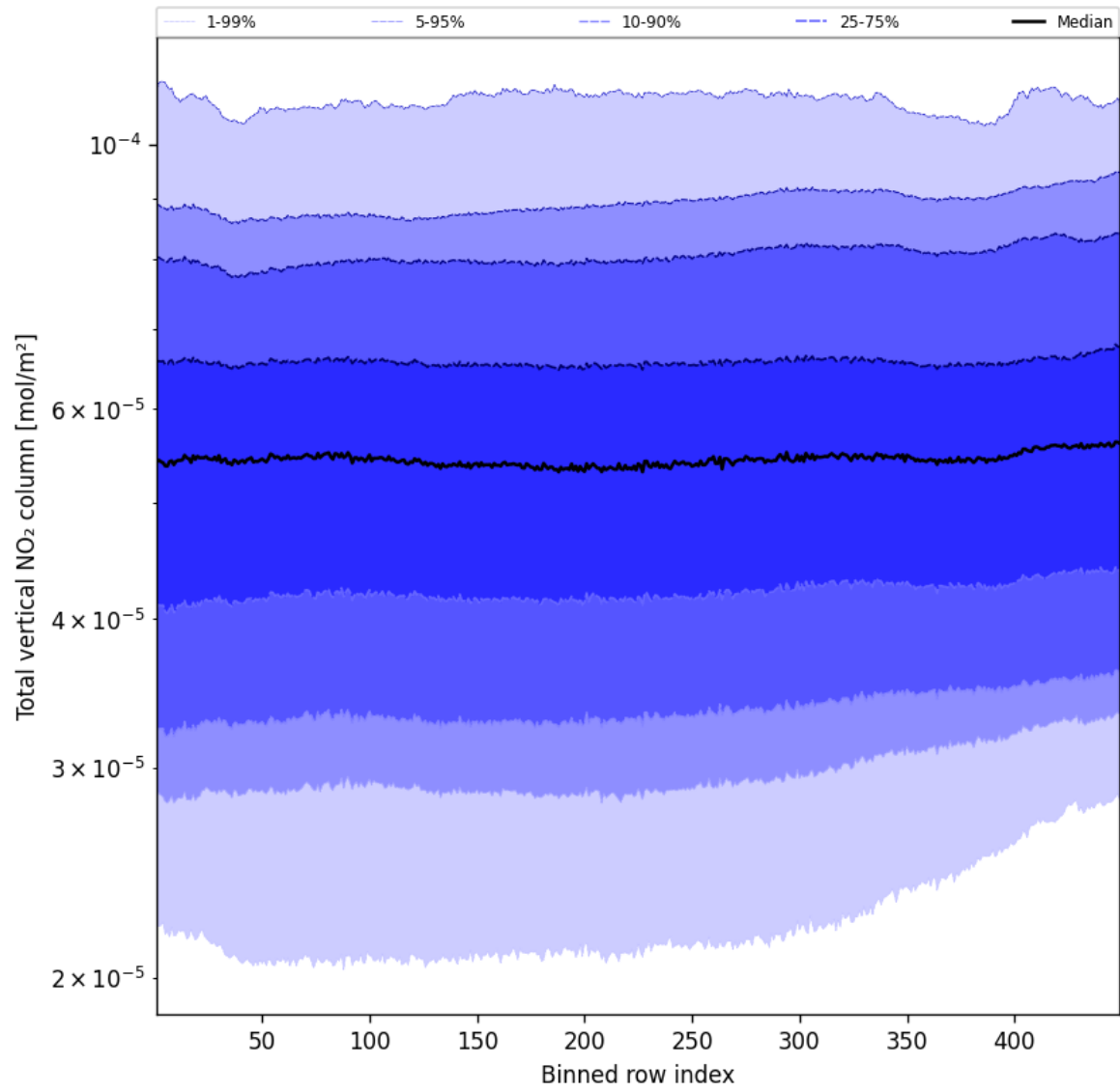
Figure 55: Along track statistics of "Total vertical NO 2 column" for 2024-11-05 to 2024-11-07
