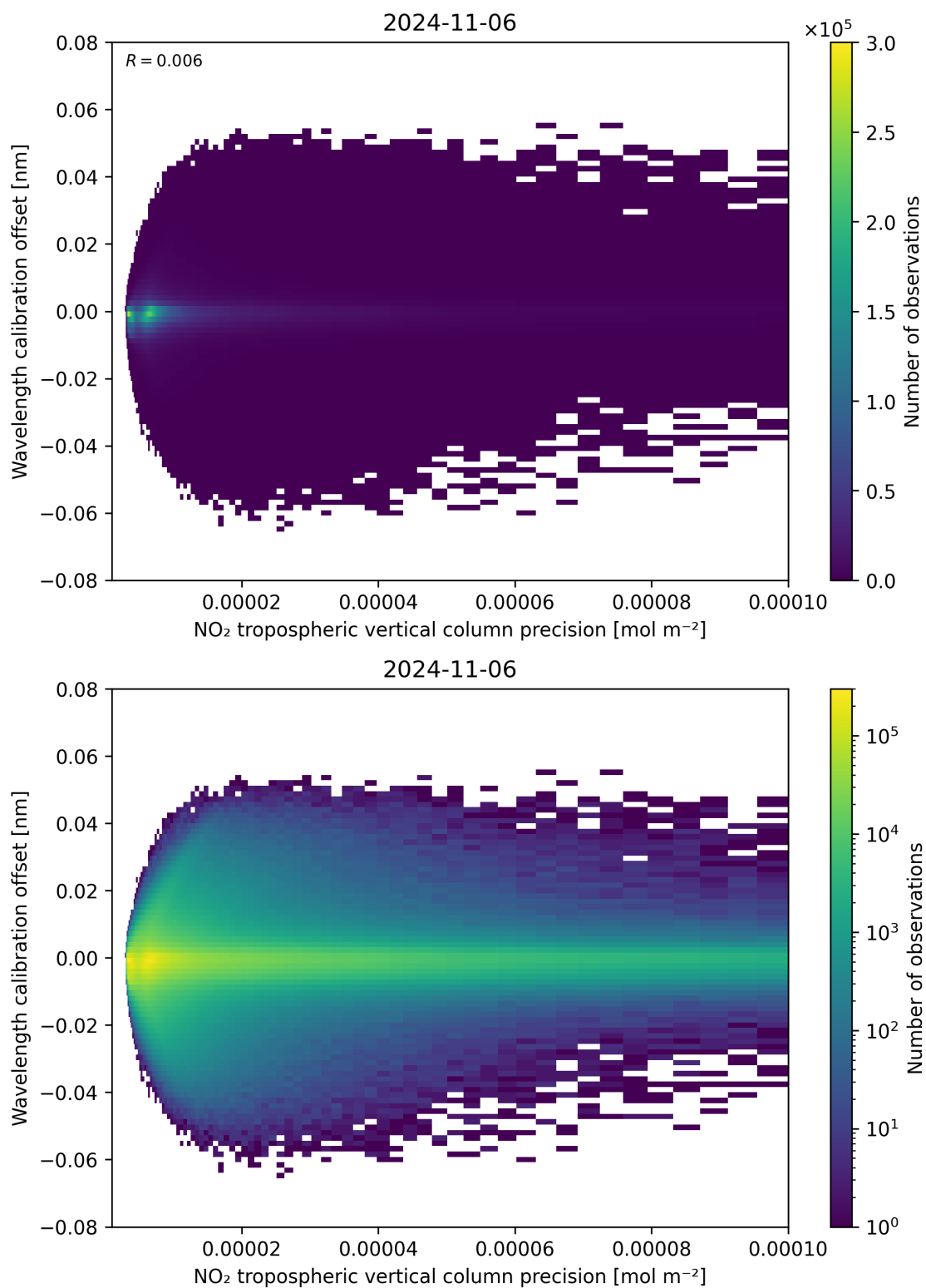
Figure 141: Scatter density plot of “NO 2 tropospheric vertical column precision” against “Wavelength calibration offset” for 2024-11-05 to 2024-11-07.
