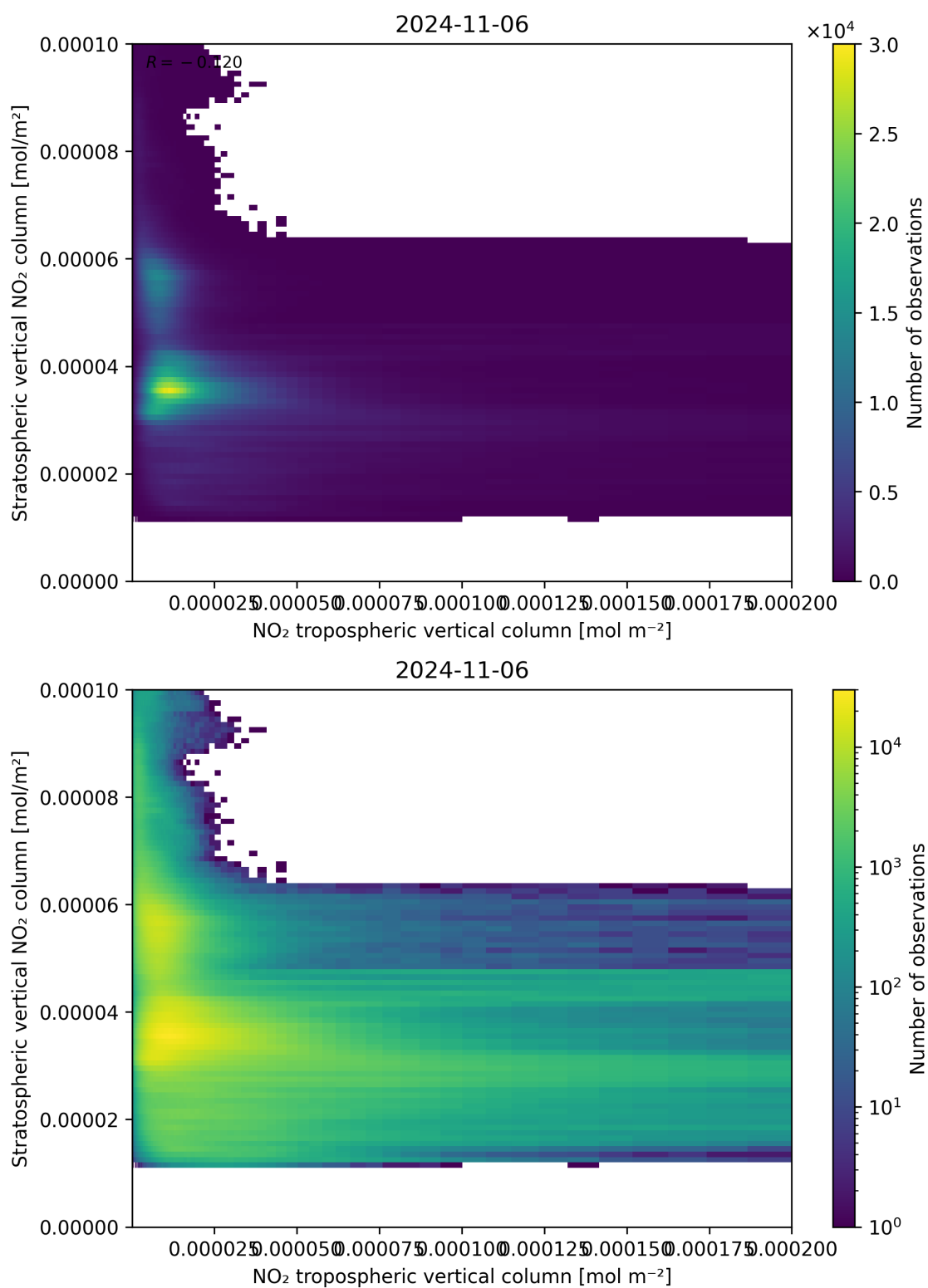
Figure 125: Scatter density plot of “NO 2 tropospheric vertical column” against “Stratospheric vertical NO 2 column” for 2024-11-05 to 2024-11-07.
