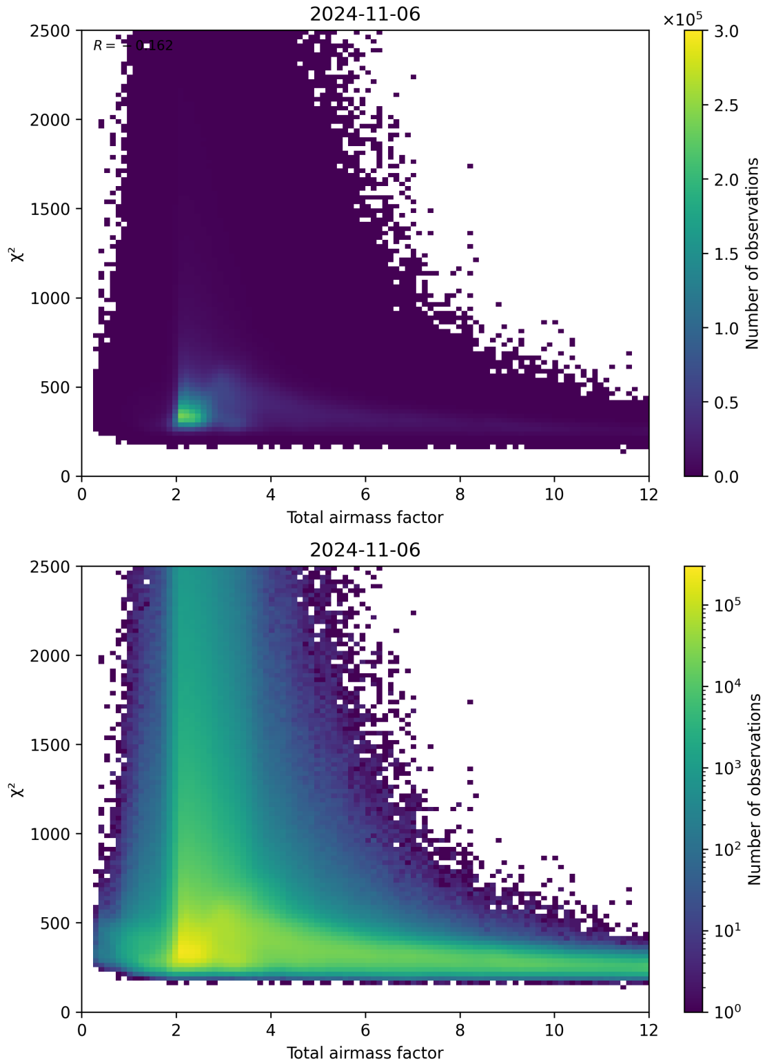
Figure 63: Scatter density plot of “Total airmass factor” against “ \chi^2 ” for 2024-11-05 to 2024-11-07.
