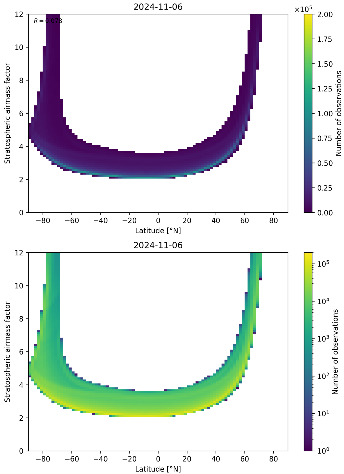
Figure 83: Scatter density plot of “Latitude” against “Stratospheric air mass factor” for 2024-11-05 to 2024-11-07.
