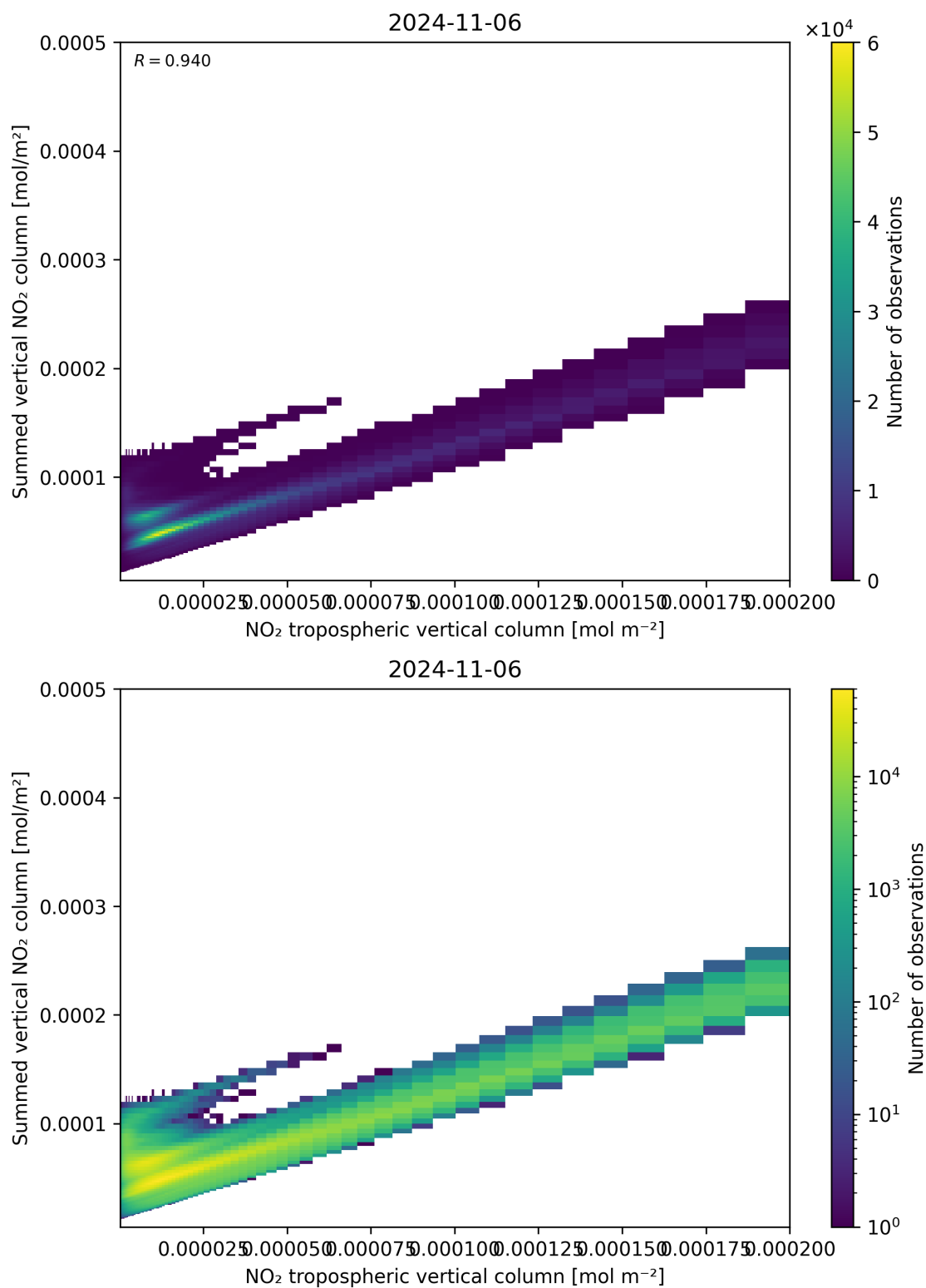
Figure 126: Scatter density plot of “NO 2 tropospheric vertical column” against “Summed vertical NO 2 column” for 2024-11-05 to 2024-11-07.
