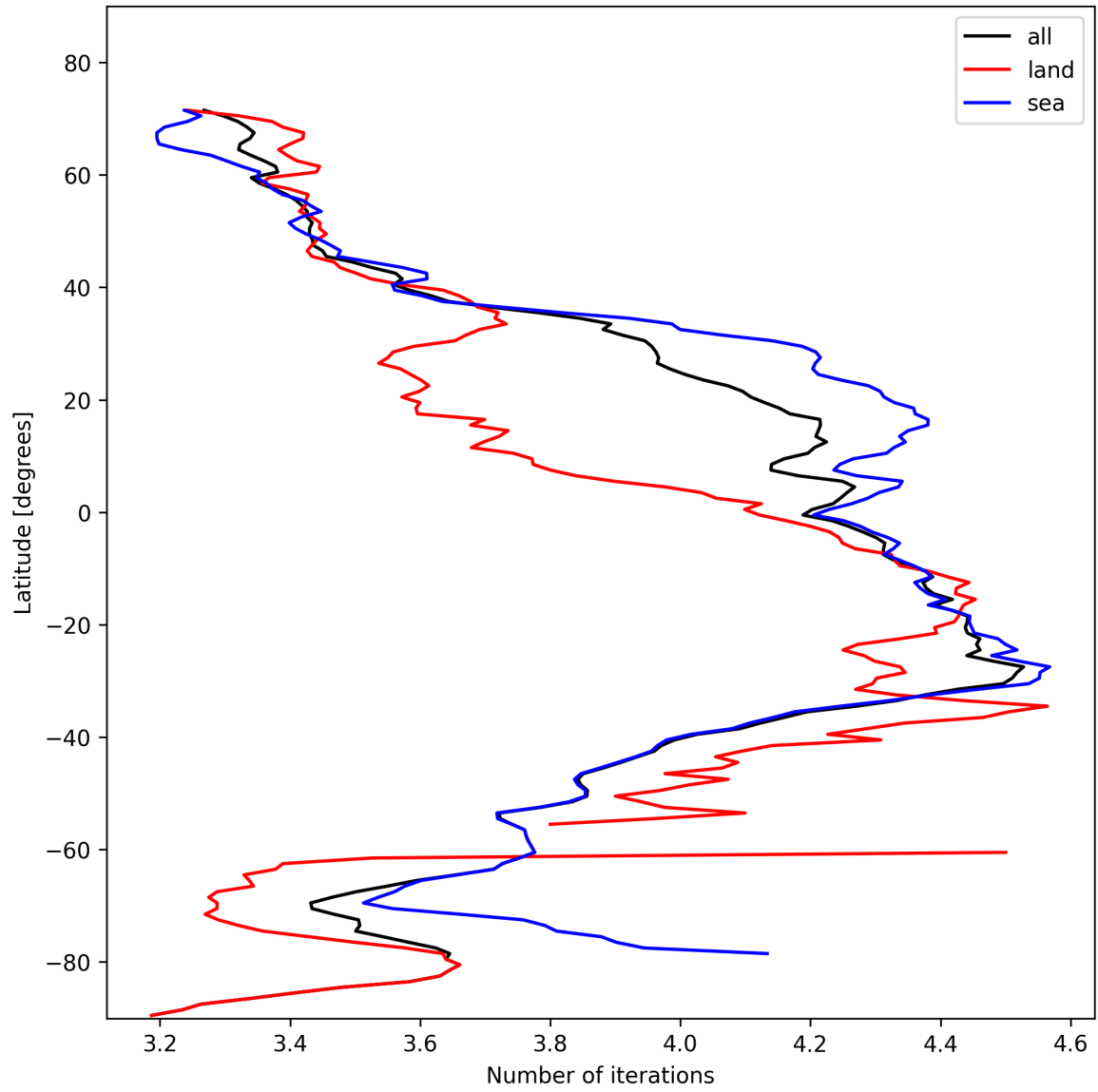
Figure 17: Zonal average of “Number of iterations” for 2024-11-05 to 2024-11-07.
