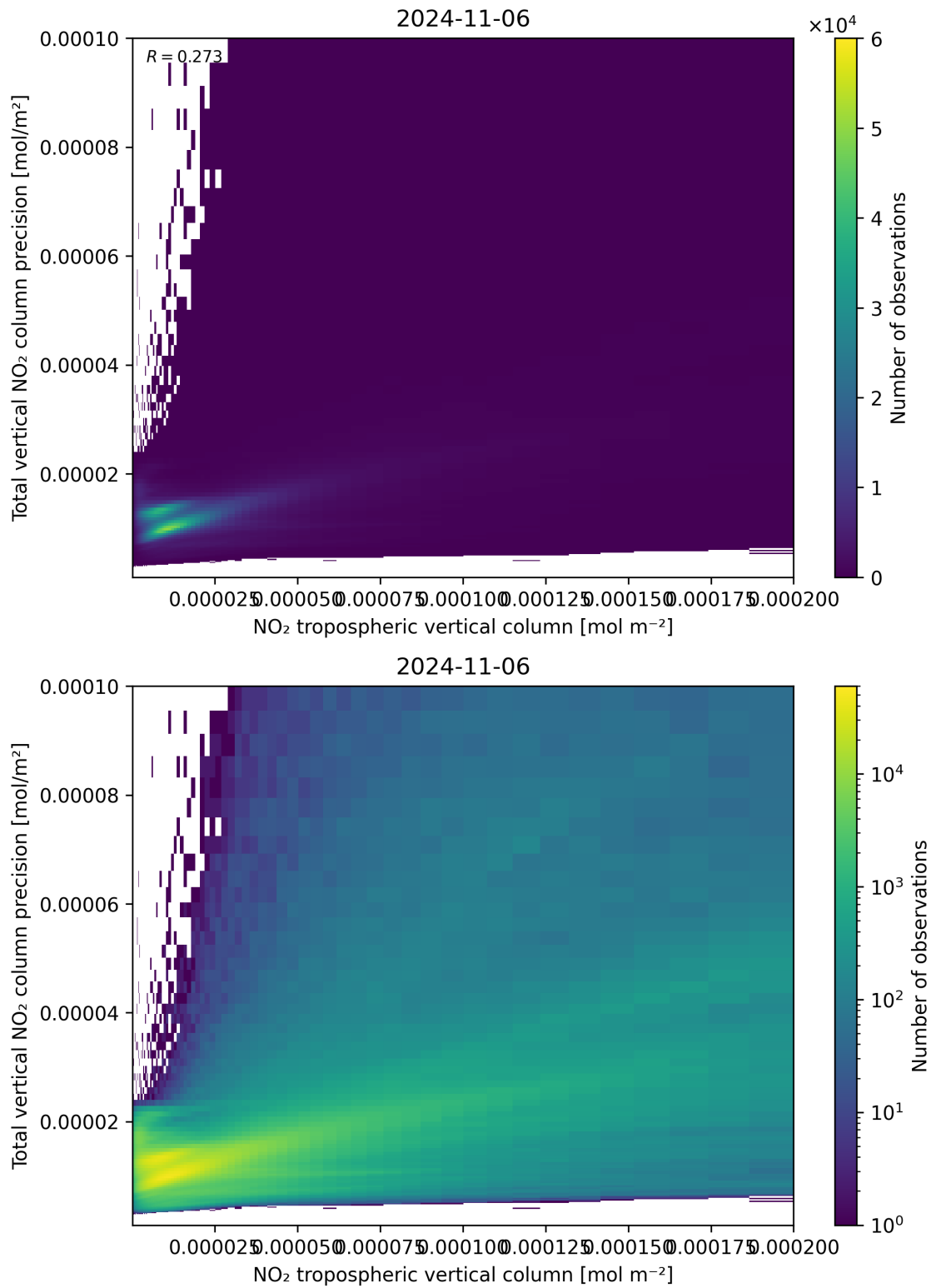
Figure 129: Scatter density plot of “NO 2 tropospheric vertical column” against “Total vertical NO 2 column precision” for 2024-11-05 to 2024-11-07.
