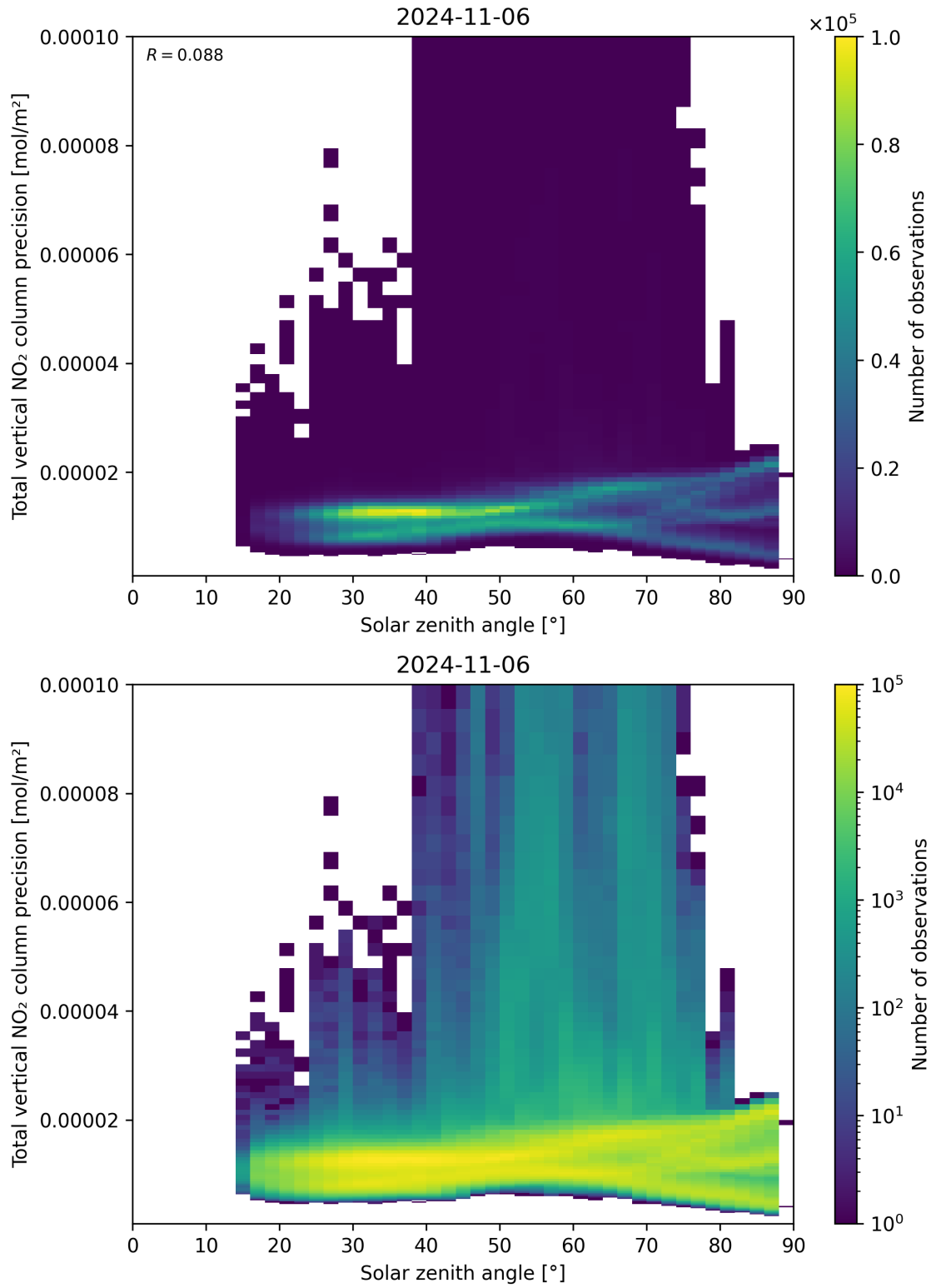
Figure 154: Scatter density plot of “Solar zenith angle” against “Total vertical NO 2 column precision” for 2024-11-05 to 2024-11-07.
