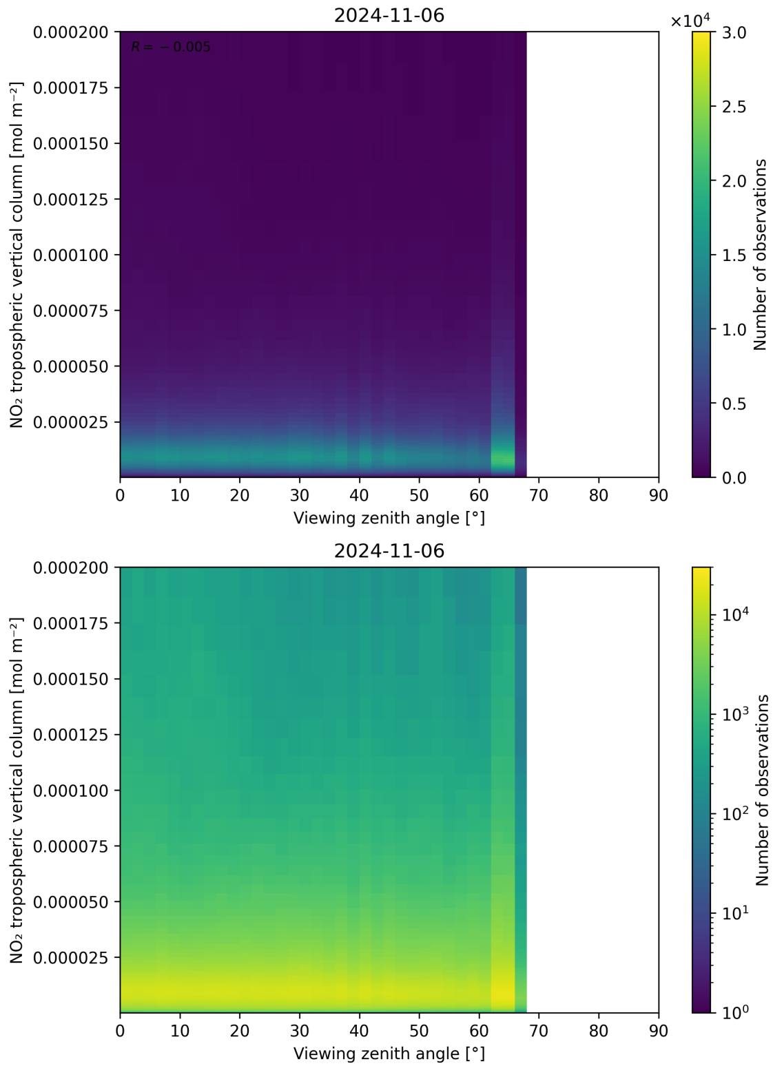
Figure 169: Scatter density plot of “Viewing zenith angle” against “NO 2 tropospheric vertical column” for 2024-11-05 to 2024-11-07.
