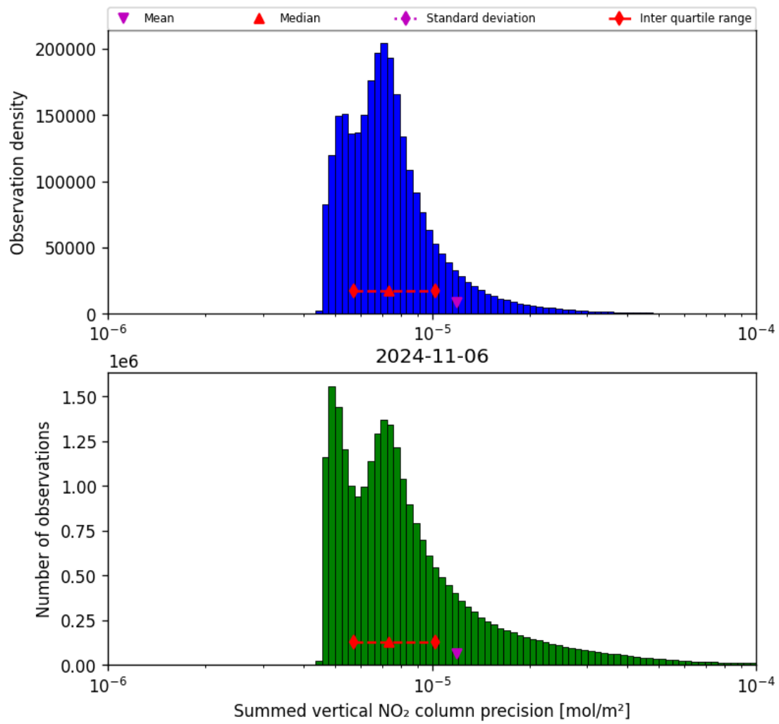
Figure 41: Histogram of "Summed vertical NO 2 column precision" for 2024-11-05 to 2024-11-07
