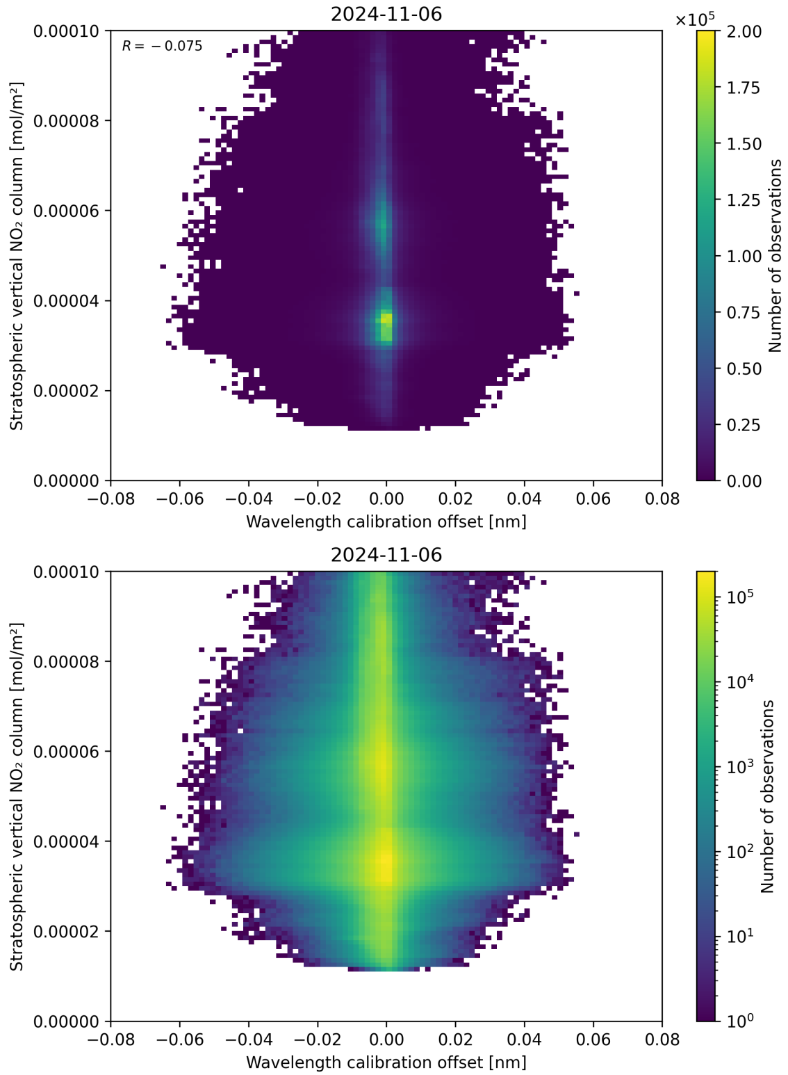
Figure 176: Scatter density plot of “Wavelength calibration offset” against “Stratospheric vertical NO 2 column” for 2024-11-05 to 2024-11-07.
