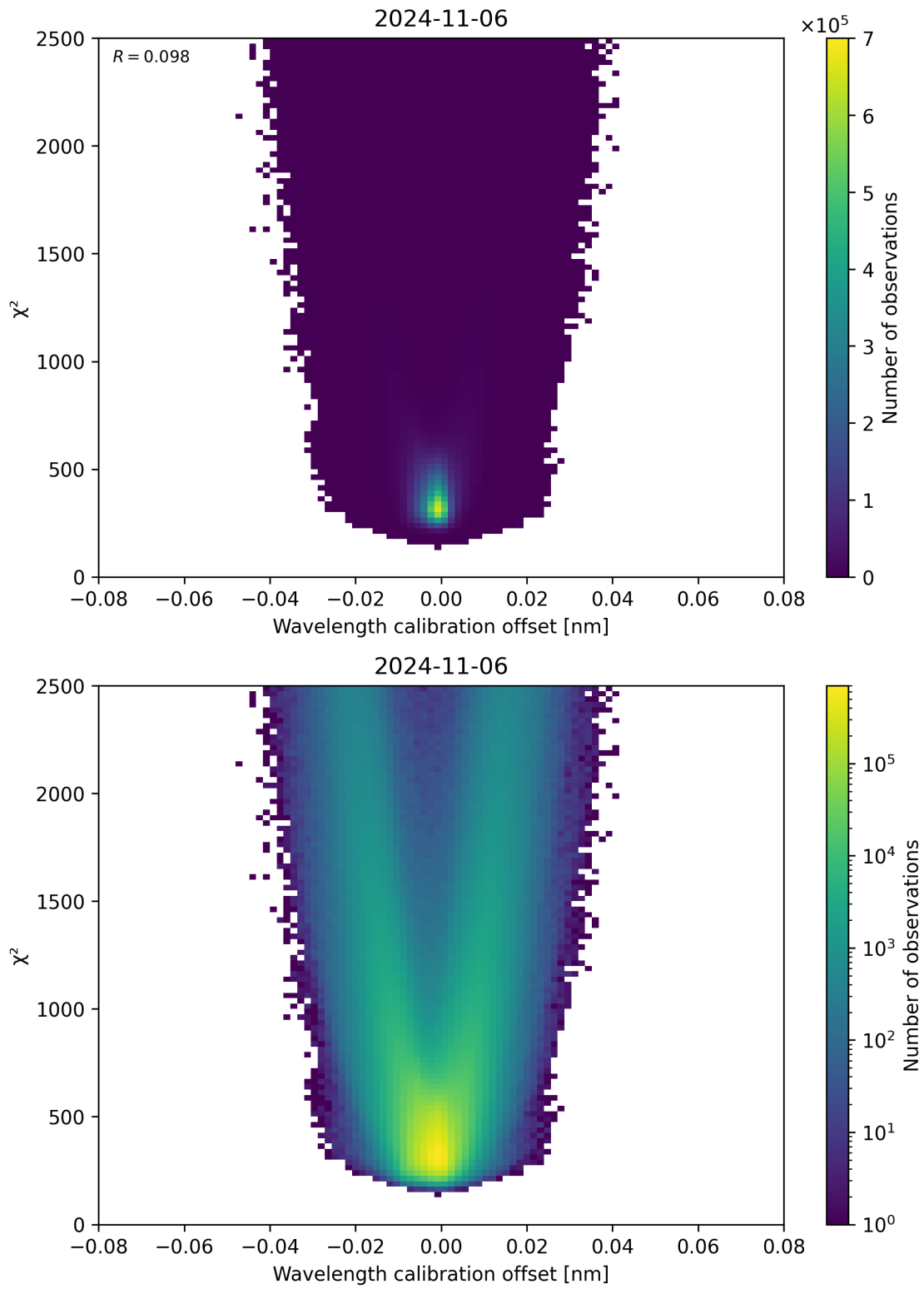
Figure 175: Scatter density plot of “Wavelength calibration offset” against “ \chi^2 ” for 2024-11-05 to 2024-11-07.
