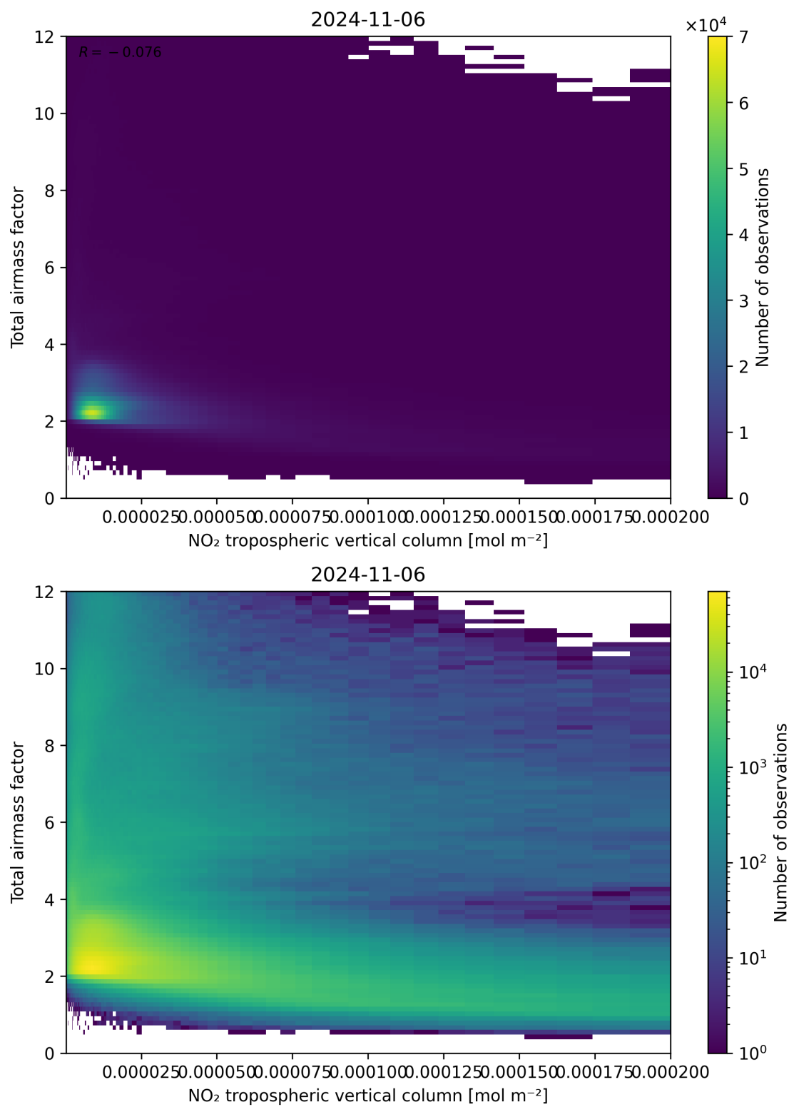
Figure 122: Scatter density plot of “NO 2 tropospheric vertical column” against “Total air mass factor” for 2024-11-05 to 2024-11-07.
