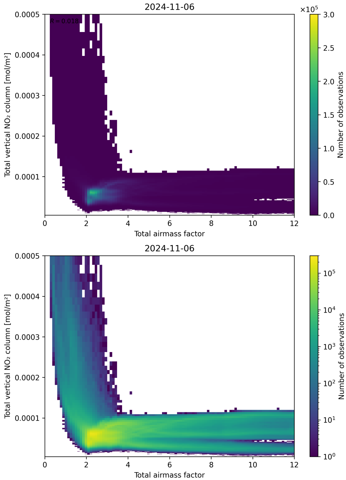
Figure 67: Scatter density plot of “Total air mass factor” against “Total vertical NO 2 column” for 2024-11-05 to 2024-11-07.
