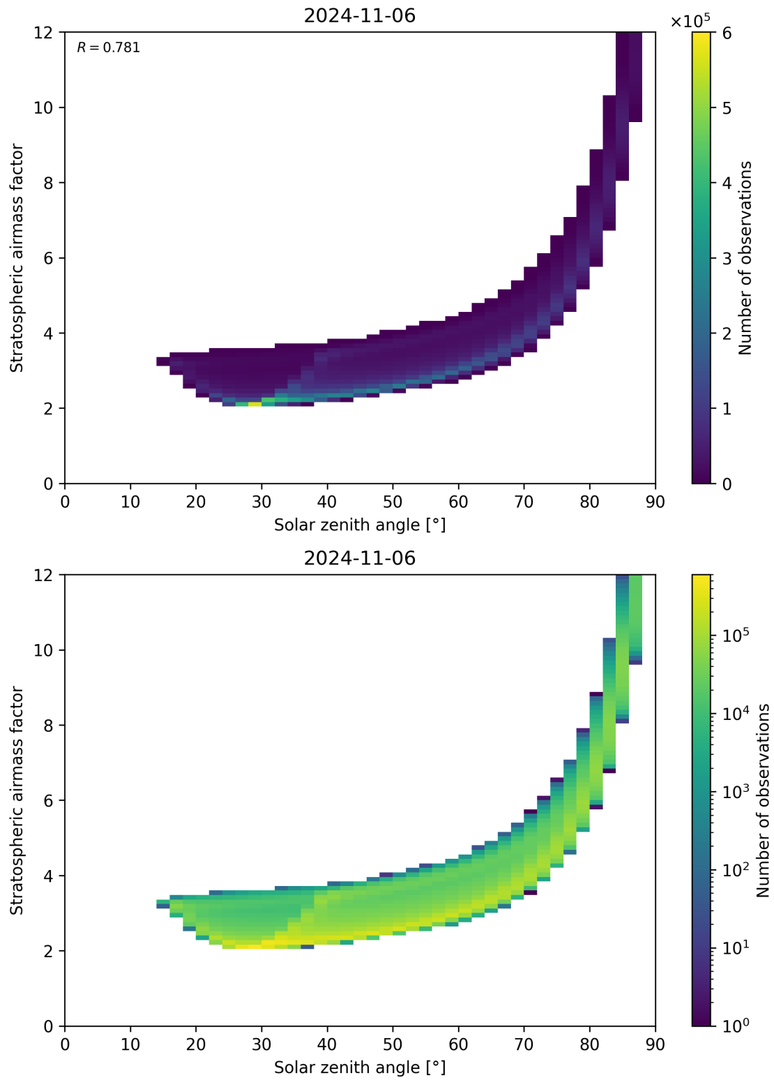
Figure 145: Scatter density plot of “Solar zenith angle” against “Stratospheric airmass factor” for 2024-11-05 to 2024-11-07.
