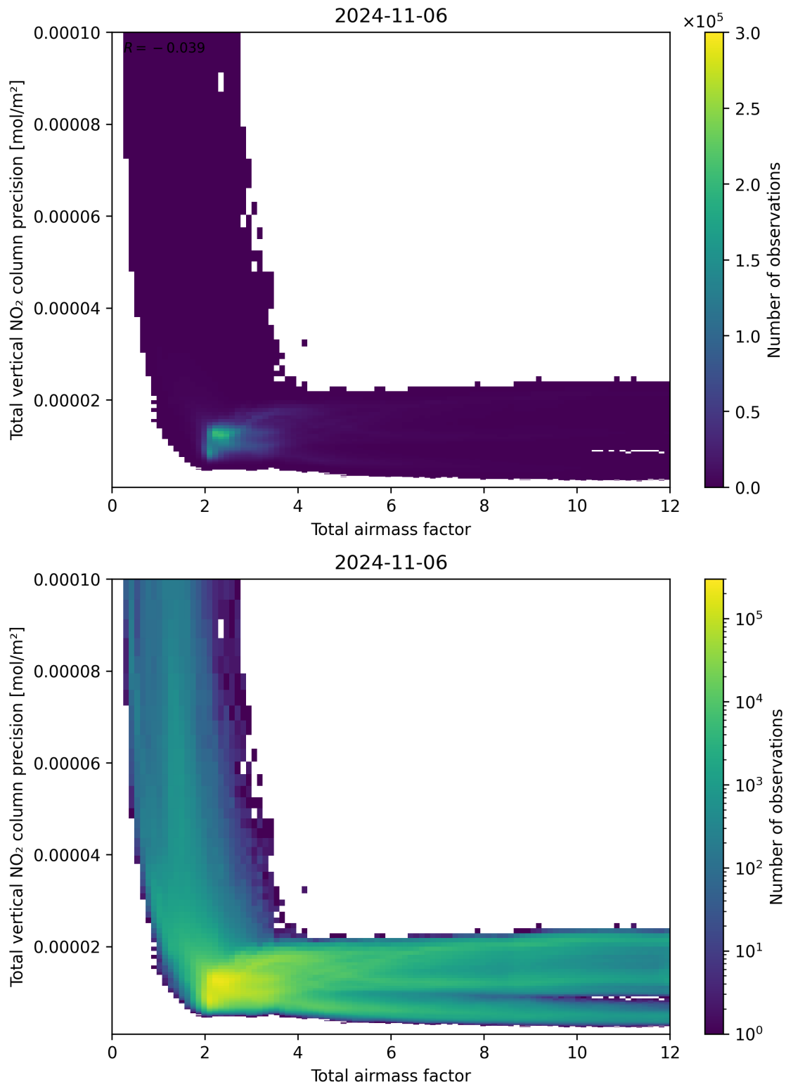
Figure 68: Scatter density plot of “Total airmass factor” against “Total vertical NO 2 column precision” for 2024-11-05 to 2024-11-07.
