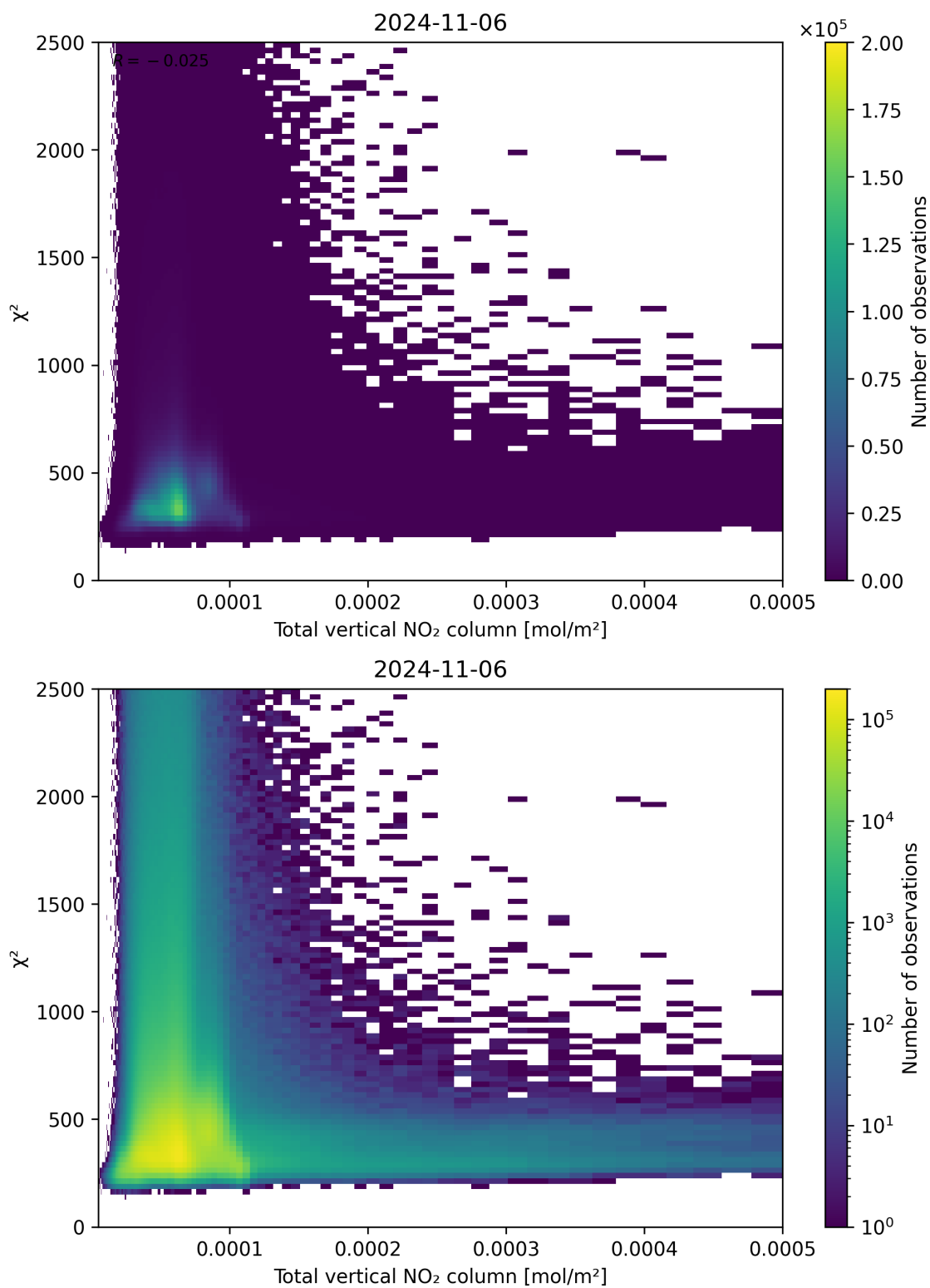
Figure 111: Scatter density plot of “Total vertical NO 2 column” against “ \chi^2 ” for 2024-11-05 to 2024-11-07.
