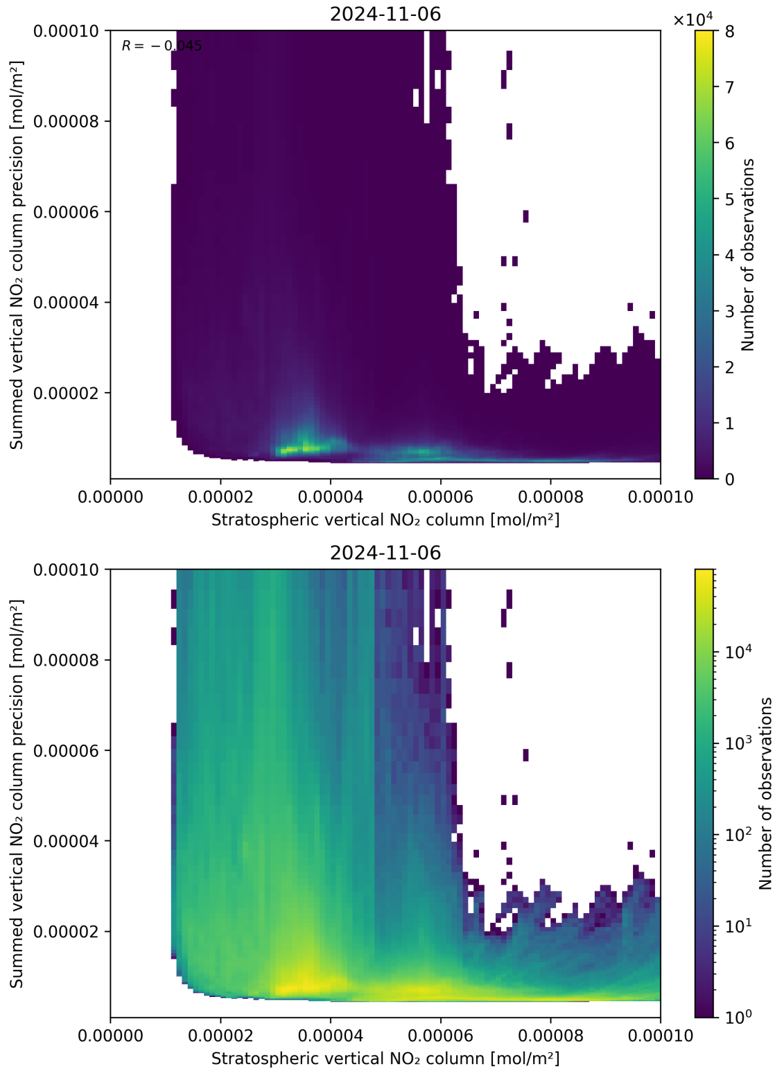
Figure 99: Scatter density plot of “Stratospheric vertical NO 2 column” against “Summed vertical NO 2 column precision” for 2024-11-05 to 2024-11-07.
