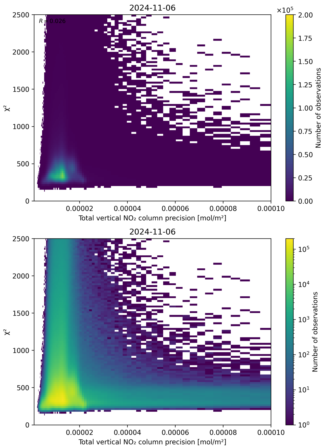
Figure 116: Scatter density plot of “Total vertical NO 2 column precision” against “ \chi^2 ” for 2024-11-05 to 2024-11-07.
