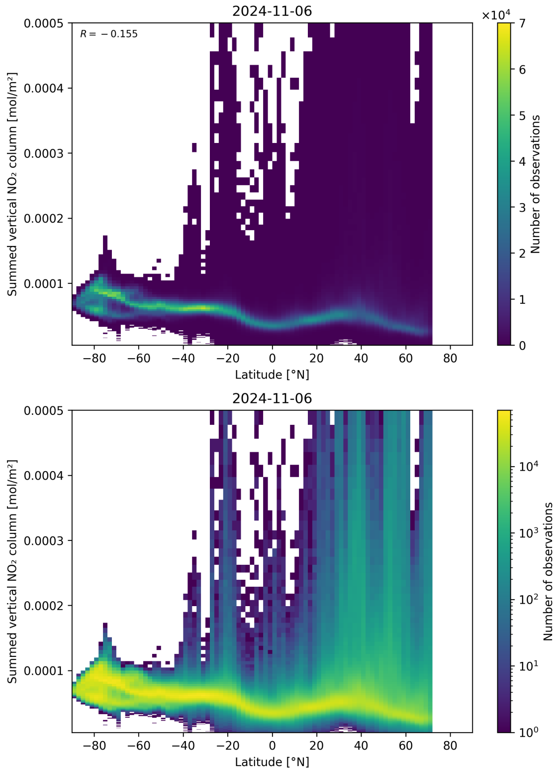
Figure 88: Scatter density plot of “Latitude” against “Summed vertical NO 2 column” for 2024-11-05 to 2024-11-07.
