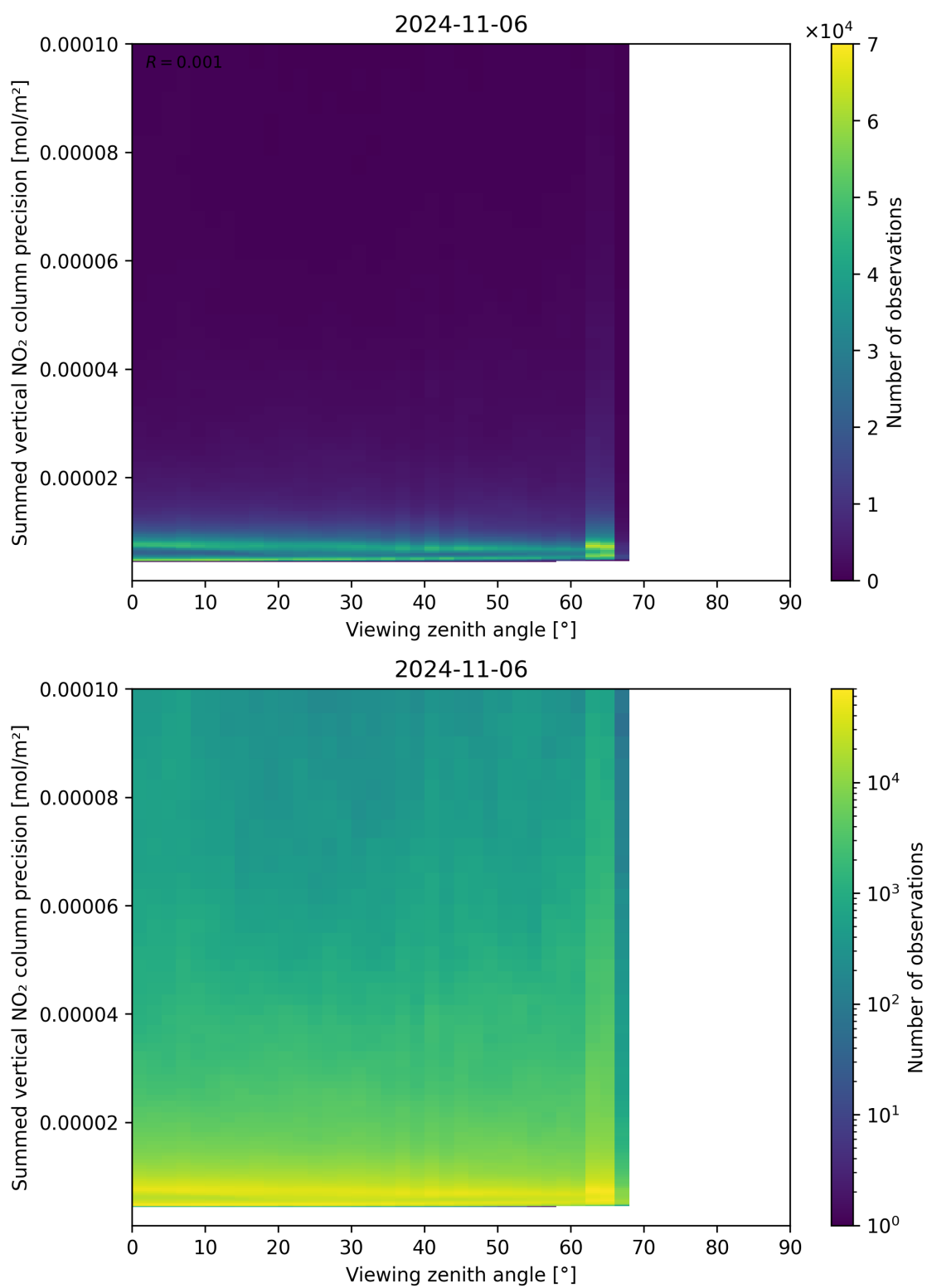
Figure 166: Scatter density plot of “Viewing zenith angle” against “Summed vertical NO 2 column precision” for 2024-11-05 to 2024-11-07.
