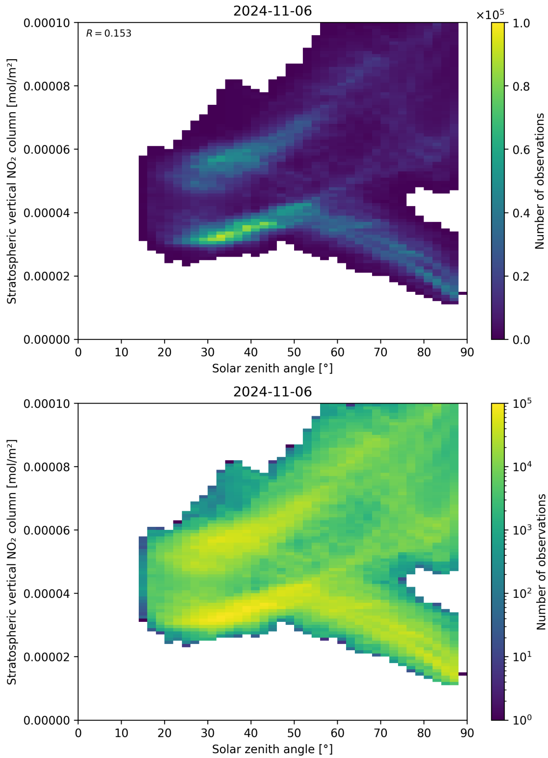
Figure 150: Scatter density plot of “Solar zenith angle” against “Stratospheric vertical NO 2 column” for 2024-11-05 to 2024-11-07.
