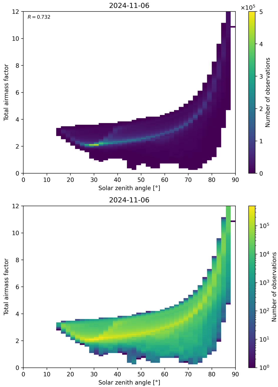
Figure 146: Scatter density plot of “Solar zenith angle” against “Total airmass factor” for 2024-11-05 to 2024-11-07.
