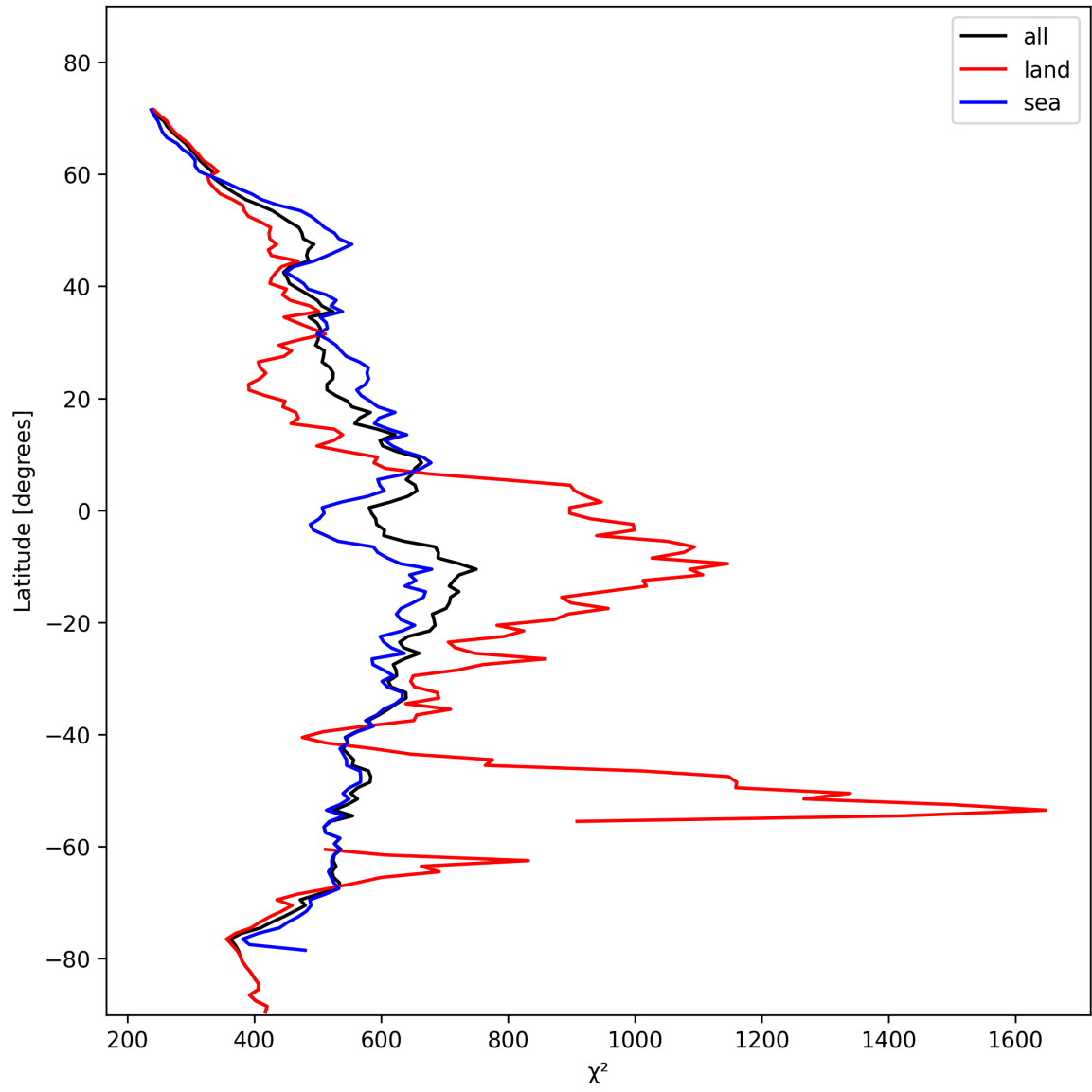
Figure 25: Zonal average of “ \chi^2 ” for 2024-11-05 to 2024-11-07.
