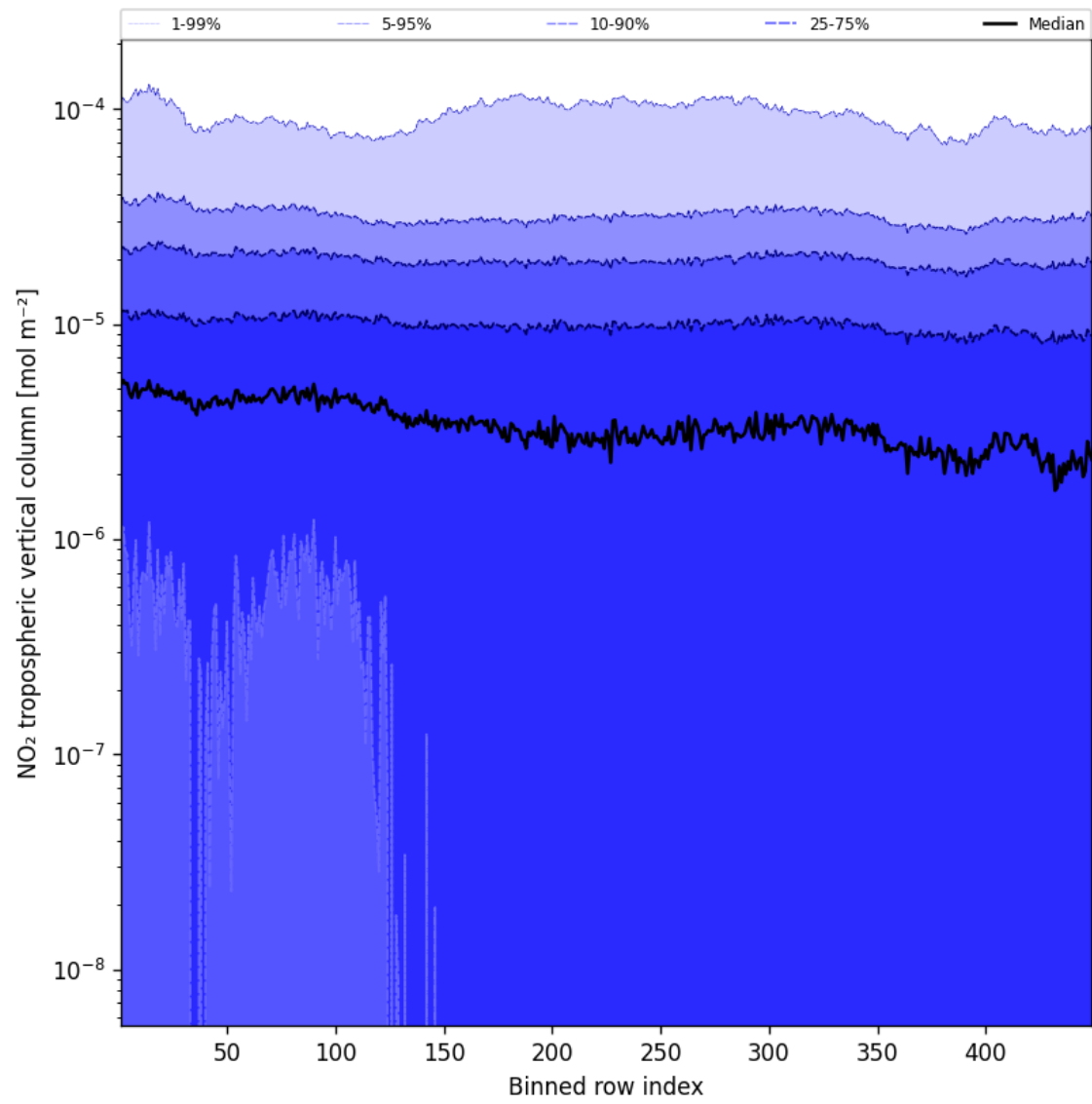
Figure 46: Along track statistics of “NO 2 tropospheric vertical column” for 2024-11-05 to 2024-11-07
