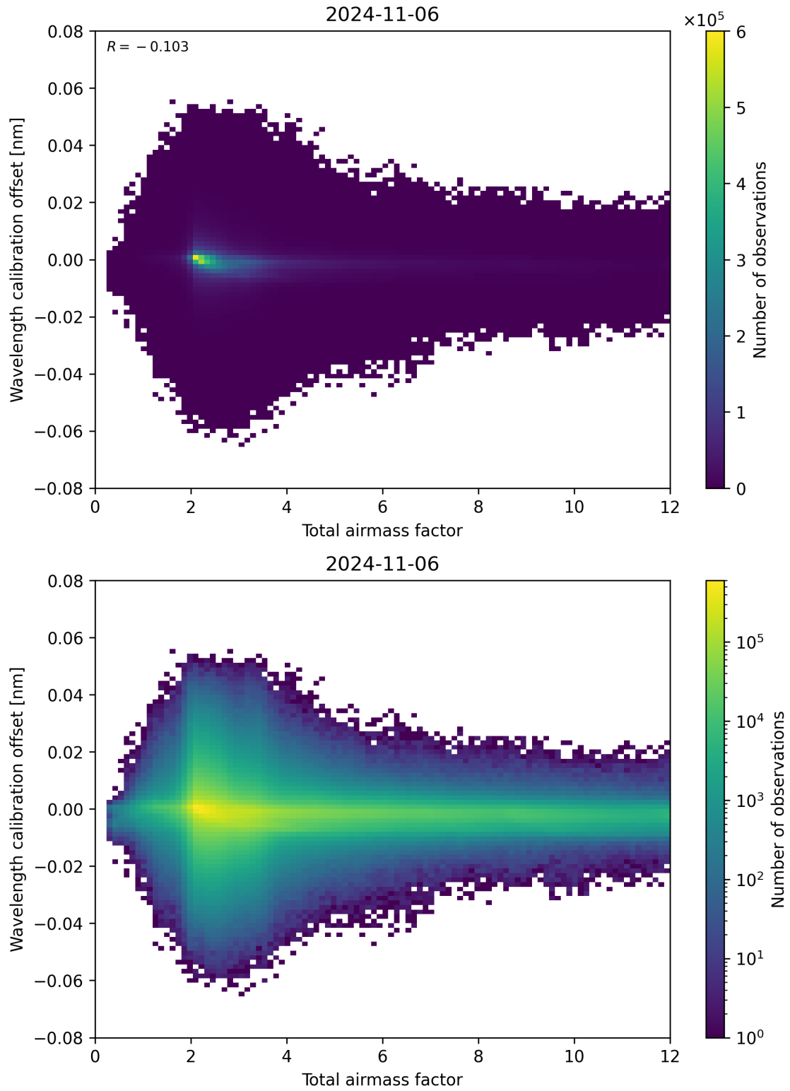
Figure 70: Scatter density plot of “Total airmass factor” against “Wavelength calibration offset” for 2024-11-05 to 2024-11-07.
