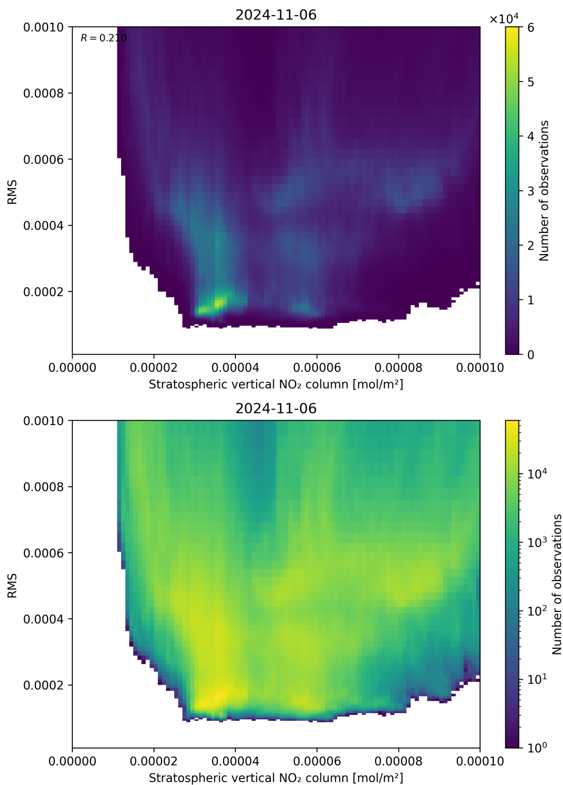
Figure 102: Scatter density plot of “Stratospheric vertical NO 2 column” against “RMS” for 2024-11-05 to 2024-11-07.
