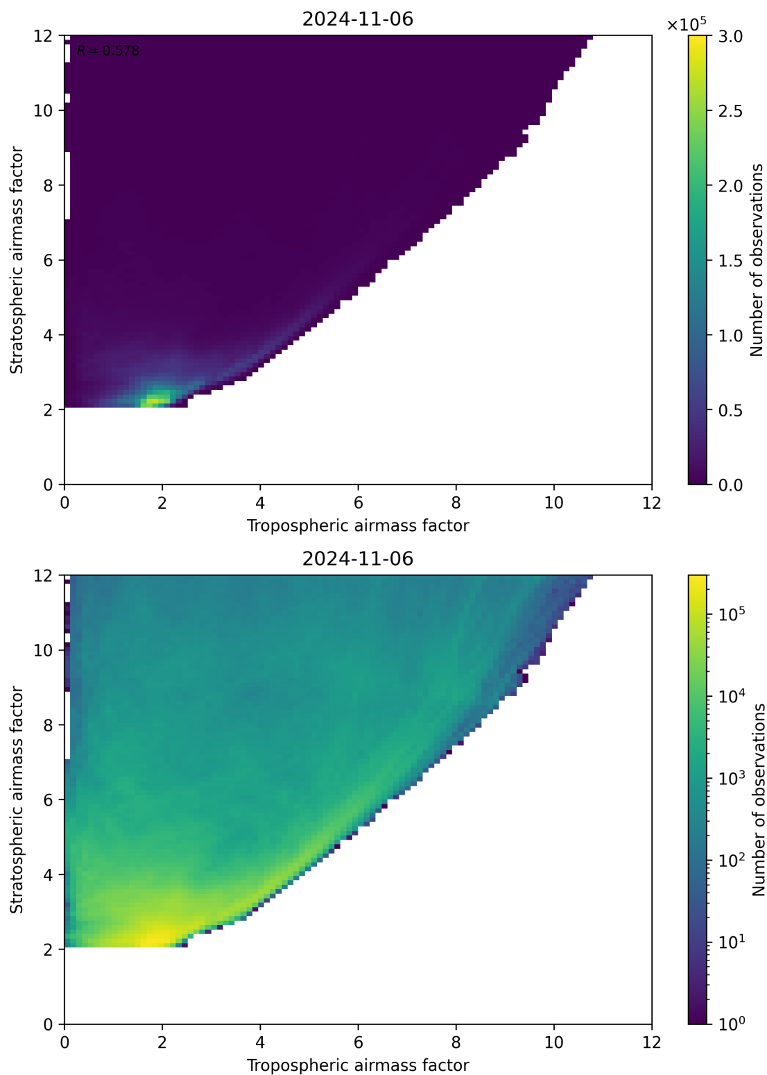
Figure 71: Scatter density plot of “Tropospheric airmass factor” against “Stratospheric airmass factor” for 2024-11-05 to 2024-11-07.
