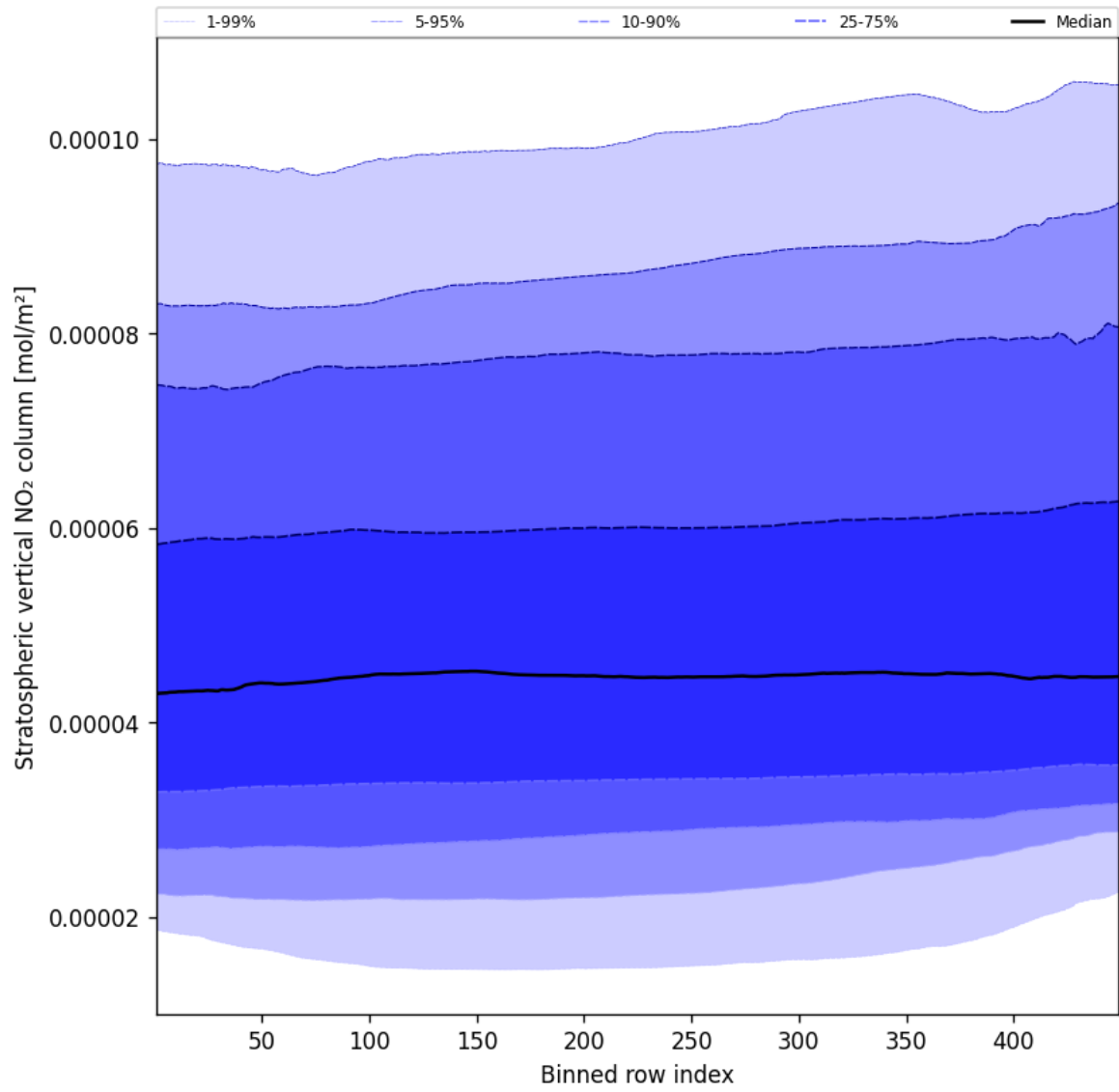
Figure 53: Along track statistics of “Stratospheric vertical NO 2 column” for 2024-11-05 to 2024-11-07
