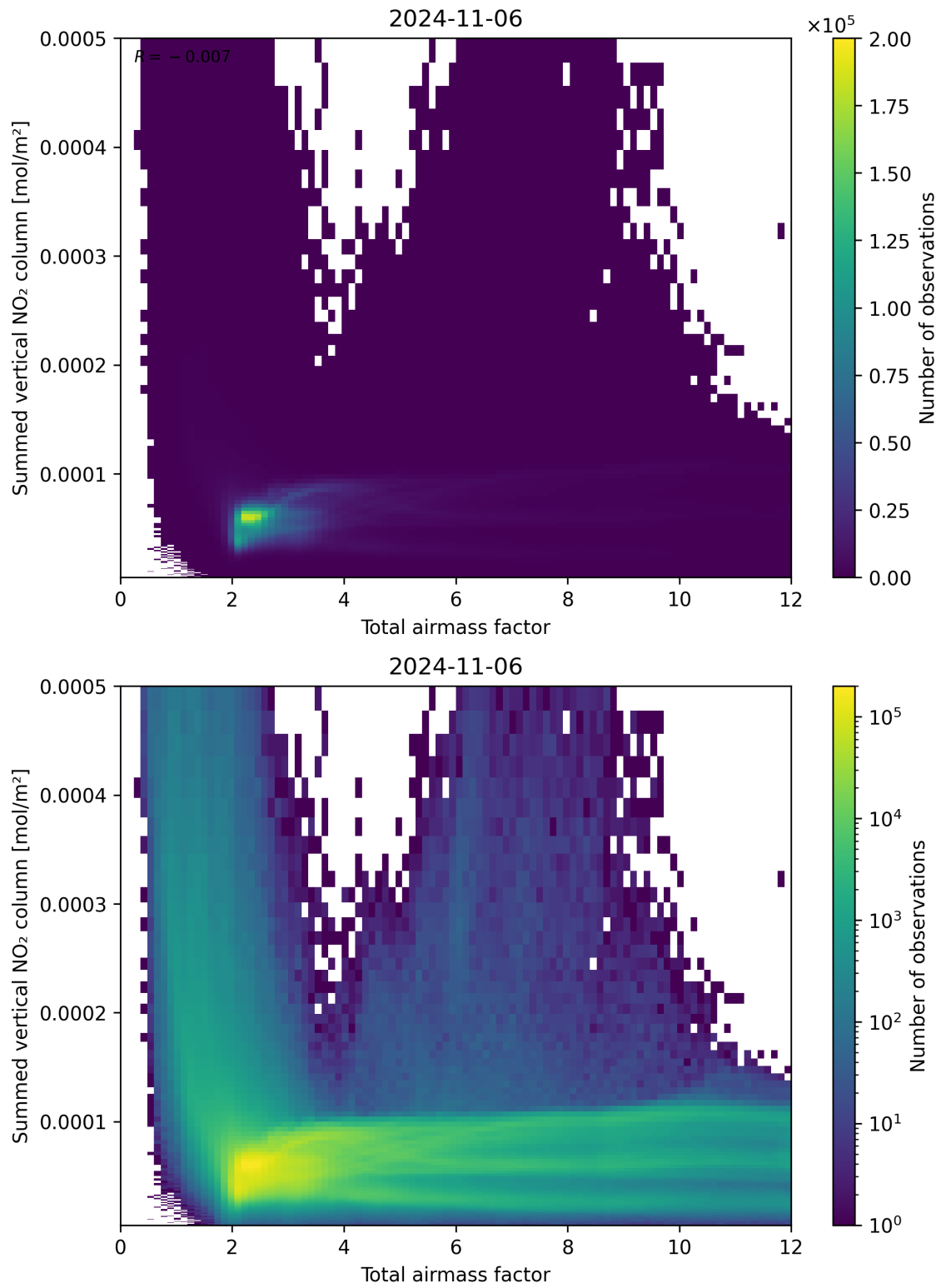
Figure 65: Scatter density plot of “Total airmass factor” against “Summed vertical NO 2 column” for 2024-11-05 to 2024-11-07.
