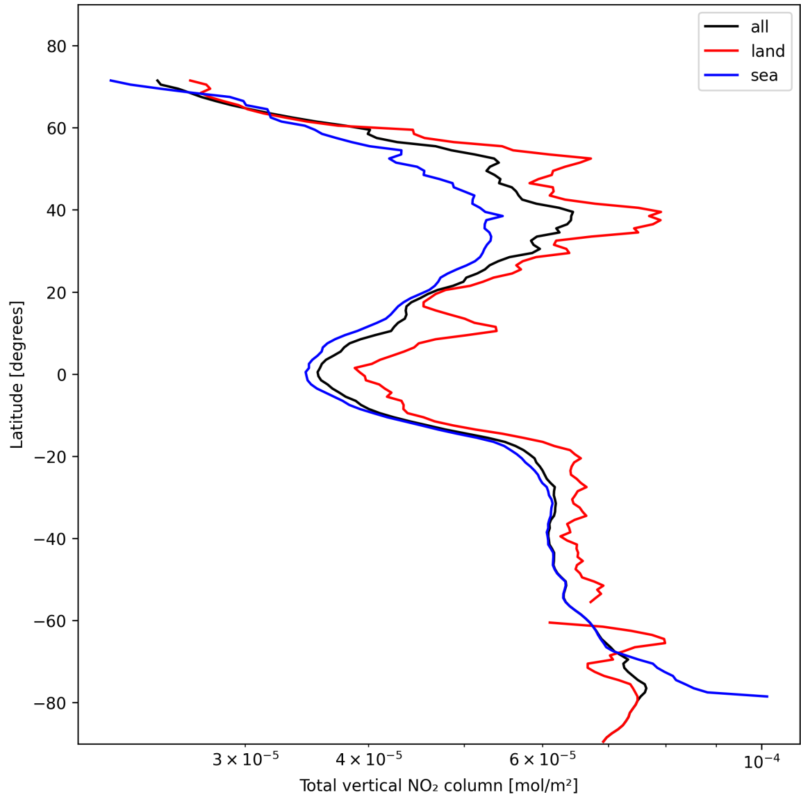
Figure 21: Zonal average of “Total vertical NO 2 column” for 2024-11-05 to 2024-11-07.
