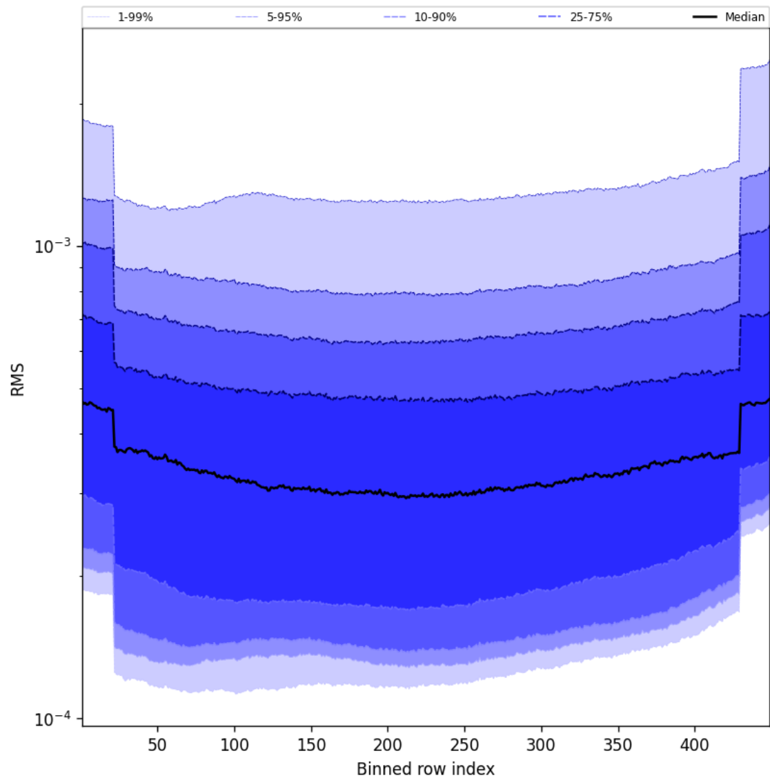
Figure 60: Along track statistics of “RMS” for 2024-11-05 to 2024-11-07
