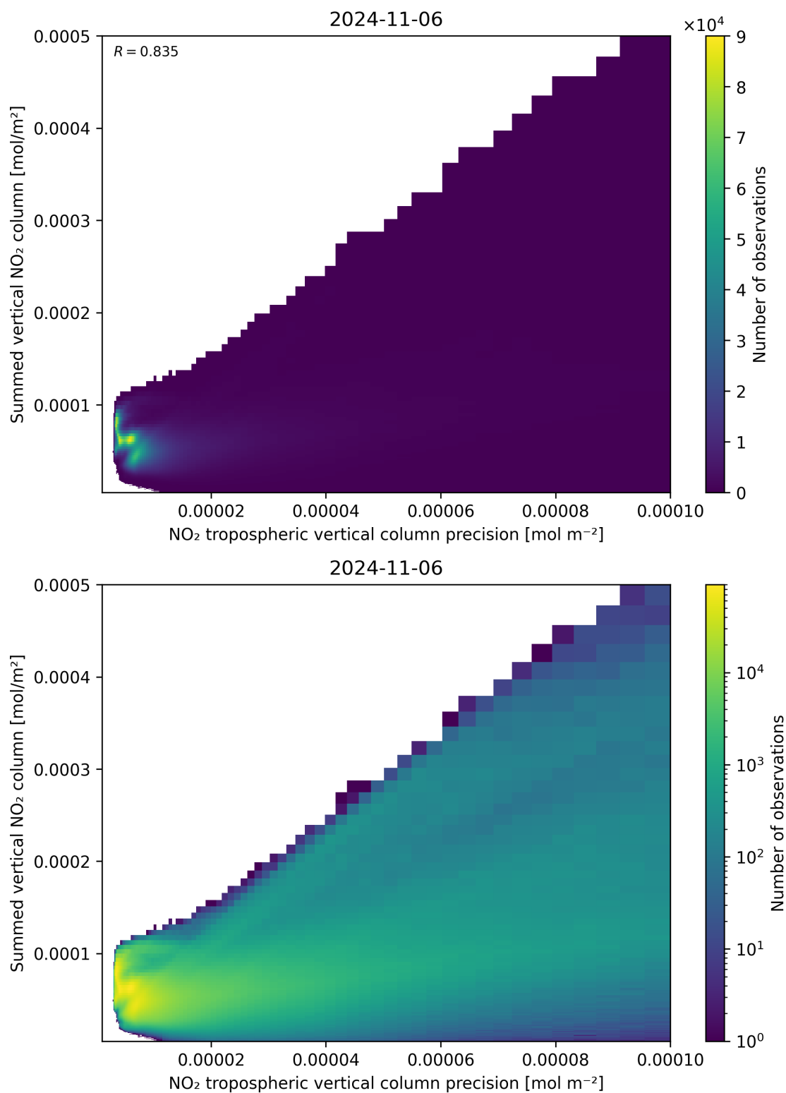
Figure 136: Scatter density plot of “NO 2 tropospheric vertical column precision” against “Summed vertical NO 2 column” for 2024-11-05 to 2024-11-07.
