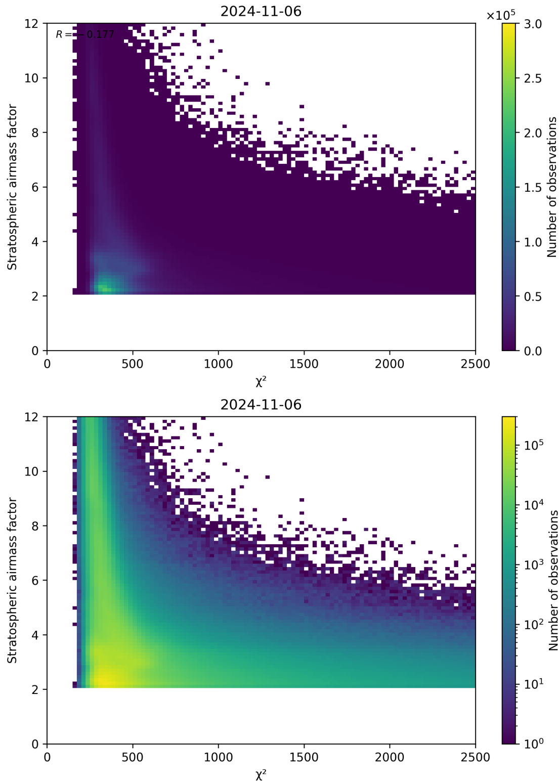
Figure 81: Scatter density plot of “ \chi^2 ” against “Stratospheric airmass factor” for 2024-11-05 to 2024-11-07.
