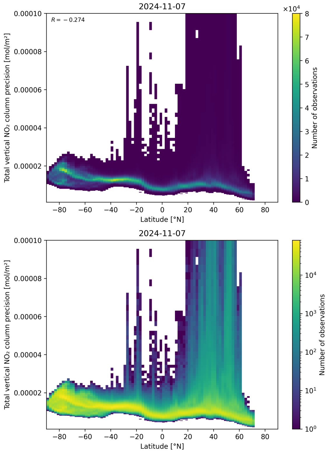
Figure 91: Scatter density plot of “Latitude” against “Total vertical NO 2 column precision” for 2024-11-06 to 2024-11-08.
