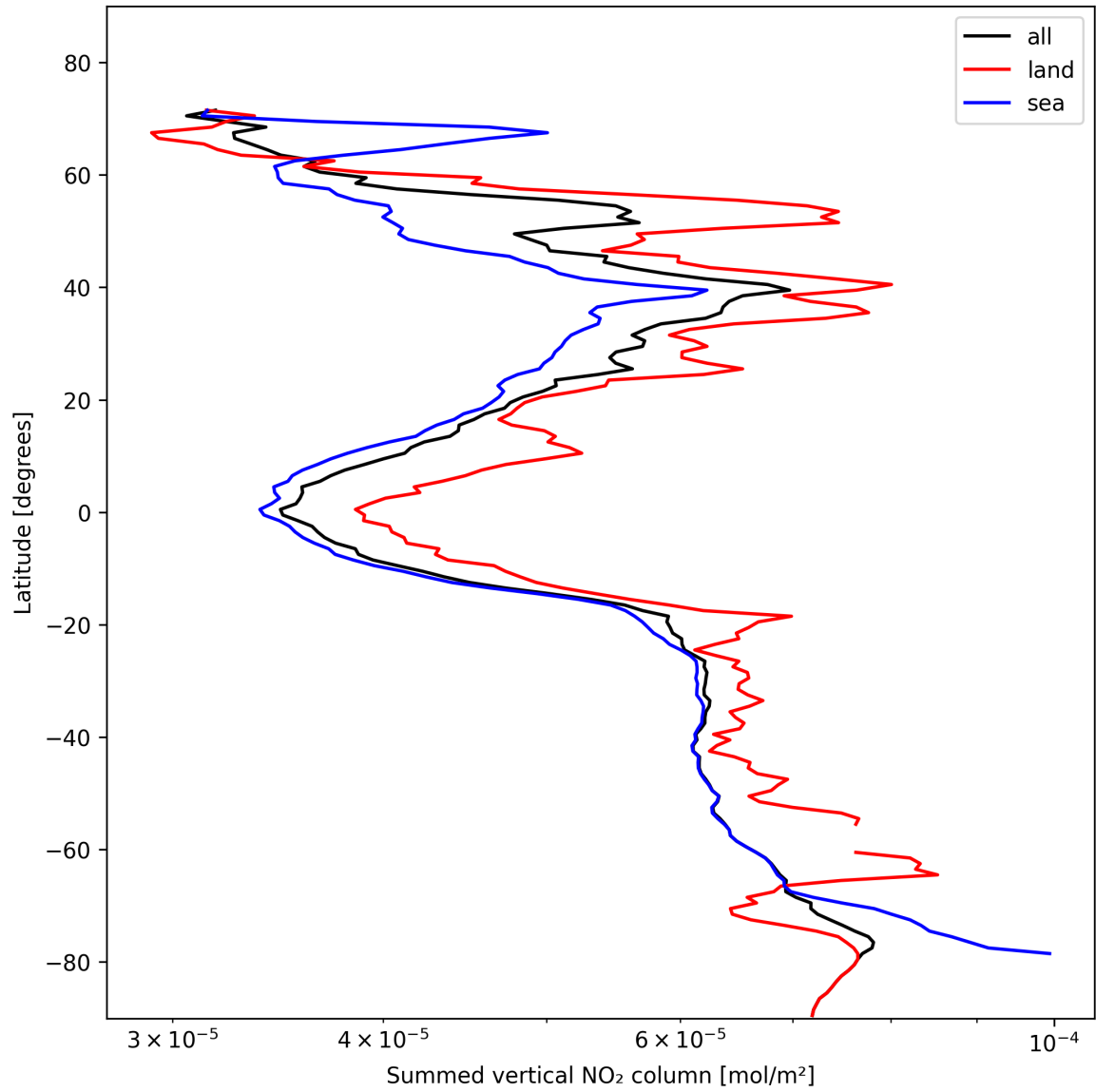
Figure 23: Zonal average of “Summed vertical NO 2 column” for 2024-11-06 to 2024-11-08.
