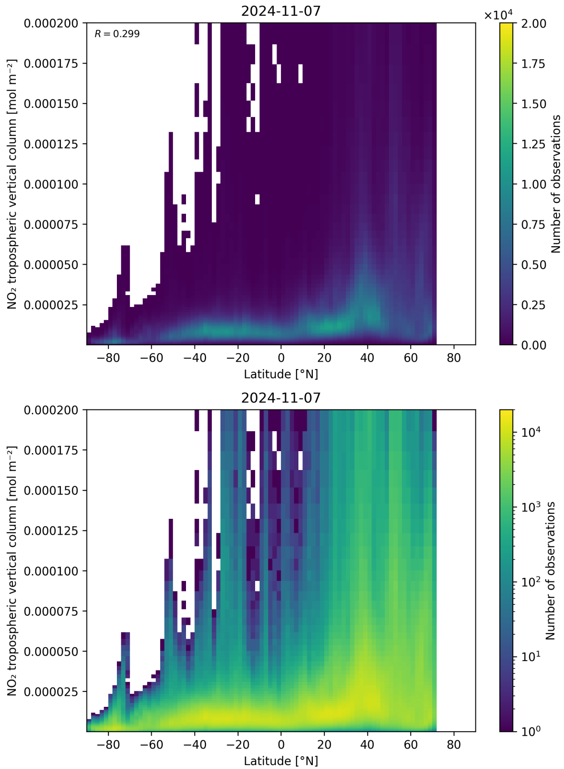
Figure 92: Scatter density plot of “Latitude” against “NO 2 tropospheric vertical column” for 2024-11-06 to 2024-11-08.
