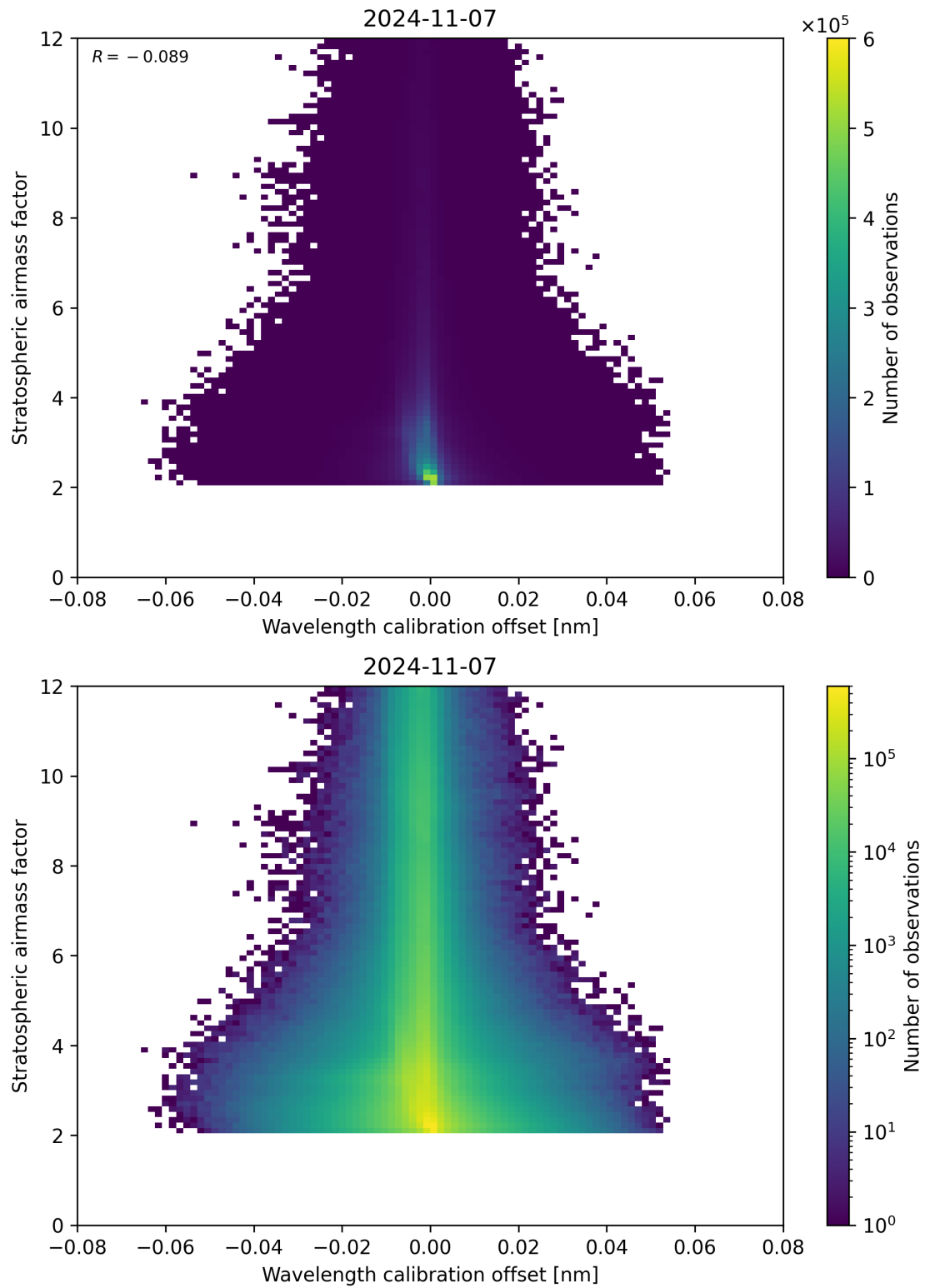
Figure 174: Scatter density plot of “Wavelength calibration offset” against “Stratospheric air mass factor” for 2024-11-06 to 2024-11-08.
