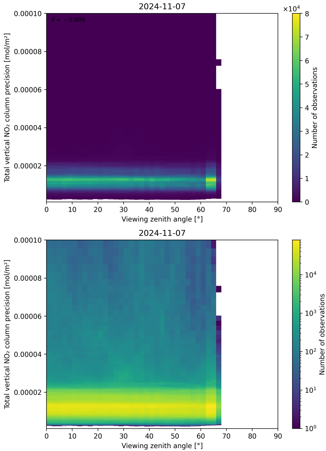
Figure 168: Scatter density plot of “Viewing zenith angle” against “Total vertical NO 2 column precision” for 2024-11-06 to 2024-11-08.
