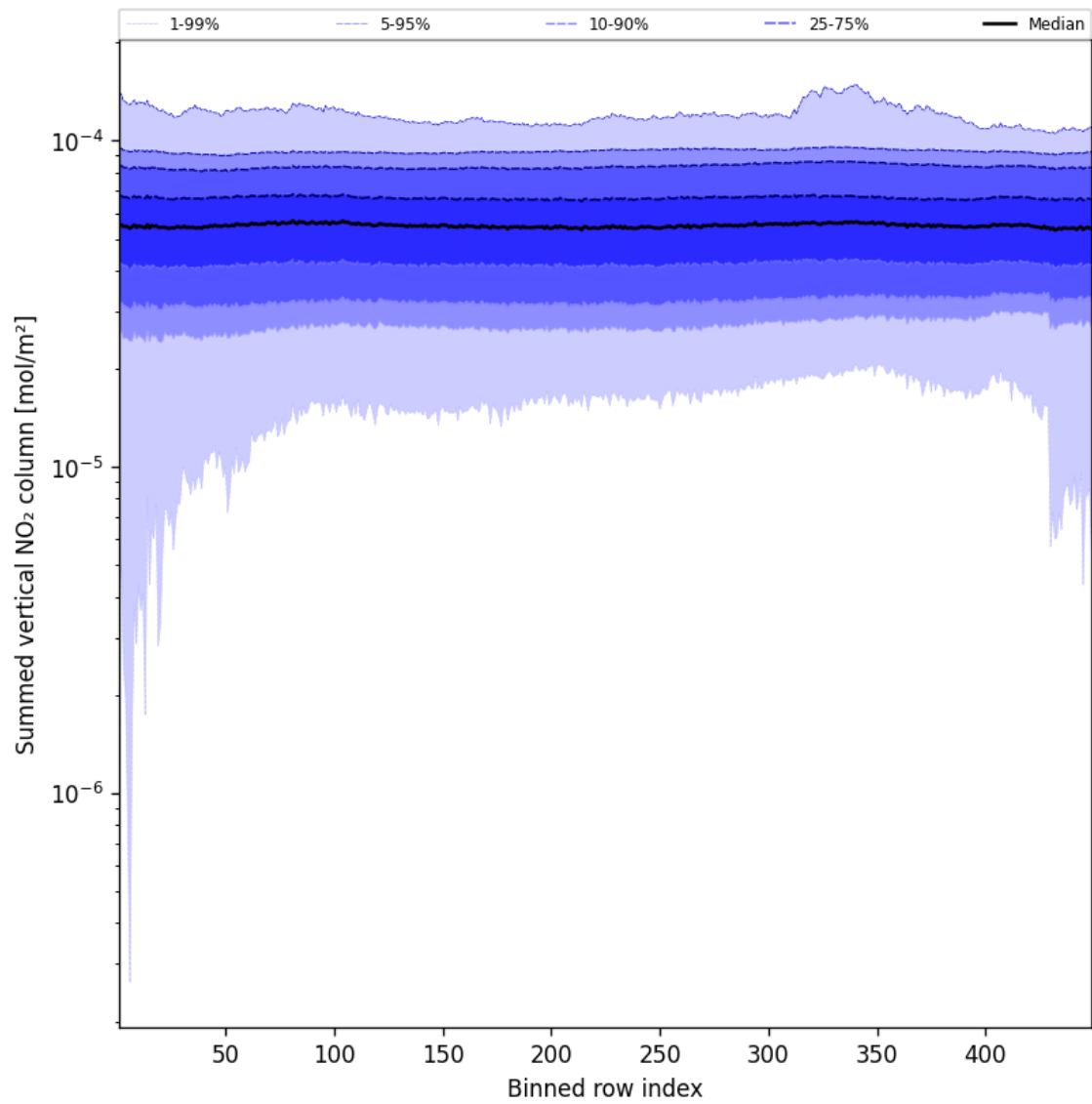
Figure 57: Along track statistics of “Summed vertical NO 2 column” for 2024-11-06 to 2024-11-08
