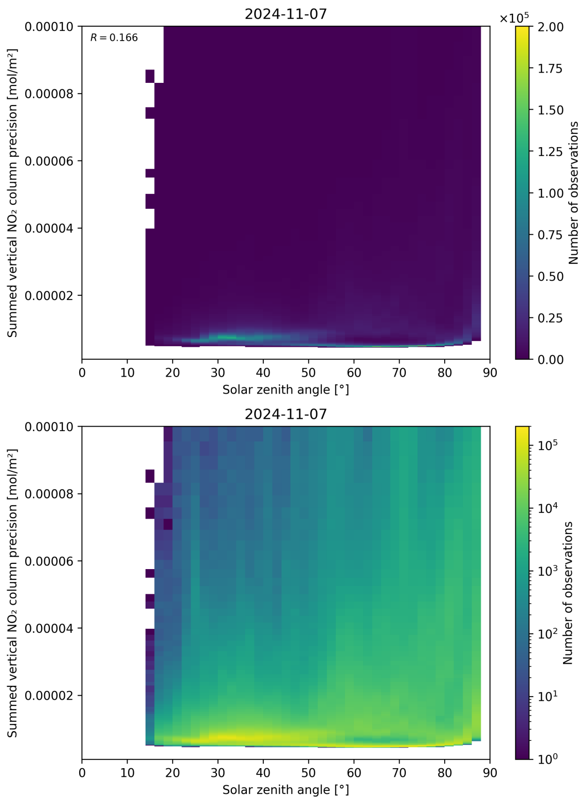
Figure 152: Scatter density plot of “Solar zenith angle” against “Summed vertical NO 2 column precision” for 2024-11-06 to 2024-11-08.
