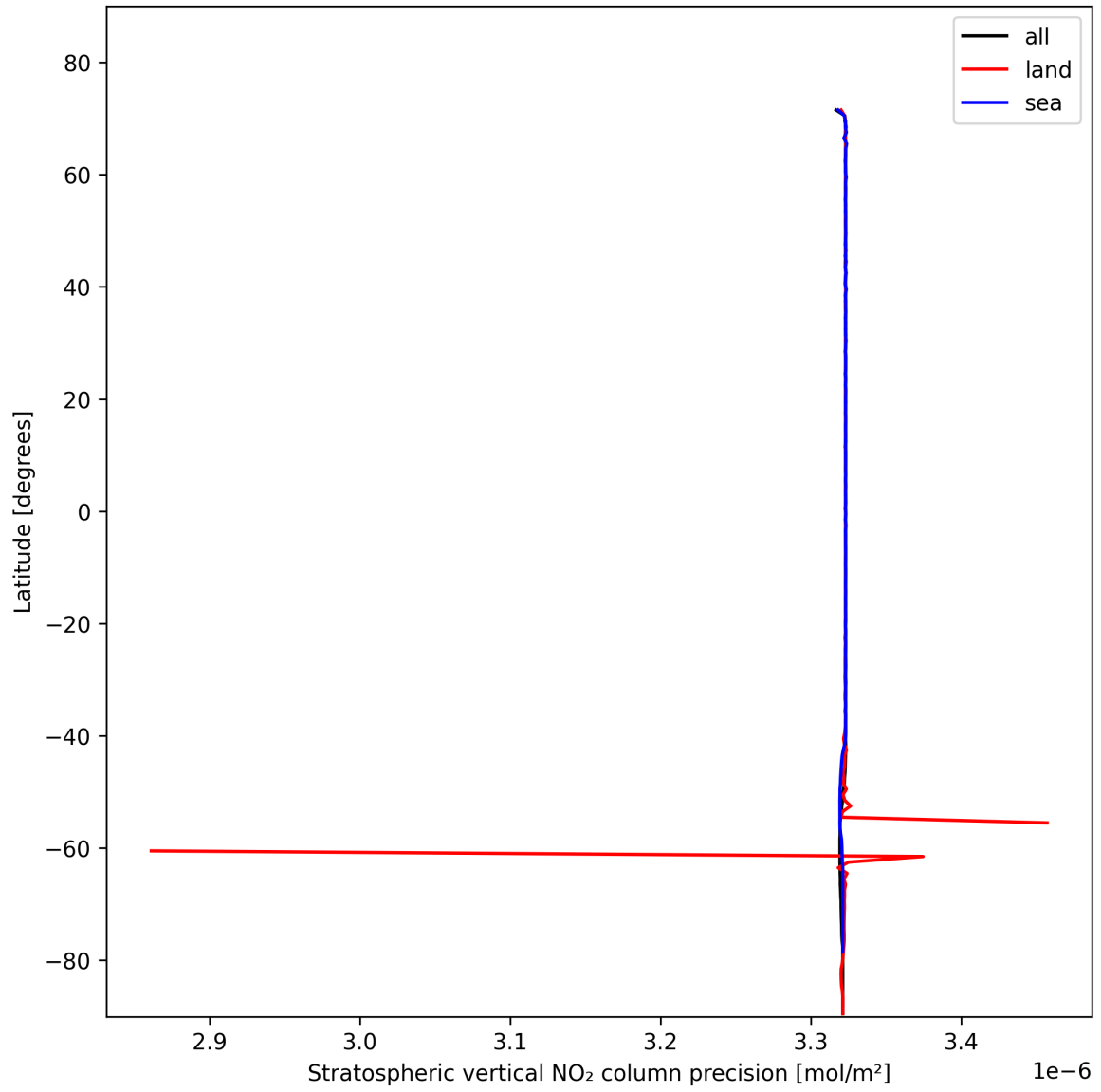
Figure 20: Zonal average of “Stratospheric vertical NO 2 column precision” for 2024-11-06 to 2024-11-08.
