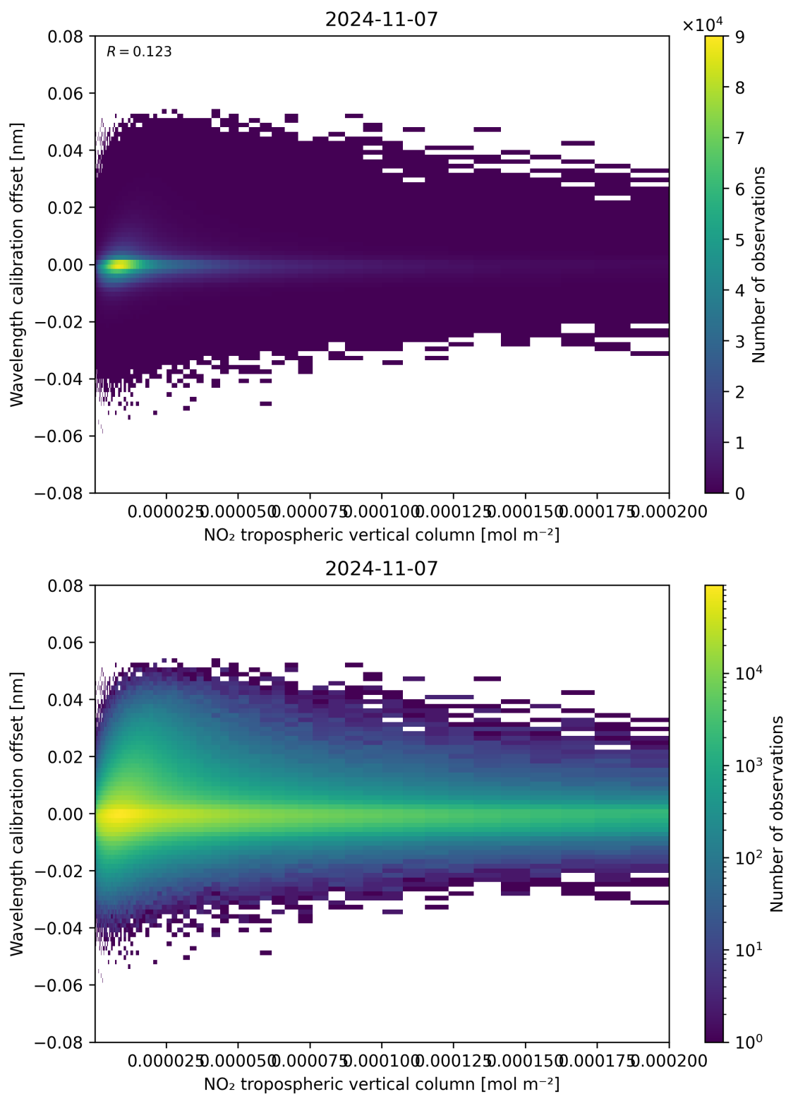
Figure 143: Scatter density plot of “NO 2 tropospheric vertical column” against “Wavelength calibration offset” for 2024-11-06 to 2024-11-08.
