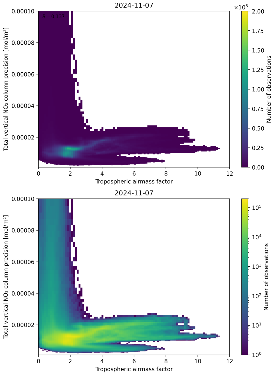
Figure 78: Scatter density plot of “Tropospheric air mass factor” against “Total vertical NO 2 column precision” for 2024-11-06 to 2024-11-08.
