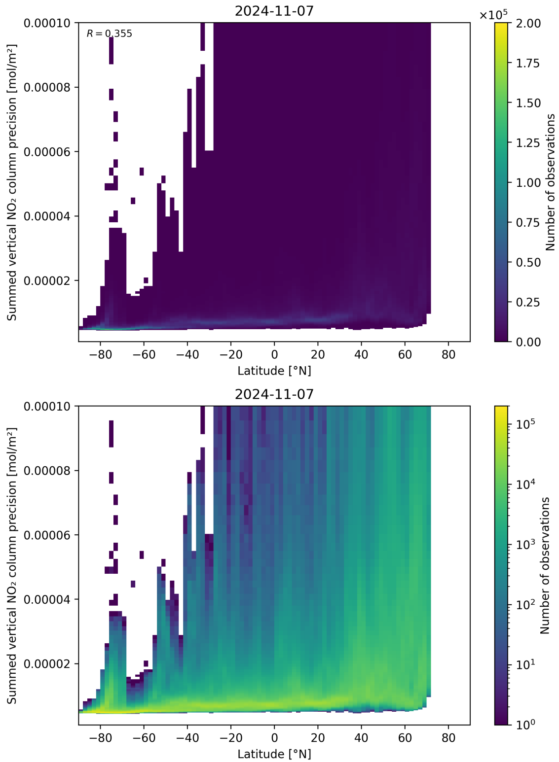
Figure 89: Scatter density plot of “Latitude” against “Summed vertical NO 2 column precision” for 2024-11-06 to 2024-11-08.
