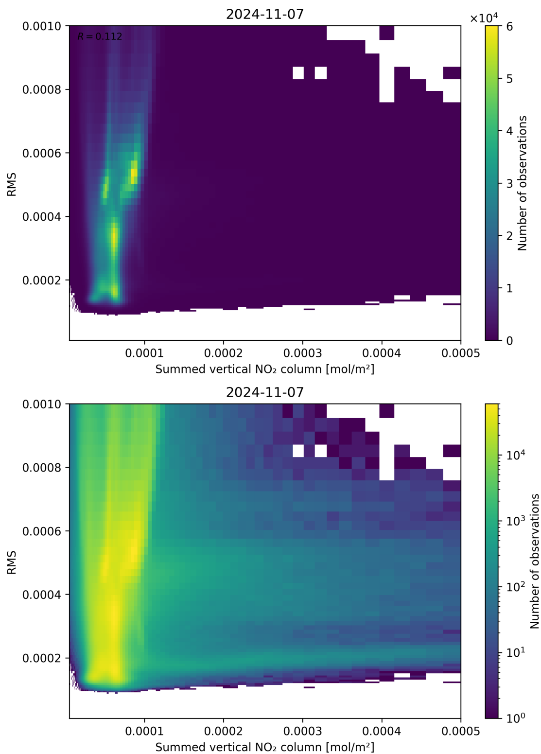
Figure 109: Scatter density plot of “Summed vertical NO 2 column” against “RMS” for 2024-11-06 to 2024-11-08.
