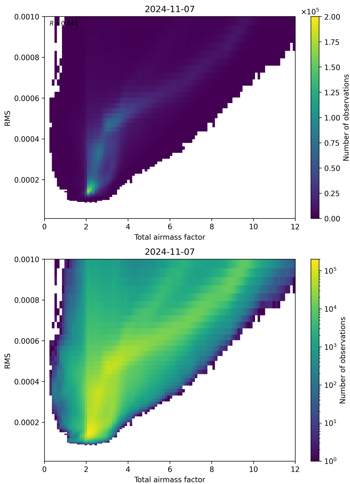
Figure 69: Scatter density plot of “Total airmass factor” against “RMS” for 2024-11-06 to 2024-11-08.
