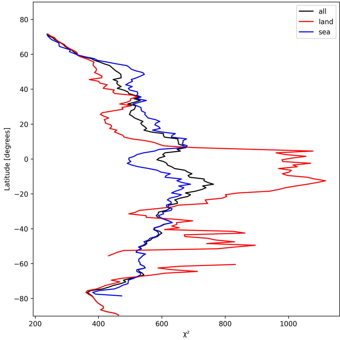
Figure 25: Zonal average of “ \chi^2 ” for 2024-11-06 to 2024-11-08.
