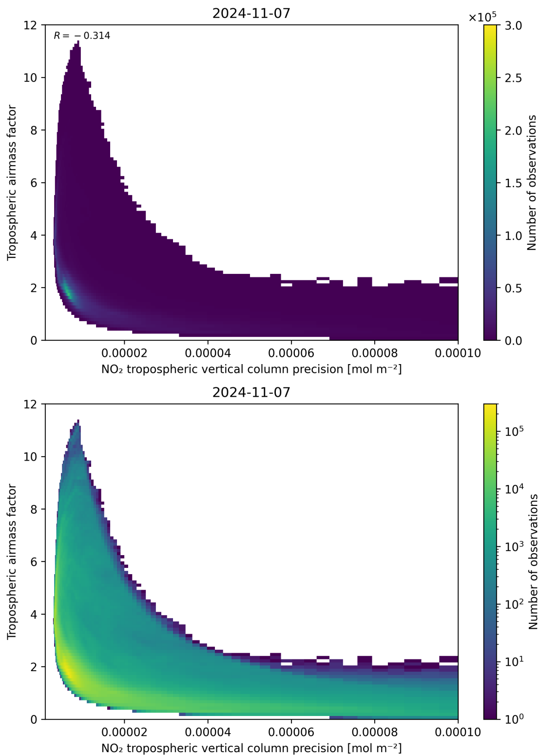
Figure 133: Scatter density plot of “NO 2 tropospheric vertical column precision” against “Tropospheric airmass factor” for 2024-11-06 to 2024-11-08.
