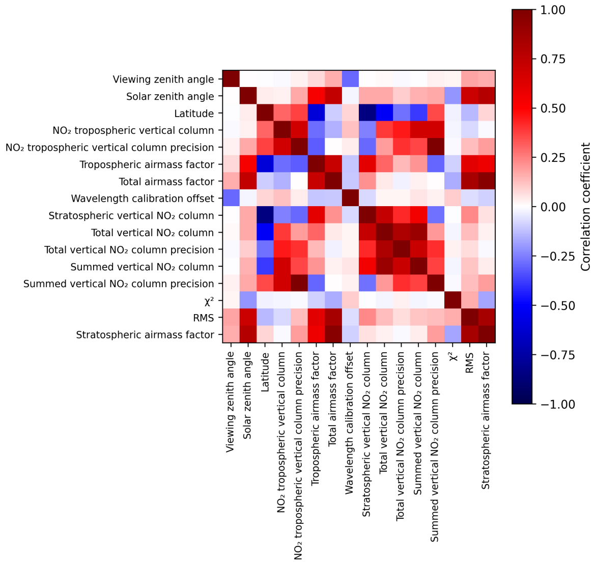
Figure 2: Map of correlation matrix for 2024-11-06 to 2024-11-08.
