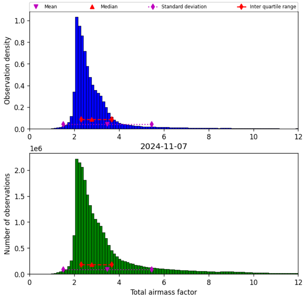
Figure 32: Histogram of “Total airmass factor” for 2024-11-06 to 2024-11-08
