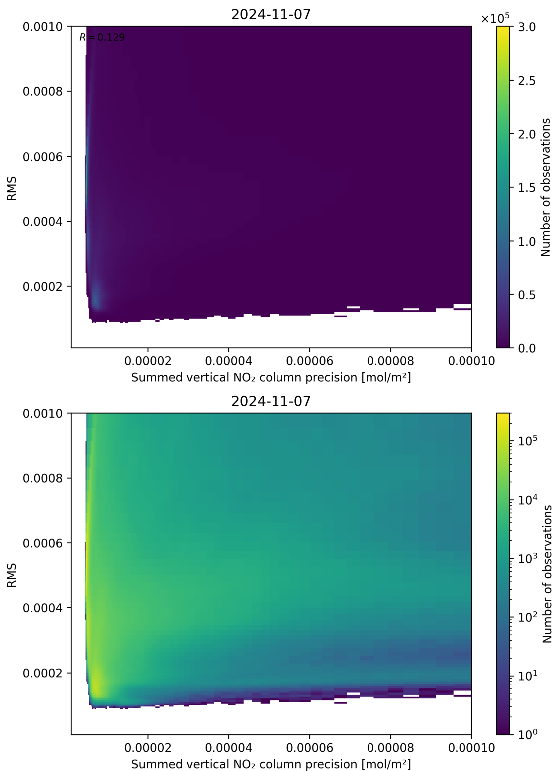
Figure 108: Scatter density plot of “Summed vertical NO 2 column precision” against “RMS” for 2024-11-06 to 2024-11-08.
