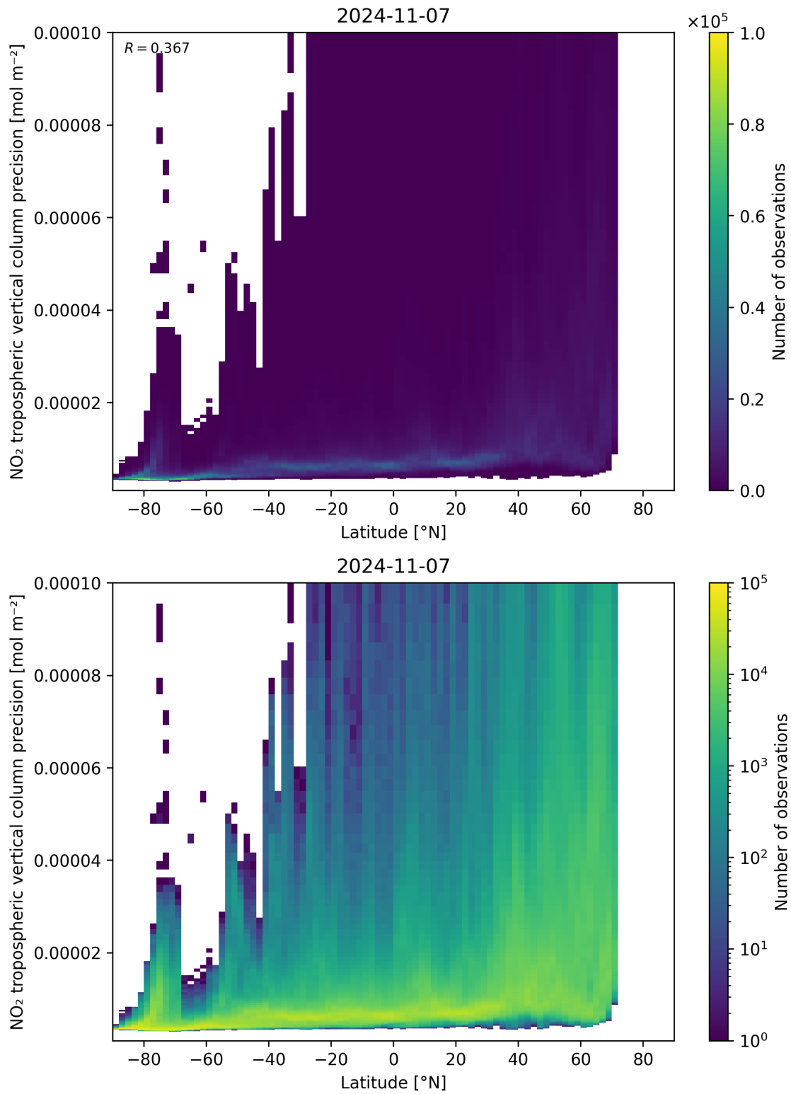
Figure 93: Scatter density plot of “Latitude” against “NO 2 tropospheric vertical column precision” for 2024-11-06 to 2024-11-08.
