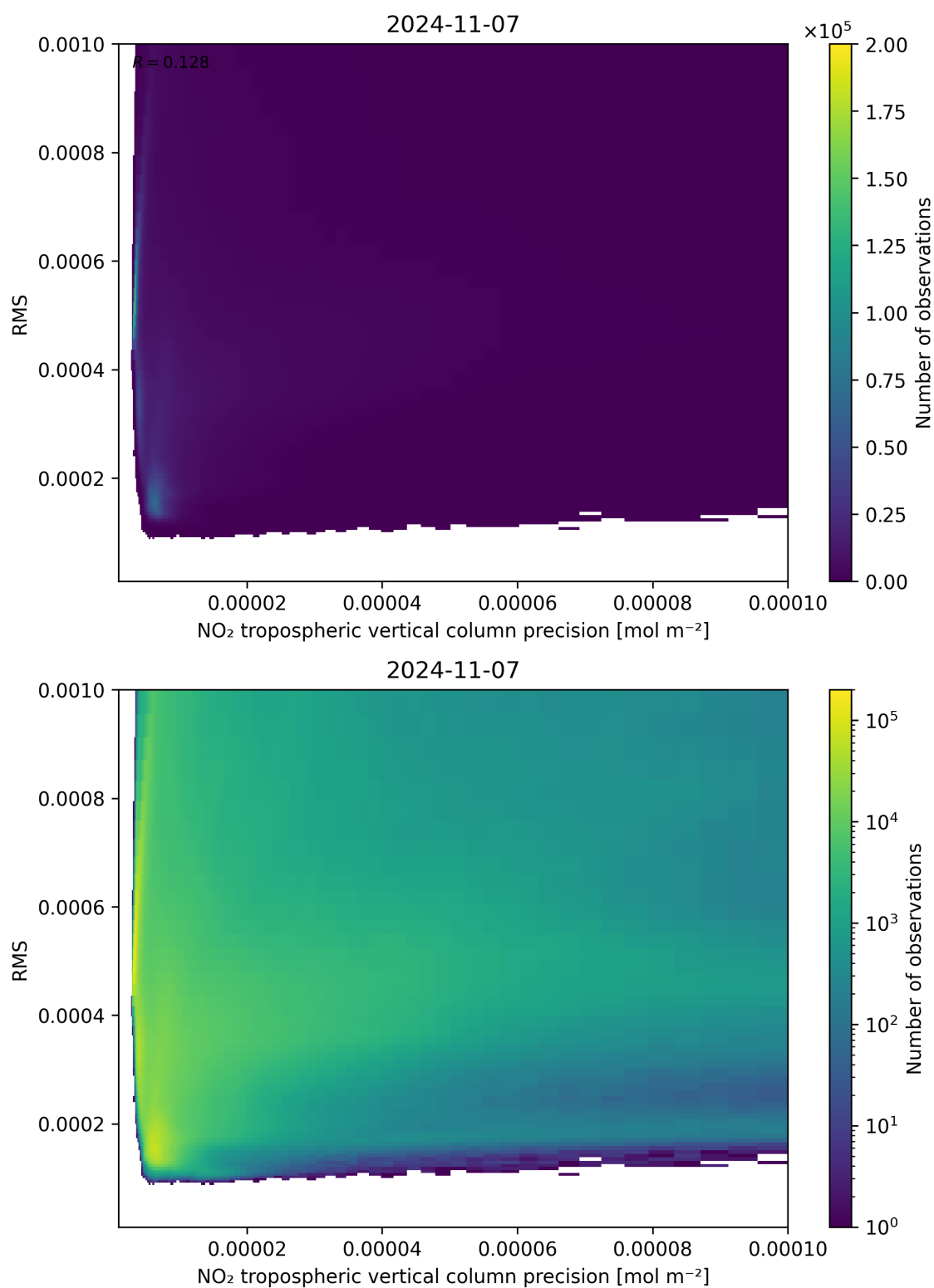
Figure 140: Scatter density plot of “NO 2 tropospheric vertical column precision” against “RMS” for 2024-11-06 to 2024-11-08.
