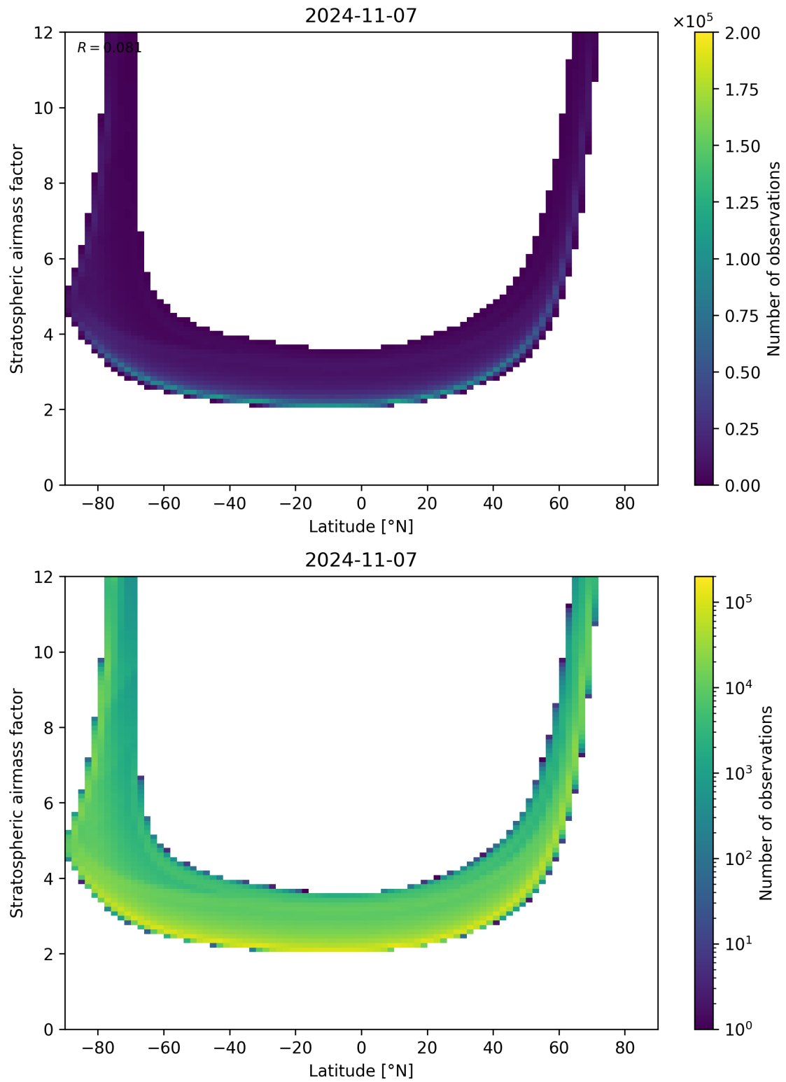
Figure 83: Scatter density plot of “Latitude” against “Stratospheric air mass factor” for 2024-11-06 to 2024-11-08.
