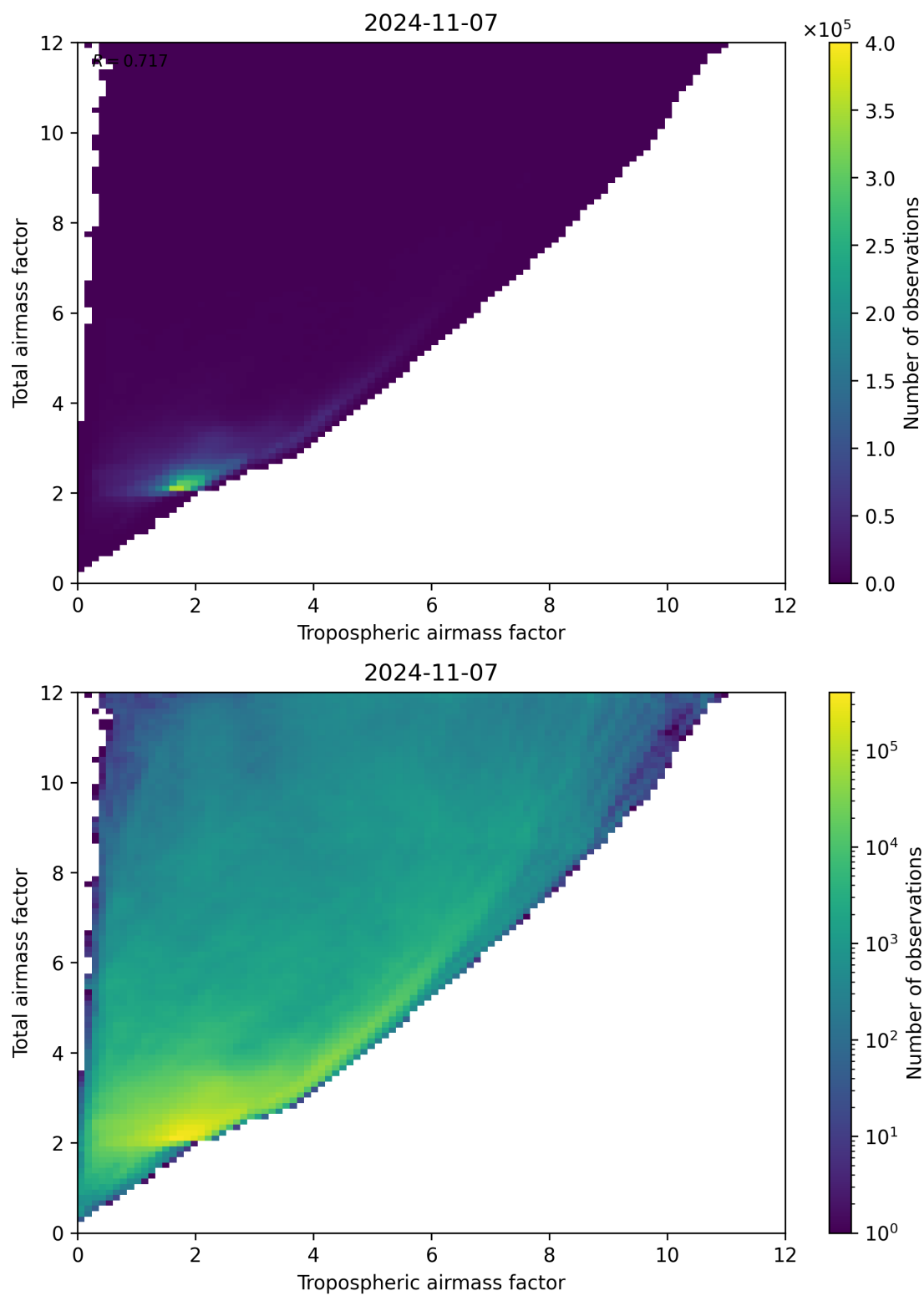
Figure 72: Scatter density plot of “Tropospheric airmass factor” against “Total airmass factor” for 2024-11-06 to 2024-11-08.
