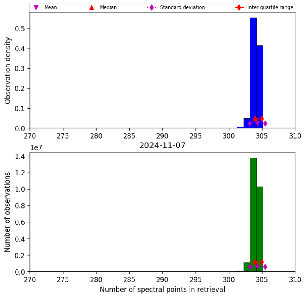
Figure 33: Histogram of “Number of spectral points in retrieval” for 2024-11-06 to 2024-11-08
