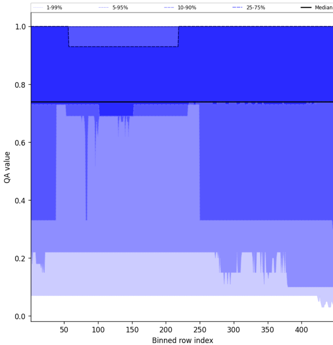
Figure 45: Along track statistics of “QA value” for 2024-11-06 to 2024-11-08
