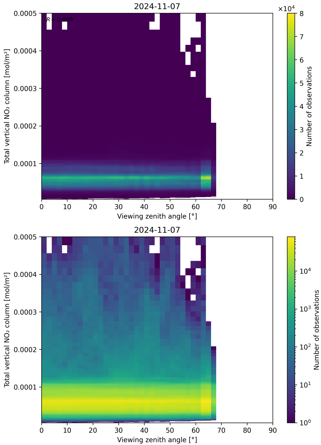
Figure 167: Scatter density plot of “Viewing zenith angle” against “Total vertical NO 2 column” for 2024-11-06 to 2024-11-08.
