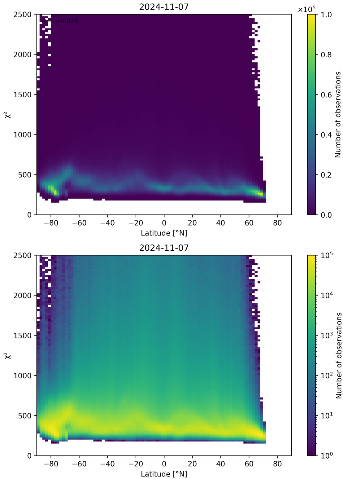
Figure 86: Scatter density plot of “Latitude” against “ \chi^2 ” for 2024-11-06 to 2024-11-08.
