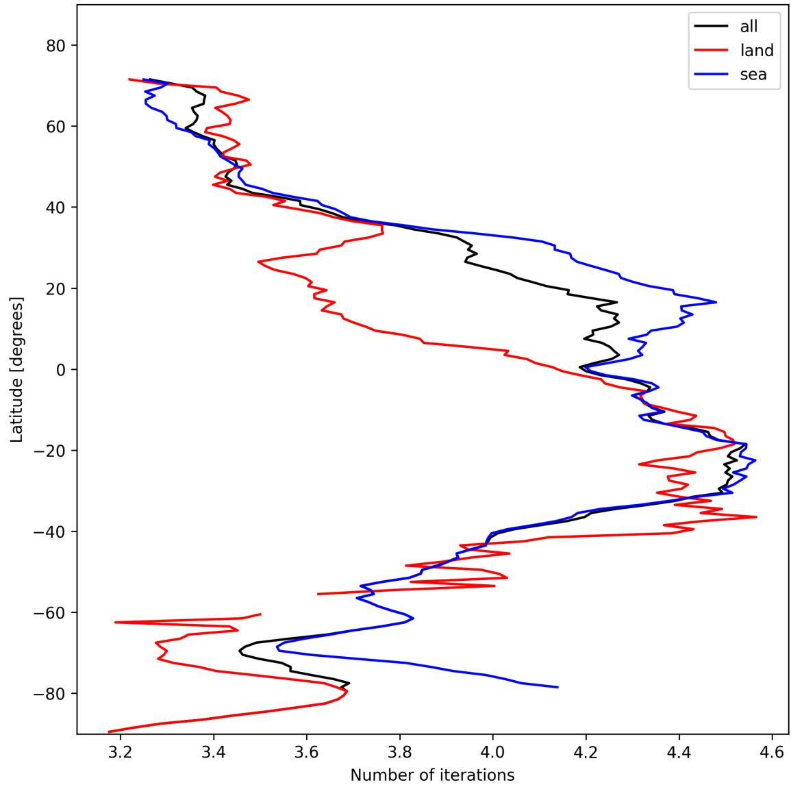
Figure 17: Zonal average of “Number of iterations” for 2024-11-06 to 2024-11-08.
