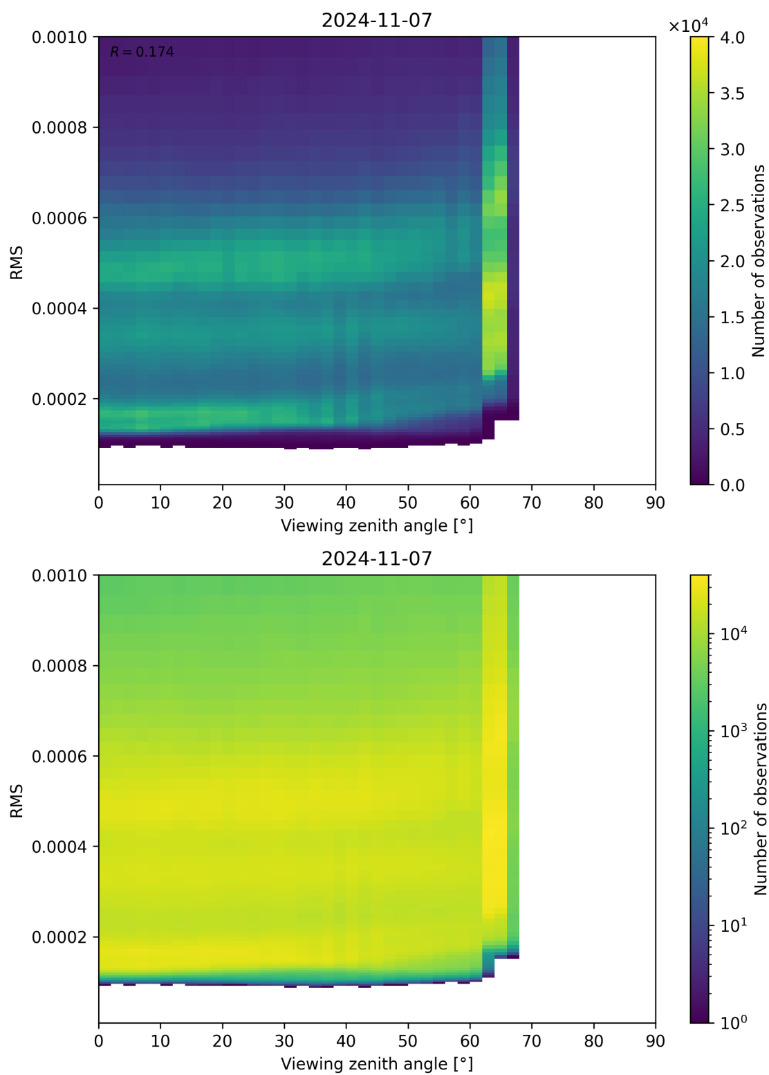
Figure 171: Scatter density plot of “Viewing zenith angle” against “RMS” for 2024-11-06 to 2024-11-08.
