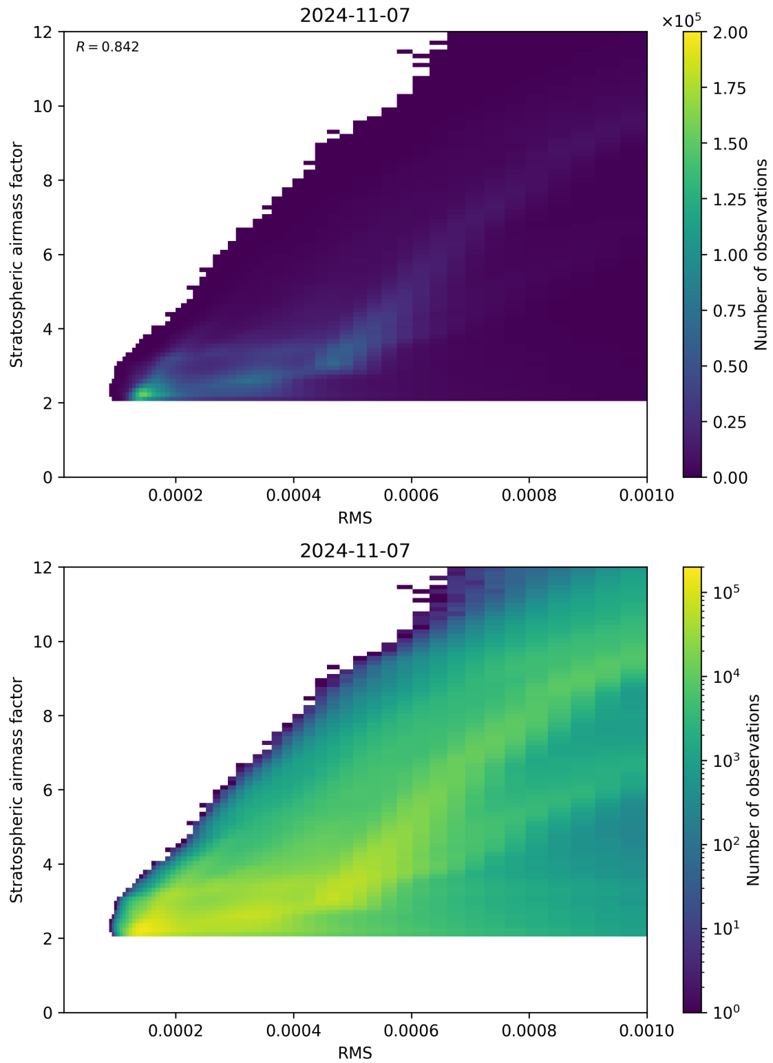
Figure 144: Scatter density plot of “RMS” against “Stratospheric airmass factor” for 2024-11-06 to 2024-11-08.
