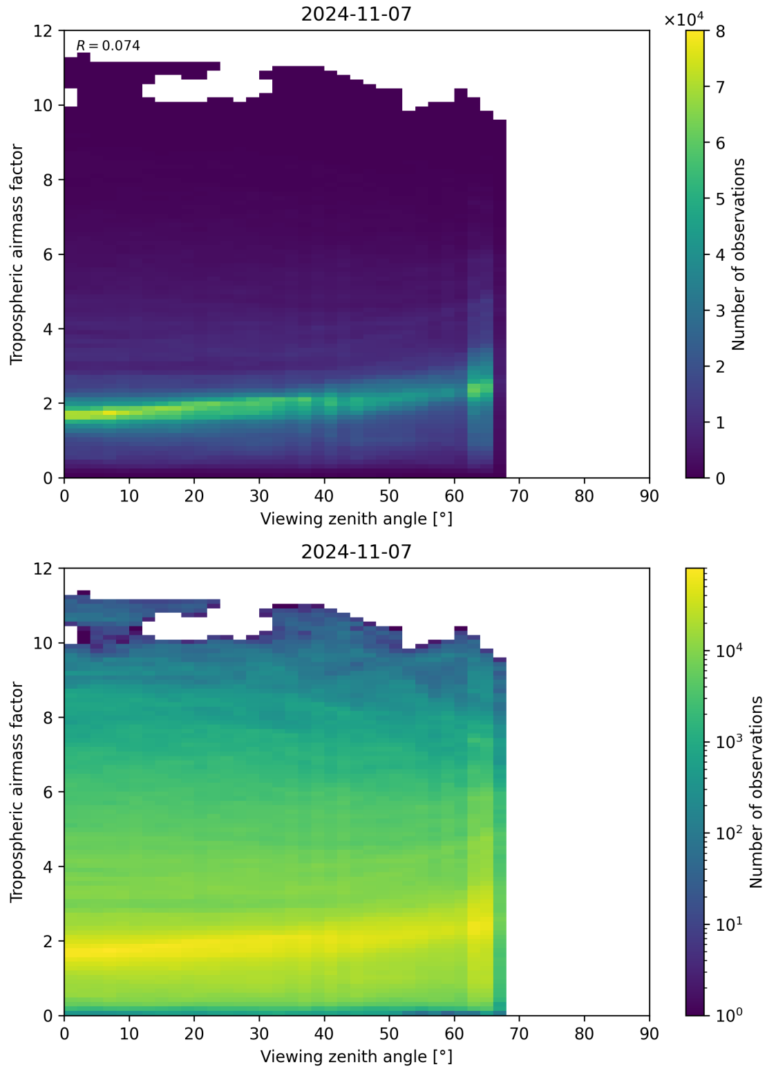
Figure 161: Scatter density plot of “Viewing zenith angle” against “Tropospheric airmass factor” for 2024-11-06 to 2024-11-08.
