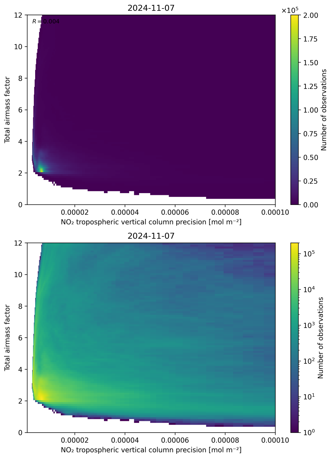
Figure 132: Scatter density plot of “NO 2 tropospheric vertical column precision” against “Total air mass factor” for 2024-11-06 to 2024-11-08.
