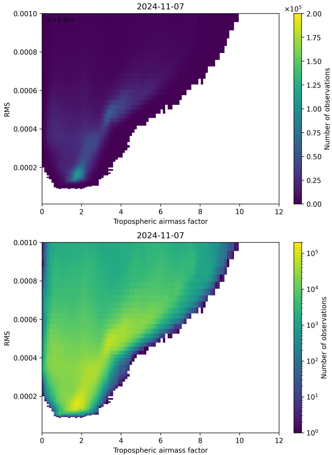
Figure 79: Scatter density plot of “Tropospheric airmass factor” against “RMS” for 2024-11-06 to 2024-11-08.
