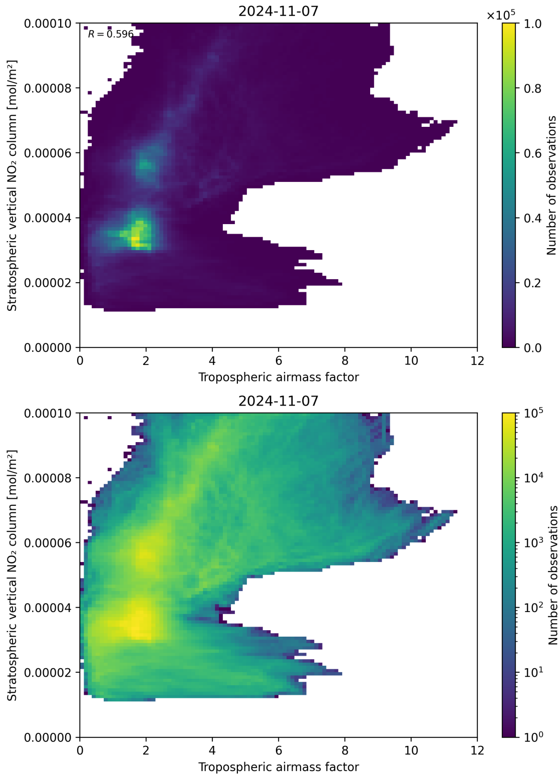
Figure 74: Scatter density plot of “Tropospheric air mass factor” against “Stratospheric vertical NO 2 column” for 2024-11-06 to 2024-11-08.
