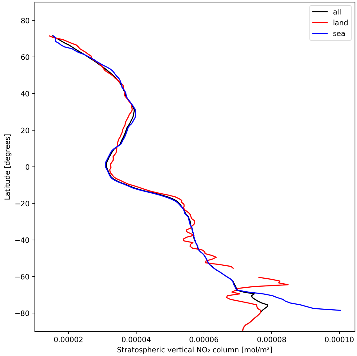
Figure 19: Zonal average of “Stratospheric vertical NO 2 column” for 2024-11-06 to 2024-11-08.
