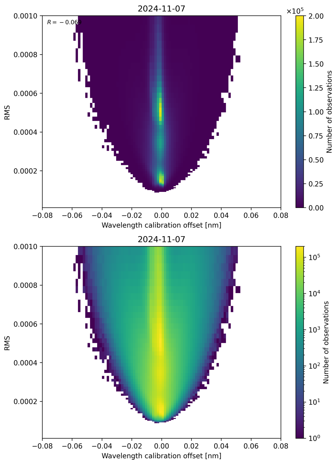
Figure 181: Scatter density plot of “Wavelength calibration offset” against “RMS” for 2024-11-06 to 2024-11-08.
