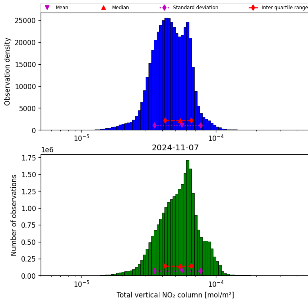
Figure 38: Histogram of “Total vertical NO 2 column” for 2024-11-06 to 2024-11-08
