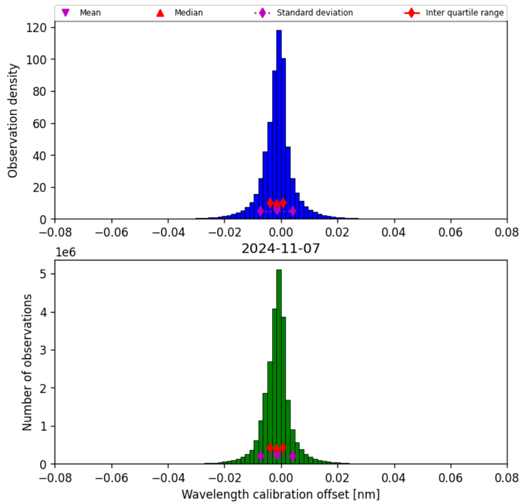
Figure 35: Histogram of “Wavelength calibration offset” for 2024-11-06 to 2024-11-08
