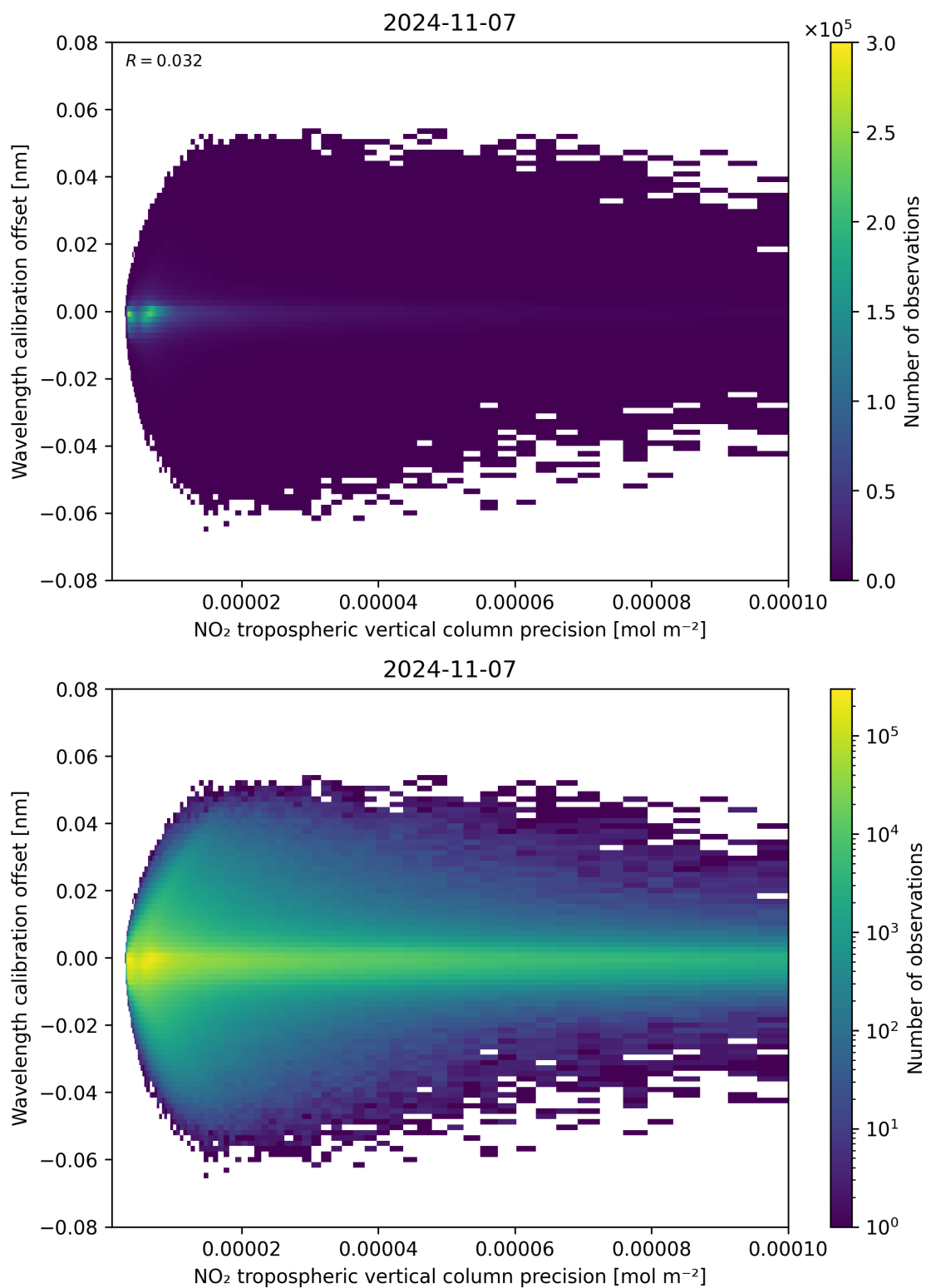
Figure 141: Scatter density plot of “NO 2 tropospheric vertical column precision” against “Wavelength calibration offset” for 2024-11-06 to 2024-11-08.
