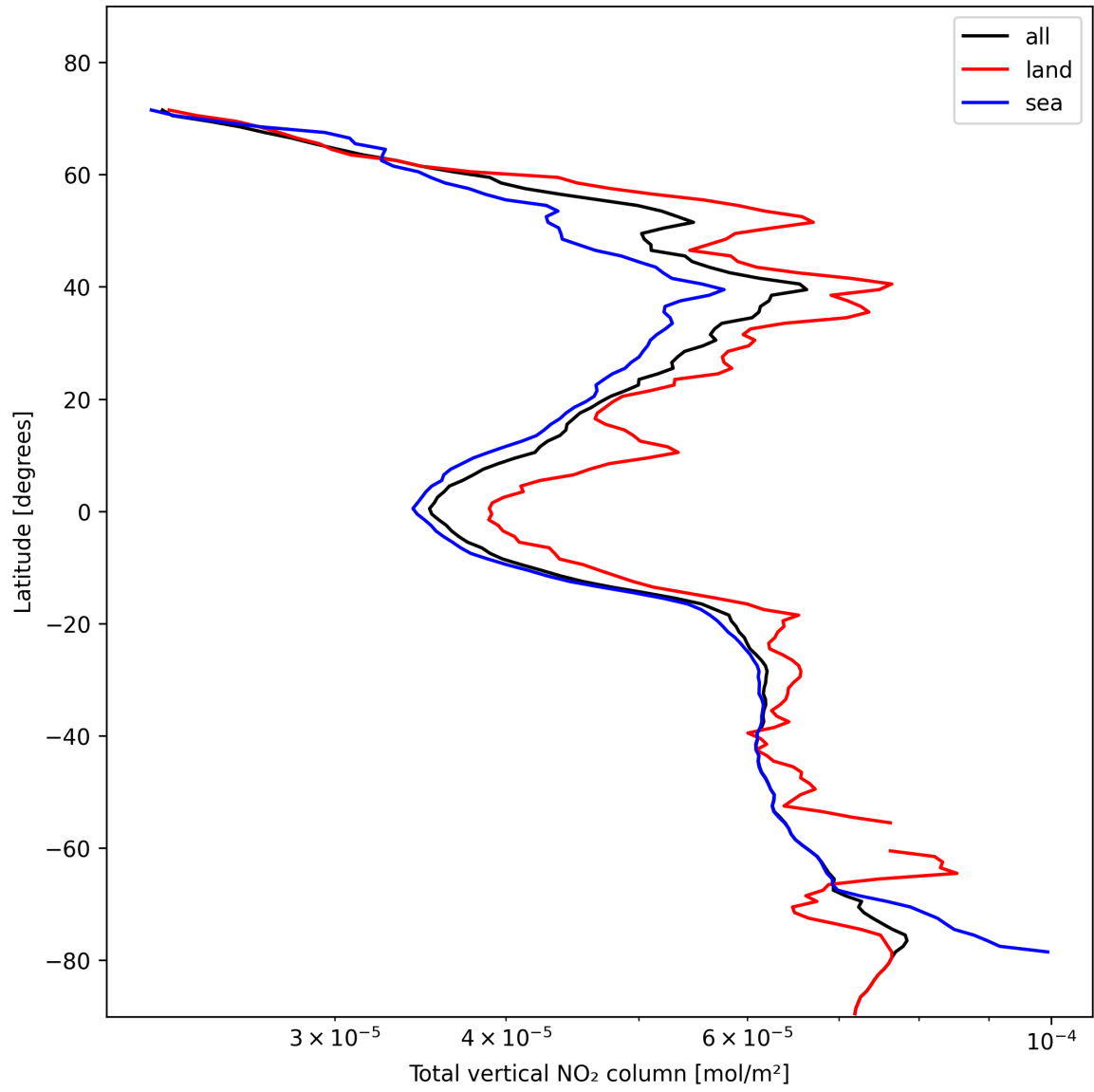
Figure 21: Zonal average of “Total vertical NO 2 column” for 2024-11-06 to 2024-11-08.
