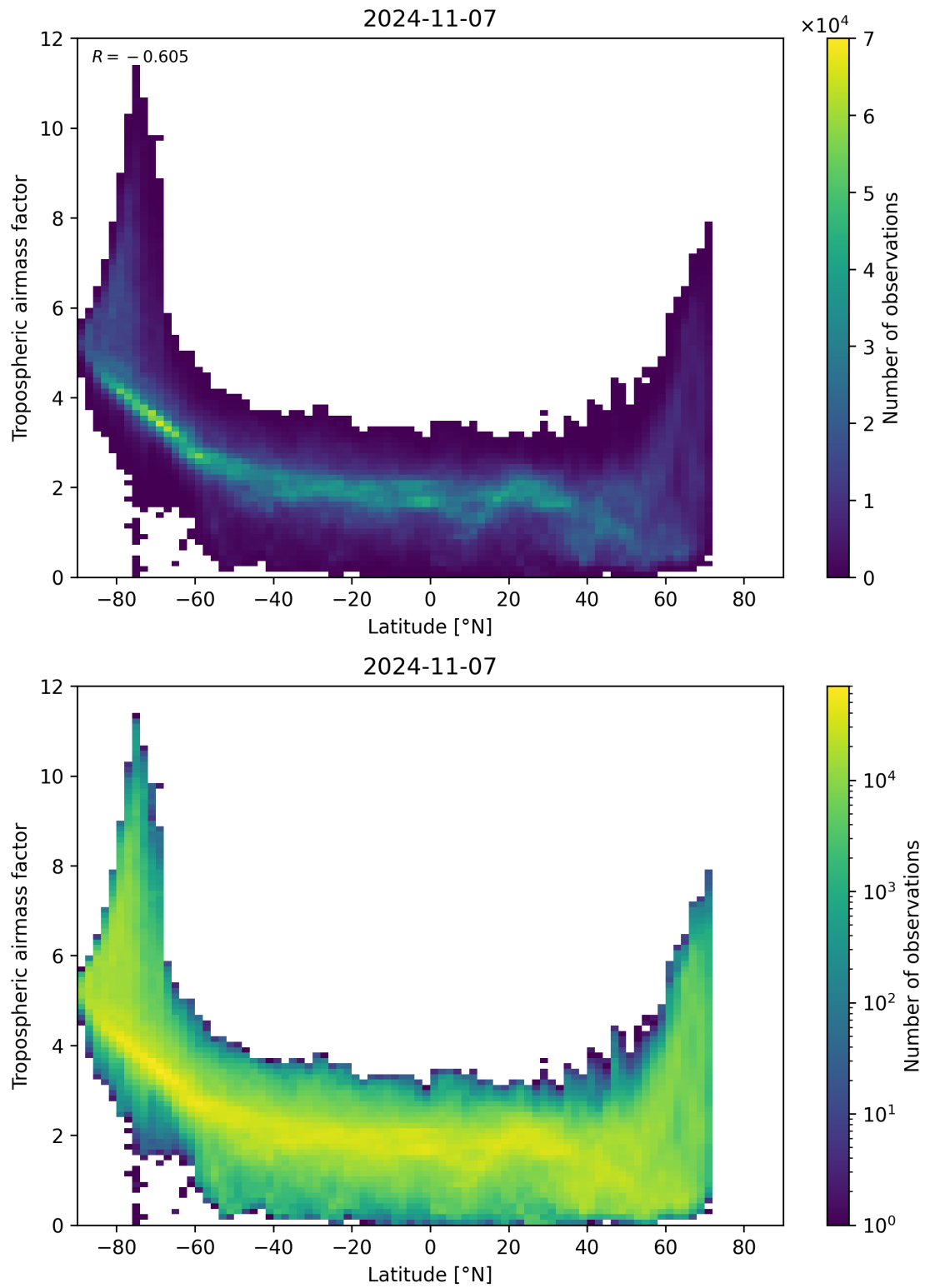
Figure 85: Scatter density plot of “Latitude” against “Tropospheric airmass factor” for 2024-11-06 to 2024-11-08.
