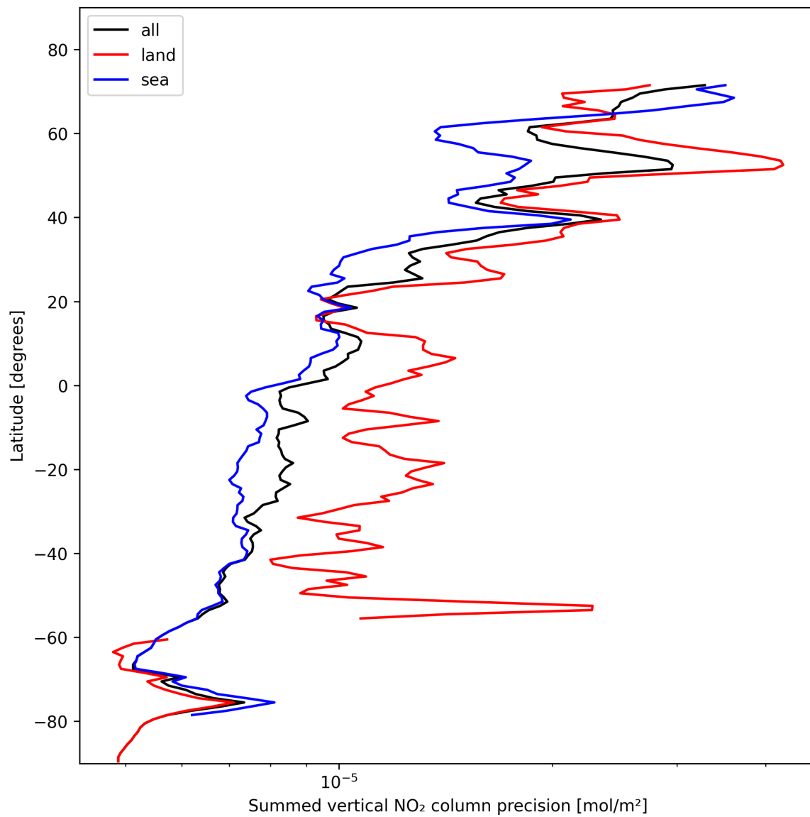
Figure 24: Zonal average of “Summed vertical NO 2 column precision” for 2024-11-06 to 2024-11-08.
