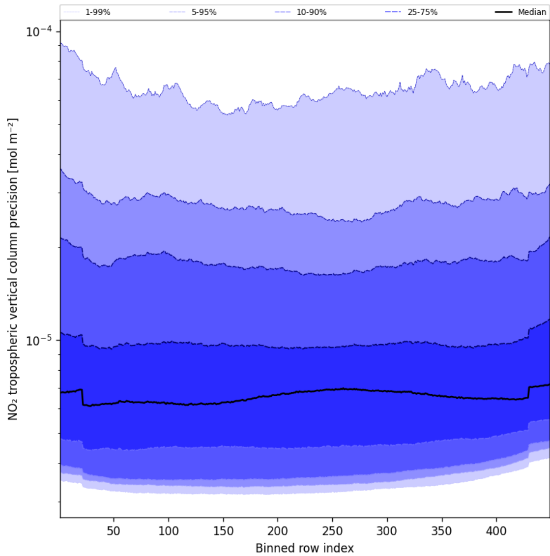
Figure 47: Along track statistics of “NO 2 tropospheric vertical column precision” for 2024-11-06 to 2024-11-08
