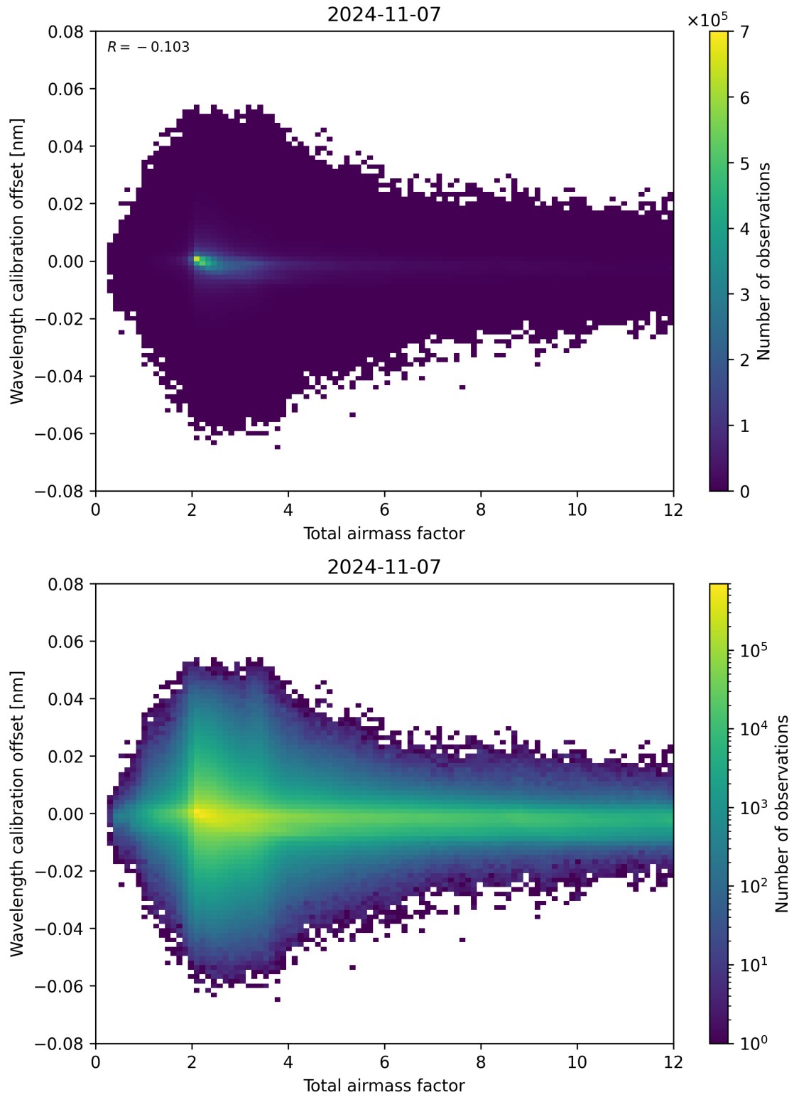
Figure 70: Scatter density plot of “Total airmass factor” against “Wavelength calibration offset” for 2024-11-06 to 2024-11-08.
