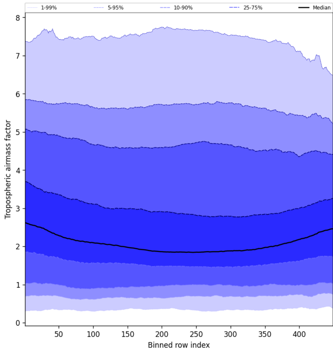
Figure 48: Along track statistics of “Tropospheric air mass factor” for 2024-11-06 to 2024-11-08
