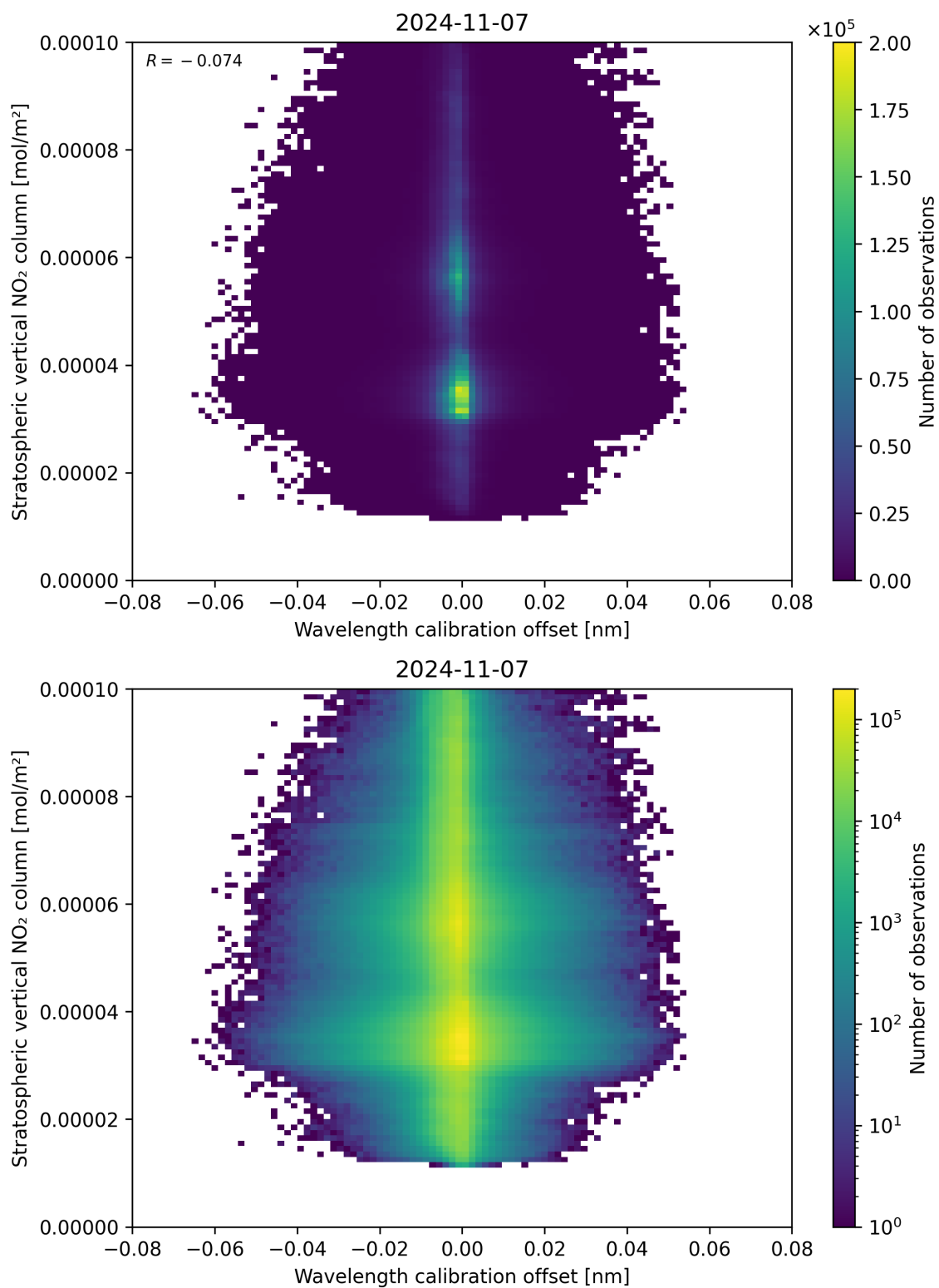
Figure 176: Scatter density plot of “Wavelength calibration offset” against “Stratospheric vertical NO 2 column” for 2024-11-06 to 2024-11-08.
