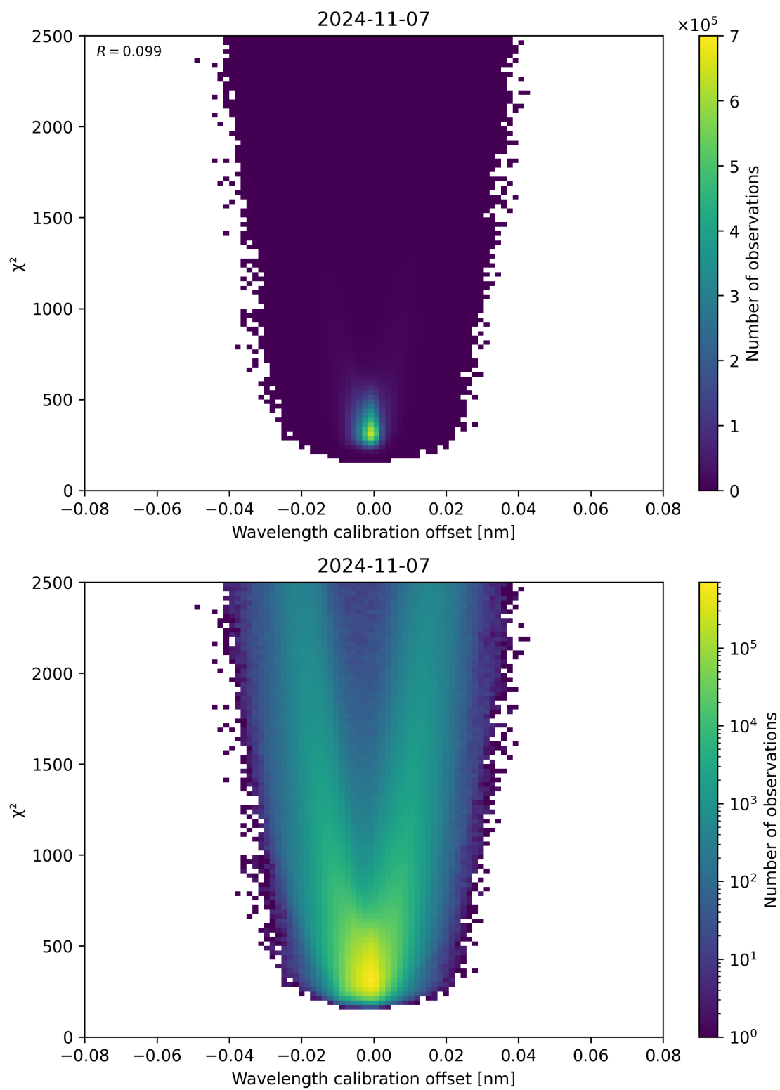
Figure 175: Scatter density plot of “Wavelength calibration offset” against “ \chi^2 ” for 2024-11-06 to 2024-11-08.
