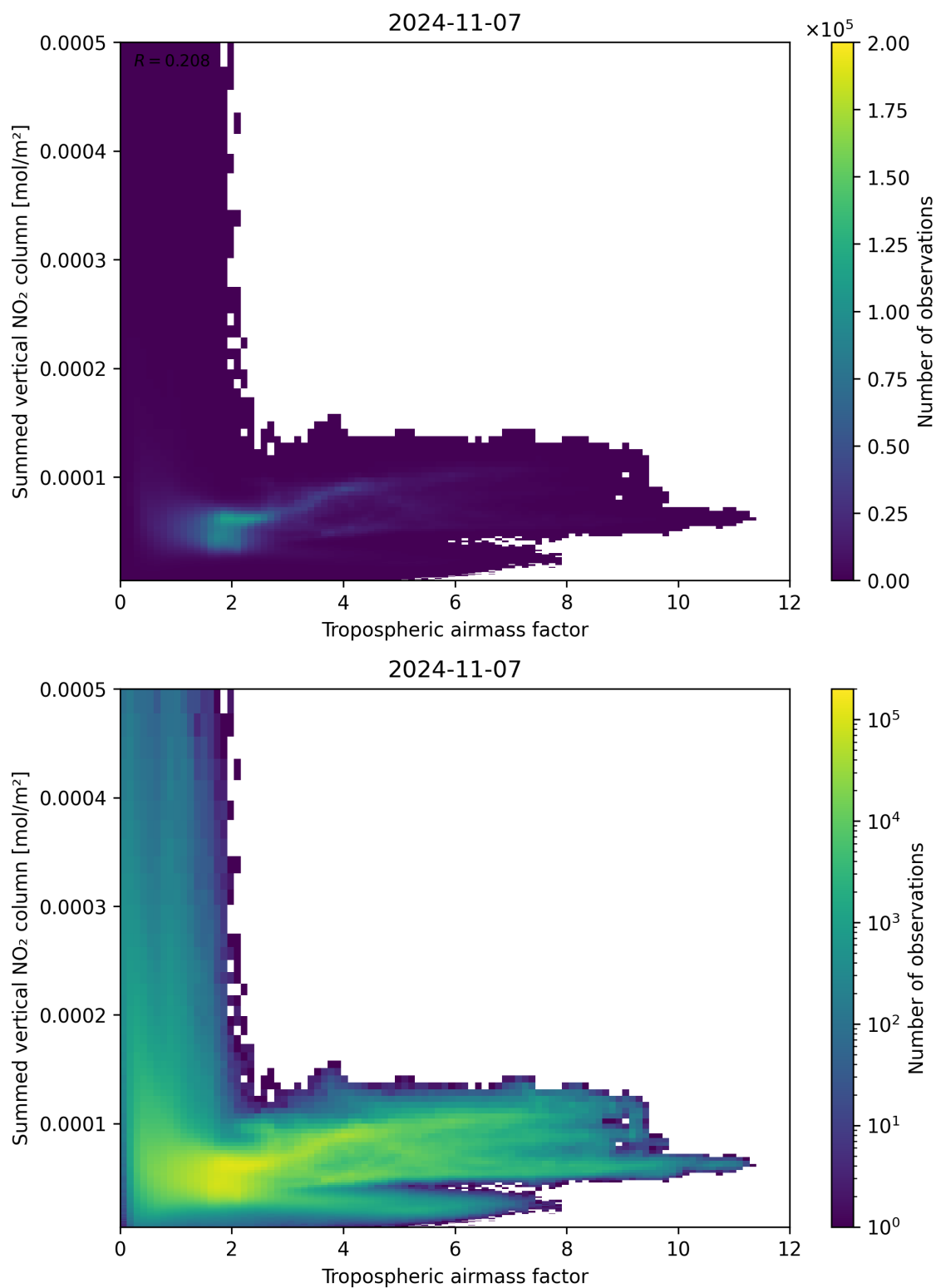
Figure 75: Scatter density plot of “Tropospheric airmass factor” against “Summed vertical NO 2 column” for 2024-11-06 to 2024-11-08.
