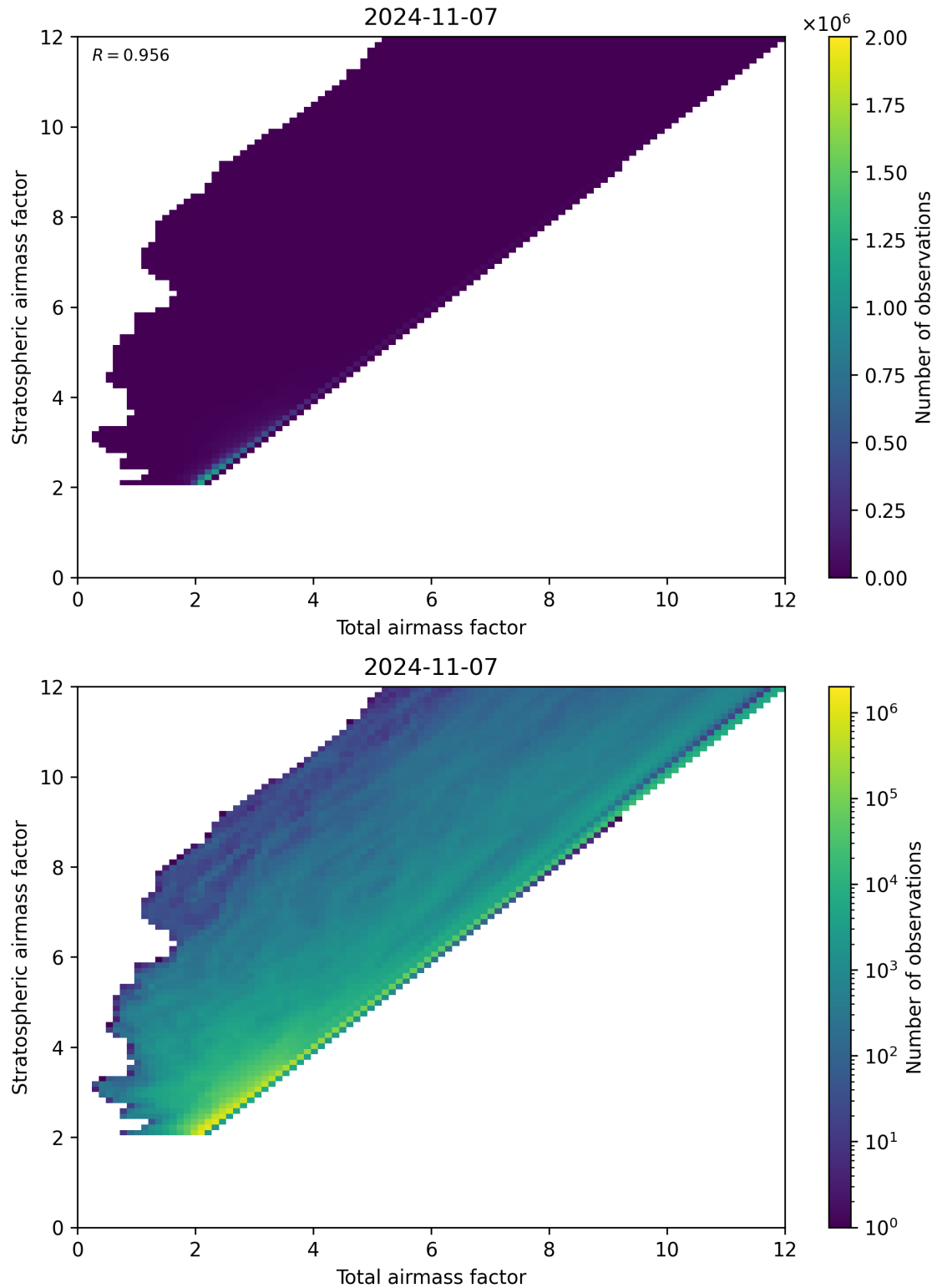
Figure 62: Scatter density plot of “Total airmass factor” against “Stratospheric airmass factor” for 2024-11-06 to 2024-11-08.
