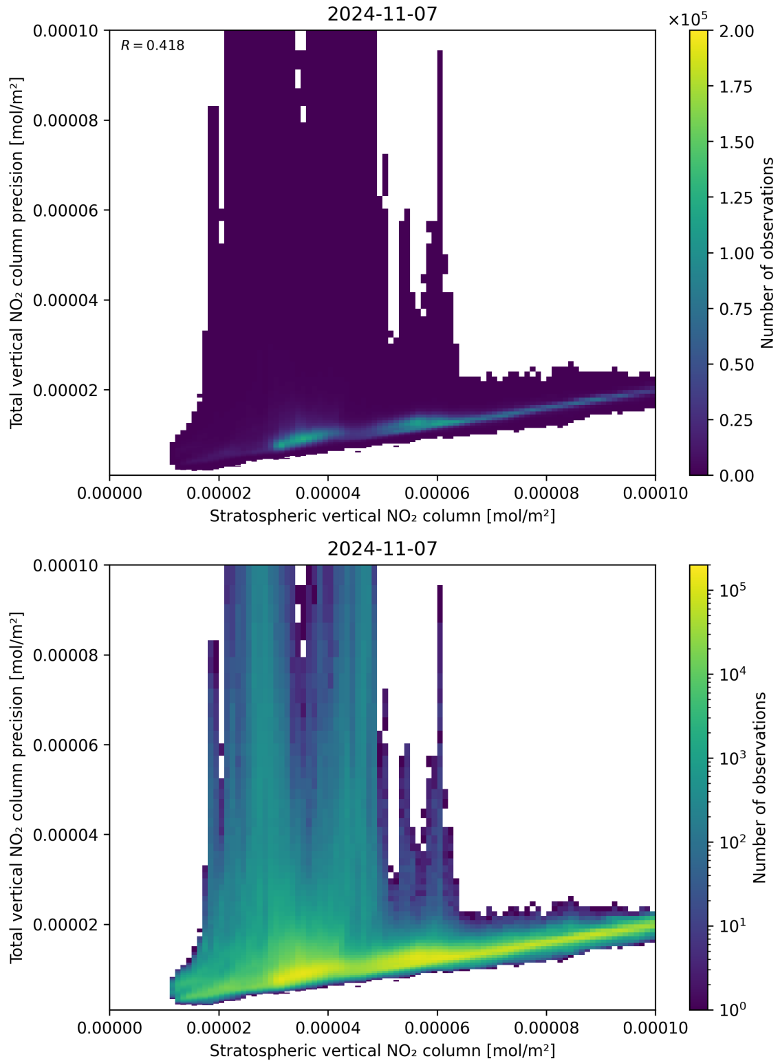
Figure 101: Scatter density plot of “Stratospheric vertical NO 2 column” against “Total vertical NO 2 column precision” for 2024-11-06 to 2024-11-08.
