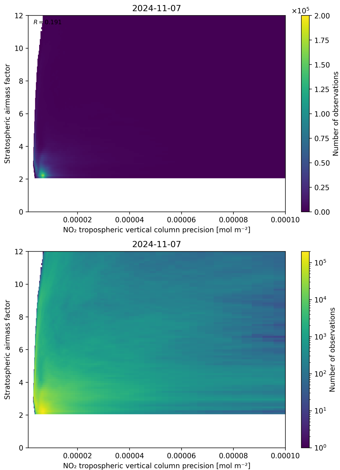
Figure 131: Scatter density plot of “NO 2 tropospheric vertical column precision” against “Stratospheric airmass factor” for 2024-11-06 to 2024-11-08.
