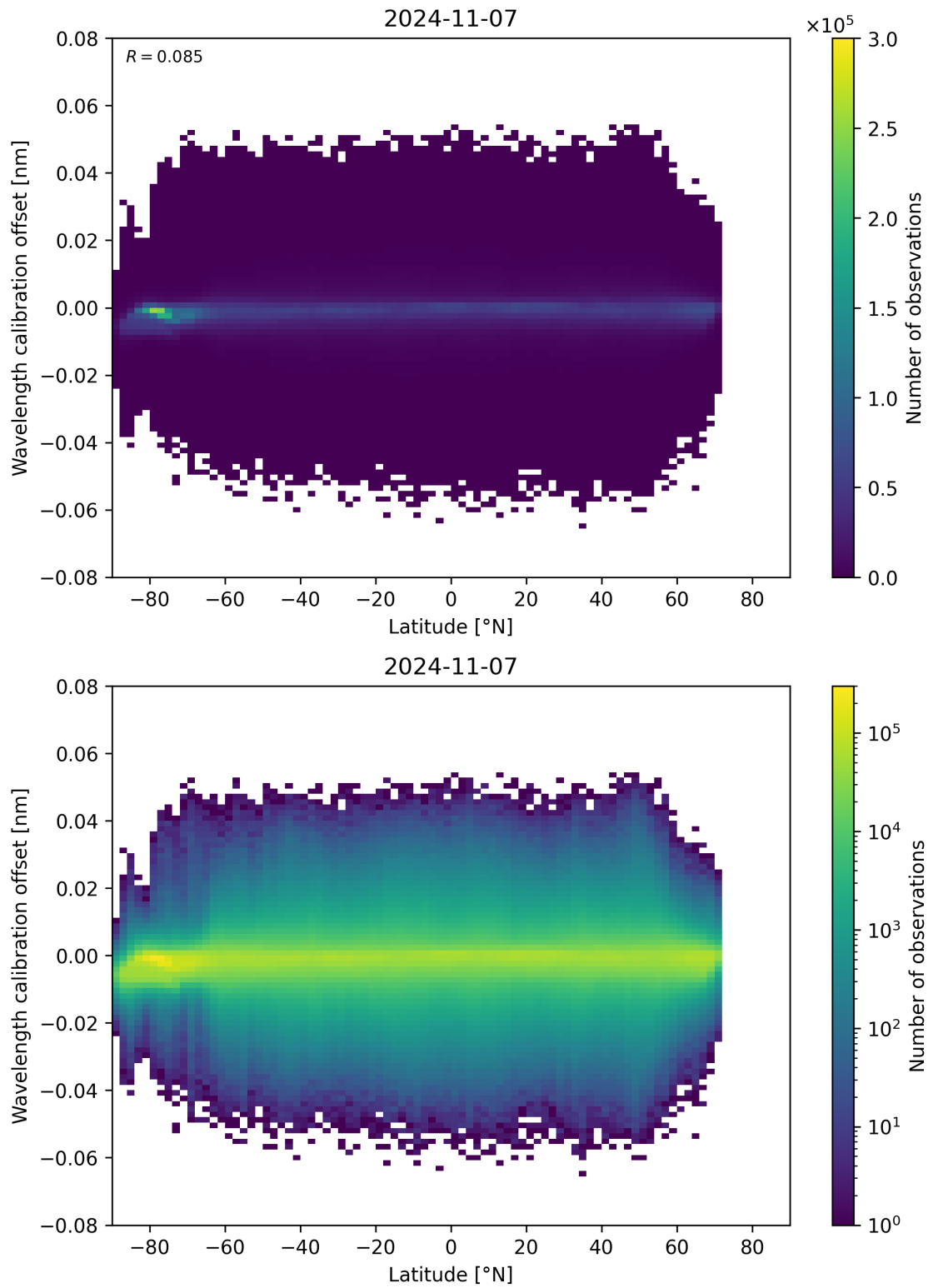
Figure 95: Scatter density plot of “Latitude” against “Wavelength calibration offset” for 2024-11-06 to 2024-11-08.
