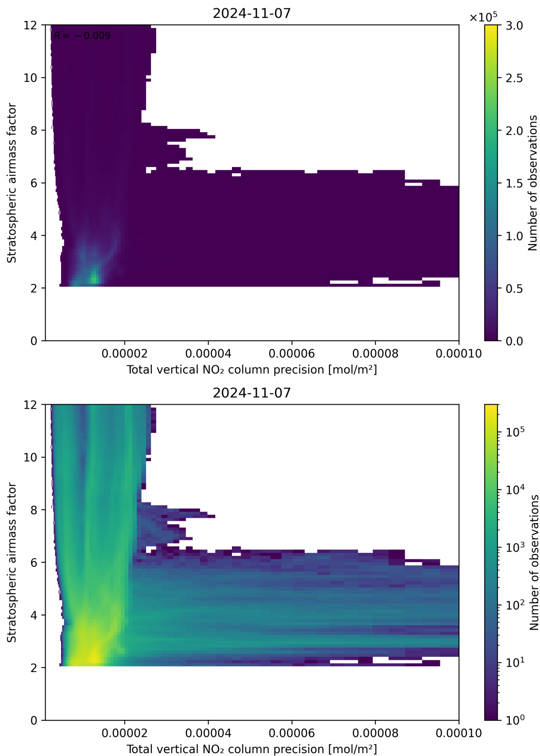
Figure 115: Scatter density plot of “Total vertical NO 2 column precision” against “Stratospheric air mass factor” for 2024-11-06 to 2024-11-08.
