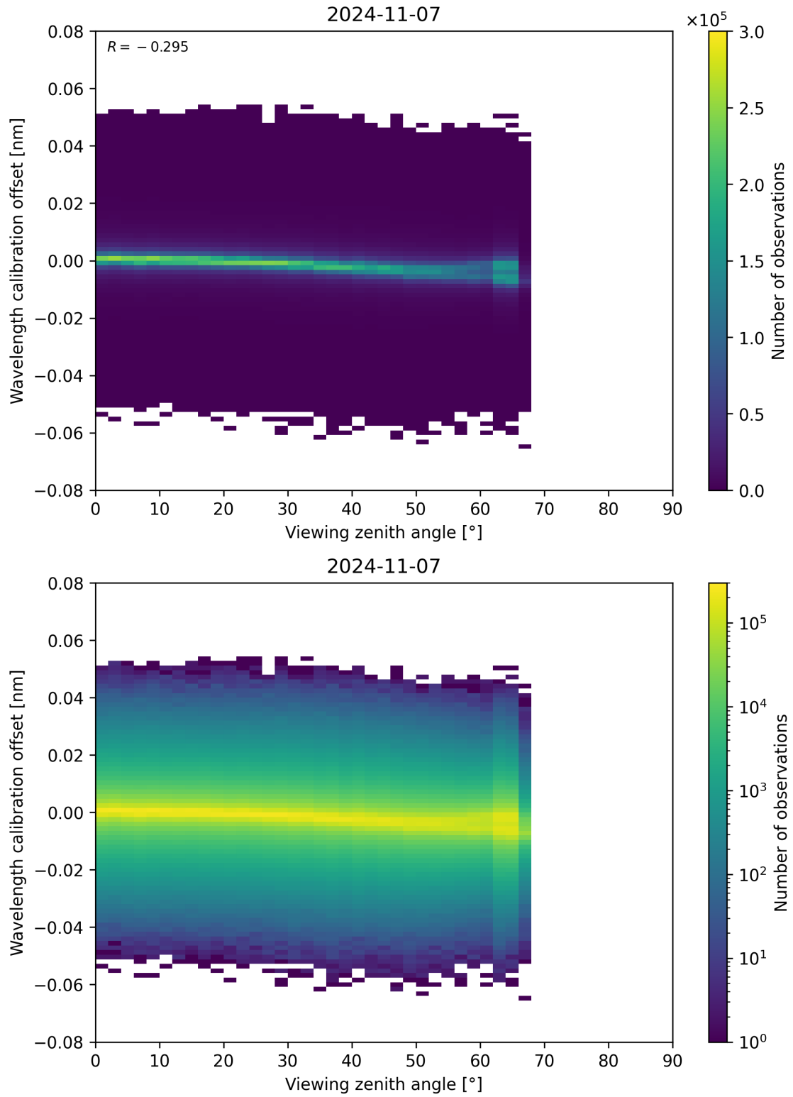
Figure 173: Scatter density plot of “Viewing zenith angle” against “Wavelength calibration offset” for 2024-11-06 to 2024-11-08.
