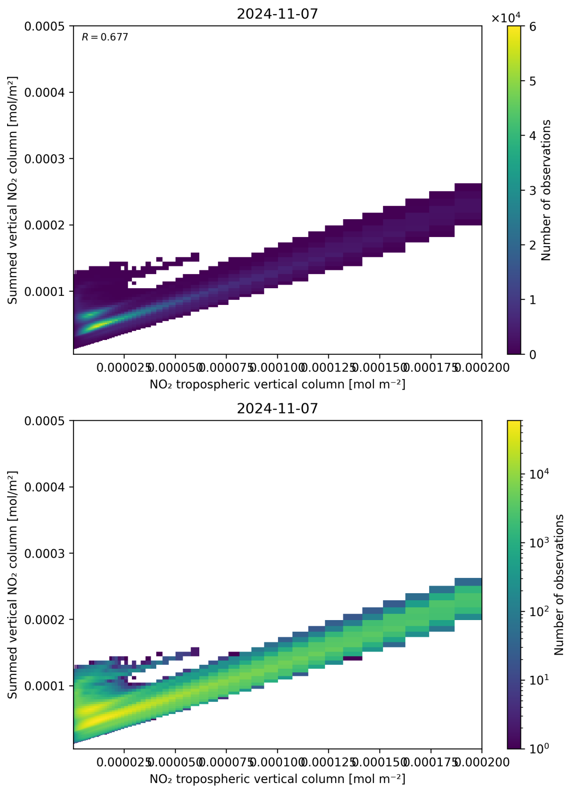
Figure 126: Scatter density plot of “NO 2 tropospheric vertical column” against “Summed vertical NO 2 column” for 2024-11-06 to 2024-11-08.
