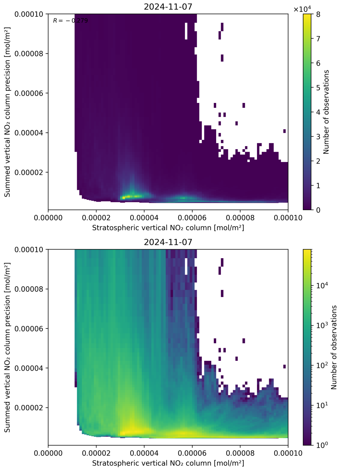
Figure 99: Scatter density plot of “Stratospheric vertical NO 2 column” against “Summed vertical NO 2 column precision” for 2024-11-06 to 2024-11-08.
