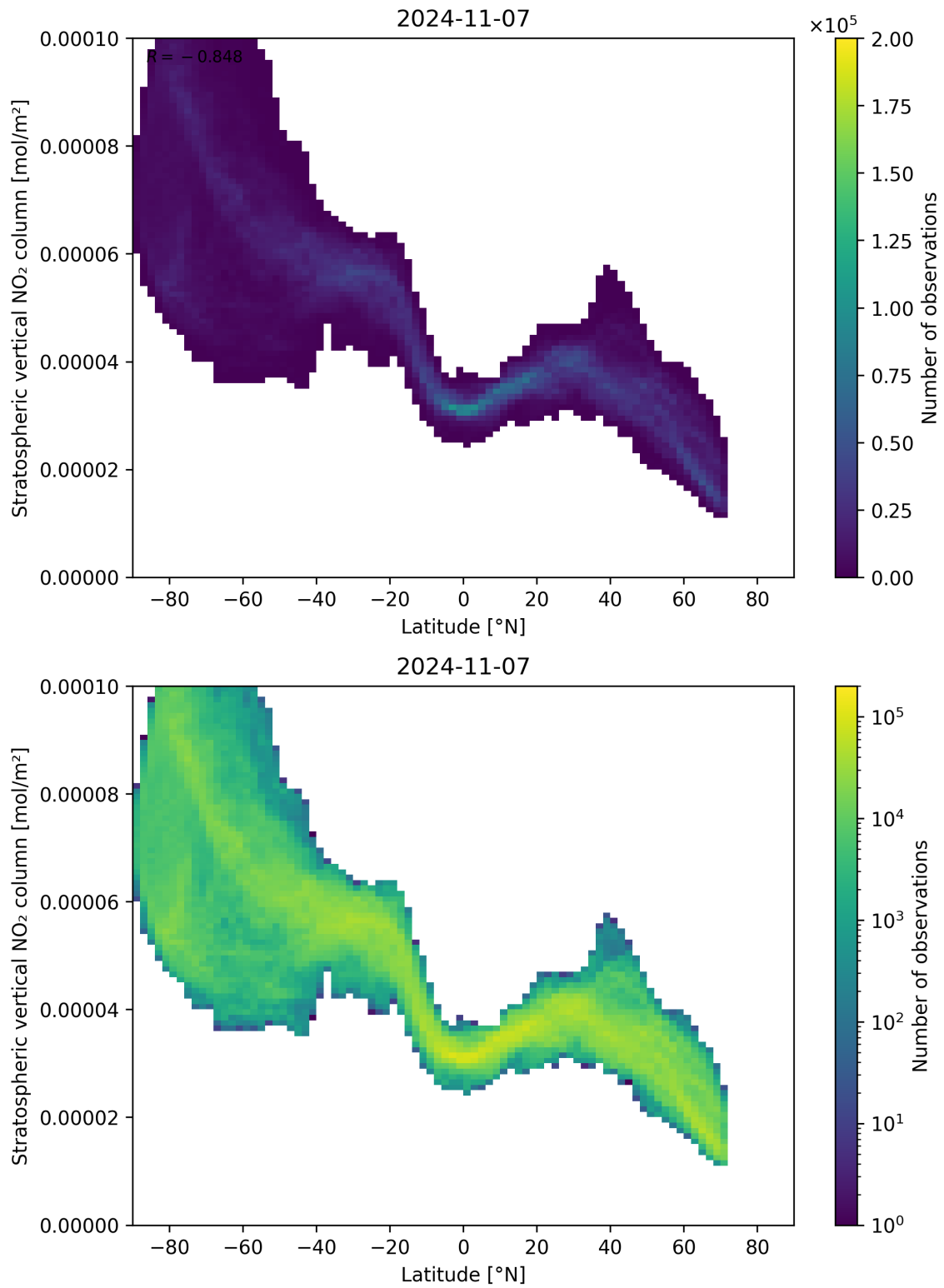
Figure 87: Scatter density plot of “Latitude” against “Stratospheric vertical NO 2 column” for 2024-11-06 to 2024-11-08.
