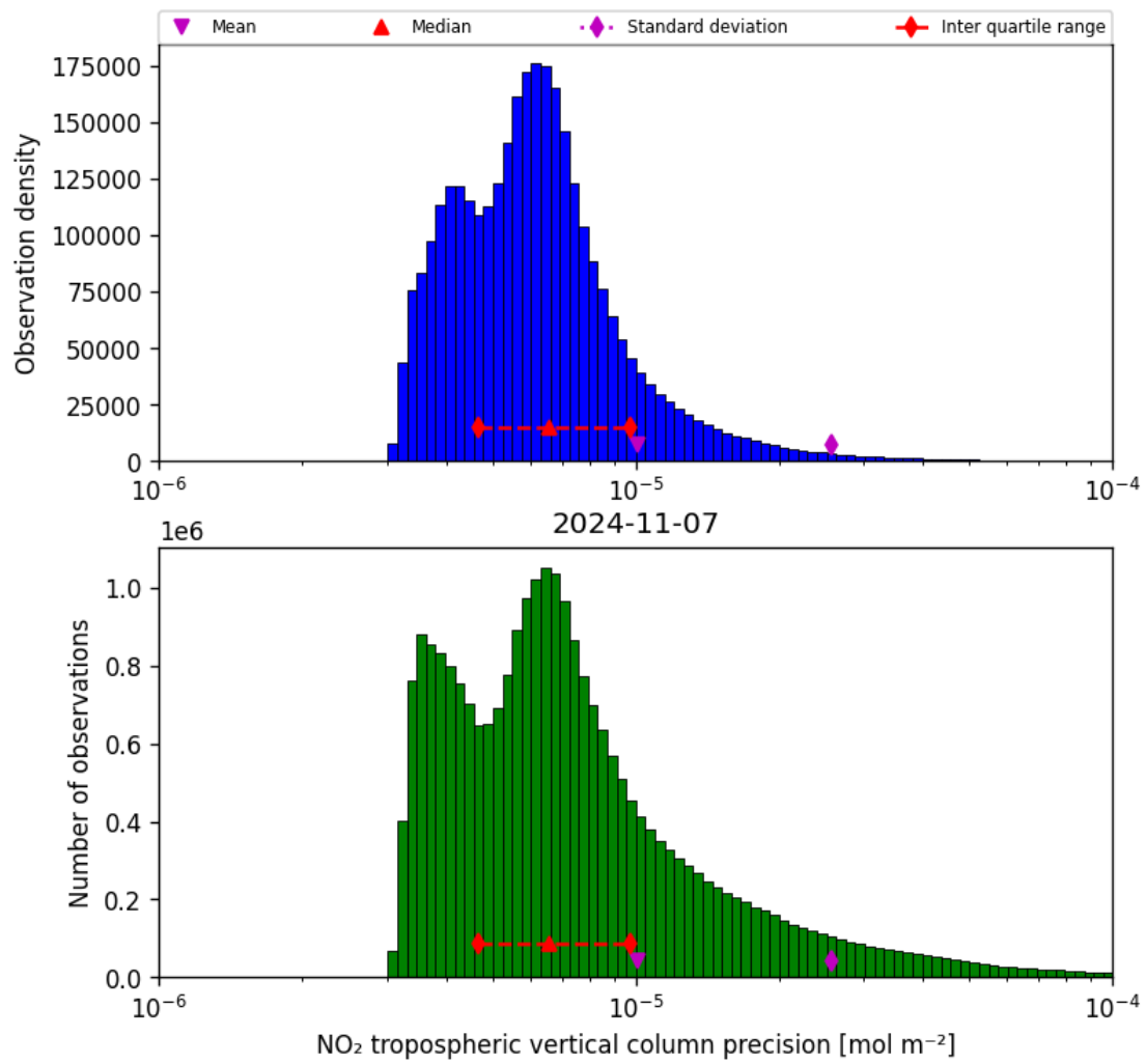
Figure 30: Histogram of “NO 2 tropospheric vertical column precision” for 2024-11-06 to 2024-11-08
