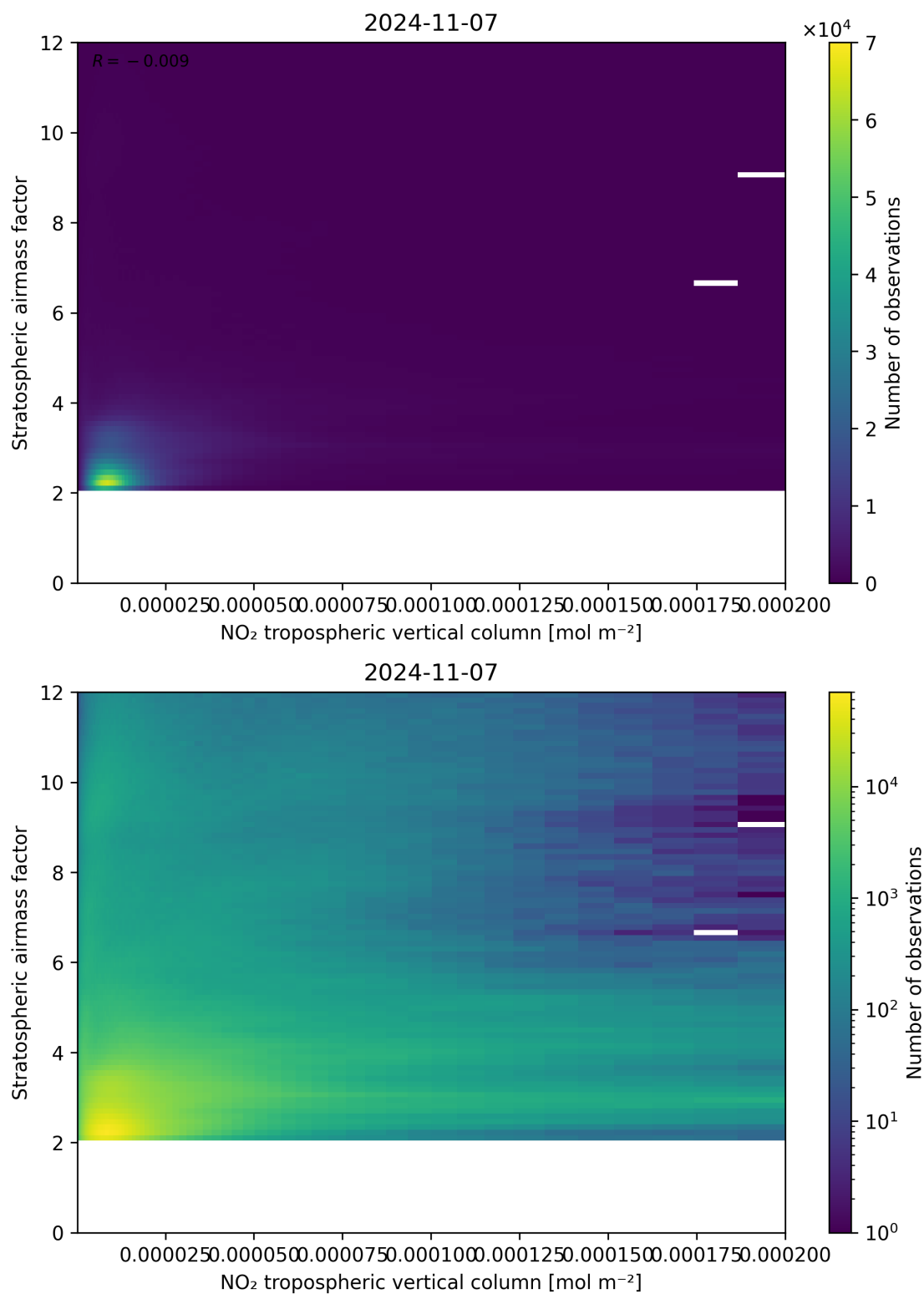
Figure 121: Scatter density plot of “NO 2 tropospheric vertical column” against “Stratospheric air mass factor” for 2024-11-06 to 2024-11-08.
