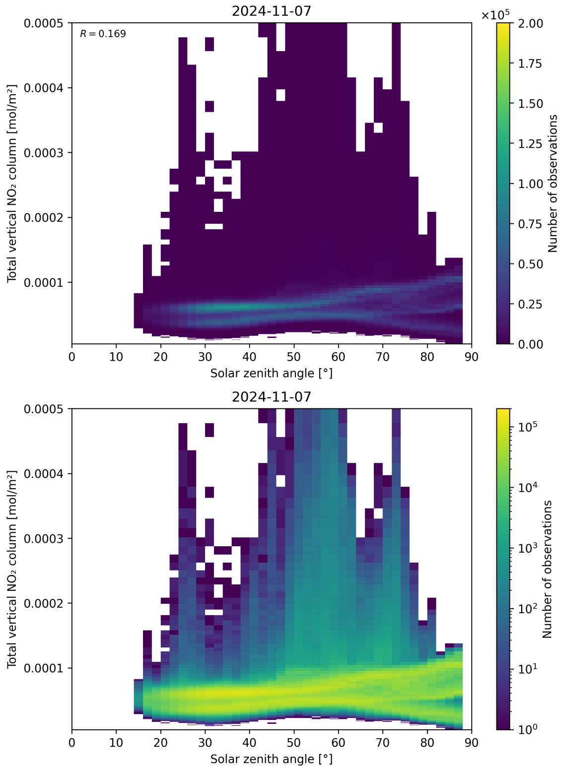
Figure 153: Scatter density plot of “Solar zenith angle” against “Total vertical NO 2 column” for 2024-11-06 to 2024-11-08.
