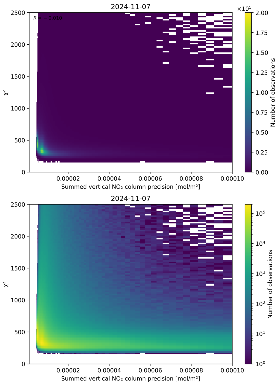
Figure 107: Scatter density plot of “Summed vertical NO 2 column precision” against “ \chi^2 ” for 2024-11-06 to 2024-11-08.
