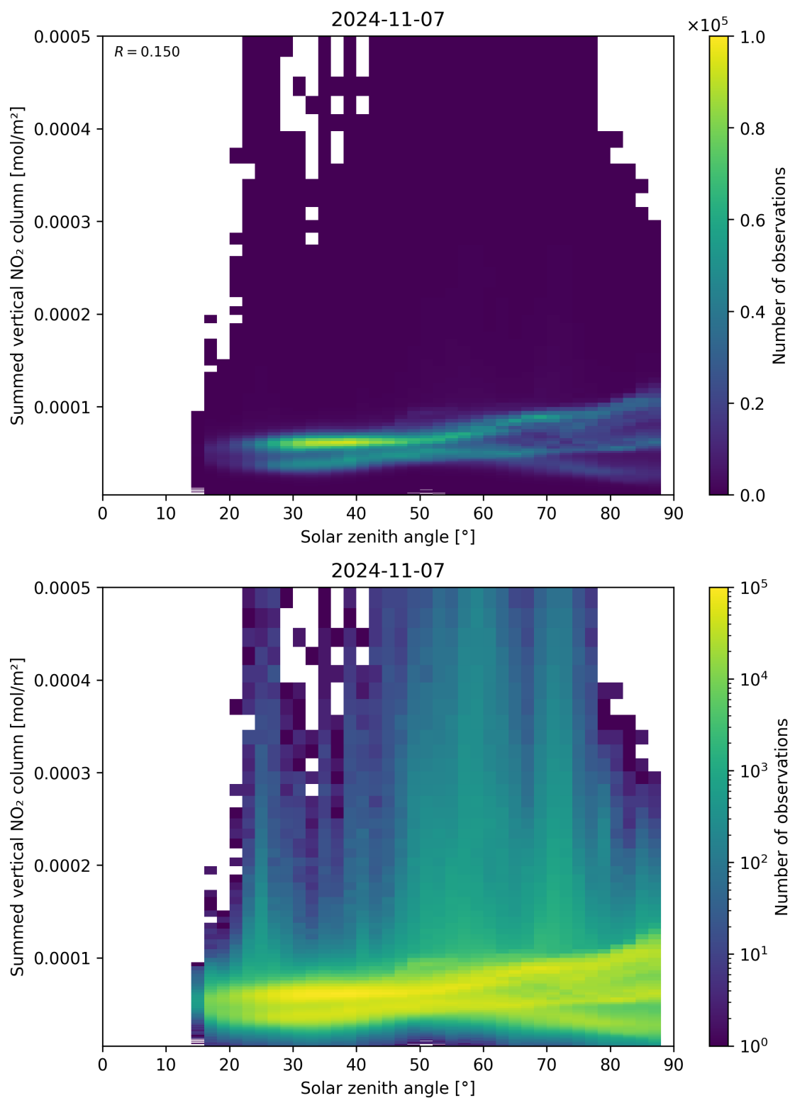
Figure 151: Scatter density plot of “Solar zenith angle” against “Summed vertical NO 2 column” for 2024-11-06 to 2024-11-08.
