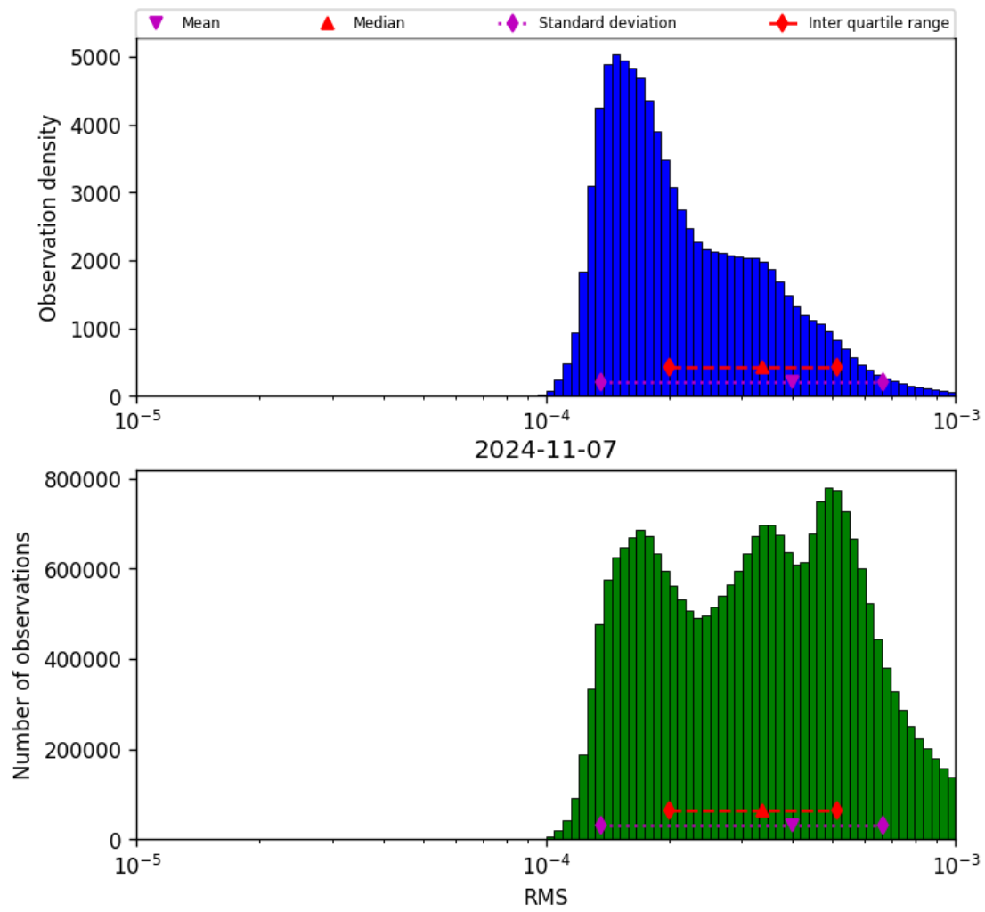
Figure 43: Histogram of “RMS” for 2024-11-06 to 2024-11-08
