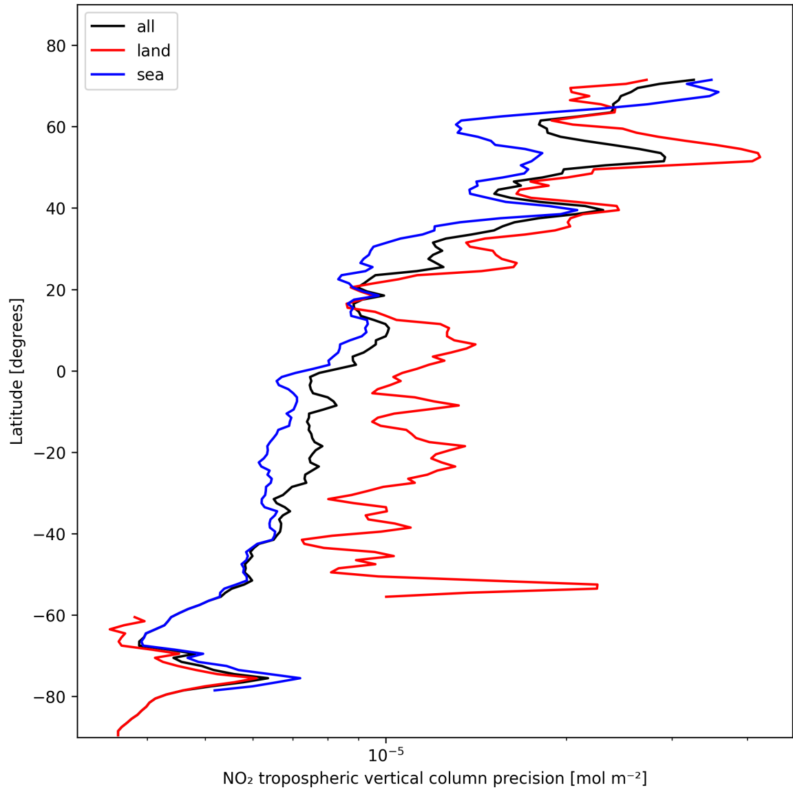
Figure 13: Zonal average of “NO 2 tropospheric vertical column precision” for 2024-11-06 to 2024-11-08.
