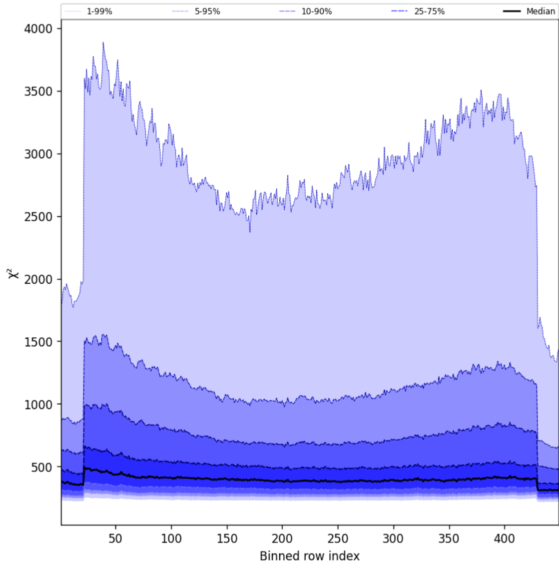
Figure 59: Along track statistics of “ \chi^2 ” for 2024-11-06 to 2024-11-08
