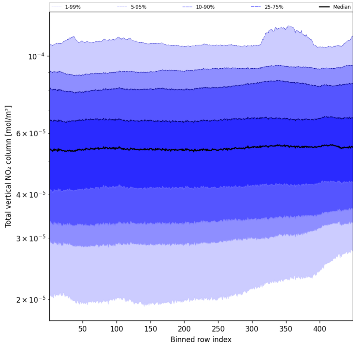
Figure 55: Along track statistics of “Total vertical NO 2 column” for 2024-11-06 to 2024-11-08
