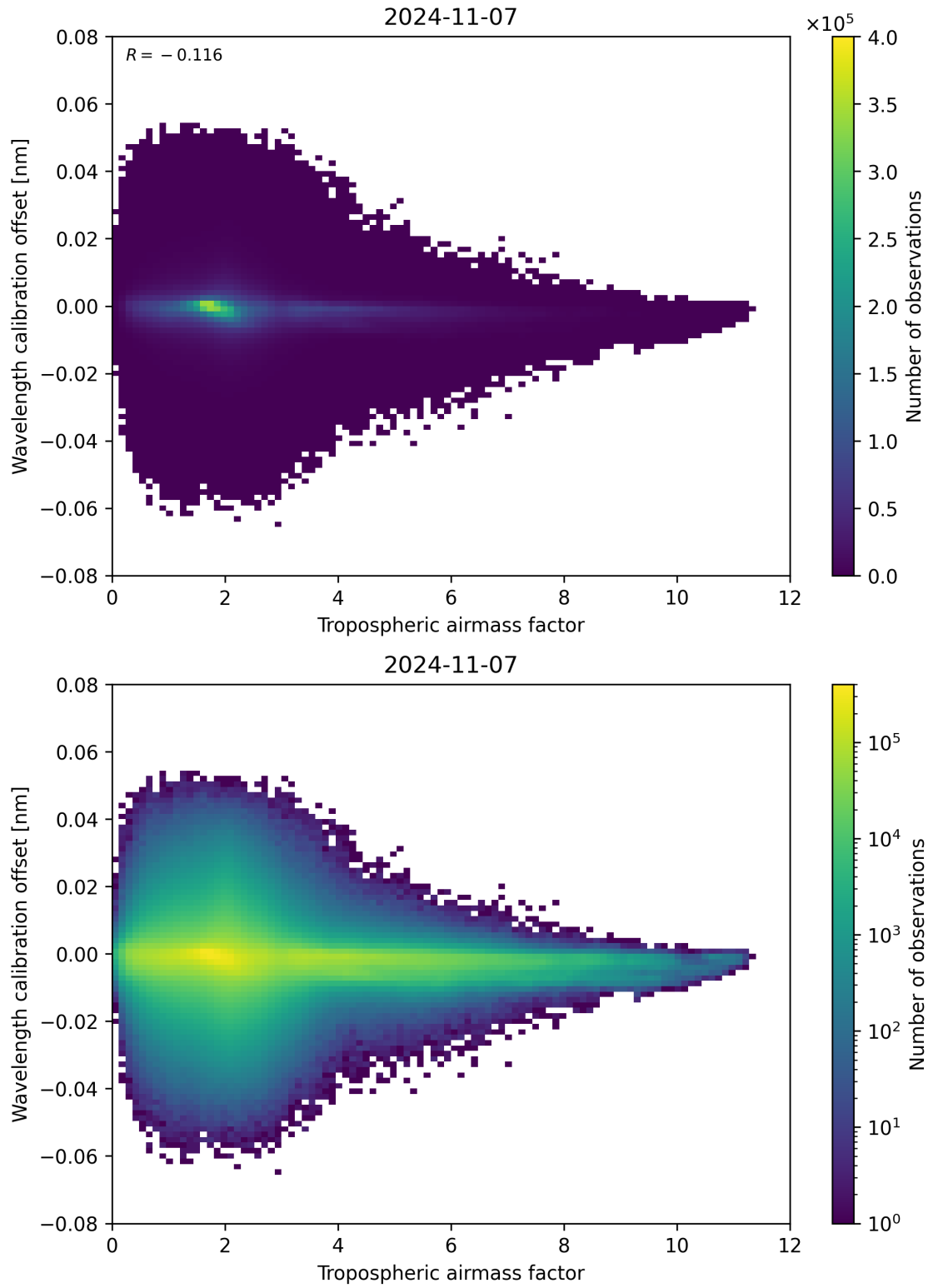
Figure 80: Scatter density plot of “Tropospheric airmass factor” against “Wavelength calibration offset” for 2024-11-06 to 2024-11-08.
