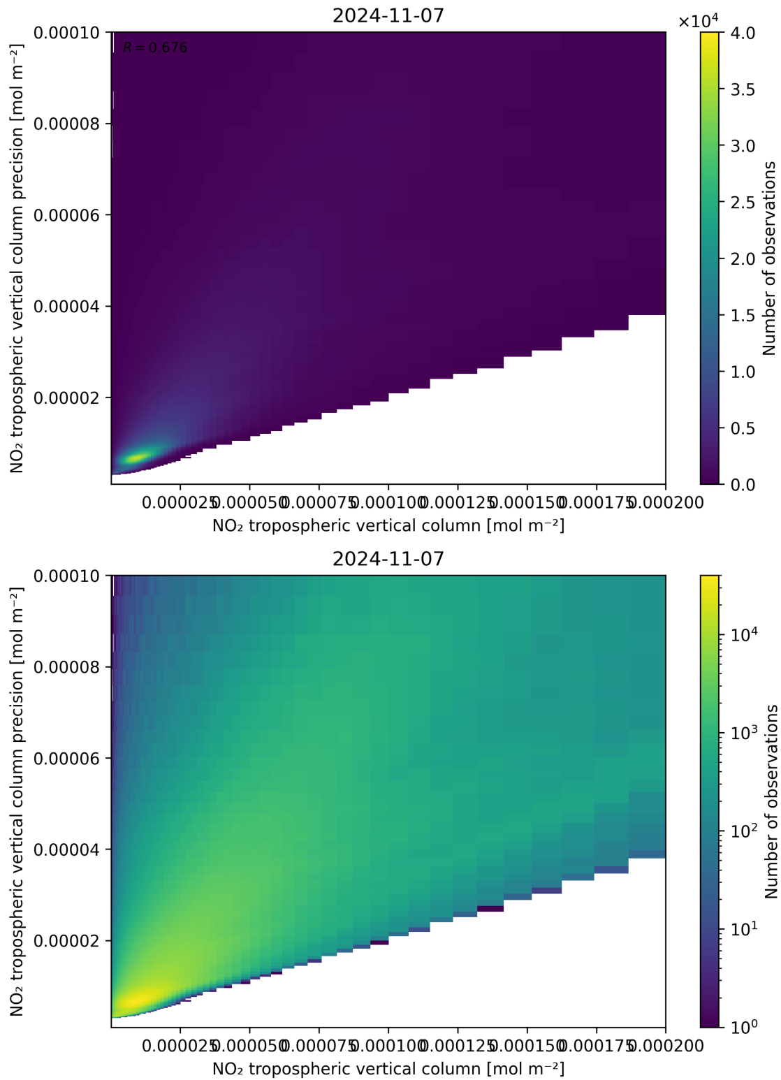
Figure 130: Scatter density plot of “NO 2 tropospheric vertical column” against “NO 2 tropospheric vertical column precision” for 2024-11-06 to 2024-11-08.
