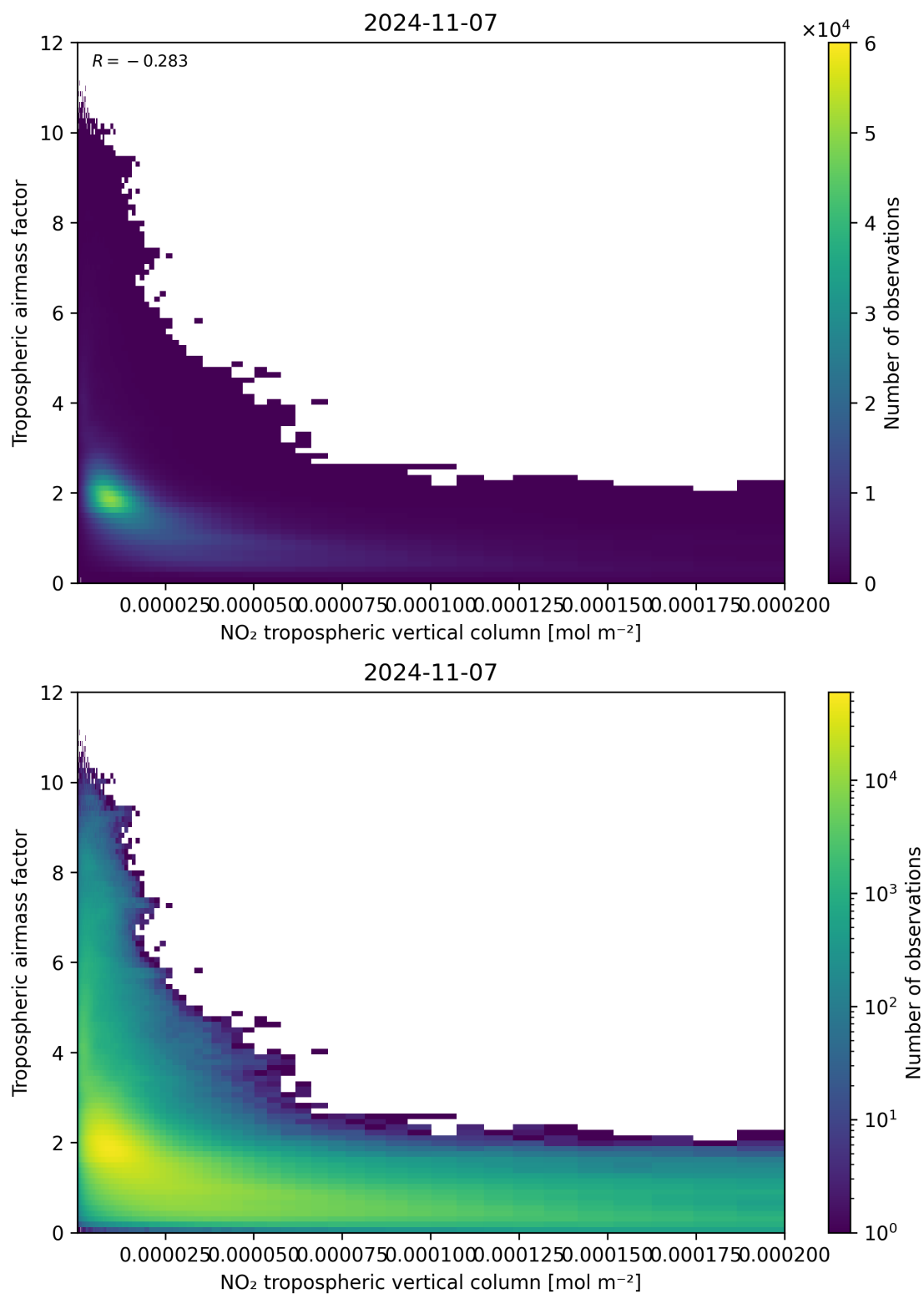
Figure 123: Scatter density plot of “NO 2 tropospheric vertical column” against “Tropospheric airmass factor” for 2024-11-06 to 2024-11-08.
