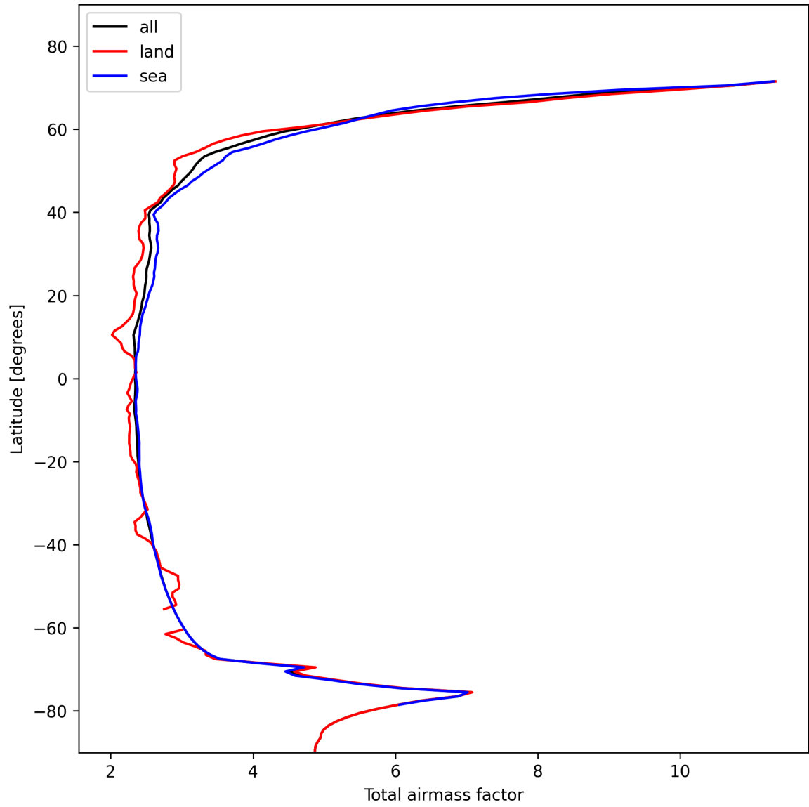
Figure 15: Zonal average of “Total airmass factor” for 2024-11-06 to 2024-11-08.
