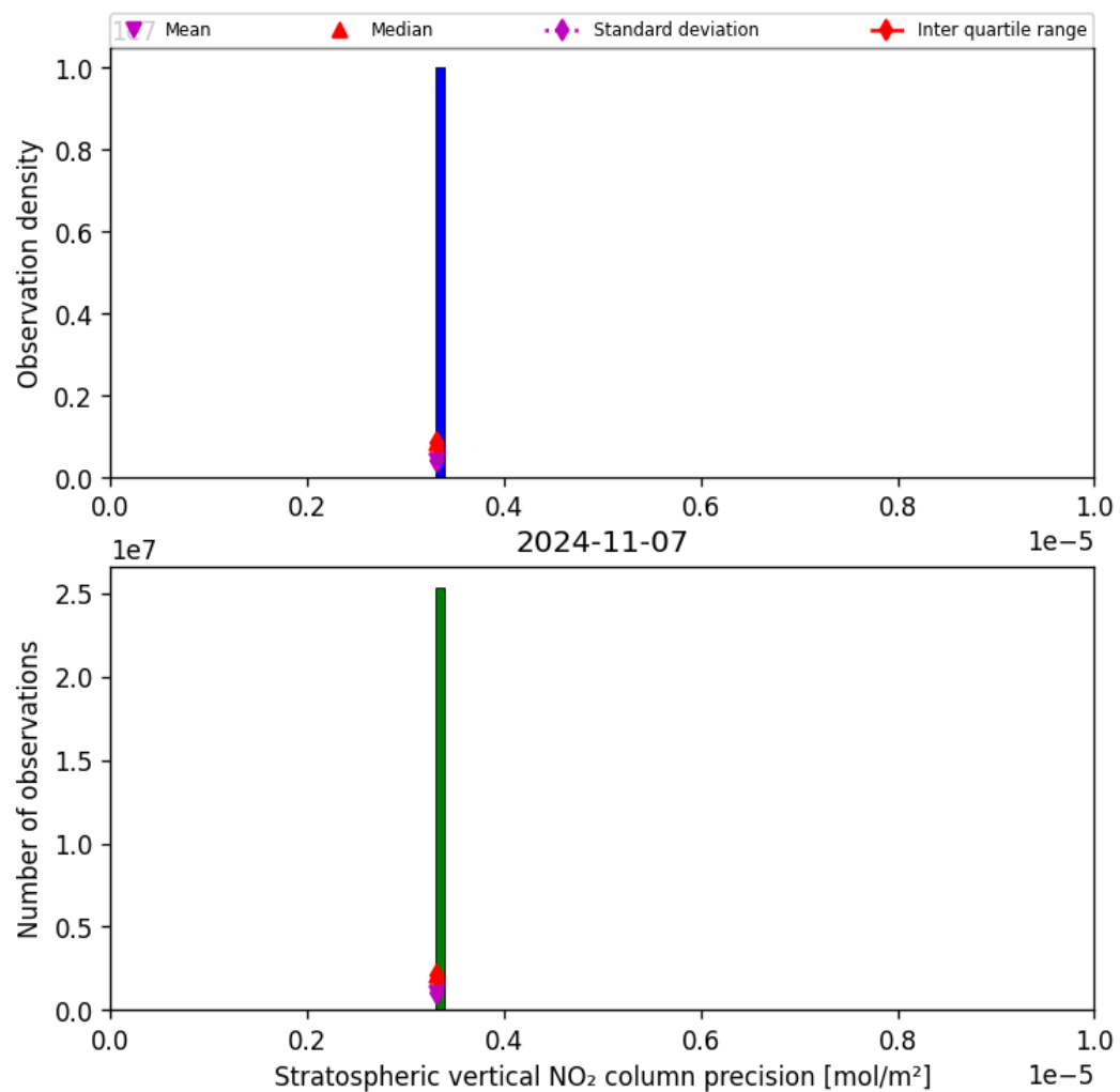
Figure 37: Histogram of “Stratospheric vertical NO 2 column precision” for 2024-11-06 to 2024-11-08
