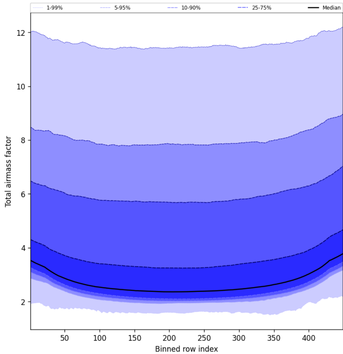
Figure 49: Along track statistics of “Total airmass factor” for 2024-11-06 to 2024-11-08
