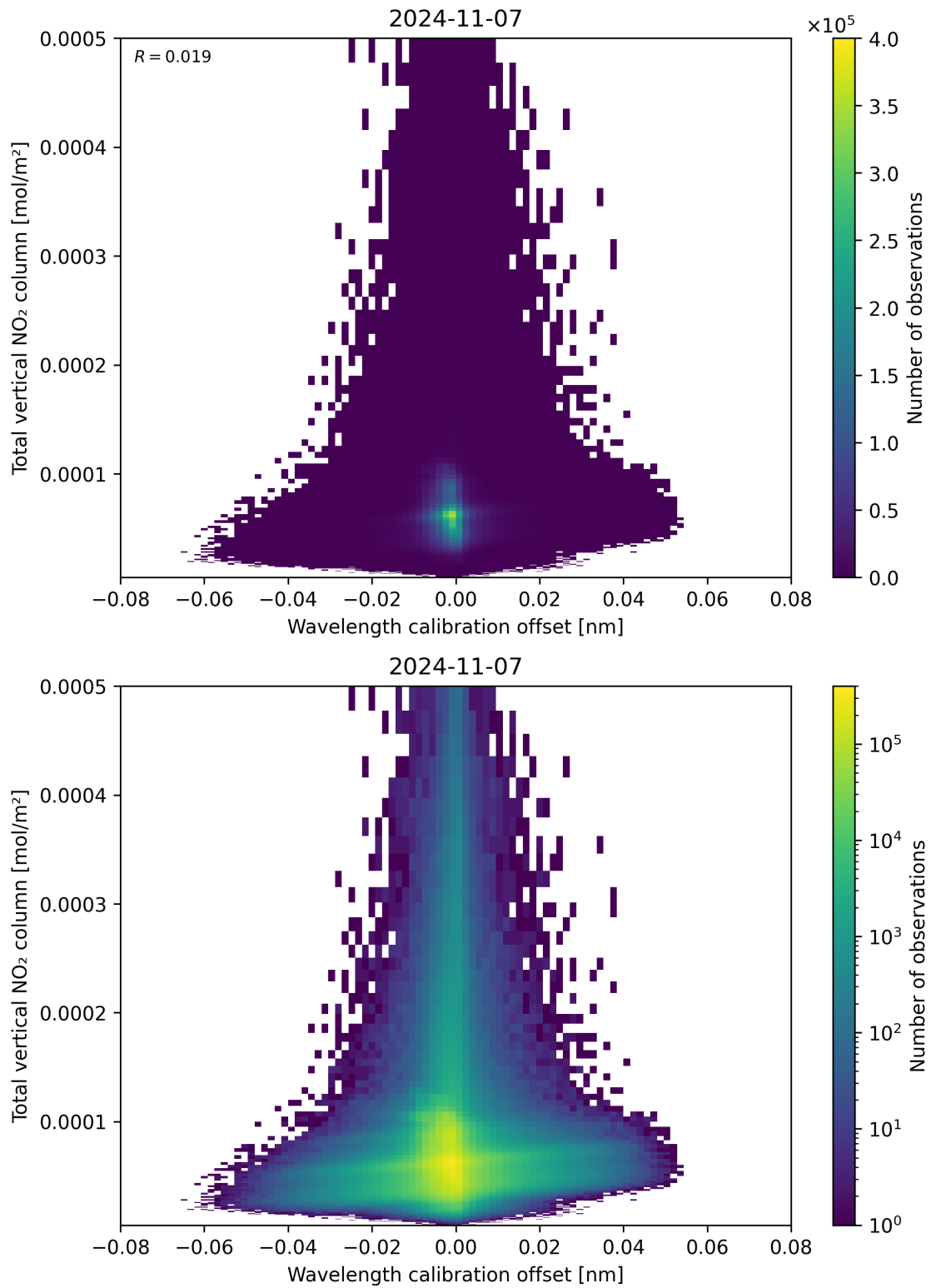
Figure 179: Scatter density plot of “Wavelength calibration offset” against “Total vertical NO 2 column” for 2024-11-06 to 2024-11-08.
