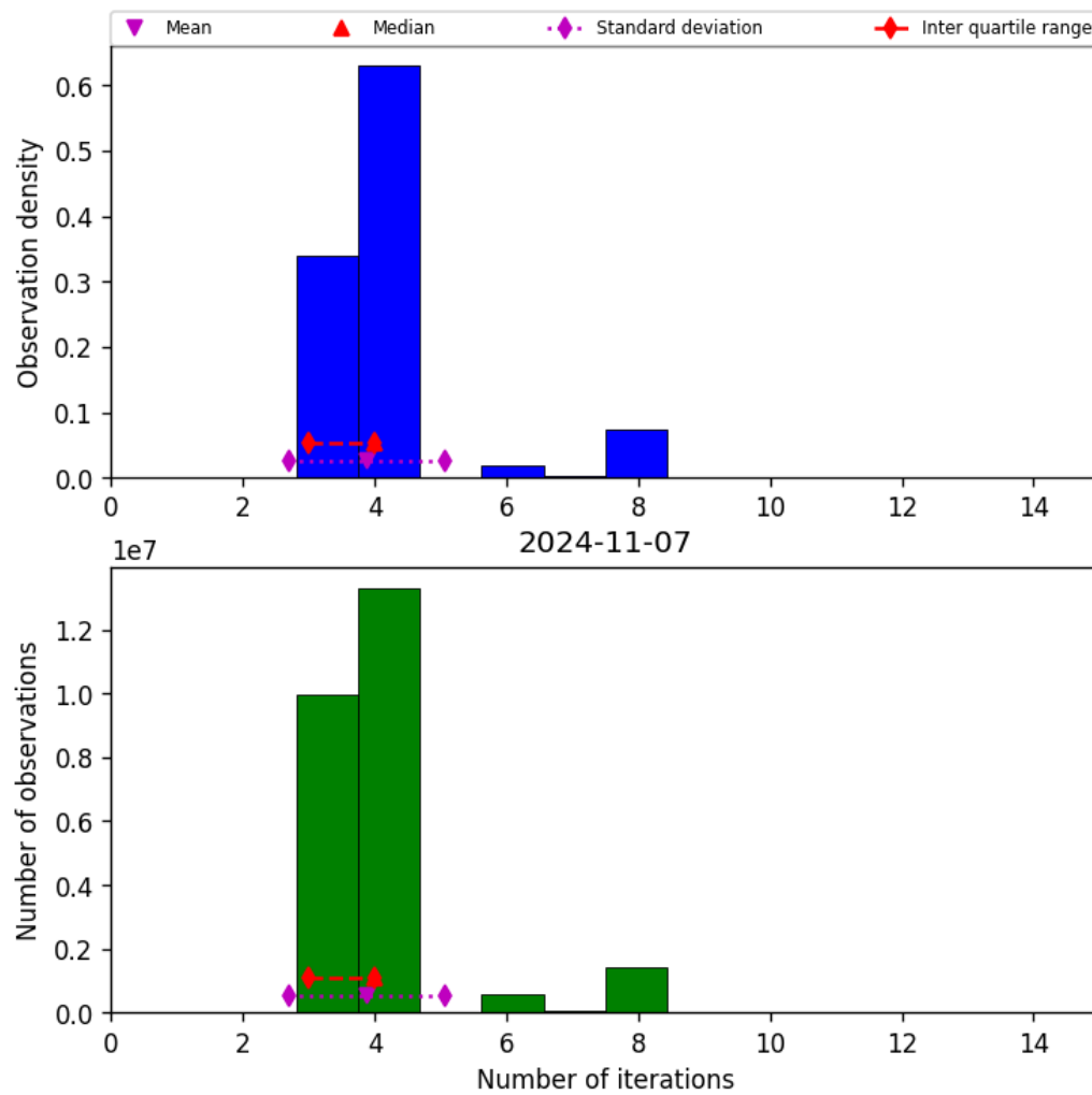
Figure 34: Histogram of “Number of iterations” for 2024-11-06 to 2024-11-08
