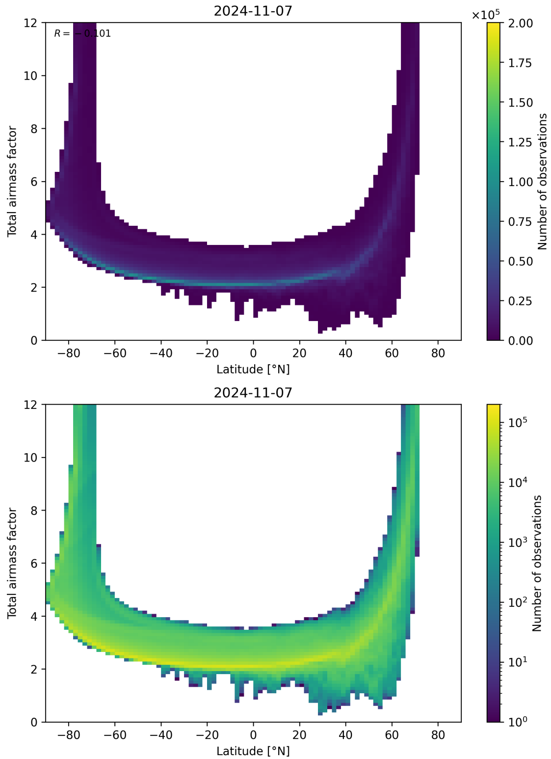
Figure 84: Scatter density plot of “Latitude” against “Total airmass factor” for 2024-11-06 to 2024-11-08.
