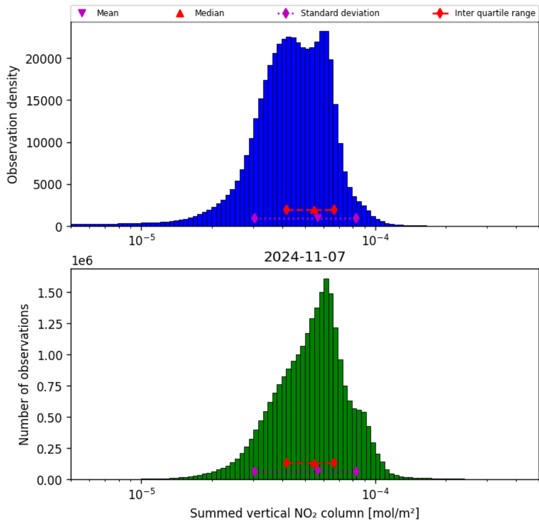
Figure 40: Histogram of “Summed vertical NO 2 column” for 2024-11-06 to 2024-11-08
