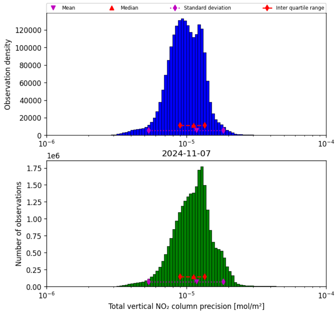
Figure 39: Histogram of “Total vertical NO 2 column precision” for 2024-11-06 to 2024-11-08
