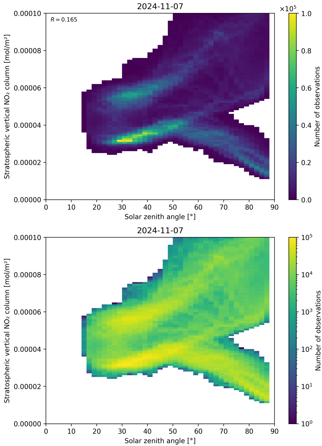
Figure 150: Scatter density plot of “Solar zenith angle” against “Stratospheric vertical NO 2 column” for 2024-11-06 to 2024-11-08.
