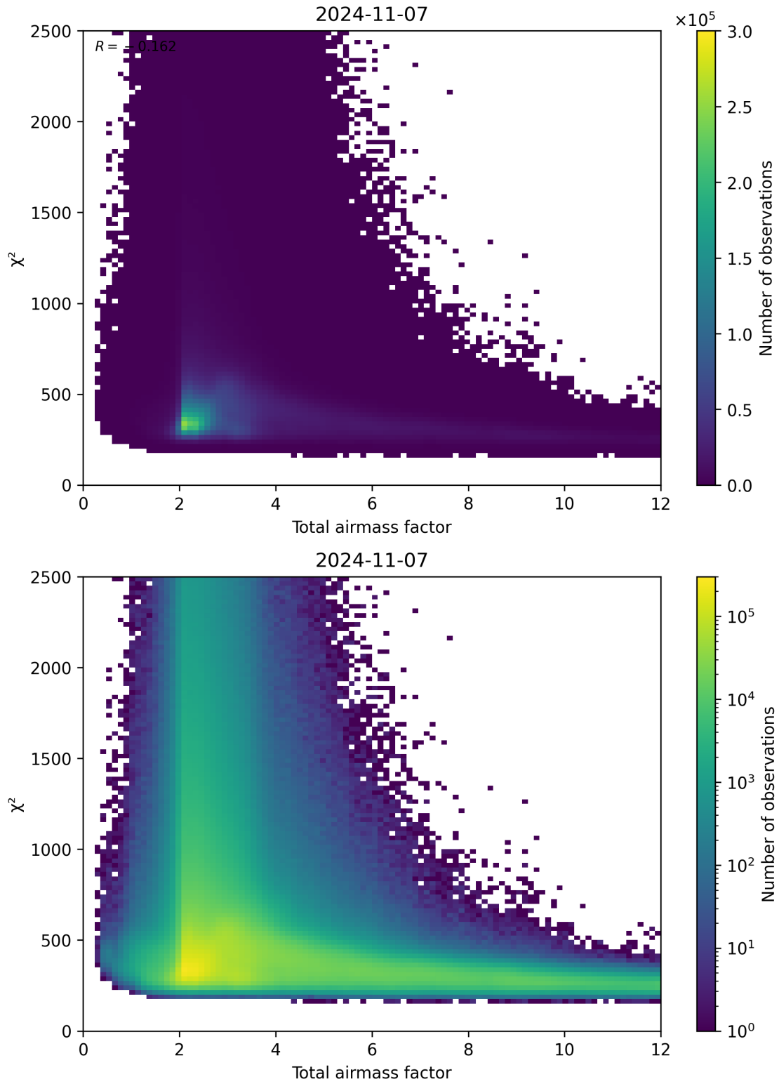
Figure 63: Scatter density plot of “Total airmass factor” against “ \chi^2 ” for 2024-11-06 to 2024-11-08.
