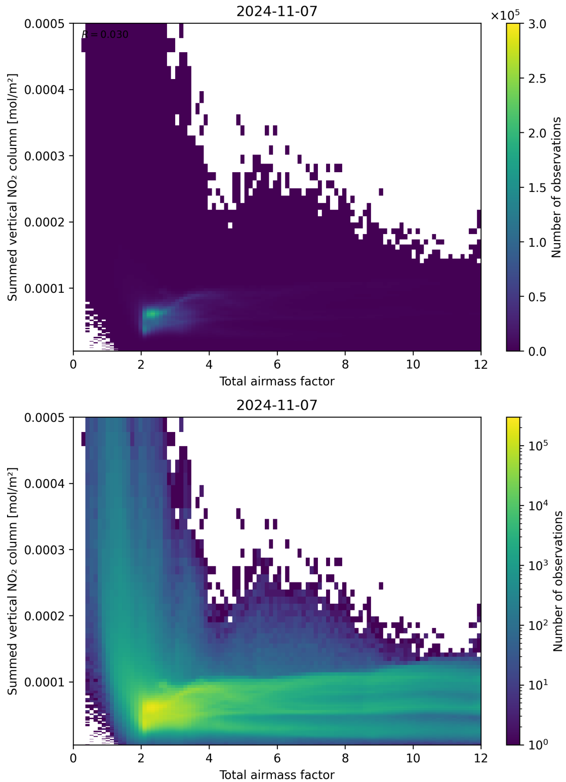
Figure 65: Scatter density plot of “Total airmass factor” against “Summed vertical NO 2 column” for 2024-11-06 to 2024-11-08.
