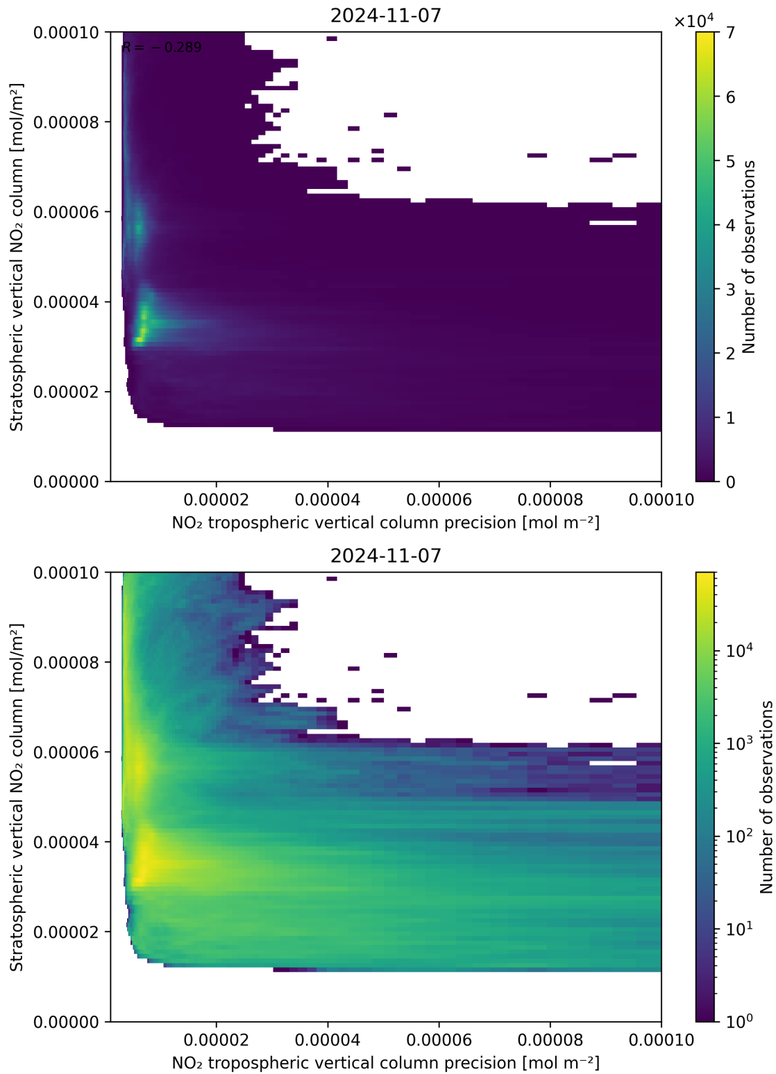
Figure 135: Scatter density plot of “NO 2 tropospheric vertical column precision” against “Stratospheric vertical NO 2 column” for 2024-11-06 to 2024-11-08.
