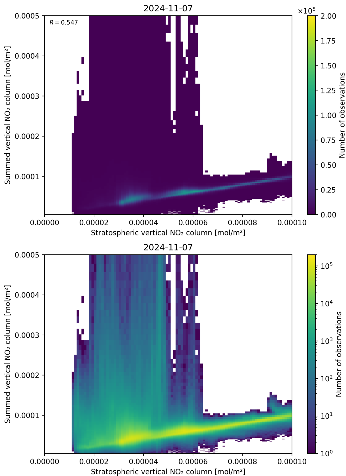
Figure 98: Scatter density plot of “Stratospheric vertical NO 2 column” against “Summed vertical NO 2 column” for 2024-11-06 to 2024-11-08.
