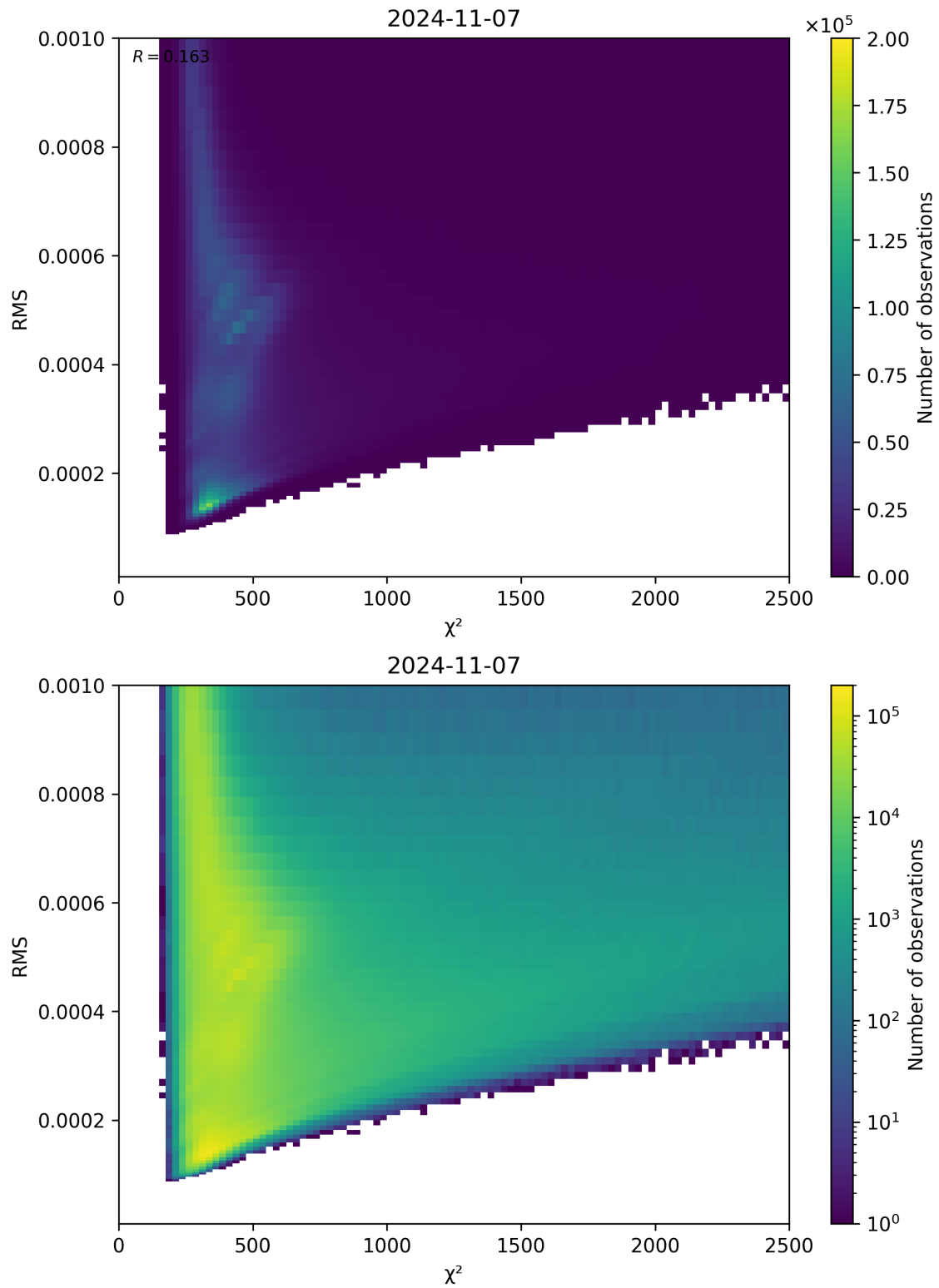
Figure 82: Scatter density plot of “ \chi^2 ” against “RMS” for 2024-11-06 to 2024-11-08.
