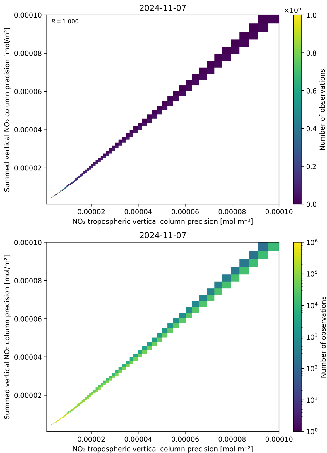
Figure 137: Scatter density plot of “NO 2 tropospheric vertical column precision” against “Summed vertical NO 2 column precision” for 2024-11-06 to 2024-11-08.
