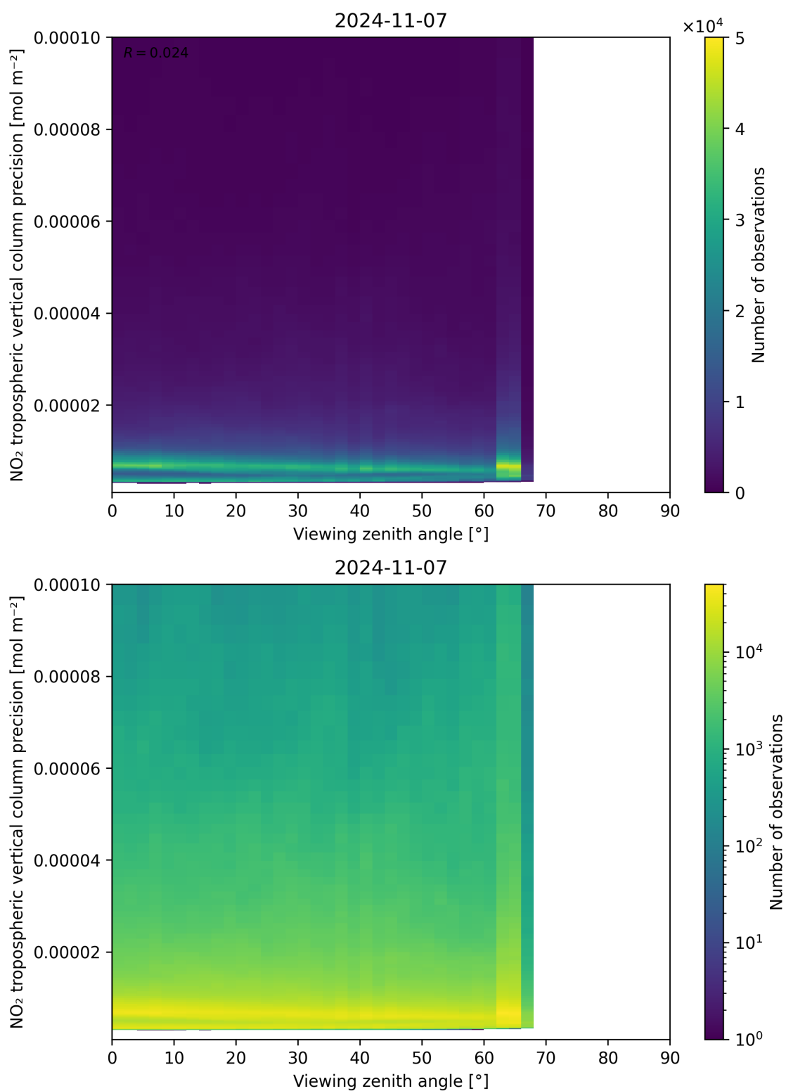
Figure 170: Scatter density plot of “Viewing zenith angle” against “NO 2 tropospheric vertical column precision” for 2024-11-06 to 2024-11-08.
