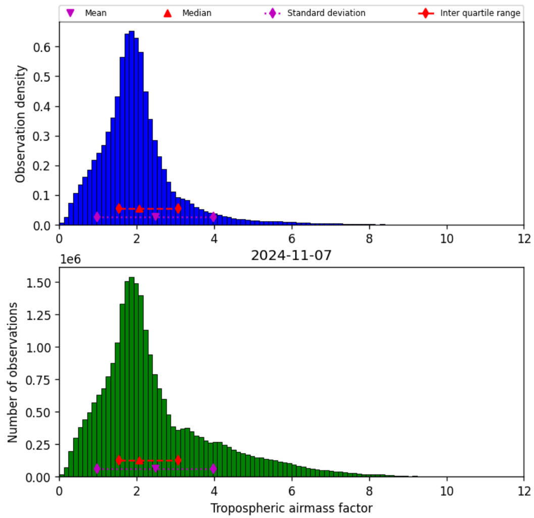
Figure 31: Histogram of “Tropospheric airmass factor” for 2024-11-06 to 2024-11-08
