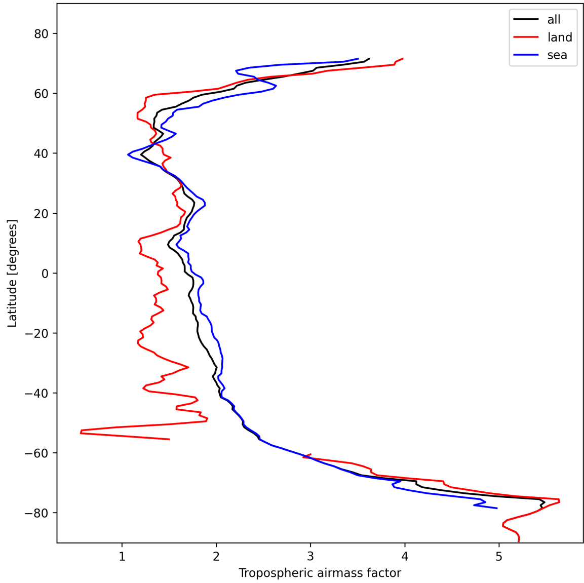
Figure 14: Zonal average of “Tropospheric airmass factor” for 2024-11-06 to 2024-11-08.
