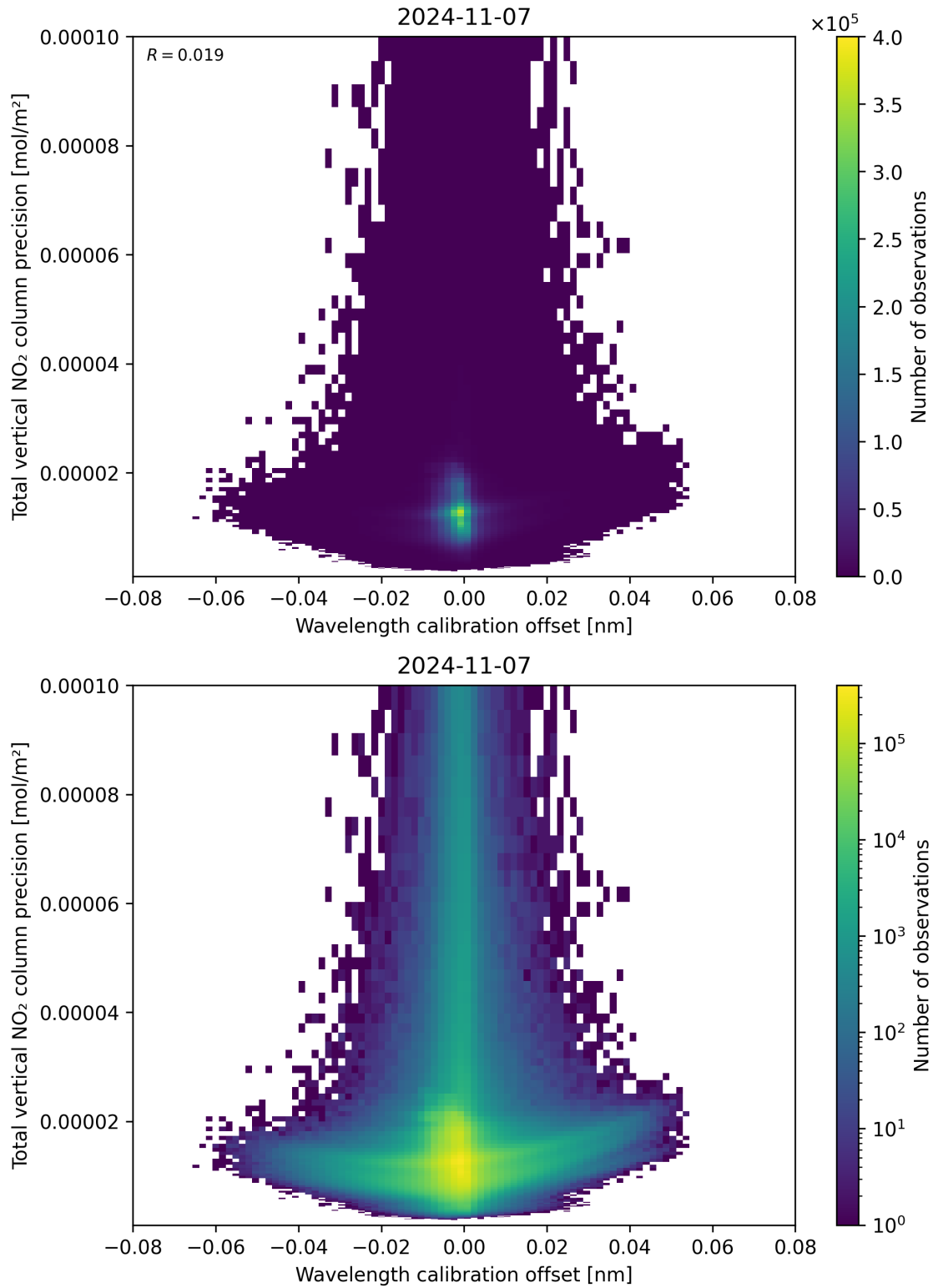
Figure 180: Scatter density plot of “Wavelength calibration offset” against “Total vertical NO 2 column precision” for 2024-11-06 to 2024-11-08.
