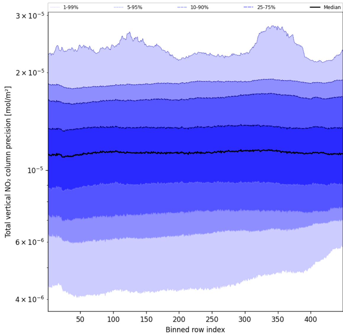
Figure 56: Along track statistics of “Total vertical NO 2 column precision” for 2024-11-06 to 2024-11-08
