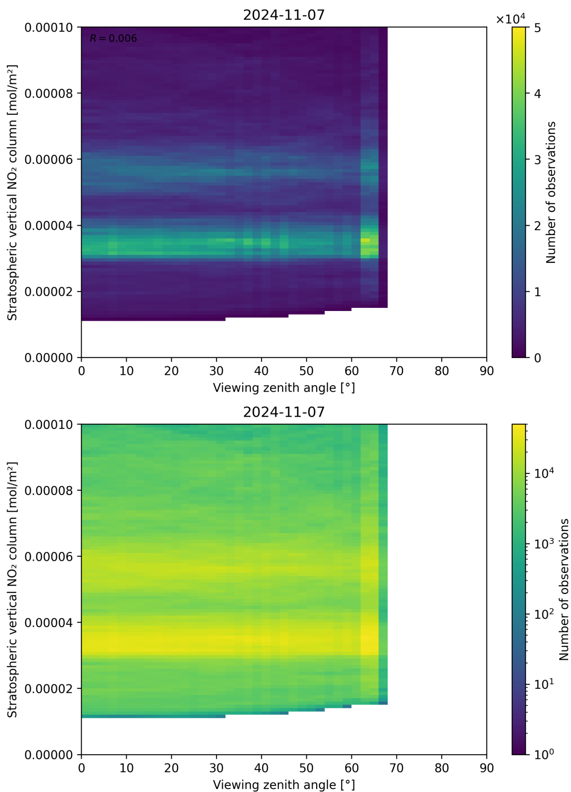
Figure 164: Scatter density plot of “Viewing zenith angle” against “Stratospheric vertical NO 2 column” for 2024-11-06 to 2024-11-08.
