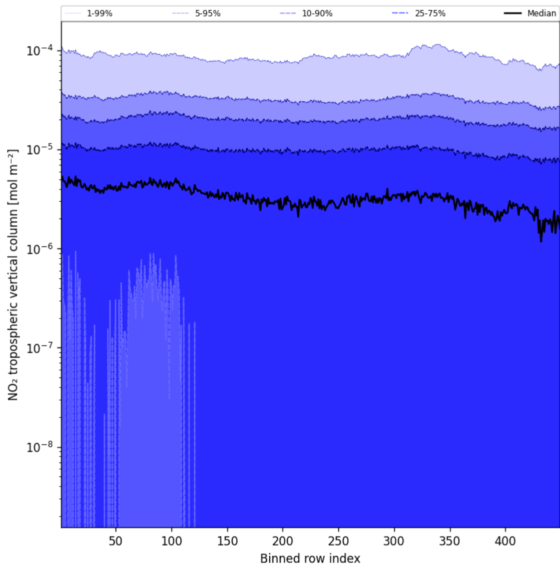
Figure 46: Along track statistics of “NO 2 tropospheric vertical column” for 2024-11-06 to 2024-11-08
