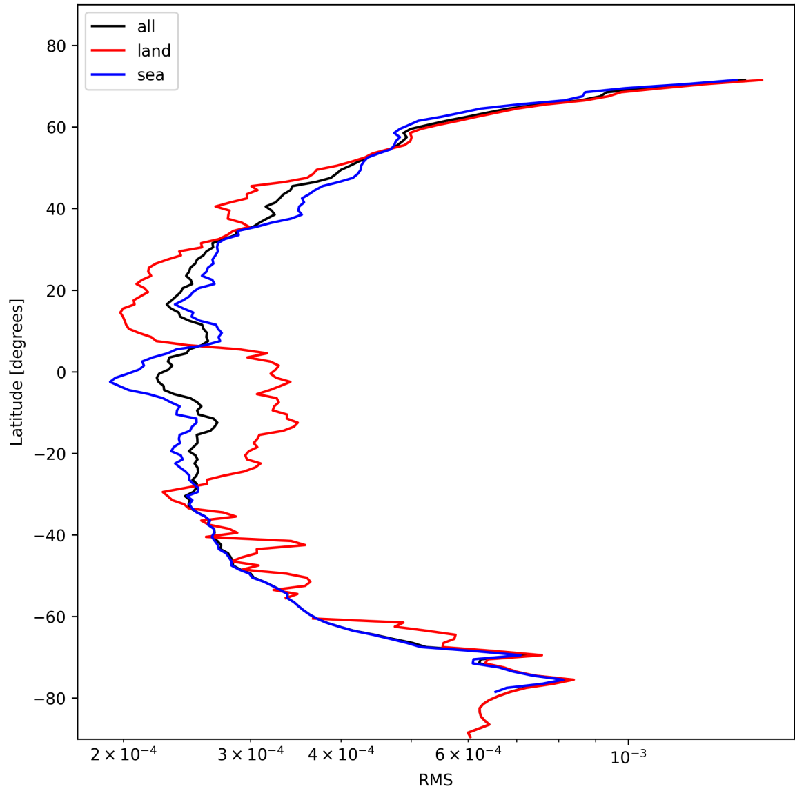
Figure 26: Zonal average of “RMS” for 2024-11-06 to 2024-11-08.
