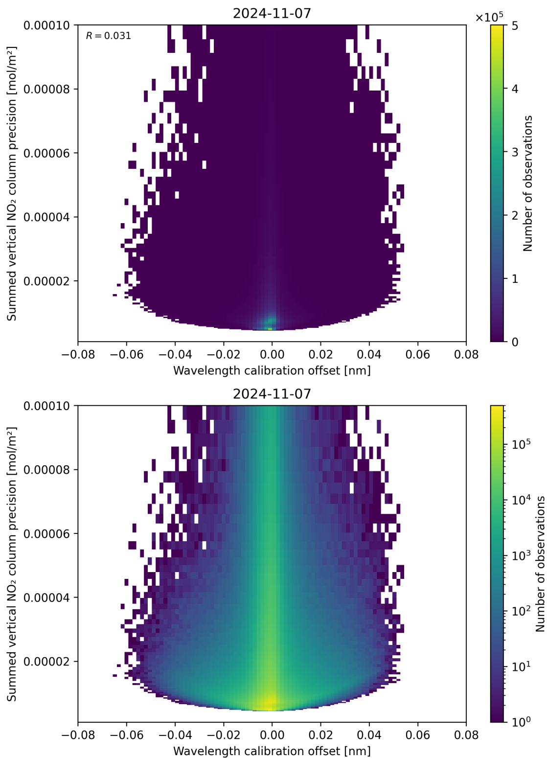
Figure 178: Scatter density plot of “Wavelength calibration offset” against “Summed vertical NO 2 column precision” for 2024-11-06 to 2024-11-08.
