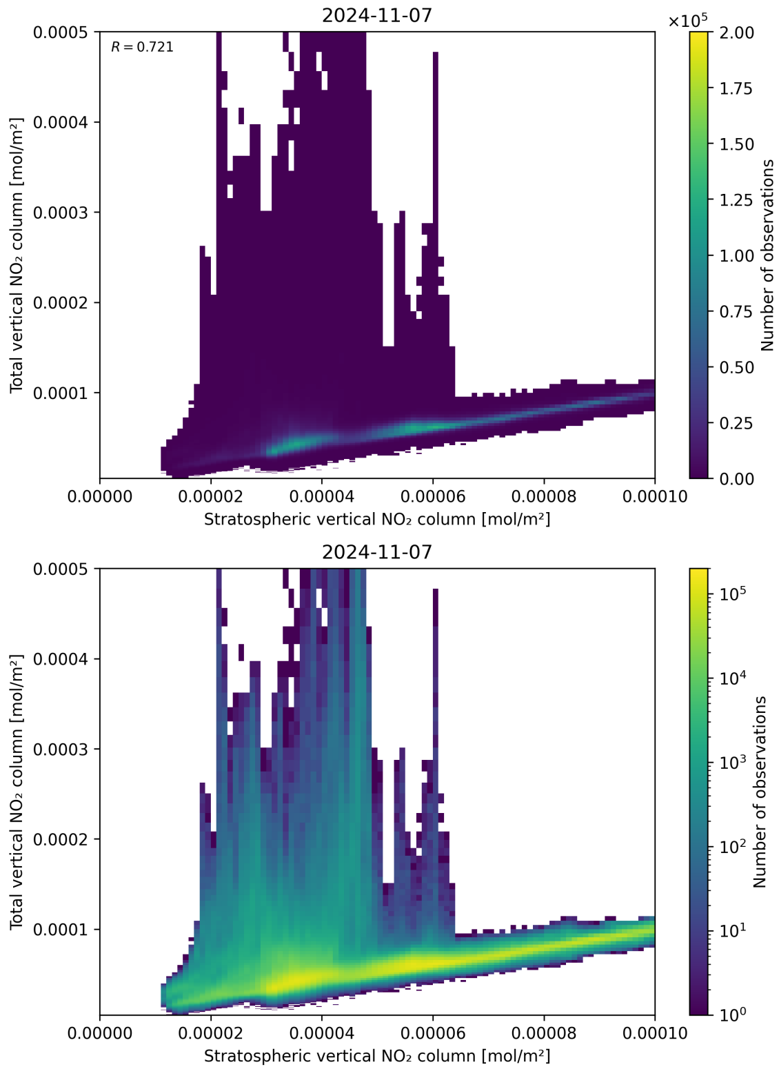
Figure 100: Scatter density plot of “Stratospheric vertical NO 2 column” against “Total vertical NO 2 column” for 2024-11-06 to 2024-11-08.
