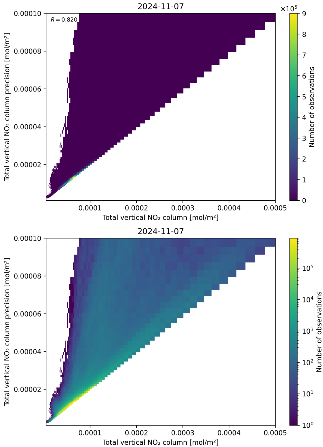
Figure 114: Scatter density plot of “Total vertical NO 2 column” against “Total vertical NO 2 column precision” for 2024-11-06 to 2024-11-08.
