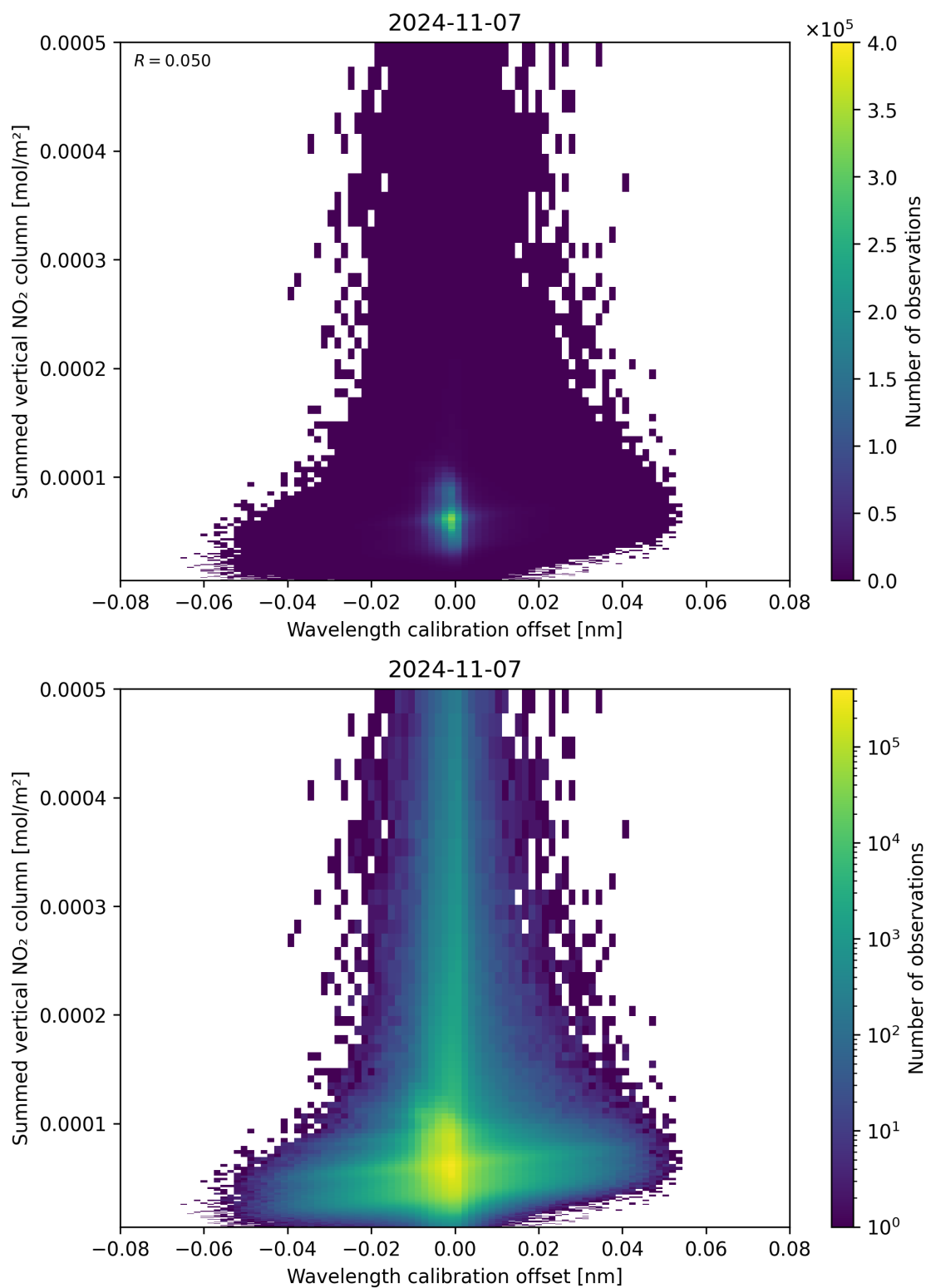
Figure 177: Scatter density plot of “Wavelength calibration offset” against “Summed vertical NO 2 column” for 2024-11-06 to 2024-11-08.
