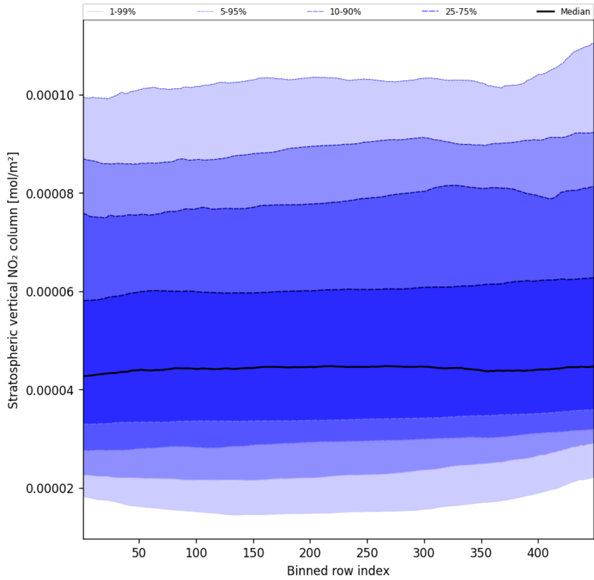
Figure 53: Along track statistics of “Stratospheric vertical NO 2 column” for 2024-11-06 to 2024-11-08
