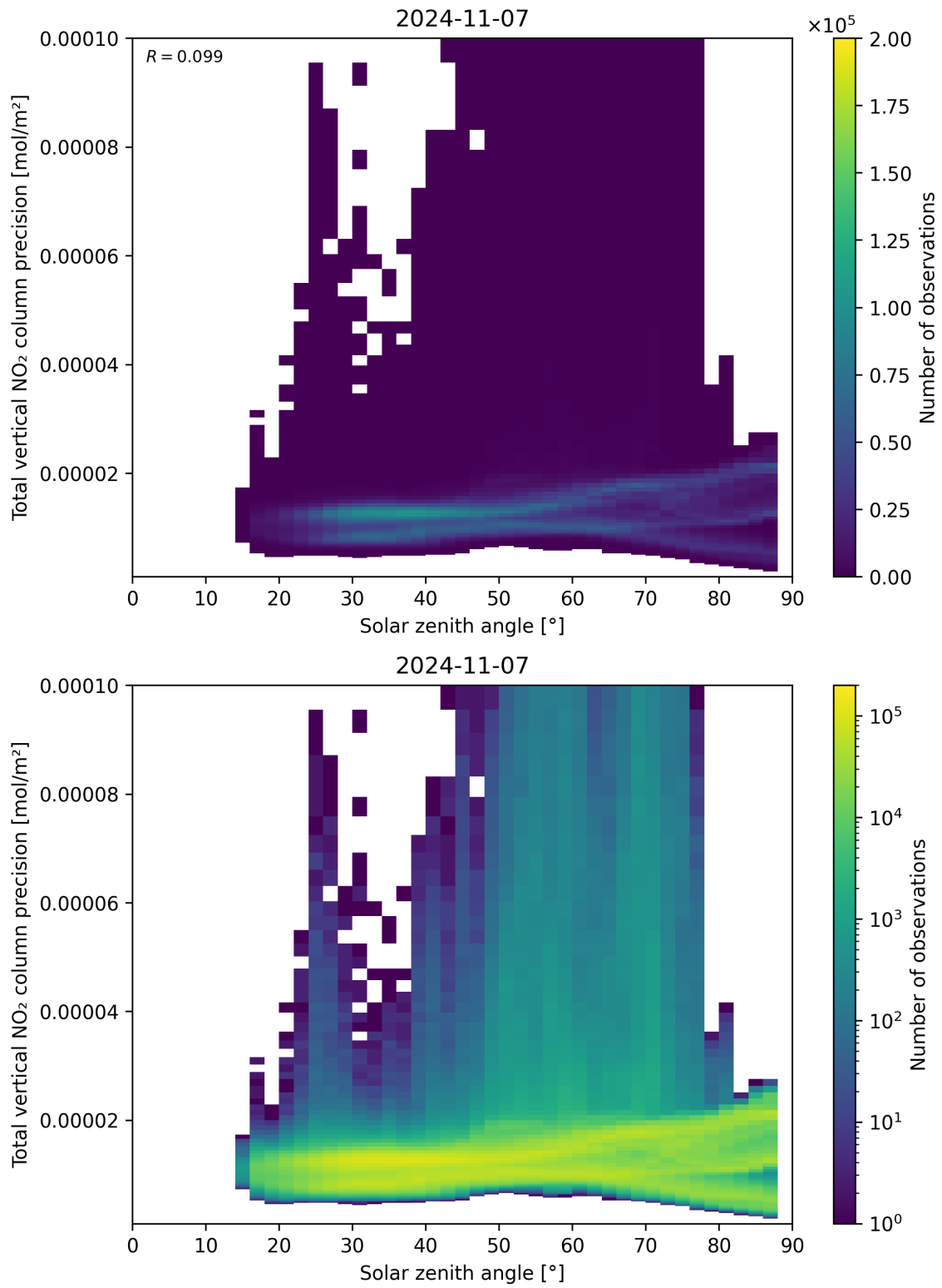
Figure 154: Scatter density plot of “Solar zenith angle” against “Total vertical NO 2 column precision” for 2024-11-06 to 2024-11-08.
