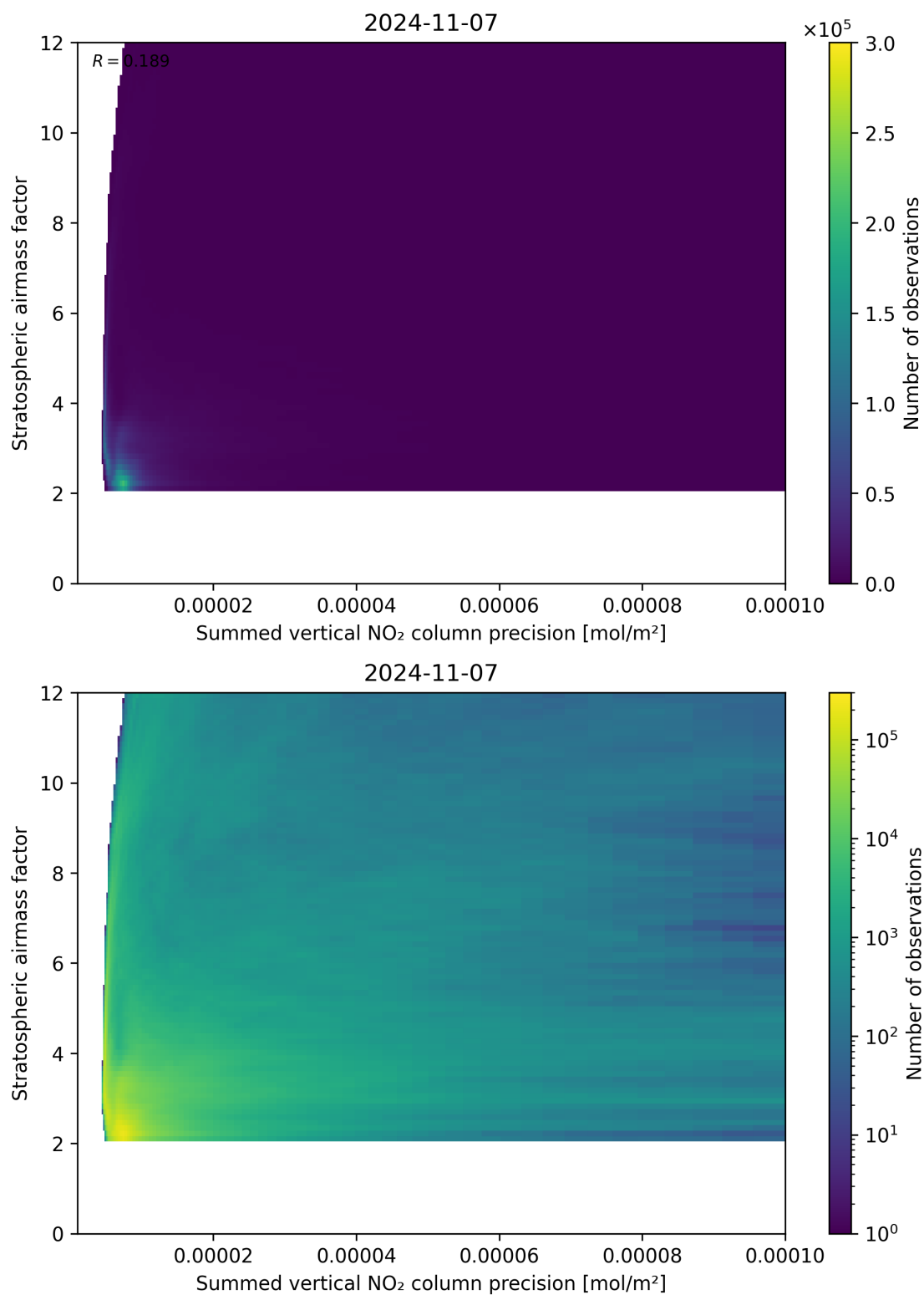
Figure 106: Scatter density plot of “Summed vertical NO 2 column precision” against “Stratospheric airmass factor” for 2024-11-06 to 2024-11-08.
