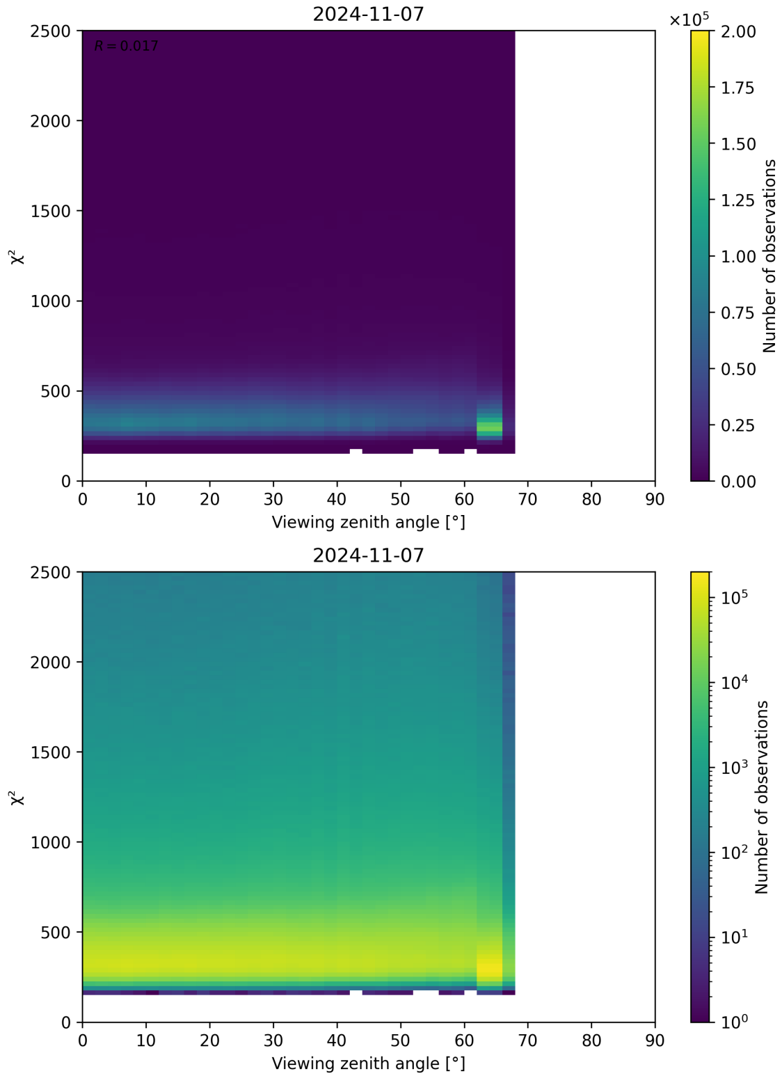
Figure 162: Scatter density plot of “Viewing zenith angle” against “ \chi^2 ” for 2024-11-06 to 2024-11-08.
