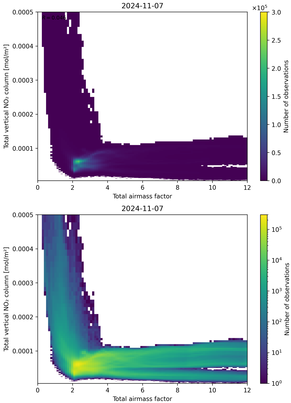
Figure 67: Scatter density plot of “Total airmass factor” against “Total vertical NO 2 column” for 2024-11-06 to 2024-11-08.
