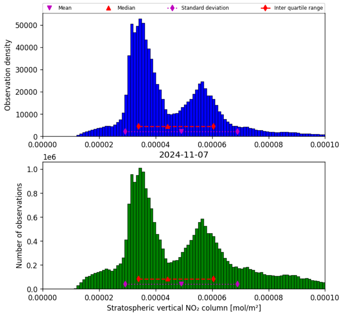
Figure 36: Histogram of “Stratospheric vertical NO 2 column” for 2024-11-06 to 2024-11-08
