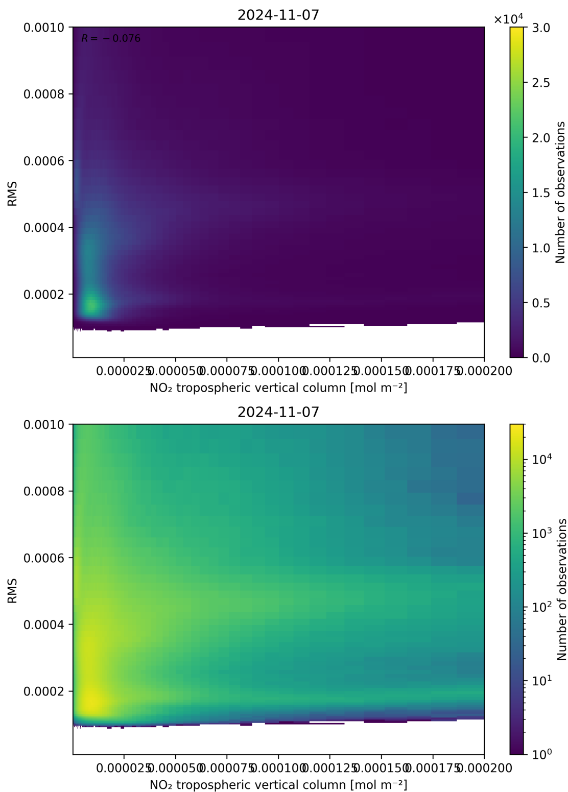
Figure 142: Scatter density plot of “NO 2 tropospheric vertical column” against “RMS” for 2024-11-06 to 2024-11-08.
