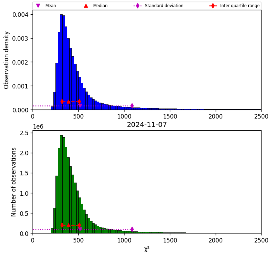
Figure 42: Histogram of “ \chi^2 ” for 2024-11-06 to 2024-11-08
