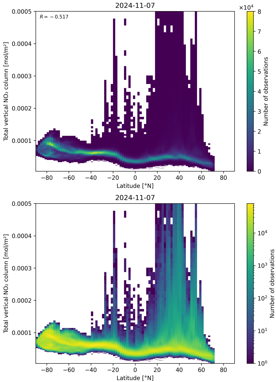
Figure 90: Scatter density plot of “Latitude” against “Total vertical NO 2 column” for 2024-11-06 to 2024-11-08.
