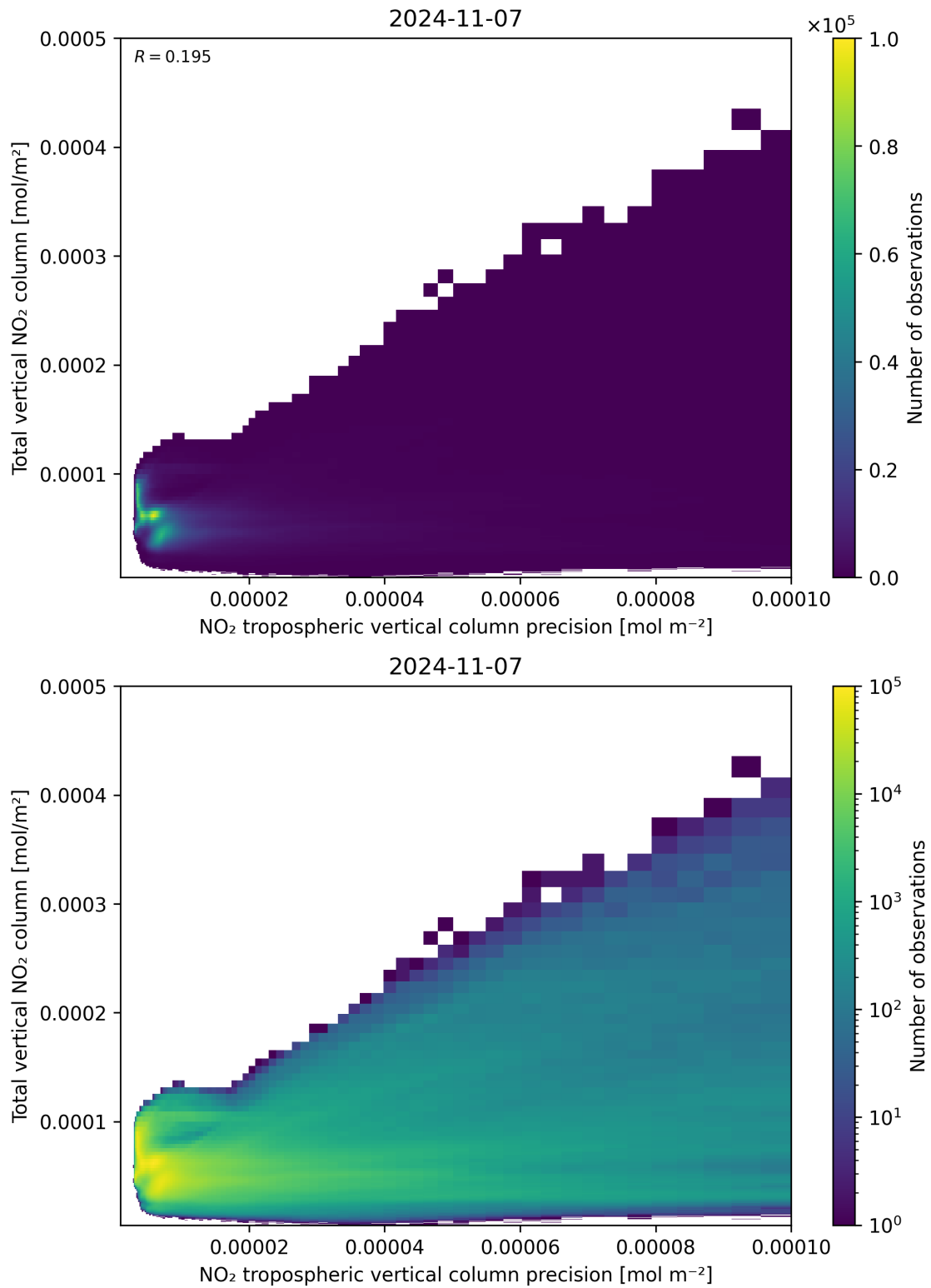
Figure 138: Scatter density plot of “NO 2 tropospheric vertical column precision” against “Total vertical NO 2 column” for 2024-11-06 to 2024-11-08.
