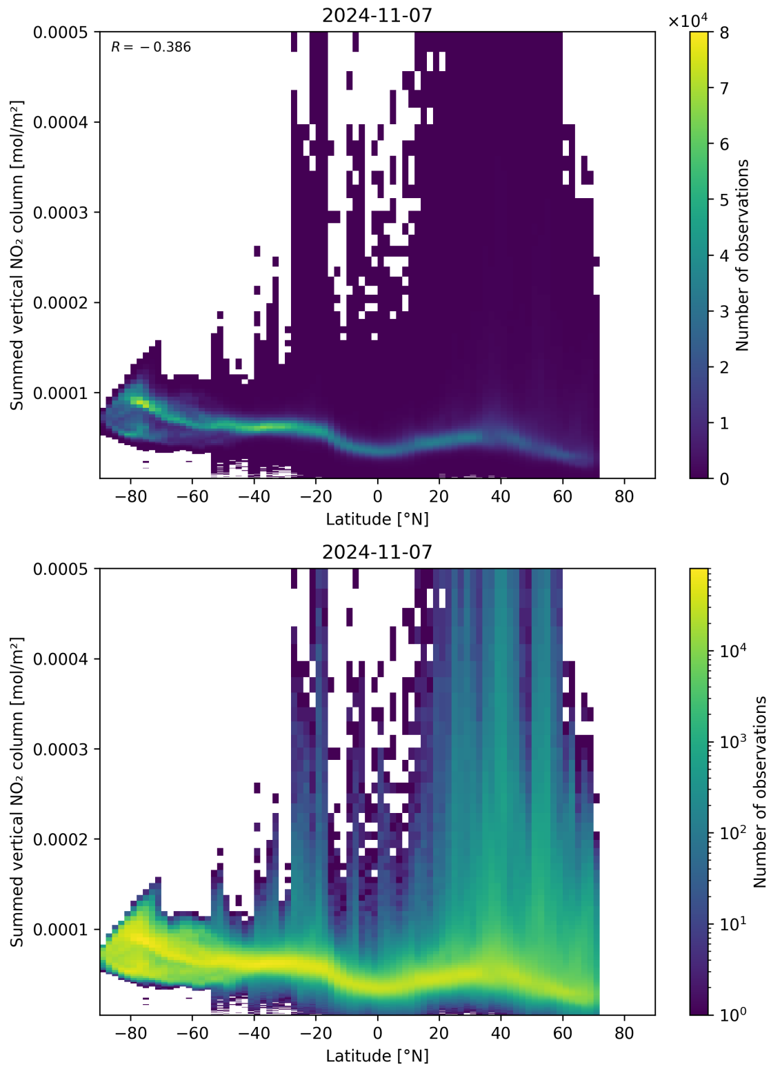
Figure 88: Scatter density plot of “Latitude” against “Summed vertical NO 2 column” for 2024-11-06 to 2024-11-08.
