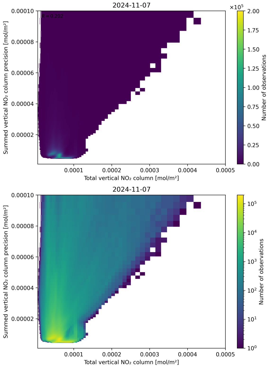
Figure 113: Scatter density plot of “Total vertical NO 2 column” against “Summed vertical NO 2 column precision” for 2024-11-06 to 2024-11-08.
