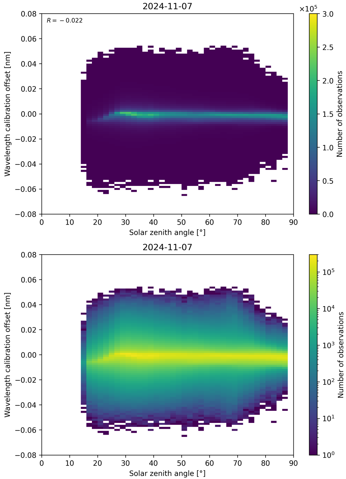
Figure 158: Scatter density plot of “Solar zenith angle” against “Wavelength calibration offset” for 2024-11-06 to 2024-11-08.
