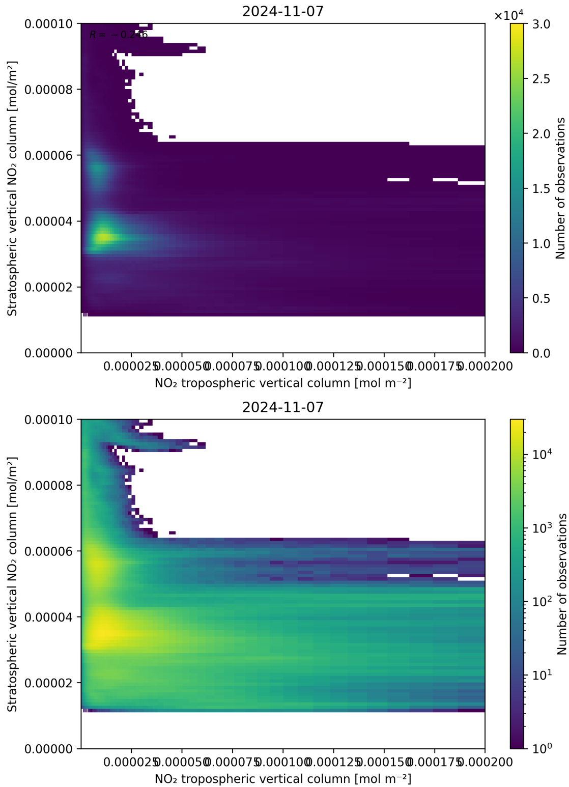
Figure 125: Scatter density plot of “NO 2 tropospheric vertical column” against “Stratospheric vertical NO 2 column” for 2024-11-06 to 2024-11-08.
