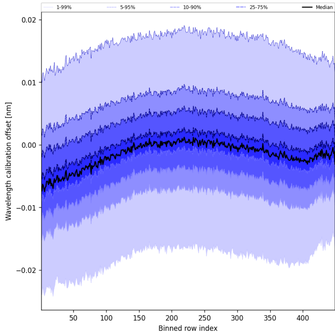
Figure 52: Along track statistics of “Wavelength calibration offset” for 2024-11-06 to 2024-11-08
