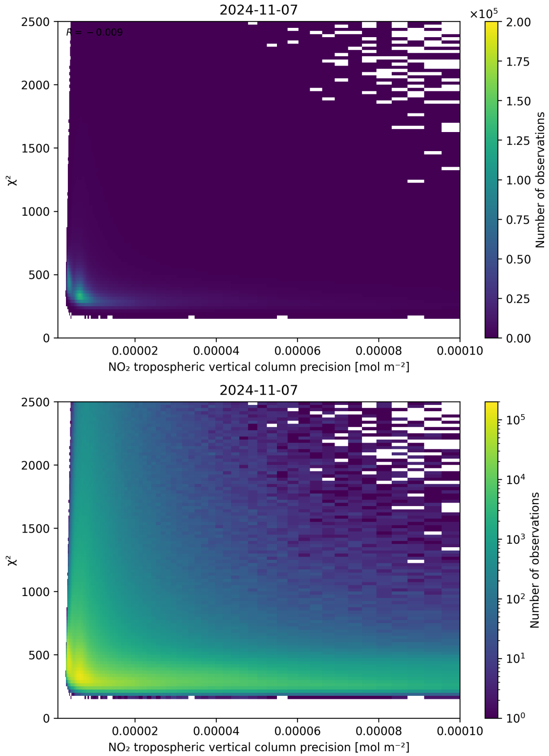
Figure 134: Scatter density plot of “NO 2 tropospheric vertical column precision” against “ \chi^2 ” for 2024-11-06 to 2024-11-08.
