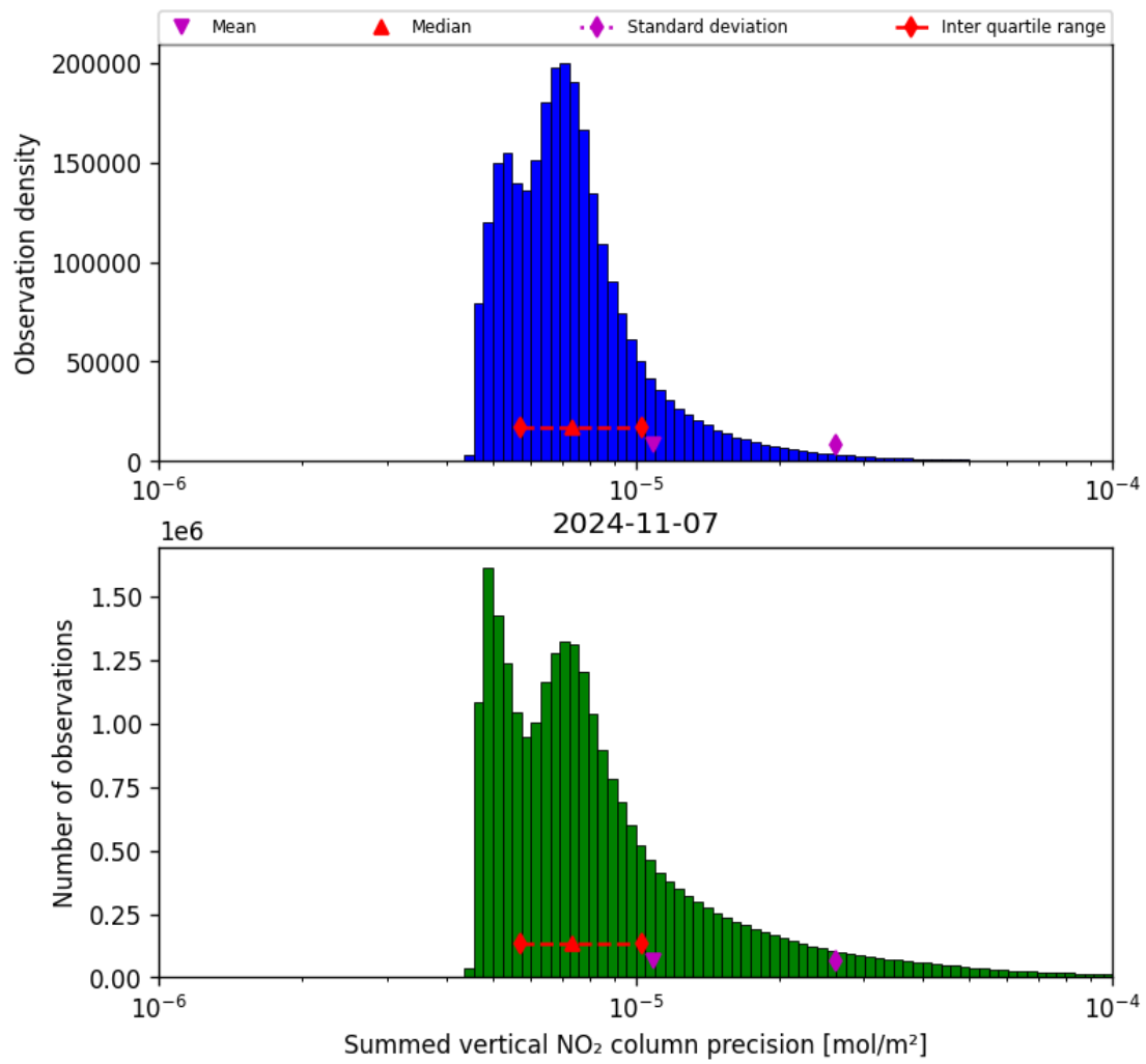
Figure 41: Histogram of "Summed vertical NO 2 column precision" for 2024-11-06 to 2024-11-08
