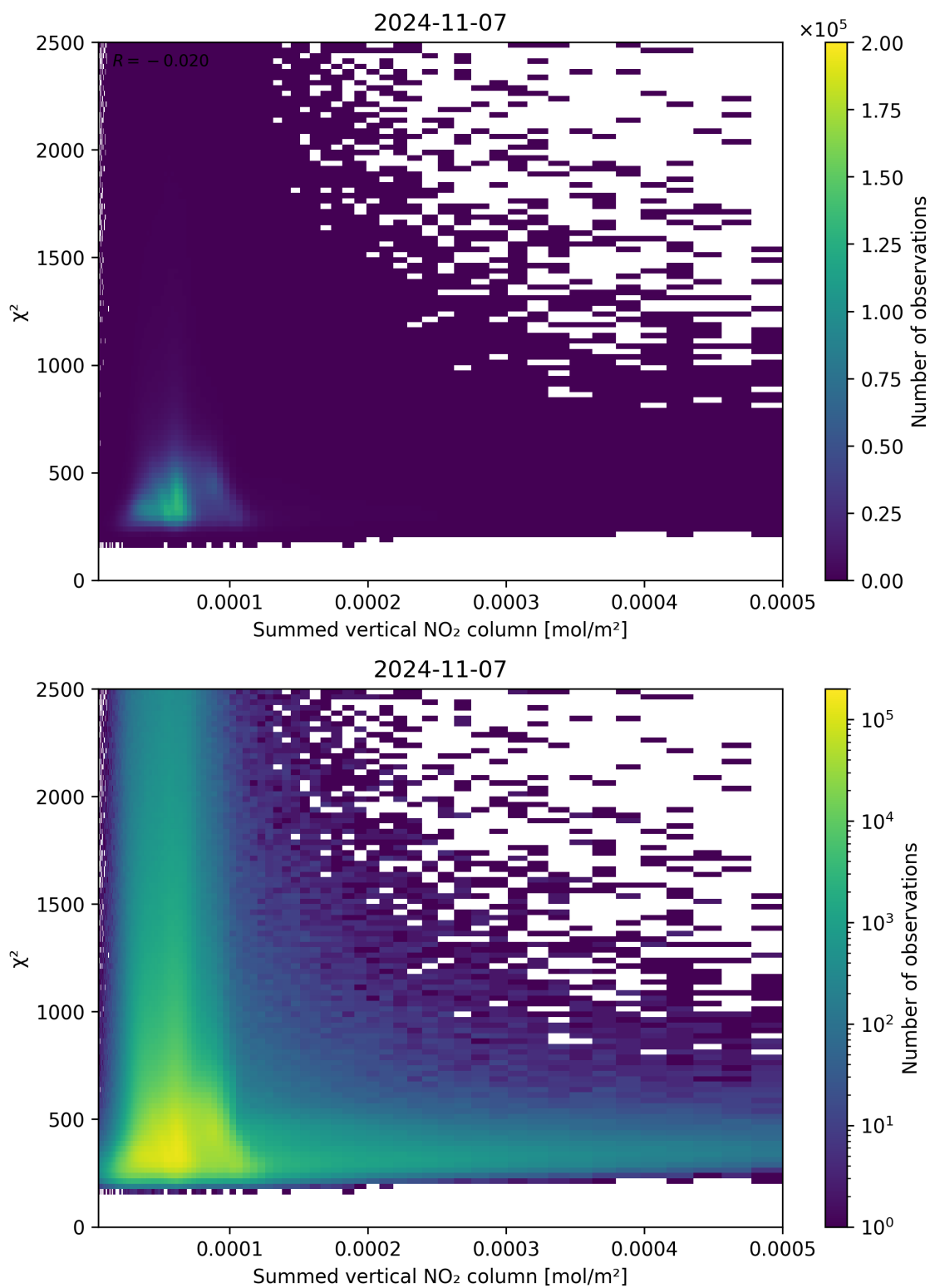
Figure 104: Scatter density plot of “Summed vertical NO 2 column” against “ \chi^2 ” for 2024-11-06 to 2024-11-08.
