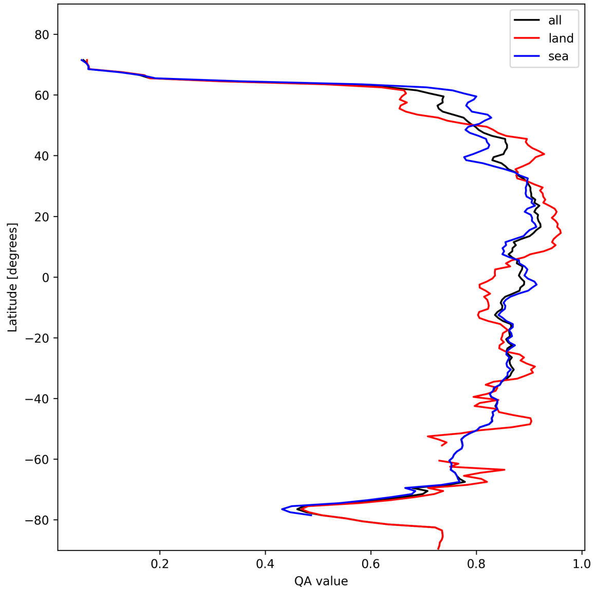
Figure 11: Zonal average of “QA value” for 2024-11-06 to 2024-11-08.
