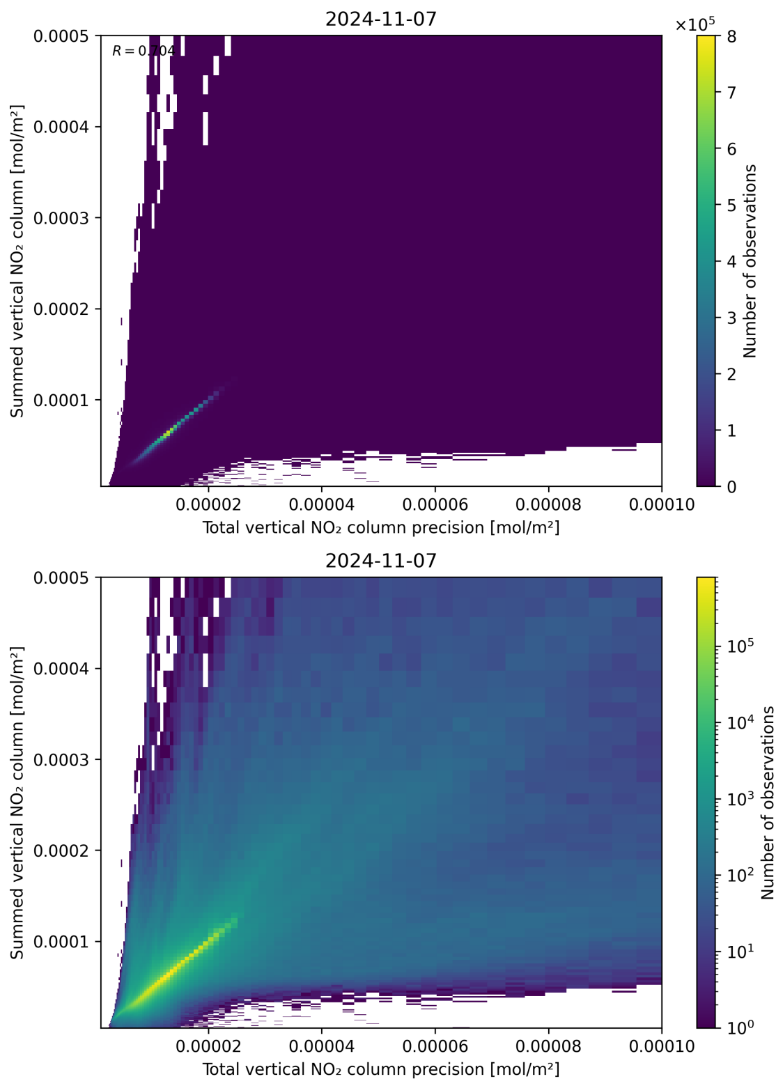
Figure 117: Scatter density plot of “Total vertical NO 2 column precision” against “Summed vertical NO 2 column” for 2024-11-06 to 2024-11-08.
