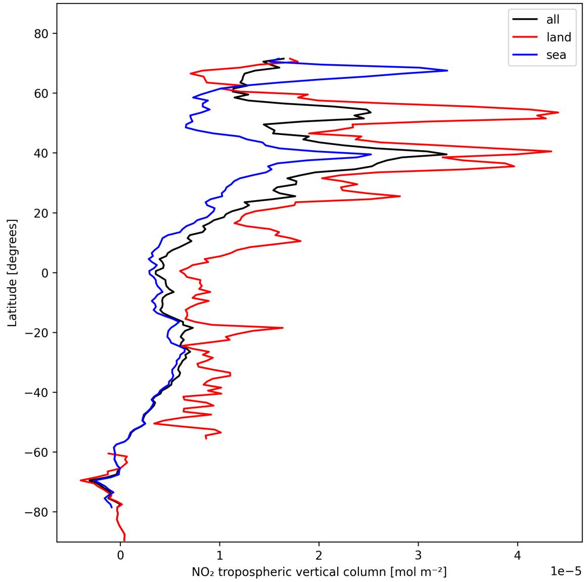
Figure 12: Zonal average of “NO 2 tropospheric vertical column” for 2024-11-06 to 2024-11-08.
