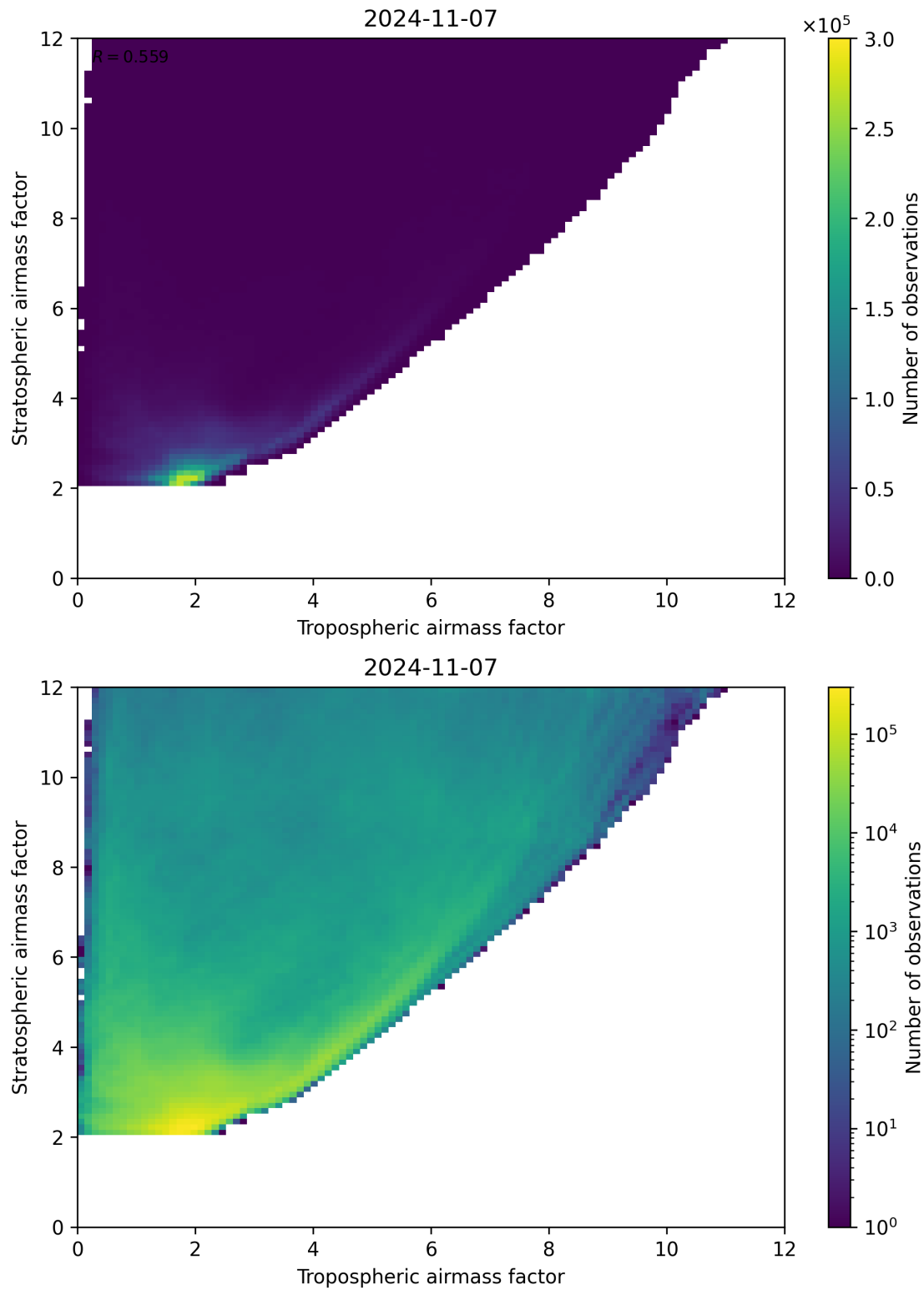
Figure 71: Scatter density plot of “Tropospheric airmass factor” against “Stratospheric airmass factor” for 2024-11-06 to 2024-11-08.
