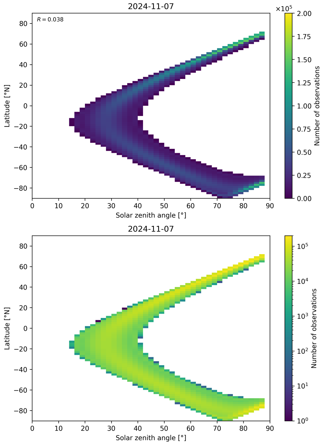
Figure 149: Scatter density plot of “Solar zenith angle” against “Latitude” for 2024-11-06 to 2024-11-08.
