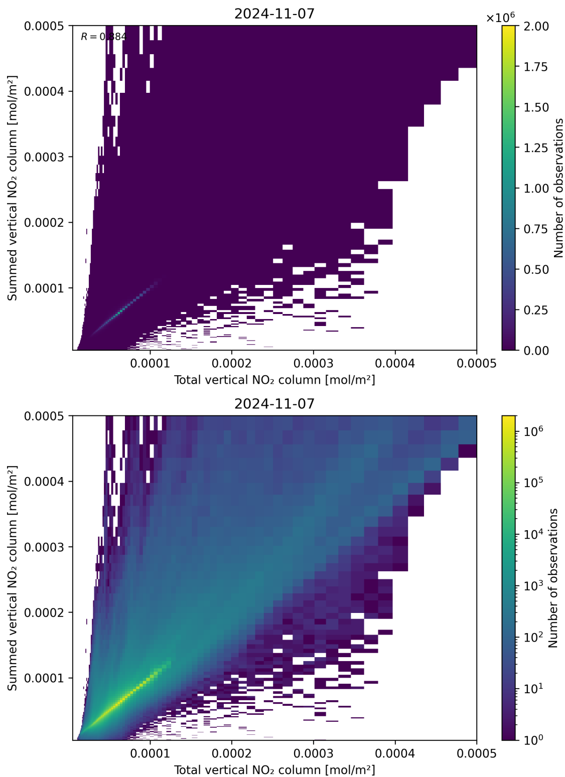
Figure 112: Scatter density plot of “Total vertical NO 2 column” against “Summed vertical NO 2 column” for 2024-11-06 to 2024-11-08.
