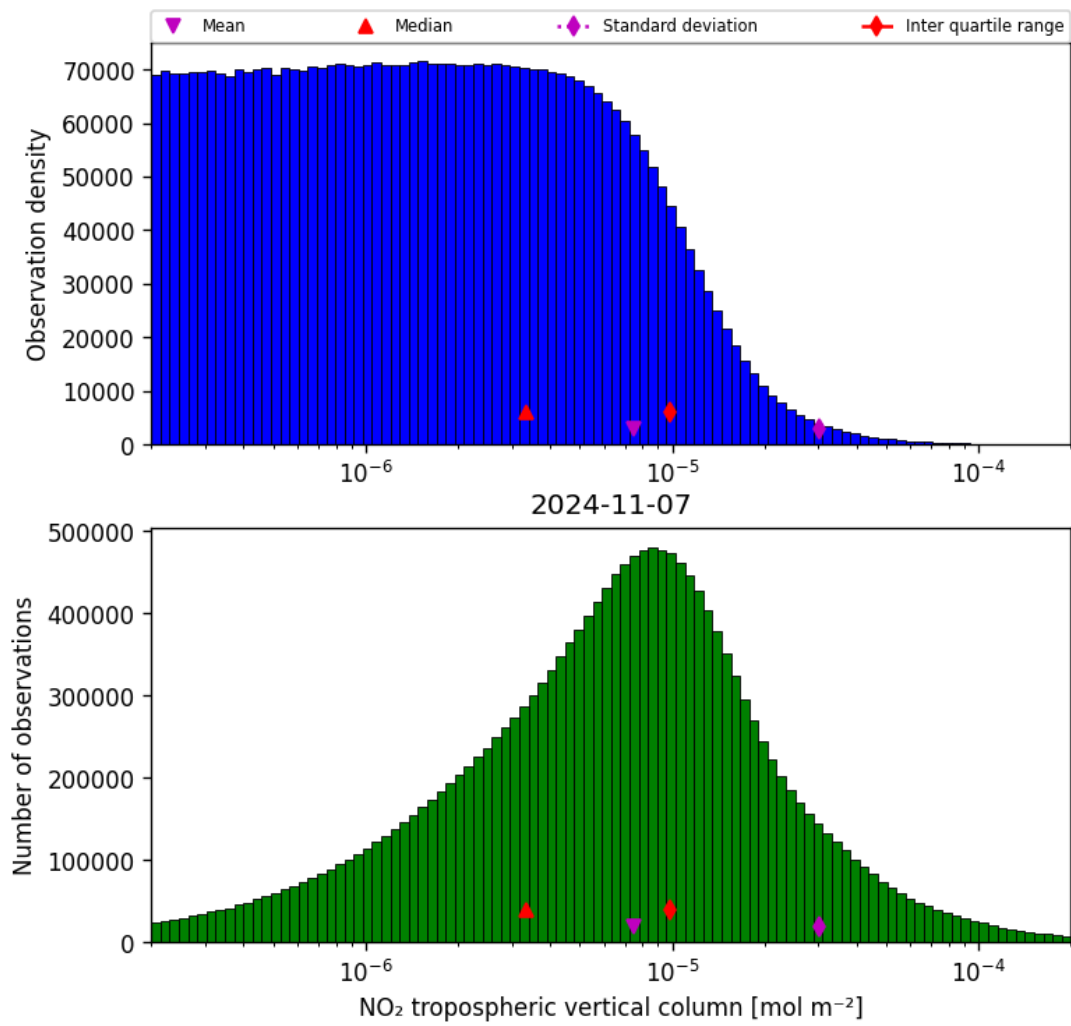
Figure 29: Histogram of “NO 2 tropospheric vertical column” for 2024-11-06 to 2024-11-08
