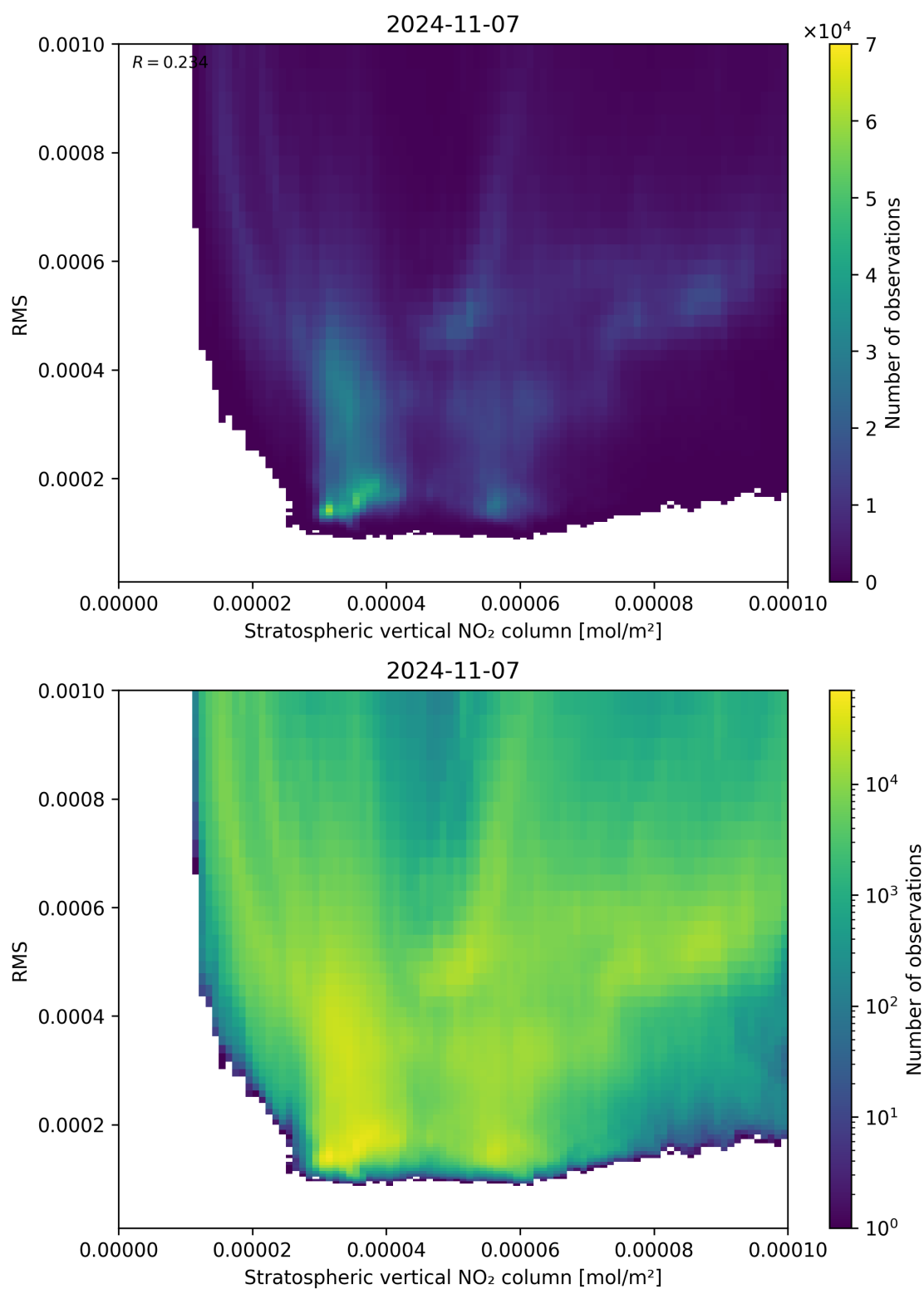
Figure 102: Scatter density plot of “Stratospheric vertical NO 2 column” against “RMS” for 2024-11-06 to 2024-11-08.
