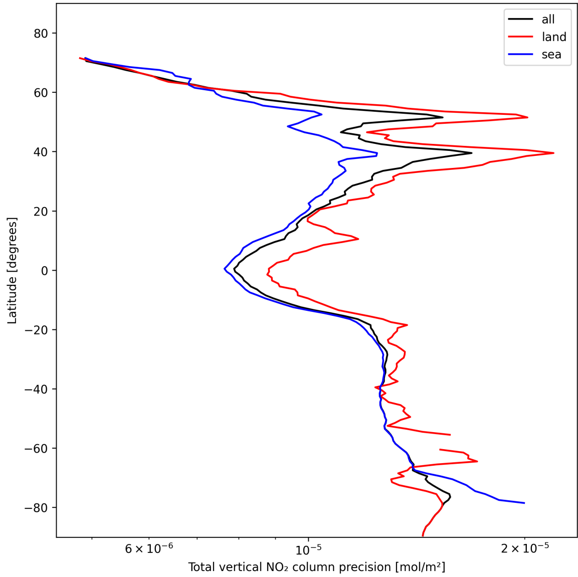
Figure 22: Zonal average of “Total vertical NO 2 column precision” for 2024-11-06 to 2024-11-08.
