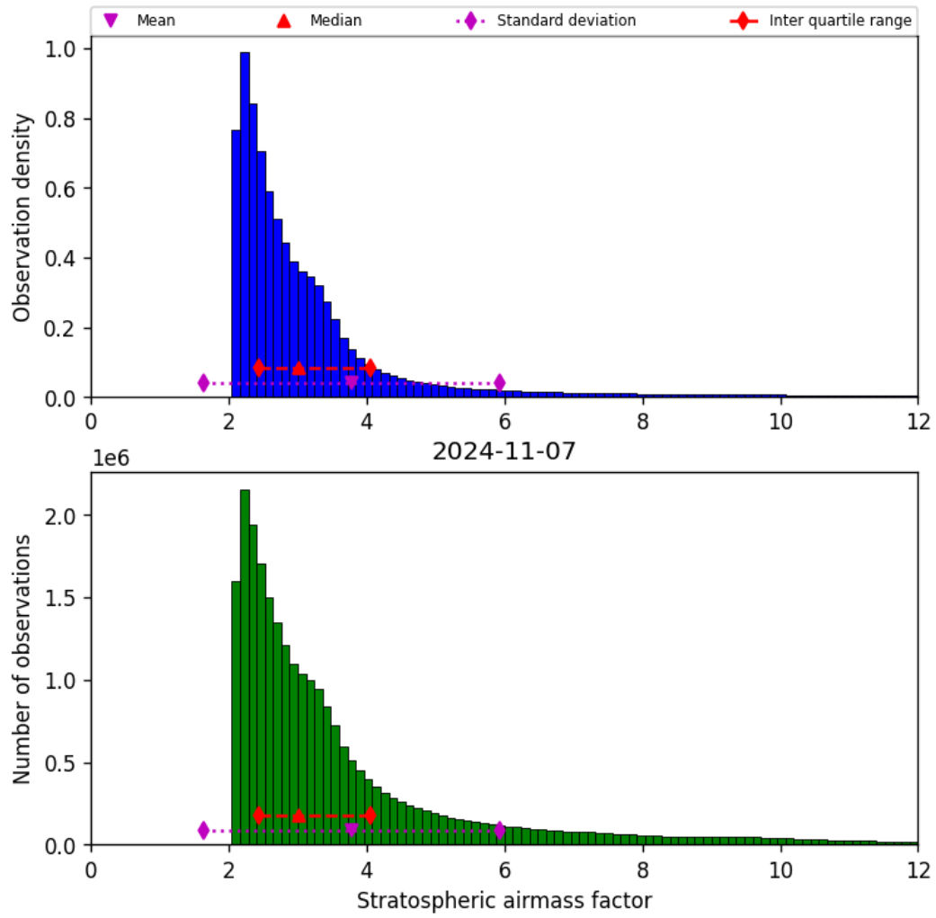
Figure 44: Histogram of “Stratospheric airmass factor” for 2024-11-06 to 2024-11-08
