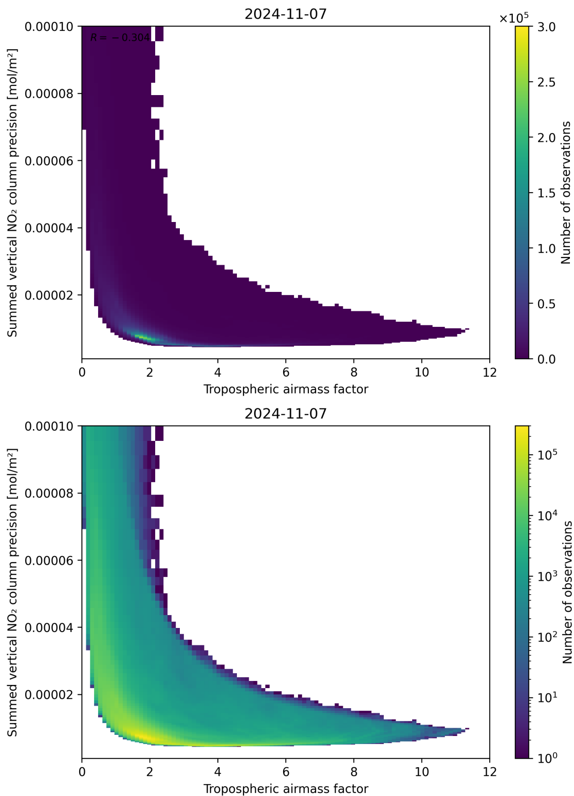
Figure 76: Scatter density plot of “Tropospheric air mass factor” against “Summed vertical NO 2 column precision” for 2024-11-06 to 2024-11-08.
