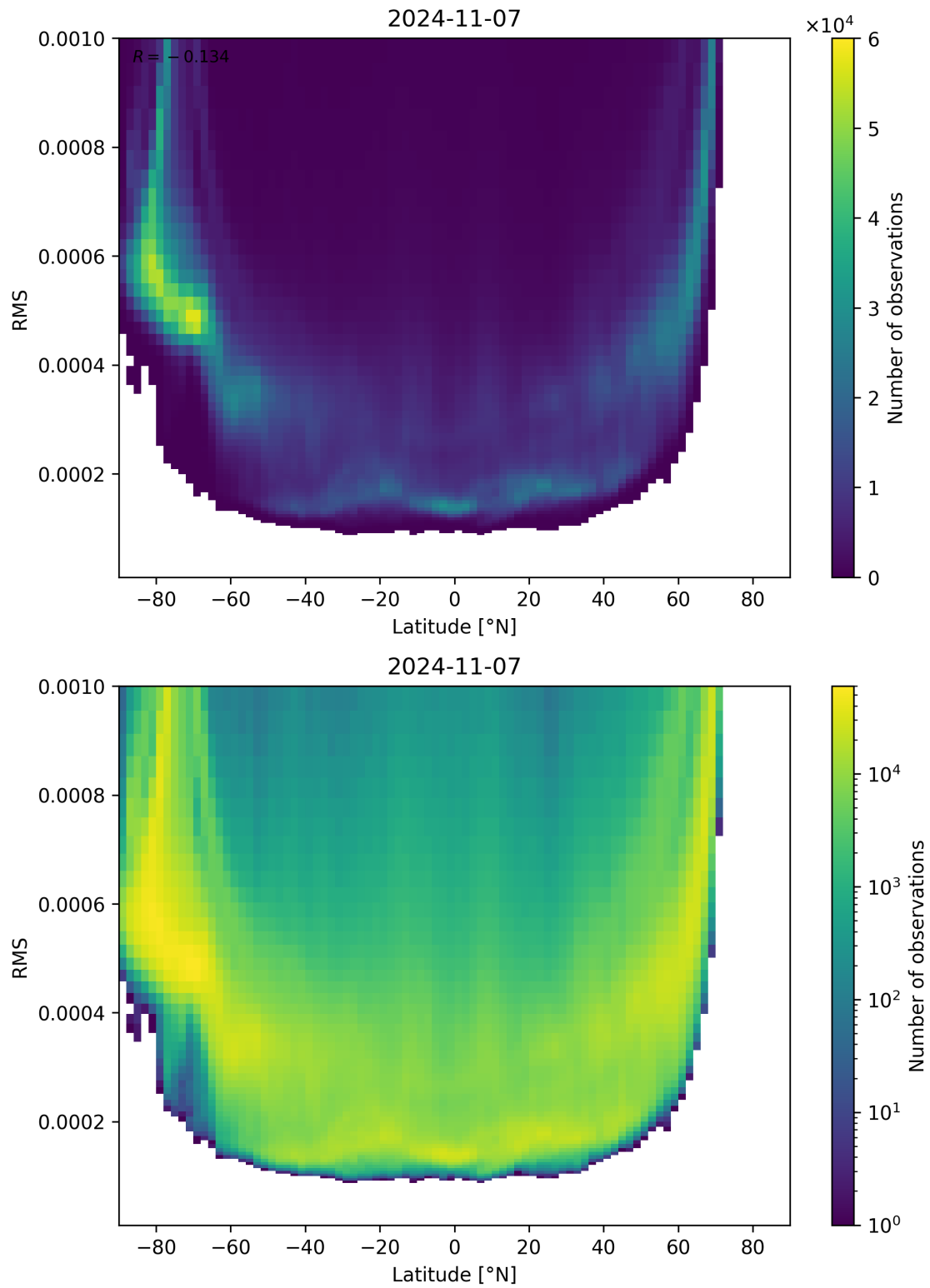
Figure 94: Scatter density plot of “Latitude” against “RMS” for 2024-11-06 to 2024-11-08.
