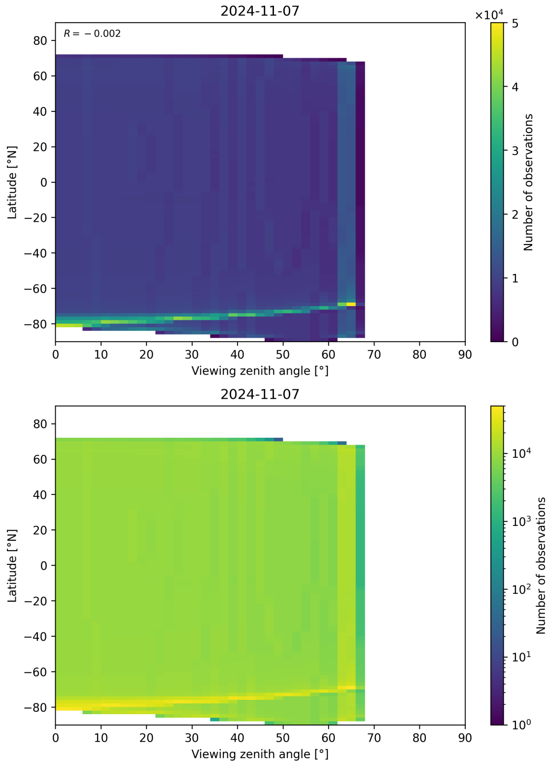
Figure 163: Scatter density plot of “Viewing zenith angle” against “Latitude” for 2024-11-06 to 2024-11-08.
