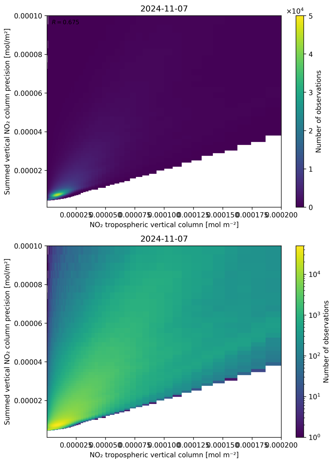
Figure 127: Scatter density plot of “NO 2 tropospheric vertical column” against “Summed vertical NO 2 column precision” for 2024-11-06 to 2024-11-08.
