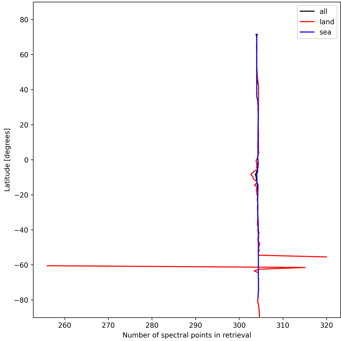
Figure 16: Zonal average of “Number of spectral points in retrieval” for 2024-11-06 to 2024-11-08.
