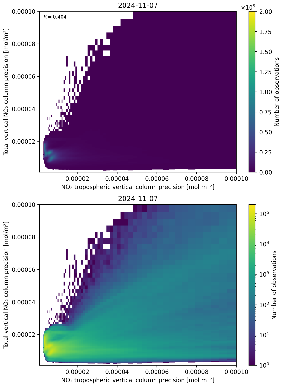
Figure 139: Scatter density plot of “NO 2 tropospheric vertical column precision” against “Total vertical NO 2 column precision” for 2024-11-06 to 2024-11-08.
