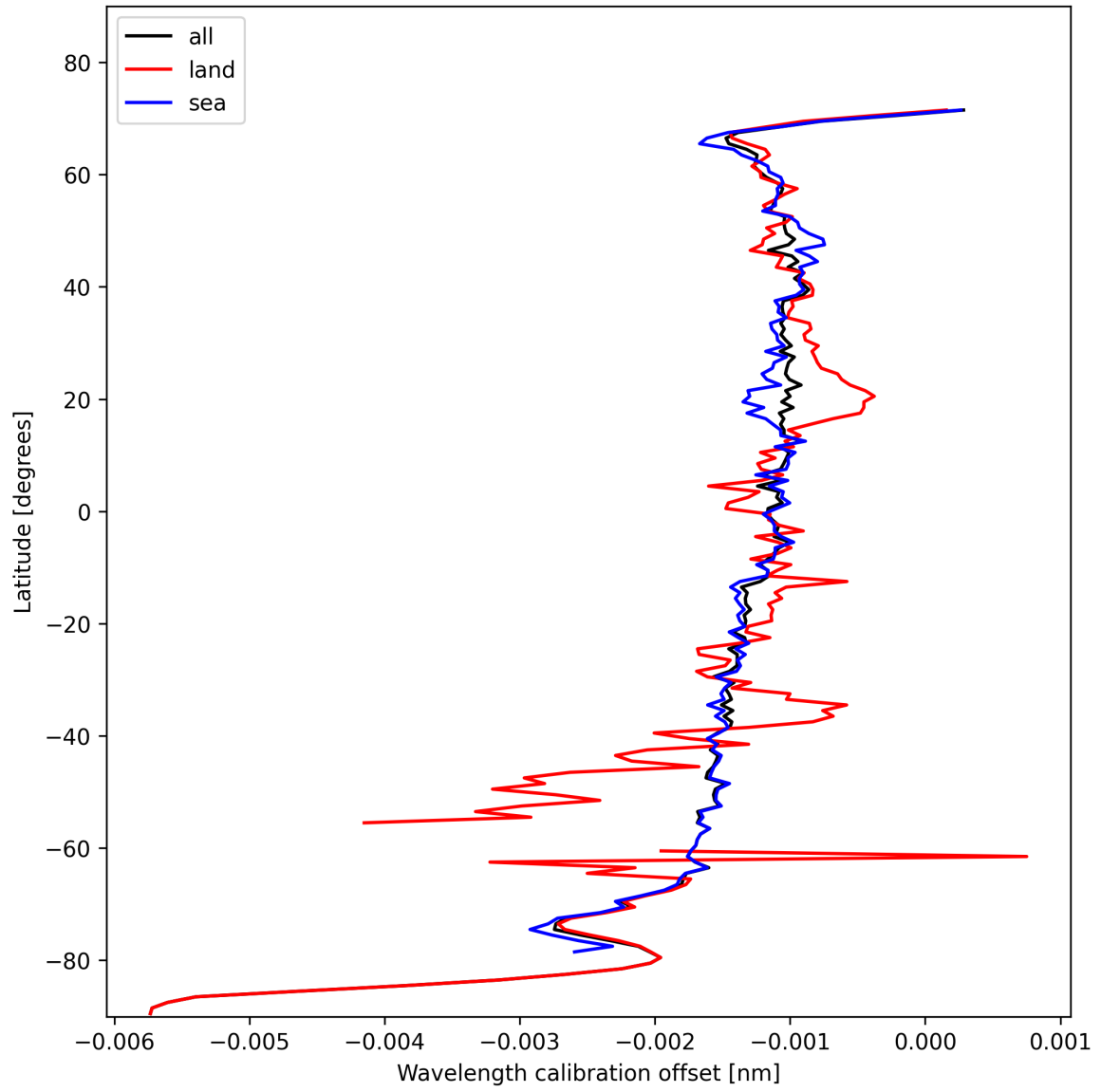
Figure 18: Zonal average of “Wavelength calibration offset” for 2024-11-06 to 2024-11-08.
