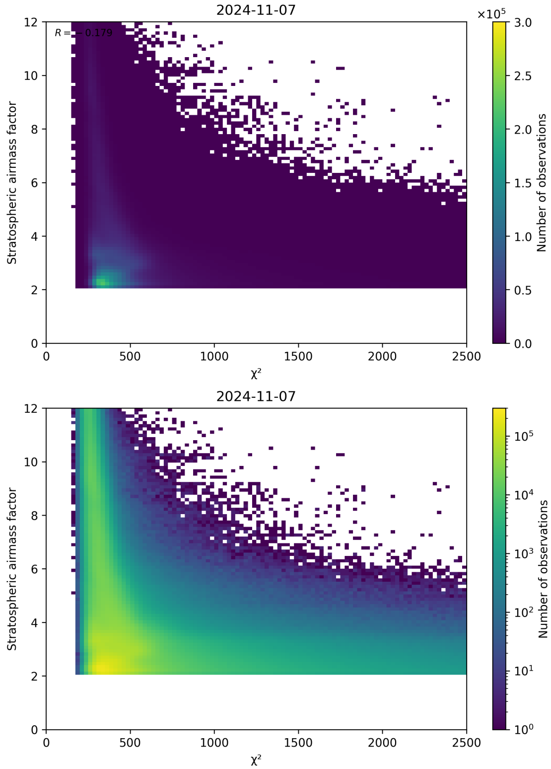
Figure 81: Scatter density plot of “ \chi^2 ” against “Stratospheric airmass factor” for 2024-11-06 to 2024-11-08.
