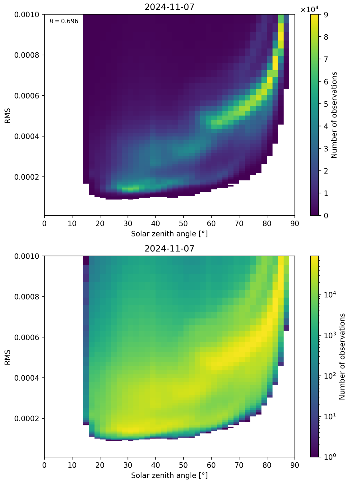
Figure 157: Scatter density plot of “Solar zenith angle” against “RMS” for 2024-11-06 to 2024-11-08.
