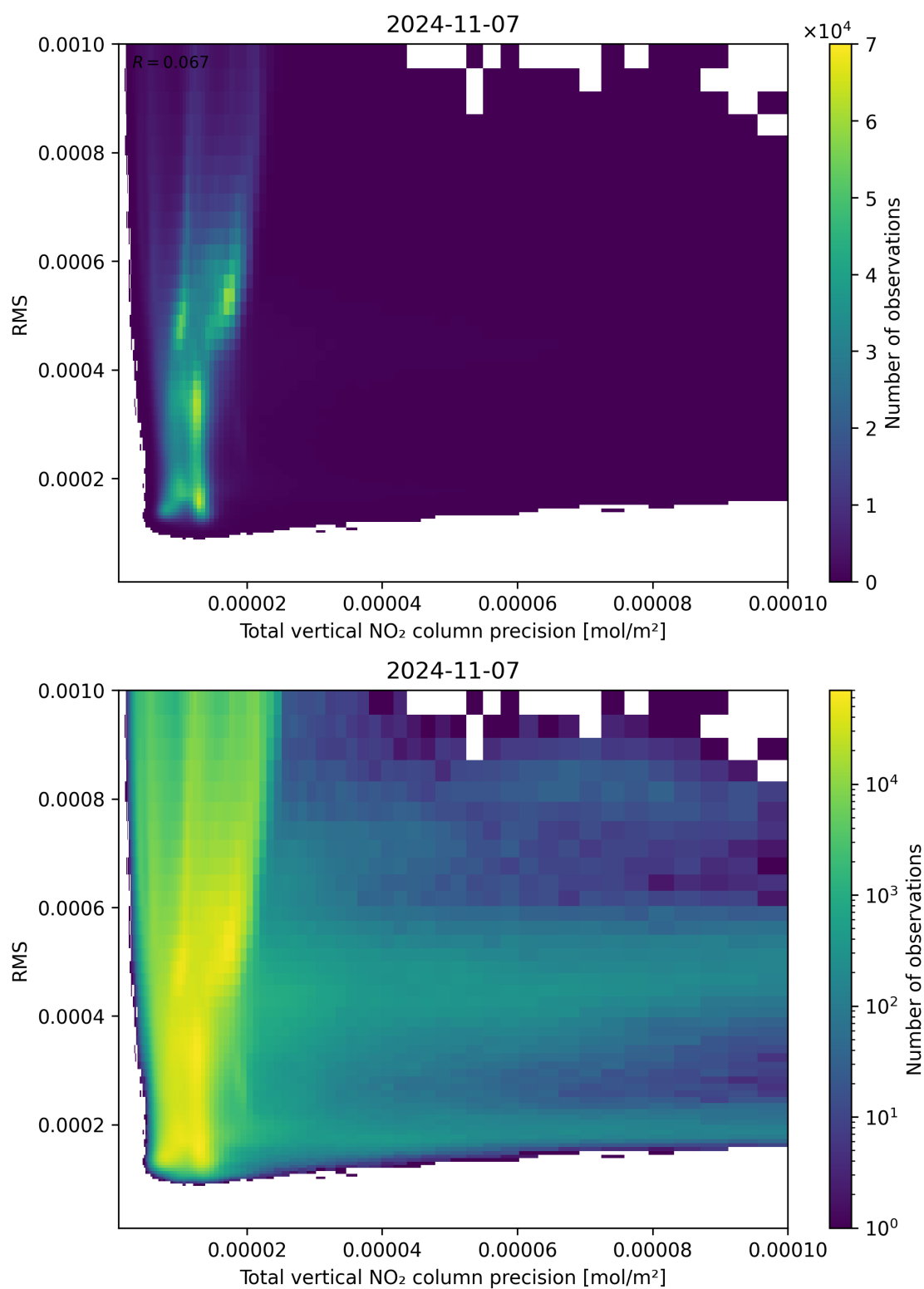
Figure 119: Scatter density plot of “Total vertical NO 2 column precision” against “RMS” for 2024-11-06 to 2024-11-08.
