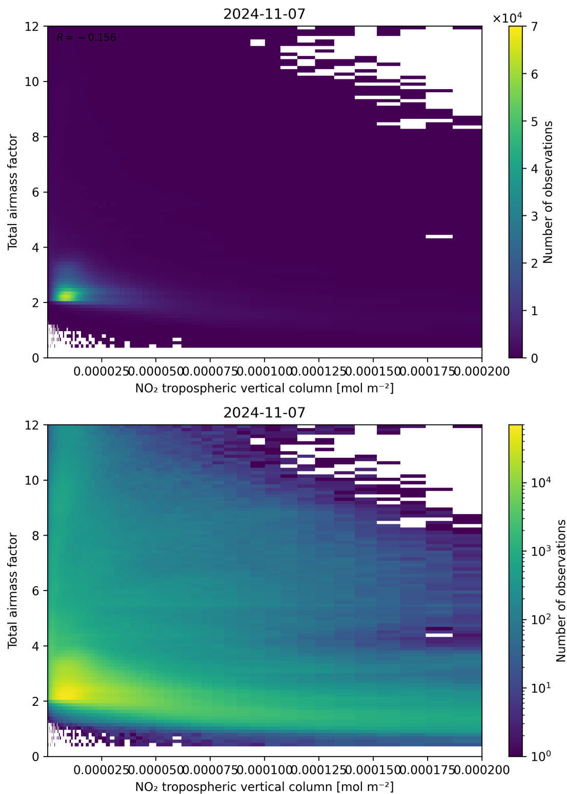
Figure 122: Scatter density plot of “NO 2 tropospheric vertical column” against “Total air mass factor” for 2024-11-06 to 2024-11-08.
