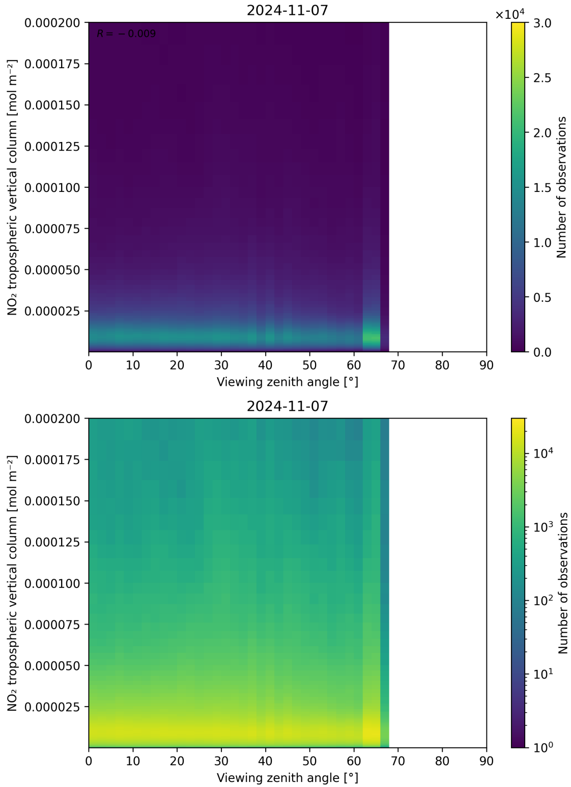
Figure 169: Scatter density plot of “Viewing zenith angle” against “NO 2 tropospheric vertical column” for 2024-11-06 to 2024-11-08.
