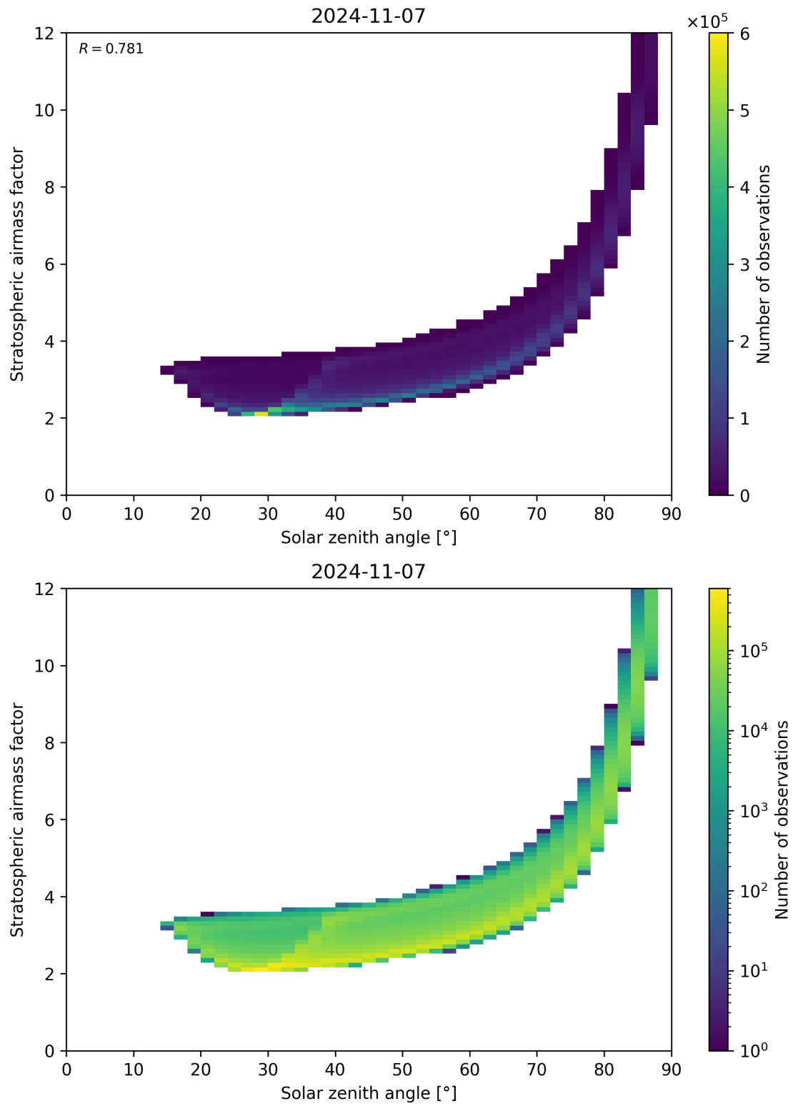
Figure 145: Scatter density plot of “Solar zenith angle” against “Stratospheric airmass factor” for 2024-11-06 to 2024-11-08.
