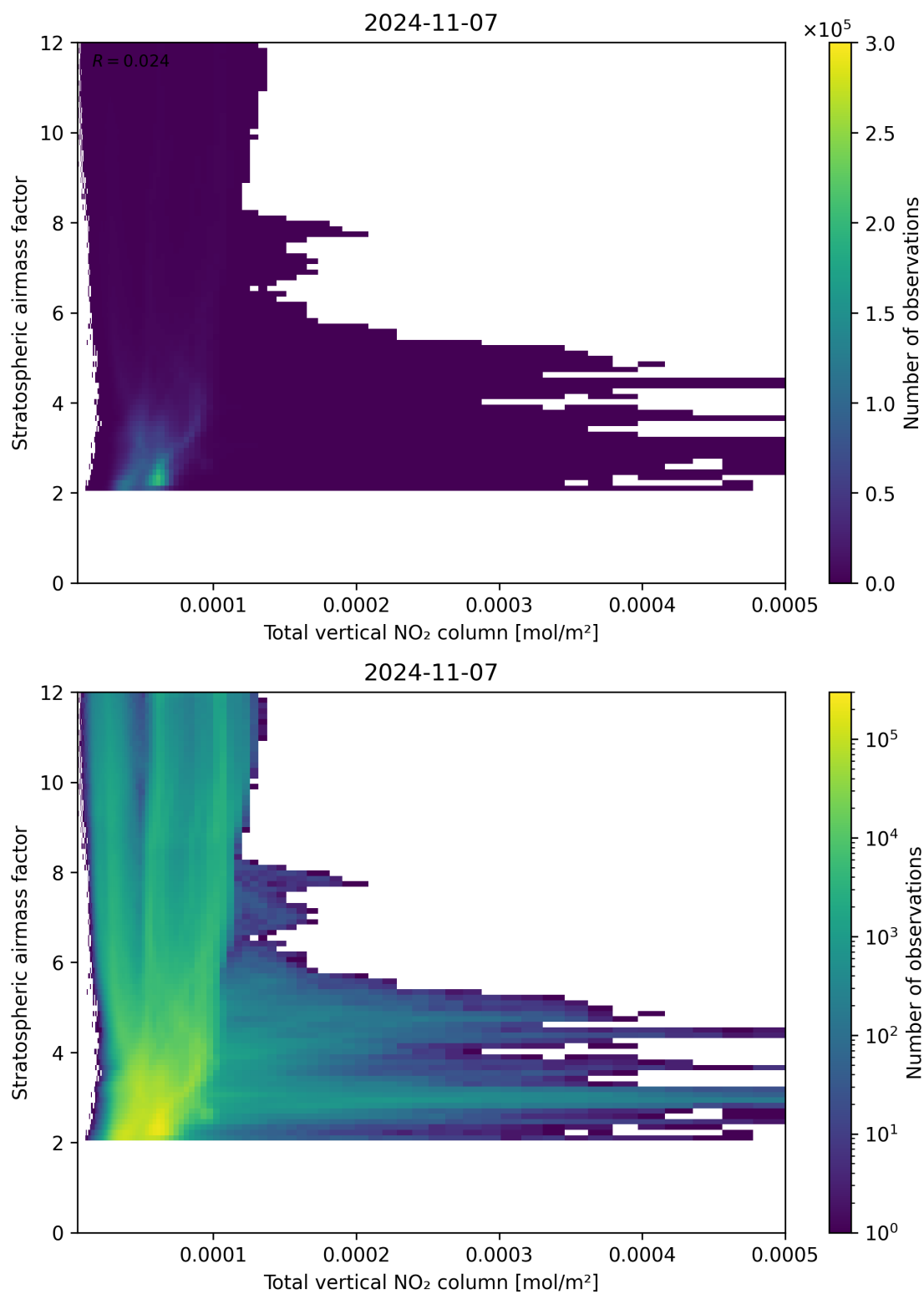
Figure 110: Scatter density plot of “Total vertical NO 2 column” against “Stratospheric airmass factor” for 2024-11-06 to 2024-11-08.
