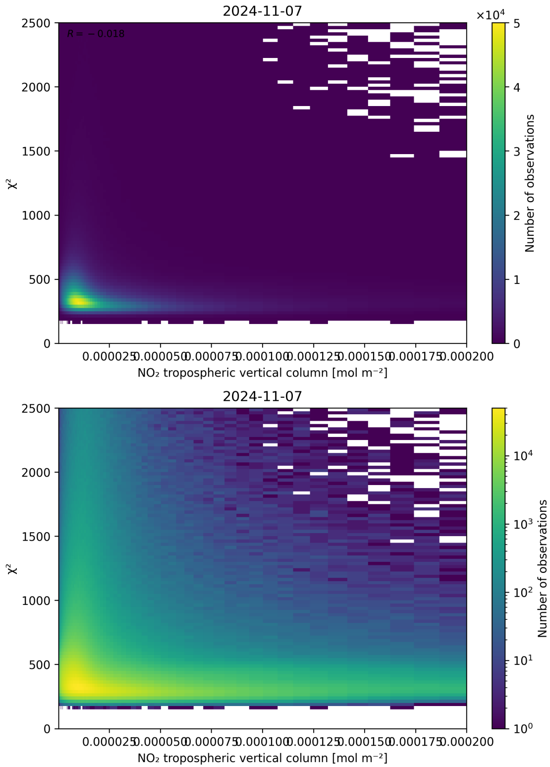
Figure 124: Scatter density plot of “NO 2 tropospheric vertical column” against “ \chi^2 ” for 2024-11-06 to 2024-11-08.
