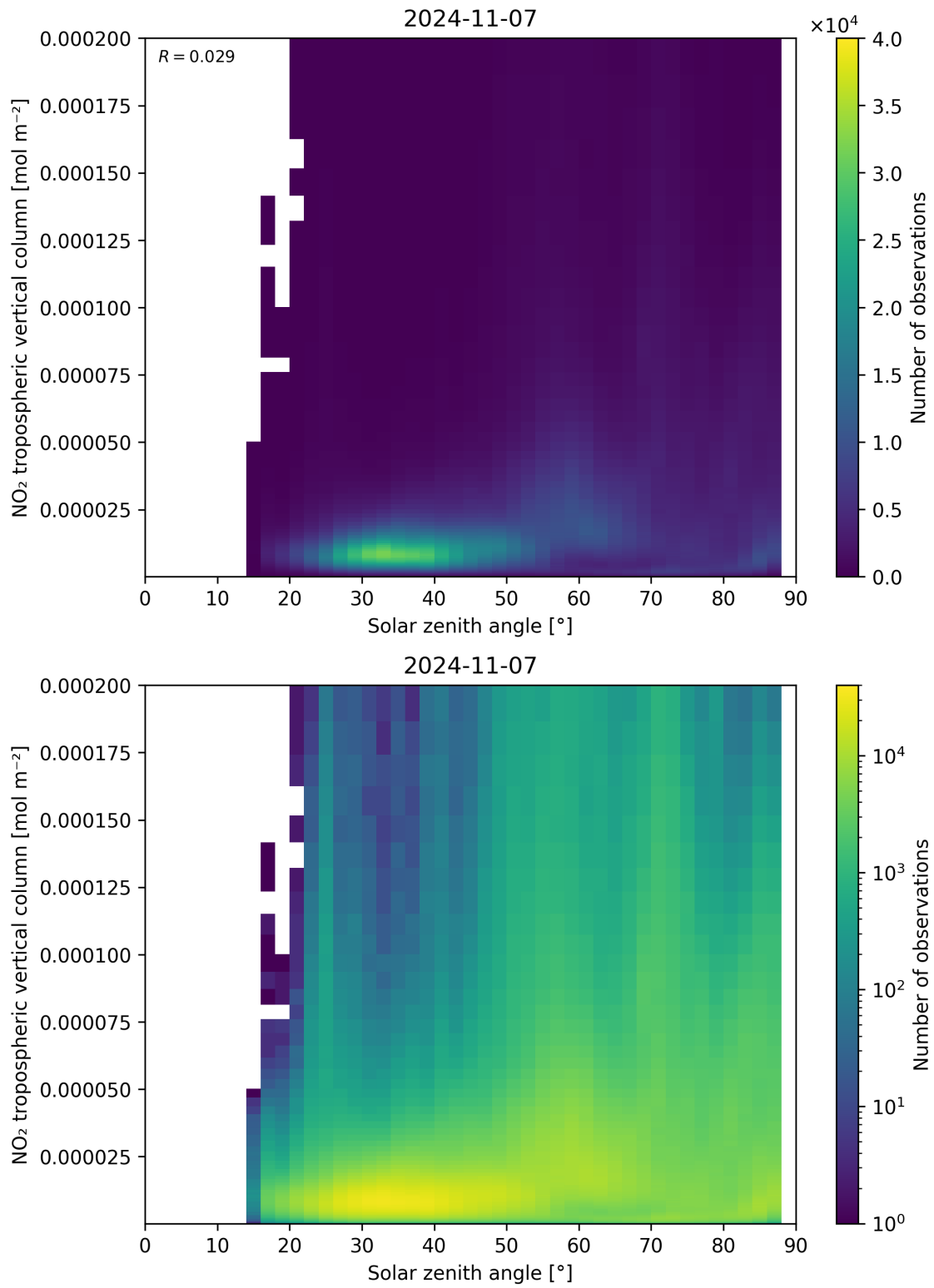
Figure 155: Scatter density plot of “Solar zenith angle” against “NO 2 tropospheric vertical column” for 2024-11-06 to 2024-11-08.
