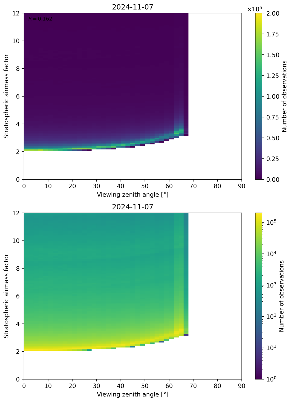
Figure 159: Scatter density plot of “Viewing zenith angle” against “Stratospheric airmass factor” for 2024-11-06 to 2024-11-08.
