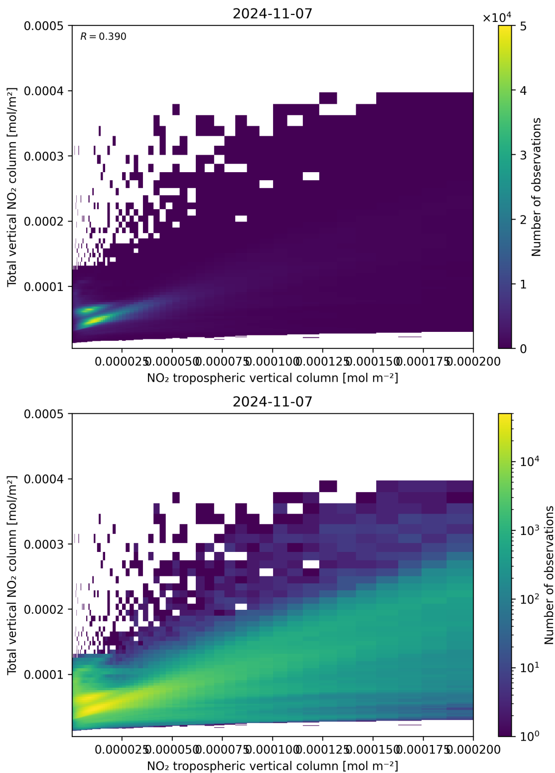
Figure 128: Scatter density plot of “NO 2 tropospheric vertical column” against “Total vertical NO 2 column” for 2024-11-06 to 2024-11-08.
