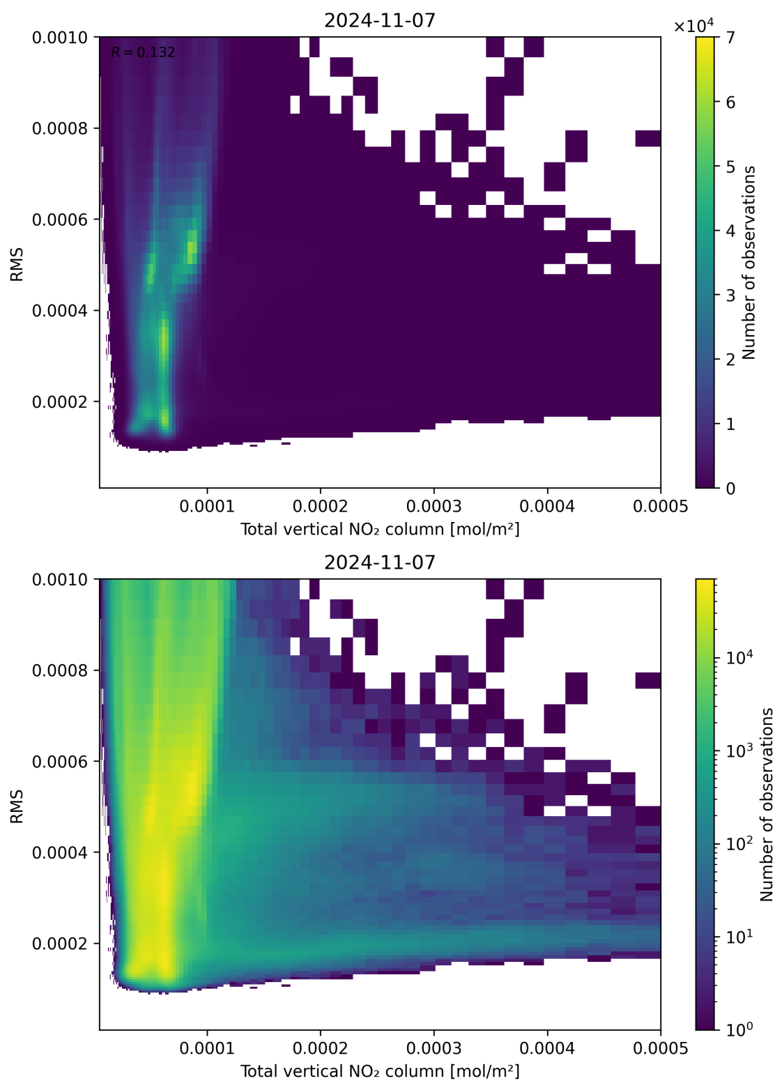
Figure 120: Scatter density plot of “Total vertical NO 2 column” against “RMS” for 2024-11-06 to 2024-11-08.
