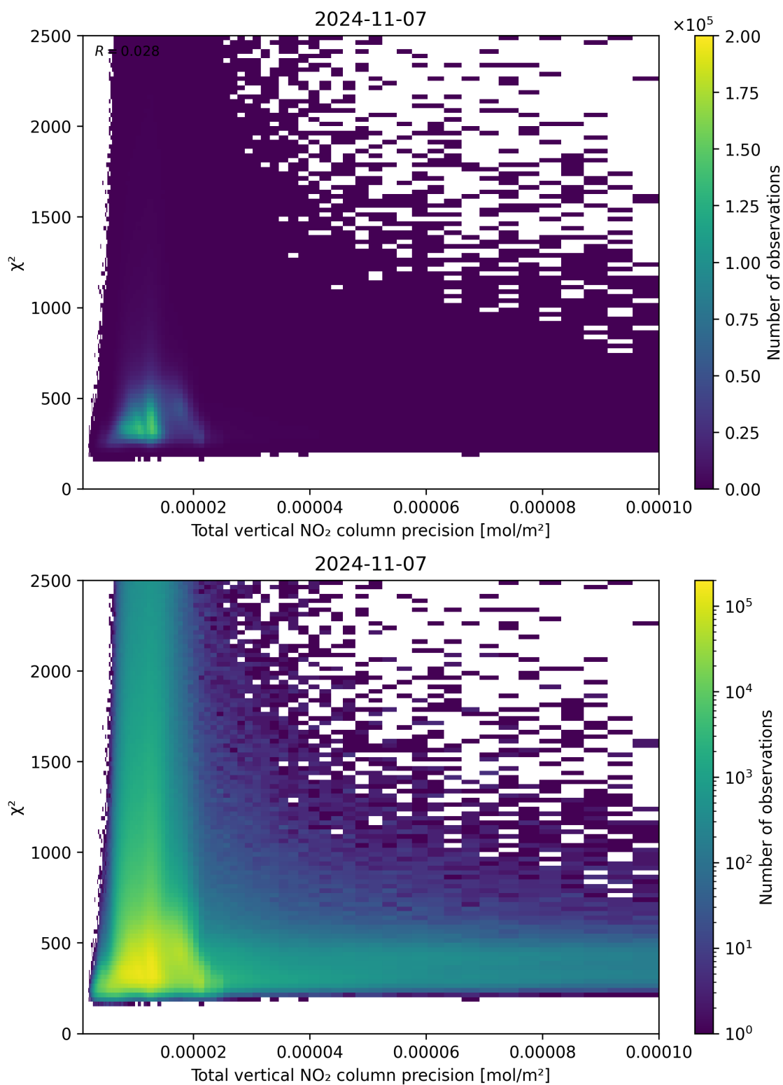
Figure 116: Scatter density plot of “Total vertical NO 2 column precision” against “ \chi^2 ” for 2024-11-06 to 2024-11-08.
