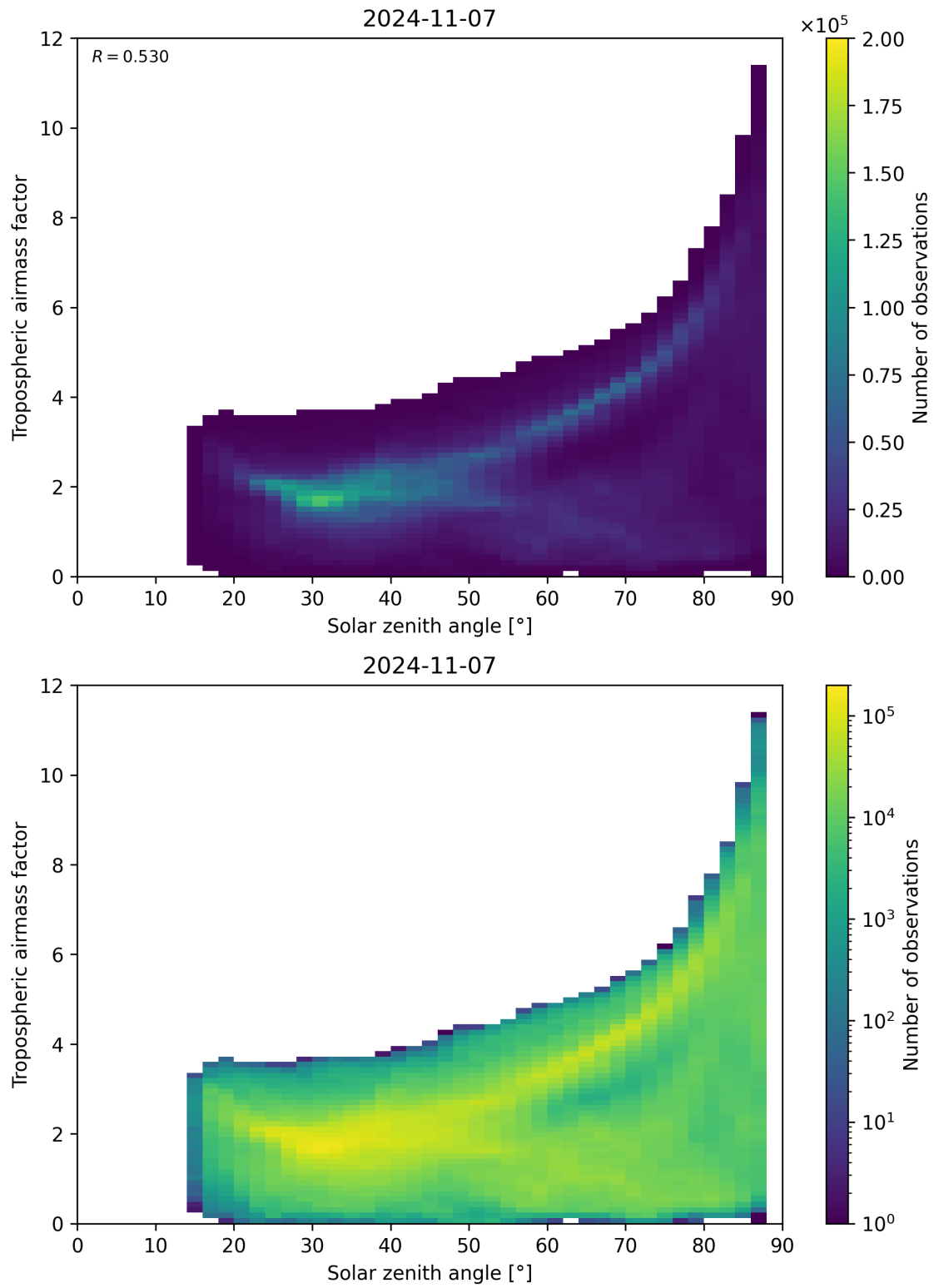
Figure 147: Scatter density plot of “Solar zenith angle” against “Tropospheric airmass factor” for 2024-11-06 to 2024-11-08.
