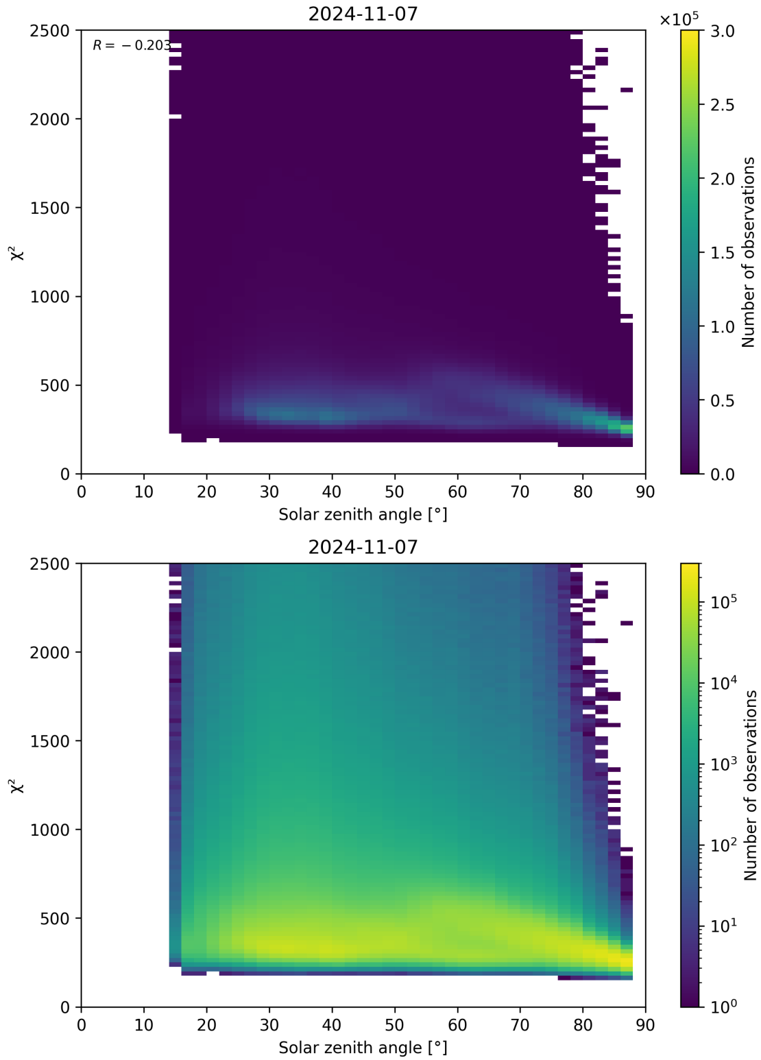
Figure 148: Scatter density plot of “Solar zenith angle” against “ \chi^2 ” for 2024-11-06 to 2024-11-08.
