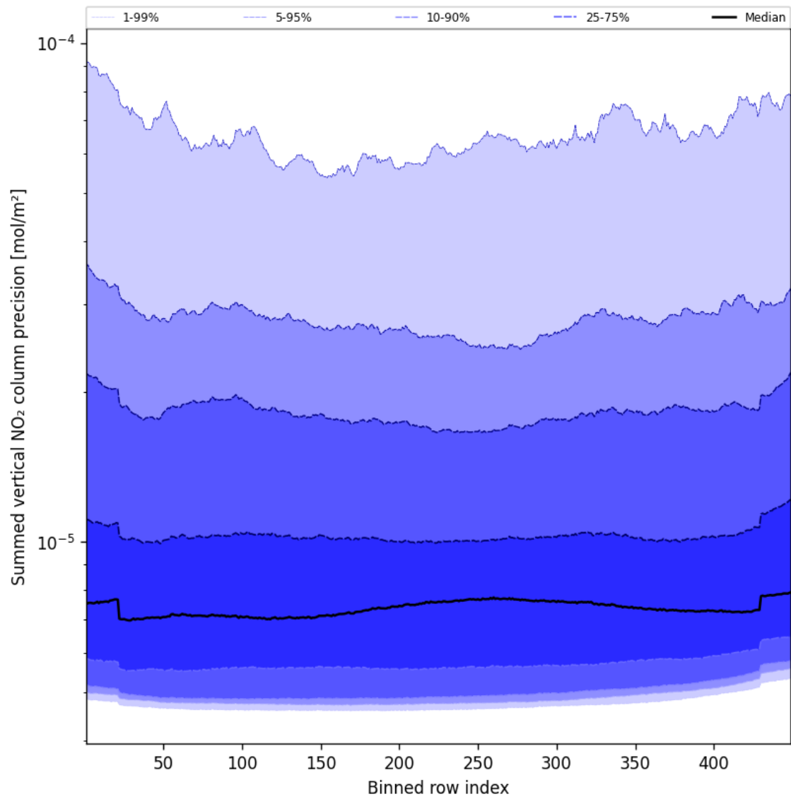
Figure 58: Along track statistics of “Summed vertical NO 2 column precision” for 2024-11-06 to 2024-11-08
