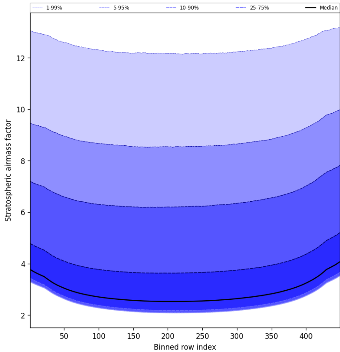
Figure 61: Along track statistics of “Stratospheric air mass factor” for 2024-11-06 to 2024-11-08
