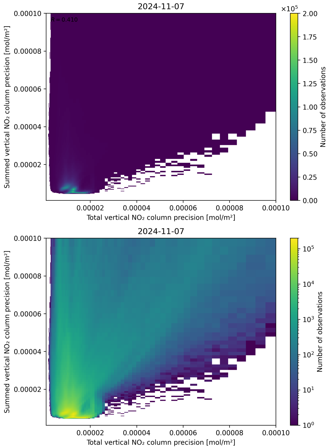
Figure 118: Scatter density plot of “Total vertical NO 2 column precision” against “Summed vertical NO 2 column precision” for 2024-11-06 to 2024-11-08.
