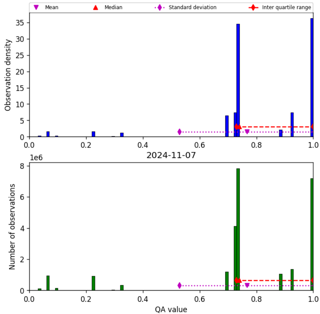
Figure 28: Histogram of “QA value” for 2024-11-06 to 2024-11-08
