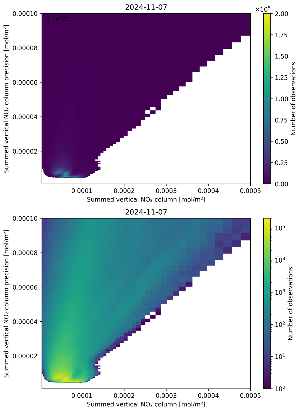
Figure 105: Scatter density plot of “Summed vertical NO 2 column” against “Summed vertical NO 2 column precision” for 2024-11-06 to 2024-11-08.
