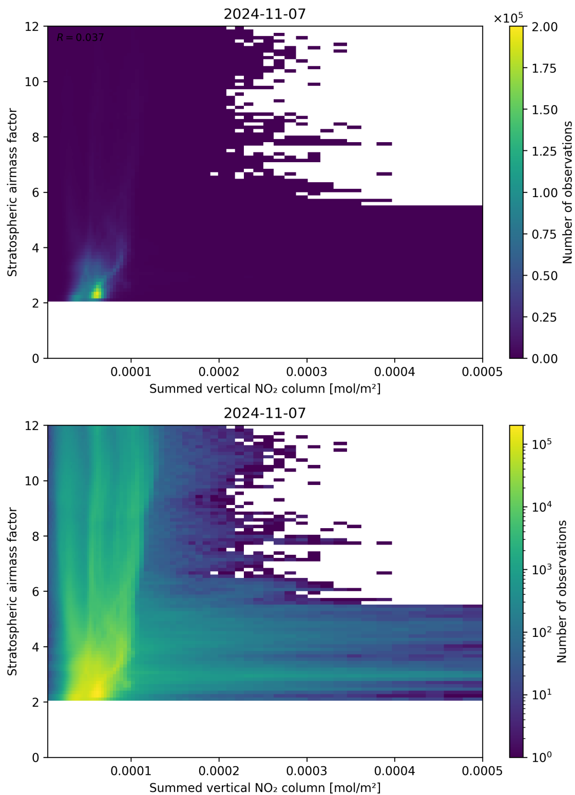
Figure 103: Scatter density plot of “Summed vertical NO 2 column” against “Stratospheric air mass factor” for 2024-11-06 to 2024-11-08.
