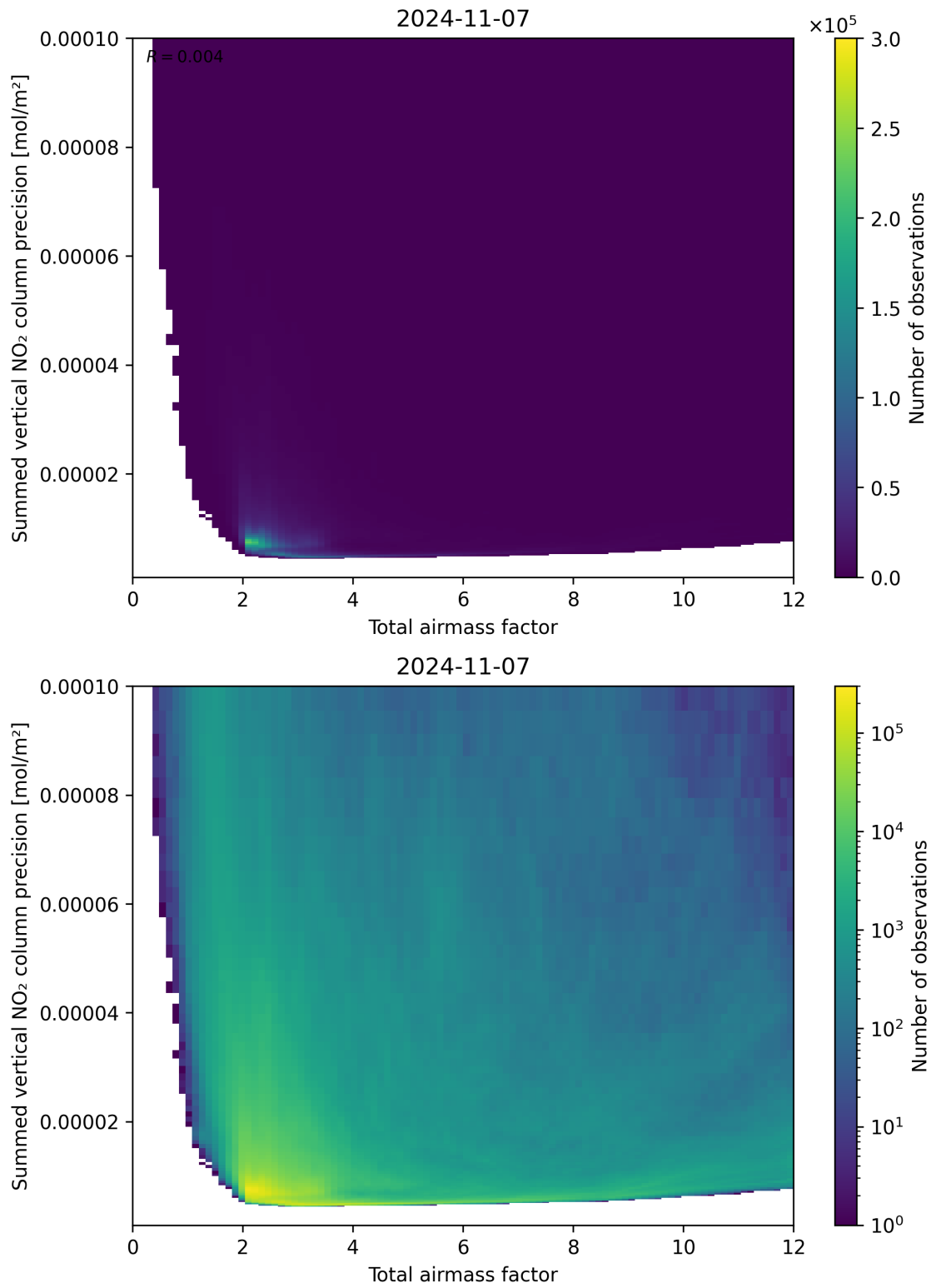
Figure 66: Scatter density plot of “Total airmass factor” against “Summed vertical NO 2 column precision” for 2024-11-06 to 2024-11-08.
