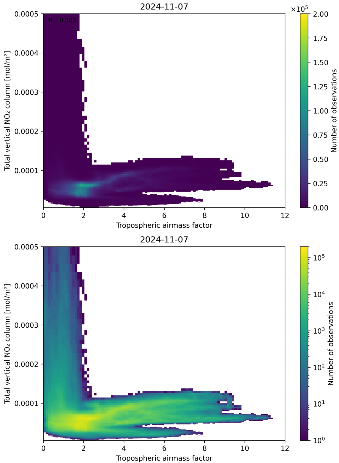
Figure 77: Scatter density plot of “Tropospheric airmass factor” against “Total vertical NO 2 column” for 2024-11-06 to 2024-11-08.
