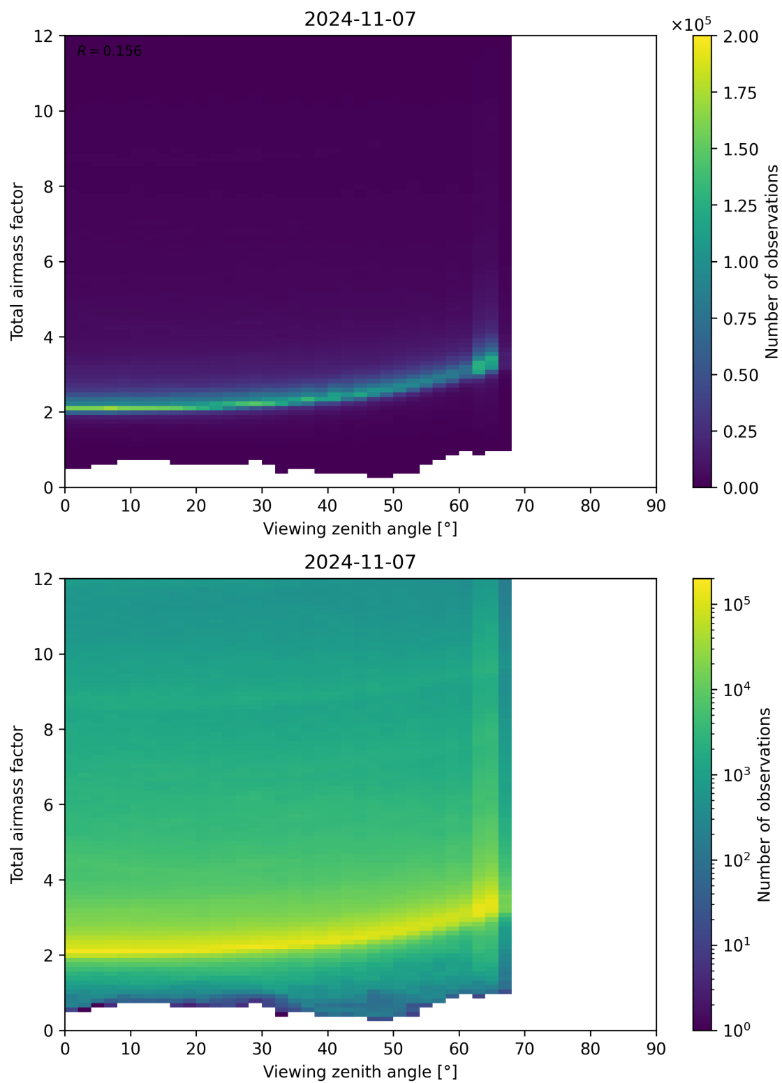
Figure 160: Scatter density plot of “Viewing zenith angle” against “Total airmass factor” for 2024-11-06 to 2024-11-08.
