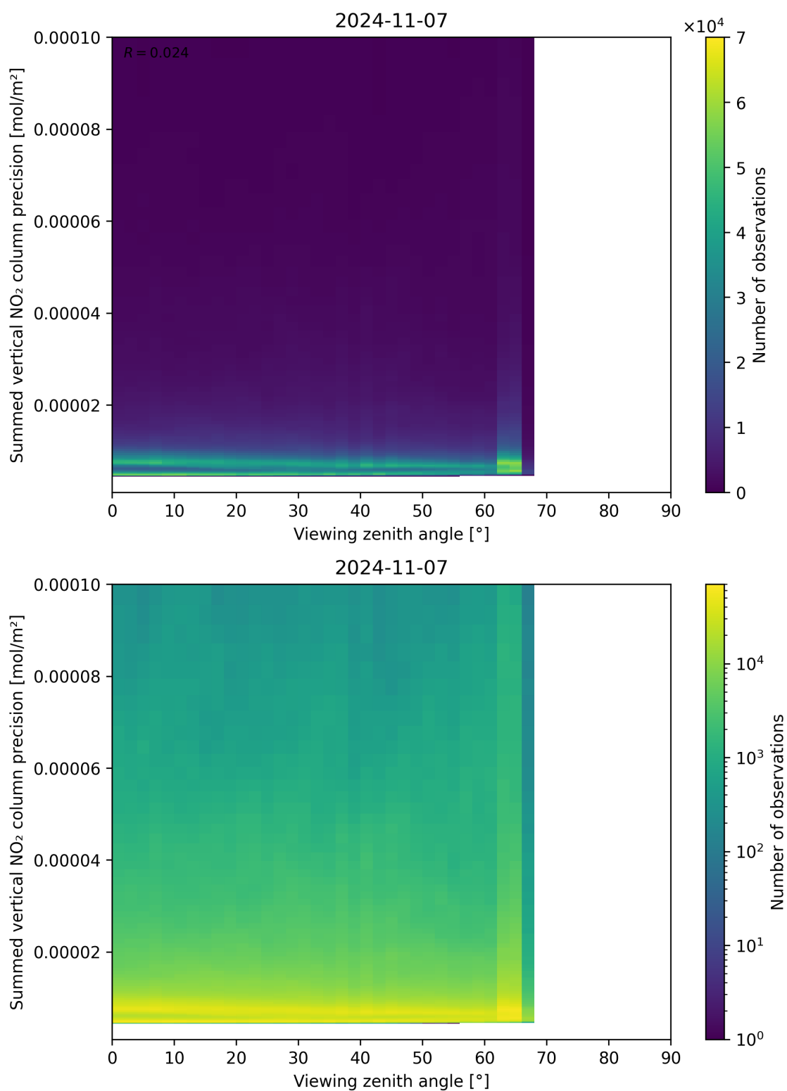
Figure 166: Scatter density plot of “Viewing zenith angle” against “Summed vertical NO 2 column precision” for 2024-11-06 to 2024-11-08.
