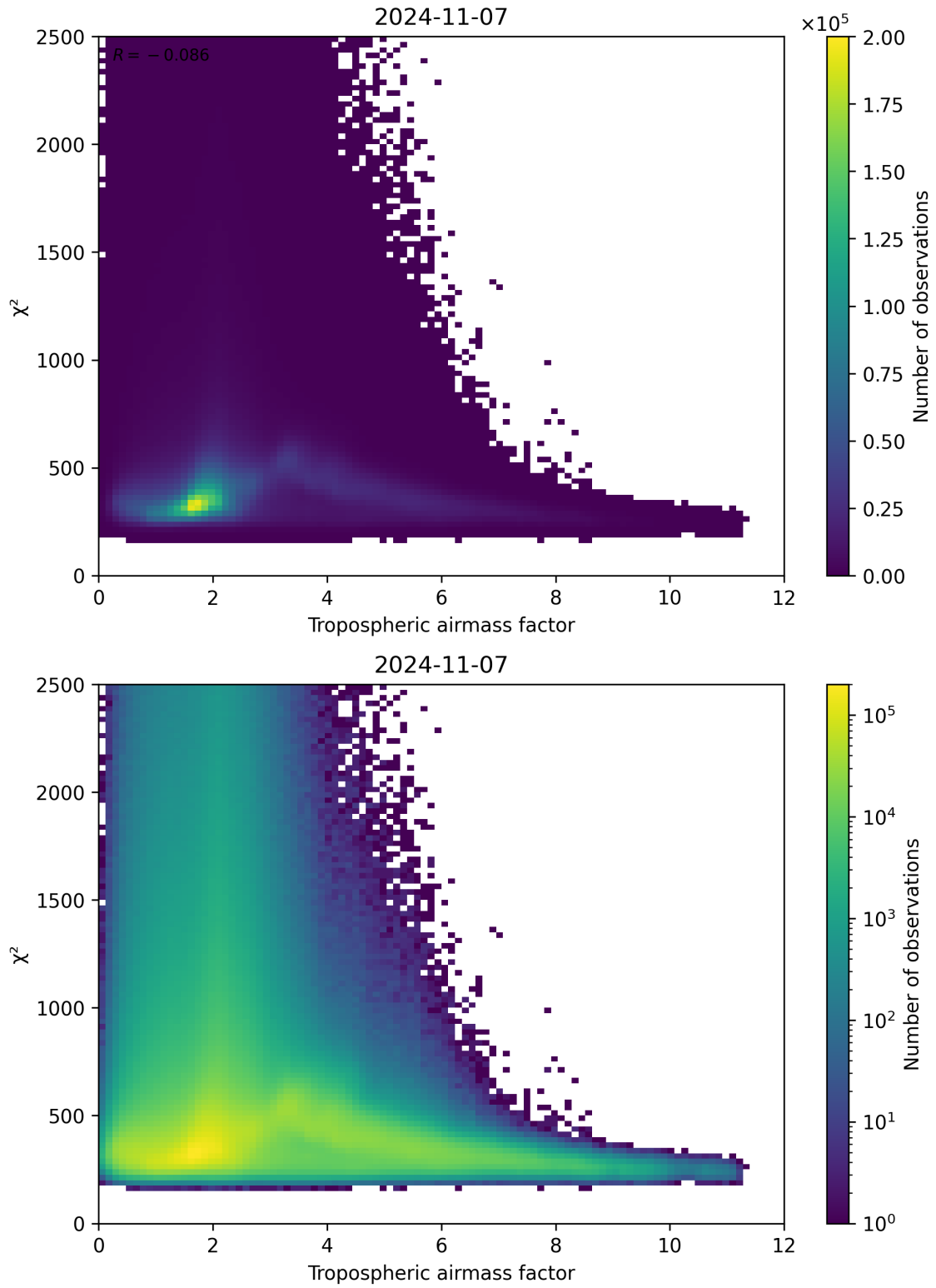
Figure 73: Scatter density plot of “Tropospheric airmass factor” against “ \chi^2 ” for 2024-11-06 to 2024-11-08.
