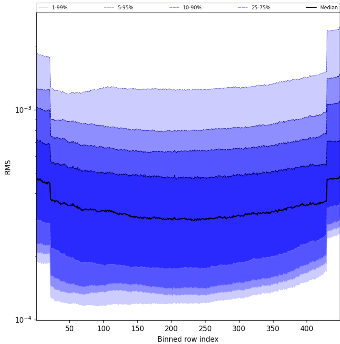
Figure 60: Along track statistics of “RMS” for 2024-11-06 to 2024-11-08
