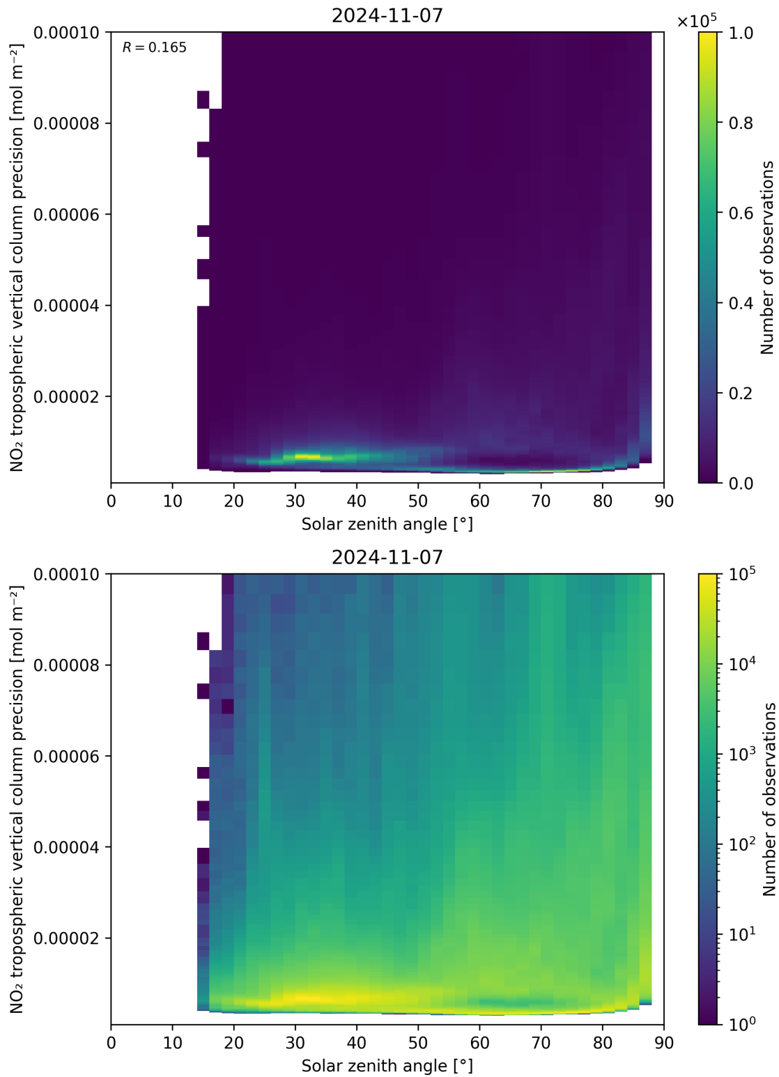
Figure 156: Scatter density plot of “Solar zenith angle” against “NO 2 tropospheric vertical column precision” for 2024-11-06 to 2024-11-08.
