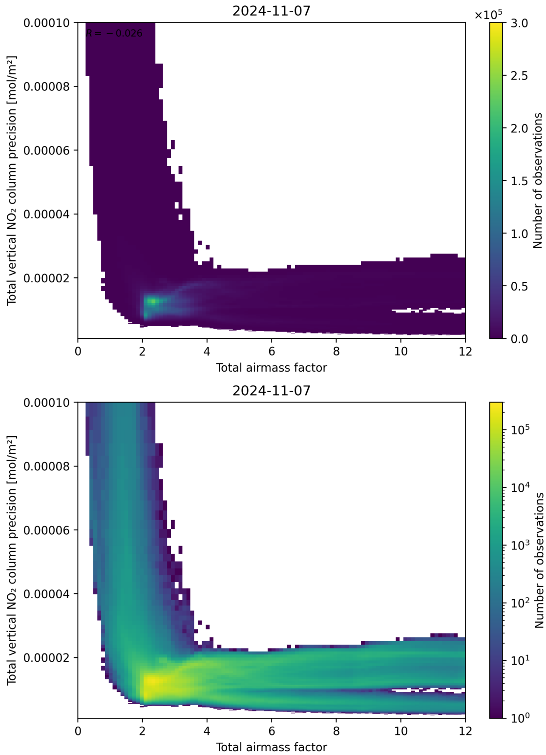
Figure 68: Scatter density plot of “Total airmass factor” against “Total vertical NO 2 column precision” for 2024-11-06 to 2024-11-08.
