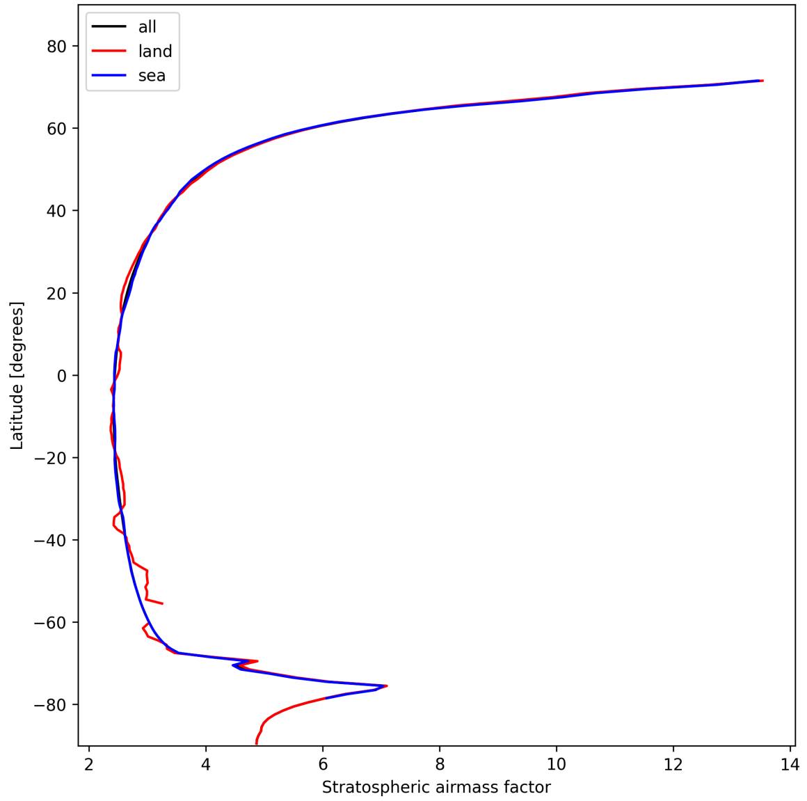
Figure 27: Zonal average of “Stratospheric air mass factor” for 2024-11-06 to 2024-11-08.
