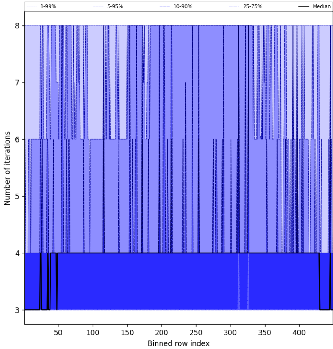
Figure 51: Along track statistics of “Number of iterations” for 2024-11-06 to 2024-11-08
