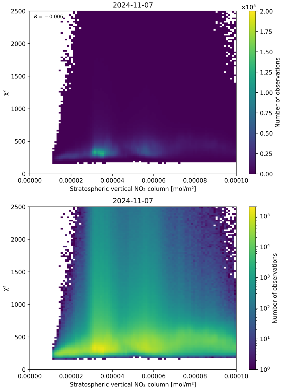
Figure 97: Scatter density plot of “Stratospheric vertical NO 2 column” against “ \chi^2 ” for 2024-11-06 to 2024-11-08.
