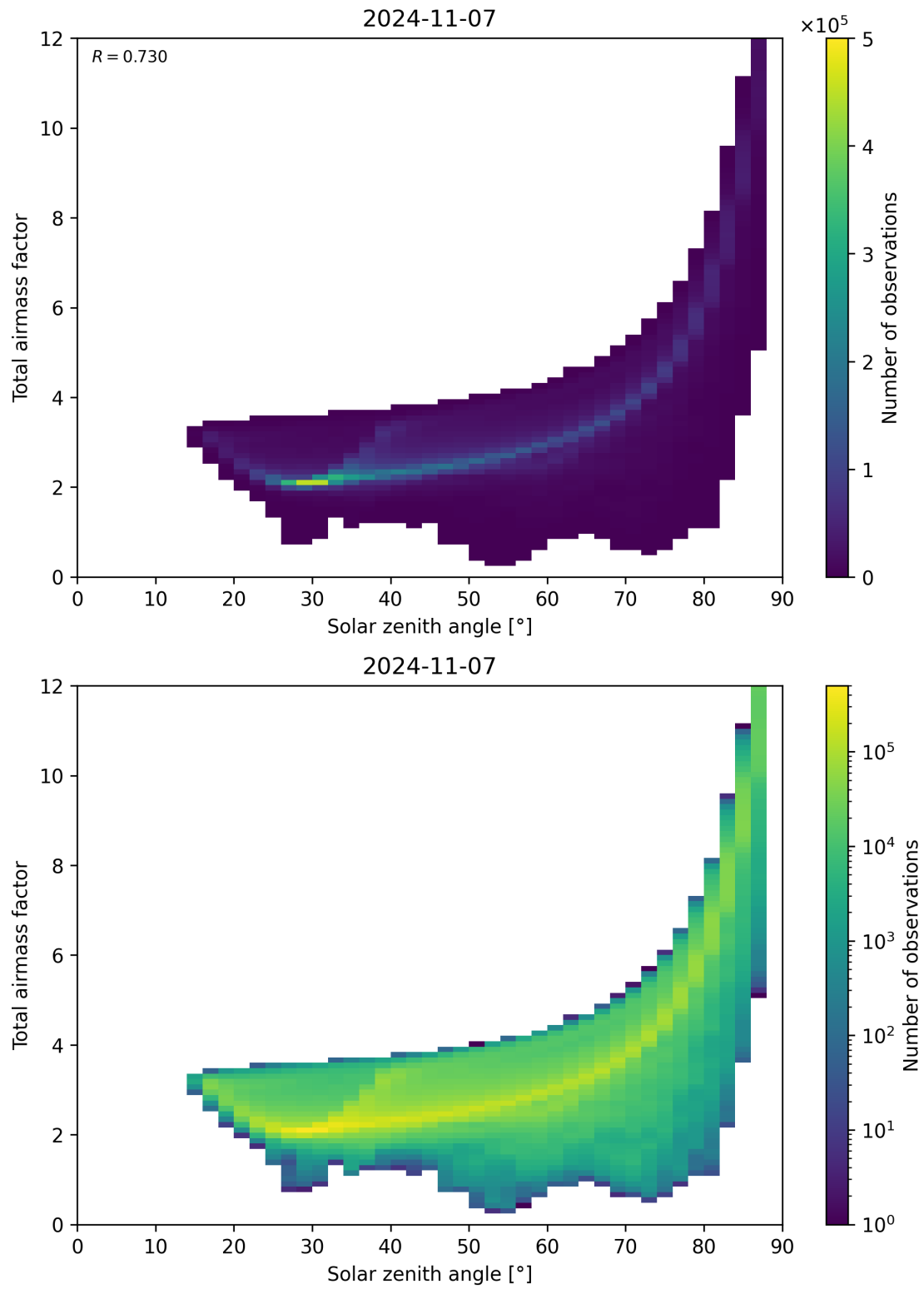
Figure 146: Scatter density plot of “Solar zenith angle” against “Total airmass factor” for 2024-11-06 to 2024-11-08.
