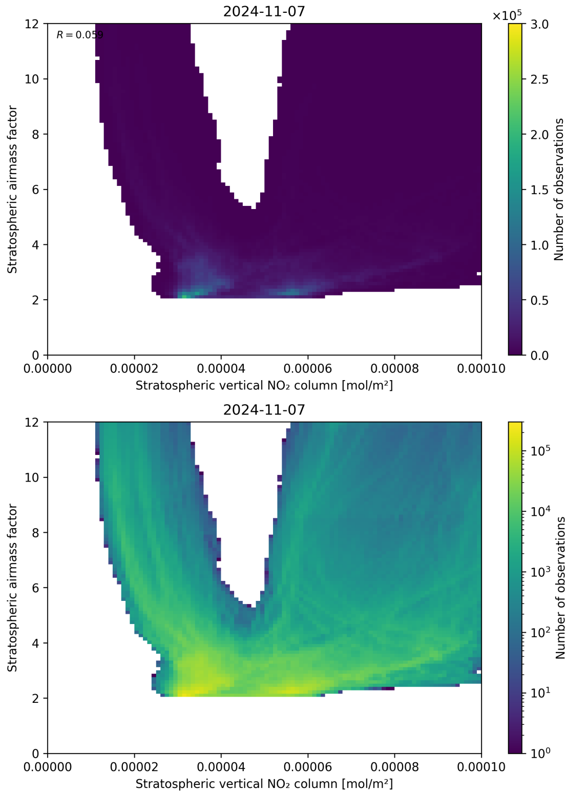
Figure 96: Scatter density plot of “Stratospheric vertical NO 2 column” against “Stratospheric airmass factor” for 2024-11-06 to 2024-11-08.
