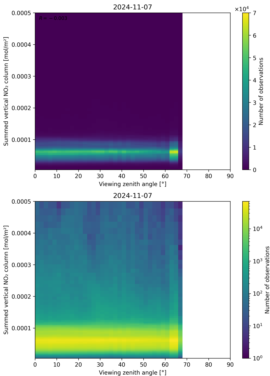
Figure 165: Scatter density plot of “Viewing zenith angle” against “Summed vertical NO 2 column” for 2024-11-06 to 2024-11-08.
