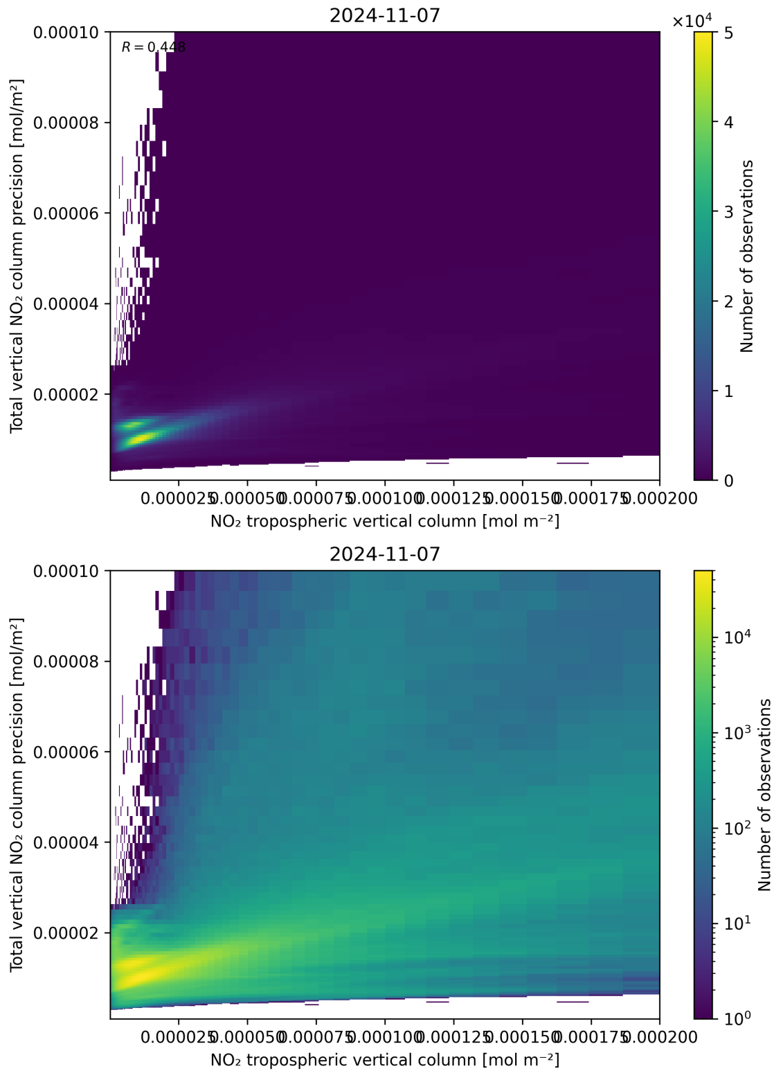
Figure 129: Scatter density plot of “NO 2 tropospheric vertical column” against “Total vertical NO 2 column precision” for 2024-11-06 to 2024-11-08.
