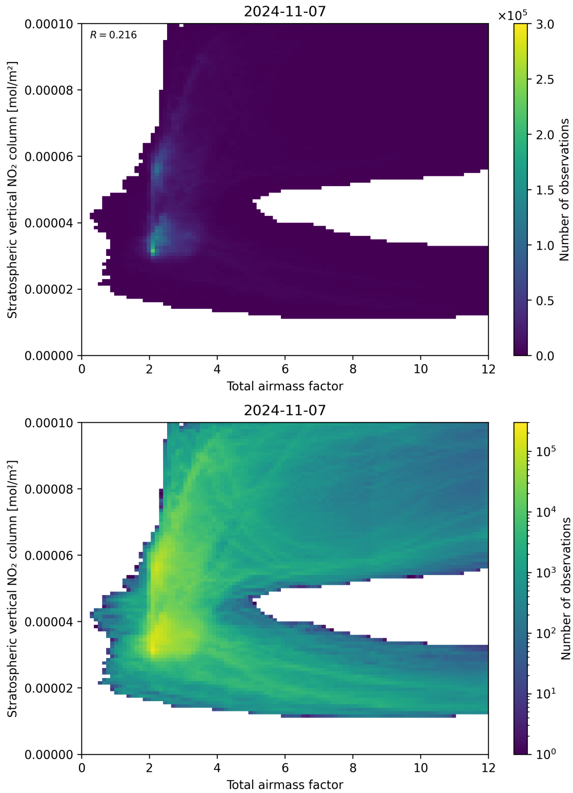
Figure 64: Scatter density plot of “Total airmass factor” against “Stratospheric vertical NO 2 column” for 2024-11-06 to 2024-11-08.
