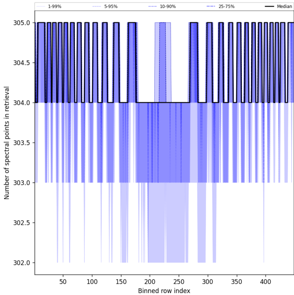
Figure 50: Along track statistics of “Number of spectral points in retrieval” for 2024-11-06 to 2024-11-08
