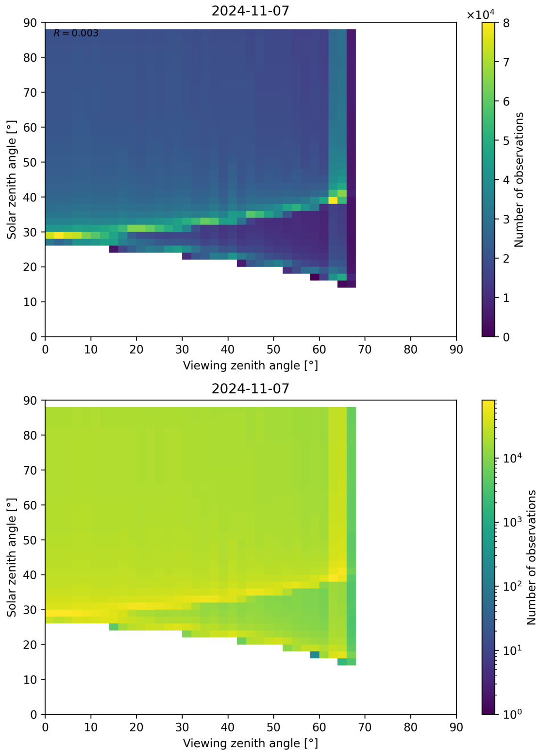
Figure 172: Scatter density plot of “Viewing zenith angle” against “Solar zenith angle” for 2024-11-06 to 2024-11-08.
