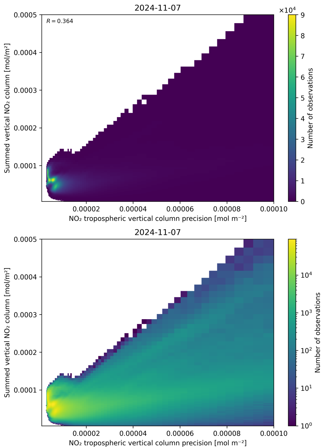
Figure 136: Scatter density plot of “NO 2 tropospheric vertical column precision” against “Summed vertical NO 2 column” for 2024-11-06 to 2024-11-08.
