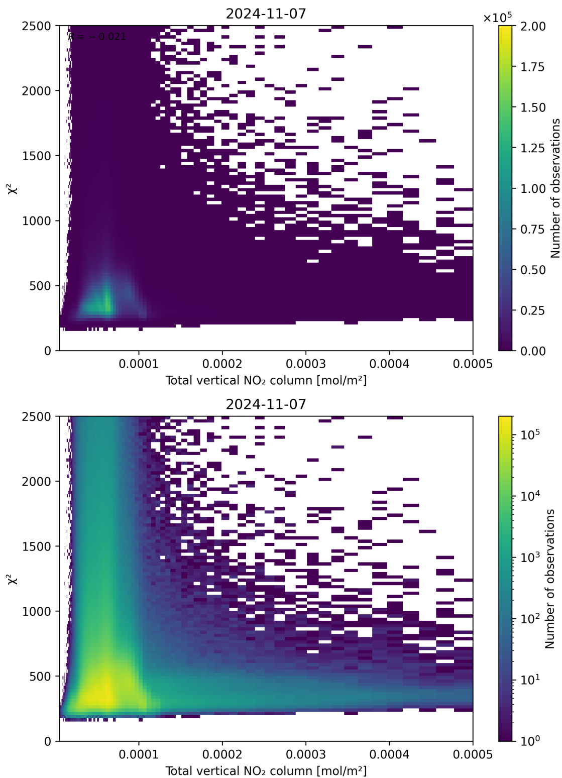
Figure 111: Scatter density plot of “Total vertical NO 2 column” against “ \chi^2 ” for 2024-11-06 to 2024-11-08.
