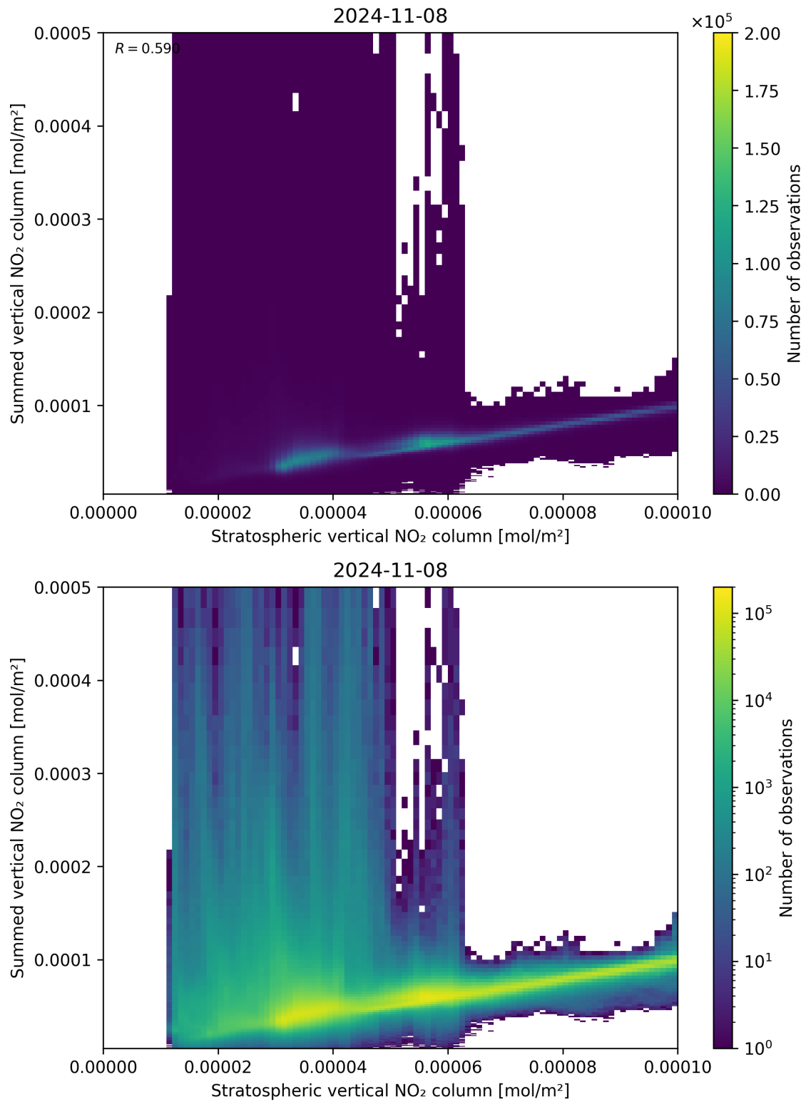
Figure 98: Scatter density plot of “Stratospheric vertical NO 2 column” against “Summed vertical NO 2 column” for 2024-11-07 to 2024-11-09.
