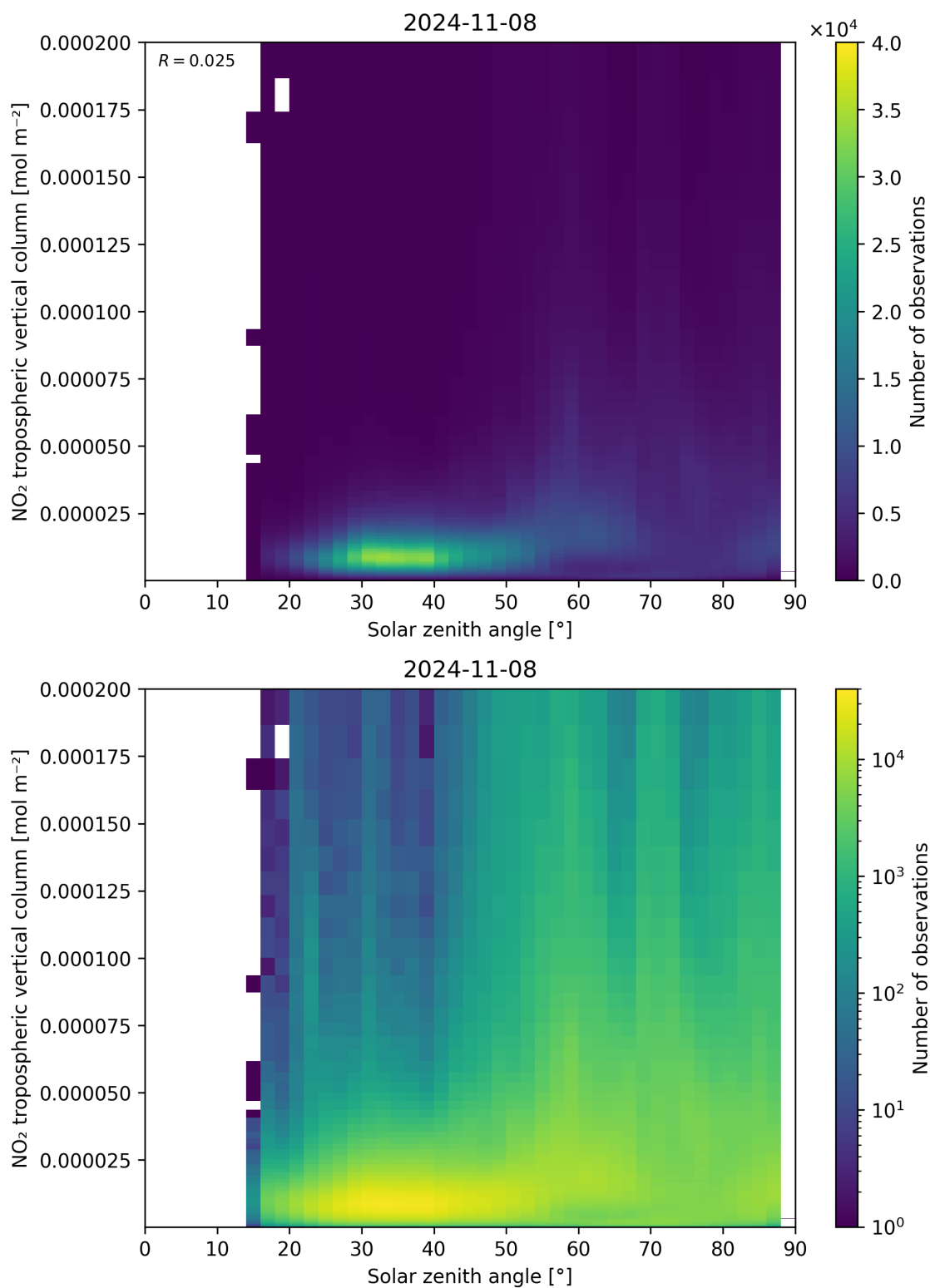
Figure 155: Scatter density plot of “Solar zenith angle” against “NO 2 tropospheric vertical column” for 2024-11-07 to 2024-11-09.
