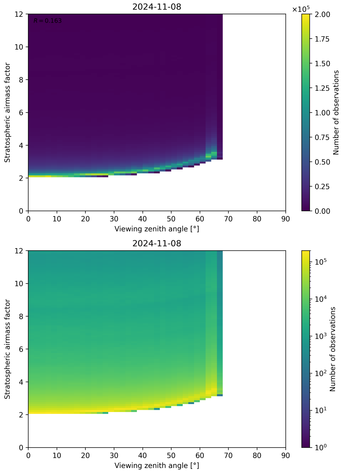
Figure 159: Scatter density plot of “Viewing zenith angle” against “Stratospheric airmass factor” for 2024-11-07 to 2024-11-09.
