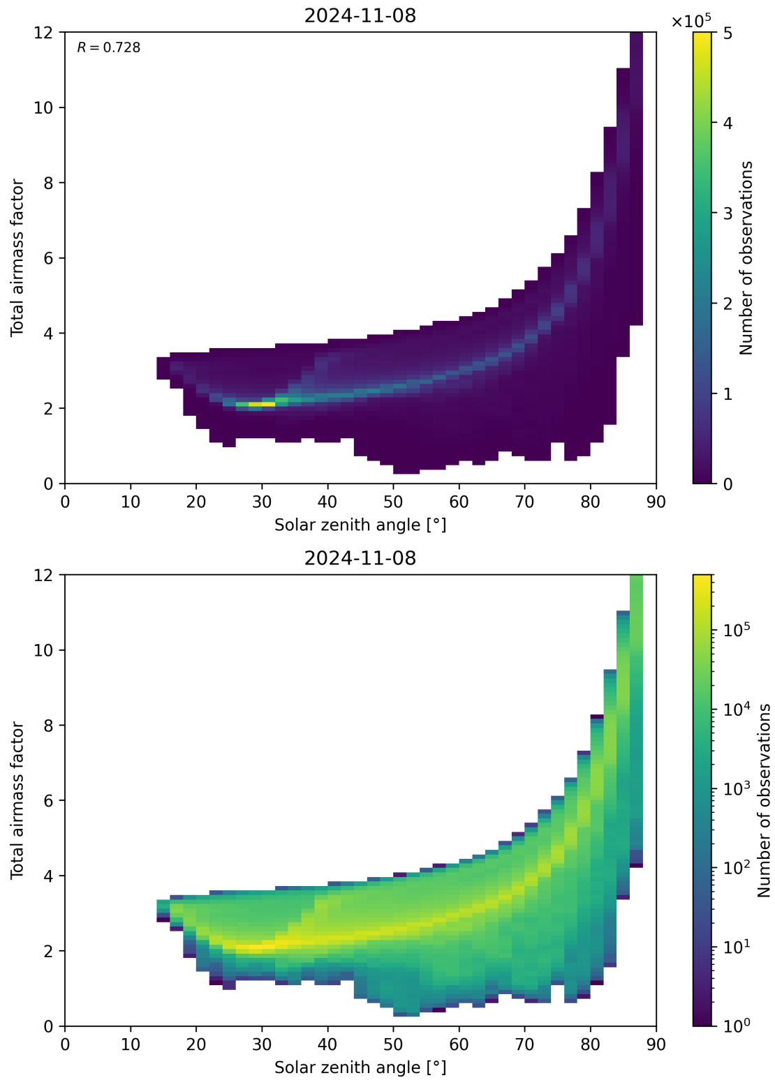
Figure 146: Scatter density plot of “Solar zenith angle” against “Total air mass factor” for 2024-11-07 to 2024-11-09.
