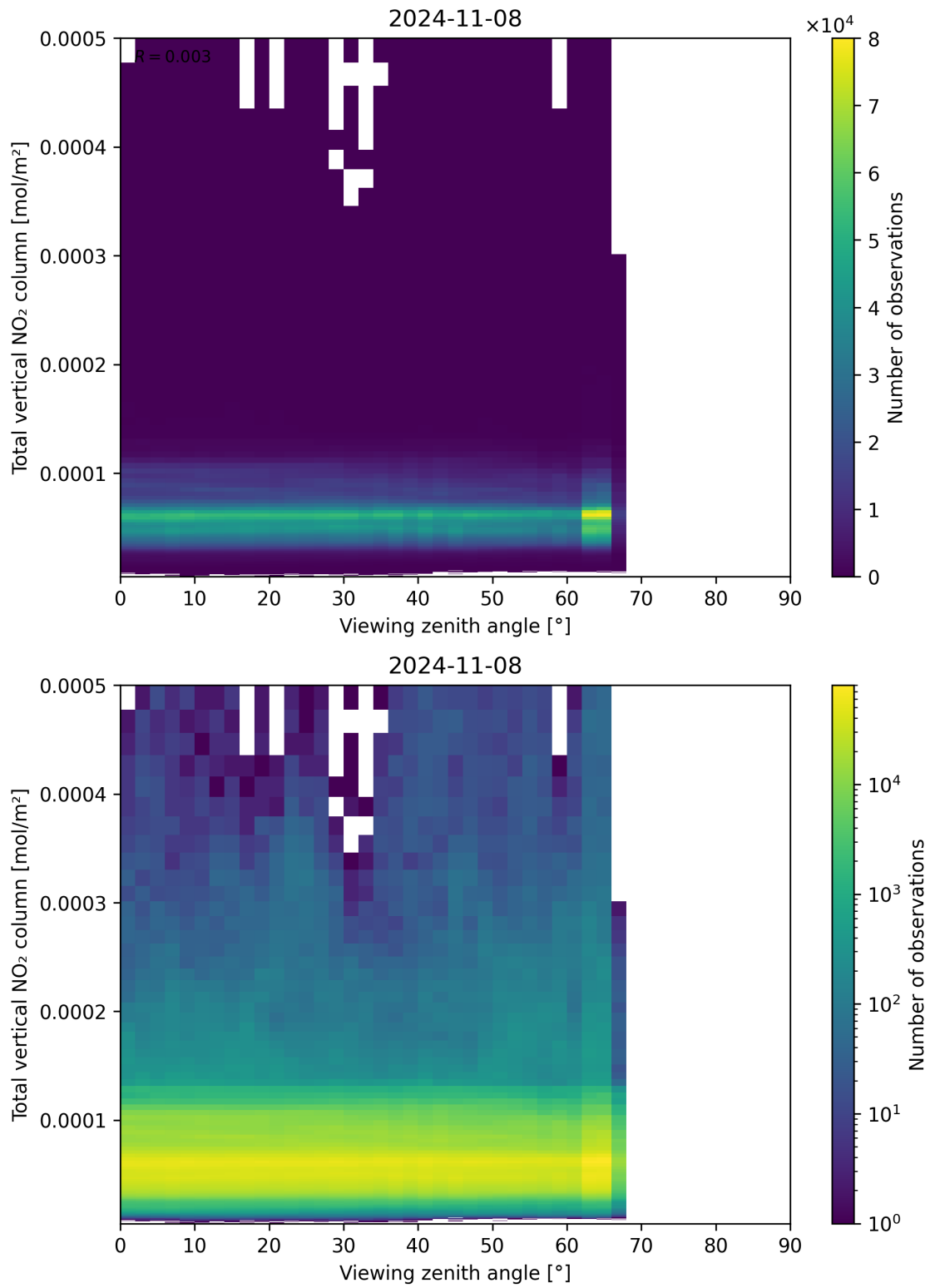
Figure 167: Scatter density plot of “Viewing zenith angle” against “Total vertical NO 2 column” for 2024-11-07 to 2024-11-09.
