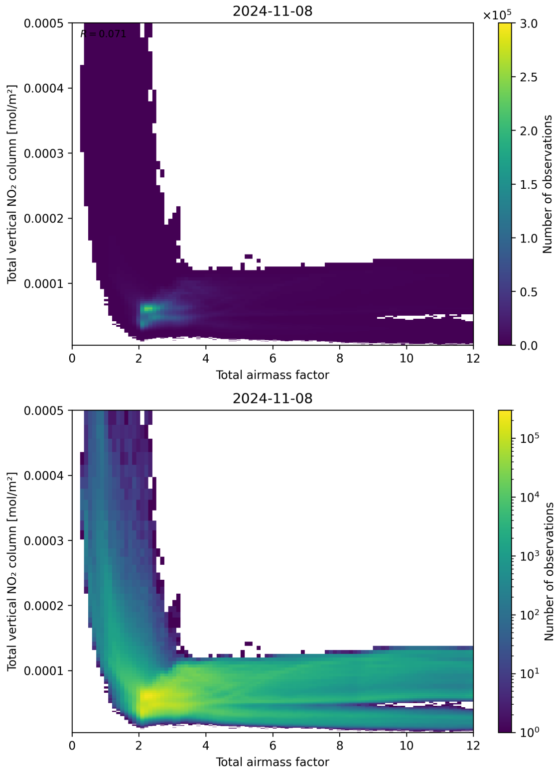
Figure 67: Scatter density plot of “Total airmass factor” against “Total vertical NO 2 column” for 2024-11-07 to 2024-11-09.
