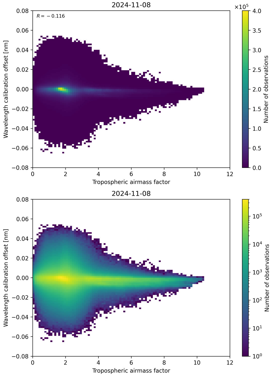
Figure 80: Scatter density plot of “Tropospheric airmass factor” against “Wavelength calibration offset” for 2024-11-07 to 2024-11-09.
