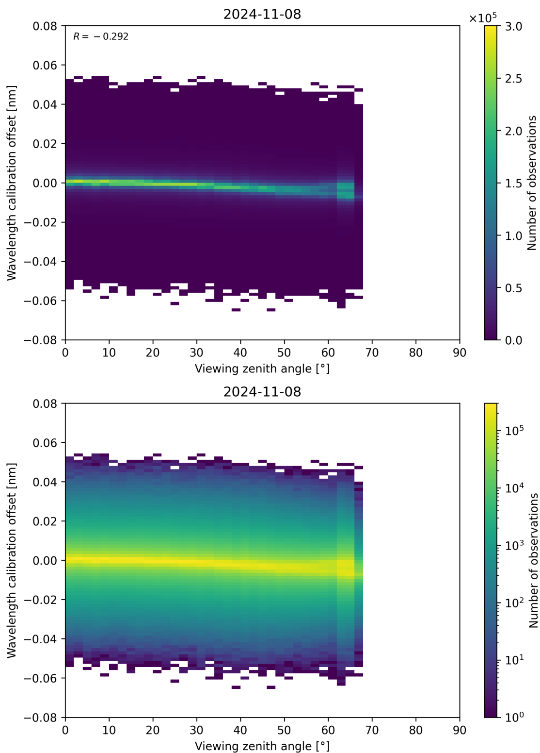
Figure 173: Scatter density plot of “Viewing zenith angle” against “Wavelength calibration offset” for 2024-11-07 to 2024-11-09.
