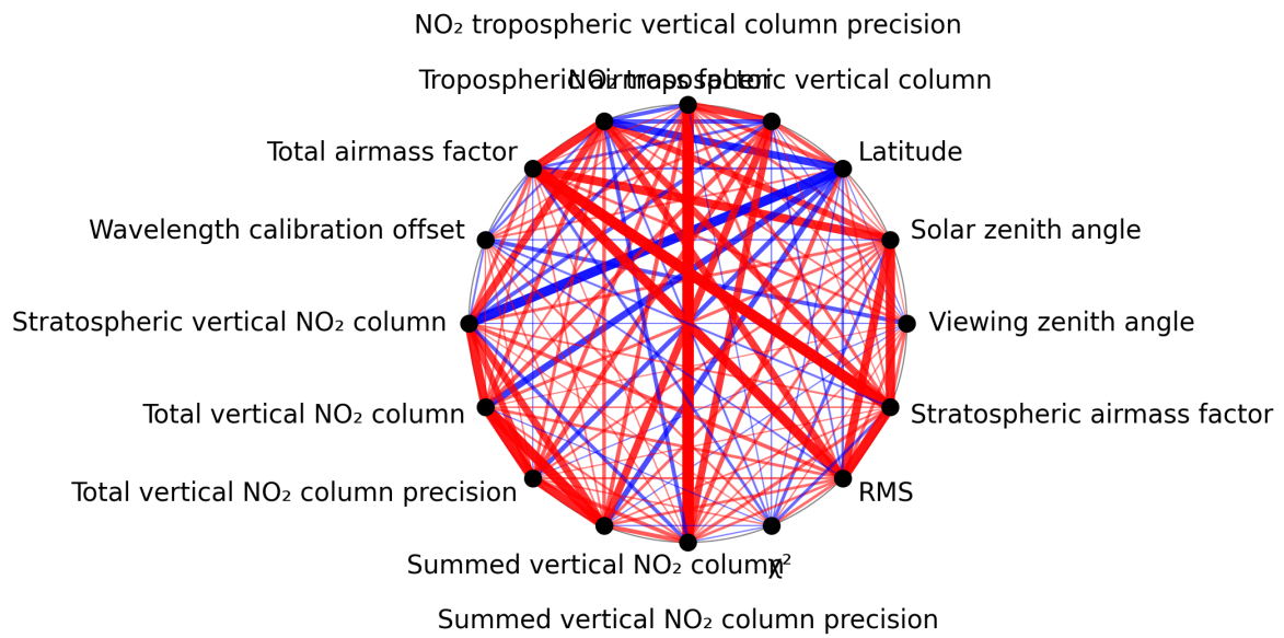
Figure 1: Map of correlation graph for 2024-11-07 to 2024-11-09.
