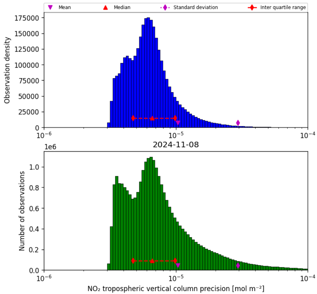
Figure 30: Histogram of “NO 2 tropospheric vertical column precision” for 2024-11-07 to 2024-11-09
