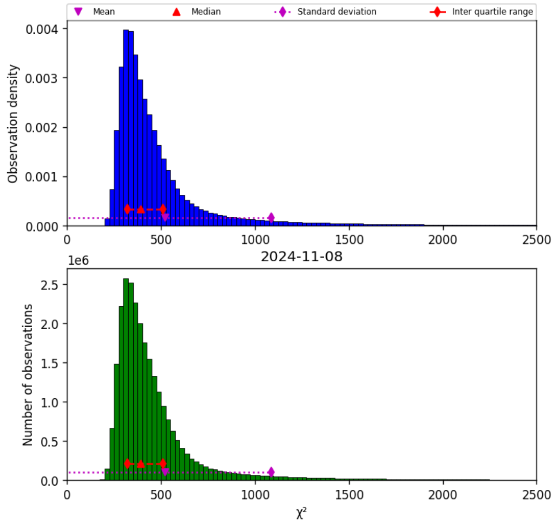
Figure 42: Histogram of “ \chi^2 ” for 2024-11-07 to 2024-11-09
