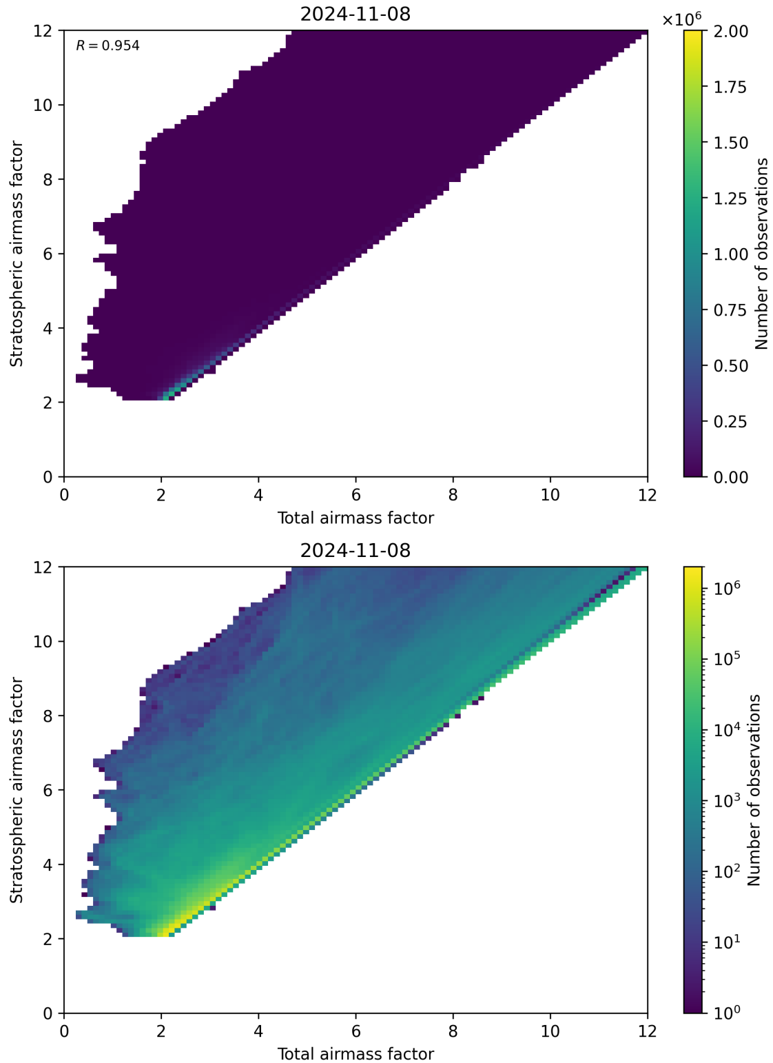
Figure 62: Scatter density plot of “Total airmass factor” against “Stratospheric airmass factor” for 2024-11-07 to 2024-11-09.
