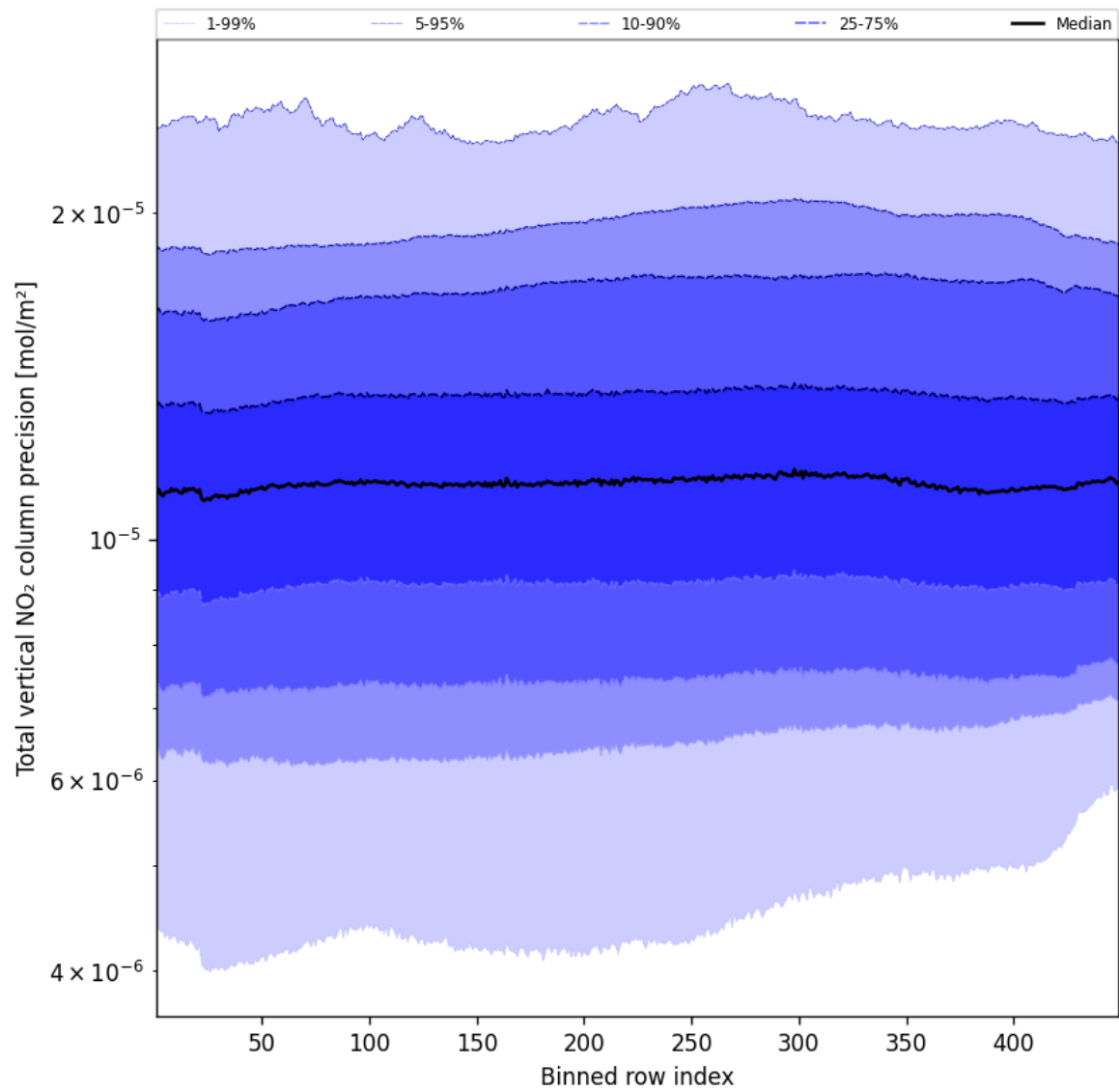
Figure 56: Along track statistics of "Total vertical NO 2 column precision" for 2024-11-07 to 2024-11-09
