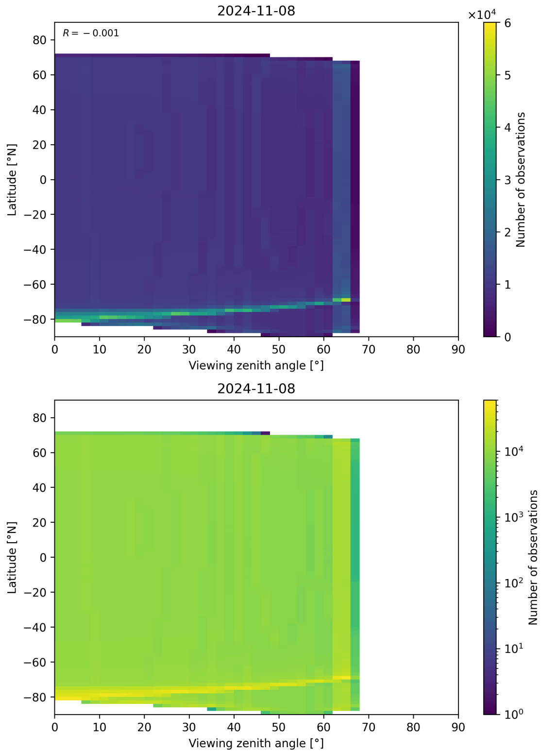
Figure 163: Scatter density plot of “Viewing zenith angle” against “Latitude” for 2024-11-07 to 2024-11-09.
