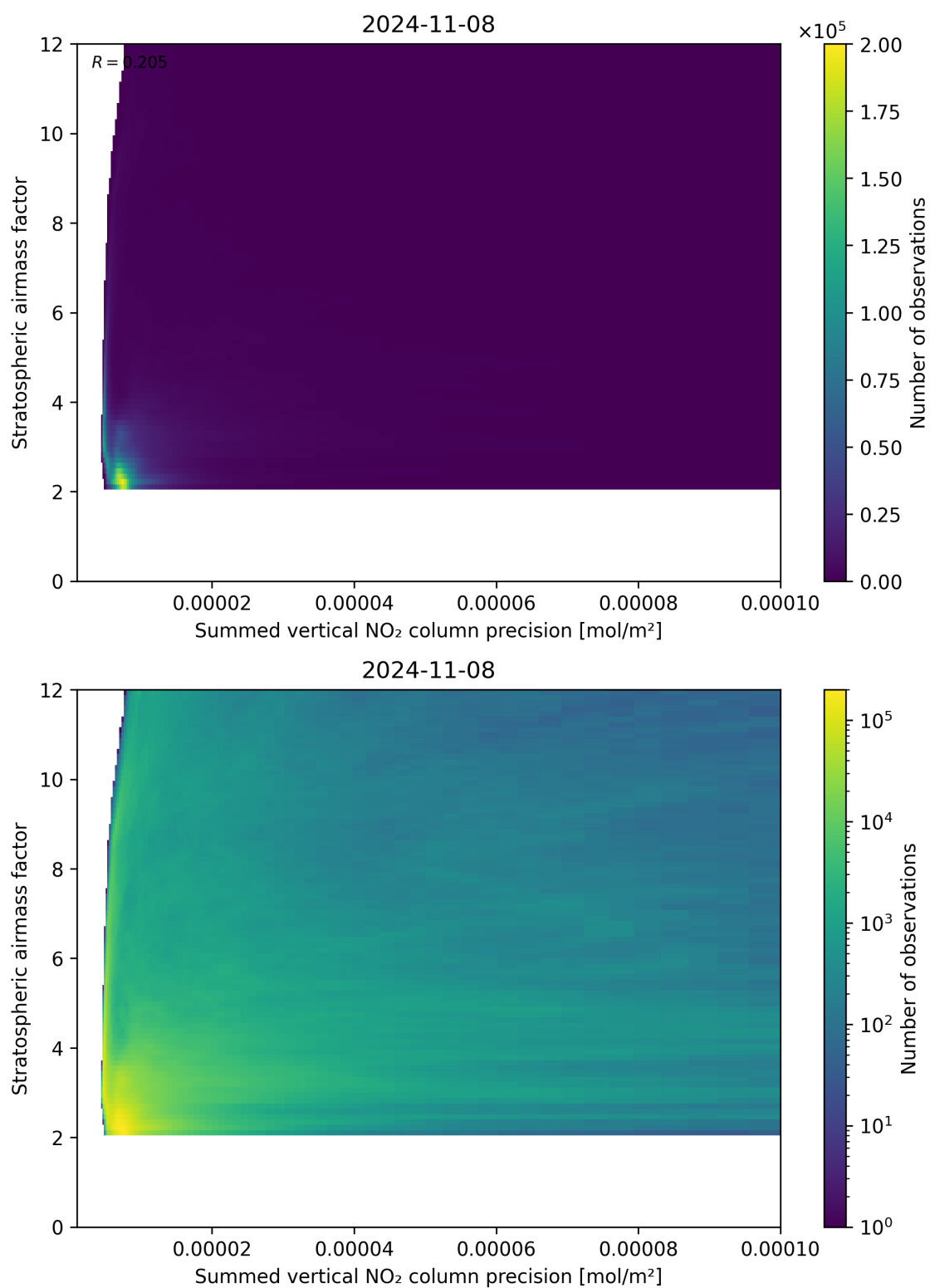
Figure 106: Scatter density plot of “Summed vertical NO 2 column precision” against “Stratospheric airmass factor” for 2024-11-07 to 2024-11-09.
