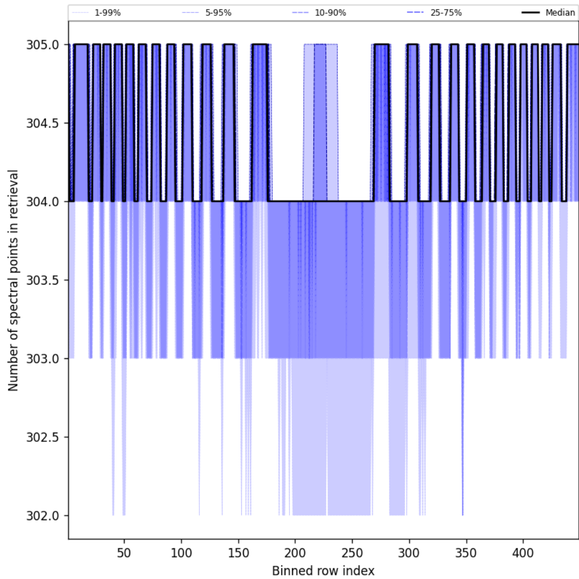
Figure 50: Along track statistics of “Number of spectral points in retrieval” for 2024-11-07 to 2024-11-09
