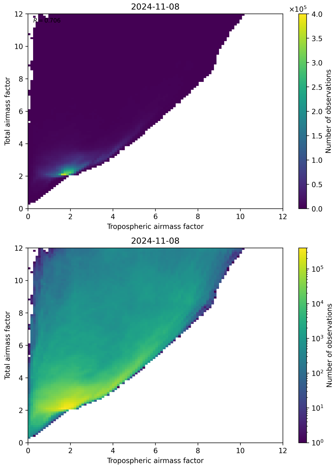
Figure 72: Scatter density plot of “Tropospheric airmass factor” against “Total airmass factor” for 2024-11-07 to 2024-11-09.
