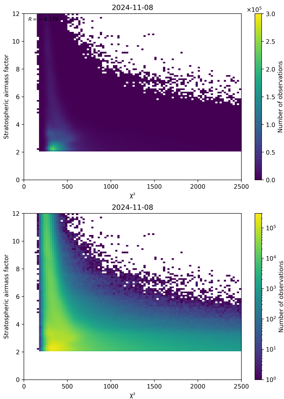
Figure 81: Scatter density plot of “ \chi^2 ” against “Stratospheric airmass factor” for 2024-11-07 to 2024-11-09.
