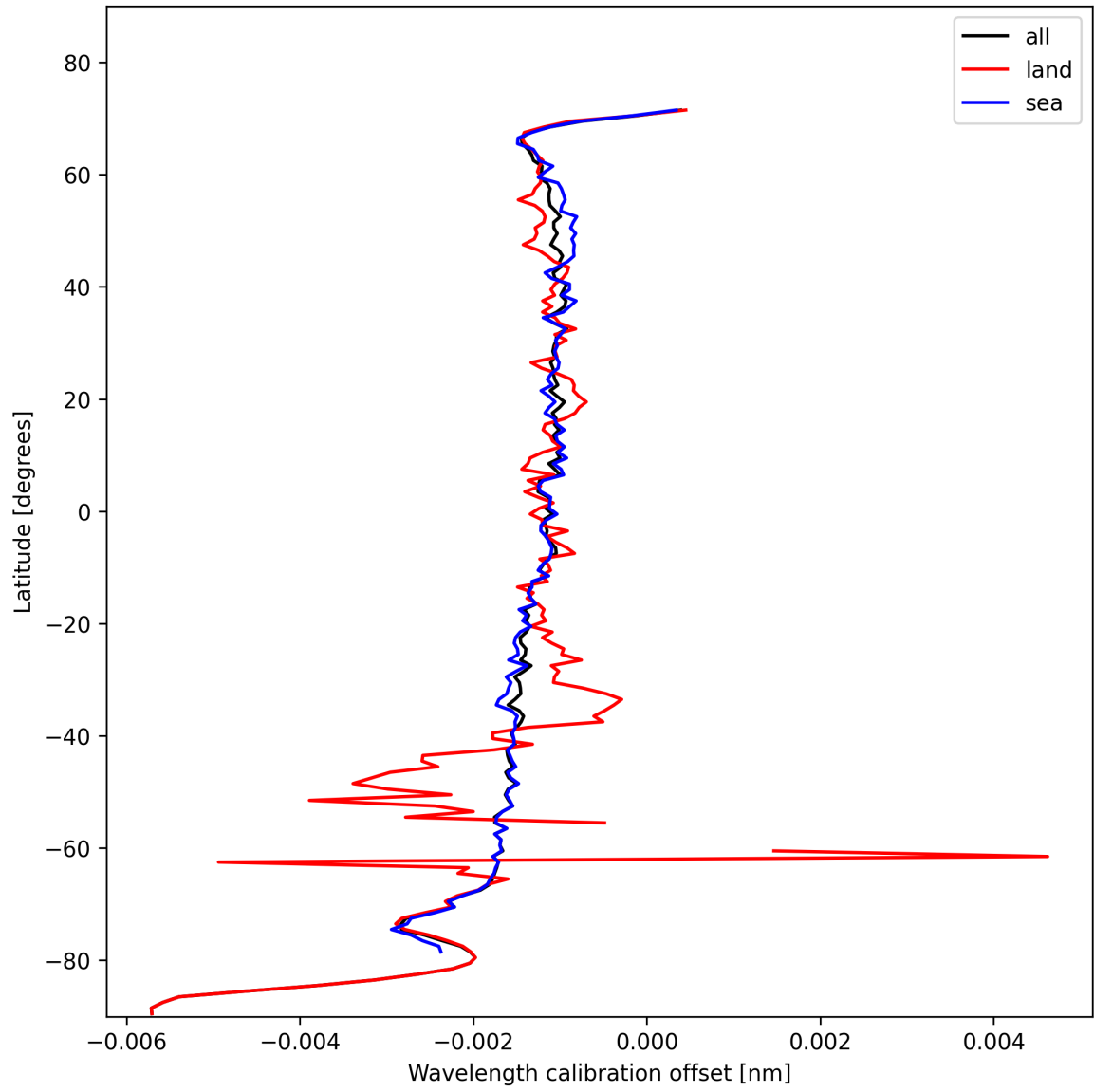
Figure 18: Zonal average of “Wavelength calibration offset” for 2024-11-07 to 2024-11-09.
