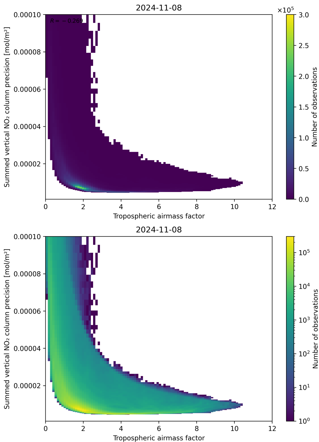
Figure 76: Scatter density plot of “Tropospheric air mass factor” against “Summed vertical NO 2 column precision” for 2024-11-07 to 2024-11-09.
