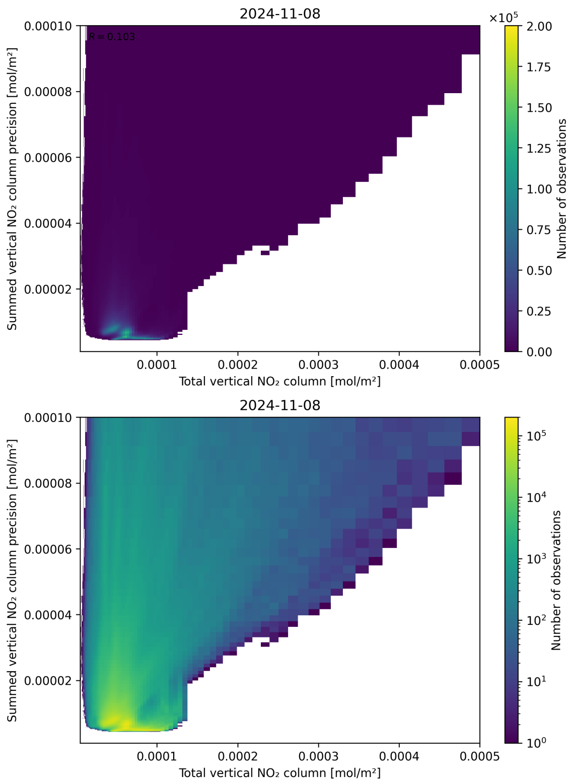
Figure 113: Scatter density plot of “Total vertical NO 2 column” against “Summed vertical NO 2 column precision” for 2024-11-07 to 2024-11-09.
