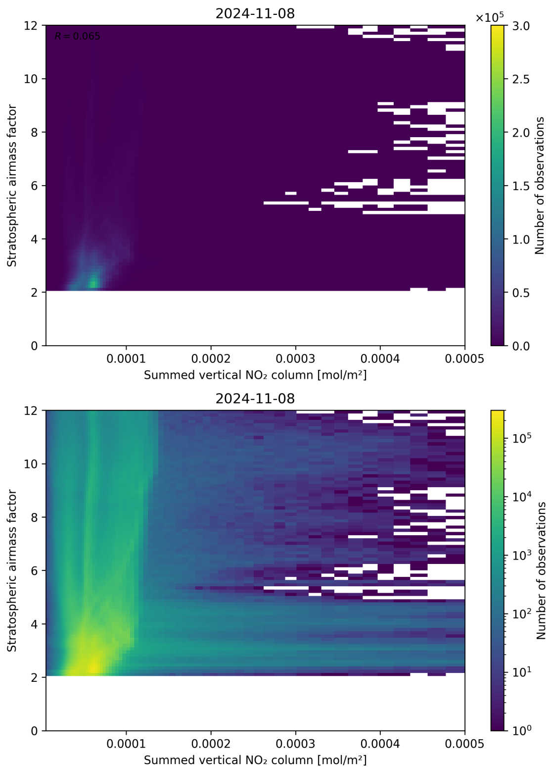
Figure 103: Scatter density plot of “Summed vertical NO 2 column” against “Stratospheric airmass factor” for 2024-11-07 to 2024-11-09.
