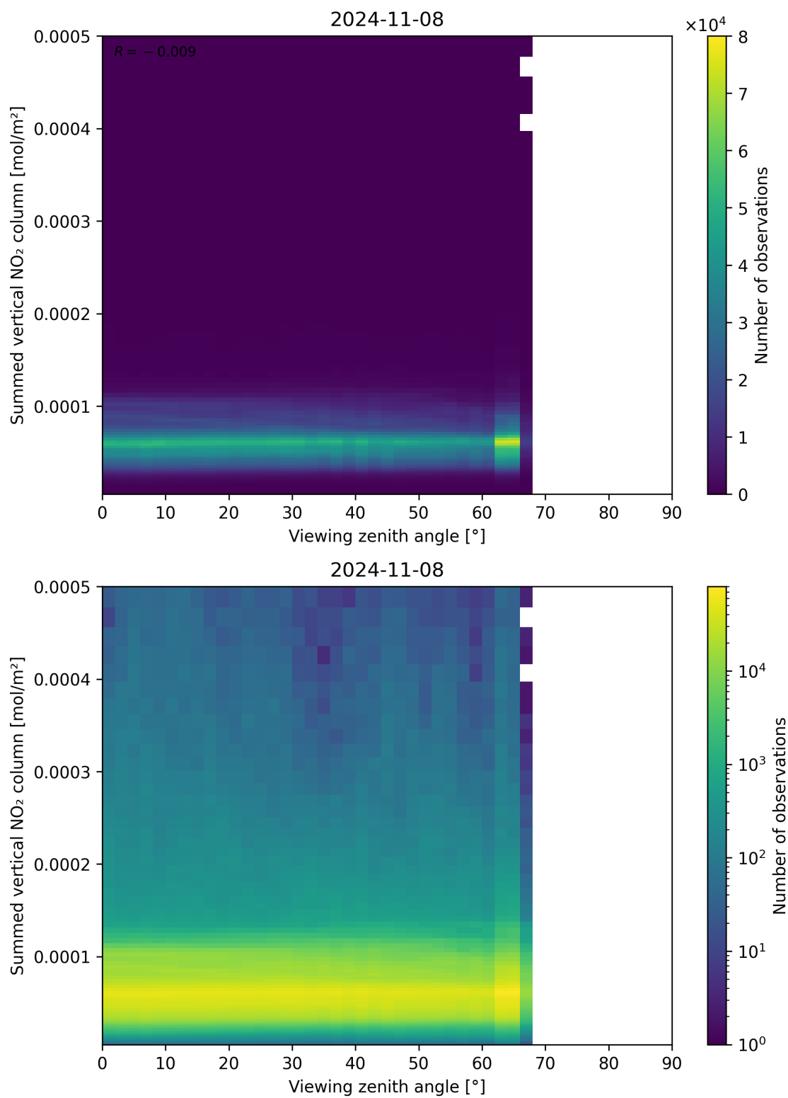
Figure 165: Scatter density plot of “Viewing zenith angle” against “Summed vertical NO 2 column” for 2024-11-07 to 2024-11-09.
