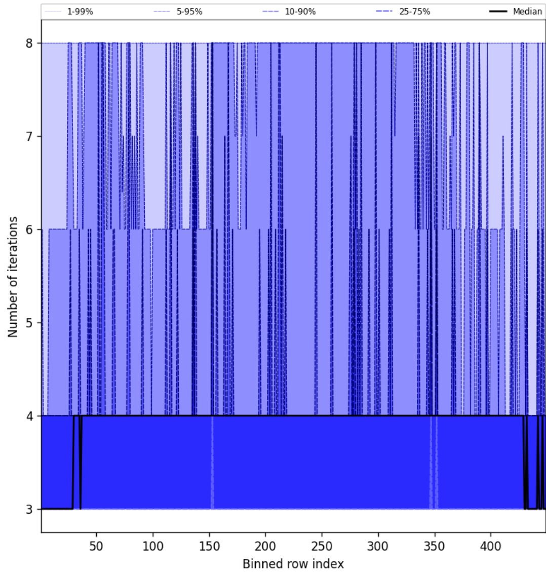
Figure 51: Along track statistics of “Number of iterations” for 2024-11-07 to 2024-11-09
