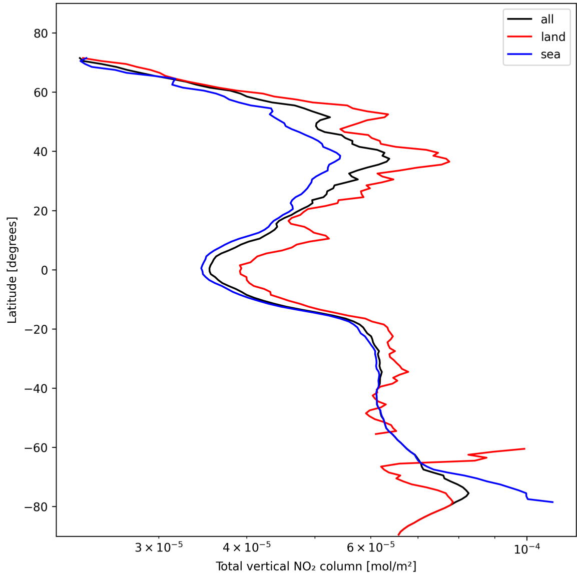
Figure 21: Zonal average of “Total vertical NO 2 column” for 2024-11-07 to 2024-11-09.
