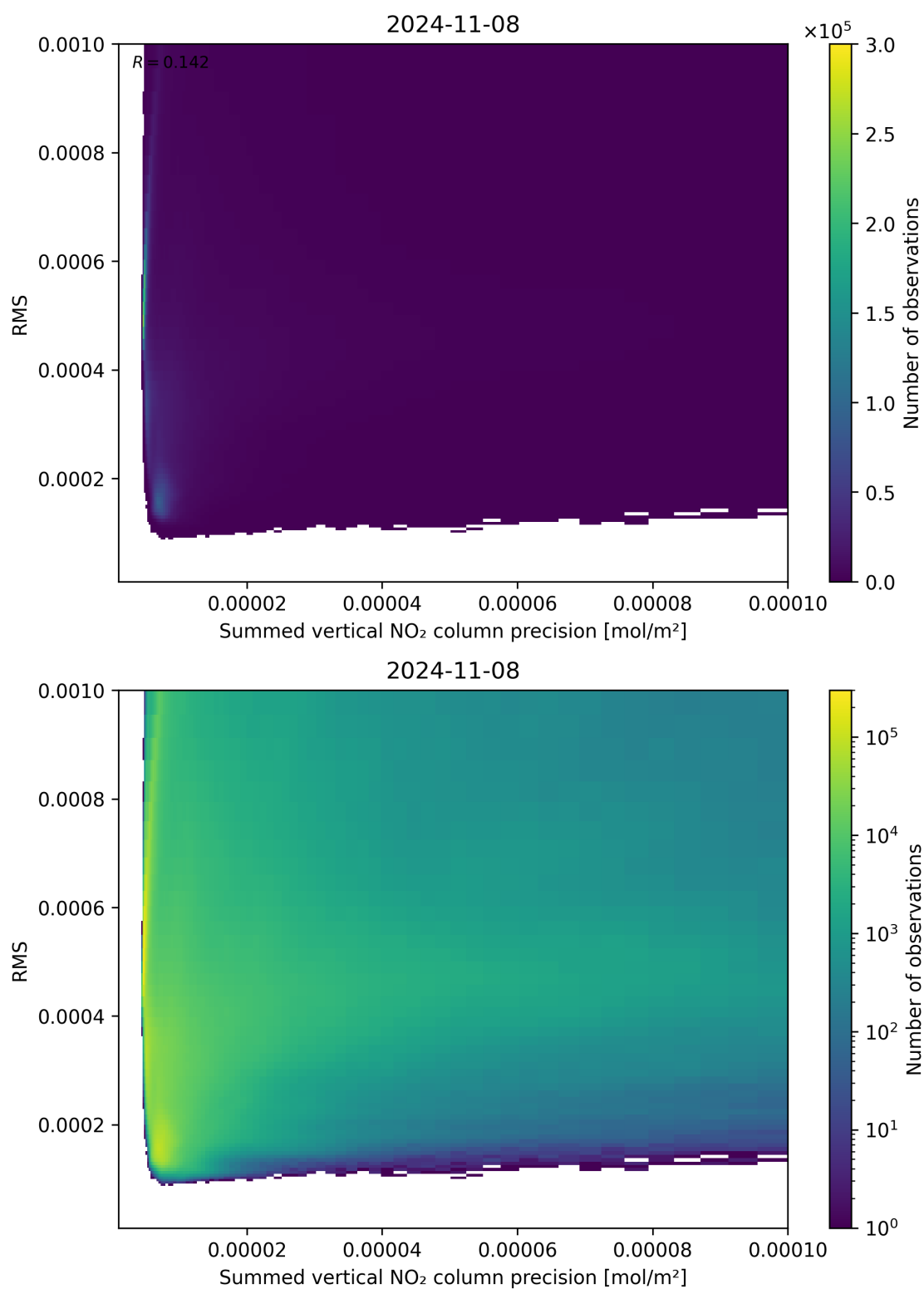
Figure 108: Scatter density plot of “Summed vertical NO 2 column precision” against “RMS” for 2024-11-07 to 2024-11-09.
