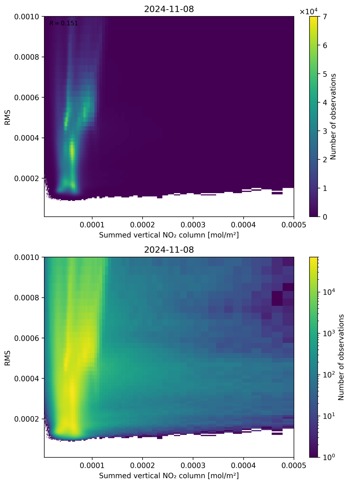
Figure 109: Scatter density plot of “Summed vertical NO 2 column” against “RMS” for 2024-11-07 to 2024-11-09.
