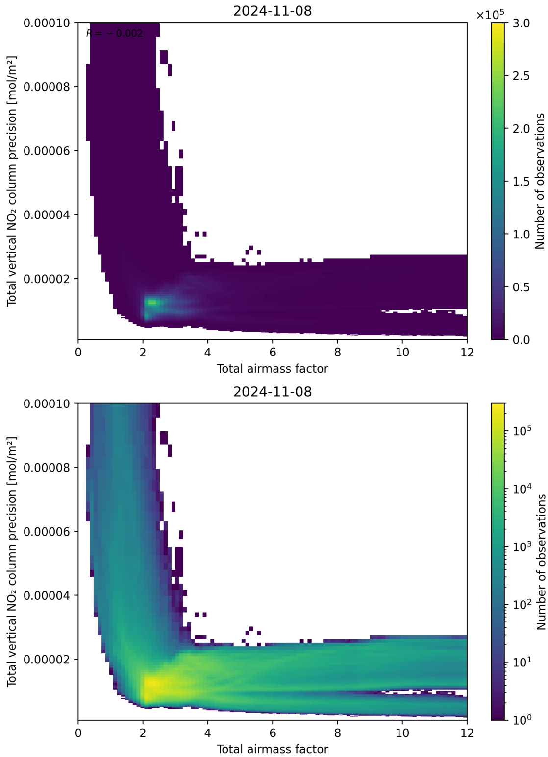
Figure 68: Scatter density plot of “Total airmass factor” against “Total vertical NO 2 column precision” for 2024-11-07 to 2024-11-09.
