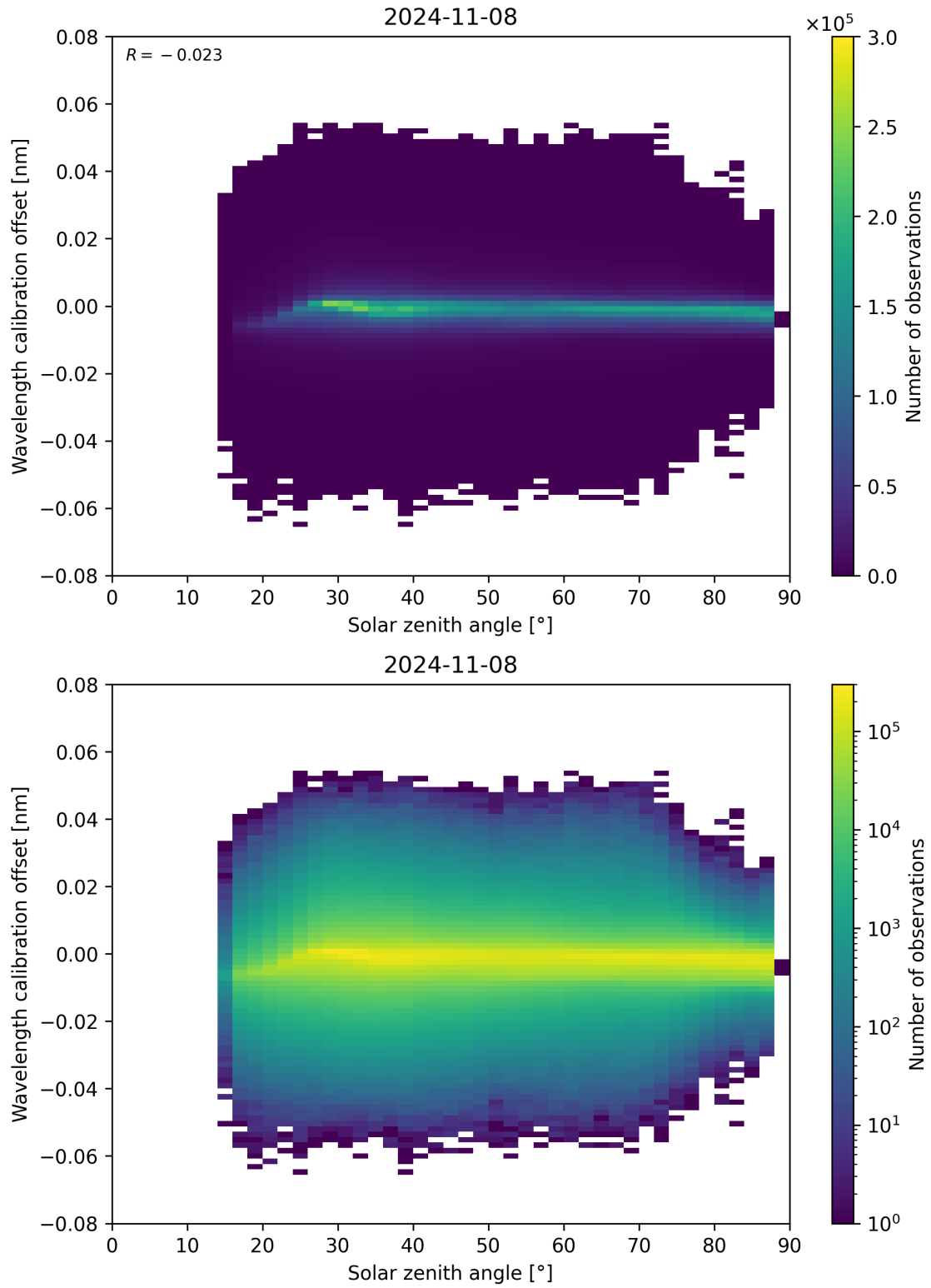
Figure 158: Scatter density plot of “Solar zenith angle” against “Wavelength calibration offset” for 2024-11-07 to 2024-11-09.
