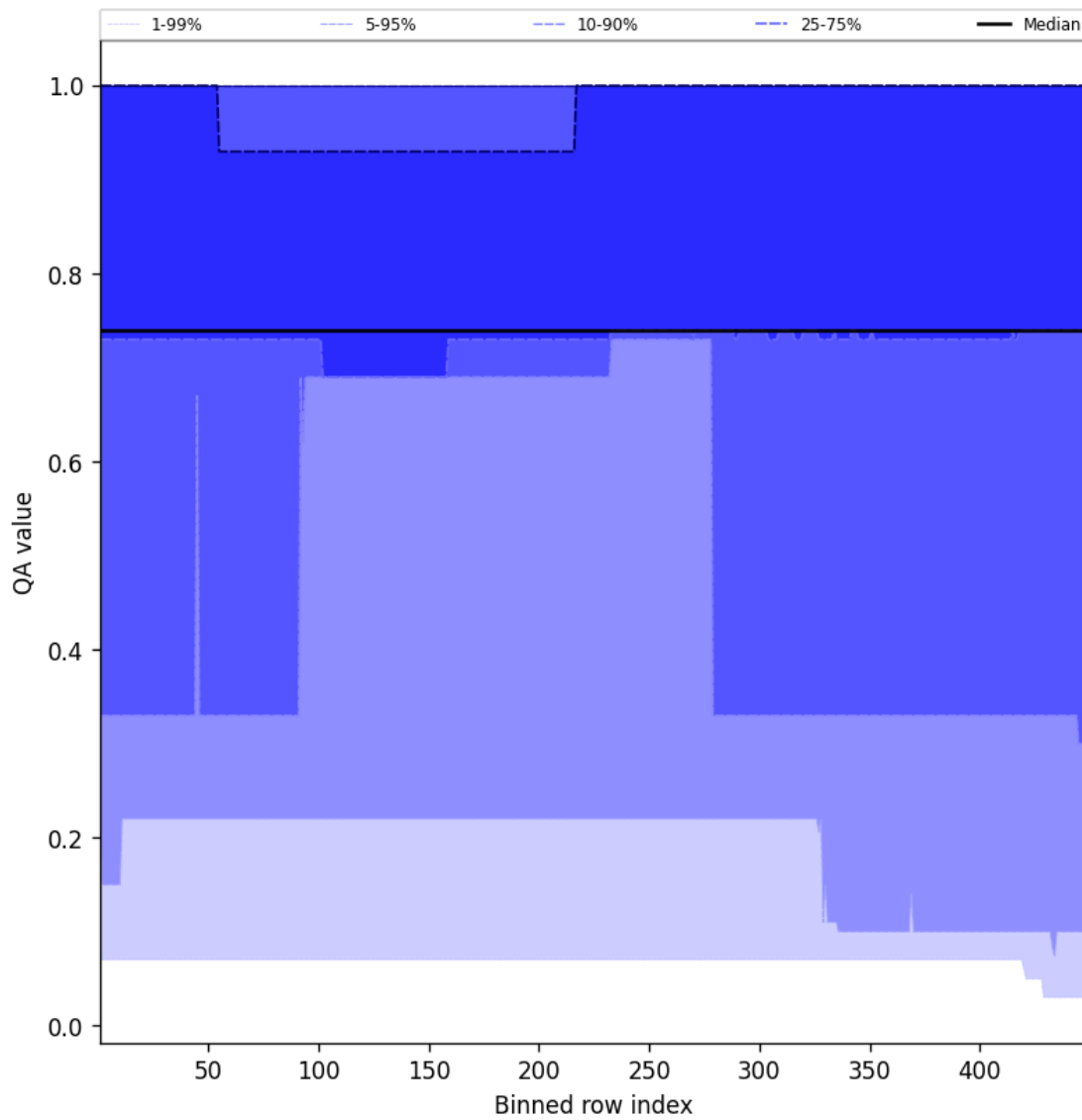
Figure 45: Along track statistics of “QA value” for 2024-11-07 to 2024-11-09
