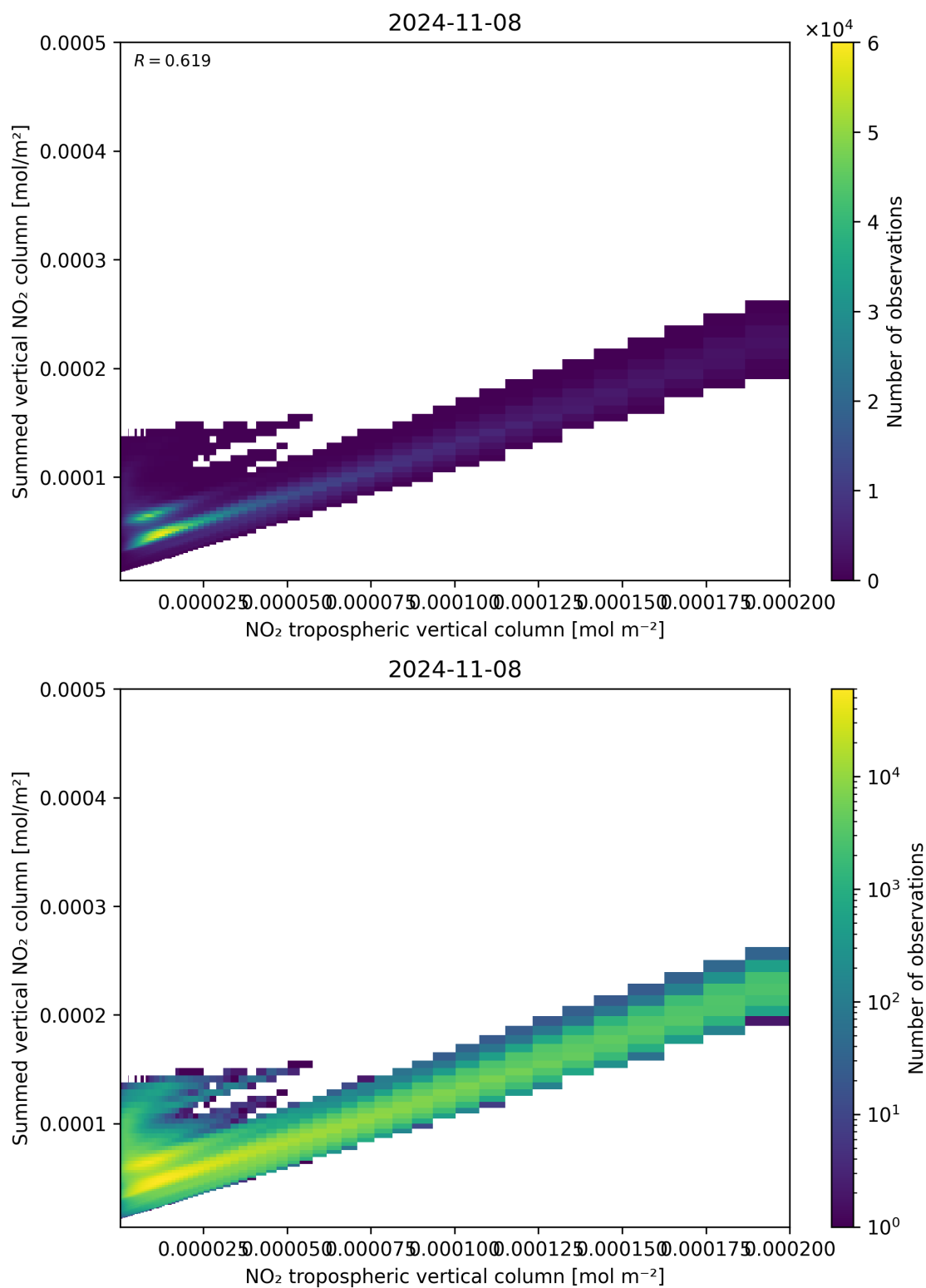
Figure 126: Scatter density plot of “NO 2 tropospheric vertical column” against “Summed vertical NO 2 column” for 2024-11-07 to 2024-11-09.
