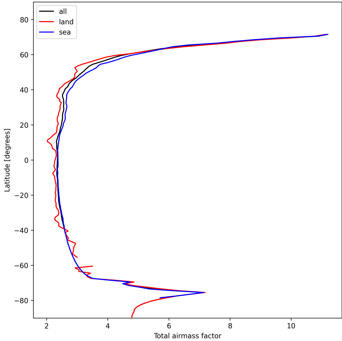
Figure 15: Zonal average of “Total airmass factor” for 2024-11-07 to 2024-11-09.
