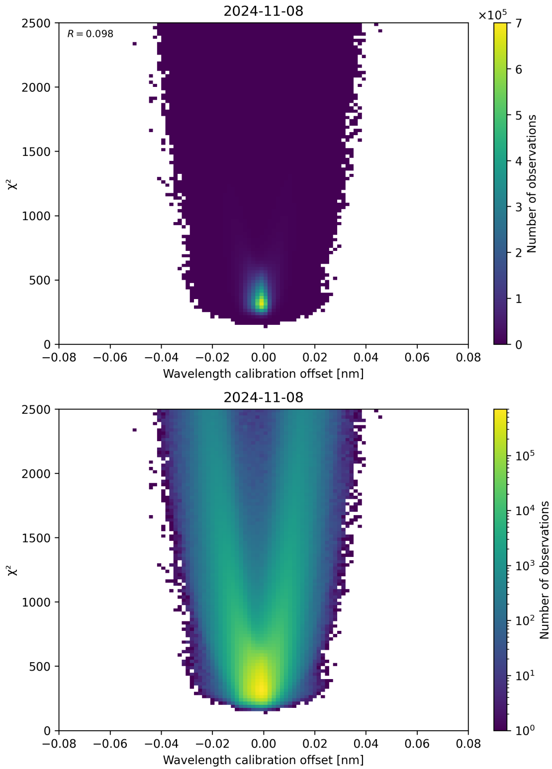
Figure 175: Scatter density plot of “Wavelength calibration offset” against “ \chi^2 ” for 2024-11-07 to 2024-11-09.
