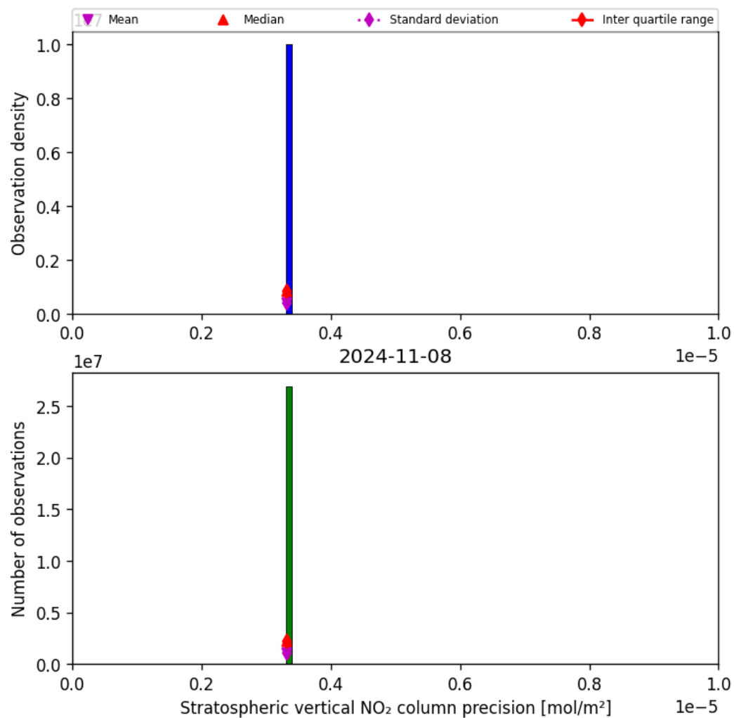
Figure 37: Histogram of “Stratospheric vertical NO 2 column precision” for 2024-11-07 to 2024-11-09
