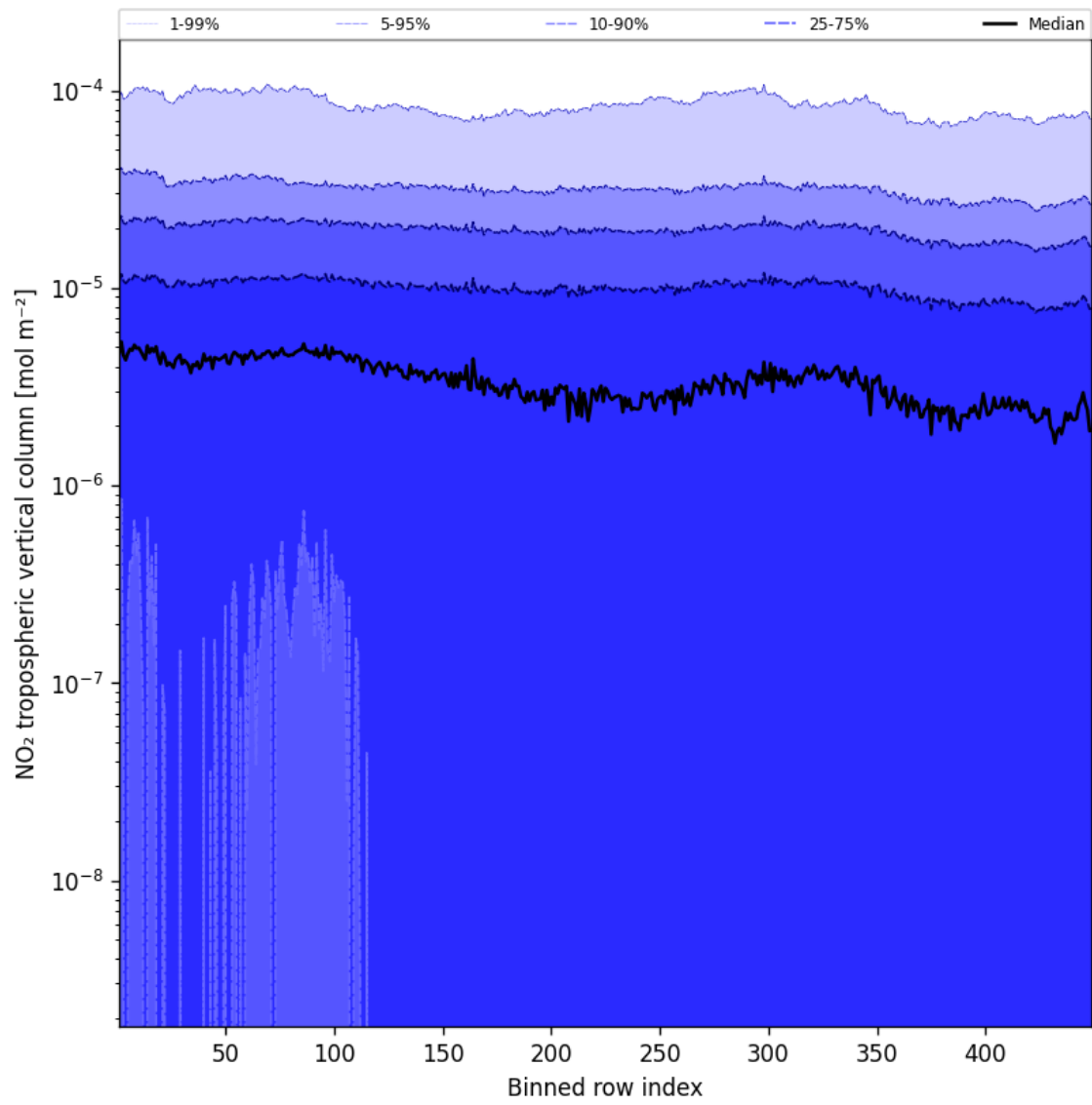
Figure 46: Along track statistics of “NO 2 tropospheric vertical column” for 2024-11-07 to 2024-11-09
