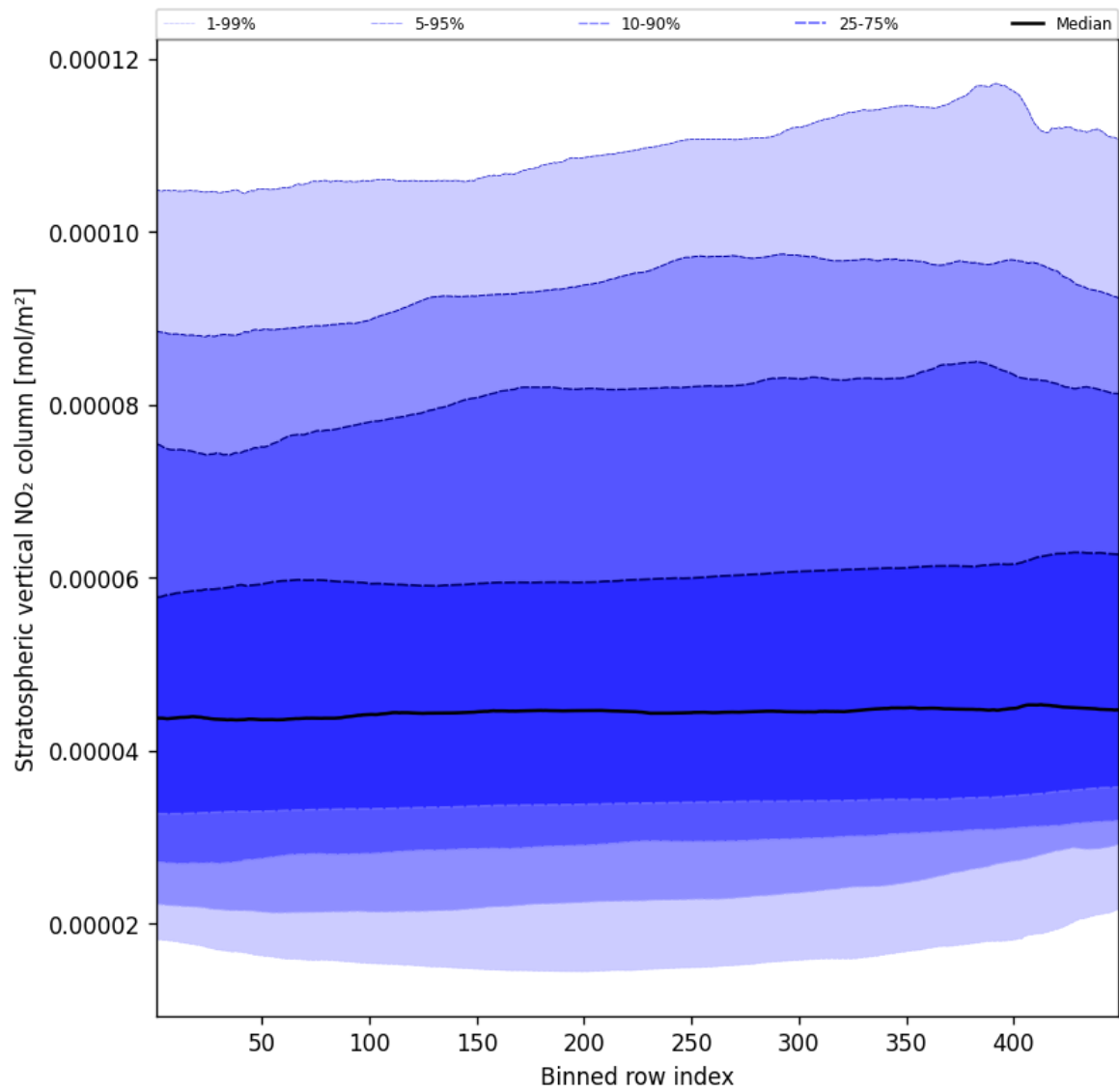
Figure 53: Along track statistics of “Stratospheric vertical NO 2 column” for 2024-11-07 to 2024-11-09
