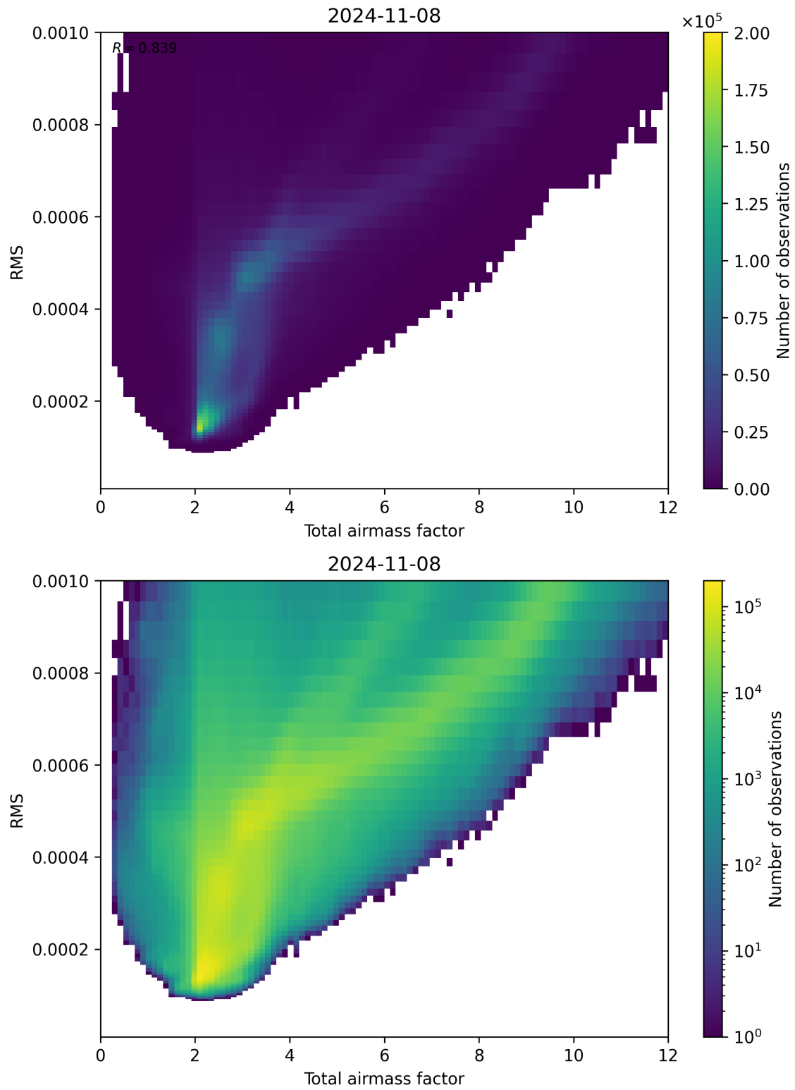
Figure 69: Scatter density plot of “Total airmass factor” against “RMS” for 2024-11-07 to 2024-11-09.
