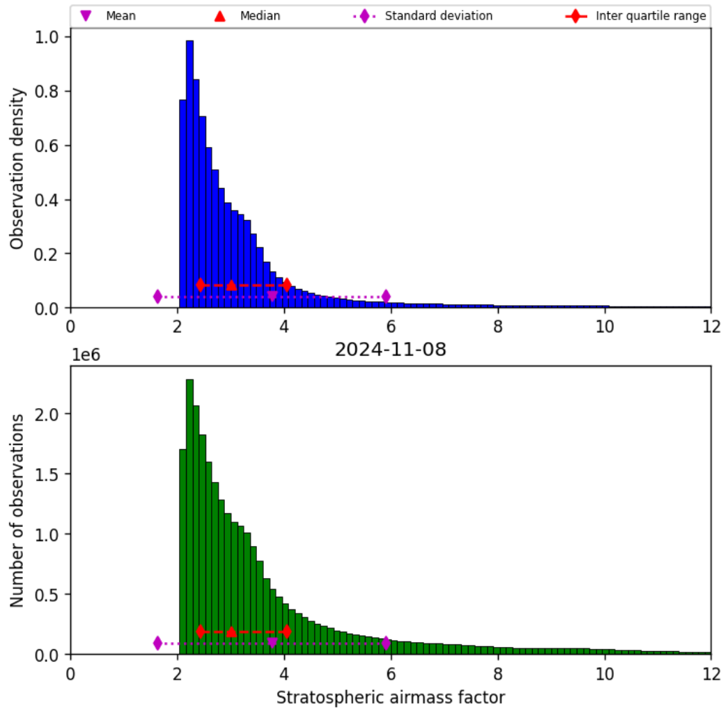
Figure 44: Histogram of “Stratospheric airmass factor” for 2024-11-07 to 2024-11-09
