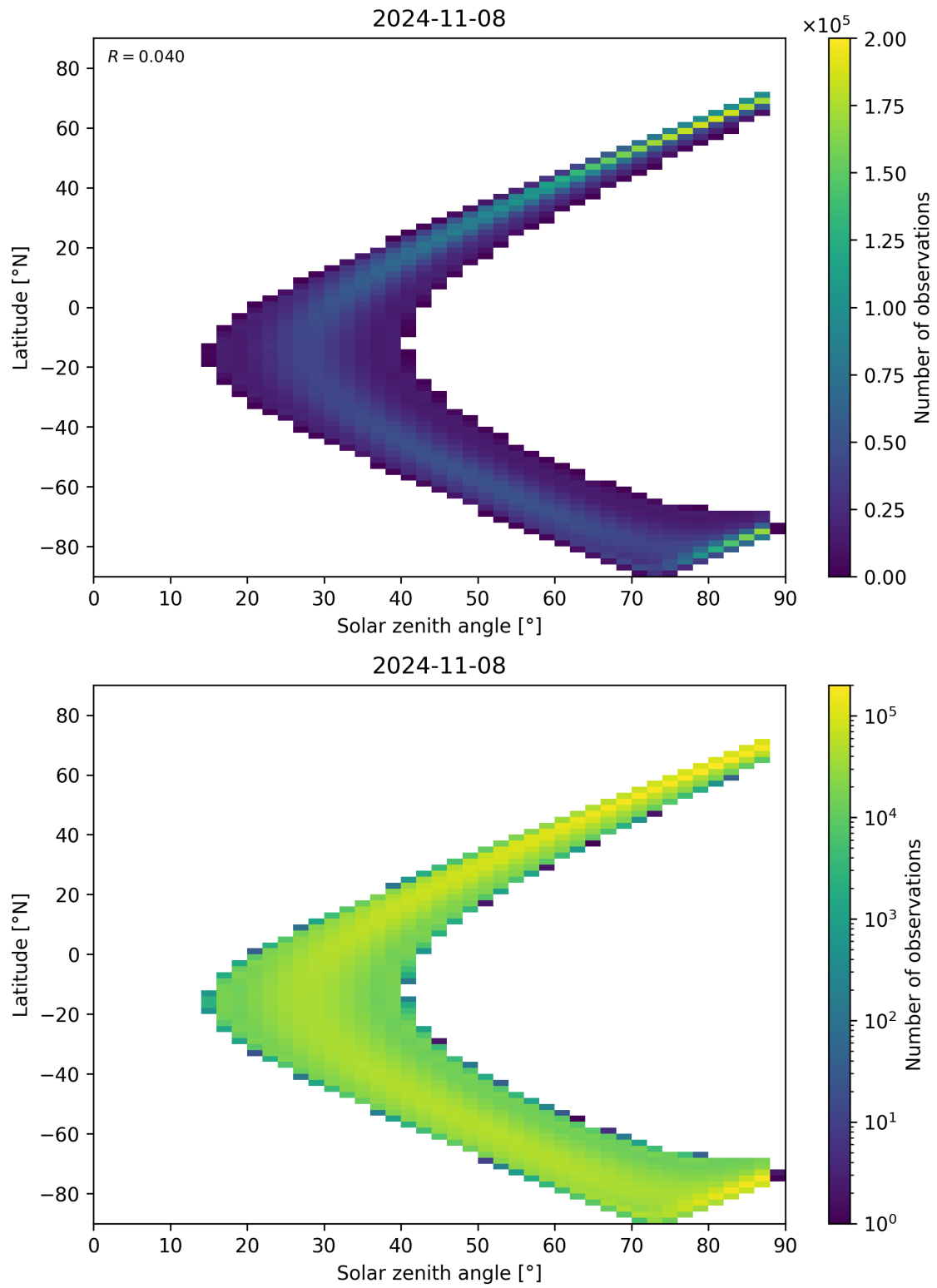
Figure 149: Scatter density plot of “Solar zenith angle” against “Latitude” for 2024-11-07 to 2024-11-09.
