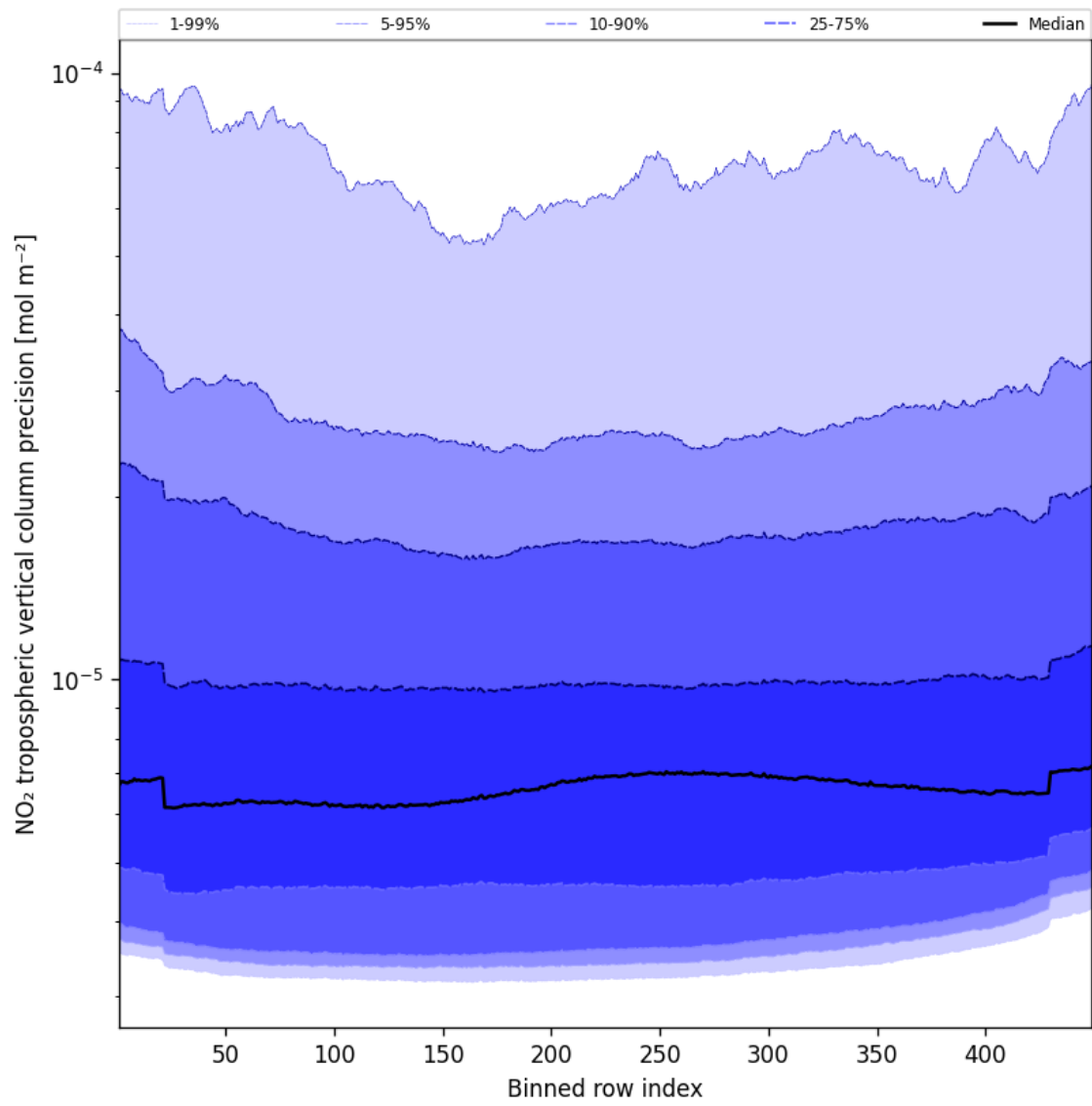
Figure 47: Along track statistics of “NO 2 tropospheric vertical column precision” for 2024-11-07 to 2024-11-09
