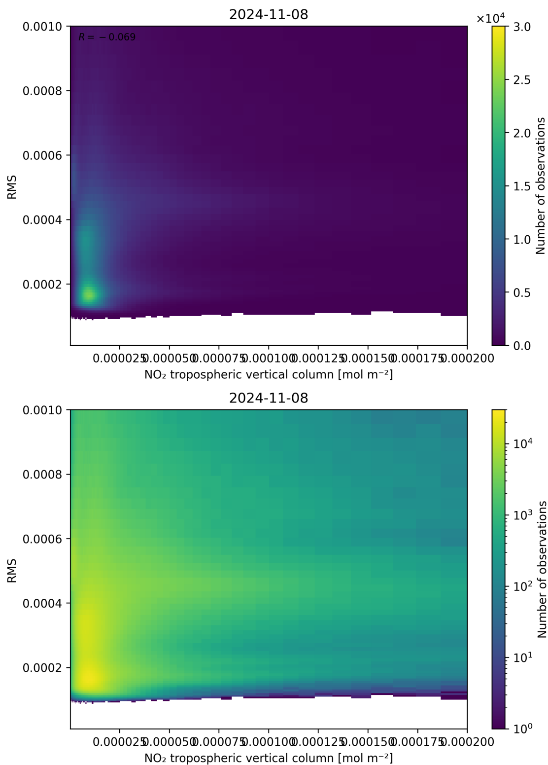
Figure 142: Scatter density plot of “NO 2 tropospheric vertical column” against “RMS” for 2024-11-07 to 2024-11-09.
