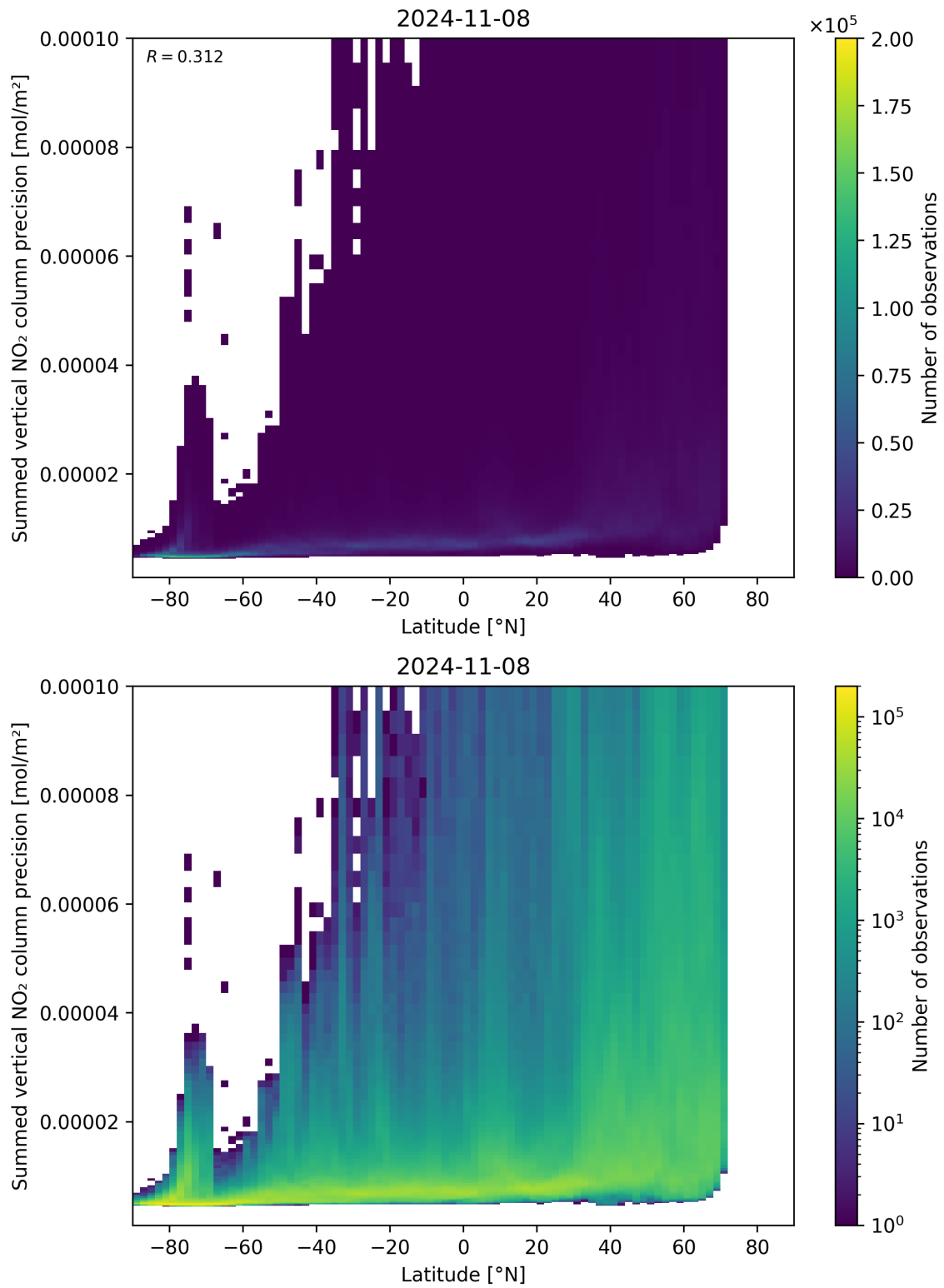
Figure 89: Scatter density plot of “Latitude” against “Summed vertical NO 2 column precision” for 2024-11-07 to 2024-11-09.
