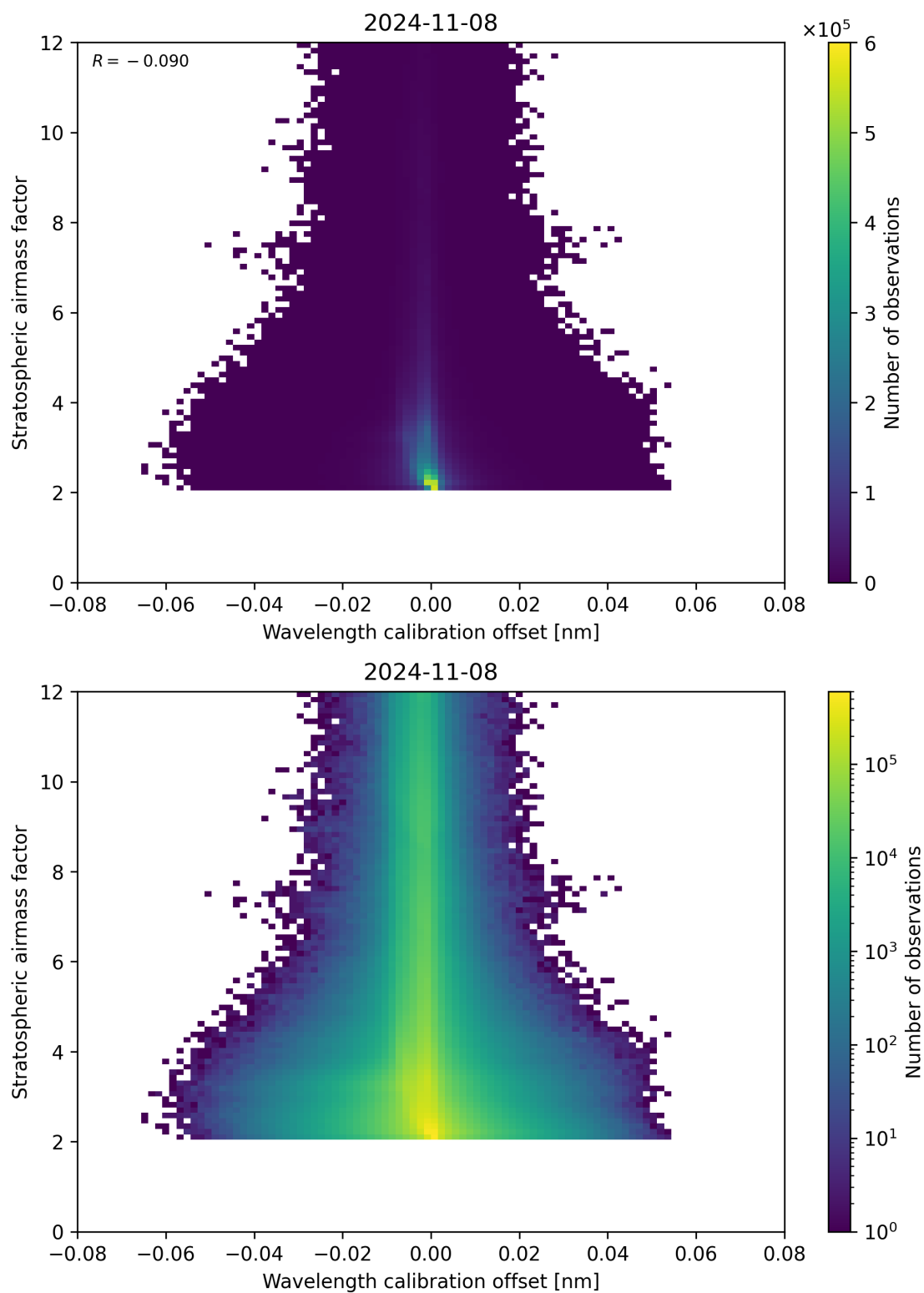
Figure 174: Scatter density plot of “Wavelength calibration offset” against “Stratospheric airmass factor” for 2024-11-07 to 2024-11-09.
