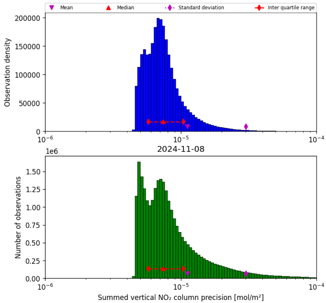
Figure 41: Histogram of “Summed vertical NO 2 column precision” for 2024-11-07 to 2024-11-09
