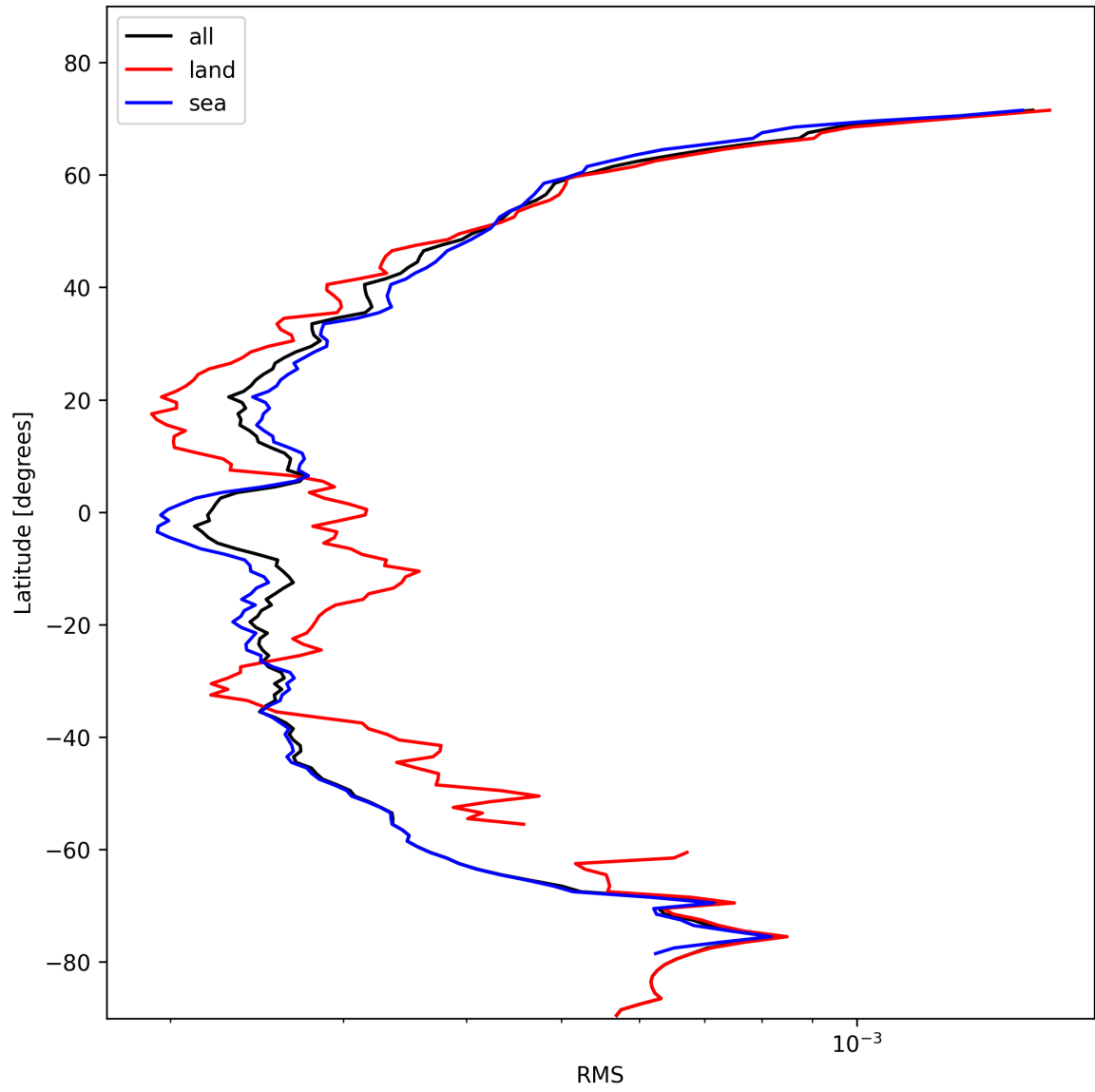
Figure 26: Zonal average of “RMS” for 2024-11-07 to 2024-11-09.
