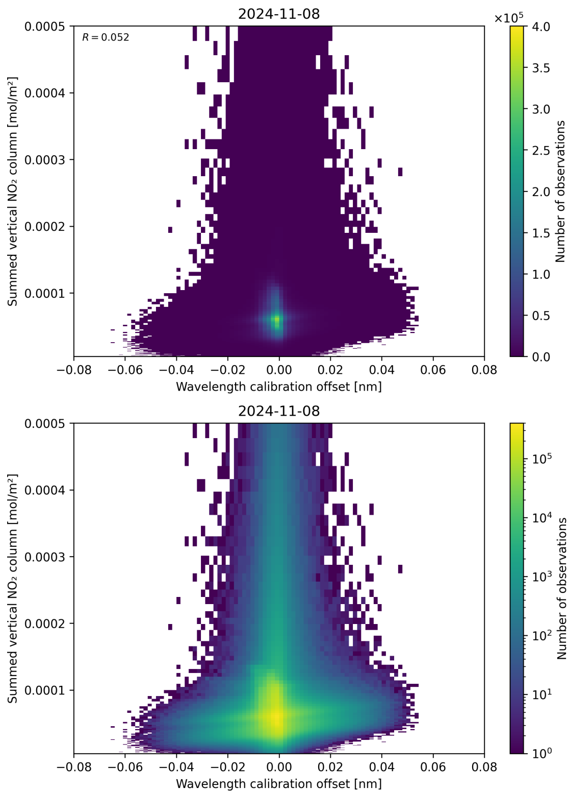
Figure 177: Scatter density plot of “Wavelength calibration offset” against “Summed vertical NO 2 column” for 2024-11-07 to 2024-11-09.
