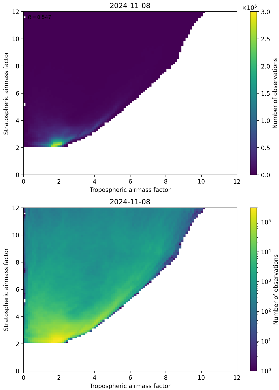
Figure 71: Scatter density plot of “Tropospheric airmass factor” against “Stratospheric airmass factor” for 2024-11-07 to 2024-11-09.
