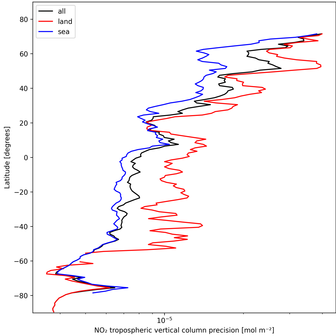
Figure 13: Zonal average of “NO 2 tropospheric vertical column precision” for 2024-11-07 to 2024-11-09.
