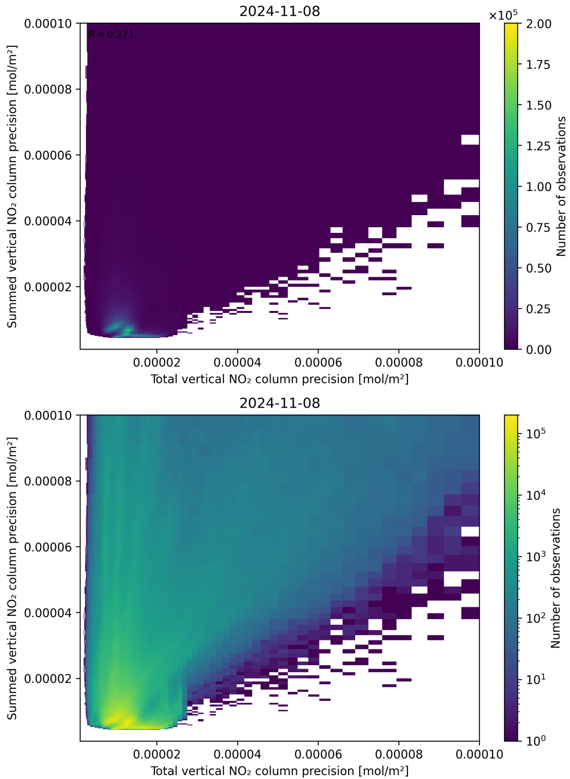
Figure 118: Scatter density plot of “Total vertical NO 2 column precision” against “Summed vertical NO 2 column precision” for 2024-11-07 to 2024-11-09.
