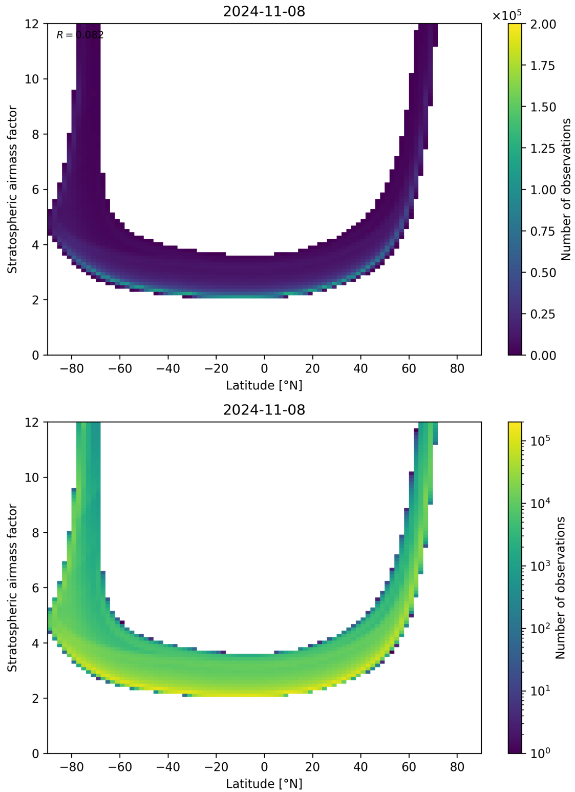
Figure 83: Scatter density plot of “Latitude” against “Stratospheric air mass factor” for 2024-11-07 to 2024-11-09.
