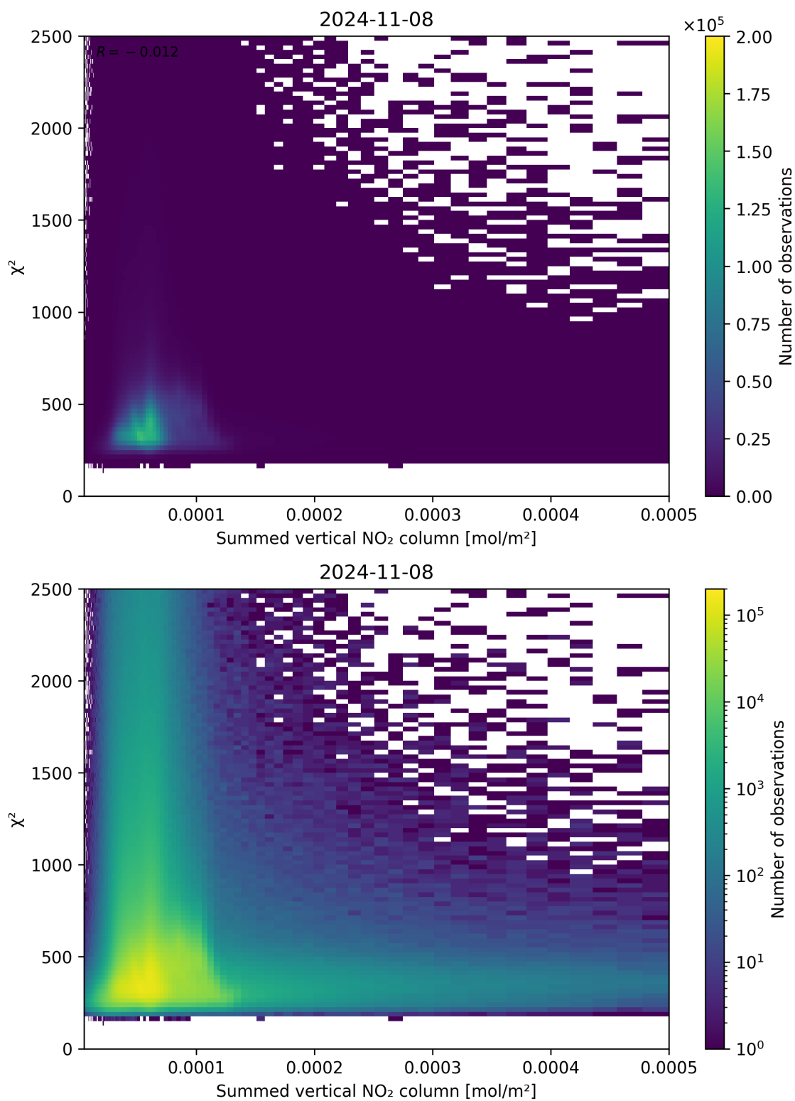
Figure 104: Scatter density plot of “Summed vertical NO 2 column” against “ \chi^2 ” for 2024-11-07 to 2024-11-09.
