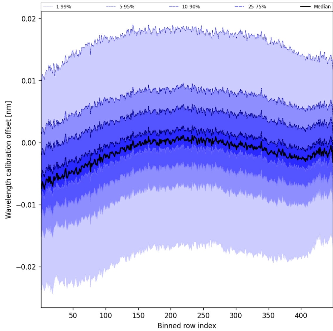
Figure 52: Along track statistics of “Wavelength calibration offset” for 2024-11-07 to 2024-11-09
