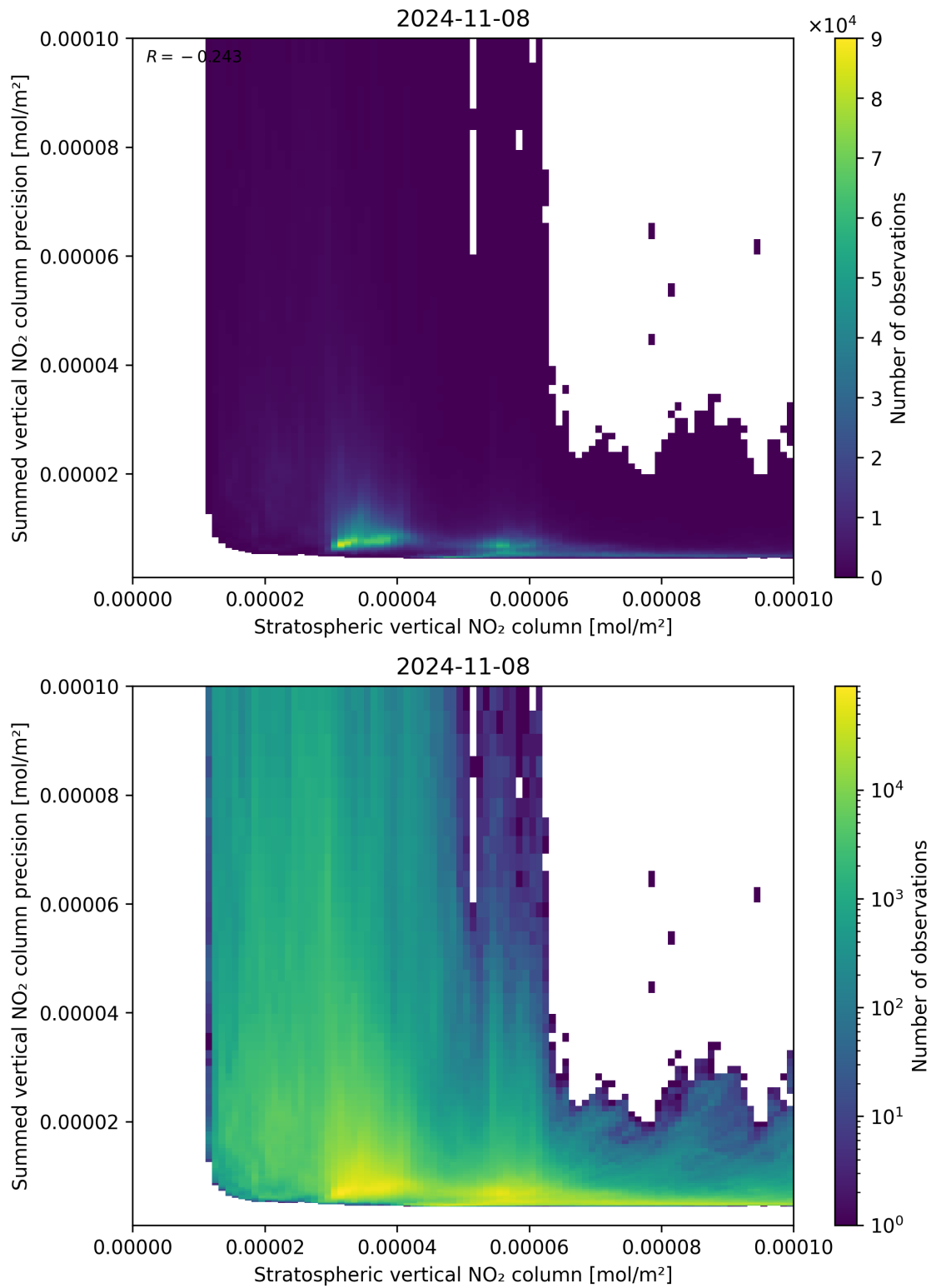
Figure 99: Scatter density plot of “Stratospheric vertical NO 2 column” against “Summed vertical NO 2 column precision” for 2024-11-07 to 2024-11-09.
