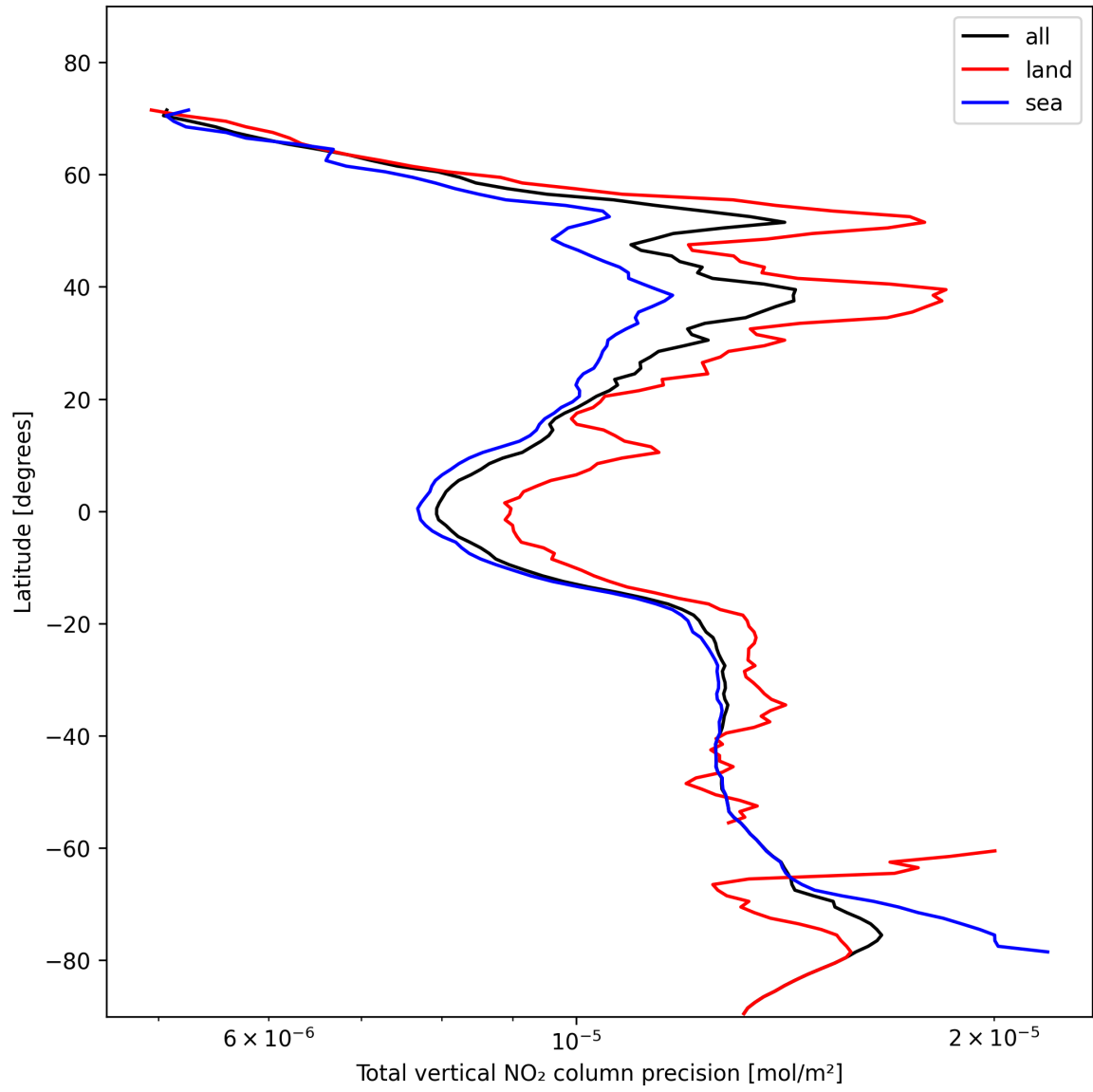
Figure 22: Zonal average of “Total vertical NO 2 column precision” for 2024-11-07 to 2024-11-09.
