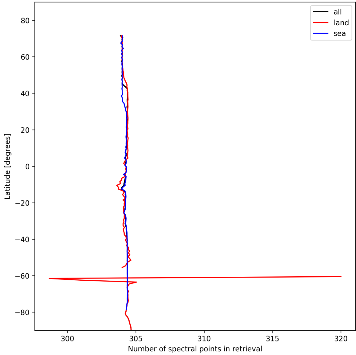
Figure 16: Zonal average of “Number of spectral points in retrieval” for 2024-11-07 to 2024-11-09.
