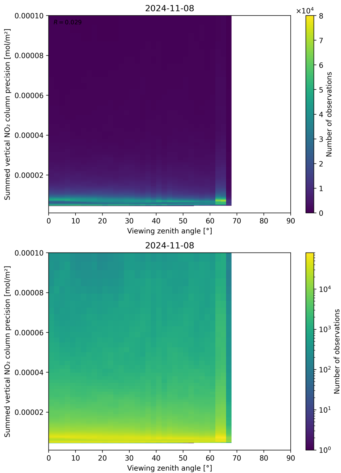
Figure 166: Scatter density plot of “Viewing zenith angle” against “Summed vertical NO 2 column precision” for 2024-11-07 to 2024-11-09.
