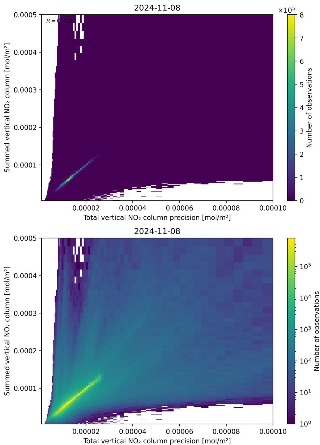
Figure 117: Scatter density plot of “Total vertical NO 2 column precision” against “Summed vertical NO 2 column” for 2024-11-07 to 2024-11-09.
