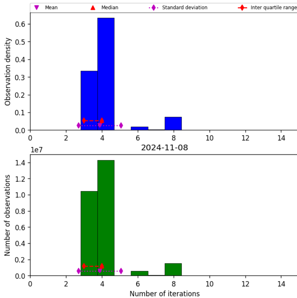
Figure 34: Histogram of “Number of iterations” for 2024-11-07 to 2024-11-09
