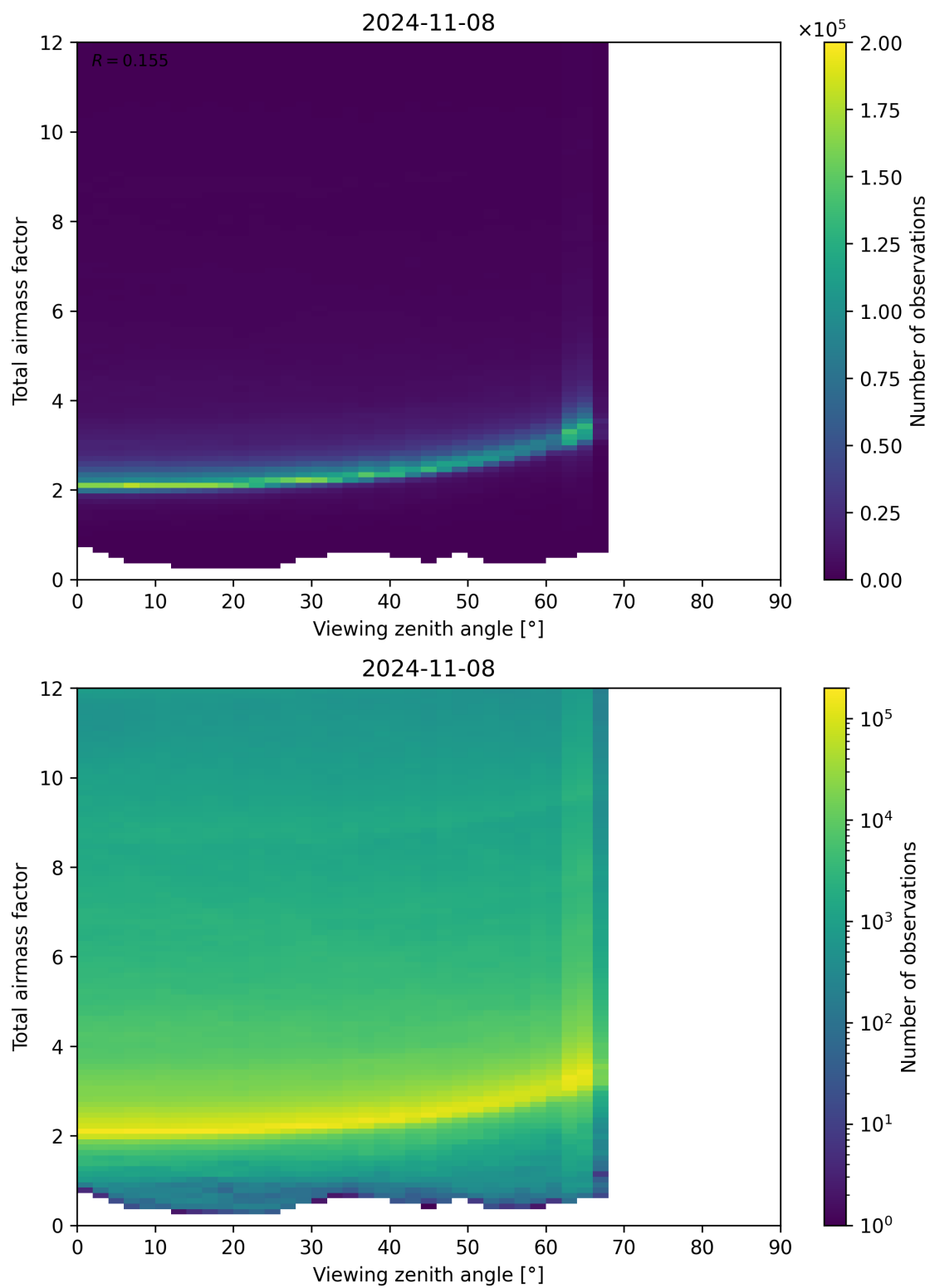
Figure 160: Scatter density plot of “Viewing zenith angle” against “Total airmass factor” for 2024-11-07 to 2024-11-09.
