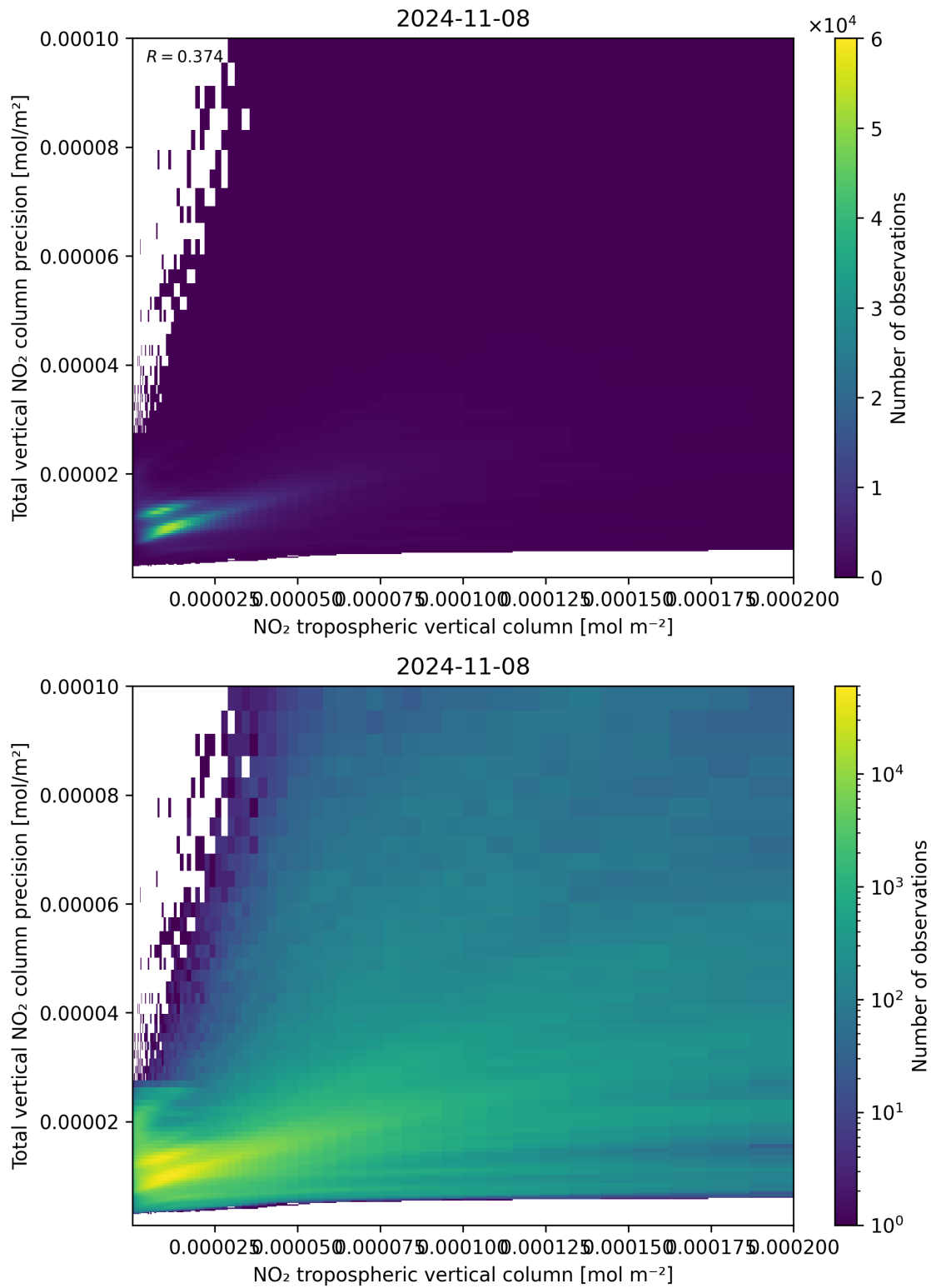
Figure 129: Scatter density plot of “NO 2 tropospheric vertical column” against “Total vertical NO 2 column precision” for 2024-11-07 to 2024-11-09.
