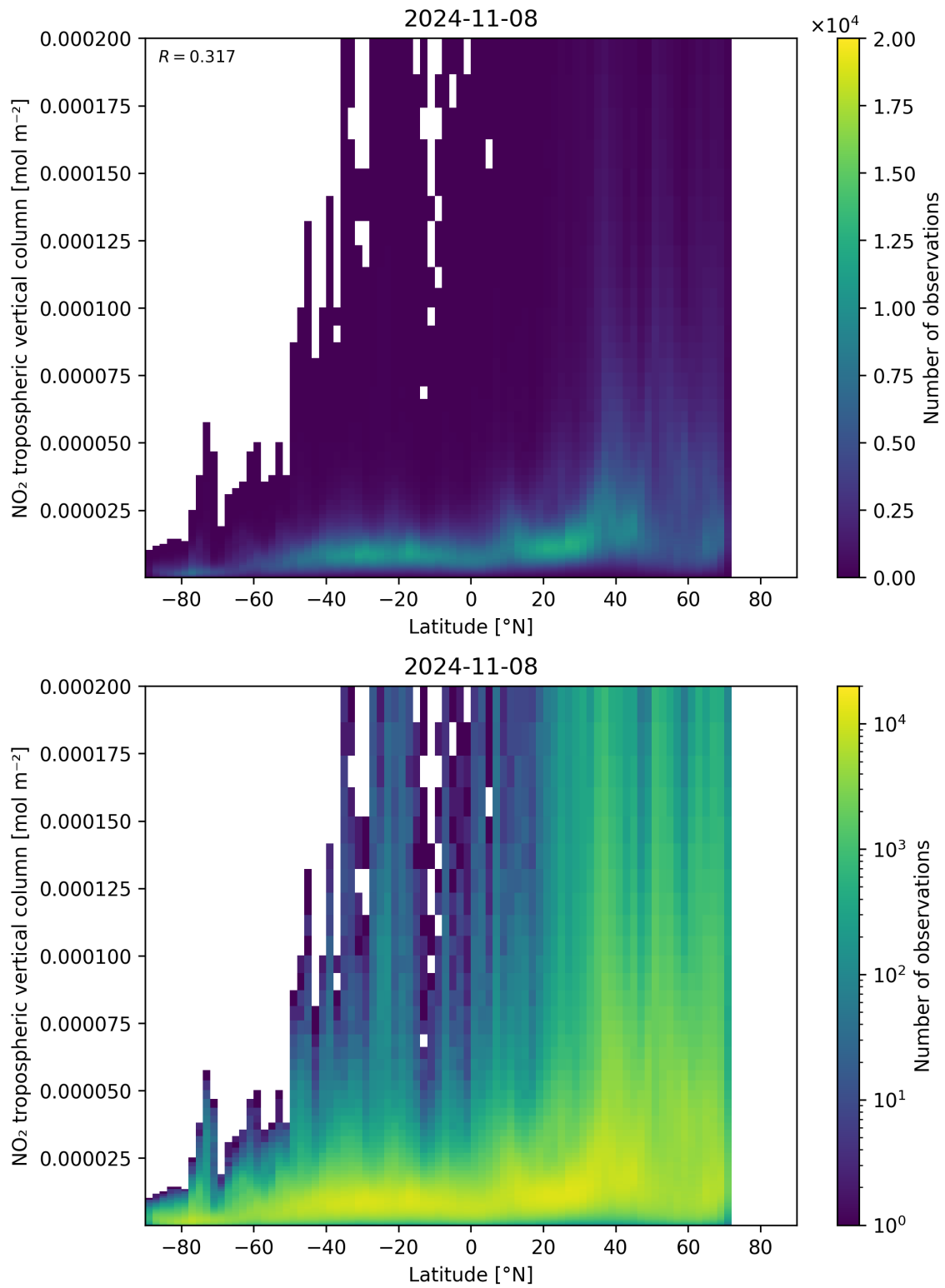
Figure 92: Scatter density plot of “Latitude” against “NO 2 tropospheric vertical column” for 2024-11-07 to 2024-11-09.
