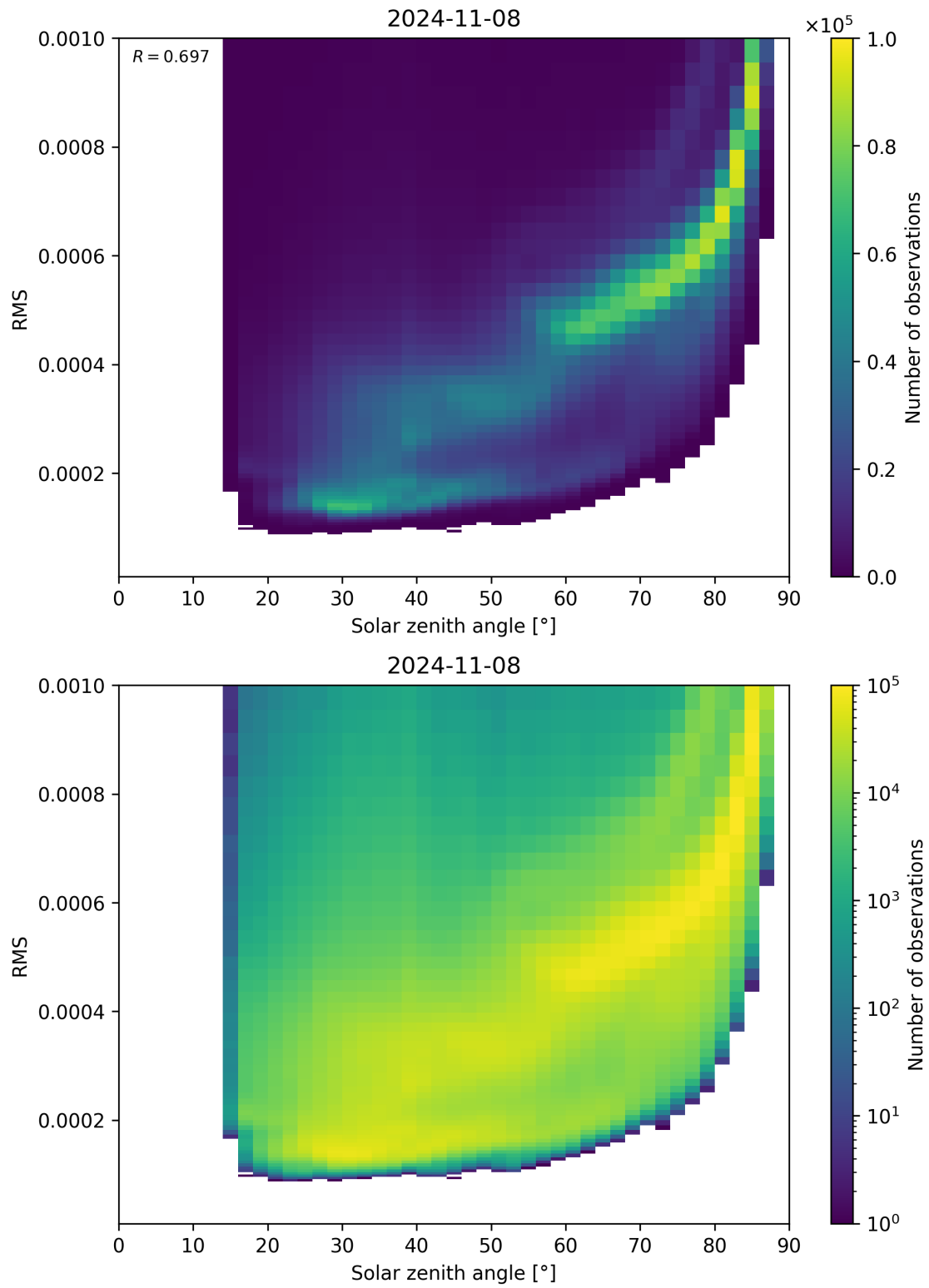
Figure 157: Scatter density plot of “Solar zenith angle” against “RMS” for 2024-11-07 to 2024-11-09.
