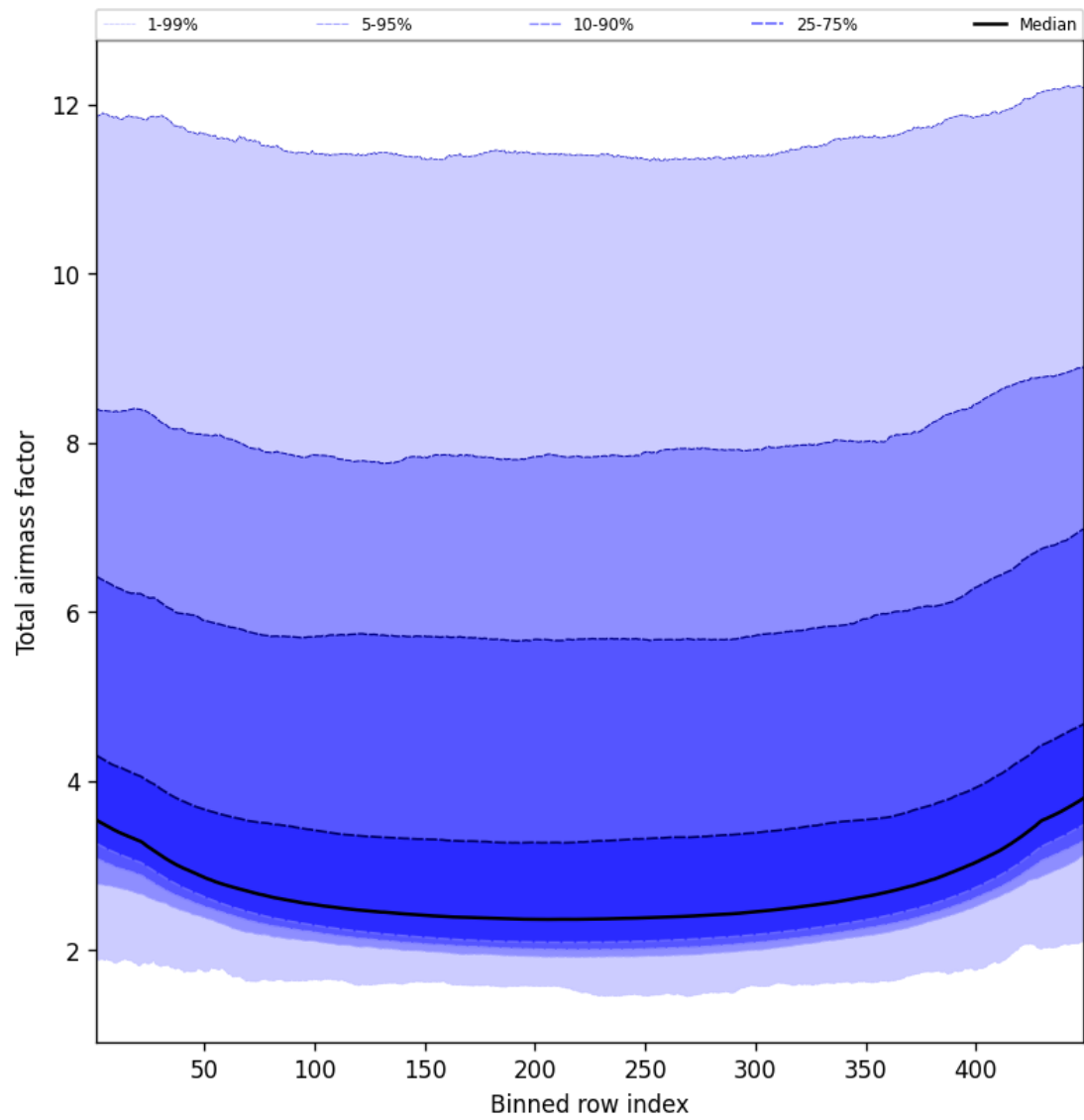
Figure 49: Along track statistics of “Total airmass factor” for 2024-11-07 to 2024-11-09
