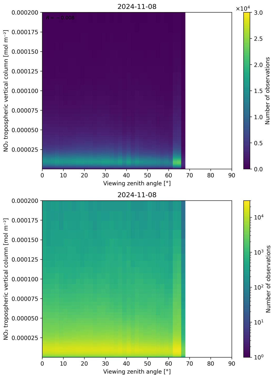
Figure 169: Scatter density plot of “Viewing zenith angle” against “NO 2 tropospheric vertical column” for 2024-11-07 to 2024-11-09.
