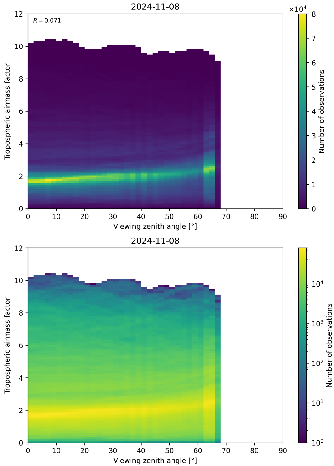
Figure 161: Scatter density plot of “Viewing zenith angle” against “Tropospheric airmass factor” for 2024-11-07 to 2024-11-09.
