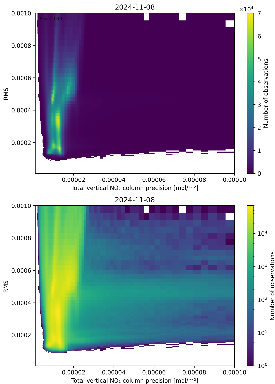
Figure 119: Scatter density plot of “Total vertical NO 2 column precision” against “RMS” for 2024-11-07 to 2024-11-09.
