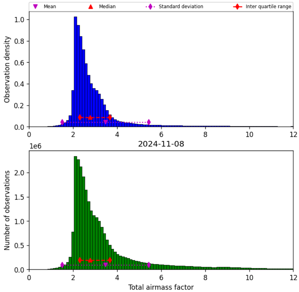
Figure 32: Histogram of “Total airmass factor” for 2024-11-07 to 2024-11-09
