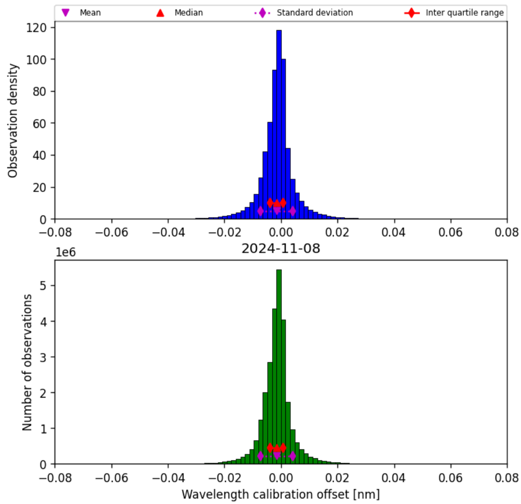
Figure 35: Histogram of “Wavelength calibration offset” for 2024-11-07 to 2024-11-09
