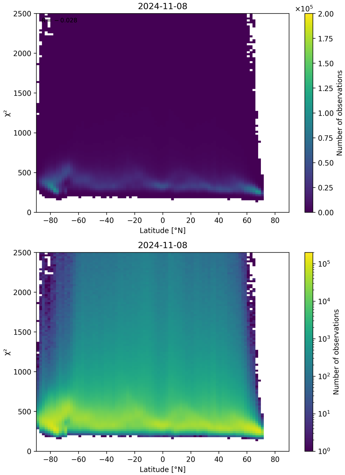
Figure 86: Scatter density plot of “Latitude” against “ \chi^2 ” for 2024-11-07 to 2024-11-09.
