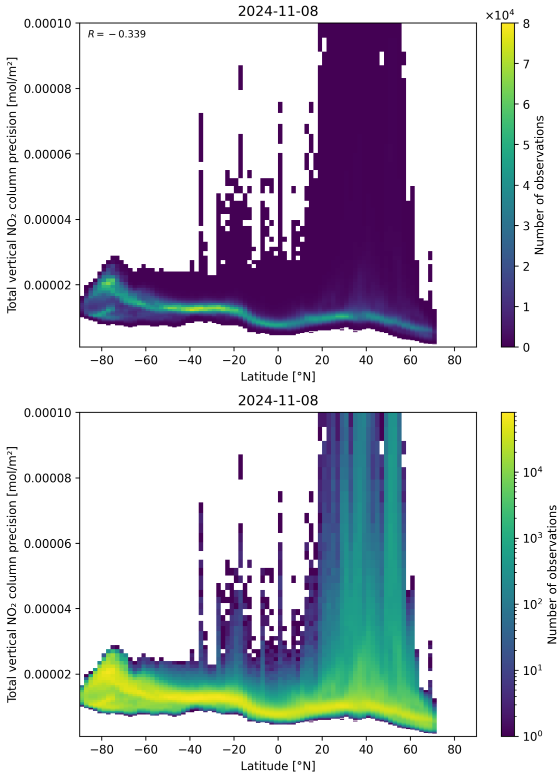
Figure 91: Scatter density plot of “Latitude” against “Total vertical NO 2 column precision” for 2024-11-07 to 2024-11-09.
