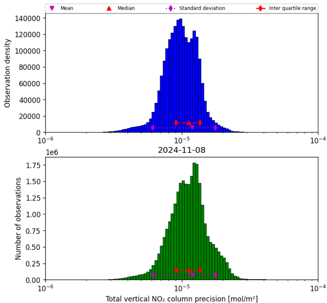
Figure 39: Histogram of “Total vertical NO 2 column precision” for 2024-11-07 to 2024-11-09
