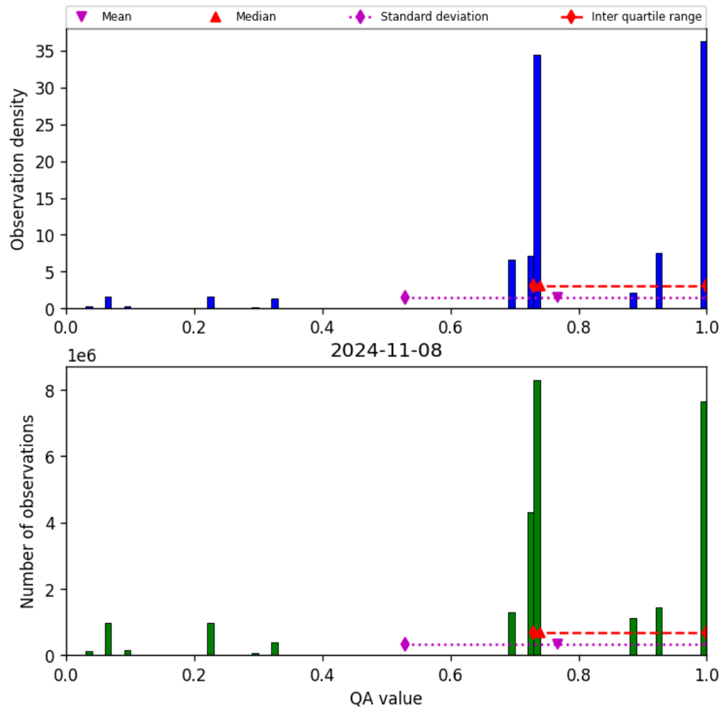
Figure 28: Histogram of “QA value” for 2024-11-07 to 2024-11-09
