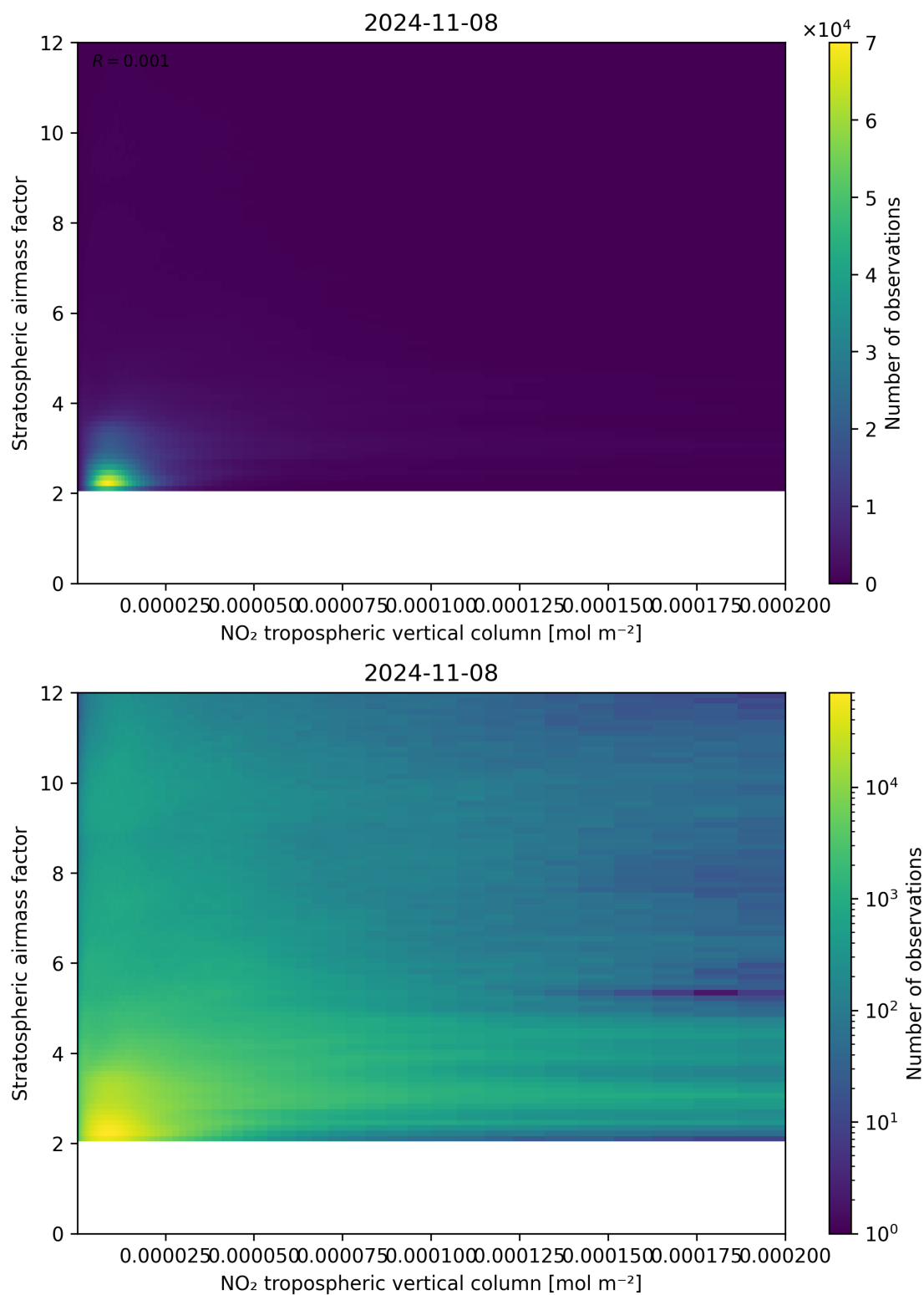
Figure 121: Scatter density plot of “NO 2 tropospheric vertical column” against “Stratospheric airmass factor” for 2024-11-07 to 2024-11-09.
