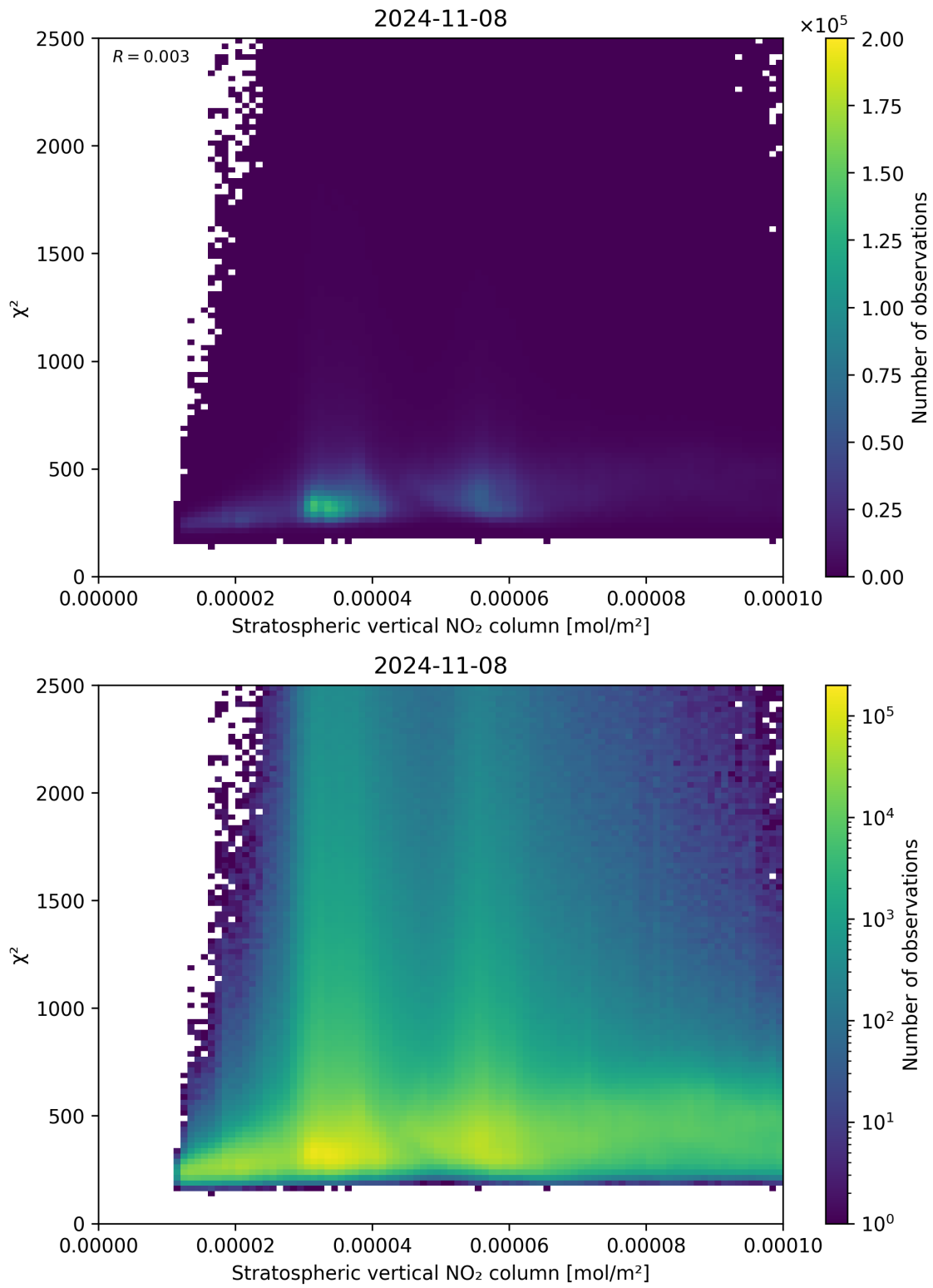
Figure 97: Scatter density plot of “Stratospheric vertical NO 2 column” against “ \chi^2 ” for 2024-11-07 to 2024-11-09.
