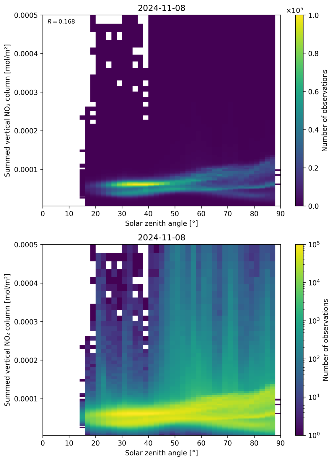
Figure 151: Scatter density plot of “Solar zenith angle” against “Summed vertical NO 2 column” for 2024-11-07 to 2024-11-09.
