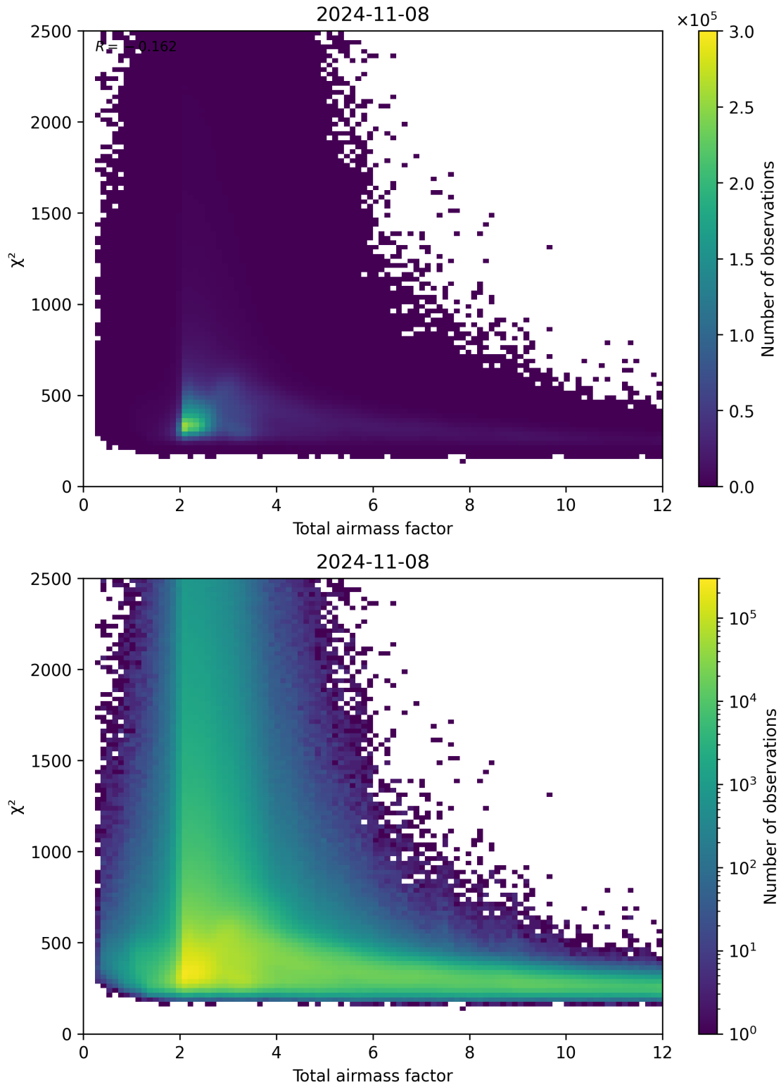
Figure 63: Scatter density plot of “Total airmass factor” against “ \chi^2 ” for 2024-11-07 to 2024-11-09.
