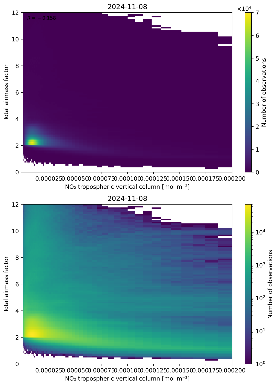
Figure 122: Scatter density plot of “NO 2 tropospheric vertical column” against “Total airmass factor” for 2024-11-07 to 2024-11-09.
