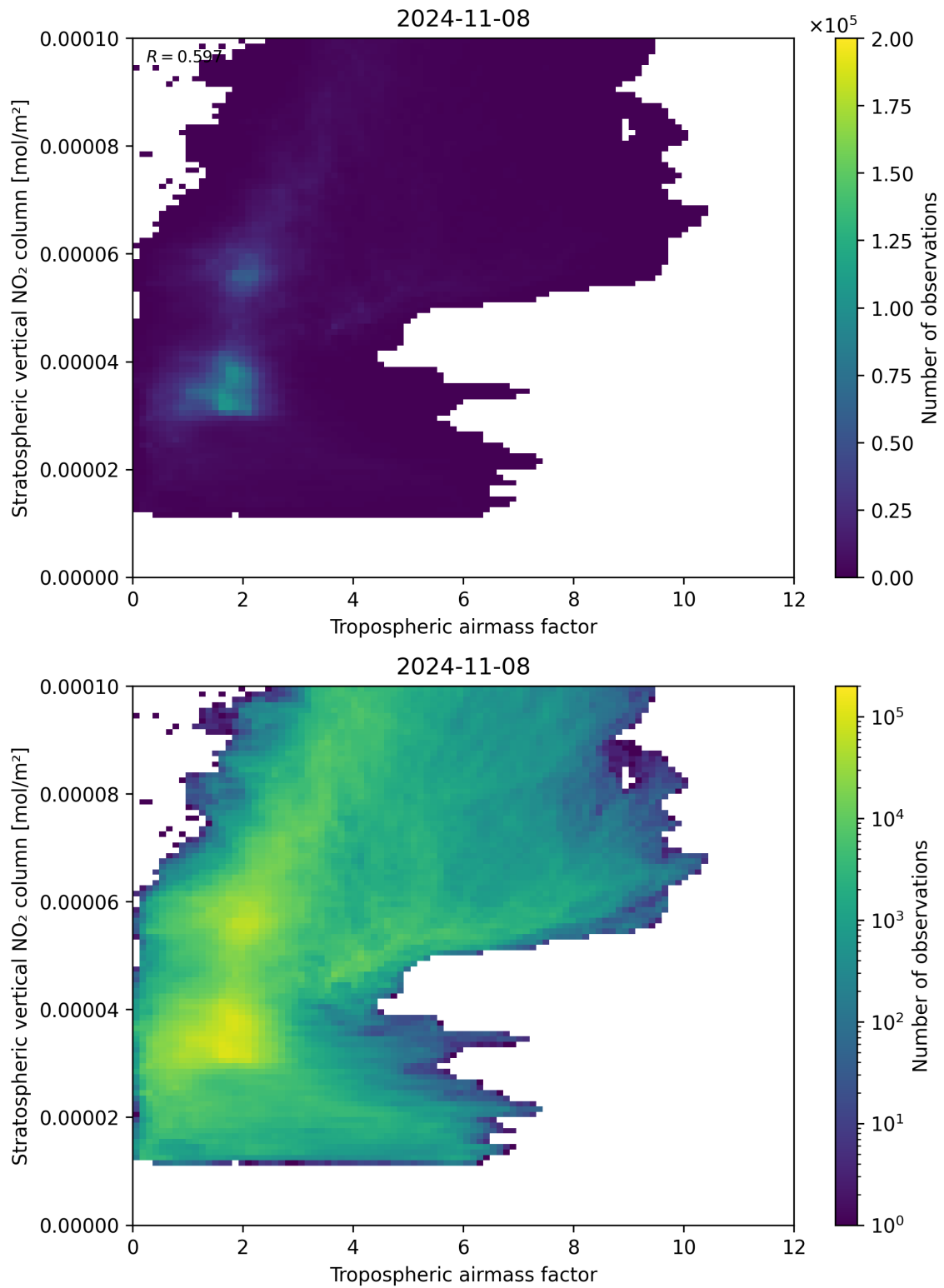
Figure 74: Scatter density plot of “Tropospheric air mass factor” against “Stratospheric vertical NO 2 column” for 2024-11-07 to 2024-11-09.
