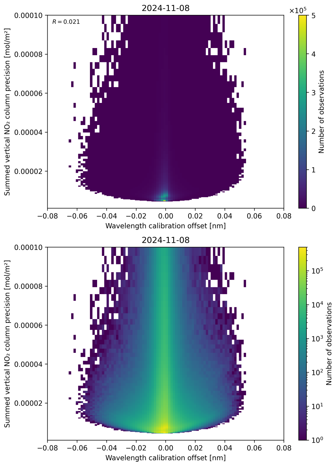
Figure 178: Scatter density plot of “Wavelength calibration offset” against “Summed vertical NO 2 column precision” for 2024-11-07 to 2024-11-09.
