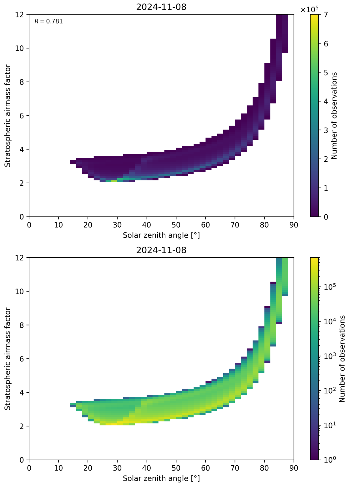
Figure 145: Scatter density plot of “Solar zenith angle” against “Stratospheric airmass factor” for 2024-11-07 to 2024-11-09.
