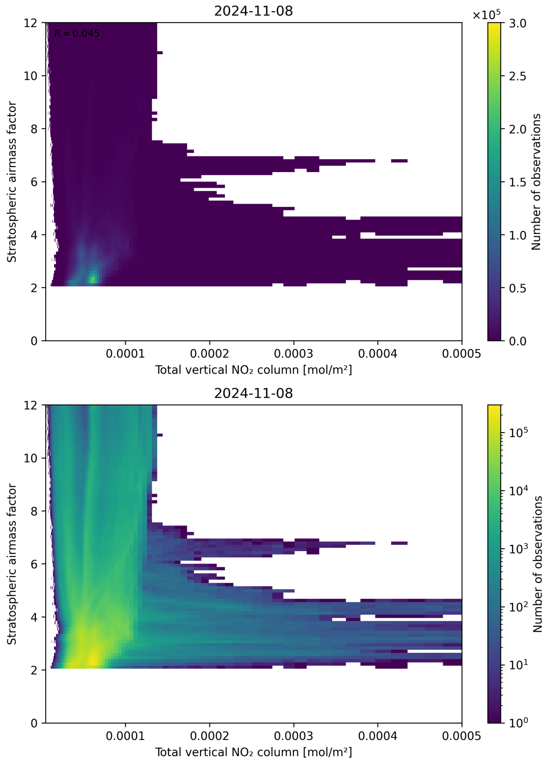
Figure 110: Scatter density plot of “Total vertical NO 2 column” against “Stratospheric airmass factor” for 2024-11-07 to 2024-11-09.
