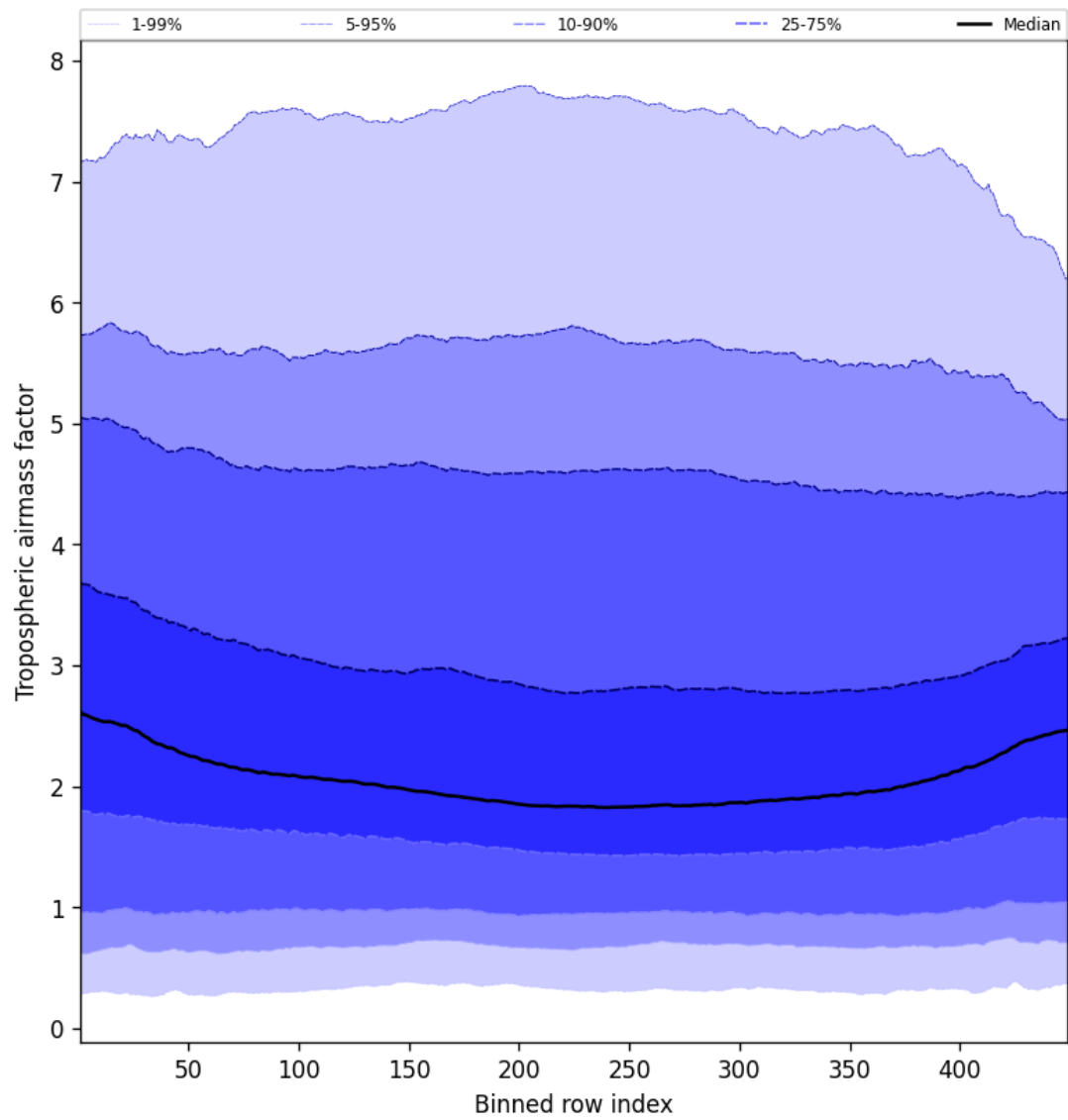
Figure 48: Along track statistics of “Tropospheric air mass factor” for 2024-11-07 to 2024-11-09
