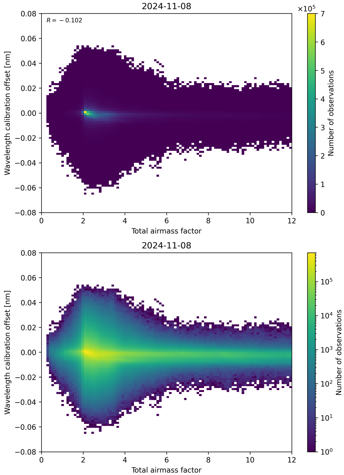
Figure 70: Scatter density plot of “Total airmass factor” against “Wavelength calibration offset” for 2024-11-07 to 2024-11-09.
