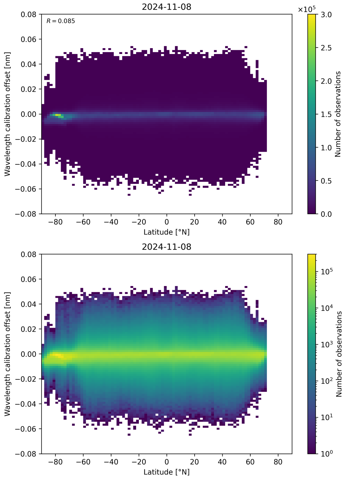
Figure 95: Scatter density plot of “Latitude” against “Wavelength calibration offset” for 2024-11-07 to 2024-11-09.
