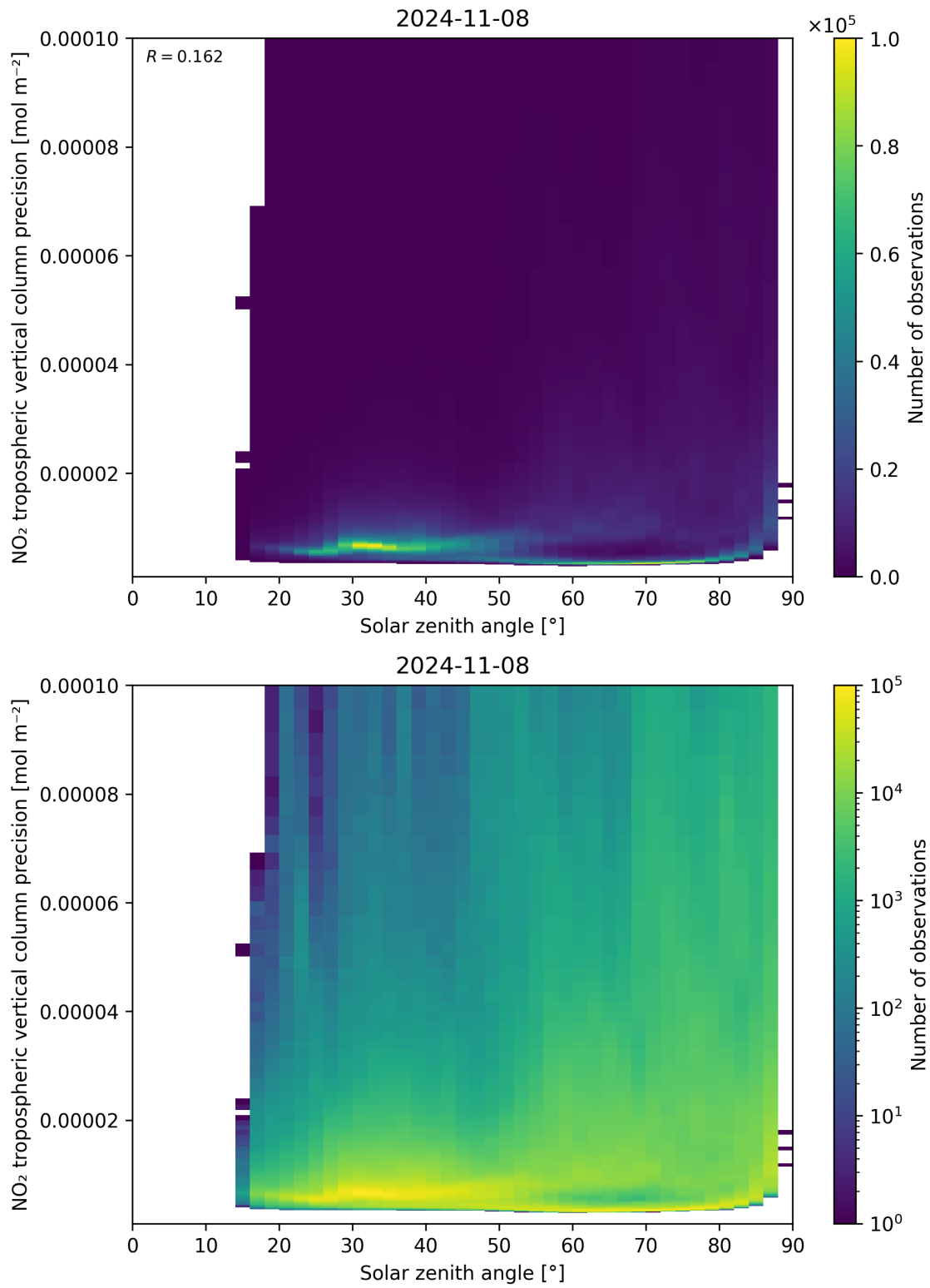
Figure 156: Scatter density plot of “Solar zenith angle” against “NO 2 tropospheric vertical column precision” for 2024-11-07 to 2024-11-09.
