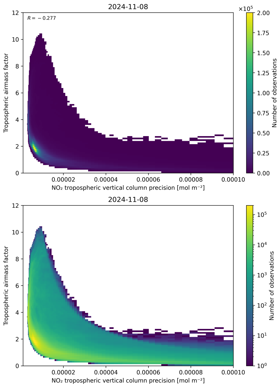
Figure 133: Scatter density plot of “NO 2 tropospheric vertical column precision” against “Tropospheric air mass factor” for 2024-11-07 to 2024-11-09.
