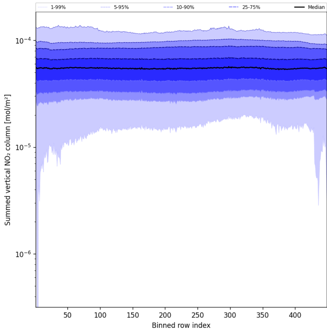
Figure 57: Along track statistics of “Summed vertical NO 2 column” for 2024-11-07 to 2024-11-09
