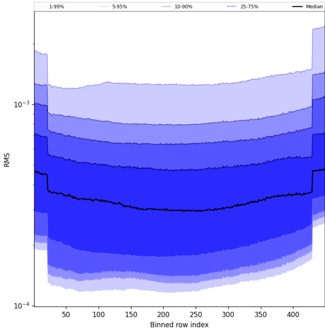
Figure 60: Along track statistics of “RMS” for 2024-11-07 to 2024-11-09
