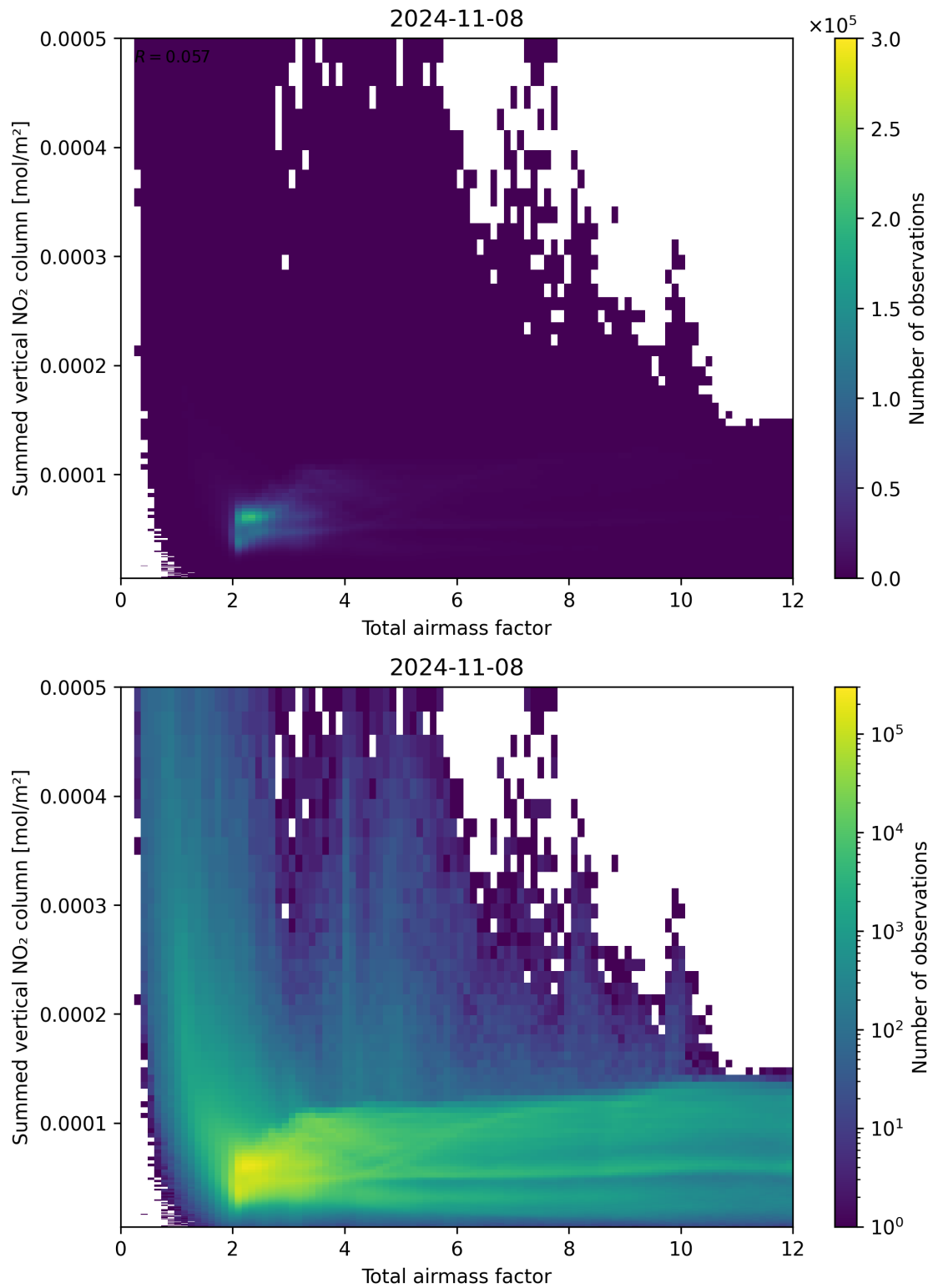
Figure 65: Scatter density plot of “Total airmass factor” against “Summed vertical NO 2 column” for 2024-11-07 to 2024-11-09.
