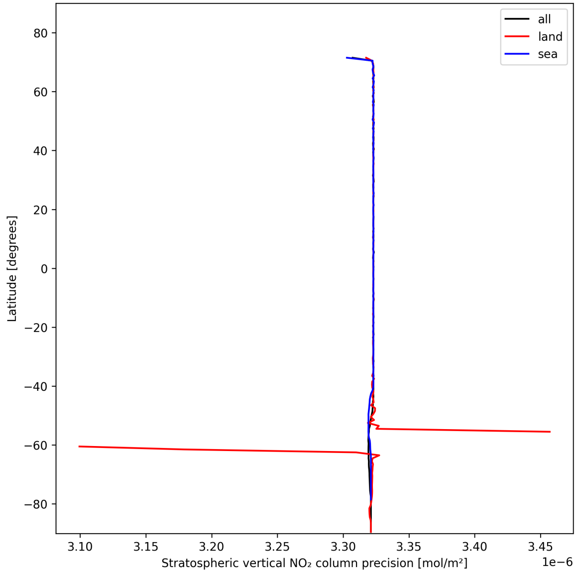
Figure 20: Zonal average of “Stratospheric vertical NO 2 column precision” for 2024-11-07 to 2024-11-09.
