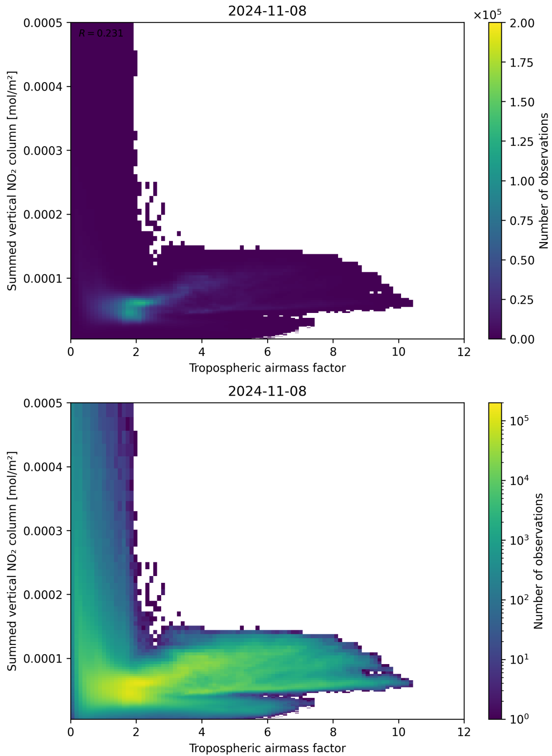
Figure 75: Scatter density plot of “Tropospheric air mass factor” against “Summed vertical NO 2 column” for 2024-11-07 to 2024-11-09.
