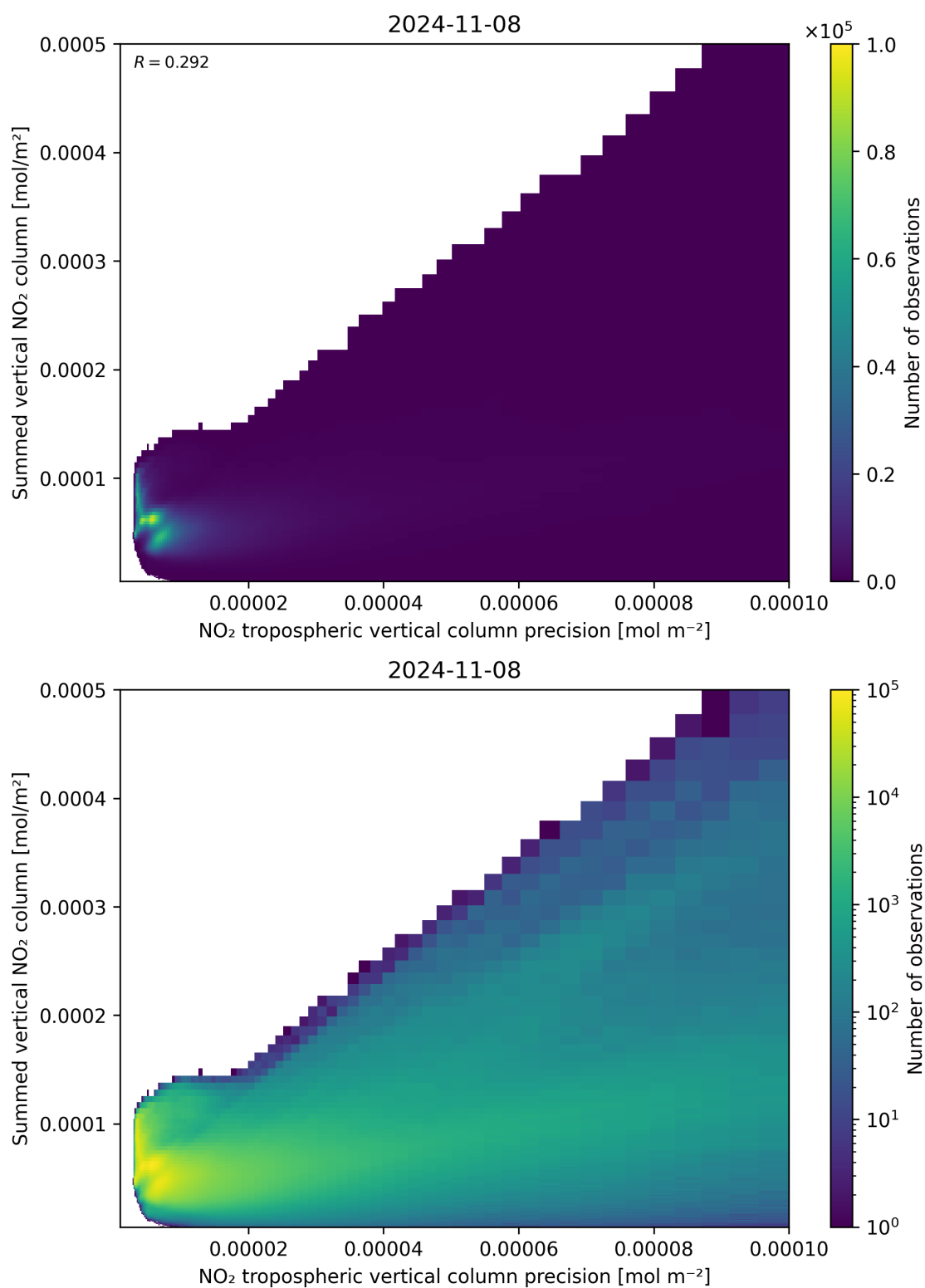
Figure 136: Scatter density plot of “NO 2 tropospheric vertical column precision” against “Summed vertical NO 2 column” for 2024-11-07 to 2024-11-09.
