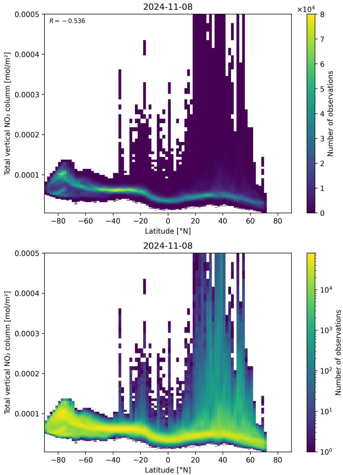
Figure 90: Scatter density plot of “Latitude” against “Total vertical NO 2 column” for 2024-11-07 to 2024-11-09.
