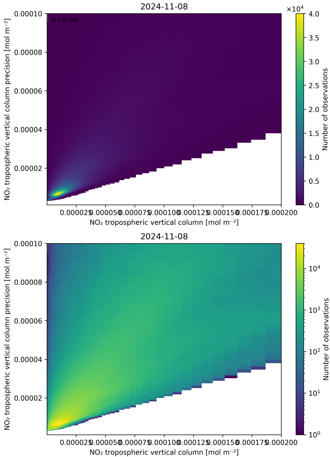
Figure 130: Scatter density plot of “NO 2 tropospheric vertical column” against “NO 2 tropospheric vertical column precision” for 2024-11-07 to 2024-11-09.
