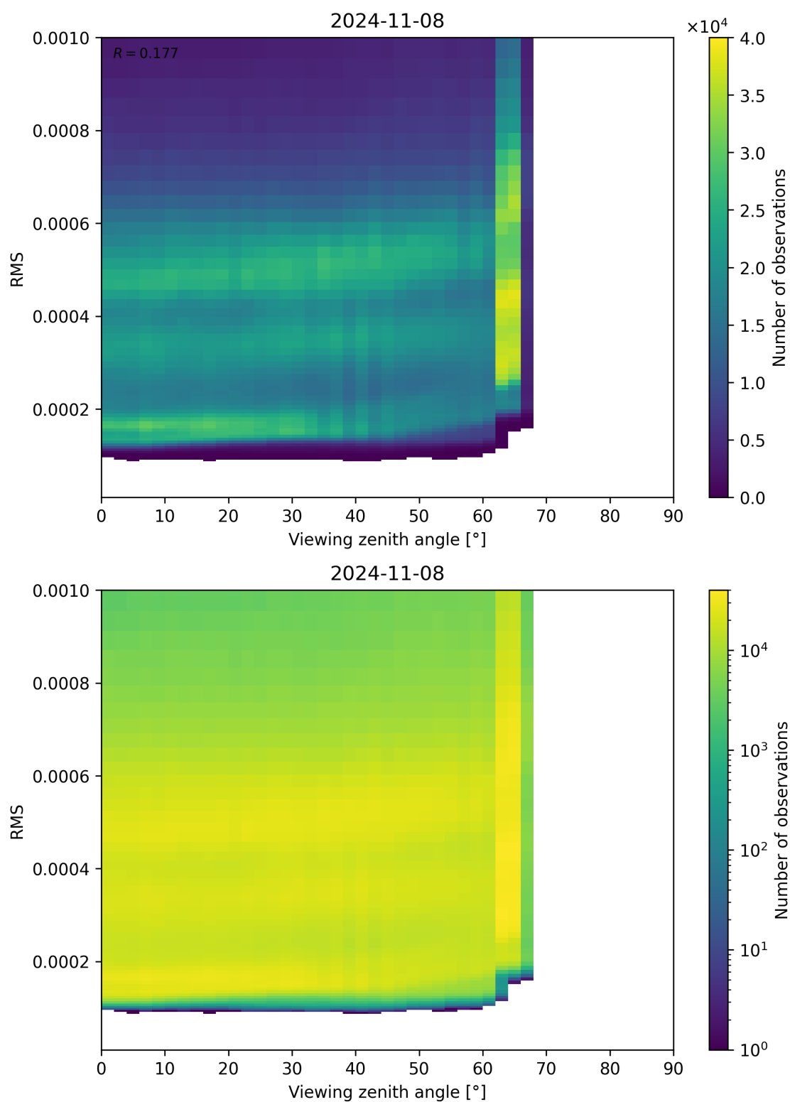
Figure 171: Scatter density plot of “Viewing zenith angle” against “RMS” for 2024-11-07 to 2024-11-09.
