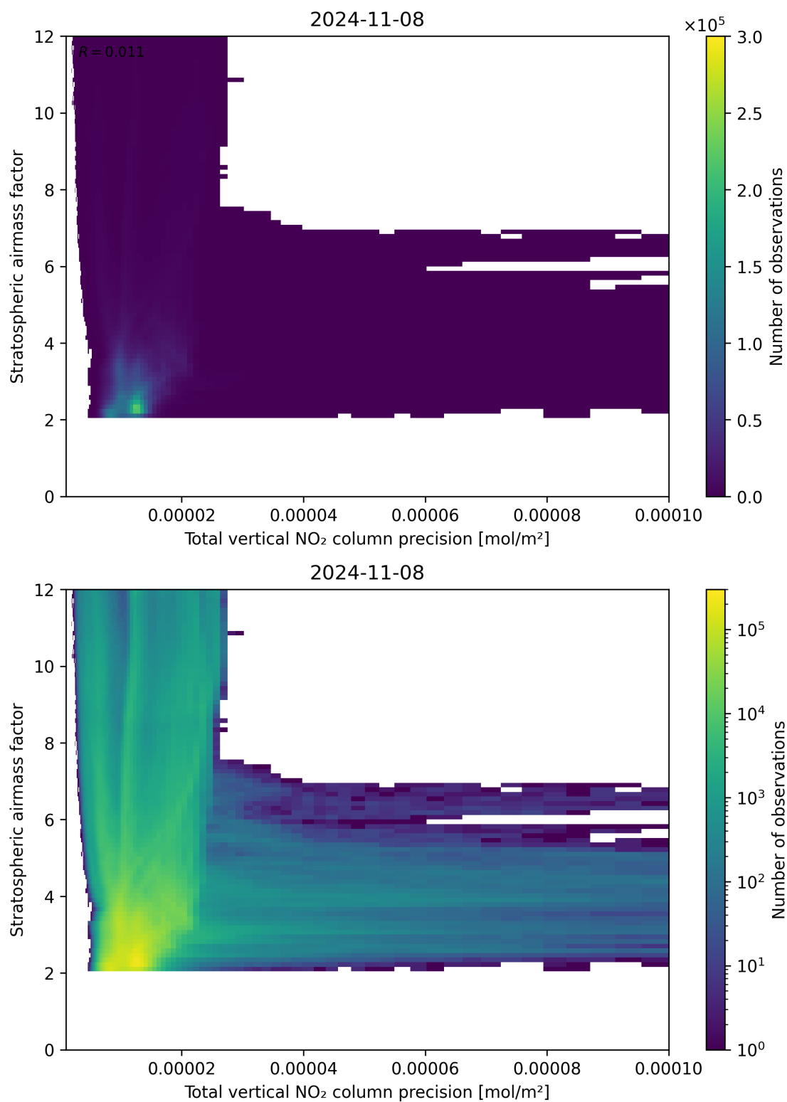
Figure 115: Scatter density plot of “Total vertical NO 2 column precision” against “Stratospheric air mass factor” for 2024-11-07 to 2024-11-09.
