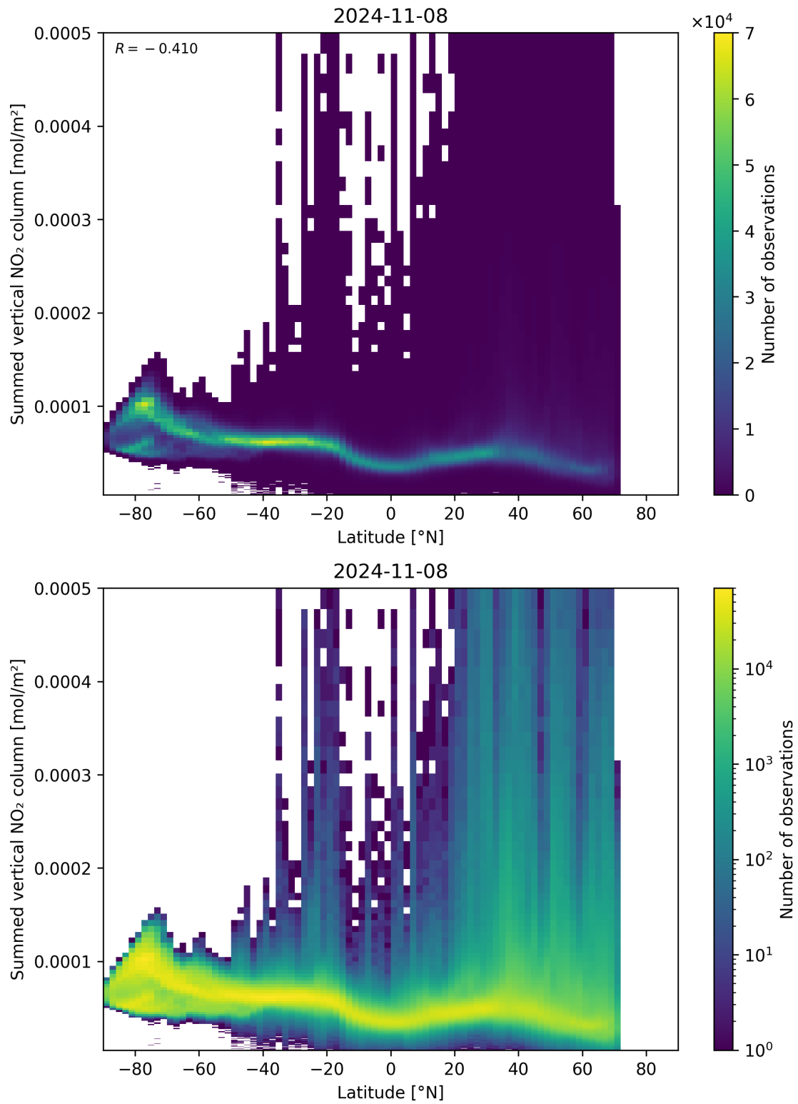
Figure 88: Scatter density plot of “Latitude” against “Summed vertical NO 2 column” for 2024-11-07 to 2024-11-09.
