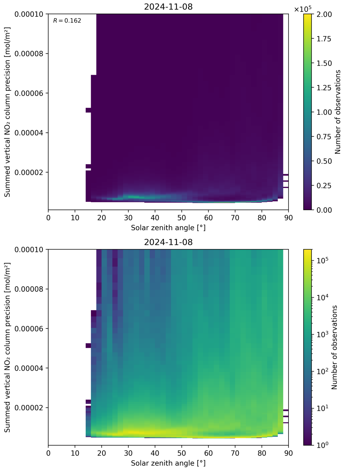
Figure 152: Scatter density plot of “Solar zenith angle” against “Summed vertical NO 2 column precision” for 2024-11-07 to 2024-11-09.
