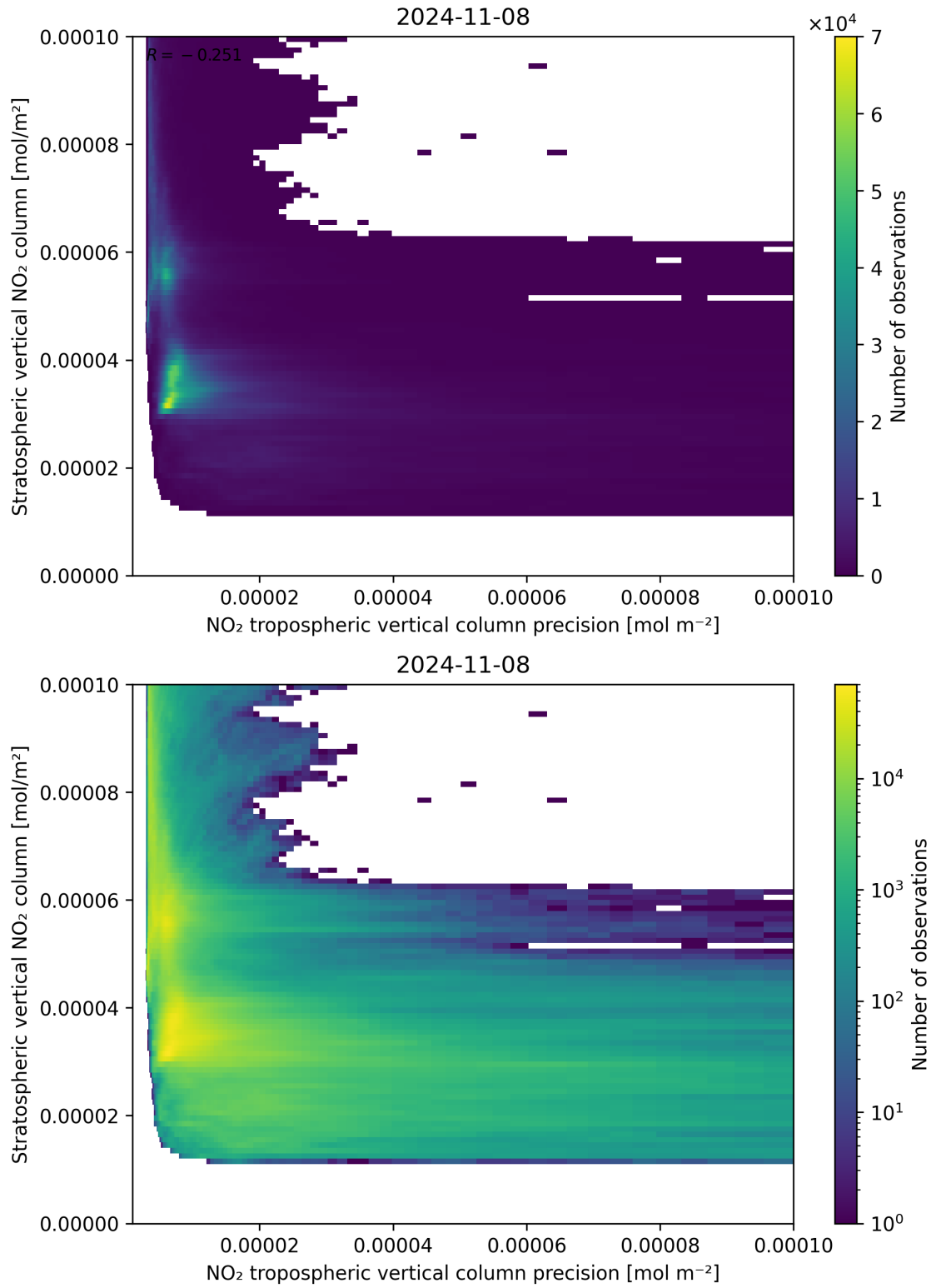
Figure 135: Scatter density plot of “NO 2 tropospheric vertical column precision” against “Stratospheric vertical NO 2 column” for 2024-11-07 to 2024-11-09.
