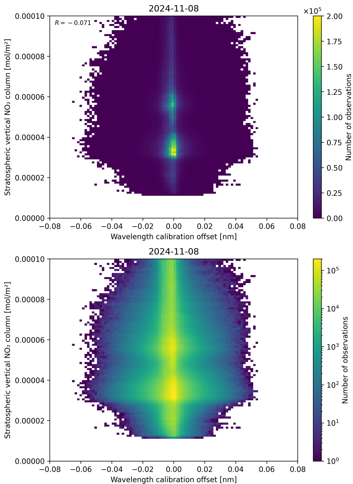
Figure 176: Scatter density plot of “Wavelength calibration offset” against “Stratospheric vertical NO 2 column” for 2024-11-07 to 2024-11-09.
