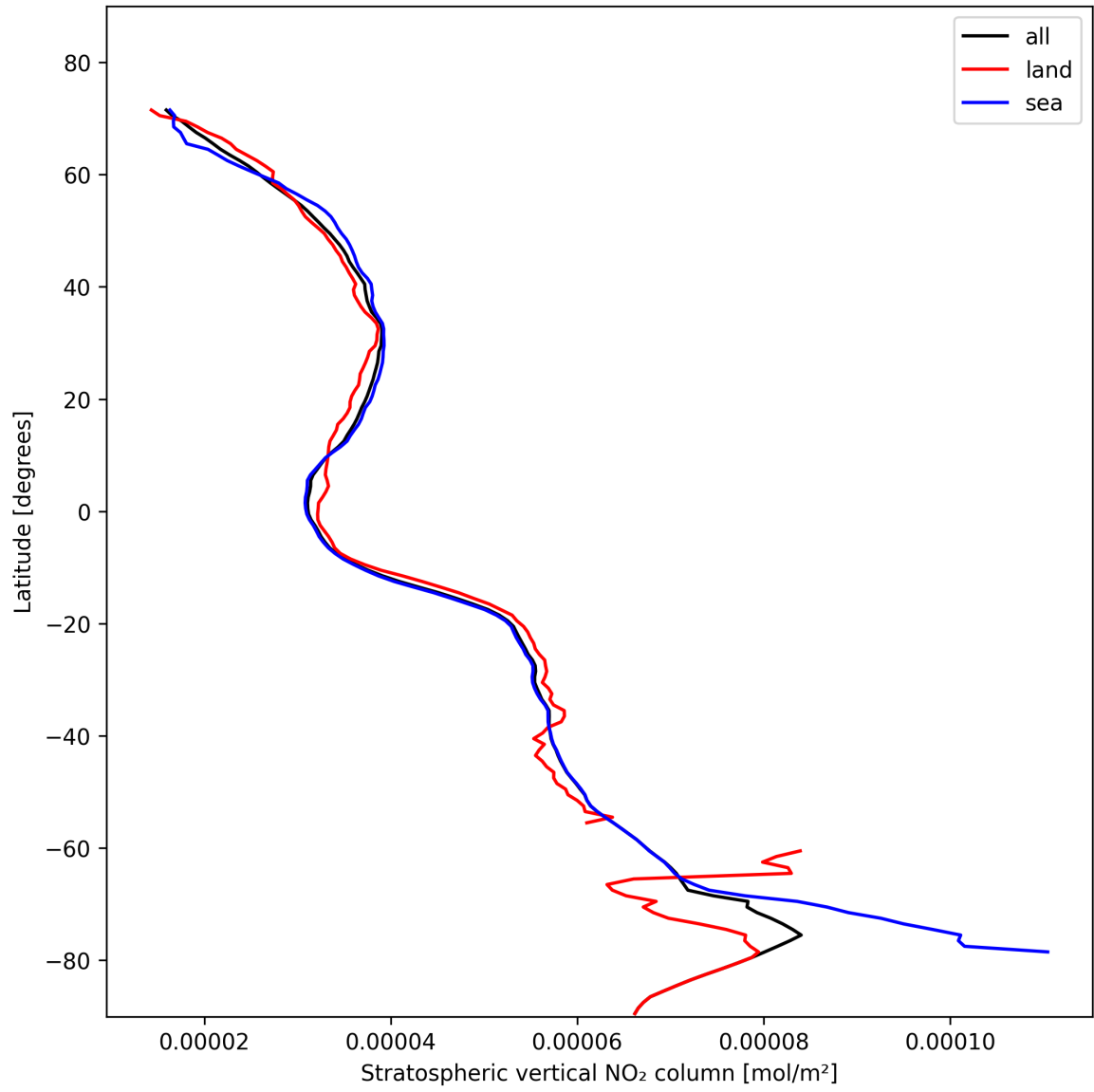
Figure 19: Zonal average of “Stratospheric vertical NO 2 column” for 2024-11-07 to 2024-11-09.
