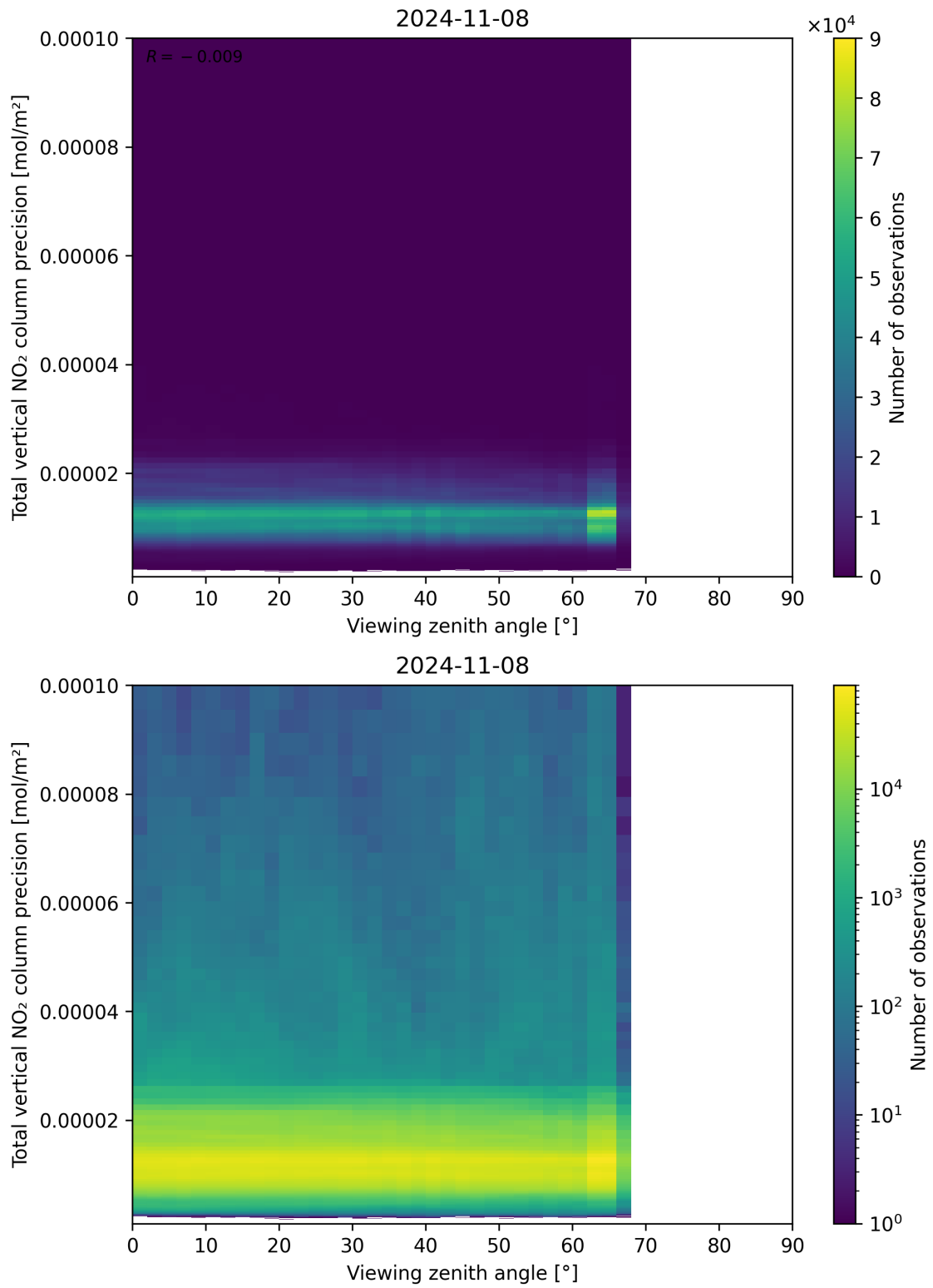
Figure 168: Scatter density plot of “Viewing zenith angle” against “Total vertical NO 2 column precision” for 2024-11-07 to 2024-11-09.
