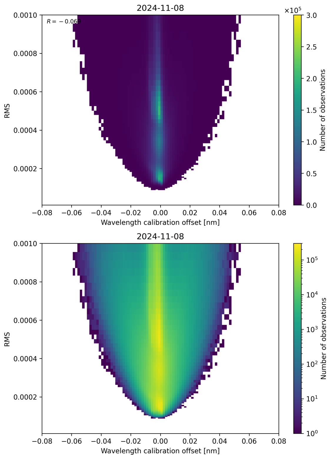
Figure 181: Scatter density plot of “Wavelength calibration offset” against “RMS” for 2024-11-07 to 2024-11-09.
