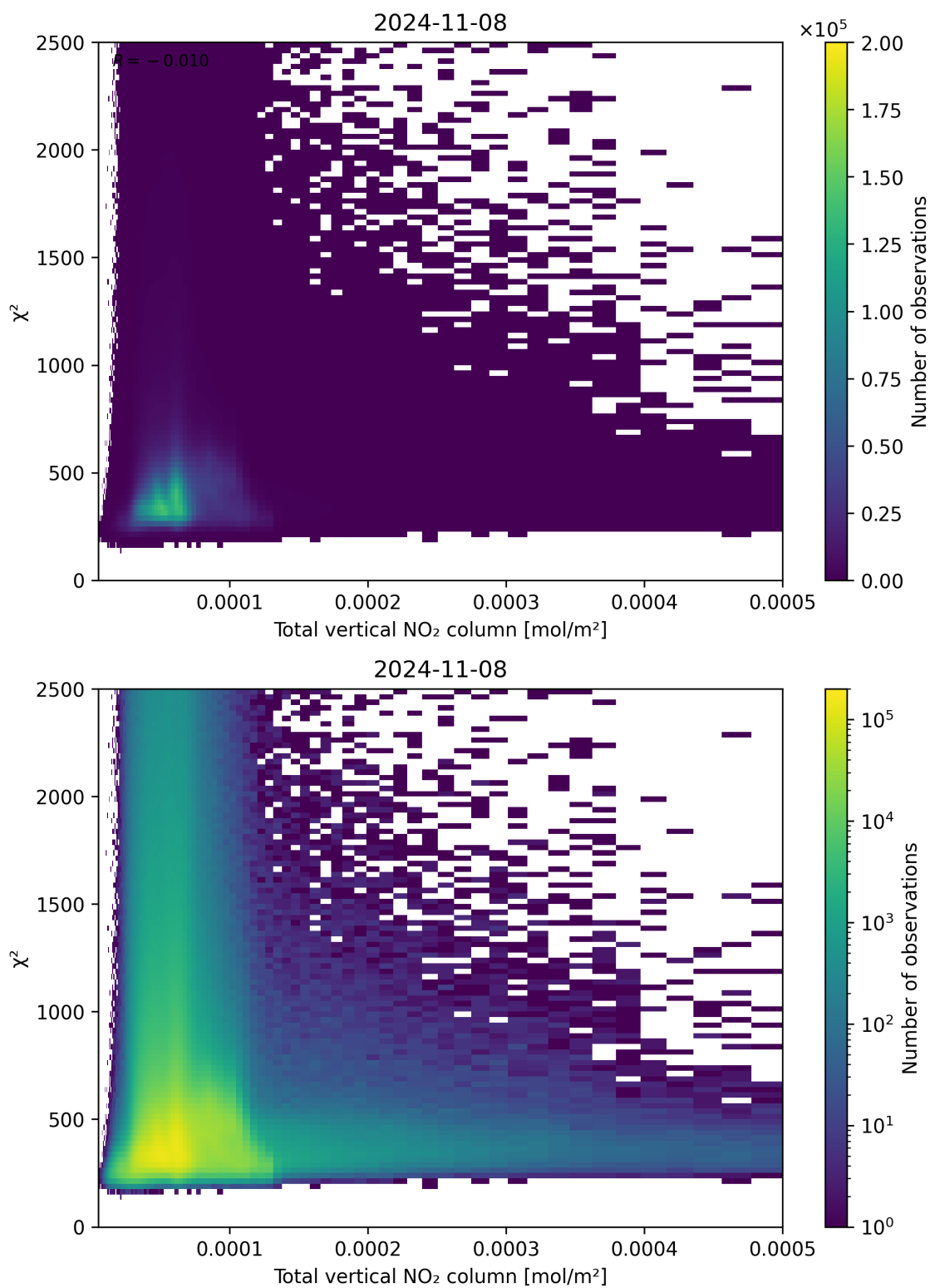
Figure 111: Scatter density plot of “Total vertical NO 2 column” against “ \chi^2 ” for 2024-11-07 to 2024-11-09.
