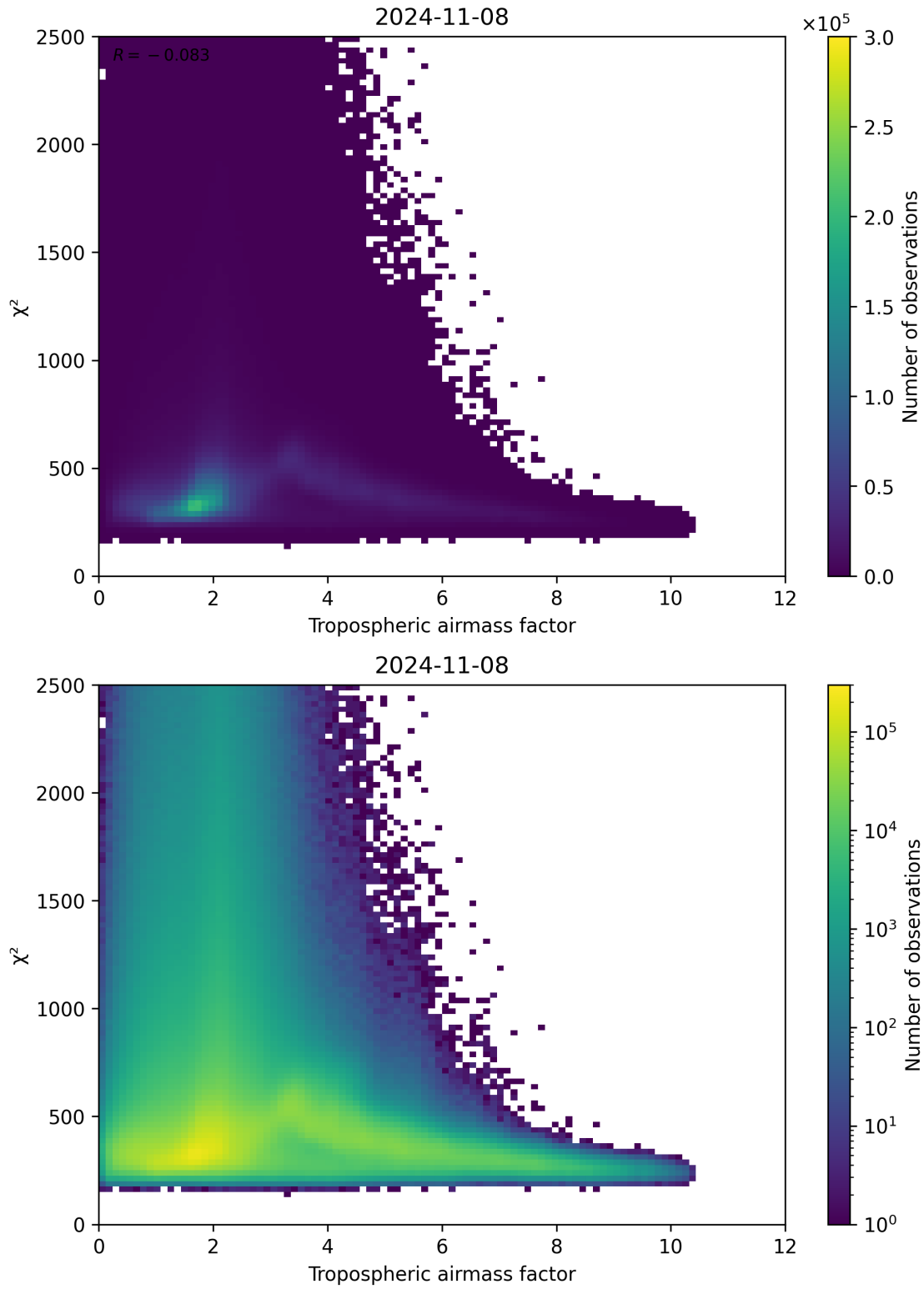
Figure 73: Scatter density plot of “Tropospheric airmass factor” against “ \chi^2 ” for 2024-11-07 to 2024-11-09.
