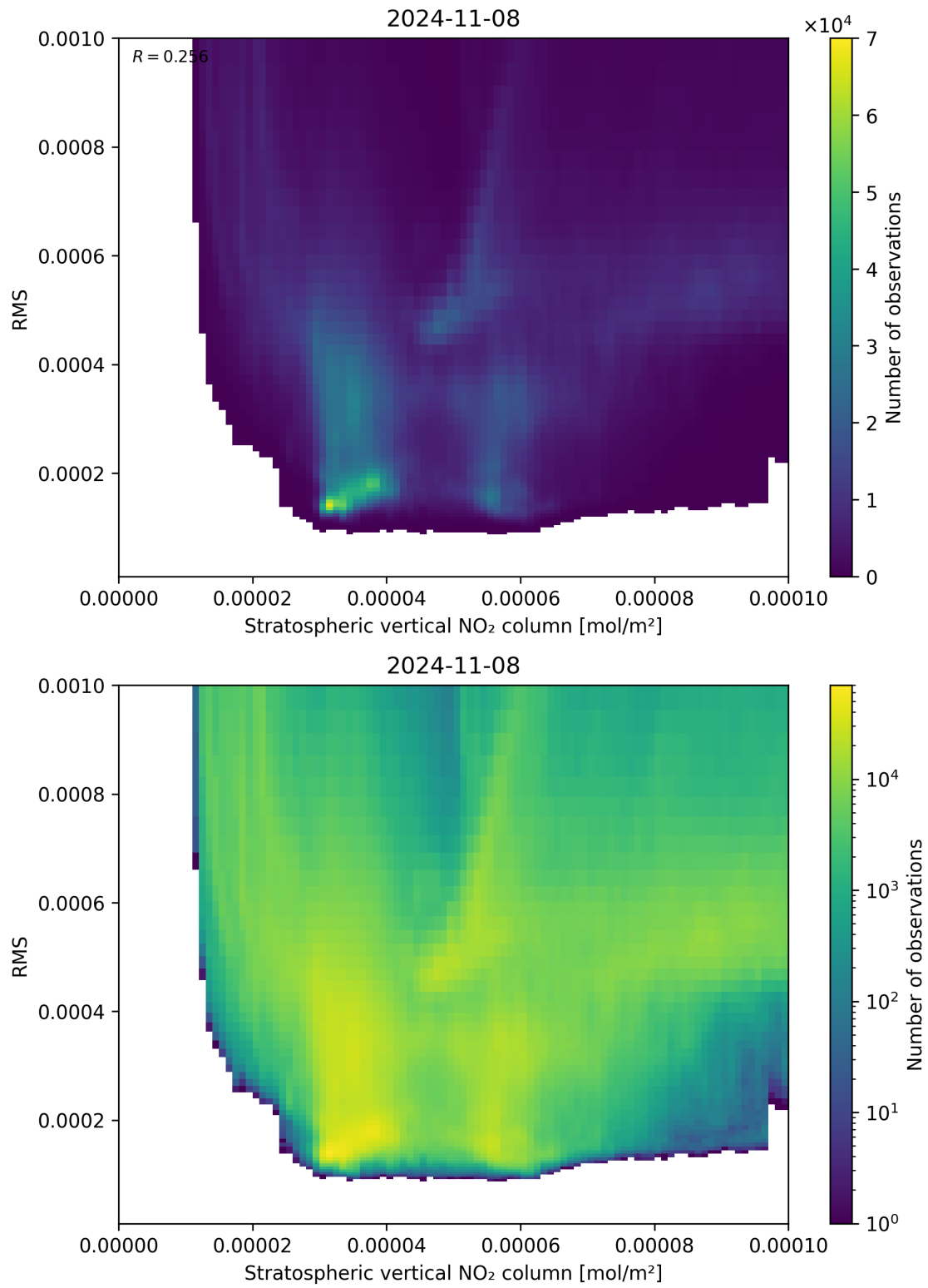
Figure 102: Scatter density plot of “Stratospheric vertical NO 2 column” against “RMS” for 2024-11-07 to 2024-11-09.
