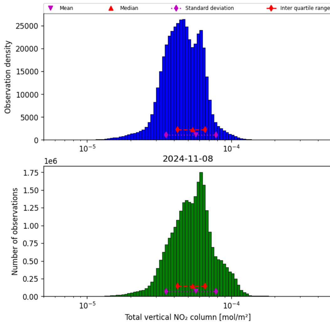
Figure 38: Histogram of “Total vertical NO 2 column” for 2024-11-07 to 2024-11-09
