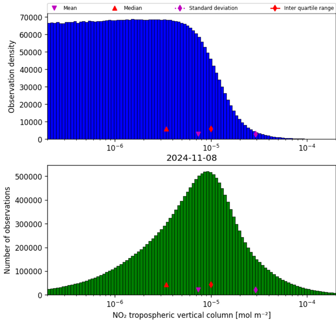
Figure 29: Histogram of “NO 2 tropospheric vertical column” for 2024-11-07 to 2024-11-09
