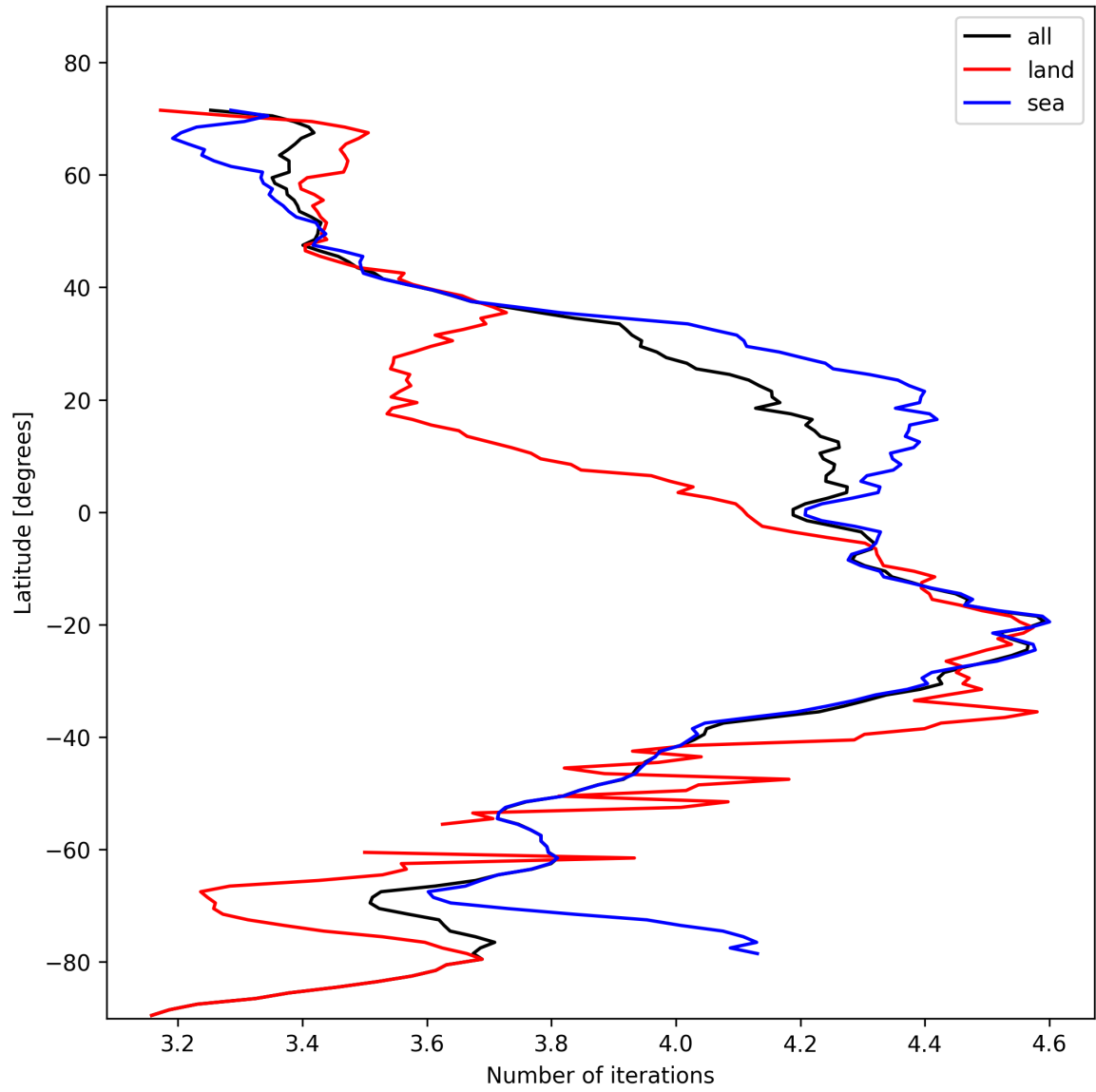
Figure 17: Zonal average of “Number of iterations” for 2024-11-07 to 2024-11-09.
