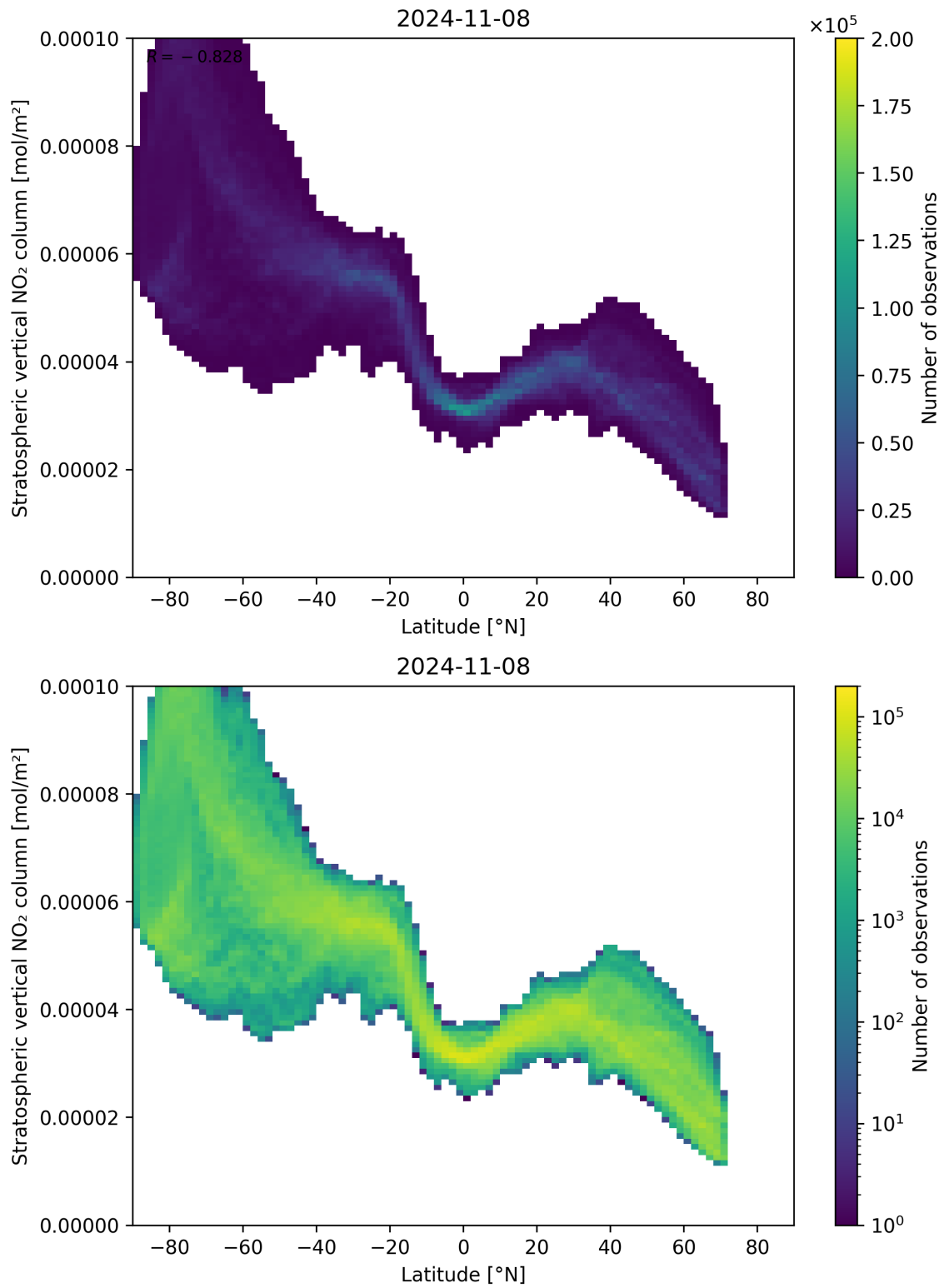
Figure 87: Scatter density plot of “Latitude” against “Stratospheric vertical NO 2 column” for 2024-11-07 to 2024-11-09.
