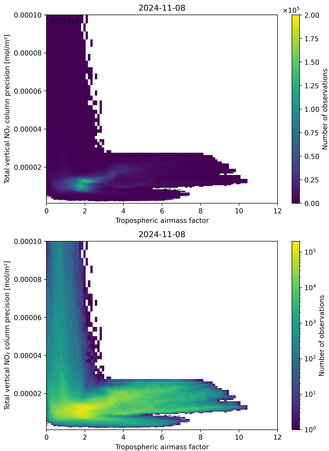
Figure 78: Scatter density plot of “Tropospheric air mass factor” against “Total vertical NO 2 column precision” for 2024-11-07 to 2024-11-09.
