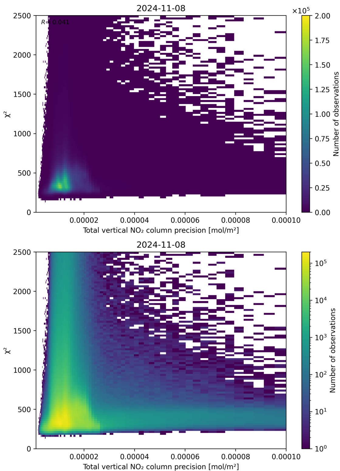
Figure 116: Scatter density plot of “Total vertical NO 2 column precision” against “ \chi^2 ” for 2024-11-07 to 2024-11-09.
