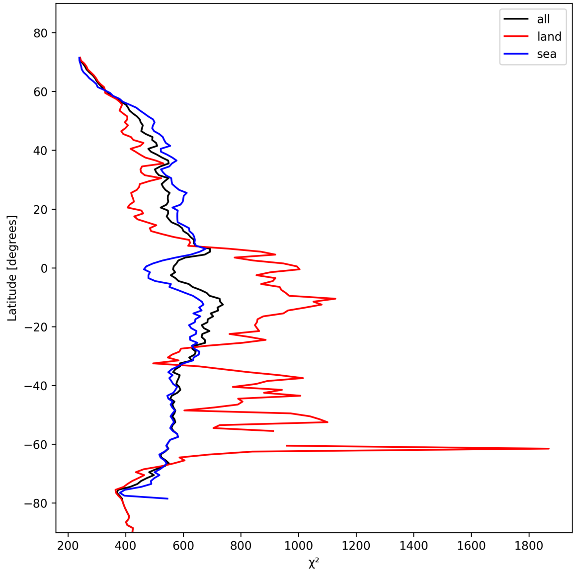
Figure 25: Zonal average of “ \chi^2 ” for 2024-11-07 to 2024-11-09.
