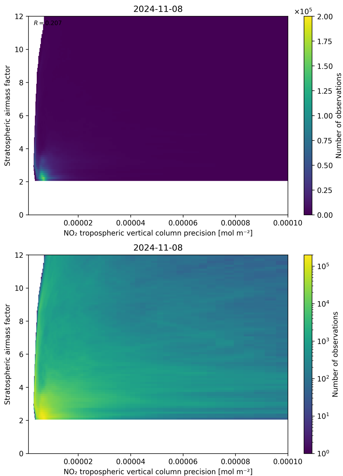
Figure 131: Scatter density plot of “NO 2 tropospheric vertical column precision” against “Stratospheric airmass factor” for 2024-11-07 to 2024-11-09.
