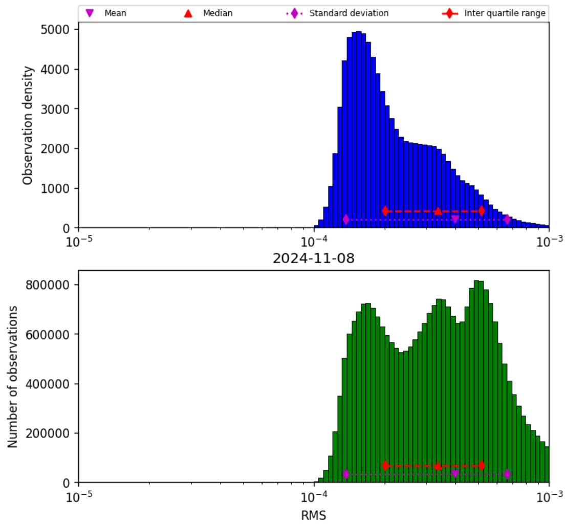
Figure 43: Histogram of “RMS” for 2024-11-07 to 2024-11-09
