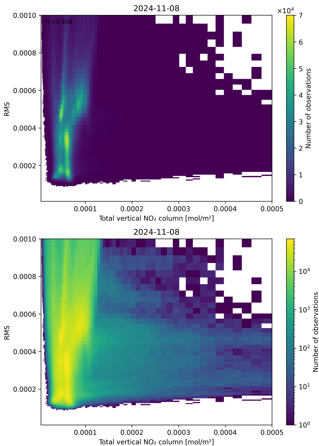
Figure 120: Scatter density plot of “Total vertical NO 2 column” against “RMS” for 2024-11-07 to 2024-11-09.
