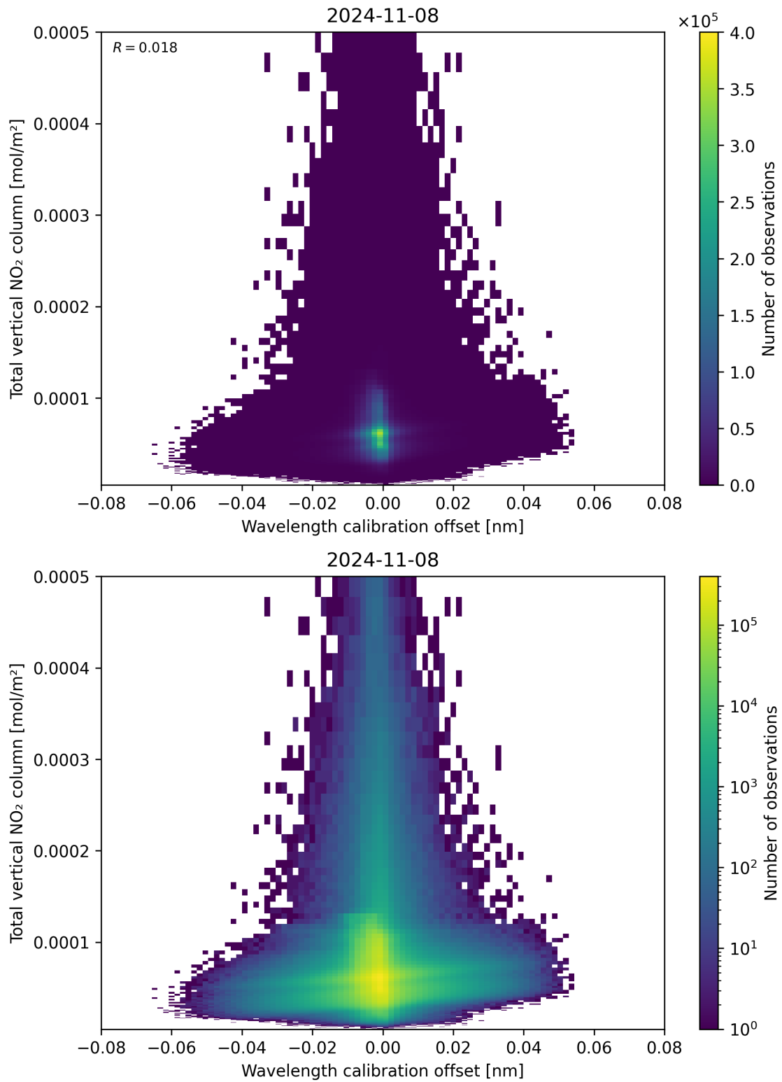
Figure 179: Scatter density plot of “Wavelength calibration offset” against “Total vertical NO 2 column” for 2024-11-07 to 2024-11-09.
