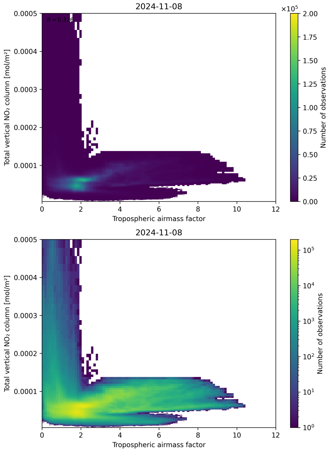
Figure 77: Scatter density plot of “Tropospheric airmass factor” against “Total vertical NO 2 column” for 2024-11-07 to 2024-11-09.
