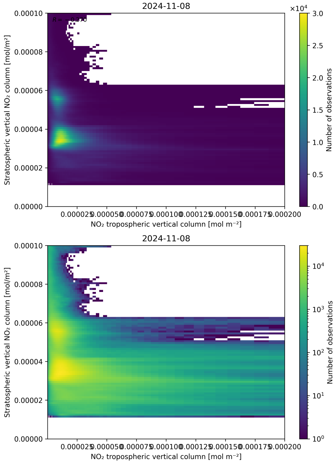
Figure 125: Scatter density plot of “NO 2 tropospheric vertical column” against “Stratospheric vertical NO 2 column” for 2024-11-07 to 2024-11-09.
