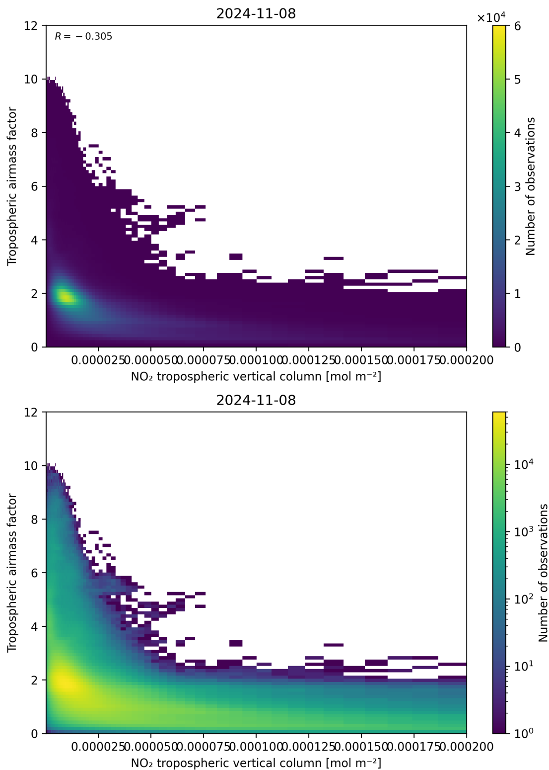
Figure 123: Scatter density plot of “NO 2 tropospheric vertical column” against “Tropospheric air mass factor” for 2024-11-07 to 2024-11-09.
