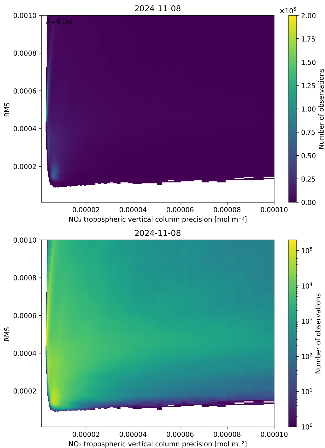
Figure 140: Scatter density plot of “NO 2 tropospheric vertical column precision” against “RMS” for 2024-11-07 to 2024-11-09.
