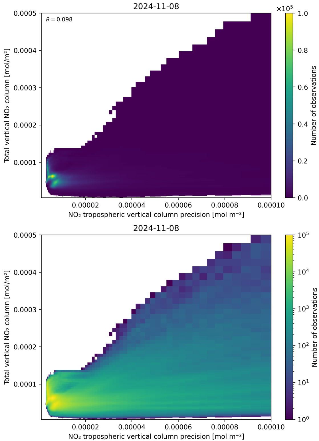
Figure 138: Scatter density plot of “NO 2 tropospheric vertical column precision” against “Total vertical NO 2 column” for 2024-11-07 to 2024-11-09.
