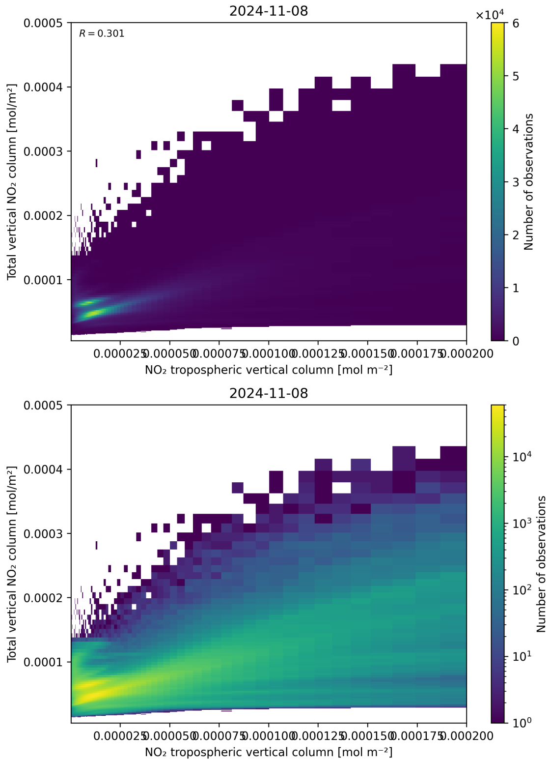
Figure 128: Scatter density plot of “NO 2 tropospheric vertical column” against “Total vertical NO 2 column” for 2024-11-07 to 2024-11-09.
