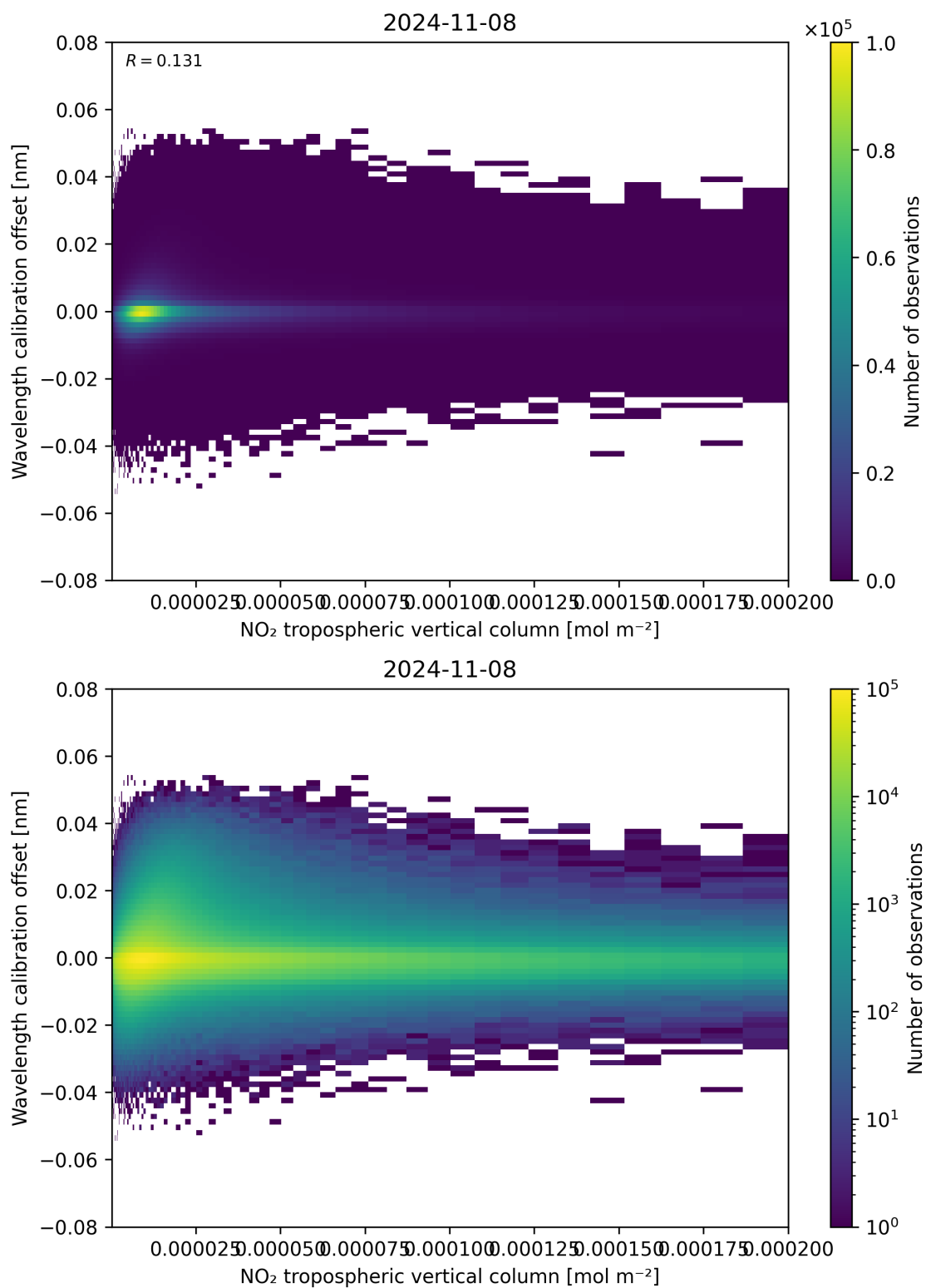
Figure 143: Scatter density plot of “NO 2 tropospheric vertical column” against “Wavelength calibration offset” for 2024-11-07 to 2024-11-09.
