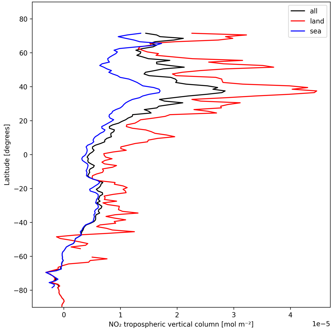
Figure 12: Zonal average of “NO 2 tropospheric vertical column” for 2024-11-07 to 2024-11-09.
