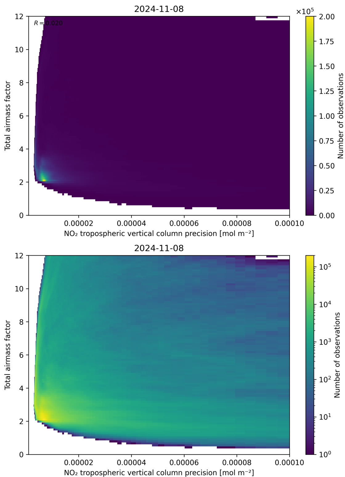
Figure 132: Scatter density plot of “NO 2 tropospheric vertical column precision” against “Total air mass factor” for 2024-11-07 to 2024-11-09.
