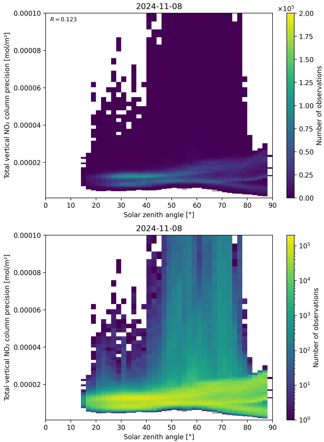
Figure 154: Scatter density plot of “Solar zenith angle” against “Total vertical NO 2 column precision” for 2024-11-07 to 2024-11-09.
