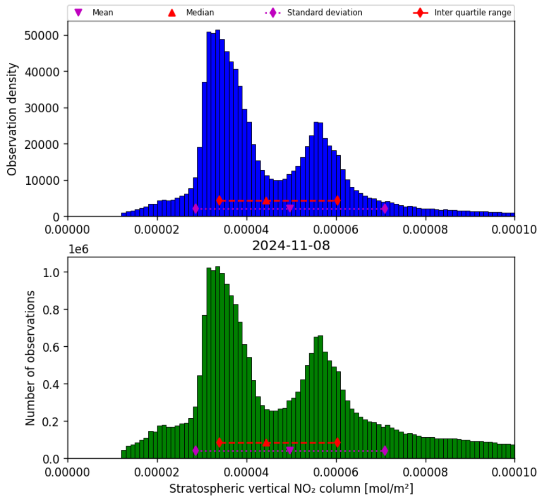
Figure 36: Histogram of “Stratospheric vertical NO 2 column” for 2024-11-07 to 2024-11-09
