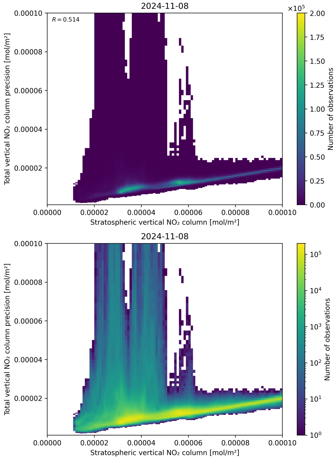
Figure 101: Scatter density plot of “Stratospheric vertical NO 2 column” against “Total vertical NO 2 column precision” for 2024-11-07 to 2024-11-09.
