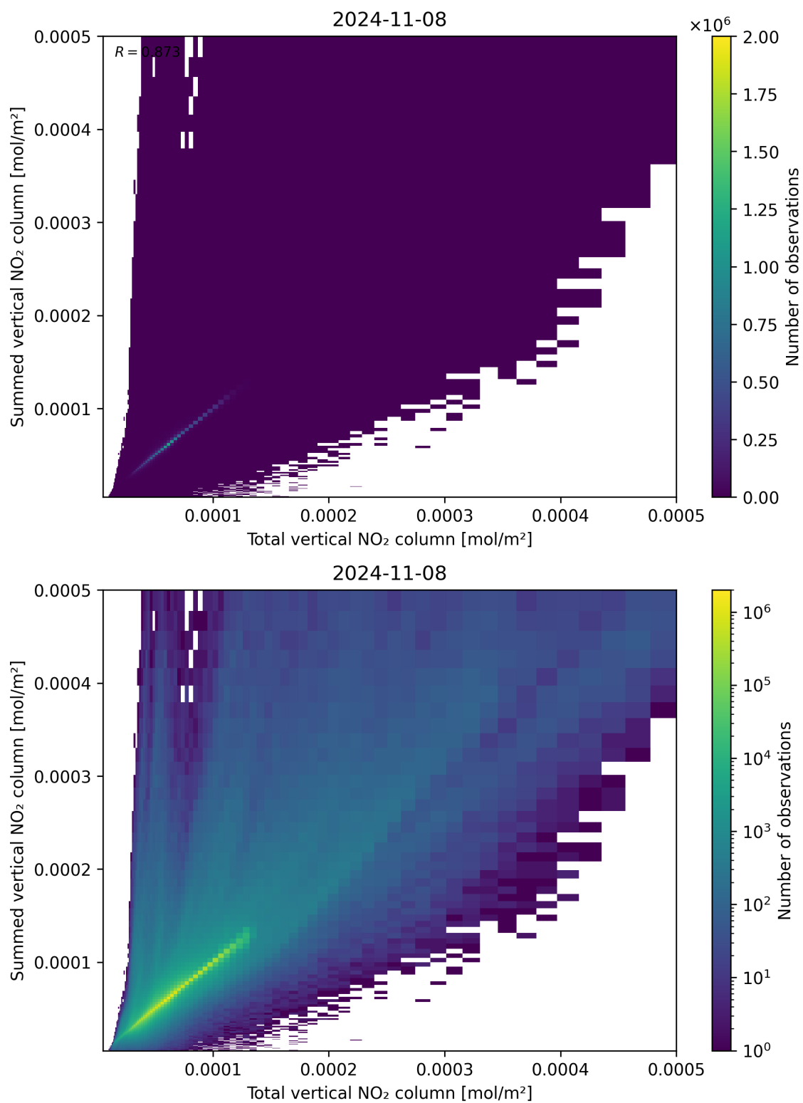
Figure 112: Scatter density plot of “Total vertical NO 2 column” against “Summed vertical NO 2 column” for 2024-11-07 to 2024-11-09.
