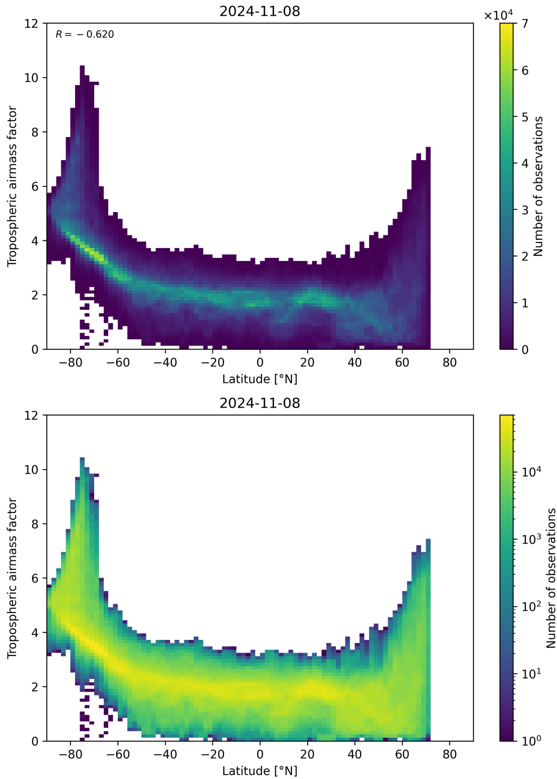
Figure 85: Scatter density plot of “Latitude” against “Tropospheric air mass factor” for 2024-11-07 to 2024-11-09.
