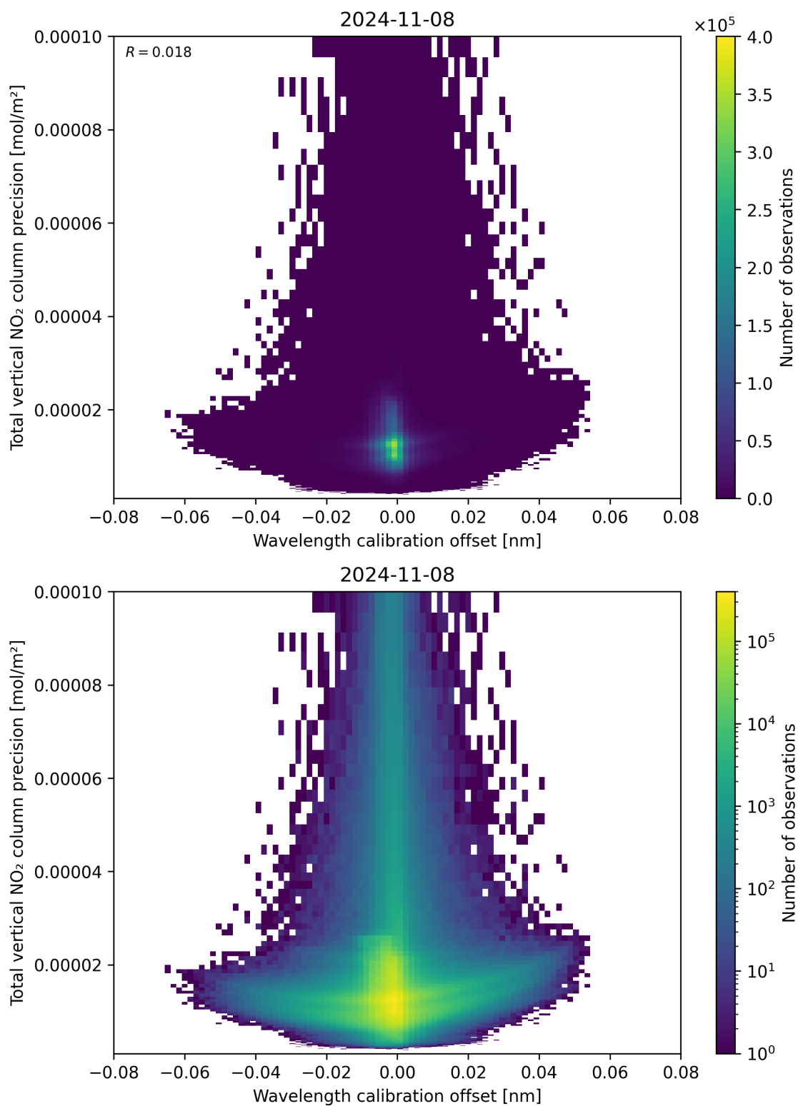
Figure 180: Scatter density plot of “Wavelength calibration offset” against “Total vertical NO 2 column precision” for 2024-11-07 to 2024-11-09.
