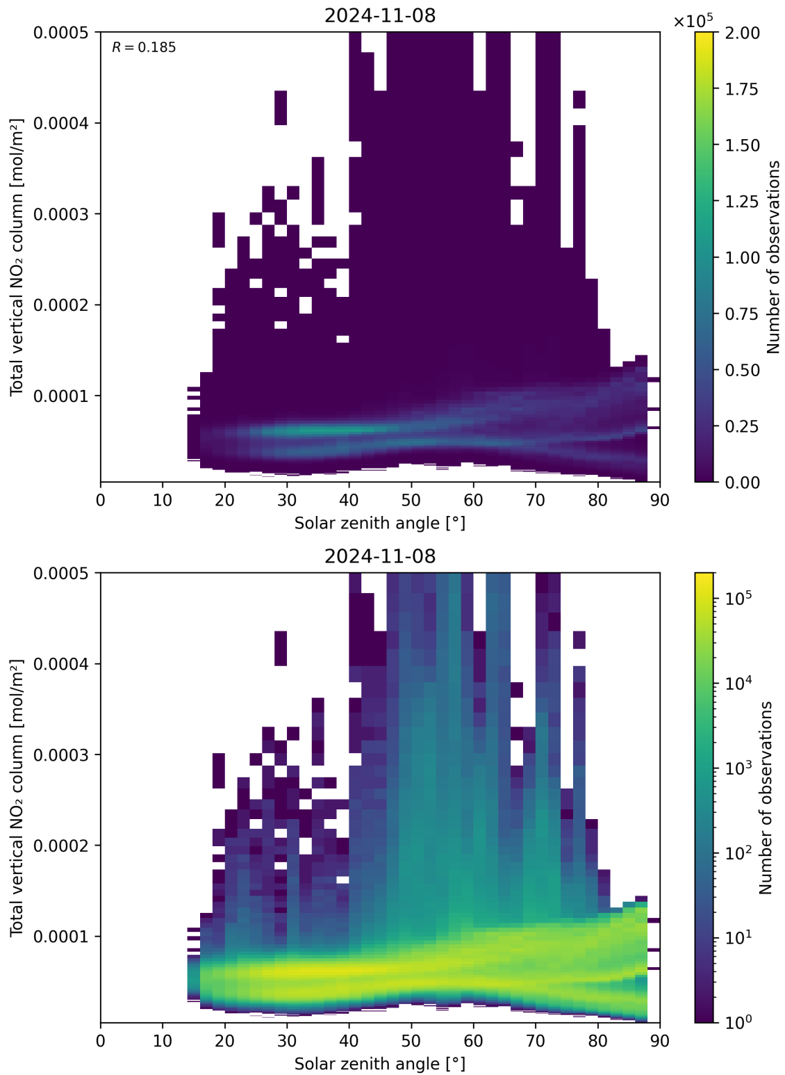
Figure 153: Scatter density plot of “Solar zenith angle” against “Total vertical NO 2 column” for 2024-11-07 to 2024-11-09.
