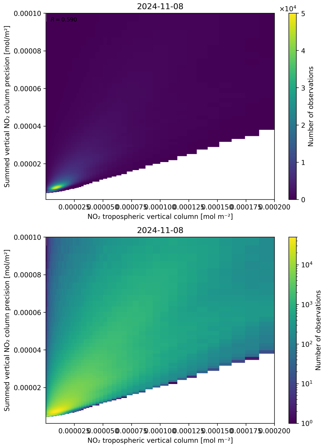
Figure 127: Scatter density plot of “NO 2 tropospheric vertical column” against “Summed vertical NO 2 column precision” for 2024-11-07 to 2024-11-09.
