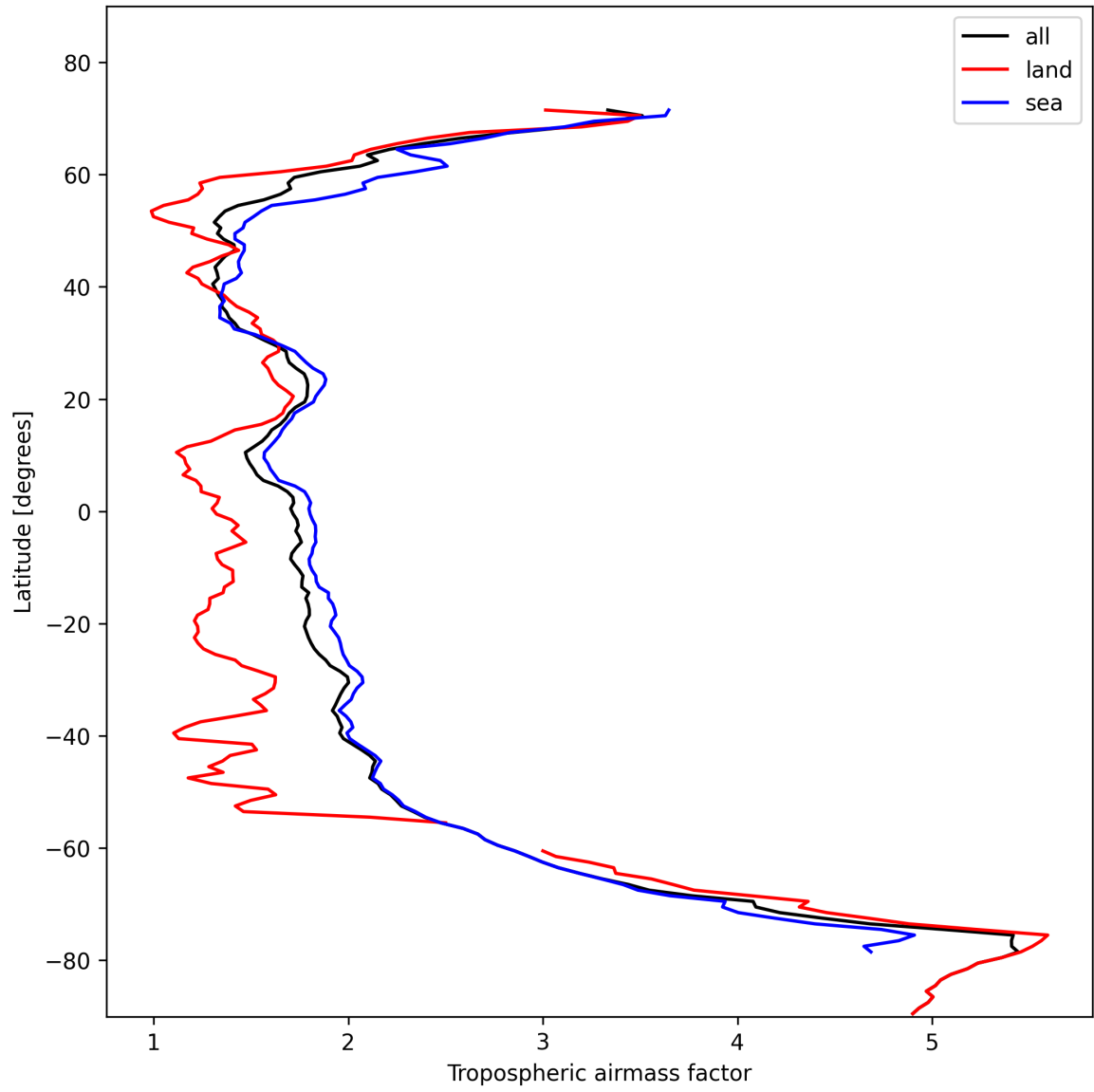
Figure 14: Zonal average of “Tropospheric airmass factor” for 2024-11-07 to 2024-11-09.
