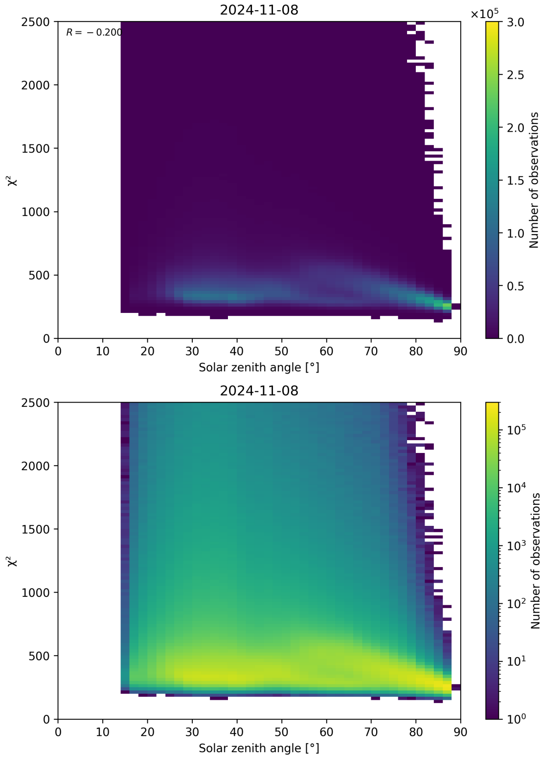
Figure 148: Scatter density plot of “Solar zenith angle” against “ \chi^2 ” for 2024-11-07 to 2024-11-09.
