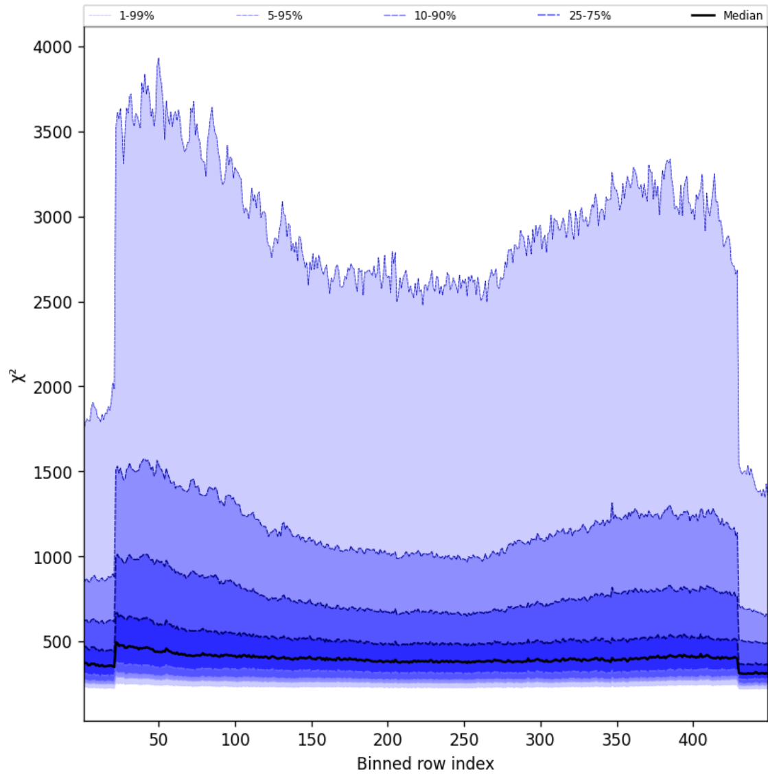
Figure 59: Along track statistics of “ \chi^2 ” for 2024-11-07 to 2024-11-09
