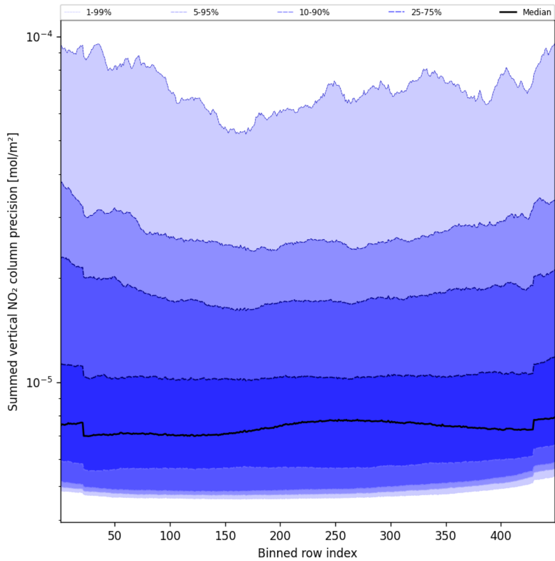
Figure 58: Along track statistics of “Summed vertical NO 2 column precision” for 2024-11-07 to 2024-11-09
