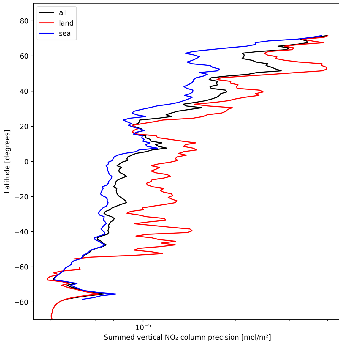
Figure 24: Zonal average of “Summed vertical NO 2 column precision” for 2024-11-07 to 2024-11-09.
