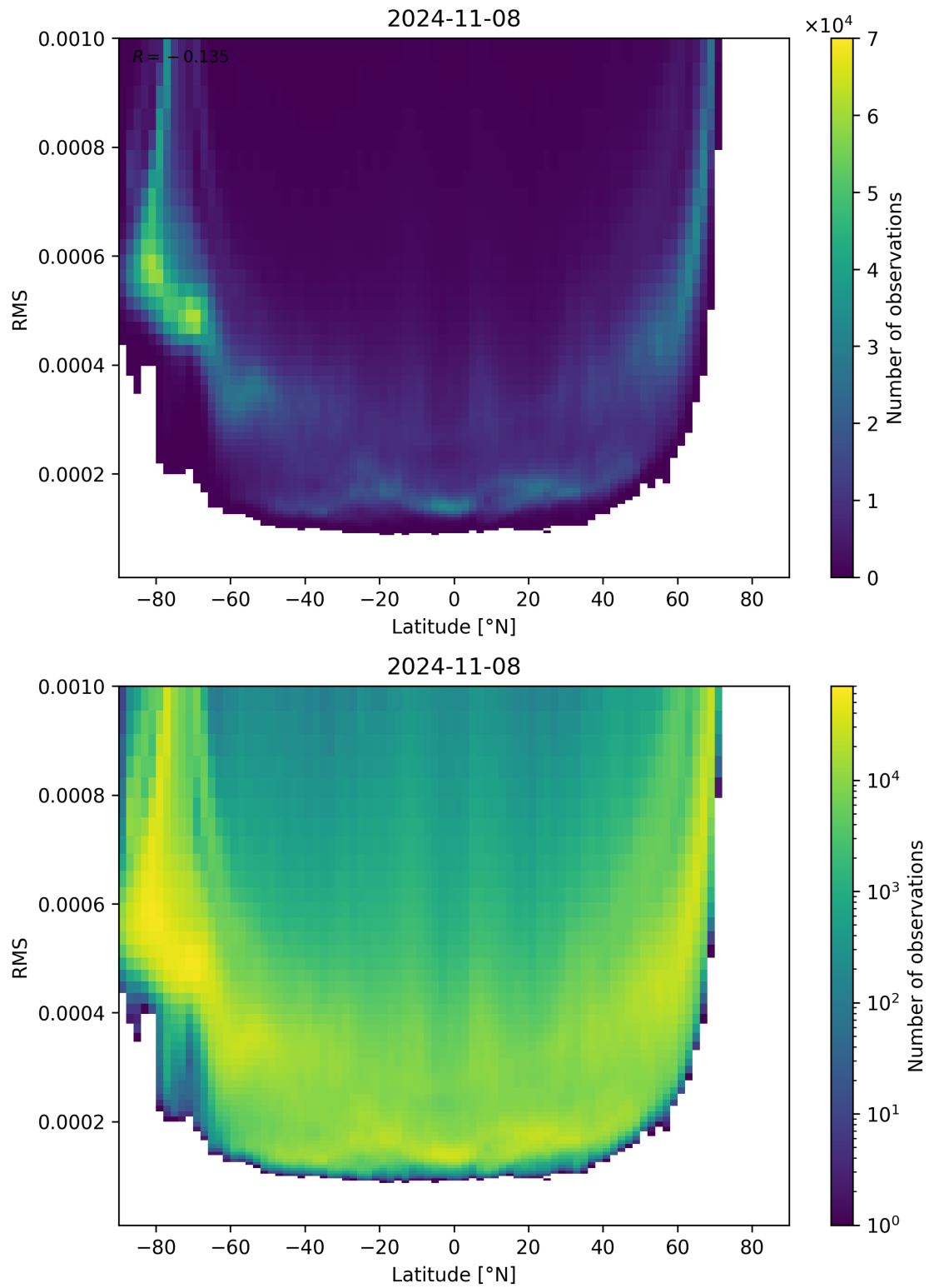
Figure 94: Scatter density plot of “Latitude” against “RMS” for 2024-11-07 to 2024-11-09.
