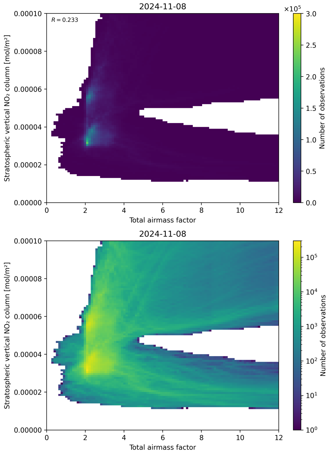
Figure 64: Scatter density plot of “Total airmass factor” against “Stratospheric vertical NO 2 column” for 2024-11-07 to 2024-11-09.
