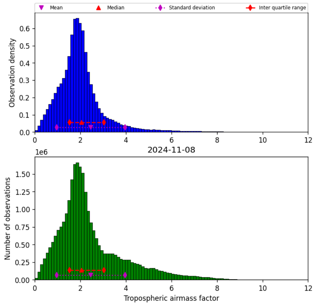
Figure 31: Histogram of “Tropospheric airmass factor” for 2024-11-07 to 2024-11-09
