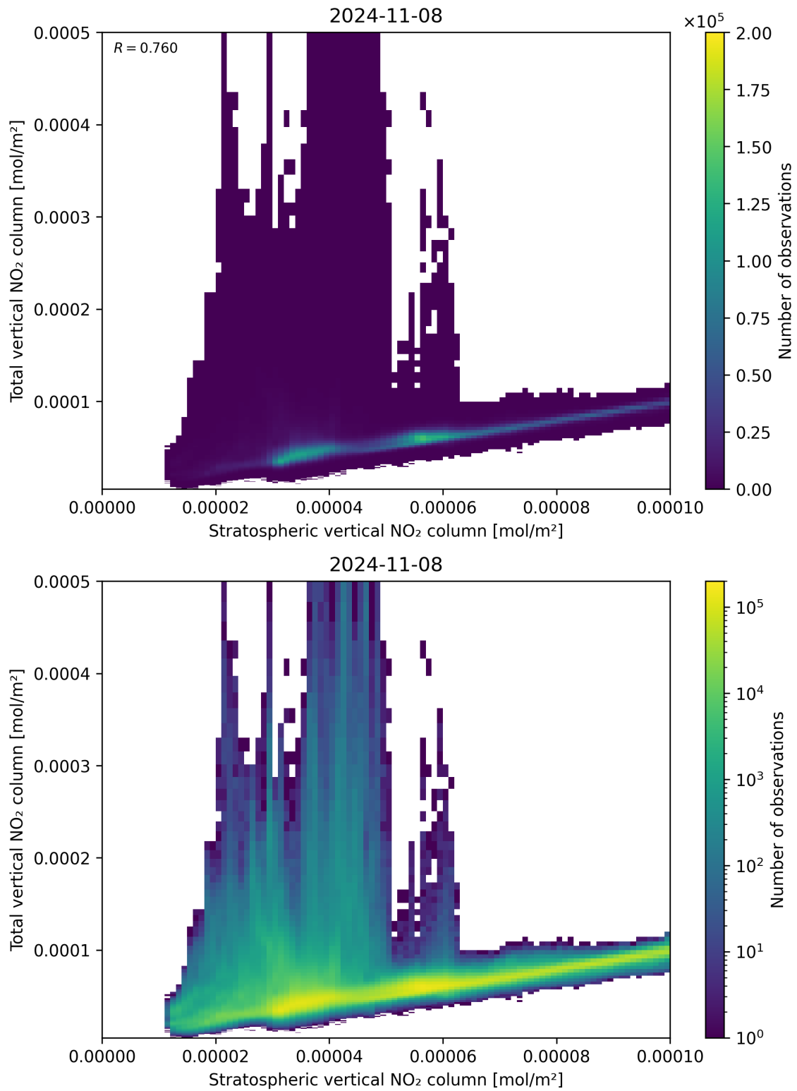
Figure 100: Scatter density plot of “Stratospheric vertical NO 2 column” against “Total vertical NO 2 column” for 2024-11-07 to 2024-11-09.
