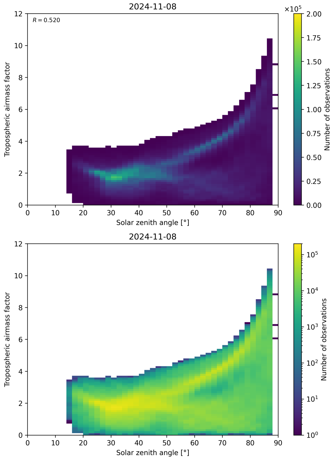
Figure 147: Scatter density plot of “Solar zenith angle” against “Tropospheric airmass factor” for 2024-11-07 to 2024-11-09.
