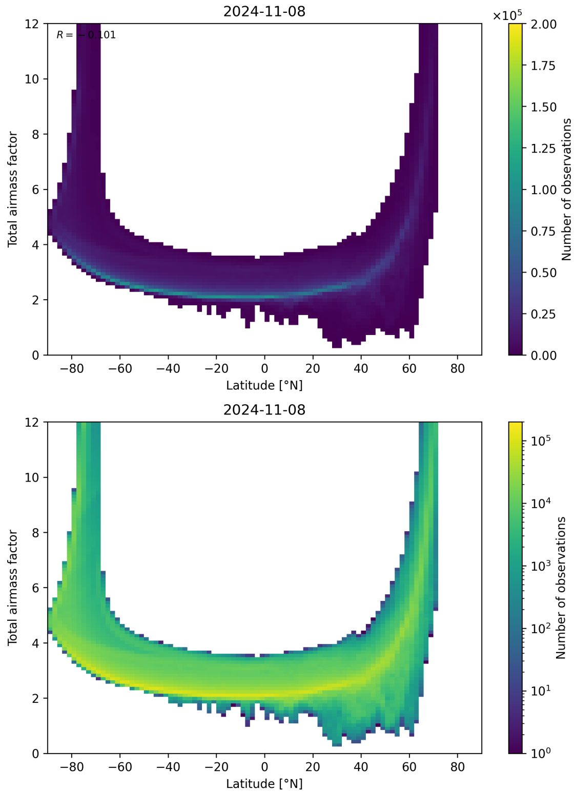
Figure 84: Scatter density plot of “Latitude” against “Total airmass factor” for 2024-11-07 to 2024-11-09.
