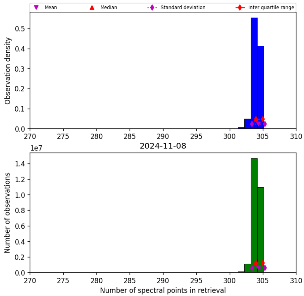
Figure 33: Histogram of “Number of spectral points in retrieval” for 2024-11-07 to 2024-11-09
