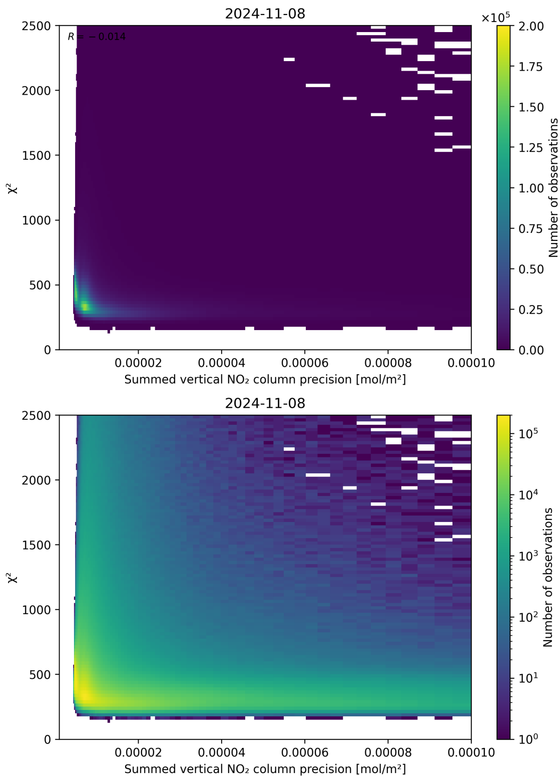
Figure 107: Scatter density plot of “Summed vertical NO 2 column precision” against “ \chi^2 ” for 2024-11-07 to 2024-11-09.
