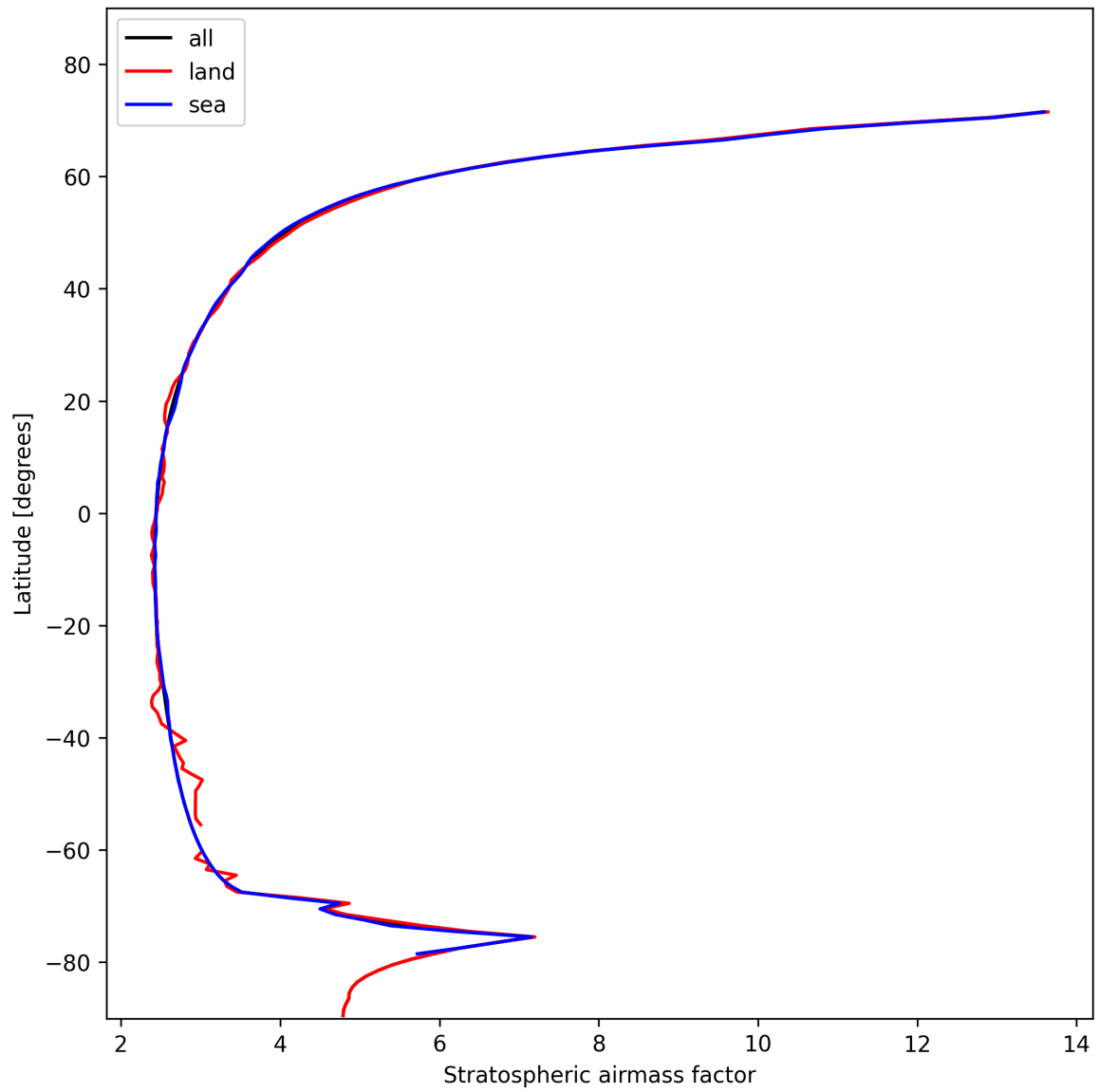
Figure 27: Zonal average of “Stratospheric air mass factor” for 2024-11-07 to 2024-11-09.
