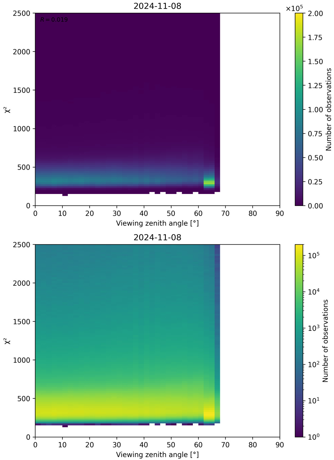
Figure 162: Scatter density plot of “Viewing zenith angle” against “ \chi^2 ” for 2024-11-07 to 2024-11-09.
