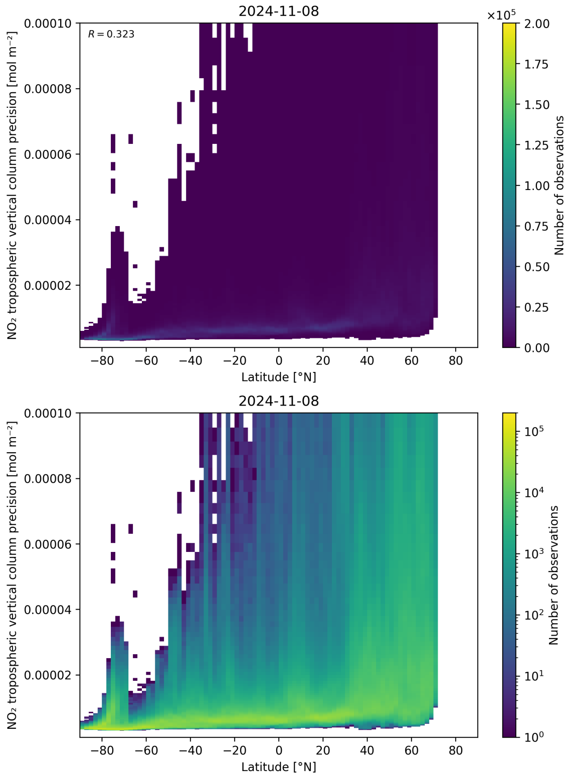
Figure 93: Scatter density plot of “Latitude” against “NO 2 tropospheric vertical column precision” for 2024-11-07 to 2024-11-09.
