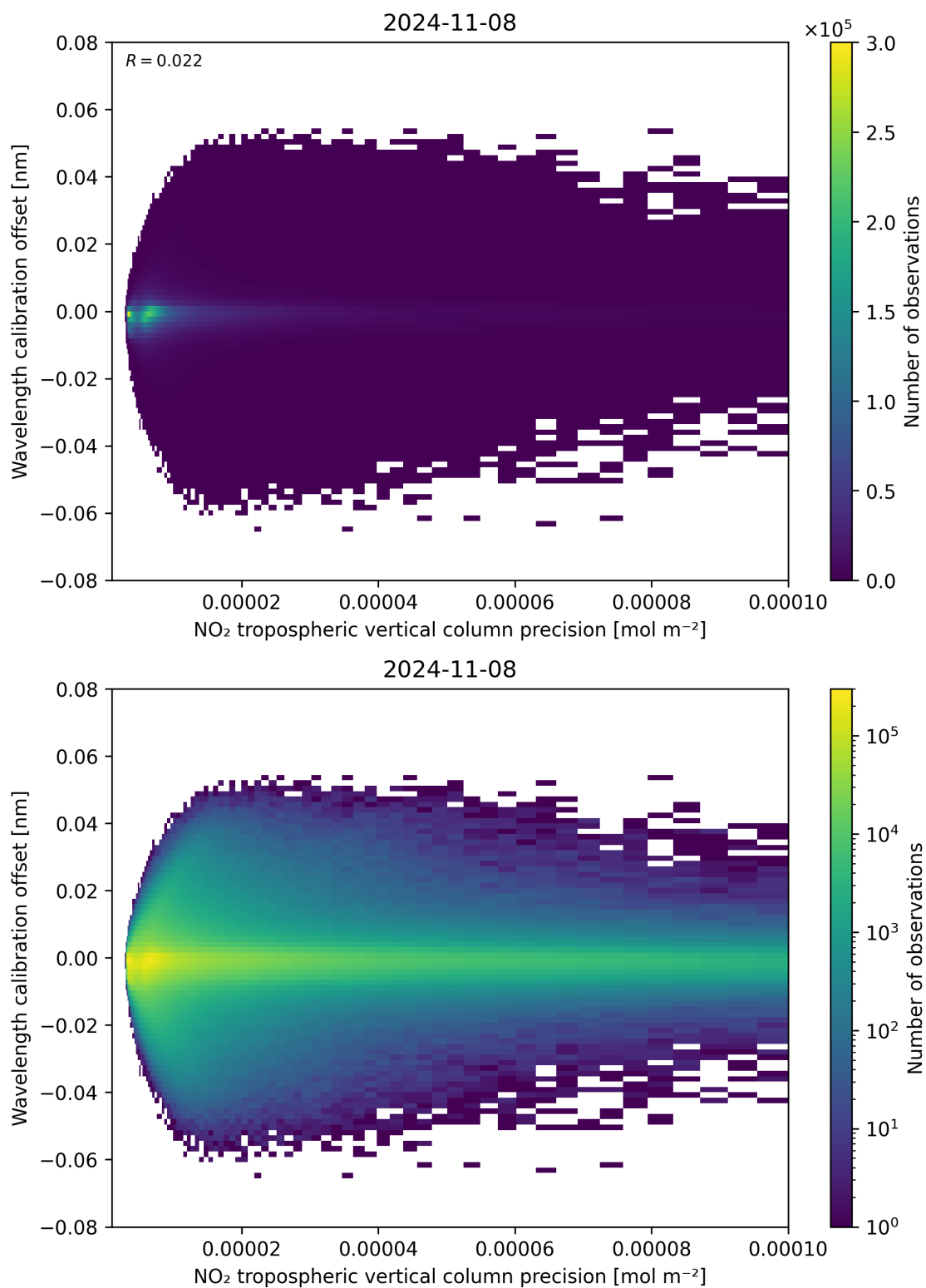
Figure 141: Scatter density plot of “NO 2 tropospheric vertical column precision” against “Wavelength calibration offset” for 2024-11-07 to 2024-11-09.
