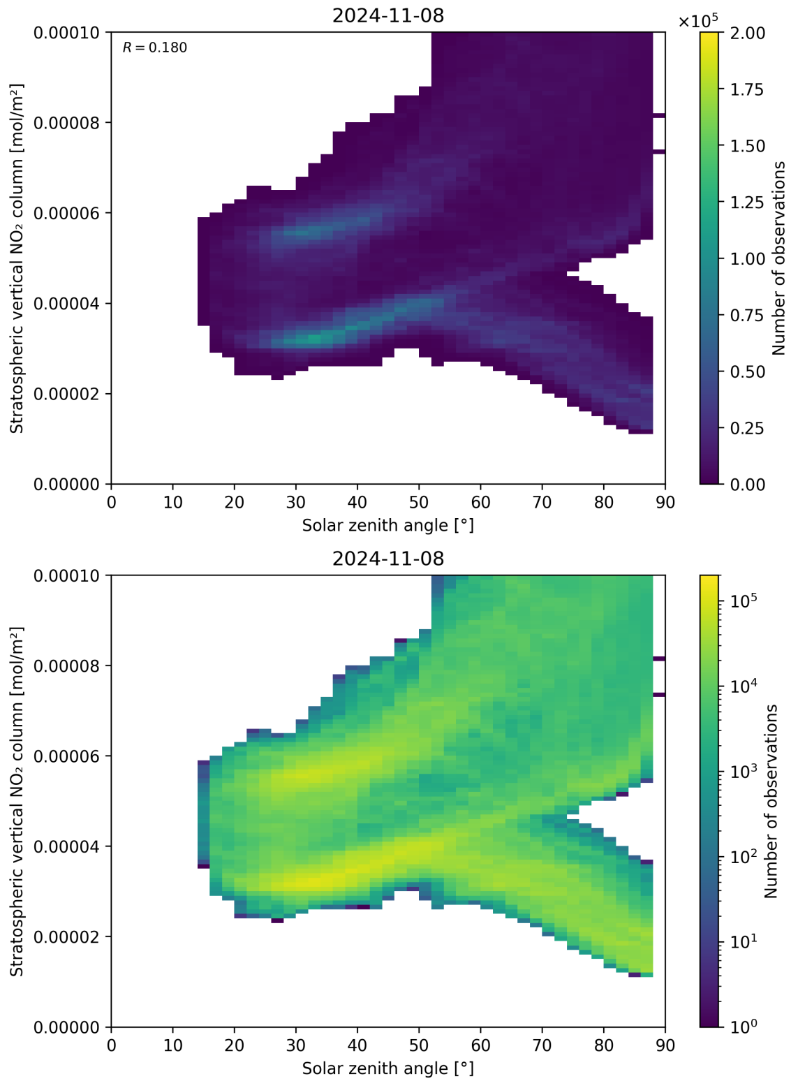
Figure 150: Scatter density plot of “Solar zenith angle” against “Stratospheric vertical \text{NO}_2 column” for 2024-11-07 to 2024-11-09.
