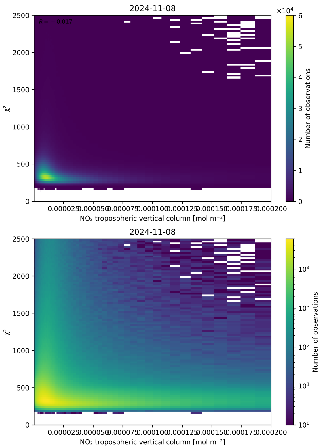
Figure 124: Scatter density plot of “NO 2 tropospheric vertical column” against “ \chi^2 ” for 2024-11-07 to 2024-11-09.
