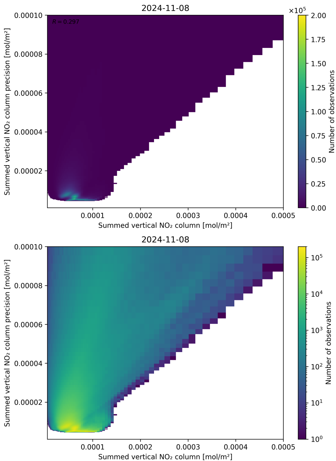
Figure 105: Scatter density plot of “Summed vertical NO 2 column” against “Summed vertical NO 2 column precision” for 2024-11-07 to 2024-11-09.
