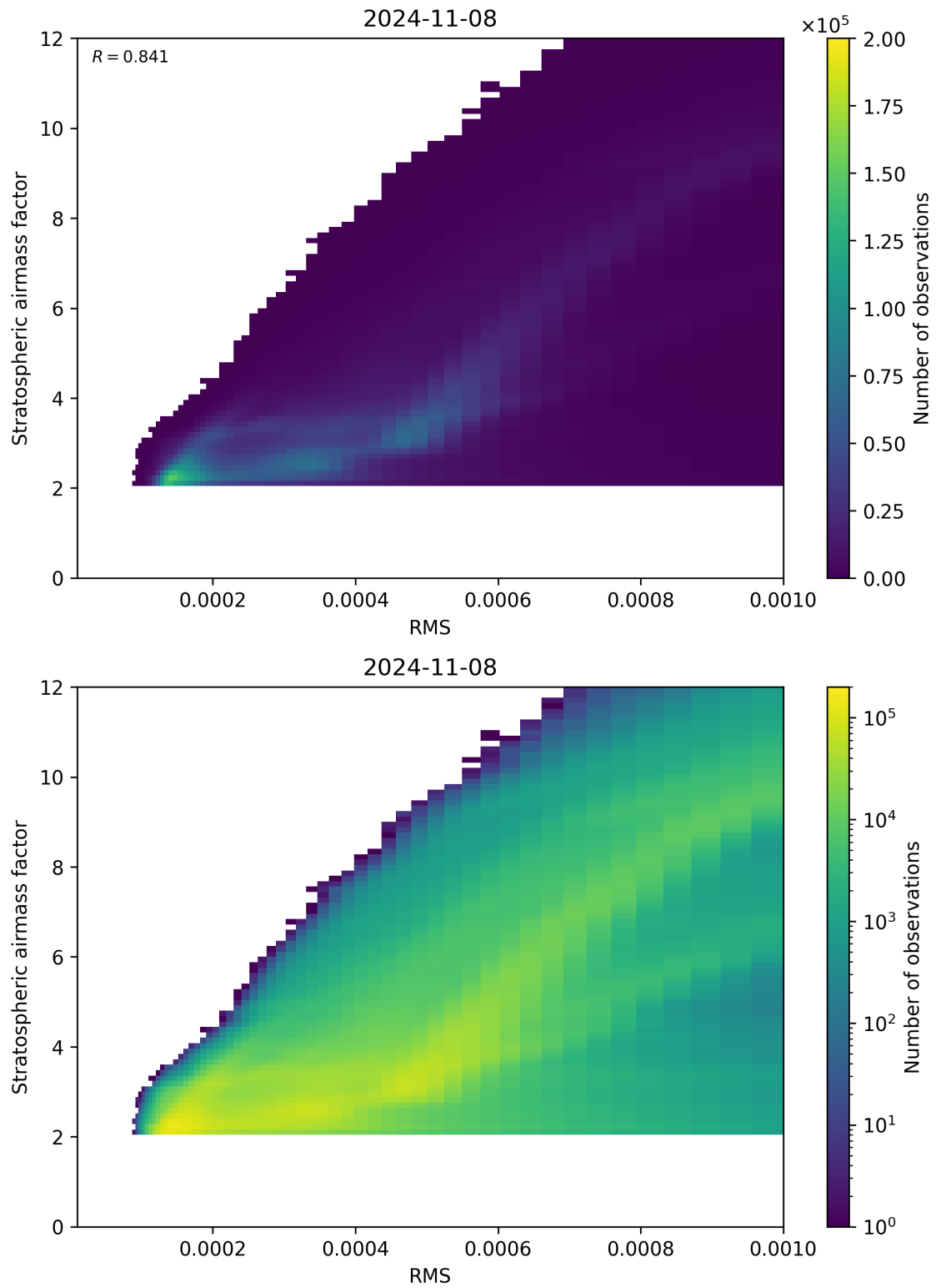
Figure 144: Scatter density plot of “RMS” against “Stratospheric airmass factor” for 2024-11-07 to 2024-11-09.
