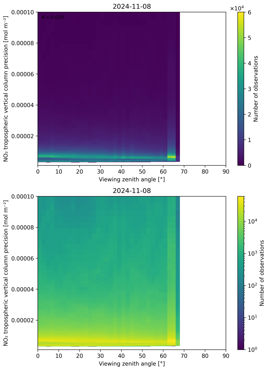
Figure 170: Scatter density plot of “Viewing zenith angle” against “NO 2 tropospheric vertical column precision” for 2024-11-07 to 2024-11-09.
