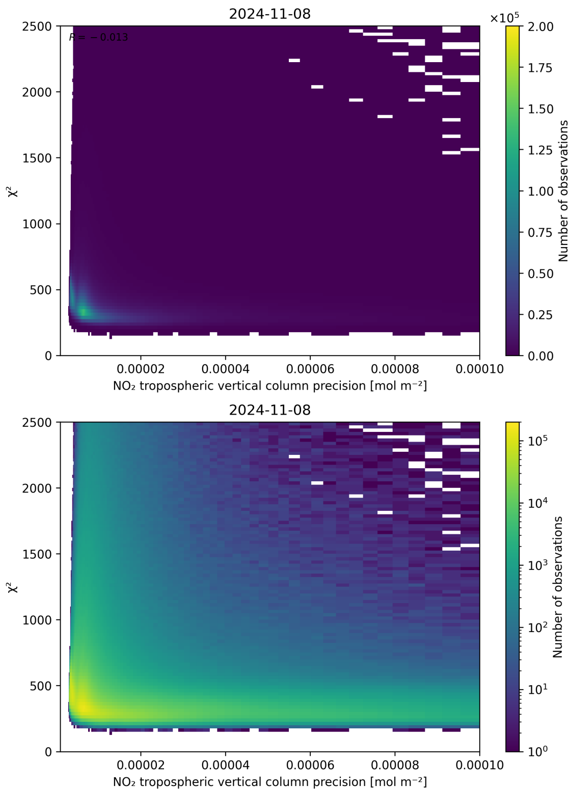
Figure 134: Scatter density plot of “NO 2 tropospheric vertical column precision” against “ \chi^2 ” for 2024-11-07 to 2024-11-09.
