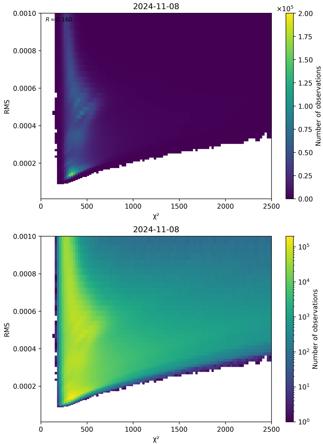
Figure 82: Scatter density plot of “ \chi^2 ” against “RMS” for 2024-11-07 to 2024-11-09.
