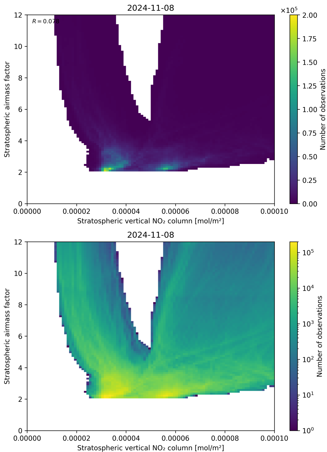
Figure 96: Scatter density plot of “Stratospheric vertical NO 2 column” against “Stratospheric airmass factor” for 2024-11-07 to 2024-11-09.
