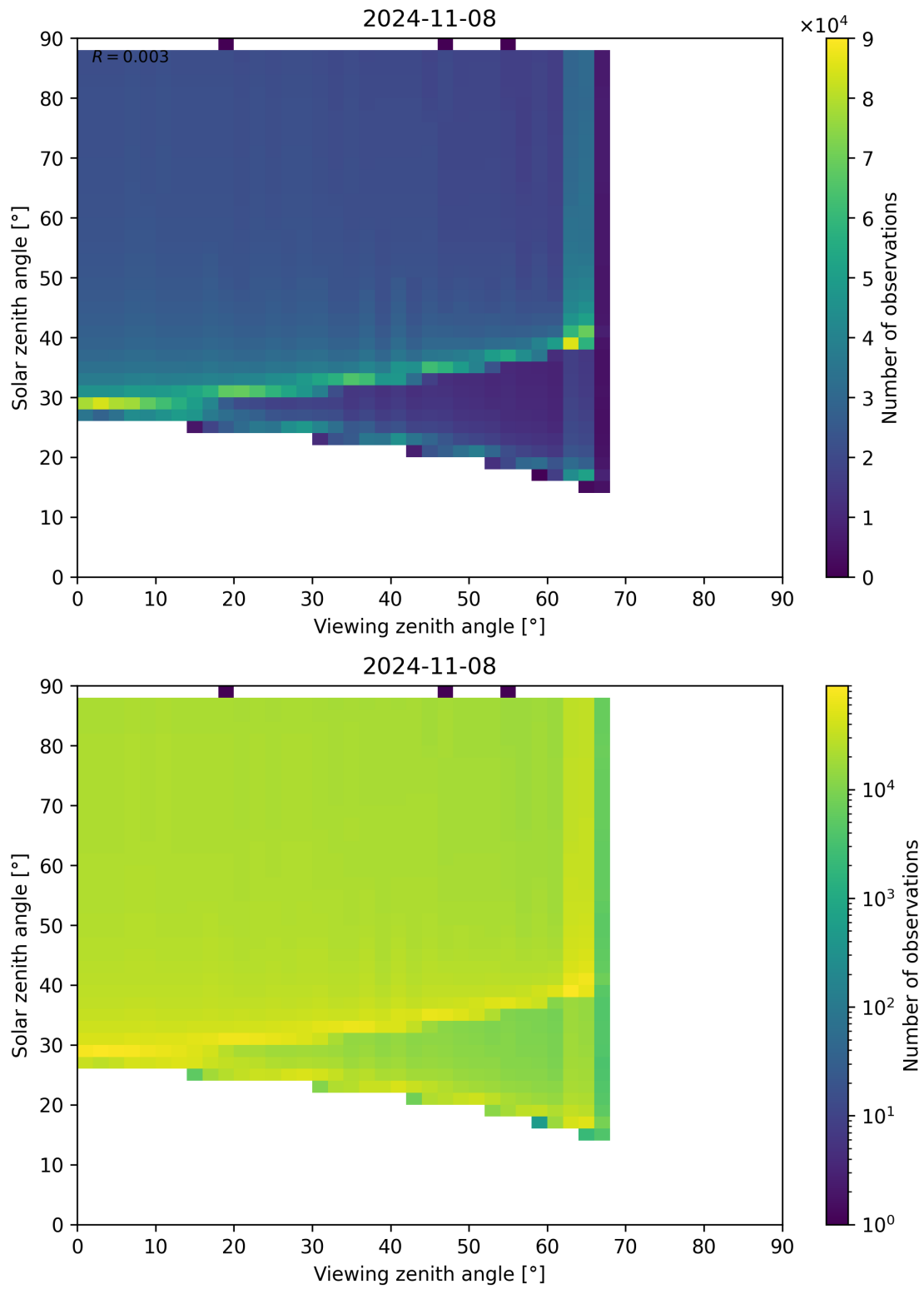
Figure 172: Scatter density plot of “Viewing zenith angle” against “Solar zenith angle” for 2024-11-07 to 2024-11-09.
