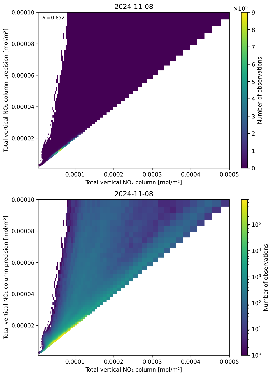
Figure 114: Scatter density plot of “Total vertical NO 2 column” against “Total vertical NO 2 column precision” for 2024-11-07 to 2024-11-09.
