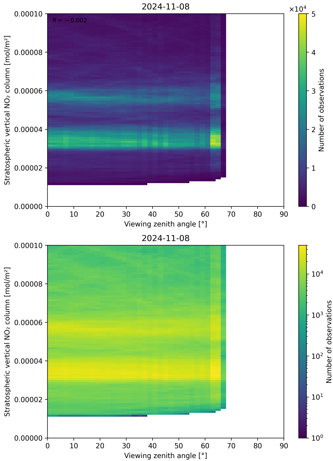
Figure 164: Scatter density plot of “Viewing zenith angle” against “Stratospheric vertical NO 2 column” for 2024-11-07 to 2024-11-09.
