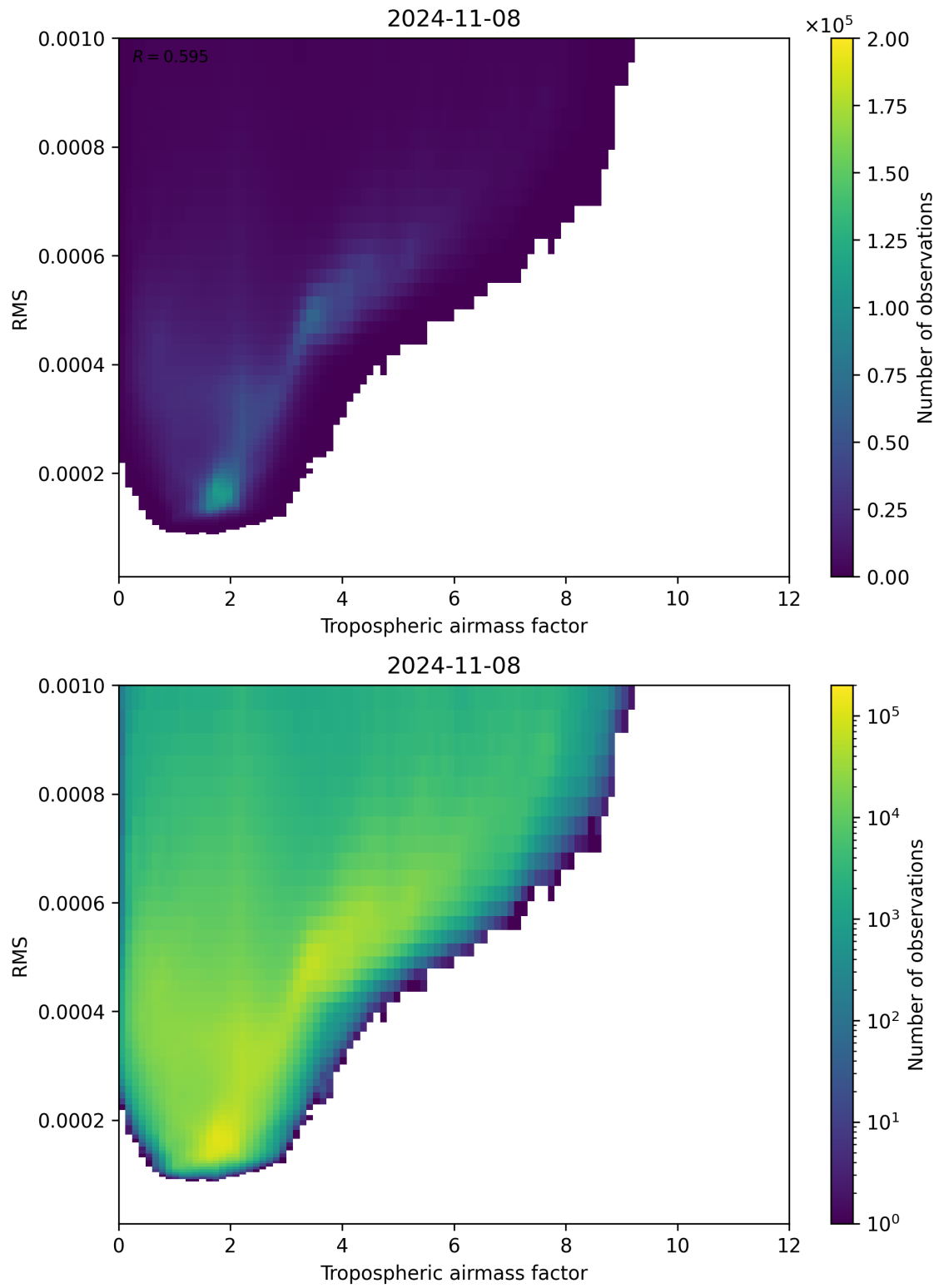
Figure 79: Scatter density plot of “Tropospheric airmass factor” against “RMS” for 2024-11-07 to 2024-11-09.
