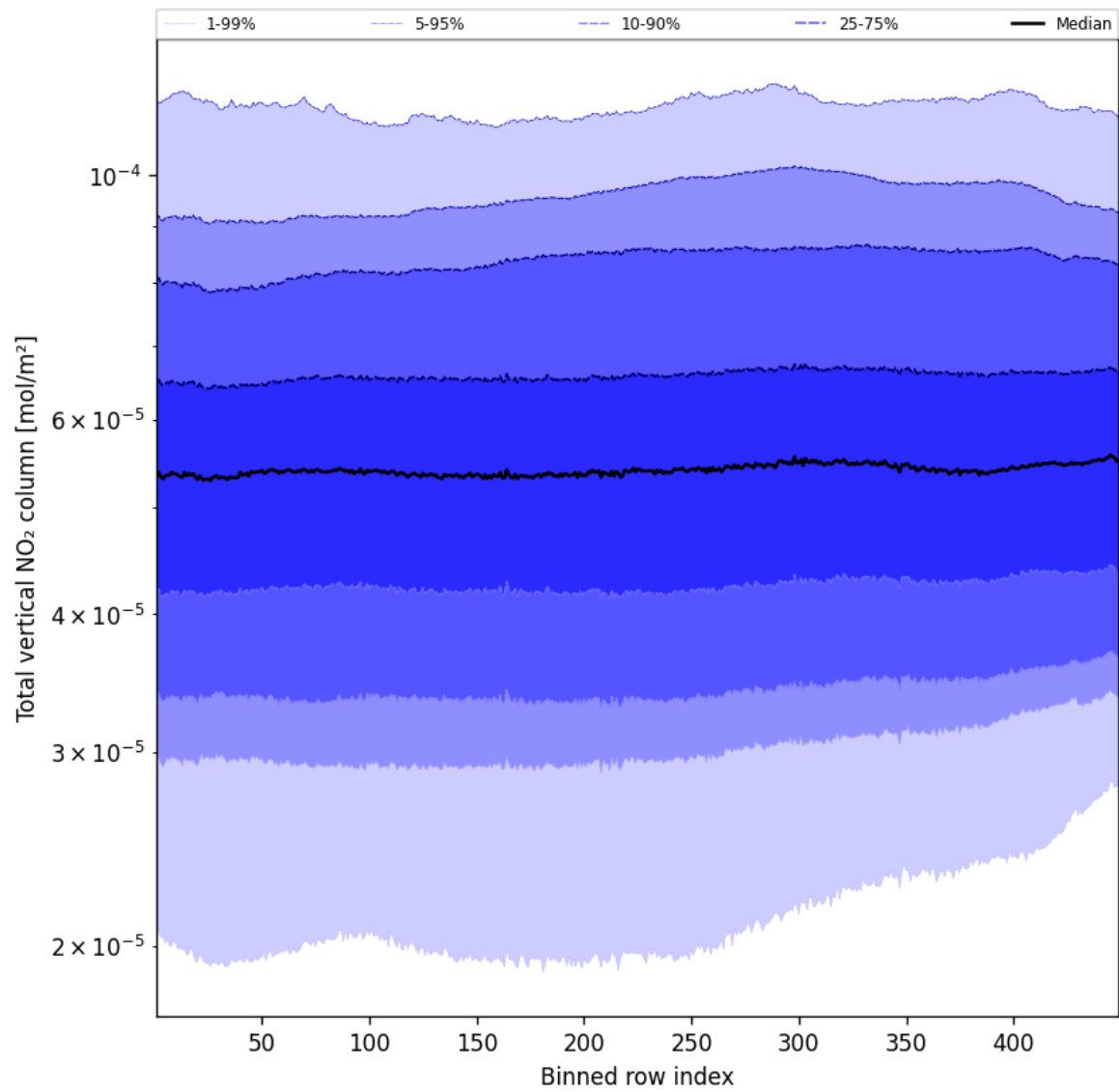
Figure 55: Along track statistics of “Total vertical NO 2 column” for 2024-11-07 to 2024-11-09
