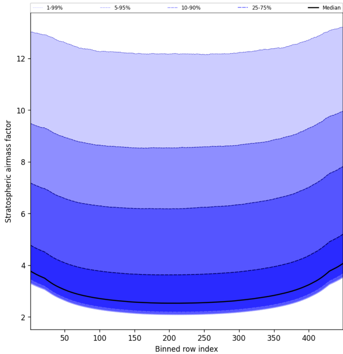
Figure 61: Along track statistics of “Stratospheric air mass factor” for 2024-11-07 to 2024-11-09
