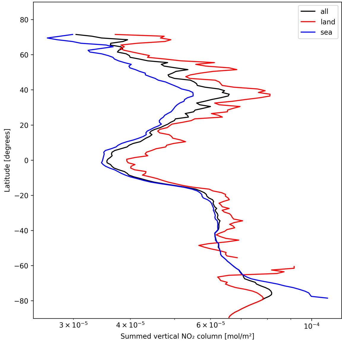
Figure 23: Zonal average of “Summed vertical NO 2 column” for 2024-11-07 to 2024-11-09.
