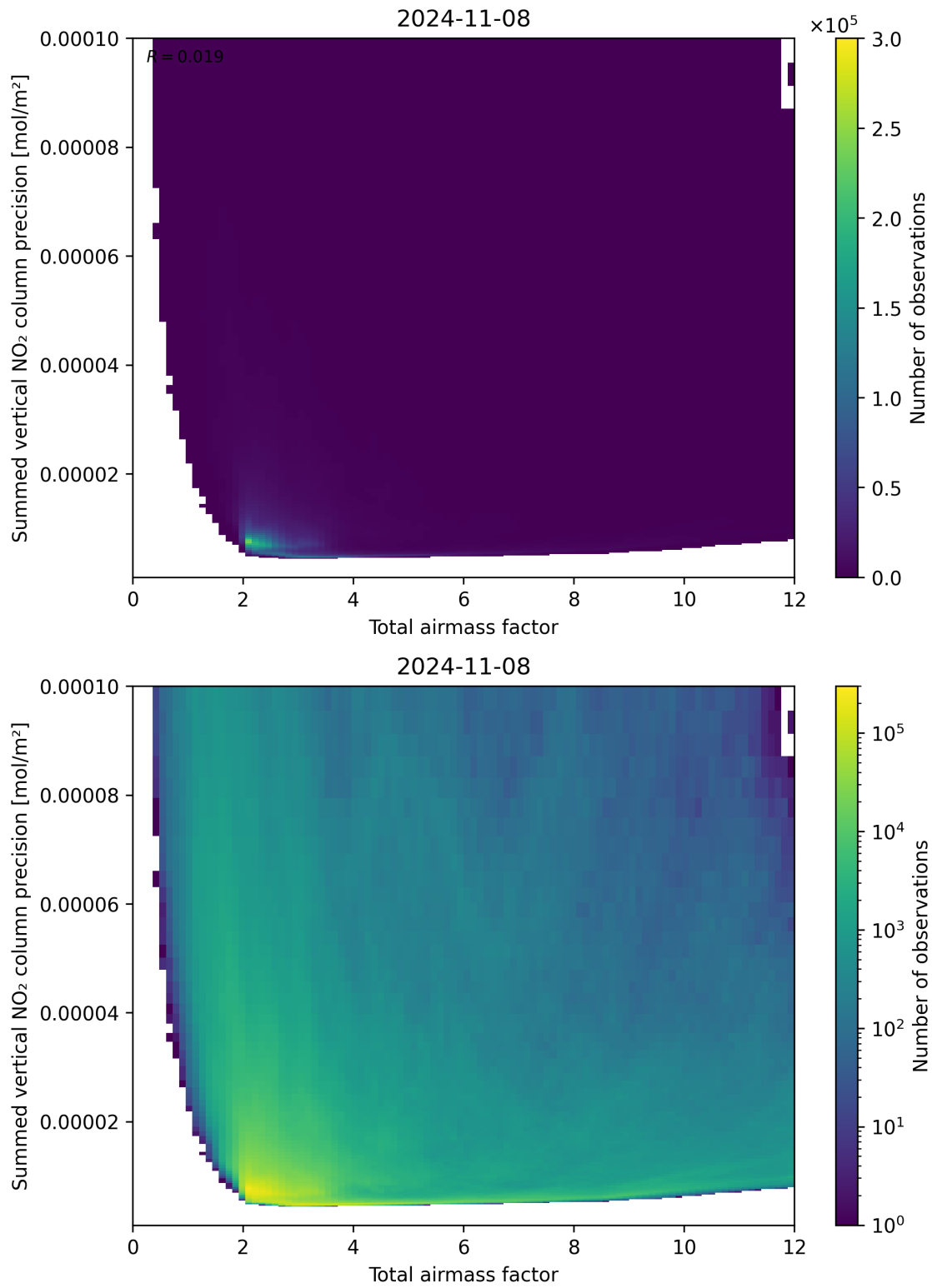
Figure 66: Scatter density plot of “Total airmass factor” against “Summed vertical NO 2 column precision” for 2024-11-07 to 2024-11-09.
