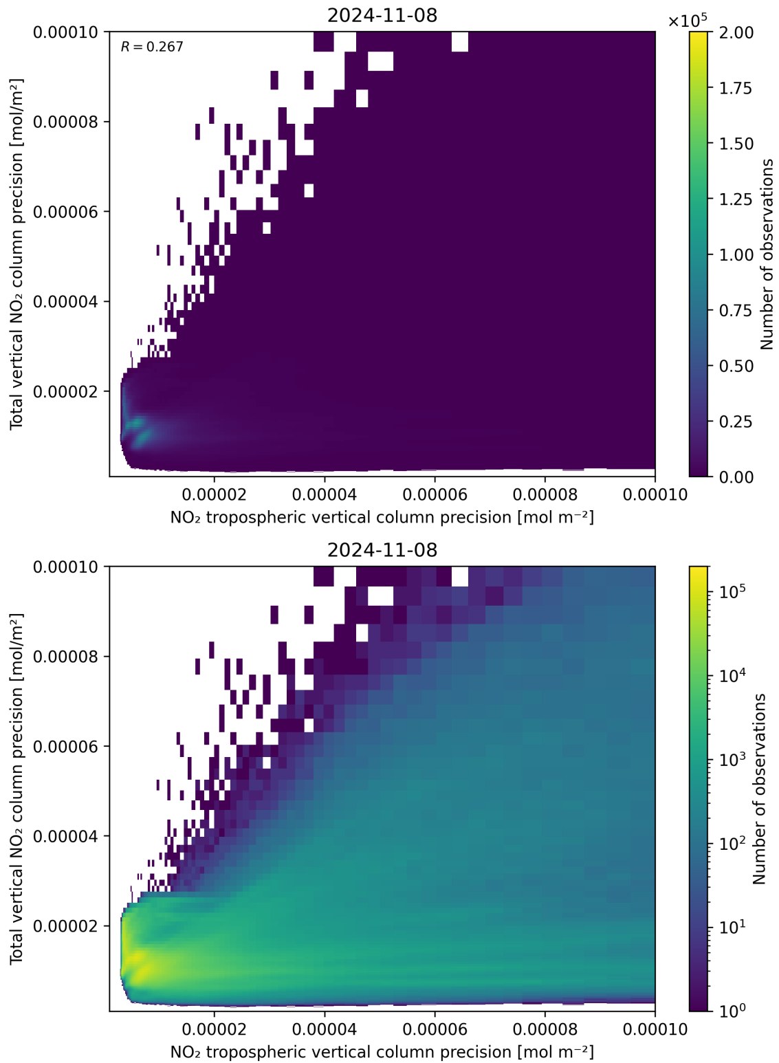
Figure 139: Scatter density plot of “NO 2 tropospheric vertical column precision” against “Total vertical NO 2 column precision” for 2024-11-07 to 2024-11-09.
