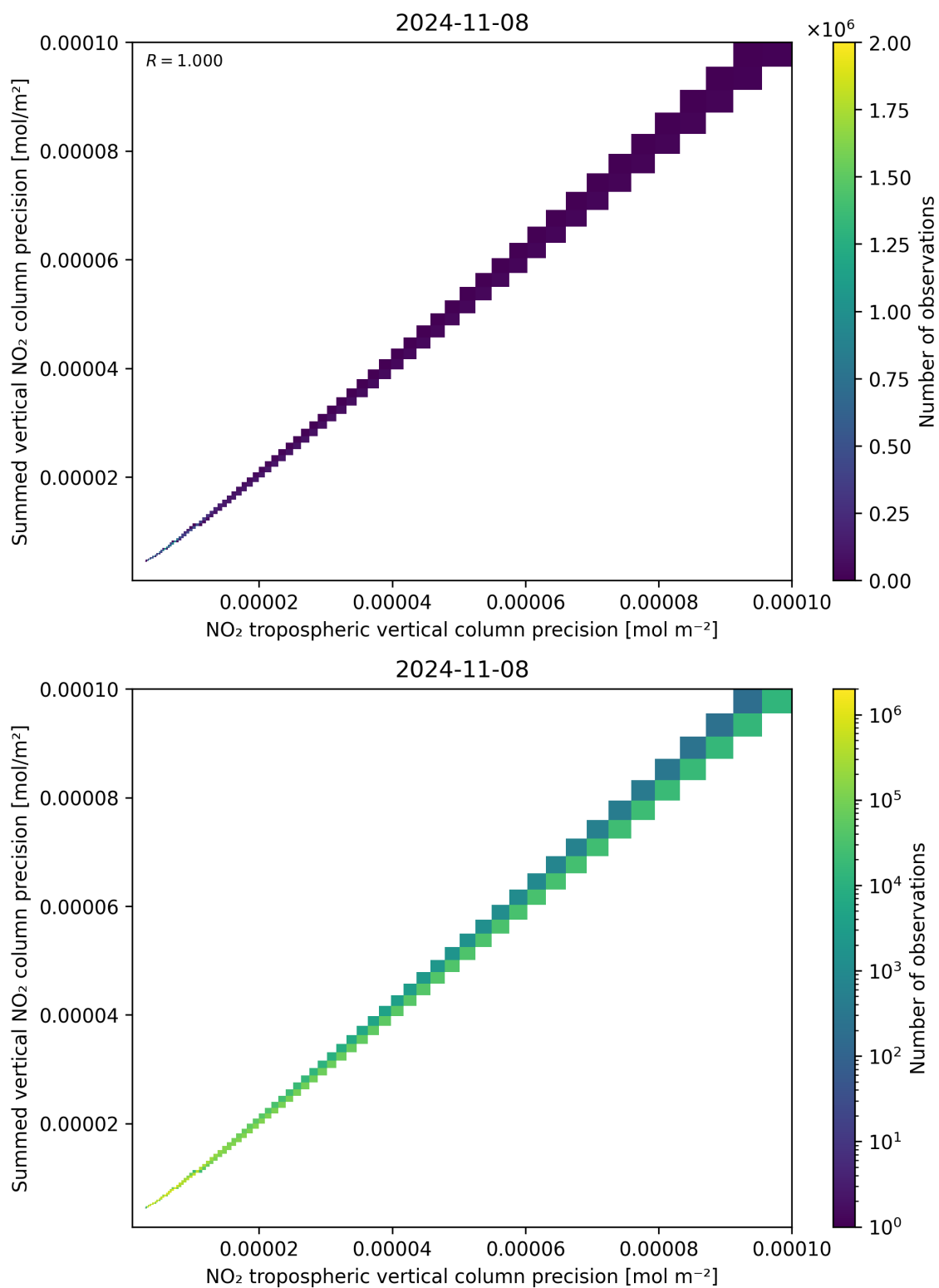
Figure 137: Scatter density plot of “NO 2 tropospheric vertical column precision” against “Summed vertical NO 2 column precision” for 2024-11-07 to 2024-11-09.
