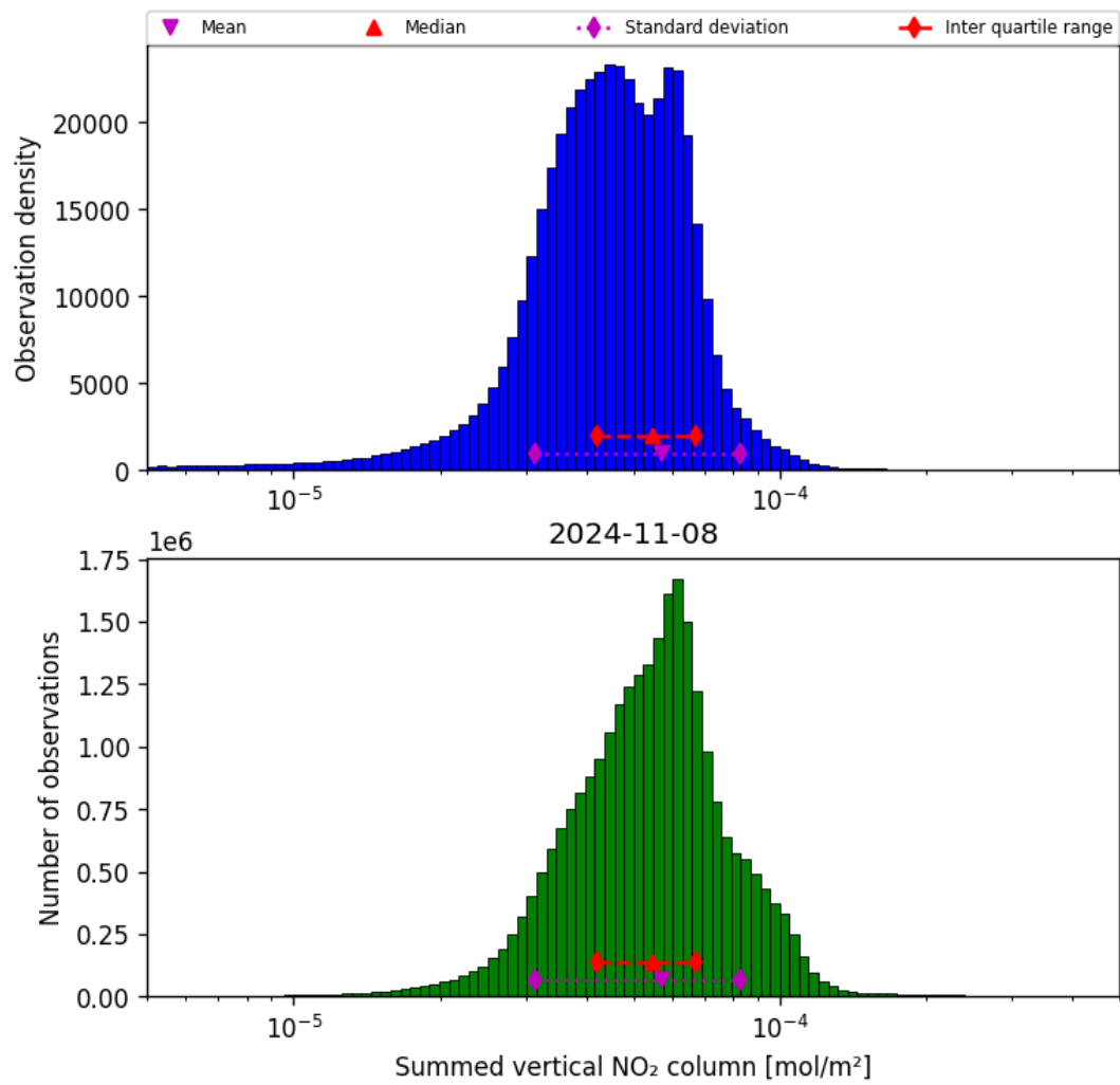
Figure 40: Histogram of “Summed vertical NO 2 column” for 2024-11-07 to 2024-11-09
