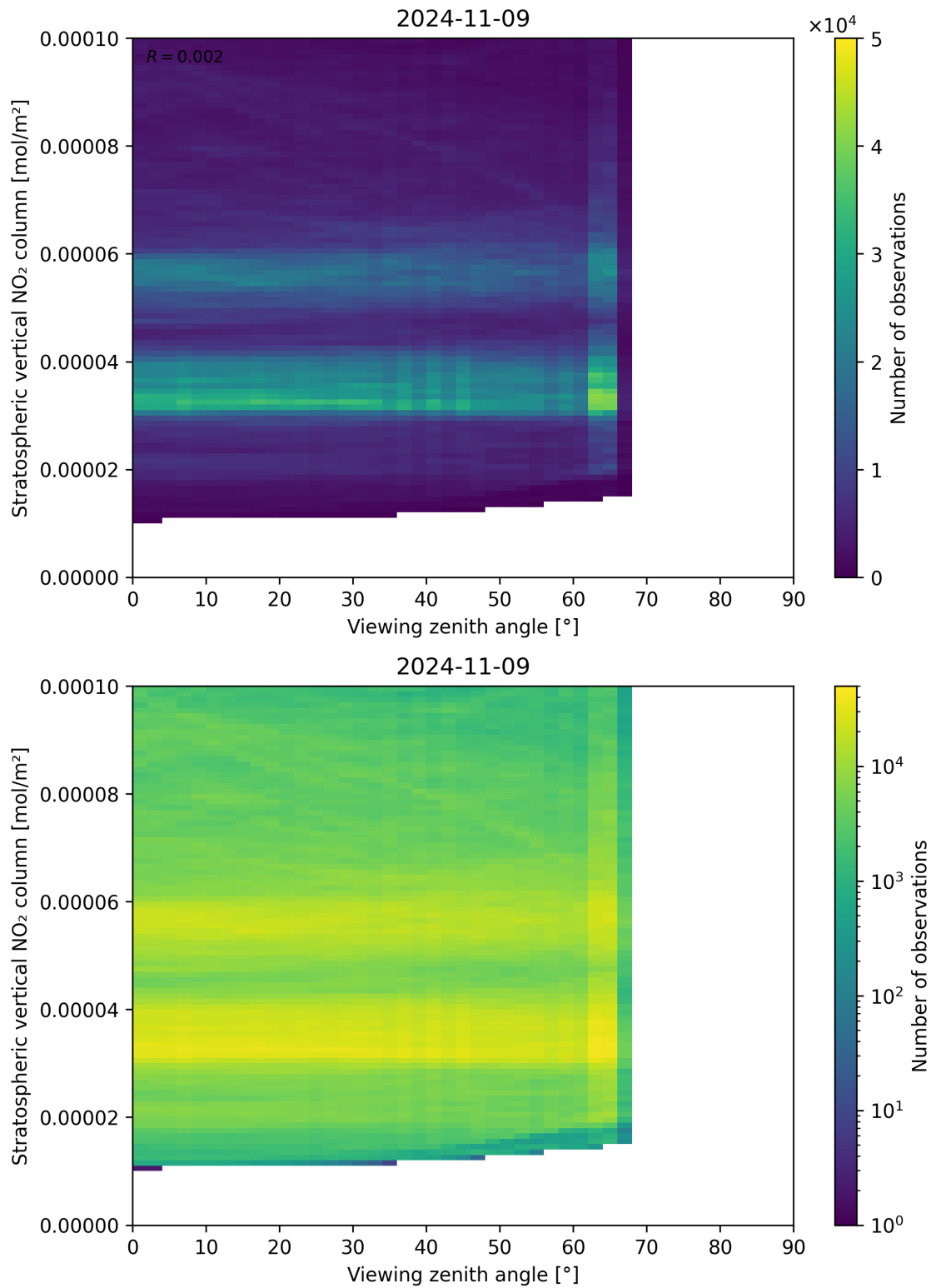
Figure 164: Scatter density plot of “Viewing zenith angle” against “Stratospheric vertical NO 2 column” for 2024-11-09 to 2024-11-10.
