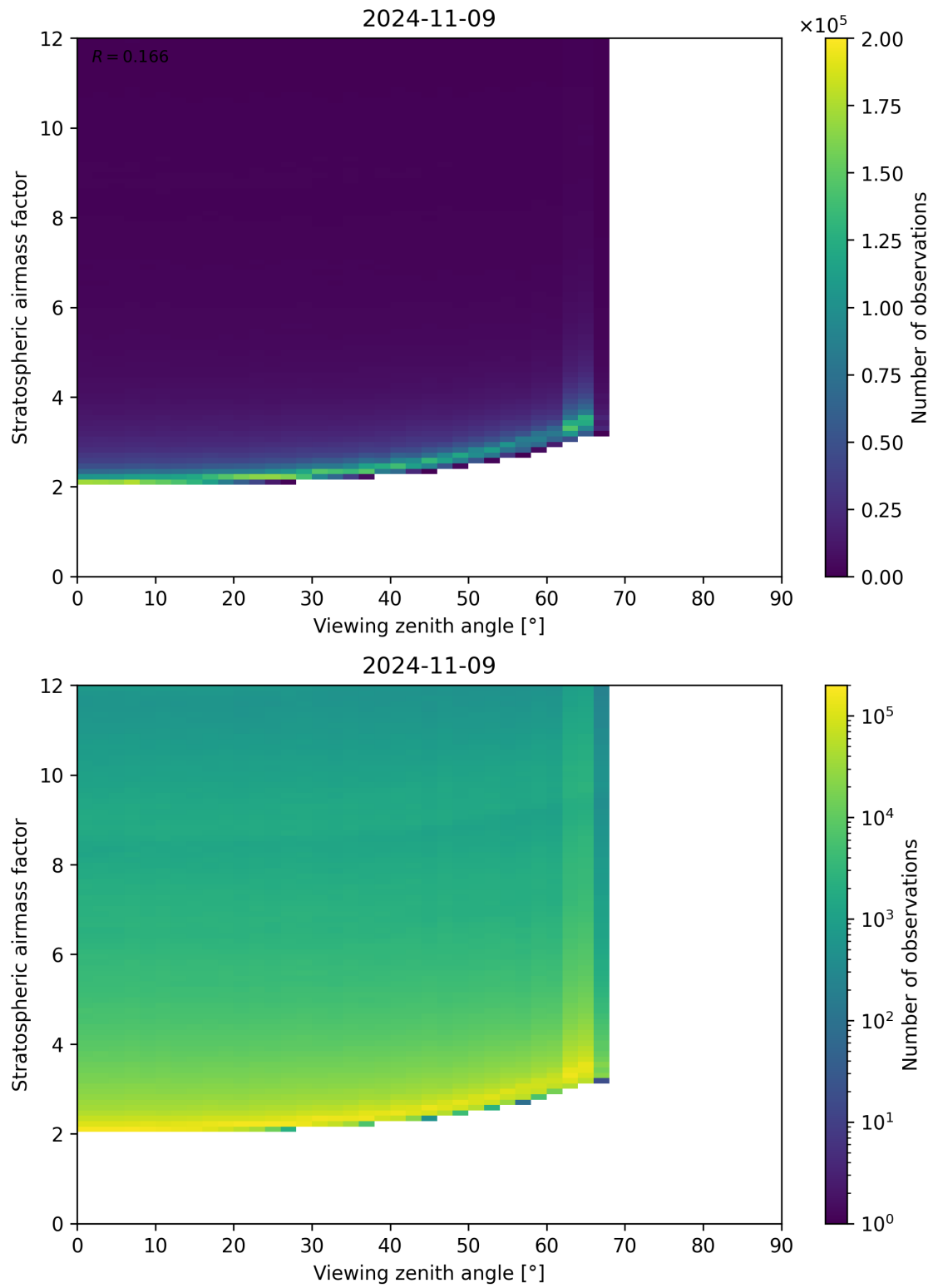
Figure 159: Scatter density plot of “Viewing zenith angle” against “Stratospheric airmass factor” for 2024-11-09 to 2024-11-10.
