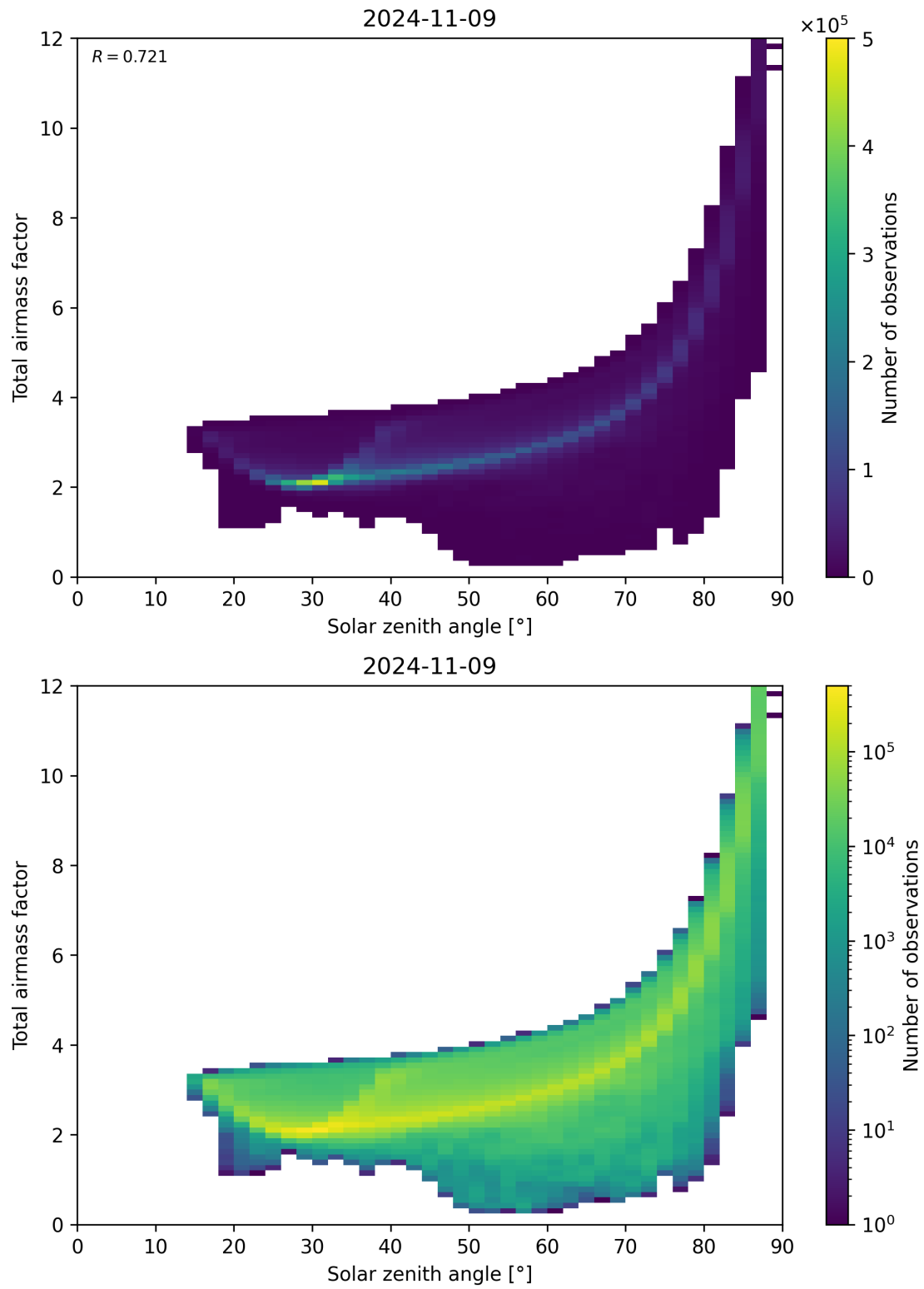
Figure 146: Scatter density plot of “Solar zenith angle” against “Total airmass factor” for 2024-11-09 to 2024-11-10.
