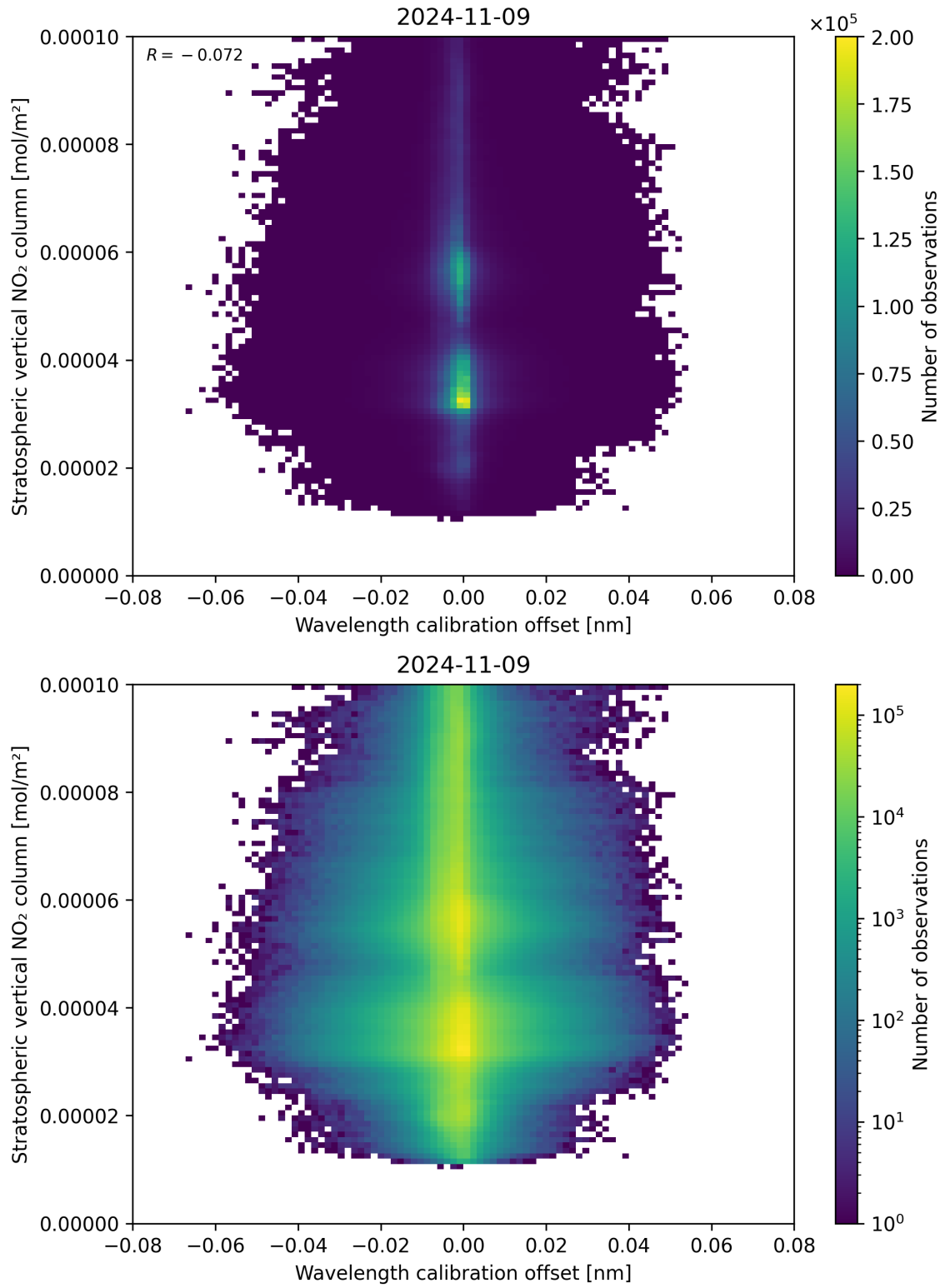
Figure 176: Scatter density plot of “Wavelength calibration offset” against “Stratospheric vertical NO 2 column” for 2024-11-09 to 2024-11-10.
