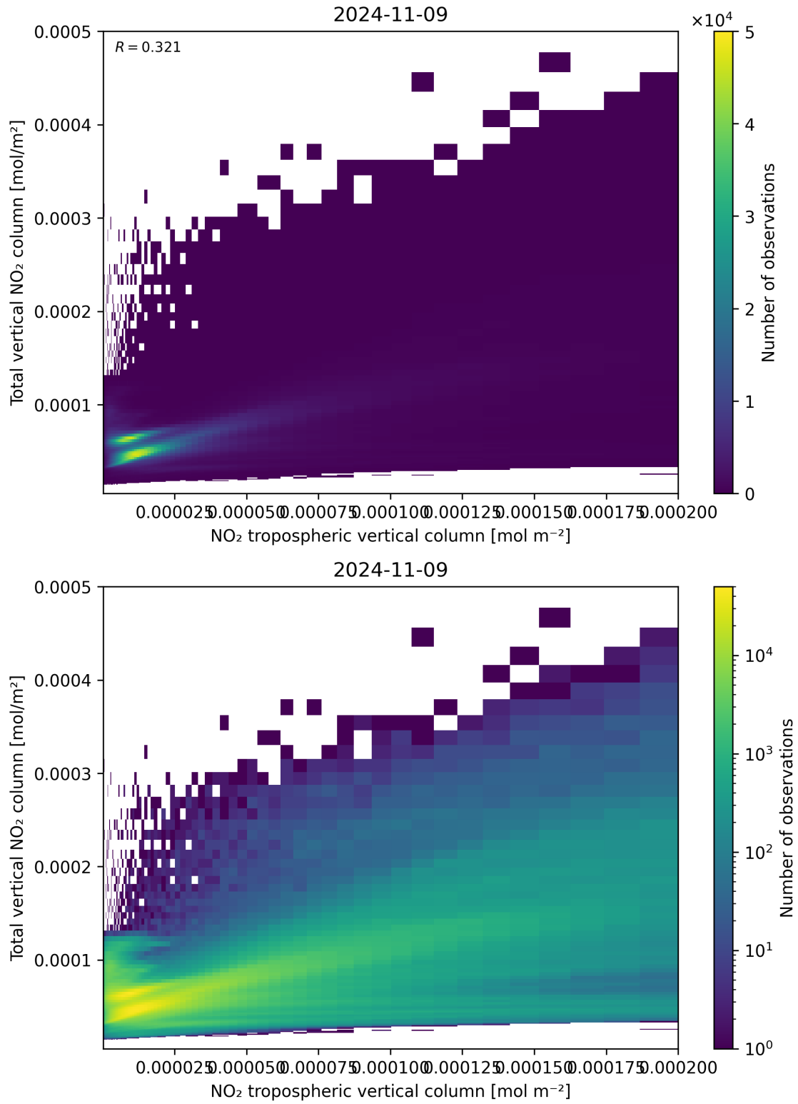
Figure 128: Scatter density plot of “NO 2 tropospheric vertical column” against “Total vertical NO 2 column” for 2024-11-09 to 2024-11-10.
