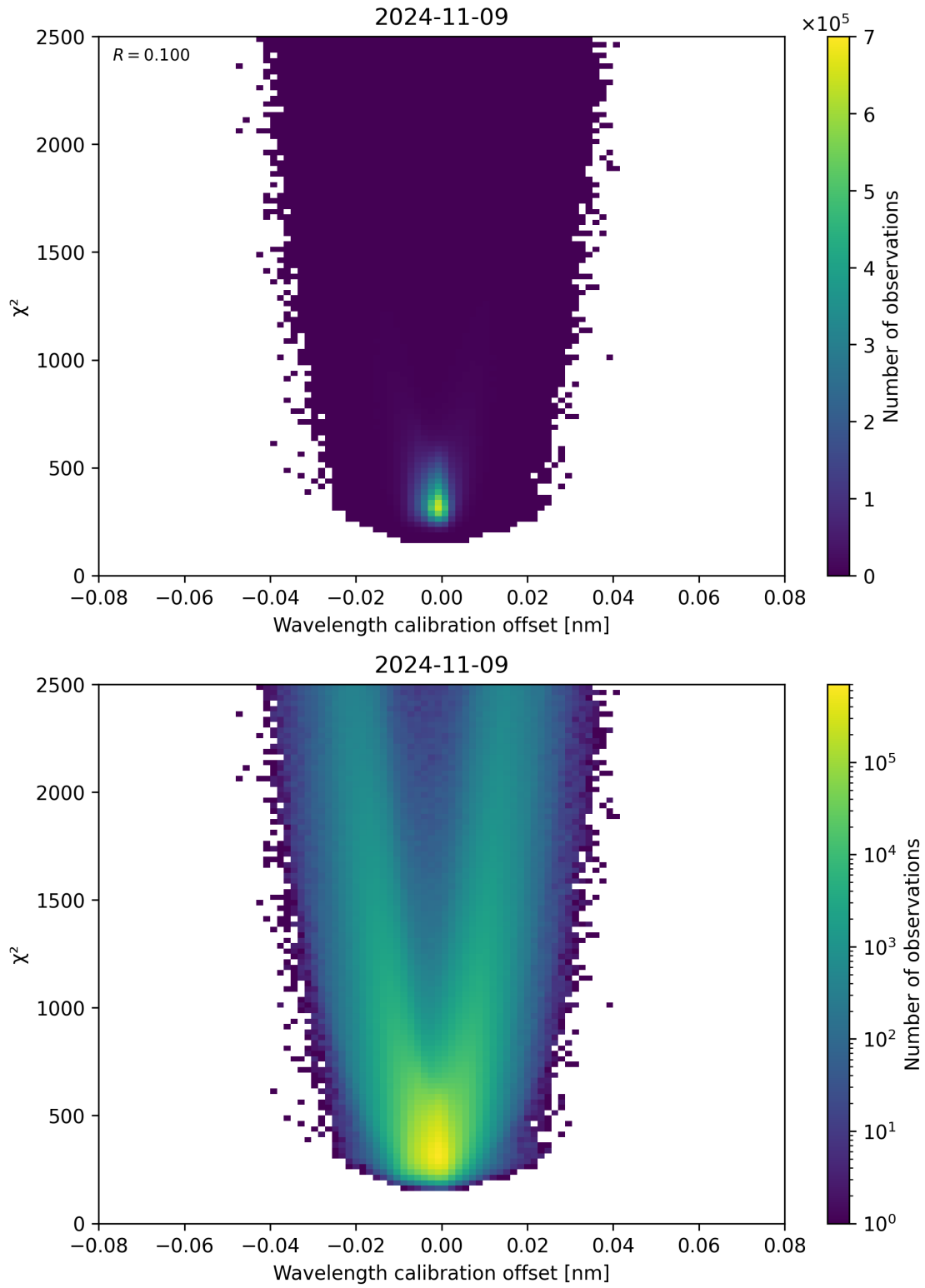
Figure 175: Scatter density plot of “Wavelength calibration offset” against “ \chi^2 ” for 2024-11-09 to 2024-11-10.
