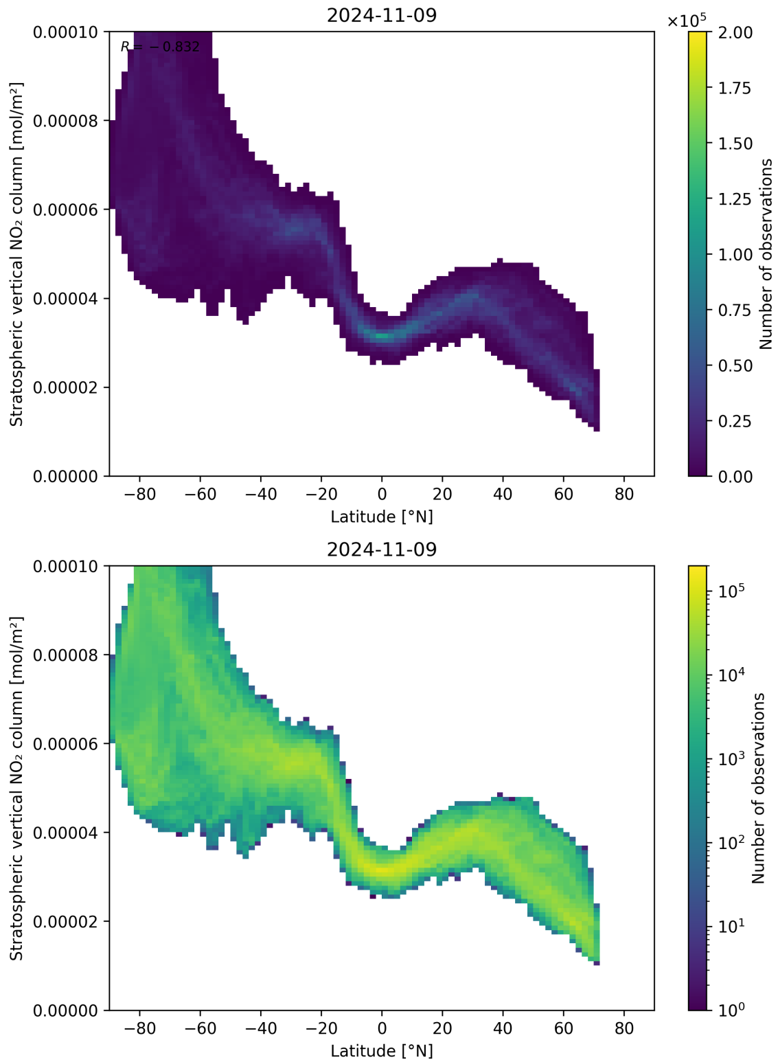
Figure 87: Scatter density plot of “Latitude” against “Stratospheric vertical NO 2 column” for 2024-11-09 to 2024-11-10.
