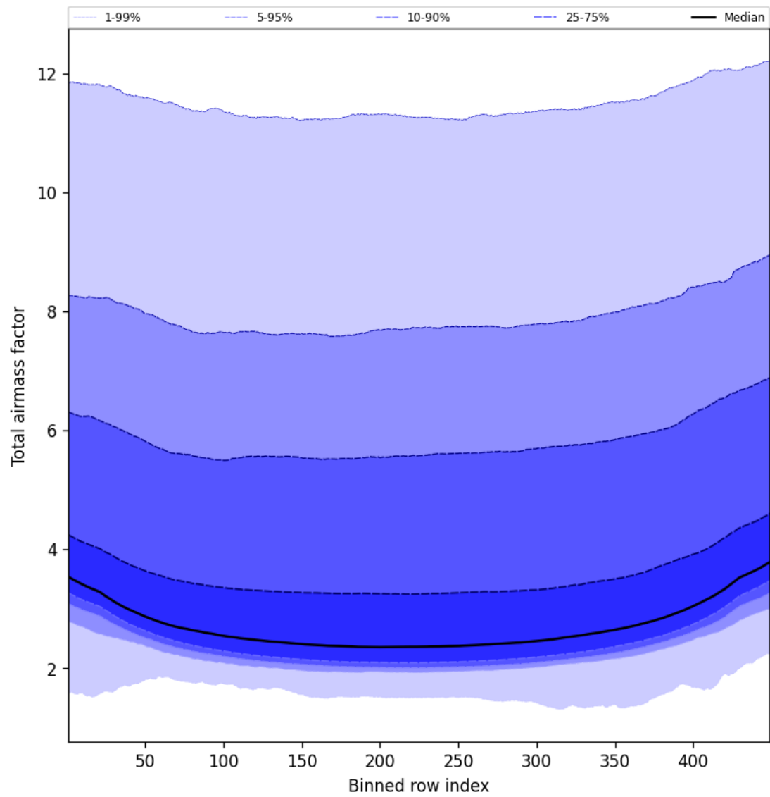
Figure 49: Along track statistics of “Total airmass factor” for 2024-11-09 to 2024-11-10
