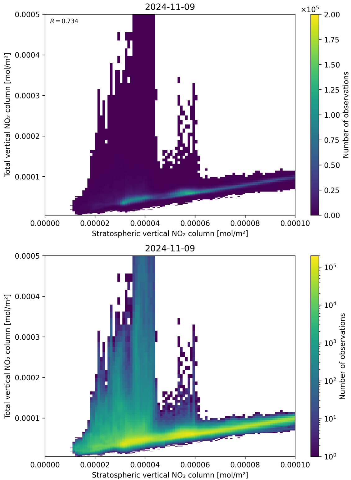
Figure 100: Scatter density plot of “Stratospheric vertical NO 2 column” against “Total vertical NO 2 column” for 2024-11-09 to 2024-11-10.
