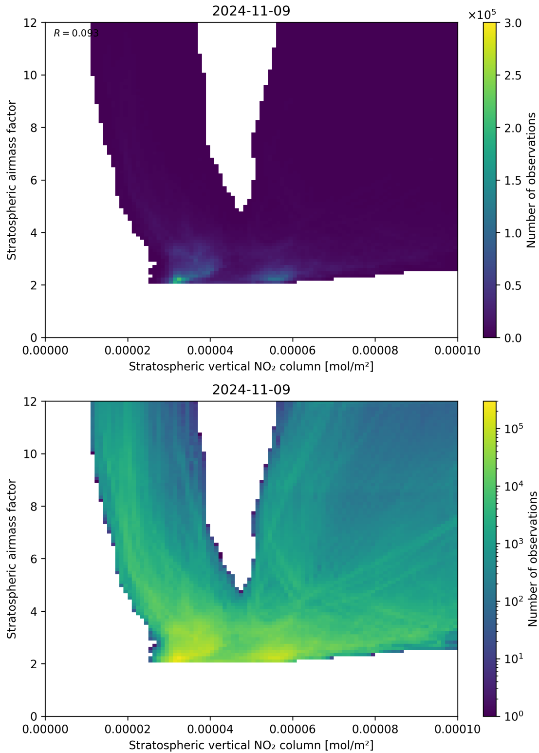
Figure 96: Scatter density plot of “Stratospheric vertical NO 2 column” against “Stratospheric airmass factor” for 2024-11-09 to 2024-11-10.
