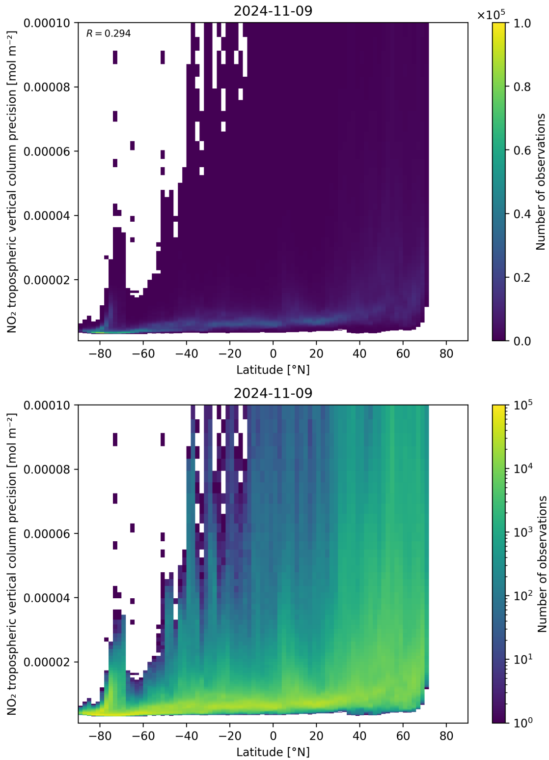
Figure 93: Scatter density plot of “Latitude” against “NO 2 tropospheric vertical column precision” for 2024-11-09 to 2024-11-10.
