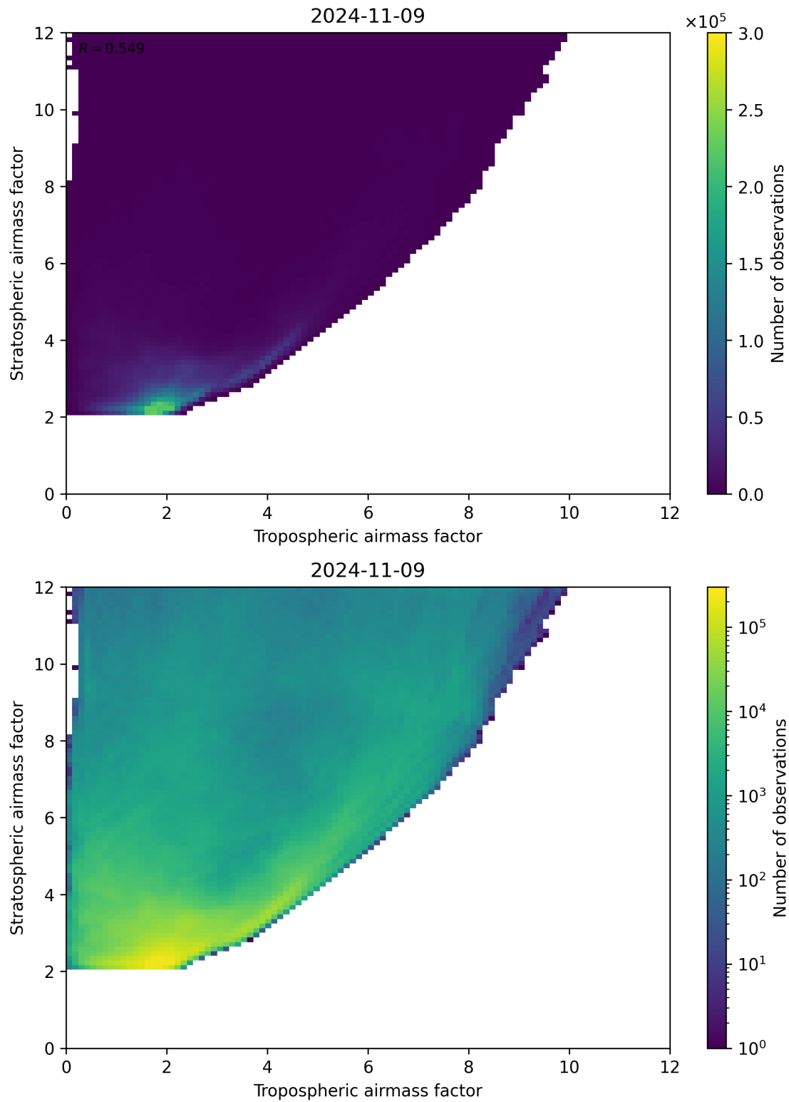
Figure 71: Scatter density plot of “Tropospheric airmass factor” against “Stratospheric airmass factor” for 2024-11-09 to 2024-11-10.
