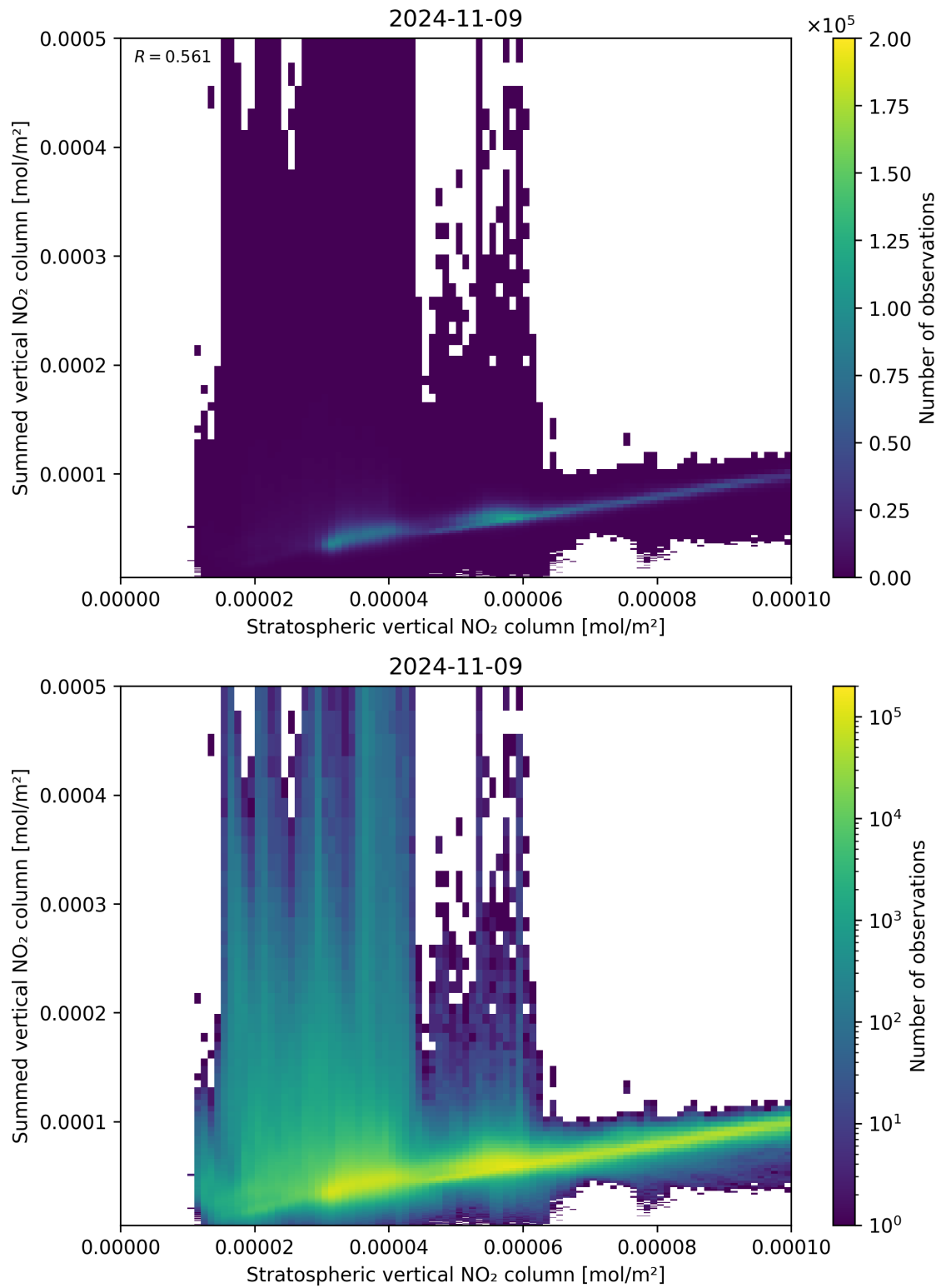
Figure 98: Scatter density plot of “Stratospheric vertical NO 2 column” against “Summed vertical NO 2 column” for 2024-11-09 to 2024-11-10.
