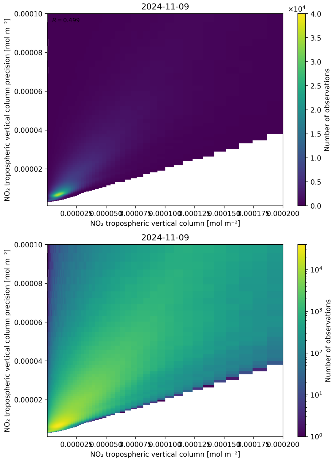
Figure 130: Scatter density plot of “NO 2 tropospheric vertical column” against “NO 2 tropospheric vertical column precision” for 2024-11-09 to 2024-11-10.
