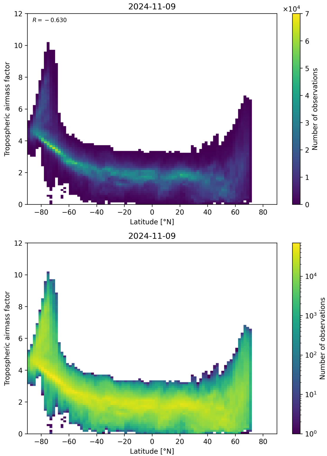
Figure 85: Scatter density plot of “Latitude” against “Tropospheric airmass factor” for 2024-11-09 to 2024-11-10.
