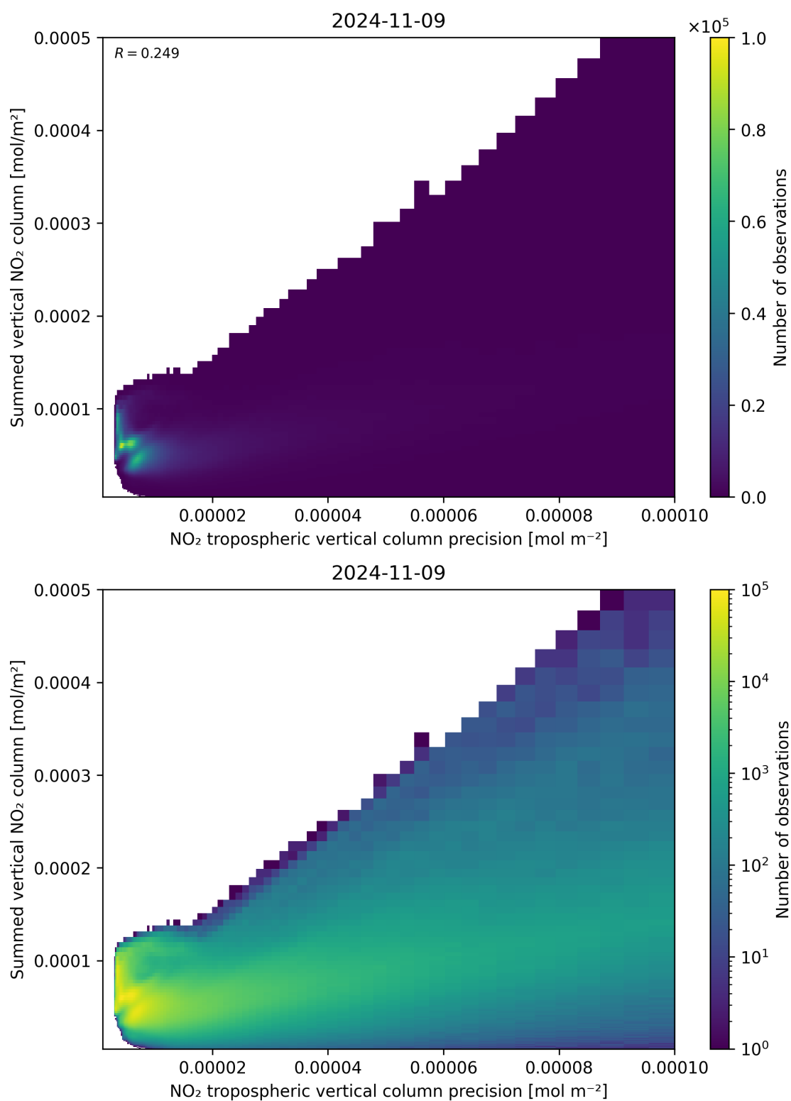
Figure 136: Scatter density plot of “NO 2 tropospheric vertical column precision” against “Summed vertical NO 2 column” for 2024-11-09 to 2024-11-10.
