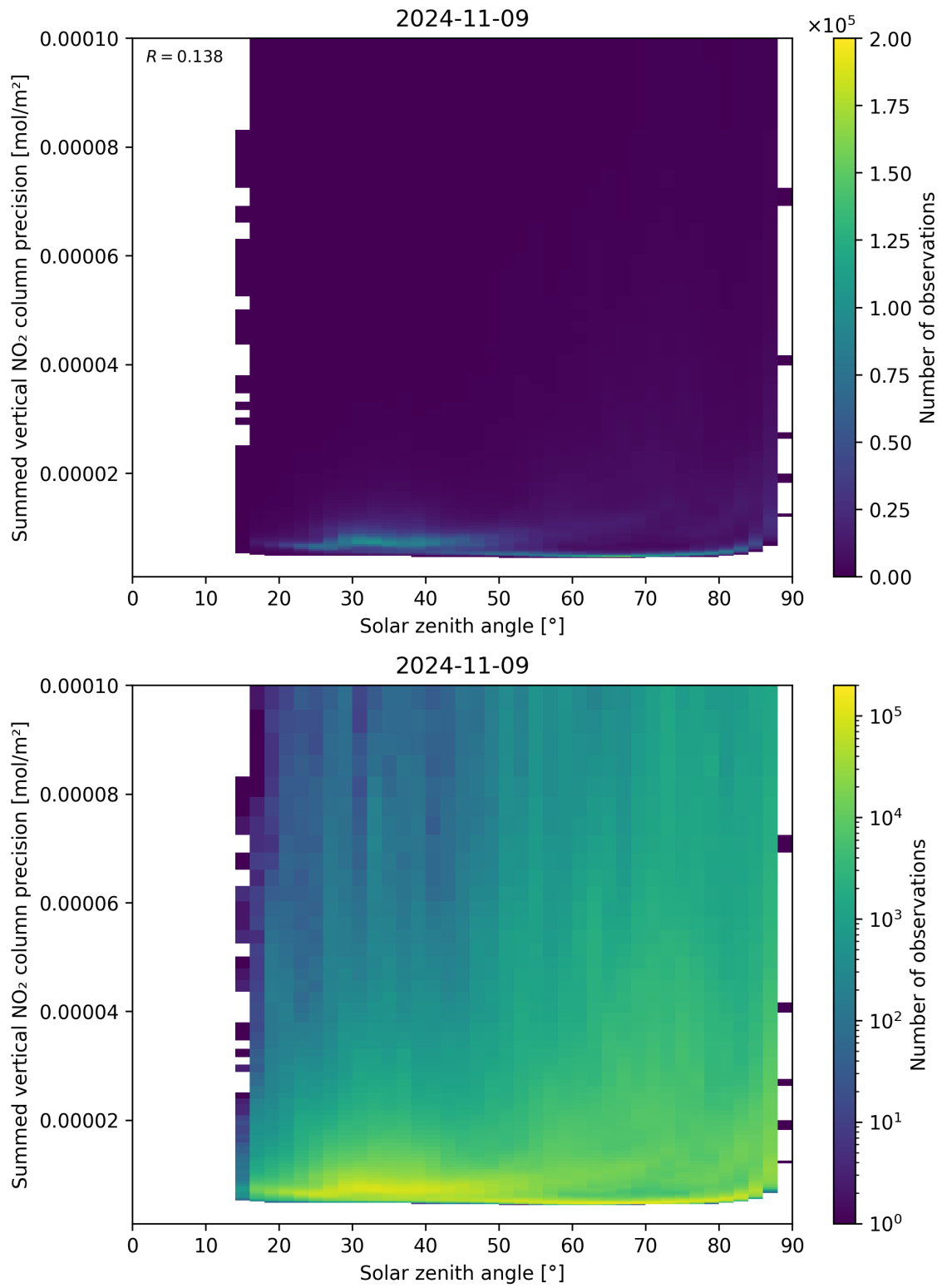
Figure 152: Scatter density plot of “Solar zenith angle” against “Summed vertical NO 2 column precision” for 2024-11-09 to 2024-11-10.
