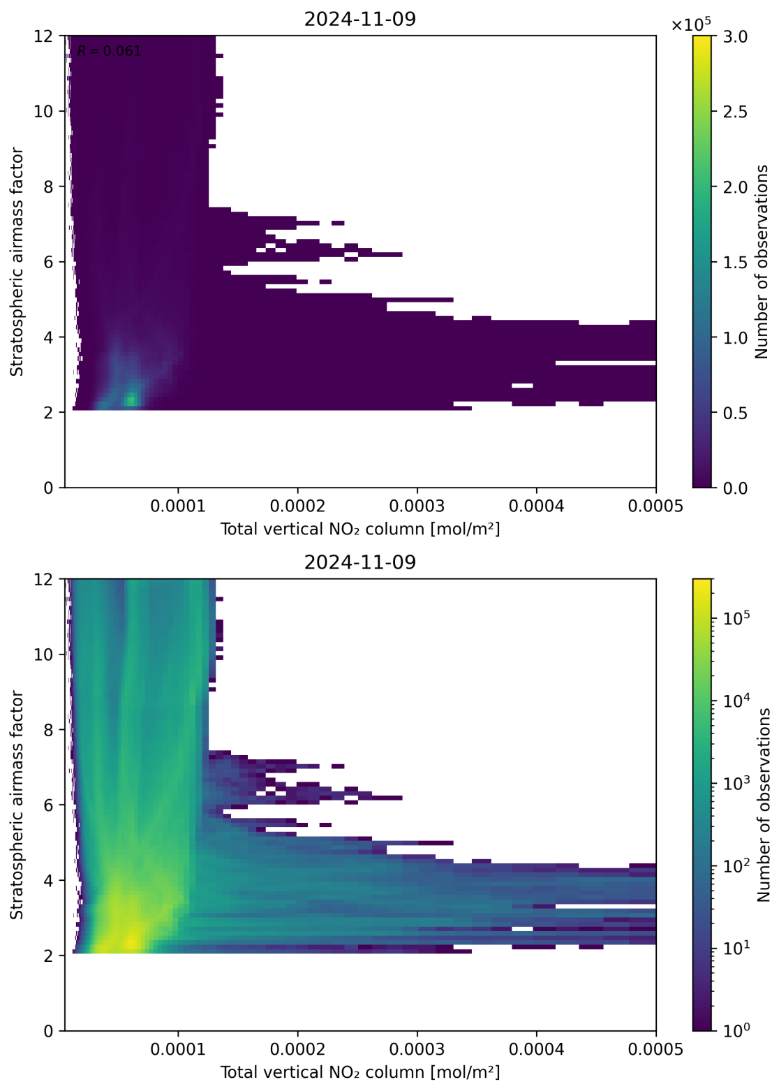
Figure 110: Scatter density plot of “Total vertical NO 2 column” against “Stratospheric airmass factor” for 2024-11-09 to 2024-11-10.
