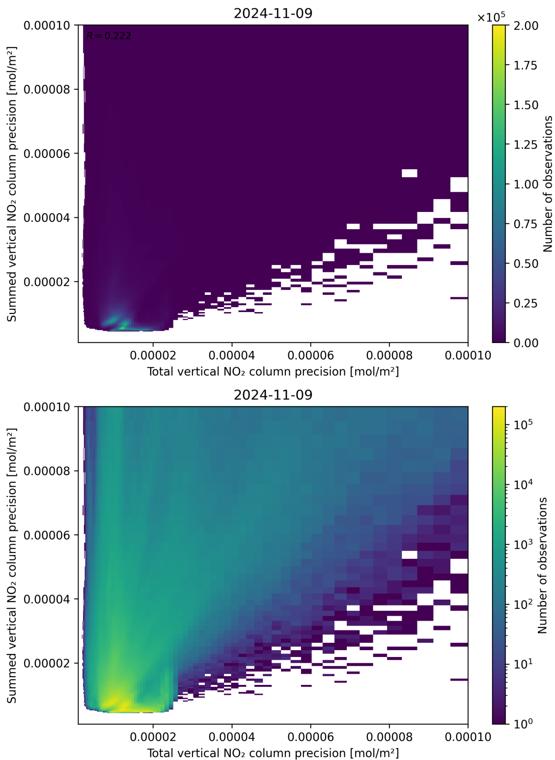
Figure 118: Scatter density plot of “Total vertical NO 2 column precision” against “Summed vertical NO 2 column precision” for 2024-11-09 to 2024-11-10.
