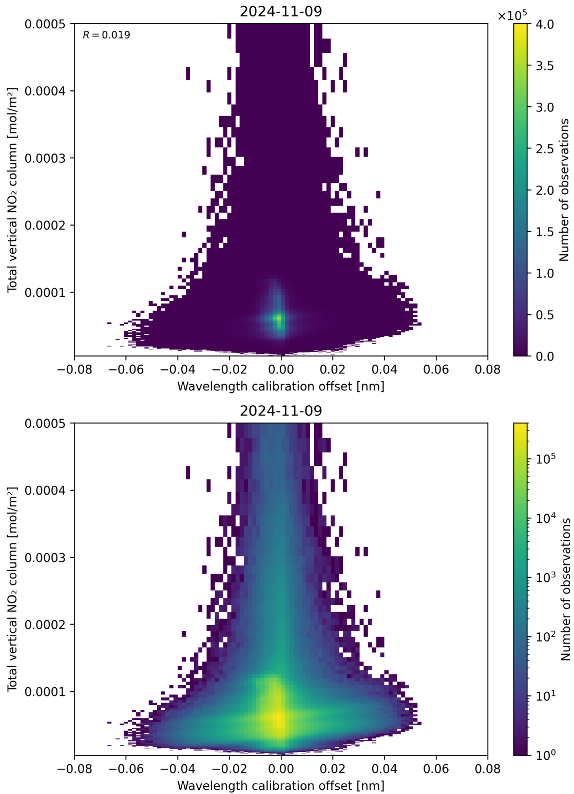
Figure 179: Scatter density plot of “Wavelength calibration offset” against “Total vertical NO 2 column” for 2024-11-09 to 2024-11-10.
