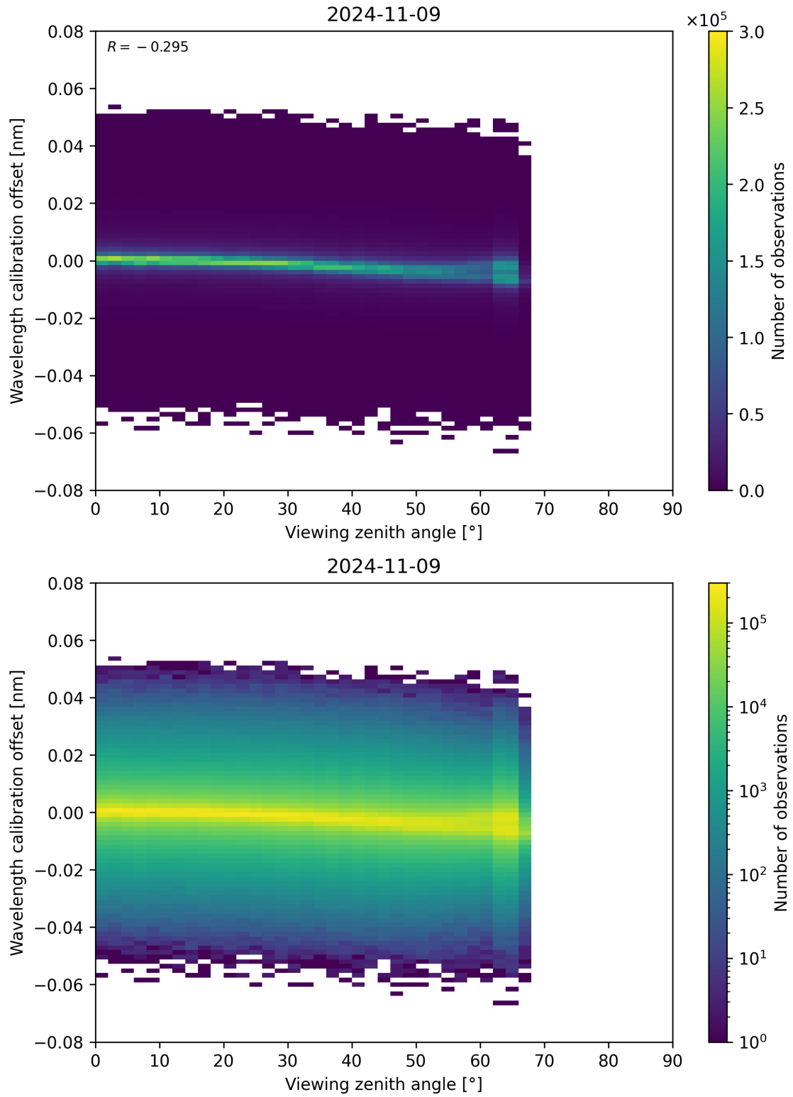
Figure 173: Scatter density plot of “Viewing zenith angle” against “Wavelength calibration offset” for 2024-11-09 to 2024-11-10.
