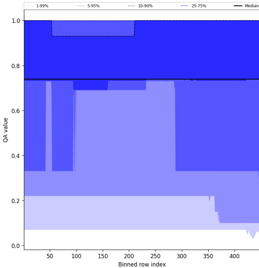
Figure 45: Along track statistics of “QA value” for 2024-11-09 to 2024-11-10
