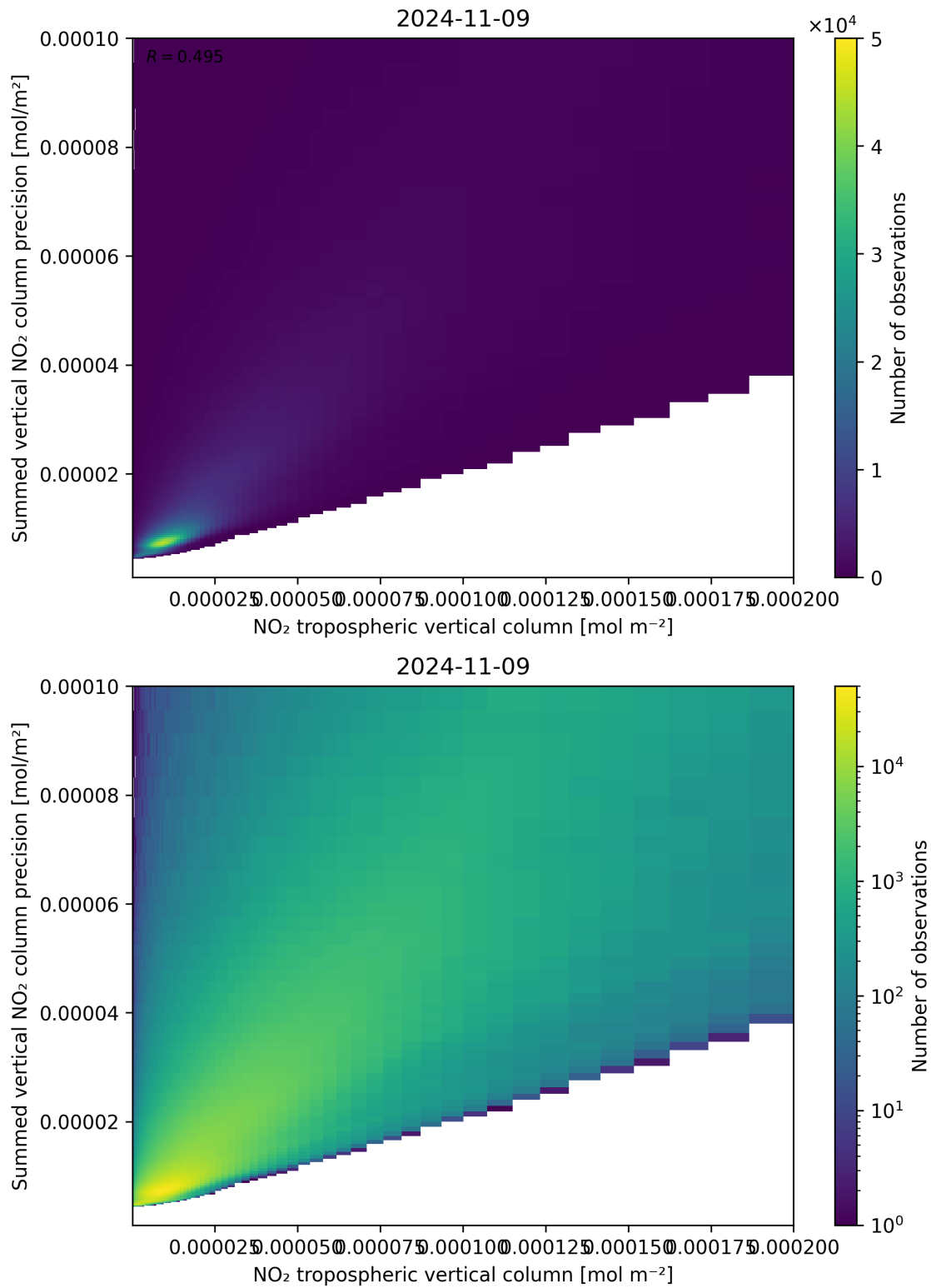
Figure 127: Scatter density plot of “NO 2 tropospheric vertical column” against “Summed vertical NO 2 column precision” for 2024-11-09 to 2024-11-10.
