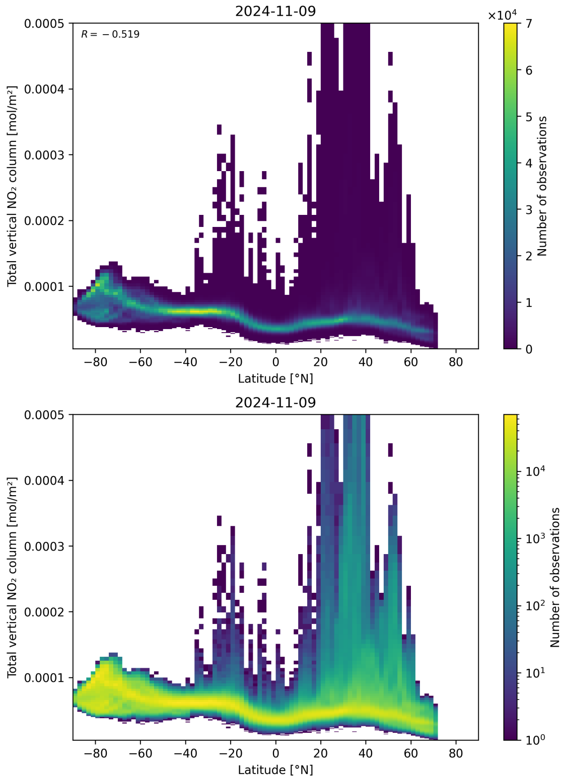
Figure 90: Scatter density plot of “Latitude” against “Total vertical NO 2 column” for 2024-11-09 to 2024-11-10.
