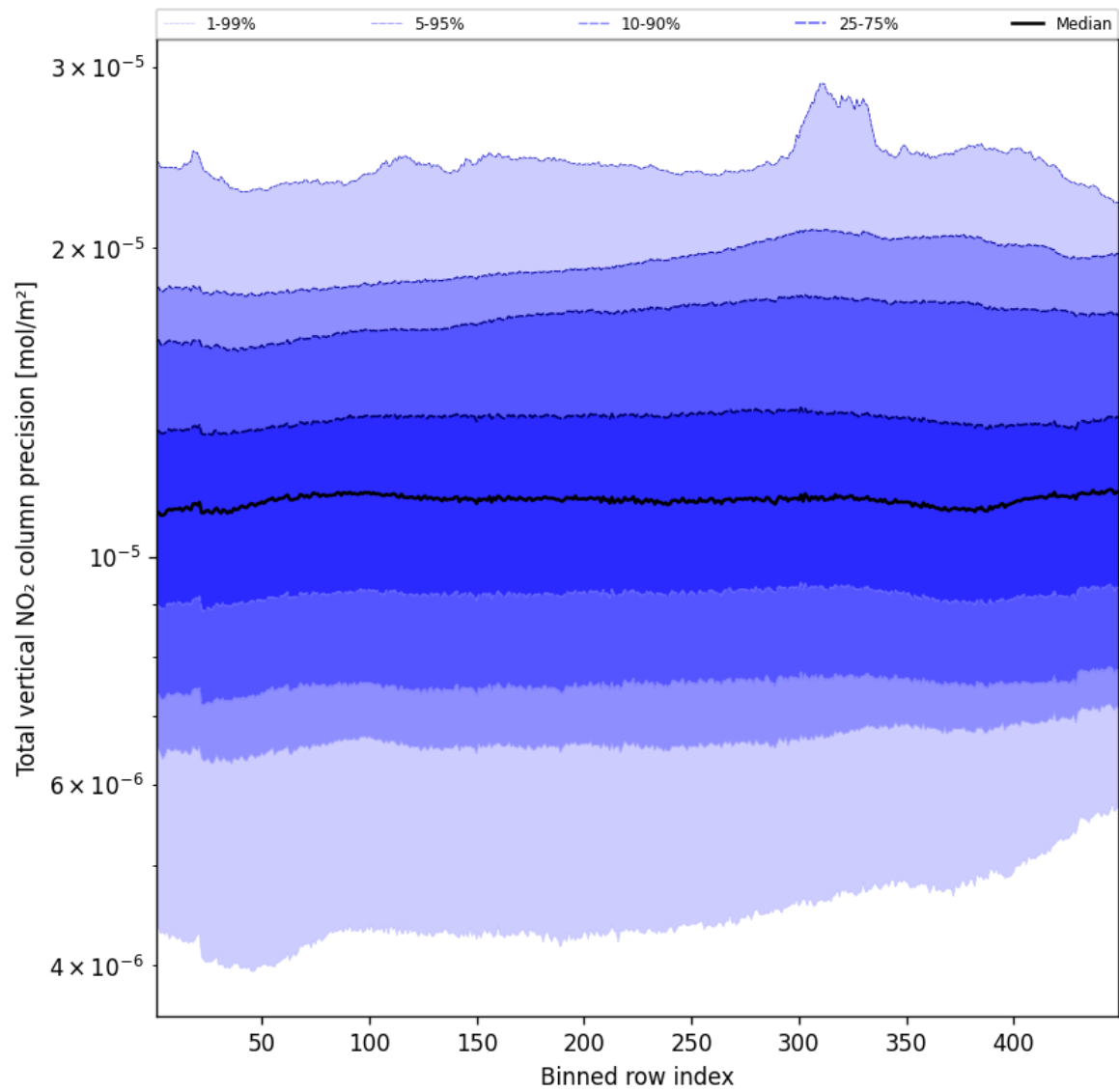
Figure 56: Along track statistics of "Total vertical NO 2 column precision" for 2024-11-09 to 2024-11-10
