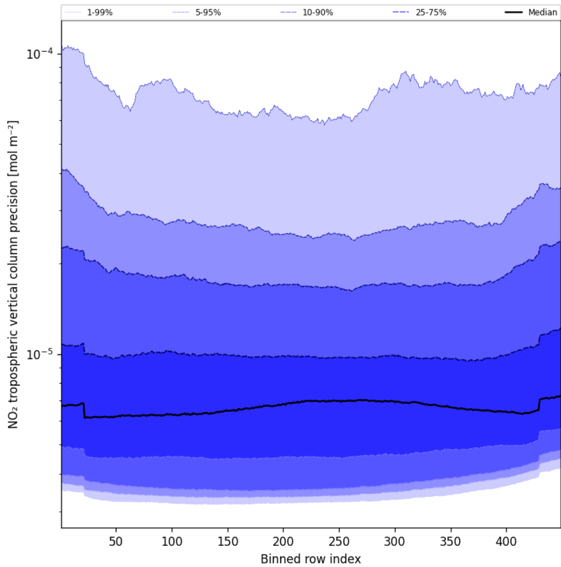
Figure 47: Along track statistics of “NO 2 tropospheric vertical column precision” for 2024-11-09 to 2024-11-10
