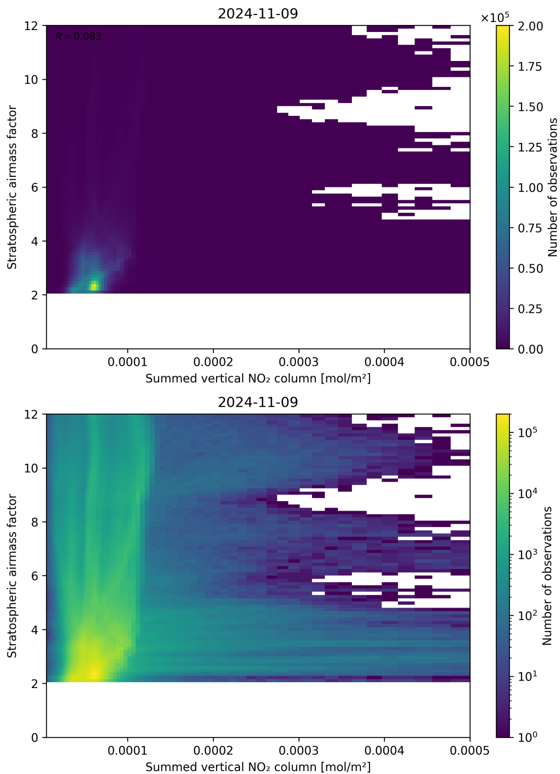
Figure 103: Scatter density plot of “Summed vertical NO 2 column” against “Stratospheric air mass factor” for 2024-11-09 to 2024-11-10.
