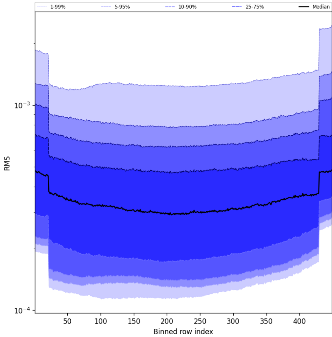
Figure 60: Along track statistics of “RMS” for 2024-11-09 to 2024-11-10
