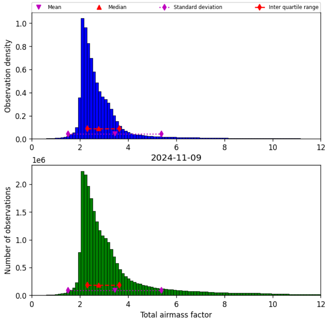
Figure 32: Histogram of “Total airmass factor” for 2024-11-09 to 2024-11-10
