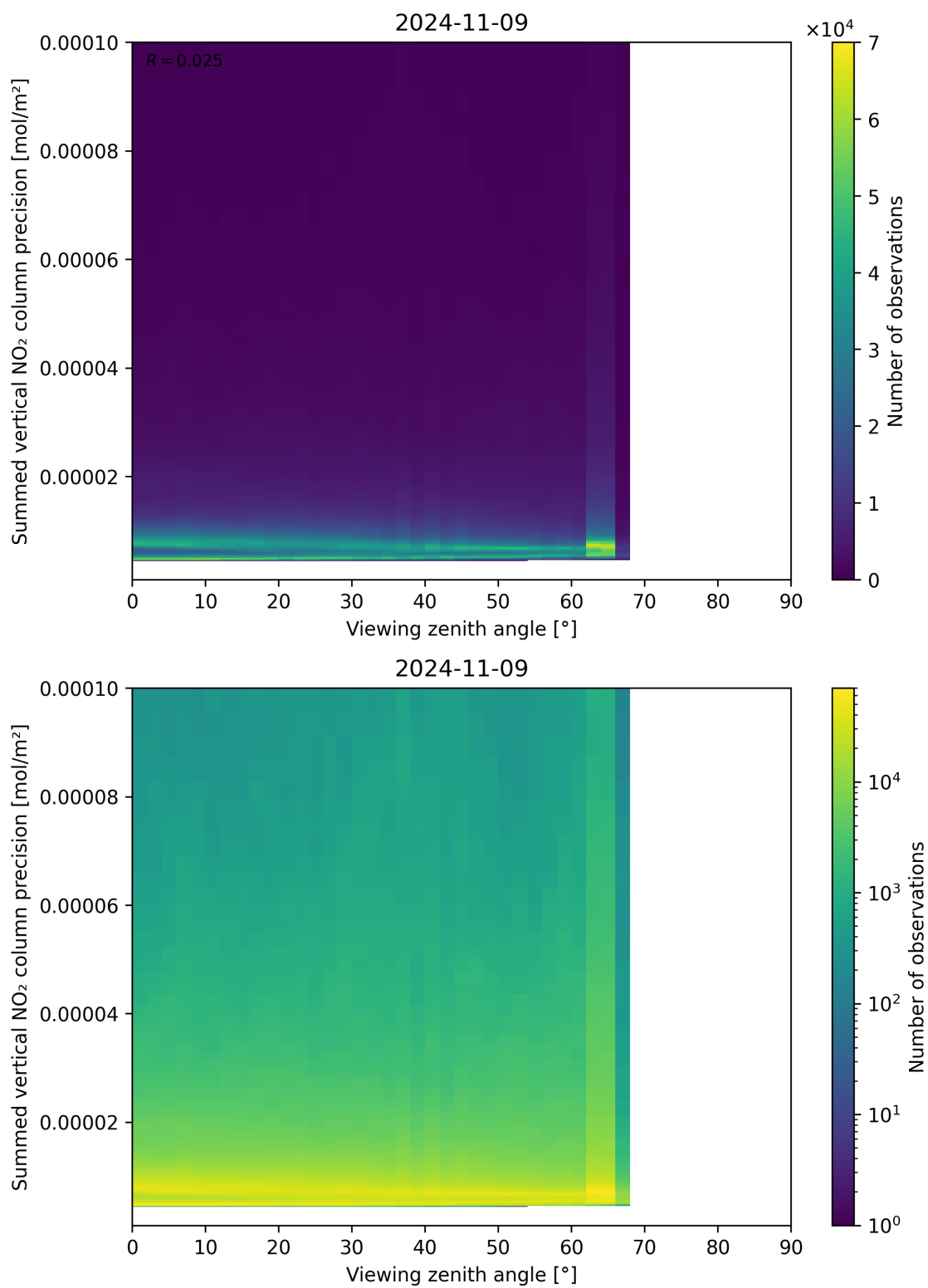
Figure 166: Scatter density plot of “Viewing zenith angle” against “Summed vertical NO 2 column precision” for 2024-11-09 to 2024-11-10.
