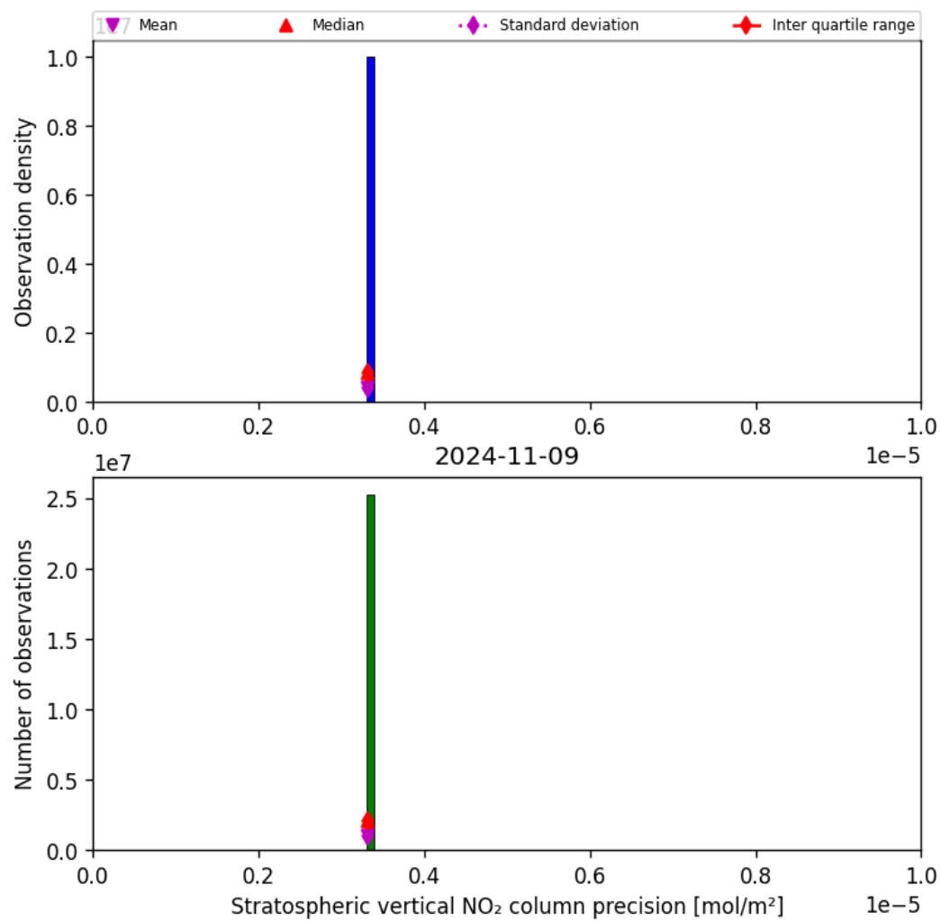
Figure 37: Histogram of “Stratospheric vertical NO 2 column precision” for 2024-11-09 to 2024-11-10
