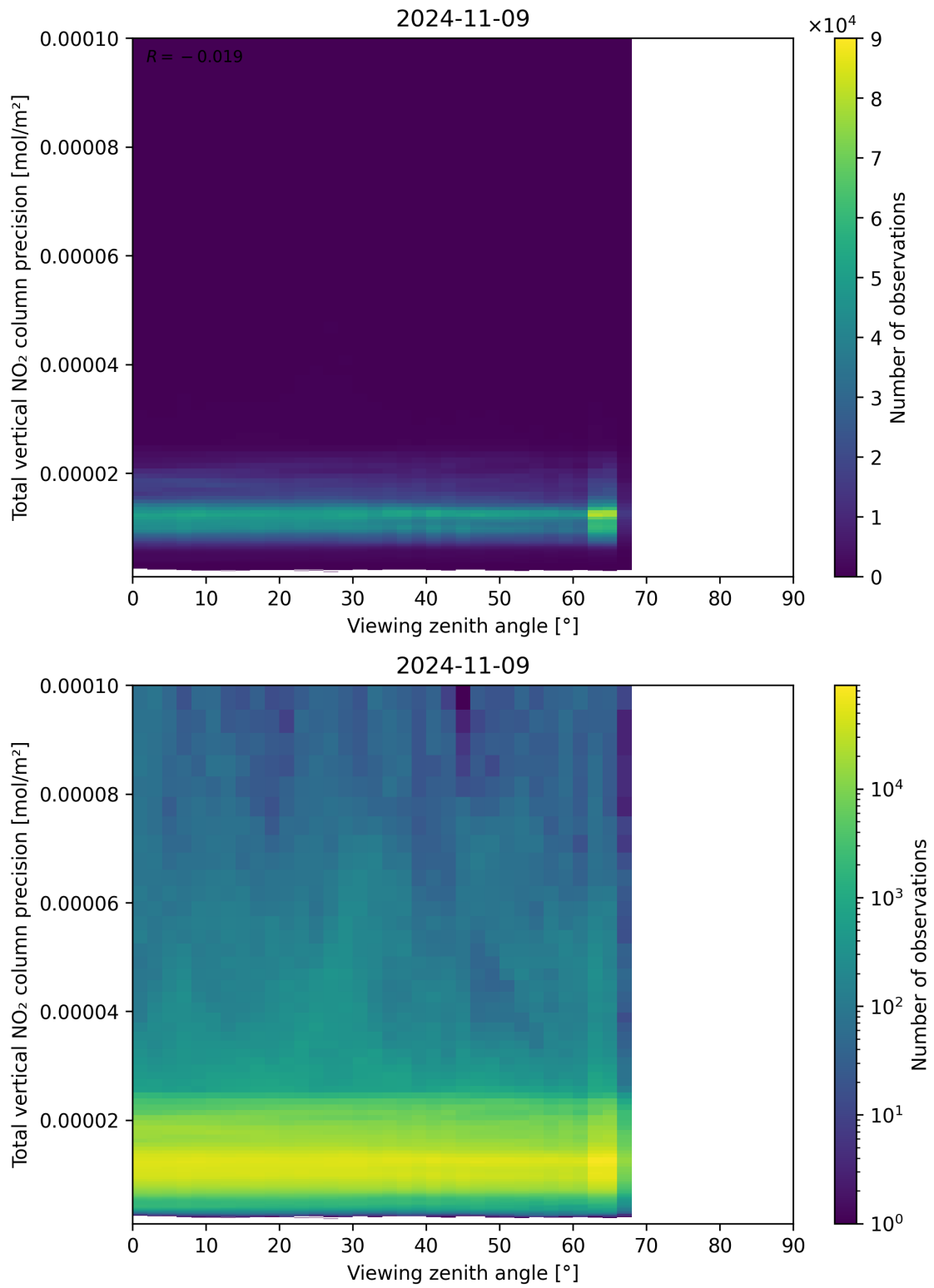
Figure 168: Scatter density plot of “Viewing zenith angle” against “Total vertical NO 2 column precision” for 2024-11-09 to 2024-11-10.
