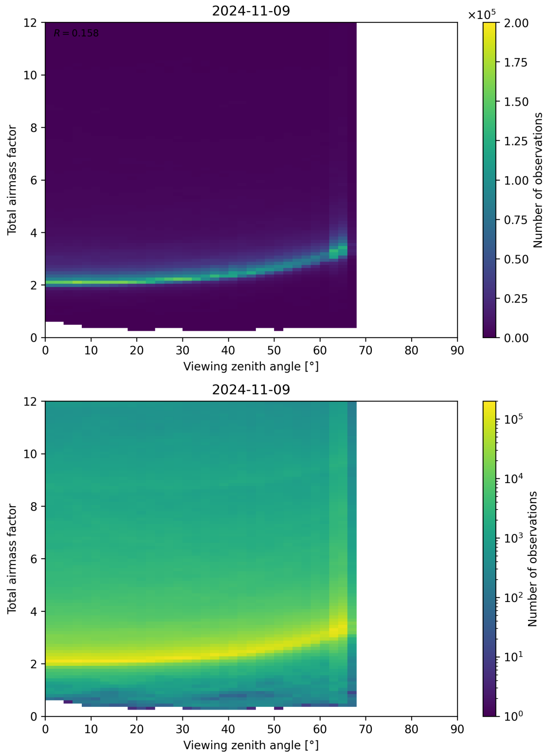
Figure 160: Scatter density plot of “Viewing zenith angle” against “Total airmass factor” for 2024-11-09 to 2024-11-10.
