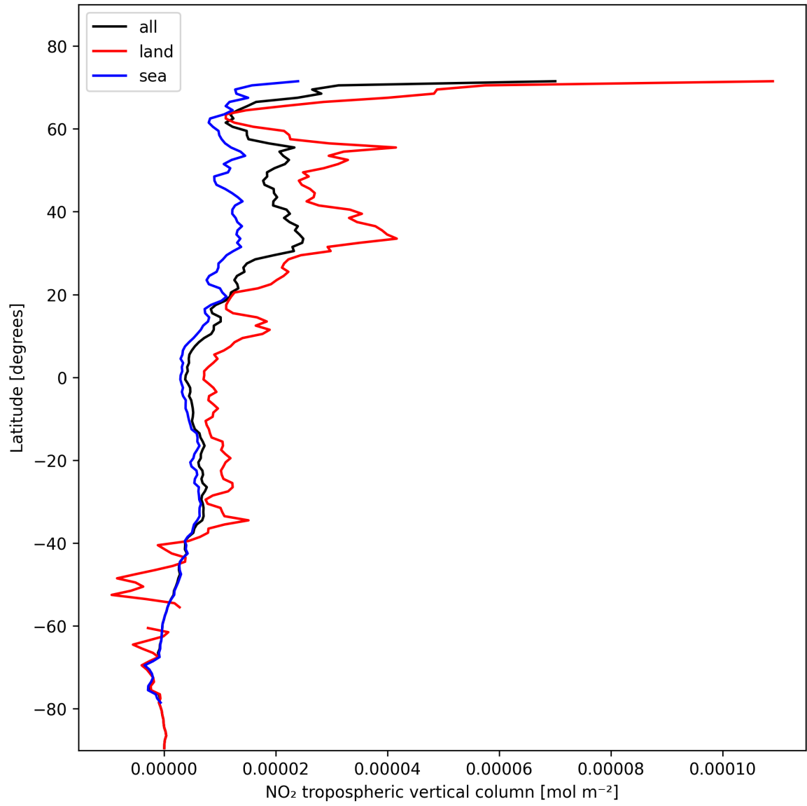
Figure 12: Zonal average of “NO 2 tropospheric vertical column” for 2024-11-09 to 2024-11-10.
