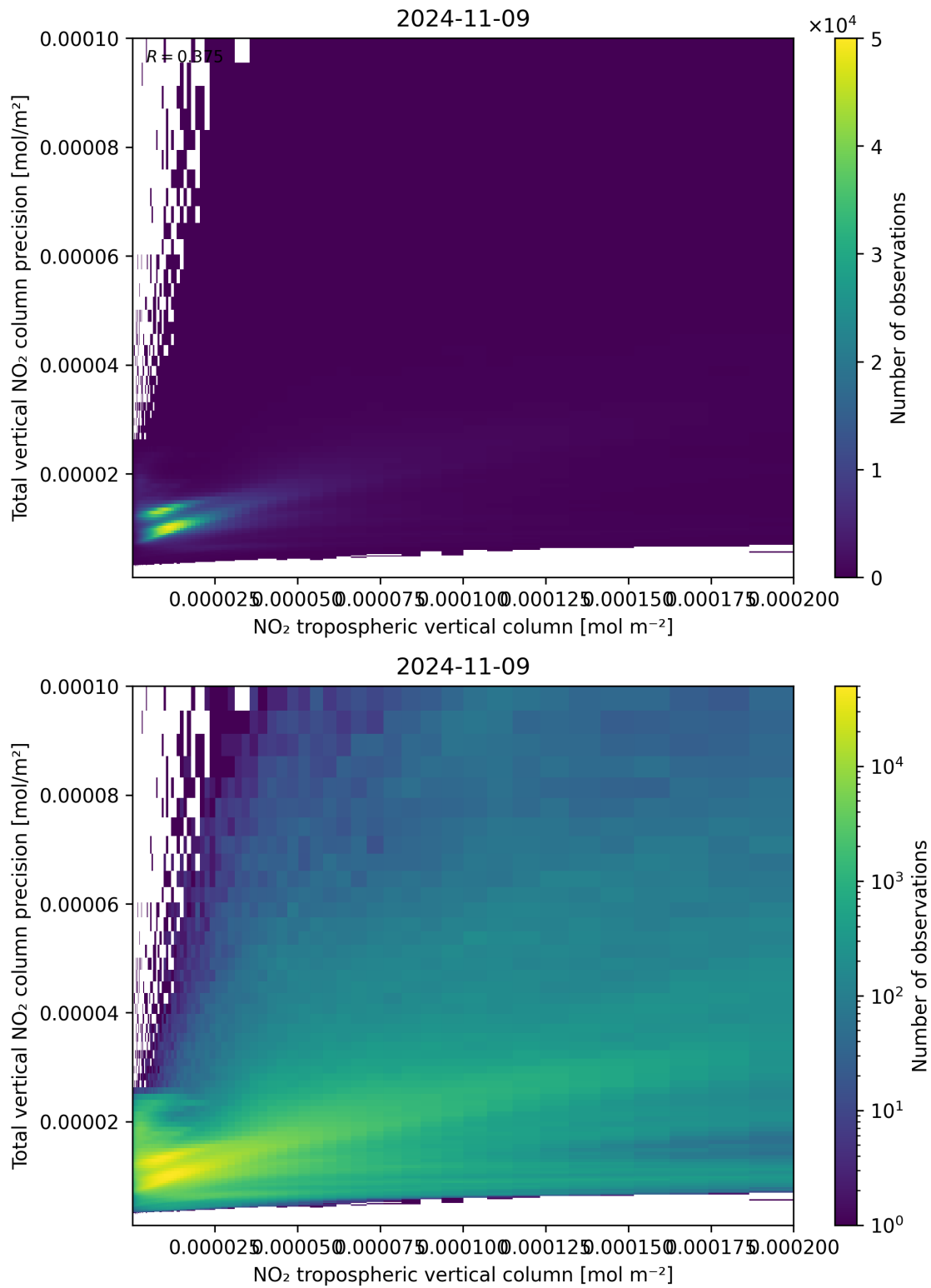
Figure 129: Scatter density plot of “NO 2 tropospheric vertical column” against “Total vertical NO 2 column precision” for 2024-11-09 to 2024-11-10.
