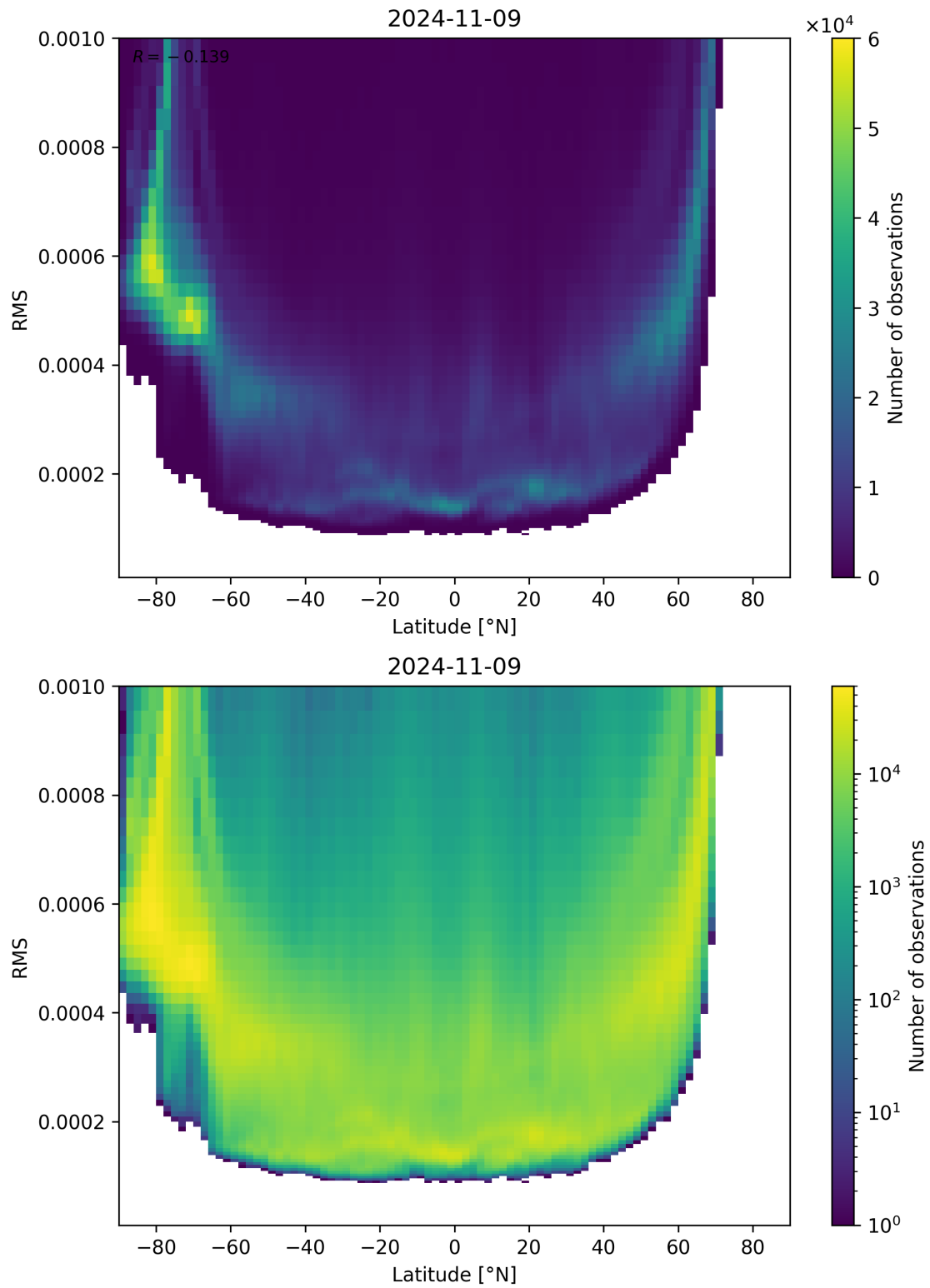
Figure 94: Scatter density plot of “Latitude” against “RMS” for 2024-11-09 to 2024-11-10.
