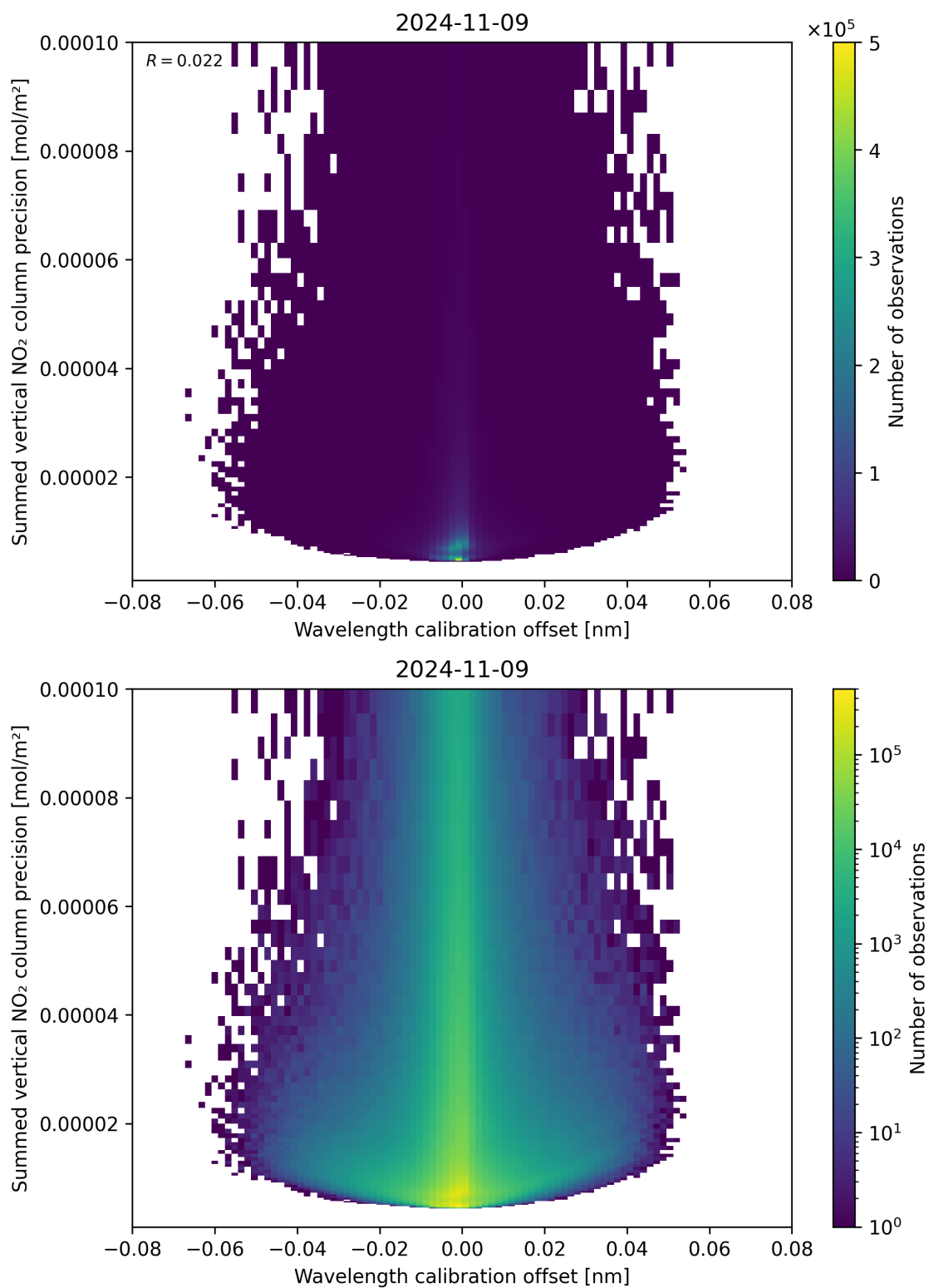
Figure 178: Scatter density plot of “Wavelength calibration offset” against “Summed vertical NO 2 column precision” for 2024-11-09 to 2024-11-10.
