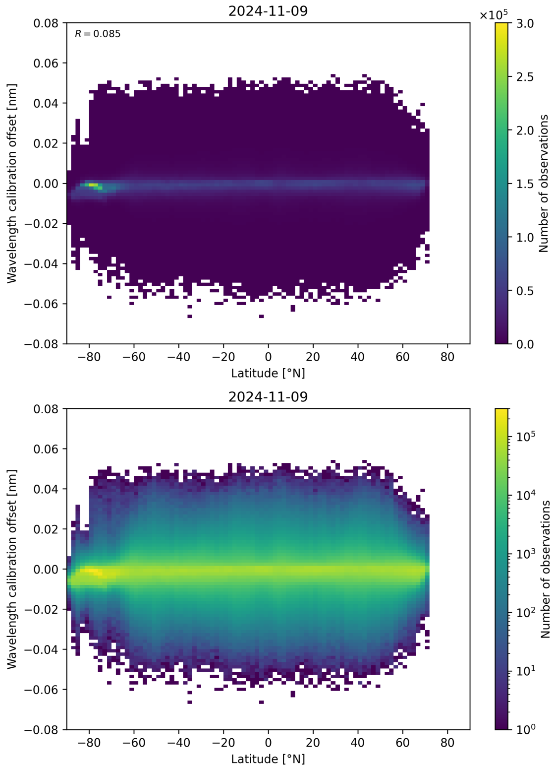
Figure 95: Scatter density plot of “Latitude” against “Wavelength calibration offset” for 2024-11-09 to 2024-11-10.
