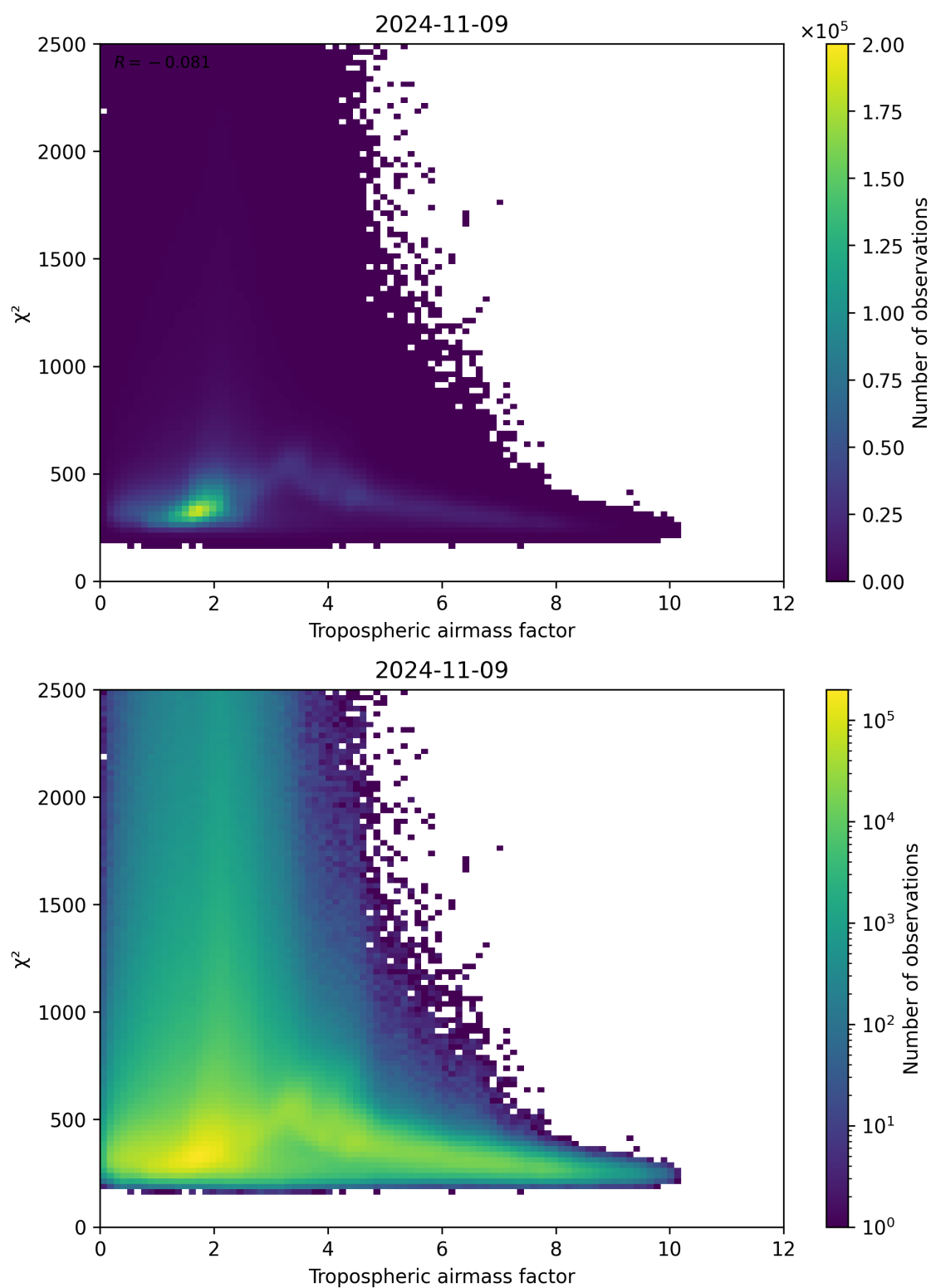
Figure 73: Scatter density plot of “Tropospheric airmass factor” against “ \chi^2 ” for 2024-11-09 to 2024-11-10.
