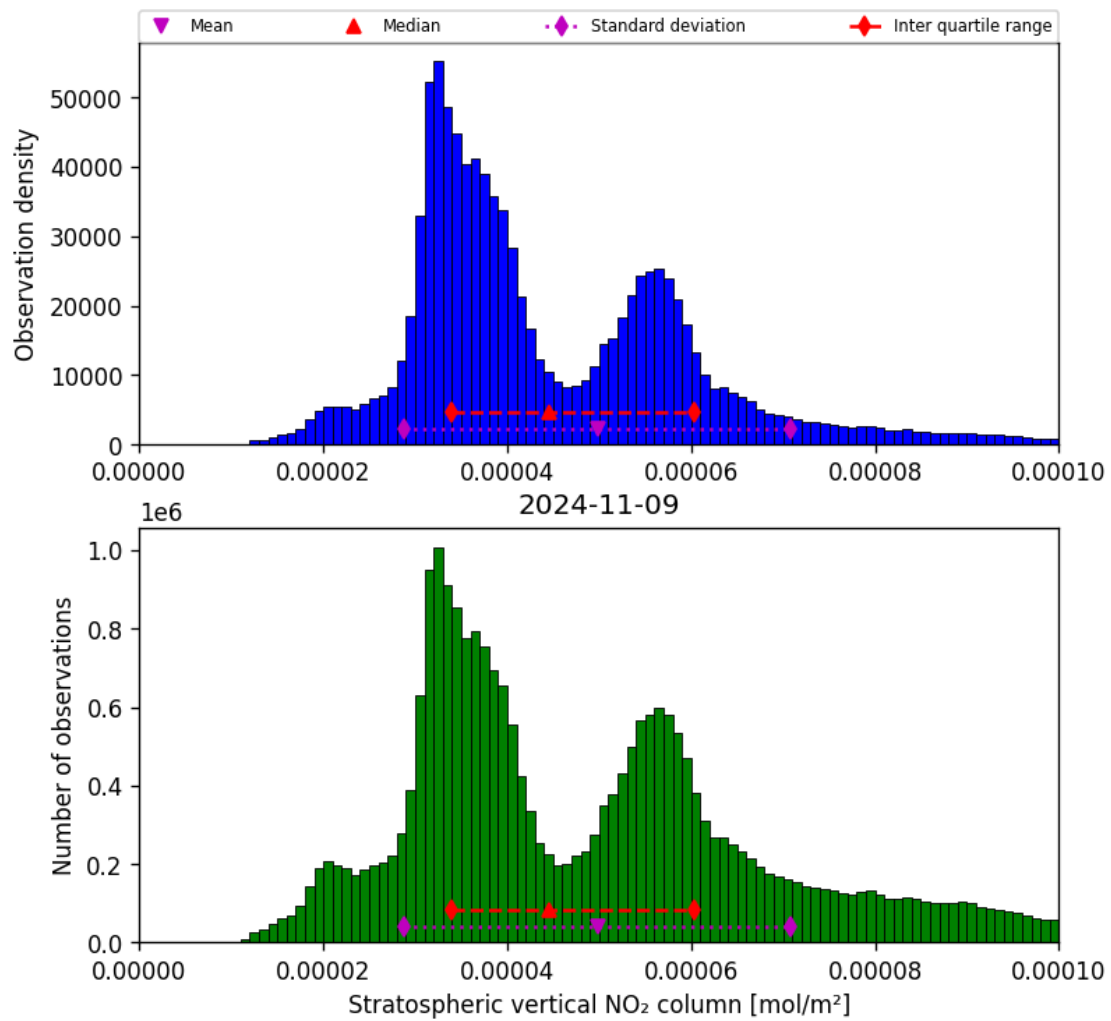
Figure 36: Histogram of “Stratospheric vertical NO 2 column” for 2024-11-09 to 2024-11-10
