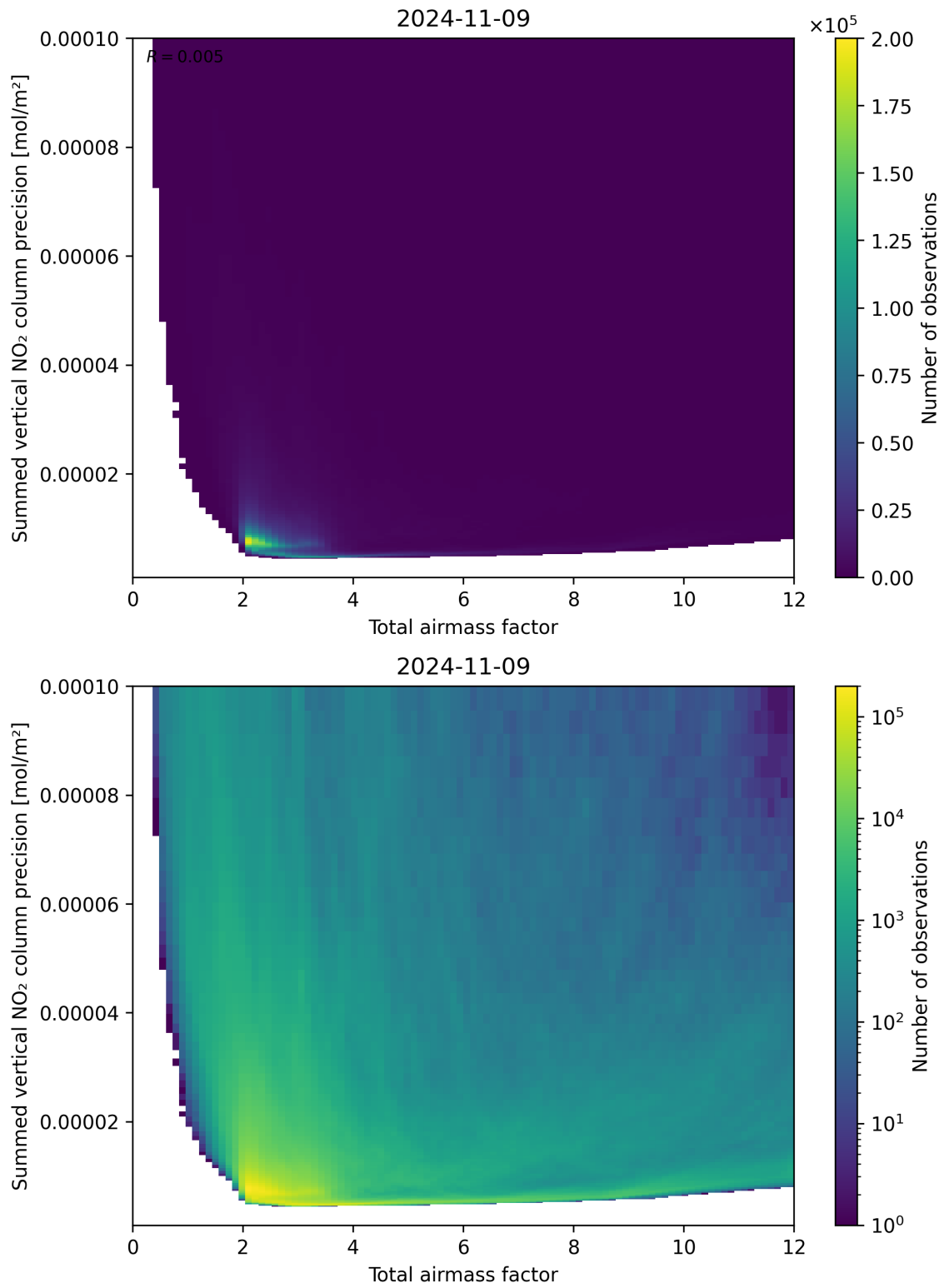
Figure 66: Scatter density plot of “Total airmass factor” against “Summed vertical NO 2 column precision” for 2024-11-09 to 2024-11-10.
