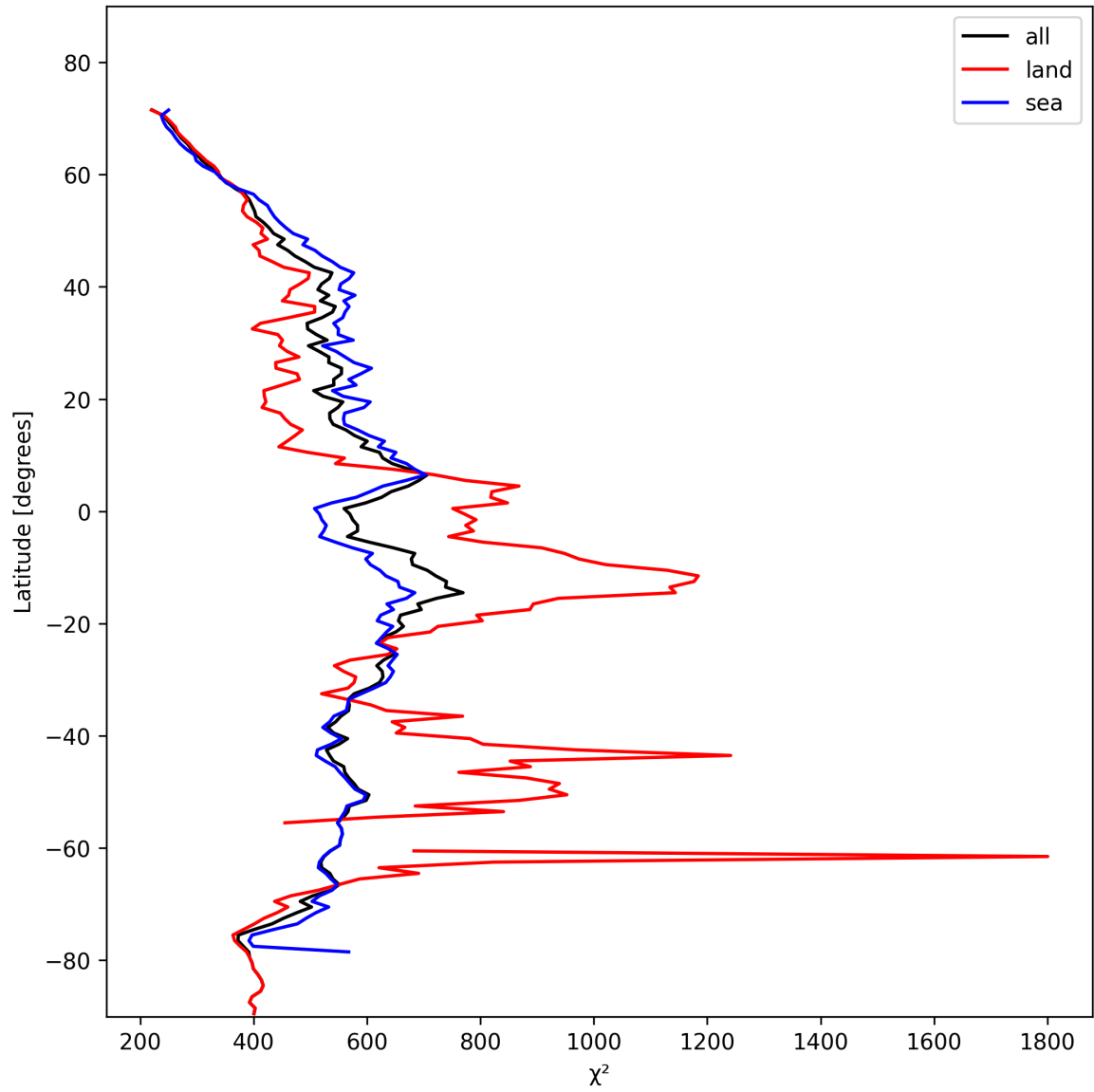
Figure 25: Zonal average of “ \chi^2 ” for 2024-11-09 to 2024-11-10.
