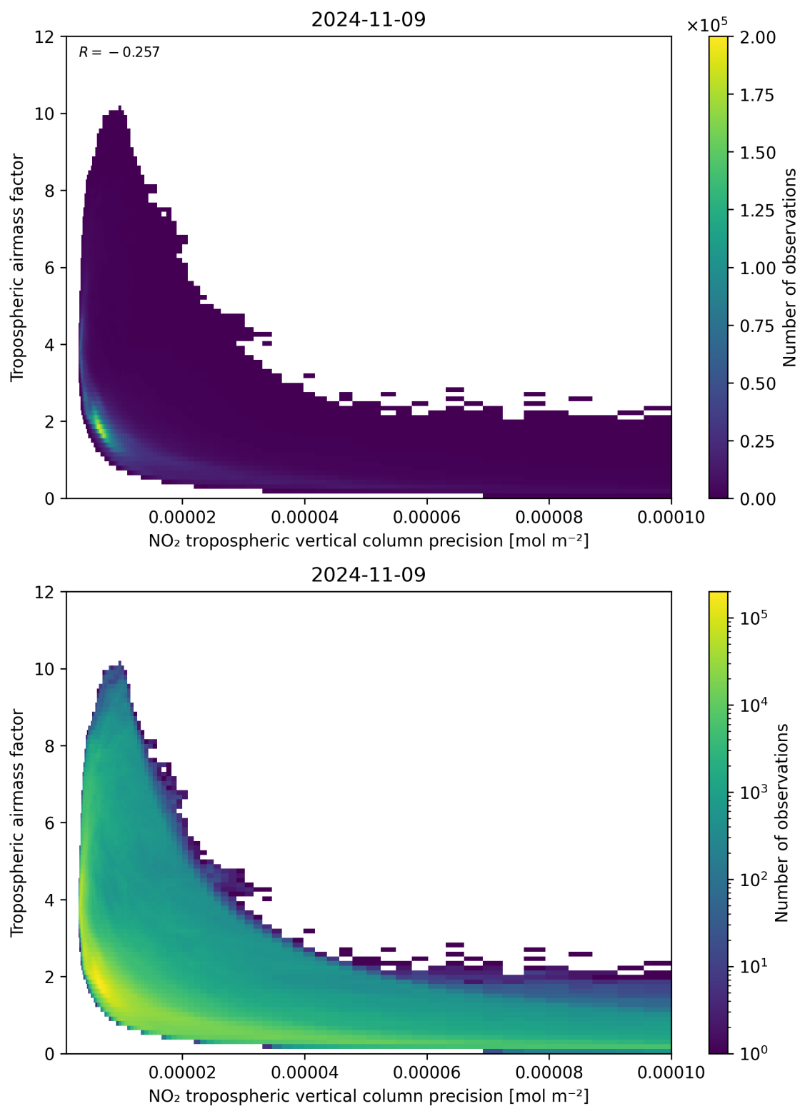
Figure 133: Scatter density plot of “NO 2 tropospheric vertical column precision” against “Tropospheric airmass factor” for 2024-11-09 to 2024-11-10.
