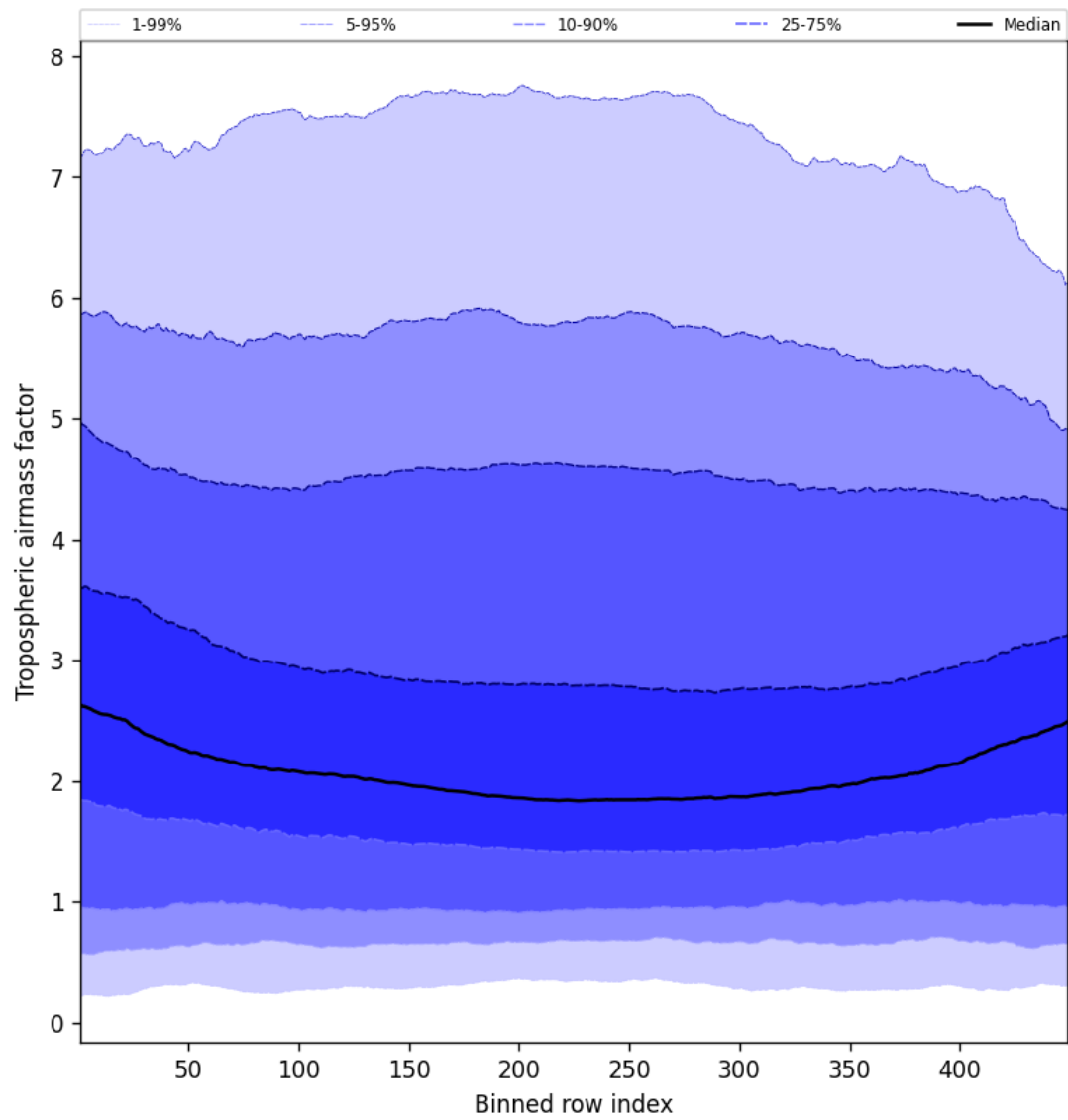
Figure 48: Along track statistics of “Tropospheric airmass factor” for 2024-11-09 to 2024-11-10
