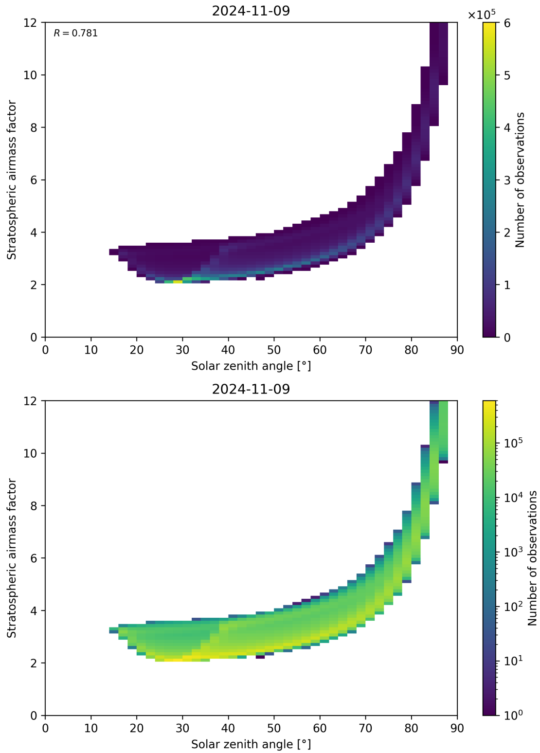
Figure 145: Scatter density plot of “Solar zenith angle” against “Stratospheric airmass factor” for 2024-11-09 to 2024-11-10.
