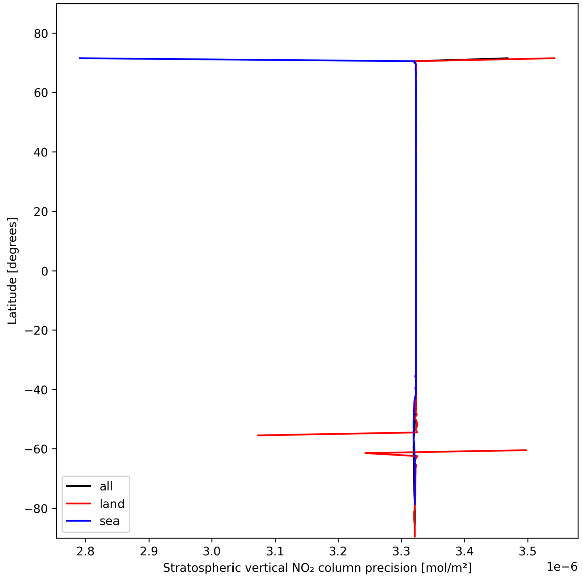
Figure 20: Zonal average of “Stratospheric vertical NO 2 column precision” for 2024-11-09 to 2024-11-10.
