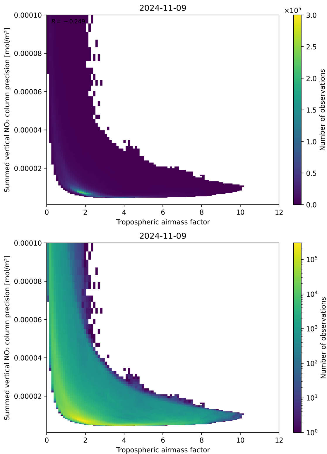
Figure 76: Scatter density plot of “Tropospheric air mass factor” against “Summed vertical NO 2 column precision” for 2024-11-09 to 2024-11-10.
