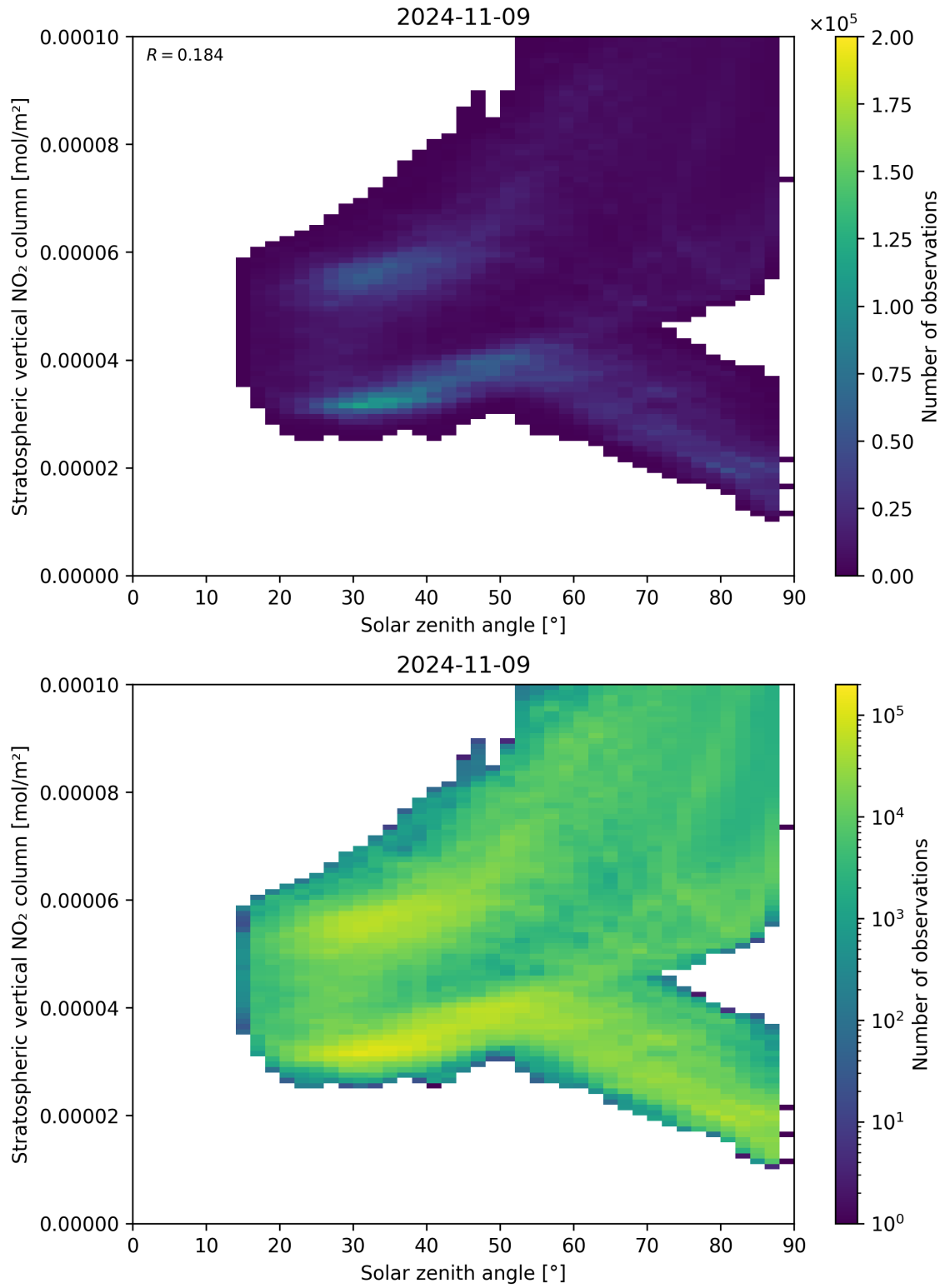
Figure 150: Scatter density plot of “Solar zenith angle” against “Stratospheric vertical NO 2 column” for 2024-11-09 to 2024-11-10.
