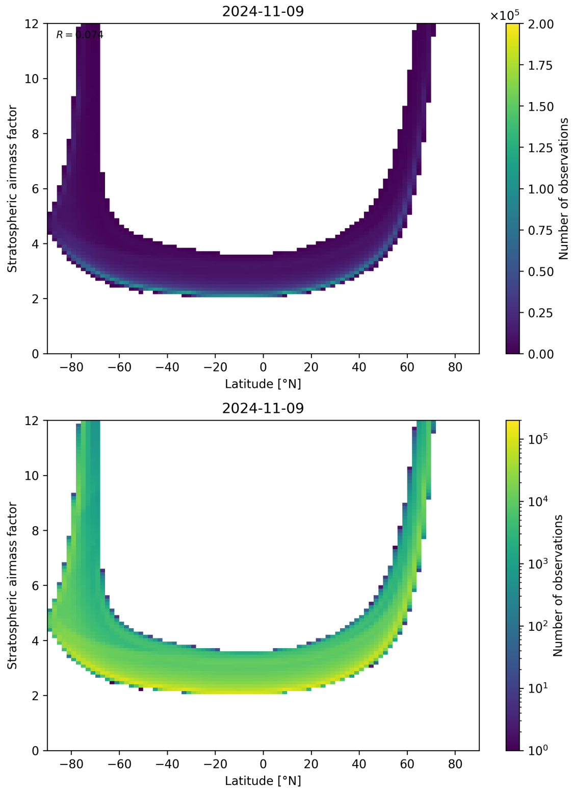
Figure 83: Scatter density plot of “Latitude” against “Stratospheric airmass factor” for 2024-11-09 to 2024-11-10.
