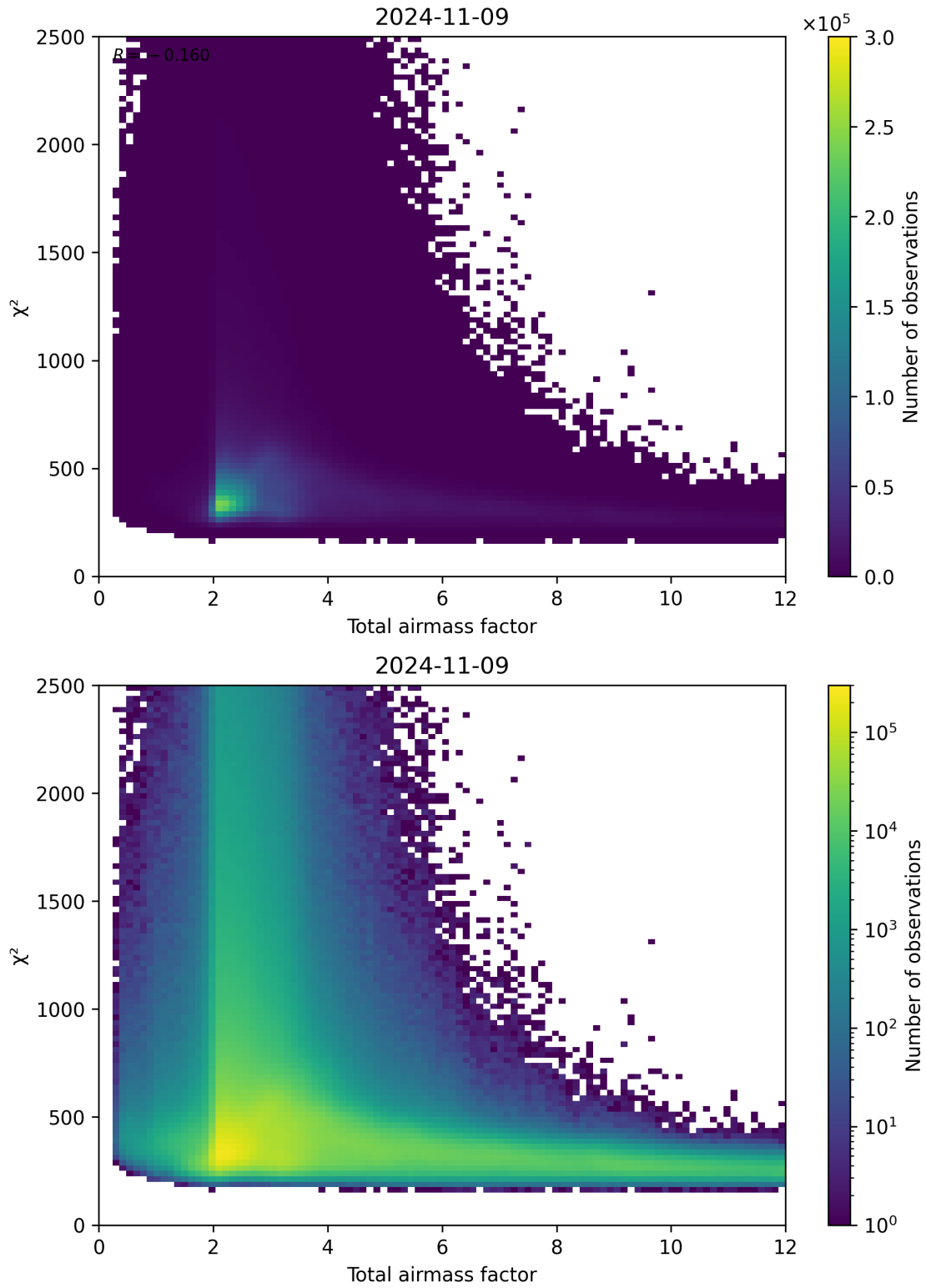
Figure 63: Scatter density plot of “Total airmass factor” against “ \chi^2 ” for 2024-11-09 to 2024-11-10.
