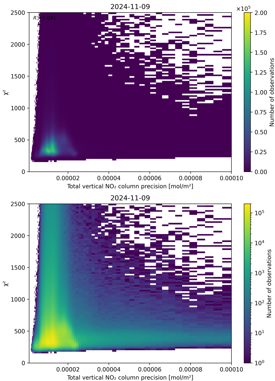
Figure 116: Scatter density plot of “Total vertical NO 2 column precision” against “ \chi^2 ” for 2024-11-09 to 2024-11-10.
