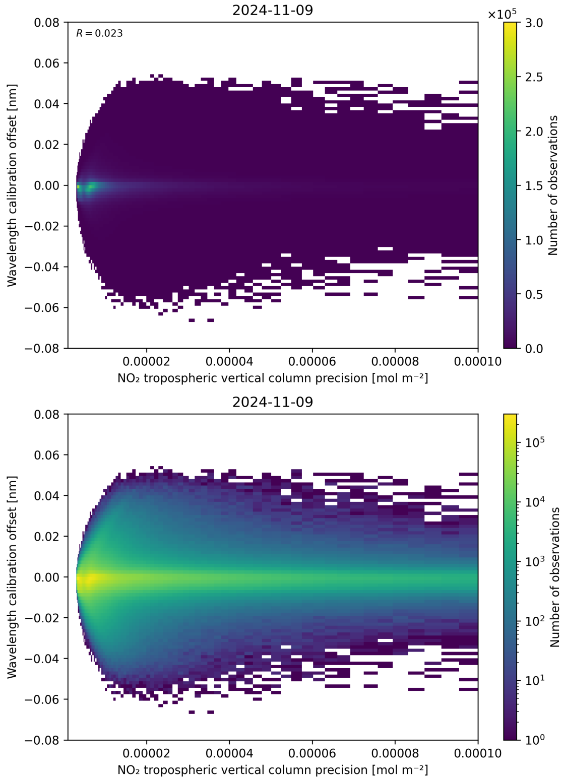
Figure 141: Scatter density plot of “NO 2 tropospheric vertical column precision” against “Wavelength calibration offset” for 2024-11-09 to 2024-11-10.
