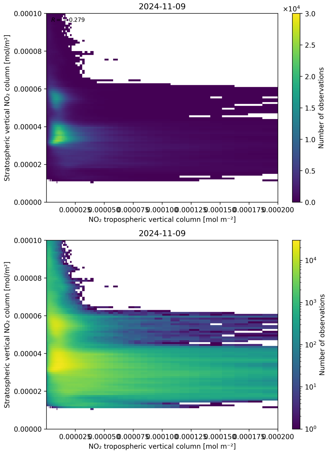
Figure 125: Scatter density plot of “NO 2 tropospheric vertical column” against “Stratospheric vertical NO 2 column” for 2024-11-09 to 2024-11-10.
