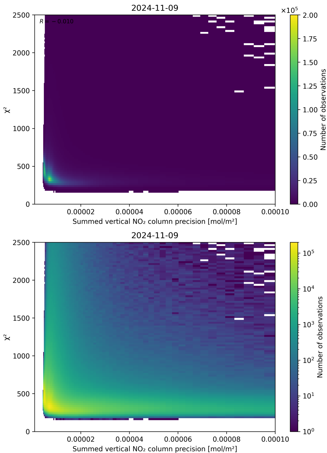
Figure 107: Scatter density plot of “Summed vertical NO 2 column precision” against “ \chi^2 ” for 2024-11-09 to 2024-11-10.
