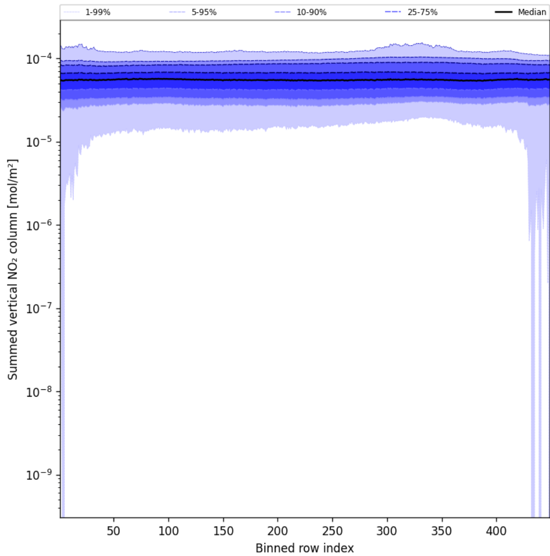
Figure 57: Along track statistics of “Summed vertical NO 2 column” for 2024-11-09 to 2024-11-10
