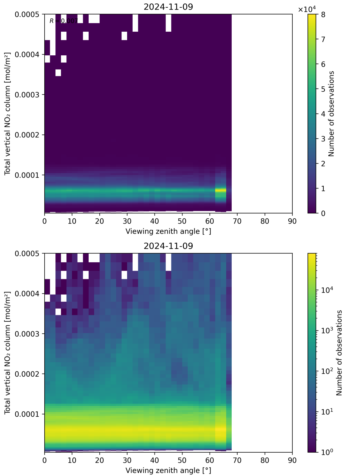
Figure 167: Scatter density plot of “Viewing zenith angle” against “Total vertical NO 2 column” for 2024-11-09 to 2024-11-10.
