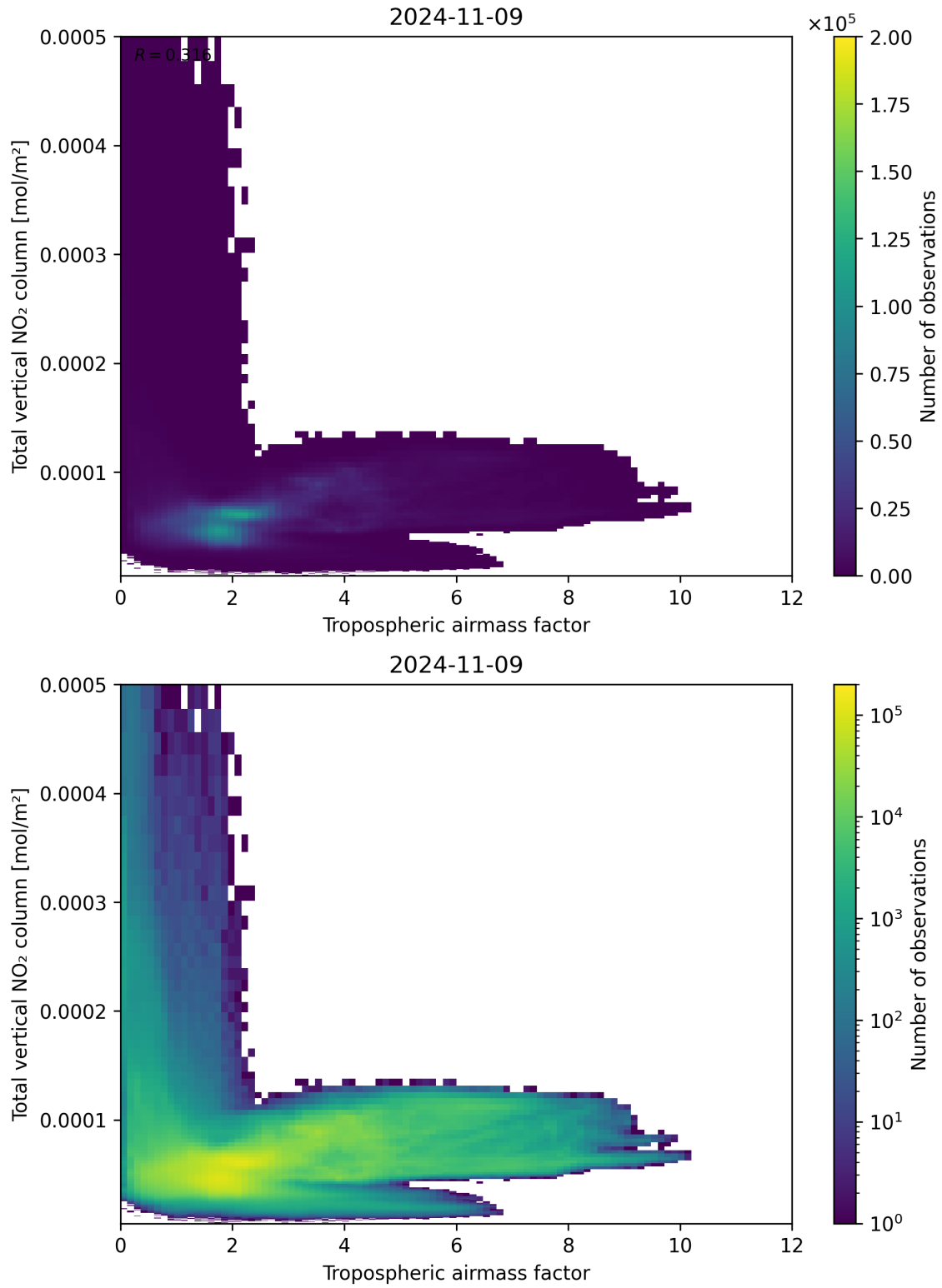
Figure 77: Scatter density plot of “Tropospheric airmass factor” against “Total vertical NO 2 column” for 2024-11-09 to 2024-11-10.
