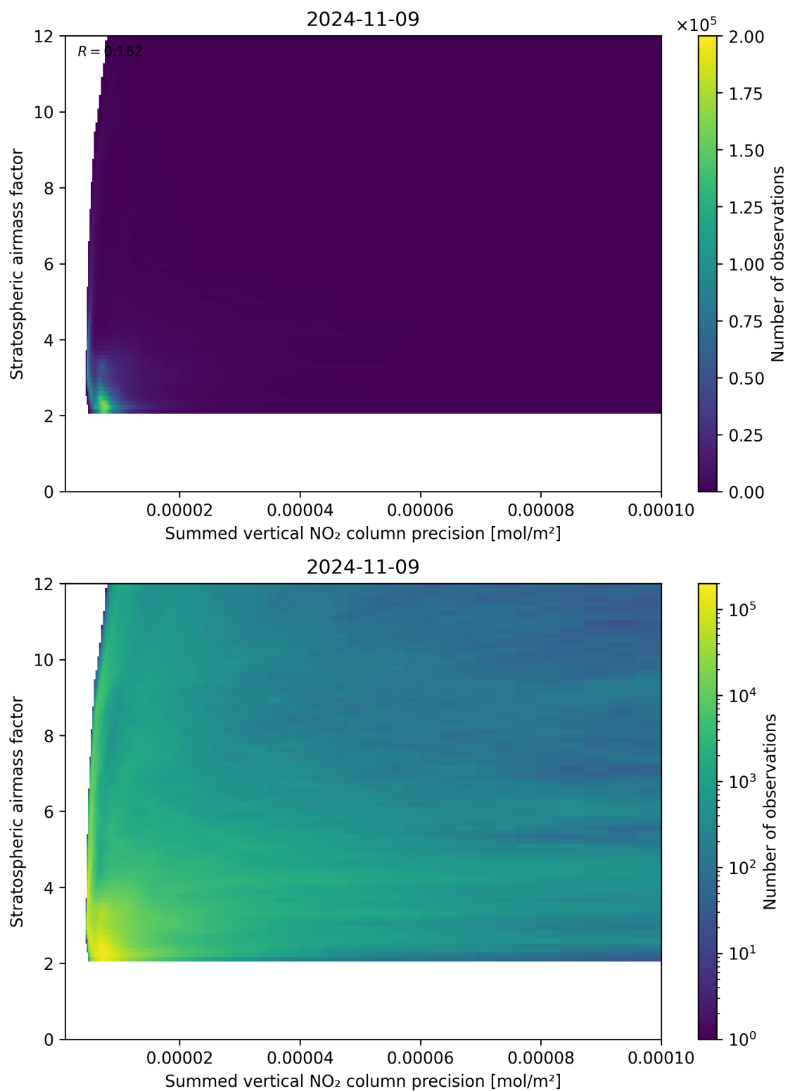
Figure 106: Scatter density plot of “Summed vertical NO 2 column precision” against “Stratospheric airmass factor” for 2024-11-09 to 2024-11-10.
