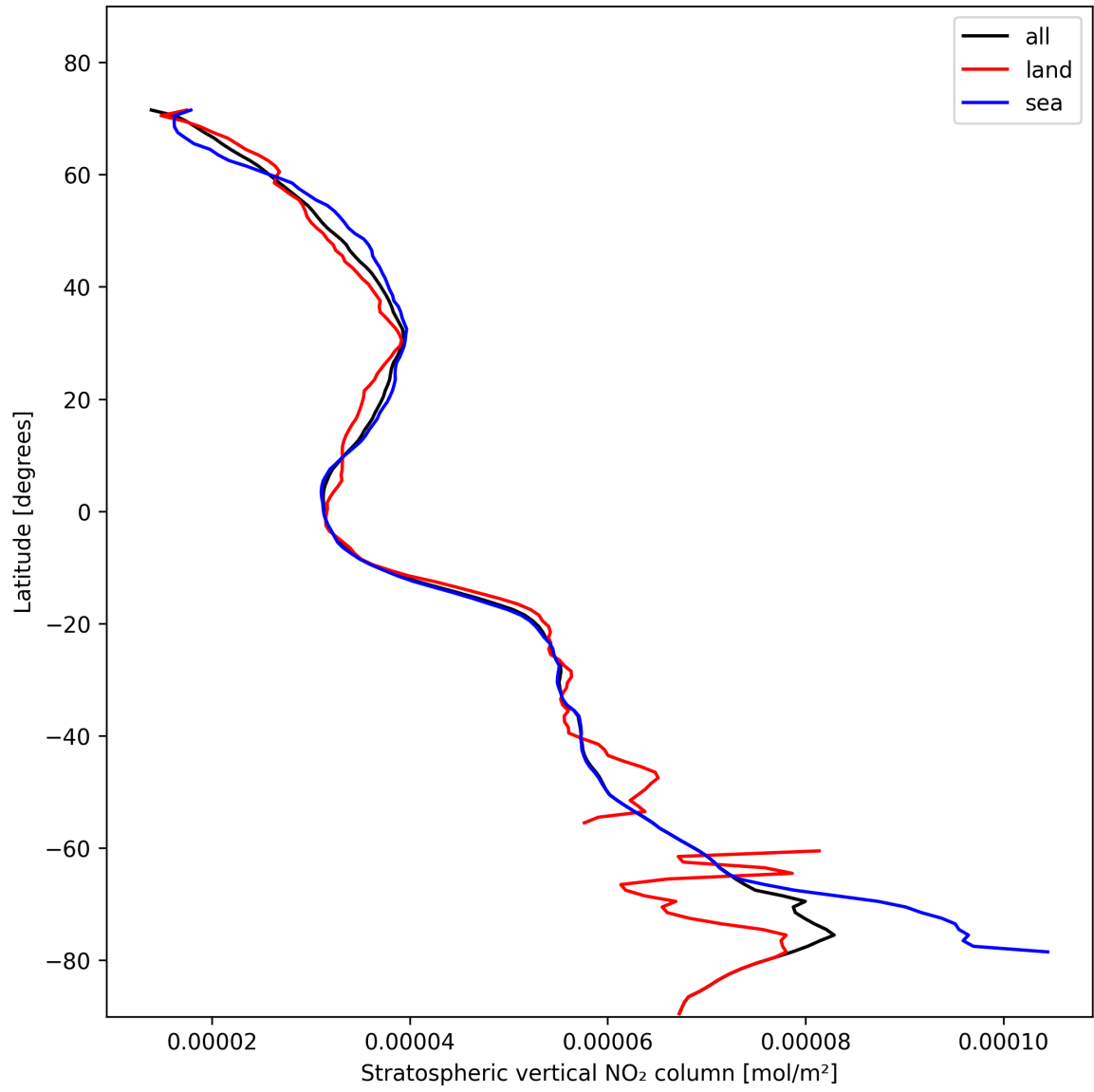
Figure 19: Zonal average of “Stratospheric vertical NO 2 column” for 2024-11-09 to 2024-11-10.
