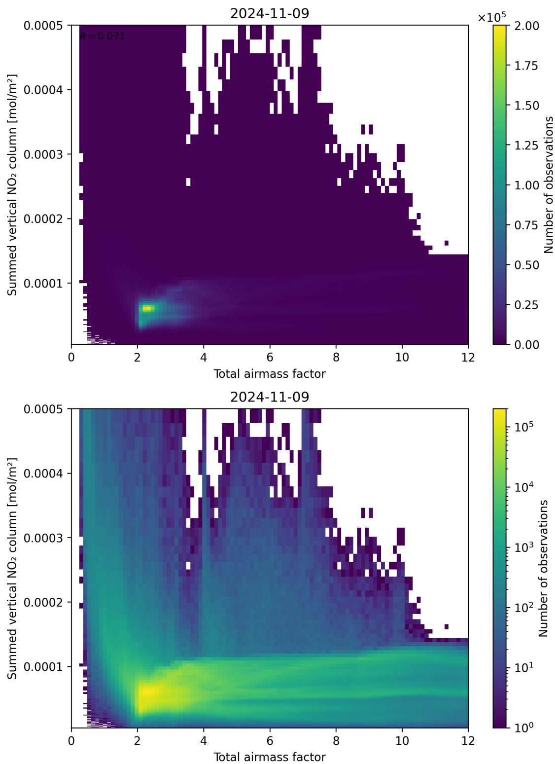
Figure 65: Scatter density plot of “Total airmass factor” against “Summed vertical NO 2 column” for 2024-11-09 to 2024-11-10.
