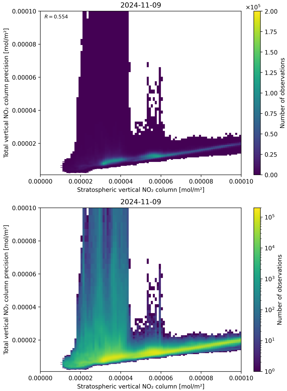
Figure 101: Scatter density plot of “Stratospheric vertical NO 2 column” against “Total vertical NO 2 column precision” for 2024-11-09 to 2024-11-10.
