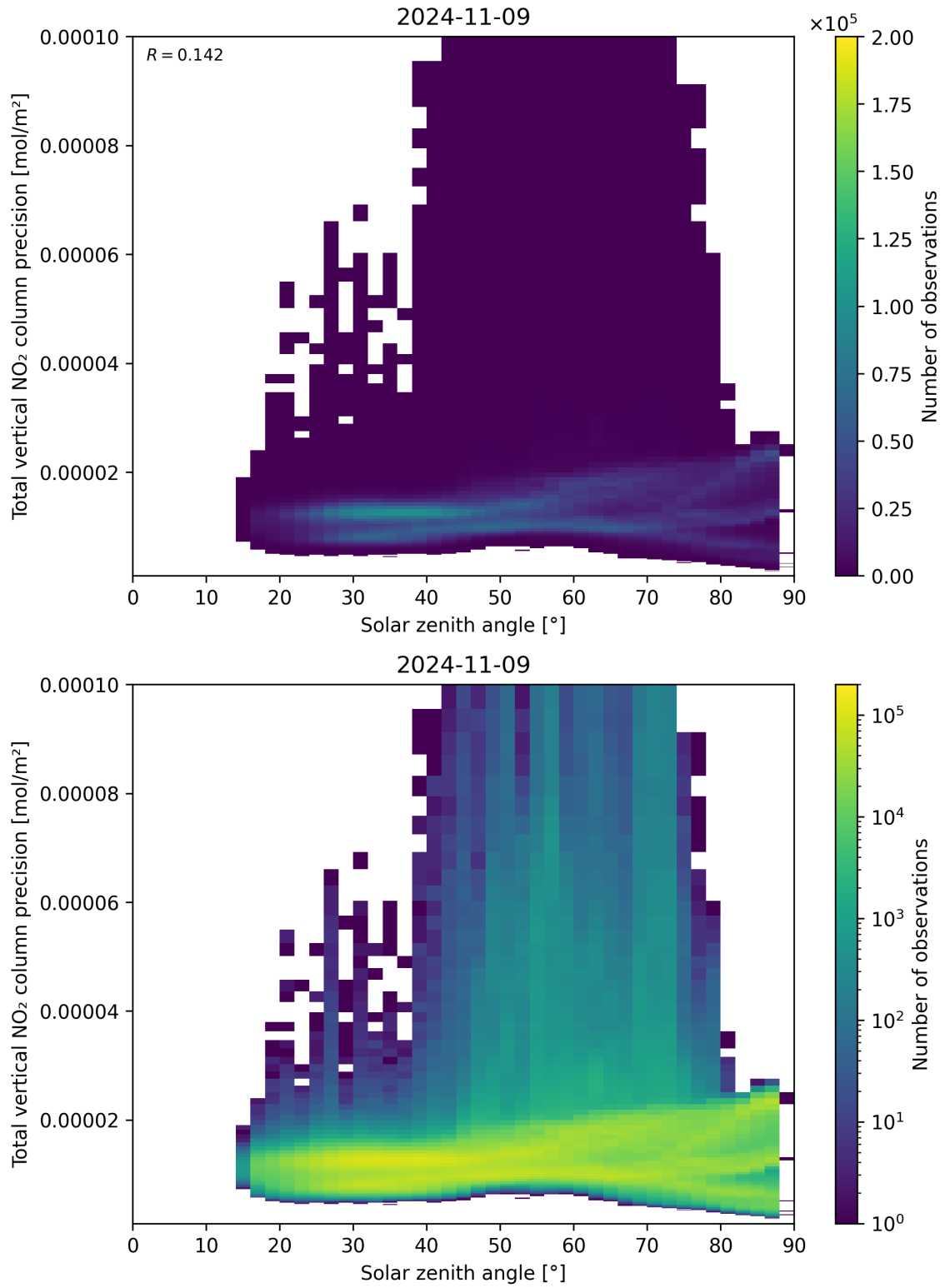
Figure 154: Scatter density plot of “Solar zenith angle” against “Total vertical NO 2 column precision” for 2024-11-09 to 2024-11-10.
