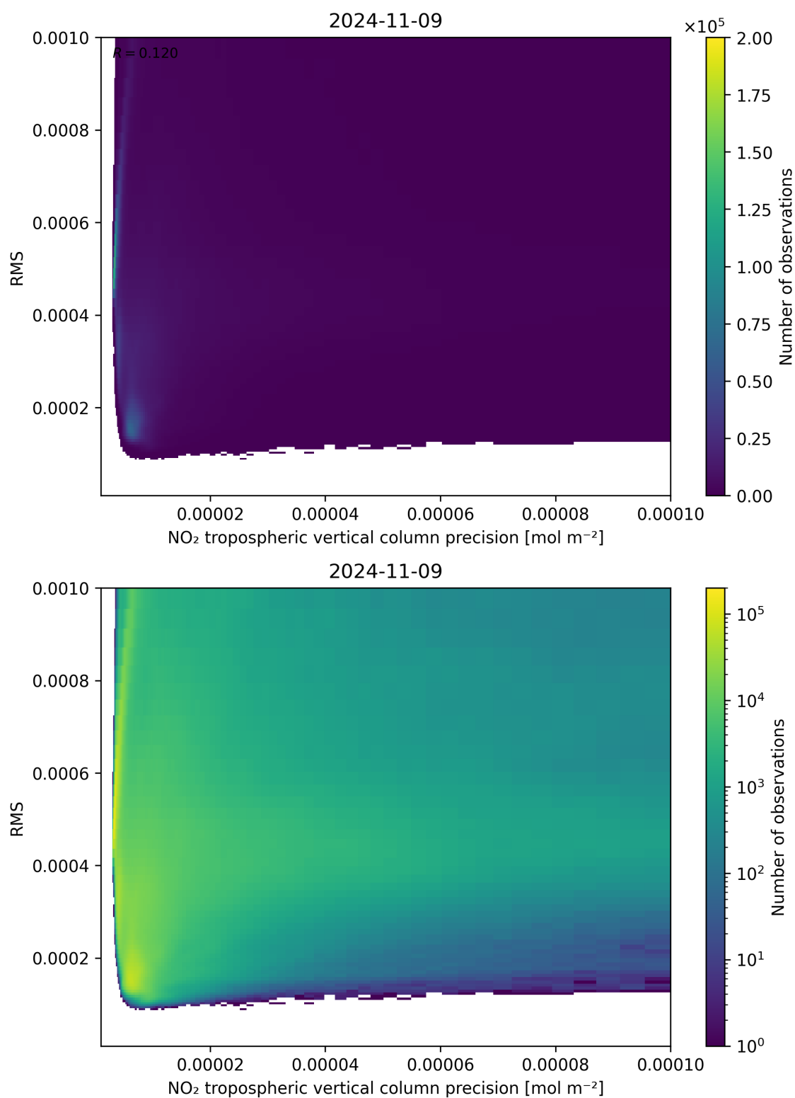
Figure 140: Scatter density plot of “NO 2 tropospheric vertical column precision” against “RMS” for 2024-11-09 to 2024-11-10.
