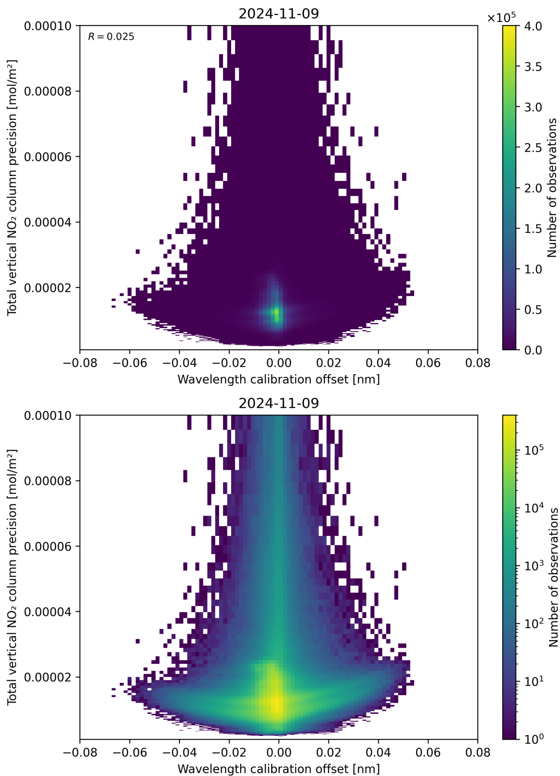
Figure 180: Scatter density plot of “Wavelength calibration offset” against “Total vertical NO 2 column precision” for 2024-11-09 to 2024-11-10.
