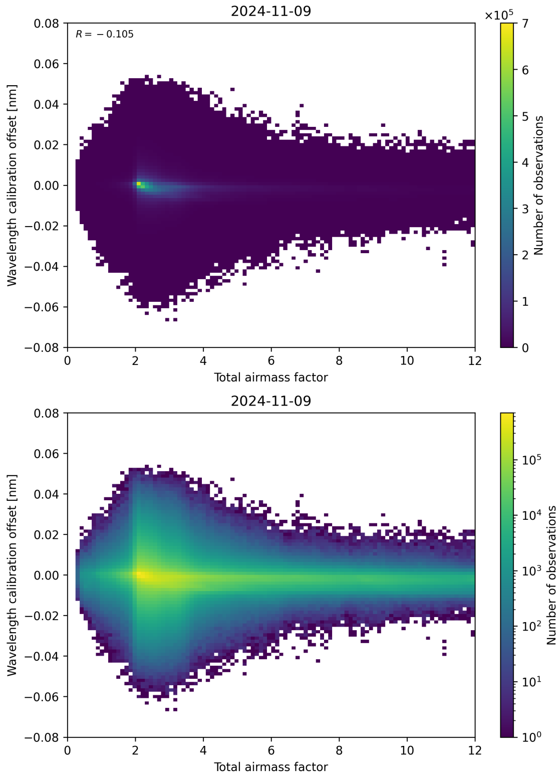
Figure 70: Scatter density plot of “Total airmass factor” against “Wavelength calibration offset” for 2024-11-09 to 2024-11-10.
