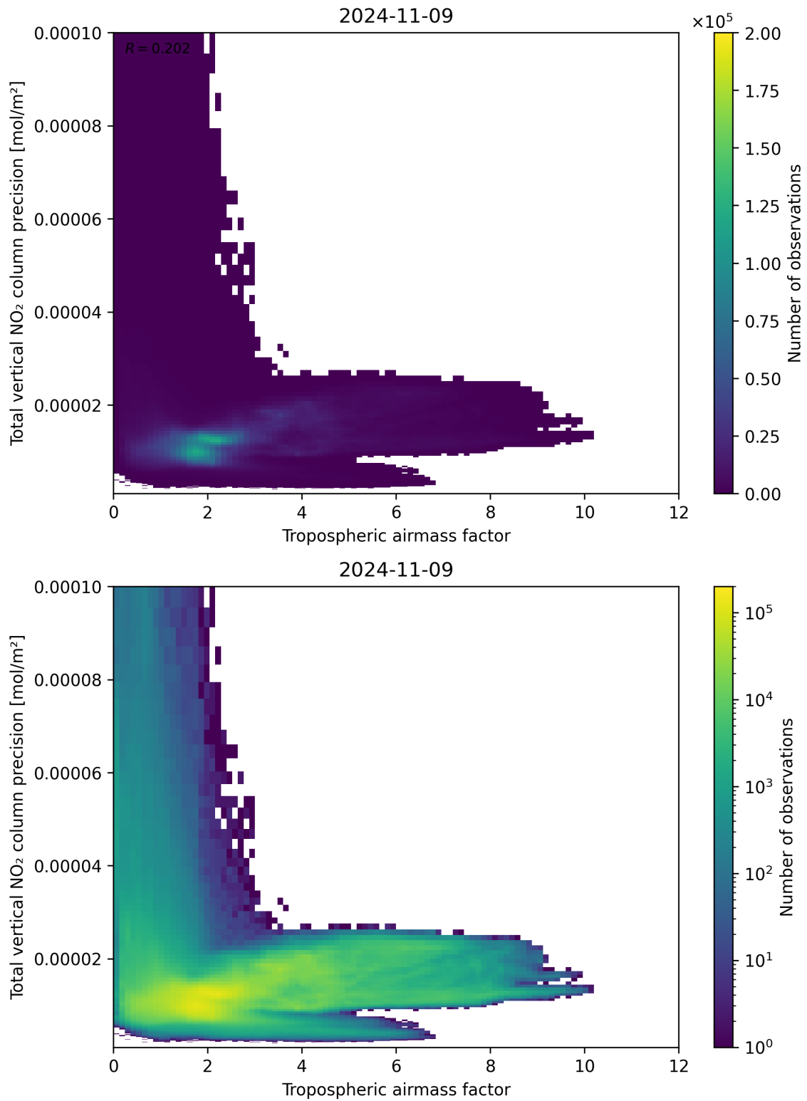
Figure 78: Scatter density plot of “Tropospheric air mass factor” against “Total vertical NO 2 column precision” for 2024-11-09 to 2024-11-10.
