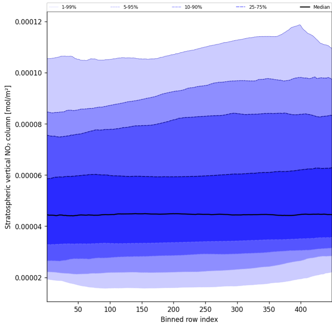
Figure 53: Along track statistics of “Stratospheric vertical NO 2 column” for 2024-11-09 to 2024-11-10
