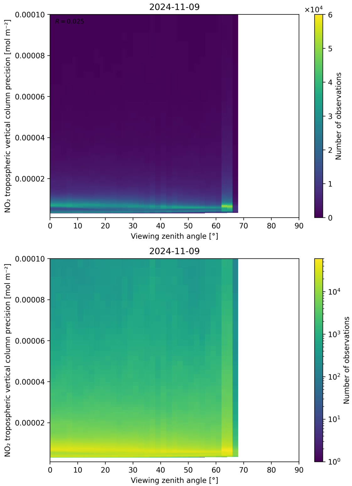
Figure 170: Scatter density plot of “Viewing zenith angle” against “NO 2 tropospheric vertical column precision” for 2024-11-09 to 2024-11-10.
