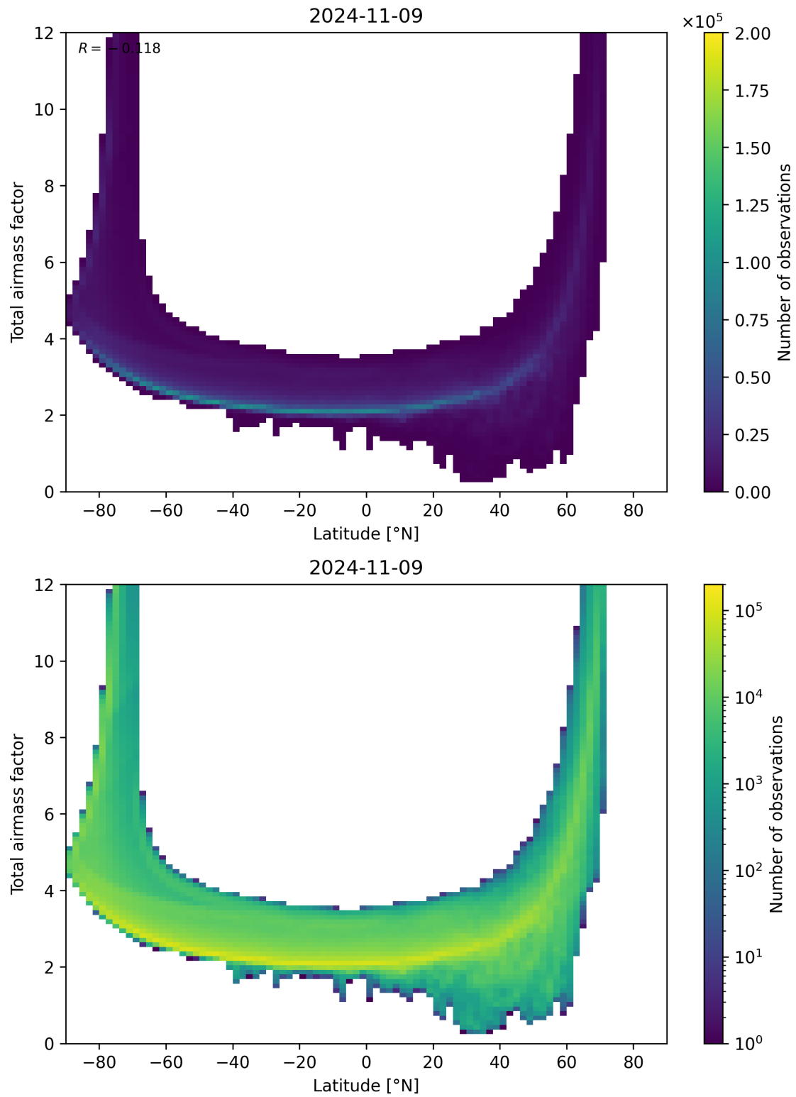
Figure 84: Scatter density plot of “Latitude” against “Total airmass factor” for 2024-11-09 to 2024-11-10.
