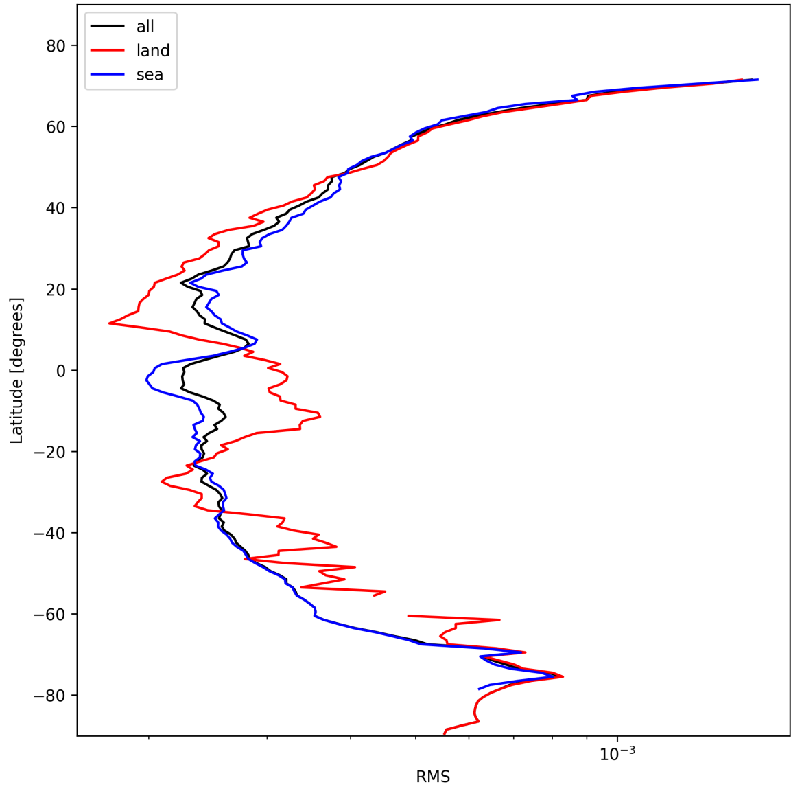
Figure 26: Zonal average of “RMS” for 2024-11-09 to 2024-11-10.
