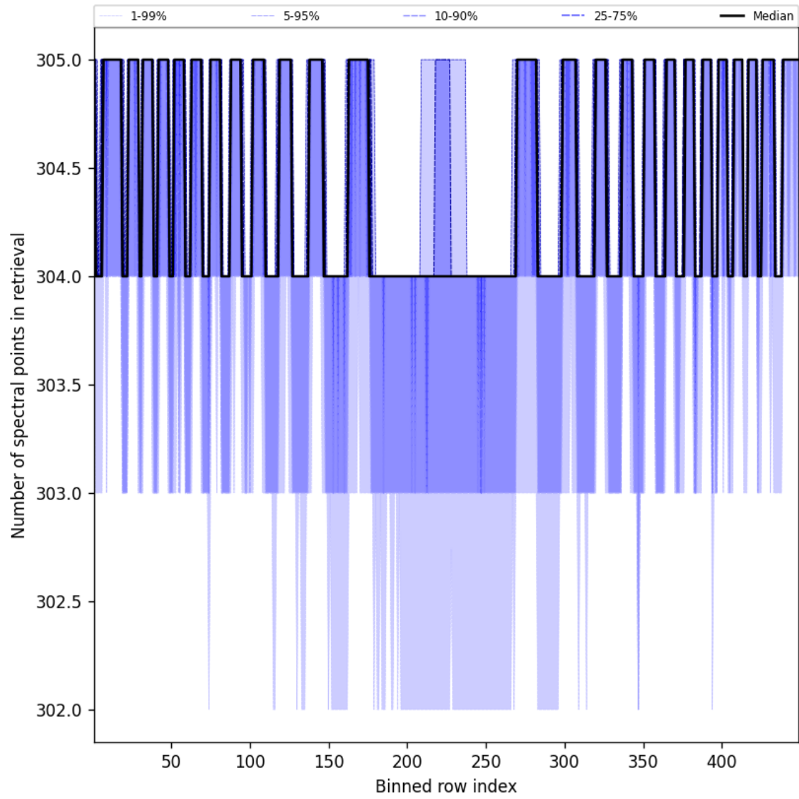
Figure 50: Along track statistics of “Number of spectral points in retrieval” for 2024-11-09 to 2024-11-10
