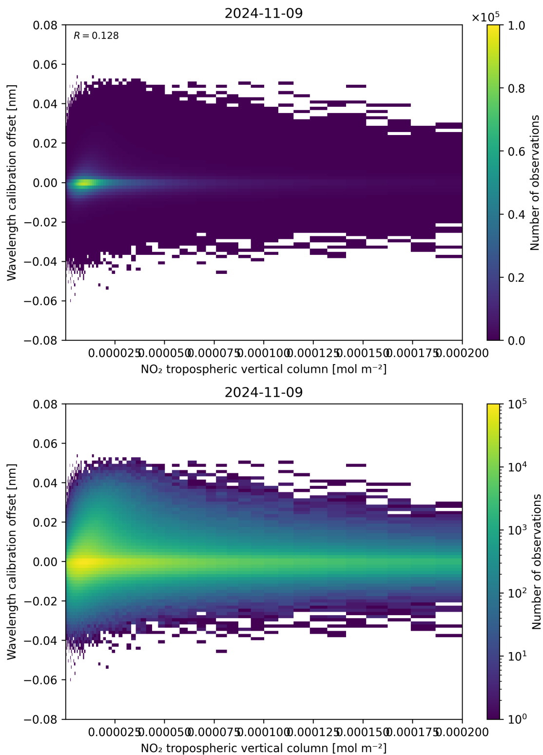
Figure 143: Scatter density plot of “NO 2 tropospheric vertical column” against “Wavelength calibration offset” for 2024-11-09 to 2024-11-10.
