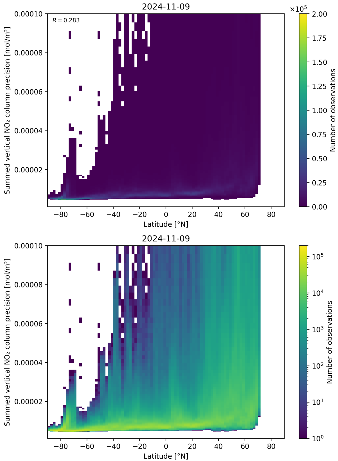
Figure 89: Scatter density plot of “Latitude” against “Summed vertical NO 2 column precision” for 2024-11-09 to 2024-11-10.
