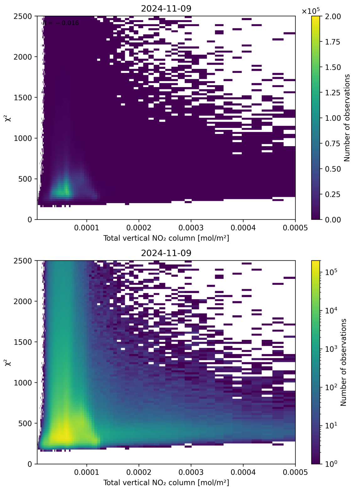
Figure 111: Scatter density plot of “Total vertical NO 2 column” against “ \chi^2 ” for 2024-11-09 to 2024-11-10.
