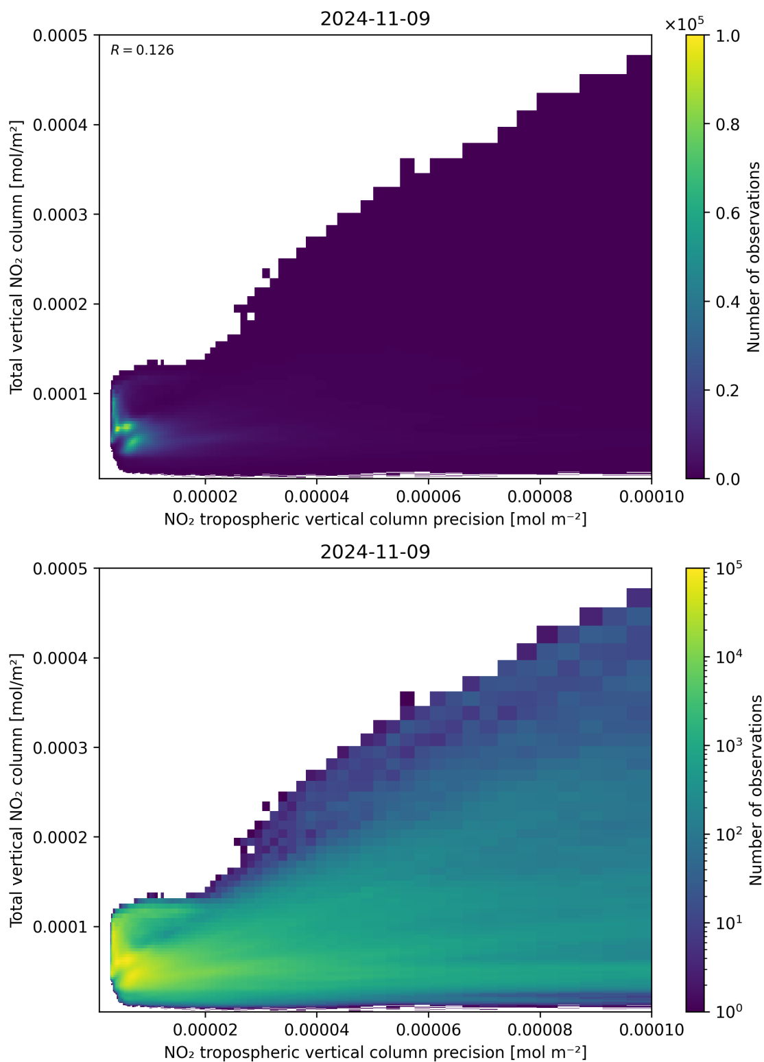
Figure 138: Scatter density plot of “NO 2 tropospheric vertical column precision” against “Total vertical NO 2 column” for 2024-11-09 to 2024-11-10.
