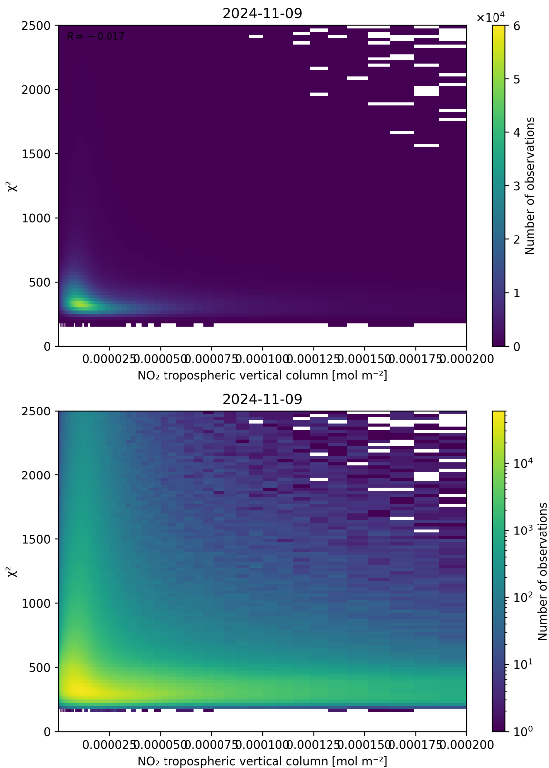
Figure 124: Scatter density plot of “NO 2 tropospheric vertical column” against “ \chi^2 ” for 2024-11-09 to 2024-11-10.
