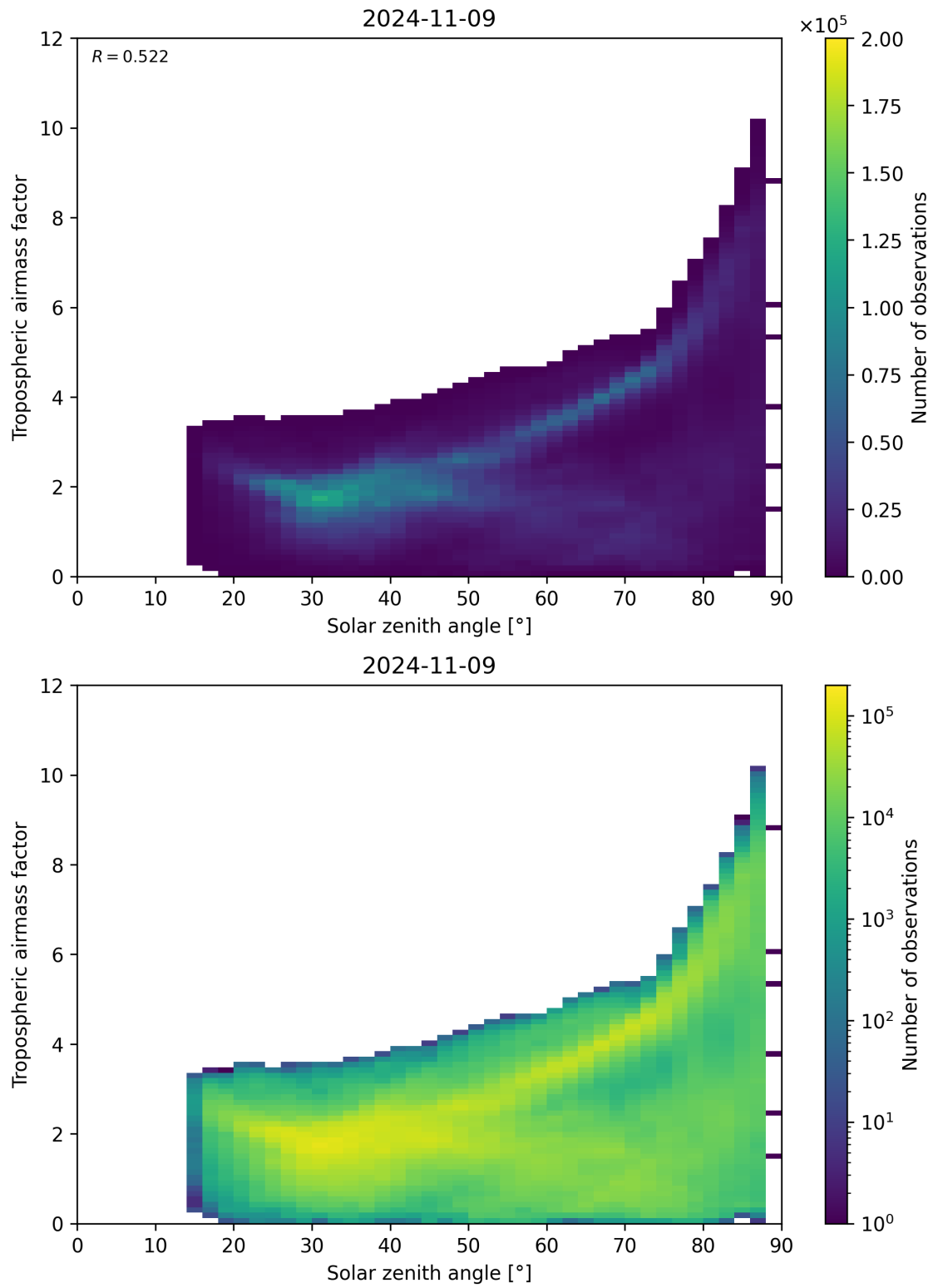
Figure 147: Scatter density plot of “Solar zenith angle” against “Tropospheric airmass factor” for 2024-11-09 to 2024-11-10.
