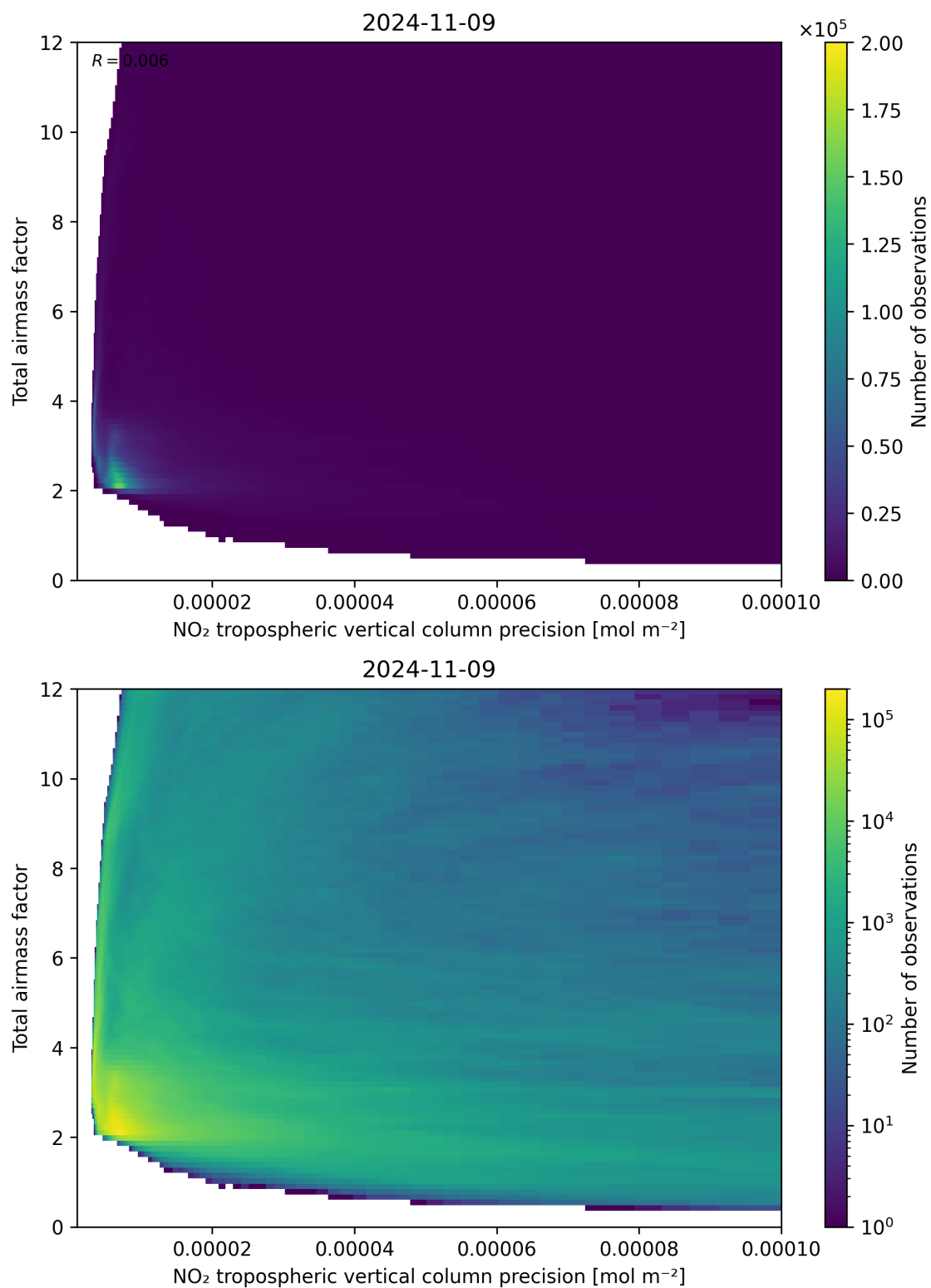
Figure 132: Scatter density plot of “NO 2 tropospheric vertical column precision” against “Total air mass factor” for 2024-11-09 to 2024-11-10.
