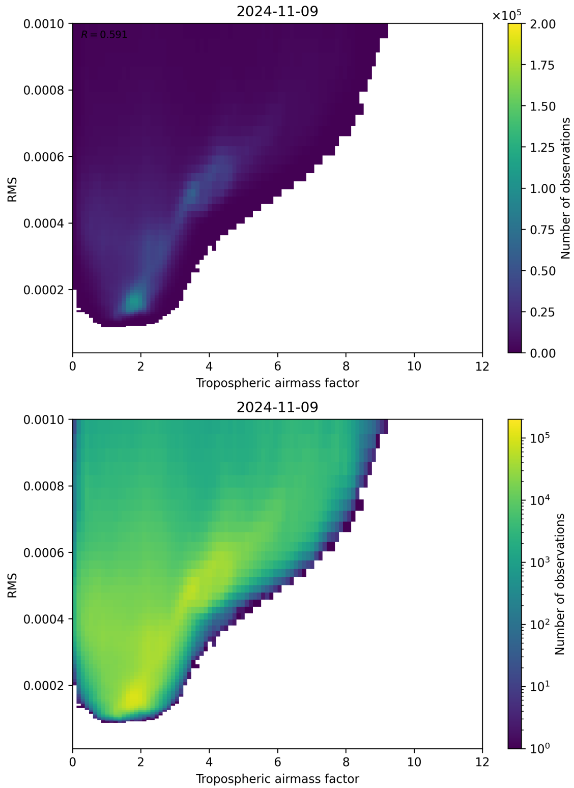
Figure 79: Scatter density plot of “Tropospheric airmass factor” against “RMS” for 2024-11-09 to 2024-11-10.
