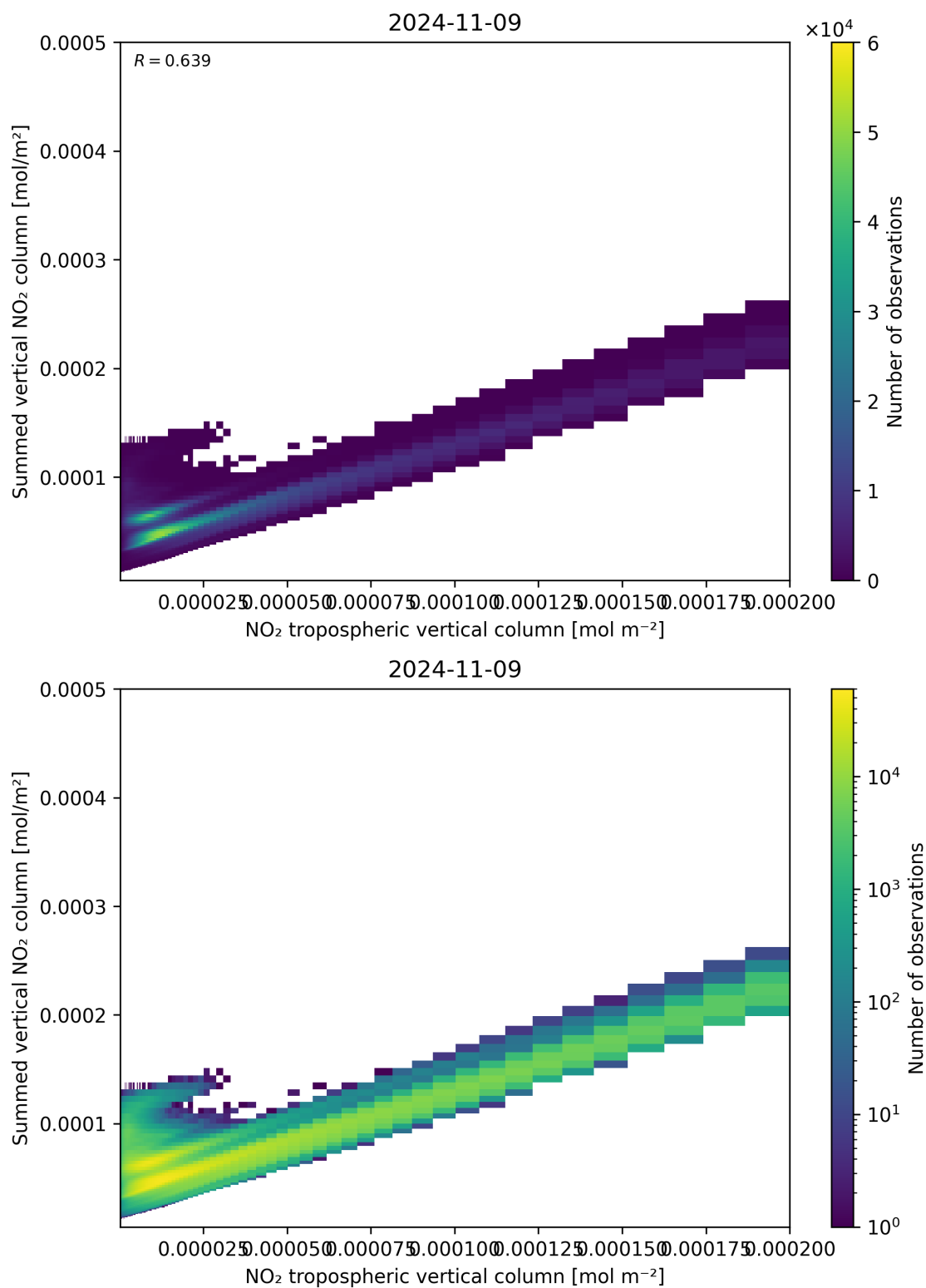
Figure 126: Scatter density plot of “NO 2 tropospheric vertical column” against “Summed vertical NO 2 column” for 2024-11-09 to 2024-11-10.
