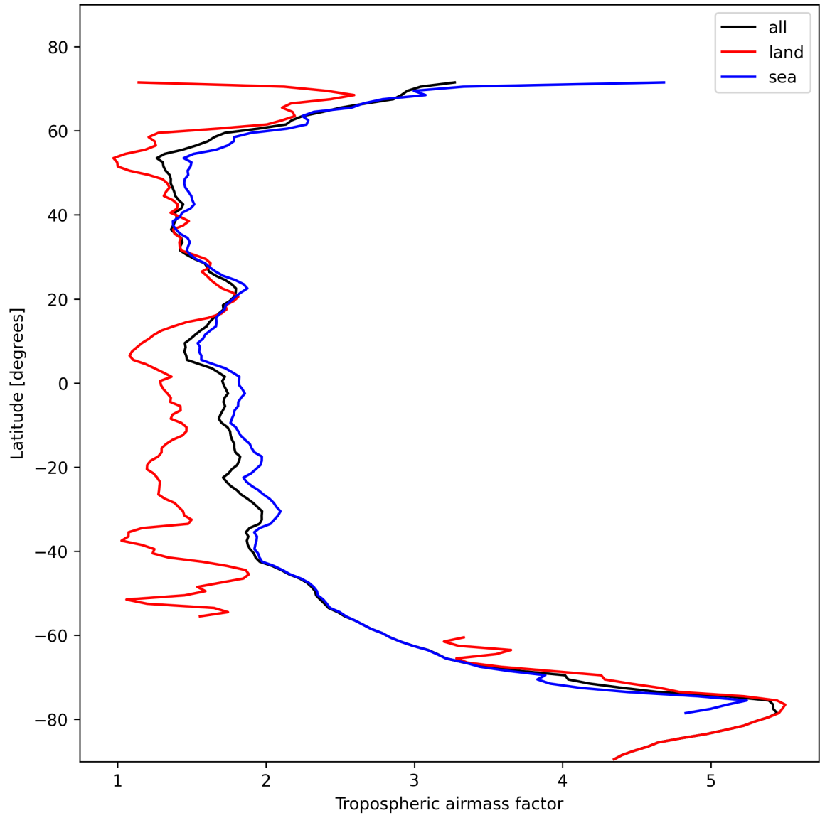
Figure 14: Zonal average of “Tropospheric airmass factor” for 2024-11-09 to 2024-11-10.
