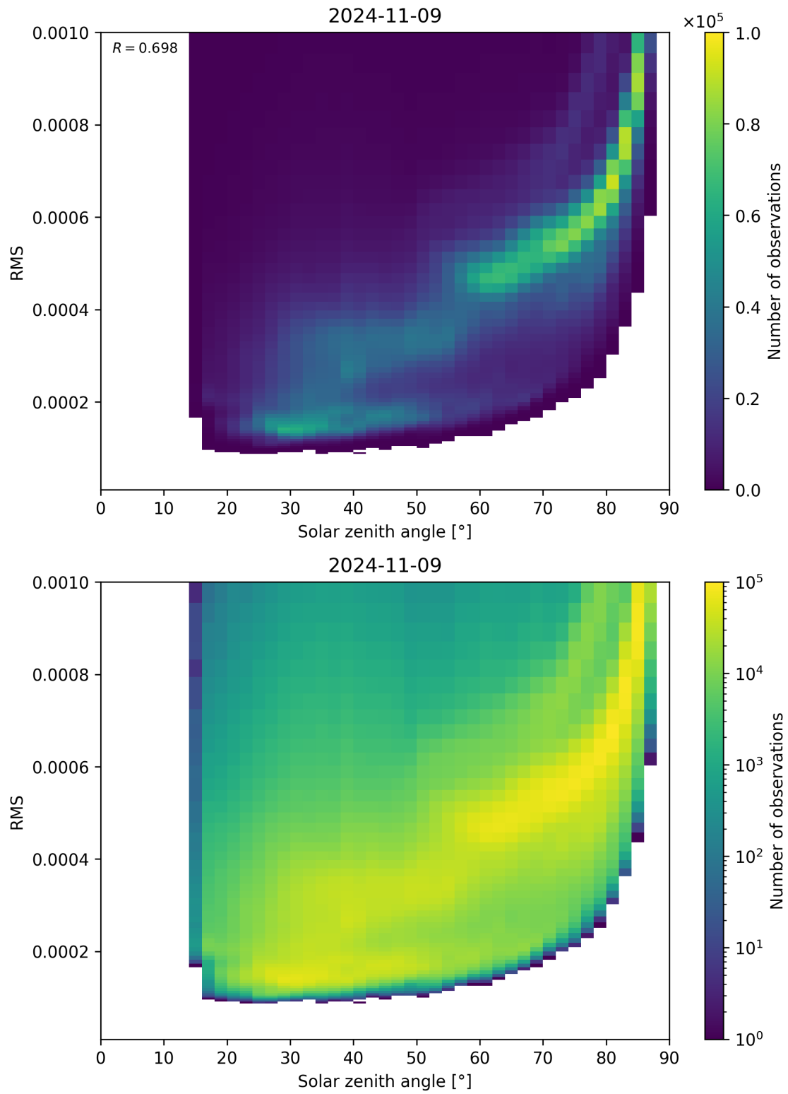
Figure 157: Scatter density plot of “Solar zenith angle” against “RMS” for 2024-11-09 to 2024-11-10.
