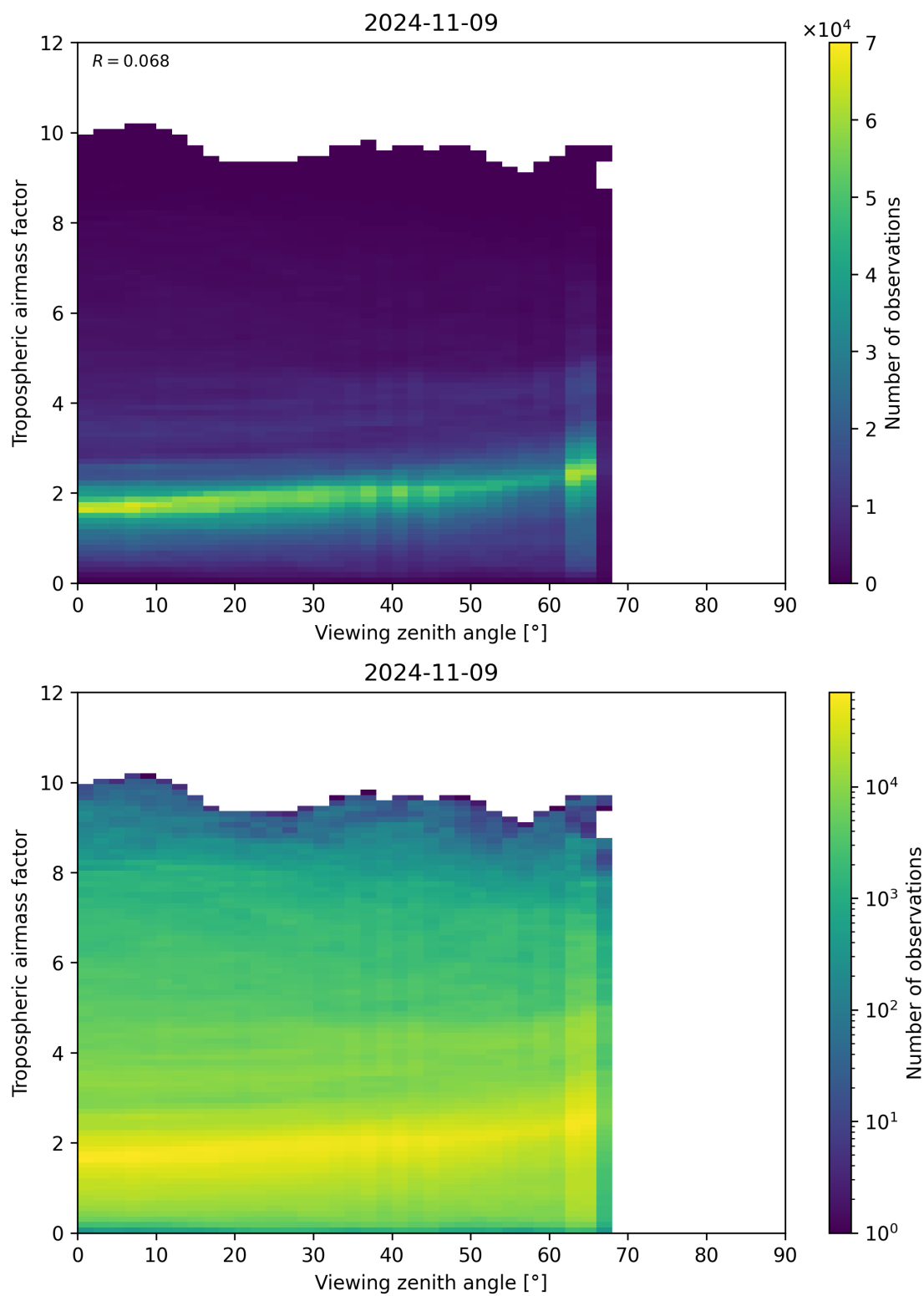
Figure 161: Scatter density plot of “Viewing zenith angle” against “Tropospheric airmass factor” for 2024-11-09 to 2024-11-10.
