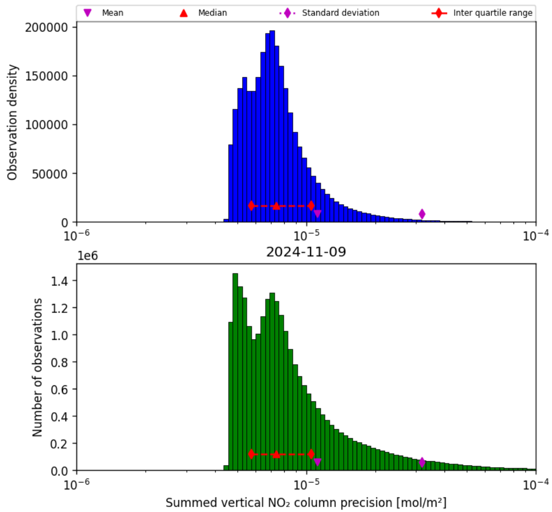
Figure 41: Histogram of “Summed vertical NO 2 column precision” for 2024-11-09 to 2024-11-10
