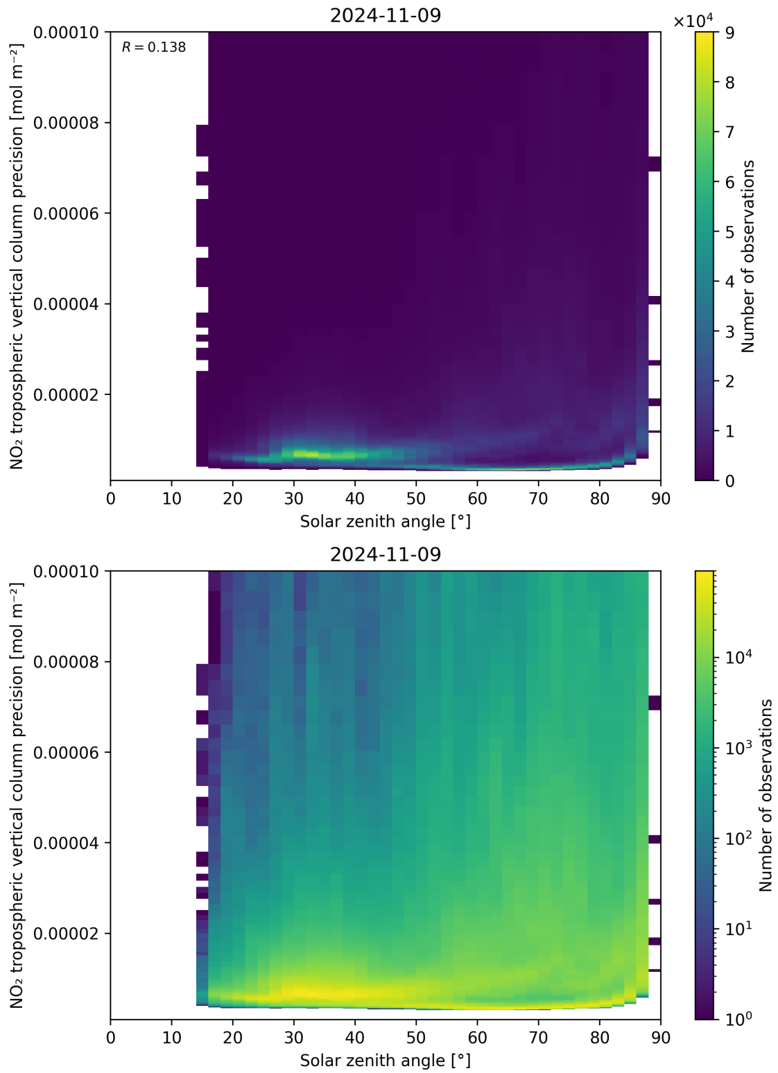
Figure 156: Scatter density plot of “Solar zenith angle” against “NO 2 tropospheric vertical column precision” for 2024-11-09 to 2024-11-10.
