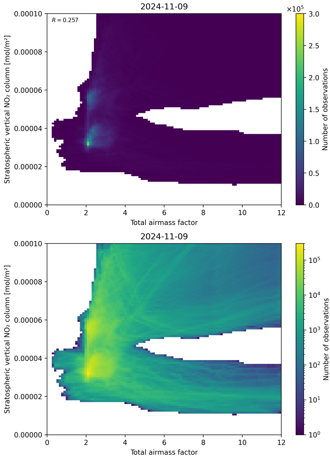
Figure 64: Scatter density plot of “Total airmass factor” against “Stratospheric vertical NO 2 column” for 2024-11-09 to 2024-11-10.
