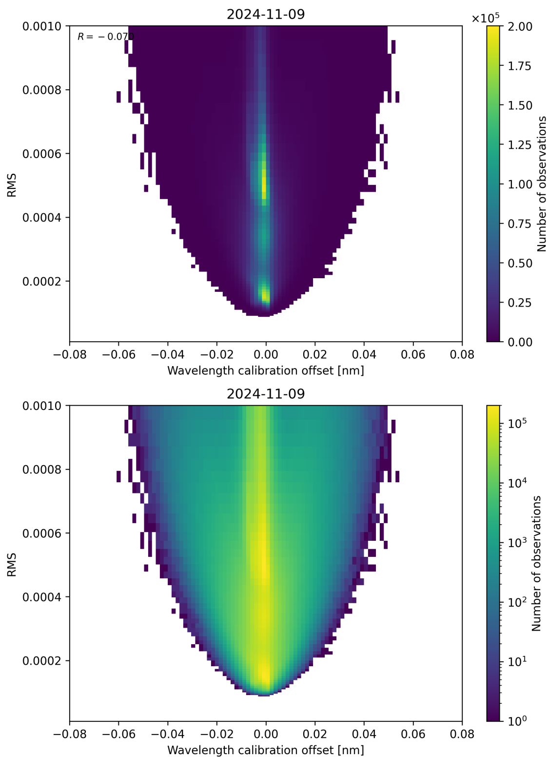
Figure 181: Scatter density plot of “Wavelength calibration offset” against “RMS” for 2024-11-09 to 2024-11-10.
