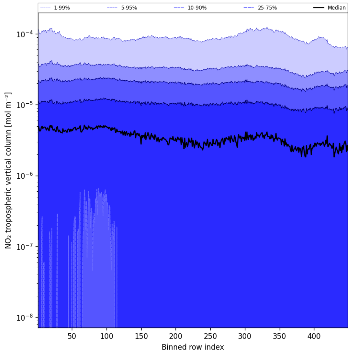
Figure 46: Along track statistics of “NO 2 tropospheric vertical column” for 2024-11-09 to 2024-11-10
