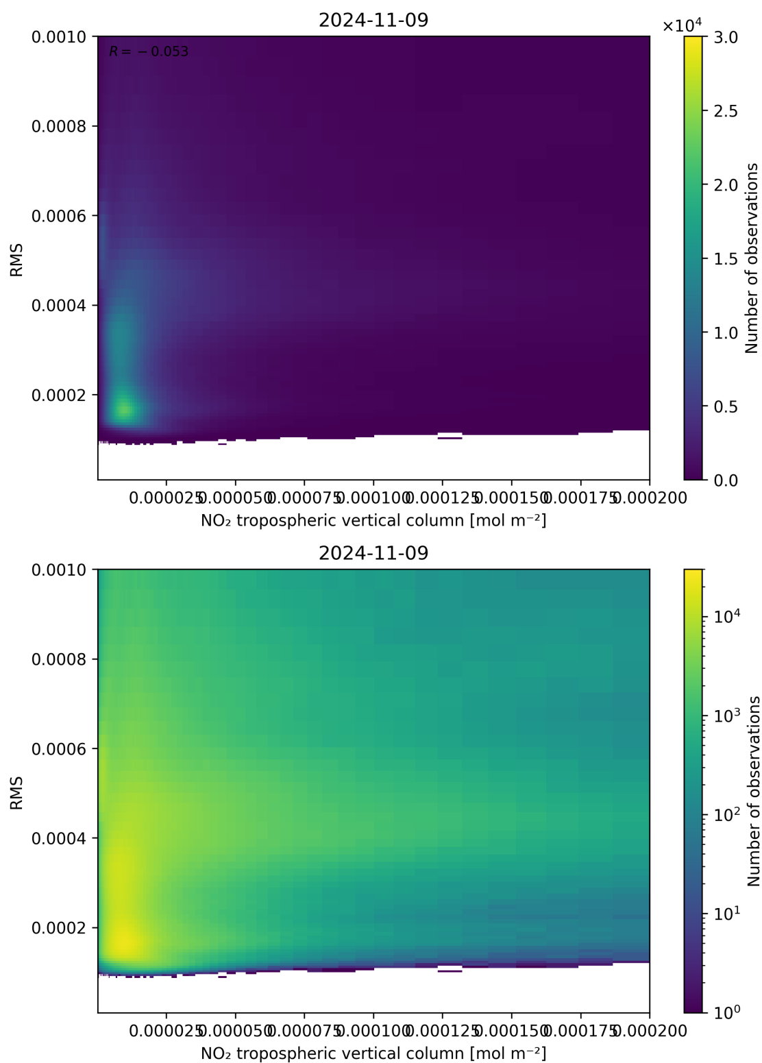
Figure 142: Scatter density plot of “NO 2 tropospheric vertical column” against “RMS” for 2024-11-09 to 2024-11-10.
