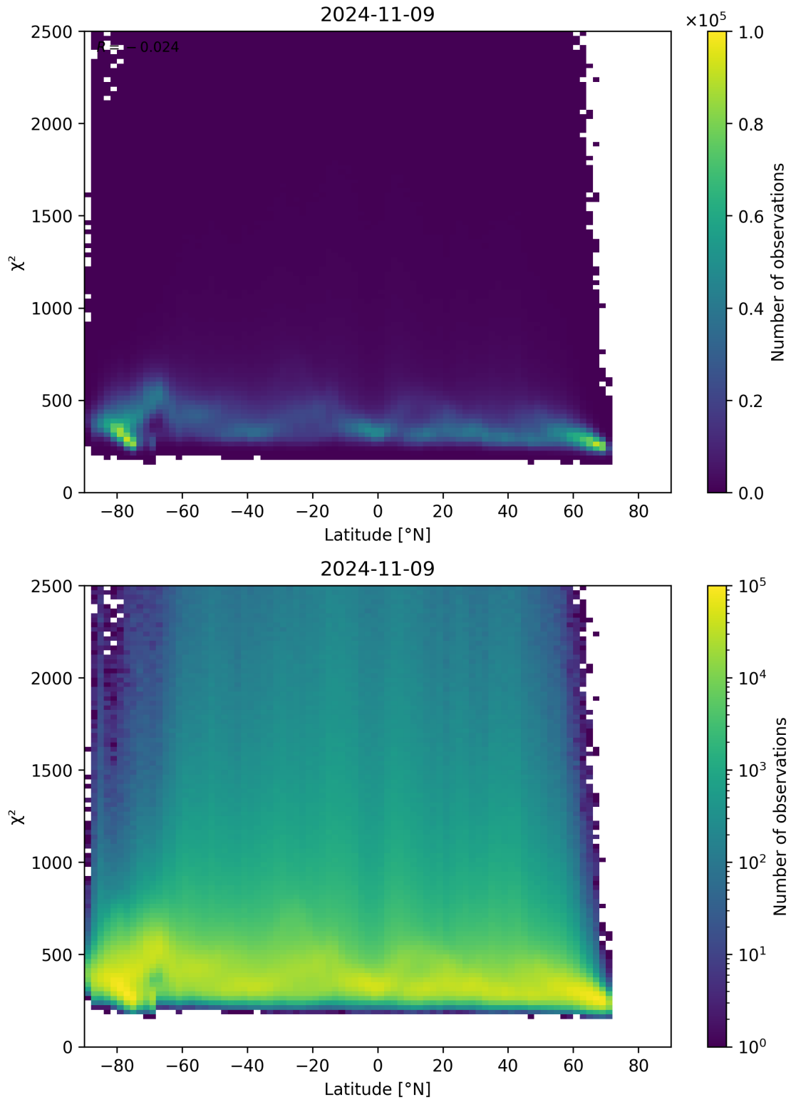
Figure 86: Scatter density plot of “Latitude” against “ \chi^2 ” for 2024-11-09 to 2024-11-10.
