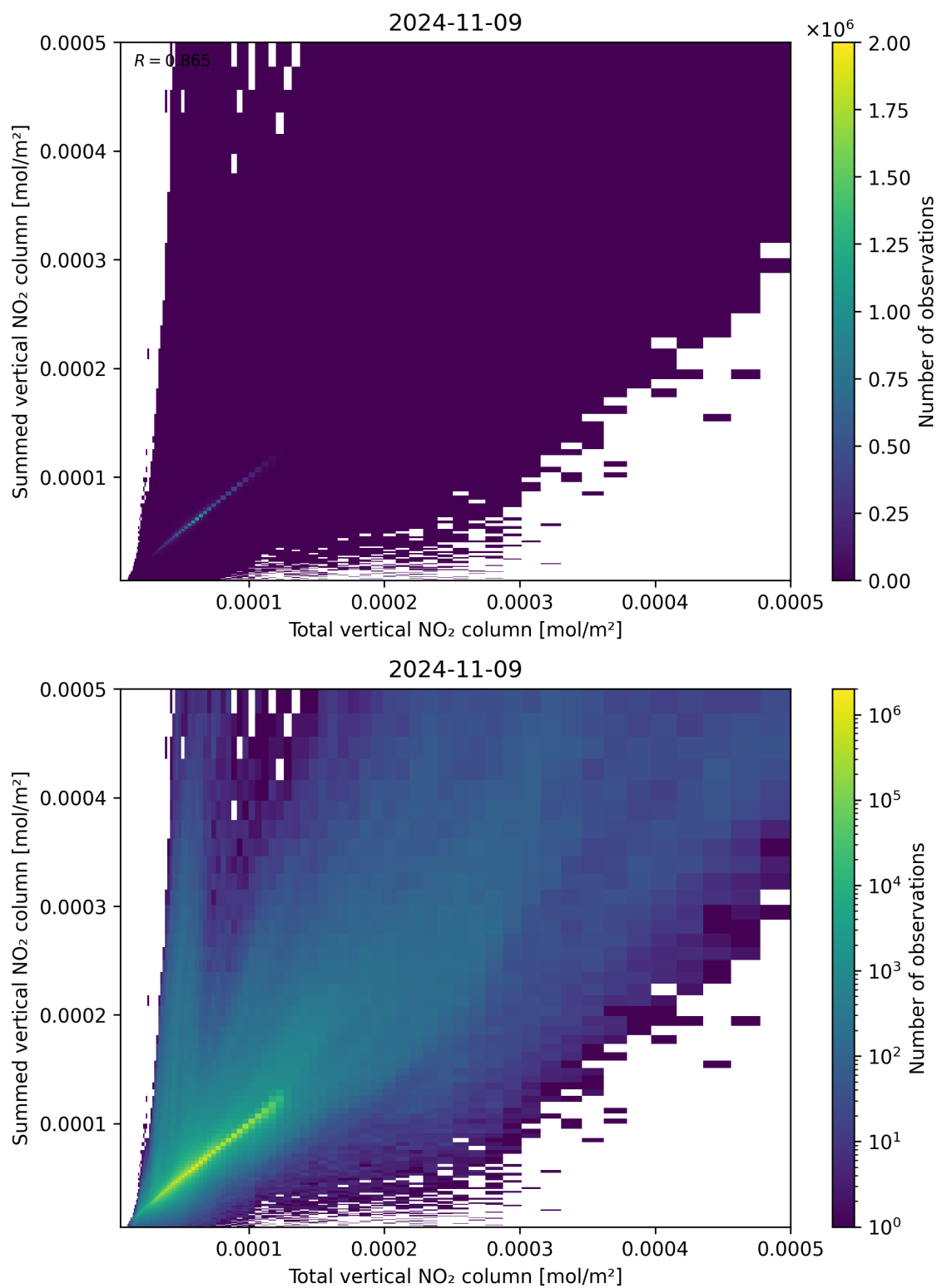
Figure 112: Scatter density plot of “Total vertical NO 2 column” against “Summed vertical NO 2 column” for 2024-11-09 to 2024-11-10.
