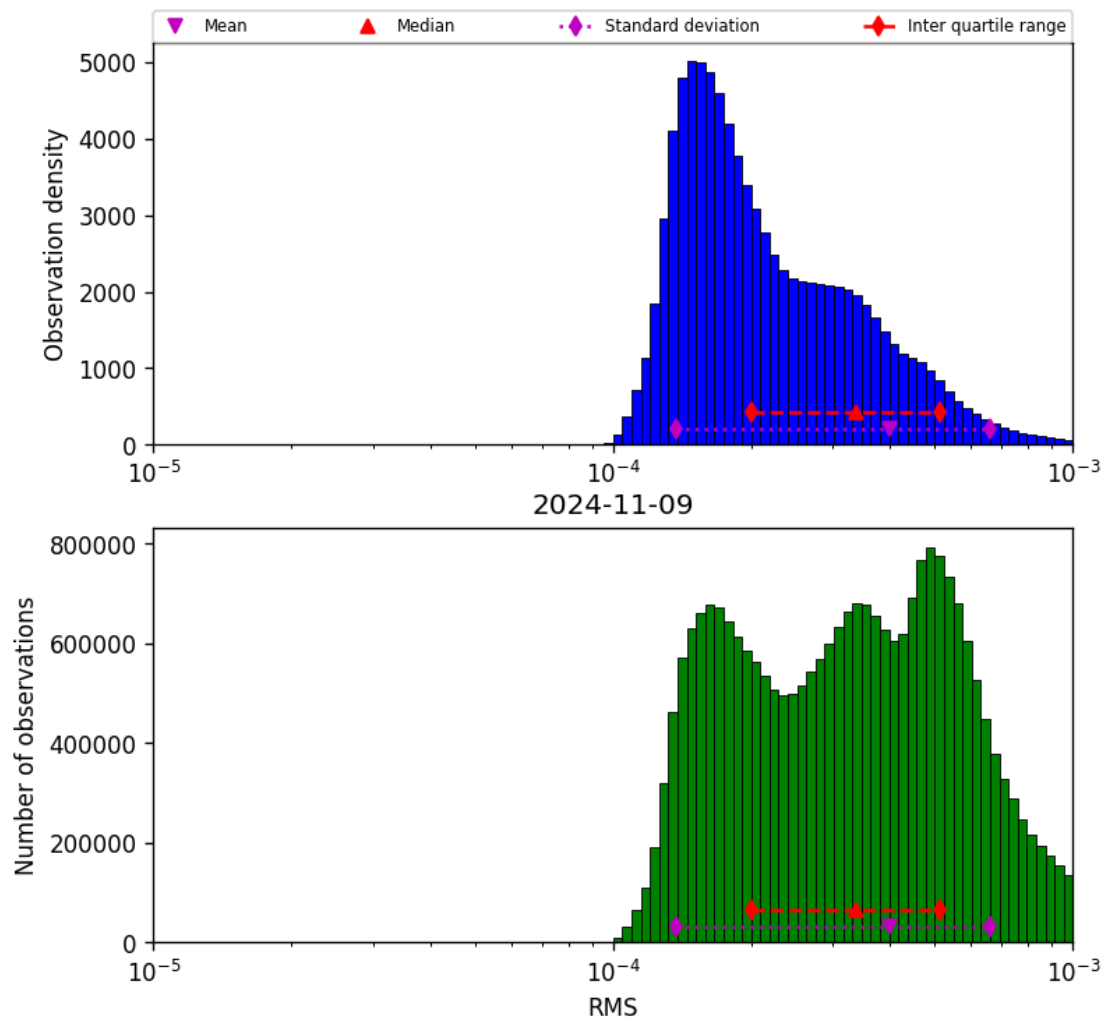
Figure 43: Histogram of “RMS” for 2024-11-09 to 2024-11-10
