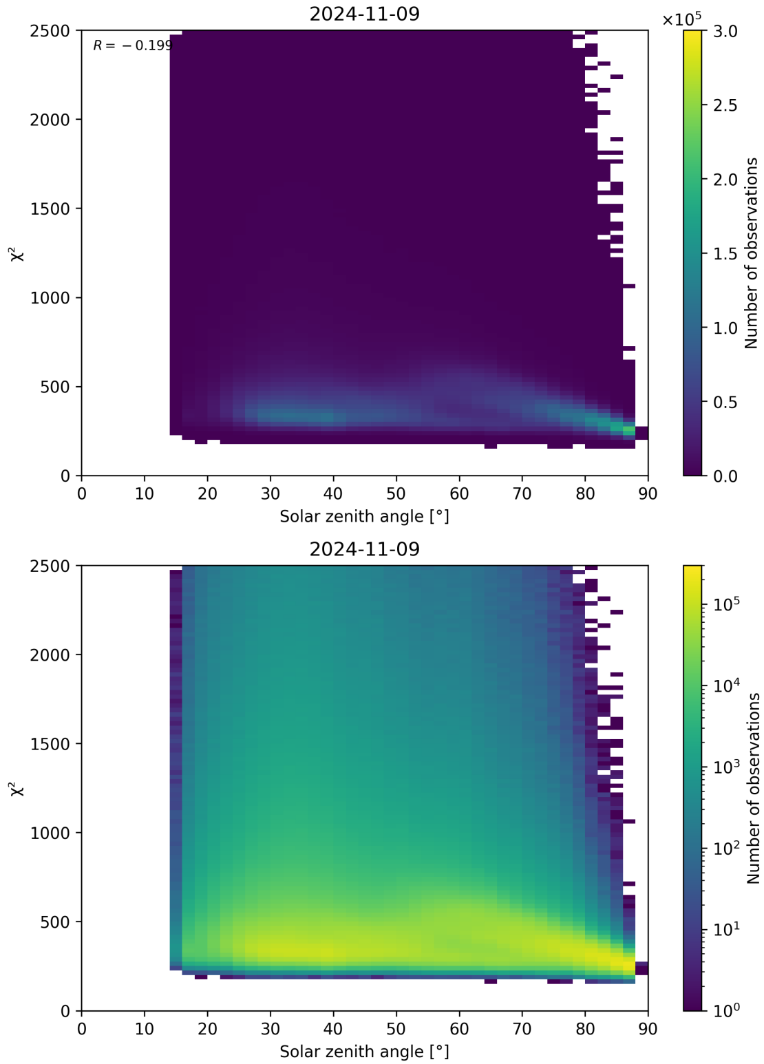
Figure 148: Scatter density plot of “Solar zenith angle” against “ \chi^2 ” for 2024-11-09 to 2024-11-10.
