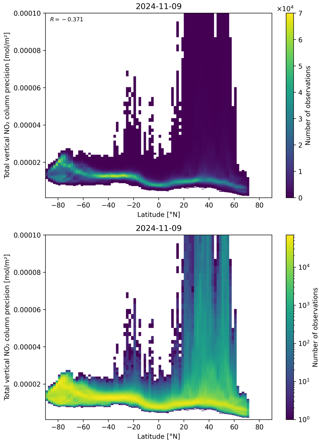
Figure 91: Scatter density plot of “Latitude” against “Total vertical NO 2 column precision” for 2024-11-09 to 2024-11-10.
