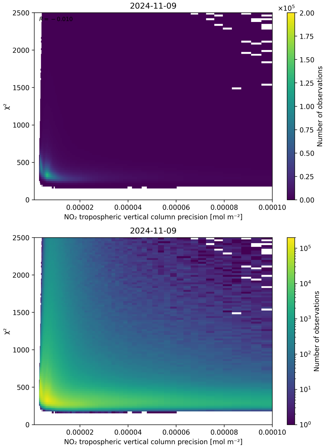
Figure 134: Scatter density plot of “NO 2 tropospheric vertical column precision” against “ \chi^2 ” for 2024-11-09 to 2024-11-10.
