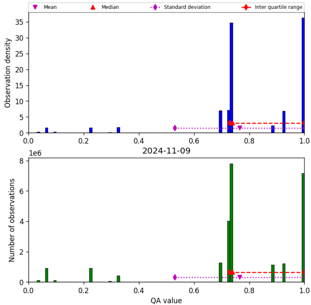
Figure 28: Histogram of “QA value” for 2024-11-09 to 2024-11-10
