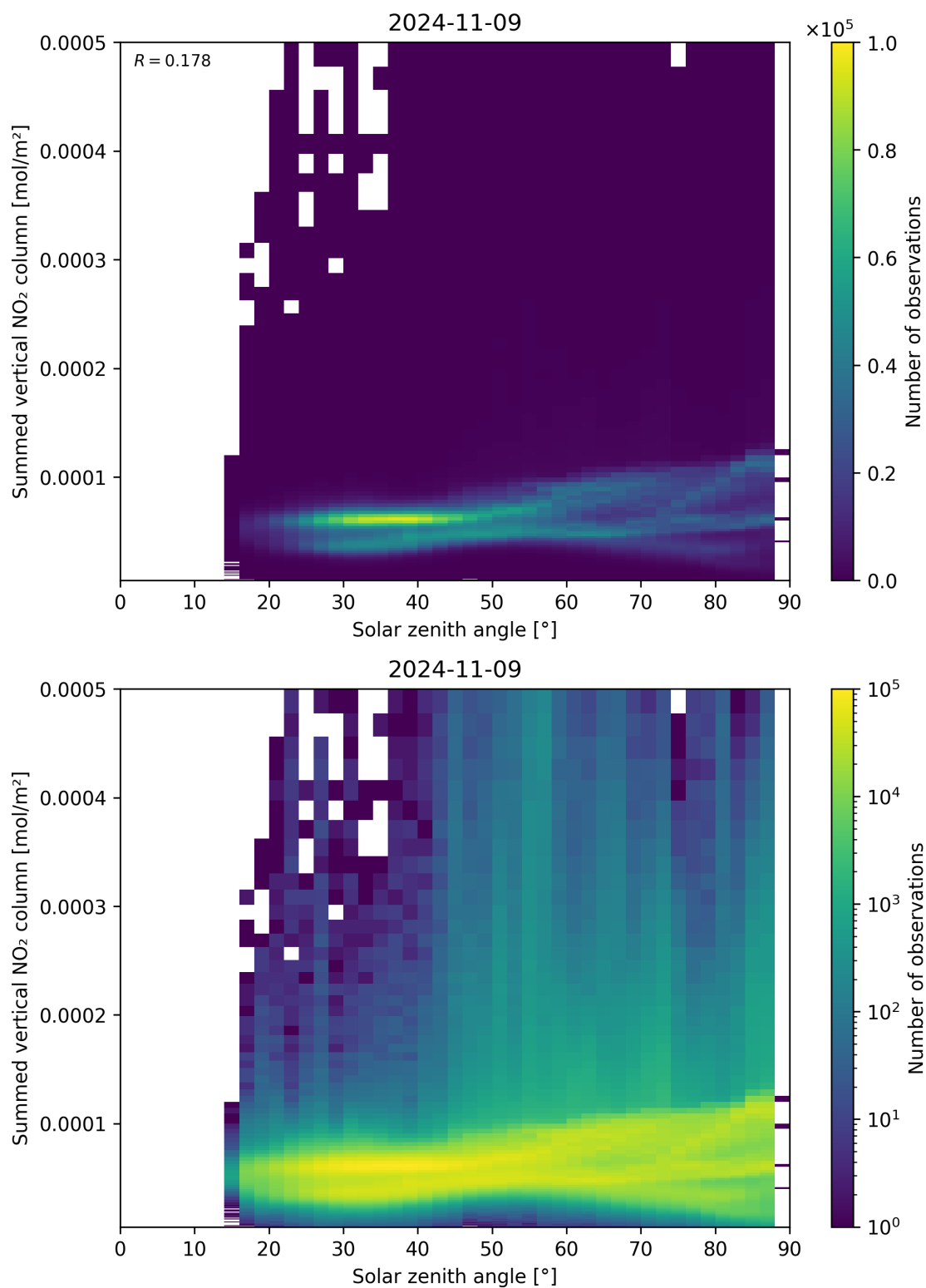
Figure 151: Scatter density plot of “Solar zenith angle” against “Summed vertical NO 2 column” for 2024-11-09 to 2024-11-10.
