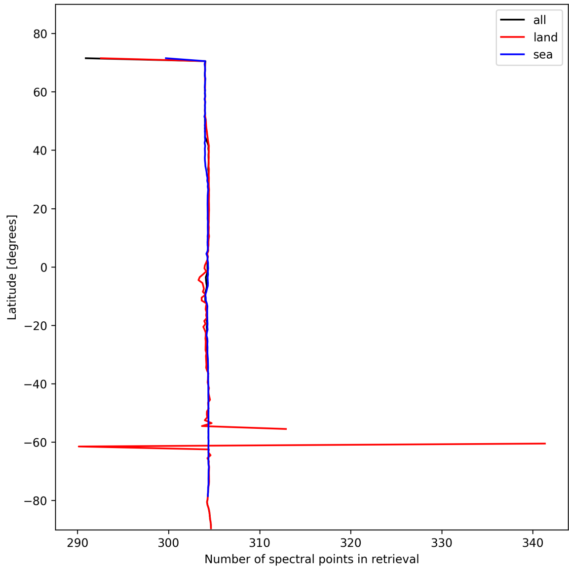
Figure 16: Zonal average of “Number of spectral points in retrieval” for 2024-11-09 to 2024-11-10.
