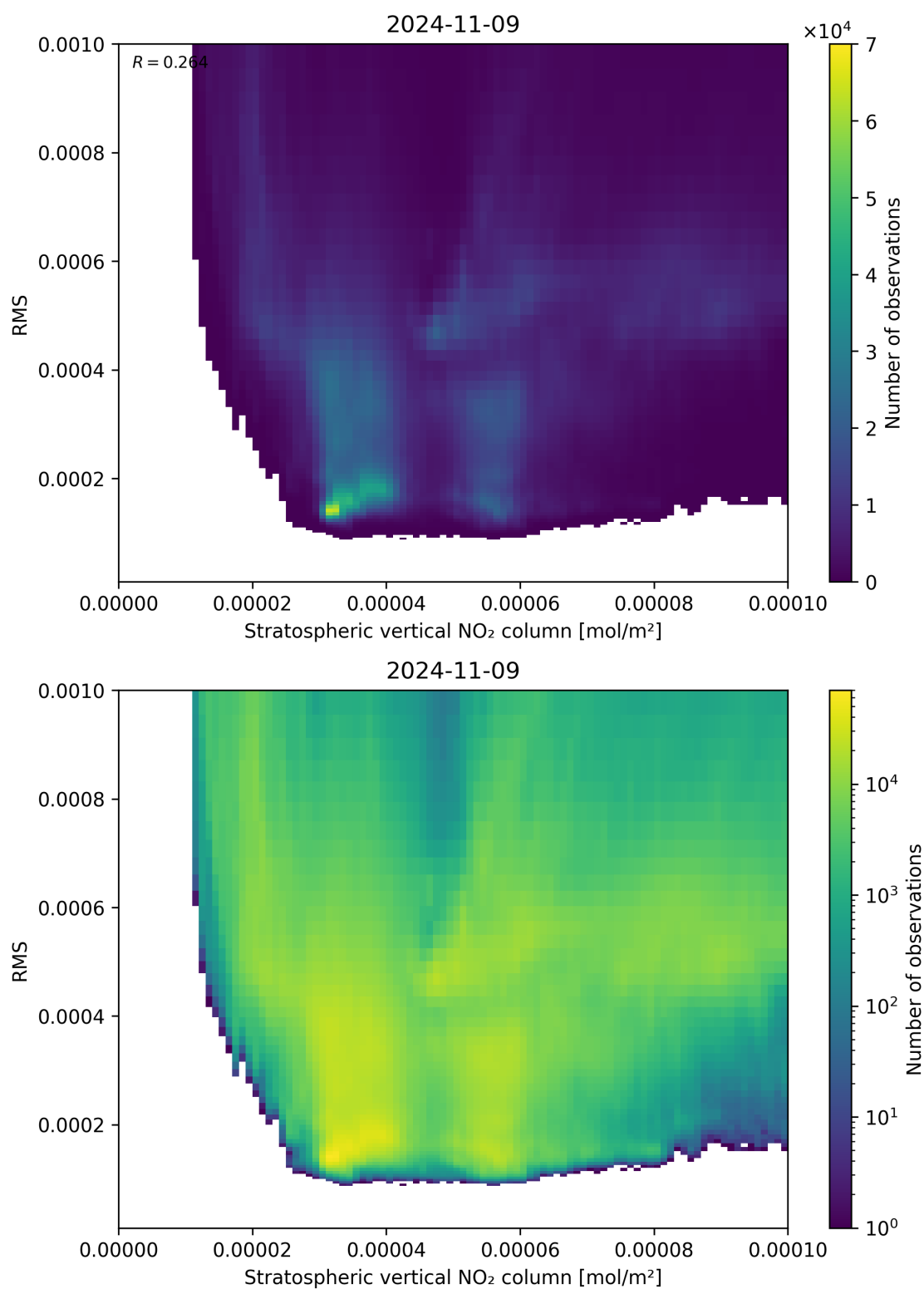
Figure 102: Scatter density plot of “Stratospheric vertical NO 2 column” against “RMS” for 2024-11-09 to 2024-11-10.
