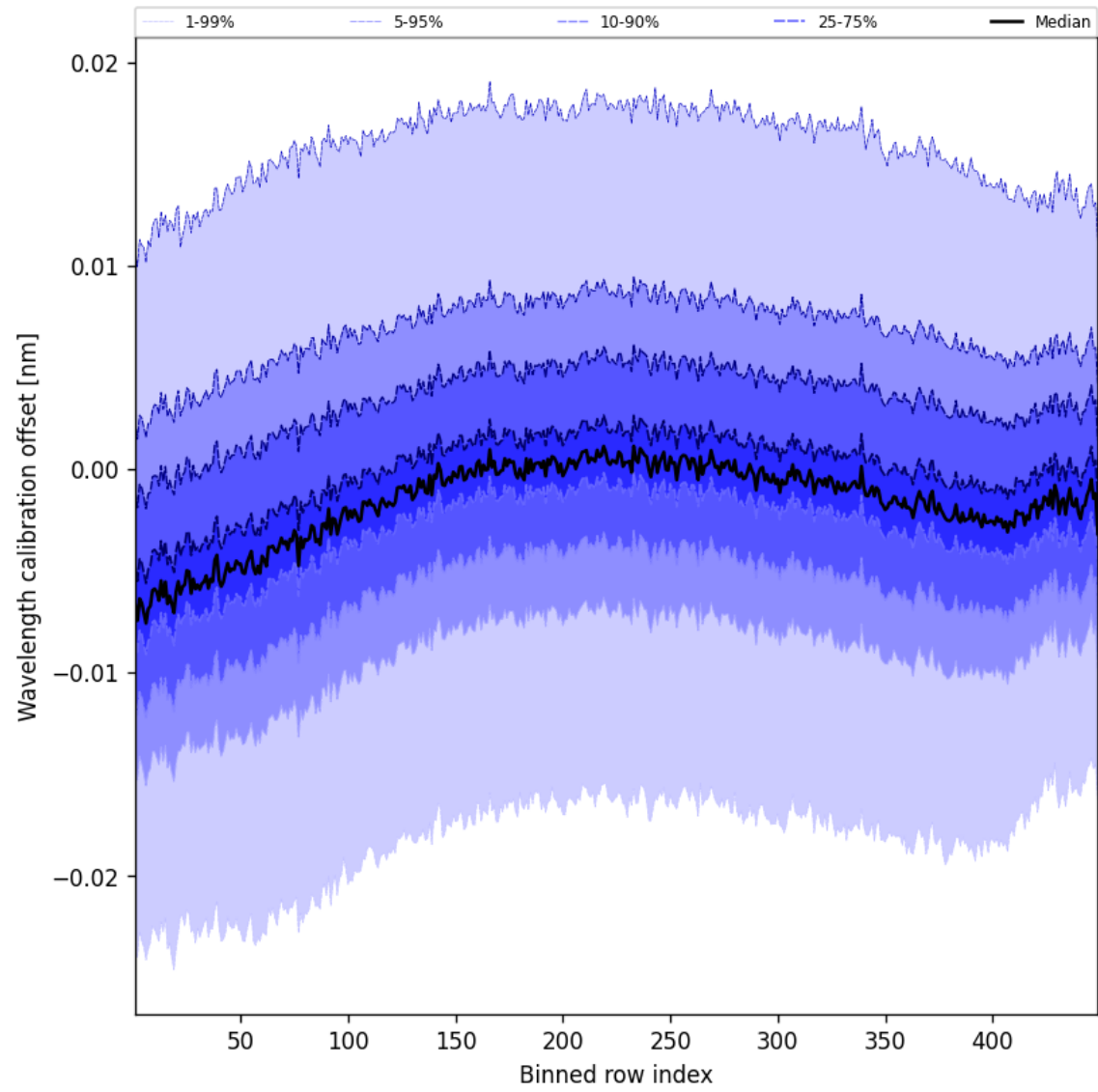
Figure 52: Along track statistics of “Wavelength calibration offset” for 2024-11-09 to 2024-11-10
