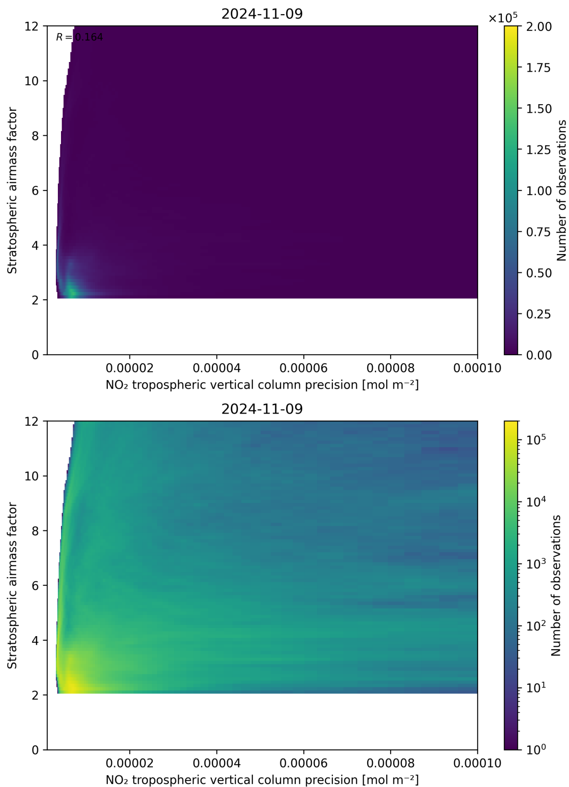
Figure 131: Scatter density plot of “NO 2 tropospheric vertical column precision” against “Stratospheric airmass factor” for 2024-11-09 to 2024-11-10.
