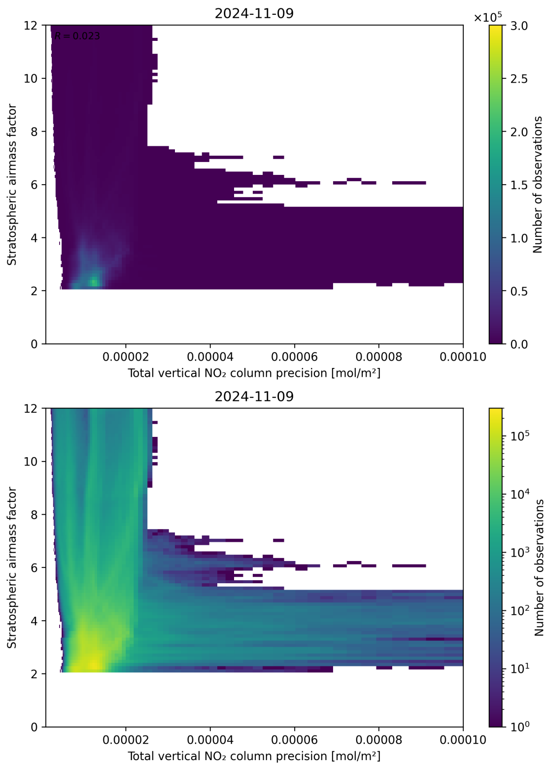
Figure 115: Scatter density plot of “Total vertical NO 2 column precision” against “Stratospheric air mass factor” for 2024-11-09 to 2024-11-10.
