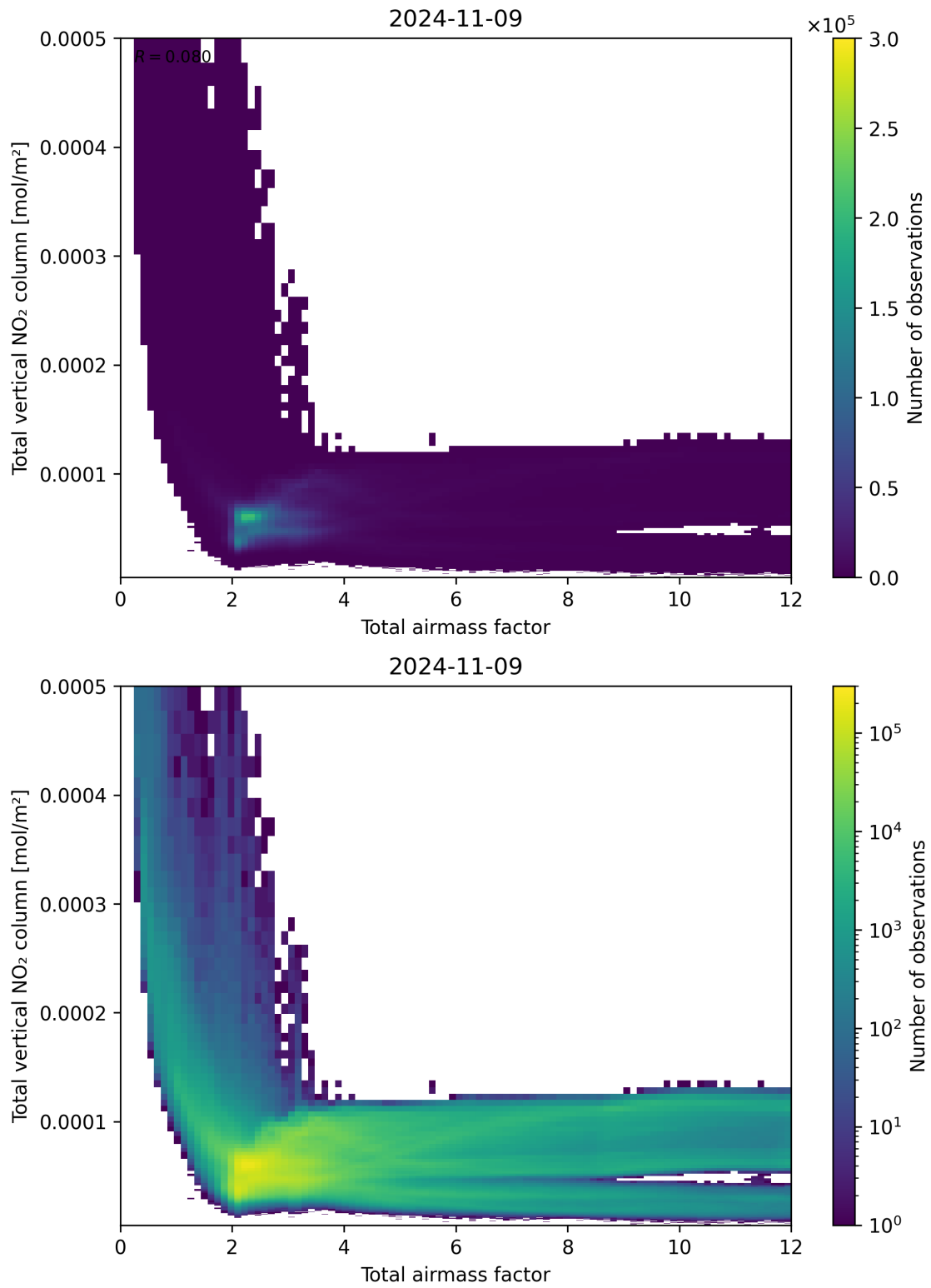
Figure 67: Scatter density plot of “Total airmass factor” against “Total vertical NO 2 column” for 2024-11-09 to 2024-11-10.
