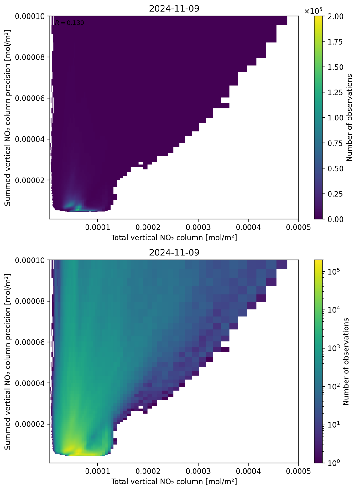
Figure 113: Scatter density plot of “Total vertical NO 2 column” against “Summed vertical NO 2 column precision” for 2024-11-09 to 2024-11-10.
