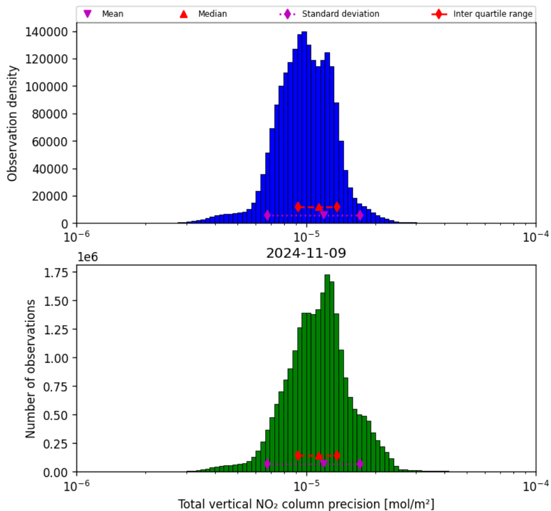
Figure 39: Histogram of “Total vertical NO 2 column precision” for 2024-11-09 to 2024-11-10
