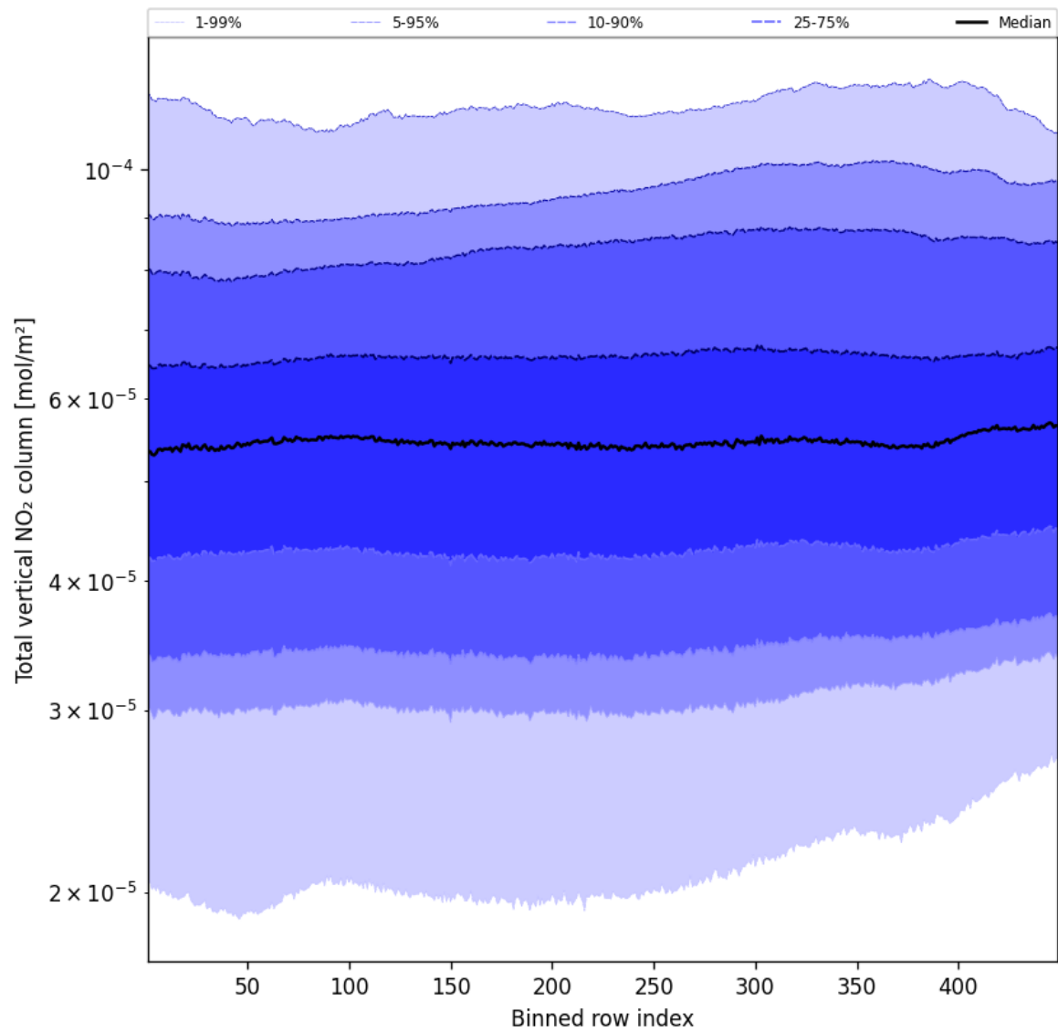
Figure 55: Along track statistics of “Total vertical NO 2 column” for 2024-11-09 to 2024-11-10
