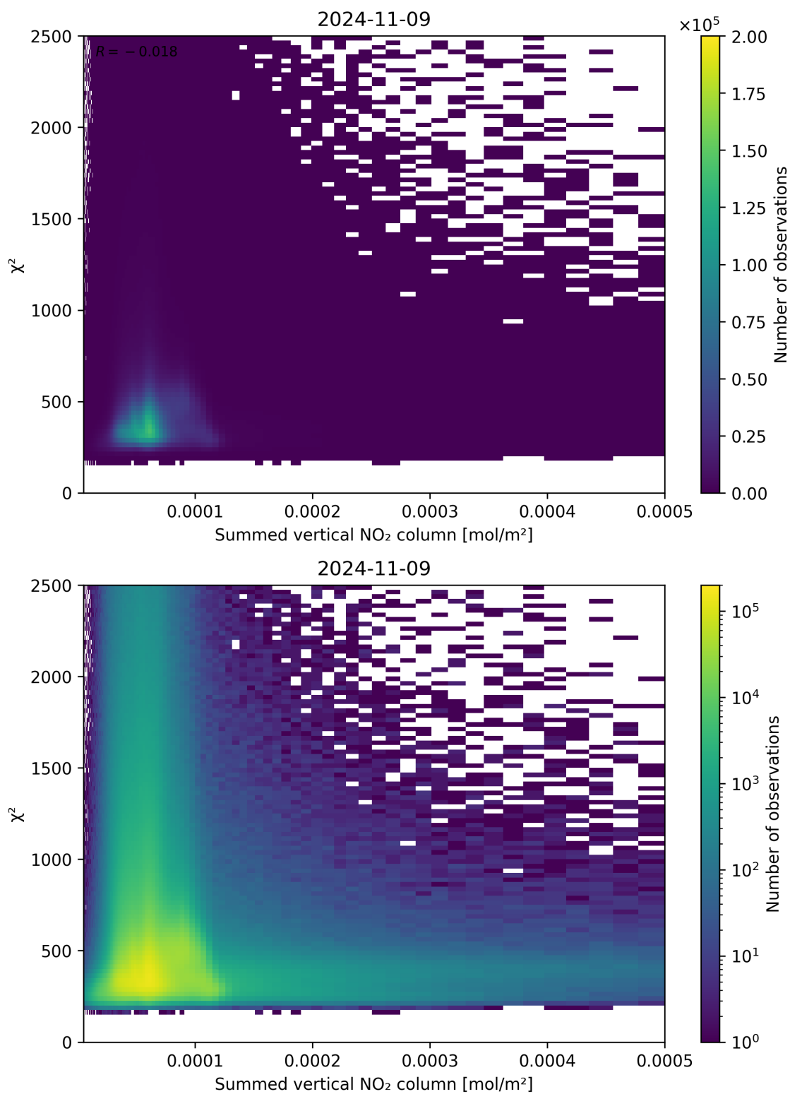
Figure 104: Scatter density plot of “Summed vertical NO 2 column” against “ \chi^2 ” for 2024-11-09 to 2024-11-10.
