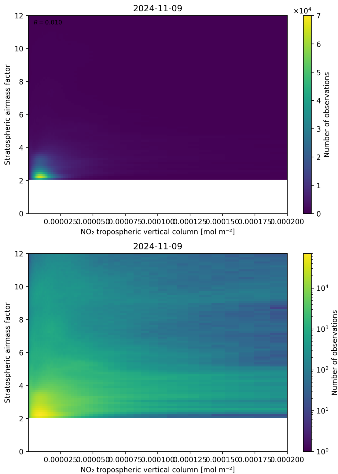
Figure 121: Scatter density plot of “NO 2 tropospheric vertical column” against “Stratospheric airmass factor” for 2024-11-09 to 2024-11-10.
