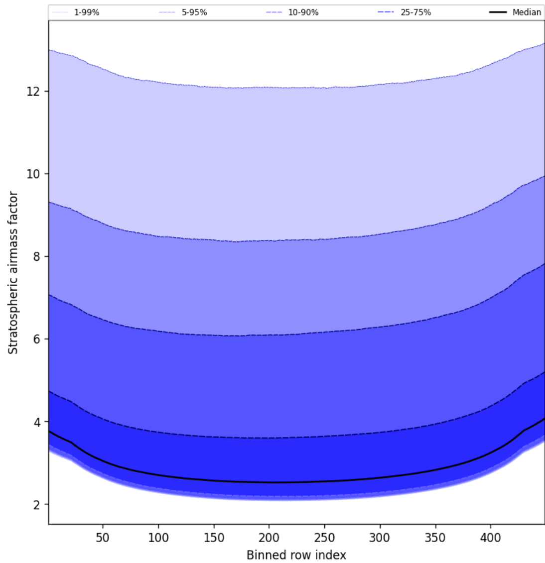
Figure 61: Along track statistics of “Stratospheric airmass factor” for 2024-11-09 to 2024-11-10
