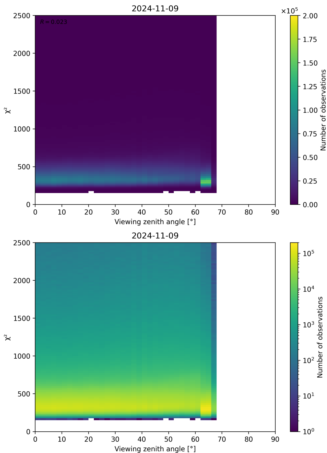
Figure 162: Scatter density plot of “Viewing zenith angle” against “ \chi^2 ” for 2024-11-09 to 2024-11-10.
