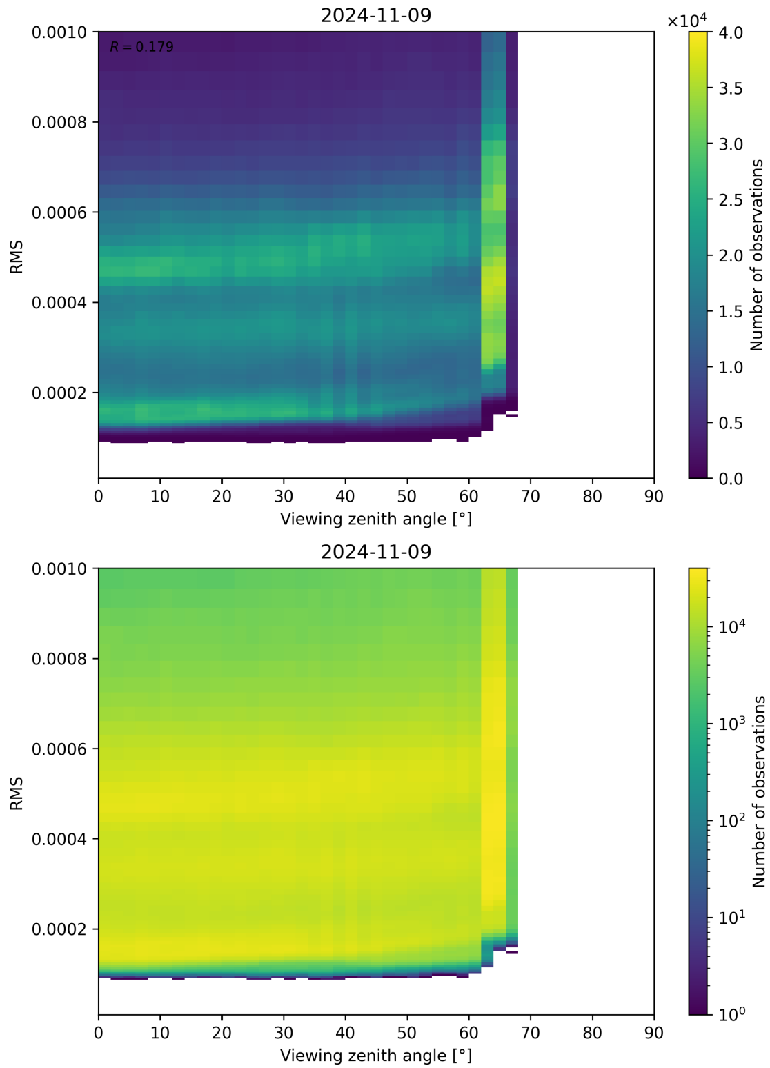
Figure 171: Scatter density plot of “Viewing zenith angle” against “RMS” for 2024-11-09 to 2024-11-10.
