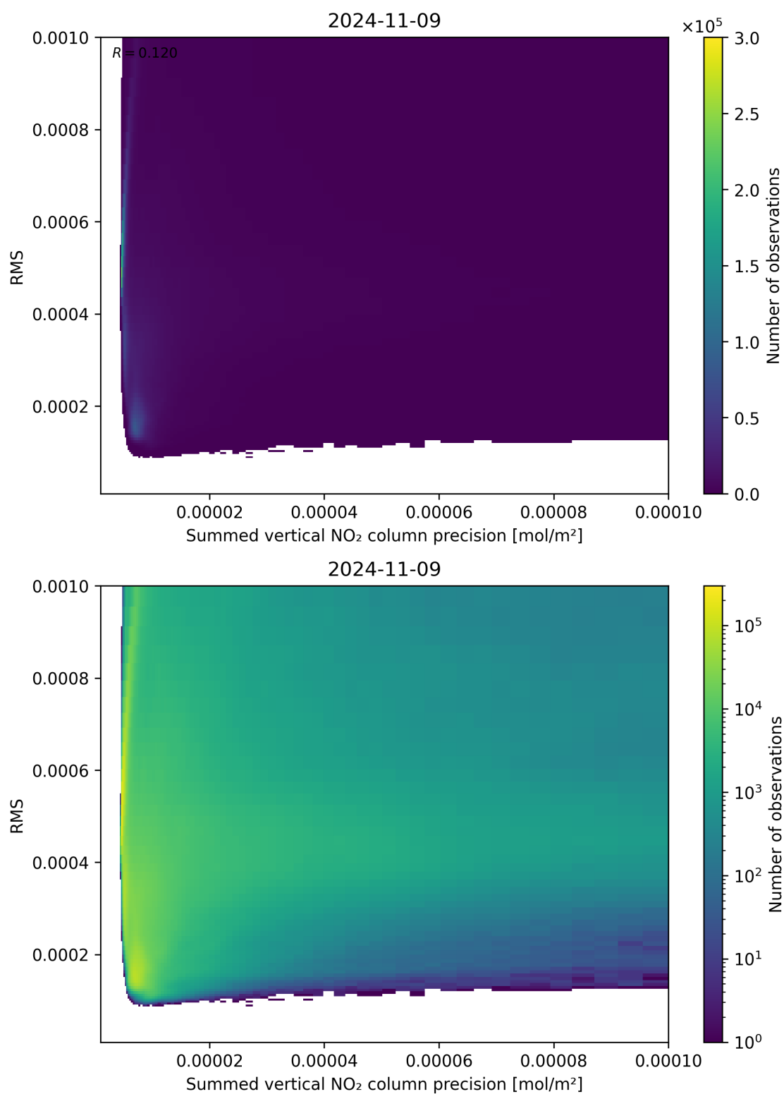
Figure 108: Scatter density plot of “Summed vertical NO 2 column precision” against “RMS” for 2024-11-09 to 2024-11-10.
