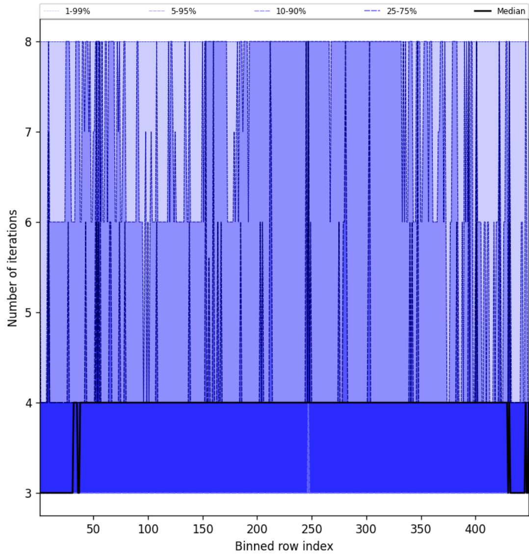
Figure 51: Along track statistics of “Number of iterations” for 2024-11-09 to 2024-11-10
