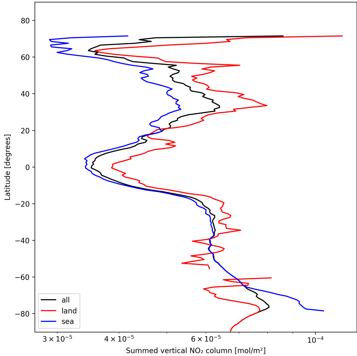
Figure 23: Zonal average of “Summed vertical NO 2 column” for 2024-11-09 to 2024-11-10.
