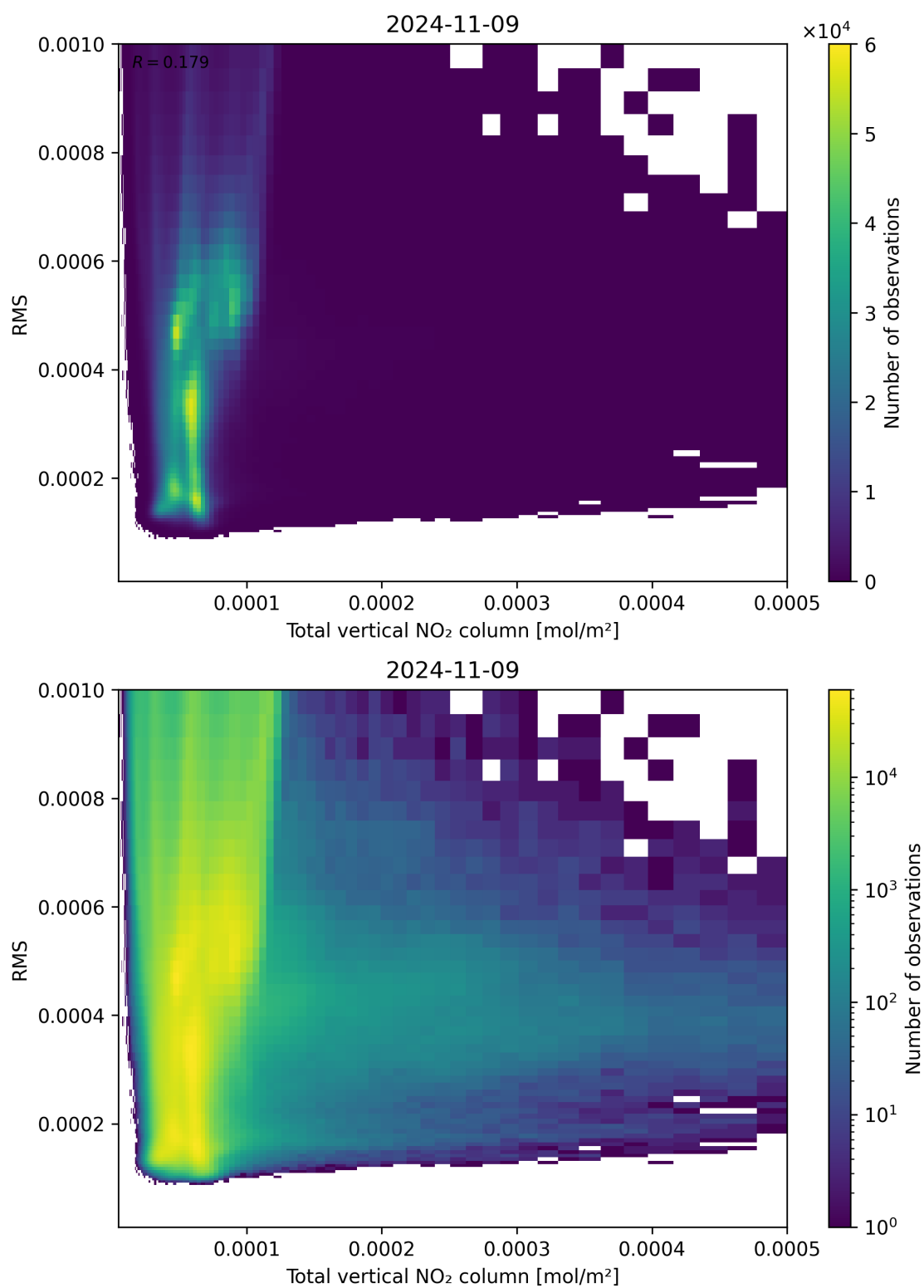
Figure 120: Scatter density plot of “Total vertical NO 2 column” against “RMS” for 2024-11-09 to 2024-11-10.
