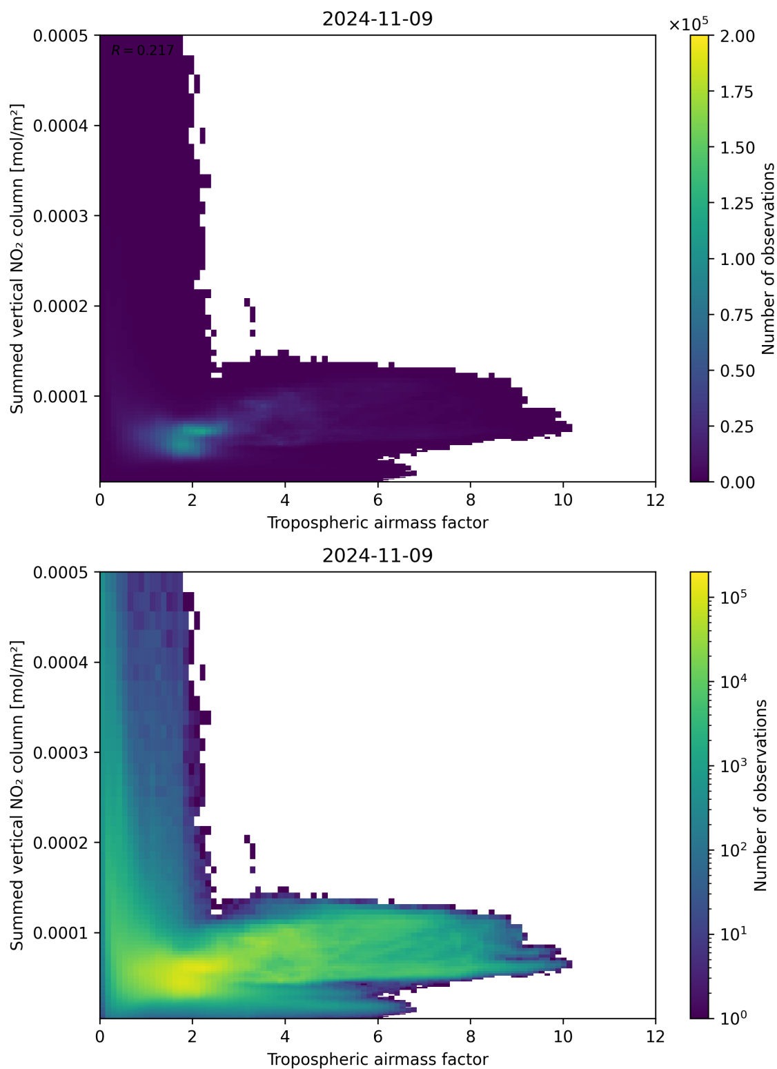
Figure 75: Scatter density plot of “Tropospheric airmass factor” against “Summed vertical NO 2 column” for 2024-11-09 to 2024-11-10.
