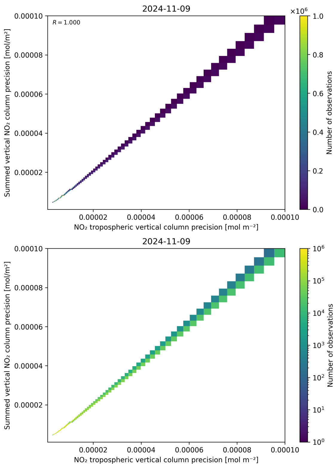
Figure 137: Scatter density plot of “NO 2 tropospheric vertical column precision” against “Summed vertical NO 2 column precision” for 2024-11-09 to 2024-11-10.
