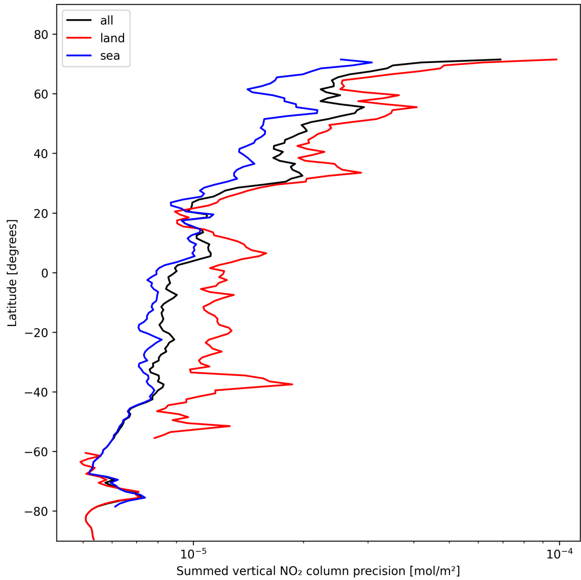
Figure 24: Zonal average of “Summed vertical NO 2 column precision” for 2024-11-09 to 2024-11-10.
