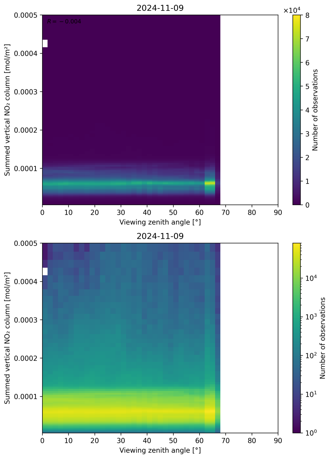
Figure 165: Scatter density plot of “Viewing zenith angle” against “Summed vertical NO 2 column” for 2024-11-09 to 2024-11-10.
