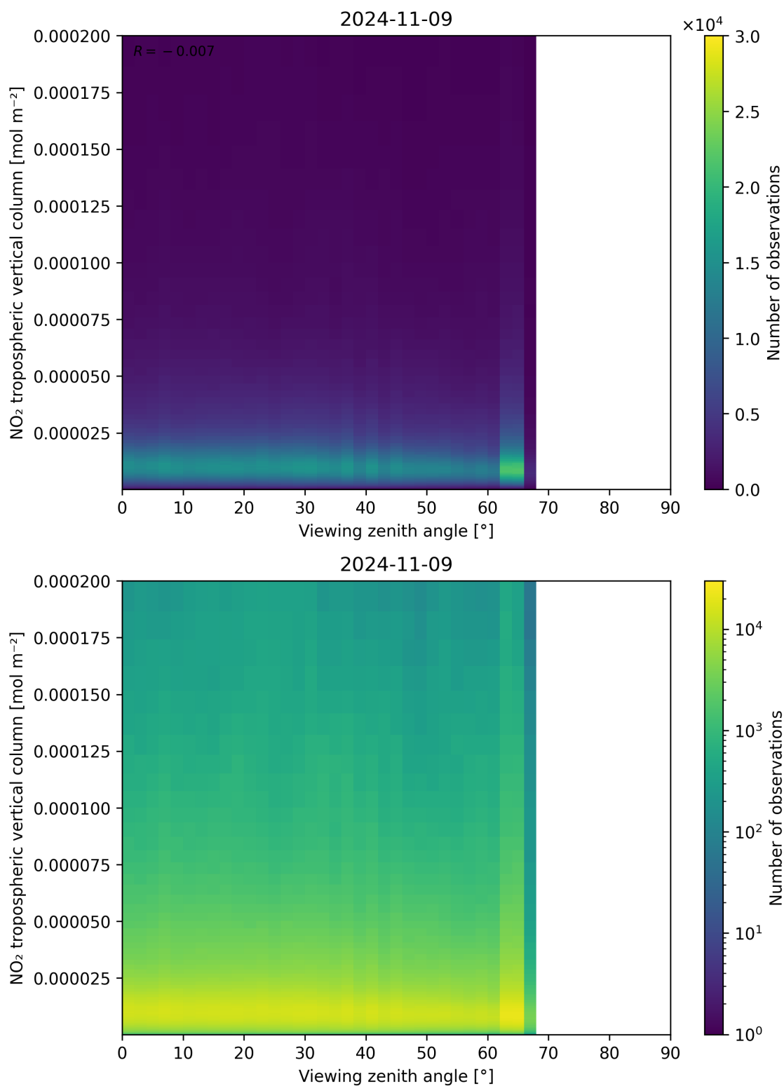
Figure 169: Scatter density plot of “Viewing zenith angle” against “NO 2 tropospheric vertical column” for 2024-11-09 to 2024-11-10.
