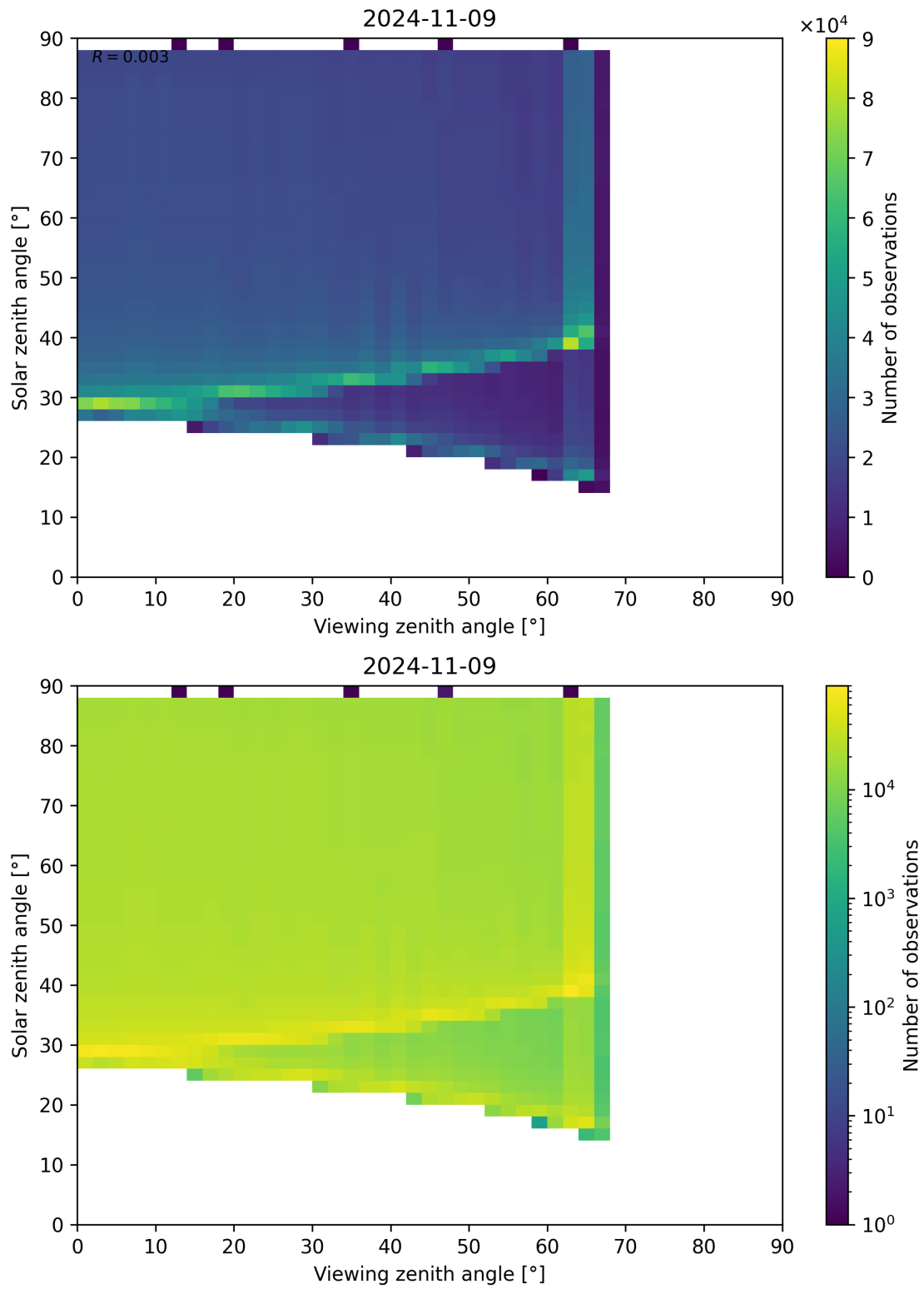
Figure 172: Scatter density plot of “Viewing zenith angle” against “Solar zenith angle” for 2024-11-09 to 2024-11-10.
