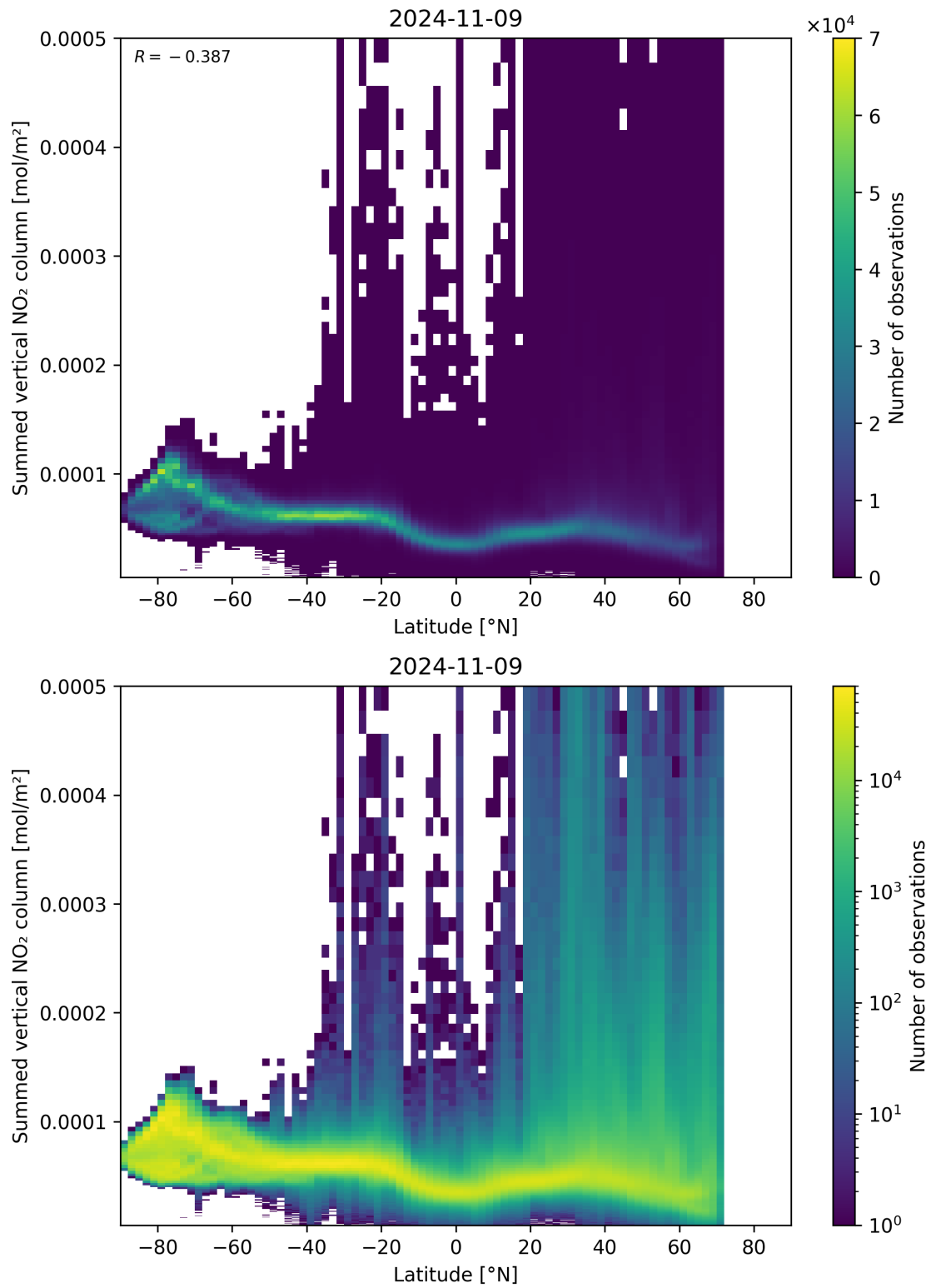
Figure 88: Scatter density plot of “Latitude” against “Summed vertical NO 2 column” for 2024-11-09 to 2024-11-10.
