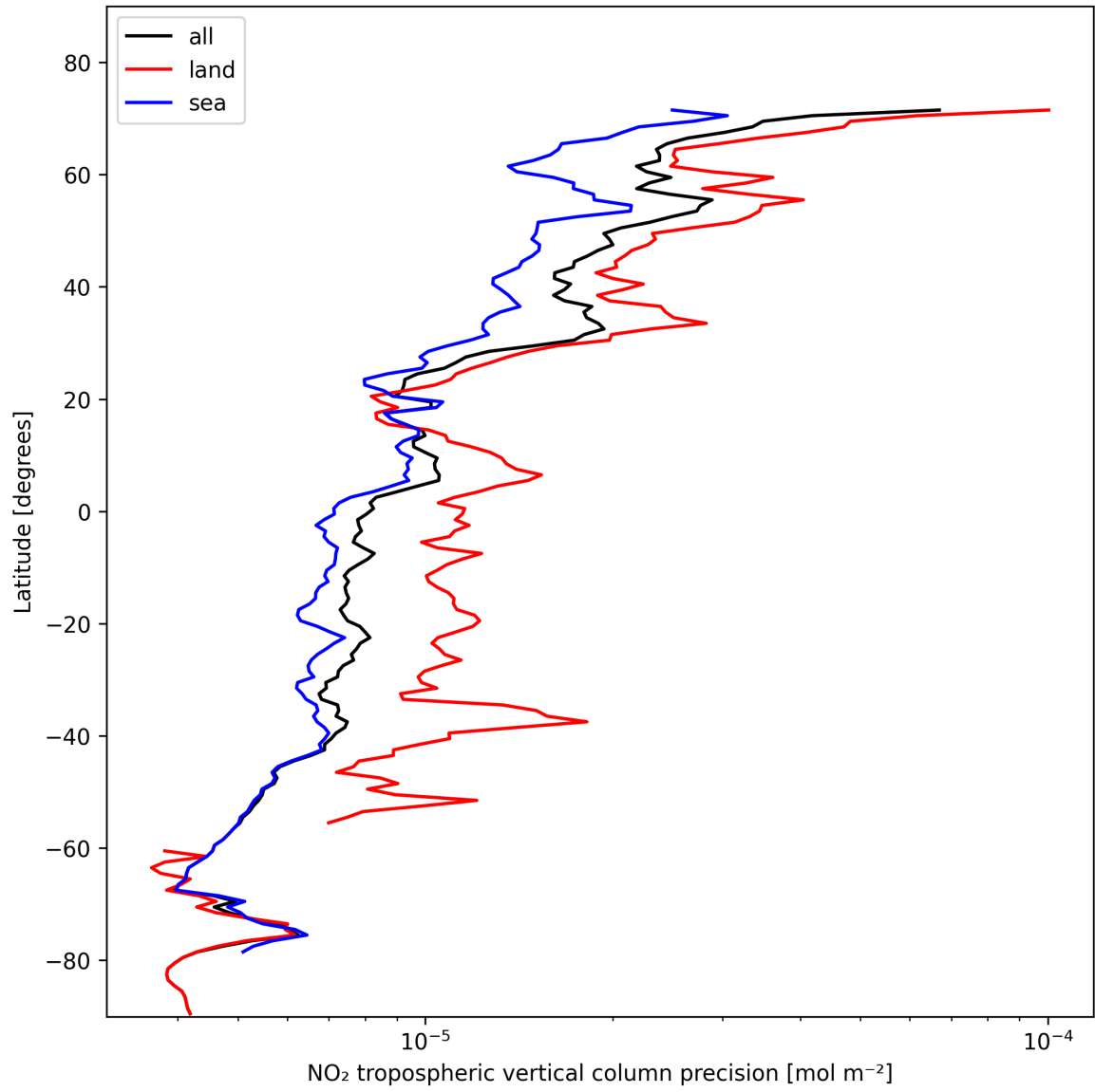
Figure 13: Zonal average of “NO 2 tropospheric vertical column precision” for 2024-11-09 to 2024-11-10.
