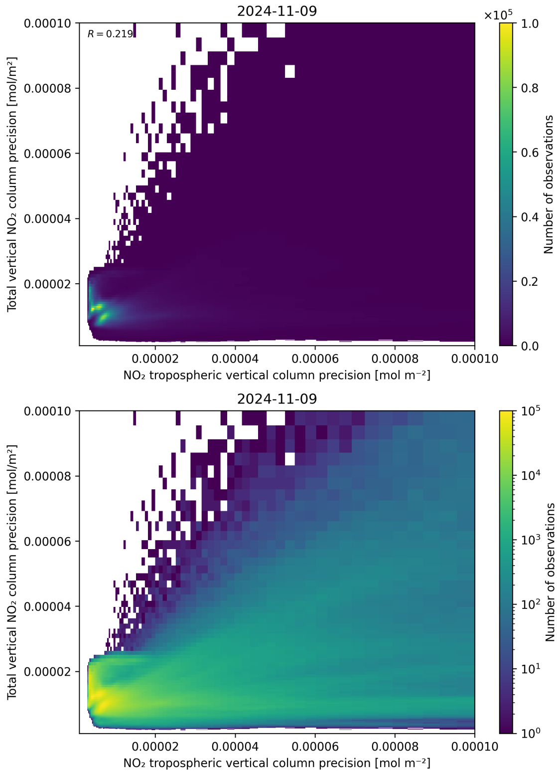
Figure 139: Scatter density plot of “NO 2 tropospheric vertical column precision” against “Total vertical NO 2 column precision” for 2024-11-09 to 2024-11-10.
