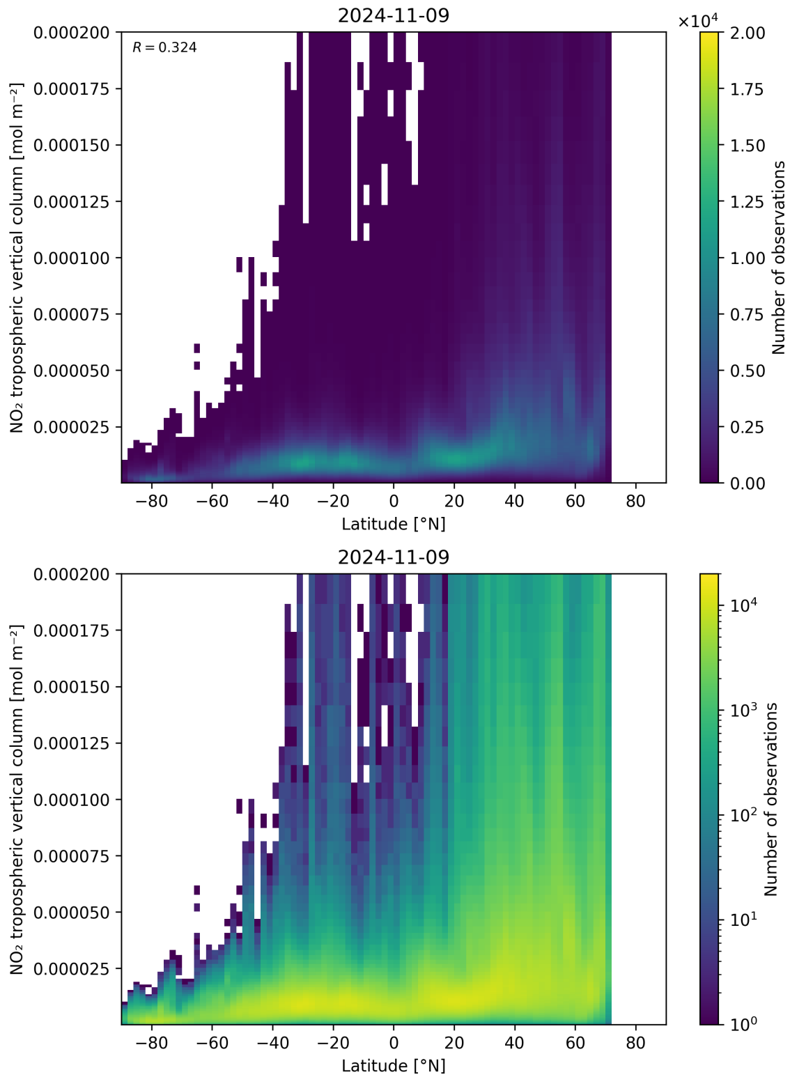
Figure 92: Scatter density plot of “Latitude” against “NO 2 tropospheric vertical column” for 2024-11-09 to 2024-11-10.
