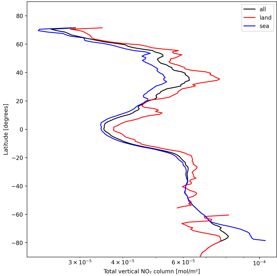
Figure 21: Zonal average of “Total vertical NO 2 column” for 2024-11-09 to 2024-11-10.
