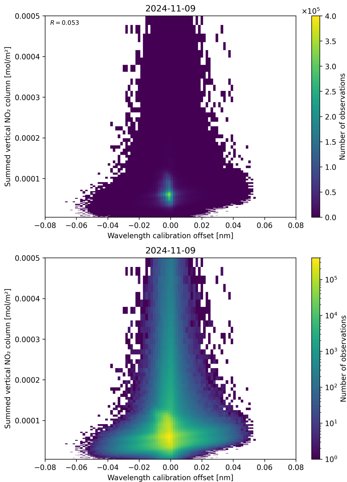
Figure 177: Scatter density plot of “Wavelength calibration offset” against “Summed vertical NO 2 column” for 2024-11-09 to 2024-11-10.
