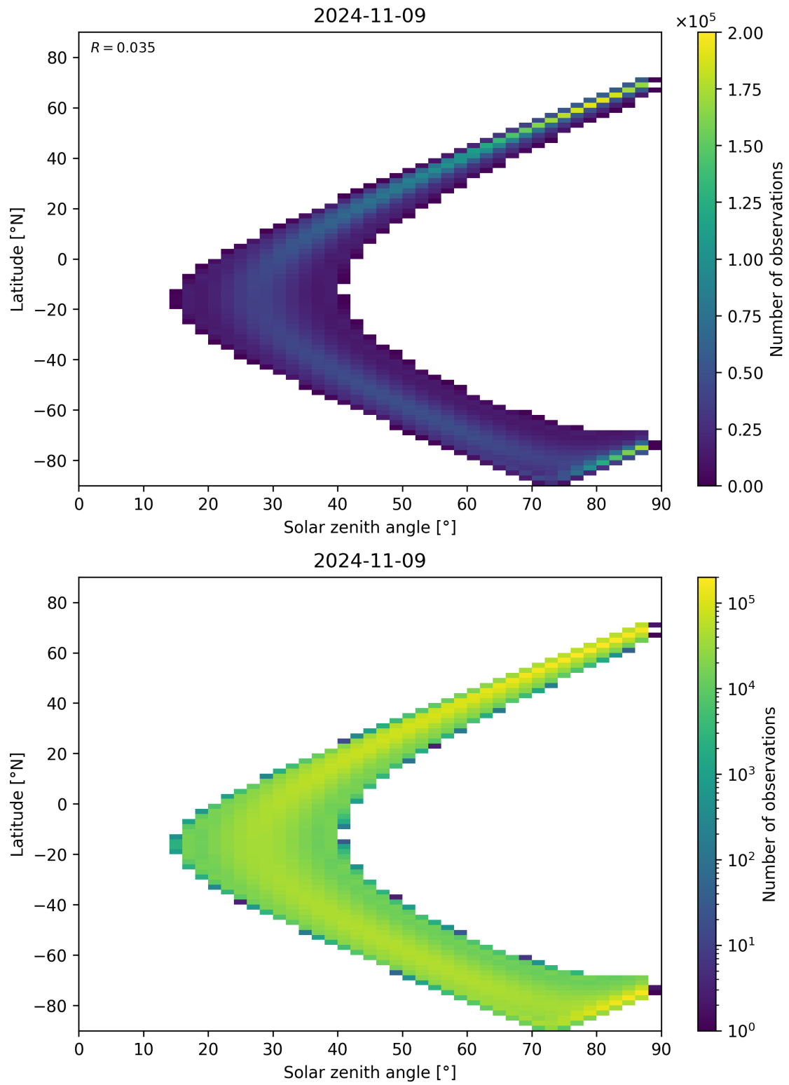
Figure 149: Scatter density plot of “Solar zenith angle” against “Latitude” for 2024-11-09 to 2024-11-10.
