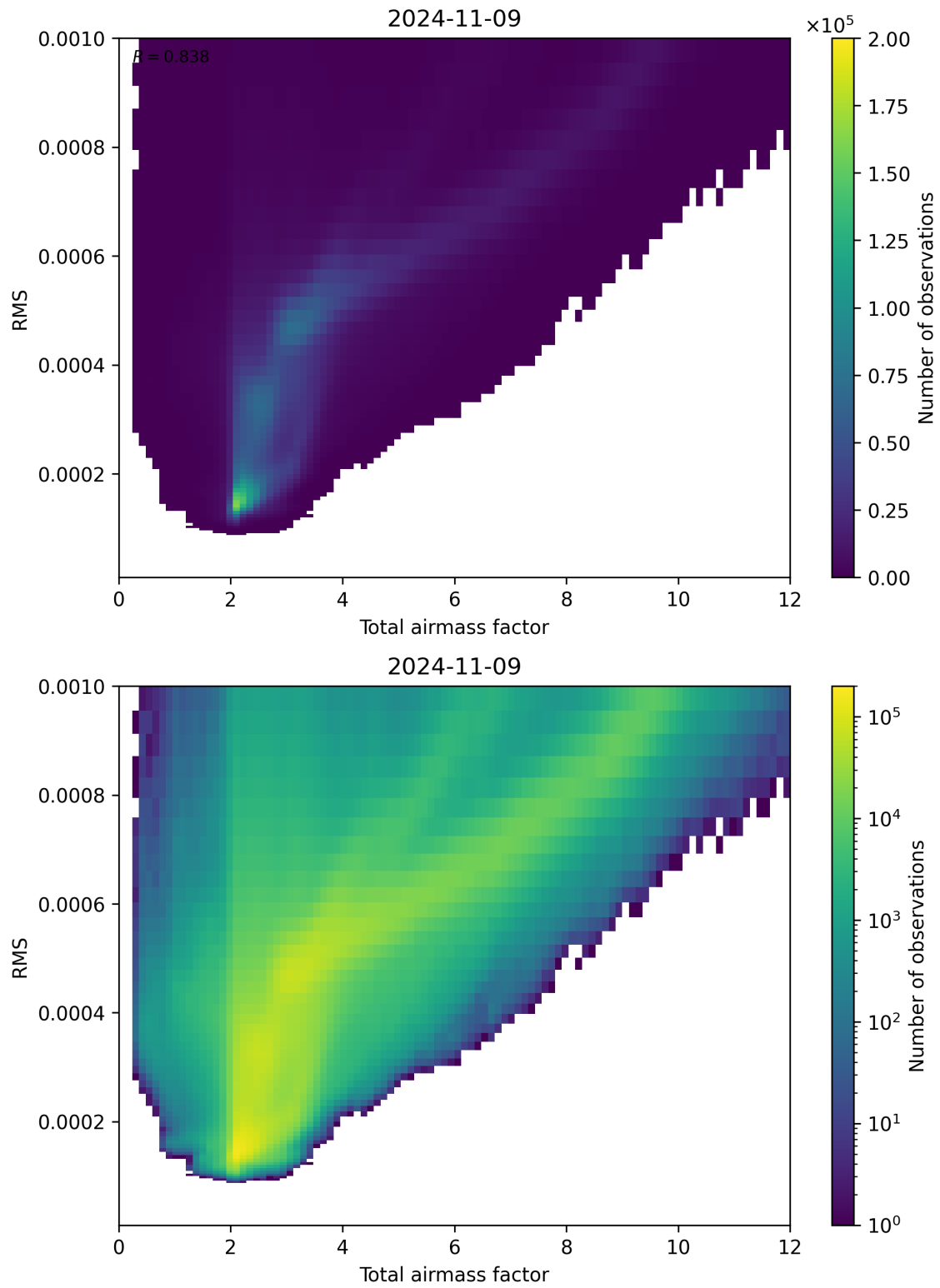
Figure 69: Scatter density plot of “Total airmass factor” against “RMS” for 2024-11-09 to 2024-11-10.
