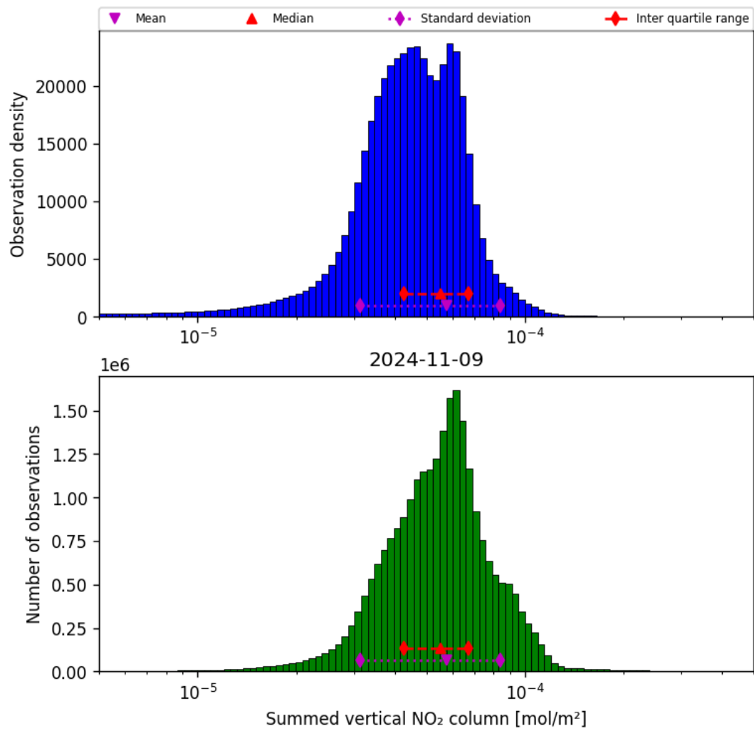
Figure 40: Histogram of “Summed vertical NO 2 column” for 2024-11-09 to 2024-11-10
