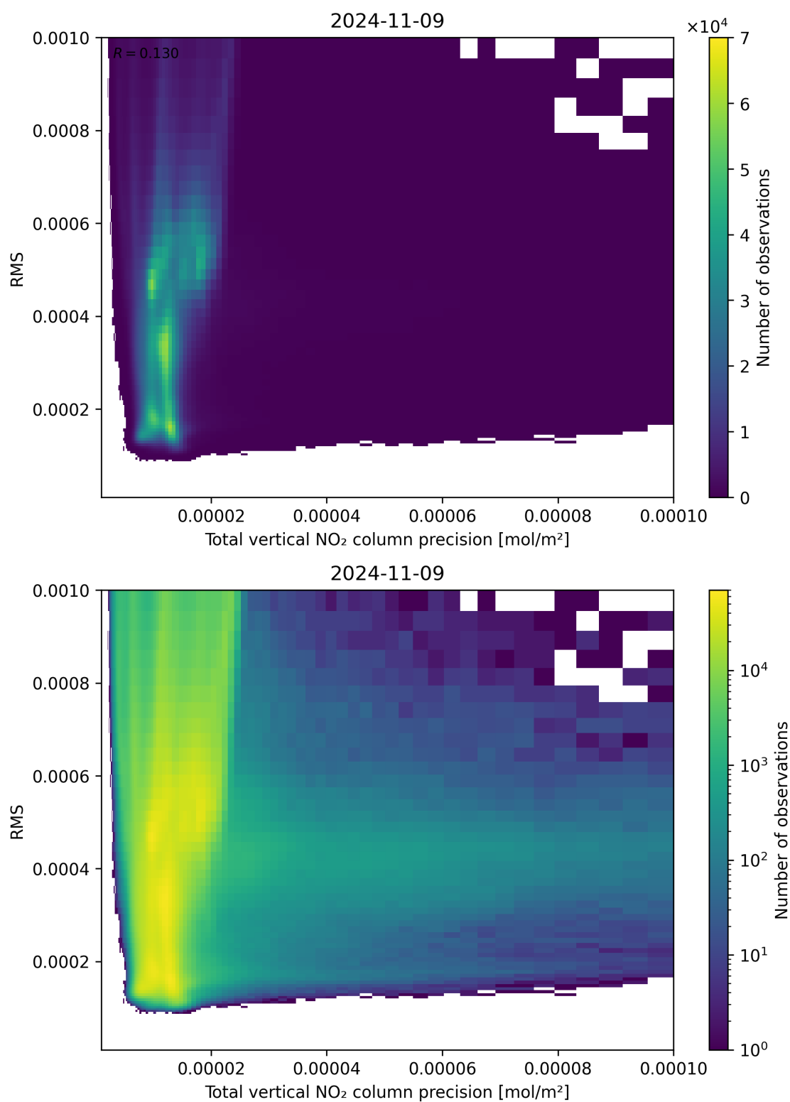
Figure 119: Scatter density plot of “Total vertical NO 2 column precision” against “RMS” for 2024-11-09 to 2024-11-10.
