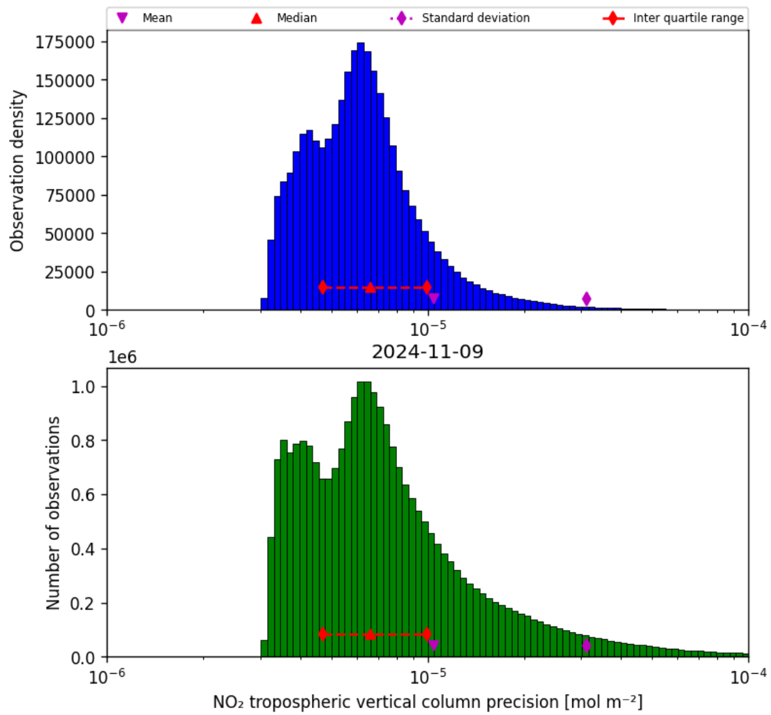
Figure 30: Histogram of “NO 2 tropospheric vertical column precision” for 2024-11-09 to 2024-11-10
