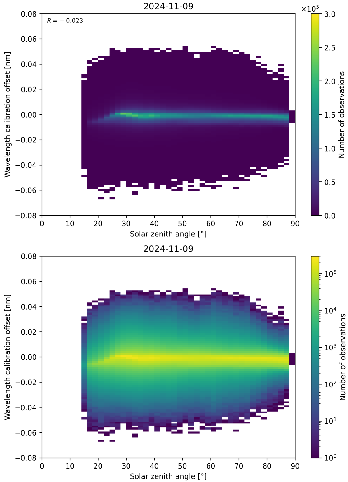
Figure 158: Scatter density plot of “Solar zenith angle” against “Wavelength calibration offset” for 2024-11-09 to 2024-11-10.
