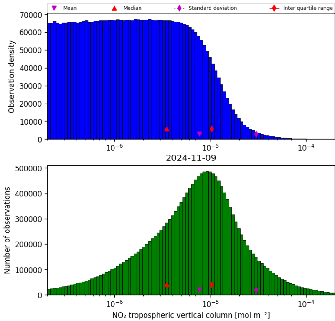
Figure 29: Histogram of “NO 2 tropospheric vertical column” for 2024-11-09 to 2024-11-10
