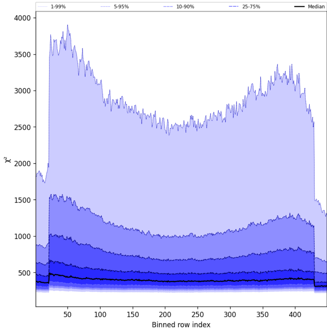
Figure 59: Along track statistics of “ \chi^2 ” for 2024-11-09 to 2024-11-10
