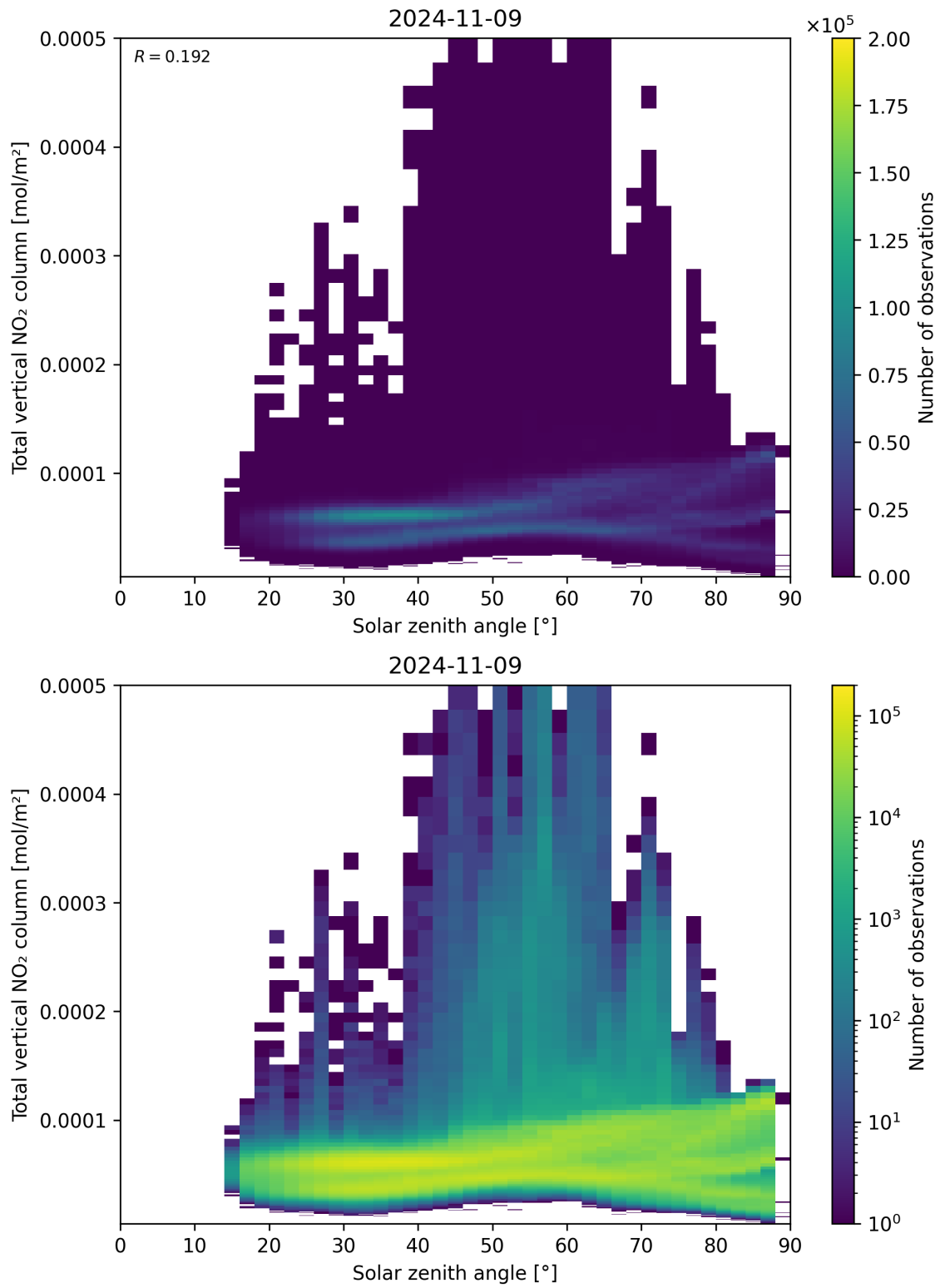
Figure 153: Scatter density plot of “Solar zenith angle” against “Total vertical NO 2 column” for 2024-11-09 to 2024-11-10.
