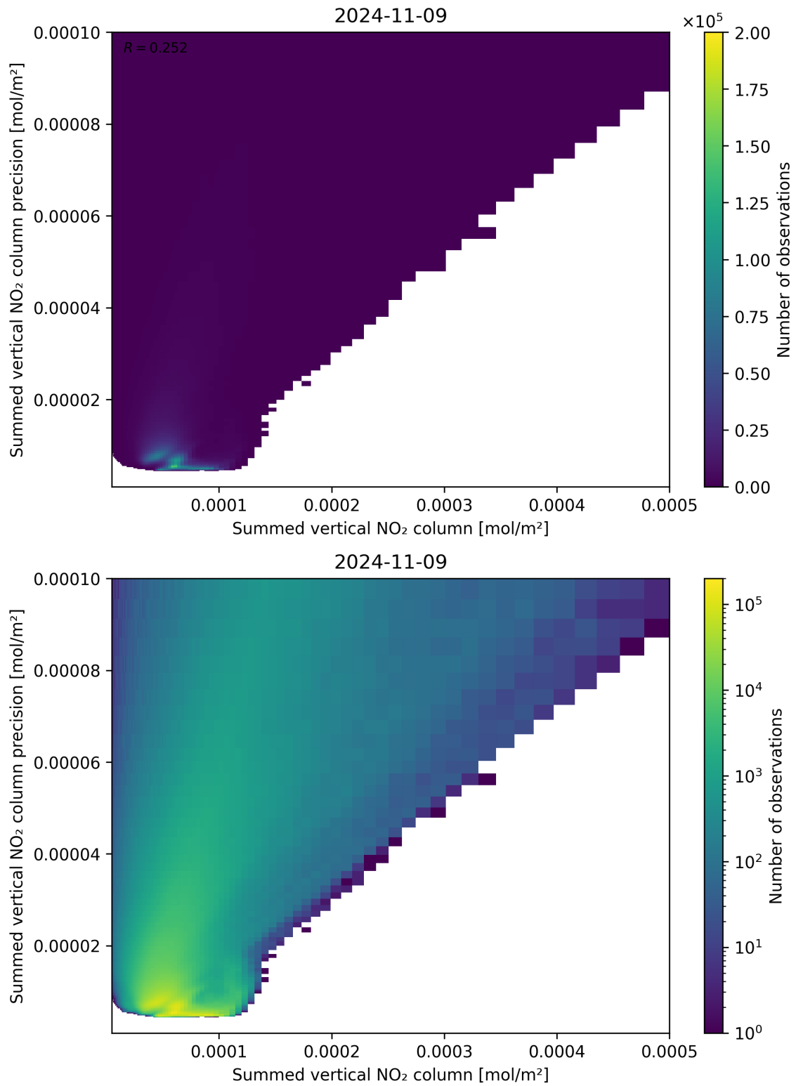
Figure 105: Scatter density plot of “Summed vertical NO 2 column” against “Summed vertical NO 2 column precision” for 2024-11-09 to 2024-11-10.
