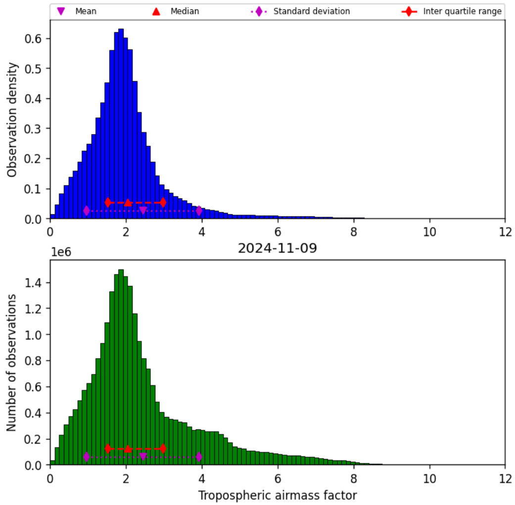
Figure 31: Histogram of “Tropospheric airmass factor” for 2024-11-09 to 2024-11-10
