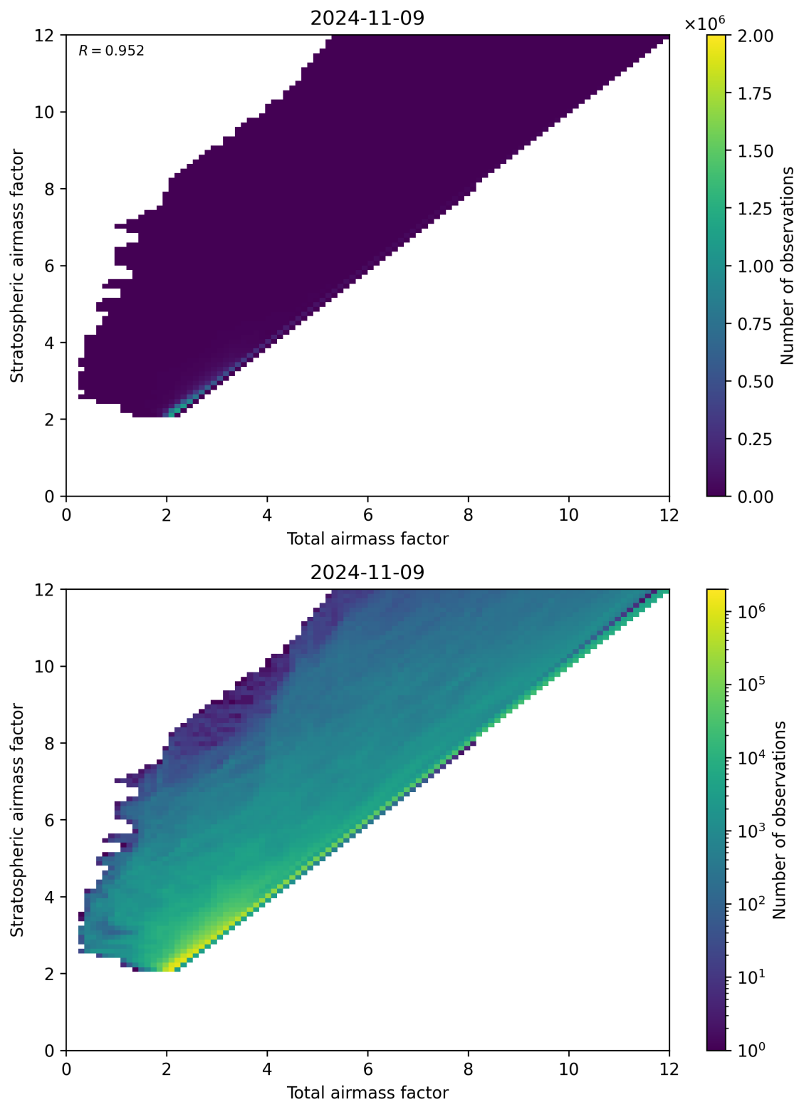
Figure 62: Scatter density plot of “Total airmass factor” against “Stratospheric airmass factor” for 2024-11-09 to 2024-11-10.
