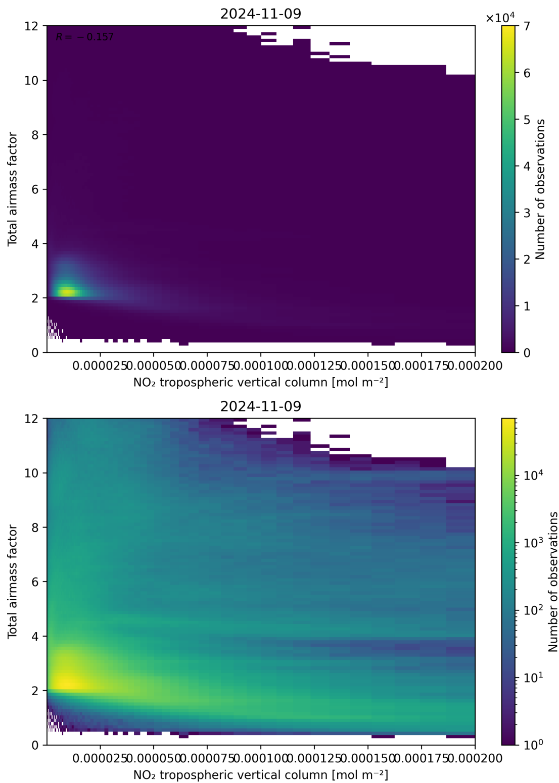
Figure 122: Scatter density plot of “NO 2 tropospheric vertical column” against “Total air mass factor” for 2024-11-09 to 2024-11-10.
