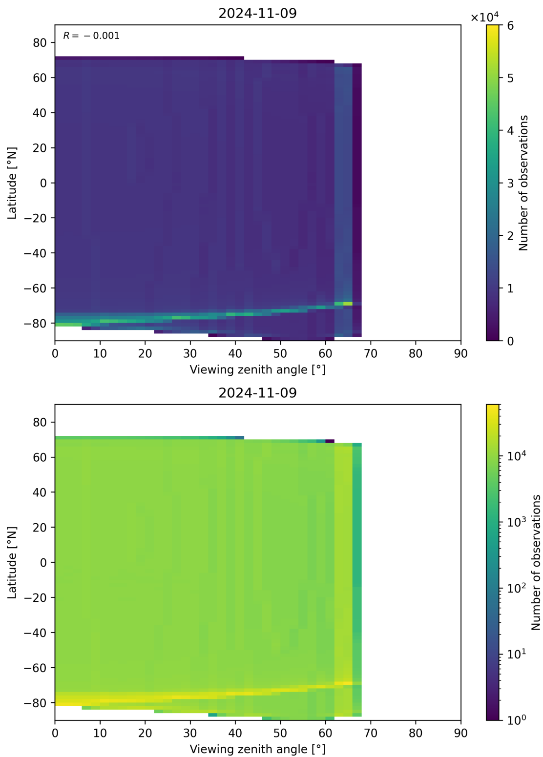
Figure 163: Scatter density plot of “Viewing zenith angle” against “Latitude” for 2024-11-09 to 2024-11-10.
