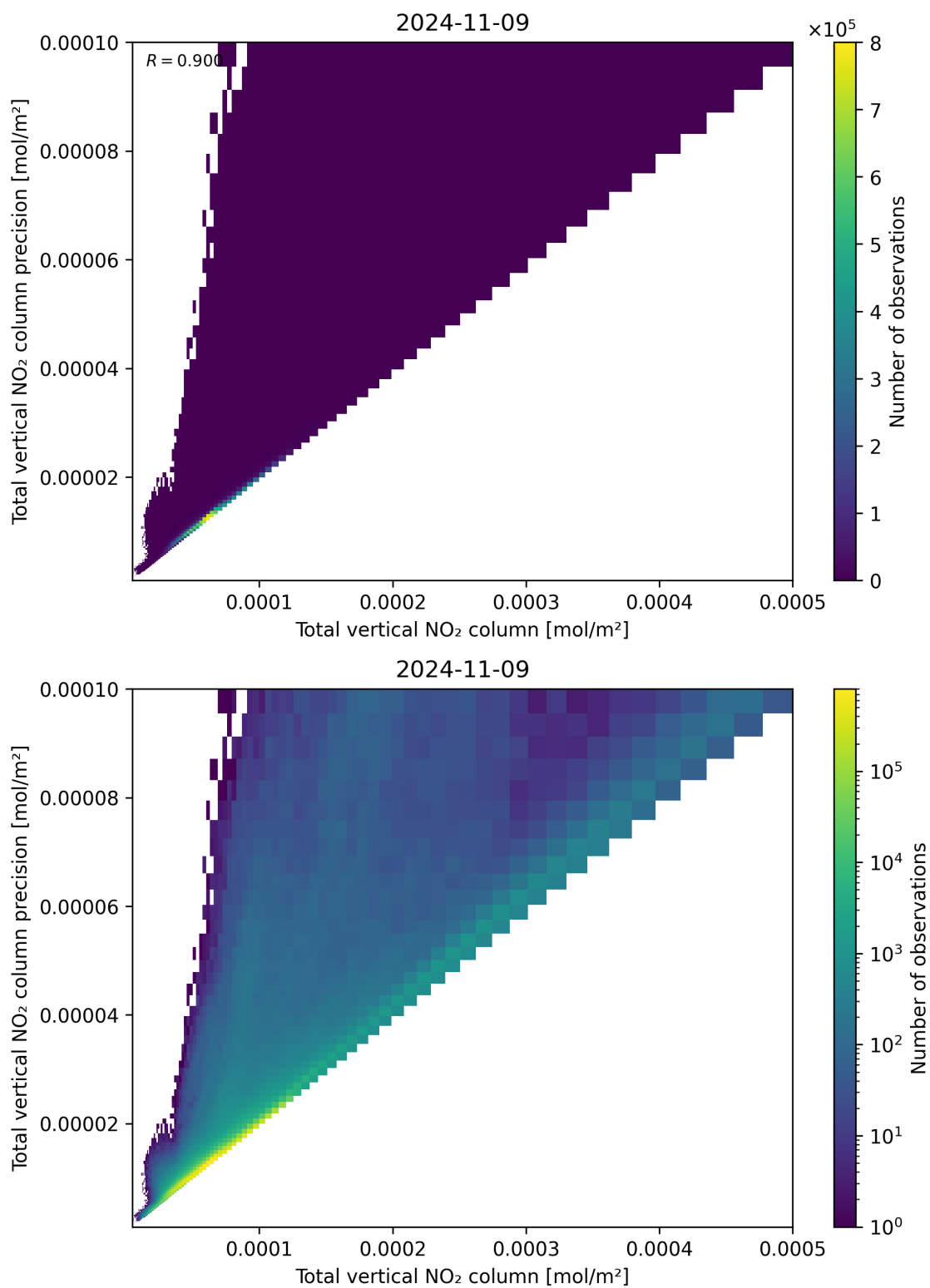
Figure 114: Scatter density plot of “Total vertical NO 2 column” against “Total vertical NO 2 column precision” for 2024-11-09 to 2024-11-10.
