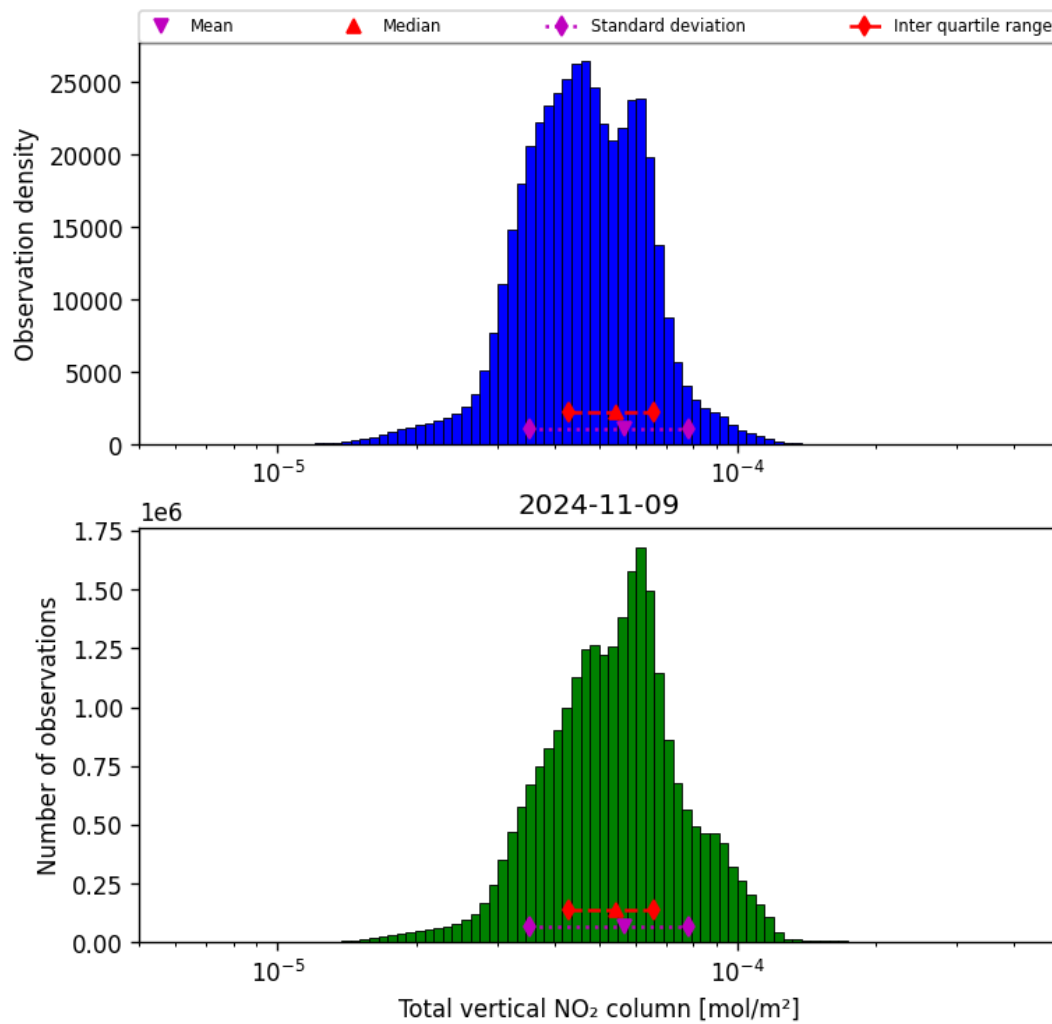
Figure 38: Histogram of “Total vertical NO 2 column” for 2024-11-09 to 2024-11-10
