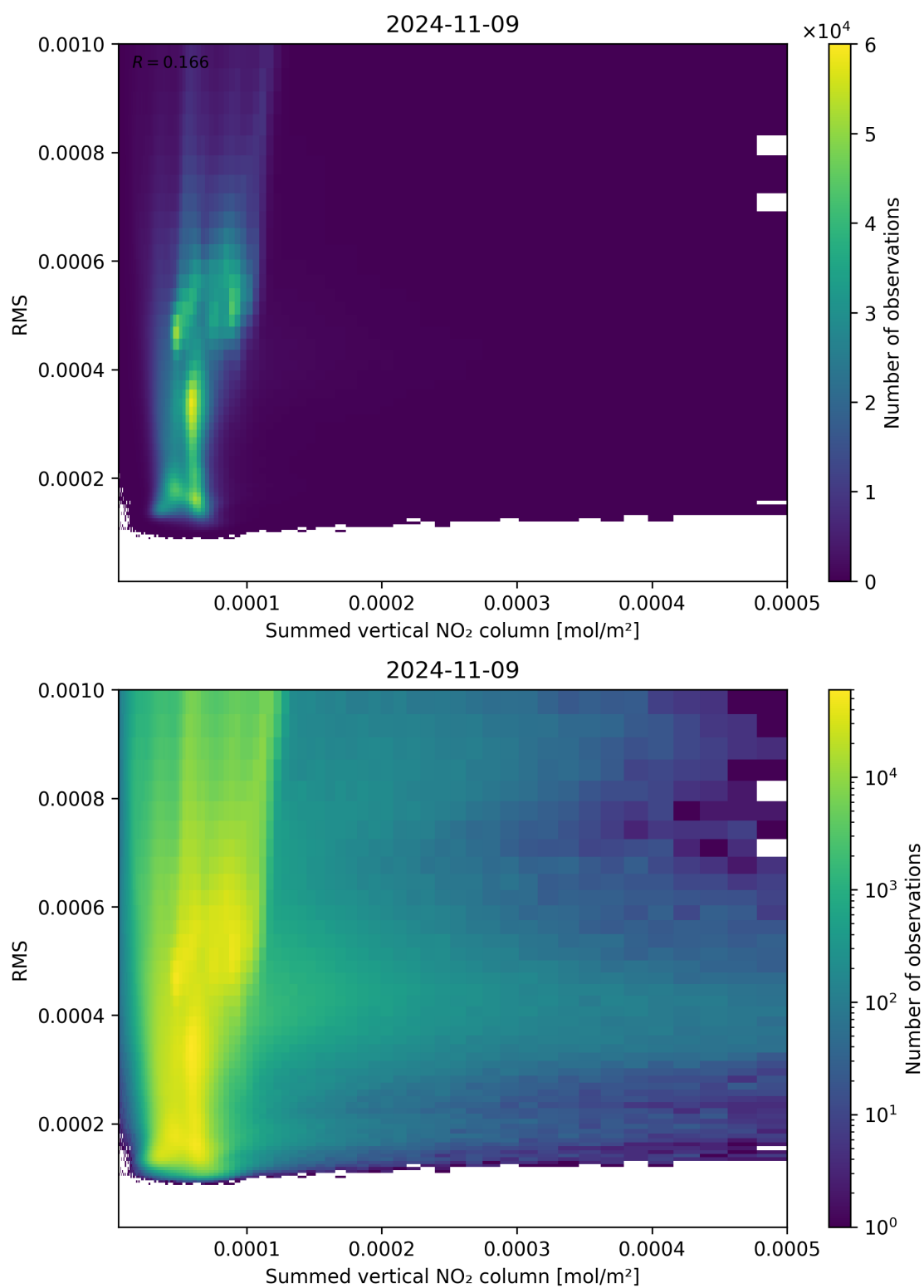
Figure 109: Scatter density plot of “Summed vertical NO 2 column” against “RMS” for 2024-11-09 to 2024-11-10.
