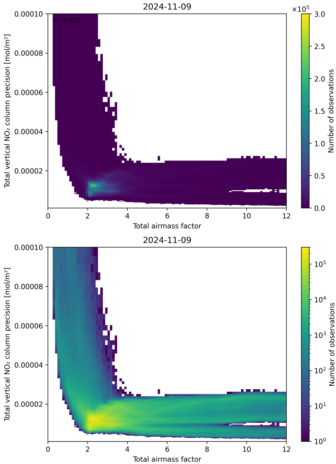
Figure 68: Scatter density plot of “Total airmass factor” against “Total vertical NO 2 column precision” for 2024-11-09 to 2024-11-10.
