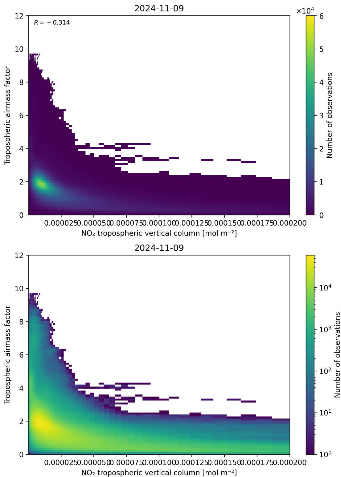
Figure 123: Scatter density plot of “NO 2 tropospheric vertical column” against “Tropospheric air mass factor” for 2024-11-09 to 2024-11-10.
