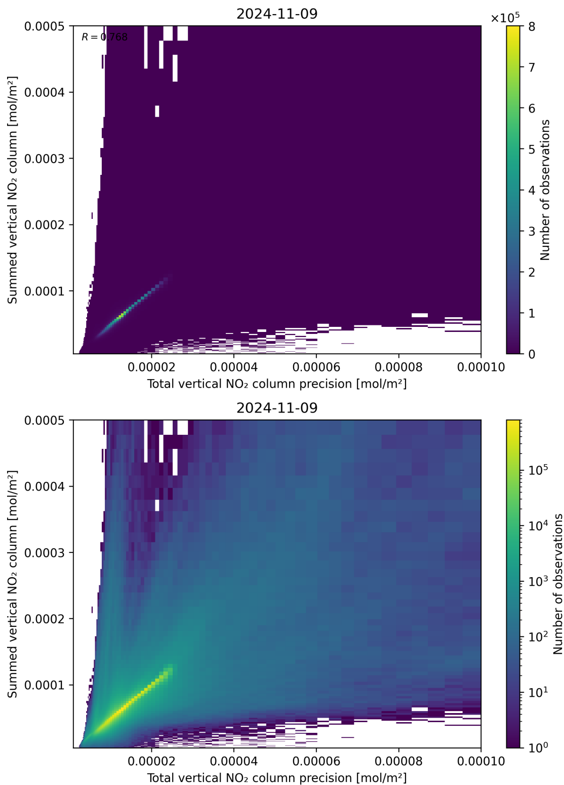
Figure 117: Scatter density plot of “Total vertical NO 2 column precision” against “Summed vertical NO 2 column” for 2024-11-09 to 2024-11-10.
