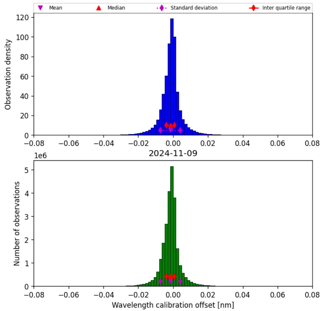
Figure 35: Histogram of “Wavelength calibration offset” for 2024-11-09 to 2024-11-10
