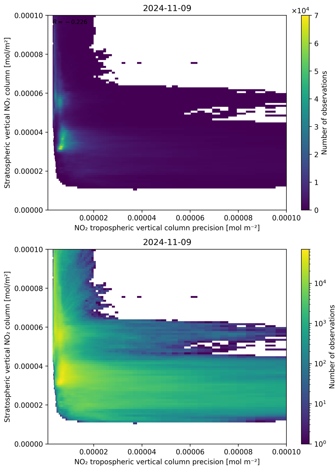
Figure 135: Scatter density plot of “NO 2 tropospheric vertical column precision” against “Stratospheric vertical NO 2 column” for 2024-11-09 to 2024-11-10.
