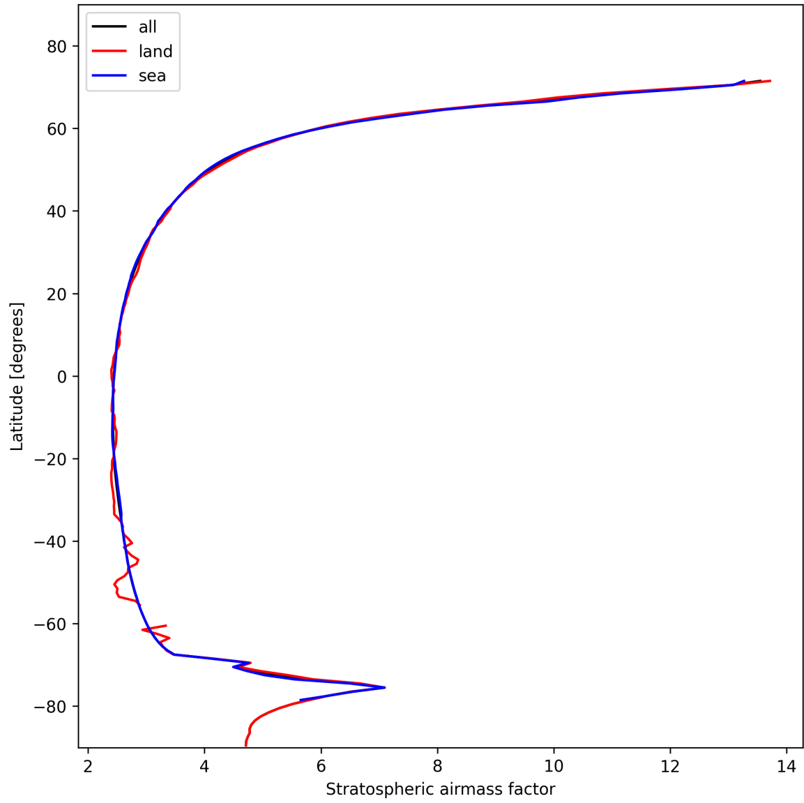
Figure 27: Zonal average of “Stratospheric air mass factor” for 2024-11-09 to 2024-11-10.
