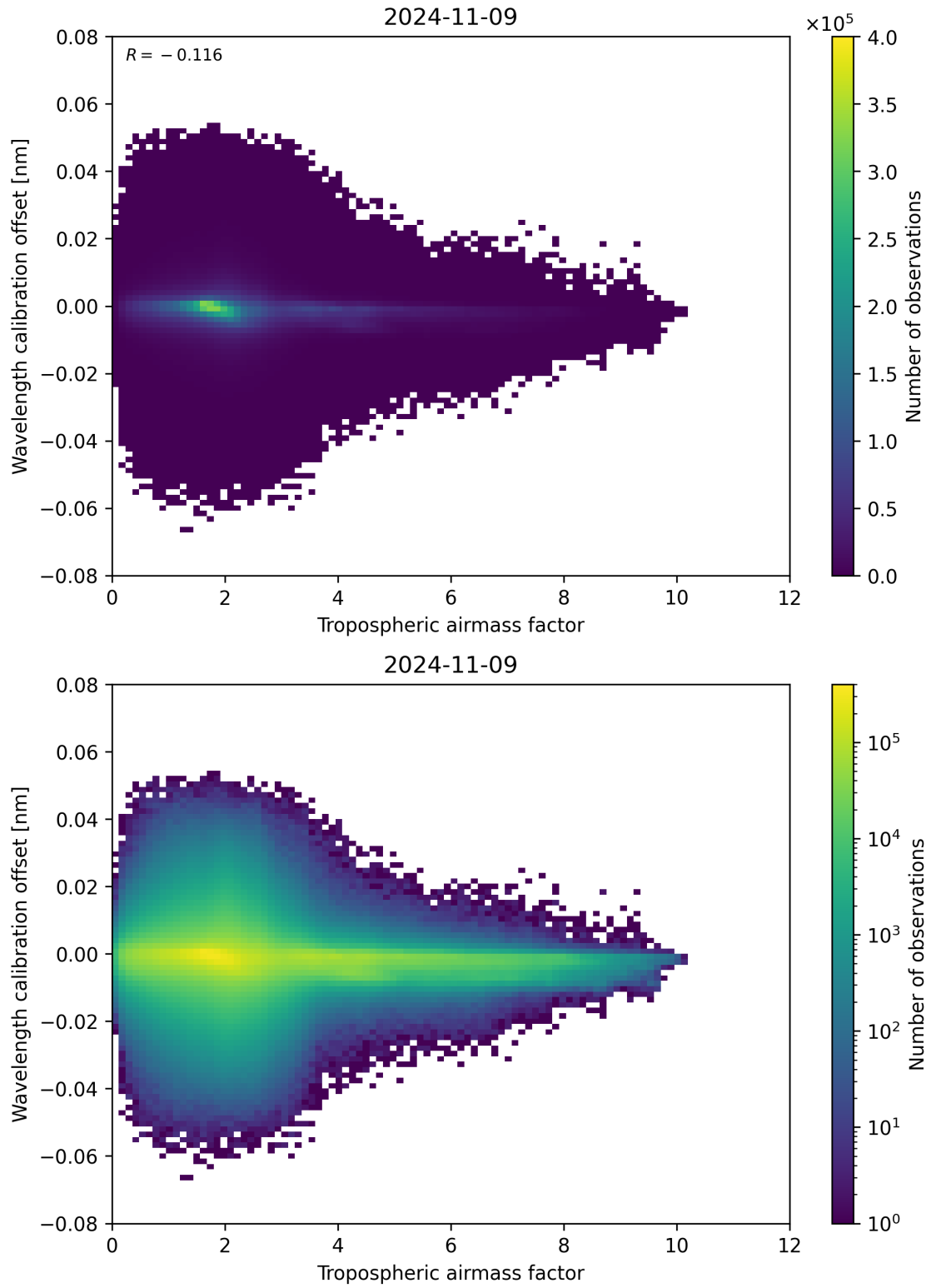
Figure 80: Scatter density plot of “Tropospheric airmass factor” against “Wavelength calibration offset” for 2024-11-09 to 2024-11-10.
