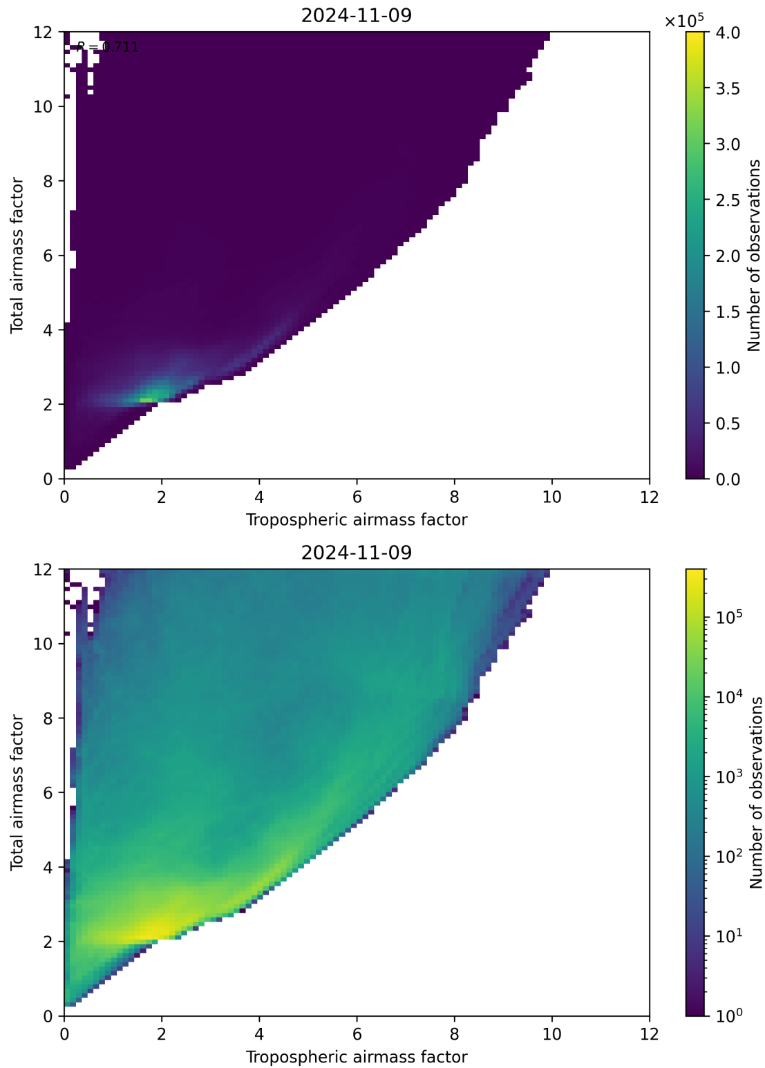
Figure 72: Scatter density plot of “Tropospheric airmass factor” against “Total airmass factor” for 2024-11-09 to 2024-11-10.
