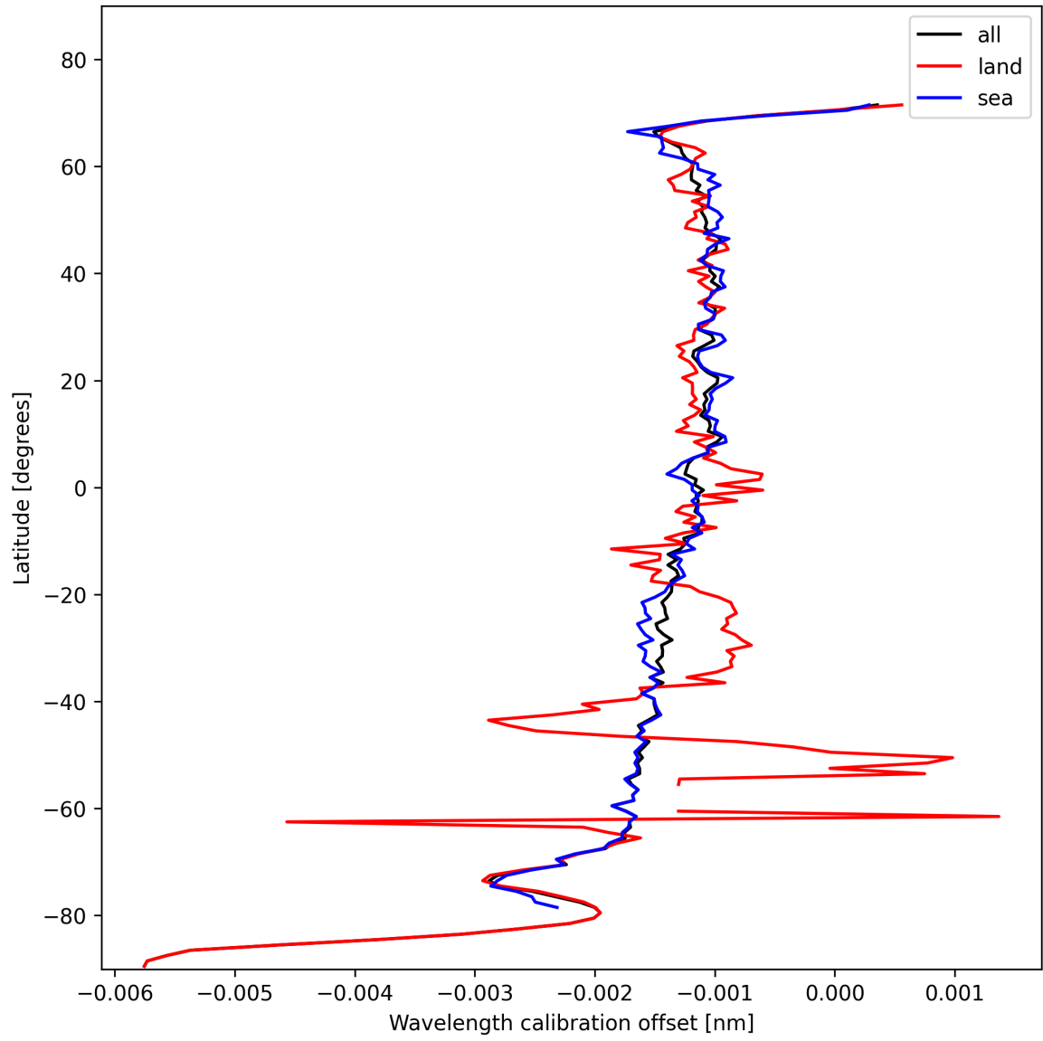
Figure 18: Zonal average of “Wavelength calibration offset” for 2024-11-09 to 2024-11-10.
