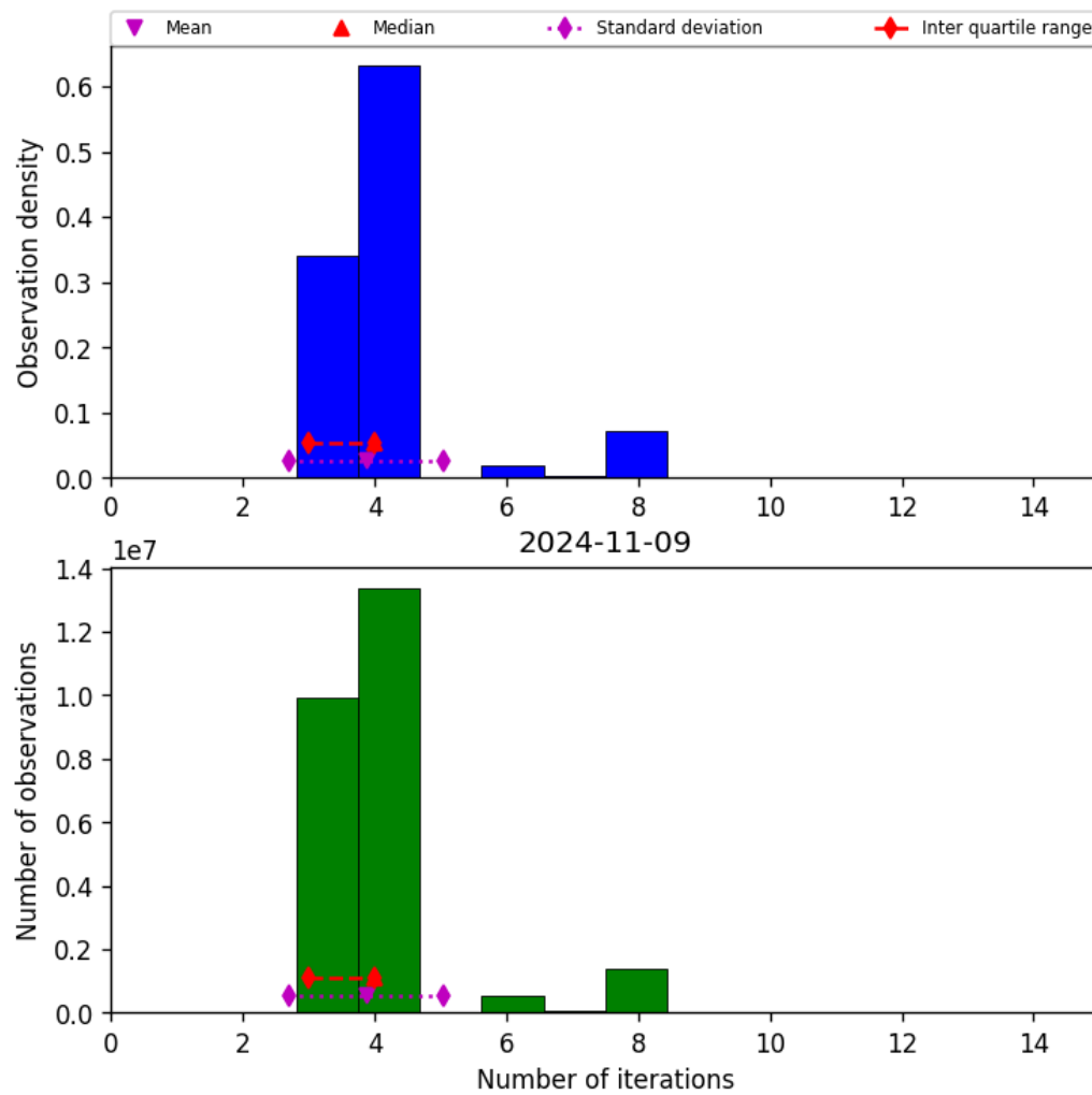
Figure 34: Histogram of “Number of iterations” for 2024-11-09 to 2024-11-10
