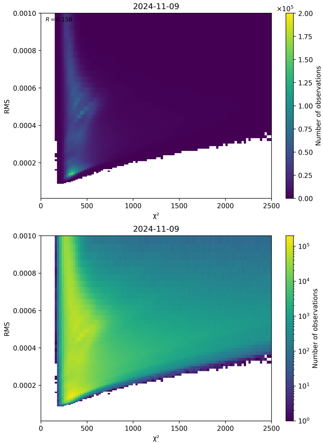
Figure 82: Scatter density plot of “ \chi^2 ” against “RMS” for 2024-11-09 to 2024-11-10.
