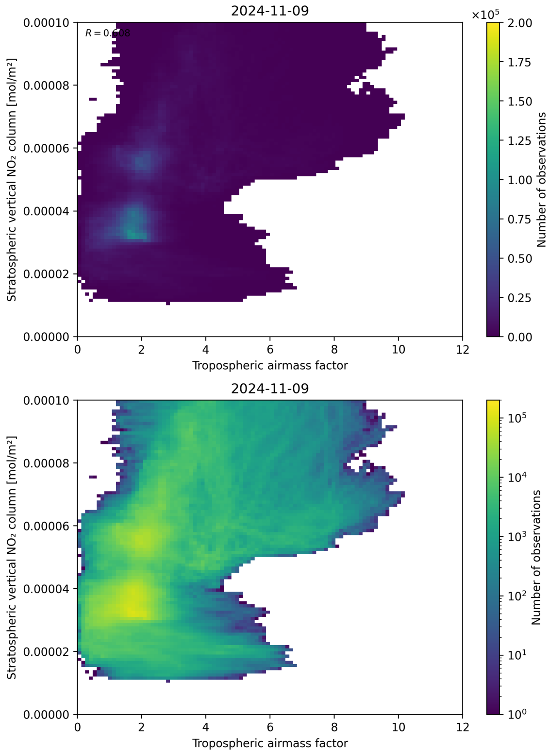
Figure 74: Scatter density plot of “Tropospheric air mass factor” against “Stratospheric vertical NO 2 column” for 2024-11-09 to 2024-11-10.
