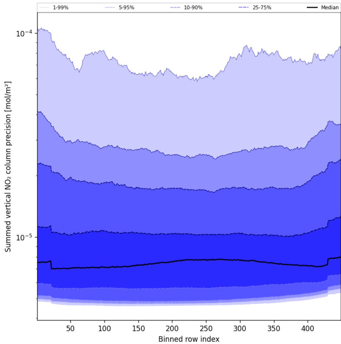
Figure 58: Along track statistics of “Summed vertical NO 2 column precision” for 2024-11-09 to 2024-11-10
