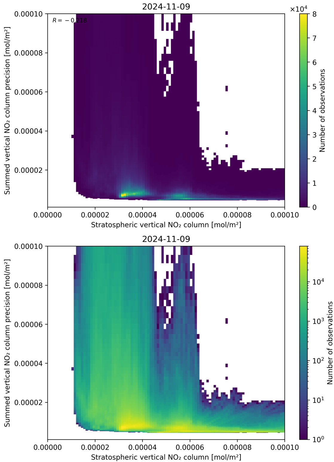
Figure 99: Scatter density plot of “Stratospheric vertical NO 2 column” against “Summed vertical NO 2 column precision” for 2024-11-09 to 2024-11-10.
