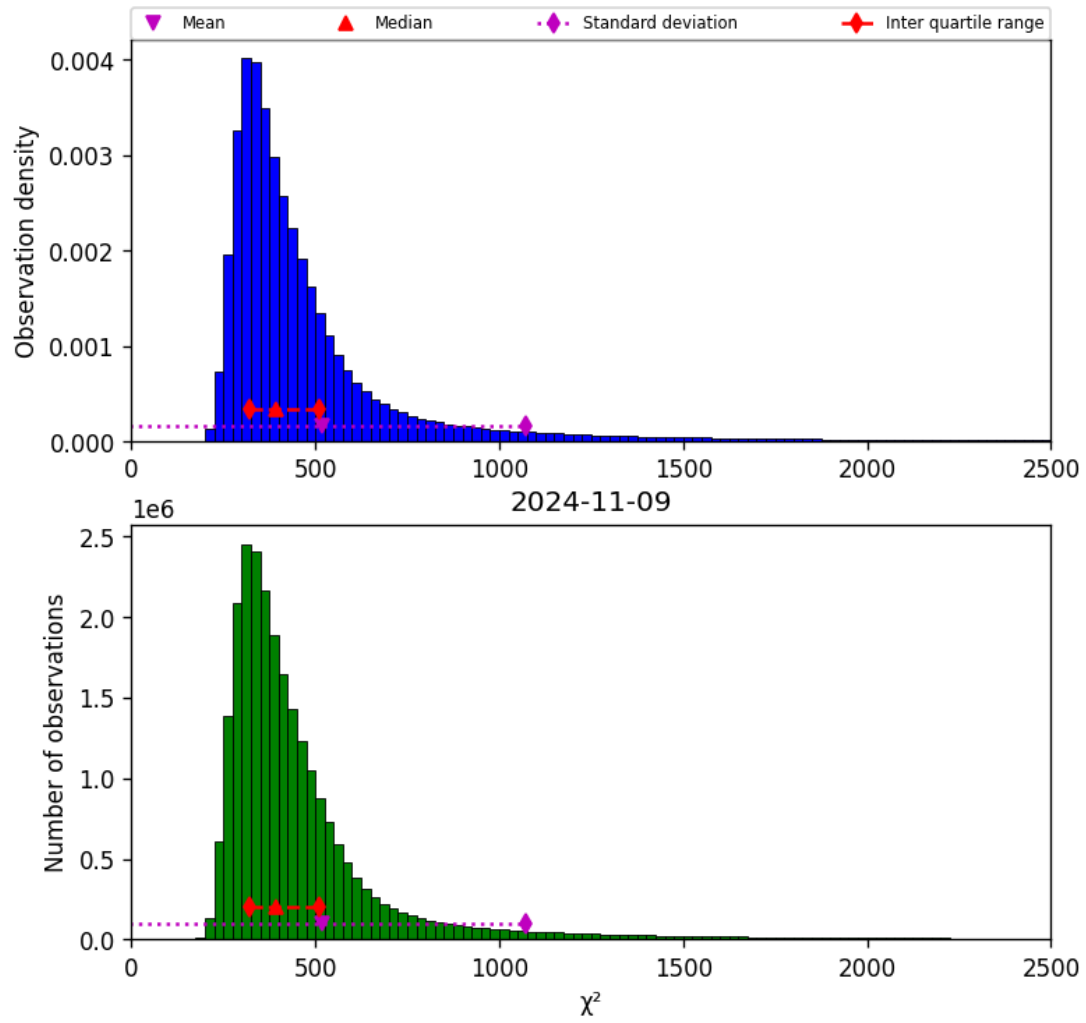
Figure 42: Histogram of “ \chi^2 ” for 2024-11-09 to 2024-11-10
