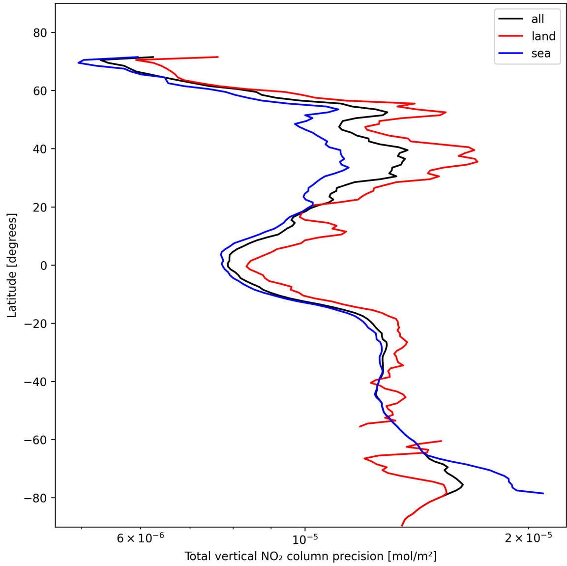
Figure 22: Zonal average of "Total vertical NO 2 column precision" for 2024-11-09 to 2024-11-10.
