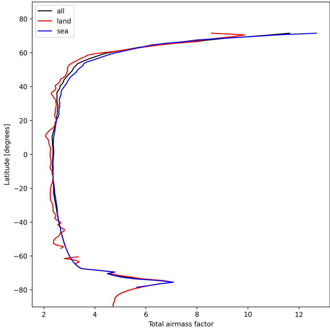
Figure 15: Zonal average of “Total airmass factor” for 2024-11-09 to 2024-11-10.
