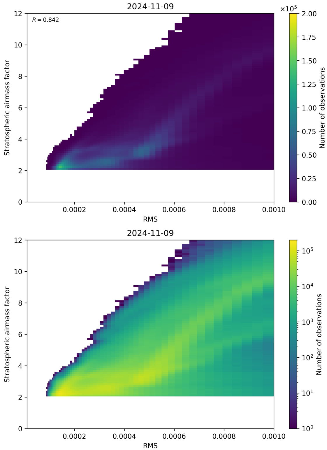
Figure 144: Scatter density plot of “RMS” against “Stratospheric airmass factor” for 2024-11-09 to 2024-11-10.
