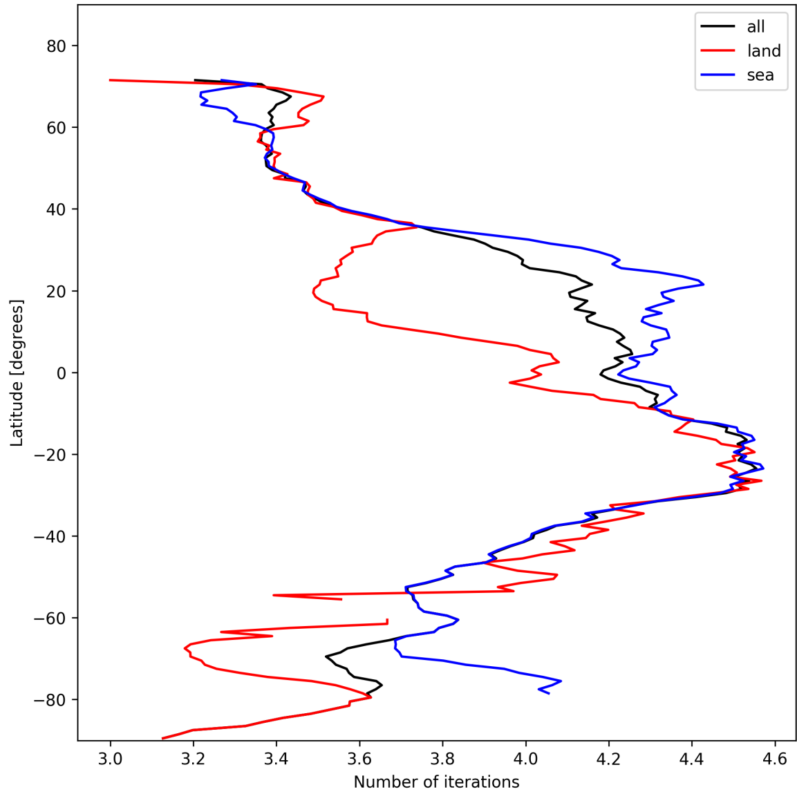
Figure 17: Zonal average of “Number of iterations” for 2024-11-09 to 2024-11-10.
