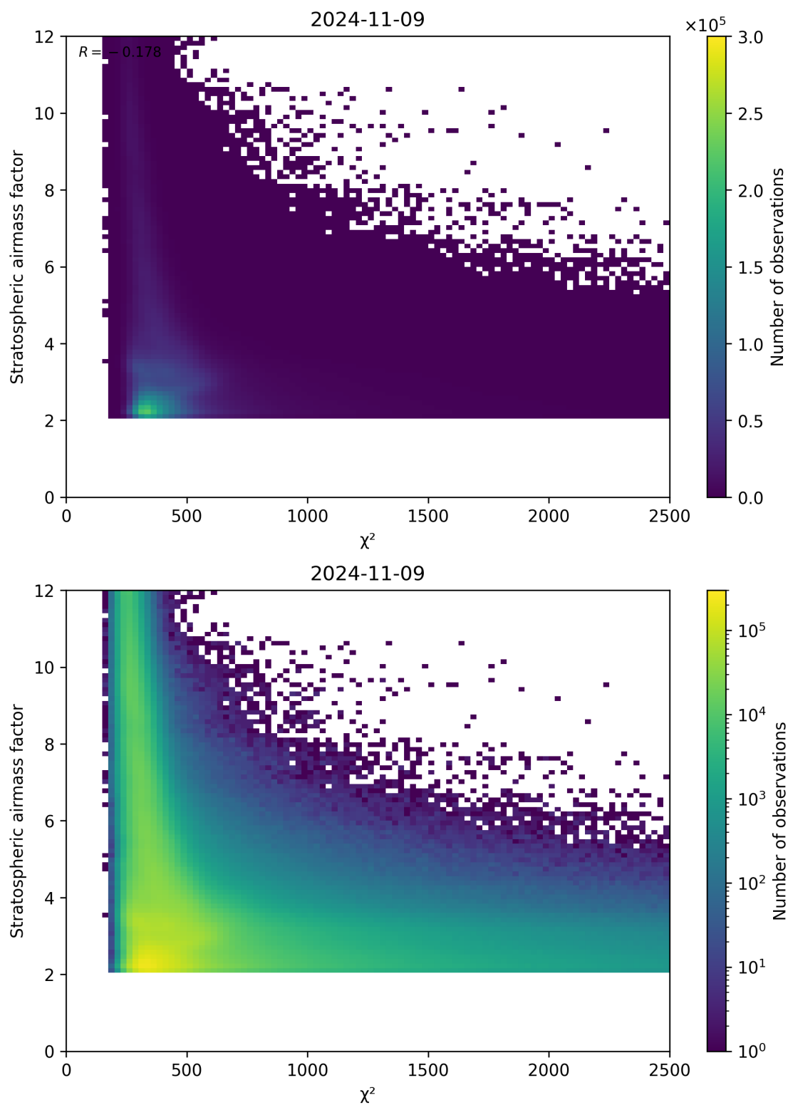
Figure 81: Scatter density plot of “ \chi^2 ” against “Stratospheric airmass factor” for 2024-11-09 to 2024-11-10.
