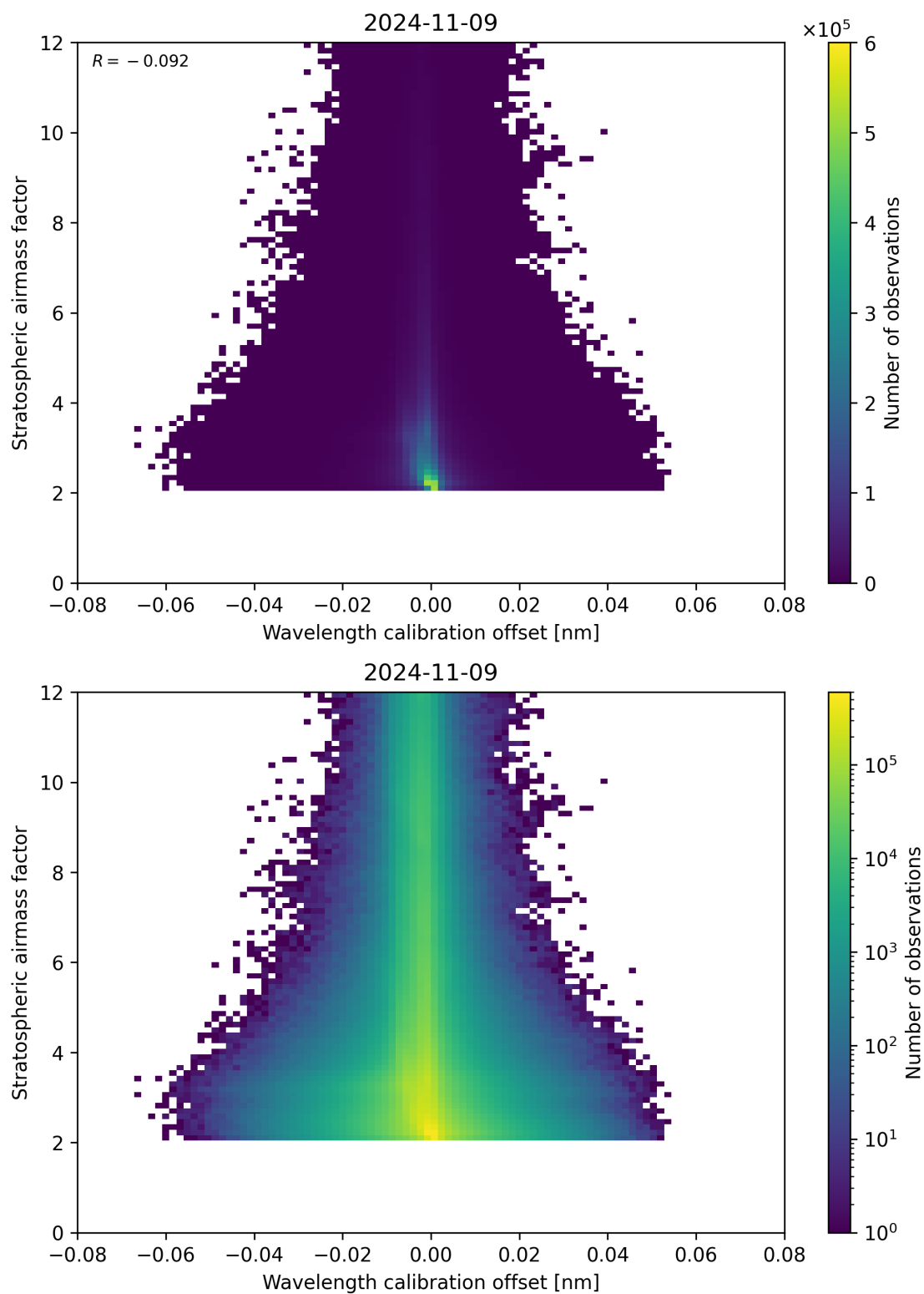
Figure 174: Scatter density plot of “Wavelength calibration offset” against “Stratospheric airmass factor” for 2024-11-09 to 2024-11-10.
