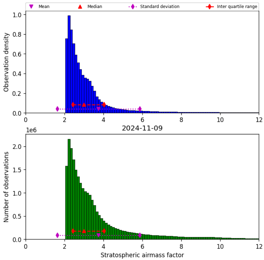
Figure 44: Histogram of “Stratospheric airmass factor” for 2024-11-09 to 2024-11-10
