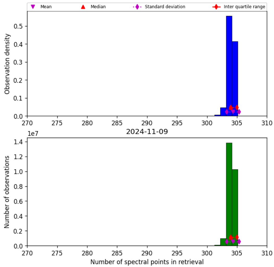
Figure 33: Histogram of “Number of spectral points in retrieval” for 2024-11-09 to 2024-11-10
