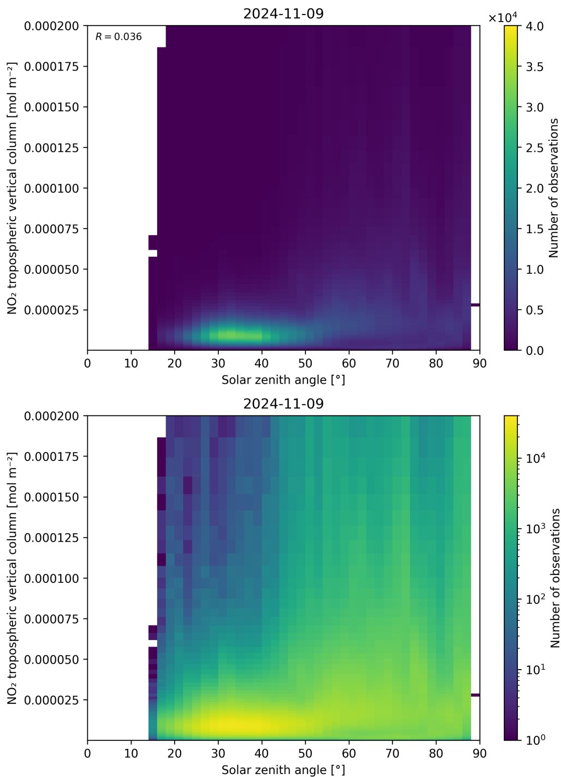
Figure 155: Scatter density plot of “Solar zenith angle” against “NO 2 tropospheric vertical column” for 2024-11-09 to 2024-11-10.
