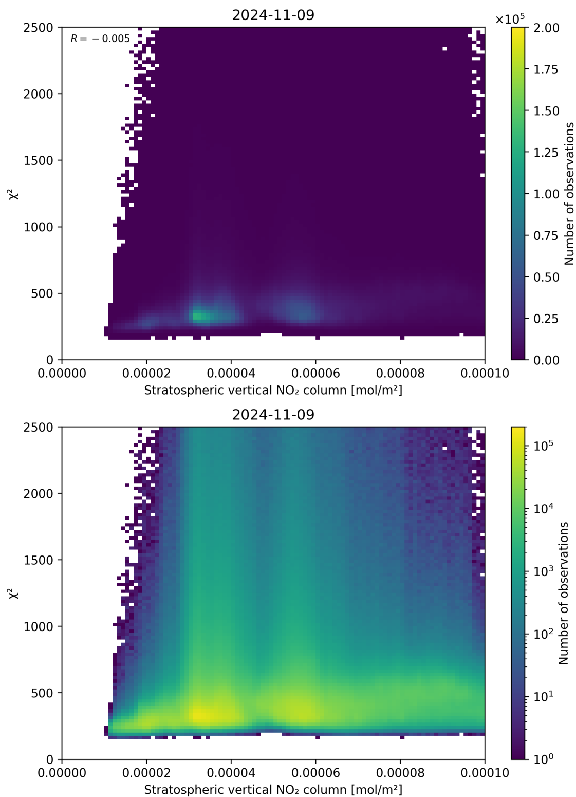
Figure 97: Scatter density plot of “Stratospheric vertical NO 2 column” against “ \chi^2 ” for 2024-11-09 to 2024-11-10.
