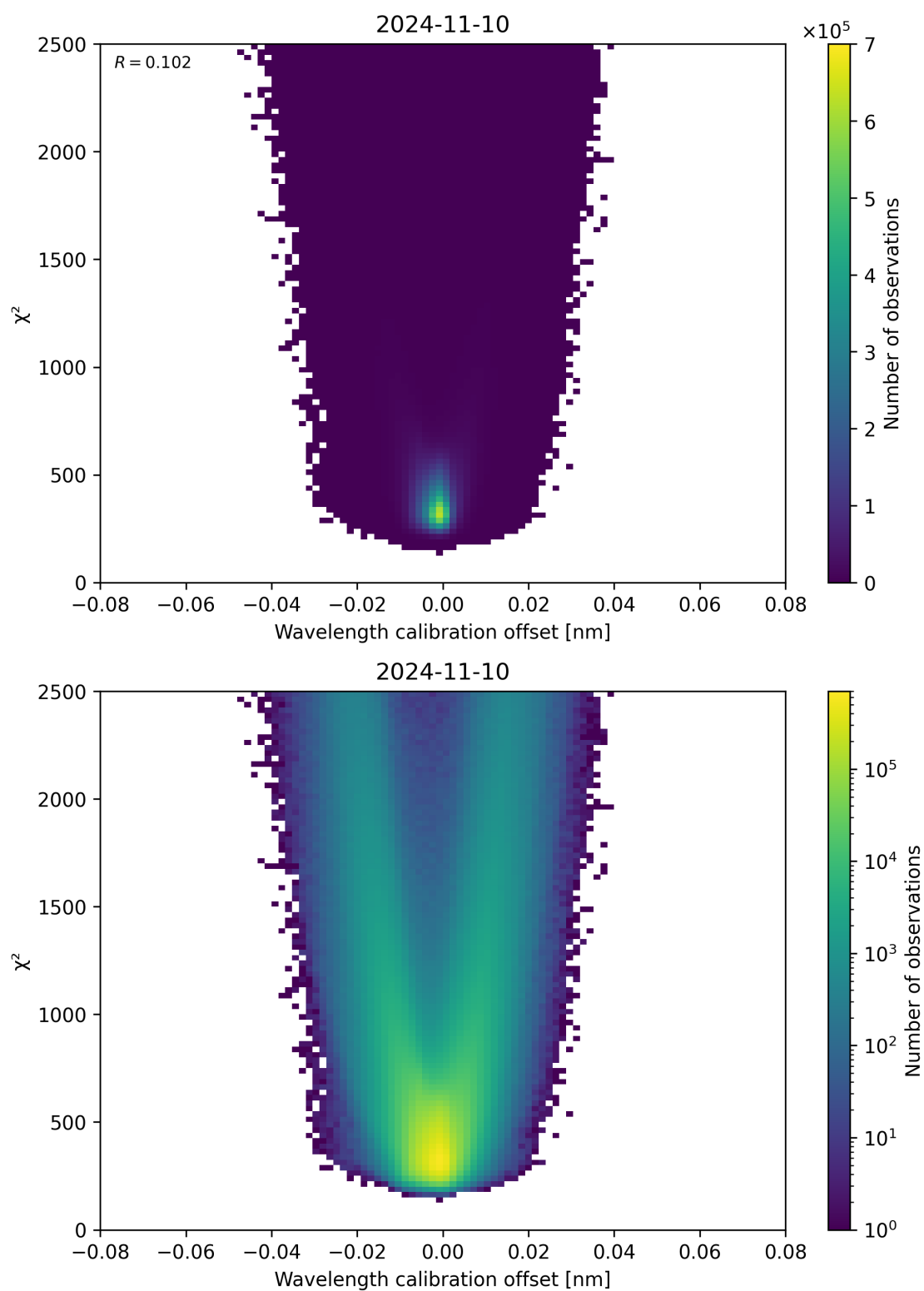
Figure 175: Scatter density plot of “Wavelength calibration offset” against “ \chi^2 ” for 2024-11-09 to 2024-11-11.
