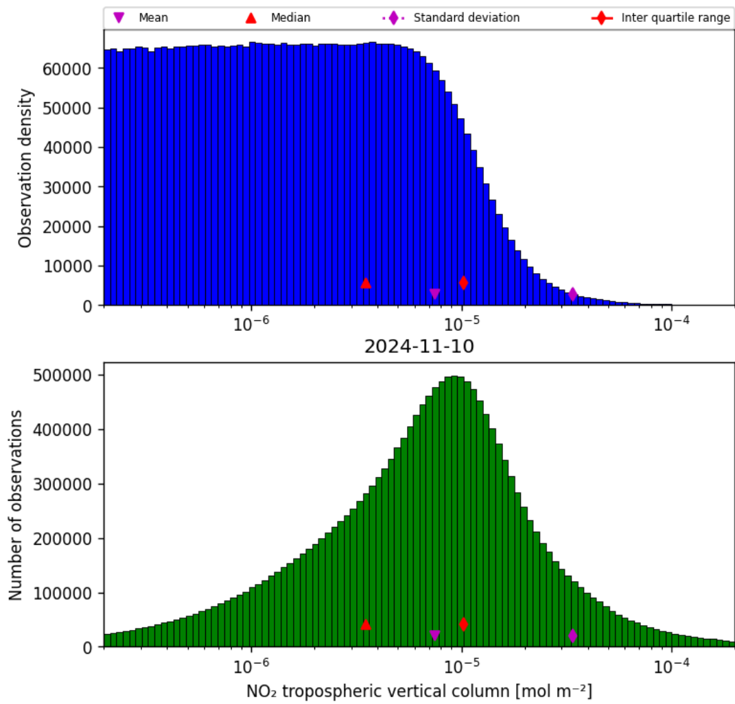
Figure 29: Histogram of “NO 2 tropospheric vertical column” for 2024-11-09 to 2024-11-11
