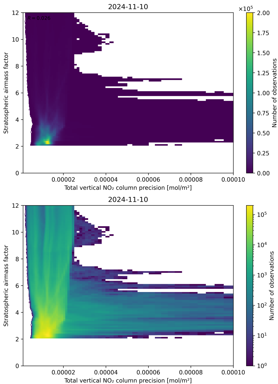
Figure 115: Scatter density plot of “Total vertical NO 2 column precision” against “Stratospheric air mass factor” for 2024-11-09 to 2024-11-11.
