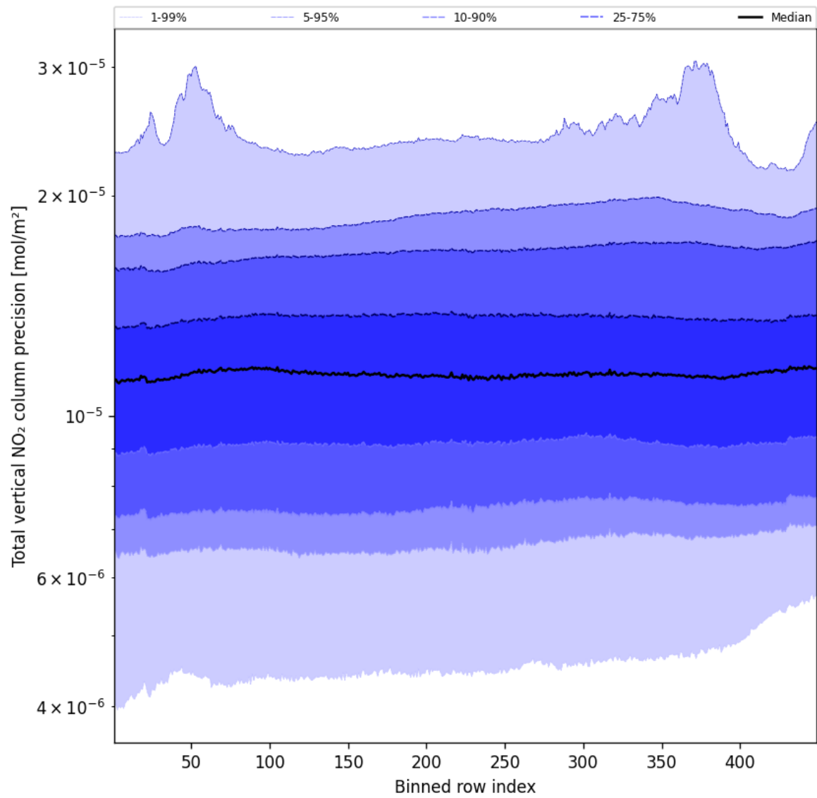
Figure 56: Along track statistics of "Total vertical NO 2 column precision" for 2024-11-09 to 2024-11-11
