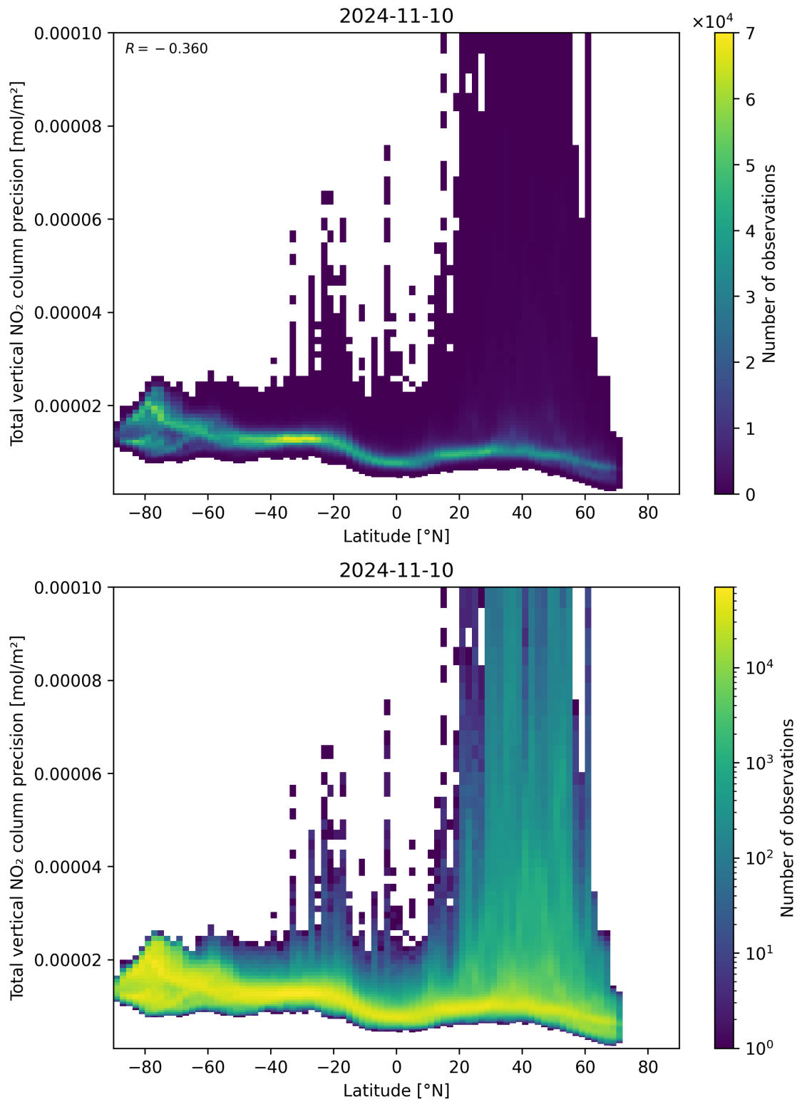
Figure 91: Scatter density plot of “Latitude” against “Total vertical NO 2 column precision” for 2024-11-09 to 2024-11-11.
