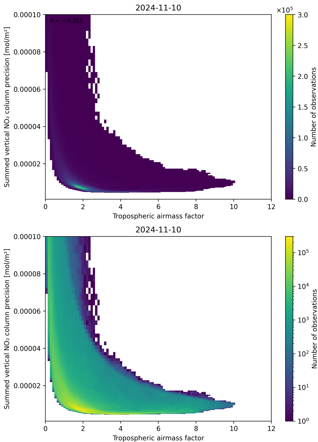
Figure 76: Scatter density plot of “Tropospheric air mass factor” against “Summed vertical NO 2 column precision” for 2024-11-09 to 2024-11-11.
