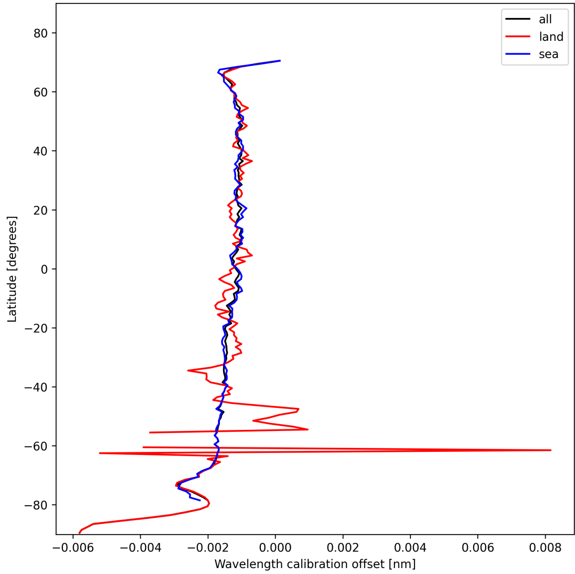
Figure 18: Zonal average of “Wavelength calibration offset” for 2024-11-09 to 2024-11-11.
