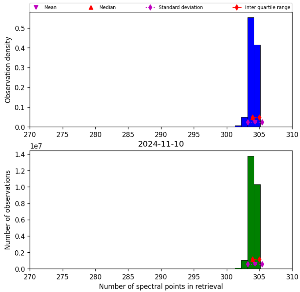
Figure 33: Histogram of “Number of spectral points in retrieval” for 2024-11-09 to 2024-11-11
