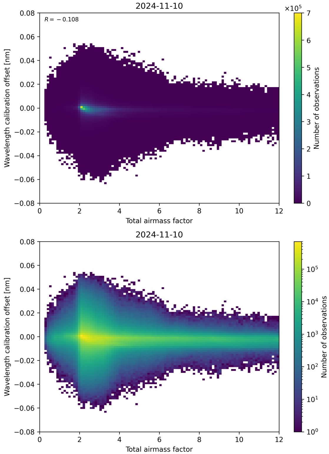
Figure 70: Scatter density plot of “Total airmass factor” against “Wavelength calibration offset” for 2024-11-09 to 2024-11-11.
