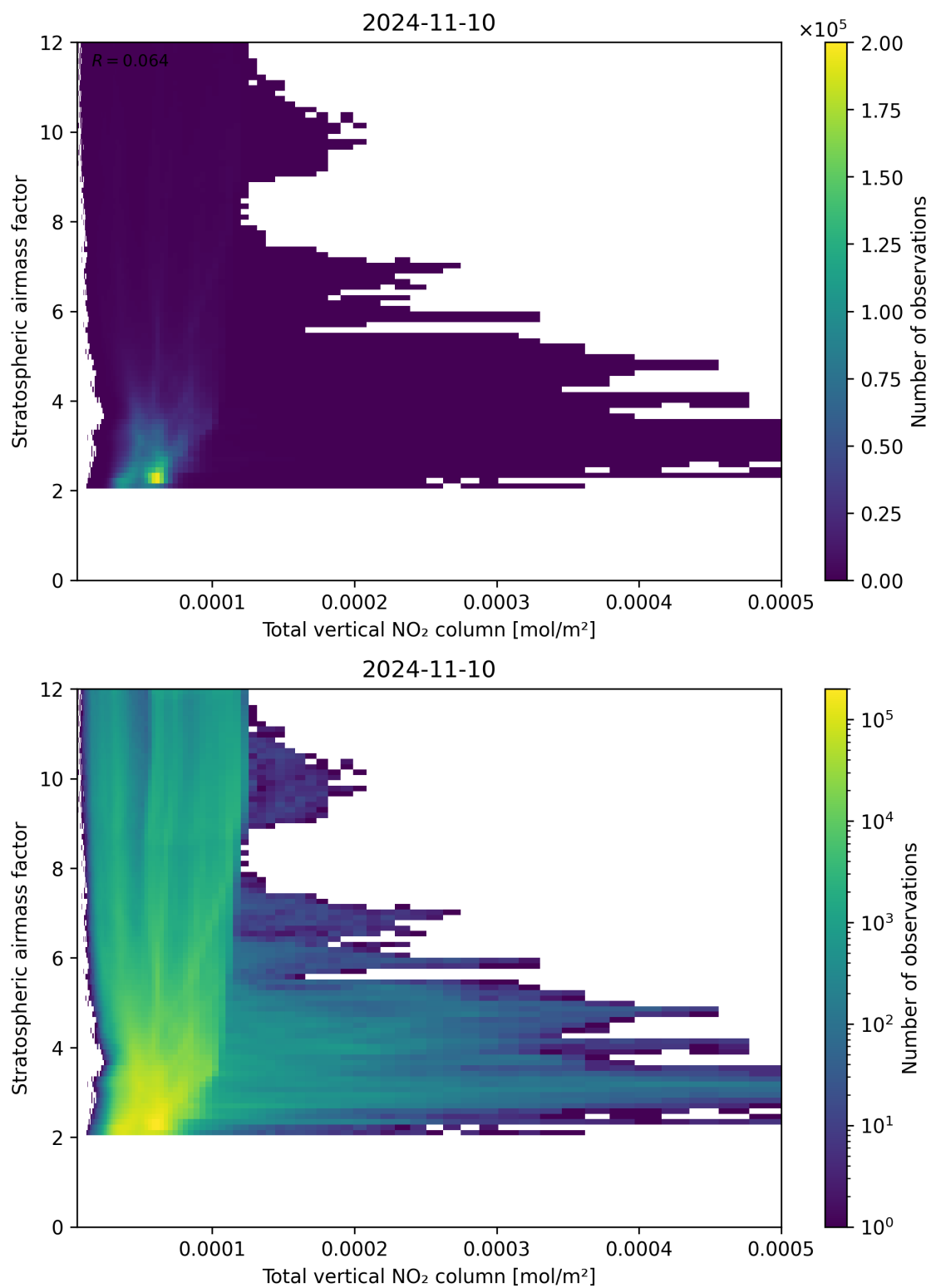
Figure 110: Scatter density plot of “Total vertical NO 2 column” against “Stratospheric airmass factor” for 2024-11-09 to 2024-11-11.
