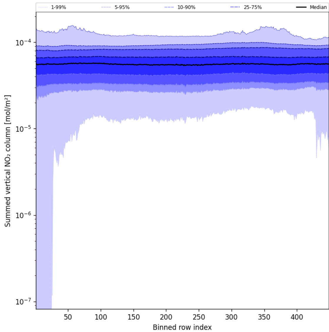
Figure 57: Along track statistics of “Summed vertical NO 2 column” for 2024-11-09 to 2024-11-11
