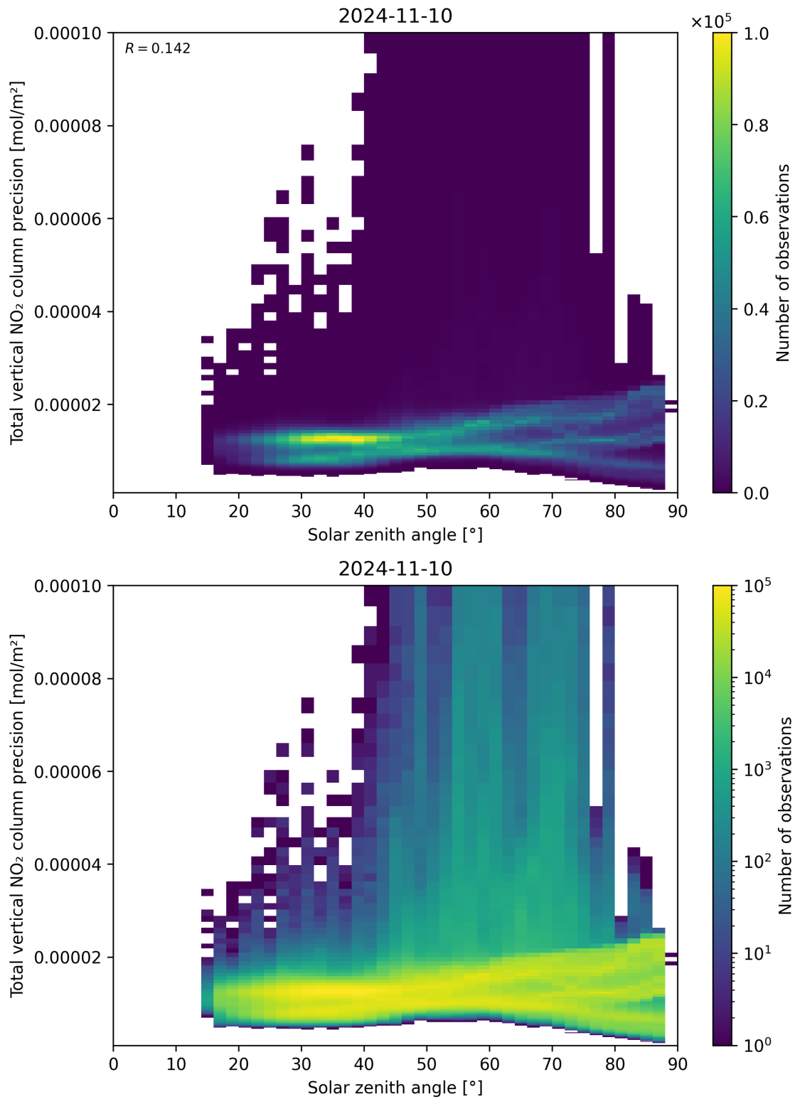
Figure 154: Scatter density plot of “Solar zenith angle” against “Total vertical NO 2 column precision” for 2024-11-09 to 2024-11-11.
