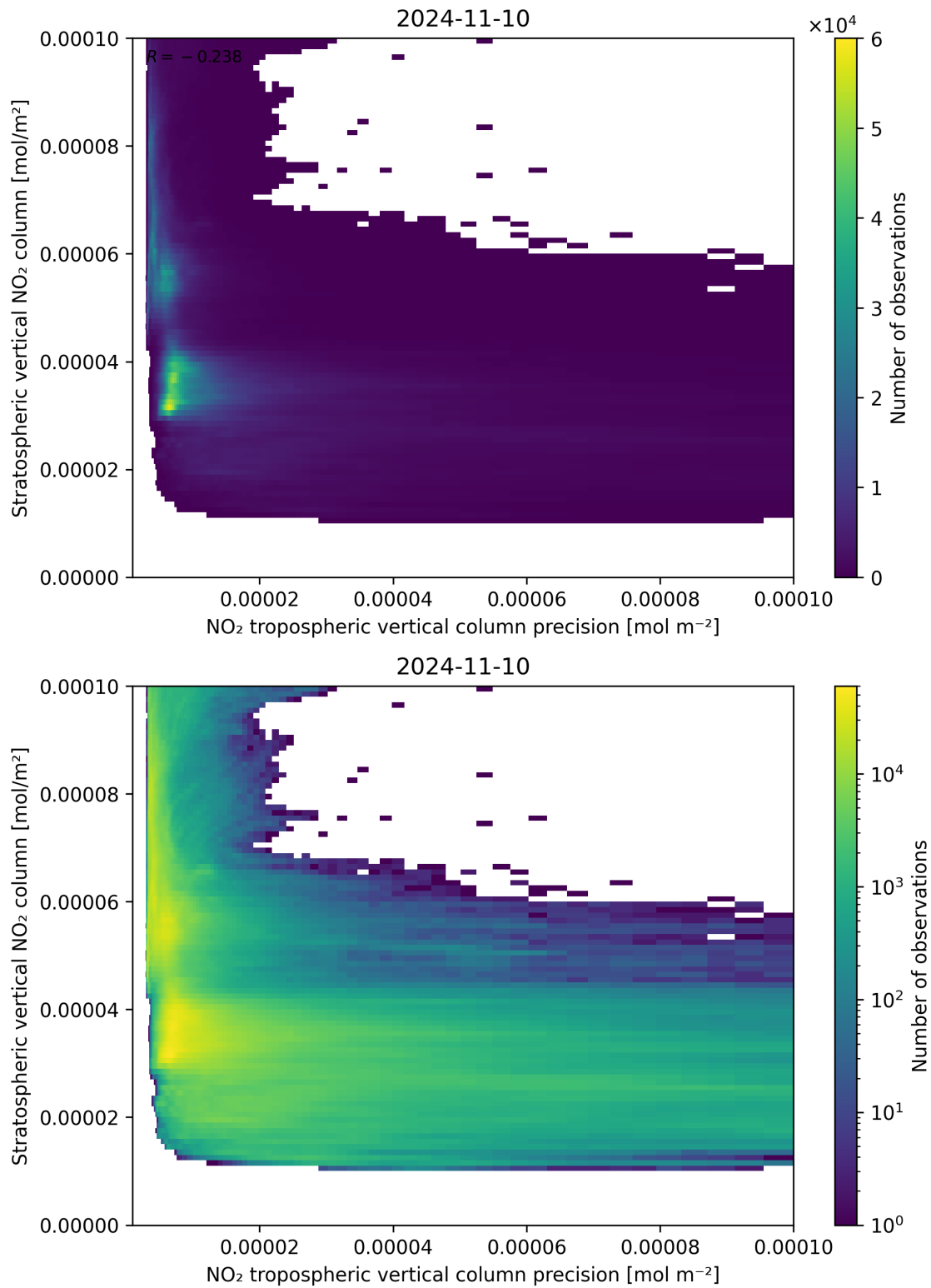
Figure 135: Scatter density plot of “NO 2 tropospheric vertical column precision” against “Stratospheric vertical NO 2 column” for 2024-11-09 to 2024-11-11.
