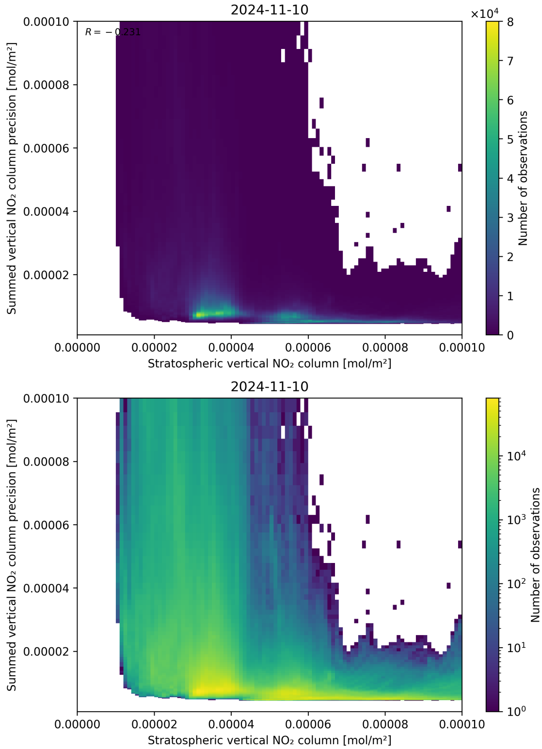
Figure 99: Scatter density plot of “Stratospheric vertical NO 2 column” against “Summed vertical NO 2 column precision” for 2024-11-09 to 2024-11-11.
