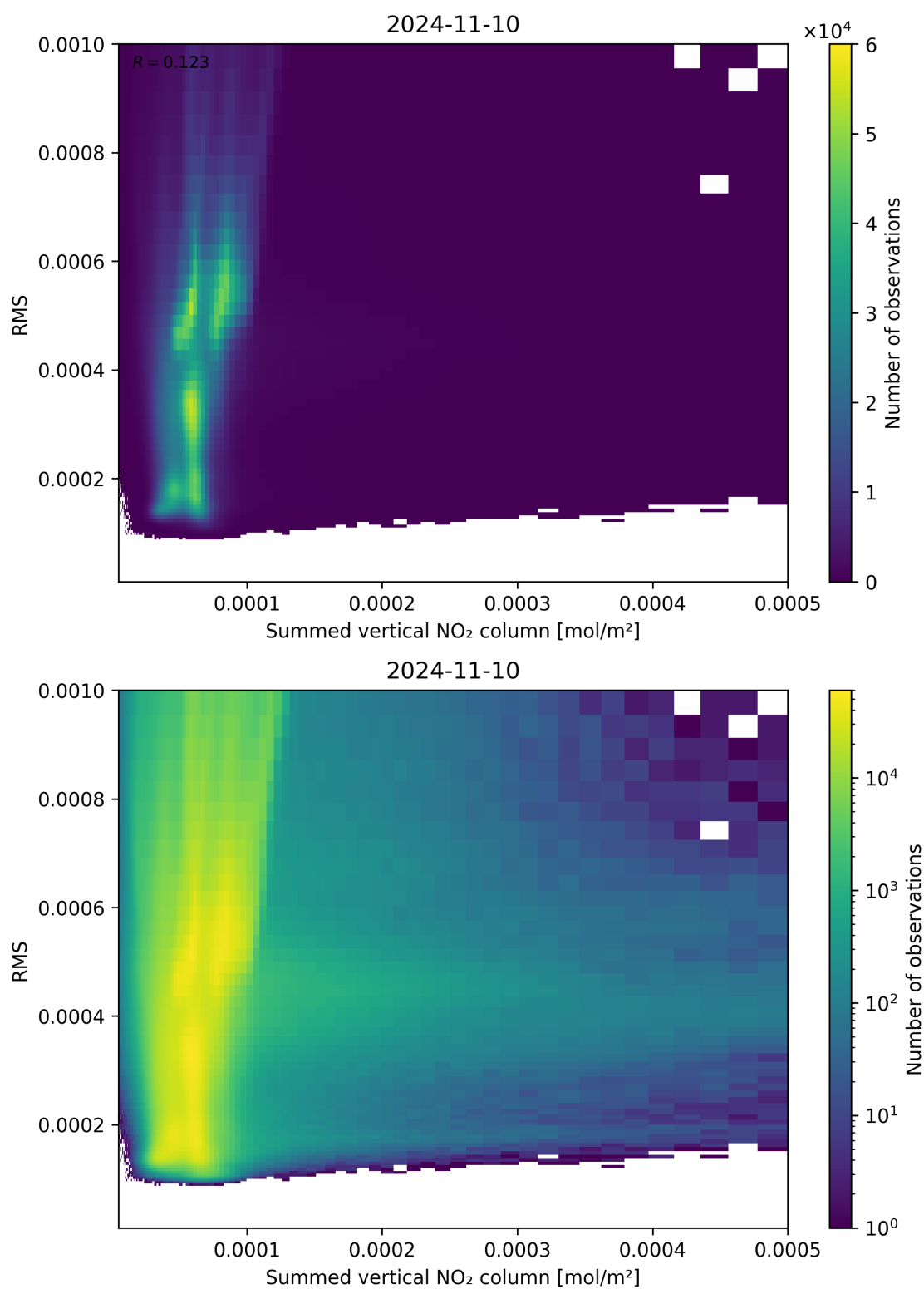
Figure 109: Scatter density plot of “Summed vertical NO 2 column” against “RMS” for 2024-11-09 to 2024-11-11.
