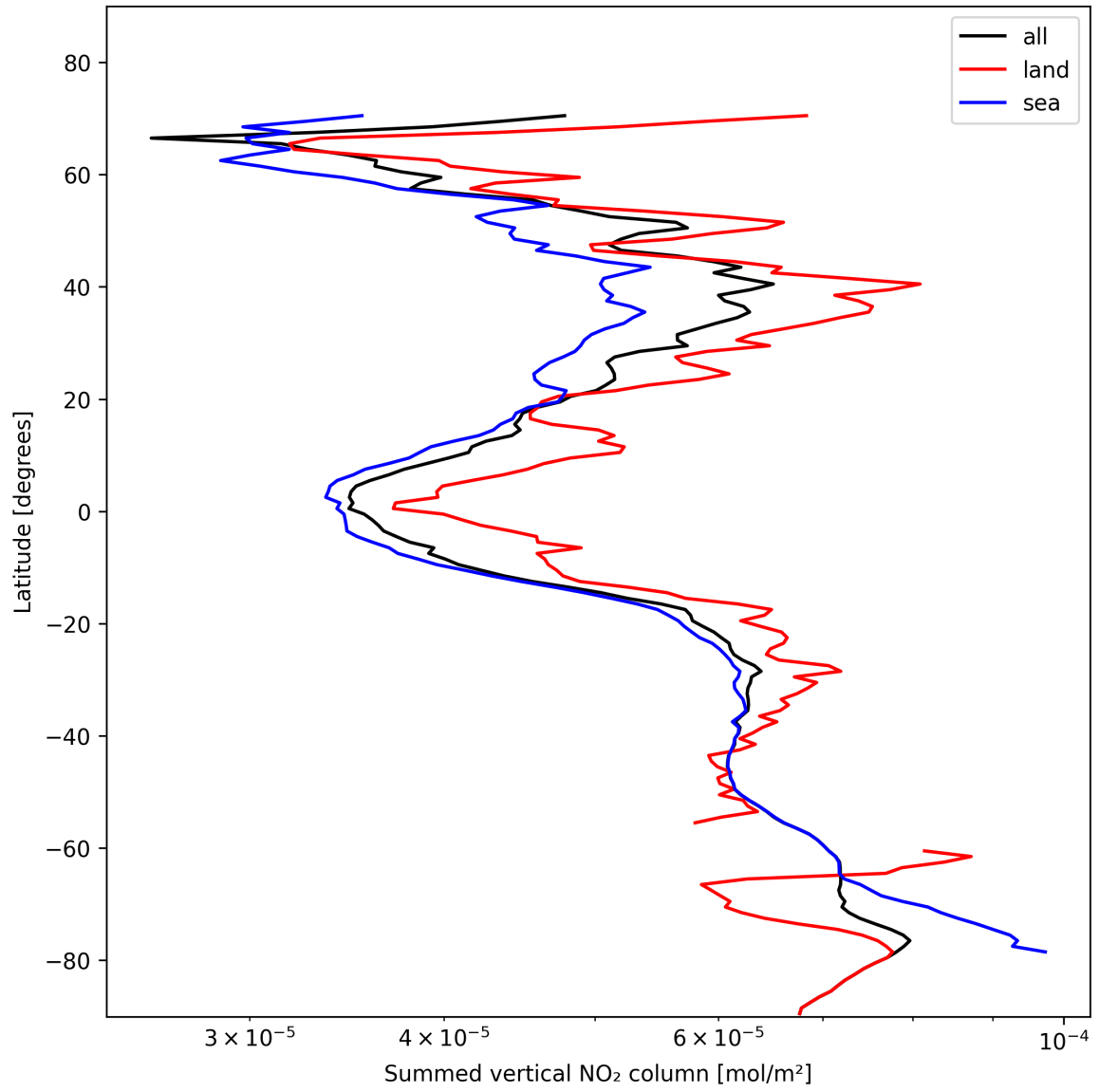
Figure 23: Zonal average of “Summed vertical NO 2 column” for 2024-11-09 to 2024-11-11.
