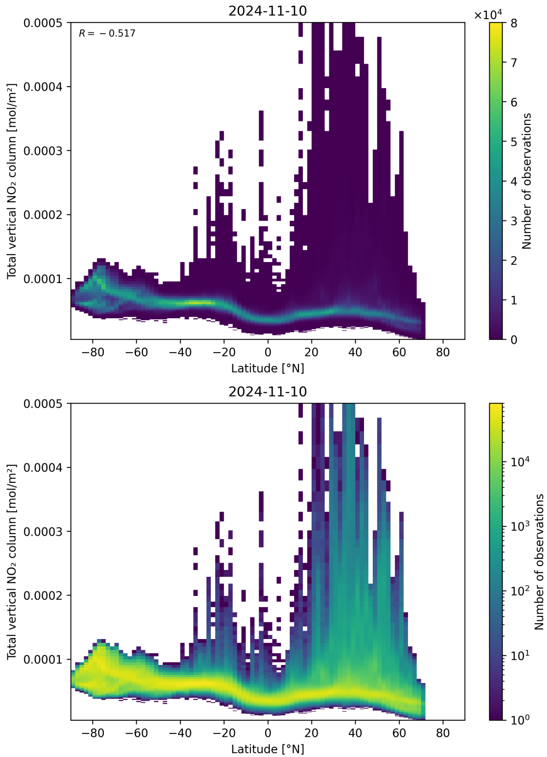
Figure 90: Scatter density plot of “Latitude” against “Total vertical NO 2 column” for 2024-11-09 to 2024-11-11.
