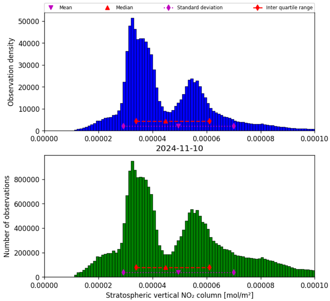
Figure 36: Histogram of “Stratospheric vertical NO 2 column” for 2024-11-09 to 2024-11-11
