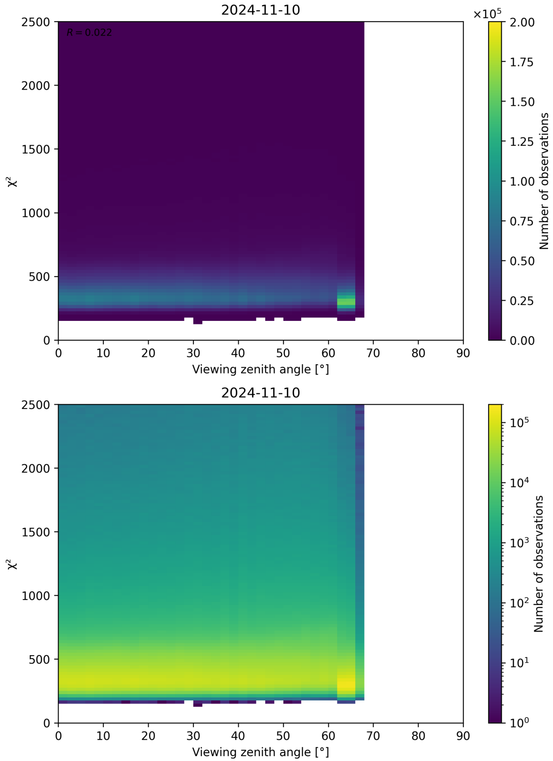
Figure 162: Scatter density plot of “Viewing zenith angle” against “ \chi^2 ” for 2024-11-09 to 2024-11-11.
