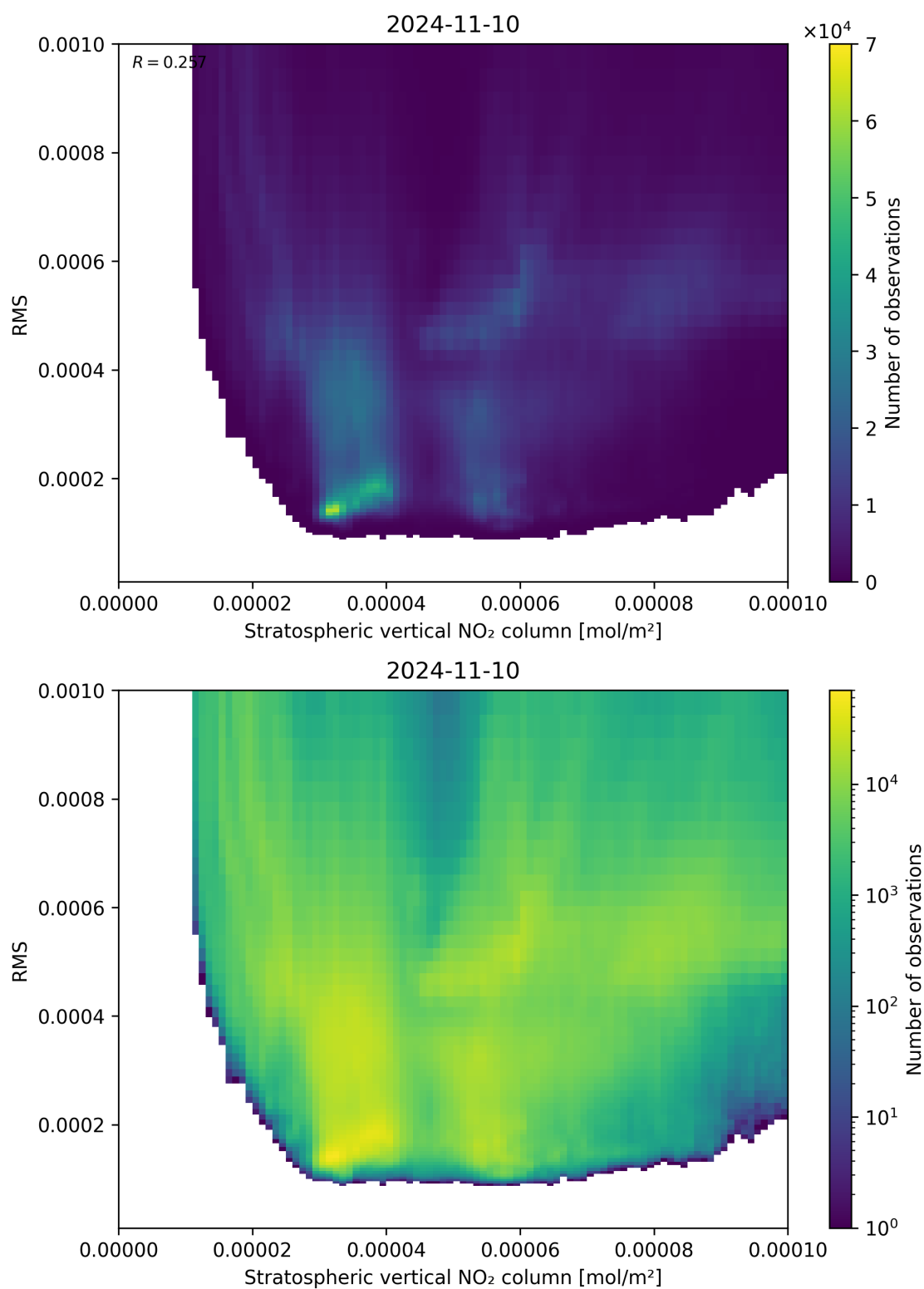
Figure 102: Scatter density plot of “Stratospheric vertical NO 2 column” against “RMS” for 2024-11-09 to 2024-11-11.
