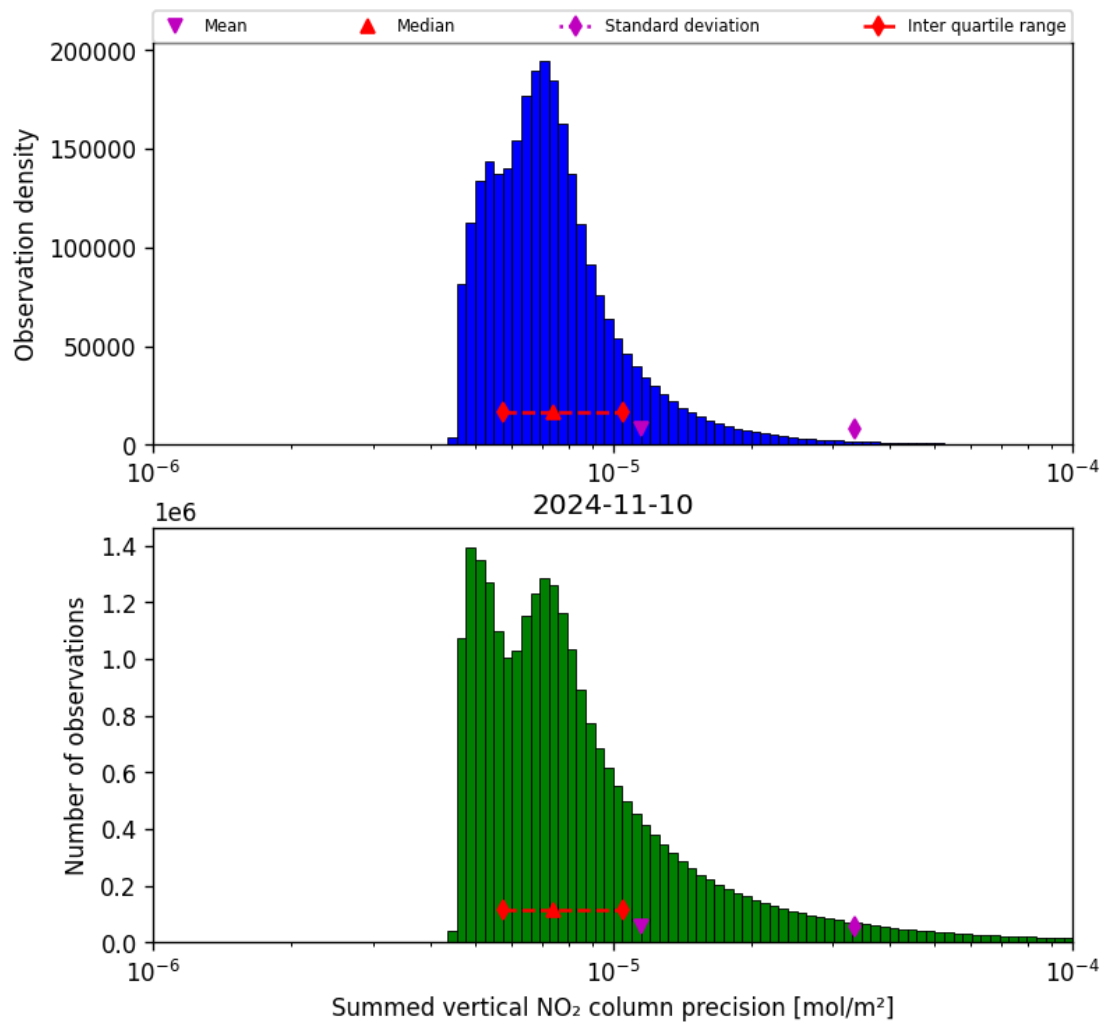
Figure 41: Histogram of "Summed vertical NO 2 column precision" for 2024-11-09 to 2024-11-11
