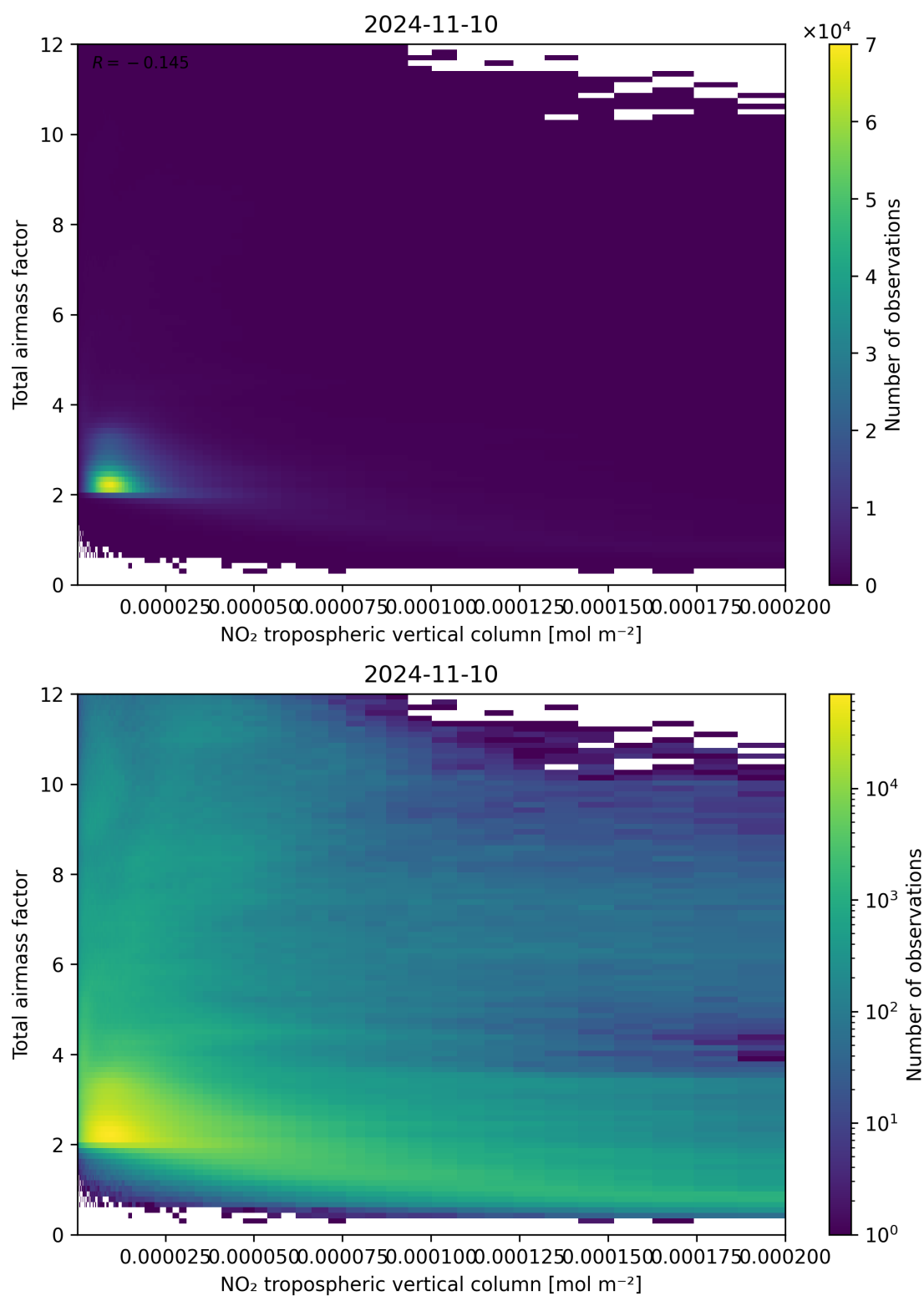
Figure 122: Scatter density plot of “NO 2 tropospheric vertical column” against “Total air mass factor” for 2024-11-09 to 2024-11-11.
