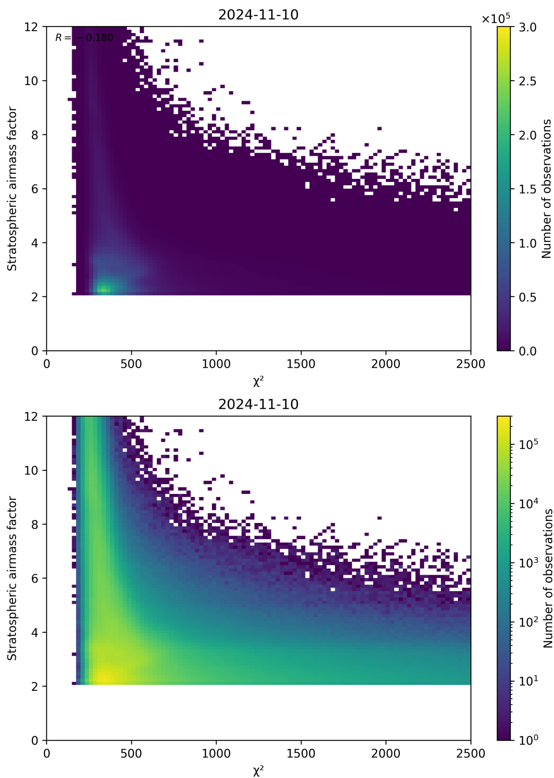
Figure 81: Scatter density plot of “ \chi^2 ” against “Stratospheric airmass factor” for 2024-11-09 to 2024-11-11.
