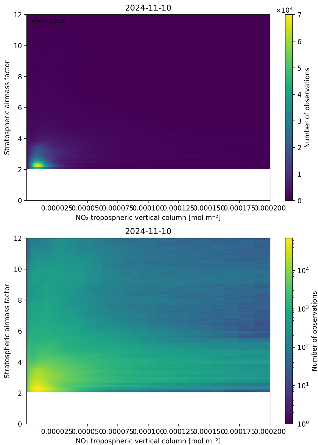
Figure 121: Scatter density plot of “NO 2 tropospheric vertical column” against “Stratospheric airmass factor” for 2024-11-09 to 2024-11-11.
