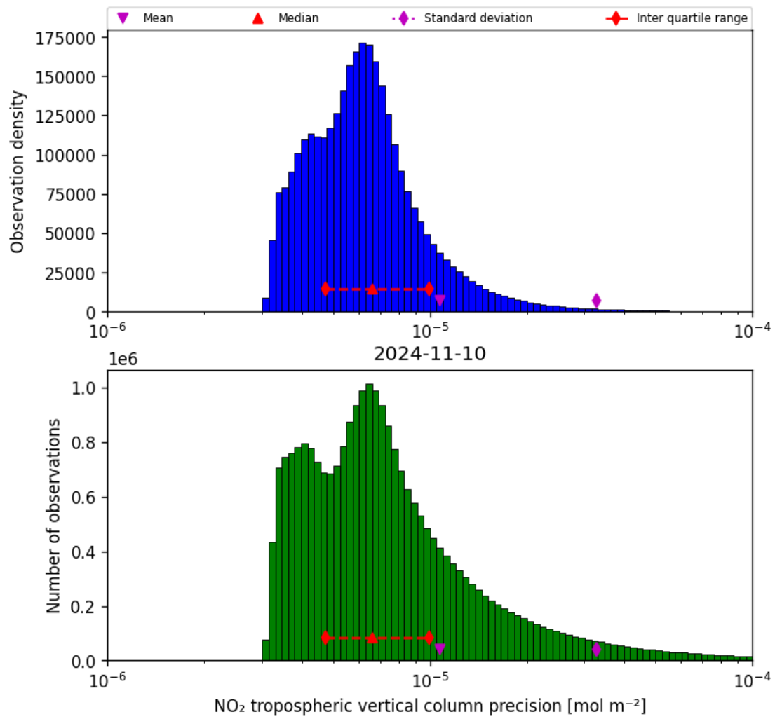
Figure 30: Histogram of “NO 2 tropospheric vertical column precision” for 2024-11-09 to 2024-11-11
