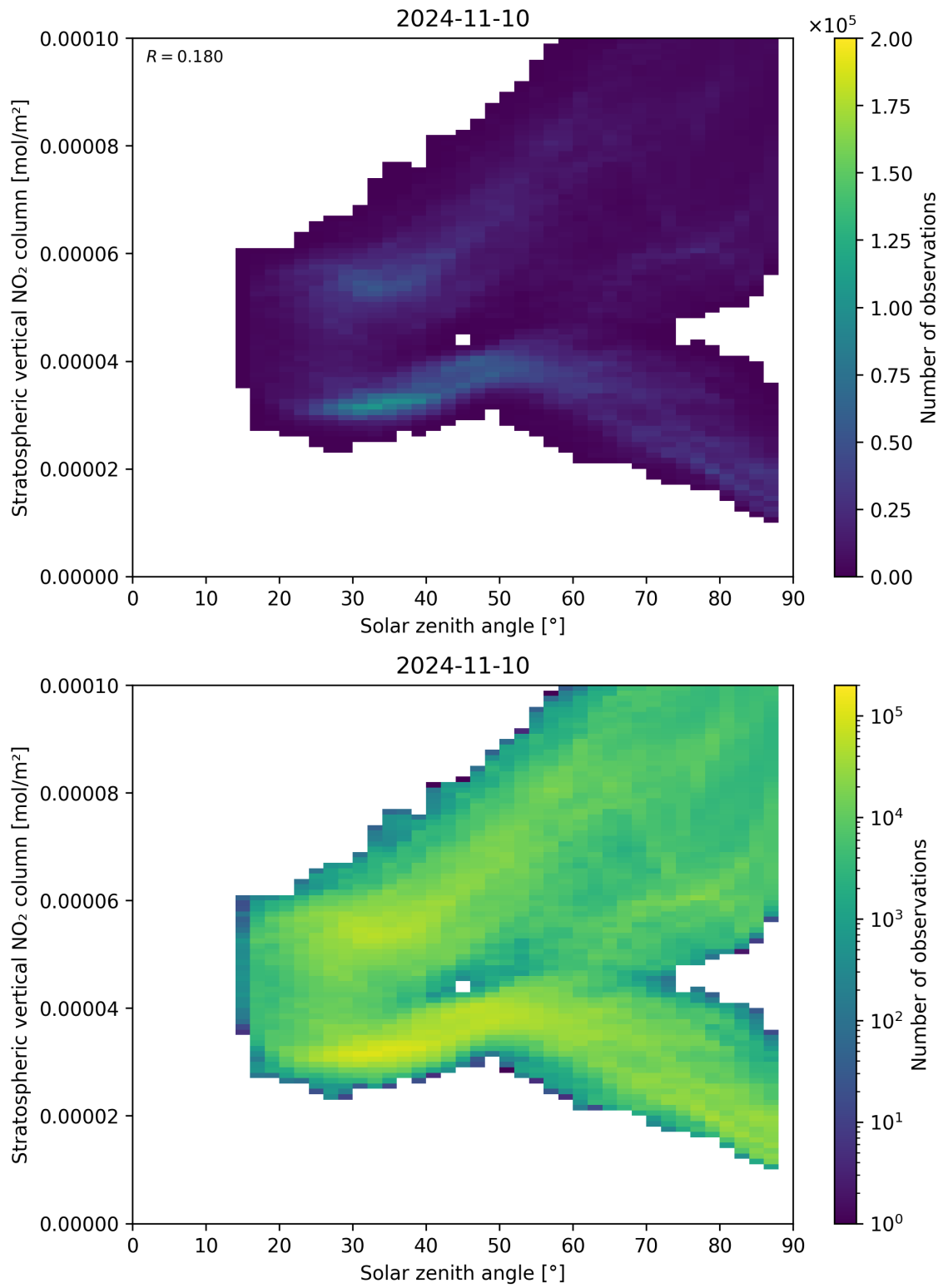
Figure 150: Scatter density plot of “Solar zenith angle” against “Stratospheric vertical NO 2 column” for 2024-11-09 to 2024-11-11.
