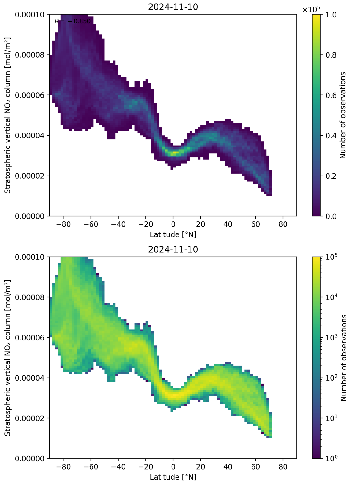
Figure 87: Scatter density plot of “Latitude” against “Stratospheric vertical NO 2 column” for 2024-11-09 to 2024-11-11.
