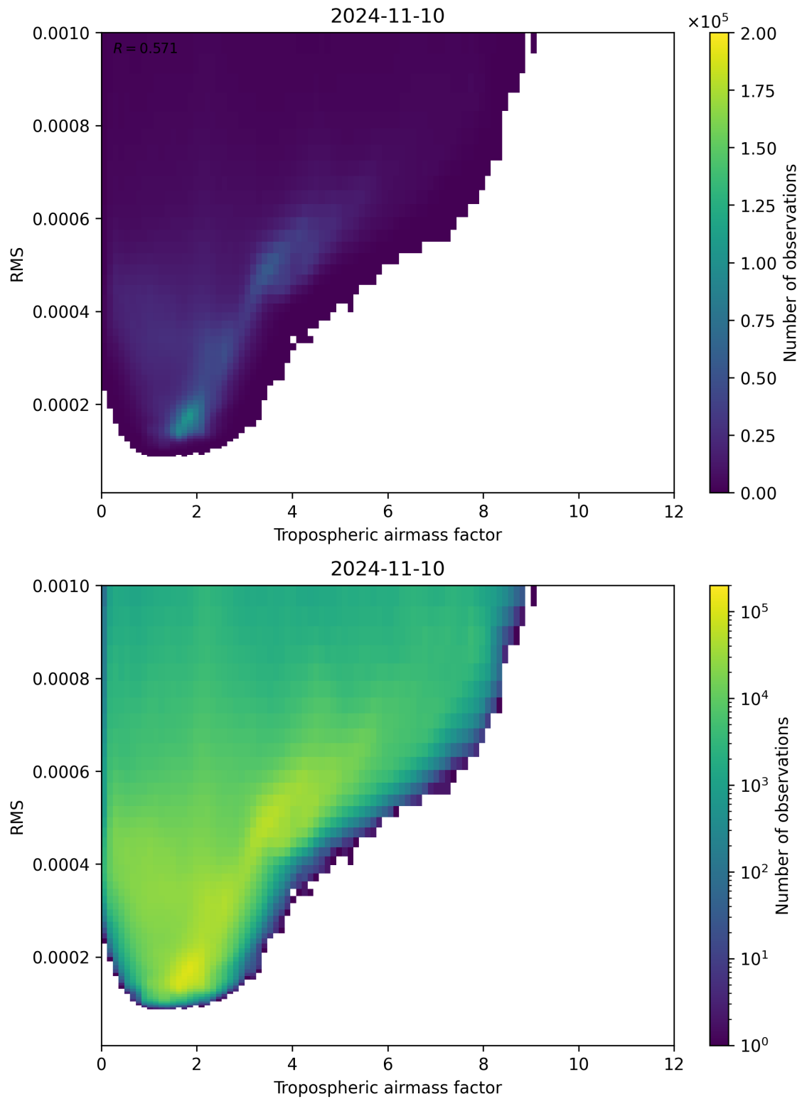
Figure 79: Scatter density plot of “Tropospheric airmass factor” against “RMS” for 2024-11-09 to 2024-11-11.
