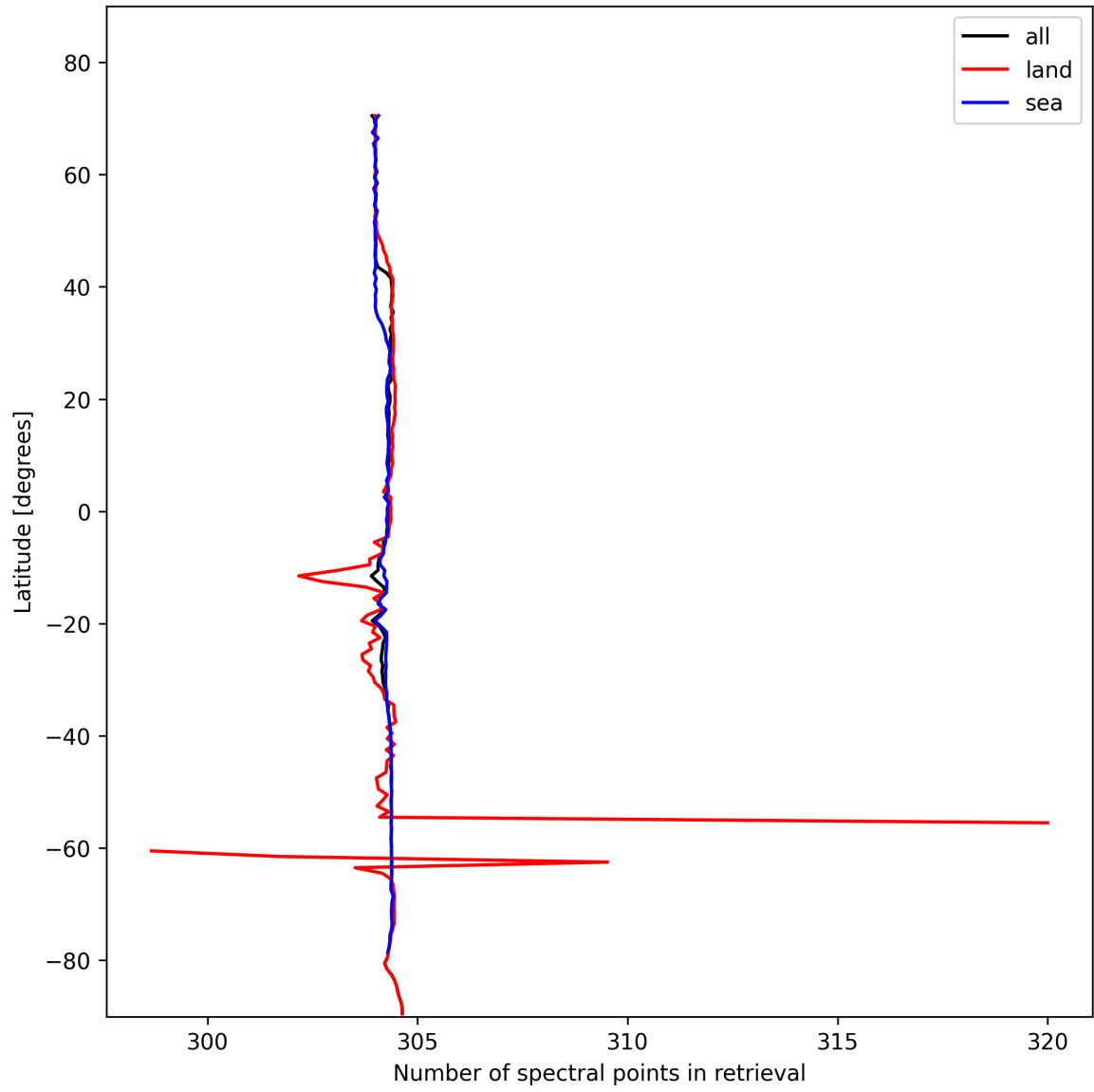
Figure 16: Zonal average of “Number of spectral points in retrieval” for 2024-11-09 to 2024-11-11.
