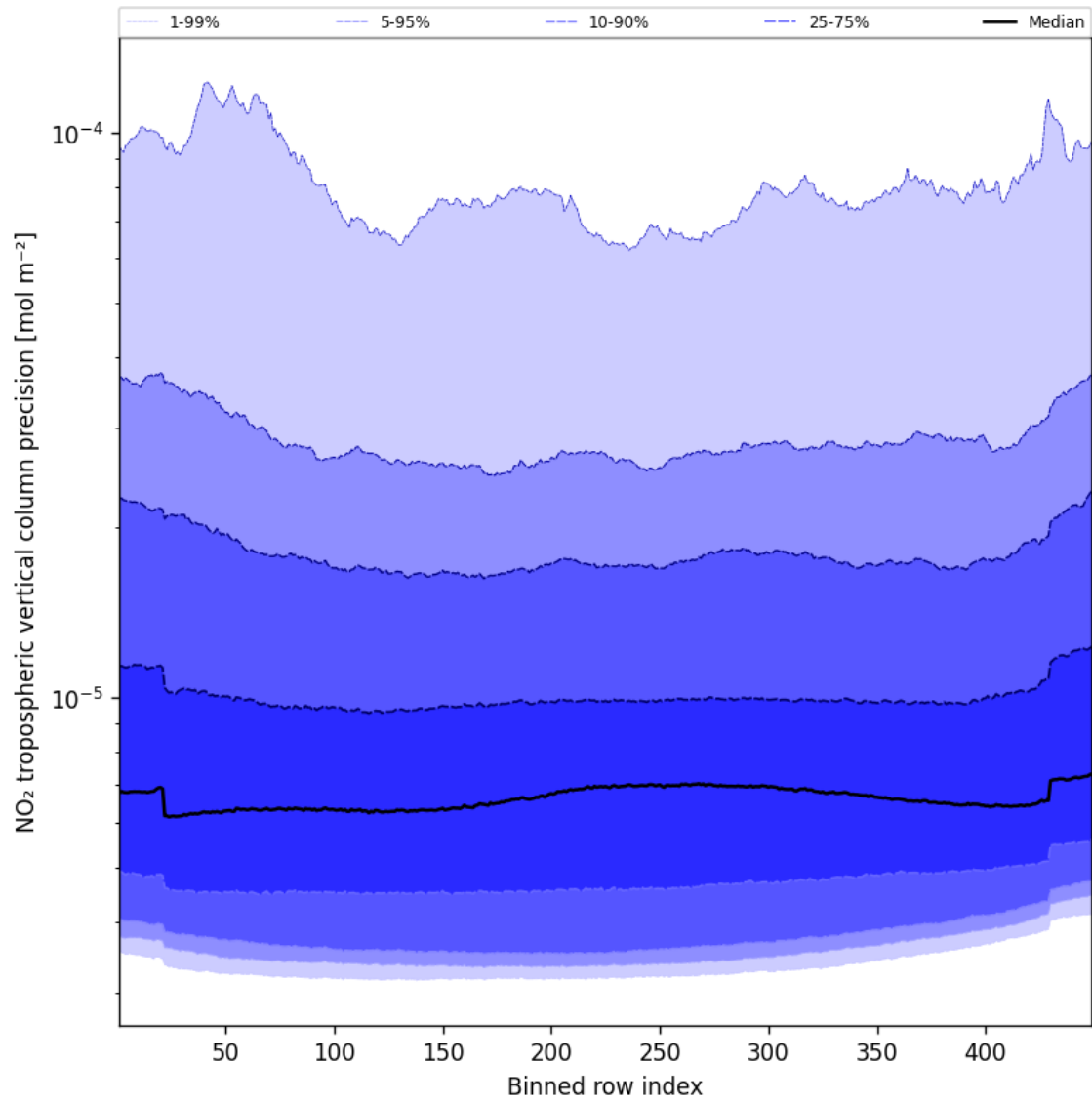
Figure 47: Along track statistics of “NO 2 tropospheric vertical column precision” for 2024-11-09 to 2024-11-11
