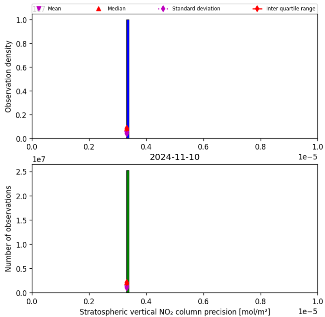
Figure 37: Histogram of “Stratospheric vertical NO 2 column precision” for 2024-11-09 to 2024-11-11
