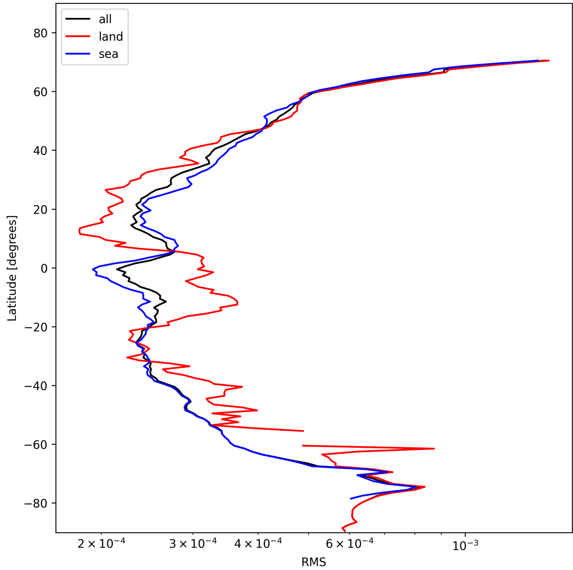
Figure 26: Zonal average of “RMS” for 2024-11-09 to 2024-11-11.
