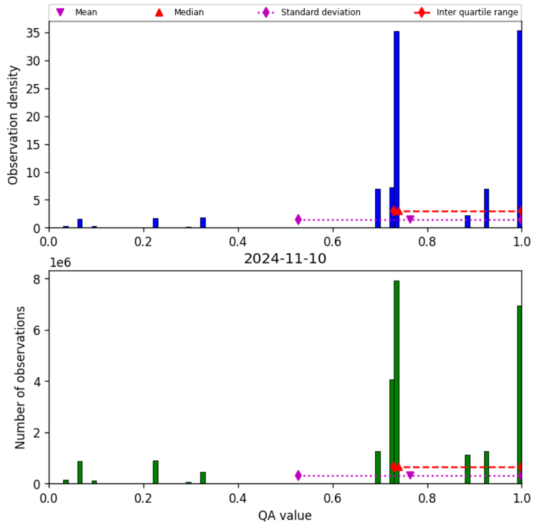
Figure 28: Histogram of “QA value” for 2024-11-09 to 2024-11-11
