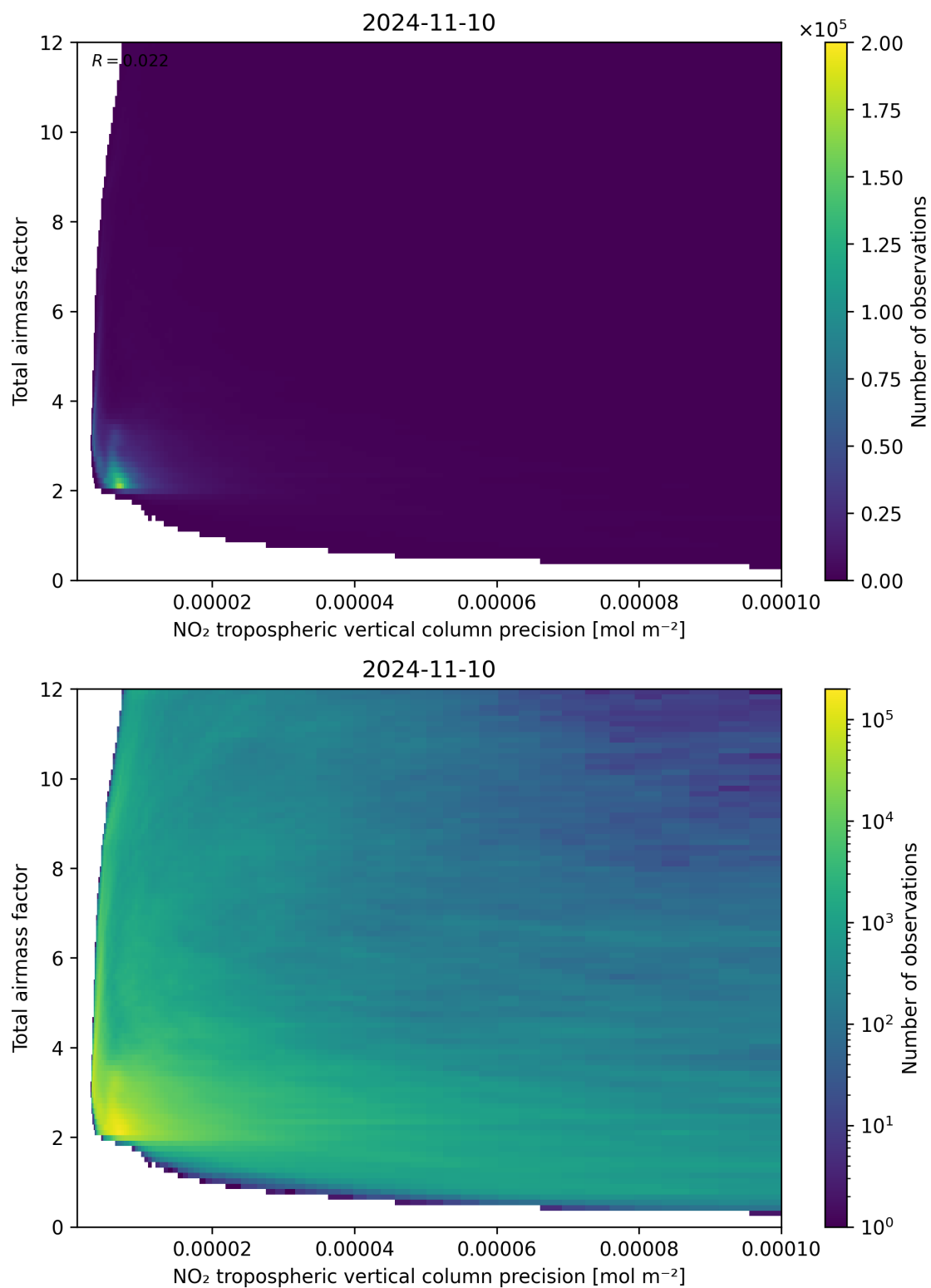
Figure 132: Scatter density plot of “NO 2 tropospheric vertical column precision” against “Total air mass factor” for 2024-11-09 to 2024-11-11.
