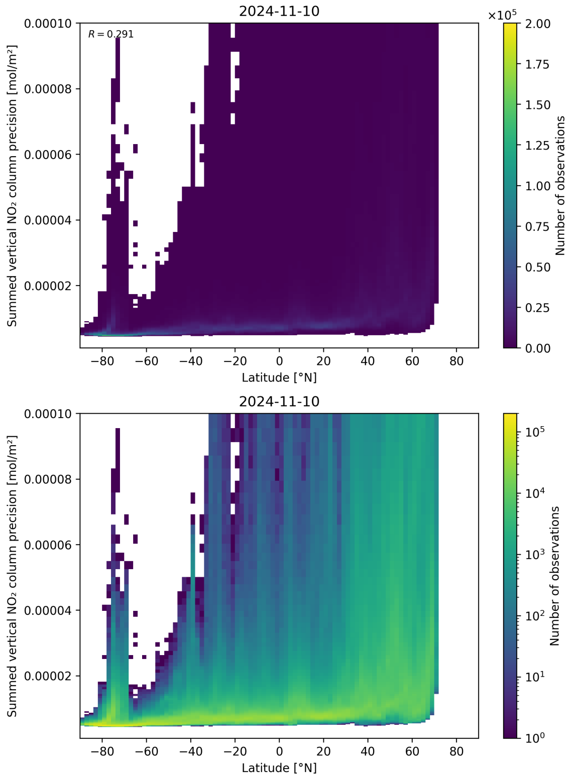
Figure 89: Scatter density plot of “Latitude” against “Summed vertical NO 2 column precision” for 2024-11-09 to 2024-11-11.
