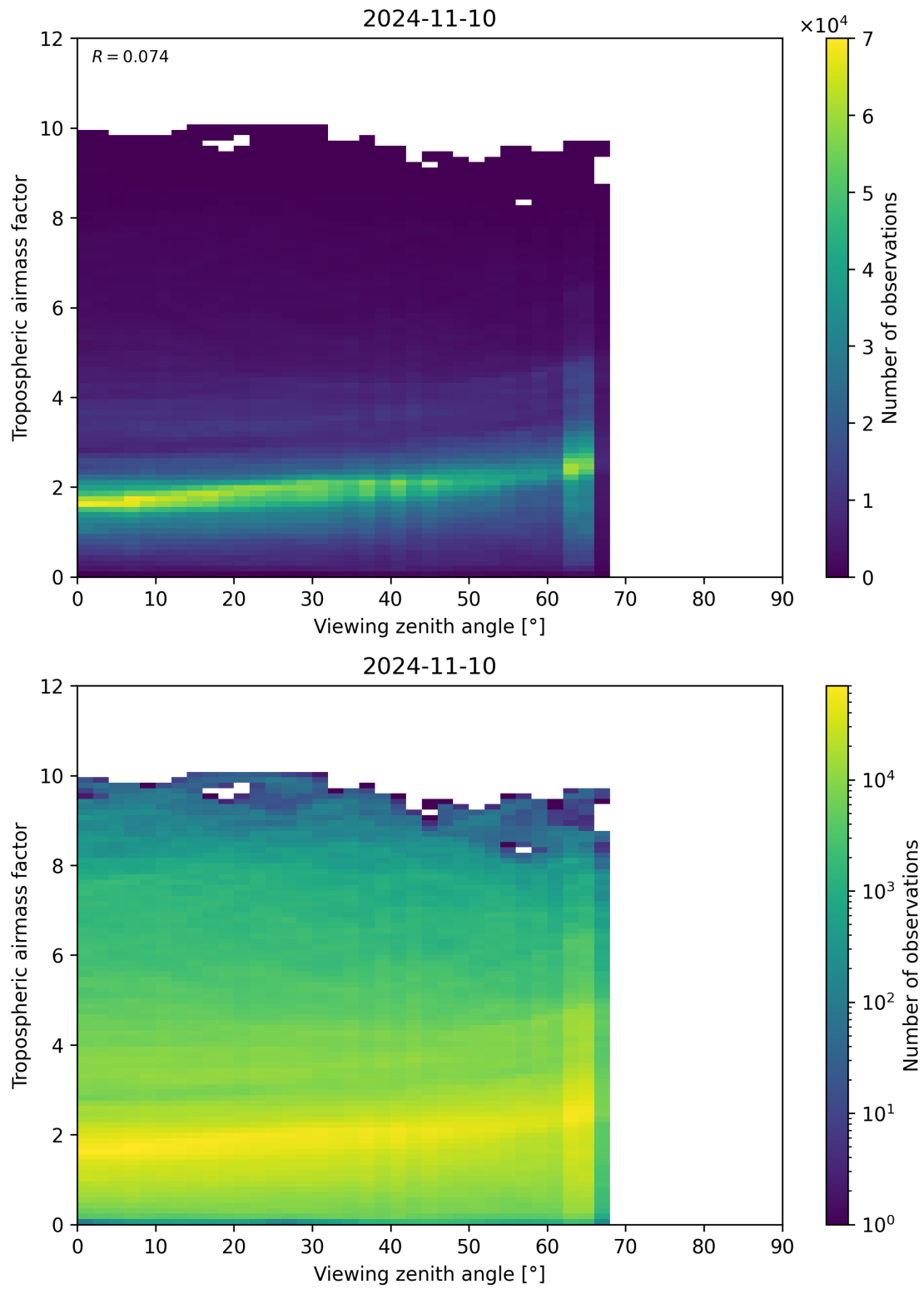
Figure 161: Scatter density plot of “Viewing zenith angle” against “Tropospheric air mass factor” for 2024-11-09 to 2024-11-11.
