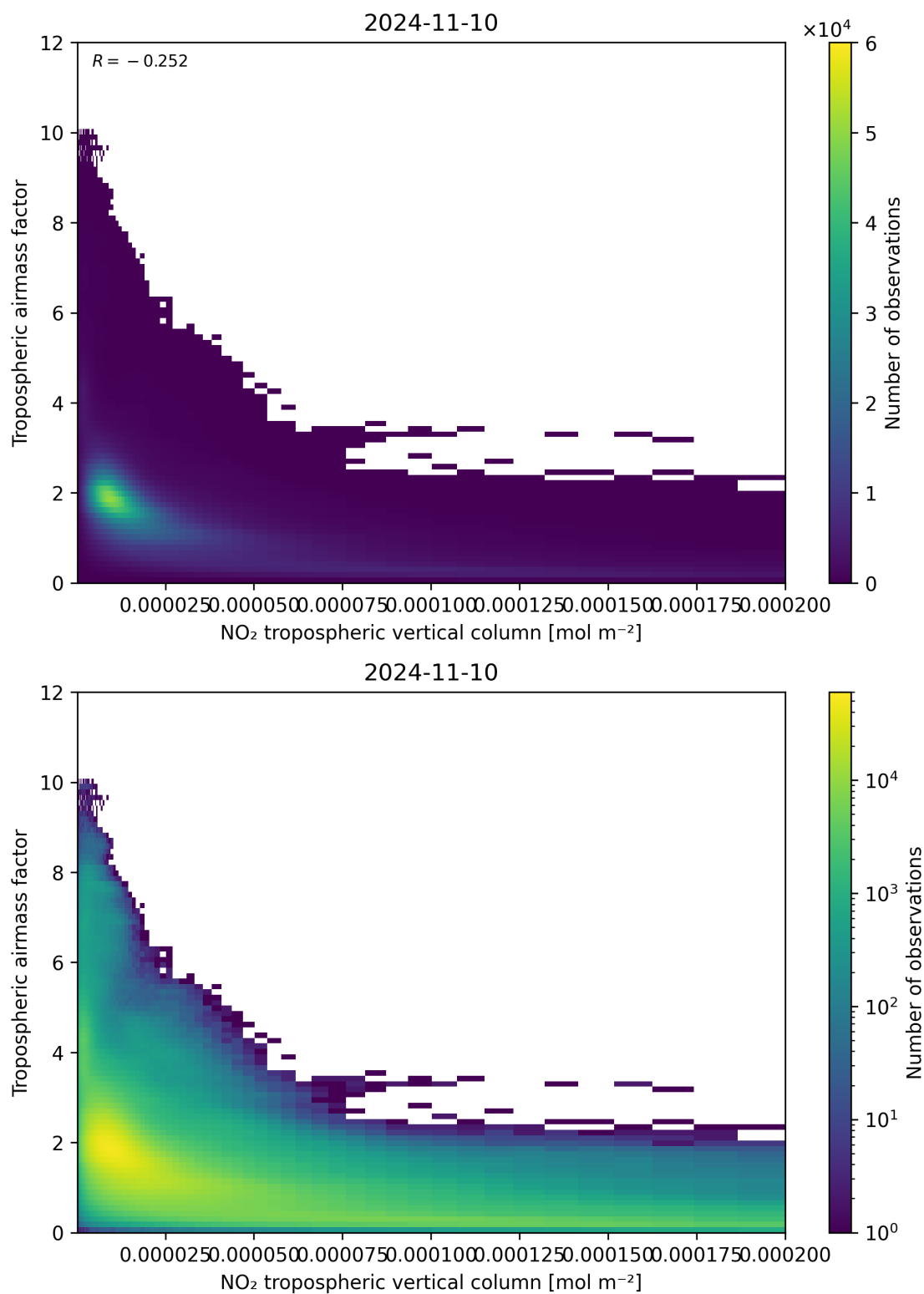
Figure 123: Scatter density plot of “NO 2 tropospheric vertical column” against “Tropospheric air mass factor” for 2024-11-09 to 2024-11-11.
