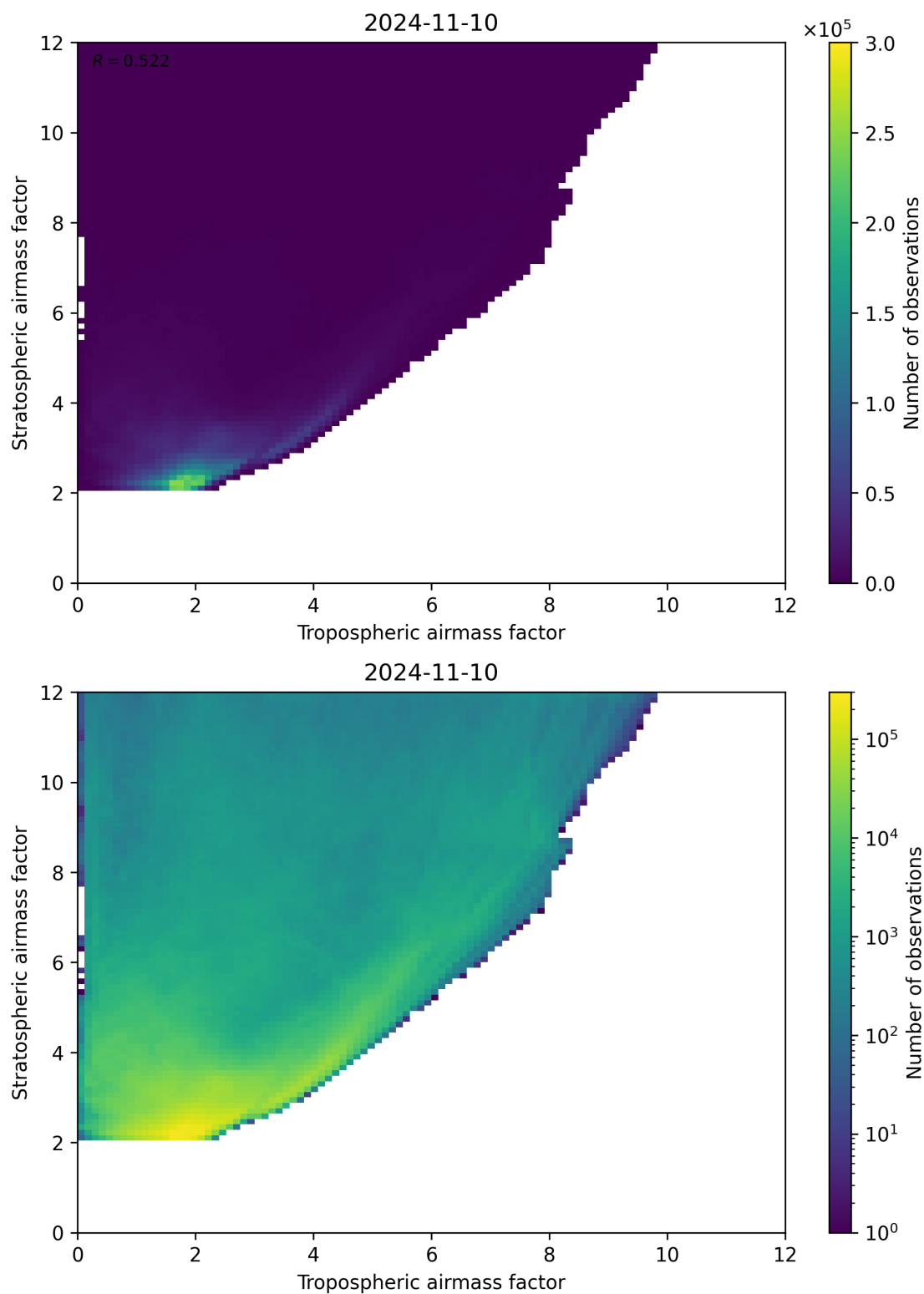
Figure 71: Scatter density plot of “Tropospheric airmass factor” against “Stratospheric airmass factor” for 2024-11-09 to 2024-11-11.
