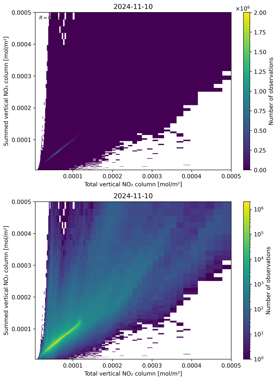
Figure 112: Scatter density plot of “Total vertical NO 2 column” against “Summed vertical NO 2 column” for 2024-11-09 to 2024-11-11.
