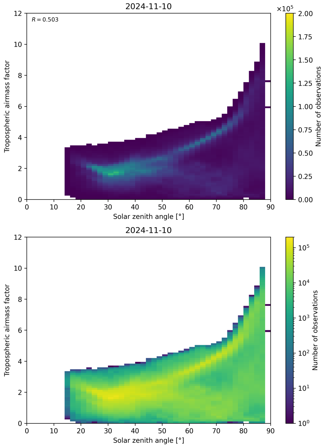
Figure 147: Scatter density plot of “Solar zenith angle” against “Tropospheric airmass factor” for 2024-11-09 to 2024-11-11.
