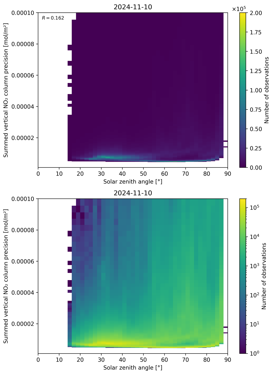
Figure 152: Scatter density plot of “Solar zenith angle” against “Summed vertical NO 2 column precision” for 2024-11-09 to 2024-11-11.
