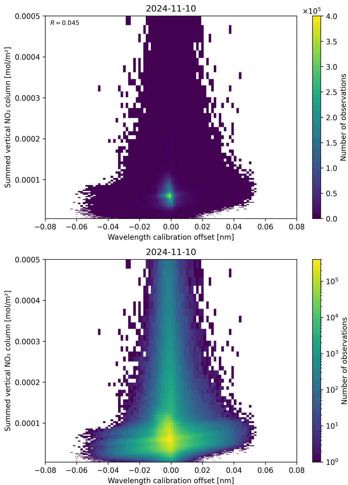
Figure 177: Scatter density plot of “Wavelength calibration offset” against “Summed vertical NO 2 column” for 2024-11-09 to 2024-11-11.
