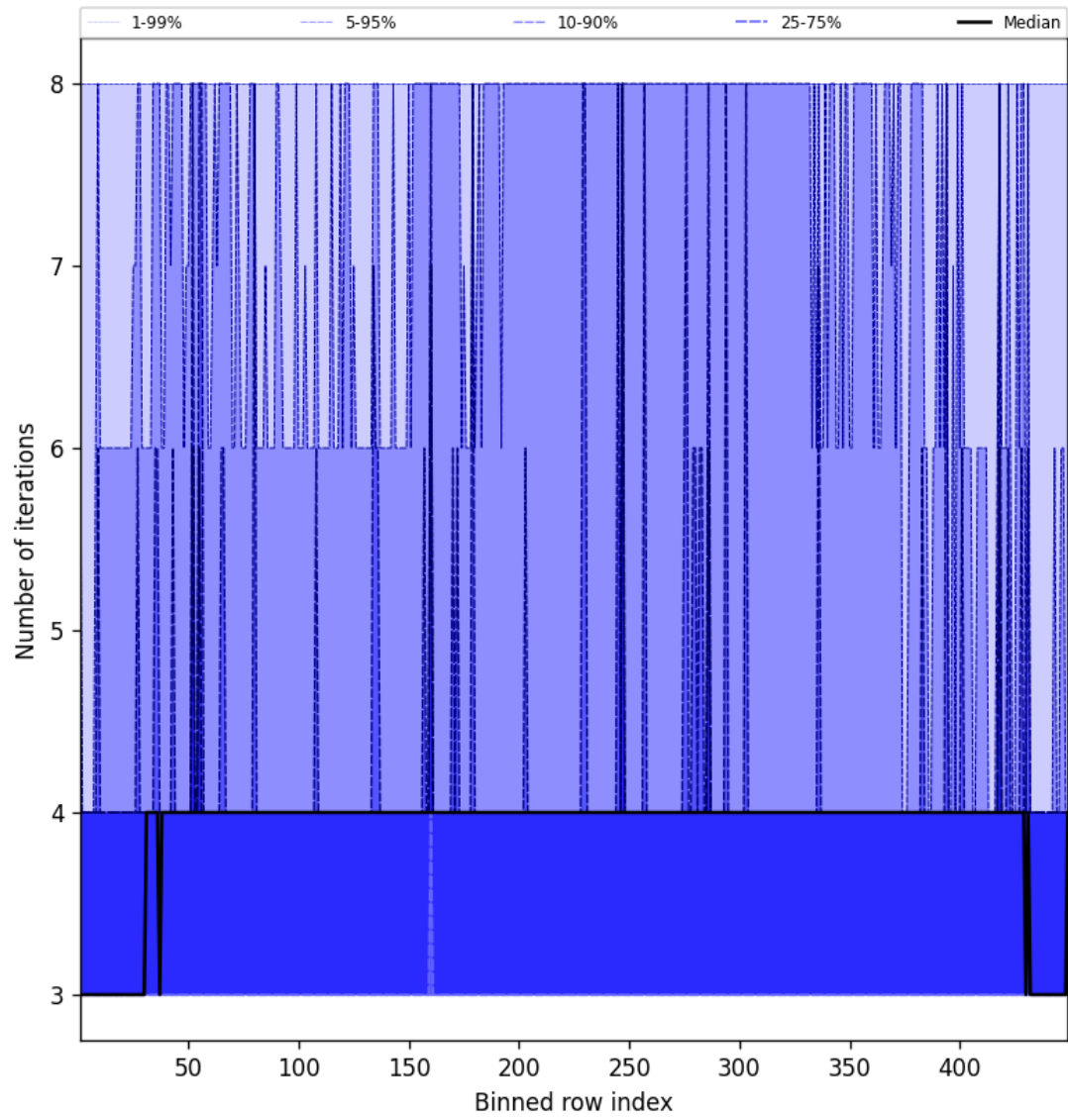
Figure 51: Along track statistics of “Number of iterations” for 2024-11-09 to 2024-11-11
