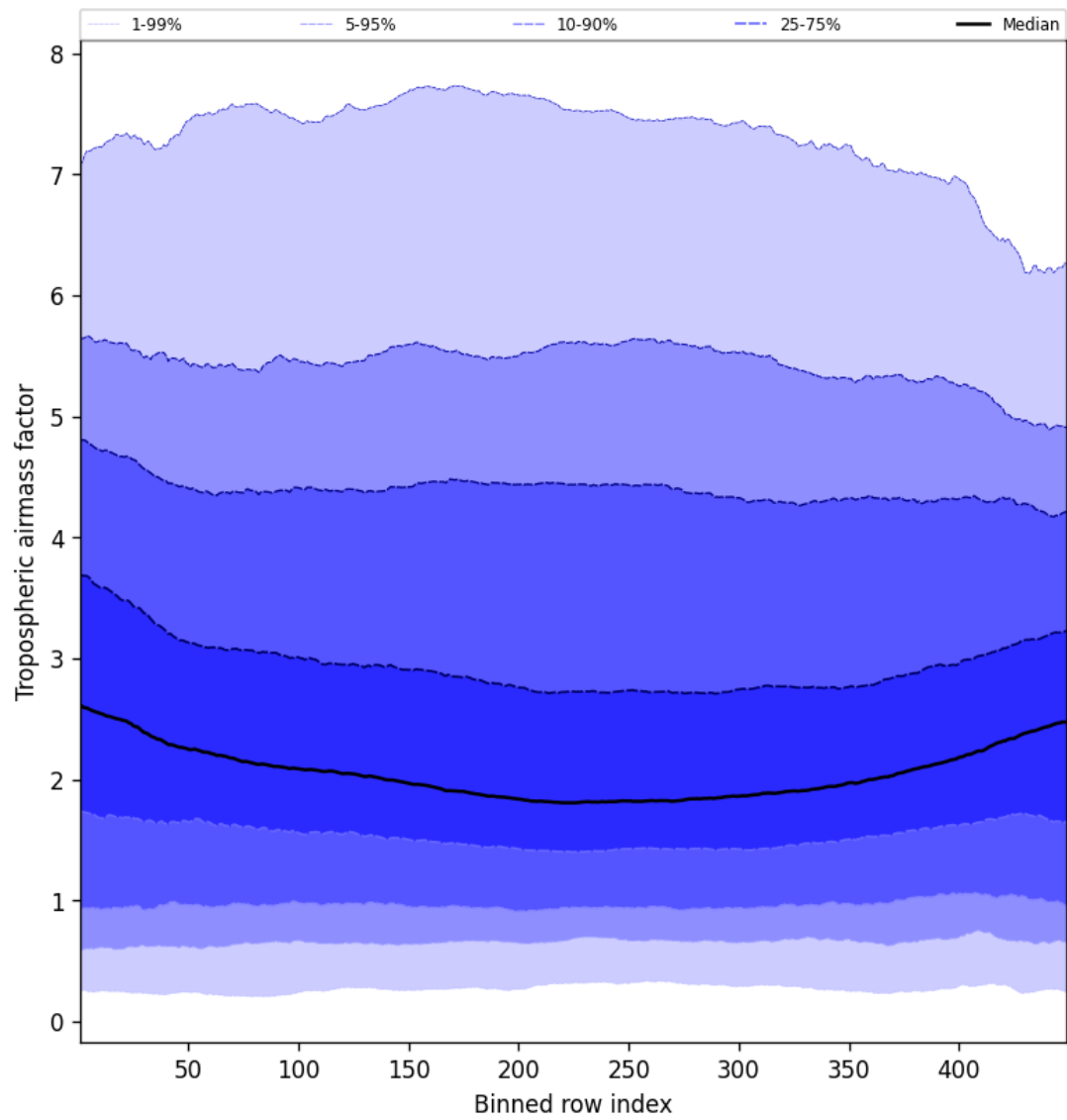
Figure 48: Along track statistics of “Tropospheric air mass factor” for 2024-11-09 to 2024-11-11
