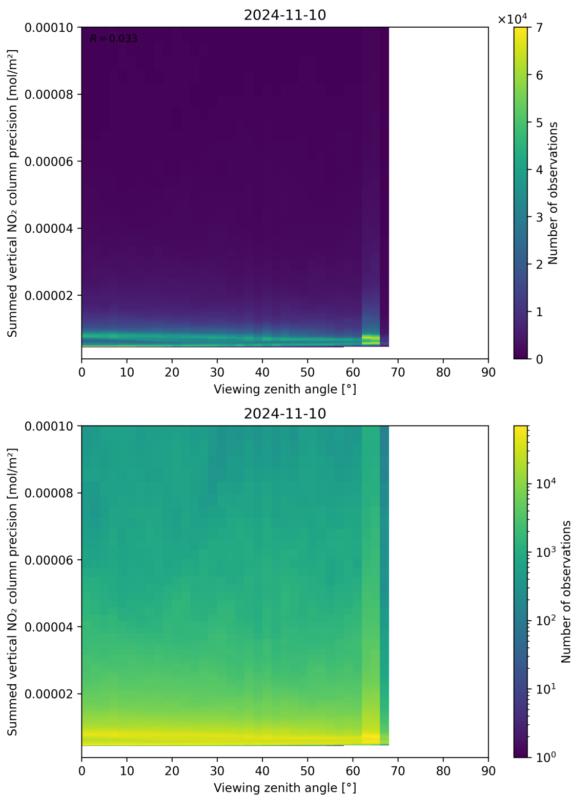
Figure 166: Scatter density plot of “Viewing zenith angle” against “Summed vertical NO 2 column precision” for 2024-11-09 to 2024-11-11.
