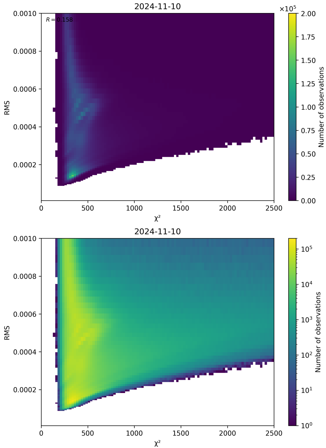
Figure 82: Scatter density plot of “ \chi^2 ” against “RMS” for 2024-11-09 to 2024-11-11.
