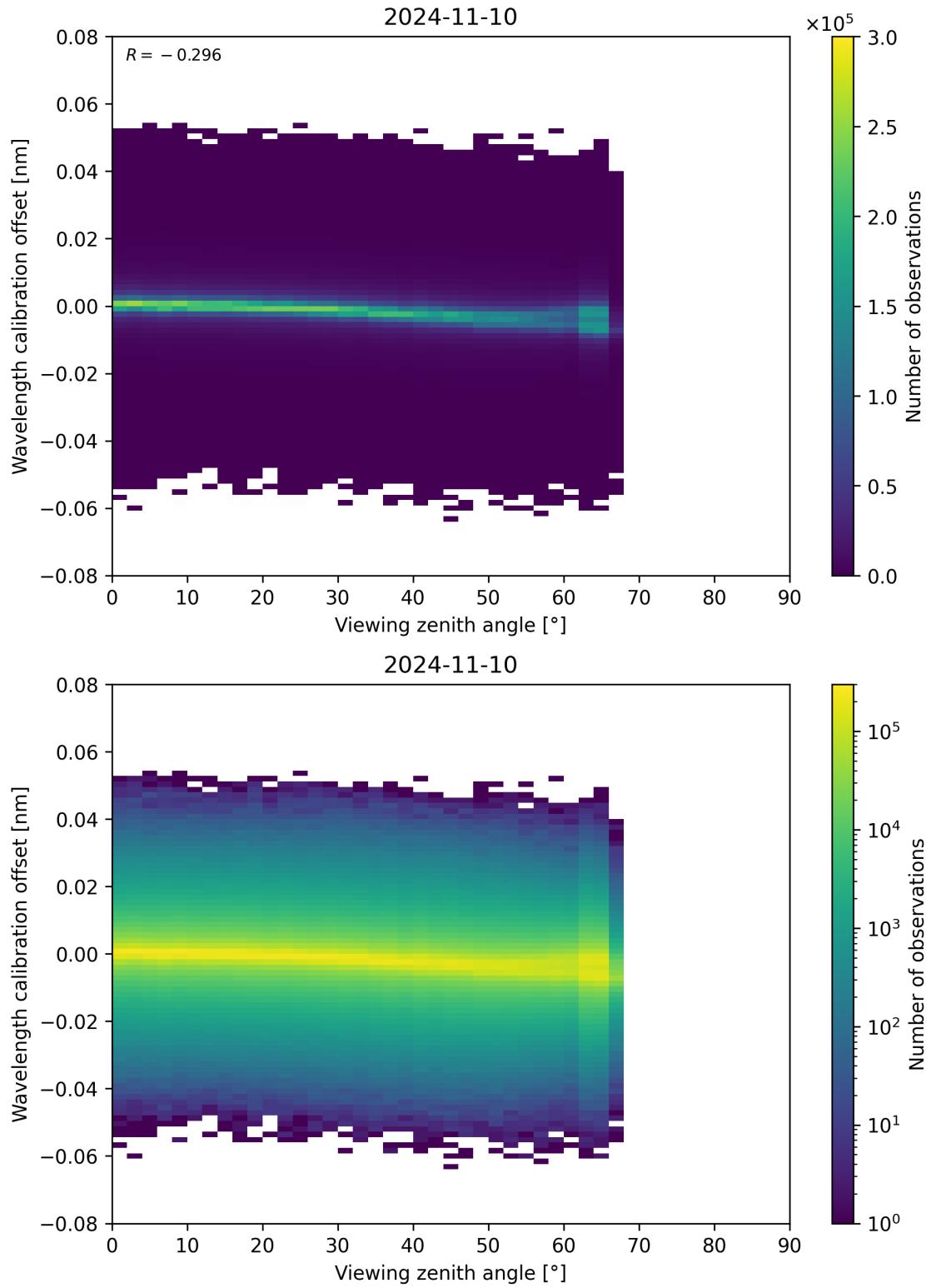
Figure 173: Scatter density plot of “Viewing zenith angle” against “Wavelength calibration offset” for 2024-11-09 to 2024-11-11.
