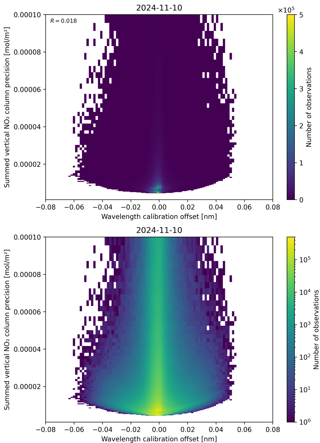
Figure 178: Scatter density plot of “Wavelength calibration offset” against “Summed vertical NO 2 column precision” for 2024-11-09 to 2024-11-11.
