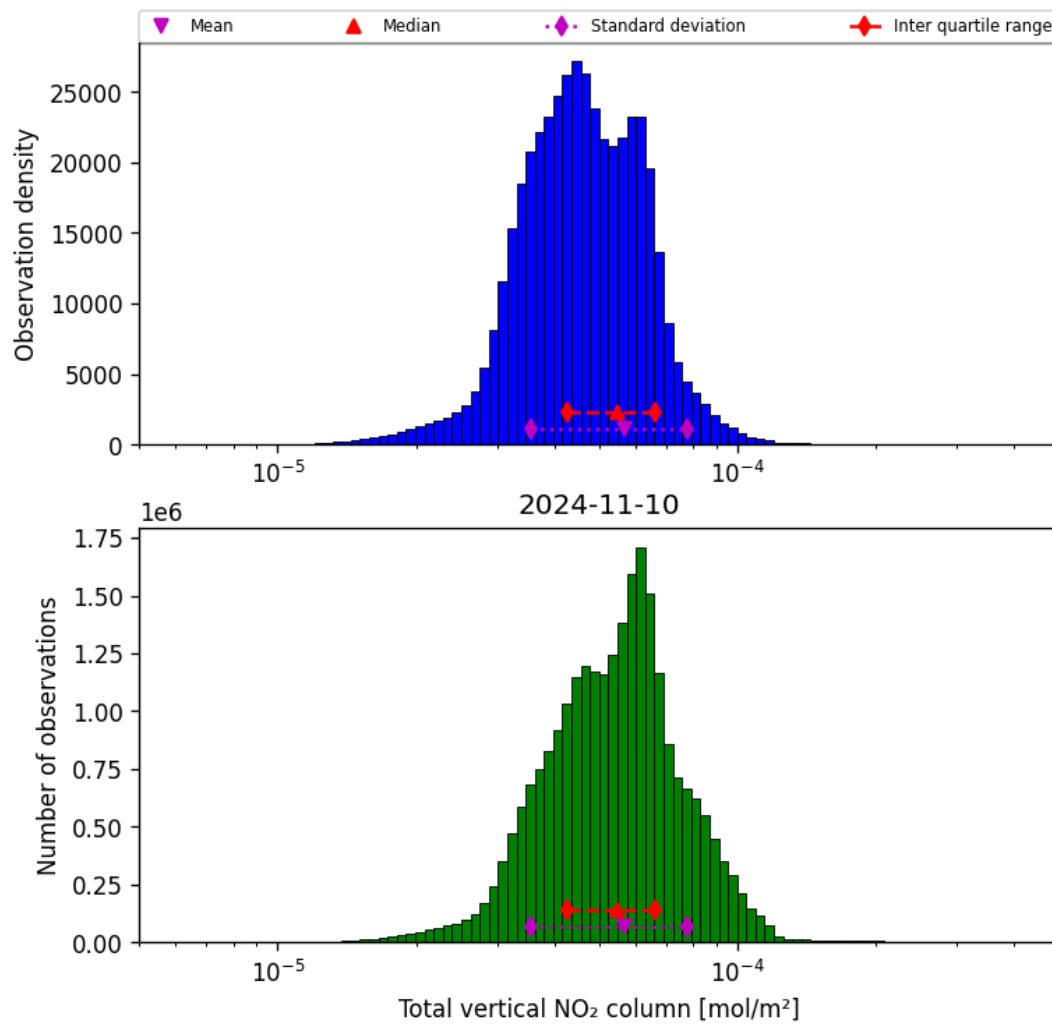
Figure 38: Histogram of “Total vertical NO 2 column” for 2024-11-09 to 2024-11-11
