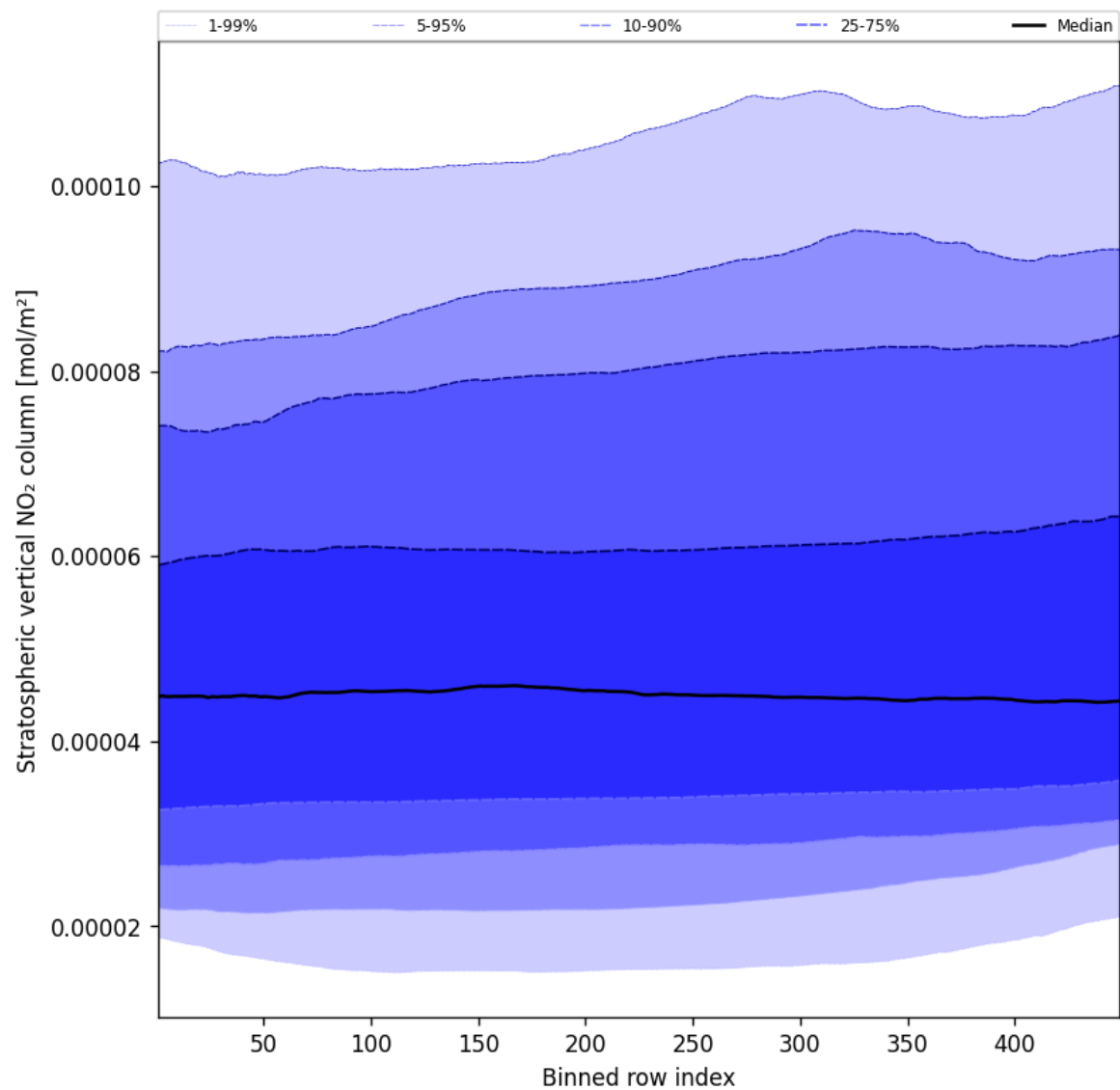
Figure 53: Along track statistics of “Stratospheric vertical NO 2 column” for 2024-11-09 to 2024-11-11
