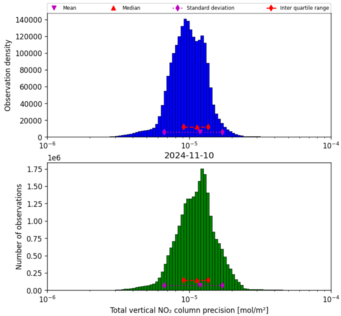
Figure 39: Histogram of “Total vertical NO 2 column precision” for 2024-11-09 to 2024-11-11
