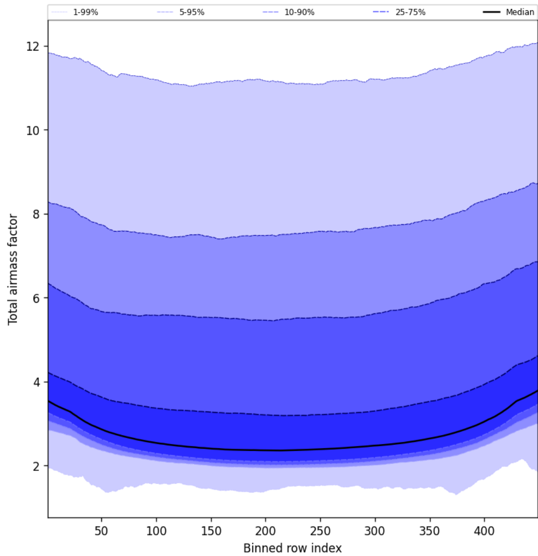
Figure 49: Along track statistics of “Total airmass factor” for 2024-11-09 to 2024-11-11
