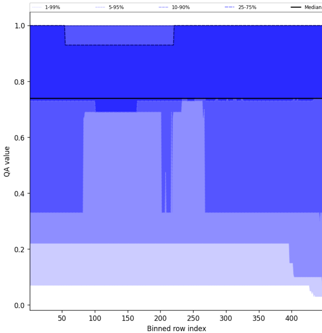
Figure 45: Along track statistics of “QA value” for 2024-11-09 to 2024-11-11
