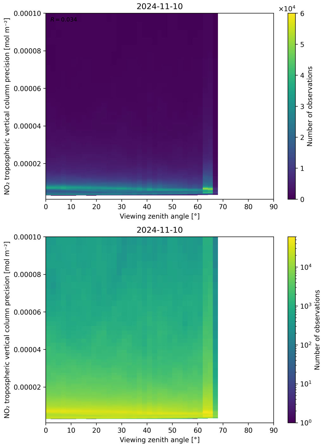
Figure 170: Scatter density plot of “Viewing zenith angle” against “NO 2 tropospheric vertical column precision” for 2024-11-09 to 2024-11-11.
