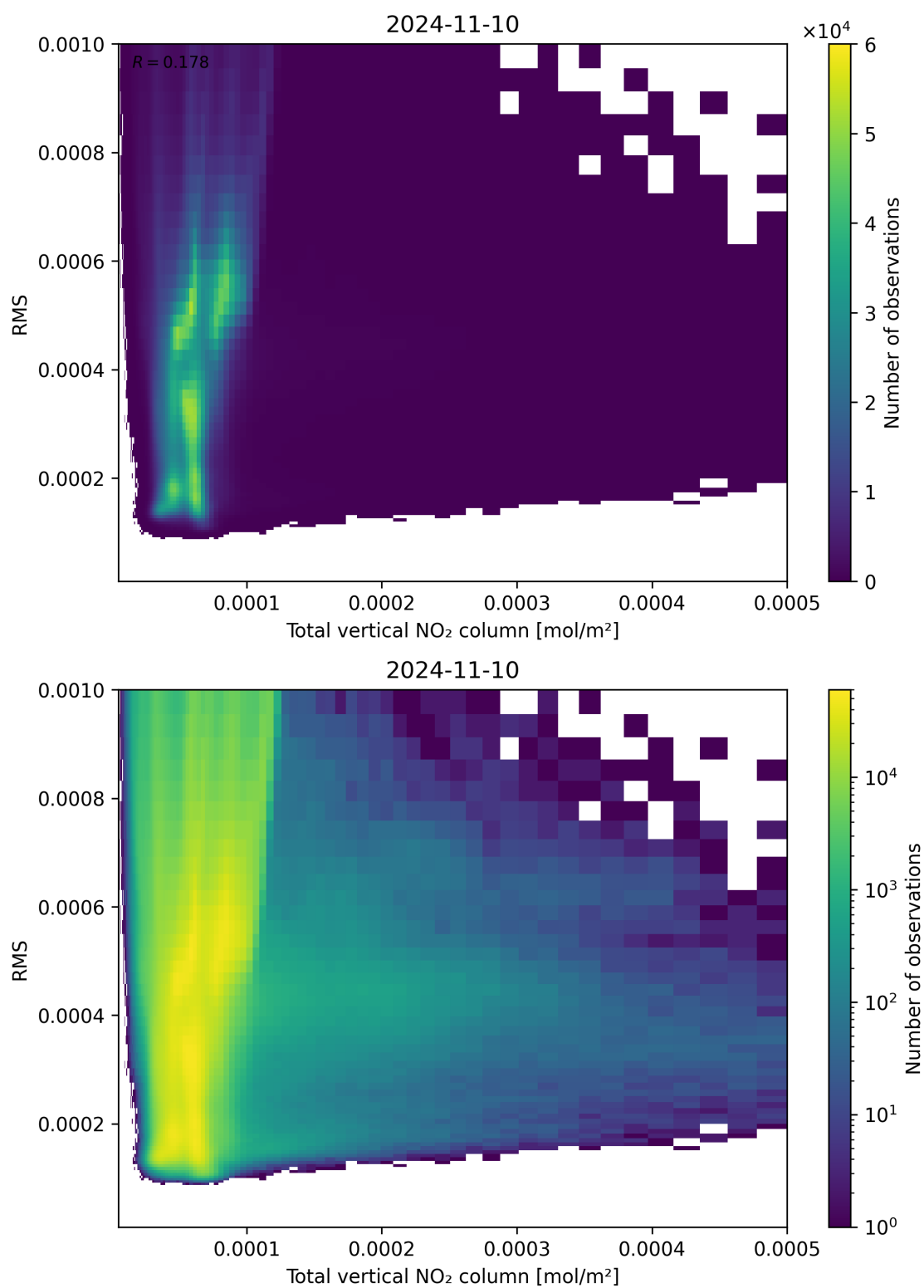
Figure 120: Scatter density plot of “Total vertical NO 2 column” against “RMS” for 2024-11-09 to 2024-11-11.
