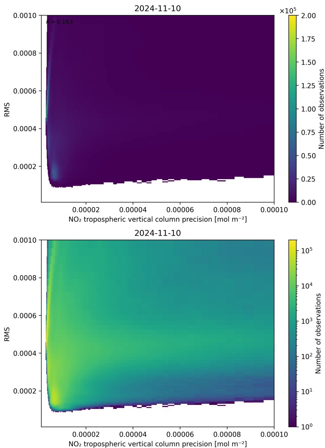
Figure 140: Scatter density plot of “NO 2 tropospheric vertical column precision” against “RMS” for 2024-11-09 to 2024-11-11.
