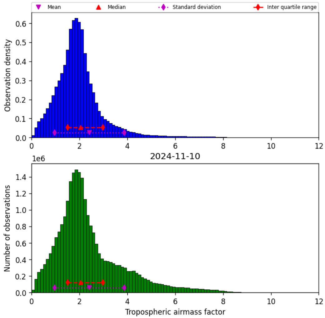
Figure 31: Histogram of “Tropospheric airmass factor” for 2024-11-09 to 2024-11-11
