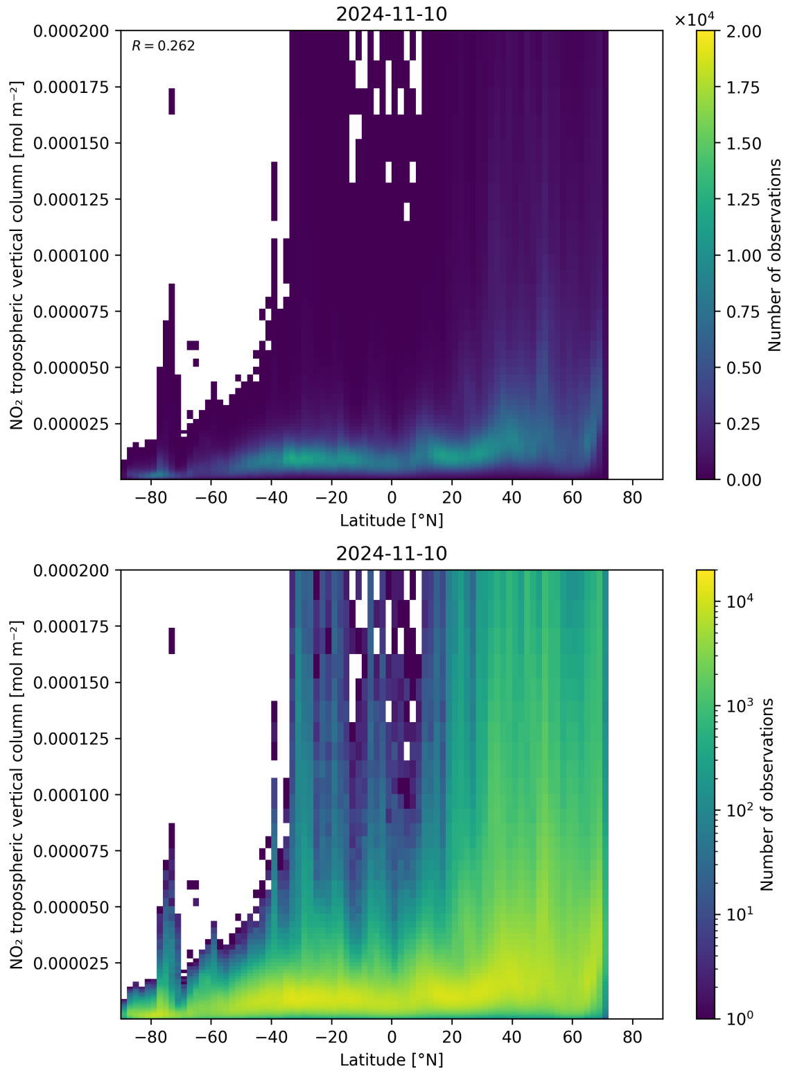
Figure 92: Scatter density plot of “Latitude” against “NO 2 tropospheric vertical column” for 2024-11-09 to 2024-11-11.
