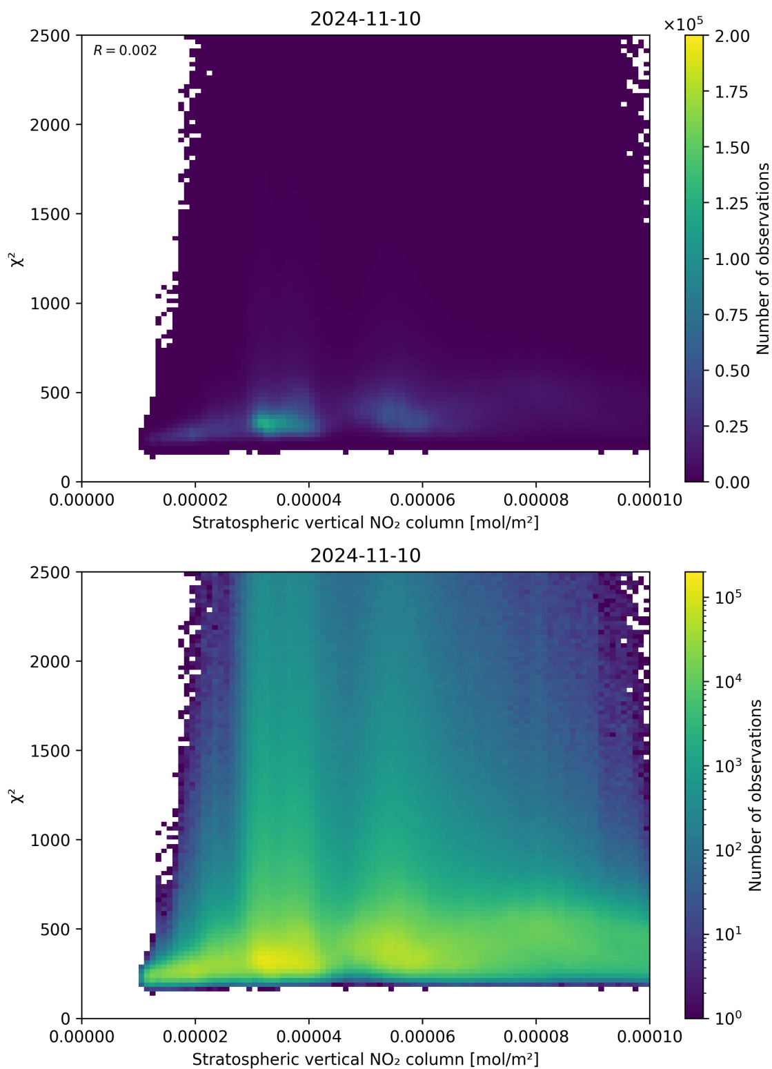
Figure 97: Scatter density plot of “Stratospheric vertical NO 2 column” against “ \chi^2 ” for 2024-11-09 to 2024-11-11.
