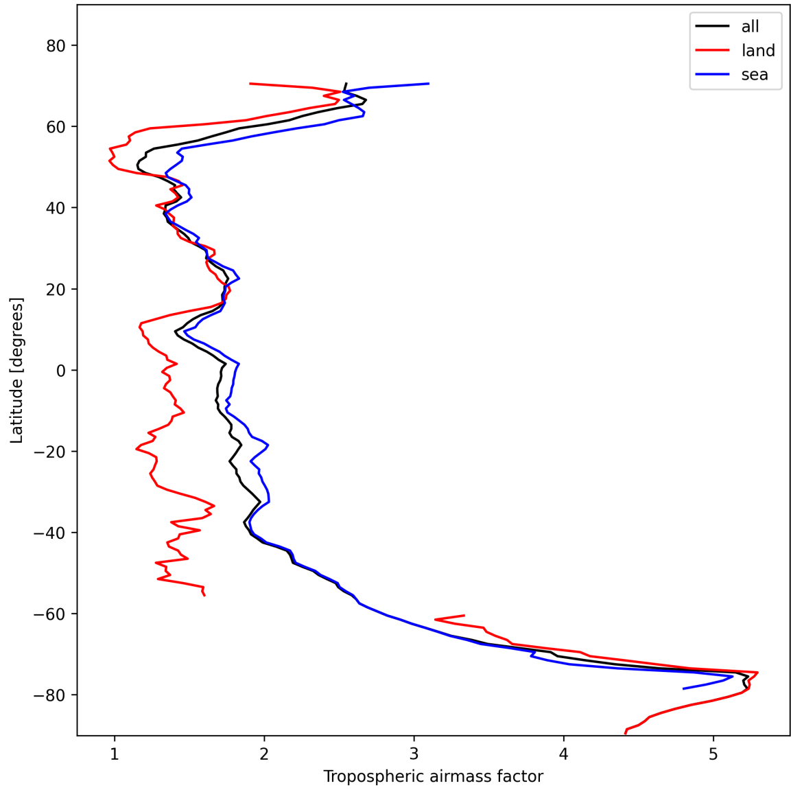
Figure 14: Zonal average of “Tropospheric airmass factor” for 2024-11-09 to 2024-11-11.
