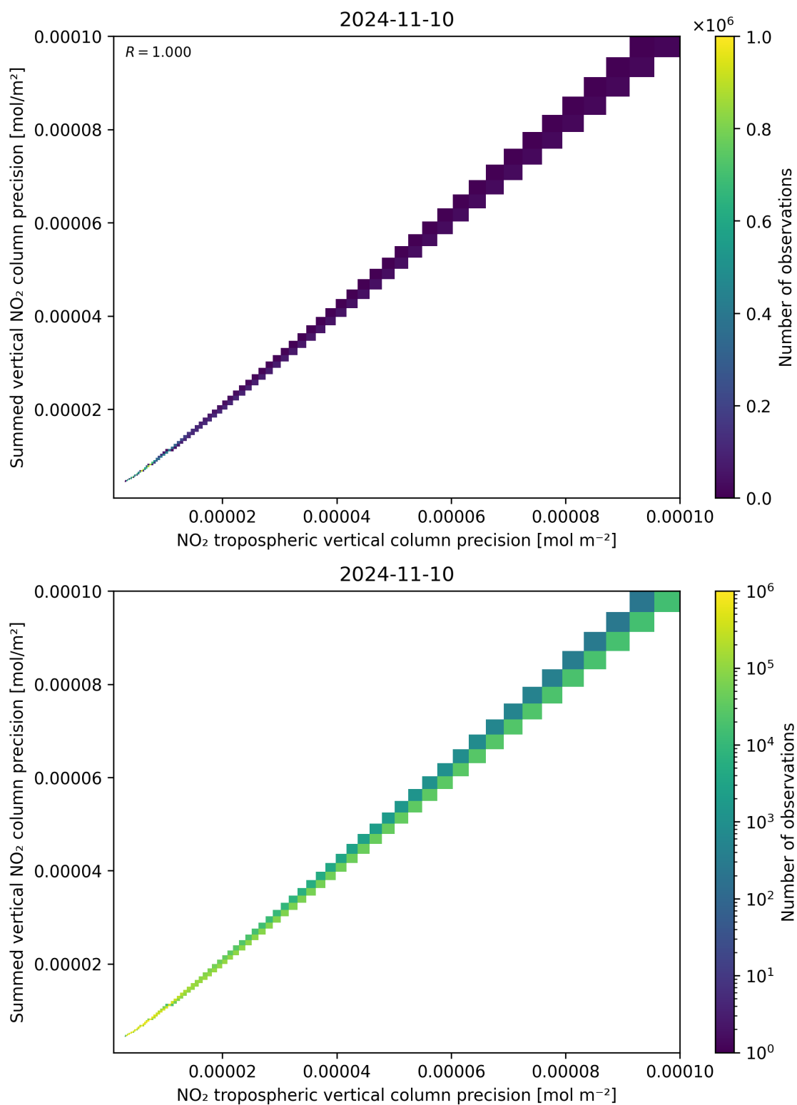
Figure 137: Scatter density plot of “NO 2 tropospheric vertical column precision” against “Summed vertical NO 2 column precision” for 2024-11-09 to 2024-11-11.
