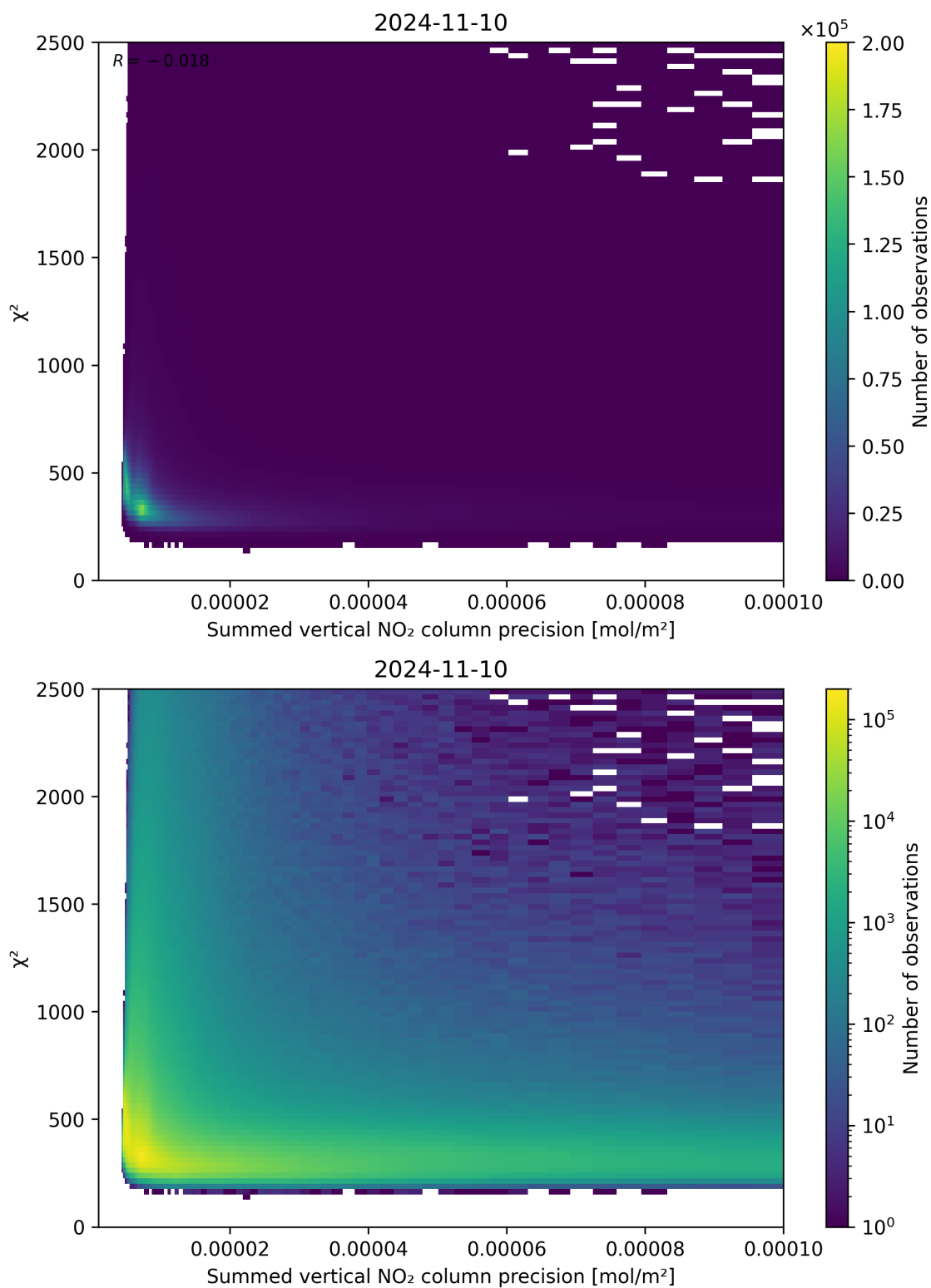
Figure 107: Scatter density plot of “Summed vertical NO 2 column precision” against “ \chi^2 ” for 2024-11-09 to 2024-11-11.
