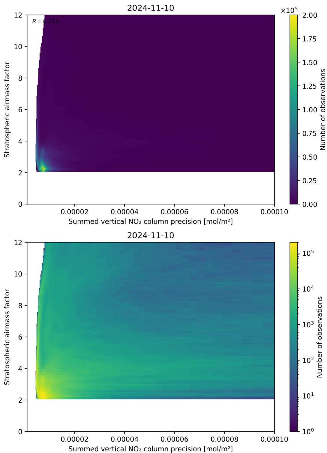
Figure 106: Scatter density plot of “Summed vertical NO 2 column precision” against “Stratospheric airmass factor” for 2024-11-09 to 2024-11-11.
