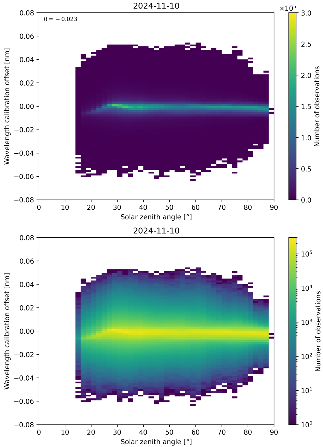
Figure 158: Scatter density plot of “Solar zenith angle” against “Wavelength calibration offset” for 2024-11-09 to 2024-11-11.
