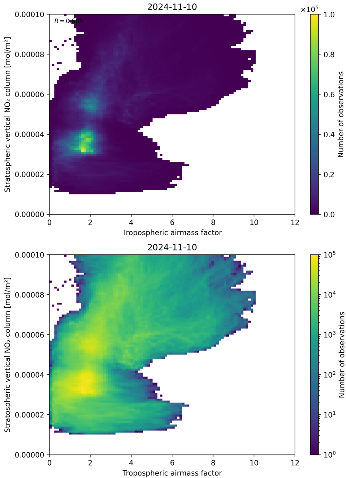
Figure 74: Scatter density plot of “Tropospheric air mass factor” against “Stratospheric vertical NO 2 column” for 2024-11-09 to 2024-11-11.
