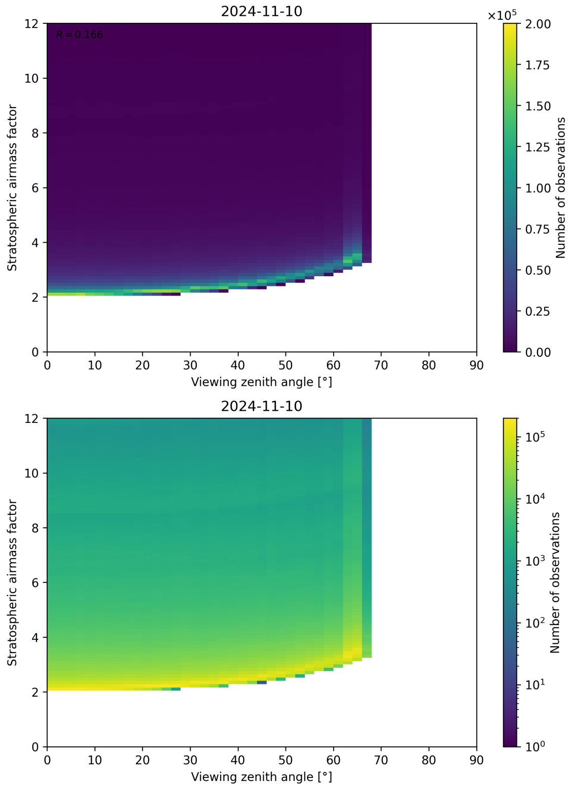
Figure 159: Scatter density plot of “Viewing zenith angle” against “Stratospheric airmass factor” for 2024-11-09 to 2024-11-11.
