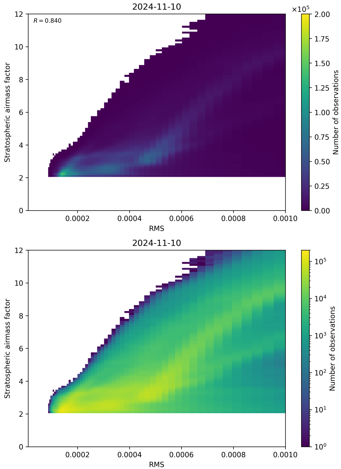
Figure 144: Scatter density plot of “RMS” against “Stratospheric airmass factor” for 2024-11-09 to 2024-11-11.
