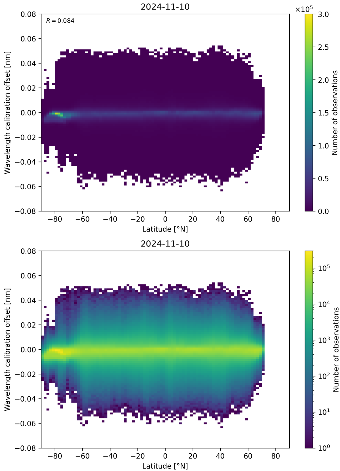
Figure 95: Scatter density plot of “Latitude” against “Wavelength calibration offset” for 2024-11-09 to 2024-11-11.
