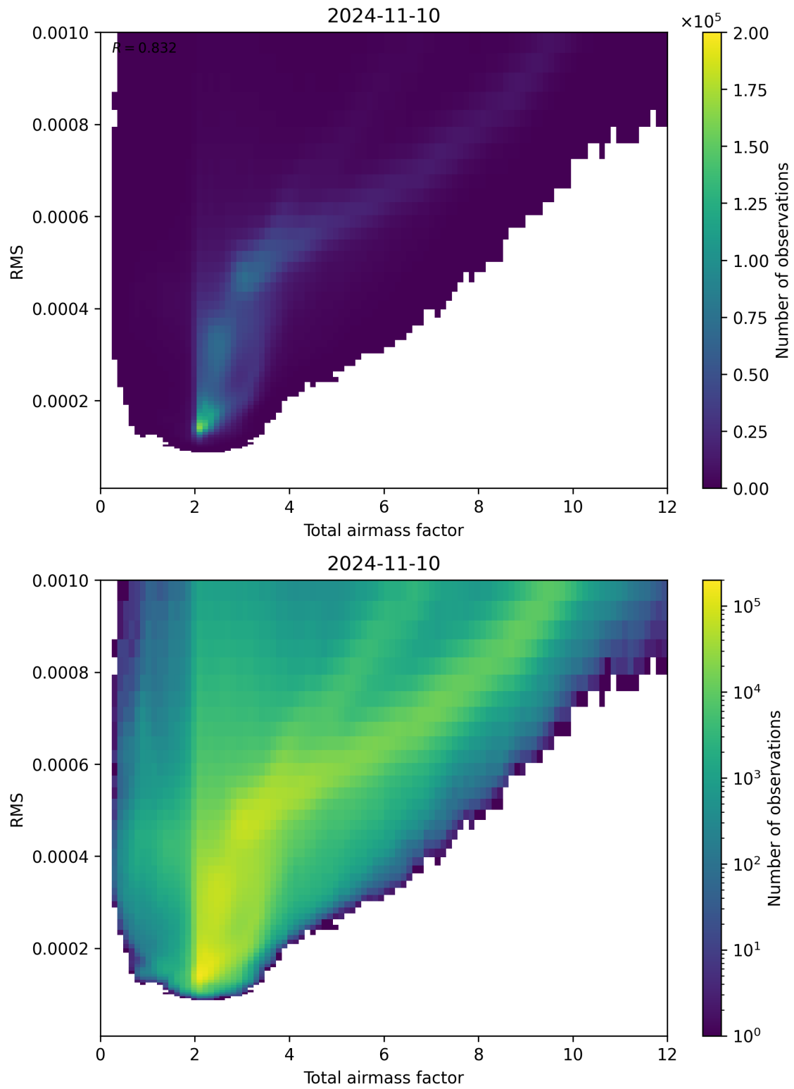
Figure 69: Scatter density plot of “Total airmass factor” against “RMS” for 2024-11-09 to 2024-11-11.
