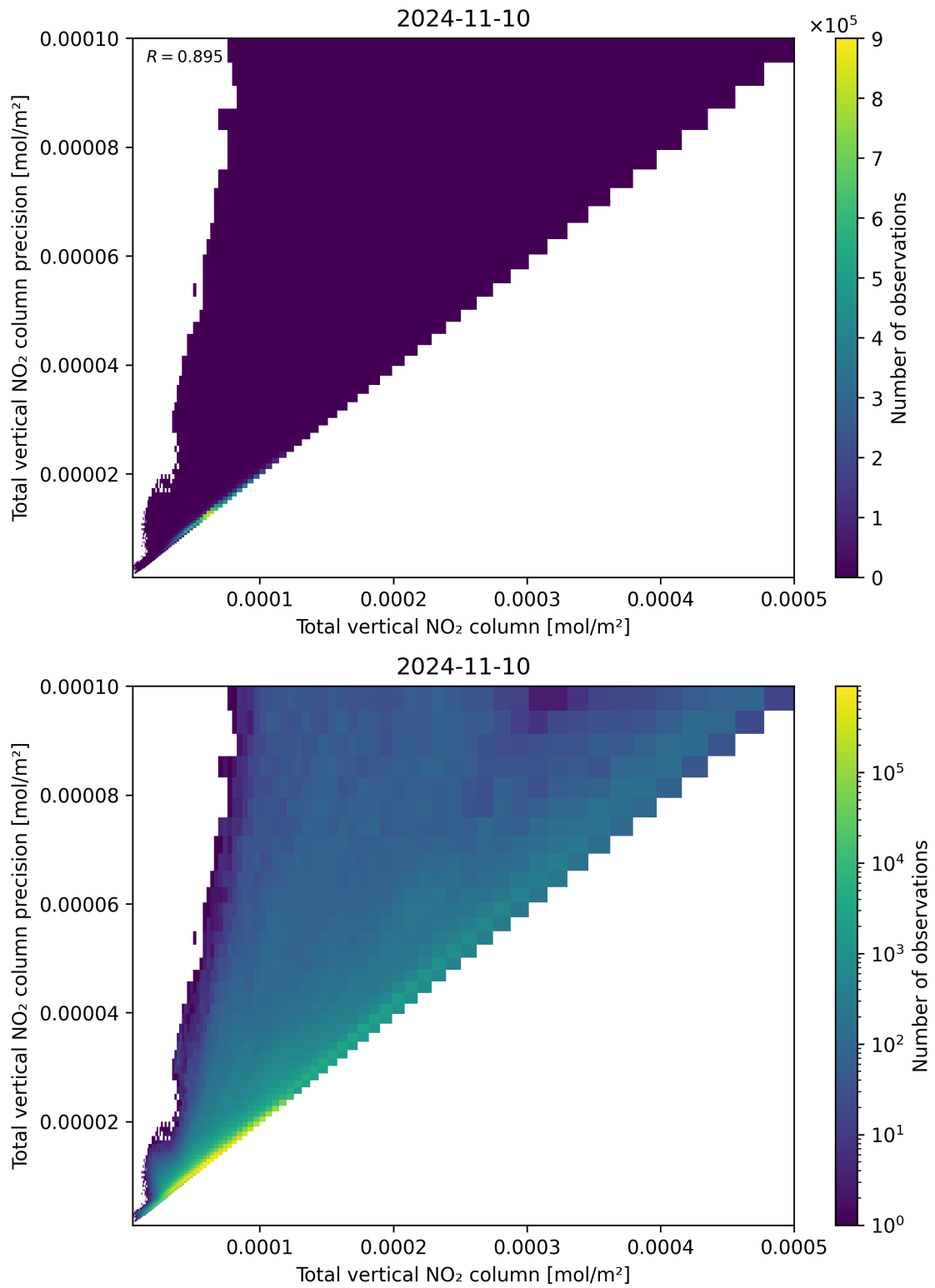
Figure 114: Scatter density plot of “Total vertical NO 2 column” against “Total vertical NO 2 column precision” for 2024-11-09 to 2024-11-11.
