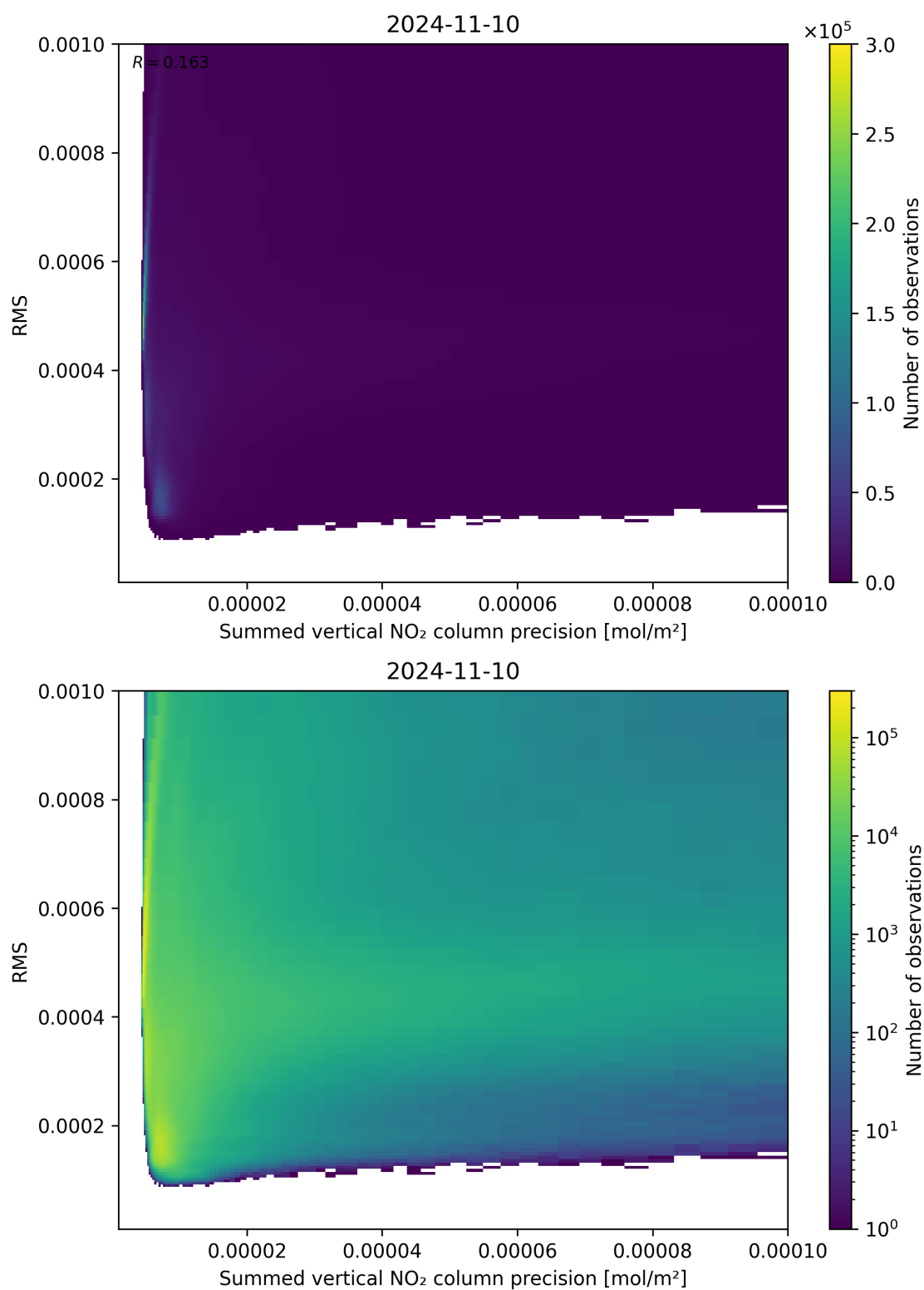
Figure 108: Scatter density plot of “Summed vertical NO 2 column precision” against “RMS” for 2024-11-09 to 2024-11-11.
