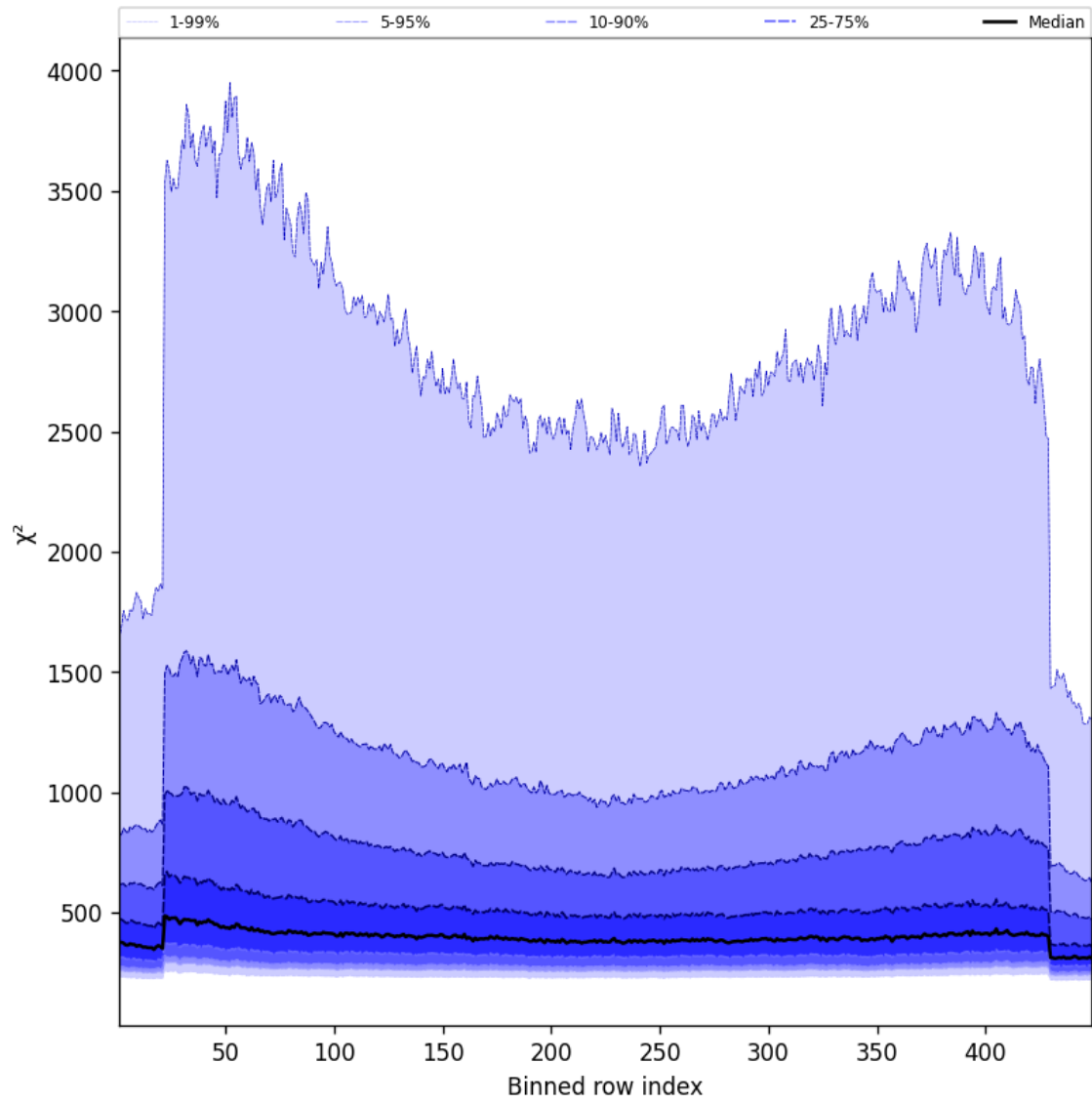
Figure 59: Along track statistics of “ \chi^2 ” for 2024-11-09 to 2024-11-11
