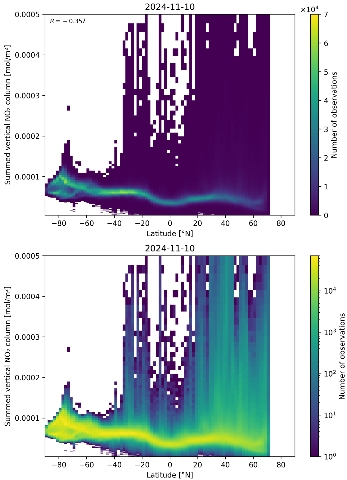
Figure 88: Scatter density plot of “Latitude” against “Summed vertical NO 2 column” for 2024-11-09 to 2024-11-11.
