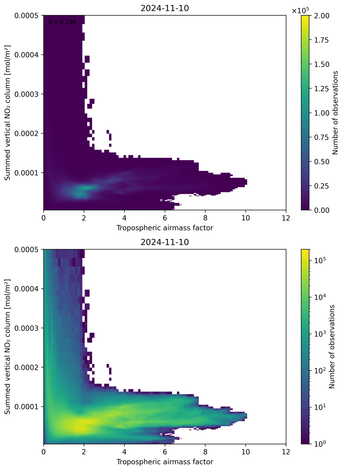
Figure 75: Scatter density plot of “Tropospheric airmass factor” against “Summed vertical NO 2 column” for 2024-11-09 to 2024-11-11.
