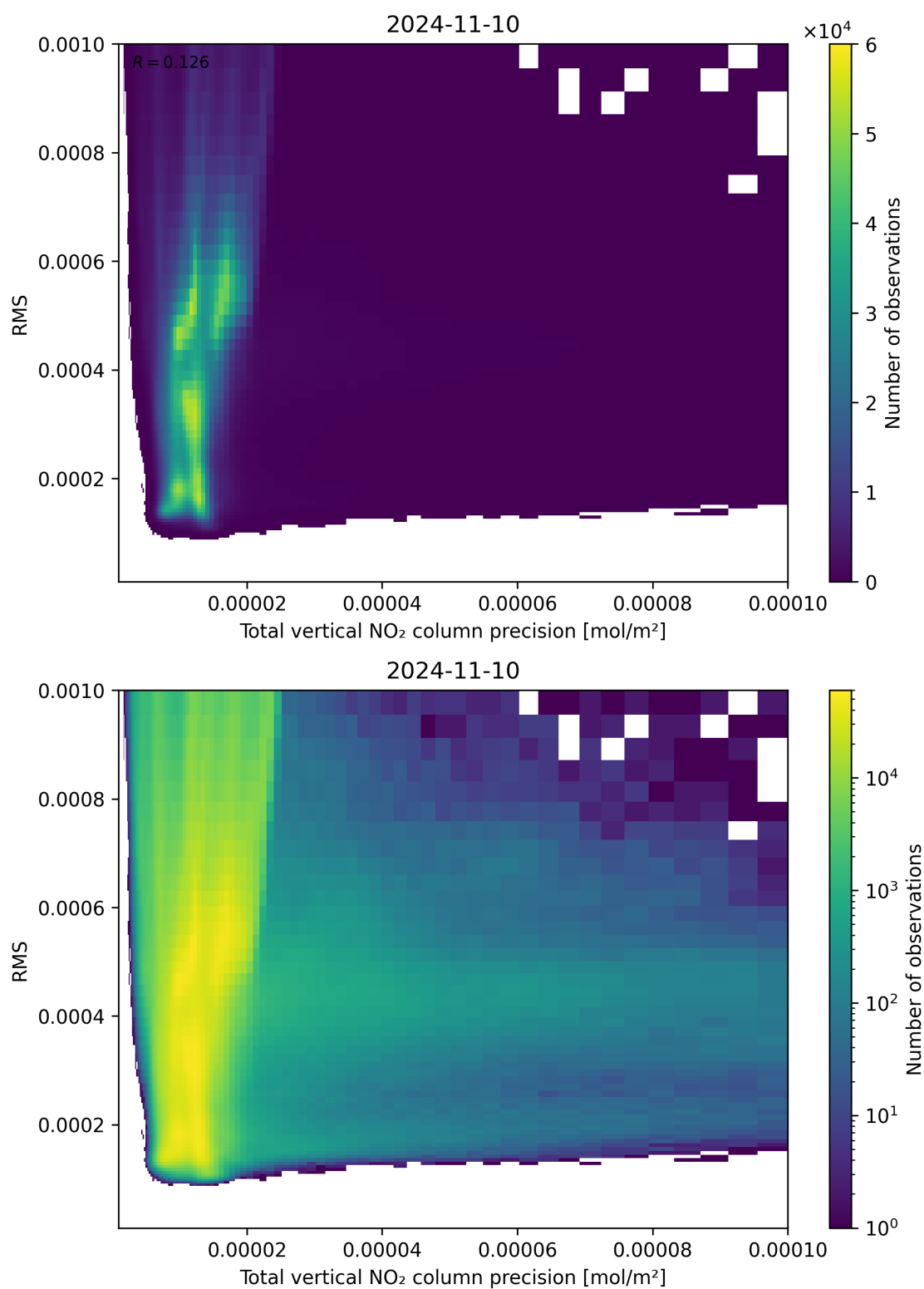
Figure 119: Scatter density plot of “Total vertical NO 2 column precision” against “RMS” for 2024-11-09 to 2024-11-11.
