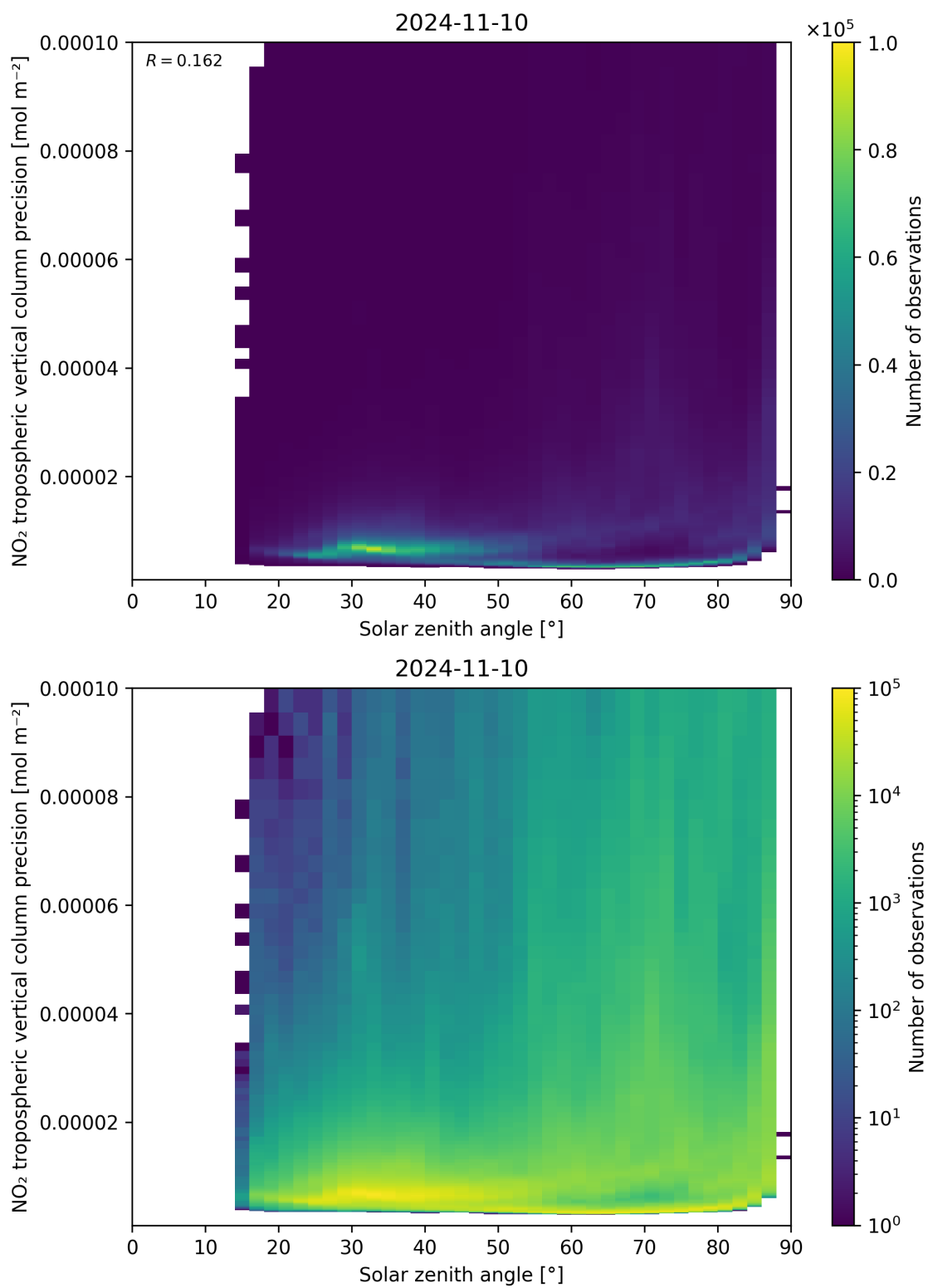
Figure 156: Scatter density plot of “Solar zenith angle” against “NO 2 tropospheric vertical column precision” for 2024-11-09 to 2024-11-11.
