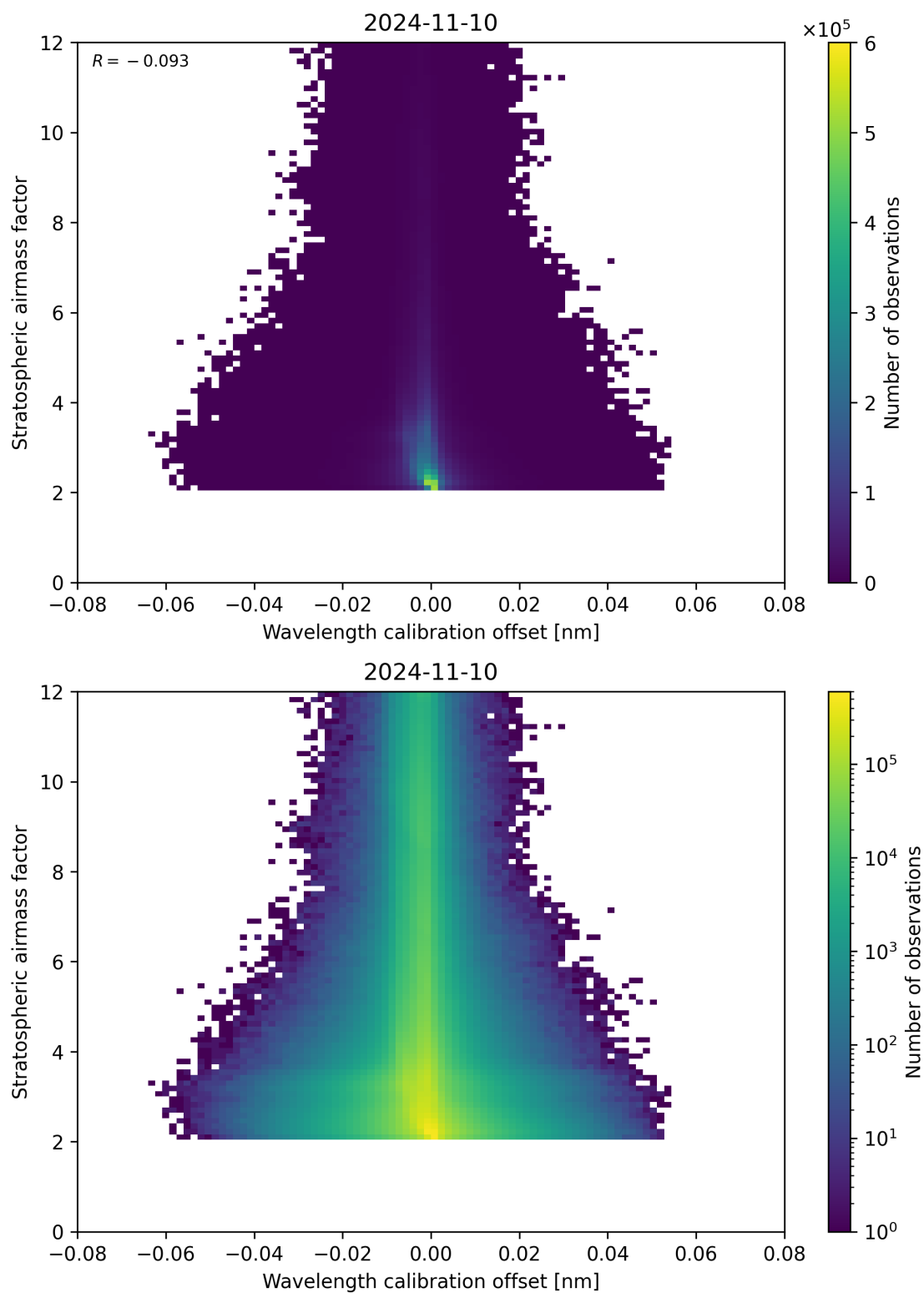
Figure 174: Scatter density plot of “Wavelength calibration offset” against “Stratospheric air mass factor” for 2024-11-09 to 2024-11-11.
