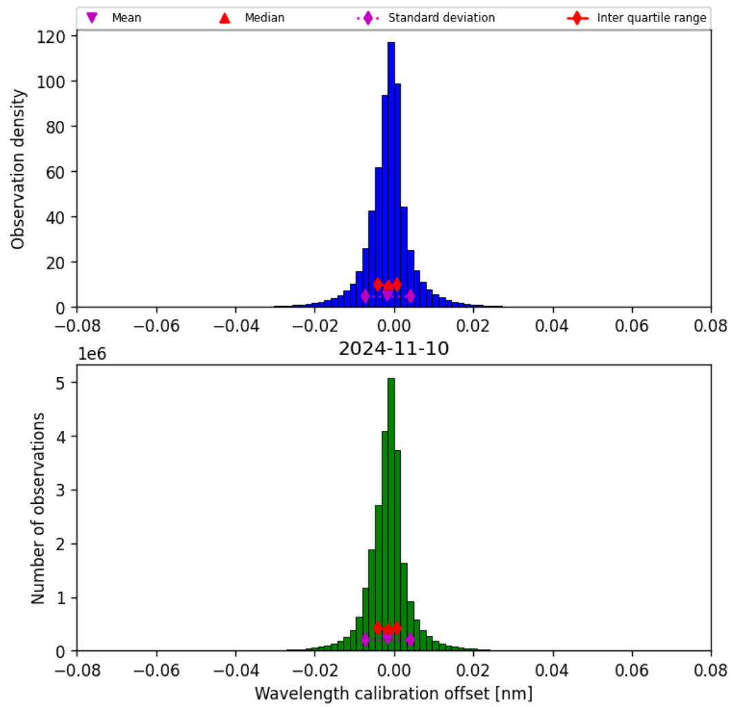
Figure 35: Histogram of “Wavelength calibration offset” for 2024-11-09 to 2024-11-11
