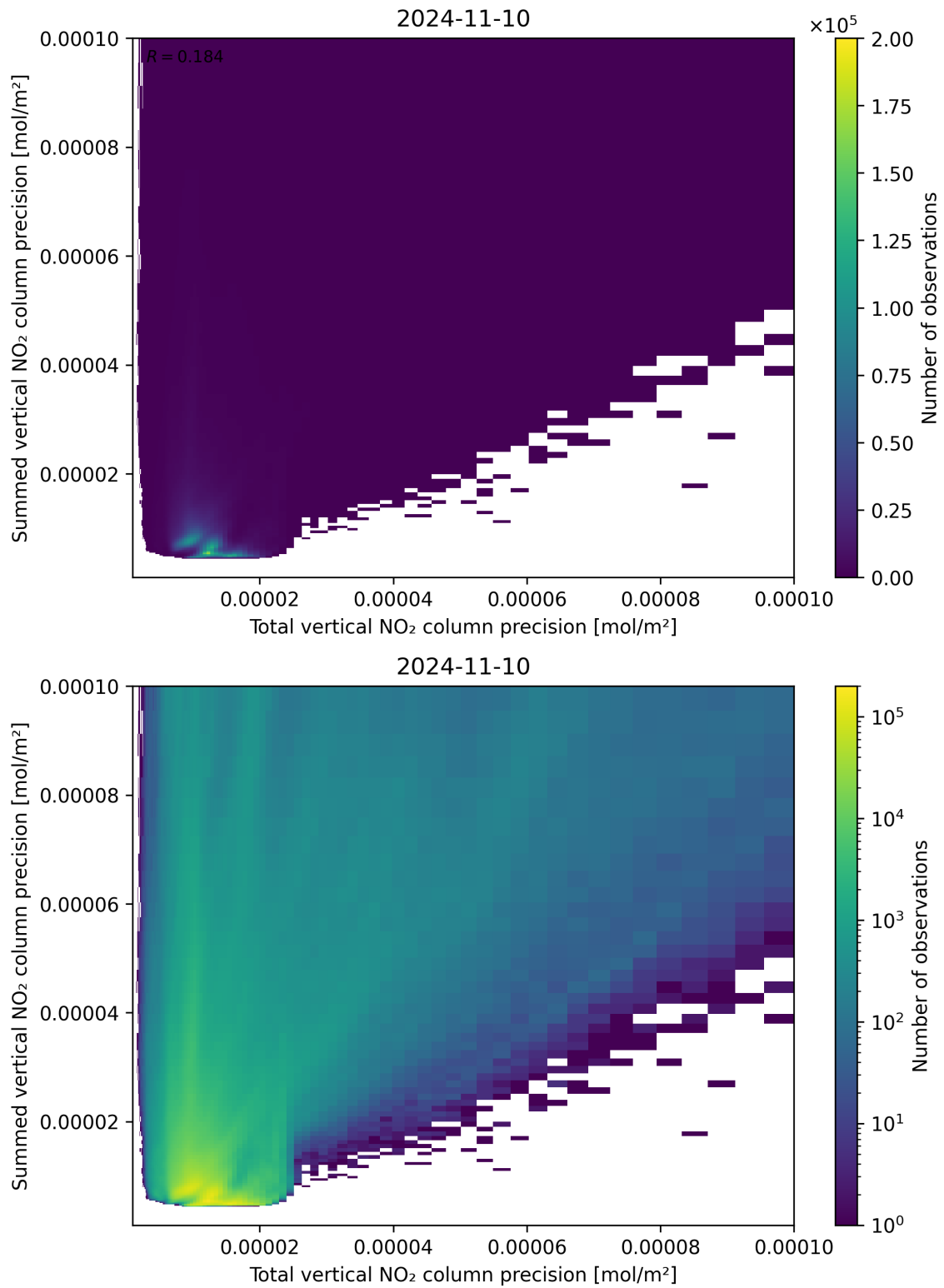
Figure 118: Scatter density plot of “Total vertical NO 2 column precision” against “Summed vertical NO 2 column precision” for 2024-11-09 to 2024-11-11.
