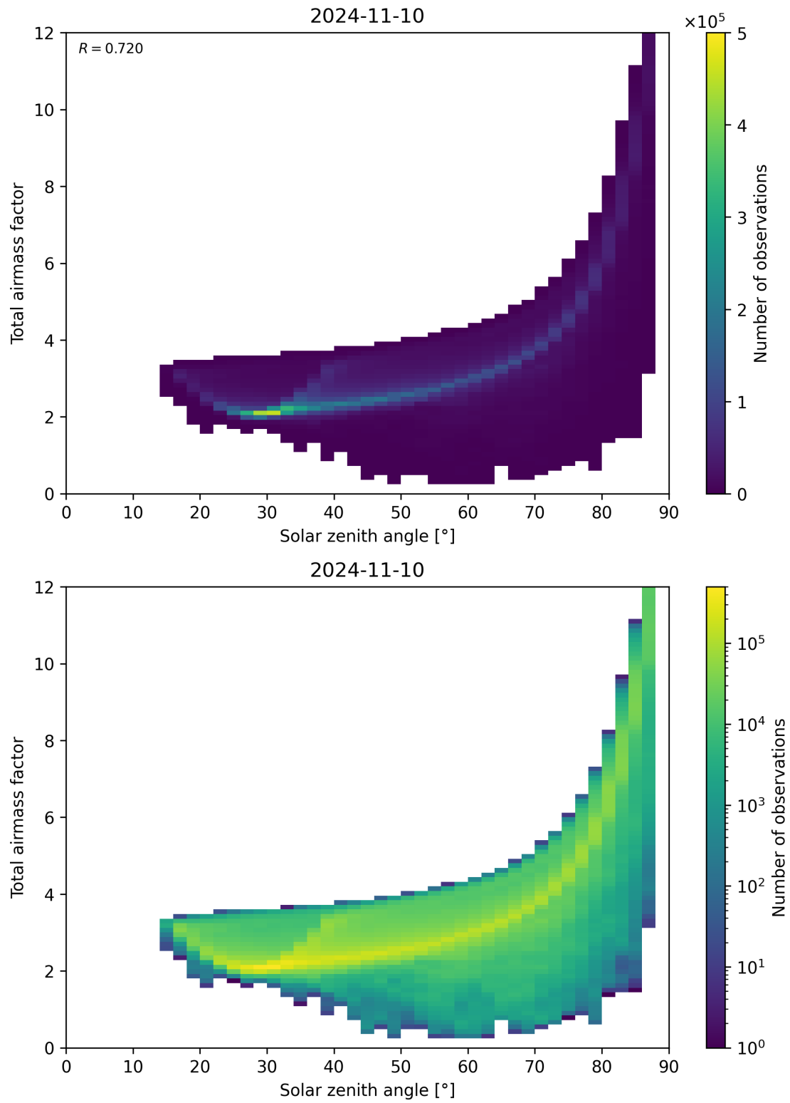
Figure 146: Scatter density plot of “Solar zenith angle” against “Total air mass factor” for 2024-11-09 to 2024-11-11.
