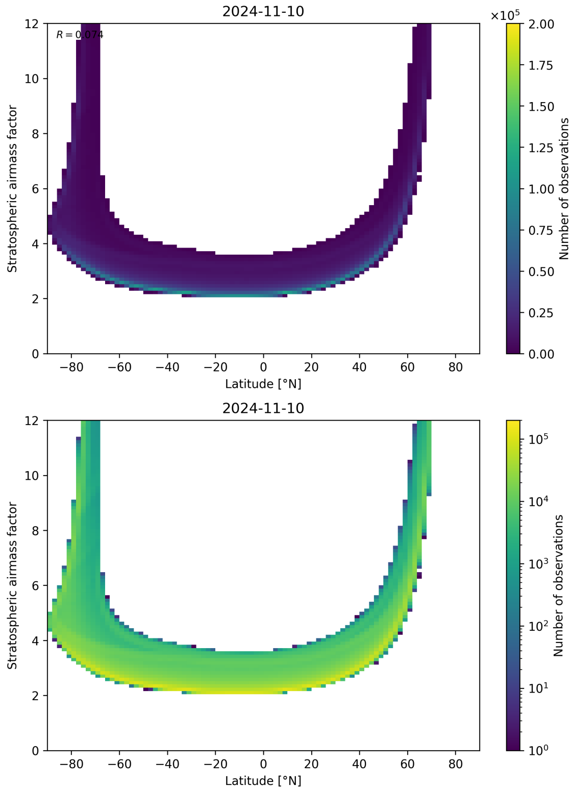
Figure 83: Scatter density plot of “Latitude” against “Stratospheric air mass factor” for 2024-11-09 to 2024-11-11.
