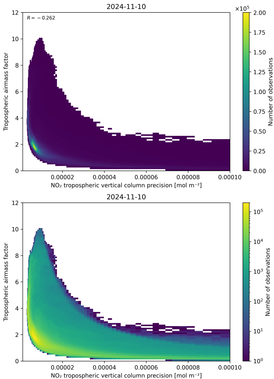
Figure 133: Scatter density plot of “NO 2 tropospheric vertical column precision” against “Tropospheric airmass factor” for 2024-11-09 to 2024-11-11.
