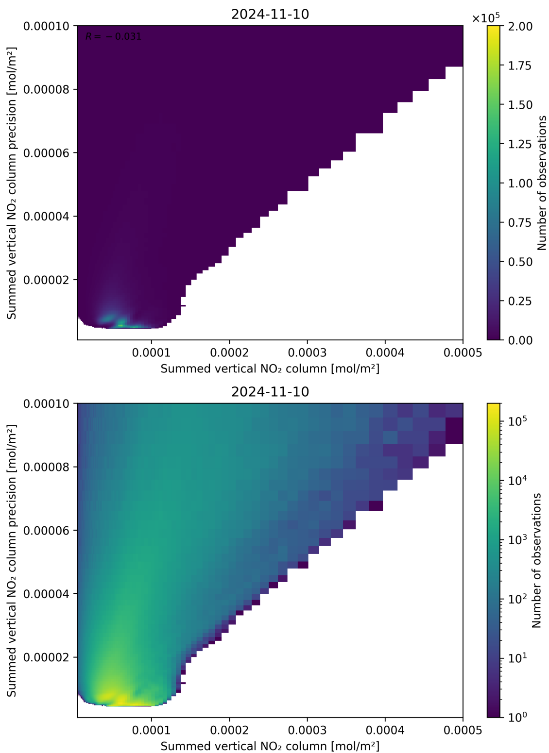
Figure 105: Scatter density plot of “Summed vertical NO 2 column” against “Summed vertical NO 2 column precision” for 2024-11-09 to 2024-11-11.
