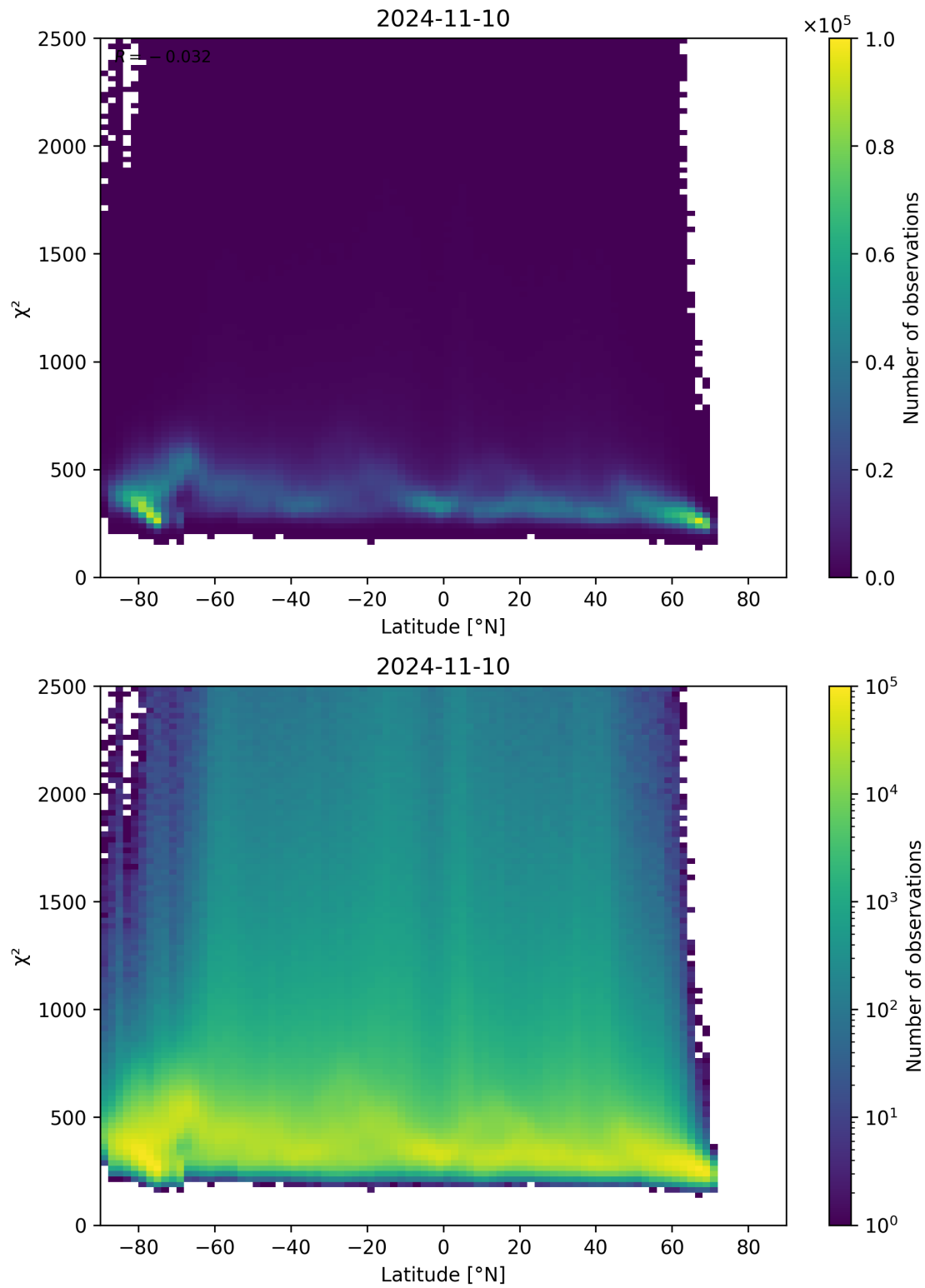
Figure 86: Scatter density plot of “Latitude” against “ \chi^2 ” for 2024-11-09 to 2024-11-11.
