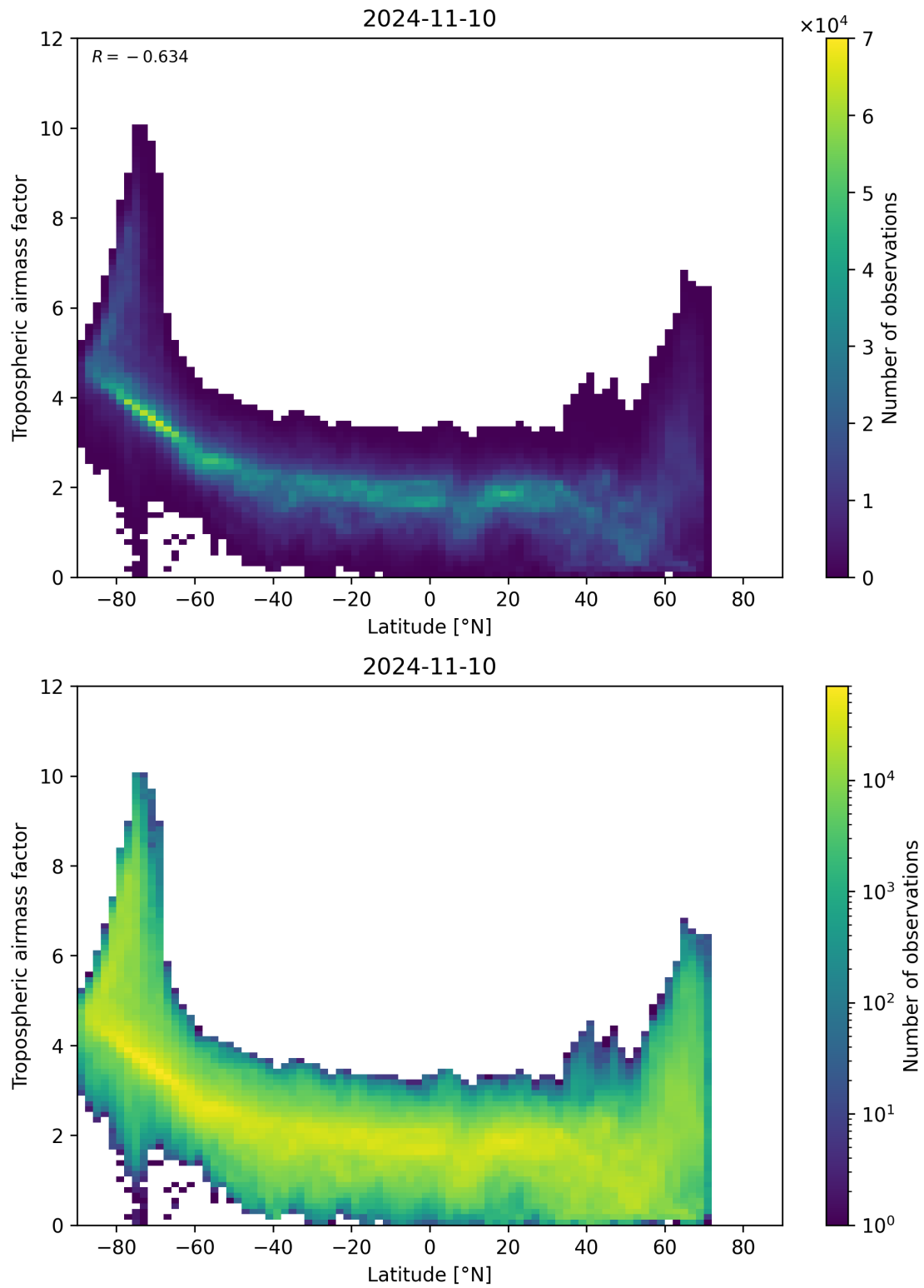
Figure 85: Scatter density plot of “Latitude” against “Tropospheric air mass factor” for 2024-11-09 to 2024-11-11.
