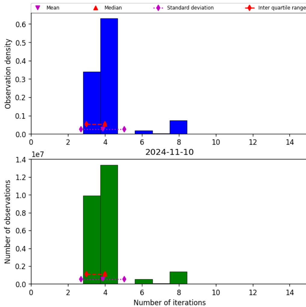
Figure 34: Histogram of “Number of iterations” for 2024-11-09 to 2024-11-11
