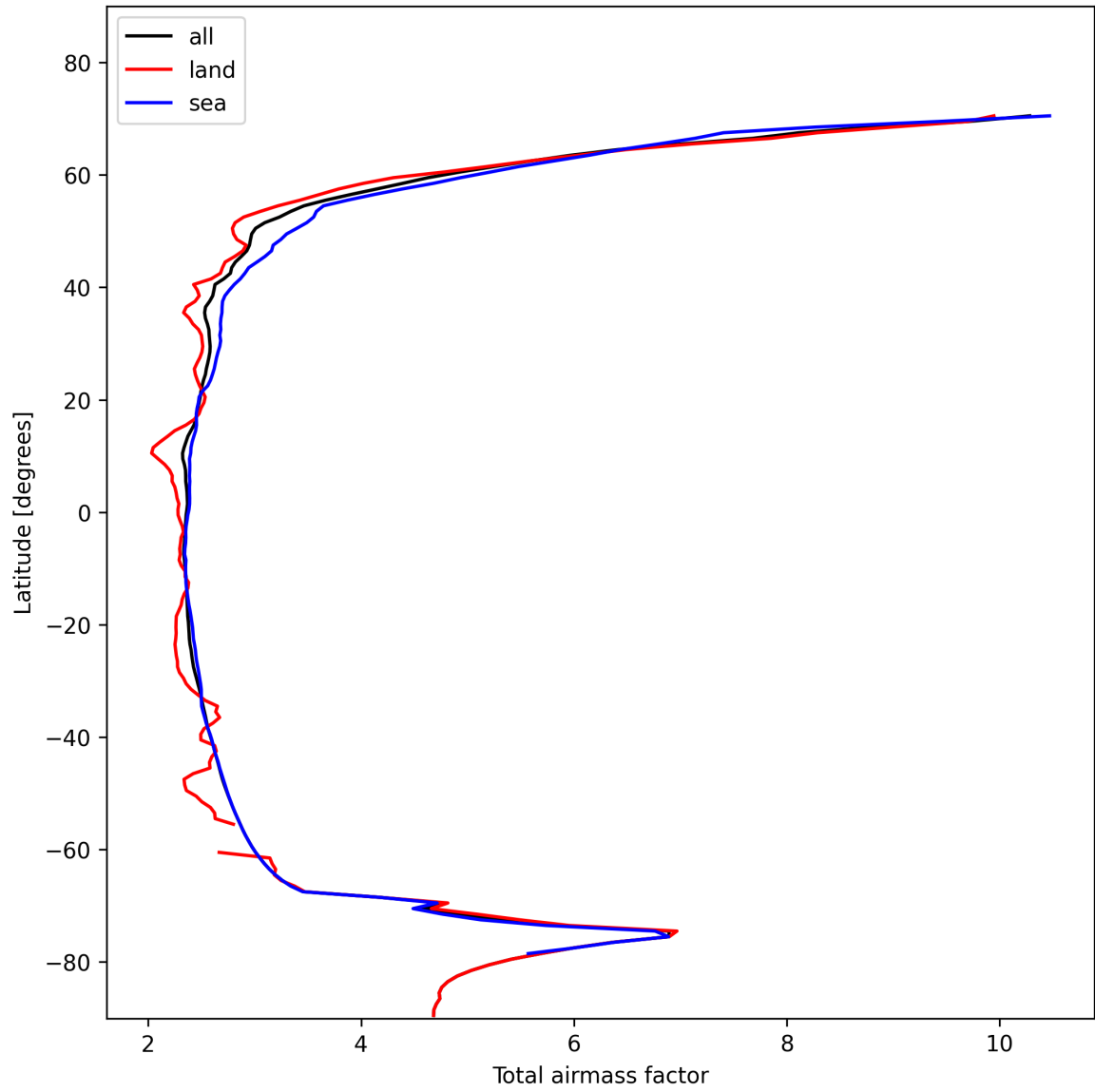
Figure 15: Zonal average of “Total airmass factor” for 2024-11-09 to 2024-11-11.
