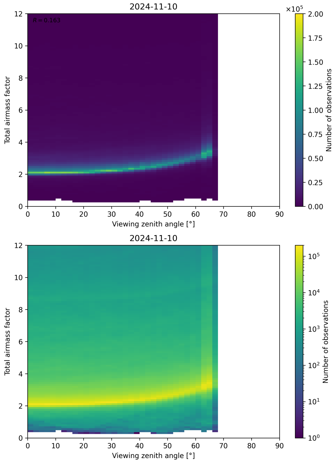
Figure 160: Scatter density plot of “Viewing zenith angle” against “Total airmass factor” for 2024-11-09 to 2024-11-11.
