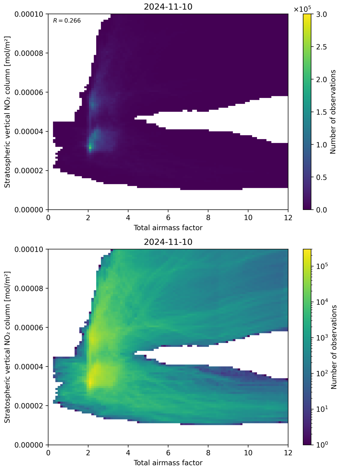
Figure 64: Scatter density plot of “Total airmass factor” against “Stratospheric vertical NO 2 column” for 2024-11-09 to 2024-11-11.
