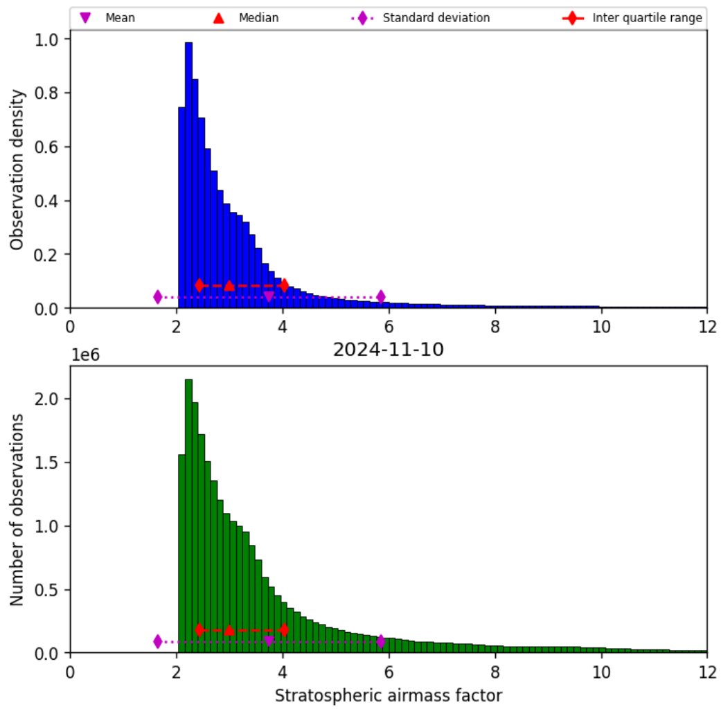
Figure 44: Histogram of “Stratospheric airmass factor” for 2024-11-09 to 2024-11-11
