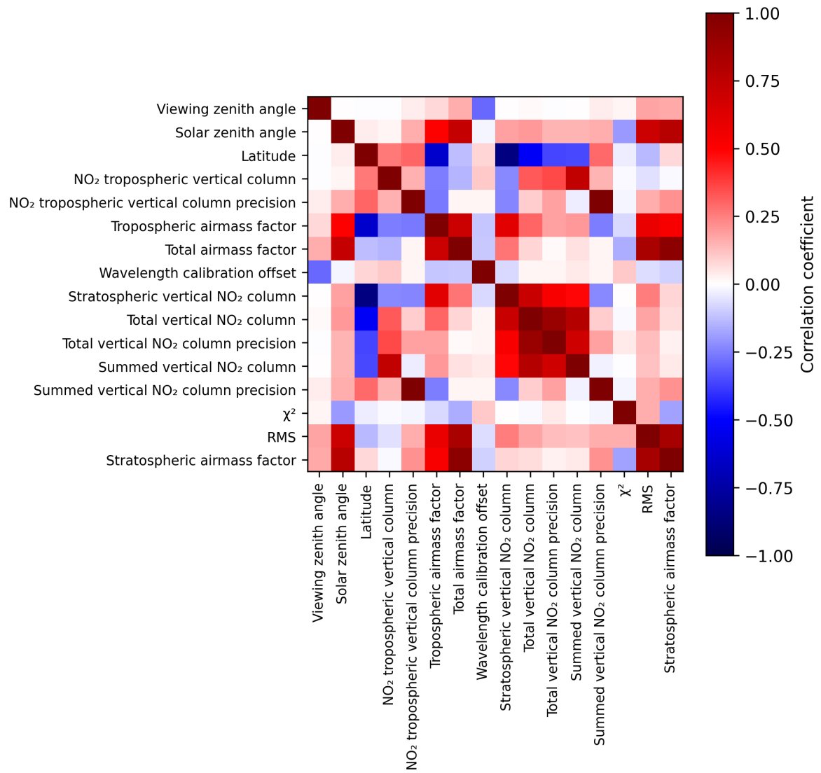
Figure 2: Map of correlation matrix for 2024-11-09 to 2024-11-11.
