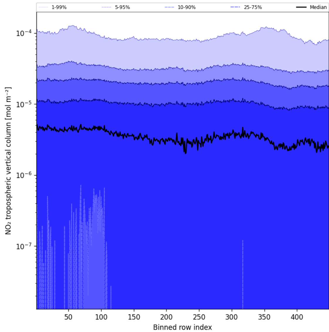
Figure 46: Along track statistics of “NO 2 tropospheric vertical column” for 2024-11-09 to 2024-11-11
