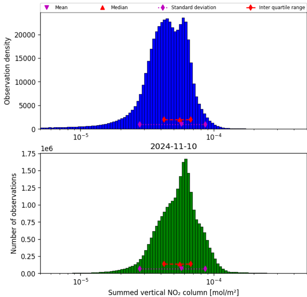
Figure 40: Histogram of “Summed vertical NO 2 column” for 2024-11-09 to 2024-11-11
