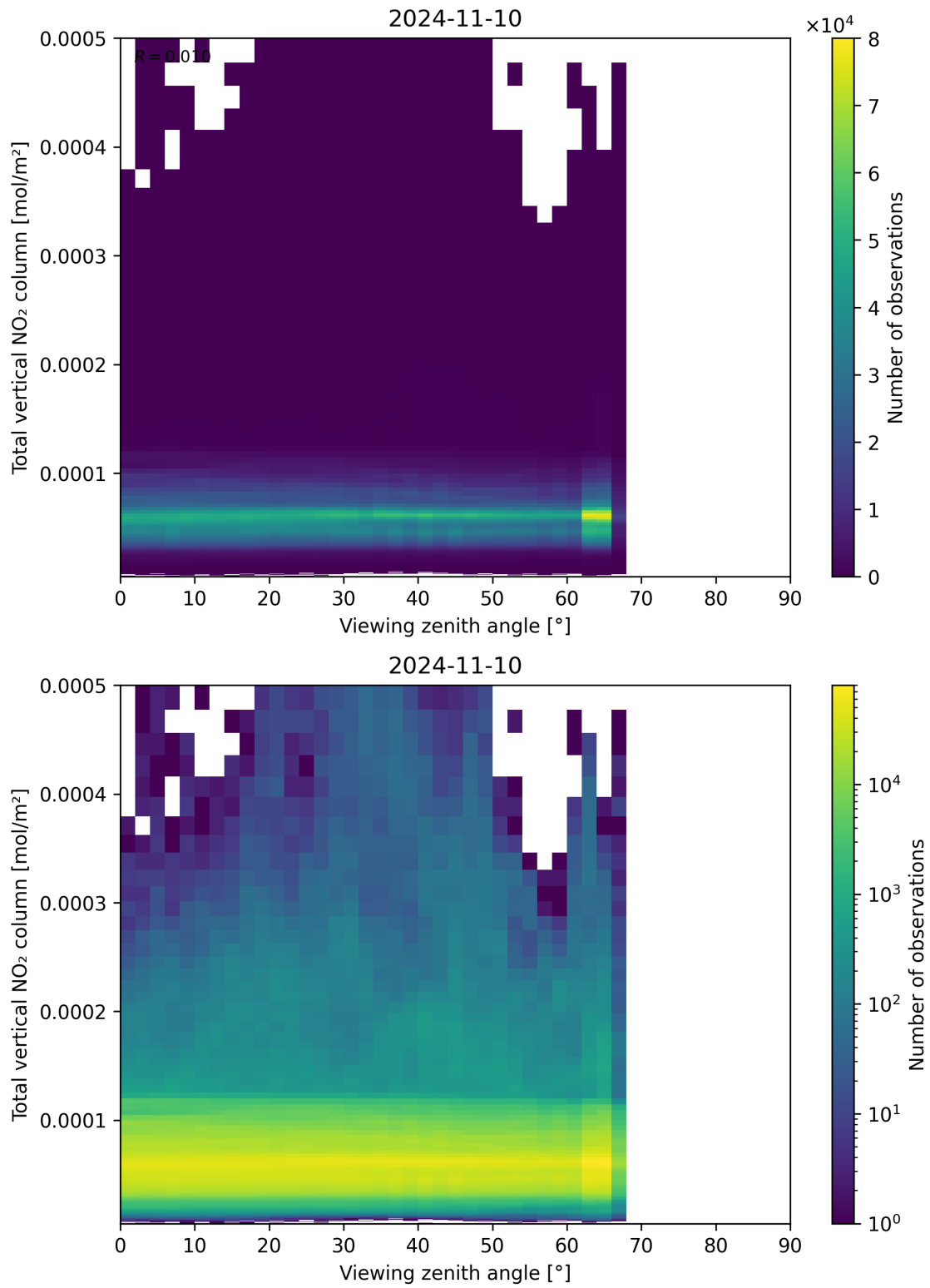
Figure 167: Scatter density plot of “Viewing zenith angle” against “Total vertical NO 2 column” for 2024-11-09 to 2024-11-11.
