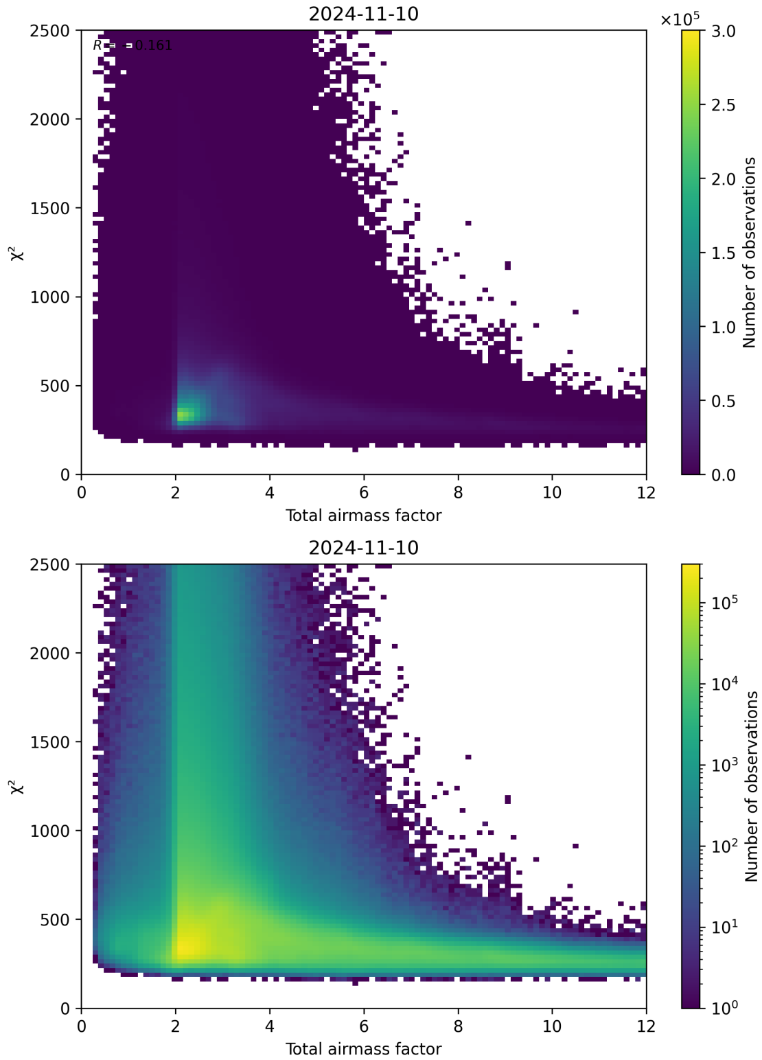
Figure 63: Scatter density plot of “Total airmass factor” against “ \chi^2 ” for 2024-11-09 to 2024-11-11.
