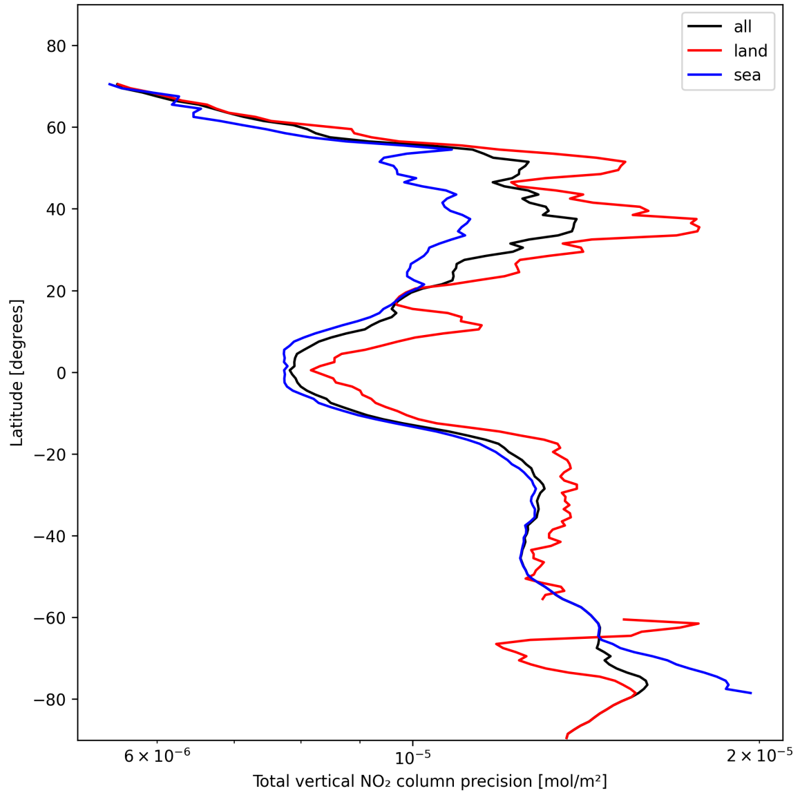
Figure 22: Zonal average of “Total vertical NO 2 column precision” for 2024-11-09 to 2024-11-11.
