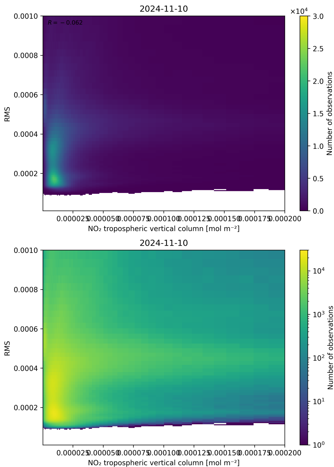
Figure 142: Scatter density plot of “NO 2 tropospheric vertical column” against “RMS” for 2024-11-09 to 2024-11-11.
