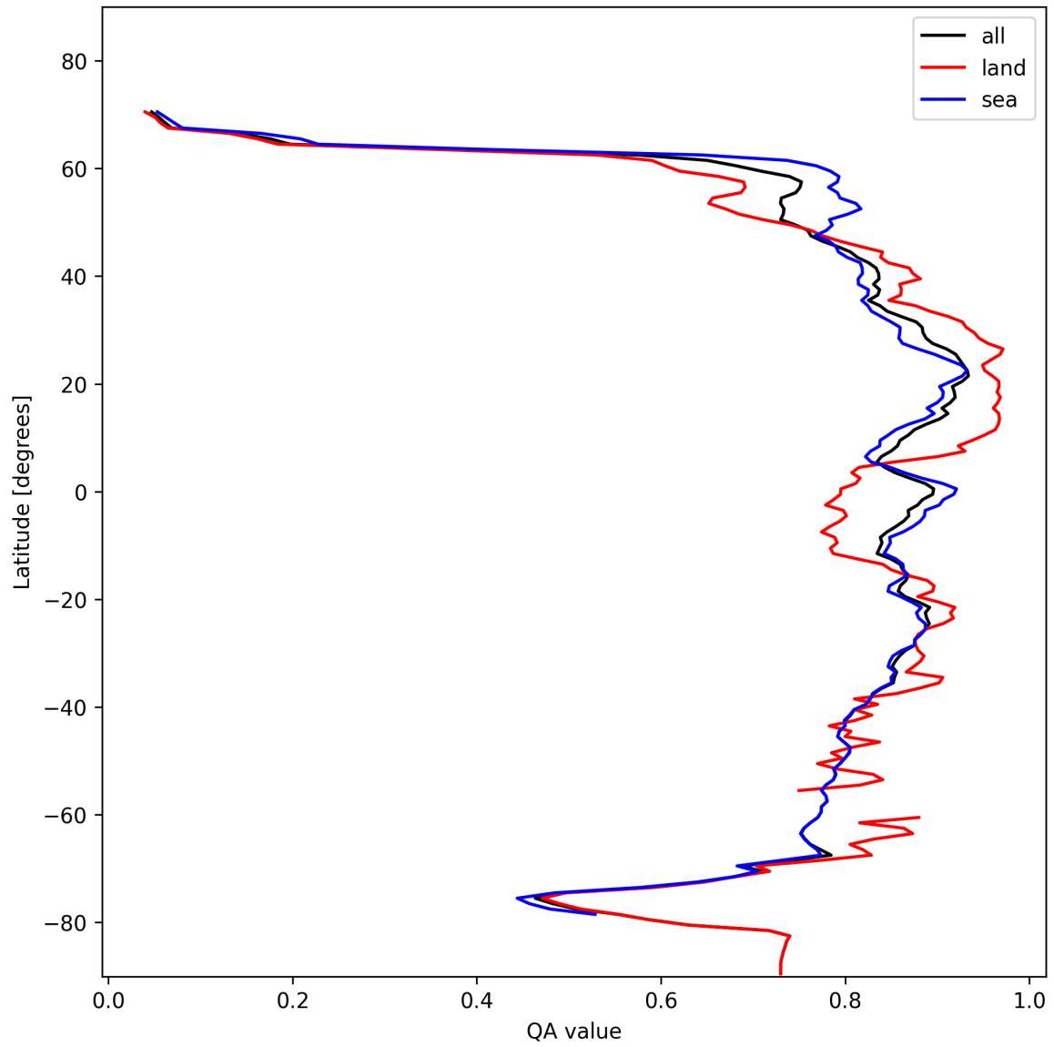
Figure 11: Zonal average of “QA value” for 2024-11-09 to 2024-11-11.
