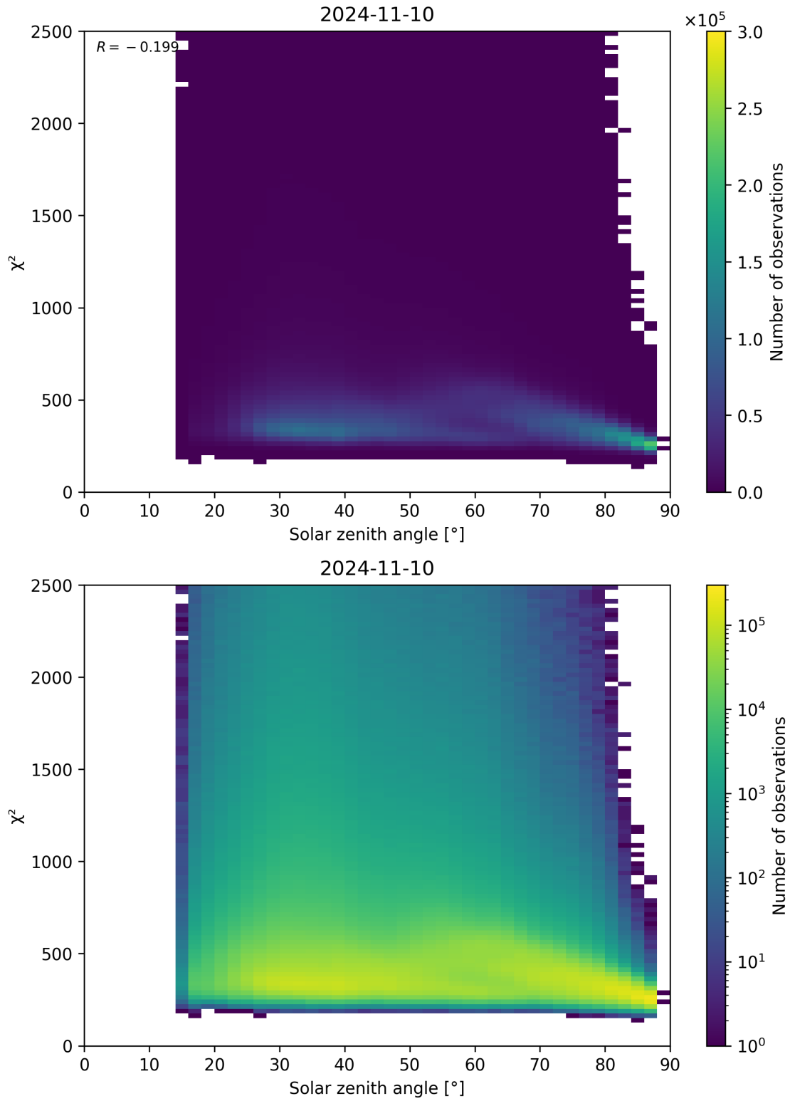
Figure 148: Scatter density plot of “Solar zenith angle” against “ \chi^2 ” for 2024-11-09 to 2024-11-11.
