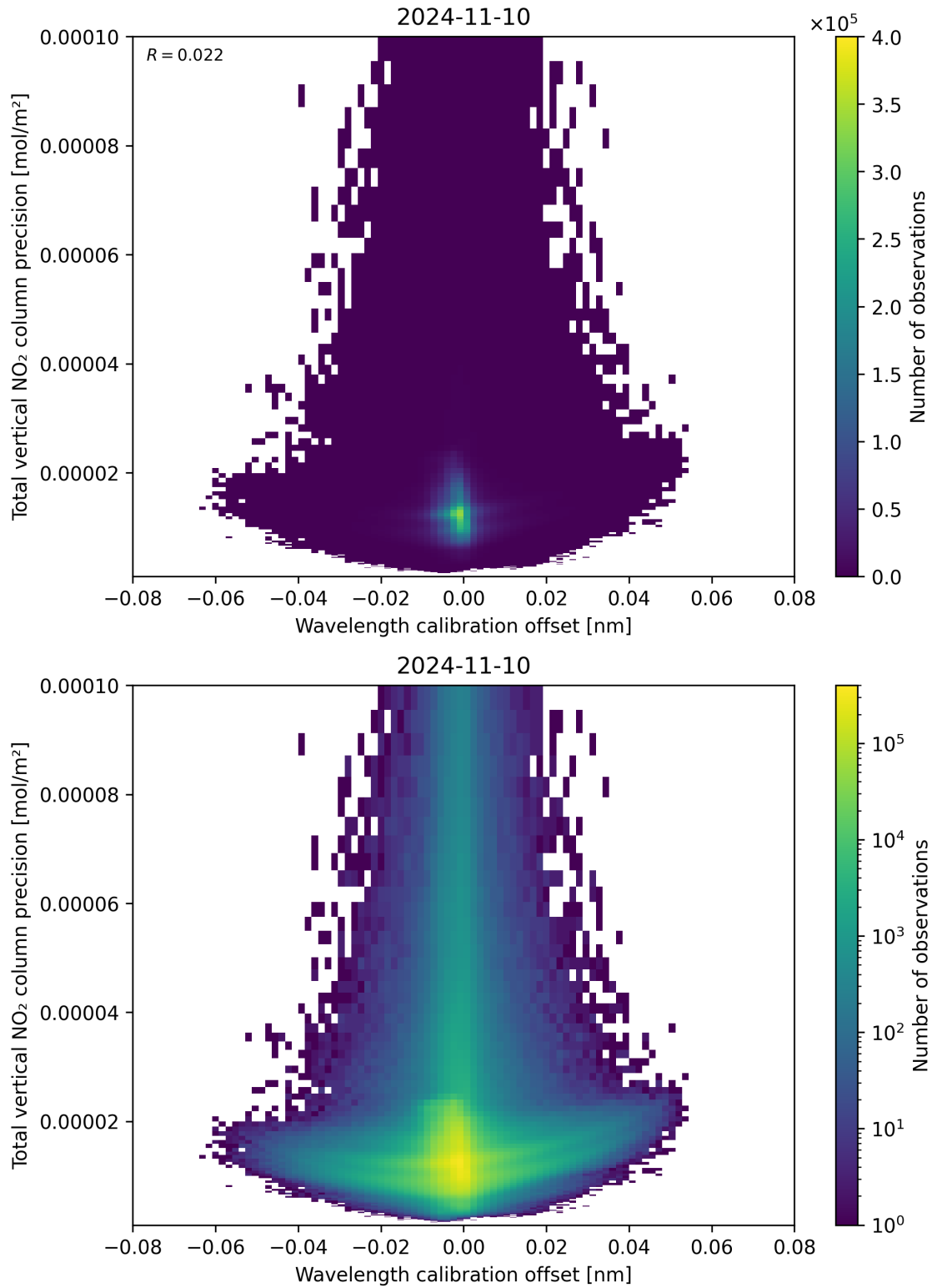
Figure 180: Scatter density plot of “Wavelength calibration offset” against “Total vertical NO 2 column precision” for 2024-11-09 to 2024-11-11.
