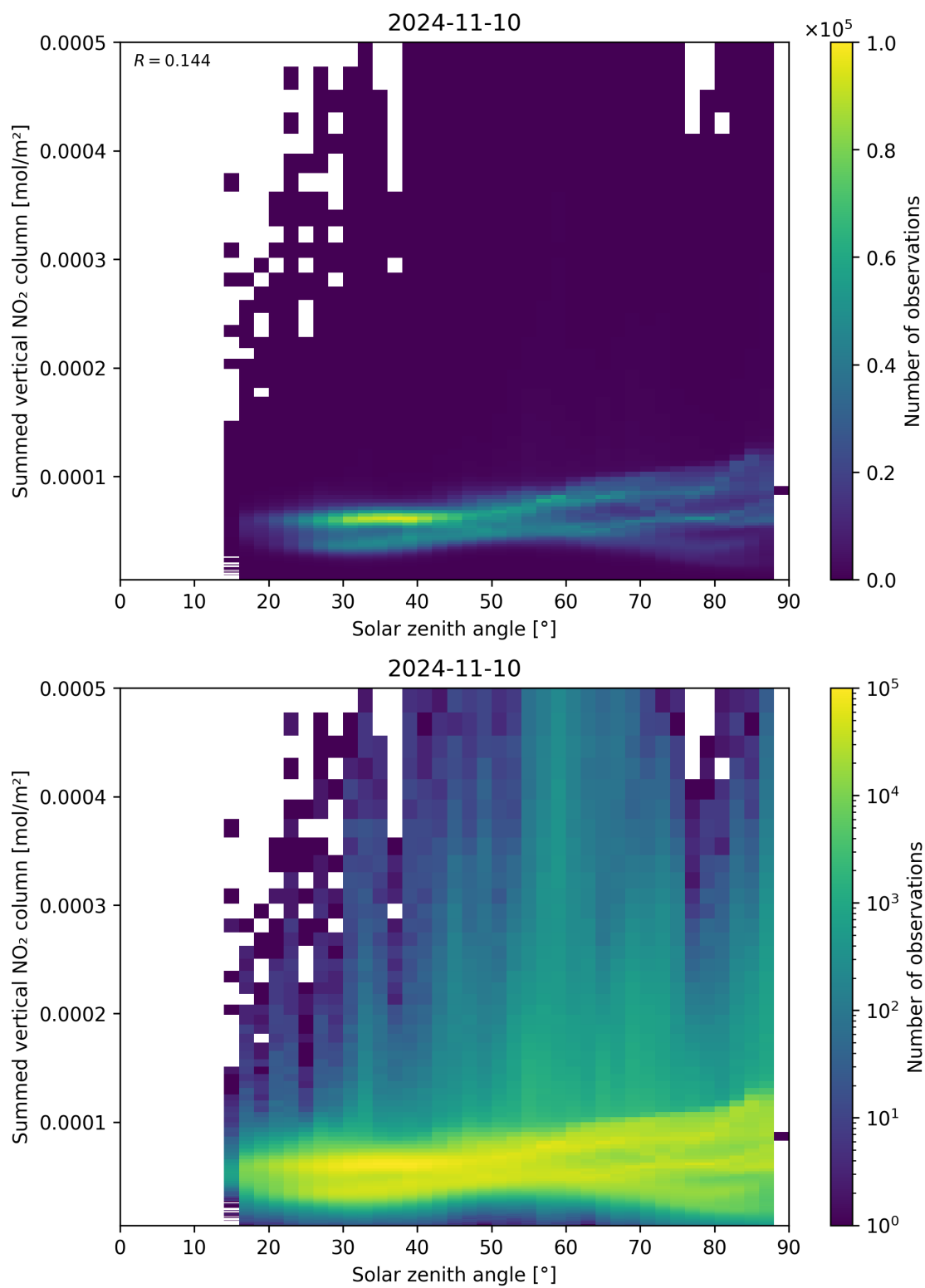
Figure 151: Scatter density plot of “Solar zenith angle” against “Summed vertical NO 2 column” for 2024-11-09 to 2024-11-11.
