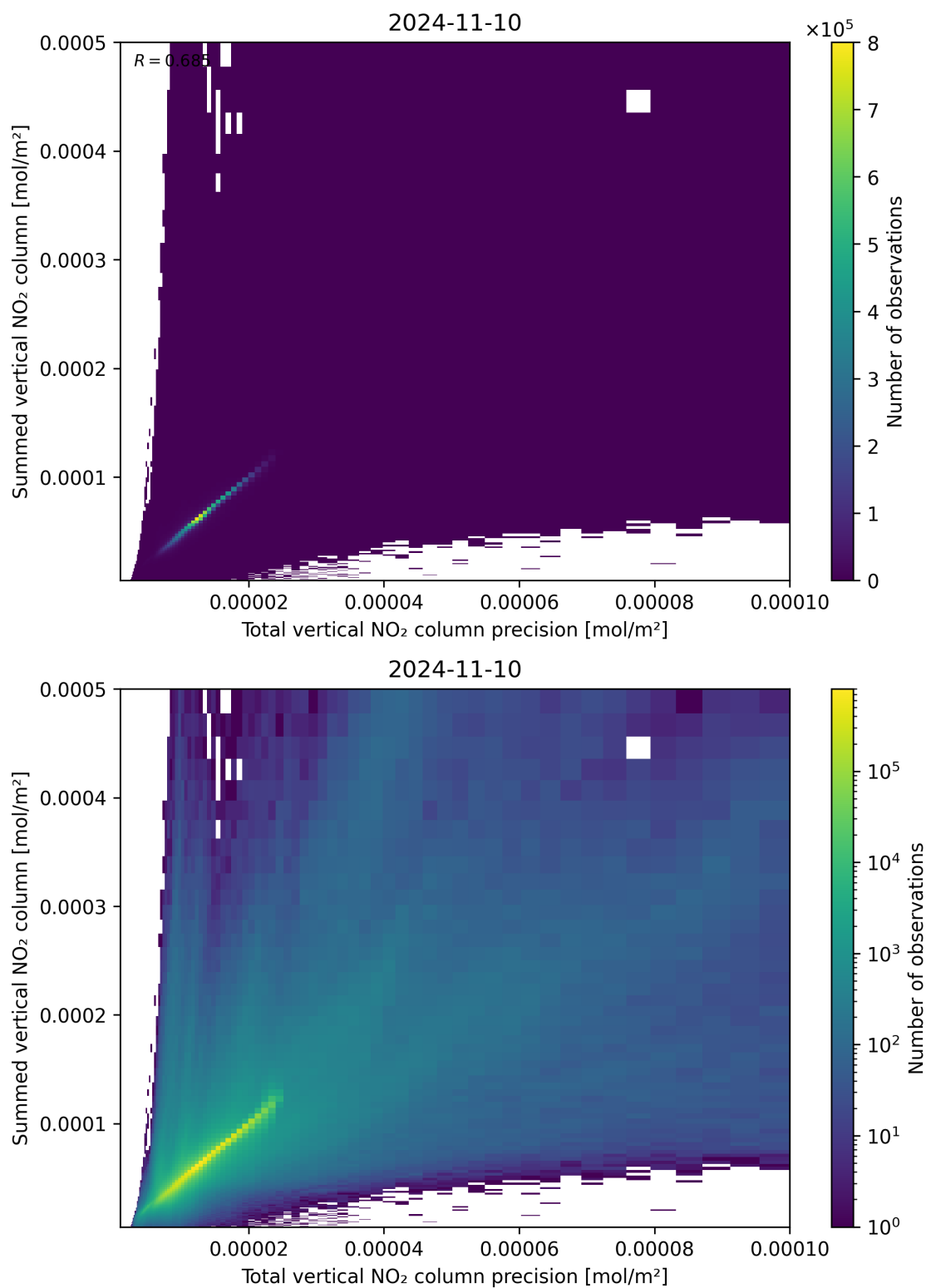
Figure 117: Scatter density plot of “Total vertical NO 2 column precision” against “Summed vertical NO 2 column” for 2024-11-09 to 2024-11-11.
