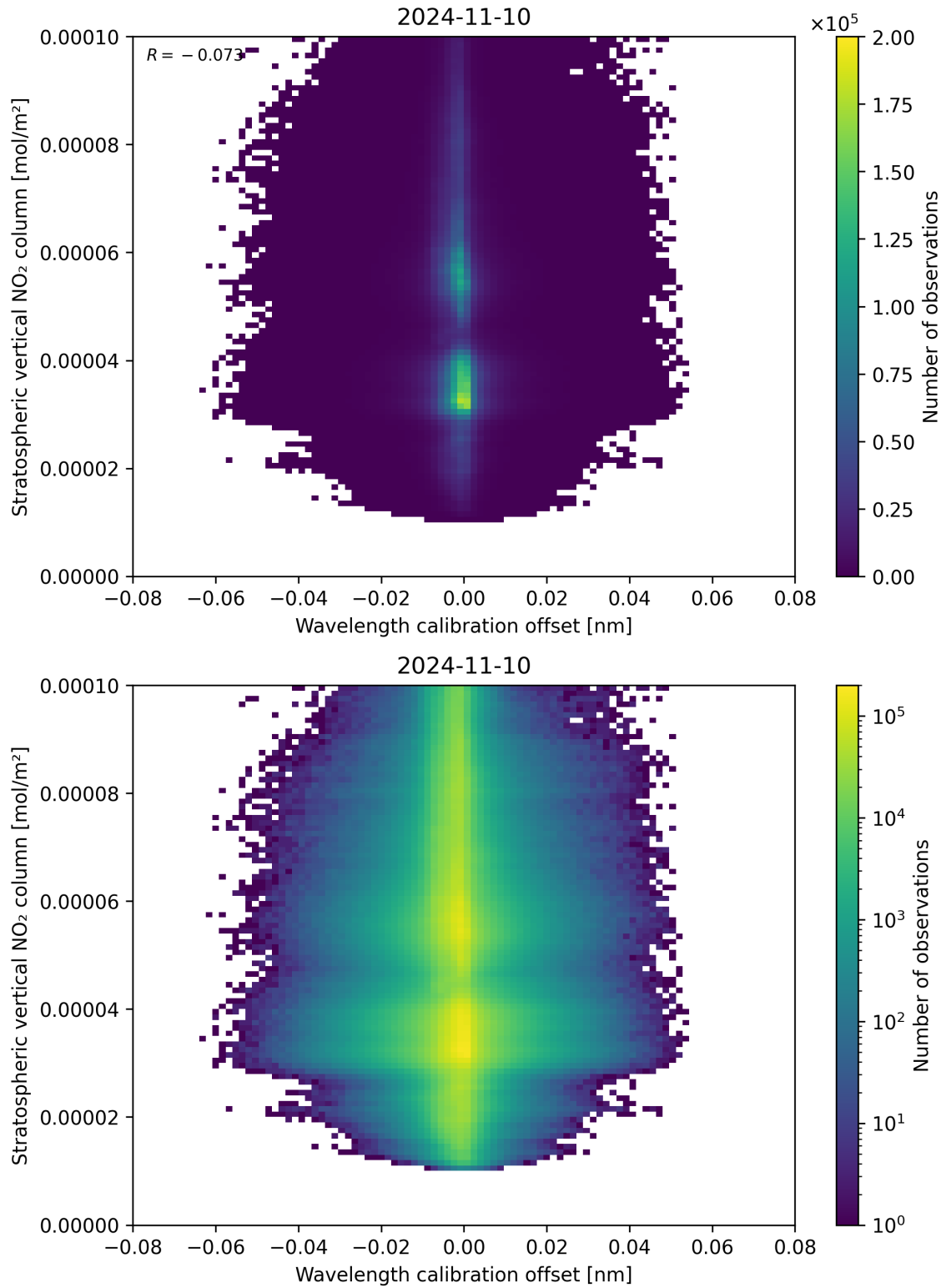
Figure 176: Scatter density plot of “Wavelength calibration offset” against “Stratospheric vertical NO 2 column” for 2024-11-09 to 2024-11-11.
