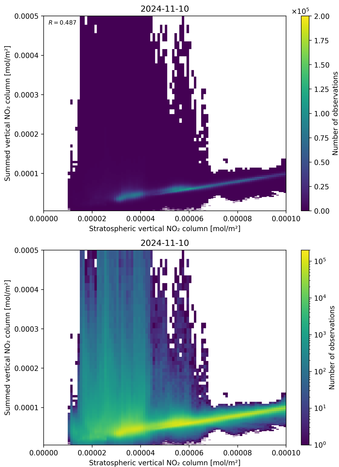
Figure 98: Scatter density plot of “Stratospheric vertical NO 2 column” against “Summed vertical NO 2 column” for 2024-11-09 to 2024-11-11.
