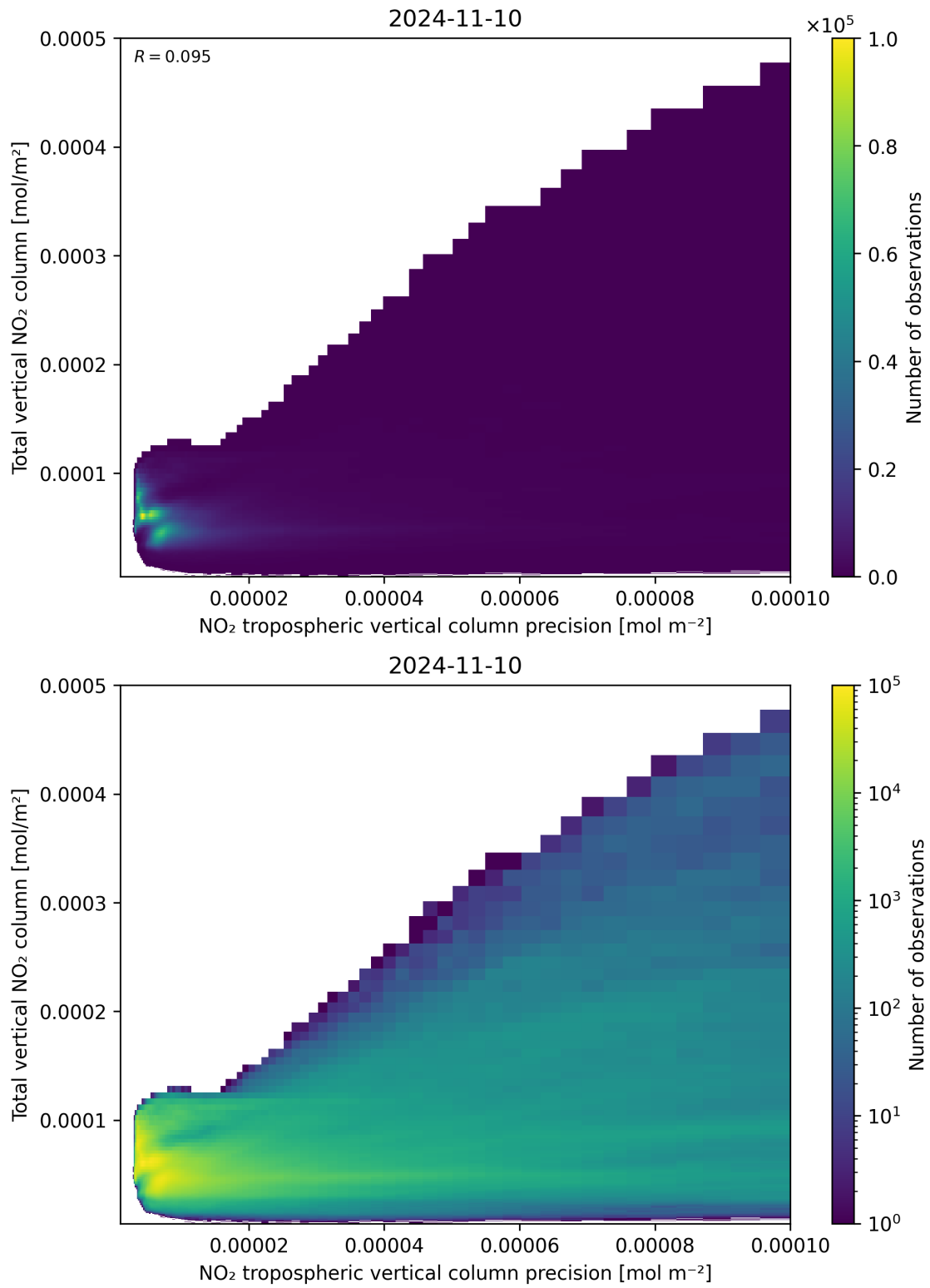
Figure 138: Scatter density plot of “NO 2 tropospheric vertical column precision” against “Total vertical NO 2 column” for 2024-11-09 to 2024-11-11.
