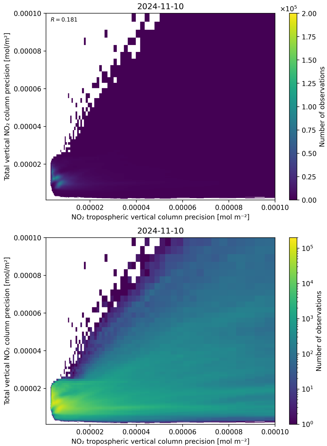
Figure 139: Scatter density plot of “NO 2 tropospheric vertical column precision” against “Total vertical NO 2 column precision” for 2024-11-09 to 2024-11-11.
