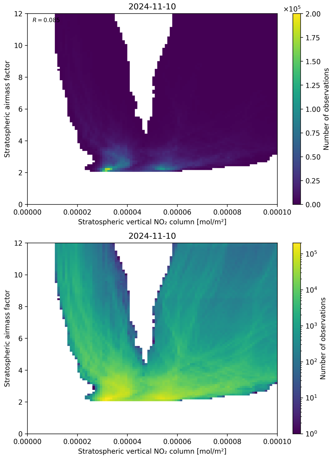
Figure 96: Scatter density plot of “Stratospheric vertical NO 2 column” against “Stratospheric airmass factor” for 2024-11-09 to 2024-11-11.
