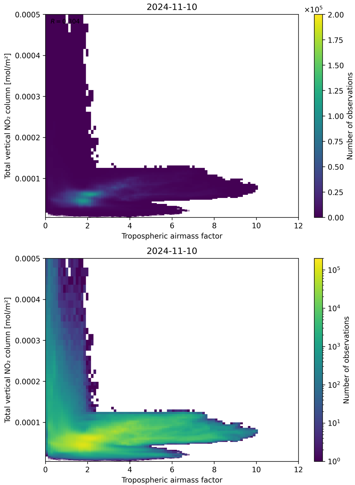
Figure 77: Scatter density plot of “Tropospheric airmass factor” against “Total vertical NO 2 column” for 2024-11-09 to 2024-11-11.
