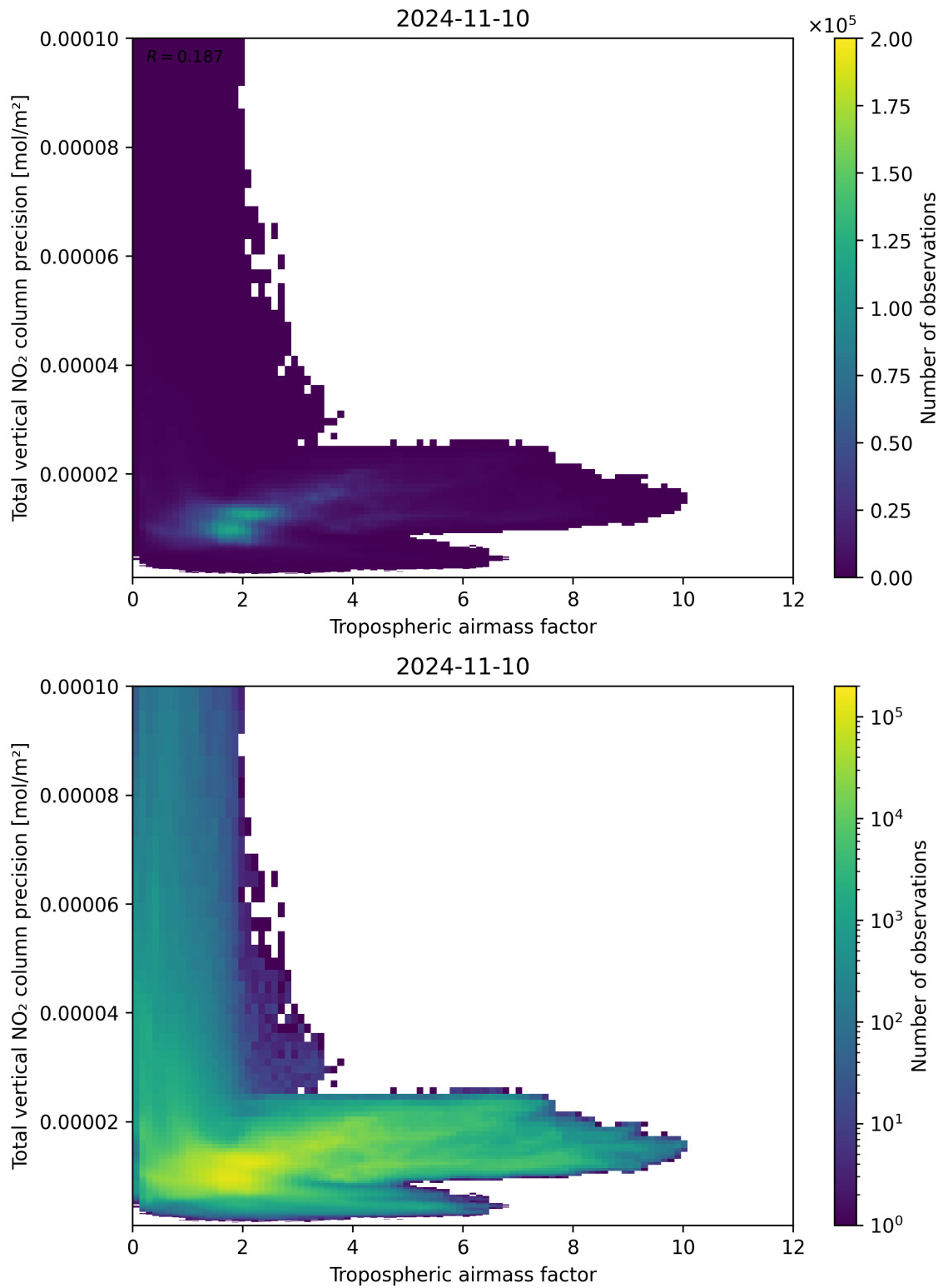
Figure 78: Scatter density plot of “Tropospheric air mass factor” against “Total vertical NO 2 column precision” for 2024-11-09 to 2024-11-11.
