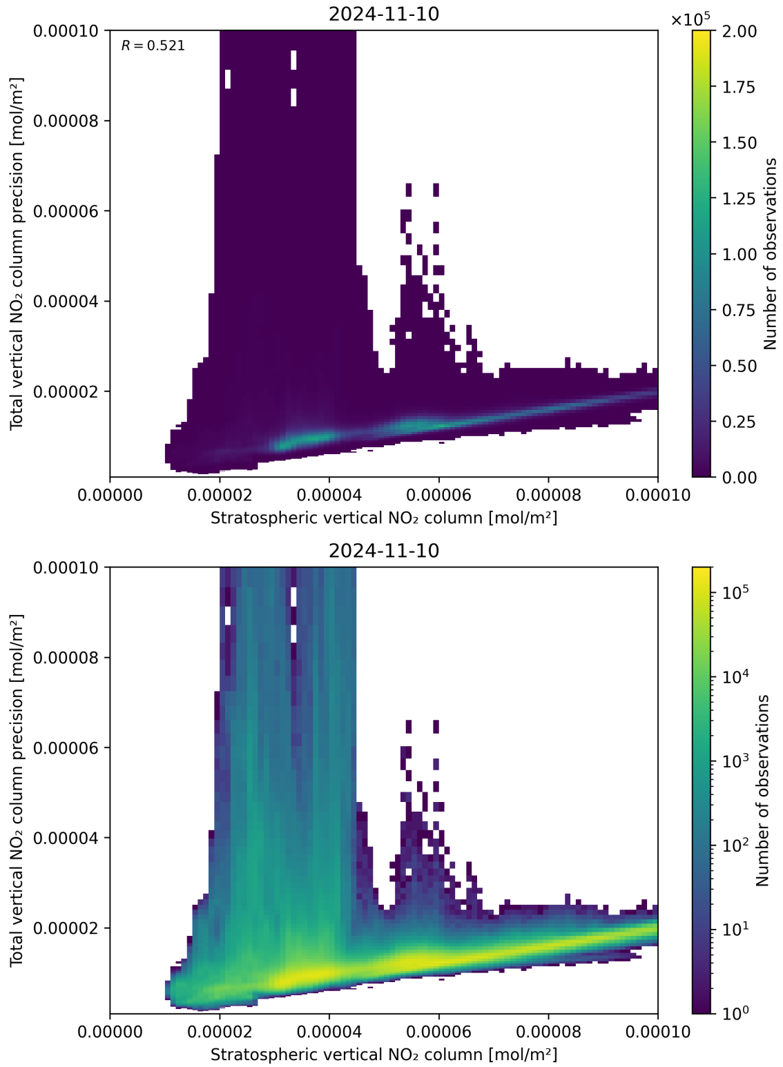
Figure 101: Scatter density plot of “Stratospheric vertical NO 2 column” against “Total vertical NO 2 column precision” for 2024-11-09 to 2024-11-11.
