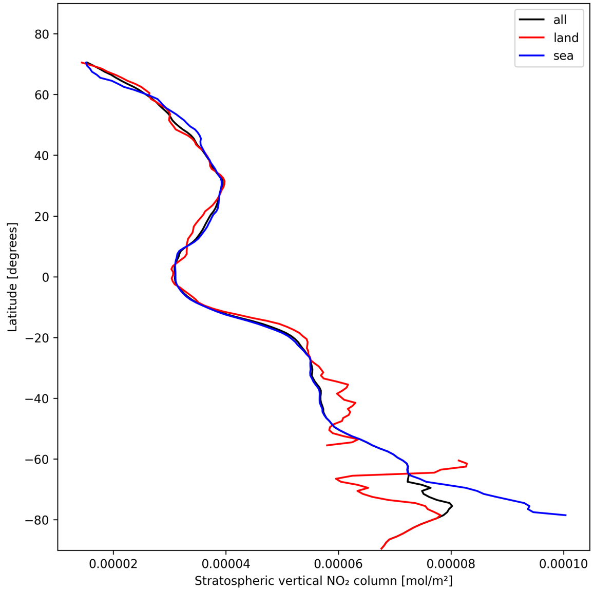
Figure 19: Zonal average of “Stratospheric vertical NO 2 column” for 2024-11-09 to 2024-11-11.
