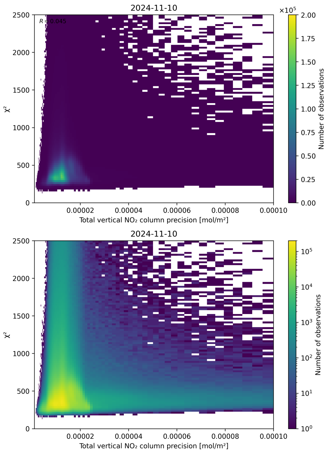
Figure 116: Scatter density plot of “Total vertical NO 2 column precision” against “ \chi^2 ” for 2024-11-09 to 2024-11-11.
