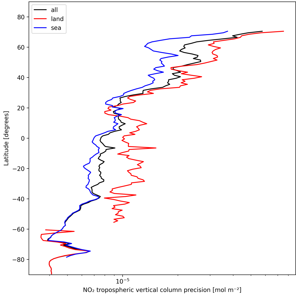
Figure 13: Zonal average of “NO 2 tropospheric vertical column precision” for 2024-11-09 to 2024-11-11.
