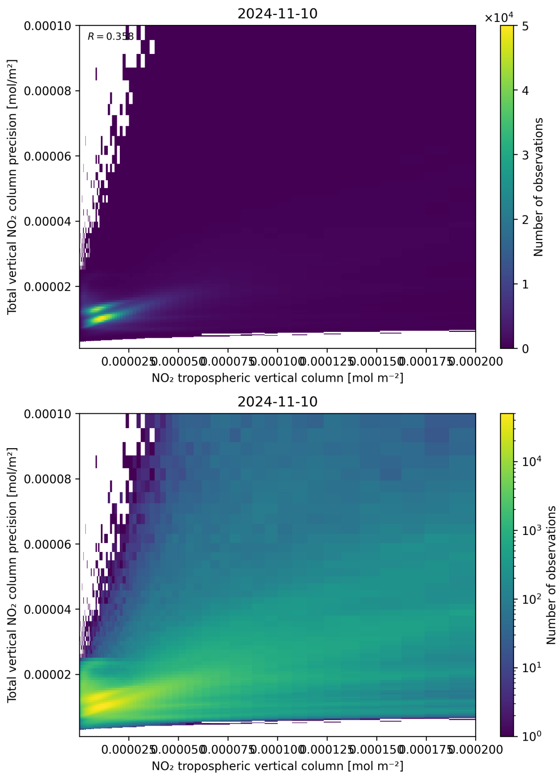
Figure 129: Scatter density plot of “NO 2 tropospheric vertical column” against “Total vertical NO 2 column precision” for 2024-11-09 to 2024-11-11.
