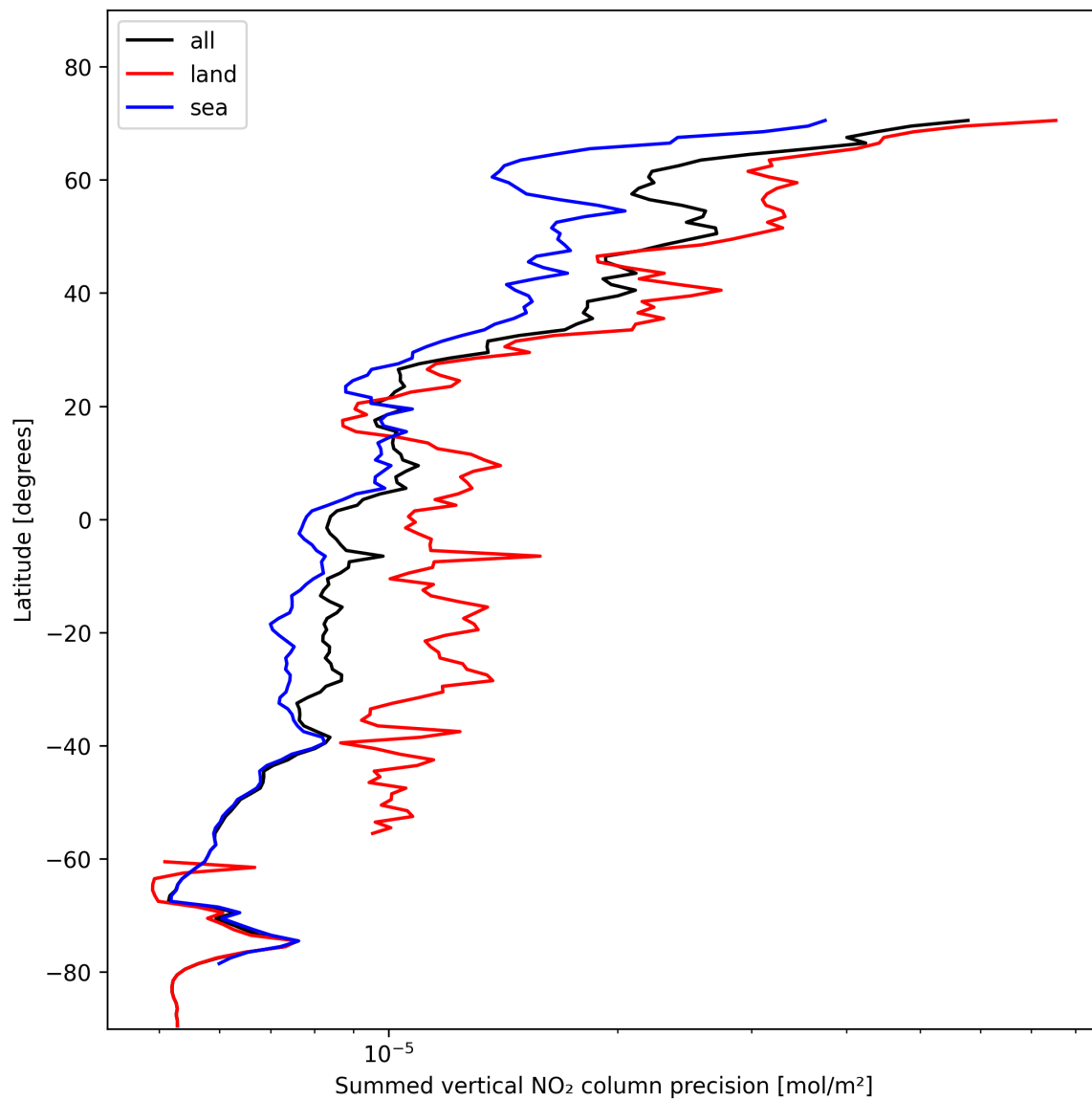
Figure 24: Zonal average of “Summed vertical NO 2 column precision” for 2024-11-09 to 2024-11-11.
