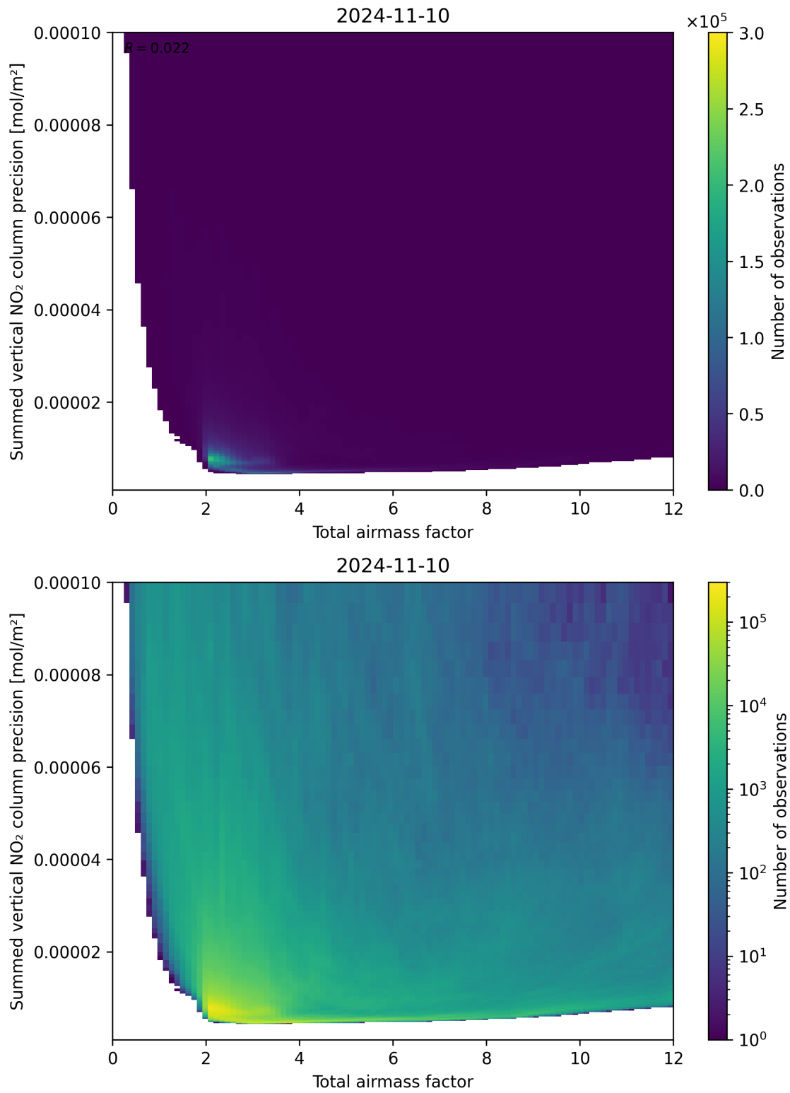
Figure 66: Scatter density plot of “Total airmass factor” against “Summed vertical NO 2 column precision” for 2024-11-09 to 2024-11-11.
