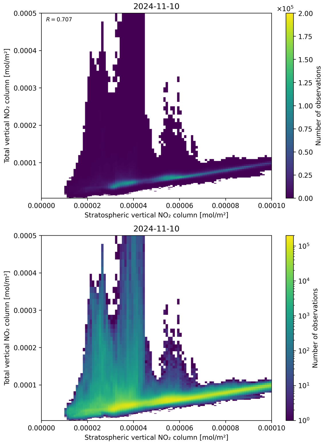
Figure 100: Scatter density plot of “Stratospheric vertical NO 2 column” against “Total vertical NO 2 column” for 2024-11-09 to 2024-11-11.
