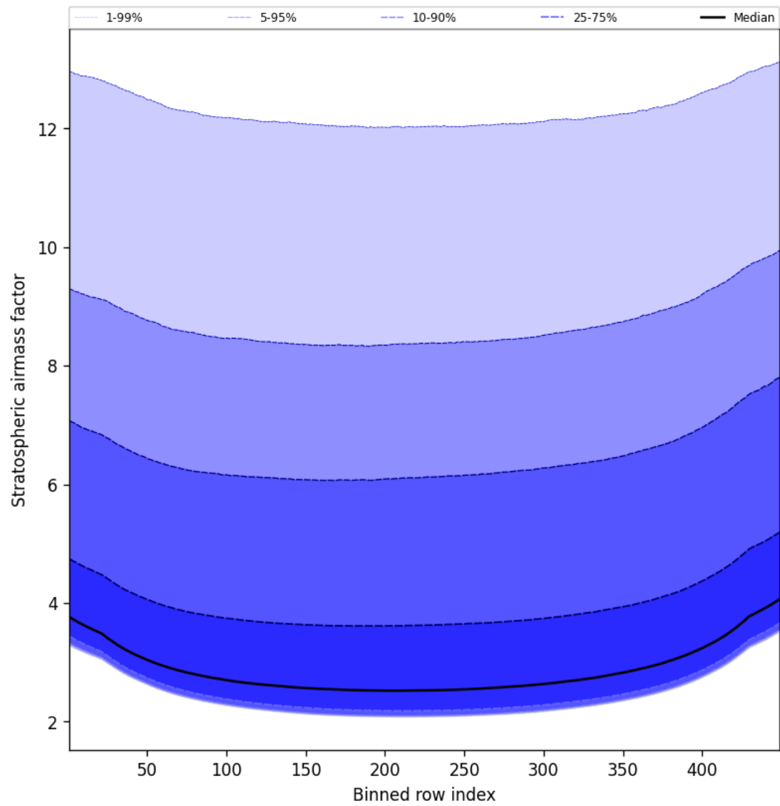
Figure 61: Along track statistics of “Stratospheric airmass factor” for 2024-11-09 to 2024-11-11
