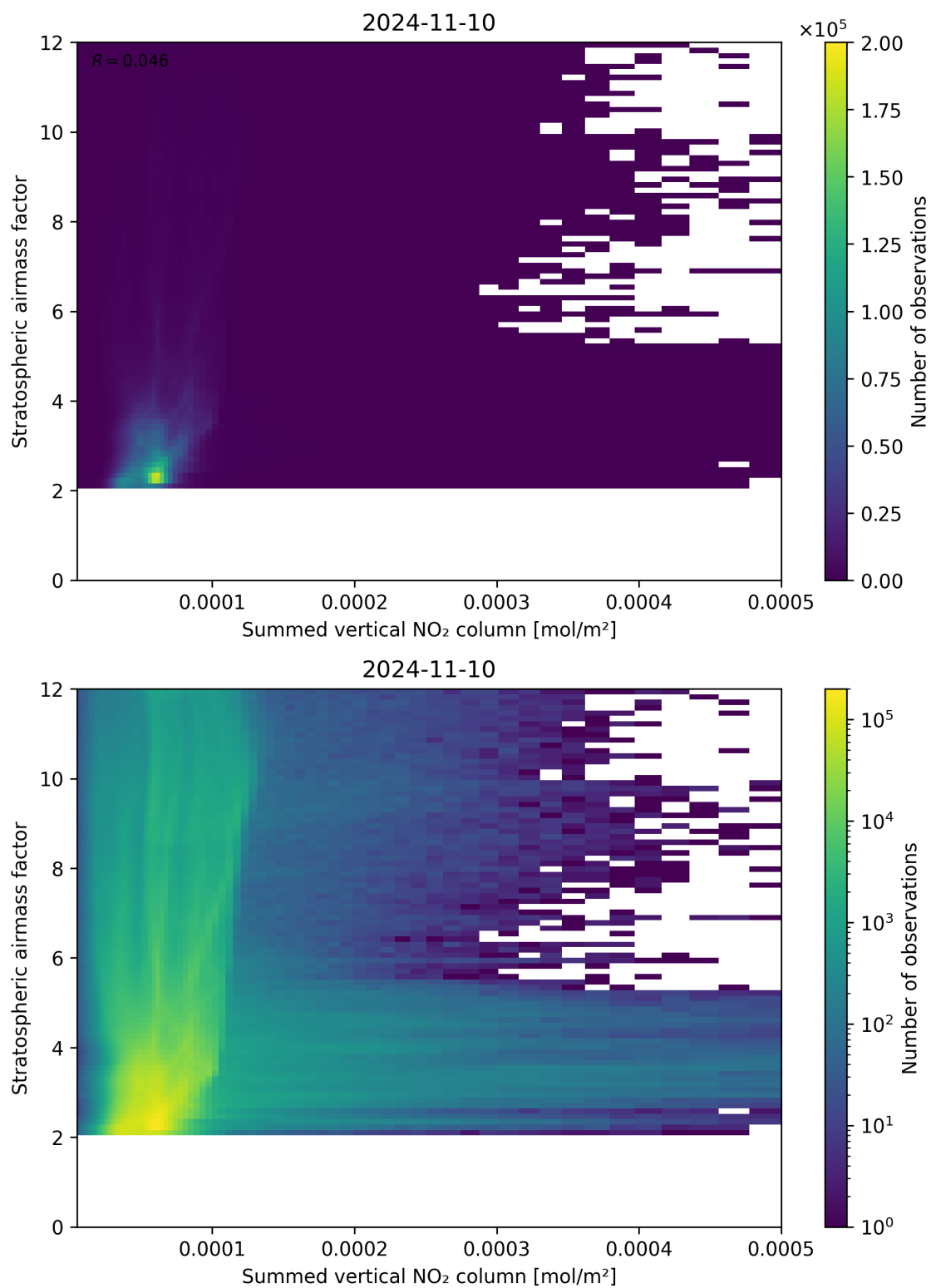
Figure 103: Scatter density plot of “Summed vertical NO 2 column” against “Stratospheric airmass factor” for 2024-11-09 to 2024-11-11.
