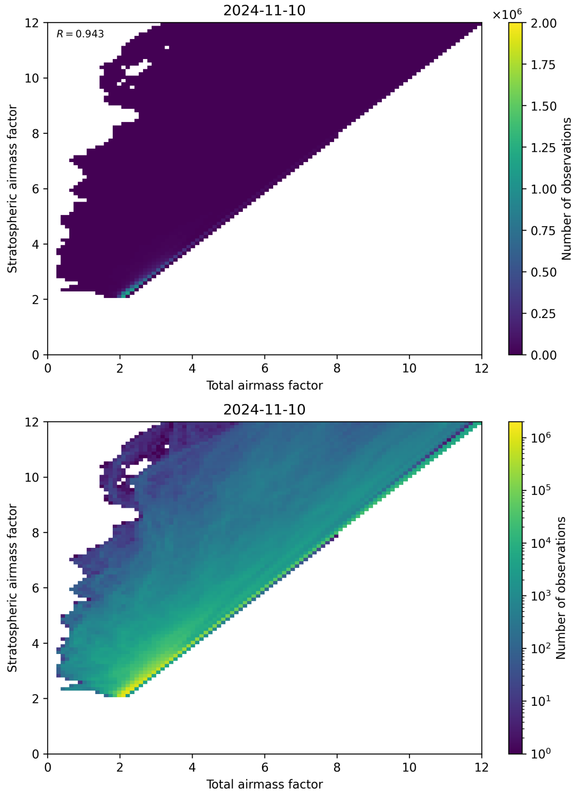
Figure 62: Scatter density plot of “Total airmass factor” against “Stratospheric airmass factor” for 2024-11-09 to 2024-11-11.
