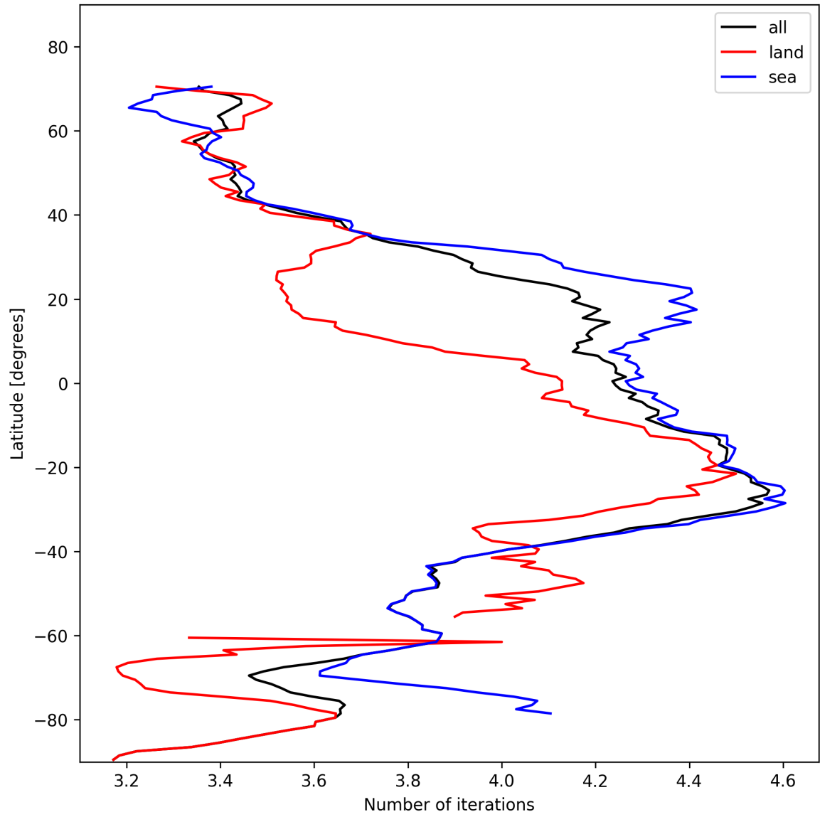
Figure 17: Zonal average of “Number of iterations” for 2024-11-09 to 2024-11-11.
