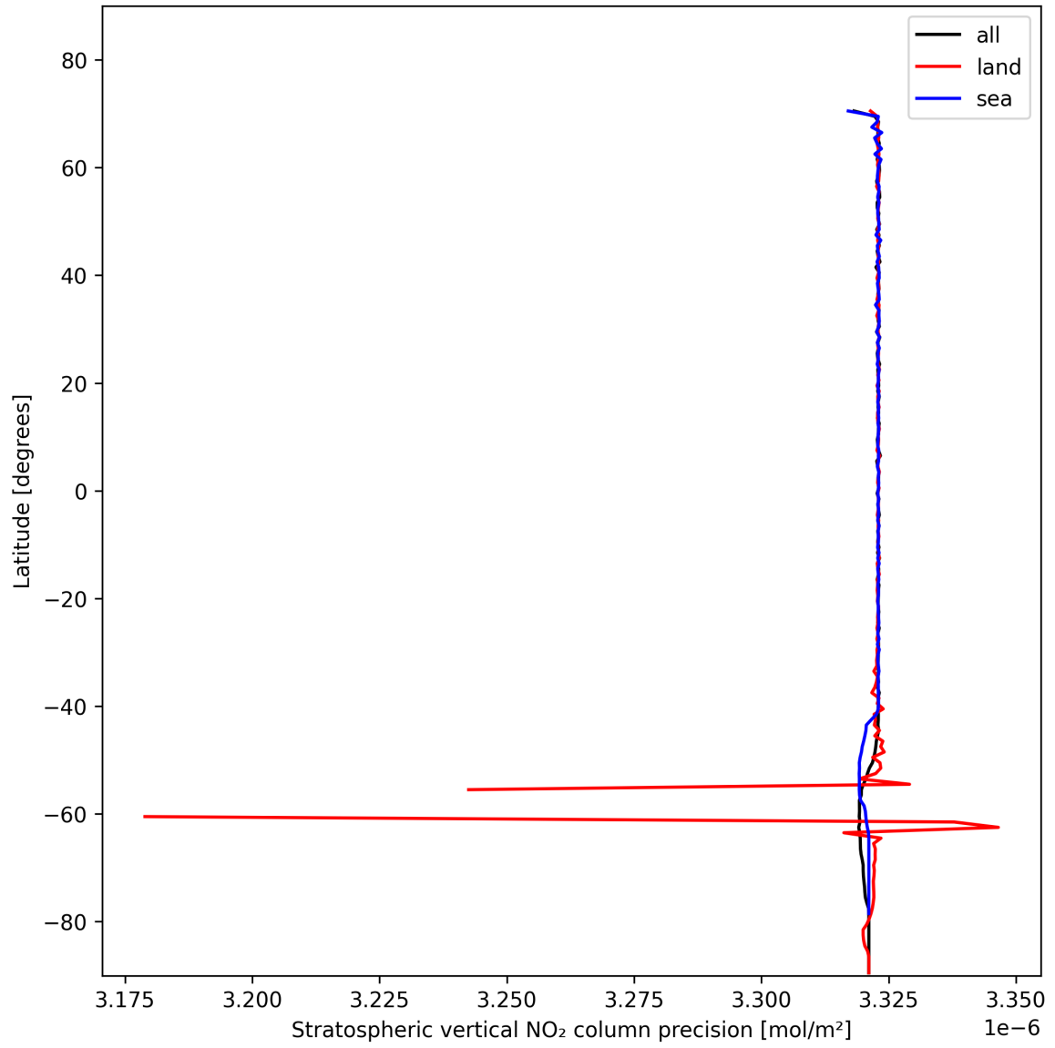
Figure 20: Zonal average of “Stratospheric vertical NO 2 column precision” for 2024-11-09 to 2024-11-11.
