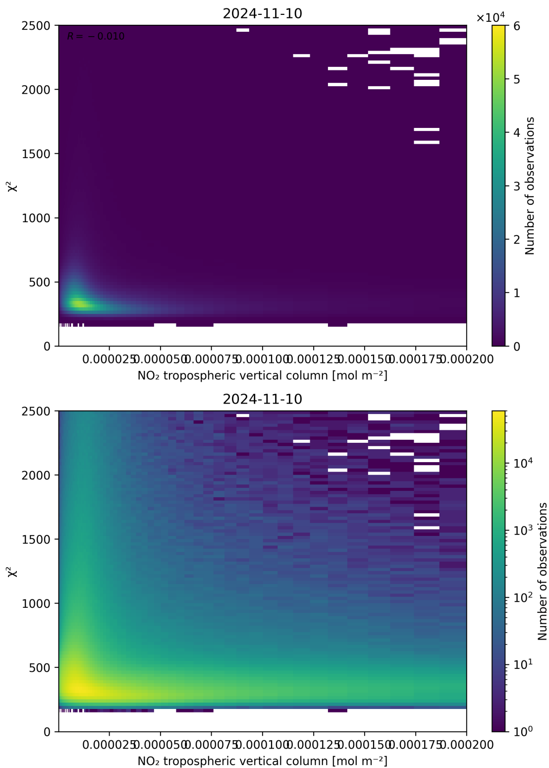
Figure 124: Scatter density plot of “NO 2 tropospheric vertical column” against “ \chi^2 ” for 2024-11-09 to 2024-11-11.
