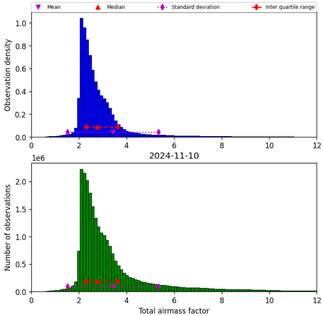
Figure 32: Histogram of “Total airmass factor” for 2024-11-09 to 2024-11-11
