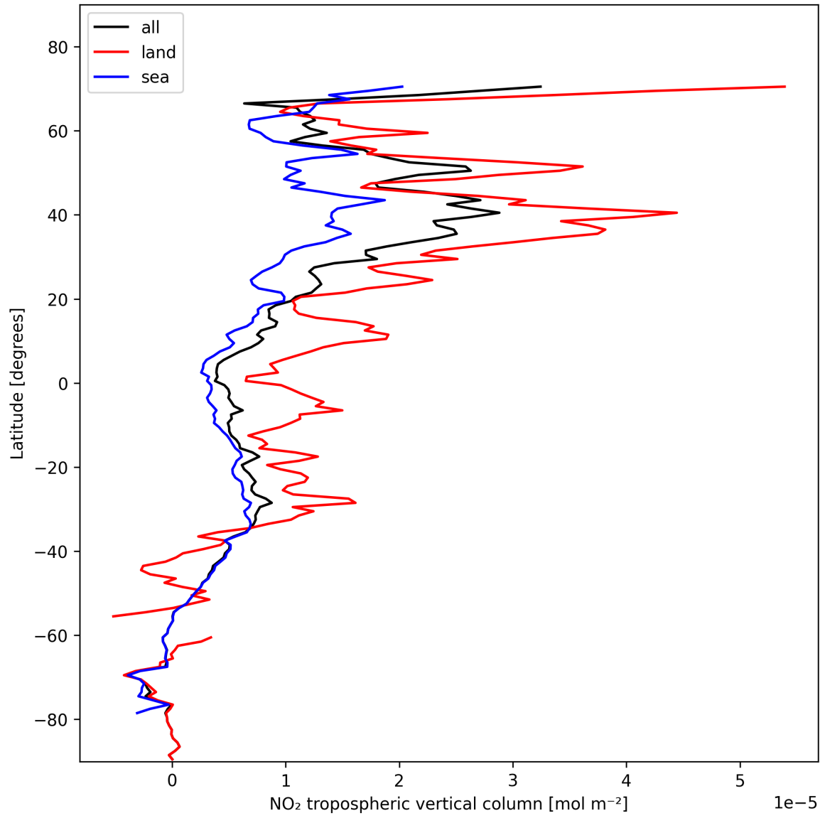
Figure 12: Zonal average of “NO 2 tropospheric vertical column” for 2024-11-09 to 2024-11-11.
