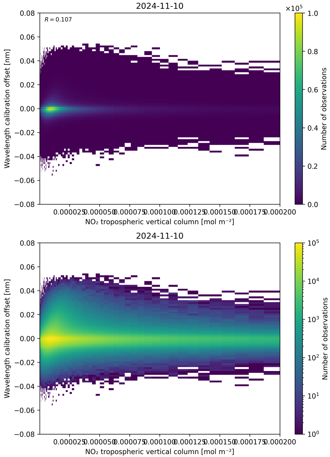
Figure 143: Scatter density plot of “NO 2 tropospheric vertical column” against “Wavelength calibration offset” for 2024-11-09 to 2024-11-11.
