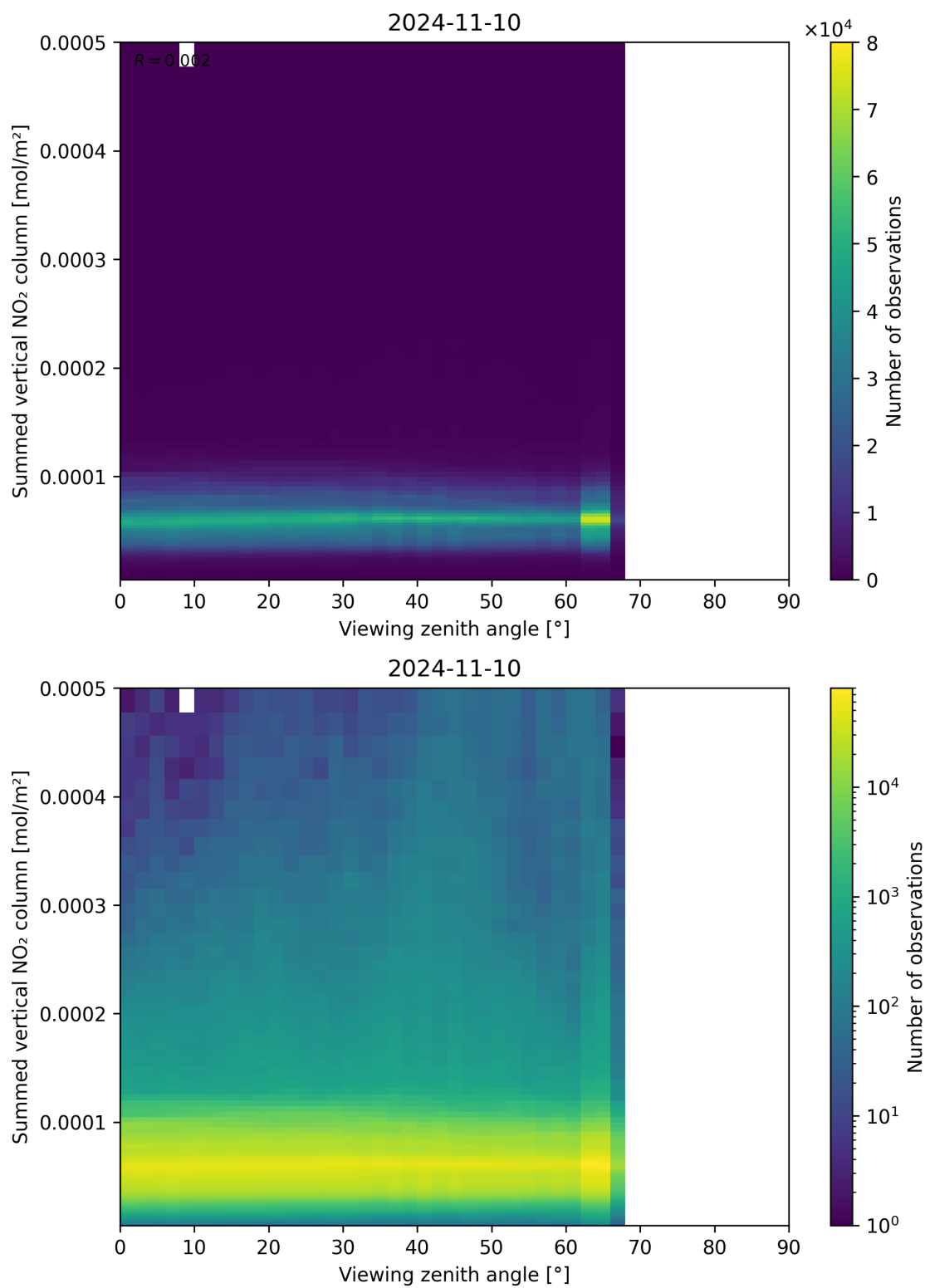
Figure 165: Scatter density plot of “Viewing zenith angle” against “Summed vertical NO 2 column” for 2024-11-09 to 2024-11-11.
