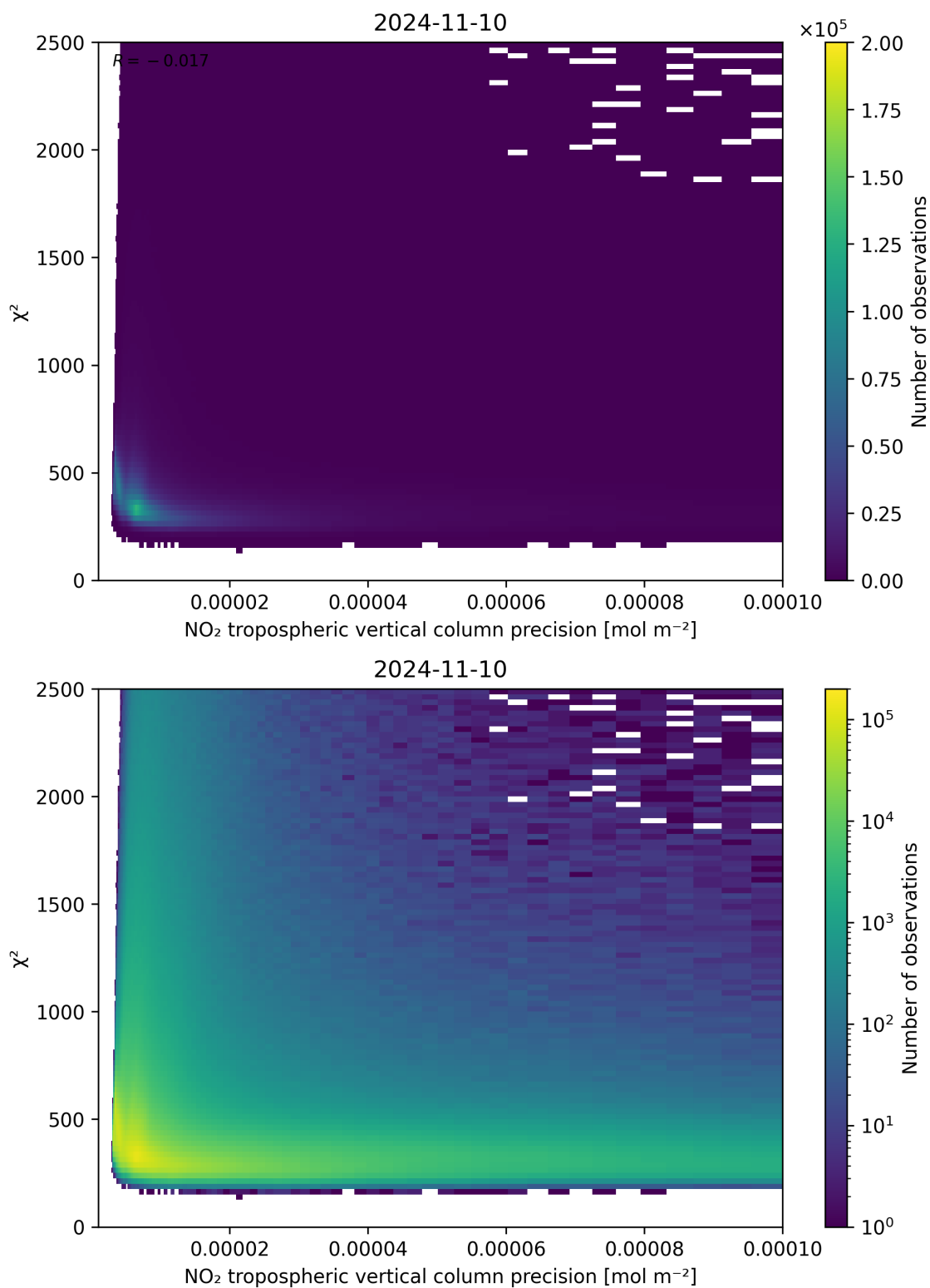
Figure 134: Scatter density plot of “NO 2 tropospheric vertical column precision” against “ \chi^2 ” for 2024-11-09 to 2024-11-11.
