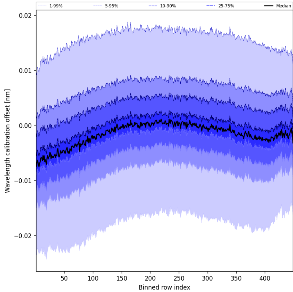
Figure 52: Along track statistics of “Wavelength calibration offset” for 2024-11-09 to 2024-11-11
