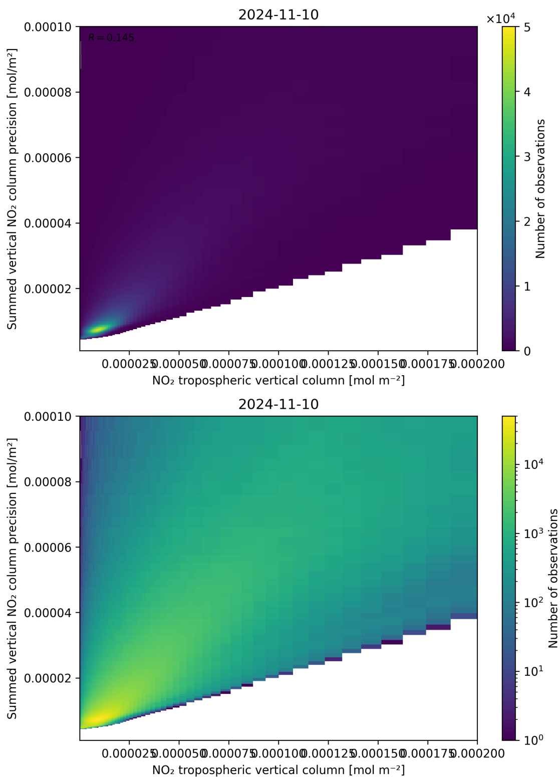
Figure 127: Scatter density plot of “NO 2 tropospheric vertical column” against “Summed vertical NO 2 column precision” for 2024-11-09 to 2024-11-11.
