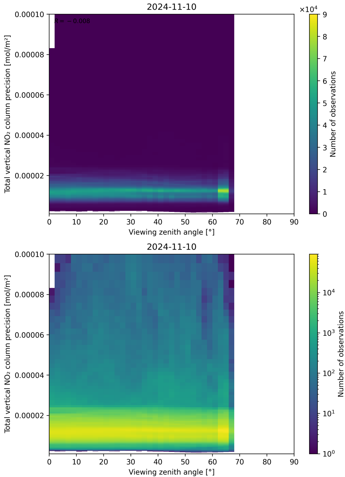
Figure 168: Scatter density plot of “Viewing zenith angle” against “Total vertical NO 2 column precision” for 2024-11-09 to 2024-11-11.
