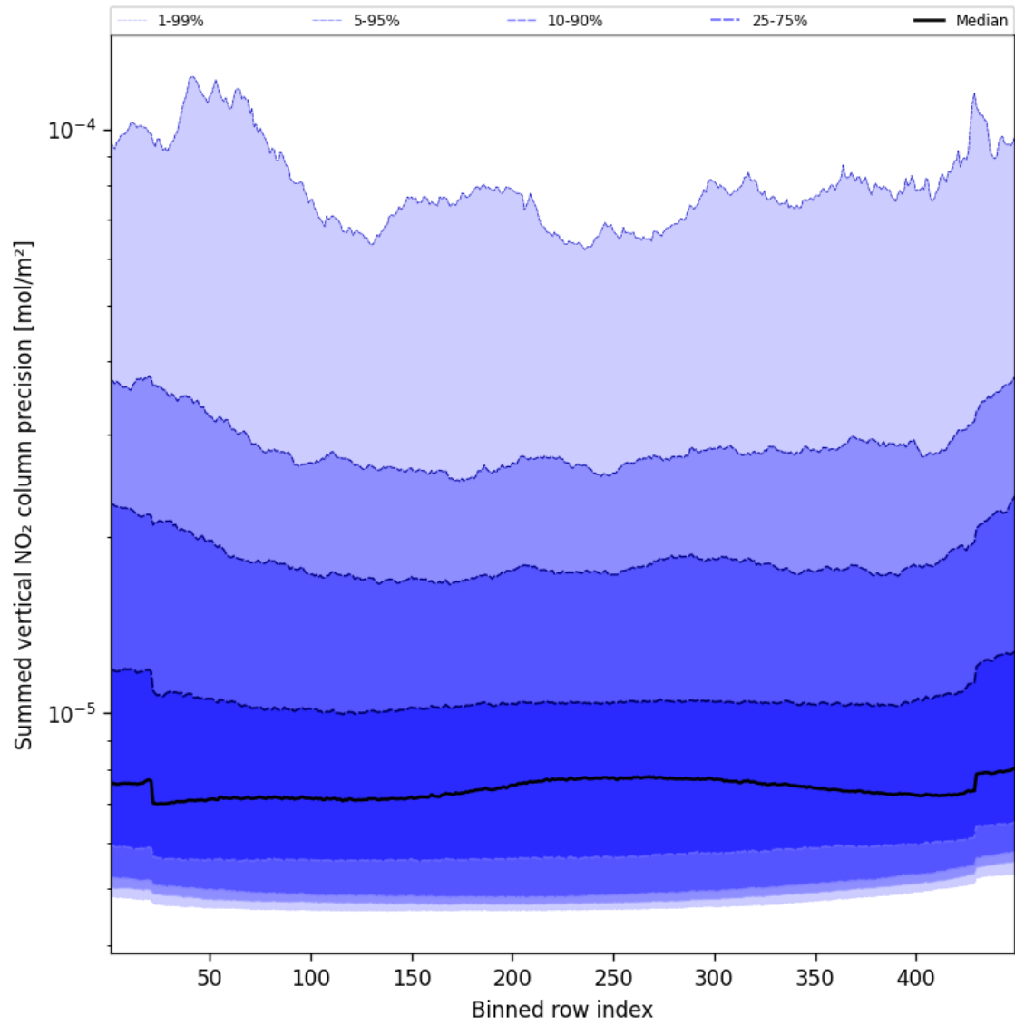
Figure 58: Along track statistics of “Summed vertical NO 2 column precision” for 2024-11-09 to 2024-11-11
