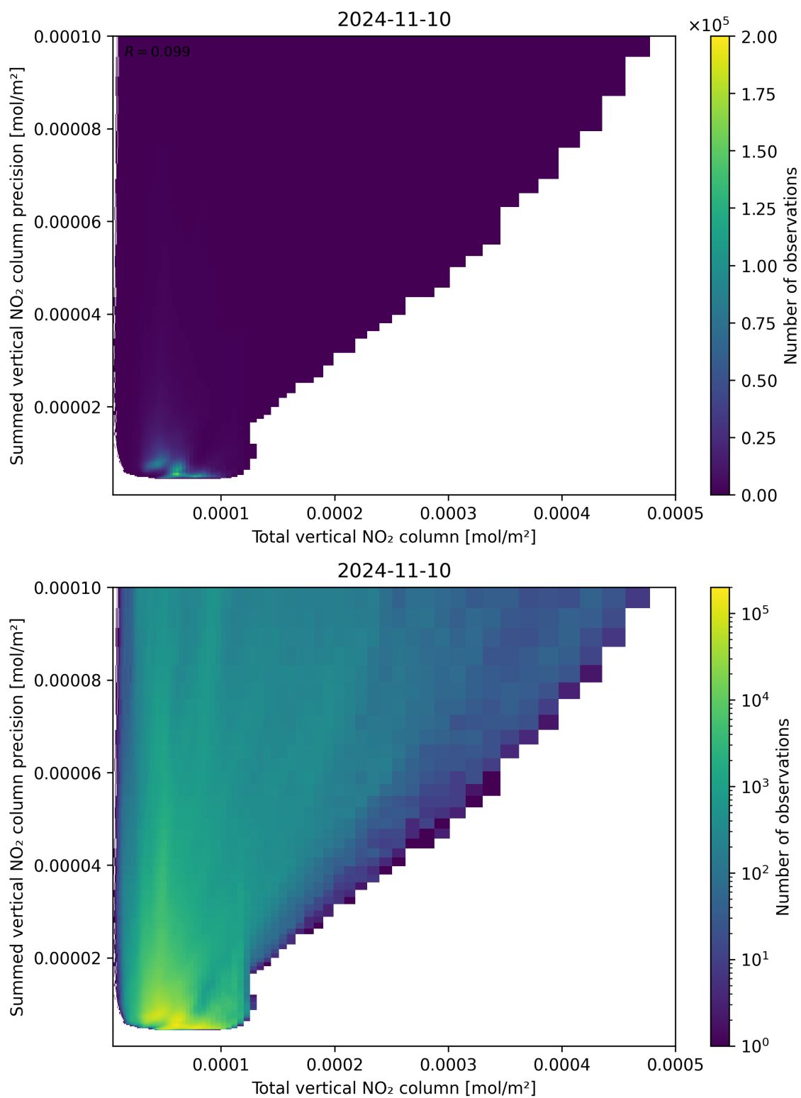
Figure 113: Scatter density plot of “Total vertical NO 2 column” against “Summed vertical NO 2 column precision” for 2024-11-09 to 2024-11-11.
