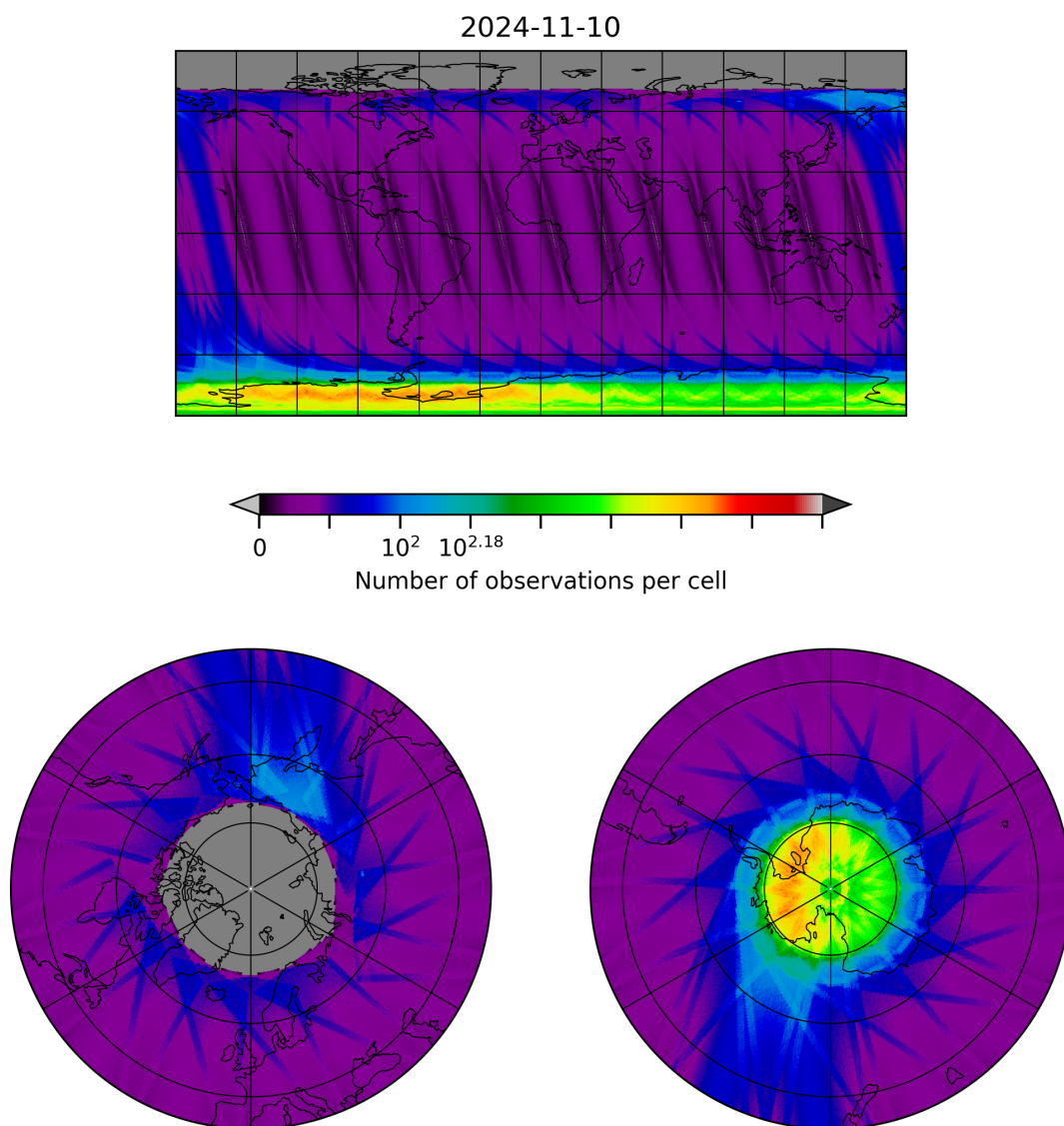
Figure 10: Map of the number of observations for 2024-11-09 to 2024-11-11
