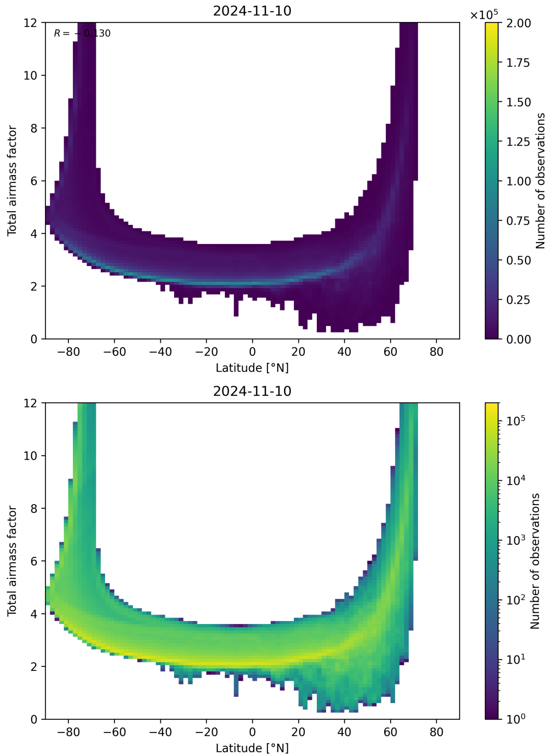
Figure 84: Scatter density plot of “Latitude” against “Total airmass factor” for 2024-11-09 to 2024-11-11.
