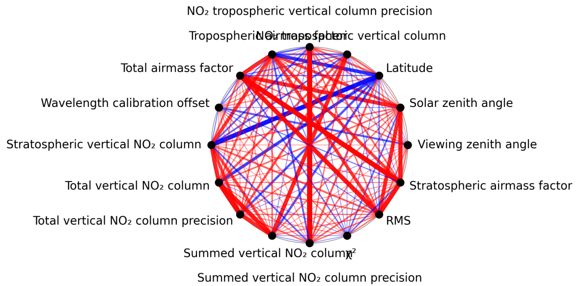
Figure 1: Map of correlation graph for 2024-11-09 to 2024-11-11.
