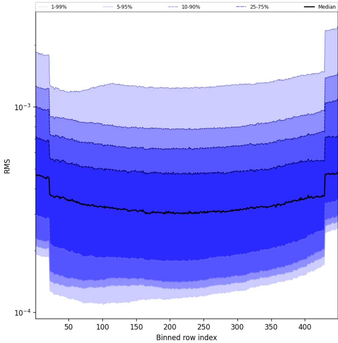
Figure 60: Along track statistics of “RMS” for 2024-11-09 to 2024-11-11
