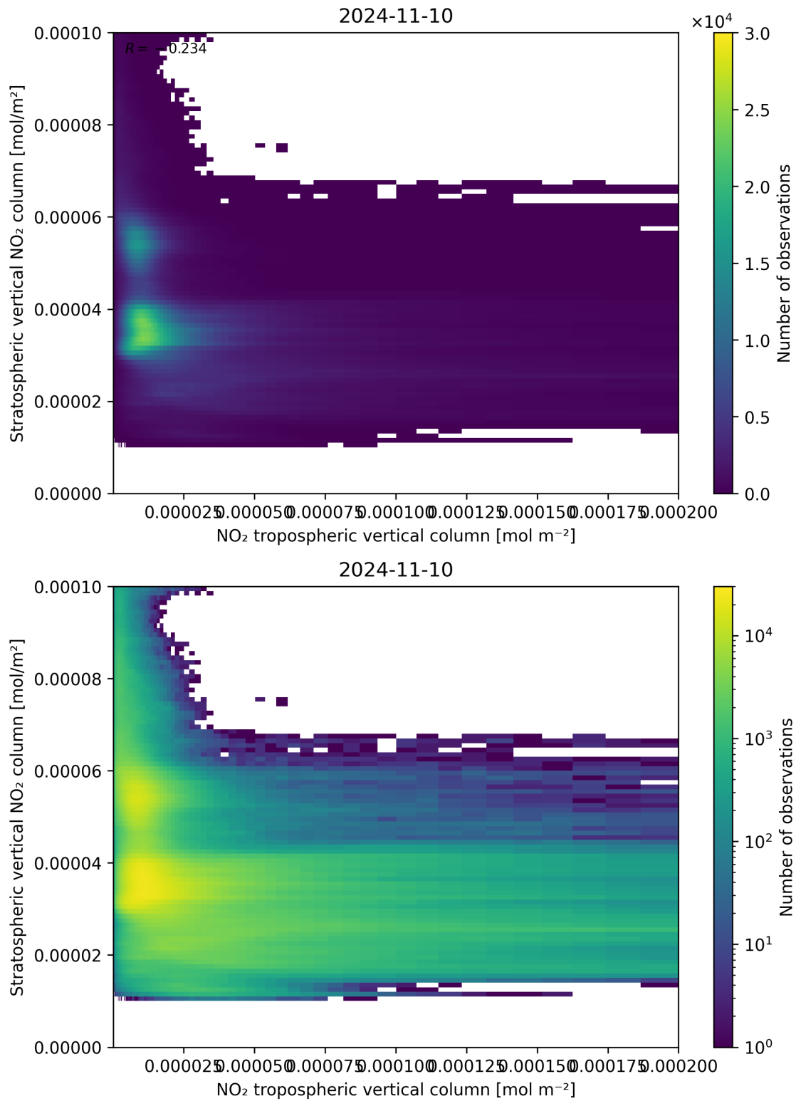
Figure 125: Scatter density plot of “NO 2 tropospheric vertical column” against “Stratospheric vertical NO 2 column” for 2024-11-09 to 2024-11-11.
