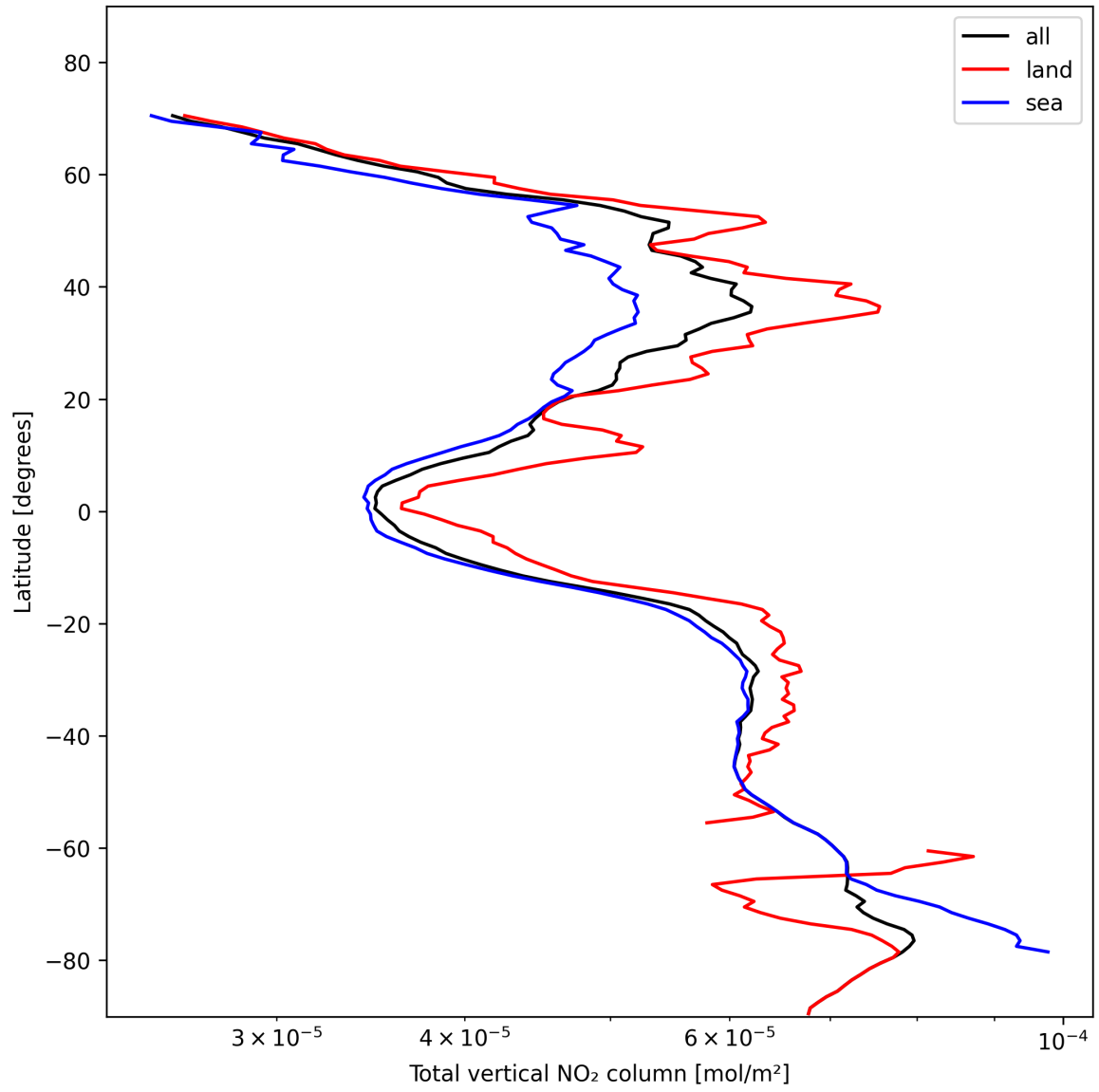
Figure 21: Zonal average of “Total vertical NO 2 column” for 2024-11-09 to 2024-11-11.
