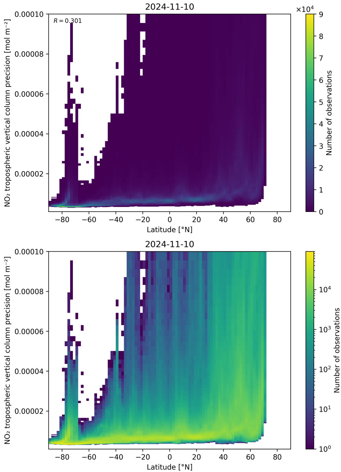
Figure 93: Scatter density plot of “Latitude” against “NO 2 tropospheric vertical column precision” for 2024-11-09 to 2024-11-11.
