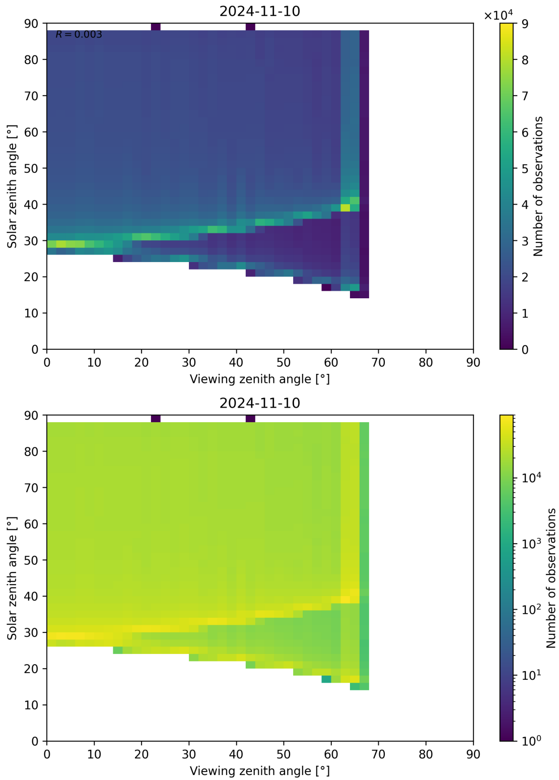
Figure 172: Scatter density plot of “Viewing zenith angle” against “Solar zenith angle” for 2024-11-09 to 2024-11-11.
