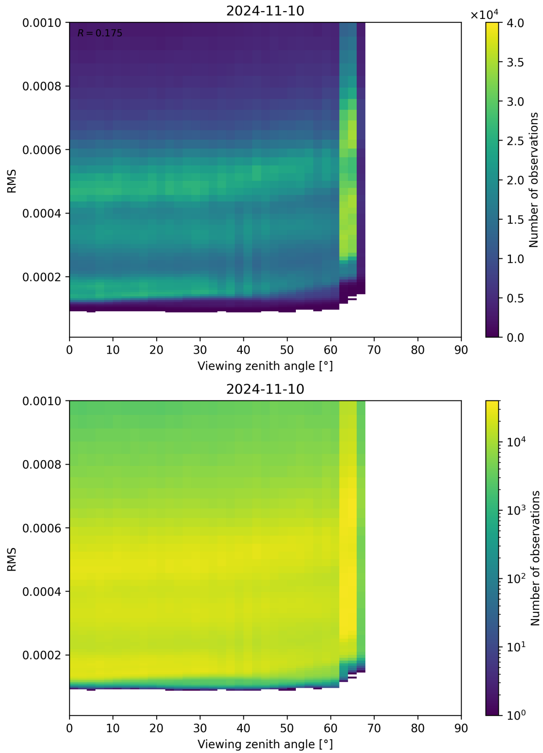
Figure 171: Scatter density plot of “Viewing zenith angle” against “RMS” for 2024-11-09 to 2024-11-11.
