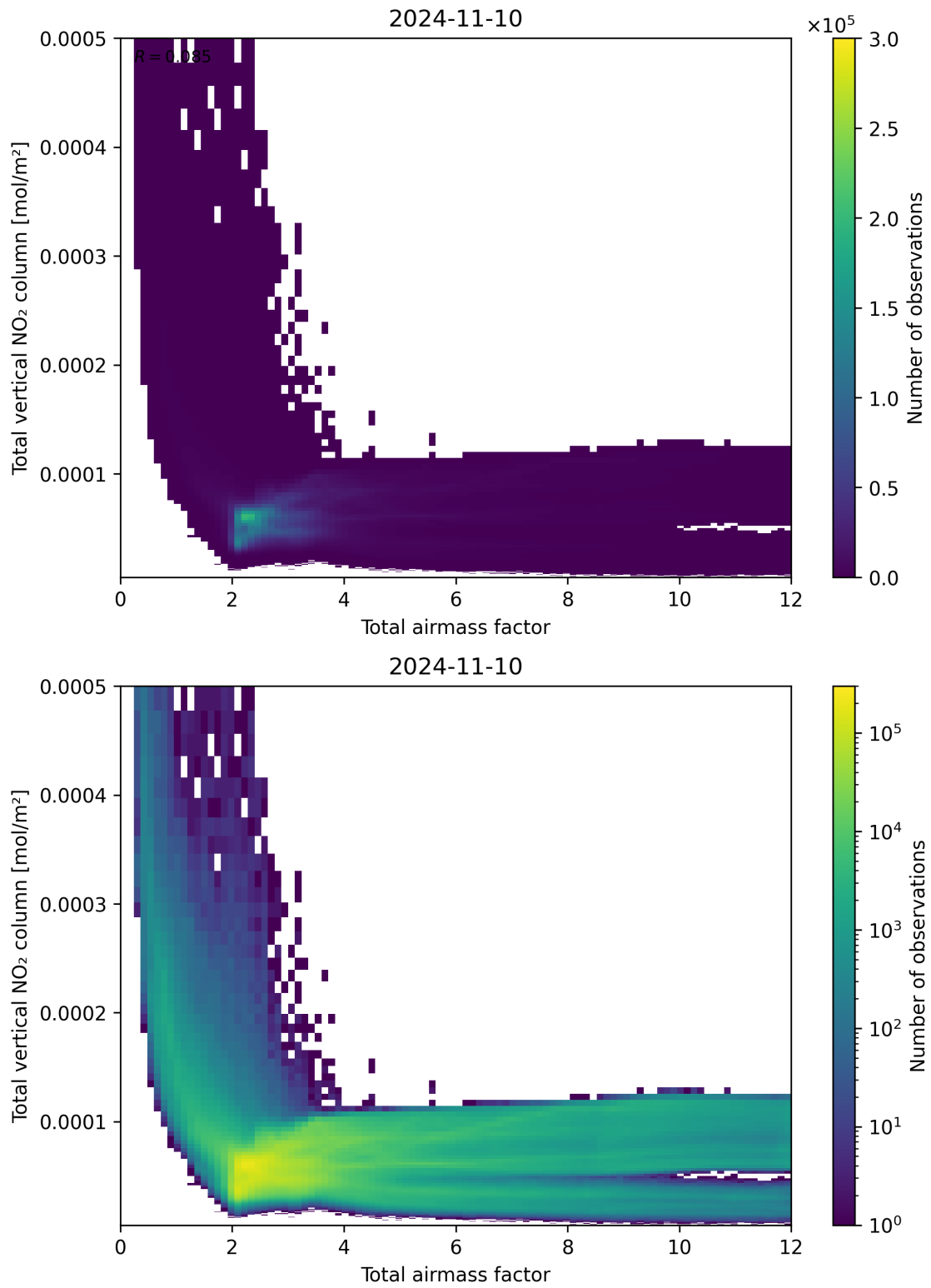
Figure 67: Scatter density plot of “Total airmass factor” against “Total vertical NO 2 column” for 2024-11-09 to 2024-11-11.
