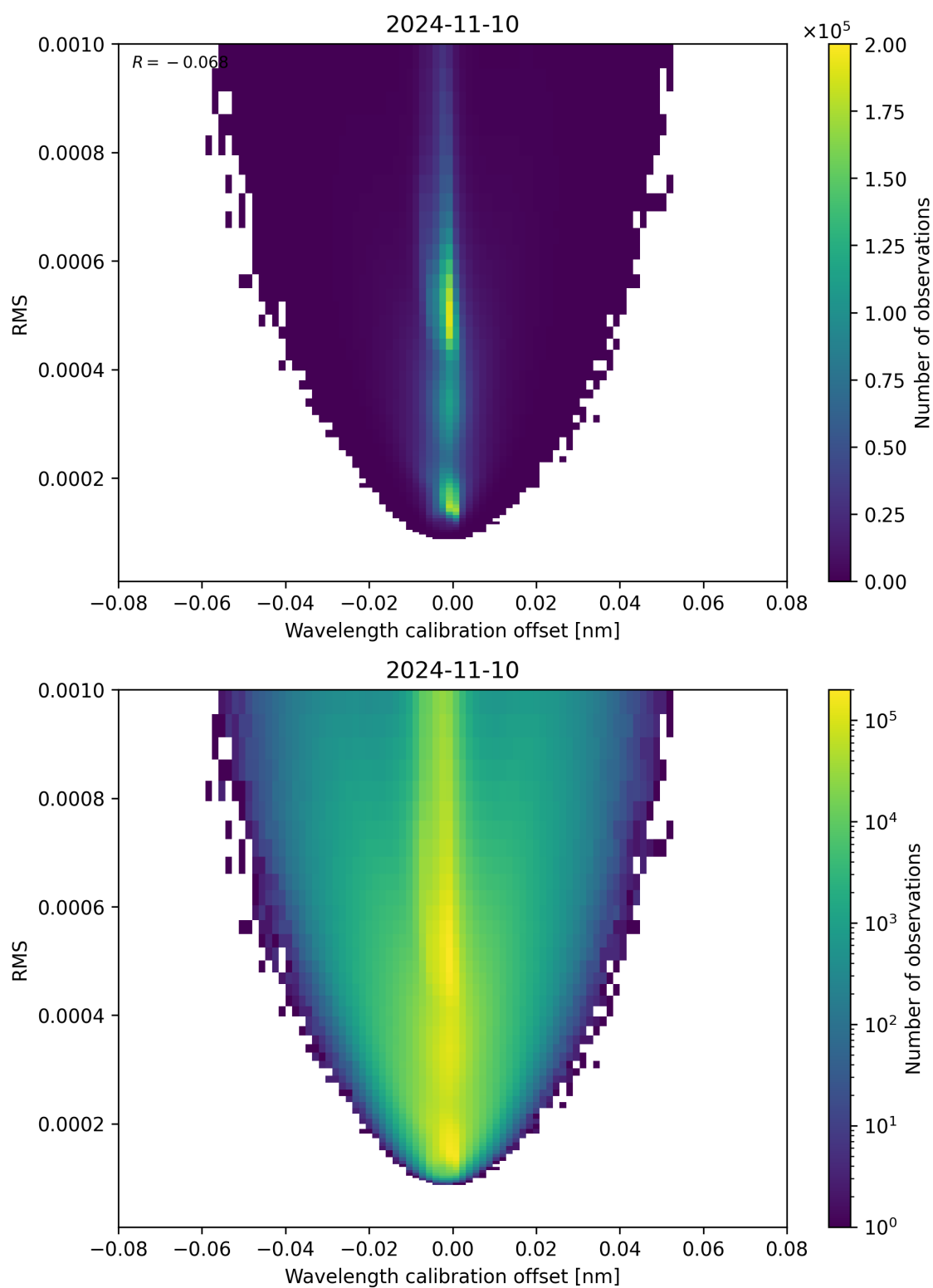
Figure 181: Scatter density plot of “Wavelength calibration offset” against “RMS” for 2024-11-09 to 2024-11-11.
