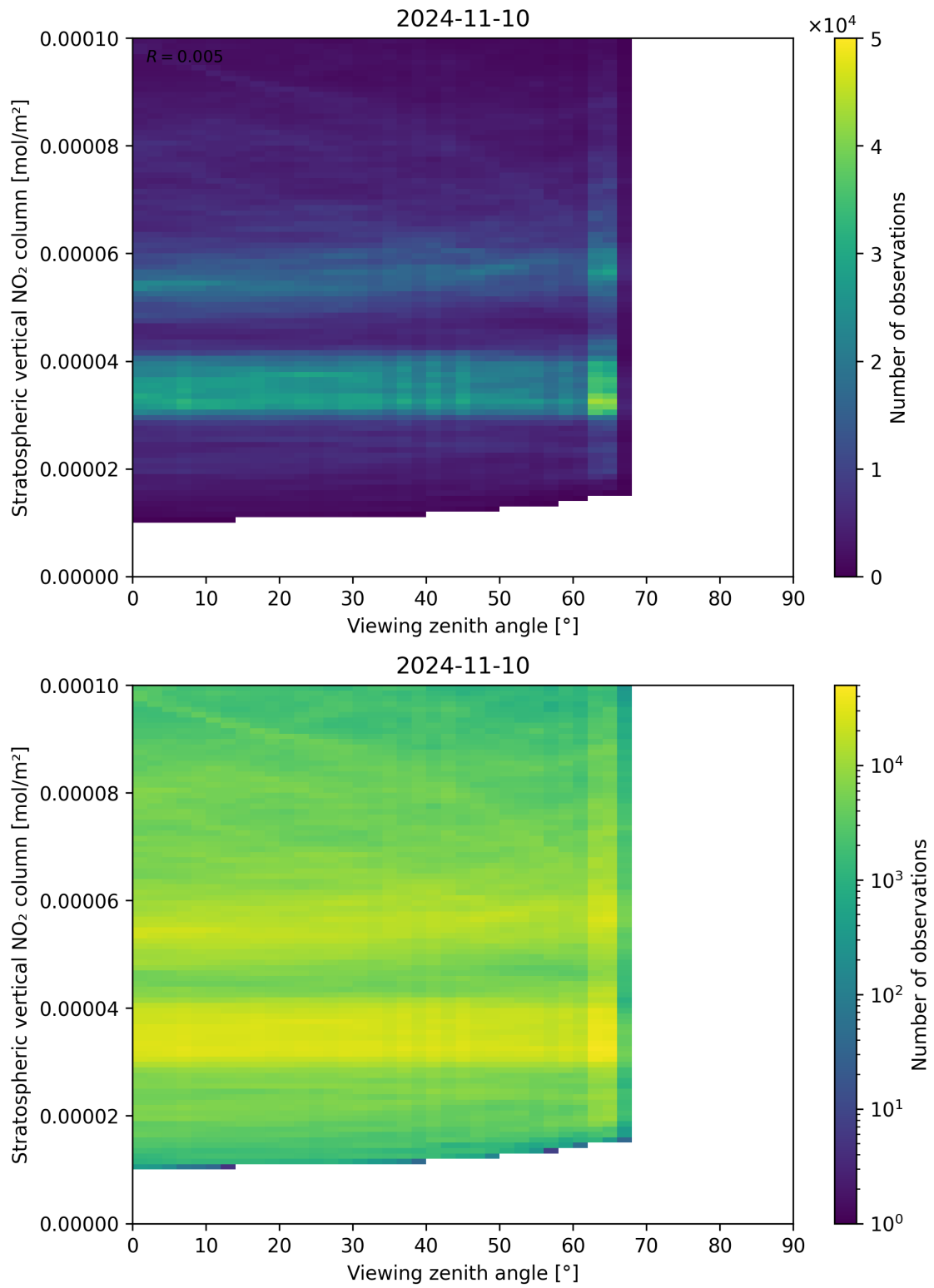
Figure 164: Scatter density plot of “Viewing zenith angle” against “Stratospheric vertical NO 2 column” for 2024-11-09 to 2024-11-11.
