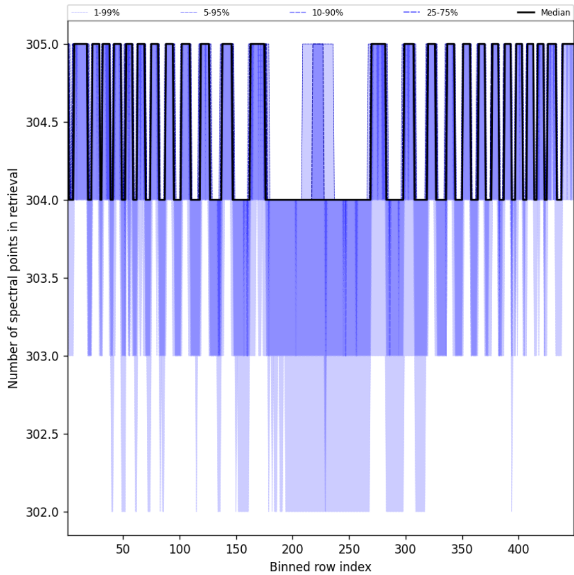
Figure 50: Along track statistics of “Number of spectral points in retrieval” for 2024-11-09 to 2024-11-11
