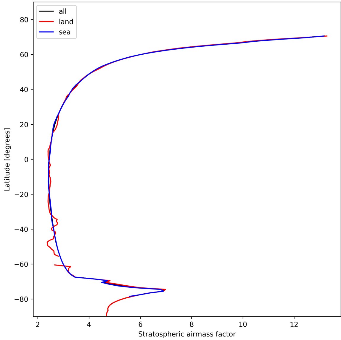
Figure 27: Zonal average of “Stratospheric air mass factor” for 2024-11-09 to 2024-11-11.
