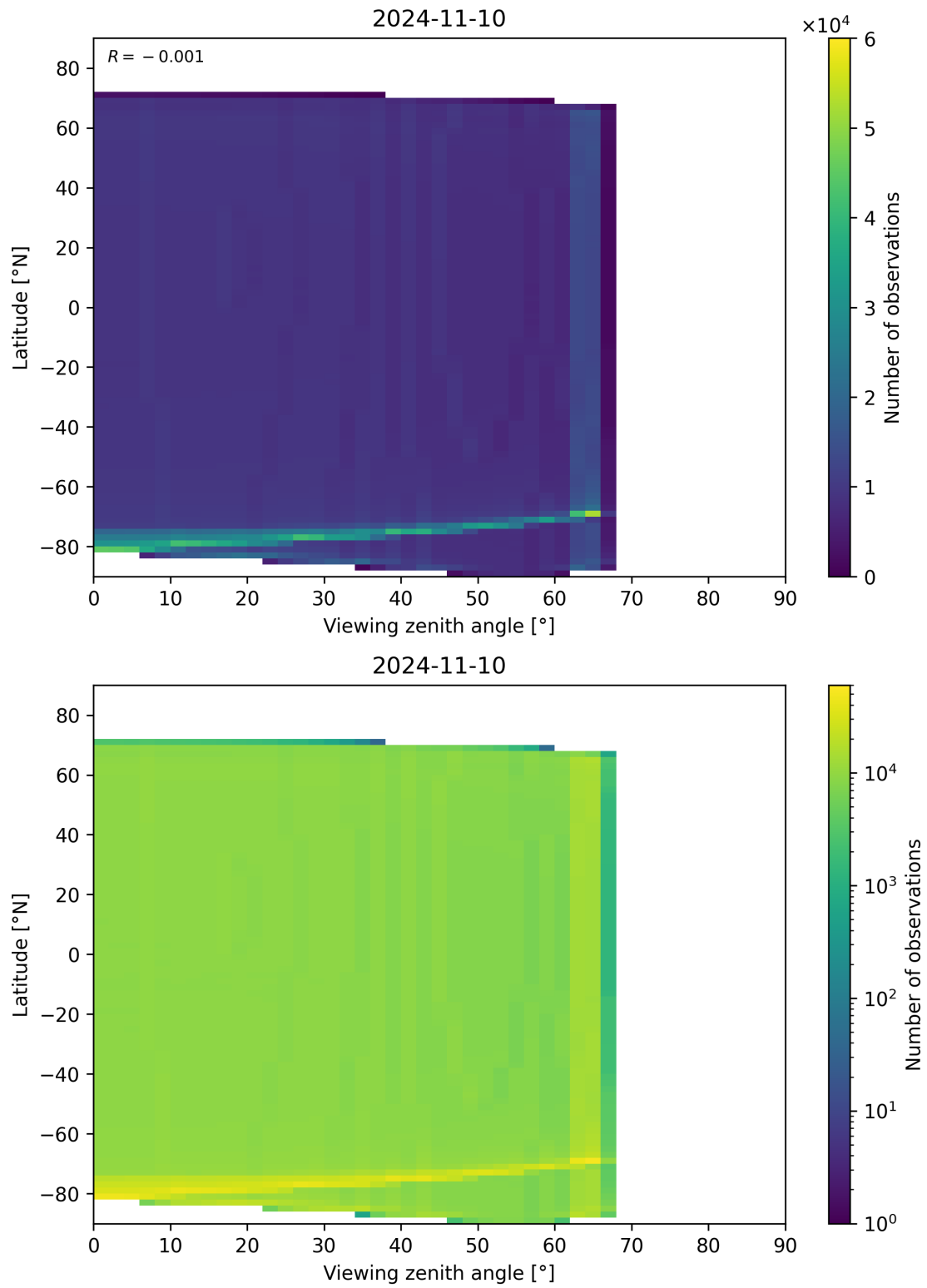
Figure 163: Scatter density plot of “Viewing zenith angle” against “Latitude” for 2024-11-09 to 2024-11-11.
