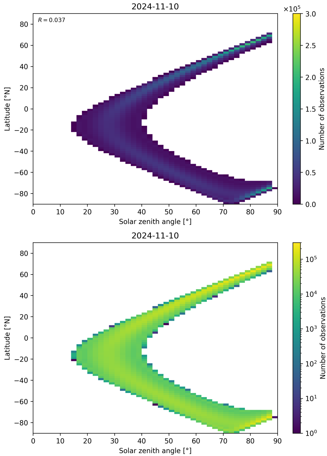
Figure 149: Scatter density plot of “Solar zenith angle” against “Latitude” for 2024-11-09 to 2024-11-11.
