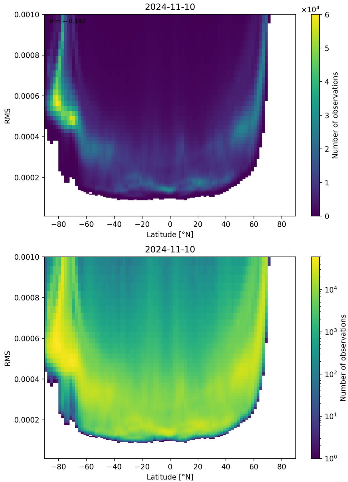
Figure 94: Scatter density plot of “Latitude” against “RMS” for 2024-11-09 to 2024-11-11.
