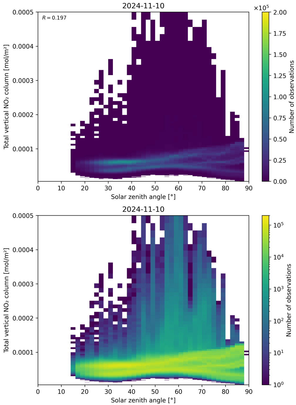
Figure 153: Scatter density plot of “Solar zenith angle” against “Total vertical NO 2 column” for 2024-11-09 to 2024-11-11.
