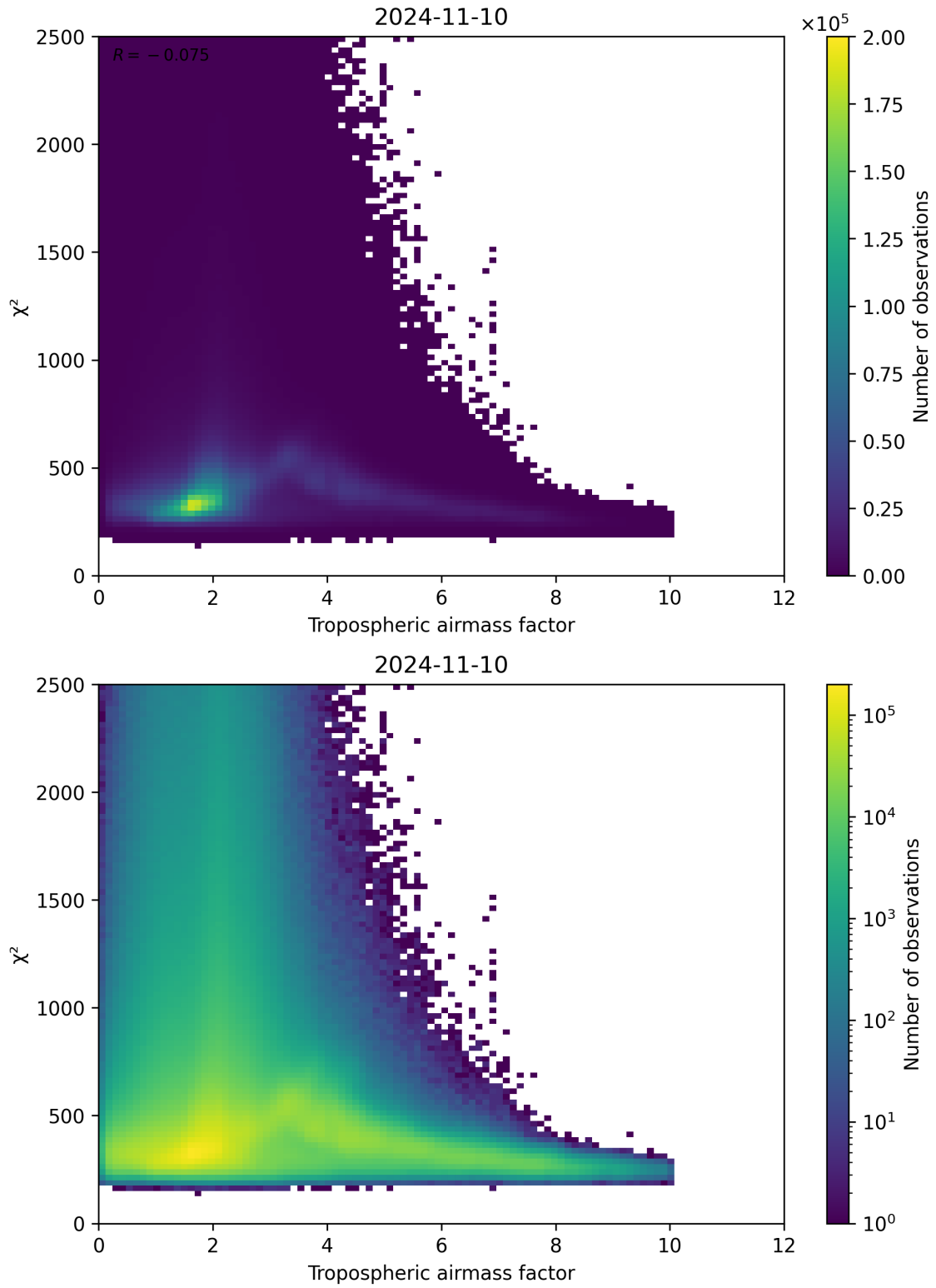
Figure 73: Scatter density plot of “Tropospheric airmass factor” against “ \chi^2 ” for 2024-11-09 to 2024-11-11.
