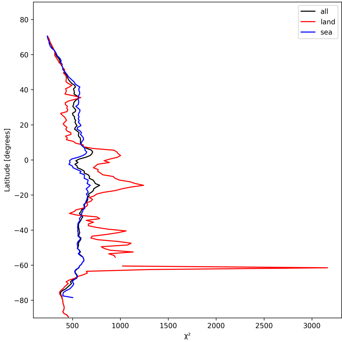
Figure 25: Zonal average of “ \chi^2 ” for 2024-11-09 to 2024-11-11.
