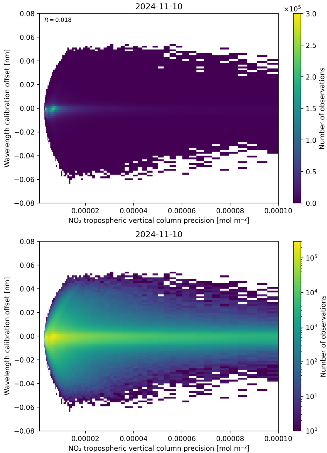
Figure 141: Scatter density plot of “NO 2 tropospheric vertical column precision” against “Wavelength calibration offset” for 2024-11-09 to 2024-11-11.
