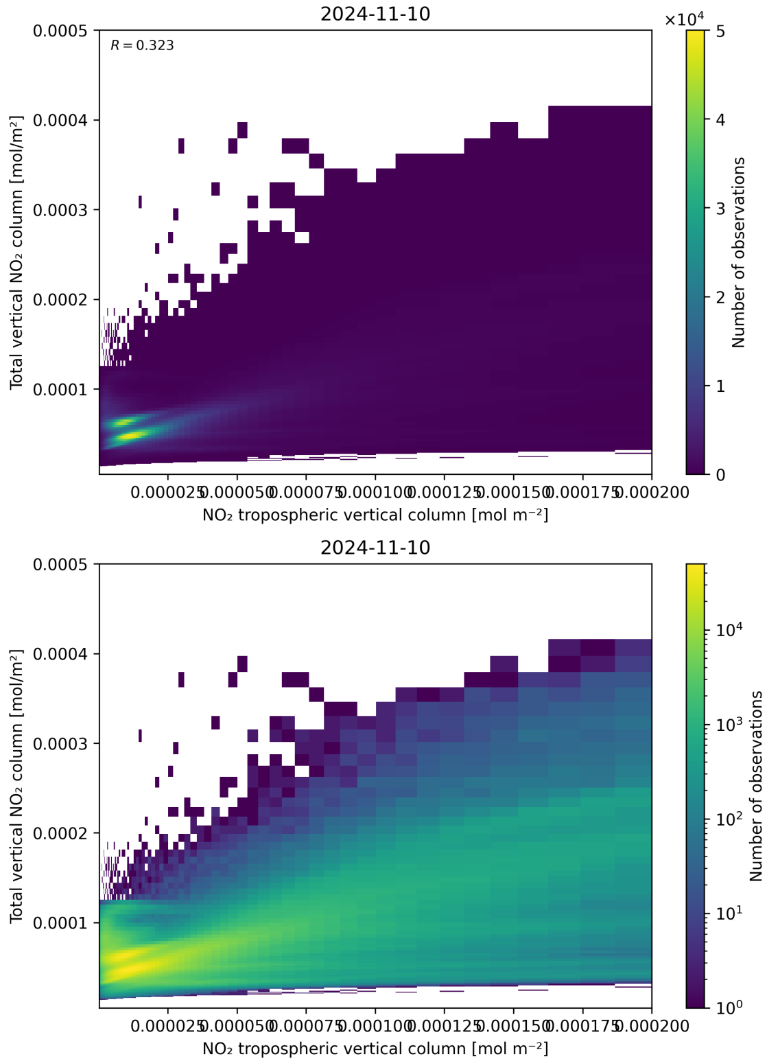
Figure 128: Scatter density plot of “NO 2 tropospheric vertical column” against “Total vertical NO 2 column” for 2024-11-09 to 2024-11-11.
