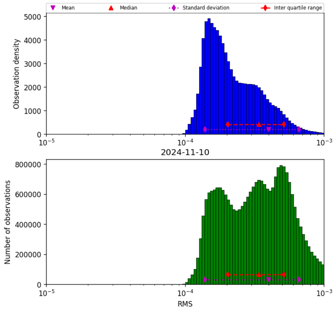
Figure 43: Histogram of “RMS” for 2024-11-09 to 2024-11-11
