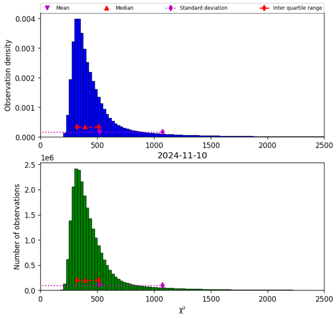
Figure 42: Histogram of “ \chi^2 ” for 2024-11-09 to 2024-11-11
