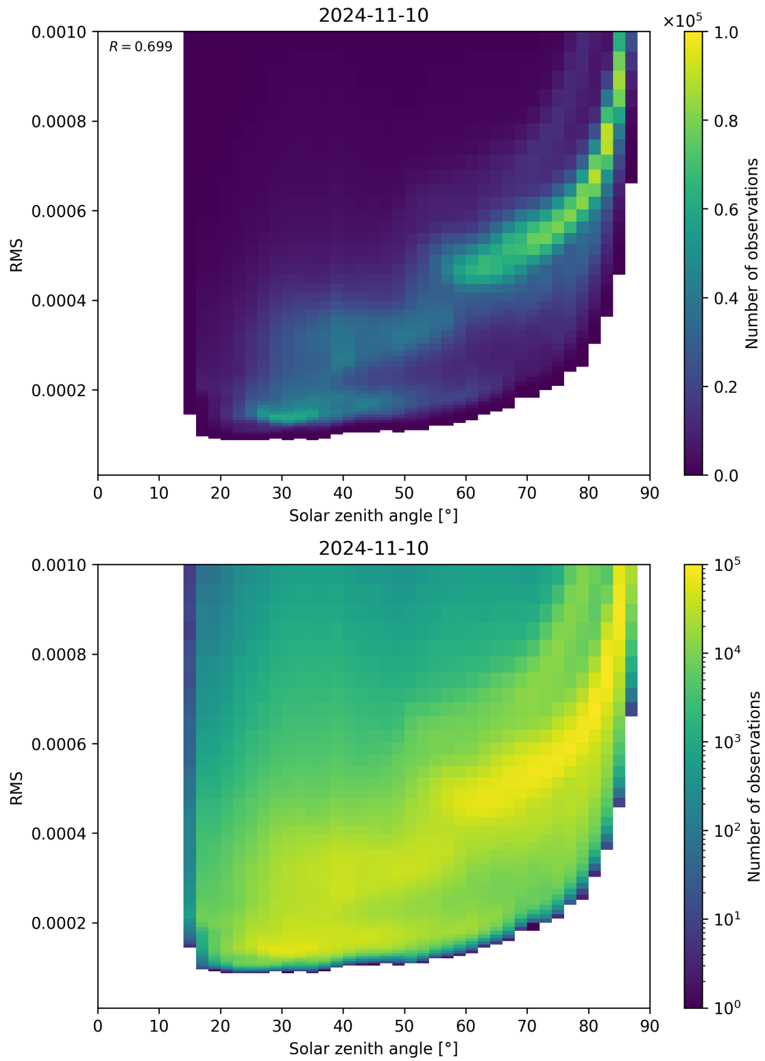
Figure 157: Scatter density plot of “Solar zenith angle” against “RMS” for 2024-11-09 to 2024-11-11.
