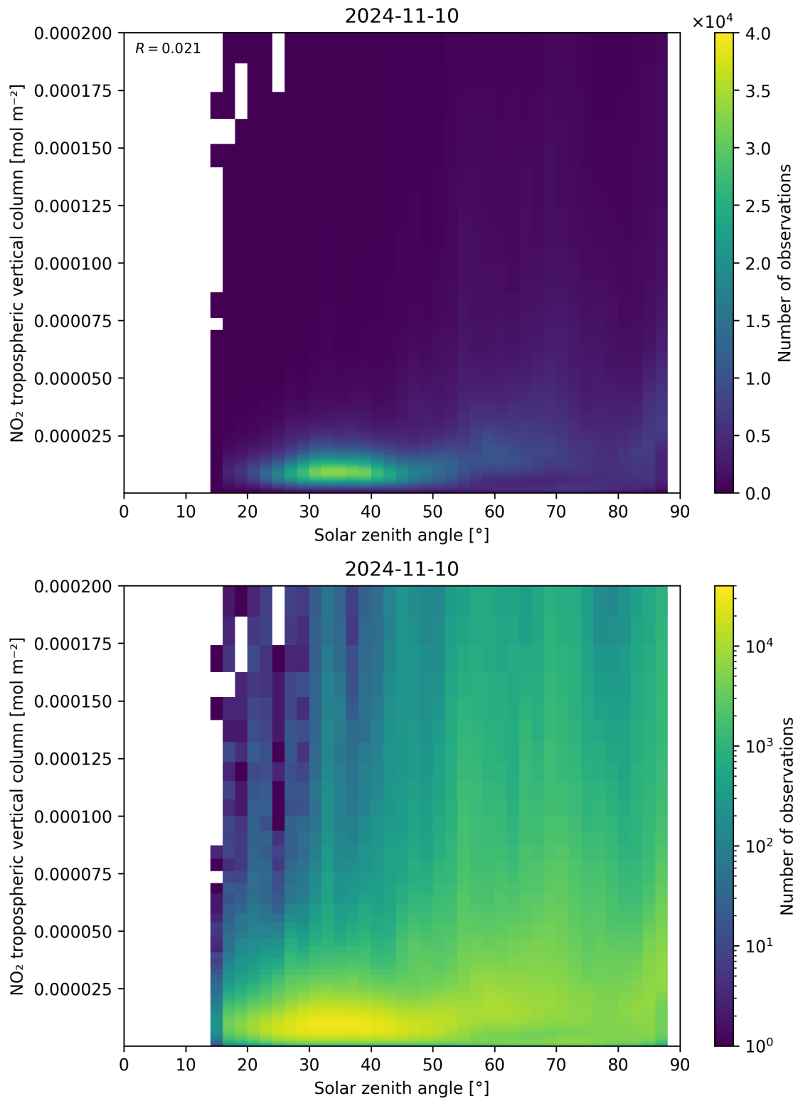
Figure 155: Scatter density plot of “Solar zenith angle” against “NO 2 tropospheric vertical column” for 2024-11-09 to 2024-11-11.
