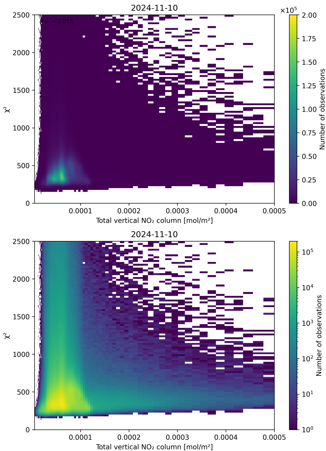
Figure 111: Scatter density plot of “Total vertical NO 2 column” against “ \chi^2 ” for 2024-11-09 to 2024-11-11.
