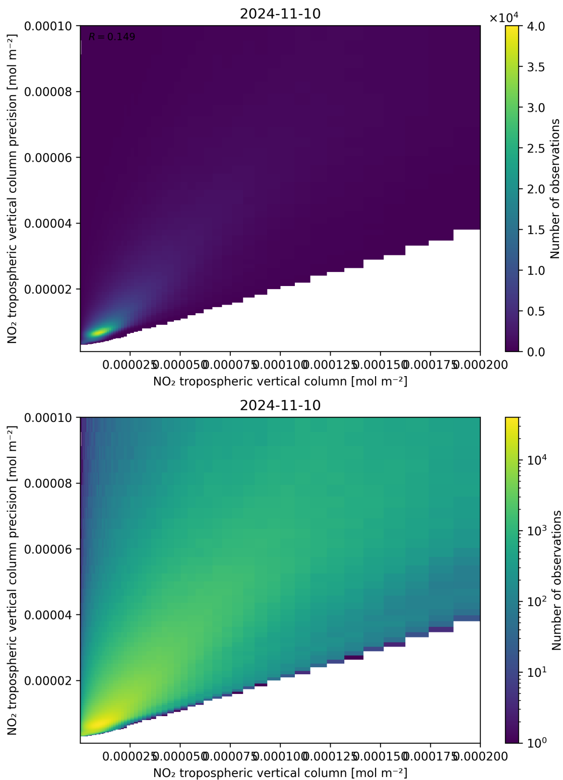
Figure 130: Scatter density plot of “NO 2 tropospheric vertical column” against “NO 2 tropospheric vertical column precision” for 2024-11-09 to 2024-11-11.
