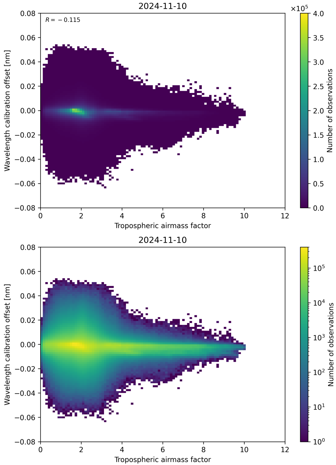
Figure 80: Scatter density plot of “Tropospheric airmass factor” against “Wavelength calibration offset” for 2024-11-09 to 2024-11-11.
