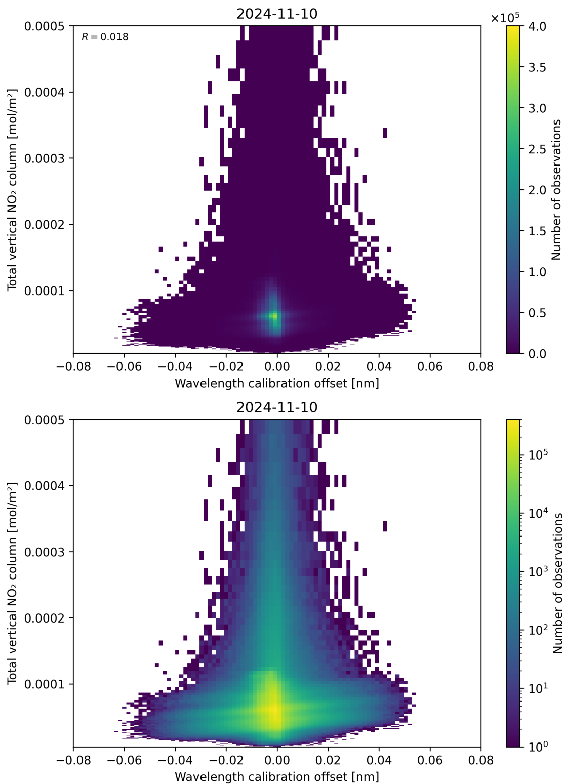
Figure 179: Scatter density plot of “Wavelength calibration offset” against “Total vertical NO 2 column” for 2024-11-09 to 2024-11-11.
