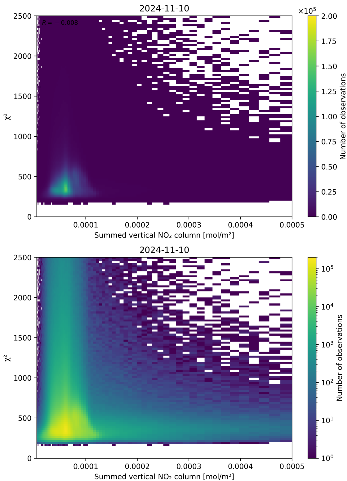
Figure 104: Scatter density plot of “Summed vertical NO 2 column” against “ \chi^2 ” for 2024-11-09 to 2024-11-11.
