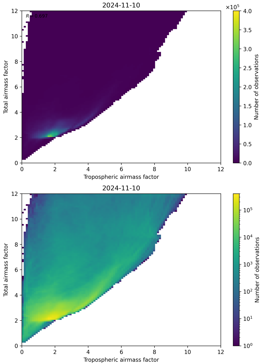
Figure 72: Scatter density plot of “Tropospheric airmass factor” against “Total airmass factor” for 2024-11-09 to 2024-11-11.
