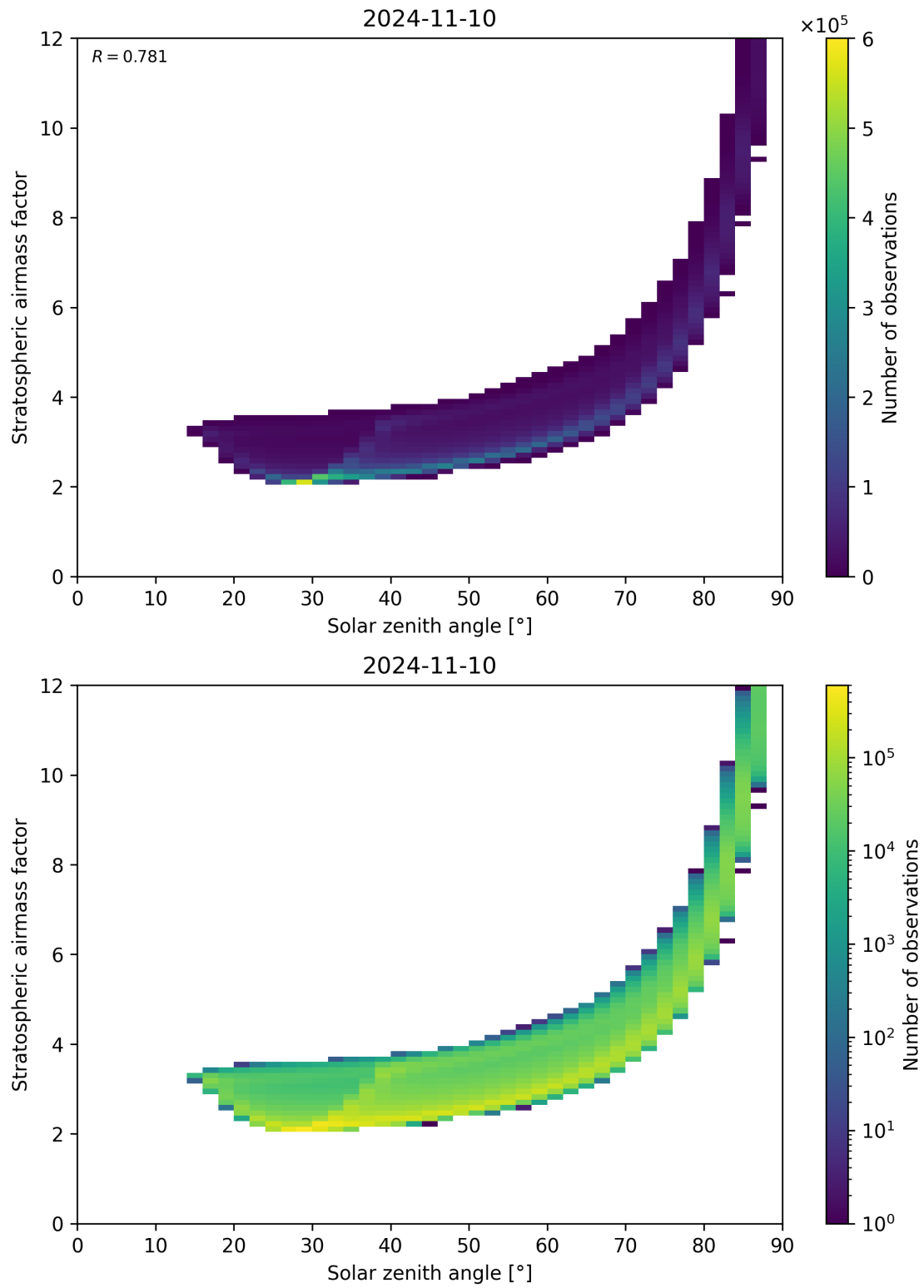
Figure 145: Scatter density plot of “Solar zenith angle” against “Stratospheric airmass factor” for 2024-11-09 to 2024-11-11.
