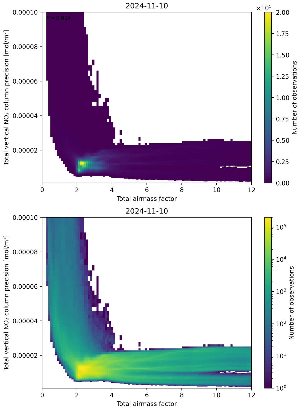
Figure 68: Scatter density plot of “Total airmass factor” against “Total vertical NO 2 column precision” for 2024-11-09 to 2024-11-11.
