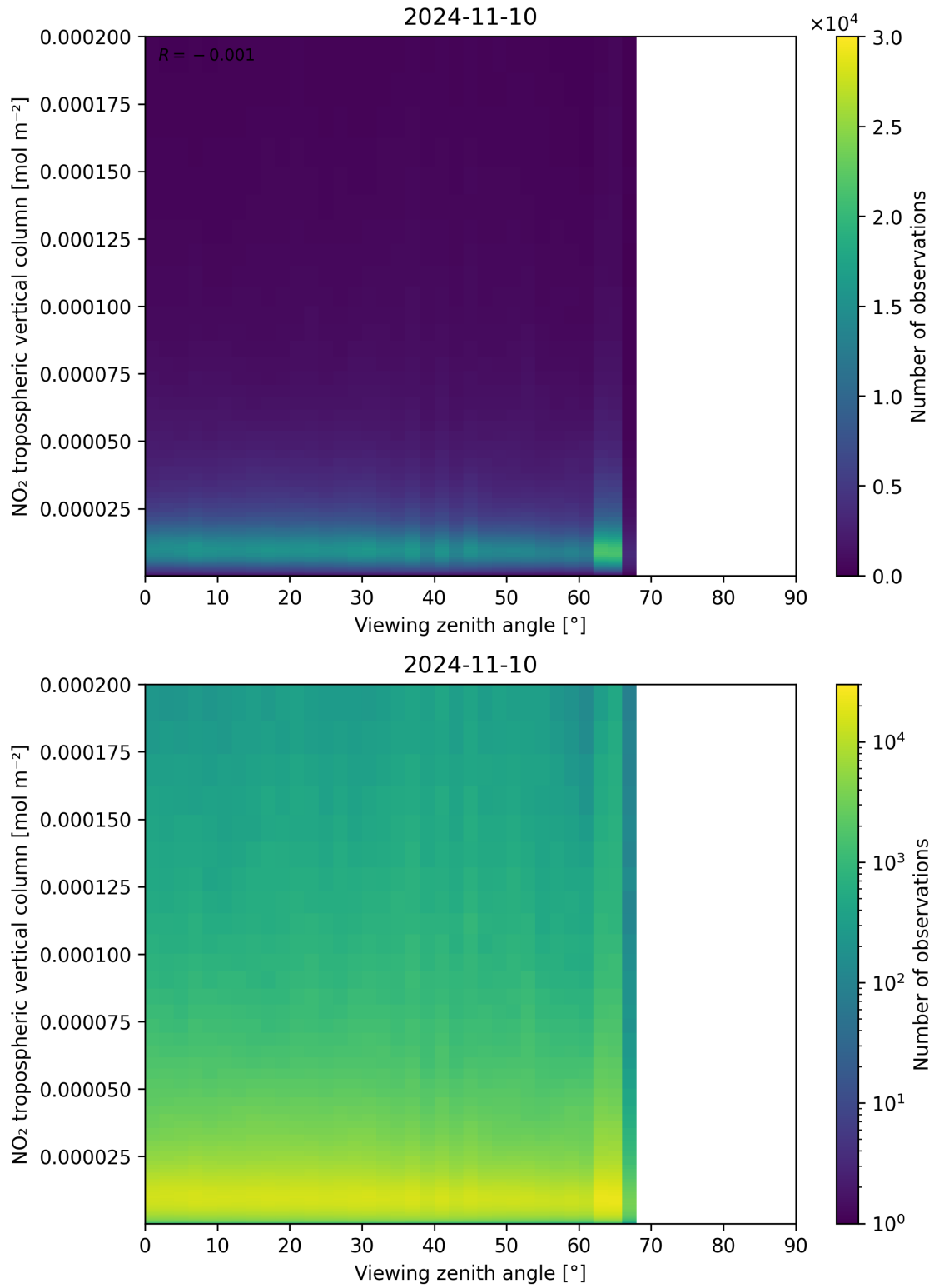
Figure 169: Scatter density plot of “Viewing zenith angle” against “NO 2 tropospheric vertical column” for 2024-11-09 to 2024-11-11.
