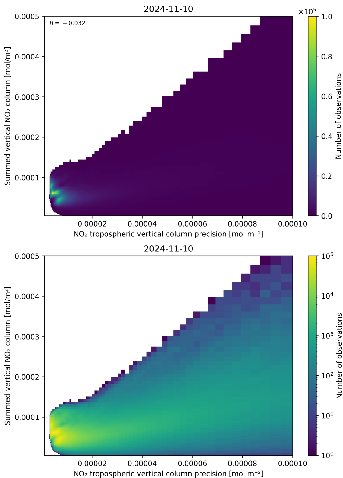
Figure 136: Scatter density plot of “NO 2 tropospheric vertical column precision” against “Summed vertical NO 2 column” for 2024-11-09 to 2024-11-11.
