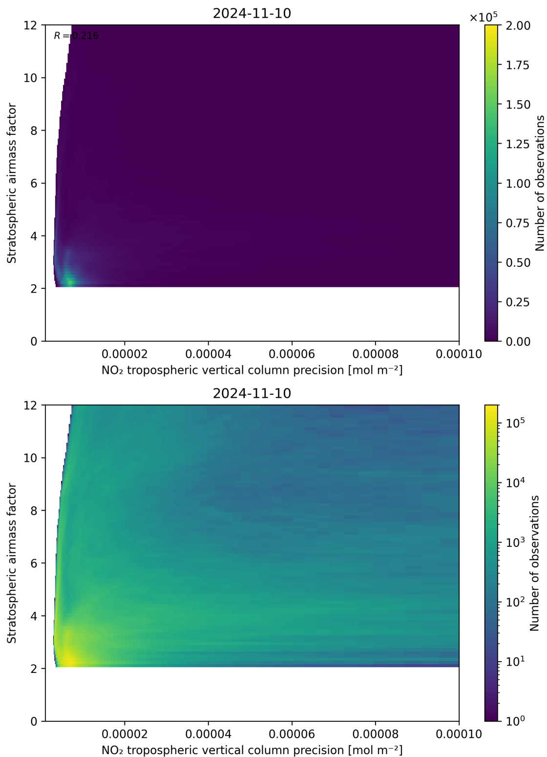
Figure 131: Scatter density plot of “NO 2 tropospheric vertical column precision” against “Stratospheric airmass factor” for 2024-11-09 to 2024-11-11.
