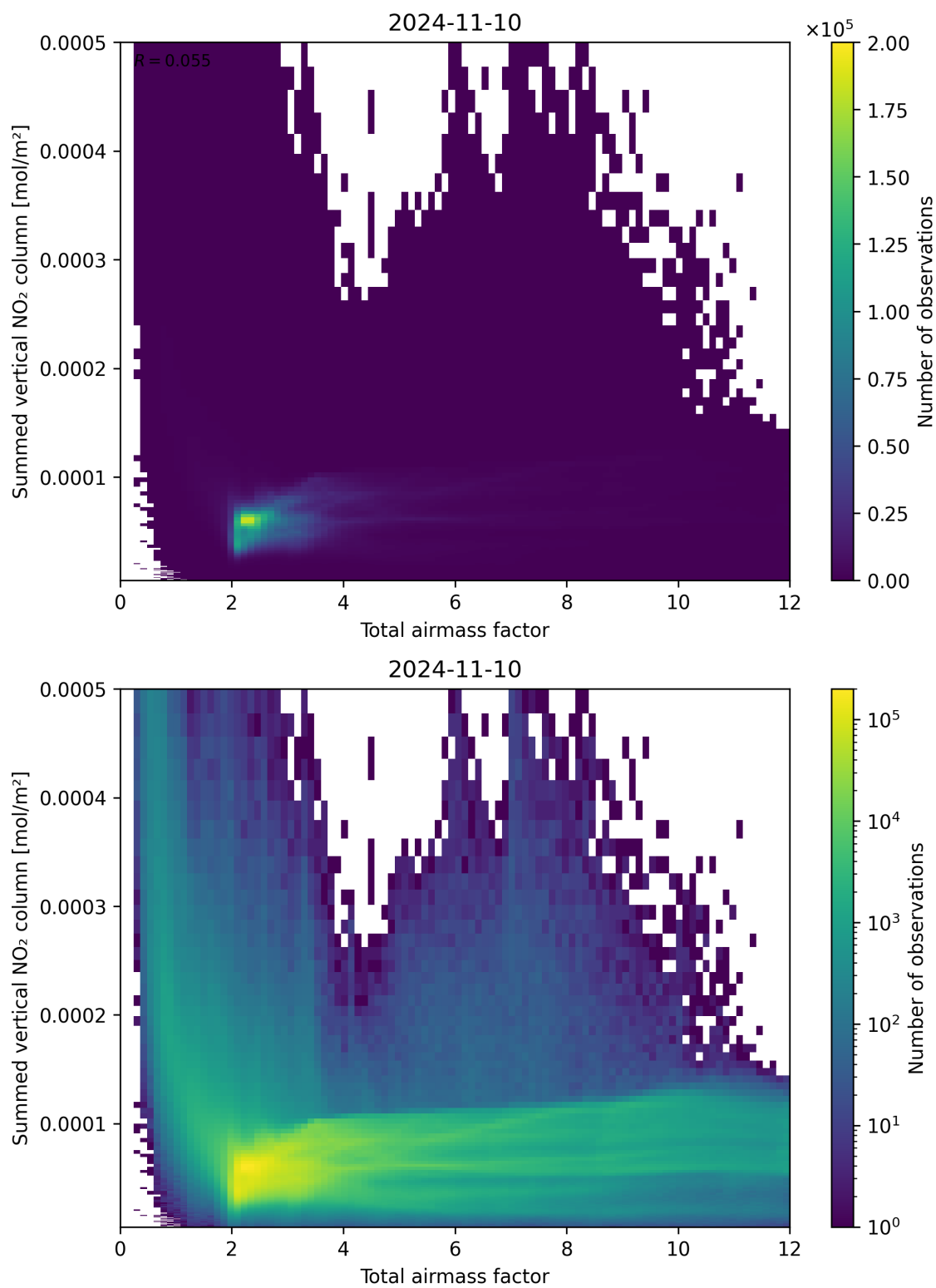
Figure 65: Scatter density plot of “Total airmass factor” against “Summed vertical NO 2 column” for 2024-11-09 to 2024-11-11.
