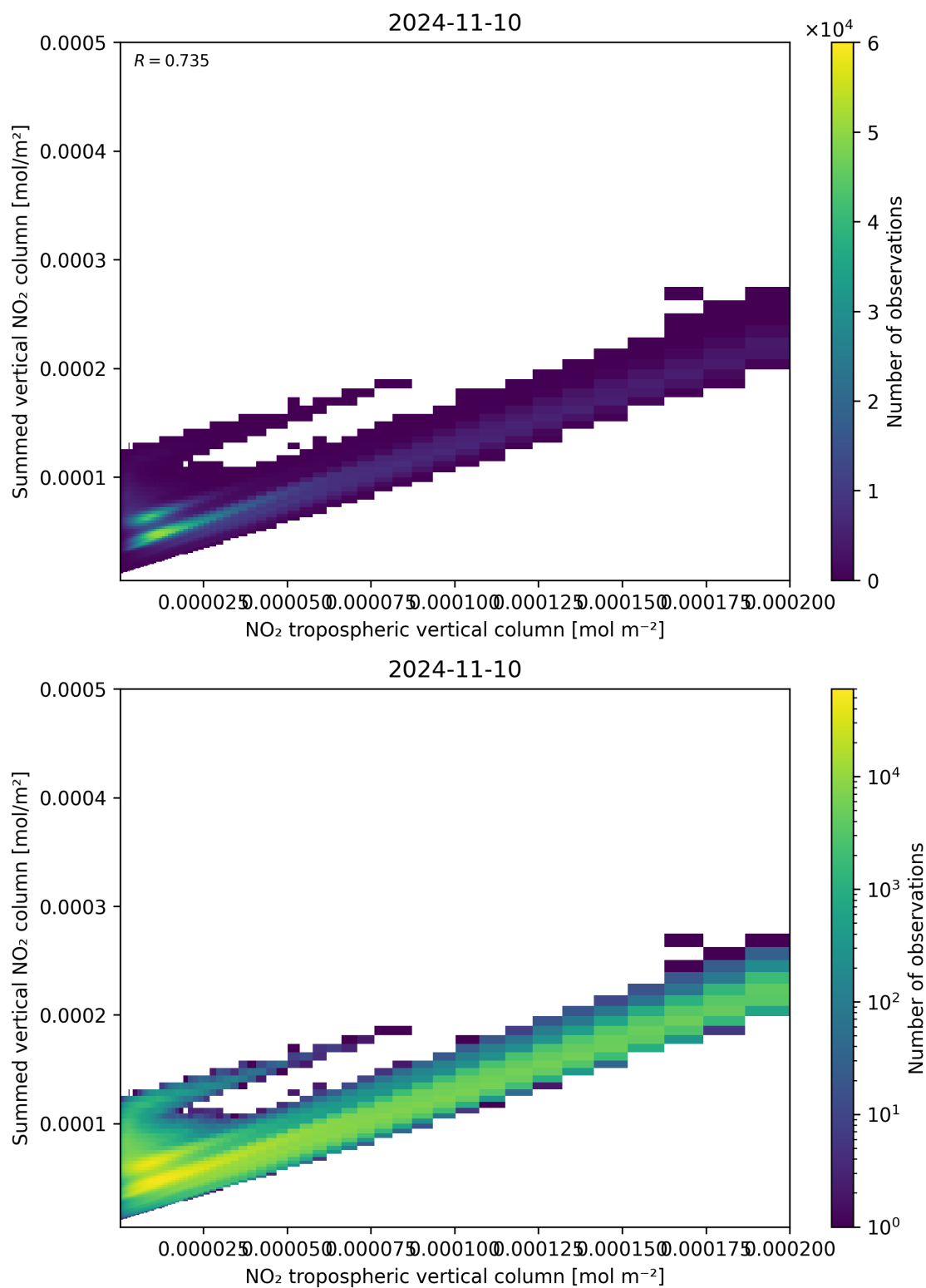
Figure 126: Scatter density plot of “NO 2 tropospheric vertical column” against “Summed vertical NO 2 column” for 2024-11-09 to 2024-11-11.
