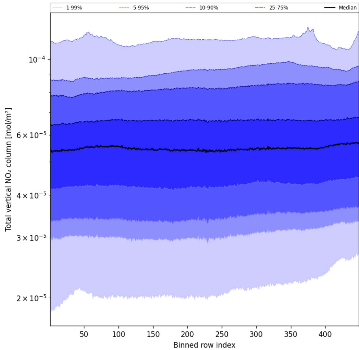
Figure 55: Along track statistics of “Total vertical NO 2 column” for 2024-11-09 to 2024-11-11
