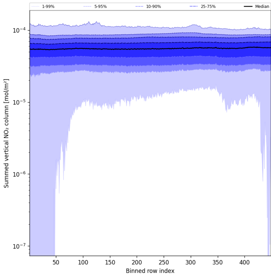
Figure 57: Along track statistics of “Summed vertical NO 2 column” for 2024-11-11 to 2024-11-13
