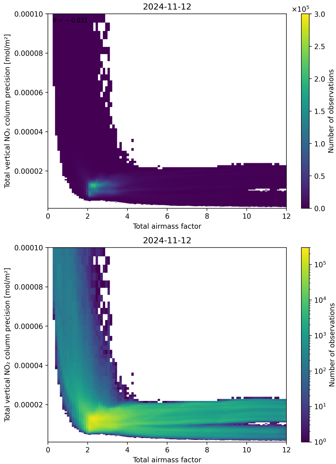
Figure 68: Scatter density plot of “Total airmass factor” against “Total vertical NO 2 column precision” for 2024-11-11 to 2024-11-13.
