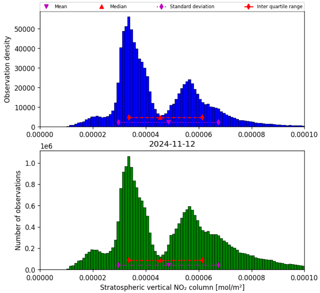
Figure 36: Histogram of “Stratospheric vertical NO 2 column” for 2024-11-11 to 2024-11-13
