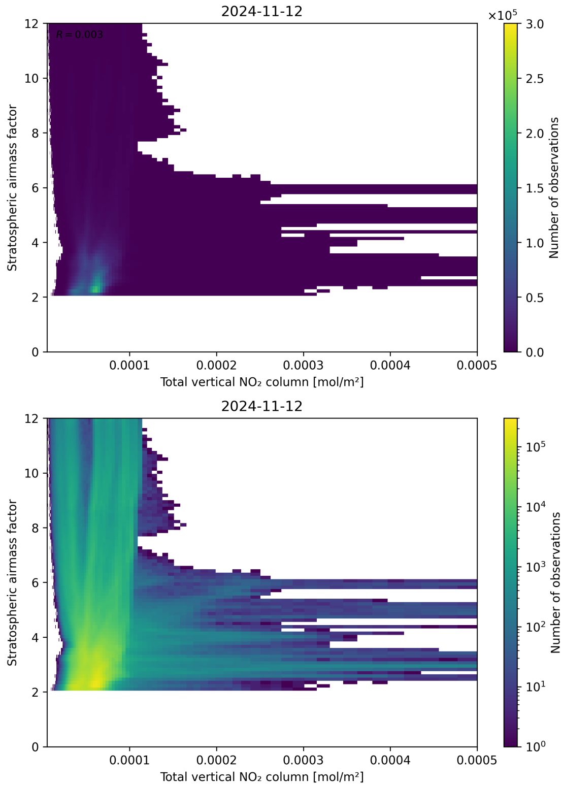
Figure 110: Scatter density plot of “Total vertical NO 2 column” against “Stratospheric airmass factor” for 2024-11-11 to 2024-11-13.
