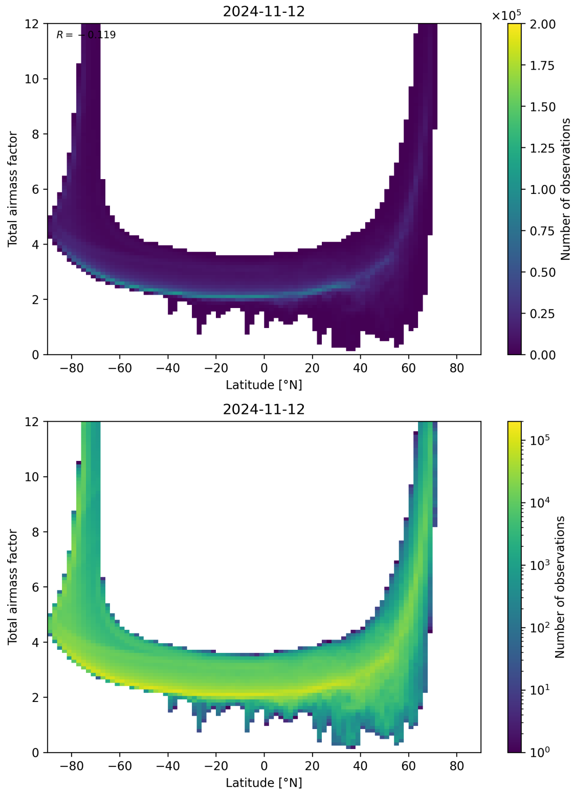
Figure 84: Scatter density plot of “Latitude” against “Total airmass factor” for 2024-11-11 to 2024-11-13.
