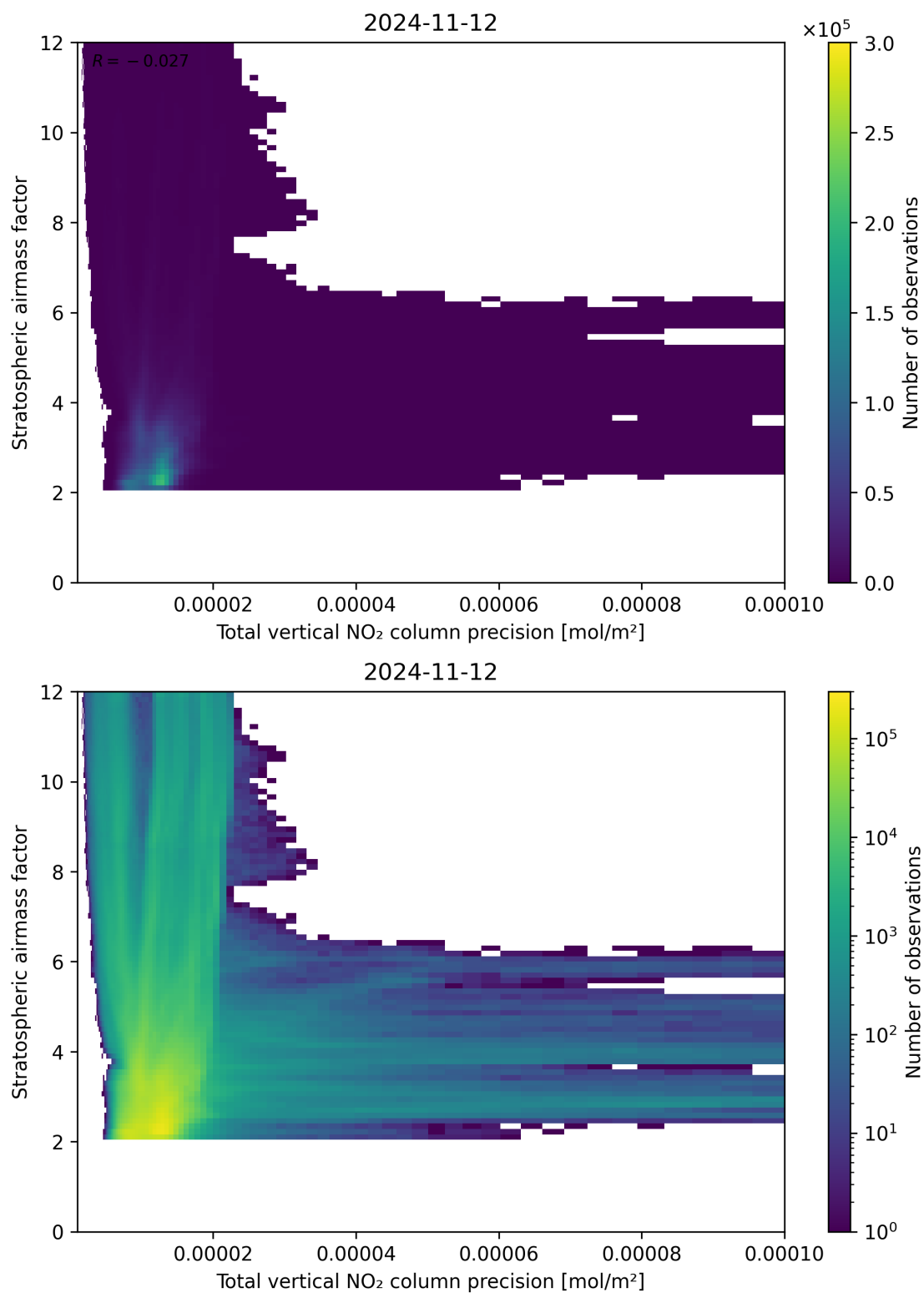
Figure 115: Scatter density plot of “Total vertical NO 2 column precision” against “Stratospheric air mass factor” for 2024-11-11 to 2024-11-13.
