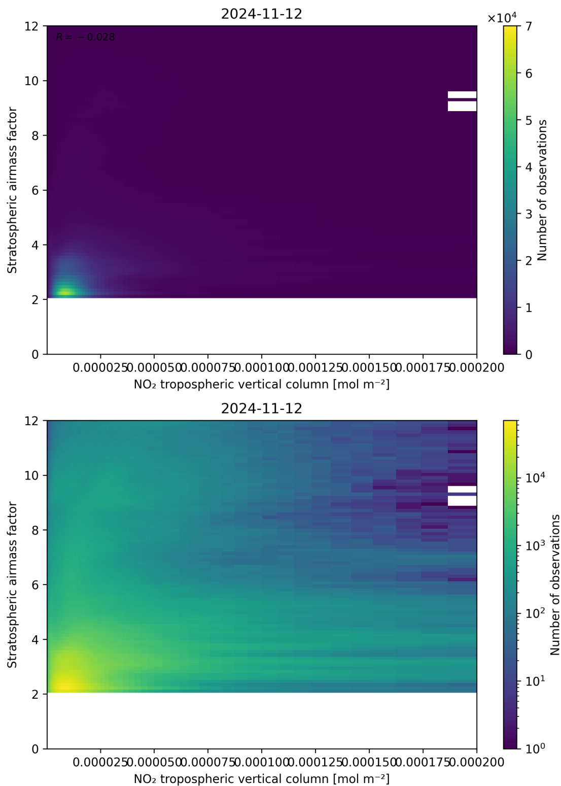
Figure 121: Scatter density plot of “NO 2 tropospheric vertical column” against “Stratospheric airmass factor” for 2024-11-11 to 2024-11-13.
