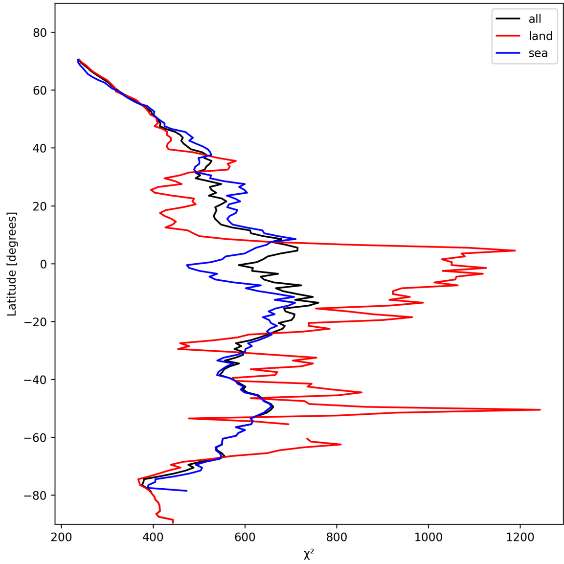
Figure 25: Zonal average of “ \chi^2 ” for 2024-11-11 to 2024-11-13.
