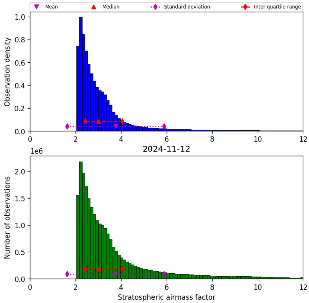
Figure 44: Histogram of “Stratospheric airmass factor” for 2024-11-11 to 2024-11-13
