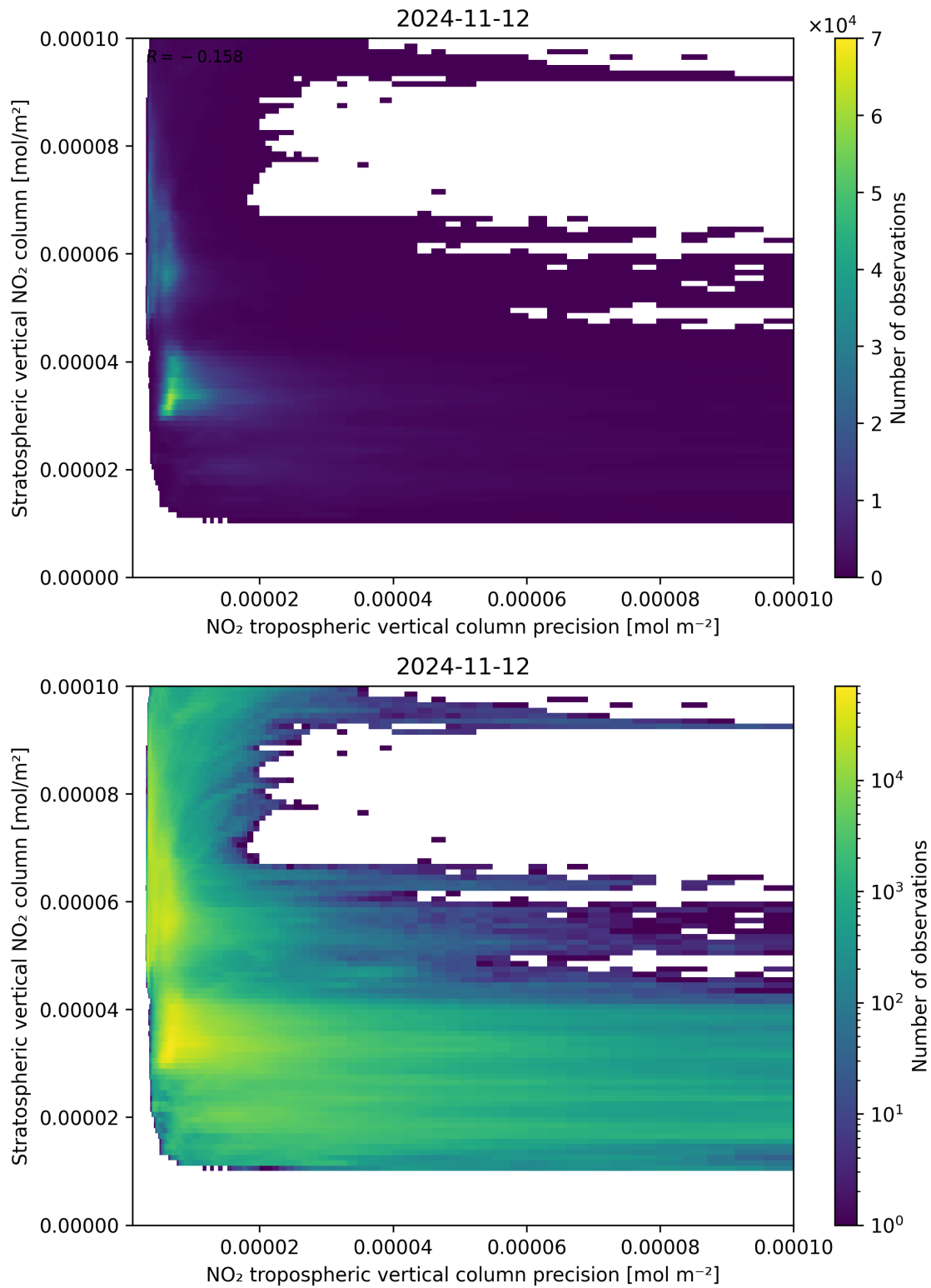
Figure 135: Scatter density plot of “NO 2 tropospheric vertical column precision” against “Stratospheric vertical NO 2 column” for 2024-11-11 to 2024-11-13.
