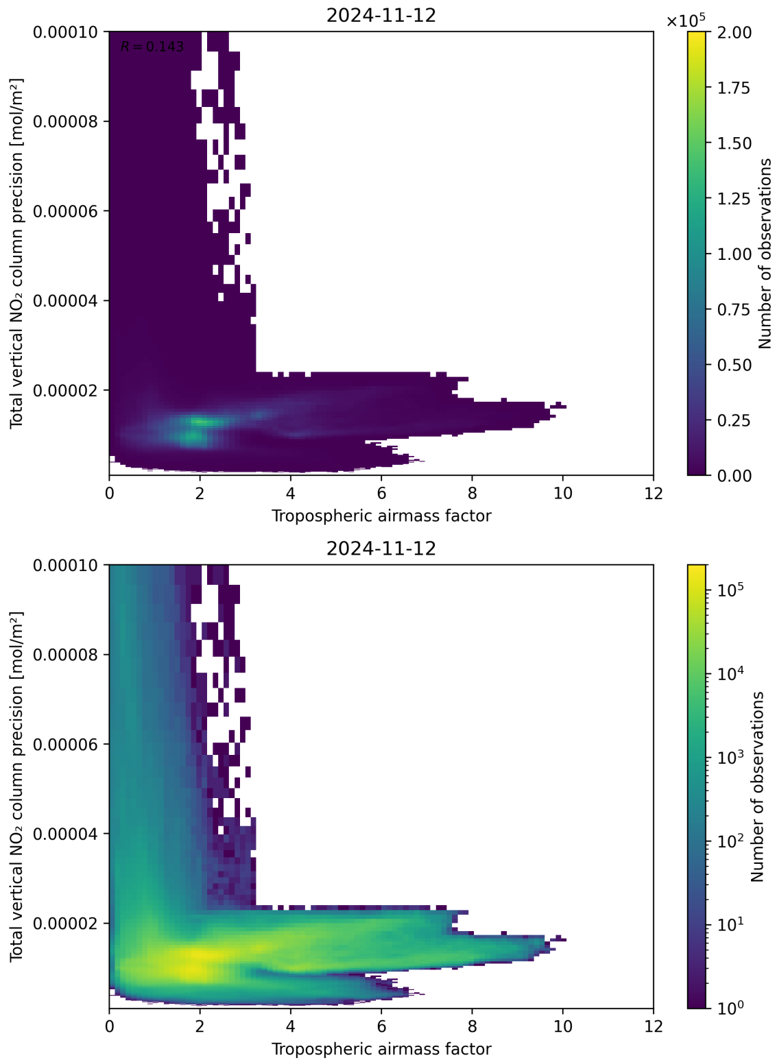
Figure 78: Scatter density plot of “Tropospheric airmass factor” against “Total vertical NO 2 column precision” for 2024-11-11 to 2024-11-13.
