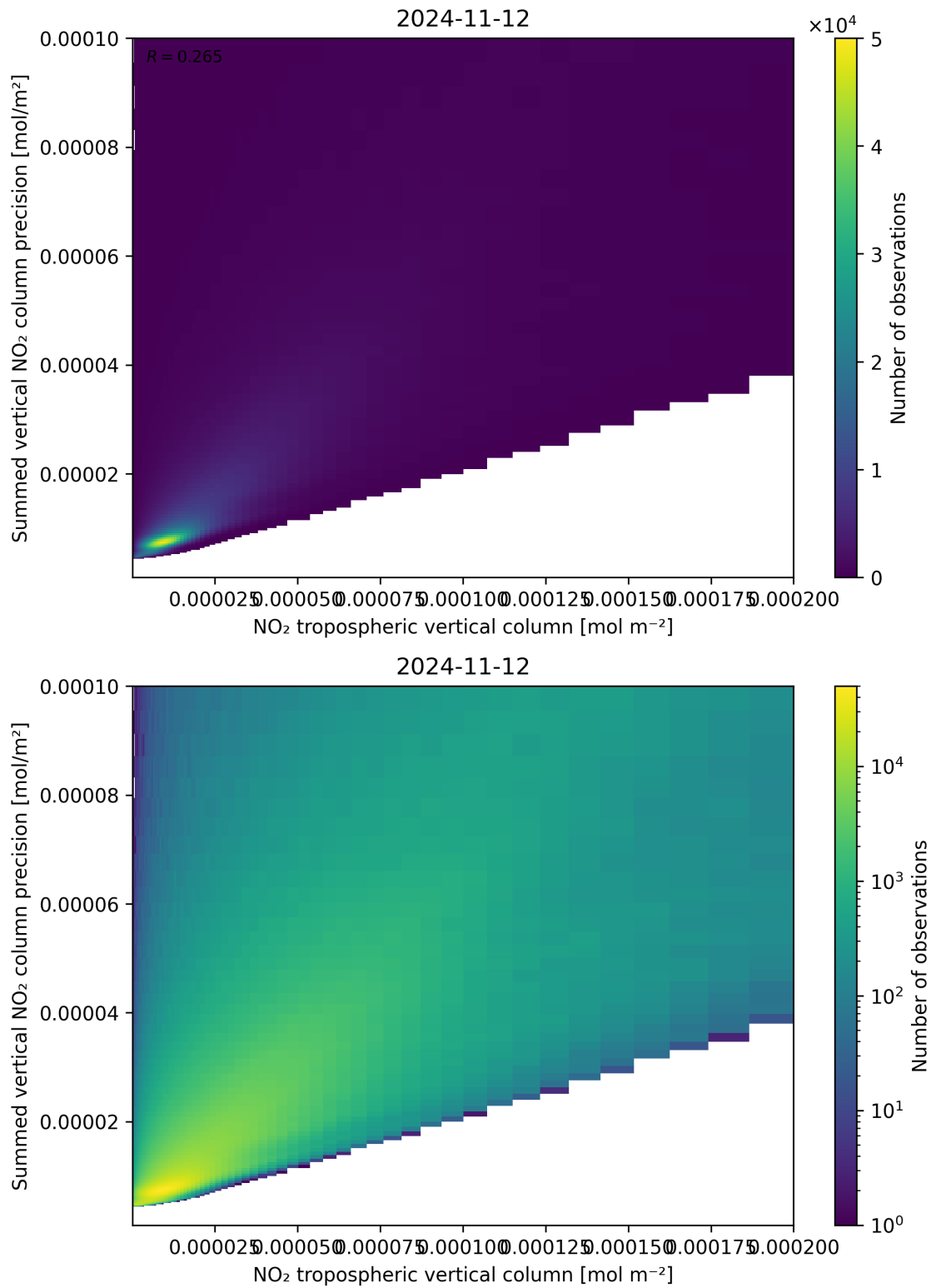
Figure 127: Scatter density plot of “NO 2 tropospheric vertical column” against “Summed vertical NO 2 column precision” for 2024-11-11 to 2024-11-13.
