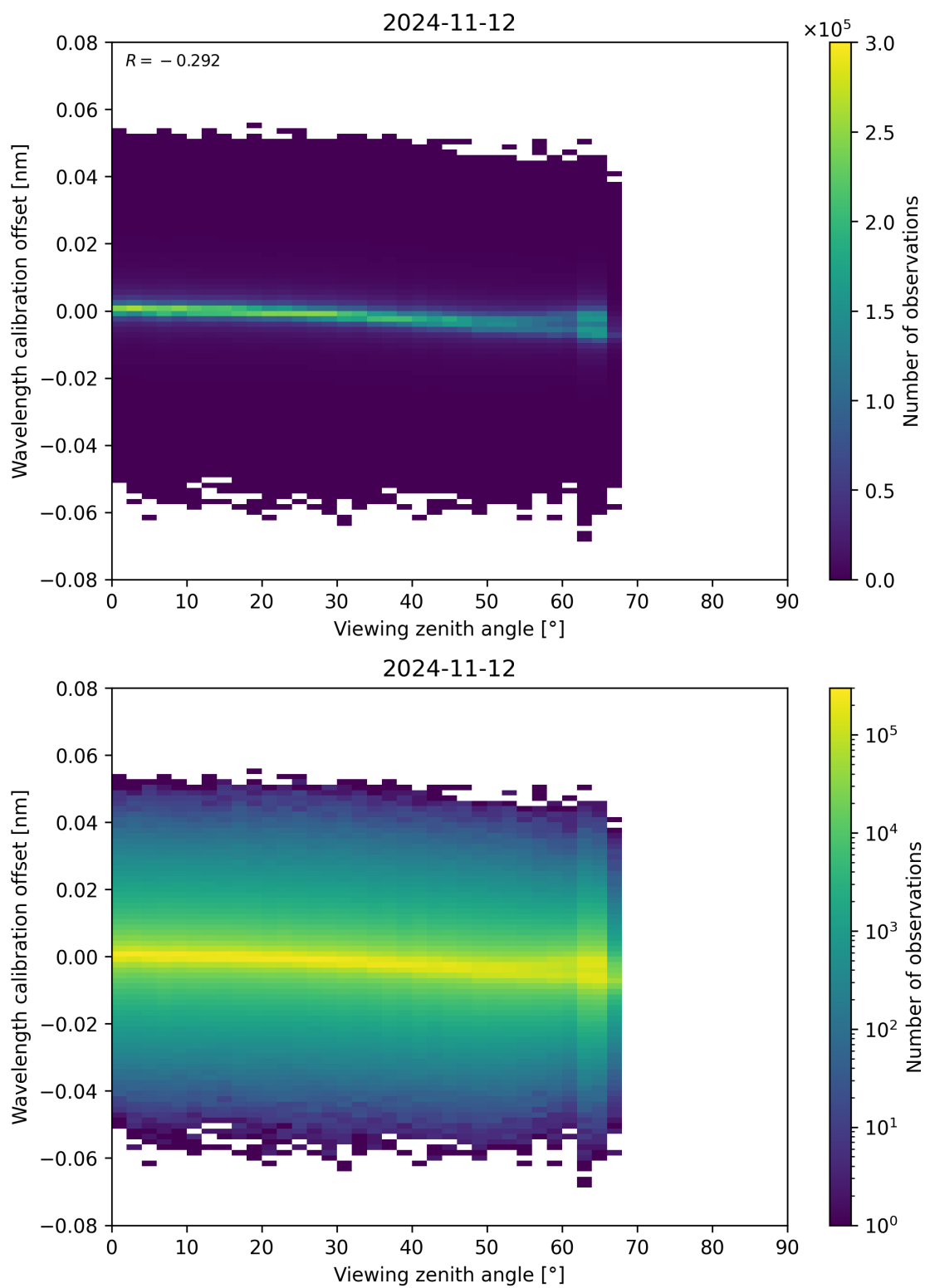
Figure 173: Scatter density plot of “Viewing zenith angle” against “Wavelength calibration offset” for 2024-11-11 to 2024-11-13.
