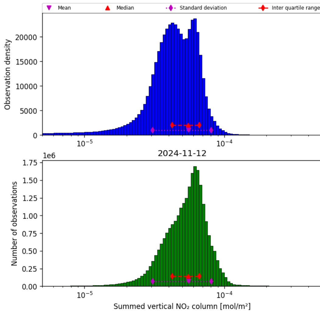
Figure 40: Histogram of “Summed vertical NO 2 column” for 2024-11-11 to 2024-11-13
