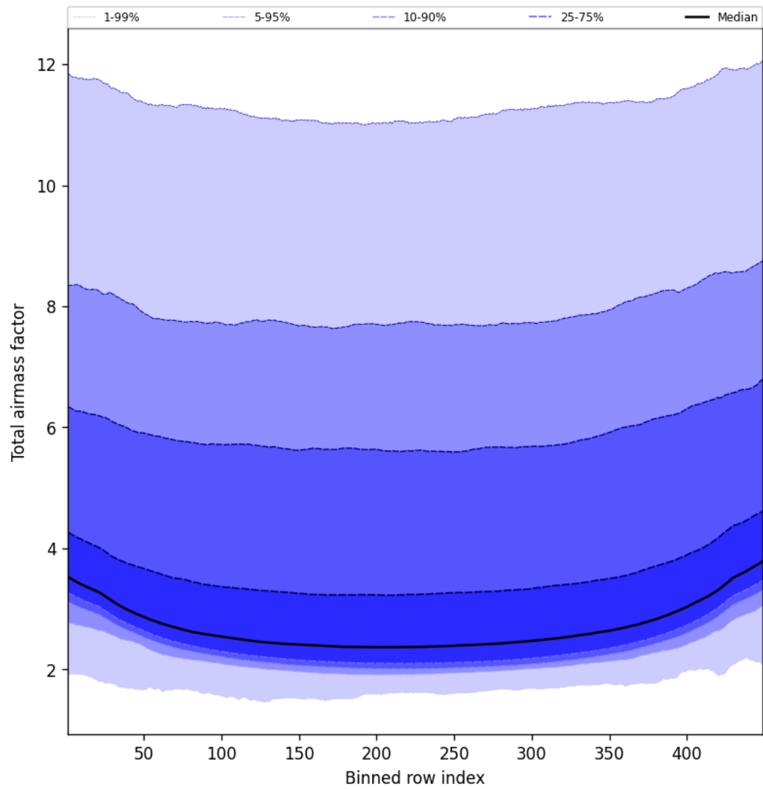
Figure 49: Along track statistics of “Total airmass factor” for 2024-11-11 to 2024-11-13
