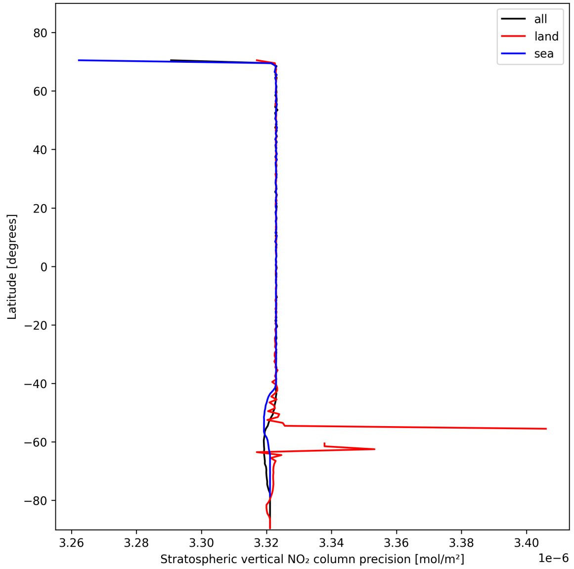
Figure 20: Zonal average of “Stratospheric vertical NO 2 column precision” for 2024-11-11 to 2024-11-13.
