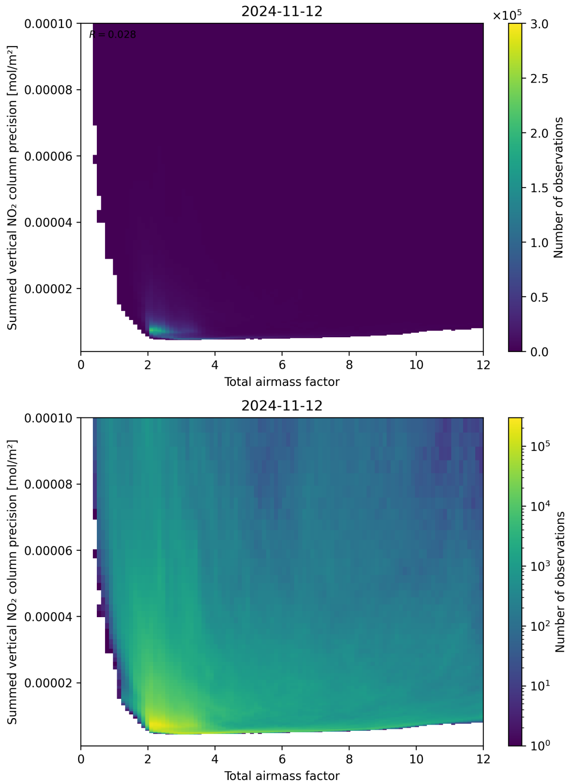
Figure 66: Scatter density plot of “Total airmass factor” against “Summed vertical NO 2 column precision” for 2024-11-11 to 2024-11-13.
