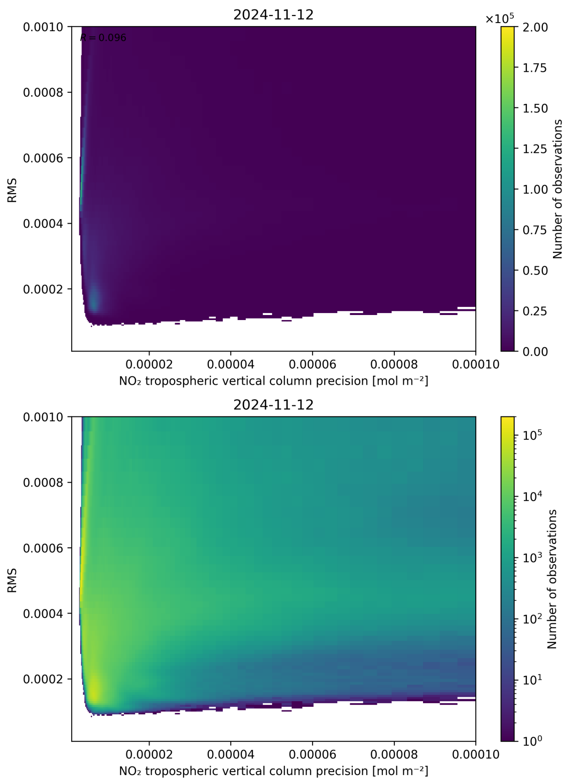
Figure 140: Scatter density plot of “NO 2 tropospheric vertical column precision” against “RMS” for 2024-11-11 to 2024-11-13.
