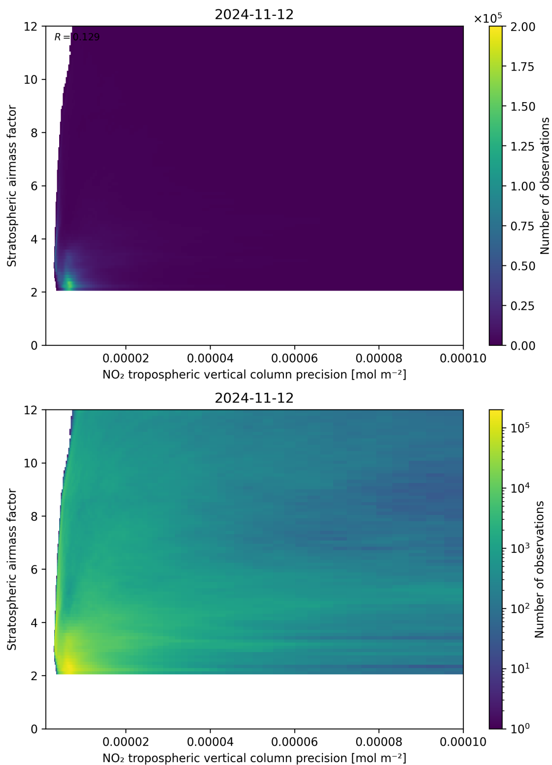
Figure 131: Scatter density plot of “NO 2 tropospheric vertical column precision” against “Stratospheric airmass factor” for 2024-11-11 to 2024-11-13.
