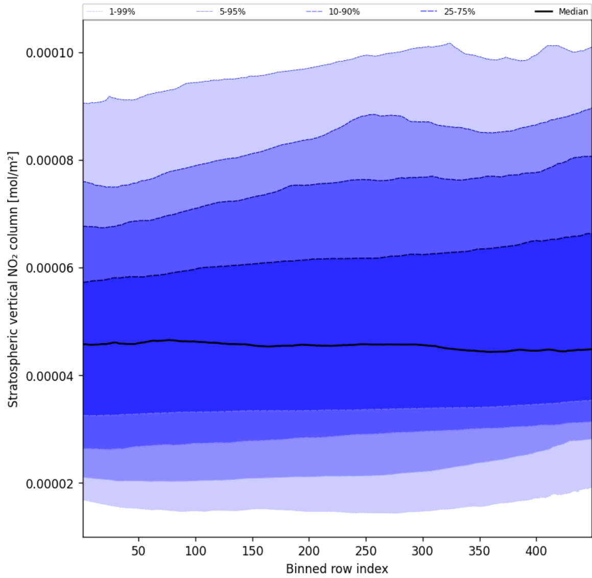
Figure 53: Along track statistics of “Stratospheric vertical NO 2 column” for 2024-11-11 to 2024-11-13
