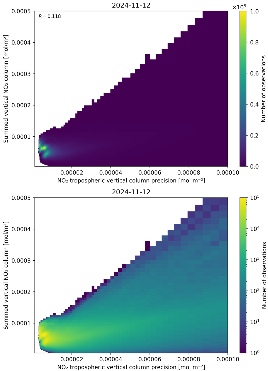
Figure 136: Scatter density plot of “NO 2 tropospheric vertical column precision” against “Summed vertical NO 2 column” for 2024-11-11 to 2024-11-13.
