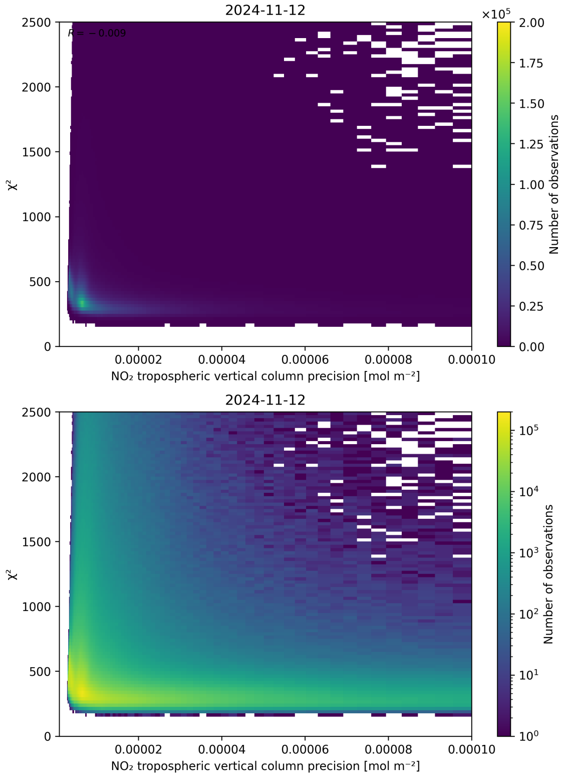
Figure 134: Scatter density plot of “NO 2 tropospheric vertical column precision” against “ \chi^2 ” for 2024-11-11 to 2024-11-13.
