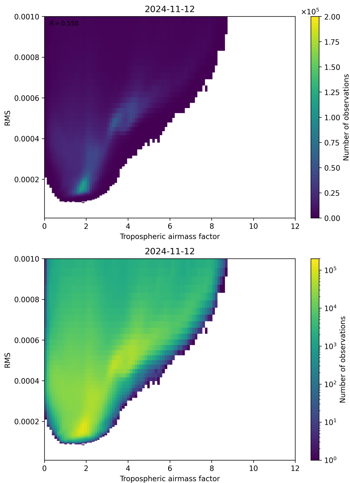
Figure 79: Scatter density plot of “Tropospheric airmass factor” against “RMS” for 2024-11-11 to 2024-11-13.
