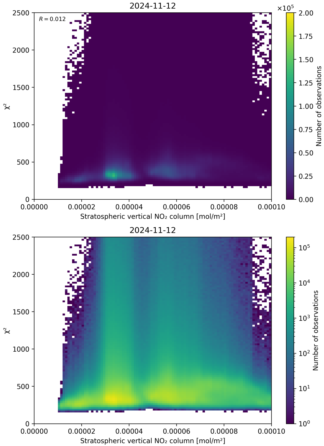
Figure 97: Scatter density plot of “Stratospheric vertical NO 2 column” against “ \chi^2 ” for 2024-11-11 to 2024-11-13.
