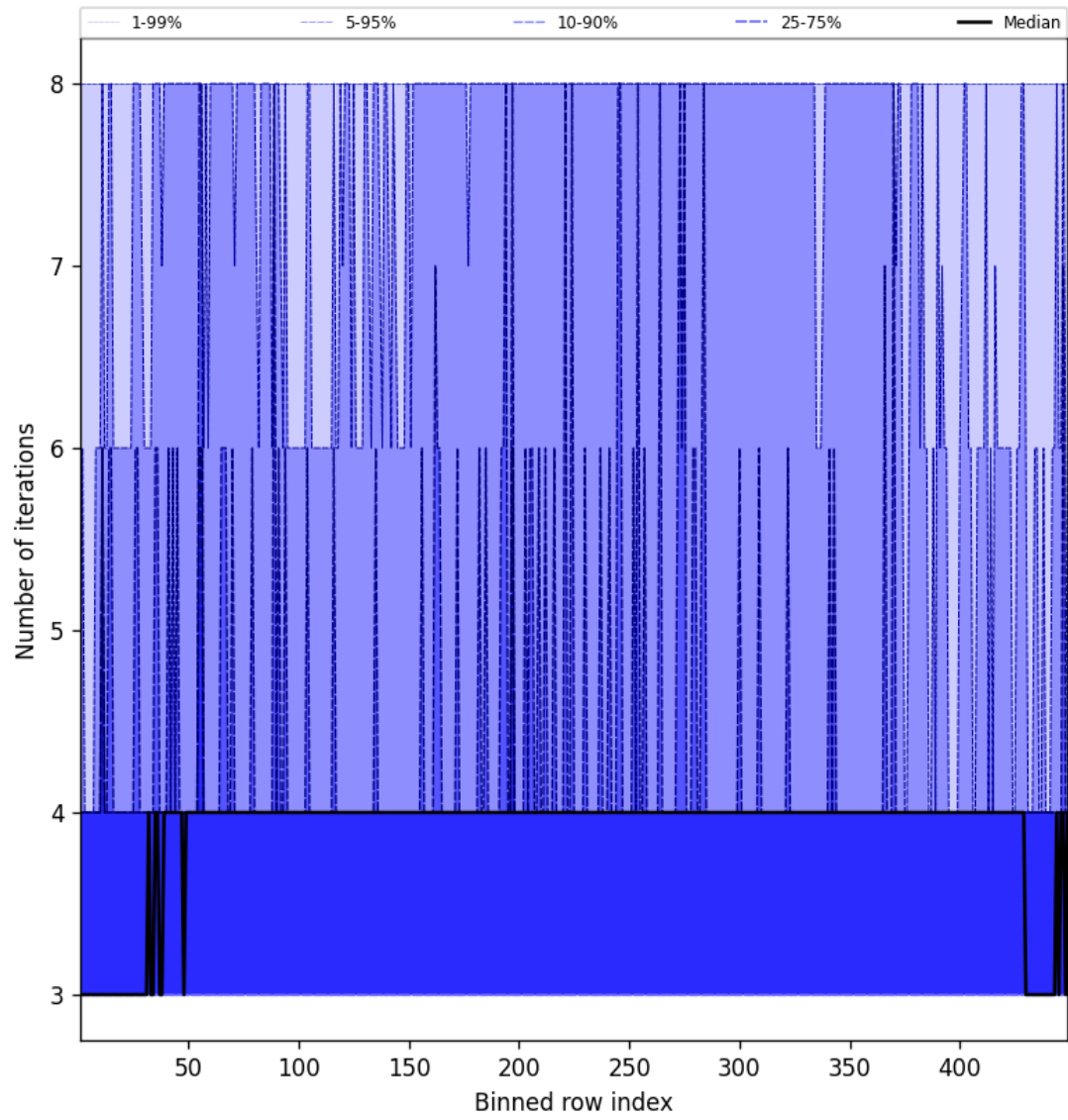
Figure 51: Along track statistics of “Number of iterations” for 2024-11-11 to 2024-11-13
