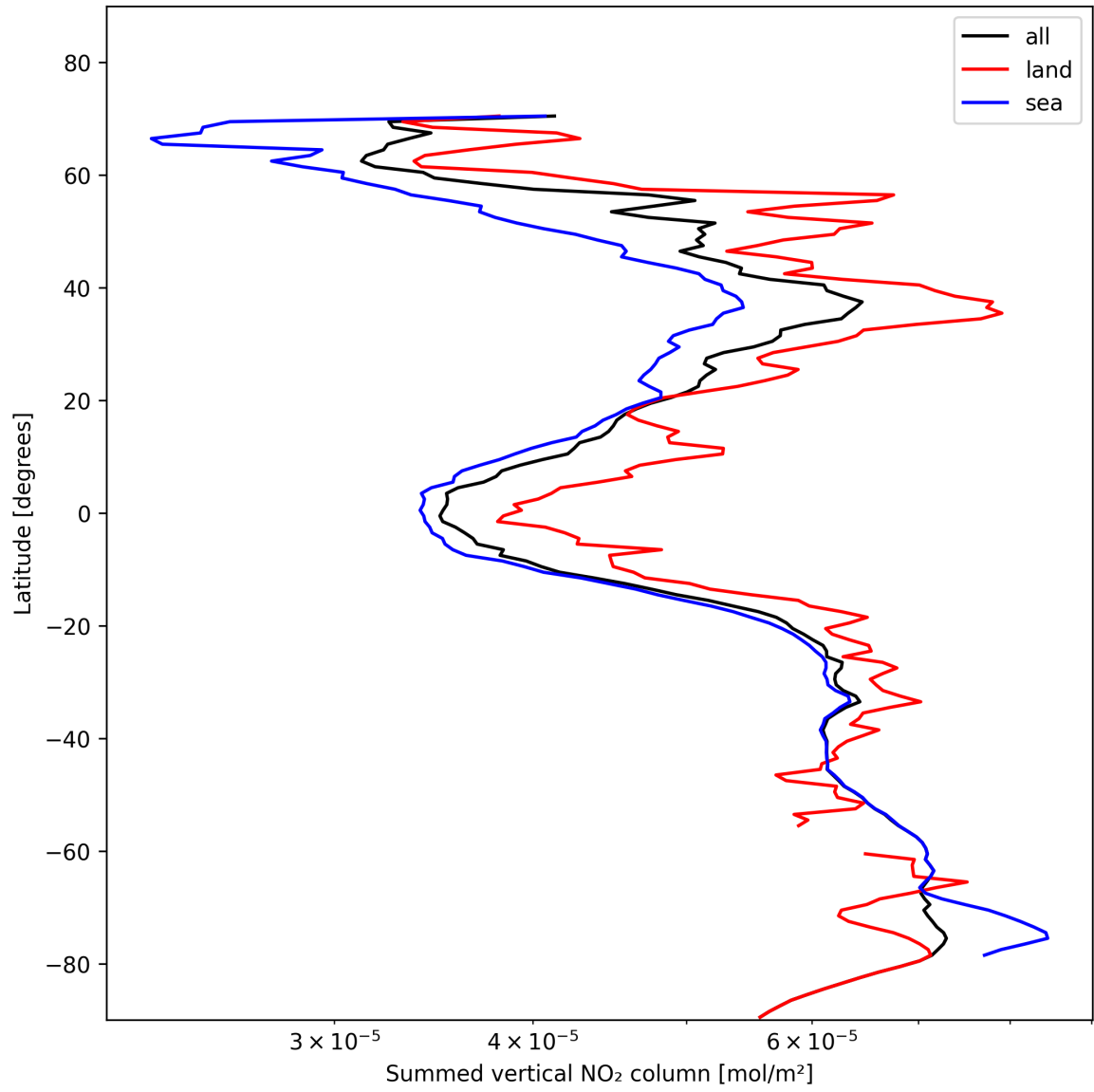
Figure 23: Zonal average of “Summed vertical NO 2 column” for 2024-11-11 to 2024-11-13.
