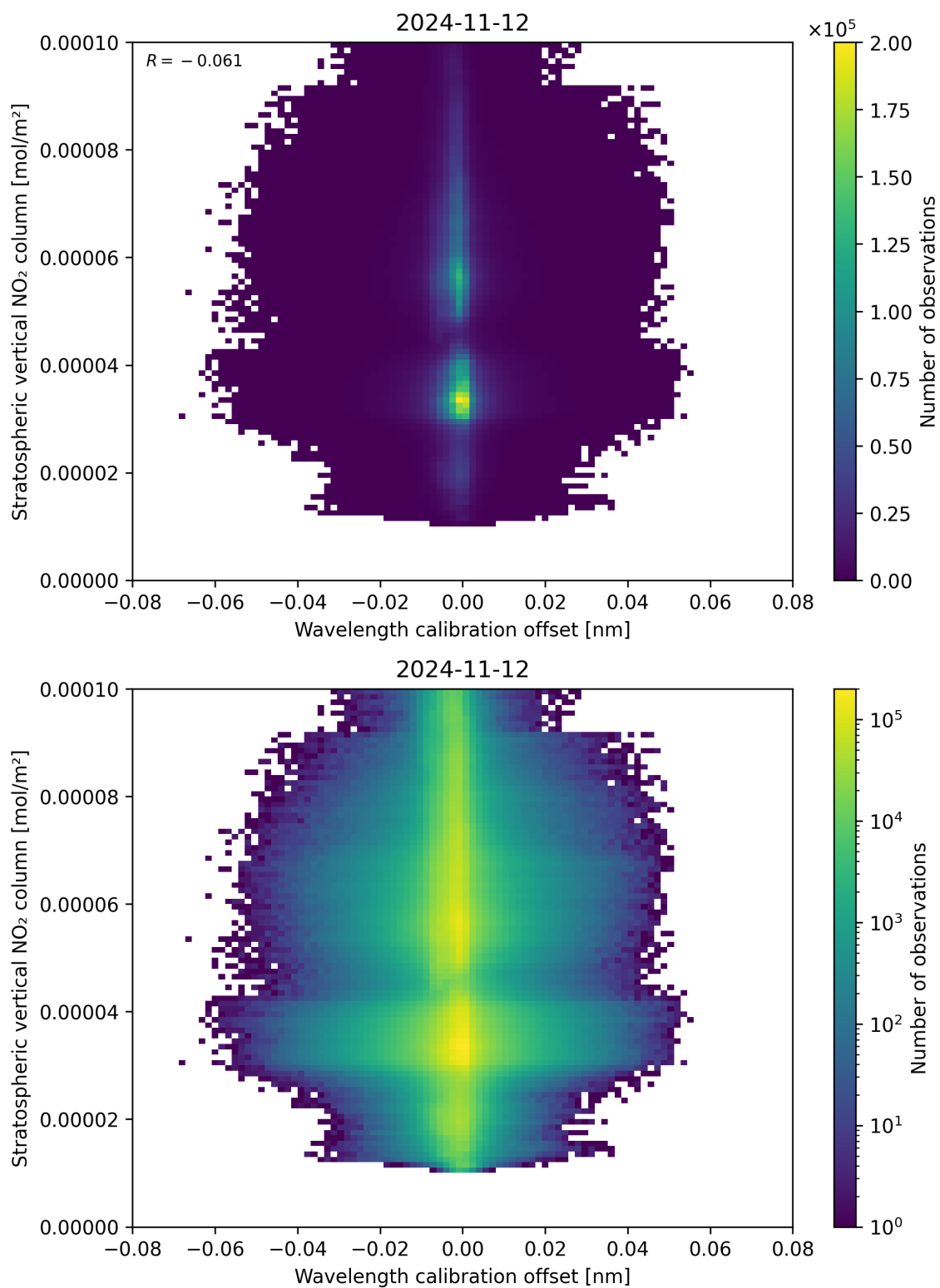
Figure 176: Scatter density plot of “Wavelength calibration offset” against “Stratospheric vertical NO 2 column” for 2024-11-11 to 2024-11-13.
