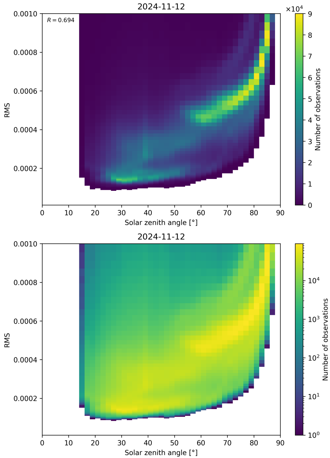
Figure 157: Scatter density plot of “Solar zenith angle” against “RMS” for 2024-11-11 to 2024-11-13.
