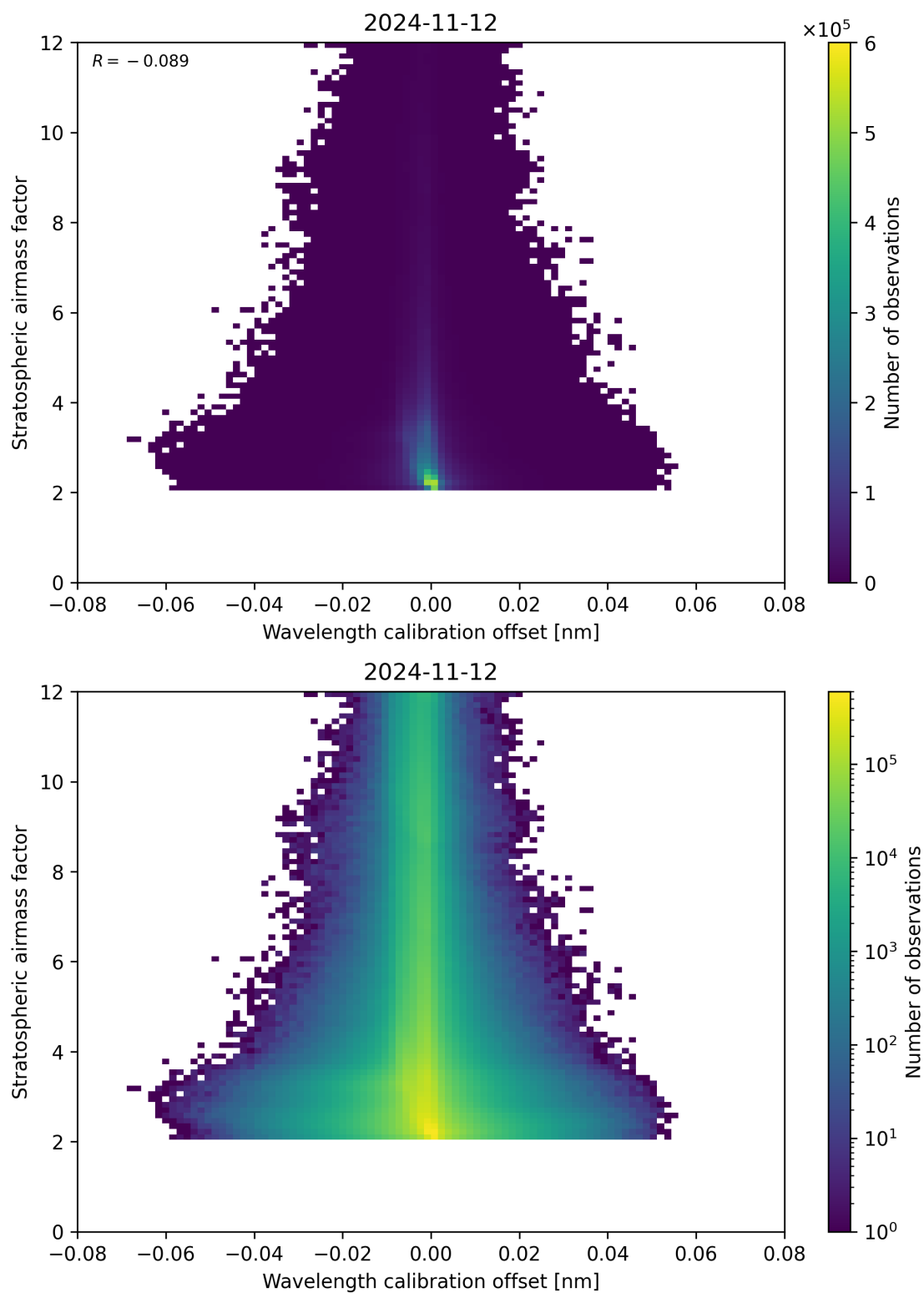
Figure 174: Scatter density plot of “Wavelength calibration offset” against “Stratospheric airmass factor” for 2024-11-11 to 2024-11-13.
