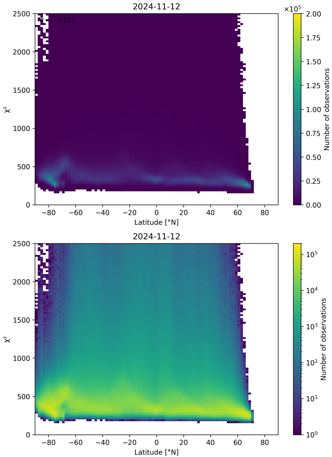
Figure 86: Scatter density plot of “Latitude” against “ \chi^2 ” for 2024-11-11 to 2024-11-13.
