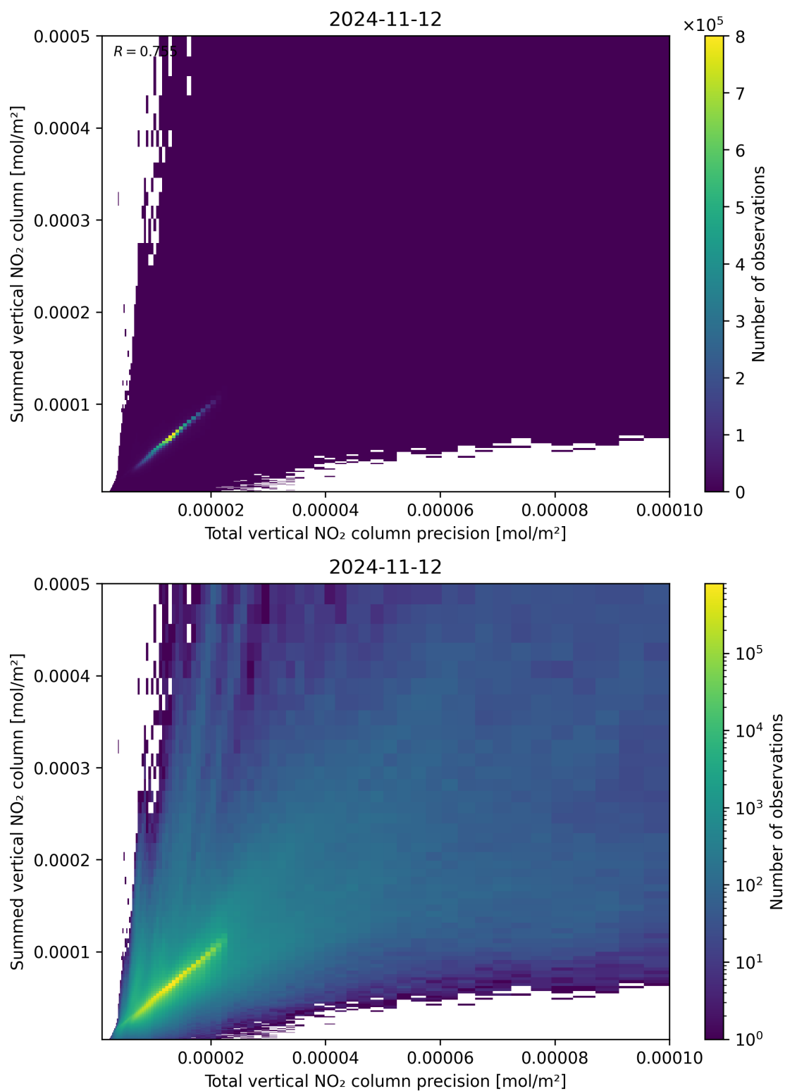
Figure 117: Scatter density plot of “Total vertical NO 2 column precision” against “Summed vertical NO 2 column” for 2024-11-11 to 2024-11-13.
