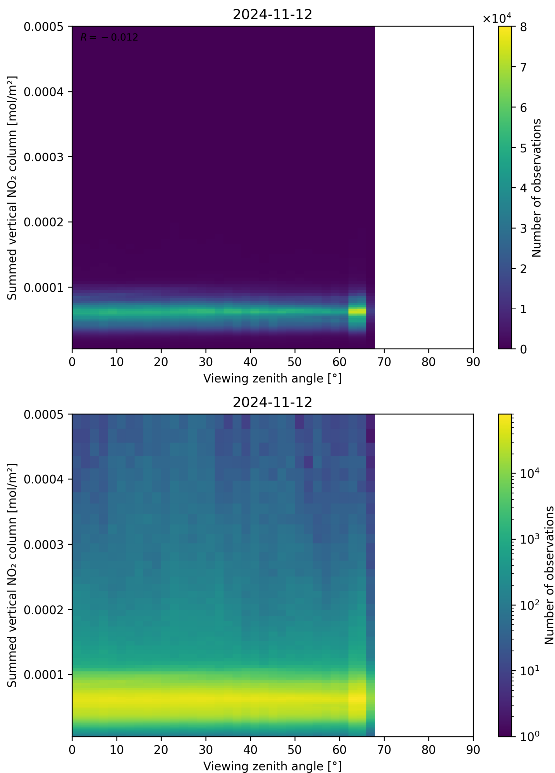
Figure 165: Scatter density plot of “Viewing zenith angle” against “Summed vertical NO 2 column” for 2024-11-11 to 2024-11-13.
