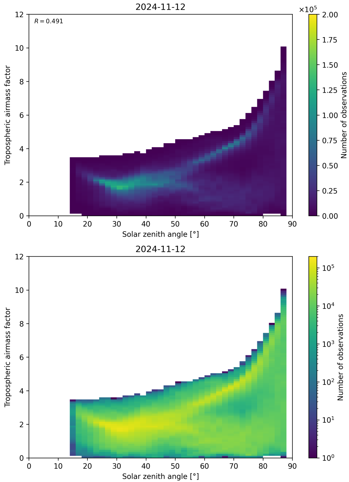
Figure 147: Scatter density plot of “Solar zenith angle” against “Tropospheric airmass factor” for 2024-11-11 to 2024-11-13.
