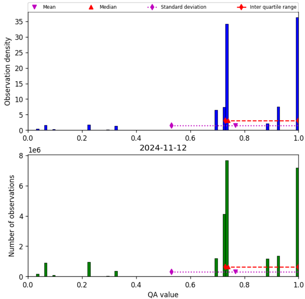
Figure 28: Histogram of “QA value” for 2024-11-11 to 2024-11-13
