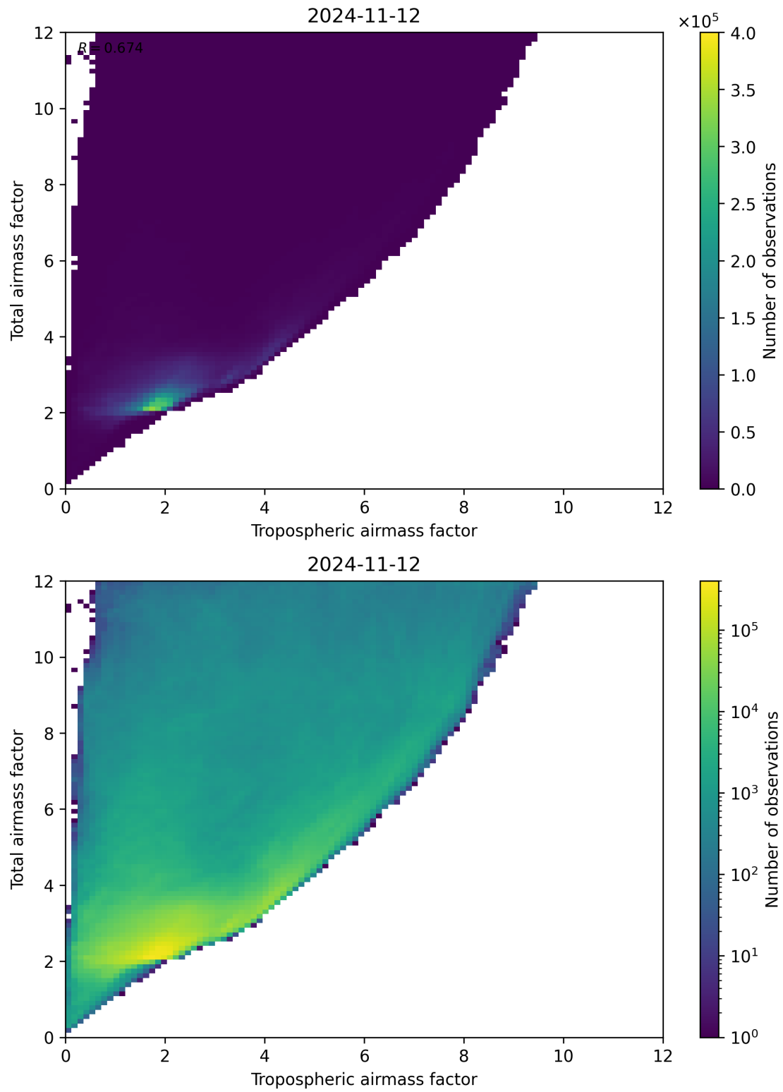
Figure 72: Scatter density plot of “Tropospheric airmass factor” against “Total airmass factor” for 2024-11-11 to 2024-11-13.
