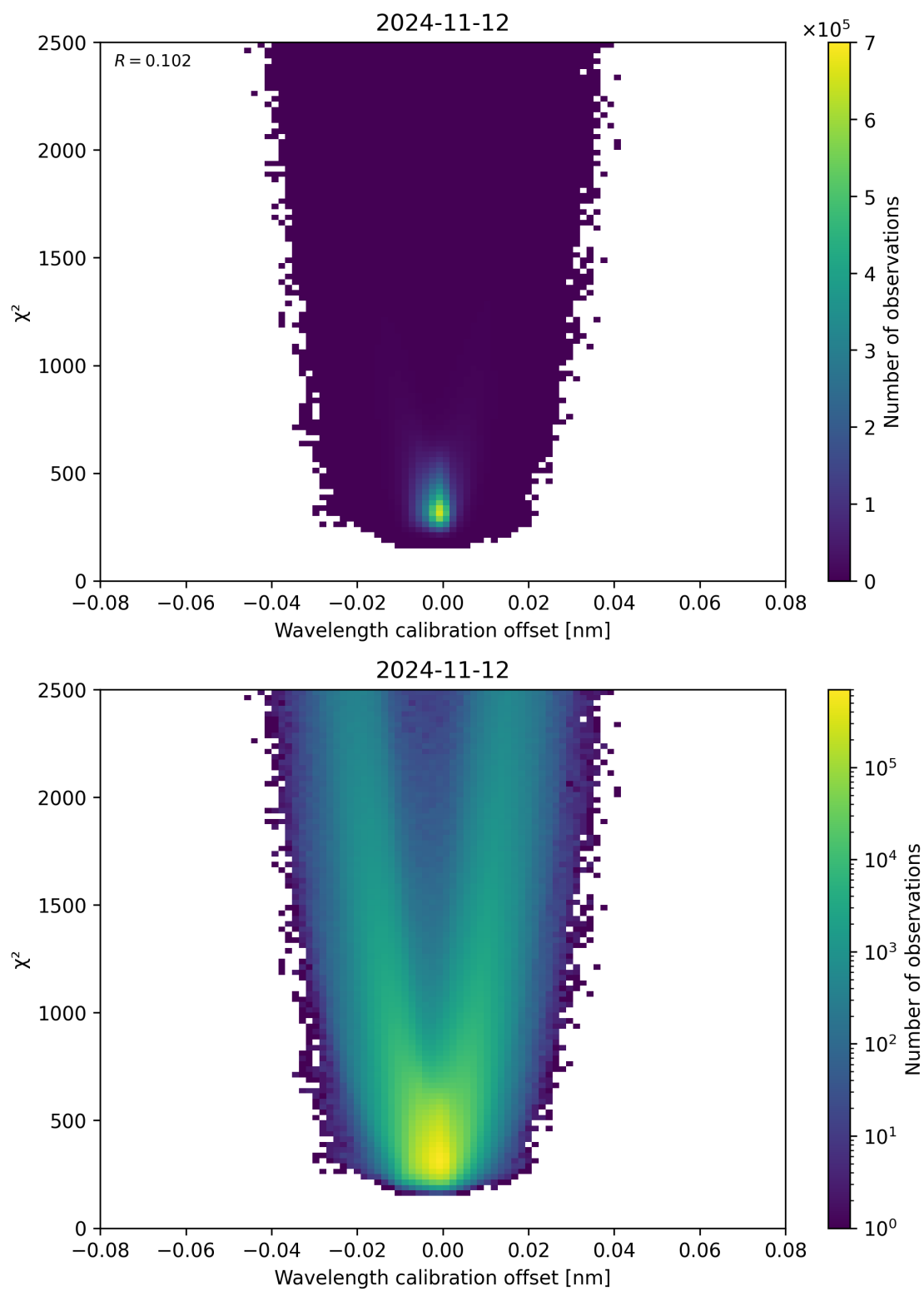
Figure 175: Scatter density plot of “Wavelength calibration offset” against “ \chi^2 ” for 2024-11-11 to 2024-11-13.
