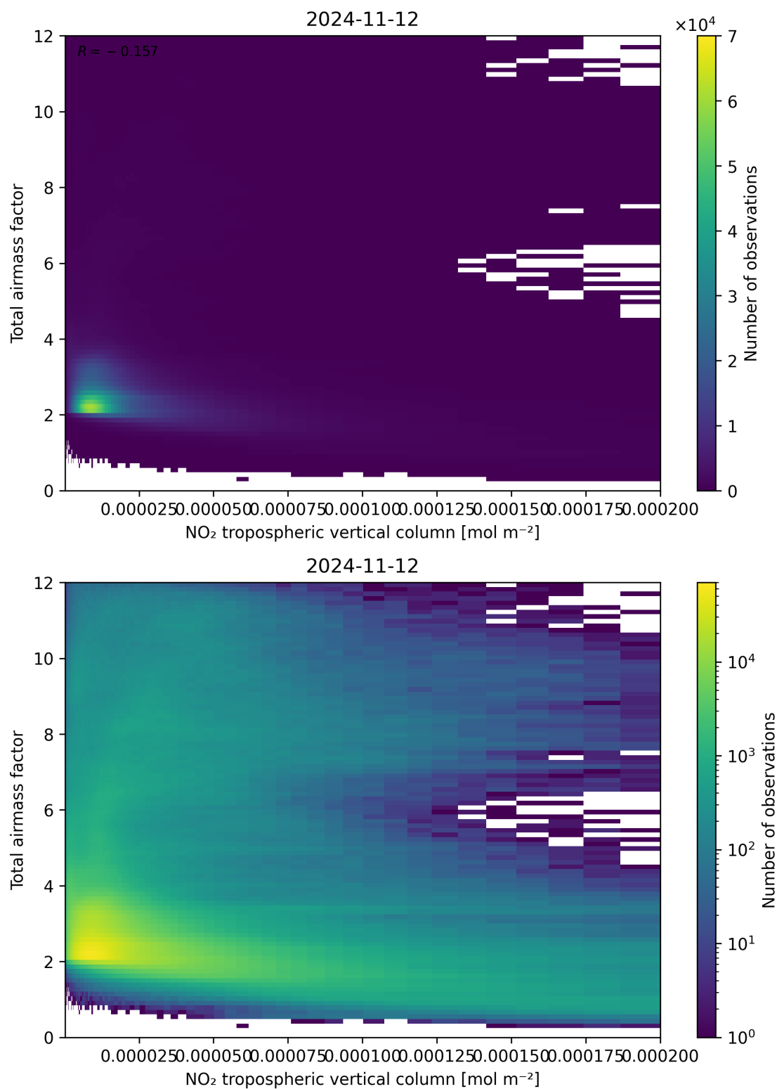
Figure 122: Scatter density plot of “NO 2 tropospheric vertical column” against “Total air mass factor” for 2024-11-11 to 2024-11-13.
