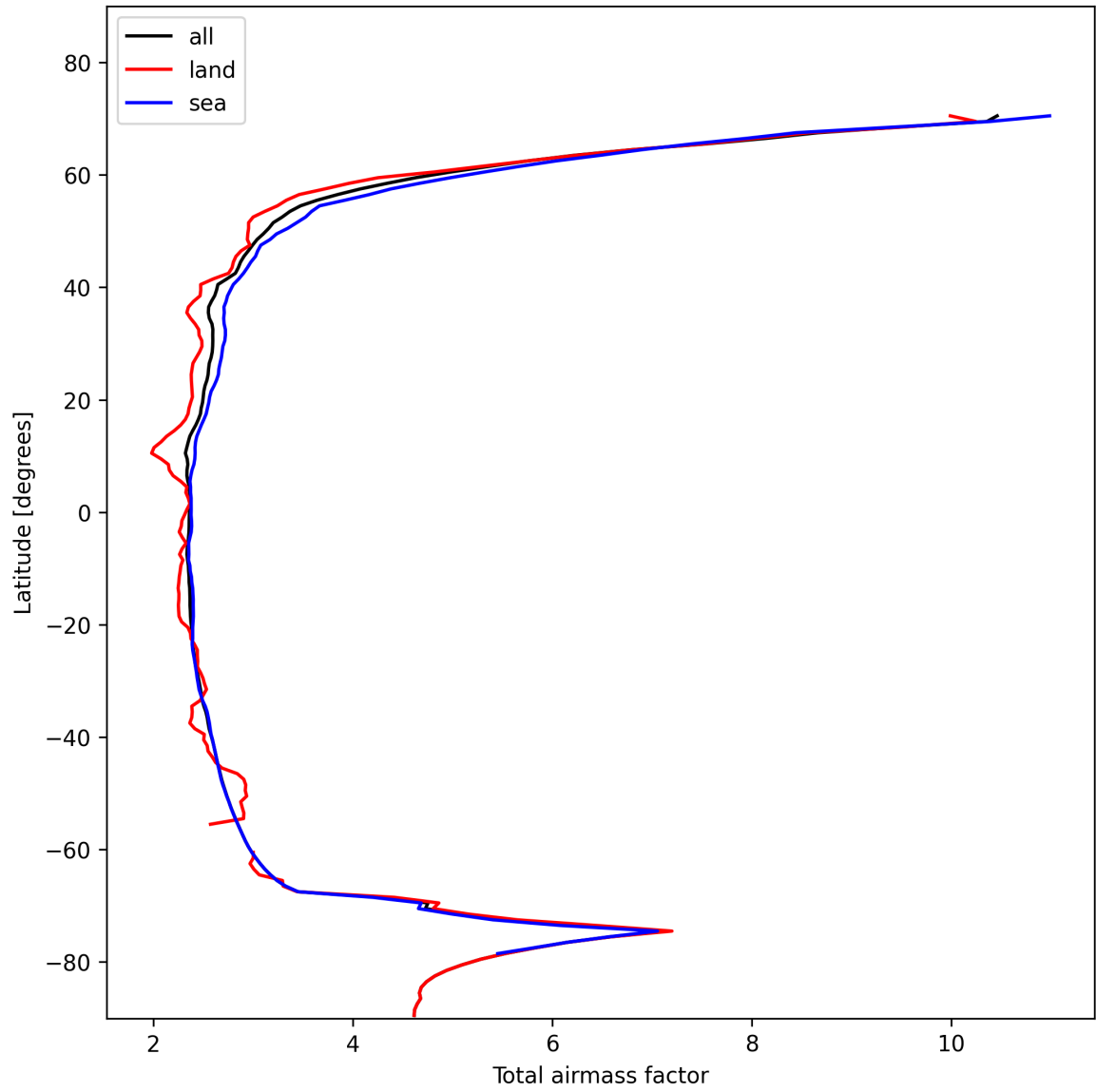
Figure 15: Zonal average of “Total airmass factor” for 2024-11-11 to 2024-11-13.
