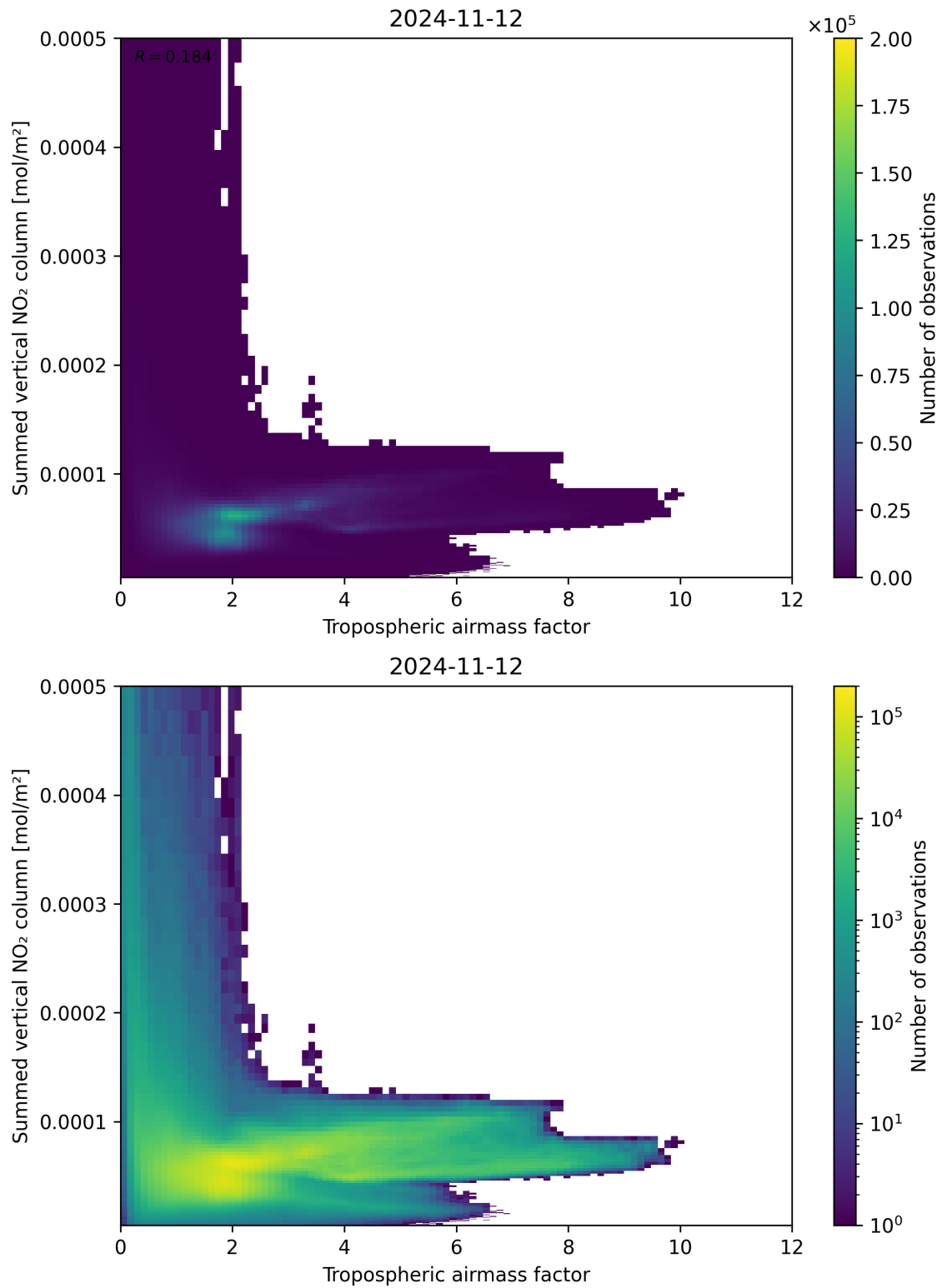
Figure 75: Scatter density plot of “Tropospheric airmass factor” against “Summed vertical NO 2 column” for 2024-11-11 to 2024-11-13.
