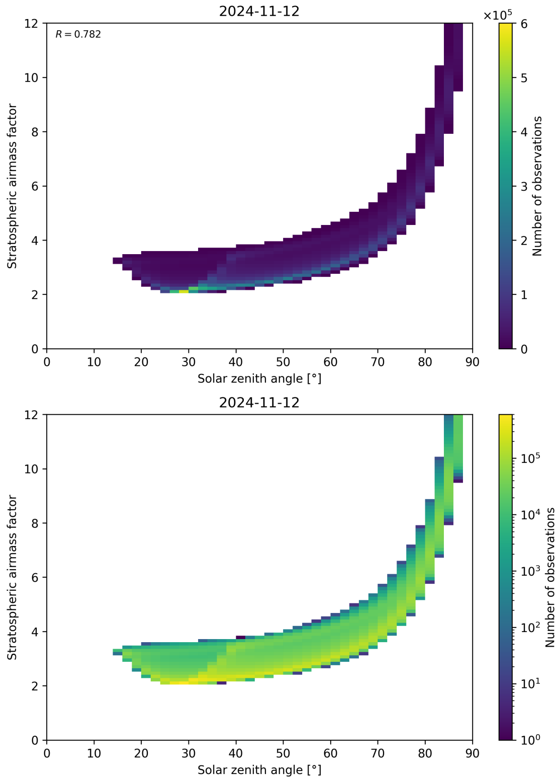
Figure 145: Scatter density plot of “Solar zenith angle” against “Stratospheric airmass factor” for 2024-11-11 to 2024-11-13.
