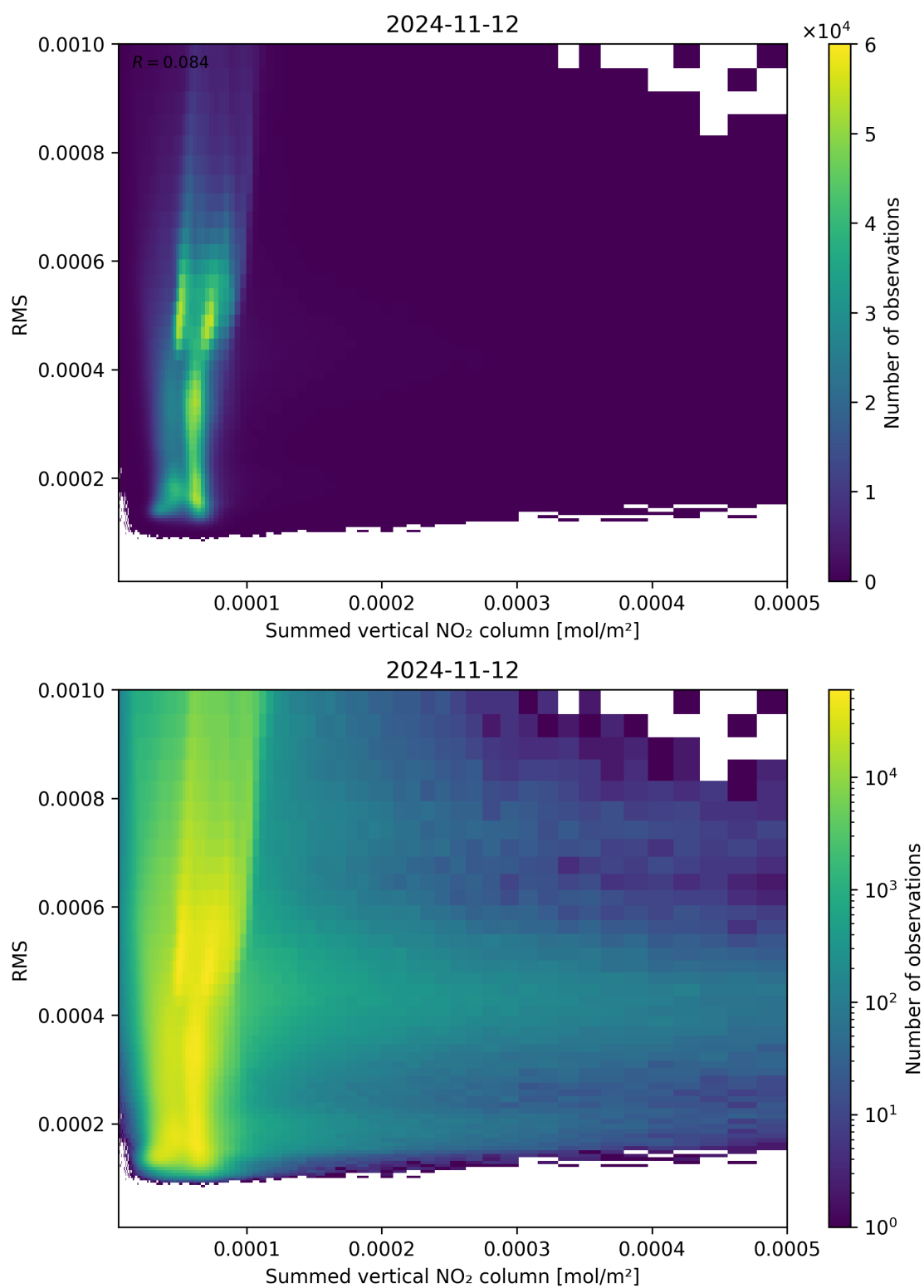
Figure 109: Scatter density plot of “Summed vertical NO 2 column” against “RMS” for 2024-11-11 to 2024-11-13.
