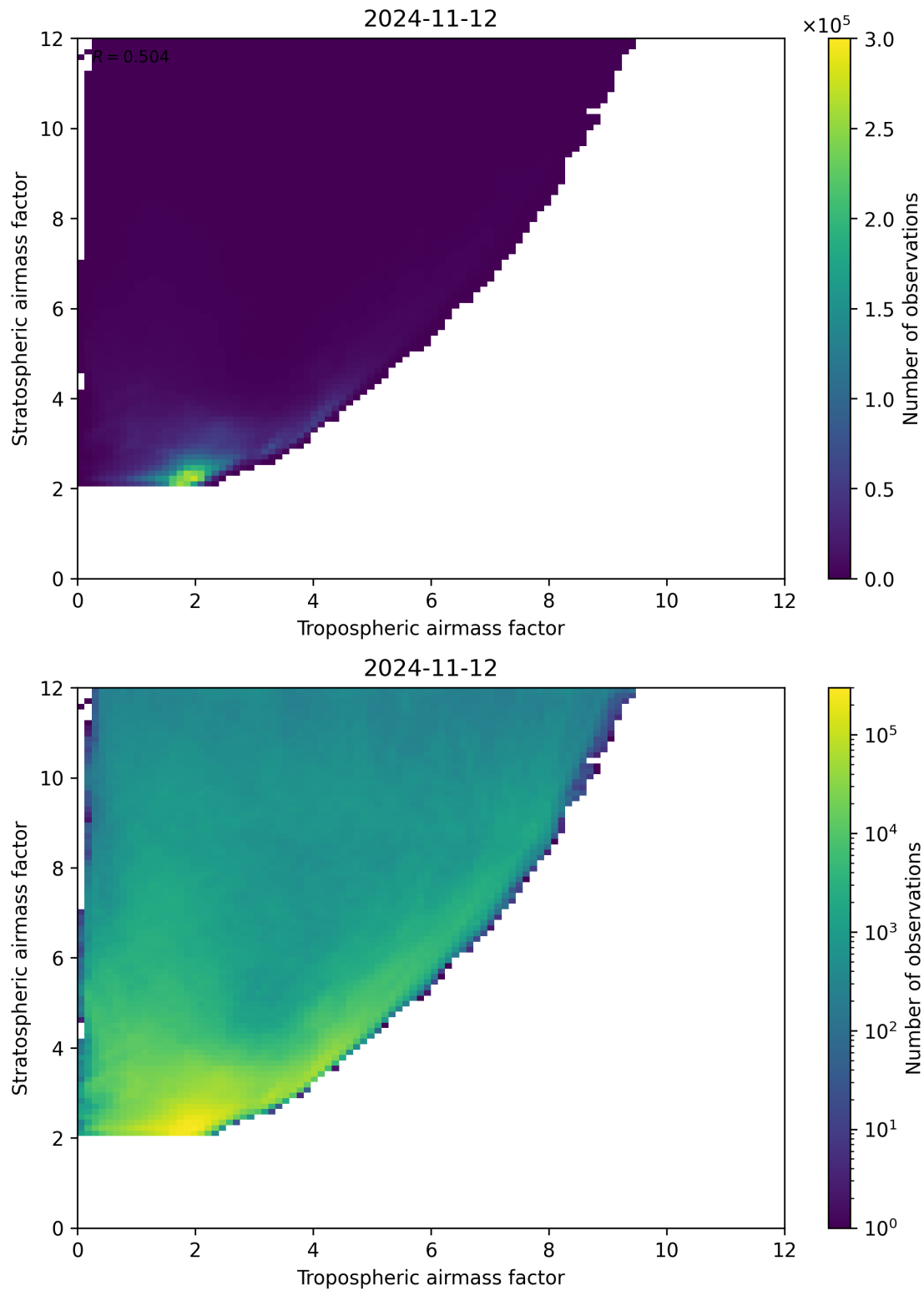
Figure 71: Scatter density plot of “Tropospheric airmass factor” against “Stratospheric airmass factor” for 2024-11-11 to 2024-11-13.
