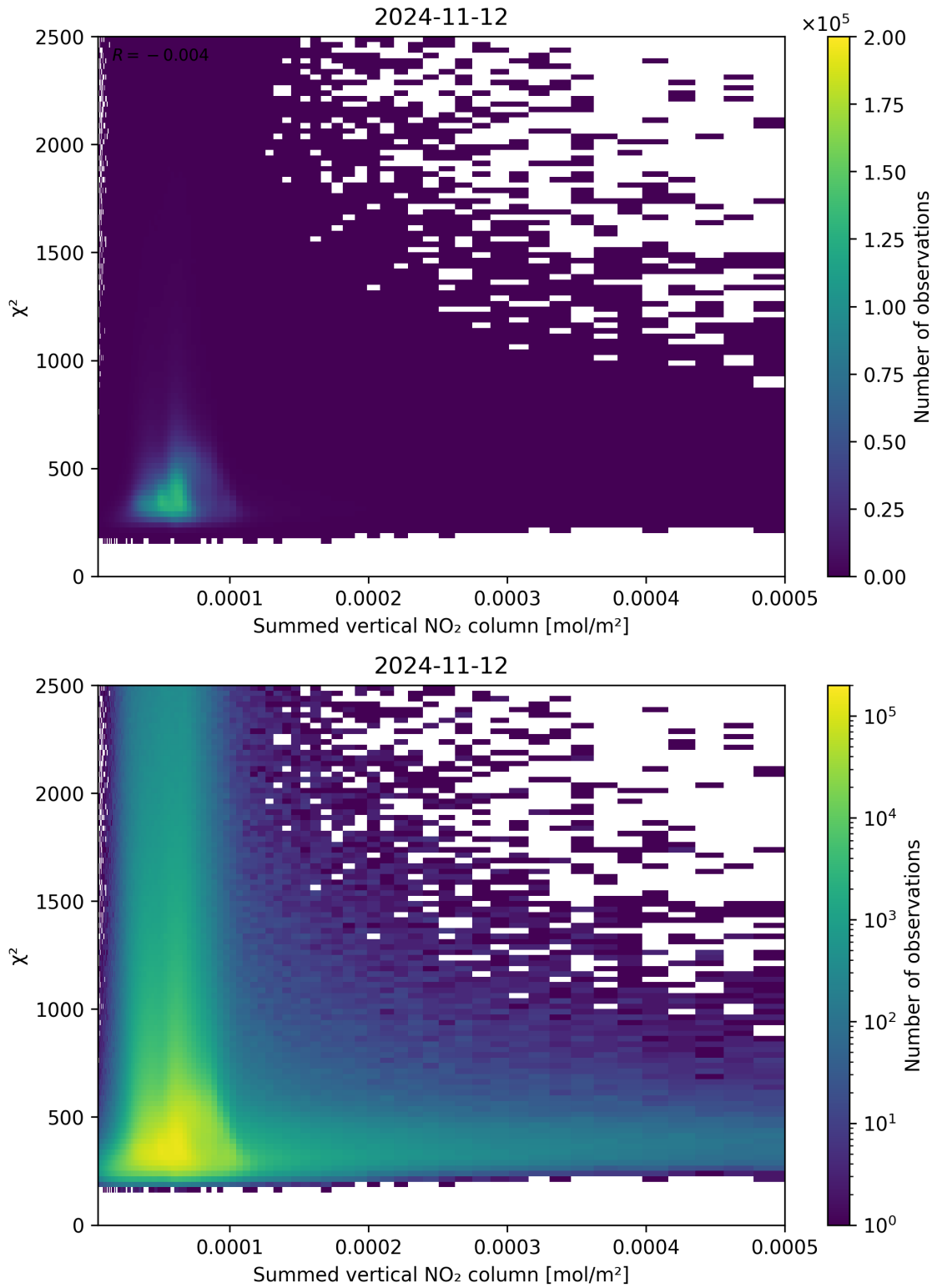
Figure 104: Scatter density plot of “Summed vertical NO 2 column” against “ \chi^2 ” for 2024-11-11 to 2024-11-13.
