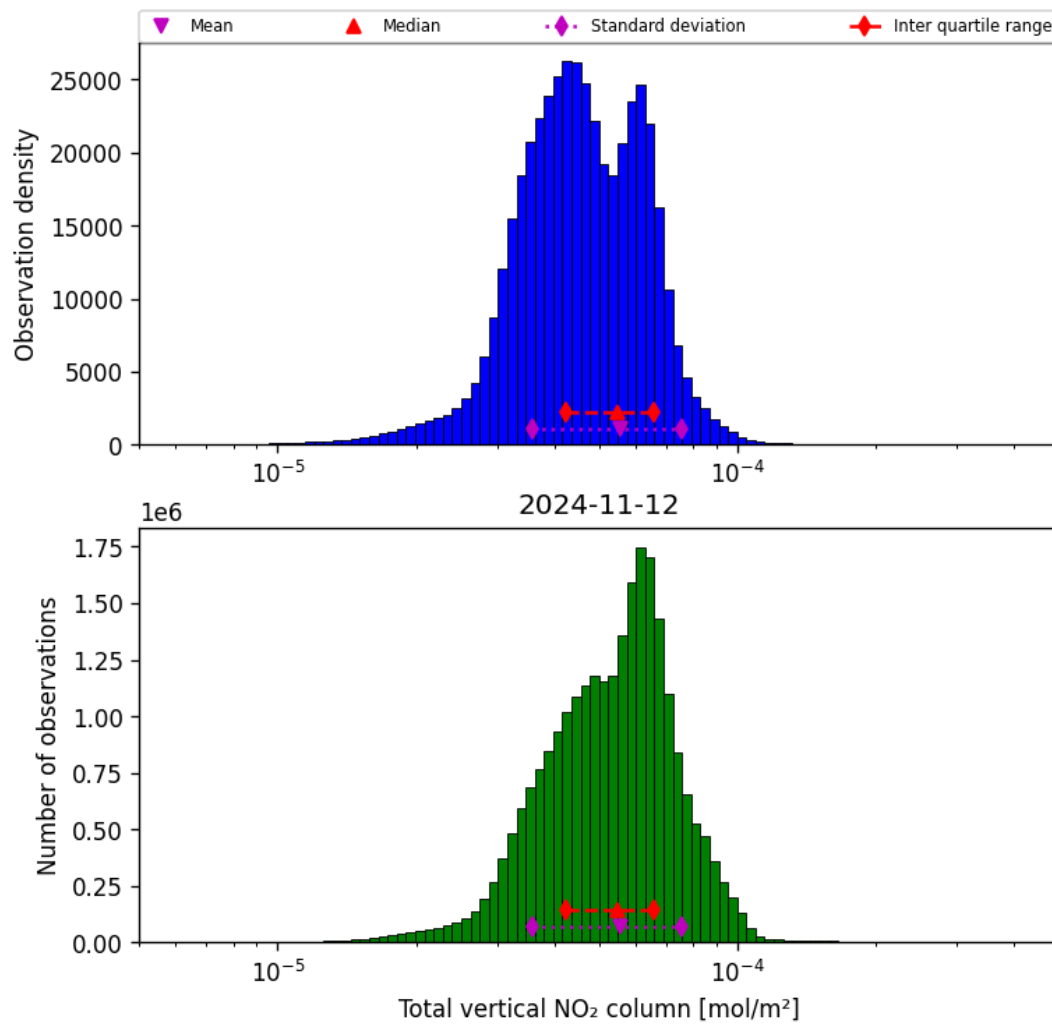
Figure 38: Histogram of “Total vertical NO 2 column” for 2024-11-11 to 2024-11-13
