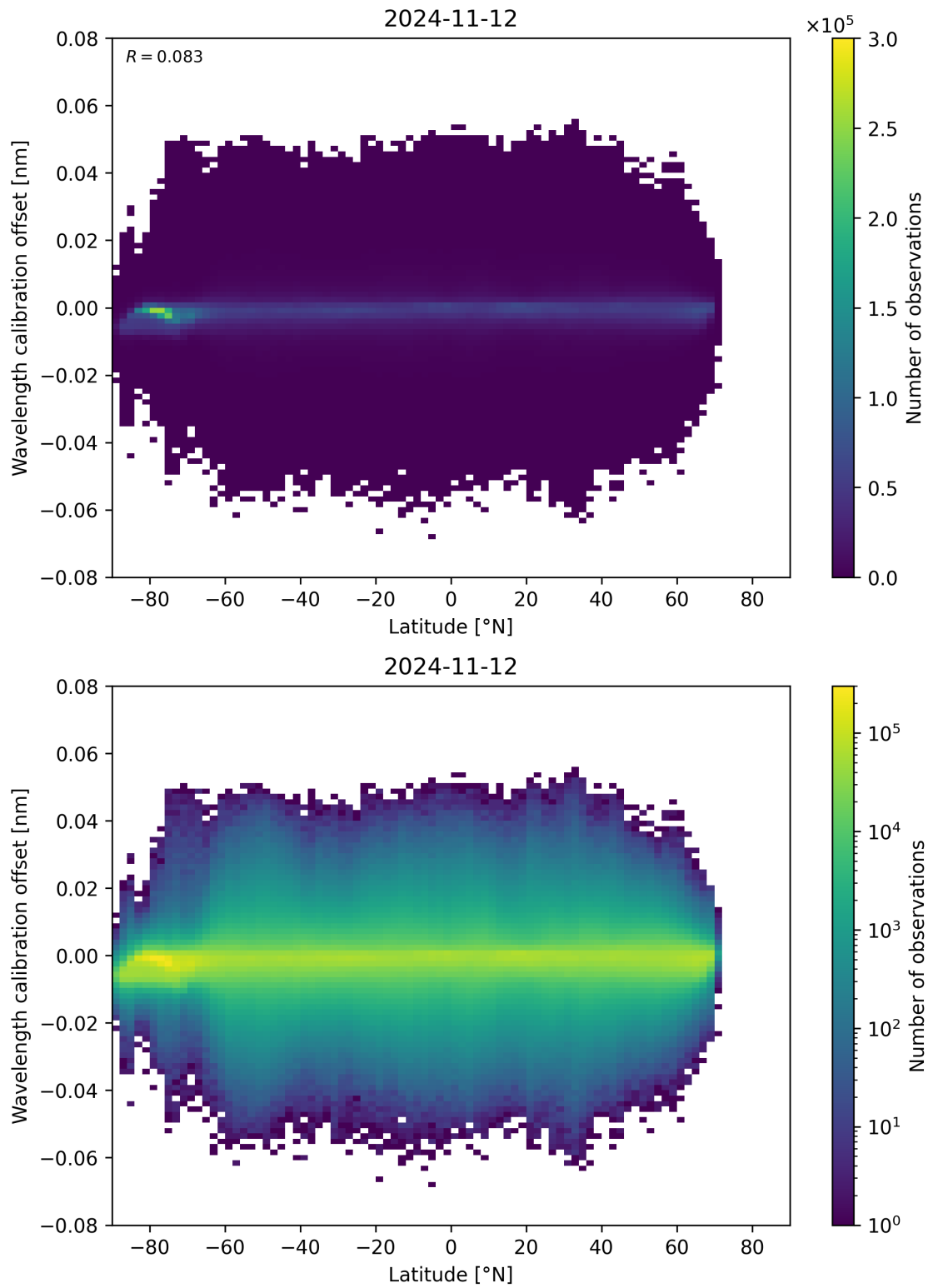
Figure 95: Scatter density plot of “Latitude” against “Wavelength calibration offset” for 2024-11-11 to 2024-11-13.
