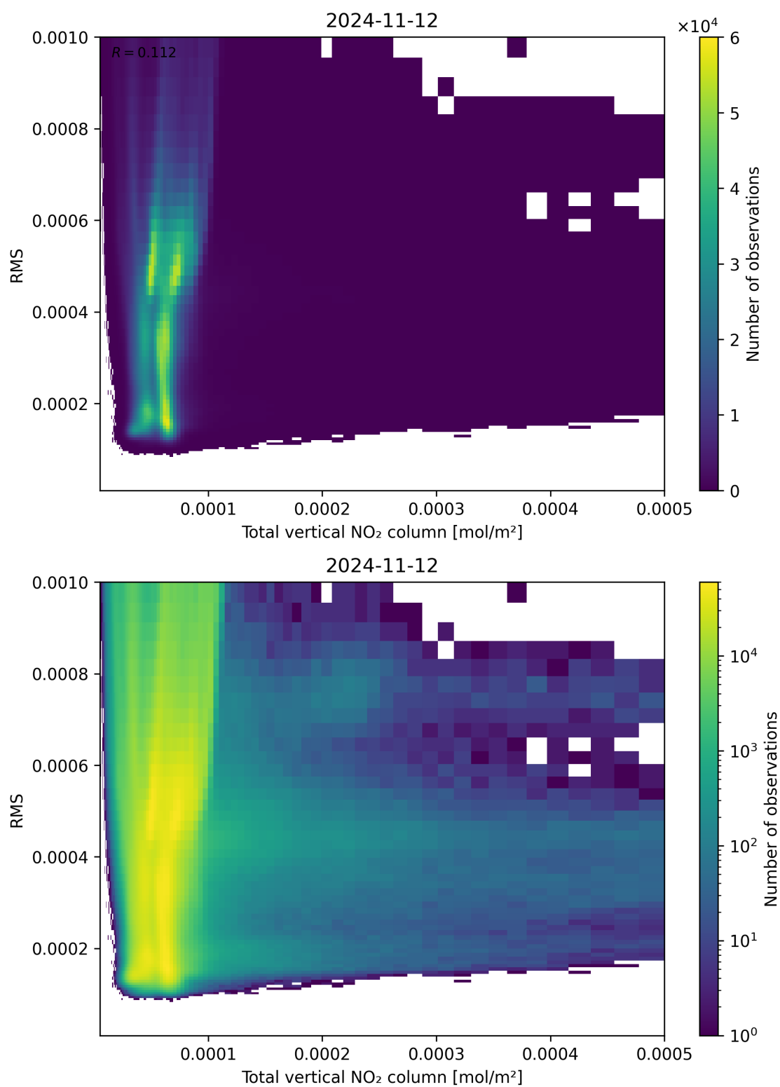
Figure 120: Scatter density plot of “Total vertical NO 2 column” against “RMS” for 2024-11-11 to 2024-11-13.
