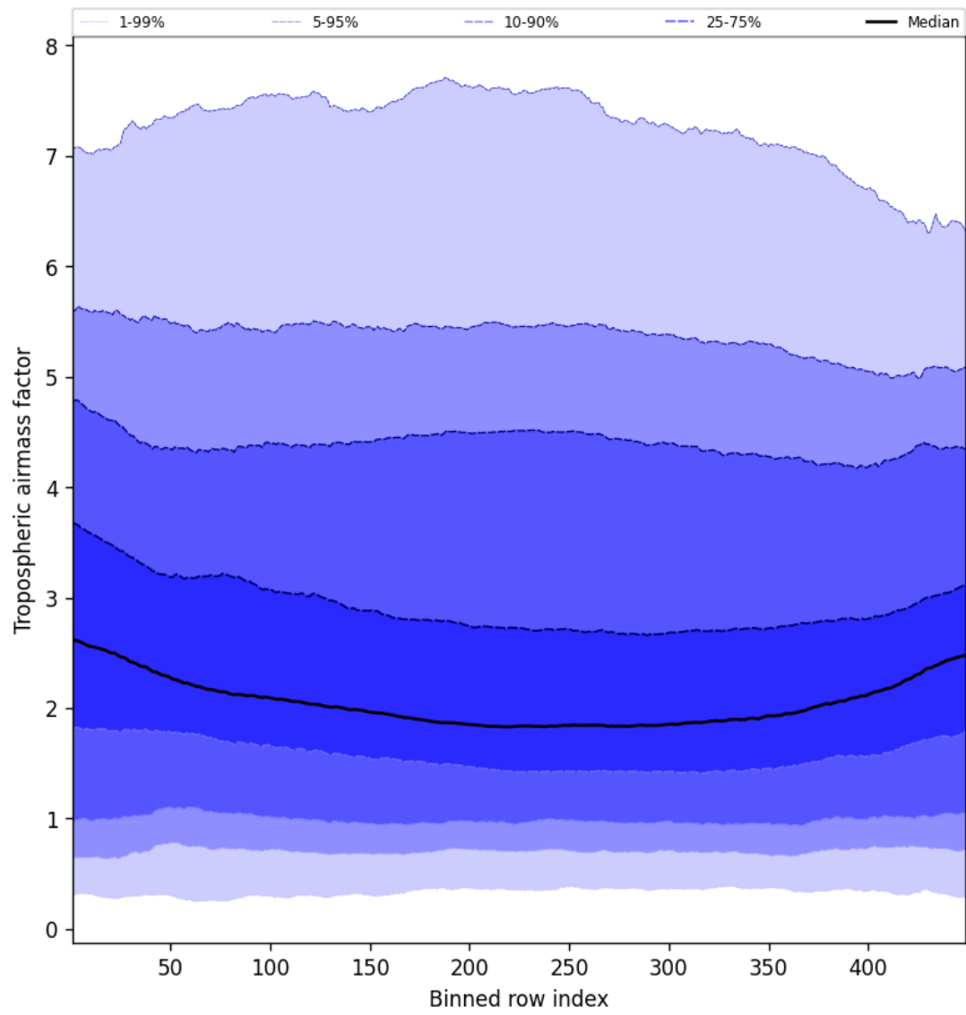
Figure 48: Along track statistics of “Tropospheric air mass factor” for 2024-11-11 to 2024-11-13
