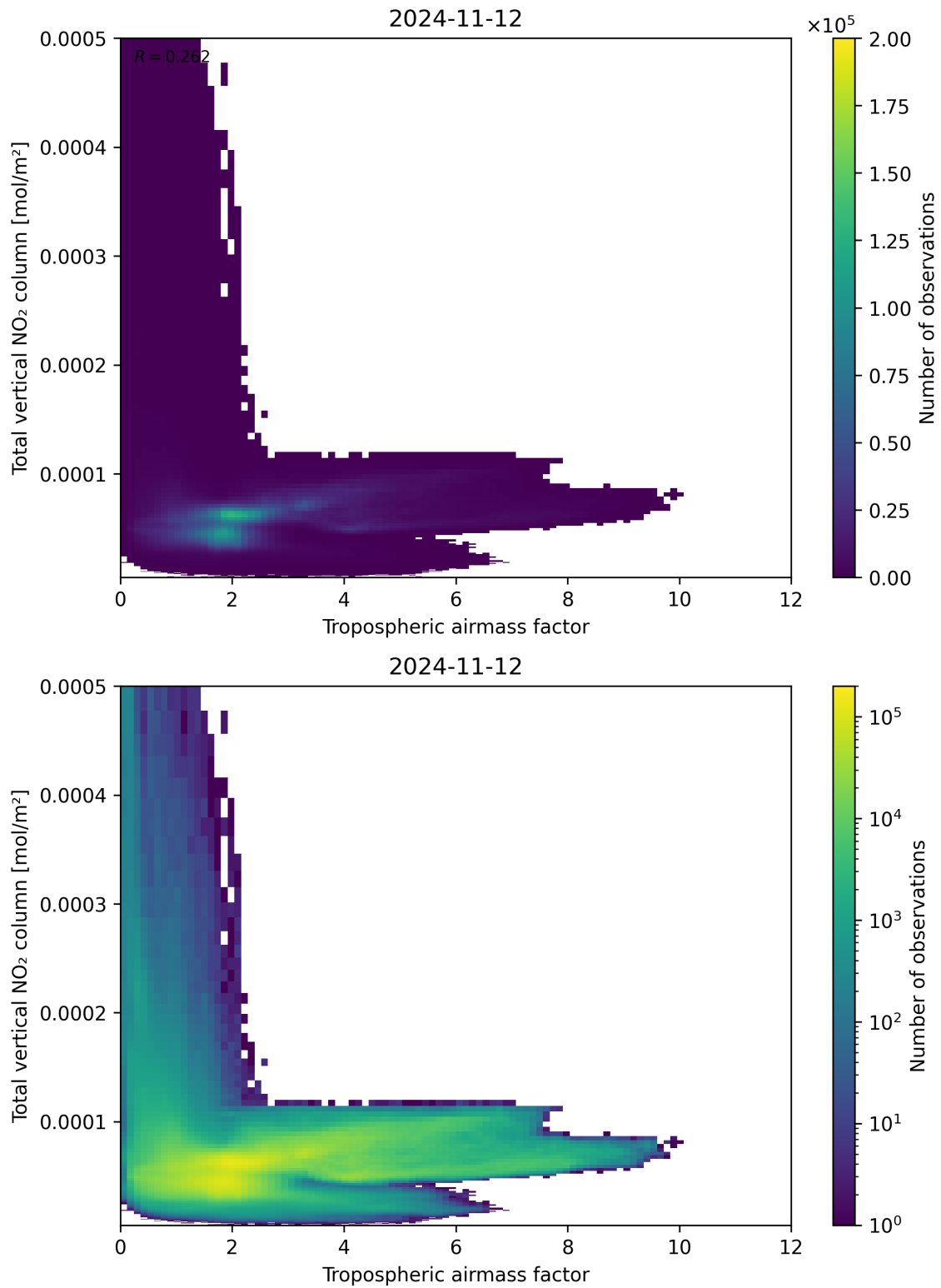
Figure 77: Scatter density plot of “Tropospheric airmass factor” against “Total vertical NO 2 column” for 2024-11-11 to 2024-11-13.
