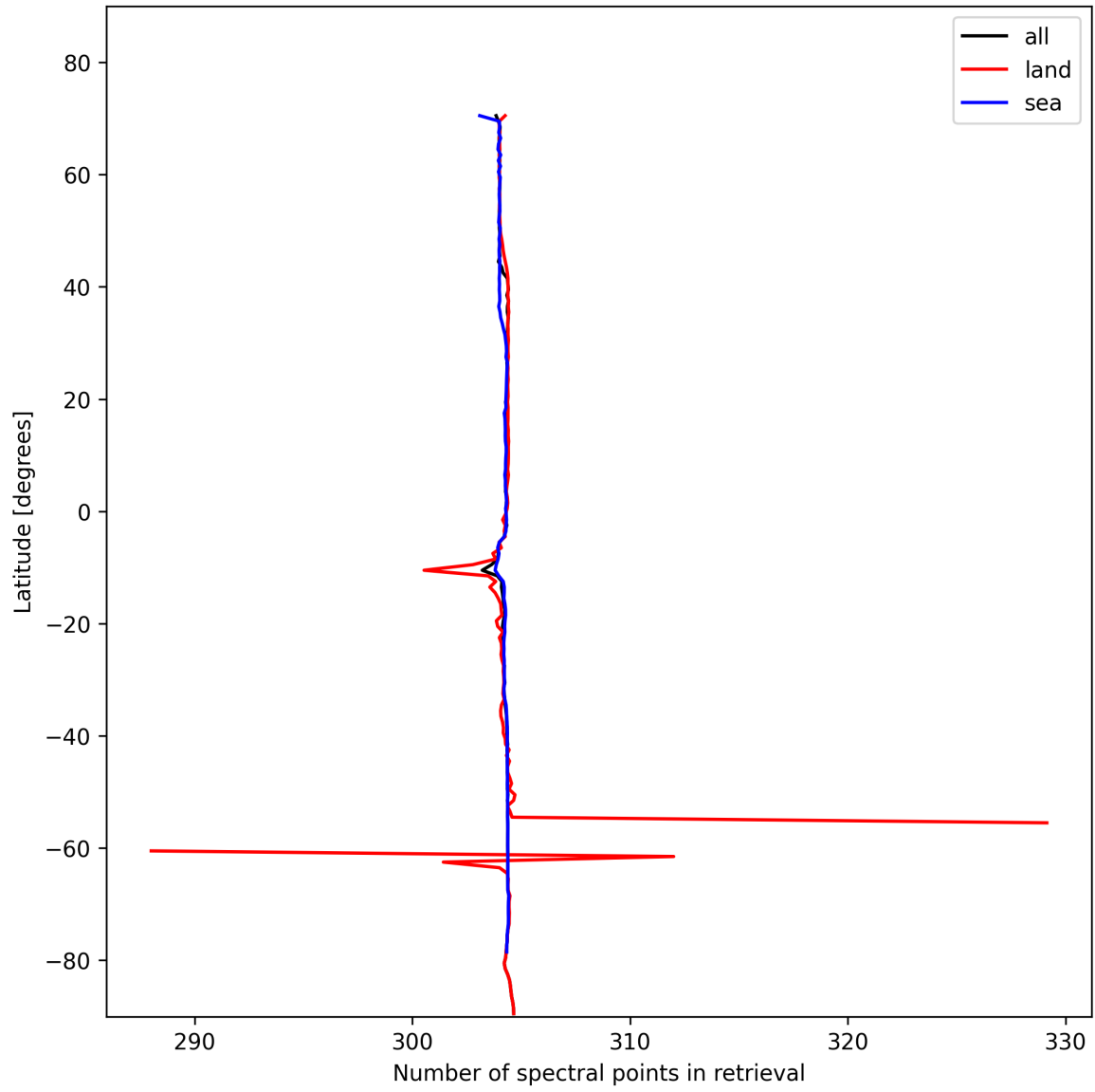
Figure 16: Zonal average of “Number of spectral points in retrieval” for 2024-11-11 to 2024-11-13.
