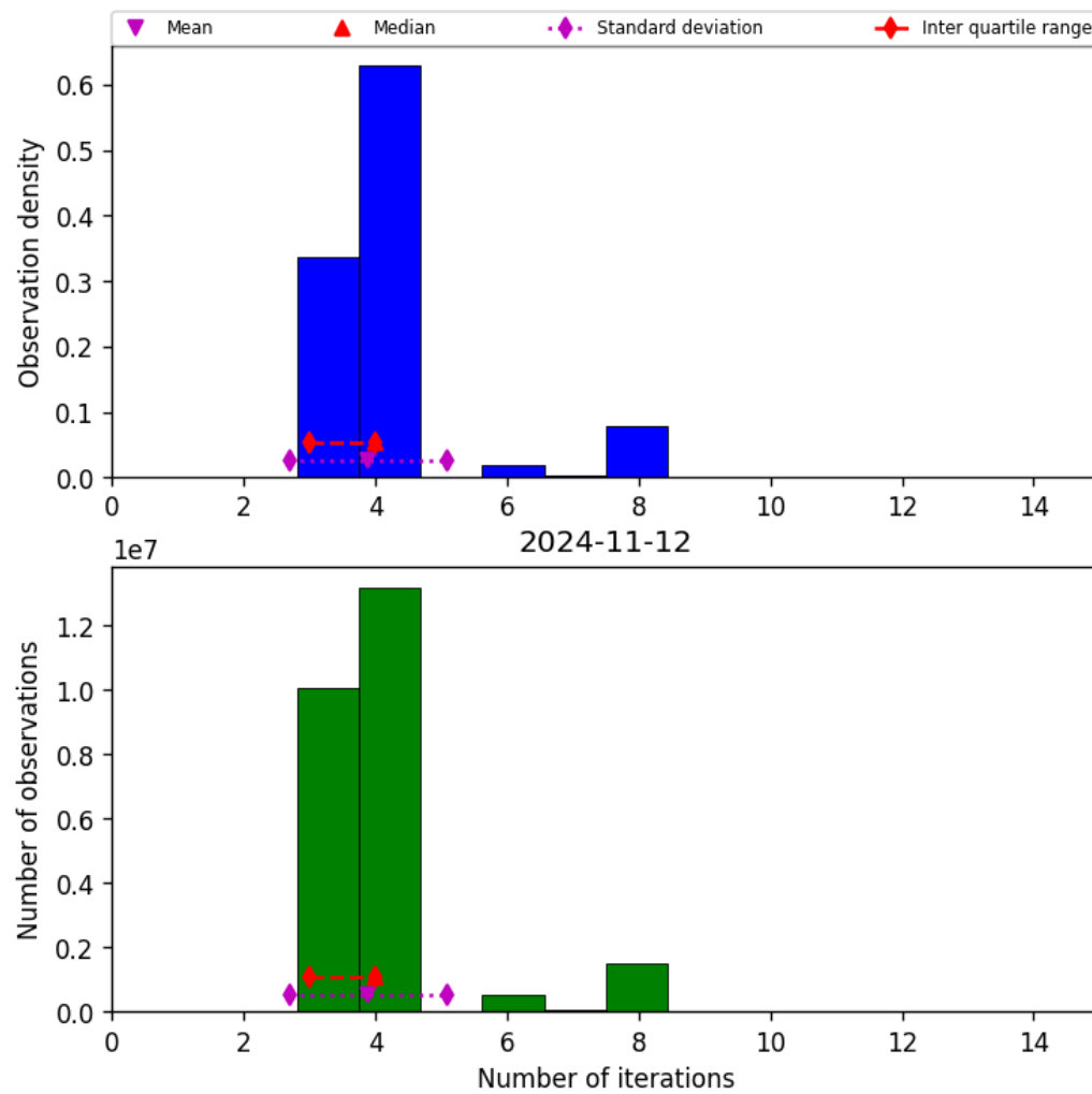
Figure 34: Histogram of “Number of iterations” for 2024-11-11 to 2024-11-13
