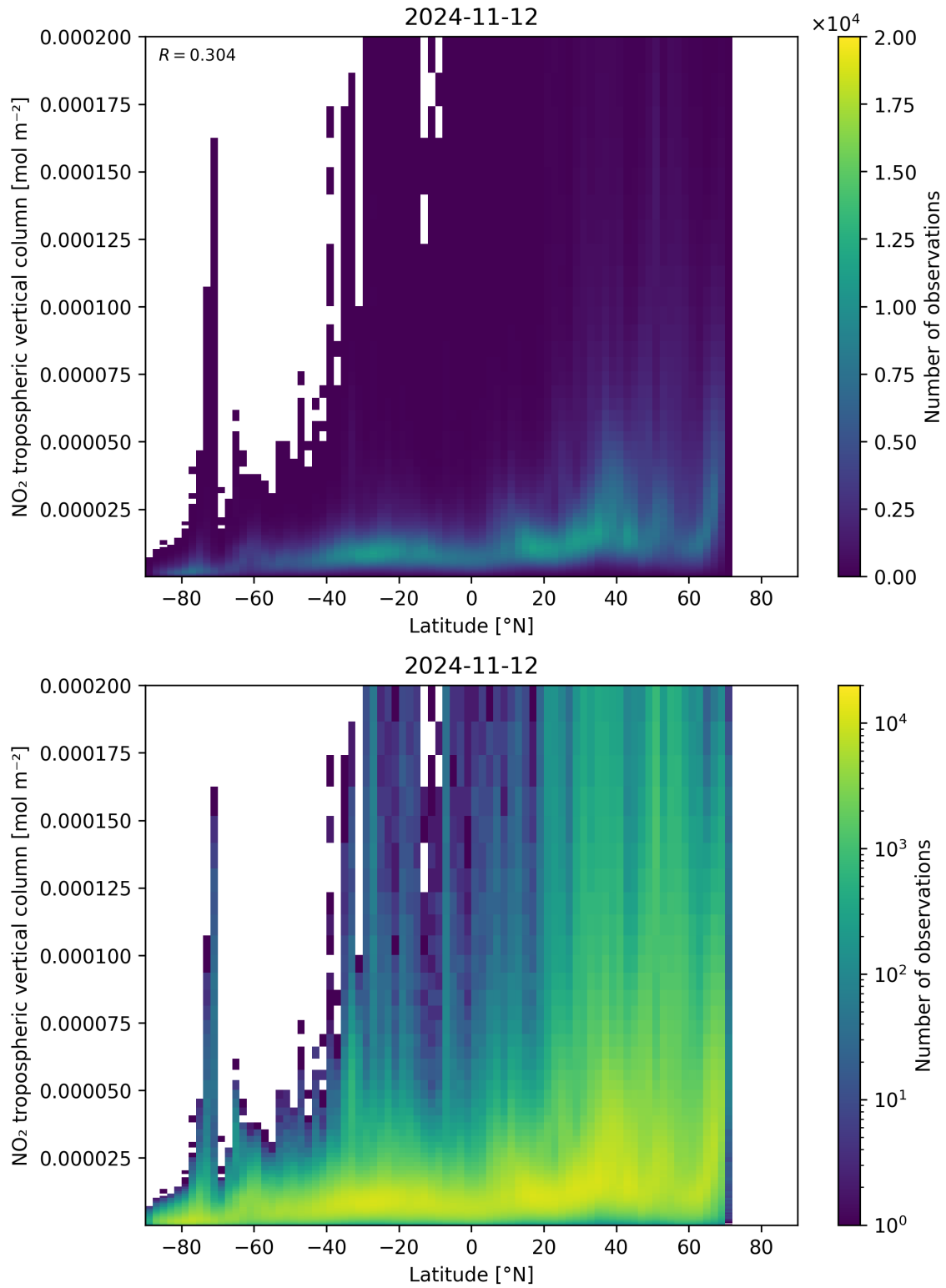
Figure 92: Scatter density plot of “Latitude” against “NO 2 tropospheric vertical column” for 2024-11-11 to 2024-11-13.
