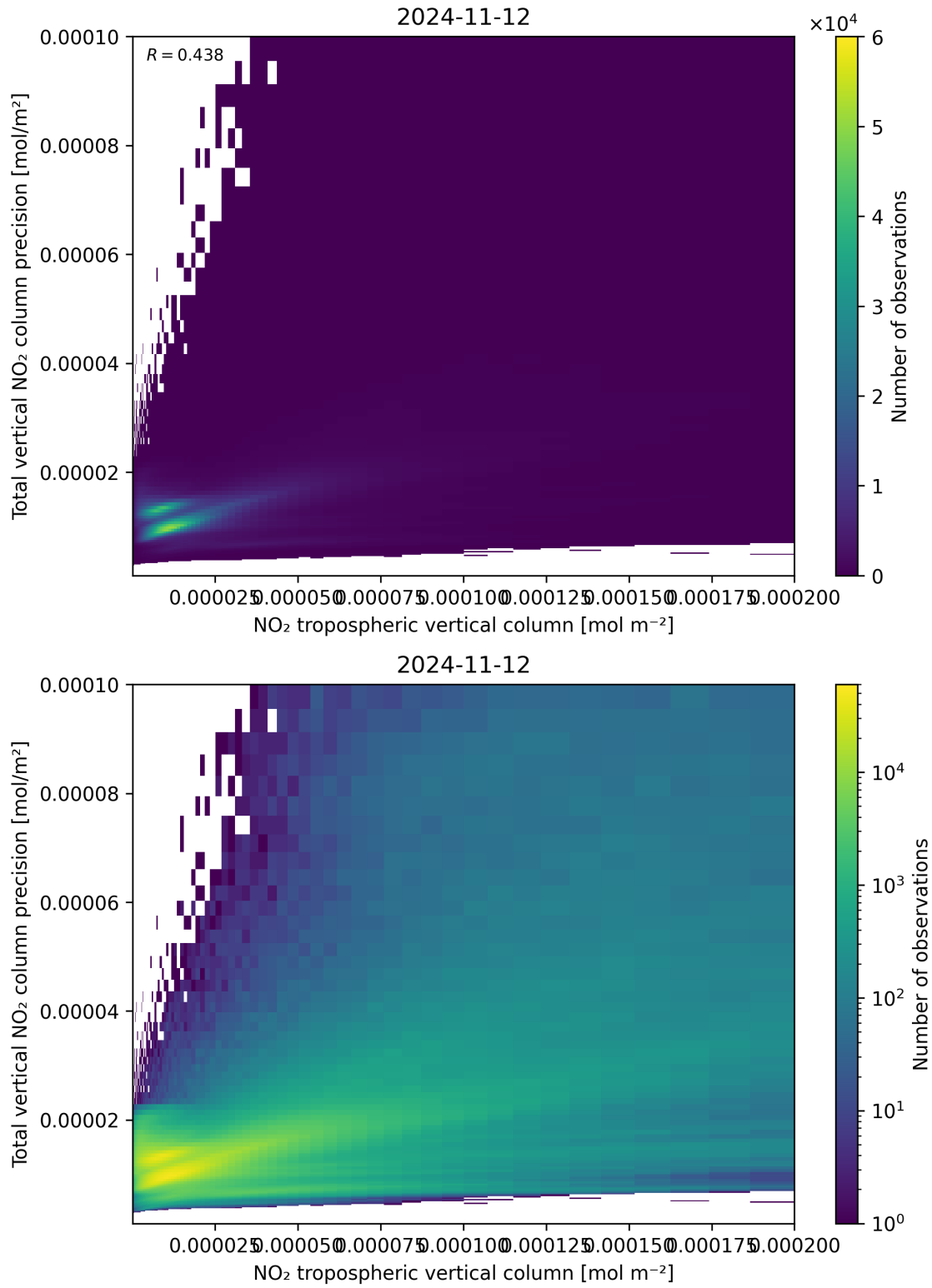
Figure 129: Scatter density plot of “NO 2 tropospheric vertical column” against “Total vertical NO 2 column precision” for 2024-11-11 to 2024-11-13.
