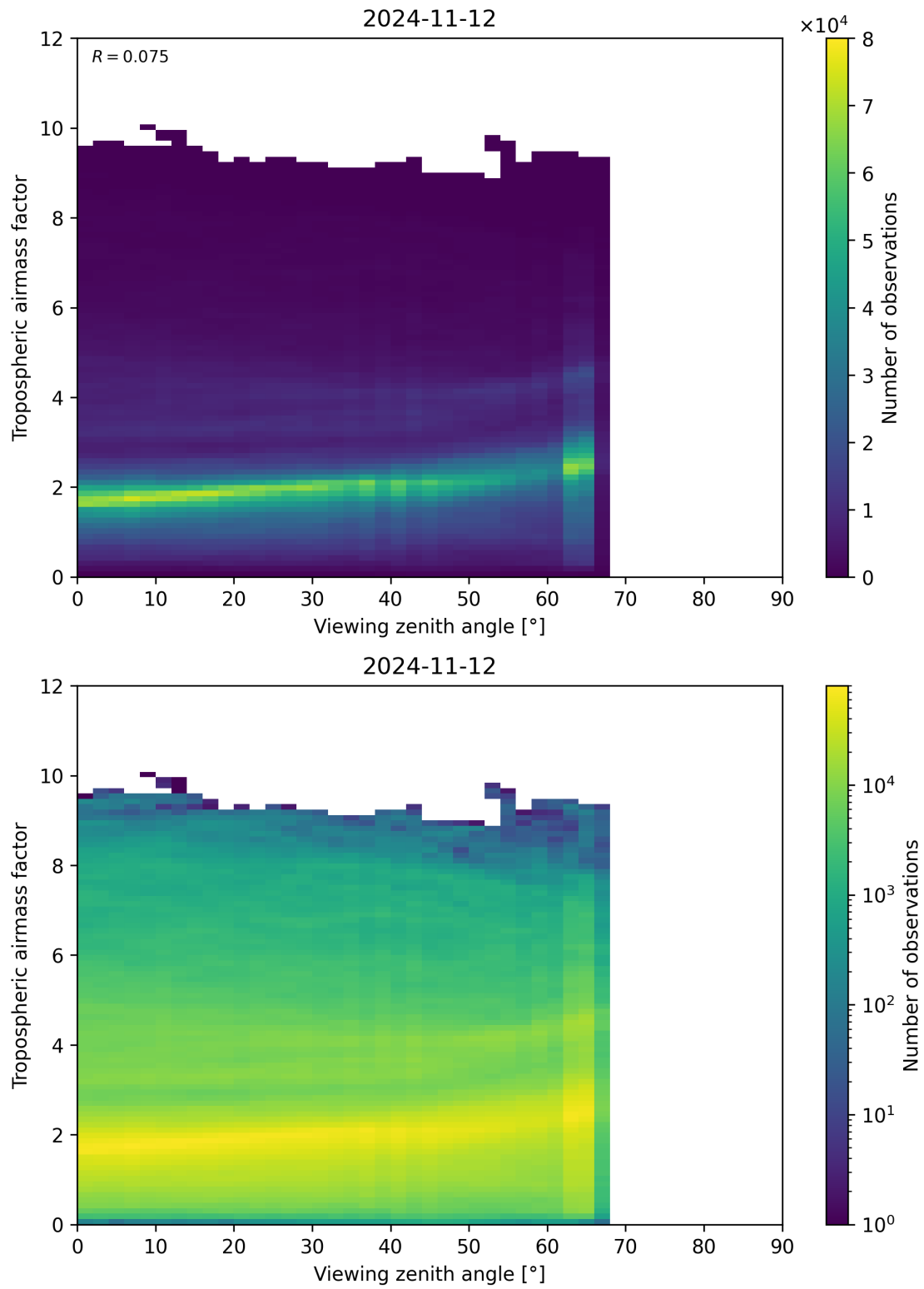
Figure 161: Scatter density plot of “Viewing zenith angle” against “Tropospheric airmass factor” for 2024-11-11 to 2024-11-13.
