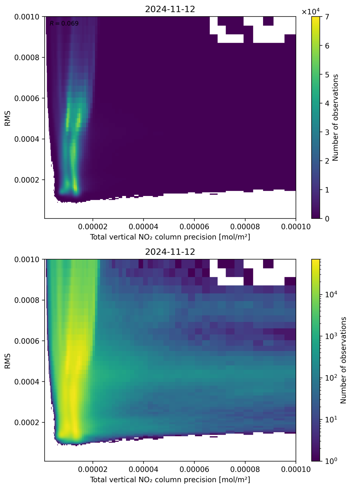
Figure 119: Scatter density plot of “Total vertical NO 2 column precision” against “RMS” for 2024-11-11 to 2024-11-13.
