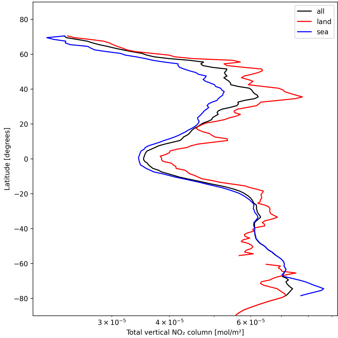
Figure 21: Zonal average of “Total vertical NO 2 column” for 2024-11-11 to 2024-11-13.
