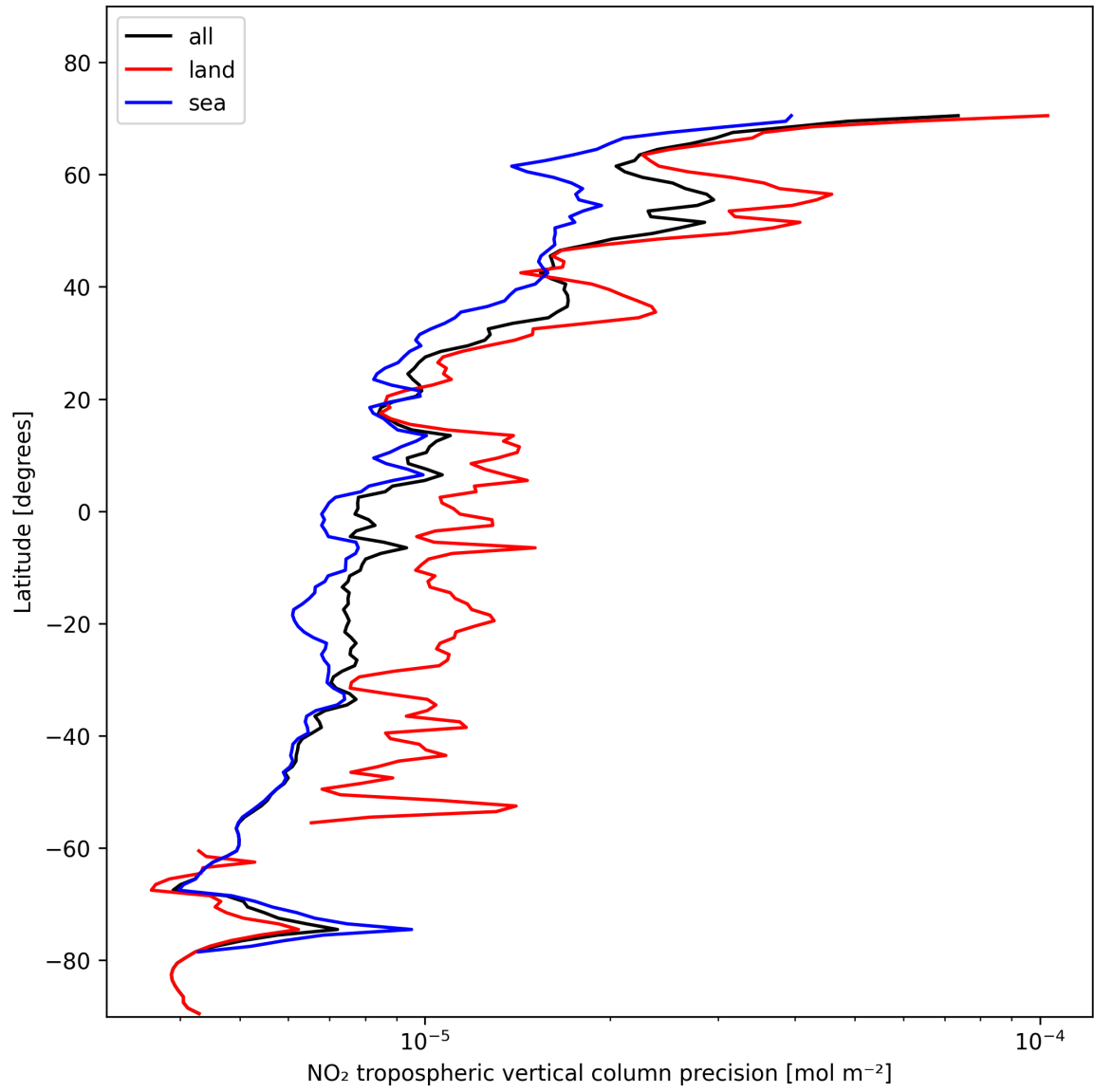
Figure 13: Zonal average of “NO 2 tropospheric vertical column precision” for 2024-11-11 to 2024-11-13.
