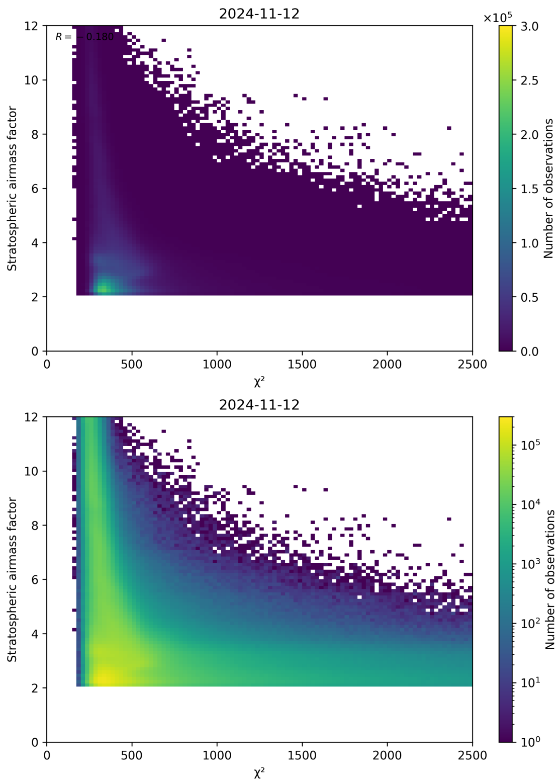
Figure 81: Scatter density plot of “ \chi^2 ” against “Stratospheric airmass factor” for 2024-11-11 to 2024-11-13.
