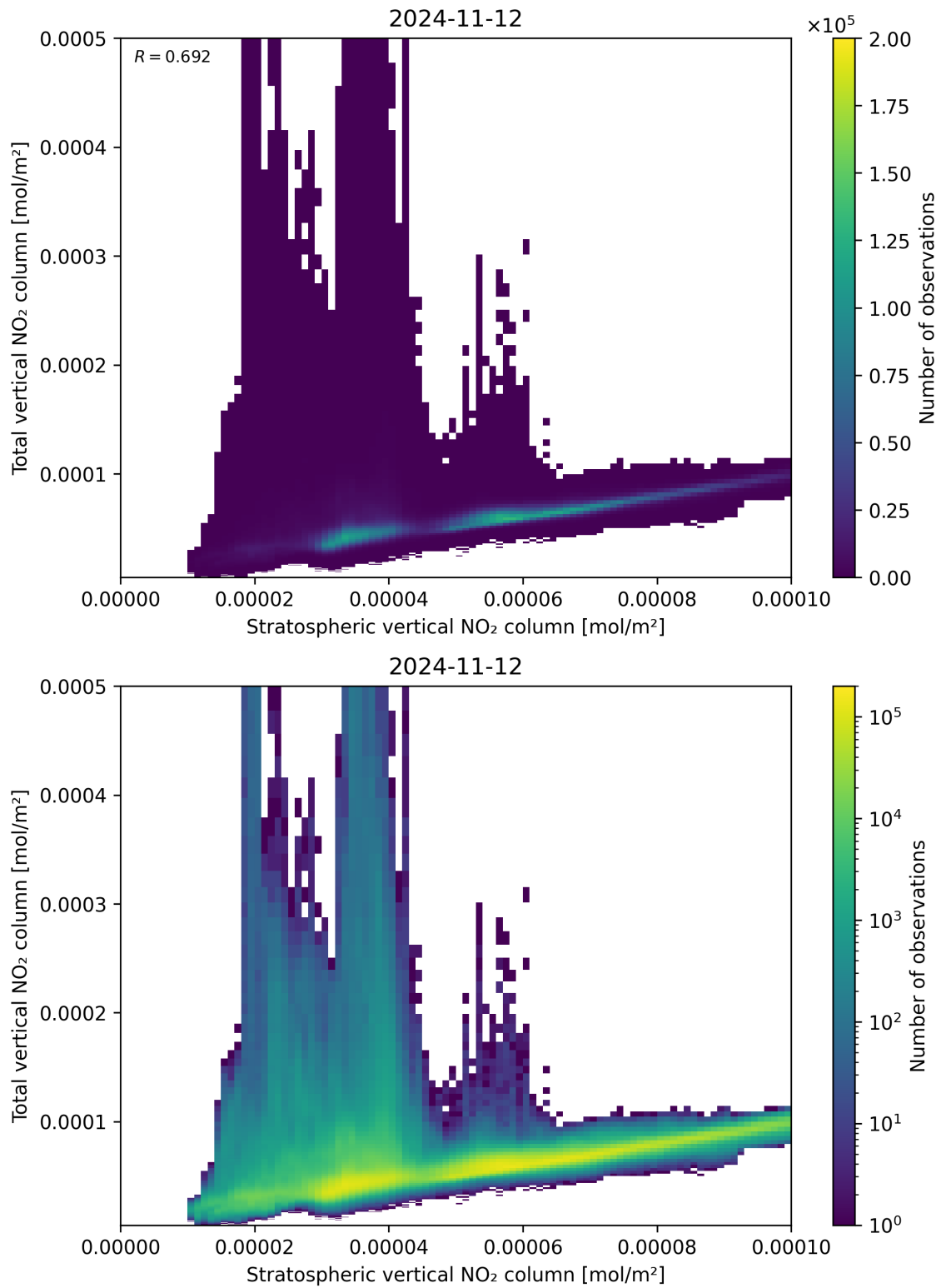
Figure 100: Scatter density plot of “Stratospheric vertical NO 2 column” against “Total vertical NO 2 column” for 2024-11-11 to 2024-11-13.
