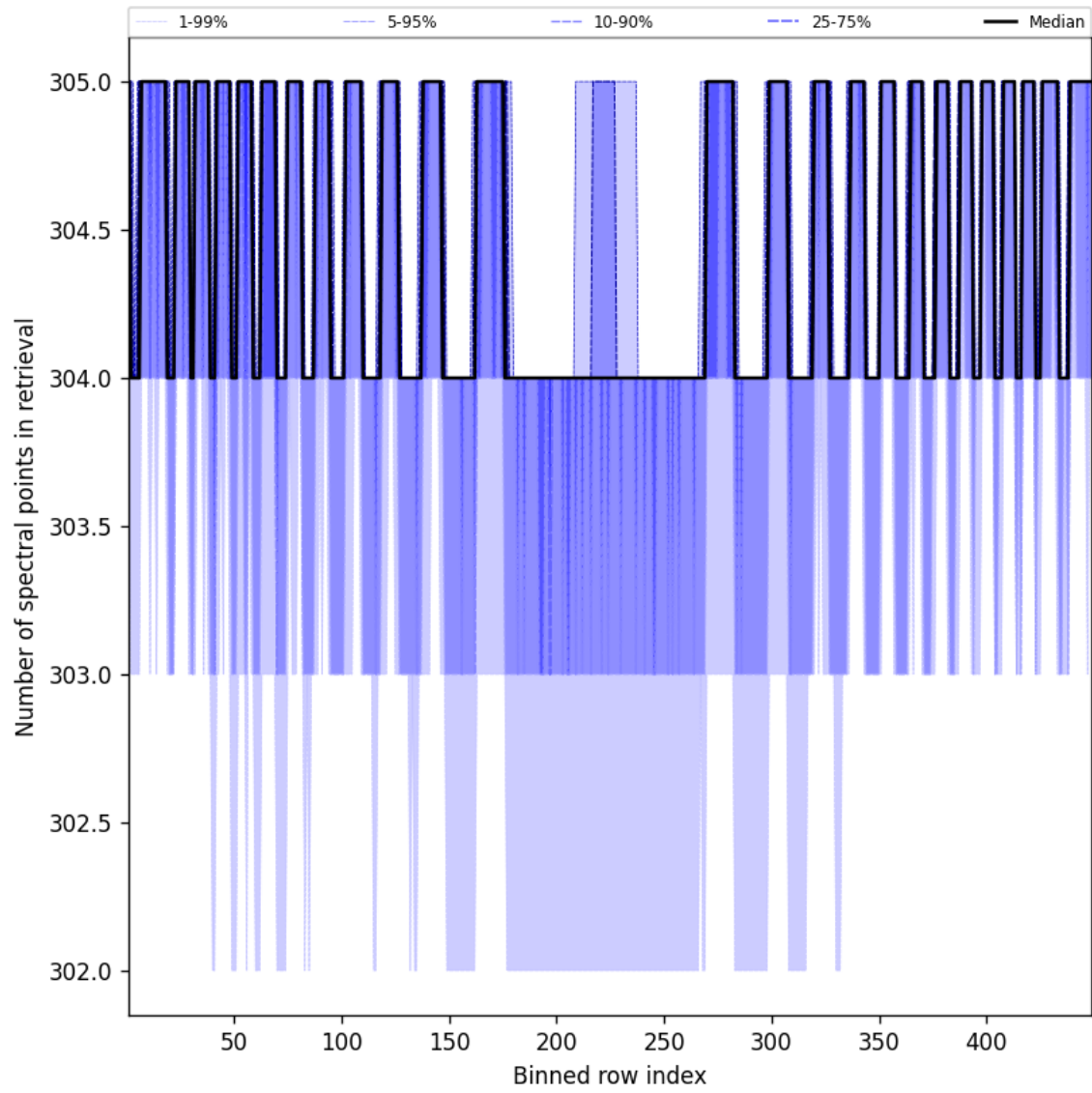
Figure 50: Along track statistics of “Number of spectral points in retrieval” for 2024-11-11 to 2024-11-13
