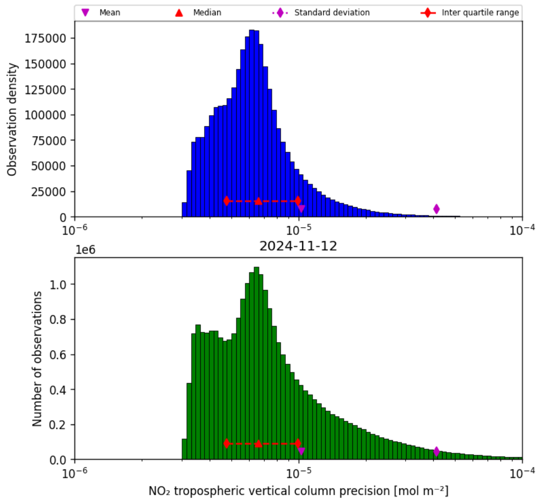
Figure 30: Histogram of “NO 2 tropospheric vertical column precision” for 2024-11-11 to 2024-11-13
