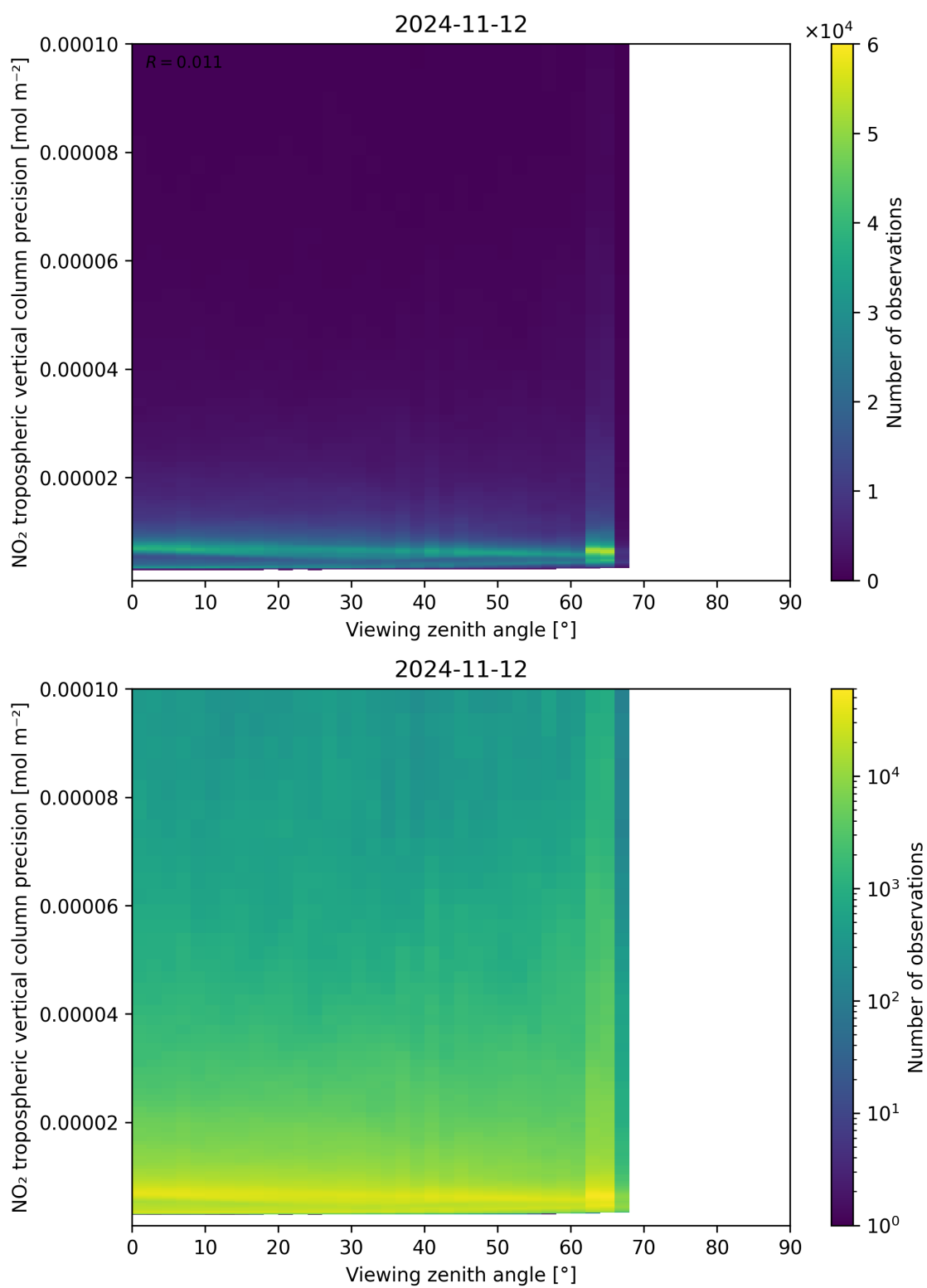
Figure 170: Scatter density plot of “Viewing zenith angle” against “NO 2 tropospheric vertical column precision” for 2024-11-11 to 2024-11-13.
