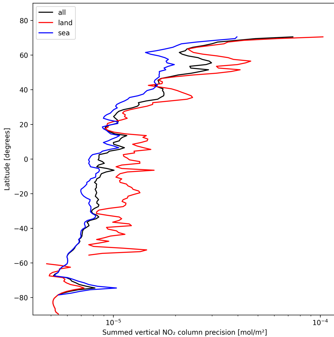
Figure 24: Zonal average of “Summed vertical NO 2 column precision” for 2024-11-11 to 2024-11-13.
