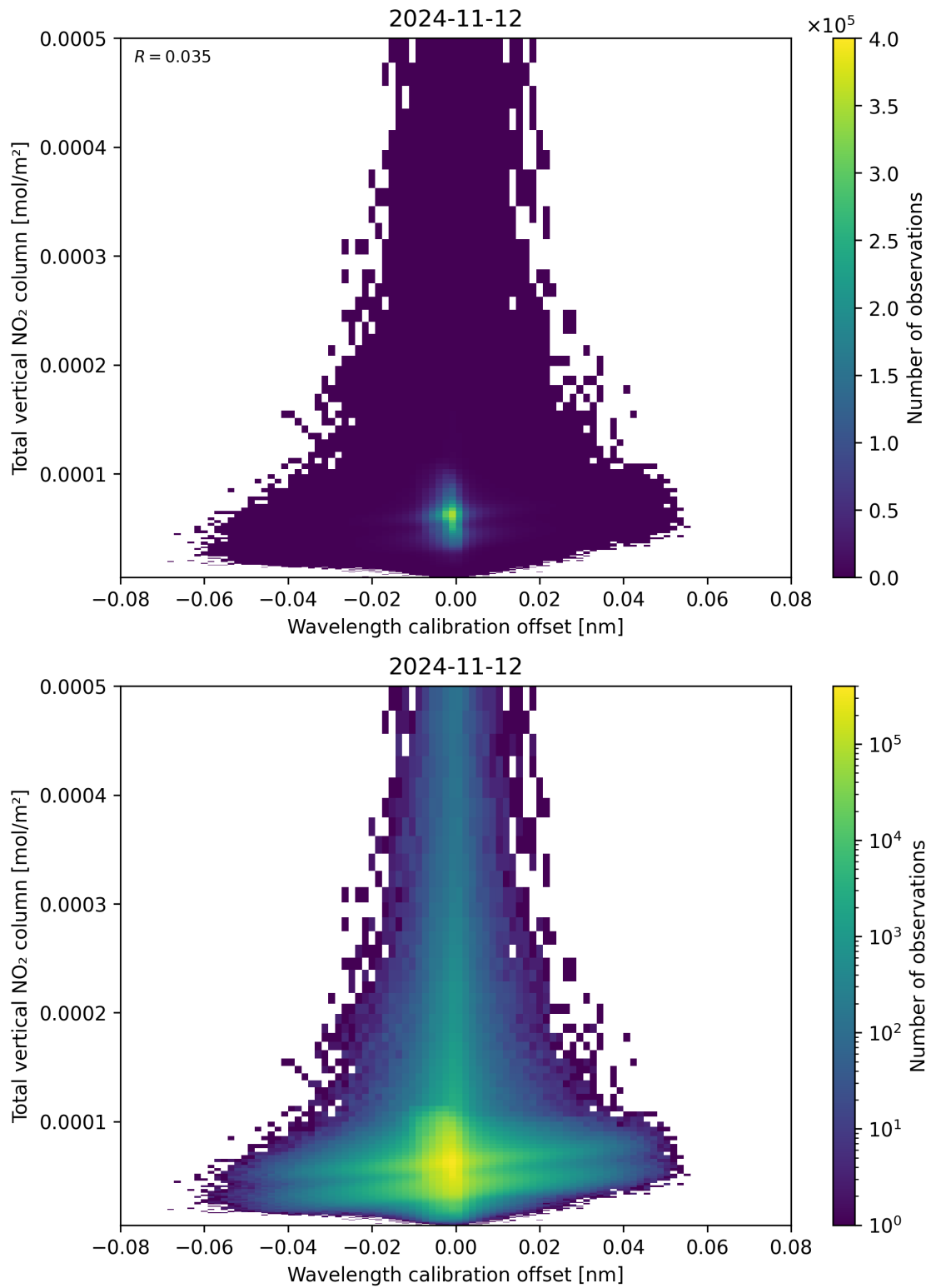
Figure 179: Scatter density plot of “Wavelength calibration offset” against “Total vertical NO 2 column” for 2024-11-11 to 2024-11-13.
