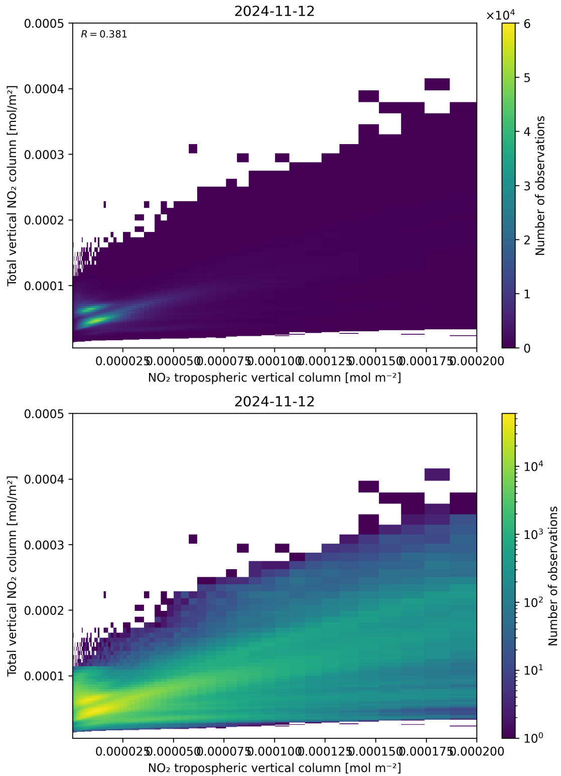
Figure 128: Scatter density plot of “NO 2 tropospheric vertical column” against “Total vertical NO 2 column” for 2024-11-11 to 2024-11-13.
