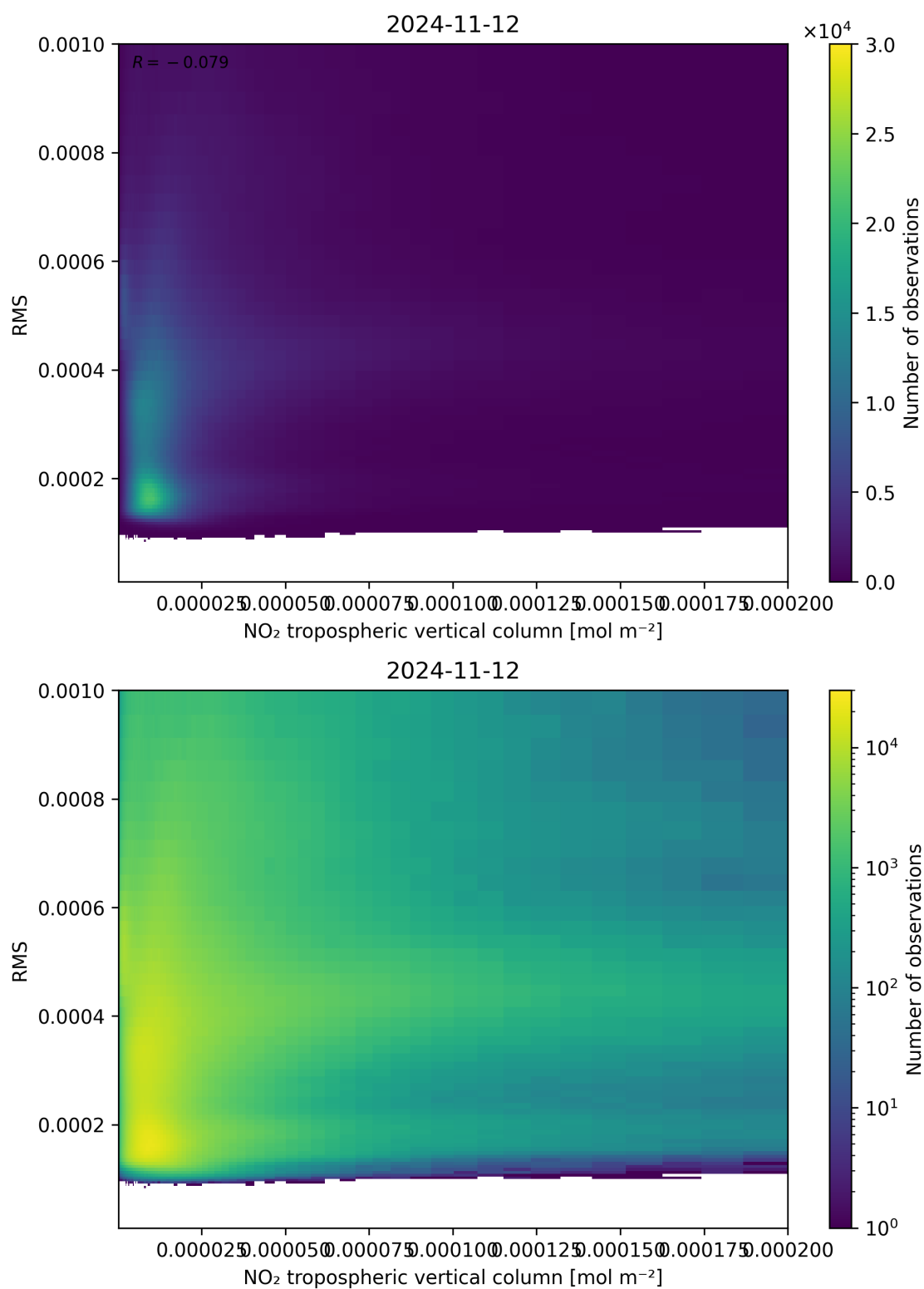
Figure 142: Scatter density plot of “NO 2 tropospheric vertical column” against “RMS” for 2024-11-11 to 2024-11-13.
