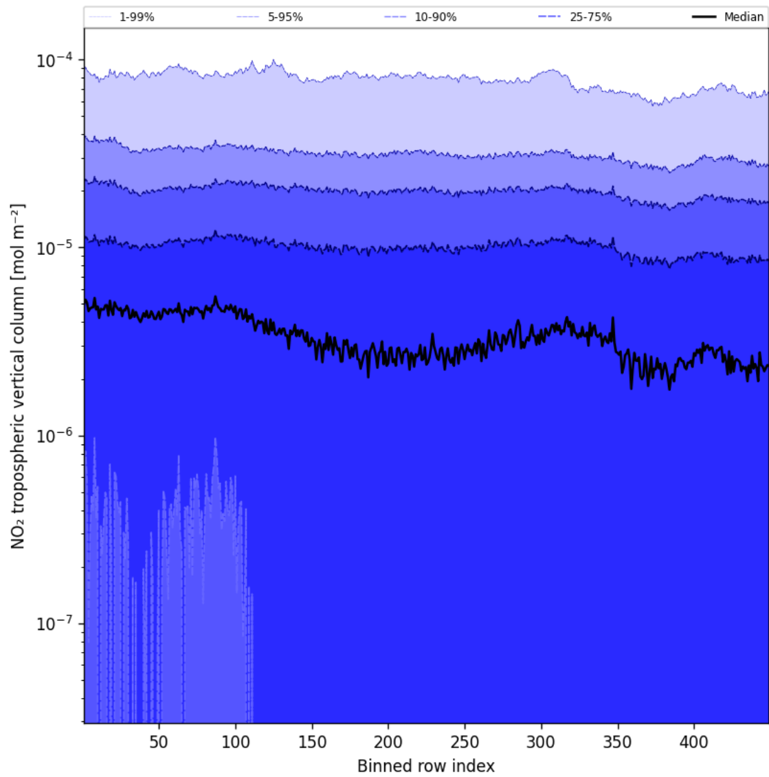
Figure 46: Along track statistics of “NO 2 tropospheric vertical column” for 2024-11-11 to 2024-11-13
