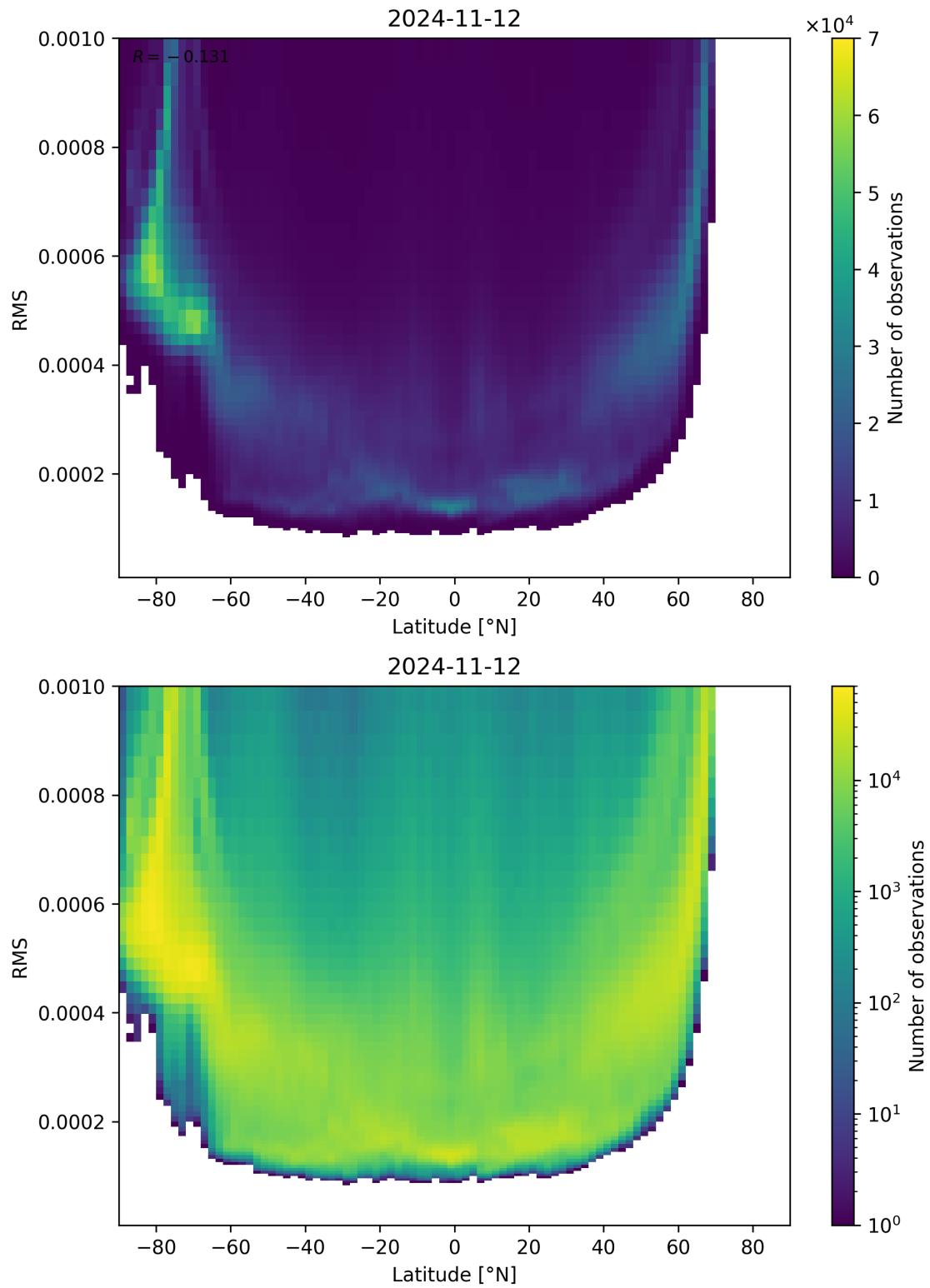
Figure 94: Scatter density plot of “Latitude” against “RMS” for 2024-11-11 to 2024-11-13.
