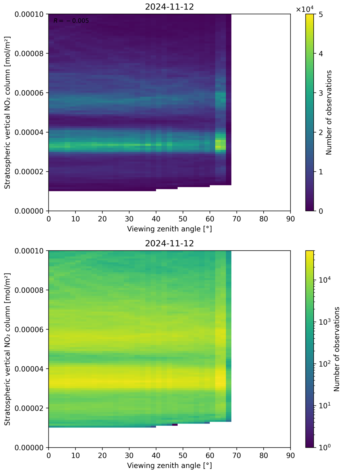
Figure 164: Scatter density plot of “Viewing zenith angle” against “Stratospheric vertical NO 2 column” for 2024-11-11 to 2024-11-13.
