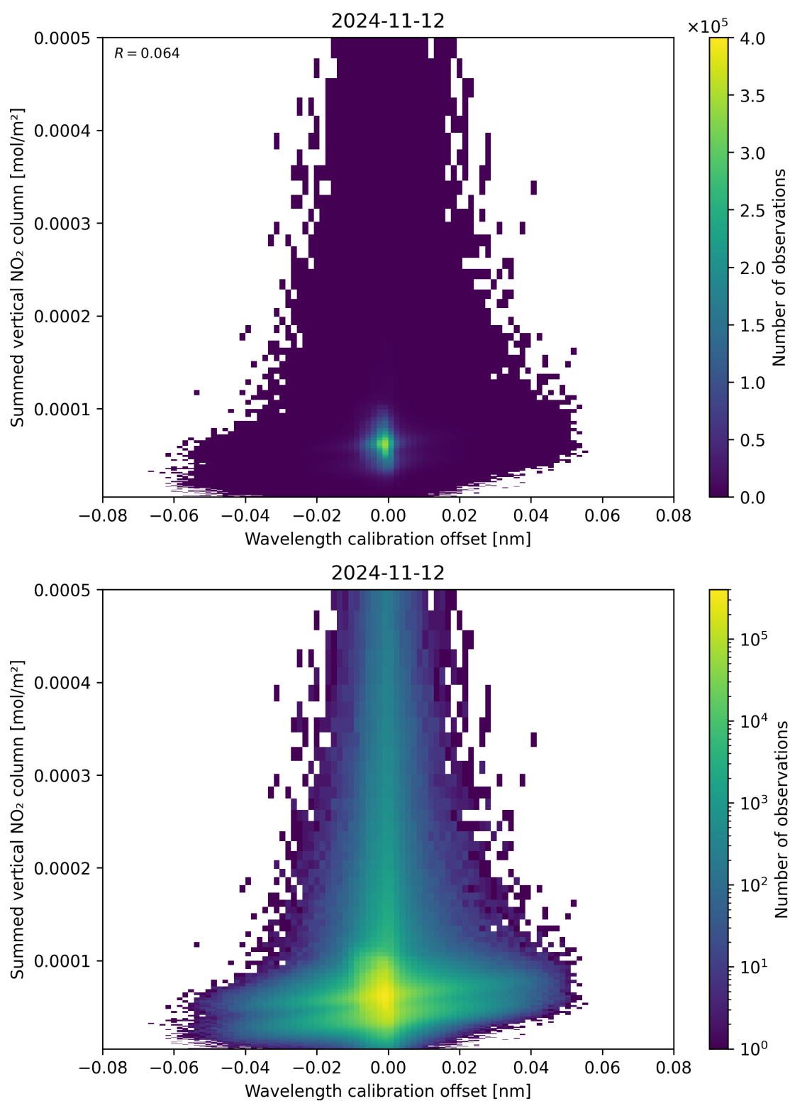
Figure 177: Scatter density plot of “Wavelength calibration offset” against “Summed vertical NO 2 column” for 2024-11-11 to 2024-11-13.
