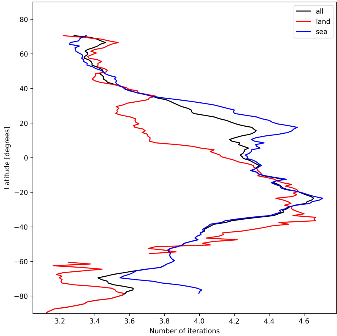
Figure 17: Zonal average of “Number of iterations” for 2024-11-11 to 2024-11-13.
