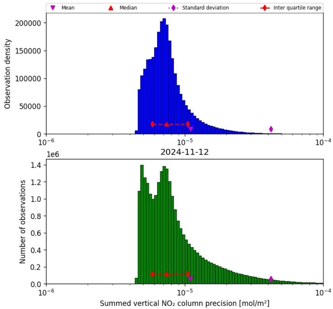
Figure 41: Histogram of "Summed vertical NO 2 column precision" for 2024-11-11 to 2024-11-13
