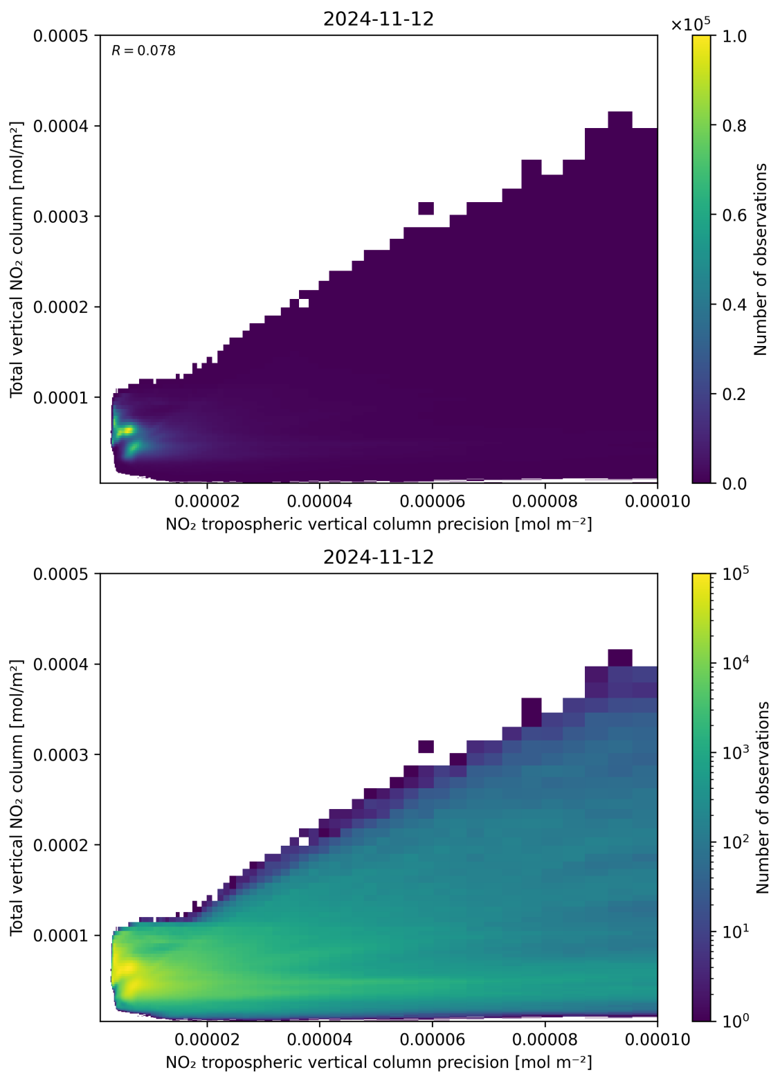
Figure 138: Scatter density plot of “NO 2 tropospheric vertical column precision” against “Total vertical NO 2 column” for 2024-11-11 to 2024-11-13.
