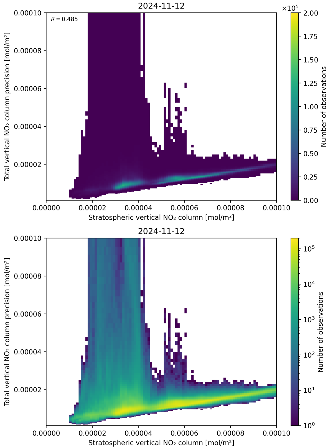
Figure 101: Scatter density plot of “Stratospheric vertical NO 2 column” against “Total vertical NO 2 column precision” for 2024-11-11 to 2024-11-13.
