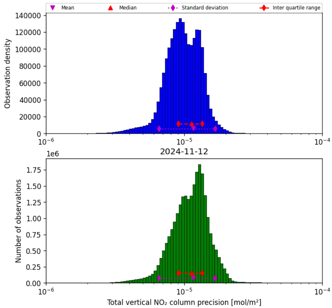
Figure 39: Histogram of “Total vertical NO 2 column precision” for 2024-11-11 to 2024-11-13
