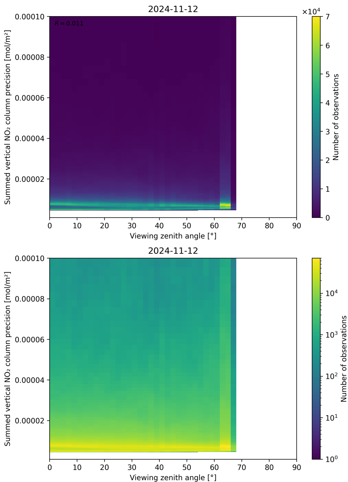
Figure 166: Scatter density plot of “Viewing zenith angle” against “Summed vertical NO 2 column precision” for 2024-11-11 to 2024-11-13.
