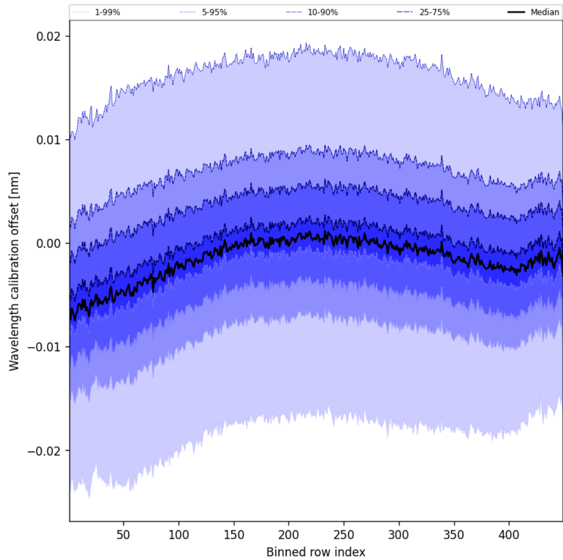
Figure 52: Along track statistics of “Wavelength calibration offset” for 2024-11-11 to 2024-11-13
