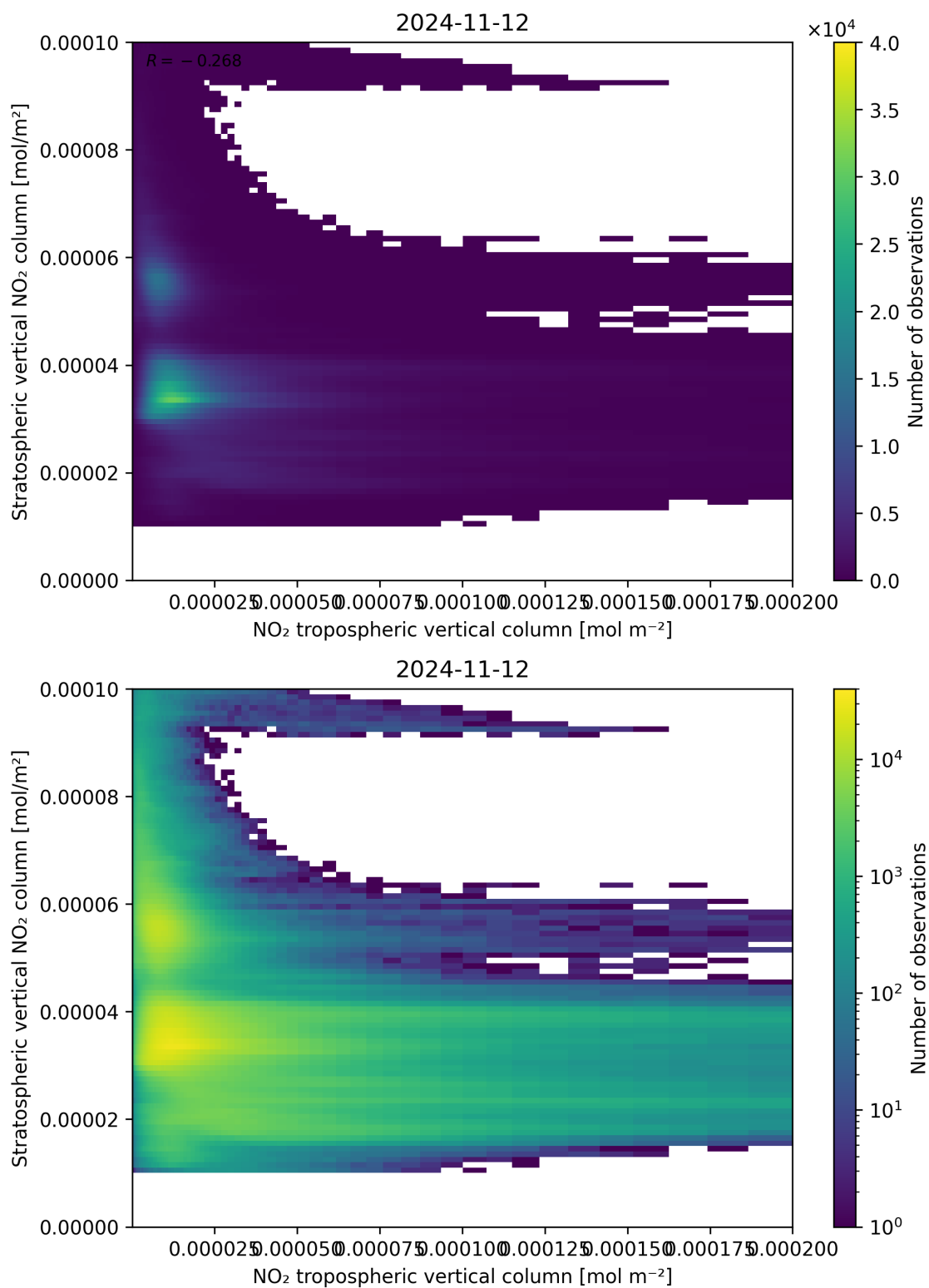
Figure 125: Scatter density plot of “NO 2 tropospheric vertical column” against “Stratospheric vertical NO 2 column” for 2024-11-11 to 2024-11-13.
