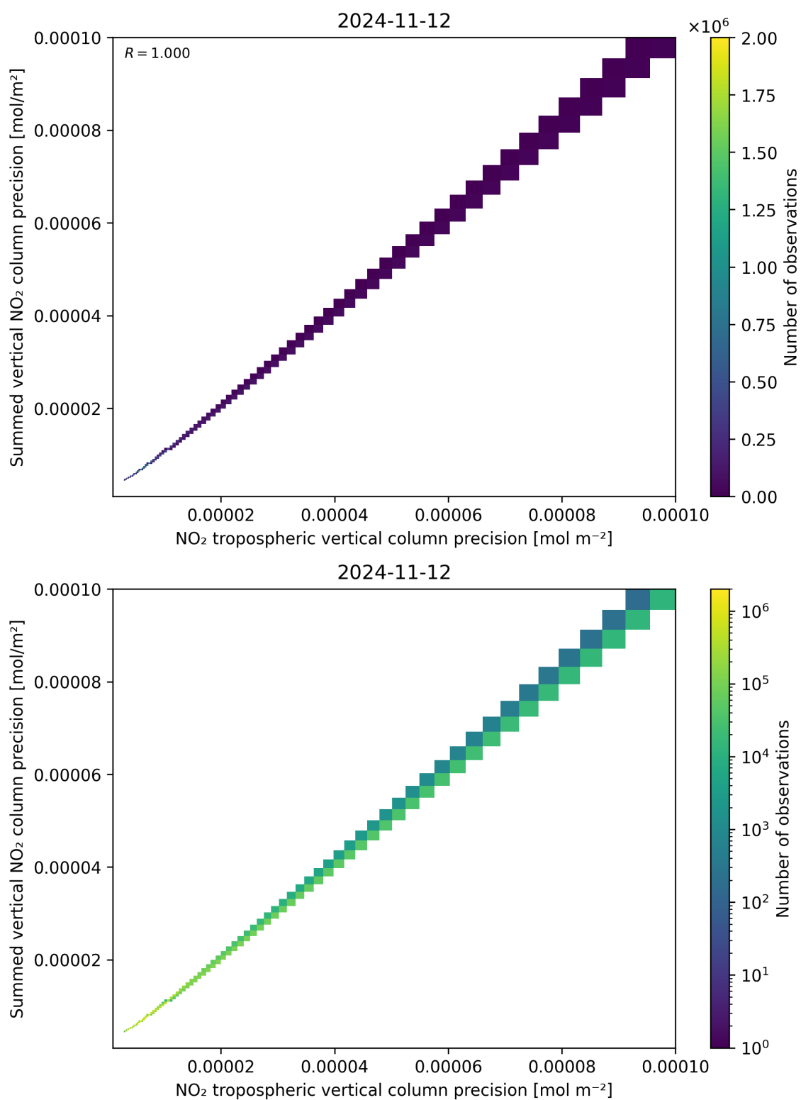
Figure 137: Scatter density plot of “NO 2 tropospheric vertical column precision” against “Summed vertical NO 2 column precision” for 2024-11-11 to 2024-11-13.
