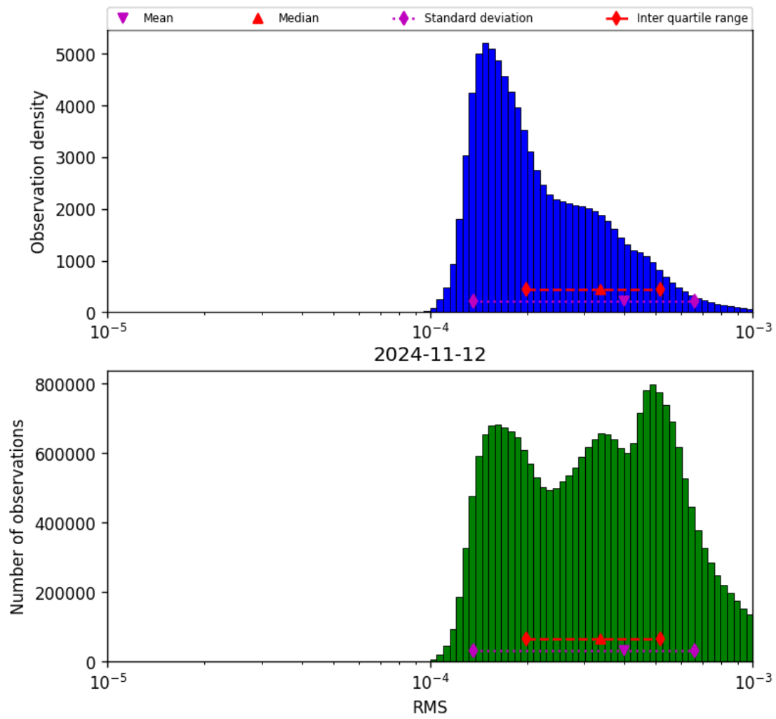
Figure 43: Histogram of “RMS” for 2024-11-11 to 2024-11-13
