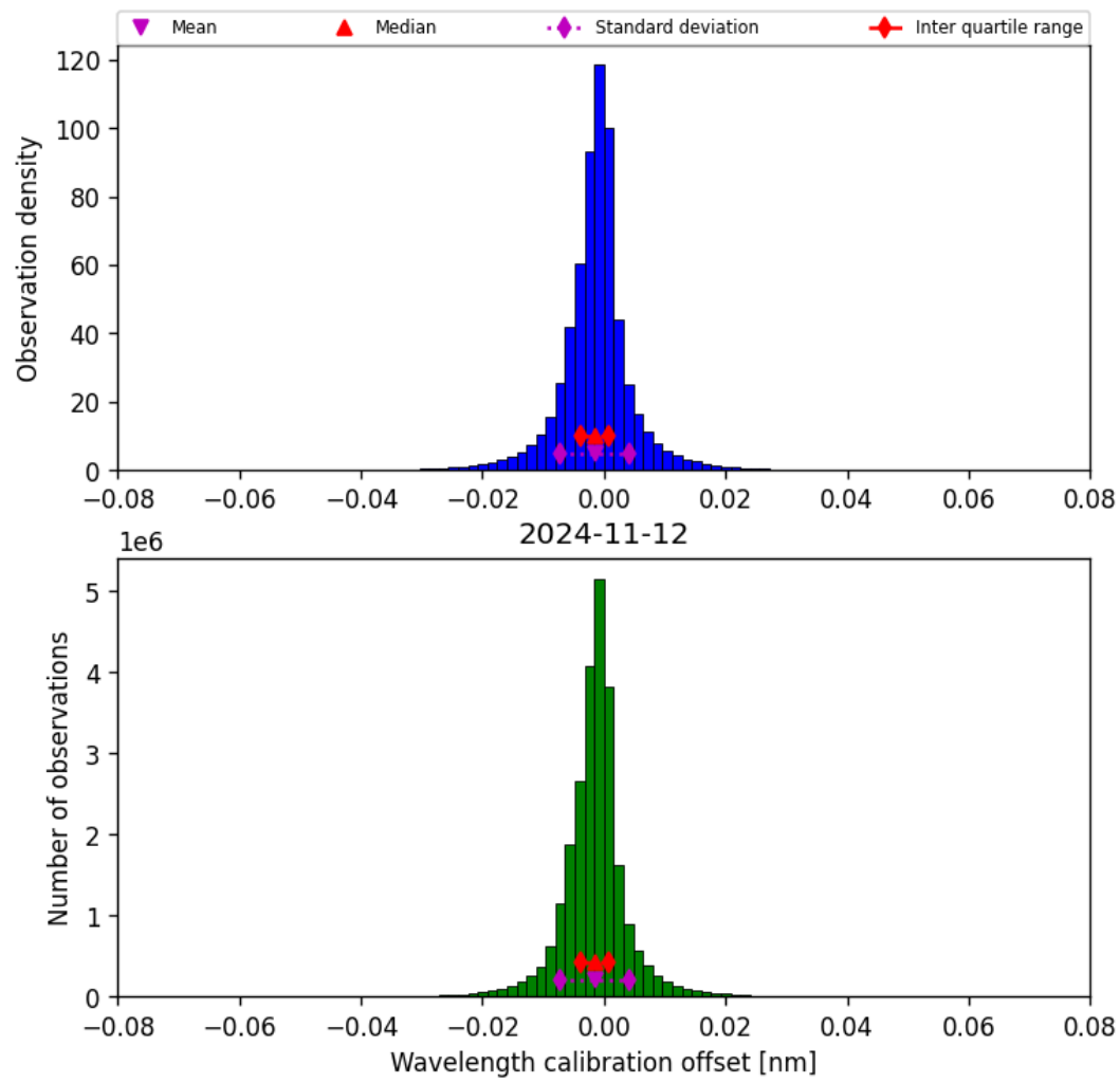
Figure 35: Histogram of “Wavelength calibration offset” for 2024-11-11 to 2024-11-13
