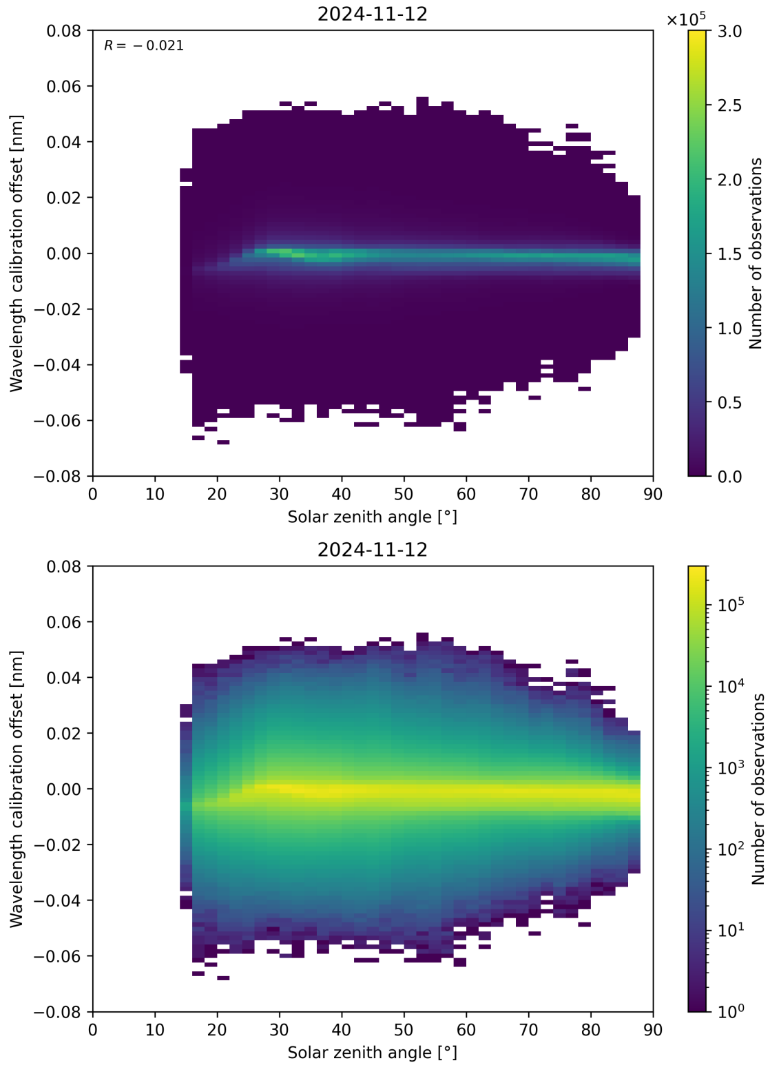
Figure 158: Scatter density plot of “Solar zenith angle” against “Wavelength calibration offset” for 2024-11-11 to 2024-11-13.
