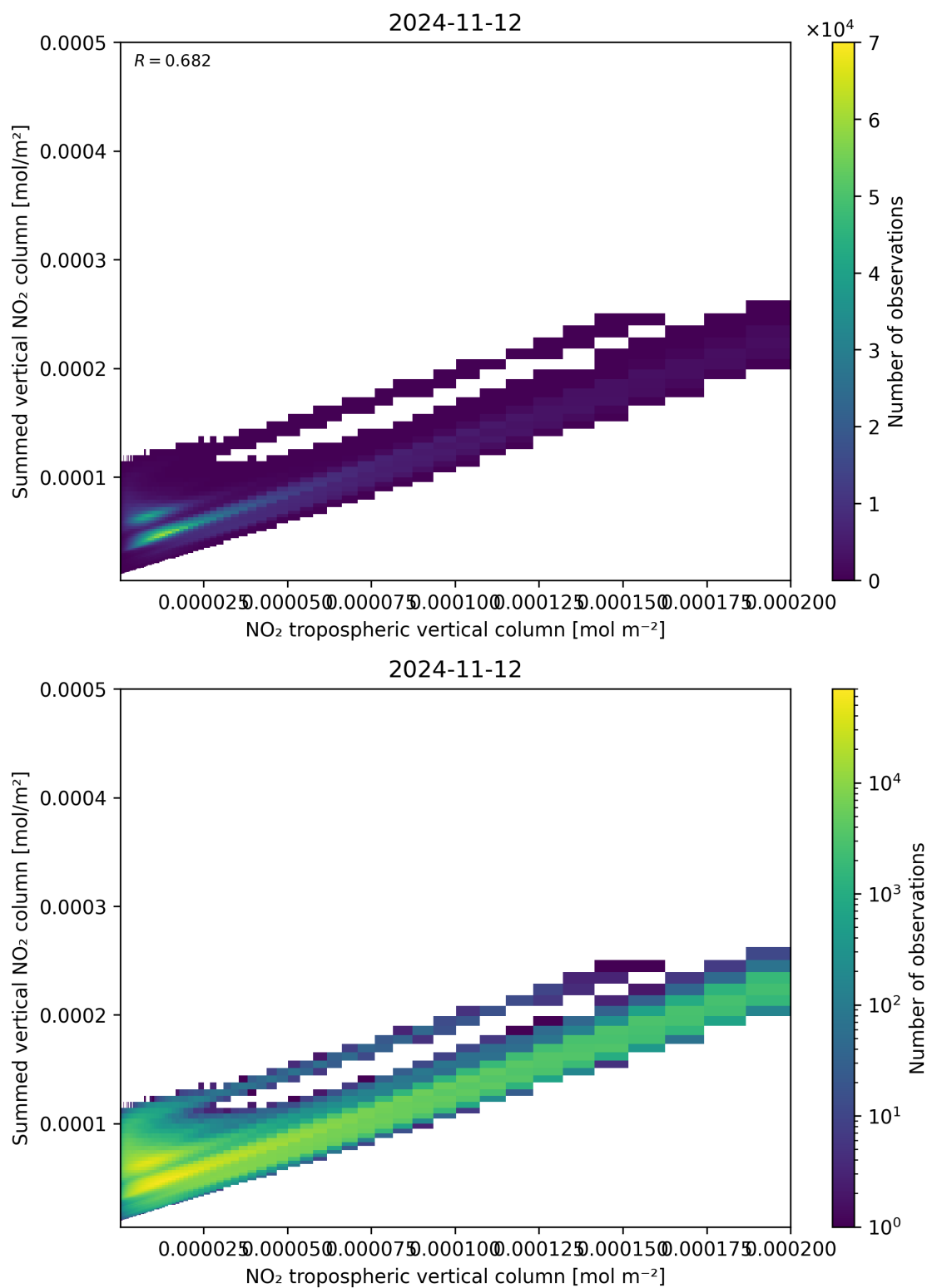
Figure 126: Scatter density plot of “NO 2 tropospheric vertical column” against “Summed vertical NO 2 column” for 2024-11-11 to 2024-11-13.
