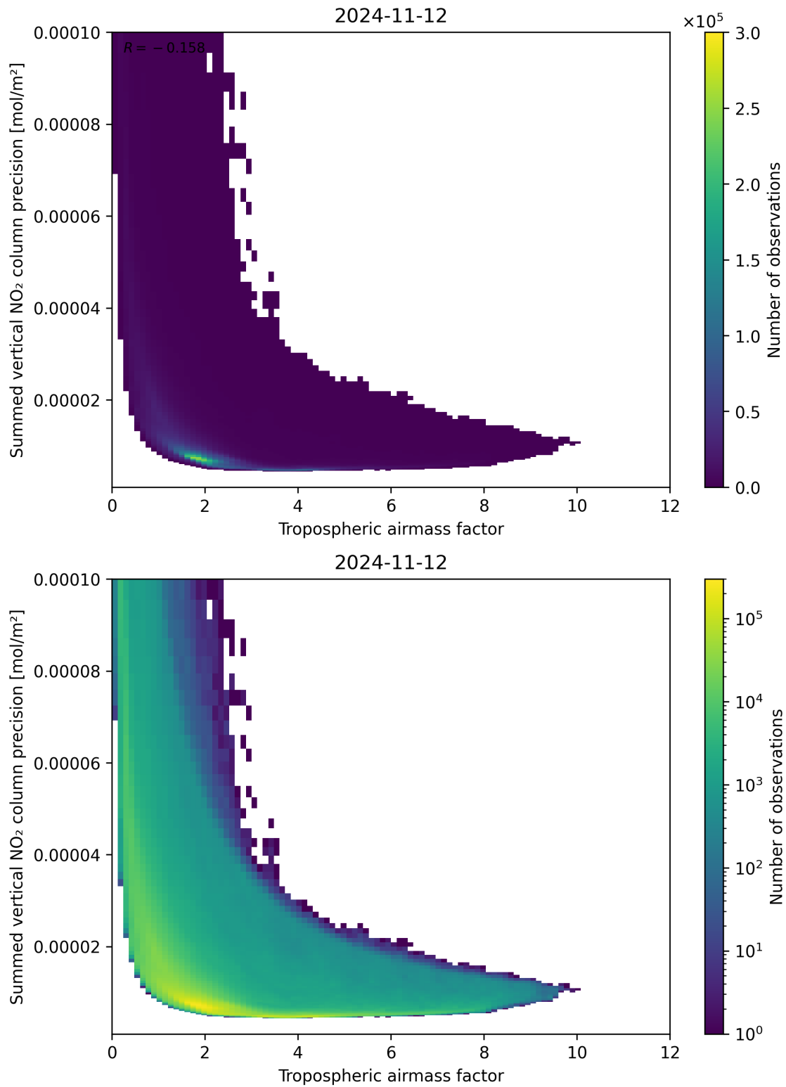
Figure 76: Scatter density plot of “Tropospheric air mass factor” against “Summed vertical NO 2 column precision” for 2024-11-11 to 2024-11-13.
