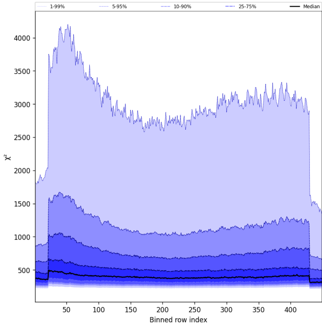
Figure 59: Along track statistics of “ \chi^2 ” for 2024-11-11 to 2024-11-13
