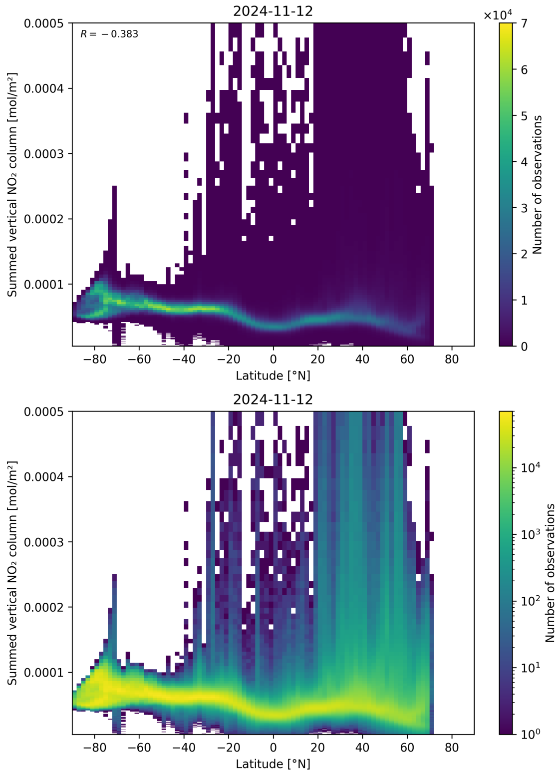
Figure 88: Scatter density plot of “Latitude” against “Summed vertical NO 2 column” for 2024-11-11 to 2024-11-13.
