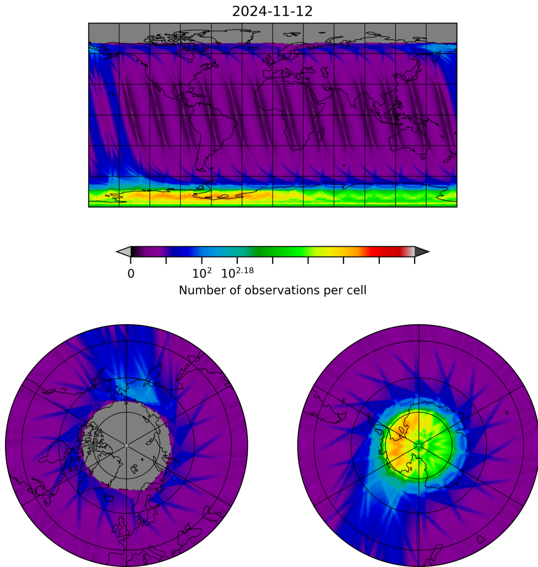
Figure 10: Map of the number of observations for 2024-11-11 to 2024-11-13
