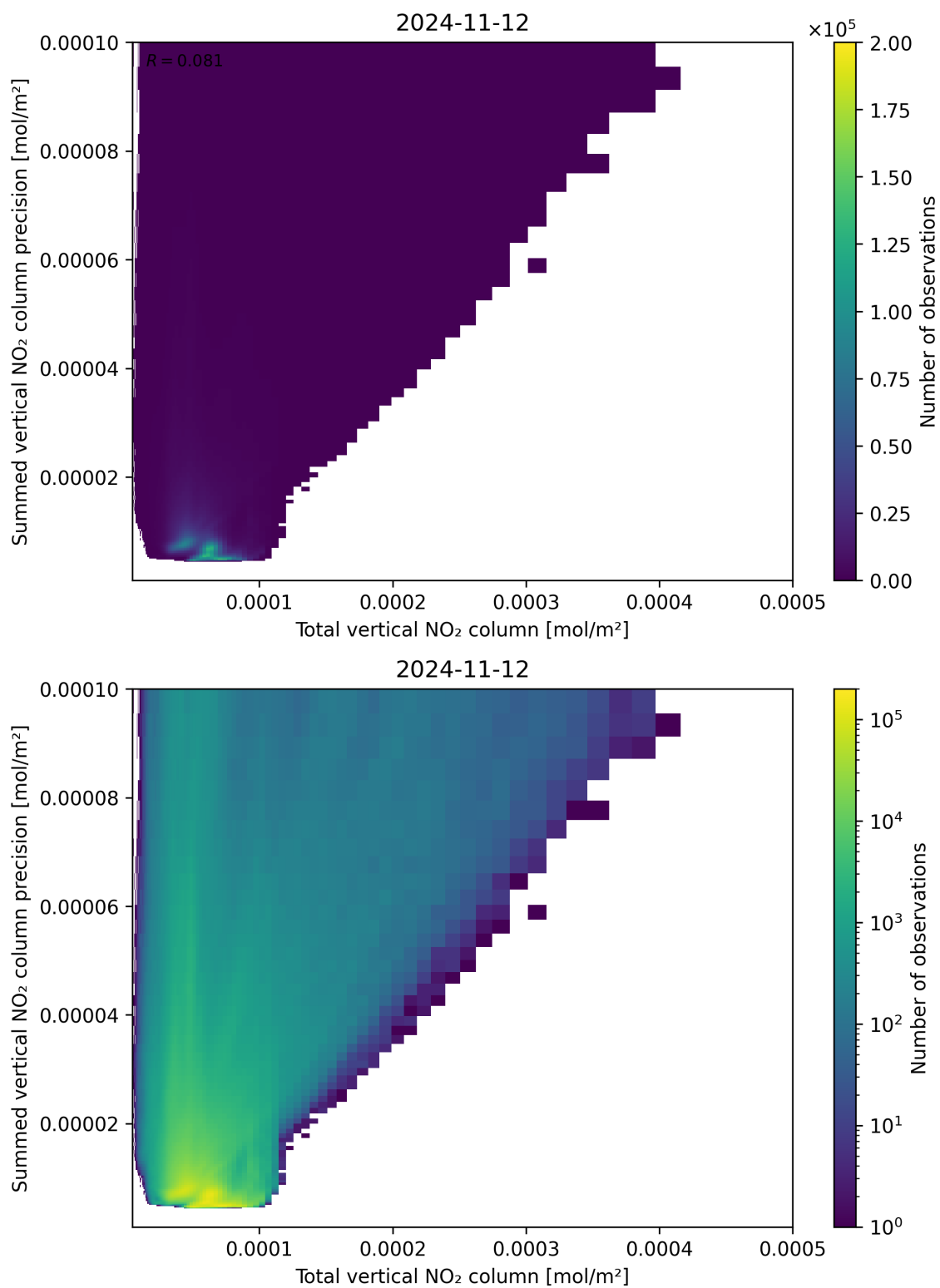
Figure 113: Scatter density plot of “Total vertical NO 2 column” against “Summed vertical NO 2 column precision” for 2024-11-11 to 2024-11-13.
