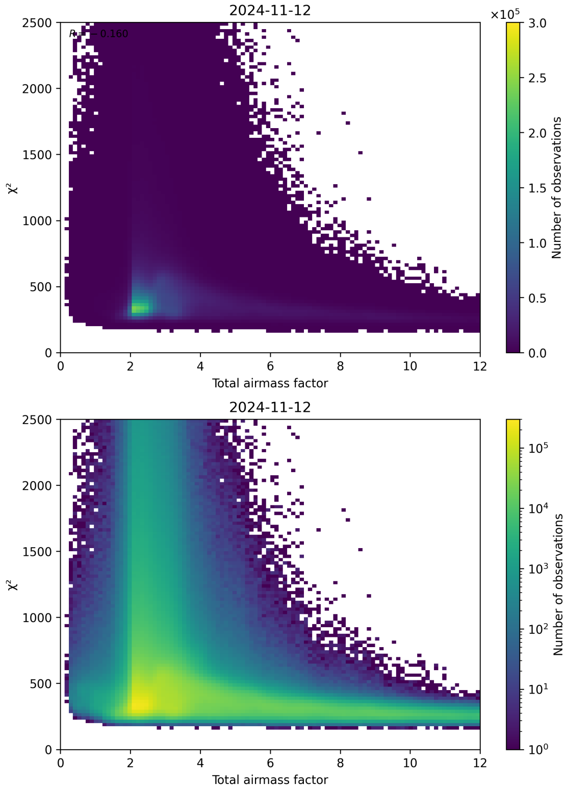
Figure 63: Scatter density plot of “Total airmass factor” against “ \chi^2 ” for 2024-11-11 to 2024-11-13.
