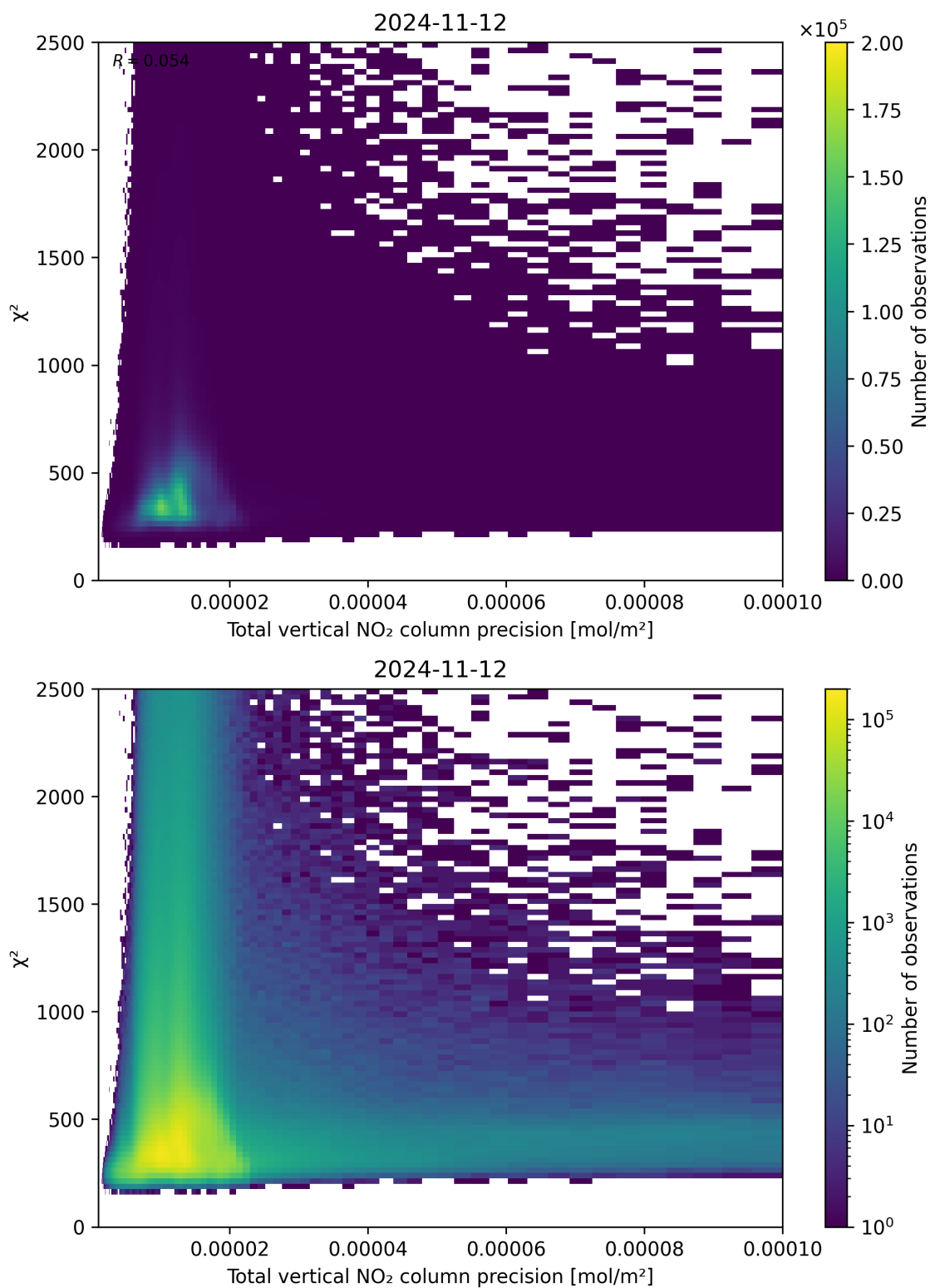
Figure 116: Scatter density plot of “Total vertical NO 2 column precision” against “ \chi^2 ” for 2024-11-11 to 2024-11-13.
