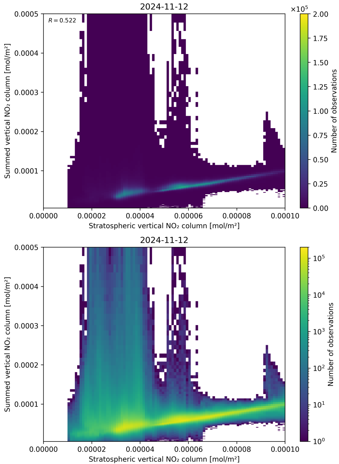
Figure 98: Scatter density plot of “Stratospheric vertical NO 2 column” against “Summed vertical NO 2 column” for 2024-11-11 to 2024-11-13.
