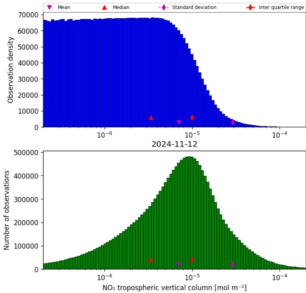
Figure 29: Histogram of “NO 2 tropospheric vertical column” for 2024-11-11 to 2024-11-13
