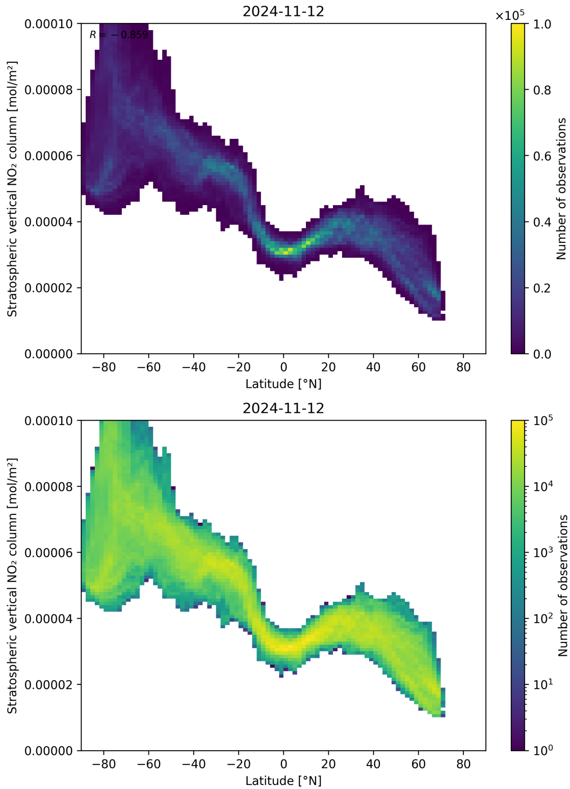
Figure 87: Scatter density plot of “Latitude” against “Stratospheric vertical NO 2 column” for 2024-11-11 to 2024-11-13.
