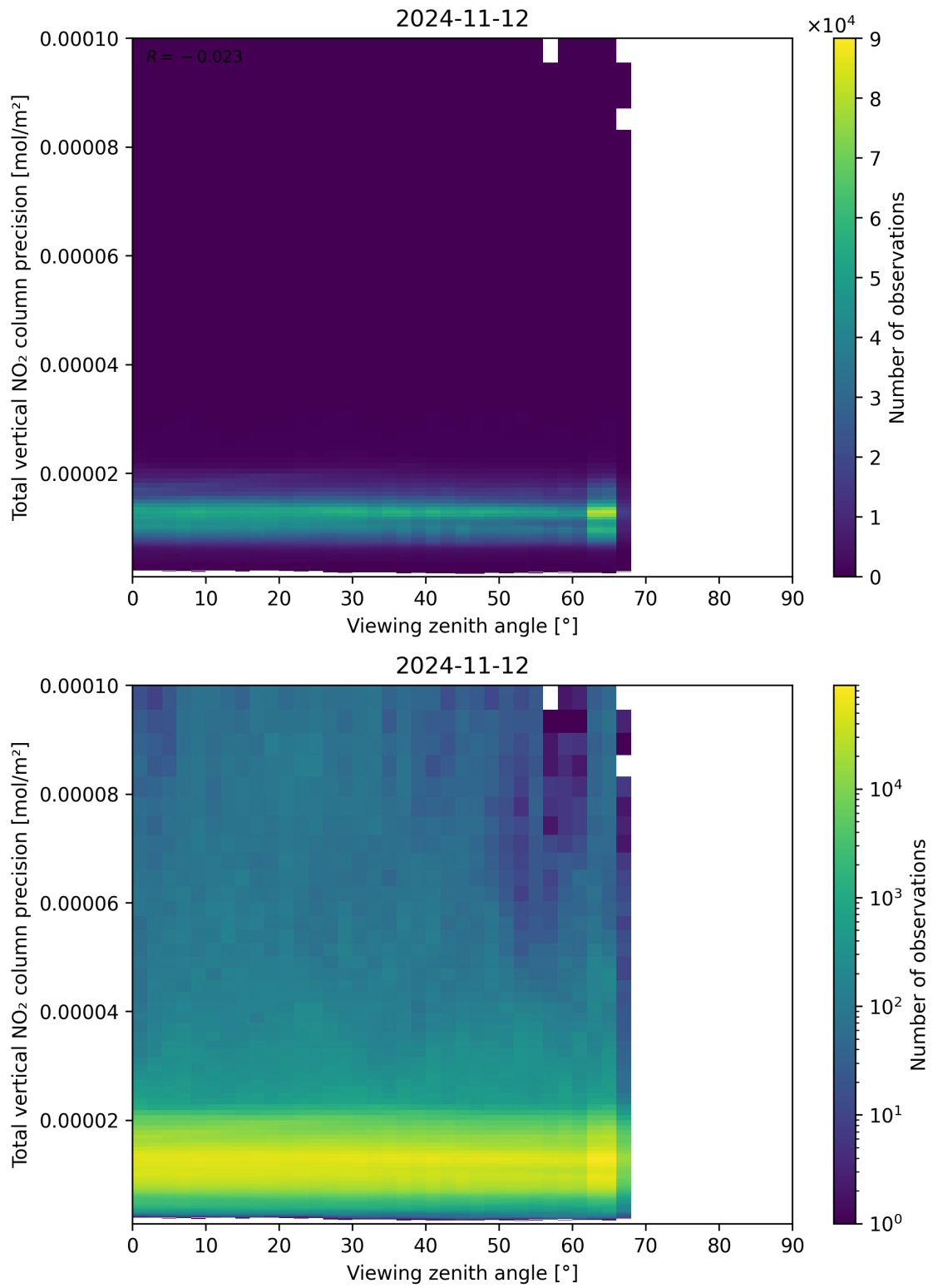
Figure 168: Scatter density plot of “Viewing zenith angle” against “Total vertical NO 2 column precision” for 2024-11-11 to 2024-11-13.
