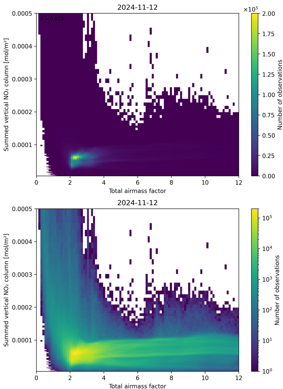
Figure 65: Scatter density plot of “Total airmass factor” against “Summed vertical NO 2 column” for 2024-11-11 to 2024-11-13.
