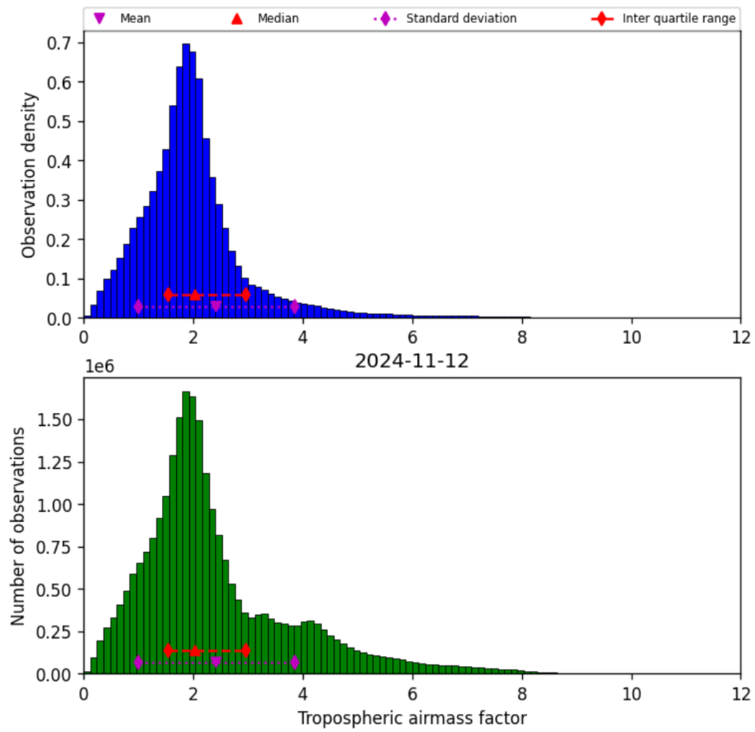
Figure 31: Histogram of “Tropospheric airmass factor” for 2024-11-11 to 2024-11-13
