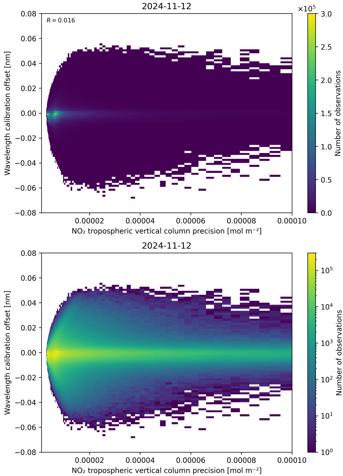
Figure 141: Scatter density plot of “NO 2 tropospheric vertical column precision” against “Wavelength calibration offset” for 2024-11-11 to 2024-11-13.
