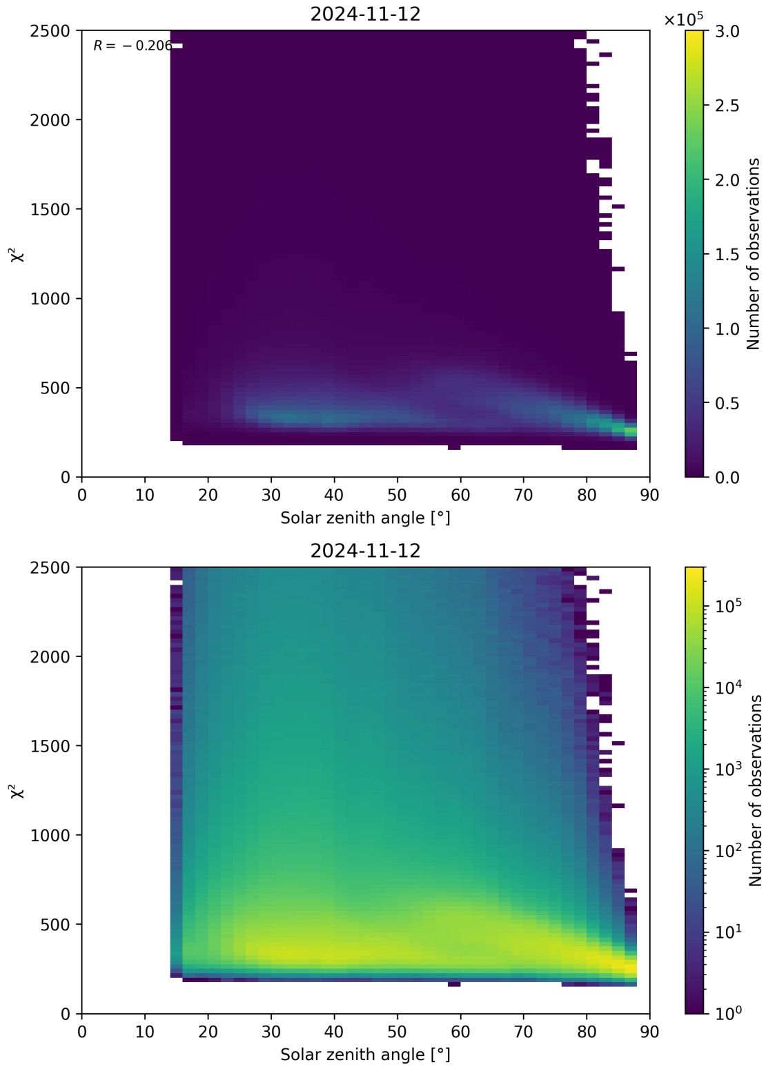
Figure 148: Scatter density plot of “Solar zenith angle” against “ \chi^2 ” for 2024-11-11 to 2024-11-13.
