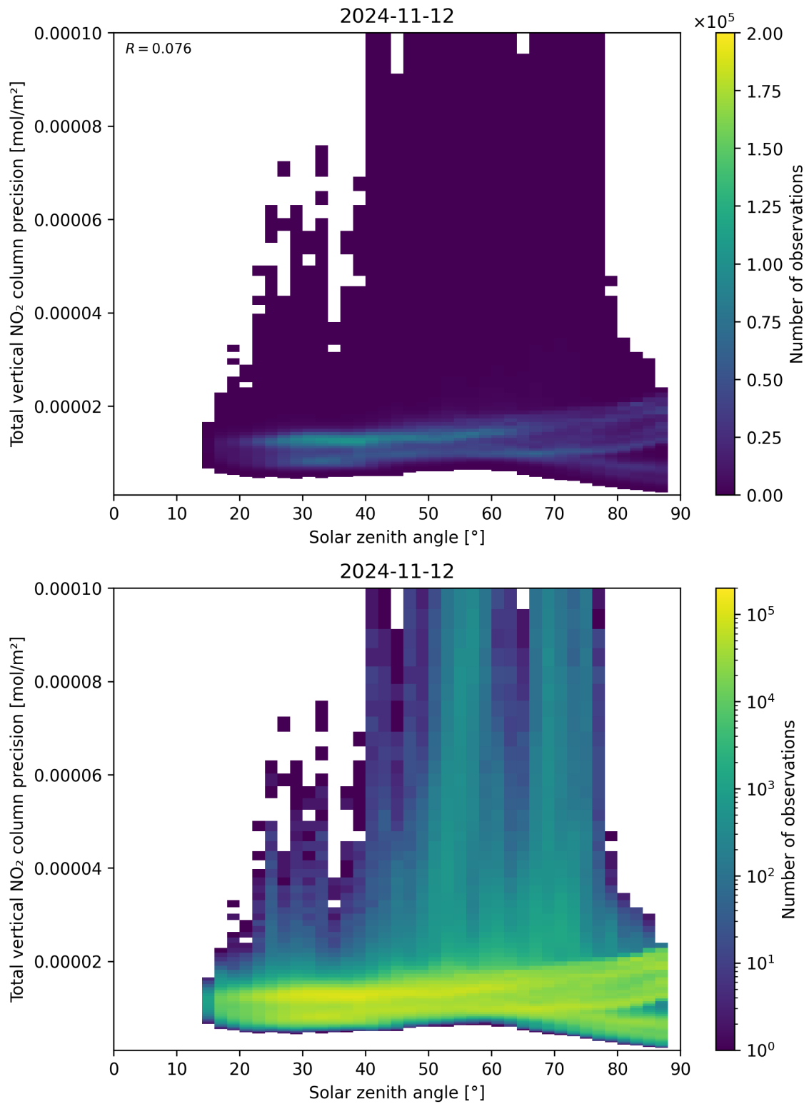
Figure 154: Scatter density plot of “Solar zenith angle” against “Total vertical NO 2 column precision” for 2024-11-11 to 2024-11-13.
