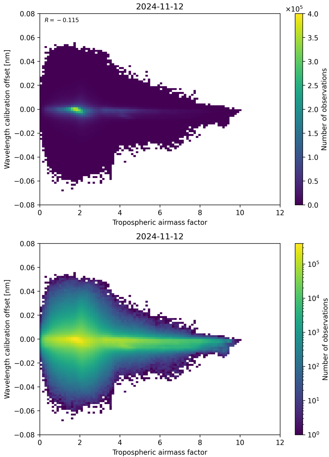
Figure 80: Scatter density plot of “Tropospheric airmass factor” against “Wavelength calibration offset” for 2024-11-11 to 2024-11-13.
