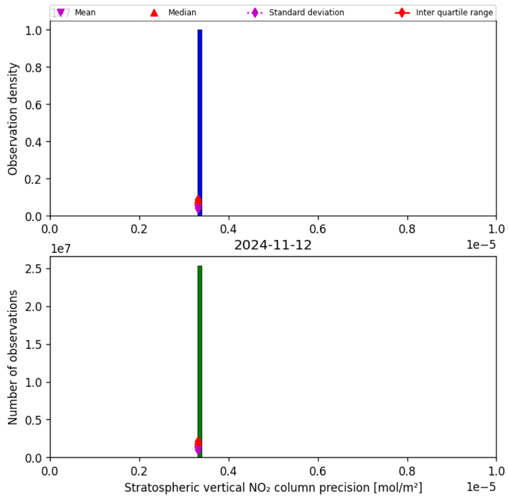
Figure 37: Histogram of “Stratospheric vertical NO 2 column precision” for 2024-11-11 to 2024-11-13
