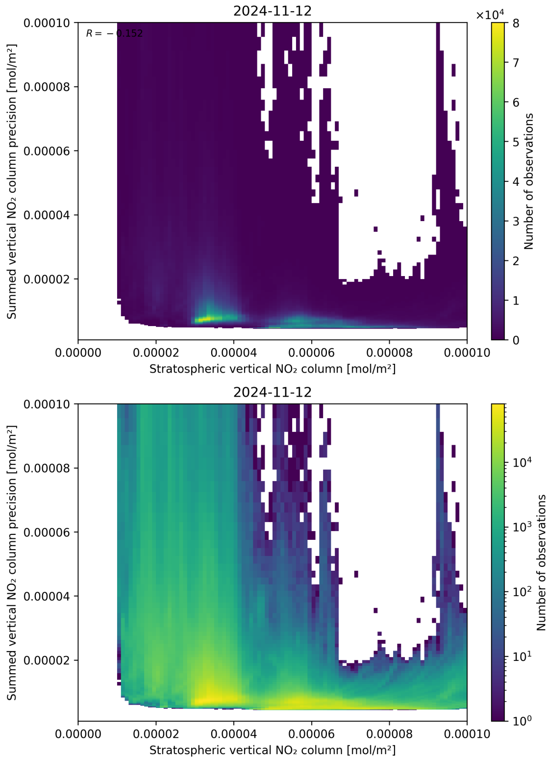
Figure 99: Scatter density plot of “Stratospheric vertical NO 2 column” against “Summed vertical NO 2 column precision” for 2024-11-11 to 2024-11-13.
