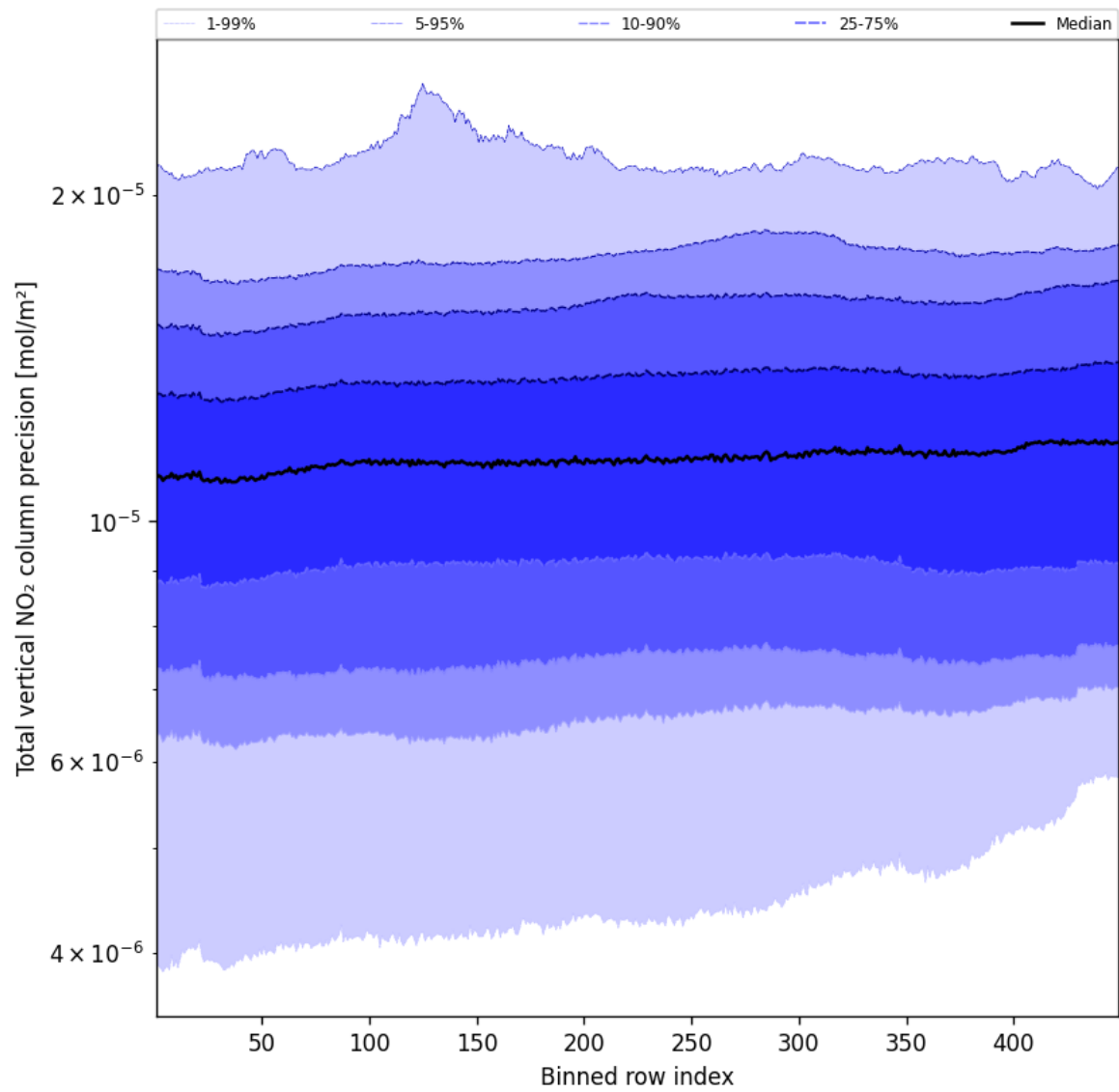
Figure 56: Along track statistics of “Total vertical NO 2 column precision” for 2024-11-11 to 2024-11-13
