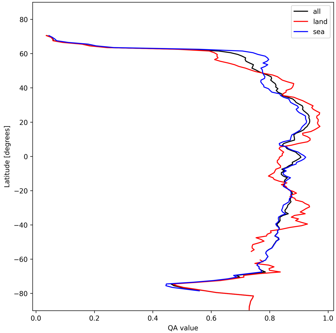
Figure 11: Zonal average of “QA value” for 2024-11-11 to 2024-11-13.
