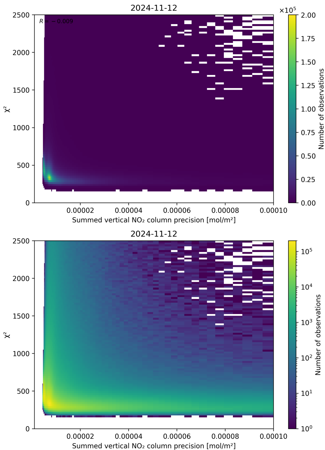
Figure 107: Scatter density plot of “Summed vertical NO 2 column precision” against “ \chi^2 ” for 2024-11-11 to 2024-11-13.
