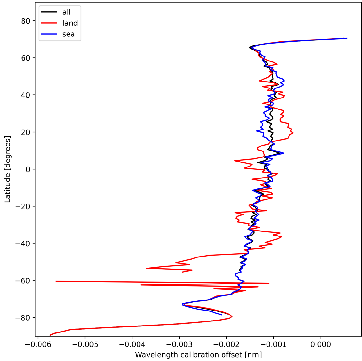
Figure 18: Zonal average of “Wavelength calibration offset” for 2024-11-11 to 2024-11-13.
