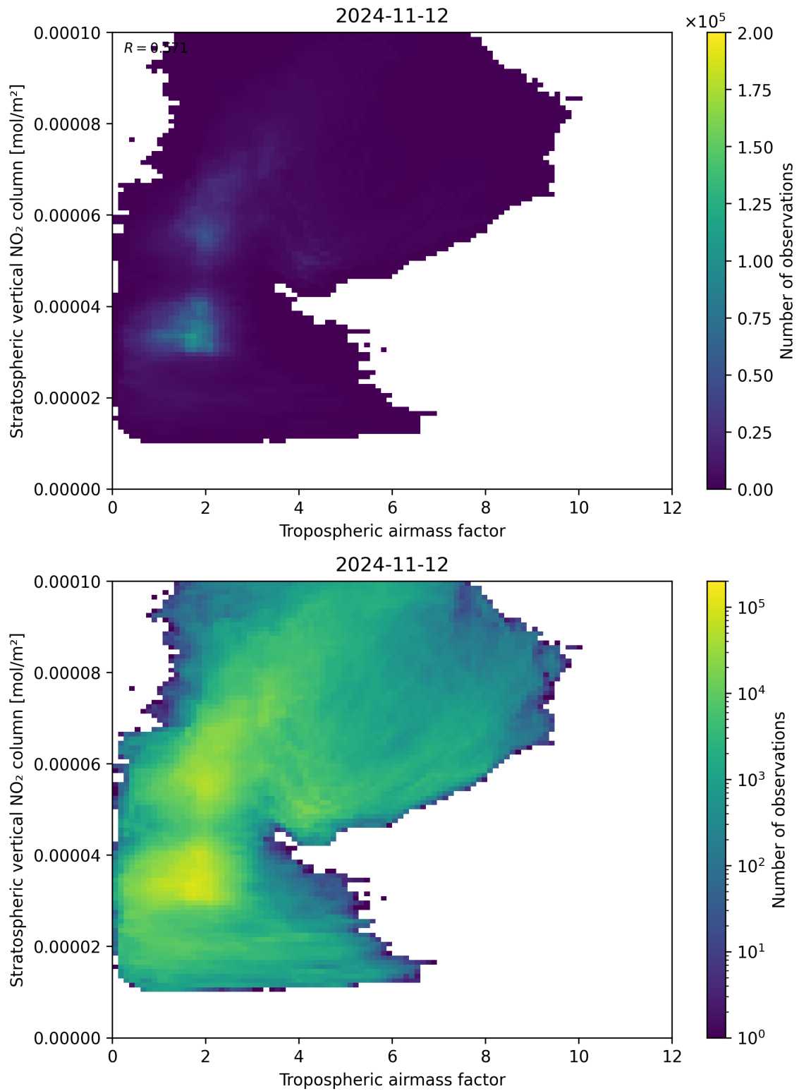
Figure 74: Scatter density plot of “Tropospheric airmass factor” against “Stratospheric vertical NO 2 column” for 2024-11-11 to 2024-11-13.
