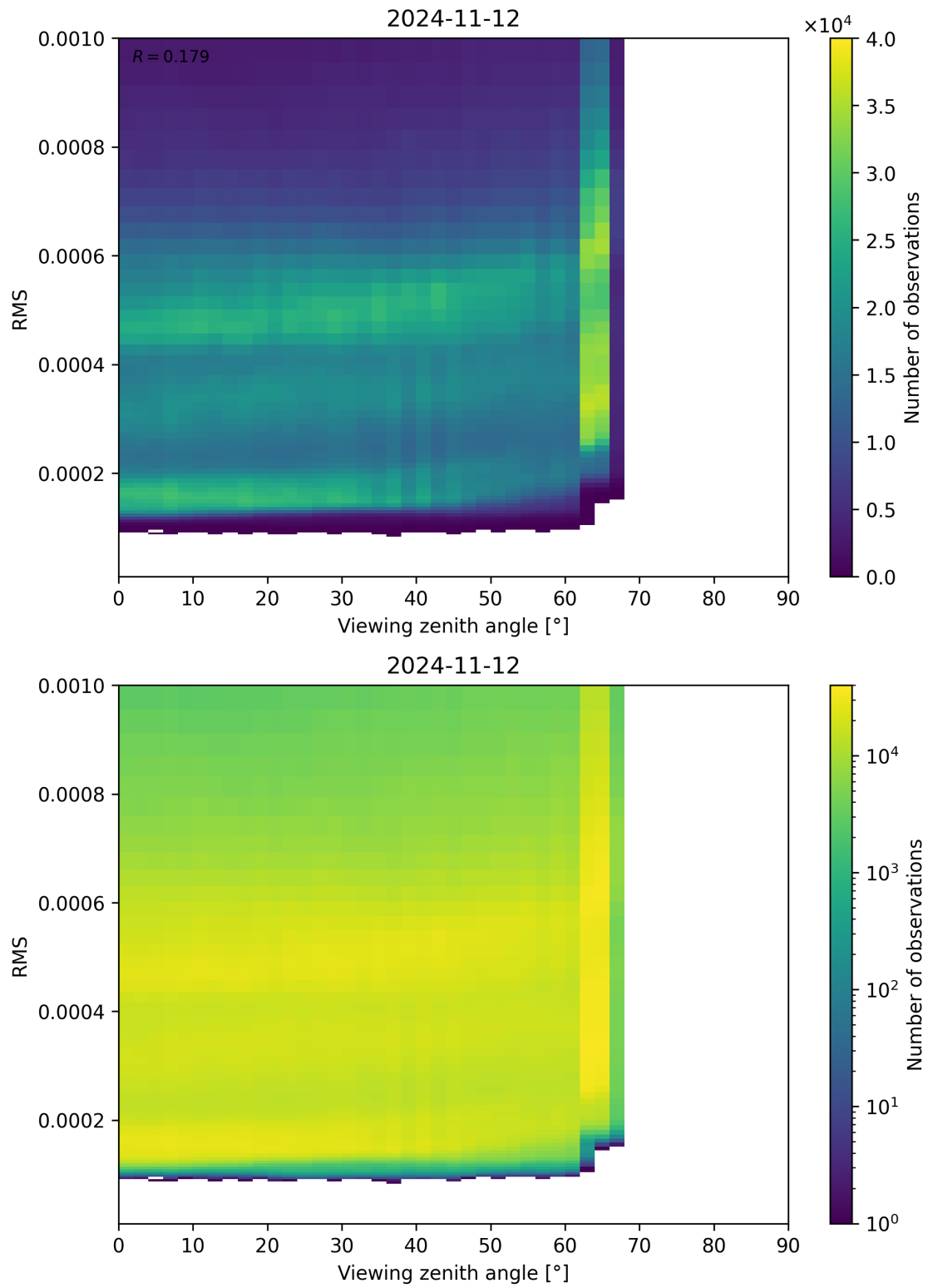
Figure 171: Scatter density plot of “Viewing zenith angle” against “RMS” for 2024-11-11 to 2024-11-13.
