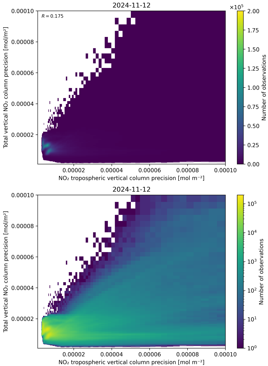
Figure 139: Scatter density plot of “NO 2 tropospheric vertical column precision” against “Total vertical NO 2 column precision” for 2024-11-11 to 2024-11-13.
