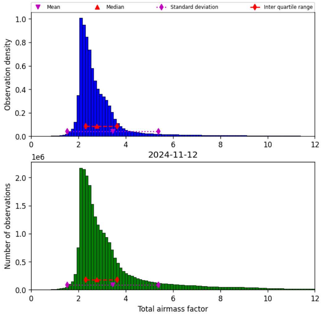
Figure 32: Histogram of “Total airmass factor” for 2024-11-11 to 2024-11-13
