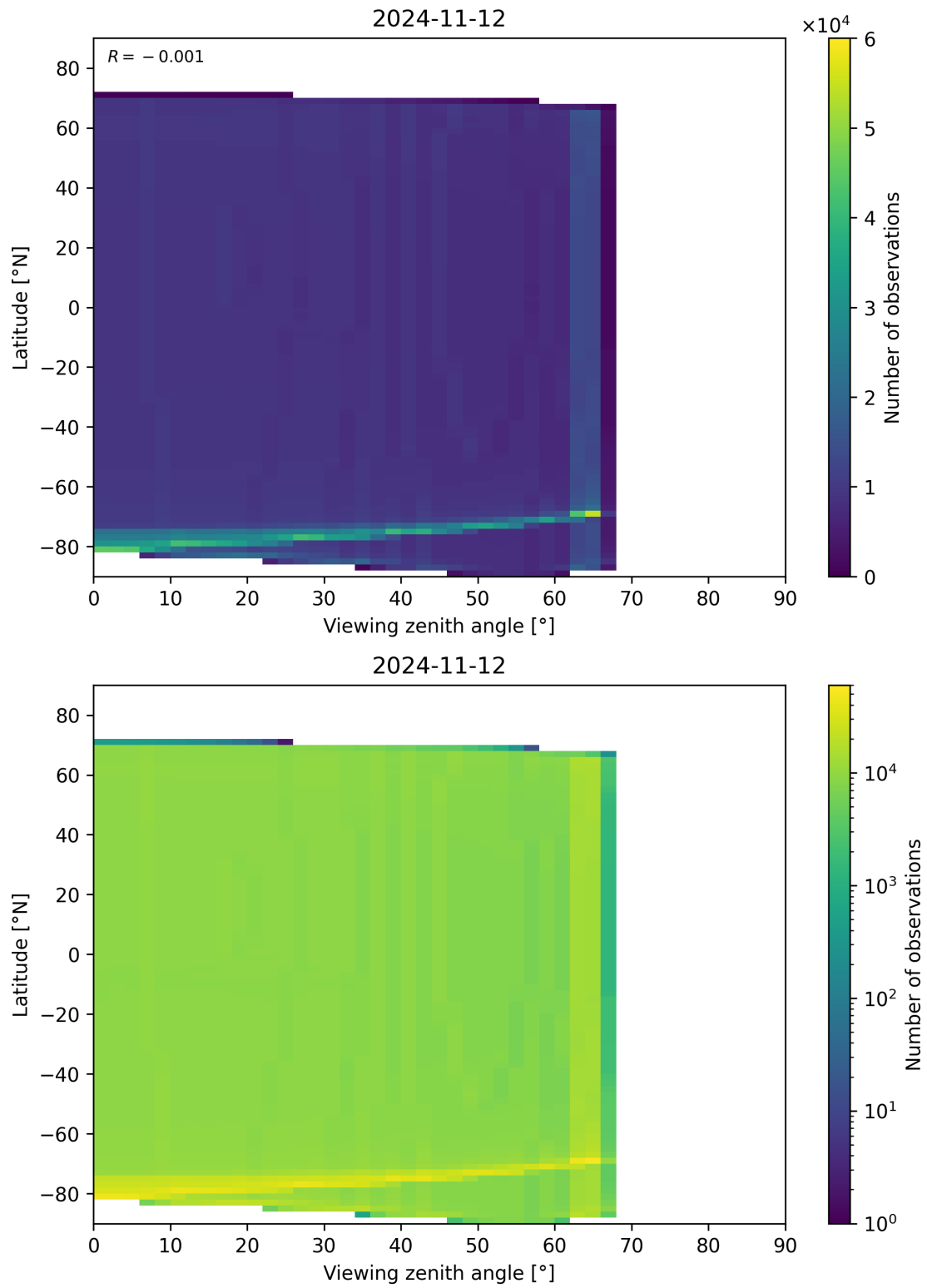
Figure 163: Scatter density plot of “Viewing zenith angle” against “Latitude” for 2024-11-11 to 2024-11-13.
