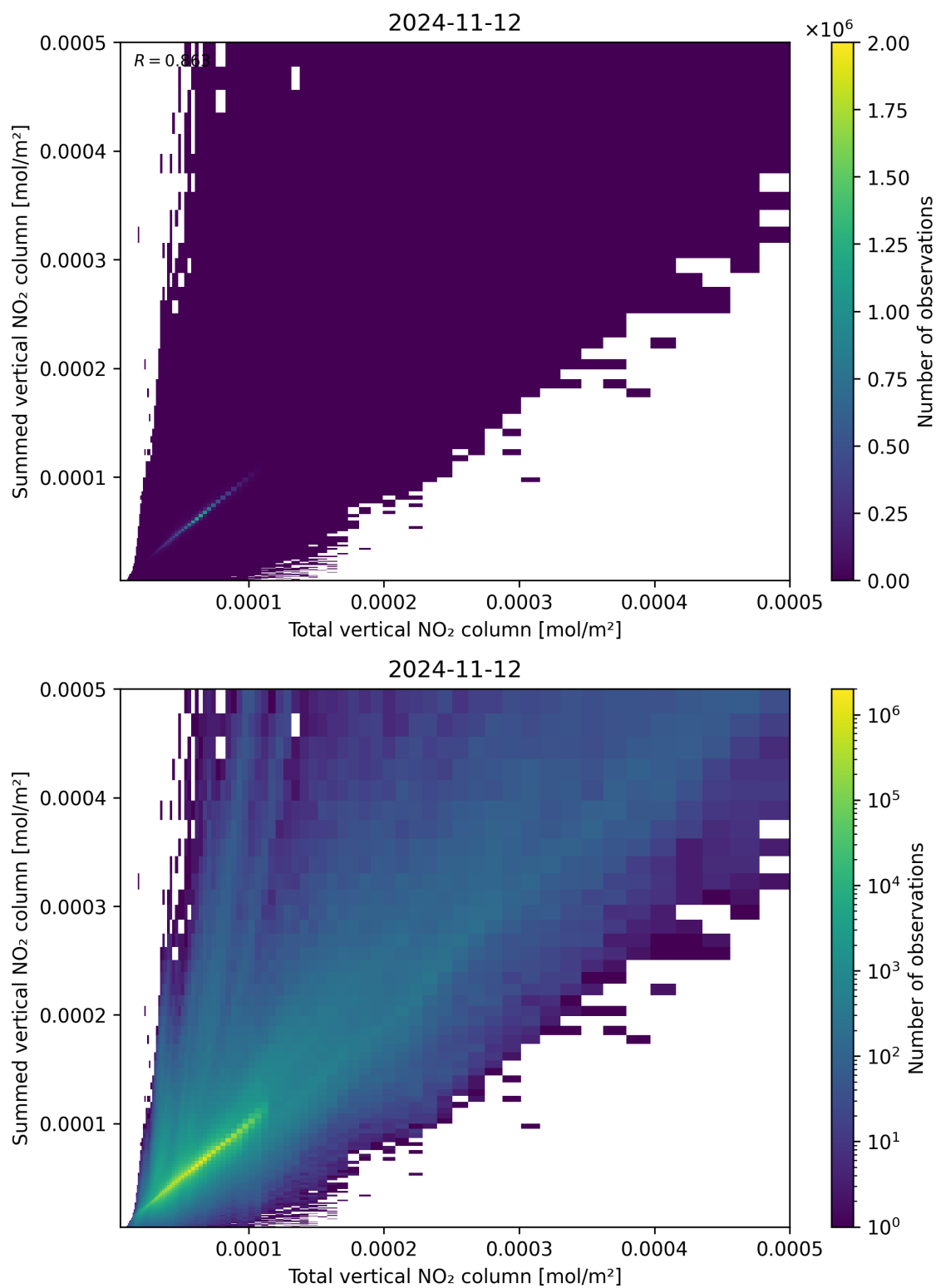
Figure 112: Scatter density plot of “Total vertical NO 2 column” against “Summed vertical NO 2 column” for 2024-11-11 to 2024-11-13.
