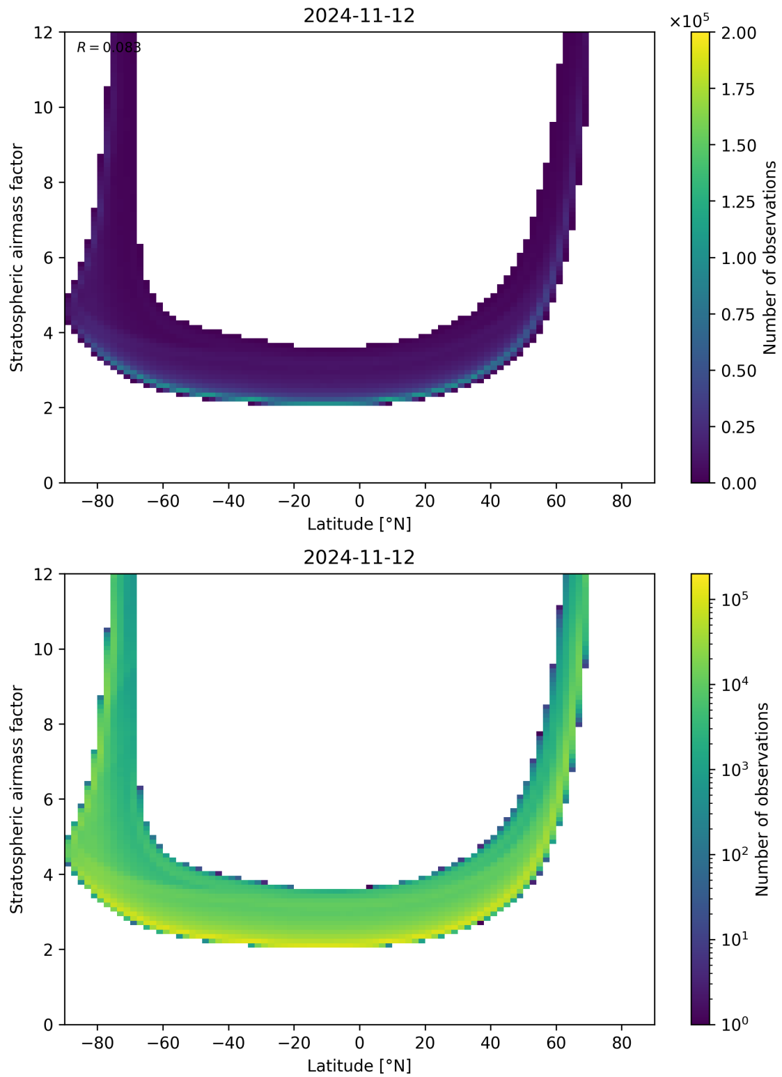
Figure 83: Scatter density plot of “Latitude” against “Stratospheric air mass factor” for 2024-11-11 to 2024-11-13.
