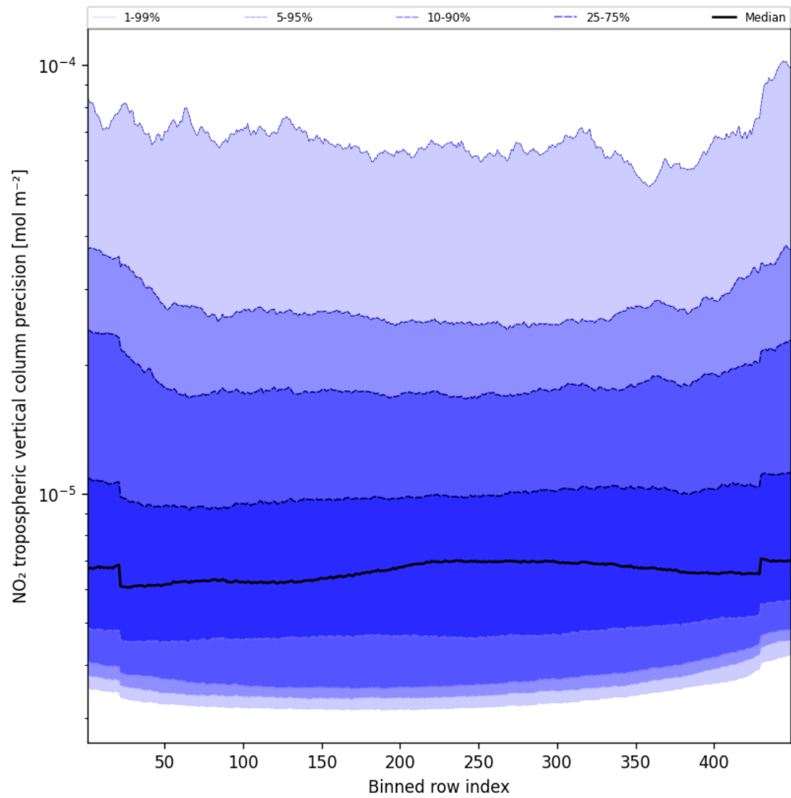
Figure 47: Along track statistics of “NO 2 tropospheric vertical column precision” for 2024-11-11 to 2024-11-13
