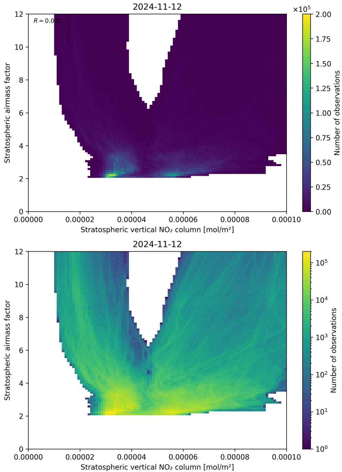
Figure 96: Scatter density plot of “Stratospheric vertical NO 2 column” against “Stratospheric airmass factor” for 2024-11-11 to 2024-11-13.
