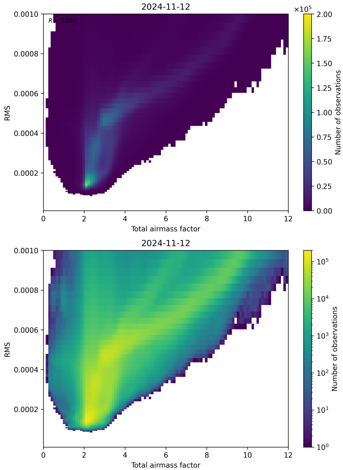
Figure 69: Scatter density plot of “Total airmass factor” against “RMS” for 2024-11-11 to 2024-11-13.
