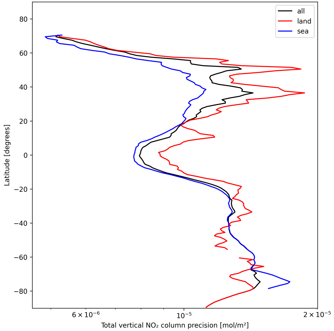
Figure 22: Zonal average of "Total vertical NO 2 column precision" for 2024-11-11 to 2024-11-13.
