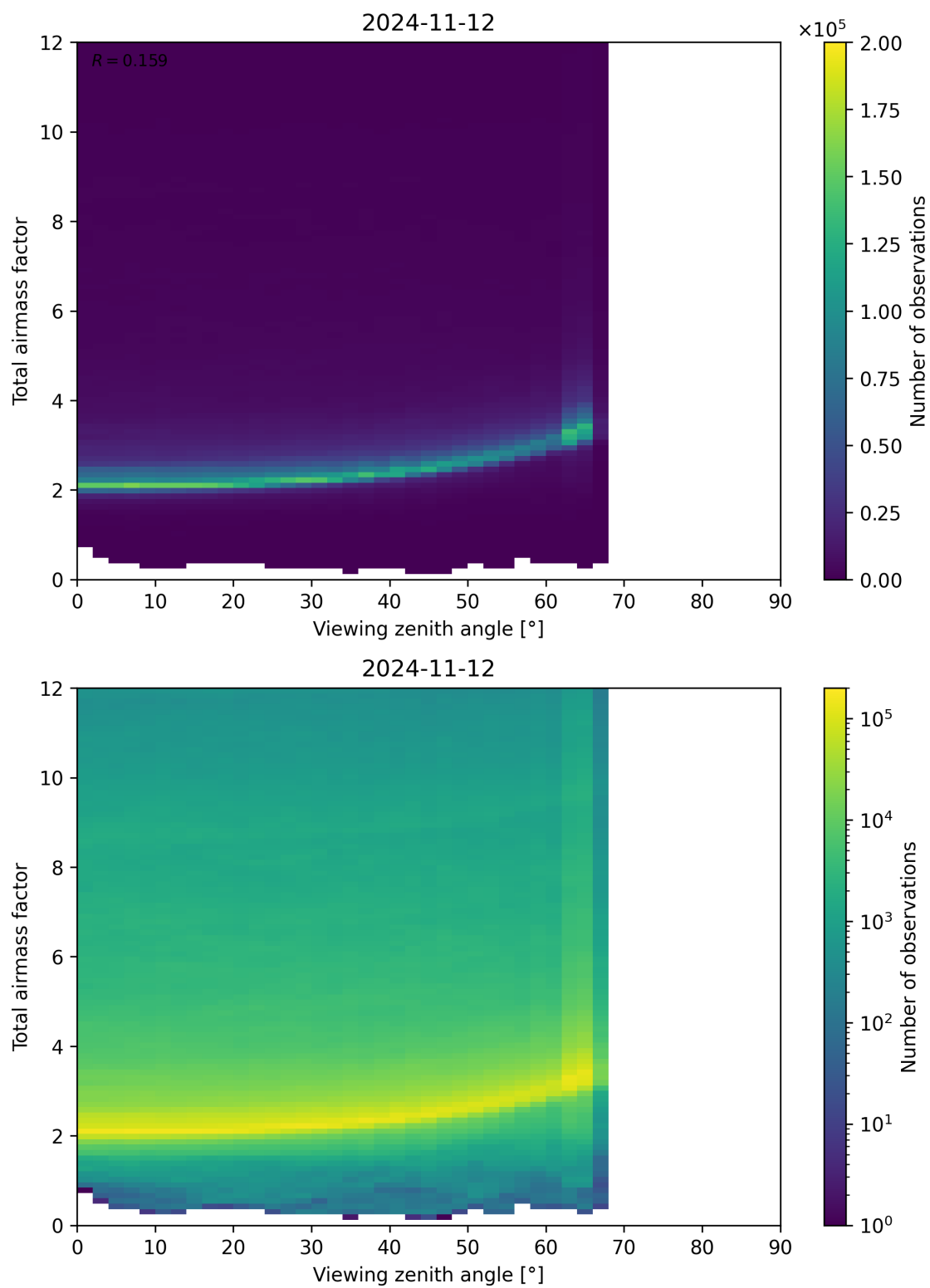
Figure 160: Scatter density plot of “Viewing zenith angle” against “Total airmass factor” for 2024-11-11 to 2024-11-13.
