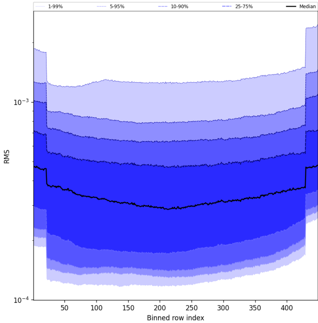
Figure 60: Along track statistics of “RMS” for 2024-11-11 to 2024-11-13
