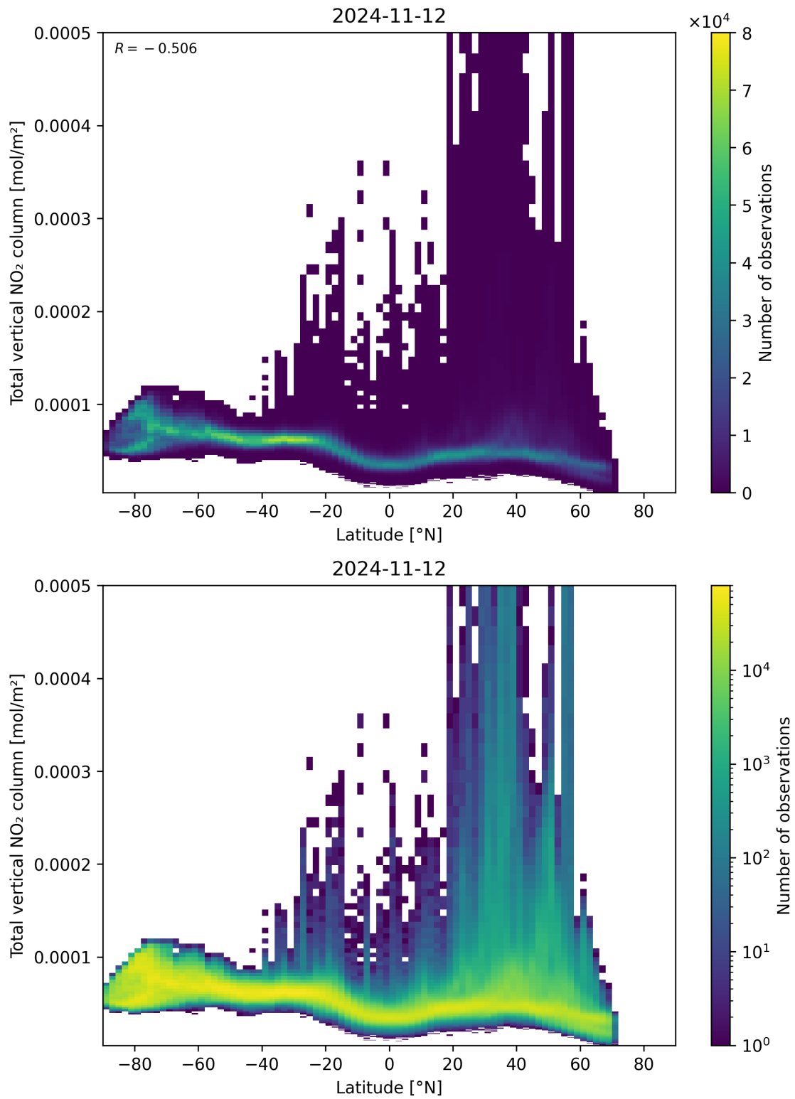
Figure 90: Scatter density plot of “Latitude” against “Total vertical NO 2 column” for 2024-11-11 to 2024-11-13.
