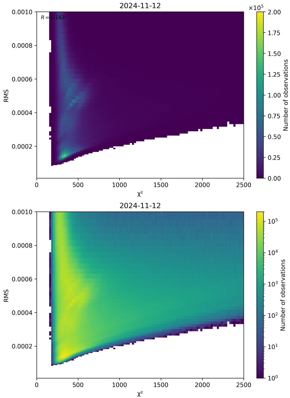
Figure 82: Scatter density plot of “ \chi^2 ” against “RMS” for 2024-11-11 to 2024-11-13.
