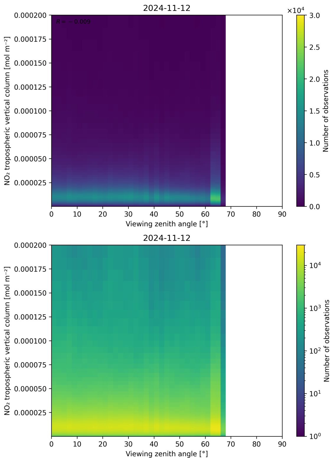
Figure 169: Scatter density plot of “Viewing zenith angle” against “NO 2 tropospheric vertical column” for 2024-11-11 to 2024-11-13.
