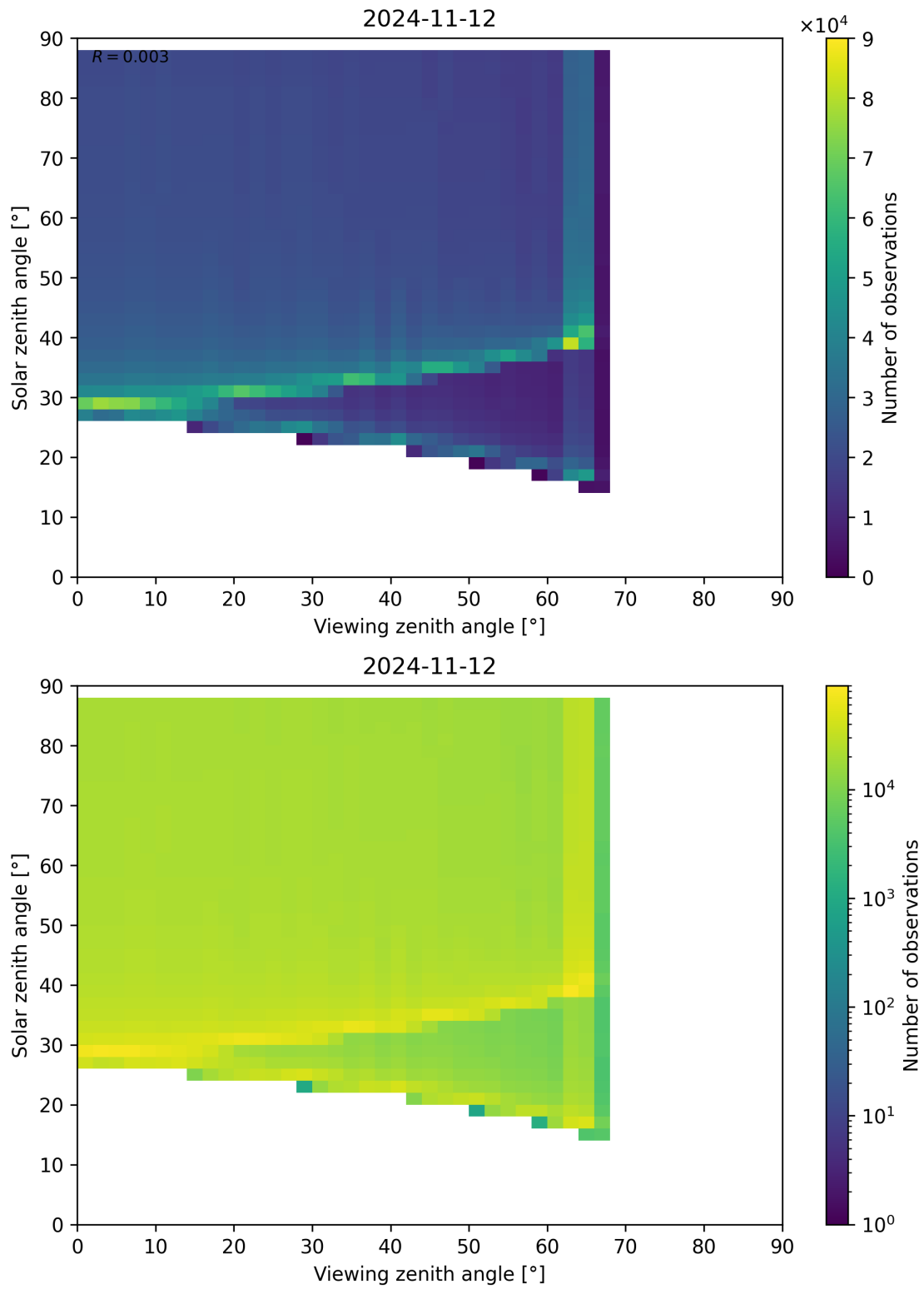
Figure 172: Scatter density plot of “Viewing zenith angle” against “Solar zenith angle” for 2024-11-11 to 2024-11-13.
