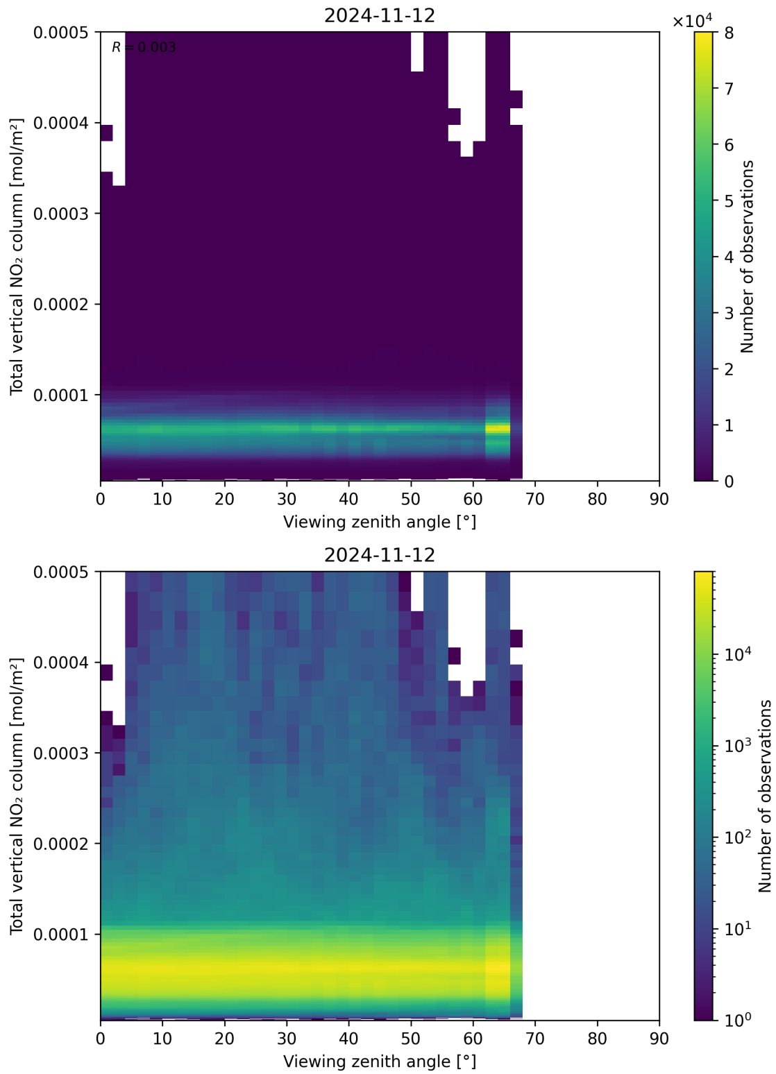
Figure 167: Scatter density plot of “Viewing zenith angle” against “Total vertical NO 2 column” for 2024-11-11 to 2024-11-13.
