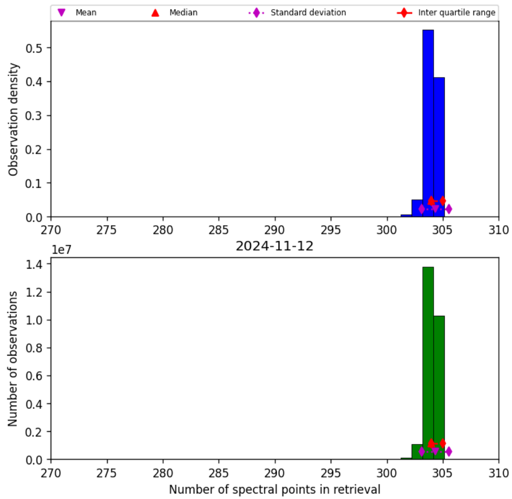
Figure 33: Histogram of “Number of spectral points in retrieval” for 2024-11-11 to 2024-11-13
