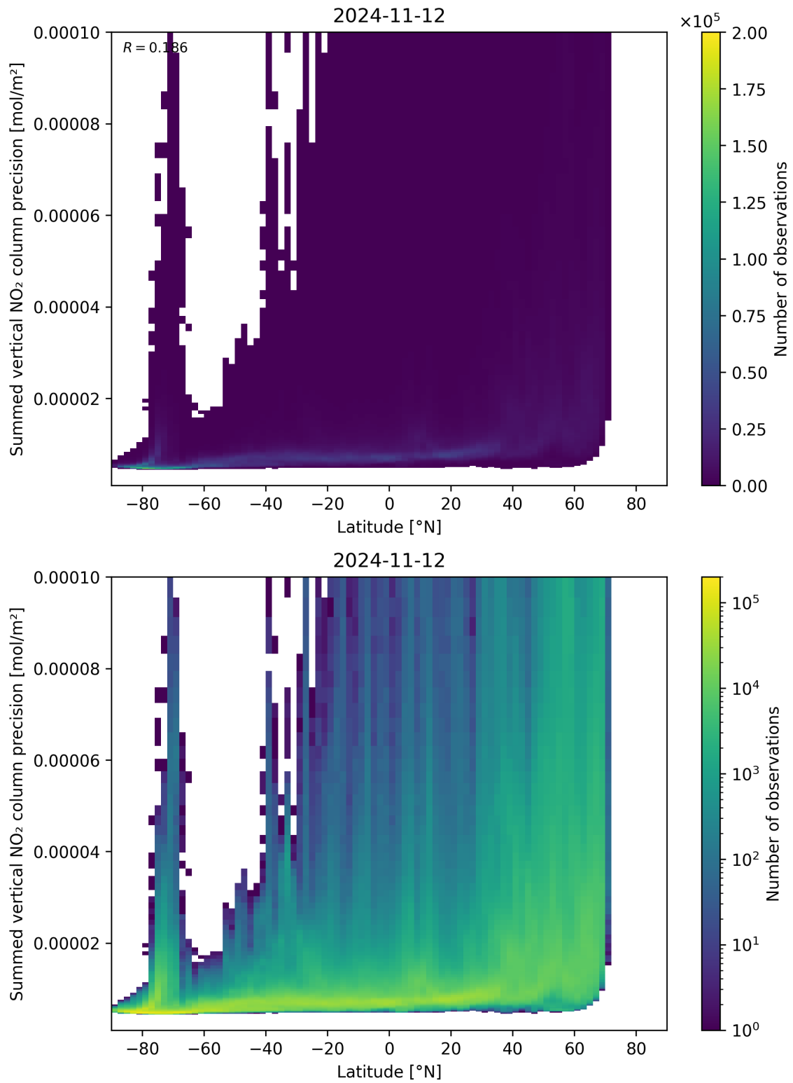
Figure 89: Scatter density plot of “Latitude” against “Summed vertical NO 2 column precision” for 2024-11-11 to 2024-11-13.
