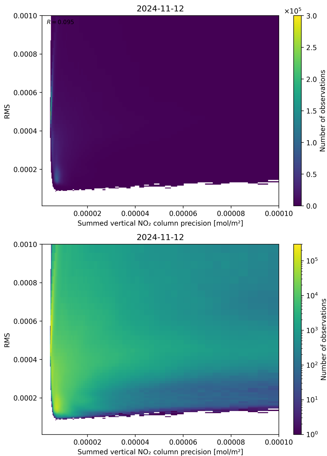
Figure 108: Scatter density plot of “Summed vertical NO 2 column precision” against “RMS” for 2024-11-11 to 2024-11-13.
