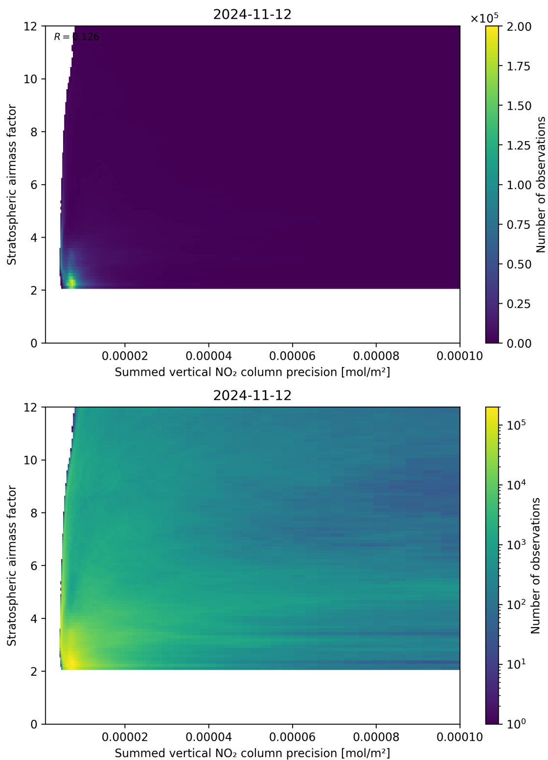
Figure 106: Scatter density plot of “Summed vertical NO 2 column precision” against “Stratospheric airmass factor” for 2024-11-11 to 2024-11-13.
