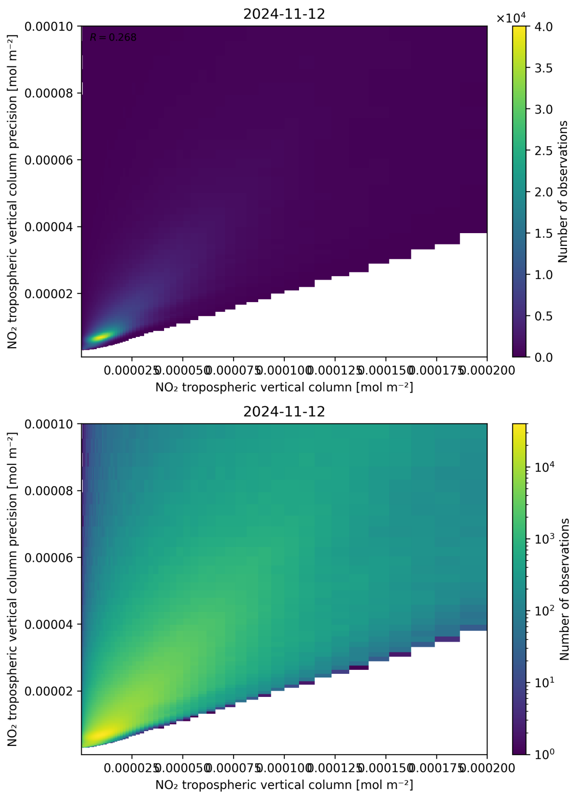
Figure 130: Scatter density plot of “NO 2 tropospheric vertical column” against “NO 2 tropospheric vertical column precision” for 2024-11-11 to 2024-11-13.
