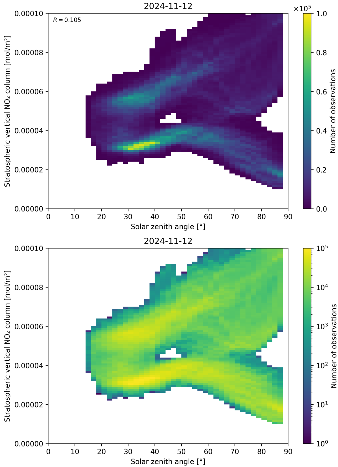
Figure 150: Scatter density plot of “Solar zenith angle” against “Stratospheric vertical NO 2 column” for 2024-11-11 to 2024-11-13.
