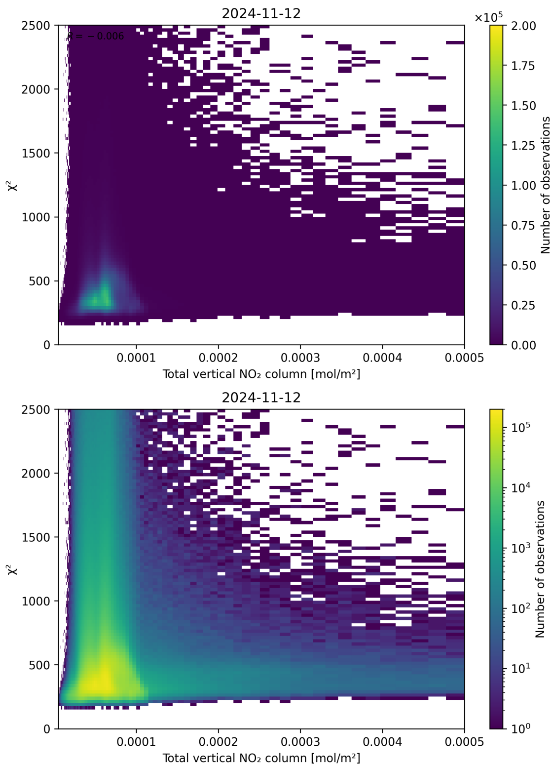
Figure 111: Scatter density plot of “Total vertical NO 2 column” against “ \chi^2 ” for 2024-11-11 to 2024-11-13.
