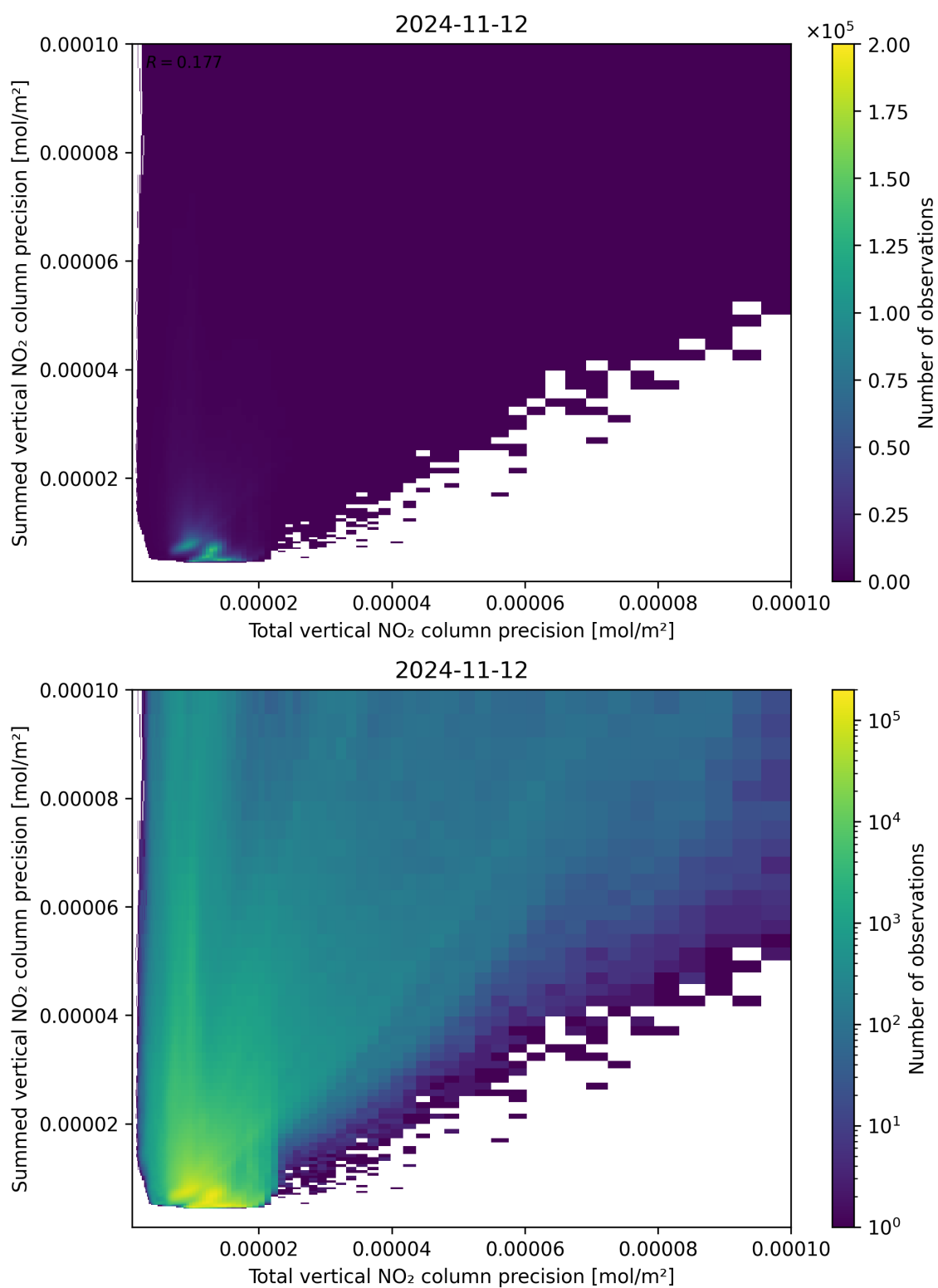
Figure 118: Scatter density plot of “Total vertical NO 2 column precision” against “Summed vertical NO 2 column precision” for 2024-11-11 to 2024-11-13.
