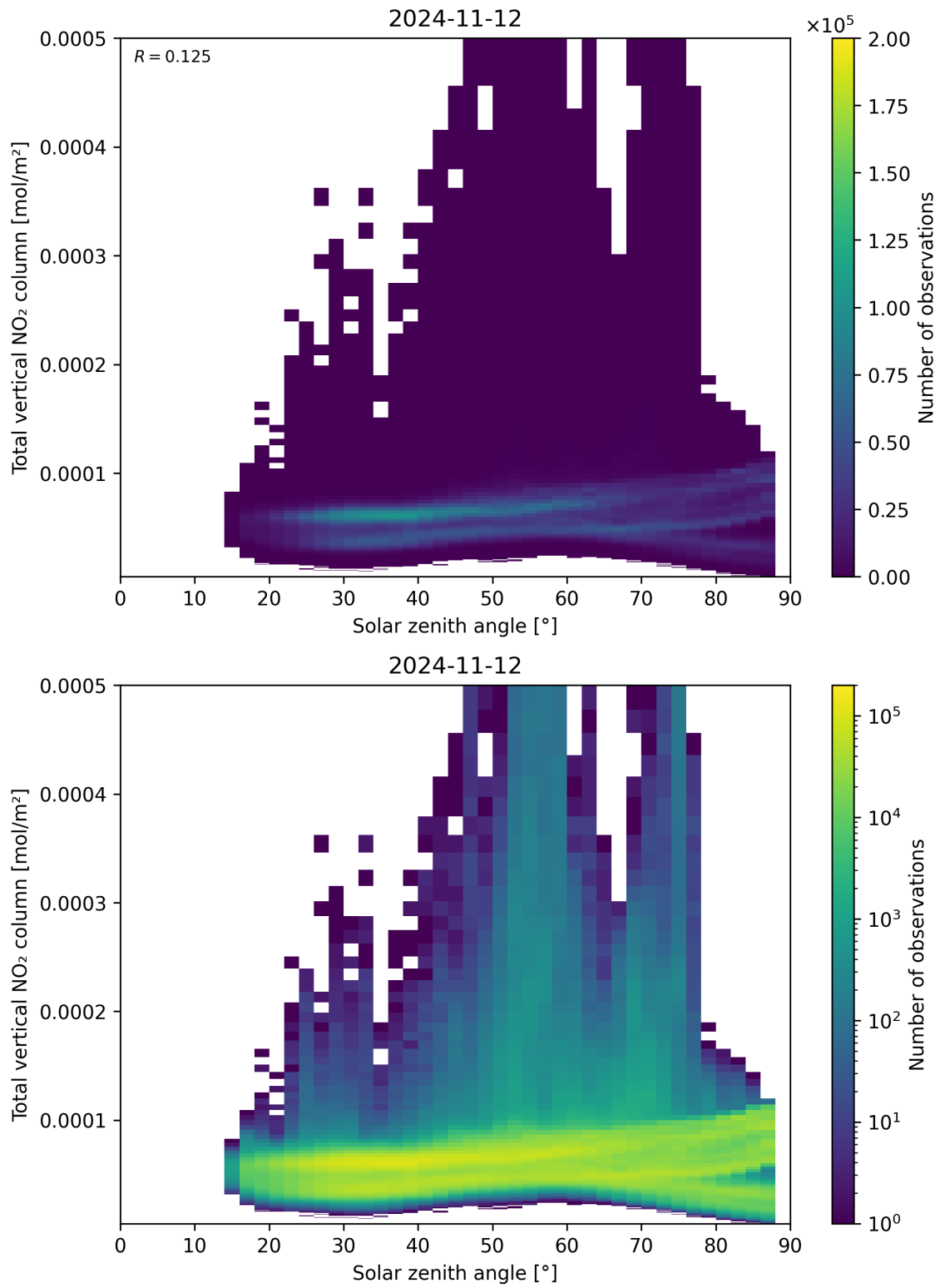
Figure 153: Scatter density plot of “Solar zenith angle” against “Total vertical NO 2 column” for 2024-11-11 to 2024-11-13.
