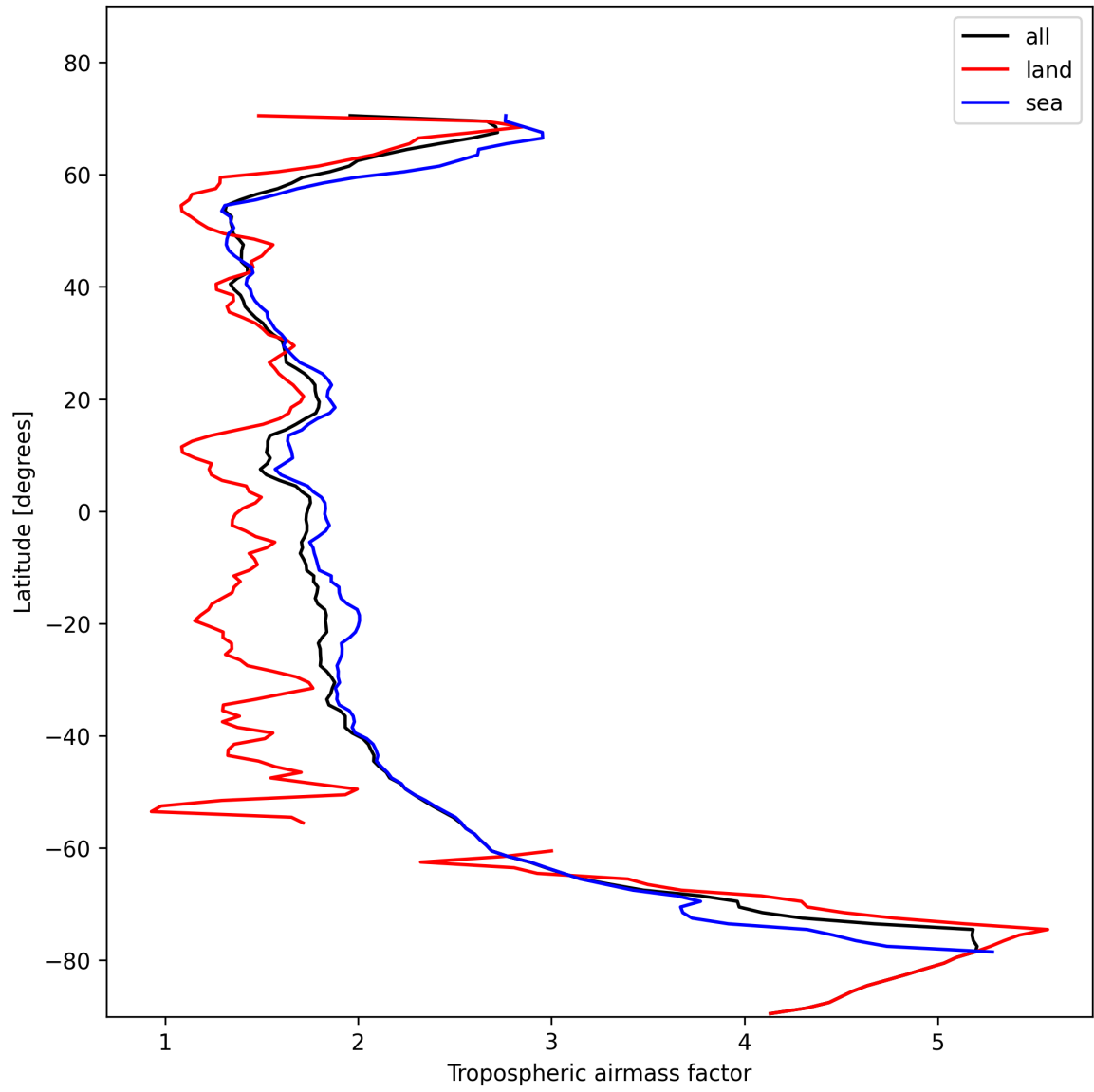
Figure 14: Zonal average of “Tropospheric airmass factor” for 2024-11-11 to 2024-11-13.
