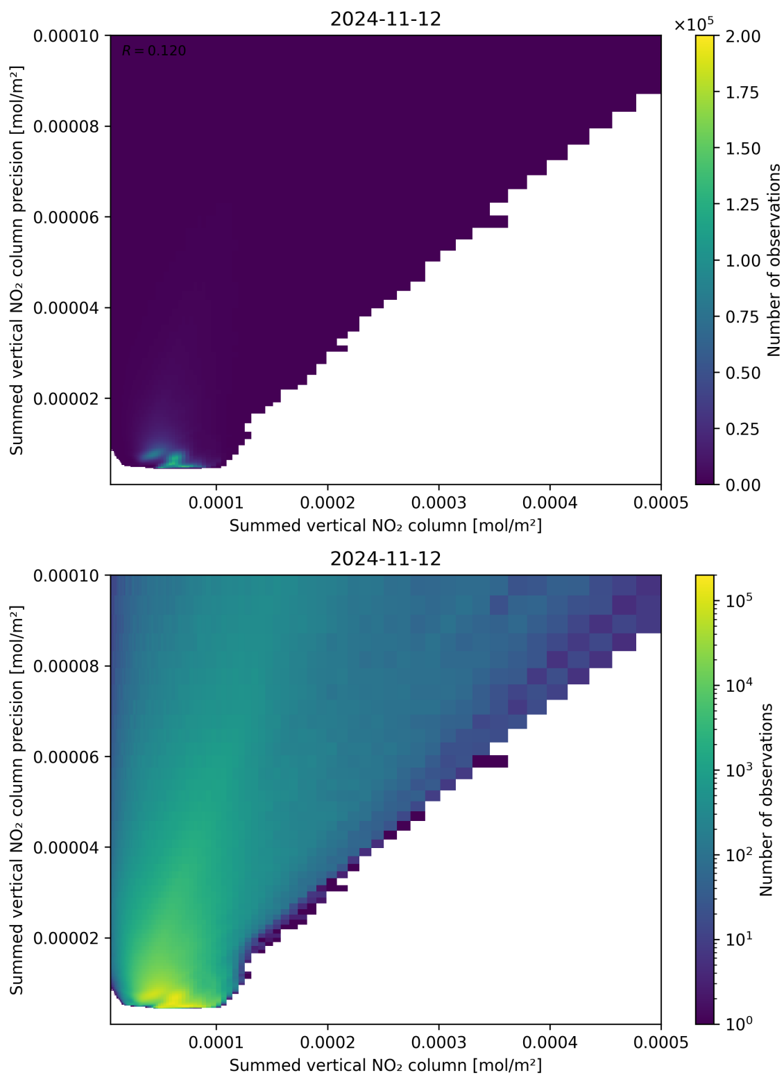
Figure 105: Scatter density plot of “Summed vertical NO 2 column” against “Summed vertical NO 2 column precision” for 2024-11-11 to 2024-11-13.
