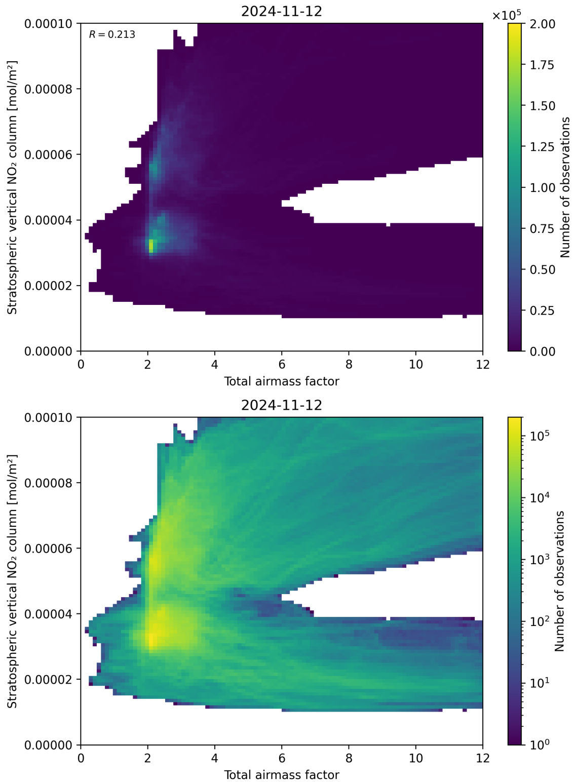
Figure 64: Scatter density plot of “Total airmass factor” against “Stratospheric vertical NO 2 column” for 2024-11-11 to 2024-11-13.
