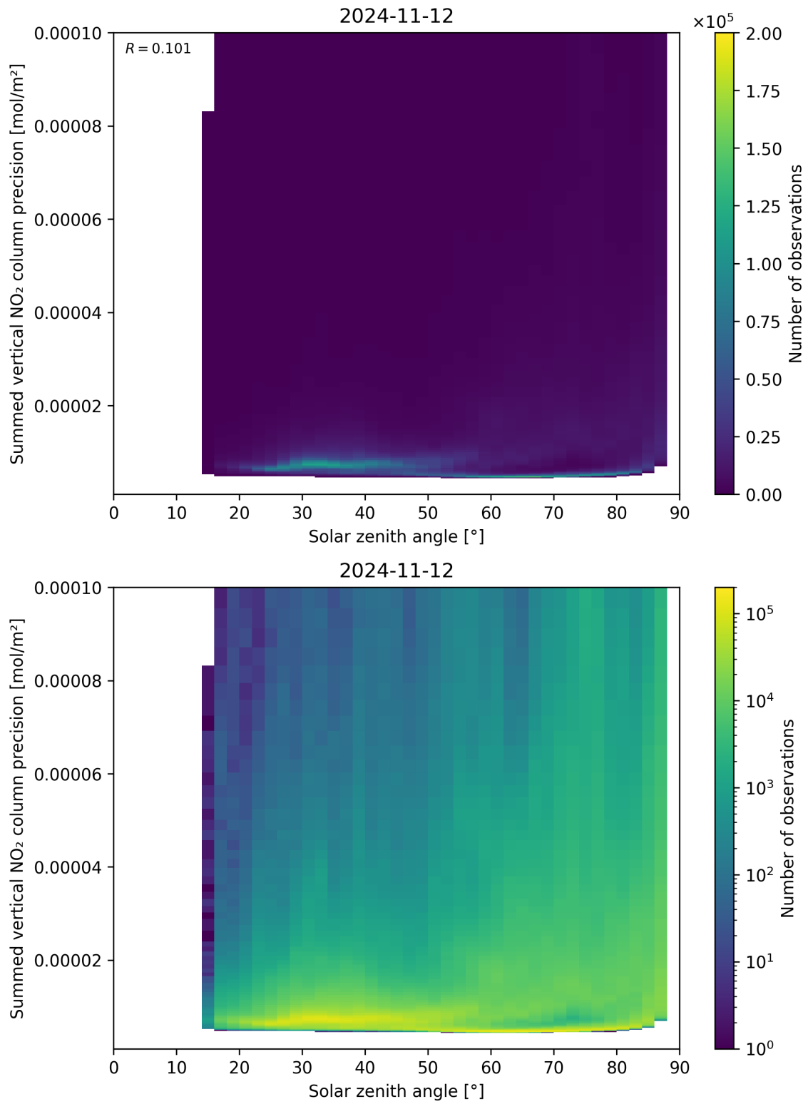
Figure 152: Scatter density plot of “Solar zenith angle” against “Summed vertical NO 2 column precision” for 2024-11-11 to 2024-11-13.
