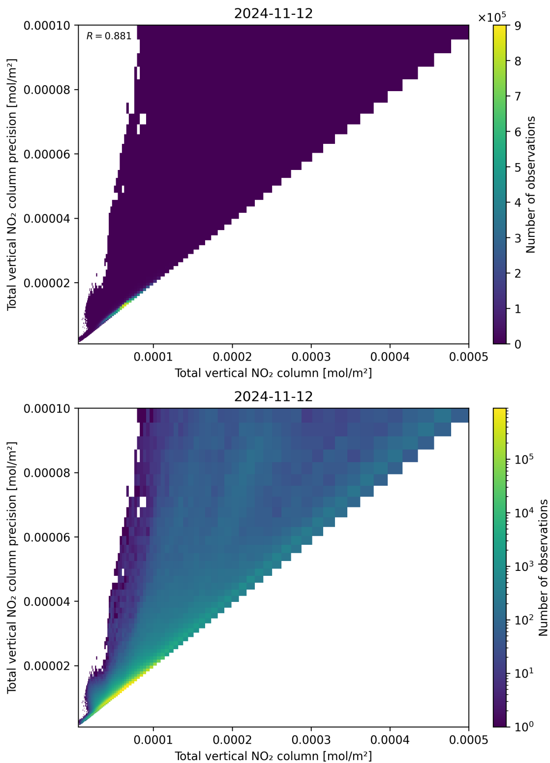
Figure 114: Scatter density plot of “Total vertical NO 2 column” against “Total vertical NO 2 column precision” for 2024-11-11 to 2024-11-13.
