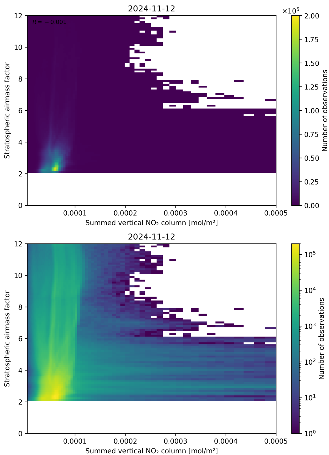
Figure 103: Scatter density plot of “Summed vertical NO 2 column” against “Stratospheric air mass factor” for 2024-11-11 to 2024-11-13.
