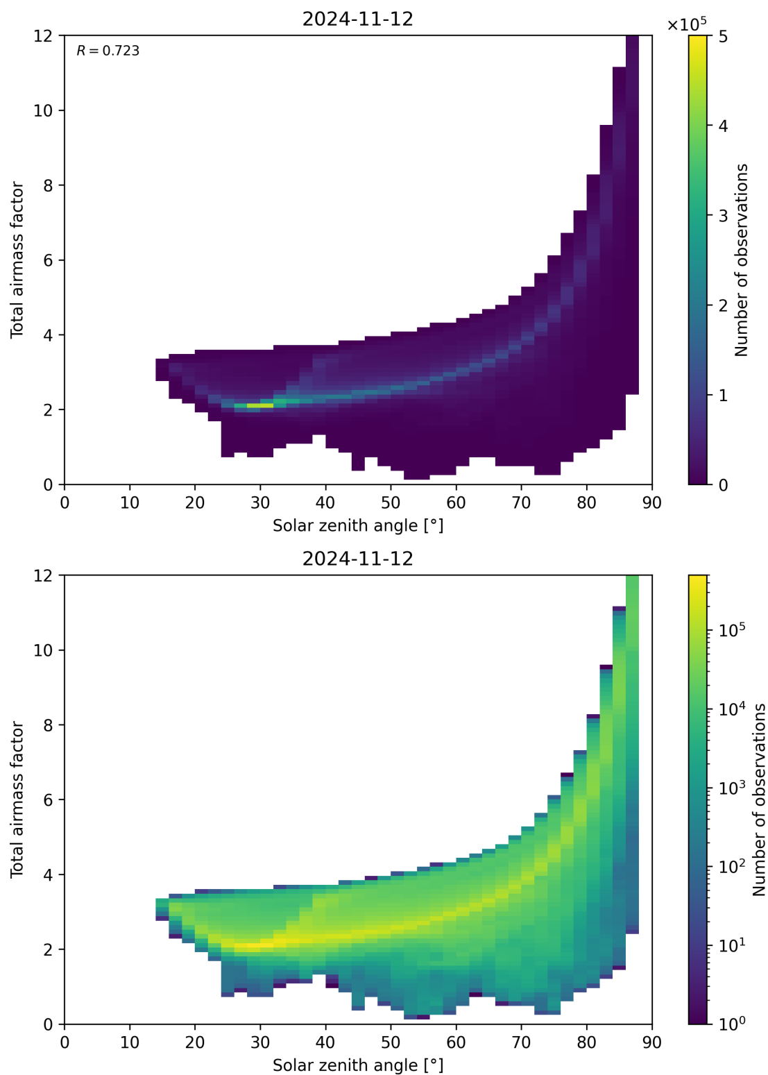
Figure 146: Scatter density plot of “Solar zenith angle” against “Total airmass factor” for 2024-11-11 to 2024-11-13.
