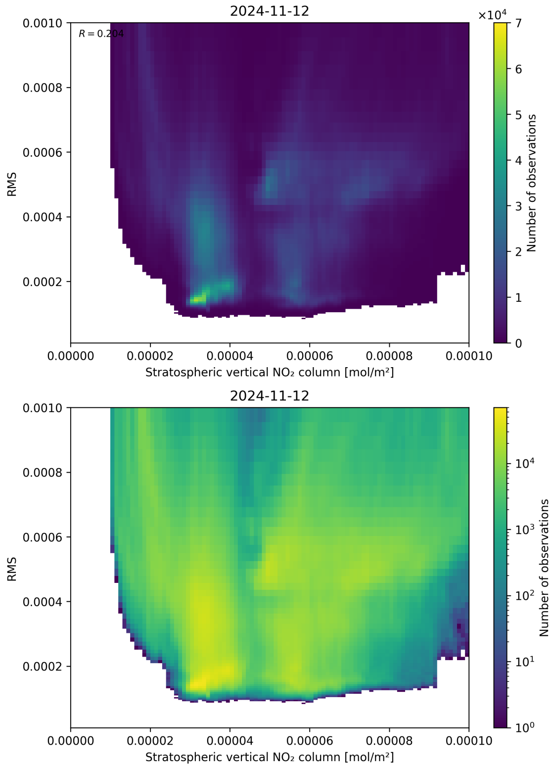
Figure 102: Scatter density plot of “Stratospheric vertical NO 2 column” against “RMS” for 2024-11-11 to 2024-11-13.
