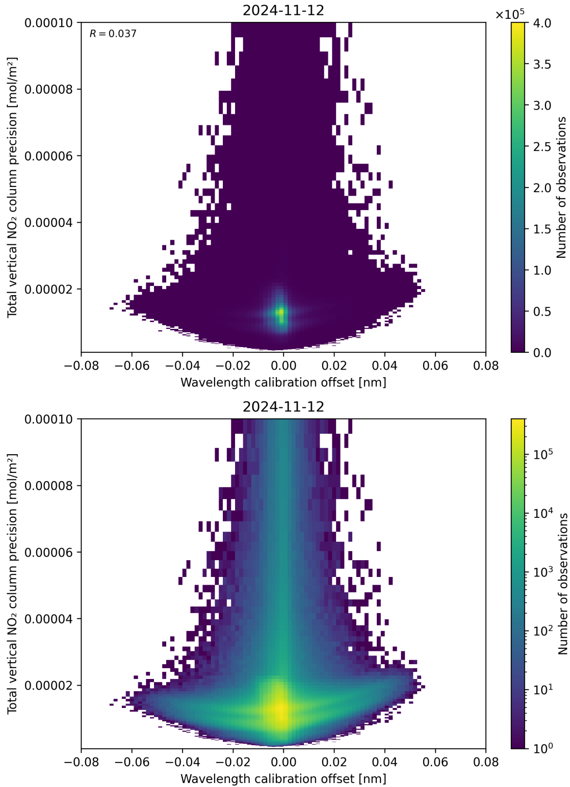
Figure 180: Scatter density plot of “Wavelength calibration offset” against “Total vertical NO 2 column precision” for 2024-11-11 to 2024-11-13.
