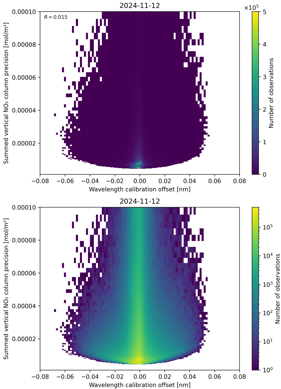
Figure 178: Scatter density plot of “Wavelength calibration offset” against “Summed vertical NO 2 column precision” for 2024-11-11 to 2024-11-13.
