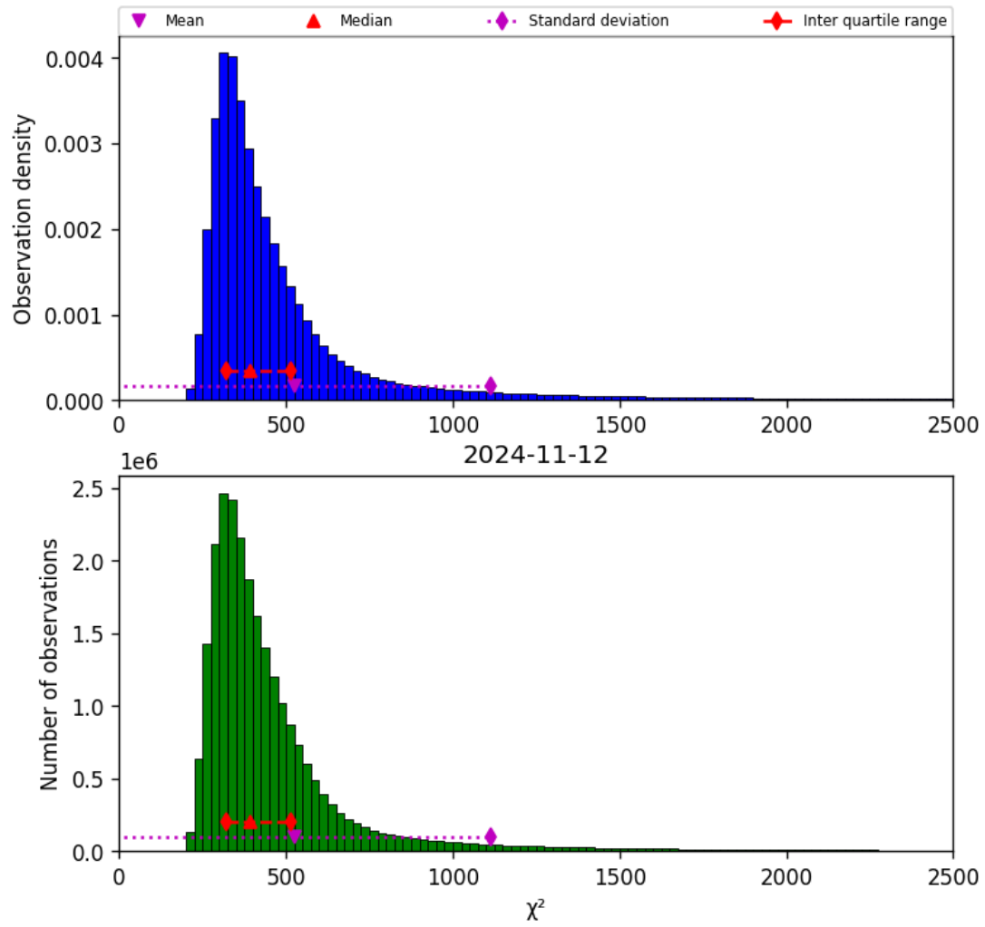
Figure 42: Histogram of “ \chi^2 ” for 2024-11-11 to 2024-11-13
