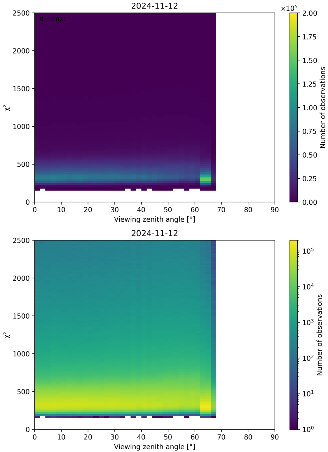
Figure 162: Scatter density plot of “Viewing zenith angle” against “ \chi^2 ” for 2024-11-11 to 2024-11-13.
