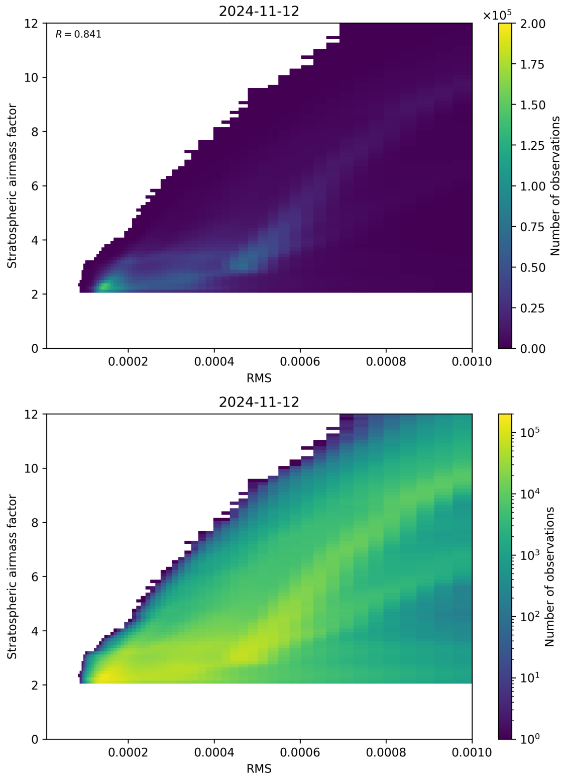
Figure 144: Scatter density plot of “RMS” against “Stratospheric airmass factor” for 2024-11-11 to 2024-11-13.
