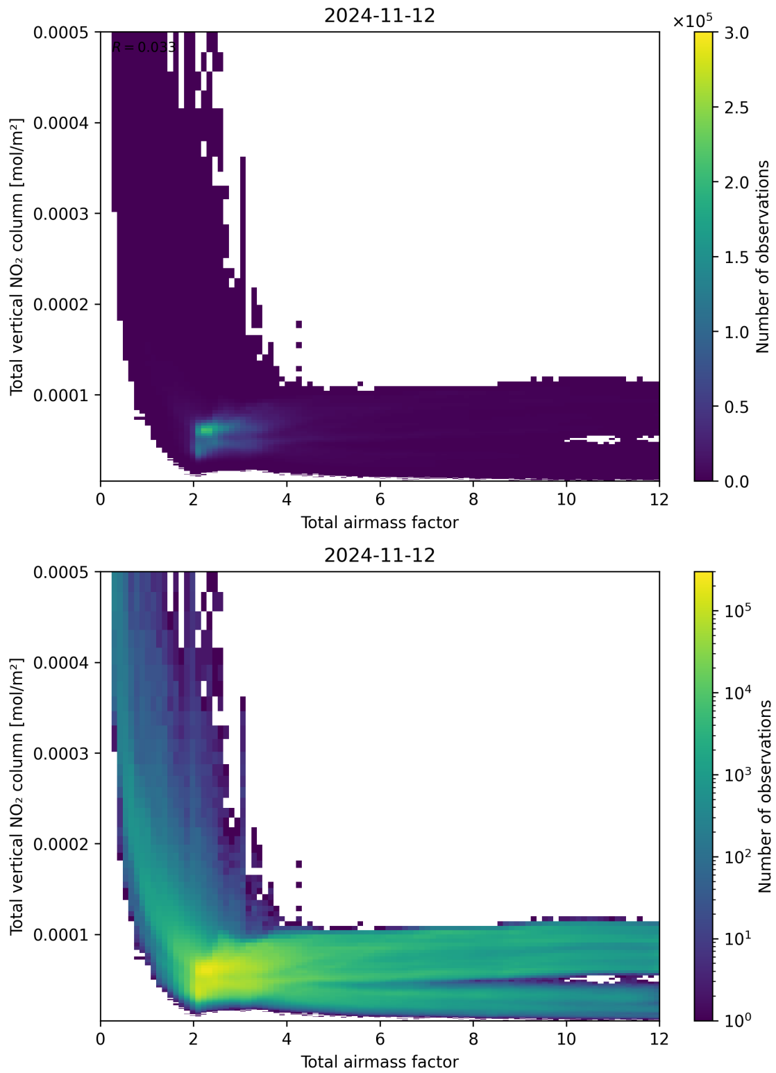
Figure 67: Scatter density plot of “Total airmass factor” against “Total vertical NO 2 column” for 2024-11-11 to 2024-11-13.
