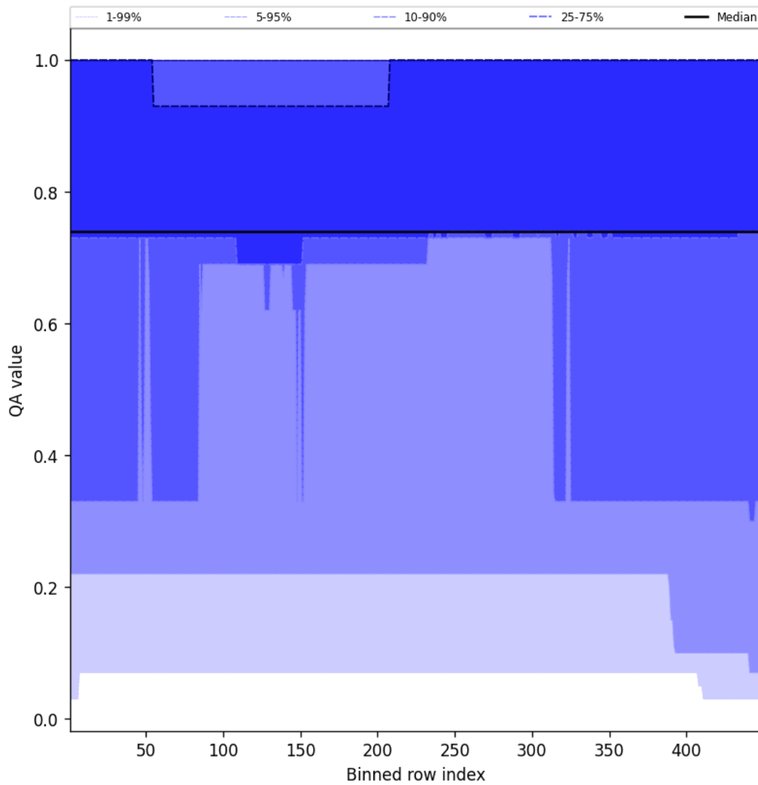
Figure 45: Along track statistics of “QA value” for 2024-11-11 to 2024-11-13
