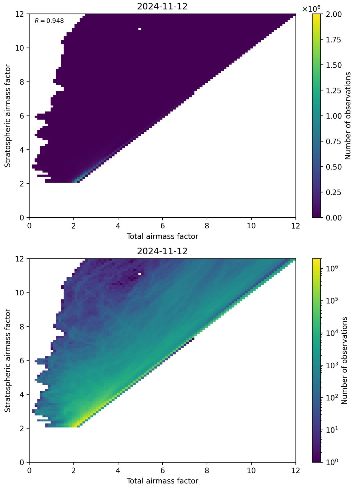
Figure 62: Scatter density plot of “Total airmass factor” against “Stratospheric airmass factor” for 2024-11-11 to 2024-11-13.
