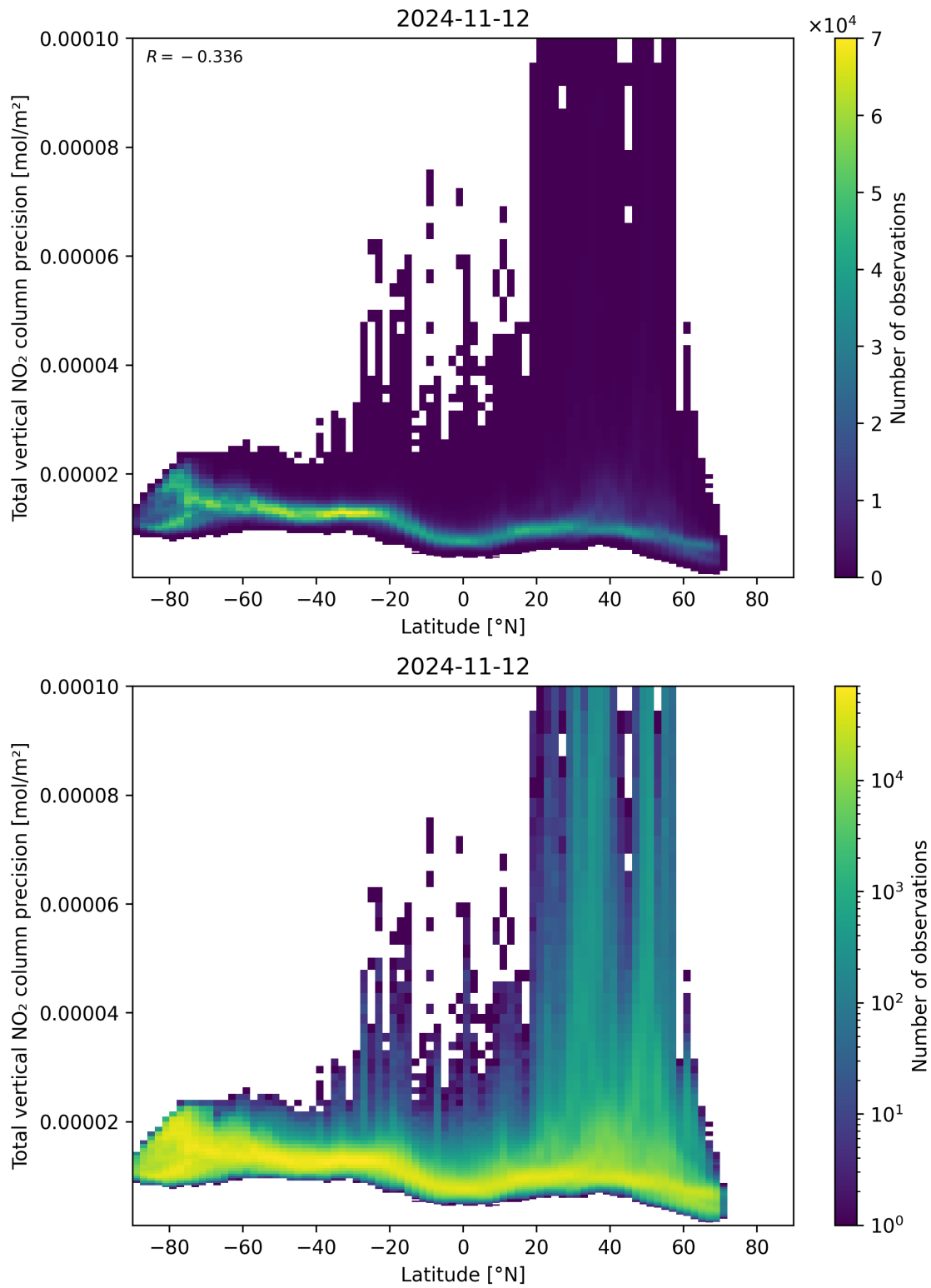
Figure 91: Scatter density plot of “Latitude” against “Total vertical NO 2 column precision” for 2024-11-11 to 2024-11-13.
