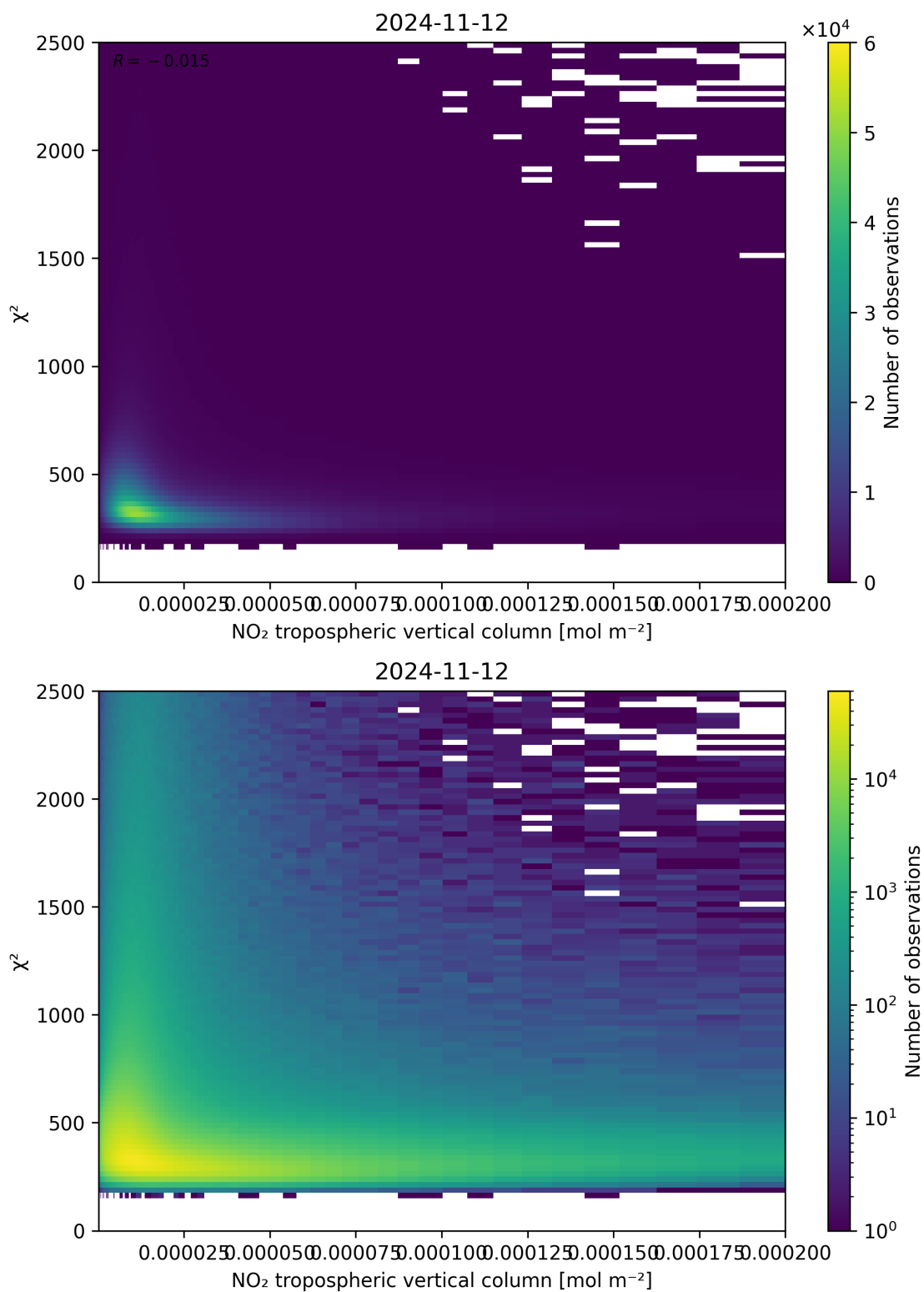
Figure 124: Scatter density plot of “NO 2 tropospheric vertical column” against “ \chi^2 ” for 2024-11-11 to 2024-11-13.
