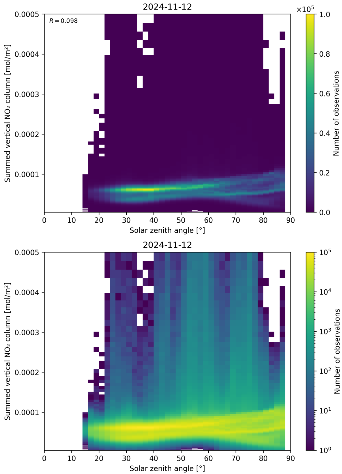
Figure 151: Scatter density plot of “Solar zenith angle” against “Summed vertical NO 2 column” for 2024-11-11 to 2024-11-13.
