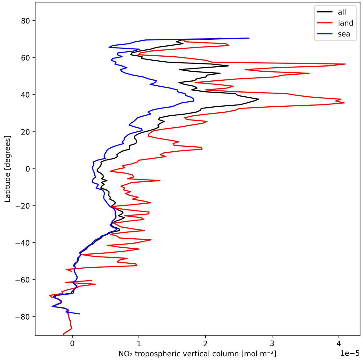
Figure 12: Zonal average of “NO 2 tropospheric vertical column” for 2024-11-11 to 2024-11-13.
