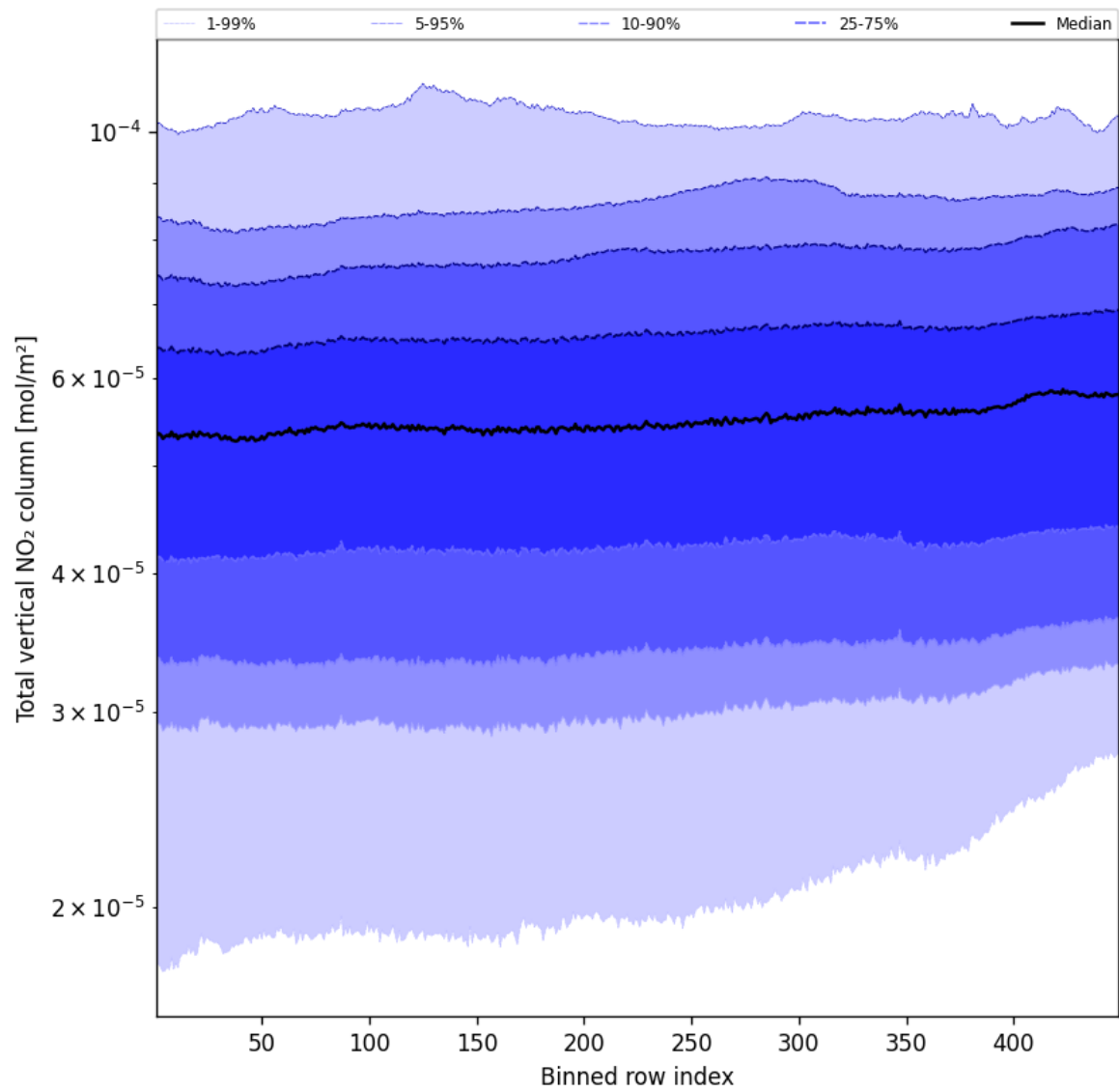
Figure 55: Along track statistics of “Total vertical NO 2 column” for 2024-11-11 to 2024-11-13
