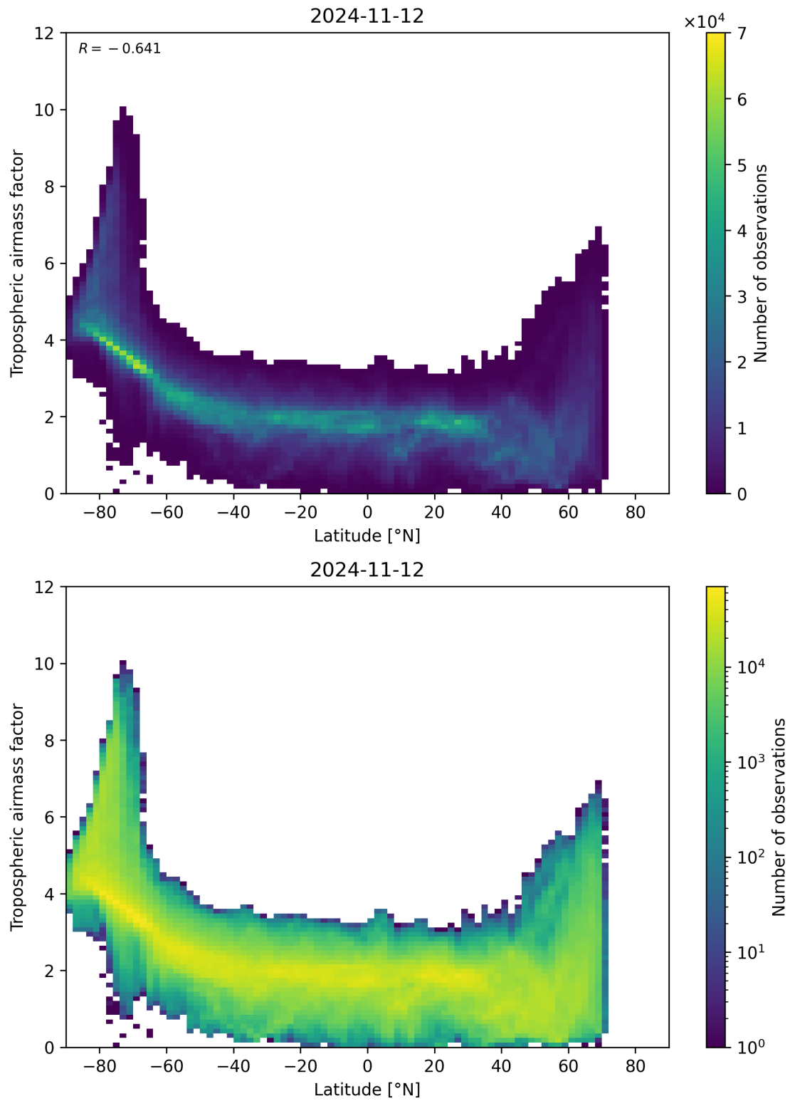
Figure 85: Scatter density plot of “Latitude” against “Tropospheric air mass factor” for 2024-11-11 to 2024-11-13.
