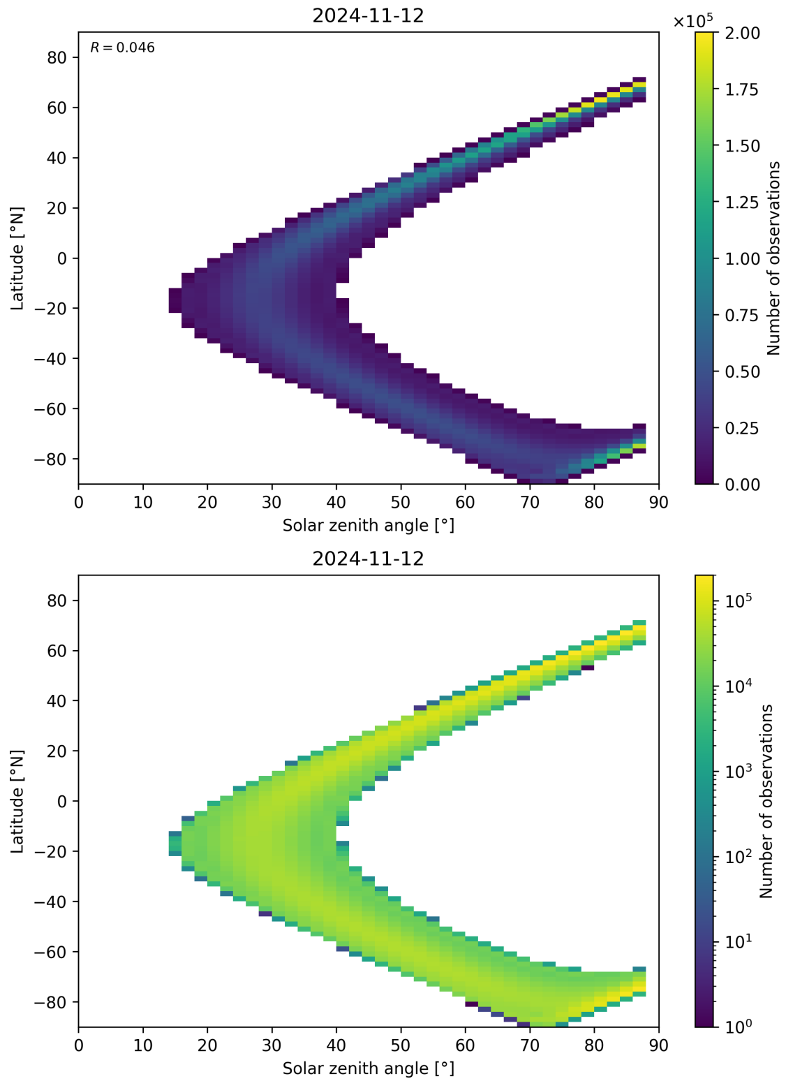
Figure 149: Scatter density plot of “Solar zenith angle” against “Latitude” for 2024-11-11 to 2024-11-13.
