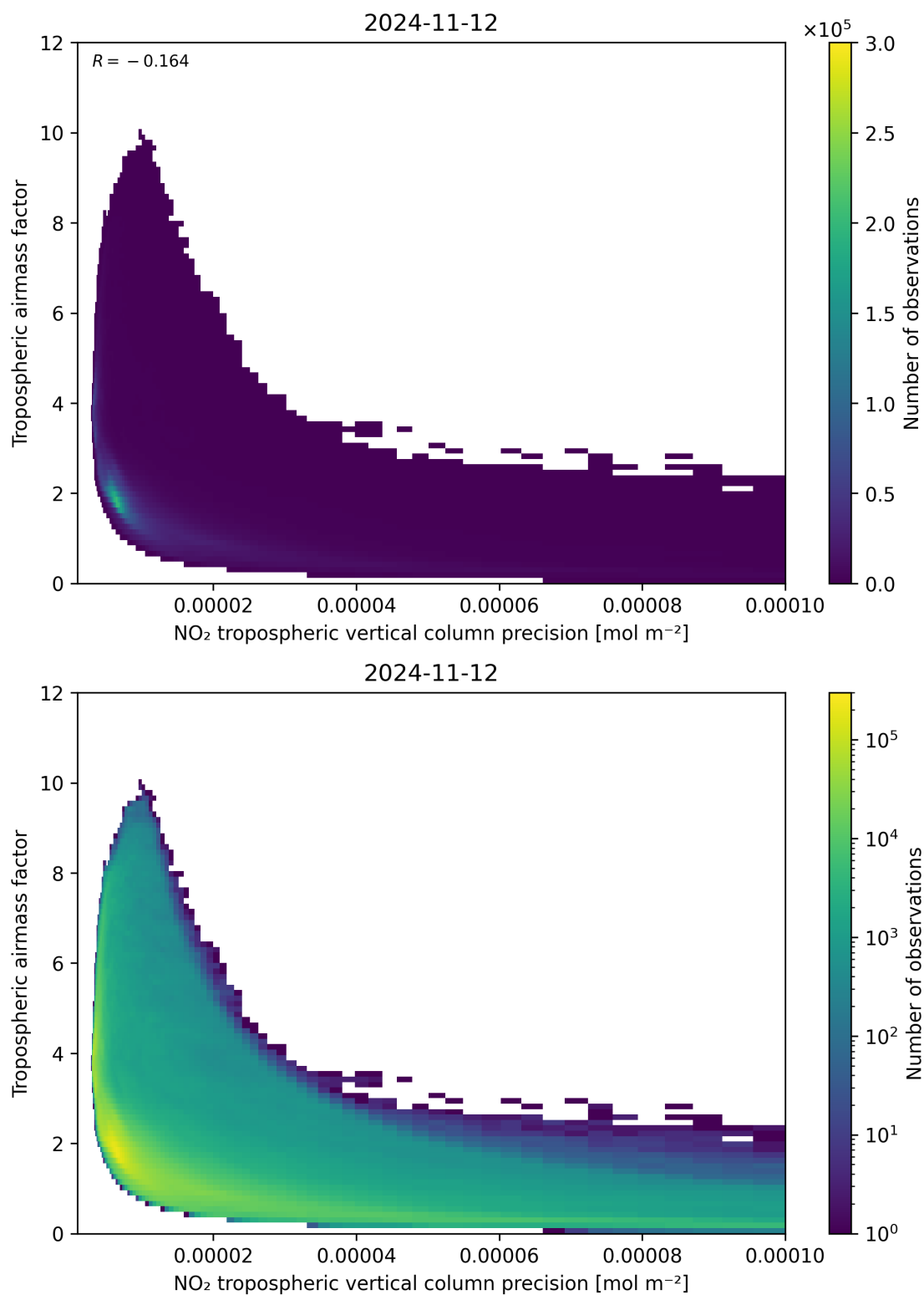
Figure 133: Scatter density plot of “NO 2 tropospheric vertical column precision” against “Tropospheric air mass factor” for 2024-11-11 to 2024-11-13.
