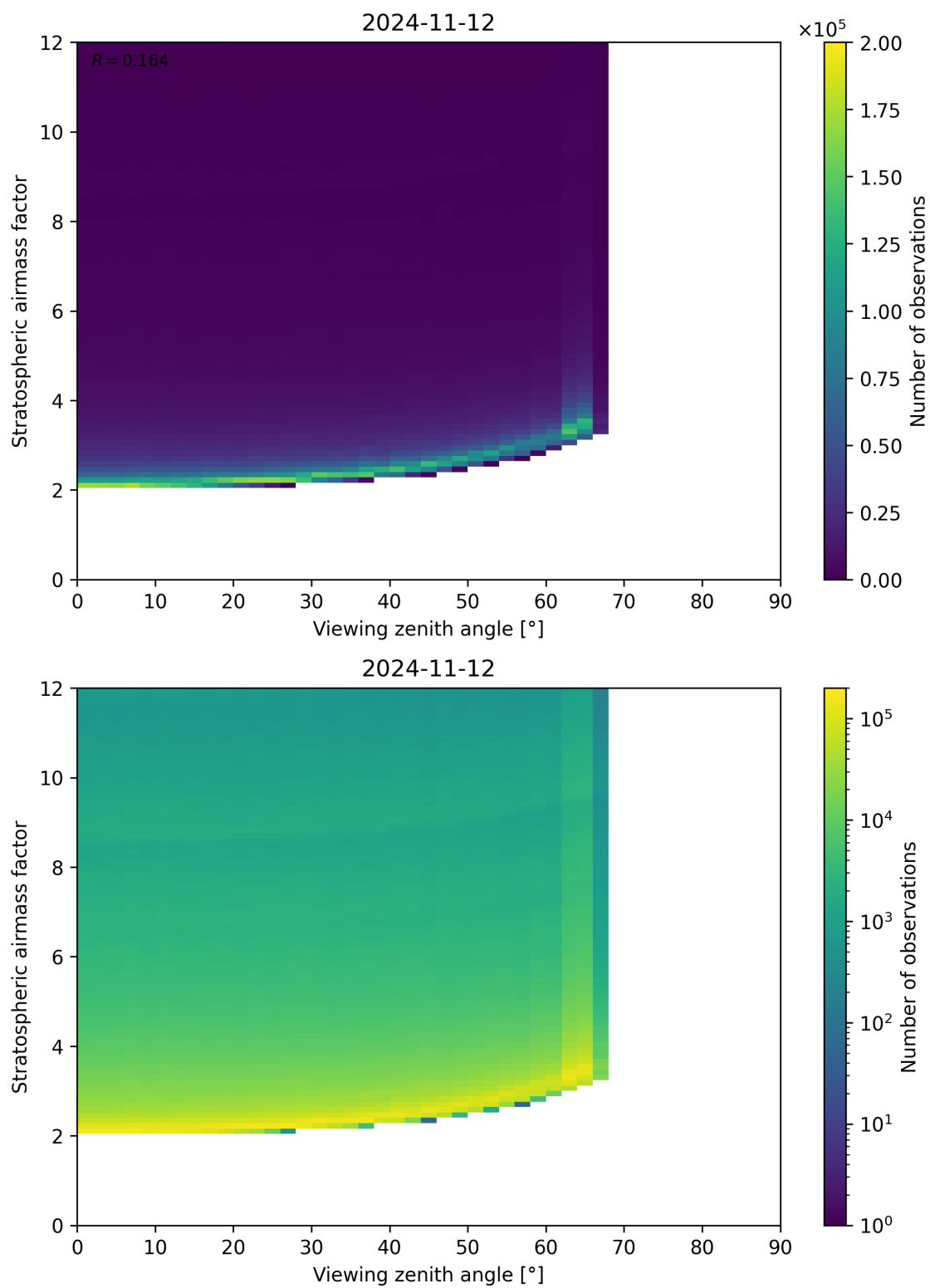
Figure 159: Scatter density plot of “Viewing zenith angle” against “Stratospheric airmass factor” for 2024-11-11 to 2024-11-13.
