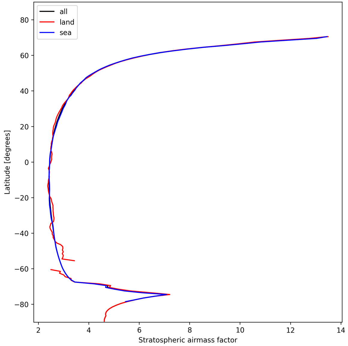
Figure 27: Zonal average of “Stratospheric air mass factor” for 2024-11-11 to 2024-11-13.
