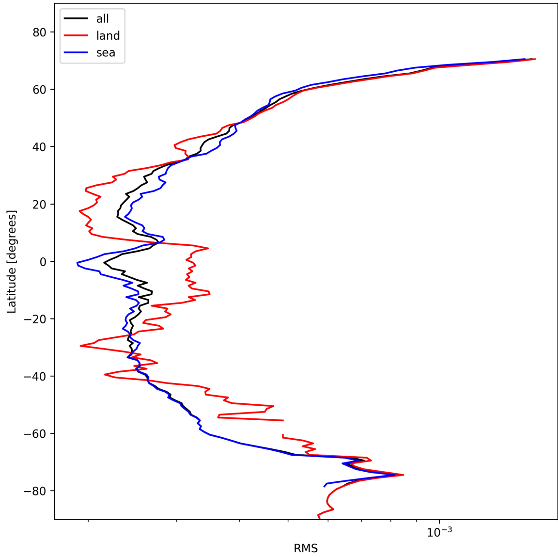
Figure 26: Zonal average of “RMS” for 2024-11-11 to 2024-11-13.
