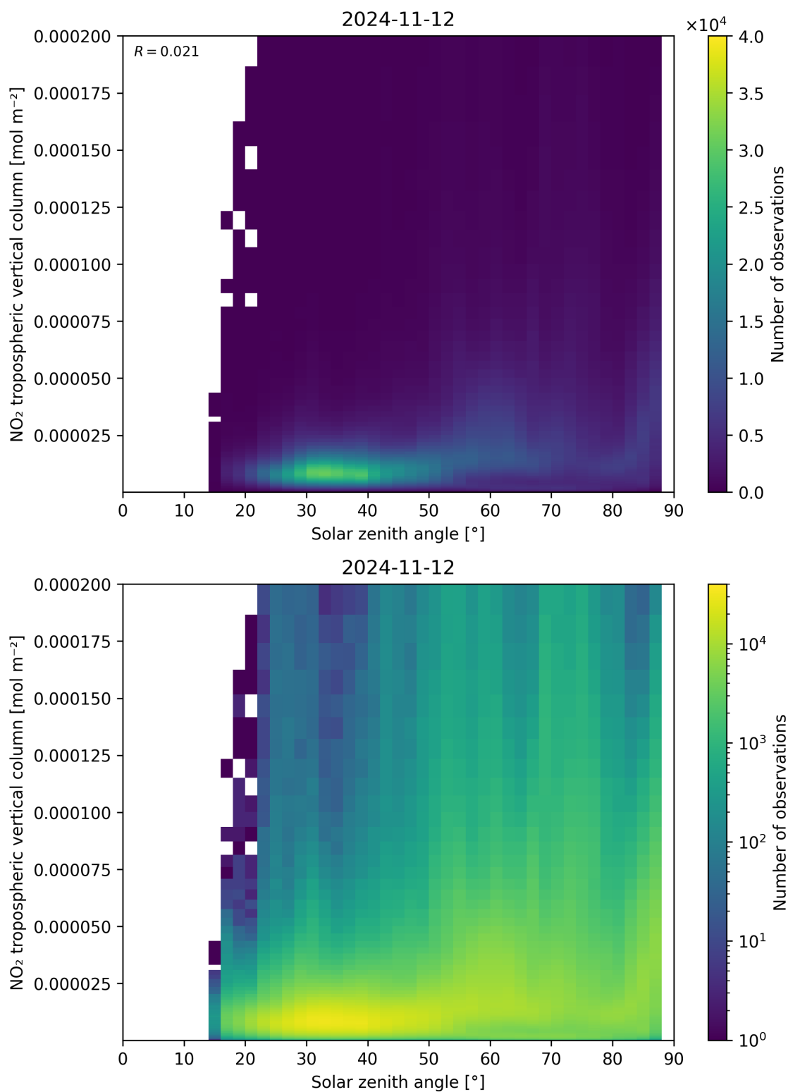
Figure 155: Scatter density plot of “Solar zenith angle” against “NO 2 tropospheric vertical column” for 2024-11-11 to 2024-11-13.
