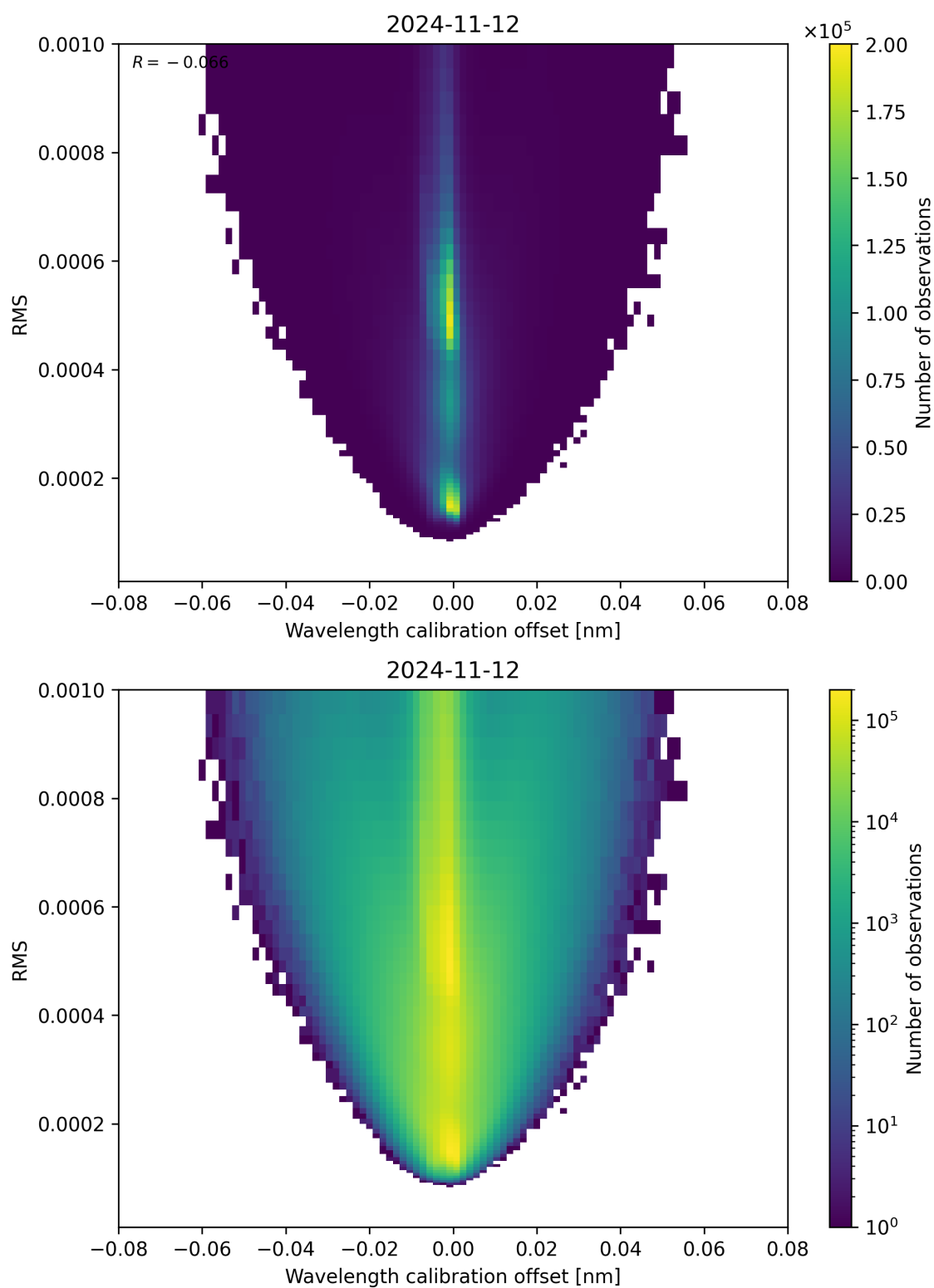
Figure 181: Scatter density plot of “Wavelength calibration offset” against “RMS” for 2024-11-11 to 2024-11-13.
