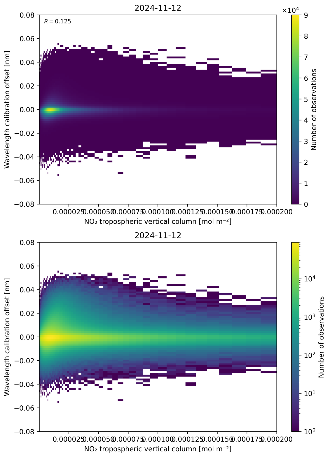
Figure 143: Scatter density plot of “NO 2 tropospheric vertical column” against “Wavelength calibration offset” for 2024-11-11 to 2024-11-13.
