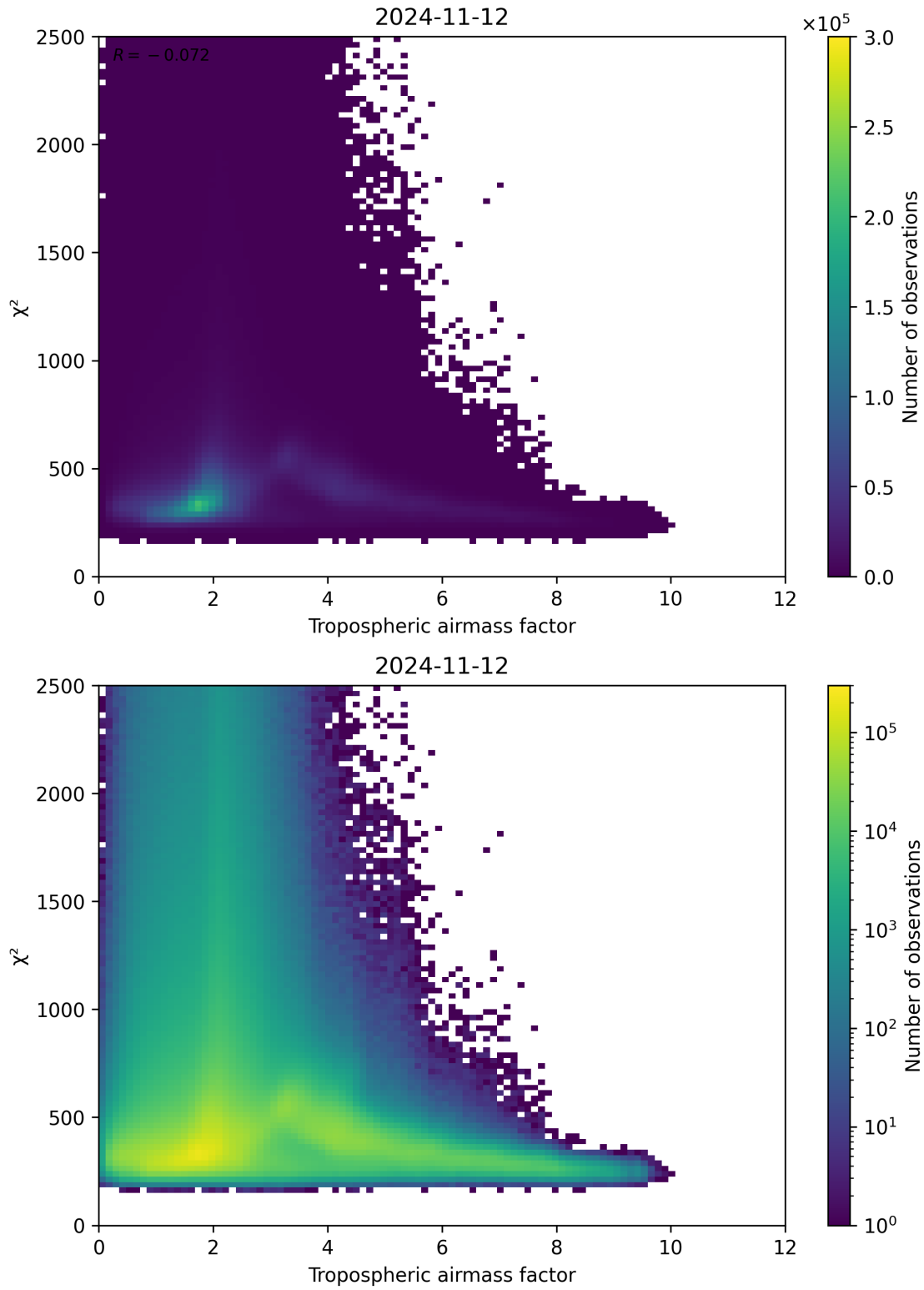
Figure 73: Scatter density plot of “Tropospheric airmass factor” against “ \chi^2 ” for 2024-11-11 to 2024-11-13.
