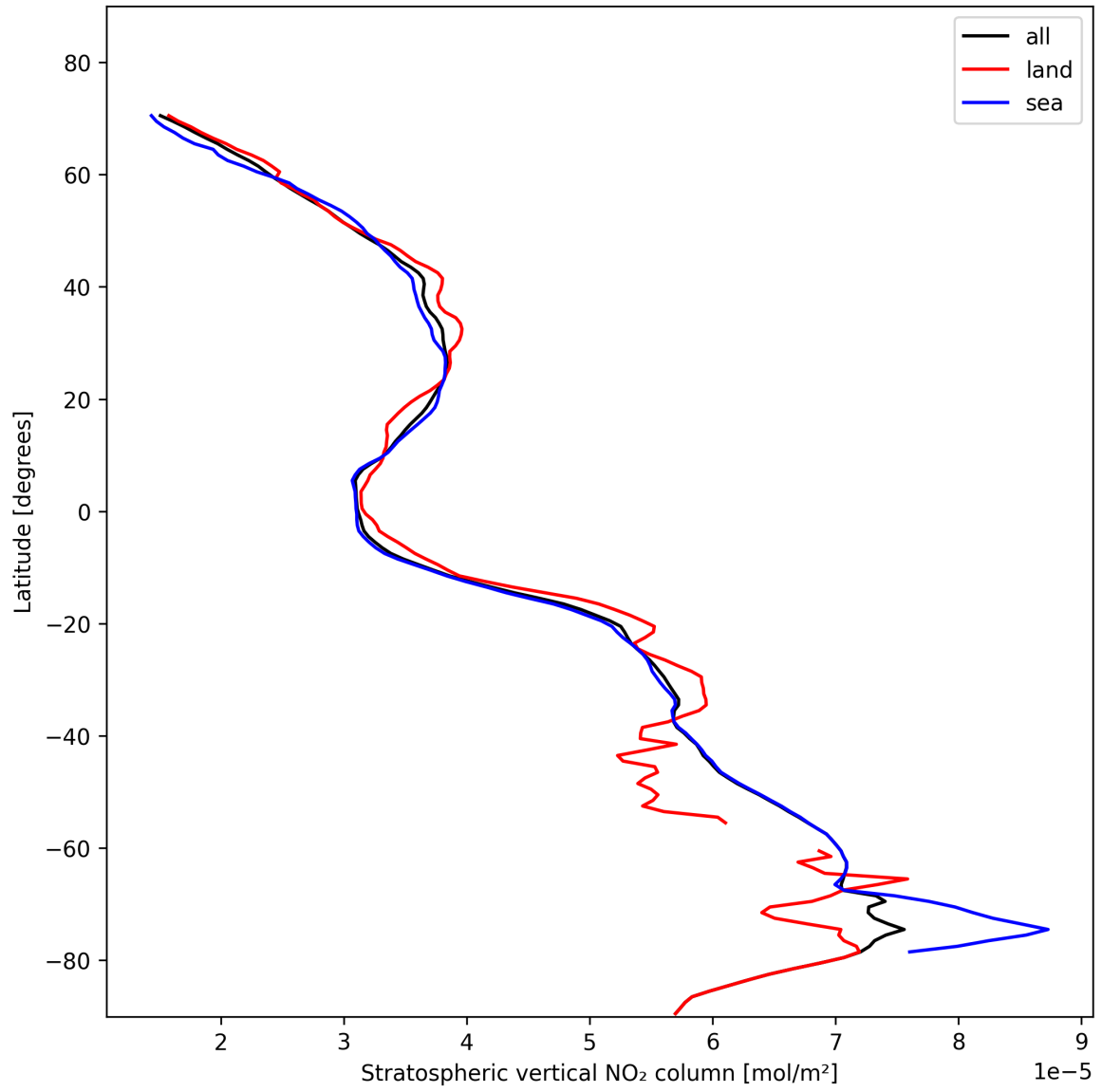
Figure 19: Zonal average of “Stratospheric vertical NO 2 column” for 2024-11-11 to 2024-11-13.
