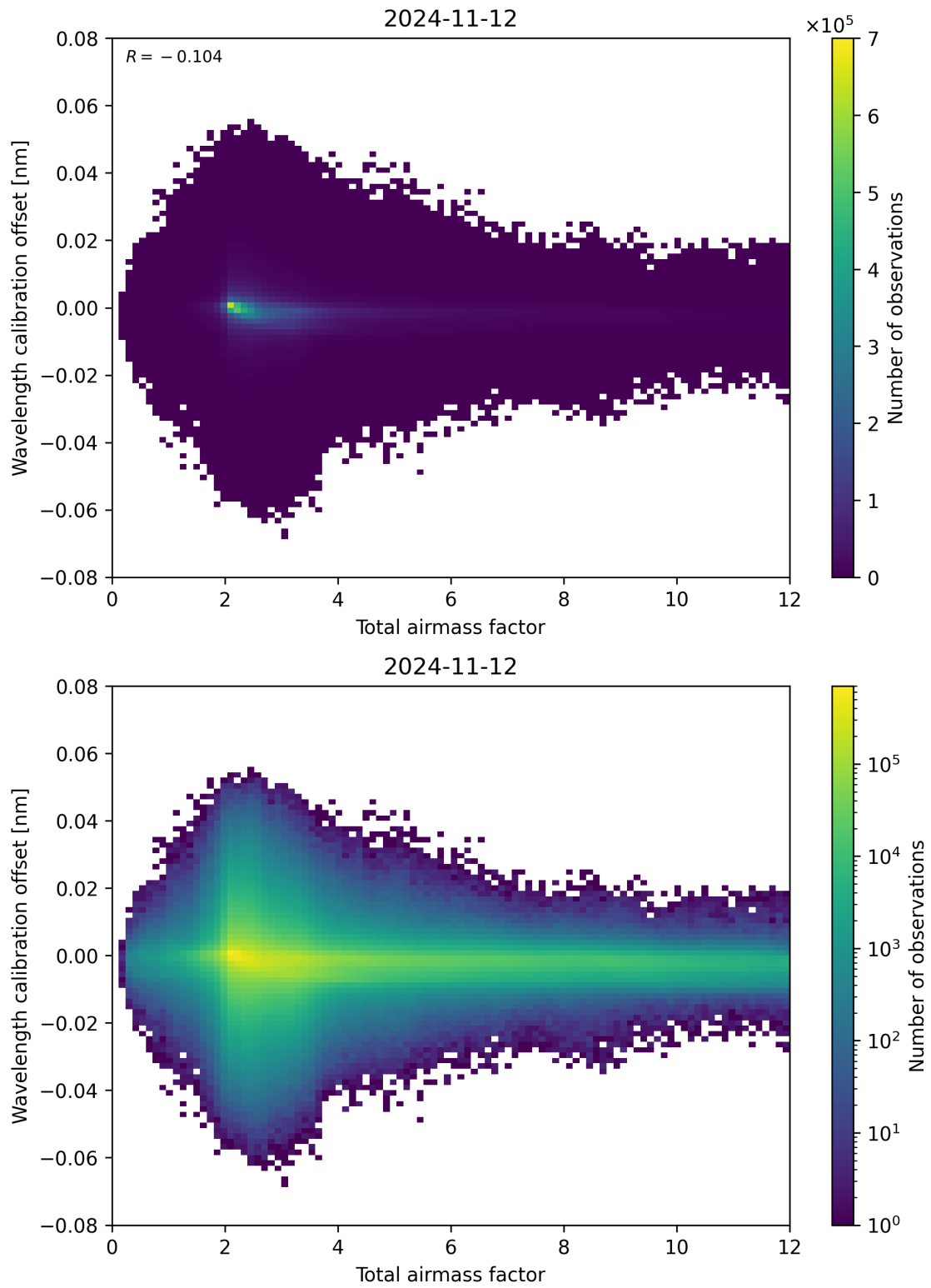
Figure 70: Scatter density plot of “Total airmass factor” against “Wavelength calibration offset” for 2024-11-11 to 2024-11-13.
