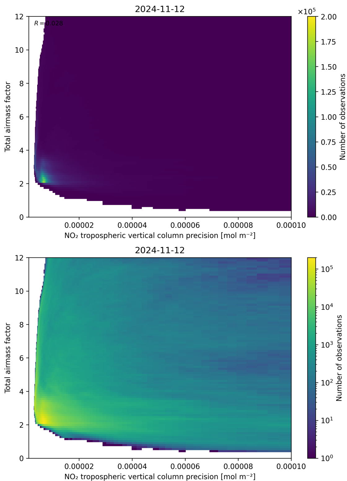
Figure 132: Scatter density plot of “NO 2 tropospheric vertical column precision” against “Total air mass factor” for 2024-11-11 to 2024-11-13.
