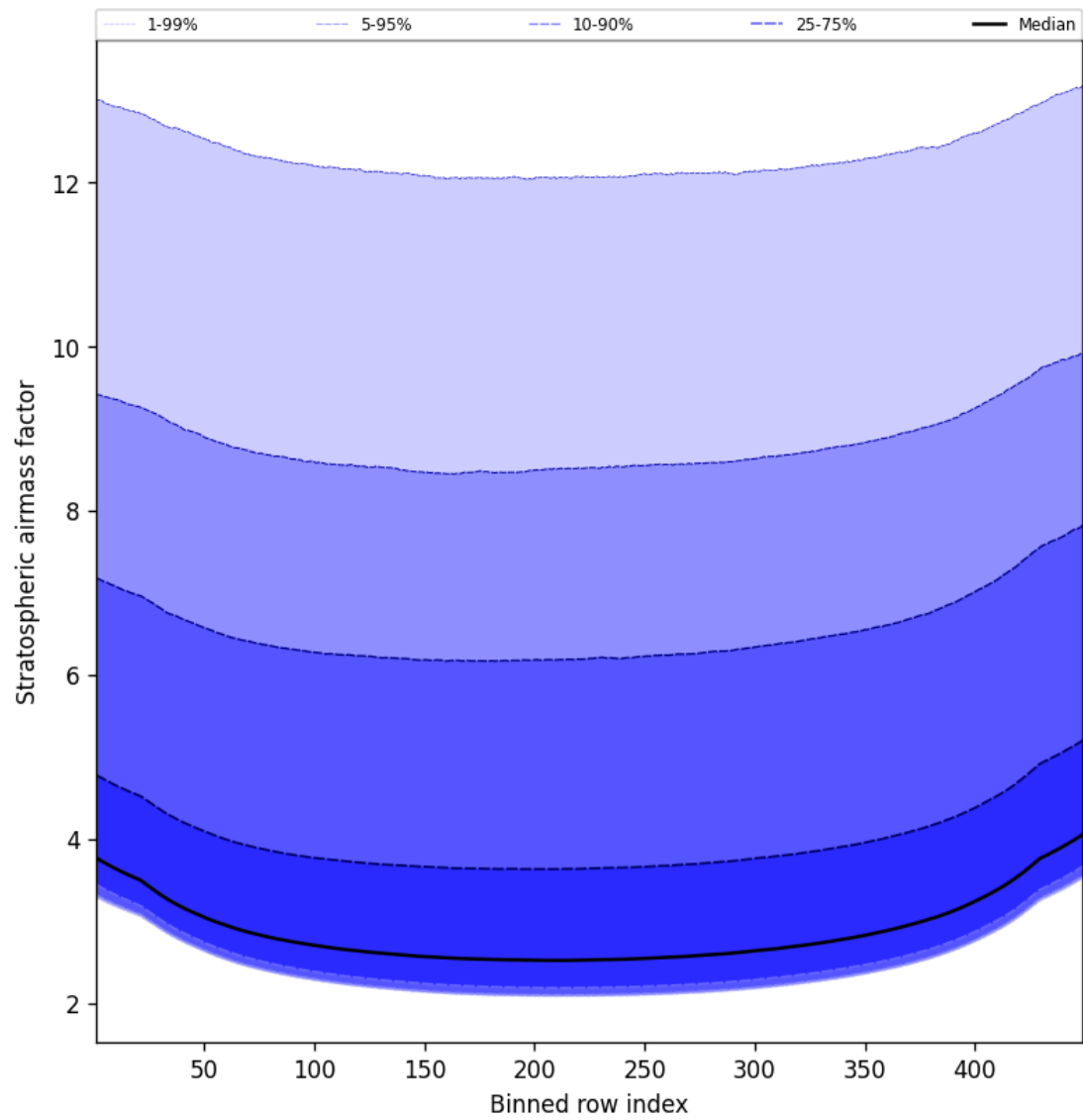
Figure 61: Along track statistics of “Stratospheric air mass factor” for 2024-11-11 to 2024-11-13
