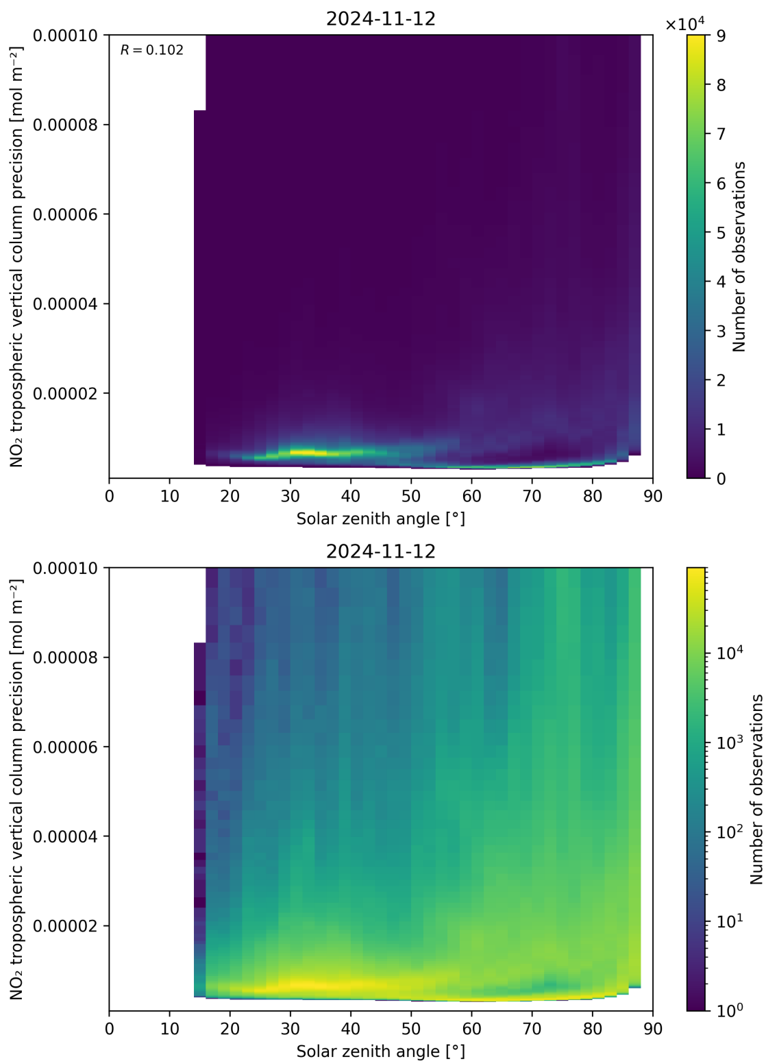
Figure 156: Scatter density plot of “Solar zenith angle” against “NO 2 tropospheric vertical column precision” for 2024-11-11 to 2024-11-13.
