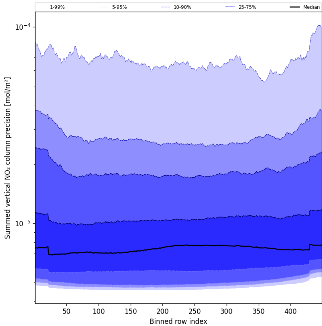
Figure 58: Along track statistics of “Summed vertical NO 2 column precision” for 2024-11-11 to 2024-11-13
