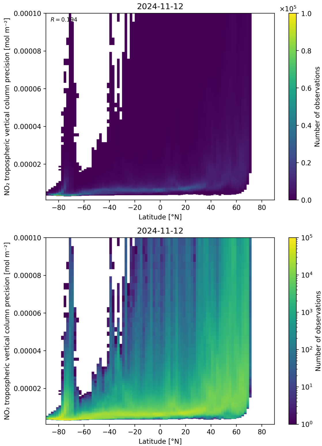
Figure 93: Scatter density plot of “Latitude” against “NO 2 tropospheric vertical column precision” for 2024-11-11 to 2024-11-13.
