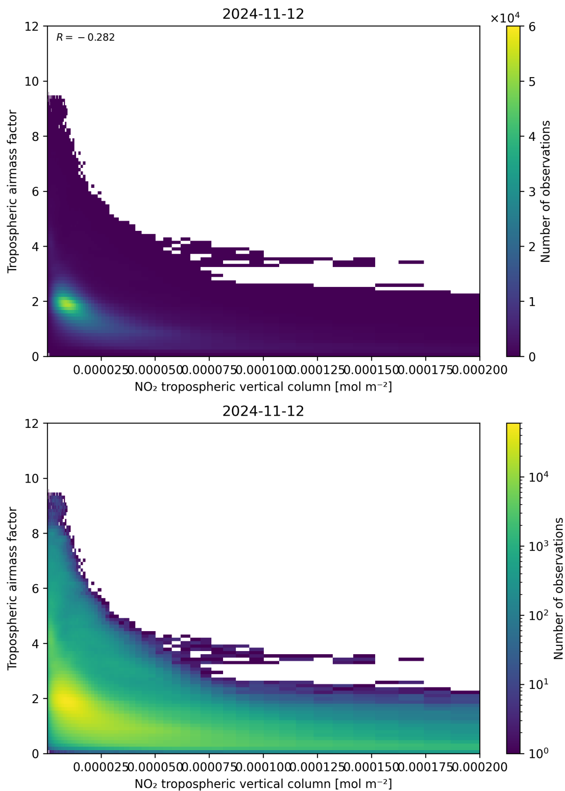
Figure 123: Scatter density plot of “NO 2 tropospheric vertical column” against “Tropospheric air mass factor” for 2024-11-11 to 2024-11-13.
