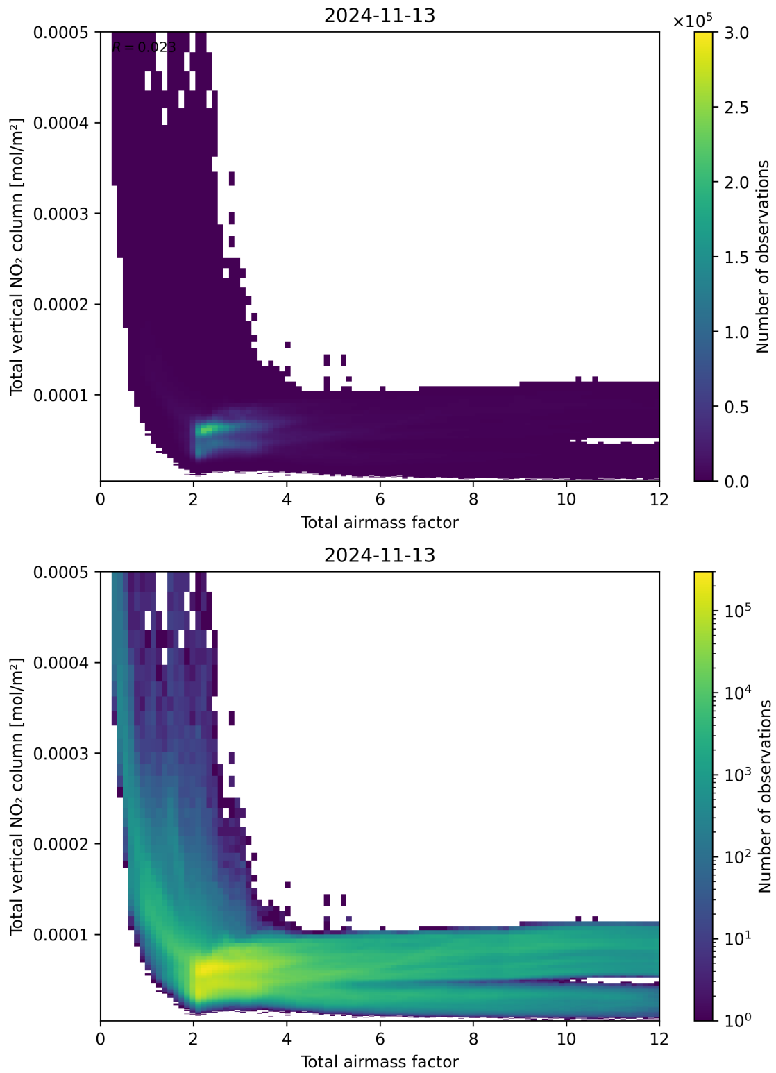
Figure 67: Scatter density plot of “Total airmass factor” against “Total vertical NO 2 column” for 2024-11-12 to 2024-11-14.
