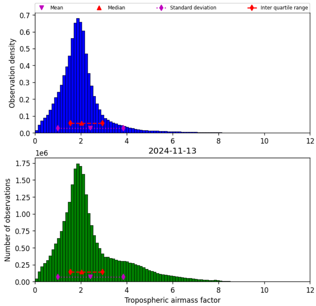
Figure 31: Histogram of “Tropospheric airmass factor” for 2024-11-12 to 2024-11-14
