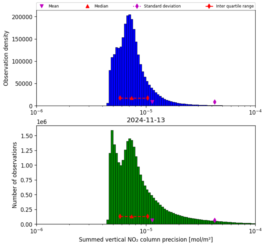
Figure 41: Histogram of “Summed vertical NO 2 column precision” for 2024-11-12 to 2024-11-14
