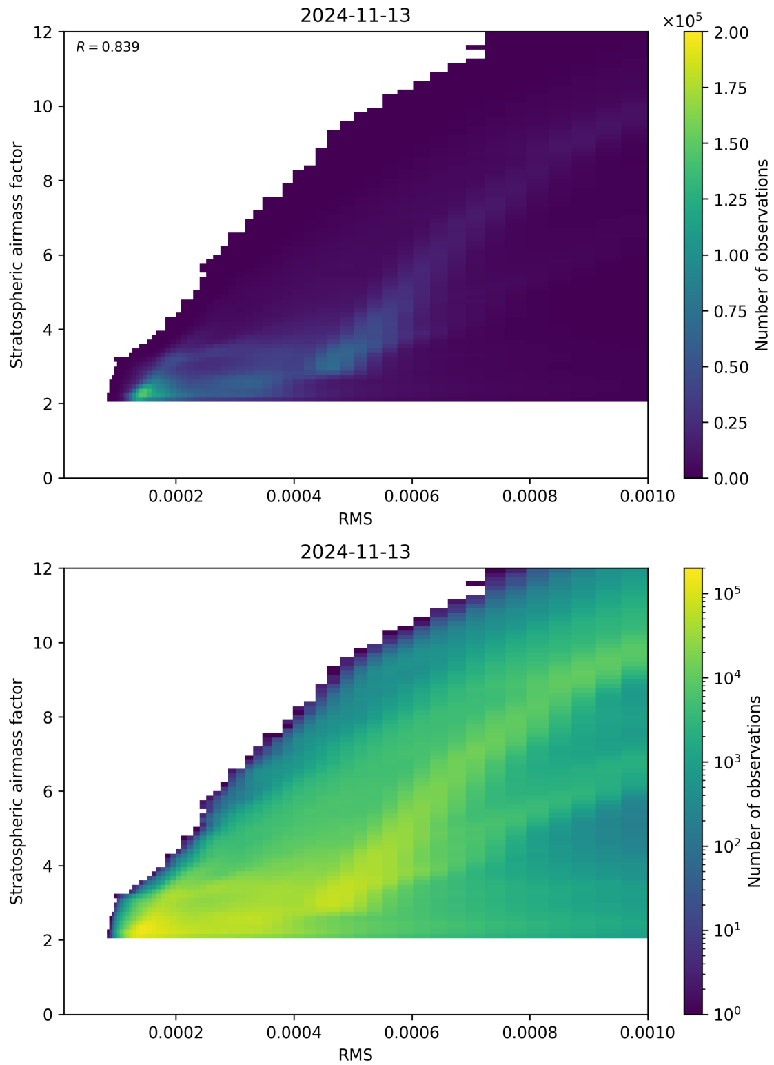
Figure 144: Scatter density plot of “RMS” against “Stratospheric airmass factor” for 2024-11-12 to 2024-11-14.
