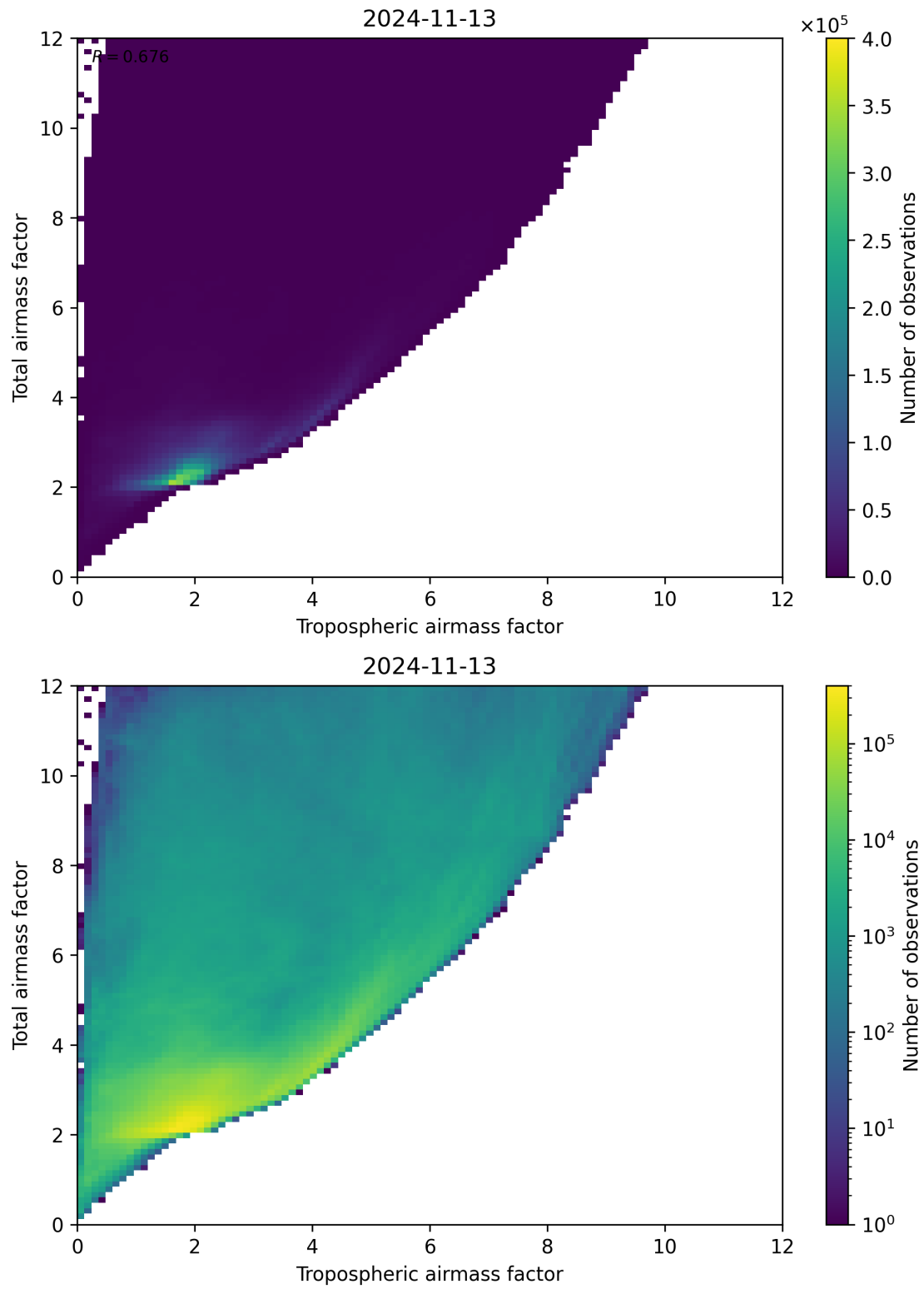
Figure 72: Scatter density plot of “Tropospheric airmass factor” against “Total airmass factor” for 2024-11-12 to 2024-11-14.
