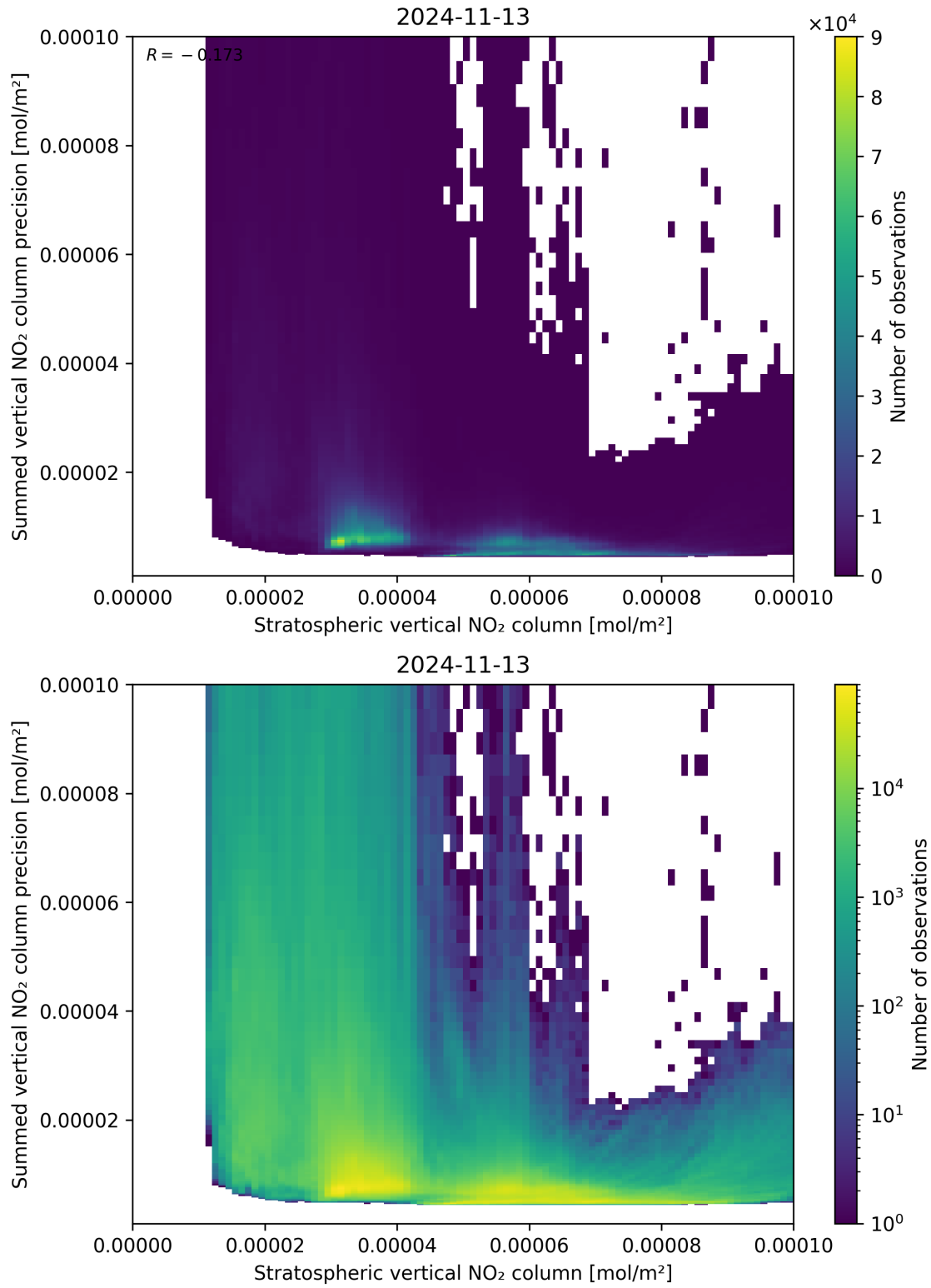
Figure 99: Scatter density plot of “Stratospheric vertical NO 2 column” against “Summed vertical NO 2 column precision” for 2024-11-12 to 2024-11-14.
