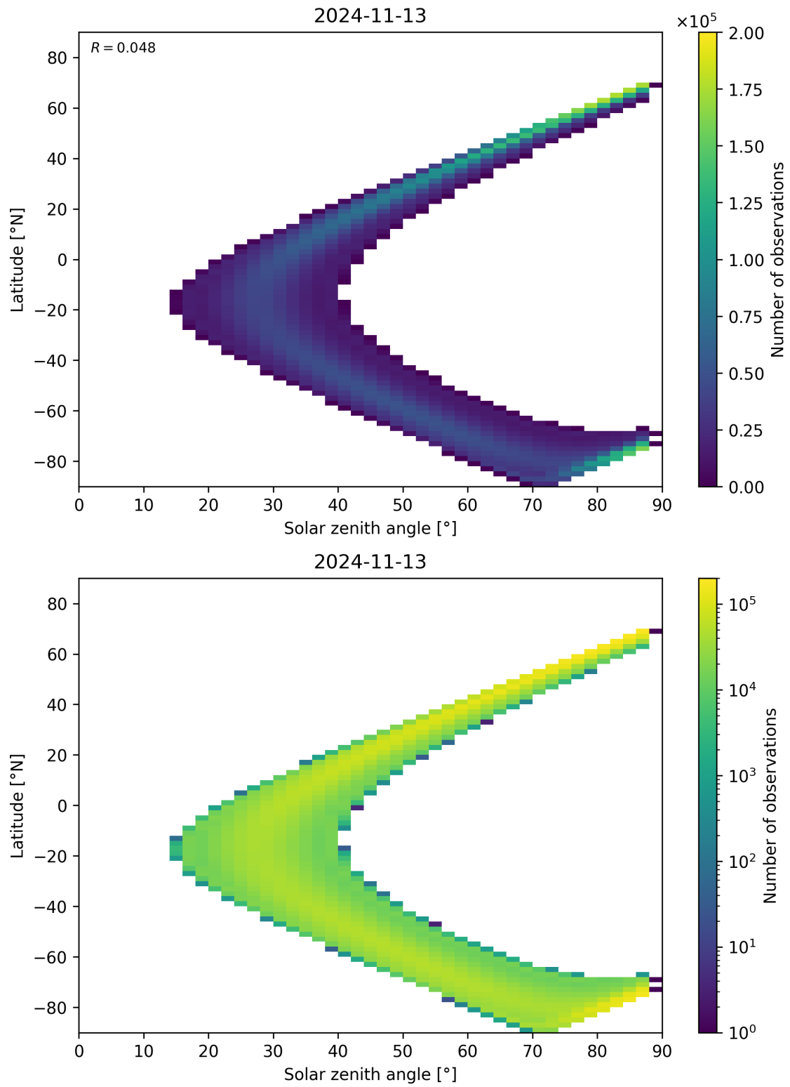
Figure 149: Scatter density plot of “Solar zenith angle” against “Latitude” for 2024-11-12 to 2024-11-14.
