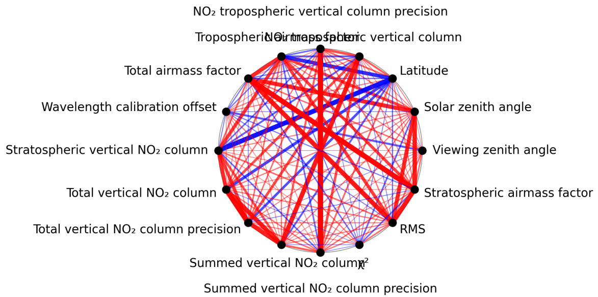
Figure 1: Map of correlation graph for 2024-11-12 to 2024-11-14.
