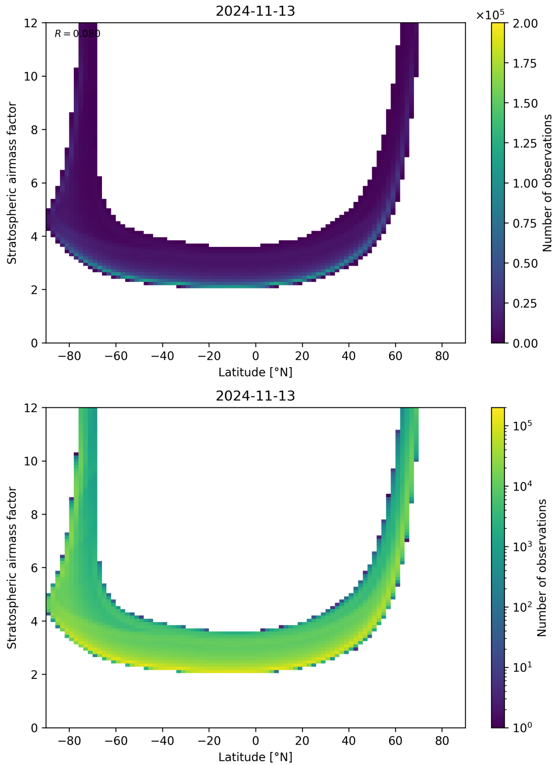
Figure 83: Scatter density plot of “Latitude” against “Stratospheric air mass factor” for 2024-11-12 to 2024-11-14.
