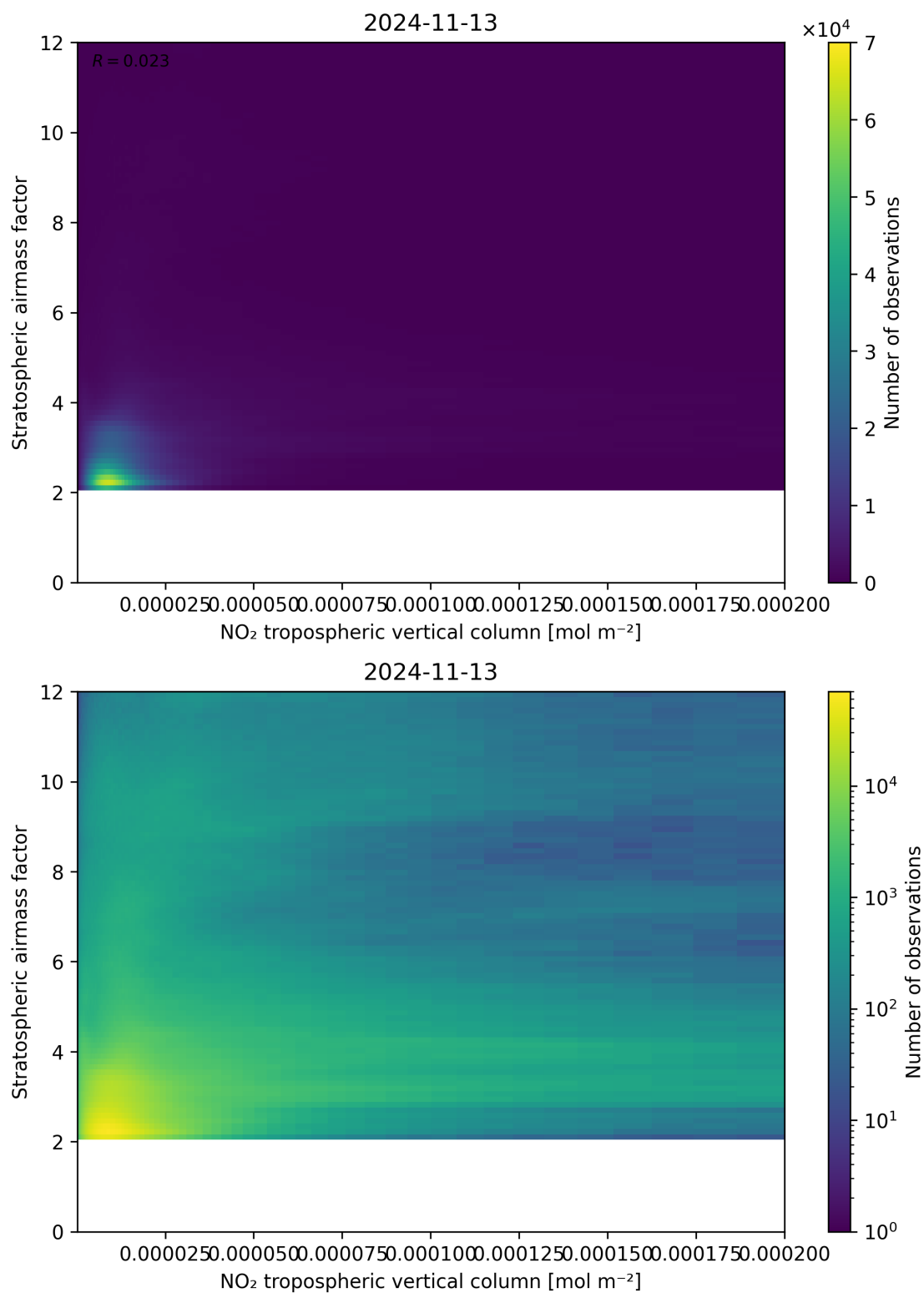
Figure 121: Scatter density plot of “NO 2 tropospheric vertical column” against “Stratospheric airmass factor” for 2024-11-12 to 2024-11-14.
