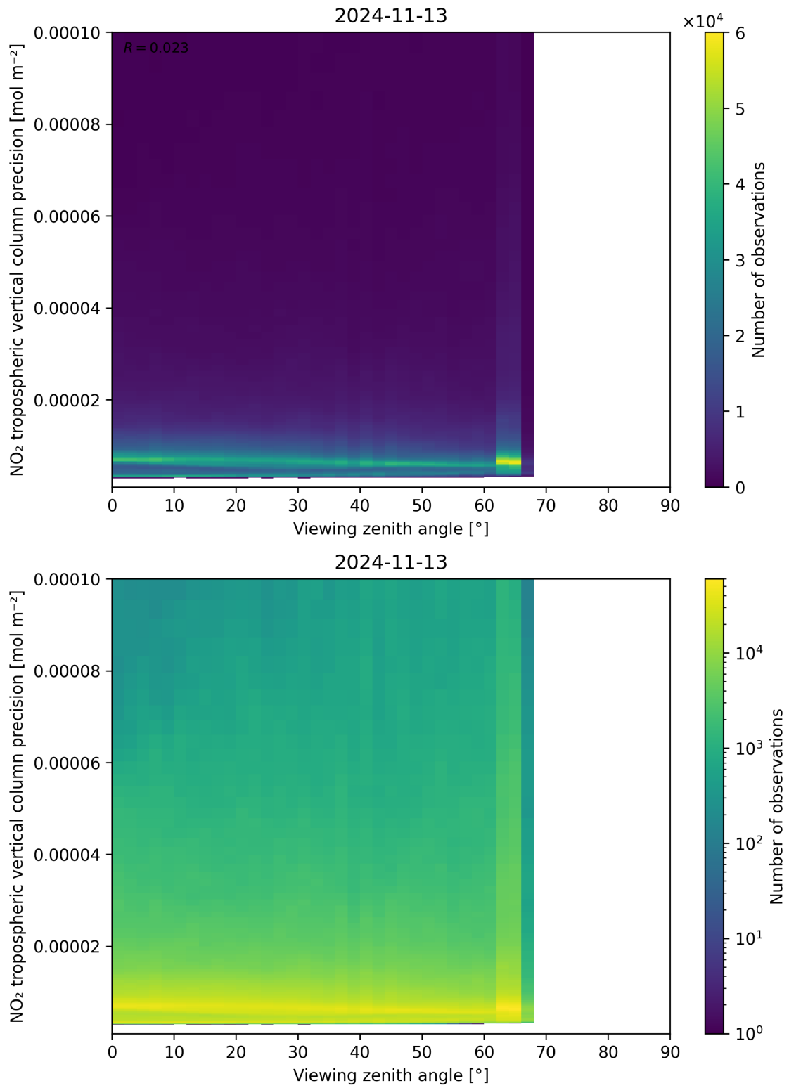
Figure 170: Scatter density plot of “Viewing zenith angle” against “NO 2 tropospheric vertical column precision” for 2024-11-12 to 2024-11-14.
