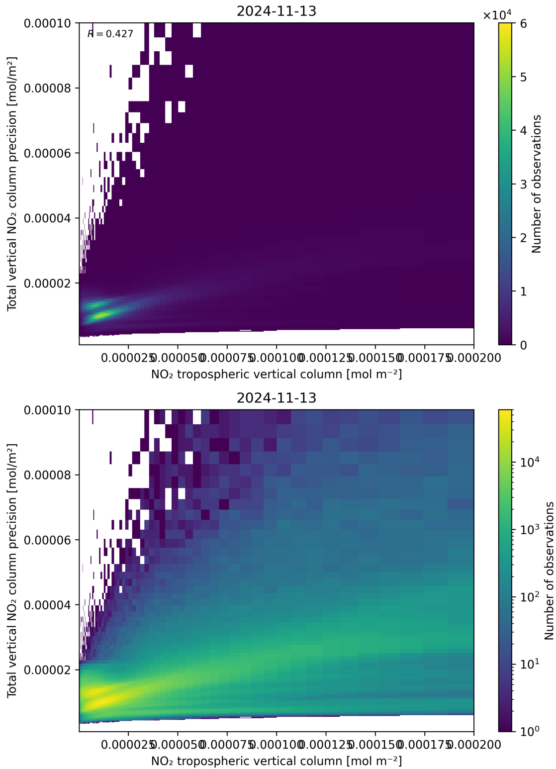
Figure 129: Scatter density plot of “NO 2 tropospheric vertical column” against “Total vertical NO 2 column precision” for 2024-11-12 to 2024-11-14.
