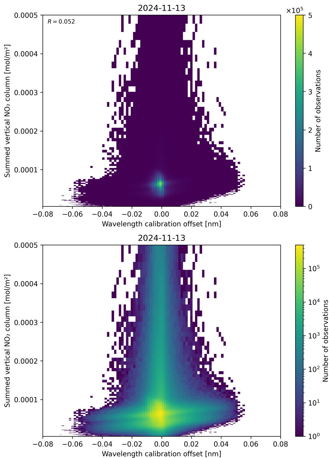
Figure 177: Scatter density plot of “Wavelength calibration offset” against “Summed vertical NO 2 column” for 2024-11-12 to 2024-11-14.
