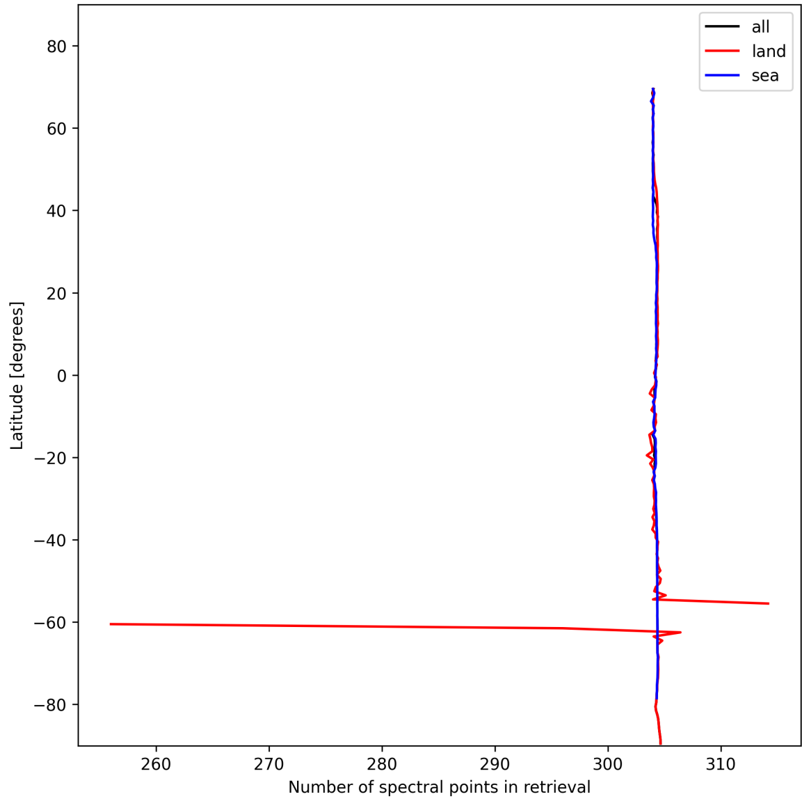
Figure 16: Zonal average of “Number of spectral points in retrieval” for 2024-11-12 to 2024-11-14.
