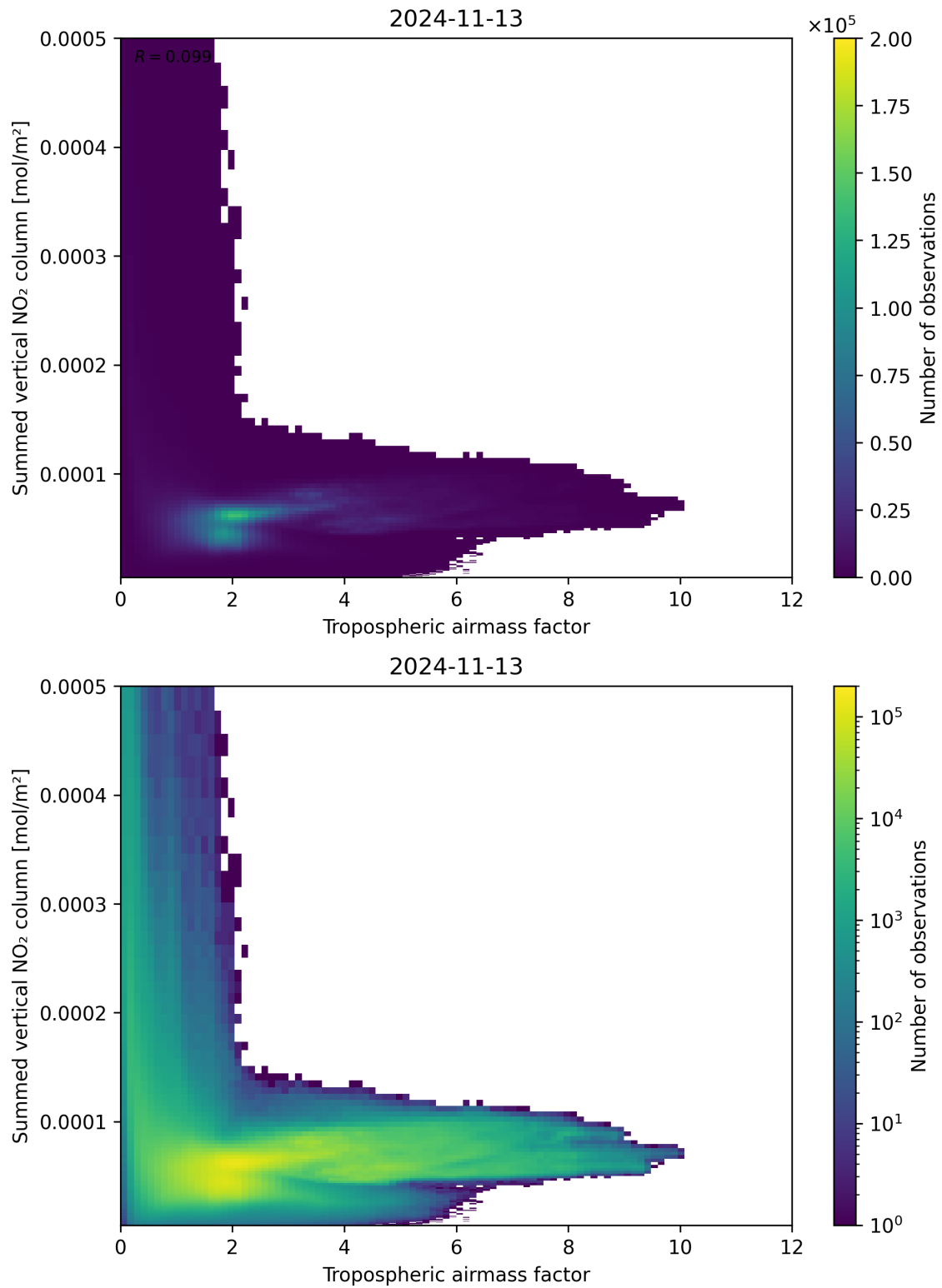
Figure 75: Scatter density plot of “Tropospheric airmass factor” against “Summed vertical NO 2 column” for 2024-11-12 to 2024-11-14.
