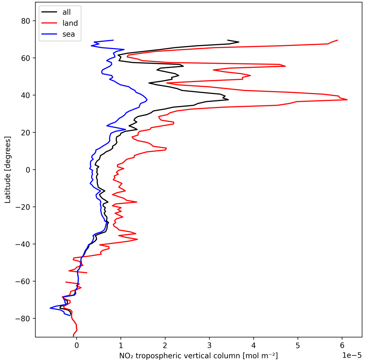
Figure 12: Zonal average of “NO 2 tropospheric vertical column” for 2024-11-12 to 2024-11-14.
