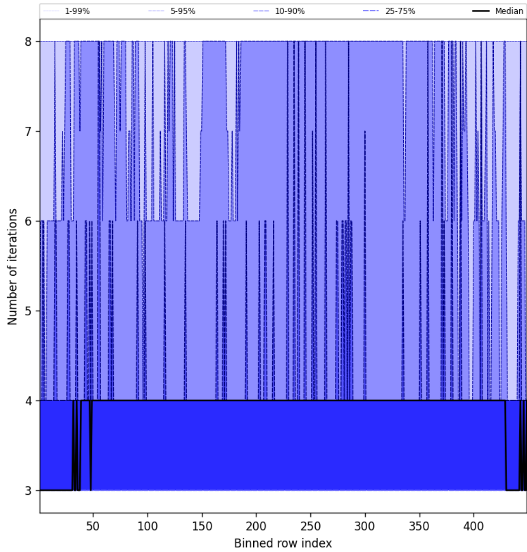
Figure 51: Along track statistics of “Number of iterations” for 2024-11-12 to 2024-11-14
