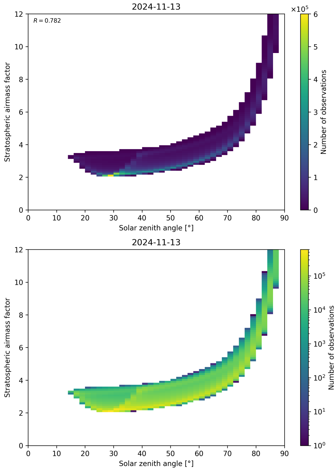
Figure 145: Scatter density plot of “Solar zenith angle” against “Stratospheric airmass factor” for 2024-11-12 to 2024-11-14.
