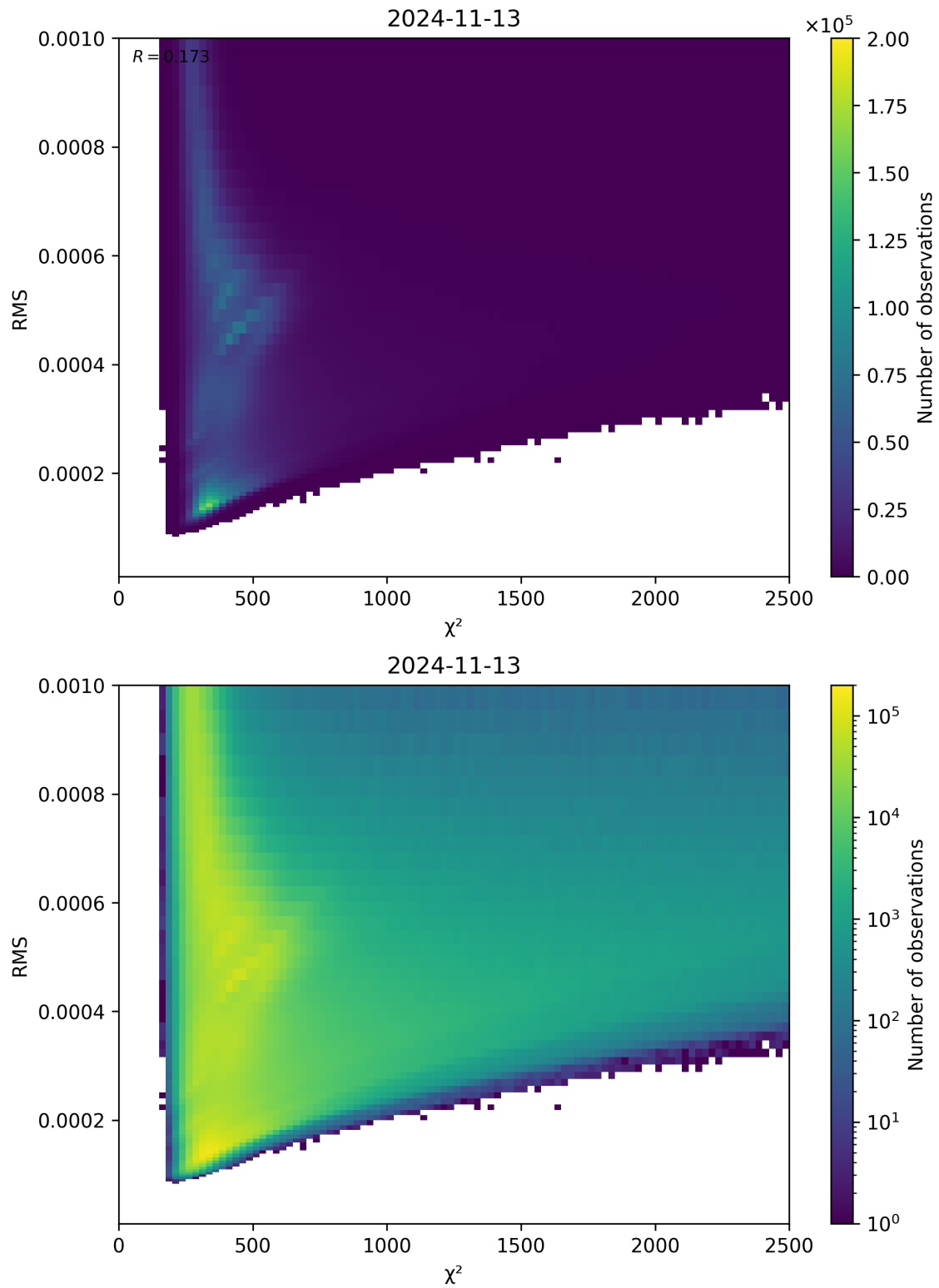
Figure 82: Scatter density plot of “ \chi^2 ” against “RMS” for 2024-11-12 to 2024-11-14.
