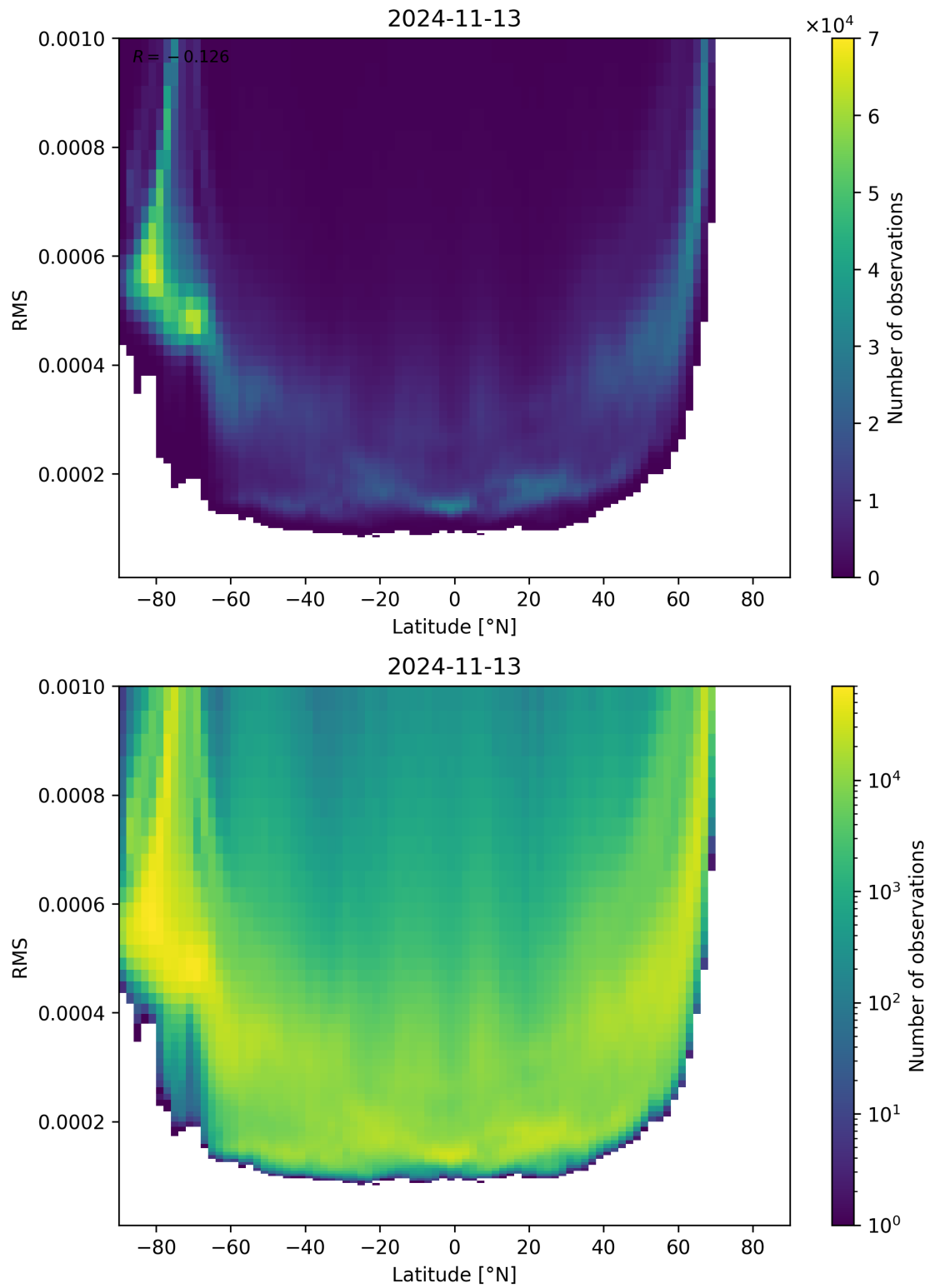
Figure 94: Scatter density plot of “Latitude” against “RMS” for 2024-11-12 to 2024-11-14.
