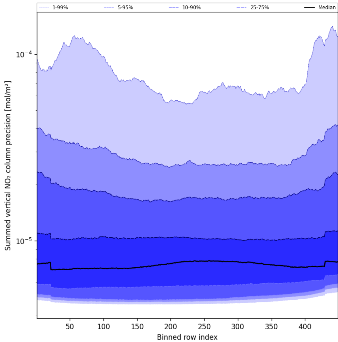
Figure 58: Along track statistics of “Summed vertical NO 2 column precision” for 2024-11-12 to 2024-11-14
