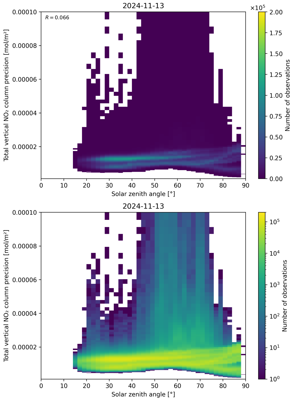
Figure 154: Scatter density plot of “Solar zenith angle” against “Total vertical NO 2 column precision” for 2024-11-12 to 2024-11-14.
