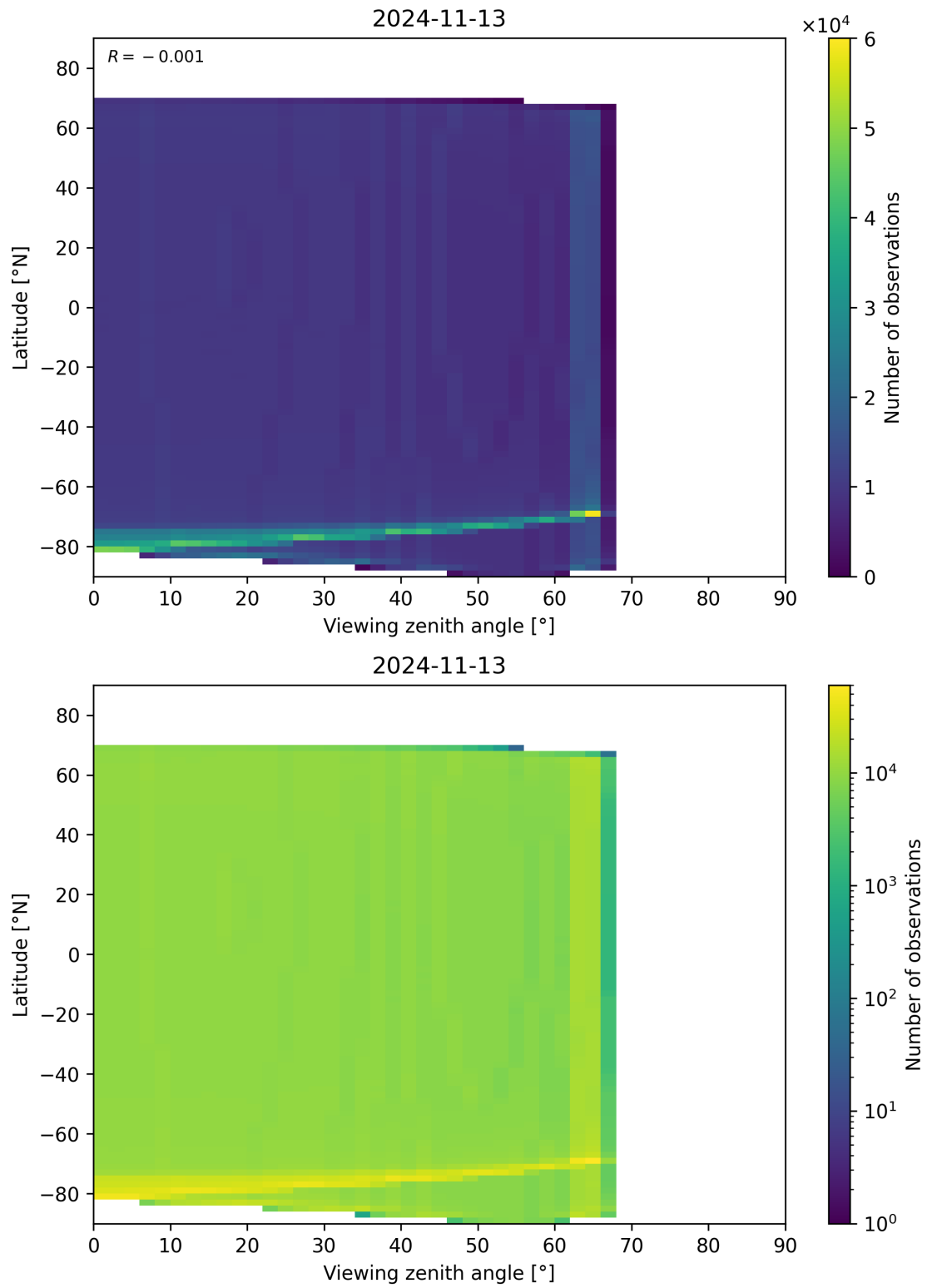
Figure 163: Scatter density plot of “Viewing zenith angle” against “Latitude” for 2024-11-12 to 2024-11-14.
