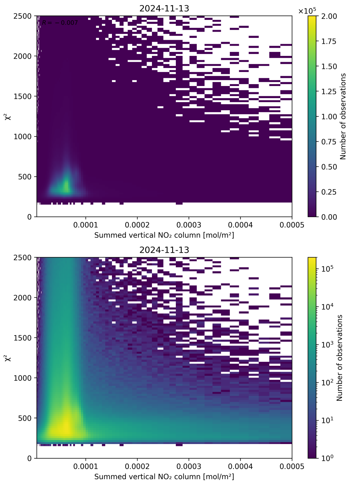
Figure 104: Scatter density plot of “Summed vertical NO 2 column” against “ \chi^2 ” for 2024-11-12 to 2024-11-14.
