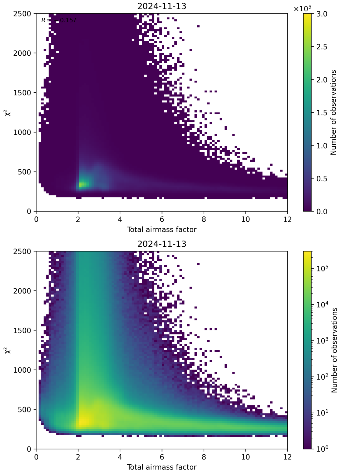
Figure 63: Scatter density plot of “Total airmass factor” against “ \chi^2 ” for 2024-11-12 to 2024-11-14.
