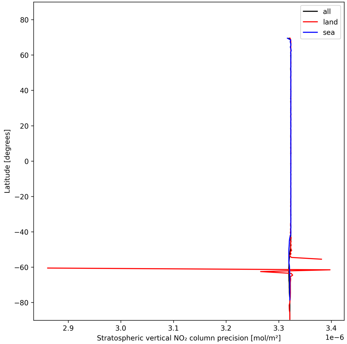
Figure 20: Zonal average of “Stratospheric vertical NO 2 column precision” for 2024-11-12 to 2024-11-14.
