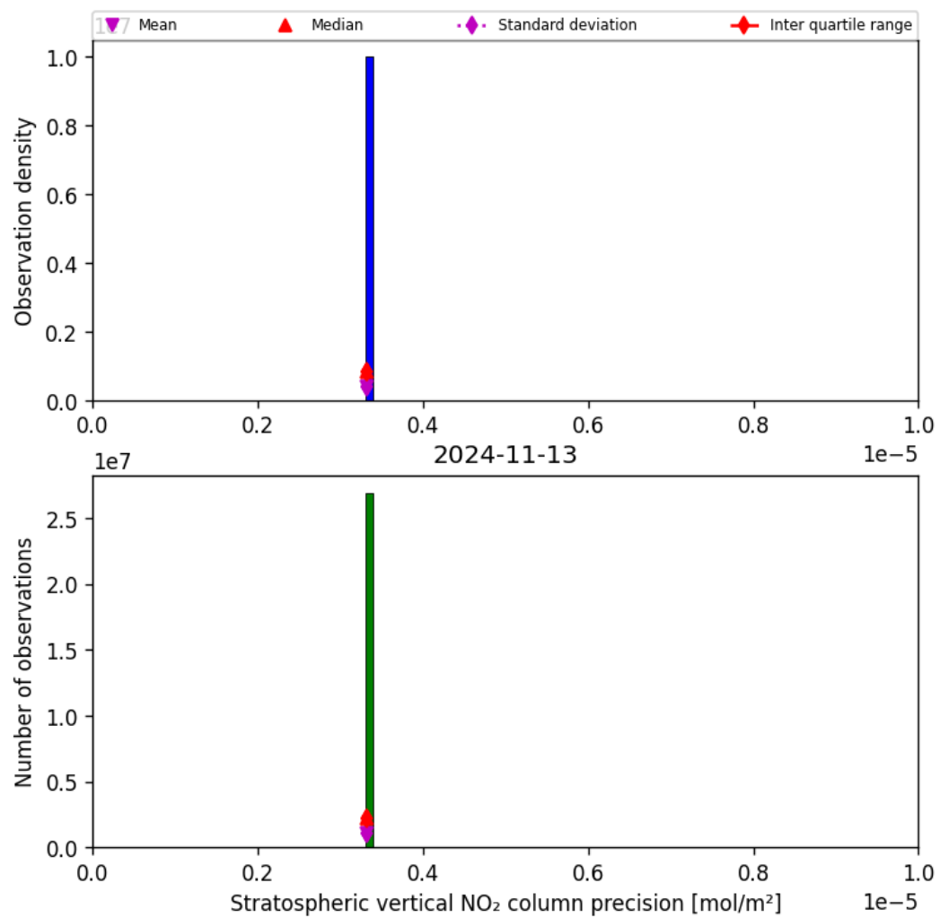
Figure 37: Histogram of “Stratospheric vertical NO 2 column precision” for 2024-11-12 to 2024-11-14
