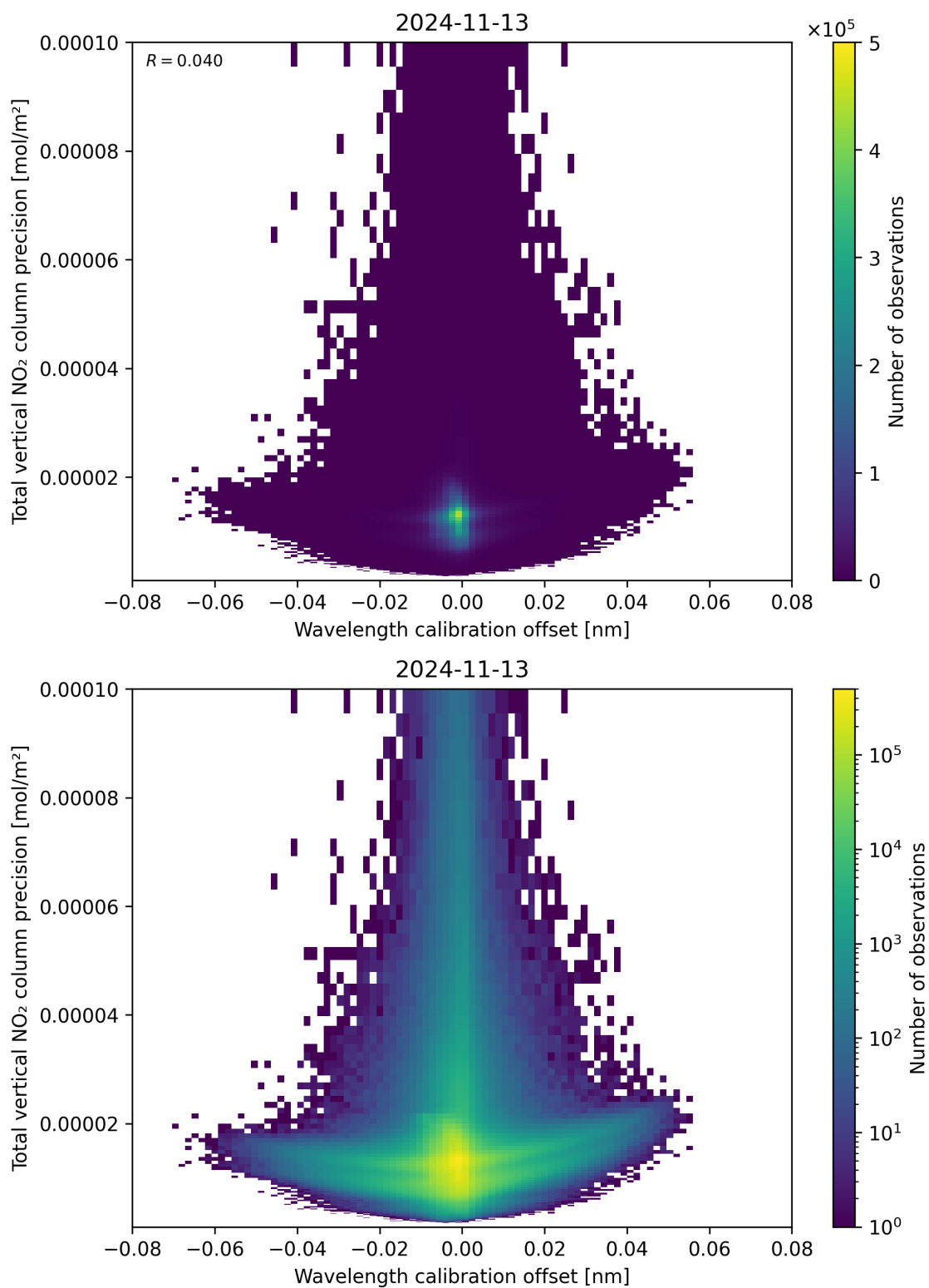
Figure 180: Scatter density plot of “Wavelength calibration offset” against “Total vertical NO 2 column precision” for 2024-11-12 to 2024-11-14.
