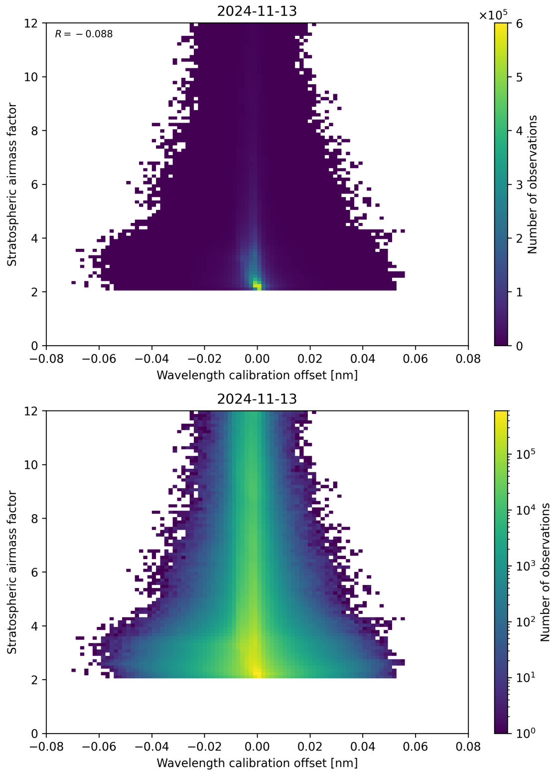
Figure 174: Scatter density plot of “Wavelength calibration offset” against “Stratospheric airmass factor” for 2024-11-12 to 2024-11-14.
