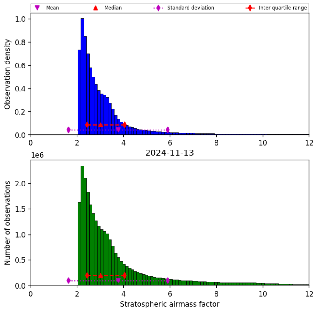
Figure 44: Histogram of “Stratospheric airmass factor” for 2024-11-12 to 2024-11-14
