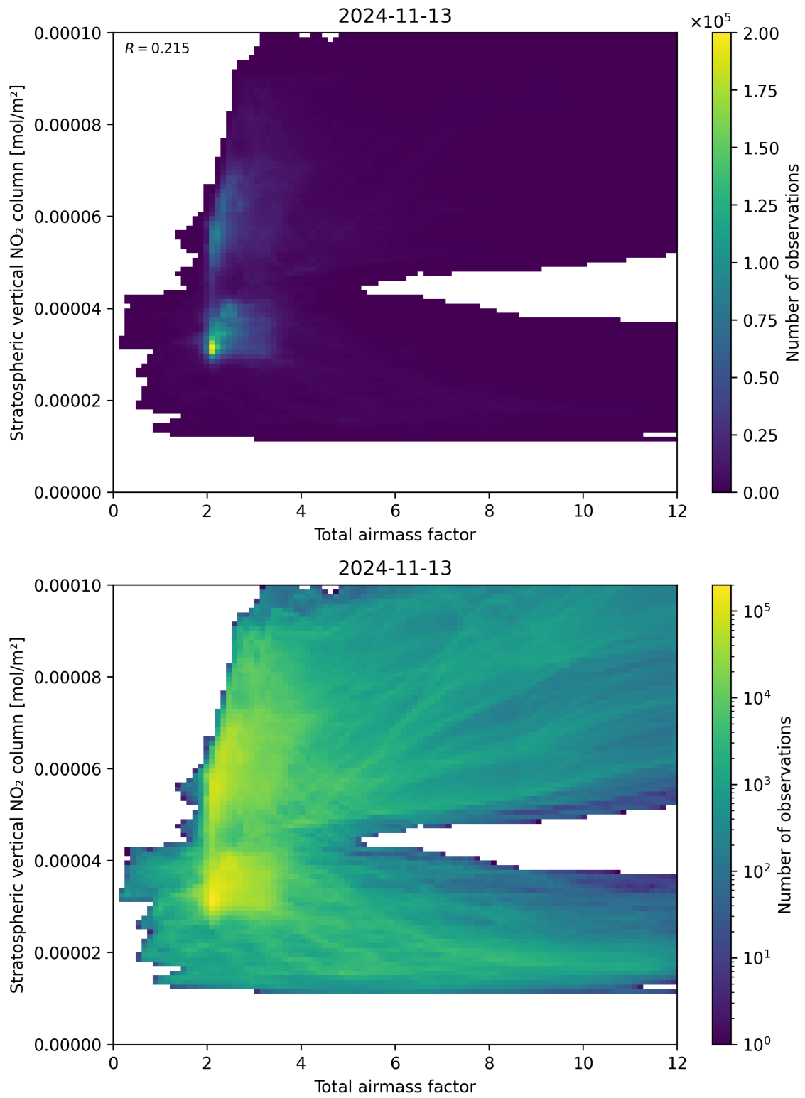
Figure 64: Scatter density plot of “Total airmass factor” against “Stratospheric vertical NO 2 column” for 2024-11-12 to 2024-11-14.
