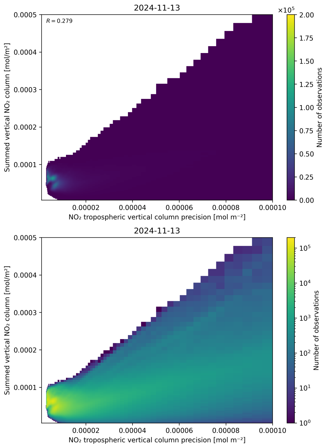
Figure 136: Scatter density plot of “NO 2 tropospheric vertical column precision” against “Summed vertical NO 2 column” for 2024-11-12 to 2024-11-14.
