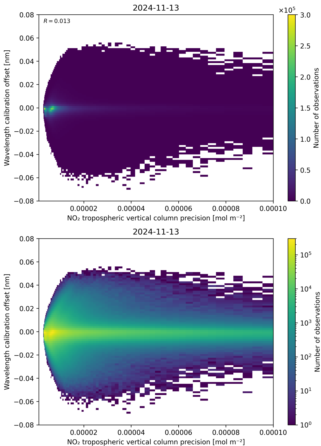
Figure 141: Scatter density plot of “NO 2 tropospheric vertical column precision” against “Wavelength calibration offset” for 2024-11-12 to 2024-11-14.
