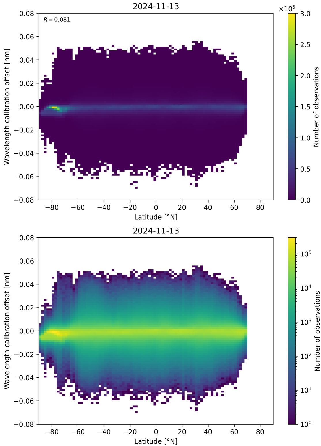
Figure 95: Scatter density plot of “Latitude” against “Wavelength calibration offset” for 2024-11-12 to 2024-11-14.
