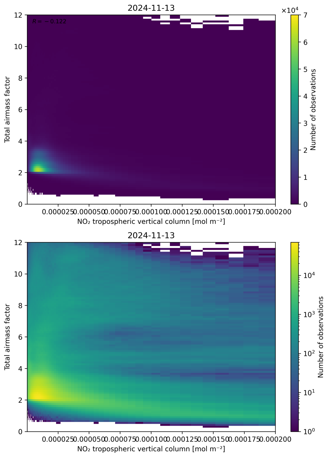
Figure 122: Scatter density plot of “NO 2 tropospheric vertical column” against “Total airmass factor” for 2024-11-12 to 2024-11-14.
