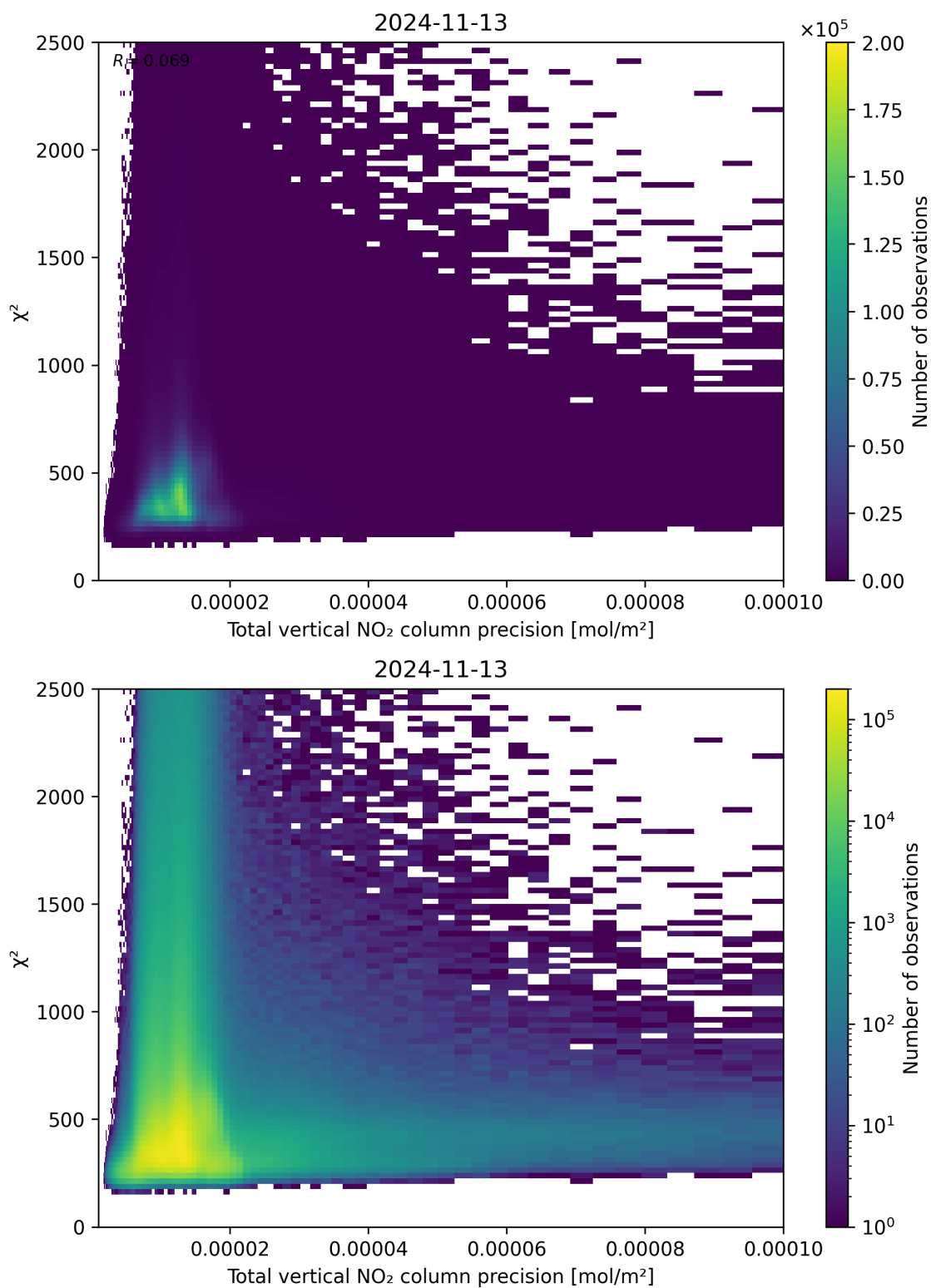
Figure 116: Scatter density plot of “Total vertical NO 2 column precision” against “ \chi^2 ” for 2024-11-12 to 2024-11-14.
