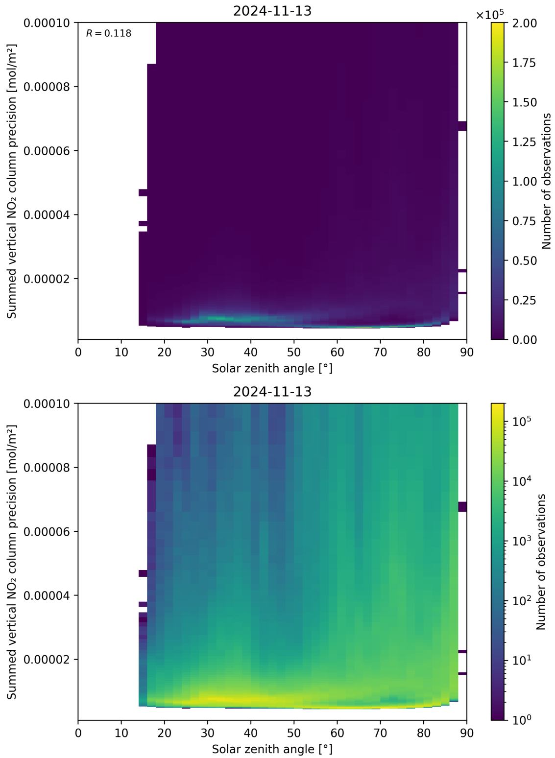
Figure 152: Scatter density plot of “Solar zenith angle” against “Summed vertical NO 2 column precision” for 2024-11-12 to 2024-11-14.
