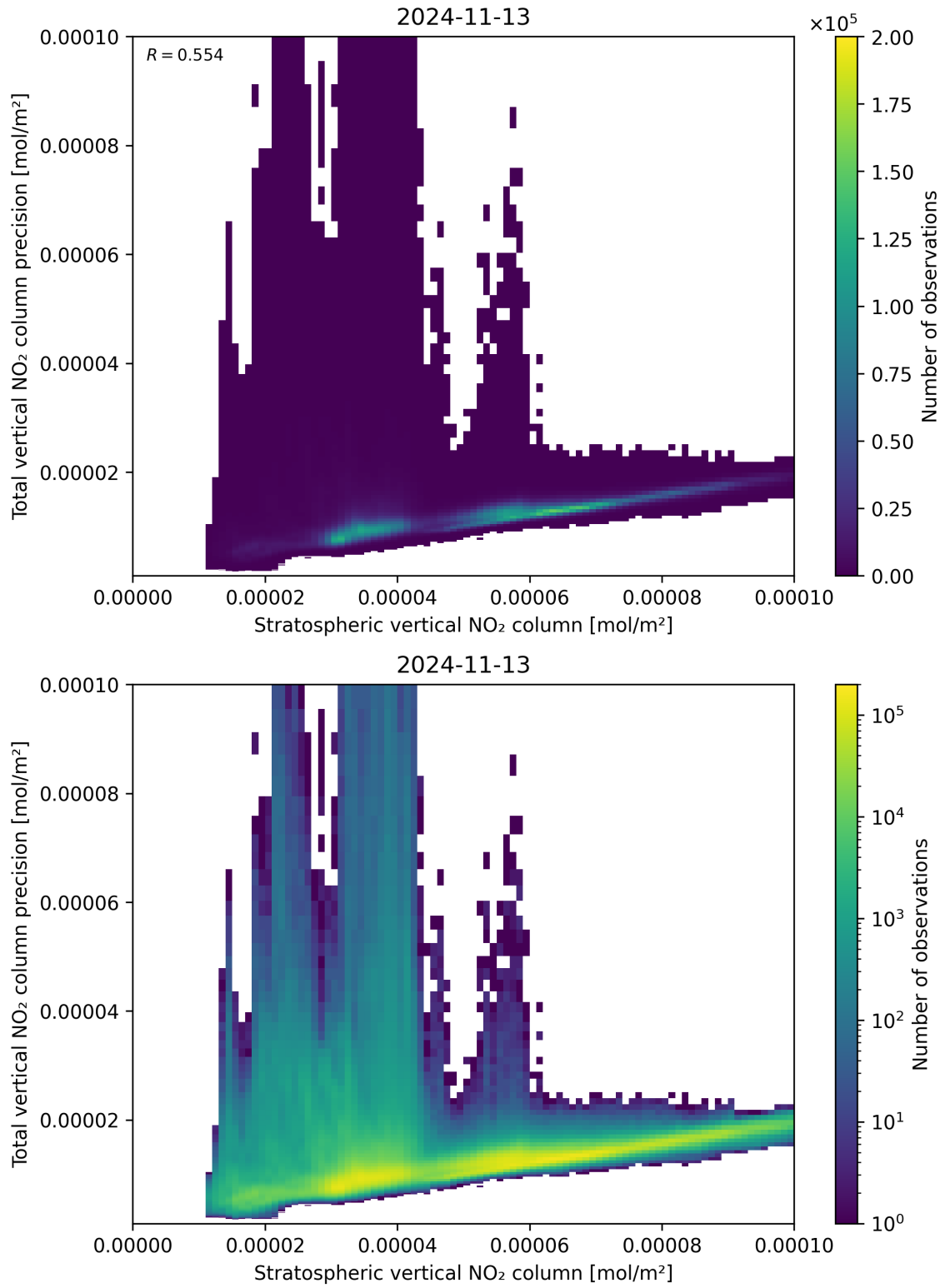
Figure 101: Scatter density plot of “Stratospheric vertical NO 2 column” against “Total vertical NO 2 column precision” for 2024-11-12 to 2024-11-14.
