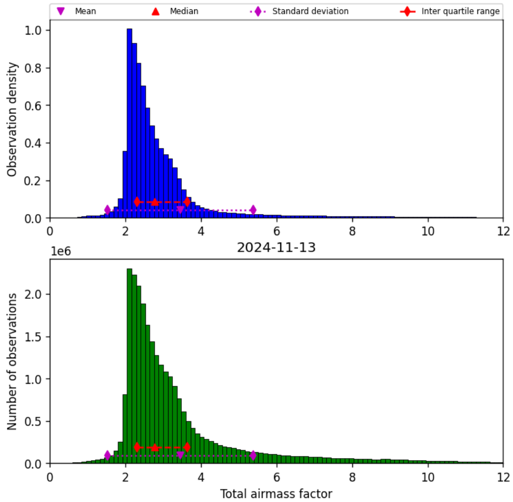
Figure 32: Histogram of “Total airmass factor” for 2024-11-12 to 2024-11-14
