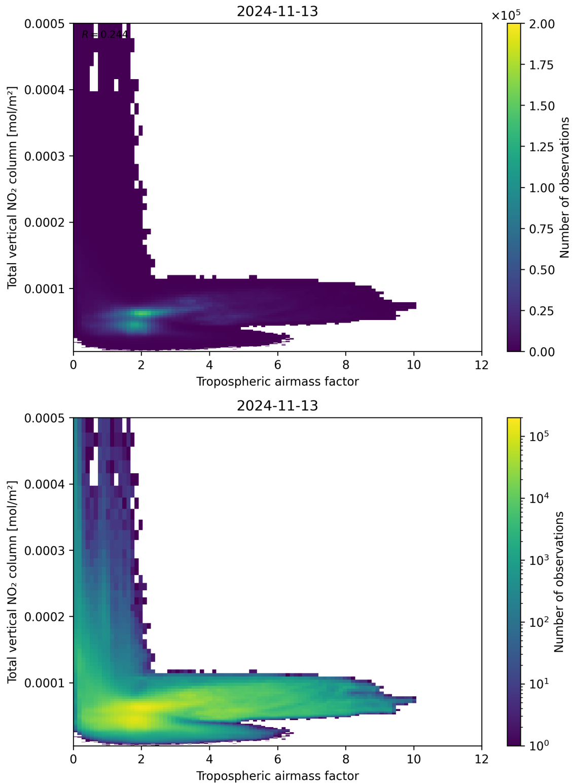
Figure 77: Scatter density plot of “Tropospheric airmass factor” against “Total vertical NO 2 column” for 2024-11-12 to 2024-11-14.
