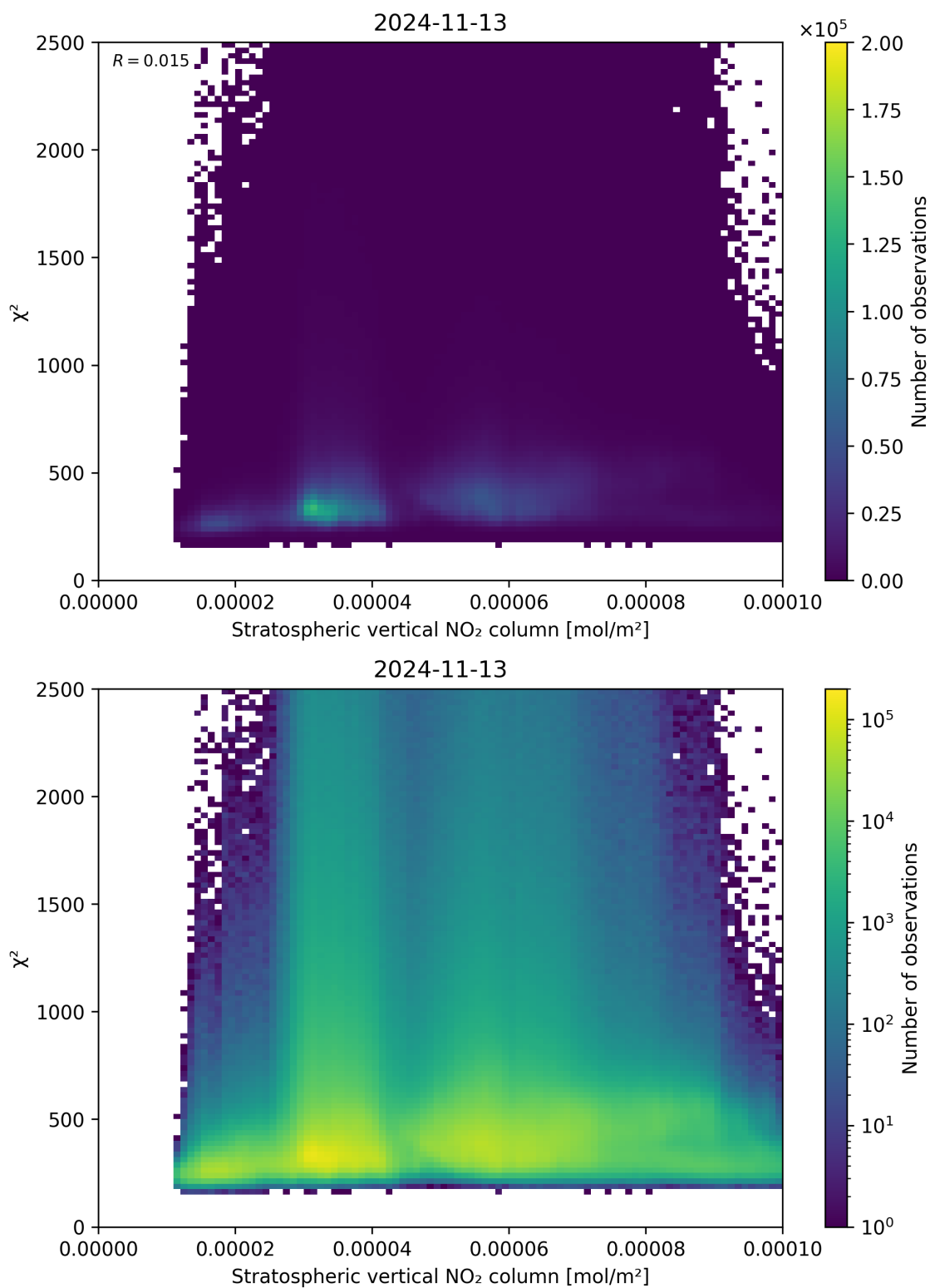
Figure 97: Scatter density plot of “Stratospheric vertical NO 2 column” against “ \chi^2 ” for 2024-11-12 to 2024-11-14.
