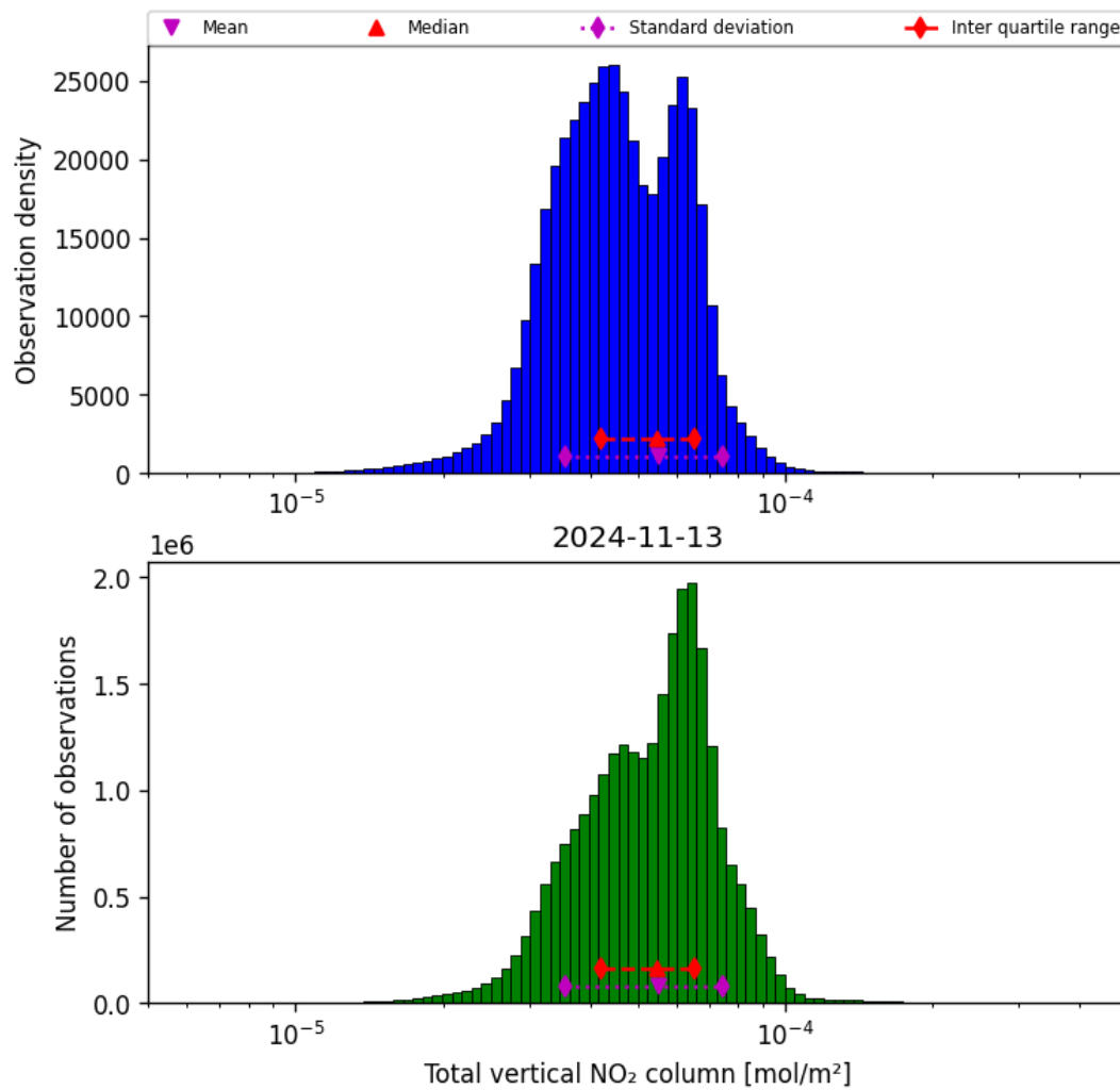
Figure 38: Histogram of “Total vertical NO 2 column” for 2024-11-12 to 2024-11-14
