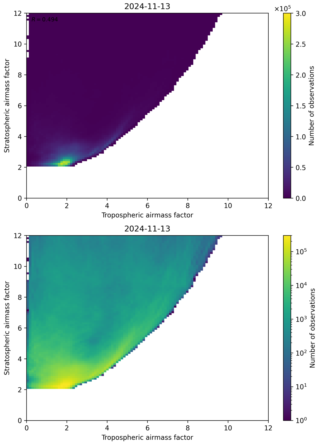
Figure 71: Scatter density plot of “Tropospheric airmass factor” against “Stratospheric airmass factor” for 2024-11-12 to 2024-11-14.
