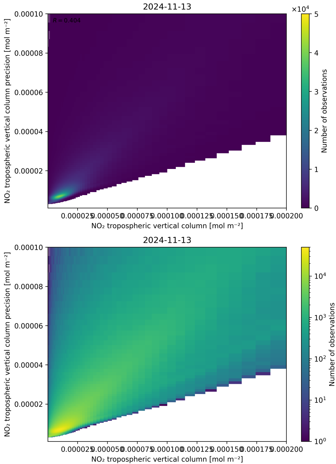
Figure 130: Scatter density plot of “NO 2 tropospheric vertical column” against “NO 2 tropospheric vertical column precision” for 2024-11-12 to 2024-11-14.
