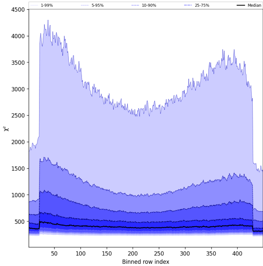
Figure 59: Along track statistics of “ \chi^2 ” for 2024-11-12 to 2024-11-14
