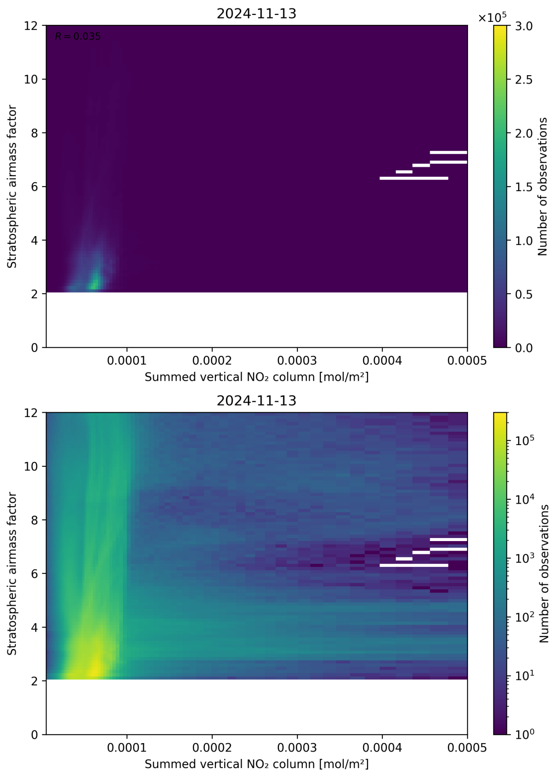
Figure 103: Scatter density plot of “Summed vertical NO 2 column” against “Stratospheric airmass factor” for 2024-11-12 to 2024-11-14.
