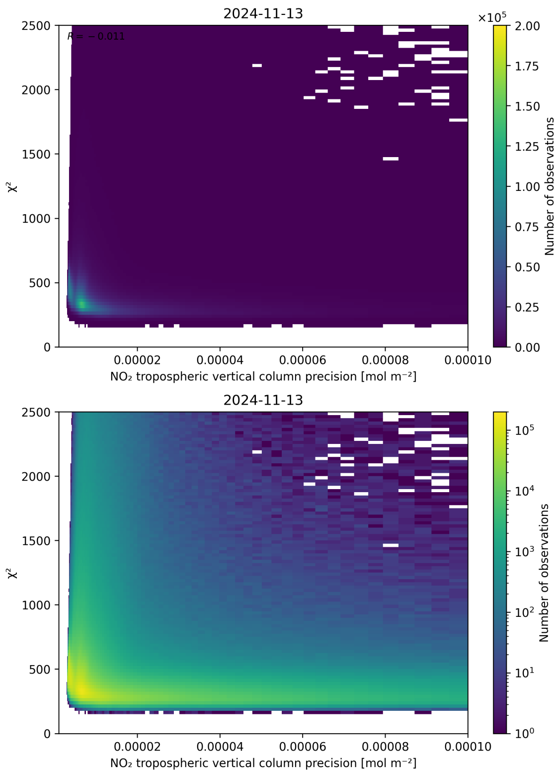
Figure 134: Scatter density plot of “NO 2 tropospheric vertical column precision” against “ \chi^2 ” for 2024-11-12 to 2024-11-14.
