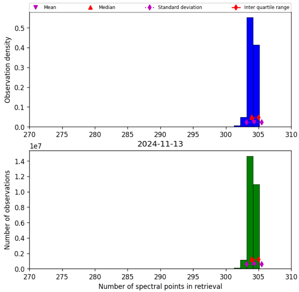
Figure 33: Histogram of “Number of spectral points in retrieval” for 2024-11-12 to 2024-11-14
