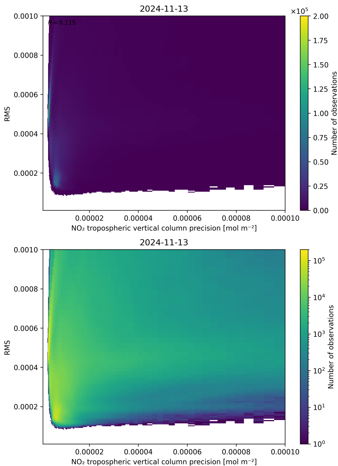
Figure 140: Scatter density plot of “NO 2 tropospheric vertical column precision” against “RMS” for 2024-11-12 to 2024-11-14.
