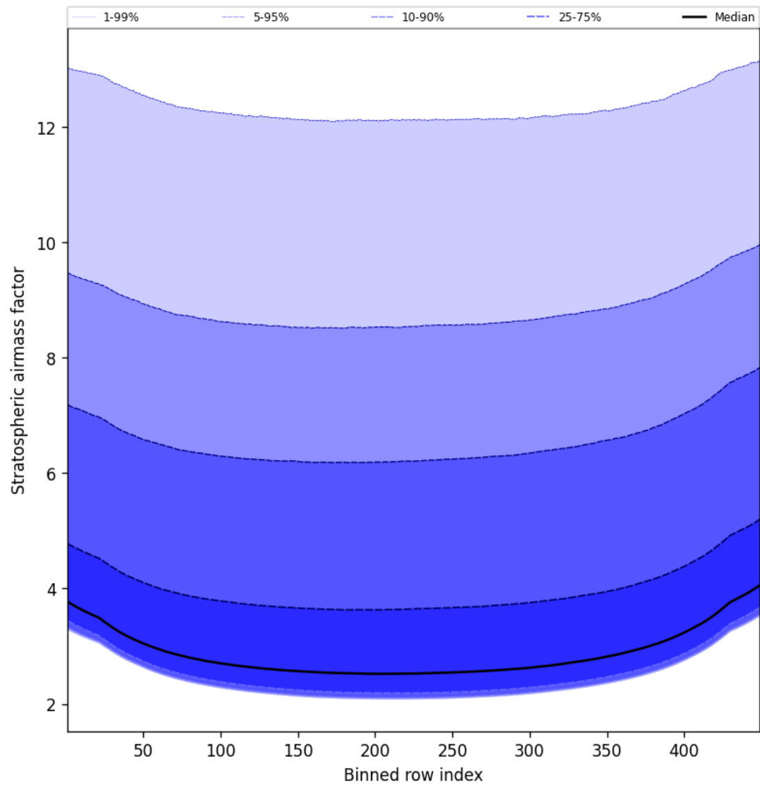
Figure 61: Along track statistics of “Stratospheric air mass factor” for 2024-11-12 to 2024-11-14
