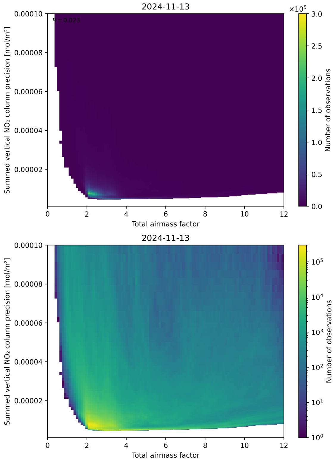
Figure 66: Scatter density plot of “Total airmass factor” against “Summed vertical NO 2 column precision” for 2024-11-12 to 2024-11-14.
