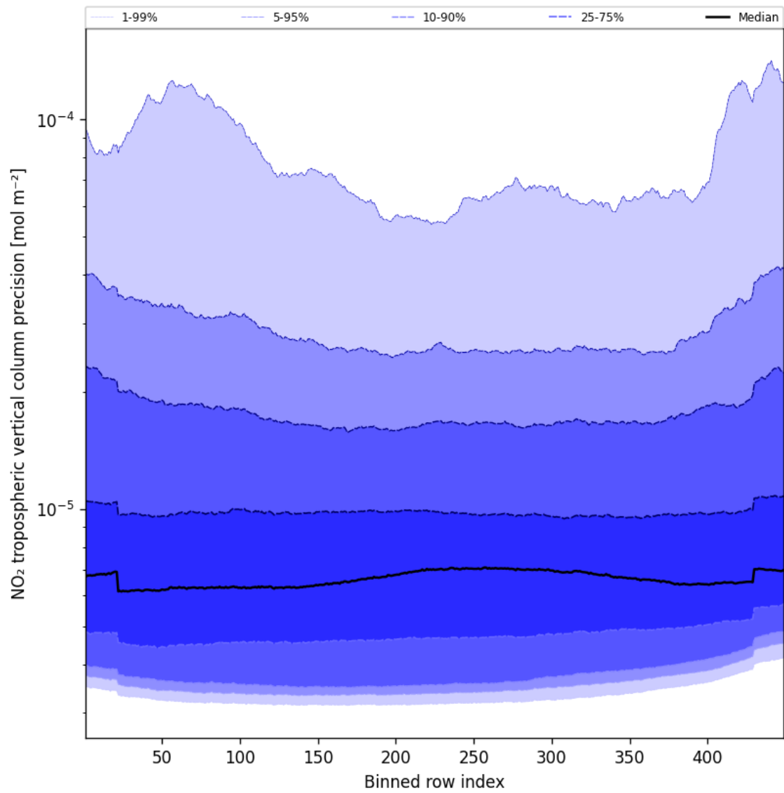
Figure 47: Along track statistics of “NO 2 tropospheric vertical column precision” for 2024-11-12 to 2024-11-14
