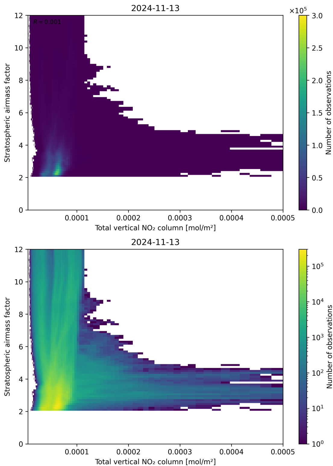
Figure 110: Scatter density plot of “Total vertical NO 2 column” against “Stratospheric airmass factor” for 2024-11-12 to 2024-11-14.
