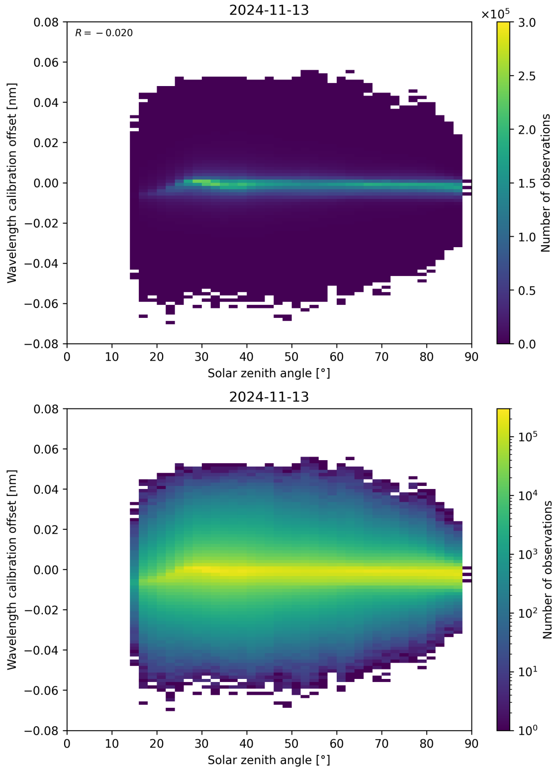
Figure 158: Scatter density plot of “Solar zenith angle” against “Wavelength calibration offset” for 2024-11-12 to 2024-11-14.
