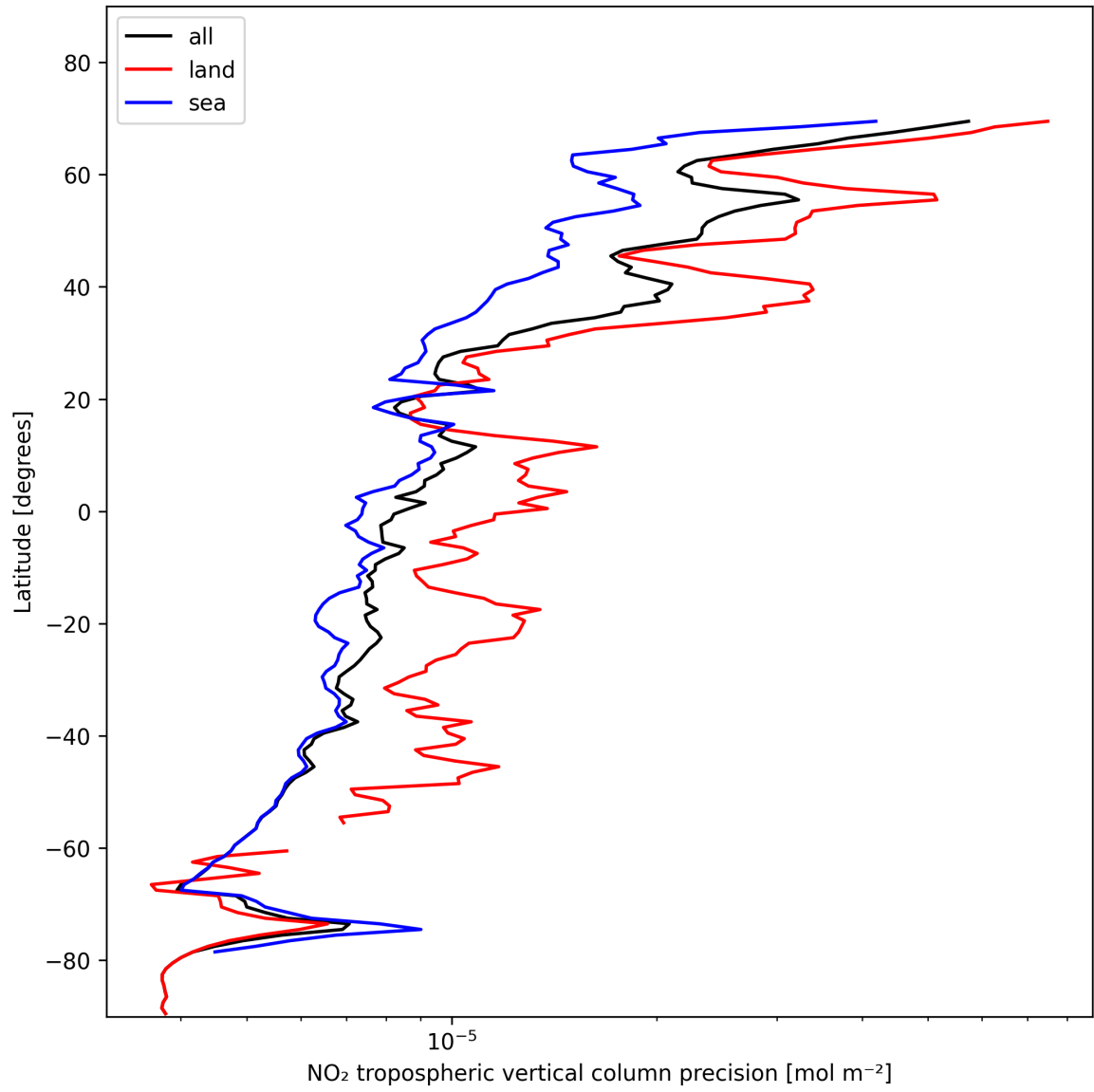
Figure 13: Zonal average of “NO 2 tropospheric vertical column precision” for 2024-11-12 to 2024-11-14.
