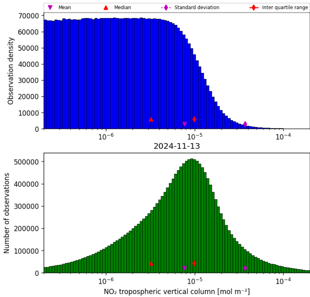
Figure 29: Histogram of “NO 2 tropospheric vertical column” for 2024-11-12 to 2024-11-14
