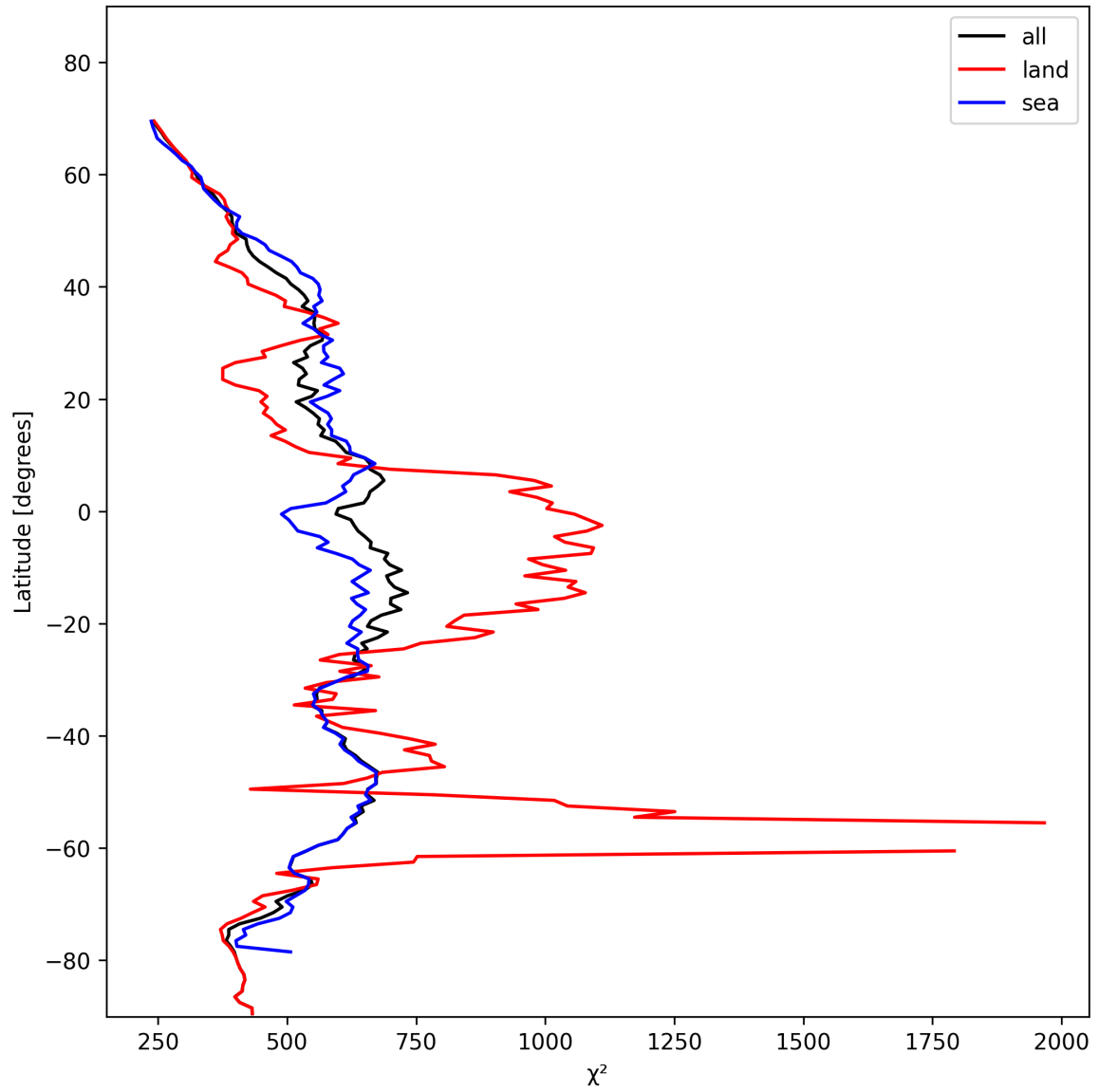
Figure 25: Zonal average of “ \chi^2 ” for 2024-11-12 to 2024-11-14.
