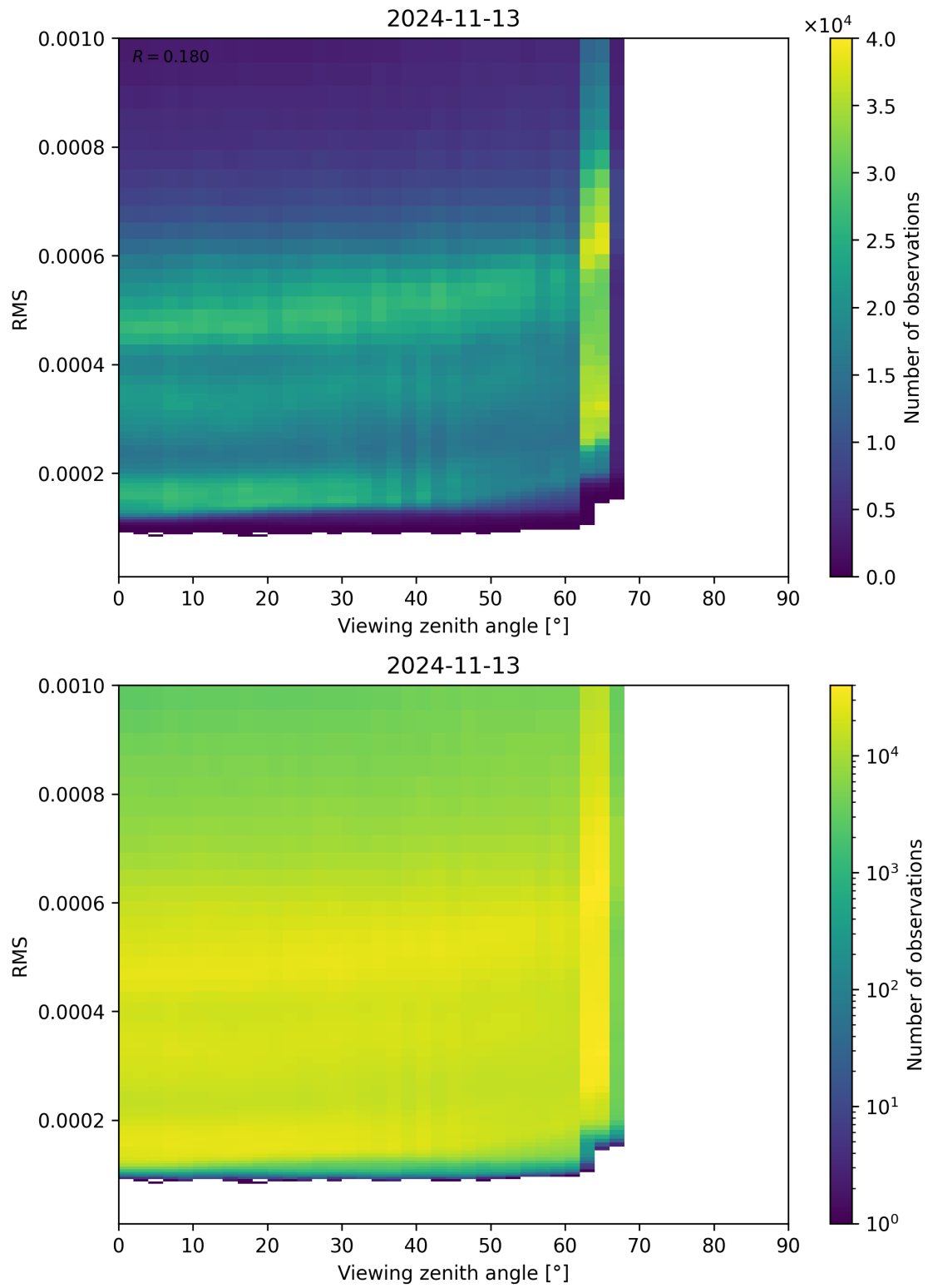
Figure 171: Scatter density plot of “Viewing zenith angle” against “RMS” for 2024-11-12 to 2024-11-14.
