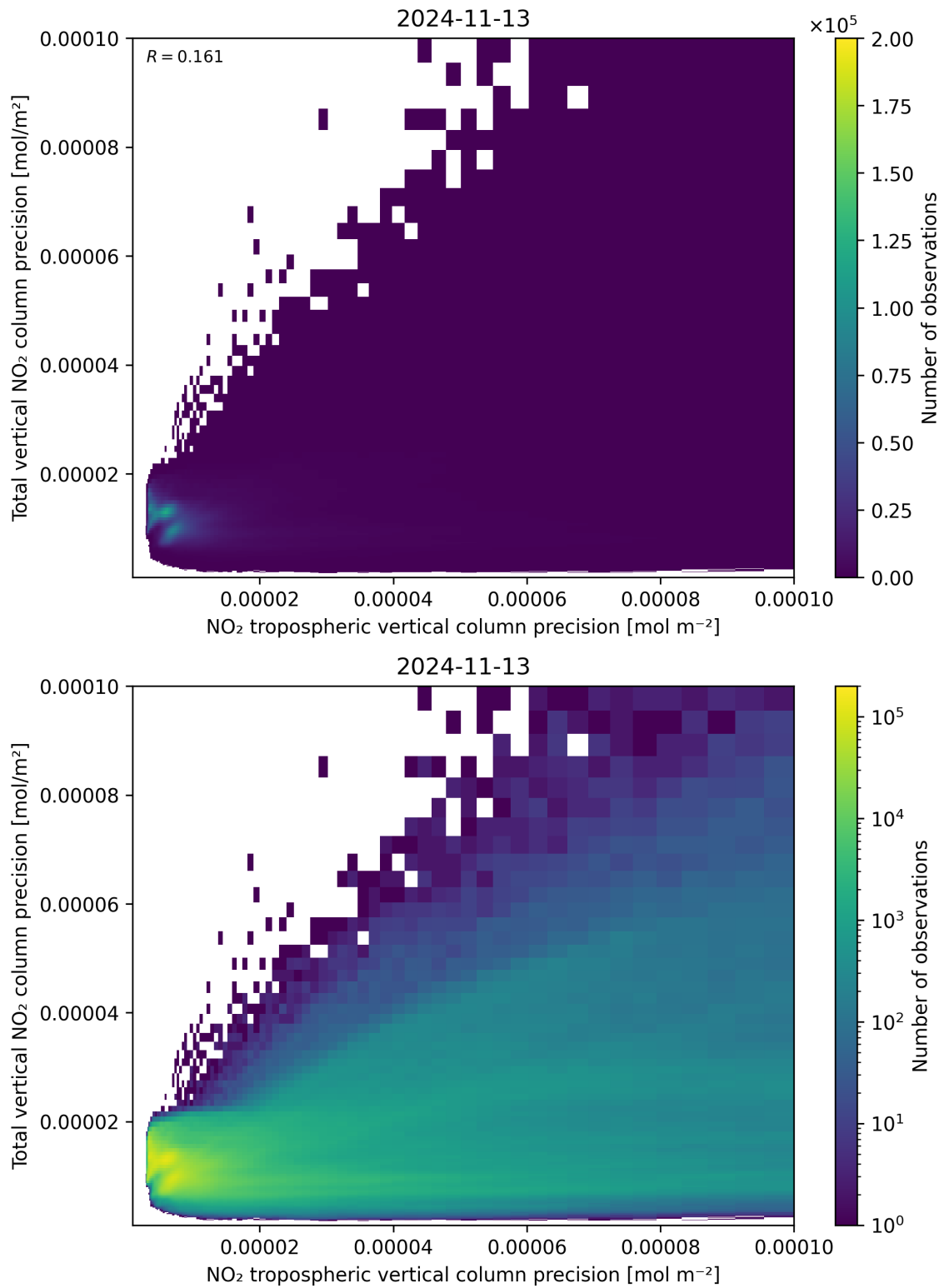
Figure 139: Scatter density plot of “NO 2 tropospheric vertical column precision” against “Total vertical NO 2 column precision” for 2024-11-12 to 2024-11-14.
