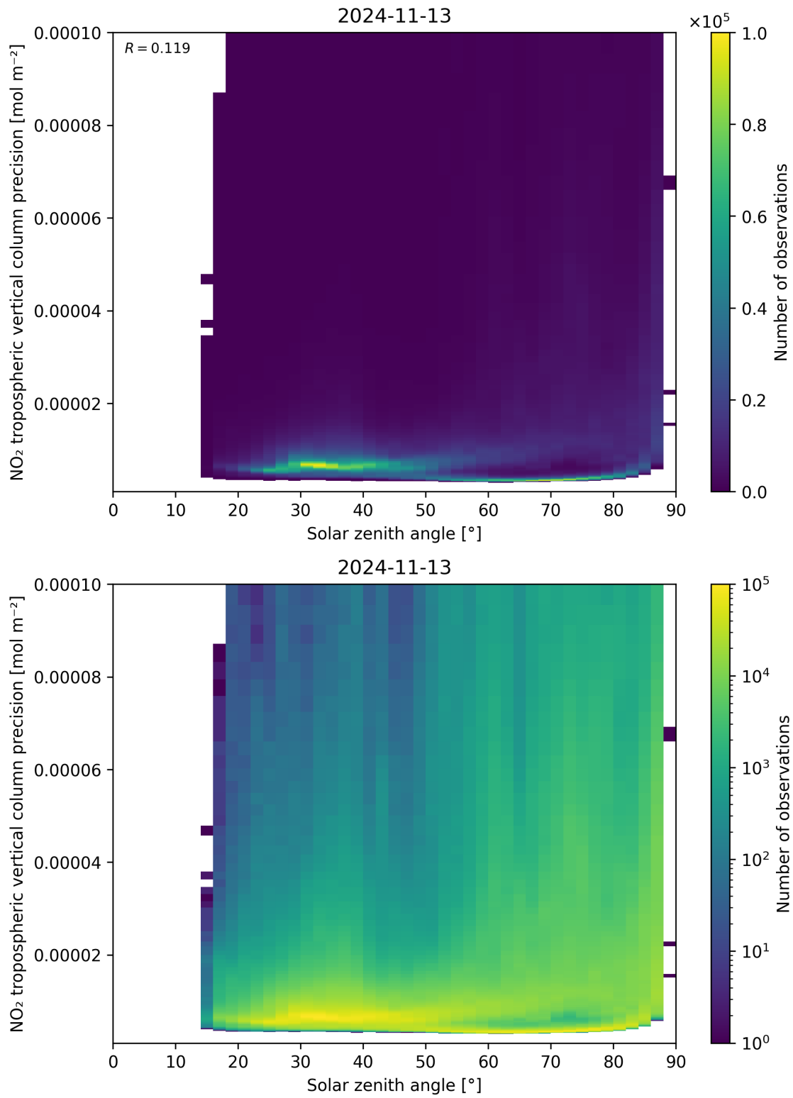
Figure 156: Scatter density plot of “Solar zenith angle” against “NO 2 tropospheric vertical column precision” for 2024-11-12 to 2024-11-14.
