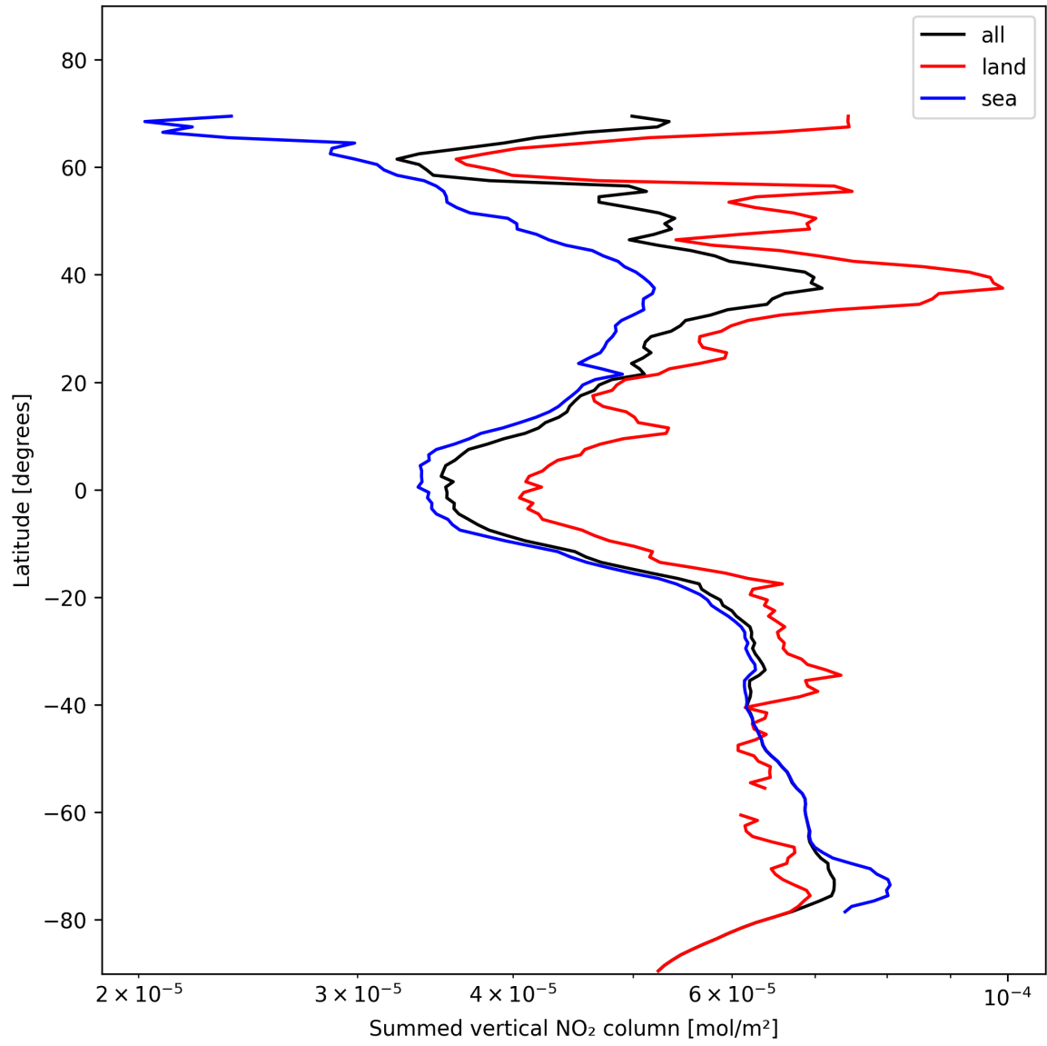
Figure 23: Zonal average of “Summed vertical NO 2 column” for 2024-11-12 to 2024-11-14.
