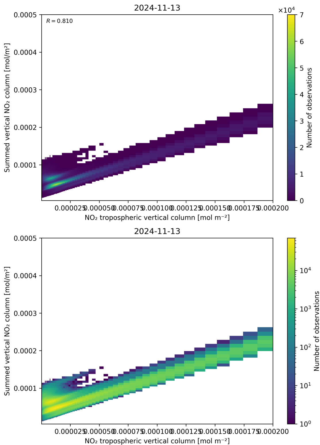
Figure 126: Scatter density plot of “NO 2 tropospheric vertical column” against “Summed vertical NO 2 column” for 2024-11-12 to 2024-11-14.
