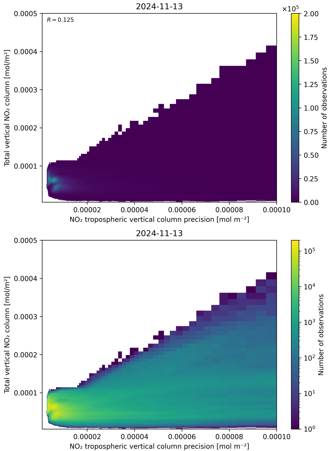
Figure 138: Scatter density plot of “NO 2 tropospheric vertical column precision” against “Total vertical NO 2 column” for 2024-11-12 to 2024-11-14.
