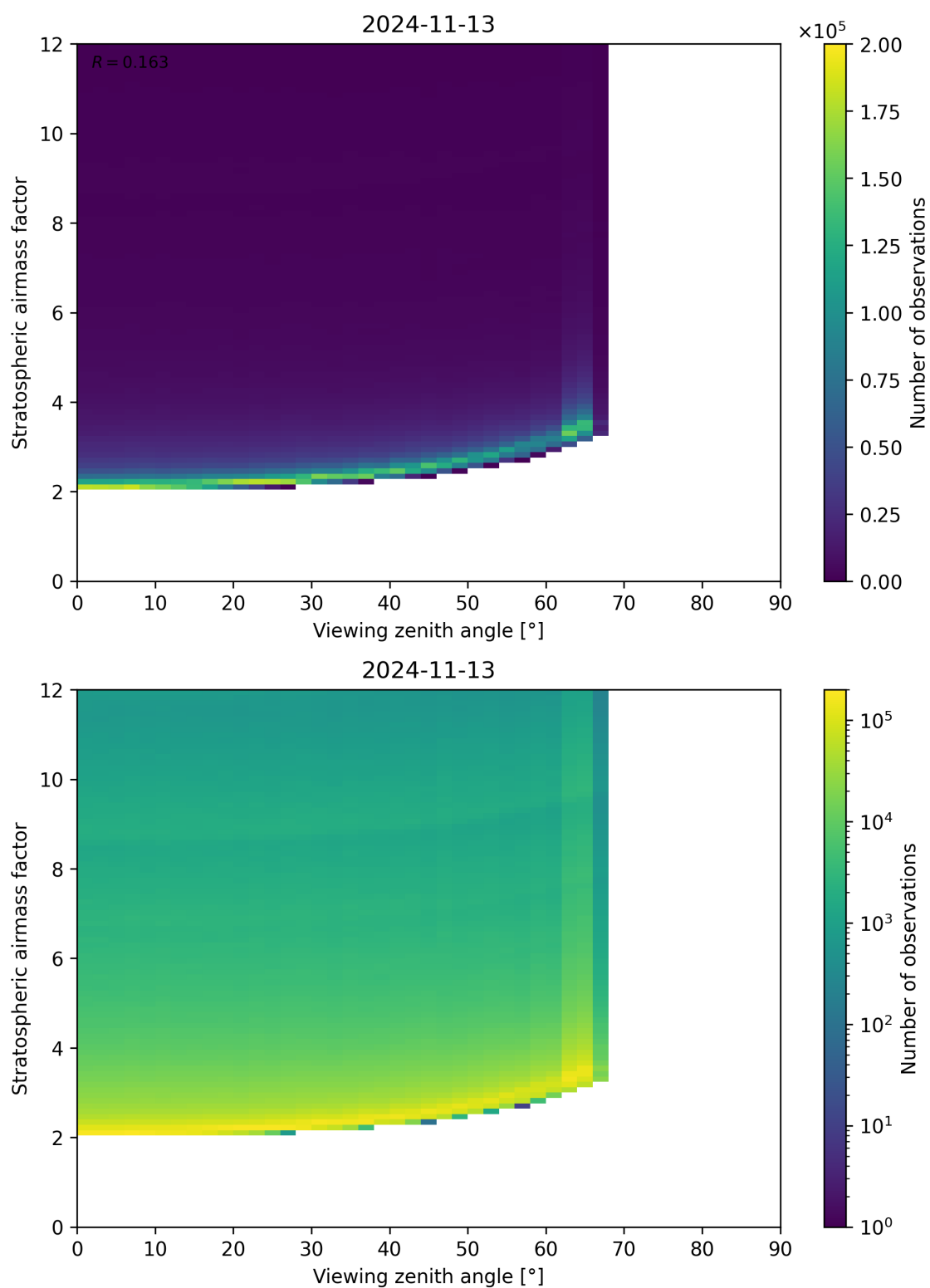
Figure 159: Scatter density plot of “Viewing zenith angle” against “Stratospheric airmass factor” for 2024-11-12 to 2024-11-14.
