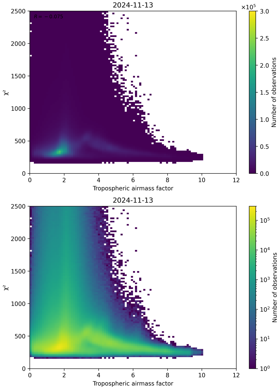
Figure 73: Scatter density plot of “Tropospheric airmass factor” against “ \chi^2 ” for 2024-11-12 to 2024-11-14.
