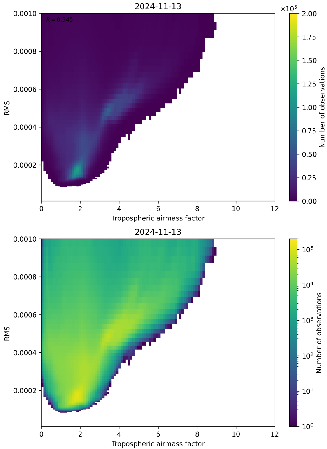
Figure 79: Scatter density plot of “Tropospheric airmass factor” against “RMS” for 2024-11-12 to 2024-11-14.
