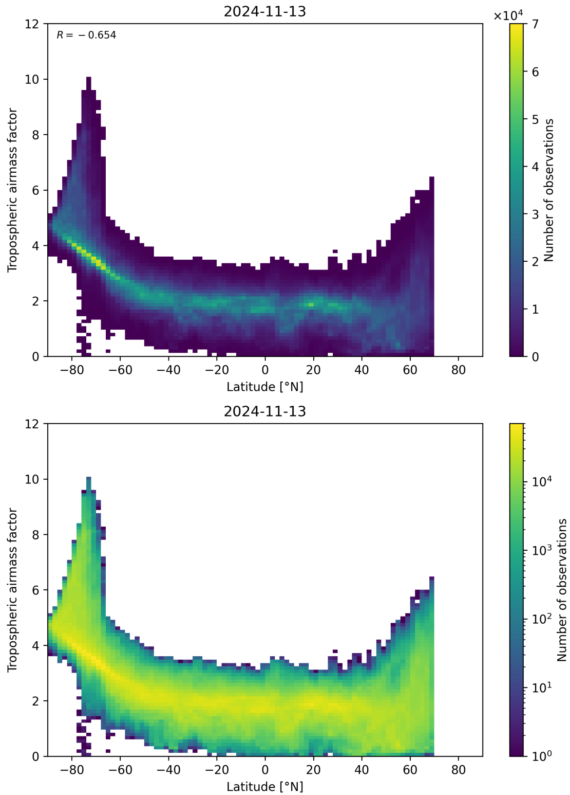
Figure 85: Scatter density plot of “Latitude” against “Tropospheric air mass factor” for 2024-11-12 to 2024-11-14.
