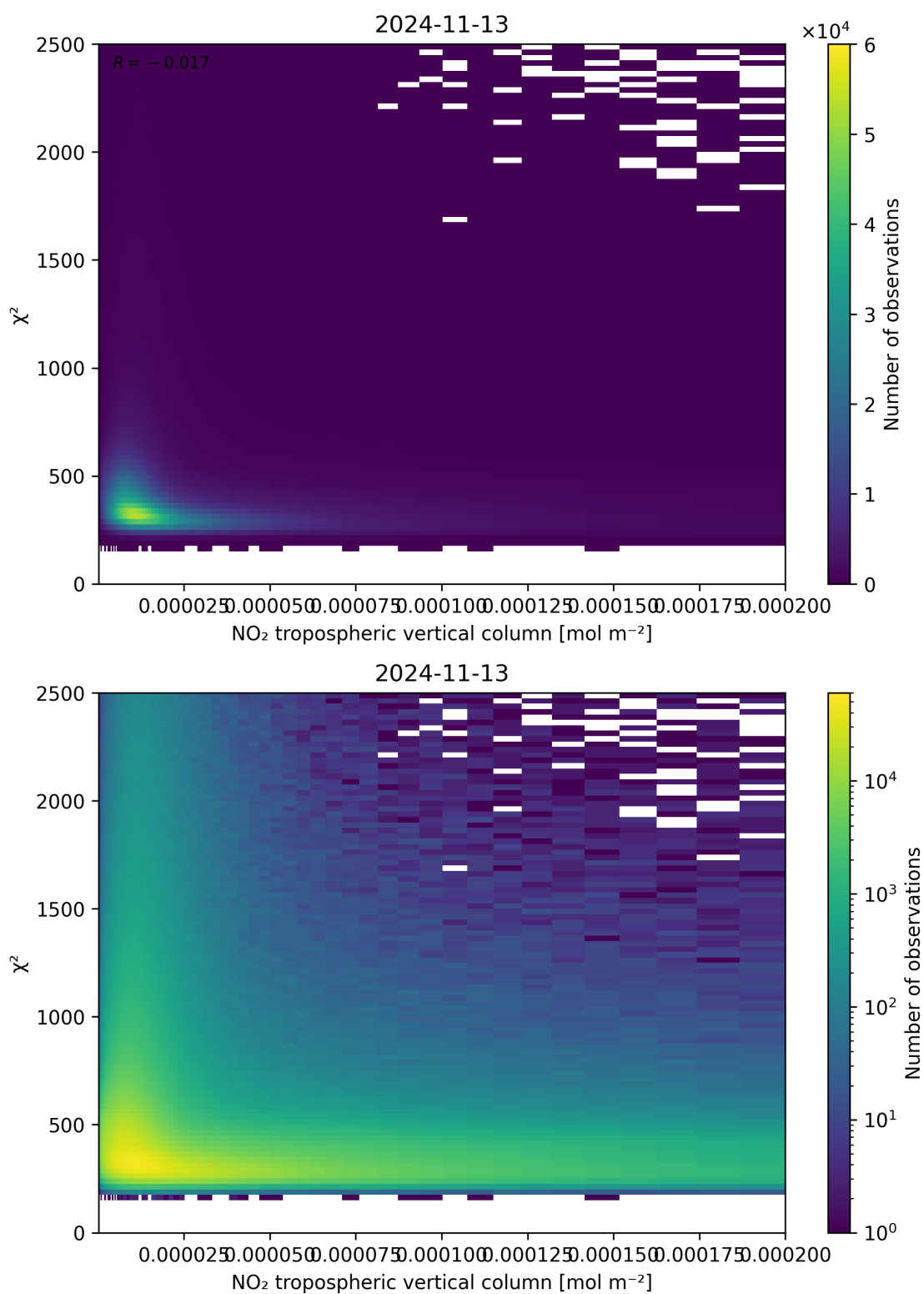
Figure 124: Scatter density plot of “NO 2 tropospheric vertical column” against “ \chi^2 ” for 2024-11-12 to 2024-11-14.
