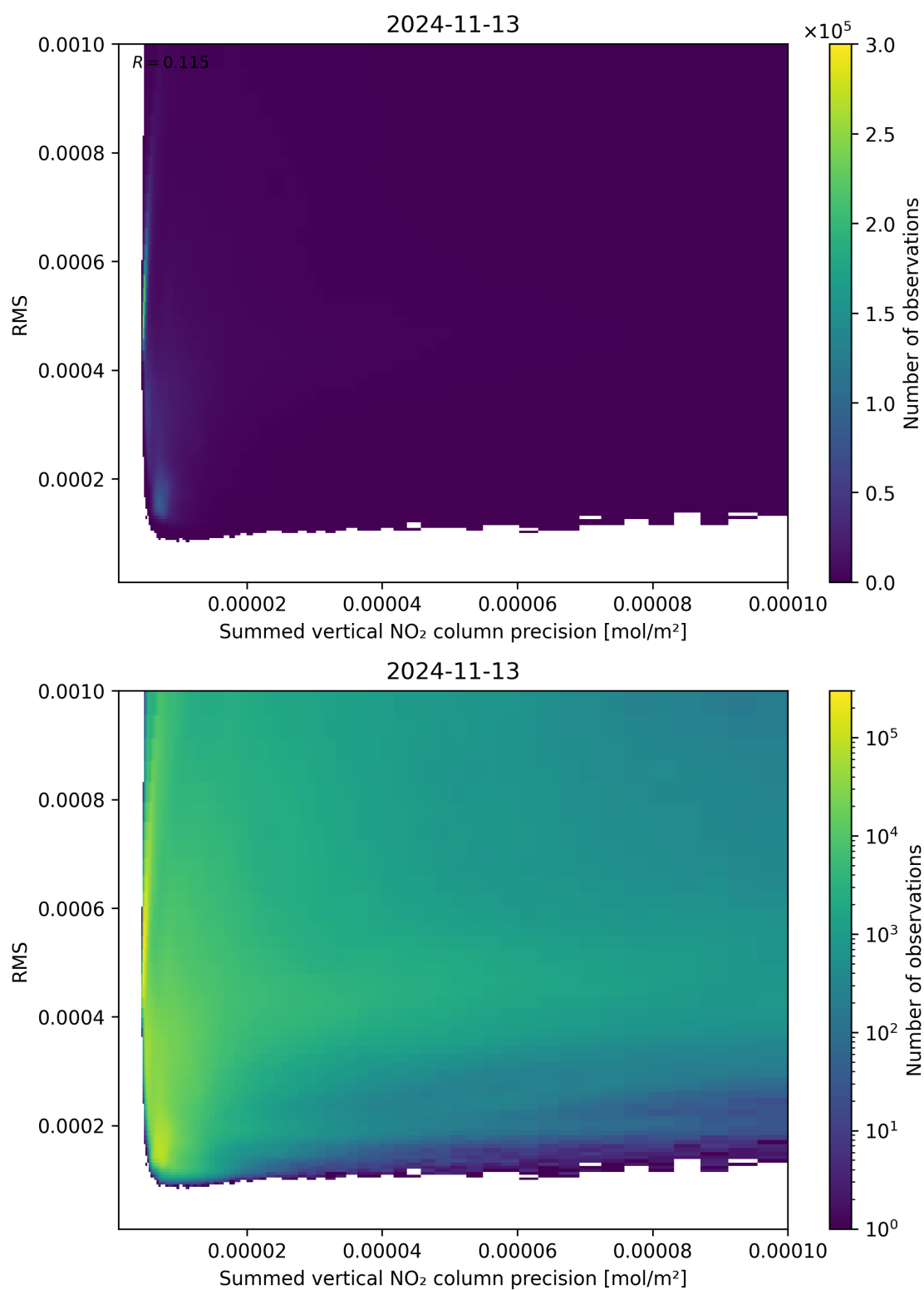
Figure 108: Scatter density plot of “Summed vertical NO 2 column precision” against “RMS” for 2024-11-12 to 2024-11-14.
