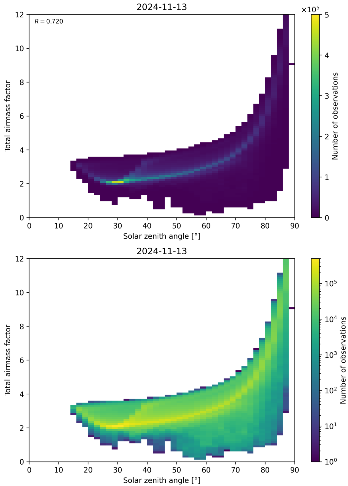
Figure 146: Scatter density plot of “Solar zenith angle” against “Total air mass factor” for 2024-11-12 to 2024-11-14.
