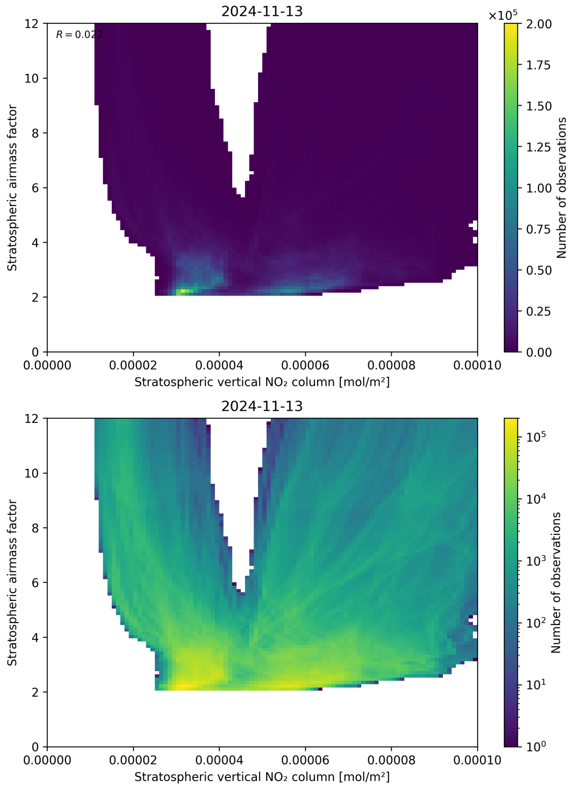
Figure 96: Scatter density plot of “Stratospheric vertical NO 2 column” against “Stratospheric airmass factor” for 2024-11-12 to 2024-11-14.
