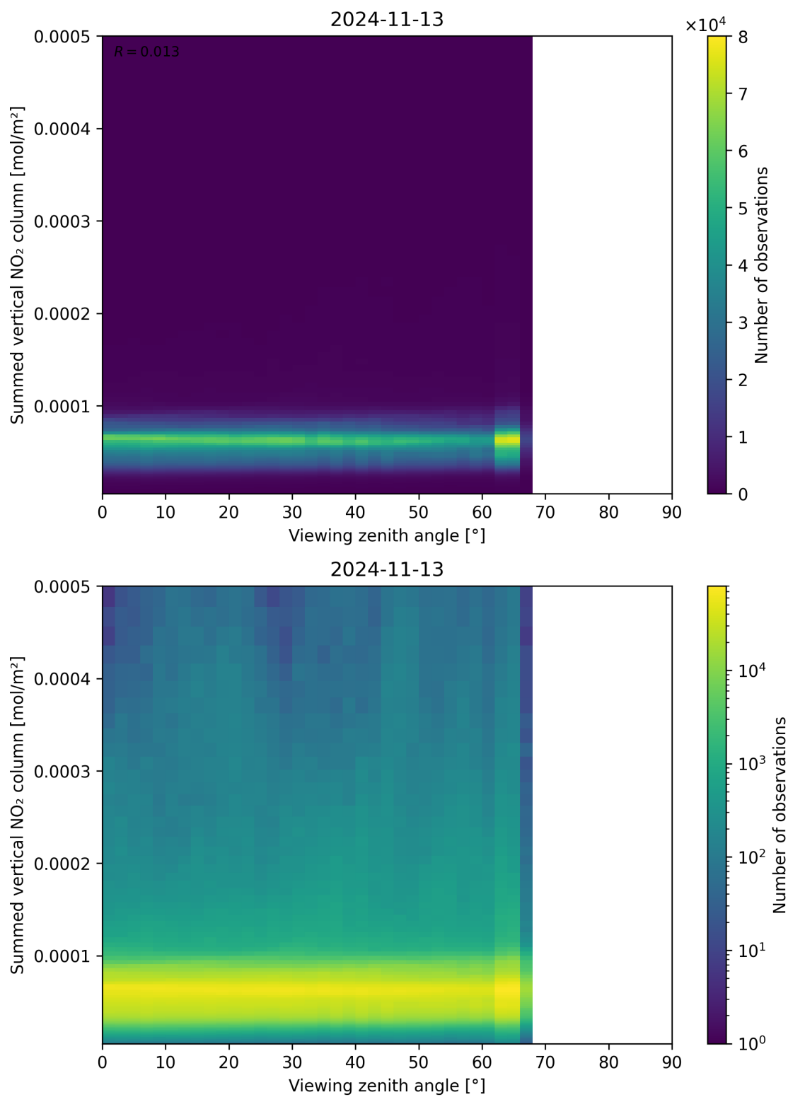
Figure 165: Scatter density plot of “Viewing zenith angle” against “Summed vertical NO 2 column” for 2024-11-12 to 2024-11-14.
