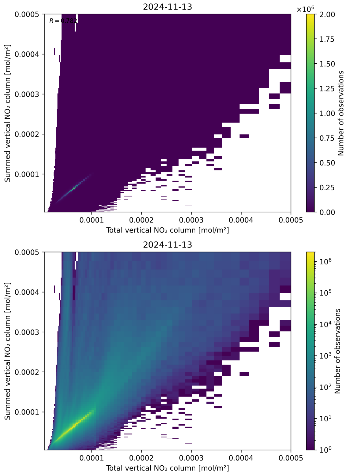
Figure 112: Scatter density plot of “Total vertical NO 2 column” against “Summed vertical NO 2 column” for 2024-11-12 to 2024-11-14.
