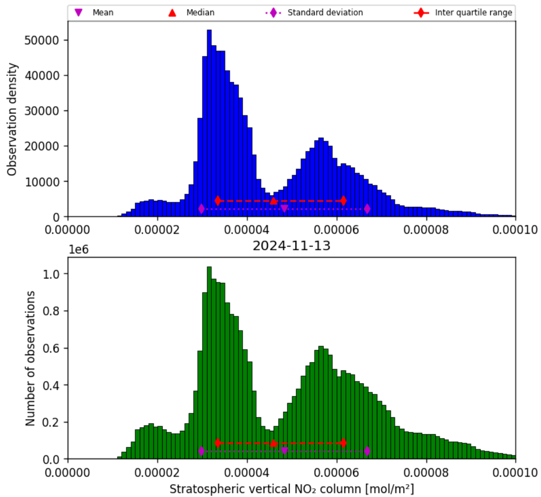
Figure 36: Histogram of “Stratospheric vertical NO 2 column” for 2024-11-12 to 2024-11-14
