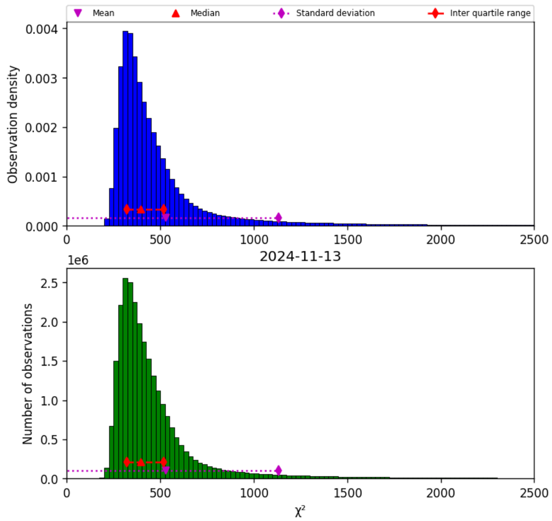
Figure 42: Histogram of “ \chi^2 ” for 2024-11-12 to 2024-11-14
