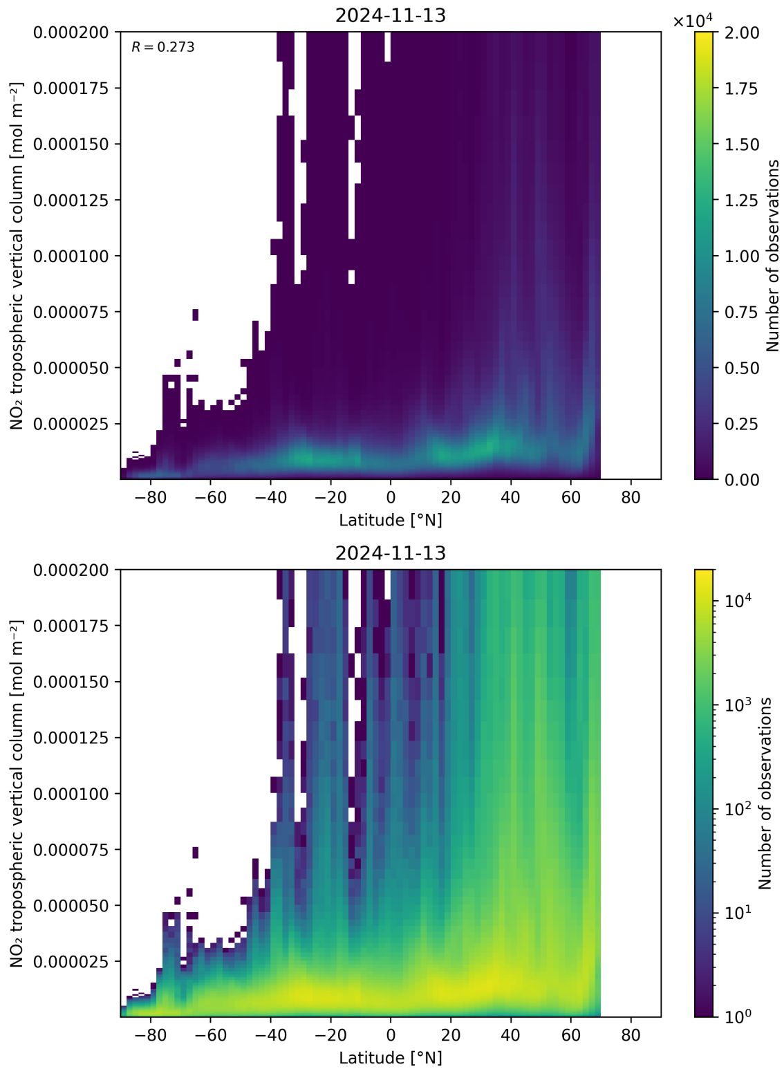
Figure 92: Scatter density plot of “Latitude” against “NO 2 tropospheric vertical column” for 2024-11-12 to 2024-11-14.
