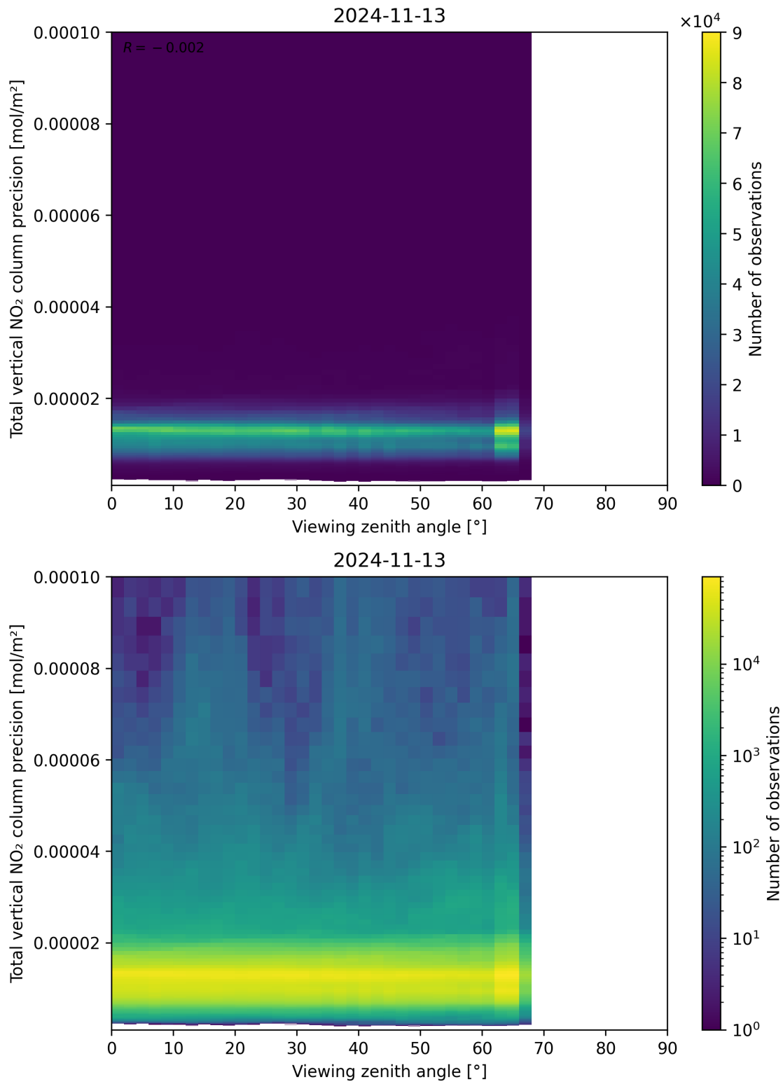
Figure 168: Scatter density plot of “Viewing zenith angle” against “Total vertical NO 2 column precision” for 2024-11-12 to 2024-11-14.
