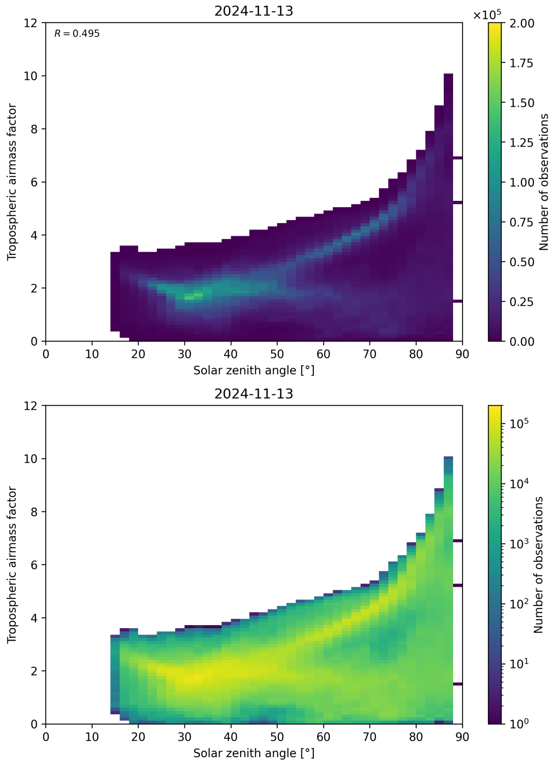
Figure 147: Scatter density plot of “Solar zenith angle” against “Tropospheric airmass factor” for 2024-11-12 to 2024-11-14.
