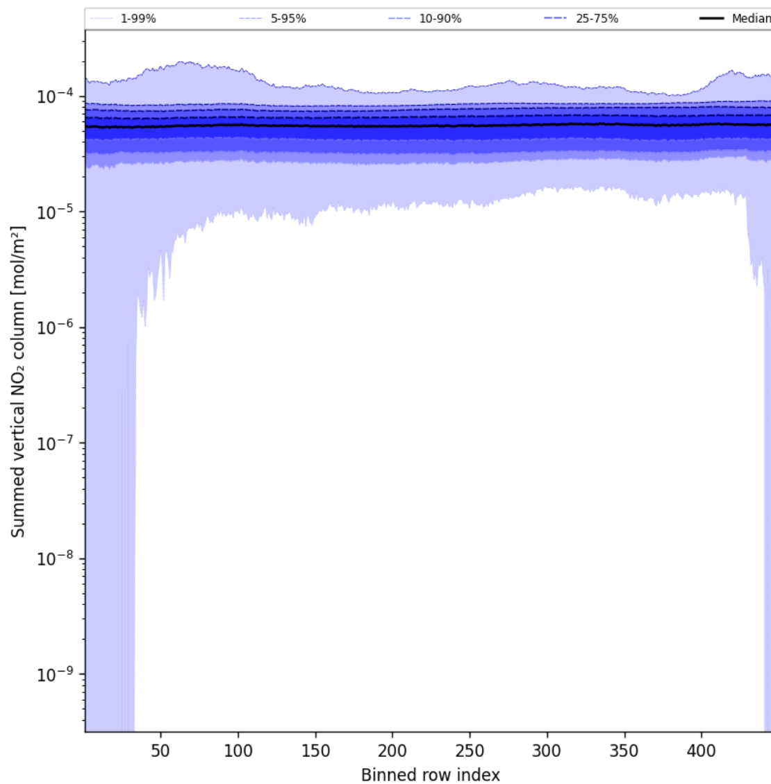
Figure 57: Along track statistics of “Summed vertical NO 2 column” for 2024-11-12 to 2024-11-14
