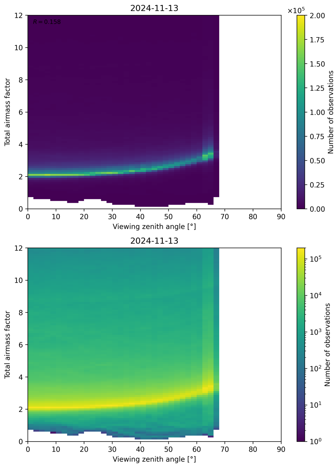
Figure 160: Scatter density plot of “Viewing zenith angle” against “Total airmass factor” for 2024-11-12 to 2024-11-14.
