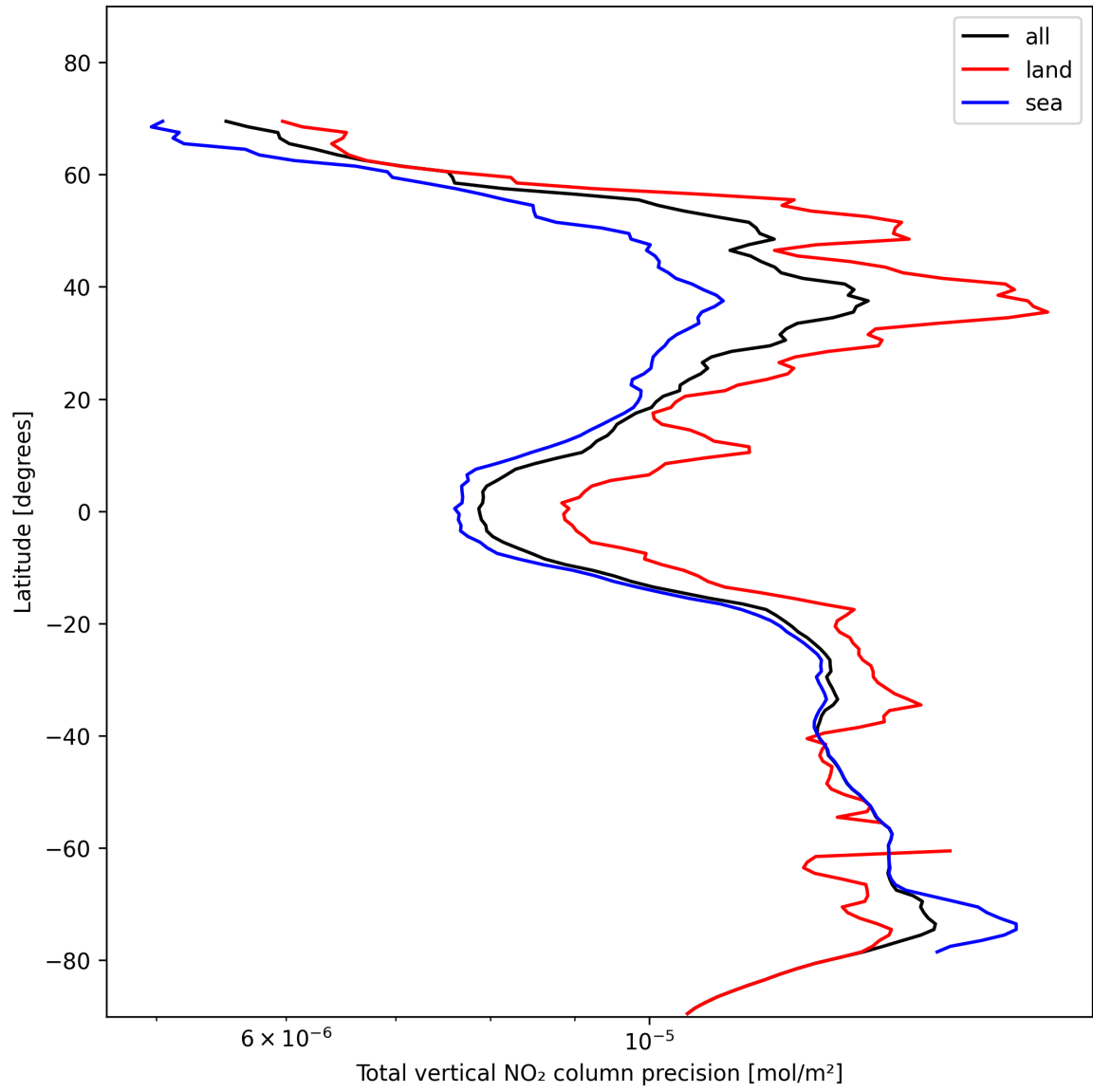
Figure 22: Zonal average of “Total vertical NO 2 column precision” for 2024-11-12 to 2024-11-14.
