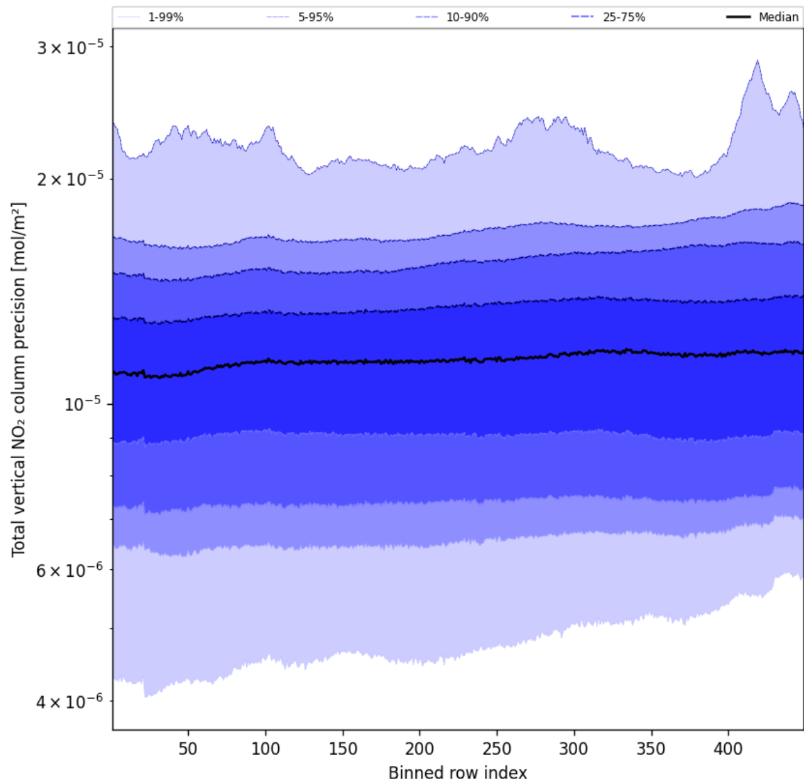
Figure 56: Along track statistics of “Total vertical NO 2 column precision” for 2024-11-12 to 2024-11-14
