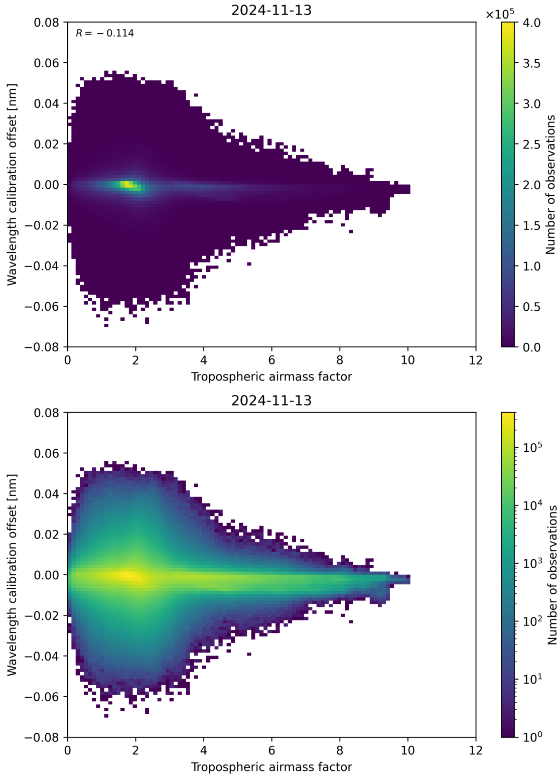
Figure 80: Scatter density plot of “Tropospheric airmass factor” against “Wavelength calibration offset” for 2024-11-12 to 2024-11-14.
