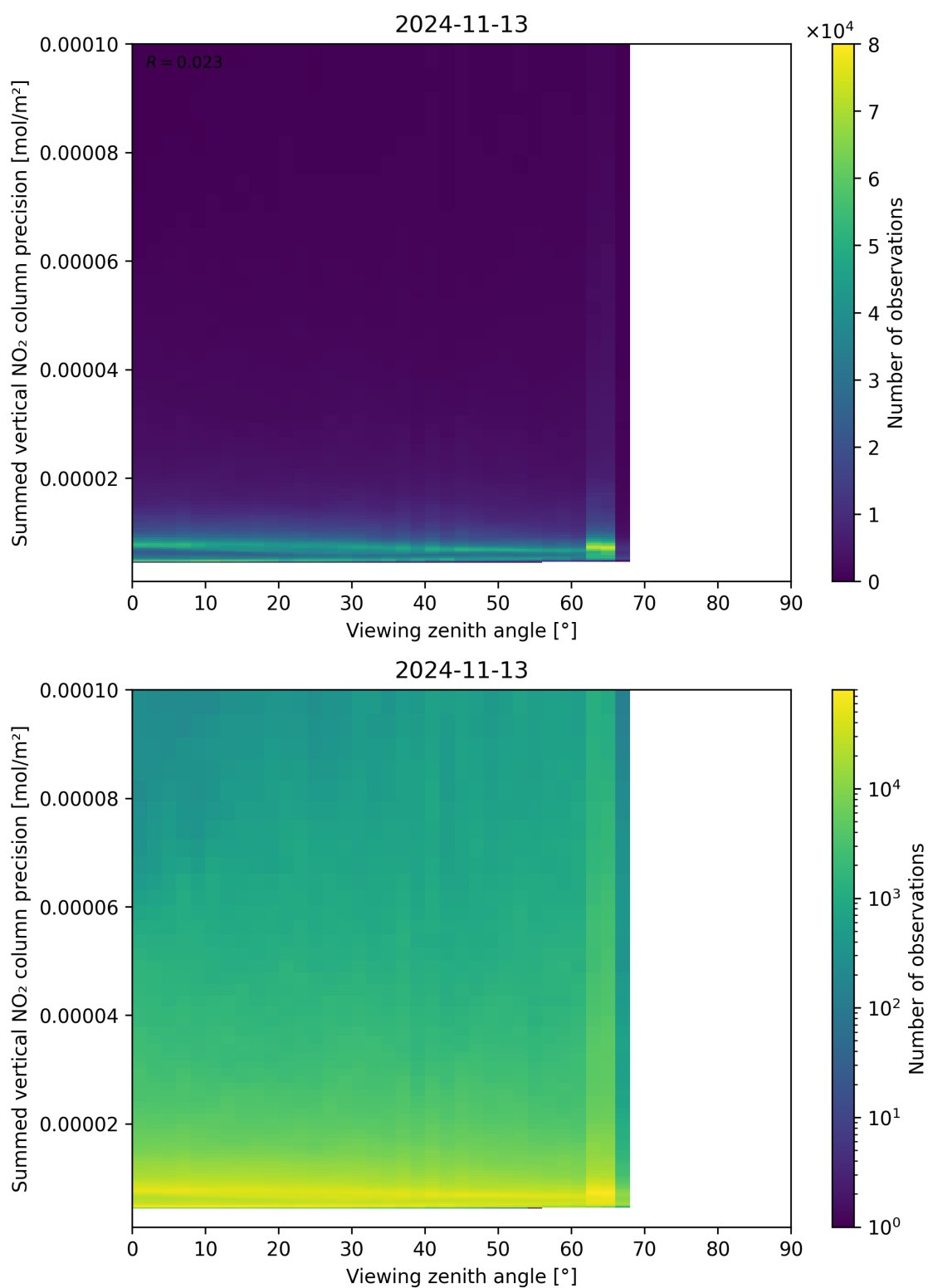
Figure 166: Scatter density plot of “Viewing zenith angle” against “Summed vertical NO 2 column precision” for 2024-11-12 to 2024-11-14.
