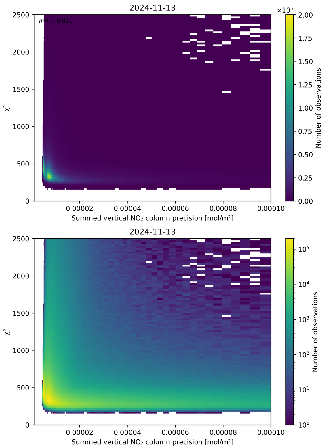
Figure 107: Scatter density plot of “Summed vertical NO 2 column precision” against “ \chi^2 ” for 2024-11-12 to 2024-11-14.
