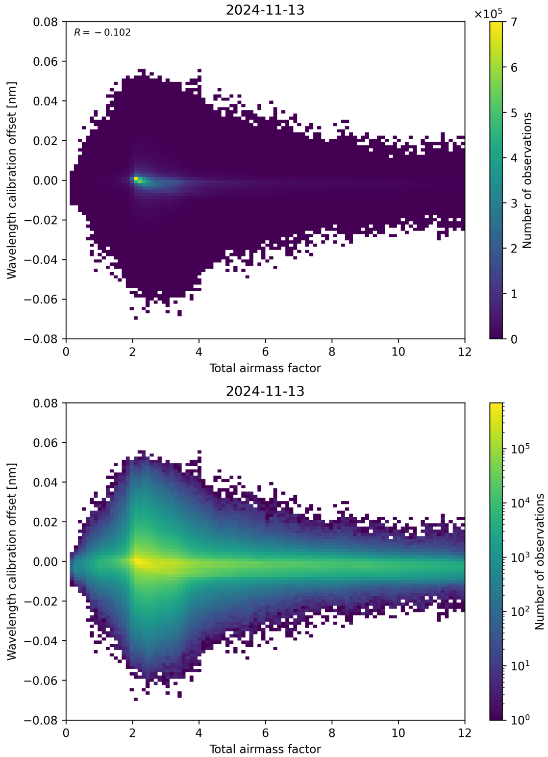
Figure 70: Scatter density plot of “Total airmass factor” against “Wavelength calibration offset” for 2024-11-12 to 2024-11-14.
