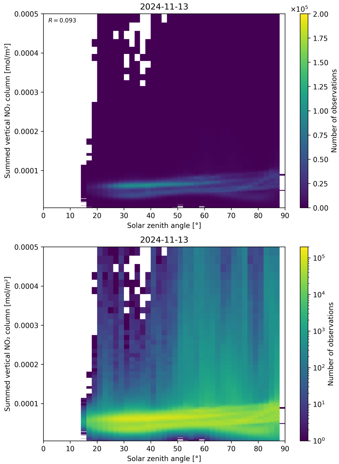
Figure 151: Scatter density plot of “Solar zenith angle” against “Summed vertical NO 2 column” for 2024-11-12 to 2024-11-14.
