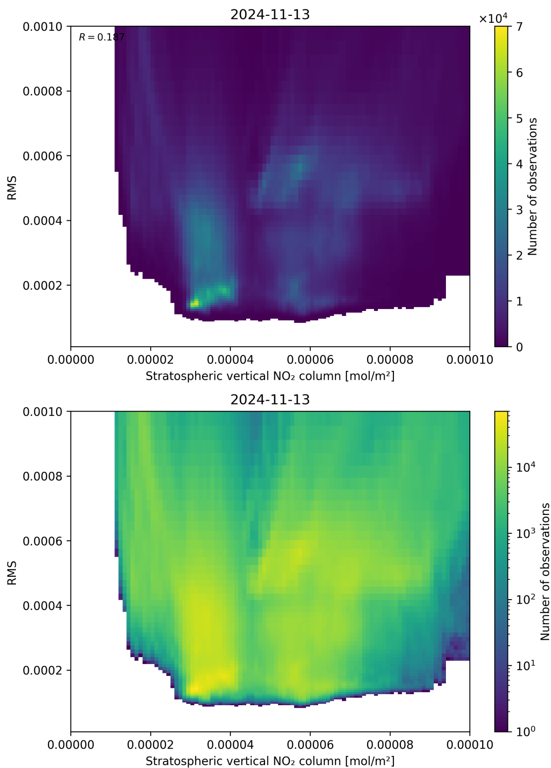
Figure 102: Scatter density plot of “Stratospheric vertical NO 2 column” against “RMS” for 2024-11-12 to 2024-11-14.
