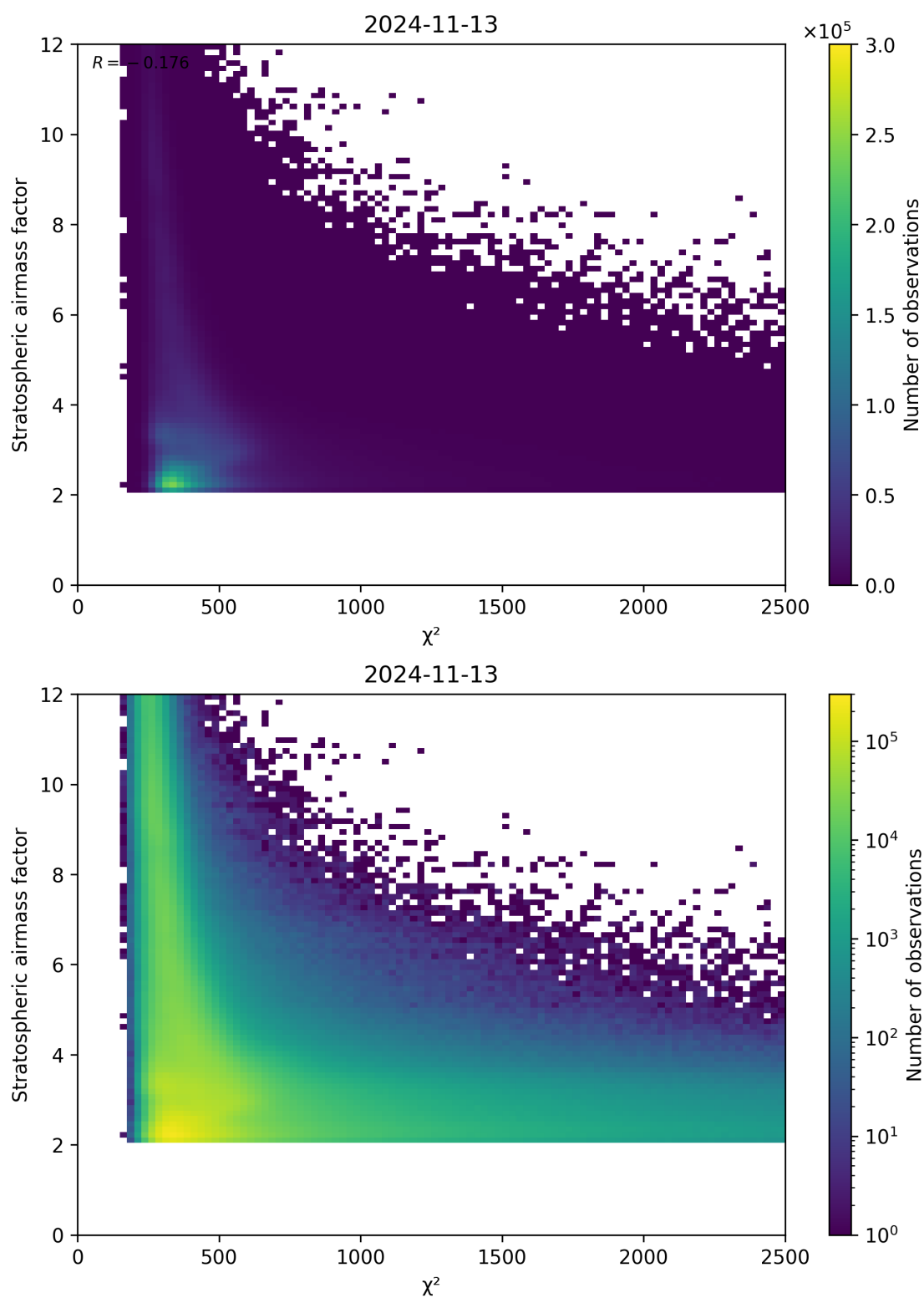
Figure 81: Scatter density plot of “ \chi^2 ” against “Stratospheric airmass factor” for 2024-11-12 to 2024-11-14.
