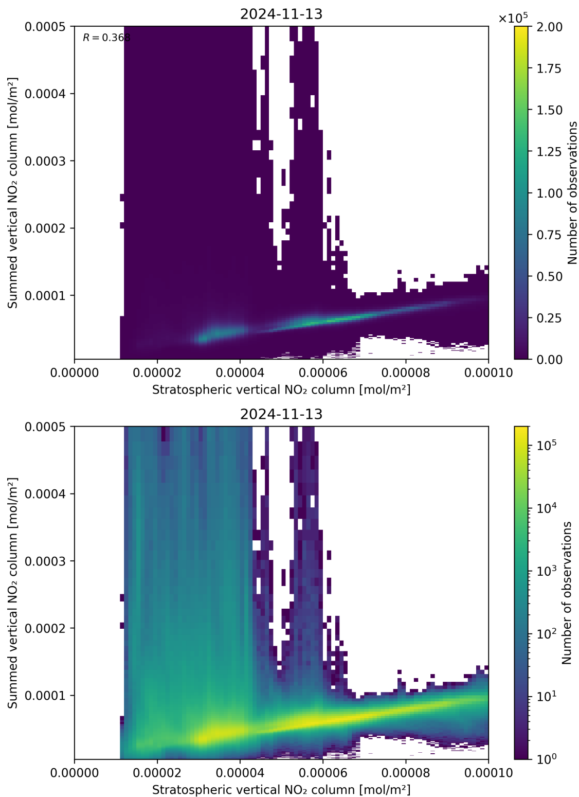
Figure 98: Scatter density plot of “Stratospheric vertical NO 2 column” against “Summed vertical NO 2 column” for 2024-11-12 to 2024-11-14.
