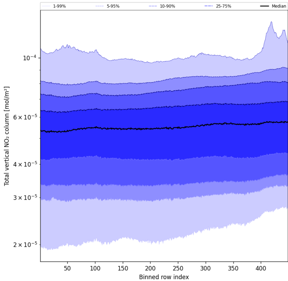
Figure 55: Along track statistics of “Total vertical NO 2 column” for 2024-11-12 to 2024-11-14
