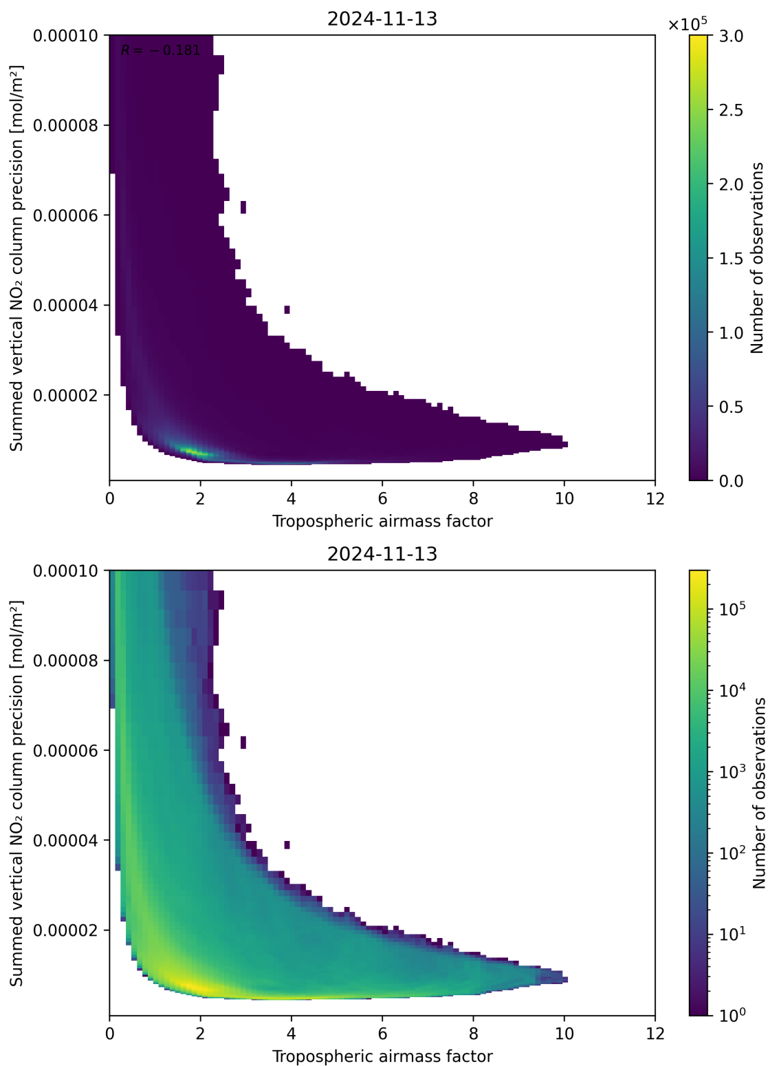
Figure 76: Scatter density plot of “Tropospheric air mass factor” against “Summed vertical NO 2 column precision” for 2024-11-12 to 2024-11-14.
