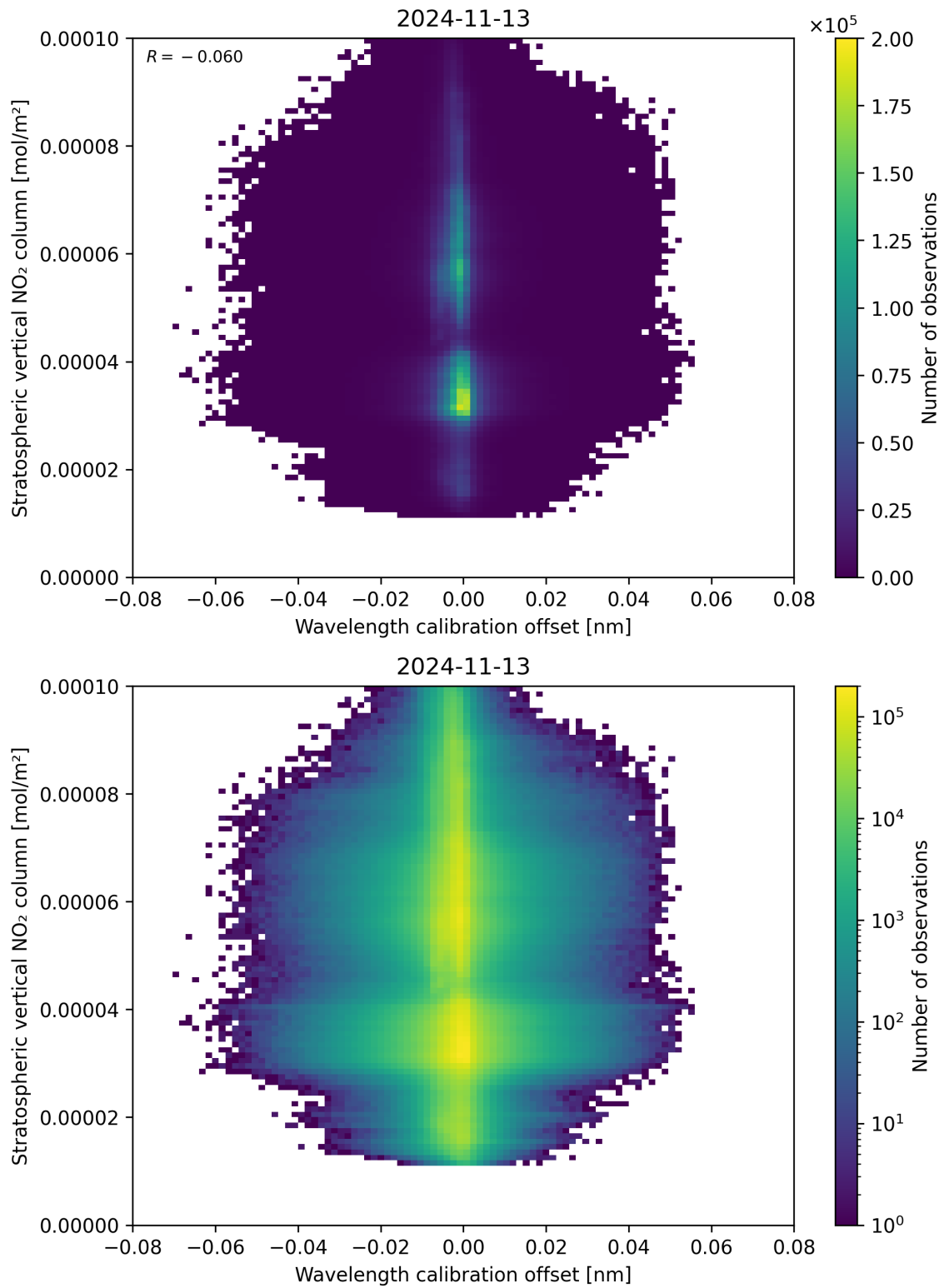
Figure 176: Scatter density plot of “Wavelength calibration offset” against “Stratospheric vertical NO 2 column” for 2024-11-12 to 2024-11-14.
