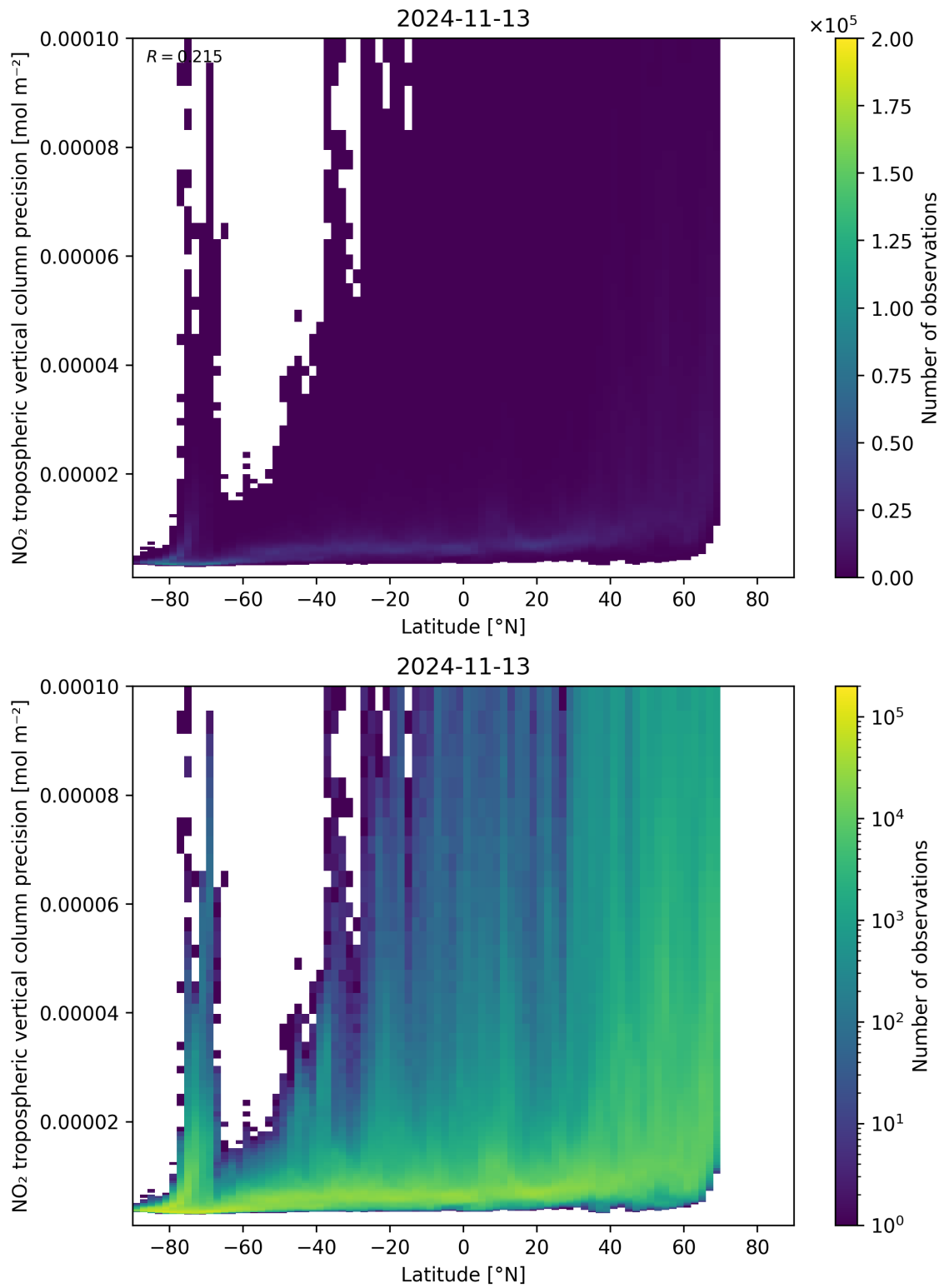
Figure 93: Scatter density plot of “Latitude” against “NO 2 tropospheric vertical column precision” for 2024-11-12 to 2024-11-14.
