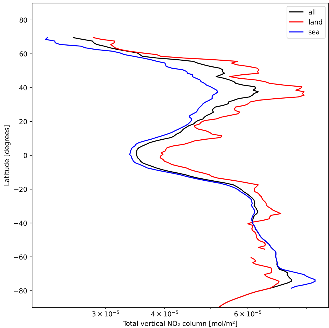
Figure 21: Zonal average of “Total vertical NO 2 column” for 2024-11-12 to 2024-11-14.
