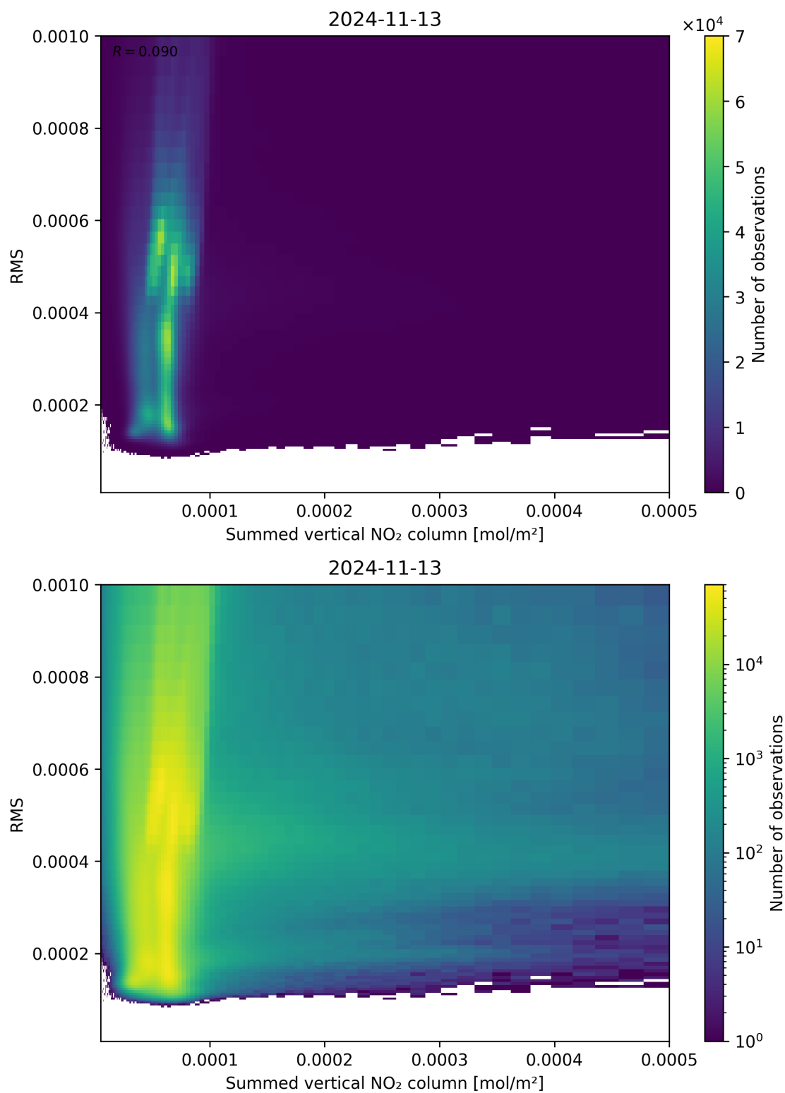
Figure 109: Scatter density plot of “Summed vertical NO 2 column” against “RMS” for 2024-11-12 to 2024-11-14.
