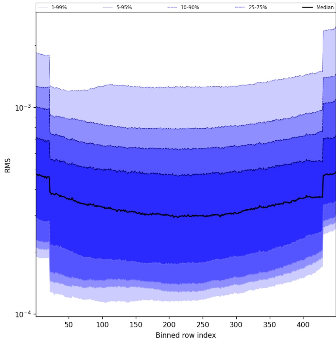
Figure 60: Along track statistics of “RMS” for 2024-11-12 to 2024-11-14
