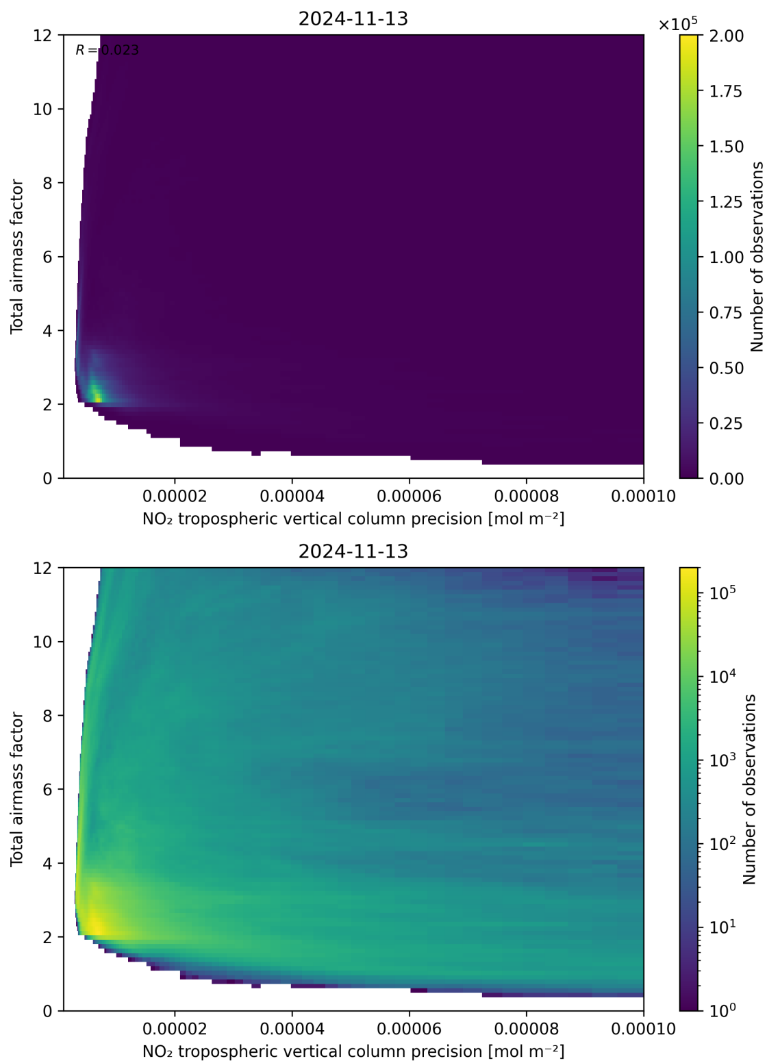
Figure 132: Scatter density plot of “NO 2 tropospheric vertical column precision” against “Total air mass factor” for 2024-11-12 to 2024-11-14.
