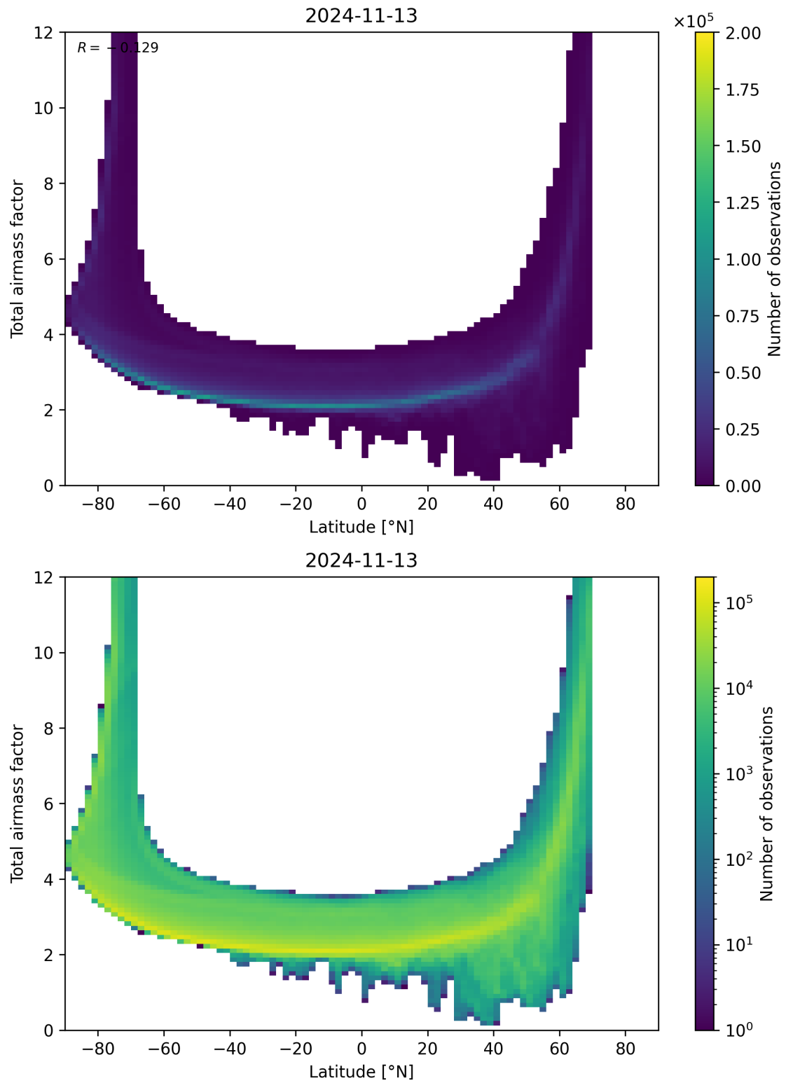
Figure 84: Scatter density plot of “Latitude” against “Total airmass factor” for 2024-11-12 to 2024-11-14.
