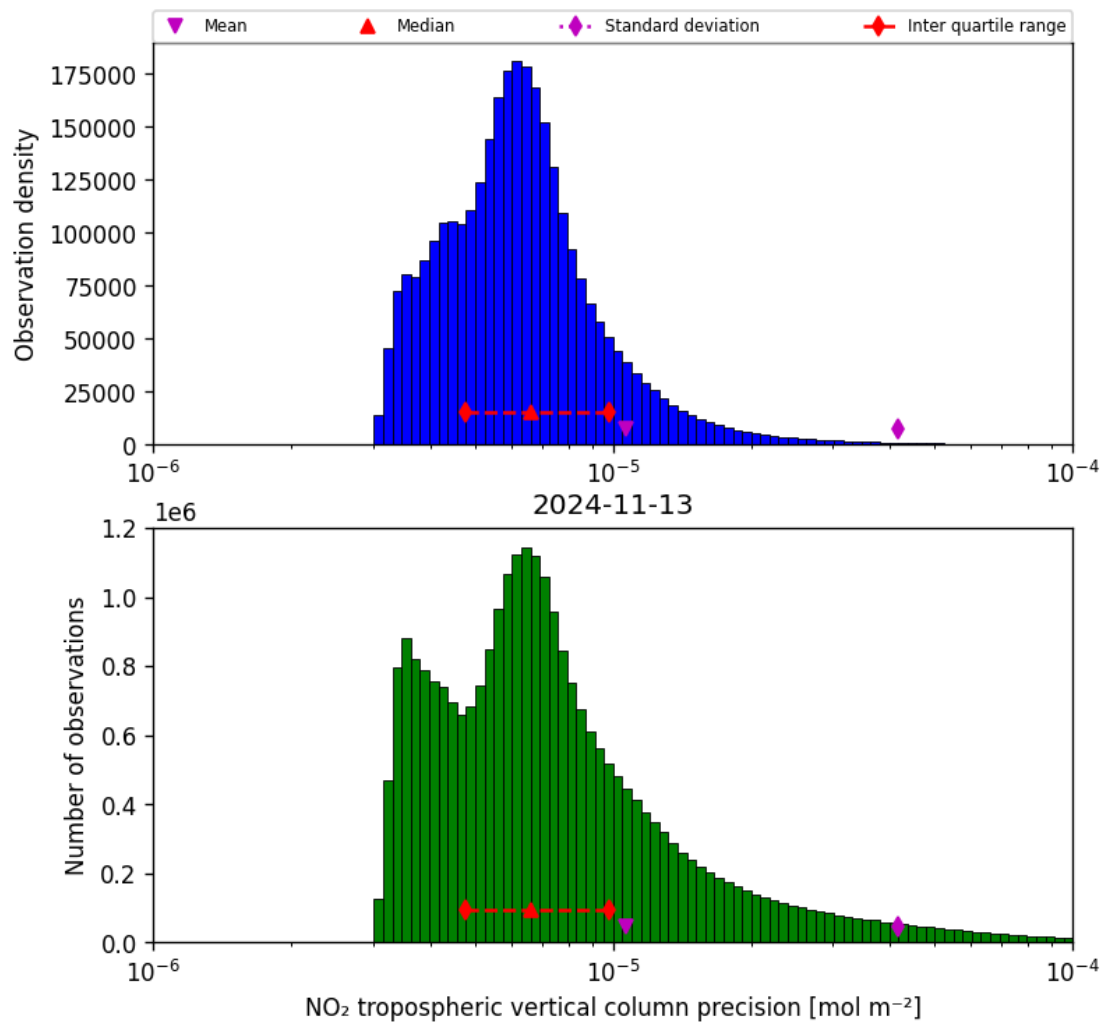
Figure 30: Histogram of “NO 2 tropospheric vertical column precision” for 2024-11-12 to 2024-11-14
