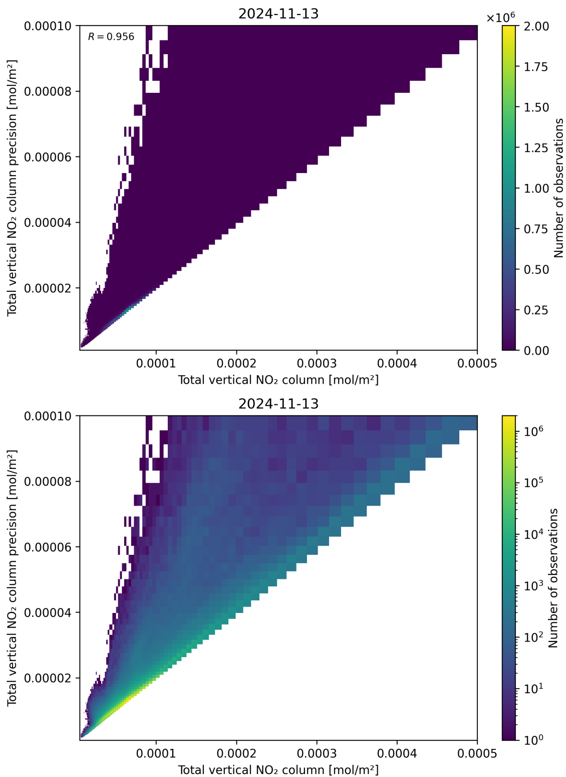
Figure 114: Scatter density plot of “Total vertical NO 2 column” against “Total vertical NO 2 column precision” for 2024-11-12 to 2024-11-14.
