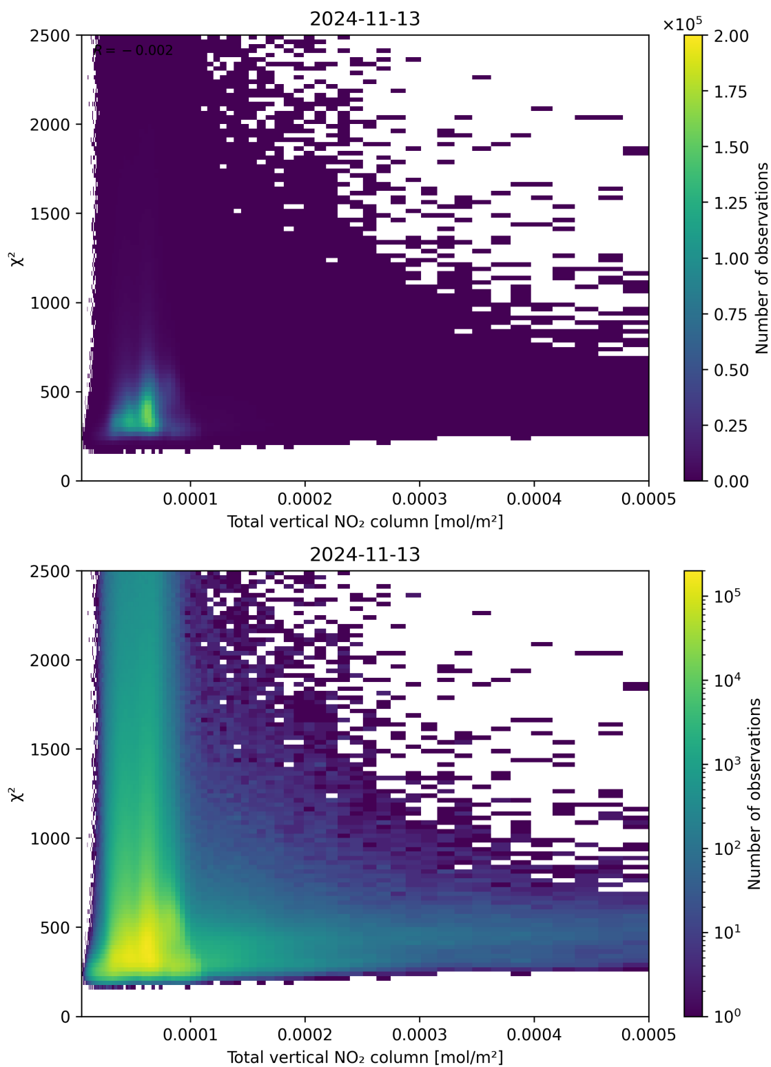
Figure 111: Scatter density plot of “Total vertical NO 2 column” against “ \chi^2 ” for 2024-11-12 to 2024-11-14.
