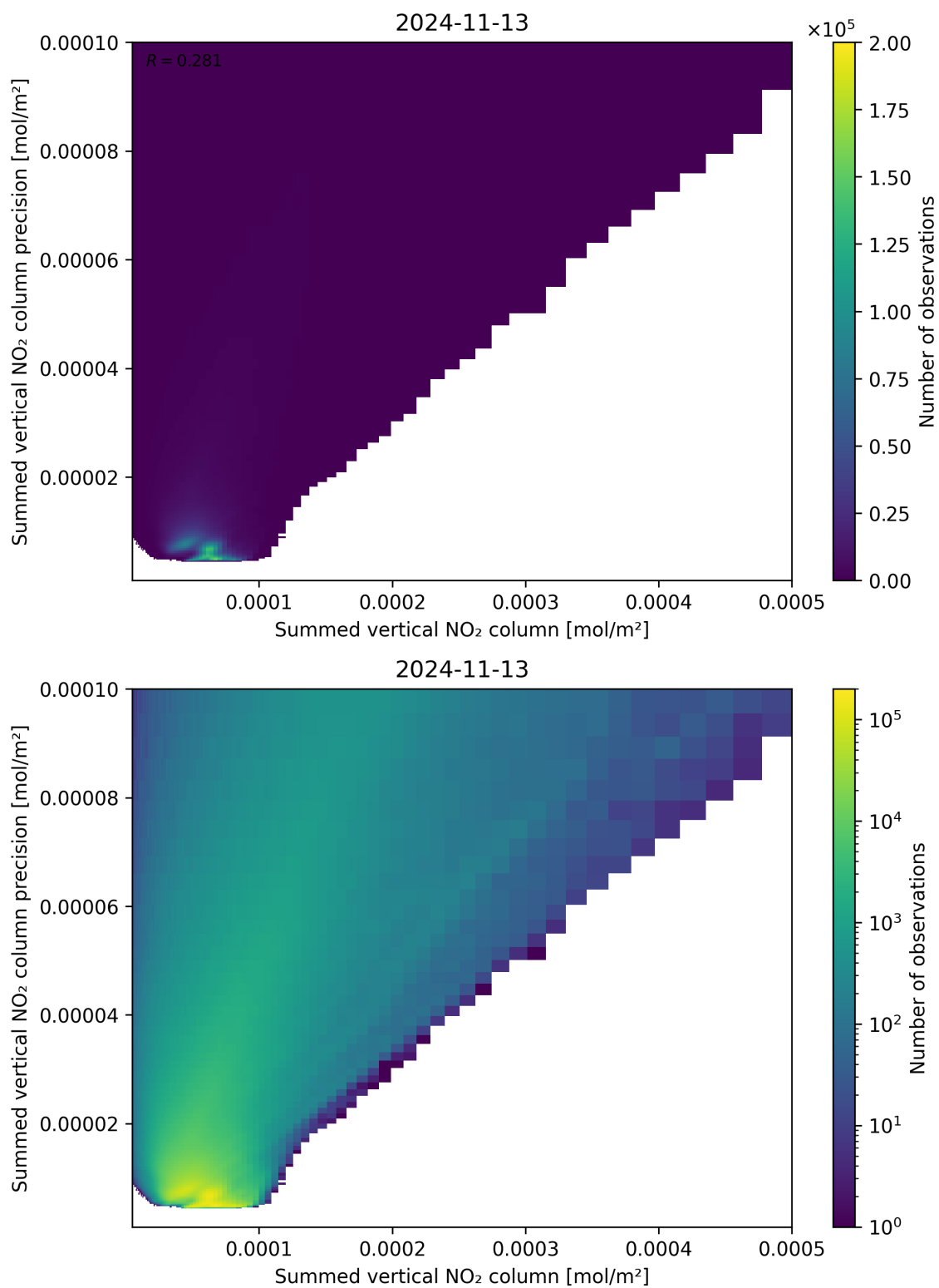
Figure 105: Scatter density plot of “Summed vertical NO 2 column” against “Summed vertical NO 2 column precision” for 2024-11-12 to 2024-11-14.
