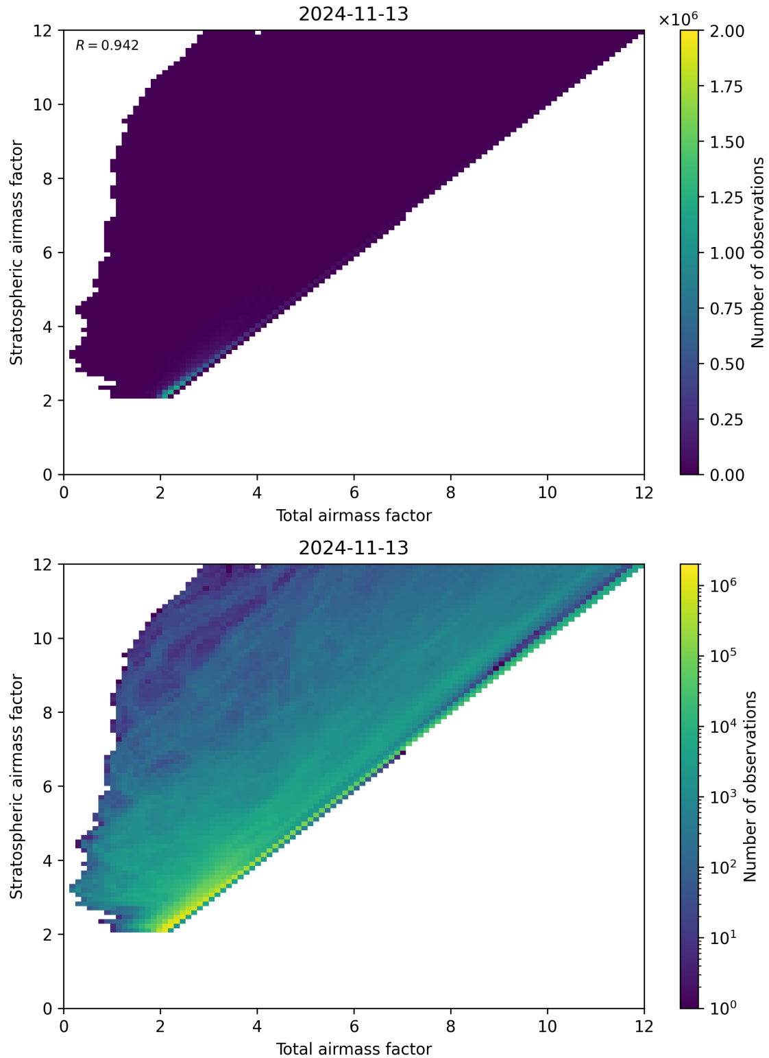
Figure 62: Scatter density plot of “Total airmass factor” against “Stratospheric airmass factor” for 2024-11-12 to 2024-11-14.
