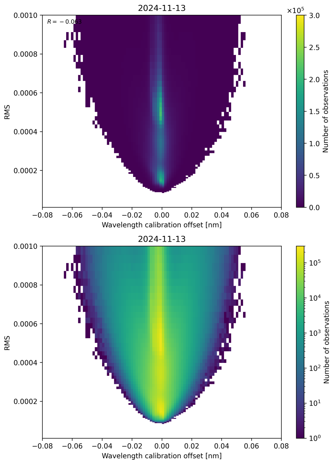
Figure 181: Scatter density plot of “Wavelength calibration offset” against “RMS” for 2024-11-12 to 2024-11-14.
