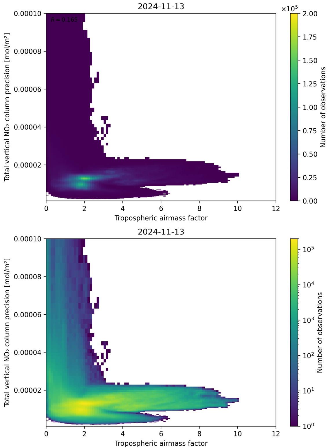
Figure 78: Scatter density plot of “Tropospheric air mass factor” against “Total vertical NO 2 column precision” for 2024-11-12 to 2024-11-14.
