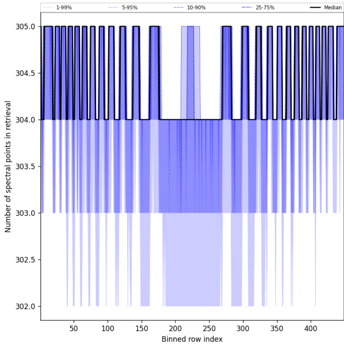
Figure 50: Along track statistics of “Number of spectral points in retrieval” for 2024-11-12 to 2024-11-14
