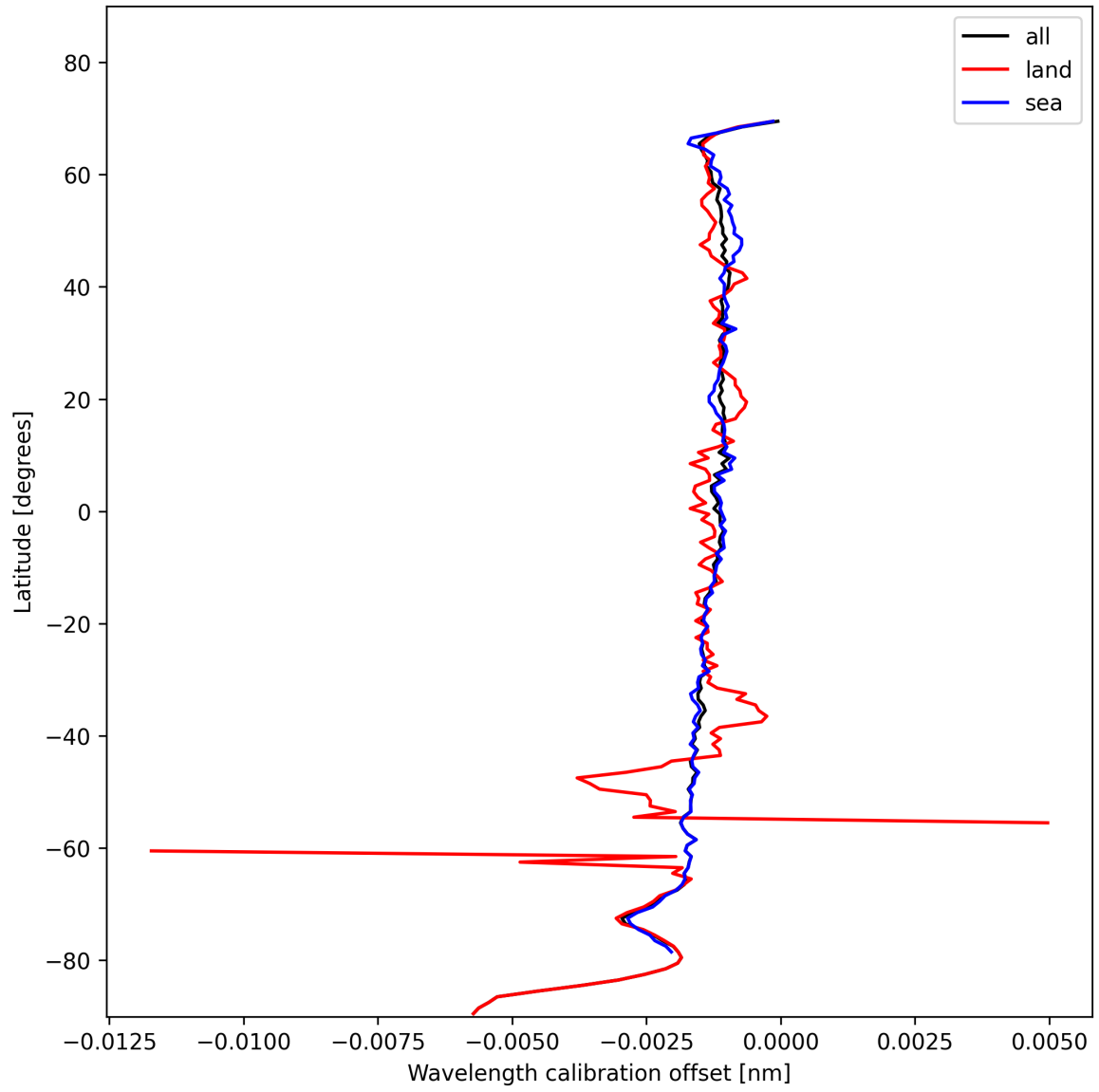
Figure 18: Zonal average of “Wavelength calibration offset” for 2024-11-12 to 2024-11-14.
