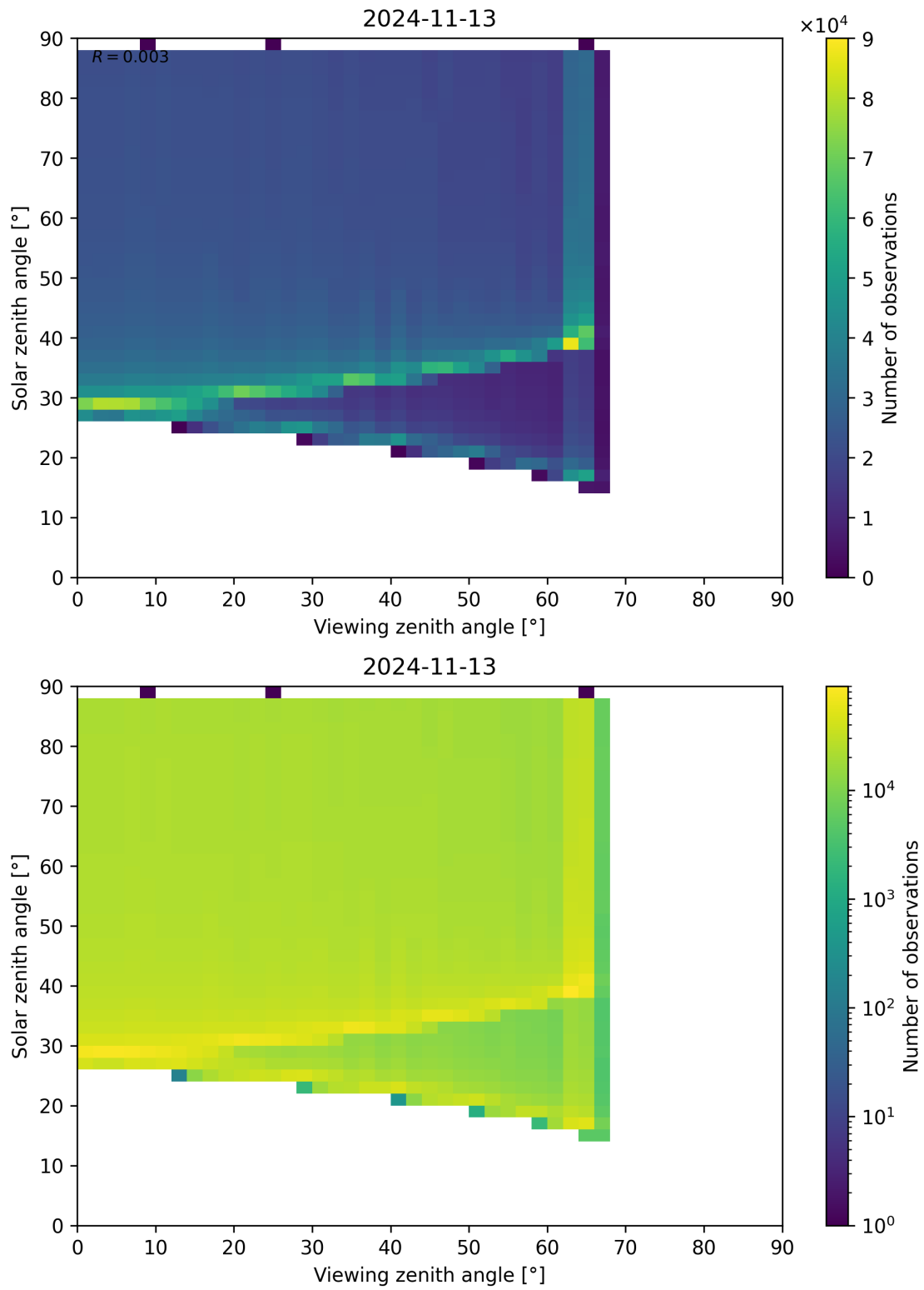
Figure 172: Scatter density plot of “Viewing zenith angle” against “Solar zenith angle” for 2024-11-12 to 2024-11-14.
