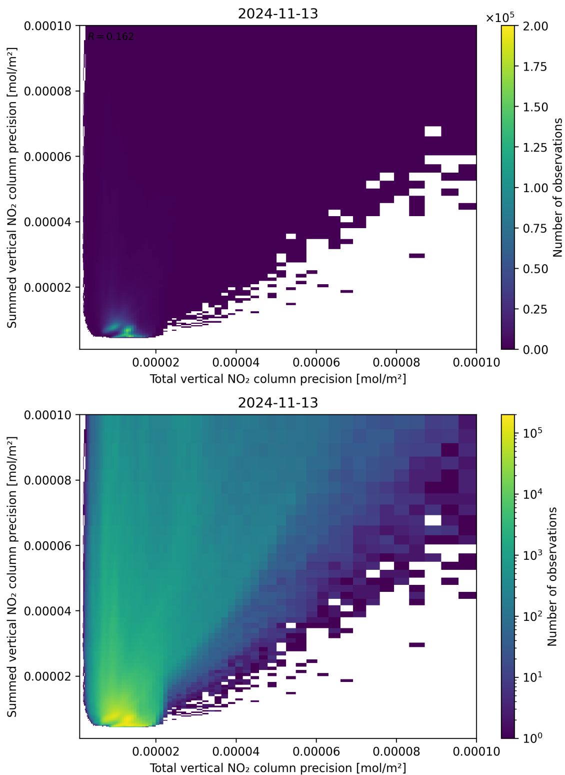
Figure 118: Scatter density plot of “Total vertical NO 2 column precision” against “Summed vertical NO 2 column precision” for 2024-11-12 to 2024-11-14.
