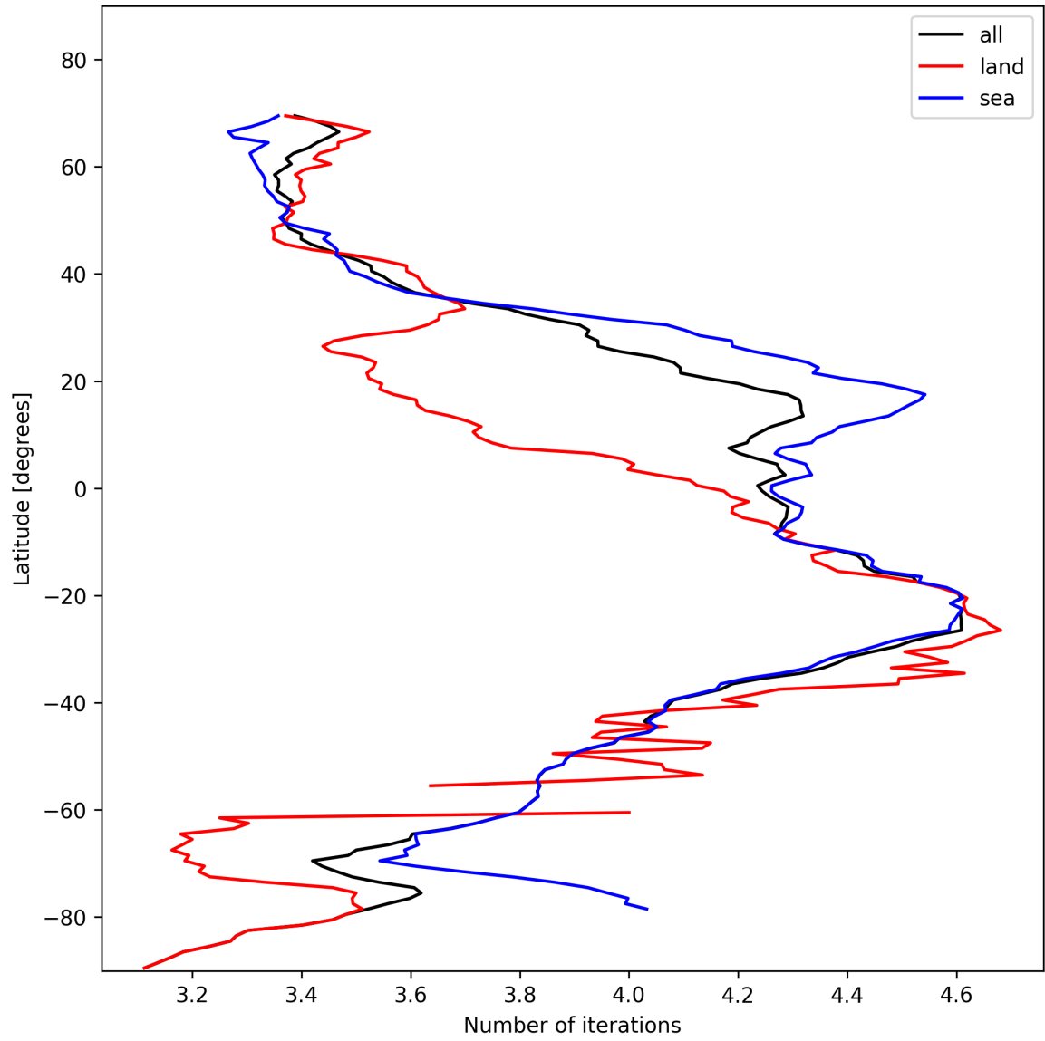
Figure 17: Zonal average of “Number of iterations” for 2024-11-12 to 2024-11-14.
