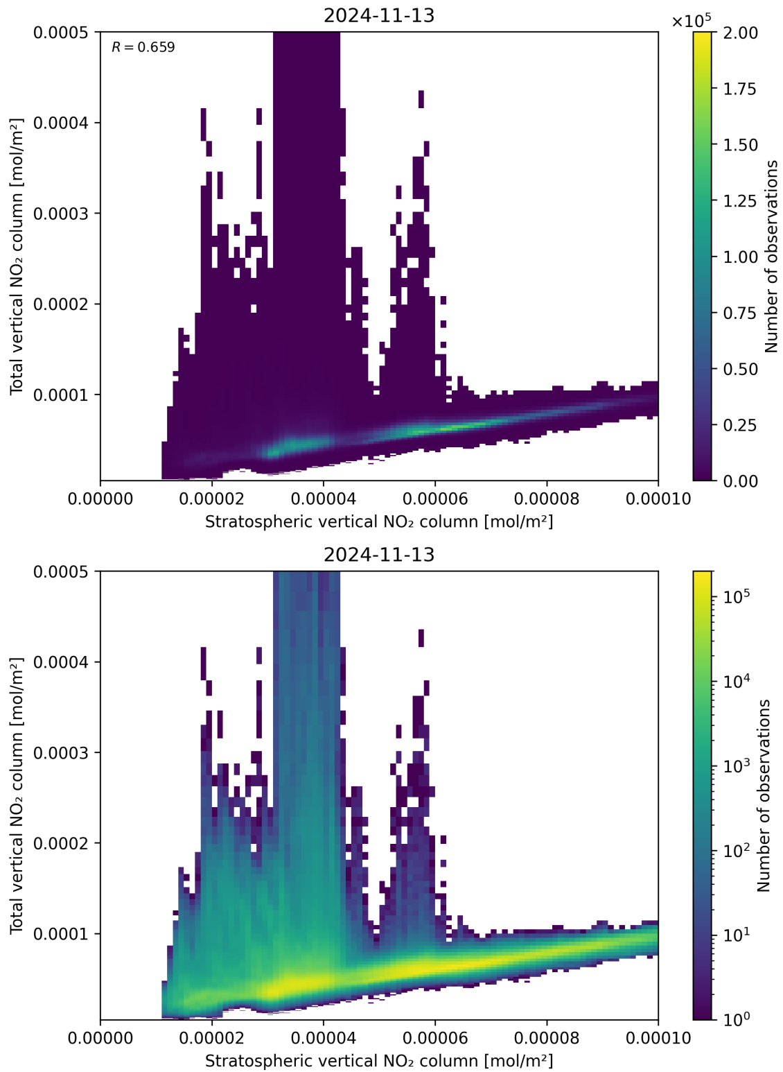
Figure 100: Scatter density plot of “Stratospheric vertical NO 2 column” against “Total vertical NO 2 column” for 2024-11-12 to 2024-11-14.
