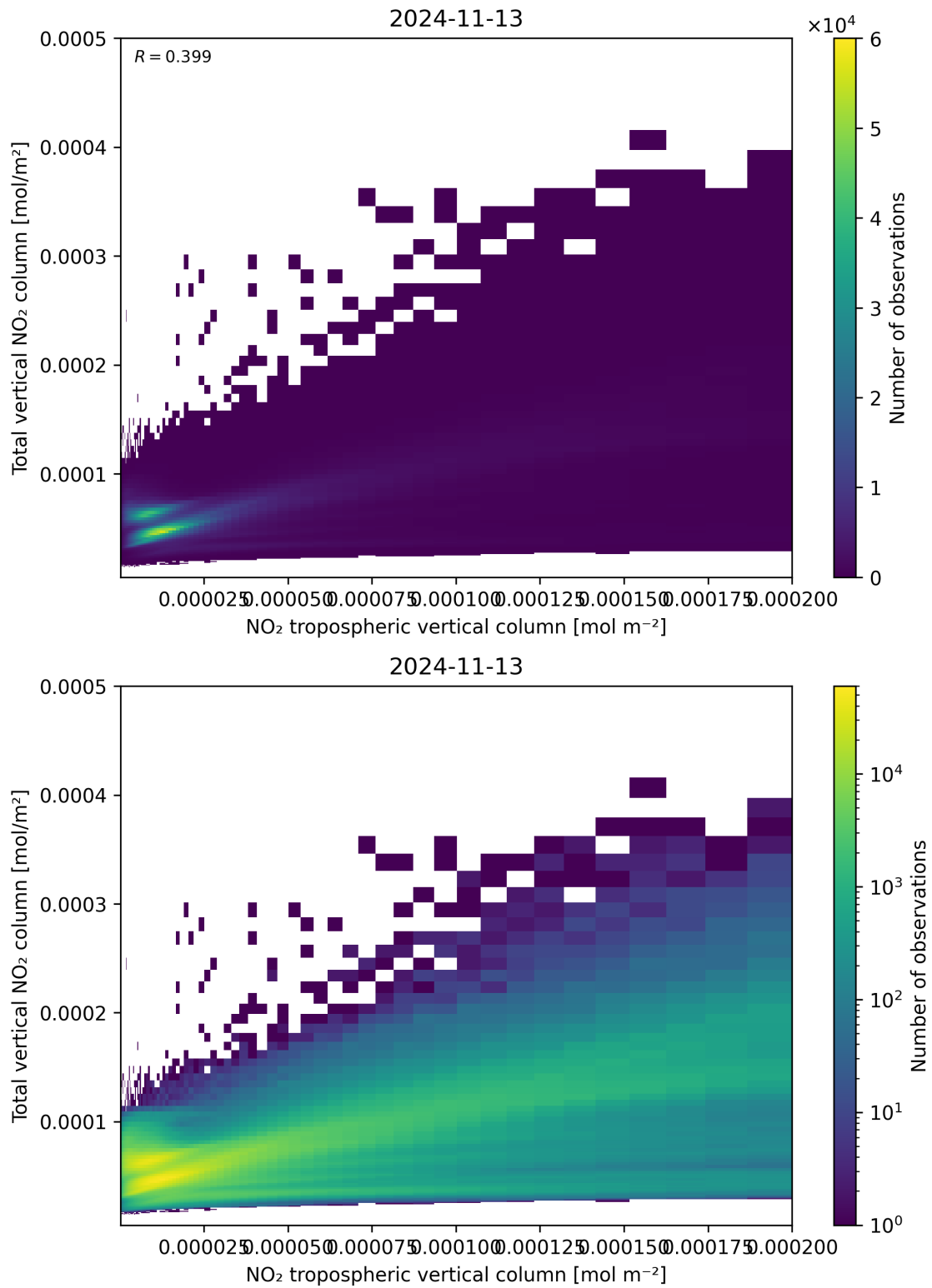
Figure 128: Scatter density plot of “NO 2 tropospheric vertical column” against “Total vertical NO 2 column” for 2024-11-12 to 2024-11-14.
