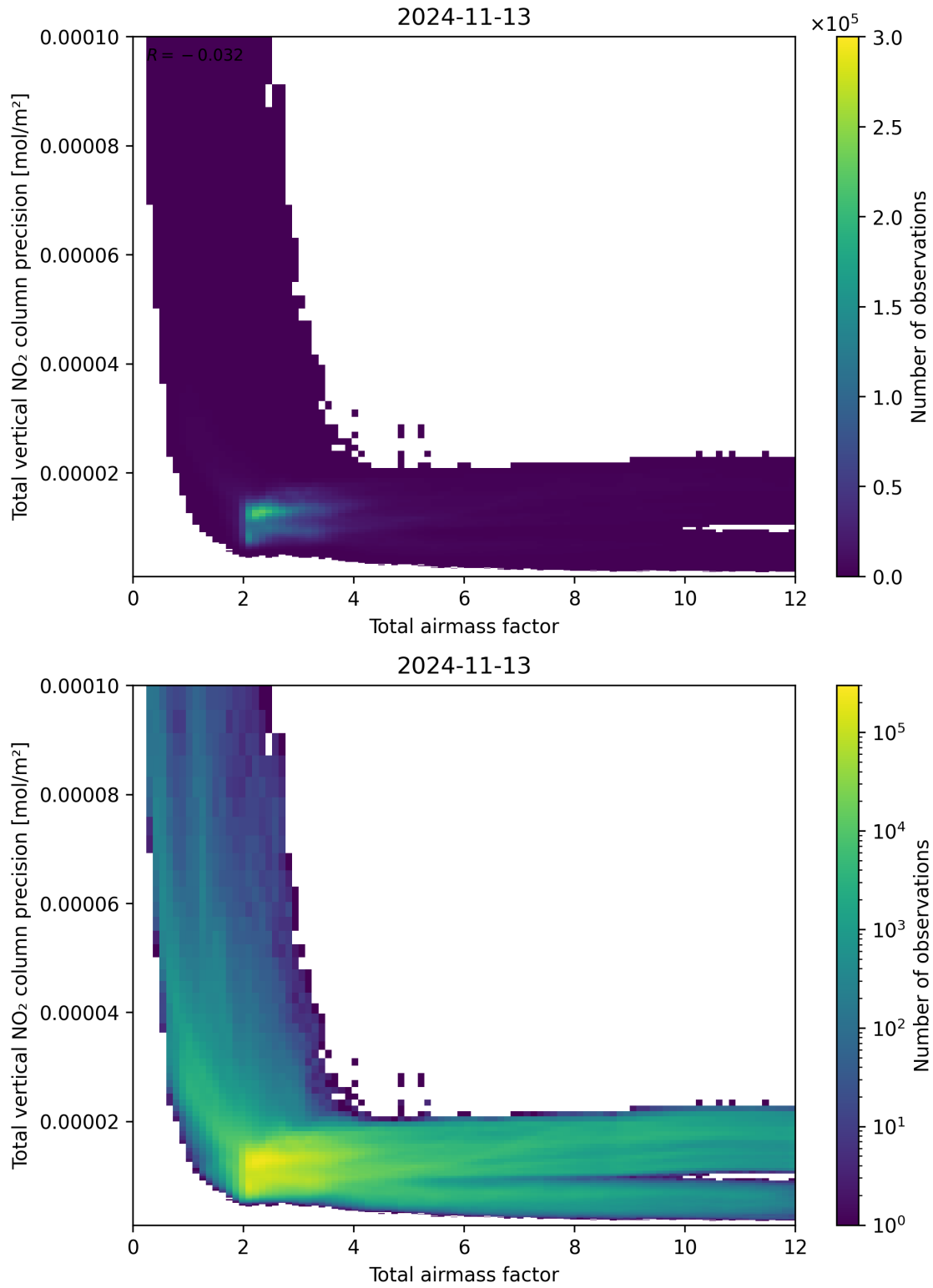
Figure 68: Scatter density plot of “Total airmass factor” against “Total vertical NO 2 column precision” for 2024-11-12 to 2024-11-14.
