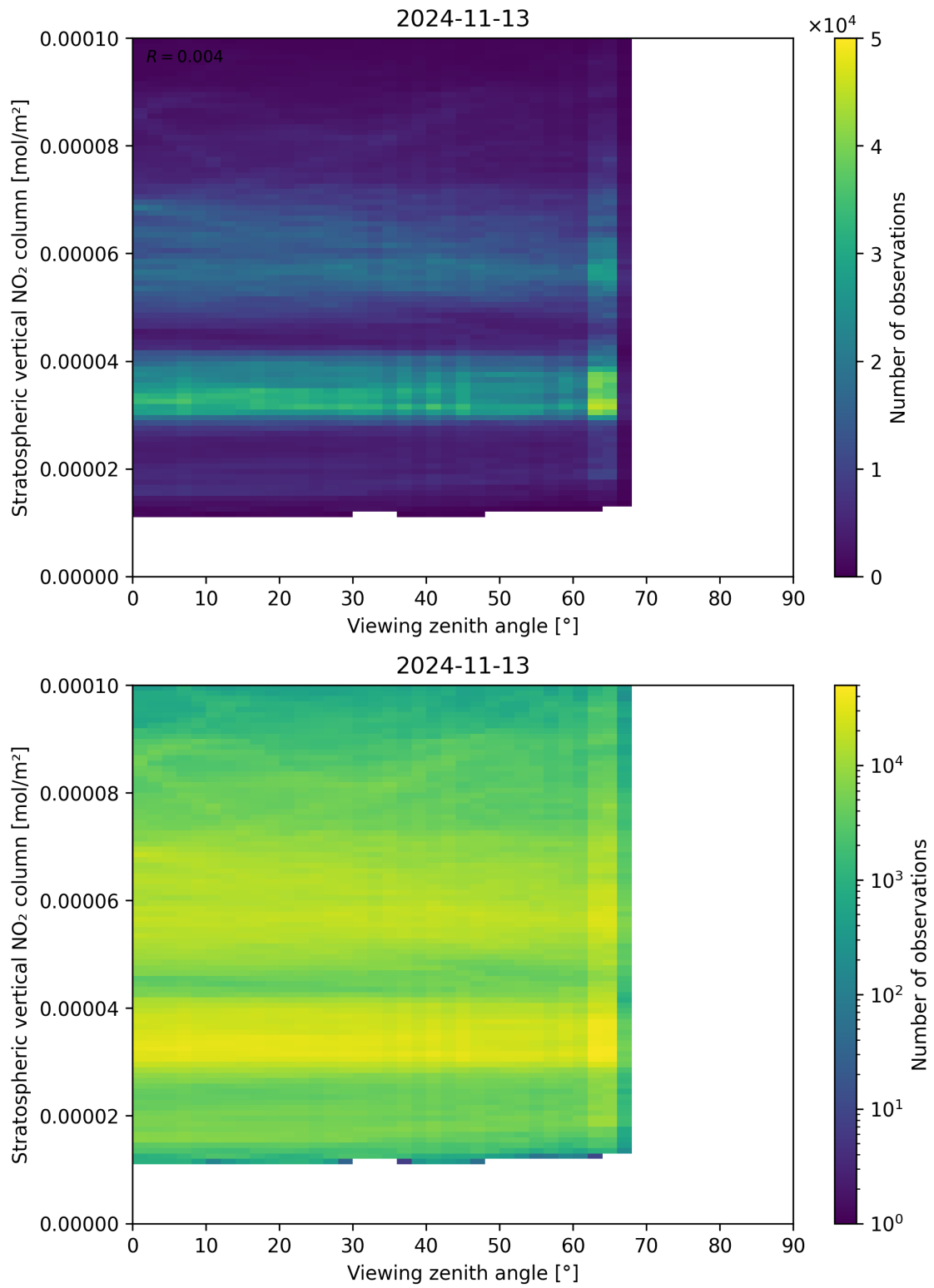
Figure 164: Scatter density plot of “Viewing zenith angle” against “Stratospheric vertical NO 2 column” for 2024-11-12 to 2024-11-14.
