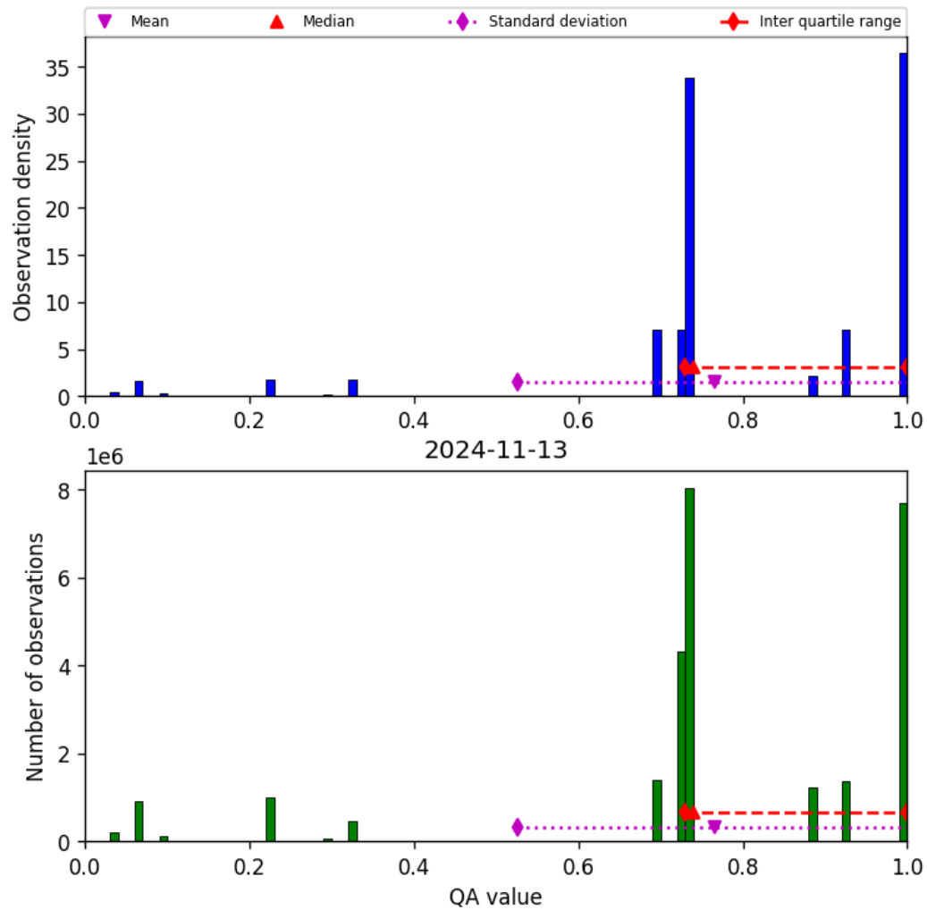
Figure 28: Histogram of “QA value” for 2024-11-12 to 2024-11-14
