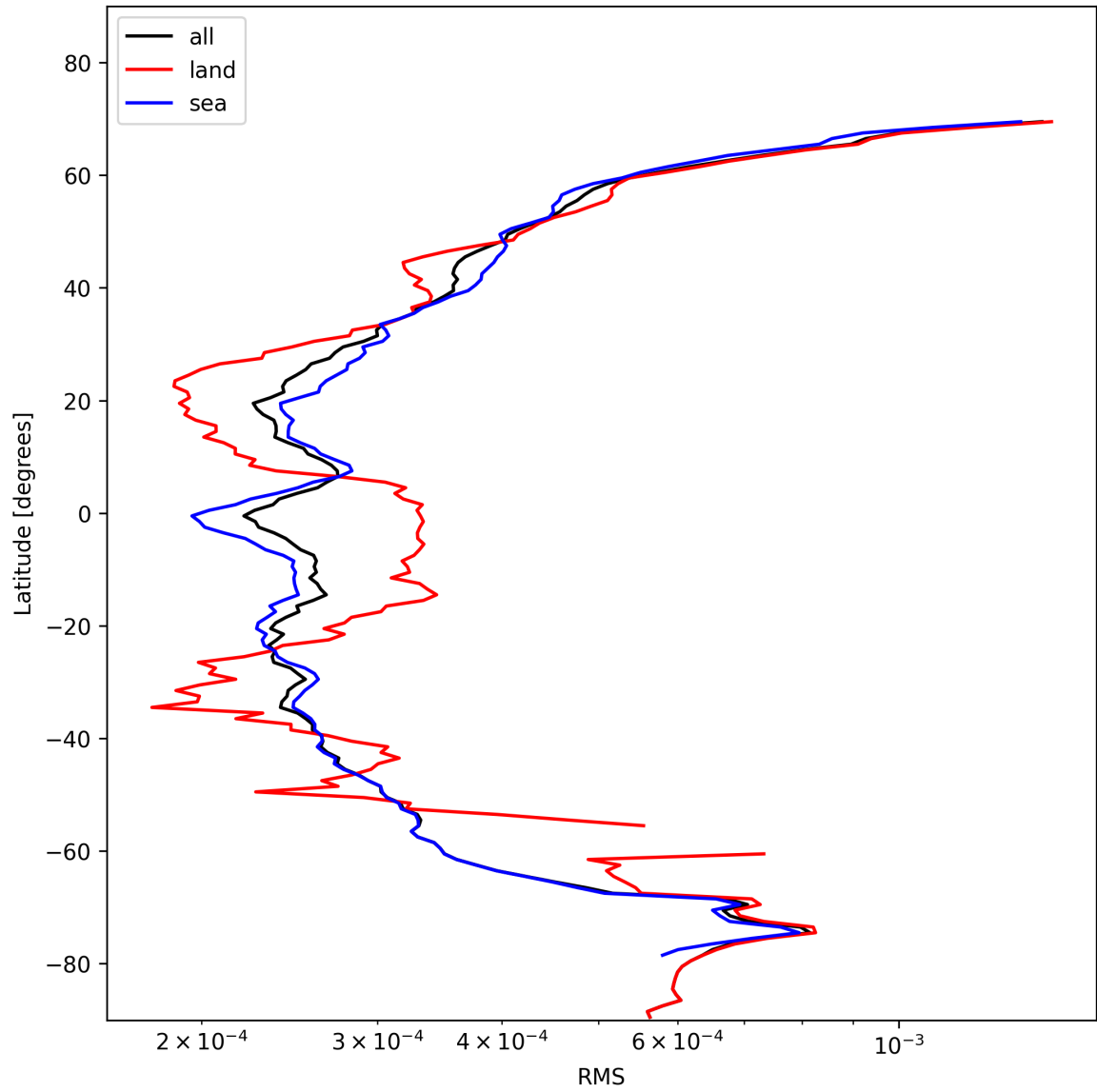
Figure 26: Zonal average of “RMS” for 2024-11-12 to 2024-11-14.
