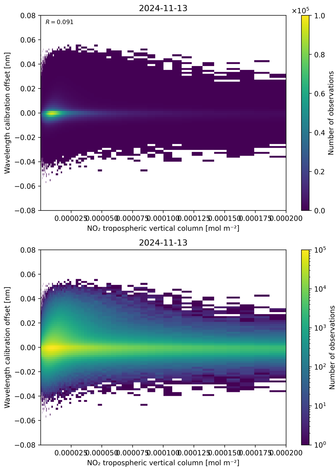
Figure 143: Scatter density plot of “NO 2 tropospheric vertical column” against “Wavelength calibration offset” for 2024-11-12 to 2024-11-14.
