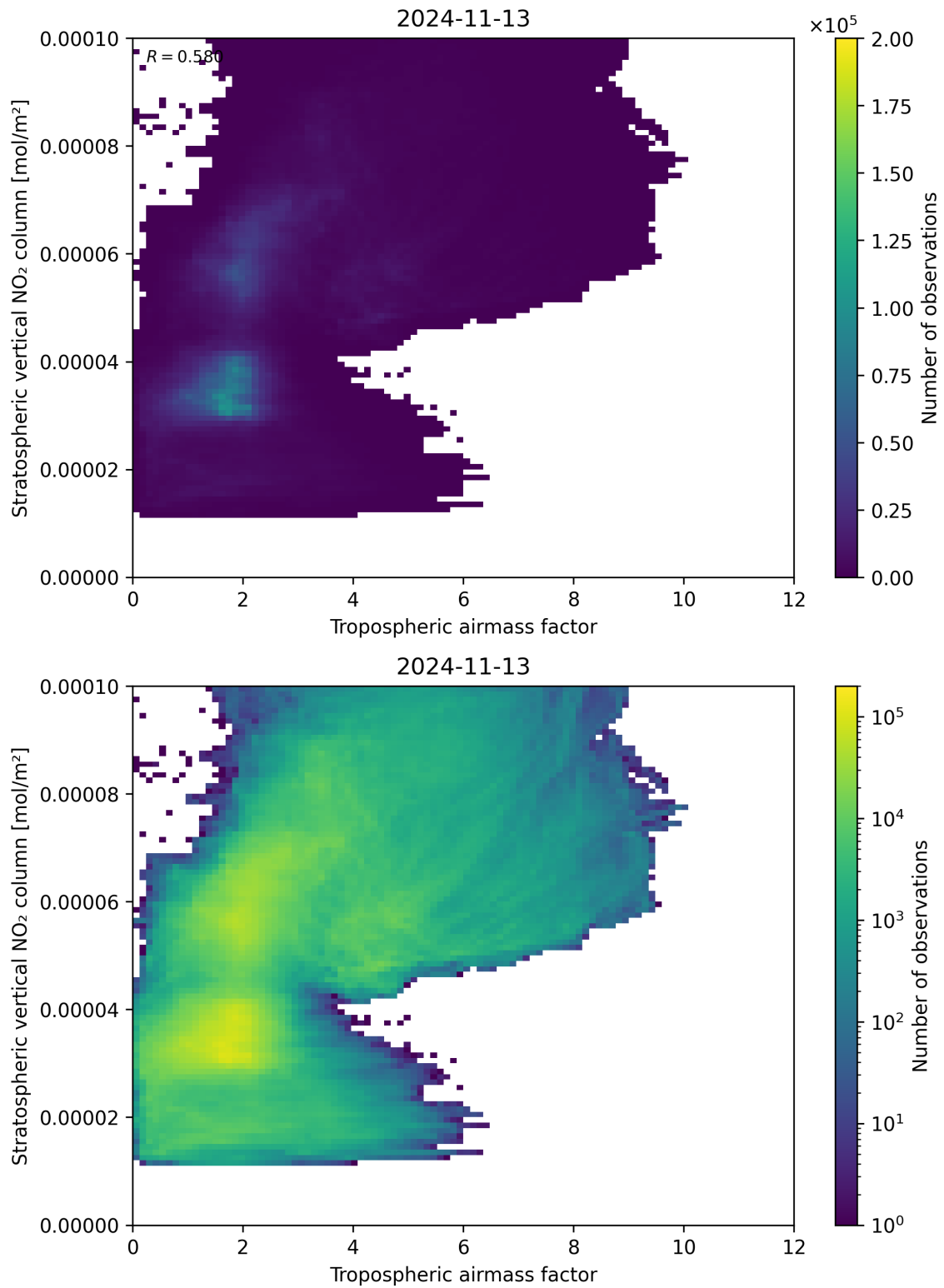
Figure 74: Scatter density plot of “Tropospheric airmass factor” against “Stratospheric vertical NO 2 column” for 2024-11-12 to 2024-11-14.
