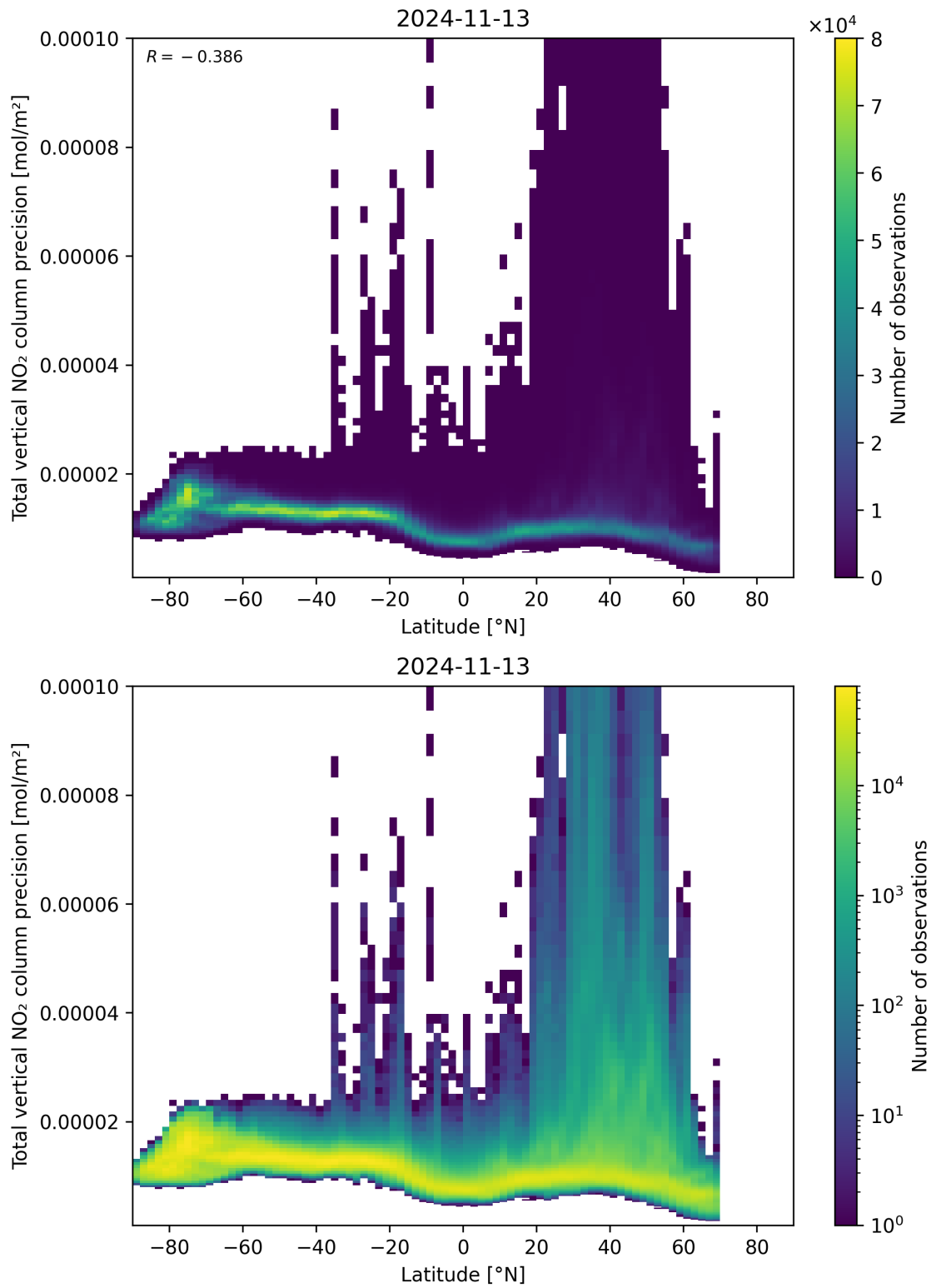
Figure 91: Scatter density plot of “Latitude” against “Total vertical NO 2 column precision” for 2024-11-12 to 2024-11-14.
