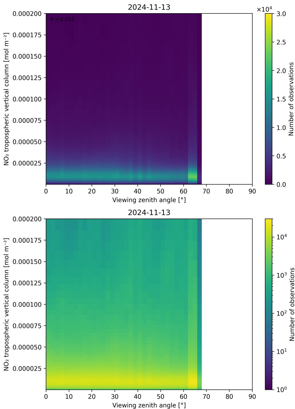
Figure 169: Scatter density plot of “Viewing zenith angle” against “NO 2 tropospheric vertical column” for 2024-11-12 to 2024-11-14.
