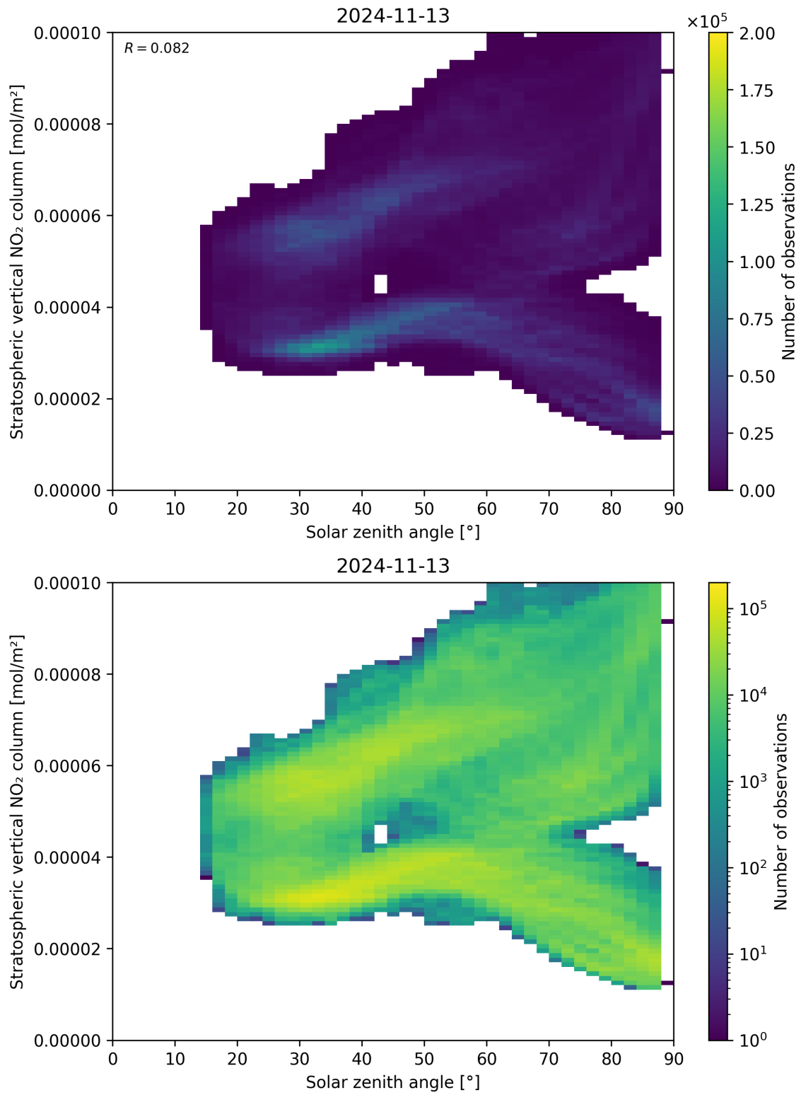
Figure 150: Scatter density plot of “Solar zenith angle” against “Stratospheric vertical NO 2 column” for 2024-11-12 to 2024-11-14.
