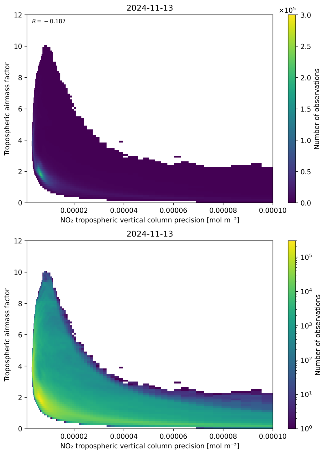
Figure 133: Scatter density plot of “NO 2 tropospheric vertical column precision” against “Tropospheric air mass factor” for 2024-11-12 to 2024-11-14.
