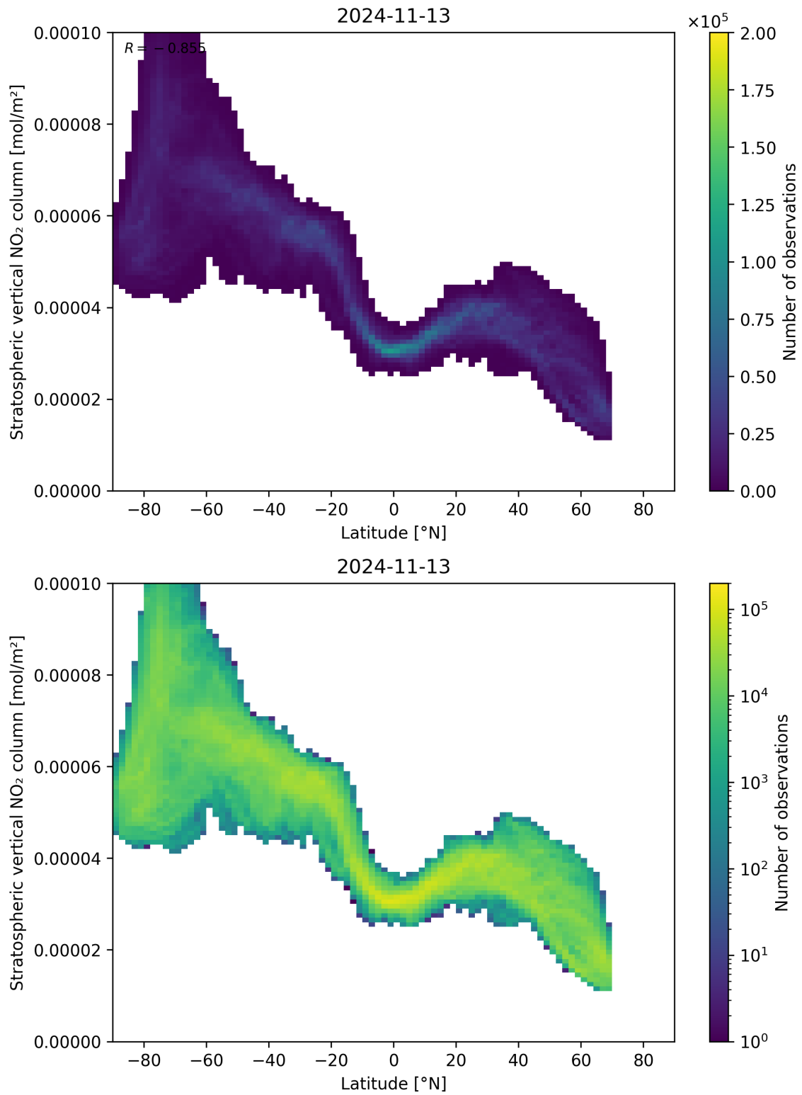
Figure 87: Scatter density plot of “Latitude” against “Stratospheric vertical NO 2 column” for 2024-11-12 to 2024-11-14.
