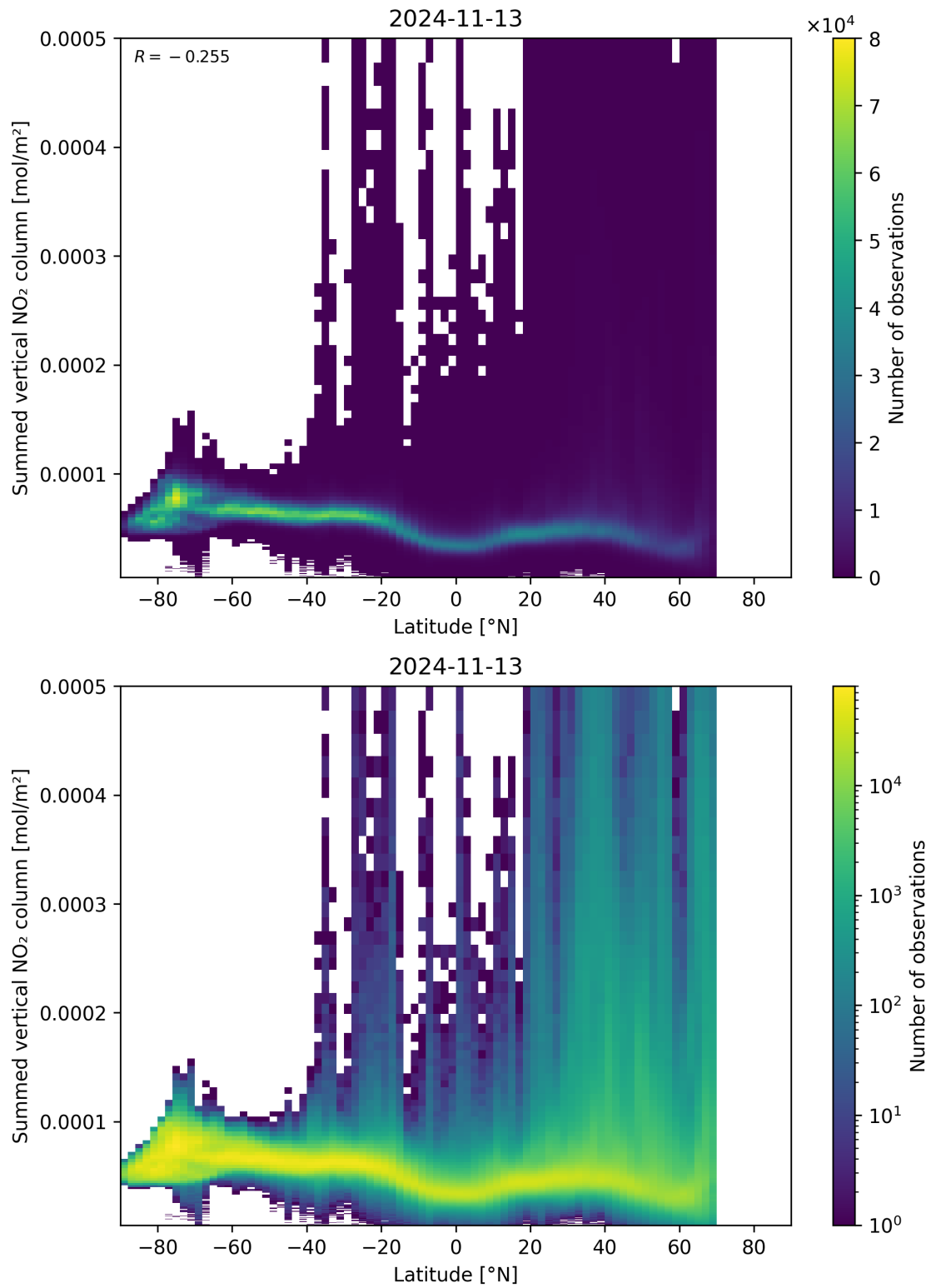
Figure 88: Scatter density plot of “Latitude” against “Summed vertical NO 2 column” for 2024-11-12 to 2024-11-14.
