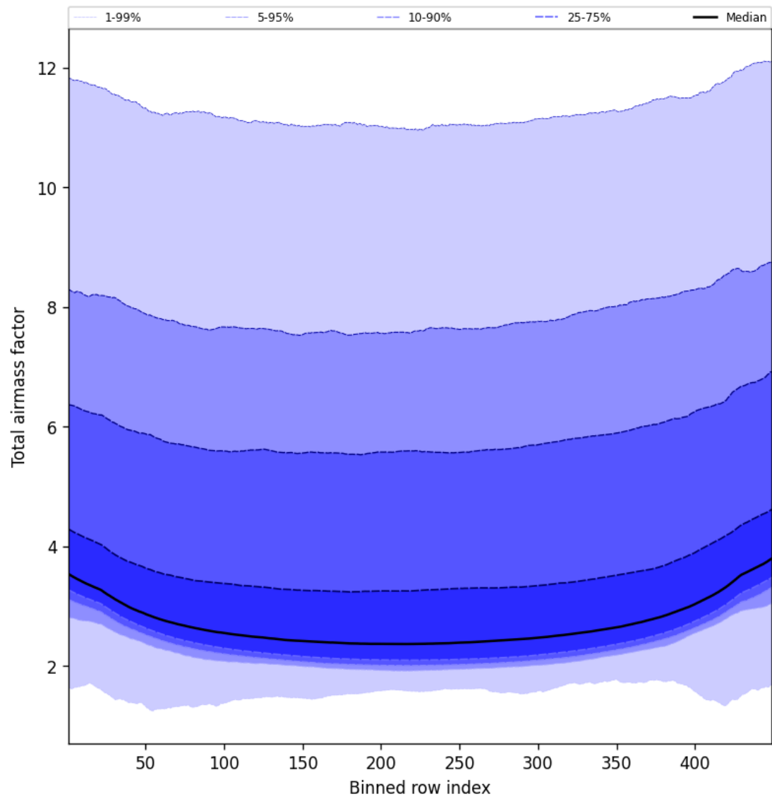
Figure 49: Along track statistics of “Total airmass factor” for 2024-11-12 to 2024-11-14
