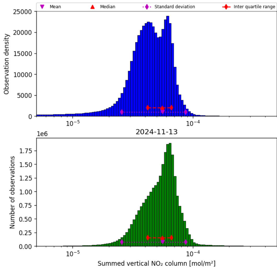
Figure 40: Histogram of “Summed vertical NO 2 column” for 2024-11-12 to 2024-11-14
