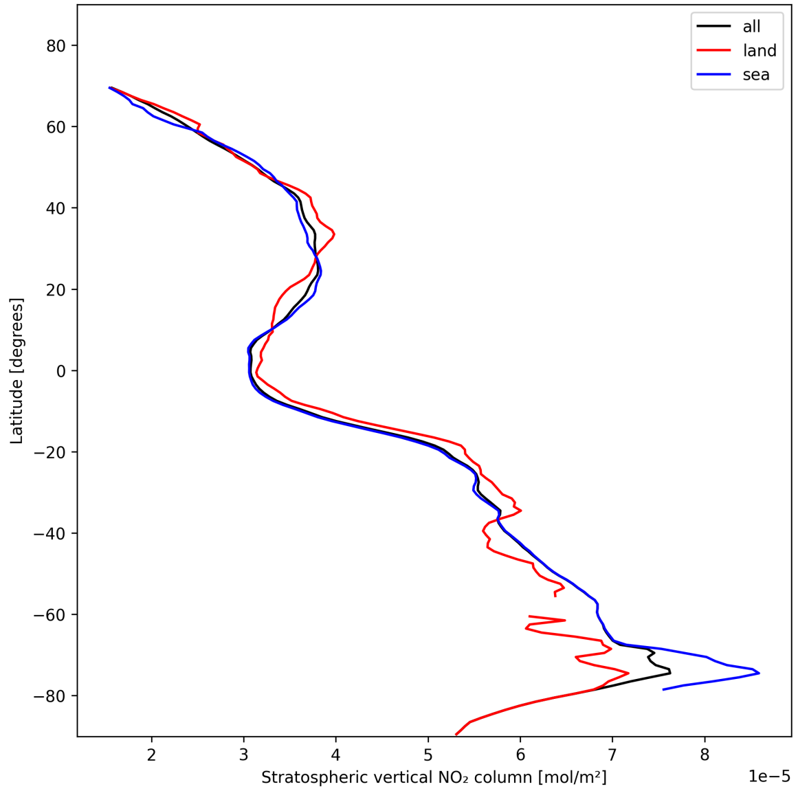
Figure 19: Zonal average of “Stratospheric vertical NO 2 column” for 2024-11-12 to 2024-11-14.
