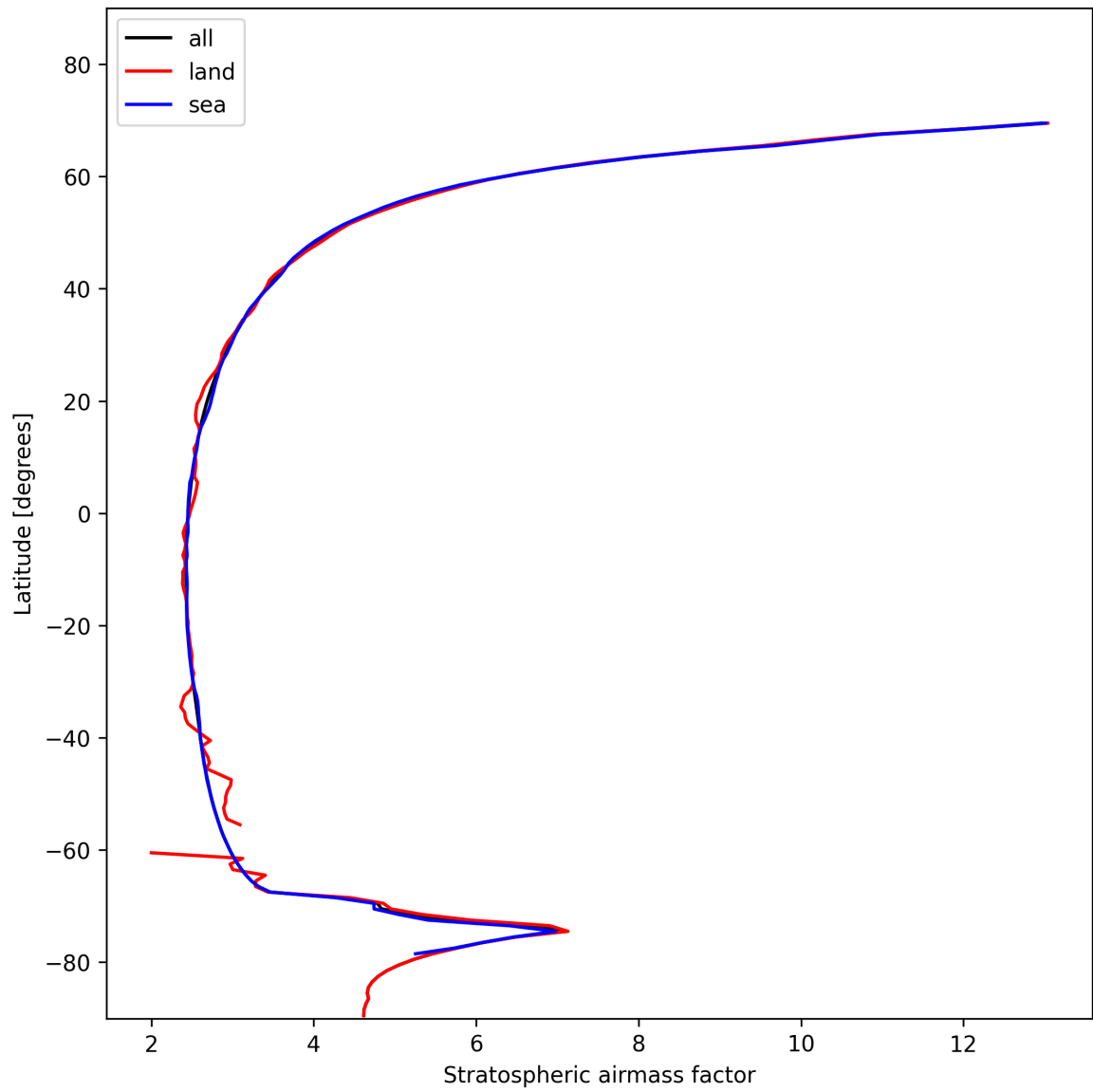
Figure 27: Zonal average of “Stratospheric air mass factor” for 2024-11-12 to 2024-11-14.
