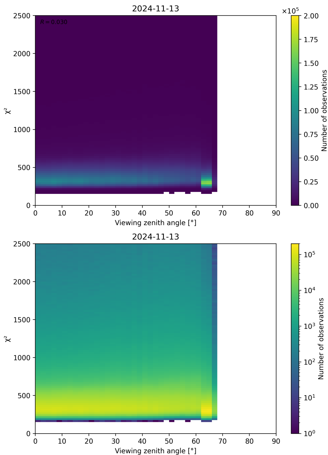
Figure 162: Scatter density plot of “Viewing zenith angle” against “ \chi^2 ” for 2024-11-12 to 2024-11-14.
