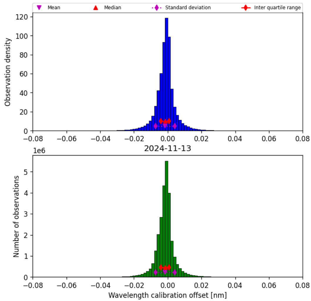
Figure 35: Histogram of “Wavelength calibration offset” for 2024-11-12 to 2024-11-14
