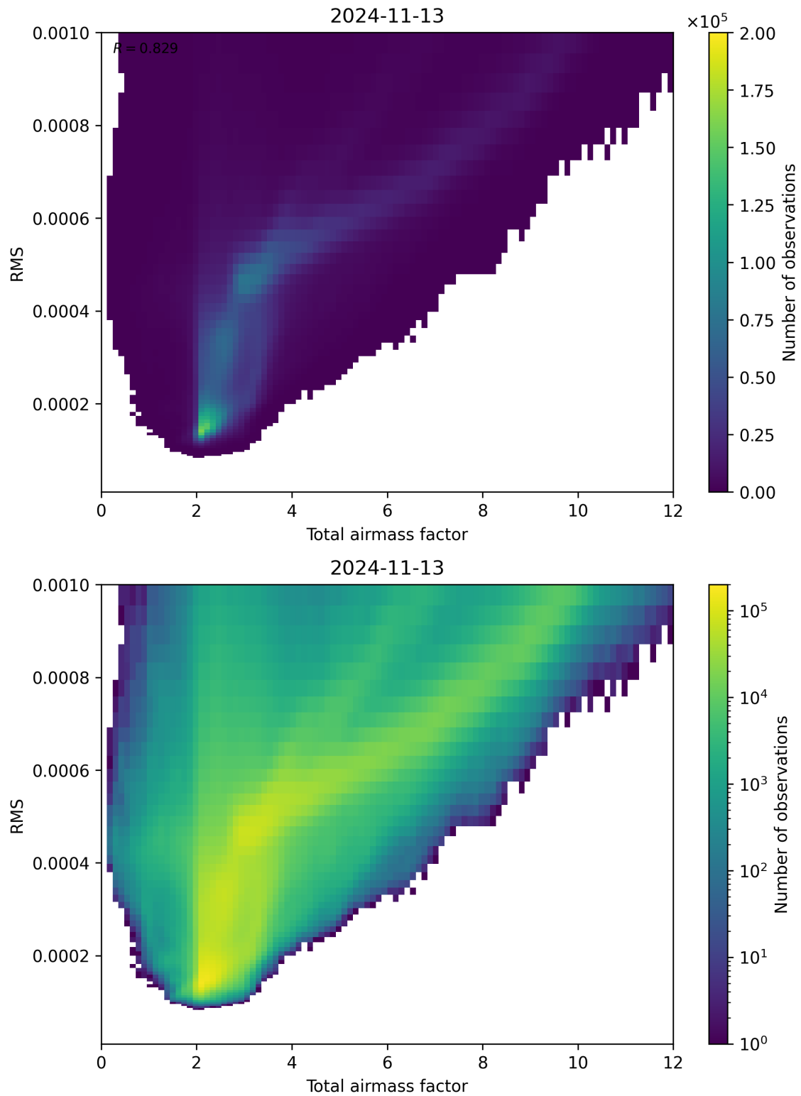
Figure 69: Scatter density plot of “Total airmass factor” against “RMS” for 2024-11-12 to 2024-11-14.
