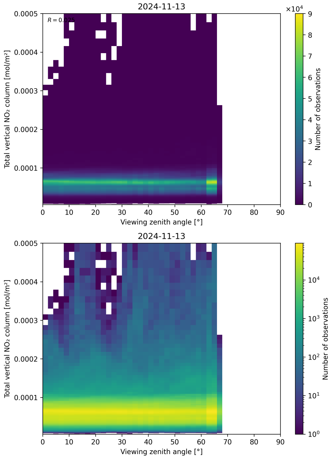
Figure 167: Scatter density plot of “Viewing zenith angle” against “Total vertical NO 2 column” for 2024-11-12 to 2024-11-14.
