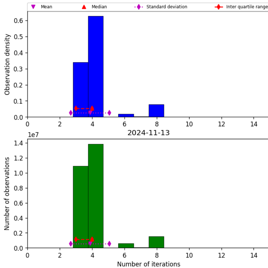
Figure 34: Histogram of “Number of iterations” for 2024-11-12 to 2024-11-14
