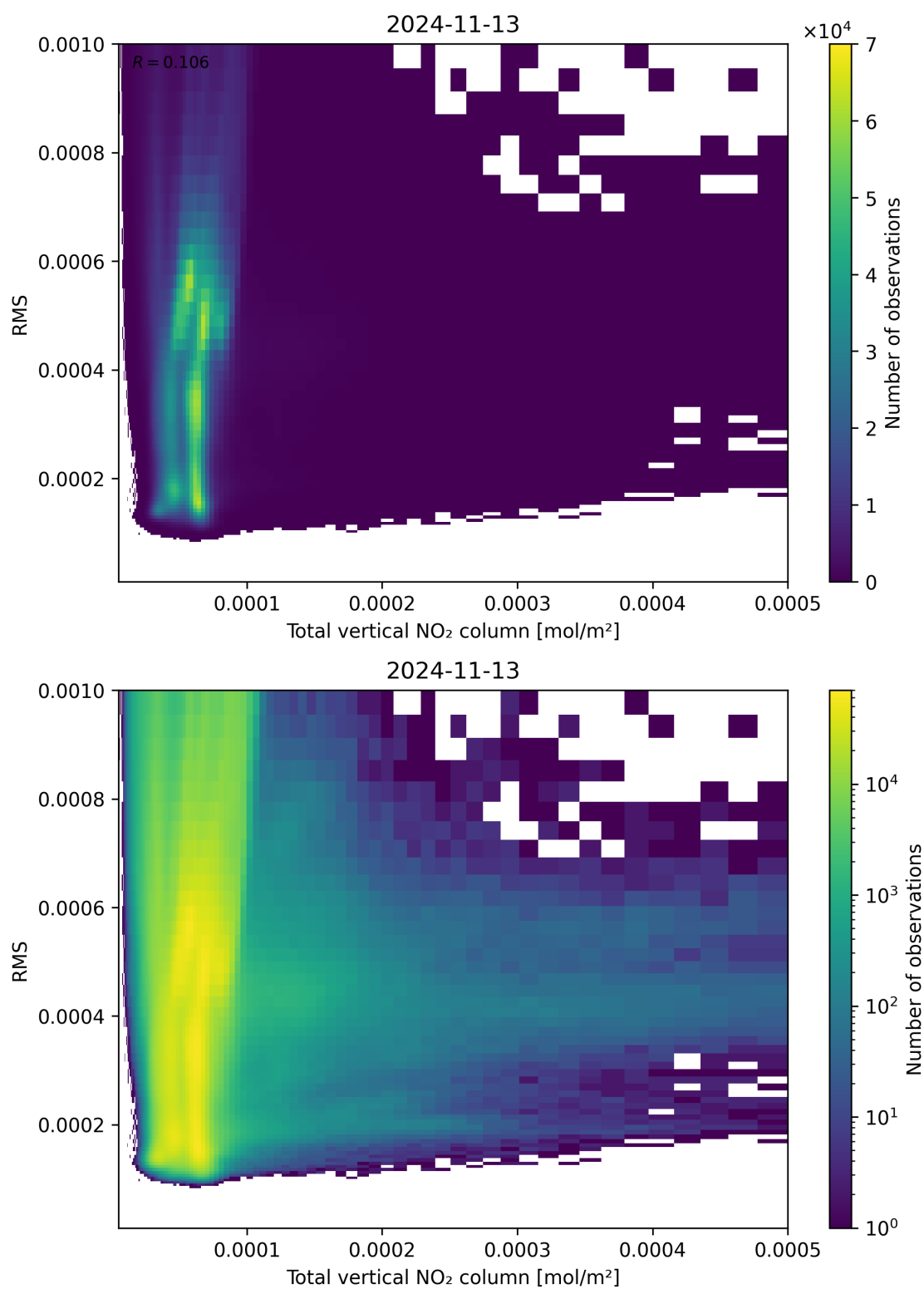
Figure 120: Scatter density plot of “Total vertical NO 2 column” against “RMS” for 2024-11-12 to 2024-11-14.
