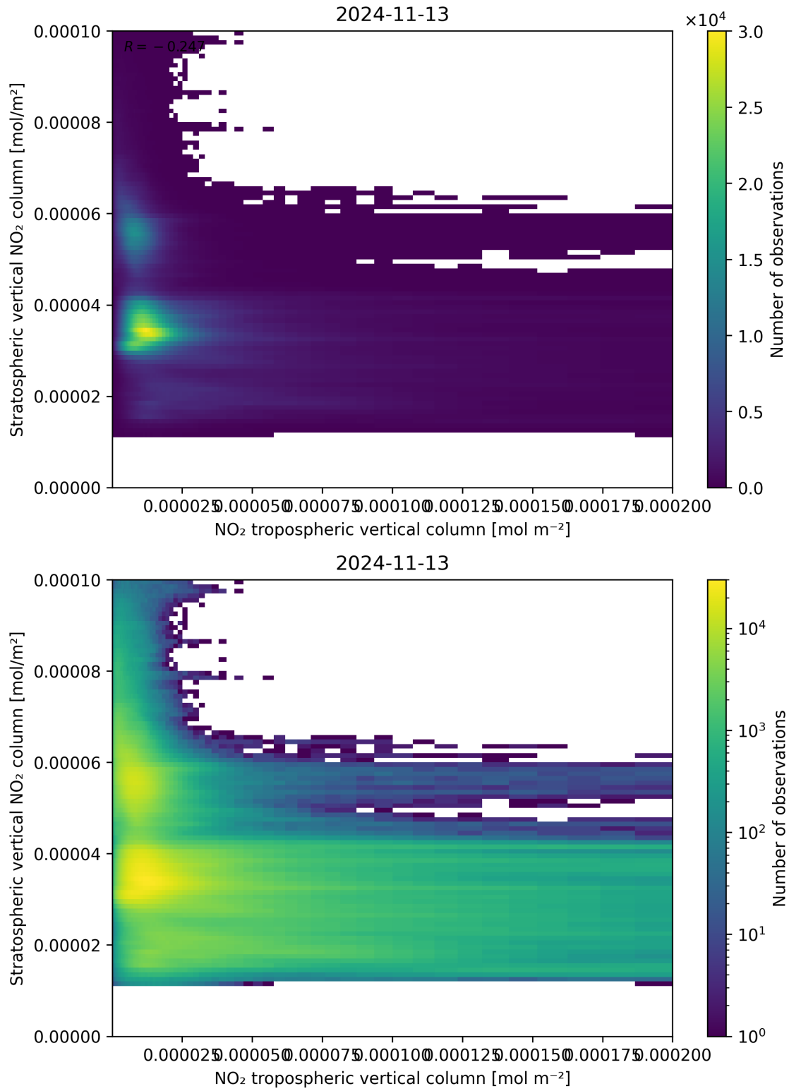
Figure 125: Scatter density plot of “NO 2 tropospheric vertical column” against “Stratospheric vertical NO 2 column” for 2024-11-12 to 2024-11-14.
