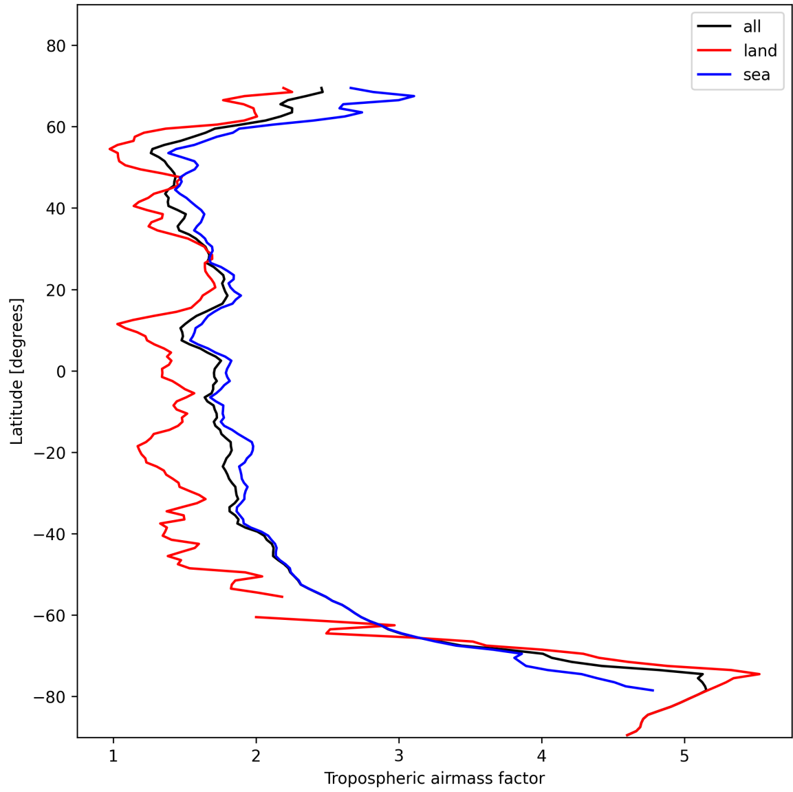
Figure 14: Zonal average of “Tropospheric airmass factor” for 2024-11-12 to 2024-11-14.
