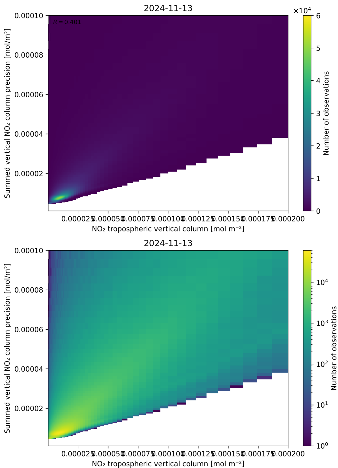
Figure 127: Scatter density plot of “NO 2 tropospheric vertical column” against “Summed vertical NO 2 column precision” for 2024-11-12 to 2024-11-14.
