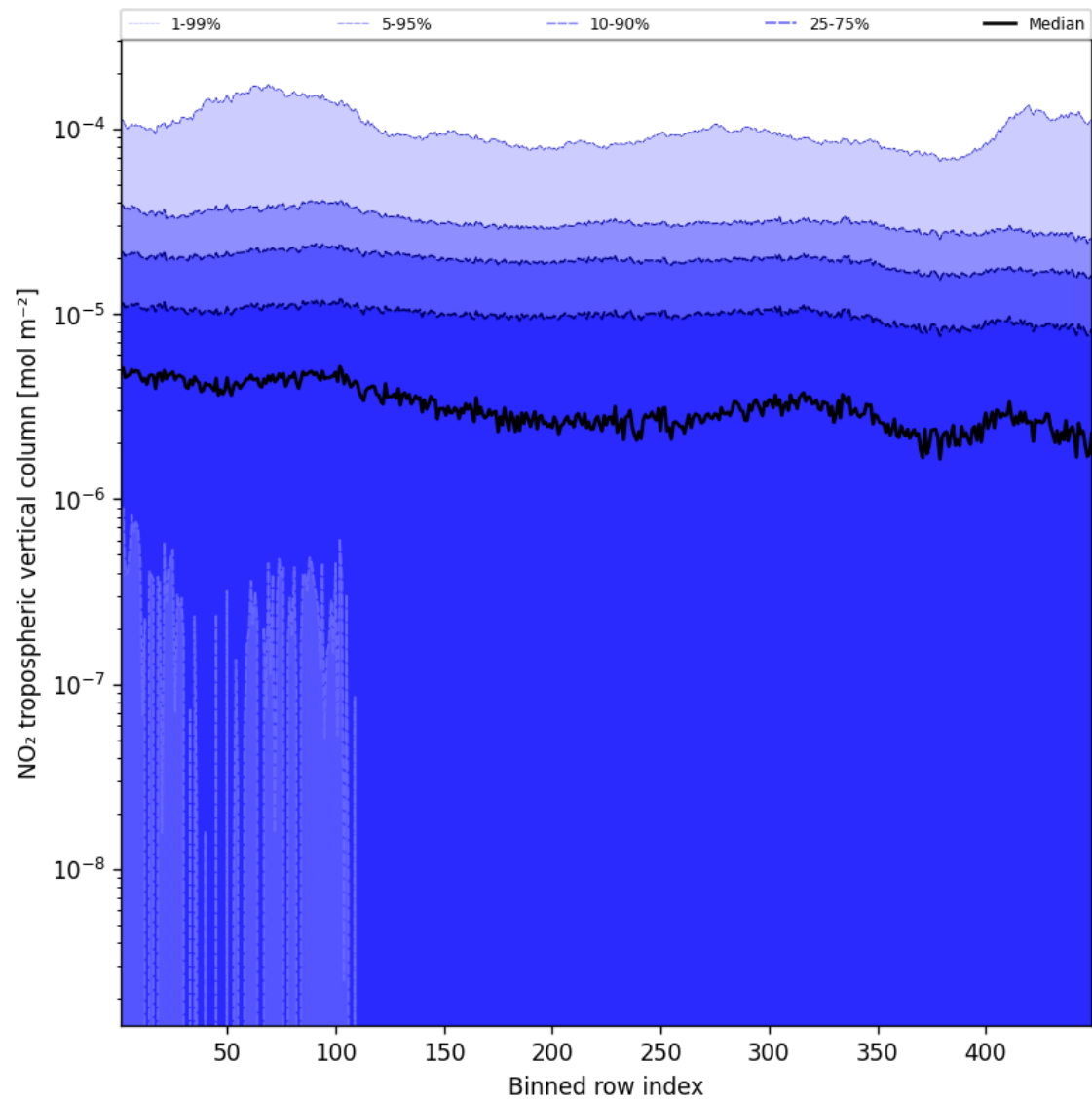
Figure 46: Along track statistics of “NO 2 tropospheric vertical column” for 2024-11-12 to 2024-11-14
