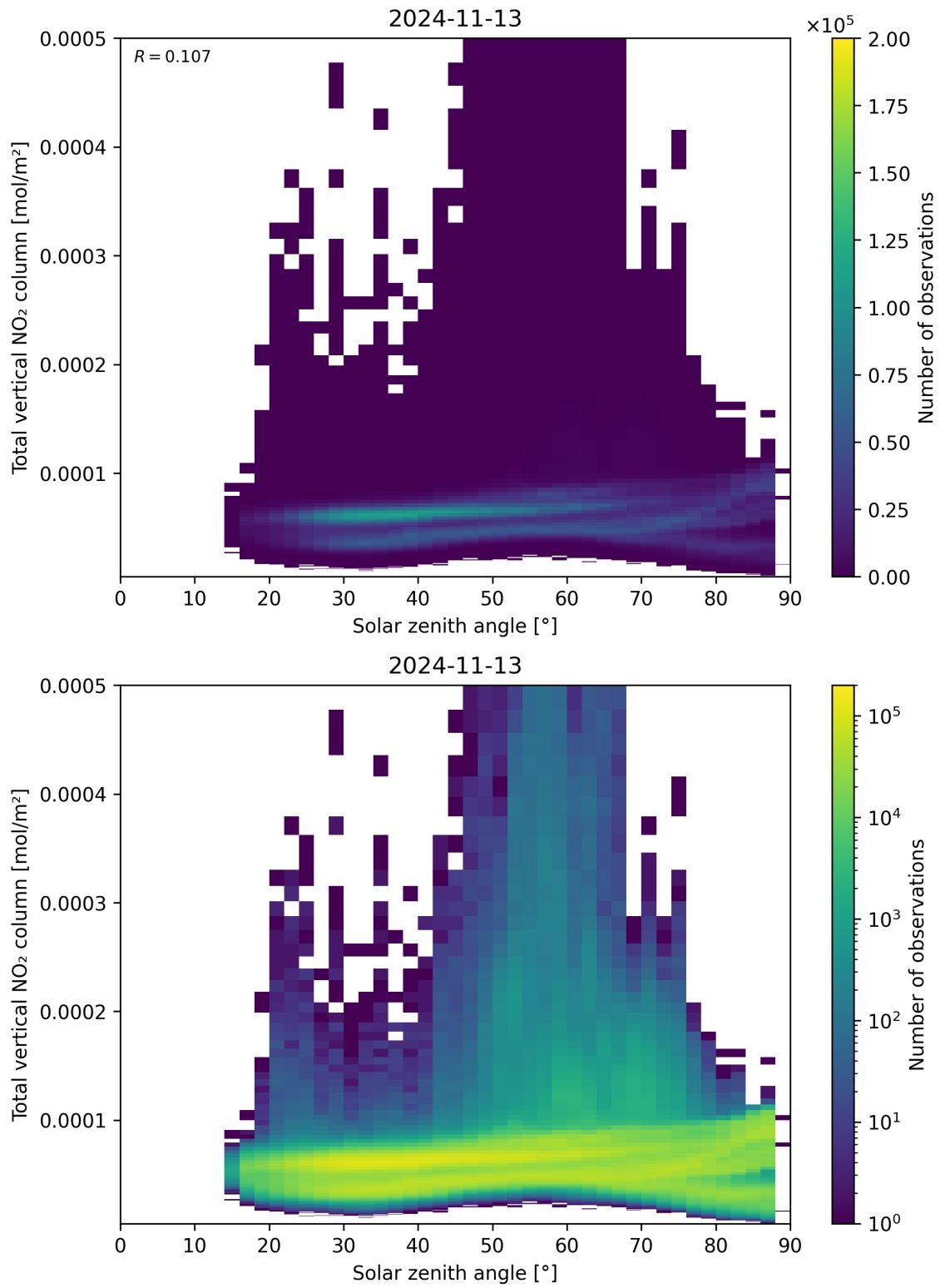
Figure 153: Scatter density plot of “Solar zenith angle” against “Total vertical NO 2 column” for 2024-11-12 to 2024-11-14.
