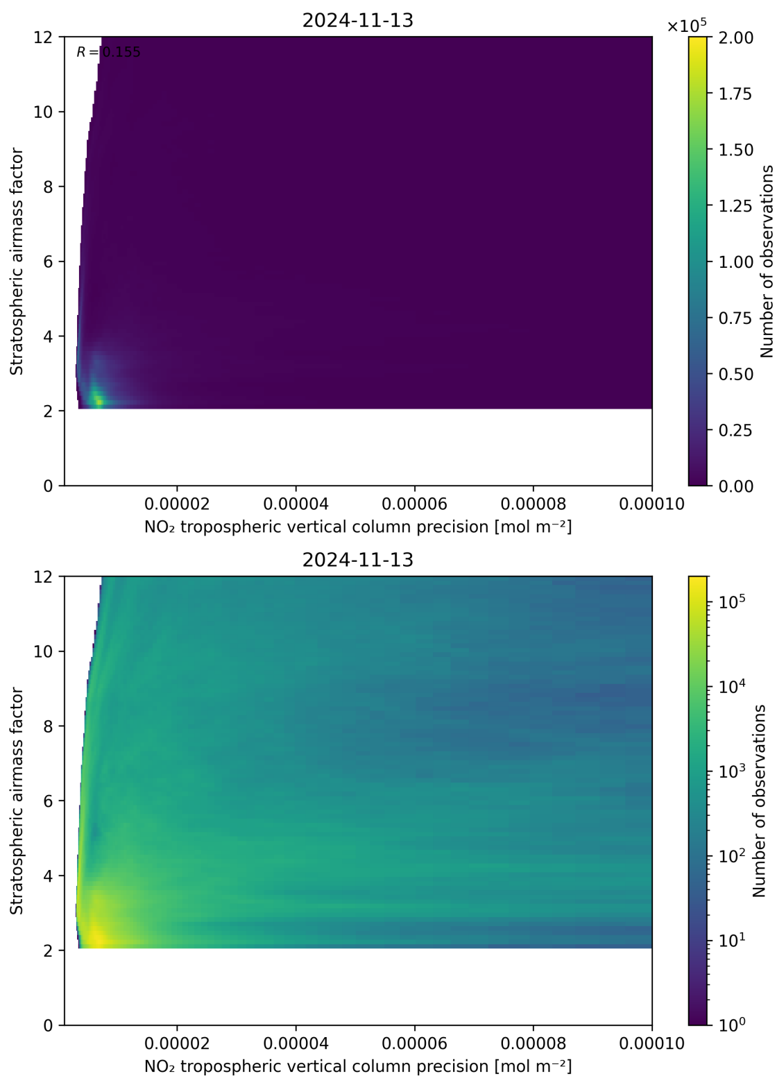
Figure 131: Scatter density plot of “NO 2 tropospheric vertical column precision” against “Stratospheric airmass factor” for 2024-11-12 to 2024-11-14.
