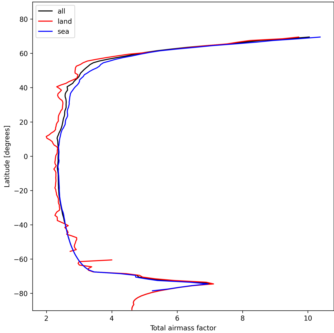
Figure 15: Zonal average of “Total airmass factor” for 2024-11-12 to 2024-11-14.
