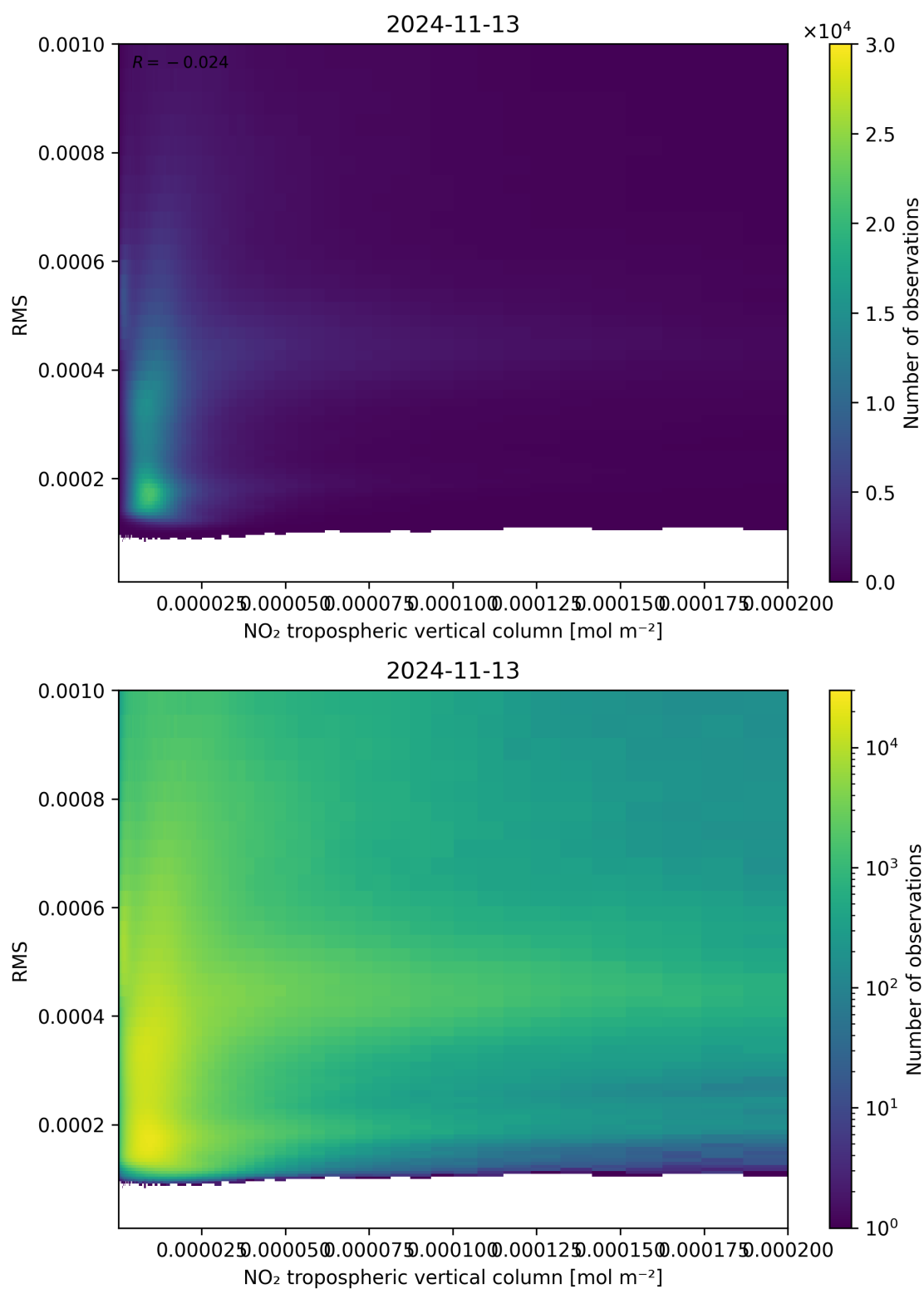
Figure 142: Scatter density plot of “NO 2 tropospheric vertical column” against “RMS” for 2024-11-12 to 2024-11-14.
