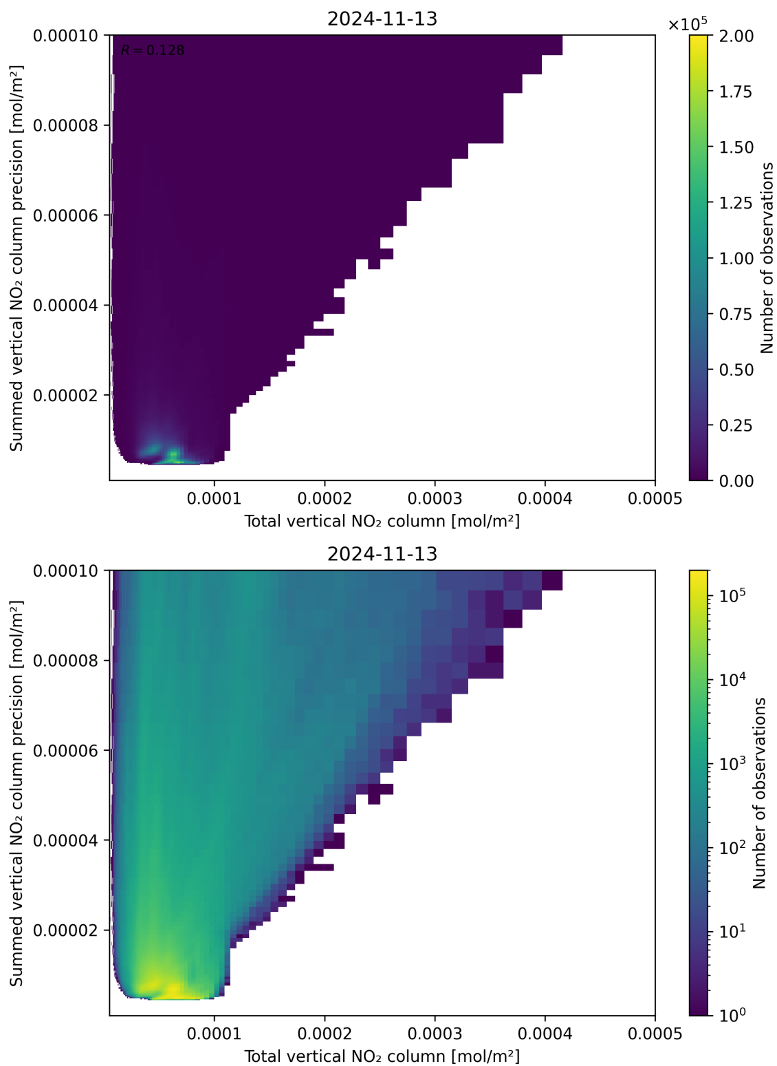
Figure 113: Scatter density plot of “Total vertical NO 2 column” against “Summed vertical NO 2 column precision” for 2024-11-12 to 2024-11-14.
