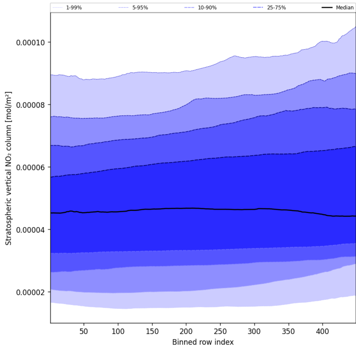
Figure 53: Along track statistics of “Stratospheric vertical NO 2 column” for 2024-11-12 to 2024-11-14
