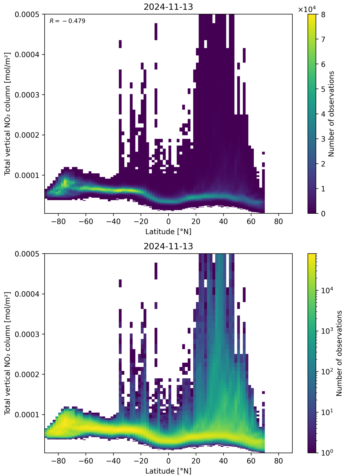
Figure 90: Scatter density plot of “Latitude” against “Total vertical NO 2 column” for 2024-11-12 to 2024-11-14.
