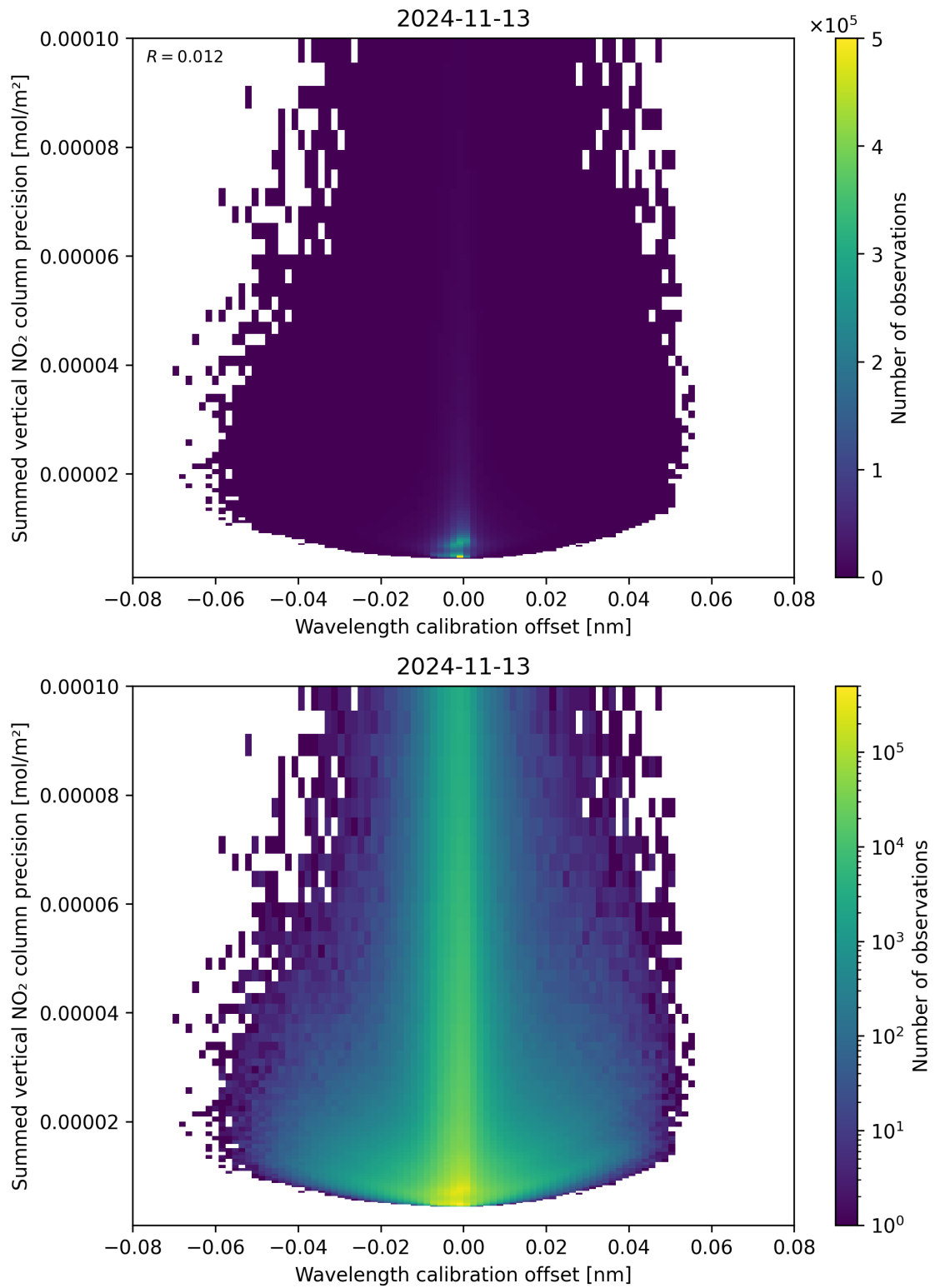
Figure 178: Scatter density plot of “Wavelength calibration offset” against “Summed vertical NO 2 column precision” for 2024-11-12 to 2024-11-14.
