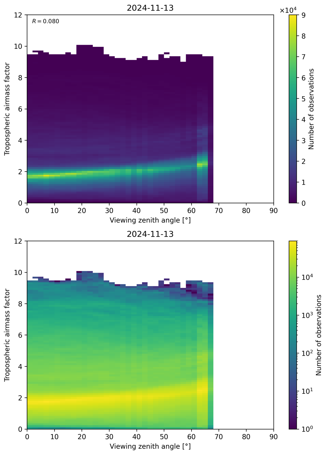
Figure 161: Scatter density plot of “Viewing zenith angle” against “Tropospheric airmass factor” for 2024-11-12 to 2024-11-14.
