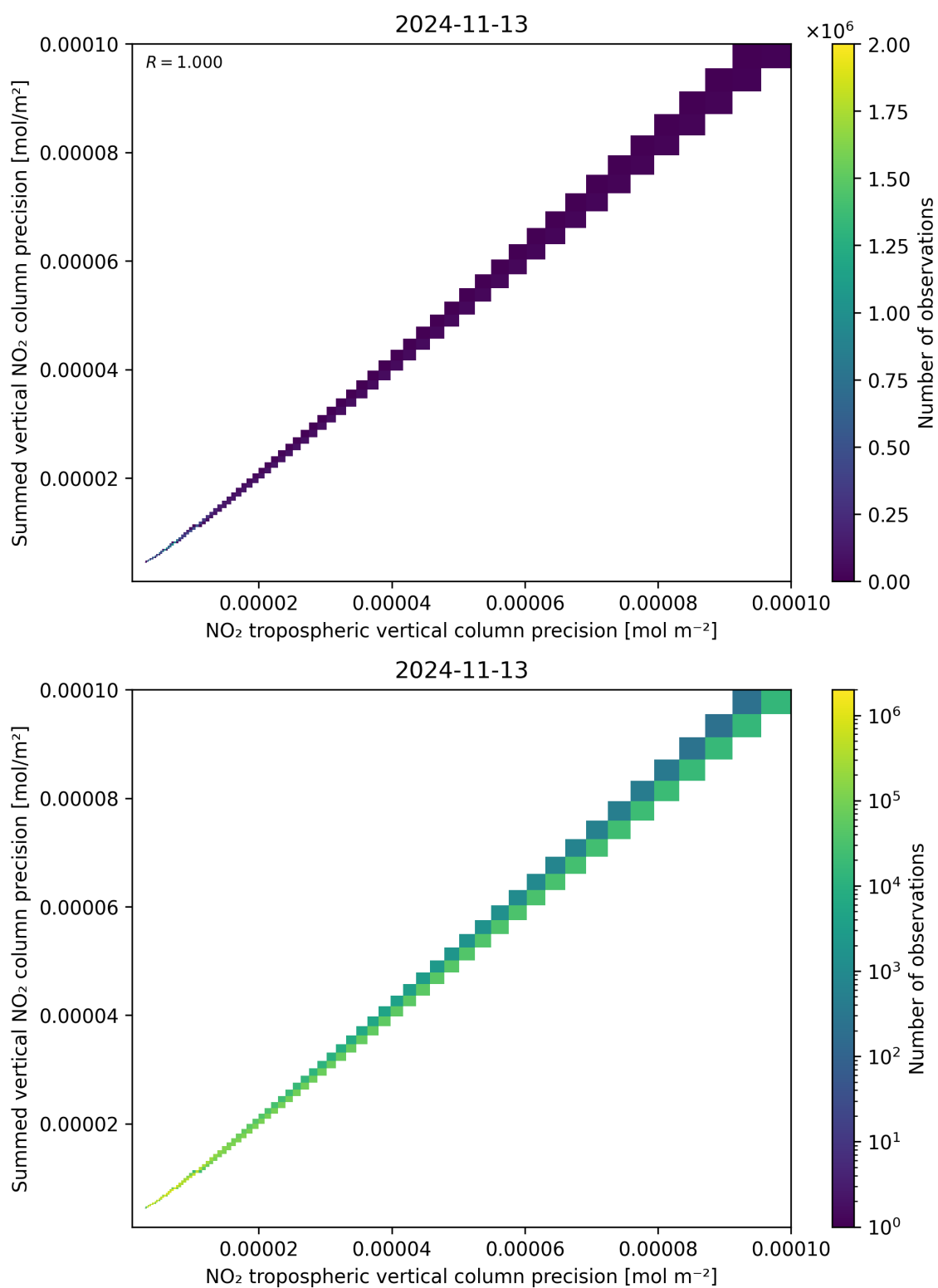
Figure 137: Scatter density plot of “NO 2 tropospheric vertical column precision” against “Summed vertical NO 2 column precision” for 2024-11-12 to 2024-11-14.
