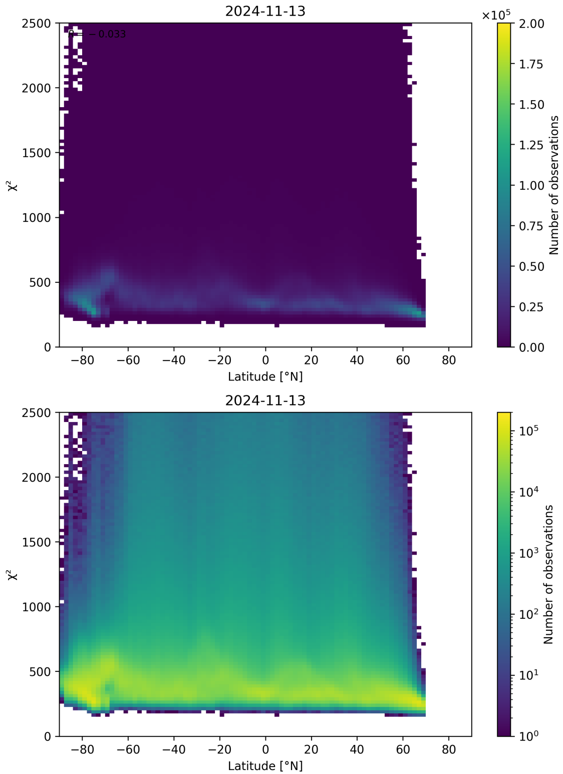
Figure 86: Scatter density plot of “Latitude” against “ \chi^2 ” for 2024-11-12 to 2024-11-14.
