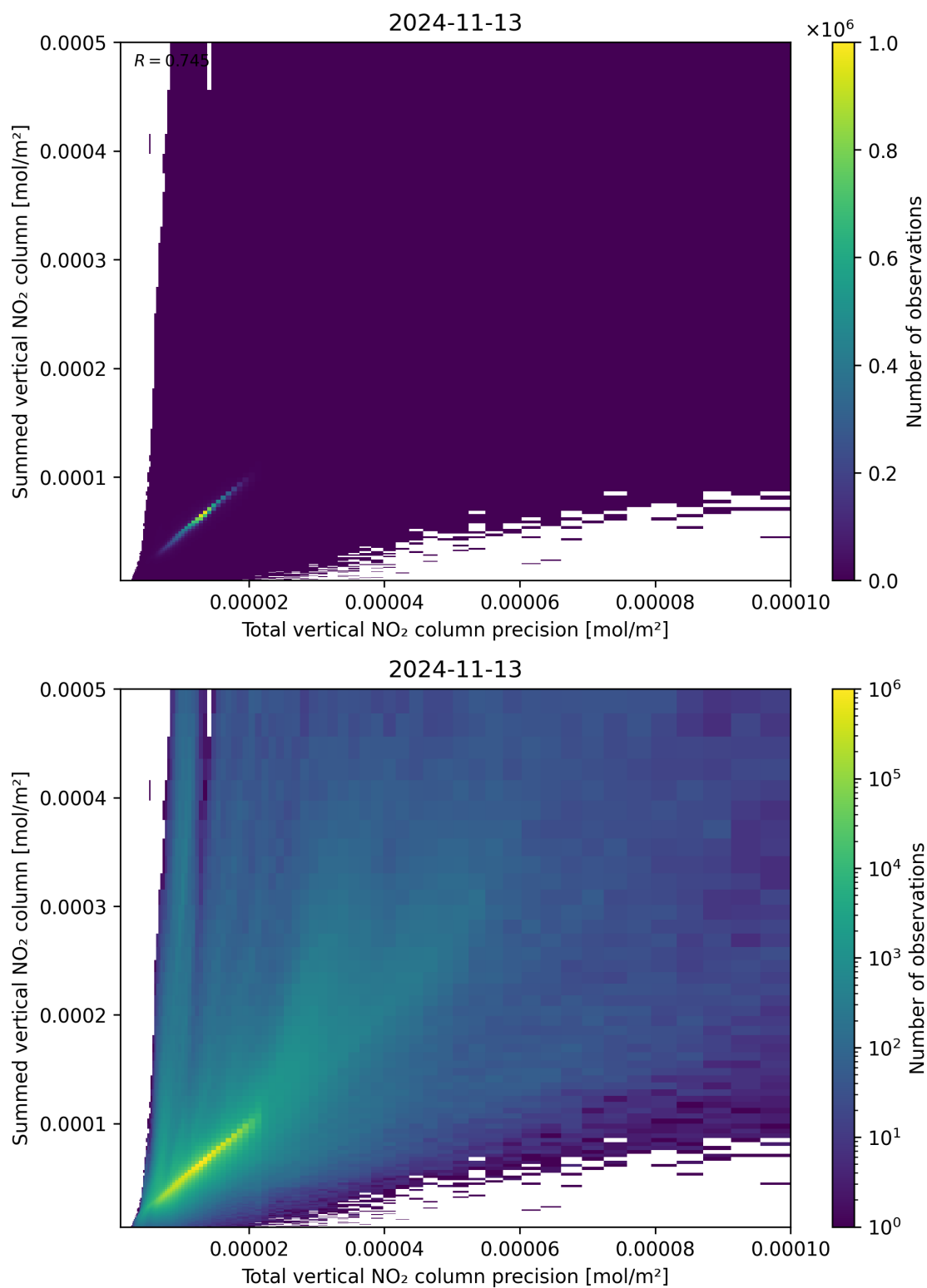
Figure 117: Scatter density plot of “Total vertical NO 2 column precision” against “Summed vertical NO 2 column” for 2024-11-12 to 2024-11-14.
