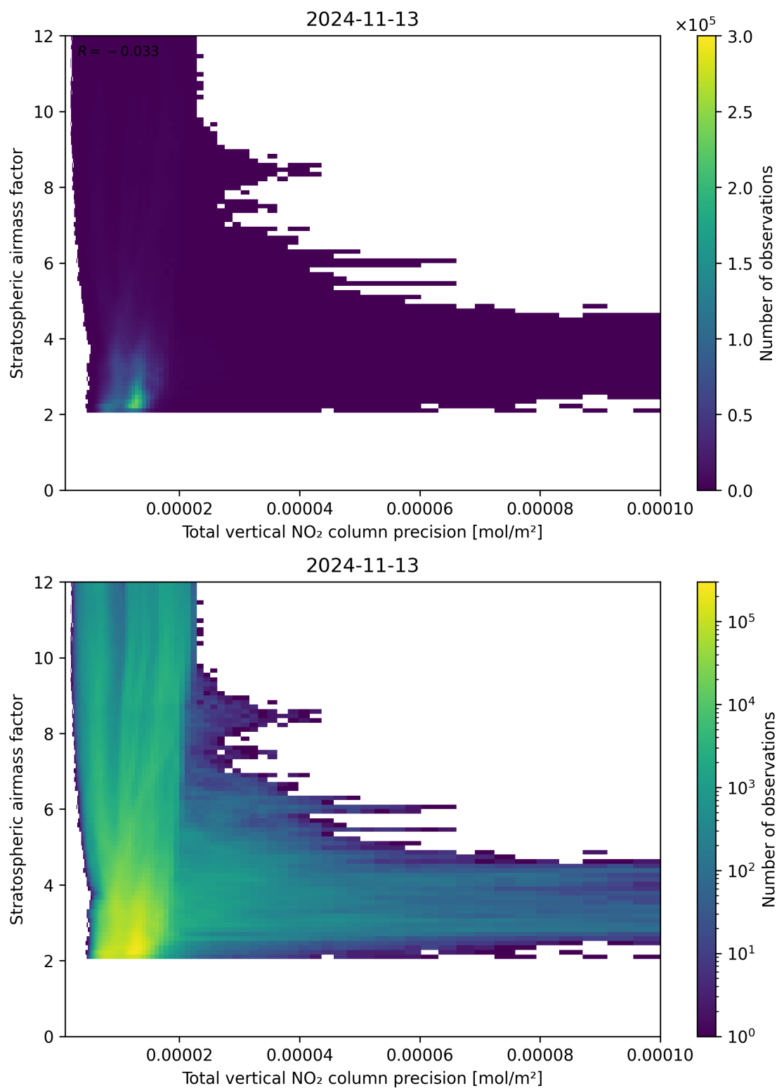
Figure 115: Scatter density plot of “Total vertical NO 2 column precision” against “Stratospheric air mass factor” for 2024-11-12 to 2024-11-14.
