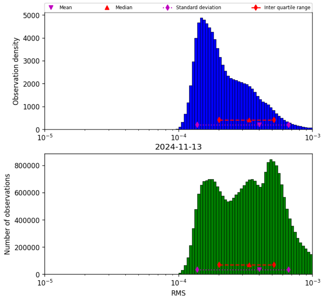
Figure 43: Histogram of “RMS” for 2024-11-12 to 2024-11-14
