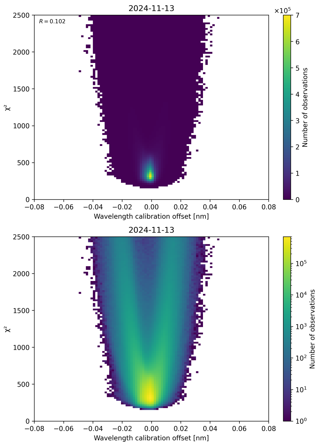
Figure 175: Scatter density plot of “Wavelength calibration offset” against “ \chi^2 ” for 2024-11-12 to 2024-11-14.
