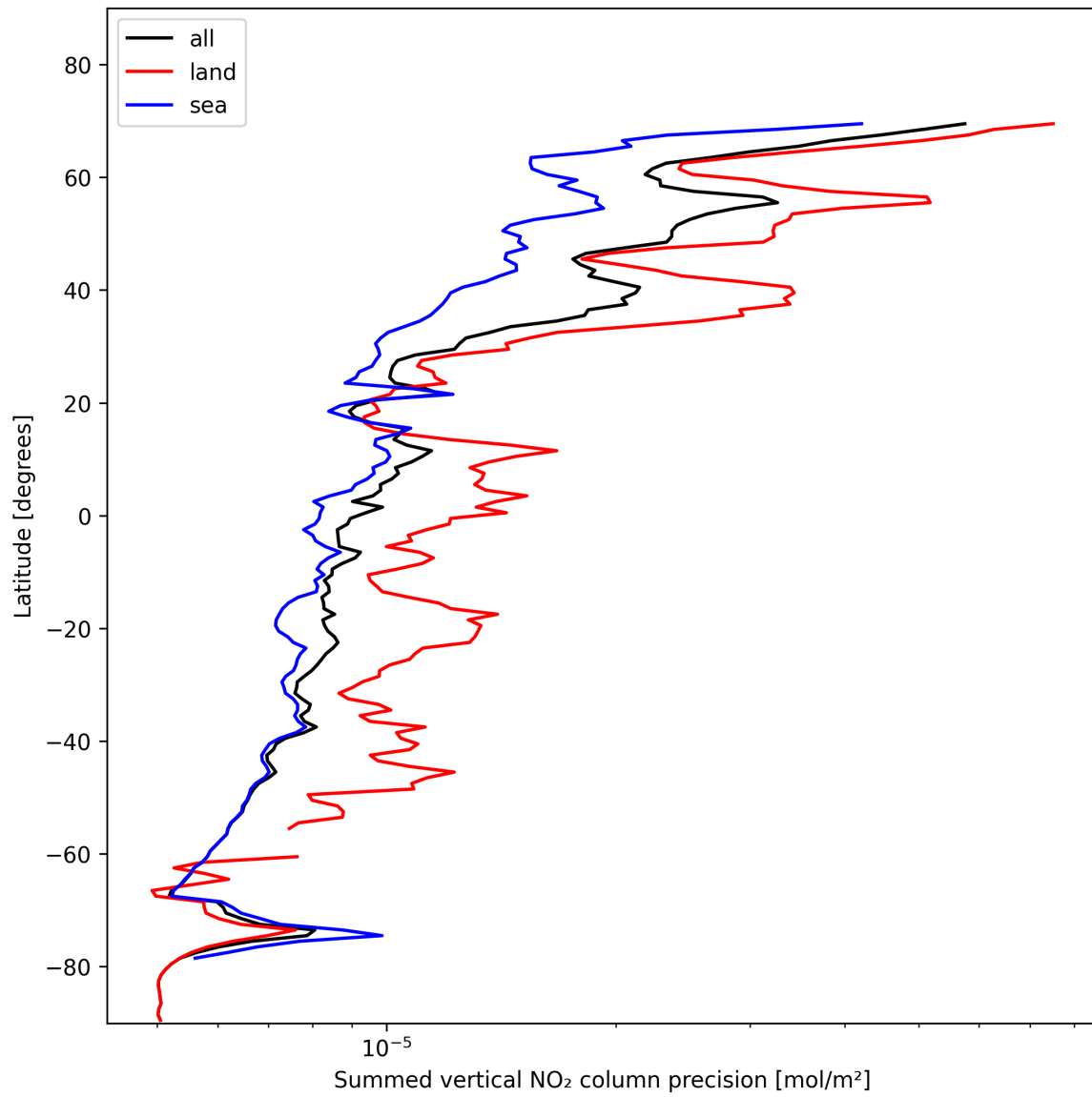
Figure 24: Zonal average of “Summed vertical NO 2 column precision” for 2024-11-12 to 2024-11-14.
