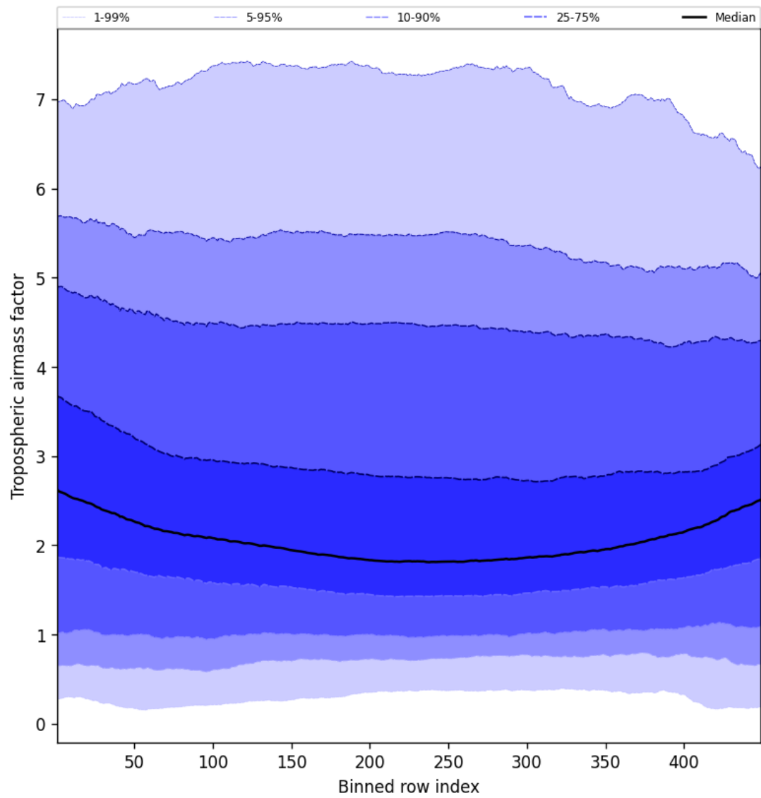
Figure 48: Along track statistics of “Tropospheric air mass factor” for 2024-11-12 to 2024-11-14
