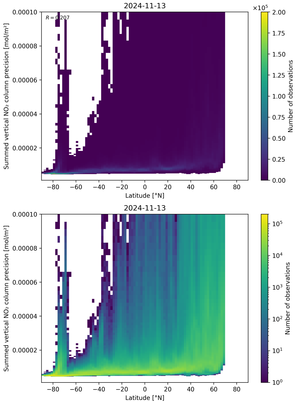
Figure 89: Scatter density plot of “Latitude” against “Summed vertical NO 2 column precision” for 2024-11-12 to 2024-11-14.
