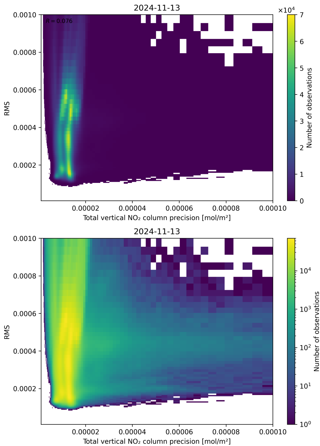
Figure 119: Scatter density plot of “Total vertical NO 2 column precision” against “RMS” for 2024-11-12 to 2024-11-14.
