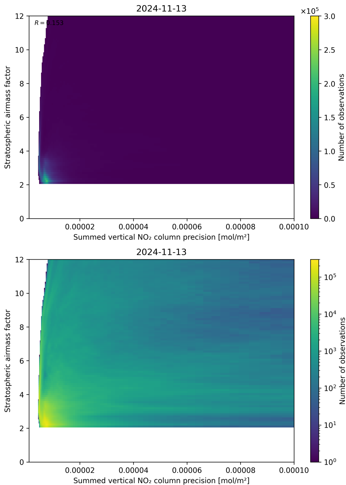
Figure 106: Scatter density plot of “Summed vertical NO 2 column precision” against “Stratospheric airmass factor” for 2024-11-12 to 2024-11-14.
