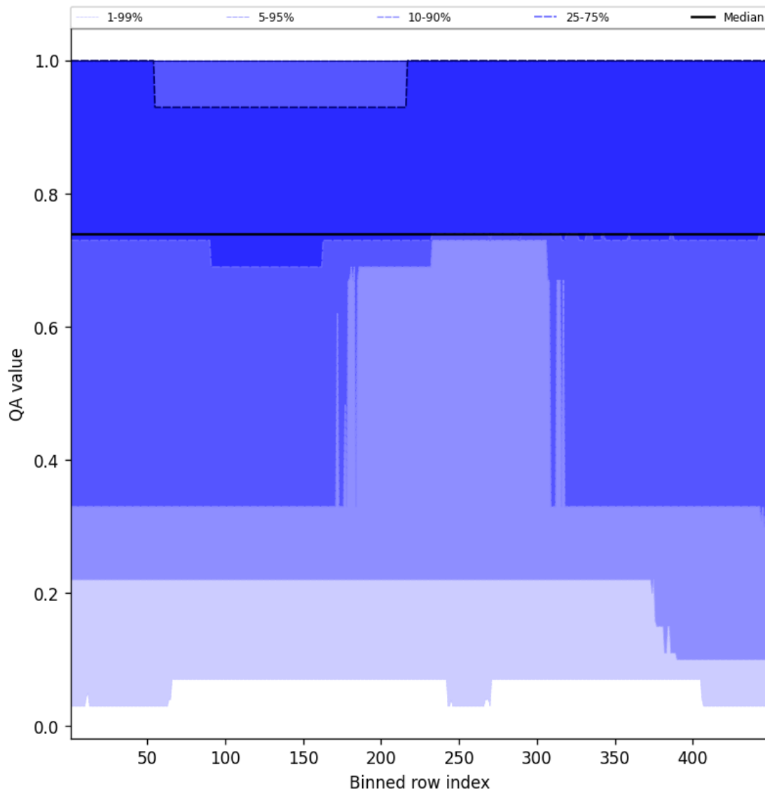
Figure 45: Along track statistics of “QA value” for 2024-11-12 to 2024-11-14
