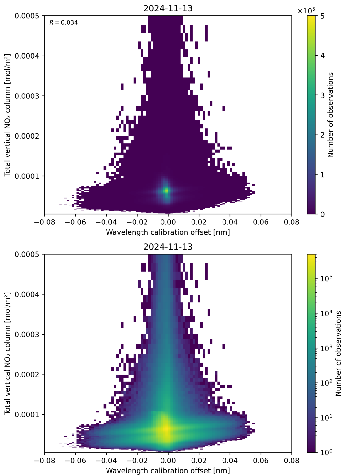
Figure 179: Scatter density plot of “Wavelength calibration offset” against “Total vertical NO 2 column” for 2024-11-12 to 2024-11-14.
