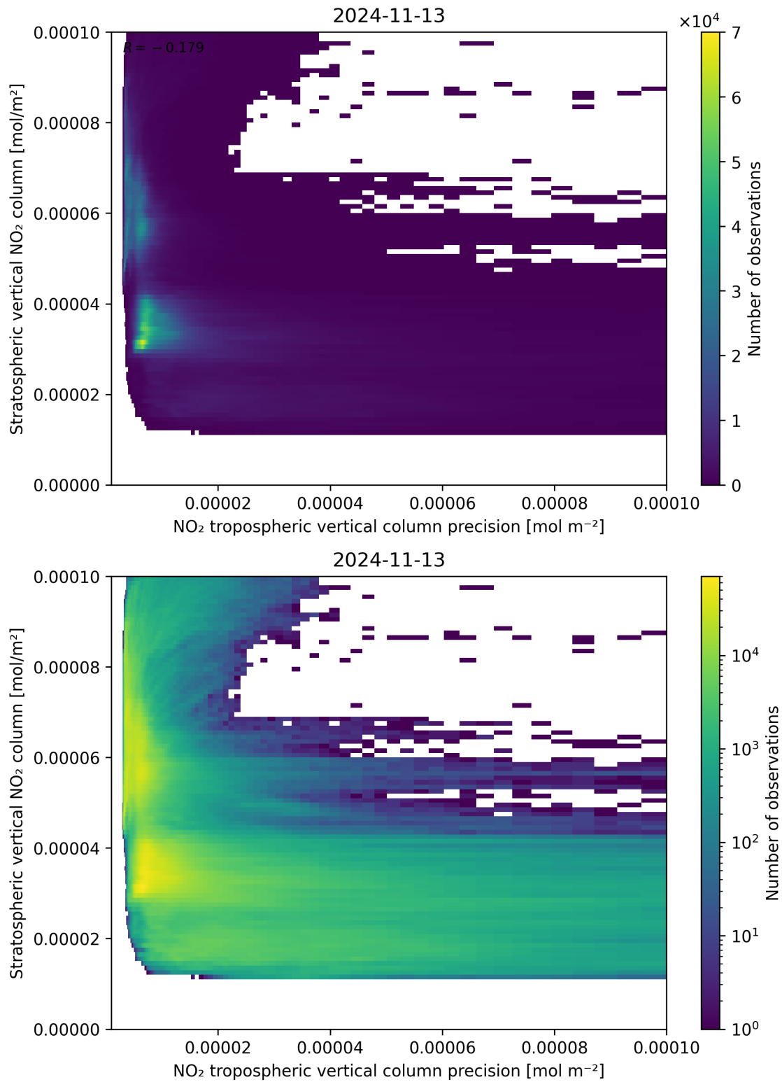
Figure 135: Scatter density plot of “NO 2 tropospheric vertical column precision” against “Stratospheric vertical NO 2 column” for 2024-11-12 to 2024-11-14.
