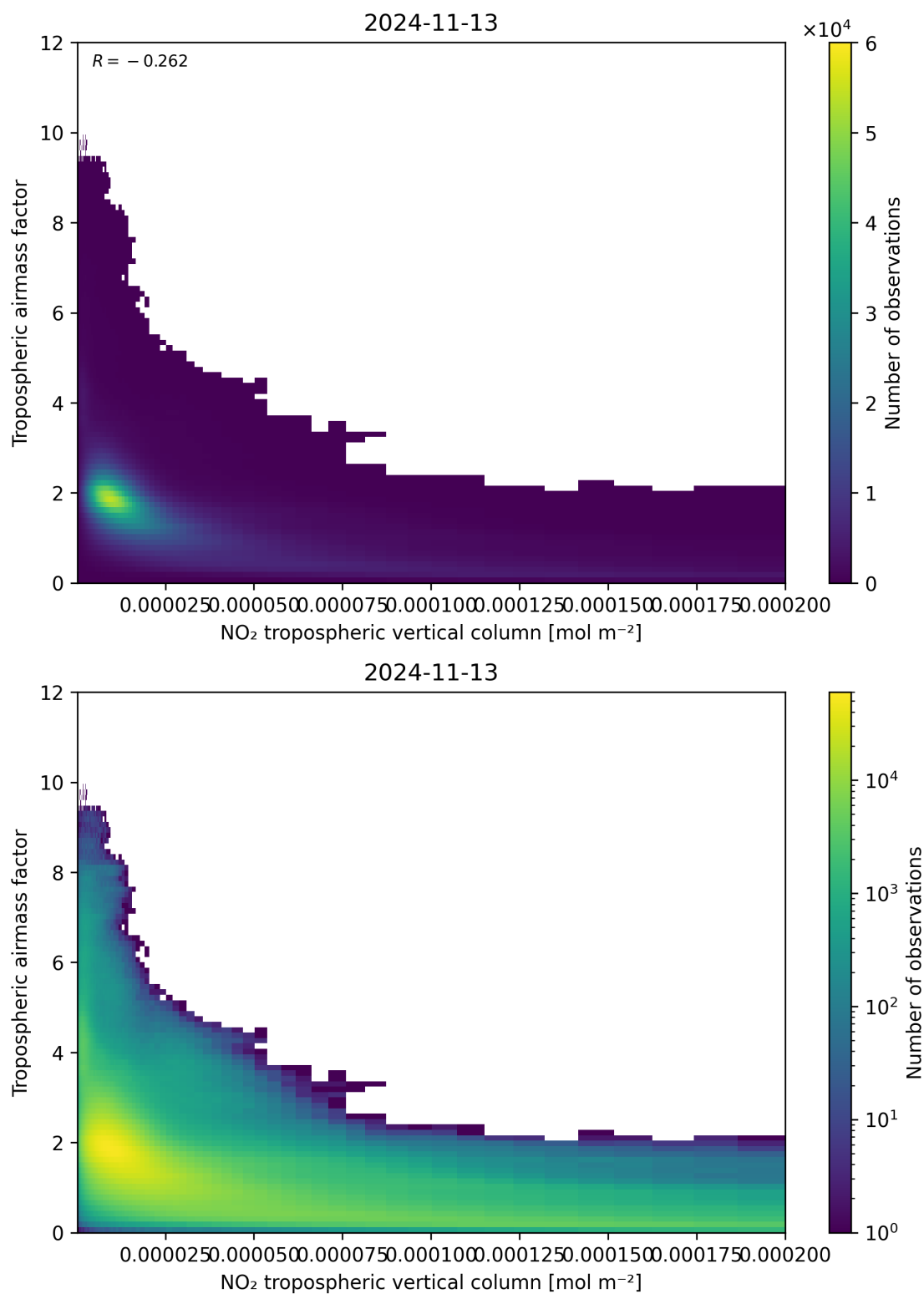
Figure 123: Scatter density plot of “NO 2 tropospheric vertical column” against “Tropospheric airmass factor” for 2024-11-12 to 2024-11-14.
