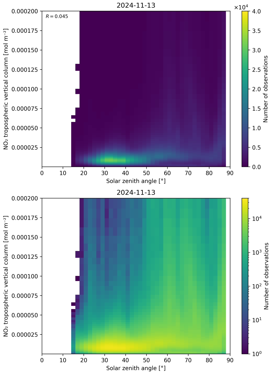
Figure 155: Scatter density plot of “Solar zenith angle” against “NO 2 tropospheric vertical column” for 2024-11-12 to 2024-11-14.
