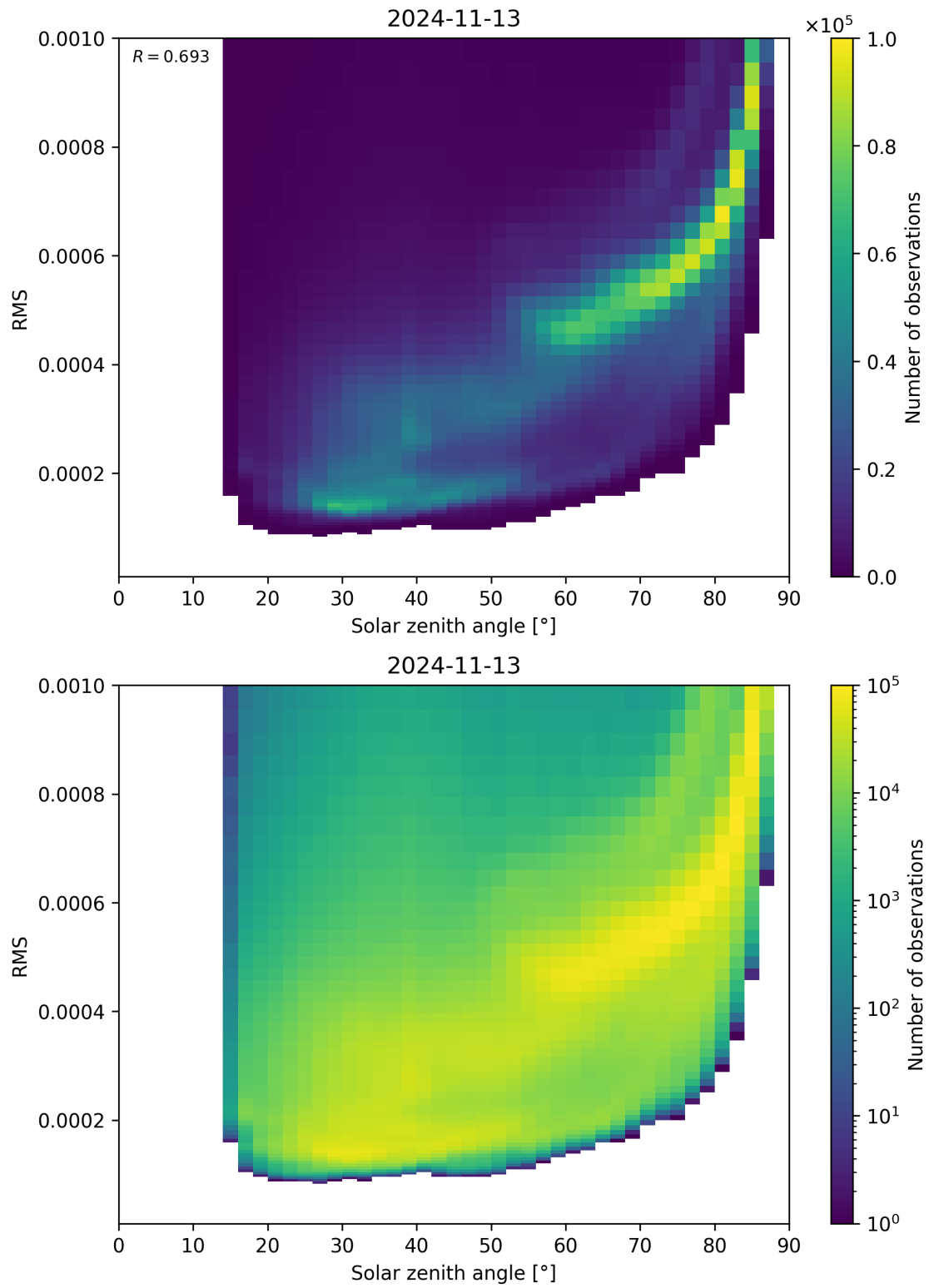
Figure 157: Scatter density plot of “Solar zenith angle” against “RMS” for 2024-11-12 to 2024-11-14.
