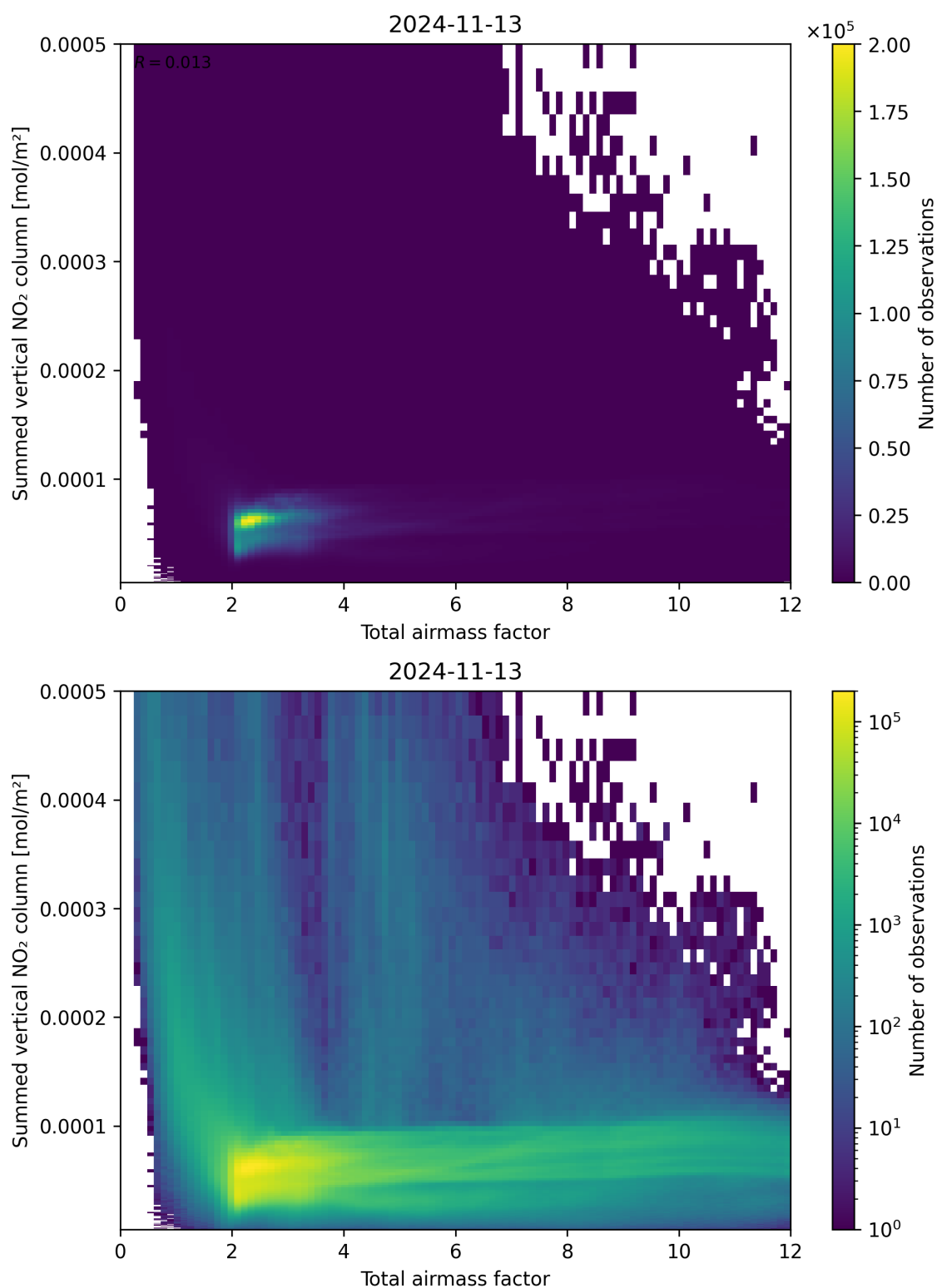
Figure 65: Scatter density plot of “Total airmass factor” against “Summed vertical NO 2 column” for 2024-11-12 to 2024-11-14.
