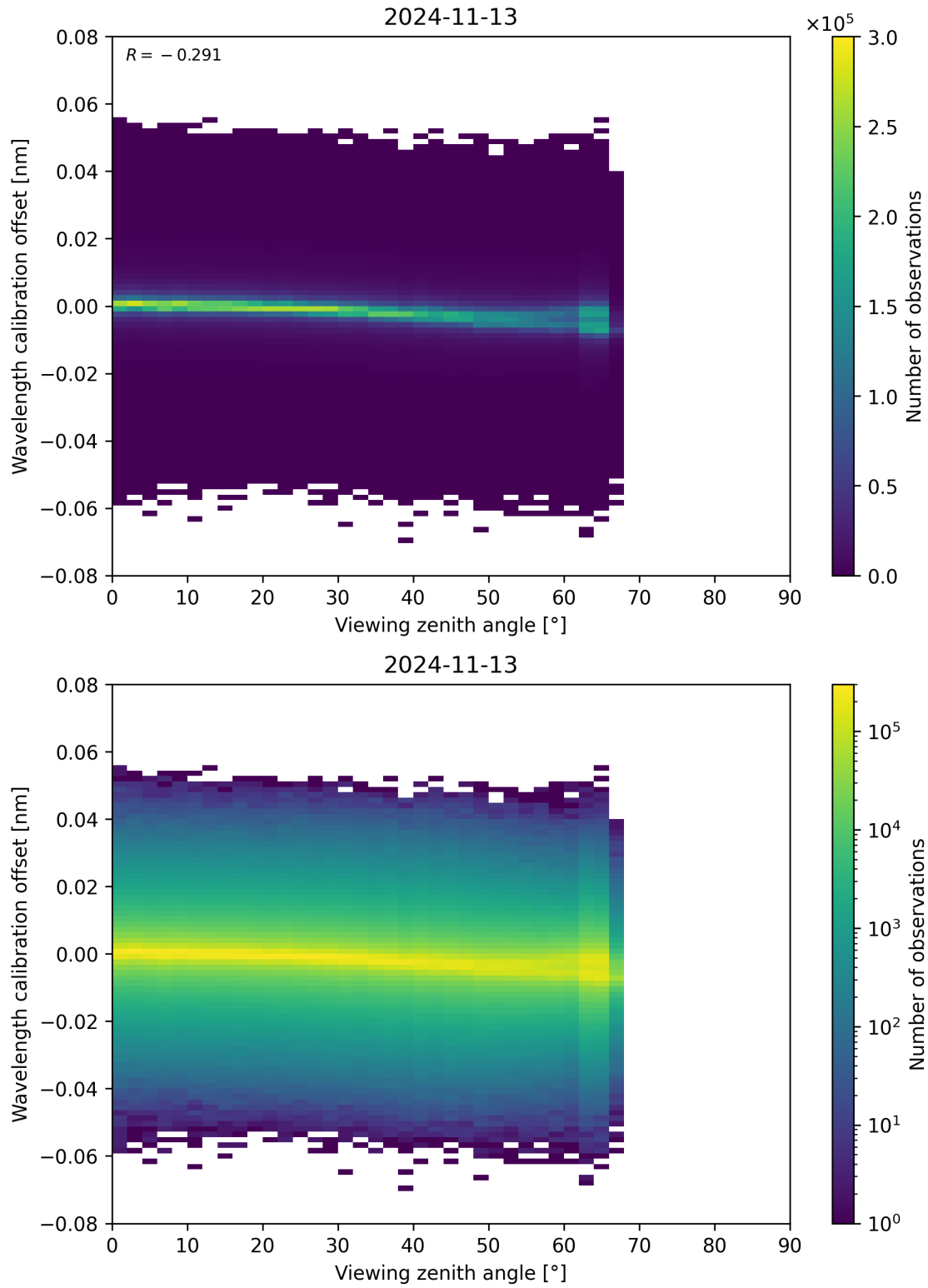
Figure 173: Scatter density plot of “Viewing zenith angle” against “Wavelength calibration offset” for 2024-11-12 to 2024-11-14.
