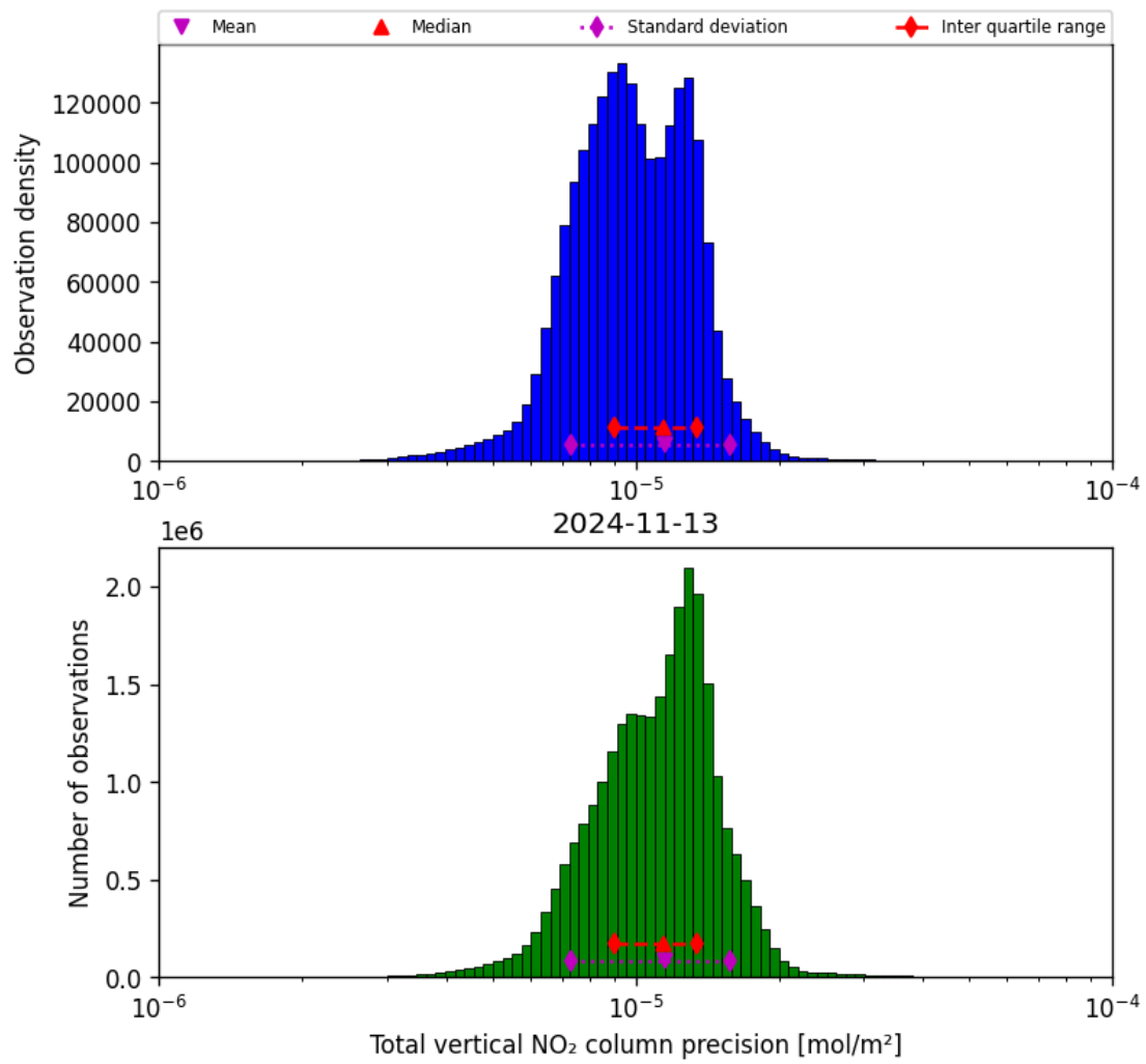
Figure 39: Histogram of “Total vertical NO 2 column precision” for 2024-11-12 to 2024-11-14
