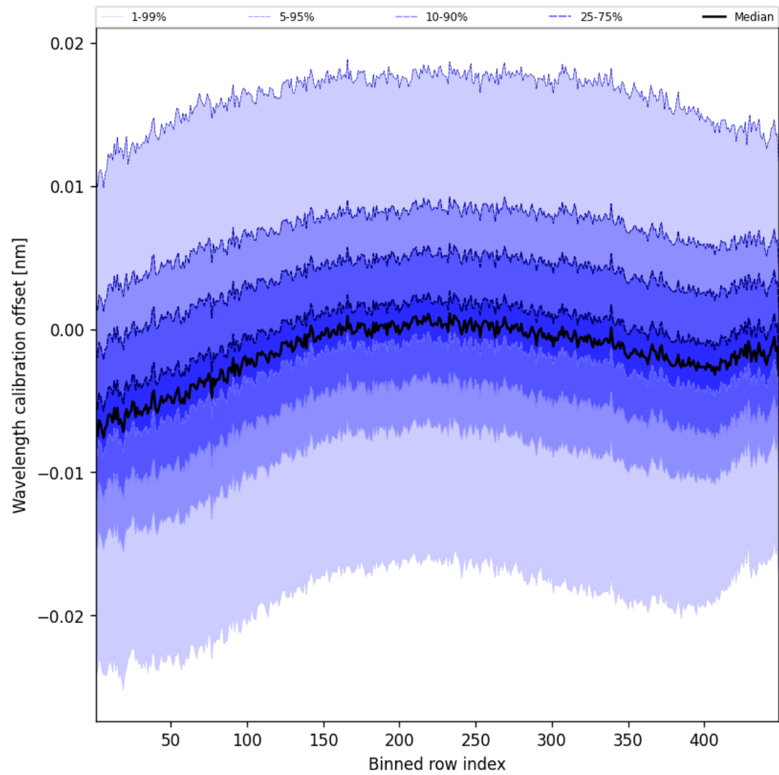
Figure 52: Along track statistics of “Wavelength calibration offset” for 2024-11-12 to 2024-11-14
