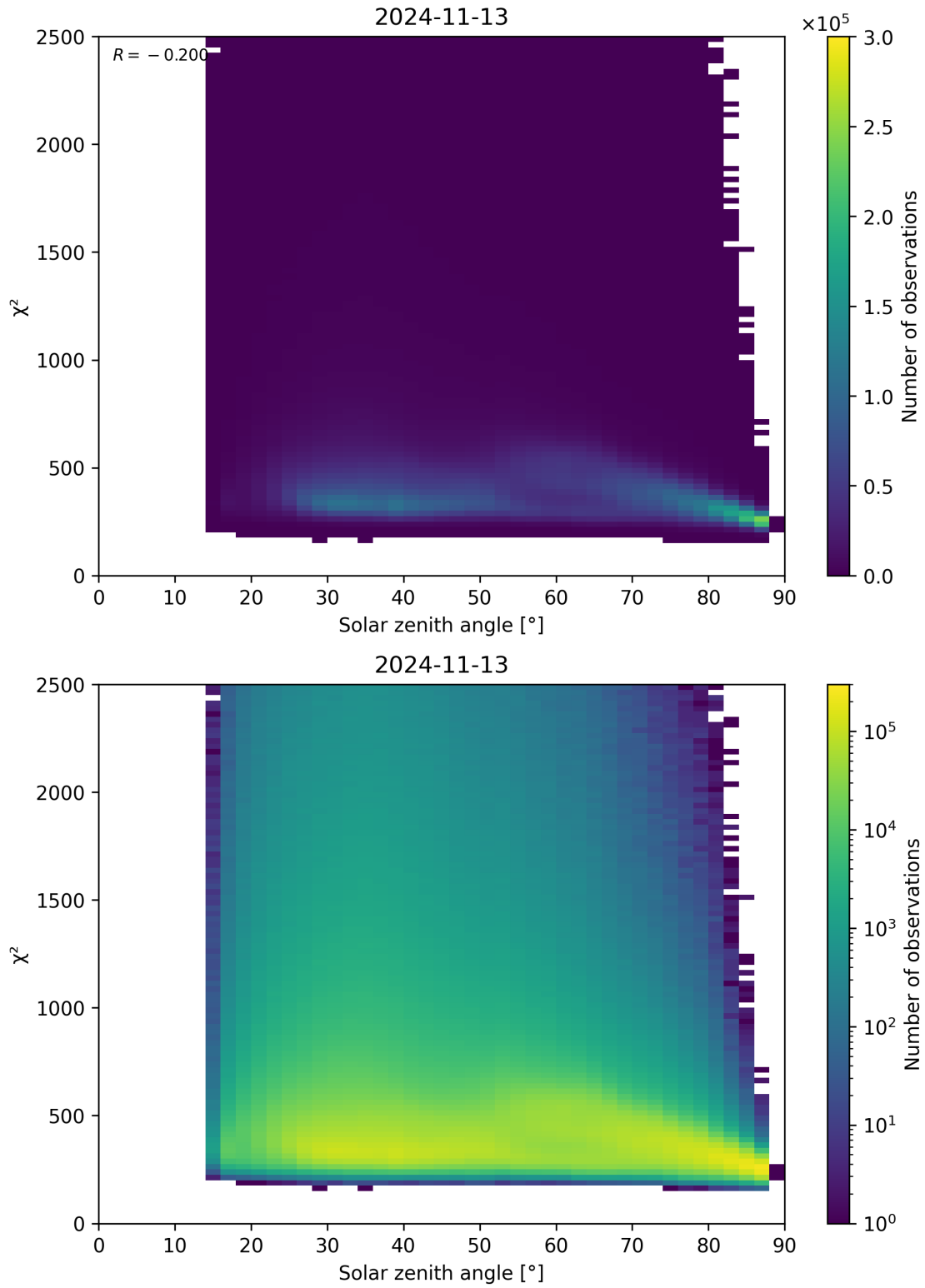
Figure 148: Scatter density plot of “Solar zenith angle” against “ \chi^2 ” for 2024-11-12 to 2024-11-14.
