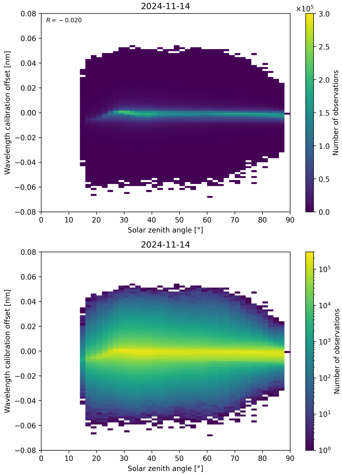
Figure 158: Scatter density plot of “Solar zenith angle” against “Wavelength calibration offset” for 2024-11-14 to 2024-11-15.
