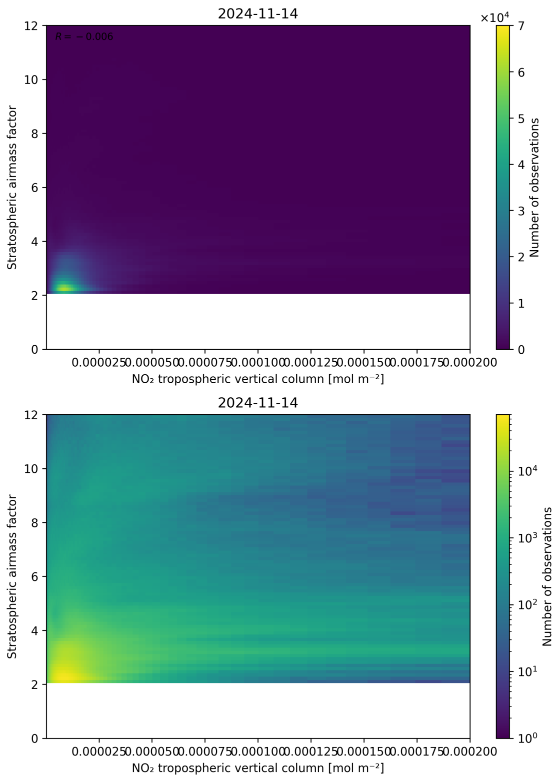
Figure 121: Scatter density plot of “NO 2 tropospheric vertical column” against “Stratospheric airmass factor” for 2024-11-14 to 2024-11-15.
