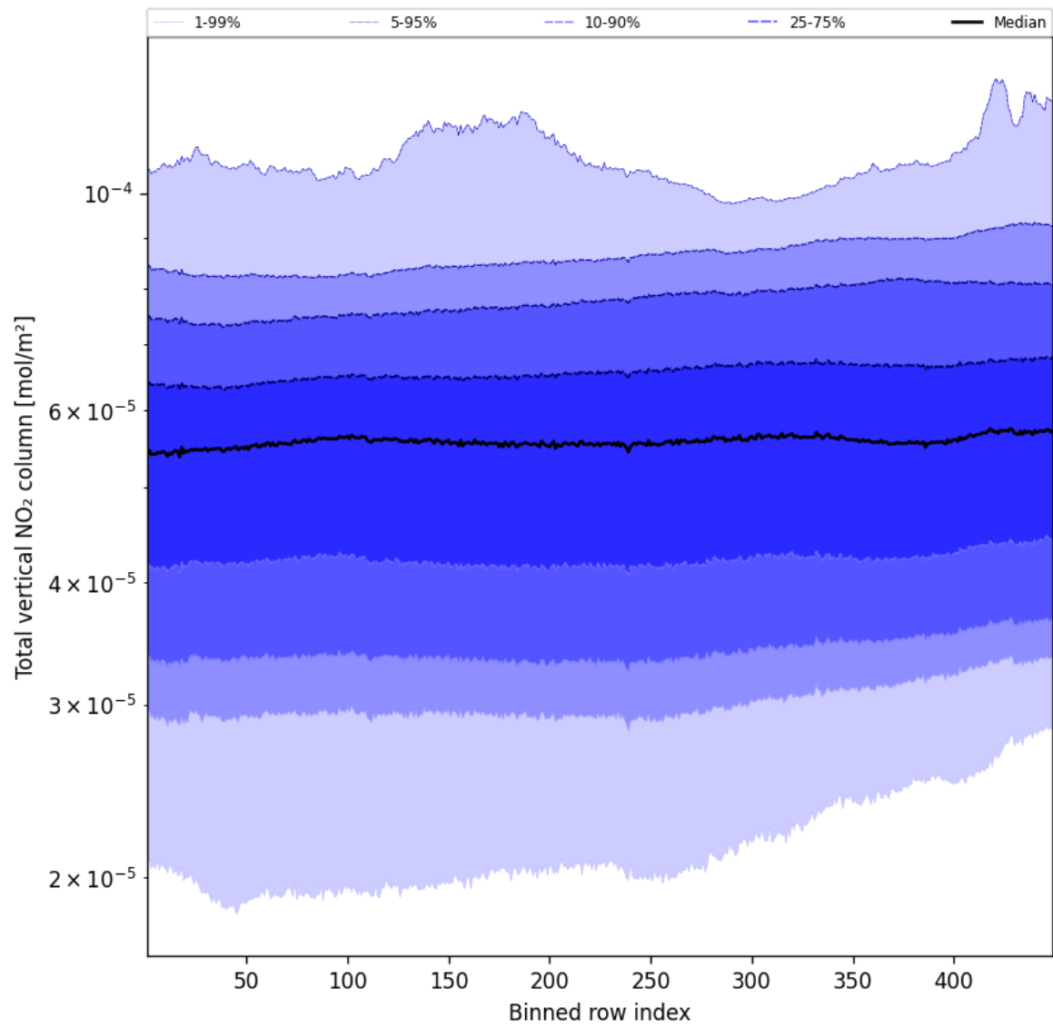
Figure 55: Along track statistics of “Total vertical NO 2 column” for 2024-11-14 to 2024-11-15
