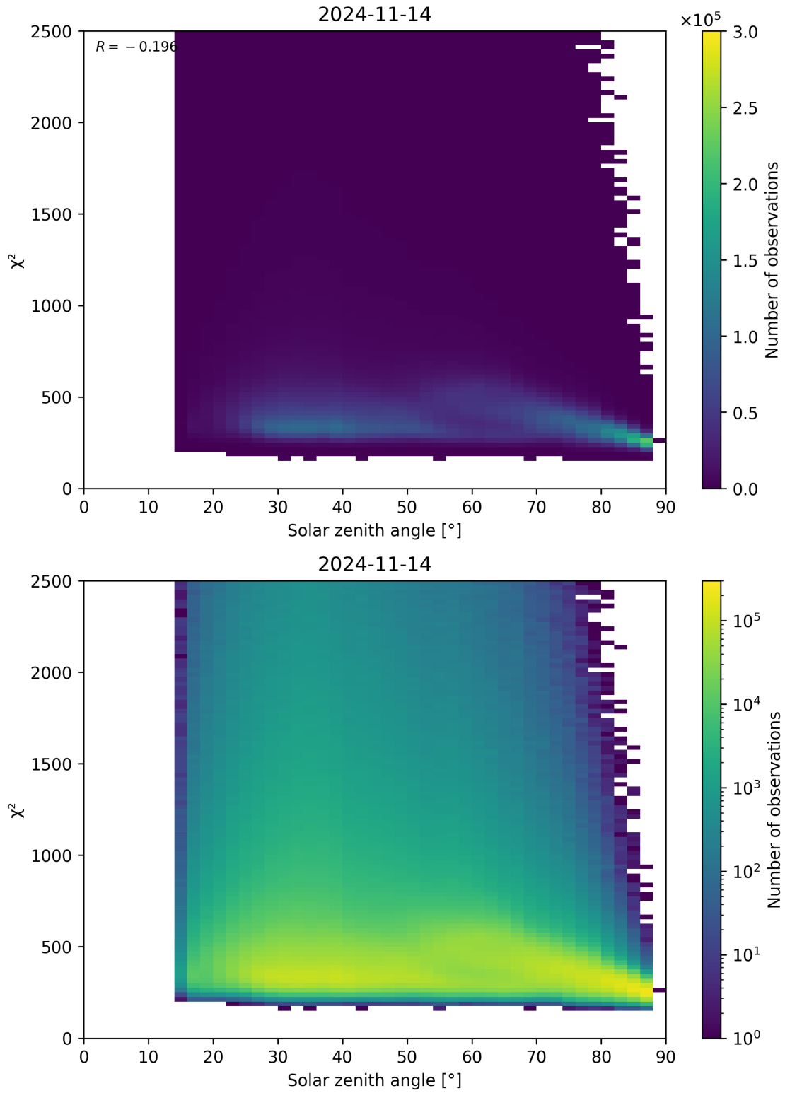
Figure 148: Scatter density plot of “Solar zenith angle” against “ \chi^2 ” for 2024-11-14 to 2024-11-15.
