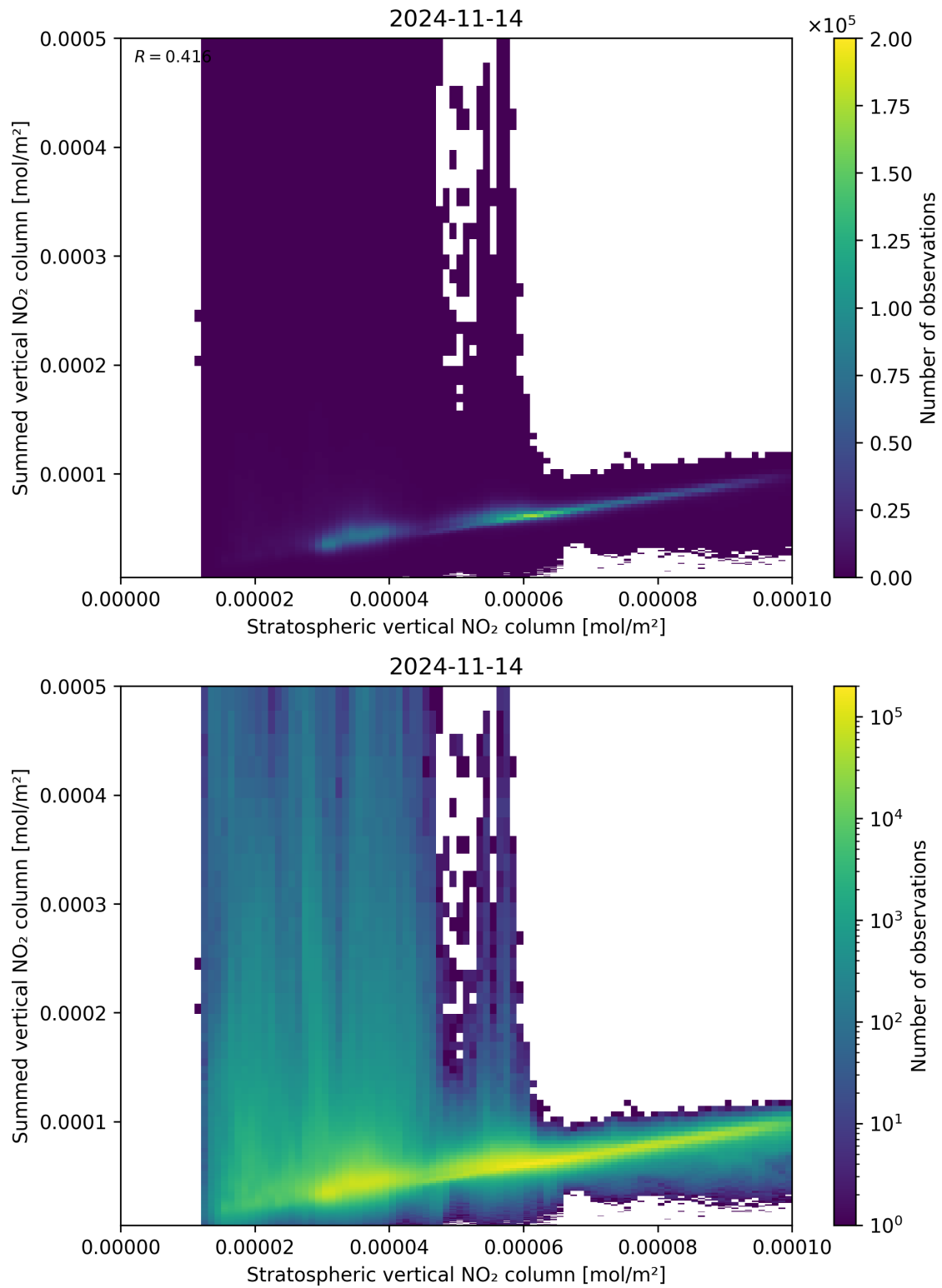
Figure 98: Scatter density plot of “Stratospheric vertical NO 2 column” against “Summed vertical NO 2 column” for 2024-11-14 to 2024-11-15.
