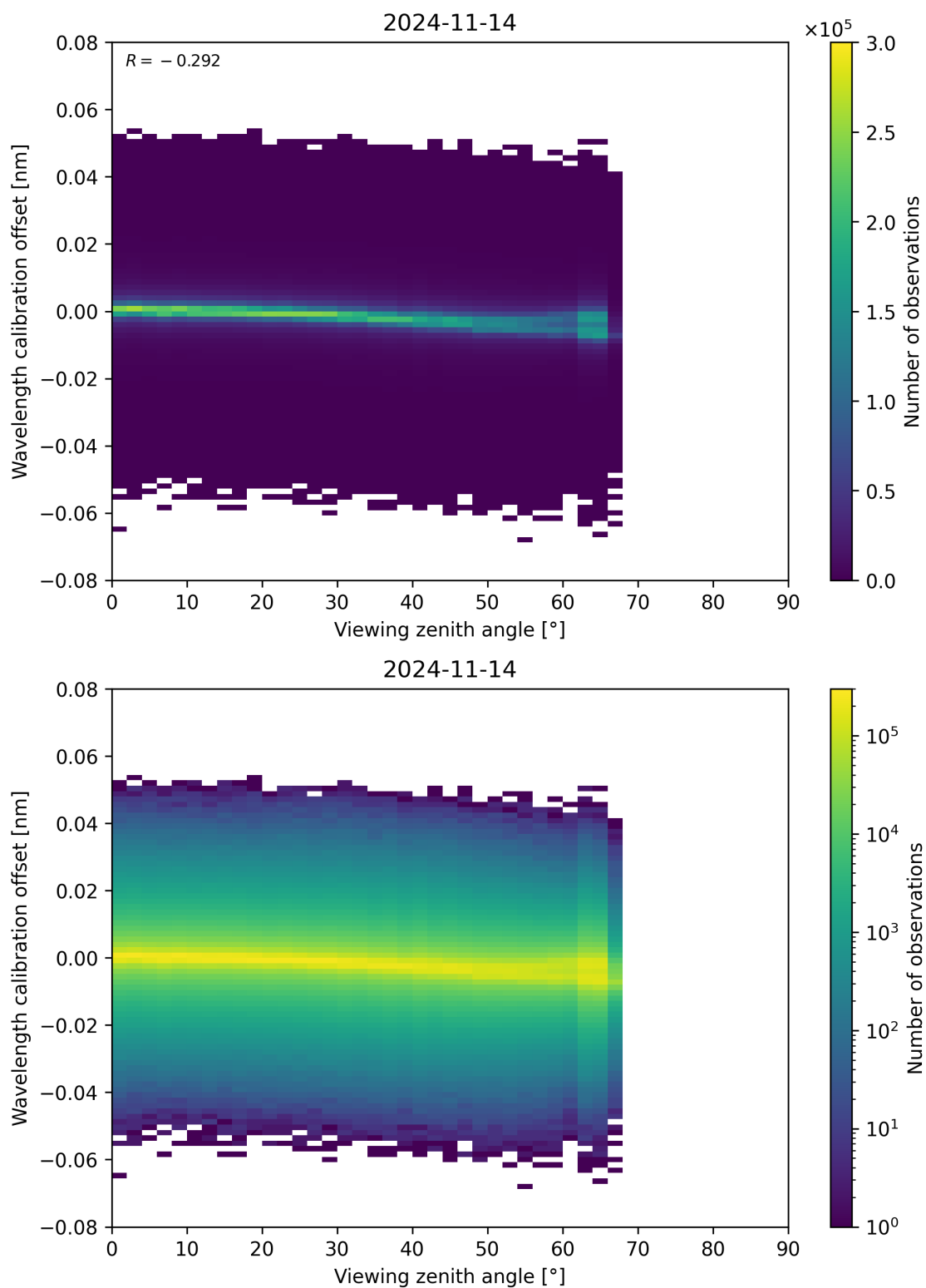
Figure 173: Scatter density plot of “Viewing zenith angle” against “Wavelength calibration offset” for 2024-11-14 to 2024-11-15.
