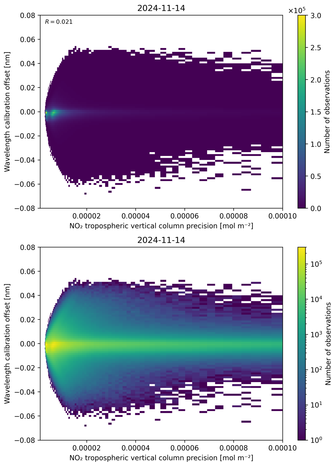
Figure 141: Scatter density plot of “NO 2 tropospheric vertical column precision” against “Wavelength calibration offset” for 2024-11-14 to 2024-11-15.
