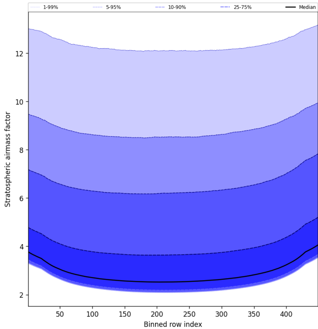
Figure 61: Along track statistics of “Stratospheric airmass factor” for 2024-11-14 to 2024-11-15
