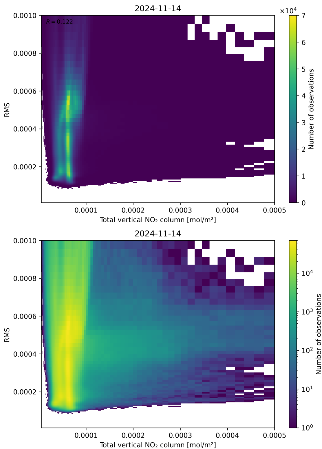
Figure 120: Scatter density plot of “Total vertical NO 2 column” against “RMS” for 2024-11-14 to 2024-11-15.
