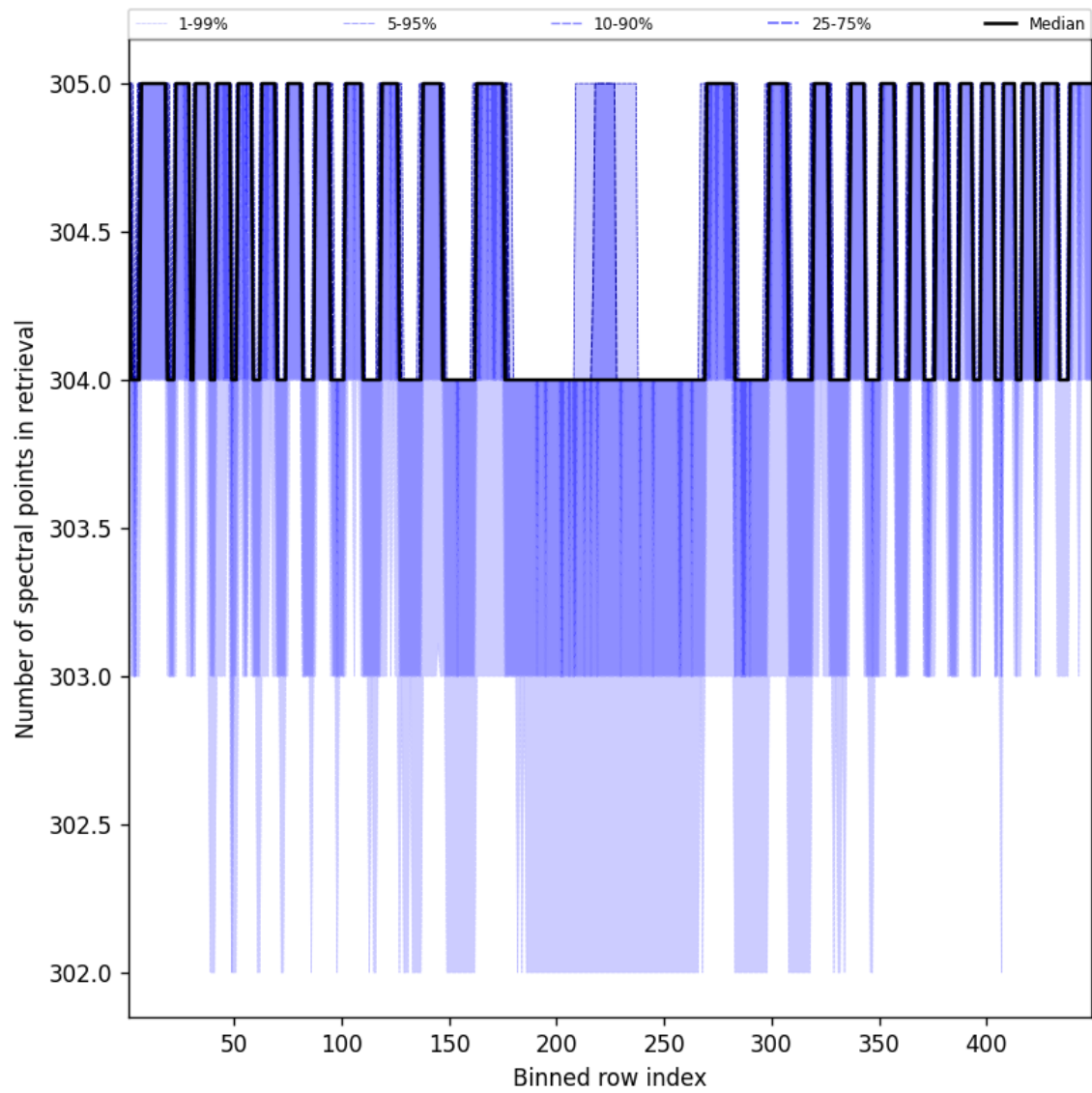
Figure 50: Along track statistics of “Number of spectral points in retrieval” for 2024-11-14 to 2024-11-15
