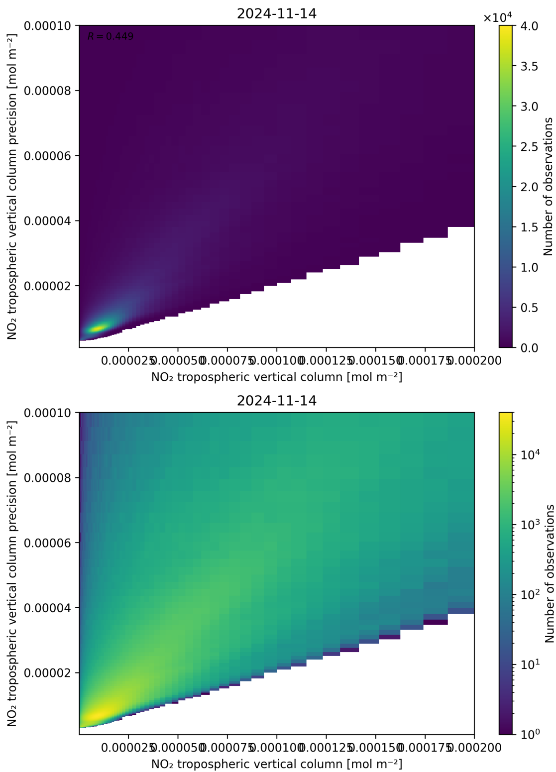
Figure 130: Scatter density plot of “NO 2 tropospheric vertical column” against “NO 2 tropospheric vertical column precision” for 2024-11-14 to 2024-11-15.
