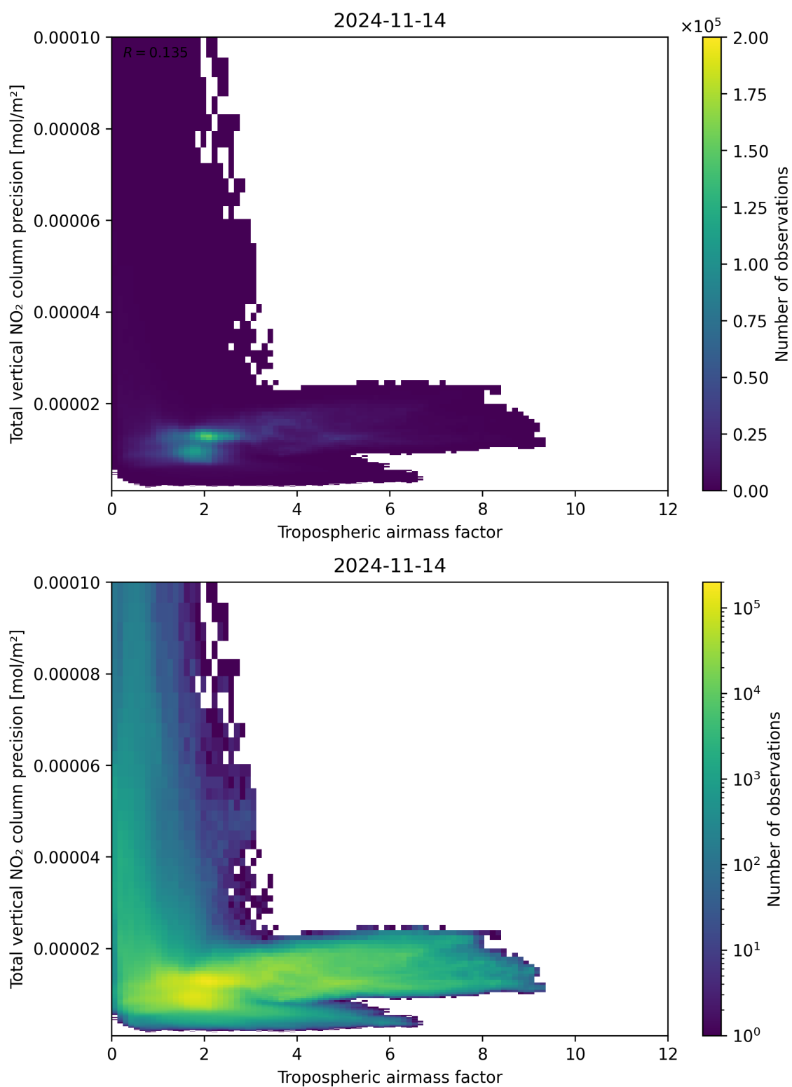
Figure 78: Scatter density plot of “Tropospheric air mass factor” against “Total vertical NO 2 column precision” for 2024-11-14 to 2024-11-15.
