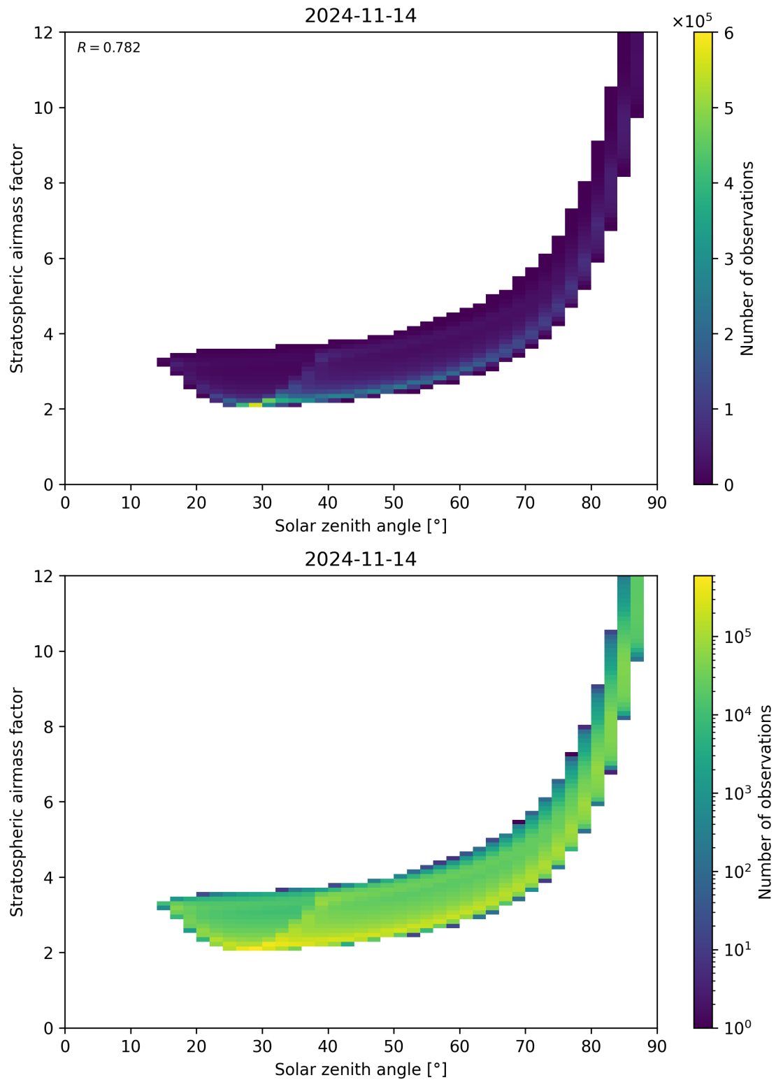
Figure 145: Scatter density plot of “Solar zenith angle” against “Stratospheric airmass factor” for 2024-11-14 to 2024-11-15.
