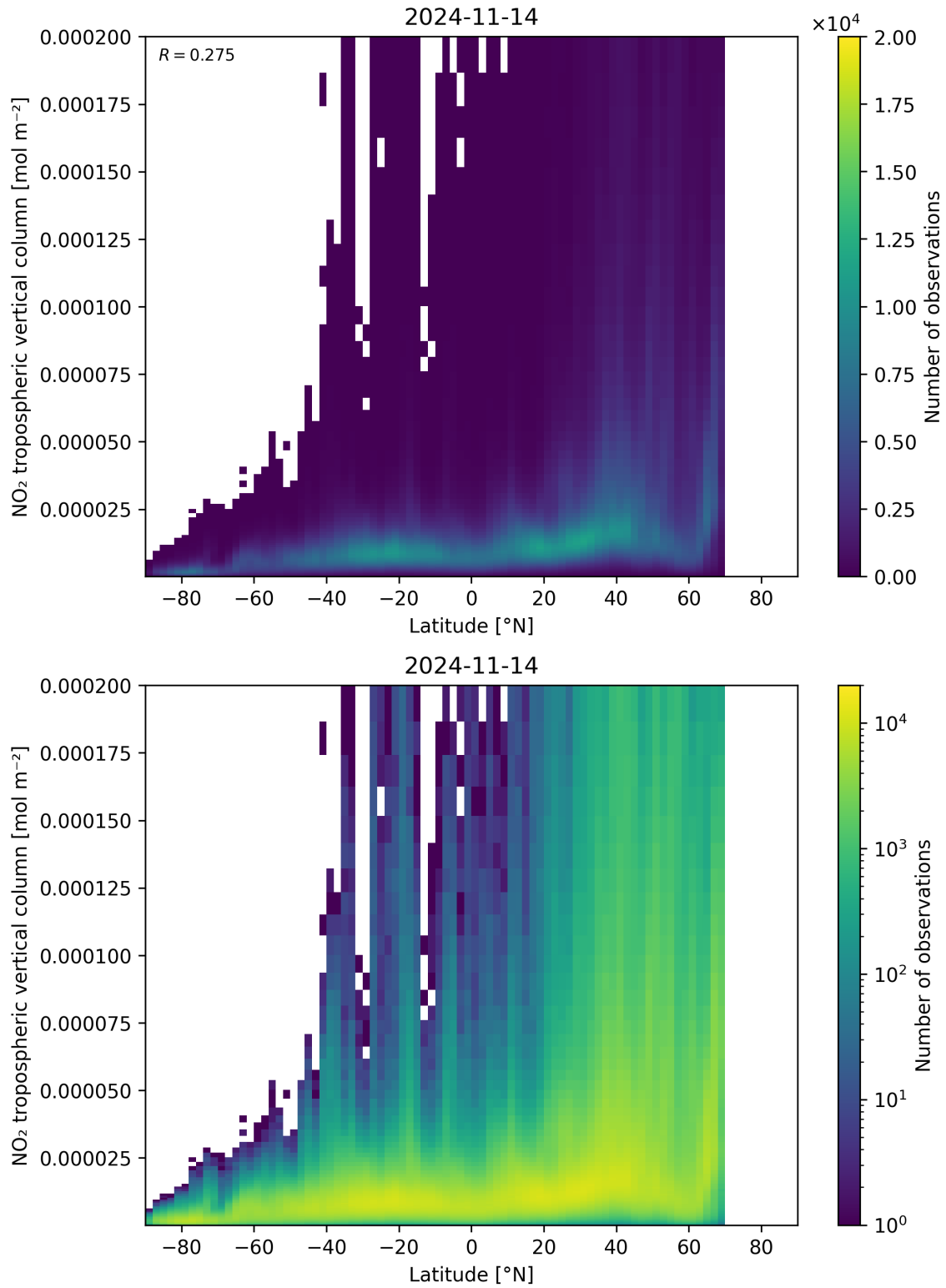
Figure 92: Scatter density plot of “Latitude” against “NO 2 tropospheric vertical column” for 2024-11-14 to 2024-11-15.
