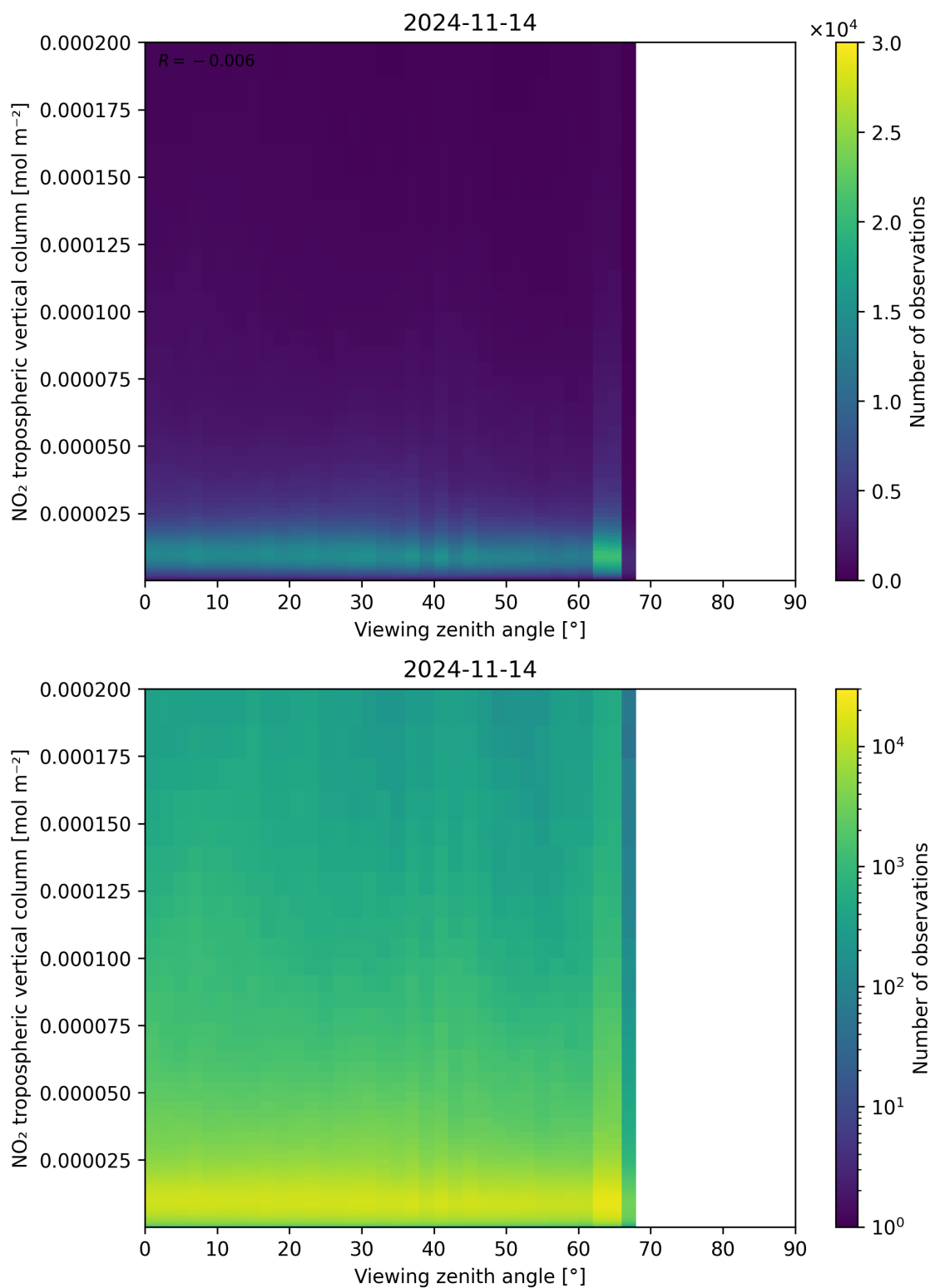
Figure 169: Scatter density plot of “Viewing zenith angle” against “NO 2 tropospheric vertical column” for 2024-11-14 to 2024-11-15.
