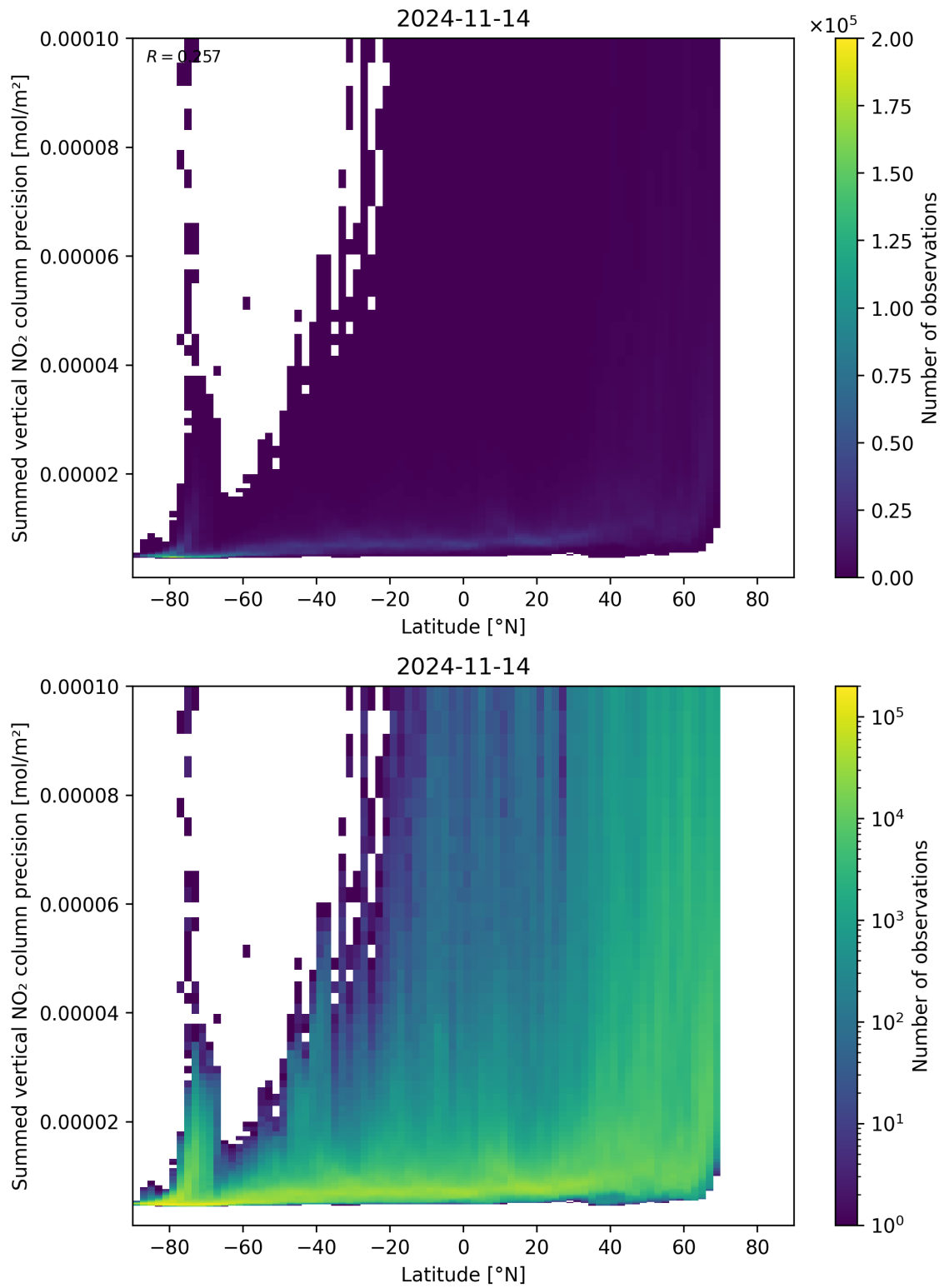
Figure 89: Scatter density plot of “Latitude” against “Summed vertical NO 2 column precision” for 2024-11-14 to 2024-11-15.
