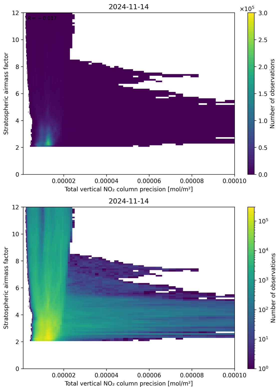
Figure 115: Scatter density plot of “Total vertical NO 2 column precision” against “Stratospheric air mass factor” for 2024-11-14 to 2024-11-15.
