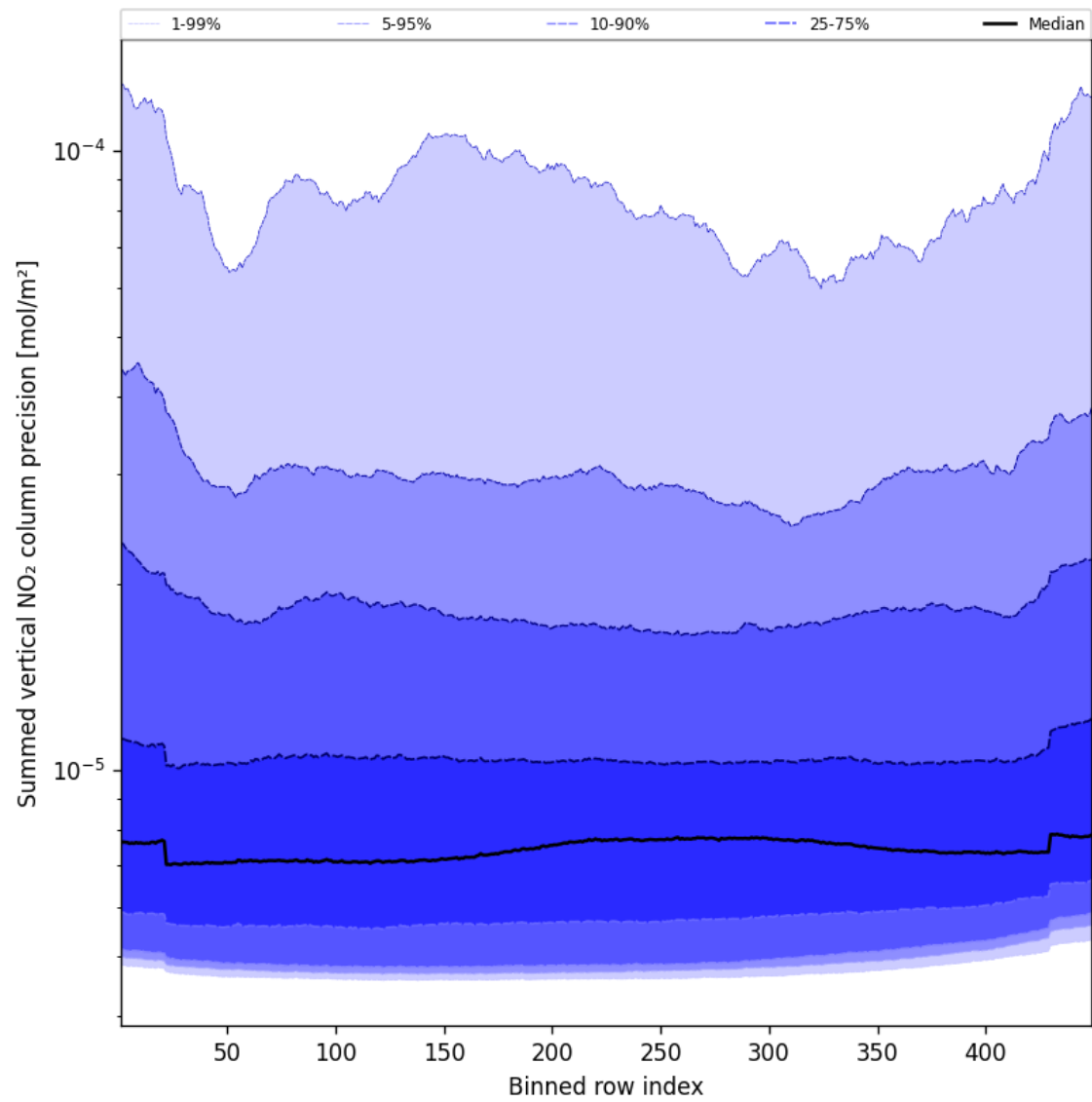
Figure 58: Along track statistics of “Summed vertical NO 2 column precision” for 2024-11-14 to 2024-11-15
