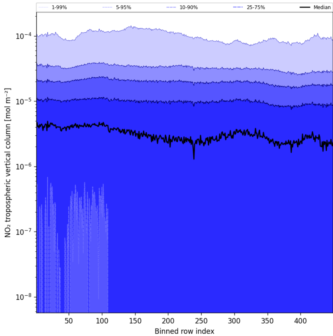
Figure 46: Along track statistics of “ \text{NO}_2 tropospheric vertical column” for 2024-11-14 to 2024-11-15
