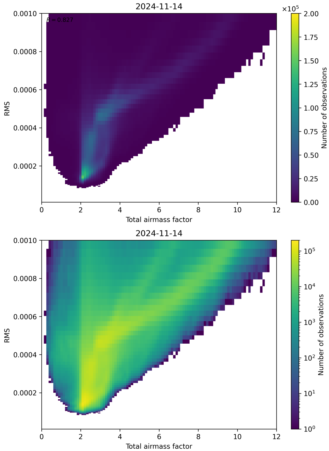
Figure 69: Scatter density plot of “Total airmass factor” against “RMS” for 2024-11-14 to 2024-11-15.
