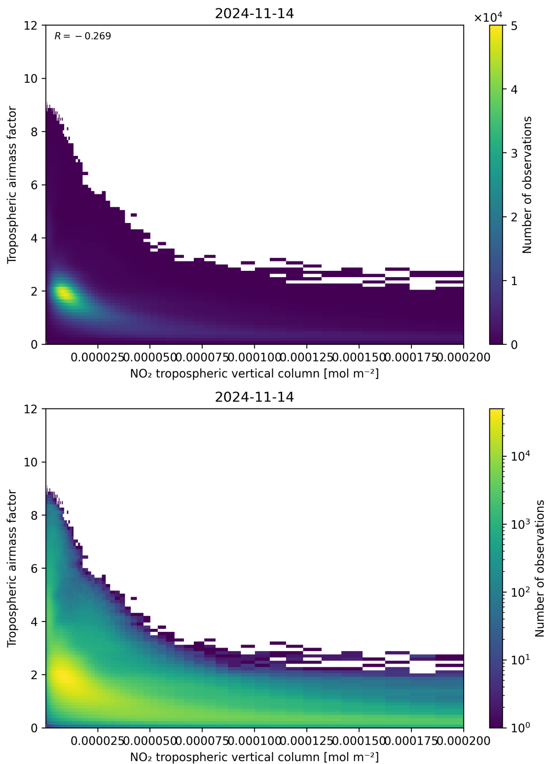
Figure 123: Scatter density plot of “NO 2 tropospheric vertical column” against “Tropospheric air mass factor” for 2024-11-14 to 2024-11-15.
