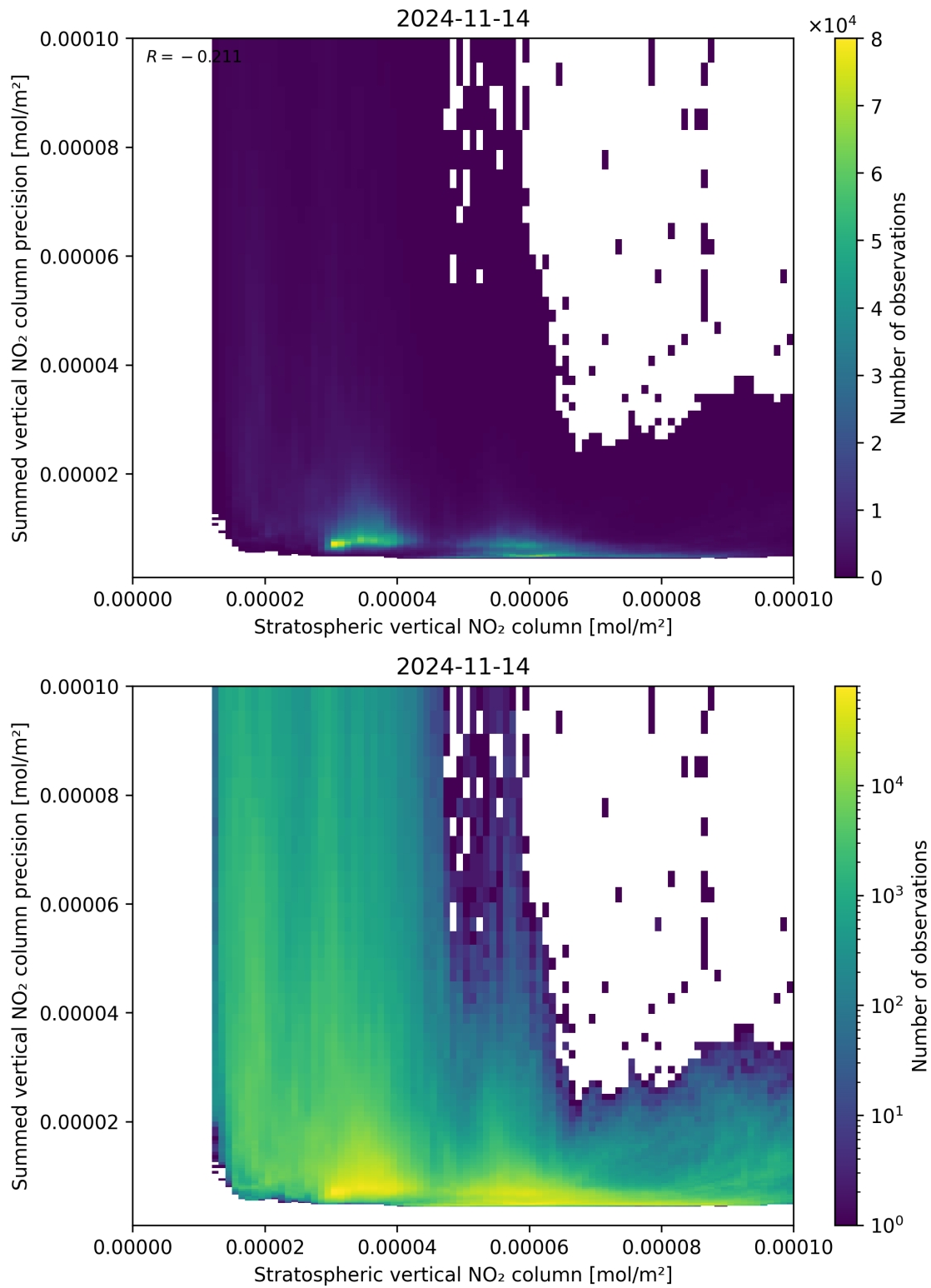
Figure 99: Scatter density plot of “Stratospheric vertical NO 2 column” against “Summed vertical NO 2 column precision” for 2024-11-14 to 2024-11-15.
