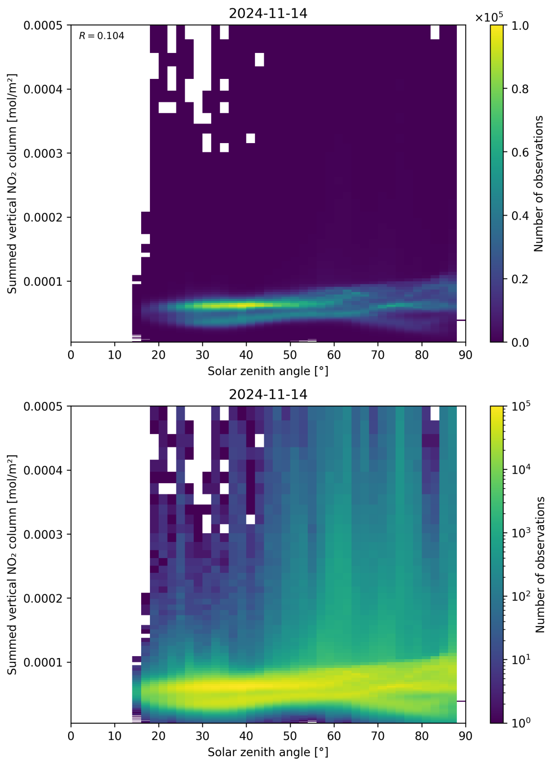
Figure 151: Scatter density plot of “Solar zenith angle” against “Summed vertical NO 2 column” for 2024-11-14 to 2024-11-15.
