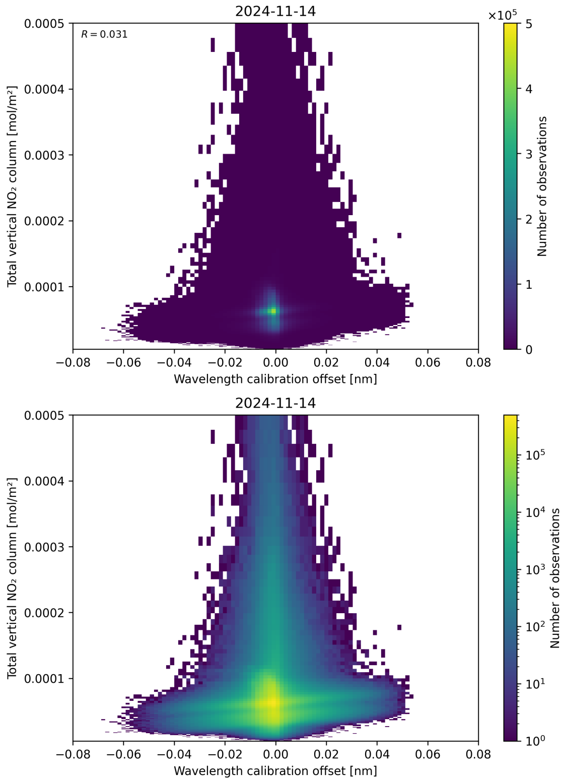
Figure 179: Scatter density plot of “Wavelength calibration offset” against “Total vertical NO 2 column” for 2024-11-14 to 2024-11-15.
