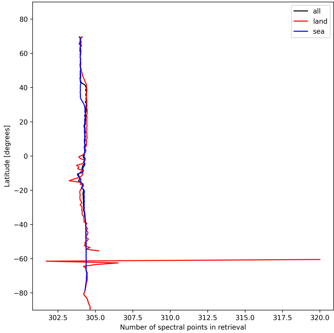
Figure 16: Zonal average of “Number of spectral points in retrieval” for 2024-11-14 to 2024-11-15.
