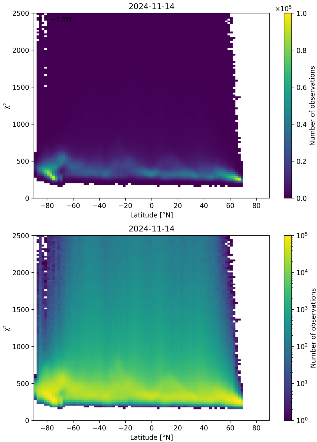
Figure 86: Scatter density plot of “Latitude” against “ \chi^2 ” for 2024-11-14 to 2024-11-15.
