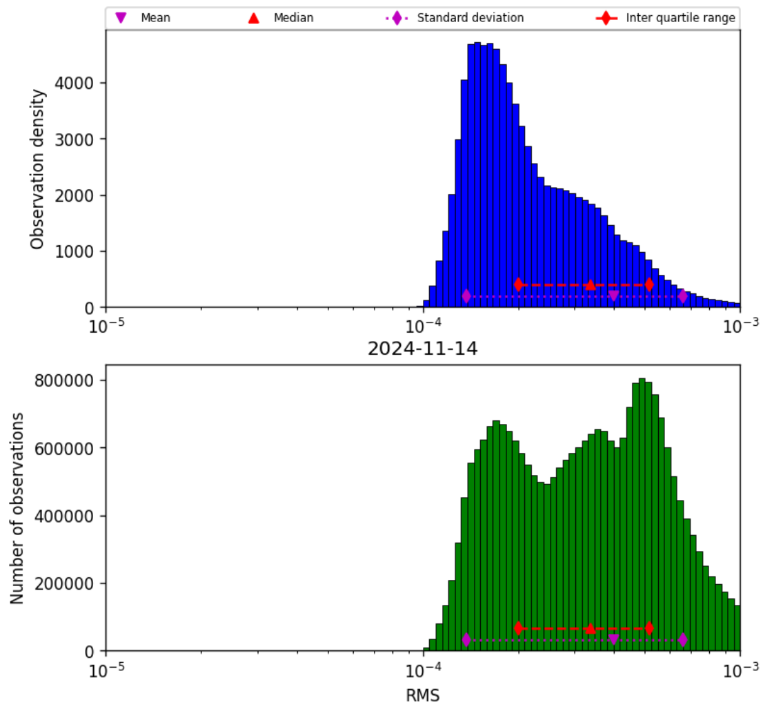
Figure 43: Histogram of “RMS” for 2024-11-14 to 2024-11-15
