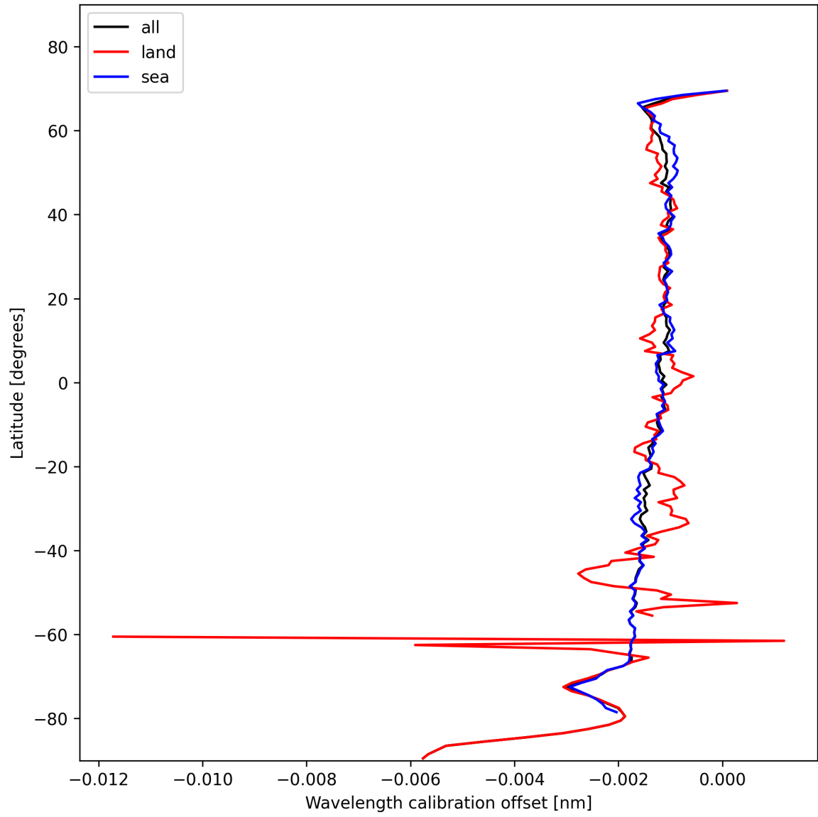
Figure 18: Zonal average of “Wavelength calibration offset” for 2024-11-14 to 2024-11-15.
