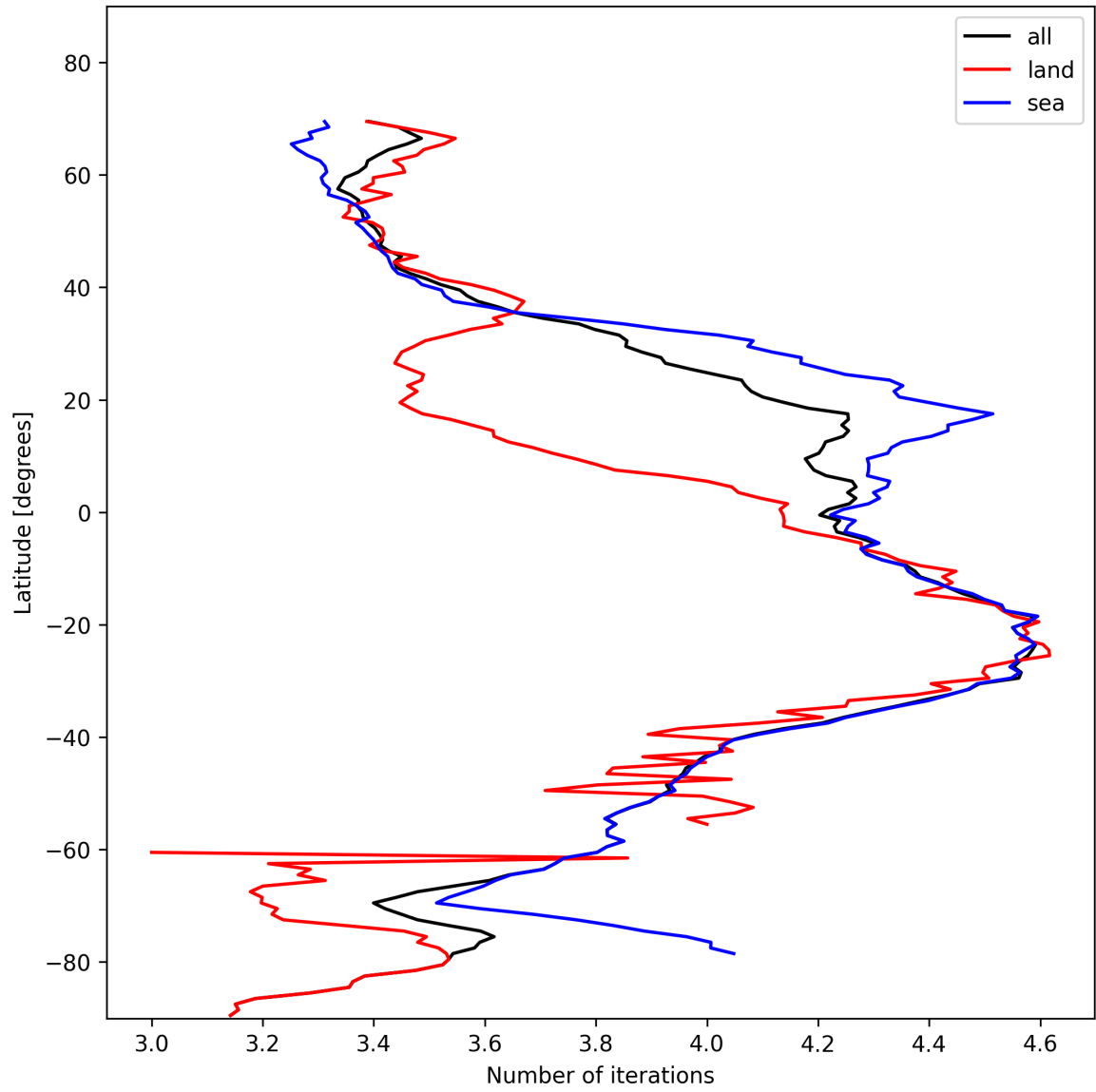
Figure 17: Zonal average of “Number of iterations” for 2024-11-14 to 2024-11-15.
