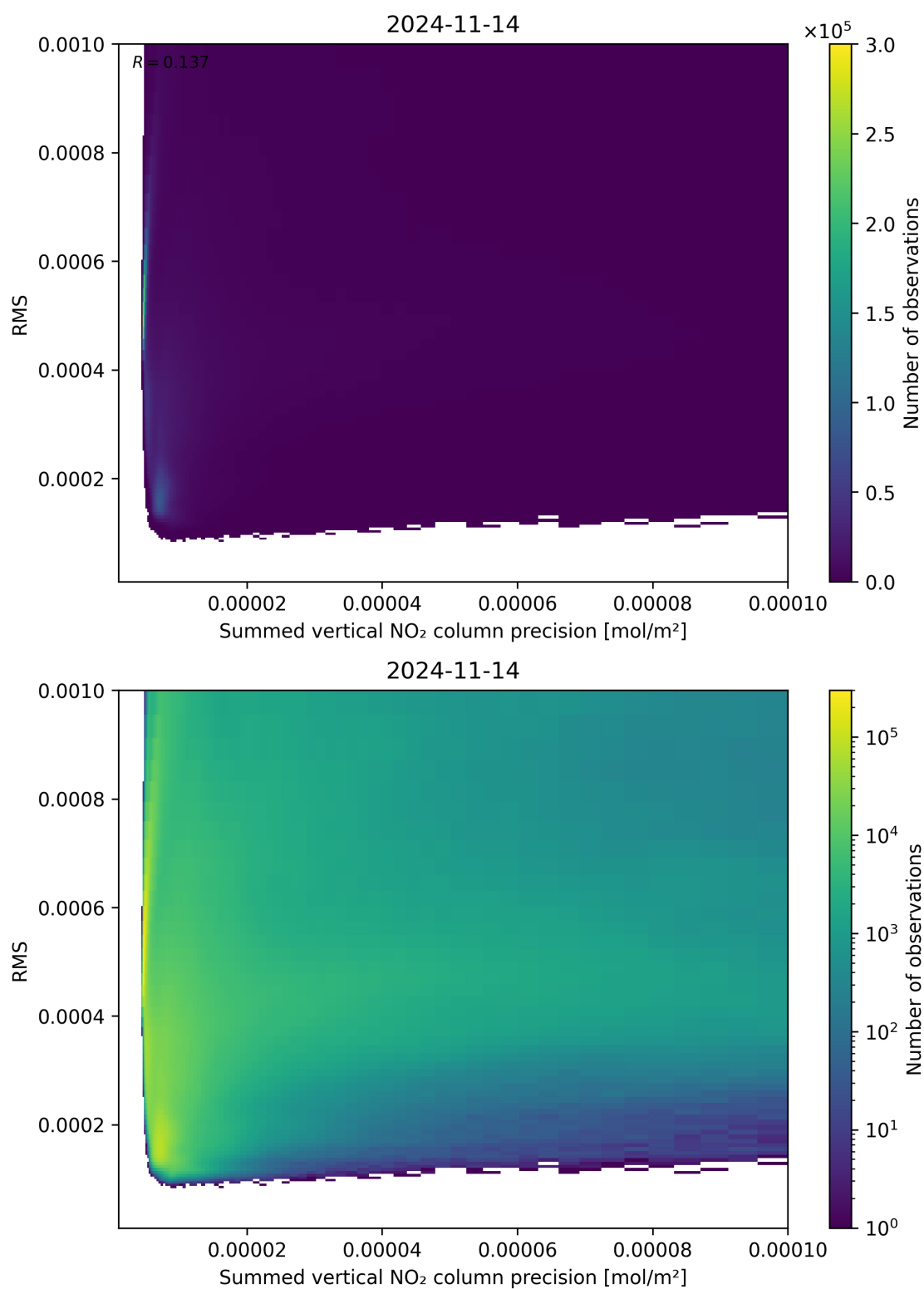
Figure 108: Scatter density plot of “Summed vertical NO 2 column precision” against “RMS” for 2024-11-14 to 2024-11-15.
