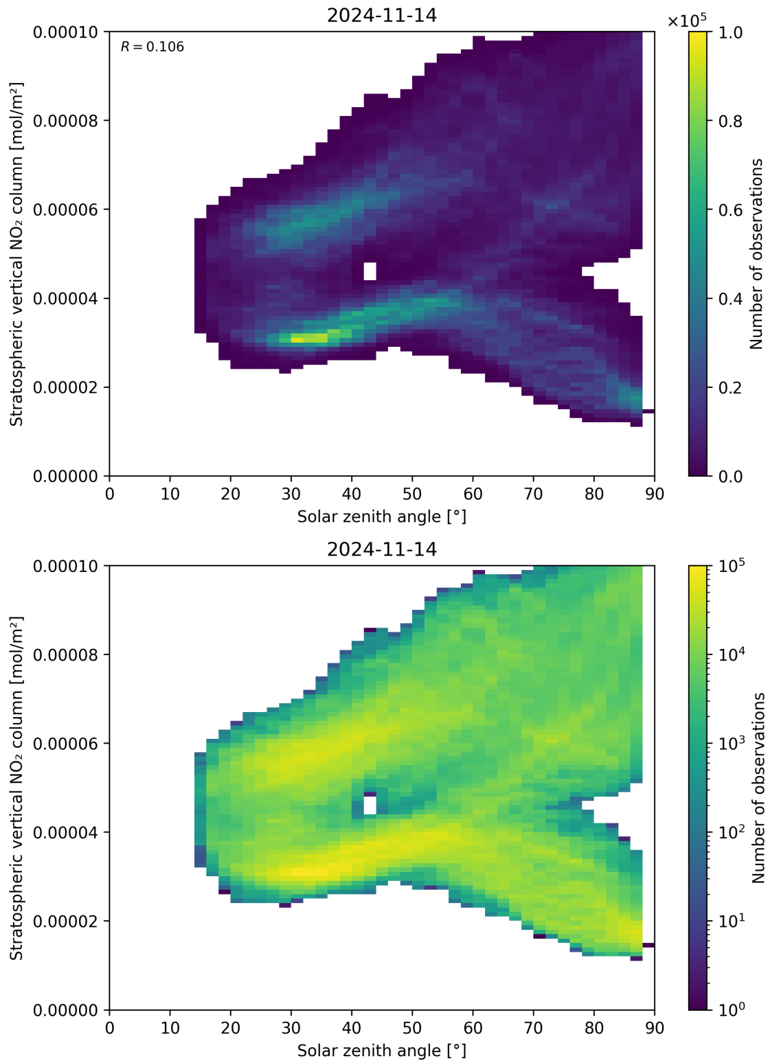
Figure 150: Scatter density plot of “Solar zenith angle” against “Stratospheric vertical NO 2 column” for 2024-11-14 to 2024-11-15.
