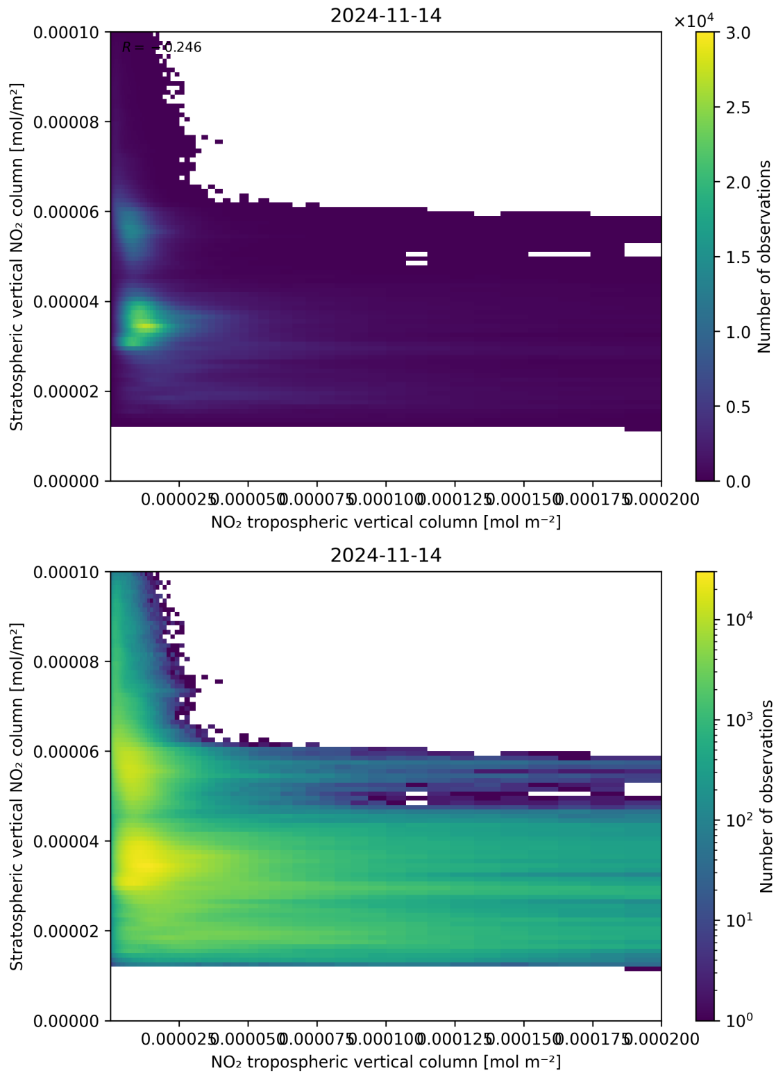
Figure 125: Scatter density plot of “NO 2 tropospheric vertical column” against “Stratospheric vertical NO 2 column” for 2024-11-14 to 2024-11-15.
