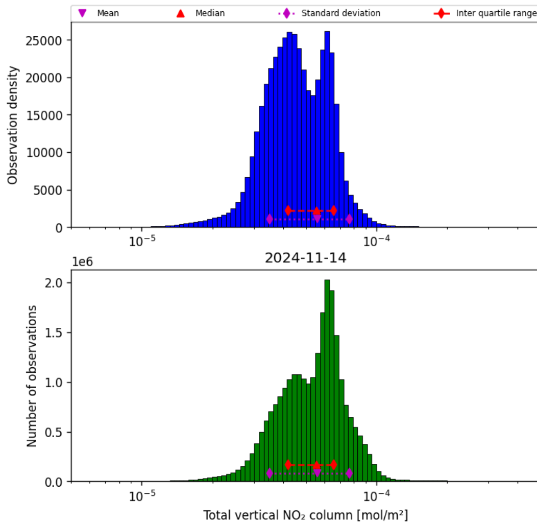
Figure 38: Histogram of “Total vertical NO 2 column” for 2024-11-14 to 2024-11-15
