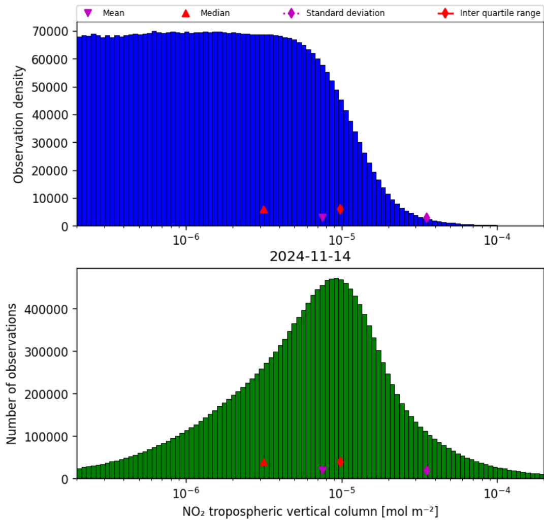
Figure 29: Histogram of “NO 2 tropospheric vertical column” for 2024-11-14 to 2024-11-15
