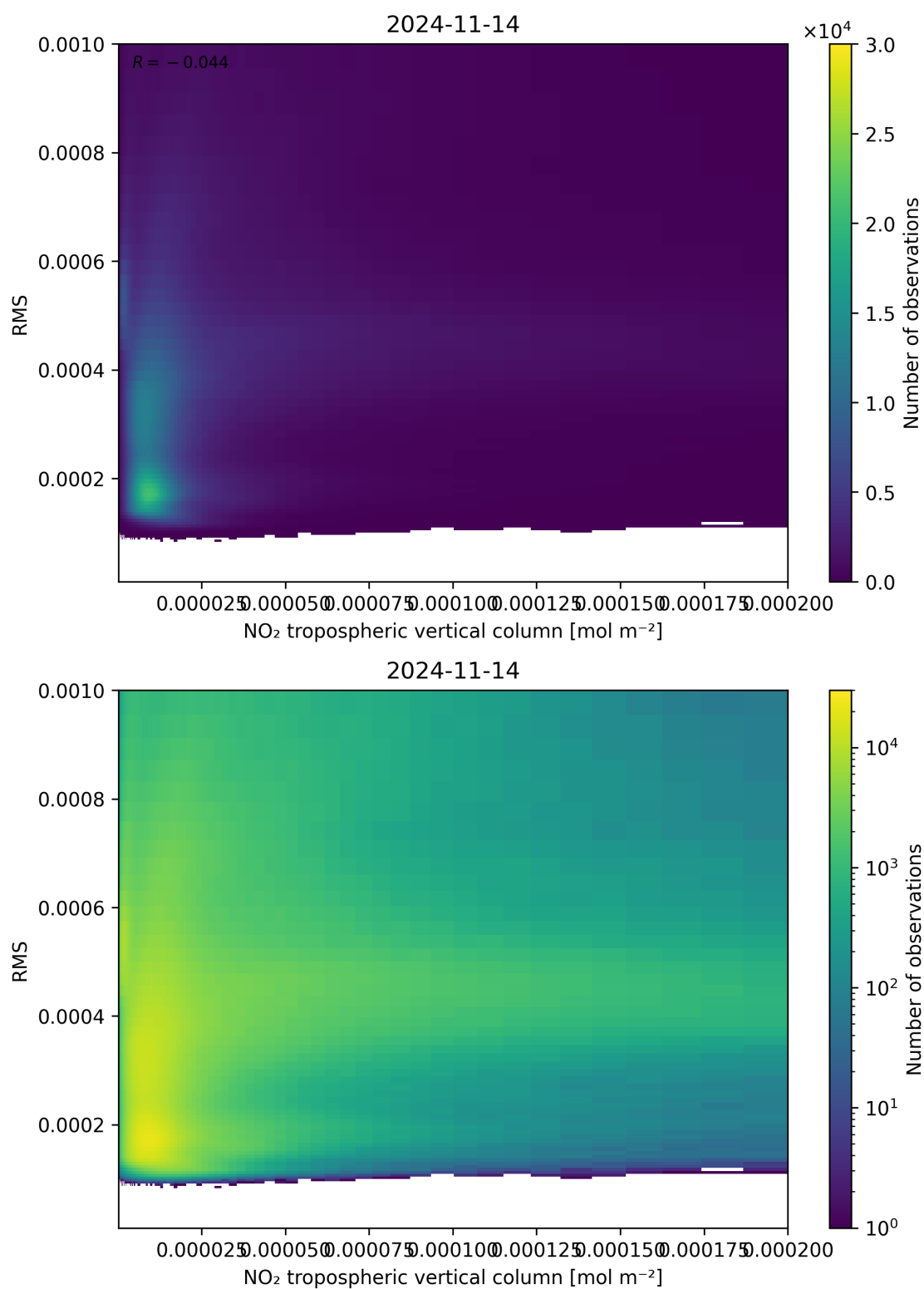
Figure 142: Scatter density plot of “NO 2 tropospheric vertical column” against “RMS” for 2024-11-14 to 2024-11-15.
