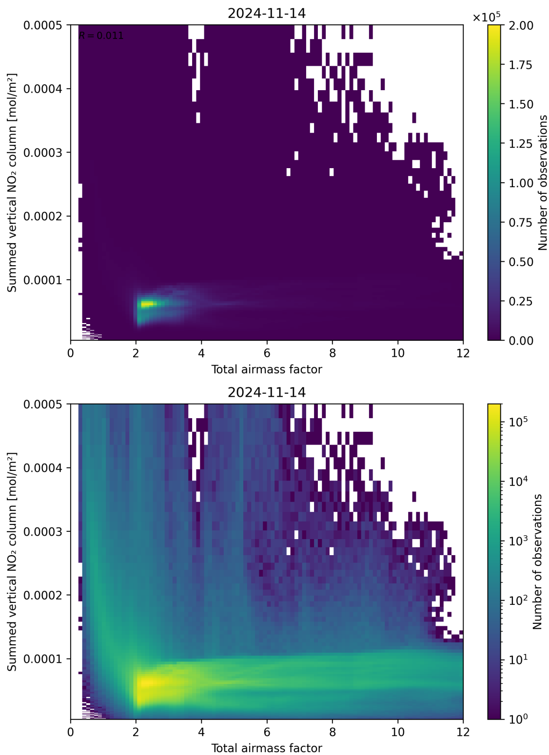
Figure 65: Scatter density plot of “Total airmass factor” against “Summed vertical NO 2 column” for 2024-11-14 to 2024-11-15.
