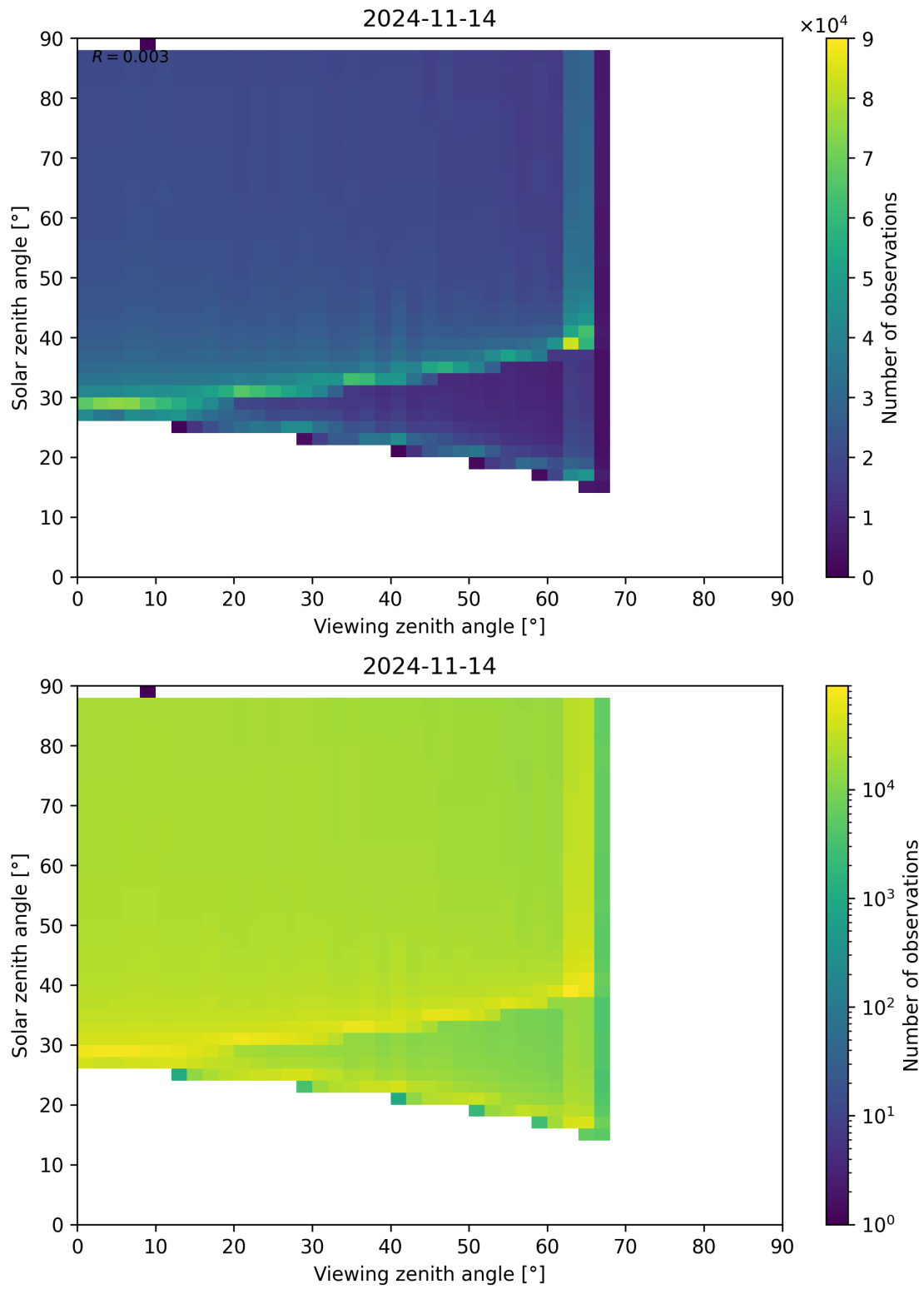
Figure 172: Scatter density plot of “Viewing zenith angle” against “Solar zenith angle” for 2024-11-14 to 2024-11-15.
