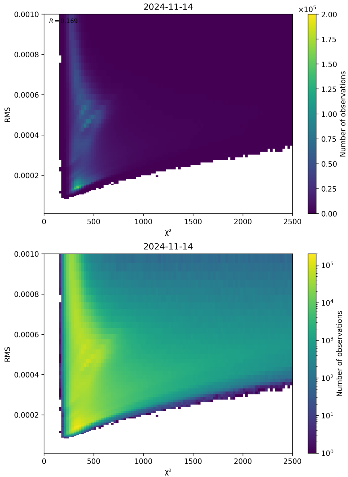
Figure 82: Scatter density plot of “ \chi^2 ” against “RMS” for 2024-11-14 to 2024-11-15.
