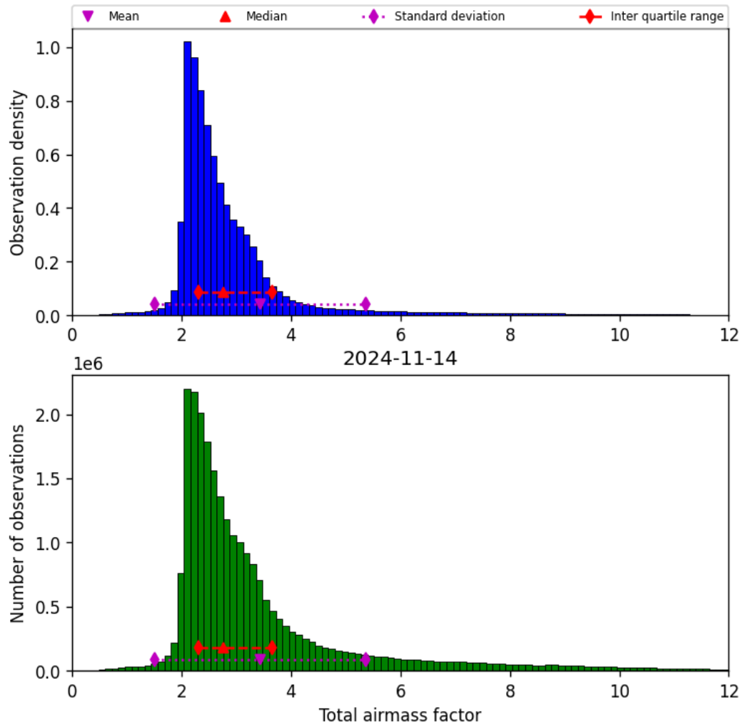
Figure 32: Histogram of “Total airmass factor” for 2024-11-14 to 2024-11-15
