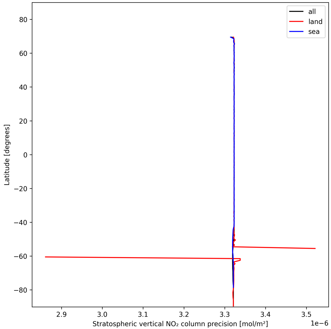
Figure 20: Zonal average of “Stratospheric vertical NO 2 column precision” for 2024-11-14 to 2024-11-15.
