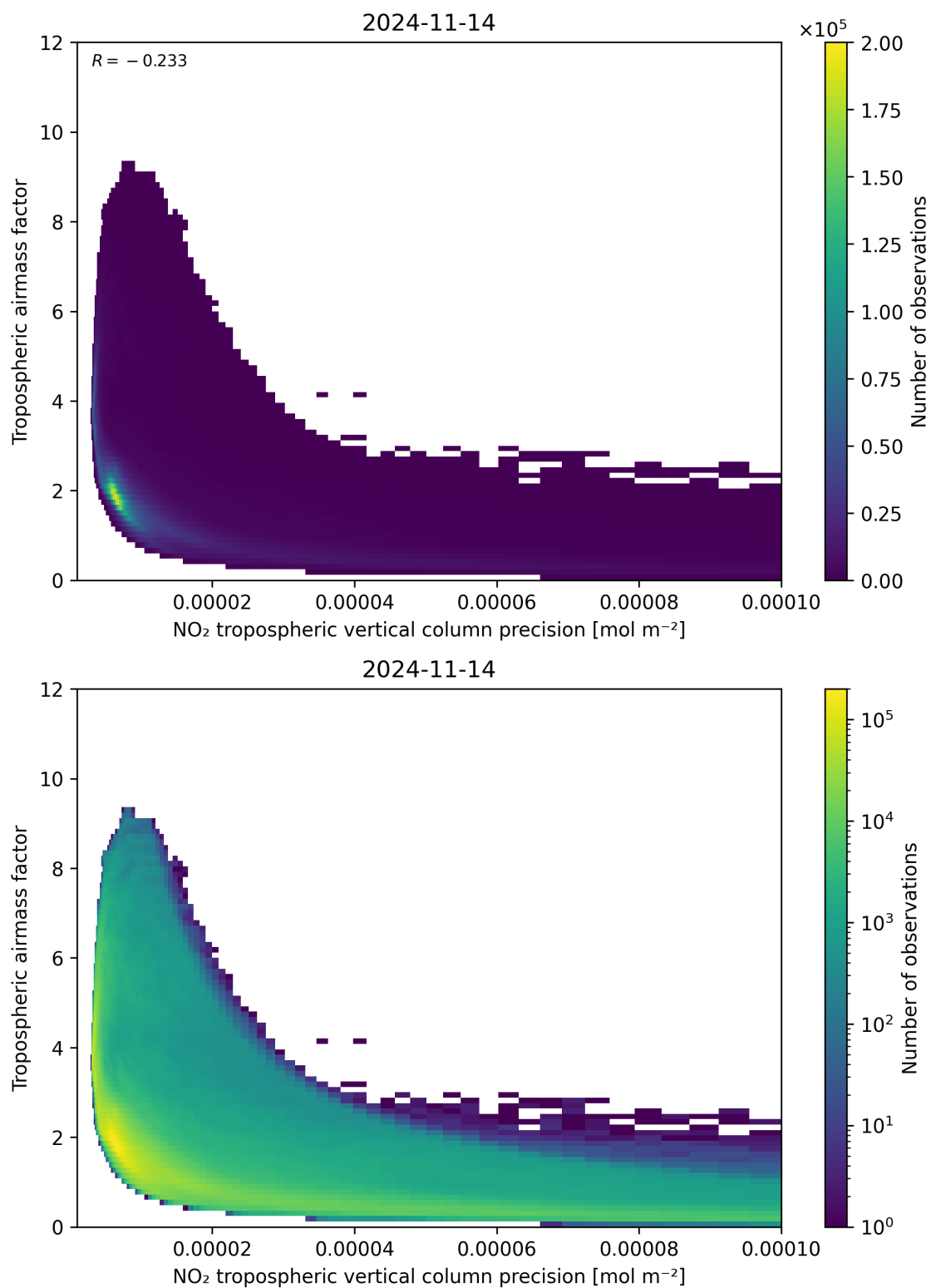
Figure 133: Scatter density plot of “NO 2 tropospheric vertical column precision” against “Tropospheric air mass factor” for 2024-11-14 to 2024-11-15.
