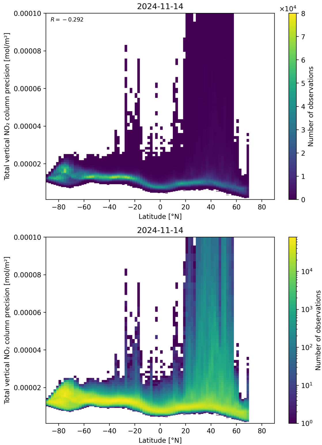
Figure 91: Scatter density plot of “Latitude” against “Total vertical NO 2 column precision” for 2024-11-14 to 2024-11-15.
