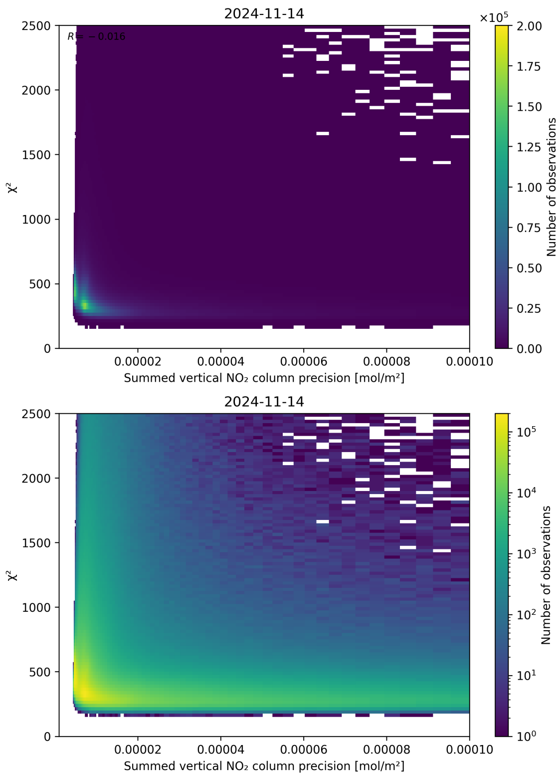
Figure 107: Scatter density plot of “Summed vertical NO 2 column precision” against “ \chi^2 ” for 2024-11-14 to 2024-11-15.
