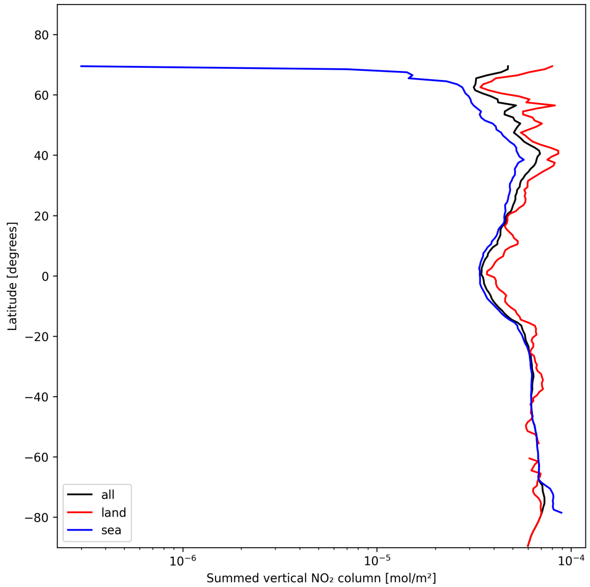
Figure 23: Zonal average of “Summed vertical NO 2 column” for 2024-11-14 to 2024-11-15.
