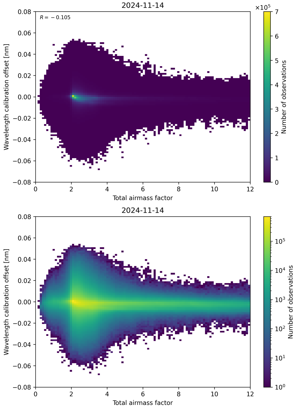
Figure 70: Scatter density plot of “Total airmass factor” against “Wavelength calibration offset” for 2024-11-14 to 2024-11-15.
