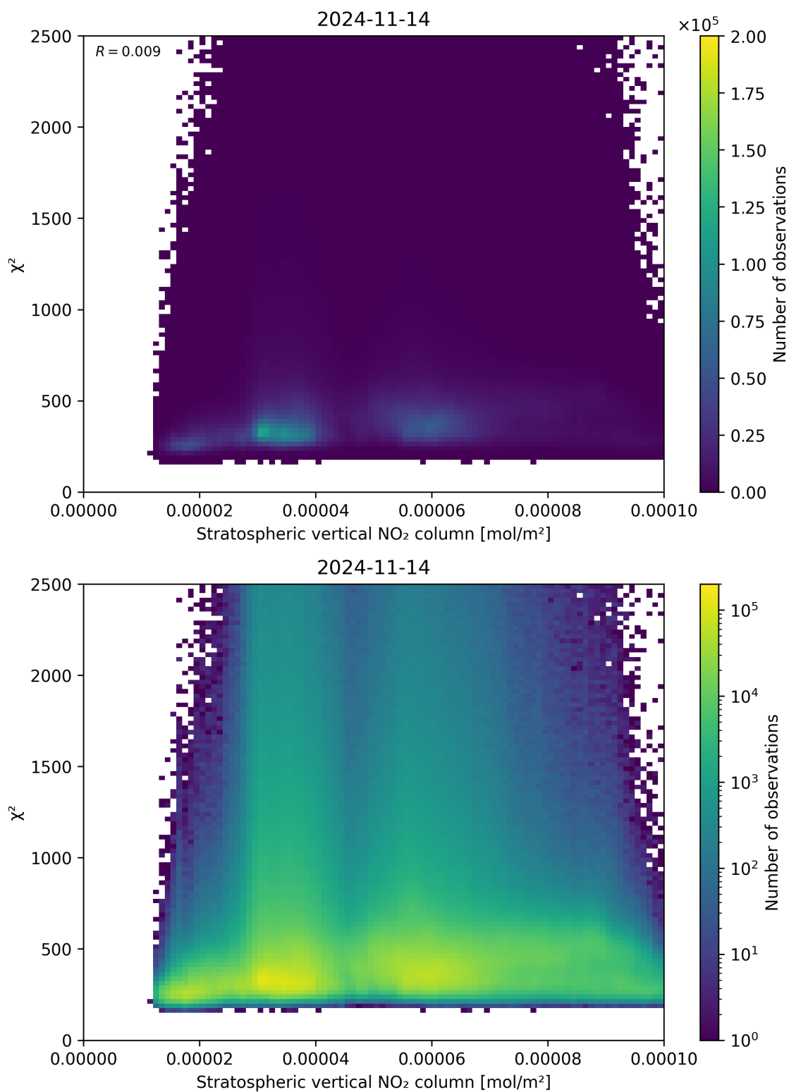
Figure 97: Scatter density plot of “Stratospheric vertical NO 2 column” against “ \chi^2 ” for 2024-11-14 to 2024-11-15.
