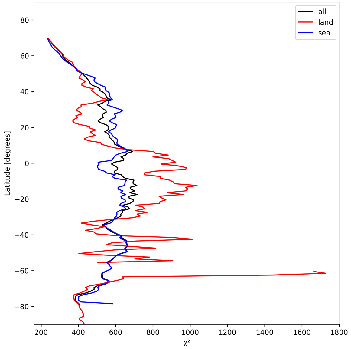
Figure 25: Zonal average of “ \chi^2 ” for 2024-11-14 to 2024-11-15.
