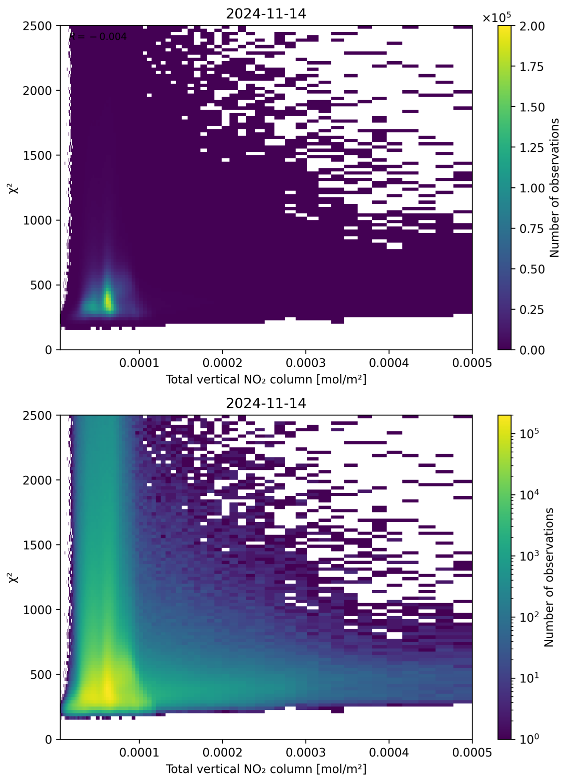
Figure 111: Scatter density plot of “Total vertical NO 2 column” against “ \chi^2 ” for 2024-11-14 to 2024-11-15.
