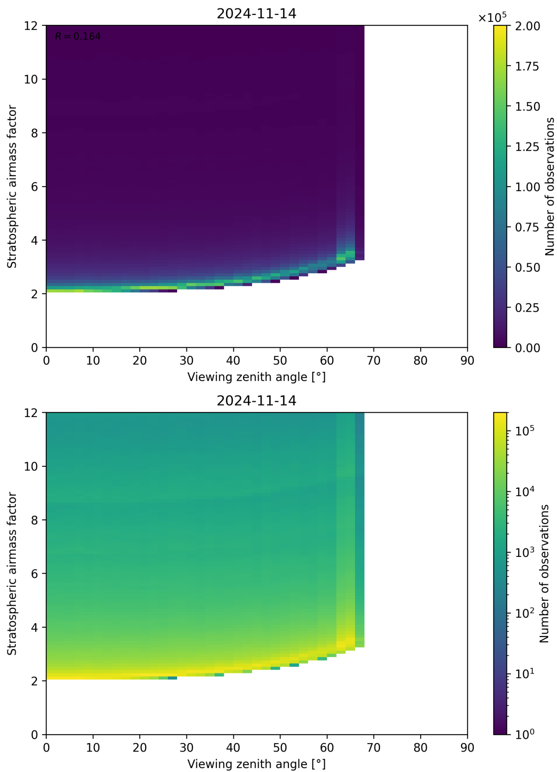
Figure 159: Scatter density plot of “Viewing zenith angle” against “Stratospheric airmass factor” for 2024-11-14 to 2024-11-15.
