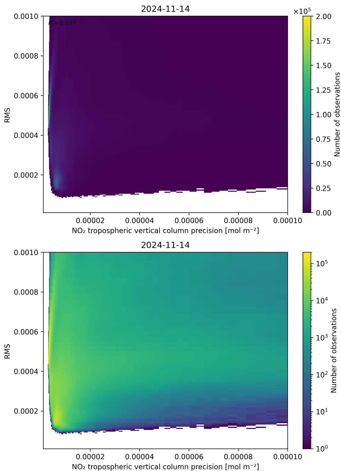
Figure 140: Scatter density plot of “NO 2 tropospheric vertical column precision” against “RMS” for 2024-11-14 to 2024-11-15.
