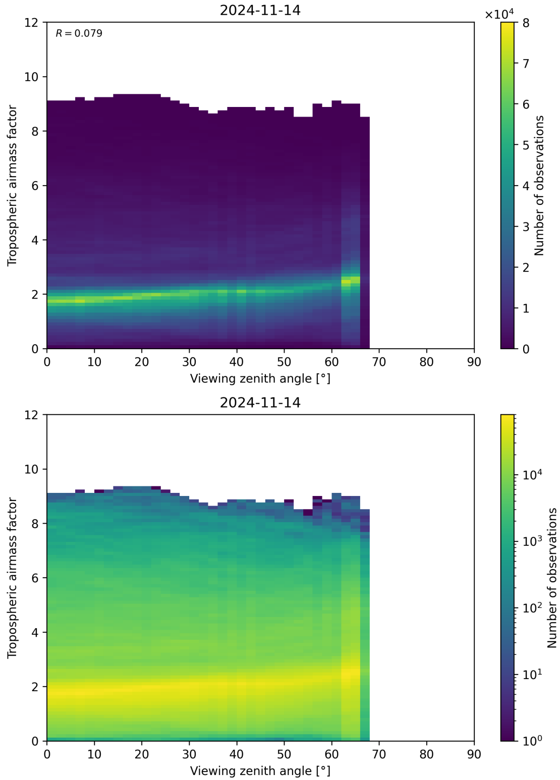
Figure 161: Scatter density plot of “Viewing zenith angle” against “Tropospheric airmass factor” for 2024-11-14 to 2024-11-15.
