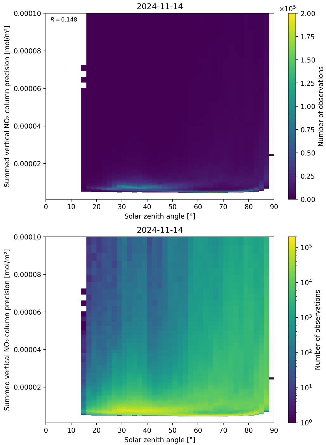
Figure 152: Scatter density plot of “Solar zenith angle” against “Summed vertical NO 2 column precision” for 2024-11-14 to 2024-11-15.
