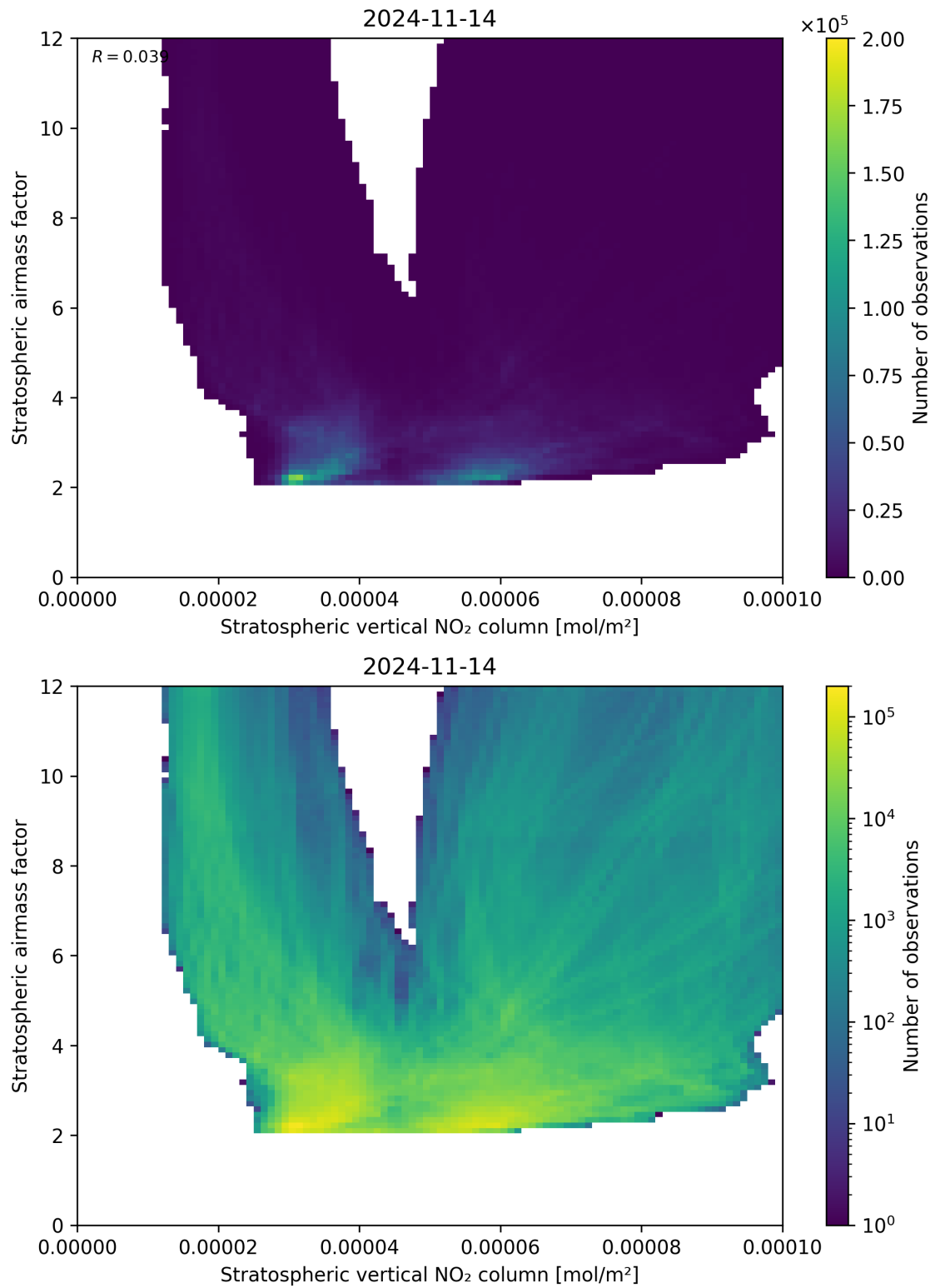
Figure 96: Scatter density plot of “Stratospheric vertical NO 2 column” against “Stratospheric airmass factor” for 2024-11-14 to 2024-11-15.
