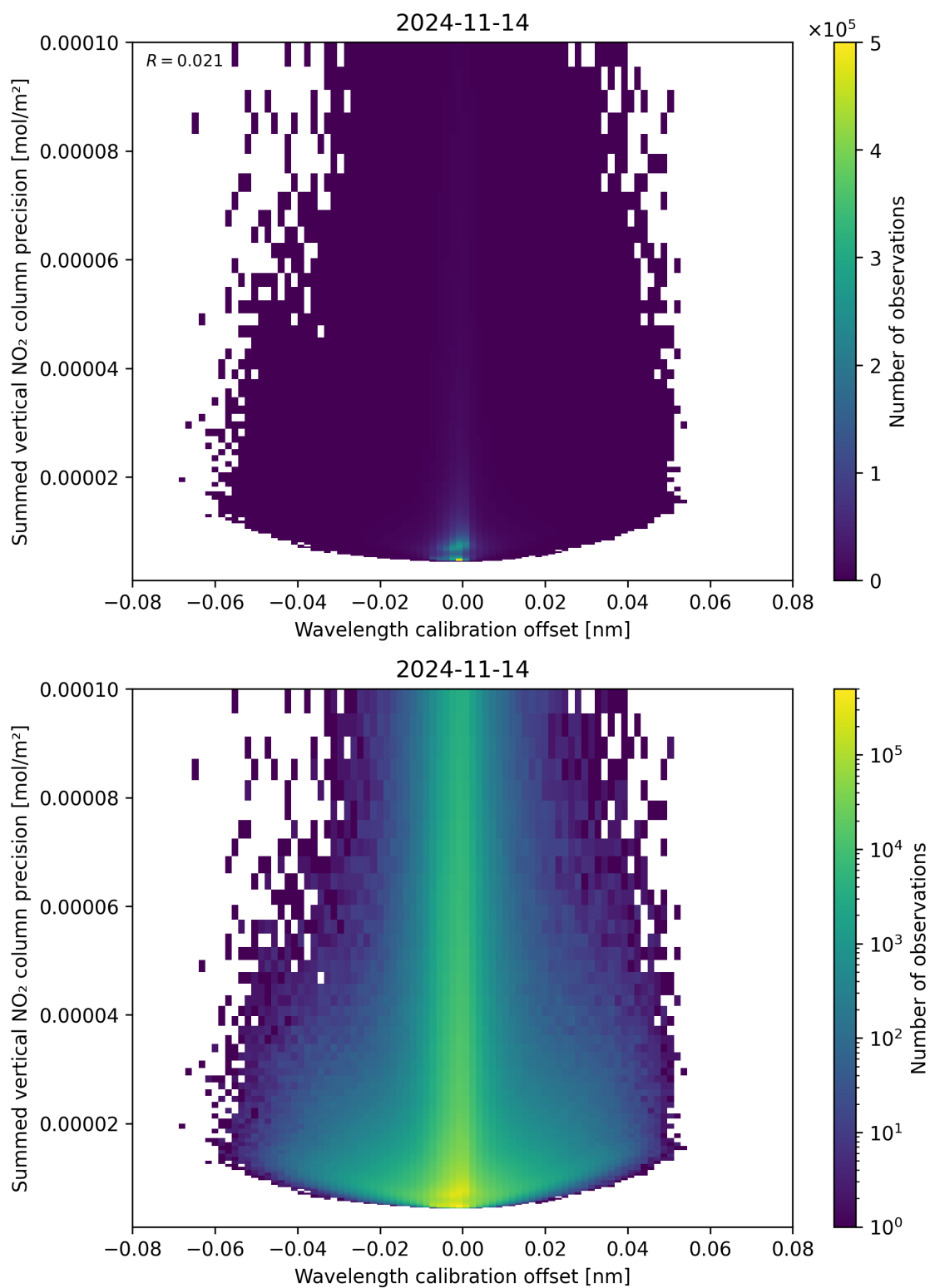
Figure 178: Scatter density plot of “Wavelength calibration offset” against “Summed vertical NO 2 column precision” for 2024-11-14 to 2024-11-15.
