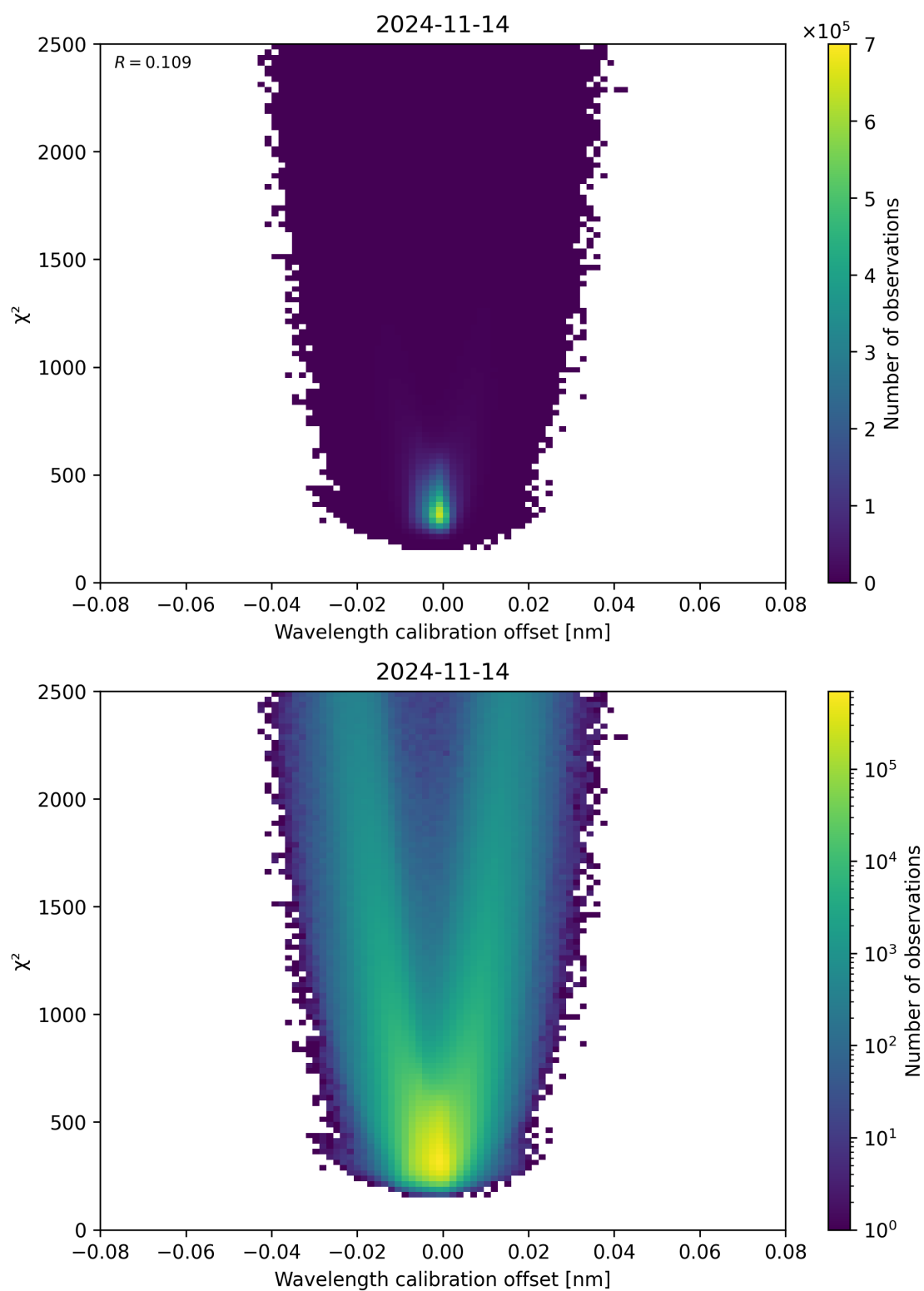
Figure 175: Scatter density plot of “Wavelength calibration offset” against “ \chi^2 ” for 2024-11-14 to 2024-11-15.
