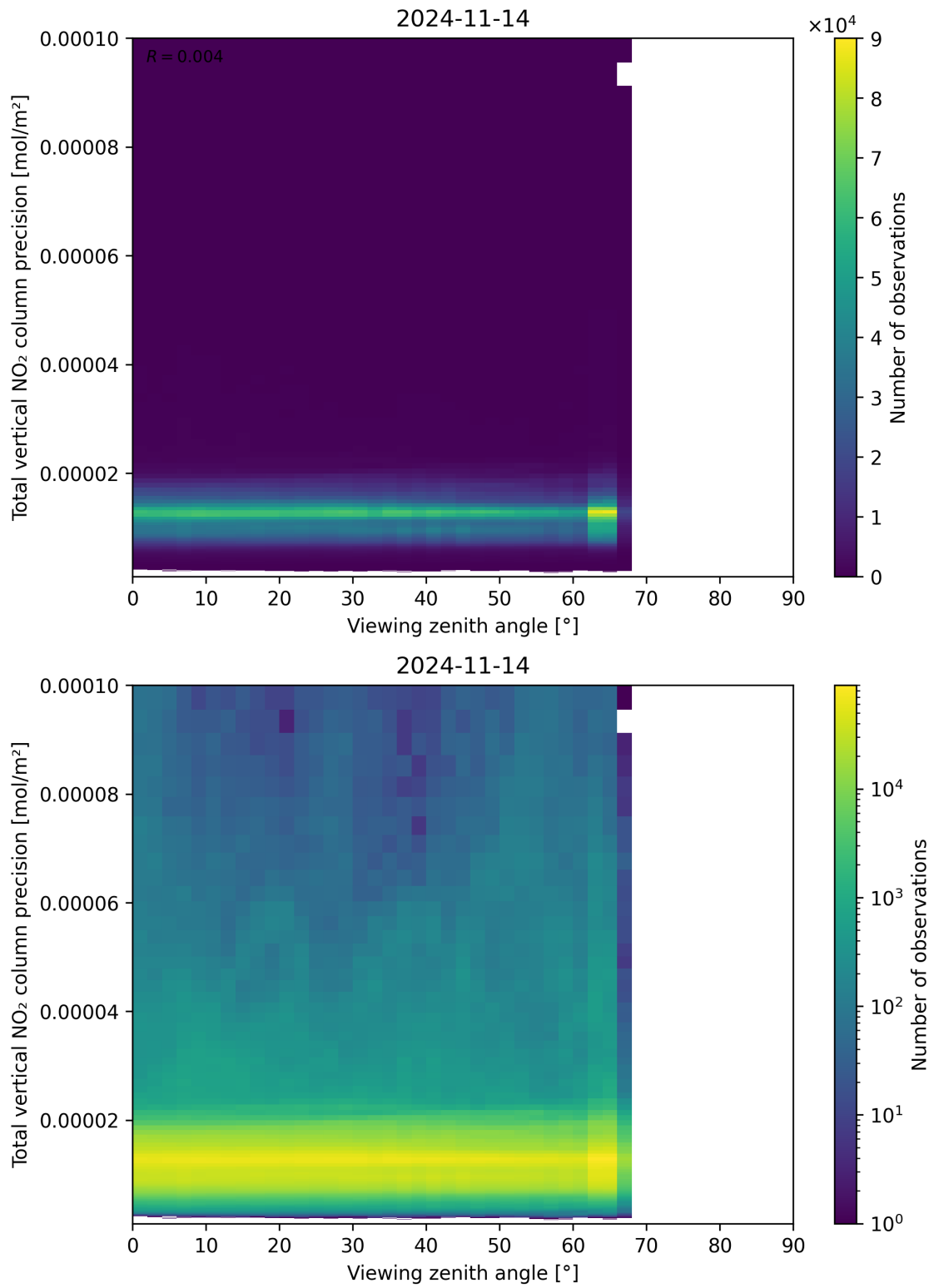
Figure 168: Scatter density plot of “Viewing zenith angle” against “Total vertical NO 2 column precision” for 2024-11-14 to 2024-11-15.
