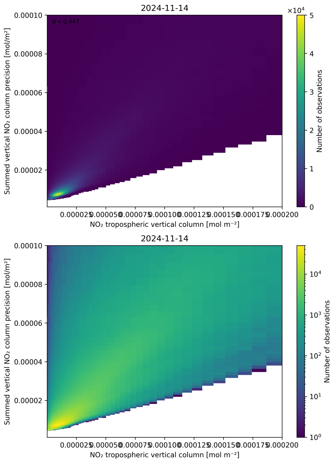
Figure 127: Scatter density plot of “NO 2 tropospheric vertical column” against “Summed vertical NO 2 column precision” for 2024-11-14 to 2024-11-15.
