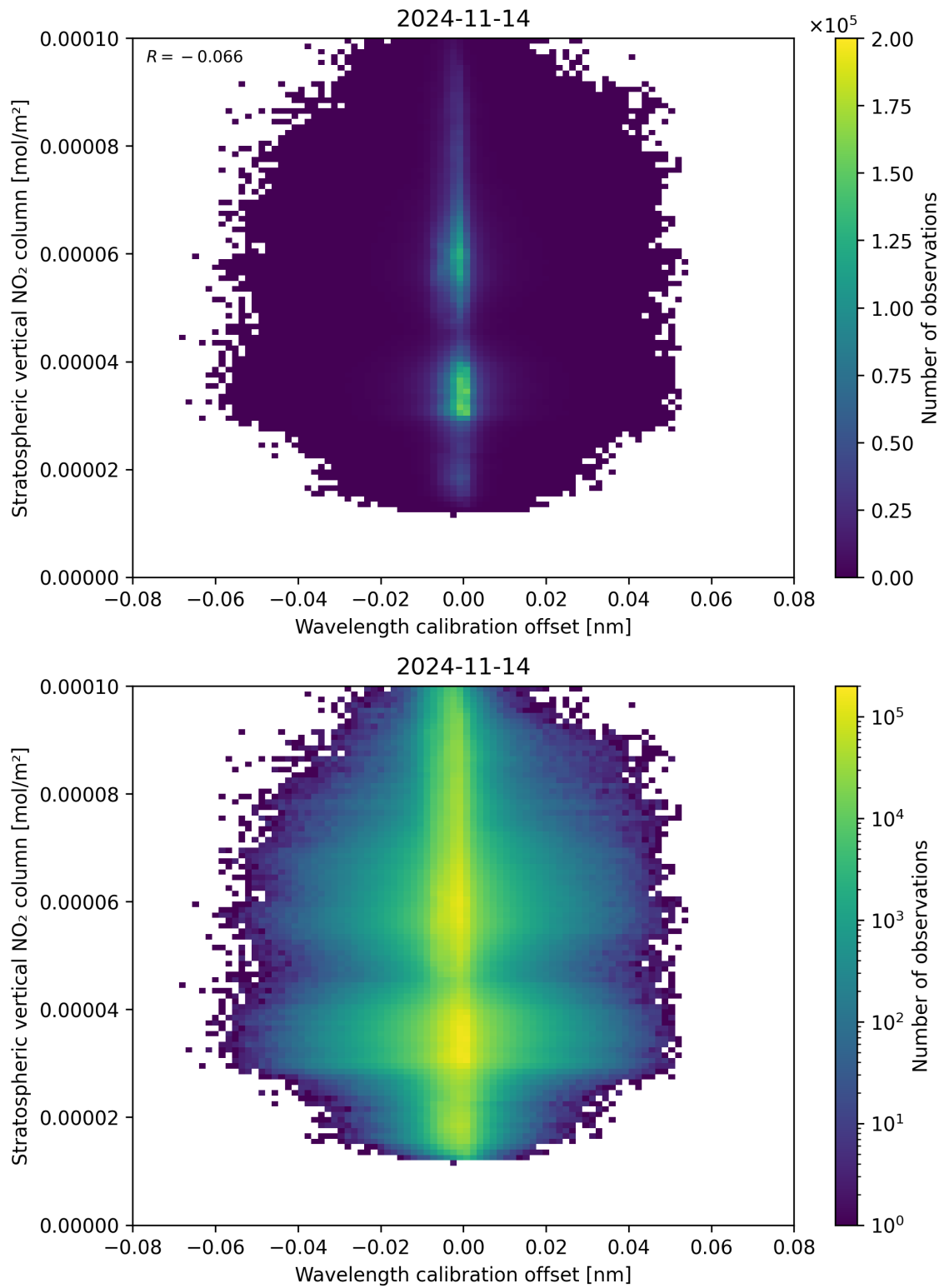
Figure 176: Scatter density plot of “Wavelength calibration offset” against “Stratospheric vertical NO 2 column” for 2024-11-14 to 2024-11-15.
