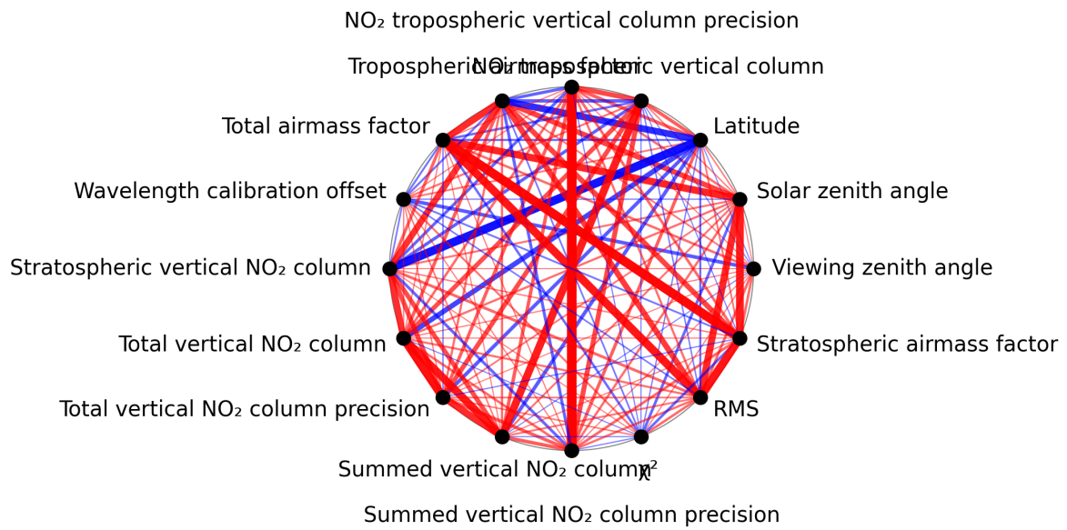
Figure 1: Map of correlation graph for 2024-11-14 to 2024-11-15.
