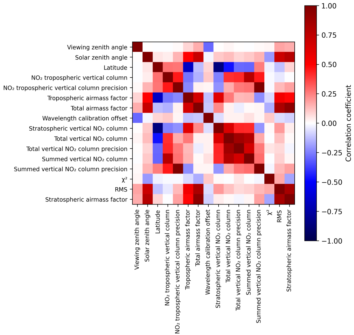
Figure 2: Map of correlation matrix for 2024-11-14 to 2024-11-15.
