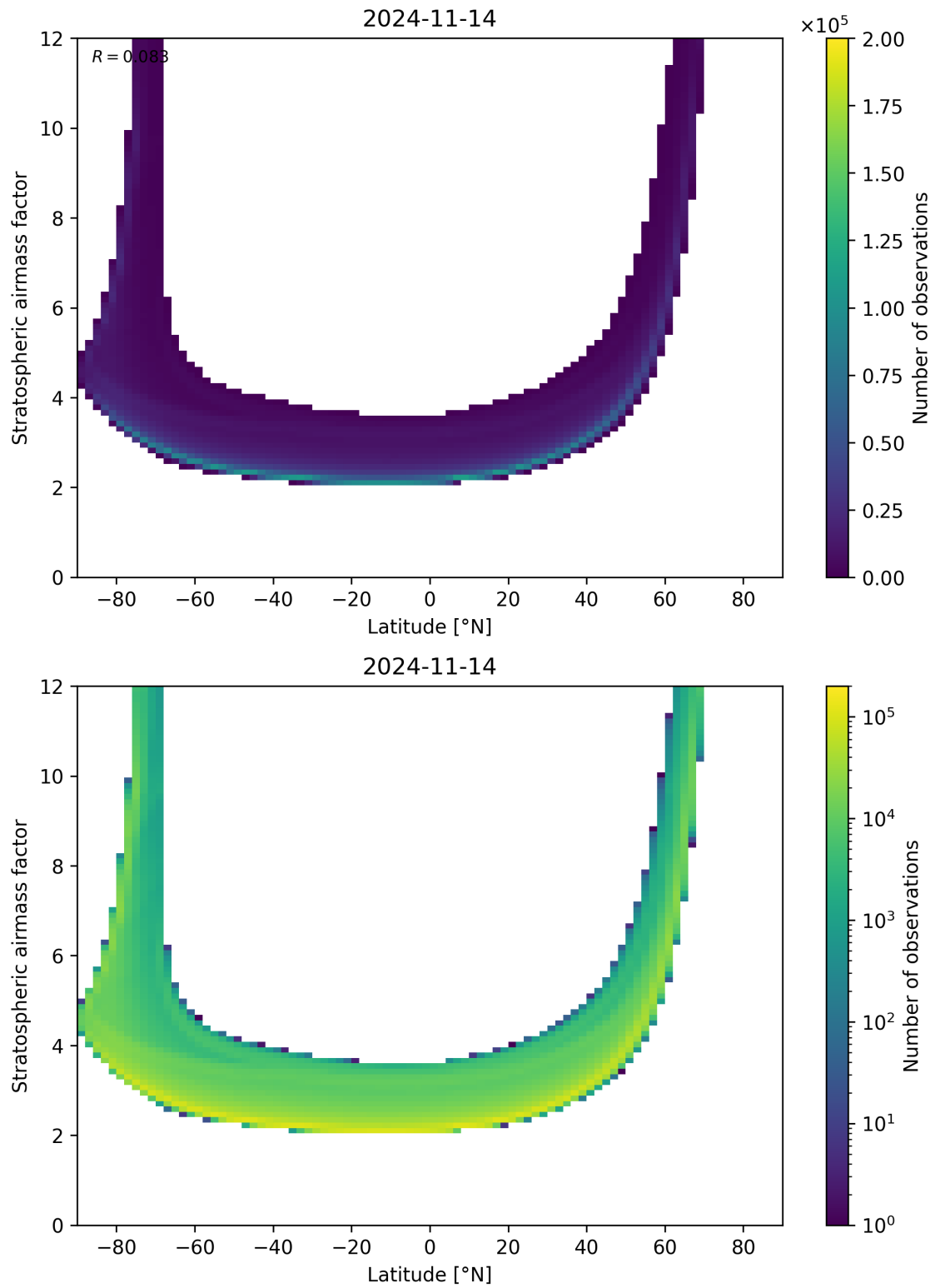
Figure 83: Scatter density plot of “Latitude” against “Stratospheric airmass factor” for 2024-11-14 to 2024-11-15.
