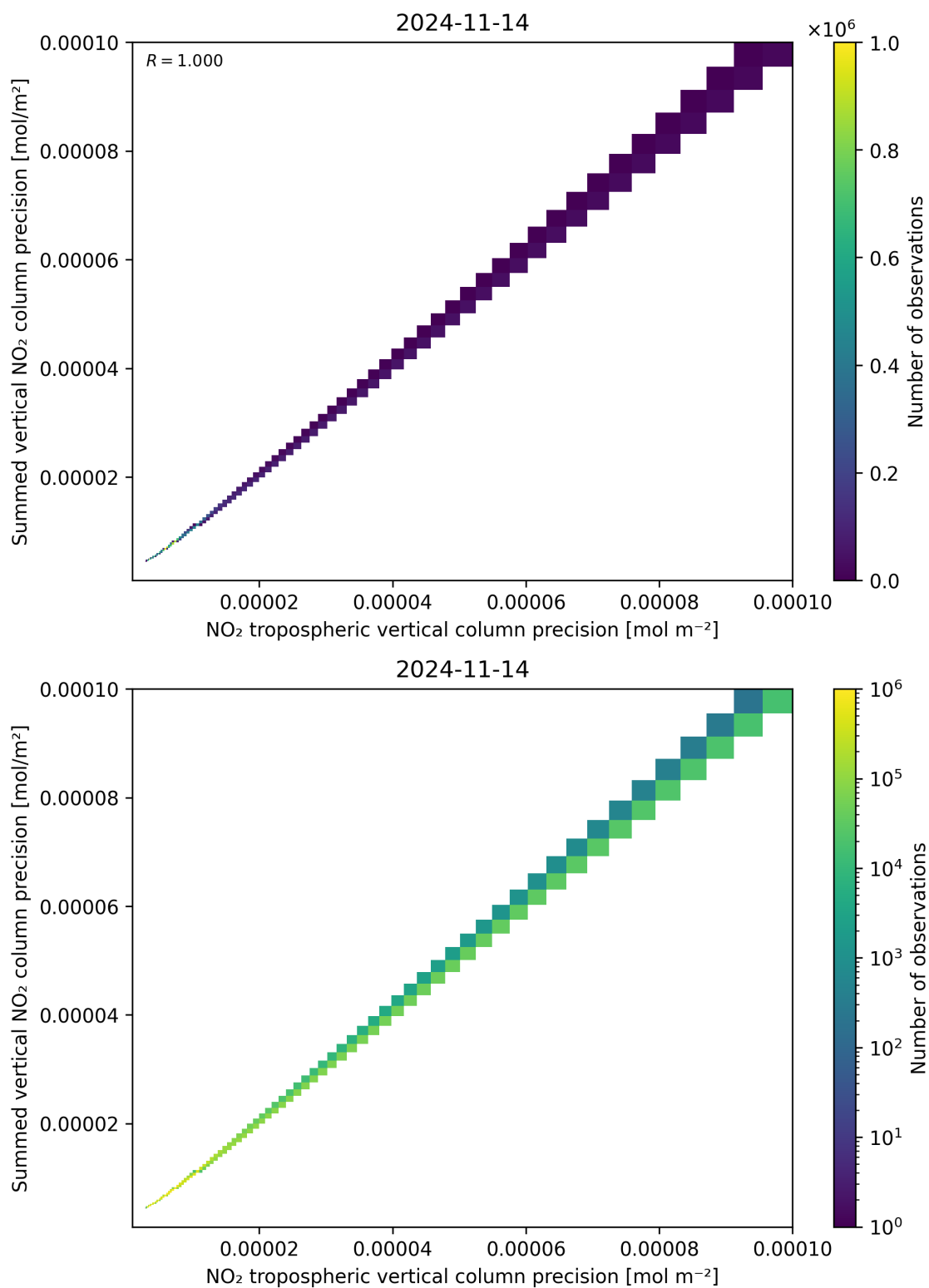
Figure 137: Scatter density plot of “NO 2 tropospheric vertical column precision” against “Summed vertical NO 2 column precision” for 2024-11-14 to 2024-11-15.
