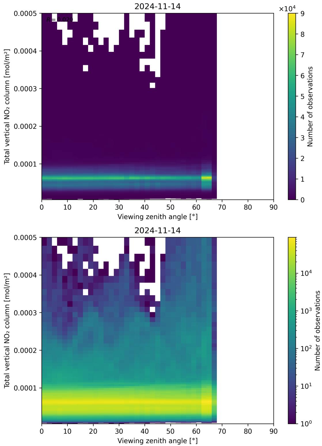
Figure 167: Scatter density plot of “Viewing zenith angle” against “Total vertical NO 2 column” for 2024-11-14 to 2024-11-15.
