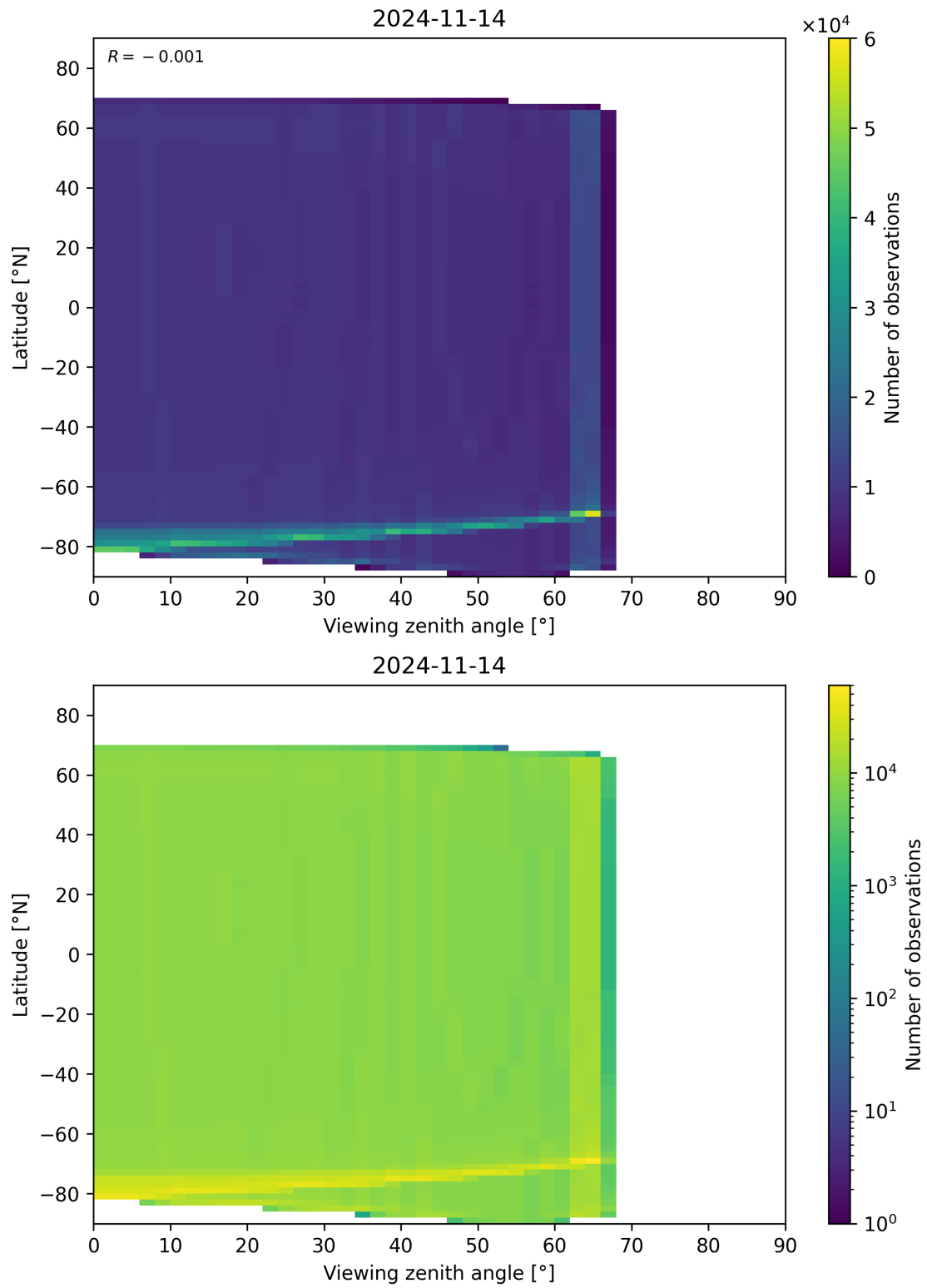
Figure 163: Scatter density plot of “Viewing zenith angle” against “Latitude” for 2024-11-14 to 2024-11-15.
