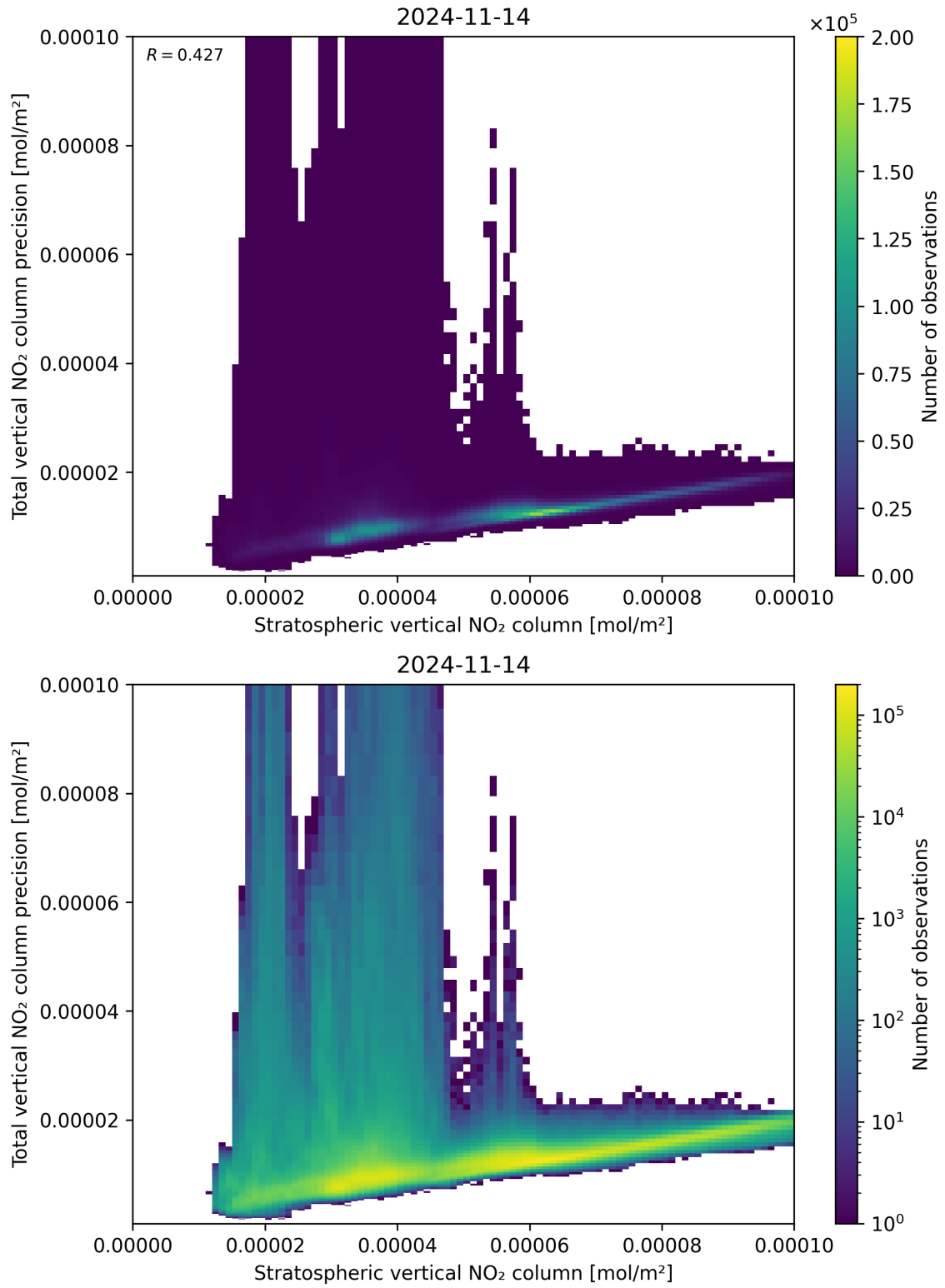
Figure 101: Scatter density plot of “Stratospheric vertical NO 2 column” against “Total vertical NO 2 column precision” for 2024-11-14 to 2024-11-15.
