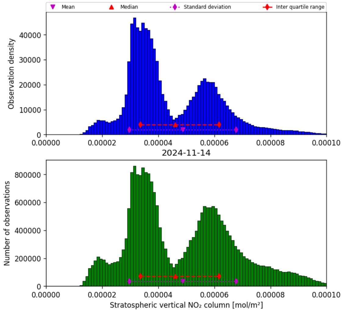
Figure 36: Histogram of “Stratospheric vertical NO 2 column” for 2024-11-14 to 2024-11-15
