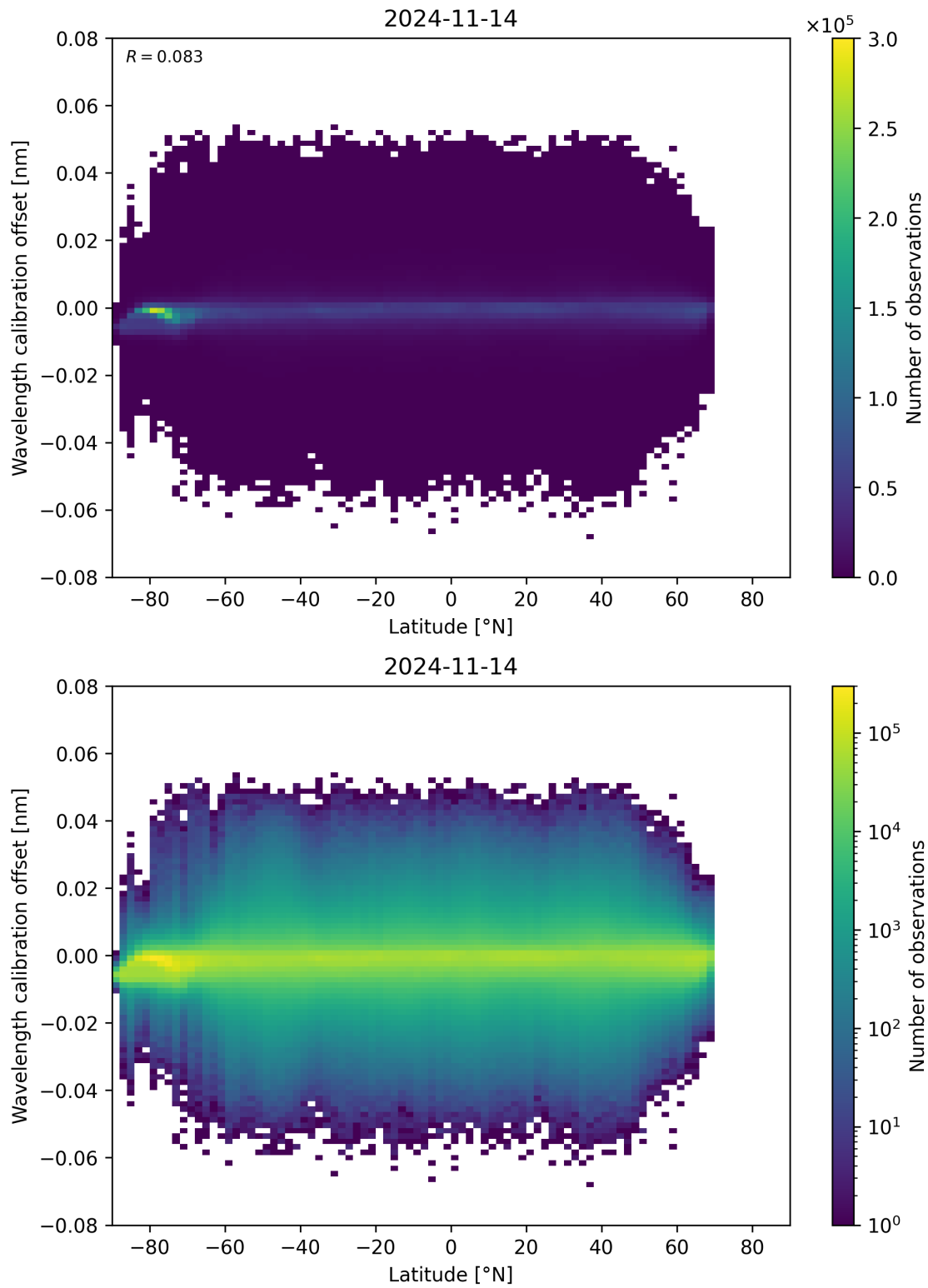
Figure 95: Scatter density plot of “Latitude” against “Wavelength calibration offset” for 2024-11-14 to 2024-11-15.
