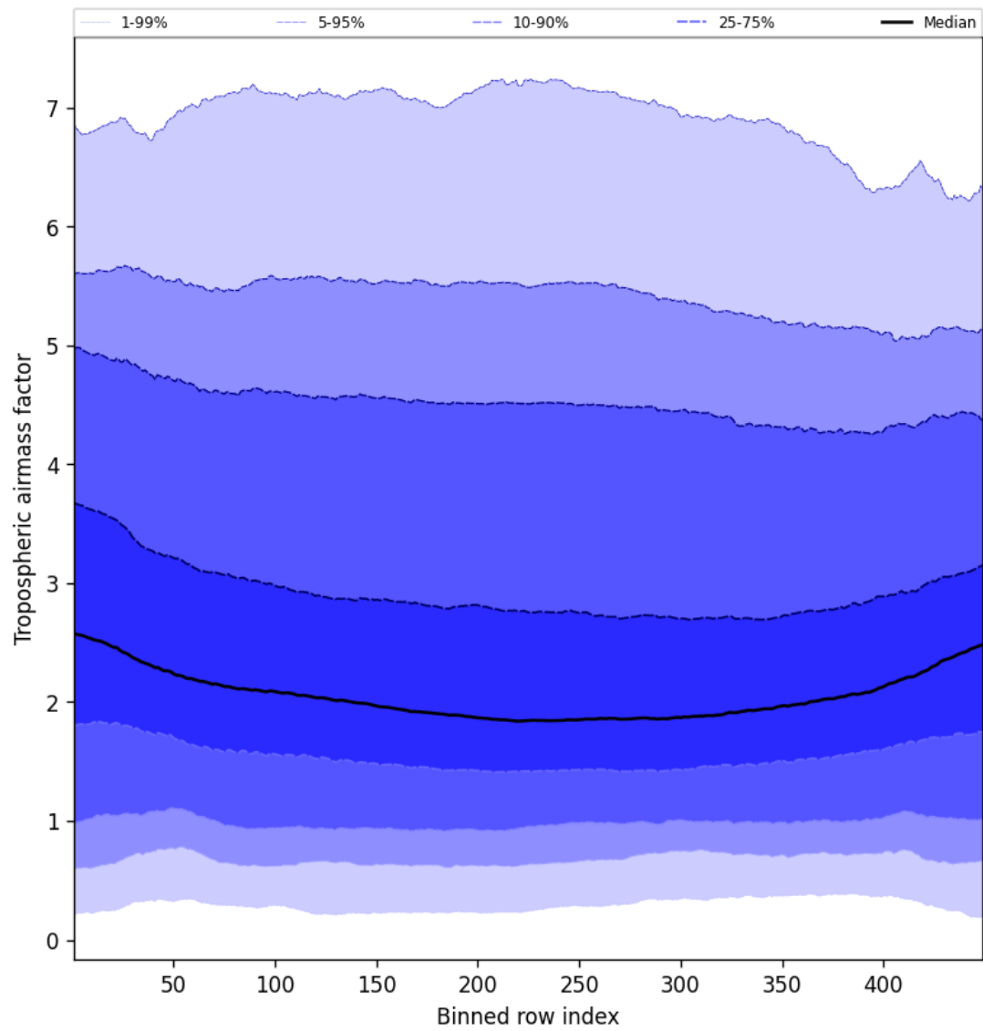
Figure 48: Along track statistics of “Tropospheric airmass factor” for 2024-11-14 to 2024-11-15
