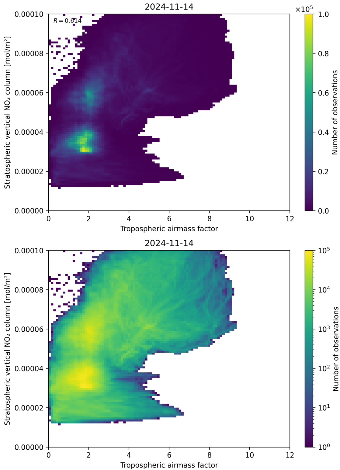
Figure 74: Scatter density plot of “Tropospheric air mass factor” against “Stratospheric vertical NO 2 column” for 2024-11-14 to 2024-11-15.
