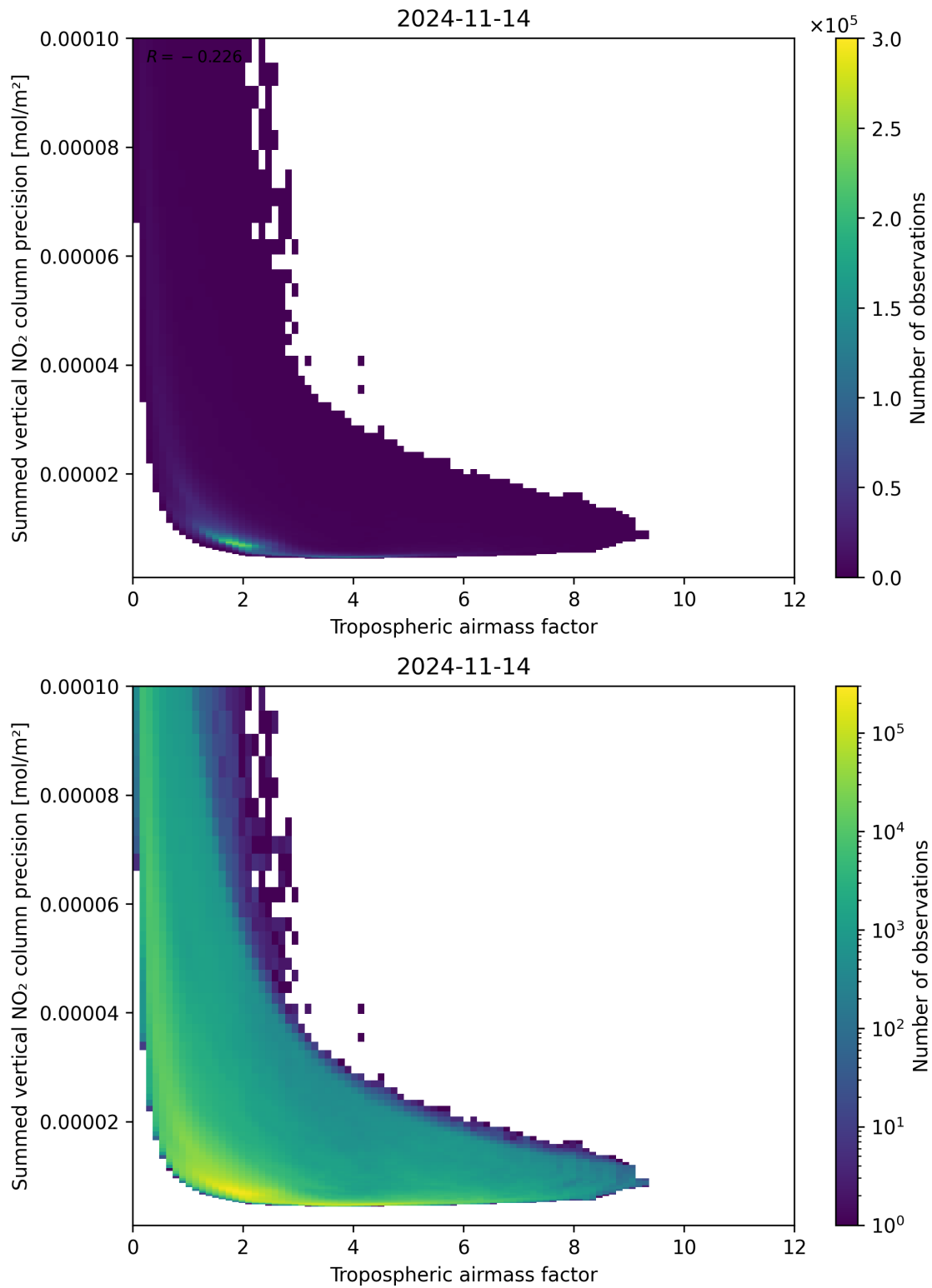
Figure 76: Scatter density plot of “Tropospheric air mass factor” against “Summed vertical NO 2 column precision” for 2024-11-14 to 2024-11-15.
