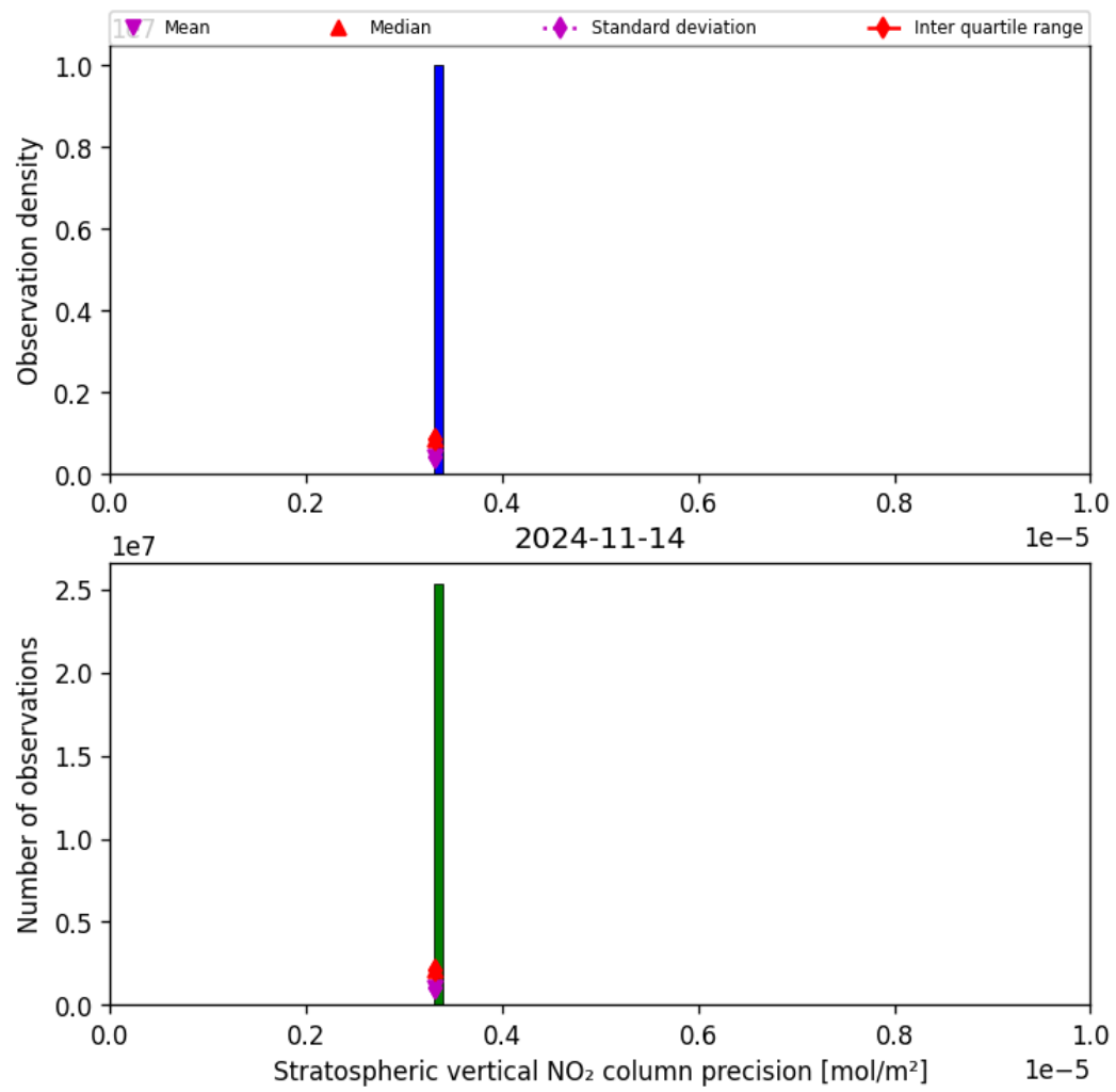
Figure 37: Histogram of “Stratospheric vertical NO 2 column precision” for 2024-11-14 to 2024-11-15
