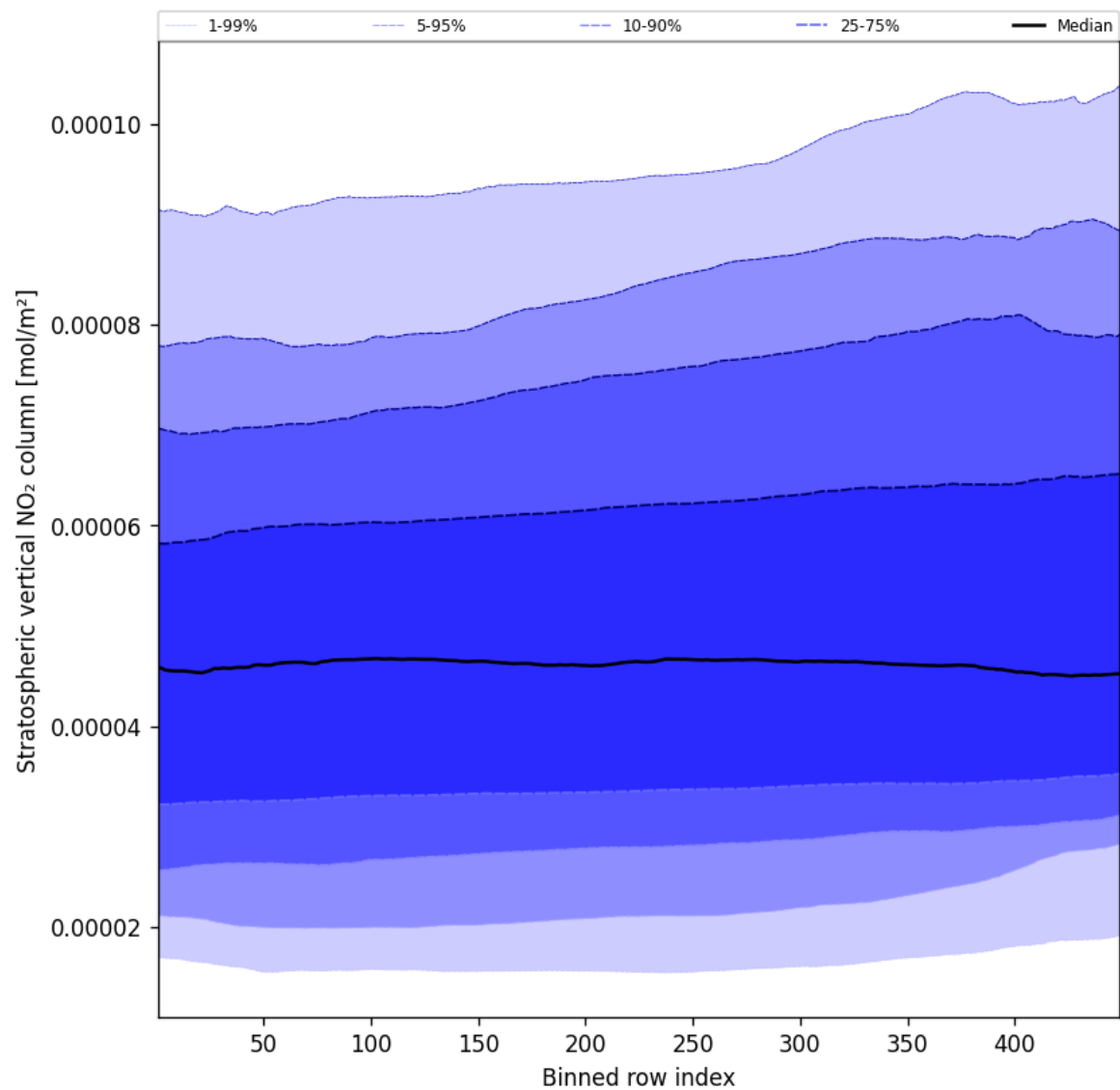
Figure 53: Along track statistics of “Stratospheric vertical NO 2 column” for 2024-11-14 to 2024-11-15
