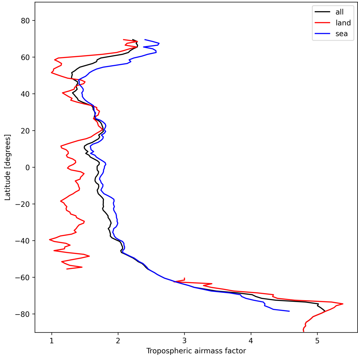
Figure 14: Zonal average of “Tropospheric airmass factor” for 2024-11-14 to 2024-11-15.
