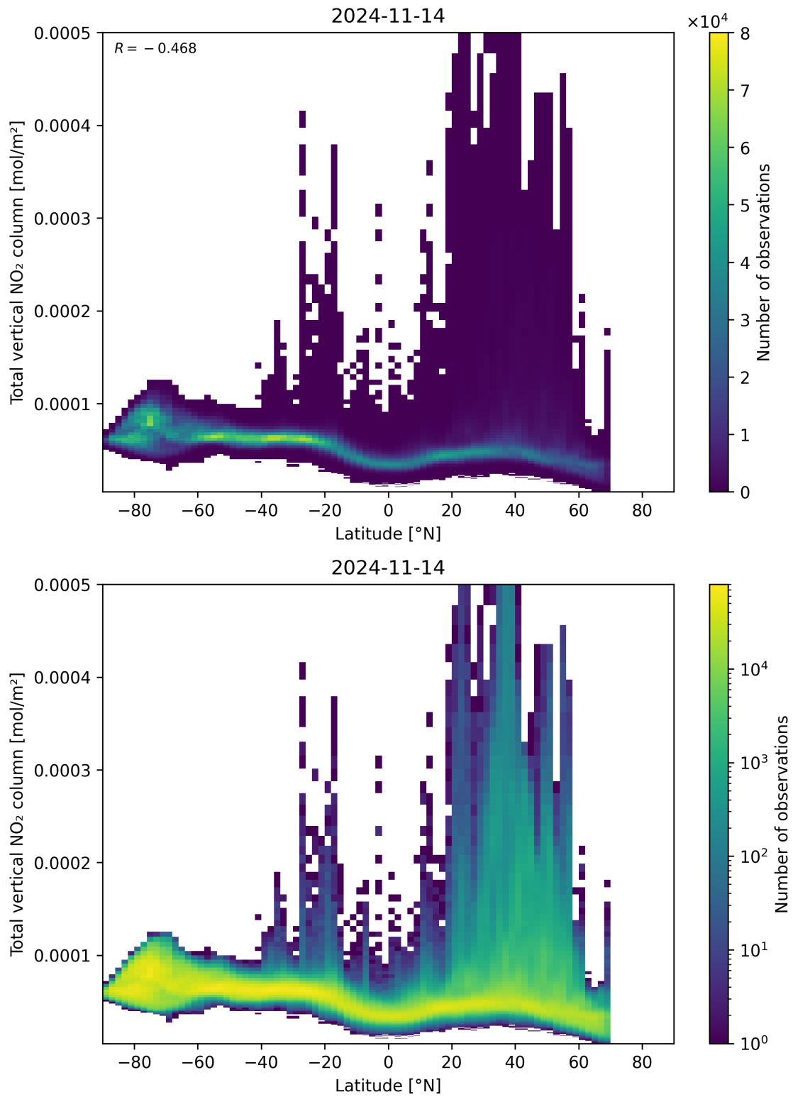
Figure 90: Scatter density plot of “Latitude” against “Total vertical NO 2 column” for 2024-11-14 to 2024-11-15.
