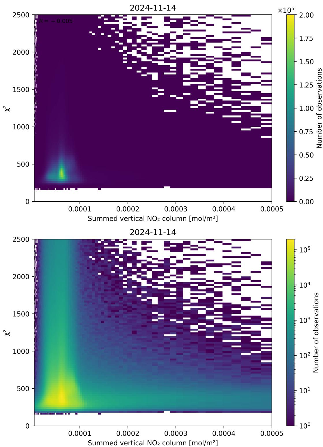
Figure 104: Scatter density plot of “Summed vertical NO 2 column” against “ \chi^2 ” for 2024-11-14 to 2024-11-15.
