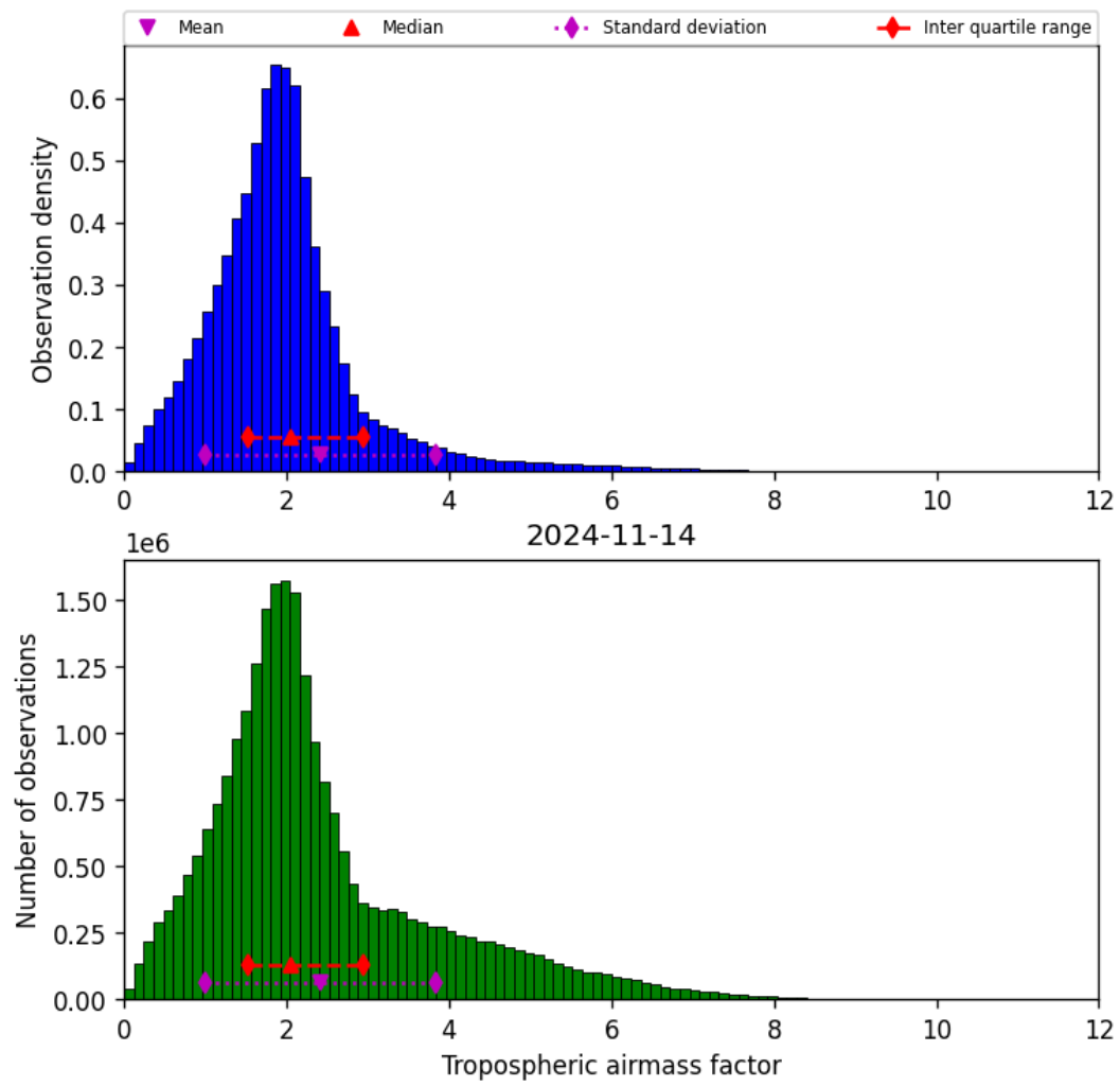
Figure 31: Histogram of “Tropospheric airmass factor” for 2024-11-14 to 2024-11-15
