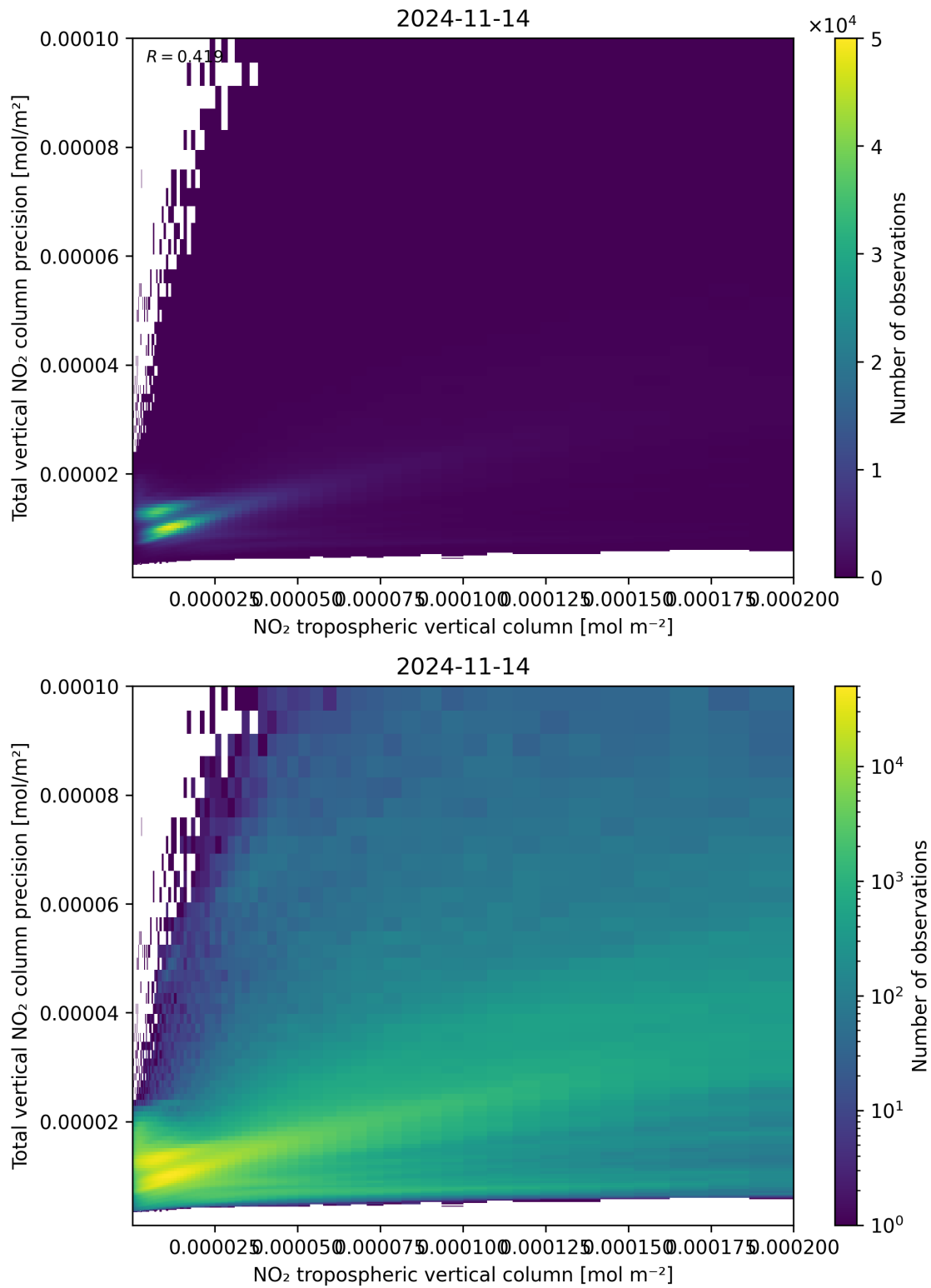
Figure 129: Scatter density plot of “NO 2 tropospheric vertical column” against “Total vertical NO 2 column precision” for 2024-11-14 to 2024-11-15.
