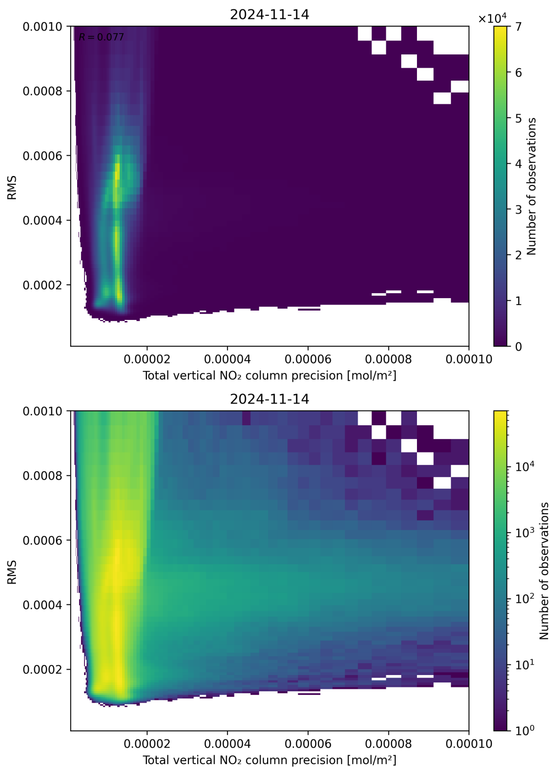
Figure 119: Scatter density plot of “Total vertical NO 2 column precision” against “RMS” for 2024-11-14 to 2024-11-15.
