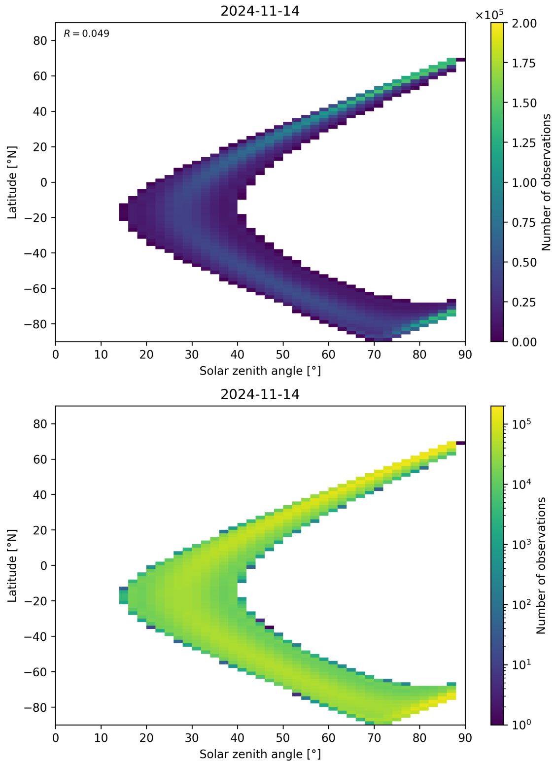
Figure 149: Scatter density plot of “Solar zenith angle” against “Latitude” for 2024-11-14 to 2024-11-15.
