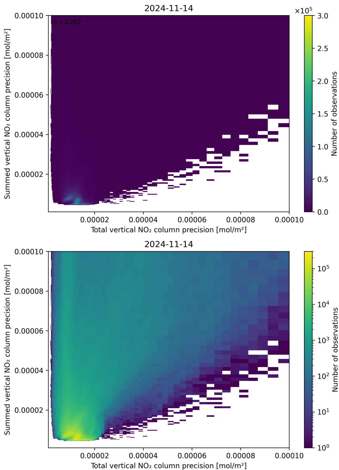
Figure 118: Scatter density plot of “Total vertical NO 2 column precision” against “Summed vertical NO 2 column precision” for 2024-11-14 to 2024-11-15.
