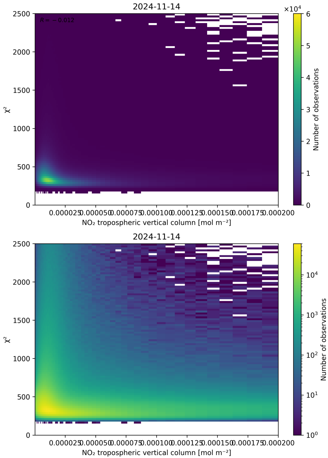
Figure 124: Scatter density plot of “NO 2 tropospheric vertical column” against “ \chi^2 ” for 2024-11-14 to 2024-11-15.
