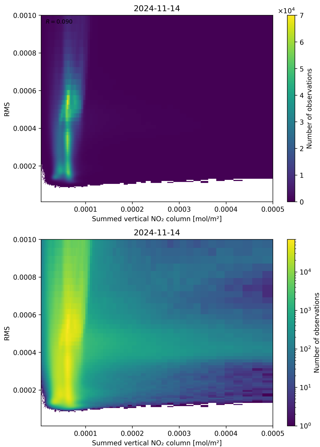
Figure 109: Scatter density plot of “Summed vertical NO 2 column” against “RMS” for 2024-11-14 to 2024-11-15.
