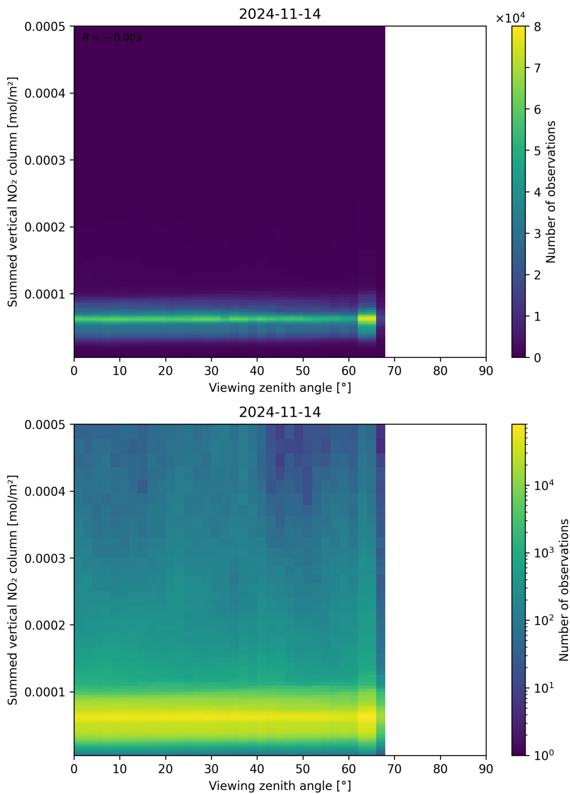
Figure 165: Scatter density plot of “Viewing zenith angle” against “Summed vertical NO 2 column” for 2024-11-14 to 2024-11-15.
