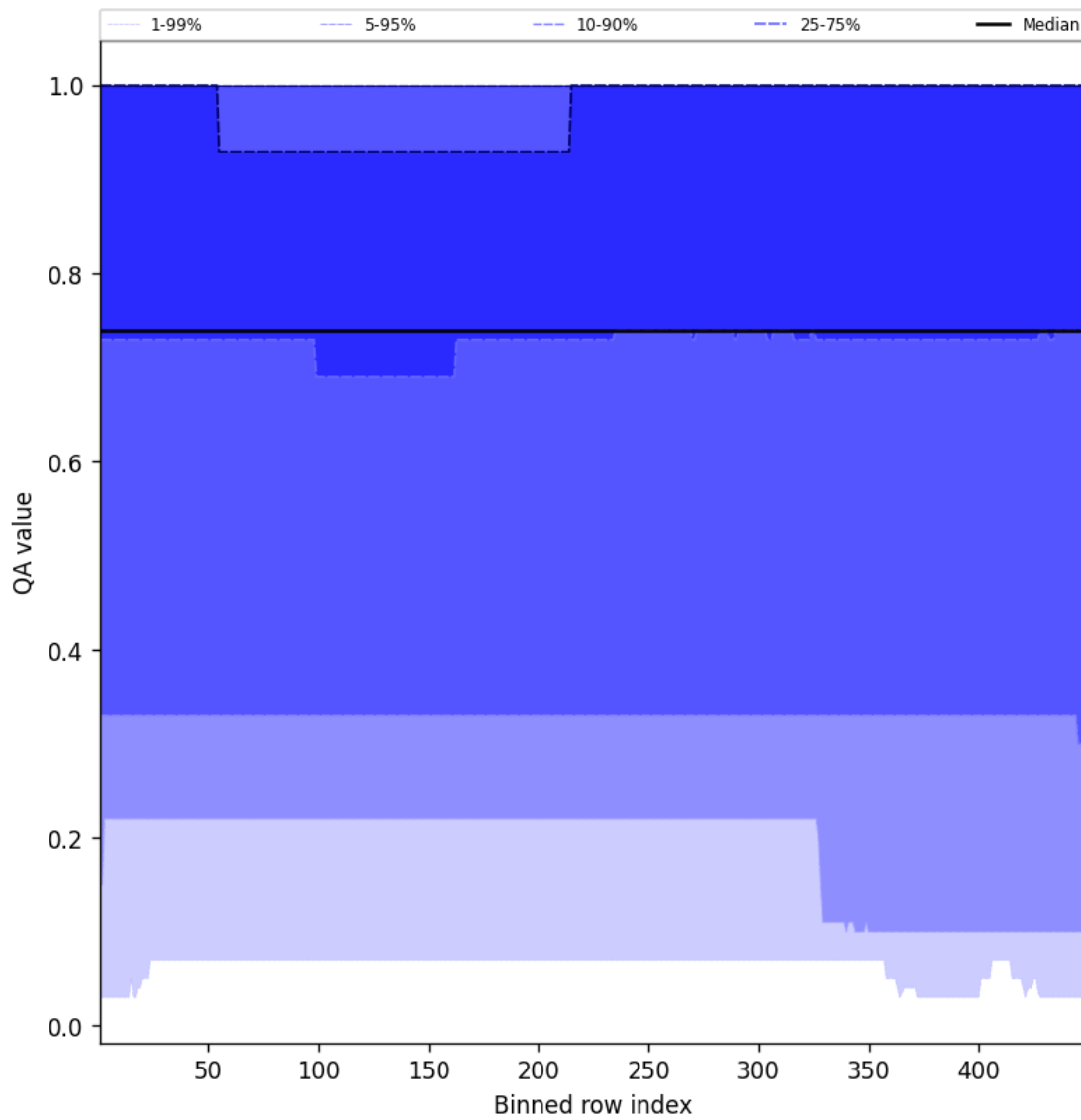
Figure 45: Along track statistics of “QA value” for 2024-11-14 to 2024-11-15
