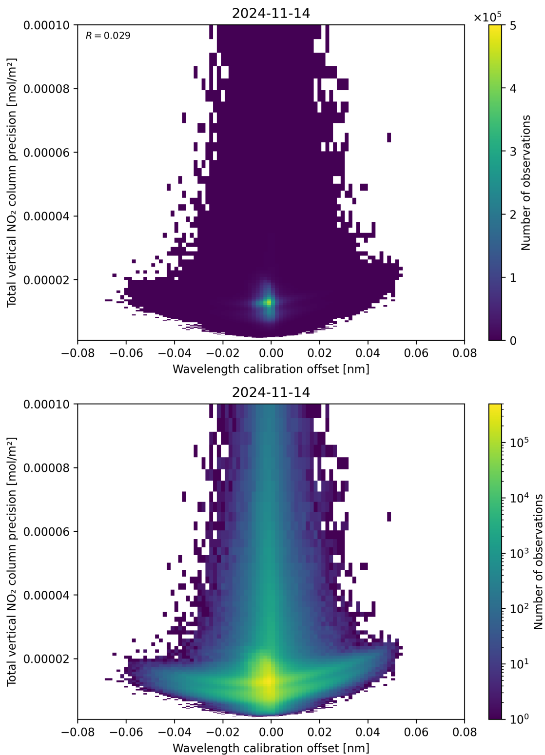
Figure 180: Scatter density plot of “Wavelength calibration offset” against “Total vertical NO 2 column precision” for 2024-11-14 to 2024-11-15.
