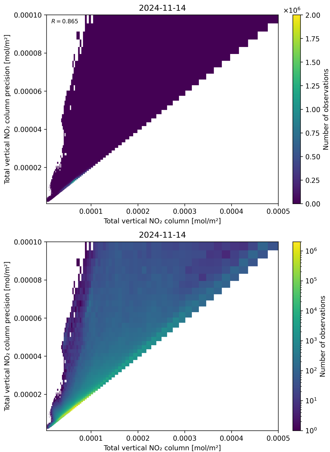
Figure 114: Scatter density plot of “Total vertical NO 2 column” against “Total vertical NO 2 column precision” for 2024-11-14 to 2024-11-15.
