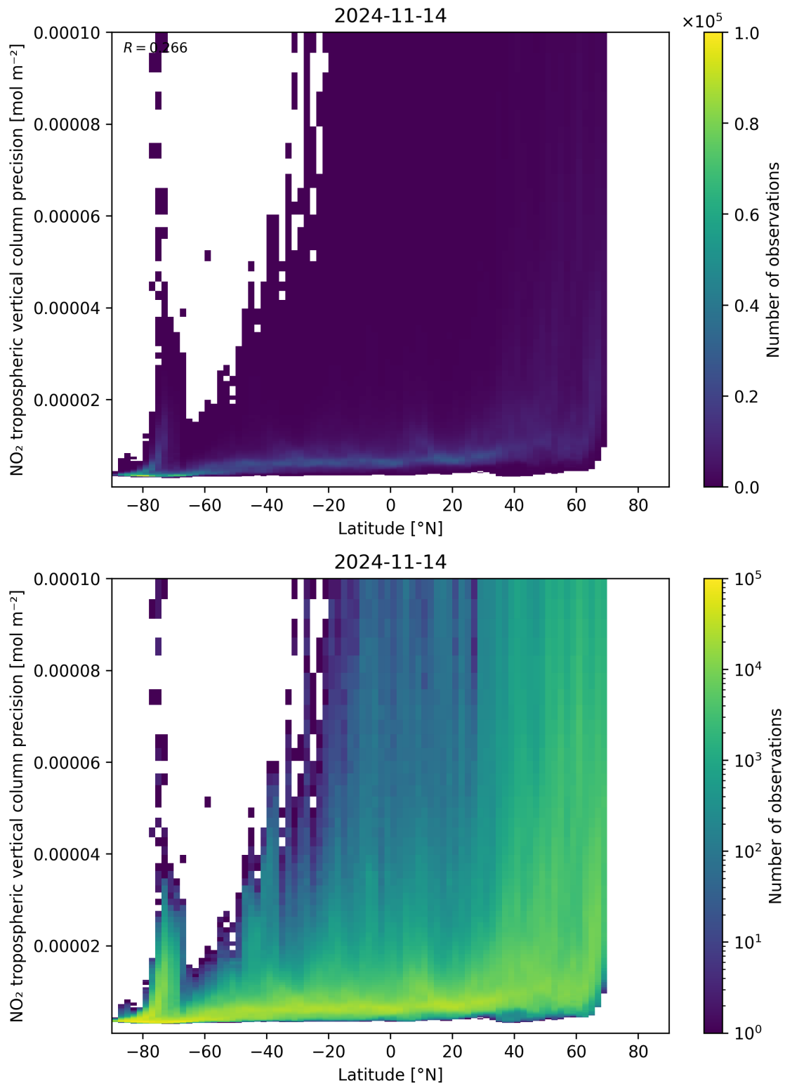
Figure 93: Scatter density plot of “Latitude” against “NO 2 tropospheric vertical column precision” for 2024-11-14 to 2024-11-15.
