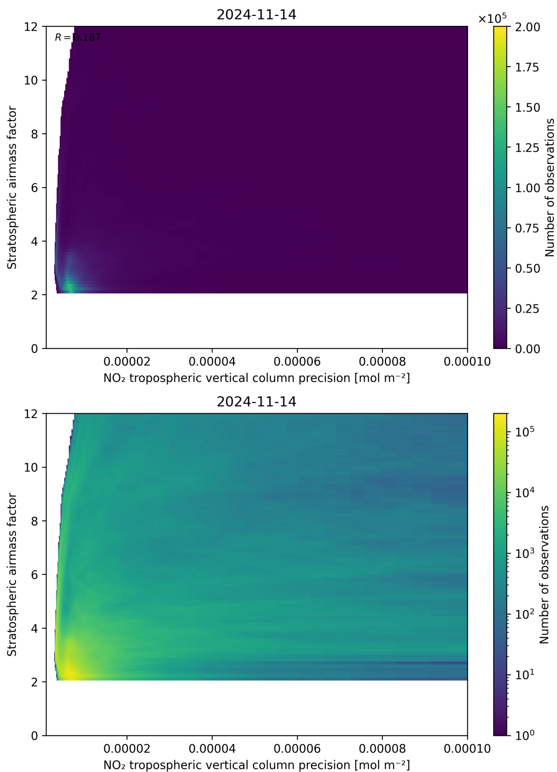
Figure 131: Scatter density plot of “NO 2 tropospheric vertical column precision” against “Stratospheric airmass factor” for 2024-11-14 to 2024-11-15.
