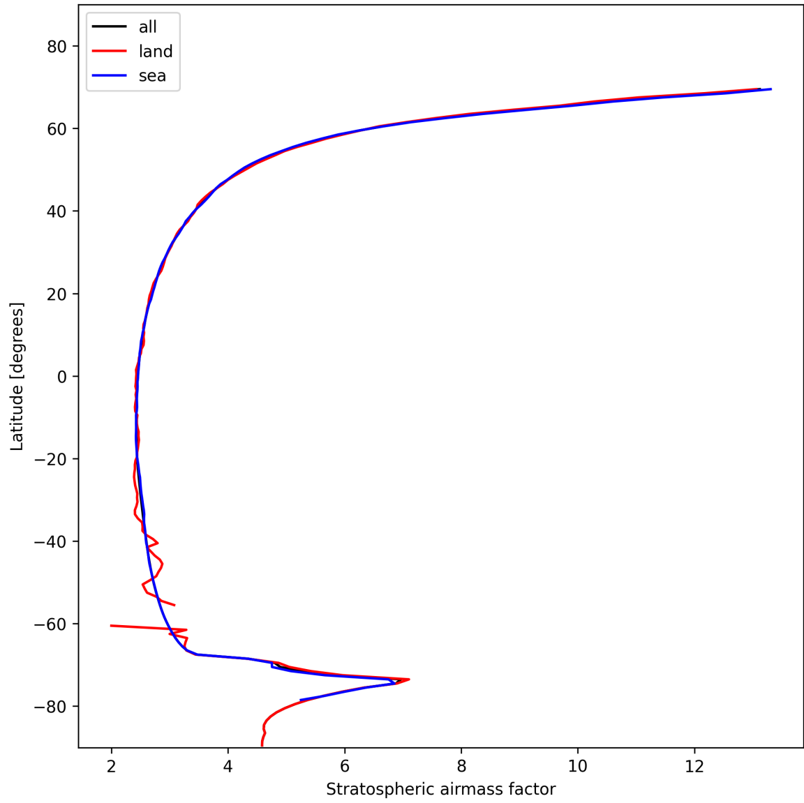
Figure 27: Zonal average of “Stratospheric air mass factor” for 2024-11-14 to 2024-11-15.
