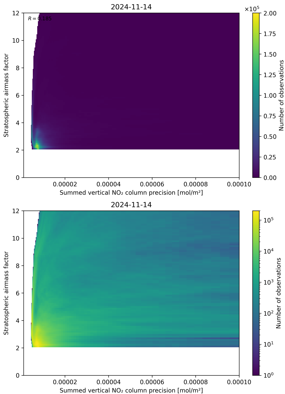
Figure 106: Scatter density plot of “Summed vertical NO 2 column precision” against “Stratospheric airmass factor” for 2024-11-14 to 2024-11-15.
