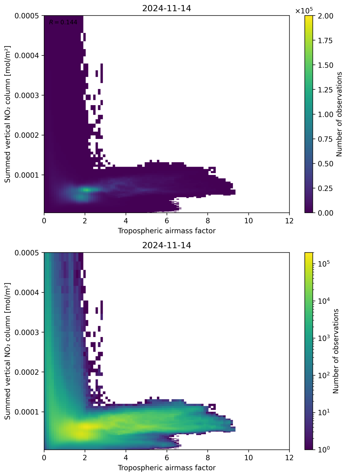
Figure 75: Scatter density plot of “Tropospheric air mass factor” against “Summed vertical NO 2 column” for 2024-11-14 to 2024-11-15.
