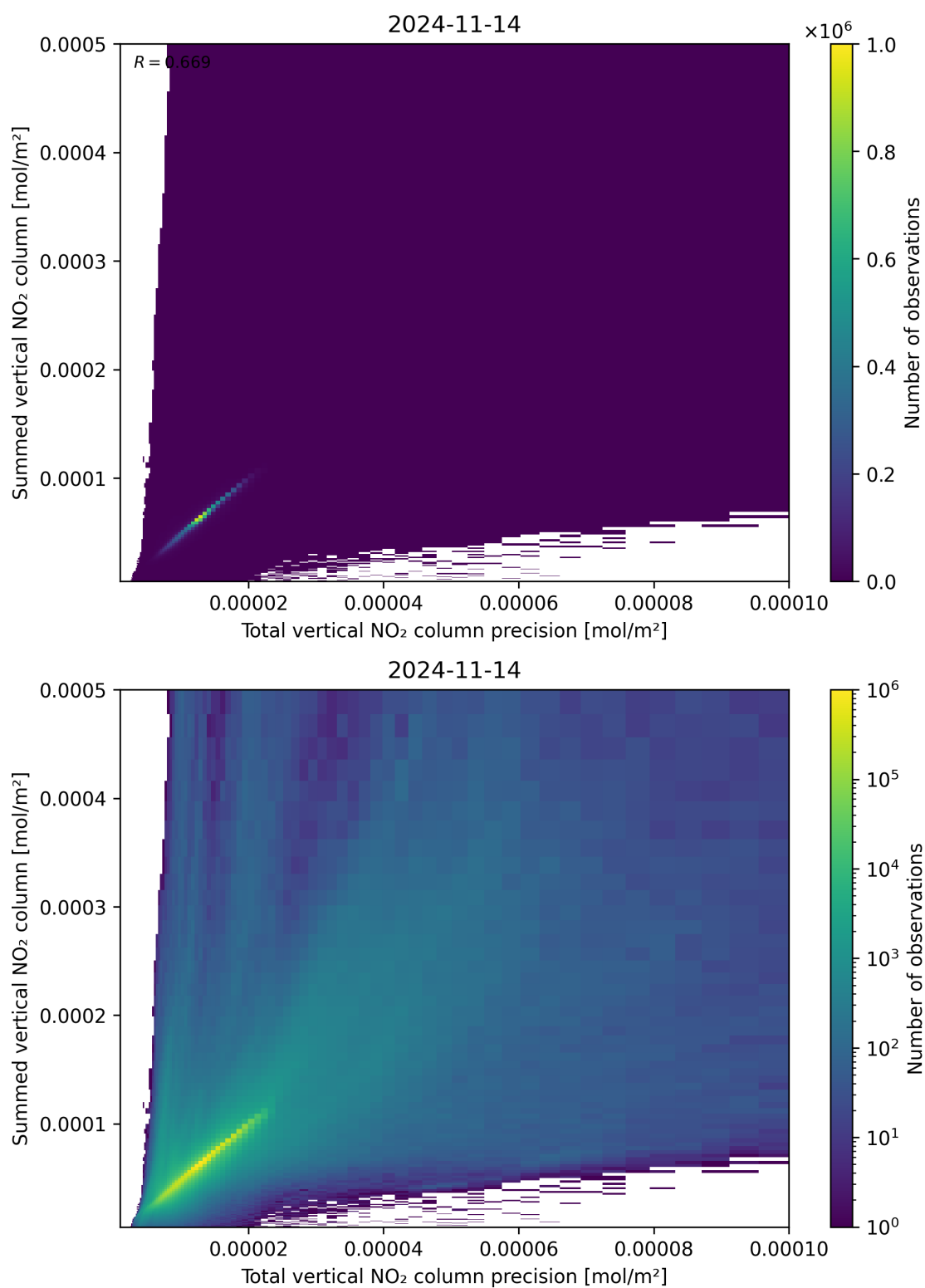
Figure 117: Scatter density plot of “Total vertical NO 2 column precision” against “Summed vertical NO 2 column” for 2024-11-14 to 2024-11-15.
