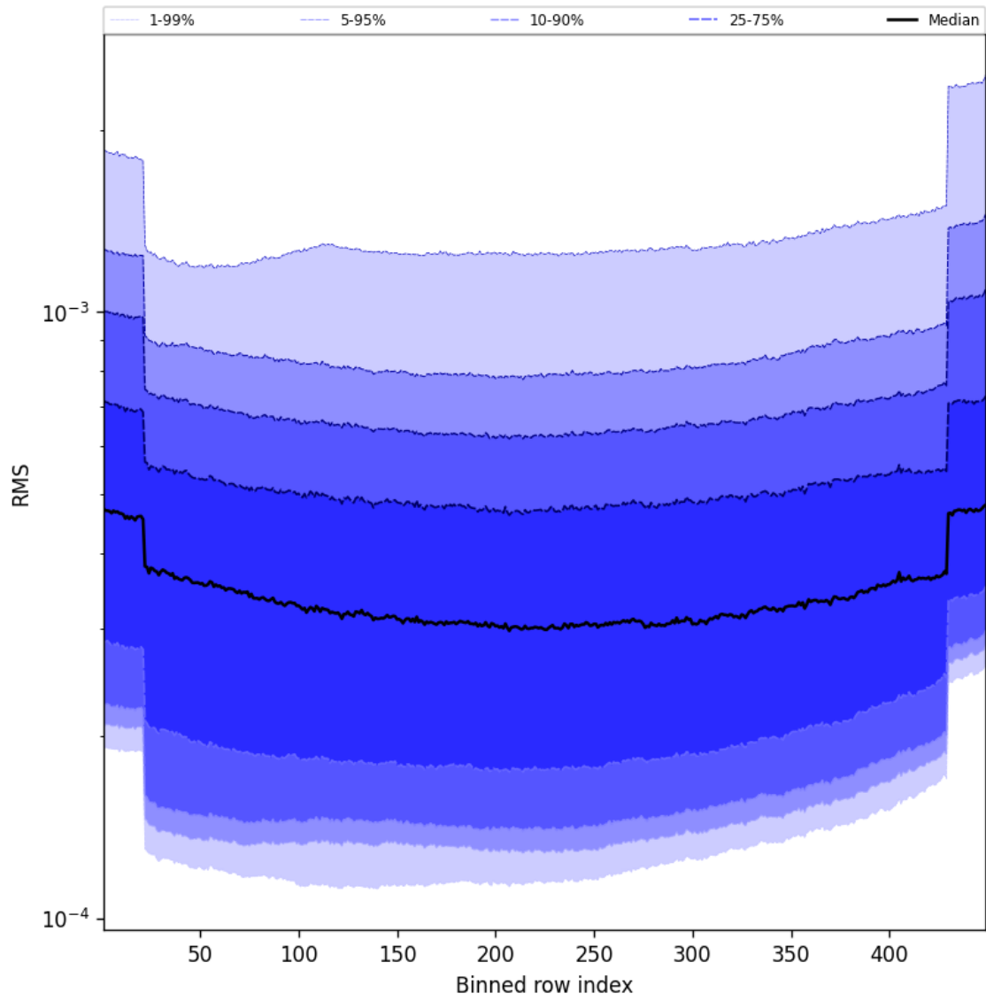
Figure 60: Along track statistics of “RMS” for 2024-11-14 to 2024-11-15
