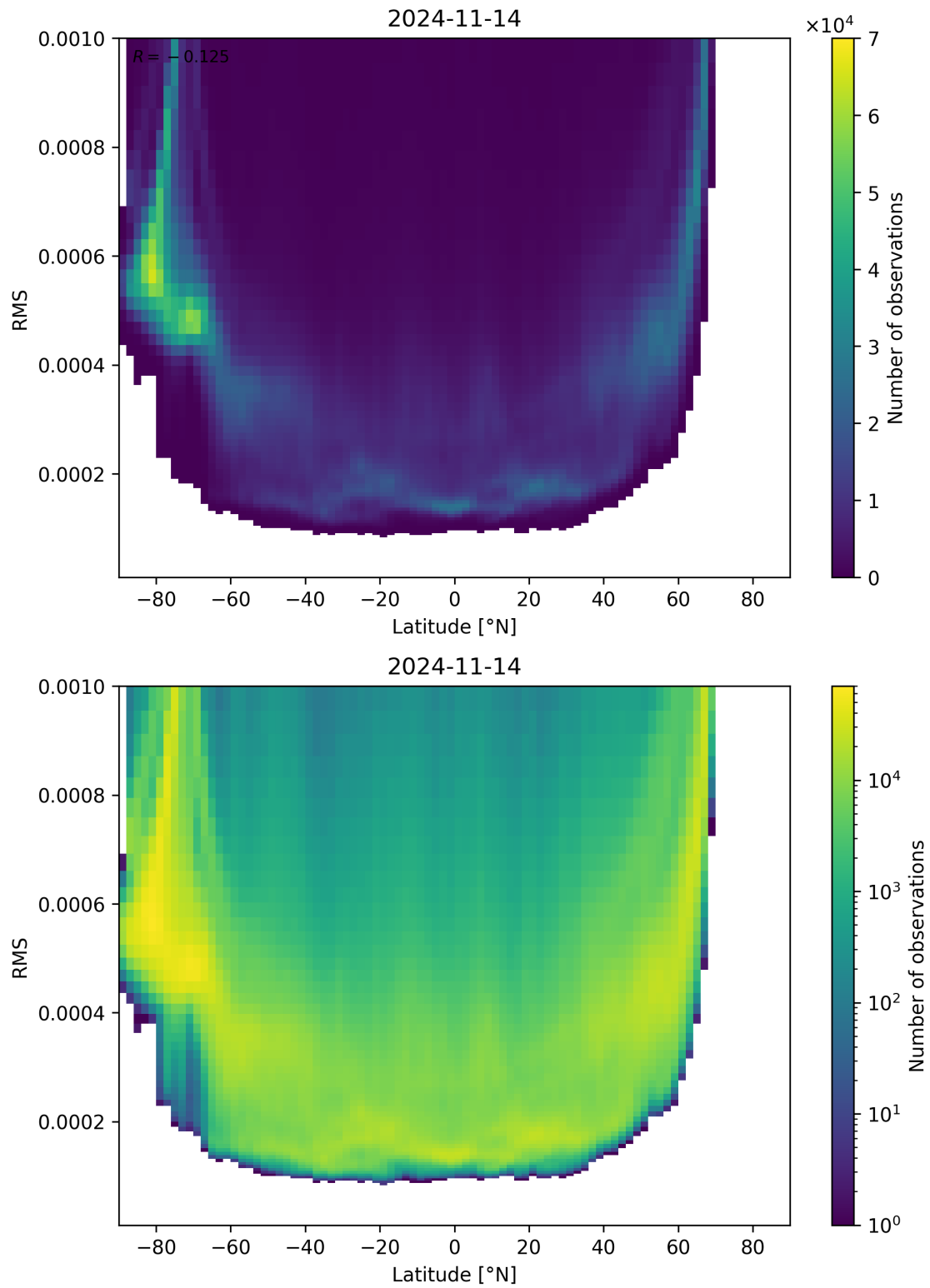
Figure 94: Scatter density plot of “Latitude” against “RMS” for 2024-11-14 to 2024-11-15.
