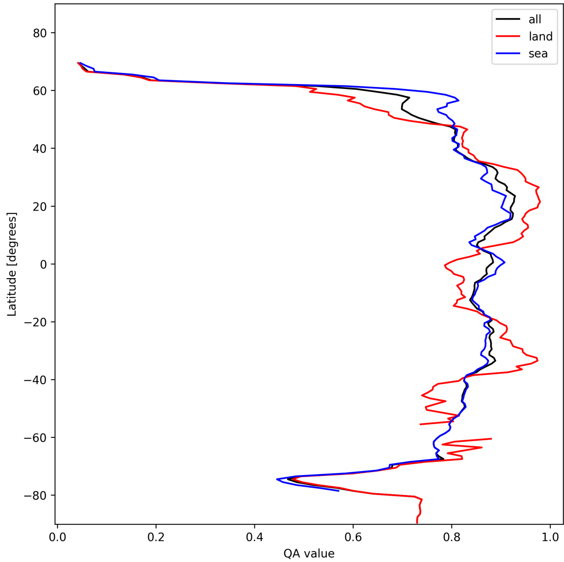
Figure 11: Zonal average of “QA value” for 2024-11-14 to 2024-11-15.
