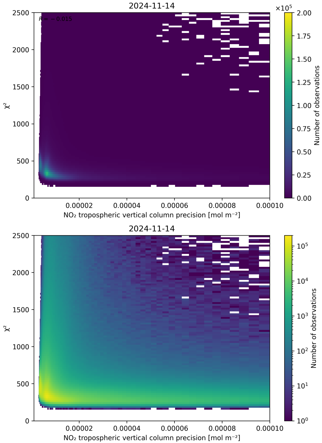
Figure 134: Scatter density plot of “NO 2 tropospheric vertical column precision” against “ \chi^2 ” for 2024-11-14 to 2024-11-15.
