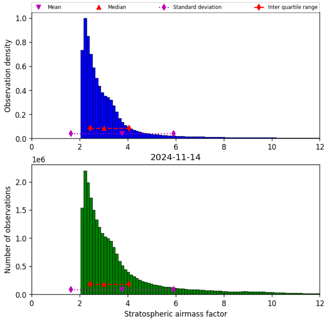
Figure 44: Histogram of “Stratospheric airmass factor” for 2024-11-14 to 2024-11-15
