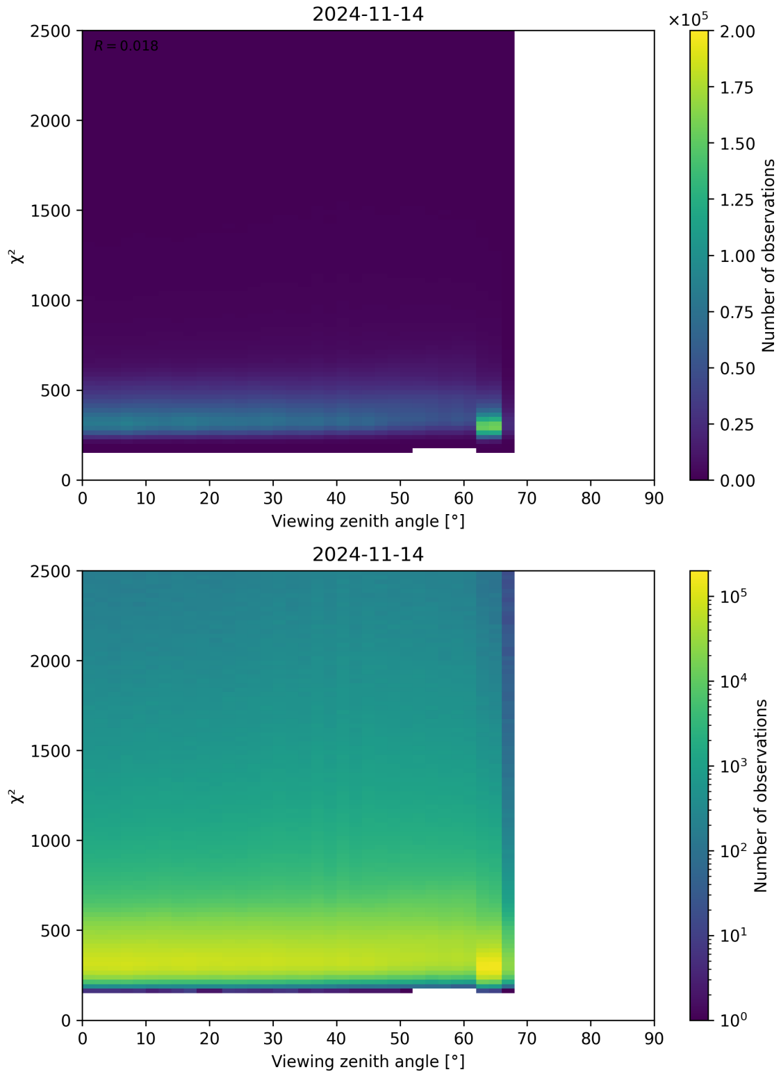
Figure 162: Scatter density plot of “Viewing zenith angle” against “ \chi^2 ” for 2024-11-14 to 2024-11-15.
