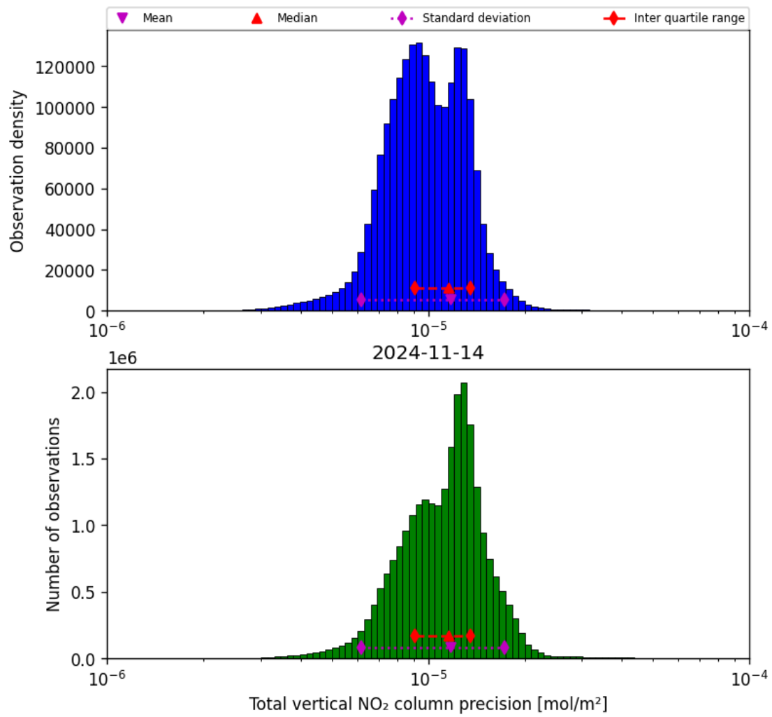
Figure 39: Histogram of “Total vertical NO 2 column precision” for 2024-11-14 to 2024-11-15
