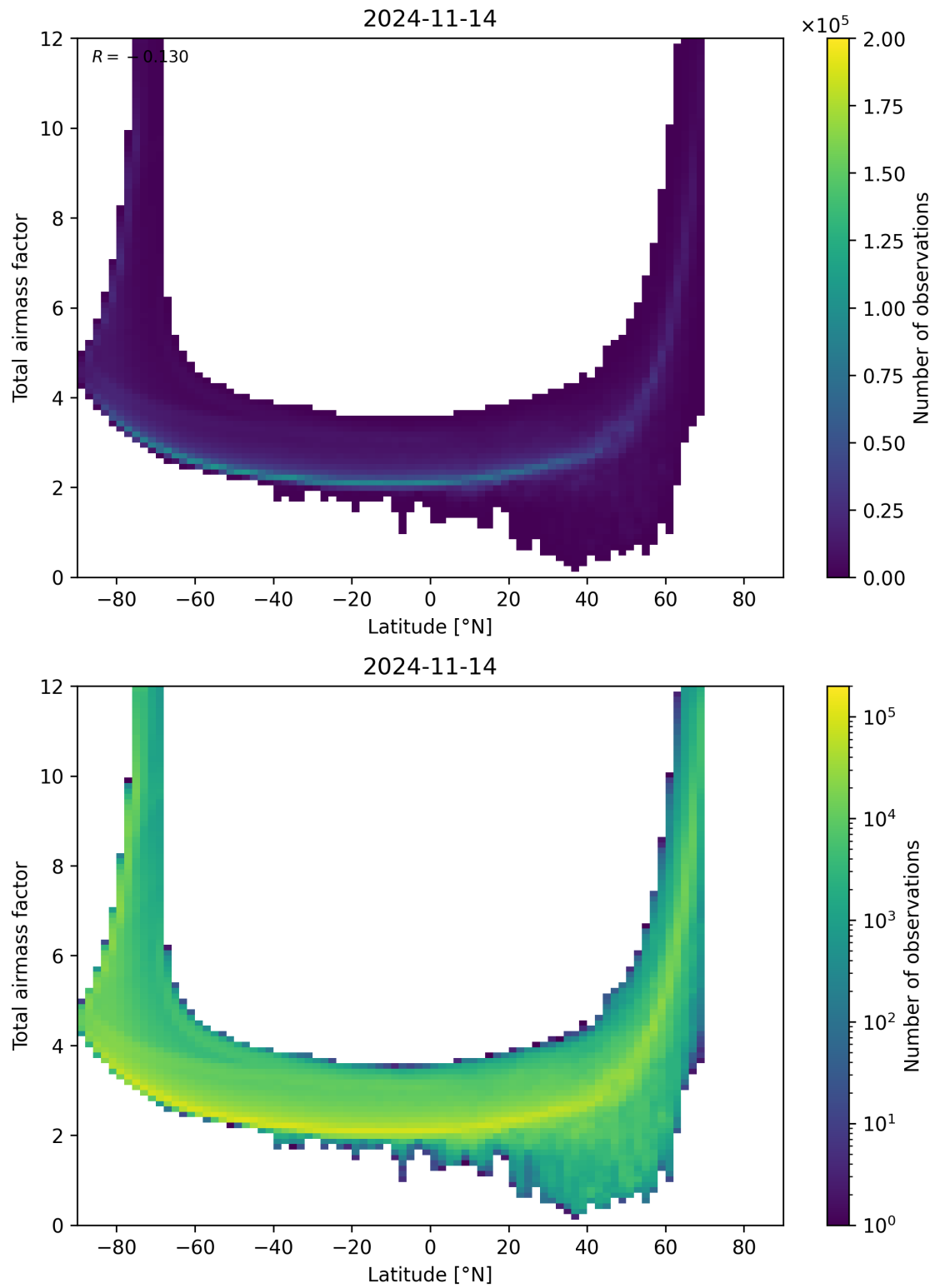
Figure 84: Scatter density plot of “Latitude” against “Total airmass factor” for 2024-11-14 to 2024-11-15.
