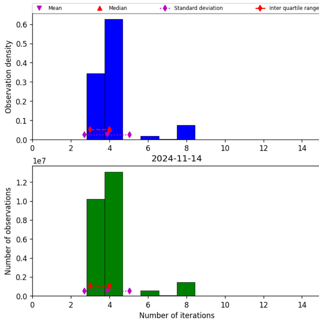
Figure 34: Histogram of “Number of iterations” for 2024-11-14 to 2024-11-15
