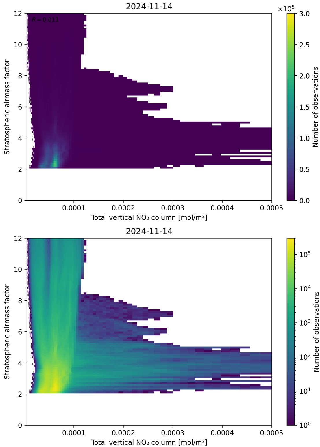
Figure 110: Scatter density plot of “Total vertical NO 2 column” against “Stratospheric airmass factor” for 2024-11-14 to 2024-11-15.
