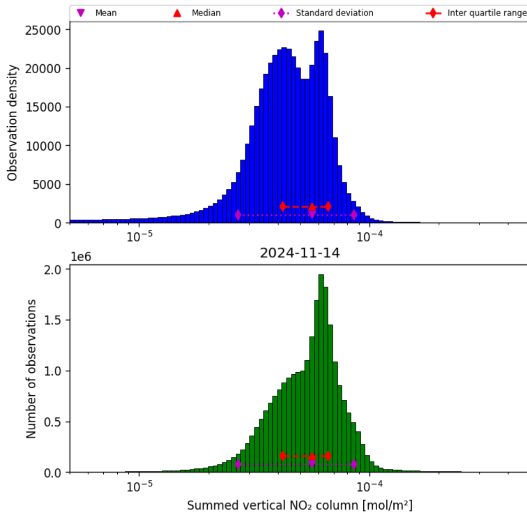
Figure 40: Histogram of “Summed vertical NO 2 column” for 2024-11-14 to 2024-11-15
