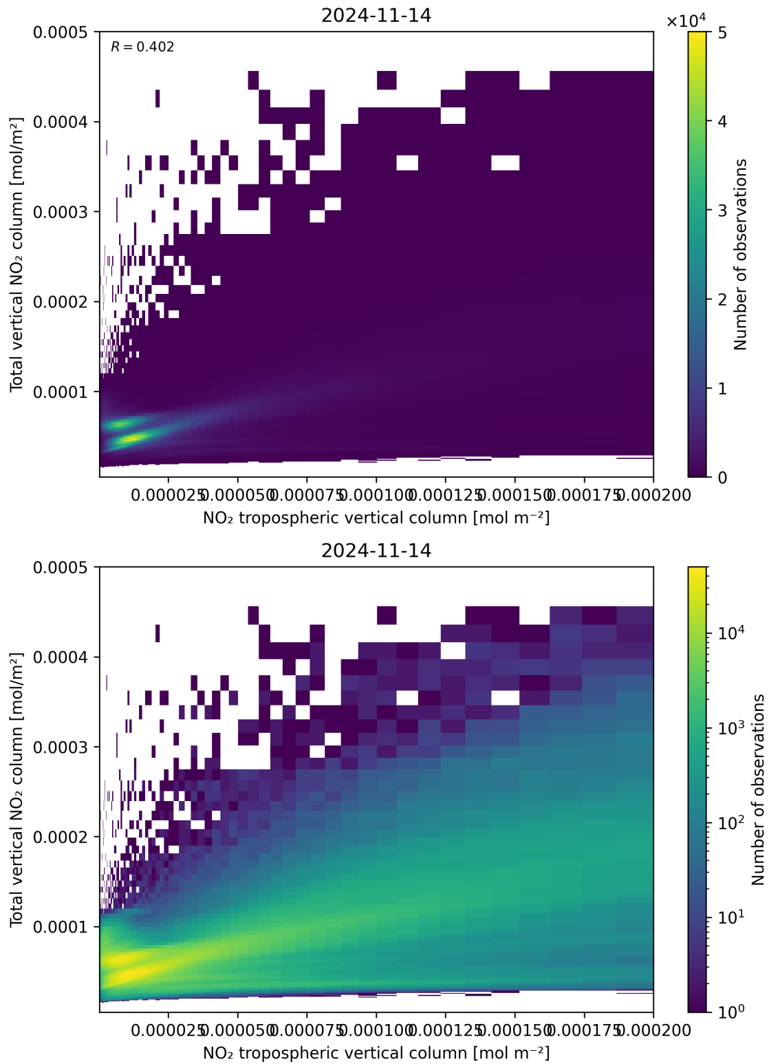
Figure 128: Scatter density plot of “NO 2 tropospheric vertical column” against “Total vertical NO 2 column” for 2024-11-14 to 2024-11-15.
