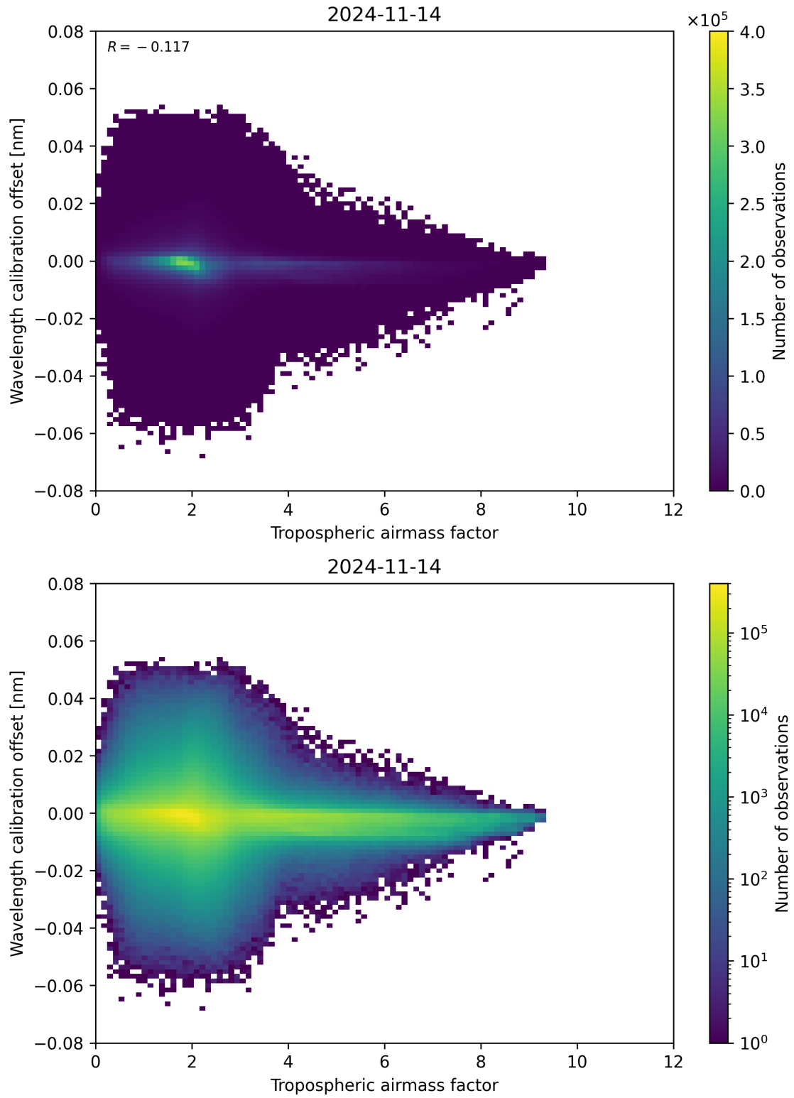
Figure 80: Scatter density plot of “Tropospheric airmass factor” against “Wavelength calibration offset” for 2024-11-14 to 2024-11-15.
