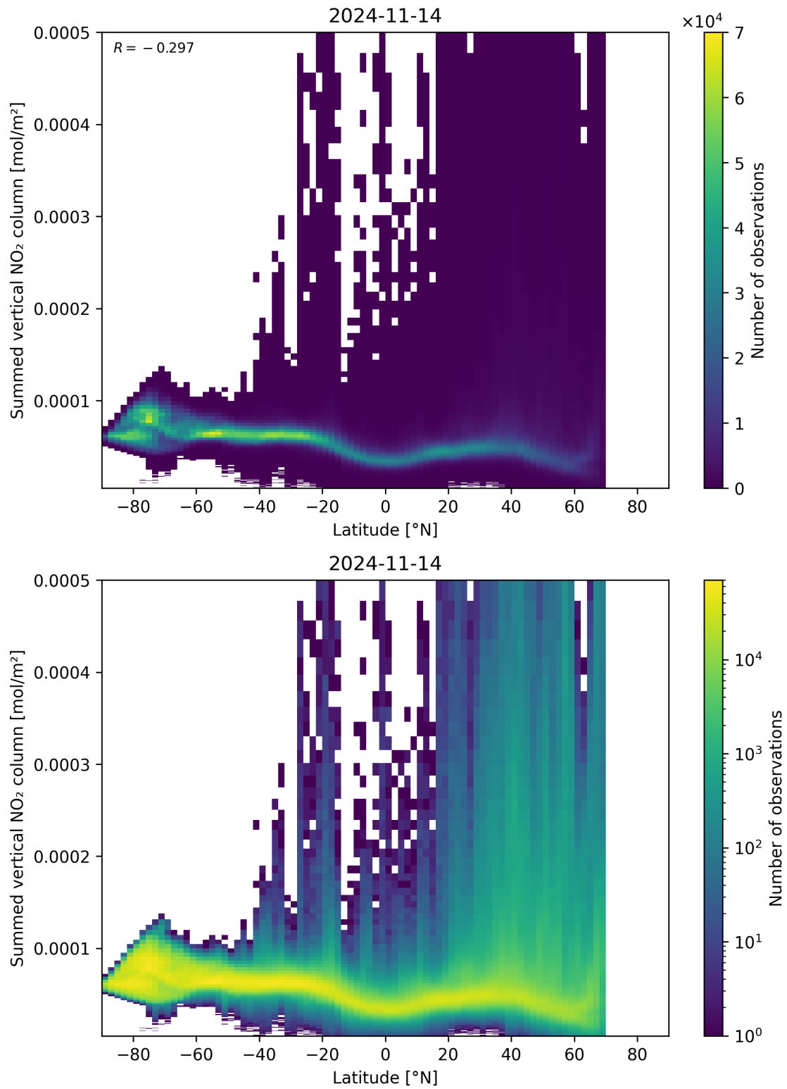
Figure 88: Scatter density plot of “Latitude” against “Summed vertical NO 2 column” for 2024-11-14 to 2024-11-15.
