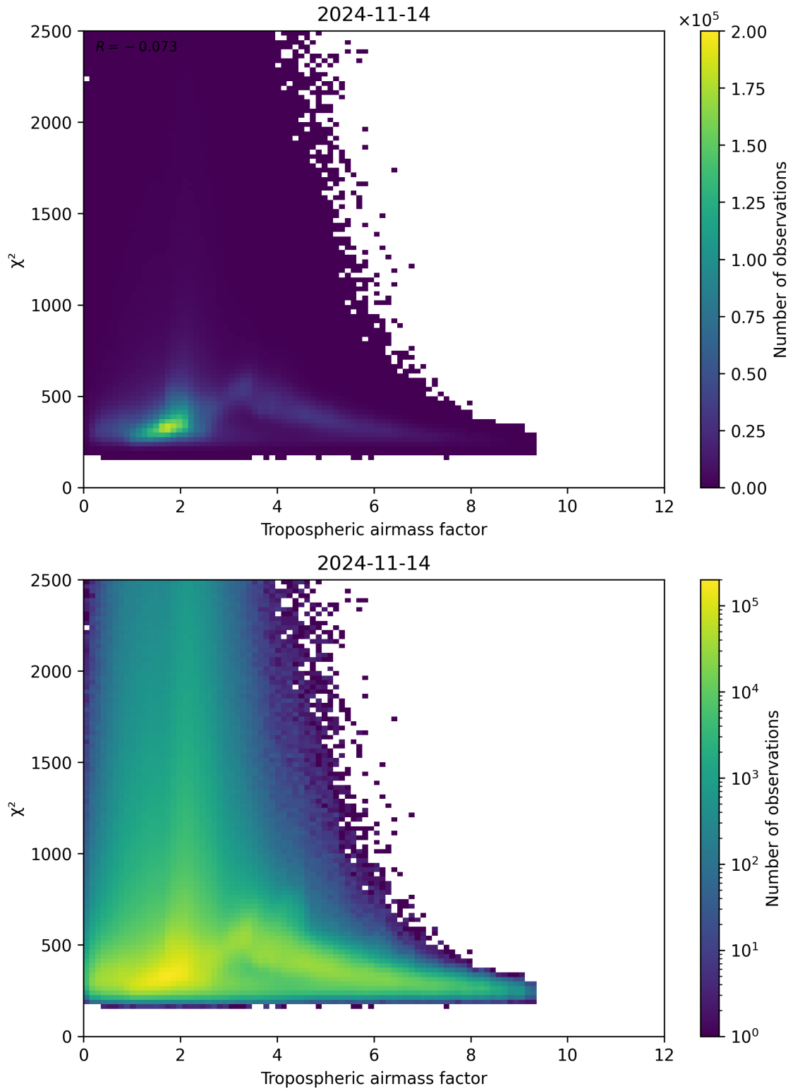
Figure 73: Scatter density plot of “Tropospheric airmass factor” against “ \chi^2 ” for 2024-11-14 to 2024-11-15.
