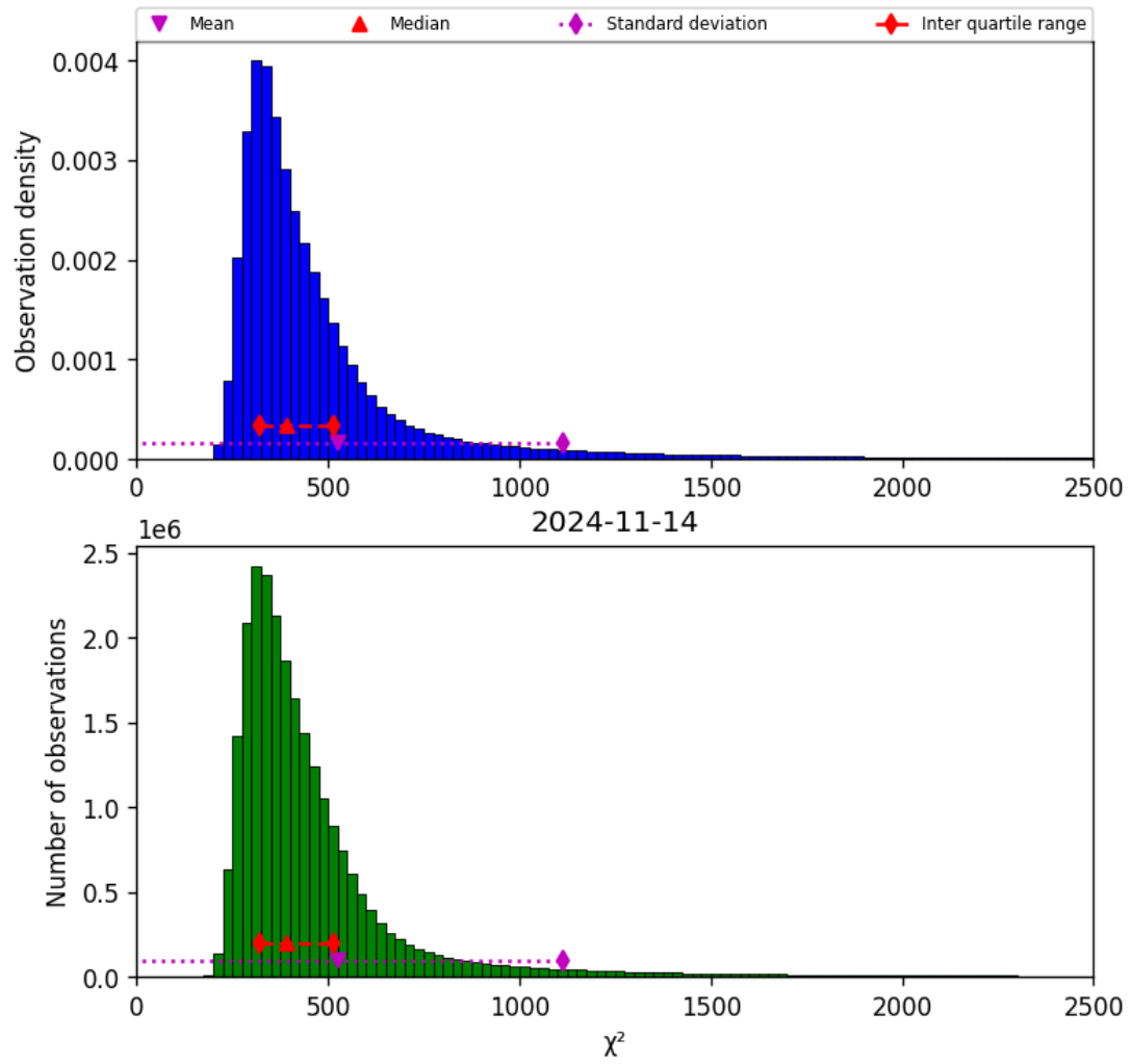
Figure 42: Histogram of “ \chi^2 ” for 2024-11-14 to 2024-11-15
