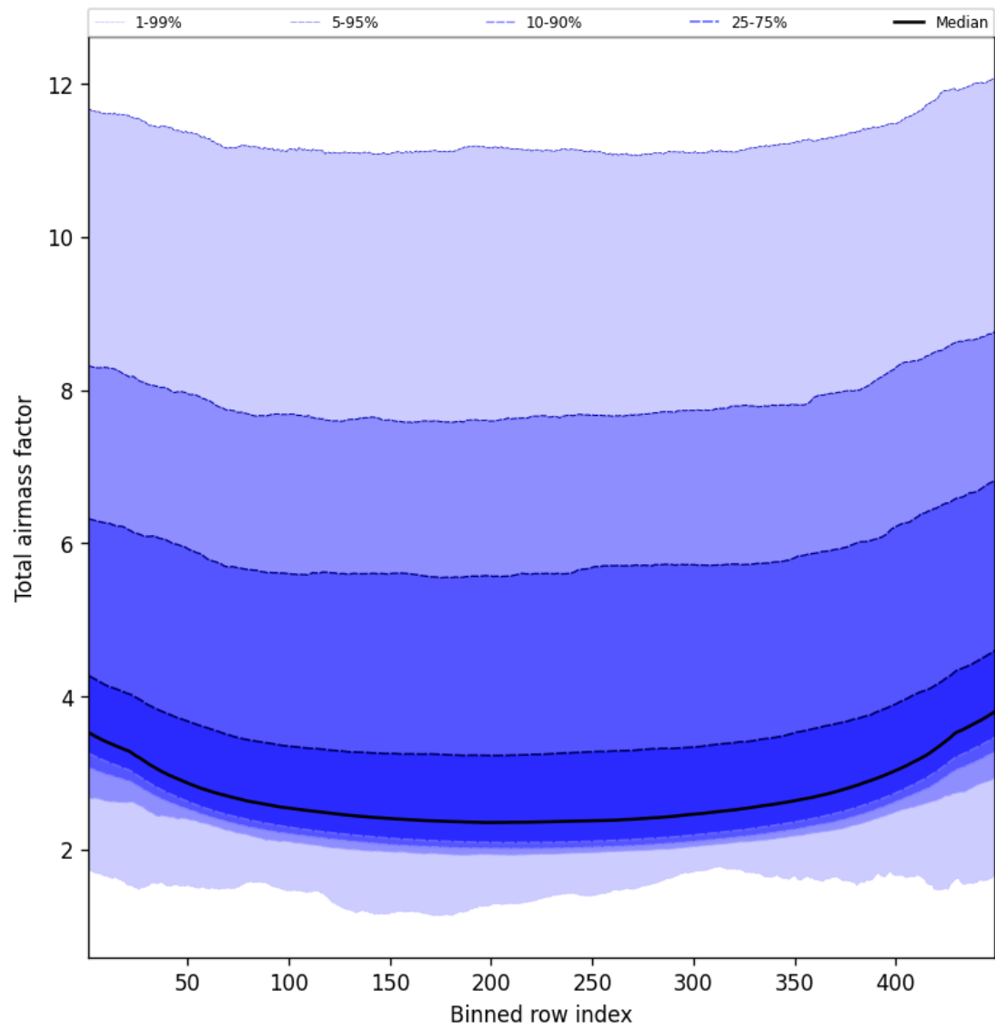
Figure 49: Along track statistics of “Total airmass factor” for 2024-11-14 to 2024-11-15
