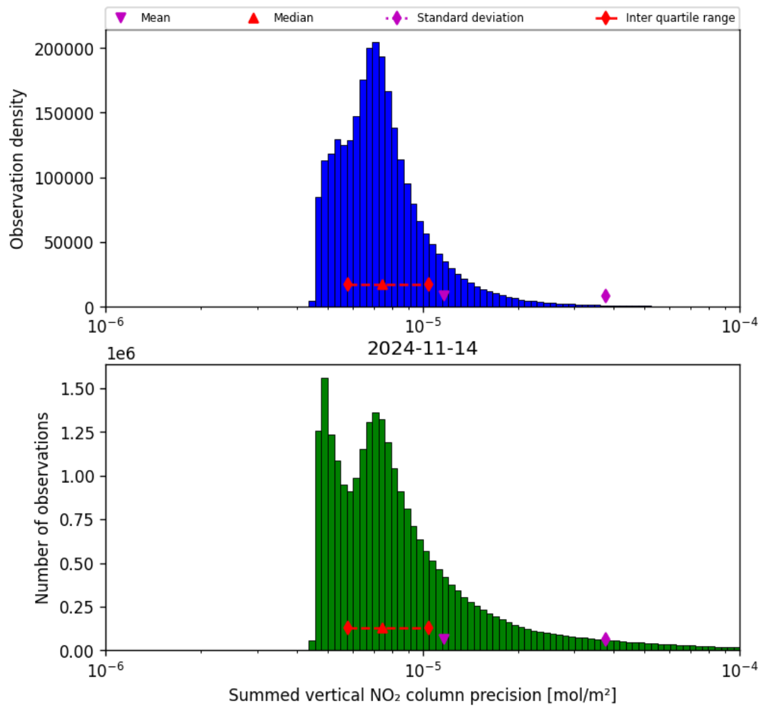
Figure 41: Histogram of “Summed vertical NO 2 column precision” for 2024-11-14 to 2024-11-15
