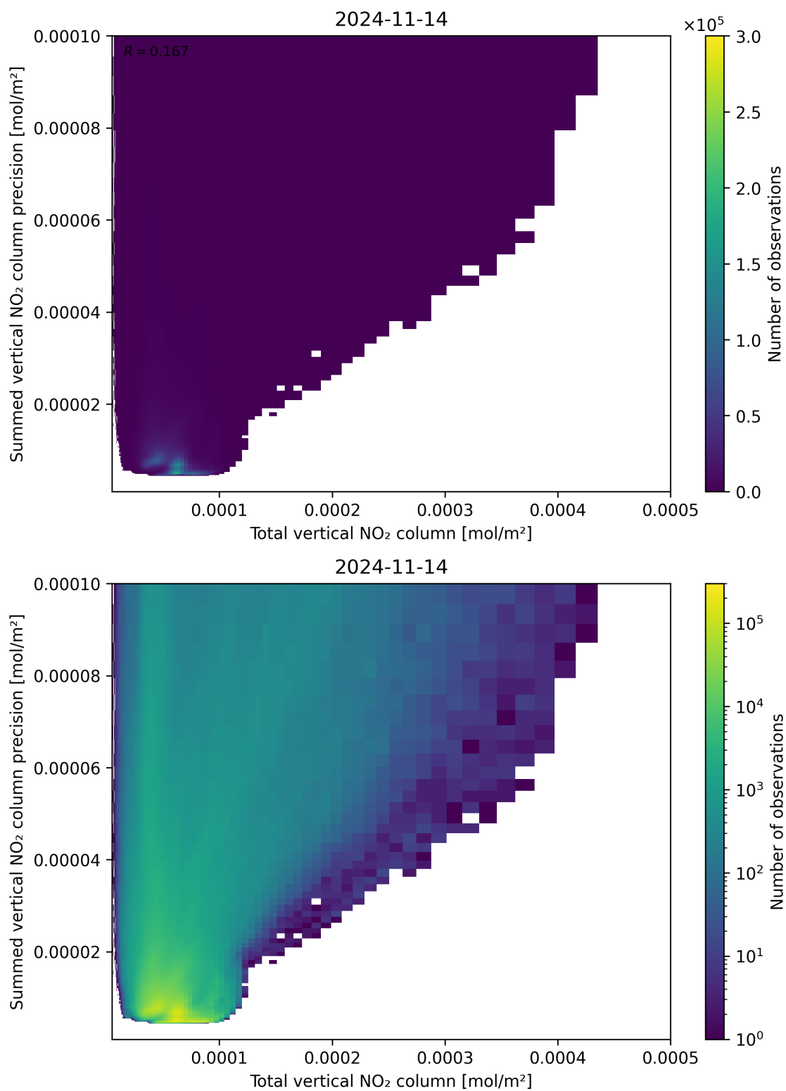
Figure 113: Scatter density plot of “Total vertical NO 2 column” against “Summed vertical NO 2 column precision” for 2024-11-14 to 2024-11-15.
