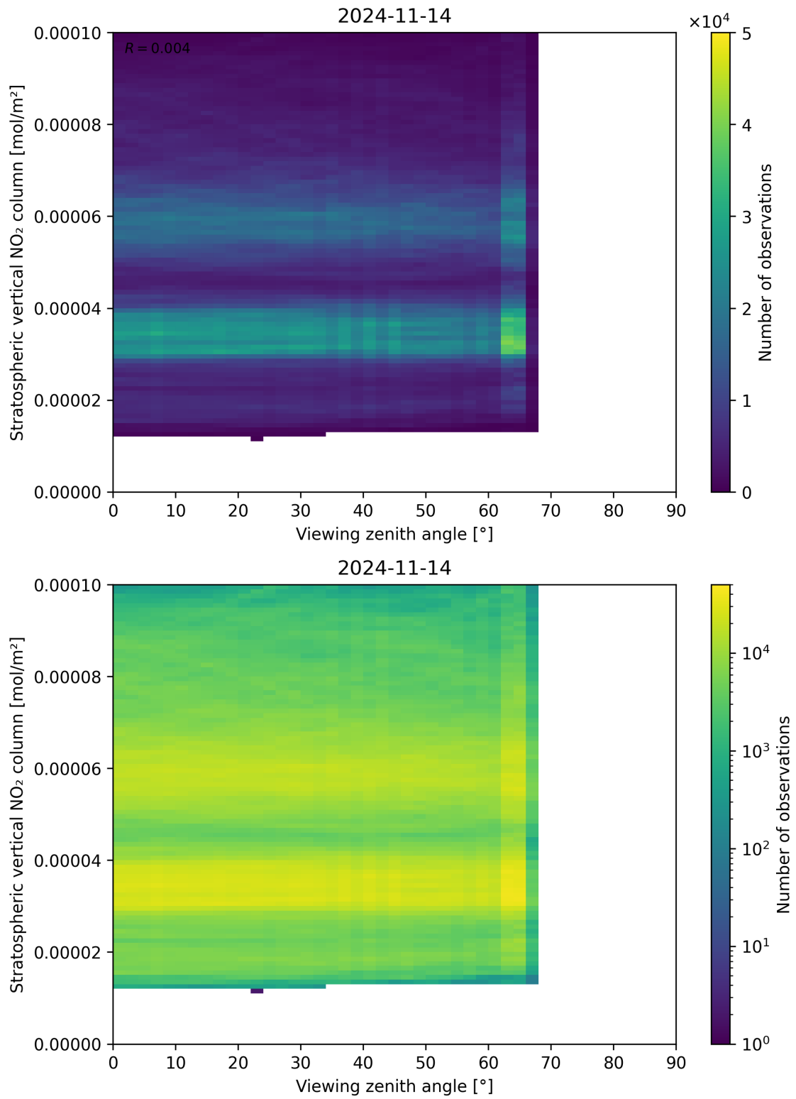
Figure 164: Scatter density plot of “Viewing zenith angle” against “Stratospheric vertical NO 2 column” for 2024-11-14 to 2024-11-15.
