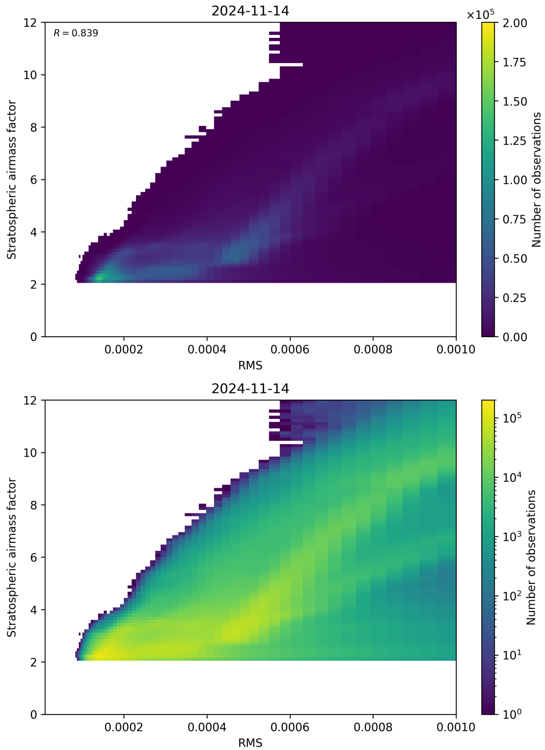
Figure 144: Scatter density plot of “RMS” against “Stratospheric airmass factor” for 2024-11-14 to 2024-11-15.
