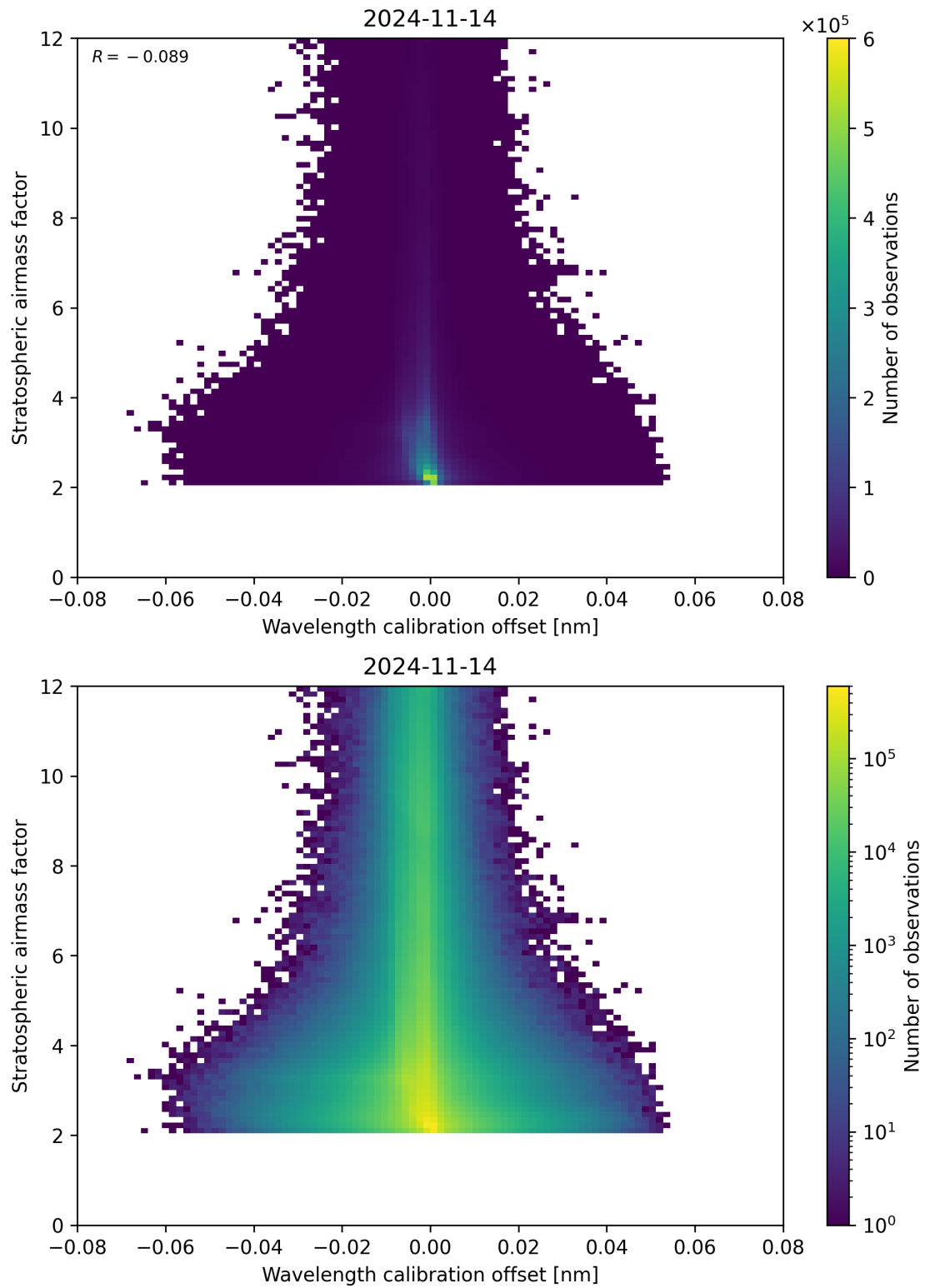
Figure 174: Scatter density plot of “Wavelength calibration offset” against “Stratospheric air mass factor” for 2024-11-14 to 2024-11-15.
