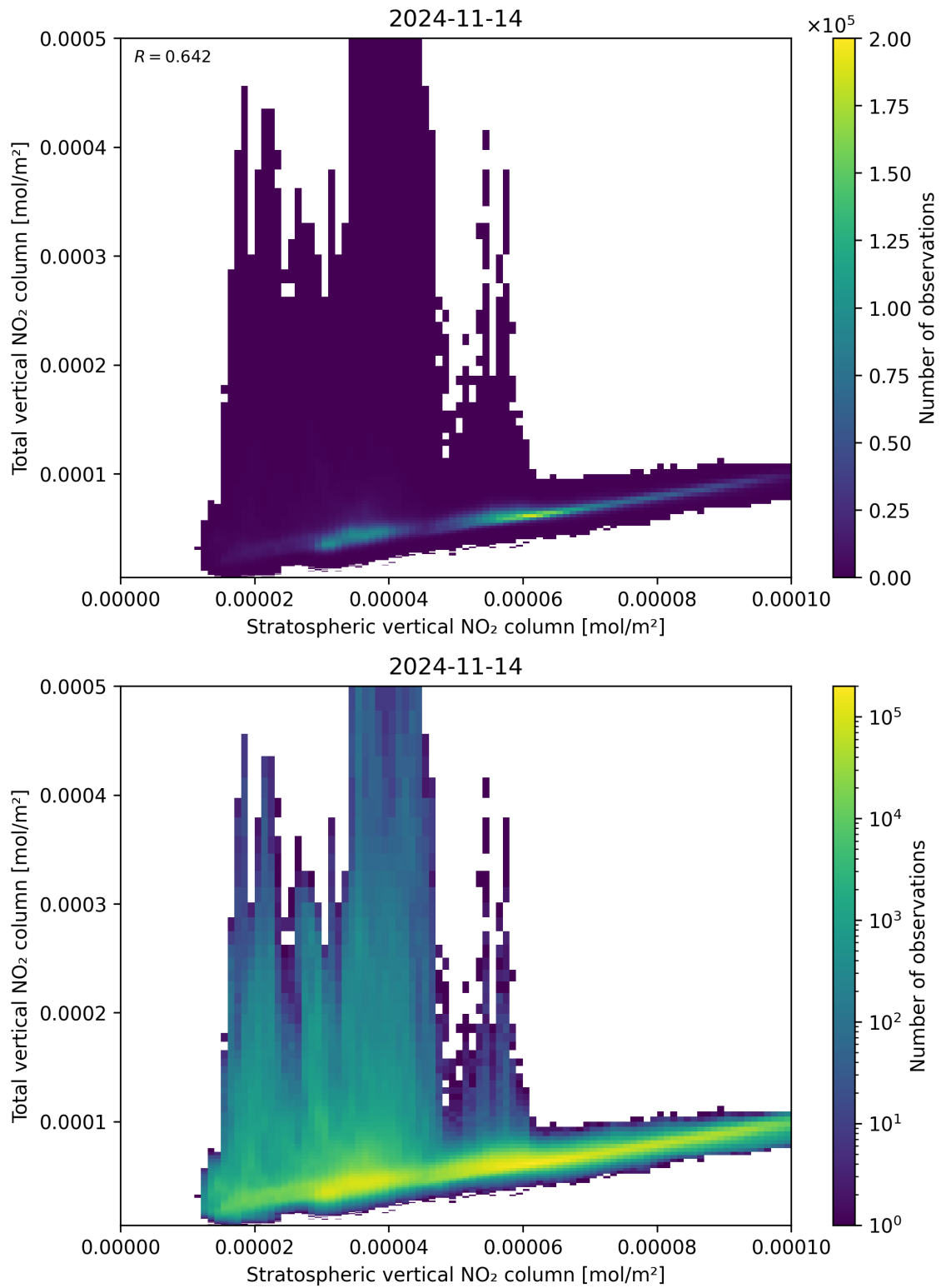
Figure 100: Scatter density plot of “Stratospheric vertical NO 2 column” against “Total vertical NO 2 column” for 2024-11-14 to 2024-11-15.
