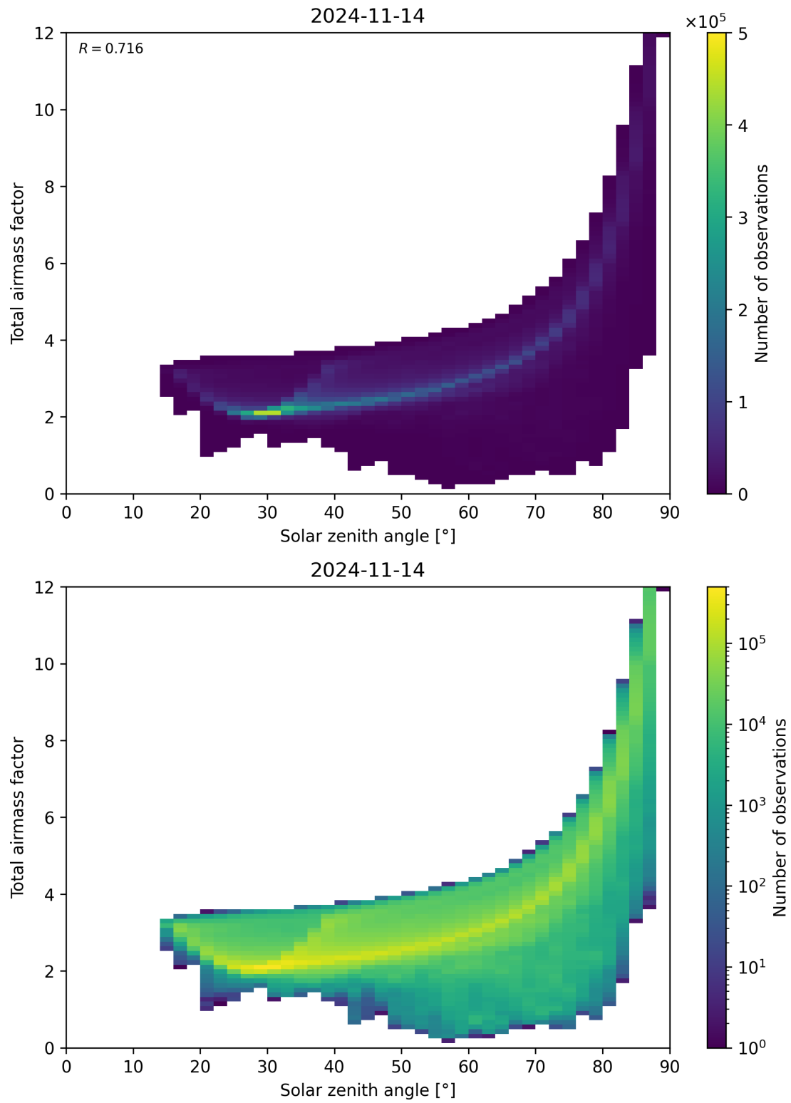
Figure 146: Scatter density plot of “Solar zenith angle” against “Total airmass factor” for 2024-11-14 to 2024-11-15.
