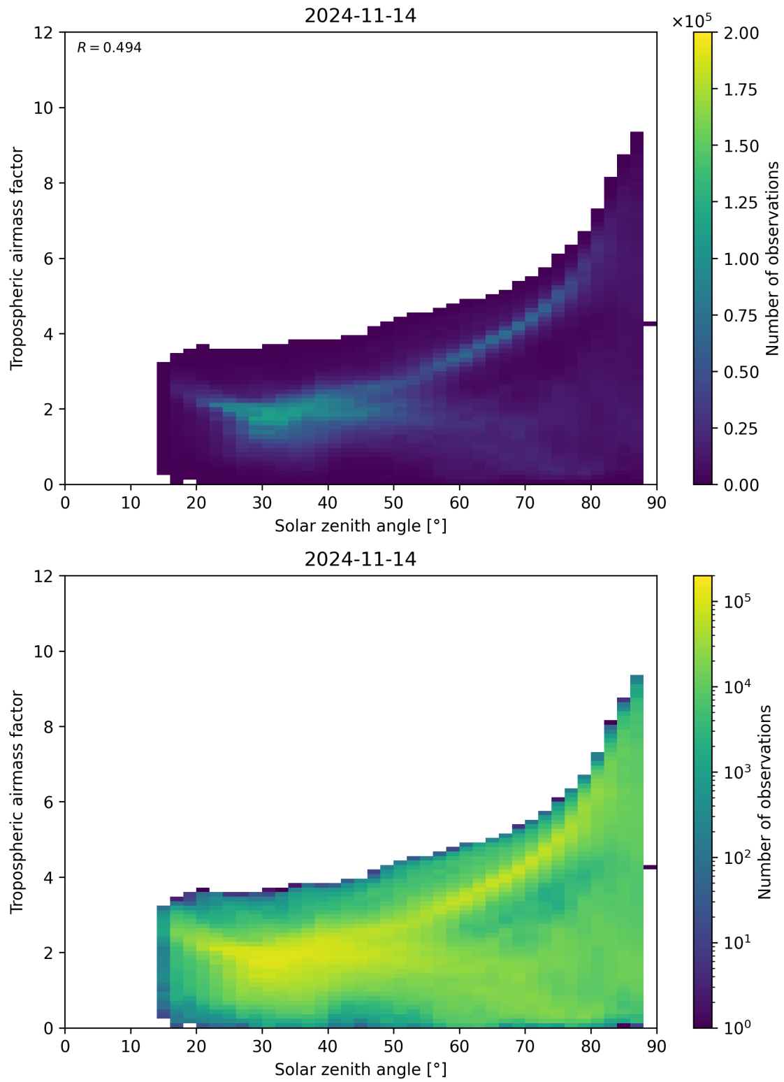
Figure 147: Scatter density plot of “Solar zenith angle” against “Tropospheric airmass factor” for 2024-11-14 to 2024-11-15.
