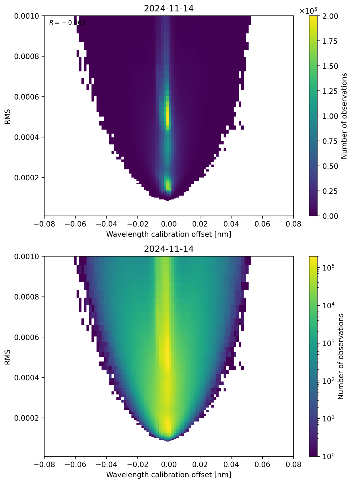
Figure 181: Scatter density plot of “Wavelength calibration offset” against “RMS” for 2024-11-14 to 2024-11-15.
