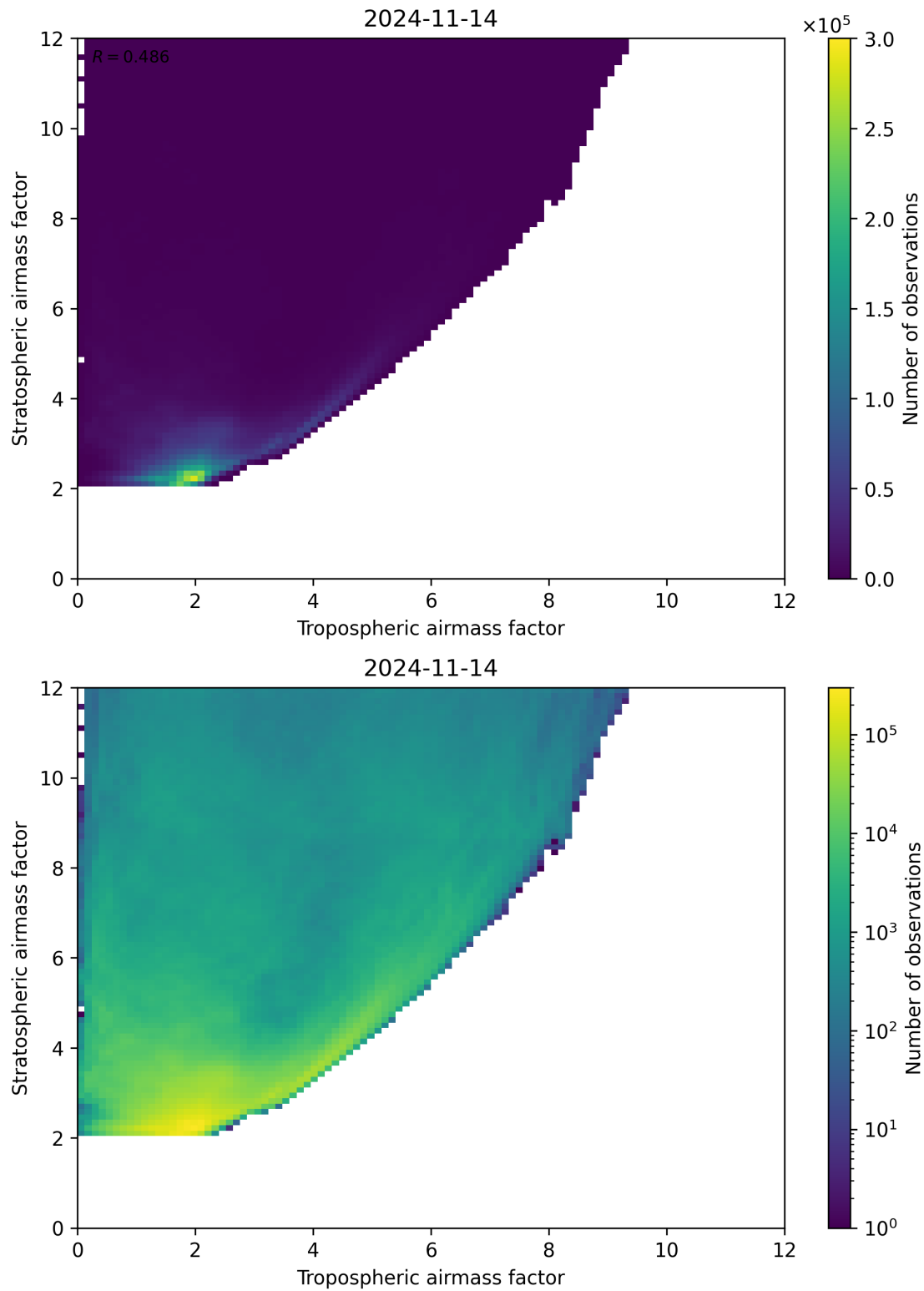
Figure 71: Scatter density plot of “Tropospheric airmass factor” against “Stratospheric airmass factor” for 2024-11-14 to 2024-11-15.
