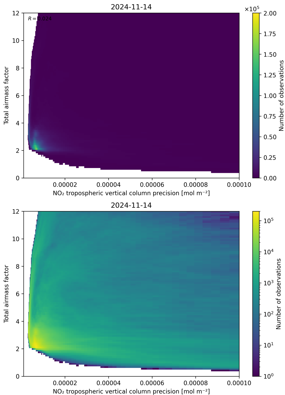
Figure 132: Scatter density plot of “NO 2 tropospheric vertical column precision” against “Total air mass factor” for 2024-11-14 to 2024-11-15.
