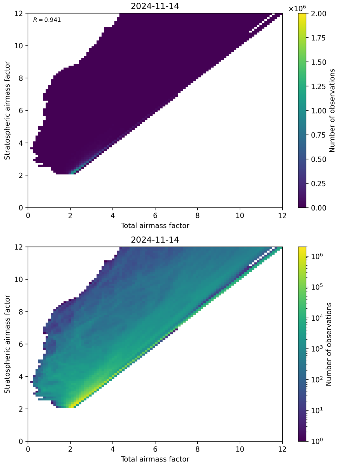
Figure 62: Scatter density plot of “Total airmass factor” against “Stratospheric airmass factor” for 2024-11-14 to 2024-11-15.
