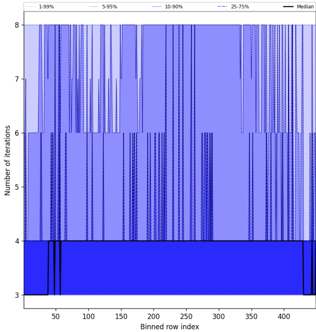
Figure 51: Along track statistics of “Number of iterations” for 2024-11-14 to 2024-11-15
