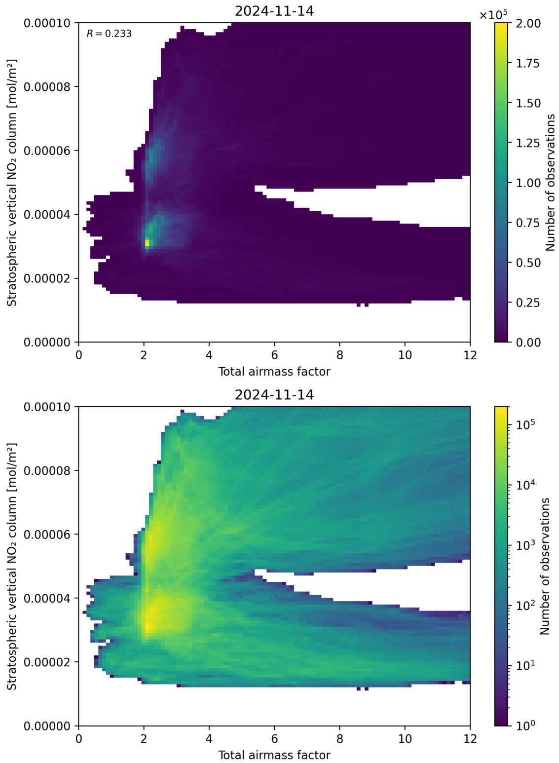
Figure 64: Scatter density plot of “Total airmass factor” against “Stratospheric vertical NO 2 column” for 2024-11-14 to 2024-11-15.
