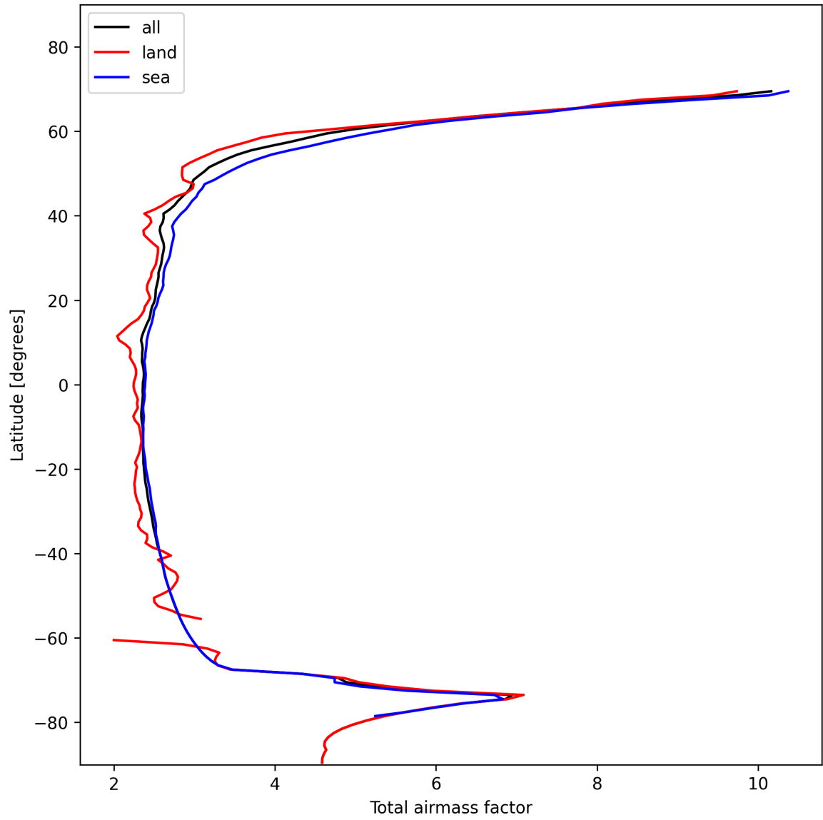
Figure 15: Zonal average of “Total airmass factor” for 2024-11-14 to 2024-11-15.
