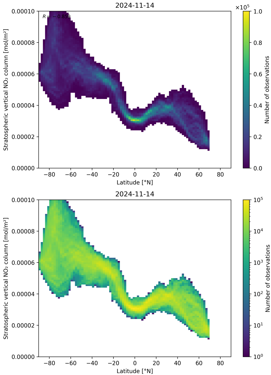
Figure 87: Scatter density plot of “Latitude” against “Stratospheric vertical NO 2 column” for 2024-11-14 to 2024-11-15.
