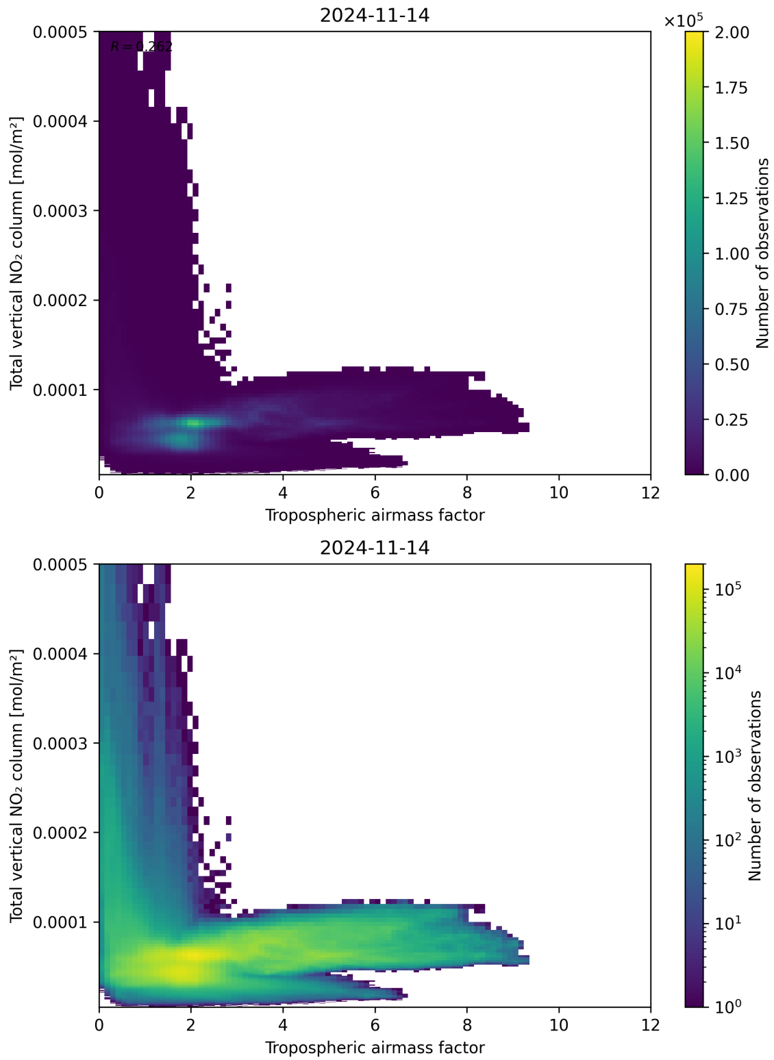
Figure 77: Scatter density plot of “Tropospheric airmass factor” against “Total vertical NO 2 column” for 2024-11-14 to 2024-11-15.
