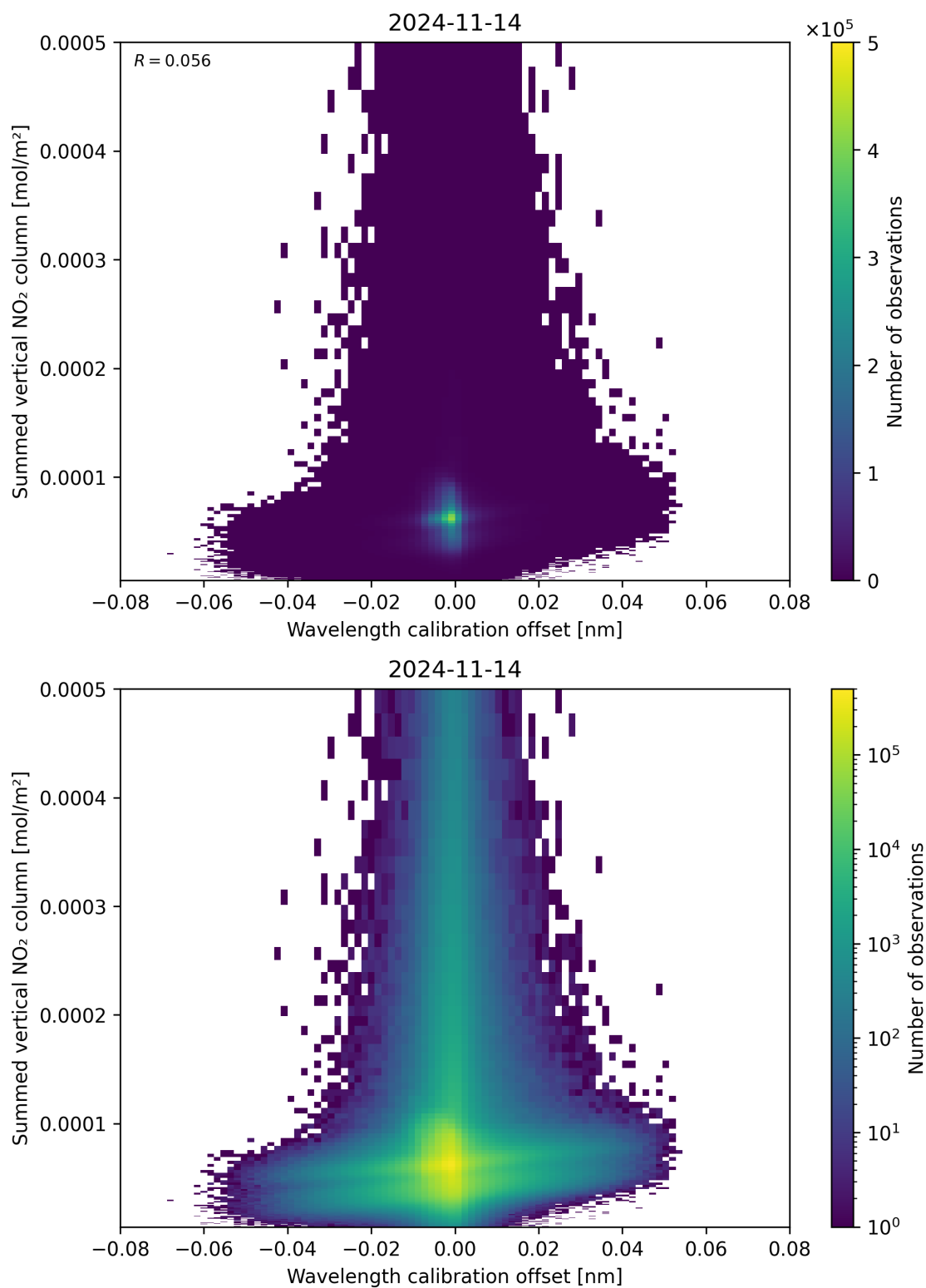
Figure 177: Scatter density plot of “Wavelength calibration offset” against “Summed vertical NO 2 column” for 2024-11-14 to 2024-11-15.
