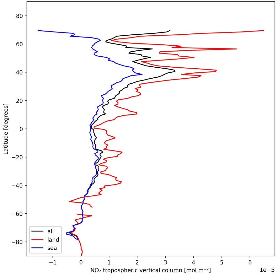
Figure 12: Zonal average of “NO 2 tropospheric vertical column” for 2024-11-14 to 2024-11-15.
