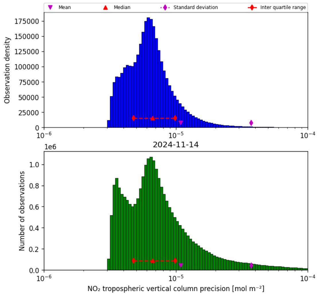
Figure 30: Histogram of “NO 2 tropospheric vertical column precision” for 2024-11-14 to 2024-11-15
