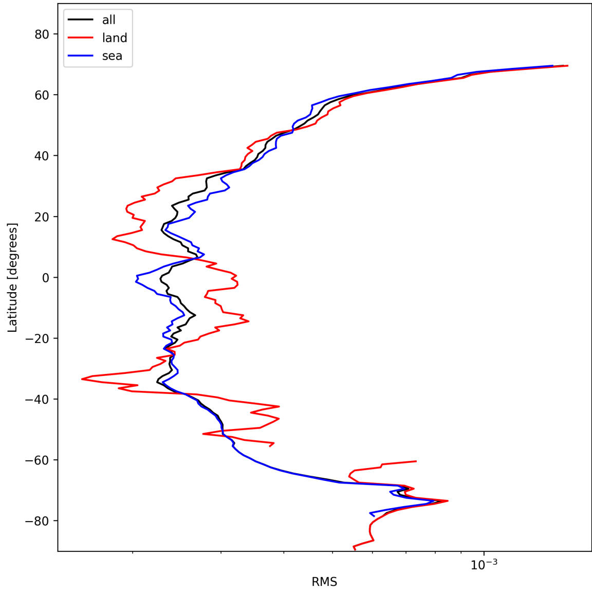
Figure 26: Zonal average of “RMS” for 2024-11-14 to 2024-11-15.
