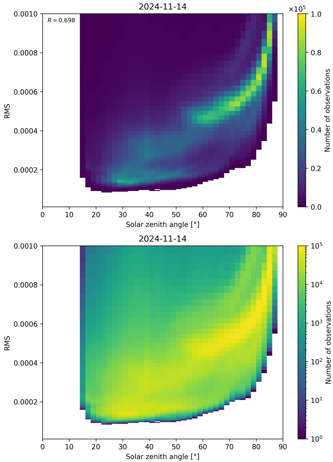
Figure 157: Scatter density plot of “Solar zenith angle” against “RMS” for 2024-11-14 to 2024-11-15.
