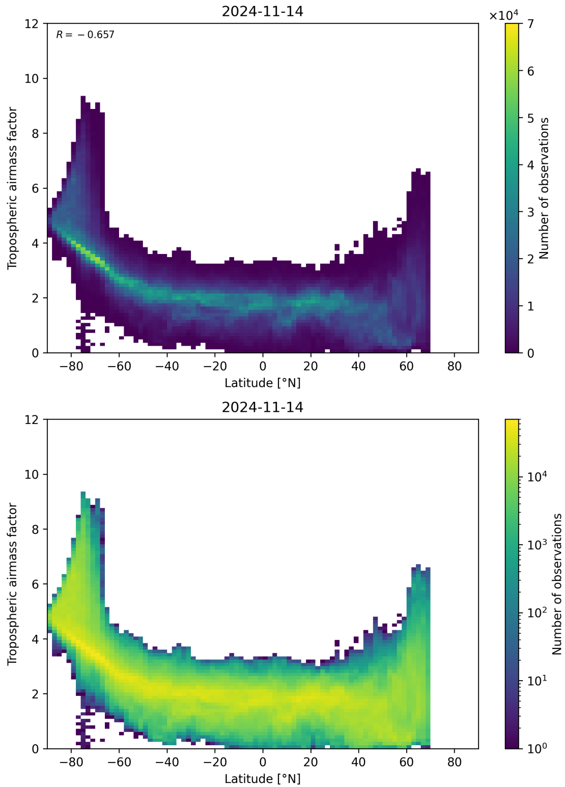
Figure 85: Scatter density plot of “Latitude” against “Tropospheric air mass factor” for 2024-11-14 to 2024-11-15.
