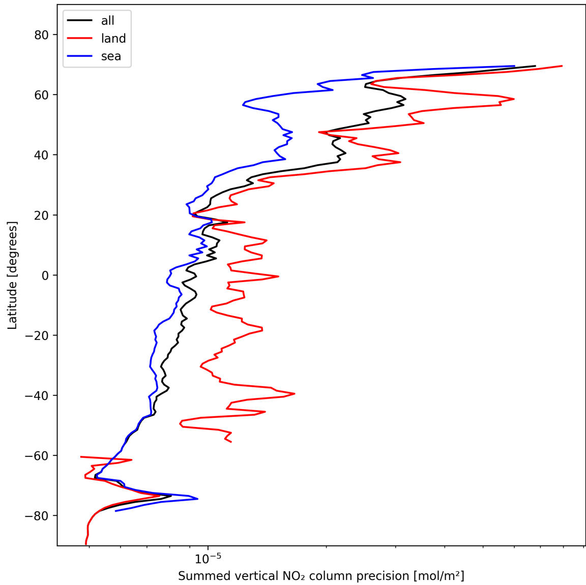
Figure 24: Zonal average of “Summed vertical NO 2 column precision” for 2024-11-14 to 2024-11-15.
