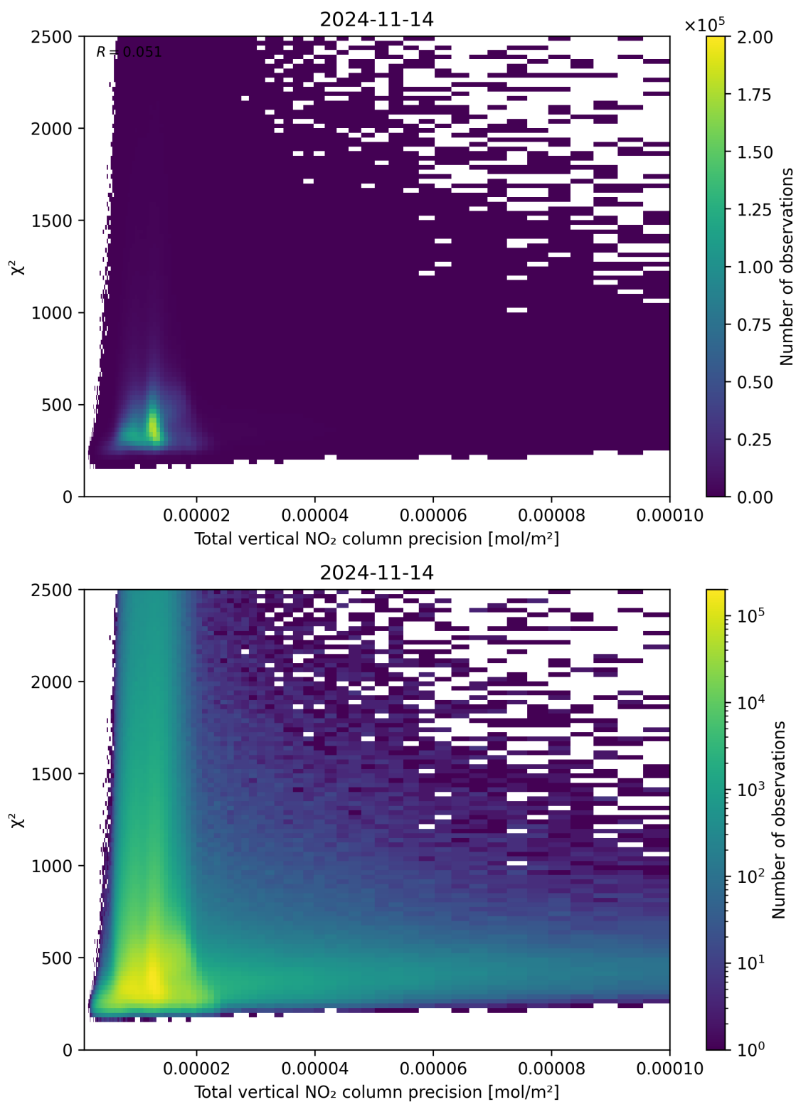
Figure 116: Scatter density plot of “Total vertical NO 2 column precision” against “ \chi^2 ” for 2024-11-14 to 2024-11-15.
