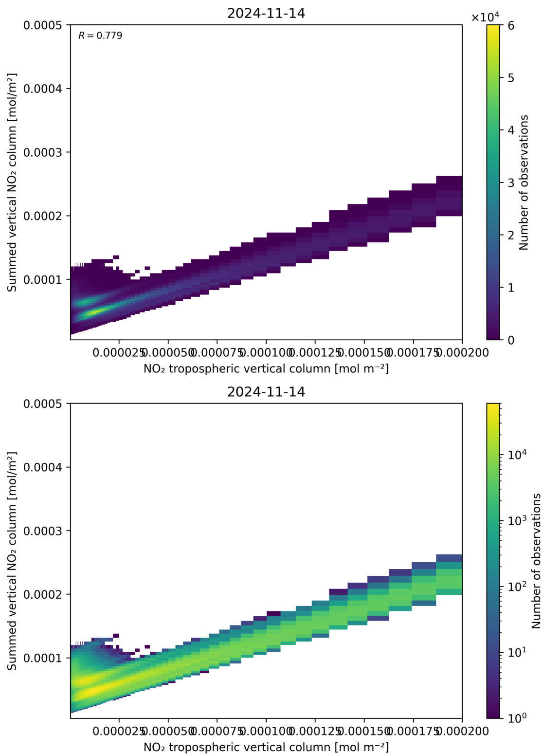
Figure 126: Scatter density plot of “NO 2 tropospheric vertical column” against “Summed vertical NO 2 column” for 2024-11-14 to 2024-11-15.
