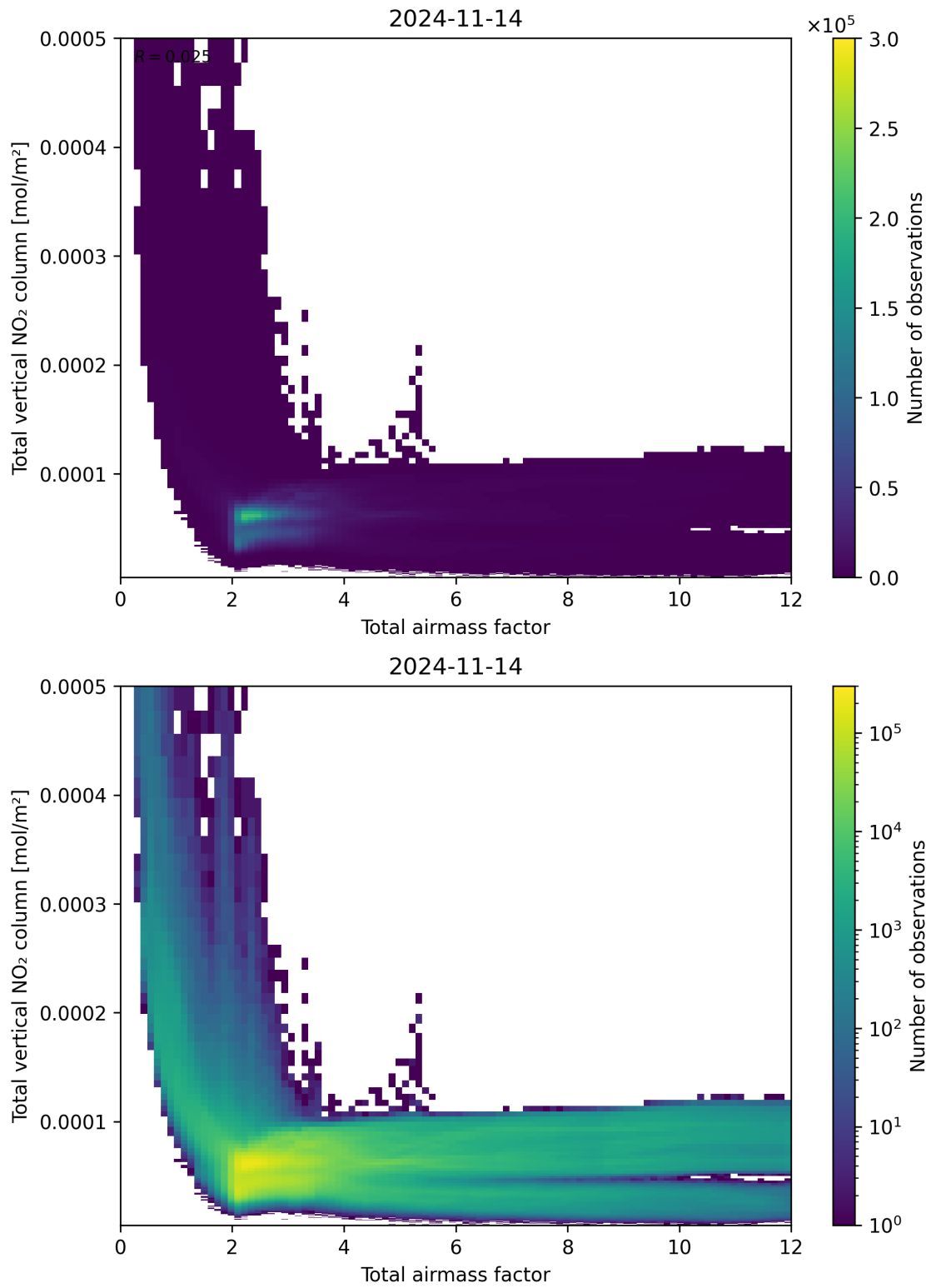
Figure 67: Scatter density plot of “Total airmass factor” against “Total vertical NO 2 column” for 2024-11-14 to 2024-11-15.
