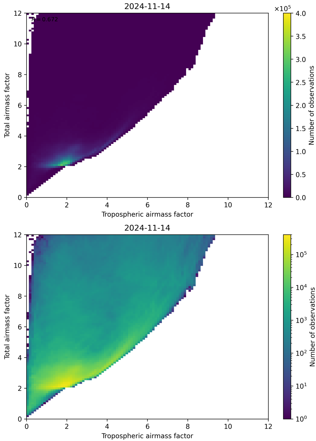
Figure 72: Scatter density plot of “Tropospheric airmass factor” against “Total airmass factor” for 2024-11-14 to 2024-11-15.
