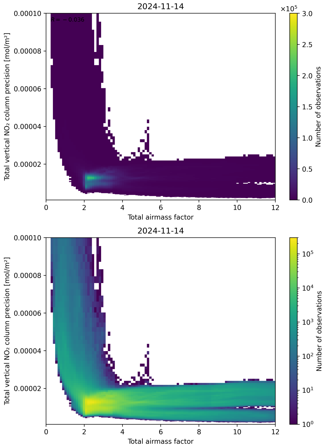
Figure 68: Scatter density plot of “Total airmass factor” against “Total vertical NO 2 column precision” for 2024-11-14 to 2024-11-15.
