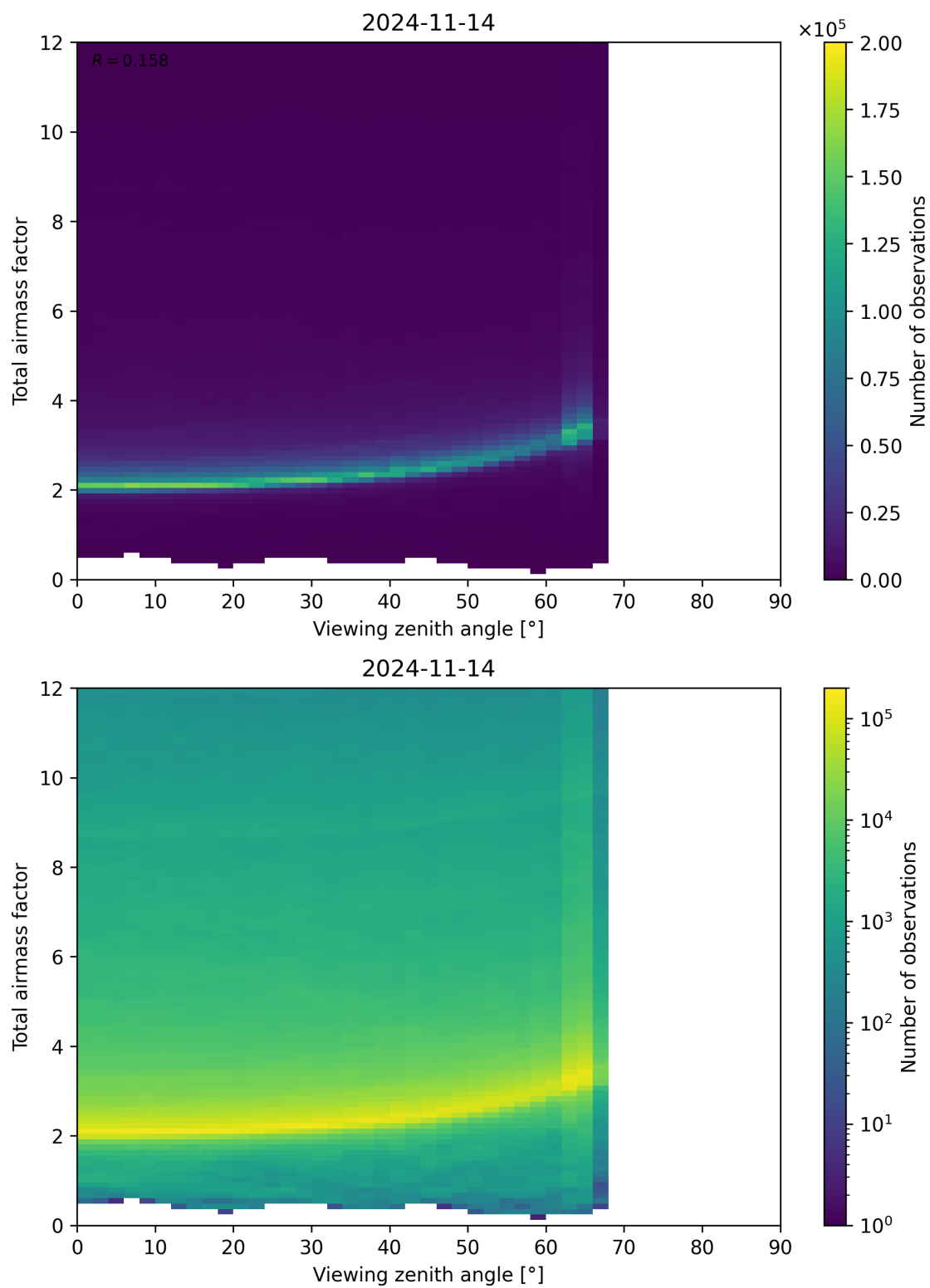
Figure 160: Scatter density plot of “Viewing zenith angle” against “Total airmass factor” for 2024-11-14 to 2024-11-15.
