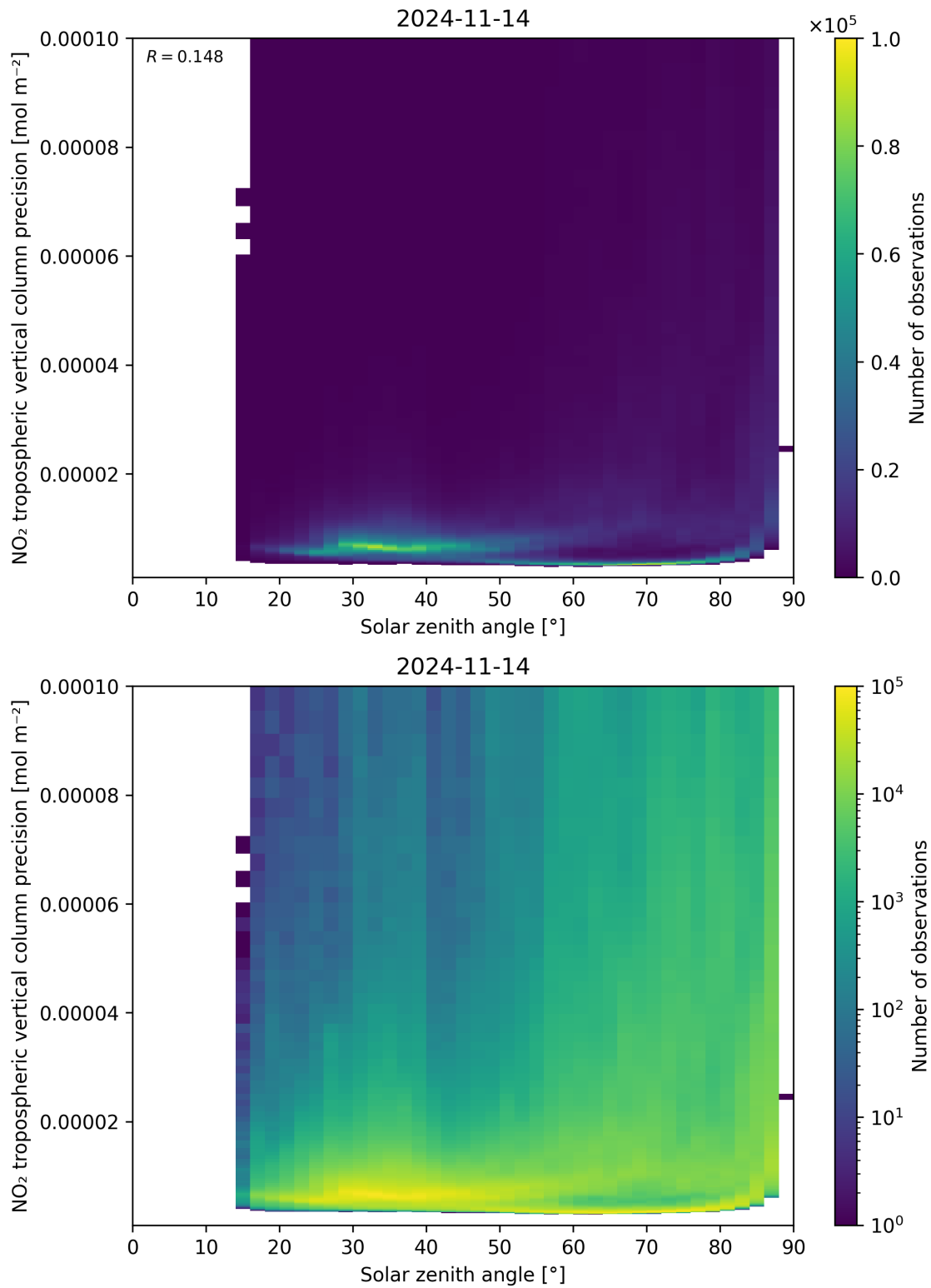
Figure 156: Scatter density plot of “Solar zenith angle” against “NO 2 tropospheric vertical column precision” for 2024-11-14 to 2024-11-15.
