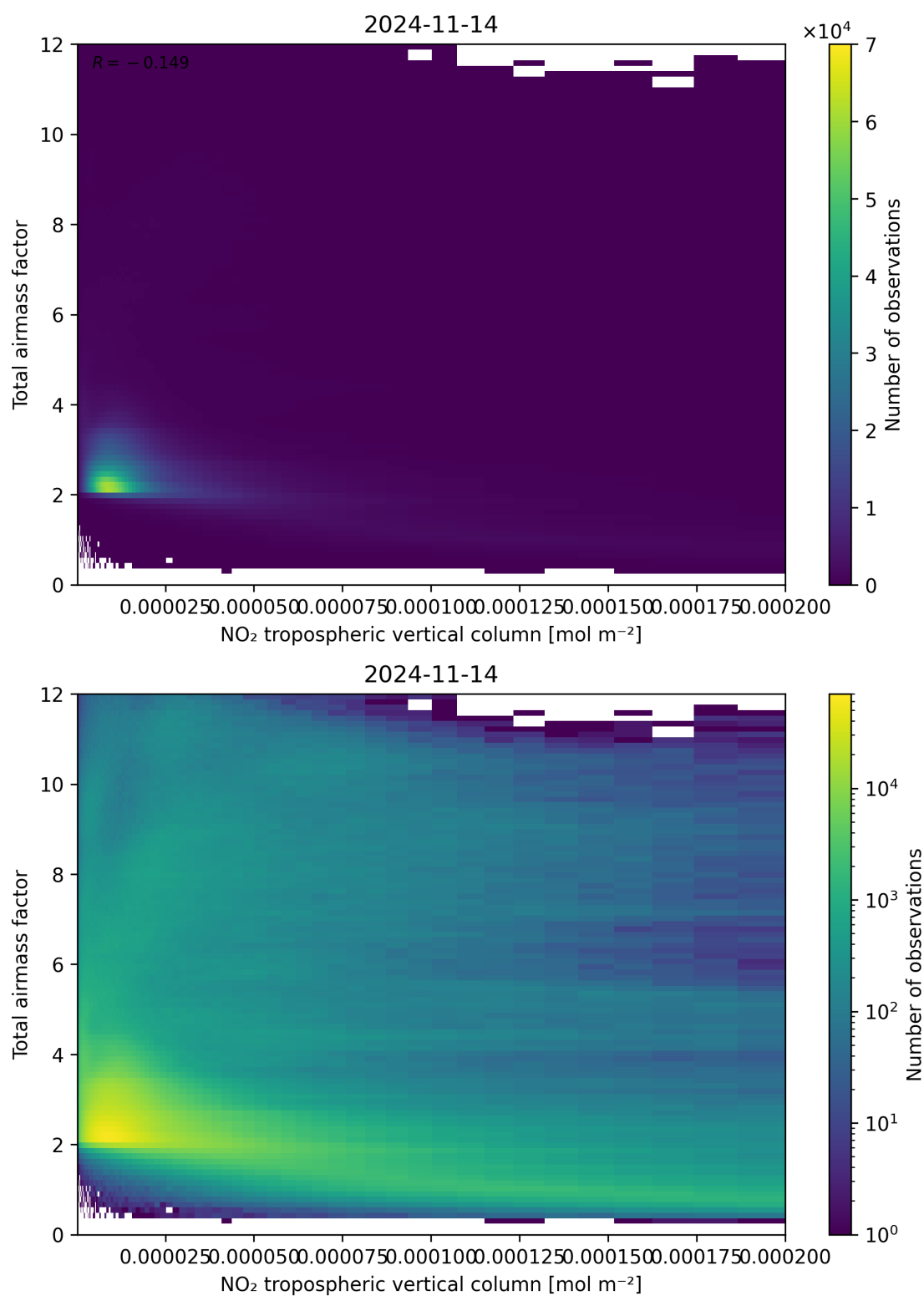
Figure 122: Scatter density plot of “NO 2 tropospheric vertical column” against “Total air mass factor” for 2024-11-14 to 2024-11-15.
