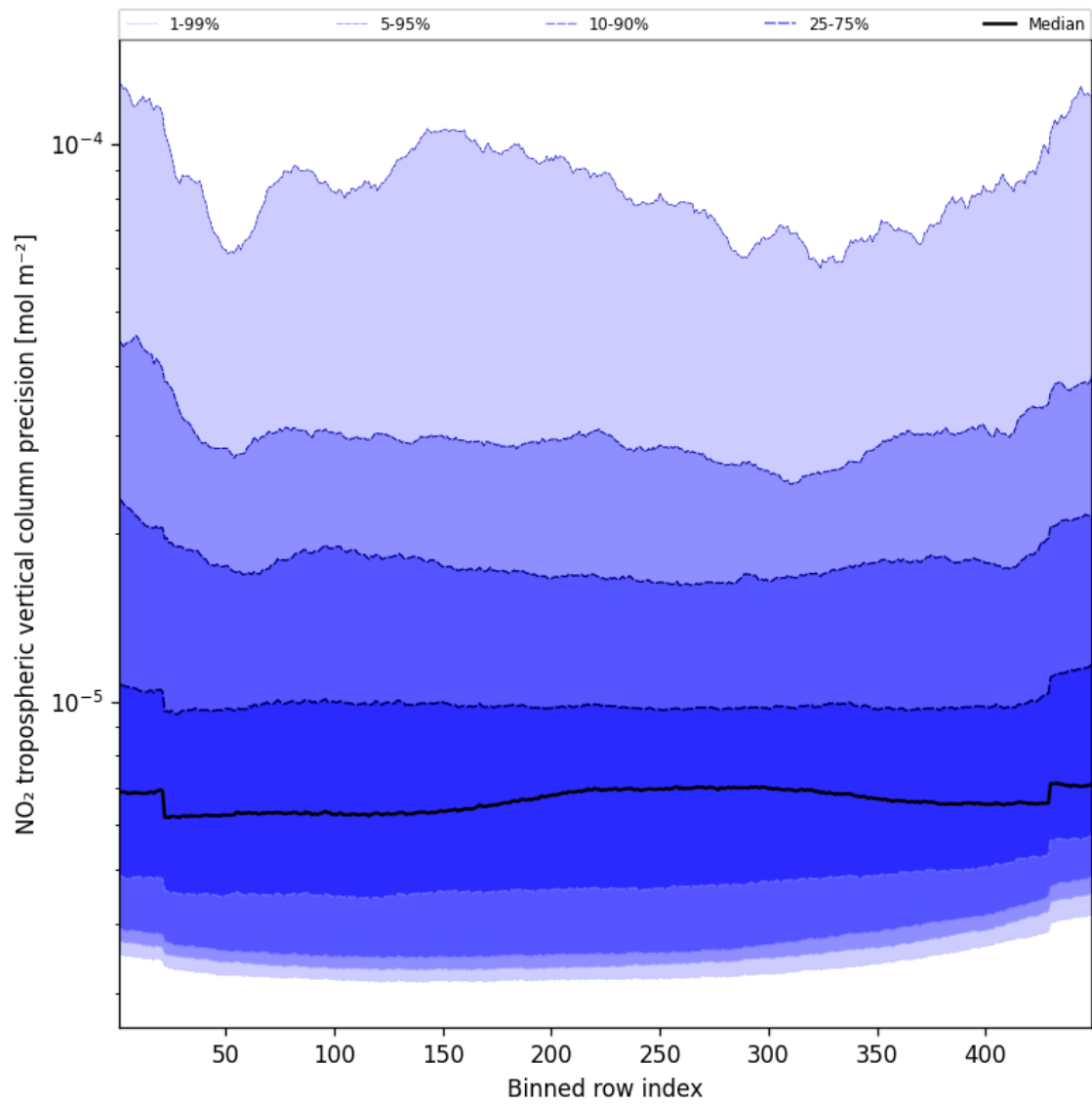
Figure 47: Along track statistics of “NO 2 tropospheric vertical column precision” for 2024-11-14 to 2024-11-15
