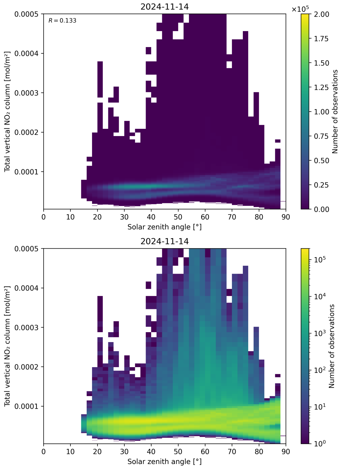
Figure 153: Scatter density plot of “Solar zenith angle” against “Total vertical NO 2 column” for 2024-11-14 to 2024-11-15.
