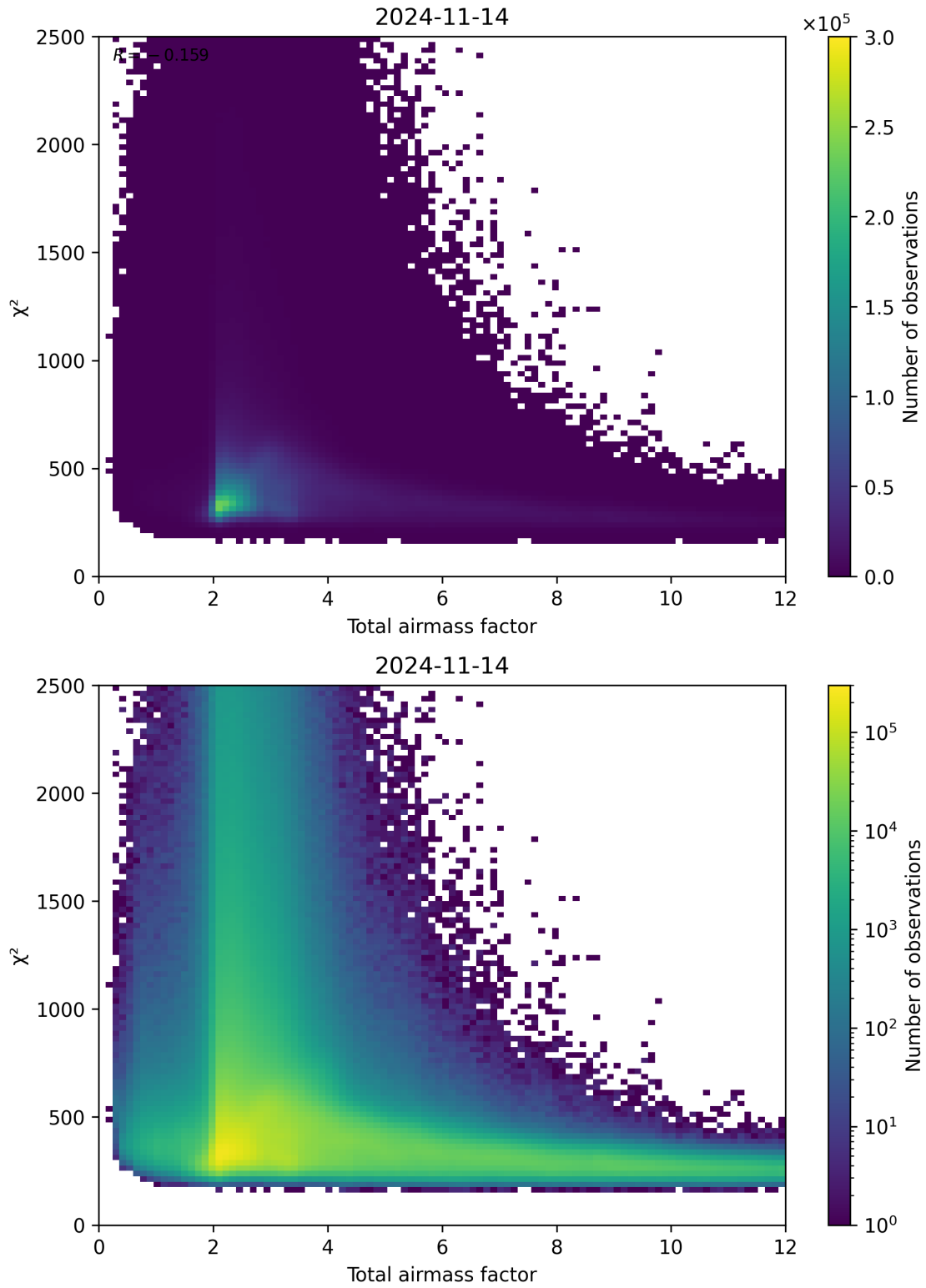
Figure 63: Scatter density plot of “Total airmass factor” against “ \chi^2 ” for 2024-11-14 to 2024-11-15.
