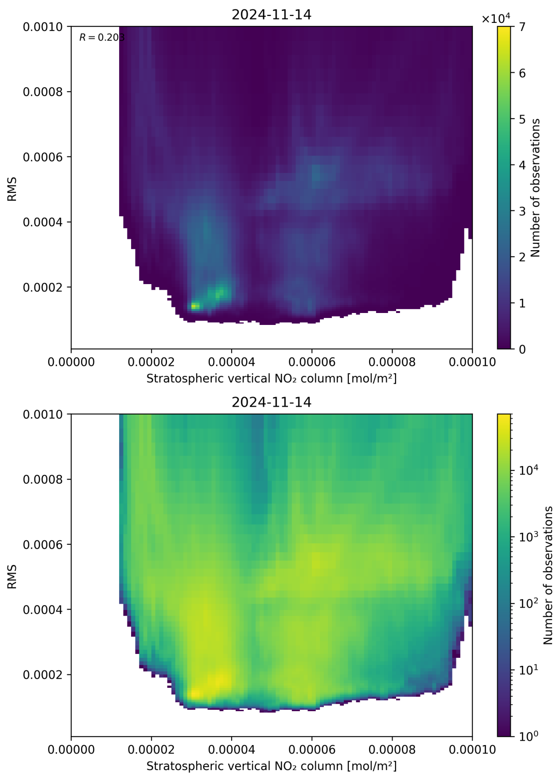
Figure 102: Scatter density plot of “Stratospheric vertical NO 2 column” against “RMS” for 2024-11-14 to 2024-11-15.
