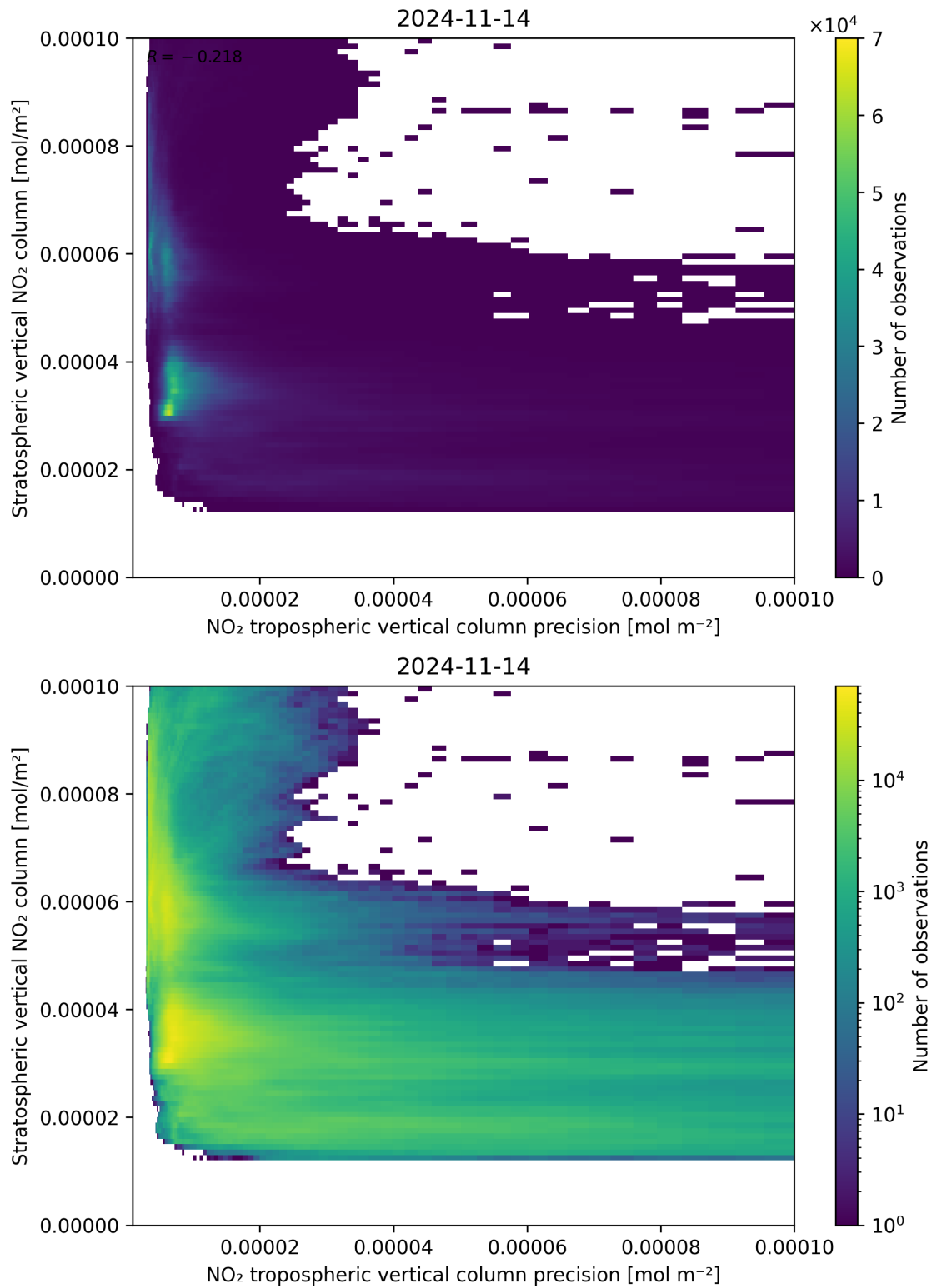
Figure 135: Scatter density plot of “NO 2 tropospheric vertical column precision” against “Stratospheric vertical NO 2 column” for 2024-11-14 to 2024-11-15.
