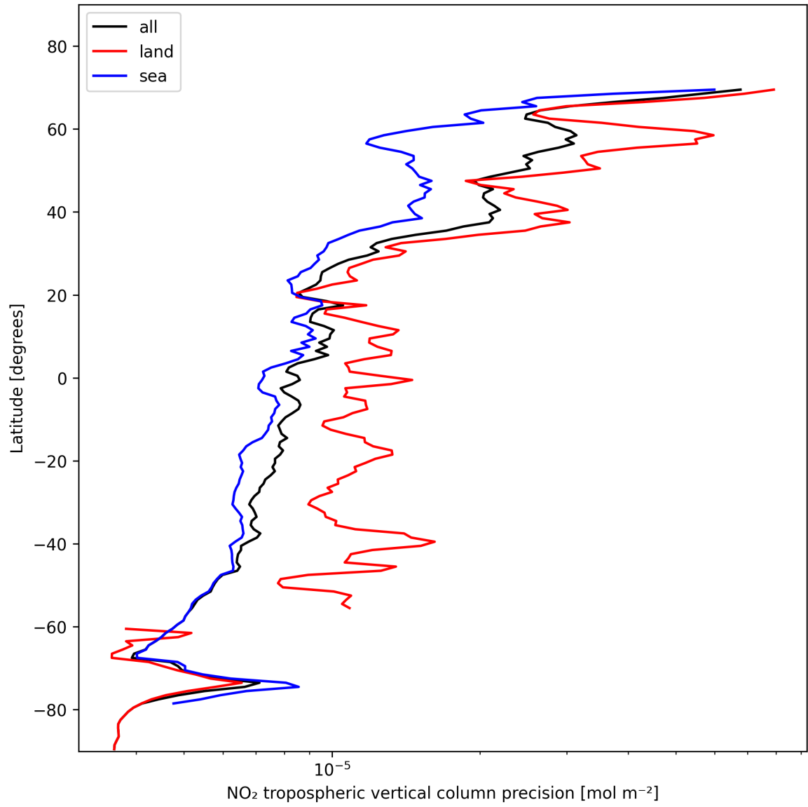
Figure 13: Zonal average of “NO 2 tropospheric vertical column precision” for 2024-11-14 to 2024-11-15.
