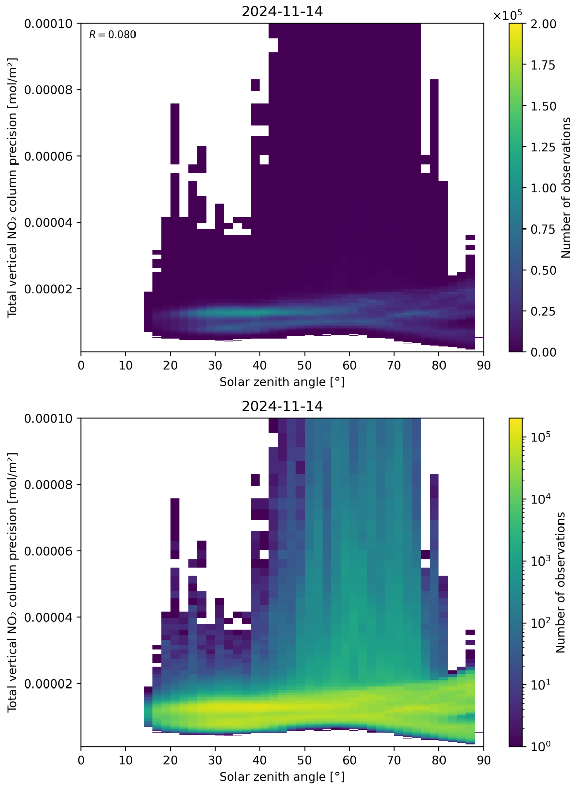
Figure 154: Scatter density plot of “Solar zenith angle” against “Total vertical NO 2 column precision” for 2024-11-14 to 2024-11-15.
