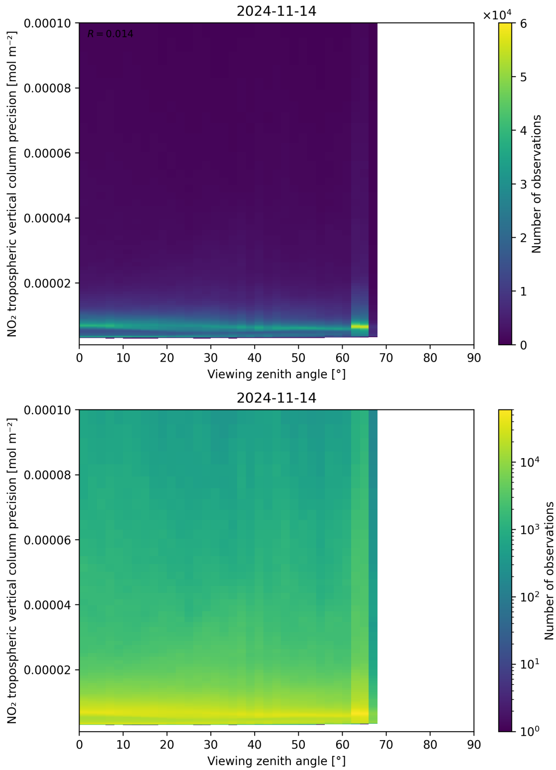
Figure 170: Scatter density plot of “Viewing zenith angle” against “NO 2 tropospheric vertical column precision” for 2024-11-14 to 2024-11-15.
