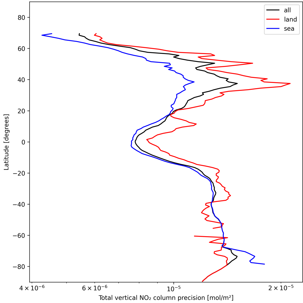
Figure 22: Zonal average of “Total vertical NO 2 column precision” for 2024-11-14 to 2024-11-15.
