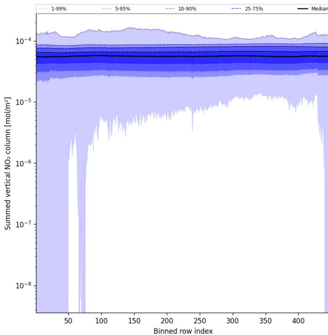
Figure 57: Along track statistics of “Summed vertical NO 2 column” for 2024-11-14 to 2024-11-15
