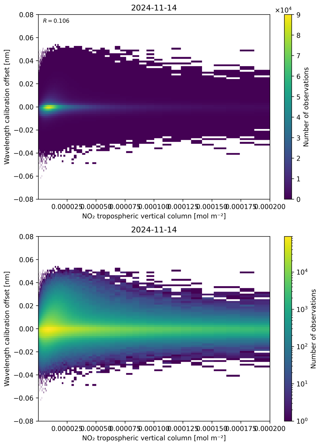
Figure 143: Scatter density plot of “NO 2 tropospheric vertical column” against “Wavelength calibration offset” for 2024-11-14 to 2024-11-15.
