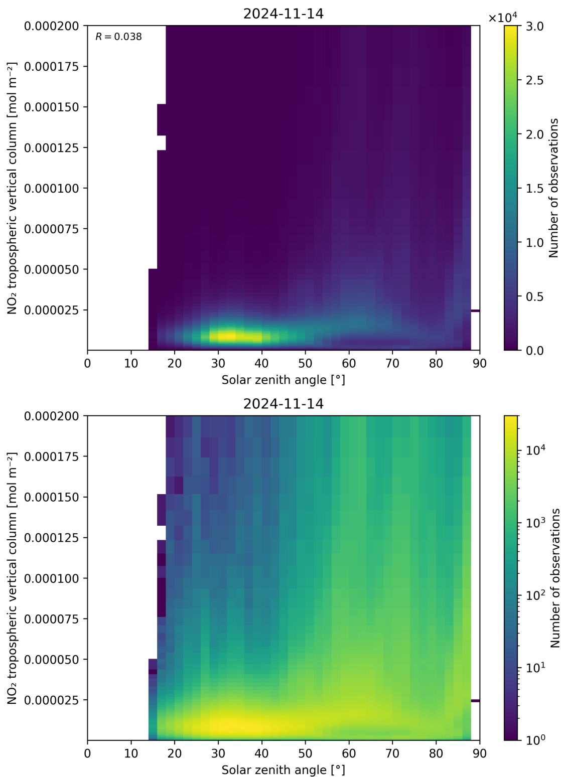
Figure 155: Scatter density plot of “Solar zenith angle” against “NO 2 tropospheric vertical column” for 2024-11-14 to 2024-11-15.
