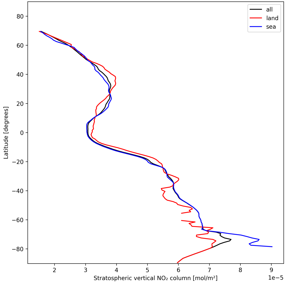
Figure 19: Zonal average of “Stratospheric vertical NO 2 column” for 2024-11-14 to 2024-11-15.
