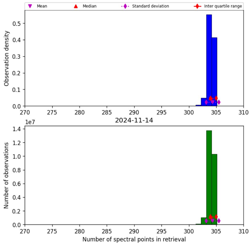
Figure 33: Histogram of “Number of spectral points in retrieval” for 2024-11-14 to 2024-11-15
