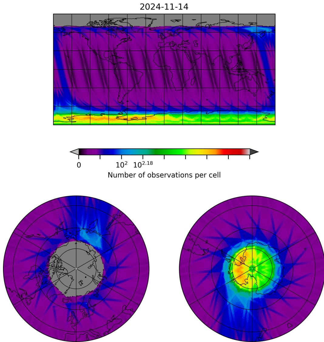
Figure 10: Map of the number of observations for 2024-11-14 to 2024-11-15
