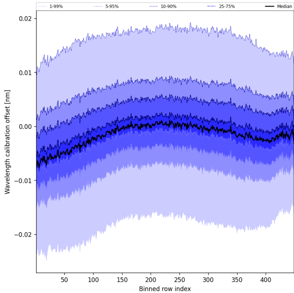
Figure 52: Along track statistics of “Wavelength calibration offset” for 2024-11-14 to 2024-11-15
