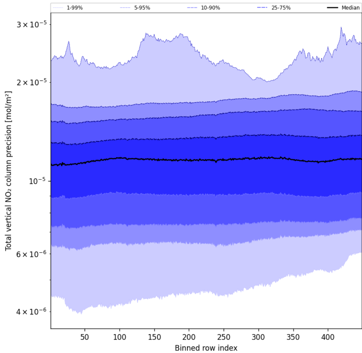
Figure 56: Along track statistics of "Total vertical NO 2 column precision" for 2024-11-14 to 2024-11-15
