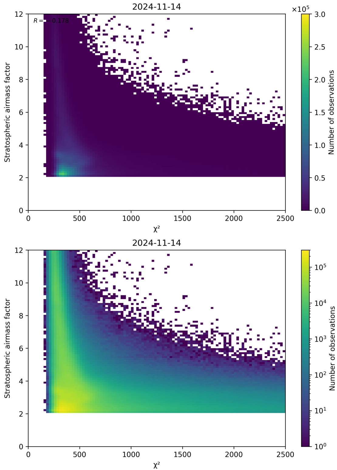
Figure 81: Scatter density plot of “ \chi^2 ” against “Stratospheric airmass factor” for 2024-11-14 to 2024-11-15.
