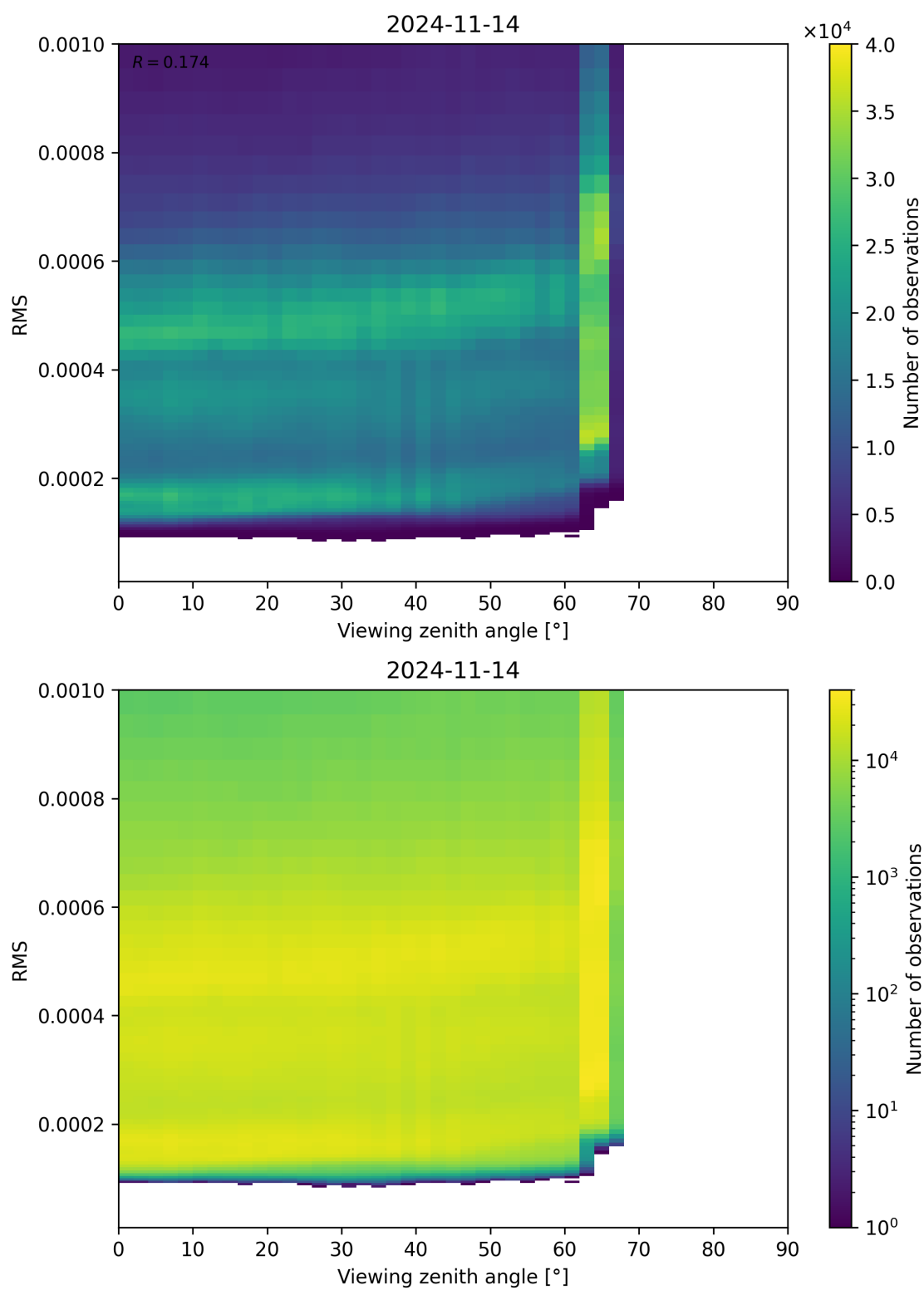
Figure 171: Scatter density plot of “Viewing zenith angle” against “RMS” for 2024-11-14 to 2024-11-15.
