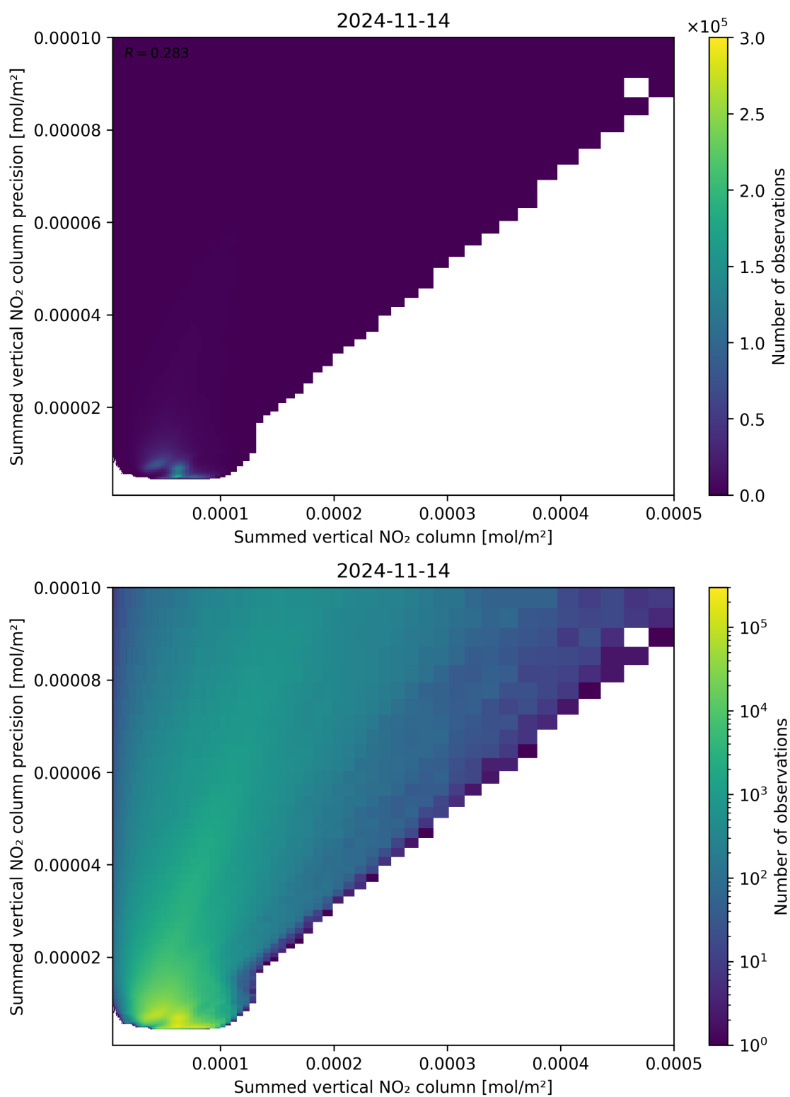
Figure 105: Scatter density plot of “Summed vertical NO 2 column” against “Summed vertical NO 2 column precision” for 2024-11-14 to 2024-11-15.
