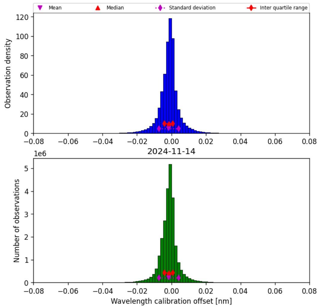
Figure 35: Histogram of “Wavelength calibration offset” for 2024-11-14 to 2024-11-15
