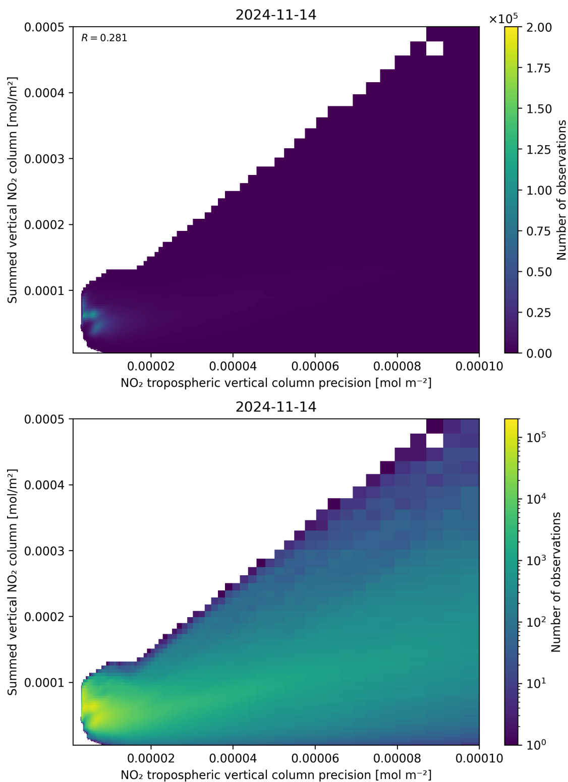
Figure 136: Scatter density plot of “NO 2 tropospheric vertical column precision” against “Summed vertical NO 2 column” for 2024-11-14 to 2024-11-15.
