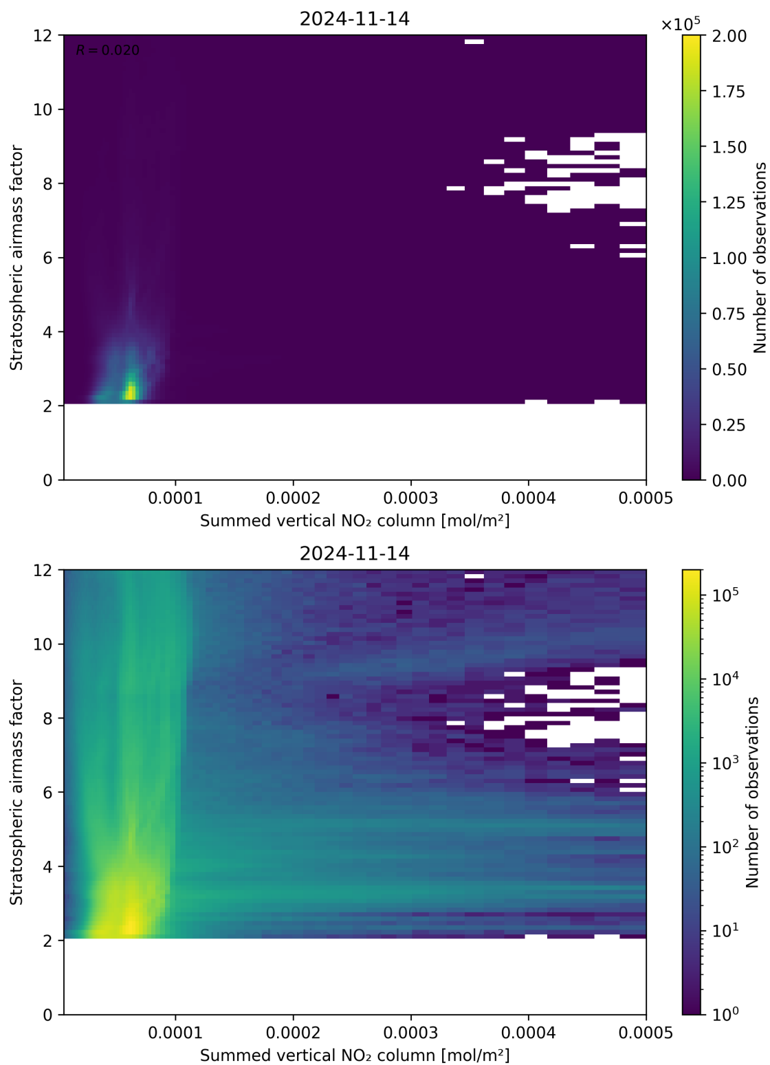
Figure 103: Scatter density plot of “Summed vertical NO 2 column” against “Stratospheric airmass factor” for 2024-11-14 to 2024-11-15.
