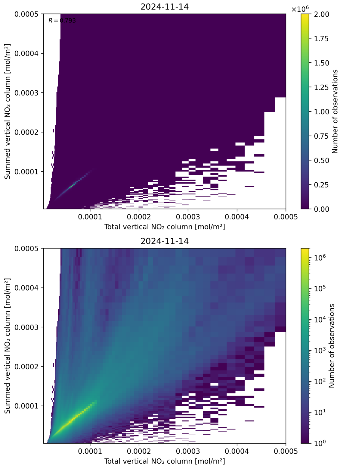
Figure 112: Scatter density plot of “Total vertical NO 2 column” against “Summed vertical NO 2 column” for 2024-11-14 to 2024-11-15.
