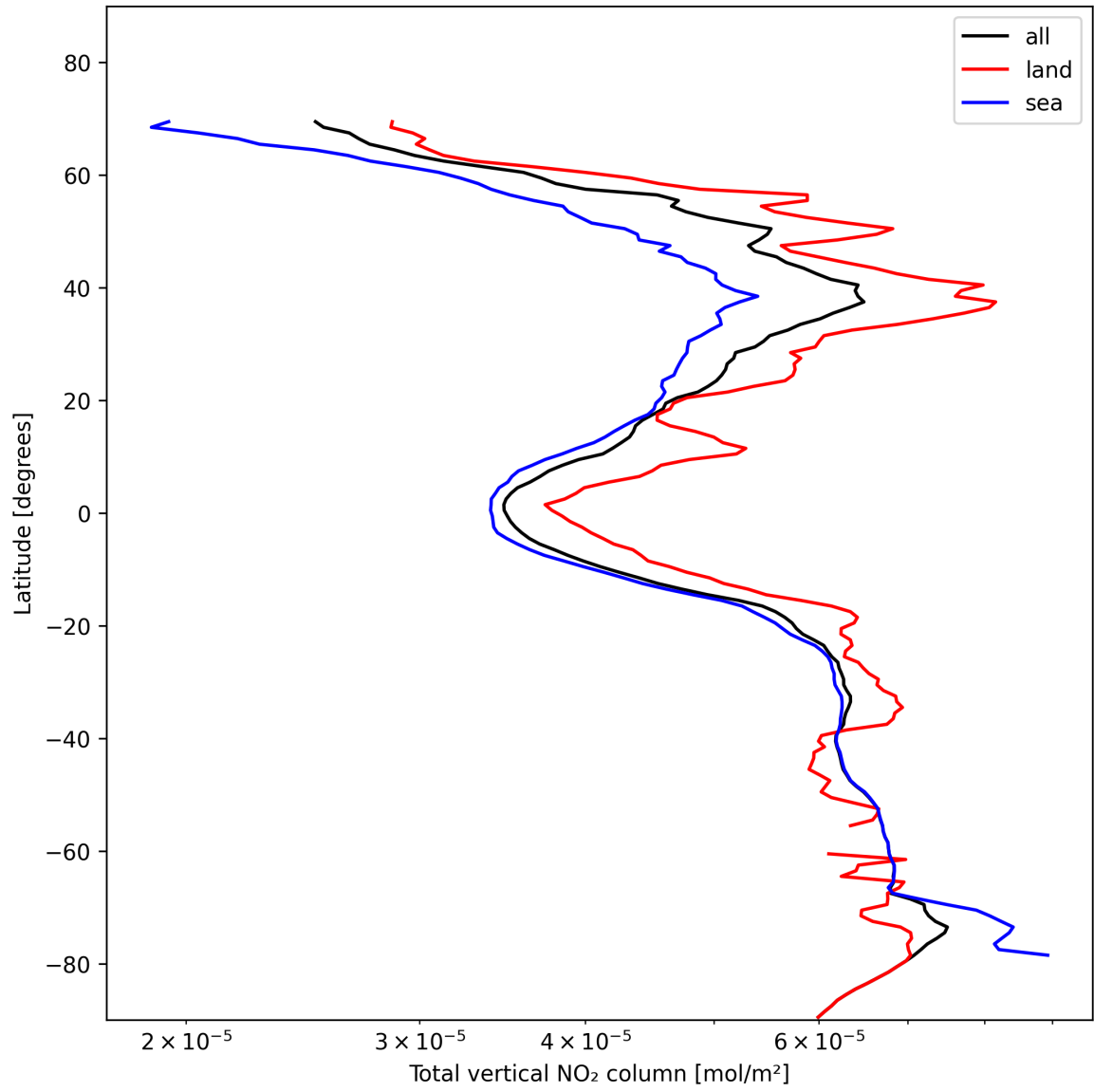
Figure 21: Zonal average of “Total vertical NO 2 column” for 2024-11-14 to 2024-11-15.
