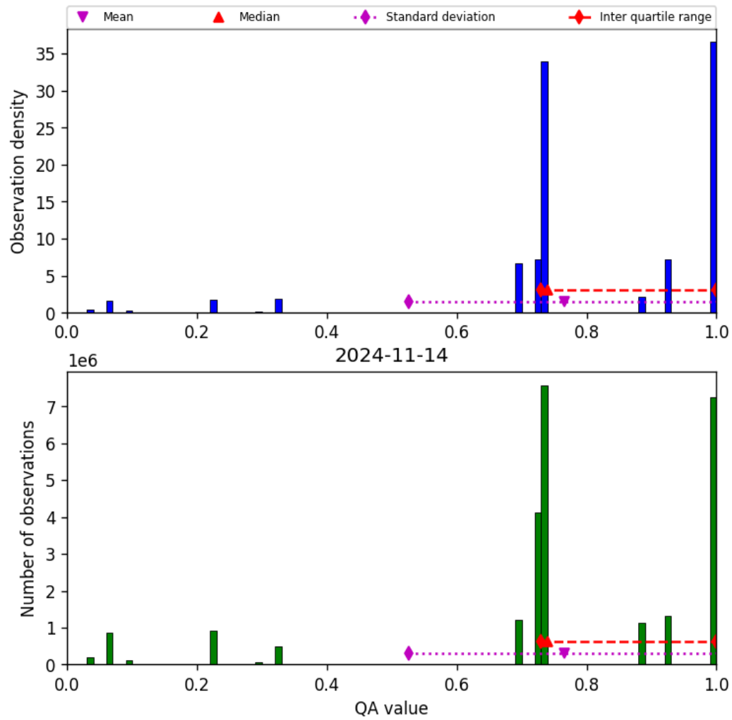
Figure 28: Histogram of “QA value” for 2024-11-14 to 2024-11-15
