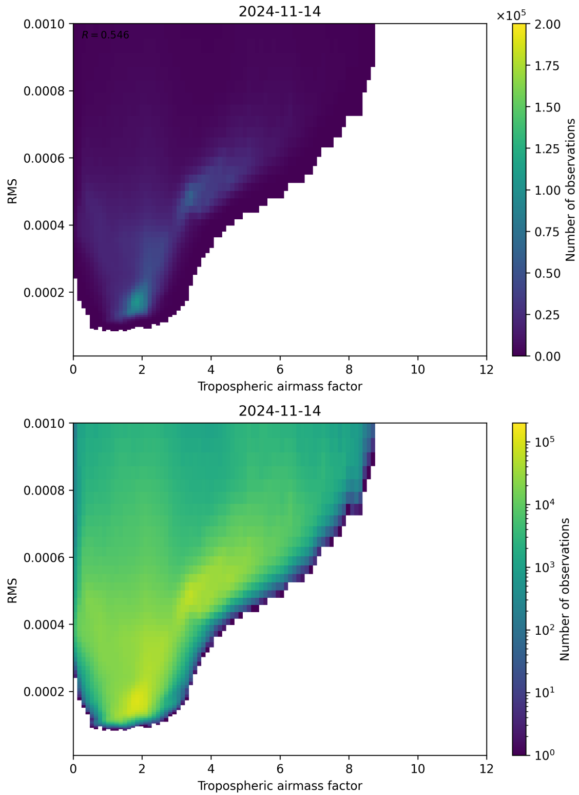
Figure 79: Scatter density plot of “Tropospheric airmass factor” against “RMS” for 2024-11-14 to 2024-11-15.
