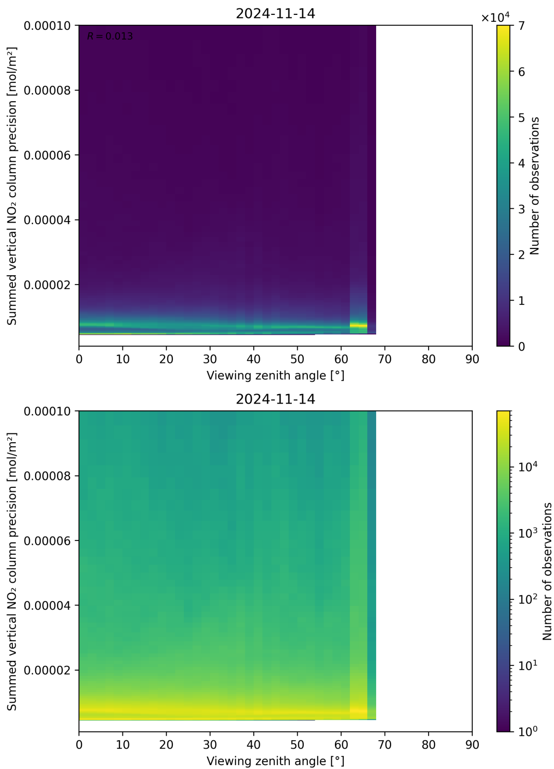
Figure 166: Scatter density plot of “Viewing zenith angle” against “Summed vertical NO 2 column precision” for 2024-11-14 to 2024-11-15.
