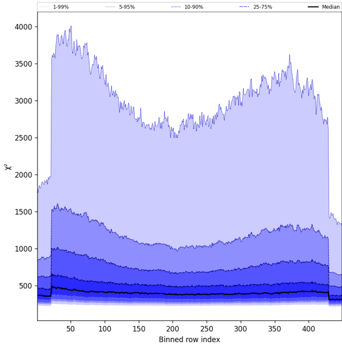
Figure 59: Along track statistics of “ \chi^2 ” for 2024-11-14 to 2024-11-15
