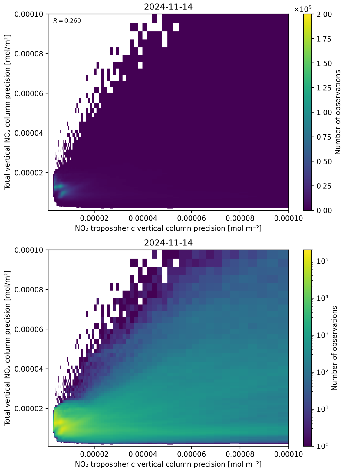
Figure 139: Scatter density plot of “NO 2 tropospheric vertical column precision” against “Total vertical NO 2 column precision” for 2024-11-14 to 2024-11-15.
