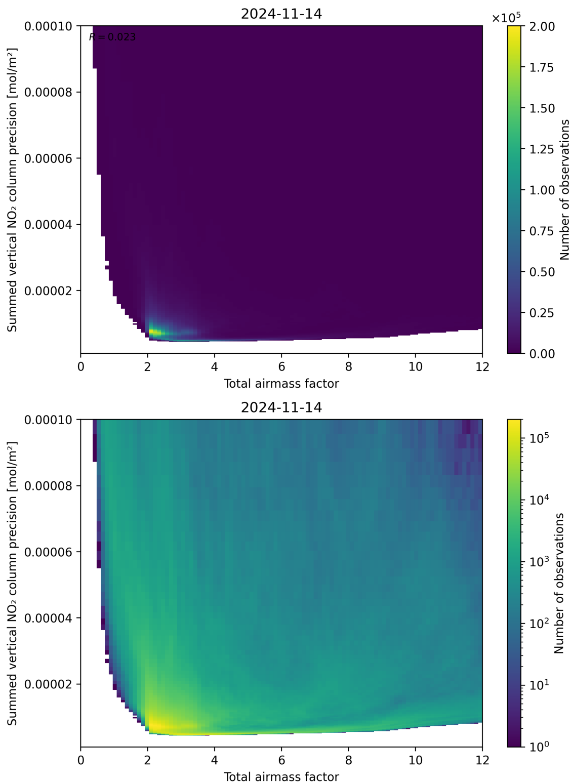
Figure 66: Scatter density plot of “Total airmass factor” against “Summed vertical NO 2 column precision” for 2024-11-14 to 2024-11-15.
