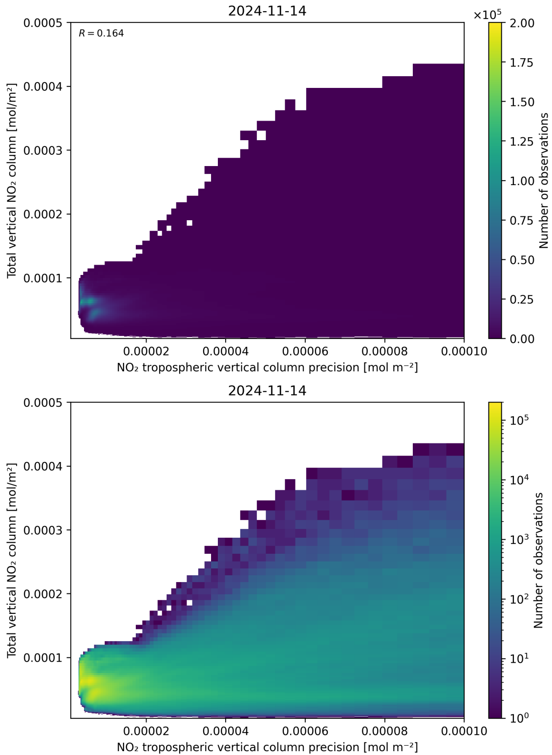
Figure 138: Scatter density plot of “NO 2 tropospheric vertical column precision” against “Total vertical NO 2 column” for 2024-11-14 to 2024-11-15.
