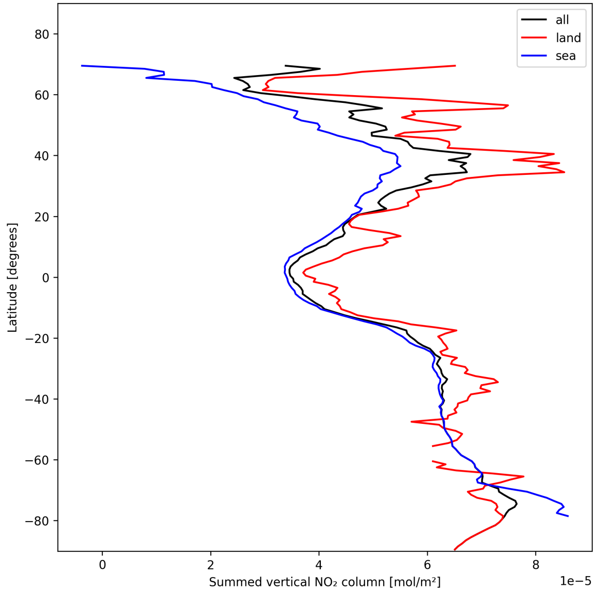
Figure 23: Zonal average of “Summed vertical NO 2 column” for 2024-11-14 to 2024-11-16.
