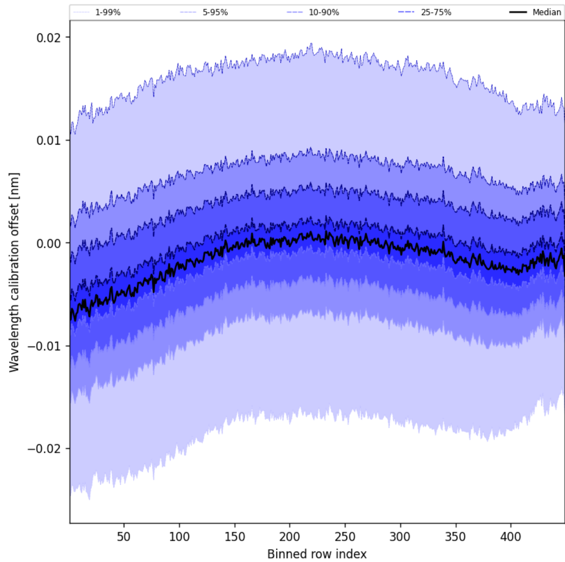
Figure 52: Along track statistics of “Wavelength calibration offset” for 2024-11-14 to 2024-11-16
