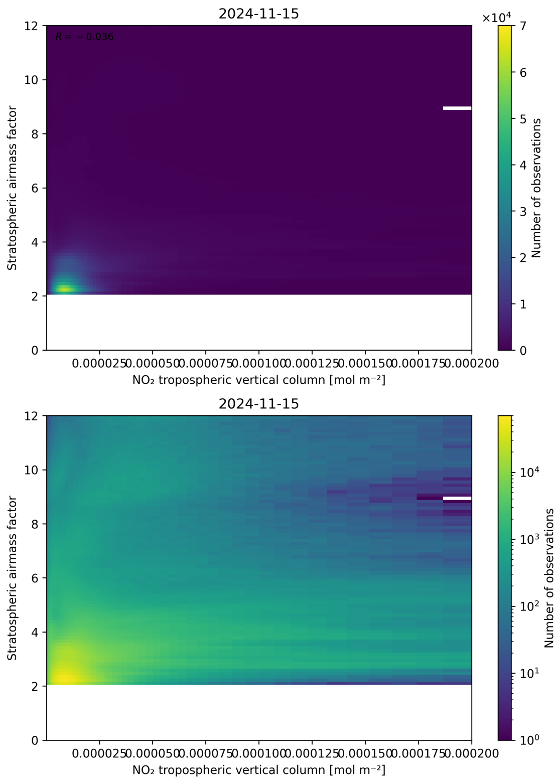
Figure 121: Scatter density plot of “NO 2 tropospheric vertical column” against “Stratospheric airmass factor” for 2024-11-14 to 2024-11-16.
