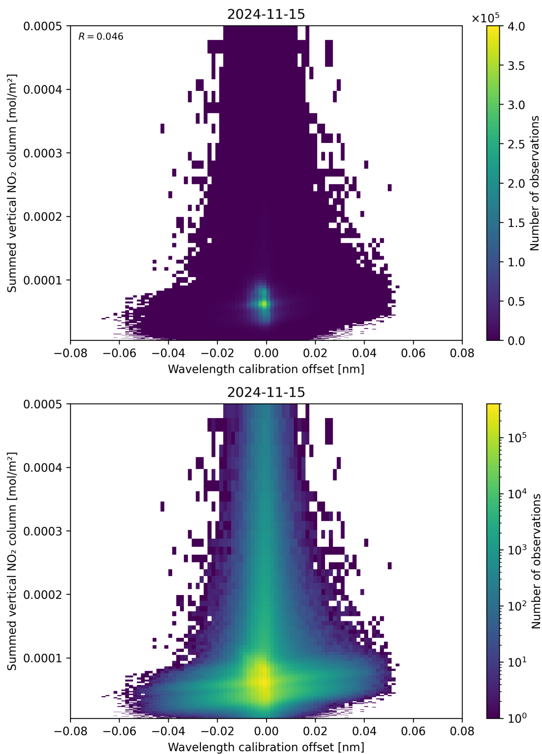
Figure 177: Scatter density plot of “Wavelength calibration offset” against “Summed vertical NO 2 column” for 2024-11-14 to 2024-11-16.
