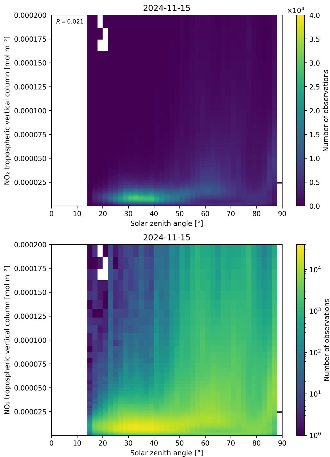
Figure 155: Scatter density plot of “Solar zenith angle” against “NO 2 tropospheric vertical column” for 2024-11-14 to 2024-11-16.
