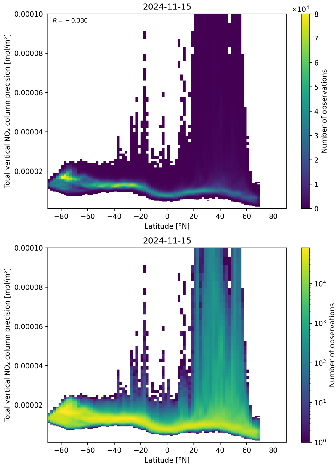
Figure 91: Scatter density plot of “Latitude” against “Total vertical NO 2 column precision” for 2024-11-14 to 2024-11-16.
