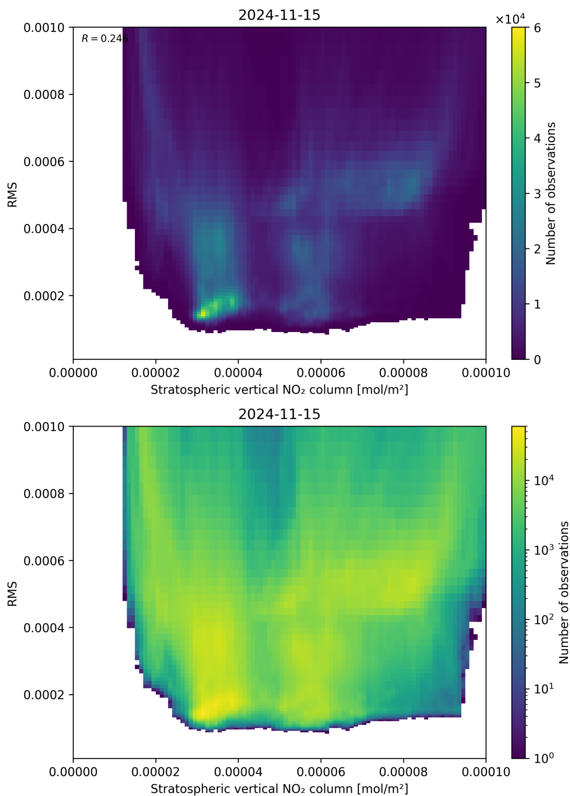
Figure 102: Scatter density plot of “Stratospheric vertical NO 2 column” against “RMS” for 2024-11-14 to 2024-11-16.
