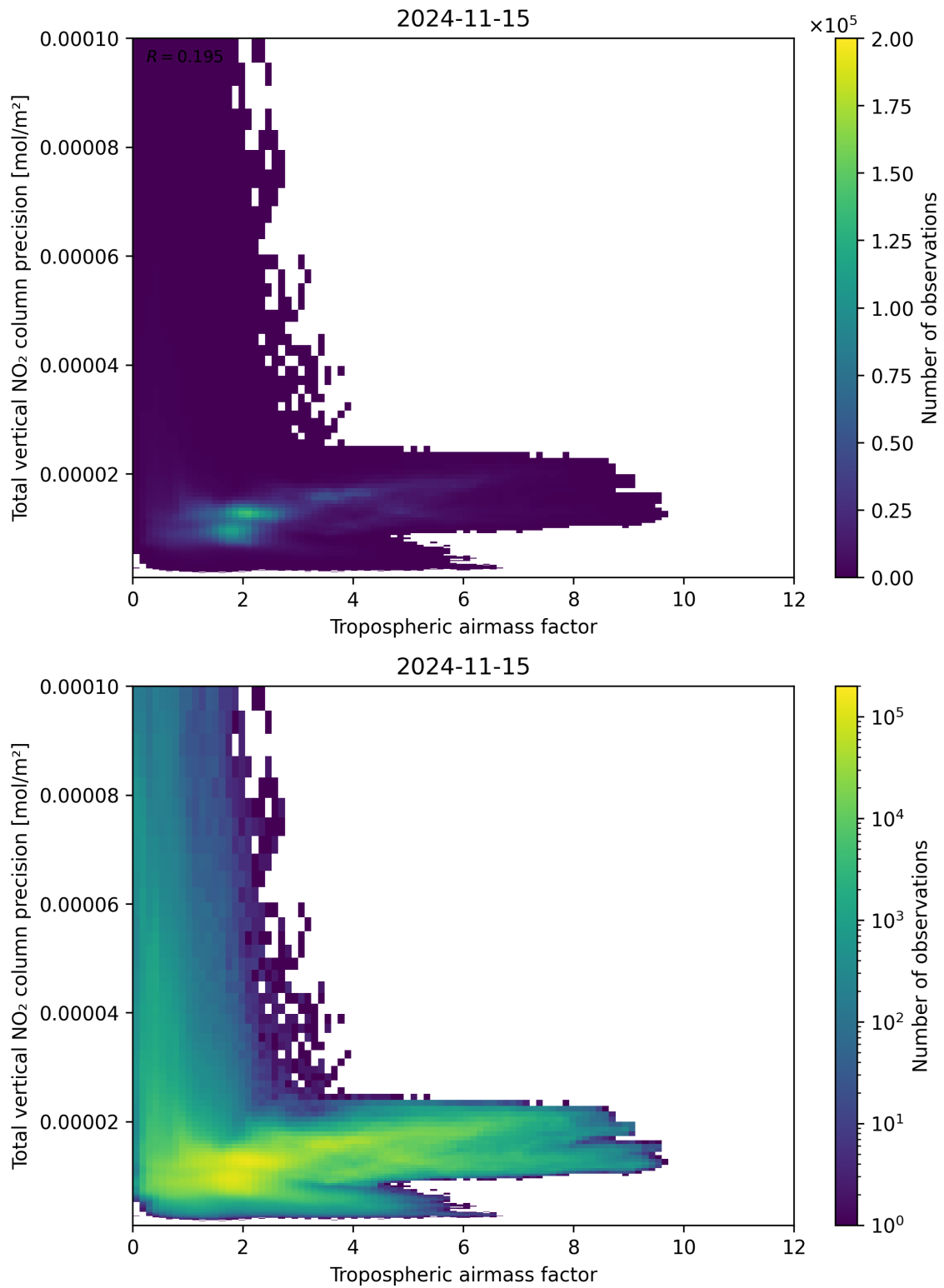
Figure 78: Scatter density plot of “Tropospheric air mass factor” against “Total vertical NO 2 column precision” for 2024-11-14 to 2024-11-16.
