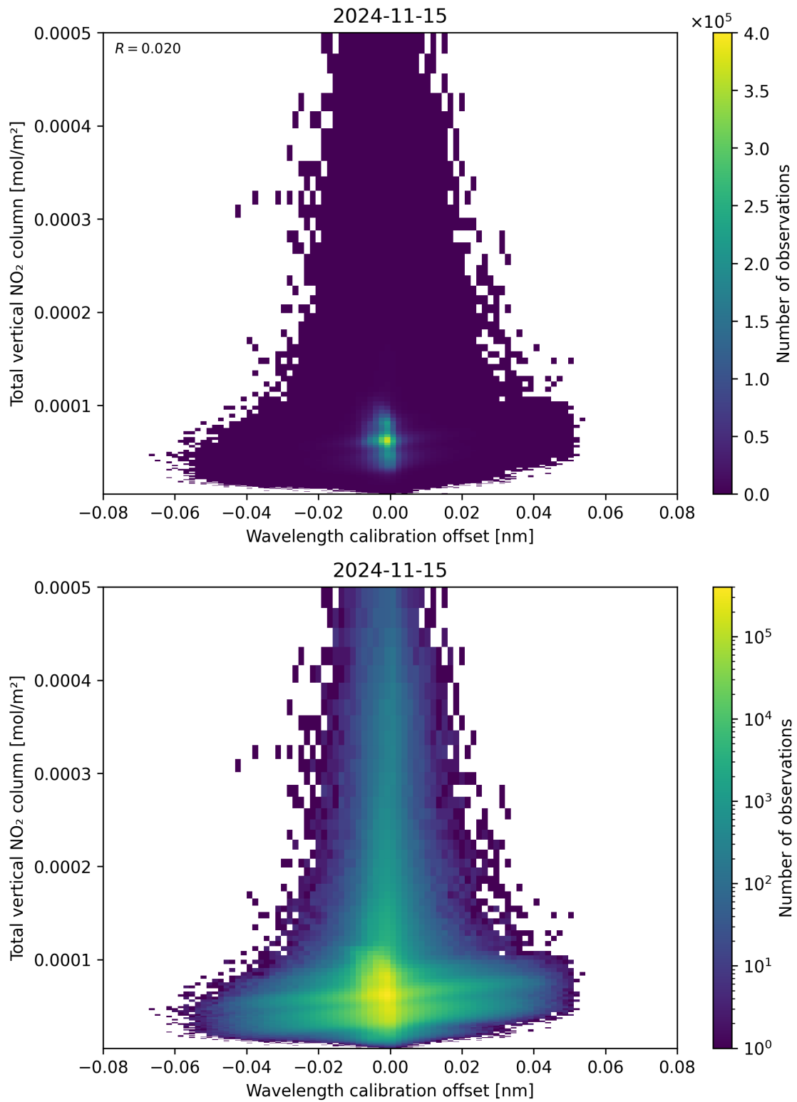
Figure 179: Scatter density plot of “Wavelength calibration offset” against “Total vertical NO 2 column” for 2024-11-14 to 2024-11-16.
