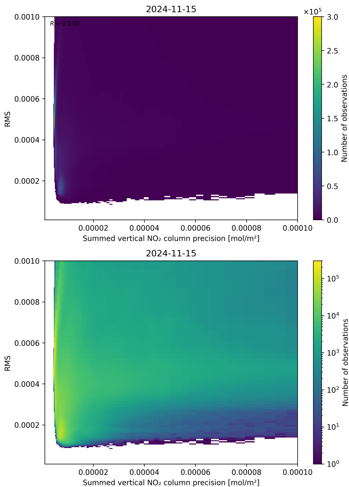
Figure 108: Scatter density plot of “Summed vertical NO 2 column precision” against “RMS” for 2024-11-14 to 2024-11-16.
