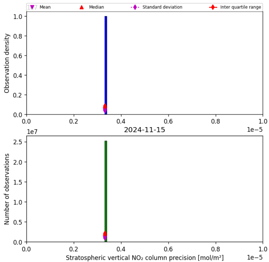
Figure 37: Histogram of “Stratospheric vertical NO 2 column precision” for 2024-11-14 to 2024-11-16
