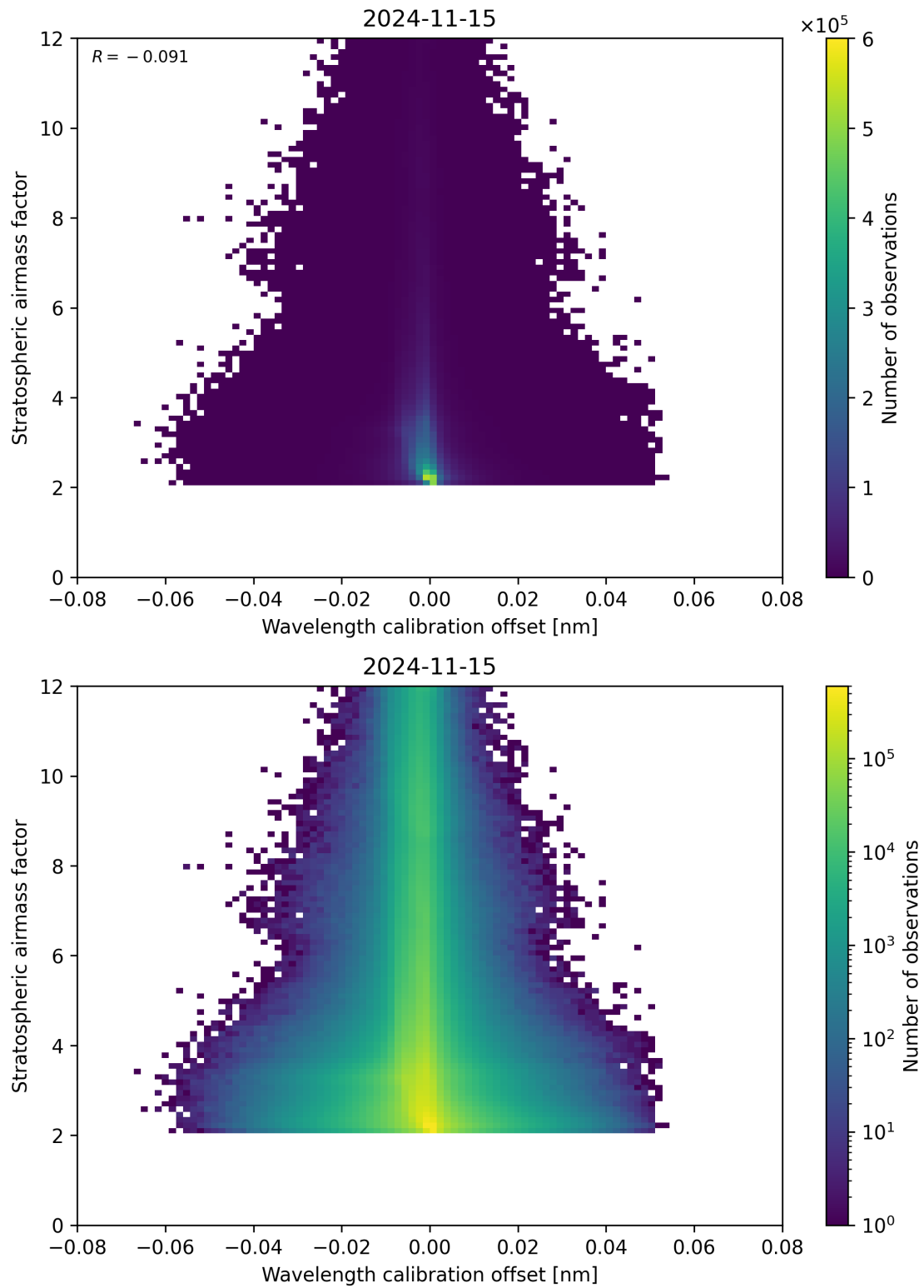
Figure 174: Scatter density plot of “Wavelength calibration offset” against “Stratospheric airmass factor” for 2024-11-14 to 2024-11-16.
