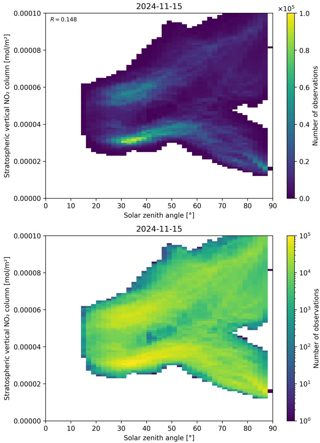
Figure 150: Scatter density plot of “Solar zenith angle” against “Stratospheric vertical NO 2 column” for 2024-11-14 to 2024-11-16.
