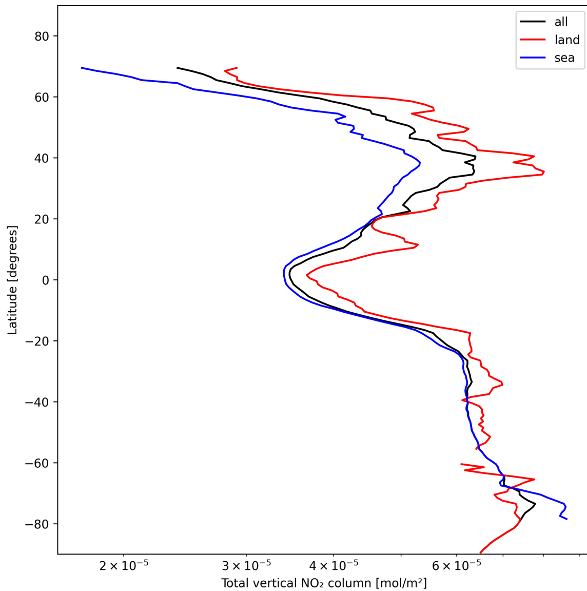
Figure 21: Zonal average of “Total vertical NO 2 column” for 2024-11-14 to 2024-11-16.
