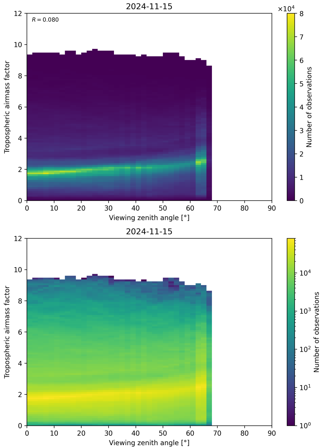
Figure 161: Scatter density plot of “Viewing zenith angle” against “Tropospheric airmass factor” for 2024-11-14 to 2024-11-16.
