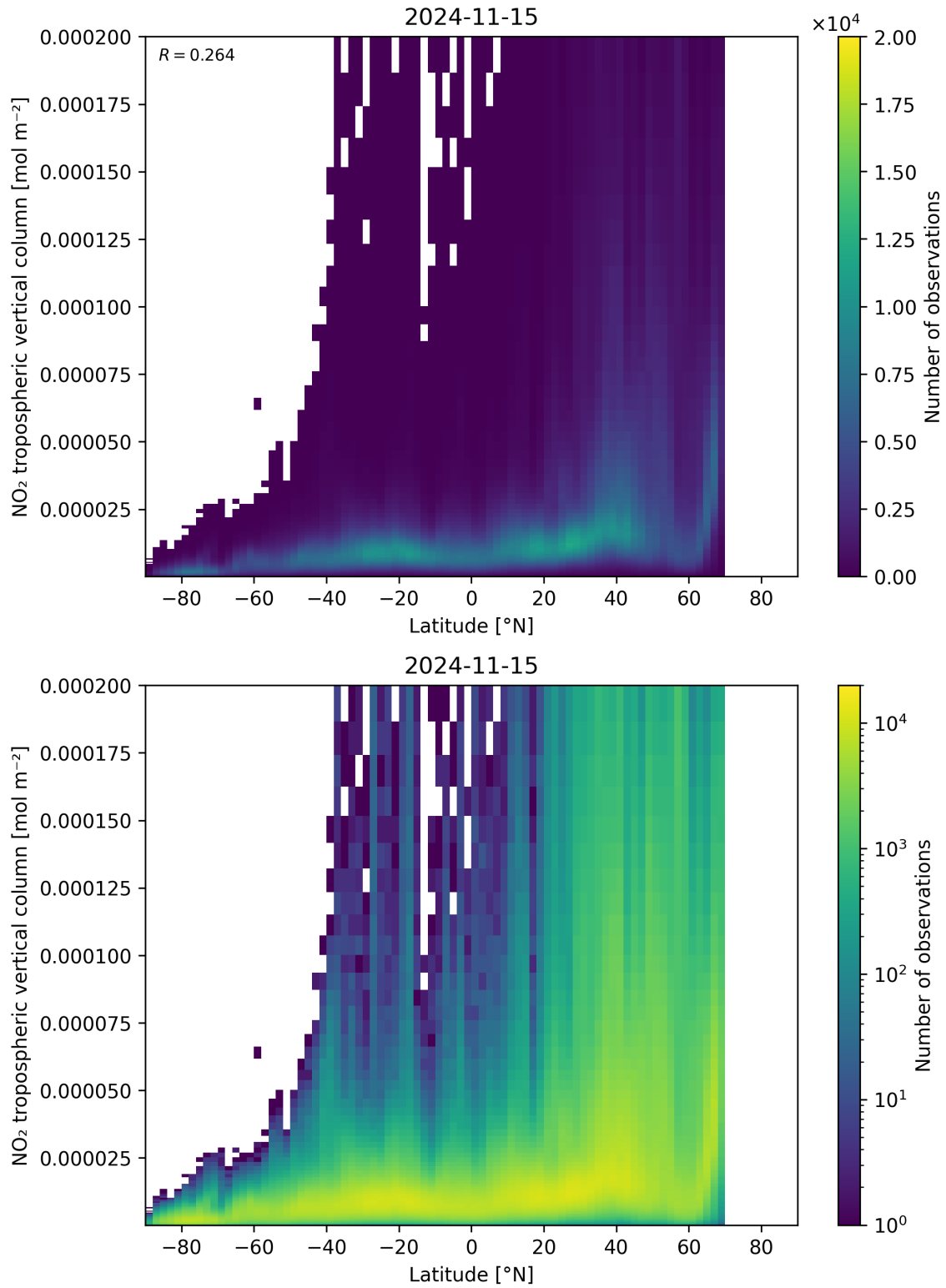
Figure 92: Scatter density plot of “Latitude” against “NO 2 tropospheric vertical column” for 2024-11-14 to 2024-11-16.
