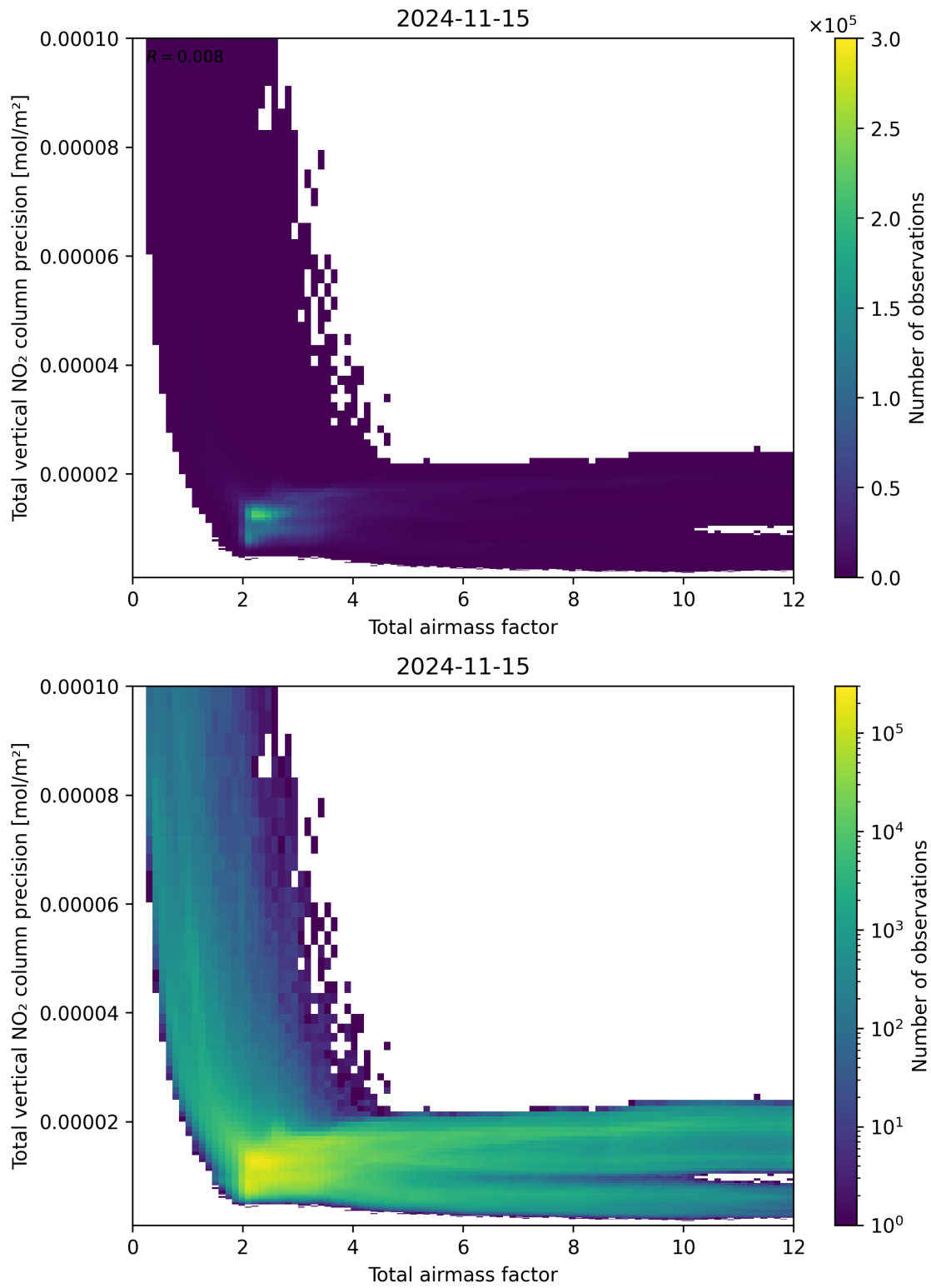
Figure 68: Scatter density plot of “Total airmass factor” against “Total vertical NO 2 column precision” for 2024-11-14 to 2024-11-16.
