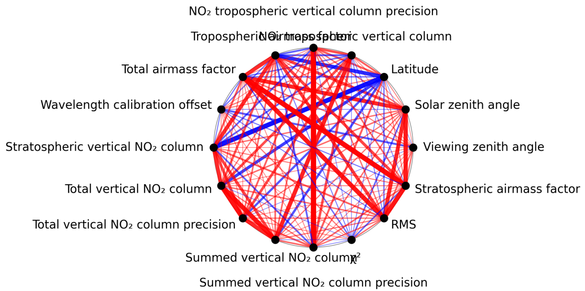
Figure 1: Map of correlation graph for 2024-11-14 to 2024-11-16.
