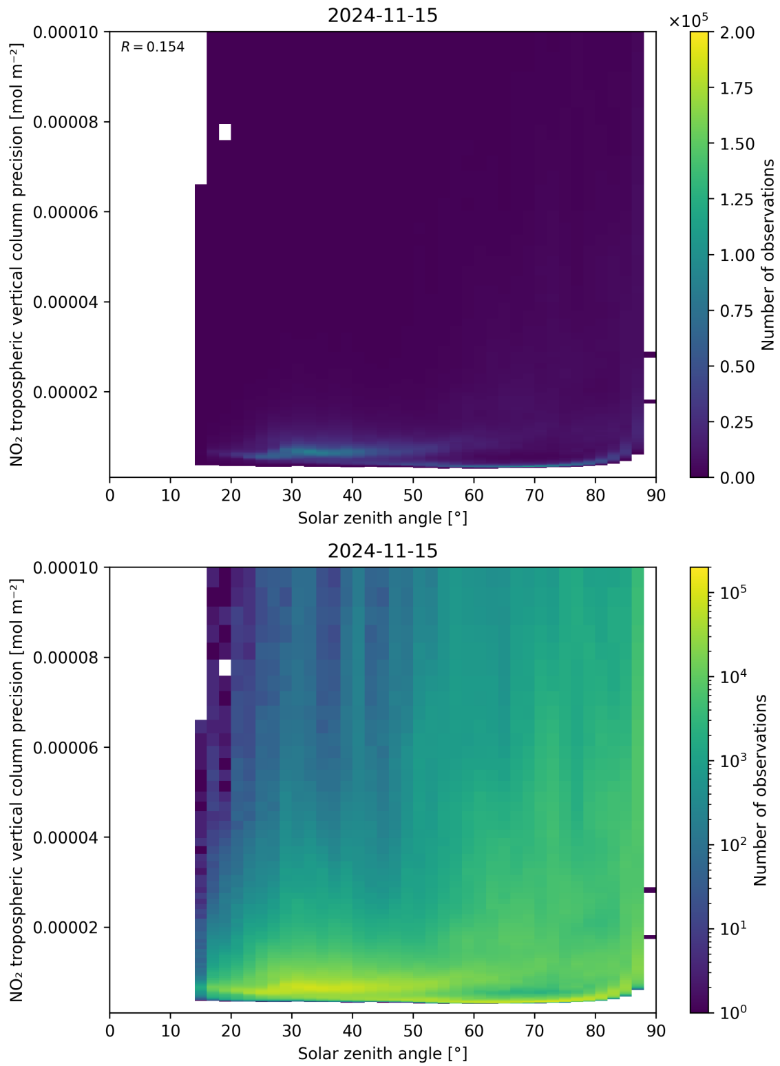
Figure 156: Scatter density plot of “Solar zenith angle” against “NO 2 tropospheric vertical column precision” for 2024-11-14 to 2024-11-16.
