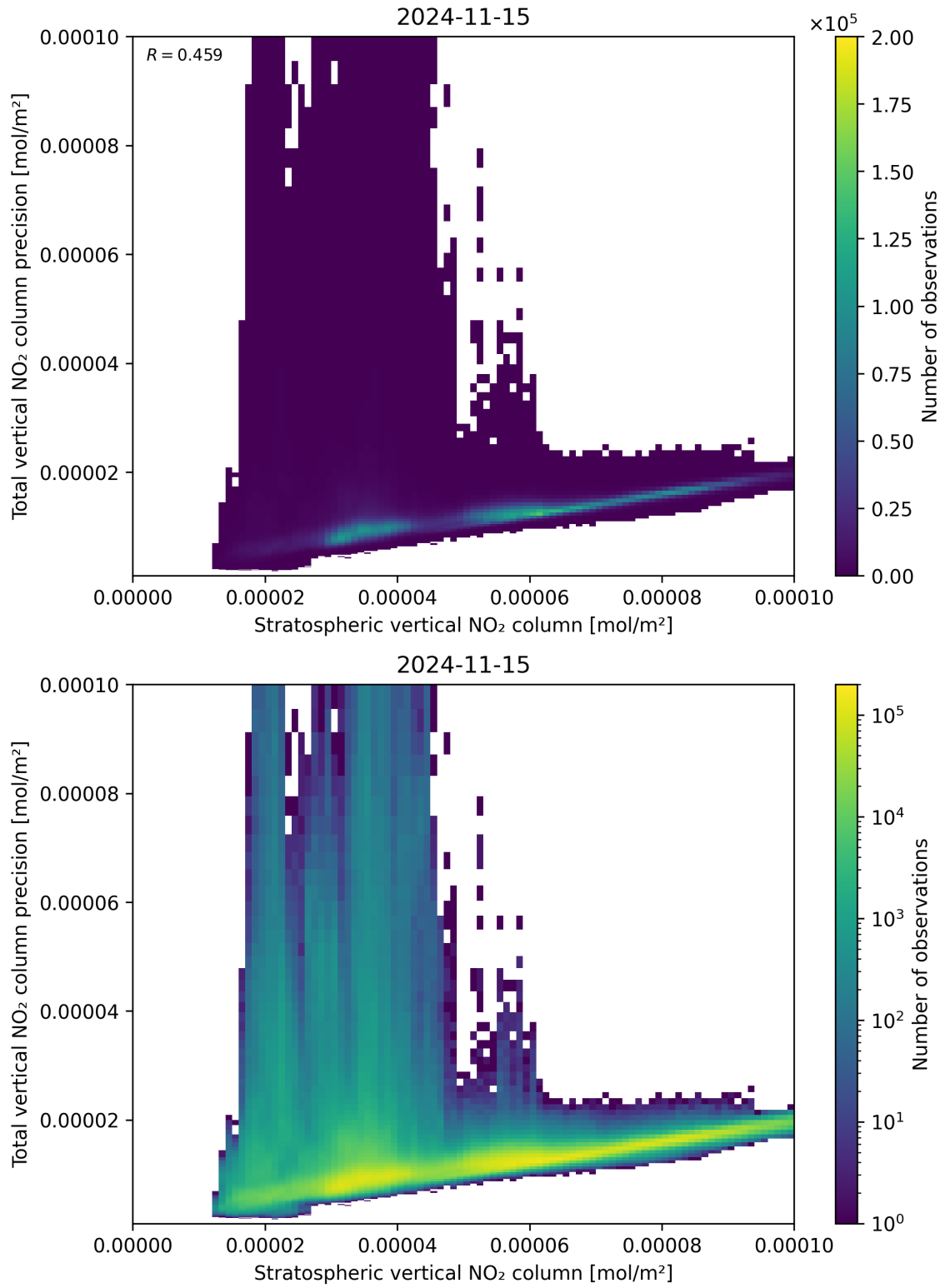
Figure 101: Scatter density plot of “Stratospheric vertical NO 2 column” against “Total vertical NO 2 column precision” for 2024-11-14 to 2024-11-16.
