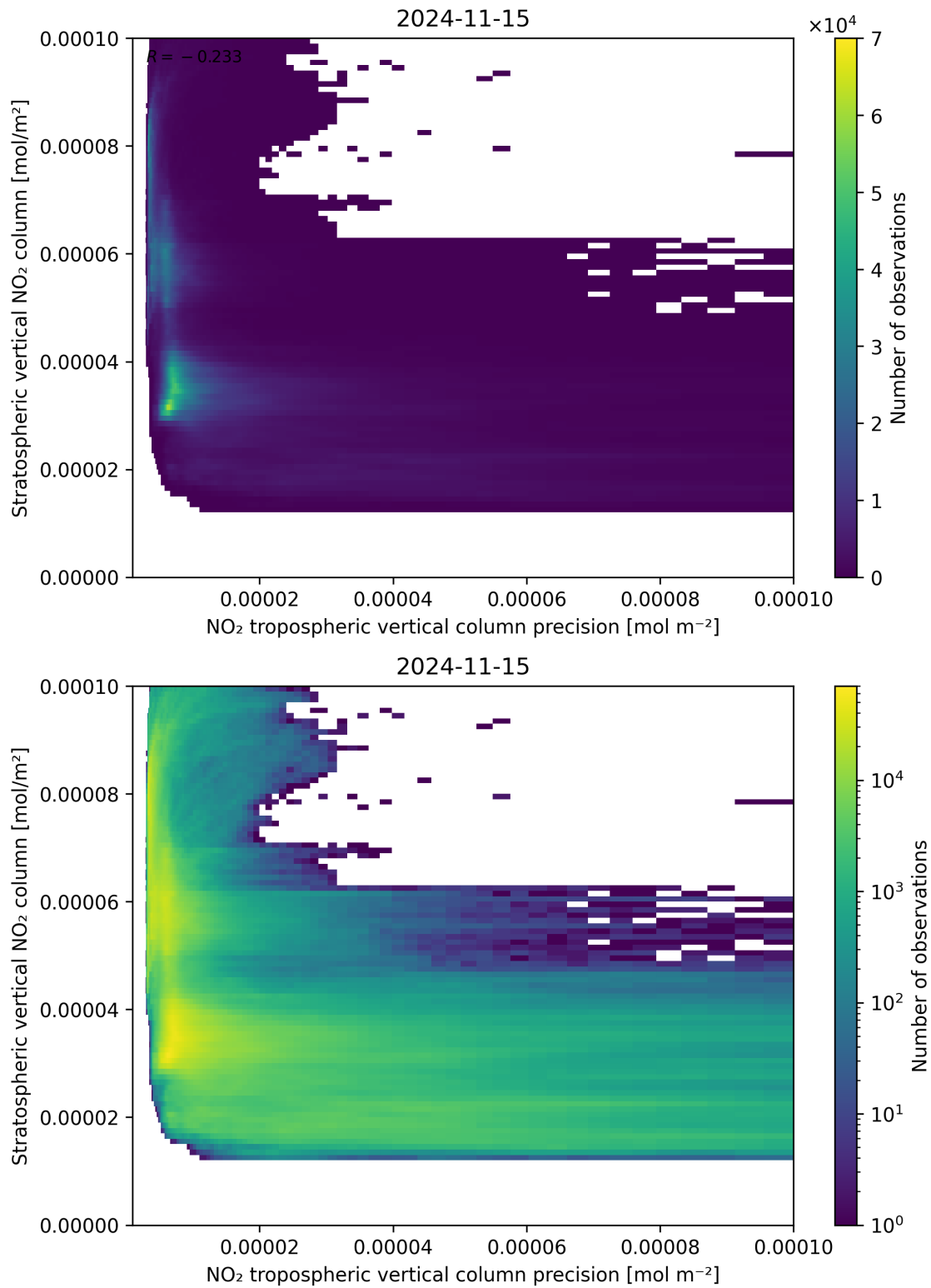
Figure 135: Scatter density plot of “NO 2 tropospheric vertical column precision” against “Stratospheric vertical NO 2 column” for 2024-11-14 to 2024-11-16.
