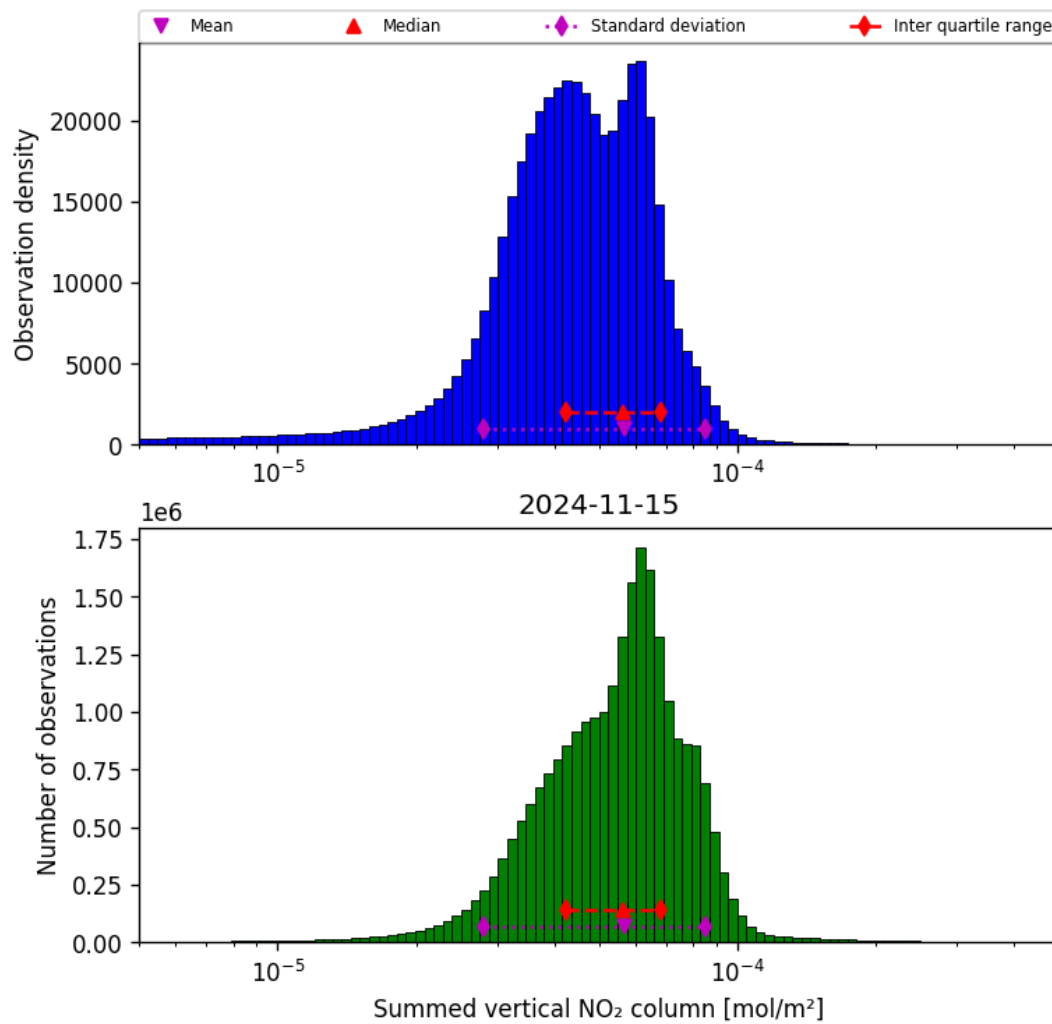
Figure 40: Histogram of “Summed vertical NO 2 column” for 2024-11-14 to 2024-11-16
