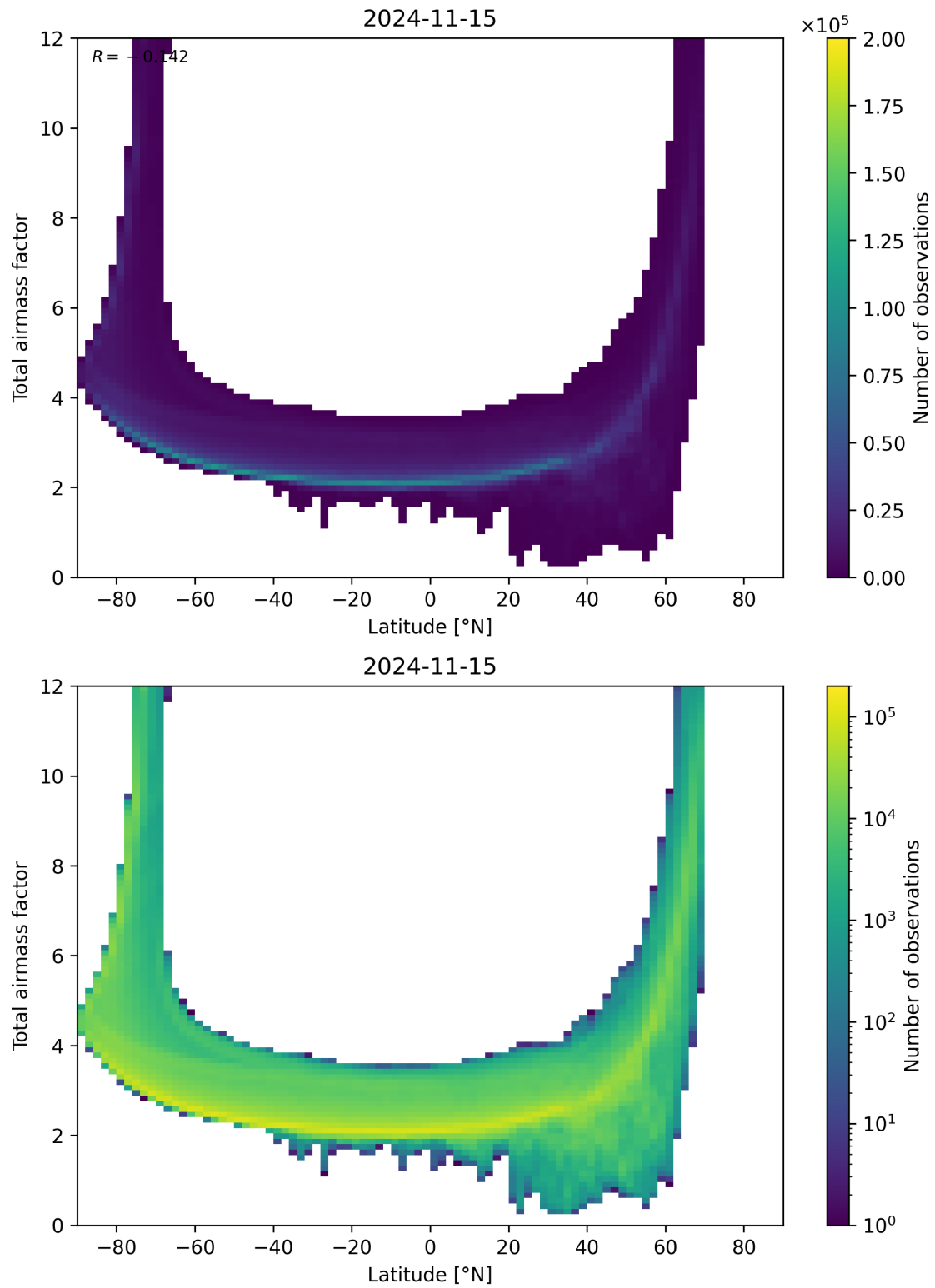
Figure 84: Scatter density plot of “Latitude” against “Total airmass factor” for 2024-11-14 to 2024-11-16.
