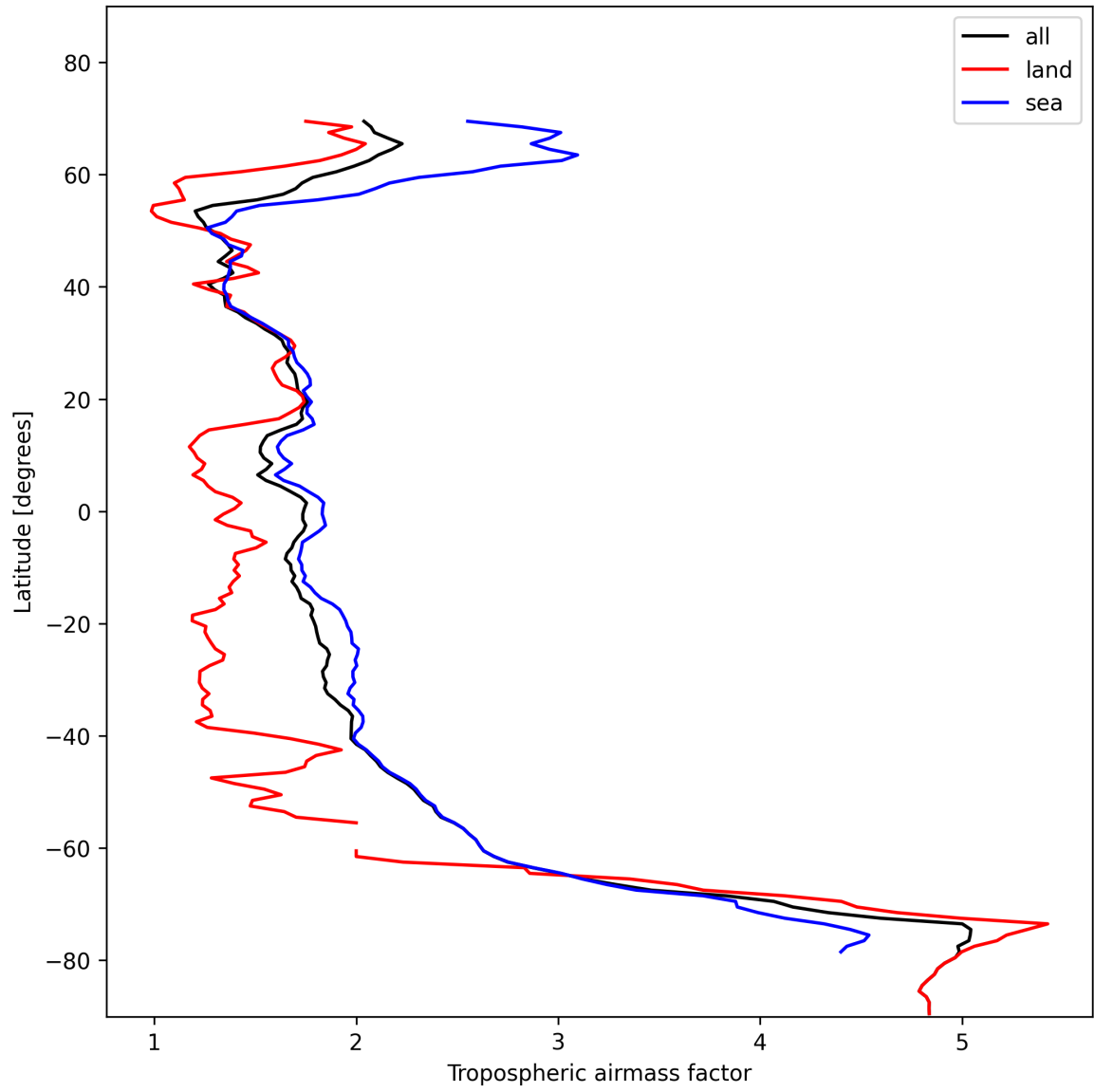
Figure 14: Zonal average of “Tropospheric airmass factor” for 2024-11-14 to 2024-11-16.
