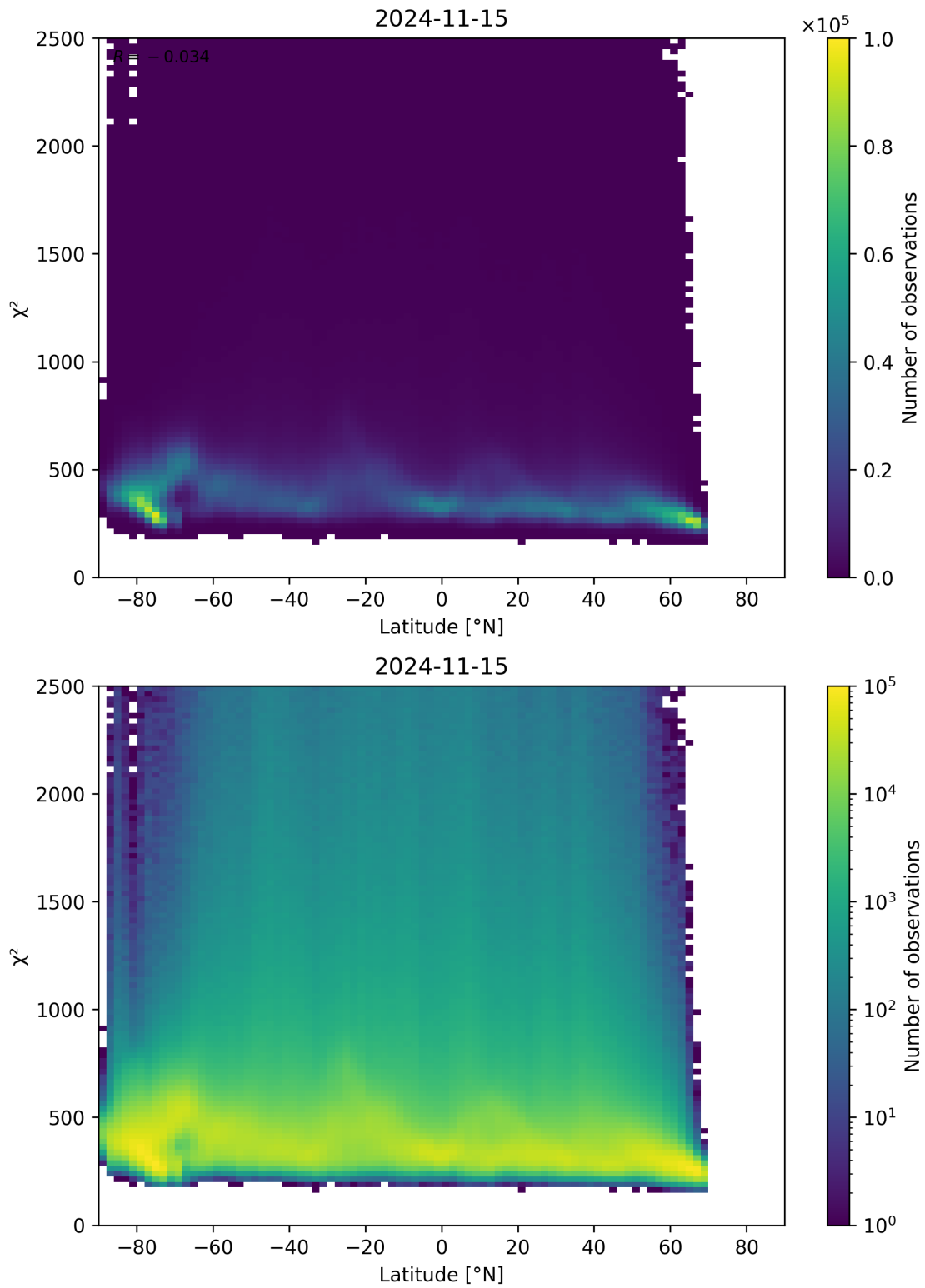
Figure 86: Scatter density plot of “Latitude” against “ \chi^2 ” for 2024-11-14 to 2024-11-16.
