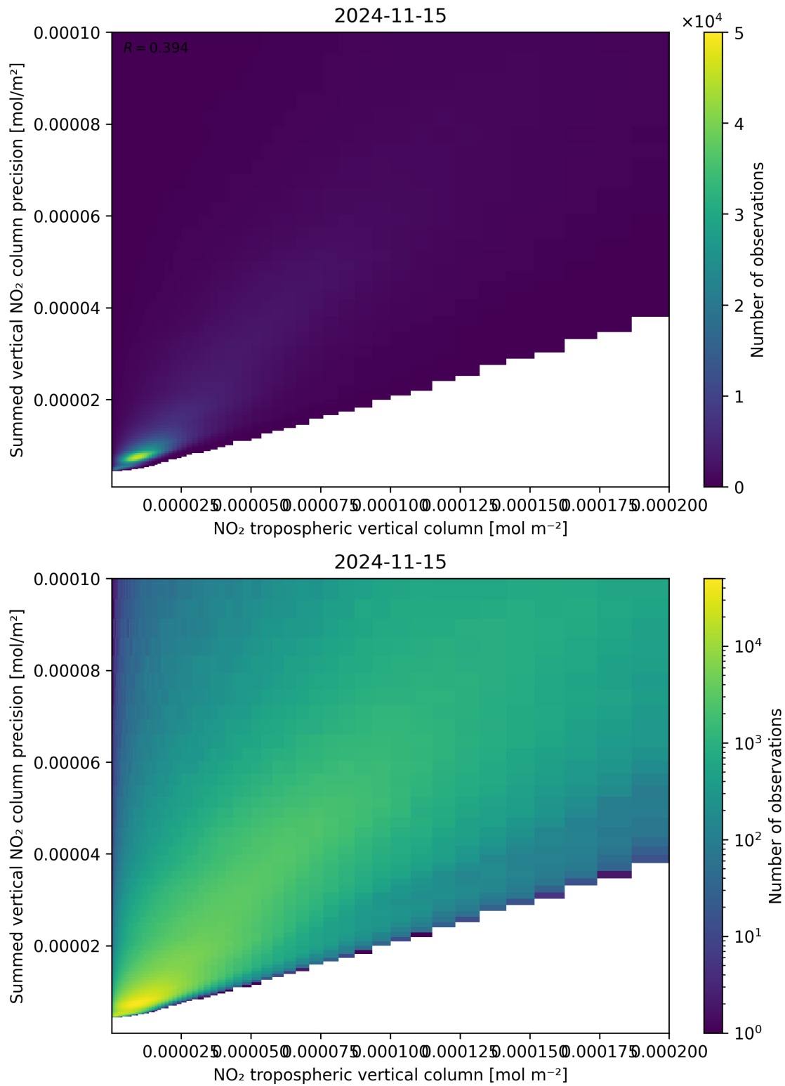
Figure 127: Scatter density plot of “NO 2 tropospheric vertical column” against “Summed vertical NO 2 column precision” for 2024-11-14 to 2024-11-16.
