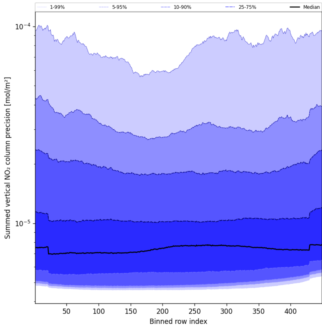
Figure 58: Along track statistics of “Summed vertical NO 2 column precision” for 2024-11-14 to 2024-11-16
