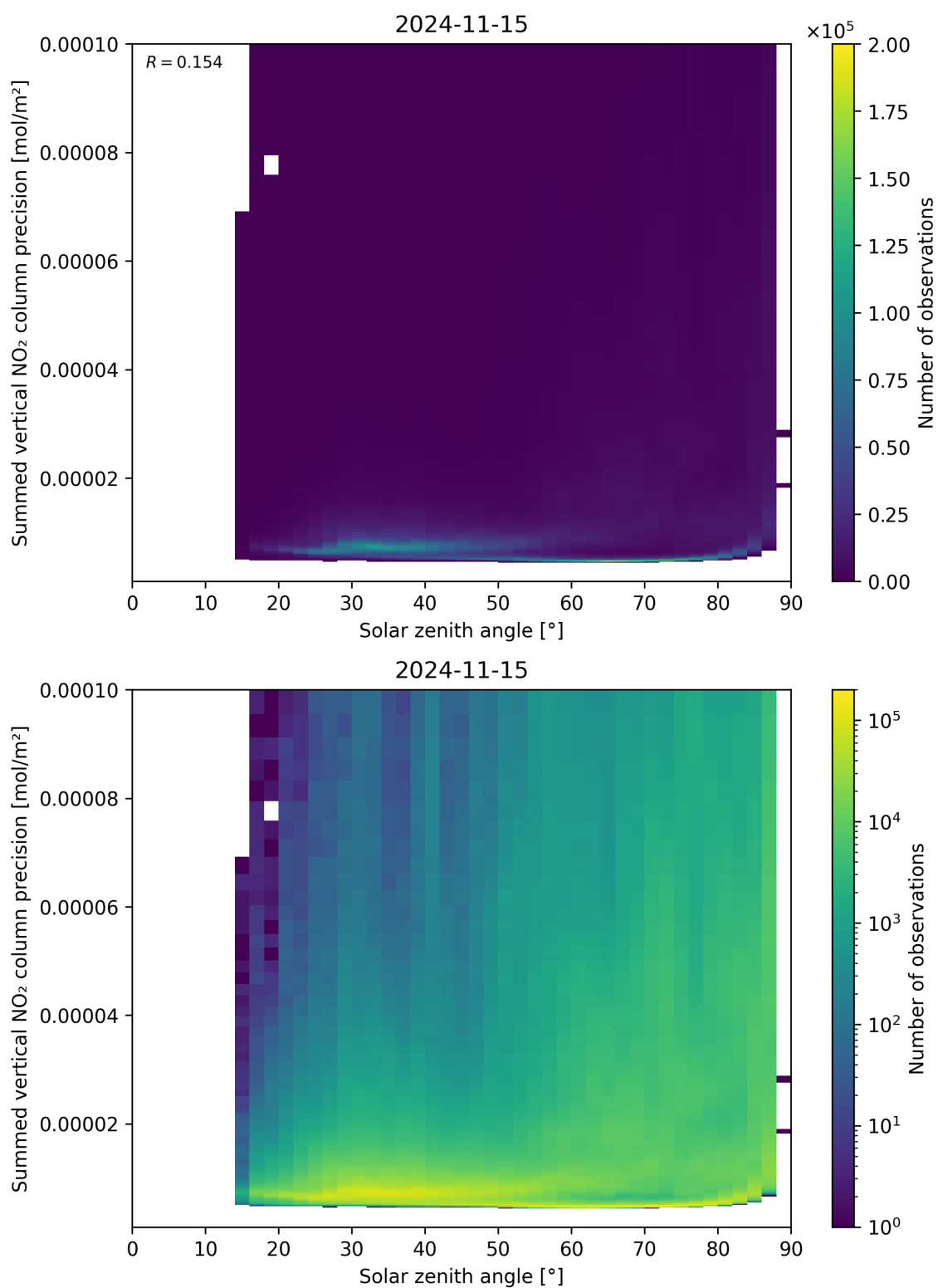
Figure 152: Scatter density plot of “Solar zenith angle” against “Summed vertical NO 2 column precision” for 2024-11-14 to 2024-11-16.
