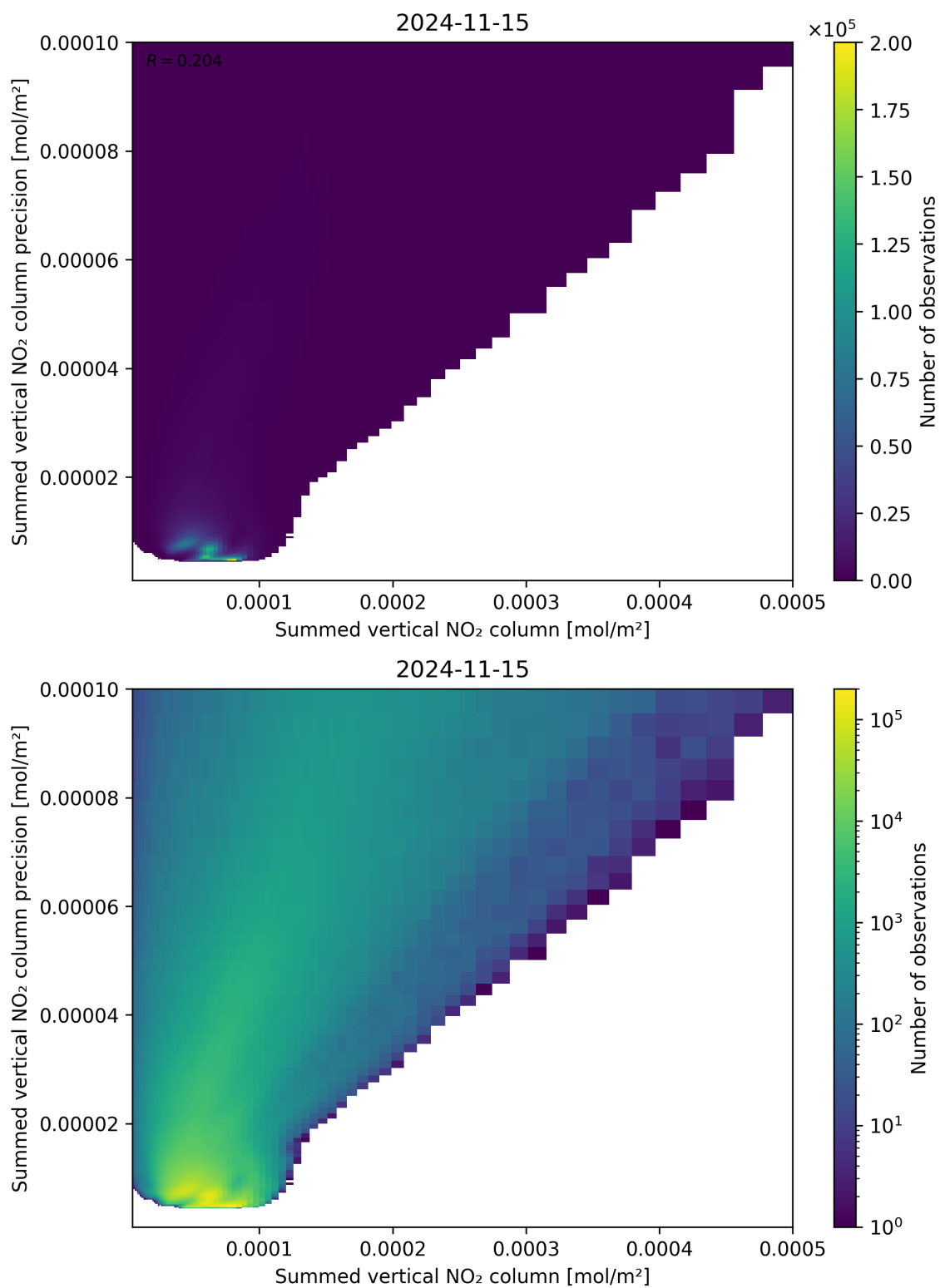
Figure 105: Scatter density plot of “Summed vertical NO 2 column” against “Summed vertical NO 2 column precision” for 2024-11-14 to 2024-11-16.
