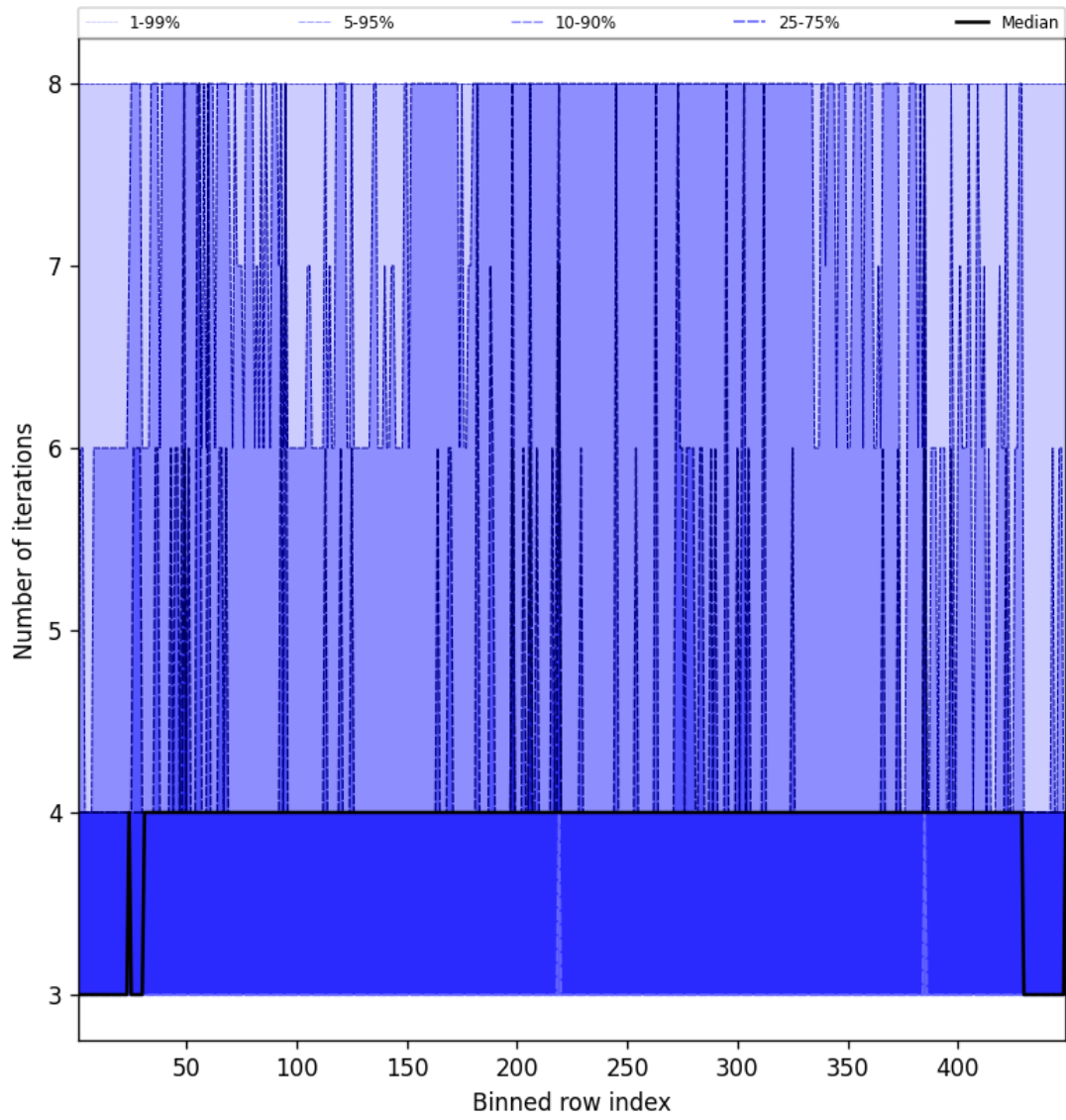
Figure 51: Along track statistics of “Number of iterations” for 2024-11-14 to 2024-11-16
