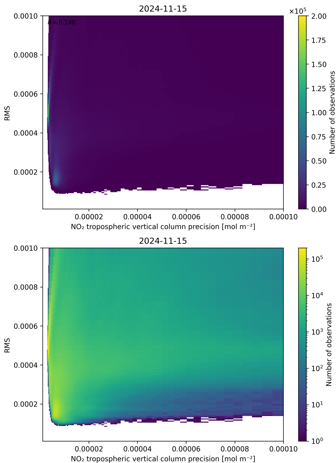
Figure 140: Scatter density plot of “NO 2 tropospheric vertical column precision” against “RMS” for 2024-11-14 to 2024-11-16.
