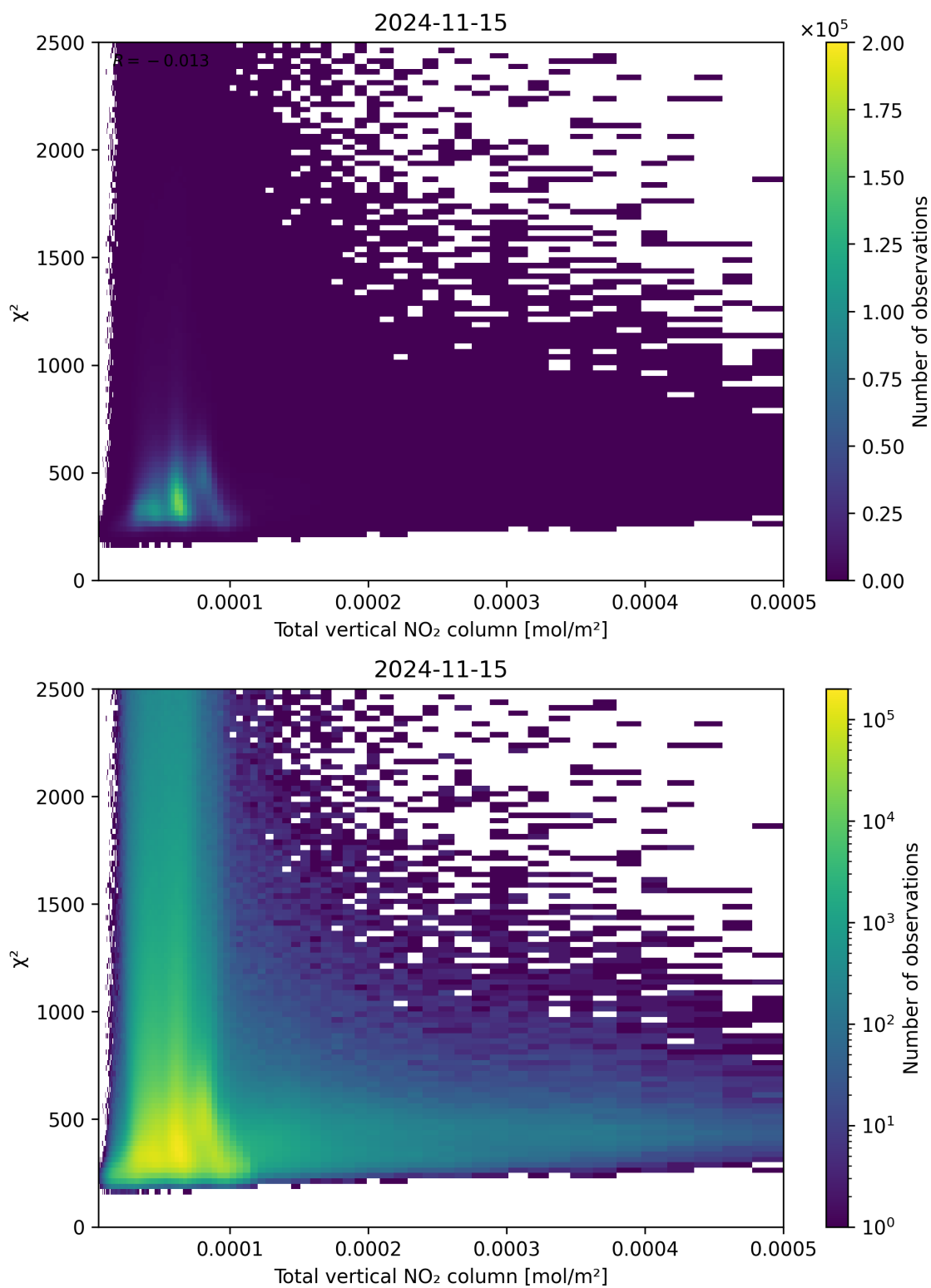
Figure 111: Scatter density plot of “Total vertical NO 2 column” against “ \chi^2 ” for 2024-11-14 to 2024-11-16.
