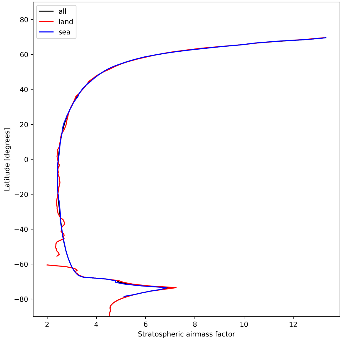
Figure 27: Zonal average of “Stratospheric airmass factor” for 2024-11-14 to 2024-11-16.
