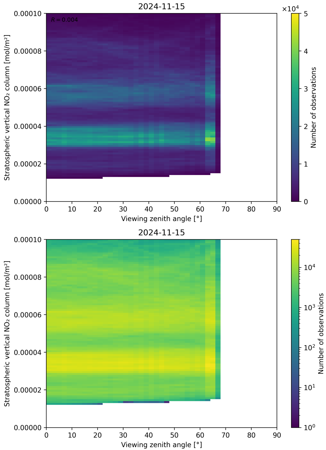
Figure 164: Scatter density plot of “Viewing zenith angle” against “Stratospheric vertical NO 2 column” for 2024-11-14 to 2024-11-16.
