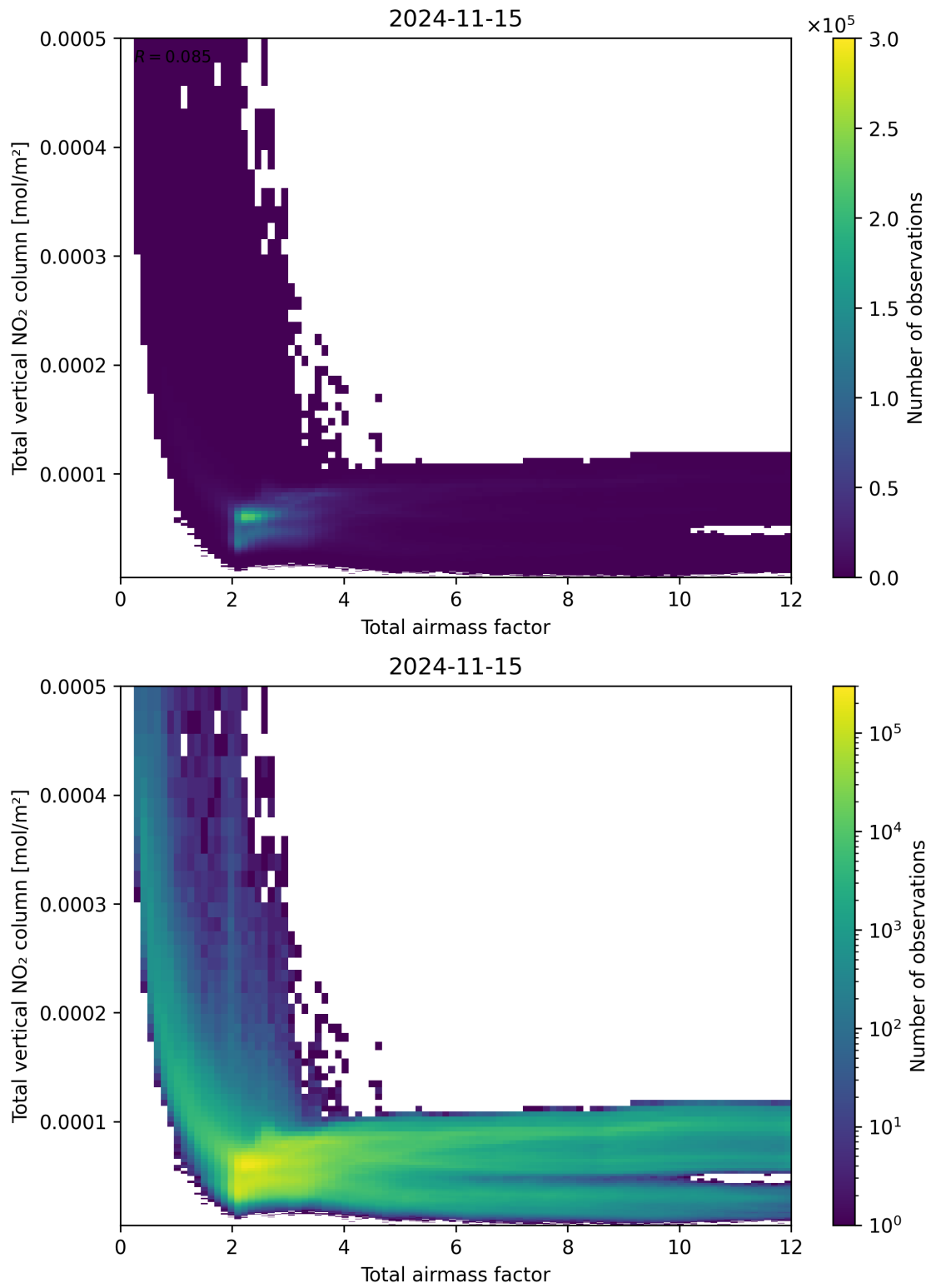
Figure 67: Scatter density plot of “Total airmass factor” against “Total vertical NO 2 column” for 2024-11-14 to 2024-11-16.
