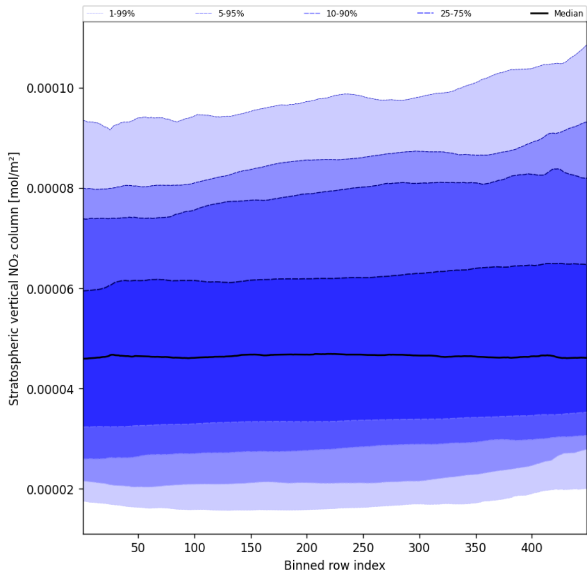
Figure 53: Along track statistics of “Stratospheric vertical NO 2 column” for 2024-11-14 to 2024-11-16
