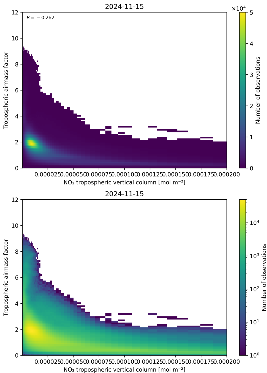
Figure 123: Scatter density plot of “NO 2 tropospheric vertical column” against “Tropospheric air mass factor” for 2024-11-14 to 2024-11-16.
