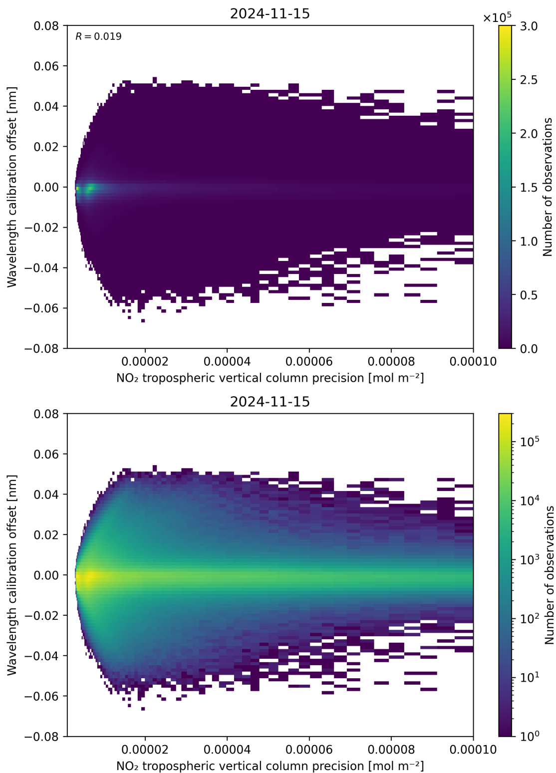
Figure 141: Scatter density plot of “NO 2 tropospheric vertical column precision” against “Wavelength calibration offset” for 2024-11-14 to 2024-11-16.
