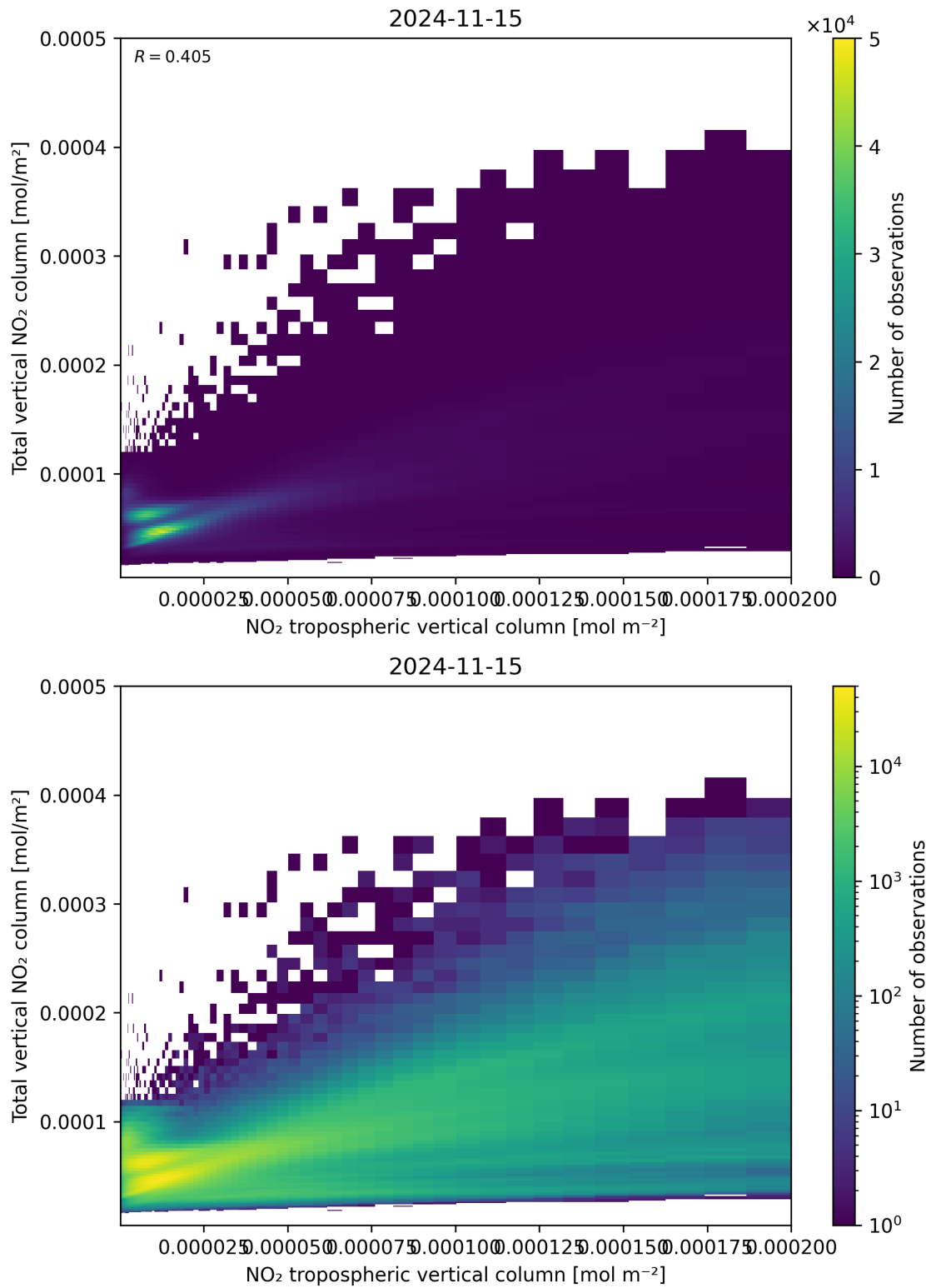
Figure 128: Scatter density plot of “NO 2 tropospheric vertical column” against “Total vertical NO 2 column” for 2024-11-14 to 2024-11-16.
