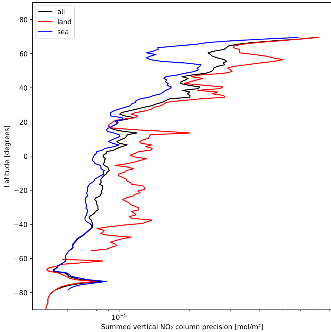
Figure 24: Zonal average of “Summed vertical NO 2 column precision” for 2024-11-14 to 2024-11-16.
