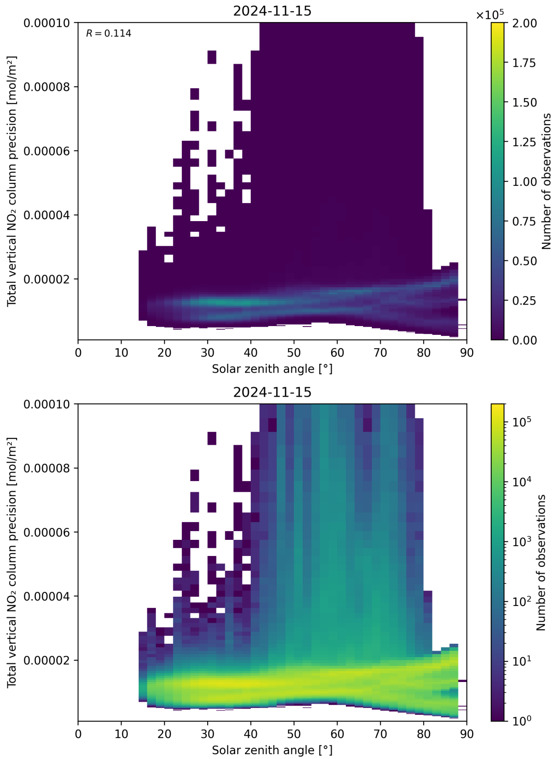
Figure 154: Scatter density plot of “Solar zenith angle” against “Total vertical NO 2 column precision” for 2024-11-14 to 2024-11-16.
