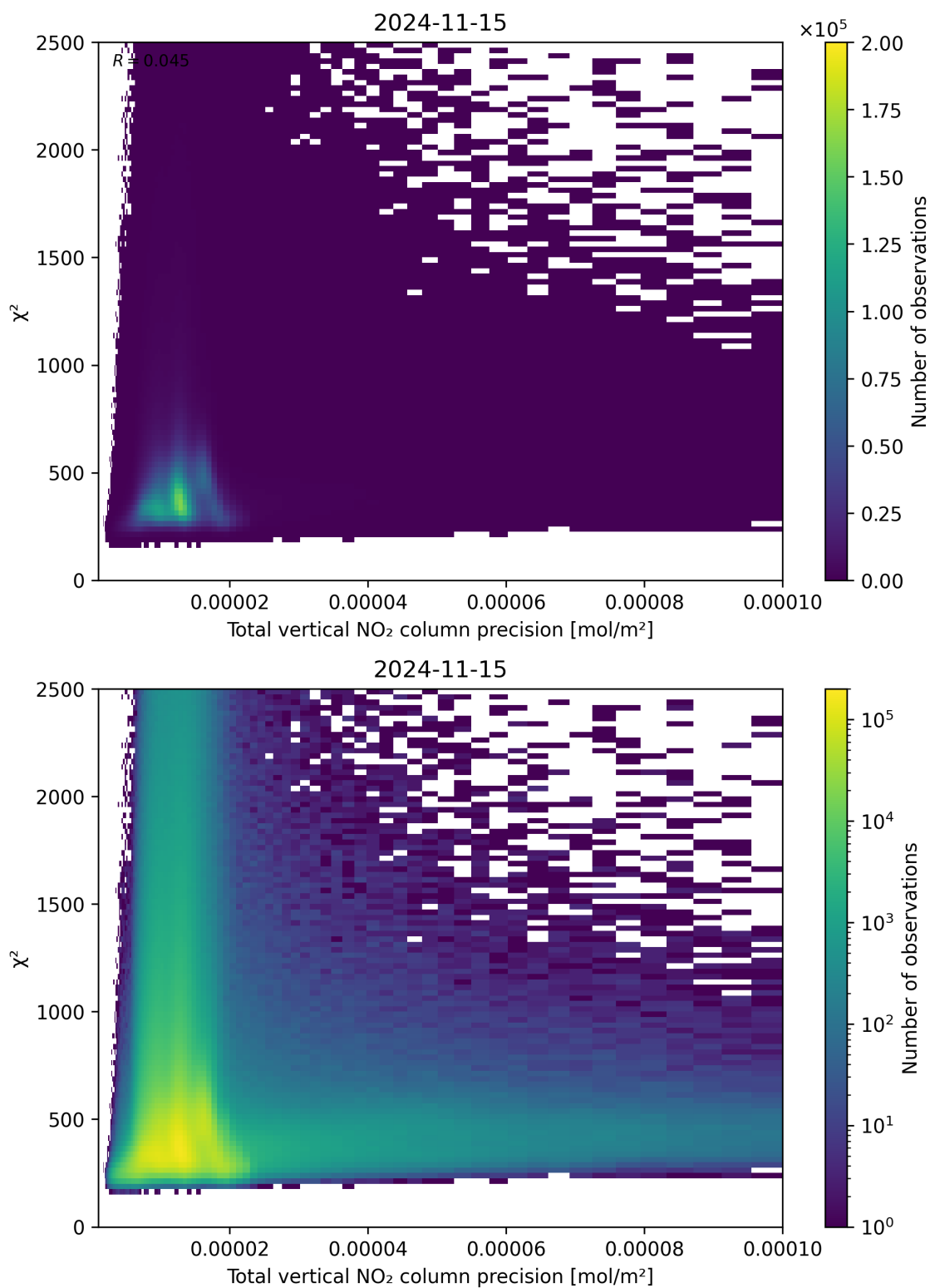
Figure 116: Scatter density plot of “Total vertical NO 2 column precision” against “ \chi^2 ” for 2024-11-14 to 2024-11-16.
