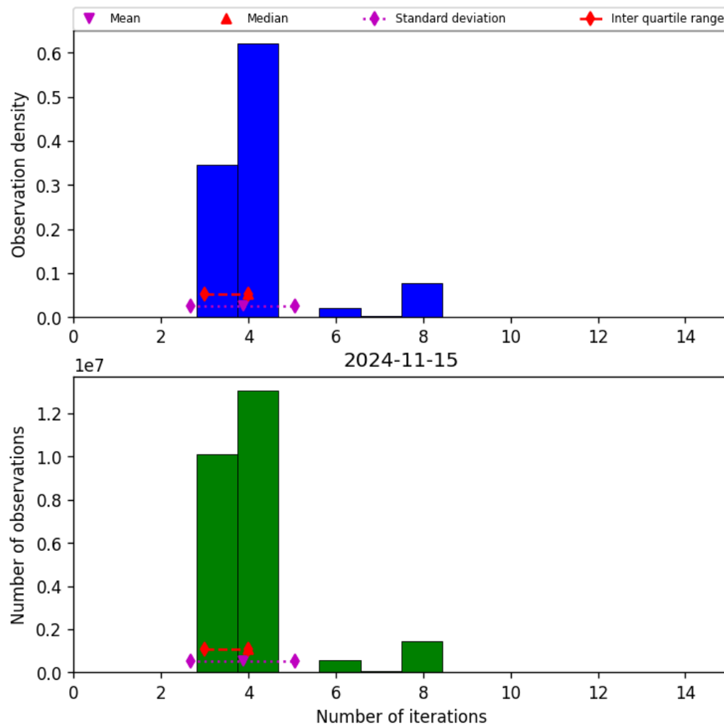
Figure 34: Histogram of “Number of iterations” for 2024-11-14 to 2024-11-16
