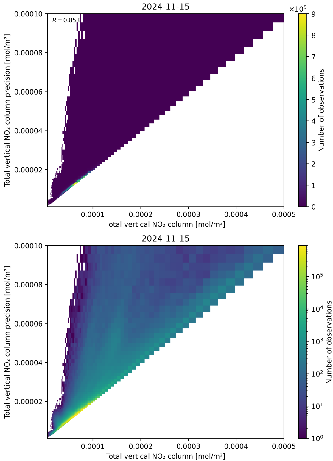
Figure 114: Scatter density plot of “Total vertical NO 2 column” against “Total vertical NO 2 column precision” for 2024-11-14 to 2024-11-16.
