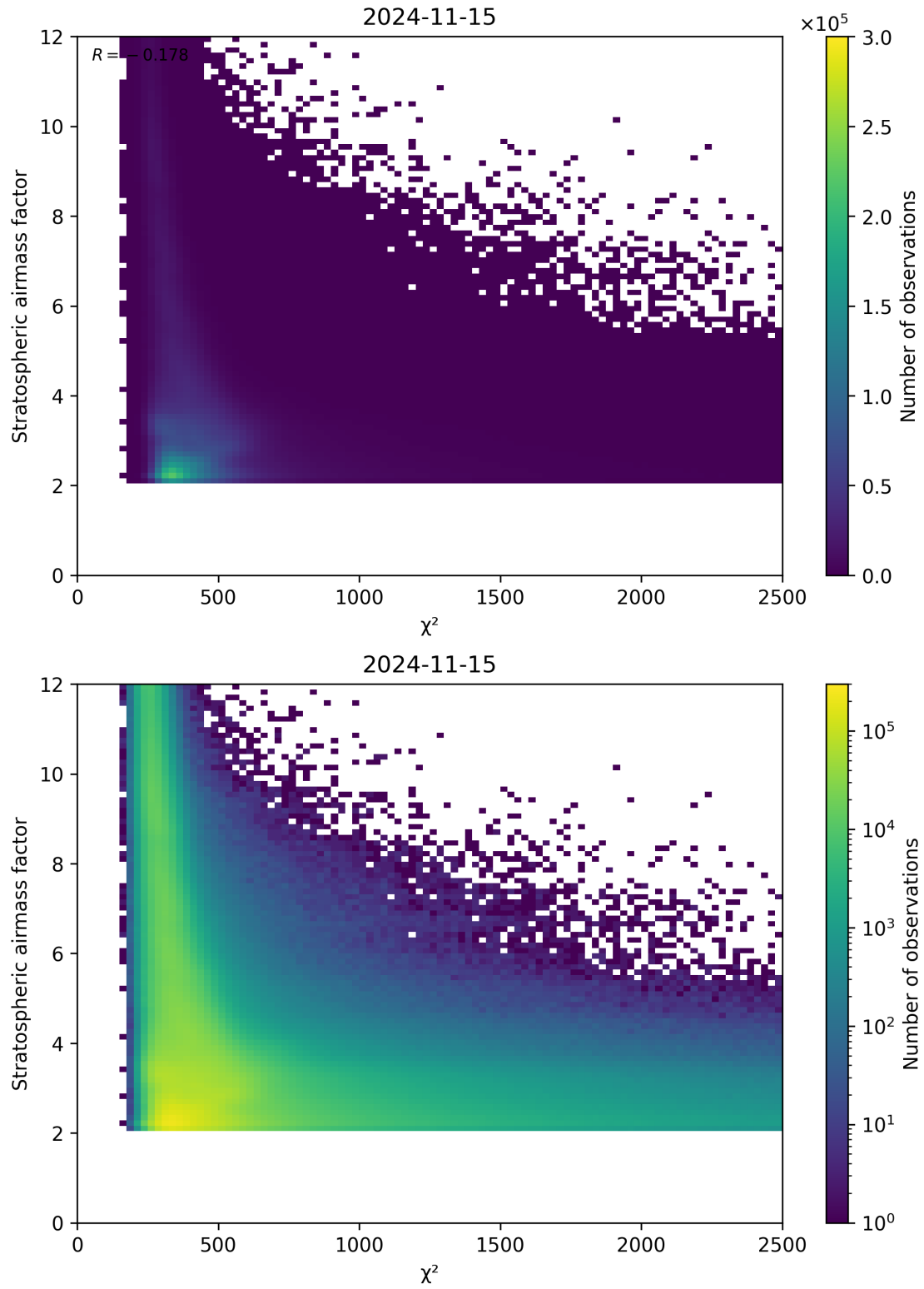
Figure 81: Scatter density plot of “ \chi^2 ” against “Stratospheric airmass factor” for 2024-11-14 to 2024-11-16.
