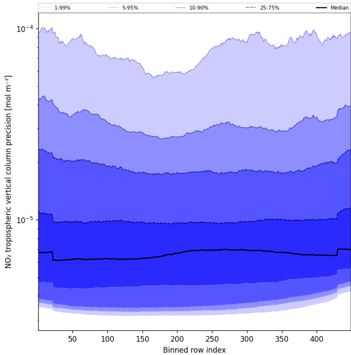
Figure 47: Along track statistics of “NO 2 tropospheric vertical column precision” for 2024-11-14 to 2024-11-16
