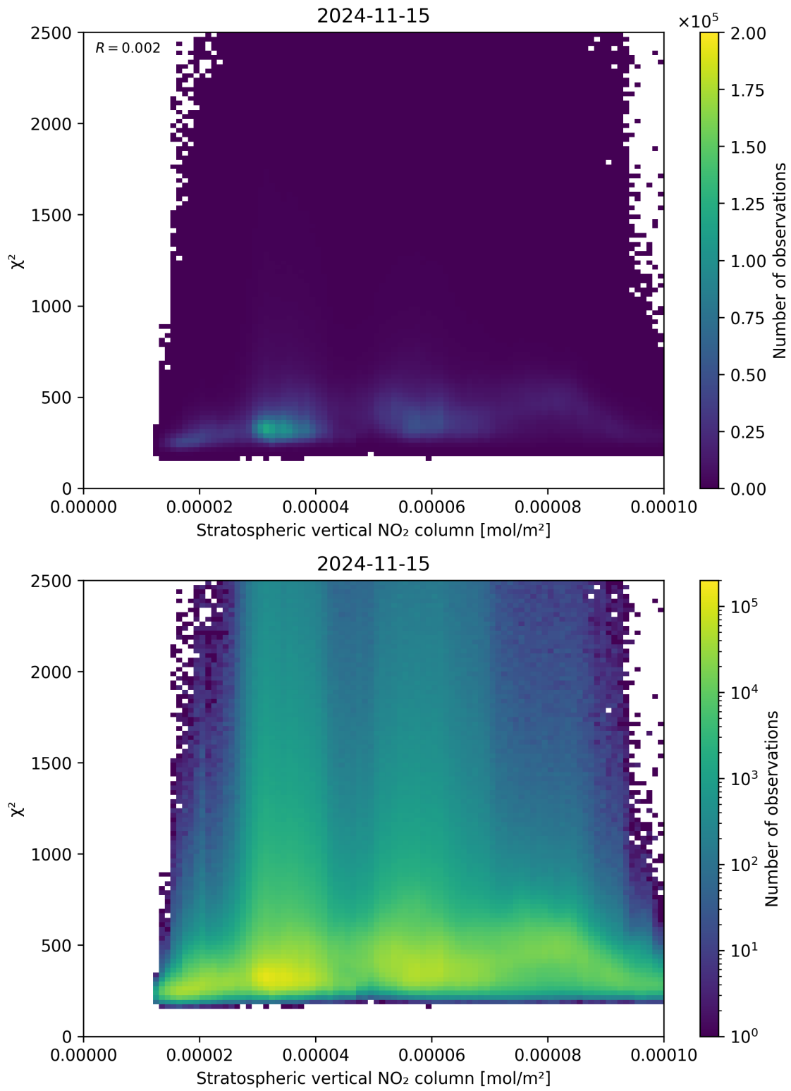
Figure 97: Scatter density plot of “Stratospheric vertical NO 2 column” against “ \chi^2 ” for 2024-11-14 to 2024-11-16.
