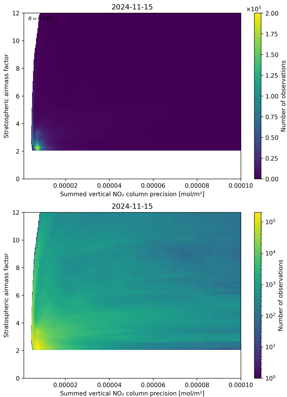
Figure 106: Scatter density plot of “Summed vertical NO 2 column precision” against “Stratospheric airmass factor” for 2024-11-14 to 2024-11-16.
