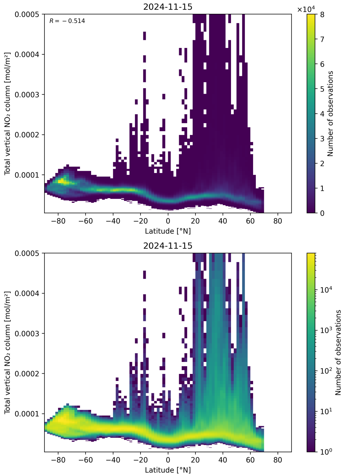
Figure 90: Scatter density plot of “Latitude” against “Total vertical NO 2 column” for 2024-11-14 to 2024-11-16.
