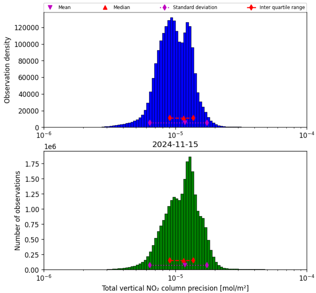
Figure 39: Histogram of “Total vertical NO 2 column precision” for 2024-11-14 to 2024-11-16
