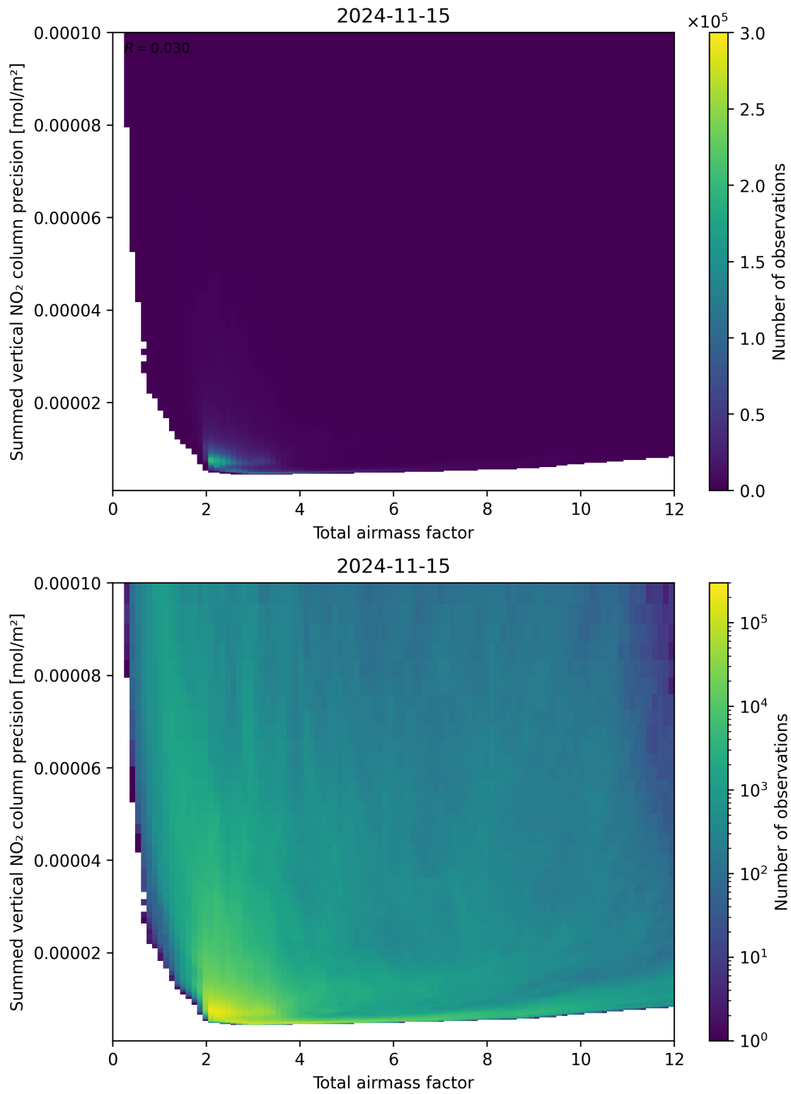
Figure 66: Scatter density plot of “Total airmass factor” against “Summed vertical NO 2 column precision” for 2024-11-14 to 2024-11-16.
