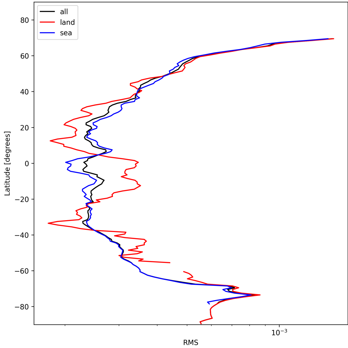
Figure 26: Zonal average of “RMS” for 2024-11-14 to 2024-11-16.
