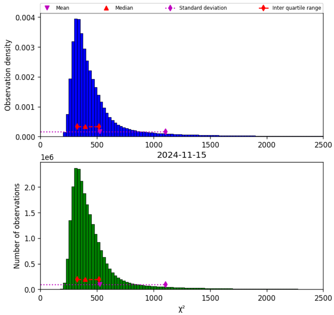
Figure 42: Histogram of “ \chi^2 ” for 2024-11-14 to 2024-11-16
