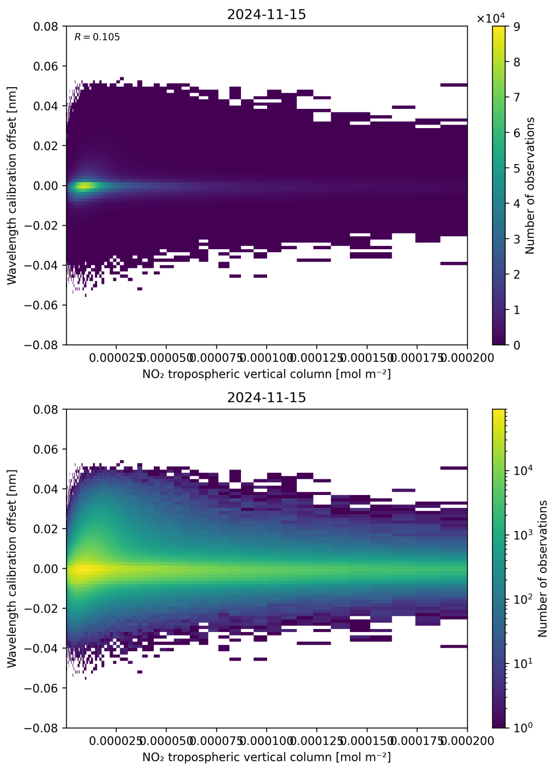
Figure 143: Scatter density plot of “NO 2 tropospheric vertical column” against “Wavelength calibration offset” for 2024-11-14 to 2024-11-16.
