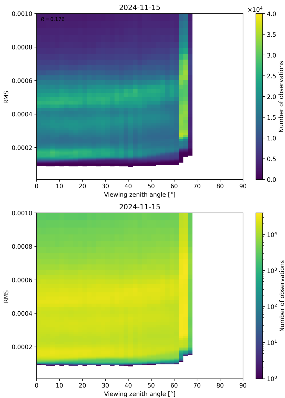
Figure 171: Scatter density plot of “Viewing zenith angle” against “RMS” for 2024-11-14 to 2024-11-16.
