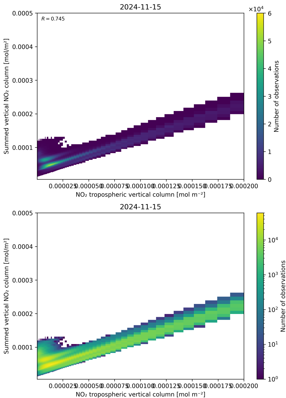
Figure 126: Scatter density plot of “NO 2 tropospheric vertical column” against “Summed vertical NO 2 column” for 2024-11-14 to 2024-11-16.
