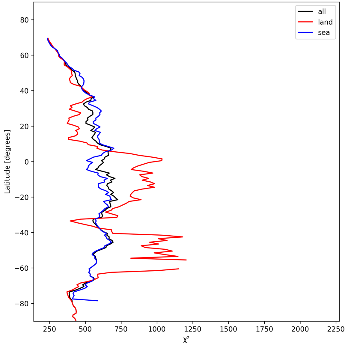
Figure 25: Zonal average of “ \chi^2 ” for 2024-11-14 to 2024-11-16.
