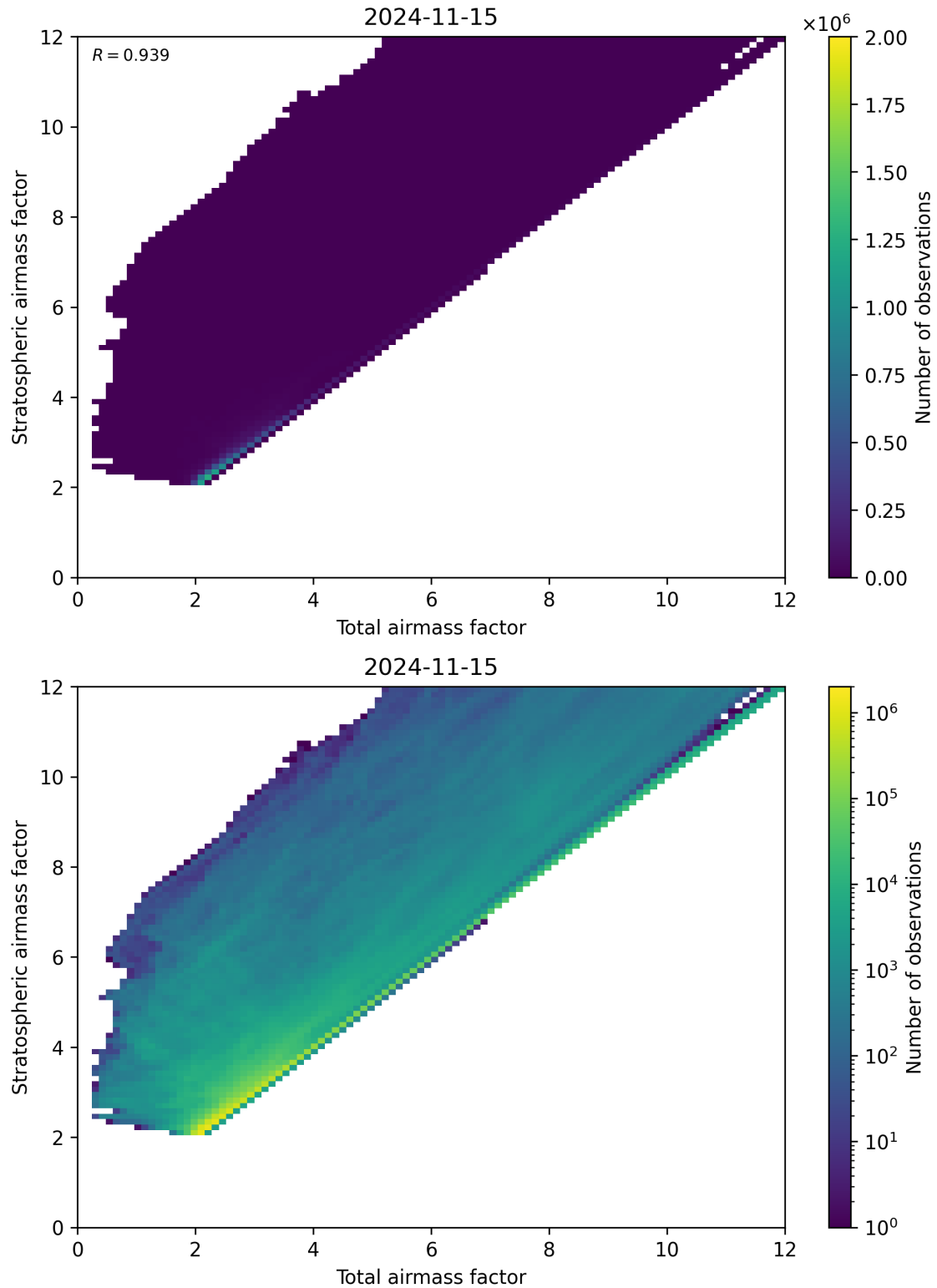
Figure 62: Scatter density plot of “Total airmass factor” against “Stratospheric airmass factor” for 2024-11-14 to 2024-11-16.
