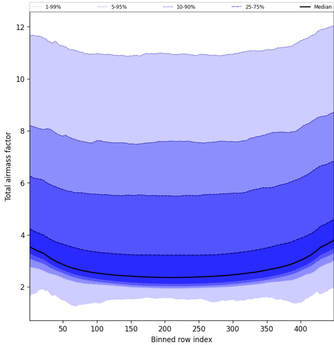
Figure 49: Along track statistics of “Total airmass factor” for 2024-11-14 to 2024-11-16
