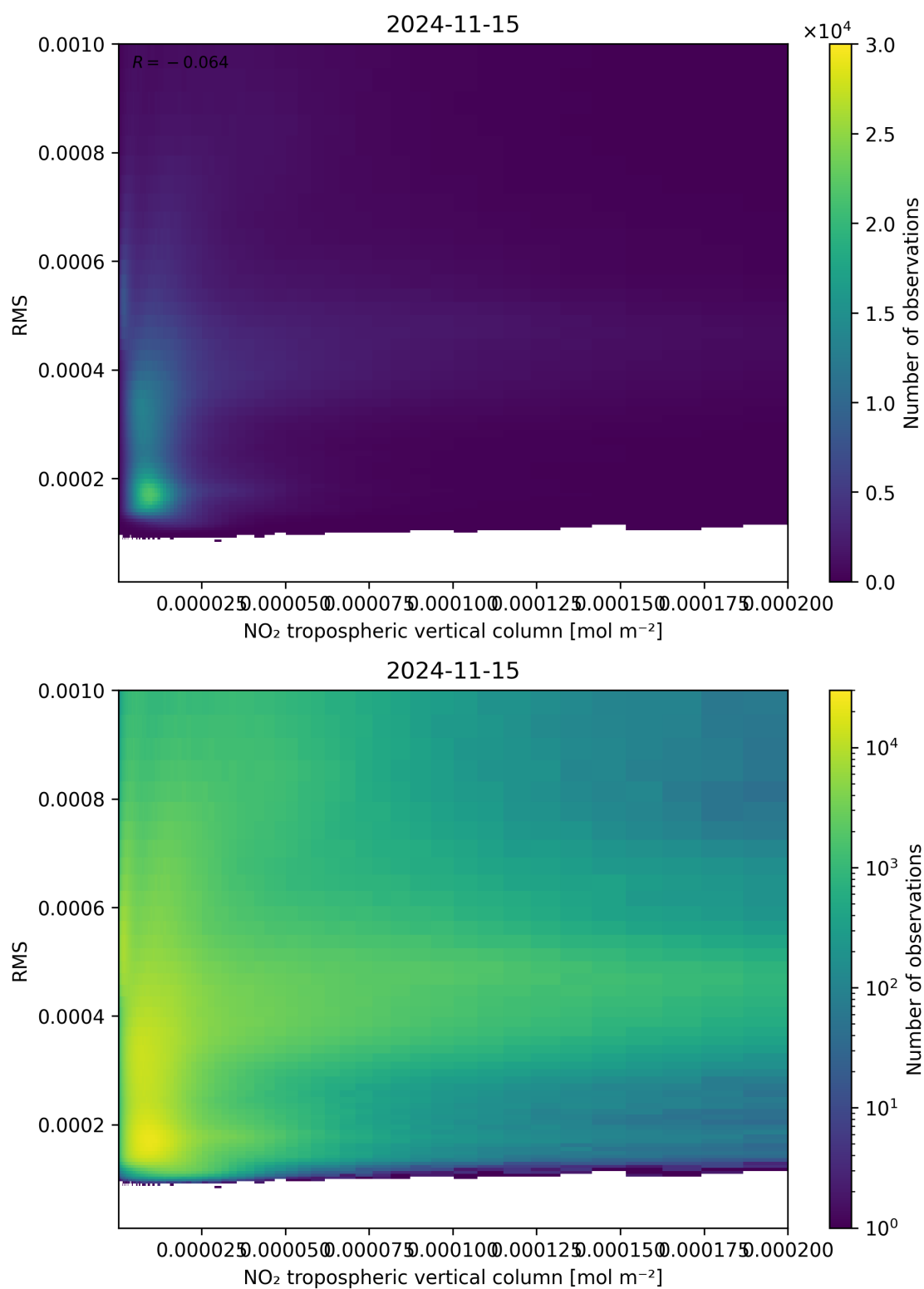
Figure 142: Scatter density plot of “NO 2 tropospheric vertical column” against “RMS” for 2024-11-14 to 2024-11-16.
