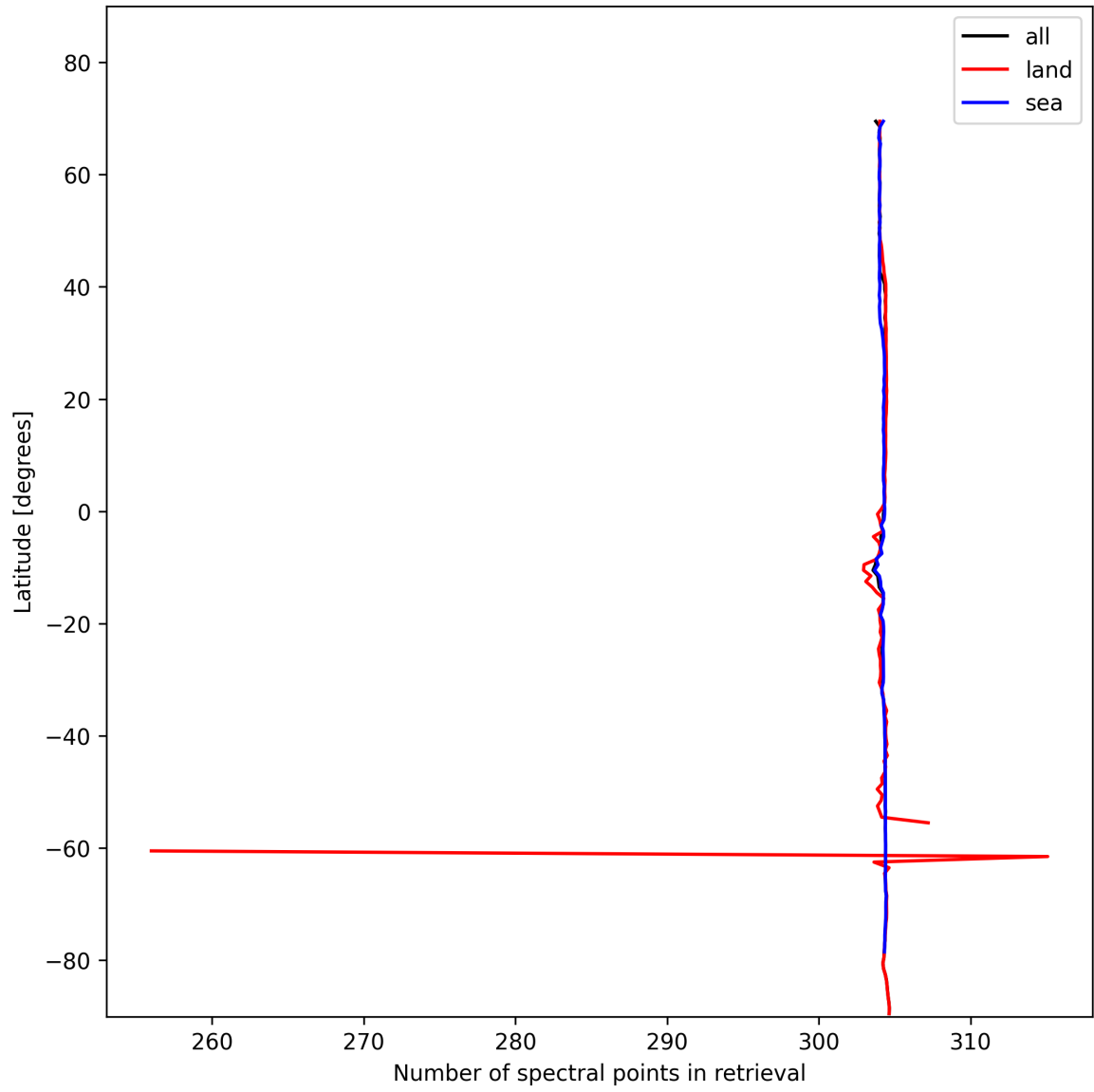
Figure 16: Zonal average of “Number of spectral points in retrieval” for 2024-11-14 to 2024-11-16.
