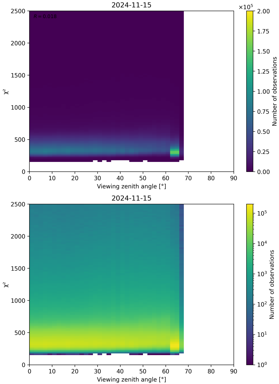
Figure 162: Scatter density plot of “Viewing zenith angle” against “ \chi^2 ” for 2024-11-14 to 2024-11-16.
