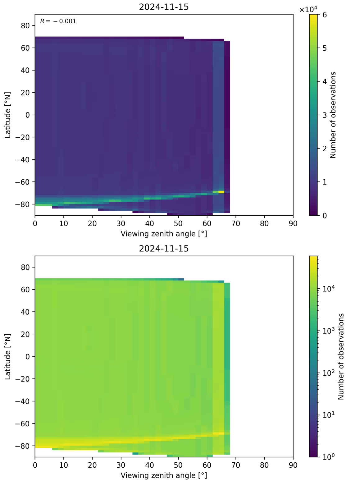
Figure 163: Scatter density plot of “Viewing zenith angle” against “Latitude” for 2024-11-14 to 2024-11-16.
