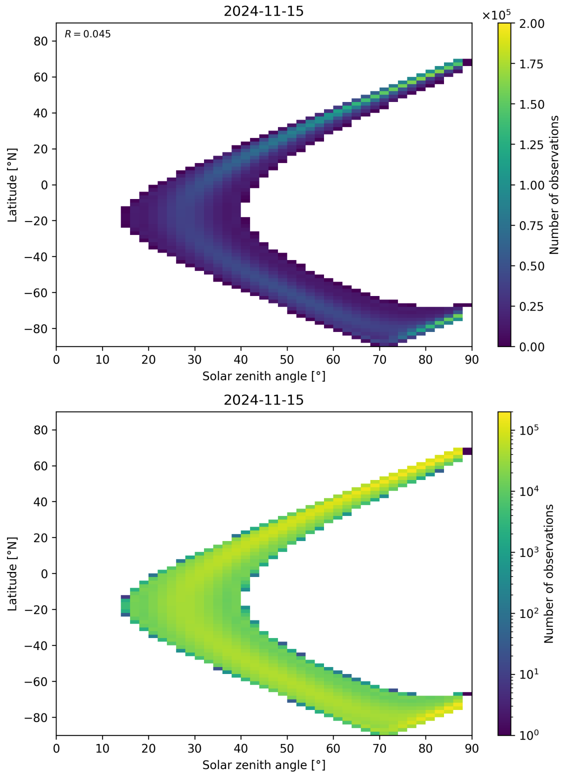
Figure 149: Scatter density plot of “Solar zenith angle” against “Latitude” for 2024-11-14 to 2024-11-16.
