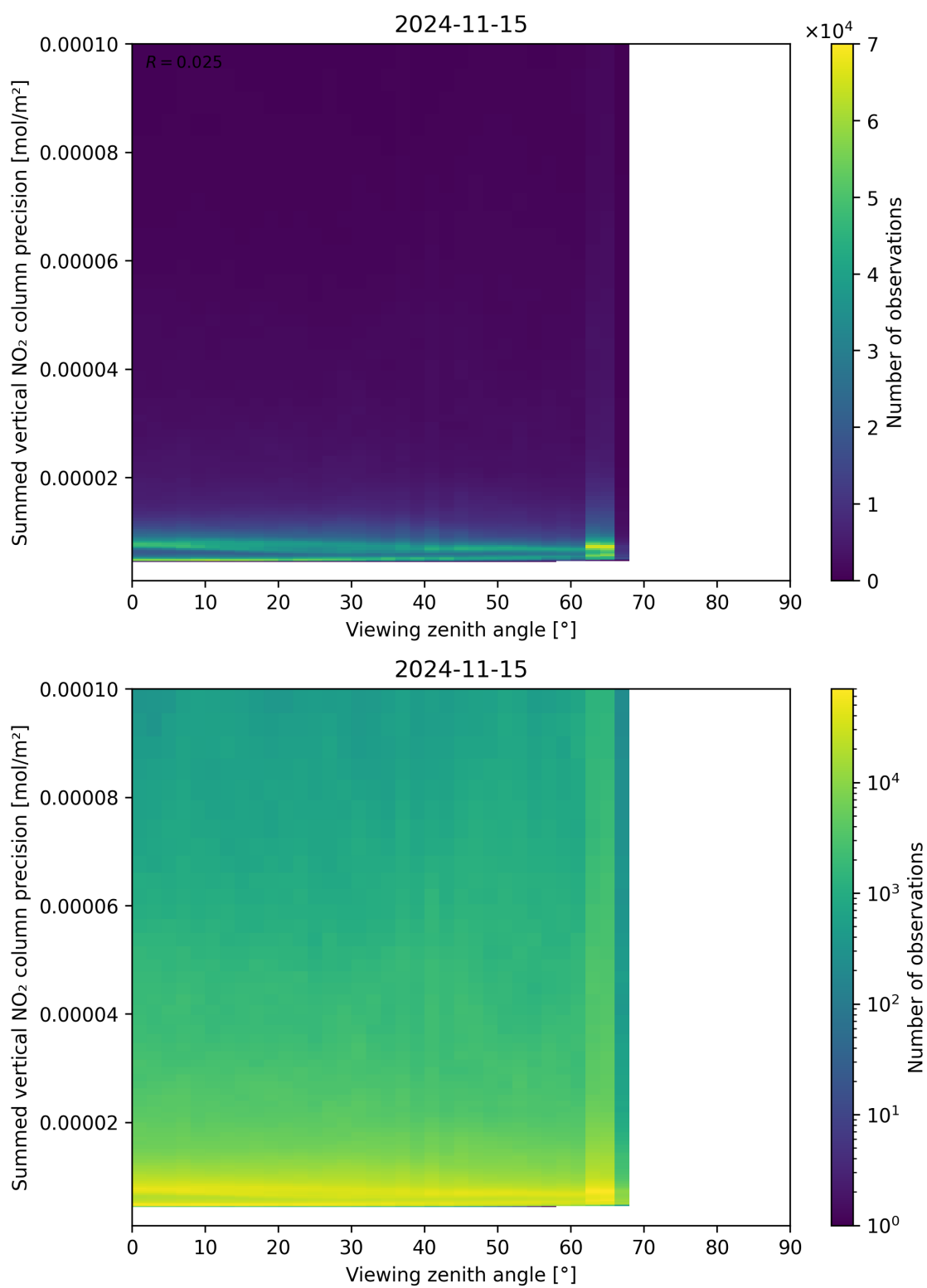
Figure 166: Scatter density plot of “Viewing zenith angle” against “Summed vertical NO 2 column precision” for 2024-11-14 to 2024-11-16.
