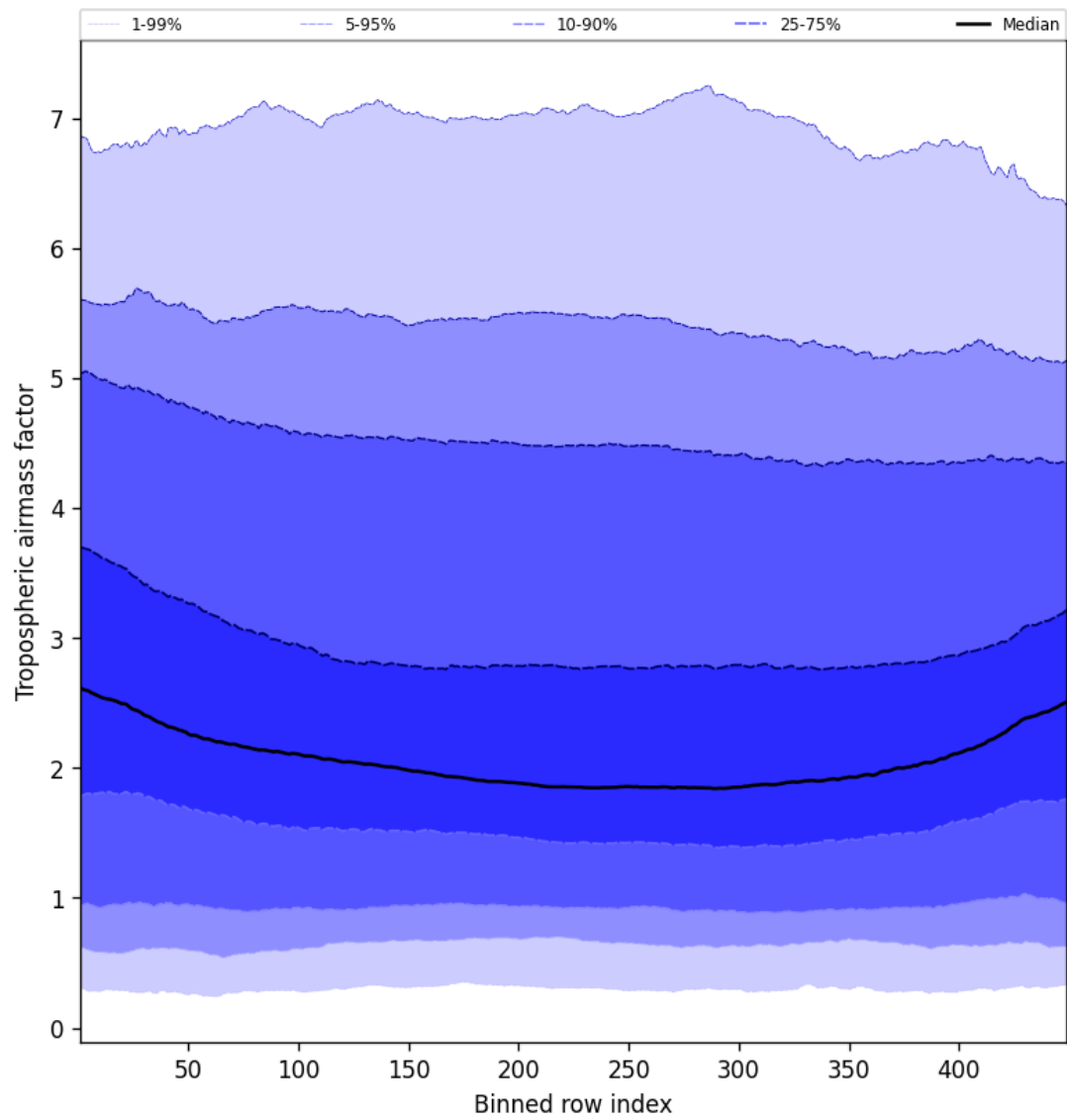
Figure 48: Along track statistics of “Tropospheric airmass factor” for 2024-11-14 to 2024-11-16
