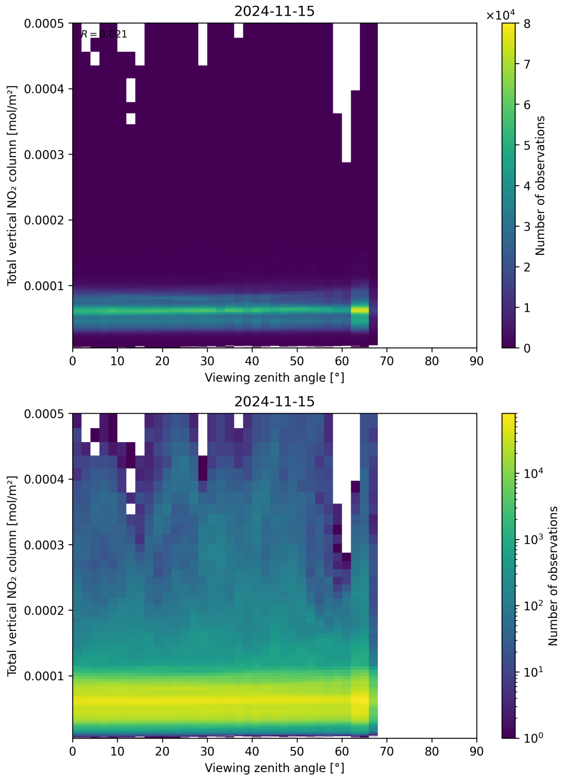
Figure 167: Scatter density plot of “Viewing zenith angle” against “Total vertical NO 2 column” for 2024-11-14 to 2024-11-16.
