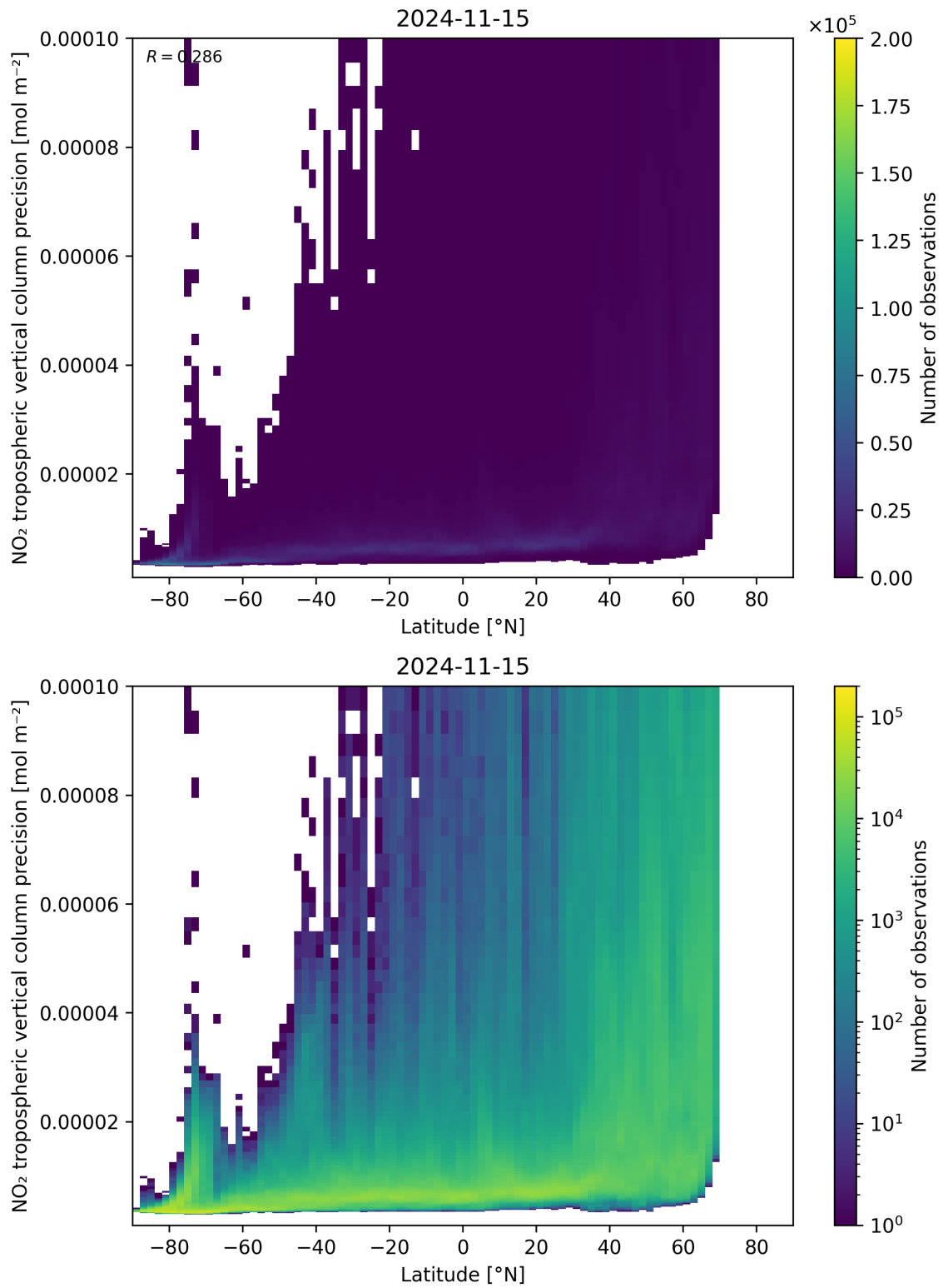
Figure 93: Scatter density plot of “Latitude” against “NO 2 tropospheric vertical column precision” for 2024-11-14 to 2024-11-16.
