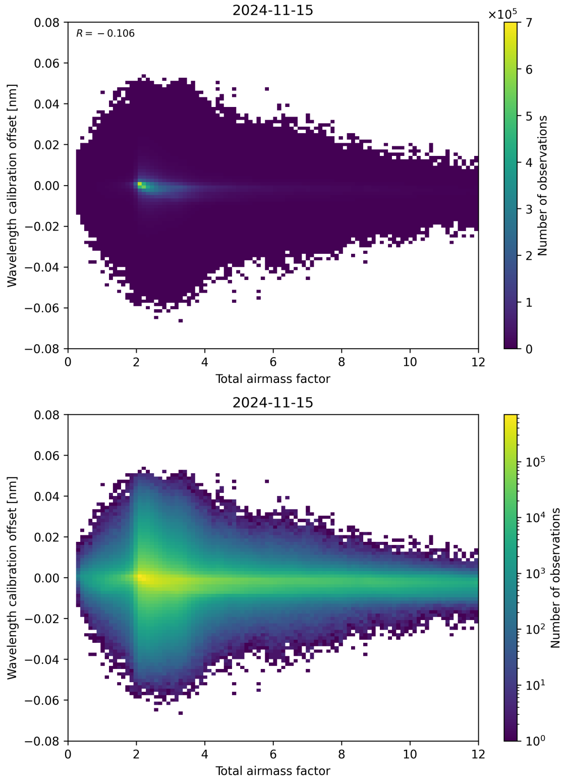
Figure 70: Scatter density plot of “Total airmass factor” against “Wavelength calibration offset” for 2024-11-14 to 2024-11-16.
