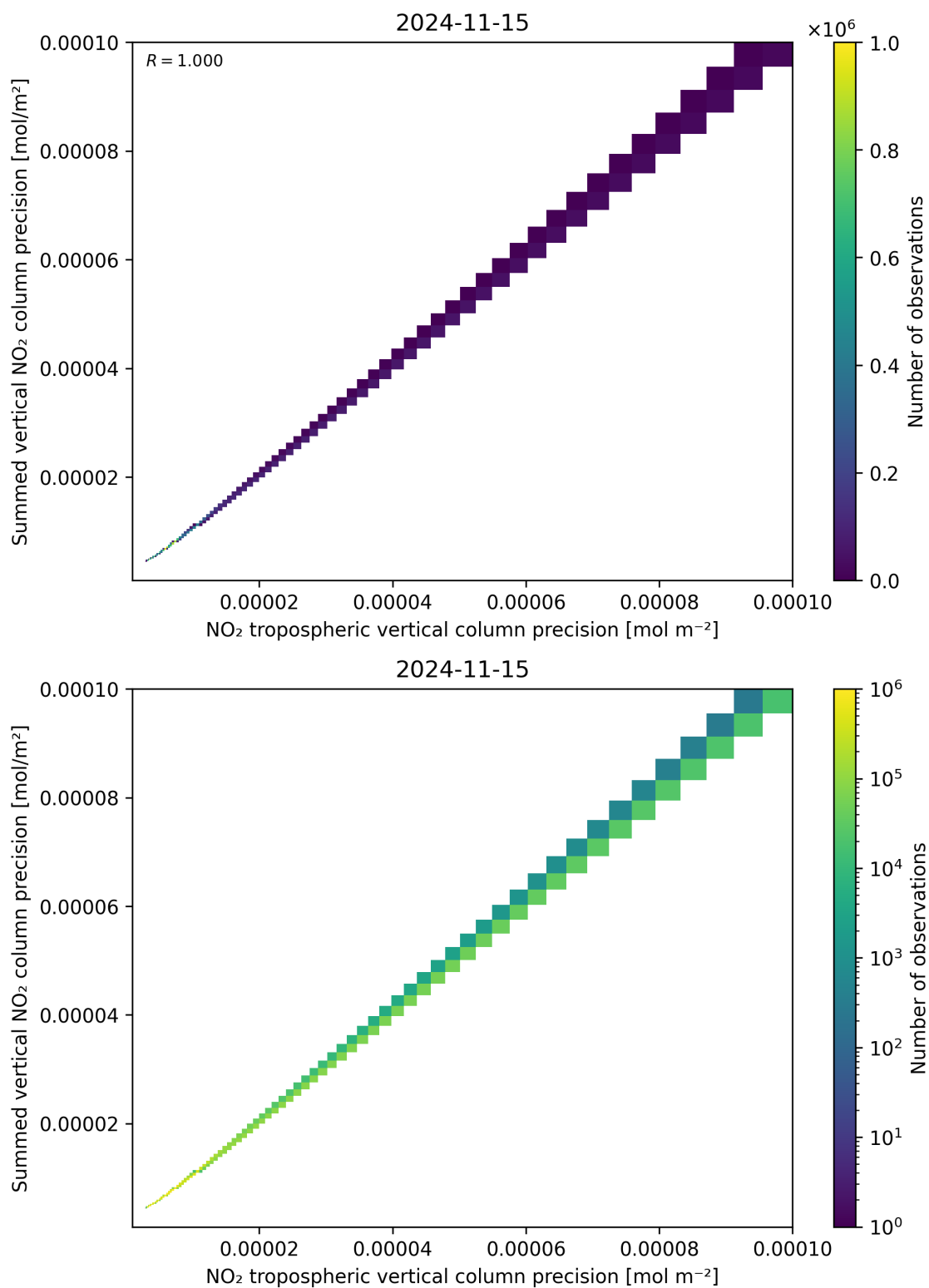
Figure 137: Scatter density plot of “NO 2 tropospheric vertical column precision” against “Summed vertical NO 2 column precision” for 2024-11-14 to 2024-11-16.
