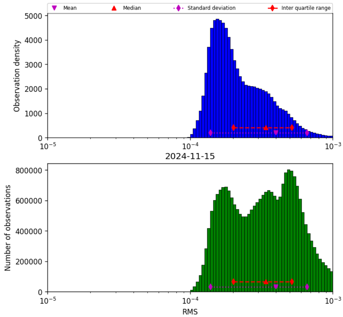
Figure 43: Histogram of “RMS” for 2024-11-14 to 2024-11-16
