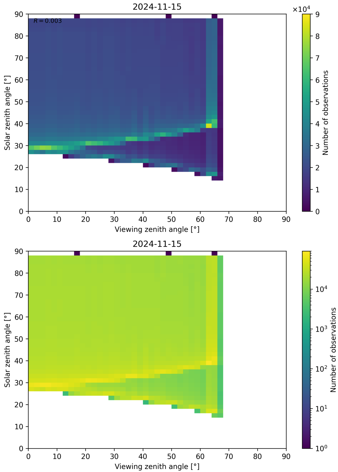
Figure 172: Scatter density plot of “Viewing zenith angle” against “Solar zenith angle” for 2024-11-14 to 2024-11-16.
