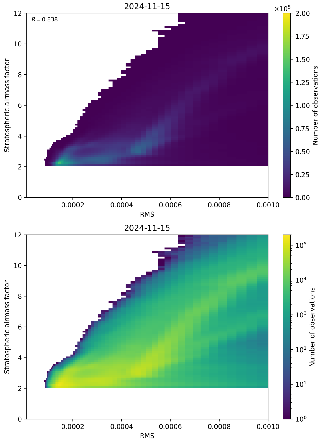
Figure 144: Scatter density plot of “RMS” against “Stratospheric airmass factor” for 2024-11-14 to 2024-11-16.
