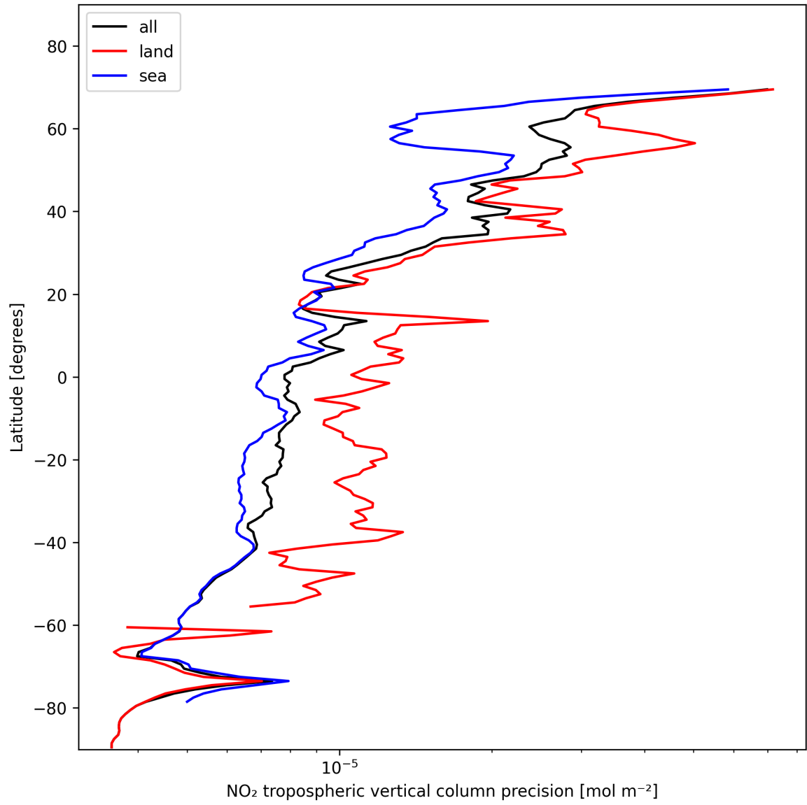
Figure 13: Zonal average of “NO 2 tropospheric vertical column precision” for 2024-11-14 to 2024-11-16.
