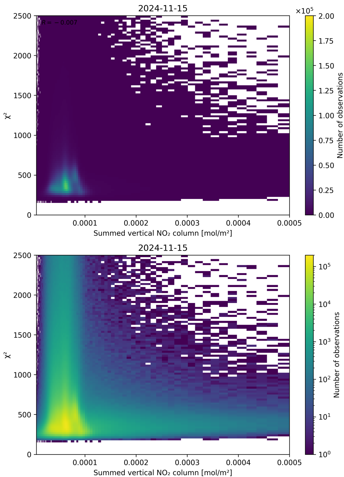
Figure 104: Scatter density plot of “Summed vertical NO 2 column” against “ \chi^2 ” for 2024-11-14 to 2024-11-16.
