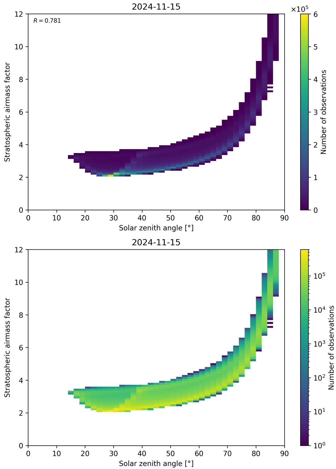
Figure 145: Scatter density plot of “Solar zenith angle” against “Stratospheric airmass factor” for 2024-11-14 to 2024-11-16.
