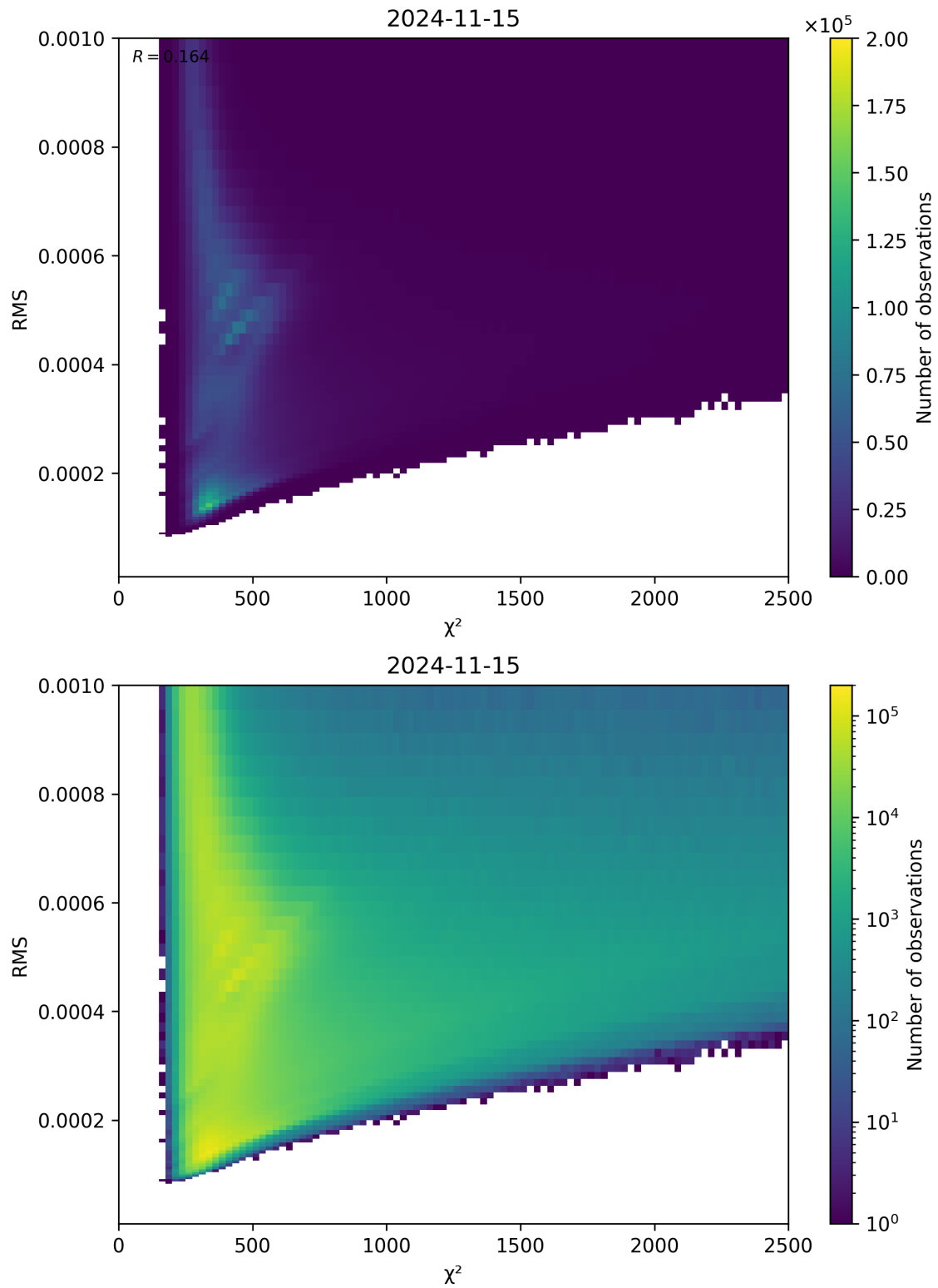
Figure 82: Scatter density plot of “ \chi^2 ” against “RMS” for 2024-11-14 to 2024-11-16.
