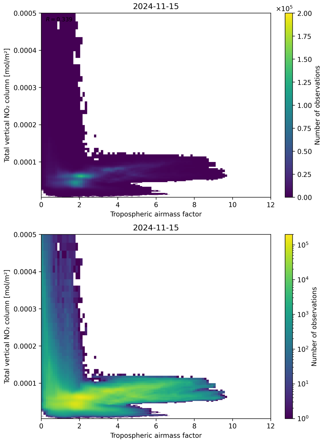
Figure 77: Scatter density plot of “Tropospheric airmass factor” against “Total vertical NO 2 column” for 2024-11-14 to 2024-11-16.
