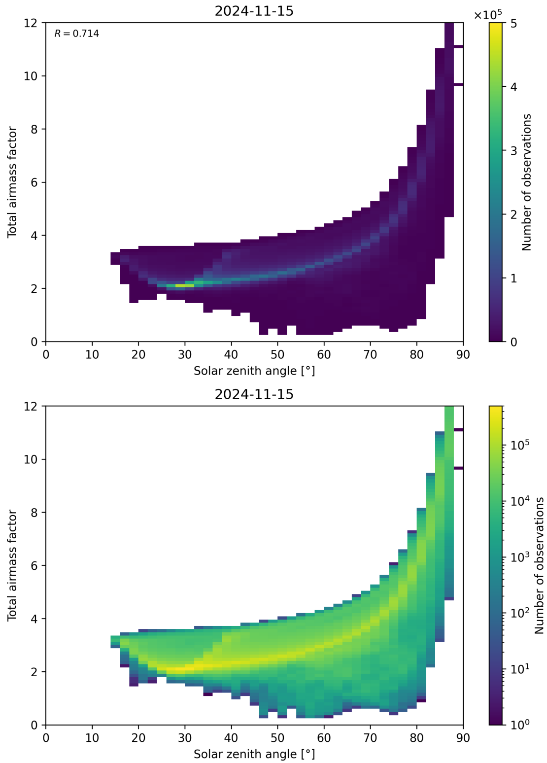
Figure 146: Scatter density plot of “Solar zenith angle” against “Total air mass factor” for 2024-11-14 to 2024-11-16.
