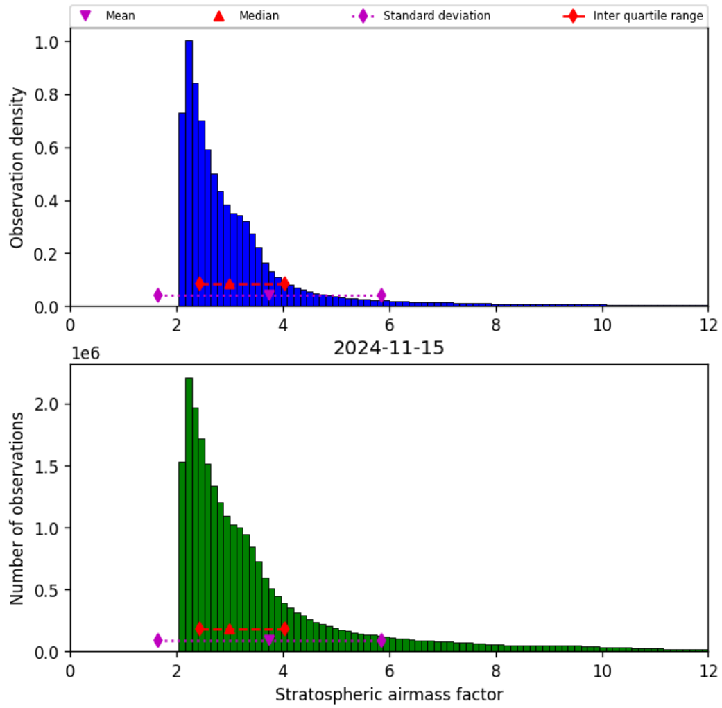
Figure 44: Histogram of “Stratospheric airmass factor” for 2024-11-14 to 2024-11-16
