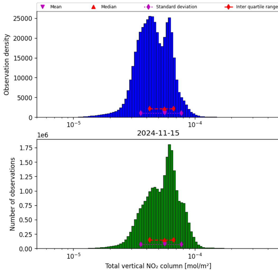
Figure 38: Histogram of “Total vertical NO 2 column” for 2024-11-14 to 2024-11-16
