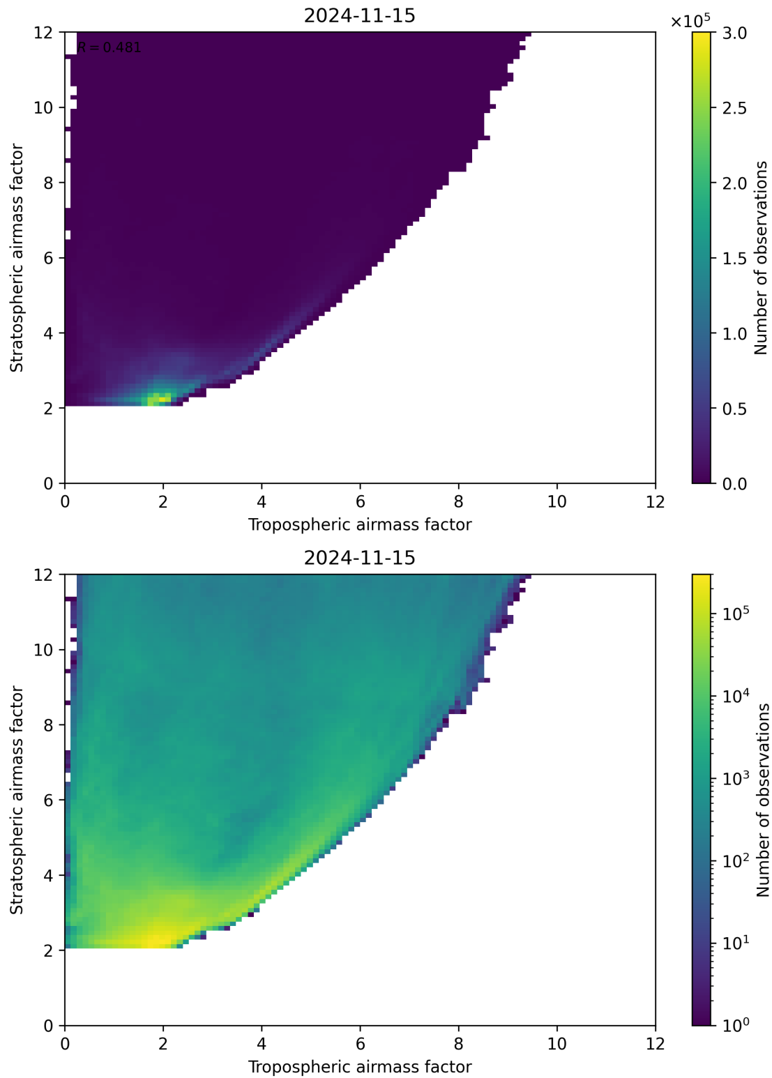
Figure 71: Scatter density plot of “Tropospheric airmass factor” against “Stratospheric airmass factor” for 2024-11-14 to 2024-11-16.
