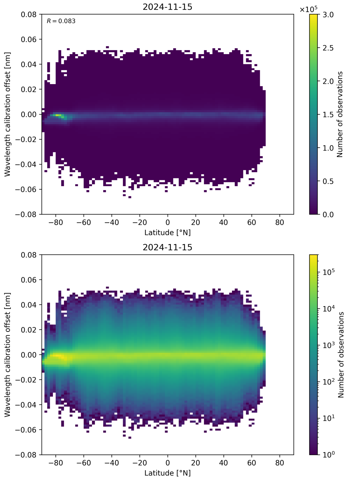
Figure 95: Scatter density plot of “Latitude” against “Wavelength calibration offset” for 2024-11-14 to 2024-11-16.
