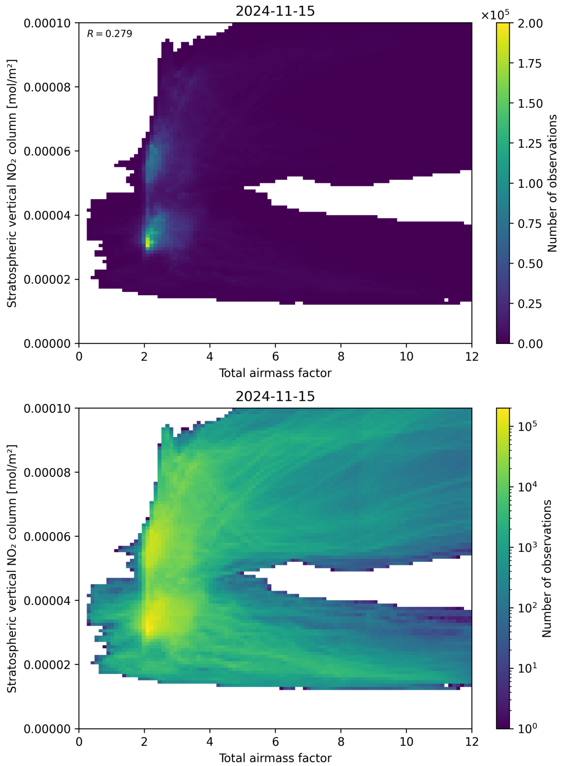
Figure 64: Scatter density plot of “Total airmass factor” against “Stratospheric vertical NO 2 column” for 2024-11-14 to 2024-11-16.
