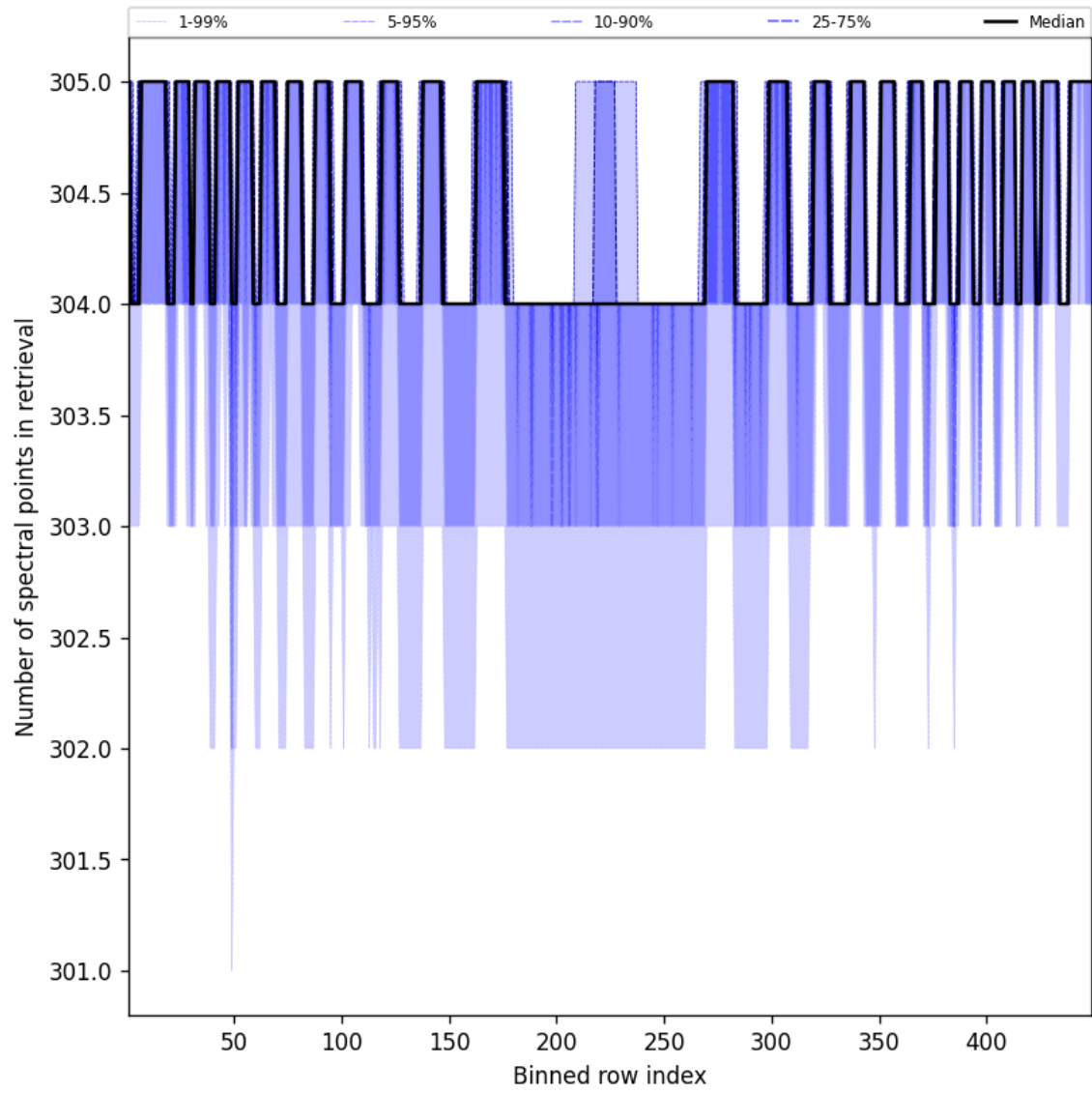
Figure 50: Along track statistics of “Number of spectral points in retrieval” for 2024-11-14 to 2024-11-16
