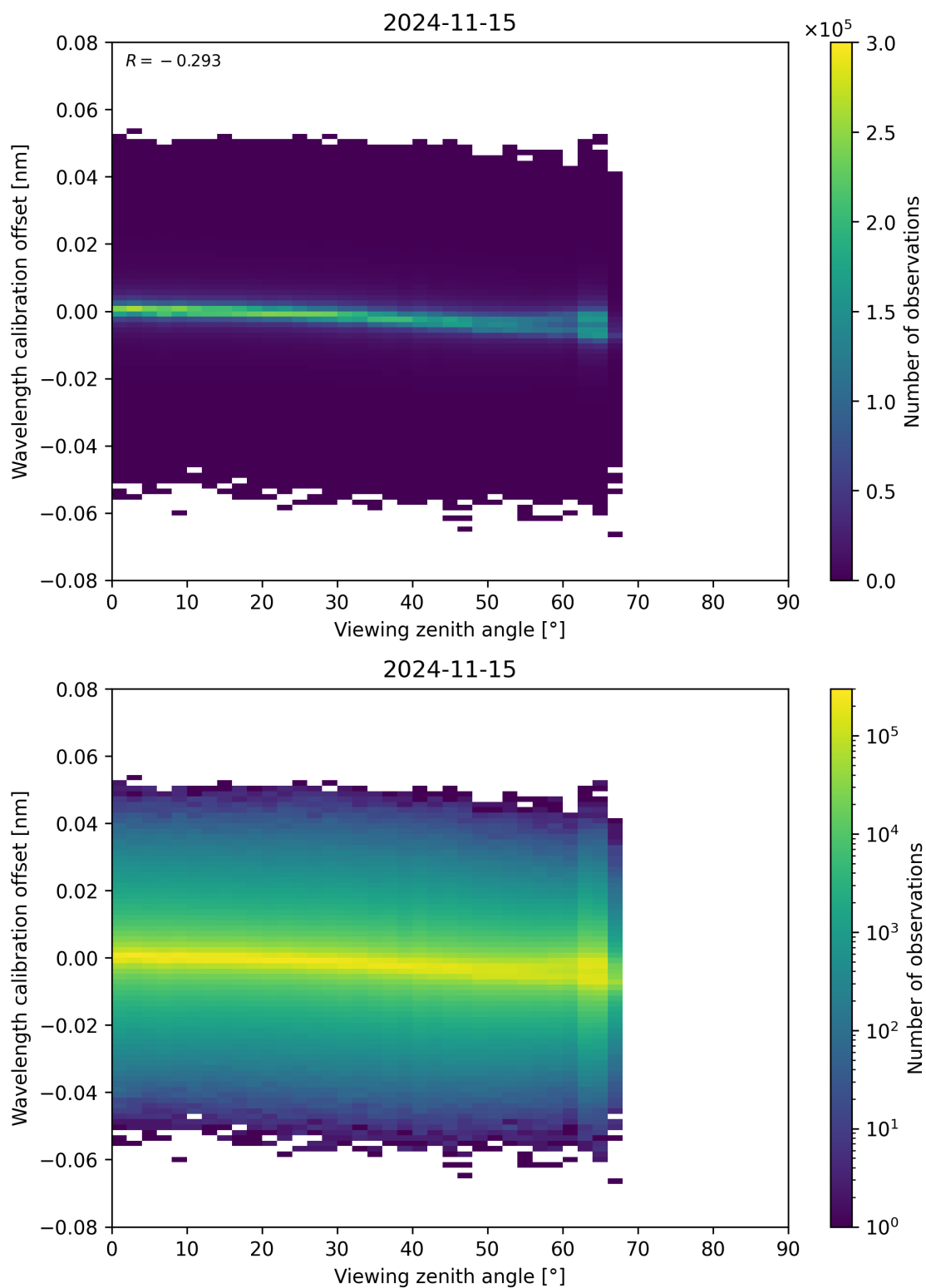
Figure 173: Scatter density plot of “Viewing zenith angle” against “Wavelength calibration offset” for 2024-11-14 to 2024-11-16.
