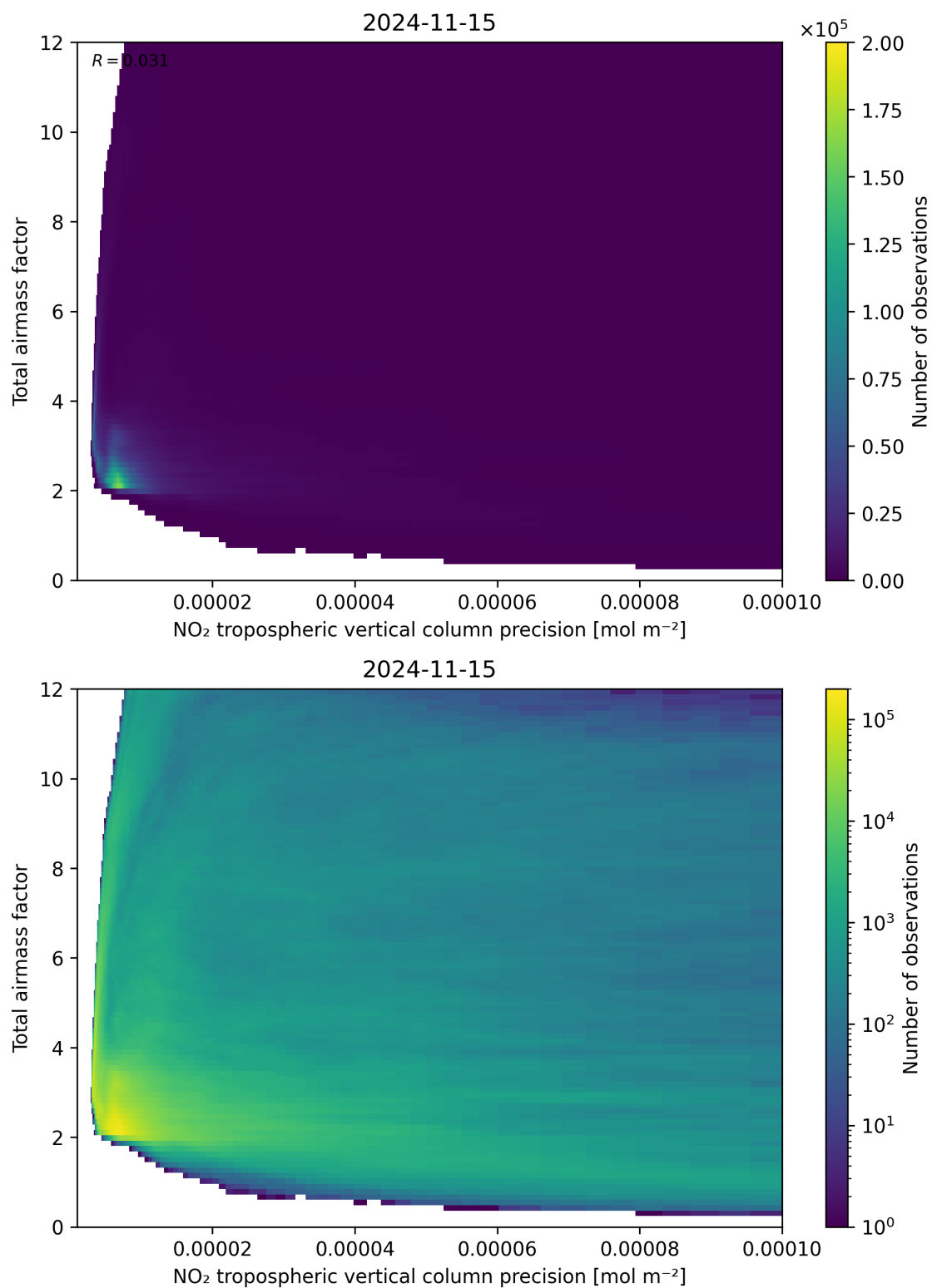
Figure 132: Scatter density plot of “NO 2 tropospheric vertical column precision” against “Total air mass factor” for 2024-11-14 to 2024-11-16.
