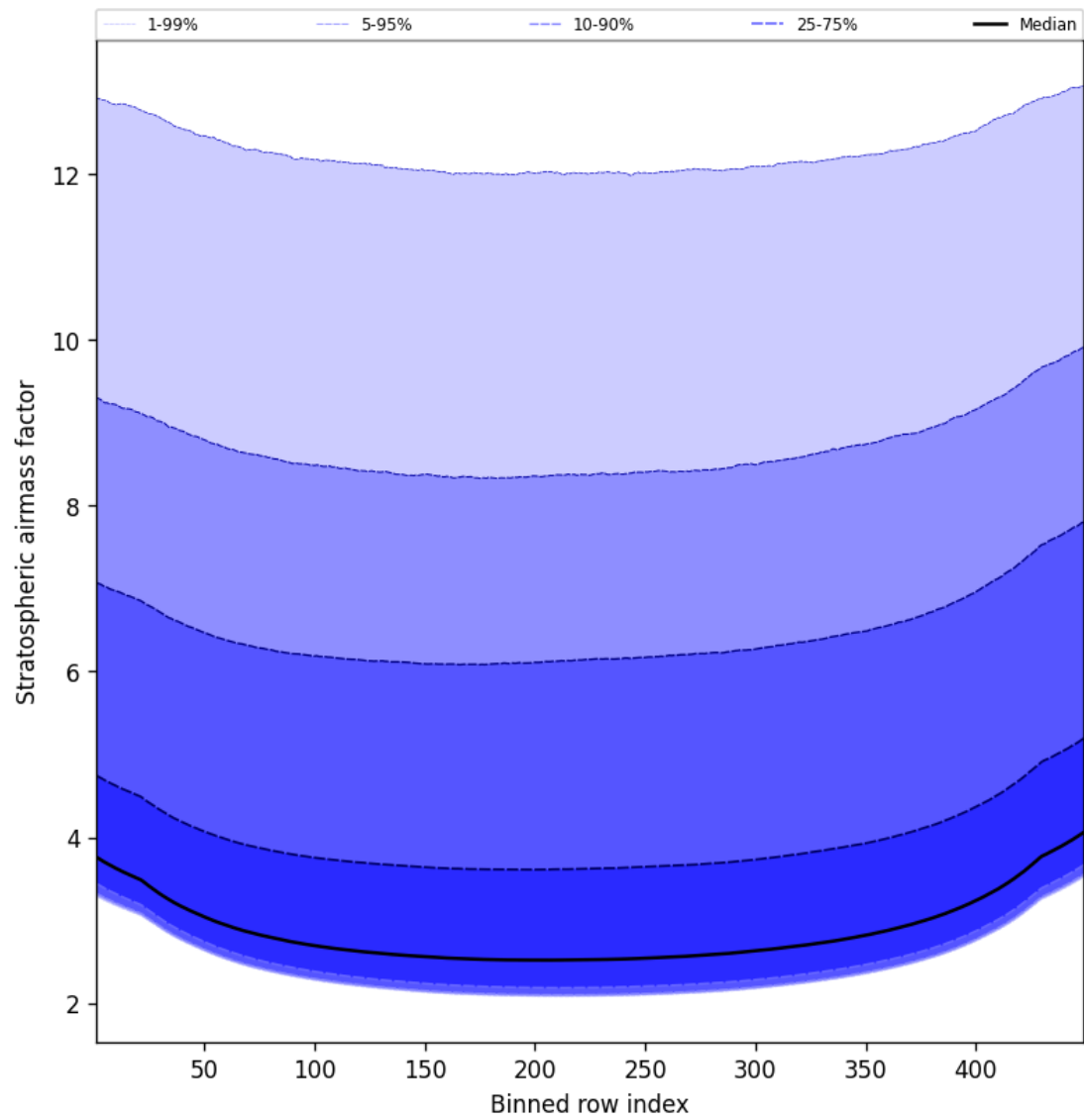
Figure 61: Along track statistics of “Stratospheric airmass factor” for 2024-11-14 to 2024-11-16
