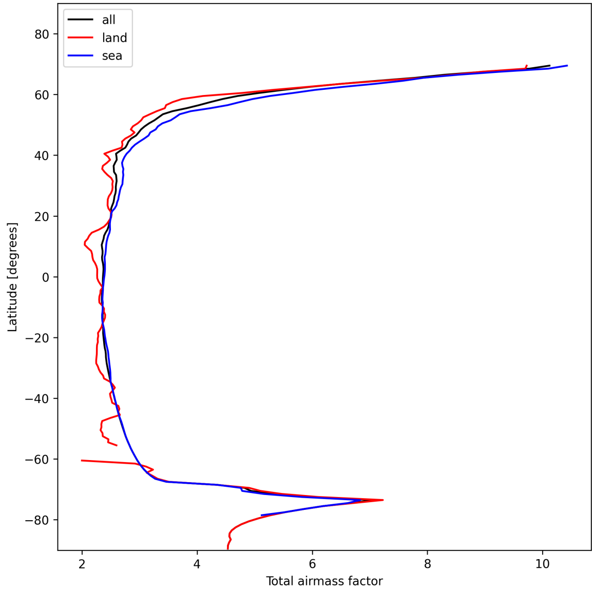
Figure 15: Zonal average of “Total airmass factor” for 2024-11-14 to 2024-11-16.
