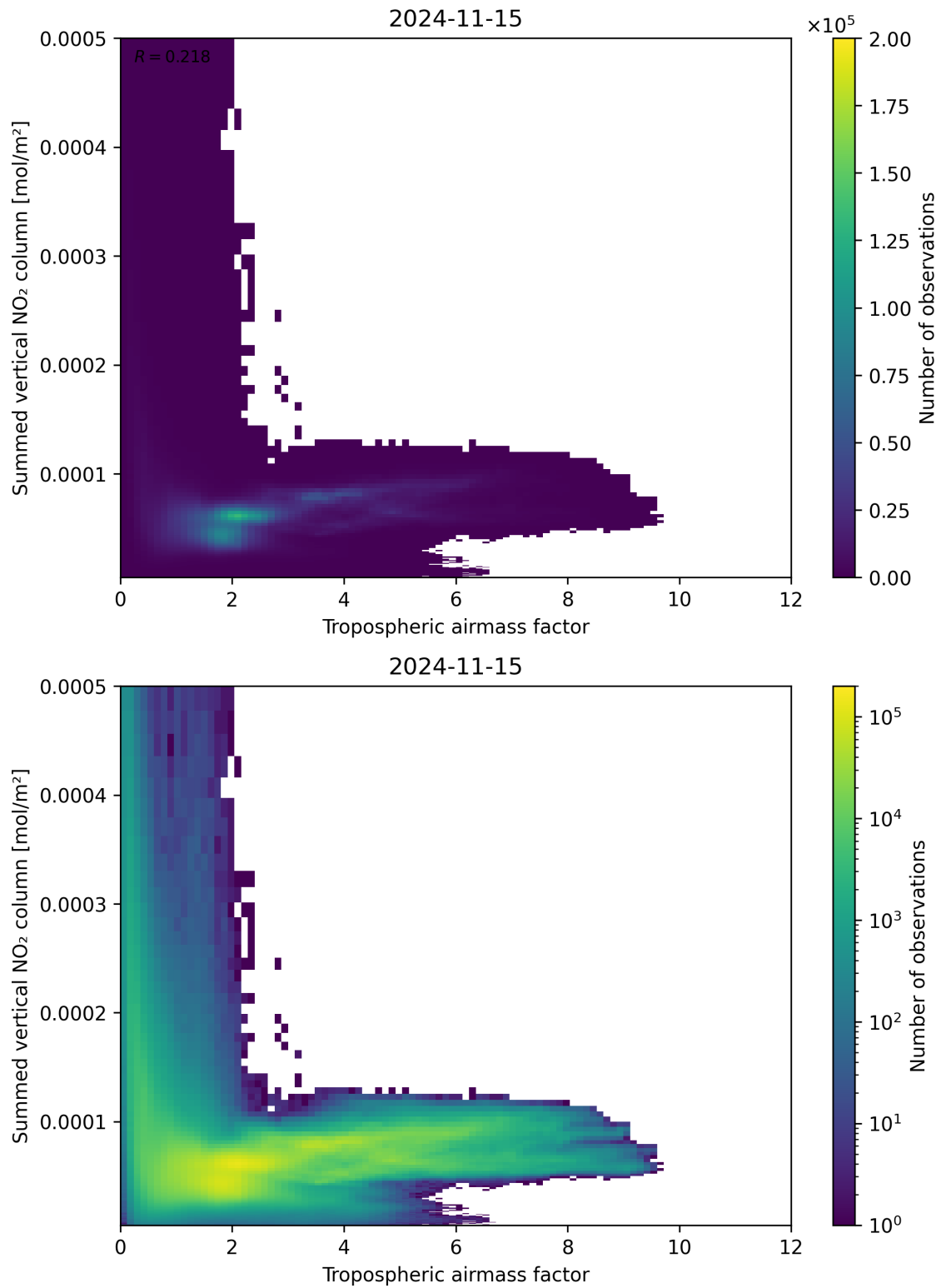
Figure 75: Scatter density plot of “Tropospheric air mass factor” against “Summed vertical NO 2 column” for 2024-11-14 to 2024-11-16.
