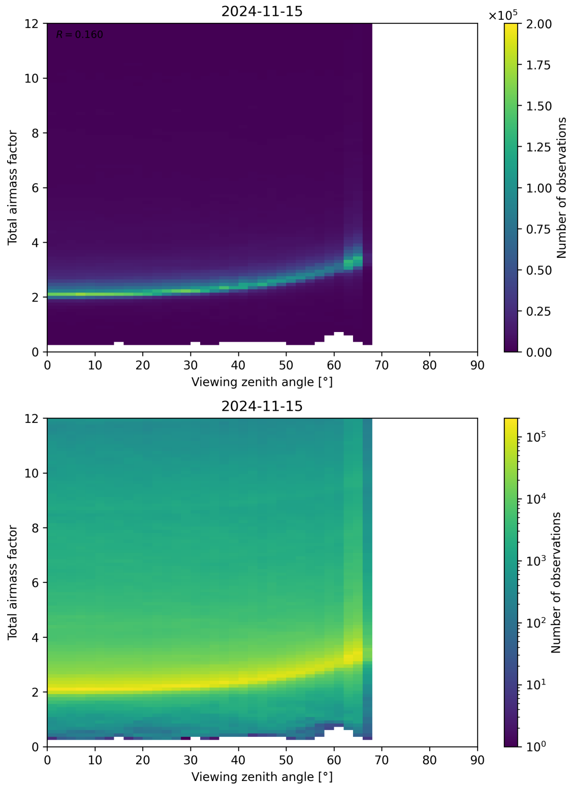
Figure 160: Scatter density plot of “Viewing zenith angle” against “Total airmass factor” for 2024-11-14 to 2024-11-16.
