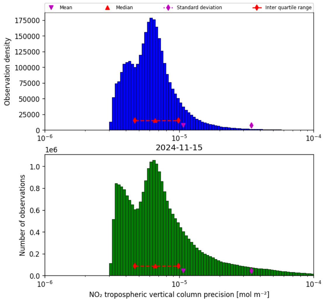
Figure 30: Histogram of “NO 2 tropospheric vertical column precision” for 2024-11-14 to 2024-11-16
