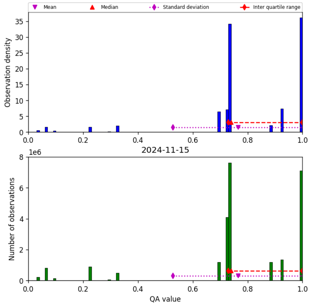
Figure 28: Histogram of “QA value” for 2024-11-14 to 2024-11-16
