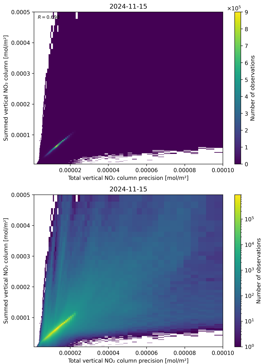
Figure 117: Scatter density plot of “Total vertical NO 2 column precision” against “Summed vertical NO 2 column” for 2024-11-14 to 2024-11-16.
