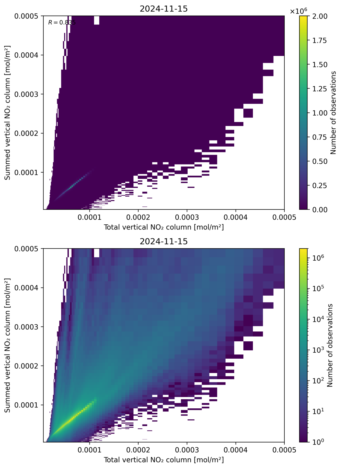
Figure 112: Scatter density plot of “Total vertical NO 2 column” against “Summed vertical NO 2 column” for 2024-11-14 to 2024-11-16.
