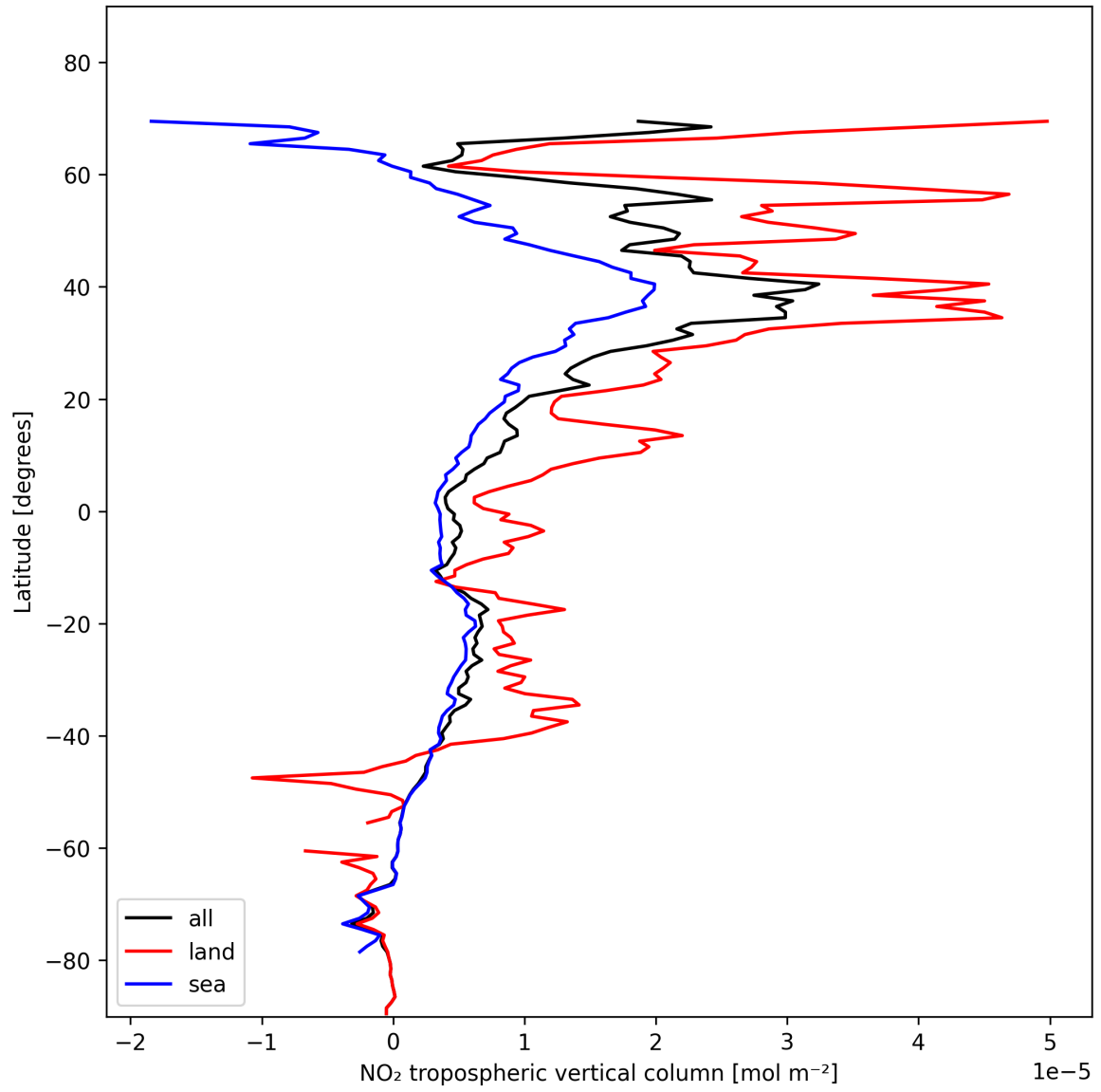
Figure 12: Zonal average of “NO 2 tropospheric vertical column” for 2024-11-14 to 2024-11-16.
