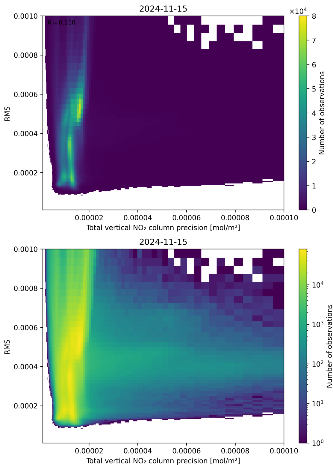
Figure 119: Scatter density plot of “Total vertical NO 2 column precision” against “RMS” for 2024-11-14 to 2024-11-16.
