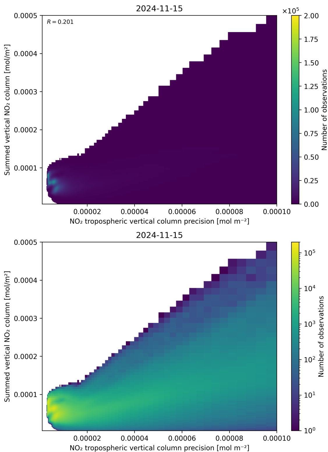
Figure 136: Scatter density plot of “NO 2 tropospheric vertical column precision” against “Summed vertical NO 2 column” for 2024-11-14 to 2024-11-16.
