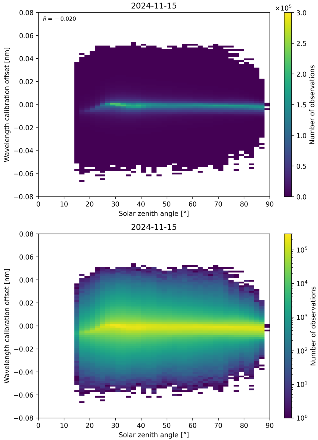
Figure 158: Scatter density plot of “Solar zenith angle” against “Wavelength calibration offset” for 2024-11-14 to 2024-11-16.
