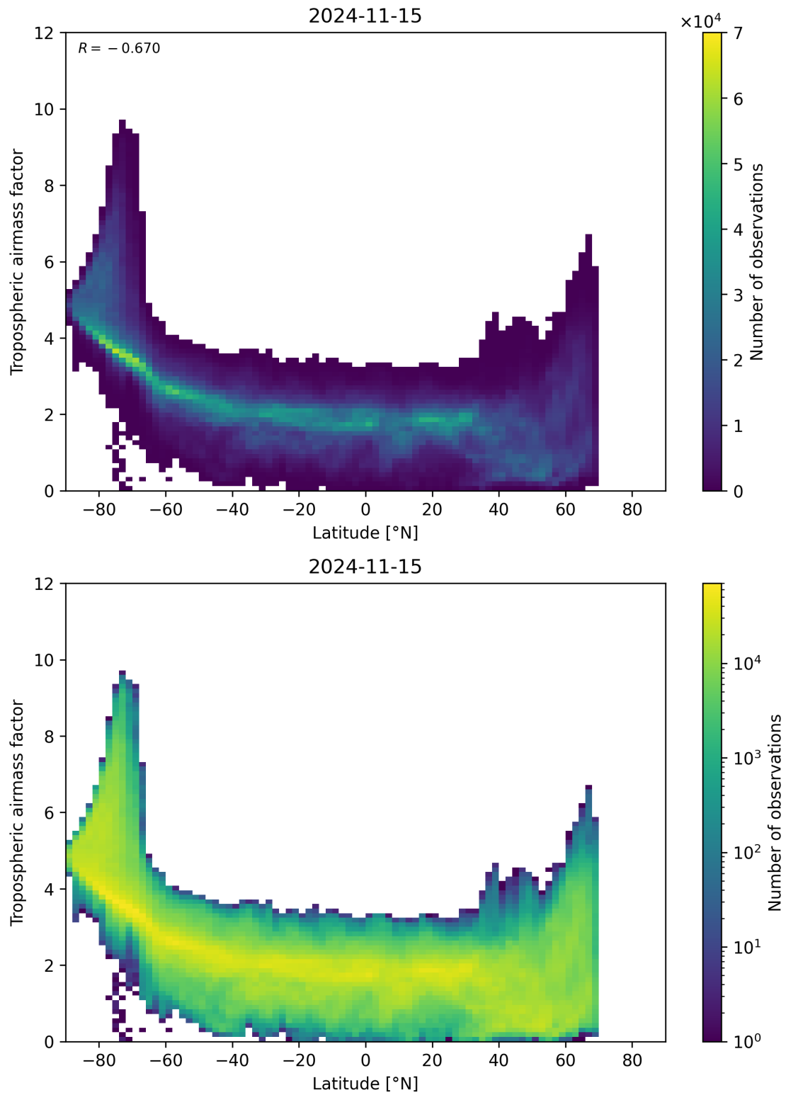
Figure 85: Scatter density plot of “Latitude” against “Tropospheric air mass factor” for 2024-11-14 to 2024-11-16.
