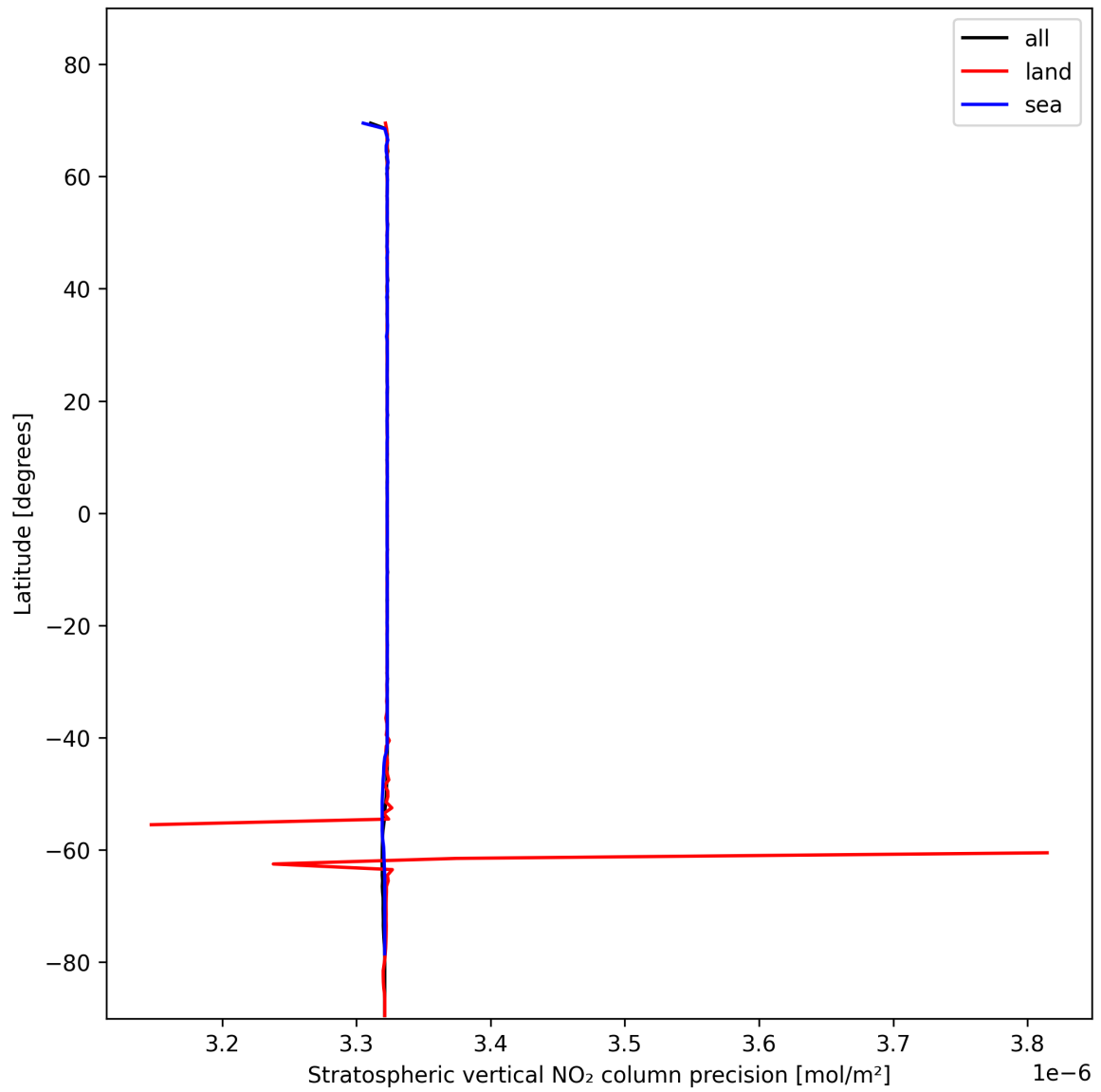
Figure 20: Zonal average of “Stratospheric vertical NO 2 column precision” for 2024-11-14 to 2024-11-16.
