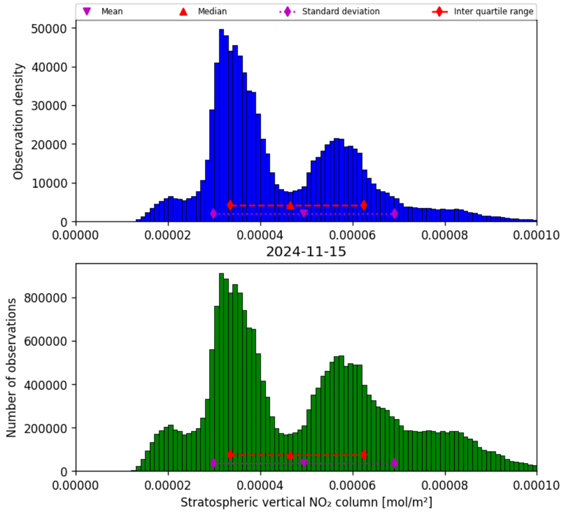
Figure 36: Histogram of “Stratospheric vertical NO 2 column” for 2024-11-14 to 2024-11-16
