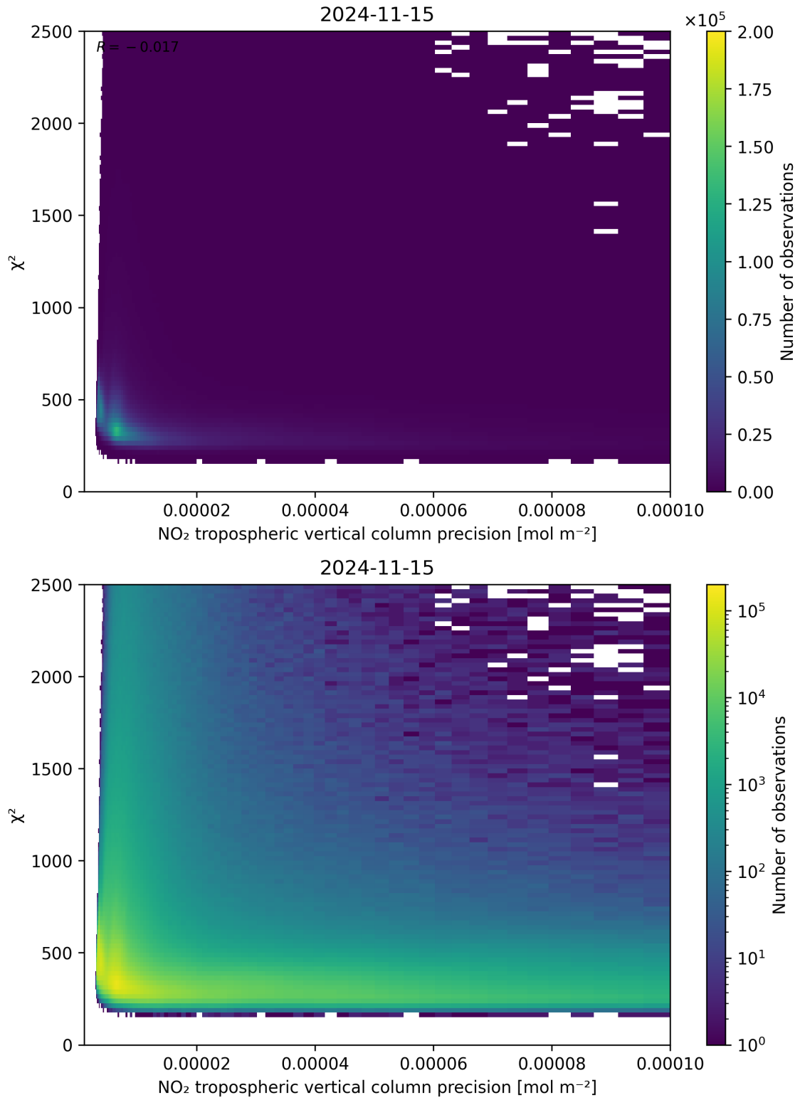
Figure 134: Scatter density plot of “NO 2 tropospheric vertical column precision” against “ \chi^2 ” for 2024-11-14 to 2024-11-16.
