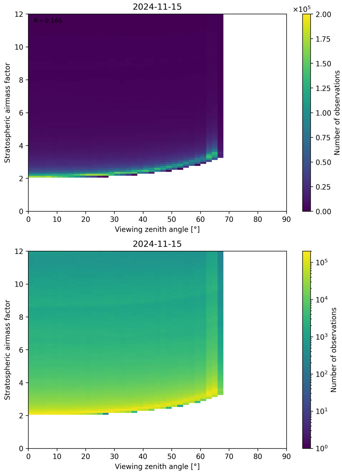
Figure 159: Scatter density plot of “Viewing zenith angle” against “Stratospheric airmass factor” for 2024-11-14 to 2024-11-16.
