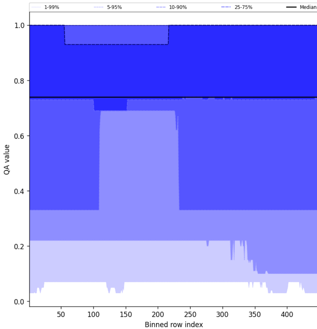
Figure 45: Along track statistics of “QA value” for 2024-11-14 to 2024-11-16
