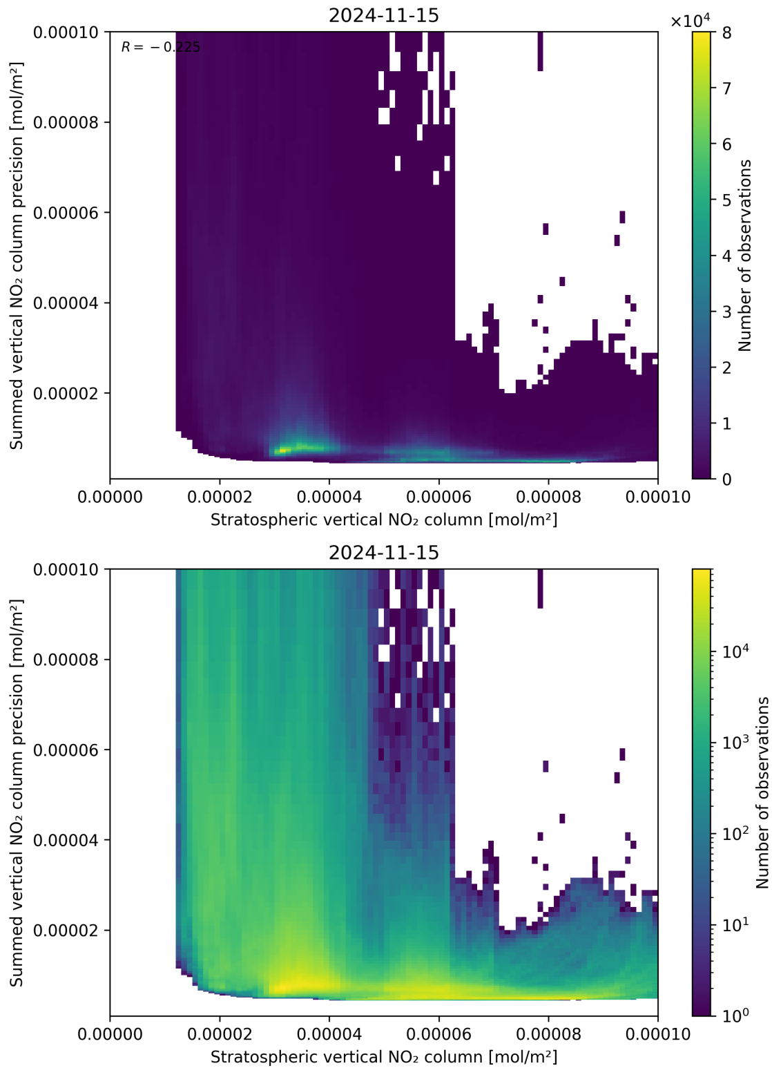
Figure 99: Scatter density plot of “Stratospheric vertical NO 2 column” against “Summed vertical NO 2 column precision” for 2024-11-14 to 2024-11-16.
