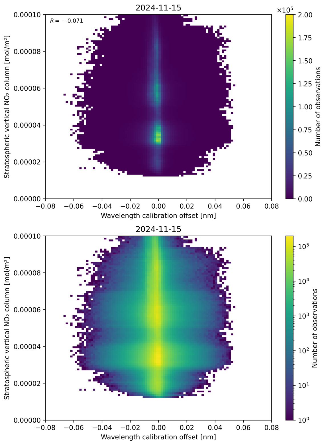
Figure 176: Scatter density plot of “Wavelength calibration offset” against “Stratospheric vertical NO 2 column” for 2024-11-14 to 2024-11-16.
