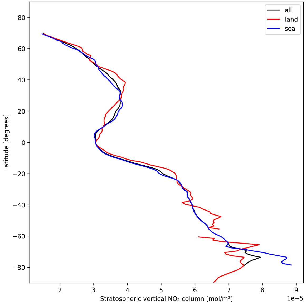
Figure 19: Zonal average of “Stratospheric vertical NO 2 column” for 2024-11-14 to 2024-11-16.
