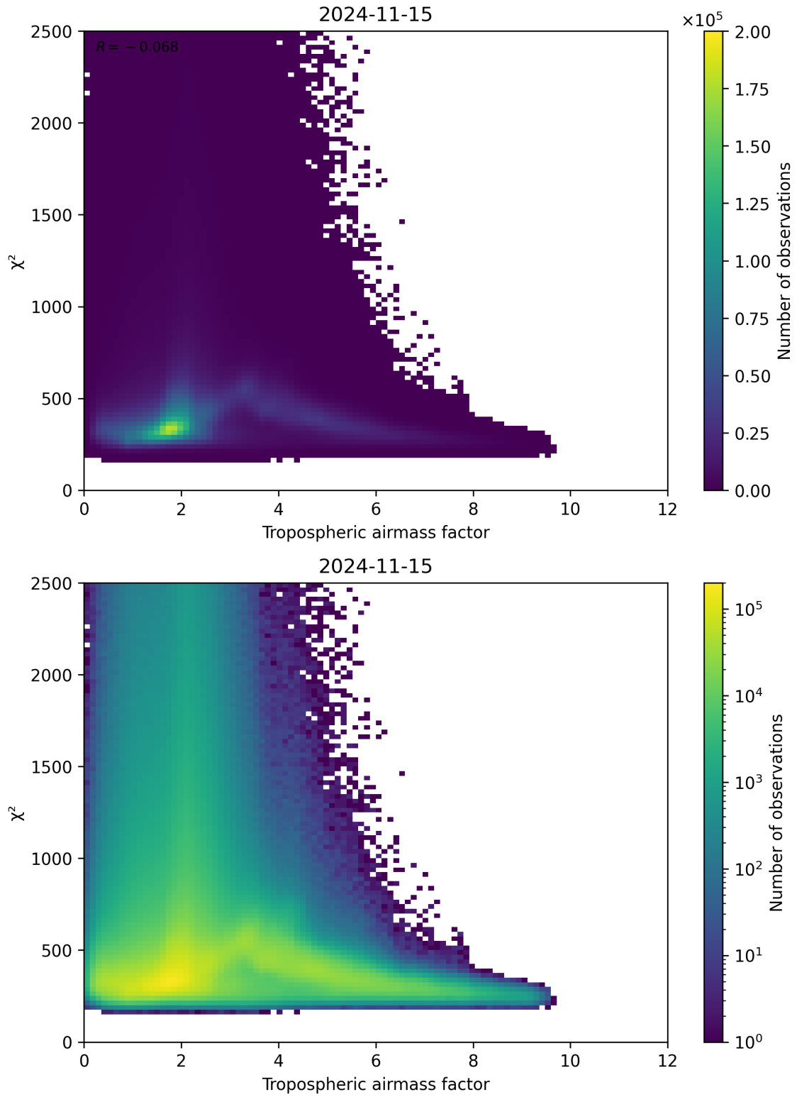
Figure 73: Scatter density plot of “Tropospheric airmass factor” against “ \chi^2 ” for 2024-11-14 to 2024-11-16.
