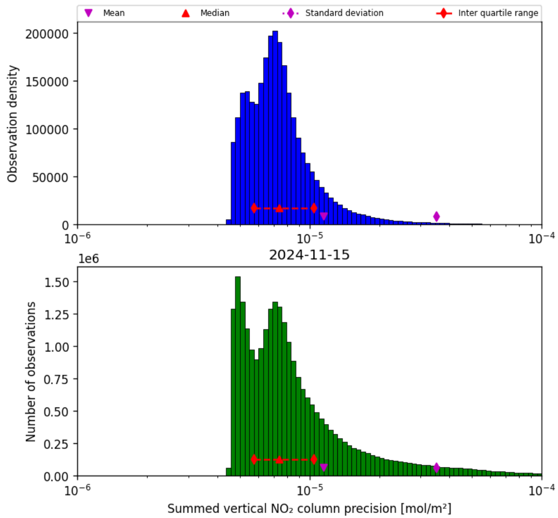
Figure 41: Histogram of “Summed vertical NO 2 column precision” for 2024-11-14 to 2024-11-16
