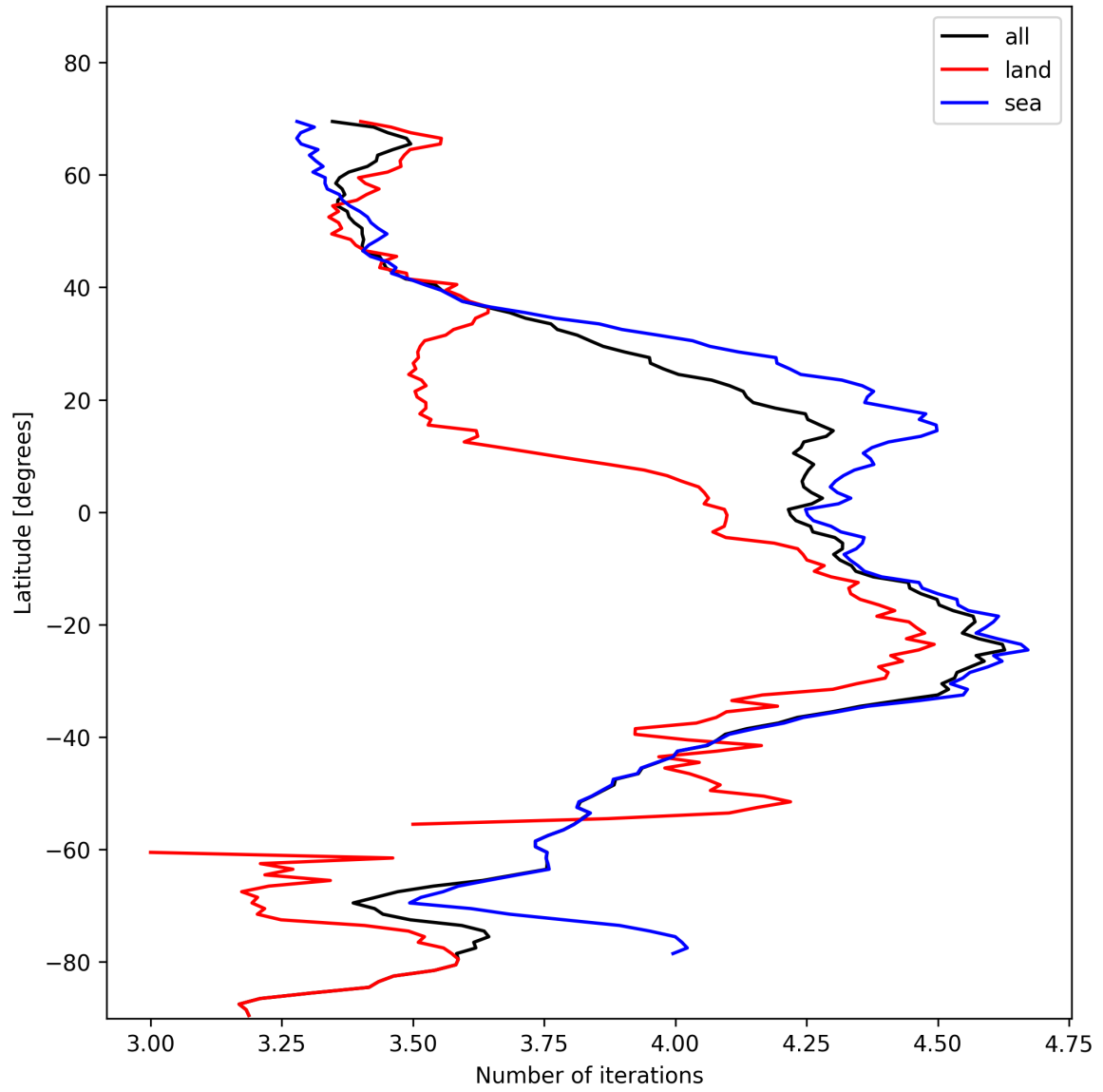
Figure 17: Zonal average of “Number of iterations” for 2024-11-14 to 2024-11-16.
