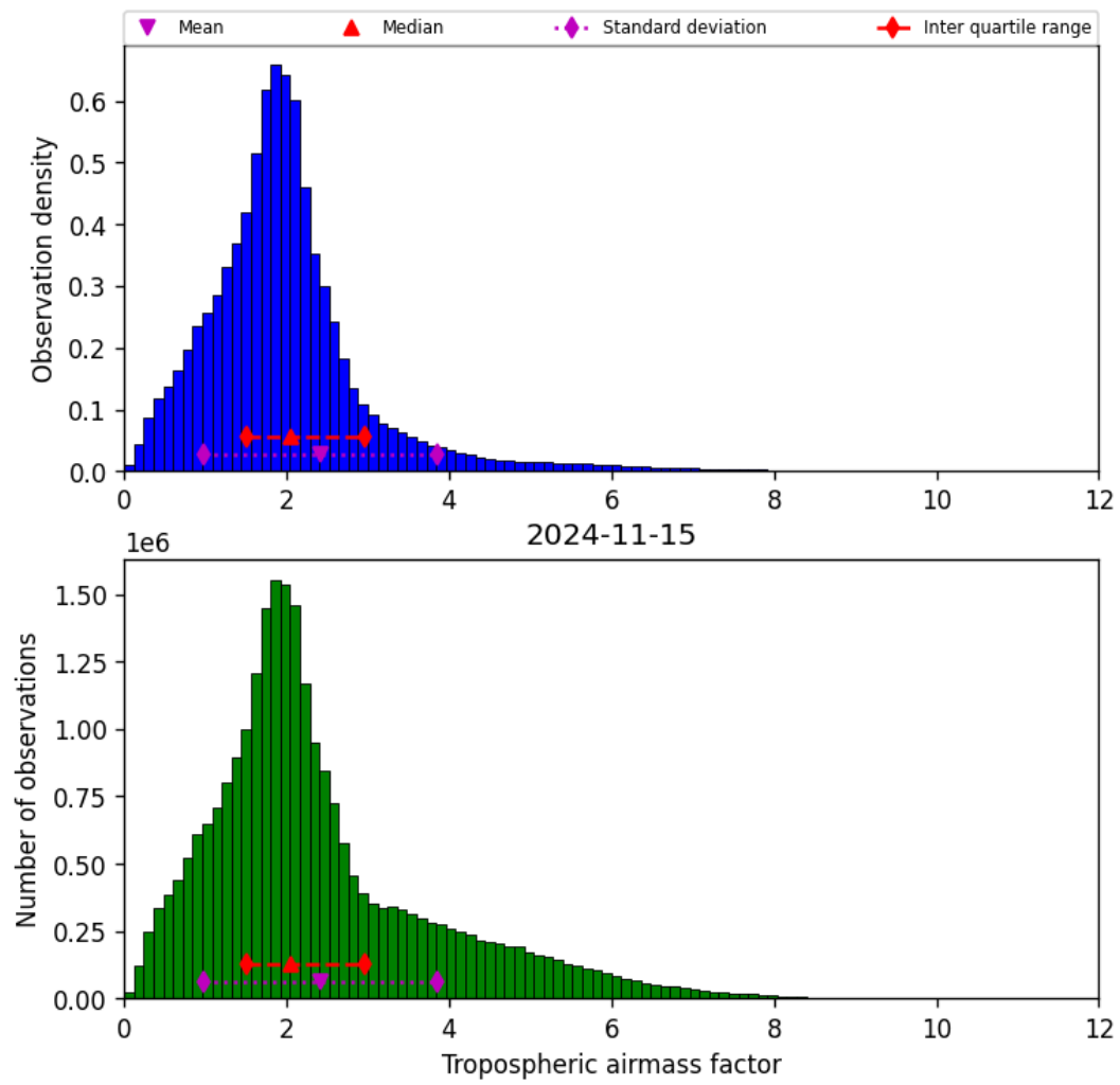
Figure 31: Histogram of “Tropospheric airmass factor” for 2024-11-14 to 2024-11-16
