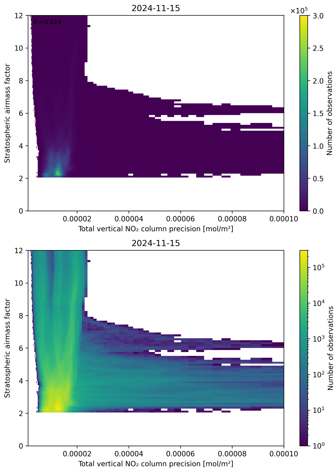
Figure 115: Scatter density plot of “Total vertical NO 2 column precision” against “Stratospheric airmass factor” for 2024-11-14 to 2024-11-16.
