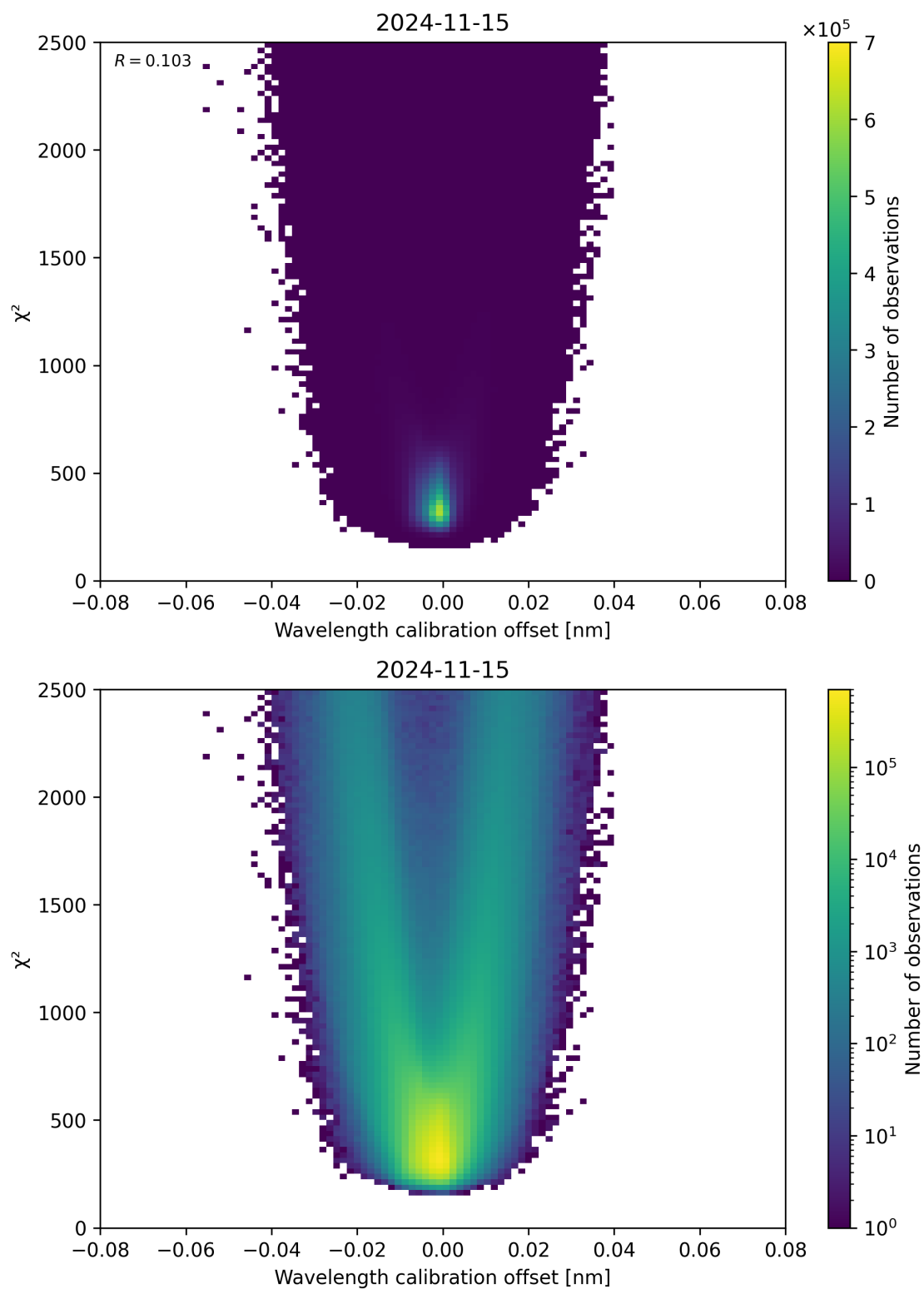
Figure 175: Scatter density plot of “Wavelength calibration offset” against “ \chi^2 ” for 2024-11-14 to 2024-11-16.
