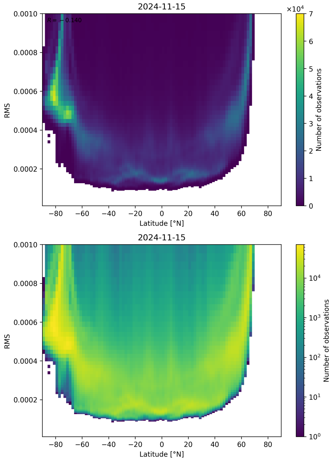
Figure 94: Scatter density plot of “Latitude” against “RMS” for 2024-11-14 to 2024-11-16.
