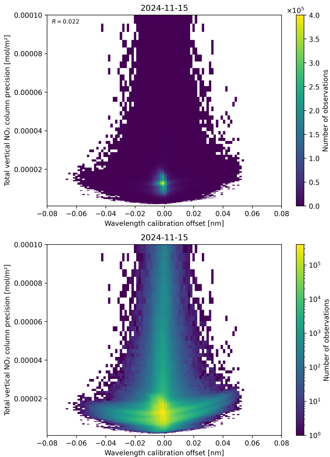
Figure 180: Scatter density plot of “Wavelength calibration offset” against “Total vertical NO 2 column precision” for 2024-11-14 to 2024-11-16.
