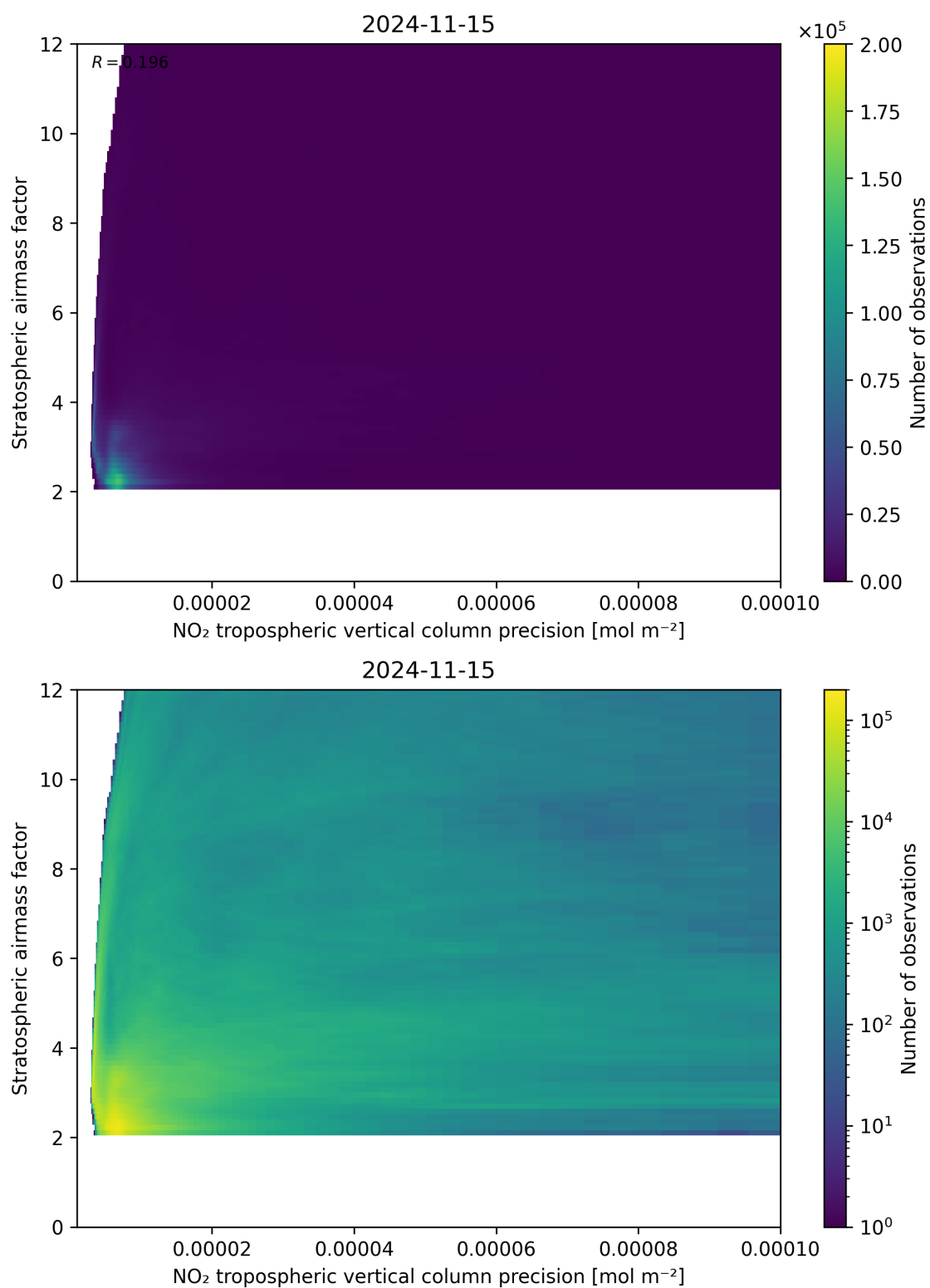
Figure 131: Scatter density plot of “NO 2 tropospheric vertical column precision” against “Stratospheric airmass factor” for 2024-11-14 to 2024-11-16.
