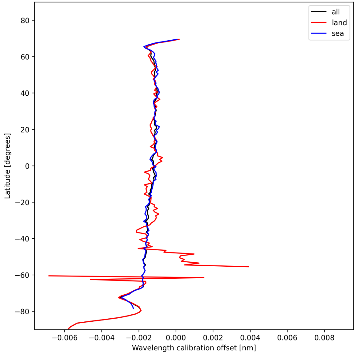
Figure 18: Zonal average of “Wavelength calibration offset” for 2024-11-14 to 2024-11-16.
