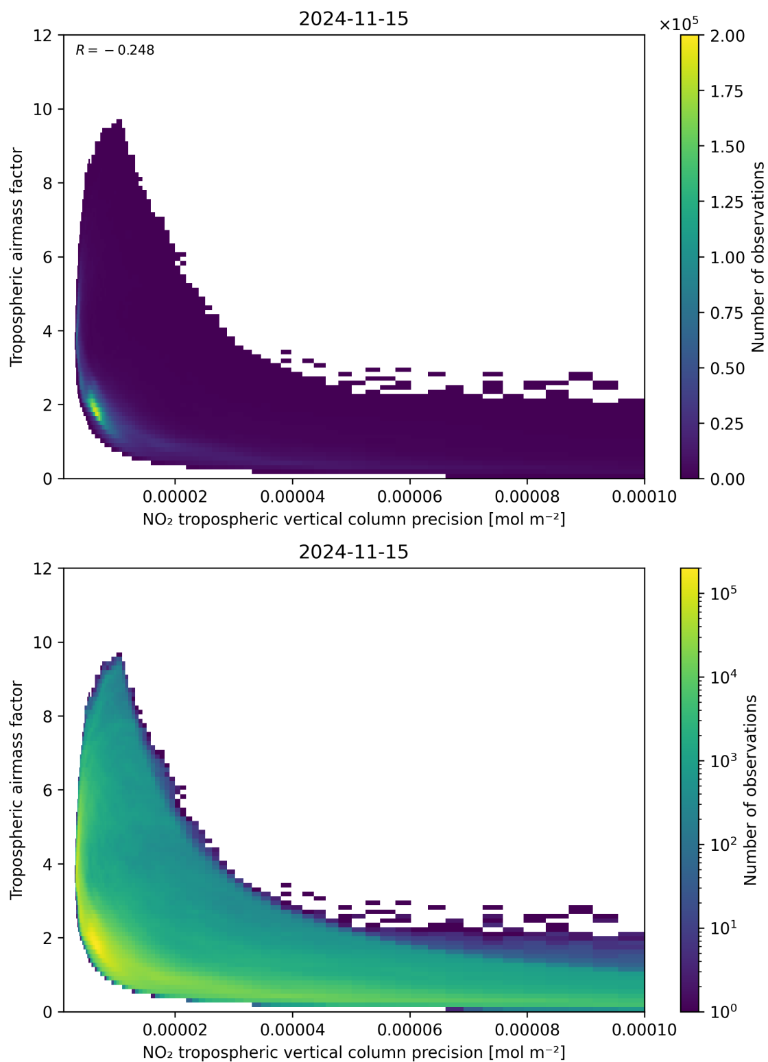
Figure 133: Scatter density plot of “NO 2 tropospheric vertical column precision” against “Tropospheric airmass factor” for 2024-11-14 to 2024-11-16.
