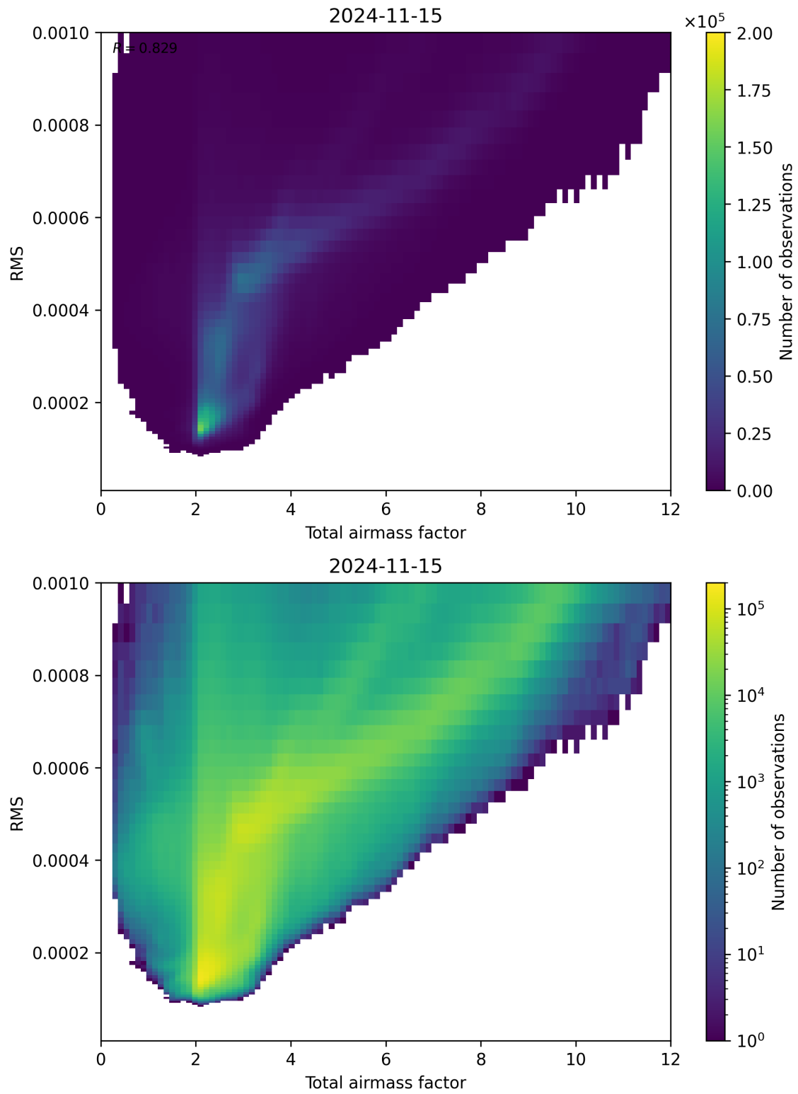
Figure 69: Scatter density plot of “Total airmass factor” against “RMS” for 2024-11-14 to 2024-11-16.
