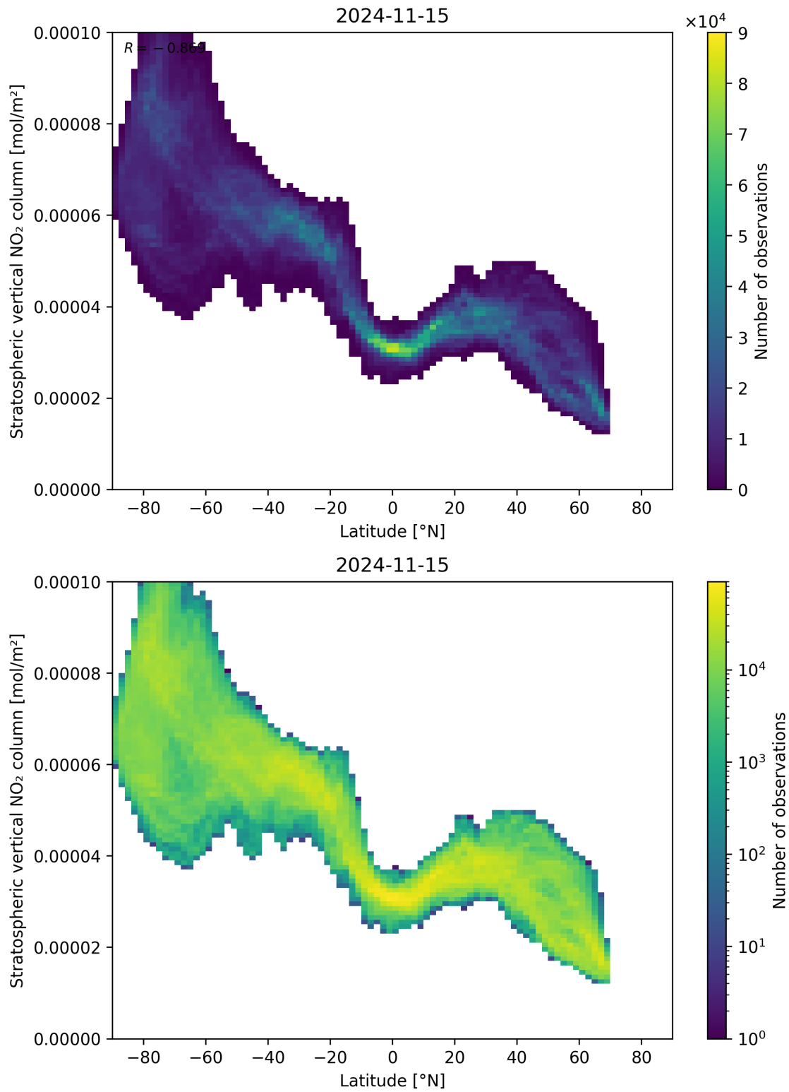
Figure 87: Scatter density plot of “Latitude” against “Stratospheric vertical NO 2 column” for 2024-11-14 to 2024-11-16.
