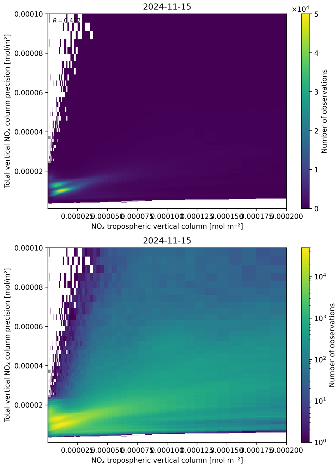
Figure 129: Scatter density plot of “NO 2 tropospheric vertical column” against “Total vertical NO 2 column precision” for 2024-11-14 to 2024-11-16.
