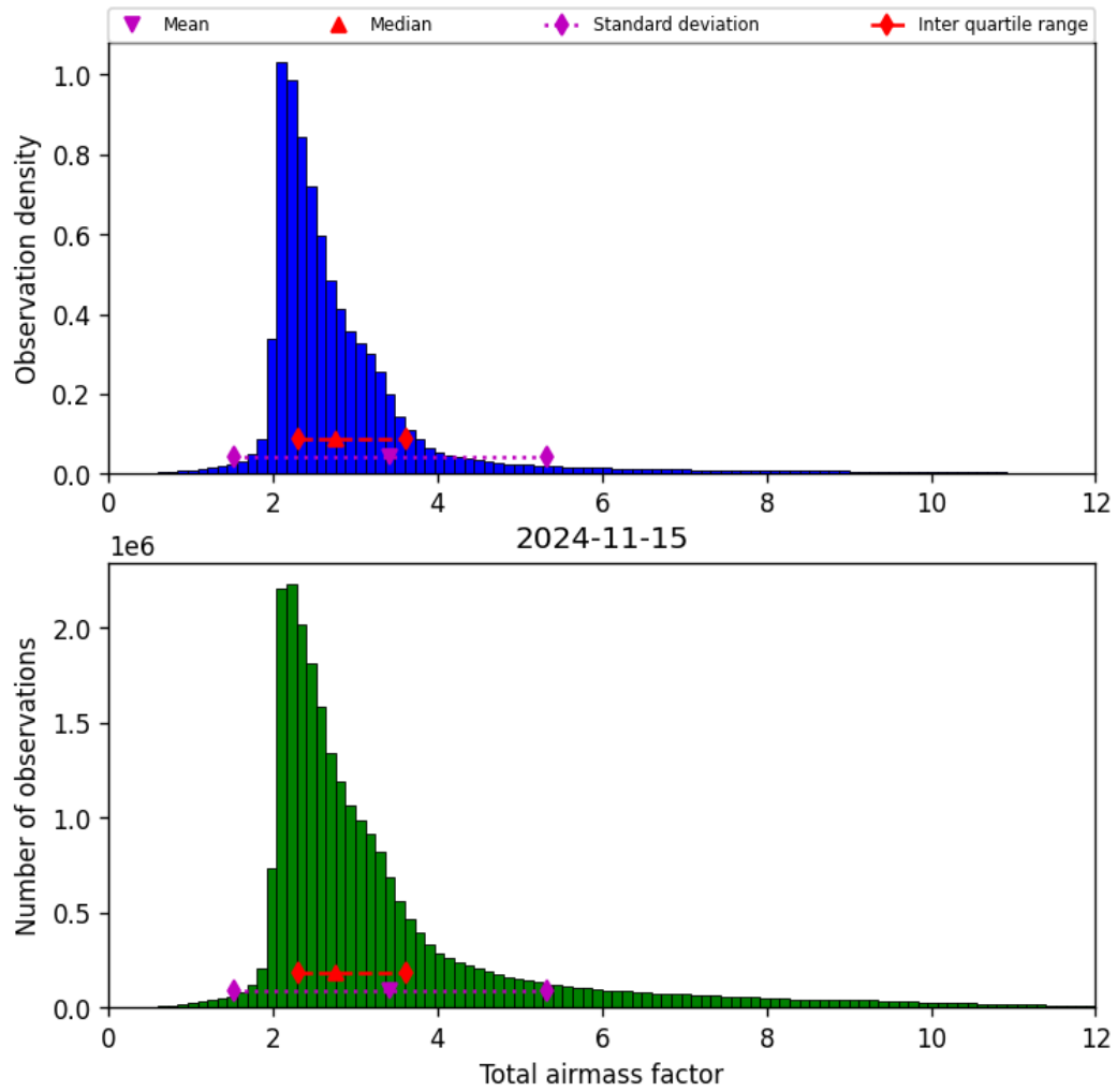
Figure 32: Histogram of “Total airmass factor” for 2024-11-14 to 2024-11-16
