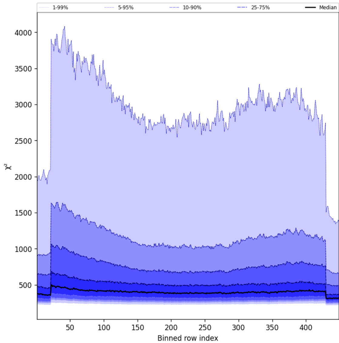
Figure 59: Along track statistics of “ \chi^2 ” for 2024-11-14 to 2024-11-16
