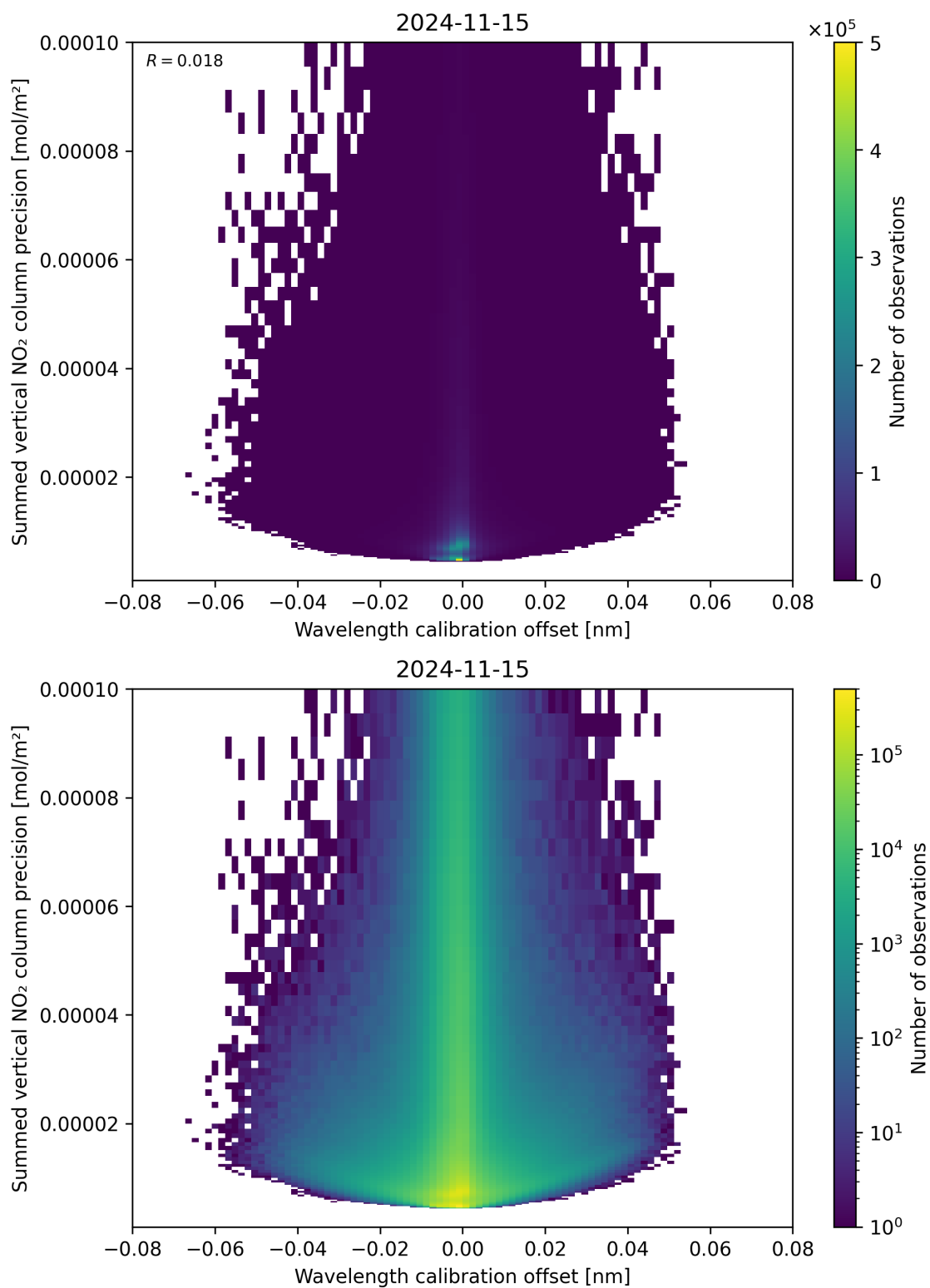
Figure 178: Scatter density plot of “Wavelength calibration offset” against “Summed vertical NO 2 column precision” for 2024-11-14 to 2024-11-16.
