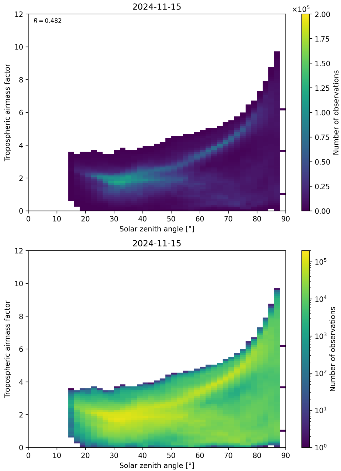
Figure 147: Scatter density plot of “Solar zenith angle” against “Tropospheric airmass factor” for 2024-11-14 to 2024-11-16.
