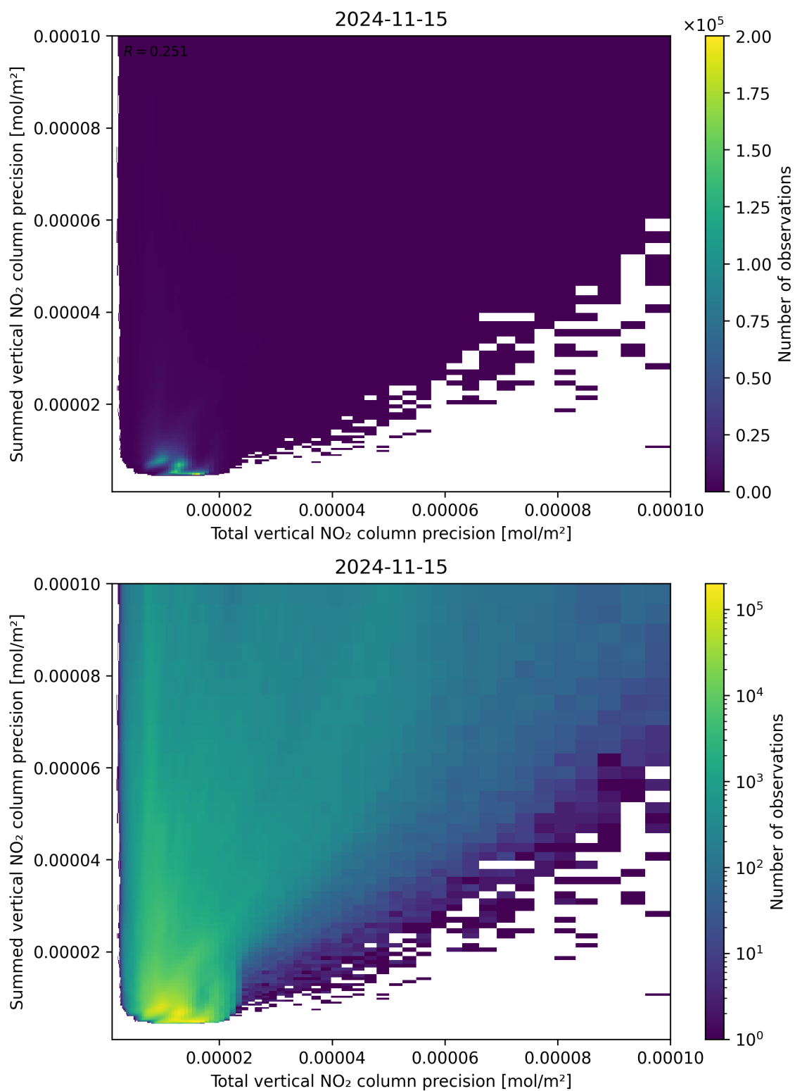
Figure 118: Scatter density plot of “Total vertical NO 2 column precision” against “Summed vertical NO 2 column precision” for 2024-11-14 to 2024-11-16.
