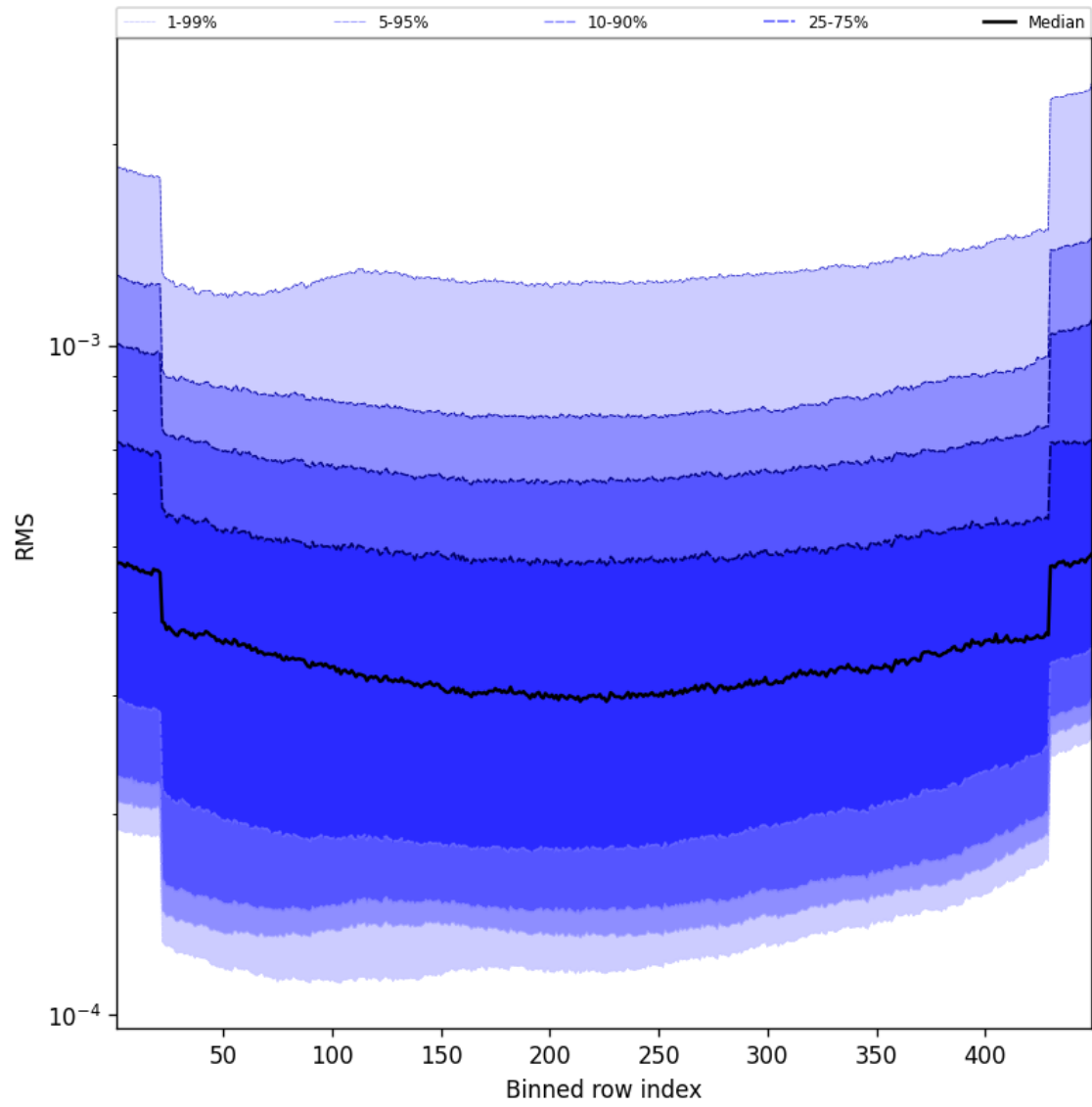
Figure 60: Along track statistics of “RMS” for 2024-11-14 to 2024-11-16
