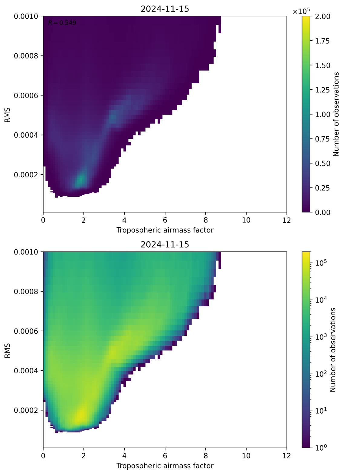
Figure 79: Scatter density plot of “Tropospheric airmass factor” against “RMS” for 2024-11-14 to 2024-11-16.
