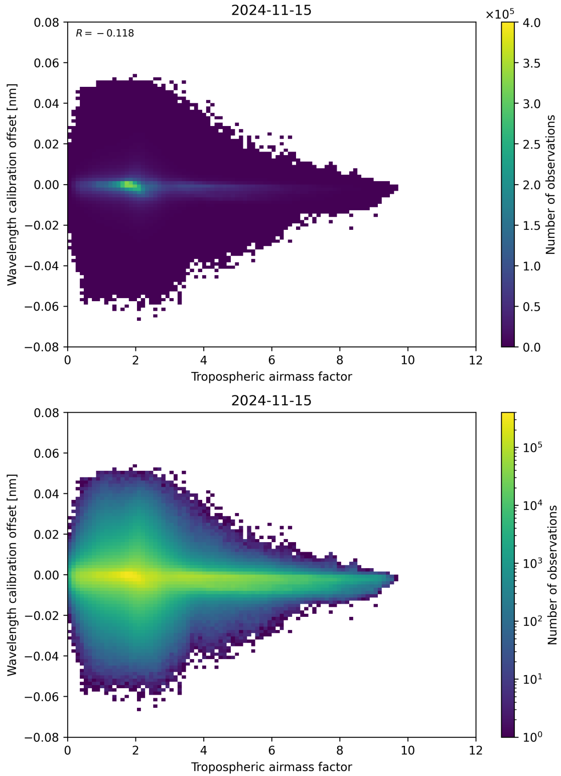
Figure 80: Scatter density plot of “Tropospheric airmass factor” against “Wavelength calibration offset” for 2024-11-14 to 2024-11-16.
