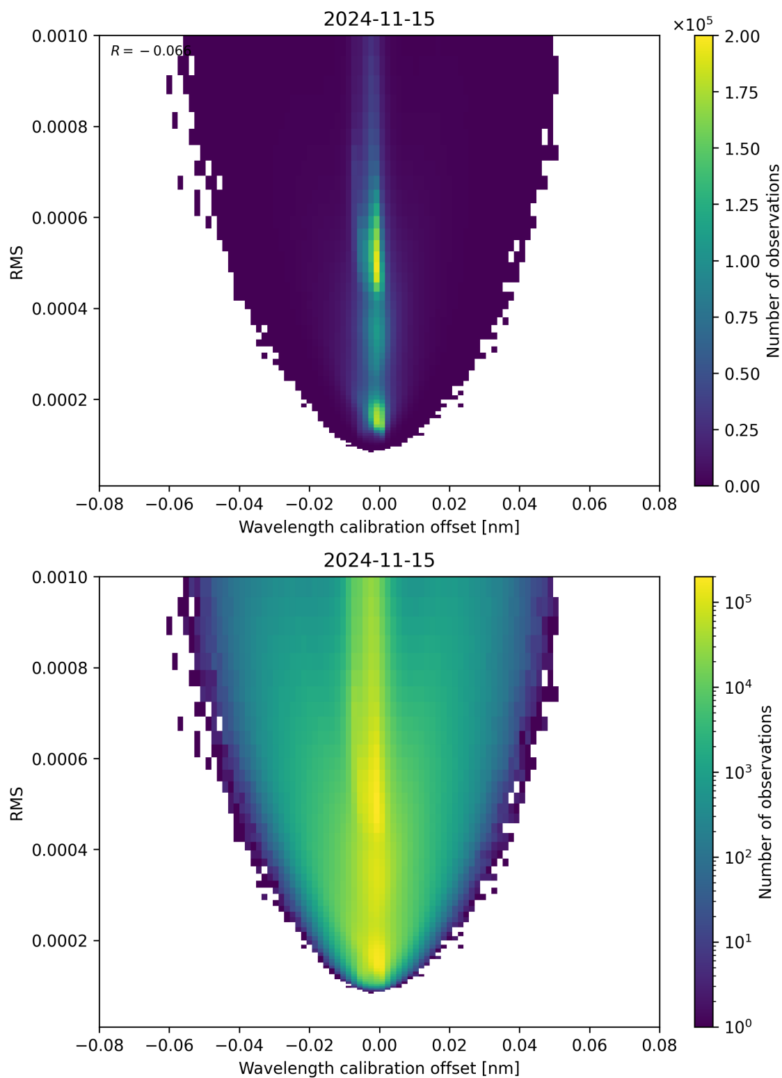
Figure 181: Scatter density plot of “Wavelength calibration offset” against “RMS” for 2024-11-14 to 2024-11-16.
