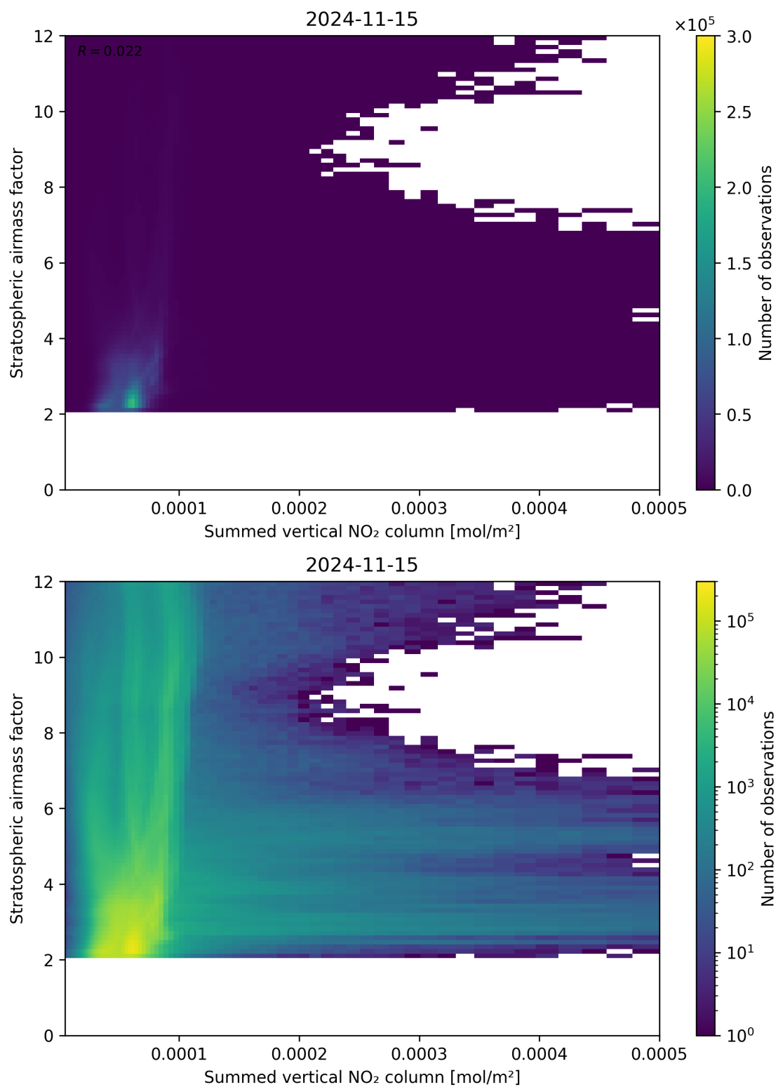
Figure 103: Scatter density plot of “Summed vertical NO 2 column” against “Stratospheric airmass factor” for 2024-11-14 to 2024-11-16.
