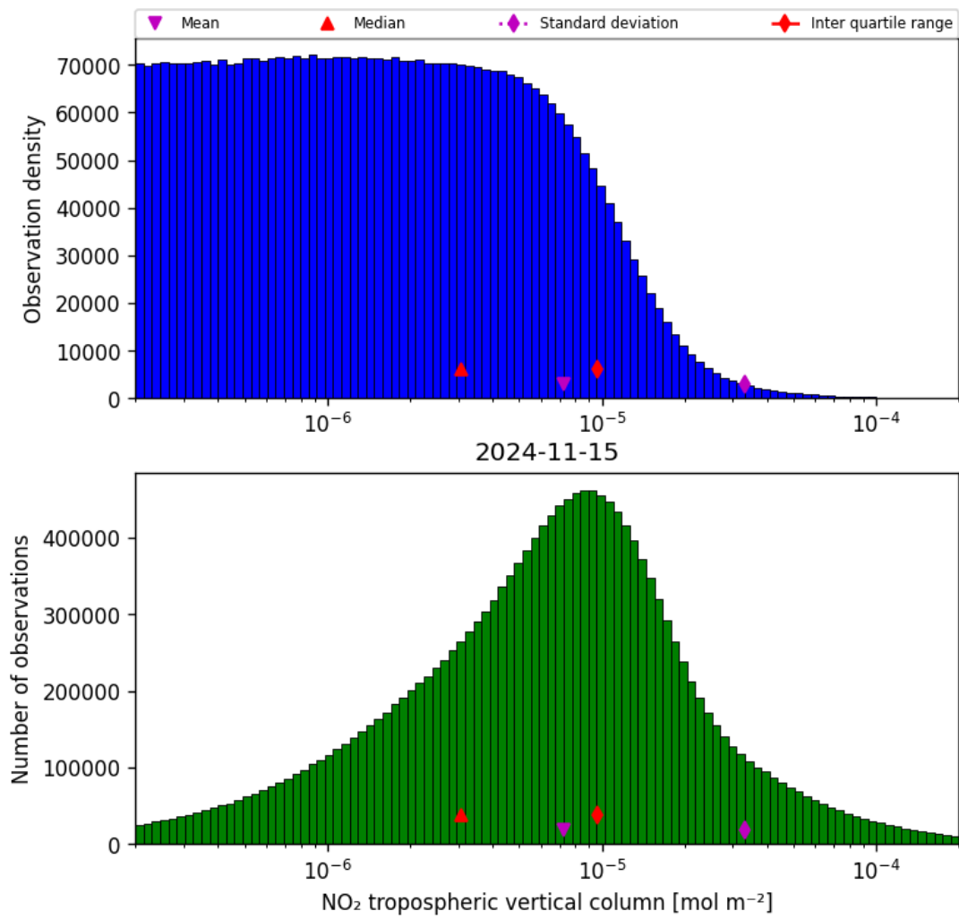
Figure 29: Histogram of “NO 2 tropospheric vertical column” for 2024-11-14 to 2024-11-16
