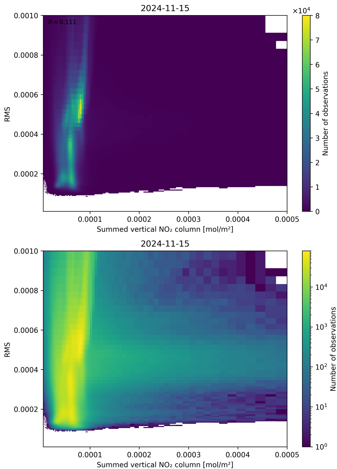
Figure 109: Scatter density plot of “Summed vertical NO 2 column” against “RMS” for 2024-11-14 to 2024-11-16.
