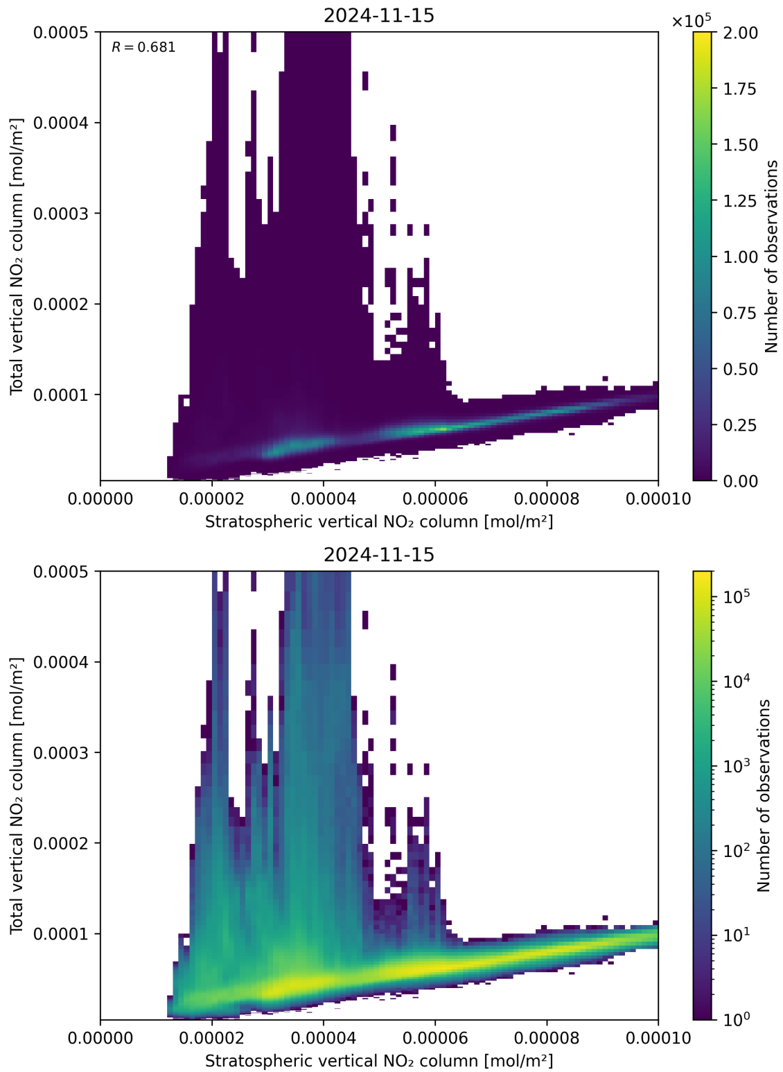
Figure 100: Scatter density plot of “Stratospheric vertical NO 2 column” against “Total vertical NO 2 column” for 2024-11-14 to 2024-11-16.
