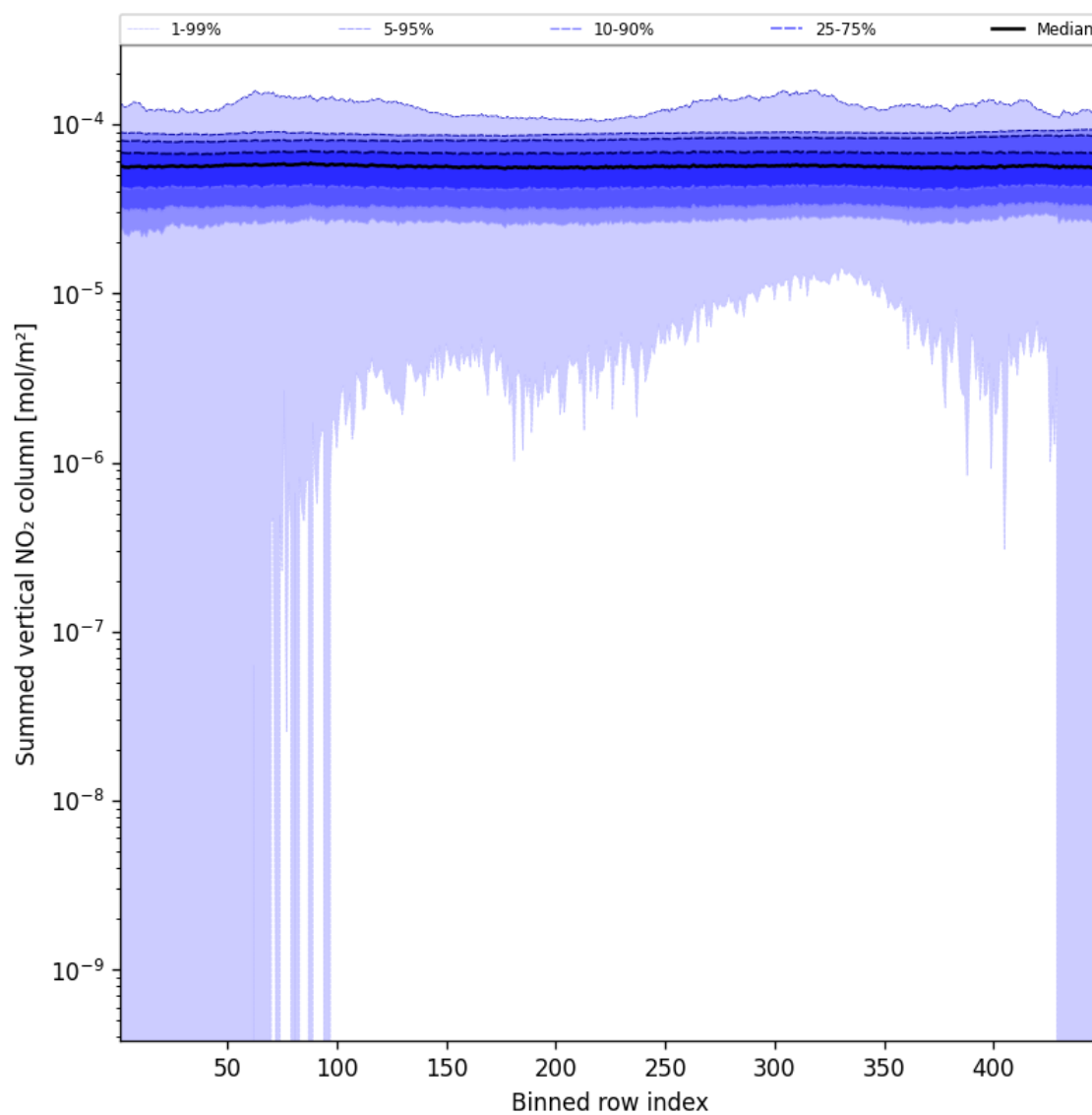
Figure 57: Along track statistics of “Summed vertical NO 2 column” for 2024-11-14 to 2024-11-16
