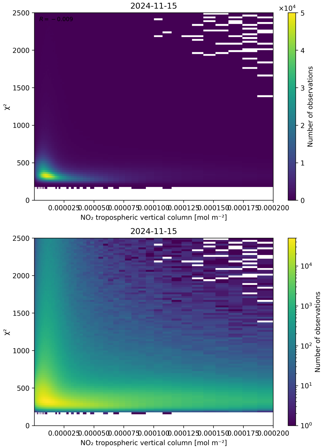
Figure 124: Scatter density plot of “NO 2 tropospheric vertical column” against “ \chi^2 ” for 2024-11-14 to 2024-11-16.
