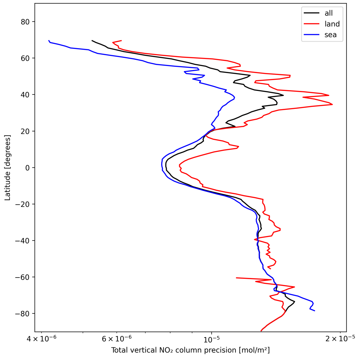
Figure 22: Zonal average of “Total vertical NO 2 column precision” for 2024-11-14 to 2024-11-16.
