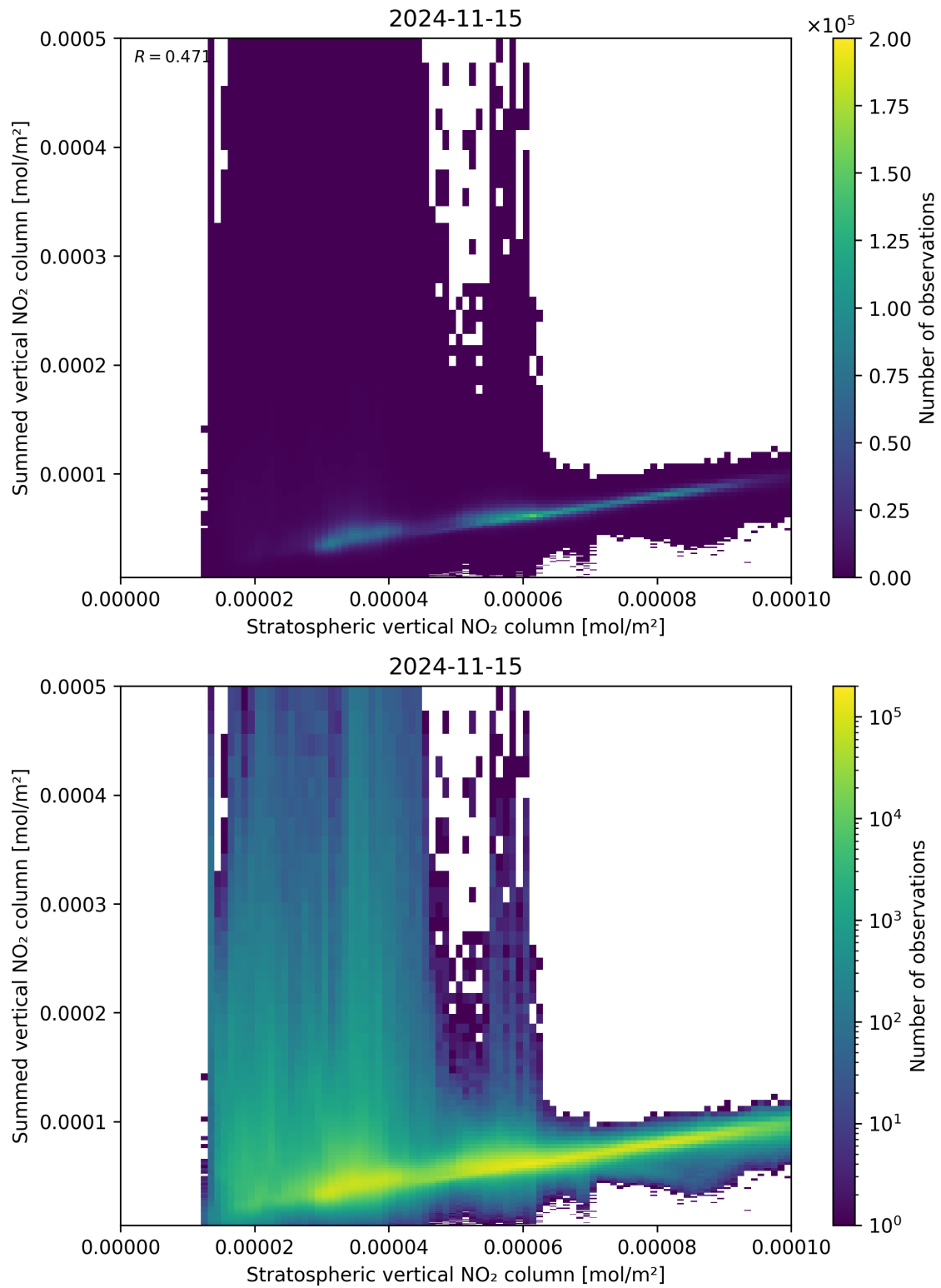
Figure 98: Scatter density plot of “Stratospheric vertical NO 2 column” against “Summed vertical NO 2 column” for 2024-11-14 to 2024-11-16.
