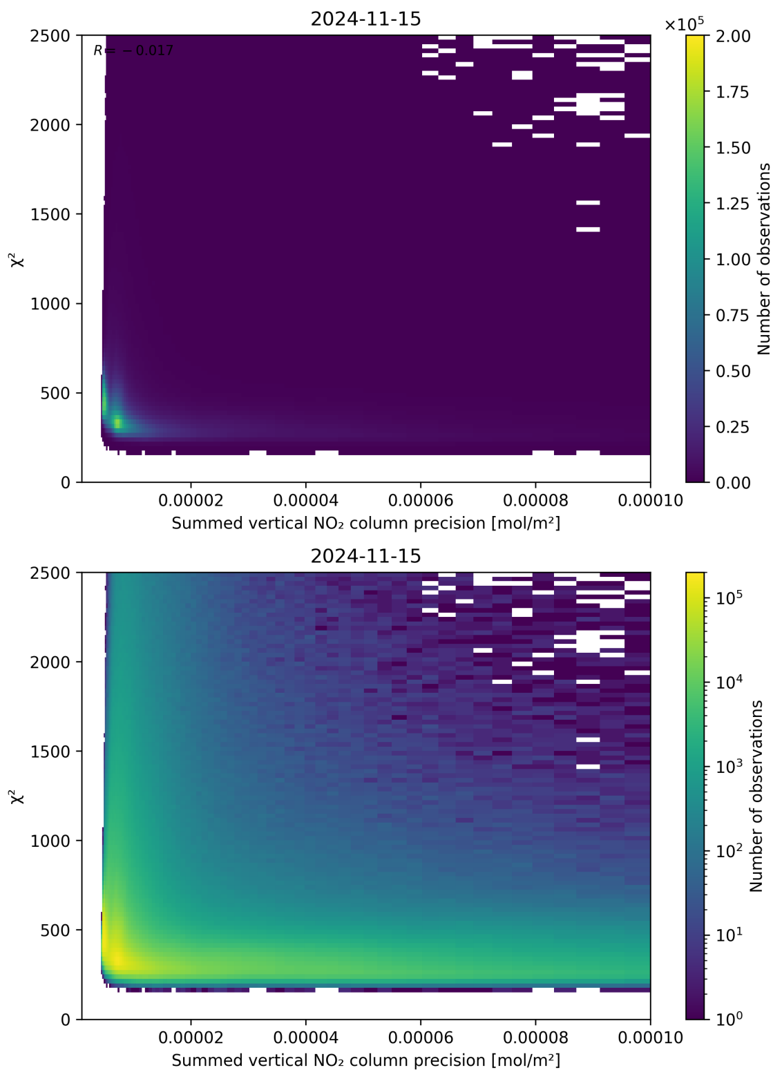
Figure 107: Scatter density plot of “Summed vertical NO 2 column precision” against “ \chi^2 ” for 2024-11-14 to 2024-11-16.
