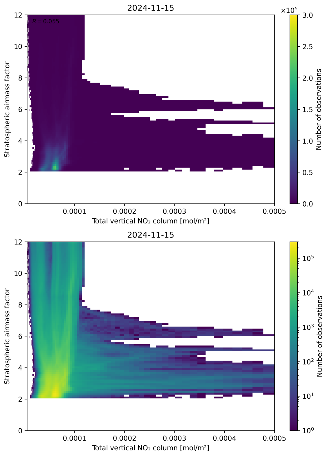
Figure 110: Scatter density plot of “Total vertical NO 2 column” against “Stratospheric airmass factor” for 2024-11-14 to 2024-11-16.
