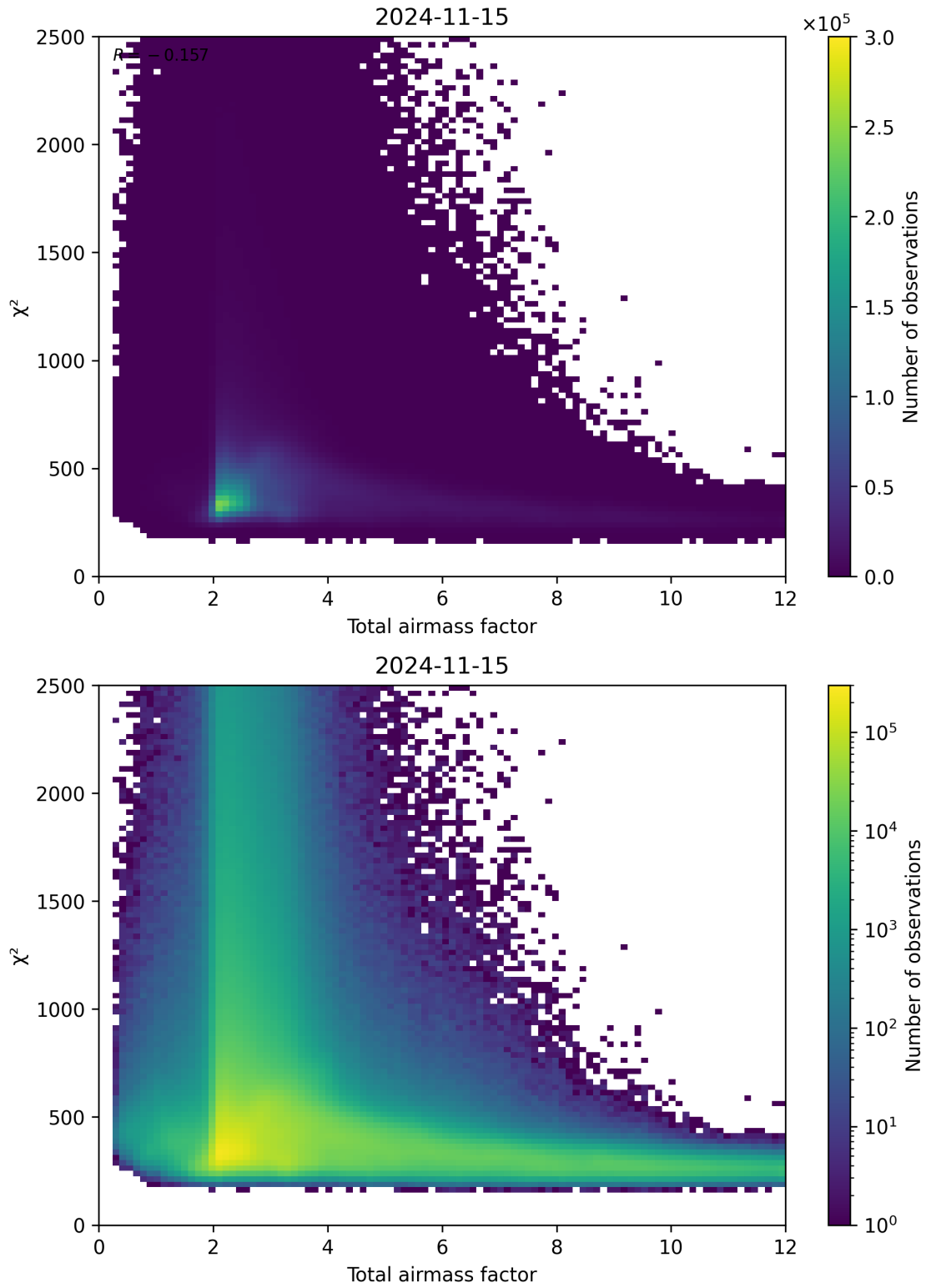
Figure 63: Scatter density plot of “Total airmass factor” against “ \chi^2 ” for 2024-11-14 to 2024-11-16.
