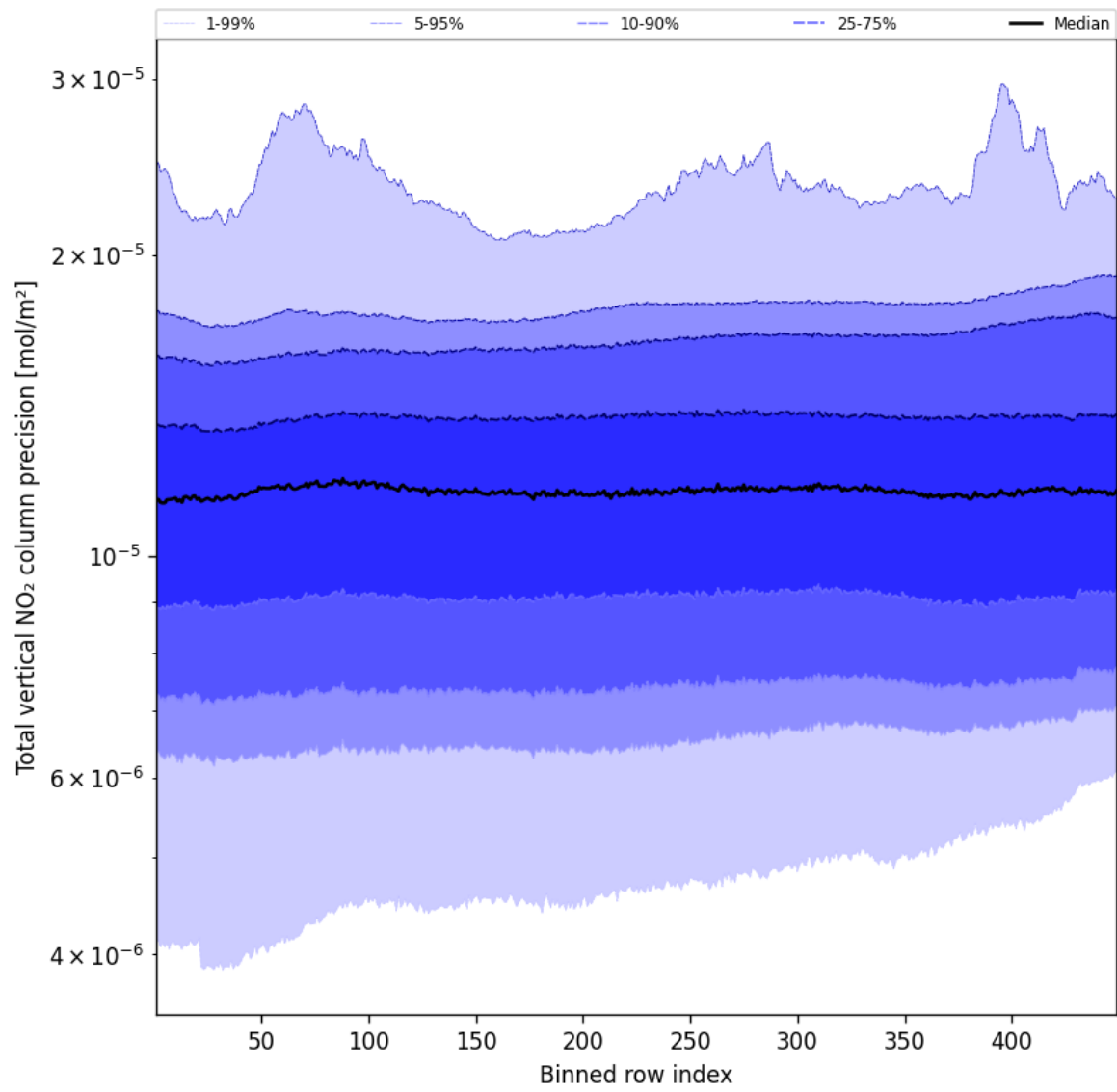
Figure 56: Along track statistics of “Total vertical NO 2 column precision” for 2024-11-14 to 2024-11-16
