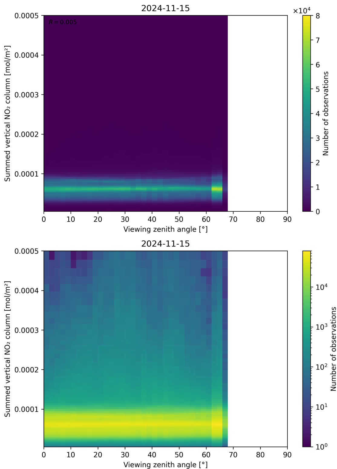
Figure 165: Scatter density plot of “Viewing zenith angle” against “Summed vertical NO 2 column” for 2024-11-14 to 2024-11-16.
