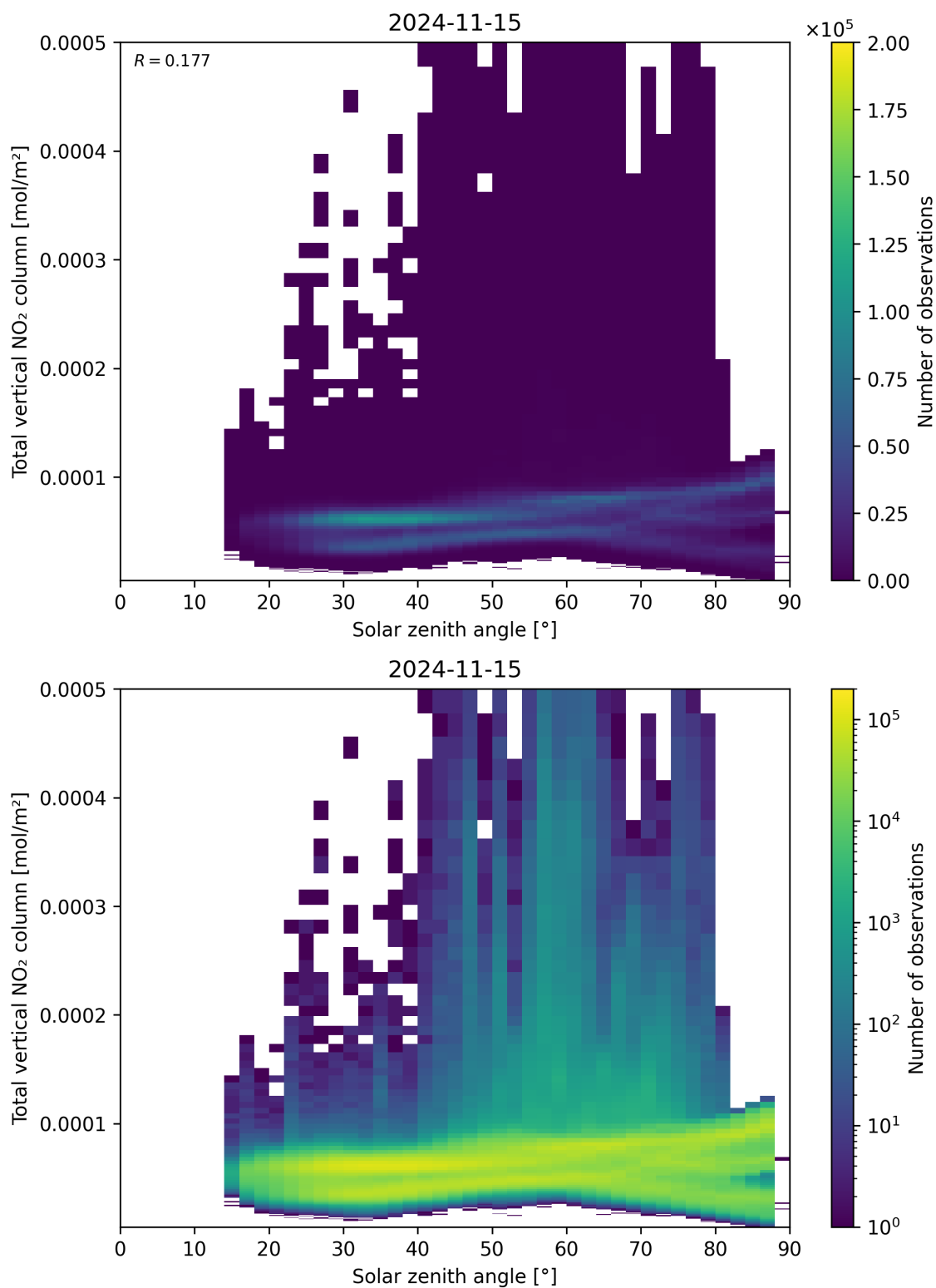
Figure 153: Scatter density plot of “Solar zenith angle” against “Total vertical NO 2 column” for 2024-11-14 to 2024-11-16.
