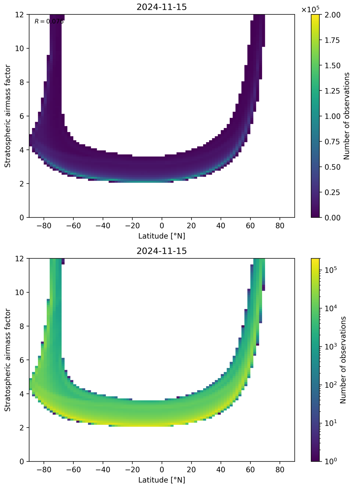
Figure 83: Scatter density plot of “Latitude” against “Stratospheric airmass factor” for 2024-11-14 to 2024-11-16.
