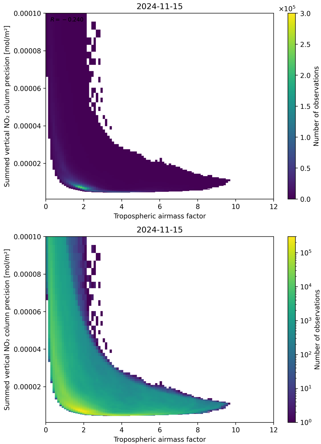
Figure 76: Scatter density plot of “Tropospheric air mass factor” against “Summed vertical NO 2 column precision” for 2024-11-14 to 2024-11-16.
