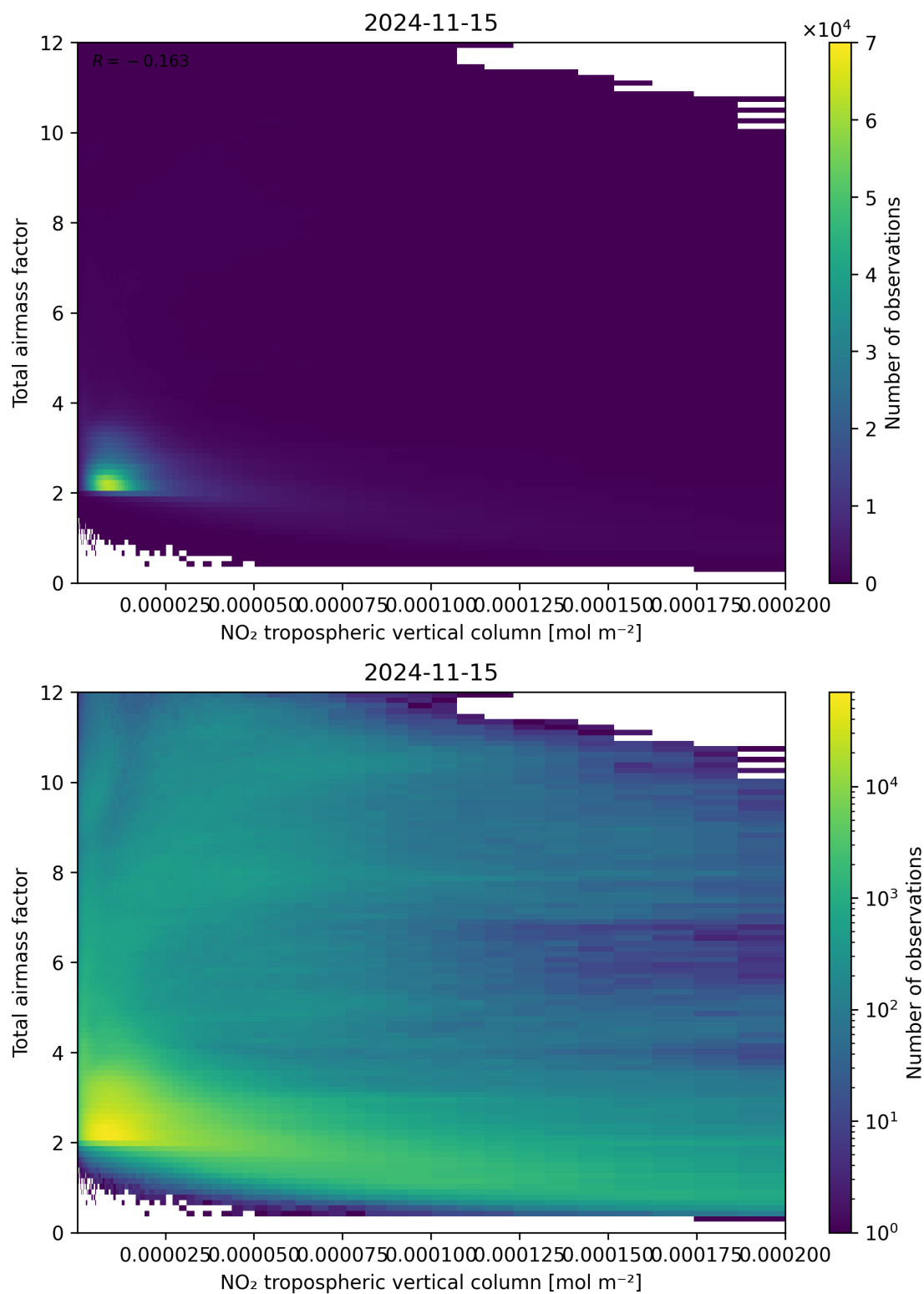
Figure 122: Scatter density plot of “NO 2 tropospheric vertical column” against “Total airmass factor” for 2024-11-14 to 2024-11-16.
