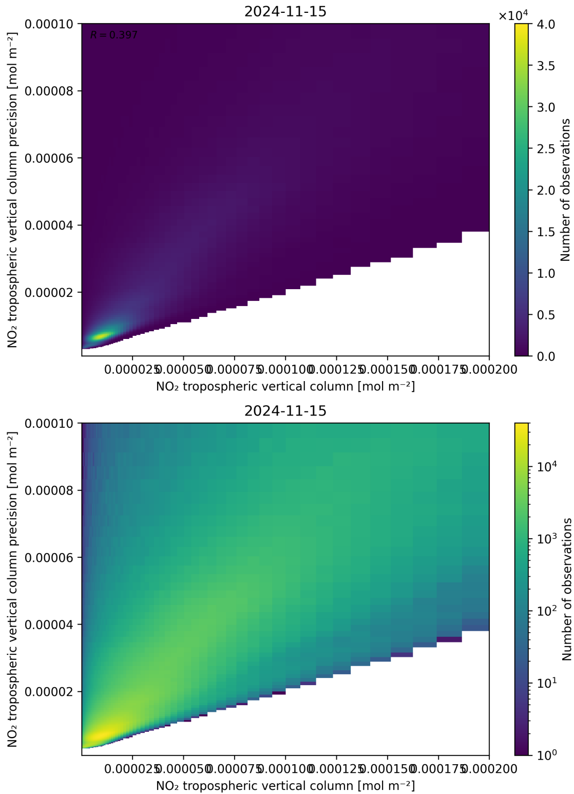
Figure 130: Scatter density plot of “NO 2 tropospheric vertical column” against “NO 2 tropospheric vertical column precision” for 2024-11-14 to 2024-11-16.
