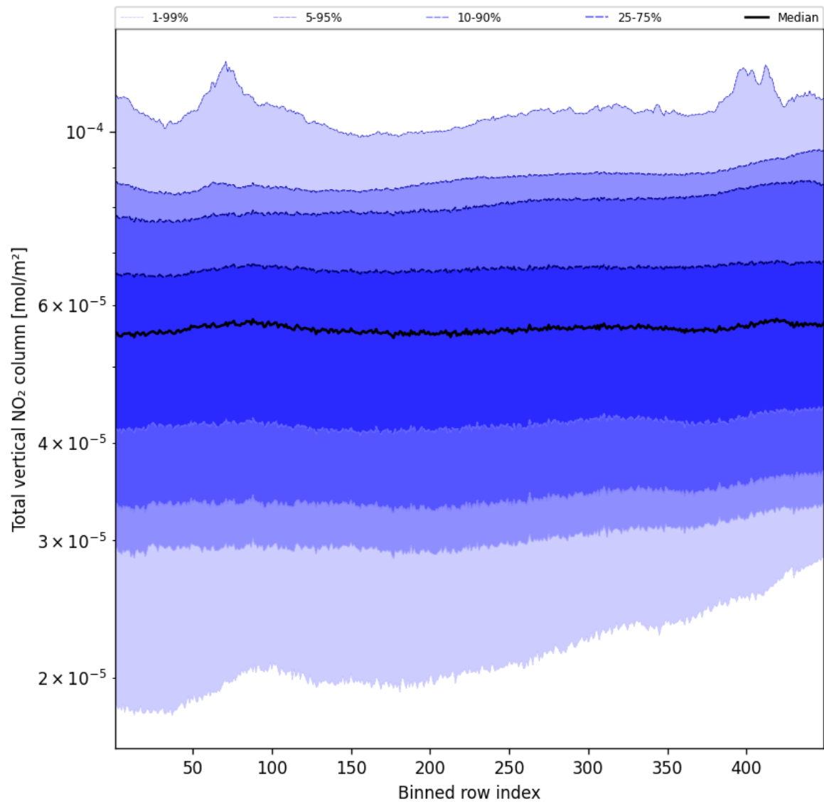
Figure 55: Along track statistics of “Total vertical NO 2 column” for 2024-11-14 to 2024-11-16
