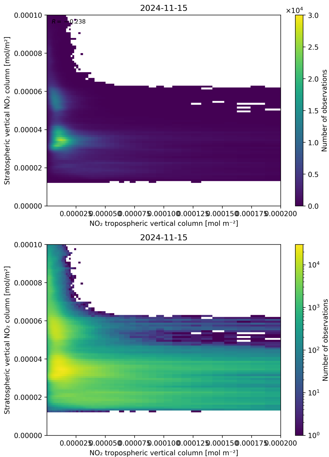
Figure 125: Scatter density plot of “NO 2 tropospheric vertical column” against “Stratospheric vertical NO 2 column” for 2024-11-14 to 2024-11-16.
