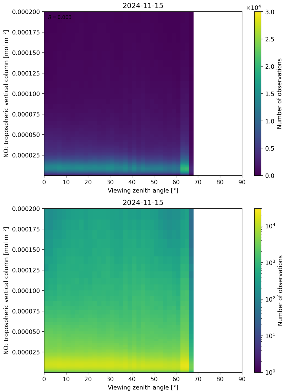
Figure 169: Scatter density plot of “Viewing zenith angle” against “NO 2 tropospheric vertical column” for 2024-11-14 to 2024-11-16.
