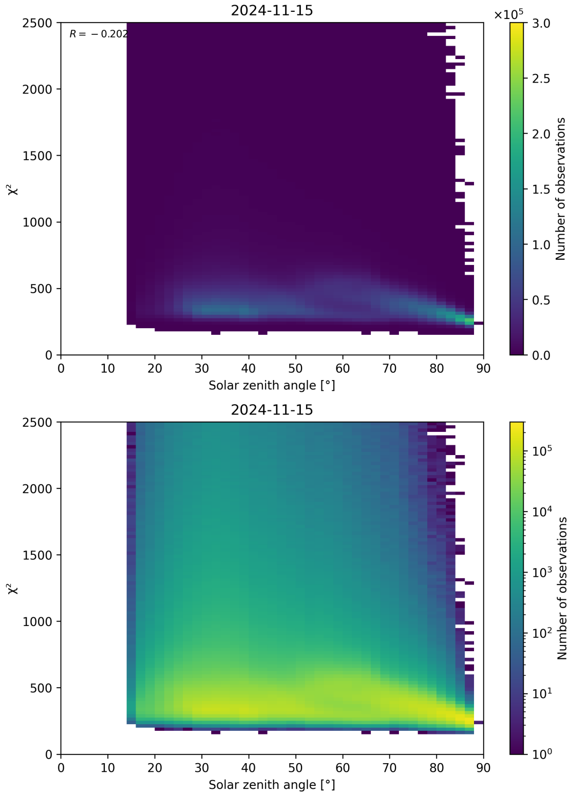
Figure 148: Scatter density plot of “Solar zenith angle” against “ \chi^2 ” for 2024-11-14 to 2024-11-16.
