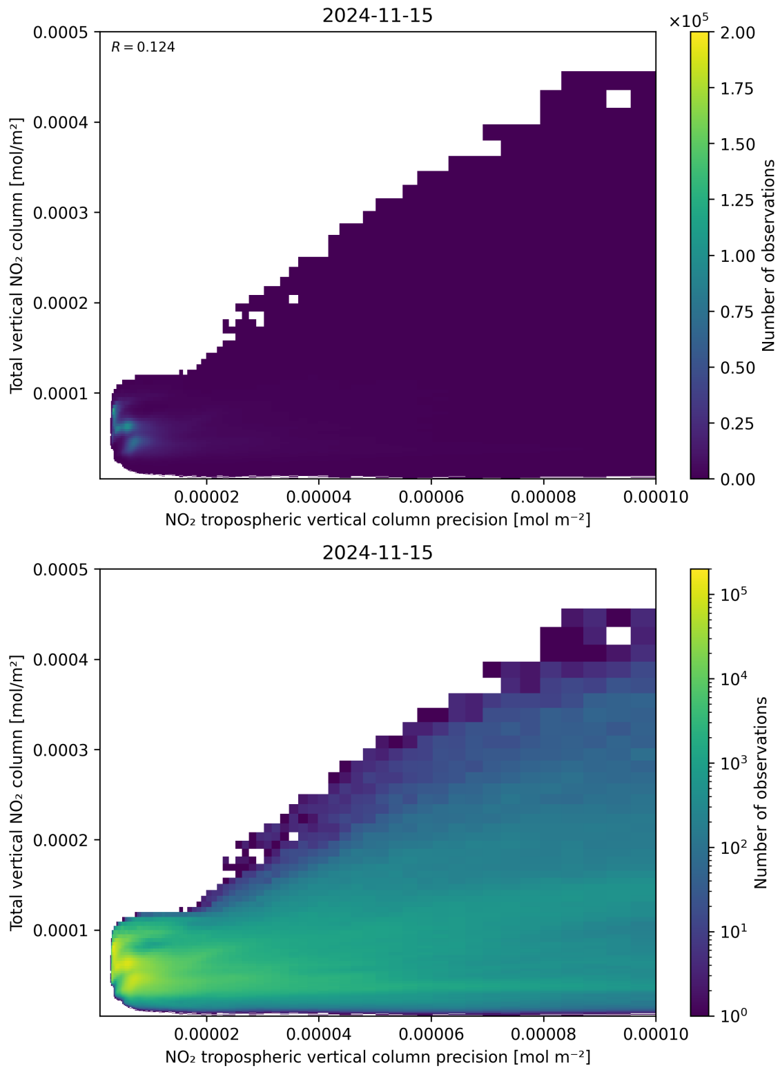
Figure 138: Scatter density plot of “NO 2 tropospheric vertical column precision” against “Total vertical NO 2 column” for 2024-11-14 to 2024-11-16.
