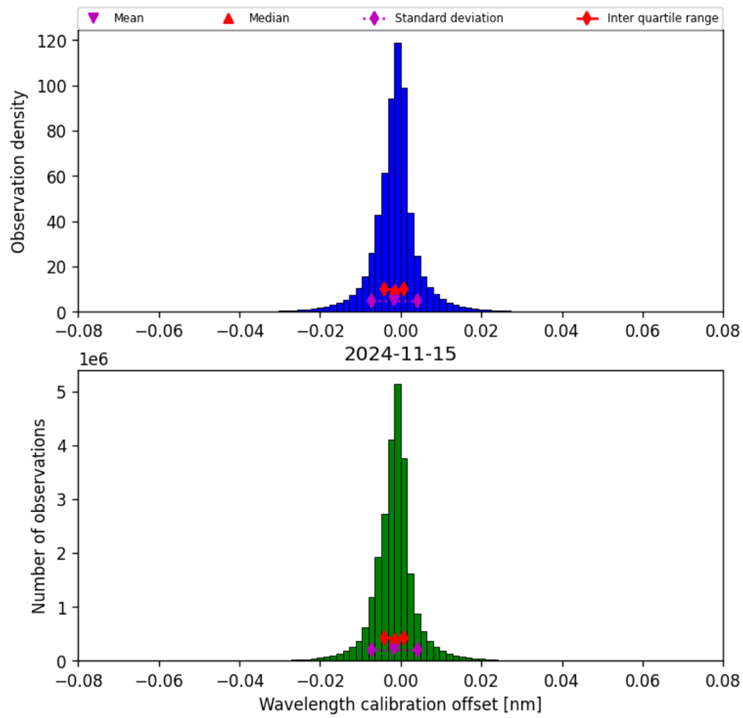
Figure 35: Histogram of “Wavelength calibration offset” for 2024-11-14 to 2024-11-16
