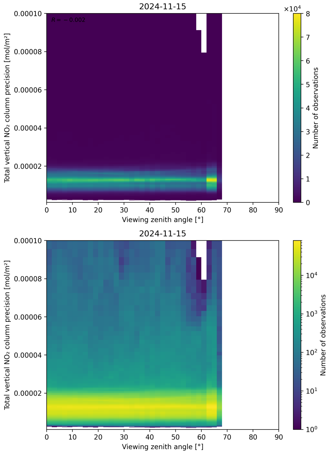
Figure 168: Scatter density plot of “Viewing zenith angle” against “Total vertical NO 2 column precision” for 2024-11-14 to 2024-11-16.
