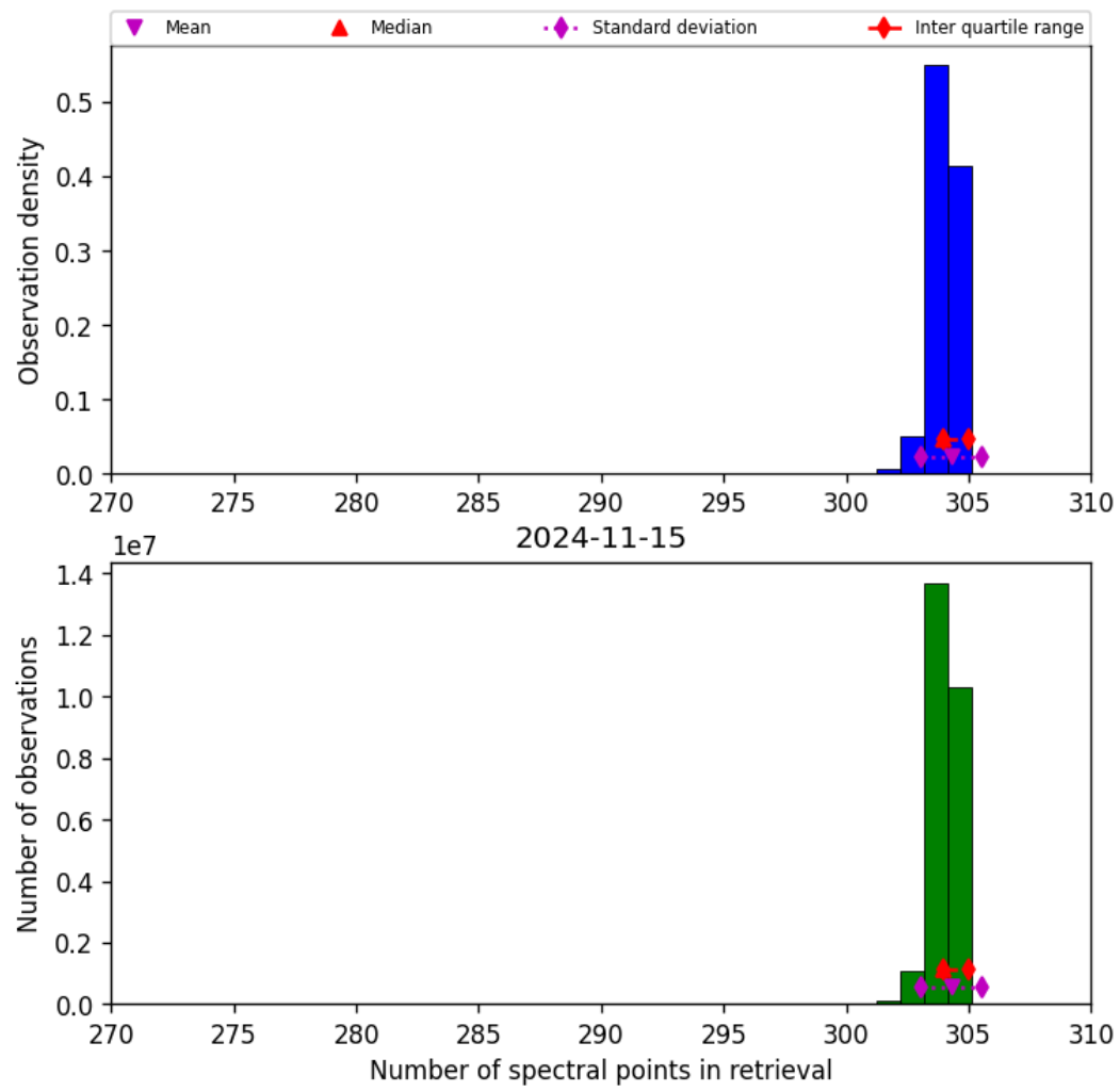
Figure 33: Histogram of “Number of spectral points in retrieval” for 2024-11-14 to 2024-11-16
