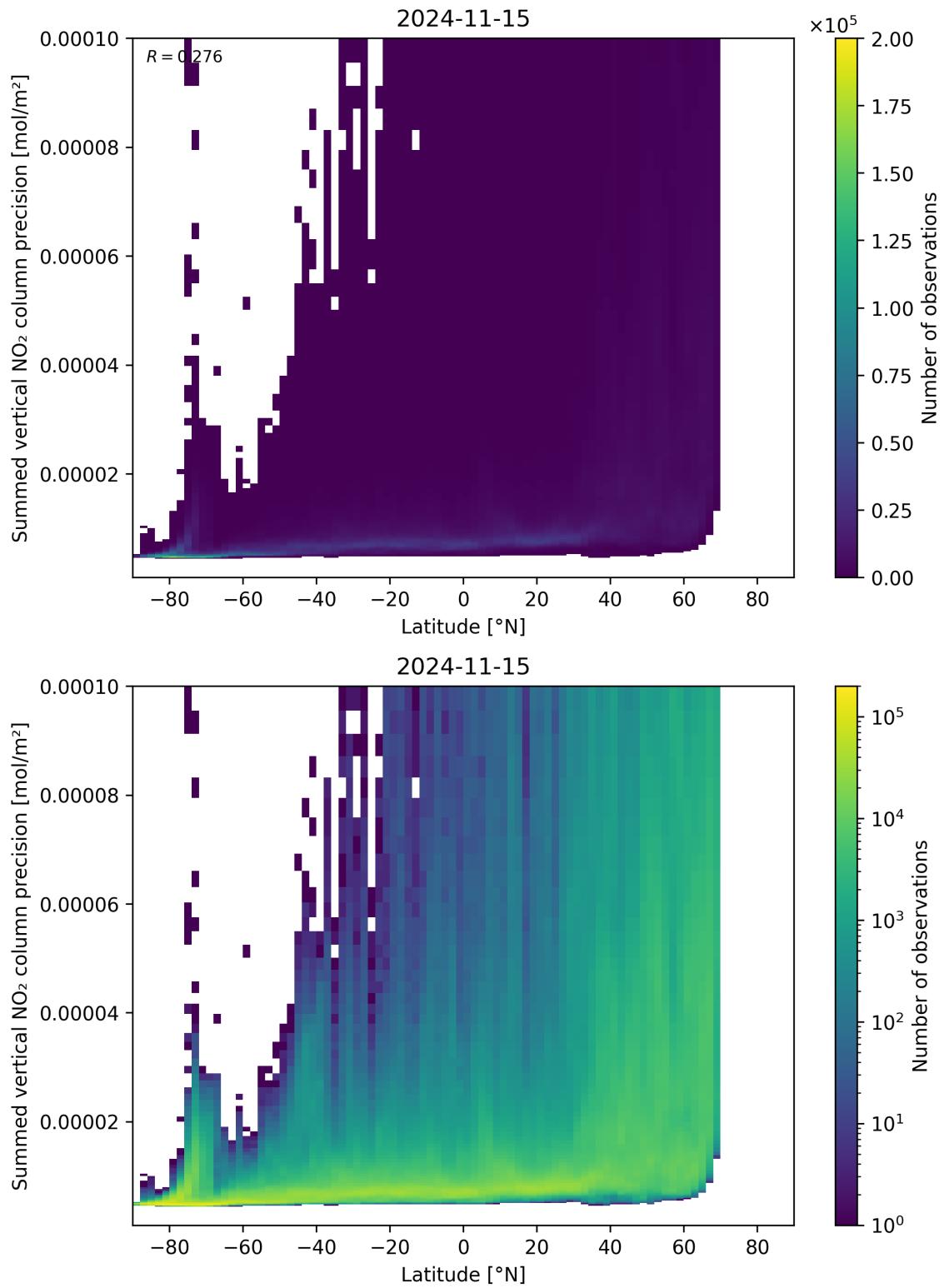
Figure 89: Scatter density plot of “Latitude” against “Summed vertical NO 2 column precision” for 2024-11-14 to 2024-11-16.
