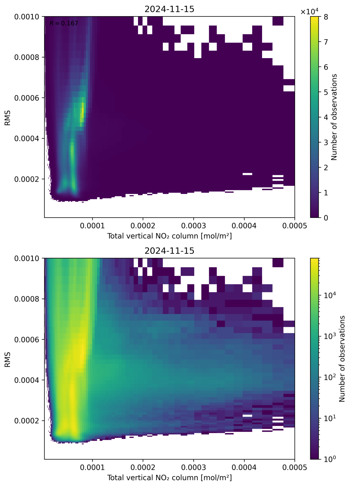
Figure 120: Scatter density plot of “Total vertical NO 2 column” against “RMS” for 2024-11-14 to 2024-11-16.
