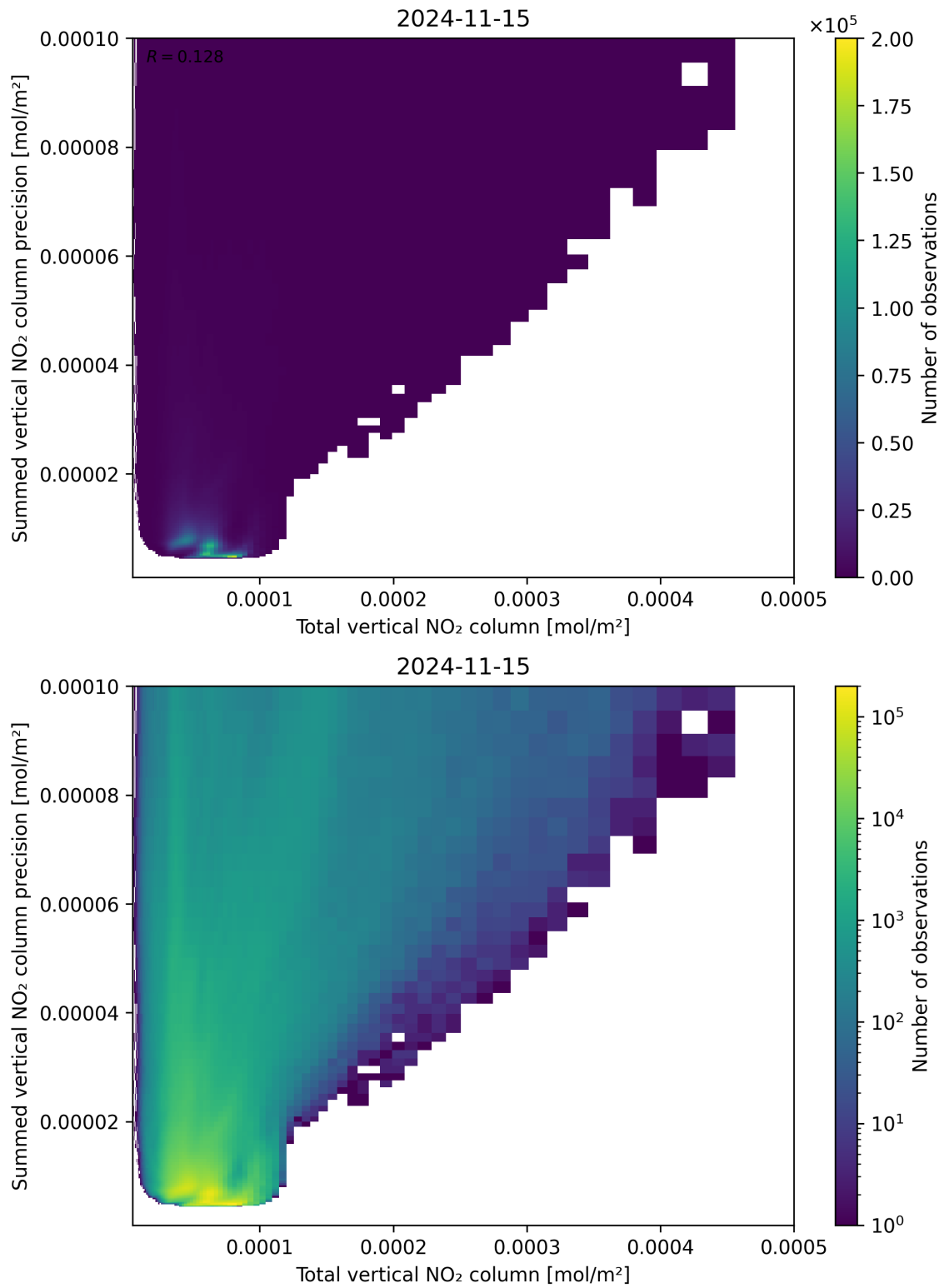
Figure 113: Scatter density plot of “Total vertical NO 2 column” against “Summed vertical NO 2 column precision” for 2024-11-14 to 2024-11-16.
