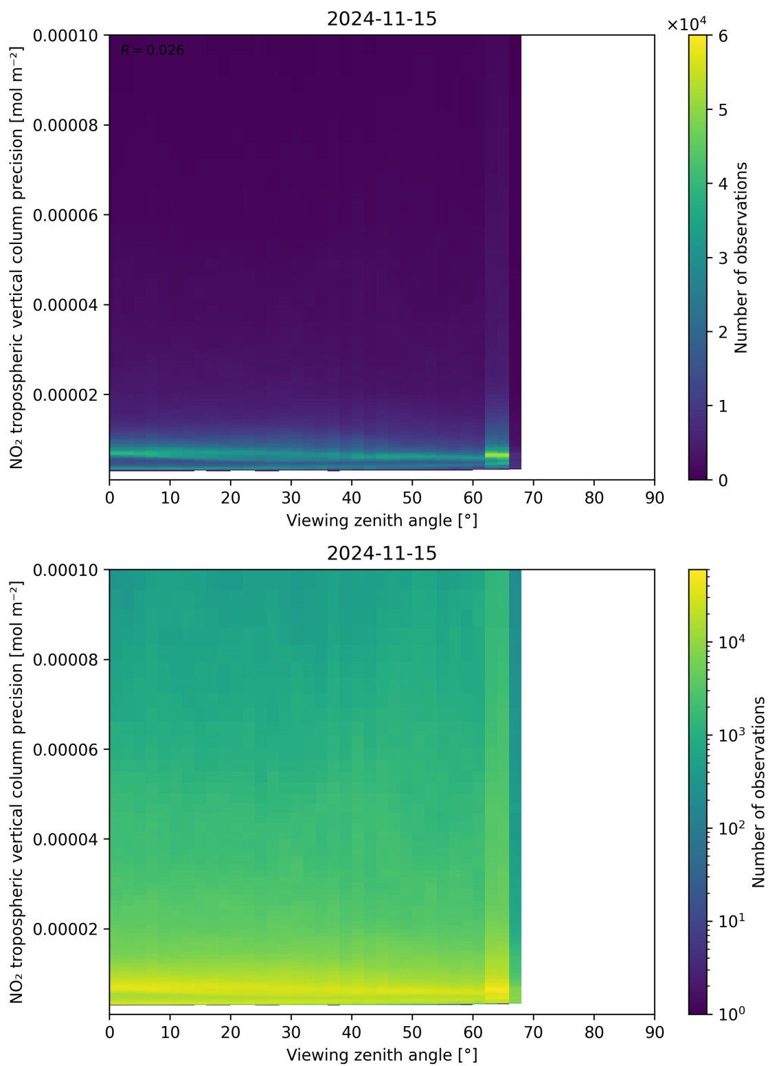
Figure 170: Scatter density plot of “Viewing zenith angle” against “NO 2 tropospheric vertical column precision” for 2024-11-14 to 2024-11-16.
