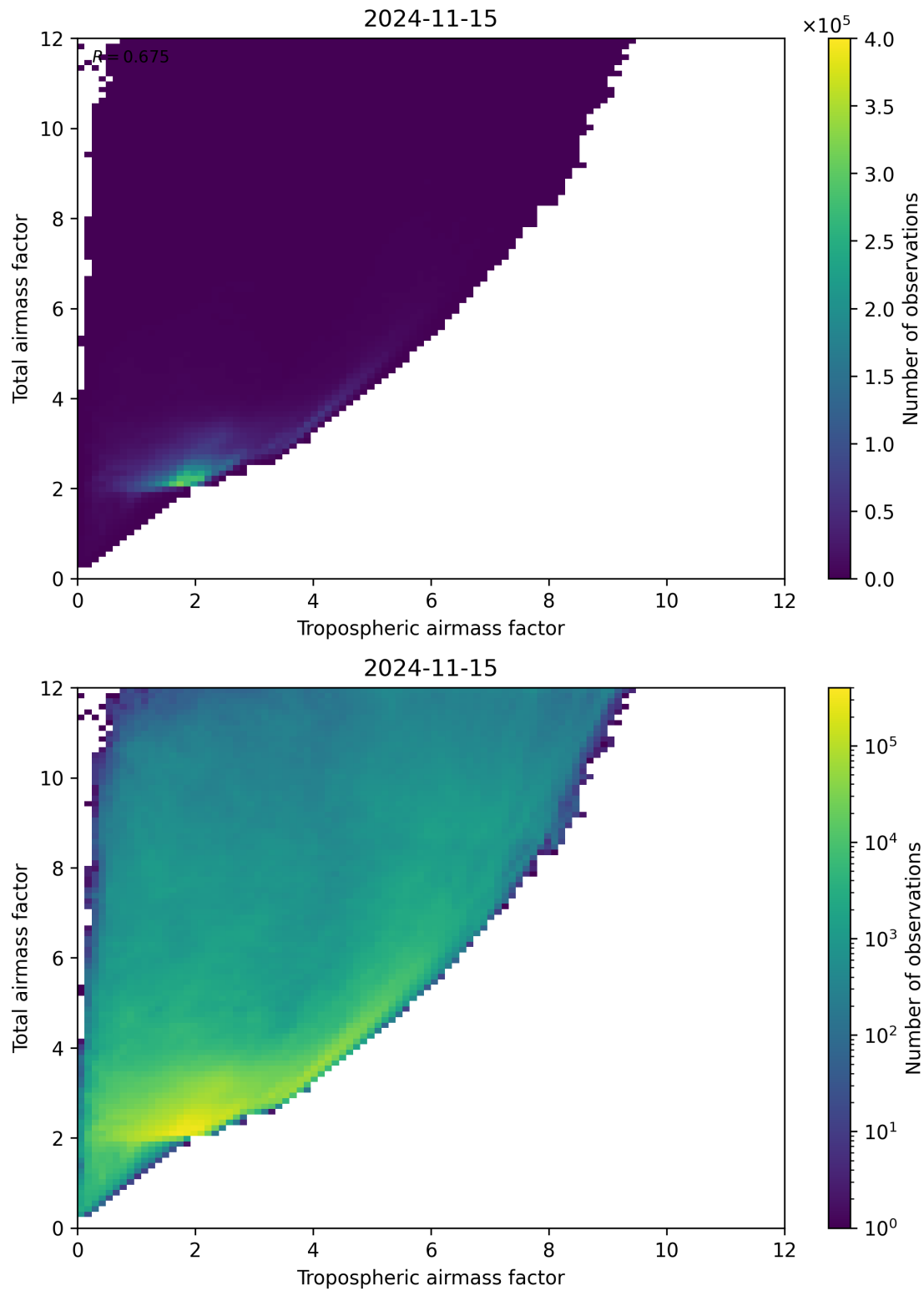
Figure 72: Scatter density plot of “Tropospheric airmass factor” against “Total airmass factor” for 2024-11-14 to 2024-11-16.
