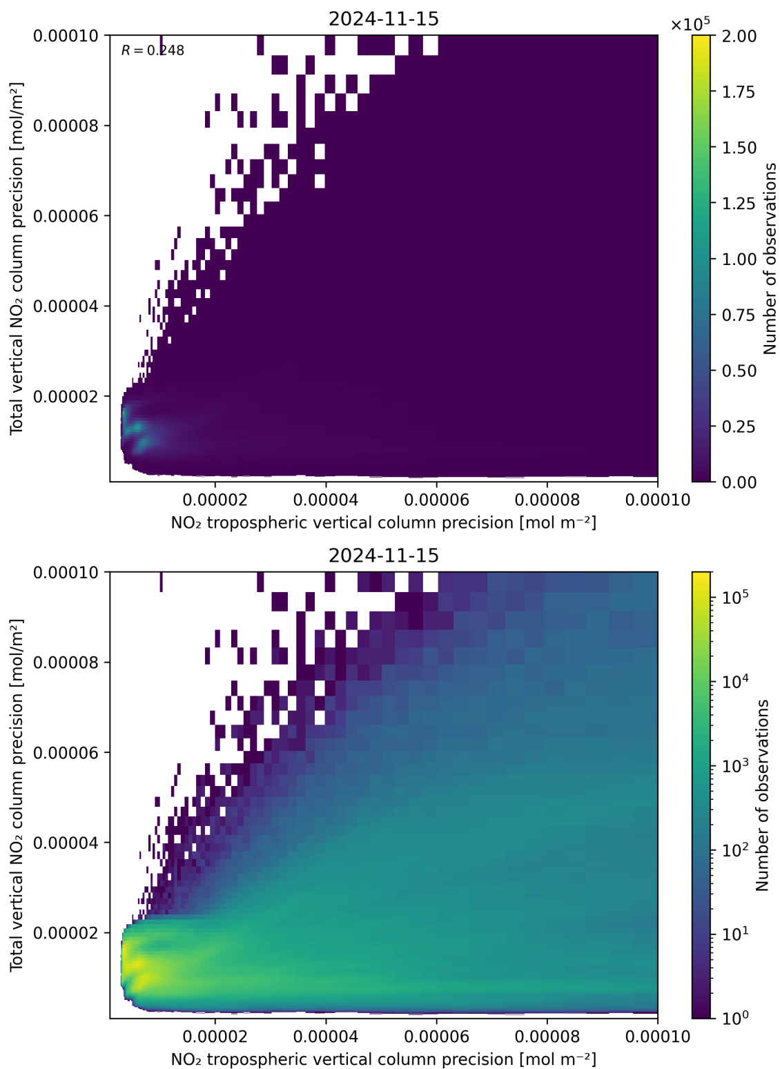
Figure 139: Scatter density plot of “NO 2 tropospheric vertical column precision” against “Total vertical NO 2 column precision” for 2024-11-14 to 2024-11-16.
