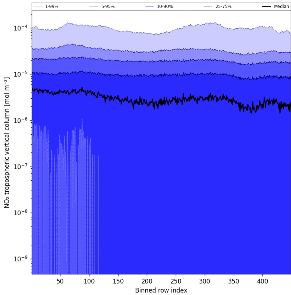
Figure 46: Along track statistics of “NO 2 tropospheric vertical column” for 2024-11-14 to 2024-11-16
