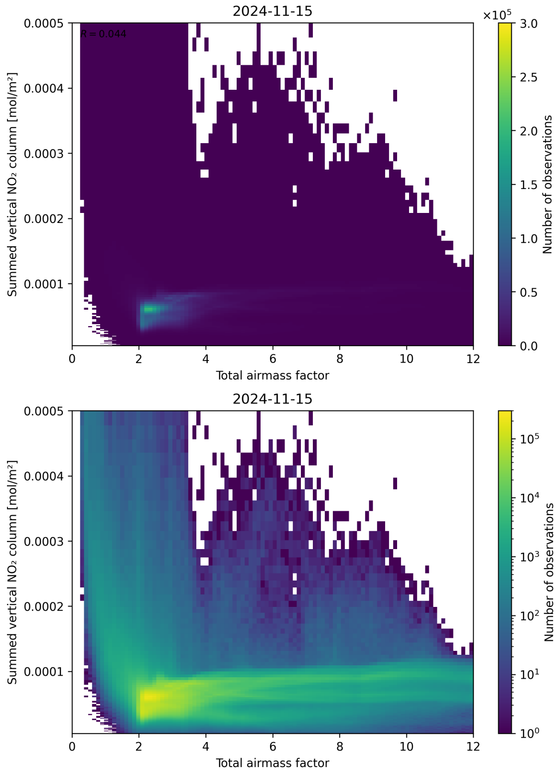
Figure 65: Scatter density plot of “Total airmass factor” against “Summed vertical NO 2 column” for 2024-11-14 to 2024-11-16.
