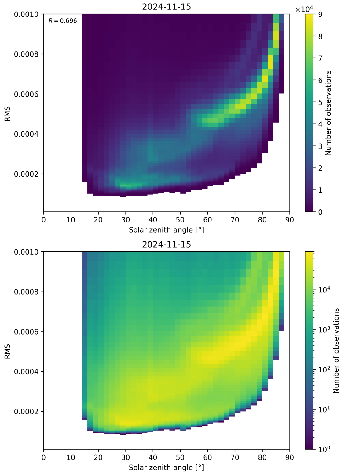
Figure 157: Scatter density plot of “Solar zenith angle” against “RMS” for 2024-11-14 to 2024-11-16.
