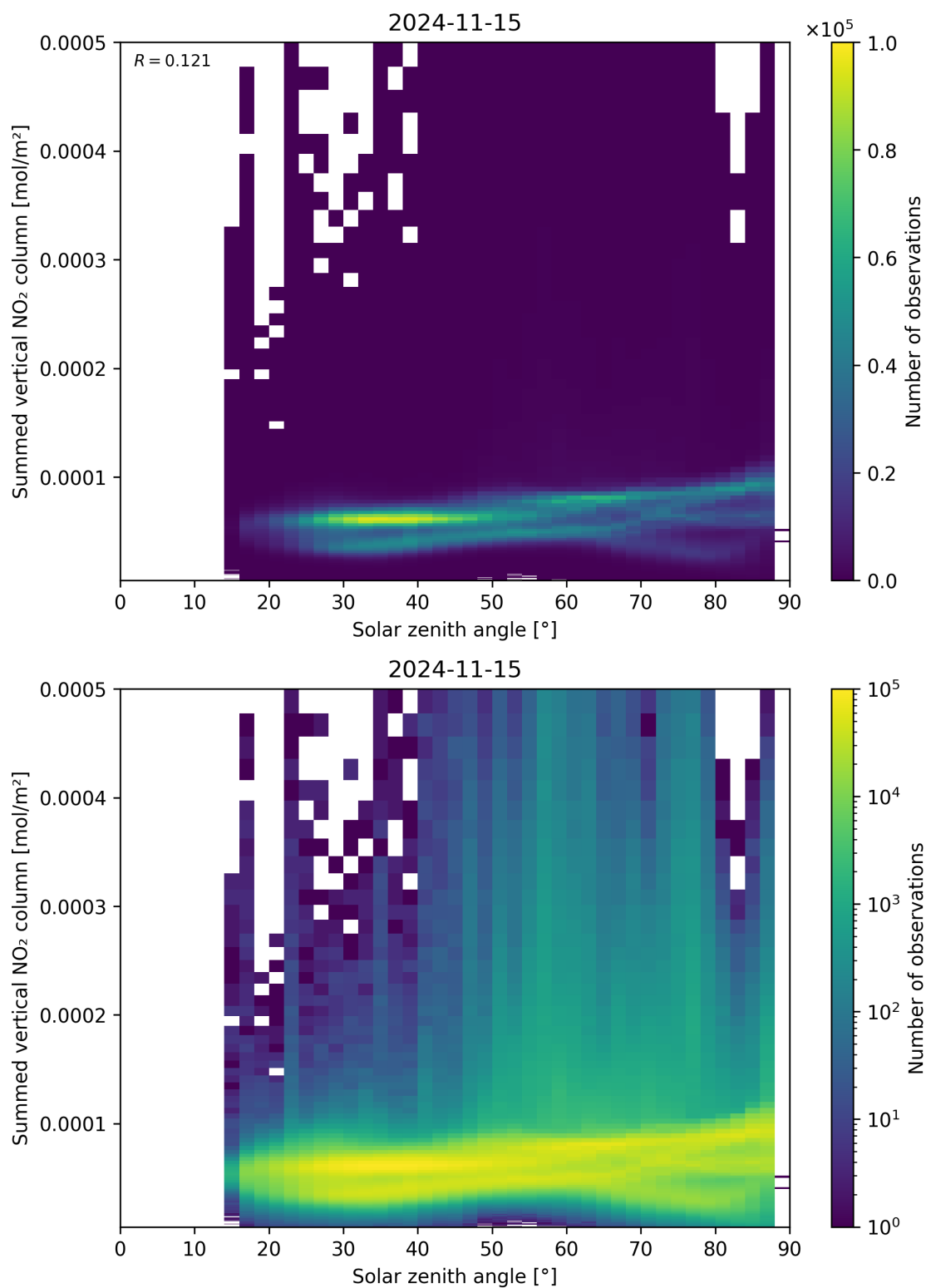
Figure 151: Scatter density plot of “Solar zenith angle” against “Summed vertical NO 2 column” for 2024-11-14 to 2024-11-16.
