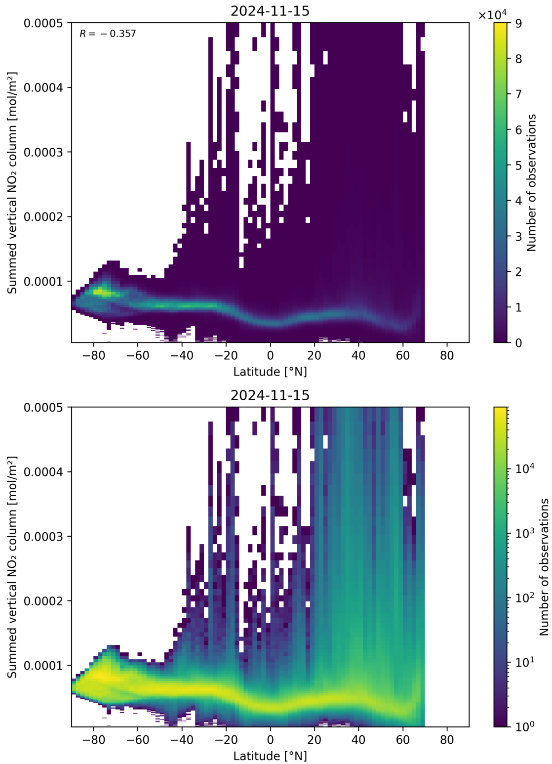
Figure 88: Scatter density plot of “Latitude” against “Summed vertical NO 2 column” for 2024-11-14 to 2024-11-16.
