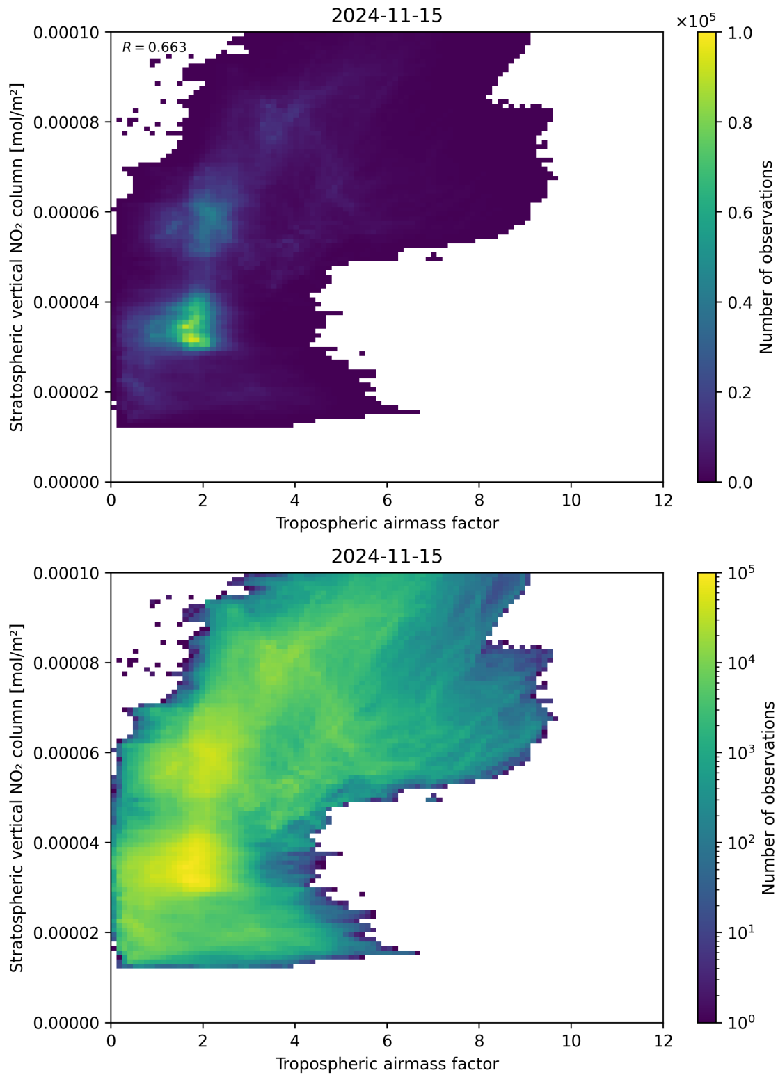
Figure 74: Scatter density plot of “Tropospheric air mass factor” against “Stratospheric vertical NO 2 column” for 2024-11-14 to 2024-11-16.
