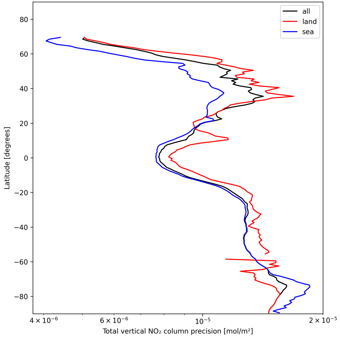
Figure 22: Zonal average of “Total vertical NO 2 column precision” for 2024-11-15 to 2024-11-17.
