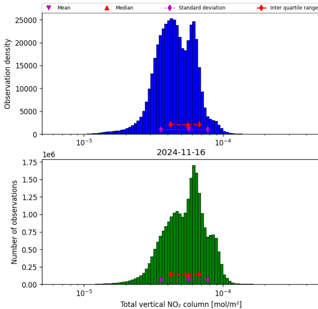
Figure 38: Histogram of “Total vertical NO 2 column” for 2024-11-15 to 2024-11-17
