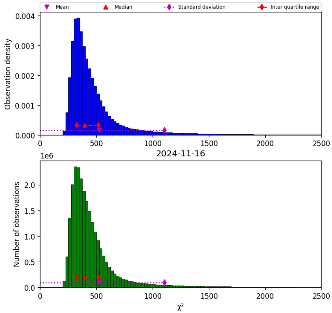
Figure 42: Histogram of “ \chi^2 ” for 2024-11-15 to 2024-11-17
