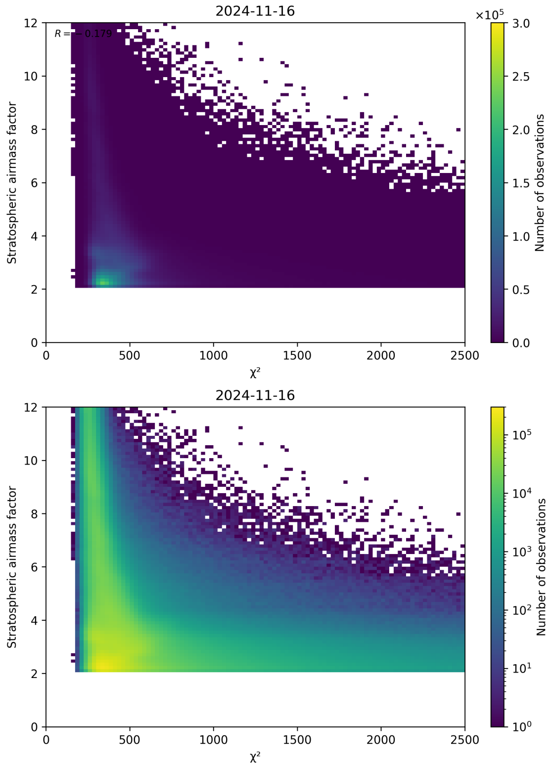
Figure 81: Scatter density plot of “ \chi^2 ” against “Stratospheric airmass factor” for 2024-11-15 to 2024-11-17.
