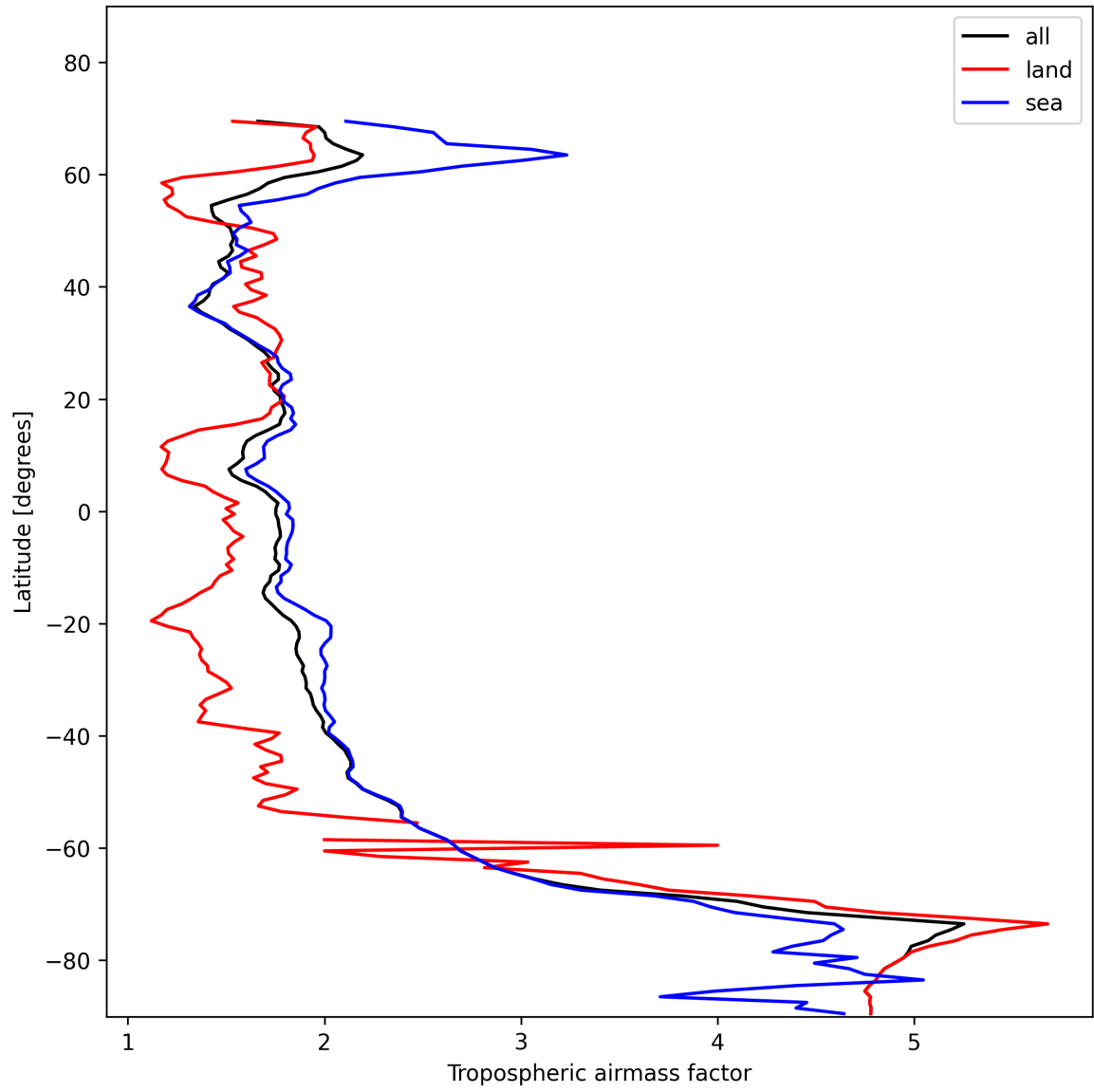
Figure 14: Zonal average of “Tropospheric airmass factor” for 2024-11-15 to 2024-11-17.
