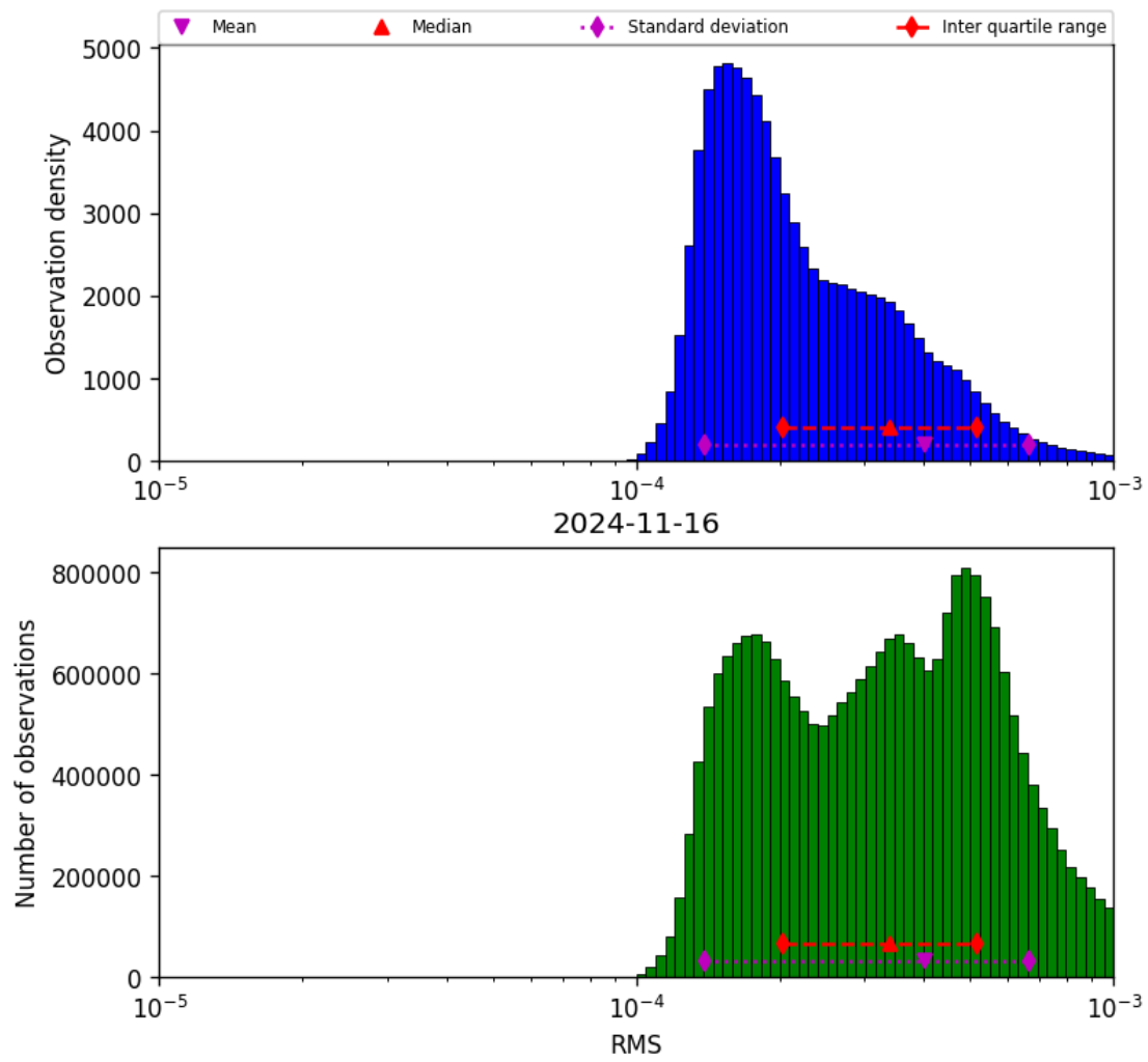
Figure 43: Histogram of “RMS” for 2024-11-15 to 2024-11-17
