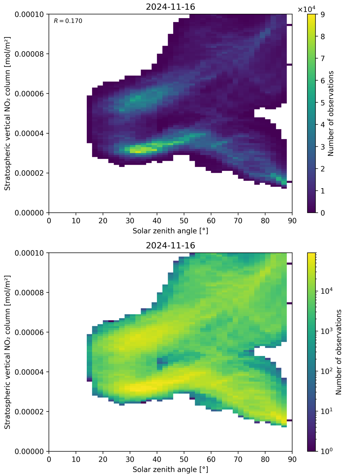
Figure 150: Scatter density plot of “Solar zenith angle” against “Stratospheric vertical NO 2 column” for 2024-11-15 to 2024-11-17.
