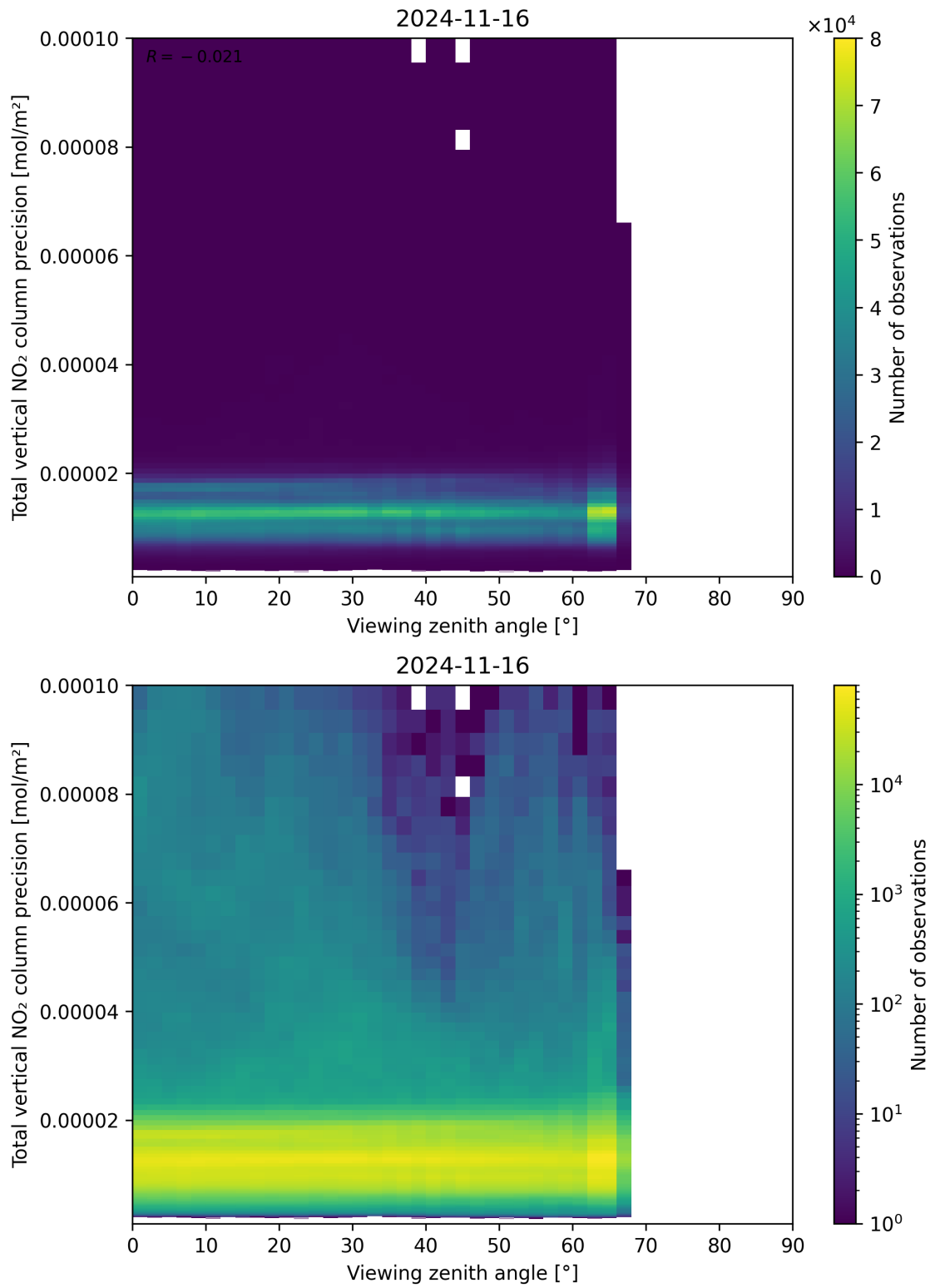
Figure 168: Scatter density plot of “Viewing zenith angle” against “Total vertical NO 2 column precision” for 2024-11-15 to 2024-11-17.
