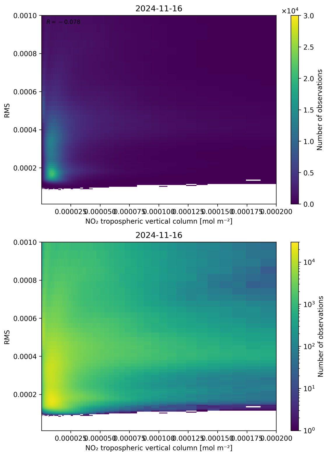
Figure 142: Scatter density plot of “NO 2 tropospheric vertical column” against “RMS” for 2024-11-15 to 2024-11-17.
