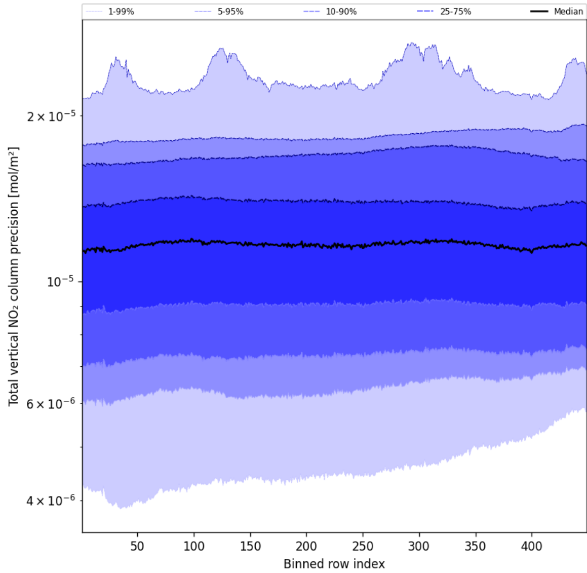
Figure 56: Along track statistics of “Total vertical NO 2 column precision” for 2024-11-15 to 2024-11-17
