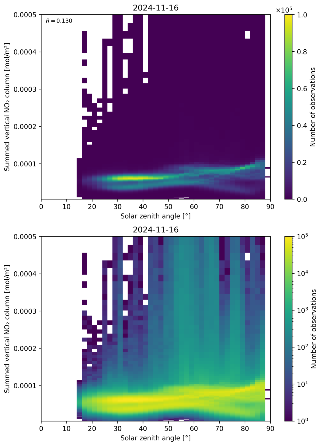
Figure 151: Scatter density plot of “Solar zenith angle” against “Summed vertical NO 2 column” for 2024-11-15 to 2024-11-17.
