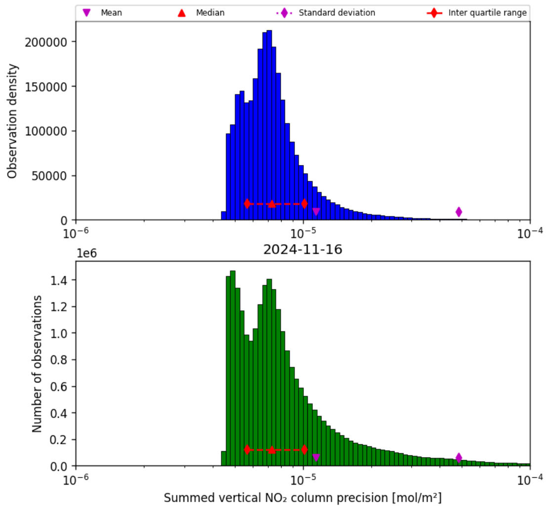
Figure 41: Histogram of "Summed vertical NO 2 column precision" for 2024-11-15 to 2024-11-17
