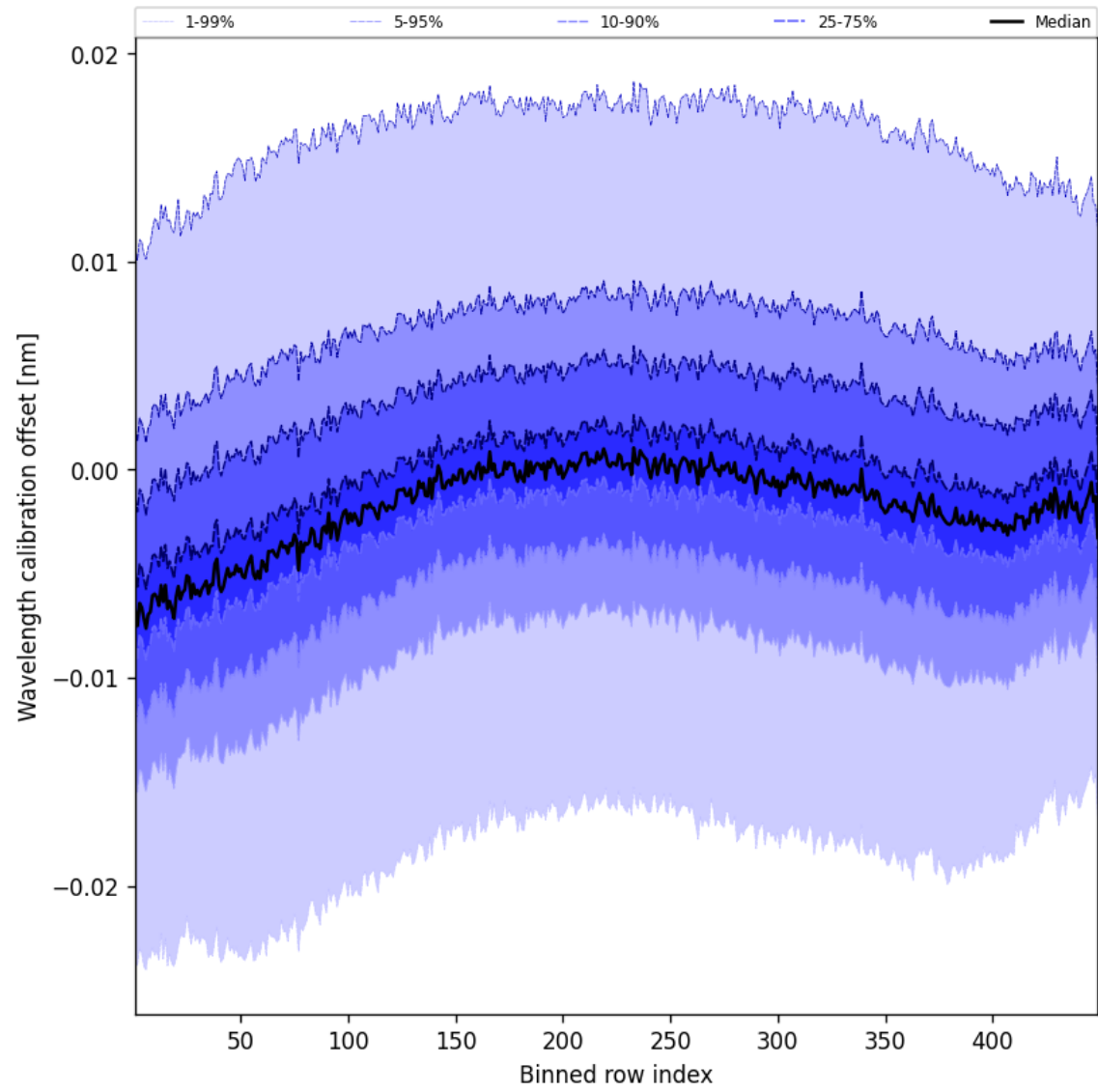
Figure 52: Along track statistics of “Wavelength calibration offset” for 2024-11-15 to 2024-11-17
