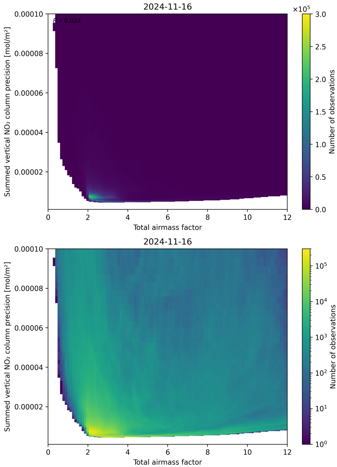
Figure 66: Scatter density plot of “Total airmass factor” against “Summed vertical NO 2 column precision” for 2024-11-15 to 2024-11-17.
