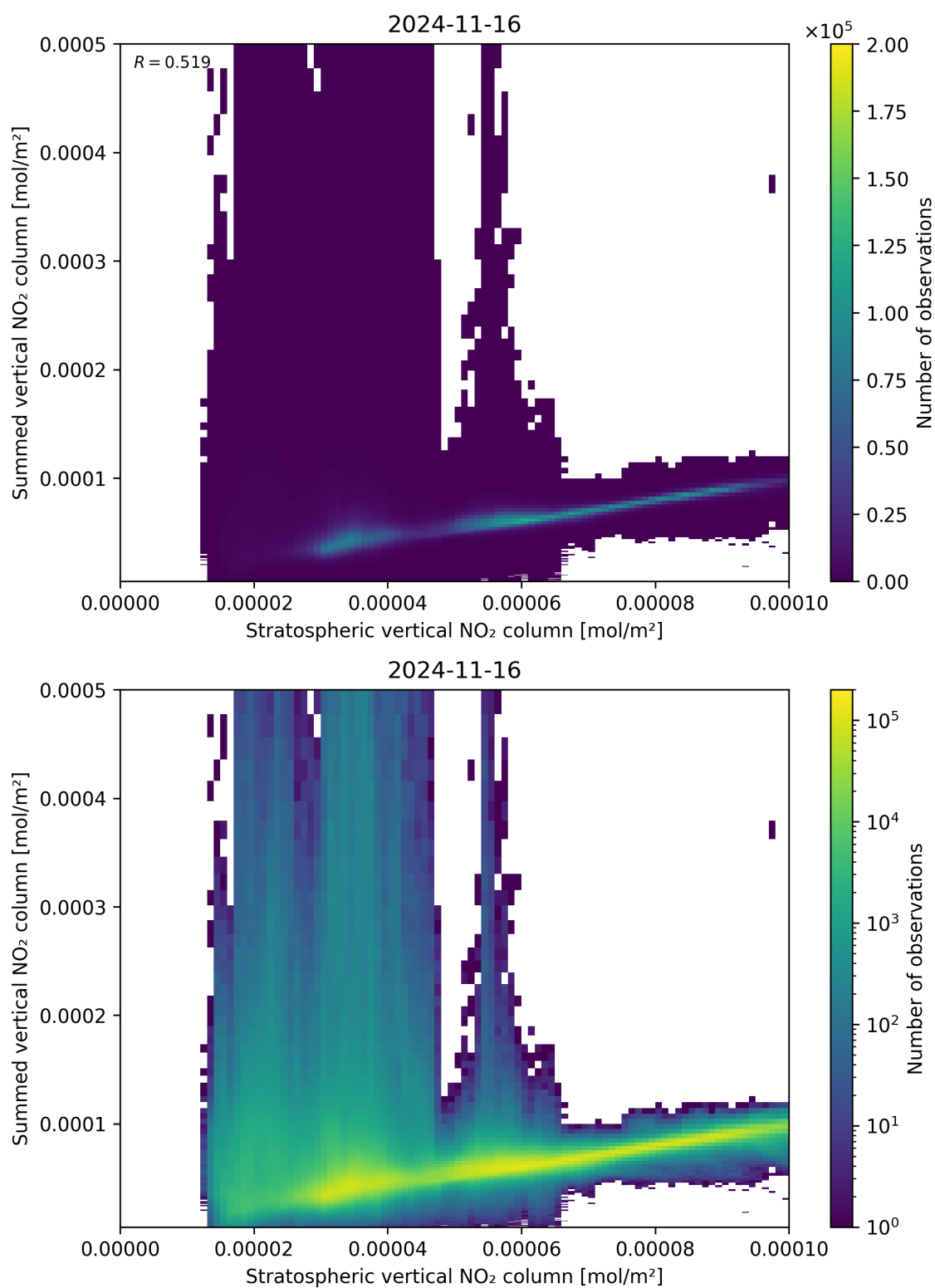
Figure 98: Scatter density plot of “Stratospheric vertical NO 2 column” against “Summed vertical NO 2 column” for 2024-11-15 to 2024-11-17.
