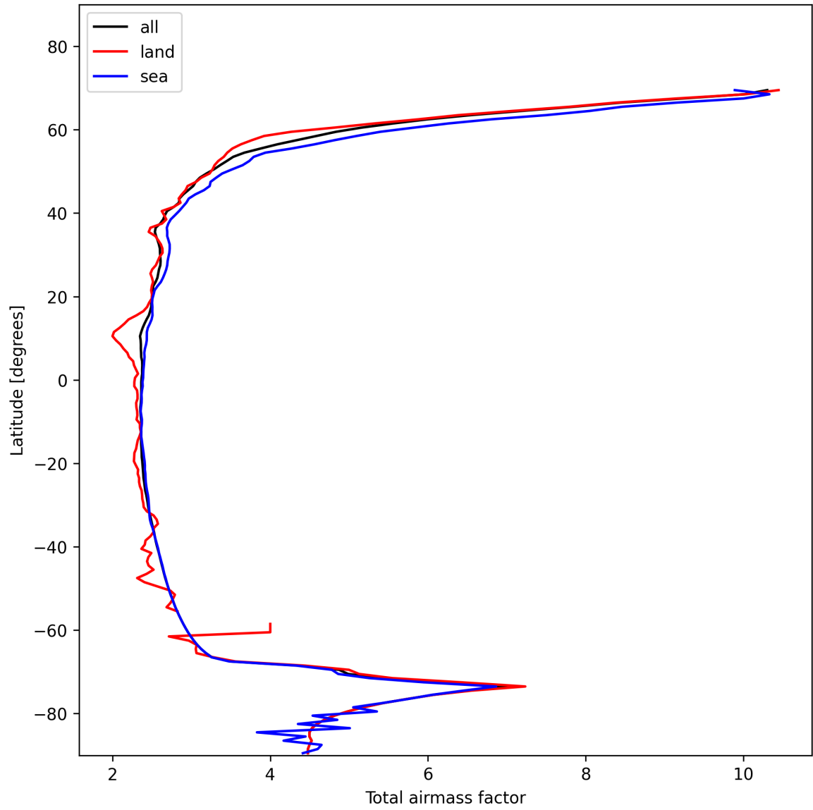
Figure 15: Zonal average of “Total airmass factor” for 2024-11-15 to 2024-11-17.
