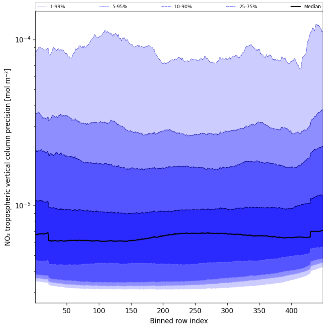
Figure 47: Along track statistics of “NO 2 tropospheric vertical column precision” for 2024-11-15 to 2024-11-17
