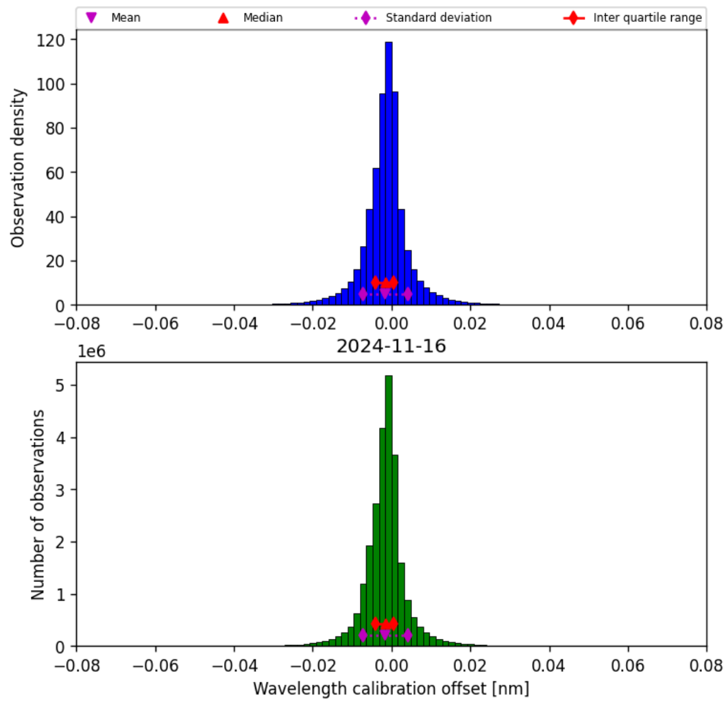
Figure 35: Histogram of “Wavelength calibration offset” for 2024-11-15 to 2024-11-17
