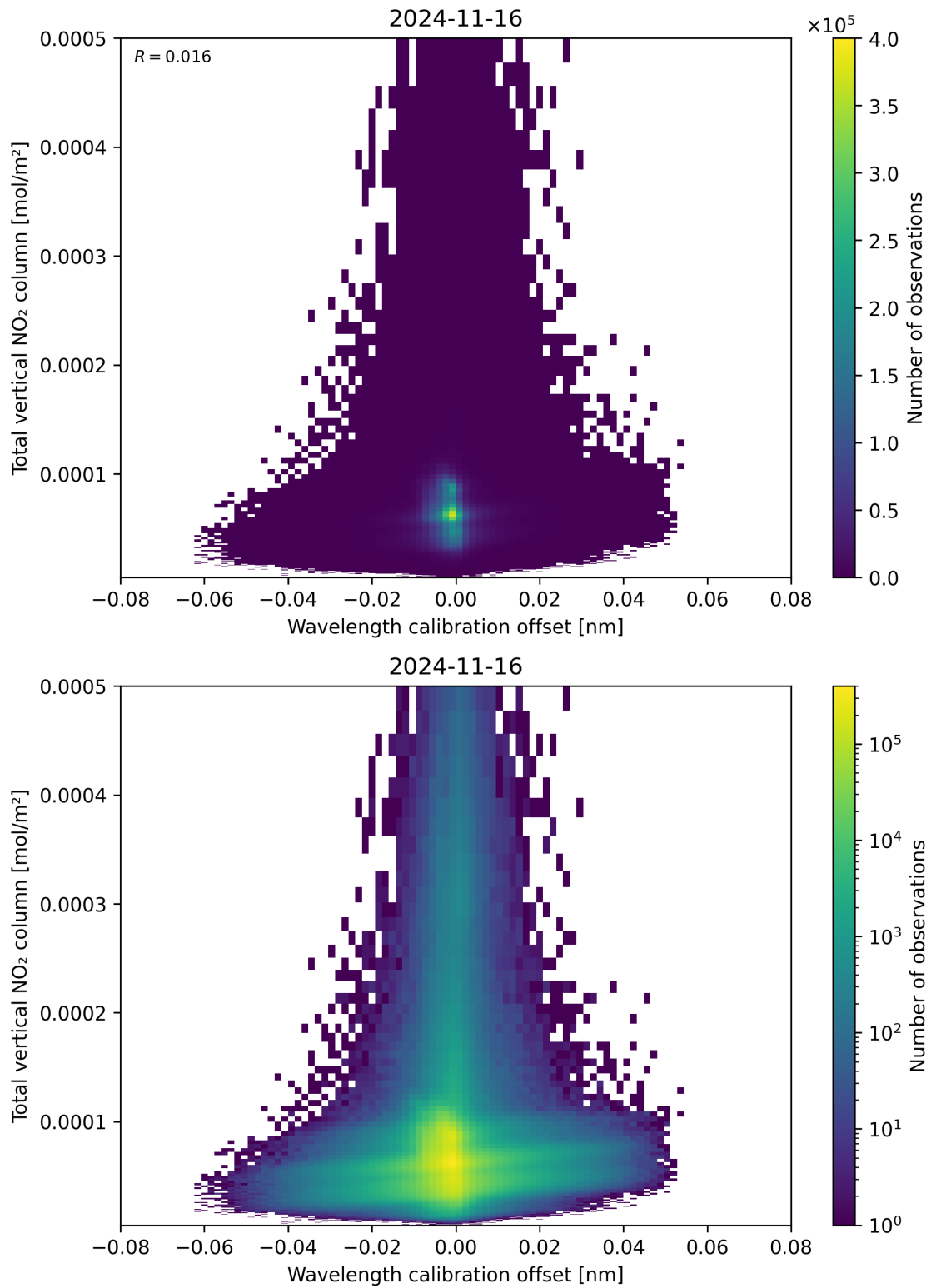
Figure 179: Scatter density plot of “Wavelength calibration offset” against “Total vertical NO 2 column” for 2024-11-15 to 2024-11-17.
