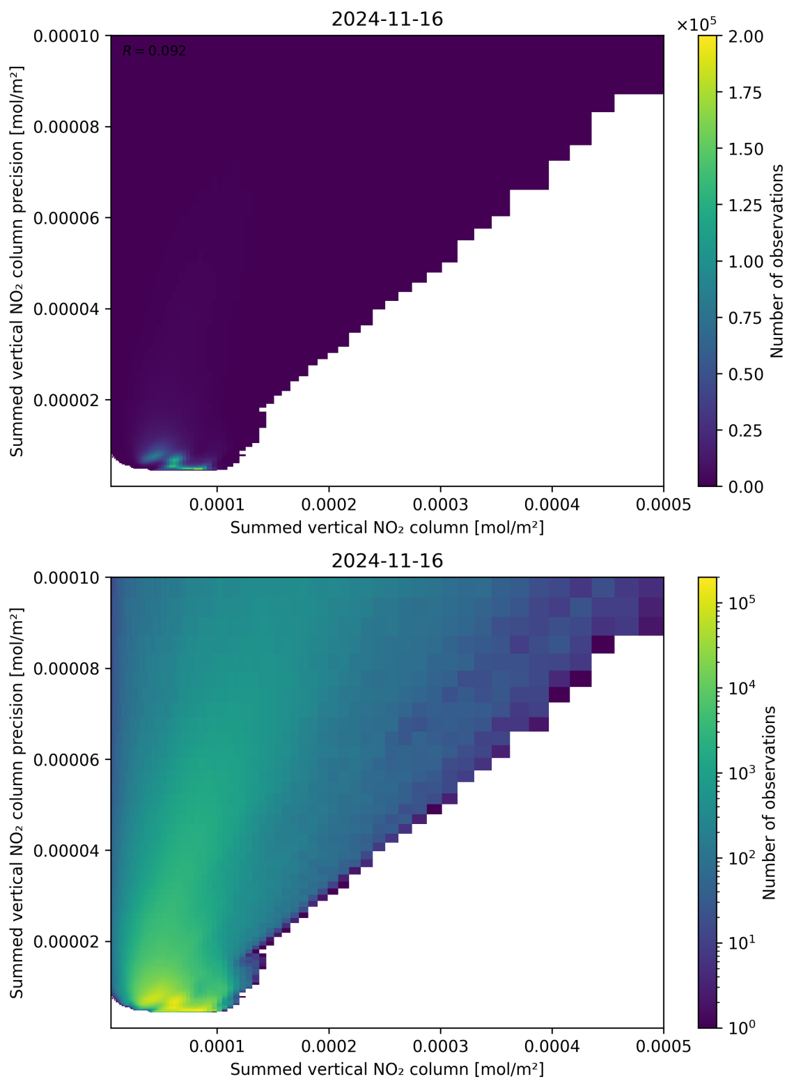
Figure 105: Scatter density plot of “Summed vertical NO 2 column” against “Summed vertical NO 2 column precision” for 2024-11-15 to 2024-11-17.
