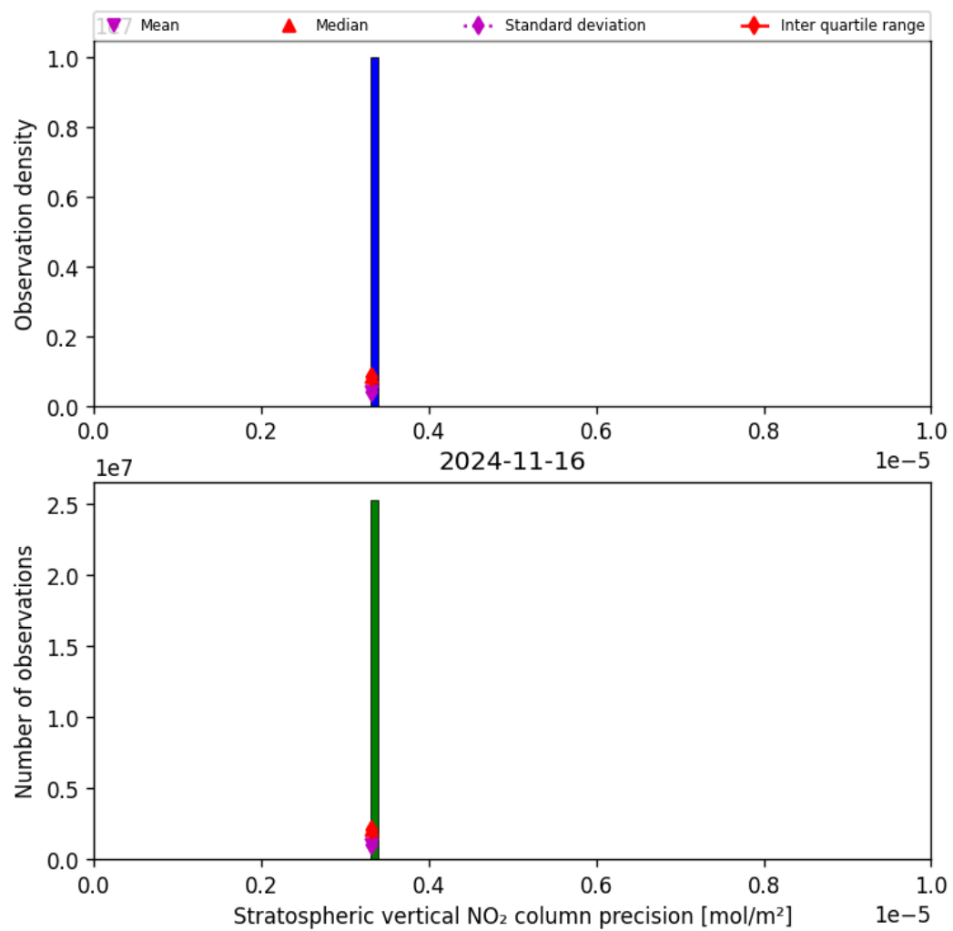
Figure 37: Histogram of “Stratospheric vertical NO 2 column precision” for 2024-11-15 to 2024-11-17
