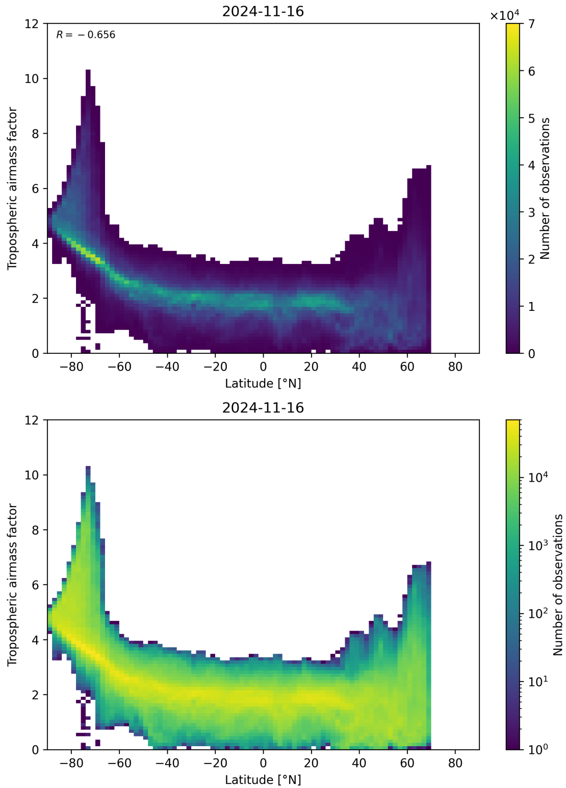
Figure 85: Scatter density plot of “Latitude” against “Tropospheric air mass factor” for 2024-11-15 to 2024-11-17.
