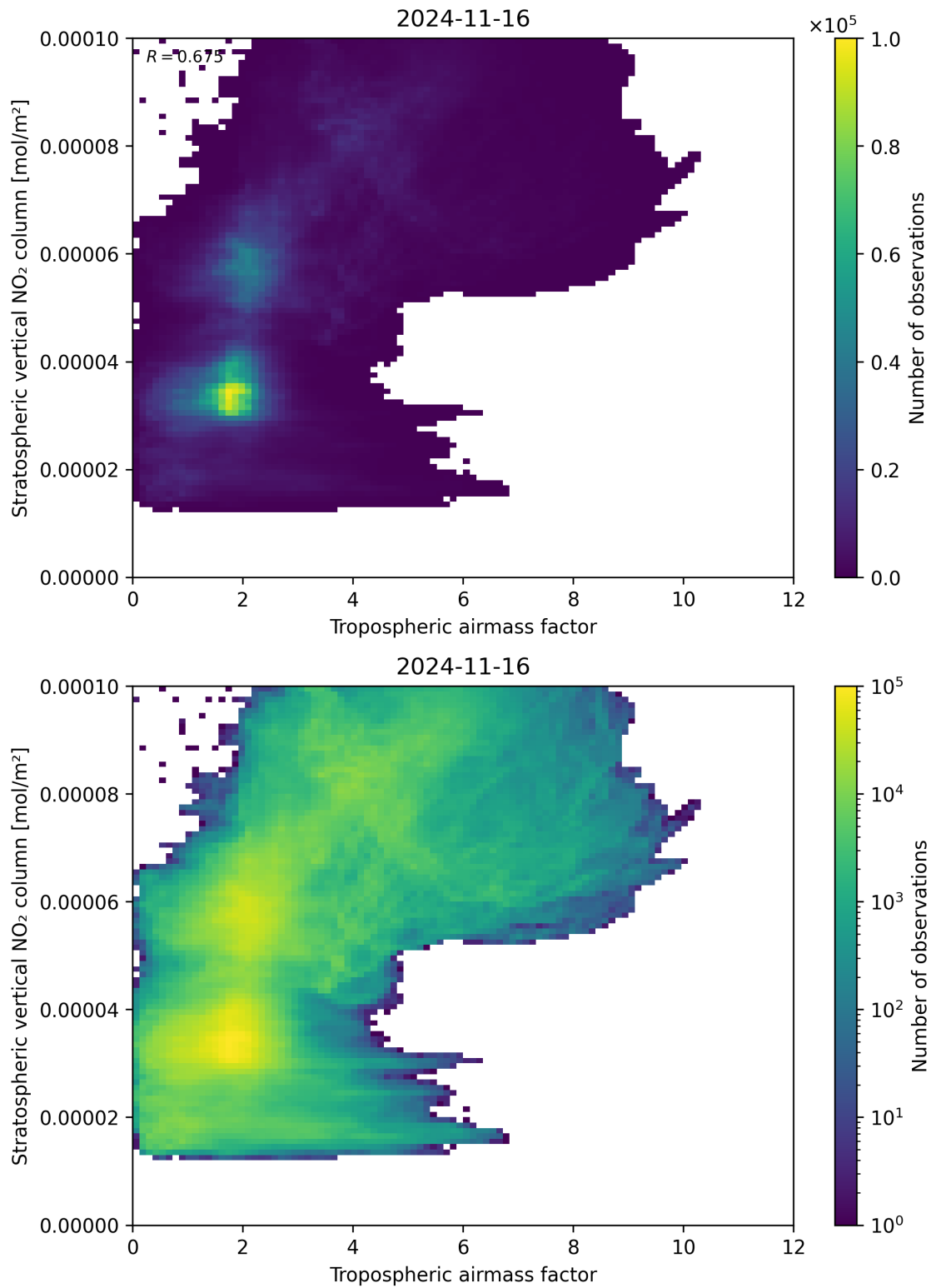
Figure 74: Scatter density plot of “Tropospheric air mass factor” against “Stratospheric vertical NO 2 column” for 2024-11-15 to 2024-11-17.
