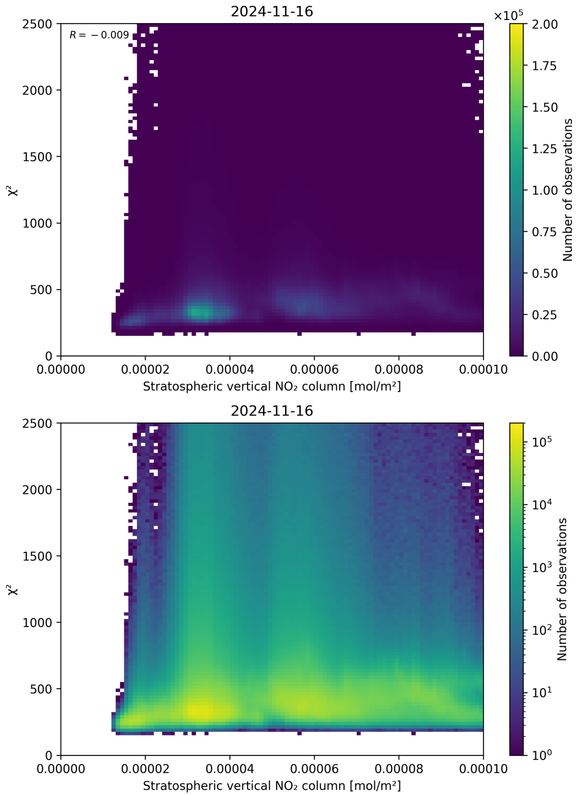
Figure 97: Scatter density plot of “Stratospheric vertical NO 2 column” against “ \chi^2 ” for 2024-11-15 to 2024-11-17.
