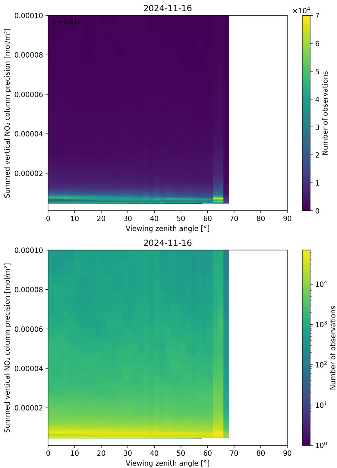
Figure 166: Scatter density plot of “Viewing zenith angle” against “Summed vertical NO 2 column precision” for 2024-11-15 to 2024-11-17.
