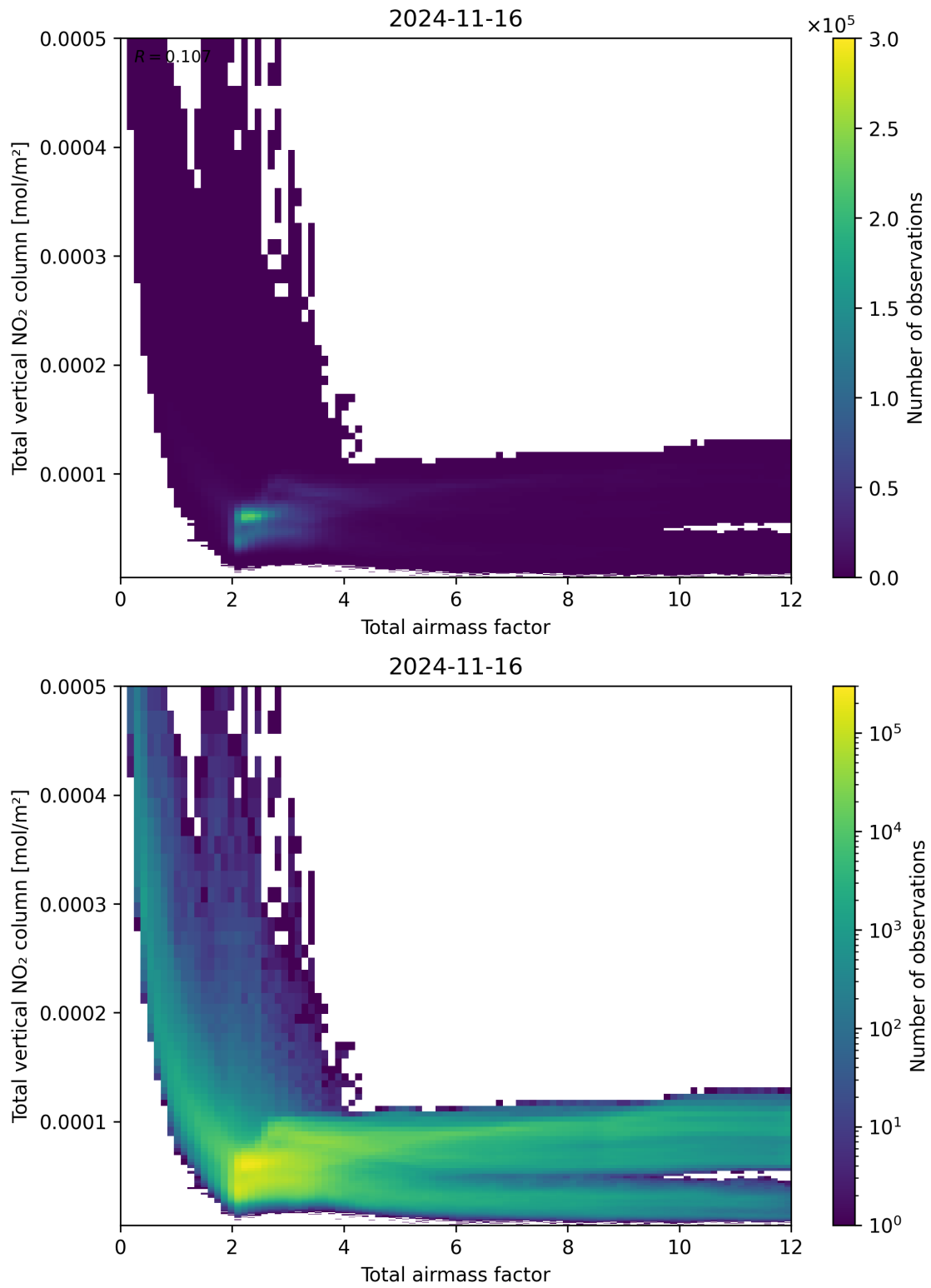
Figure 67: Scatter density plot of “Total airmass factor” against “Total vertical NO 2 column” for 2024-11-15 to 2024-11-17.
