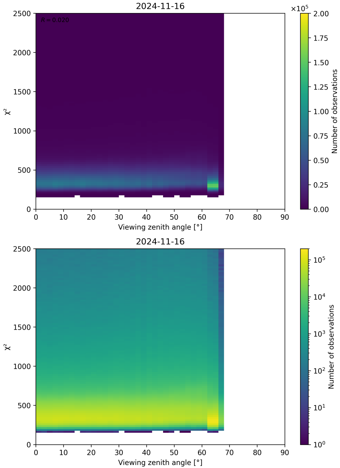
Figure 162: Scatter density plot of “Viewing zenith angle” against “ \chi^2 ” for 2024-11-15 to 2024-11-17.
