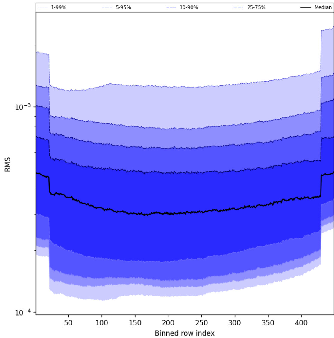
Figure 60: Along track statistics of “RMS” for 2024-11-15 to 2024-11-17
