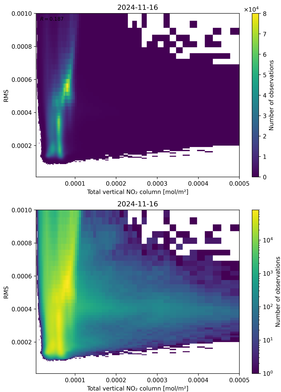
Figure 120: Scatter density plot of “Total vertical NO 2 column” against “RMS” for 2024-11-15 to 2024-11-17.
