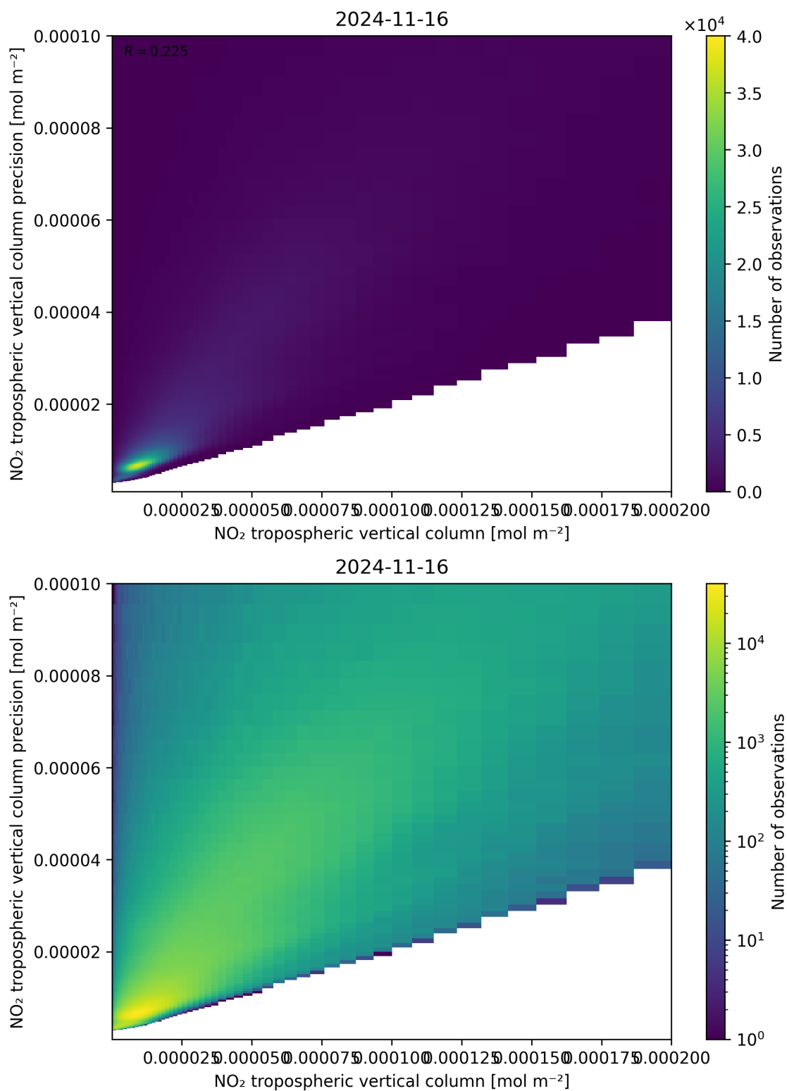
Figure 130: Scatter density plot of “NO 2 tropospheric vertical column” against “NO 2 tropospheric vertical column precision” for 2024-11-15 to 2024-11-17.
