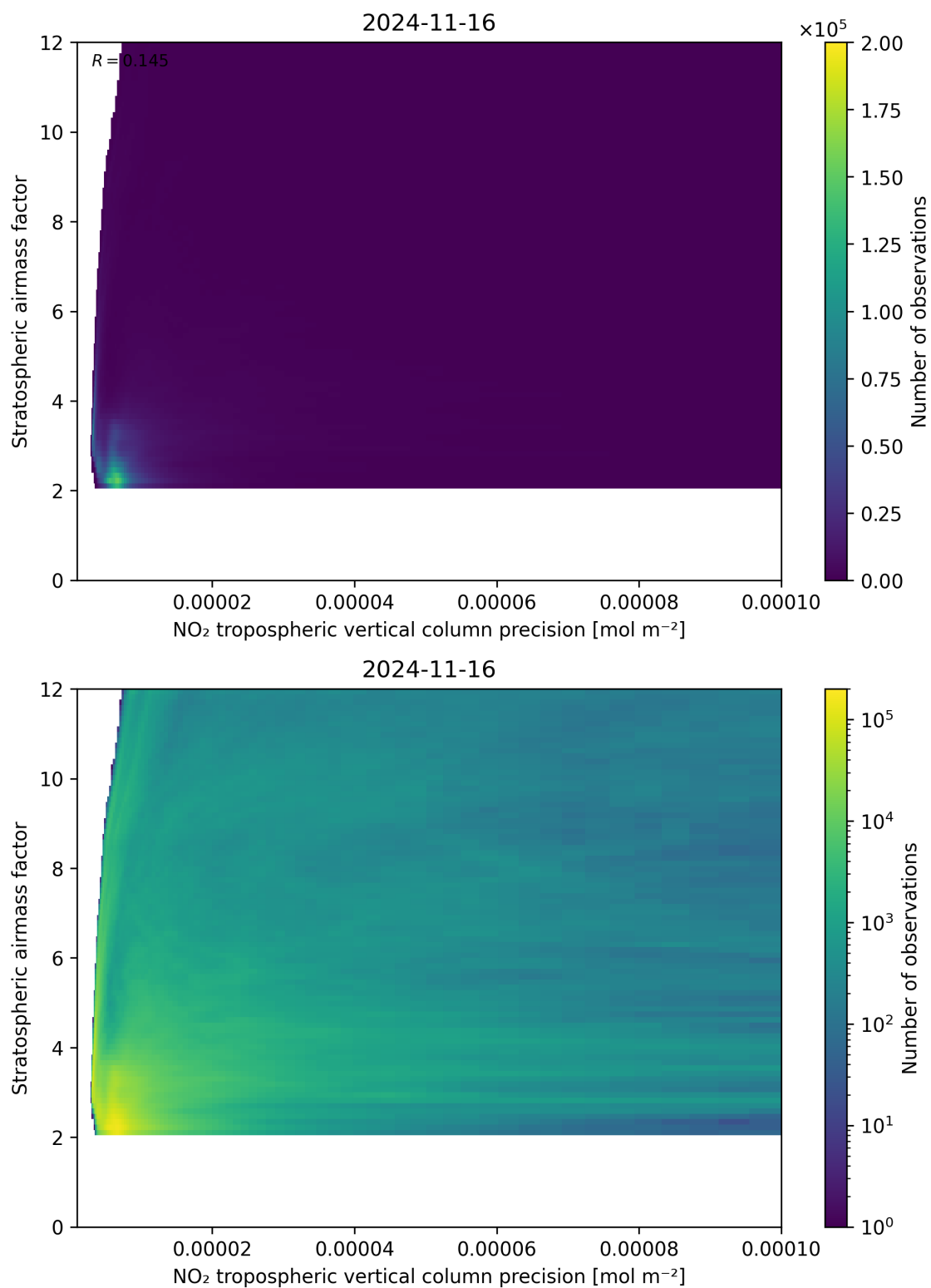
Figure 131: Scatter density plot of “NO 2 tropospheric vertical column precision” against “Stratospheric airmass factor” for 2024-11-15 to 2024-11-17.
