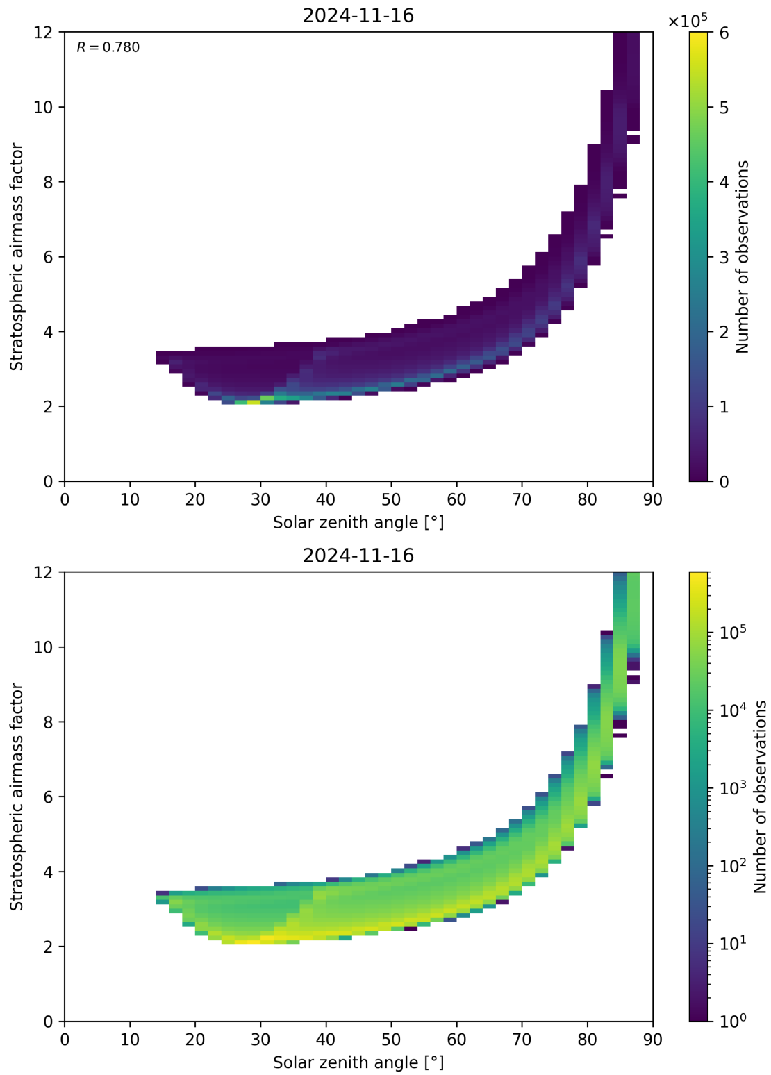
Figure 145: Scatter density plot of “Solar zenith angle” against “Stratospheric airmass factor” for 2024-11-15 to 2024-11-17.
