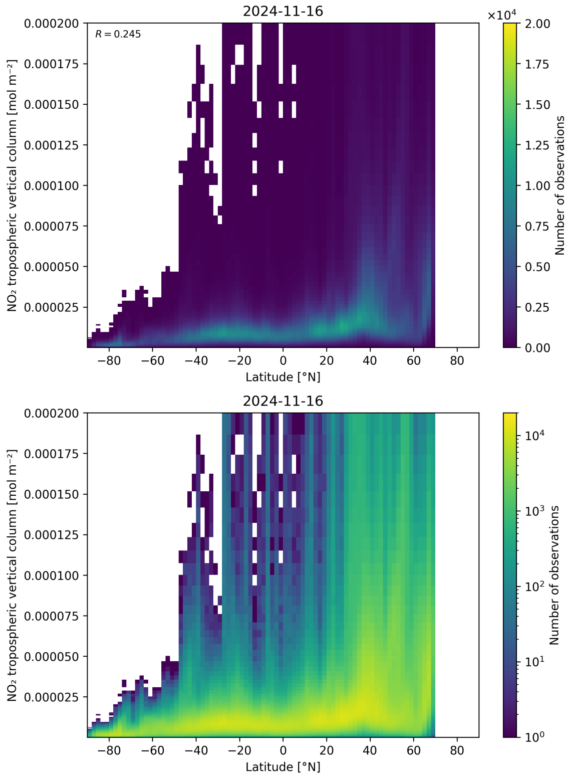
Figure 92: Scatter density plot of “Latitude” against “NO 2 tropospheric vertical column” for 2024-11-15 to 2024-11-17.
