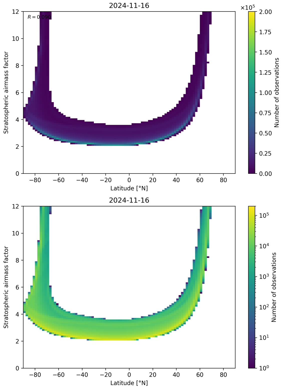
Figure 83: Scatter density plot of “Latitude” against “Stratospheric airmass factor” for 2024-11-15 to 2024-11-17.
