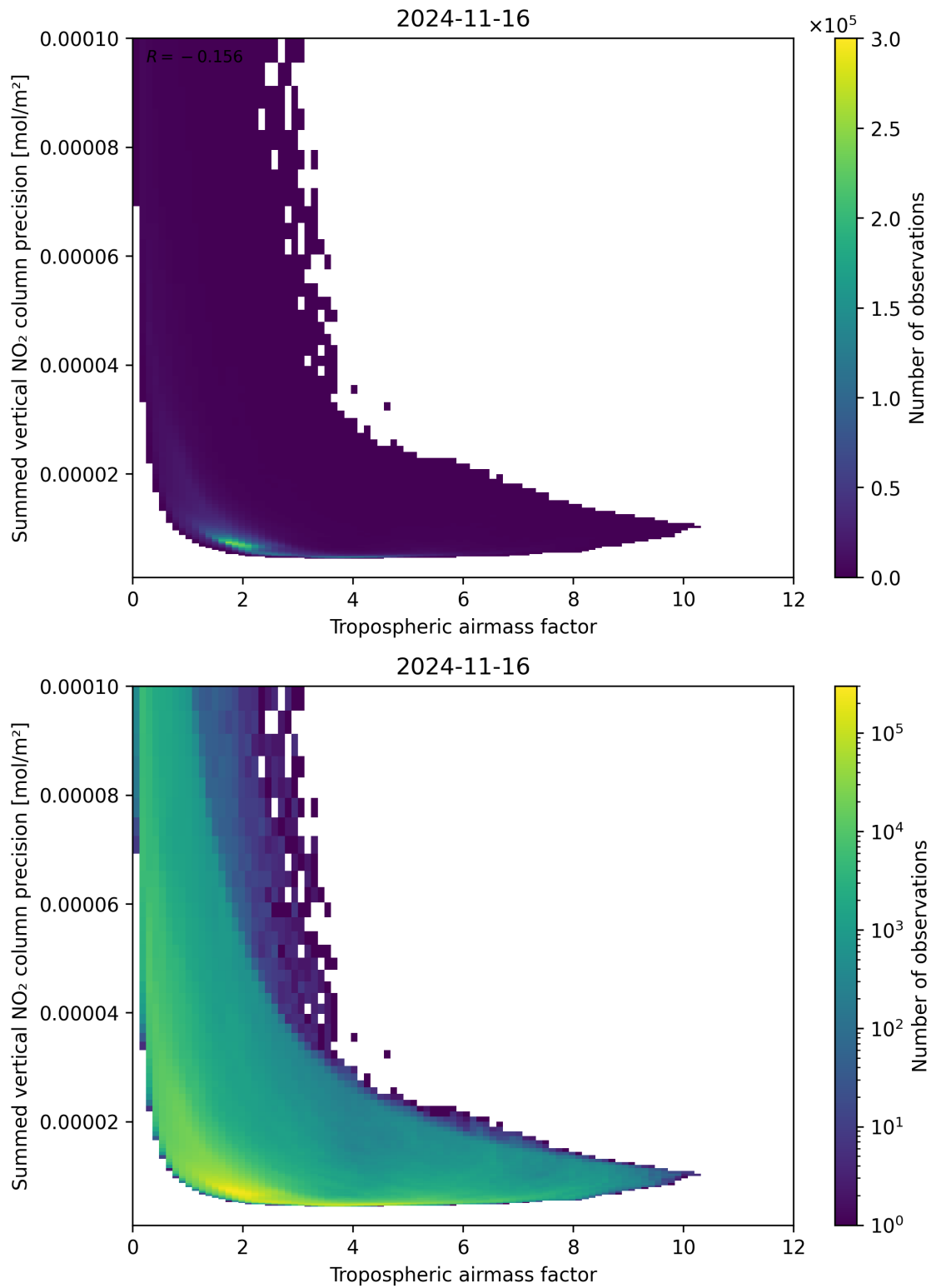
Figure 76: Scatter density plot of “Tropospheric air mass factor” against “Summed vertical NO 2 column precision” for 2024-11-15 to 2024-11-17.
