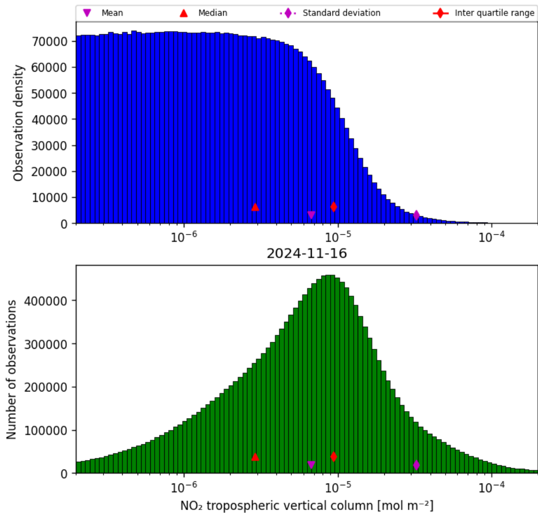
Figure 29: Histogram of “NO 2 tropospheric vertical column” for 2024-11-15 to 2024-11-17
