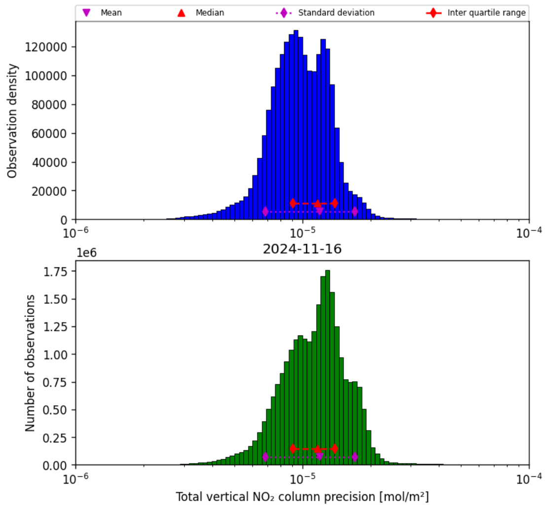
Figure 39: Histogram of “Total vertical NO 2 column precision” for 2024-11-15 to 2024-11-17
