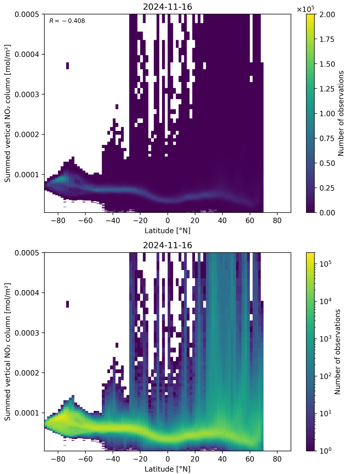
Figure 88: Scatter density plot of “Latitude” against “Summed vertical NO 2 column” for 2024-11-15 to 2024-11-17.
