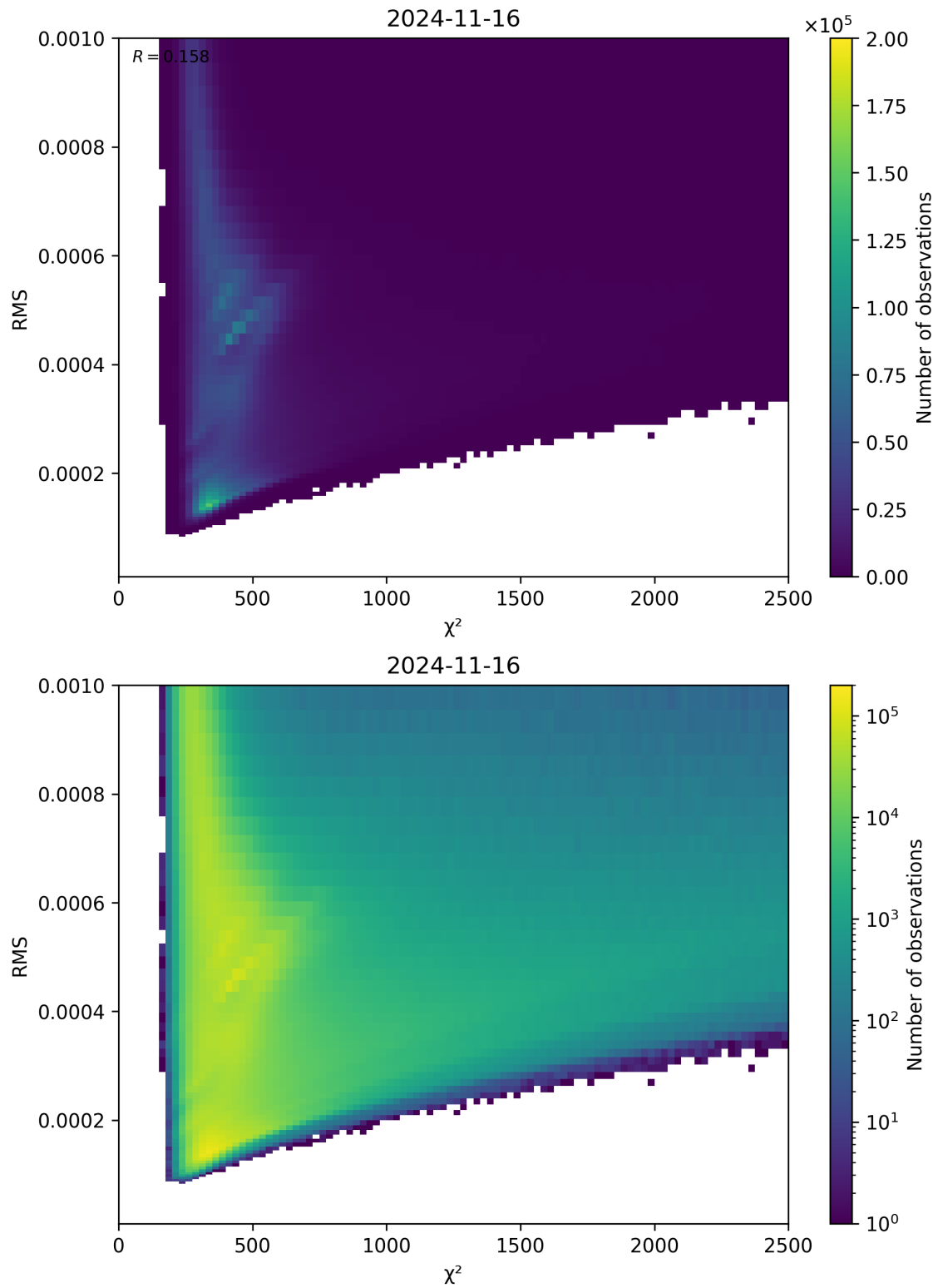
Figure 82: Scatter density plot of “ \chi^2 ” against “RMS” for 2024-11-15 to 2024-11-17.
