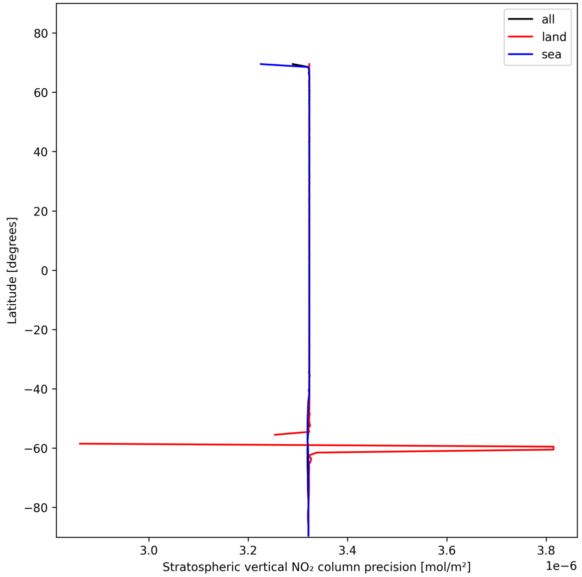
Figure 20: Zonal average of “Stratospheric vertical NO 2 column precision” for 2024-11-15 to 2024-11-17.
