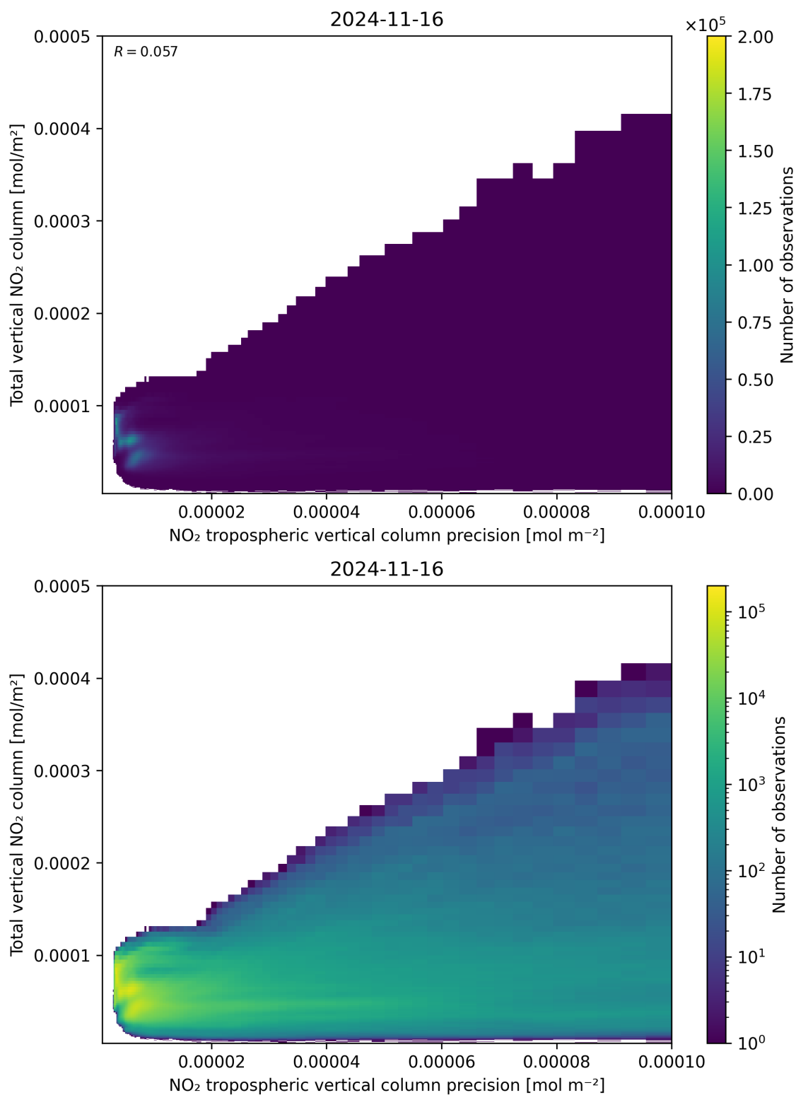
Figure 138: Scatter density plot of “NO 2 tropospheric vertical column precision” against “Total vertical NO 2 column” for 2024-11-15 to 2024-11-17.
