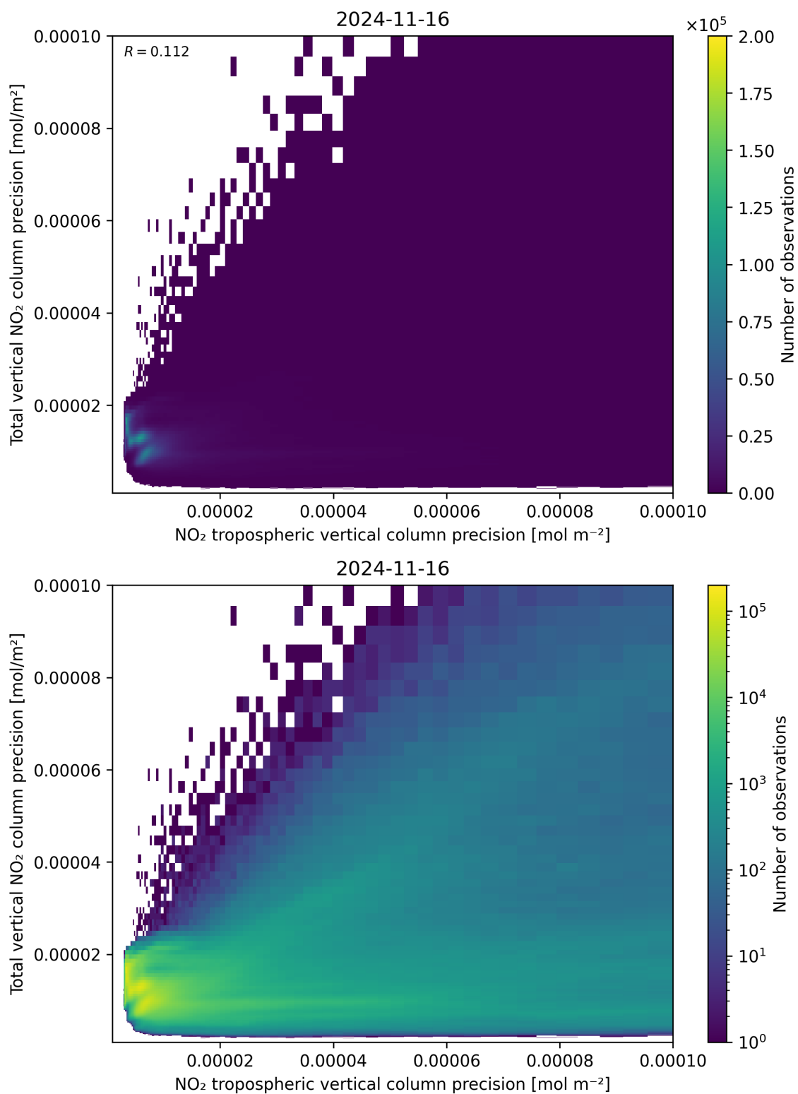
Figure 139: Scatter density plot of “NO 2 tropospheric vertical column precision” against “Total vertical NO 2 column precision” for 2024-11-15 to 2024-11-17.
