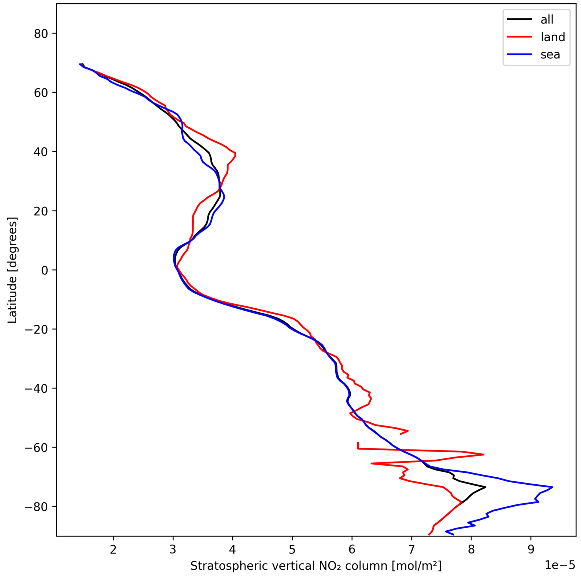
Figure 19: Zonal average of “Stratospheric vertical NO 2 column” for 2024-11-15 to 2024-11-17.
