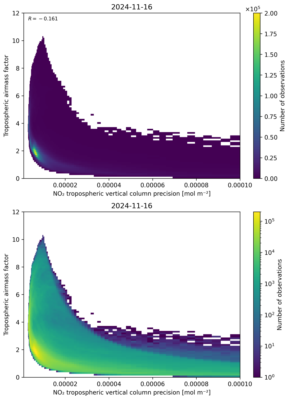
Figure 133: Scatter density plot of “NO 2 tropospheric vertical column precision” against “Tropospheric air mass factor” for 2024-11-15 to 2024-11-17.
