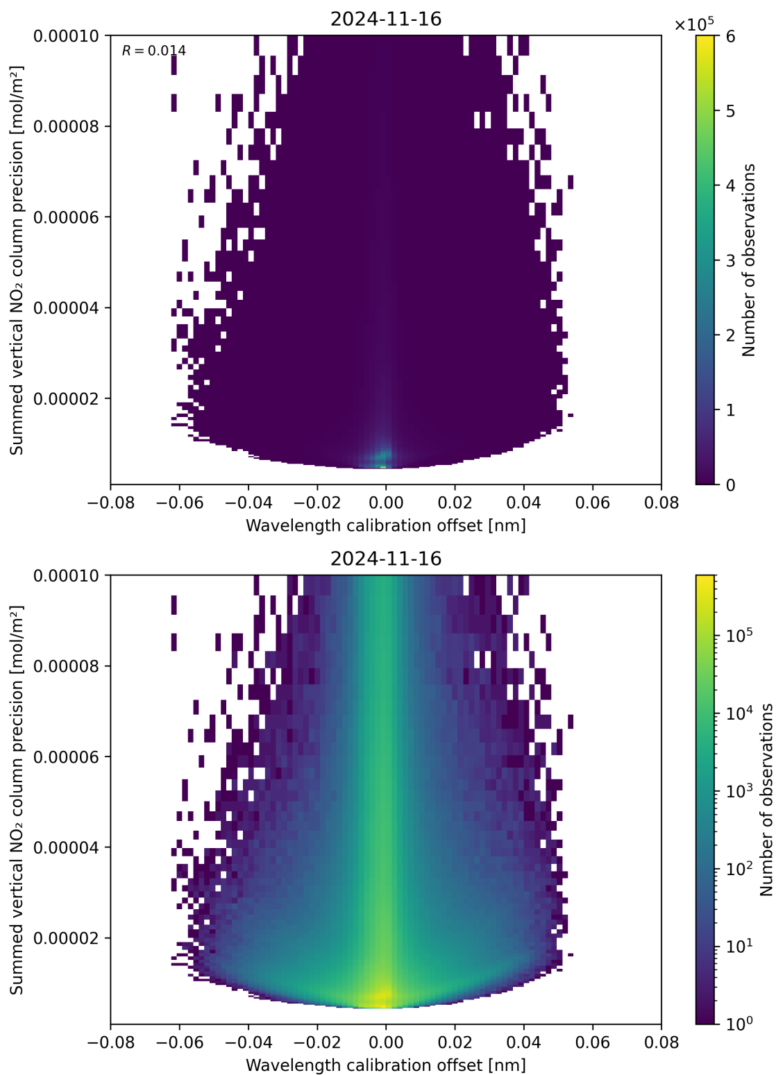
Figure 178: Scatter density plot of “Wavelength calibration offset” against “Summed vertical NO 2 column precision” for 2024-11-15 to 2024-11-17.
