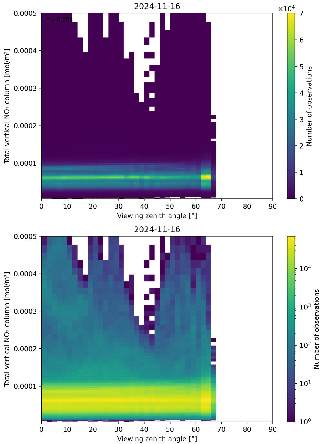
Figure 167: Scatter density plot of “Viewing zenith angle” against “Total vertical NO 2 column” for 2024-11-15 to 2024-11-17.
