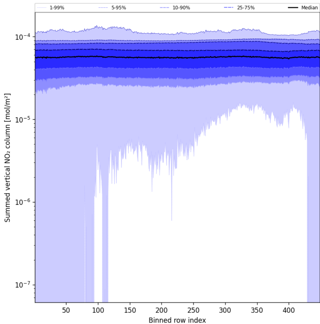
Figure 57: Along track statistics of “Summed vertical NO 2 column” for 2024-11-15 to 2024-11-17
