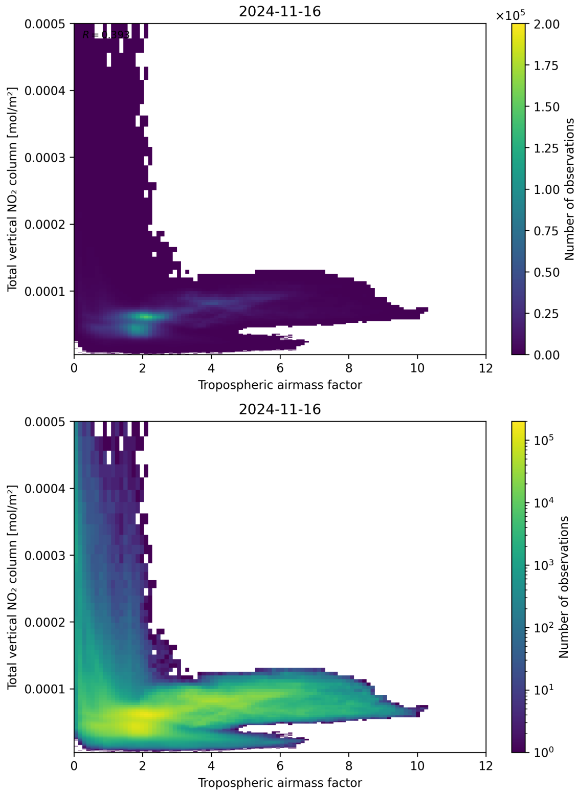
Figure 77: Scatter density plot of “Tropospheric airmass factor” against “Total vertical NO 2 column” for 2024-11-15 to 2024-11-17.
