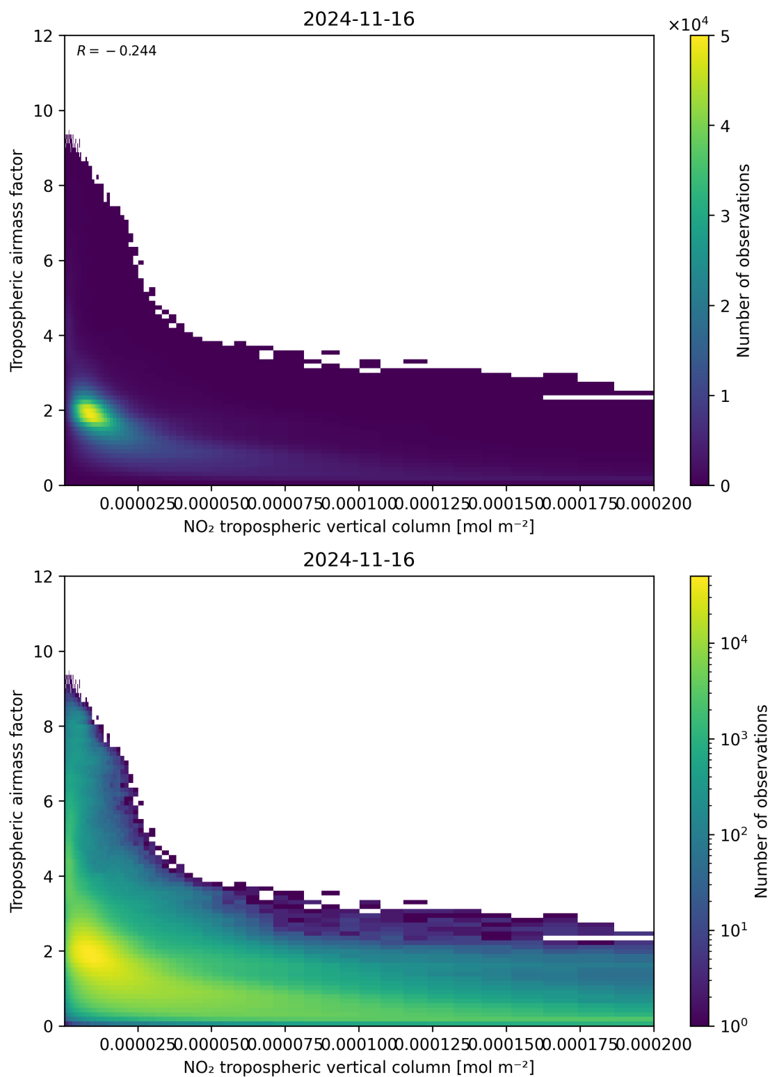
Figure 123: Scatter density plot of “NO 2 tropospheric vertical column” against “Tropospheric air mass factor” for 2024-11-15 to 2024-11-17.
