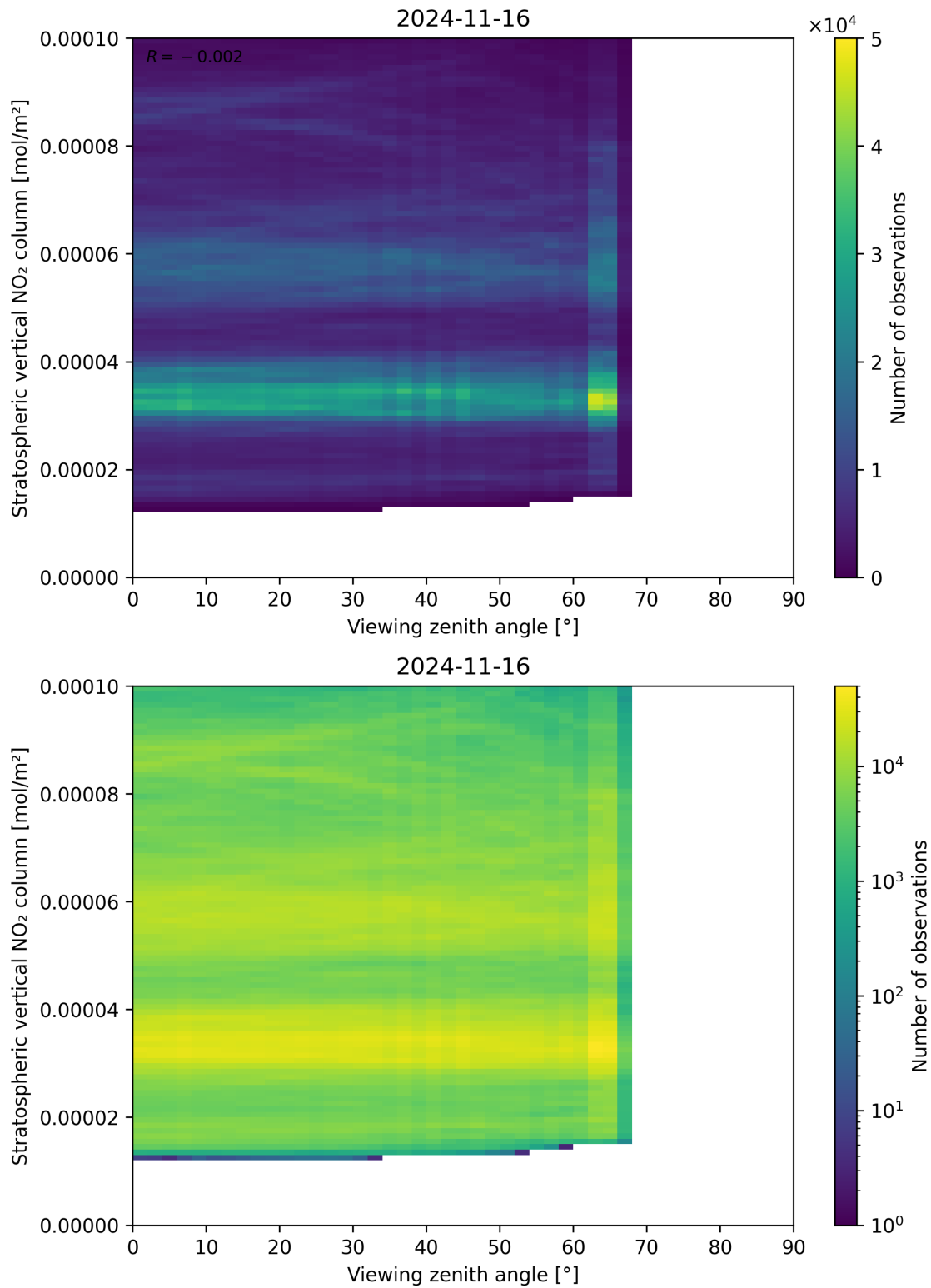
Figure 164: Scatter density plot of “Viewing zenith angle” against “Stratospheric vertical NO 2 column” for 2024-11-15 to 2024-11-17.
