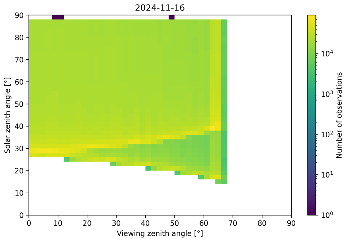
Figure 172: Scatter density plot of “Viewing zenith angle” against “Solar zenith angle” for 2024-11-15 to 2024-11-17.
