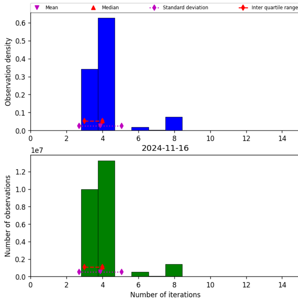
Figure 34: Histogram of “Number of iterations” for 2024-11-15 to 2024-11-17
