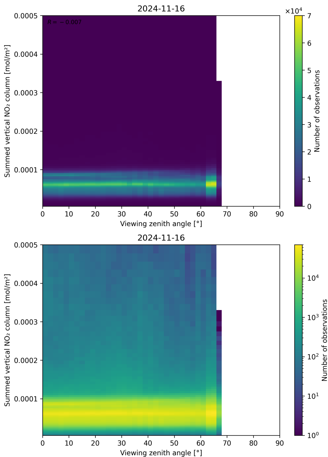
Figure 165: Scatter density plot of “Viewing zenith angle” against “Summed vertical NO 2 column” for 2024-11-15 to 2024-11-17.
