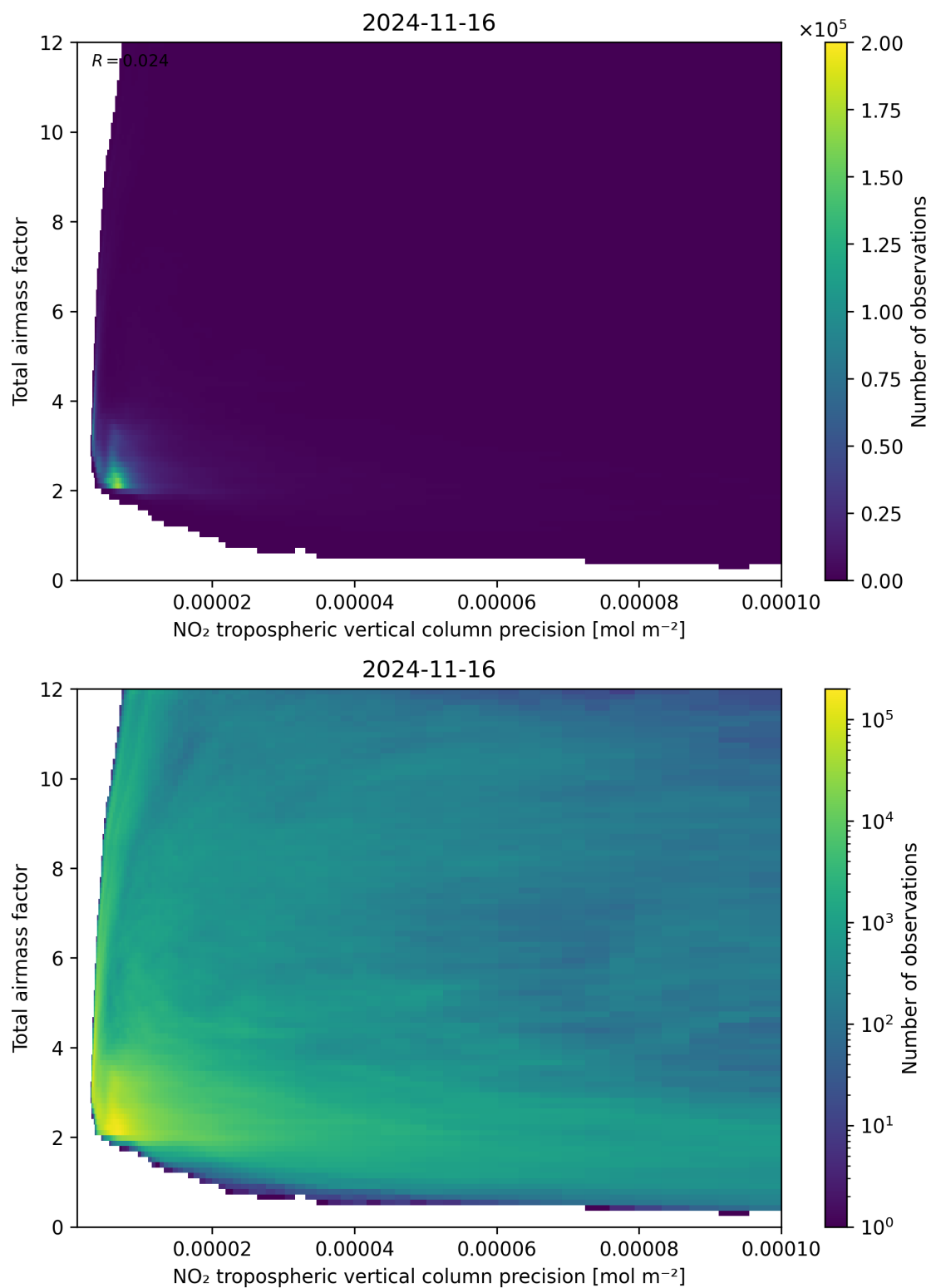
Figure 132: Scatter density plot of “NO 2 tropospheric vertical column precision” against “Total air mass factor” for 2024-11-15 to 2024-11-17.
