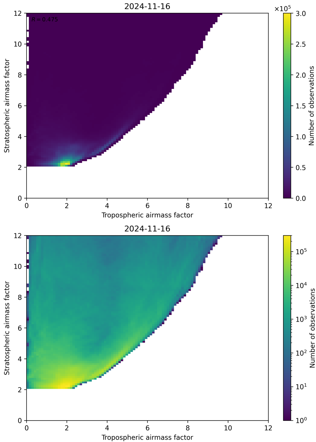
Figure 71: Scatter density plot of “Tropospheric airmass factor” against “Stratospheric airmass factor” for 2024-11-15 to 2024-11-17.
