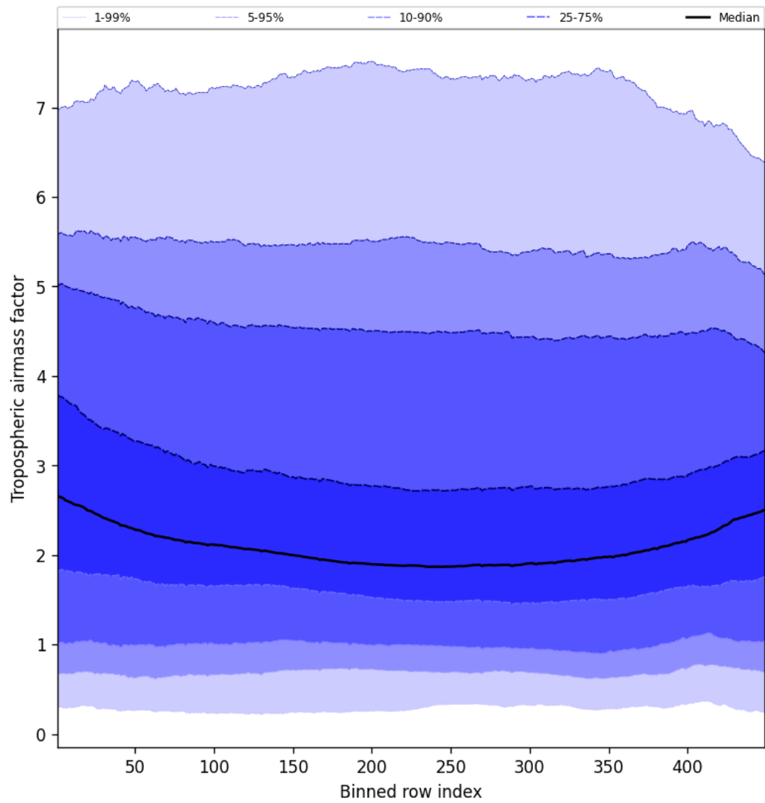
Figure 48: Along track statistics of “Tropospheric air mass factor” for 2024-11-15 to 2024-11-17
