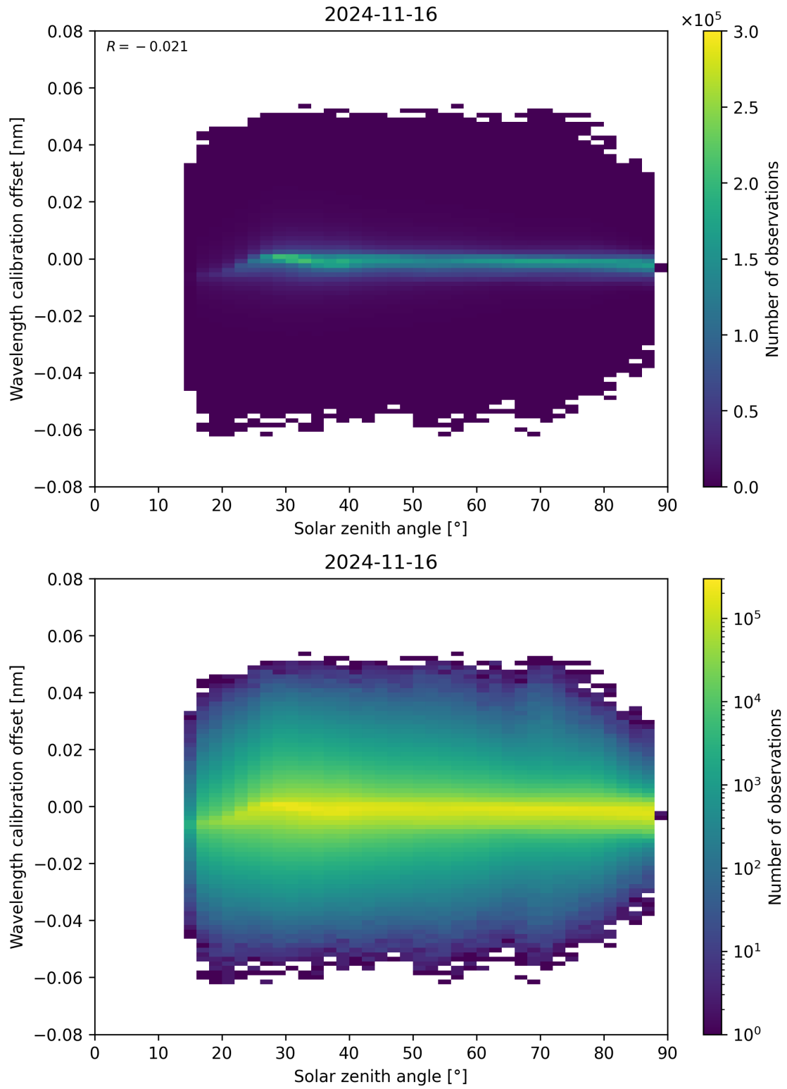
Figure 158: Scatter density plot of “Solar zenith angle” against “Wavelength calibration offset” for 2024-11-15 to 2024-11-17.
