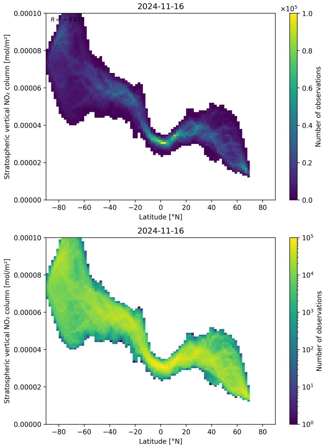
Figure 87: Scatter density plot of “Latitude” against “Stratospheric vertical NO 2 column” for 2024-11-15 to 2024-11-17.
