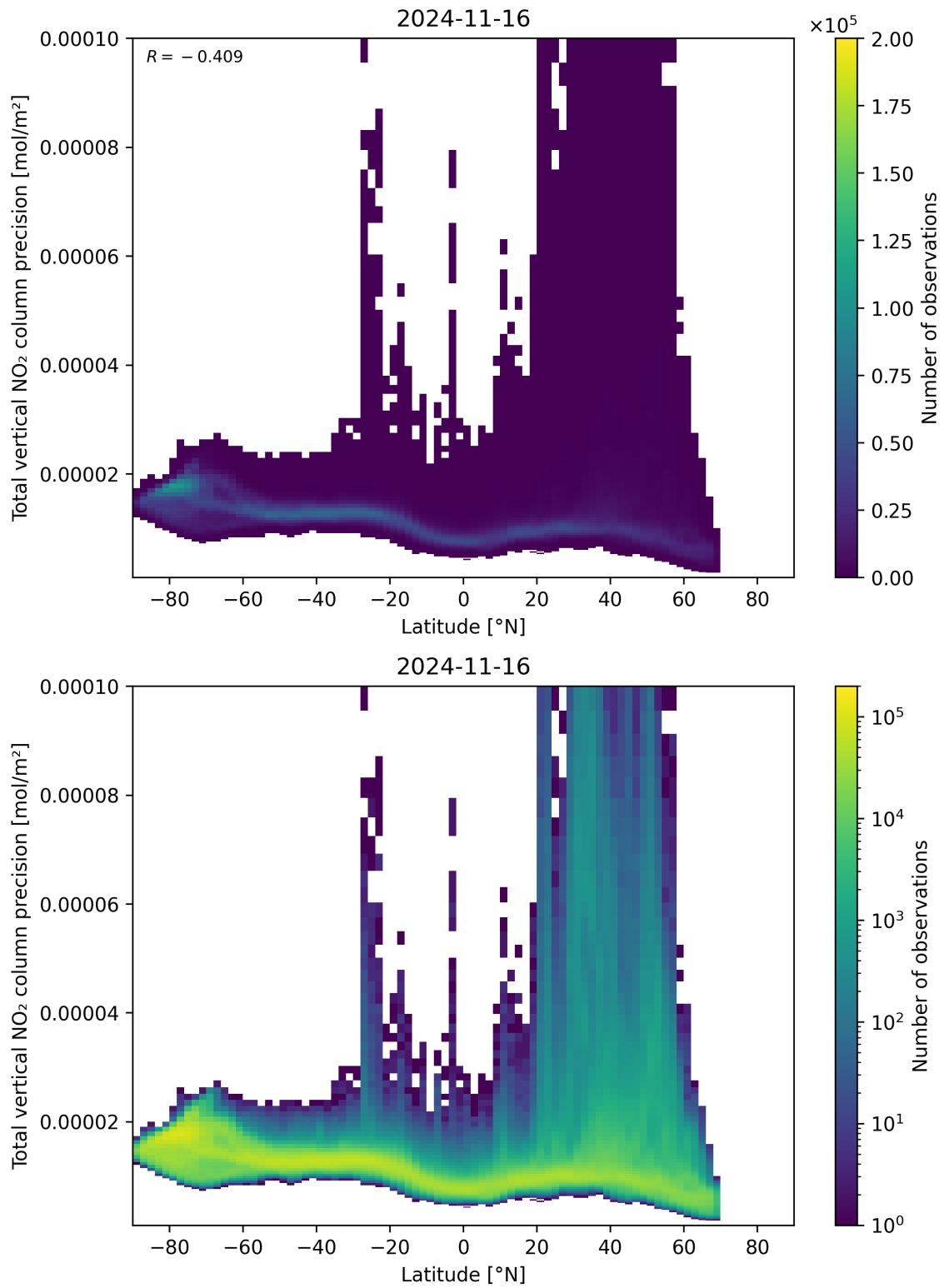
Figure 91: Scatter density plot of “Latitude” against “Total vertical NO 2 column precision” for 2024-11-15 to 2024-11-17.
