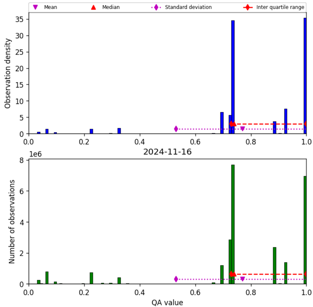
Figure 28: Histogram of “QA value” for 2024-11-15 to 2024-11-17
