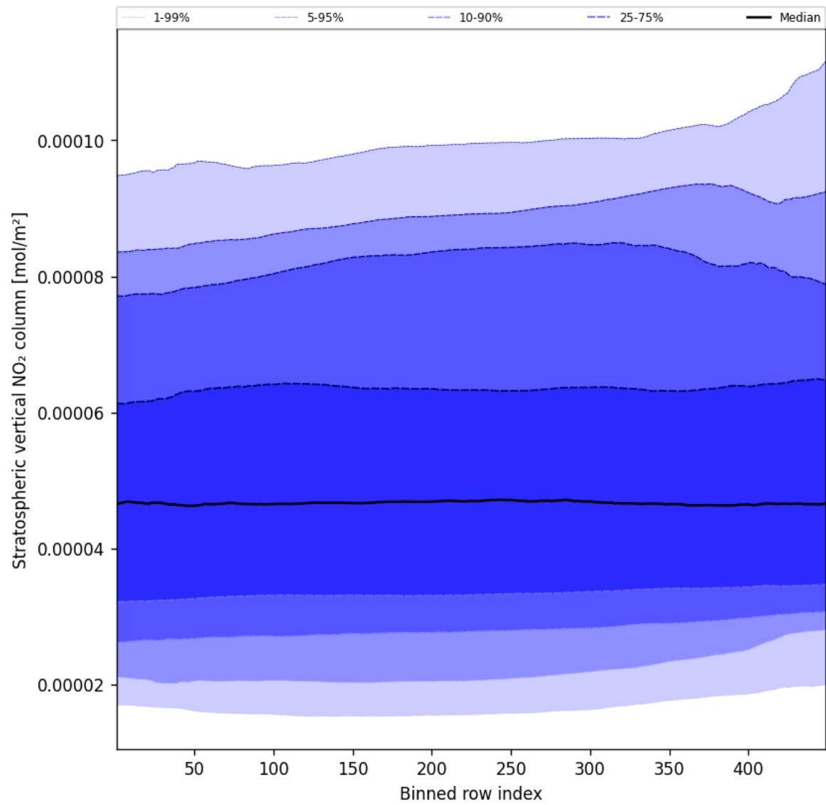
Figure 53: Along track statistics of “Stratospheric vertical NO 2 column” for 2024-11-15 to 2024-11-17
