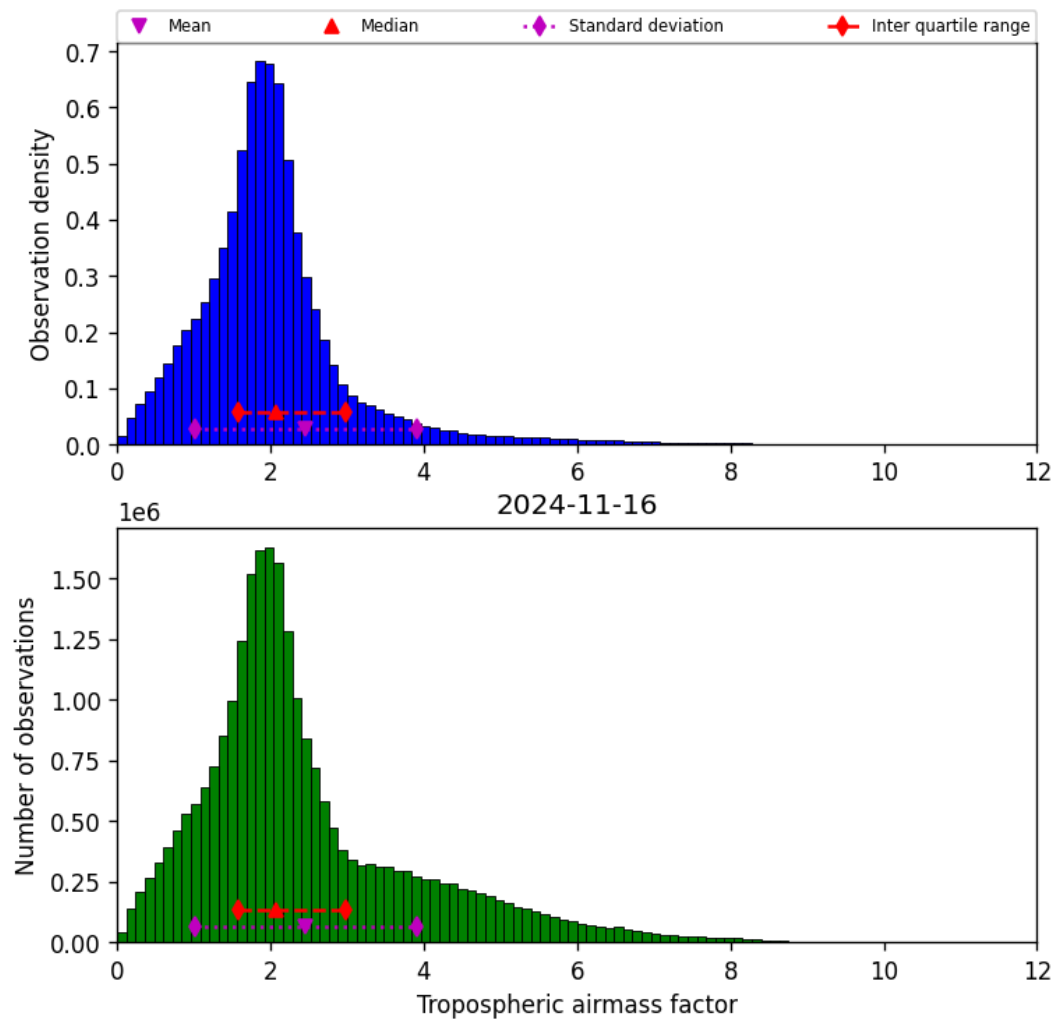
Figure 31: Histogram of “Tropospheric airmass factor” for 2024-11-15 to 2024-11-17
