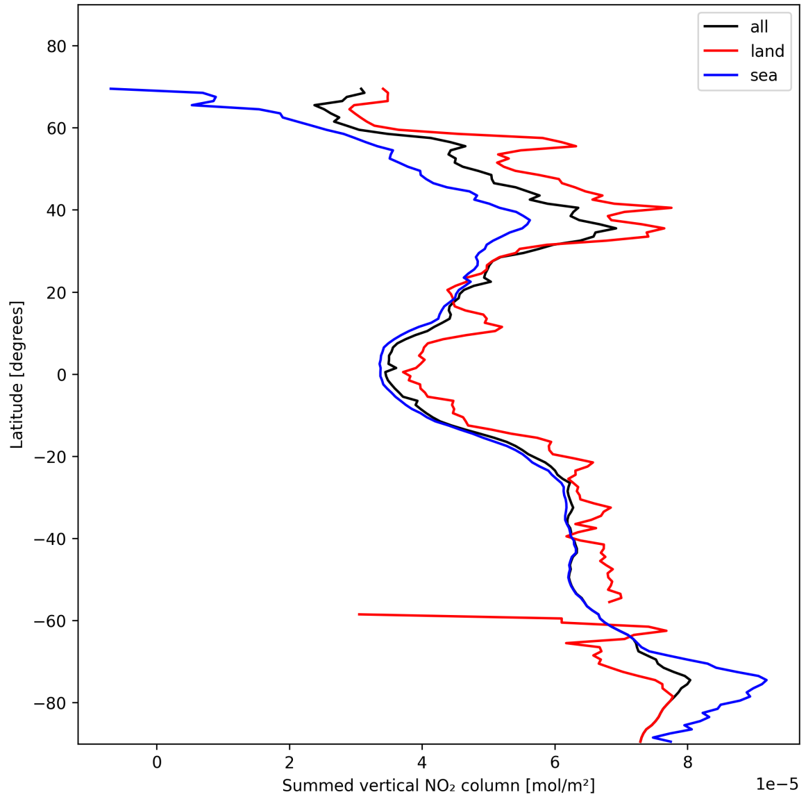
Figure 23: Zonal average of “Summed vertical NO 2 column” for 2024-11-15 to 2024-11-17.
