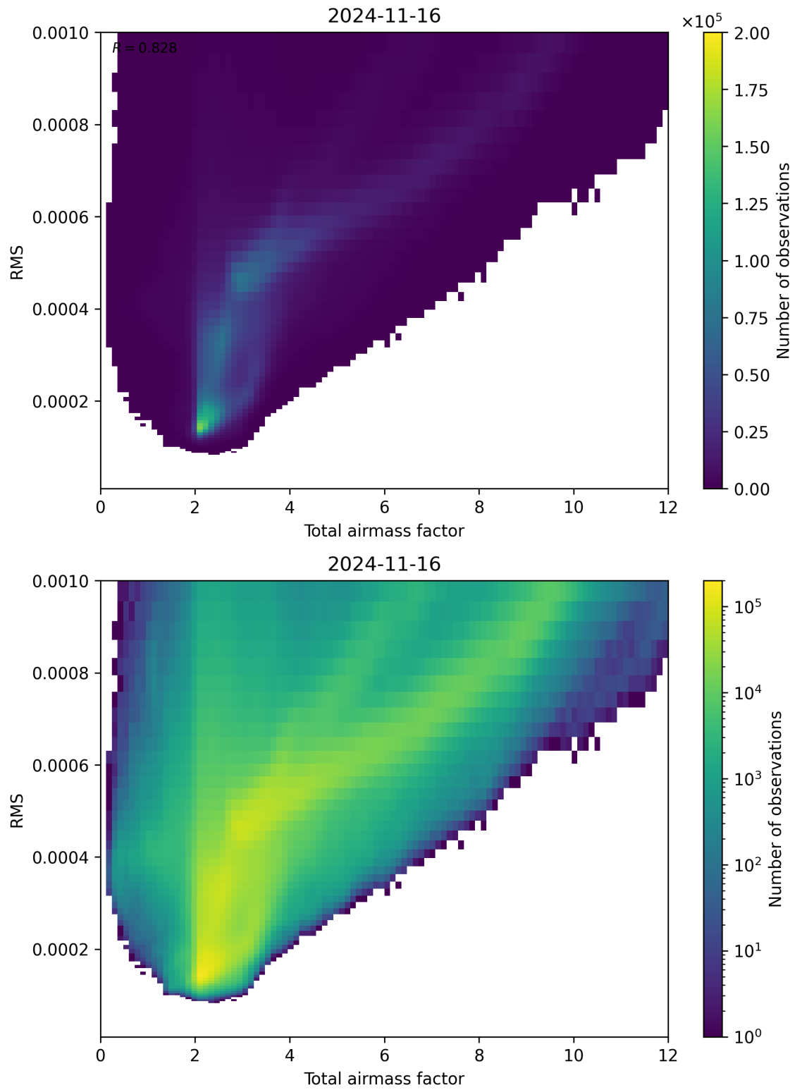
Figure 69: Scatter density plot of “Total airmass factor” against “RMS” for 2024-11-15 to 2024-11-17.
