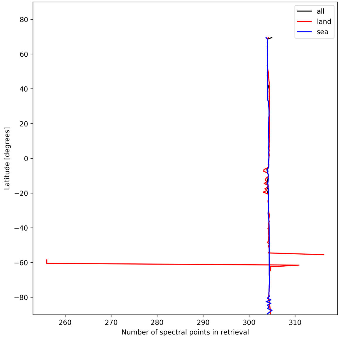
Figure 16: Zonal average of “Number of spectral points in retrieval” for 2024-11-15 to 2024-11-17.
