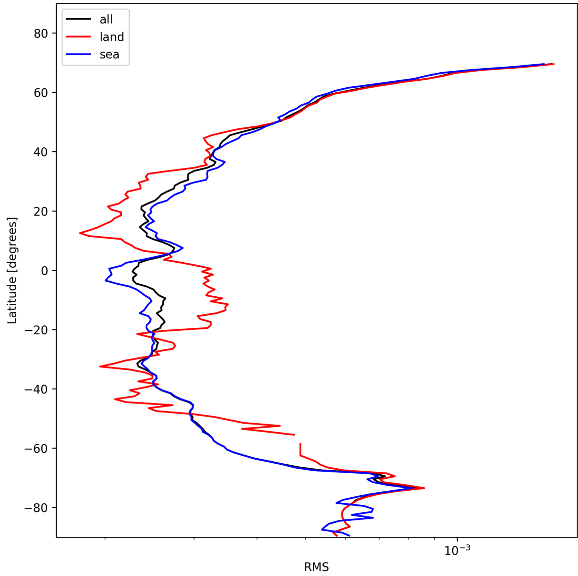
Figure 26: Zonal average of “RMS” for 2024-11-15 to 2024-11-17.
