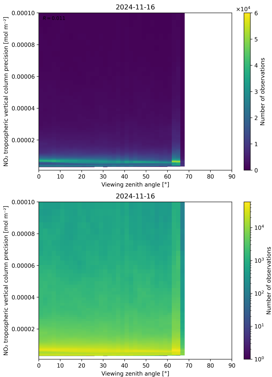
Figure 170: Scatter density plot of “Viewing zenith angle” against “NO 2 tropospheric vertical column precision” for 2024-11-15 to 2024-11-17.
