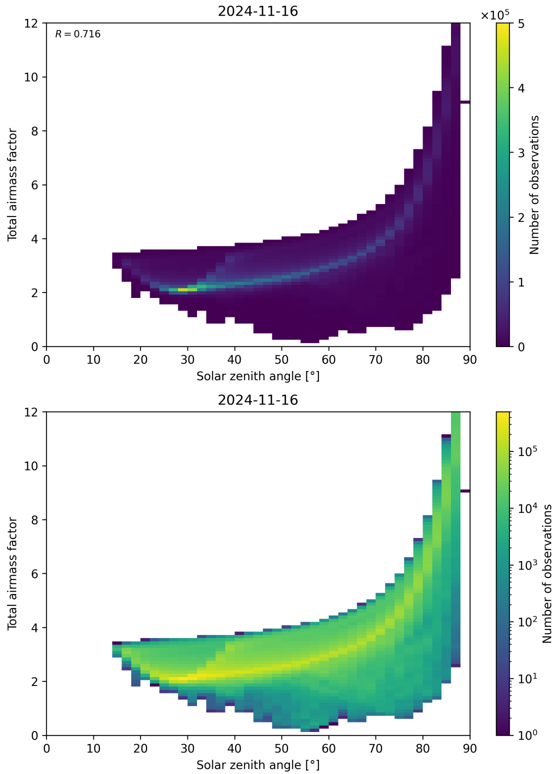
Figure 146: Scatter density plot of “Solar zenith angle” against “Total air mass factor” for 2024-11-15 to 2024-11-17.
