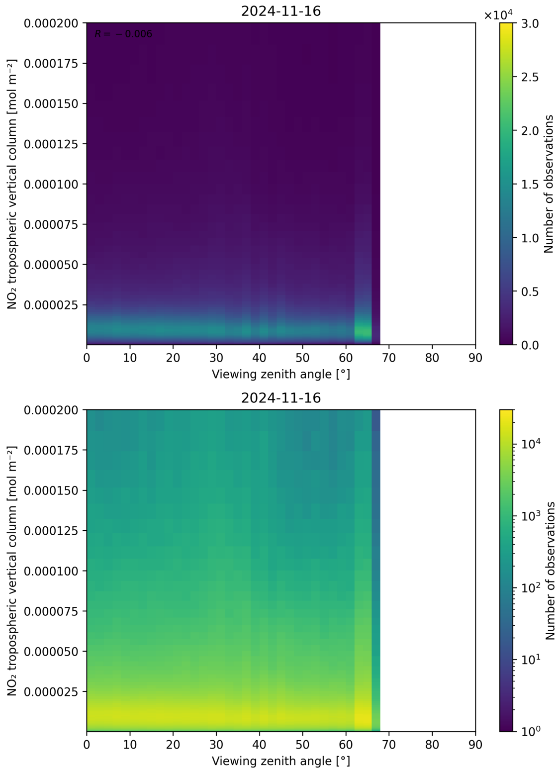
Figure 169: Scatter density plot of “Viewing zenith angle” against “NO 2 tropospheric vertical column” for 2024-11-15 to 2024-11-17.
