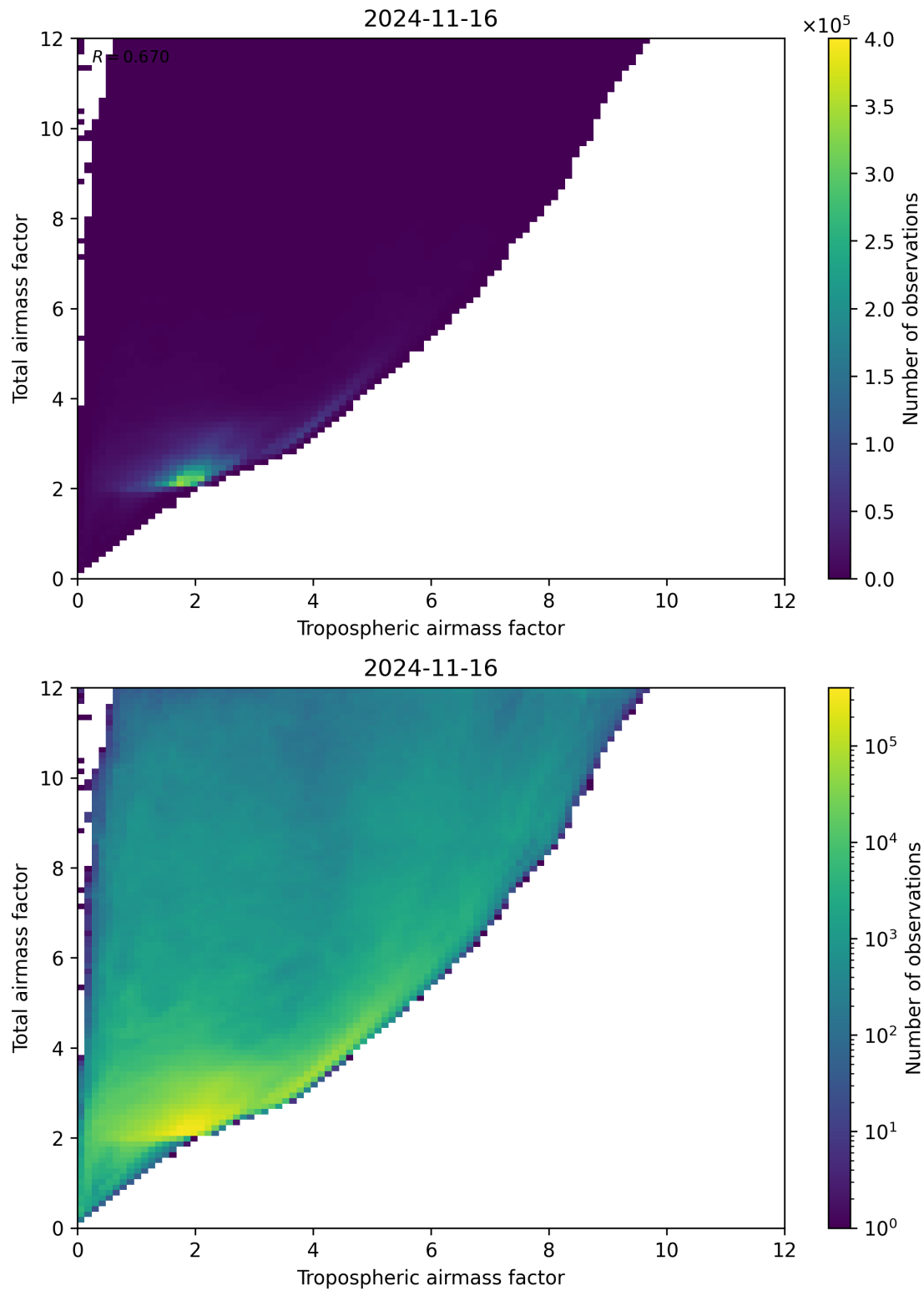
Figure 72: Scatter density plot of “Tropospheric airmass factor” against “Total airmass factor” for 2024-11-15 to 2024-11-17.
