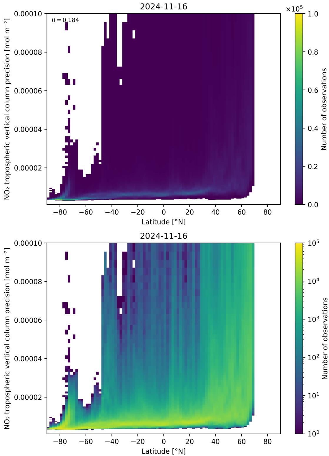
Figure 93: Scatter density plot of “Latitude” against “NO 2 tropospheric vertical column precision” for 2024-11-15 to 2024-11-17.
