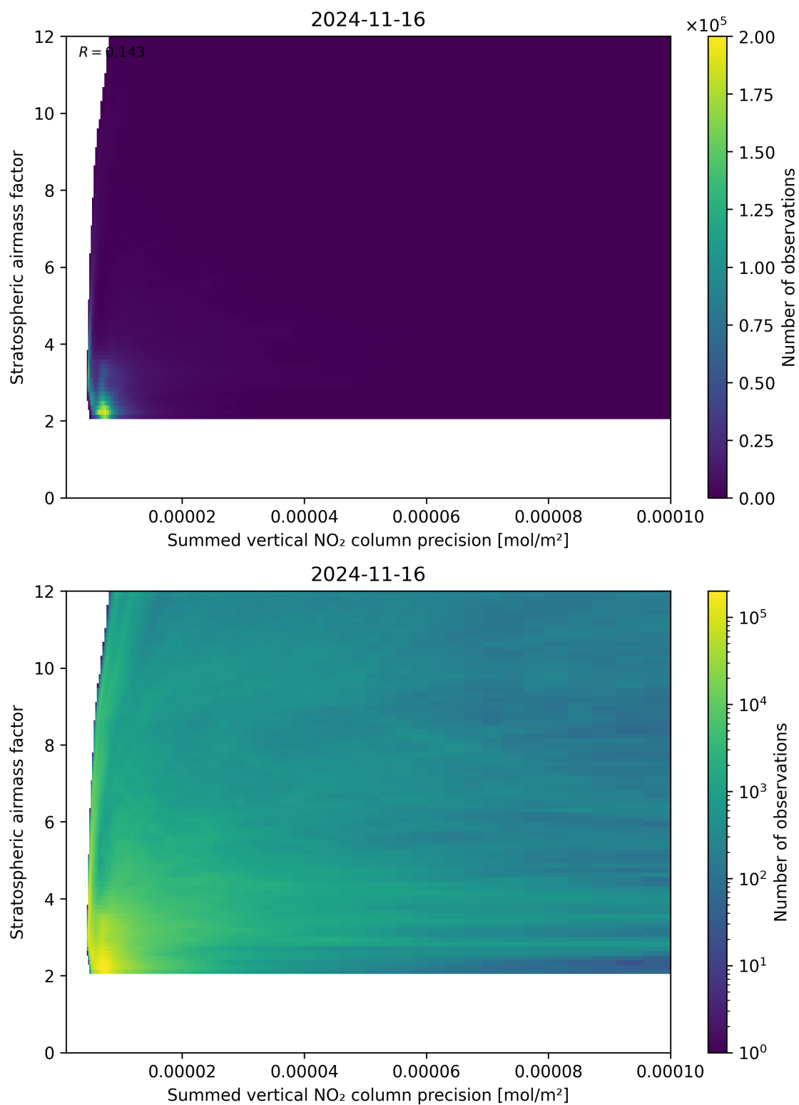
Figure 106: Scatter density plot of “Summed vertical NO 2 column precision” against “Stratospheric airmass factor” for 2024-11-15 to 2024-11-17.
