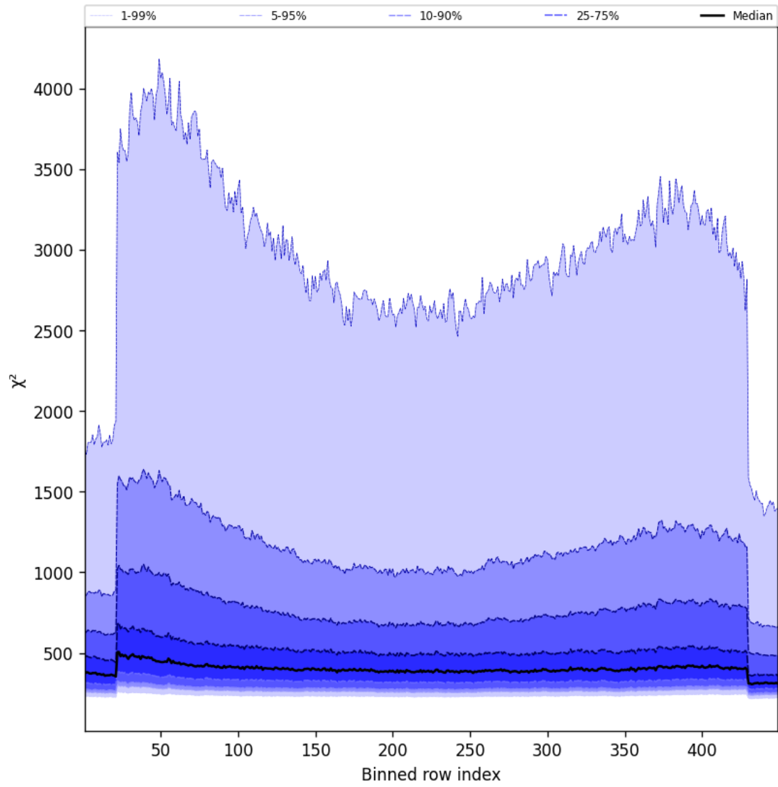
Figure 59: Along track statistics of “ \chi^2 ” for 2024-11-15 to 2024-11-17
