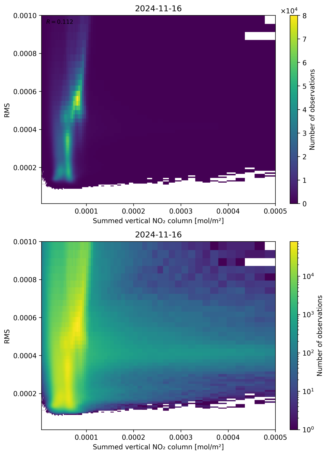
Figure 109: Scatter density plot of “Summed vertical NO 2 column” against “RMS” for 2024-11-15 to 2024-11-17.
