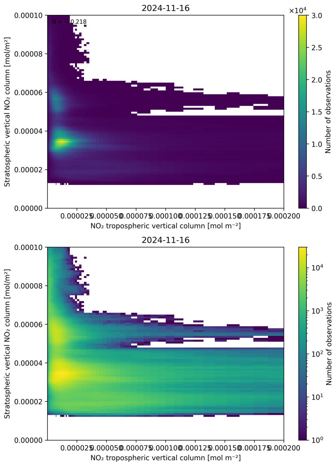
Figure 125: Scatter density plot of “NO 2 tropospheric vertical column” against “Stratospheric vertical NO 2 column” for 2024-11-15 to 2024-11-17.
