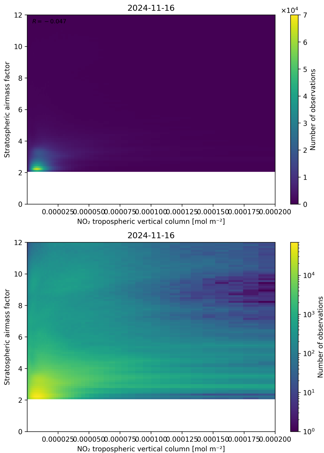
Figure 121: Scatter density plot of “NO 2 tropospheric vertical column” against “Stratospheric airmass factor” for 2024-11-15 to 2024-11-17.
