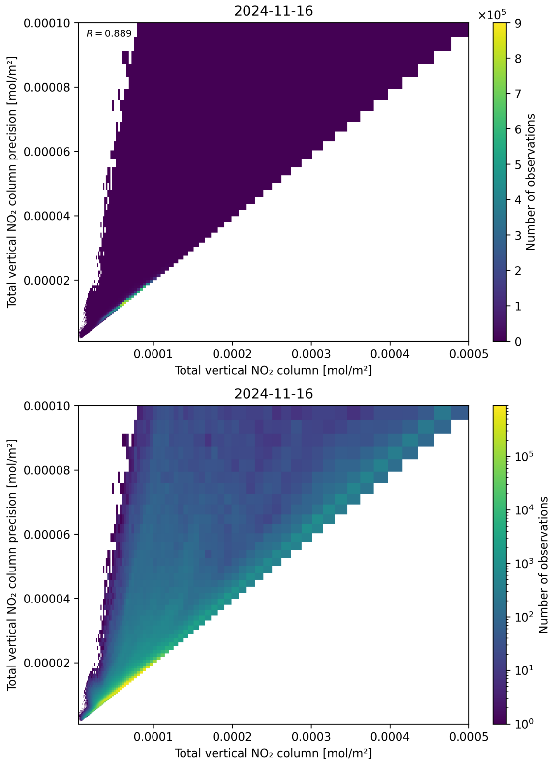
Figure 114: Scatter density plot of “Total vertical NO 2 column” against “Total vertical NO 2 column precision” for 2024-11-15 to 2024-11-17.
