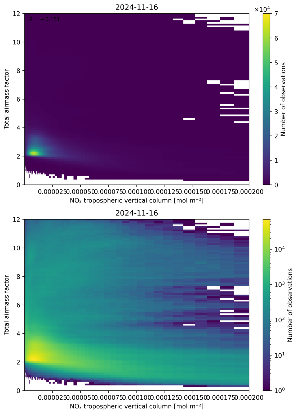
Figure 122: Scatter density plot of “NO 2 tropospheric vertical column” against “Total air mass factor” for 2024-11-15 to 2024-11-17.
