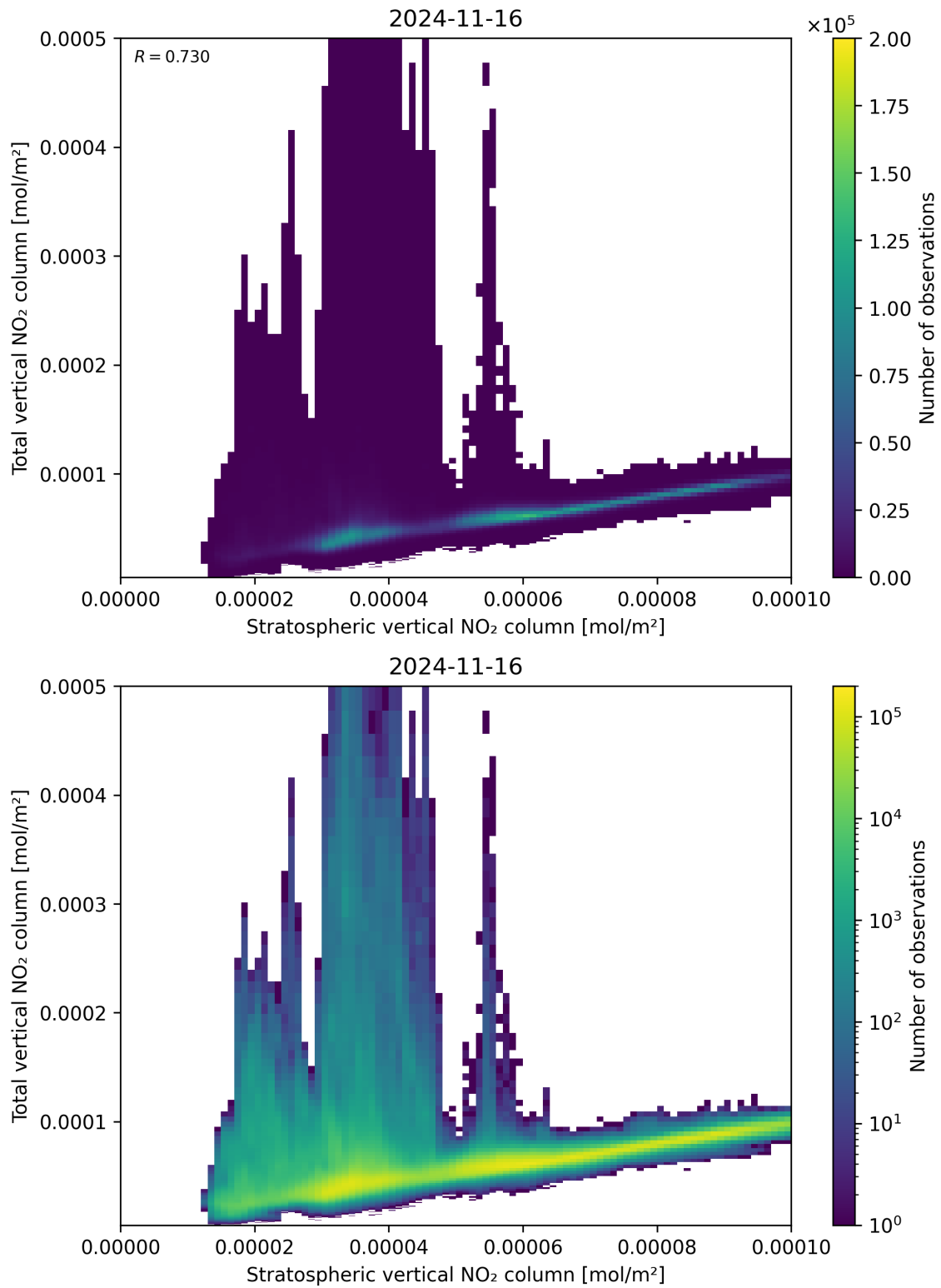
Figure 100: Scatter density plot of “Stratospheric vertical NO 2 column” against “Total vertical NO 2 column” for 2024-11-15 to 2024-11-17.
