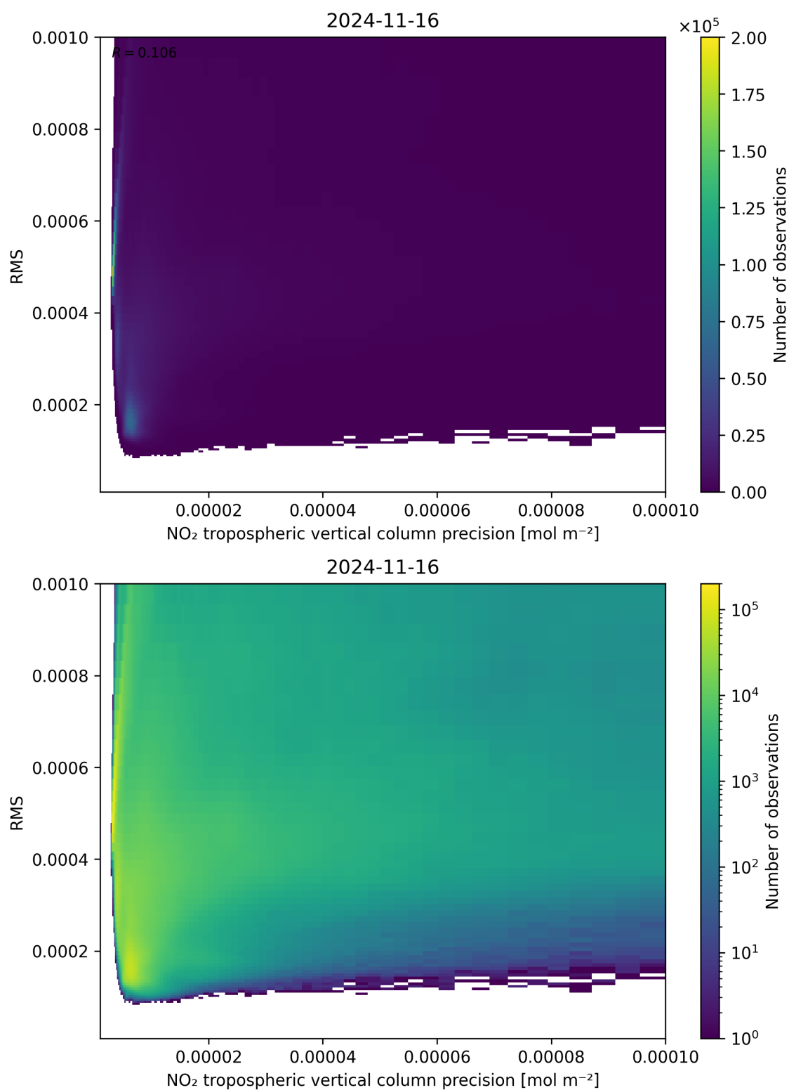
Figure 140: Scatter density plot of “NO 2 tropospheric vertical column precision” against “RMS” for 2024-11-15 to 2024-11-17.
