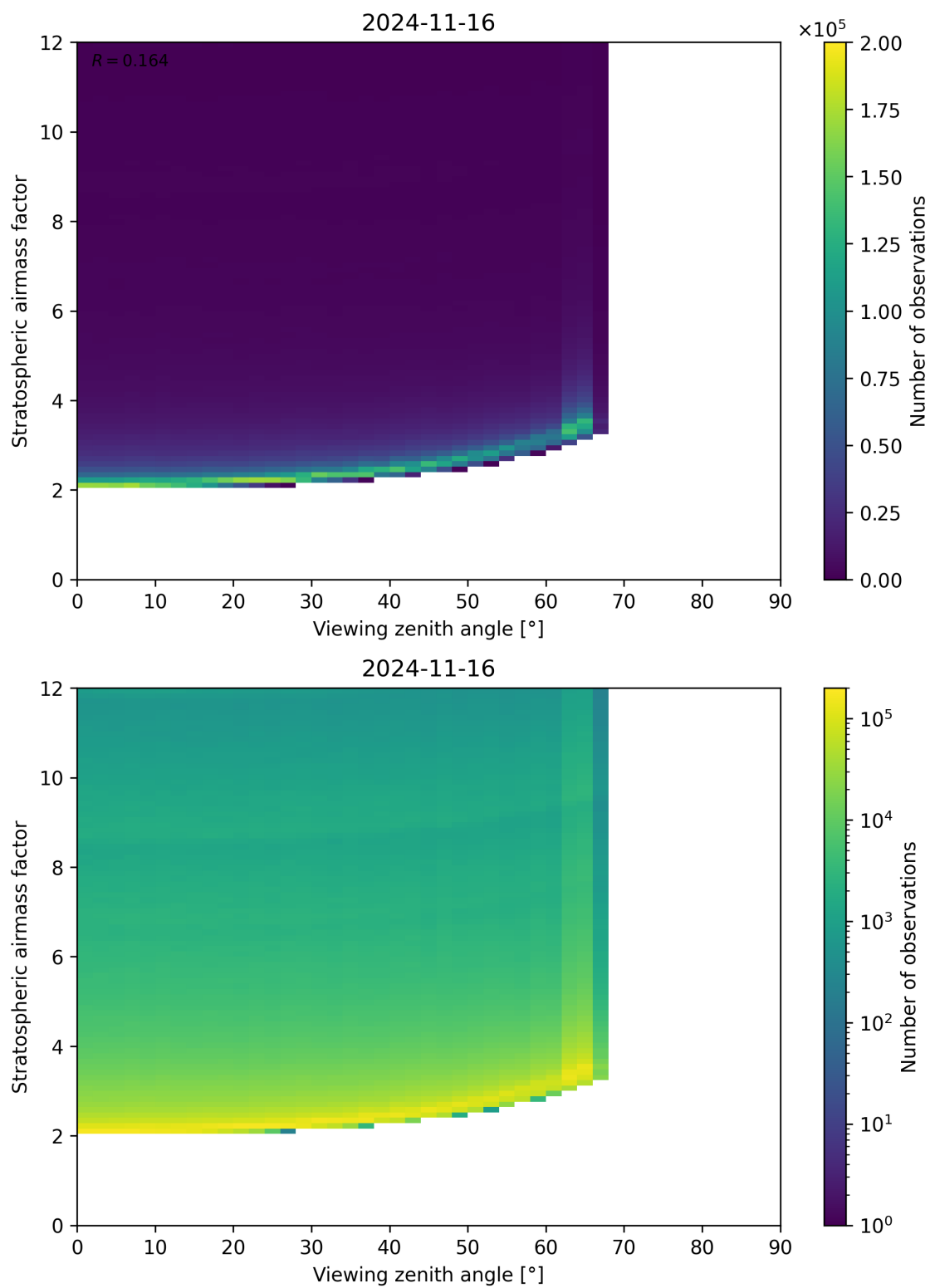
Figure 159: Scatter density plot of “Viewing zenith angle” against “Stratospheric airmass factor” for 2024-11-15 to 2024-11-17.
