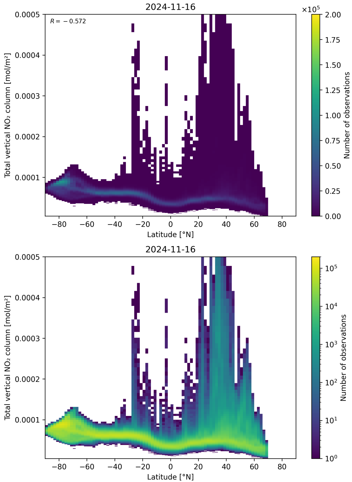
Figure 90: Scatter density plot of “Latitude” against “Total vertical NO 2 column” for 2024-11-15 to 2024-11-17.
