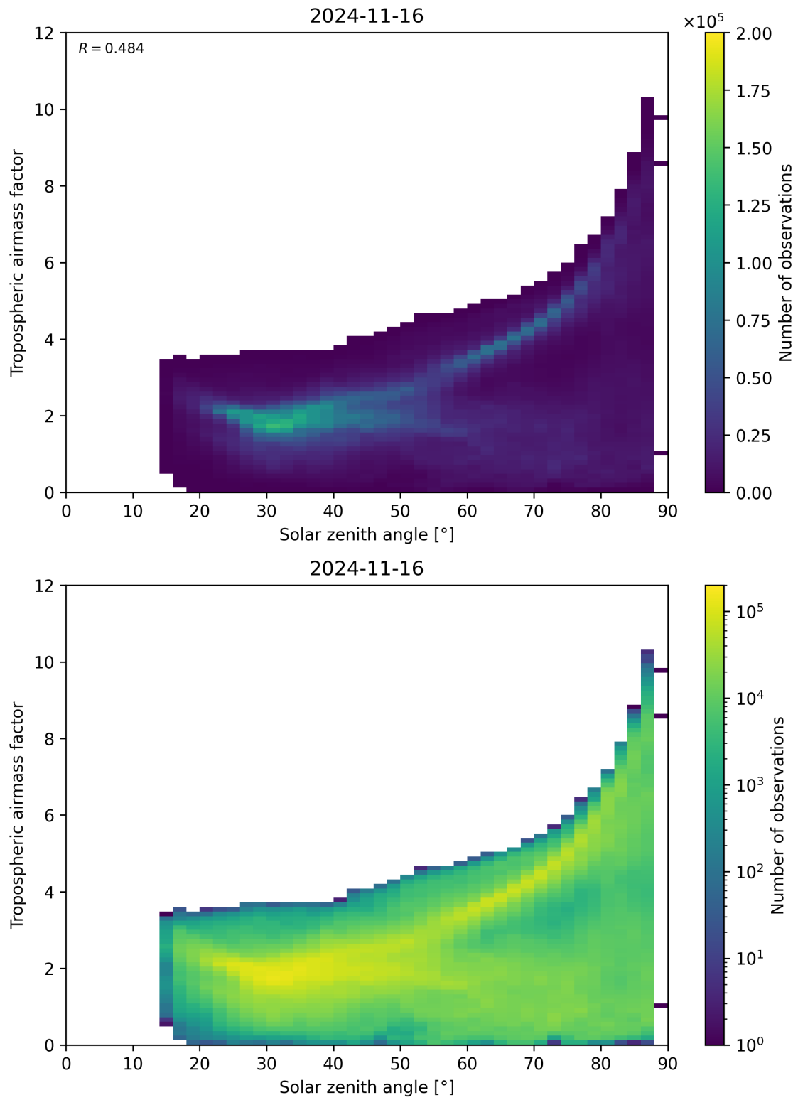
Figure 147: Scatter density plot of “Solar zenith angle” against “Tropospheric airmass factor” for 2024-11-15 to 2024-11-17.
