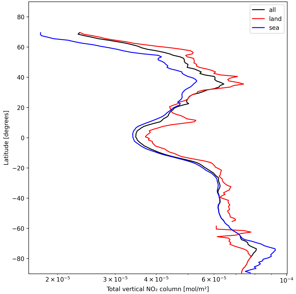
Figure 21: Zonal average of “Total vertical NO 2 column” for 2024-11-15 to 2024-11-17.
