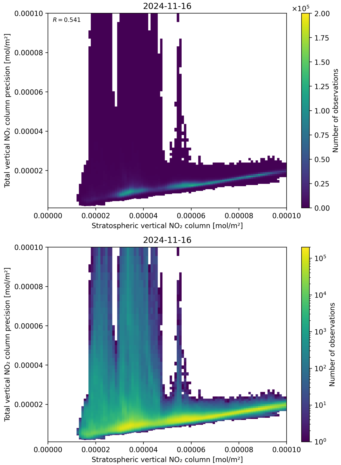
Figure 101: Scatter density plot of “Stratospheric vertical NO 2 column” against “Total vertical NO 2 column precision” for 2024-11-15 to 2024-11-17.
