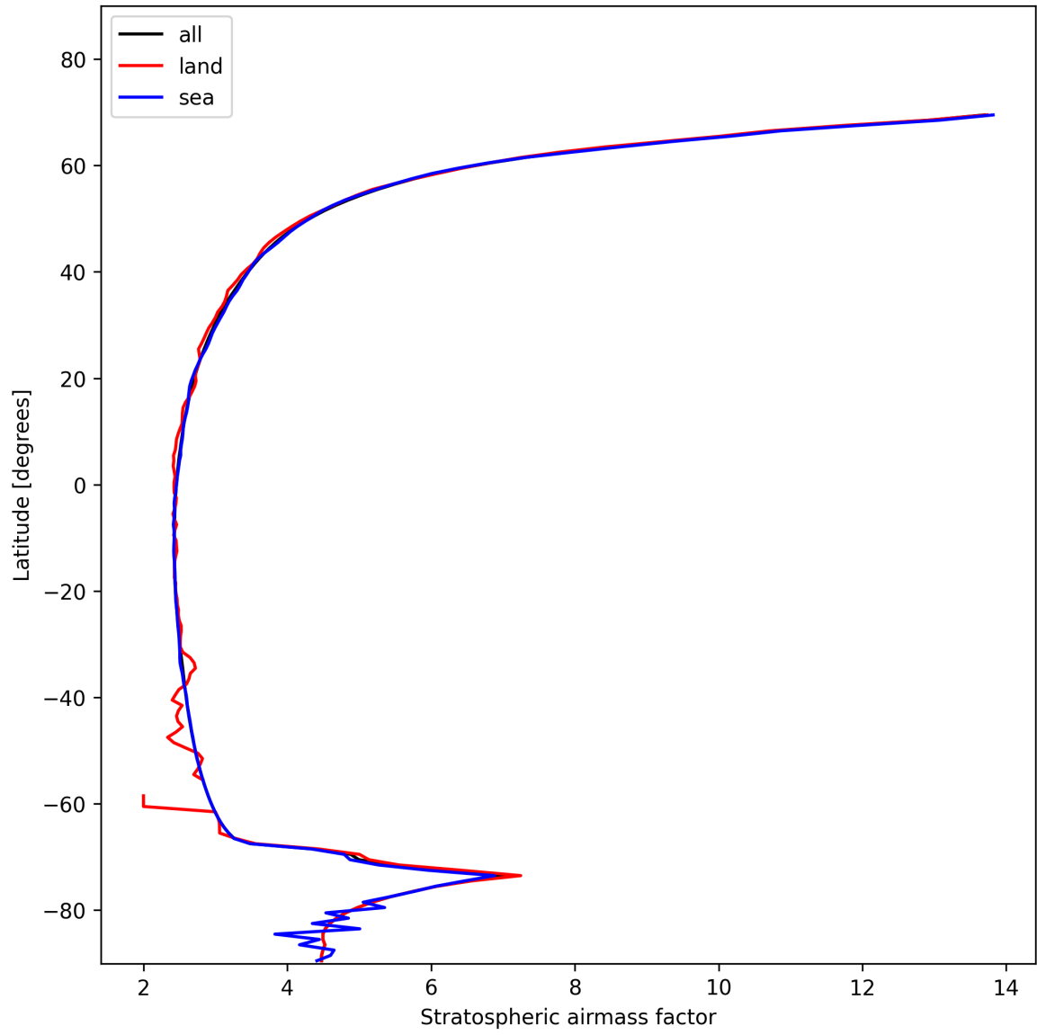
Figure 27: Zonal average of “Stratospheric air mass factor” for 2024-11-15 to 2024-11-17.
