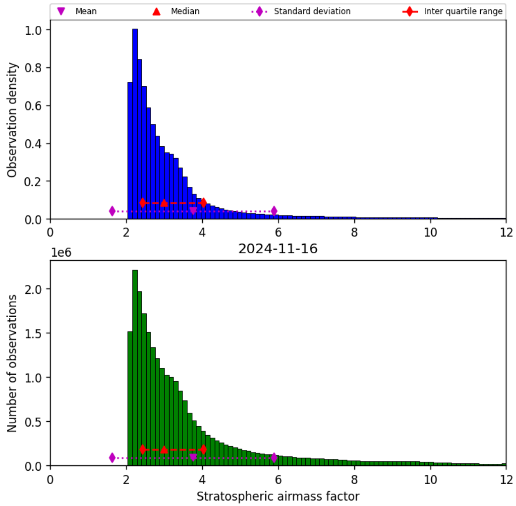
Figure 44: Histogram of “Stratospheric airmass factor” for 2024-11-15 to 2024-11-17
