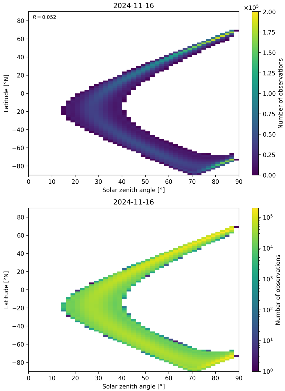
Figure 149: Scatter density plot of “Solar zenith angle” against “Latitude” for 2024-11-15 to 2024-11-17.
