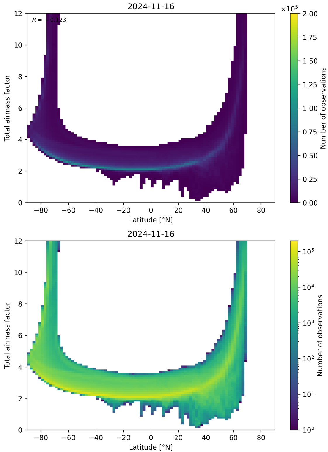
Figure 84: Scatter density plot of “Latitude” against “Total airmass factor” for 2024-11-15 to 2024-11-17.
