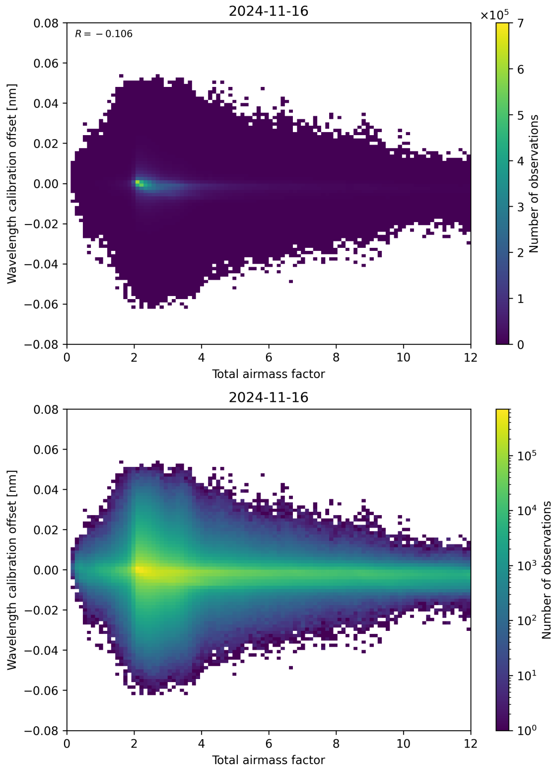
Figure 70: Scatter density plot of “Total airmass factor” against “Wavelength calibration offset” for 2024-11-15 to 2024-11-17.
