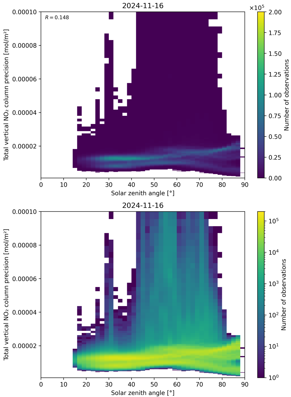
Figure 154: Scatter density plot of “Solar zenith angle” against “Total vertical NO 2 column precision” for 2024-11-15 to 2024-11-17.
