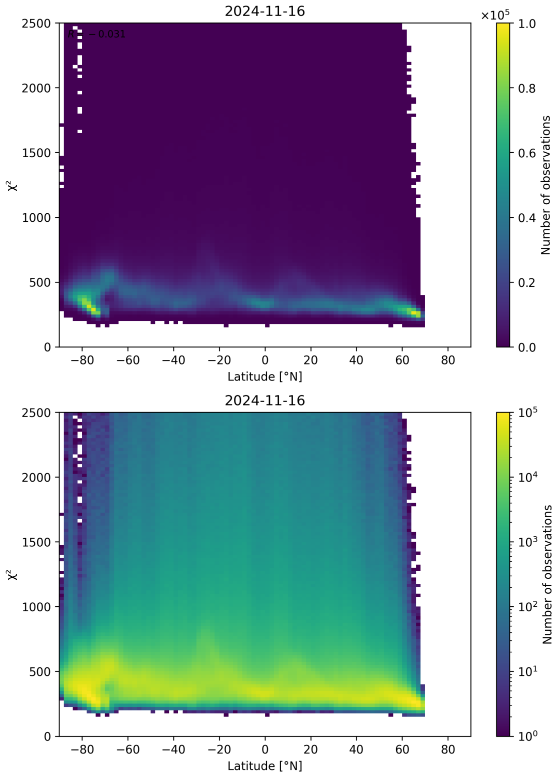
Figure 86: Scatter density plot of “Latitude” against “ \chi^2 ” for 2024-11-15 to 2024-11-17.
