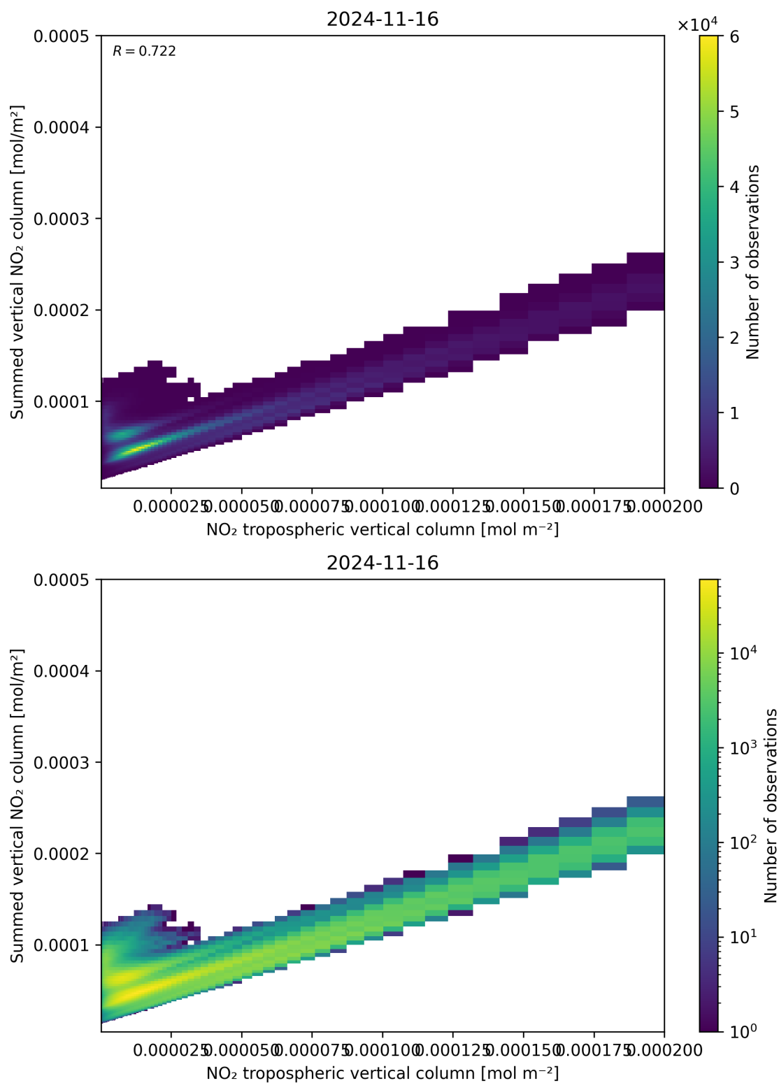
Figure 126: Scatter density plot of “NO 2 tropospheric vertical column” against “Summed vertical NO 2 column” for 2024-11-15 to 2024-11-17.
