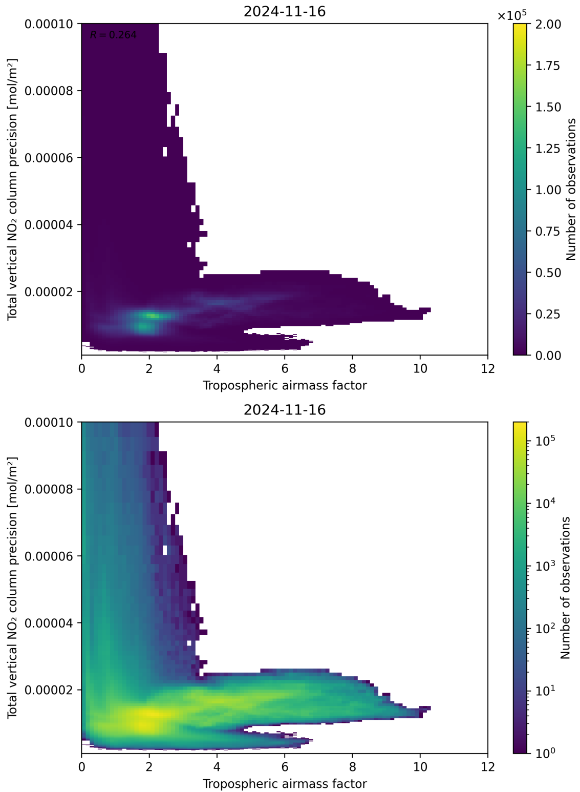
Figure 78: Scatter density plot of “Tropospheric airmass factor” against “Total vertical NO 2 column precision” for 2024-11-15 to 2024-11-17.
