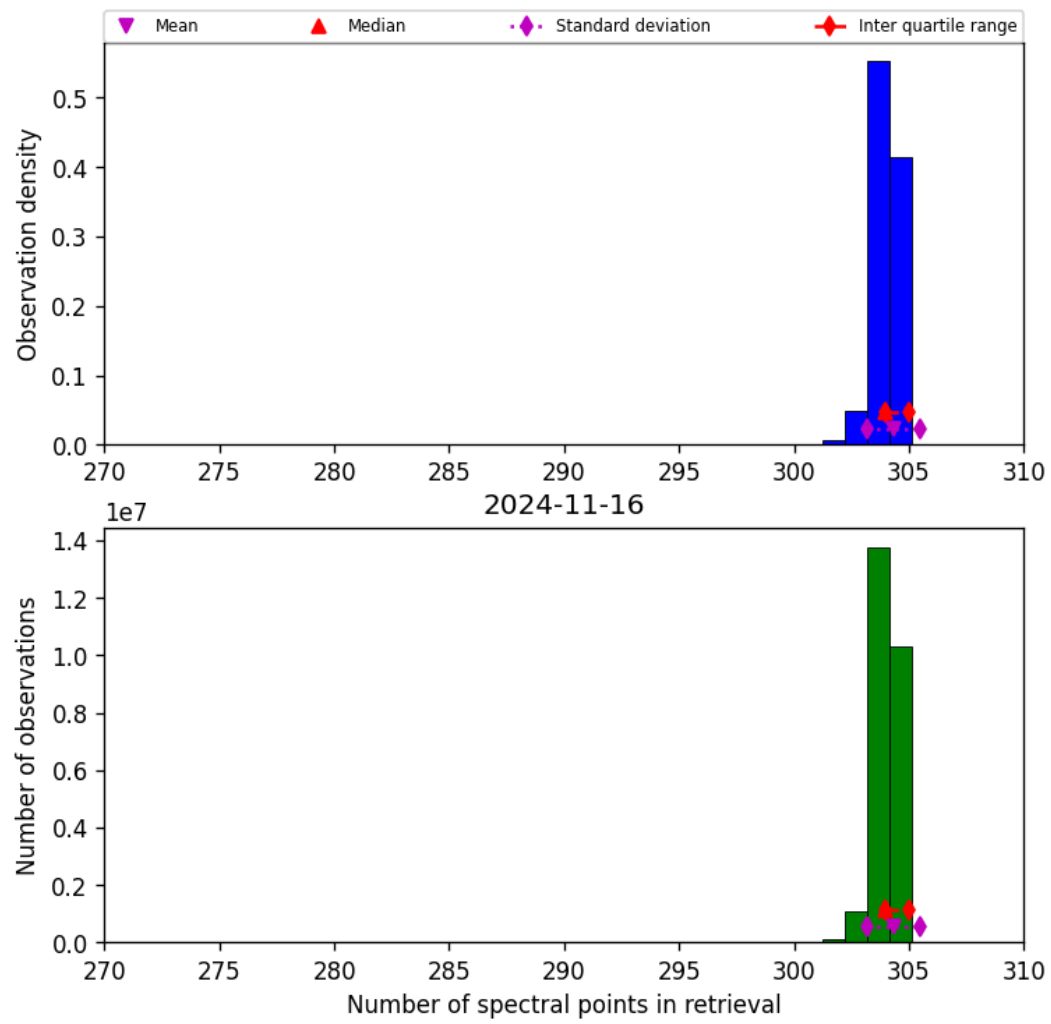
Figure 33: Histogram of “Number of spectral points in retrieval” for 2024-11-15 to 2024-11-17
