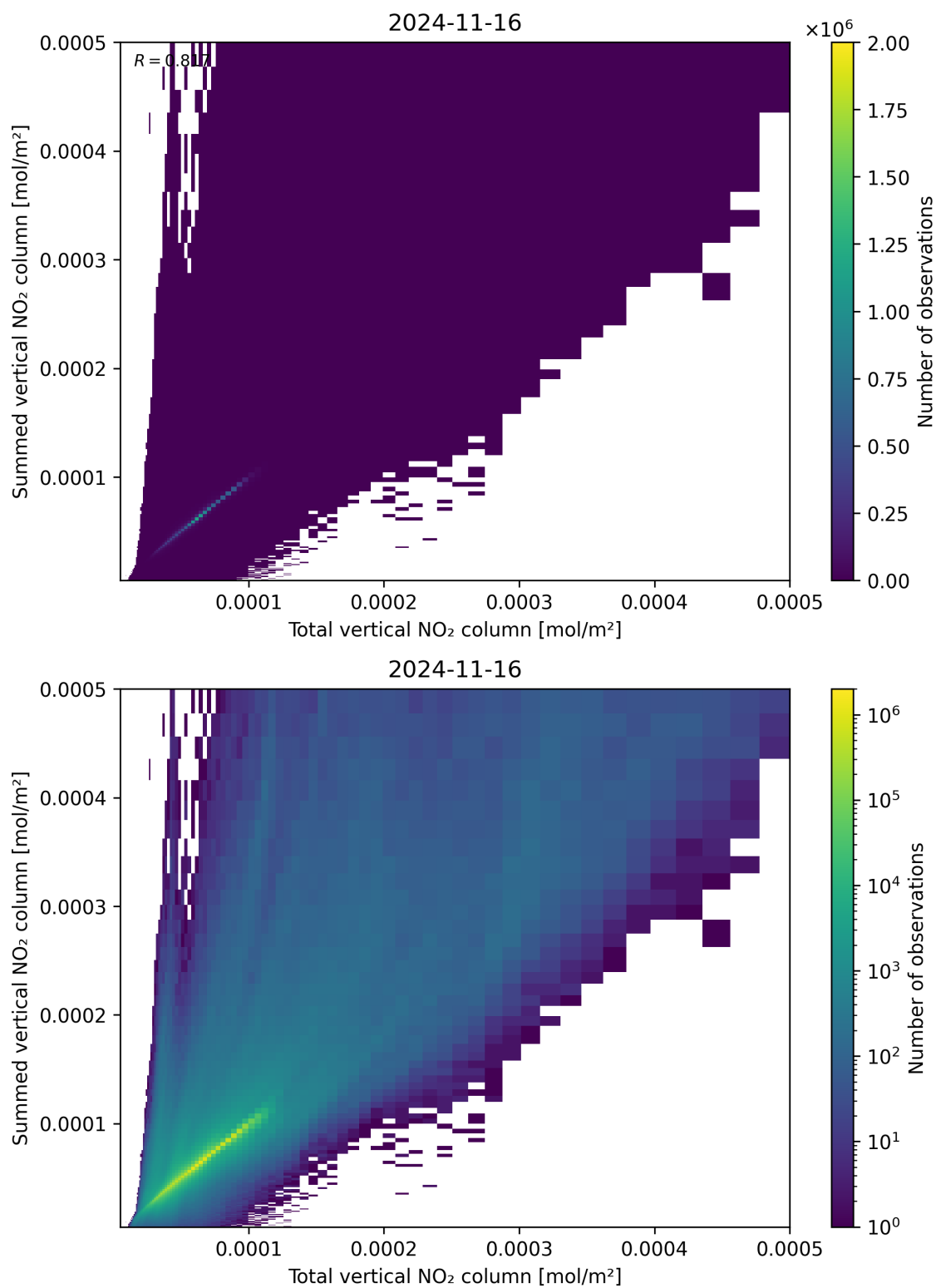
Figure 112: Scatter density plot of “Total vertical NO 2 column” against “Summed vertical NO 2 column” for 2024-11-15 to 2024-11-17.
