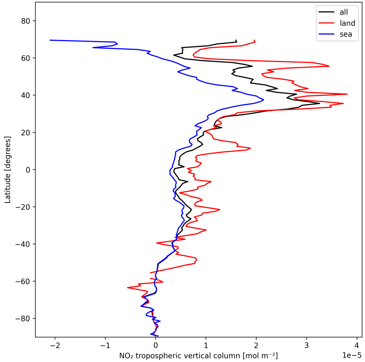
Figure 12: Zonal average of “NO 2 tropospheric vertical column” for 2024-11-15 to 2024-11-17.
