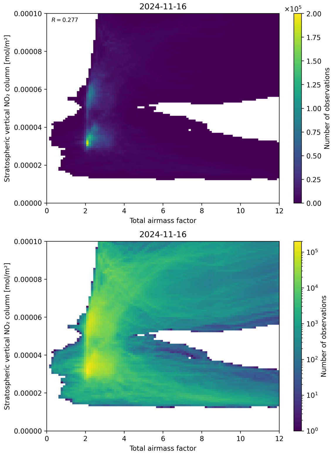
Figure 64: Scatter density plot of “Total airmass factor” against “Stratospheric vertical NO 2 column” for 2024-11-15 to 2024-11-17.
