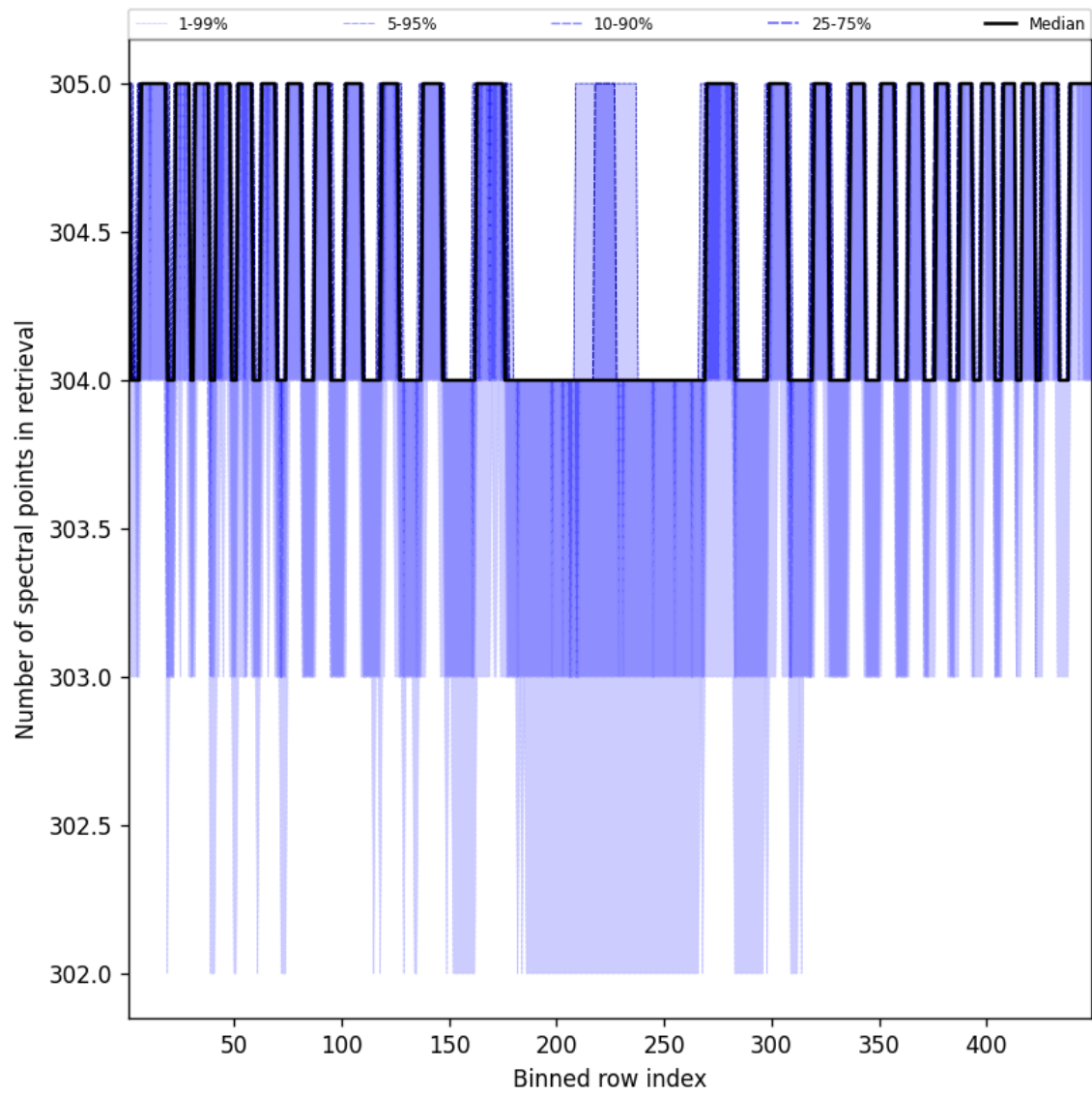
Figure 50: Along track statistics of “Number of spectral points in retrieval” for 2024-11-15 to 2024-11-17
