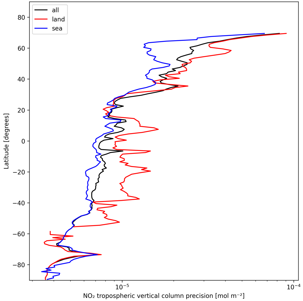
Figure 13: Zonal average of "NO 2 tropospheric vertical column precision" for 2024-11-15 to 2024-11-17.
