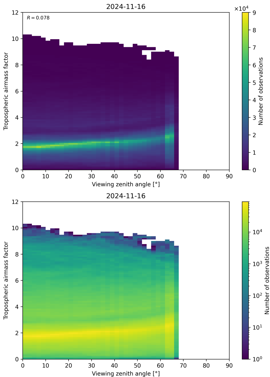
Figure 161: Scatter density plot of “Viewing zenith angle” against “Tropospheric airmass factor” for 2024-11-15 to 2024-11-17.
