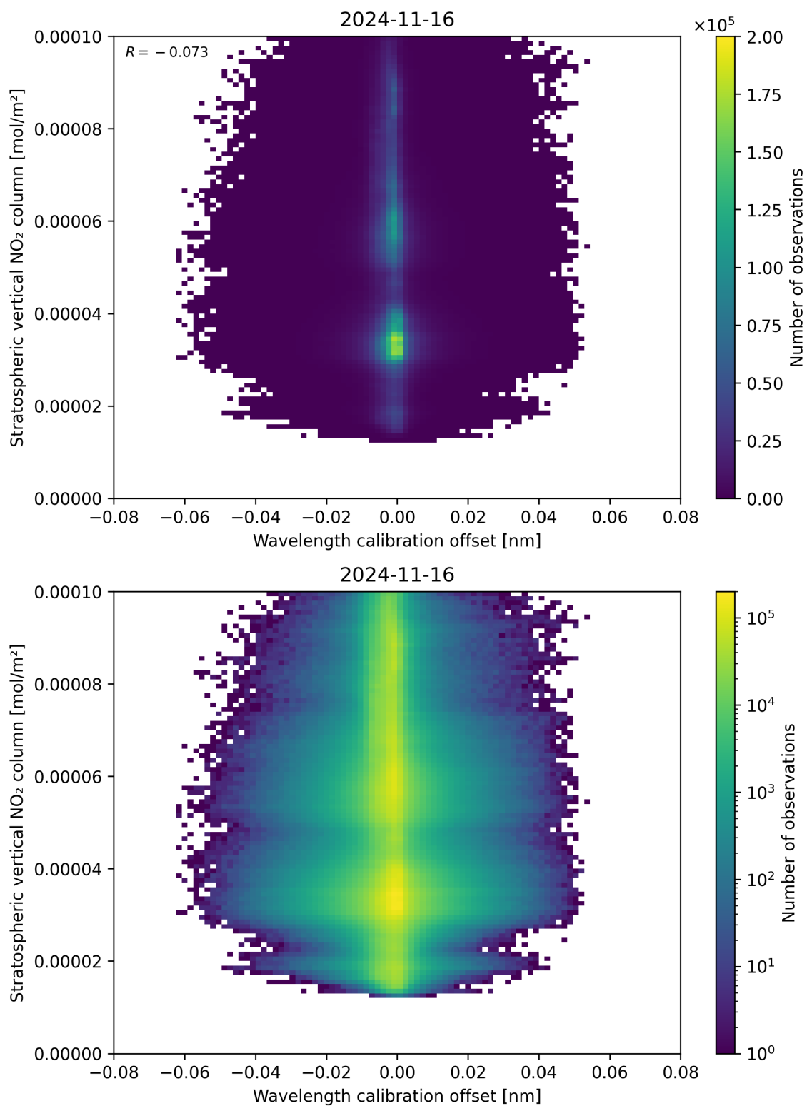
Figure 176: Scatter density plot of “Wavelength calibration offset” against “Stratospheric vertical NO 2 column” for 2024-11-15 to 2024-11-17.
