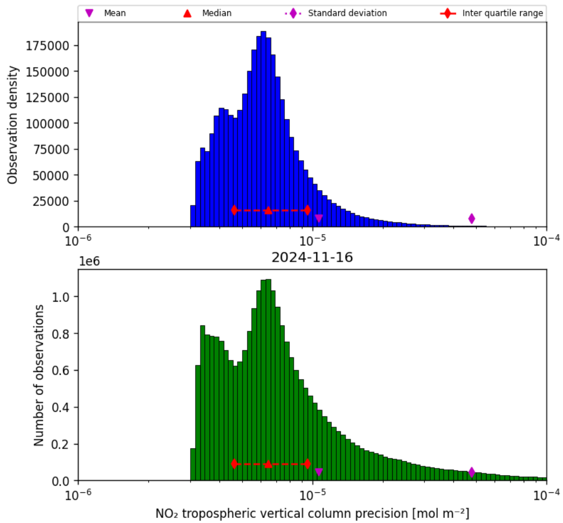
Figure 30: Histogram of "NO 2 tropospheric vertical column precision" for 2024-11-15 to 2024-11-17
