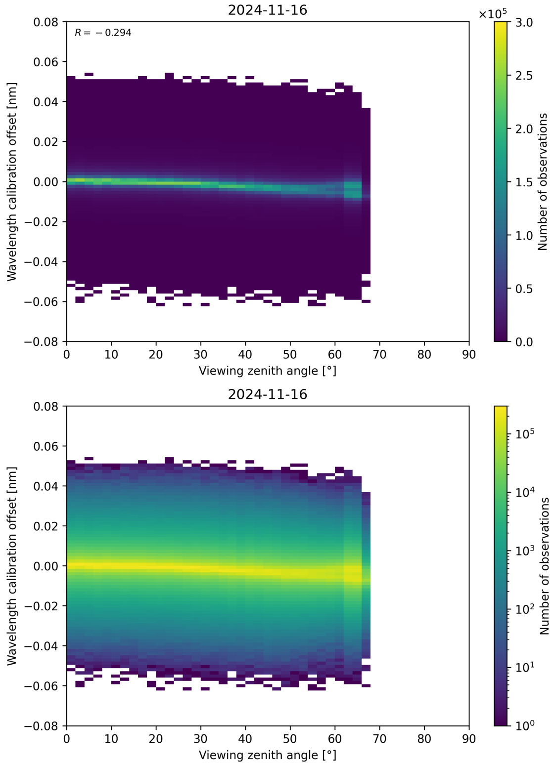
Figure 173: Scatter density plot of “Viewing zenith angle” against “Wavelength calibration offset” for 2024-11-15 to 2024-11-17.
