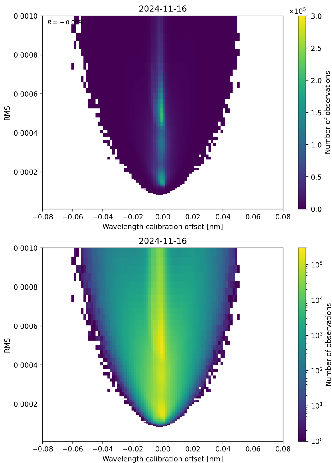
Figure 181: Scatter density plot of “Wavelength calibration offset” against “RMS” for 2024-11-15 to 2024-11-17.
