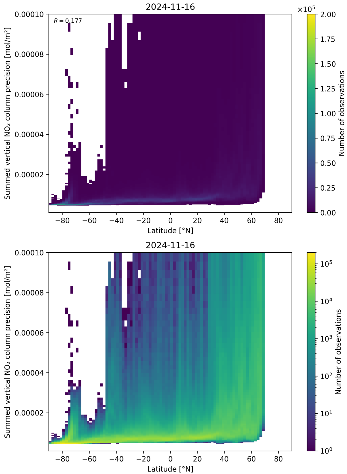
Figure 89: Scatter density plot of “Latitude” against “Summed vertical NO 2 column precision” for 2024-11-15 to 2024-11-17.
