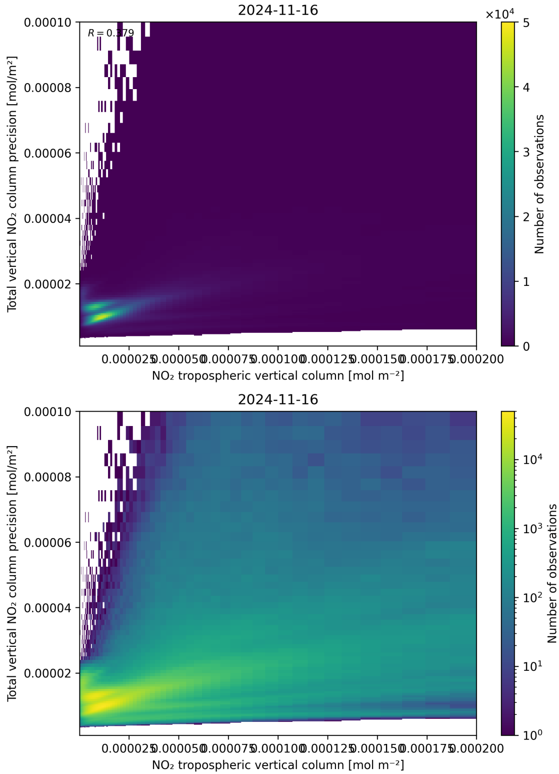
Figure 129: Scatter density plot of “NO 2 tropospheric vertical column” against “Total vertical NO 2 column precision” for 2024-11-15 to 2024-11-17.
