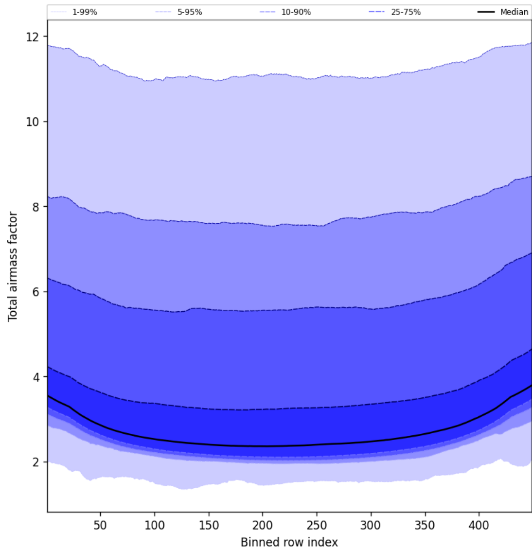
Figure 49: Along track statistics of “Total airmass factor” for 2024-11-15 to 2024-11-17
