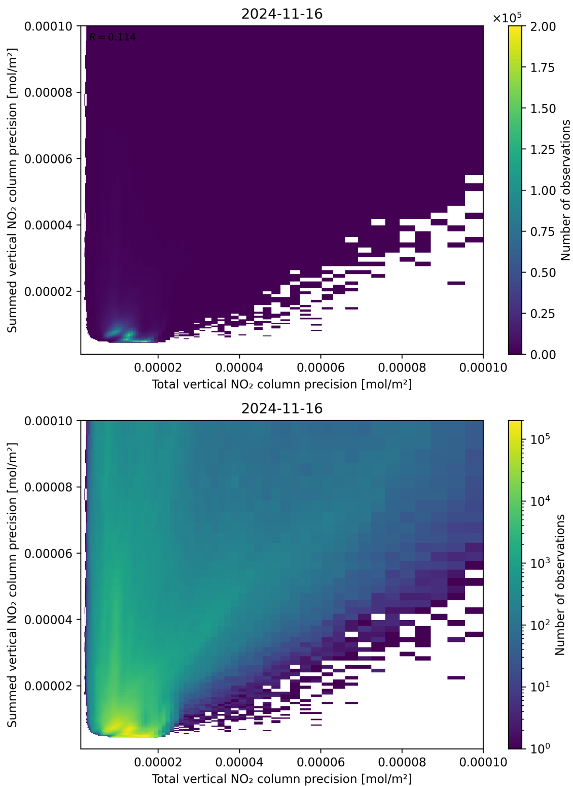
Figure 118: Scatter density plot of “Total vertical NO 2 column precision” against “Summed vertical NO 2 column precision” for 2024-11-15 to 2024-11-17.
