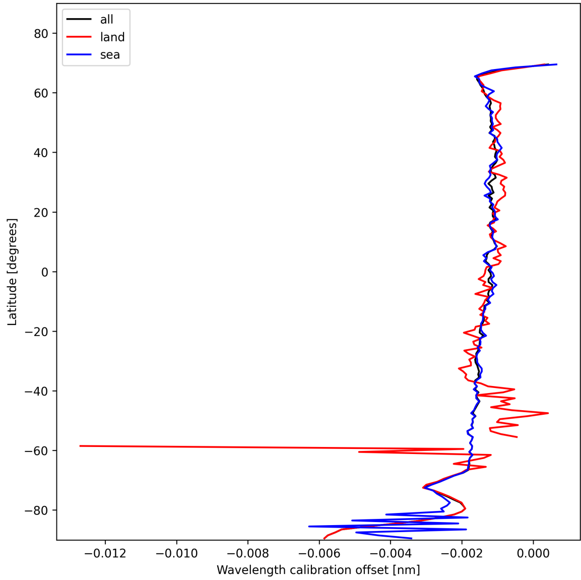
Figure 18: Zonal average of “Wavelength calibration offset” for 2024-11-15 to 2024-11-17.
