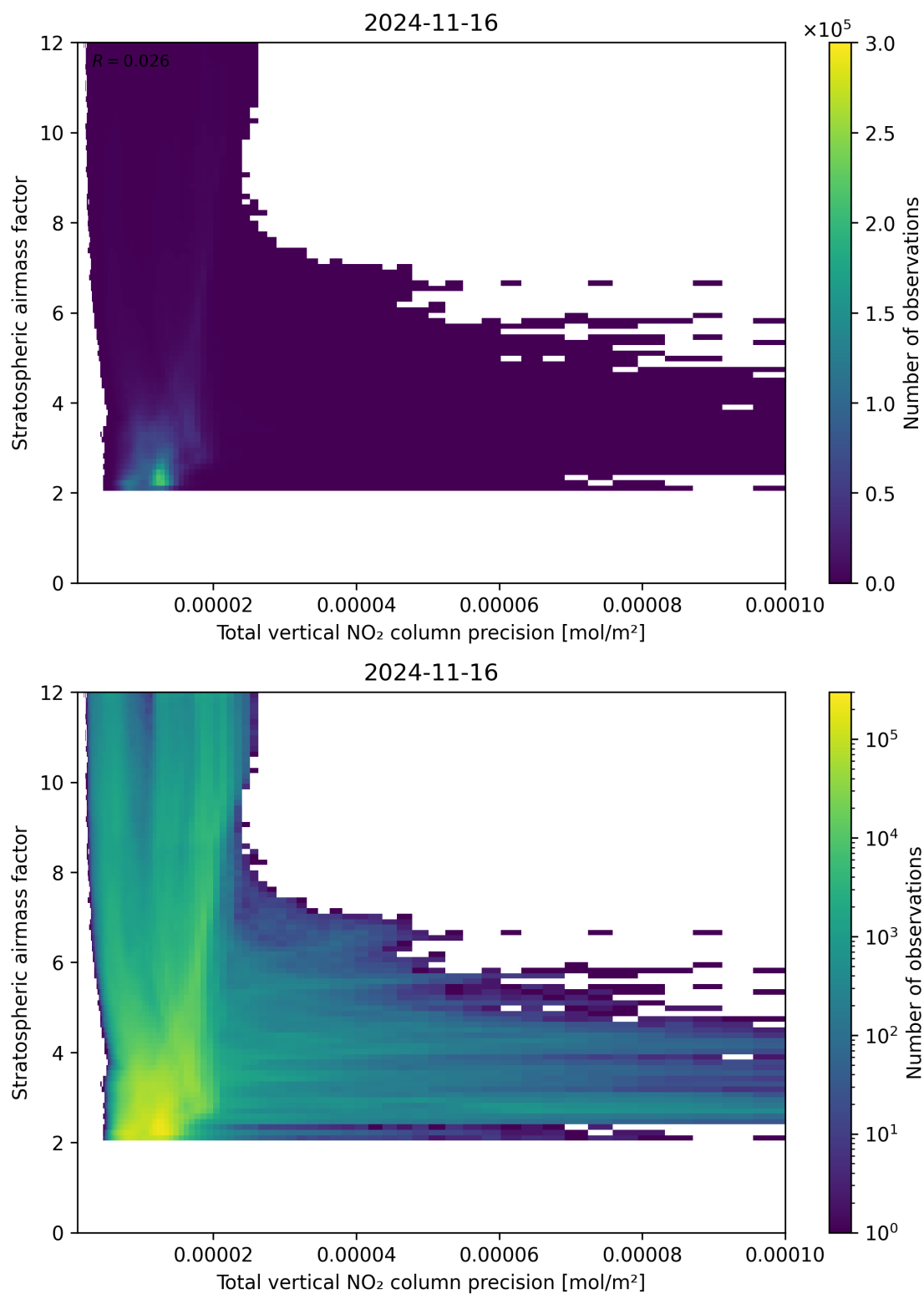
Figure 115: Scatter density plot of “Total vertical NO 2 column precision” against “Stratospheric air mass factor” for 2024-11-15 to 2024-11-17.
