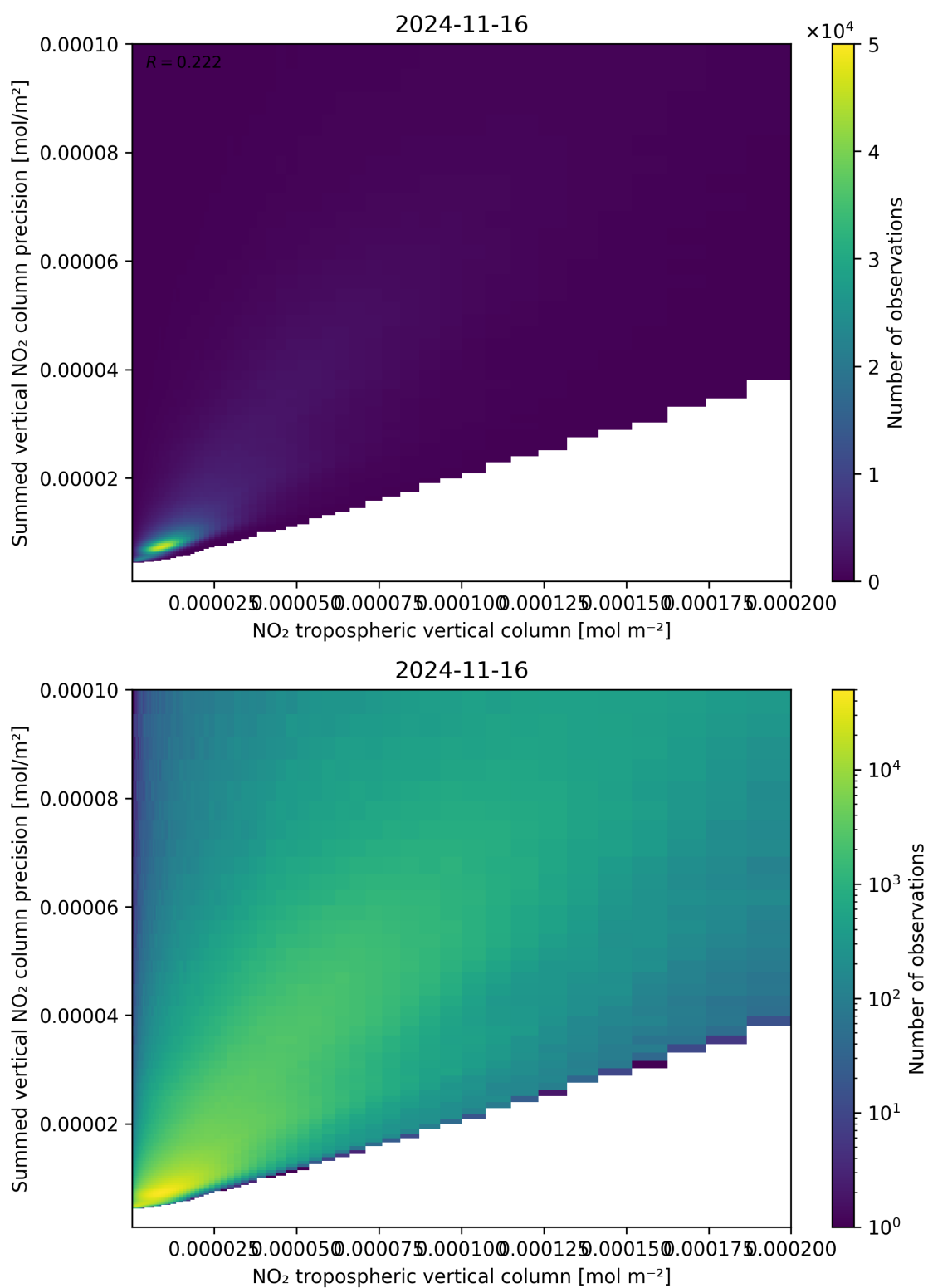
Figure 127: Scatter density plot of “NO 2 tropospheric vertical column” against “Summed vertical NO 2 column precision” for 2024-11-15 to 2024-11-17.
