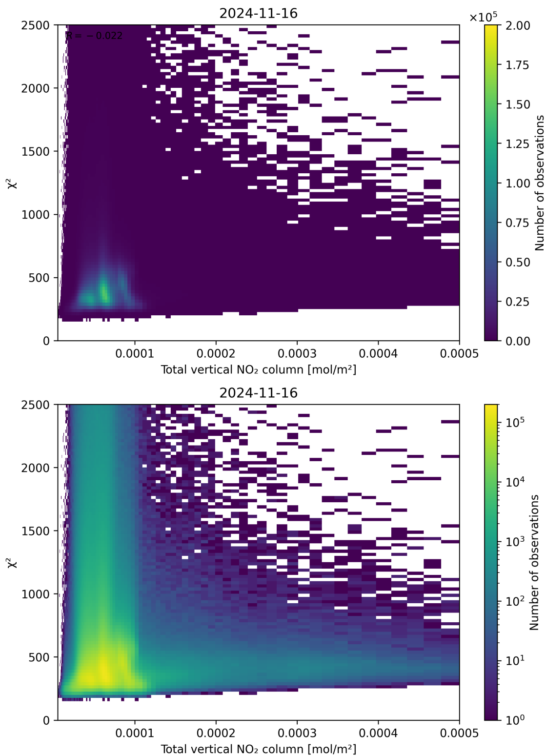
Figure 111: Scatter density plot of “Total vertical NO 2 column” against “ \chi^2 ” for 2024-11-15 to 2024-11-17.
