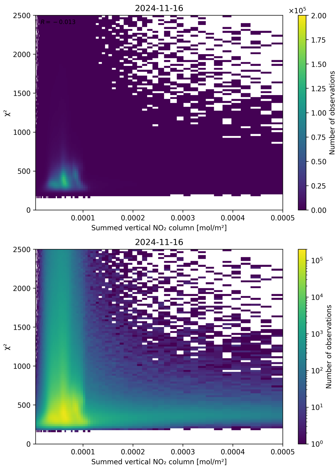
Figure 104: Scatter density plot of “Summed vertical NO 2 column” against “ \chi^2 ” for 2024-11-15 to 2024-11-17.
