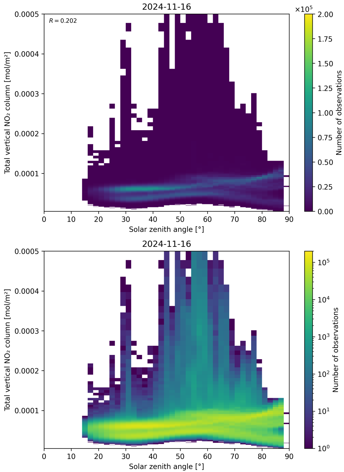
Figure 153: Scatter density plot of “Solar zenith angle” against “Total vertical NO 2 column” for 2024-11-15 to 2024-11-17.
