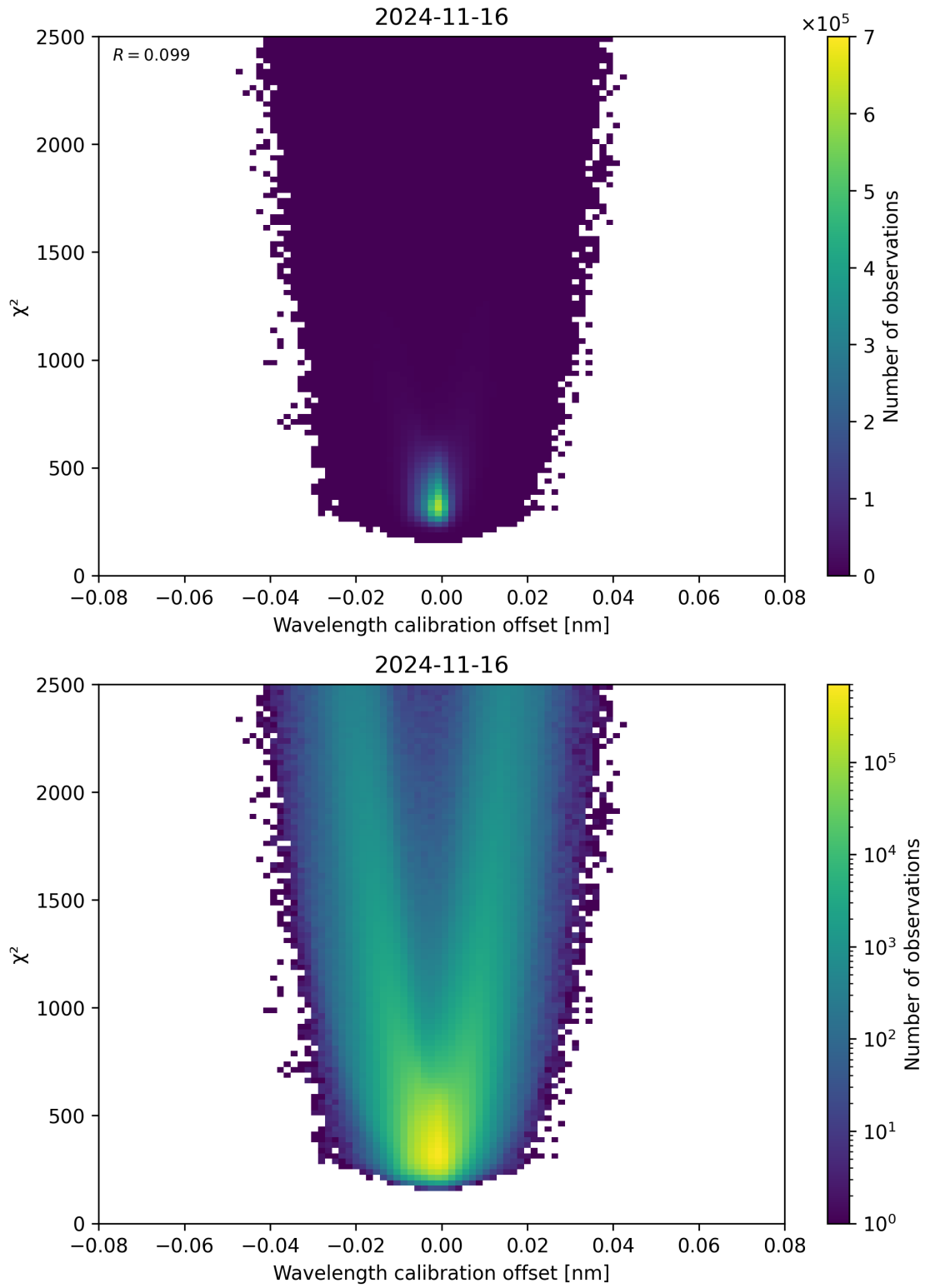
Figure 175: Scatter density plot of “Wavelength calibration offset” against “ \chi^2 ” for 2024-11-15 to 2024-11-17.
