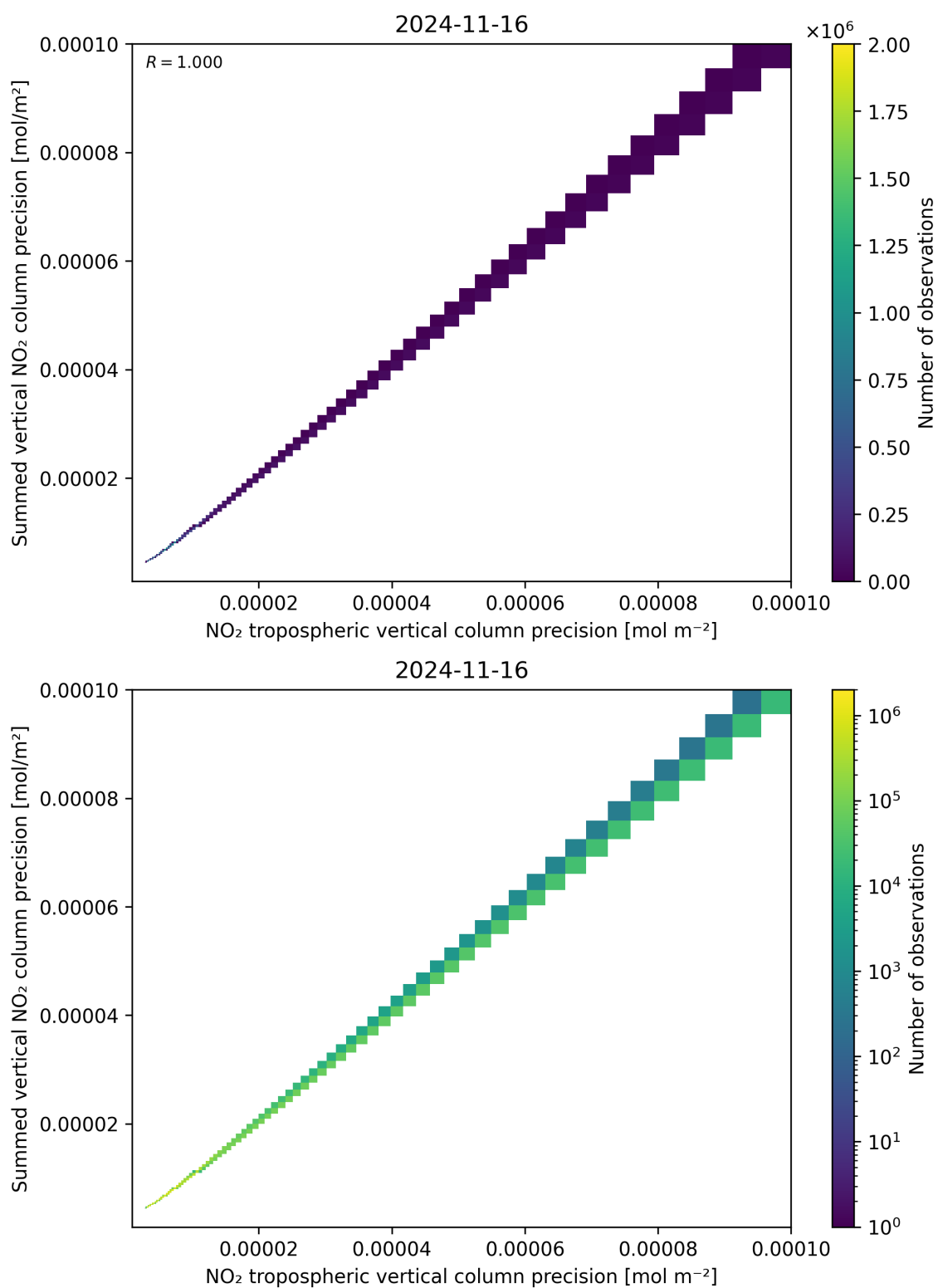
Figure 137: Scatter density plot of “NO 2 tropospheric vertical column precision” against “Summed vertical NO 2 column precision” for 2024-11-15 to 2024-11-17.
