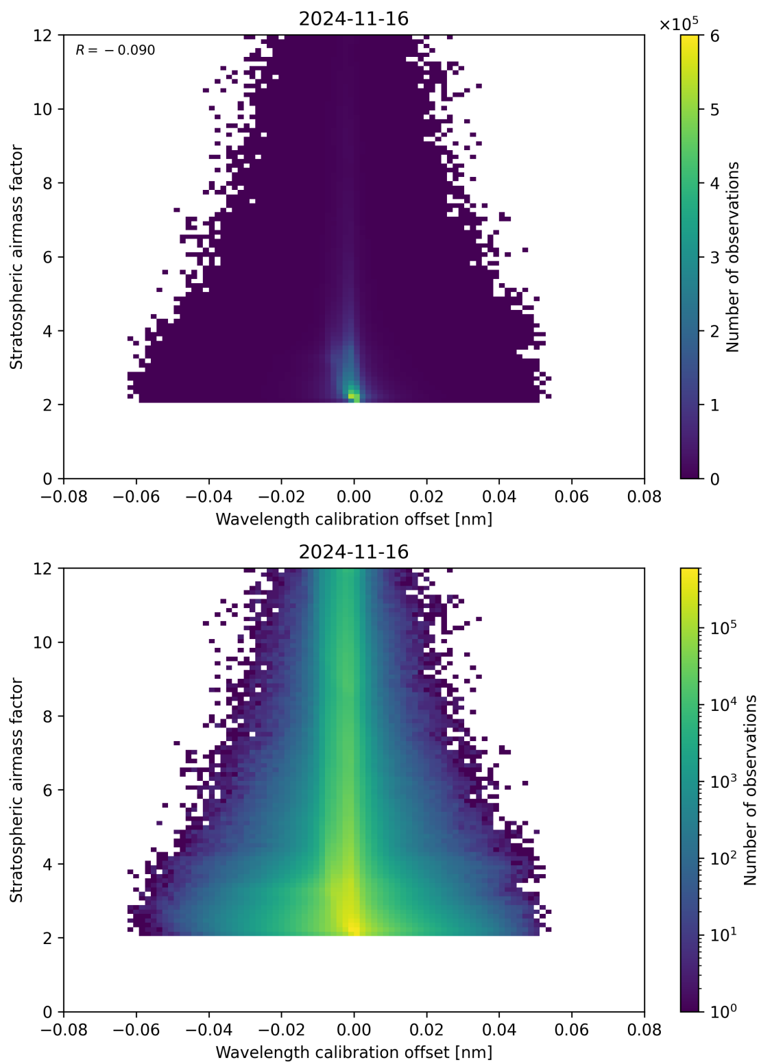
Figure 174: Scatter density plot of “Wavelength calibration offset” against “Stratospheric airmass factor” for 2024-11-15 to 2024-11-17.
