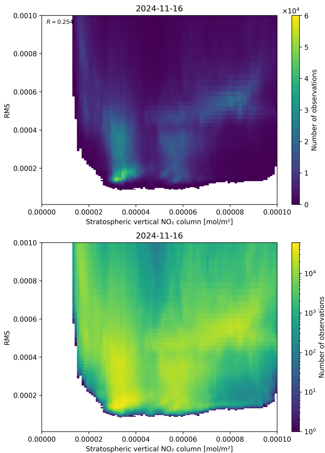
Figure 102: Scatter density plot of “Stratospheric vertical NO 2 column” against “RMS” for 2024-11-15 to 2024-11-17.
