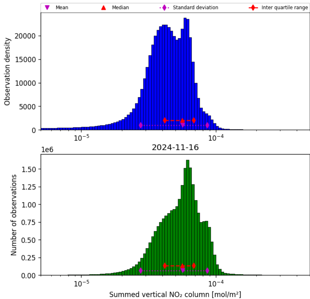
Figure 40: Histogram of “Summed vertical NO 2 column” for 2024-11-15 to 2024-11-17
