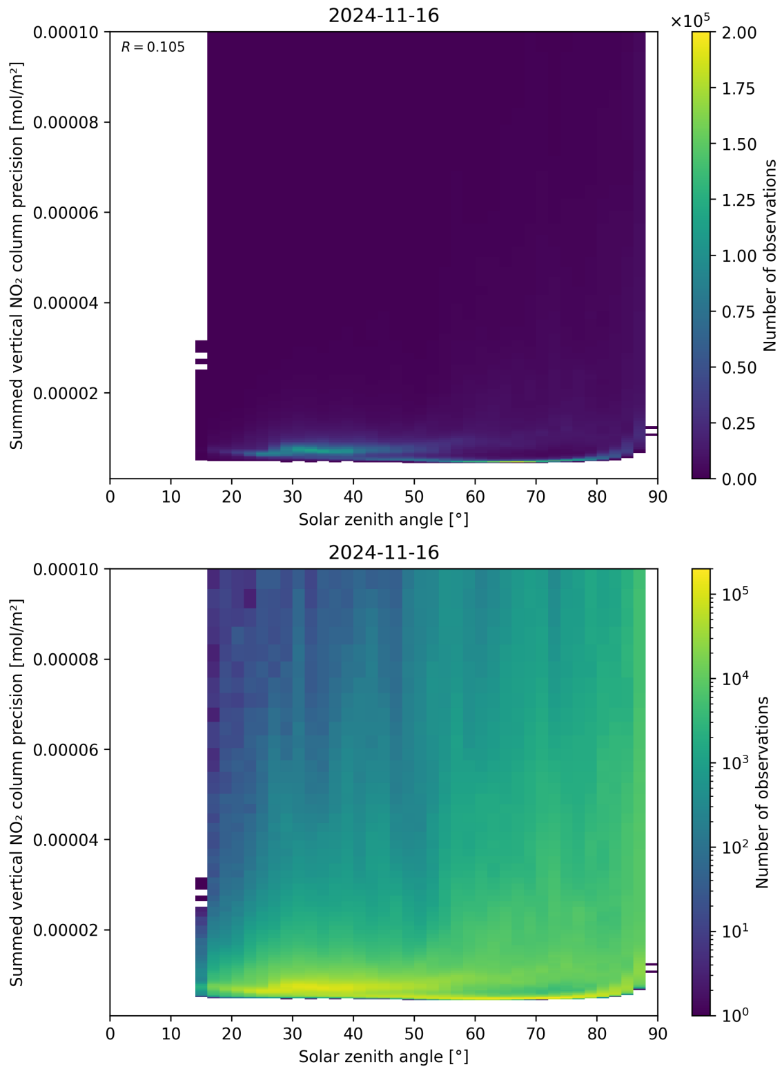
Figure 152: Scatter density plot of “Solar zenith angle” against “Summed vertical NO 2 column precision” for 2024-11-15 to 2024-11-17.
