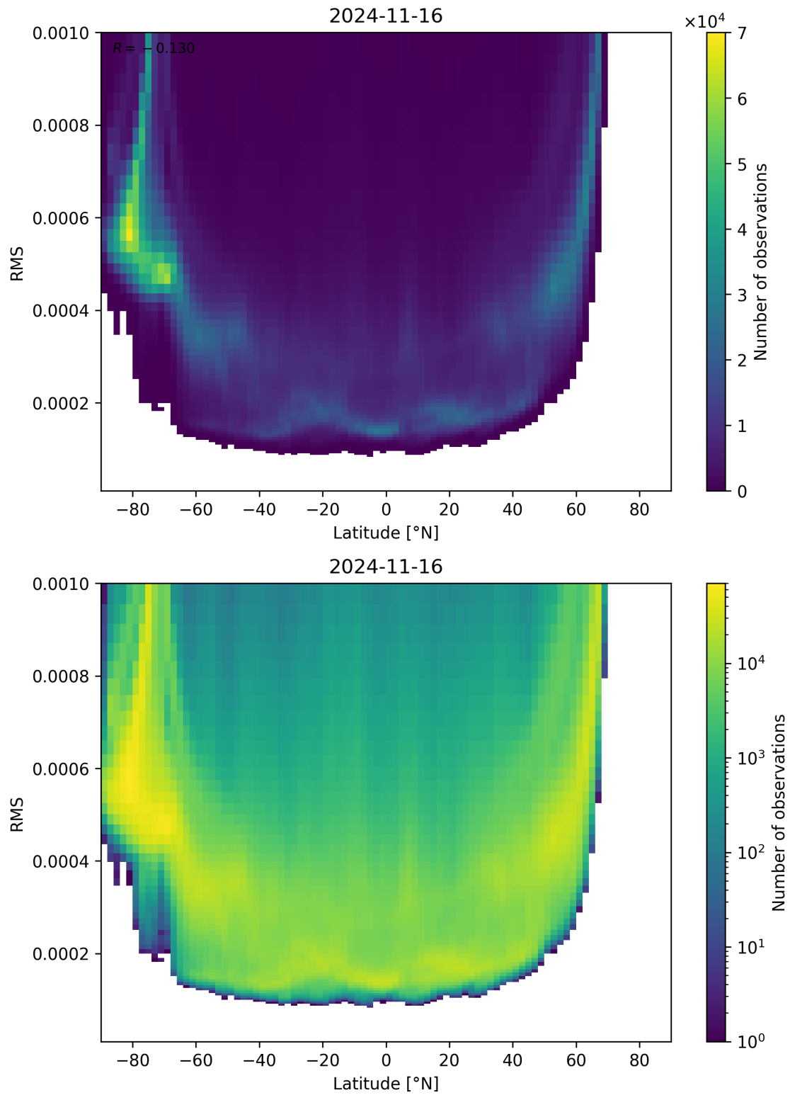
Figure 94: Scatter density plot of “Latitude” against “RMS” for 2024-11-15 to 2024-11-17.
