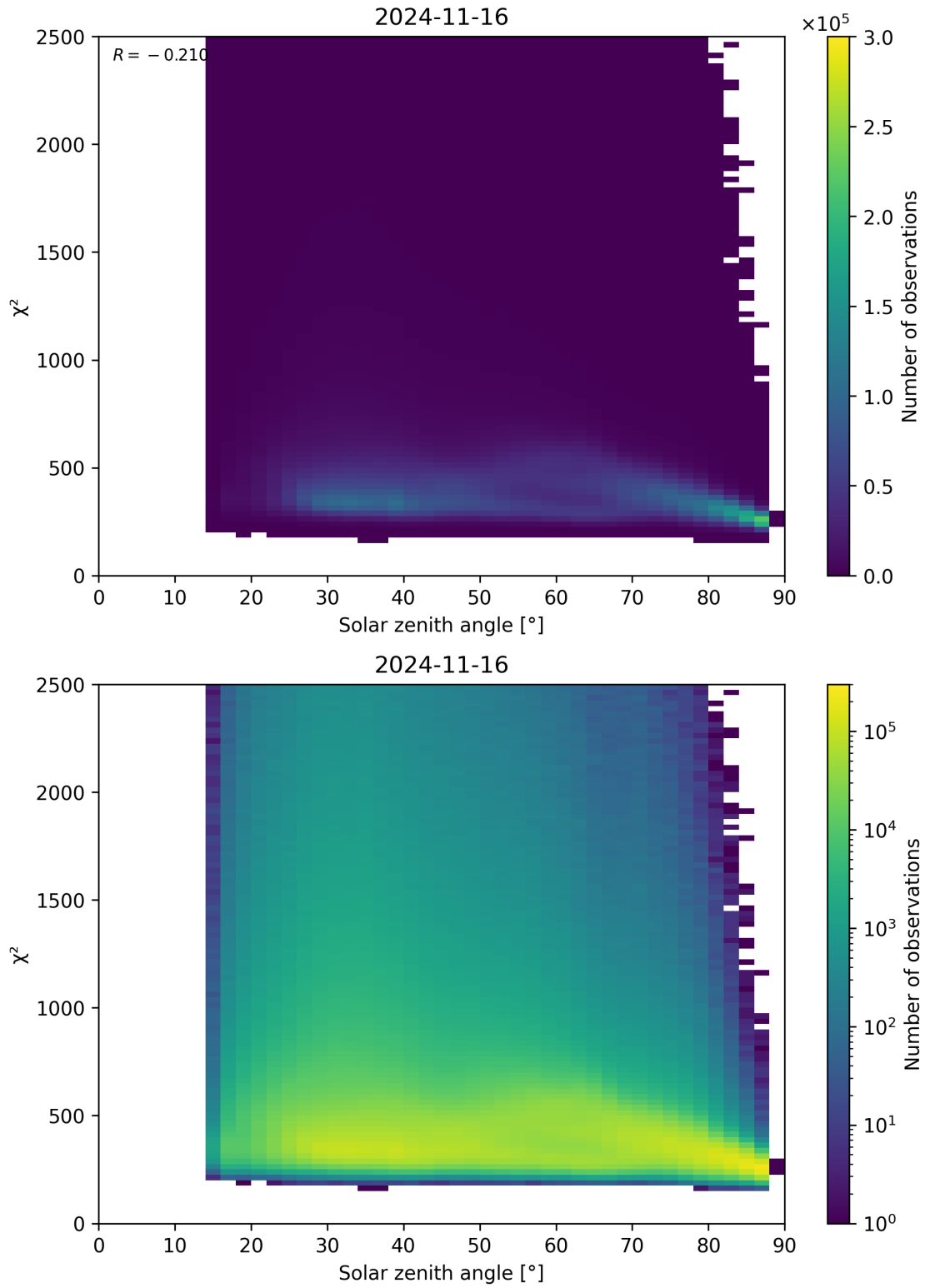
Figure 148: Scatter density plot of “Solar zenith angle” against “ \chi^2 ” for 2024-11-15 to 2024-11-17.
