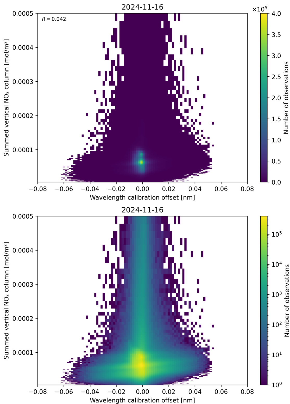
Figure 177: Scatter density plot of “Wavelength calibration offset” against “Summed vertical NO 2 column” for 2024-11-15 to 2024-11-17.
