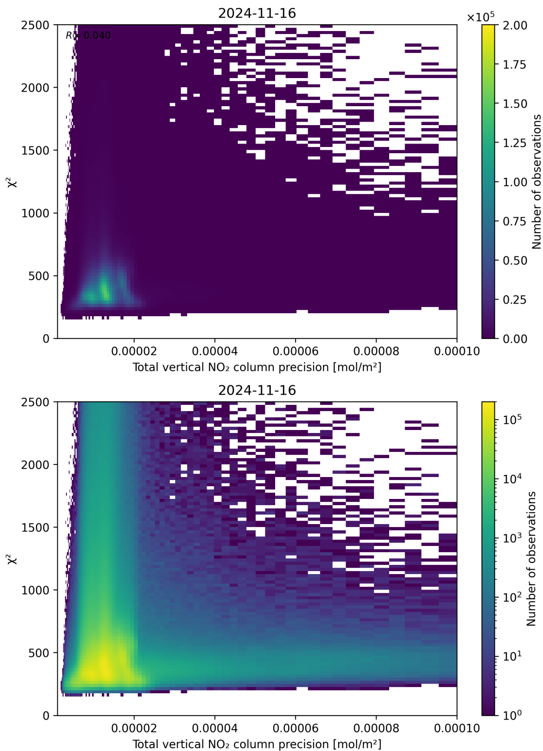
Figure 116: Scatter density plot of “Total vertical NO 2 column precision” against “ \chi^2 ” for 2024-11-15 to 2024-11-17.
