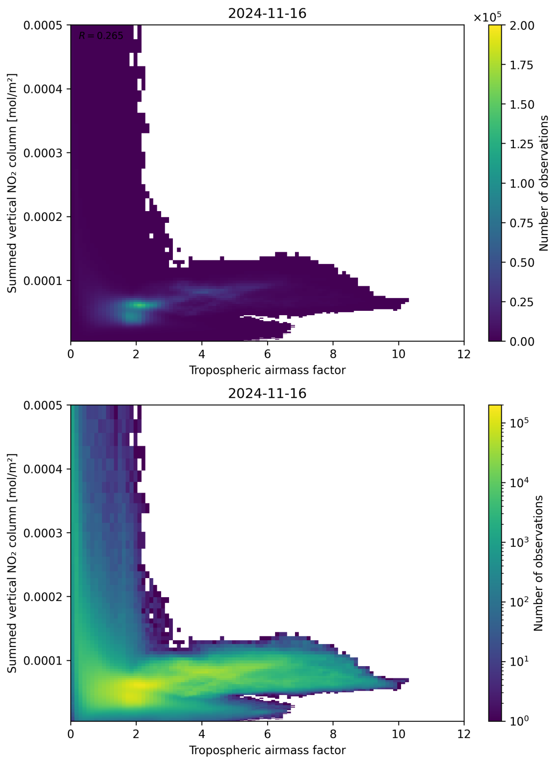
Figure 75: Scatter density plot of “Tropospheric airmass factor” against “Summed vertical NO 2 column” for 2024-11-15 to 2024-11-17.
