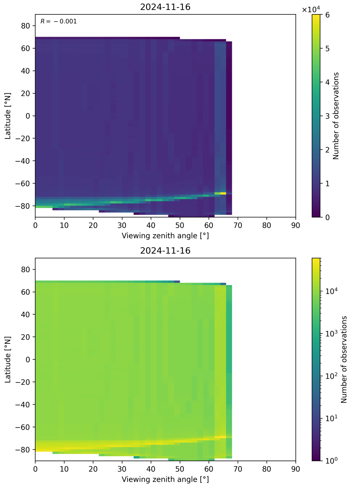
Figure 163: Scatter density plot of “Viewing zenith angle” against “Latitude” for 2024-11-15 to 2024-11-17.
