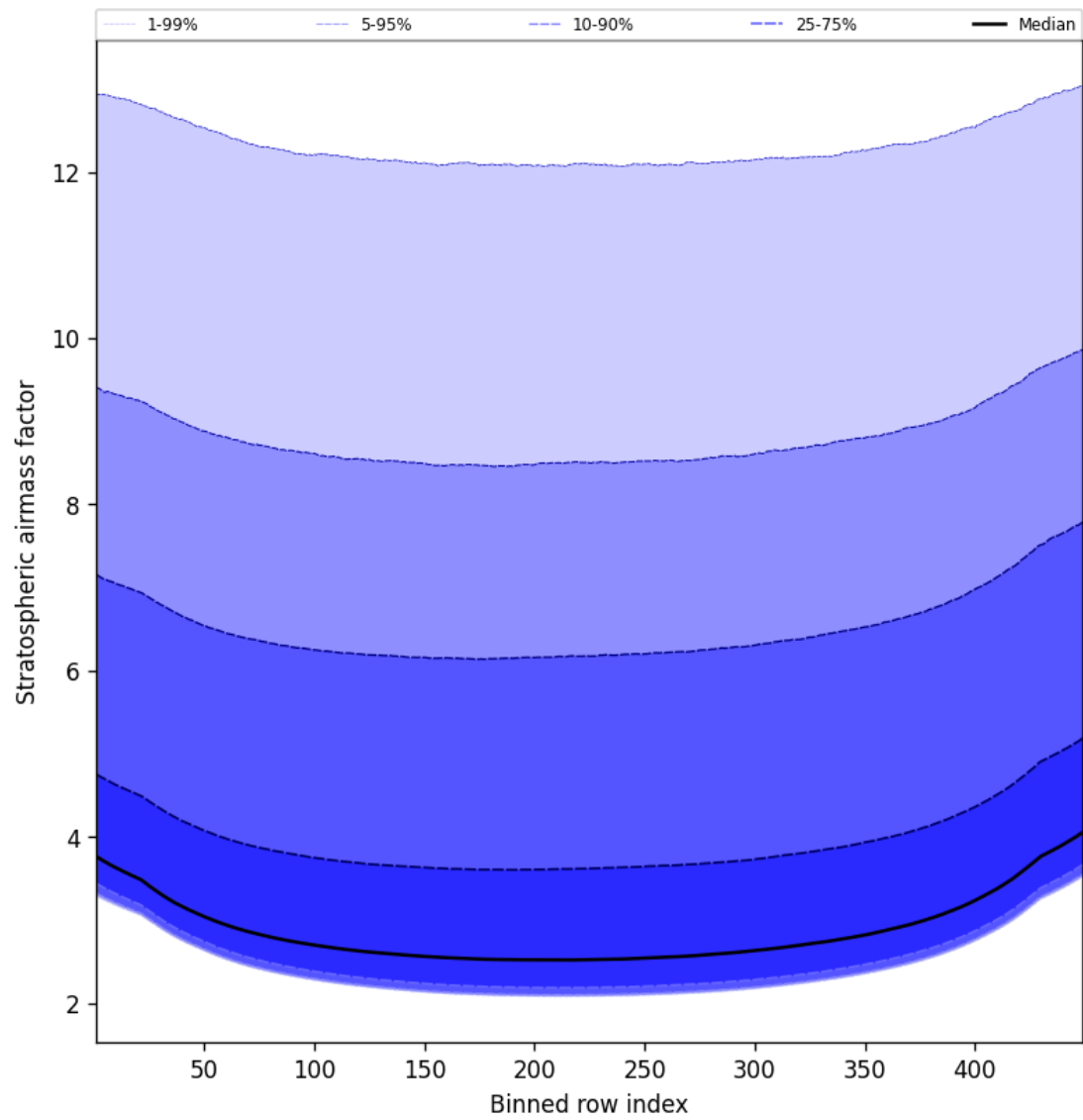
Figure 61: Along track statistics of “Stratospheric air mass factor” for 2024-11-15 to 2024-11-17
