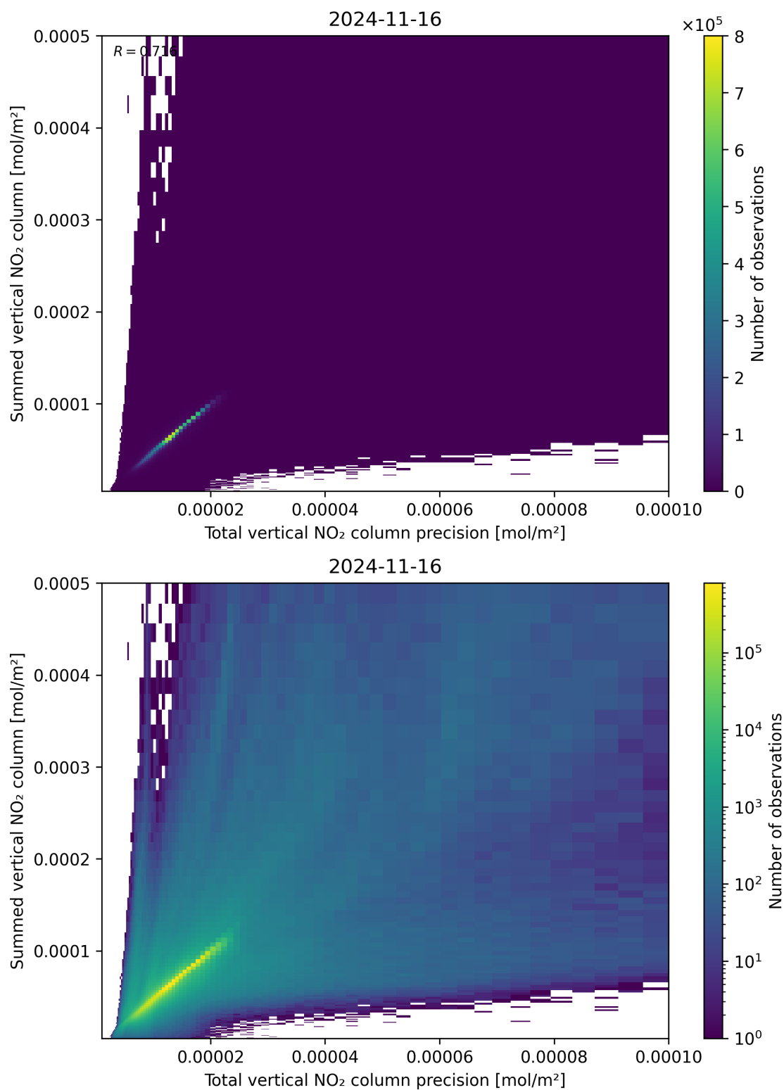
Figure 117: Scatter density plot of “Total vertical NO 2 column precision” against “Summed vertical NO 2 column” for 2024-11-15 to 2024-11-17.
