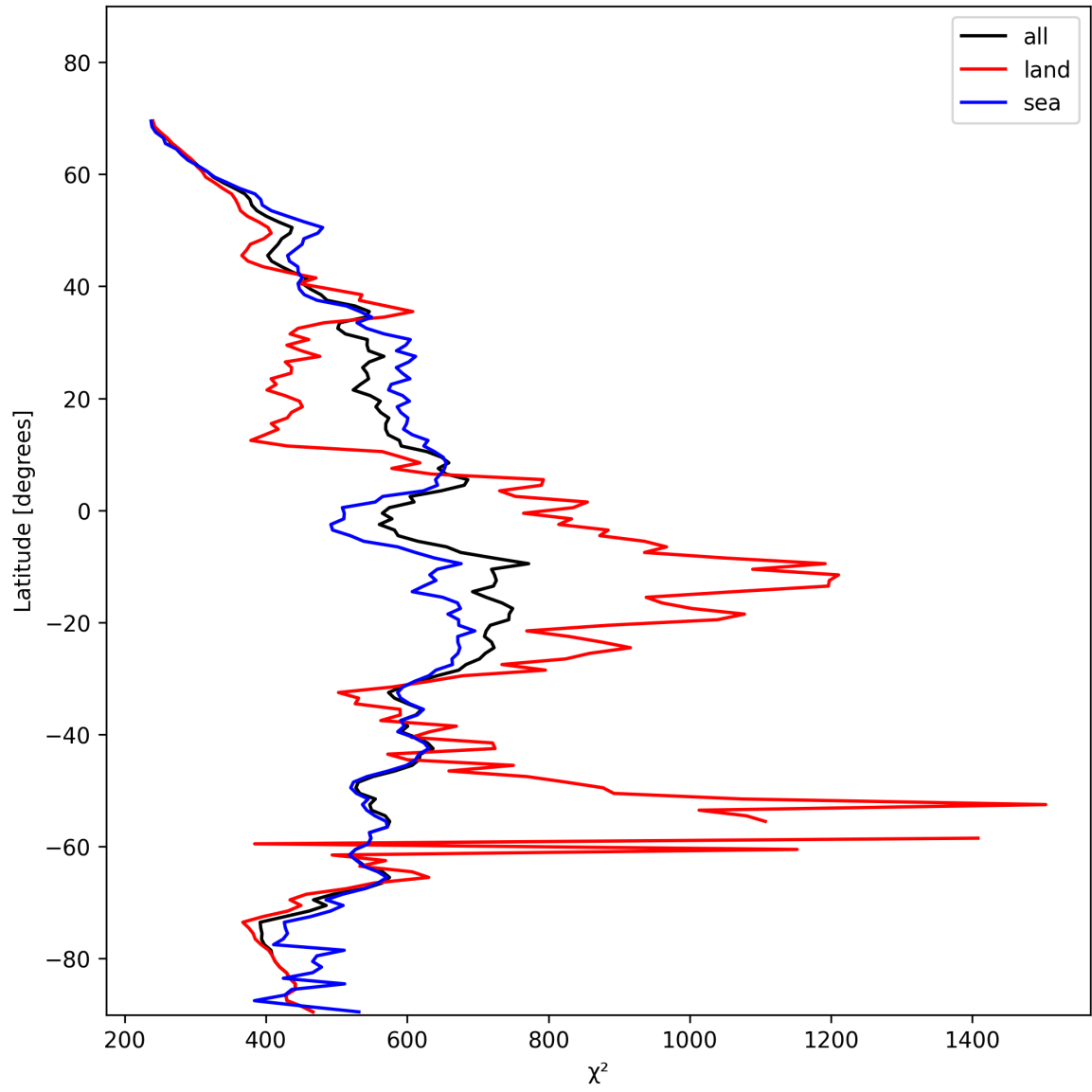
Figure 25: Zonal average of “ \chi^2 ” for 2024-11-15 to 2024-11-17.
