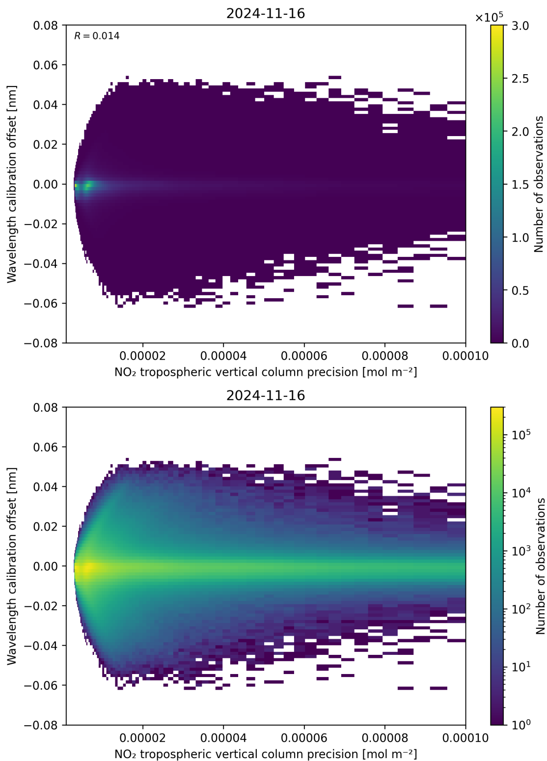
Figure 141: Scatter density plot of “NO 2 tropospheric vertical column precision” against “Wavelength calibration offset” for 2024-11-15 to 2024-11-17.
