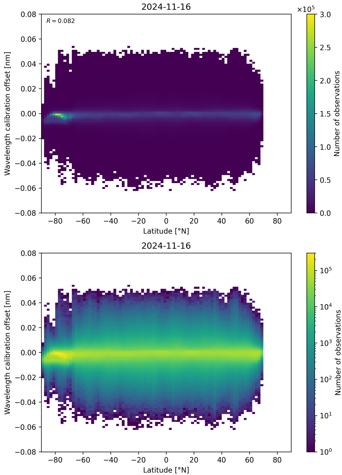
Figure 95: Scatter density plot of “Latitude” against “Wavelength calibration offset” for 2024-11-15 to 2024-11-17.
