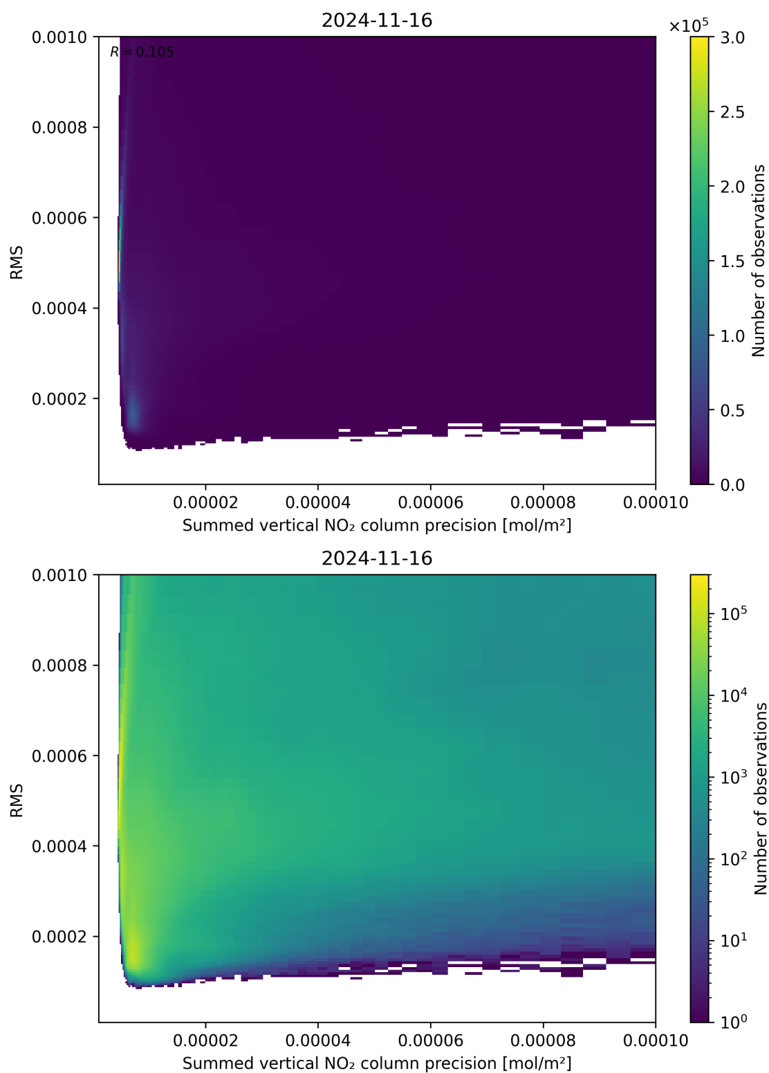
Figure 108: Scatter density plot of “Summed vertical NO 2 column precision” against “RMS” for 2024-11-15 to 2024-11-17.
