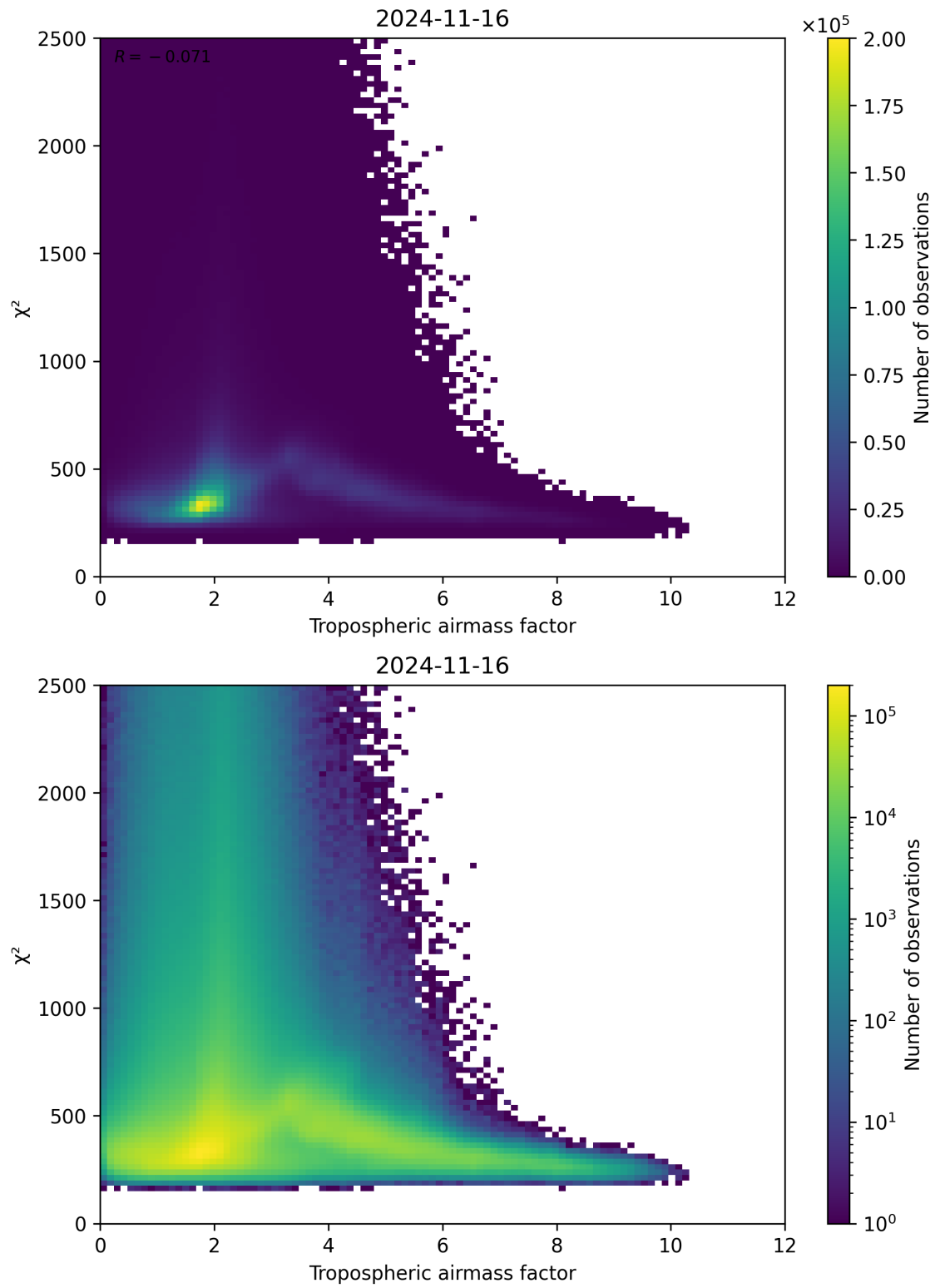
Figure 73: Scatter density plot of “Tropospheric airmass factor” against “ \chi^2 ” for 2024-11-15 to 2024-11-17.
