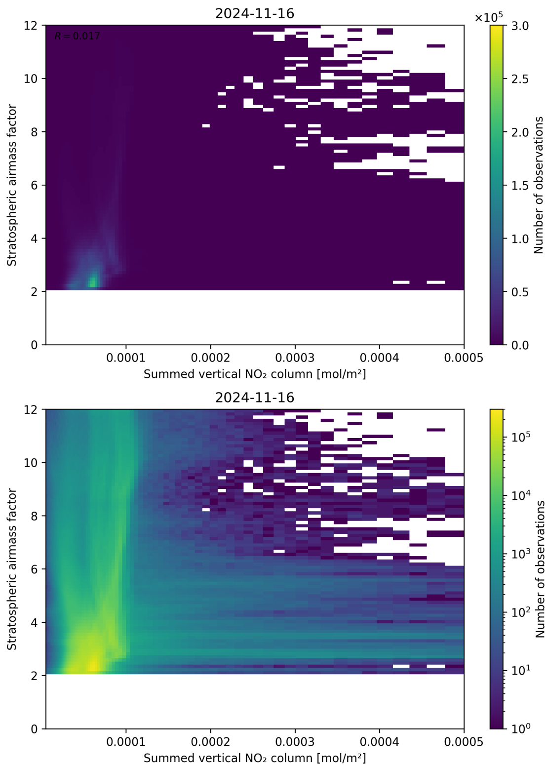
Figure 103: Scatter density plot of “Summed vertical NO 2 column” against “Stratospheric airmass factor” for 2024-11-15 to 2024-11-17.
