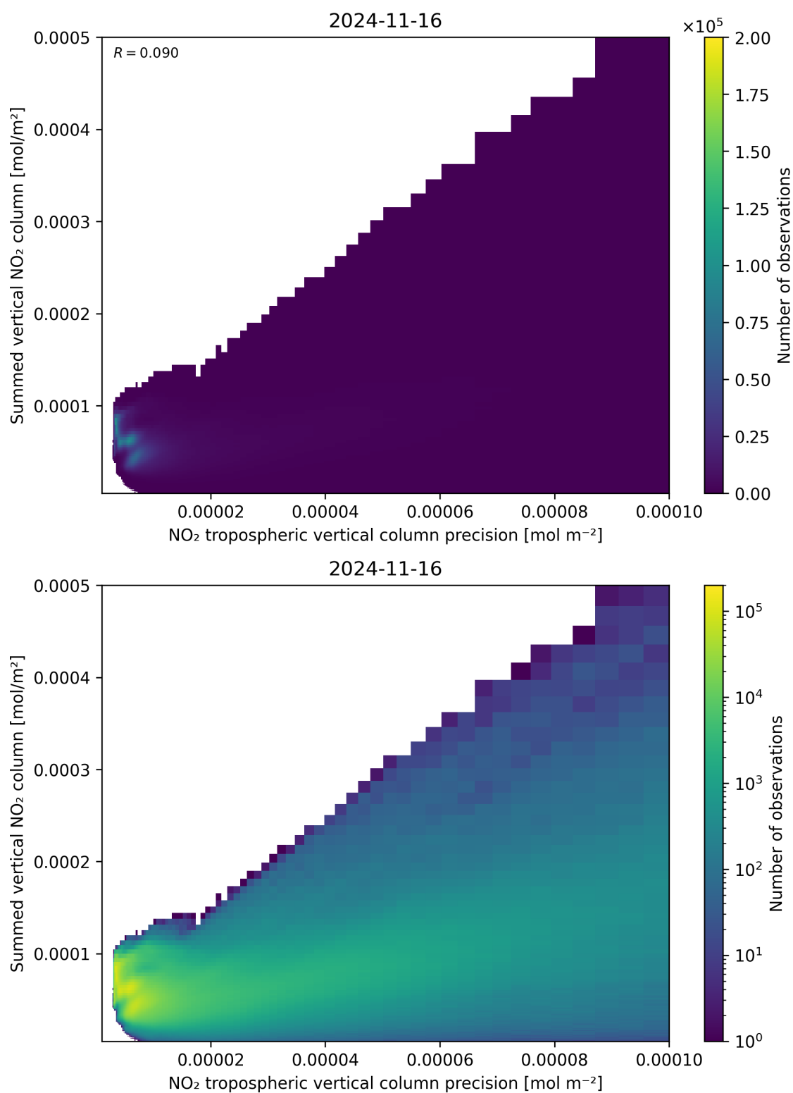
Figure 136: Scatter density plot of “NO 2 tropospheric vertical column precision” against “Summed vertical NO 2 column” for 2024-11-15 to 2024-11-17.
