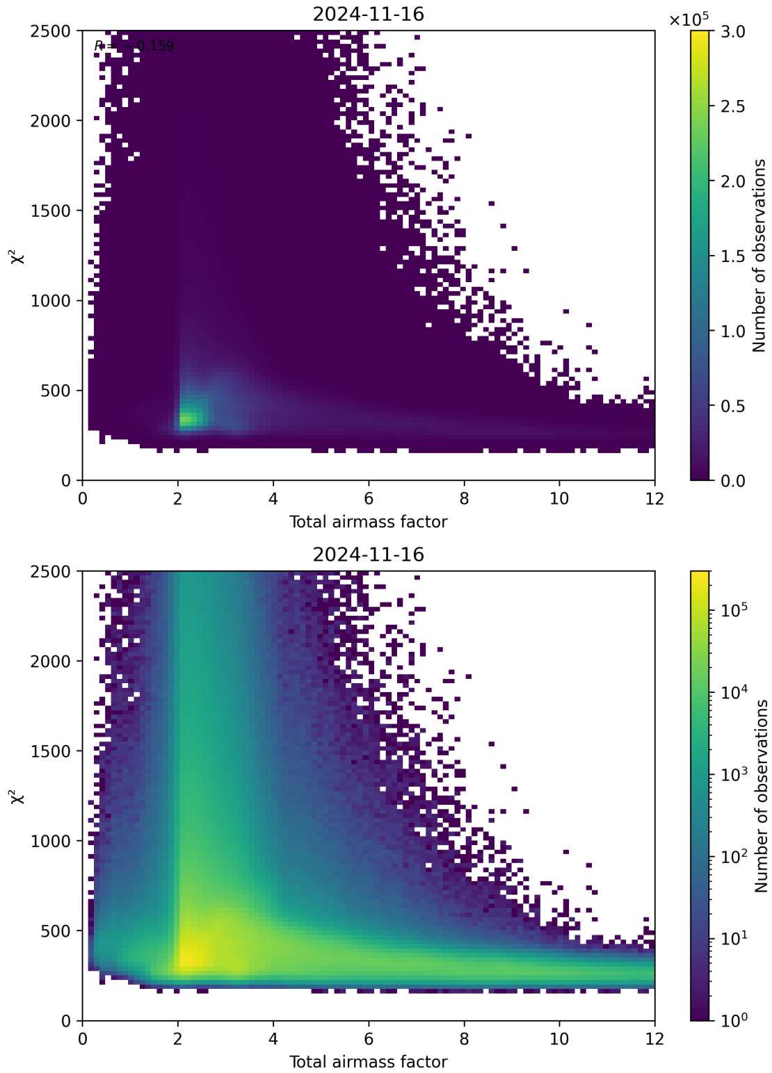
Figure 63: Scatter density plot of “Total airmass factor” against “ \chi^2 ” for 2024-11-15 to 2024-11-17.
