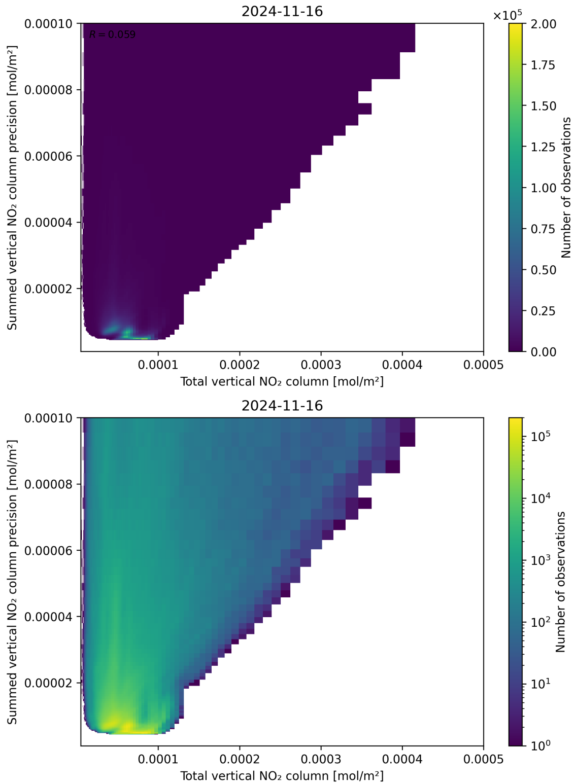
Figure 113: Scatter density plot of “Total vertical NO 2 column” against “Summed vertical NO 2 column precision” for 2024-11-15 to 2024-11-17.
