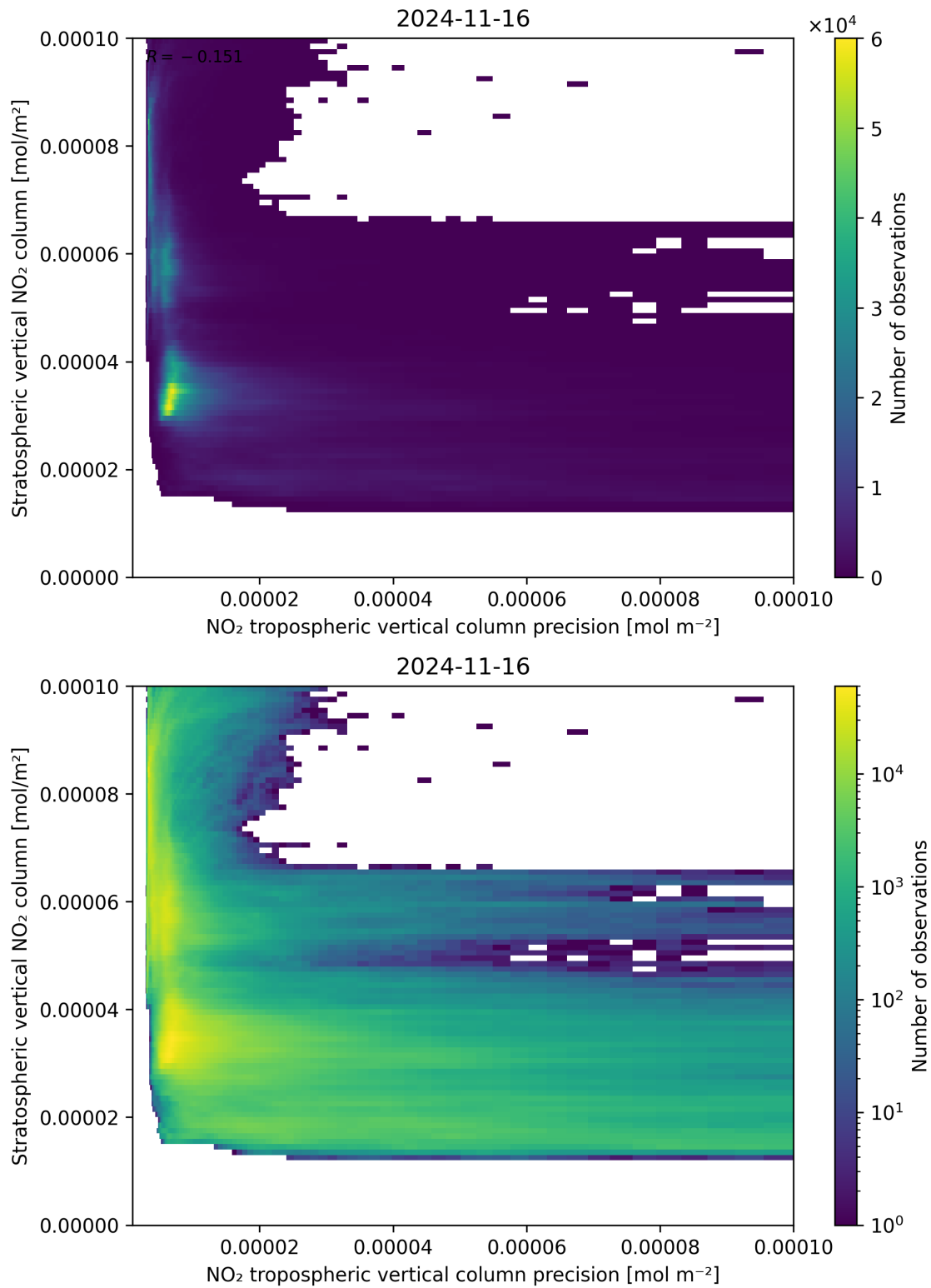
Figure 135: Scatter density plot of “NO 2 tropospheric vertical column precision” against “Stratospheric vertical NO 2 column” for 2024-11-15 to 2024-11-17.
