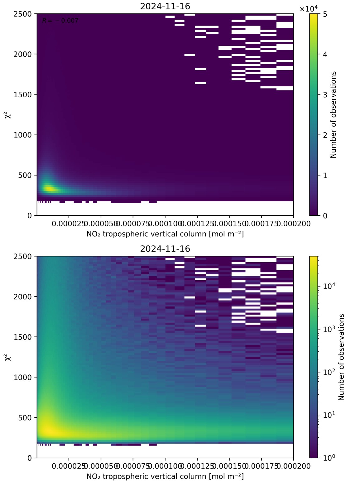
Figure 124: Scatter density plot of “NO 2 tropospheric vertical column” against “ \chi^2 ” for 2024-11-15 to 2024-11-17.
