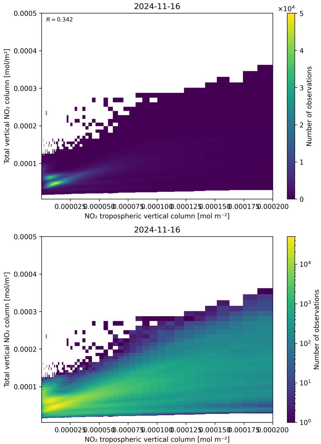
Figure 128: Scatter density plot of “NO 2 tropospheric vertical column” against “Total vertical NO 2 column” for 2024-11-15 to 2024-11-17.
