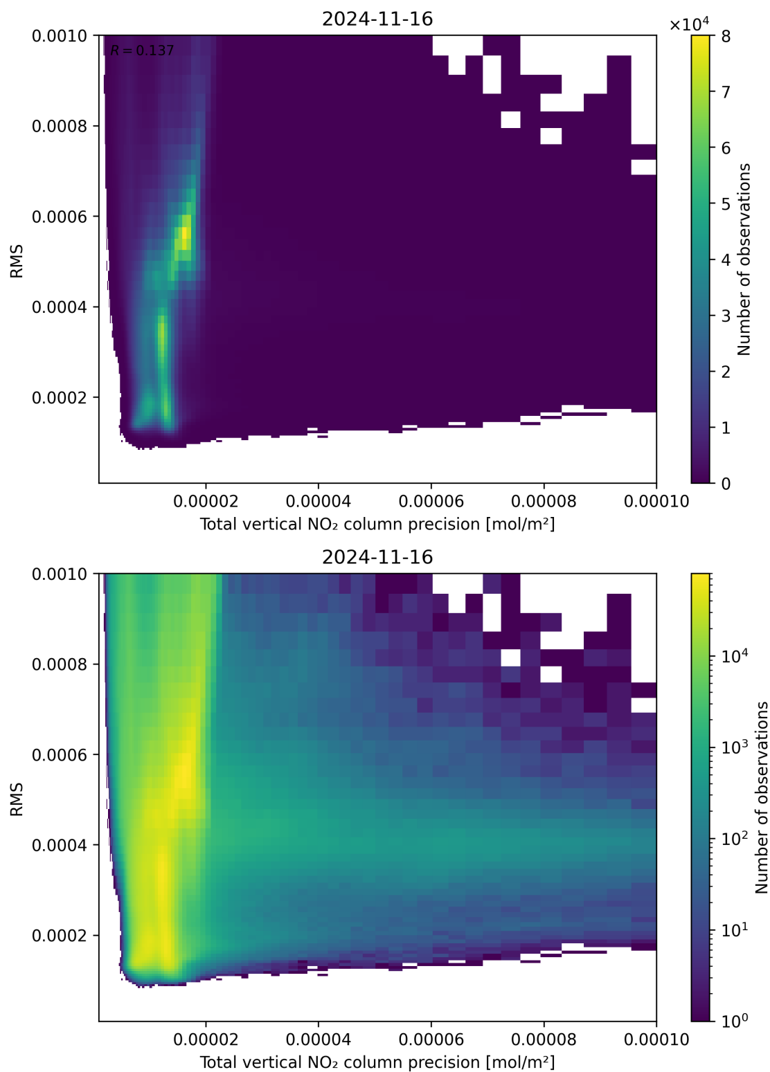
Figure 119: Scatter density plot of “Total vertical NO 2 column precision” against “RMS” for 2024-11-15 to 2024-11-17.
