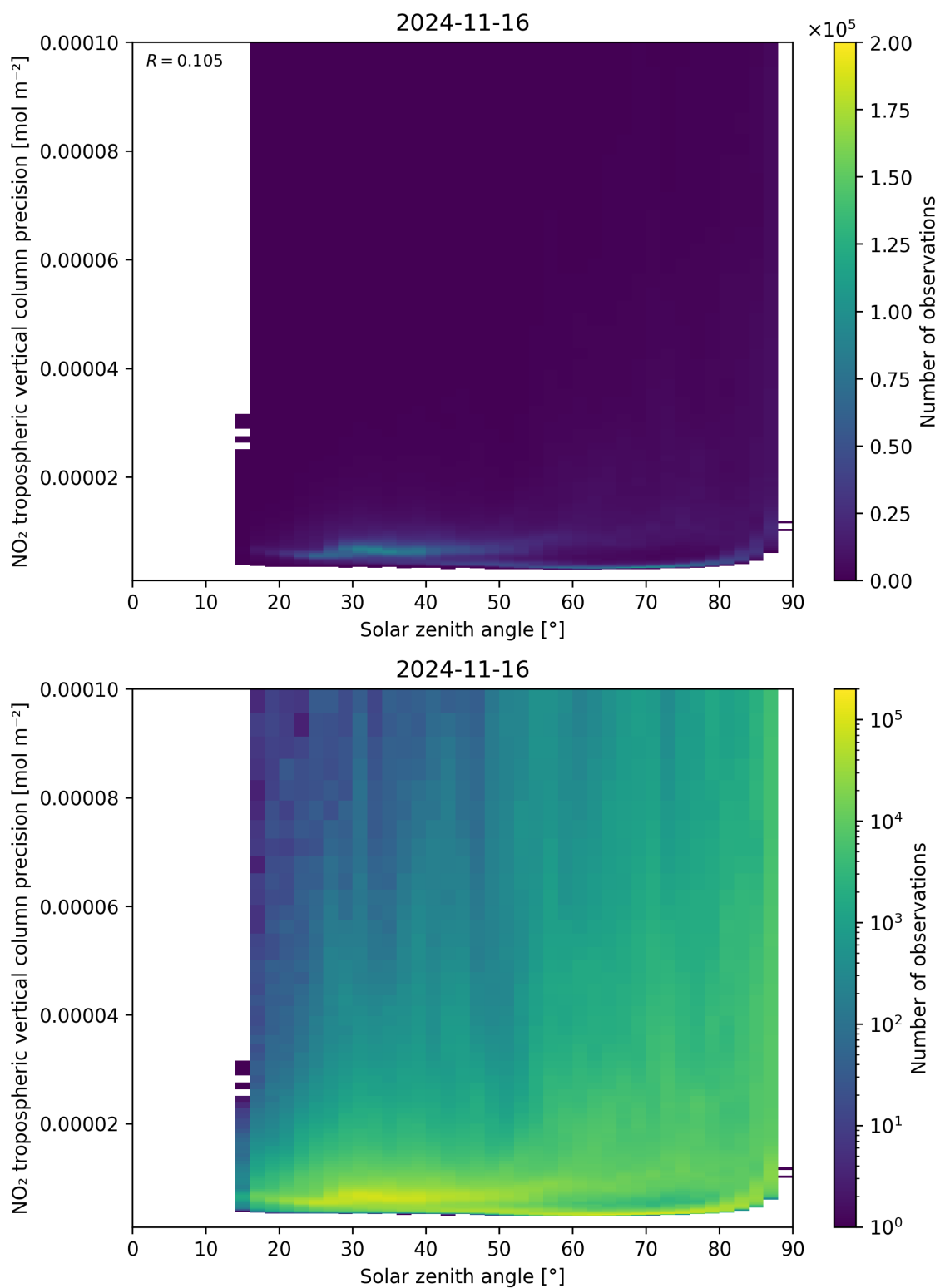
Figure 156: Scatter density plot of “Solar zenith angle” against “NO 2 tropospheric vertical column precision” for 2024-11-15 to 2024-11-17.
