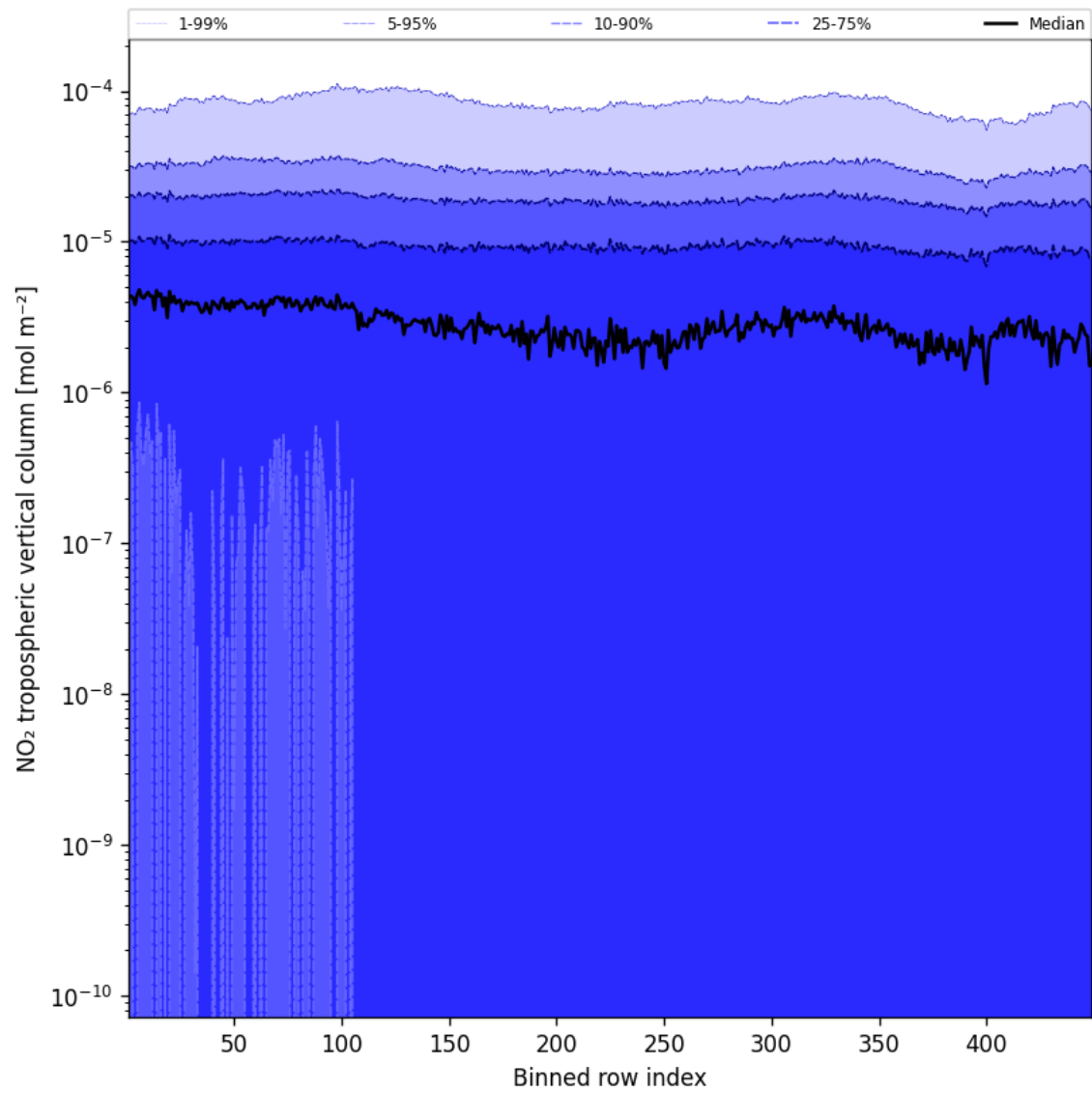
Figure 46: Along track statistics of “NO 2 tropospheric vertical column” for 2024-11-15 to 2024-11-17
