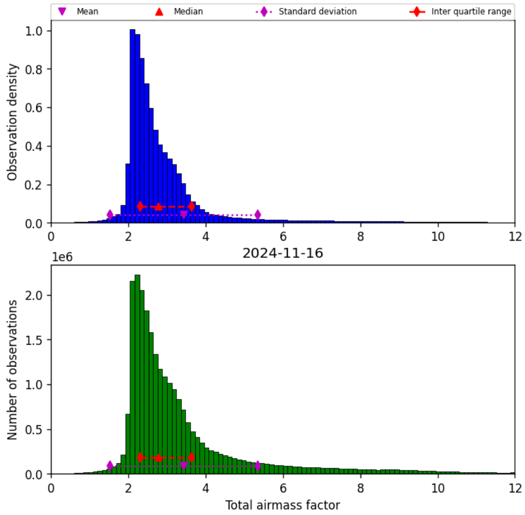
Figure 32: Histogram of “Total airmass factor” for 2024-11-15 to 2024-11-17
