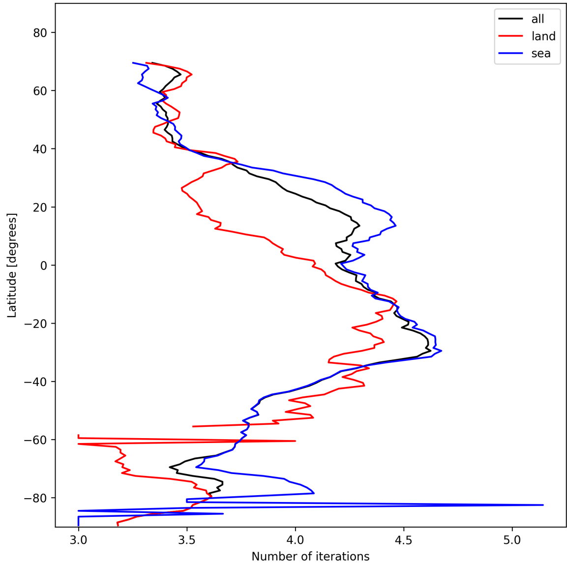
Figure 17: Zonal average of “Number of iterations” for 2024-11-15 to 2024-11-17.
