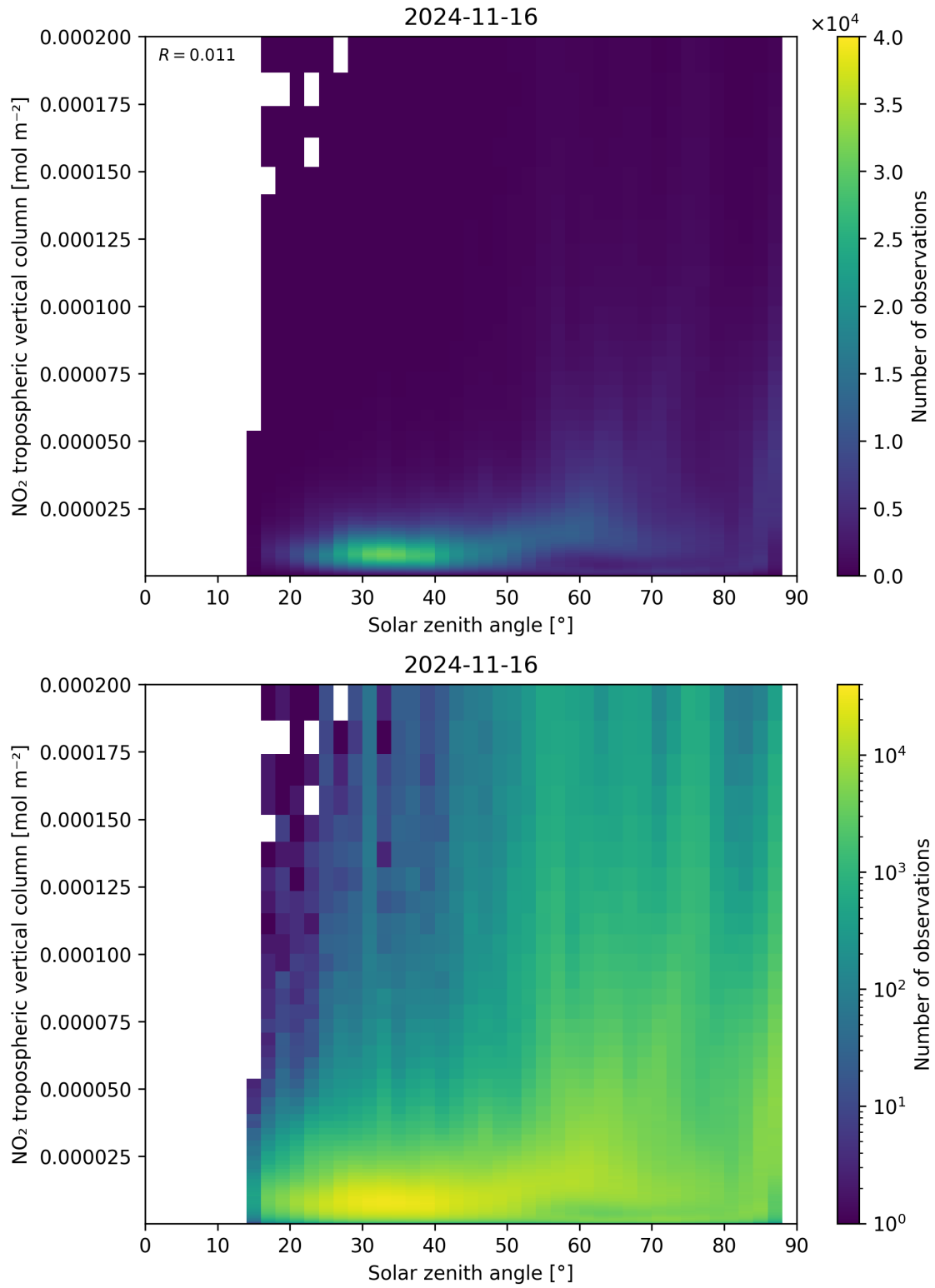
Figure 155: Scatter density plot of “Solar zenith angle” against “NO 2 tropospheric vertical column” for 2024-11-15 to 2024-11-17.
