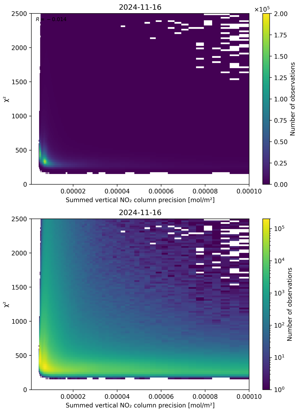
Figure 107: Scatter density plot of “Summed vertical NO 2 column precision” against “ \chi^2 ” for 2024-11-15 to 2024-11-17.
