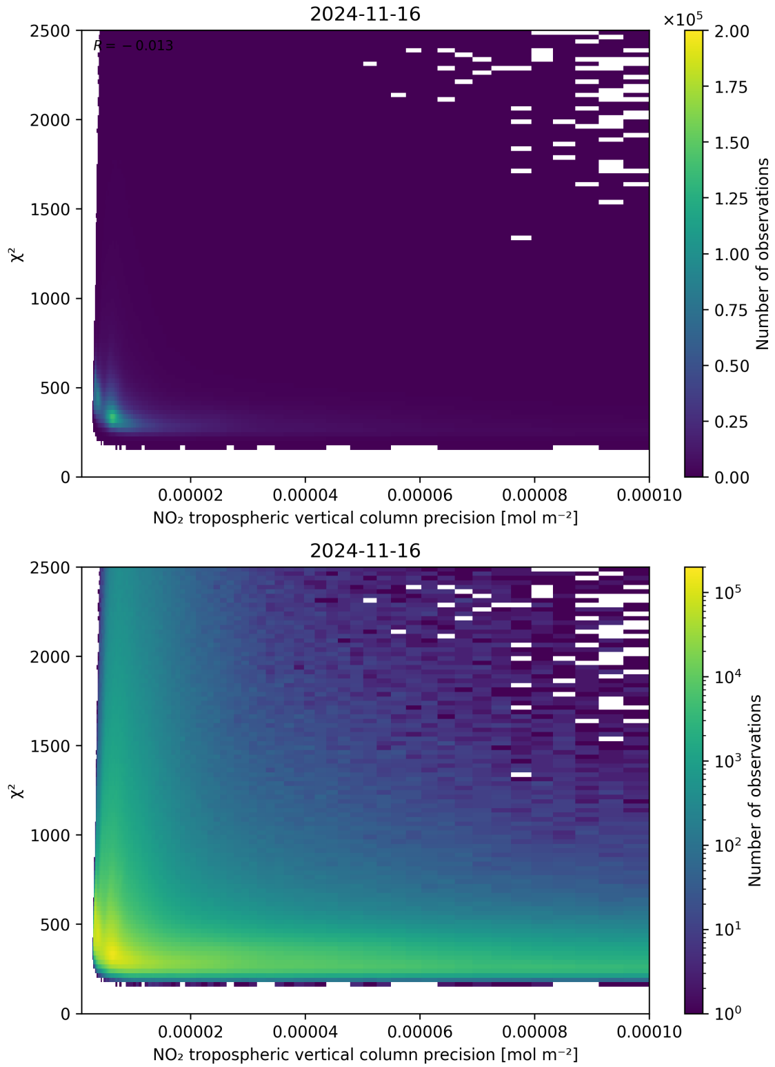
Figure 134: Scatter density plot of “NO 2 tropospheric vertical column precision” against “ \chi^2 ” for 2024-11-15 to 2024-11-17.
