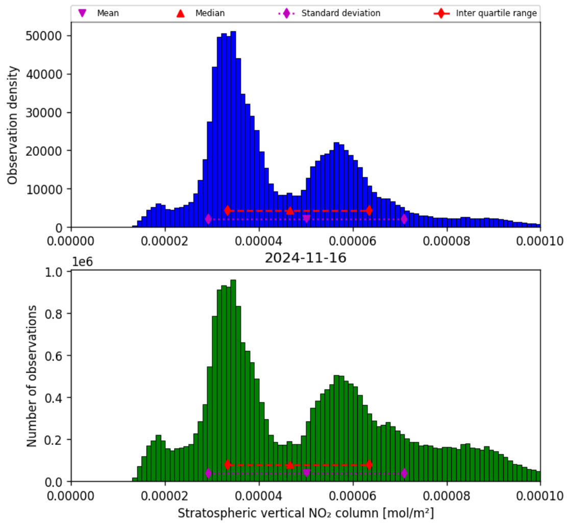
Figure 36: Histogram of “Stratospheric vertical NO 2 column” for 2024-11-15 to 2024-11-17
