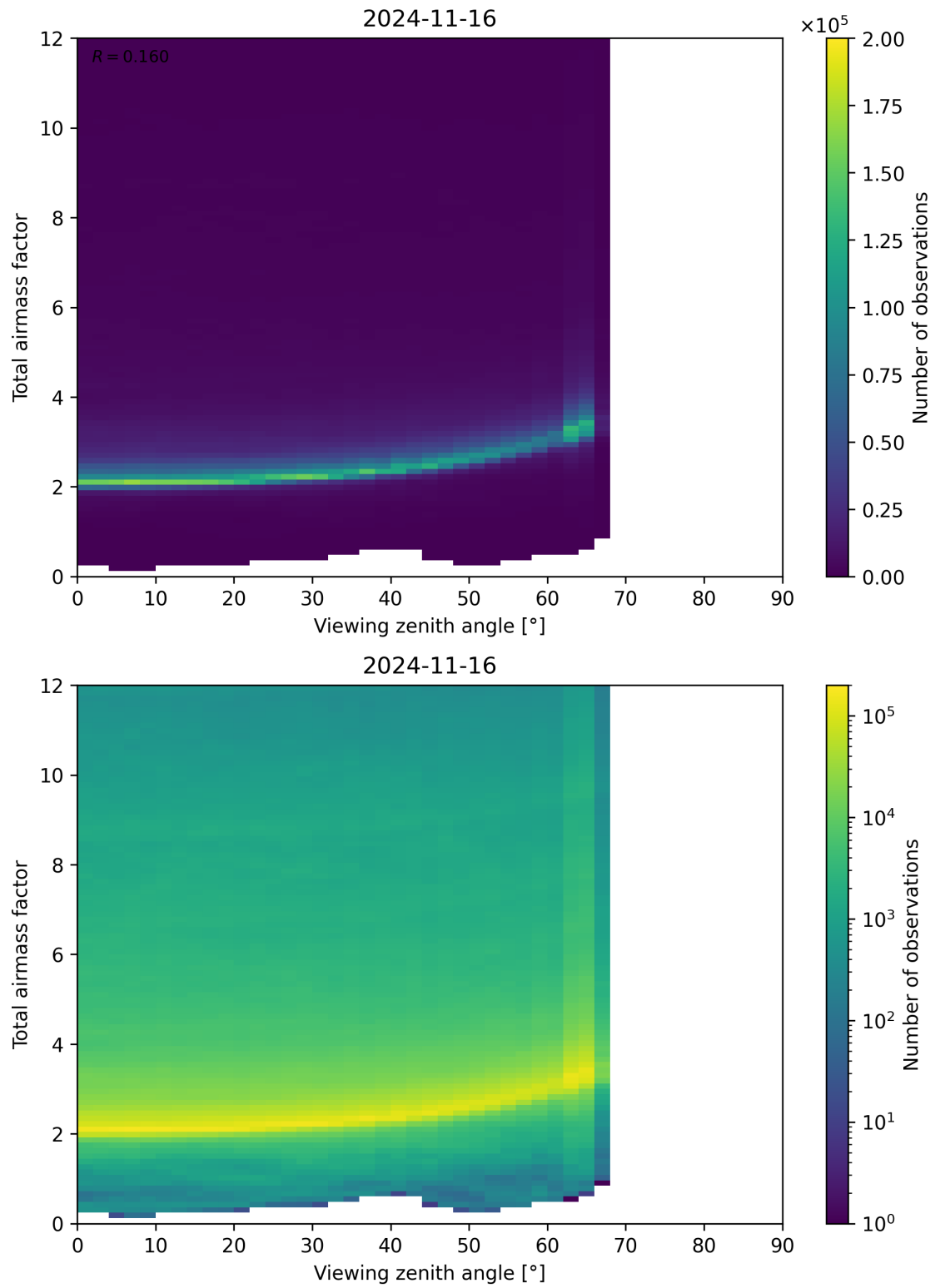
Figure 160: Scatter density plot of “Viewing zenith angle” against “Total airmass factor” for 2024-11-15 to 2024-11-17.
