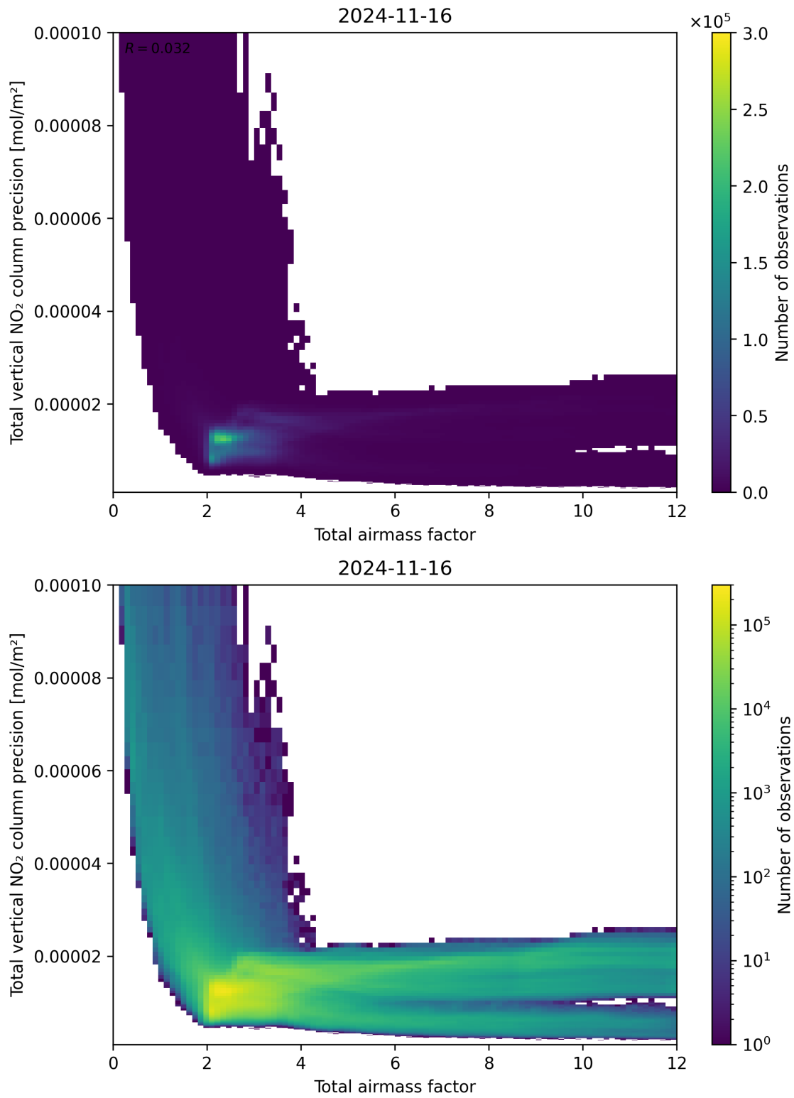
Figure 68: Scatter density plot of “Total airmass factor” against “Total vertical NO 2 column precision” for 2024-11-15 to 2024-11-17.
