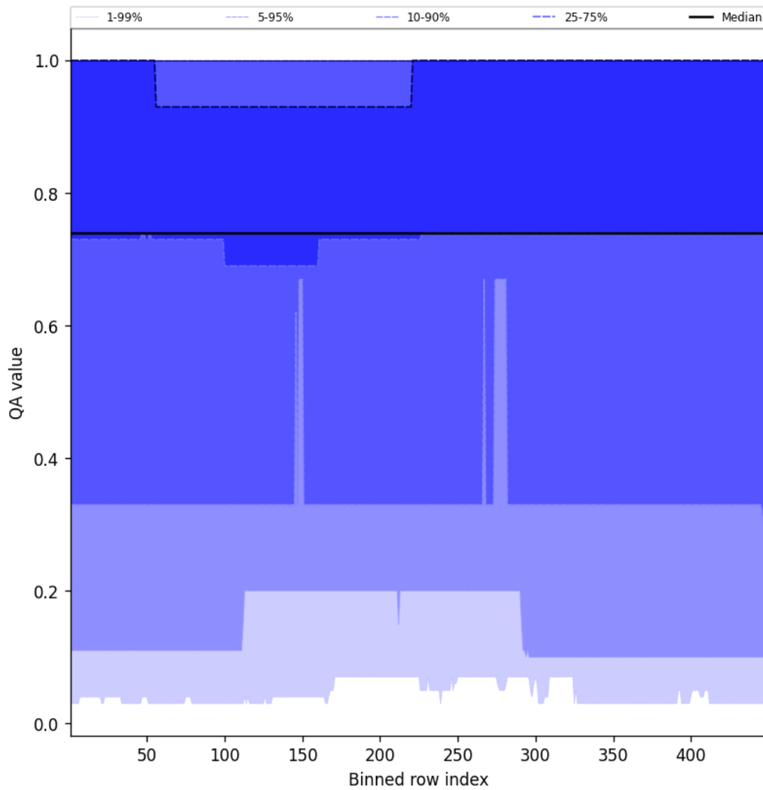
Figure 45: Along track statistics of “QA value” for 2024-11-15 to 2024-11-17
