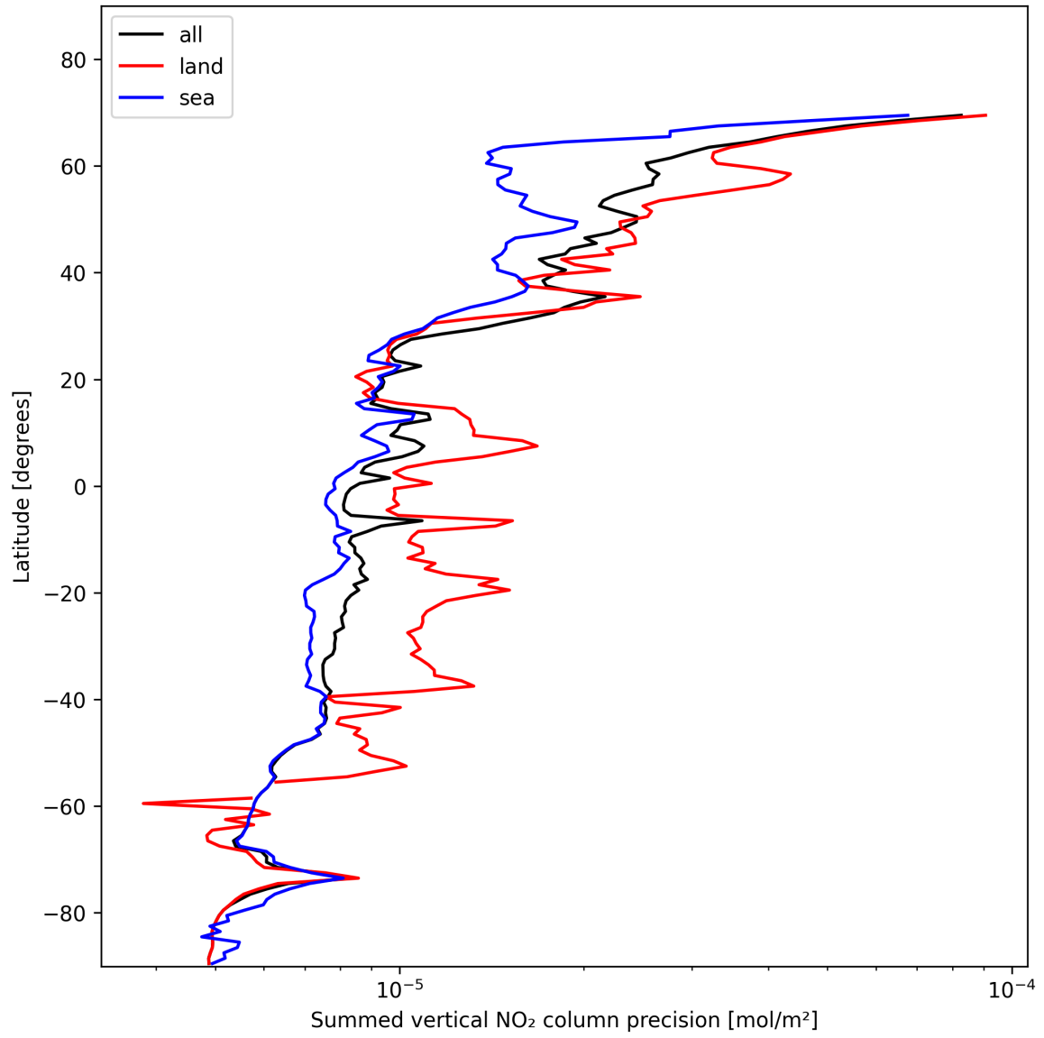
Figure 24: Zonal average of “Summed vertical NO 2 column precision” for 2024-11-15 to 2024-11-17.
