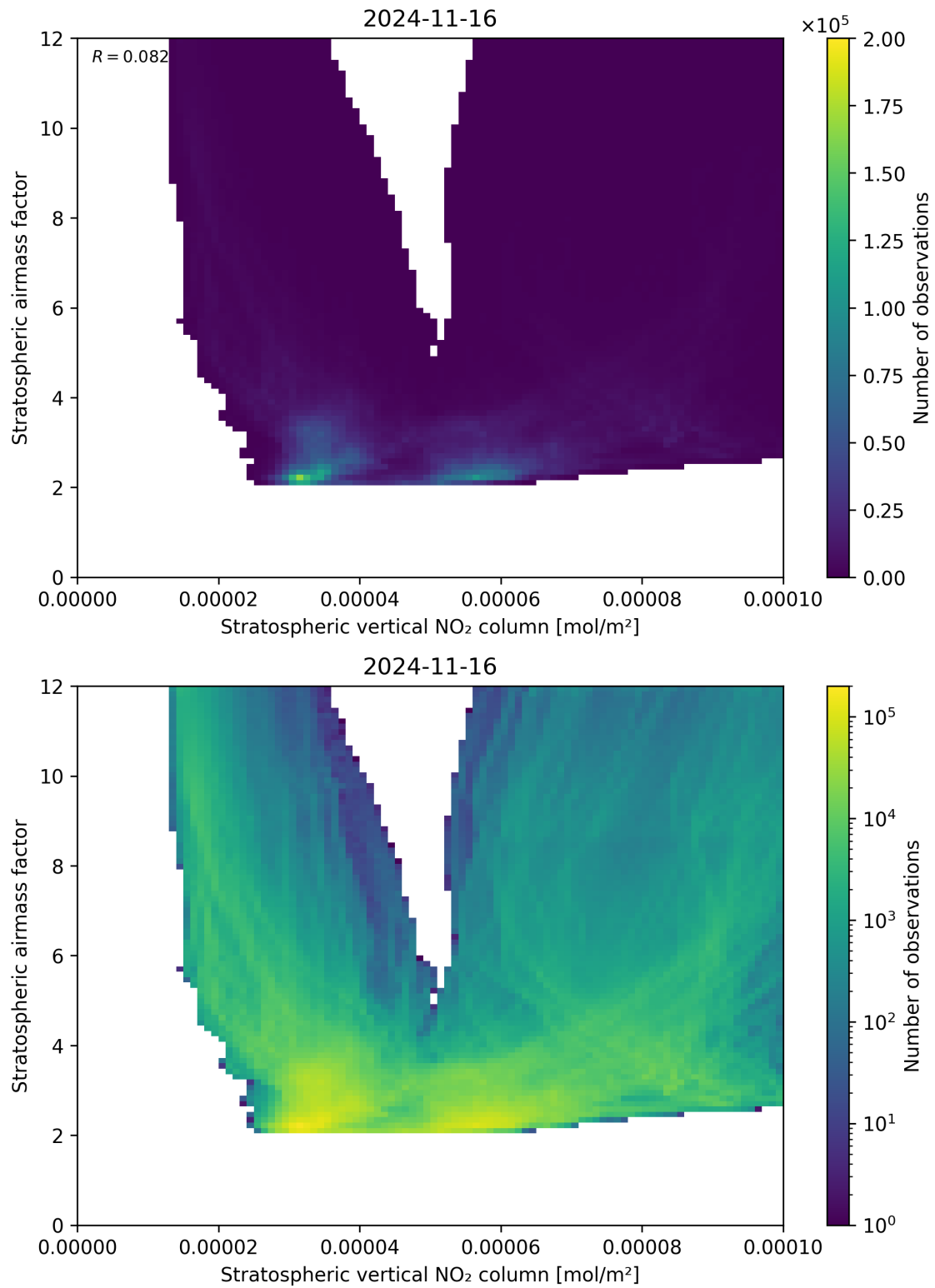
Figure 96: Scatter density plot of “Stratospheric vertical NO 2 column” against “Stratospheric airmass factor” for 2024-11-15 to 2024-11-17.
