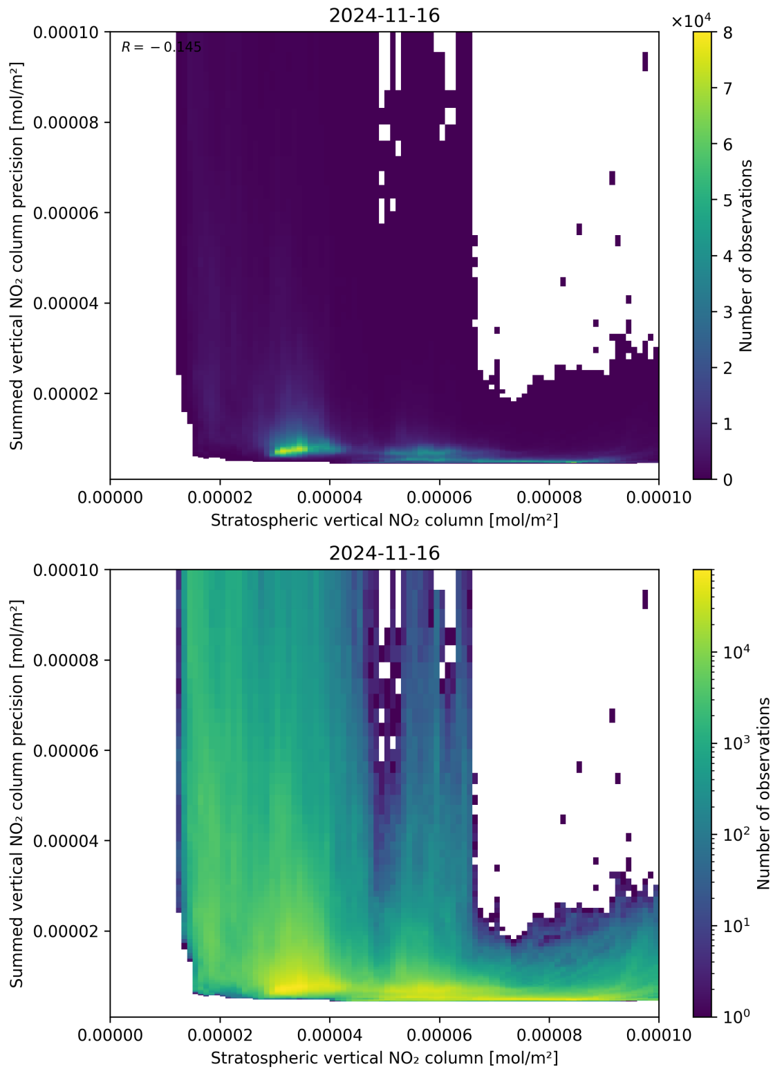
Figure 99: Scatter density plot of “Stratospheric vertical NO 2 column” against “Summed vertical NO 2 column precision” for 2024-11-15 to 2024-11-17.
