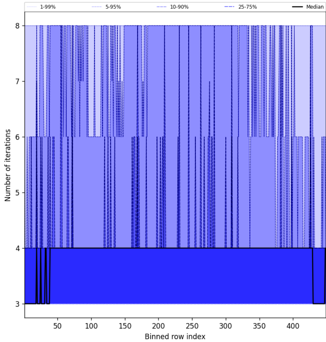
Figure 51: Along track statistics of “Number of iterations” for 2024-11-15 to 2024-11-17
