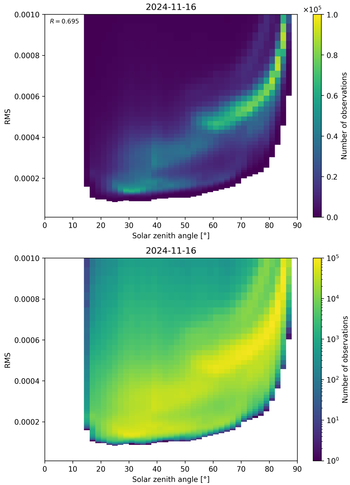
Figure 157: Scatter density plot of “Solar zenith angle” against “RMS” for 2024-11-15 to 2024-11-17.
