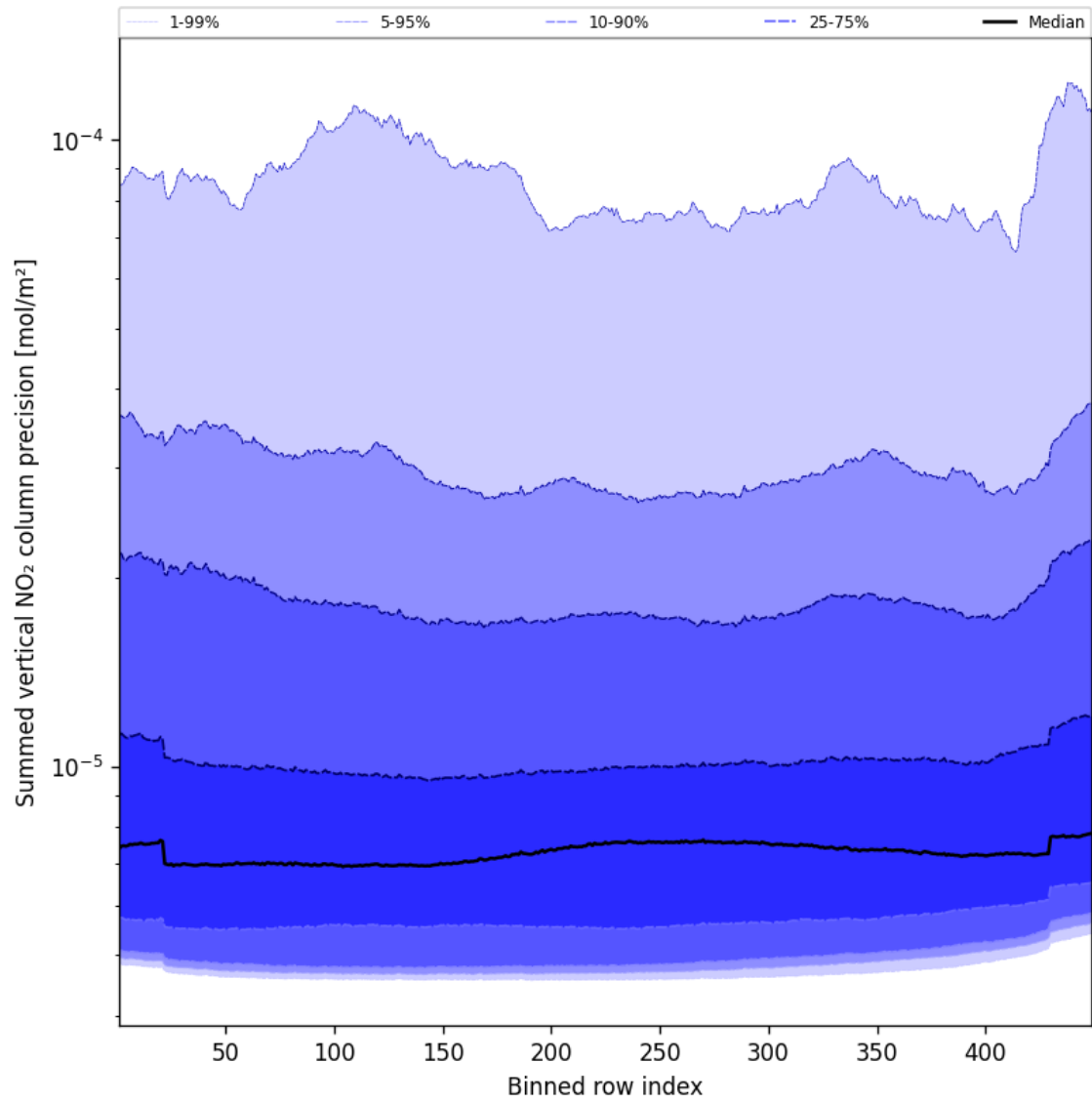
Figure 58: Along track statistics of “Summed vertical NO 2 column precision” for 2024-11-15 to 2024-11-17
