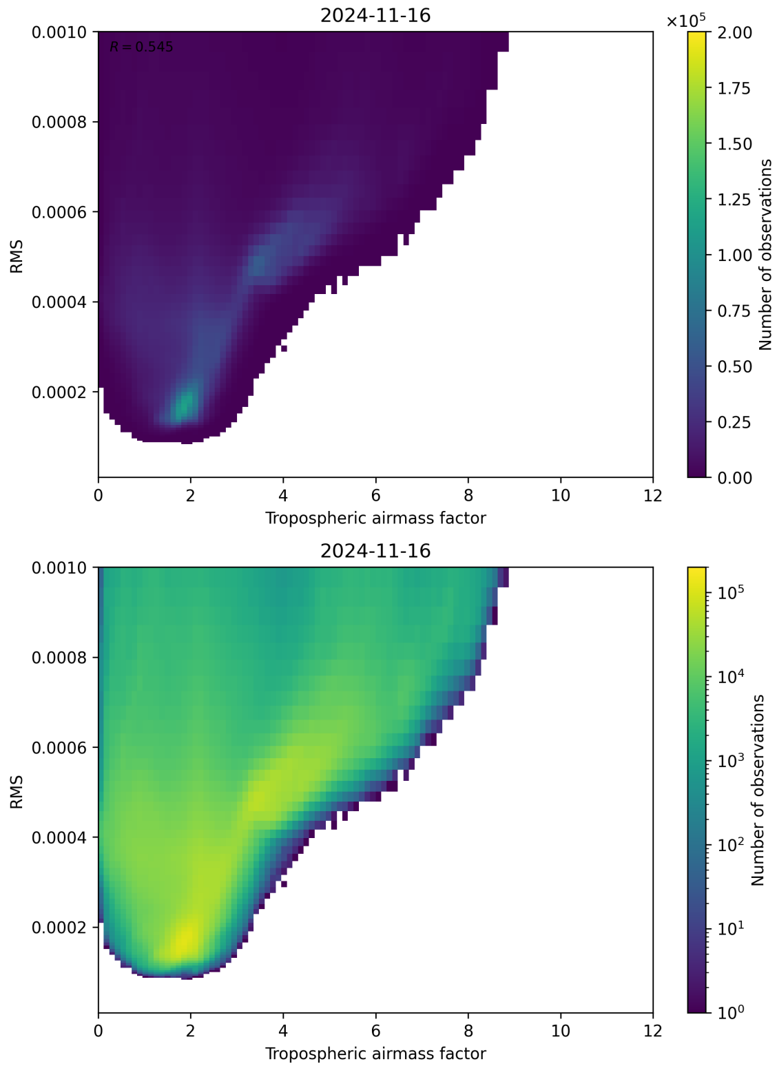
Figure 79: Scatter density plot of “Tropospheric airmass factor” against “RMS” for 2024-11-15 to 2024-11-17.
