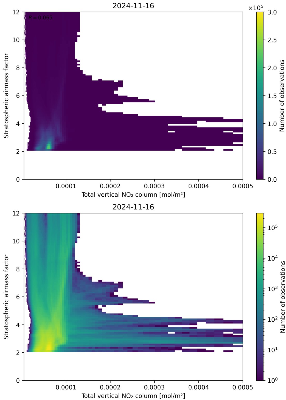
Figure 110: Scatter density plot of “Total vertical NO 2 column” against “Stratospheric air mass factor” for 2024-11-15 to 2024-11-17.
