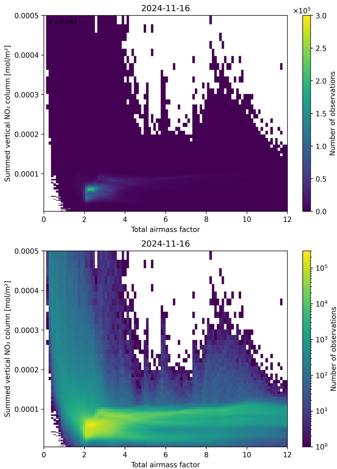
Figure 65: Scatter density plot of “Total airmass factor” against “Summed vertical NO 2 column” for 2024-11-15 to 2024-11-17.
