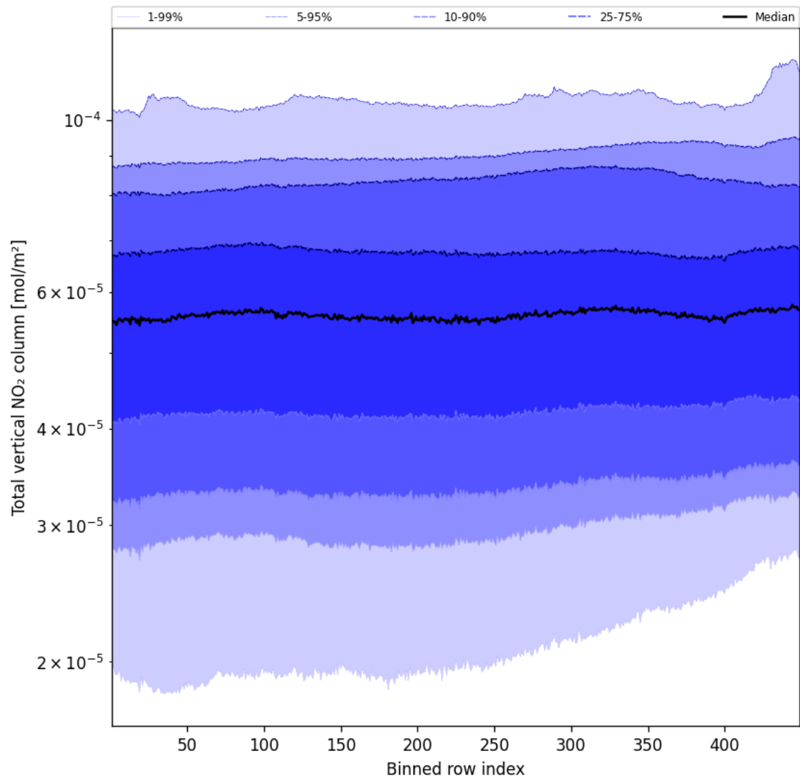
Figure 55: Along track statistics of “Total vertical NO 2 column” for 2024-11-15 to 2024-11-17
