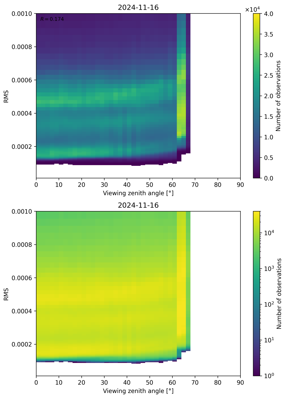
Figure 171: Scatter density plot of “Viewing zenith angle” against “RMS” for 2024-11-15 to 2024-11-17.
