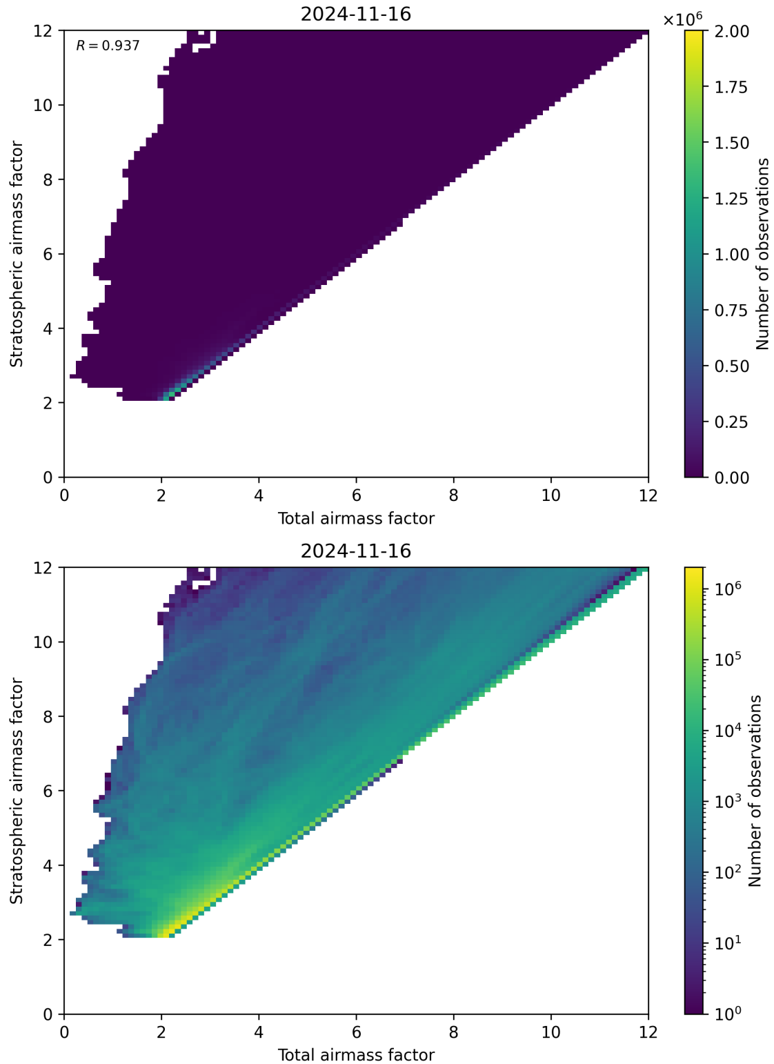
Figure 62: Scatter density plot of “Total airmass factor” against “Stratospheric airmass factor” for 2024-11-15 to 2024-11-17.
