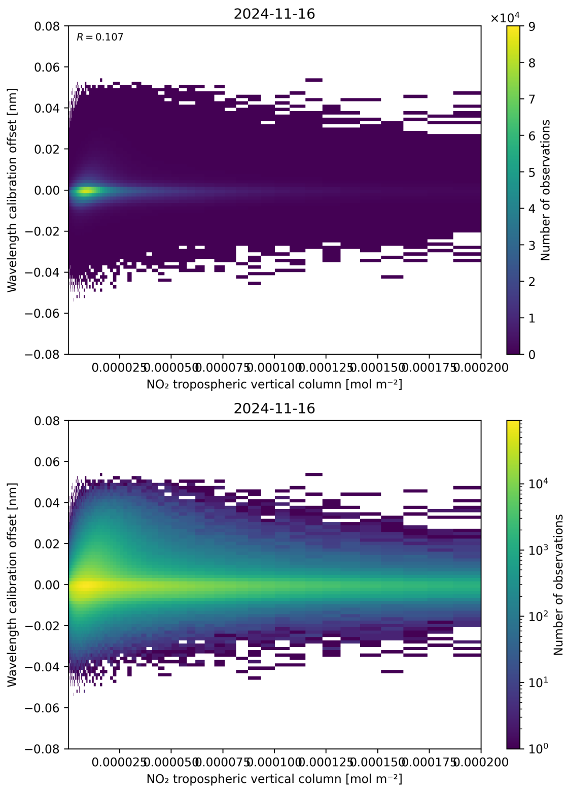
Figure 143: Scatter density plot of “NO 2 tropospheric vertical column” against “Wavelength calibration offset” for 2024-11-15 to 2024-11-17.
