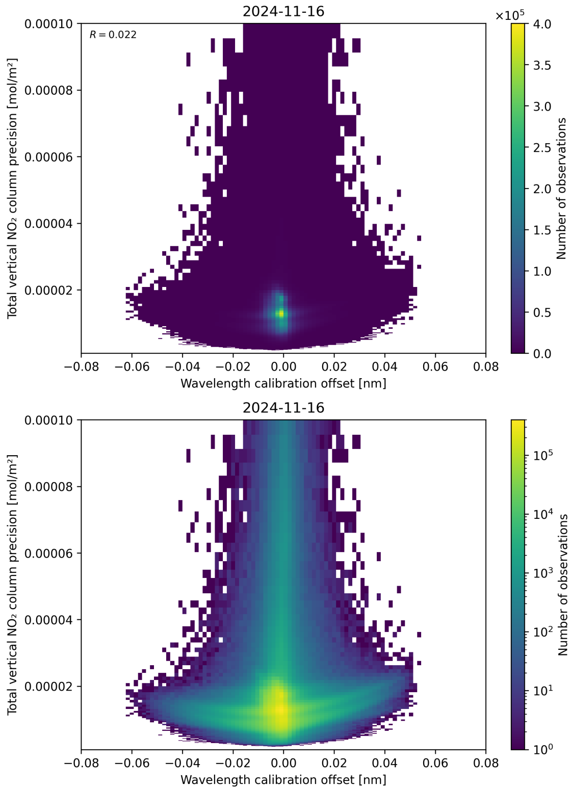
Figure 180: Scatter density plot of “Wavelength calibration offset” against “Total vertical NO 2 column precision” for 2024-11-15 to 2024-11-17.
