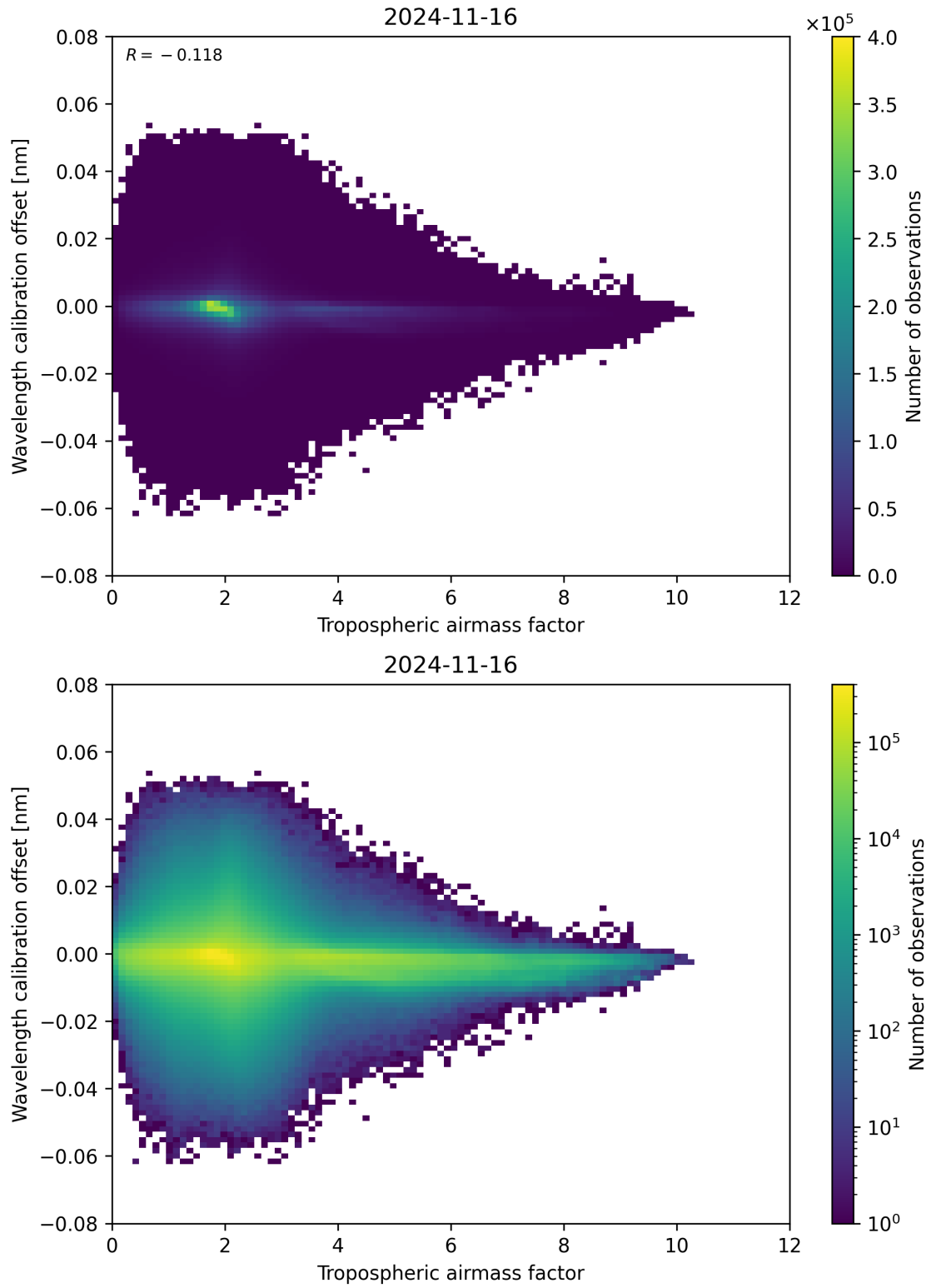
Figure 80: Scatter density plot of “Tropospheric airmass factor” against “Wavelength calibration offset” for 2024-11-15 to 2024-11-17.
