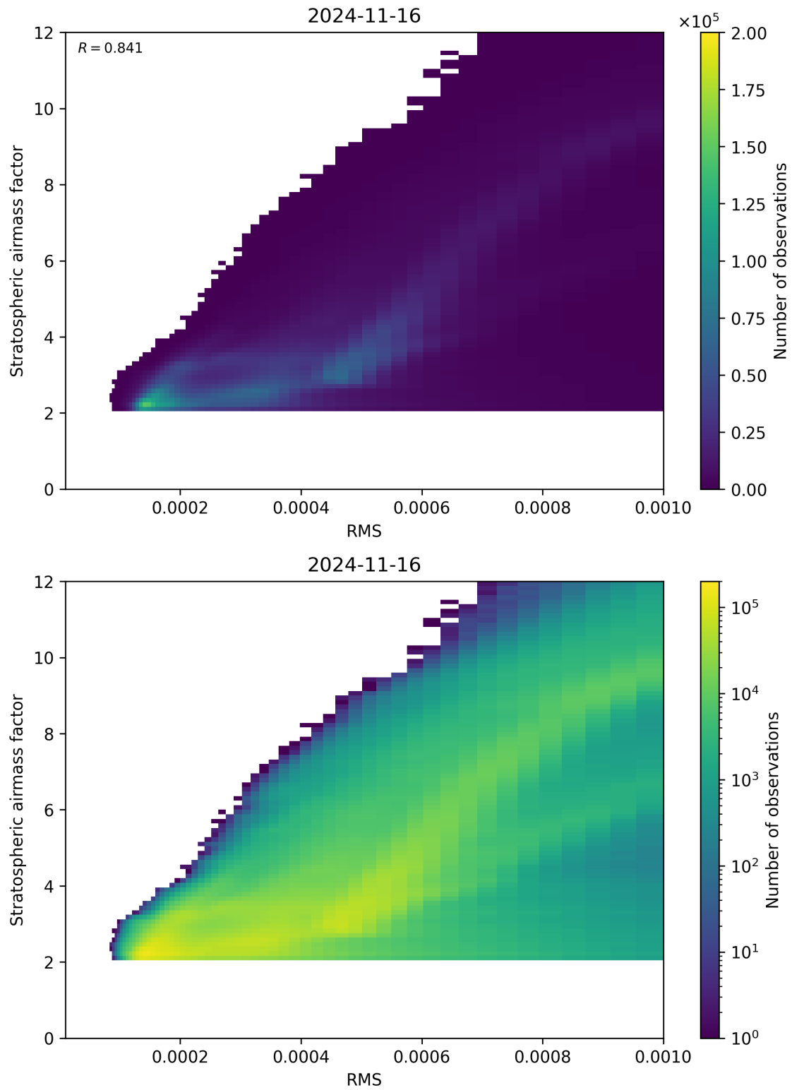
Figure 144: Scatter density plot of “RMS” against “Stratospheric airmass factor” for 2024-11-15 to 2024-11-17.
