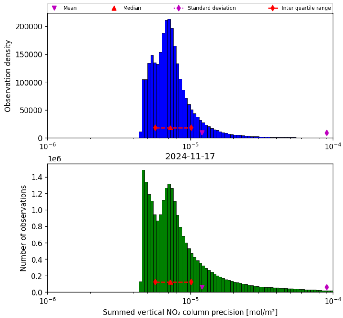
Figure 41: Histogram of “Summed vertical NO 2 column precision” for 2024-11-17 to 2024-11-18
