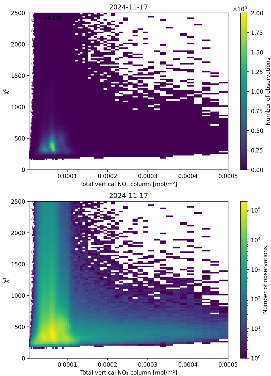
Figure 111: Scatter density plot of “Total vertical NO 2 column” against “ \chi^2 ” for 2024-11-17 to 2024-11-18.
