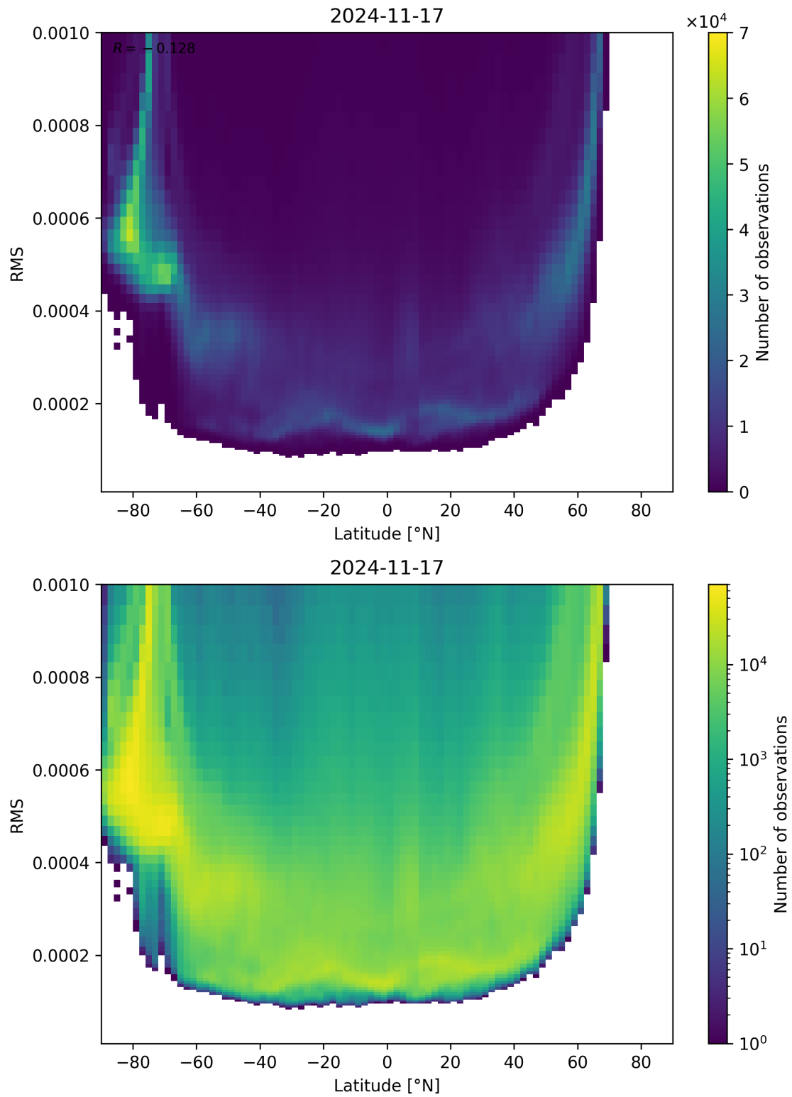
Figure 94: Scatter density plot of “Latitude” against “RMS” for 2024-11-17 to 2024-11-18.
