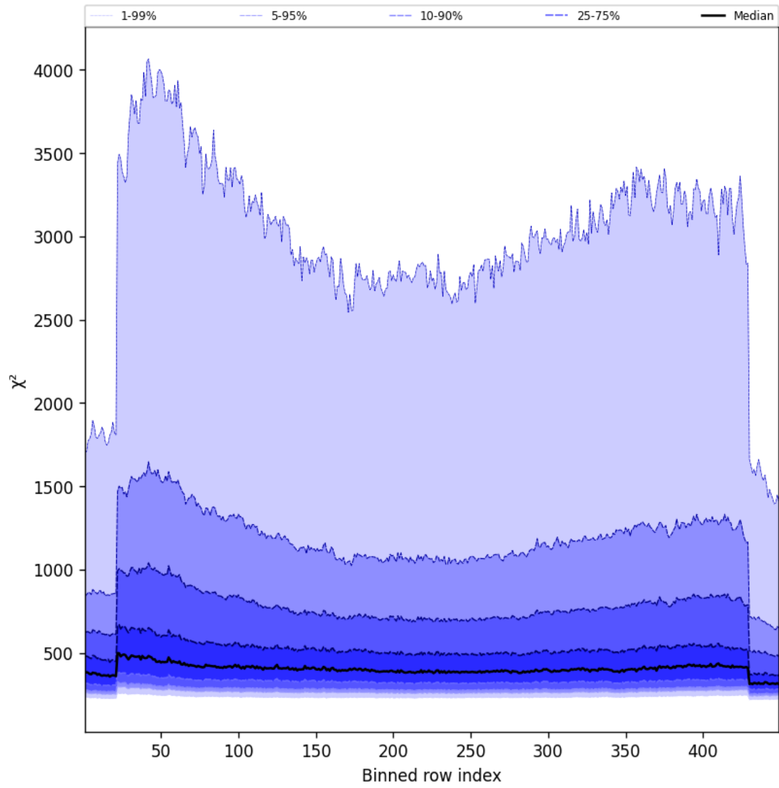
Figure 59: Along track statistics of “ \chi^2 ” for 2024-11-17 to 2024-11-18
