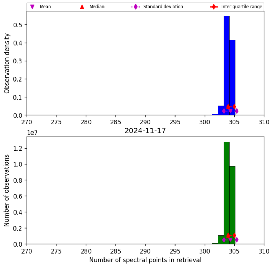
Figure 33: Histogram of “Number of spectral points in retrieval” for 2024-11-17 to 2024-11-18
