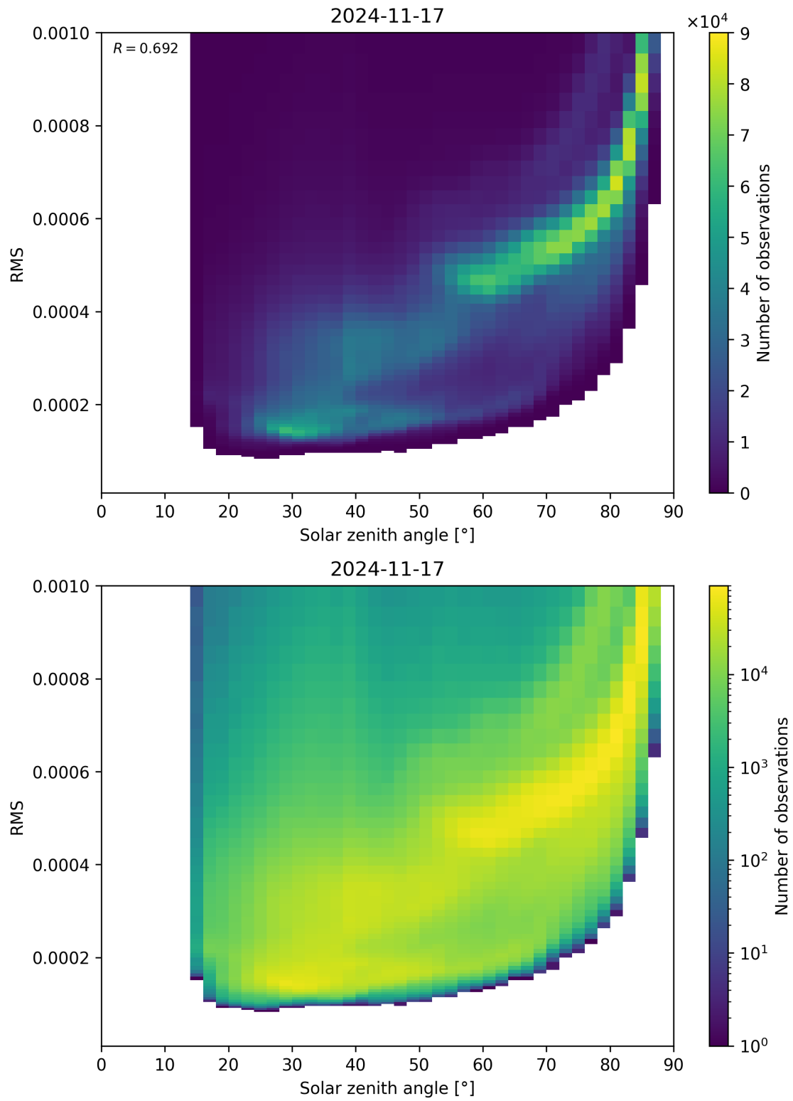
Figure 157: Scatter density plot of “Solar zenith angle” against “RMS” for 2024-11-17 to 2024-11-18.
