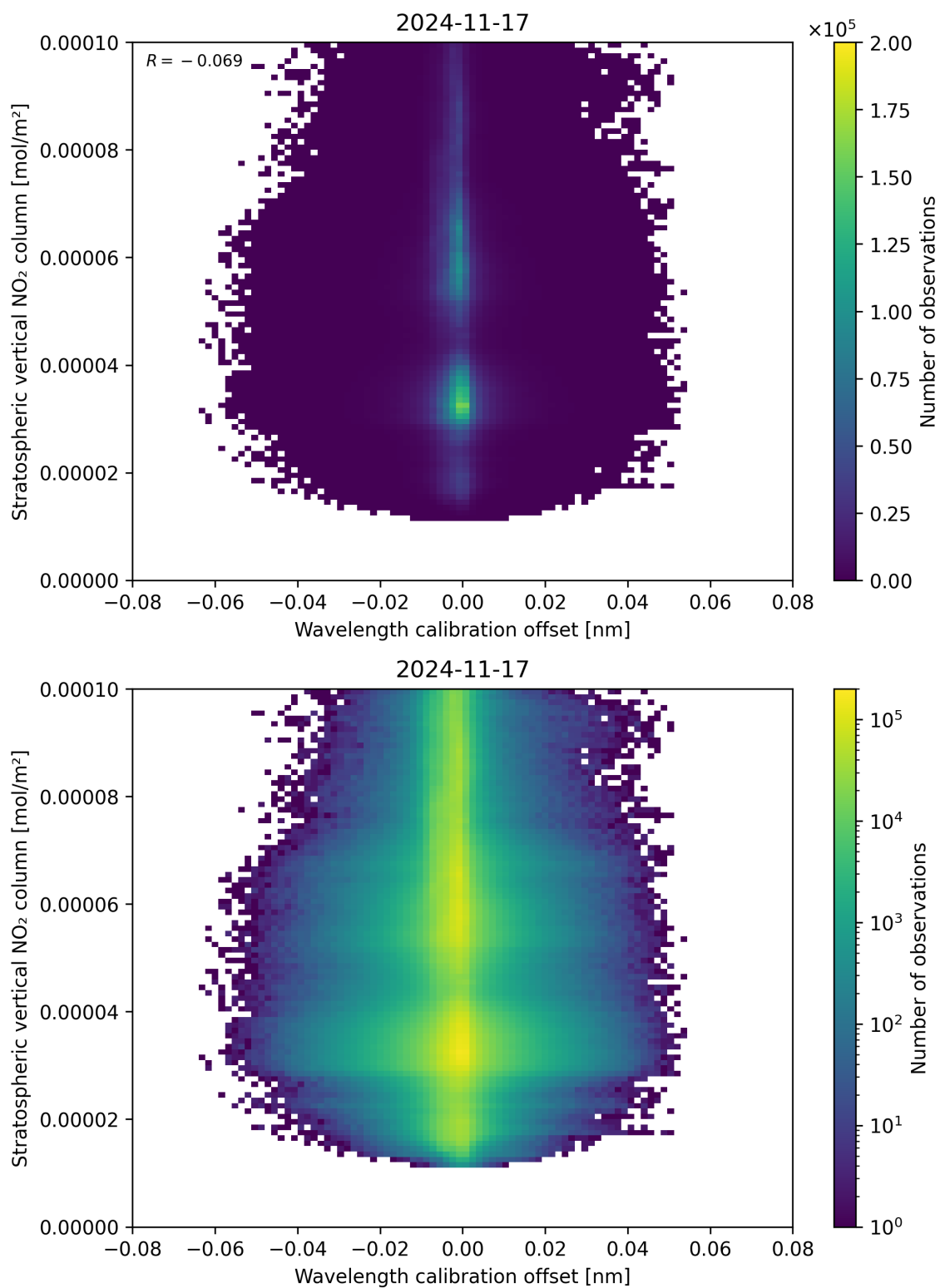
Figure 176: Scatter density plot of “Wavelength calibration offset” against “Stratospheric vertical NO 2 column” for 2024-11-17 to 2024-11-18.
