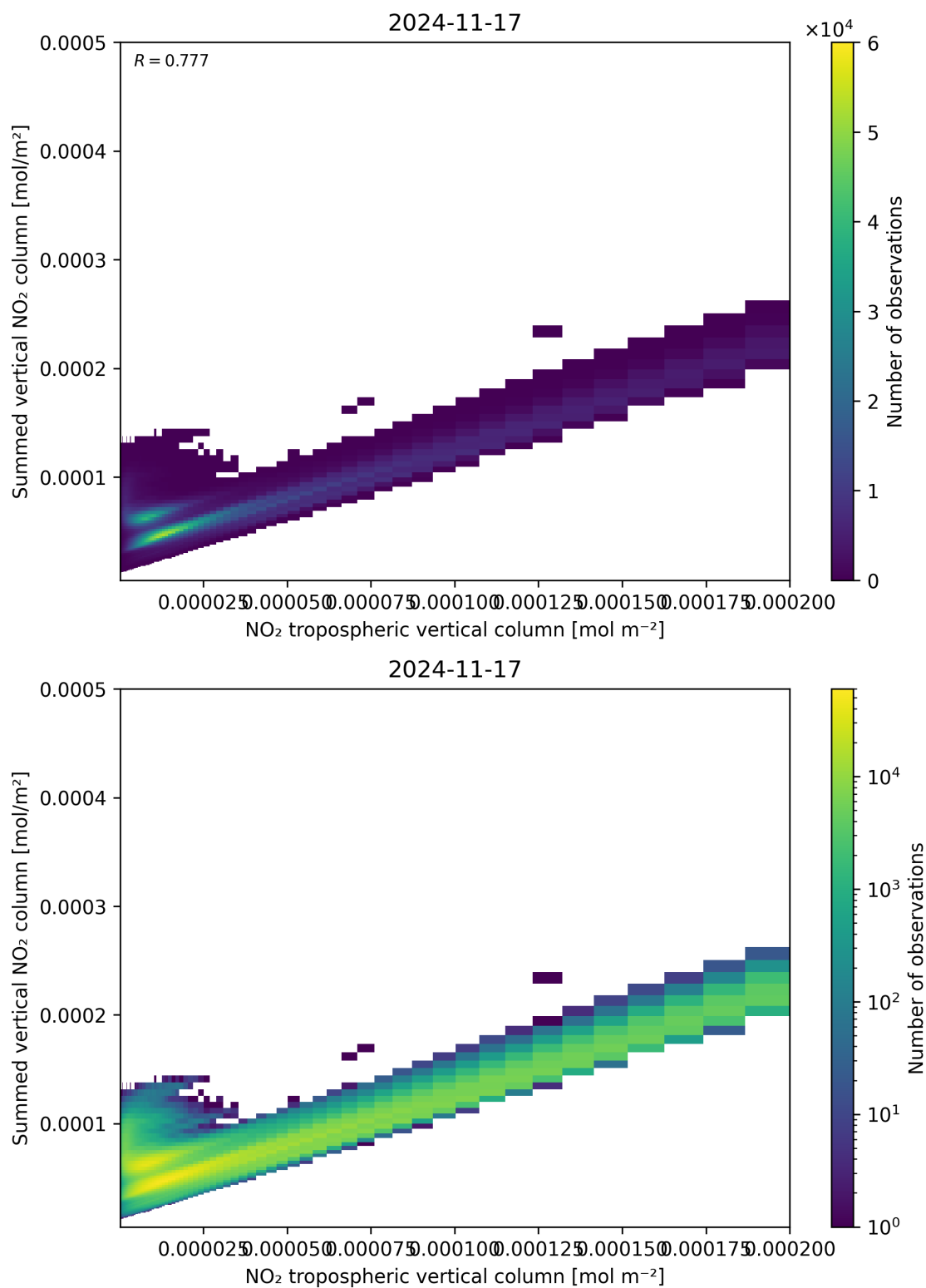
Figure 126: Scatter density plot of “NO 2 tropospheric vertical column” against “Summed vertical NO 2 column” for 2024-11-17 to 2024-11-18.
