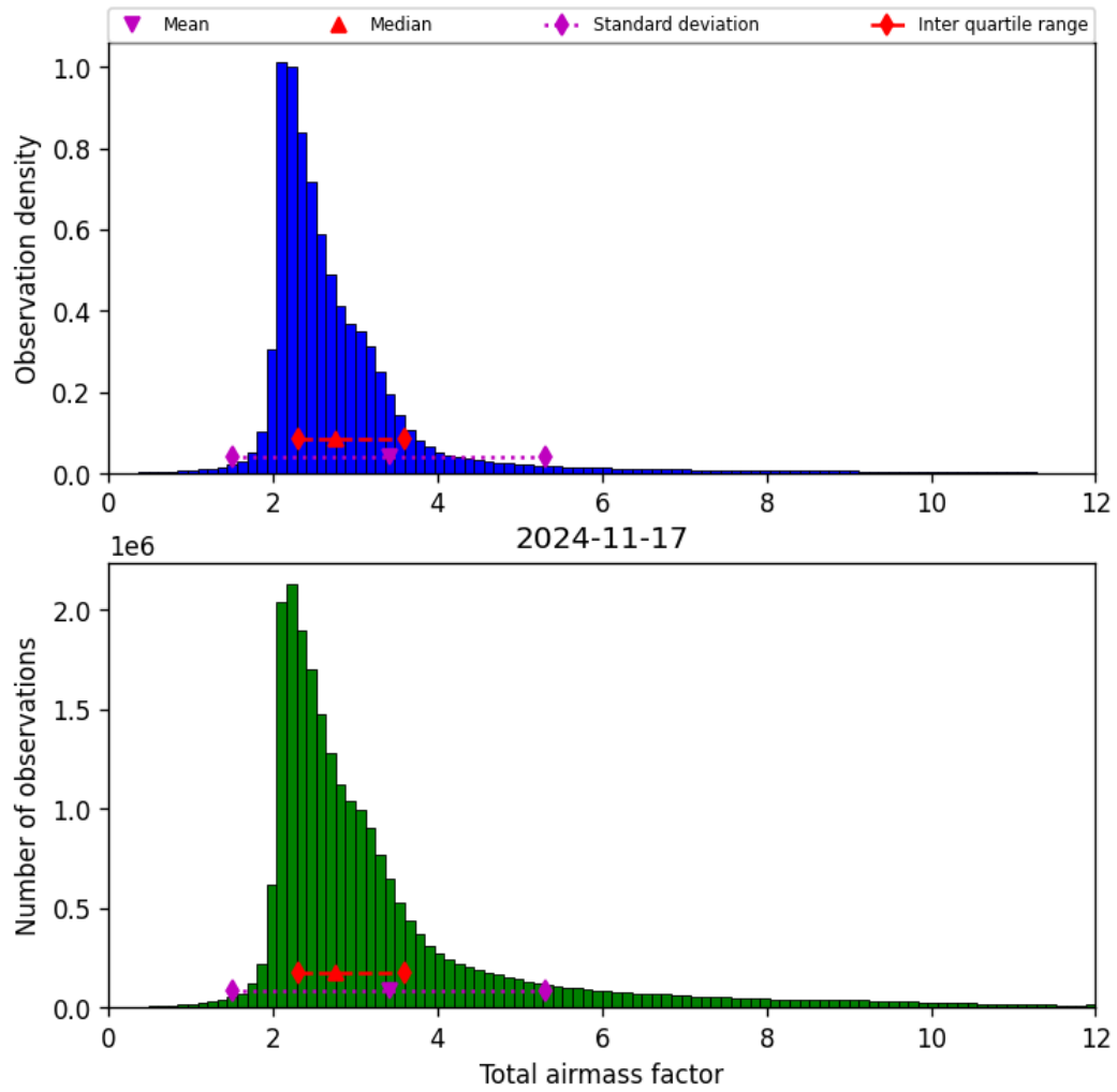
Figure 32: Histogram of “Total airmass factor” for 2024-11-17 to 2024-11-18
