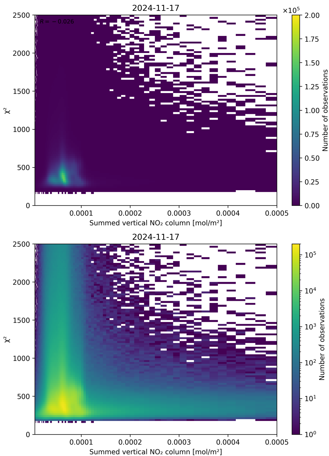
Figure 104: Scatter density plot of “Summed vertical NO 2 column” against “ \chi^2 ” for 2024-11-17 to 2024-11-18.
