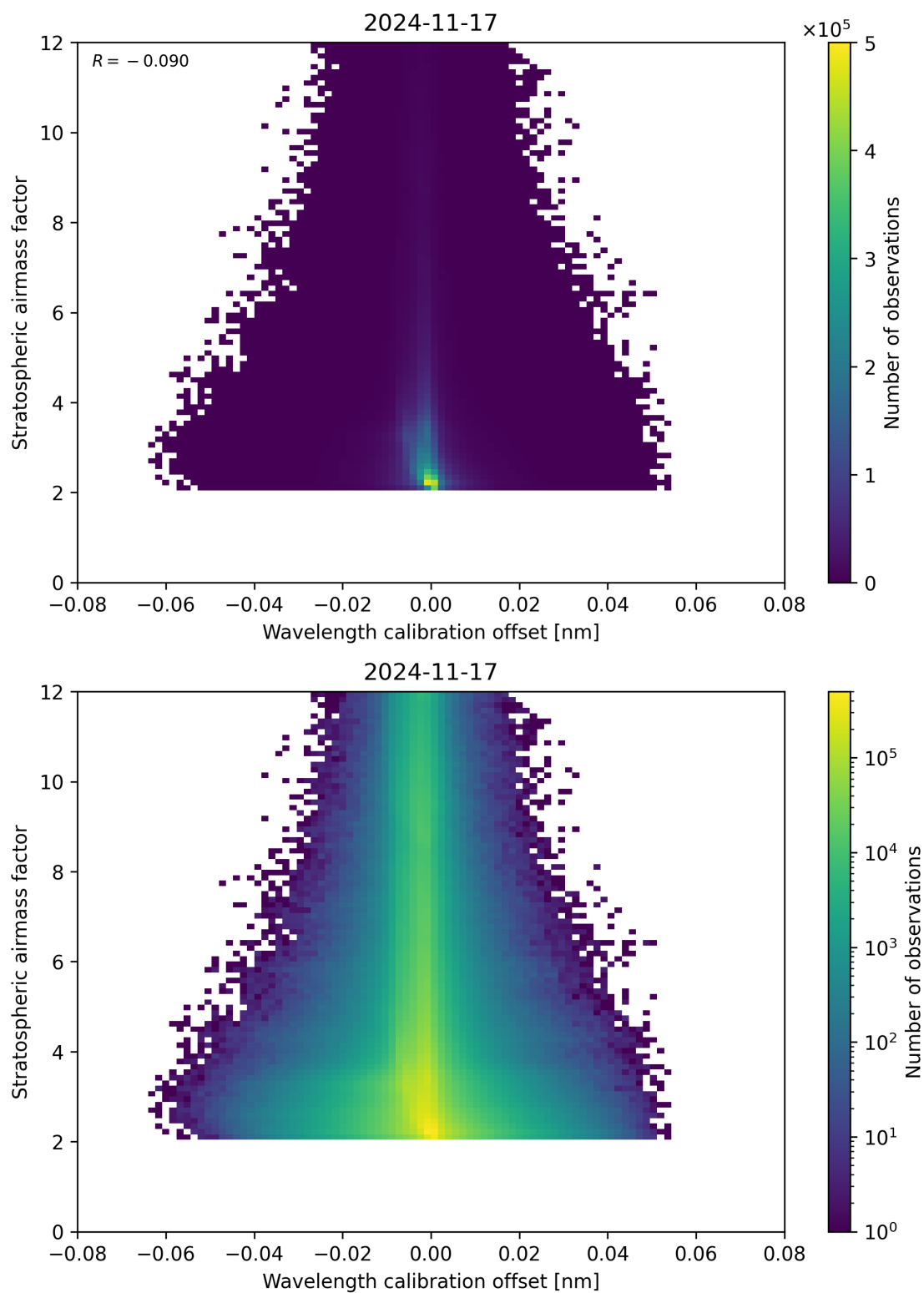
Figure 174: Scatter density plot of “Wavelength calibration offset” against “Stratospheric airmass factor” for 2024-11-17 to 2024-11-18.
