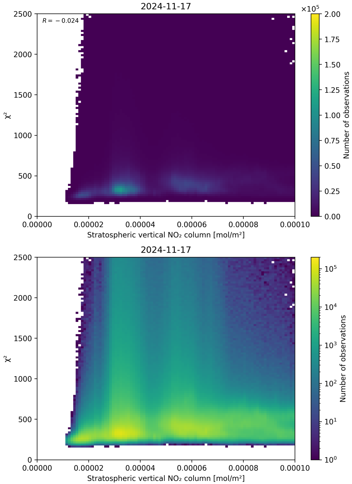
Figure 97: Scatter density plot of “Stratospheric vertical NO 2 column” against “ \chi^2 ” for 2024-11-17 to 2024-11-18.
