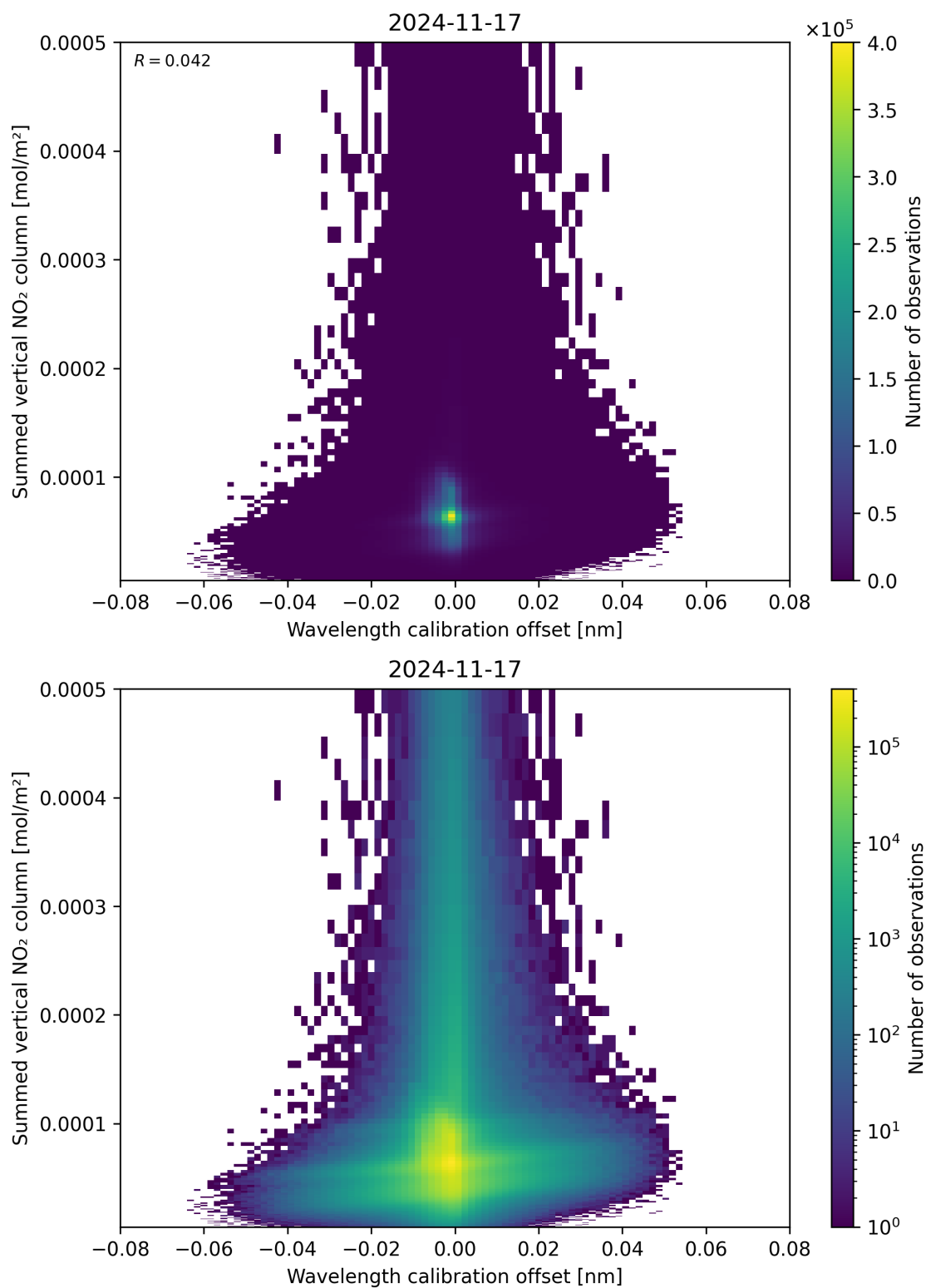
Figure 177: Scatter density plot of “Wavelength calibration offset” against “Summed vertical NO 2 column” for 2024-11-17 to 2024-11-18.
