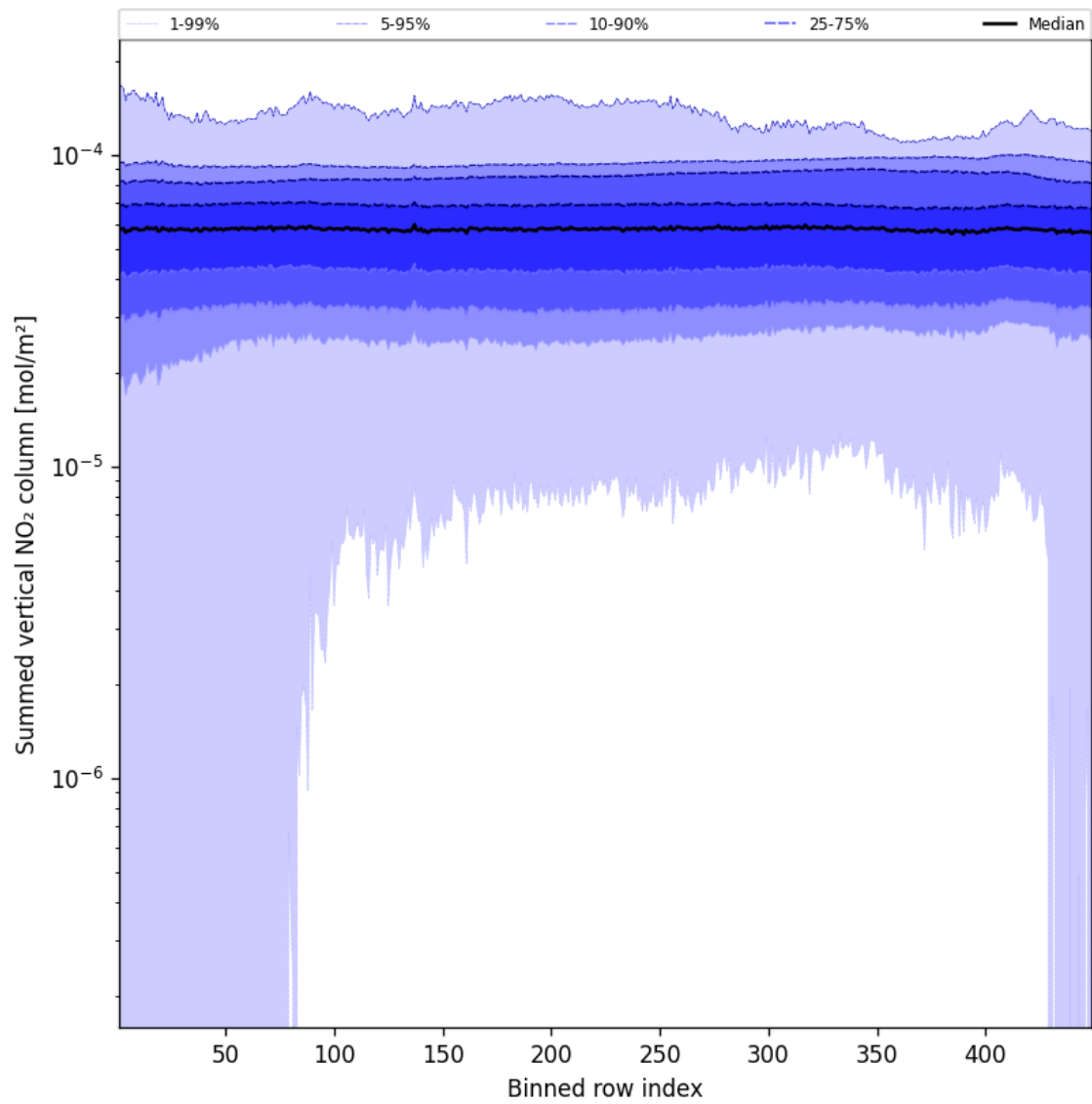
Figure 57: Along track statistics of “Summed vertical NO 2 column” for 2024-11-17 to 2024-11-18
