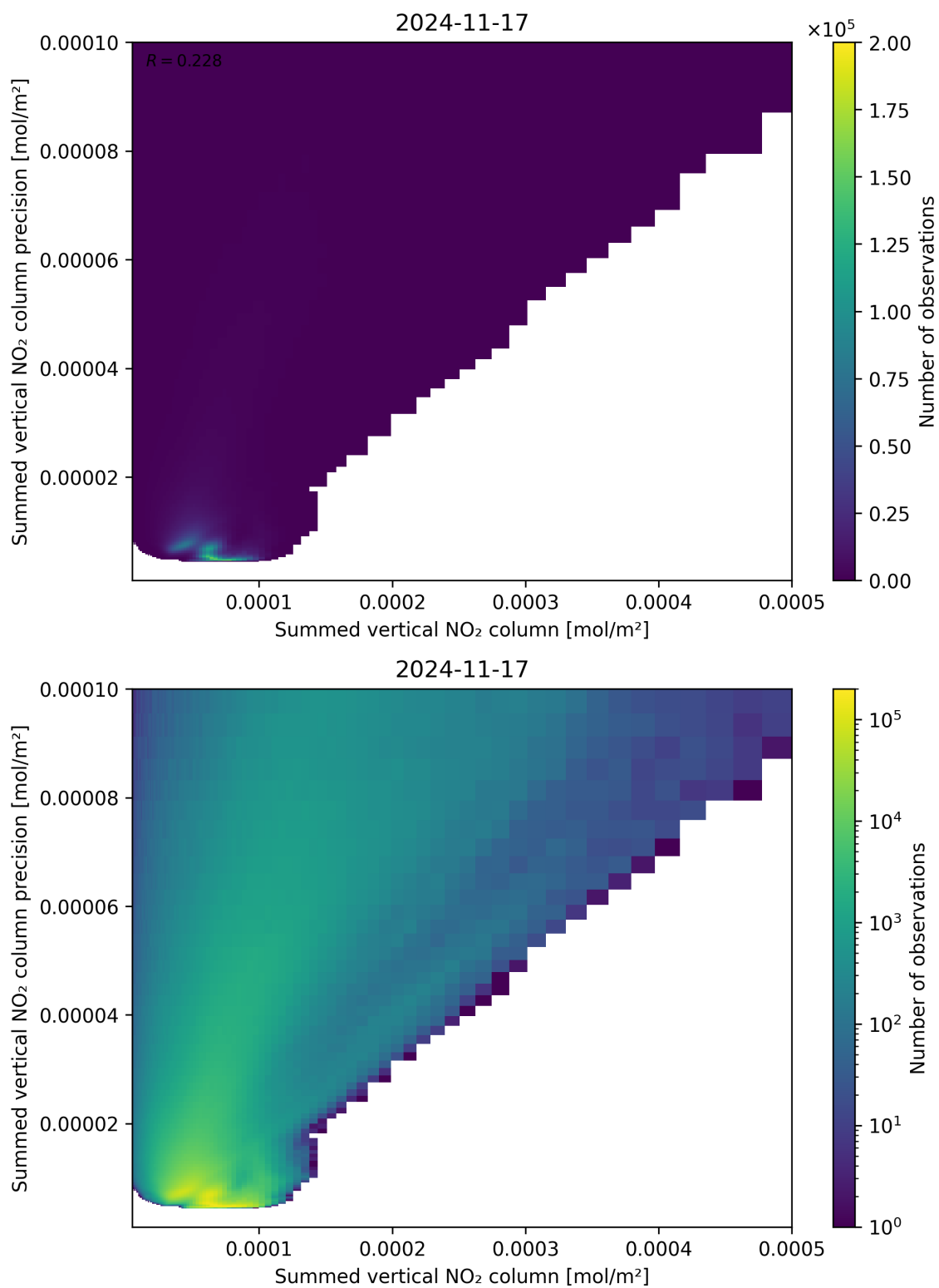
Figure 105: Scatter density plot of “Summed vertical NO 2 column” against “Summed vertical NO 2 column precision” for 2024-11-17 to 2024-11-18.
