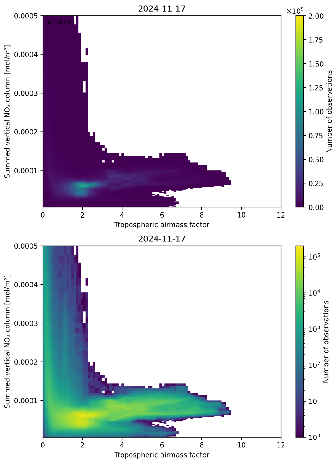
Figure 75: Scatter density plot of “Tropospheric air mass factor” against “Summed vertical NO 2 column” for 2024-11-17 to 2024-11-18.
