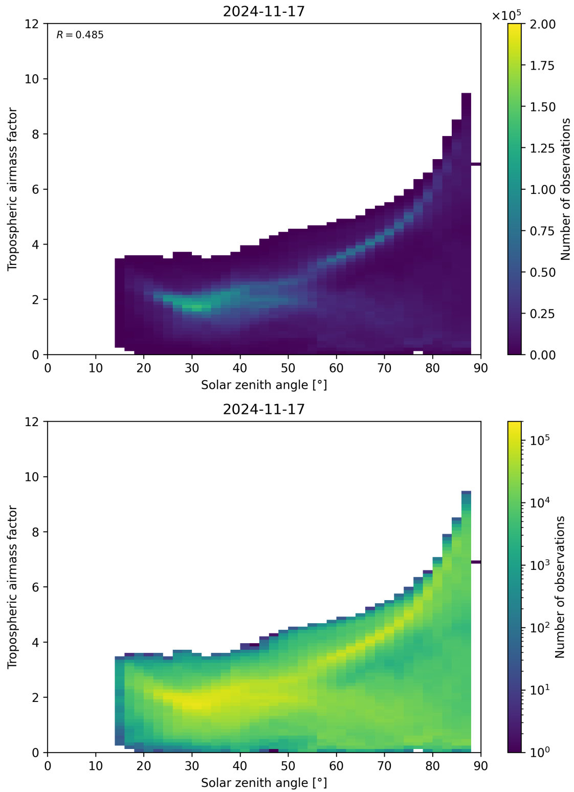
Figure 147: Scatter density plot of “Solar zenith angle” against “Tropospheric airmass factor” for 2024-11-17 to 2024-11-18.
