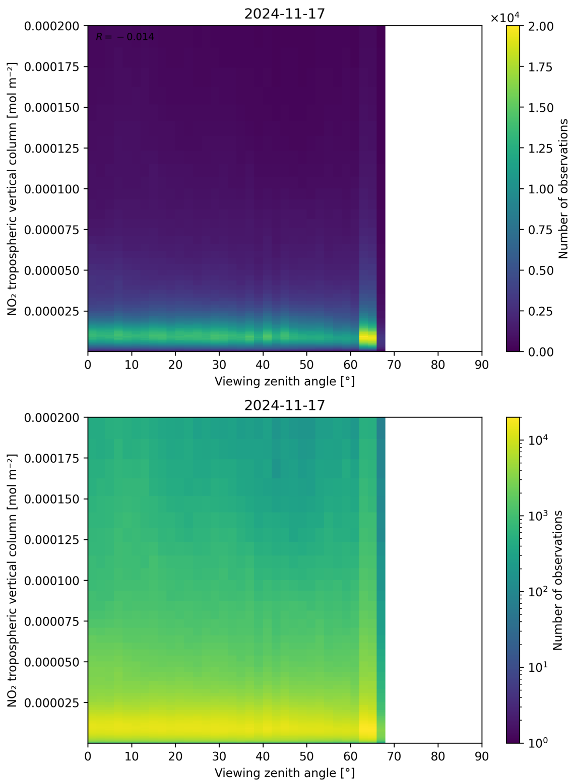
Figure 169: Scatter density plot of “Viewing zenith angle” against “NO 2 tropospheric vertical column” for 2024-11-17 to 2024-11-18.
