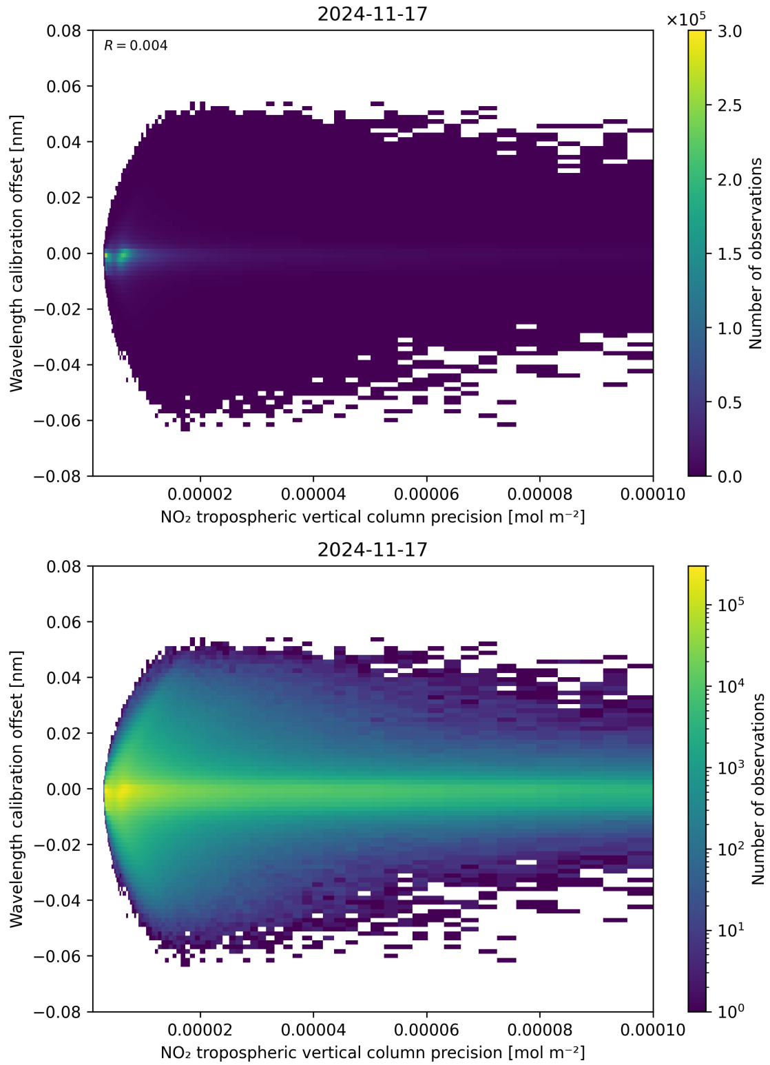
Figure 141: Scatter density plot of “NO 2 tropospheric vertical column precision” against “Wavelength calibration offset” for 2024-11-17 to 2024-11-18.
