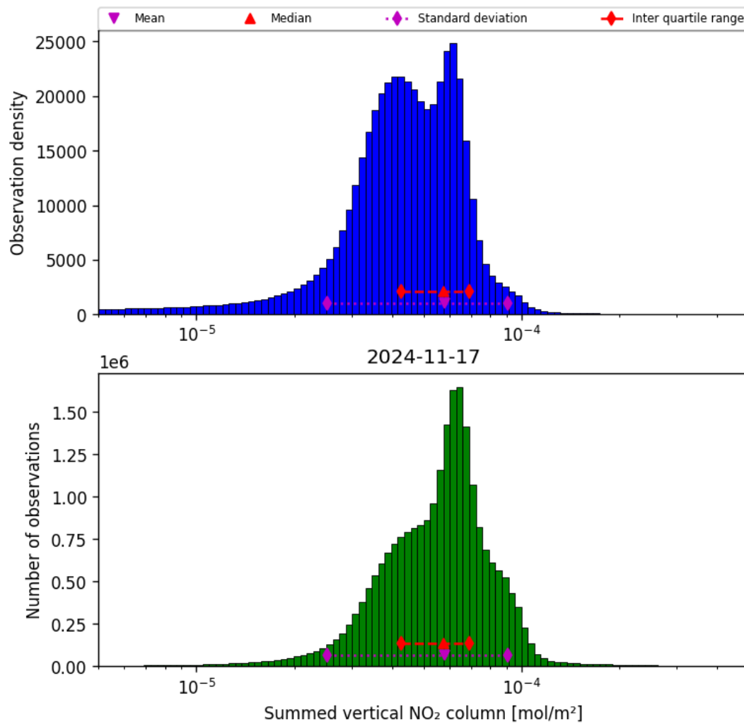
Figure 40: Histogram of “Summed vertical NO 2 column” for 2024-11-17 to 2024-11-18
