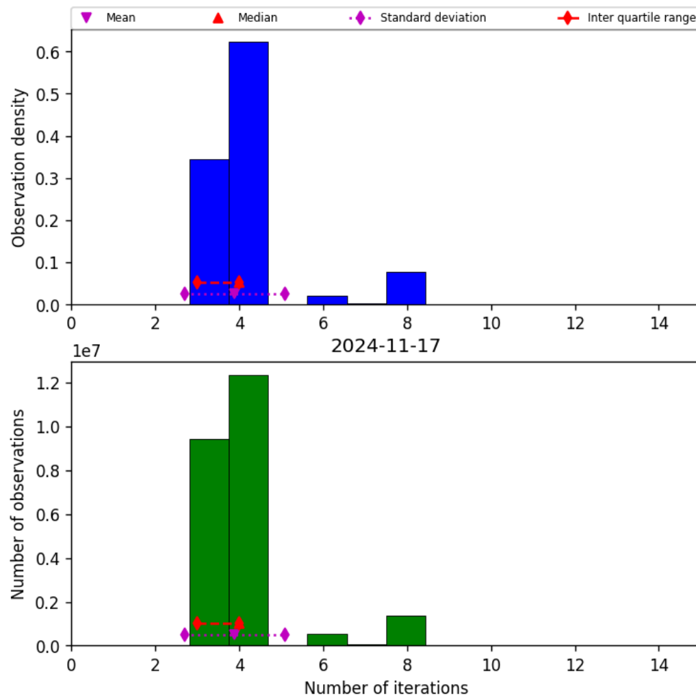
Figure 34: Histogram of “Number of iterations” for 2024-11-17 to 2024-11-18
