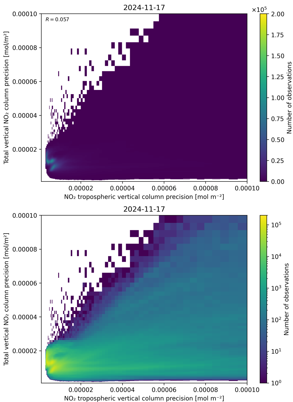
Figure 139: Scatter density plot of “NO 2 tropospheric vertical column precision” against “Total vertical NO 2 column precision” for 2024-11-17 to 2024-11-18.
