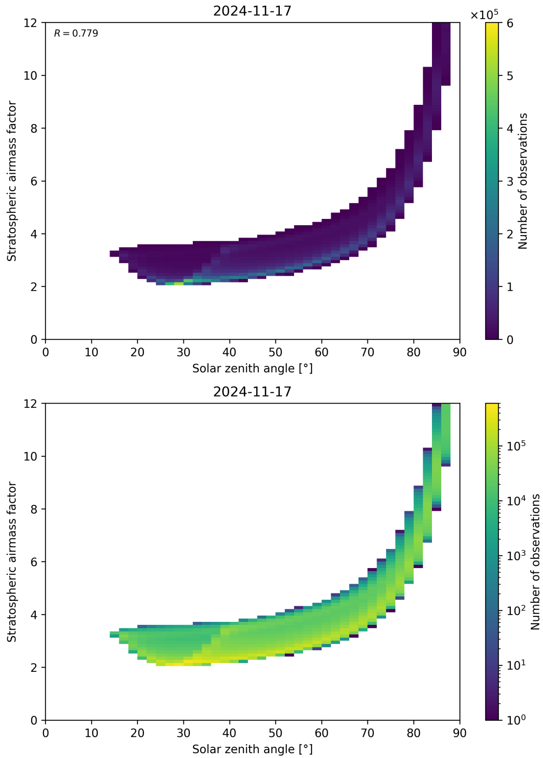
Figure 145: Scatter density plot of “Solar zenith angle” against “Stratospheric airmass factor” for 2024-11-17 to 2024-11-18.
