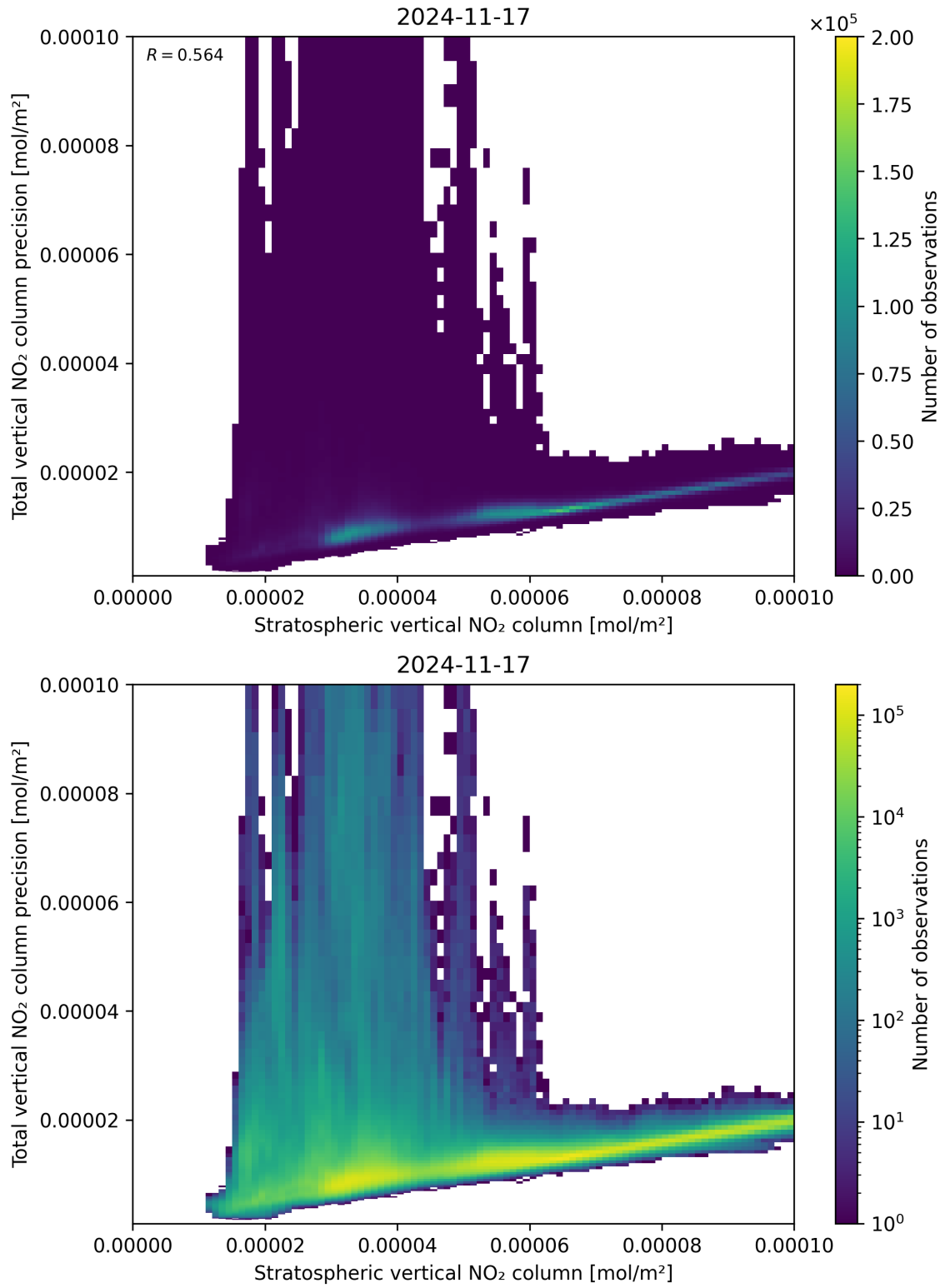
Figure 101: Scatter density plot of “Stratospheric vertical NO 2 column” against “Total vertical NO 2 column precision” for 2024-11-17 to 2024-11-18.
