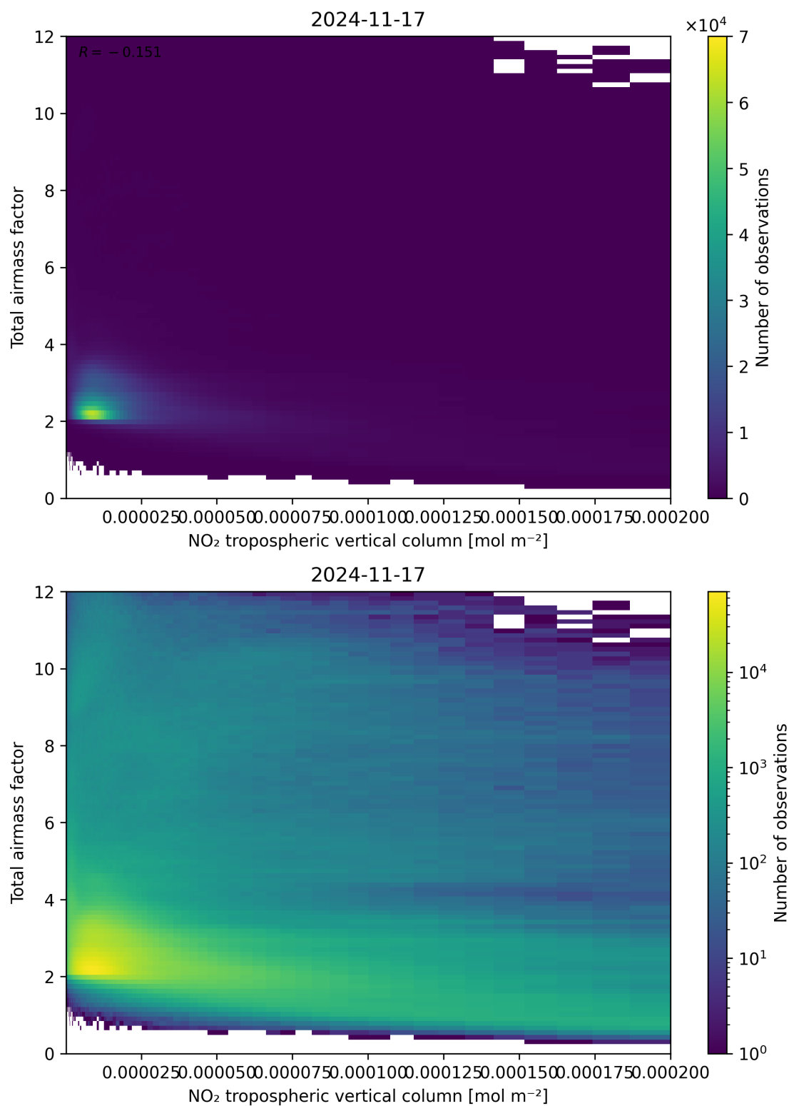
Figure 122: Scatter density plot of “NO 2 tropospheric vertical column” against “Total air mass factor” for 2024-11-17 to 2024-11-18.
