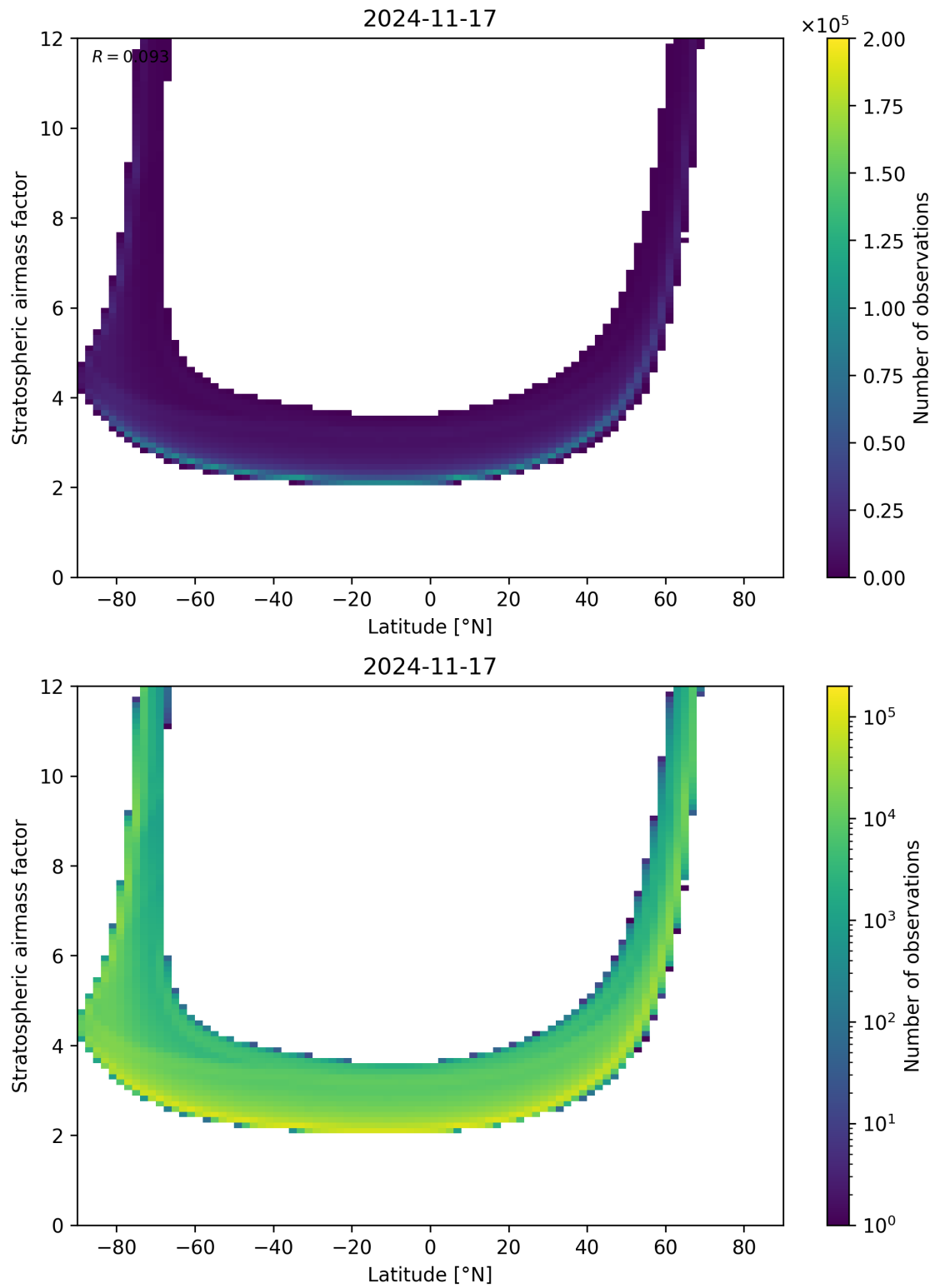
Figure 83: Scatter density plot of “Latitude” against “Stratospheric airmass factor” for 2024-11-17 to 2024-11-18.
