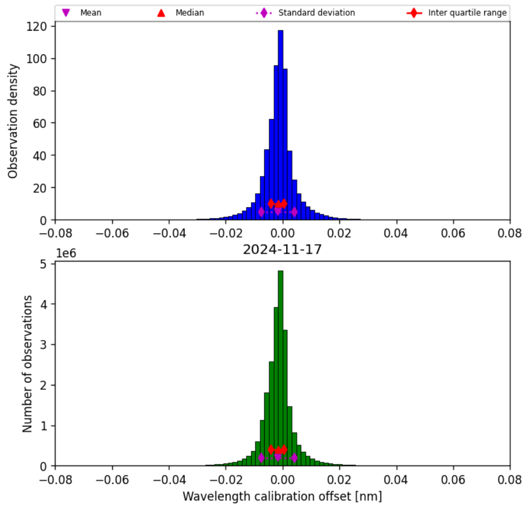
Figure 35: Histogram of “Wavelength calibration offset” for 2024-11-17 to 2024-11-18
