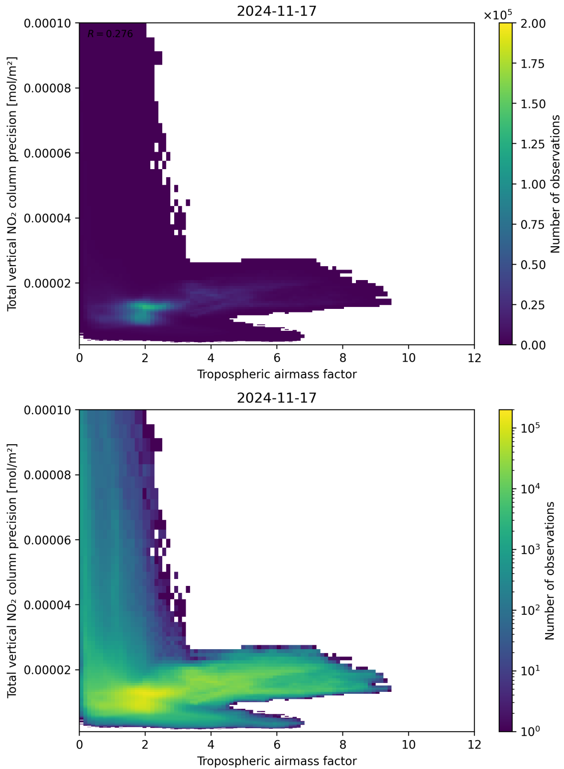
Figure 78: Scatter density plot of “Tropospheric air mass factor” against “Total vertical NO 2 column precision” for 2024-11-17 to 2024-11-18.
