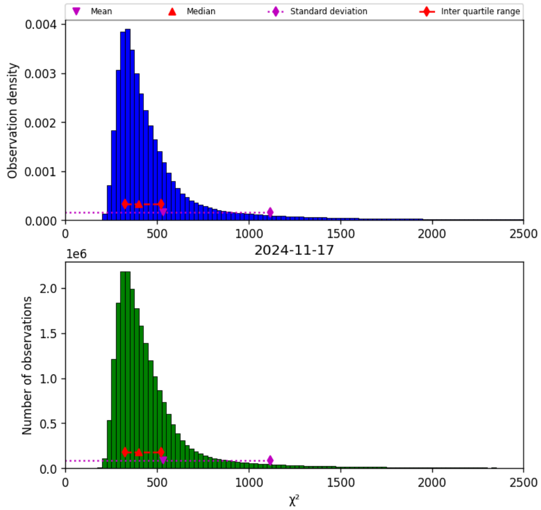
Figure 42: Histogram of “ \chi^2 ” for 2024-11-17 to 2024-11-18
