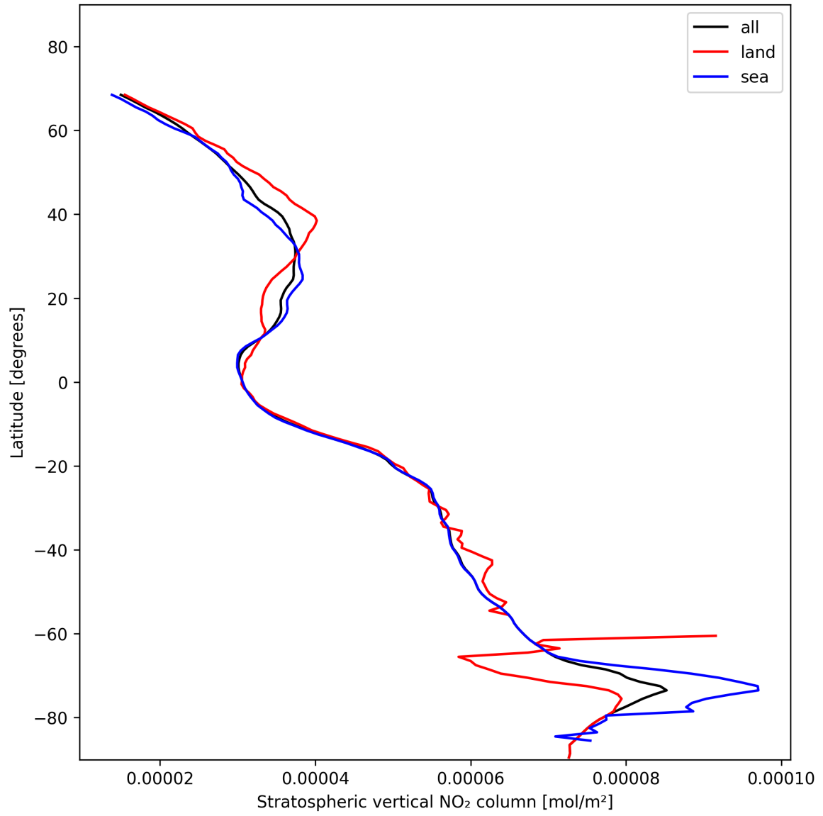
Figure 19: Zonal average of “Stratospheric vertical NO 2 column” for 2024-11-17 to 2024-11-18.
