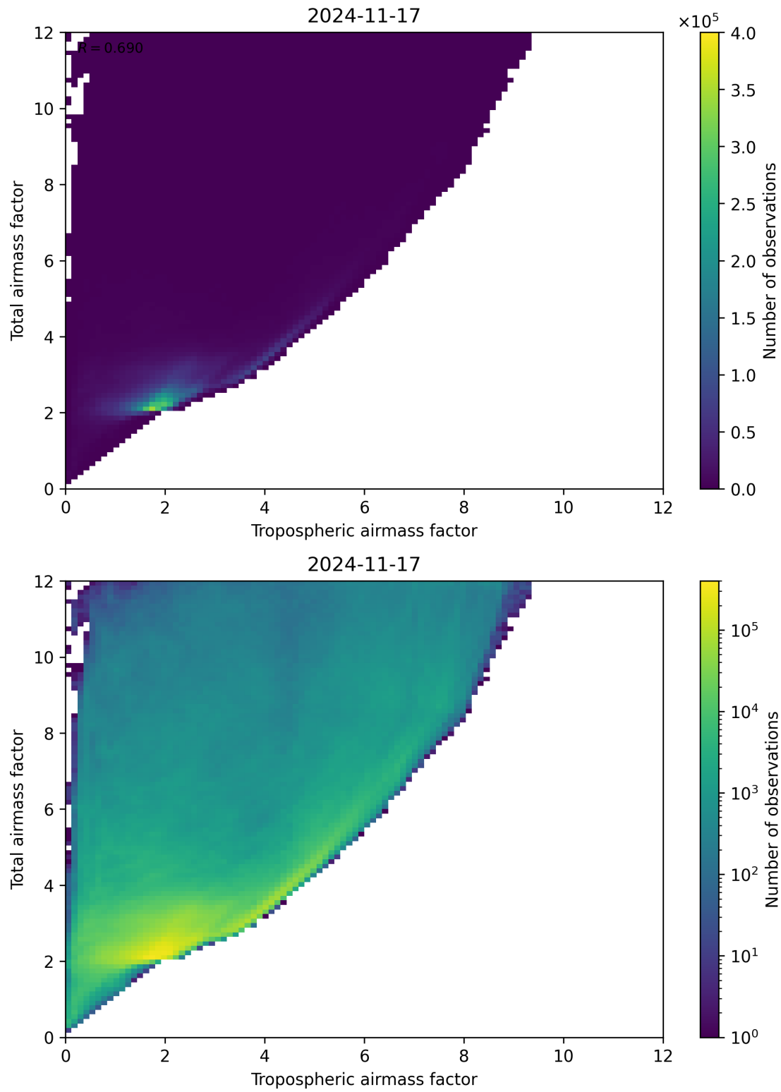
Figure 72: Scatter density plot of “Tropospheric airmass factor” against “Total airmass factor” for 2024-11-17 to 2024-11-18.
