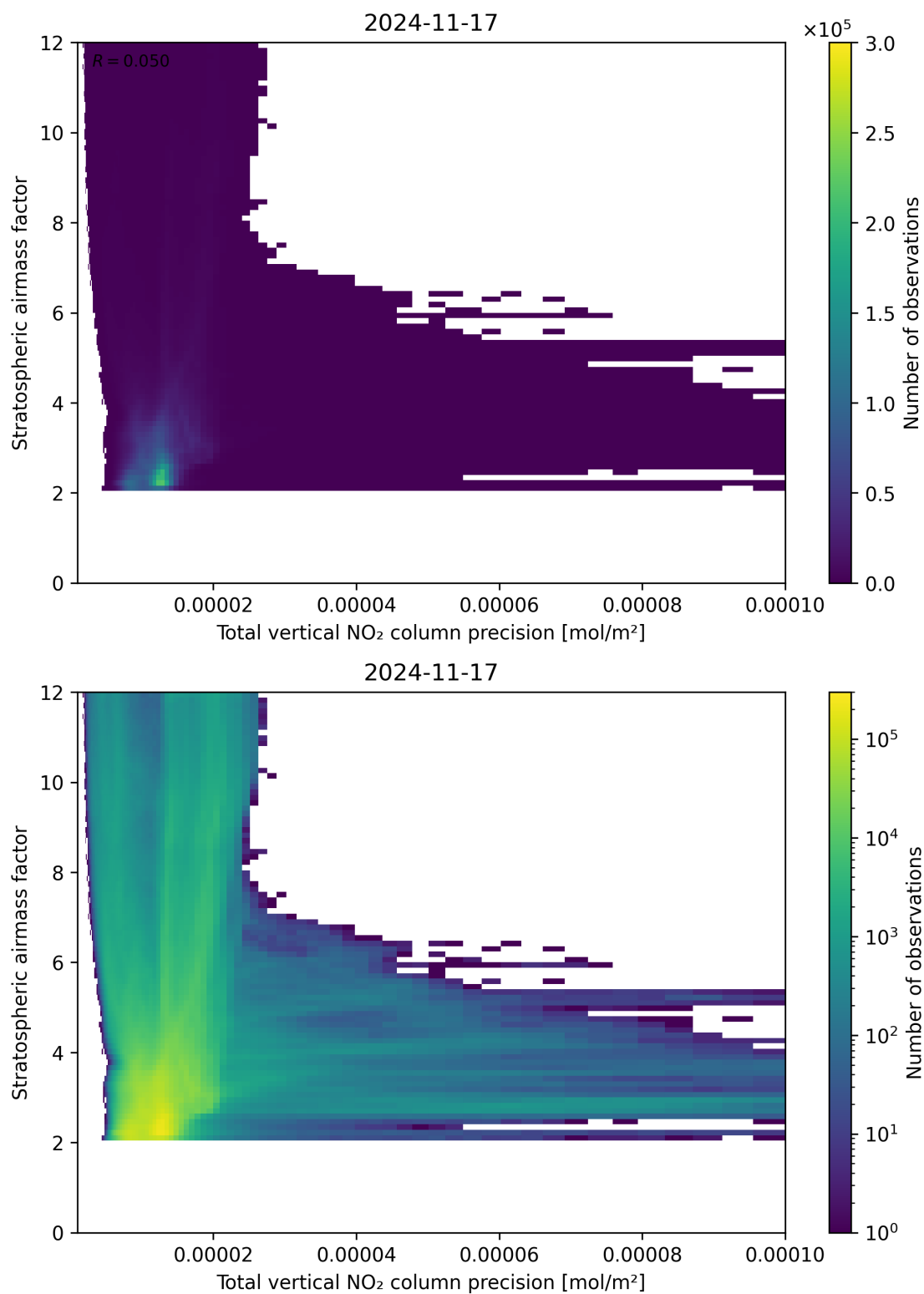
Figure 115: Scatter density plot of “Total vertical NO 2 column precision” against “Stratospheric air mass factor” for 2024-11-17 to 2024-11-18.
