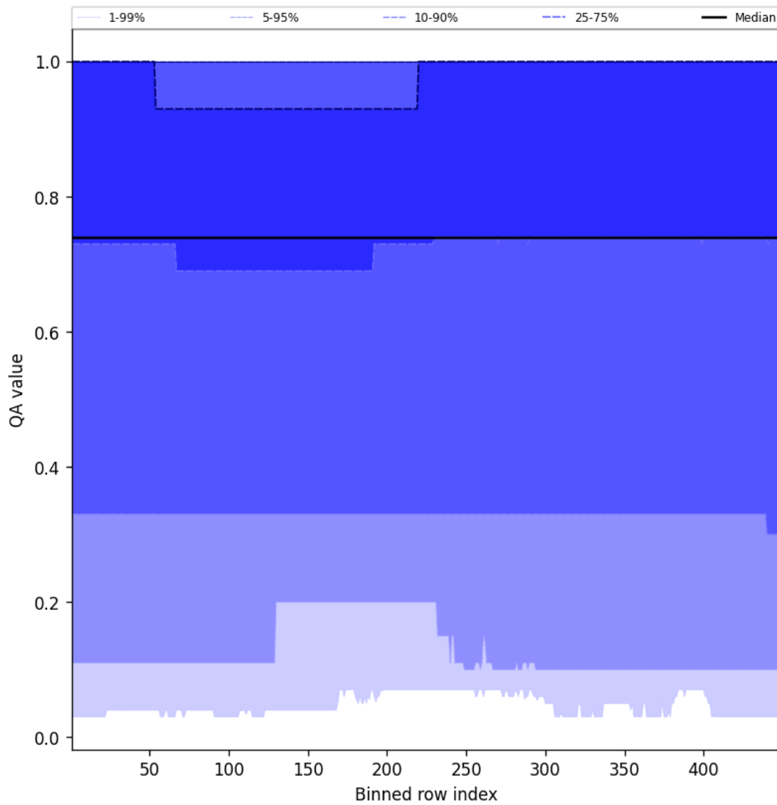
Figure 45: Along track statistics of “QA value” for 2024-11-17 to 2024-11-18
