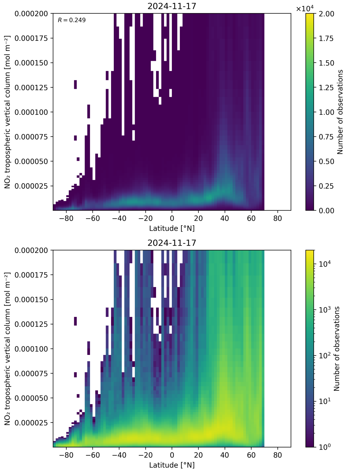
Figure 92: Scatter density plot of “Latitude” against “NO 2 tropospheric vertical column” for 2024-11-17 to 2024-11-18.
