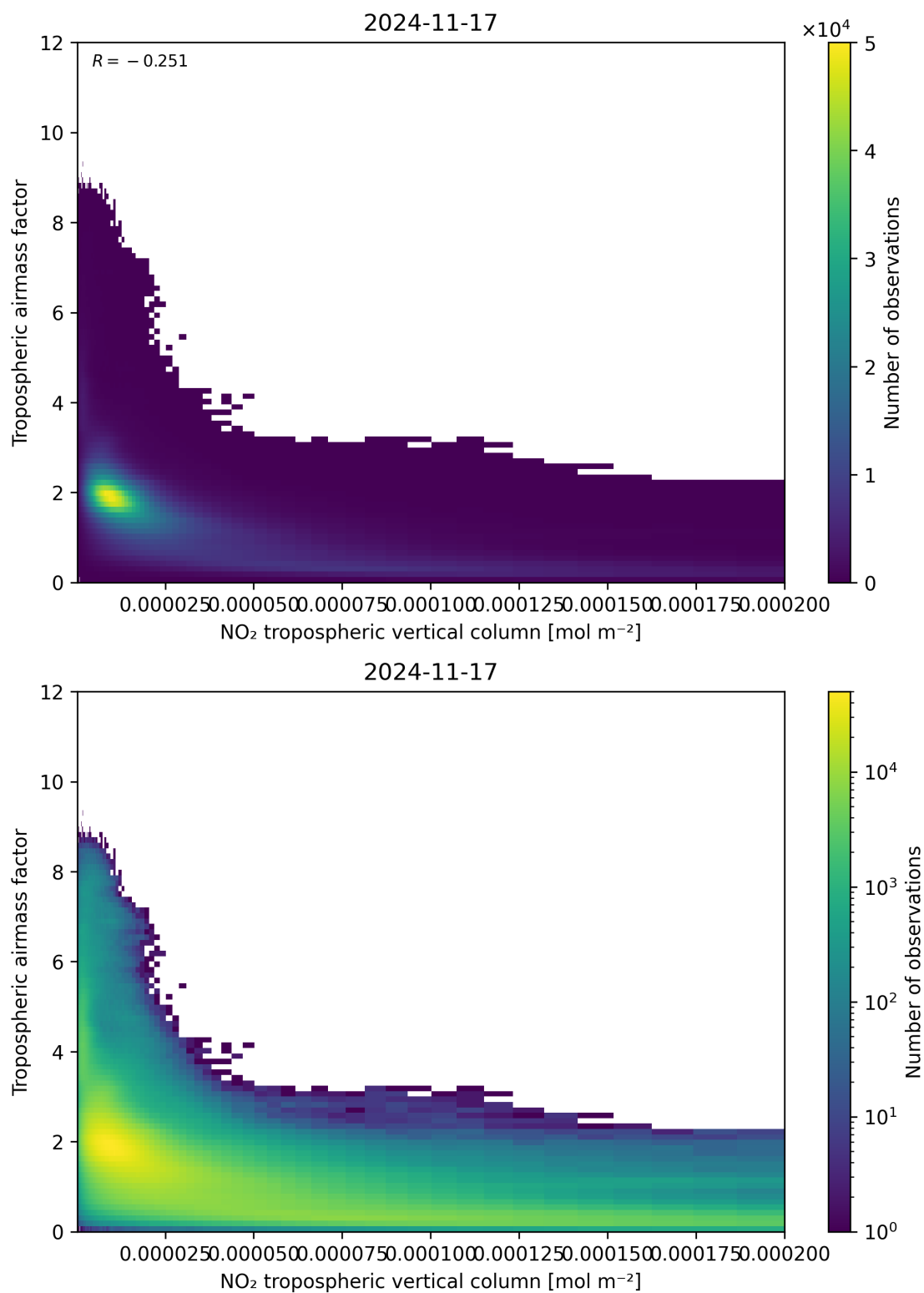
Figure 123: Scatter density plot of “NO 2 tropospheric vertical column” against “Tropospheric air mass factor” for 2024-11-17 to 2024-11-18.
