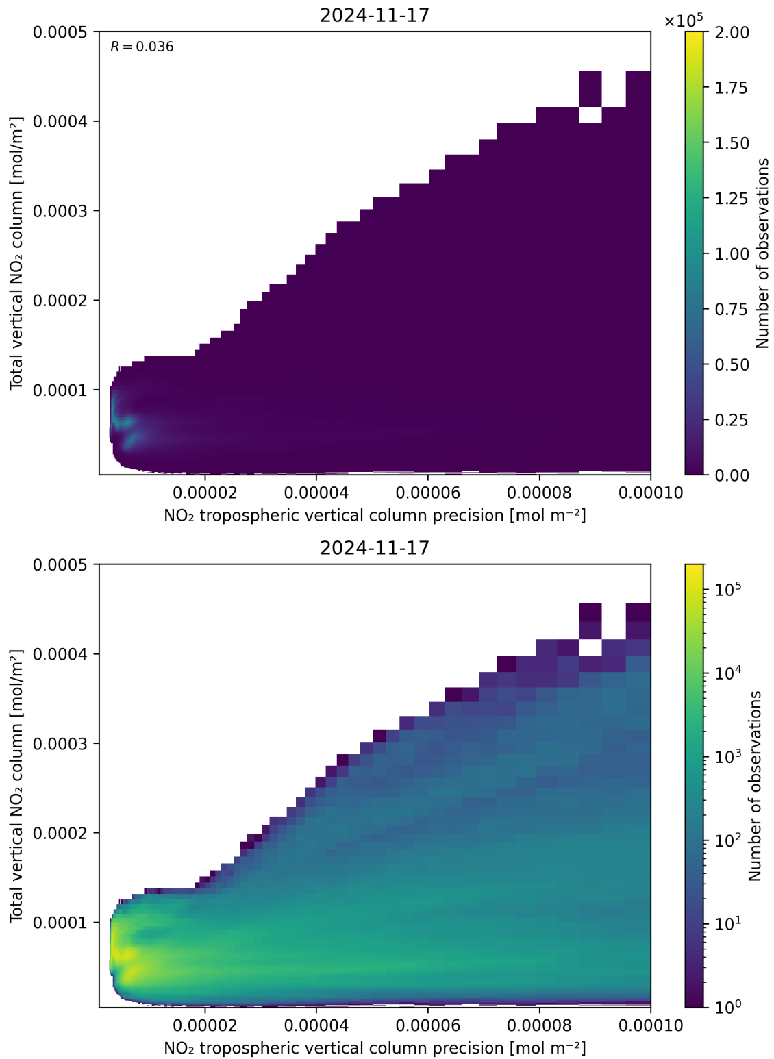
Figure 138: Scatter density plot of “NO 2 tropospheric vertical column precision” against “Total vertical NO 2 column” for 2024-11-17 to 2024-11-18.
