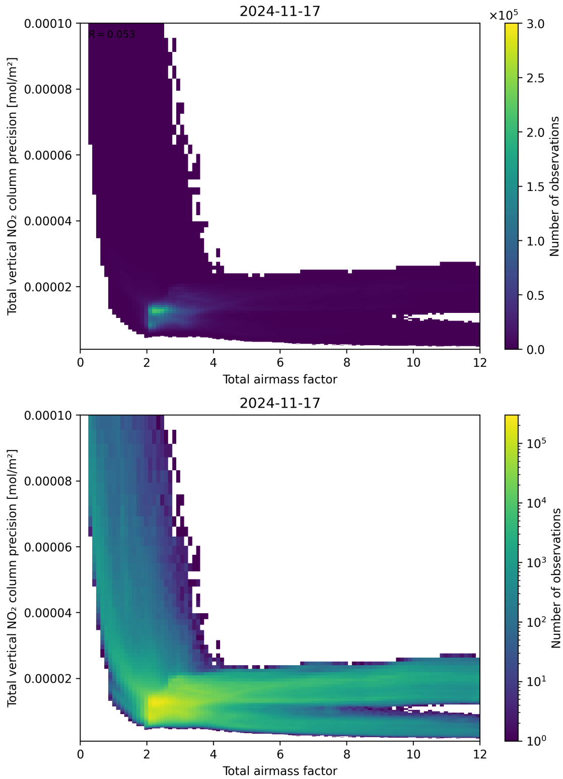
Figure 68: Scatter density plot of “Total airmass factor” against “Total vertical NO 2 column precision” for 2024-11-17 to 2024-11-18.
