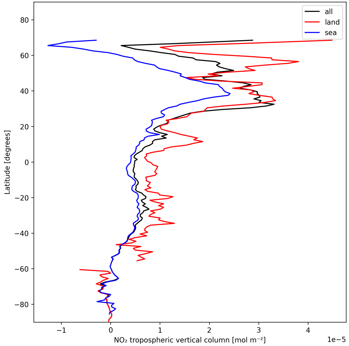
Figure 12: Zonal average of “NO 2 tropospheric vertical column” for 2024-11-17 to 2024-11-18.
