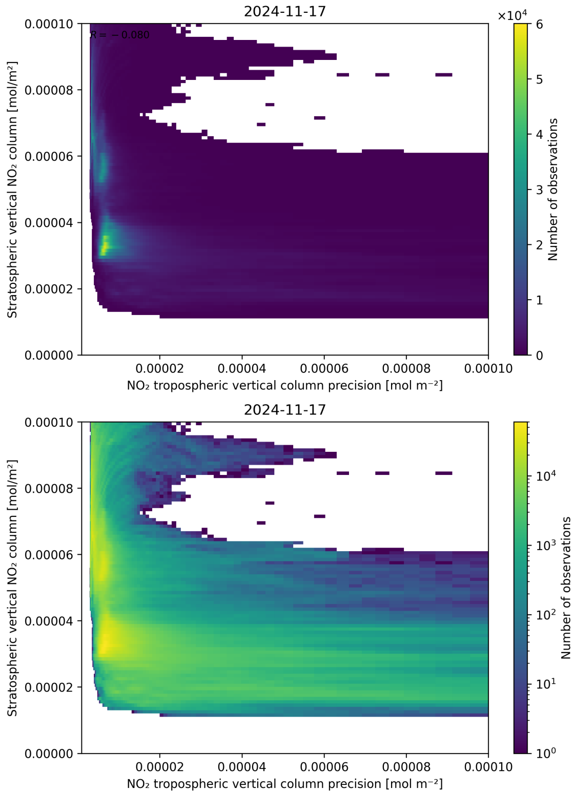
Figure 135: Scatter density plot of “NO 2 tropospheric vertical column precision” against “Stratospheric vertical NO 2 column” for 2024-11-17 to 2024-11-18.
