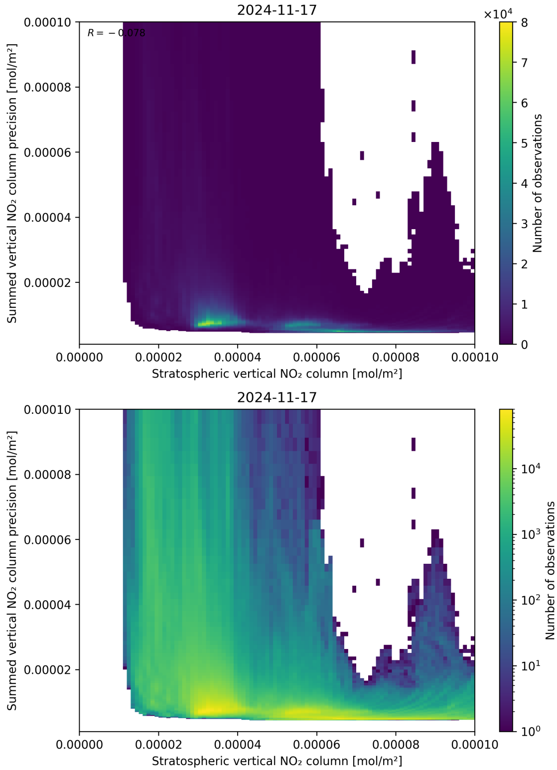
Figure 99: Scatter density plot of “Stratospheric vertical NO 2 column” against “Summed vertical NO 2 column precision” for 2024-11-17 to 2024-11-18.
