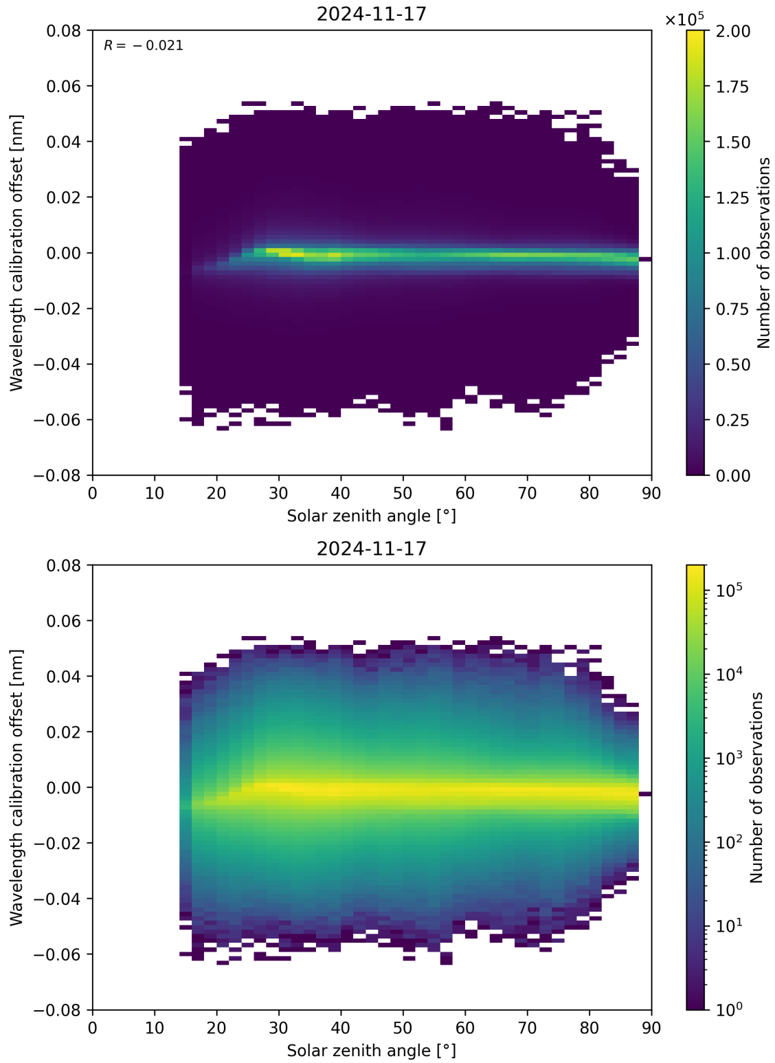
Figure 158: Scatter density plot of “Solar zenith angle” against “Wavelength calibration offset” for 2024-11-17 to 2024-11-18.
