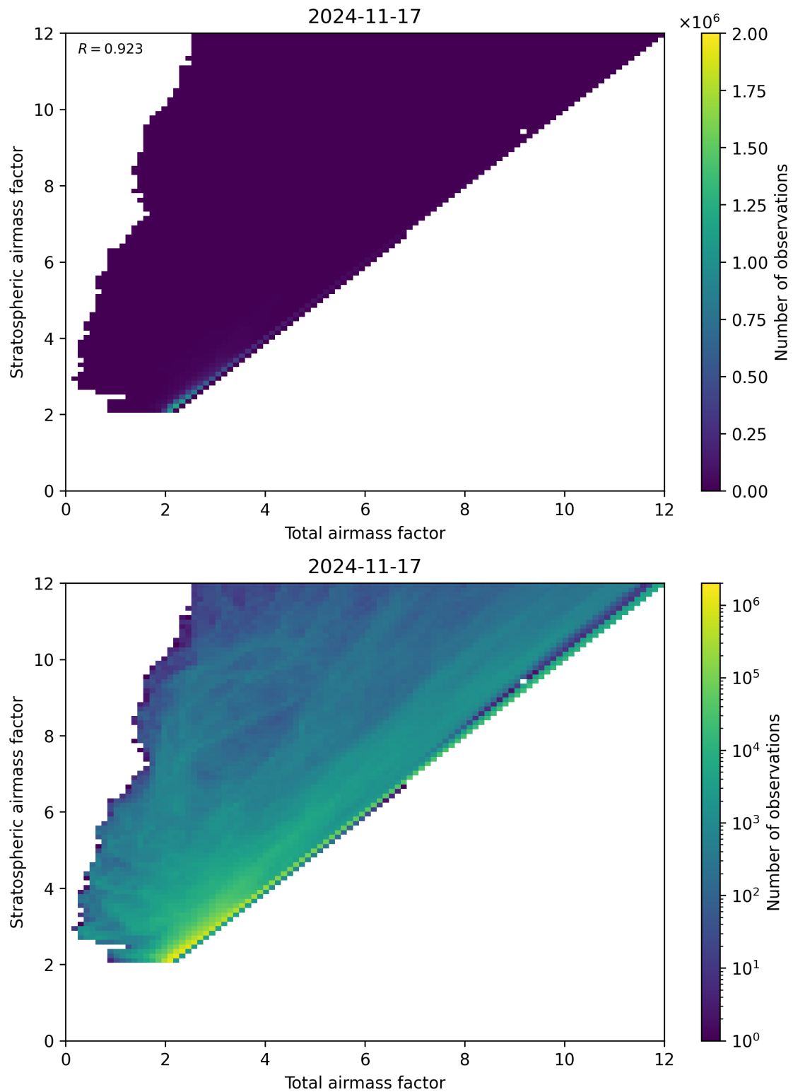
Figure 62: Scatter density plot of “Total air mass factor” against “Stratospheric air mass factor” for 2024-11-17 to 2024-11-18.
