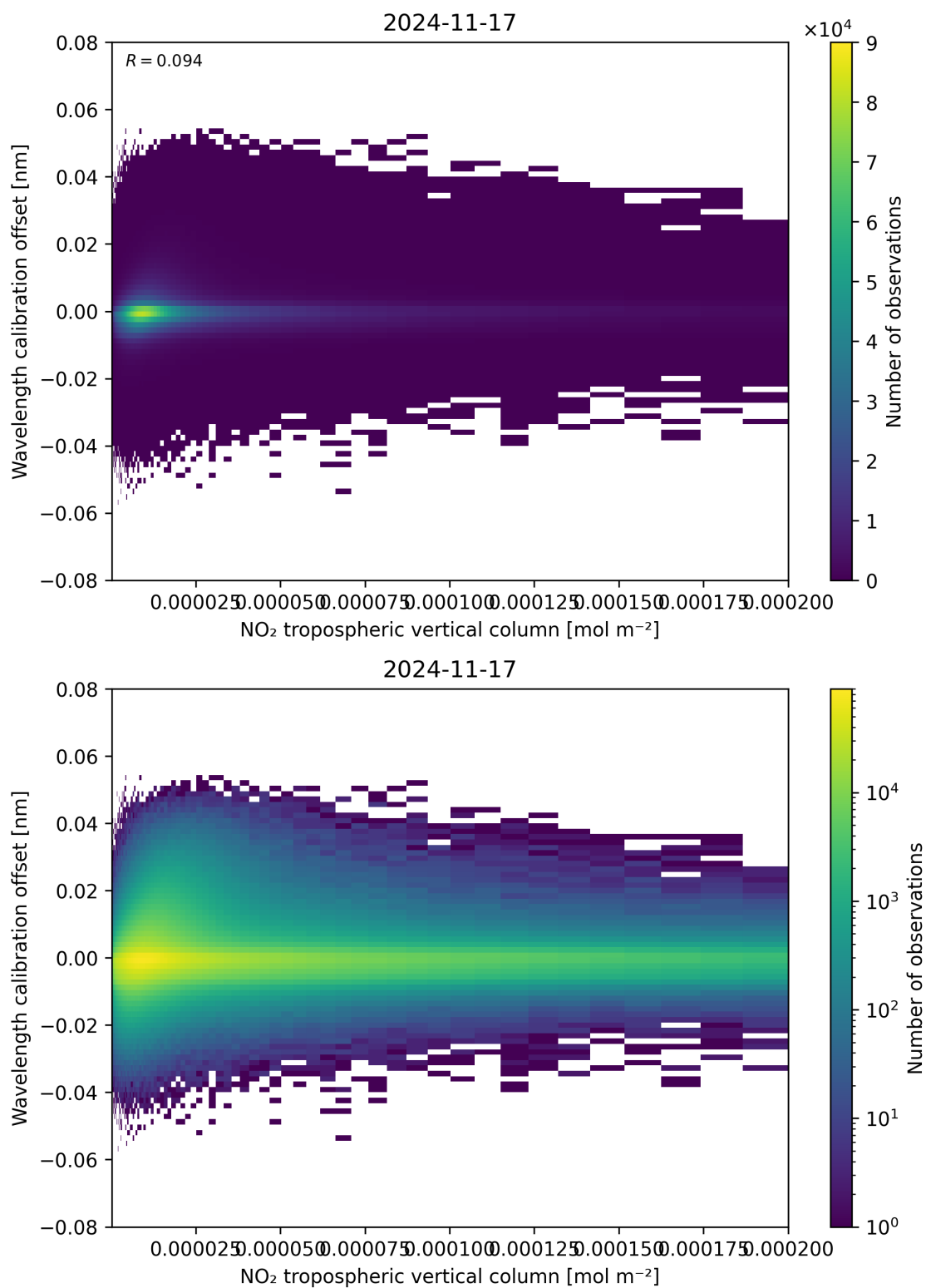
Figure 143: Scatter density plot of “NO 2 tropospheric vertical column” against “Wavelength calibration offset” for 2024-11-17 to 2024-11-18.
