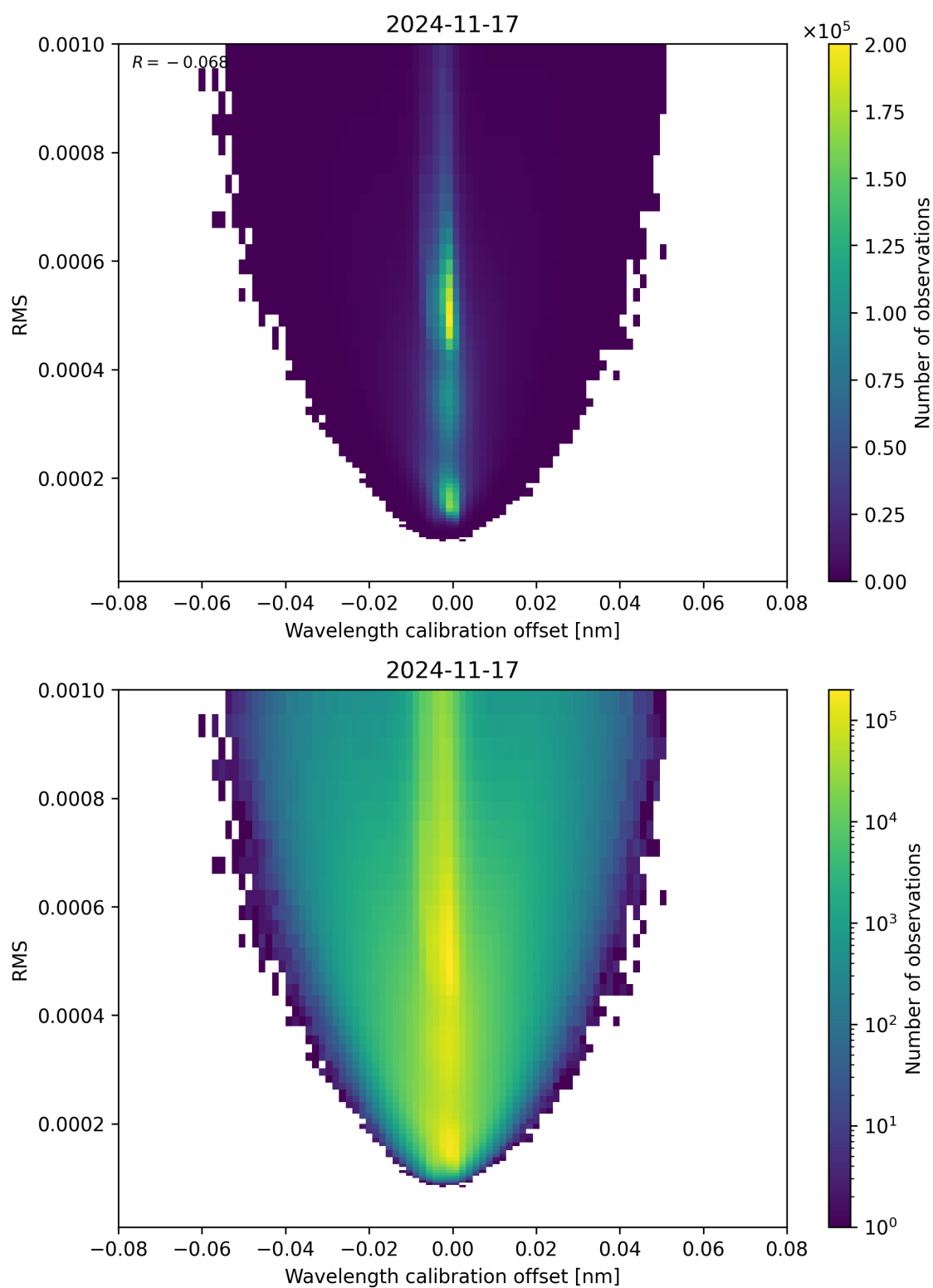
Figure 181: Scatter density plot of “Wavelength calibration offset” against “RMS” for 2024-11-17 to 2024-11-18.
