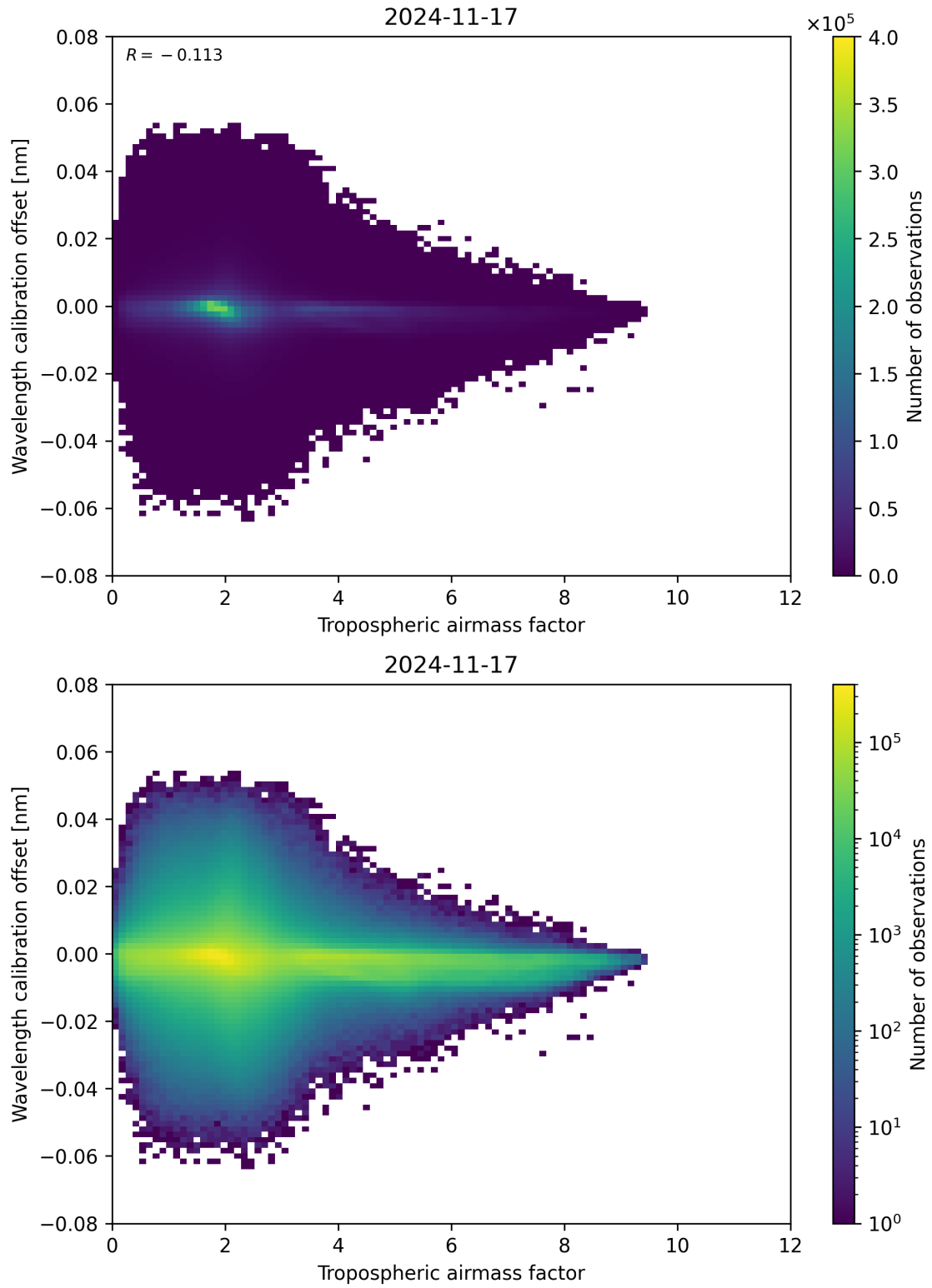
Figure 80: Scatter density plot of “Tropospheric airmass factor” against “Wavelength calibration offset” for 2024-11-17 to 2024-11-18.
