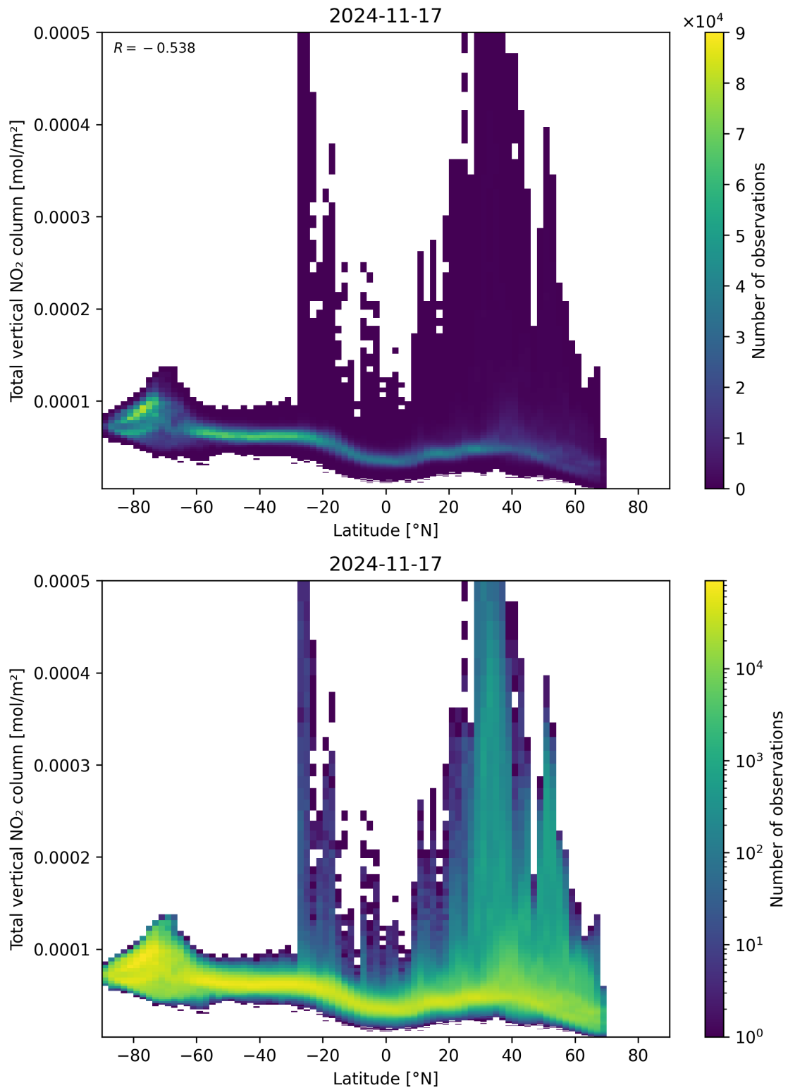
Figure 90: Scatter density plot of “Latitude” against “Total vertical NO 2 column” for 2024-11-17 to 2024-11-18.
