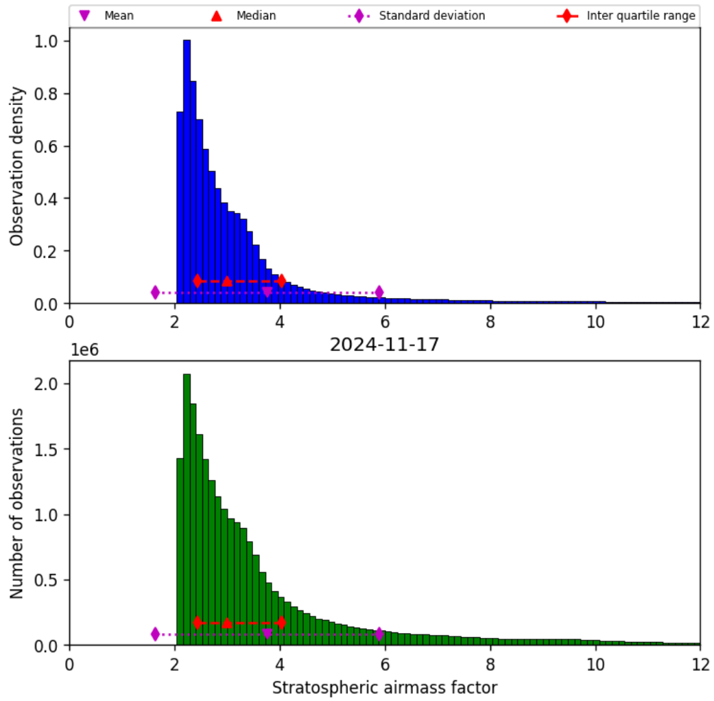
Figure 44: Histogram of “Stratospheric airmass factor” for 2024-11-17 to 2024-11-18
