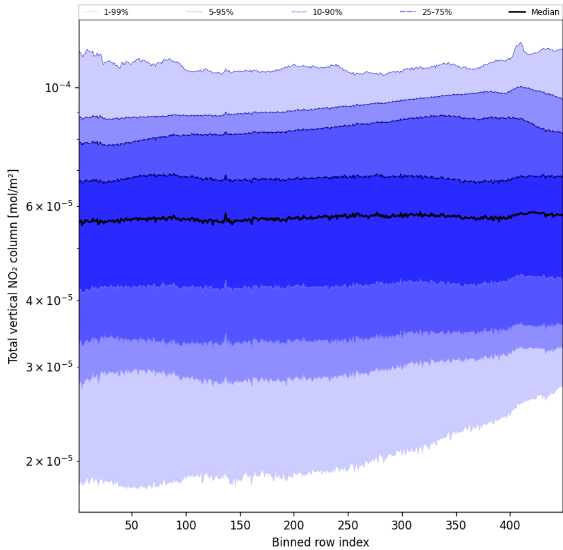
Figure 55: Along track statistics of “Total vertical NO 2 column” for 2024-11-17 to 2024-11-18
