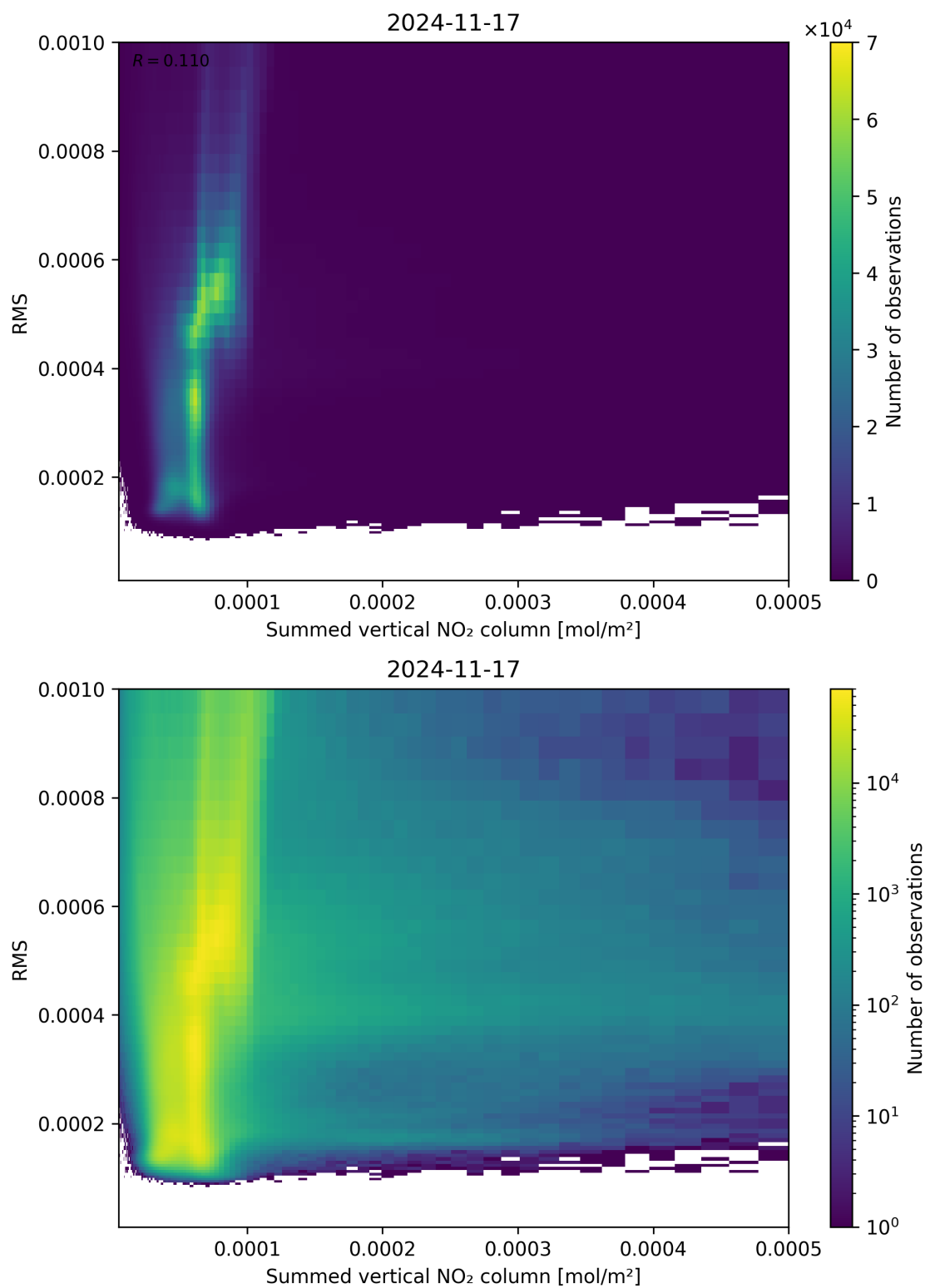
Figure 109: Scatter density plot of “Summed vertical NO 2 column” against “RMS” for 2024-11-17 to 2024-11-18.
