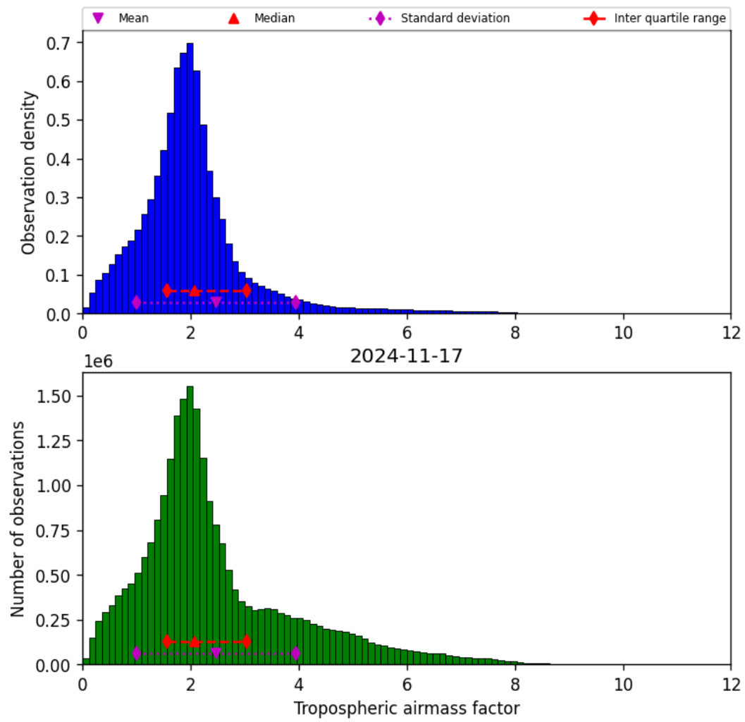
Figure 31: Histogram of “Tropospheric airmass factor” for 2024-11-17 to 2024-11-18
