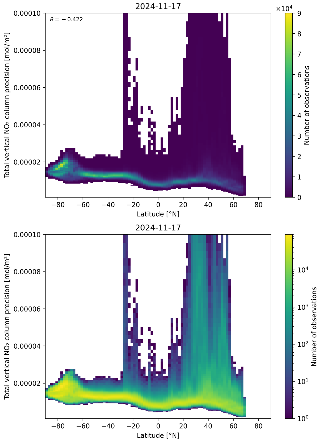
Figure 91: Scatter density plot of “Latitude” against “Total vertical NO 2 column precision” for 2024-11-17 to 2024-11-18.
