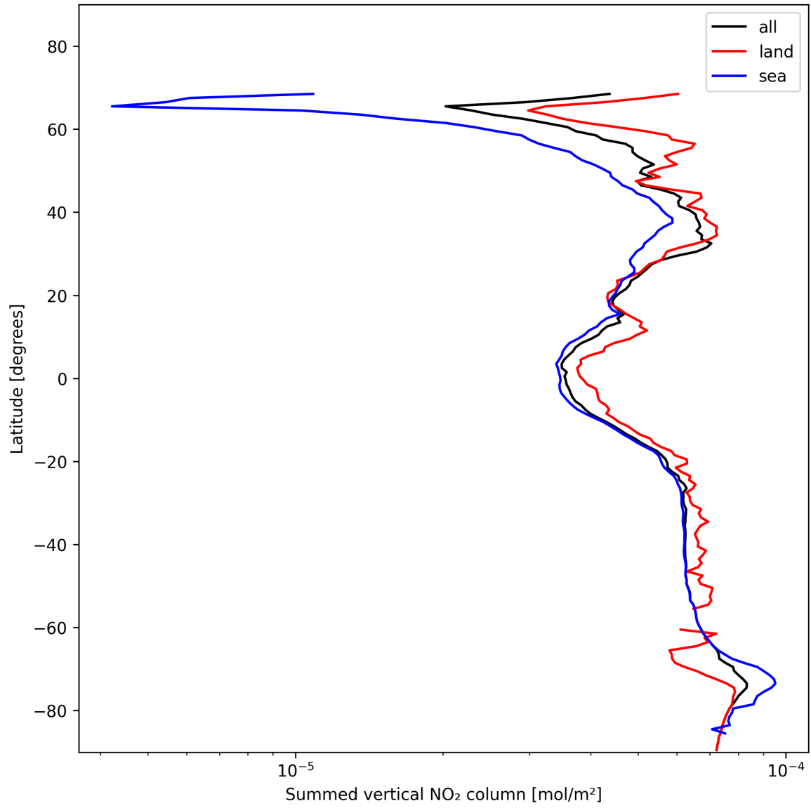
Figure 23: Zonal average of “Summed vertical NO 2 column” for 2024-11-17 to 2024-11-18.
