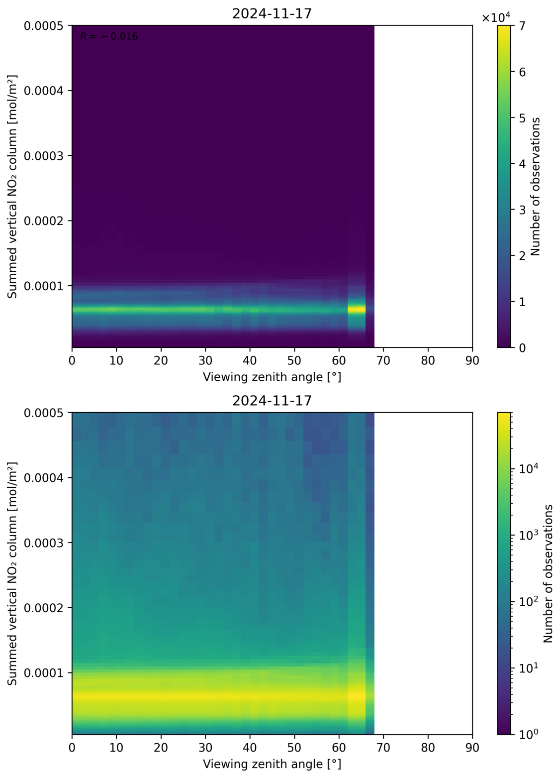
Figure 165: Scatter density plot of “Viewing zenith angle” against “Summed vertical NO 2 column” for 2024-11-17 to 2024-11-18.
