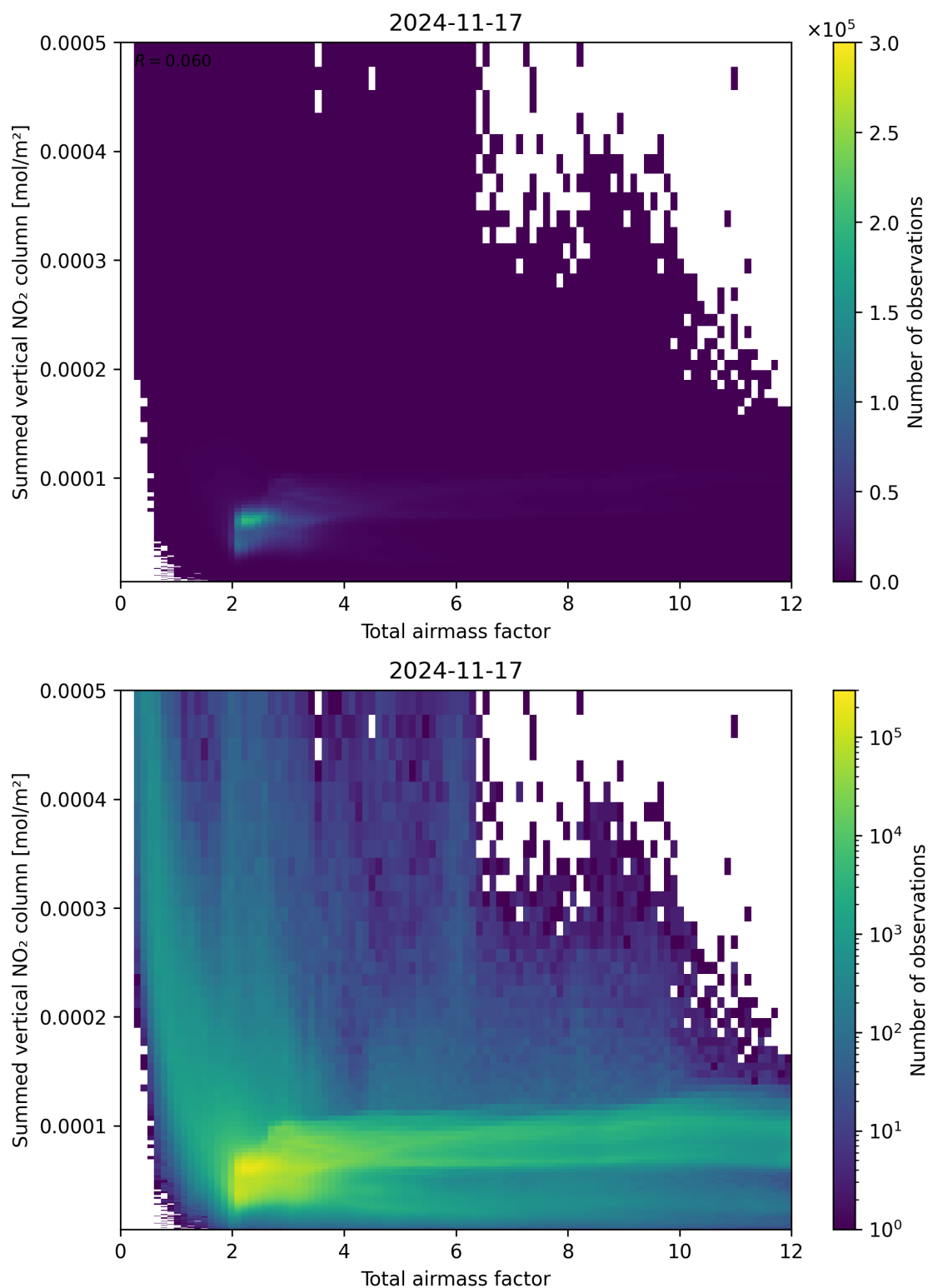
Figure 65: Scatter density plot of “Total airmass factor” against “Summed vertical NO 2 column” for 2024-11-17 to 2024-11-18.
