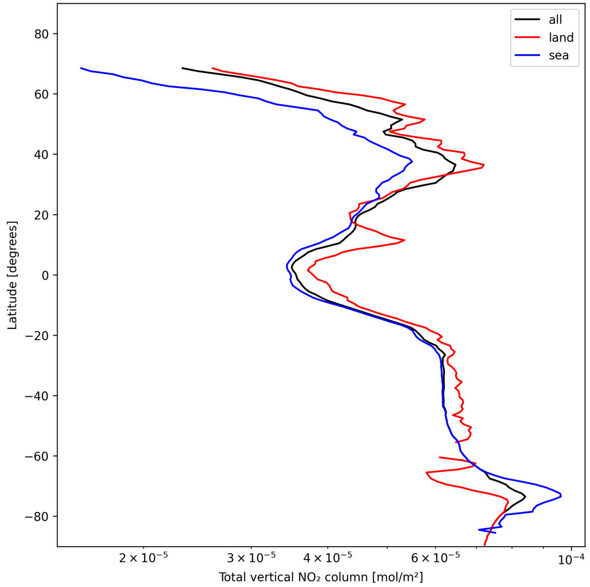
Figure 21: Zonal average of “Total vertical NO 2 column” for 2024-11-17 to 2024-11-18.
