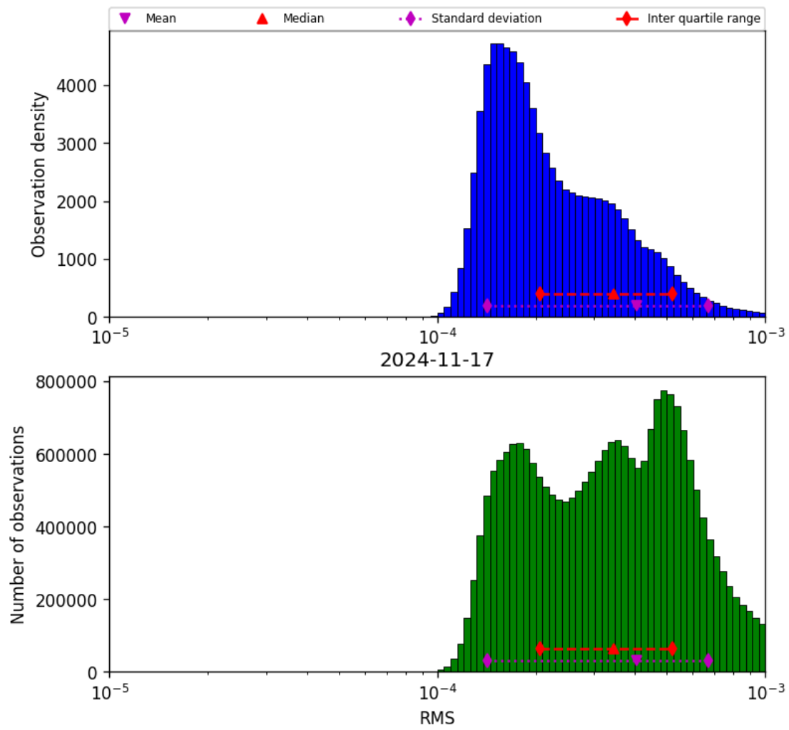
Figure 43: Histogram of “RMS” for 2024-11-17 to 2024-11-18
