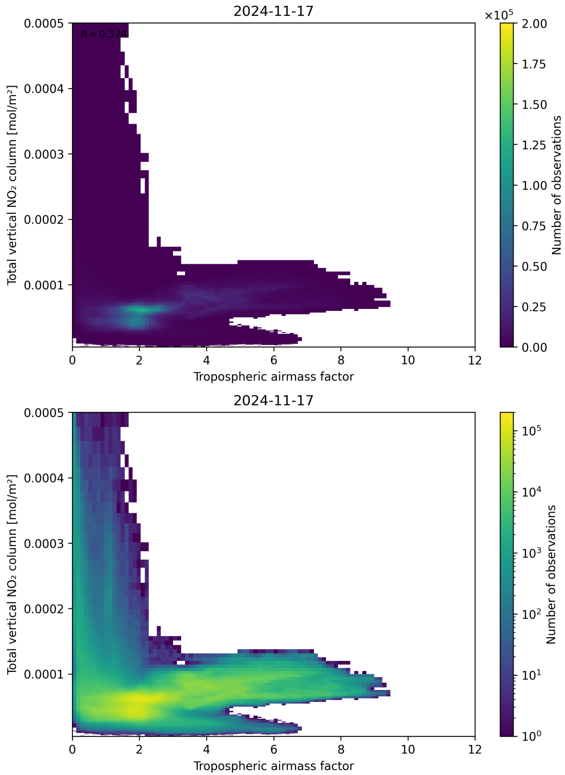
Figure 77: Scatter density plot of “Tropospheric airmass factor” against “Total vertical NO 2 column” for 2024-11-17 to 2024-11-18.
