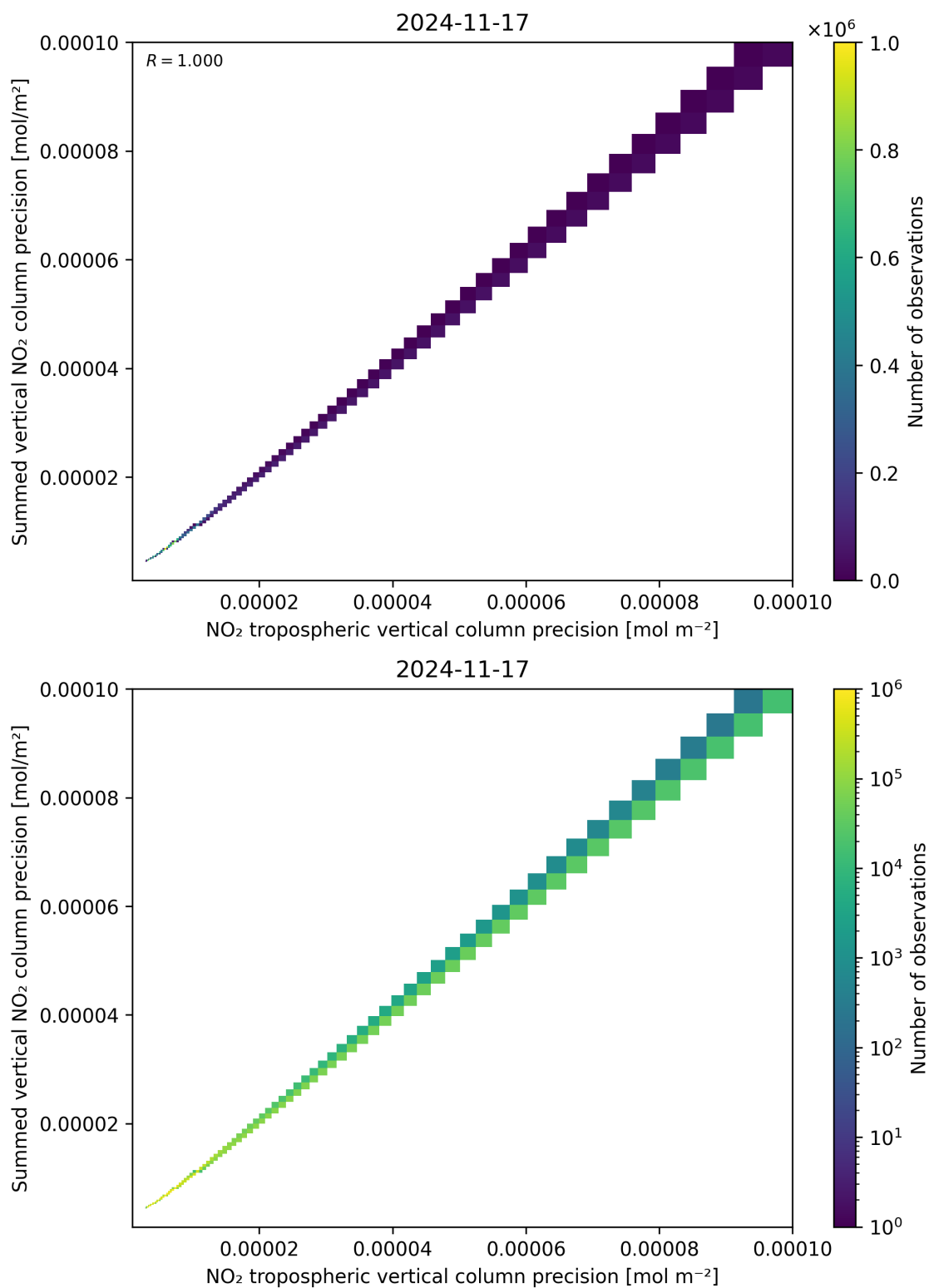
Figure 137: Scatter density plot of “NO 2 tropospheric vertical column precision” against “Summed vertical NO 2 column precision” for 2024-11-17 to 2024-11-18.
