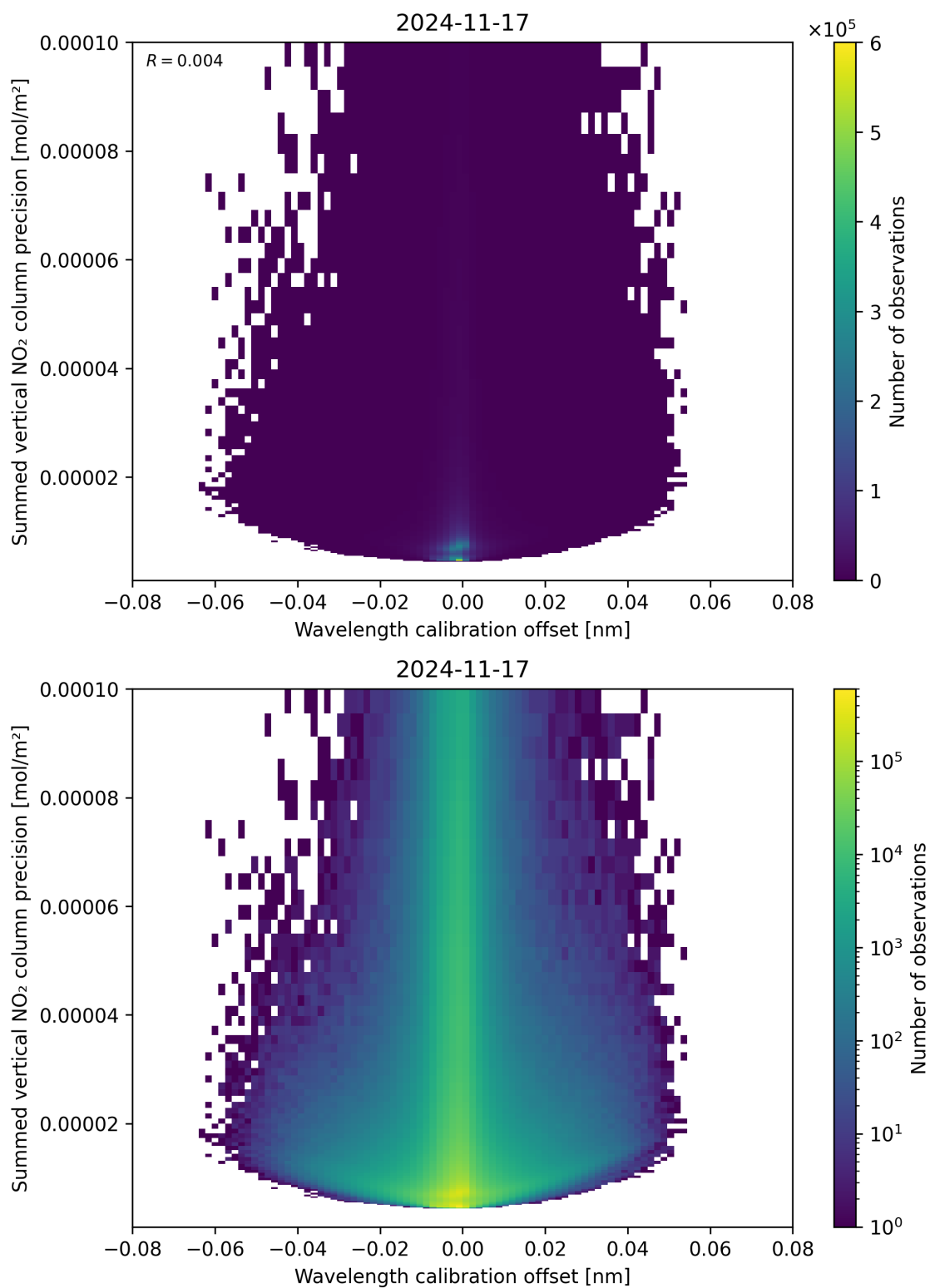
Figure 178: Scatter density plot of “Wavelength calibration offset” against “Summed vertical NO 2 column precision” for 2024-11-17 to 2024-11-18.
