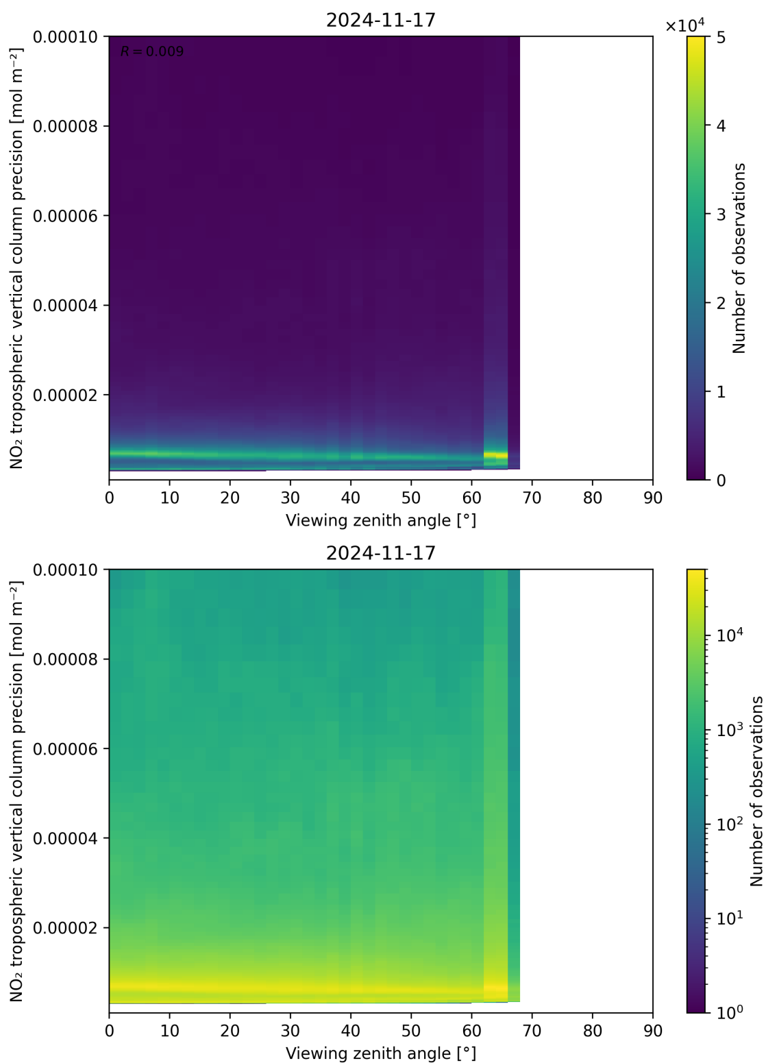
Figure 170: Scatter density plot of “Viewing zenith angle” against “NO 2 tropospheric vertical column precision” for 2024-11-17 to 2024-11-18.
