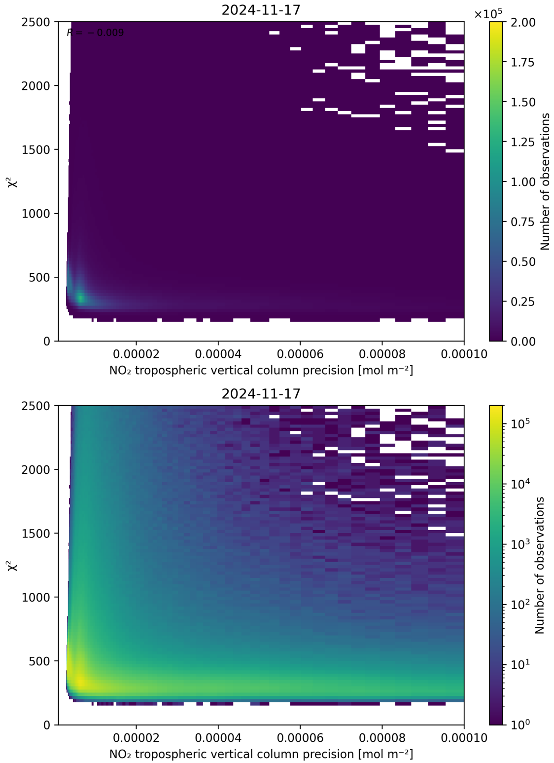
Figure 134: Scatter density plot of “NO 2 tropospheric vertical column precision” against “ \chi^2 ” for 2024-11-17 to 2024-11-18.
