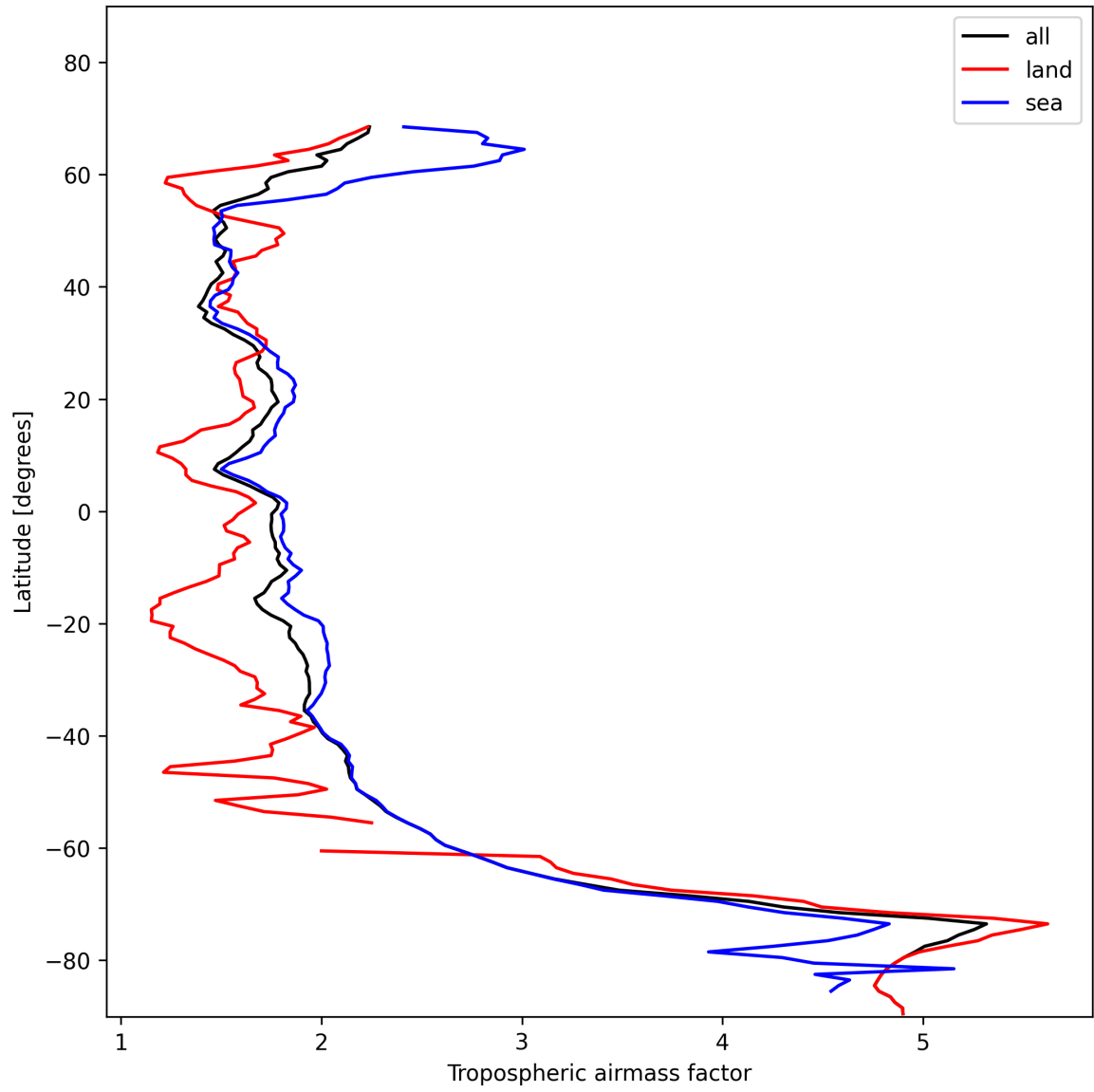
Figure 14: Zonal average of “Tropospheric airmass factor” for 2024-11-17 to 2024-11-18.
