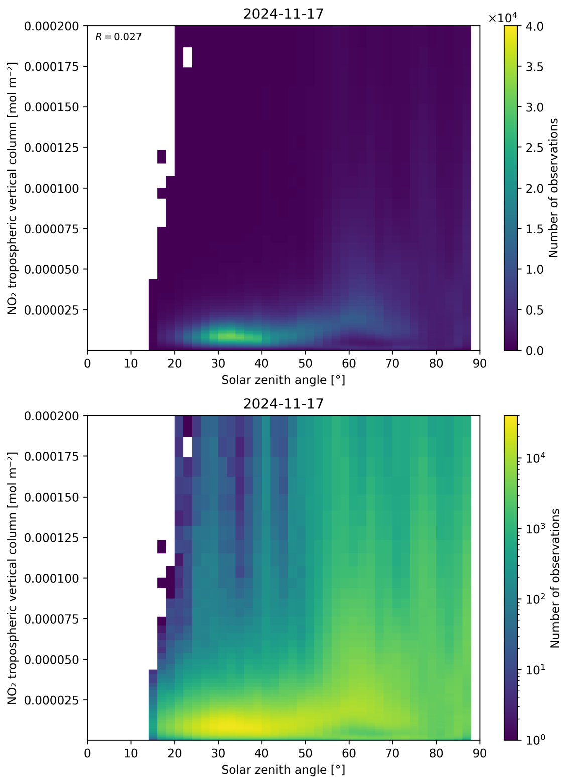
Figure 155: Scatter density plot of “Solar zenith angle” against “NO 2 tropospheric vertical column” for 2024-11-17 to 2024-11-18.
