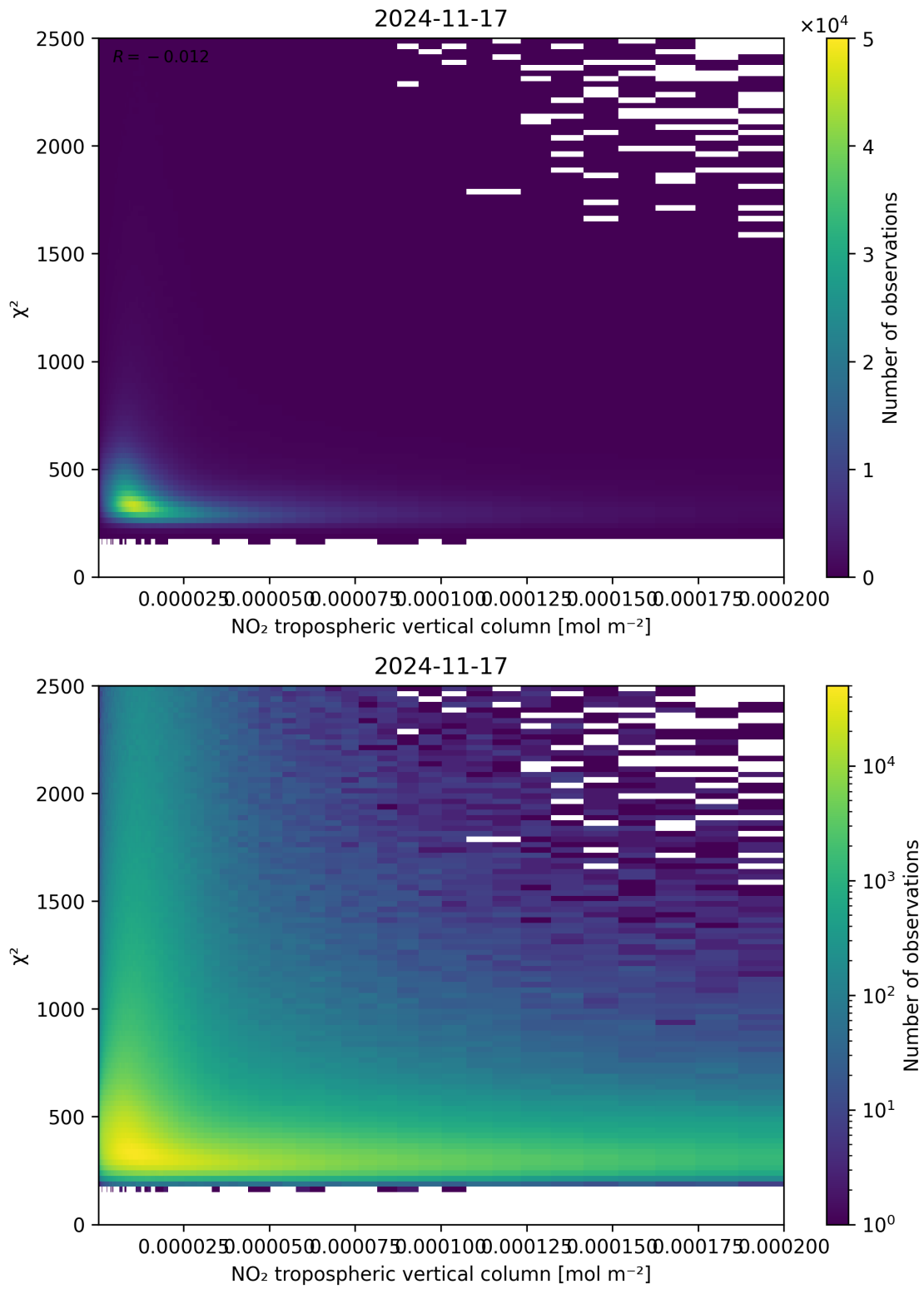
Figure 124: Scatter density plot of “NO 2 tropospheric vertical column” against “ \chi^2 ” for 2024-11-17 to 2024-11-18.
