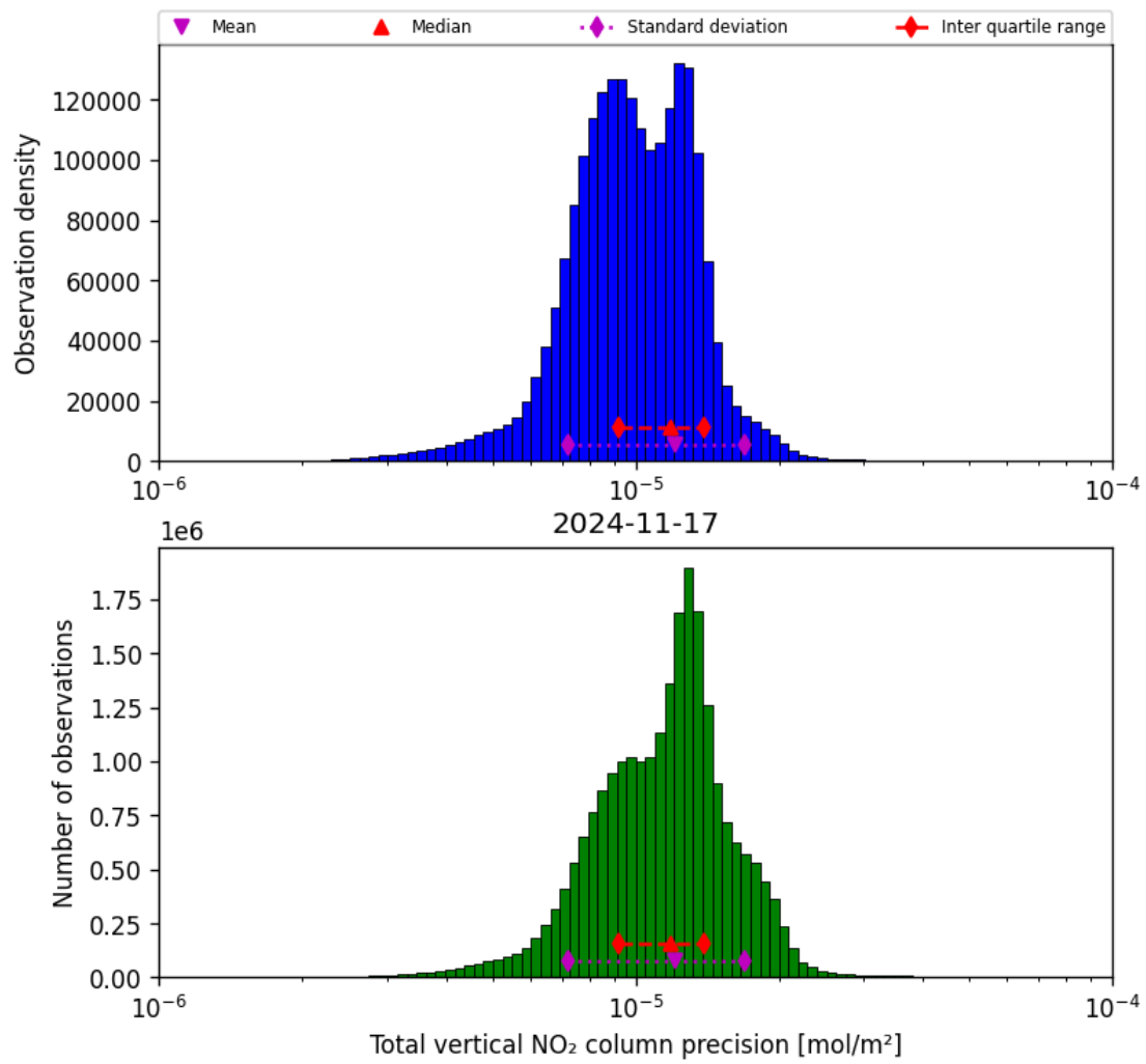
Figure 39: Histogram of “Total vertical NO 2 column precision” for 2024-11-17 to 2024-11-18
