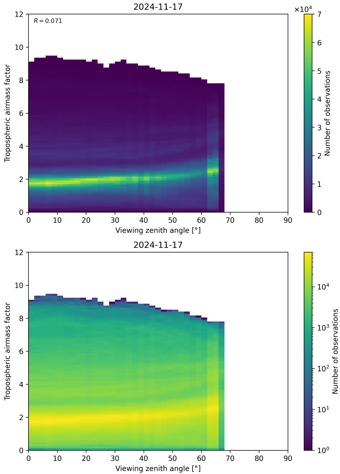
Figure 161: Scatter density plot of “Viewing zenith angle” against “Tropospheric airmass factor” for 2024-11-17 to 2024-11-18.
