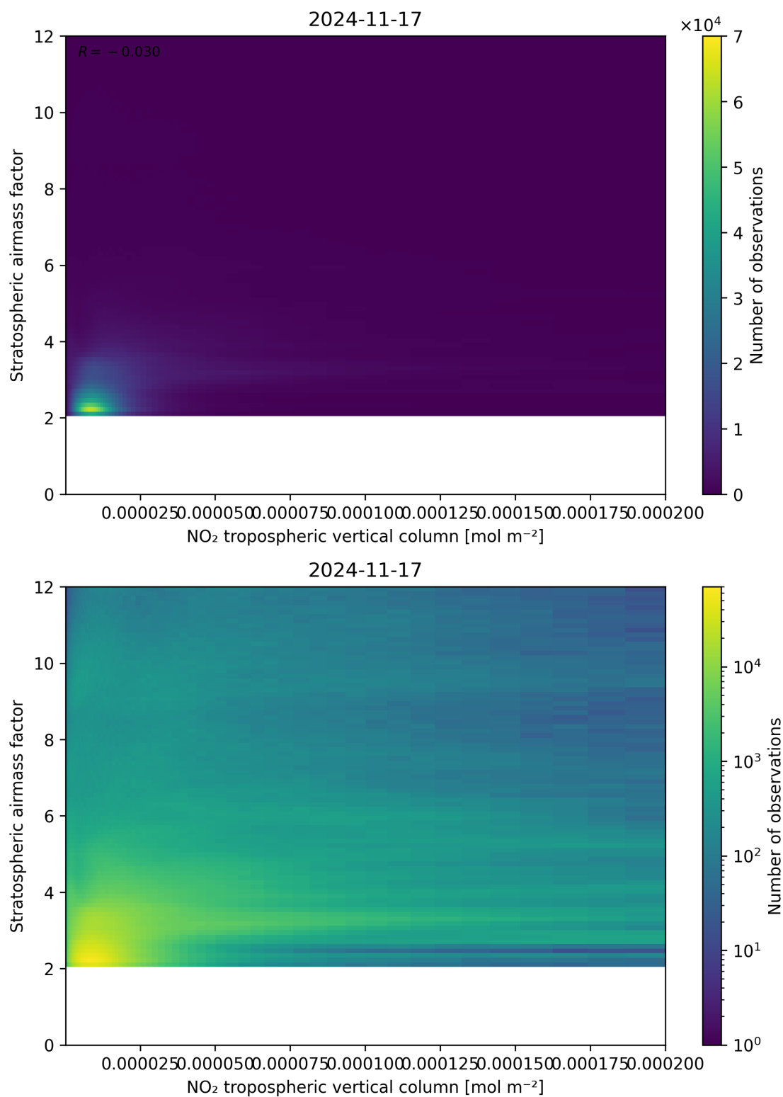
Figure 121: Scatter density plot of “NO 2 tropospheric vertical column” against “Stratospheric airmass factor” for 2024-11-17 to 2024-11-18.
