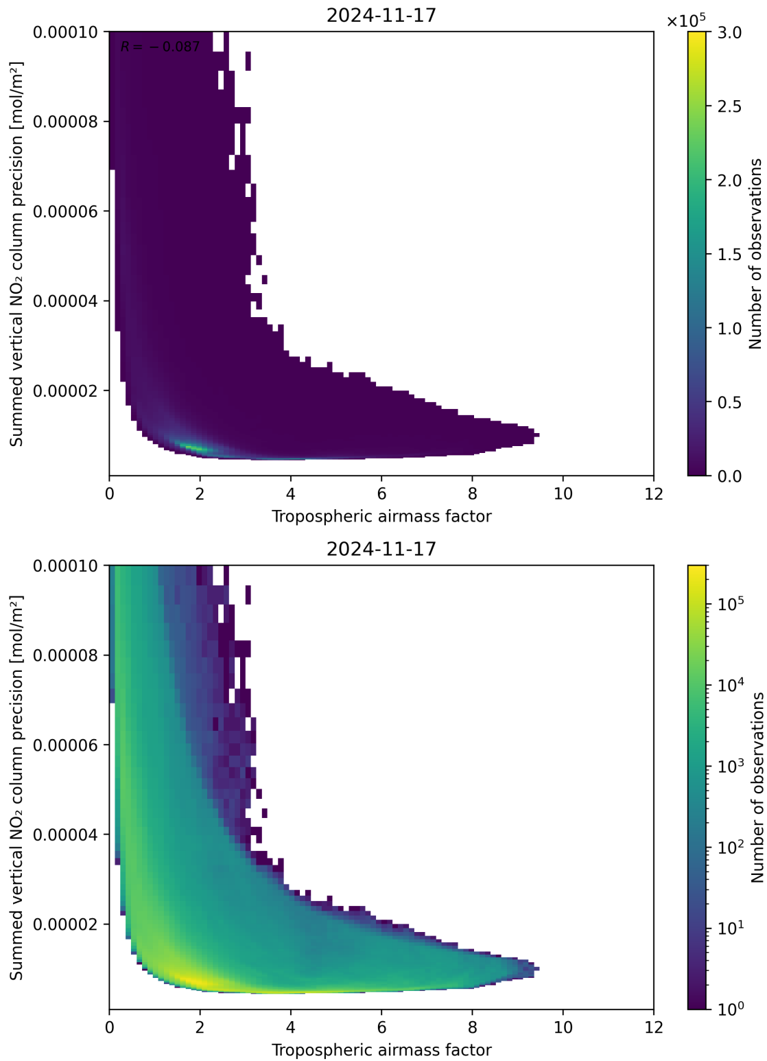
Figure 76: Scatter density plot of “Tropospheric air mass factor” against “Summed vertical NO 2 column precision” for 2024-11-17 to 2024-11-18.
