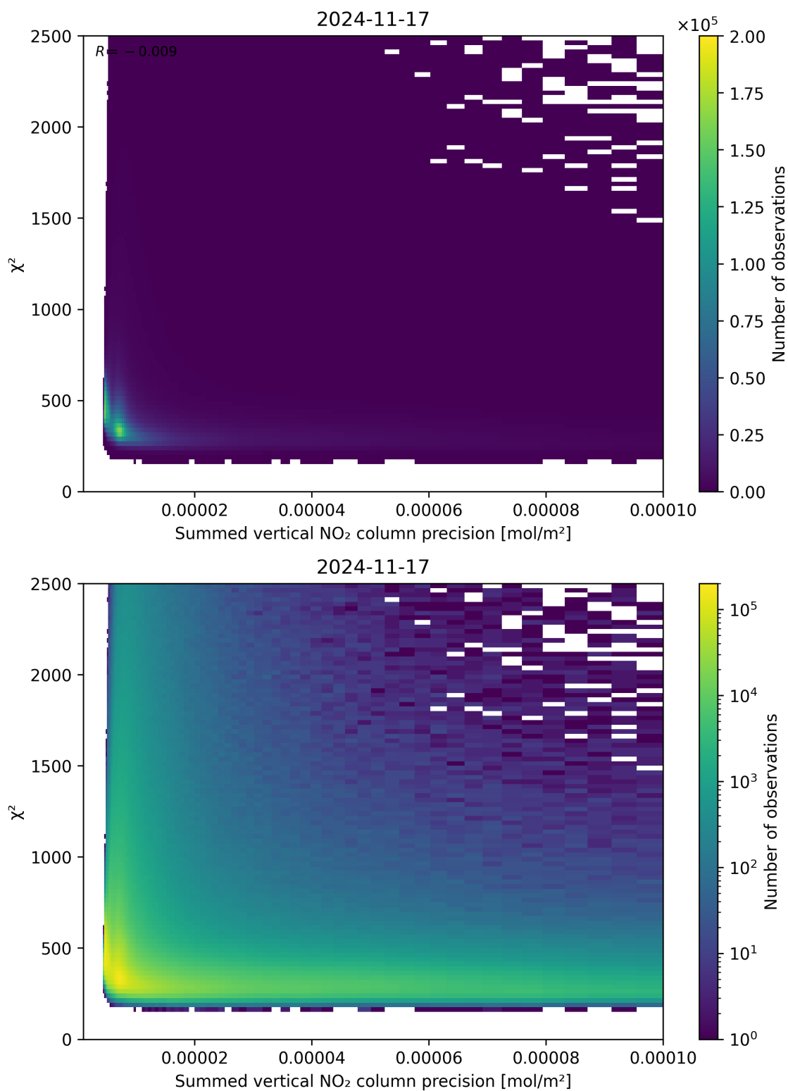
Figure 107: Scatter density plot of “Summed vertical NO 2 column precision” against “ \chi^2 ” for 2024-11-17 to 2024-11-18.
