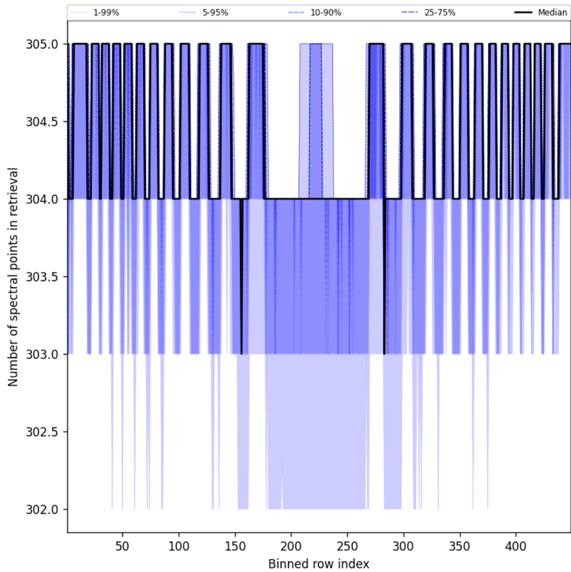
Figure 50: Along track statistics of “Number of spectral points in retrieval” for 2024-11-17 to 2024-11-18
