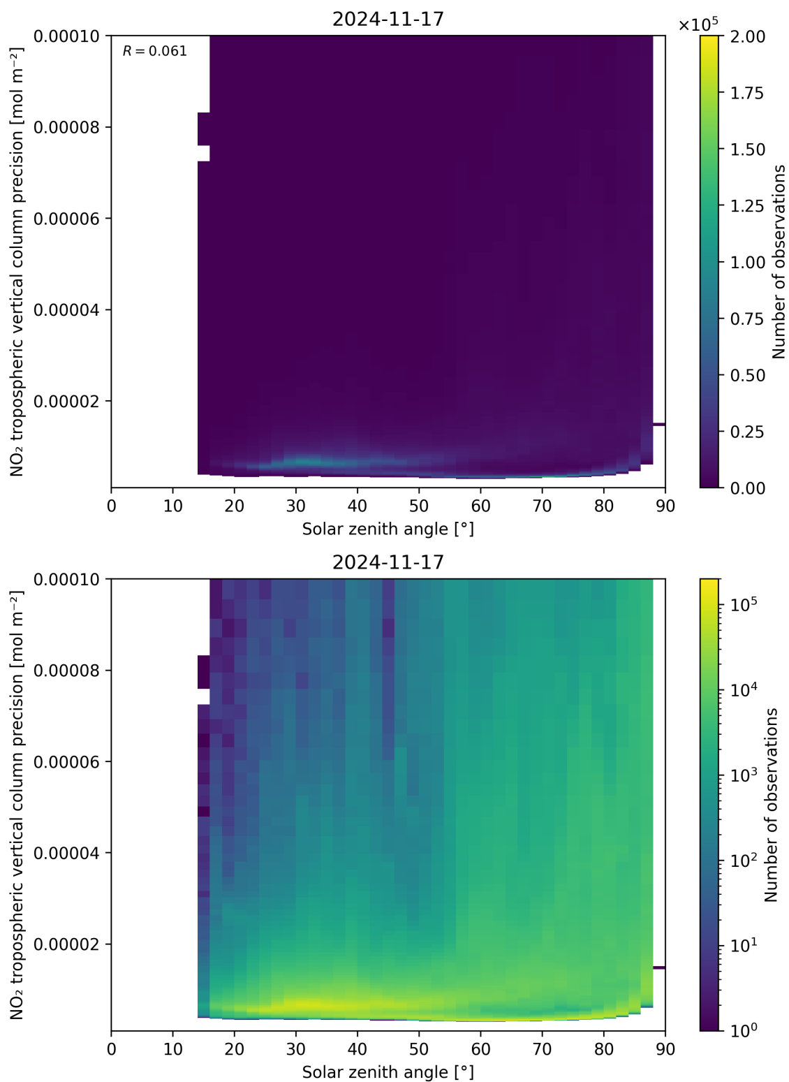
Figure 156: Scatter density plot of “Solar zenith angle” against “NO 2 tropospheric vertical column precision” for 2024-11-17 to 2024-11-18.
