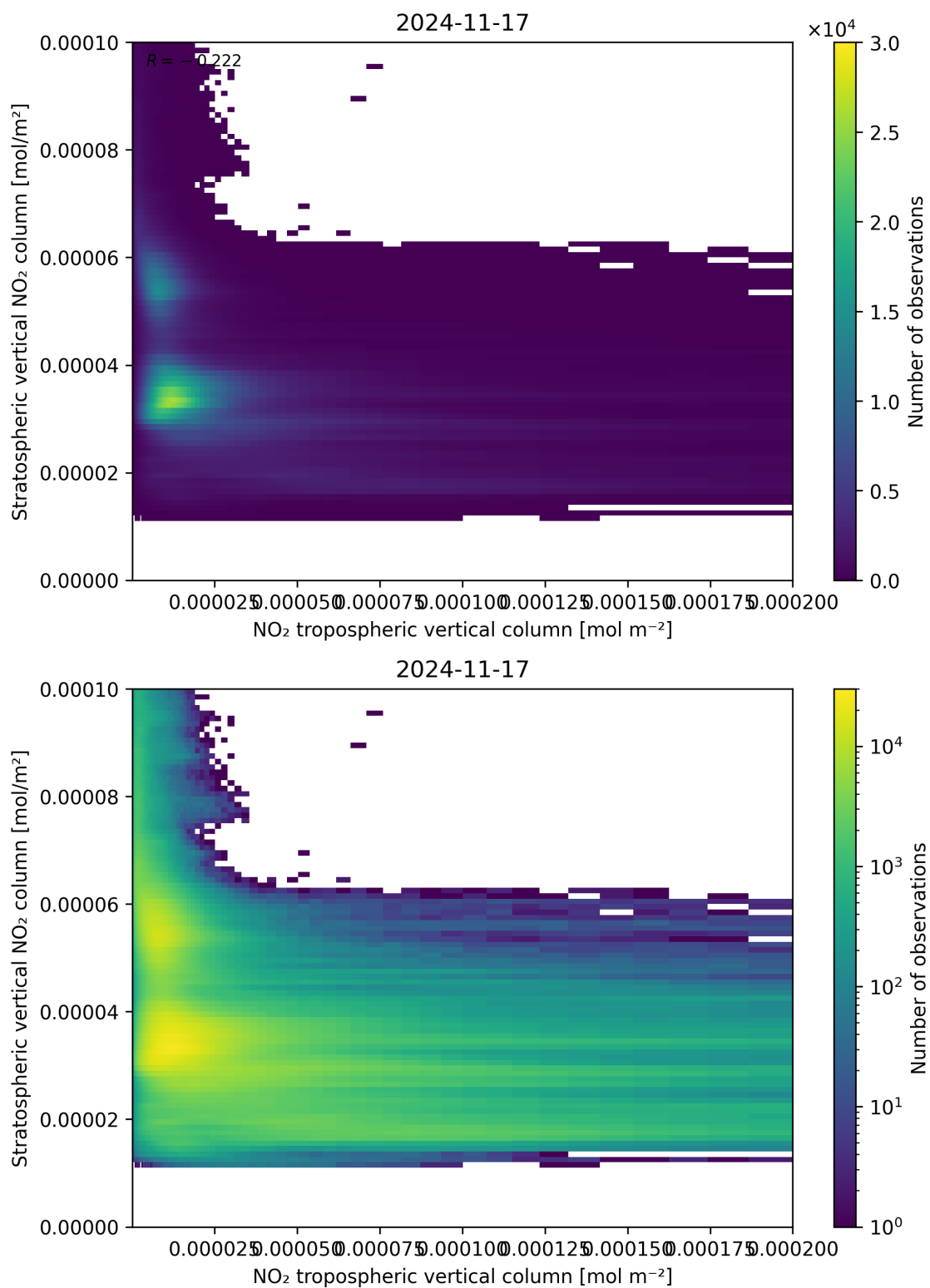
Figure 125: Scatter density plot of “NO 2 tropospheric vertical column” against “Stratospheric vertical NO 2 column” for 2024-11-17 to 2024-11-18.
