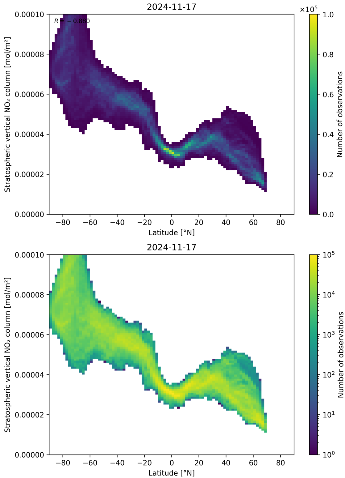
Figure 87: Scatter density plot of “Latitude” against “Stratospheric vertical NO 2 column” for 2024-11-17 to 2024-11-18.
