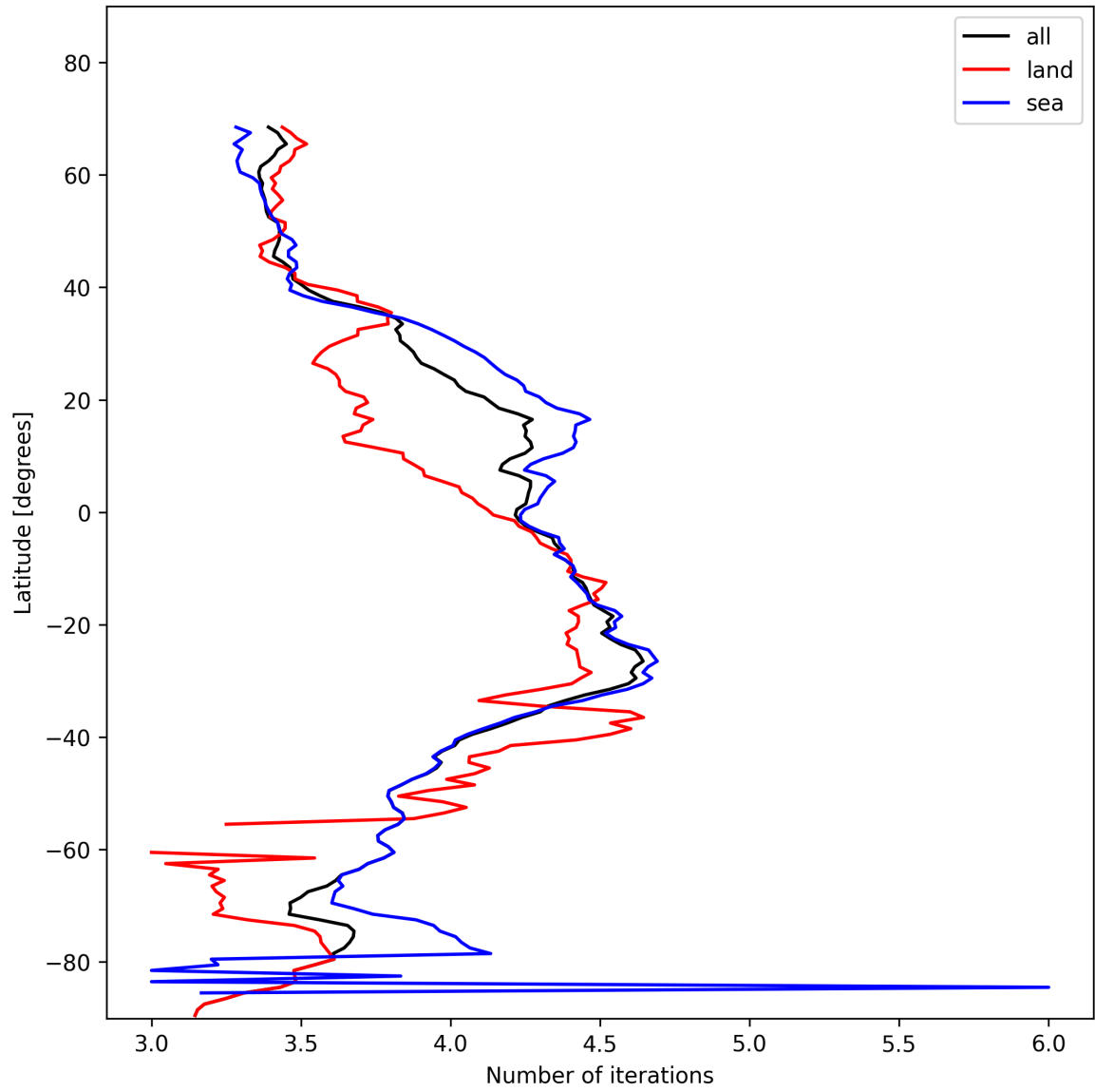
Figure 17: Zonal average of “Number of iterations” for 2024-11-17 to 2024-11-18.
