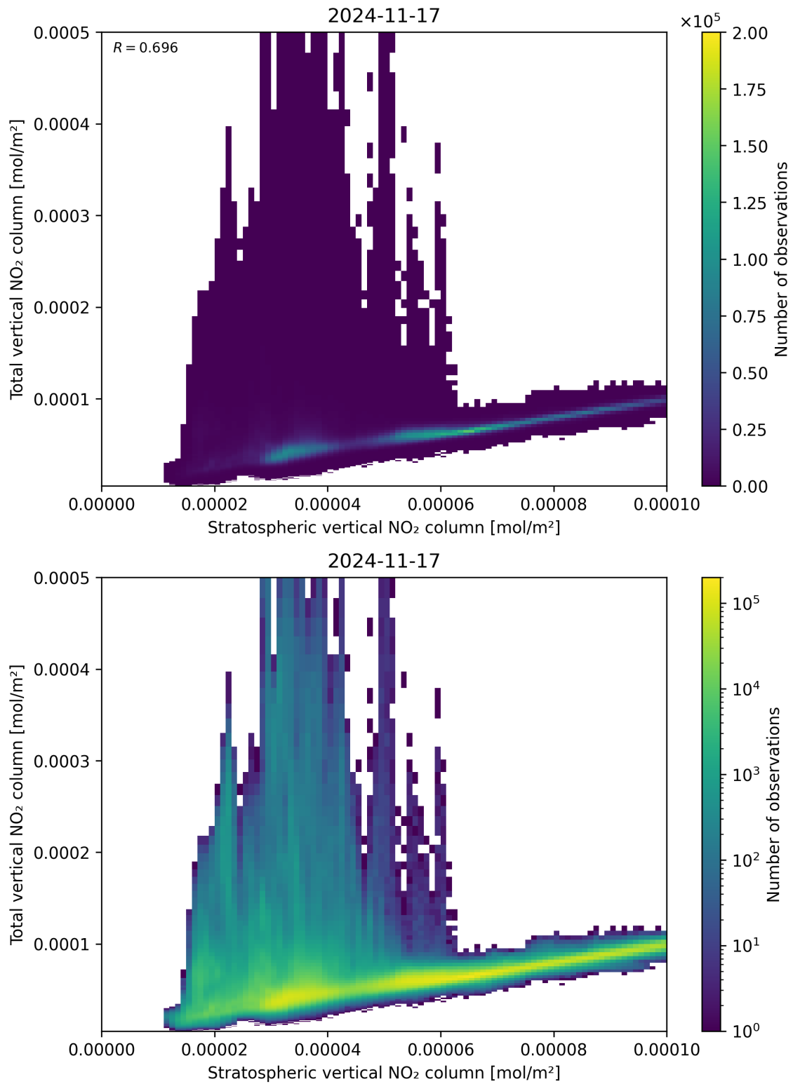
Figure 100: Scatter density plot of “Stratospheric vertical NO 2 column” against “Total vertical NO 2 column” for 2024-11-17 to 2024-11-18.
