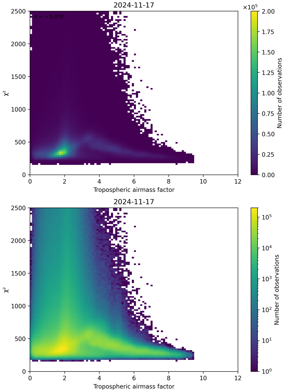
Figure 73: Scatter density plot of “Tropospheric airmass factor” against “ \chi^2 ” for 2024-11-17 to 2024-11-18.
