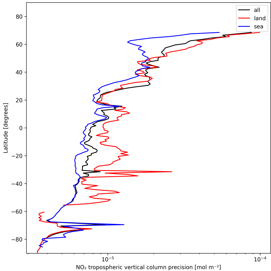
Figure 13: Zonal average of “NO 2 tropospheric vertical column precision” for 2024-11-17 to 2024-11-18.
