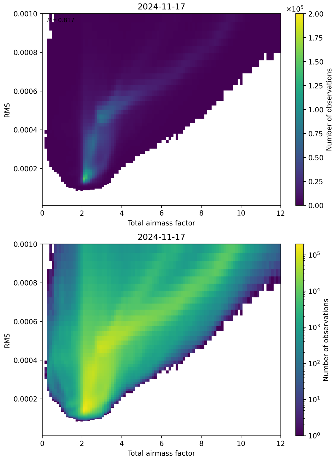
Figure 69: Scatter density plot of “Total airmass factor” against “RMS” for 2024-11-17 to 2024-11-18.
