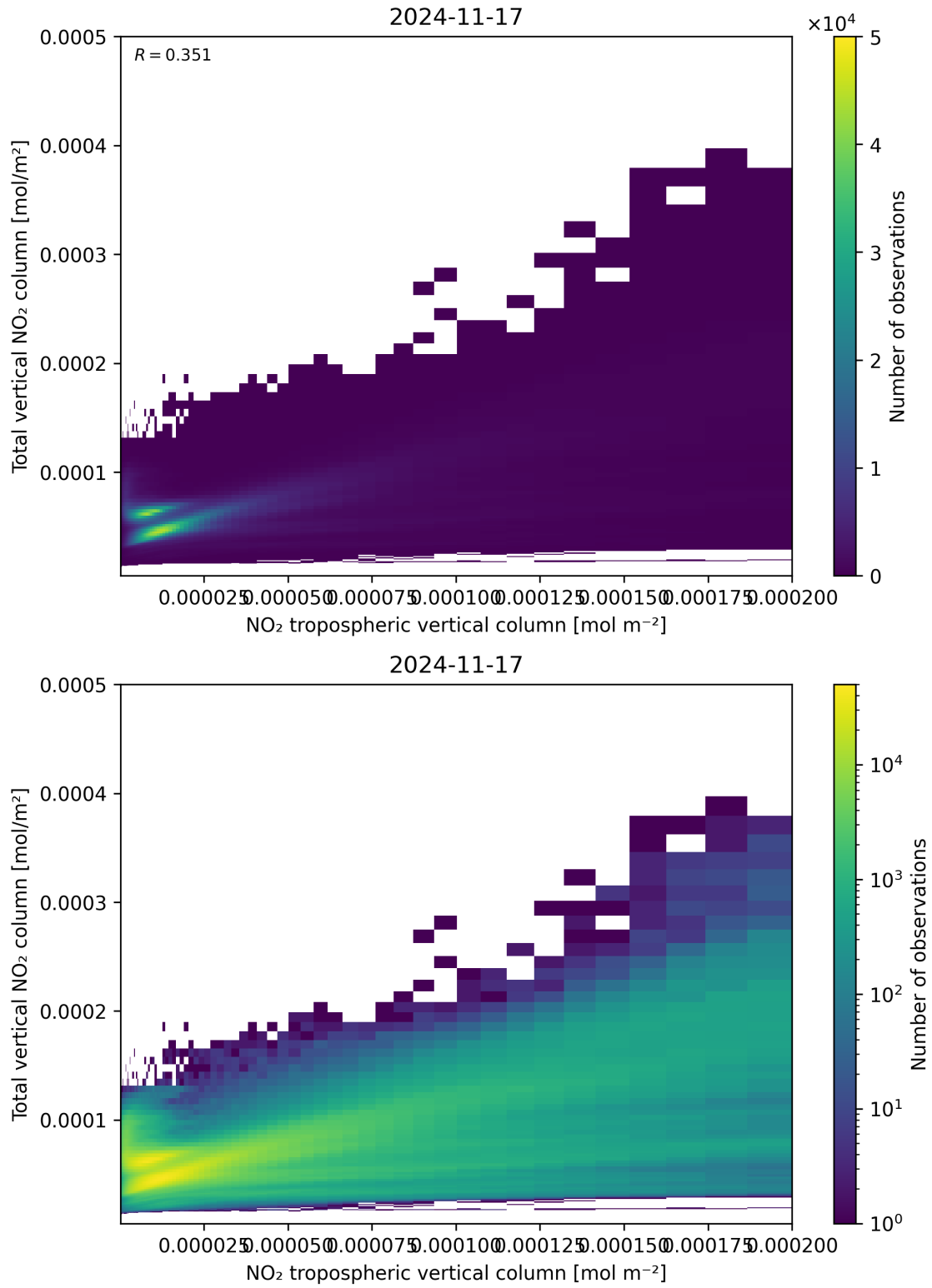
Figure 128: Scatter density plot of “NO 2 tropospheric vertical column” against “Total vertical NO 2 column” for 2024-11-17 to 2024-11-18.
