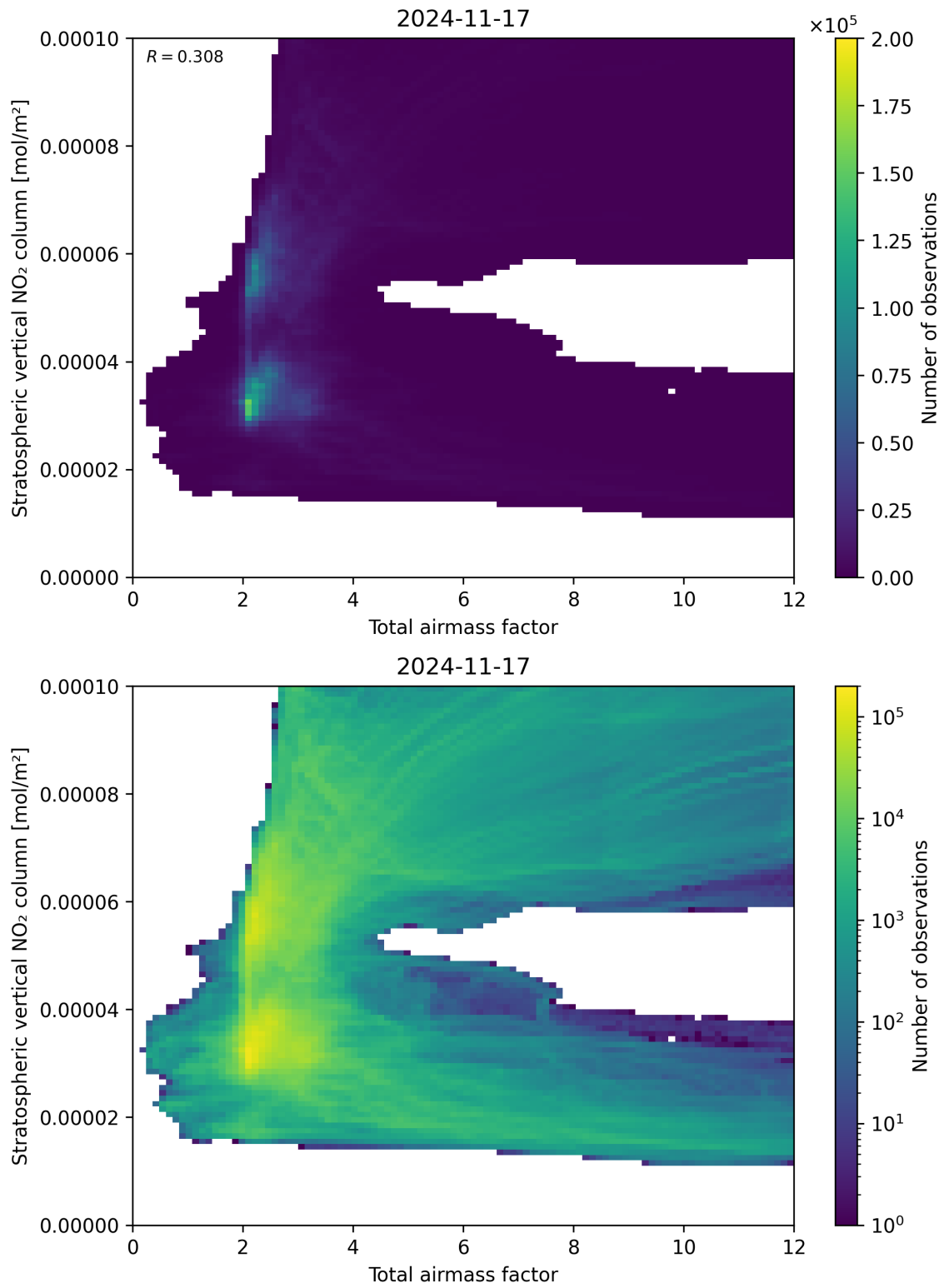
Figure 64: Scatter density plot of “Total airmass factor” against “Stratospheric vertical \text{NO}_2 column” for 2024-11-17 to 2024-11-18.
