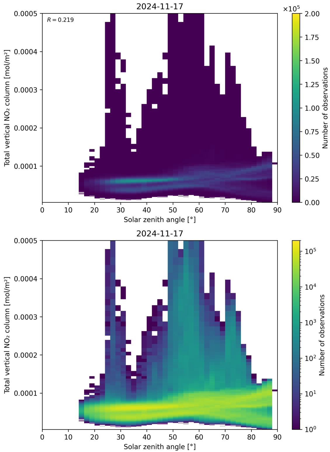
Figure 153: Scatter density plot of “Solar zenith angle” against “Total vertical NO 2 column” for 2024-11-17 to 2024-11-18.
