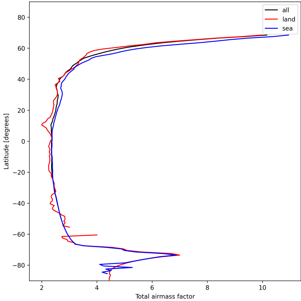
Figure 15: Zonal average of “Total airmass factor” for 2024-11-17 to 2024-11-18.
