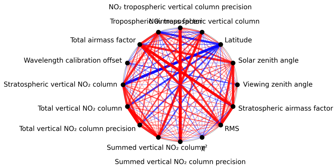
Figure 1: Map of correlation graph for 2024-11-17 to 2024-11-18.
