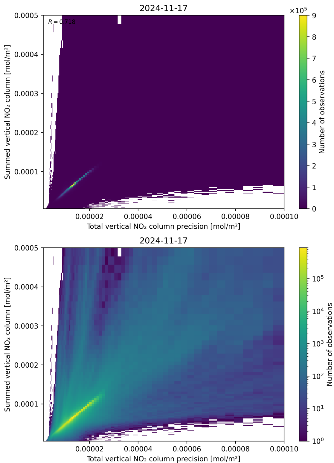
Figure 117: Scatter density plot of “Total vertical NO 2 column precision” against “Summed vertical NO 2 column” for 2024-11-17 to 2024-11-18.
