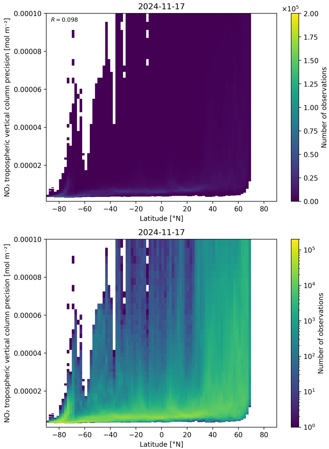
Figure 93: Scatter density plot of “Latitude” against “NO 2 tropospheric vertical column precision” for 2024-11-17 to 2024-11-18.
