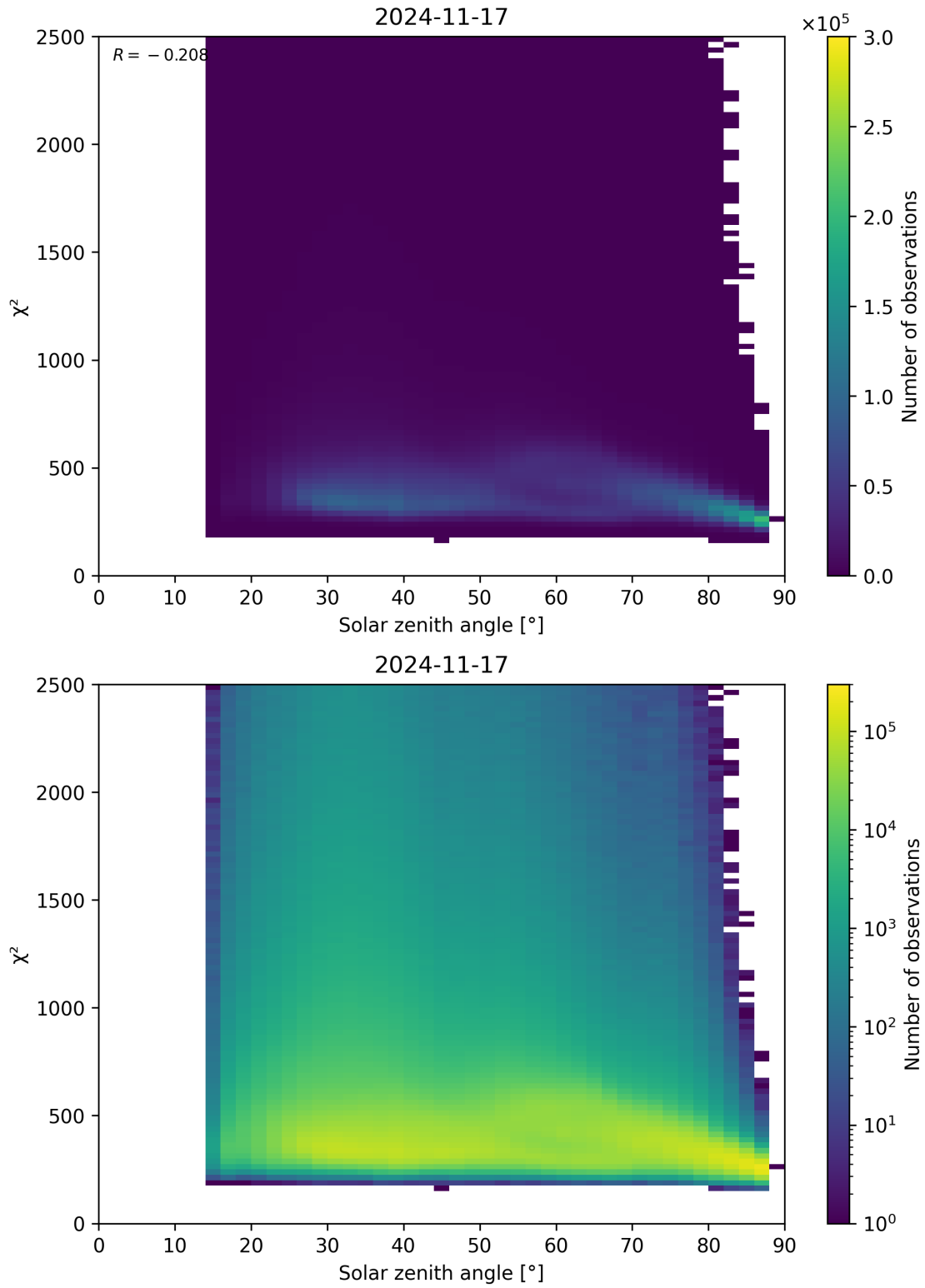
Figure 148: Scatter density plot of “Solar zenith angle” against “ \chi^2 ” for 2024-11-17 to 2024-11-18.
