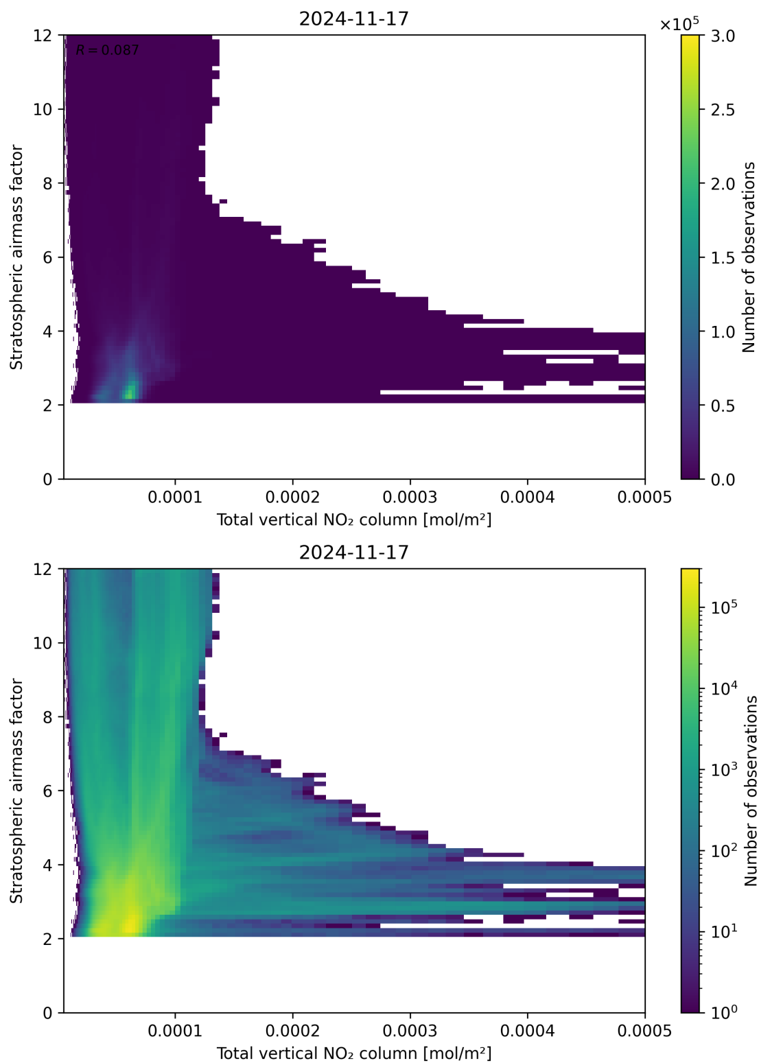
Figure 110: Scatter density plot of “Total vertical NO 2 column” against “Stratospheric air mass factor” for 2024-11-17 to 2024-11-18.
