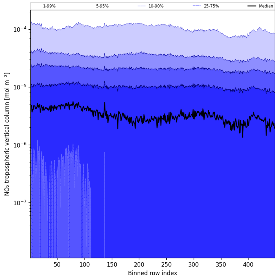
Figure 46: Along track statistics of “NO 2 tropospheric vertical column” for 2024-11-17 to 2024-11-18
