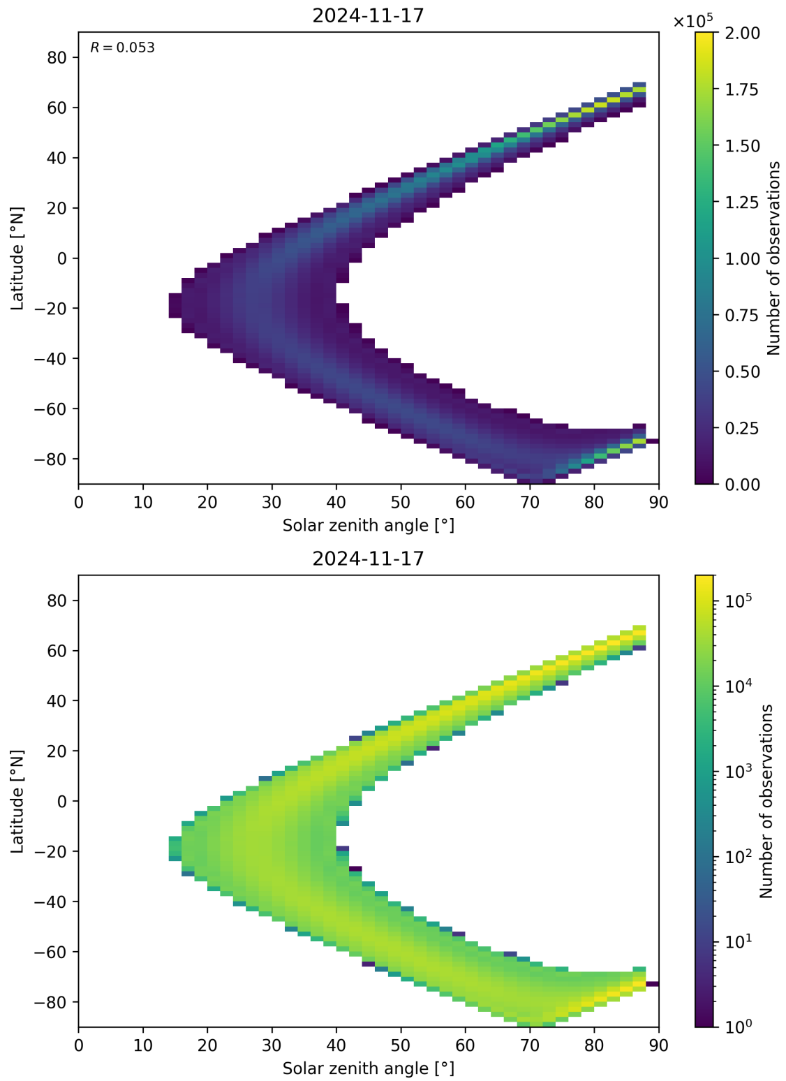
Figure 149: Scatter density plot of “Solar zenith angle” against “Latitude” for 2024-11-17 to 2024-11-18.
