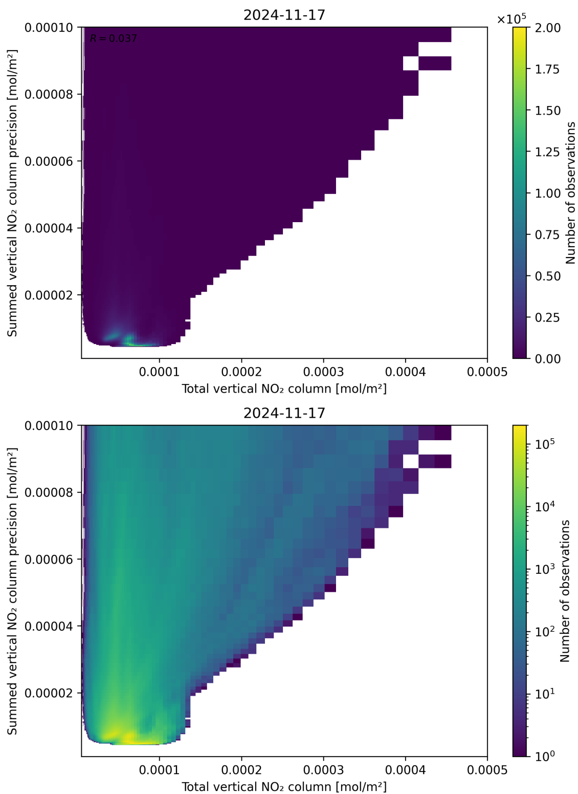
Figure 113: Scatter density plot of “Total vertical NO 2 column” against “Summed vertical NO 2 column precision” for 2024-11-17 to 2024-11-18.
