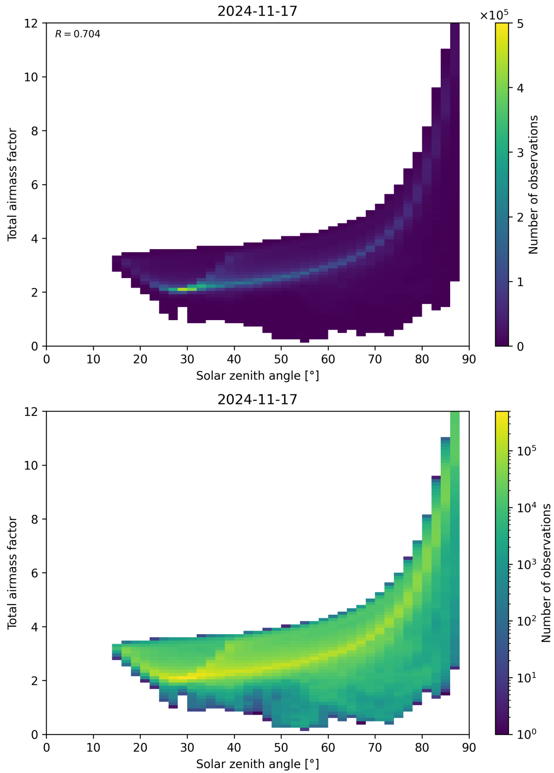
Figure 146: Scatter density plot of “Solar zenith angle” against “Total airmass factor” for 2024-11-17 to 2024-11-18.
