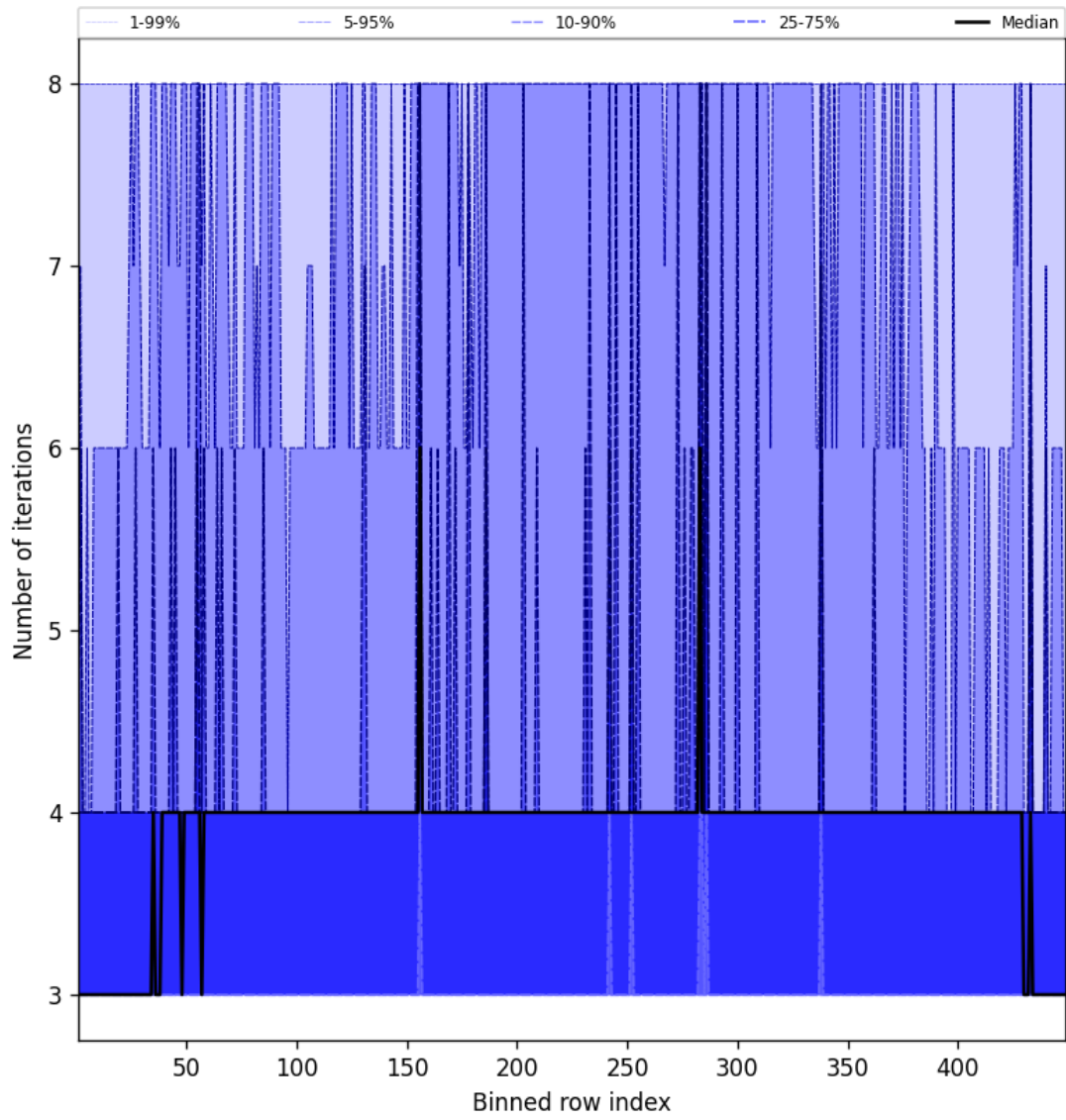
Figure 51: Along track statistics of “Number of iterations” for 2024-11-17 to 2024-11-18
