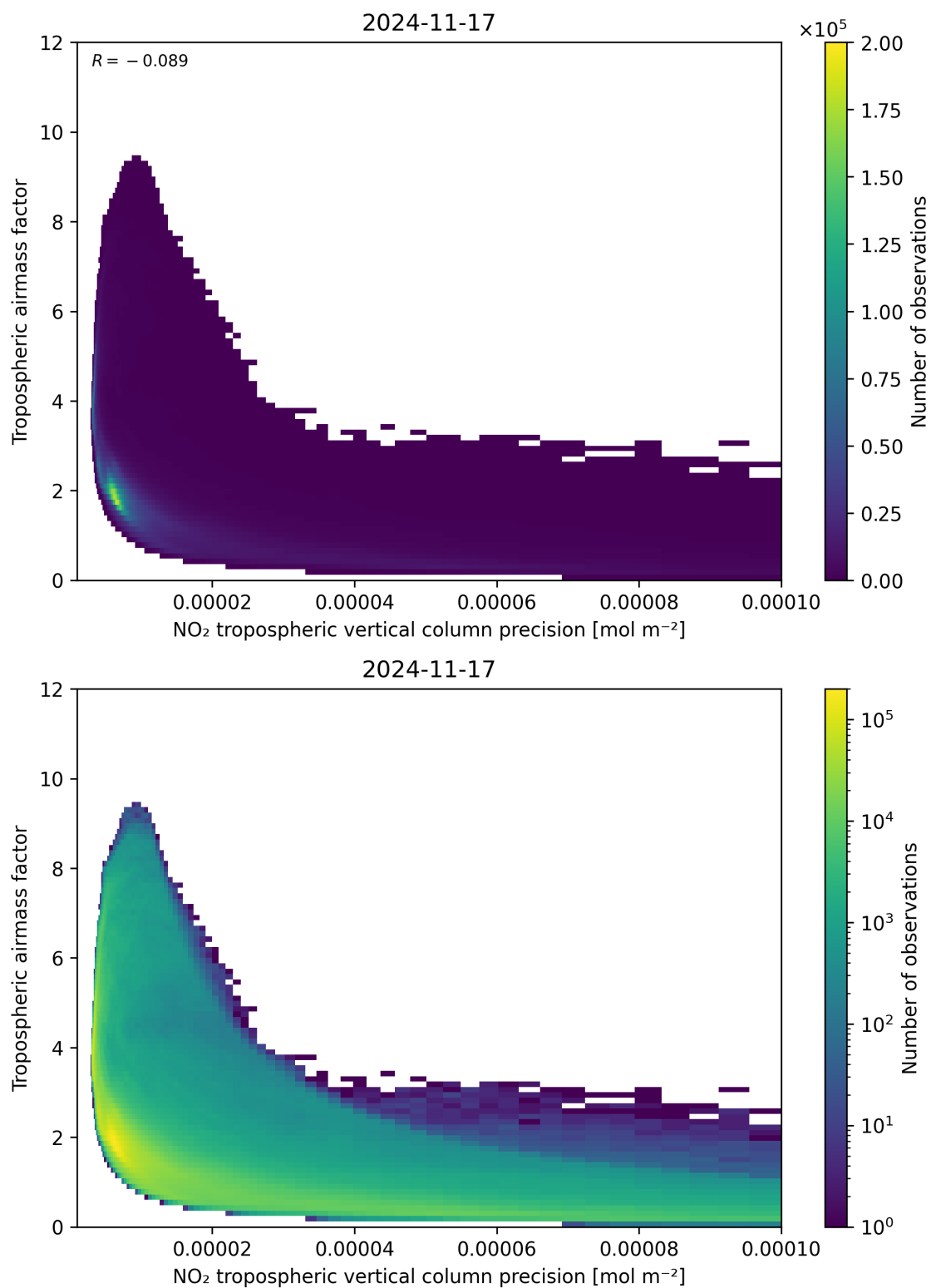
Figure 133: Scatter density plot of “NO 2 tropospheric vertical column precision” against “Tropospheric air mass factor” for 2024-11-17 to 2024-11-18.
