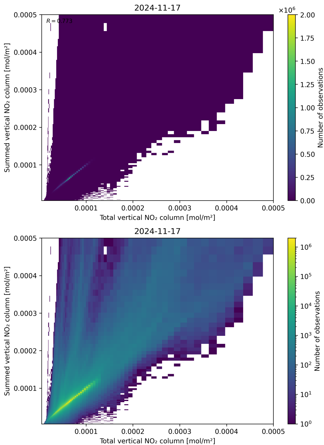
Figure 112: Scatter density plot of “Total vertical NO 2 column” against “Summed vertical NO 2 column” for 2024-11-17 to 2024-11-18.
