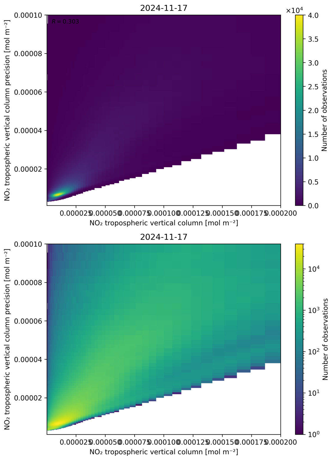
Figure 130: Scatter density plot of “NO 2 tropospheric vertical column” against “NO 2 tropospheric vertical column precision” for 2024-11-17 to 2024-11-18.
