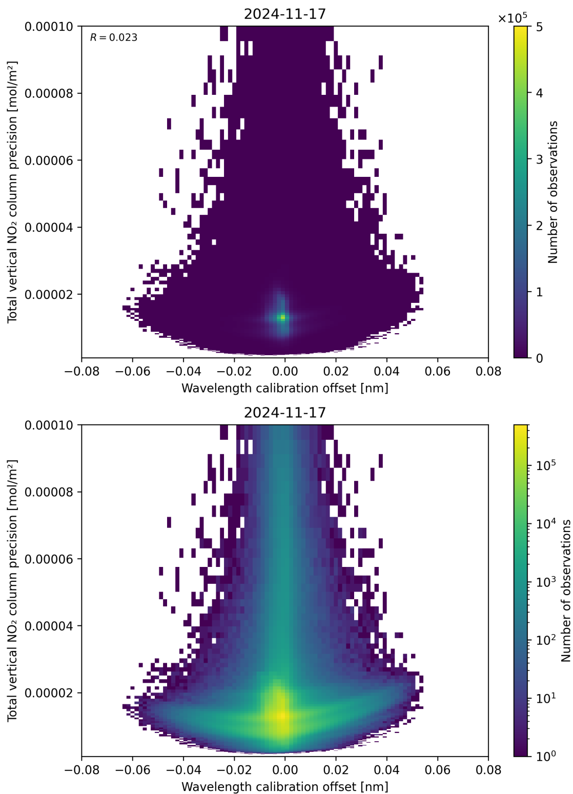
Figure 180: Scatter density plot of “Wavelength calibration offset” against “Total vertical NO 2 column precision” for 2024-11-17 to 2024-11-18.
