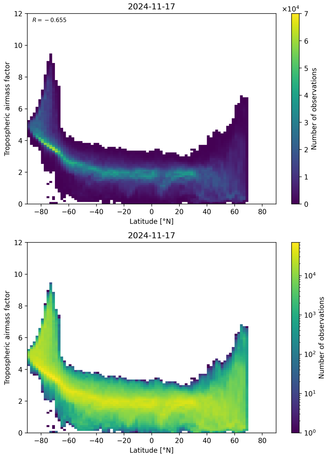
Figure 85: Scatter density plot of “Latitude” against “Tropospheric air mass factor” for 2024-11-17 to 2024-11-18.
