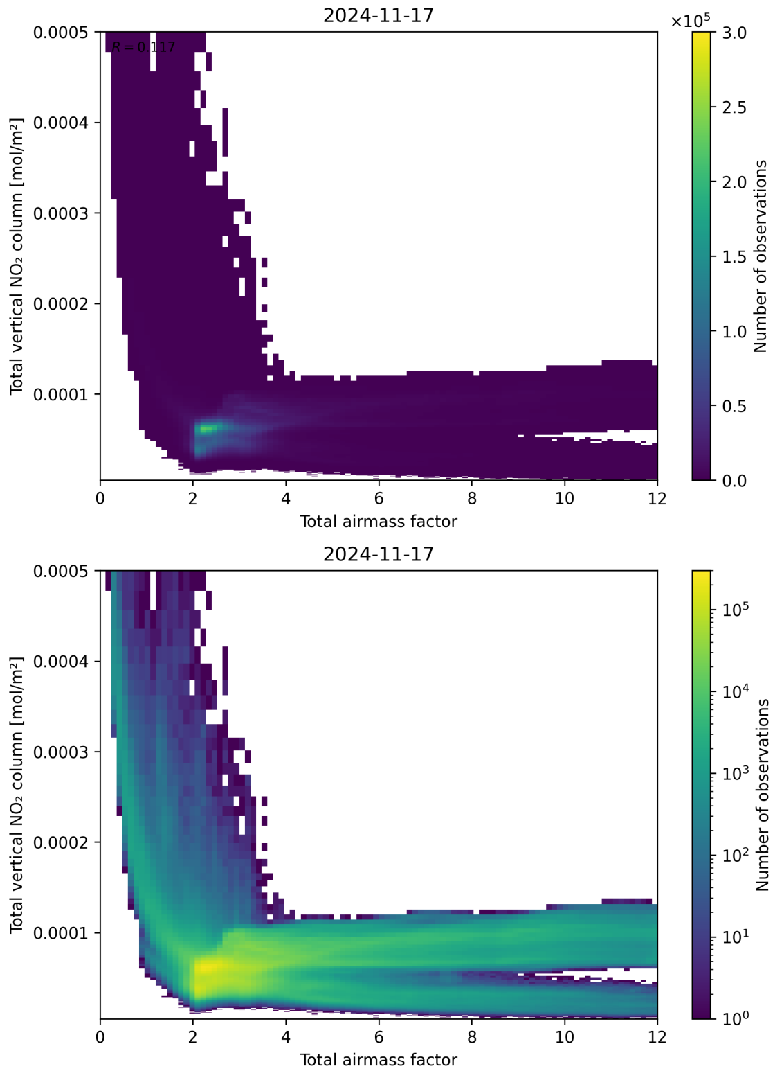
Figure 67: Scatter density plot of “Total airmass factor” against “Total vertical NO 2 column” for 2024-11-17 to 2024-11-18.
