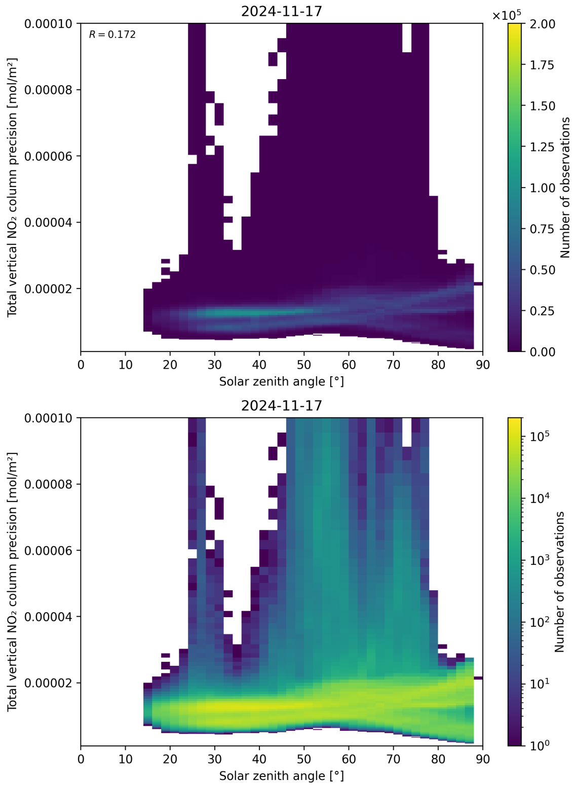
Figure 154: Scatter density plot of “Solar zenith angle” against “Total vertical NO 2 column precision” for 2024-11-17 to 2024-11-18.
