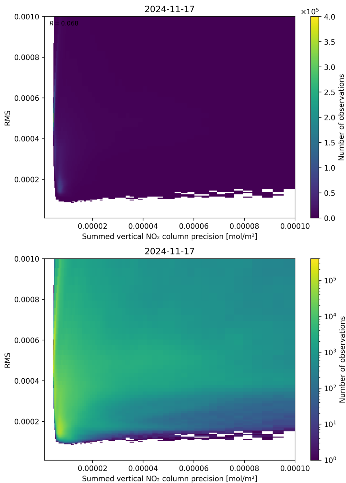
Figure 108: Scatter density plot of “Summed vertical NO 2 column precision” against “RMS” for 2024-11-17 to 2024-11-18.
