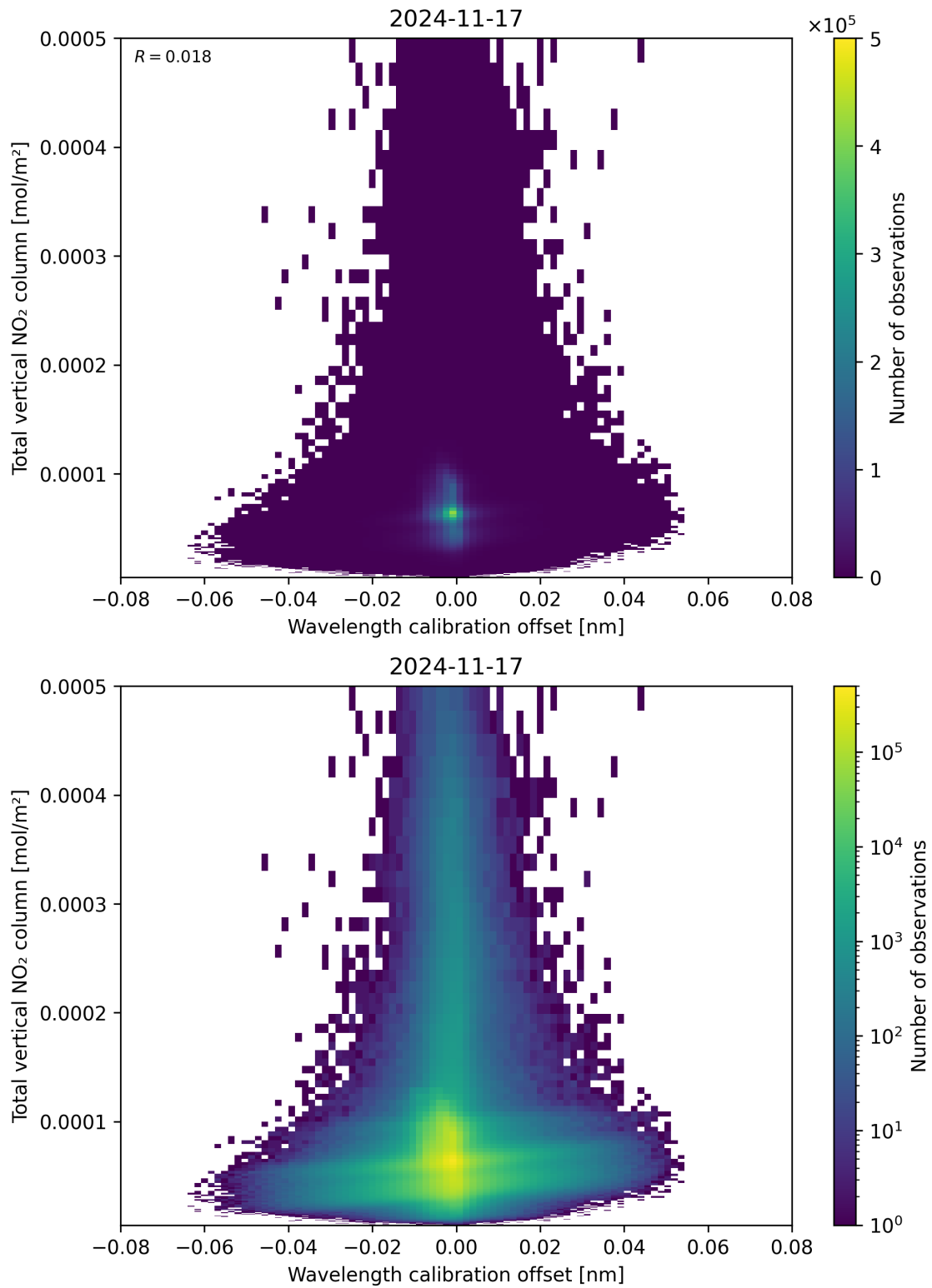
Figure 179: Scatter density plot of “Wavelength calibration offset” against “Total vertical NO 2 column” for 2024-11-17 to 2024-11-18.
