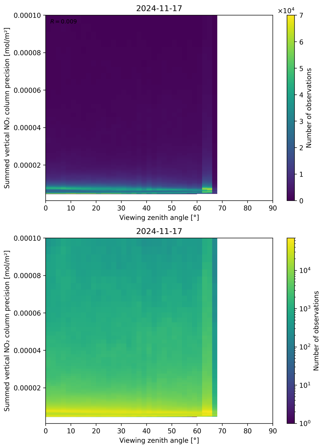
Figure 166: Scatter density plot of “Viewing zenith angle” against “Summed vertical NO 2 column precision” for 2024-11-17 to 2024-11-18.
