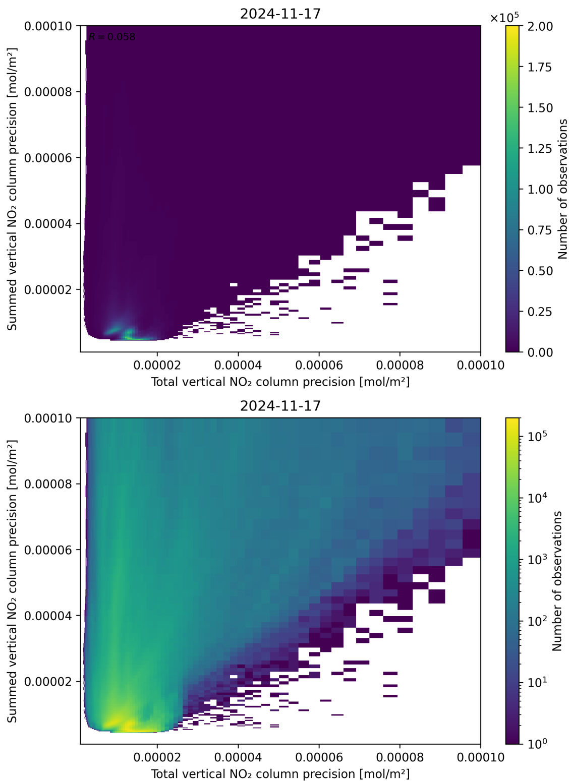
Figure 118: Scatter density plot of “Total vertical NO 2 column precision” against “Summed vertical NO 2 column precision” for 2024-11-17 to 2024-11-18.
