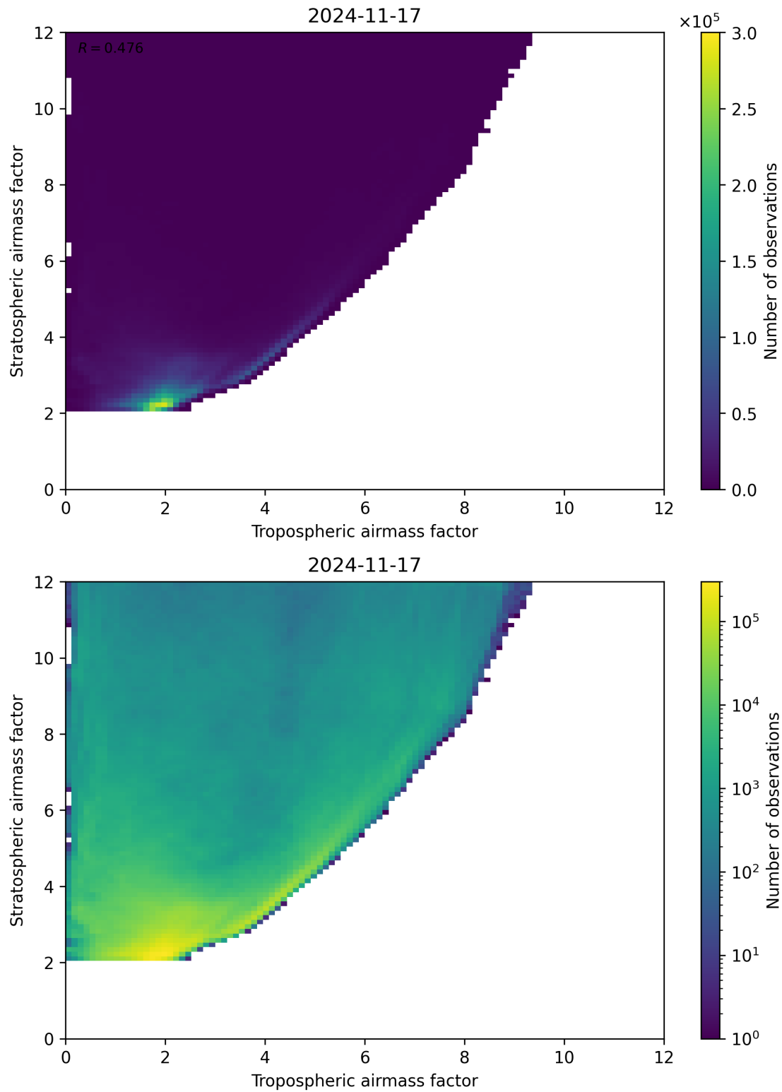
Figure 71: Scatter density plot of “Tropospheric airmass factor” against “Stratospheric airmass factor” for 2024-11-17 to 2024-11-18.
