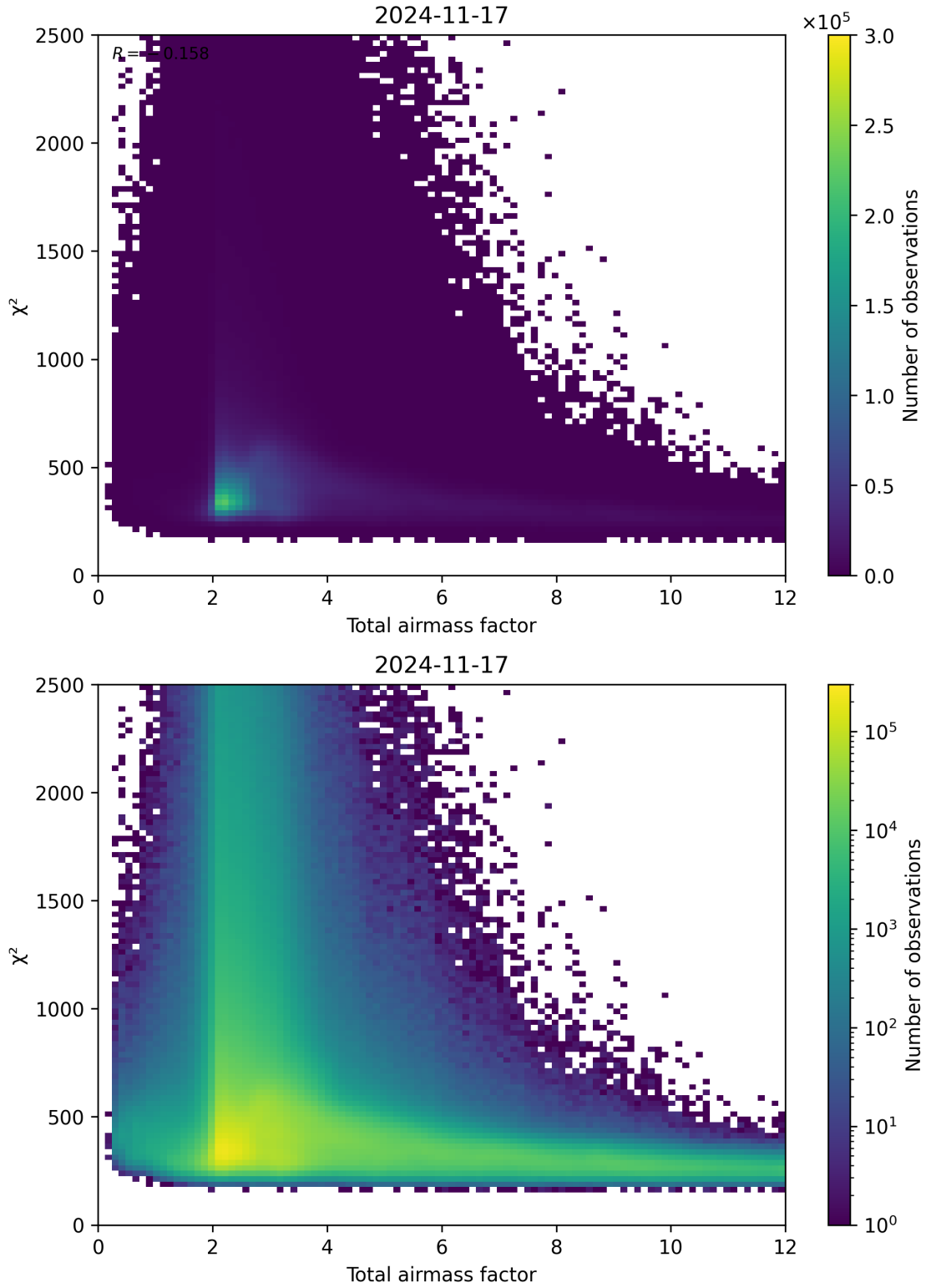
Figure 63: Scatter density plot of “Total airmass factor” against “ \chi^2 ” for 2024-11-17 to 2024-11-18.
