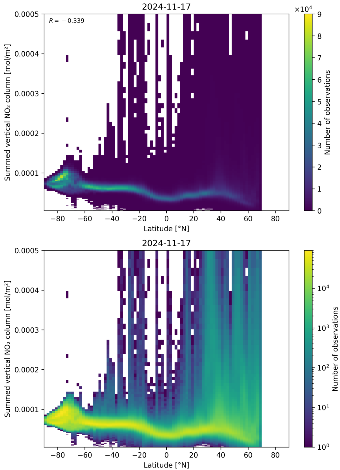
Figure 88: Scatter density plot of “Latitude” against “Summed vertical NO 2 column” for 2024-11-17 to 2024-11-18.
