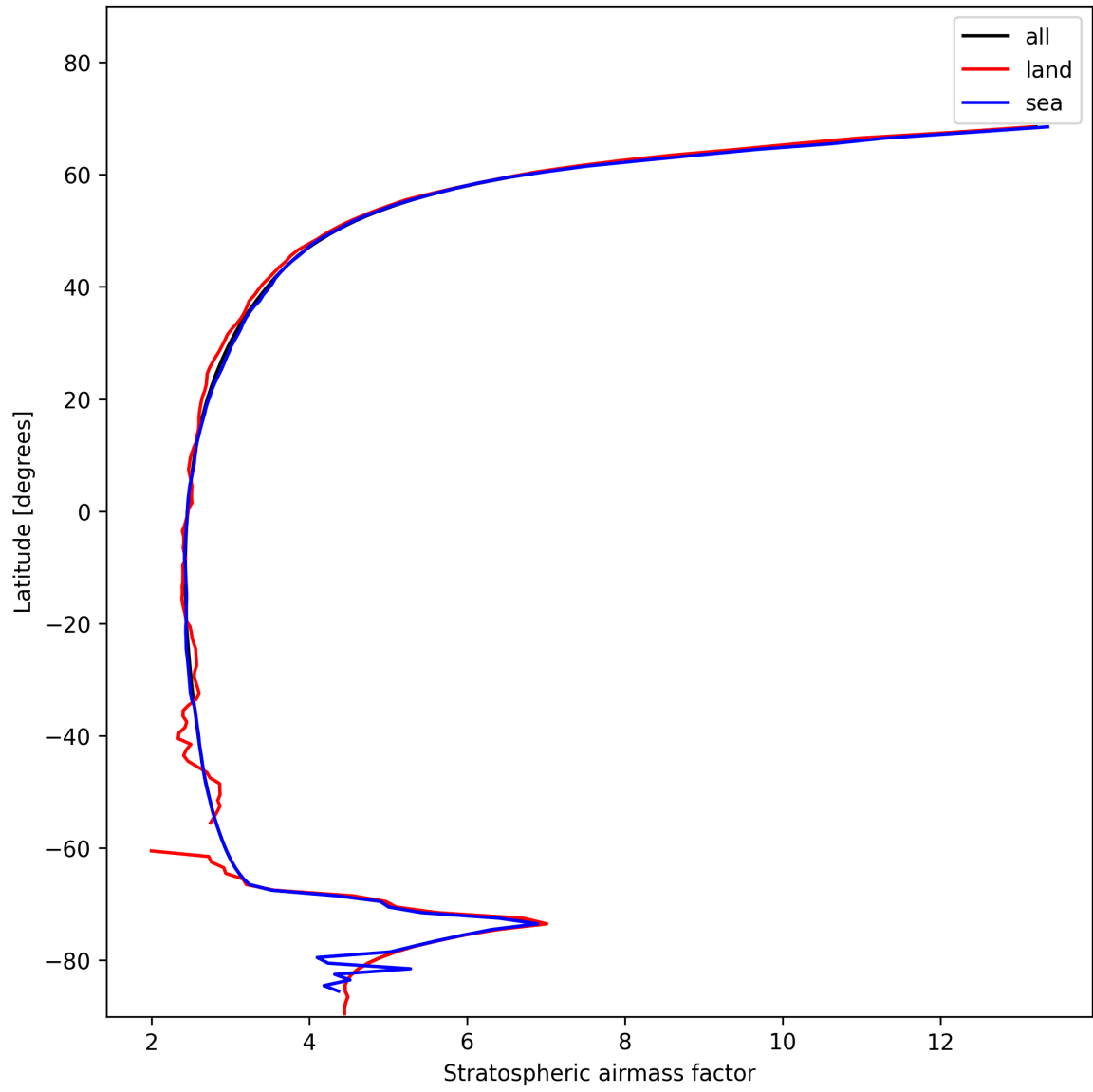
Figure 27: Zonal average of “Stratospheric airmass factor” for 2024-11-17 to 2024-11-18.
