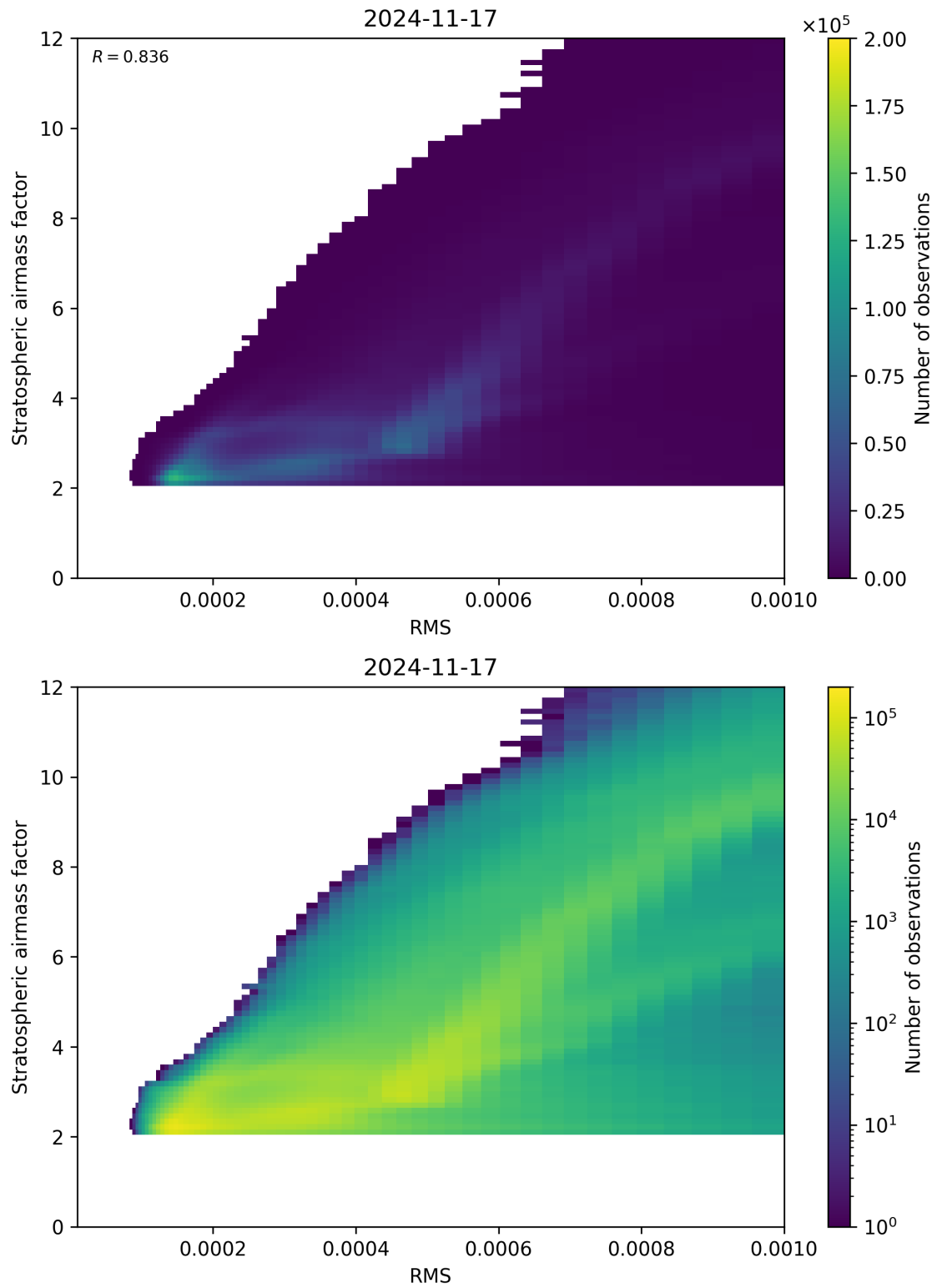
Figure 144: Scatter density plot of “RMS” against “Stratospheric airmass factor” for 2024-11-17 to 2024-11-18.
