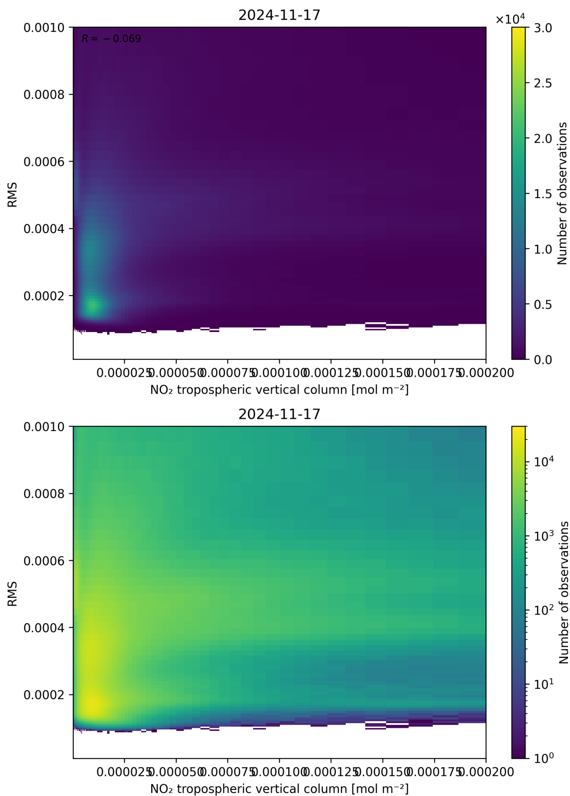
Figure 142: Scatter density plot of “NO 2 tropospheric vertical column” against “RMS” for 2024-11-17 to 2024-11-18.
