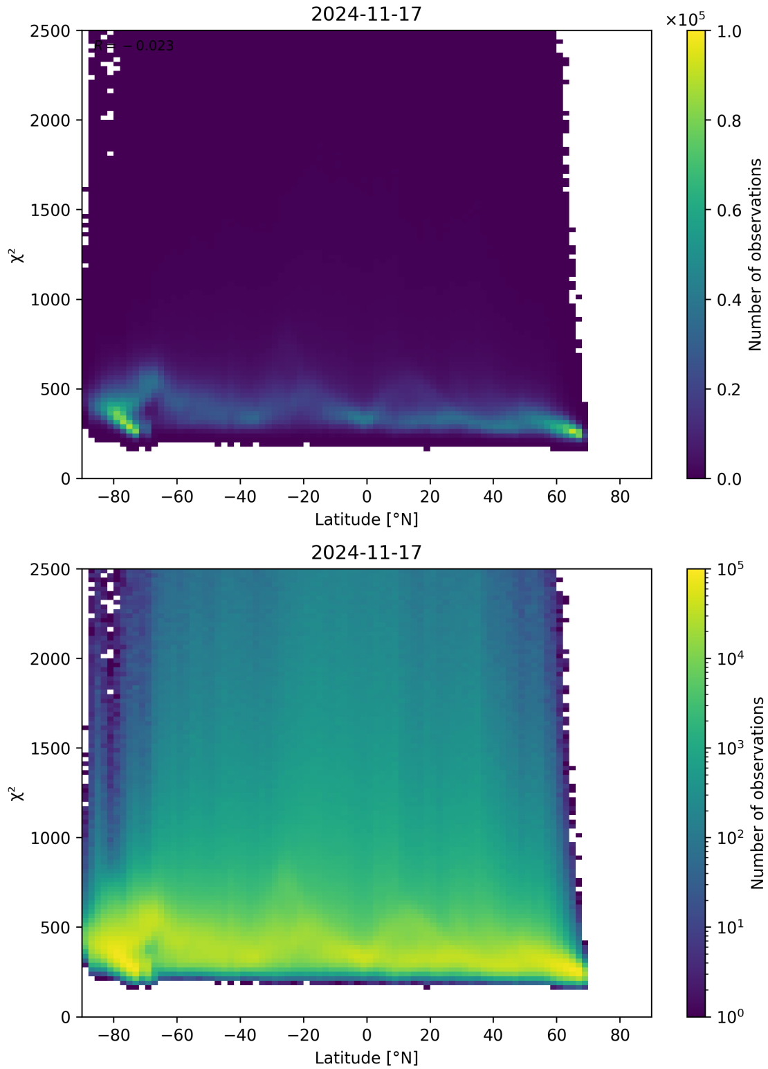
Figure 86: Scatter density plot of “Latitude” against “ \chi^2 ” for 2024-11-17 to 2024-11-18.
