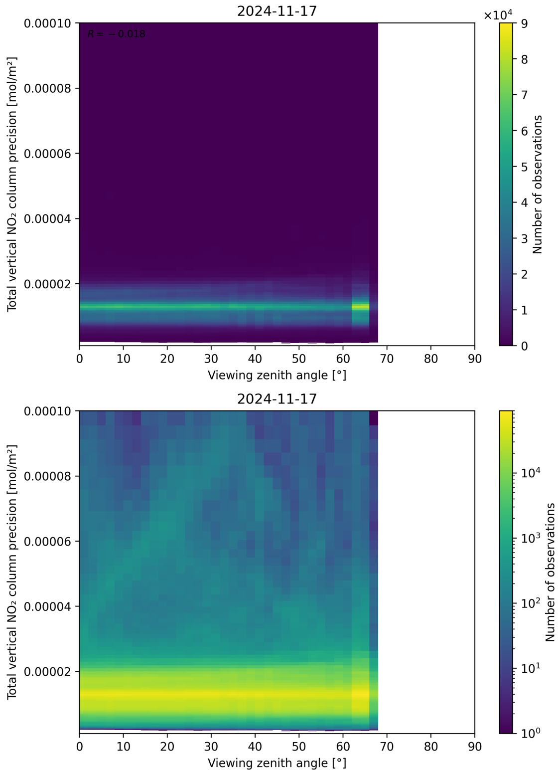
Figure 168: Scatter density plot of “Viewing zenith angle” against “Total vertical NO 2 column precision” for 2024-11-17 to 2024-11-18.
