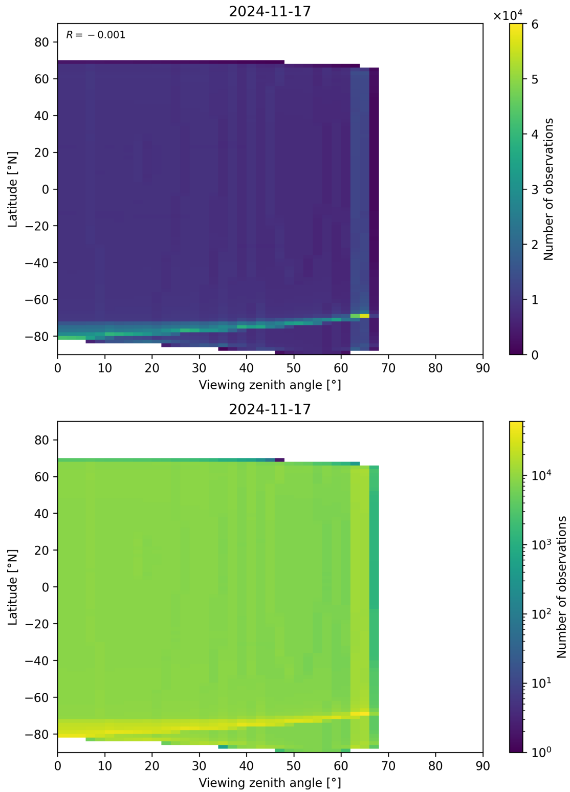
Figure 163: Scatter density plot of “Viewing zenith angle” against “Latitude” for 2024-11-17 to 2024-11-18.
