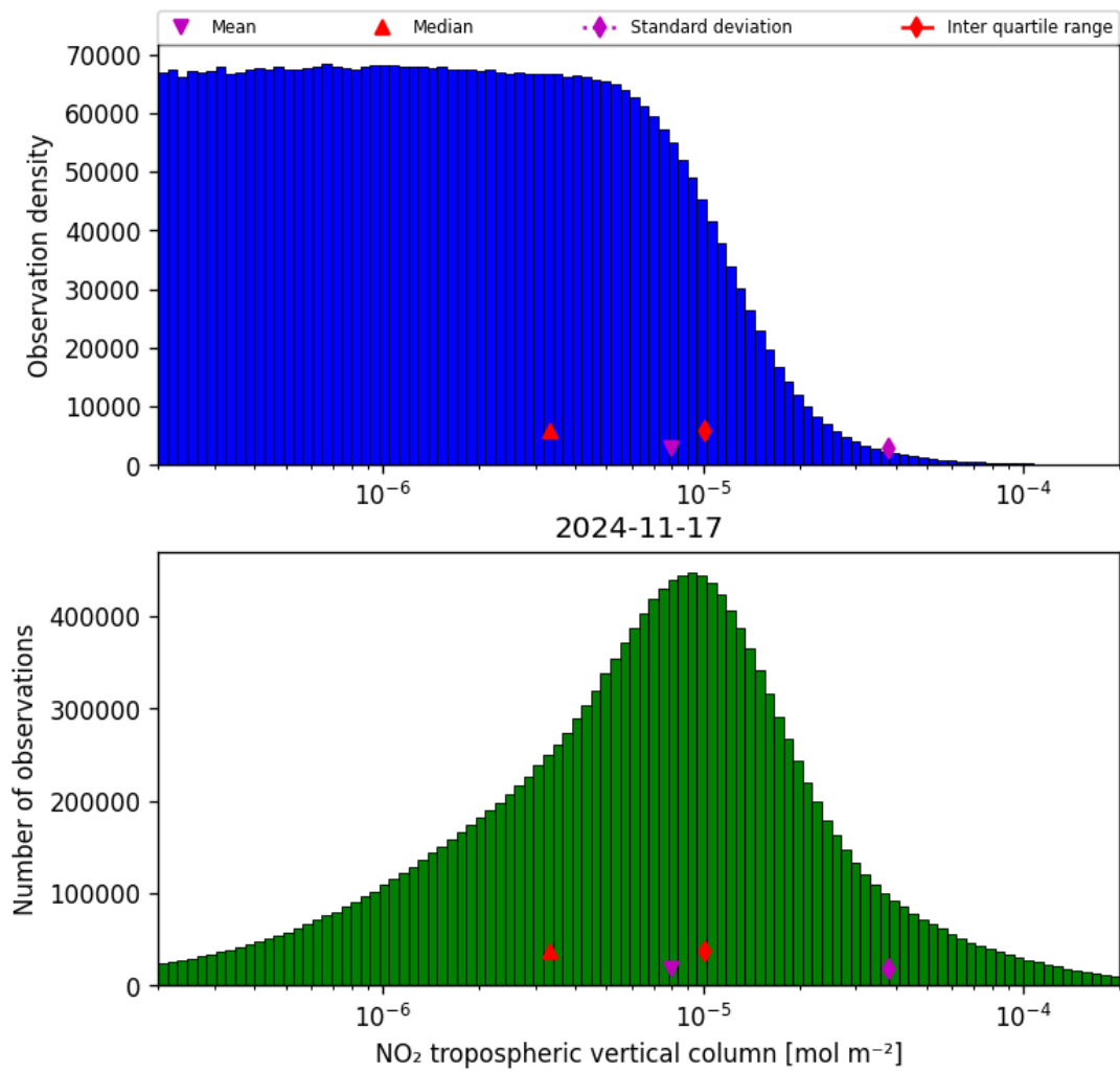
Figure 29: Histogram of “NO 2 tropospheric vertical column” for 2024-11-17 to 2024-11-18
