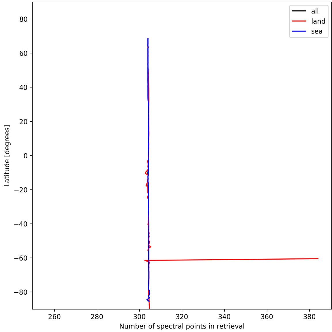
Figure 16: Zonal average of “Number of spectral points in retrieval” for 2024-11-17 to 2024-11-18.
