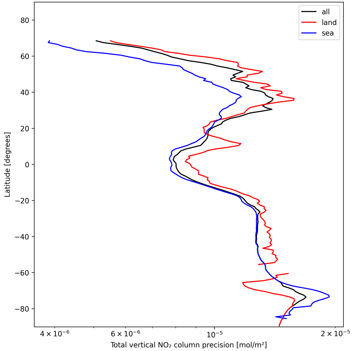
Figure 22: Zonal average of “Total vertical NO 2 column precision” for 2024-11-17 to 2024-11-18.
