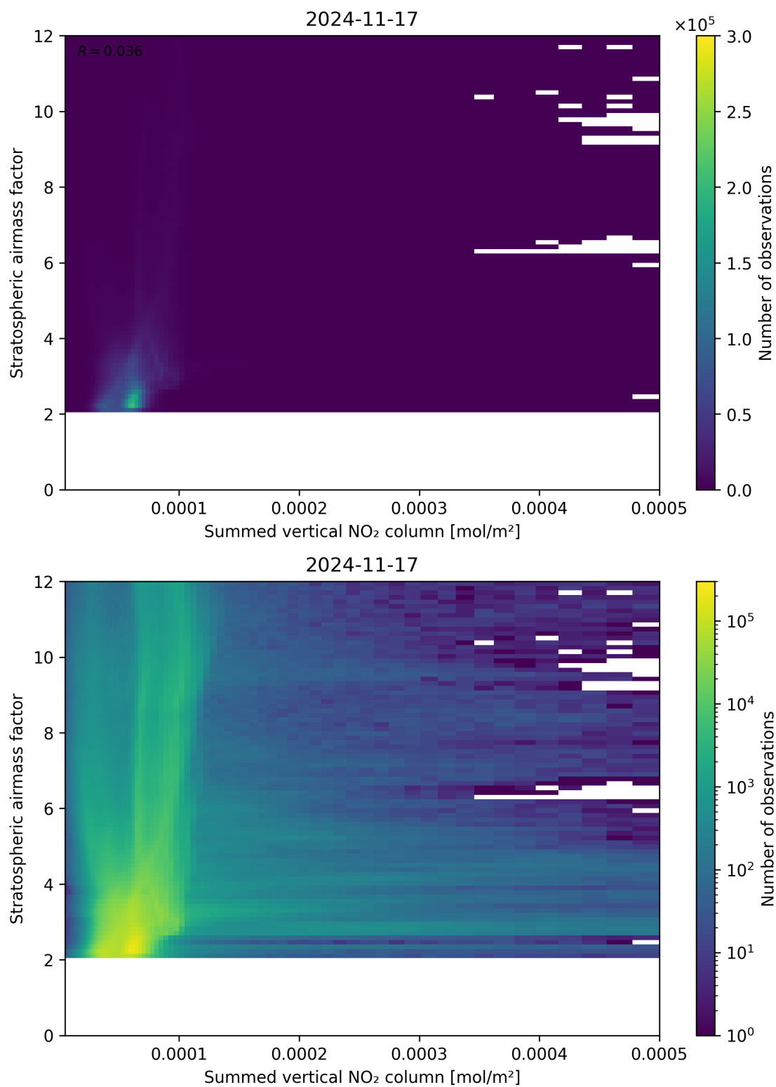
Figure 103: Scatter density plot of “Summed vertical NO 2 column” against “Stratospheric air mass factor” for 2024-11-17 to 2024-11-18.
