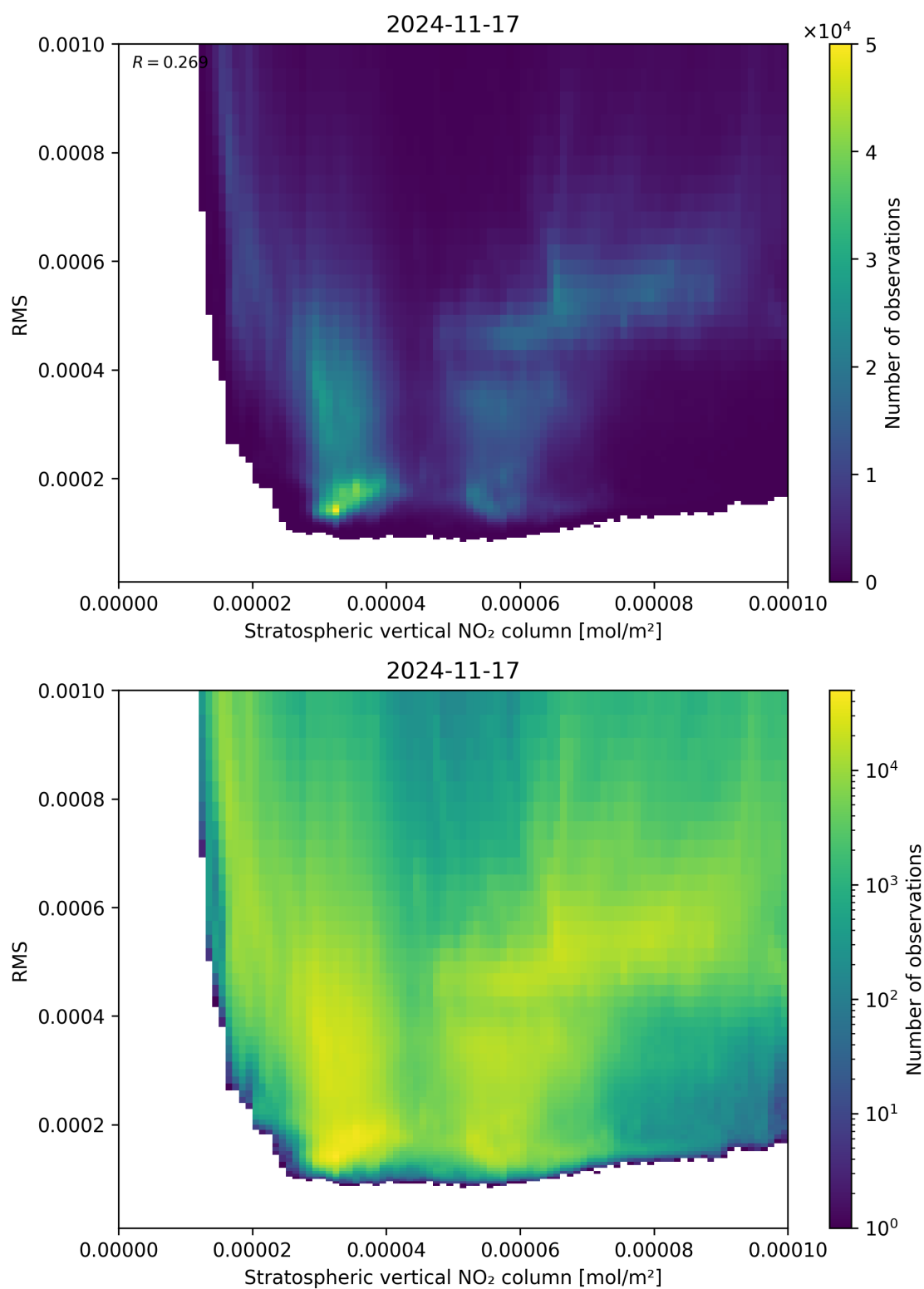
Figure 102: Scatter density plot of “Stratospheric vertical NO 2 column” against “RMS” for 2024-11-17 to 2024-11-18.
