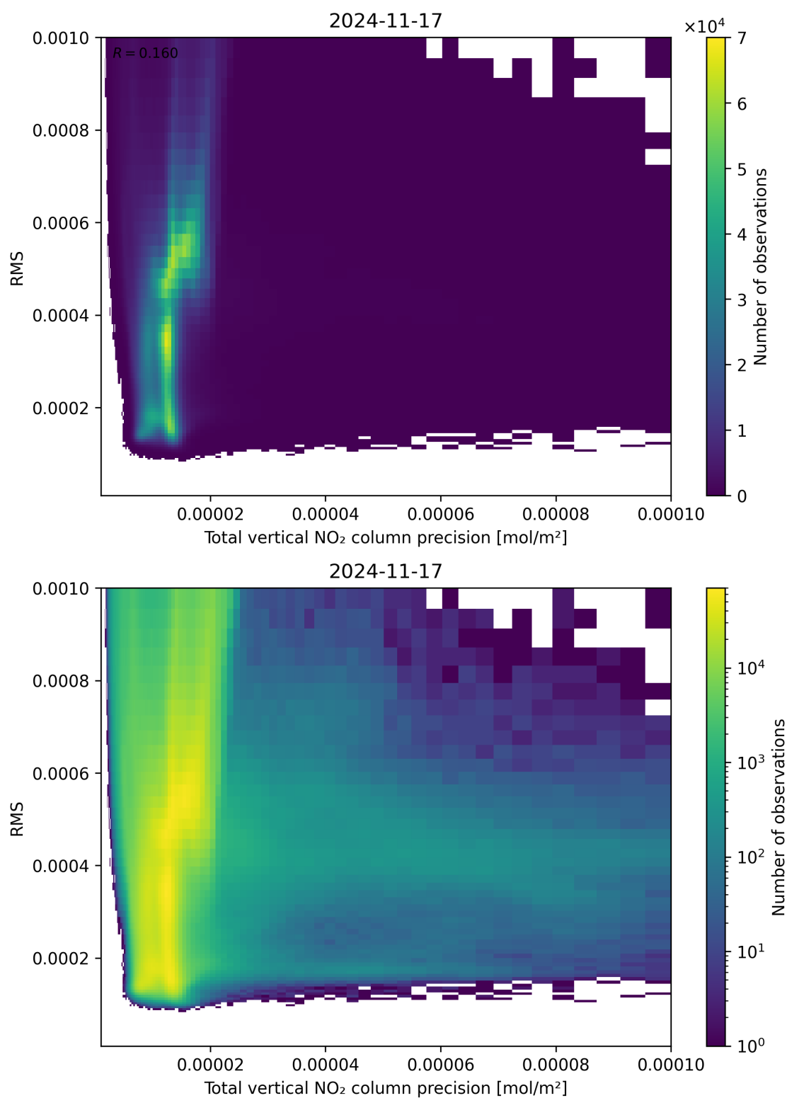
Figure 119: Scatter density plot of “Total vertical NO 2 column precision” against “RMS” for 2024-11-17 to 2024-11-18.
