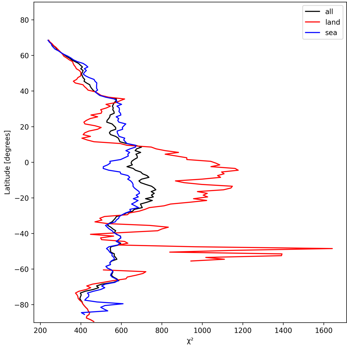
Figure 25: Zonal average of “ \chi^2 ” for 2024-11-17 to 2024-11-18.
