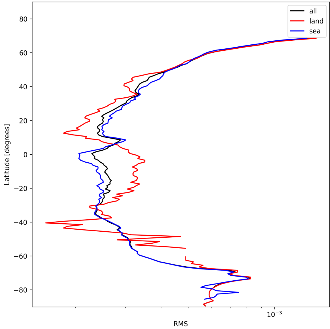
Figure 26: Zonal average of “RMS” for 2024-11-17 to 2024-11-18.
