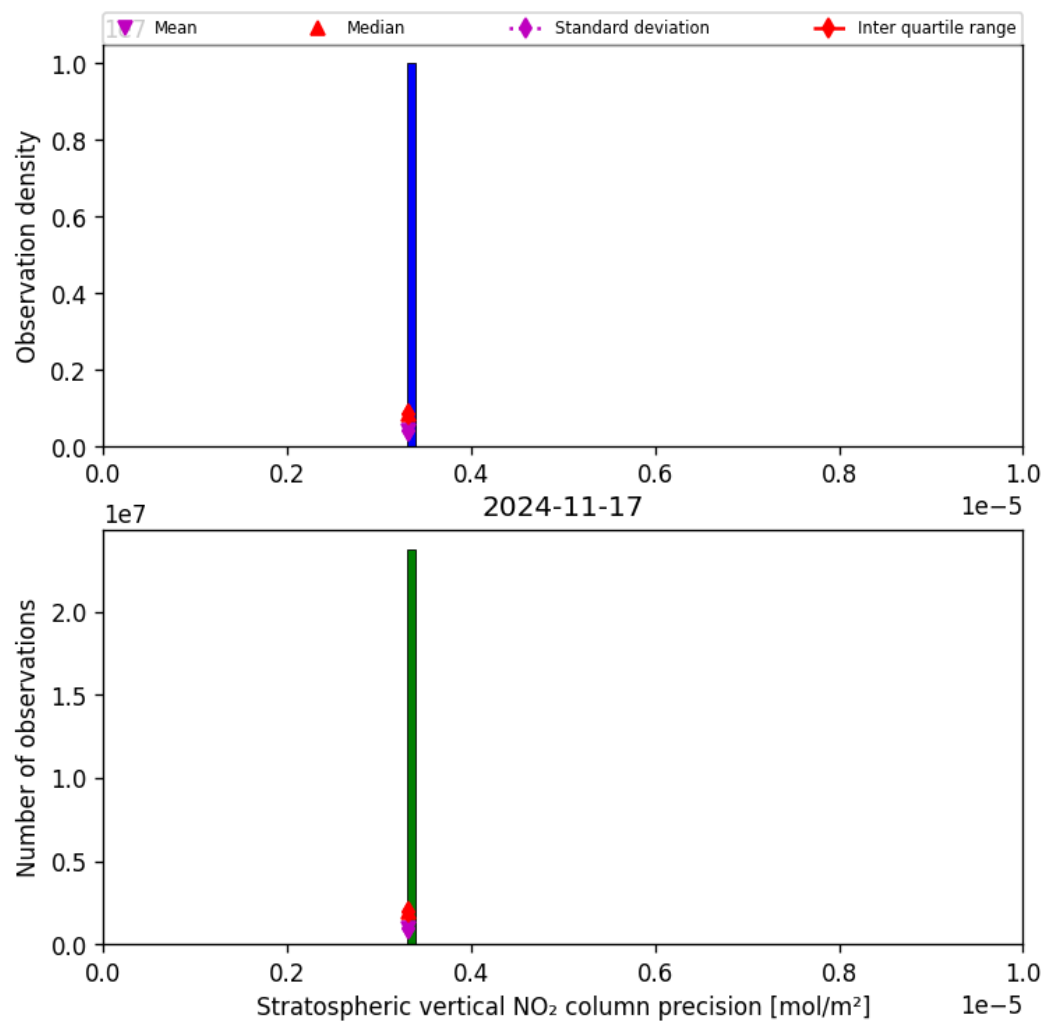
Figure 37: Histogram of “Stratospheric vertical NO 2 column precision” for 2024-11-17 to 2024-11-18
