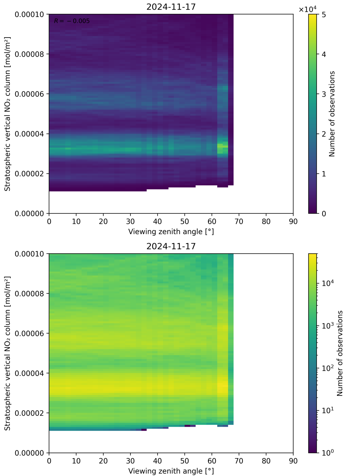
Figure 164: Scatter density plot of “Viewing zenith angle” against “Stratospheric vertical NO 2 column” for 2024-11-17 to 2024-11-18.
