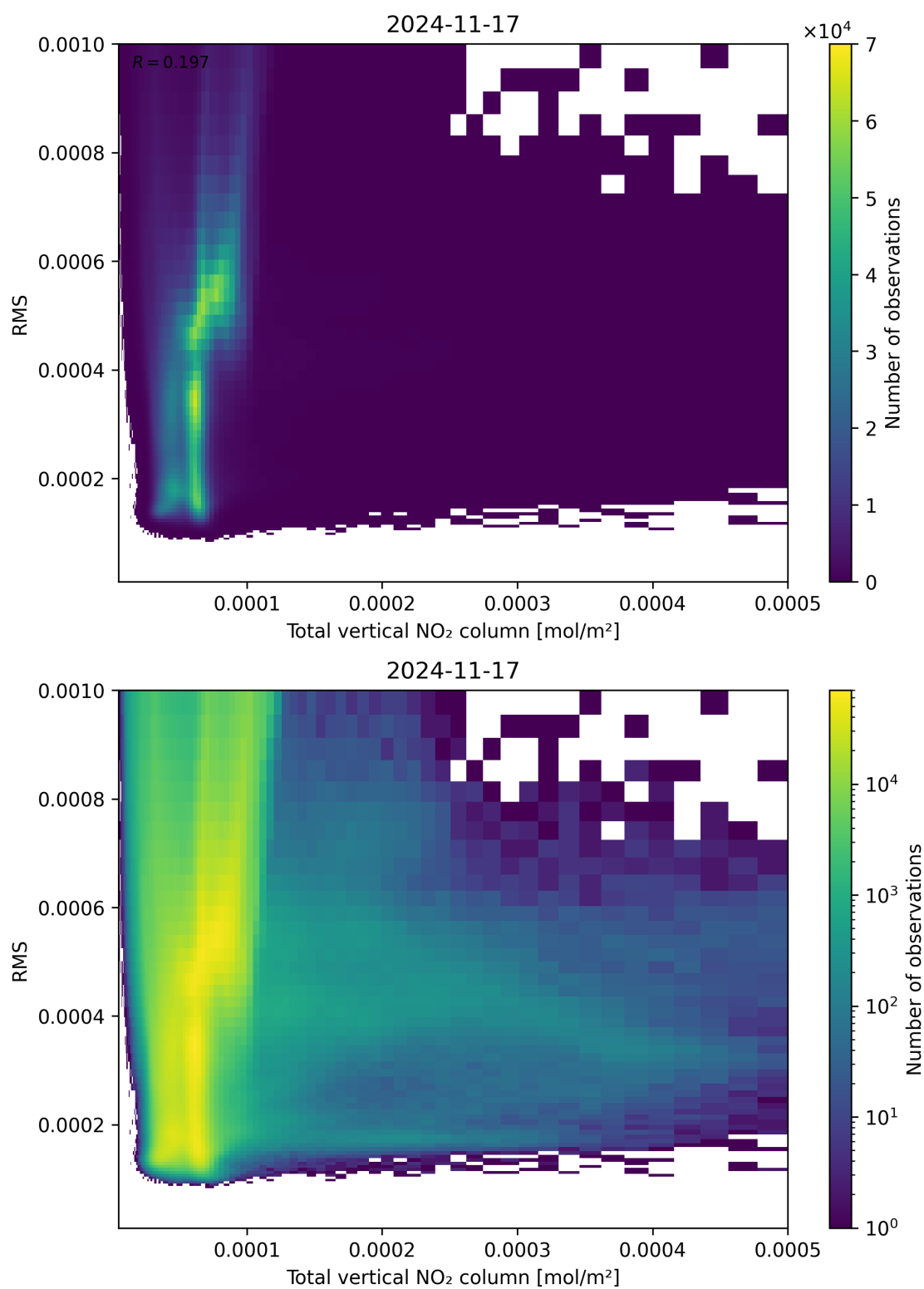
Figure 120: Scatter density plot of “Total vertical NO 2 column” against “RMS” for 2024-11-17 to 2024-11-18.
