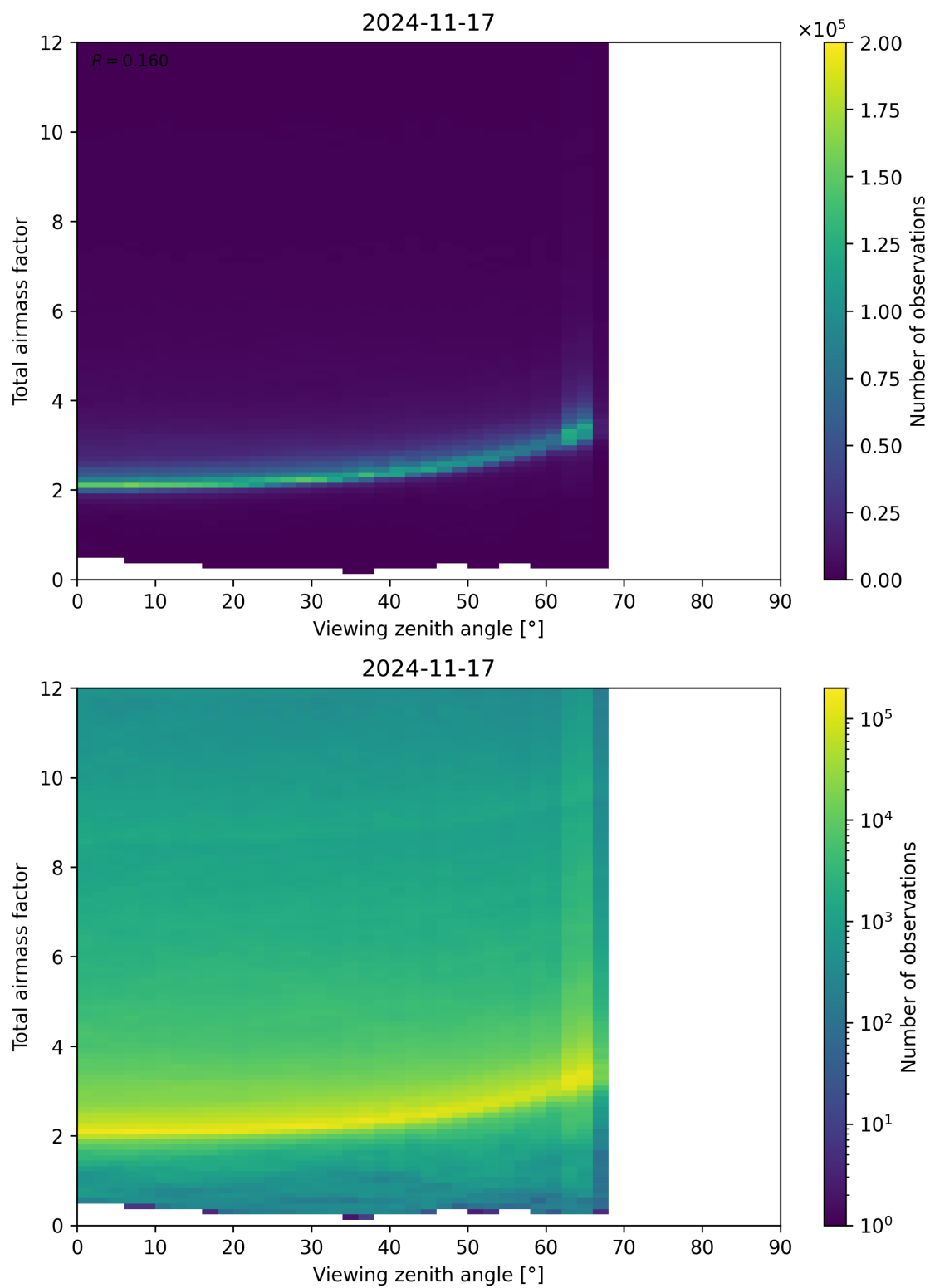
Figure 160: Scatter density plot of “Viewing zenith angle” against “Total airmass factor” for 2024-11-17 to 2024-11-18.
