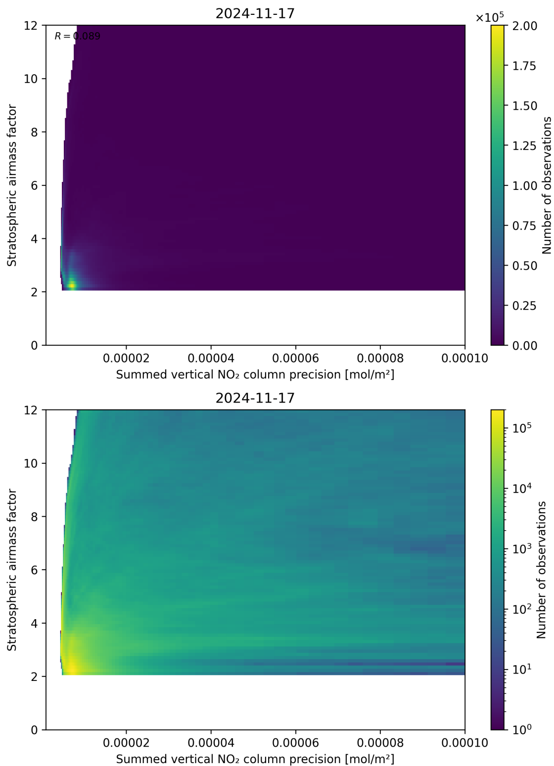
Figure 106: Scatter density plot of “Summed vertical NO 2 column precision” against “Stratospheric airmass factor” for 2024-11-17 to 2024-11-18.
