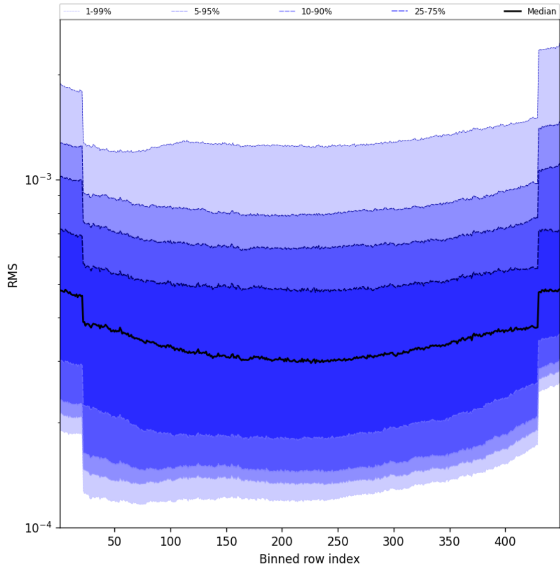
Figure 60: Along track statistics of “RMS” for 2024-11-17 to 2024-11-18
