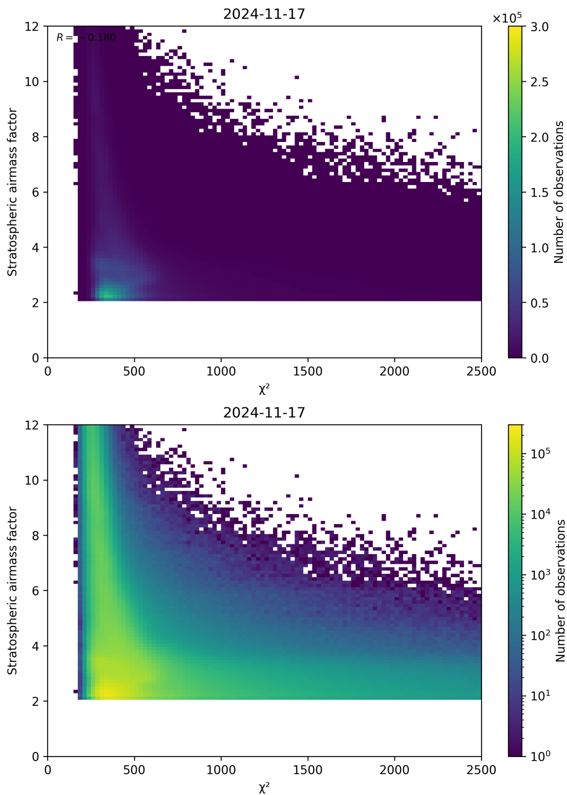
Figure 81: Scatter density plot of “ \chi^2 ” against “Stratospheric airmass factor” for 2024-11-17 to 2024-11-18.
