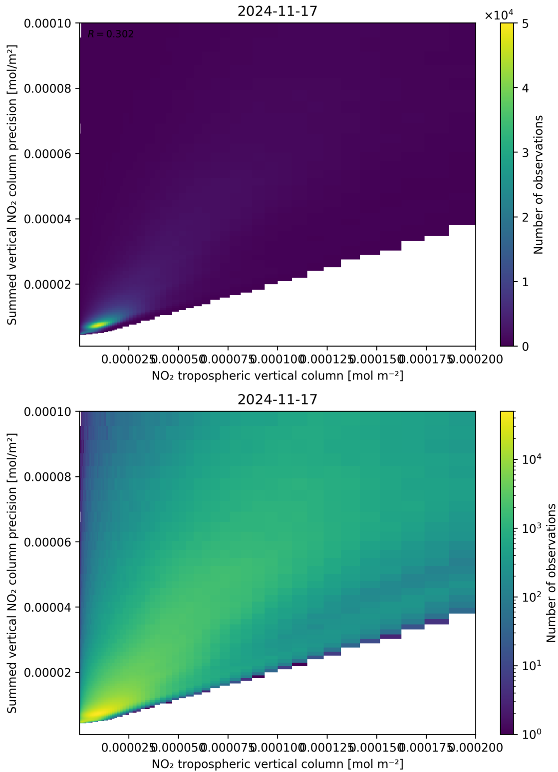
Figure 127: Scatter density plot of “NO 2 tropospheric vertical column” against “Summed vertical NO 2 column precision” for 2024-11-17 to 2024-11-18.
