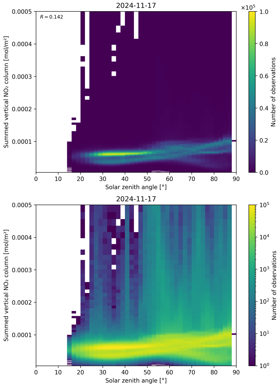
Figure 151: Scatter density plot of “Solar zenith angle” against “Summed vertical NO 2 column” for 2024-11-17 to 2024-11-18.
