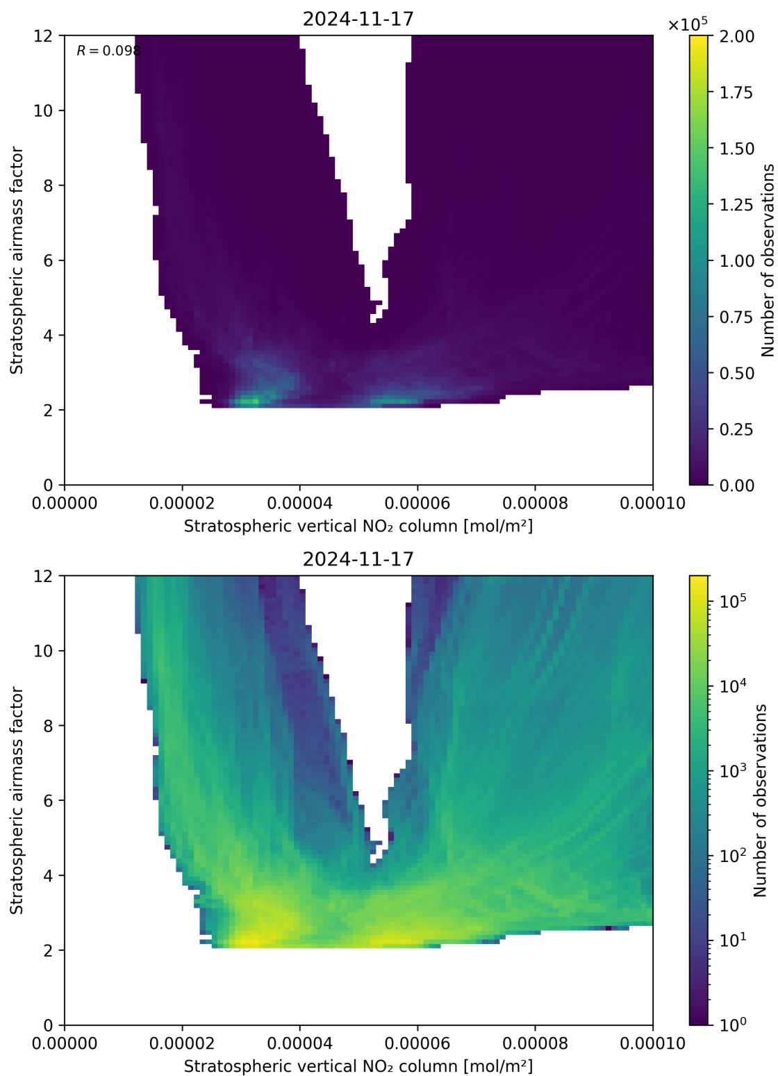
Figure 96: Scatter density plot of “Stratospheric vertical NO 2 column” against “Stratospheric airmass factor” for 2024-11-17 to 2024-11-18.
