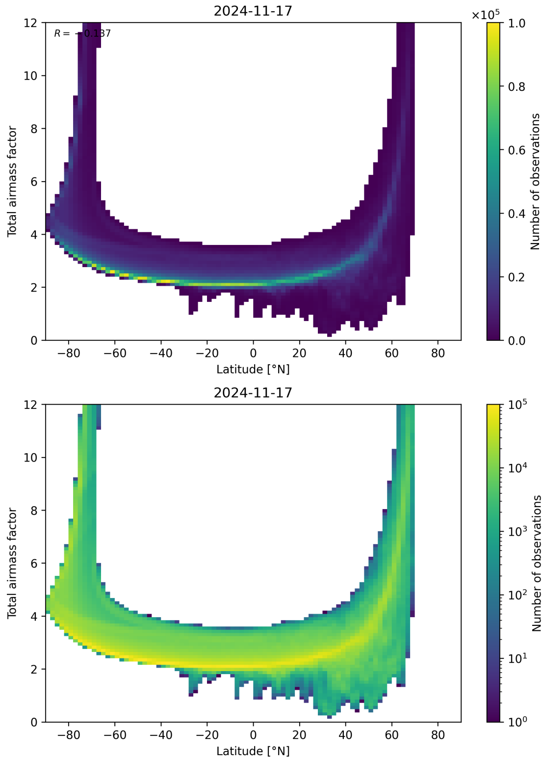
Figure 84: Scatter density plot of “Latitude” against “Total airmass factor” for 2024-11-17 to 2024-11-18.
