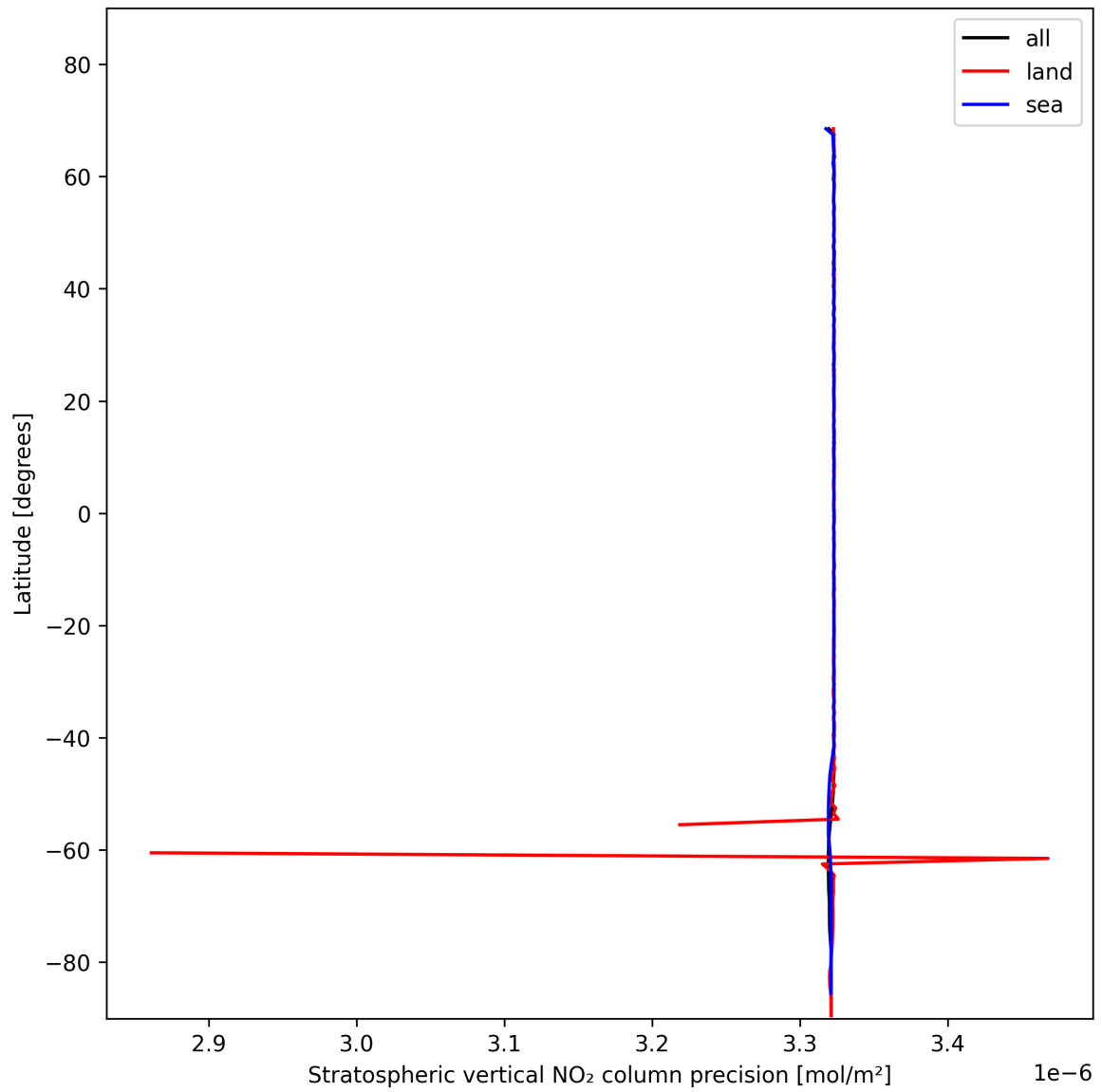
Figure 20: Zonal average of “Stratospheric vertical NO 2 column precision” for 2024-11-17 to 2024-11-18.
