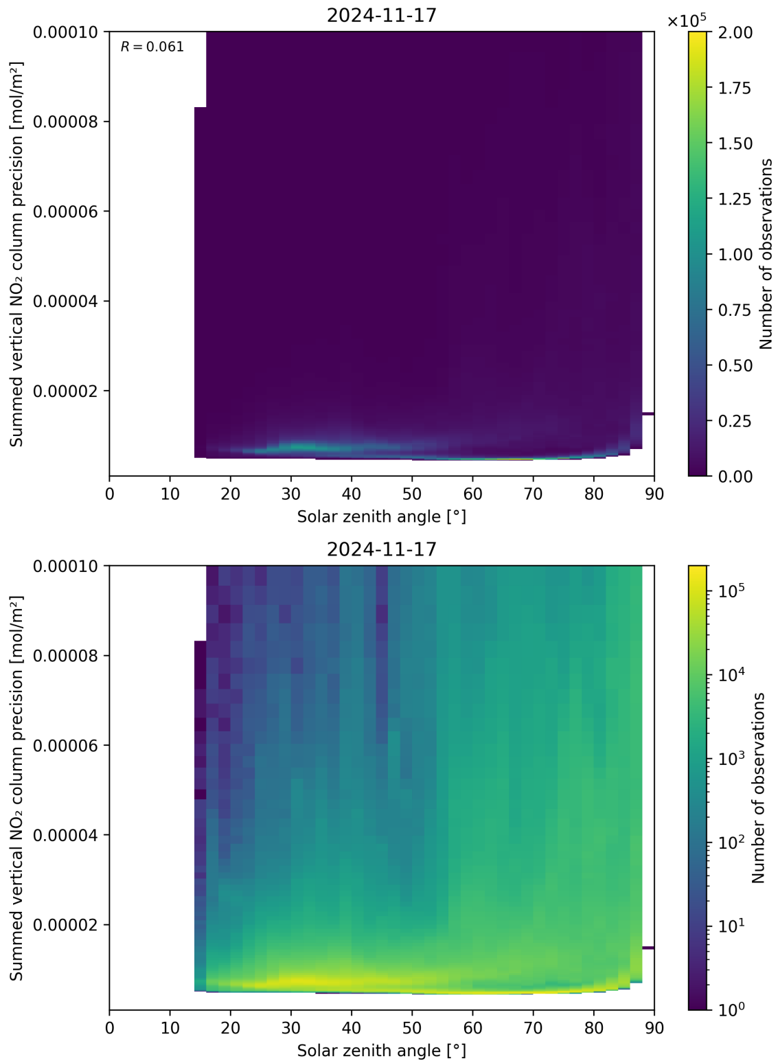
Figure 152: Scatter density plot of “Solar zenith angle” against “Summed vertical NO 2 column precision” for 2024-11-17 to 2024-11-18.
