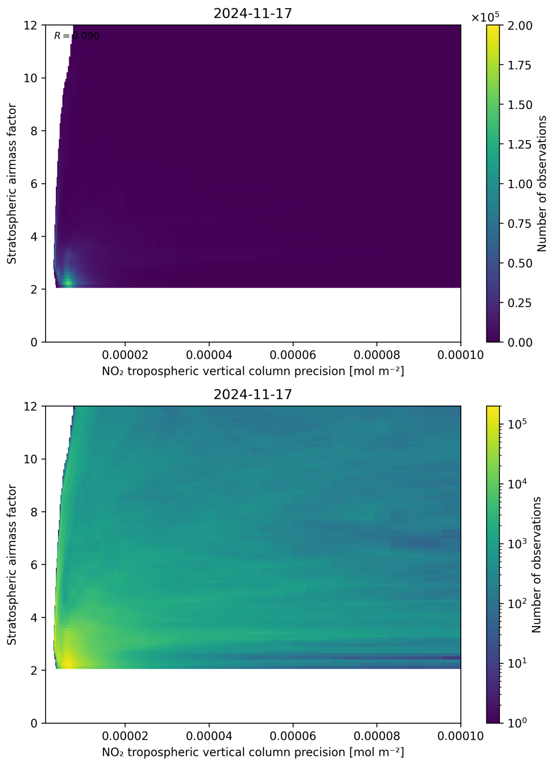
Figure 131: Scatter density plot of “NO 2 tropospheric vertical column precision” against “Stratospheric airmass factor” for 2024-11-17 to 2024-11-18.
