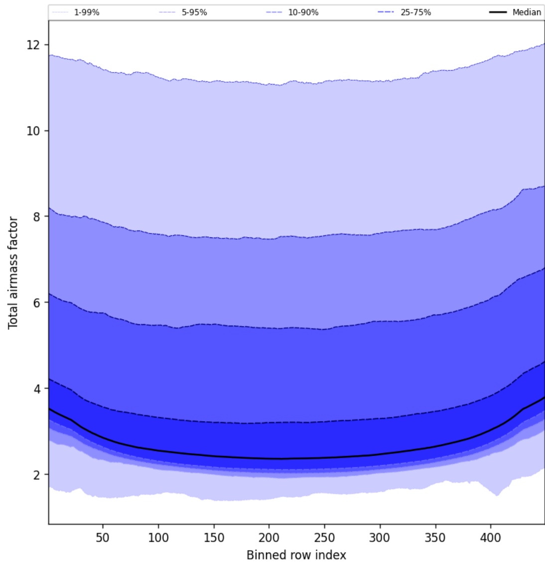
Figure 49: Along track statistics of “Total airmass factor” for 2024-11-17 to 2024-11-18
