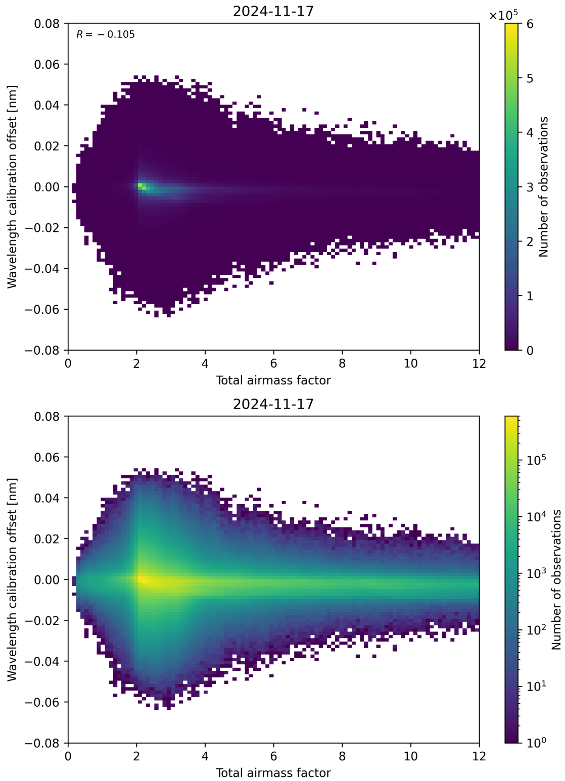
Figure 70: Scatter density plot of “Total airmass factor” against “Wavelength calibration offset” for 2024-11-17 to 2024-11-18.
