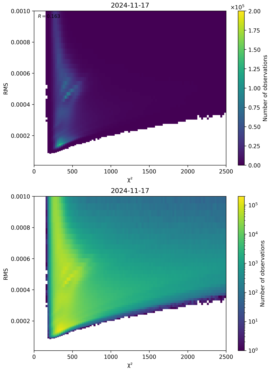
Figure 82: Scatter density plot of “ \chi^2 ” against “RMS” for 2024-11-17 to 2024-11-18.
