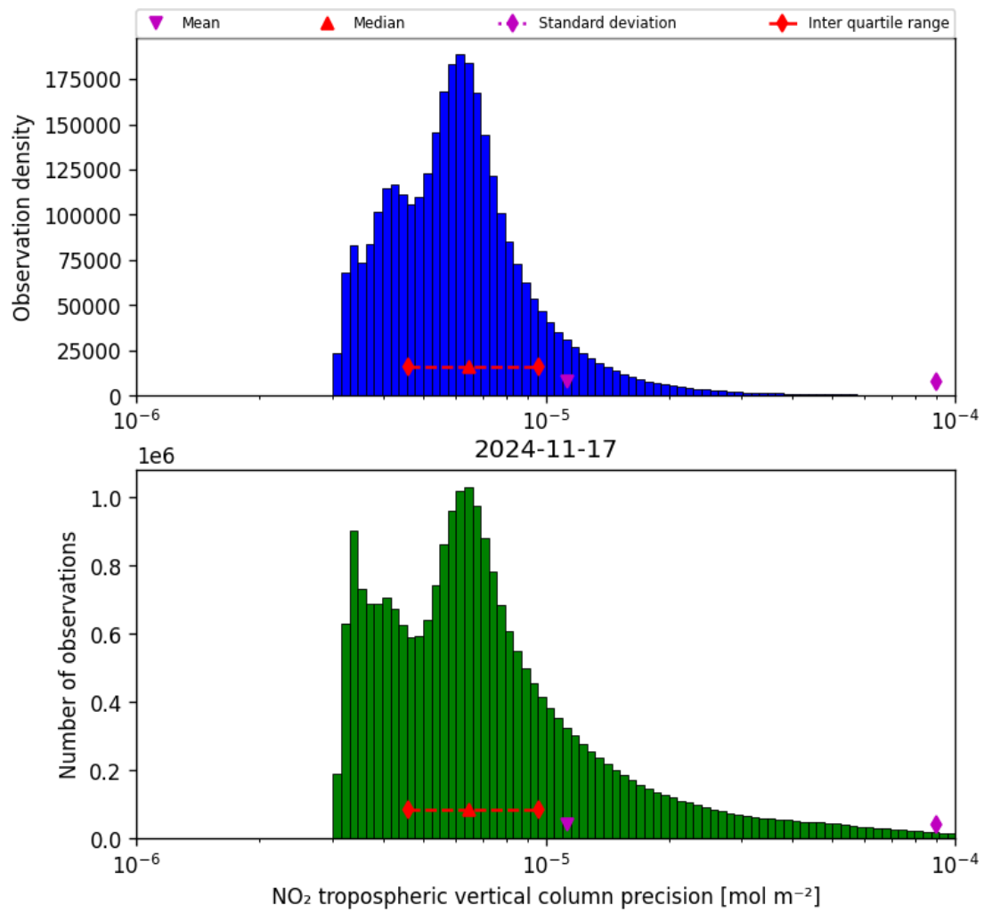
Figure 30: Histogram of “NO 2 tropospheric vertical column precision” for 2024-11-17 to 2024-11-18
