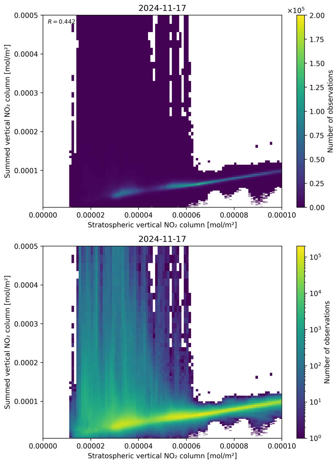
Figure 98: Scatter density plot of “Stratospheric vertical NO 2 column” against “Summed vertical NO 2 column” for 2024-11-17 to 2024-11-18.
