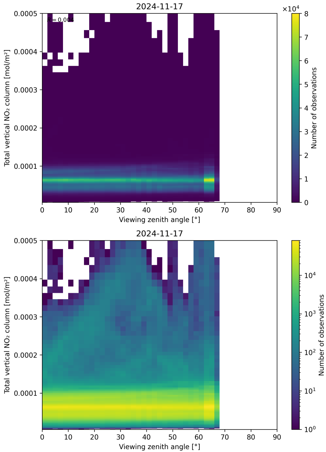
Figure 167: Scatter density plot of “Viewing zenith angle” against “Total vertical NO 2 column” for 2024-11-17 to 2024-11-18.
