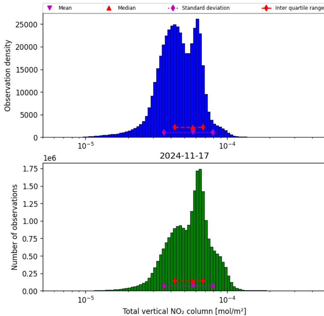
Figure 38: Histogram of “Total vertical NO 2 column” for 2024-11-17 to 2024-11-18
