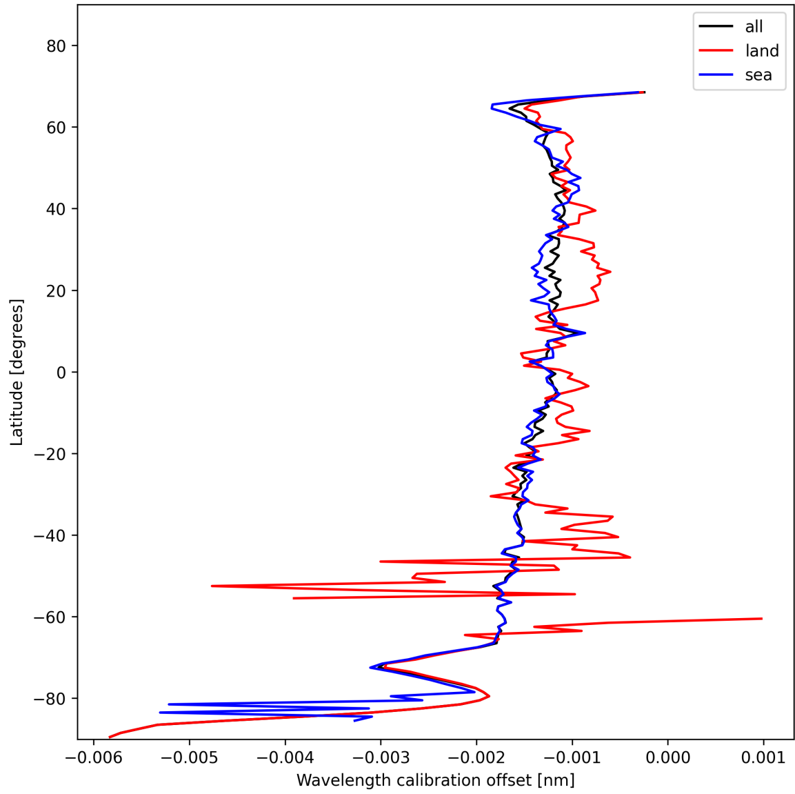
Figure 18: Zonal average of “Wavelength calibration offset” for 2024-11-17 to 2024-11-18.
