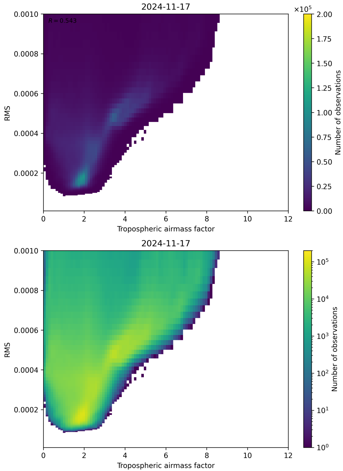
Figure 79: Scatter density plot of “Tropospheric airmass factor” against “RMS” for 2024-11-17 to 2024-11-18.
