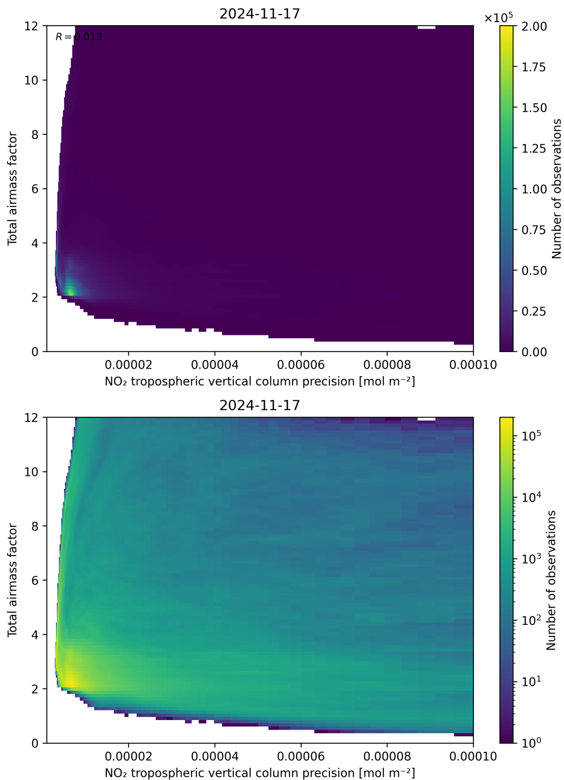
Figure 132: Scatter density plot of “NO 2 tropospheric vertical column precision” against “Total air mass factor” for 2024-11-17 to 2024-11-18.
