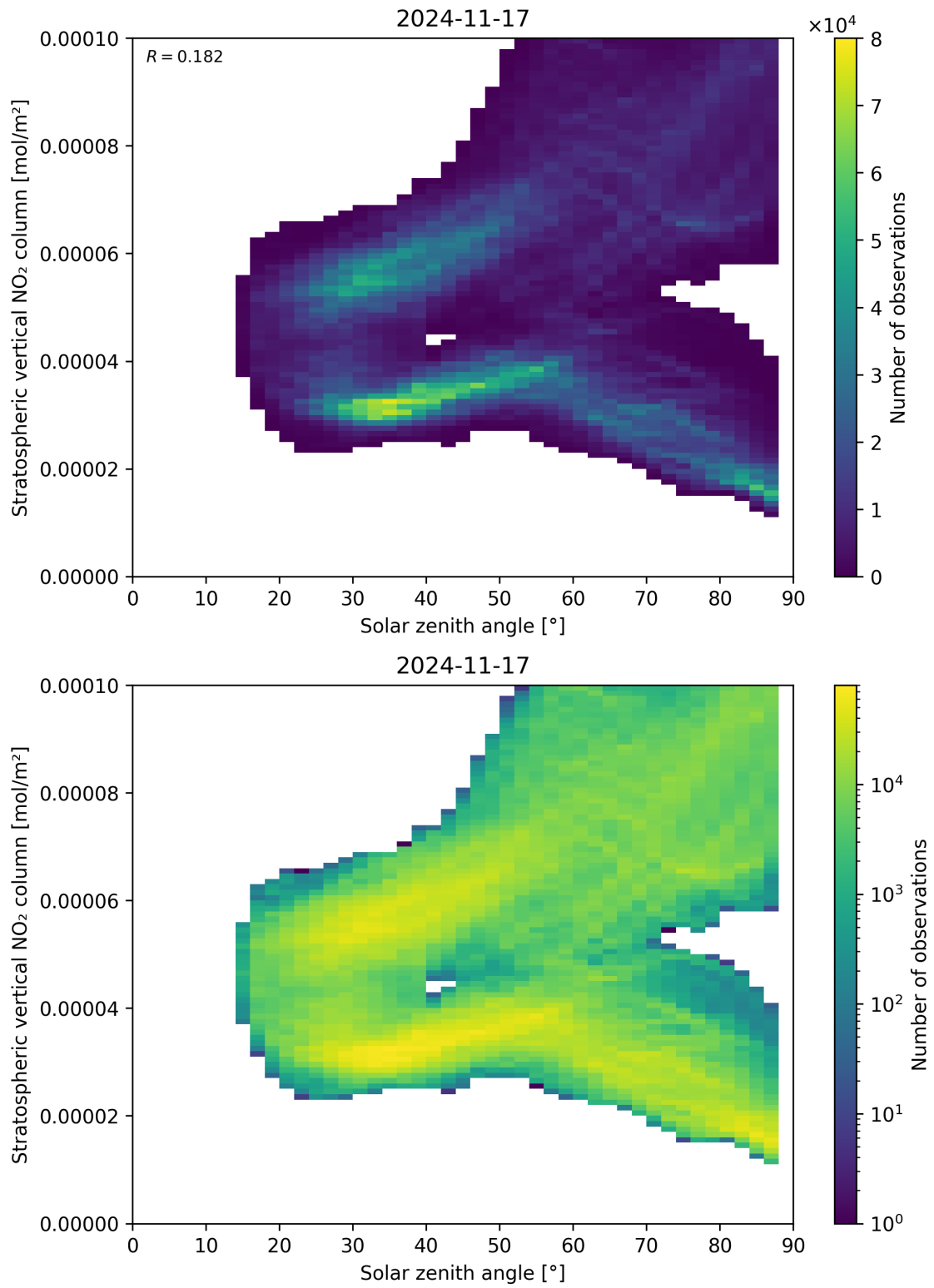
Figure 150: Scatter density plot of “Solar zenith angle” against “Stratospheric vertical NO 2 column” for 2024-11-17 to 2024-11-18.
