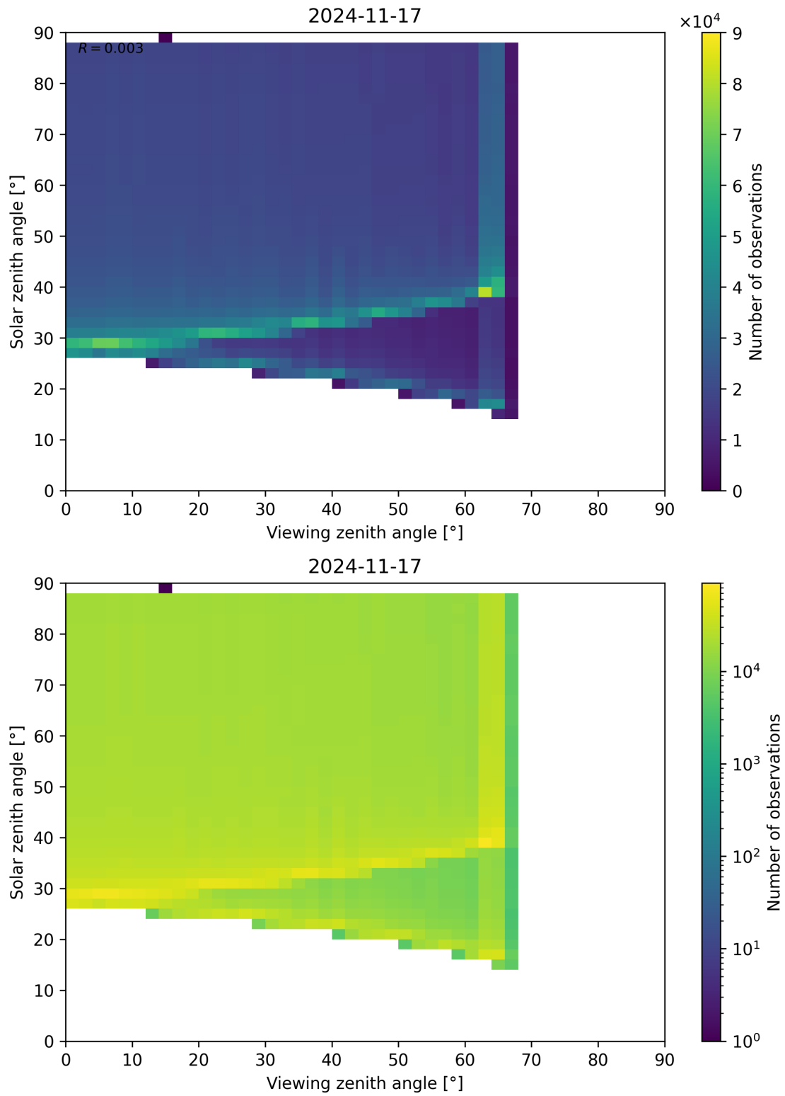
Figure 172: Scatter density plot of “Viewing zenith angle” against “Solar zenith angle” for 2024-11-17 to 2024-11-18.
