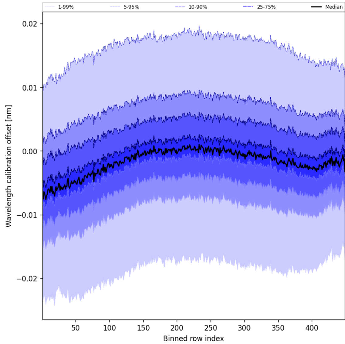
Figure 52: Along track statistics of “Wavelength calibration offset” for 2024-11-17 to 2024-11-18
