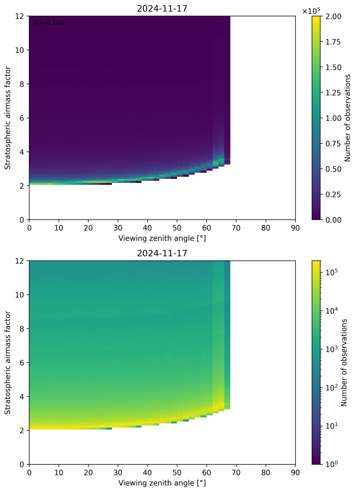
Figure 159: Scatter density plot of “Viewing zenith angle” against “Stratospheric airmass factor” for 2024-11-17 to 2024-11-18.
