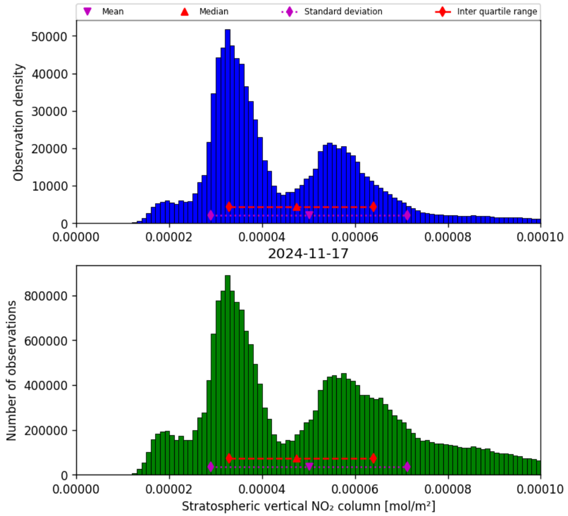
Figure 36: Histogram of “Stratospheric vertical NO 2 column” for 2024-11-17 to 2024-11-18
