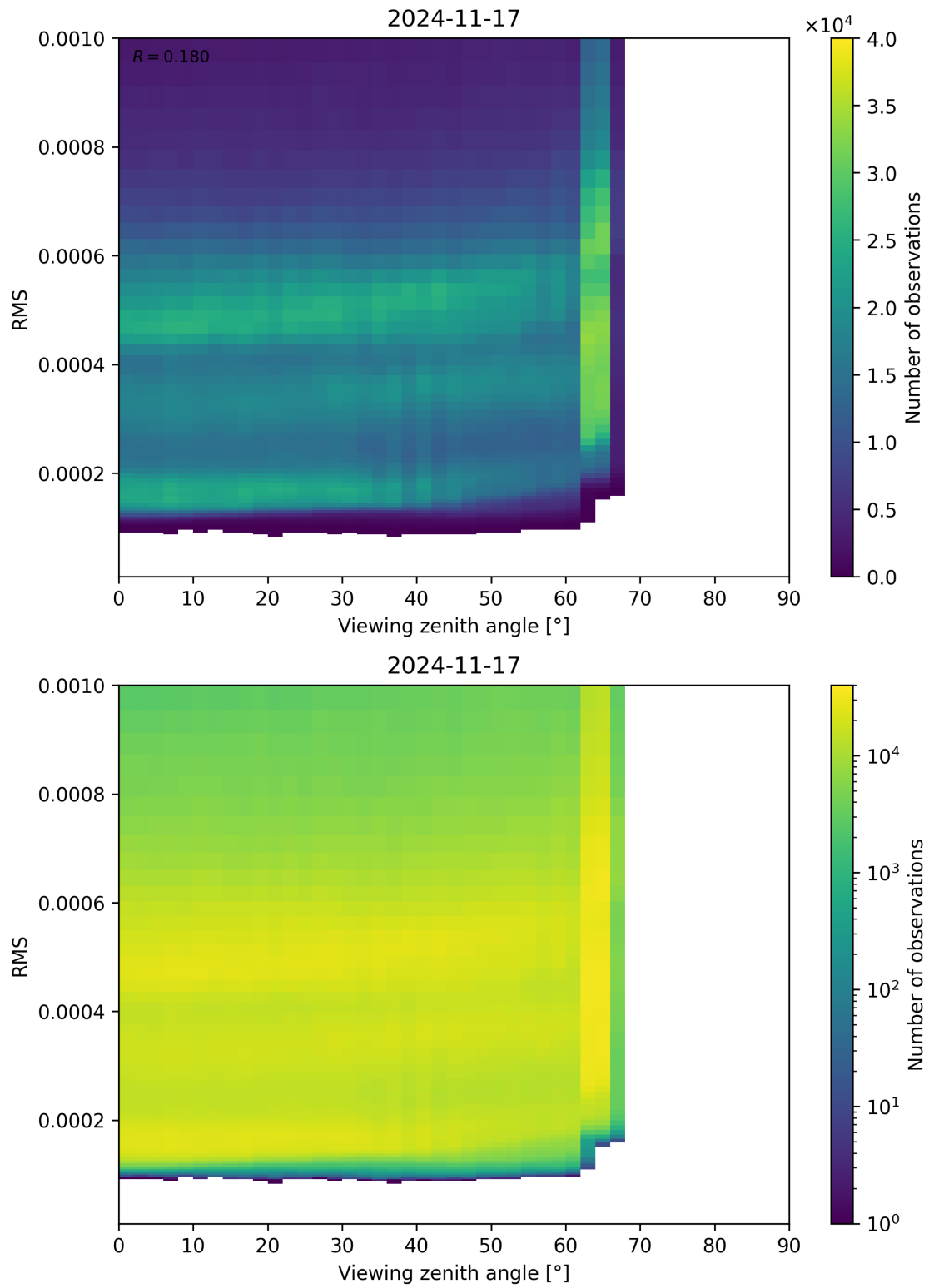
Figure 171: Scatter density plot of “Viewing zenith angle” against “RMS” for 2024-11-17 to 2024-11-18.
