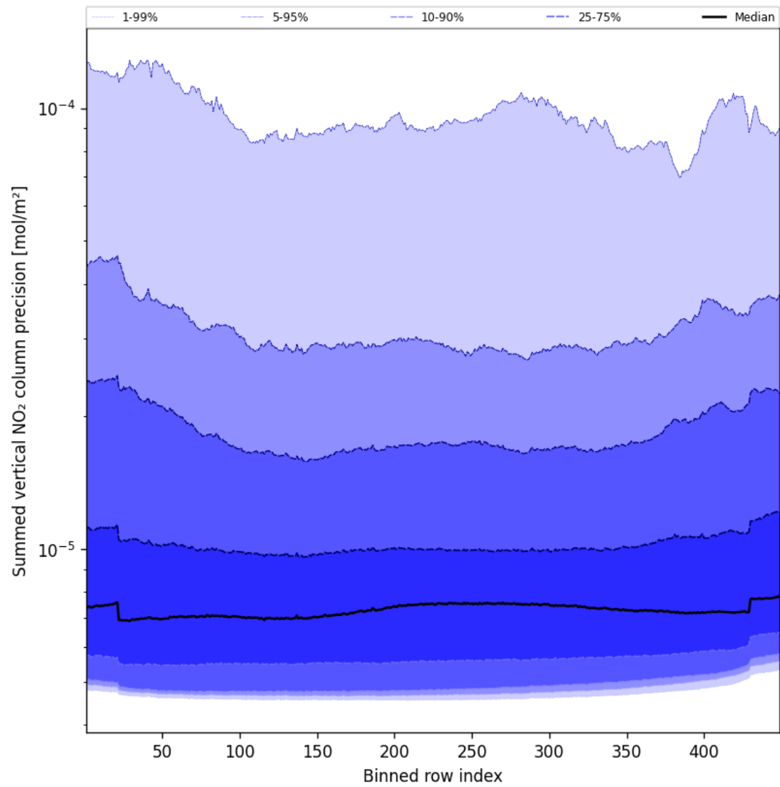
Figure 58: Along track statistics of “Summed vertical NO 2 column precision” for 2024-11-17 to 2024-11-18
