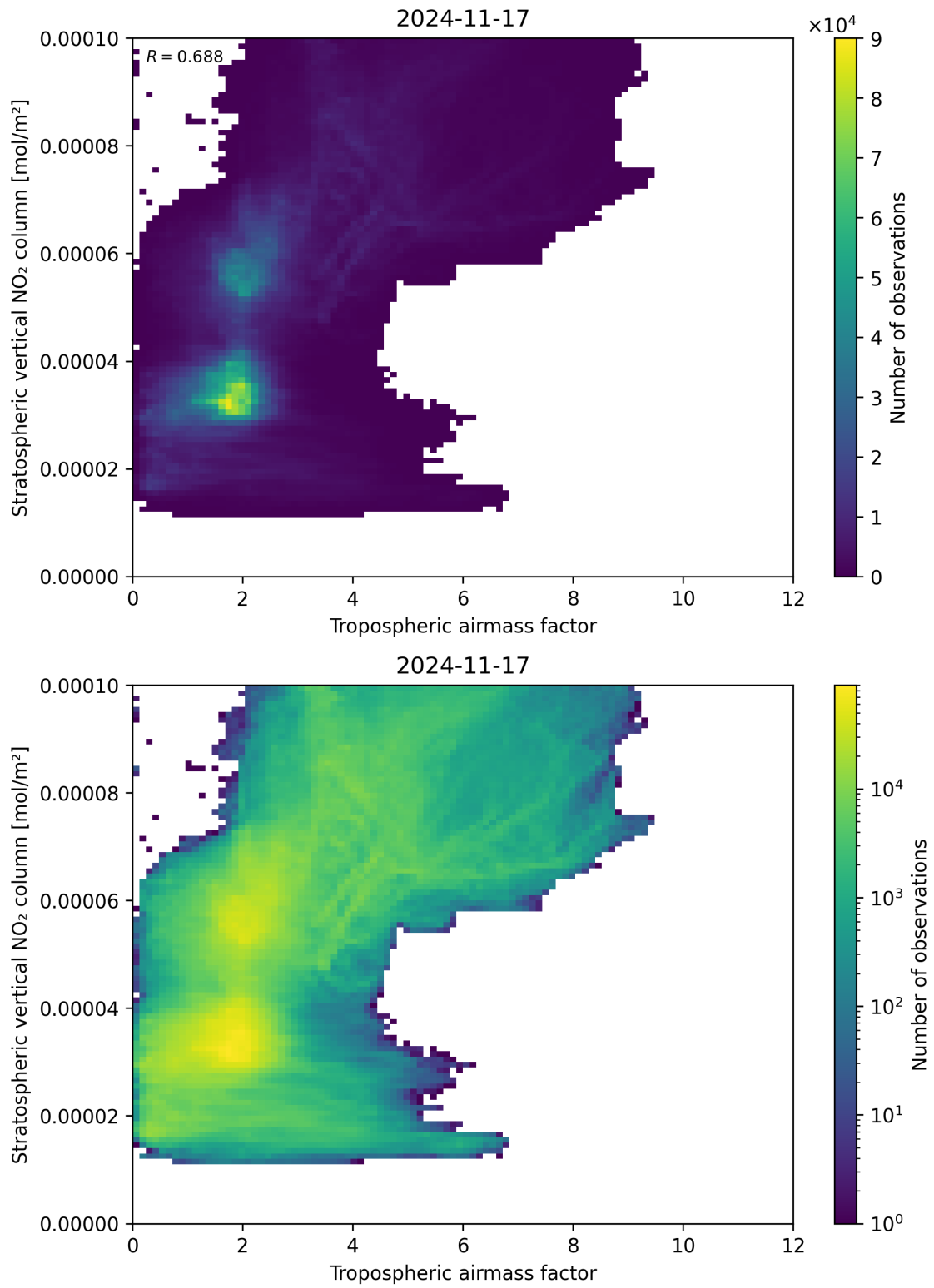
Figure 74: Scatter density plot of “Tropospheric airmass factor” against “Stratospheric vertical NO 2 column” for 2024-11-17 to 2024-11-18.
