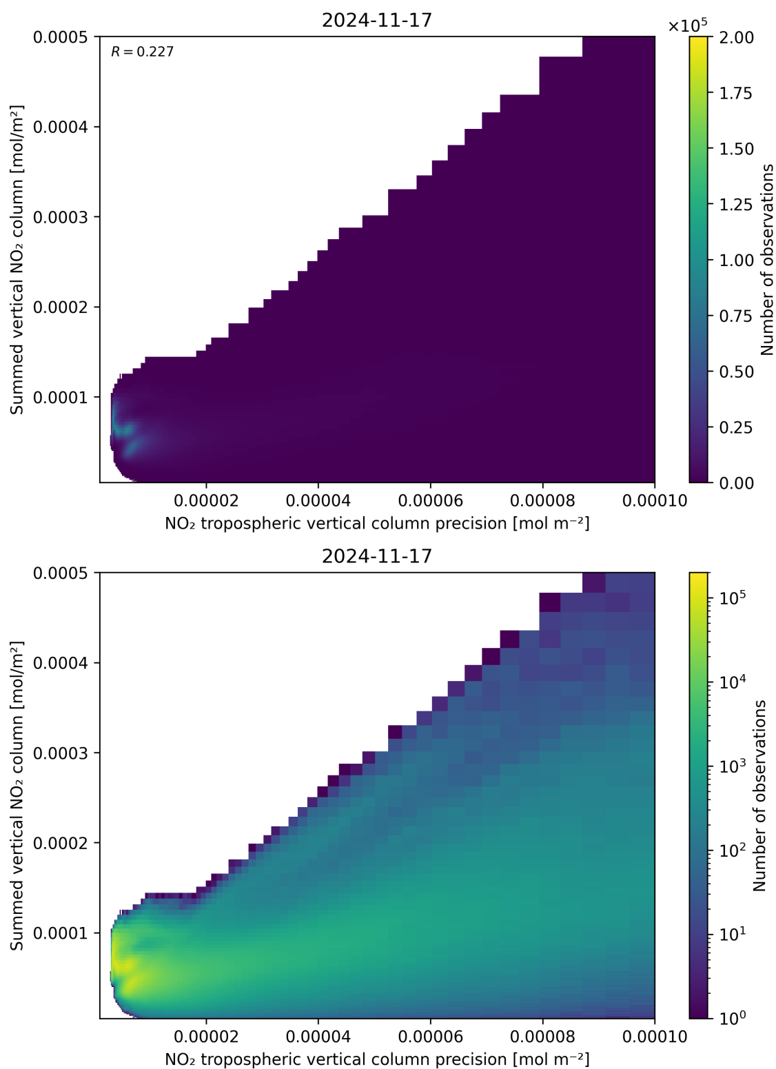
Figure 136: Scatter density plot of “NO 2 tropospheric vertical column precision” against “Summed vertical NO 2 column” for 2024-11-17 to 2024-11-18.
