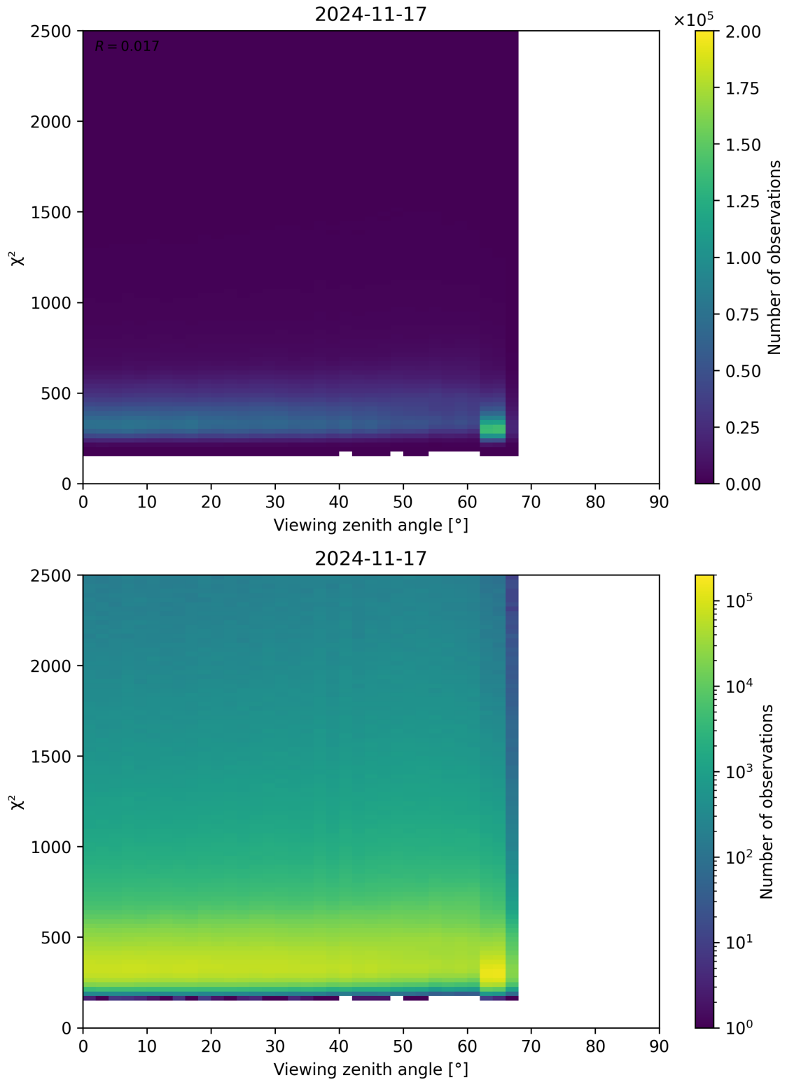
Figure 162: Scatter density plot of “Viewing zenith angle” against “ \chi^2 ” for 2024-11-17 to 2024-11-18.
