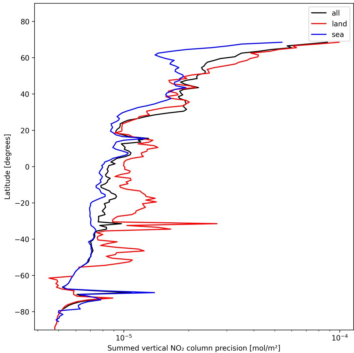
Figure 24: Zonal average of “Summed vertical NO 2 column precision” for 2024-11-17 to 2024-11-18.
