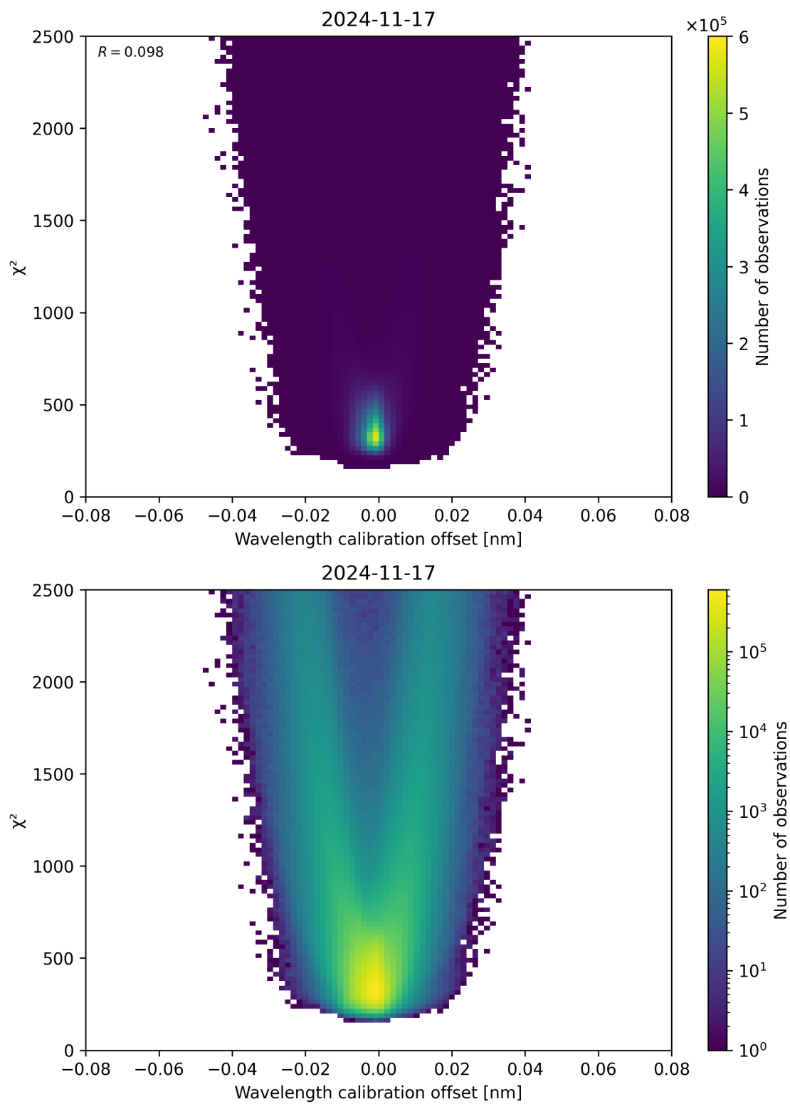
Figure 175: Scatter density plot of “Wavelength calibration offset” against “ \chi^2 ” for 2024-11-17 to 2024-11-18.
