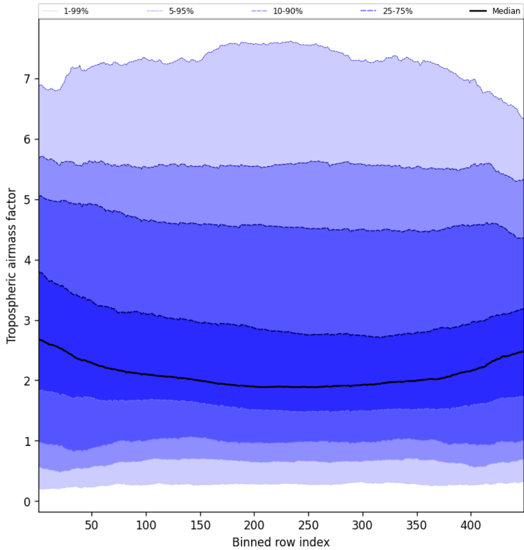
Figure 48: Along track statistics of “Tropospheric airmass factor” for 2024-11-17 to 2024-11-18
