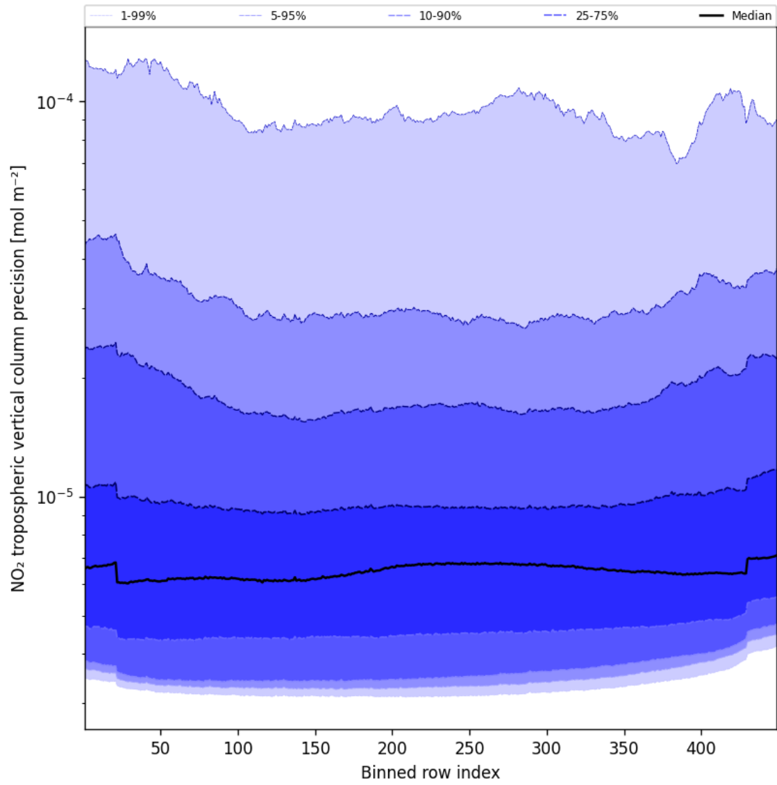
Figure 47: Along track statistics of “NO 2 tropospheric vertical column precision” for 2024-11-17 to 2024-11-18
