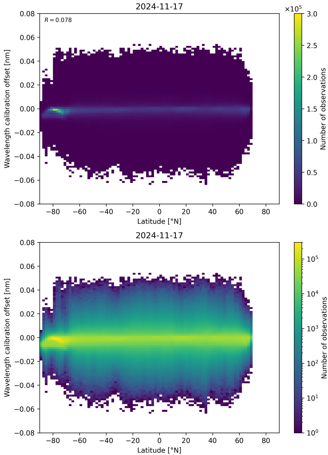
Figure 95: Scatter density plot of “Latitude” against “Wavelength calibration offset” for 2024-11-17 to 2024-11-18.
