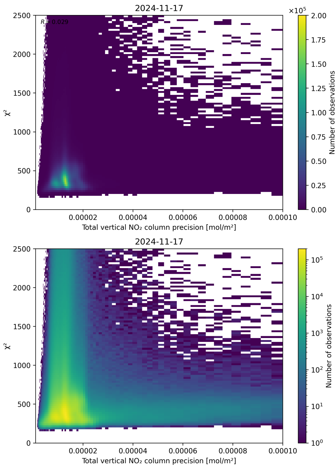
Figure 116: Scatter density plot of “Total vertical NO 2 column precision” against “ \chi^2 ” for 2024-11-17 to 2024-11-18.
