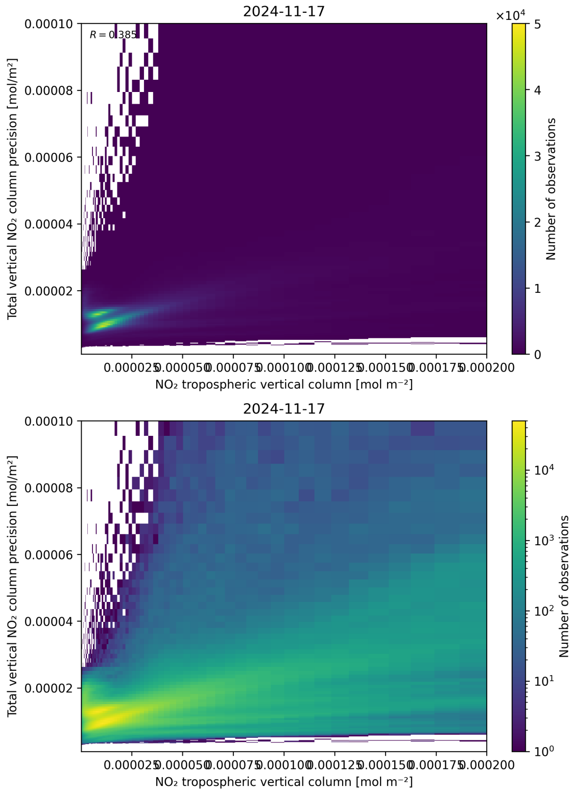
Figure 129: Scatter density plot of “NO 2 tropospheric vertical column” against “Total vertical NO 2 column precision” for 2024-11-17 to 2024-11-18.
