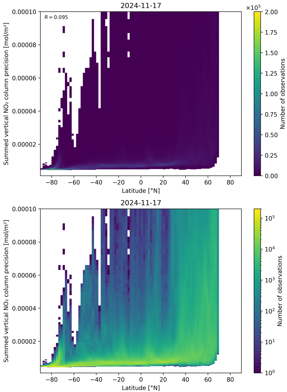
Figure 89: Scatter density plot of “Latitude” against “Summed vertical NO 2 column precision” for 2024-11-17 to 2024-11-18.
