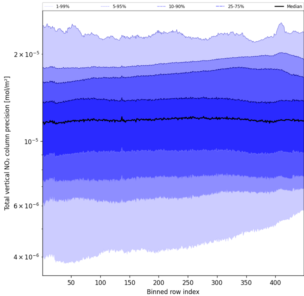
Figure 56: Along track statistics of “Total vertical NO 2 column precision” for 2024-11-17 to 2024-11-18
