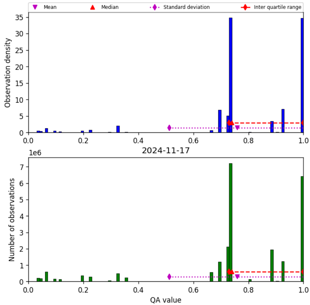
Figure 28: Histogram of “QA value” for 2024-11-17 to 2024-11-18
