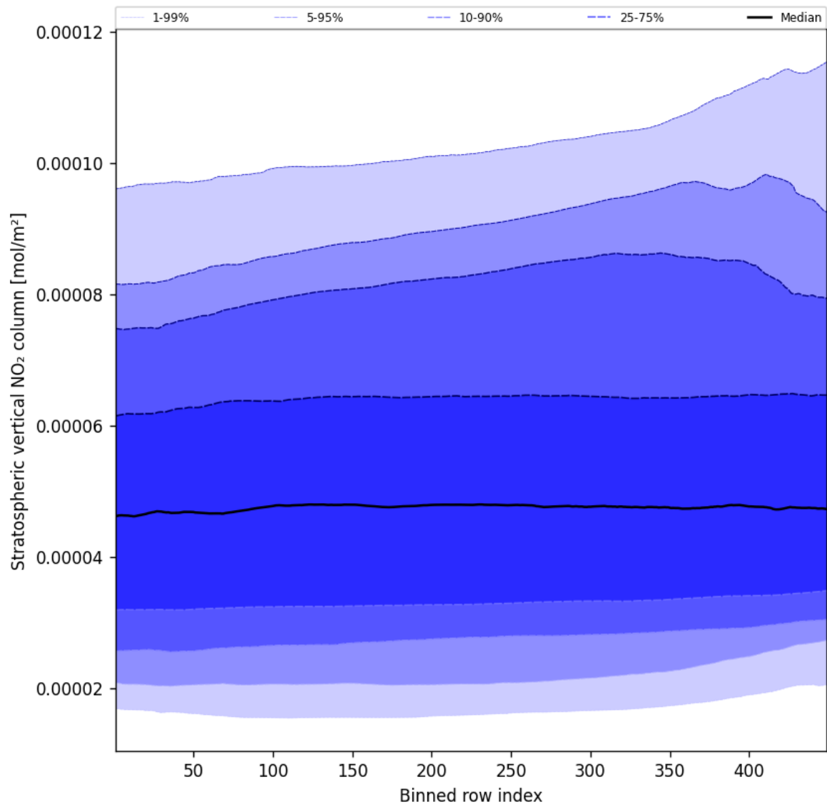
Figure 53: Along track statistics of “Stratospheric vertical NO 2 column” for 2024-11-17 to 2024-11-18
