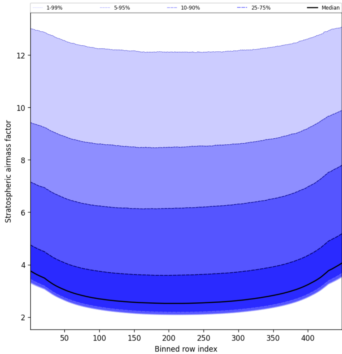
Figure 61: Along track statistics of “Stratospheric airmass factor” for 2024-11-17 to 2024-11-18
