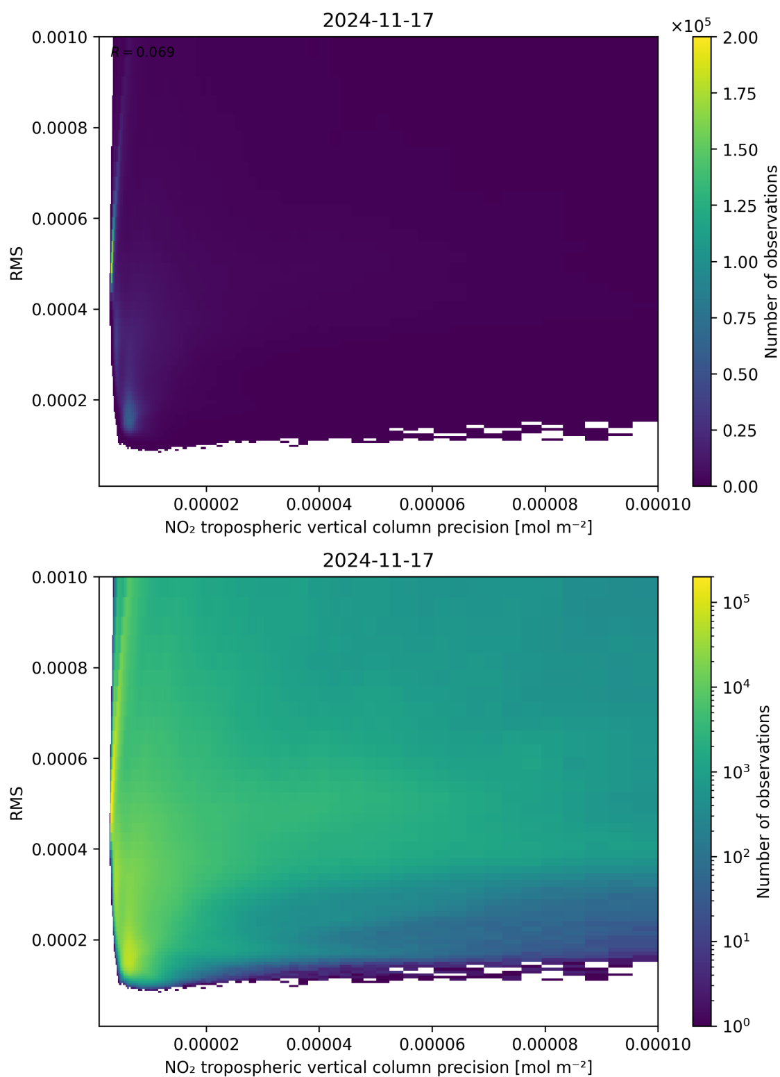
Figure 140: Scatter density plot of “NO 2 tropospheric vertical column precision” against “RMS” for 2024-11-17 to 2024-11-18.
