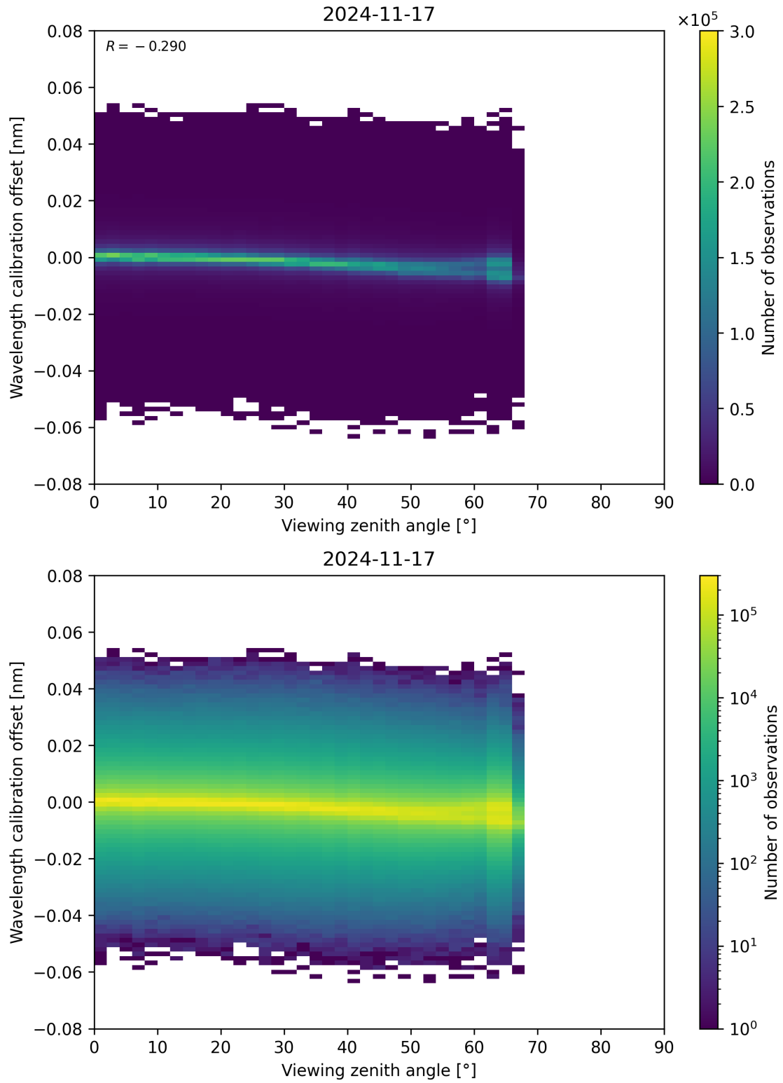
Figure 173: Scatter density plot of “Viewing zenith angle” against “Wavelength calibration offset” for 2024-11-17 to 2024-11-18.
