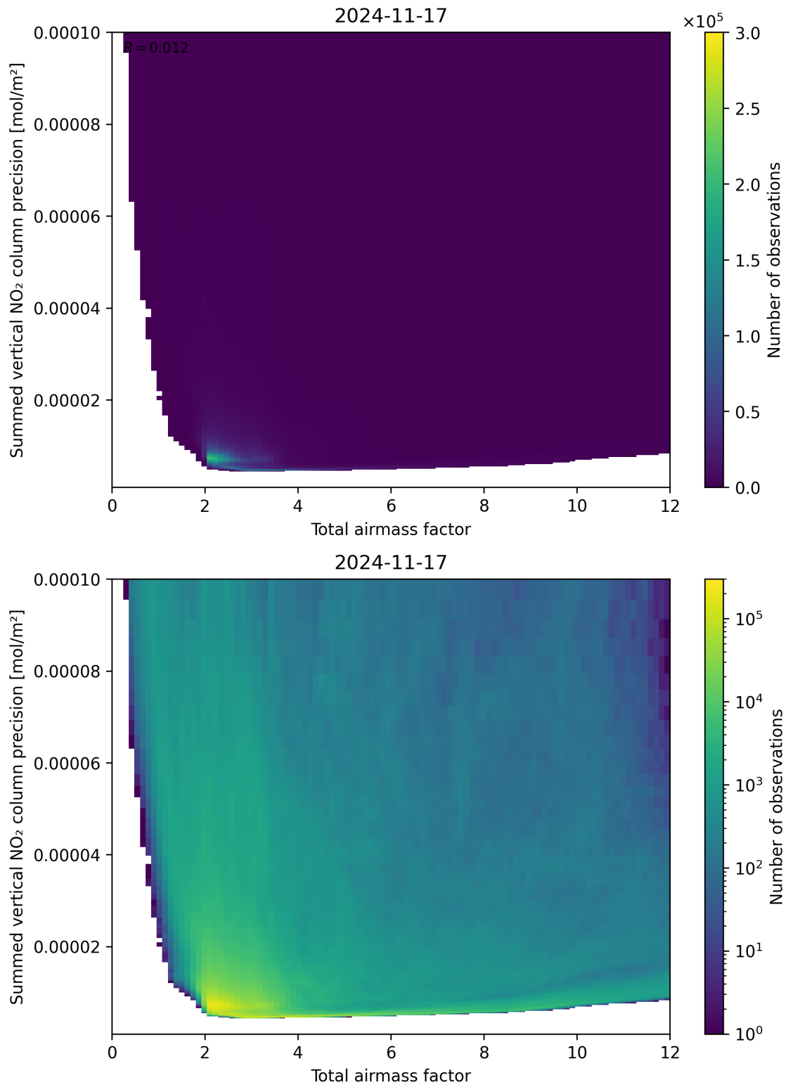
Figure 66: Scatter density plot of “Total airmass factor” against “Summed vertical NO 2 column precision” for 2024-11-17 to 2024-11-18.
