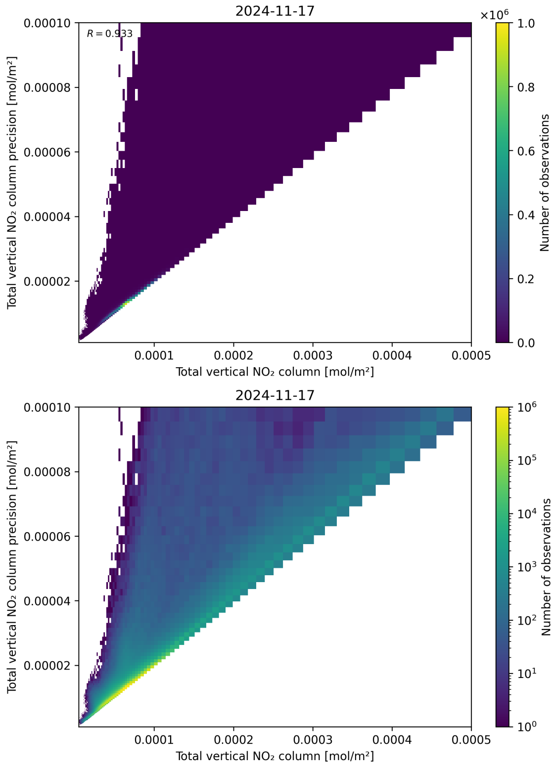
Figure 114: Scatter density plot of “Total vertical NO 2 column” against “Total vertical NO 2 column precision” for 2024-11-17 to 2024-11-18.
