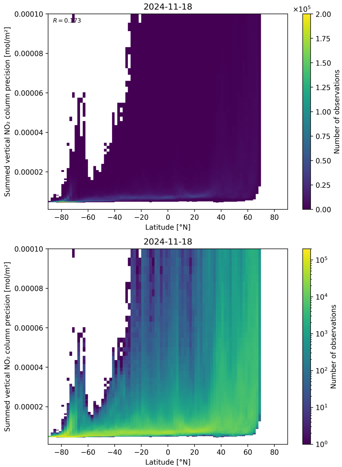
Figure 89: Scatter density plot of “Latitude” against “Summed vertical NO 2 column precision” for 2024-11-17 to 2024-11-19.
