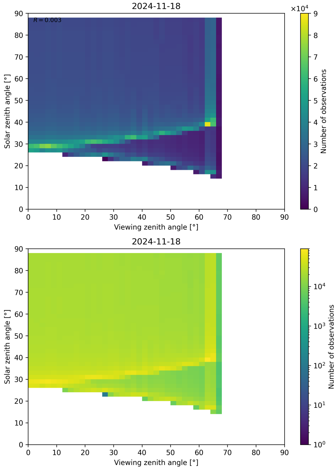
Figure 172: Scatter density plot of “Viewing zenith angle” against “Solar zenith angle” for 2024-11-17 to 2024-11-19.
