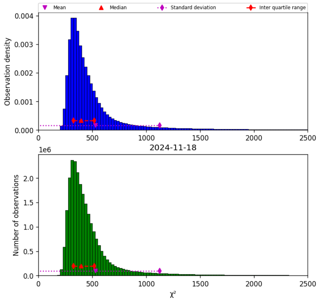
Figure 42: Histogram of “ \chi^2 ” for 2024-11-17 to 2024-11-19
