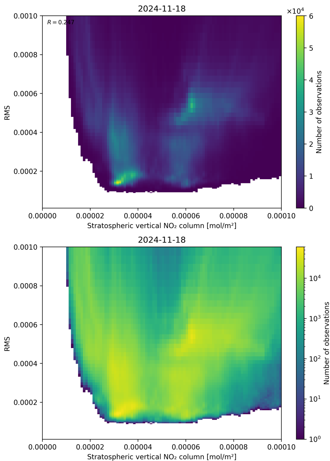
Figure 102: Scatter density plot of “Stratospheric vertical NO 2 column” against “RMS” for 2024-11-17 to 2024-11-19.
