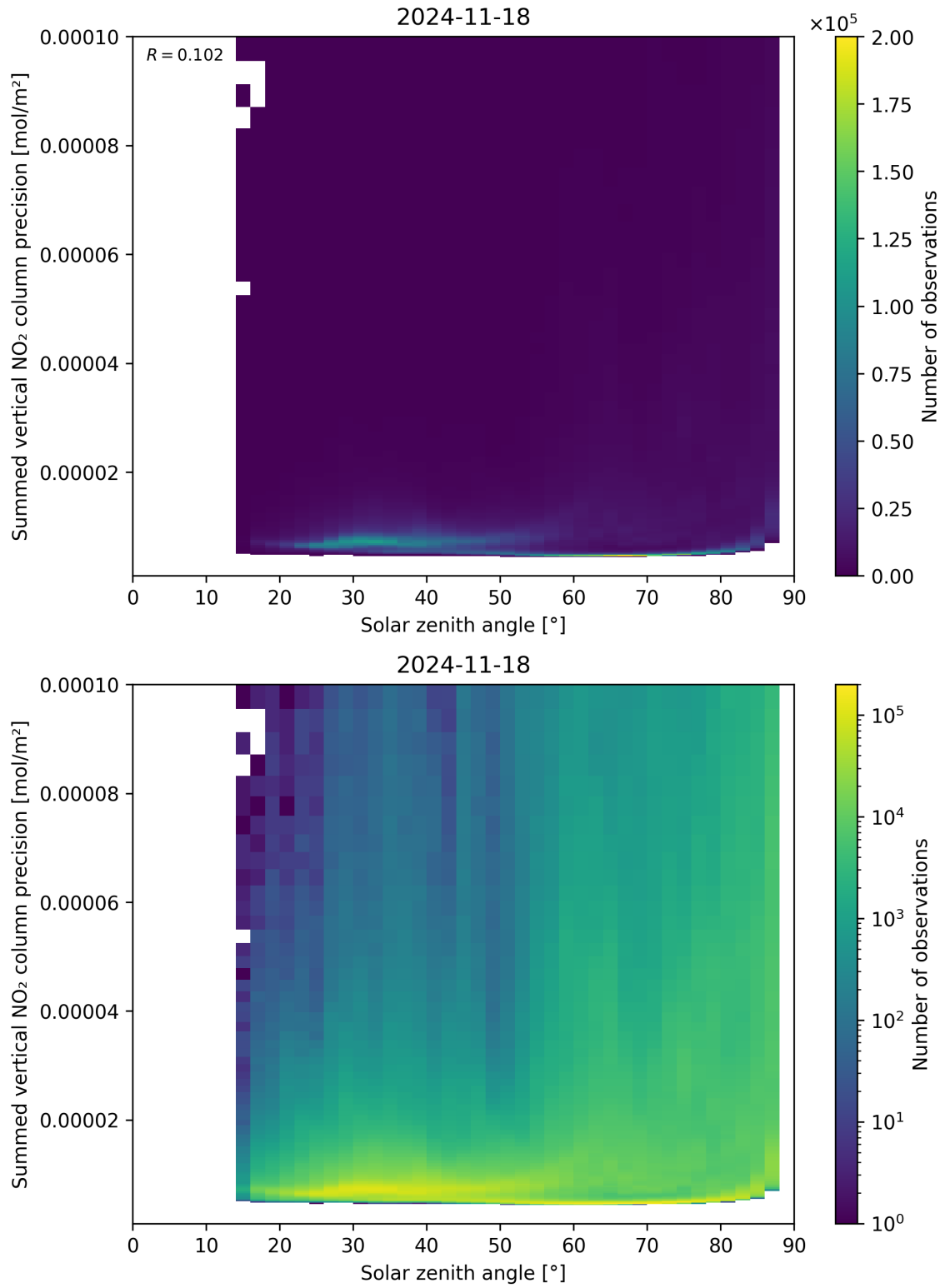
Figure 152: Scatter density plot of “Solar zenith angle” against “Summed vertical NO 2 column precision” for 2024-11-17 to 2024-11-19.
