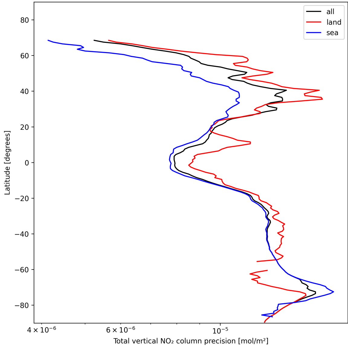
Figure 22: Zonal average of “Total vertical NO 2 column precision” for 2024-11-17 to 2024-11-19.
