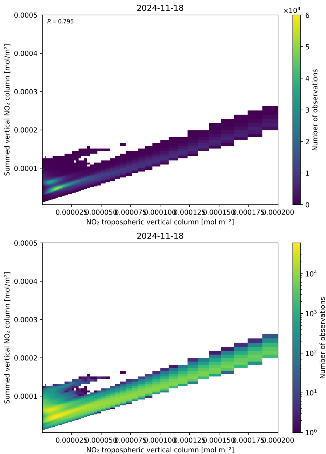
Figure 126: Scatter density plot of “NO 2 tropospheric vertical column” against “Summed vertical NO 2 column” for 2024-11-17 to 2024-11-19.
