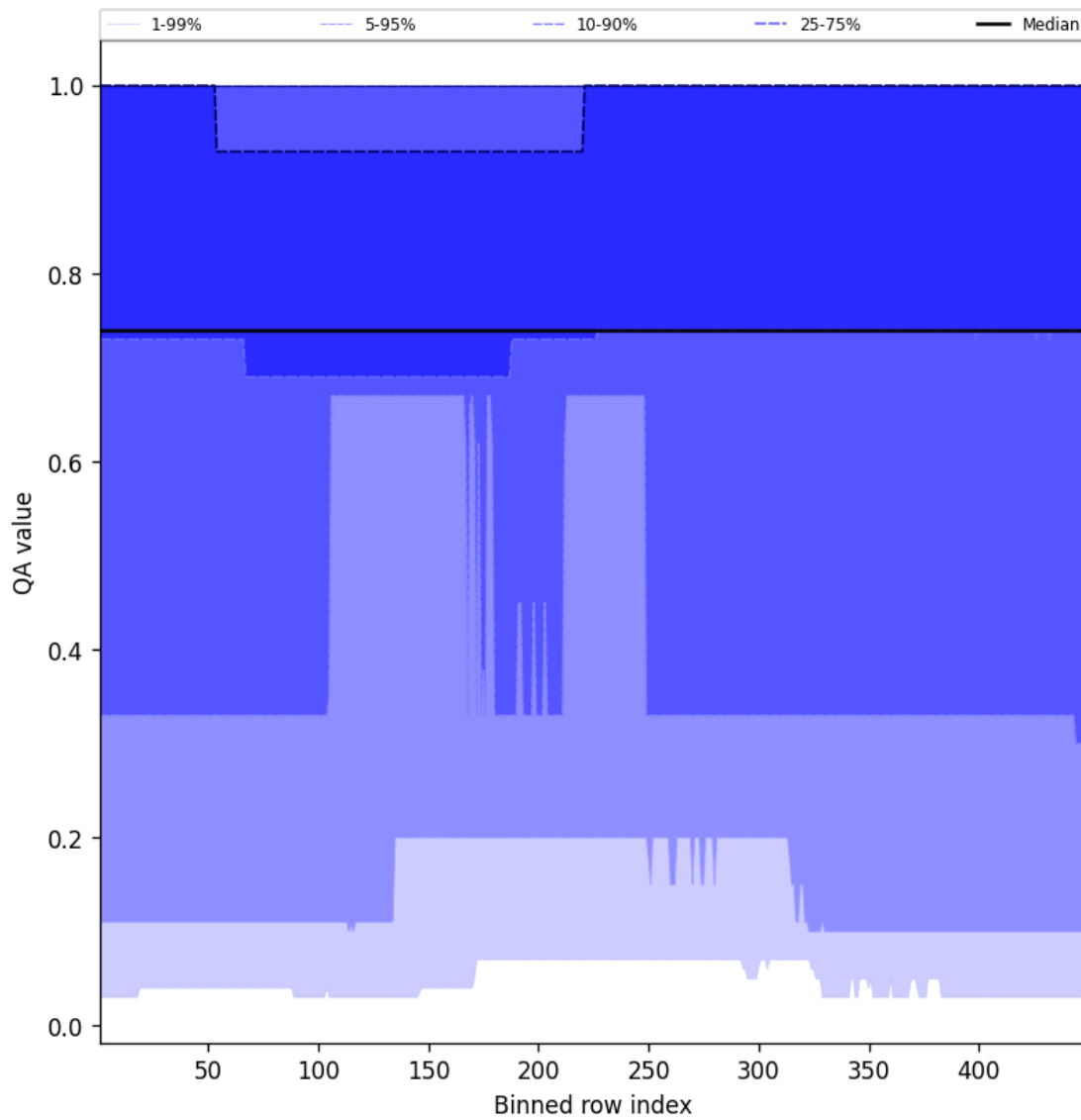
Figure 45: Along track statistics of “QA value” for 2024-11-17 to 2024-11-19
