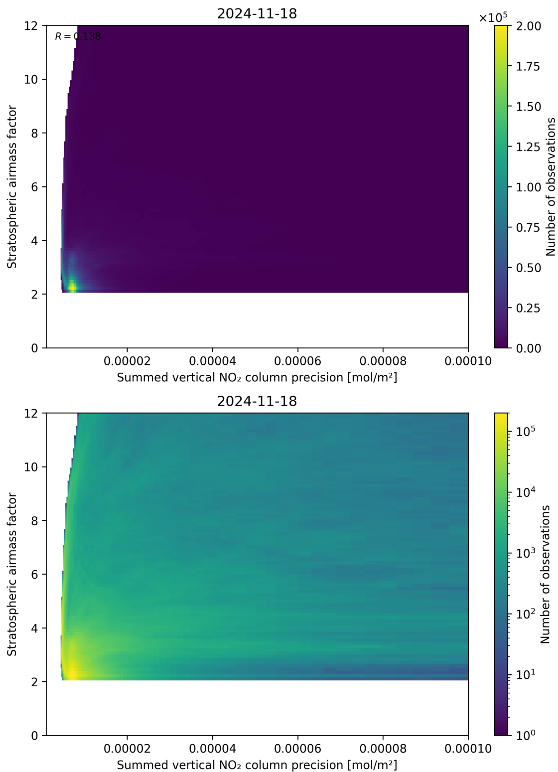
Figure 106: Scatter density plot of “Summed vertical NO 2 column precision” against “Stratospheric airmass factor” for 2024-11-17 to 2024-11-19.
