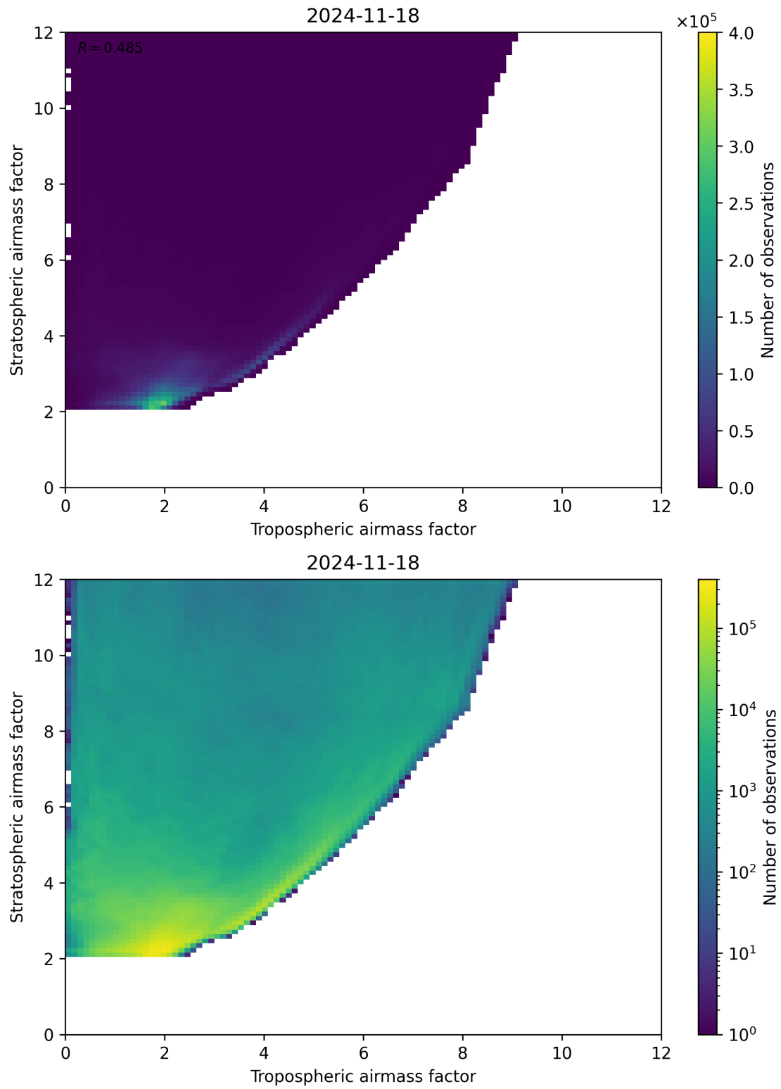
Figure 71: Scatter density plot of “Tropospheric airmass factor” against “Stratospheric airmass factor” for 2024-11-17 to 2024-11-19.
