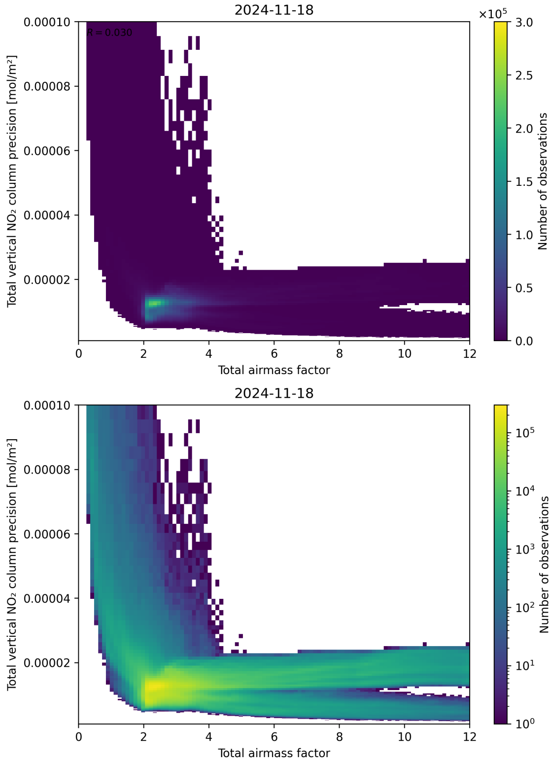
Figure 68: Scatter density plot of “Total airmass factor” against “Total vertical NO 2 column precision” for 2024-11-17 to 2024-11-19.
