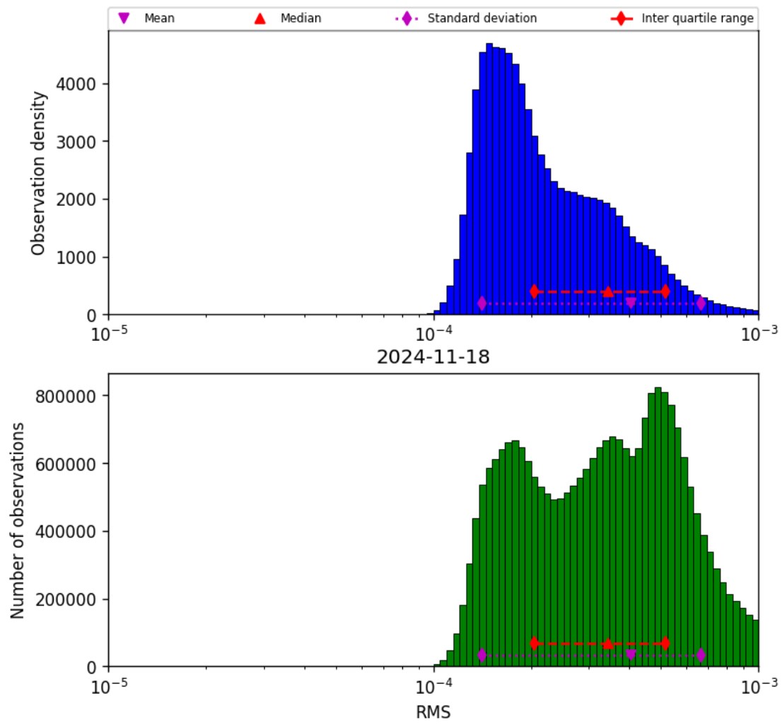
Figure 43: Histogram of “RMS” for 2024-11-17 to 2024-11-19
