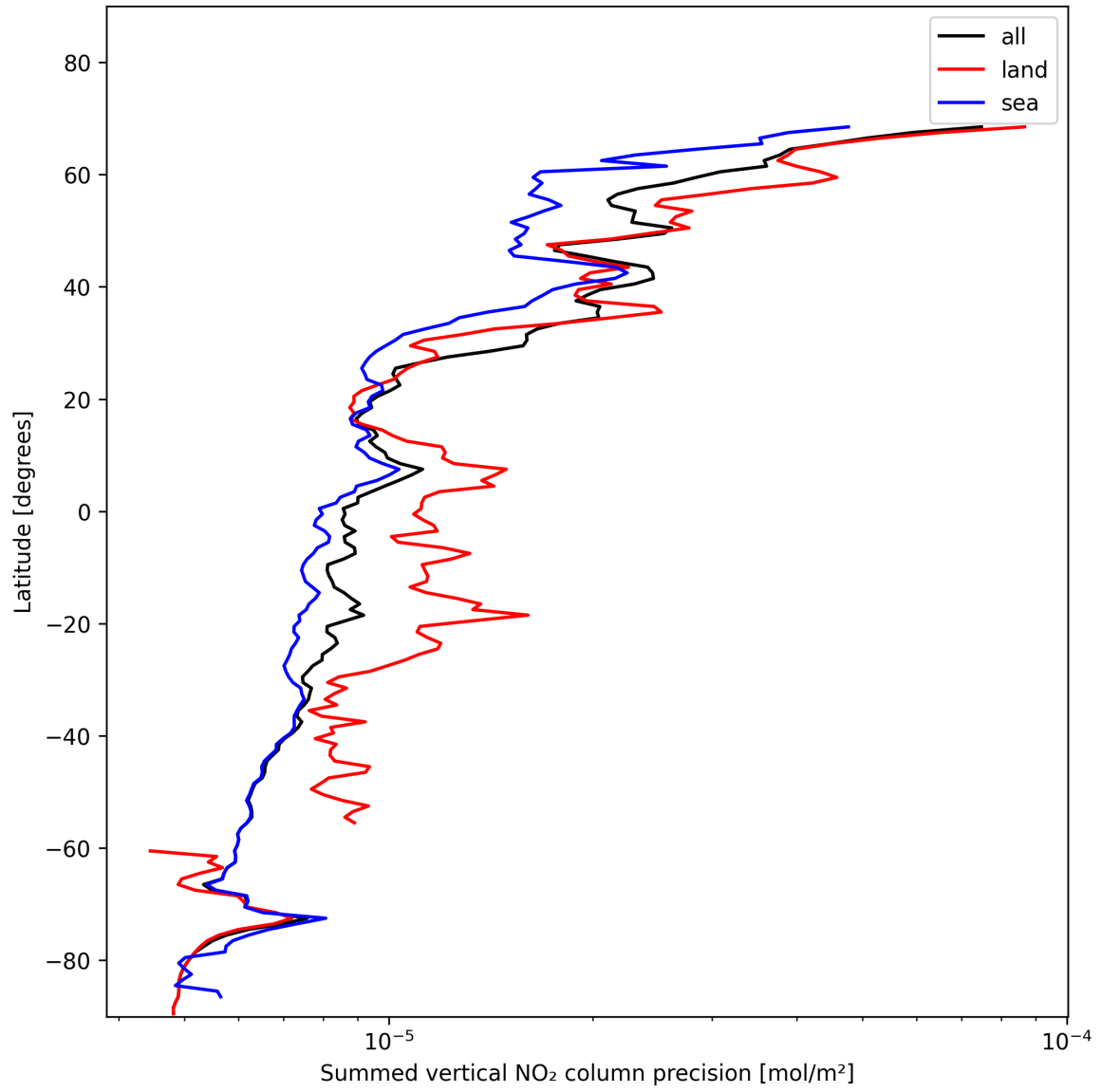
Figure 24: Zonal average of “Summed vertical NO 2 column precision” for 2024-11-17 to 2024-11-19.
