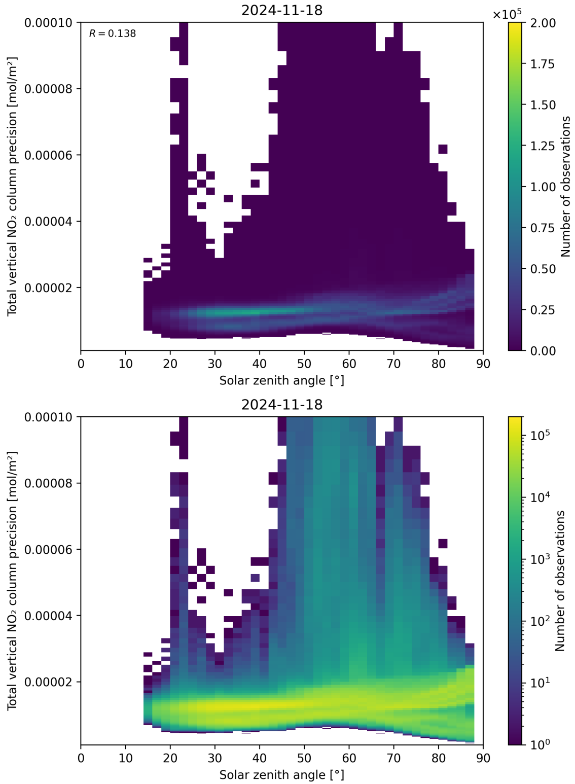
Figure 154: Scatter density plot of “Solar zenith angle” against “Total vertical NO 2 column precision” for 2024-11-17 to 2024-11-19.
