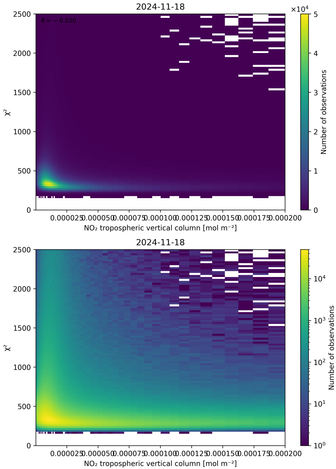
Figure 124: Scatter density plot of “NO 2 tropospheric vertical column” against “ \chi^2 ” for 2024-11-17 to 2024-11-19.
