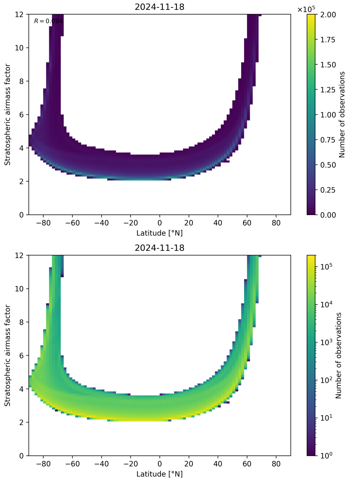
Figure 83: Scatter density plot of “Latitude” against “Stratospheric airmass factor” for 2024-11-17 to 2024-11-19.
