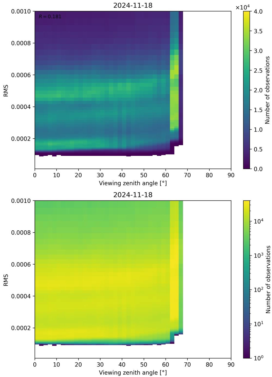
Figure 171: Scatter density plot of “Viewing zenith angle” against “RMS” for 2024-11-17 to 2024-11-19.
