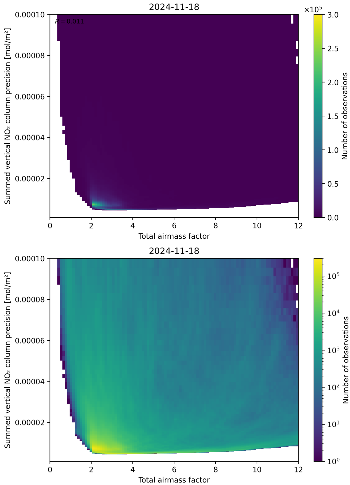
Figure 66: Scatter density plot of “Total airmass factor” against “Summed vertical NO 2 column precision” for 2024-11-17 to 2024-11-19.
