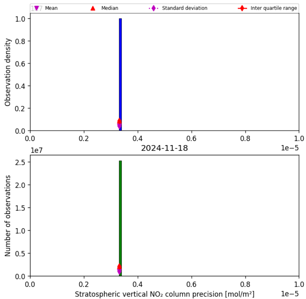
Figure 37: Histogram of “Stratospheric vertical NO 2 column precision” for 2024-11-17 to 2024-11-19
