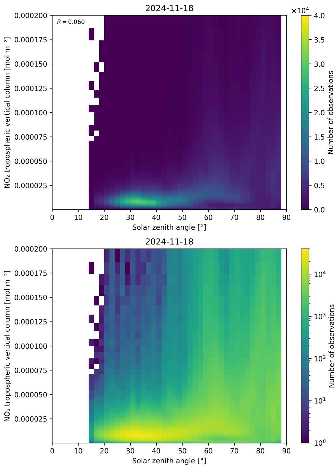
Figure 155: Scatter density plot of “Solar zenith angle” against “NO 2 tropospheric vertical column” for 2024-11-17 to 2024-11-19.
