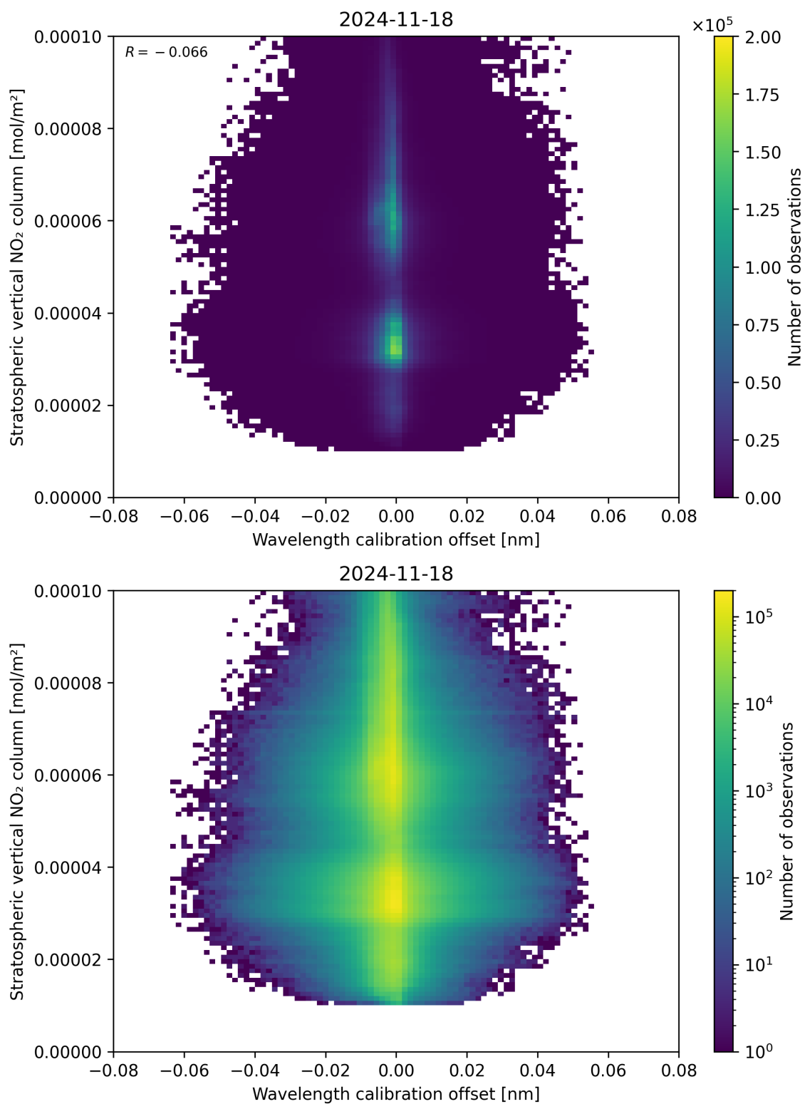
Figure 176: Scatter density plot of “Wavelength calibration offset” against “Stratospheric vertical NO 2 column” for 2024-11-17 to 2024-11-19.
