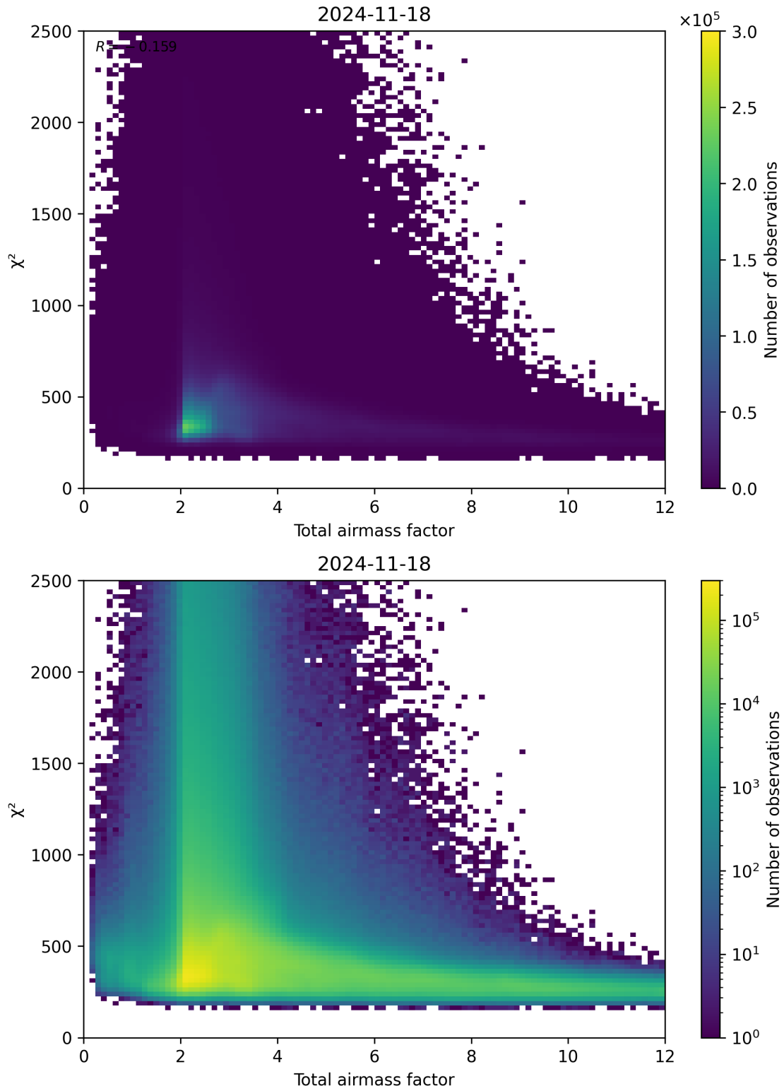
Figure 63: Scatter density plot of “Total airmass factor” against “ \chi^2 ” for 2024-11-17 to 2024-11-19.
