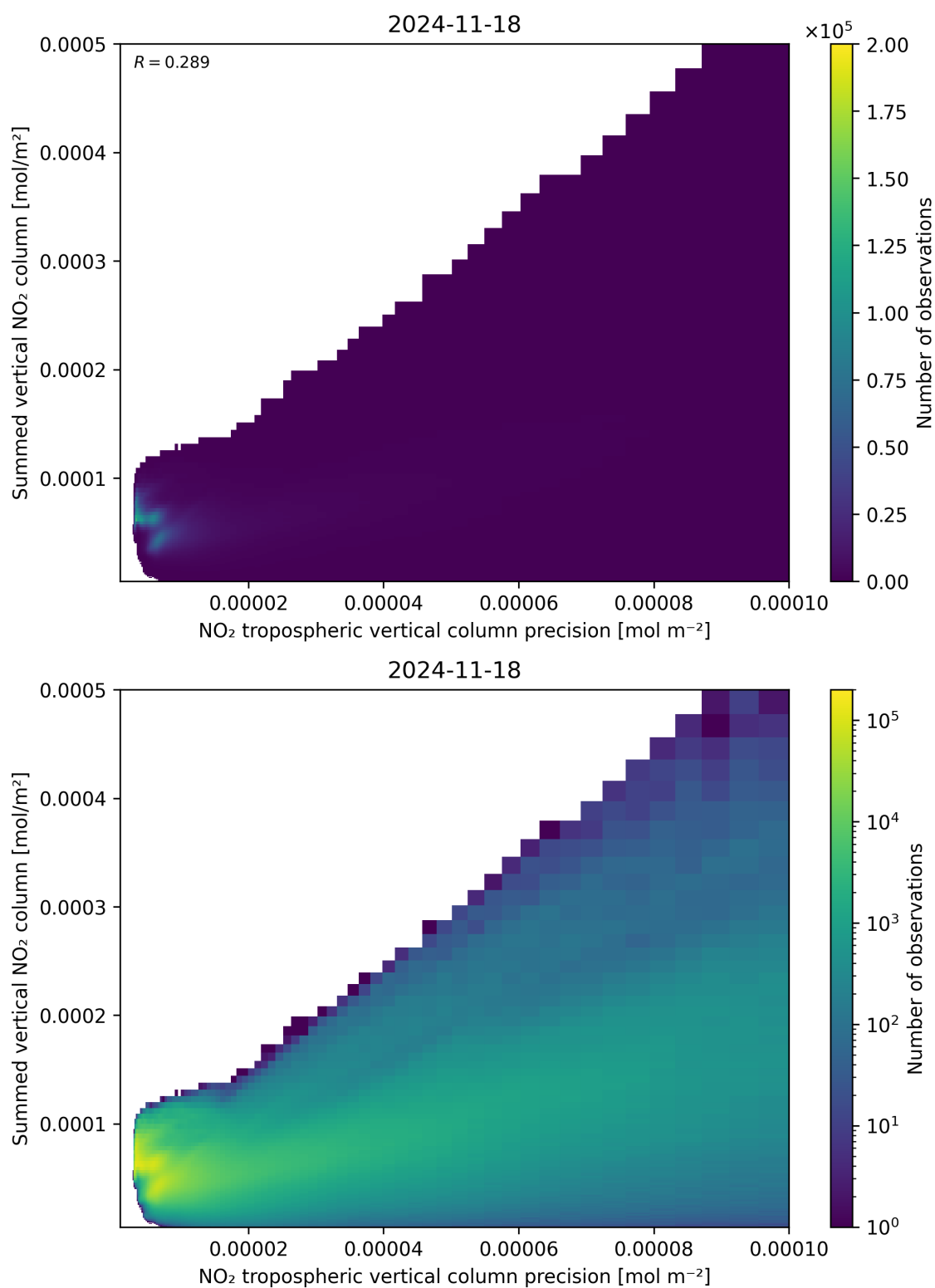
Figure 136: Scatter density plot of “NO 2 tropospheric vertical column precision” against “Summed vertical NO 2 column” for 2024-11-17 to 2024-11-19.
