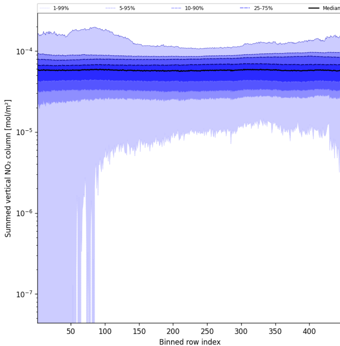
Figure 57: Along track statistics of “Summed vertical NO 2 column” for 2024-11-17 to 2024-11-19
