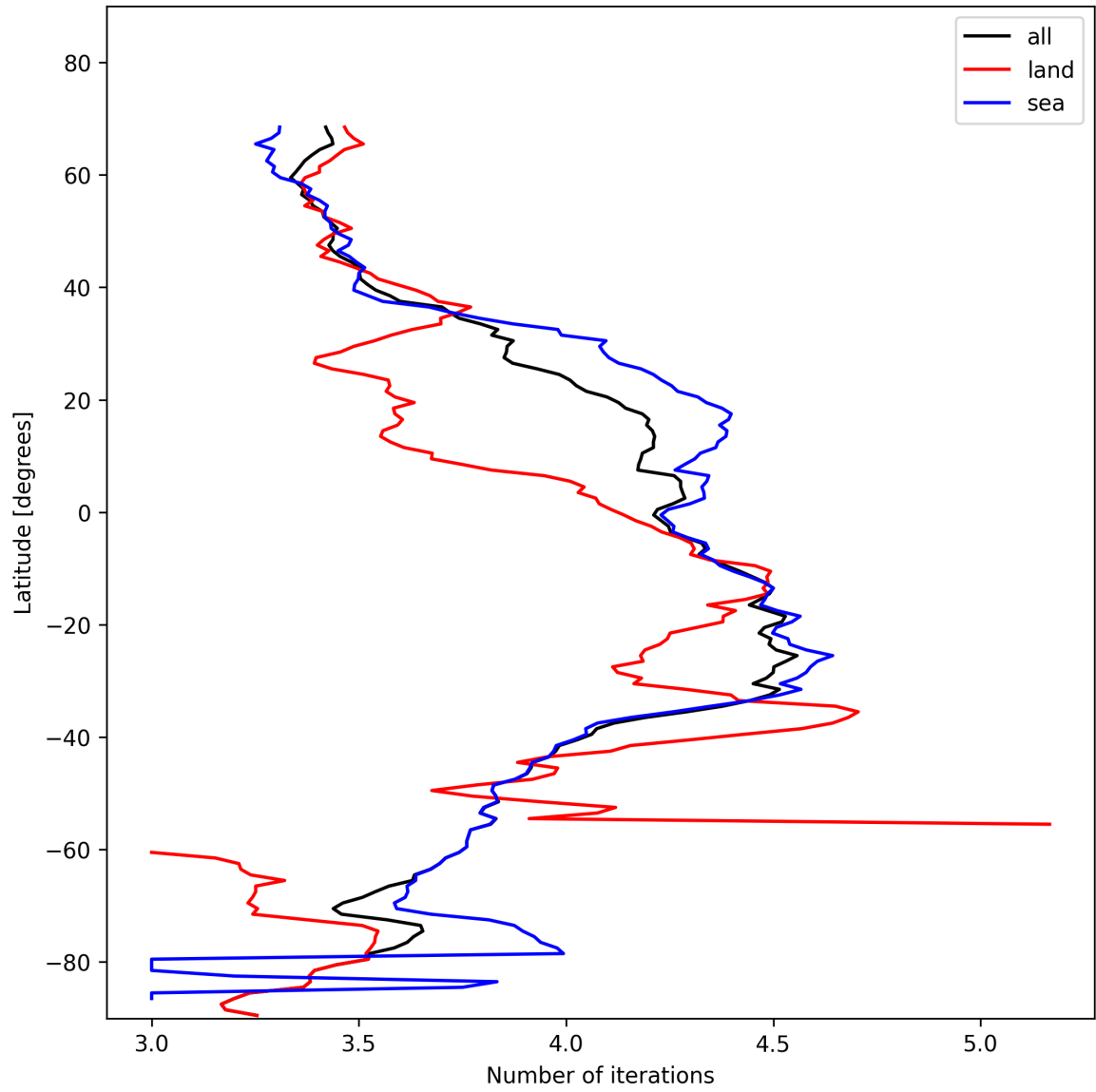
Figure 17: Zonal average of “Number of iterations” for 2024-11-17 to 2024-11-19.
