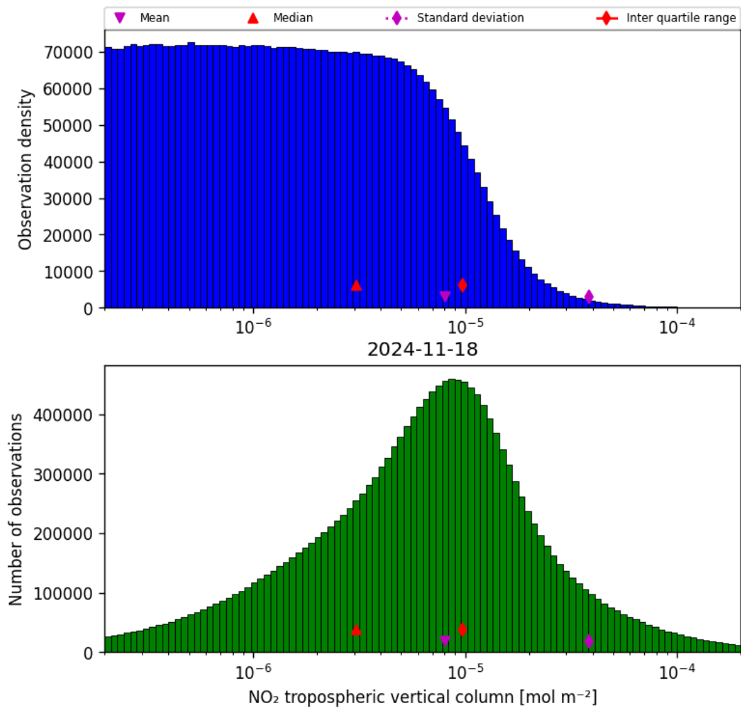
Figure 29: Histogram of “NO 2 tropospheric vertical column” for 2024-11-17 to 2024-11-19
