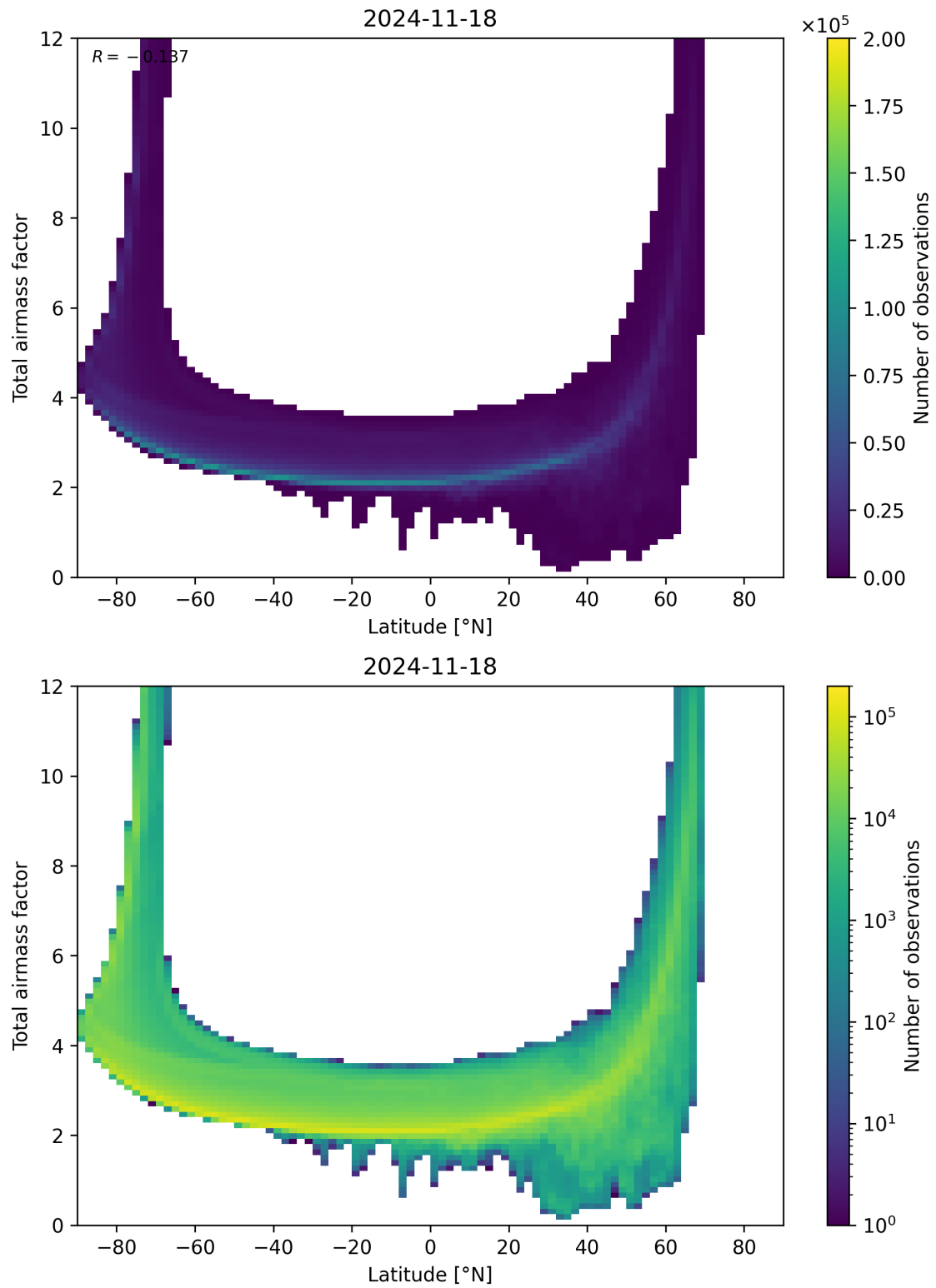
Figure 84: Scatter density plot of “Latitude” against “Total airmass factor” for 2024-11-17 to 2024-11-19.
