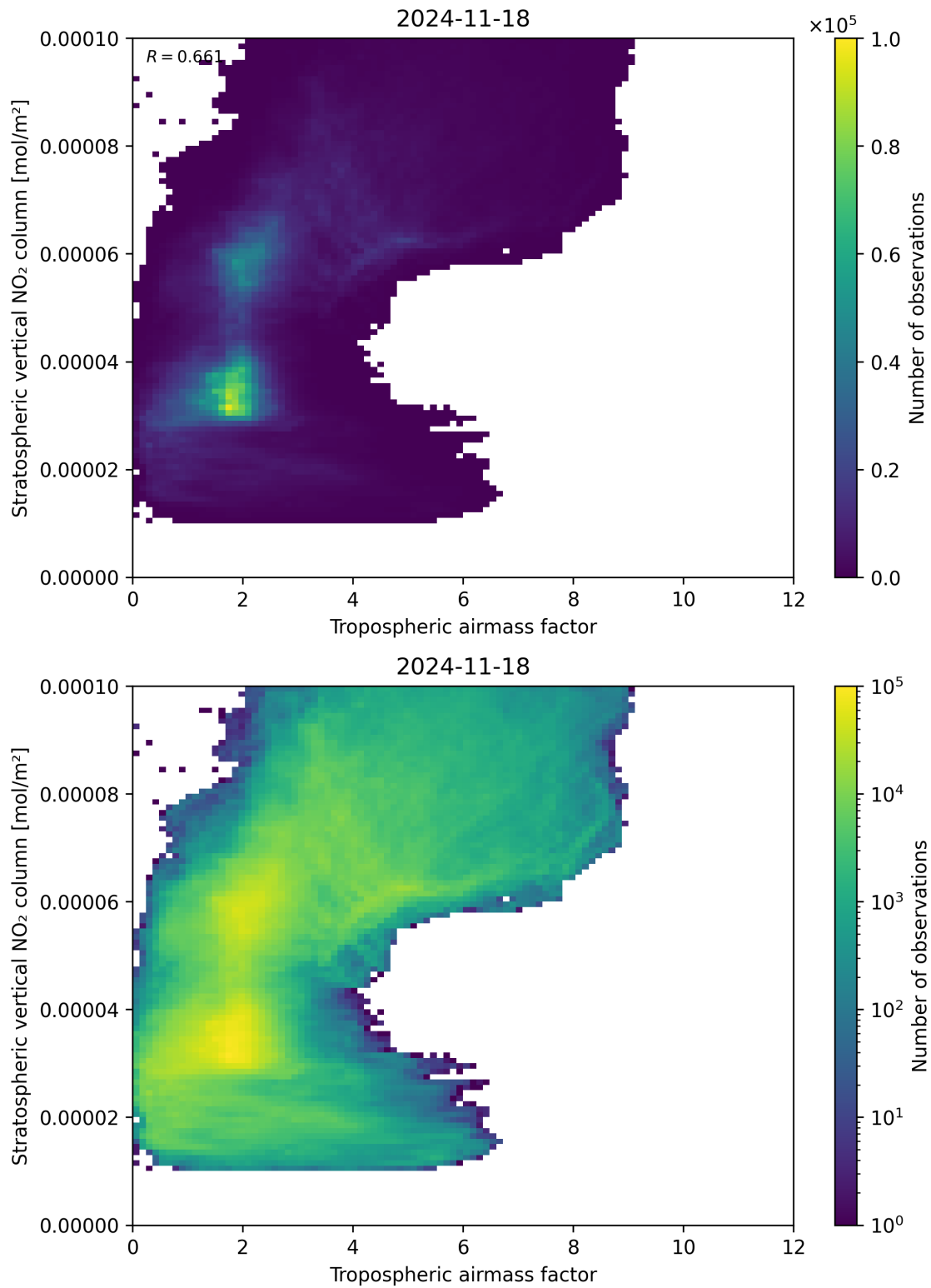
Figure 74: Scatter density plot of “Tropospheric air mass factor” against “Stratospheric vertical NO 2 column” for 2024-11-17 to 2024-11-19.
