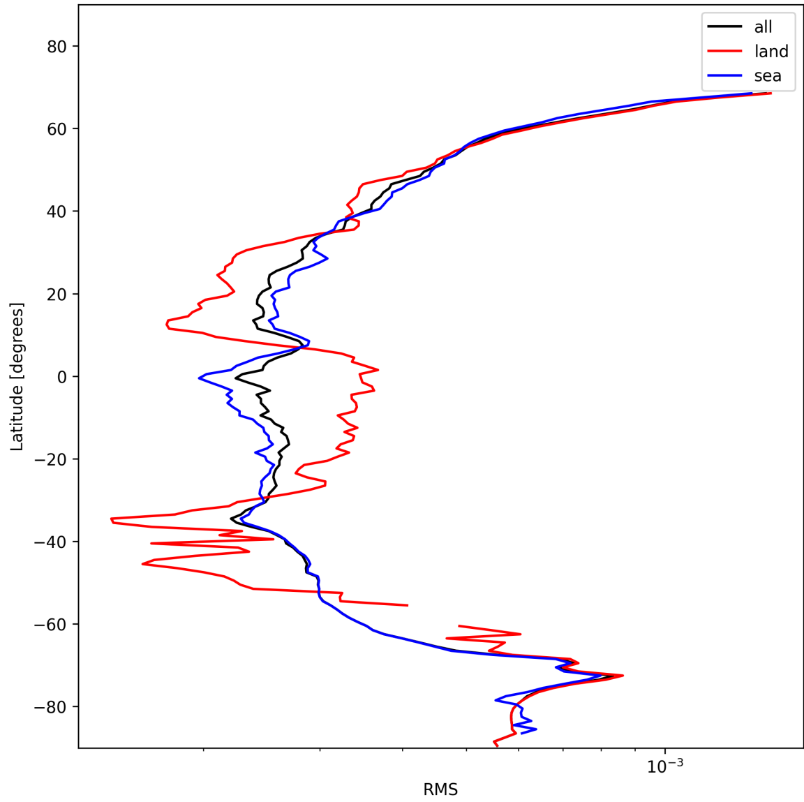
Figure 26: Zonal average of “RMS” for 2024-11-17 to 2024-11-19.
