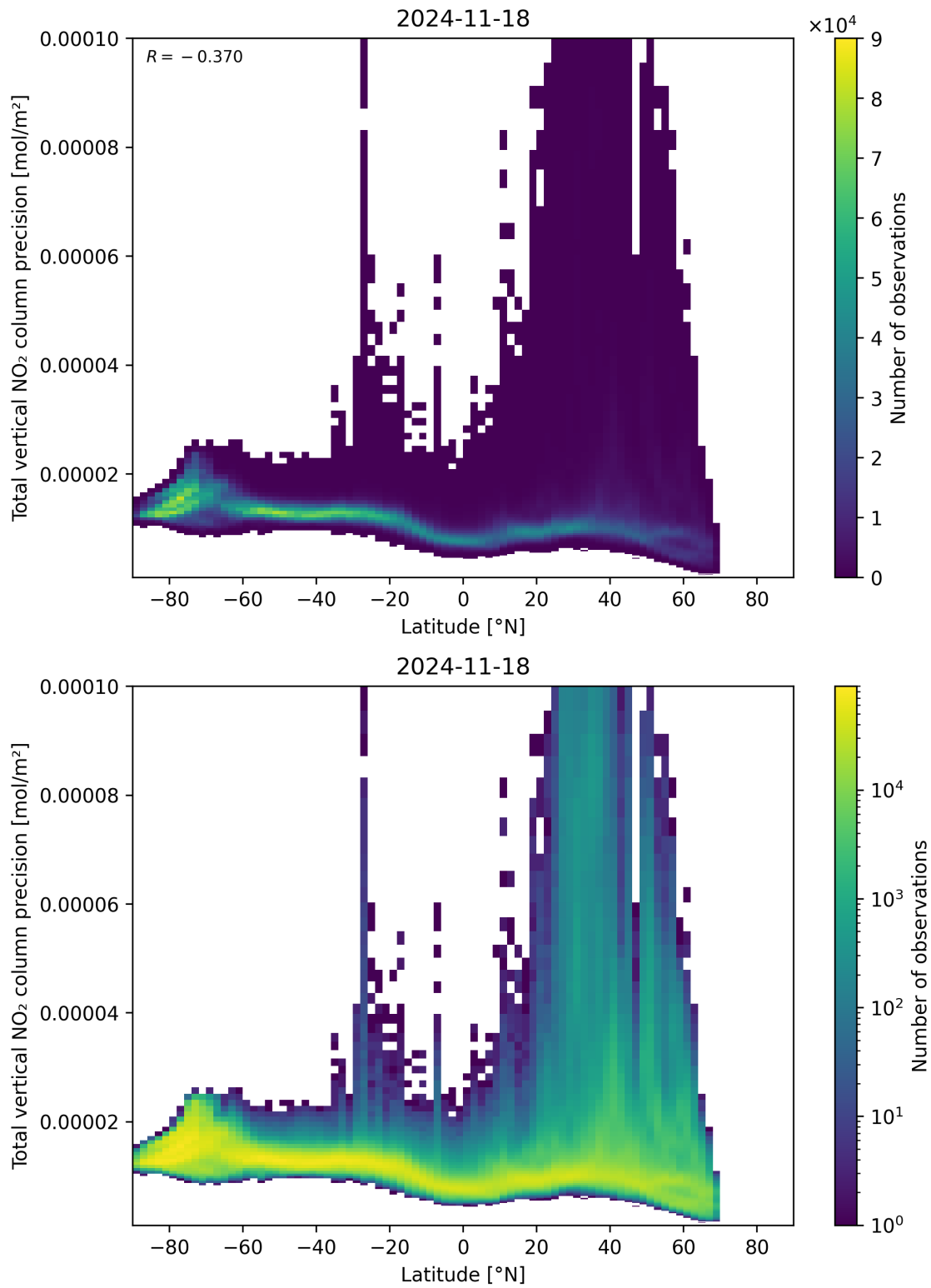
Figure 91: Scatter density plot of “Latitude” against “Total vertical NO 2 column precision” for 2024-11-17 to 2024-11-19.
