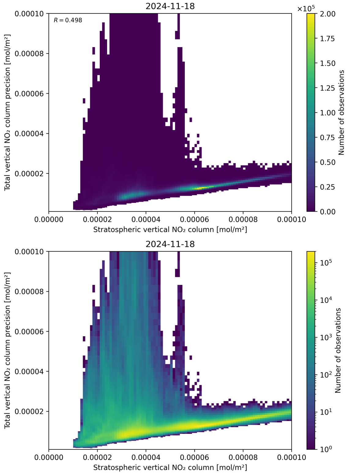
Figure 101: Scatter density plot of “Stratospheric vertical NO 2 column” against “Total vertical NO 2 column precision” for 2024-11-17 to 2024-11-19.
