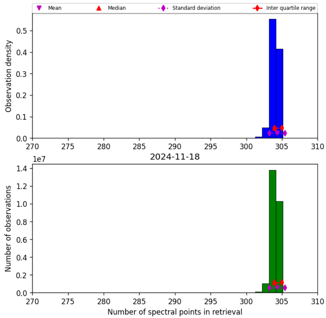
Figure 33: Histogram of “Number of spectral points in retrieval” for 2024-11-17 to 2024-11-19
