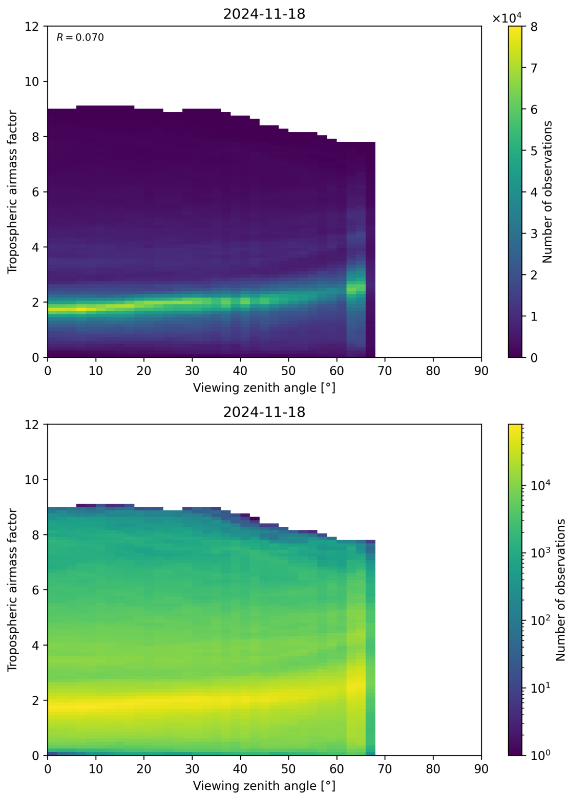
Figure 161: Scatter density plot of “Viewing zenith angle” against “Tropospheric airmass factor” for 2024-11-17 to 2024-11-19.
