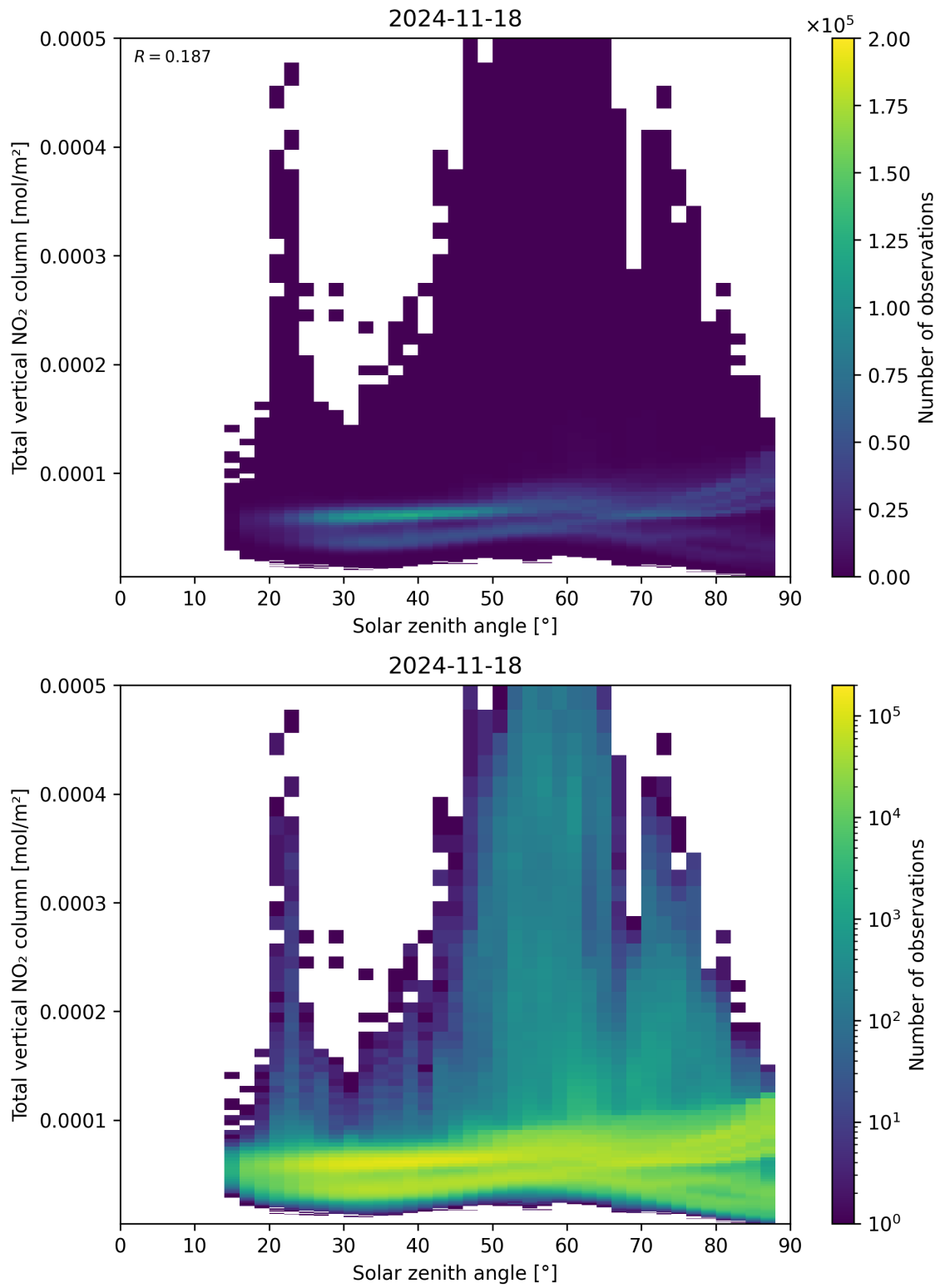
Figure 153: Scatter density plot of “Solar zenith angle” against “Total vertical \text{NO}_2 column” for 2024-11-17 to 2024-11-19.
