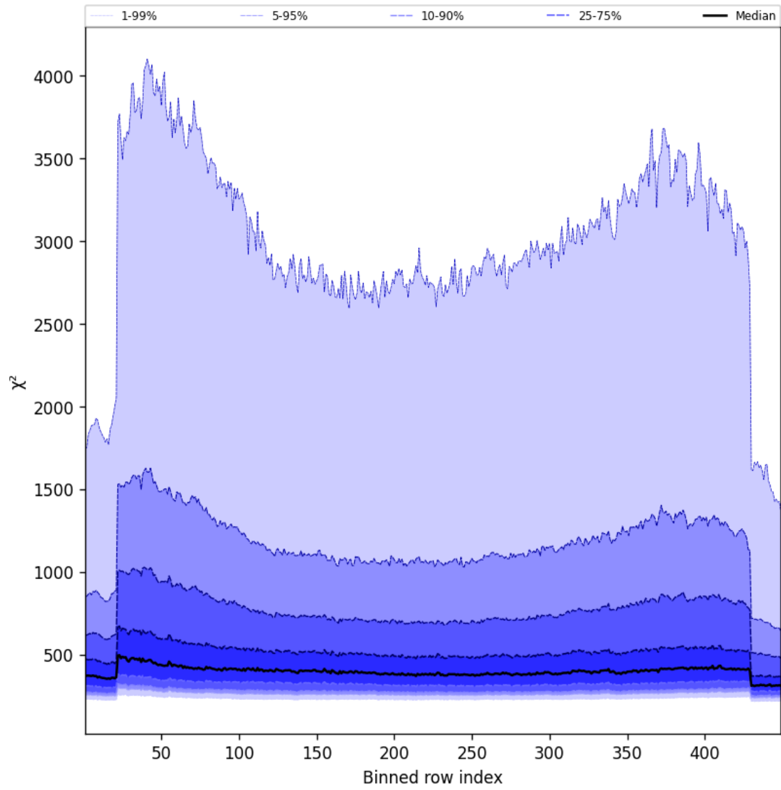
Figure 59: Along track statistics of “ \chi^2 ” for 2024-11-17 to 2024-11-19
