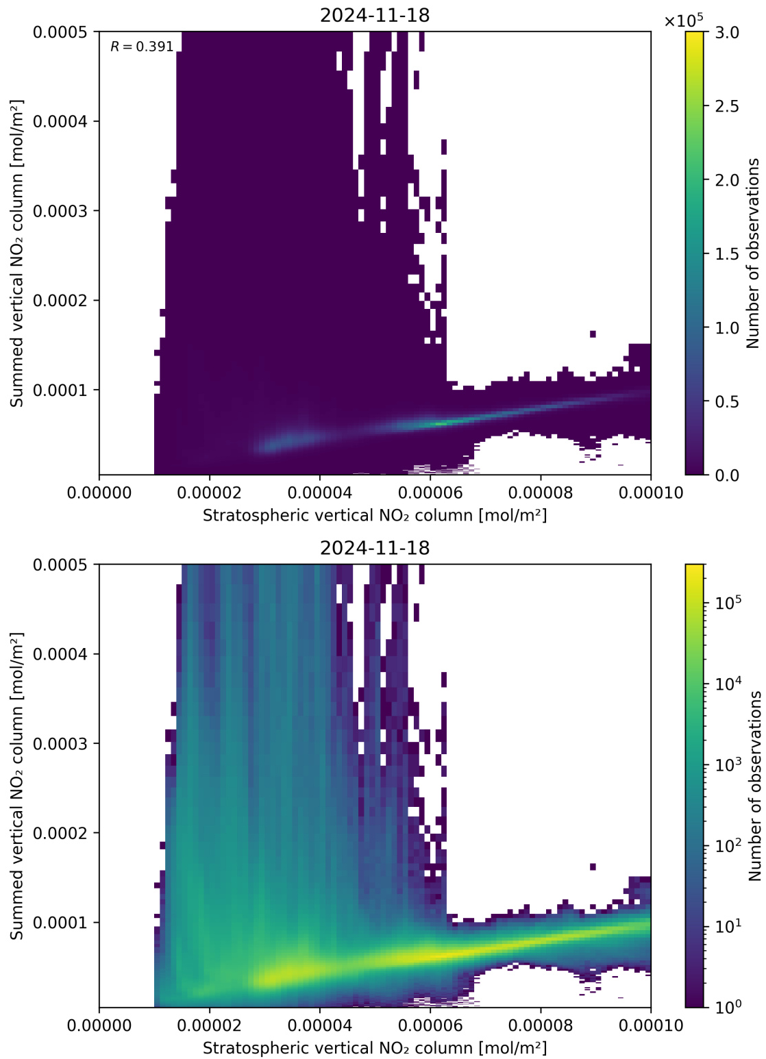
Figure 98: Scatter density plot of “Stratospheric vertical NO 2 column” against “Summed vertical NO 2 column” for 2024-11-17 to 2024-11-19.
