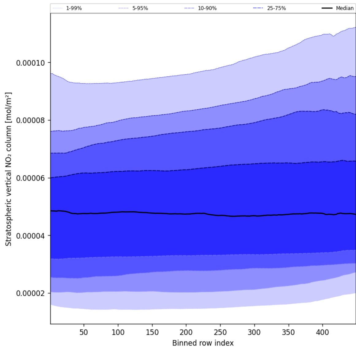
Figure 53: Along track statistics of “Stratospheric vertical NO 2 column” for 2024-11-17 to 2024-11-19
