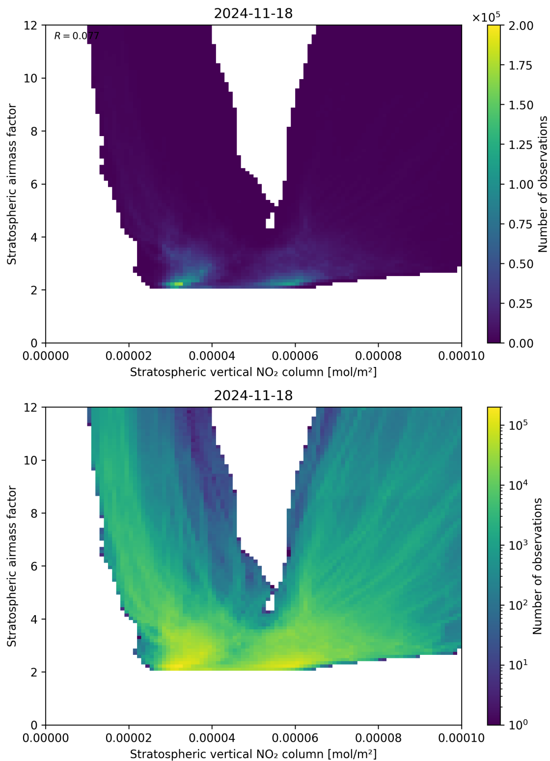
Figure 96: Scatter density plot of “Stratospheric vertical NO 2 column” against “Stratospheric airmass factor” for 2024-11-17 to 2024-11-19.
