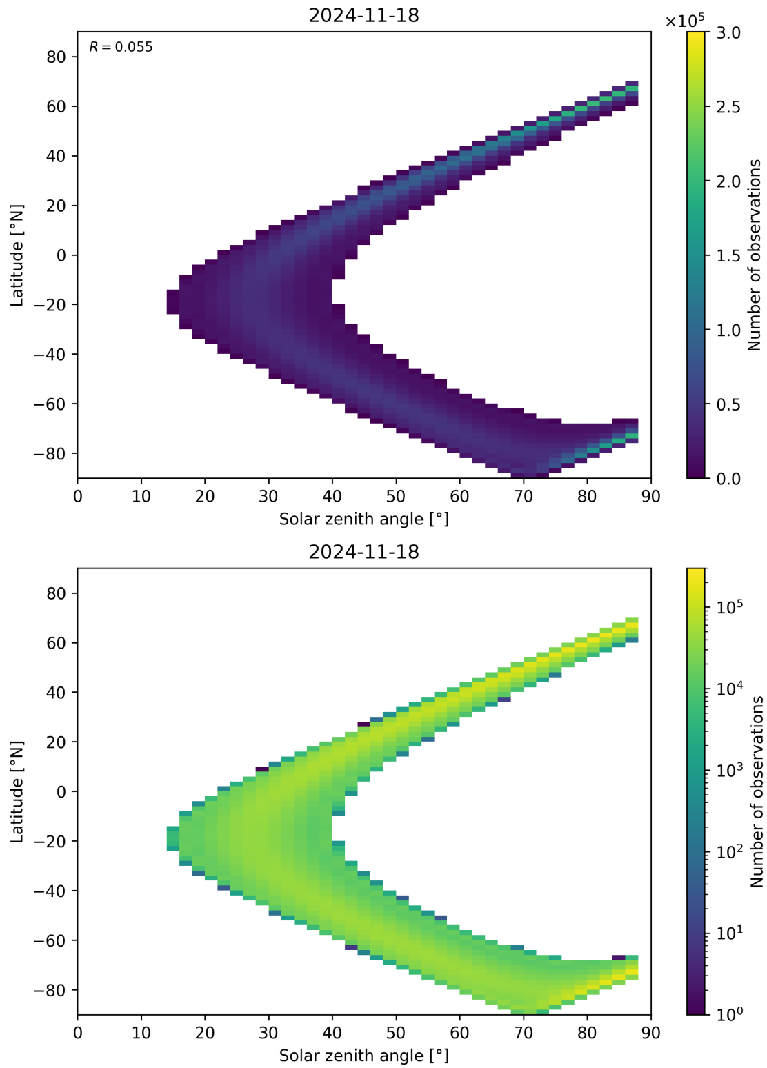
Figure 149: Scatter density plot of “Solar zenith angle” against “Latitude” for 2024-11-17 to 2024-11-19.
