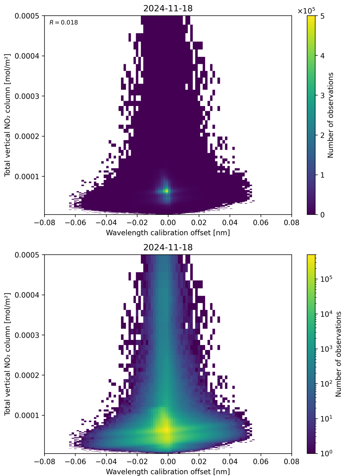
Figure 179: Scatter density plot of “Wavelength calibration offset” against “Total vertical NO 2 column” for 2024-11-17 to 2024-11-19.
