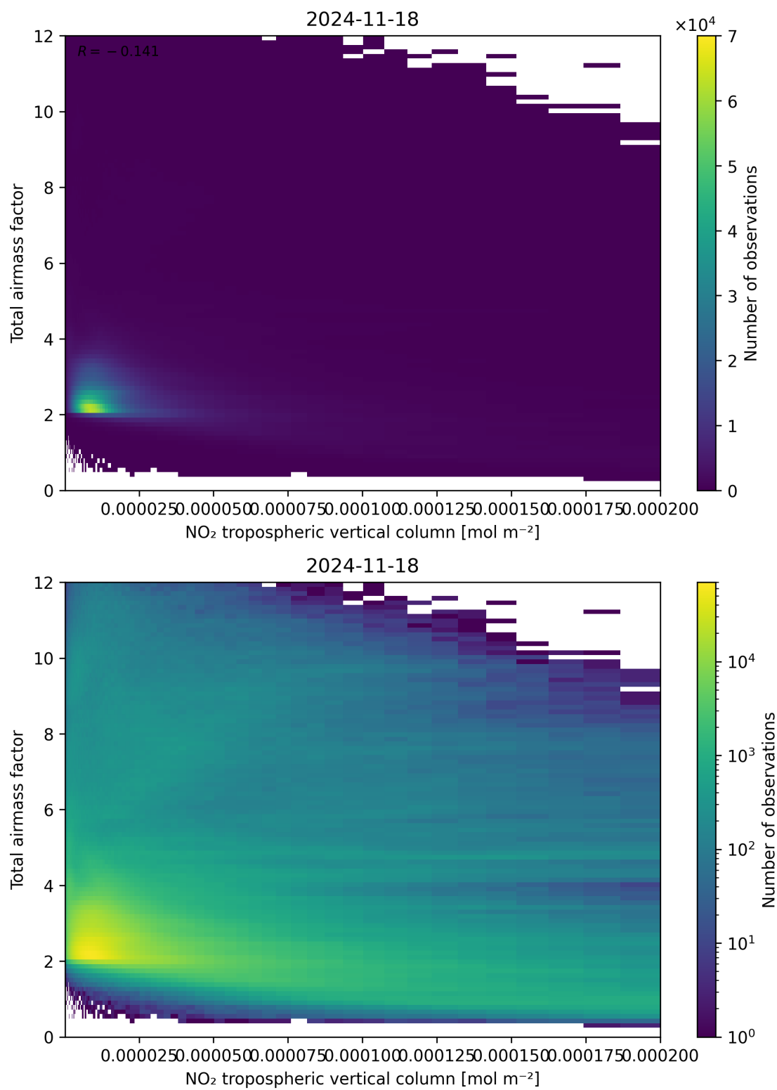
Figure 122: Scatter density plot of “NO 2 tropospheric vertical column” against “Total airmass factor” for 2024-11-17 to 2024-11-19.
