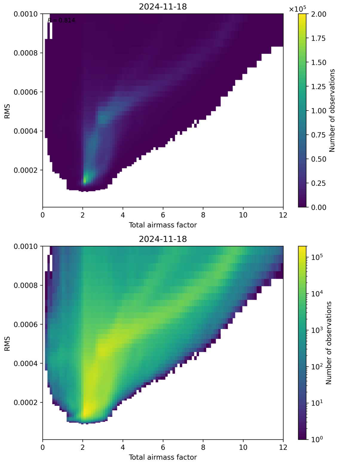
Figure 69: Scatter density plot of “Total airmass factor” against “RMS” for 2024-11-17 to 2024-11-19.
