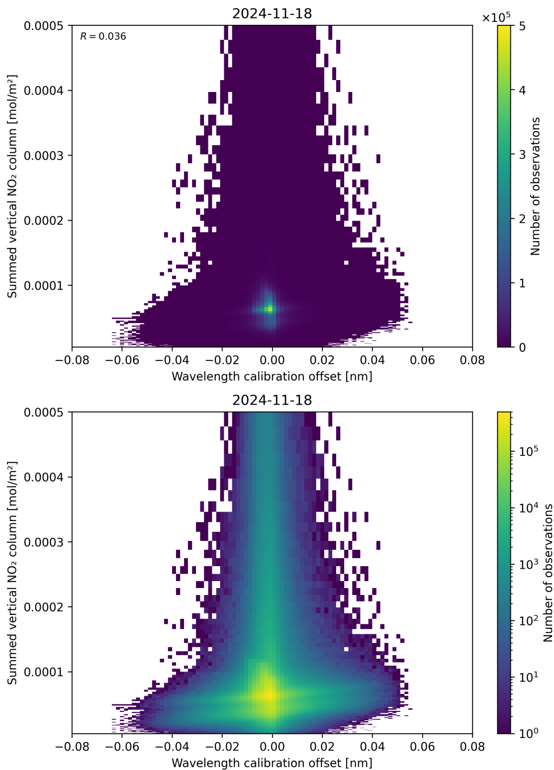
Figure 177: Scatter density plot of “Wavelength calibration offset” against “Summed vertical NO 2 column” for 2024-11-17 to 2024-11-19.
