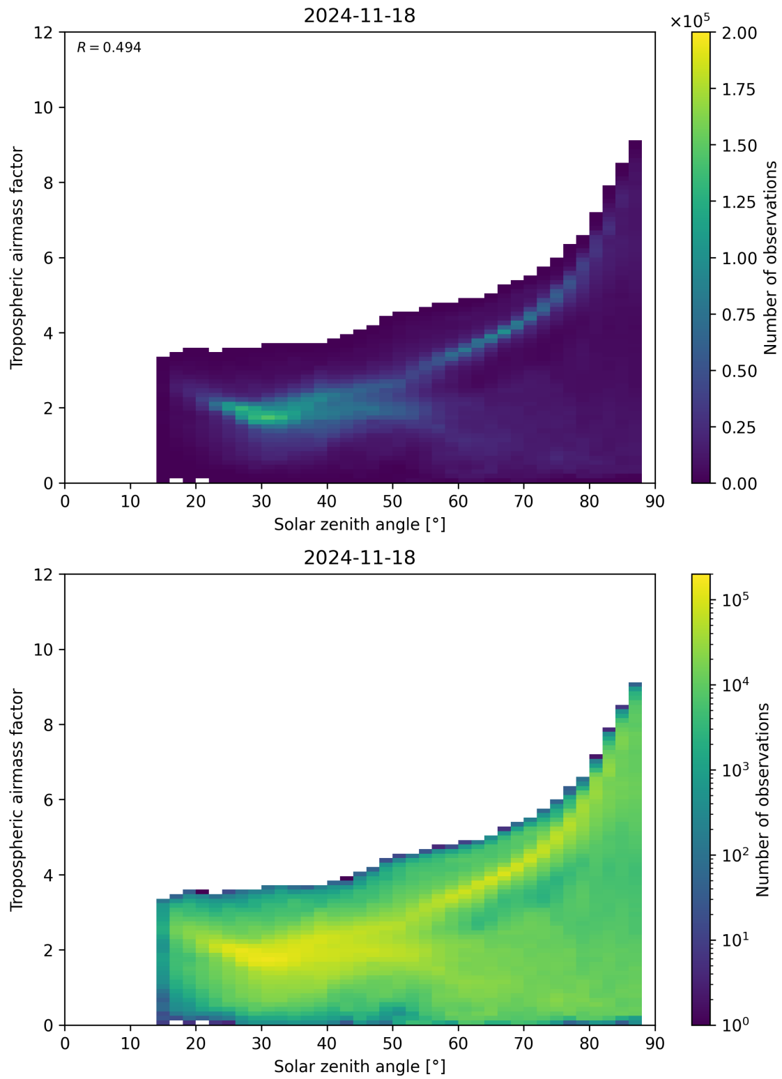
Figure 147: Scatter density plot of “Solar zenith angle” against “Tropospheric airmass factor” for 2024-11-17 to 2024-11-19.
