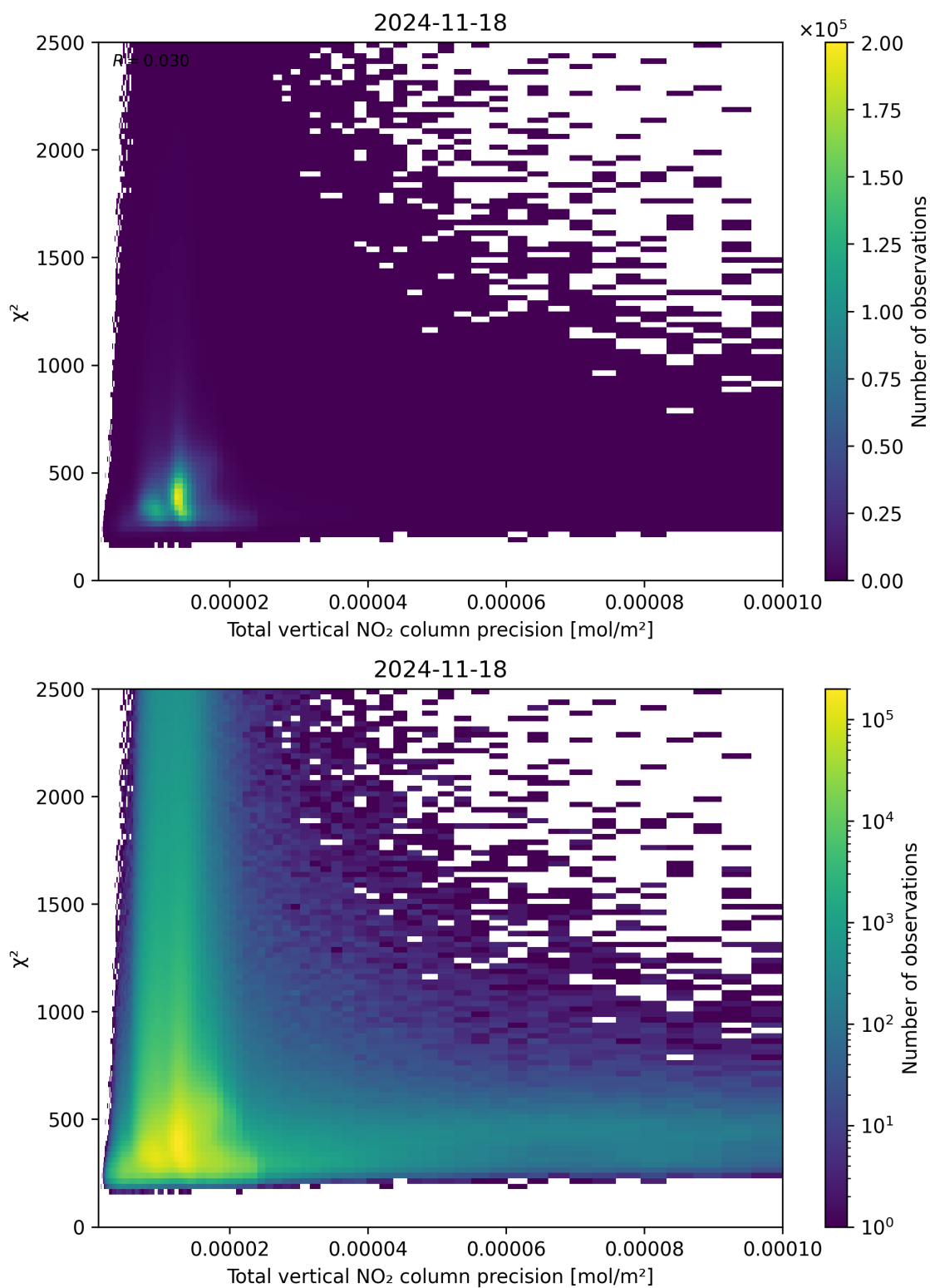
Figure 116: Scatter density plot of “Total vertical NO 2 column precision” against “ \chi^2 ” for 2024-11-17 to 2024-11-19.
