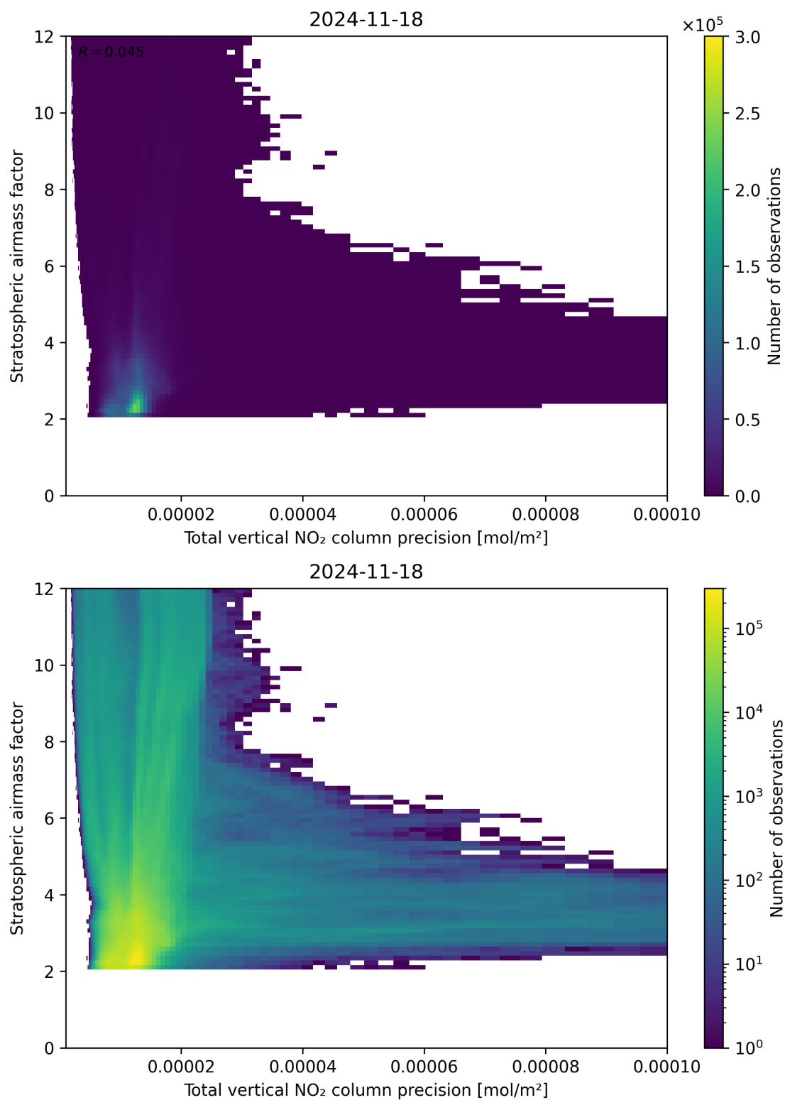
Figure 115: Scatter density plot of “Total vertical NO 2 column precision” against “Stratospheric air mass factor” for 2024-11-17 to 2024-11-19.
