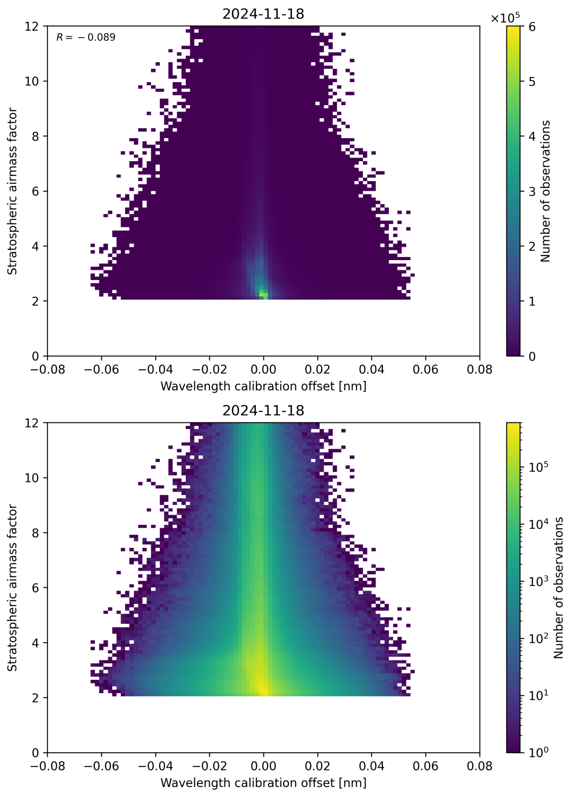
Figure 174: Scatter density plot of “Wavelength calibration offset” against “Stratospheric airmass factor” for 2024-11-17 to 2024-11-19.
