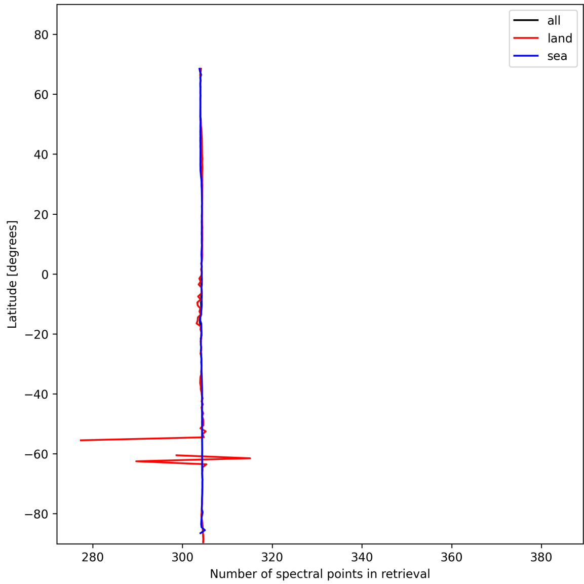
Figure 16: Zonal average of “Number of spectral points in retrieval” for 2024-11-17 to 2024-11-19.
