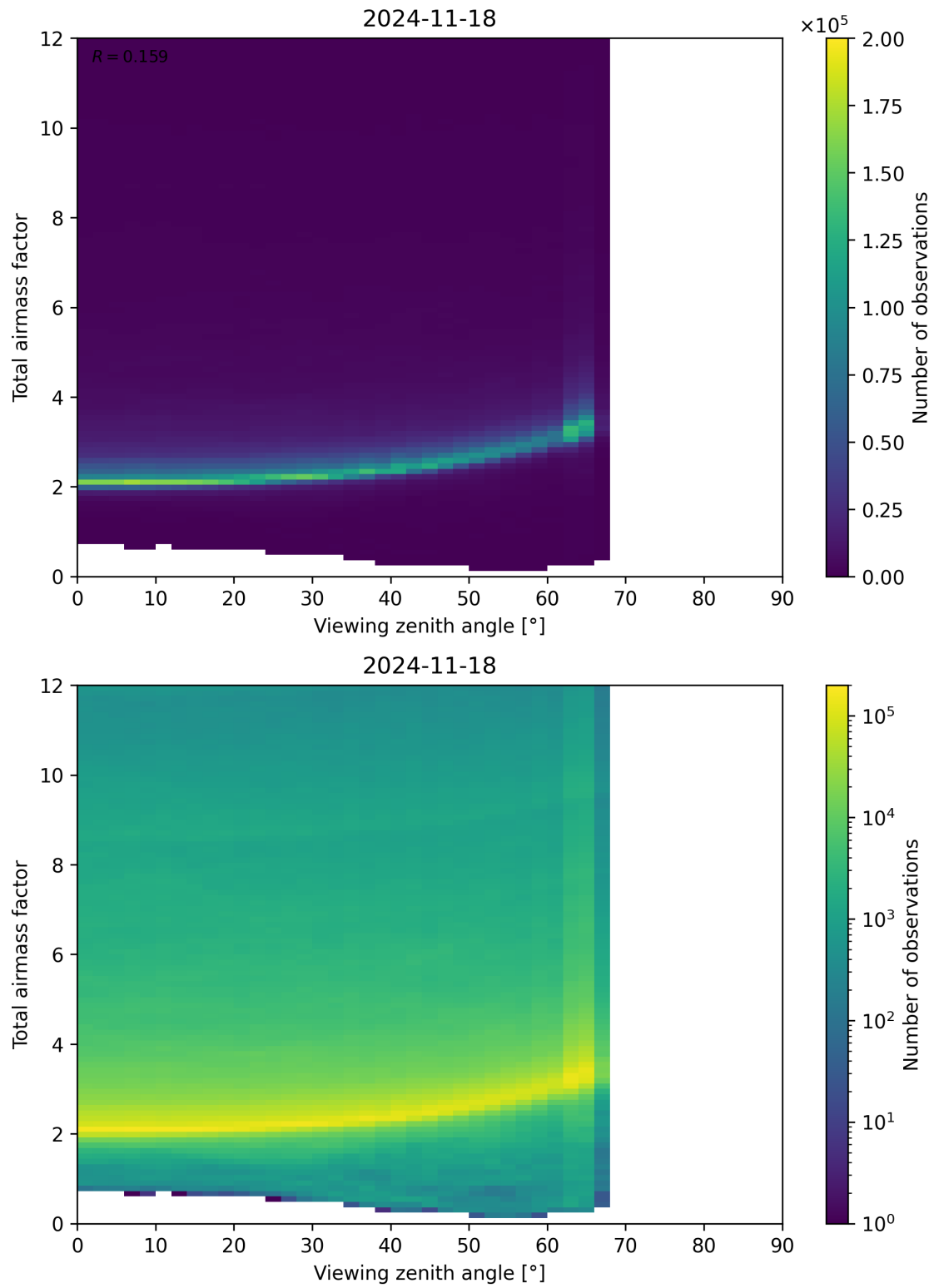
Figure 160: Scatter density plot of “Viewing zenith angle” against “Total airmass factor” for 2024-11-17 to 2024-11-19.
