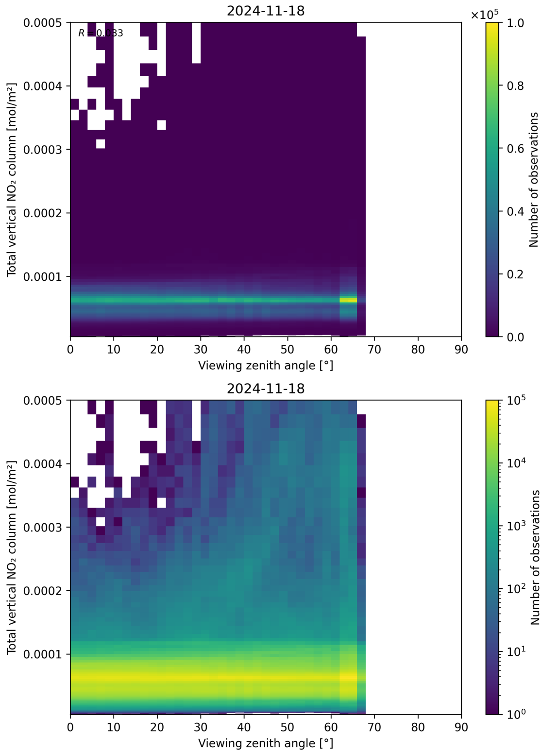
Figure 167: Scatter density plot of “Viewing zenith angle” against “Total vertical NO 2 column” for 2024-11-17 to 2024-11-19.
