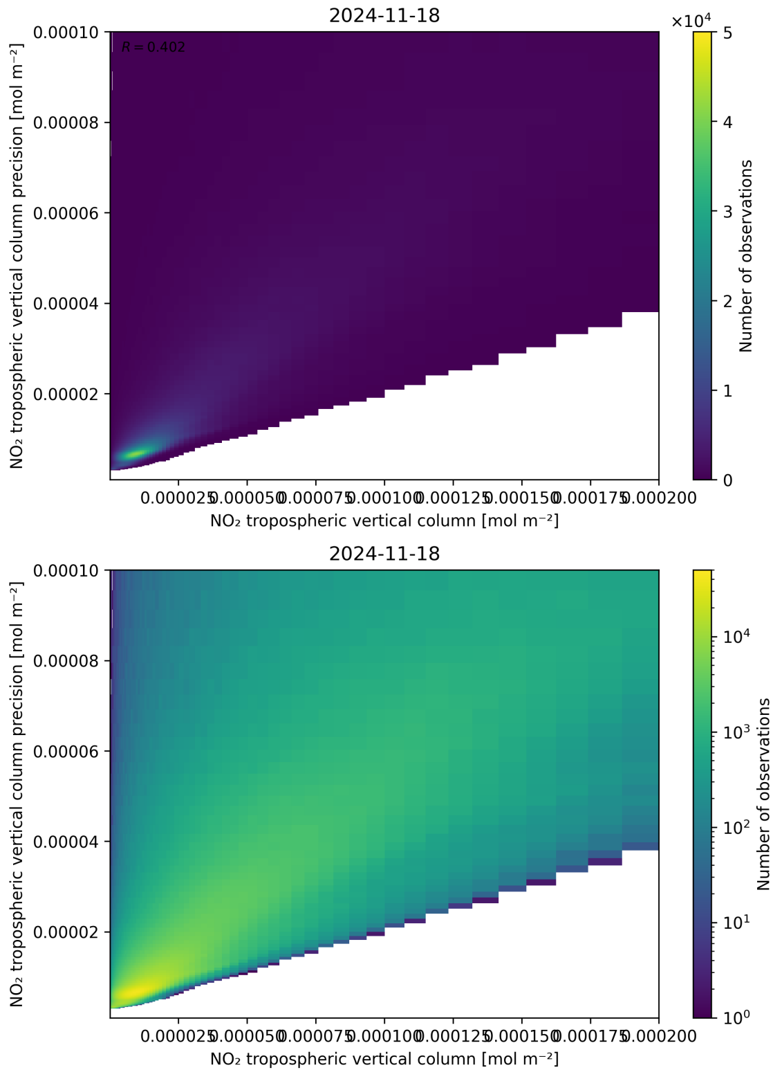
Figure 130: Scatter density plot of “NO 2 tropospheric vertical column” against “NO 2 tropospheric vertical column precision” for 2024-11-17 to 2024-11-19.
