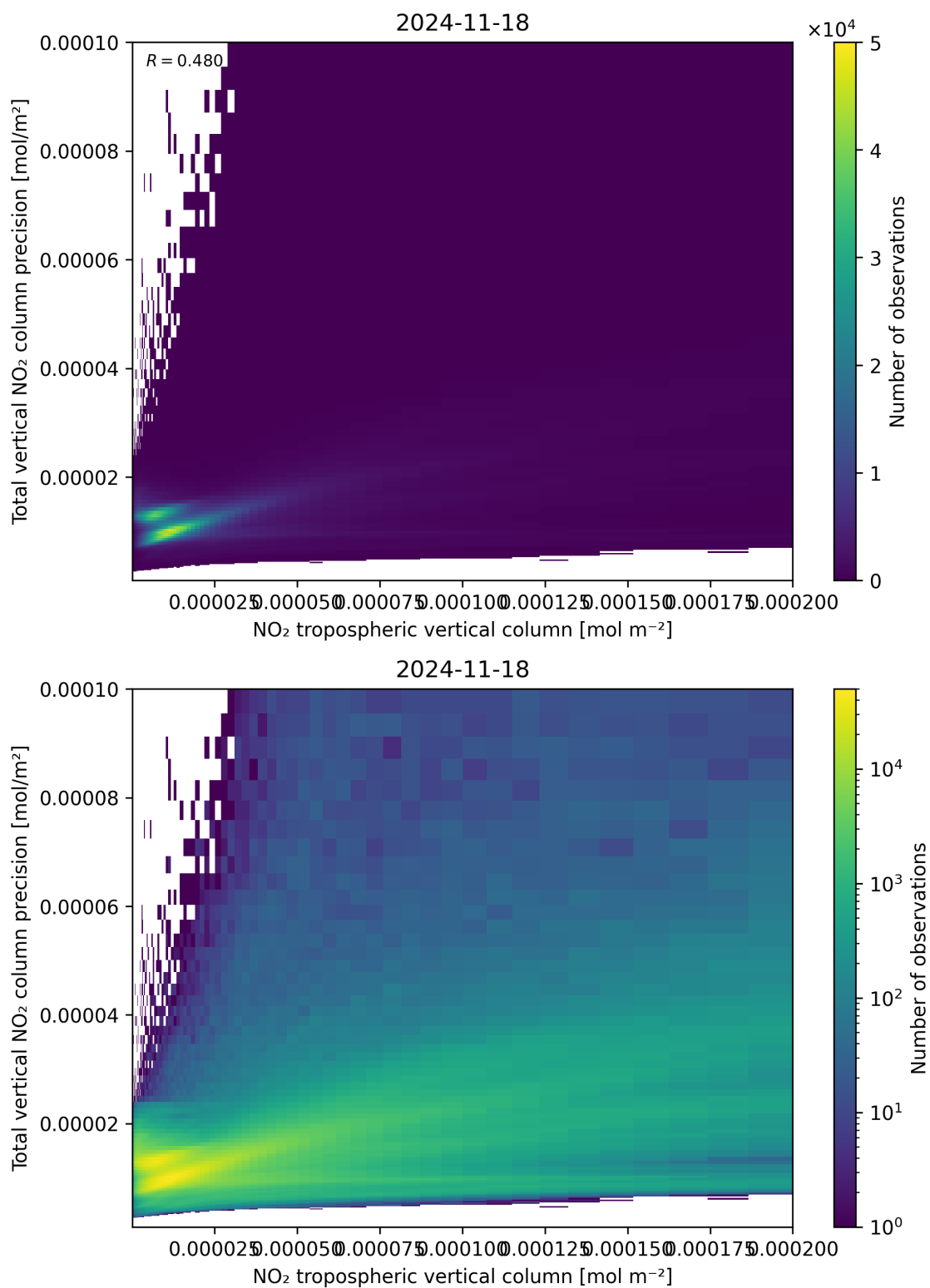
Figure 129: Scatter density plot of “NO 2 tropospheric vertical column” against “Total vertical NO 2 column precision” for 2024-11-17 to 2024-11-19.
