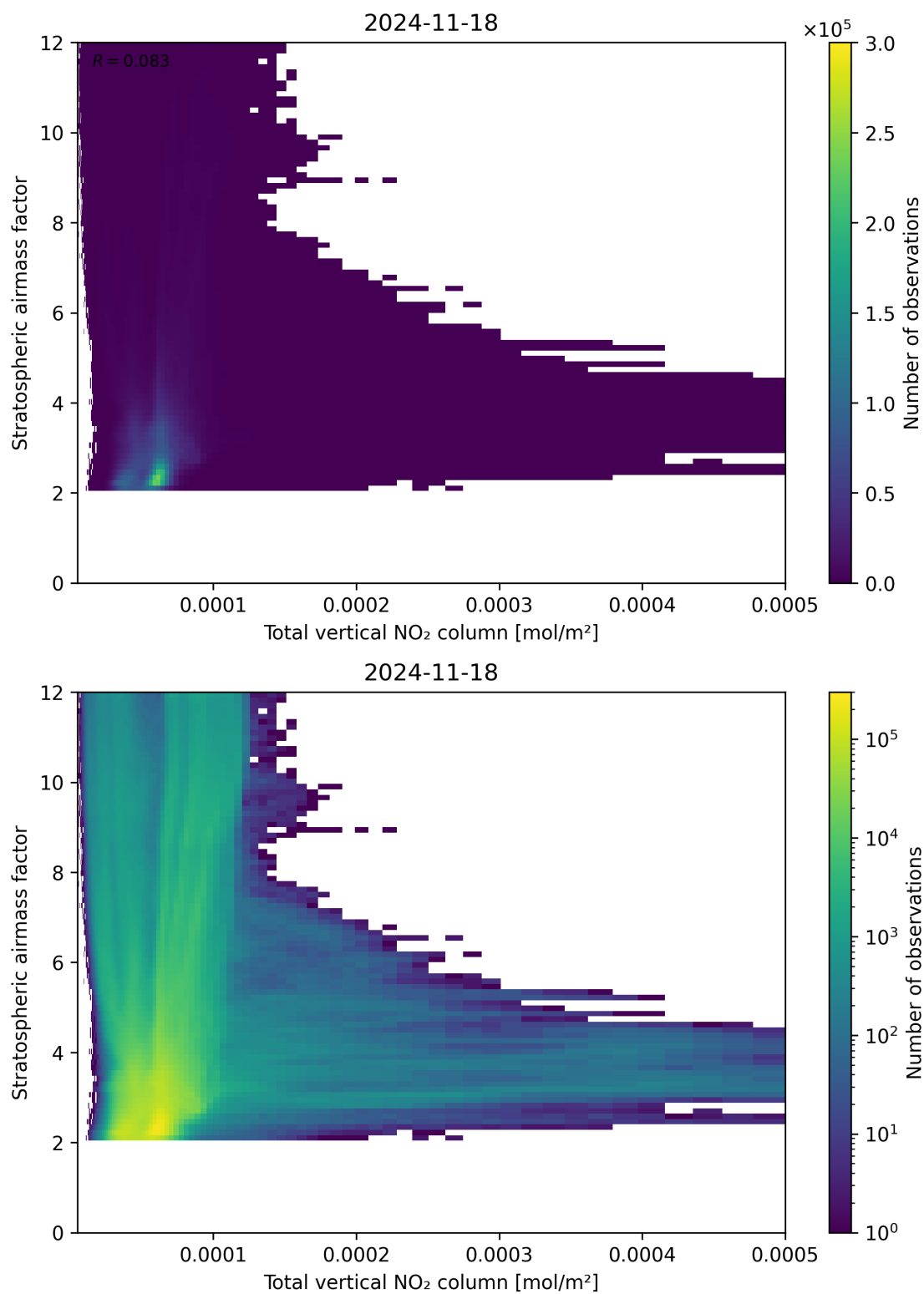
Figure 110: Scatter density plot of “Total vertical NO 2 column” against “Stratospheric air mass factor” for 2024-11-17 to 2024-11-19.
