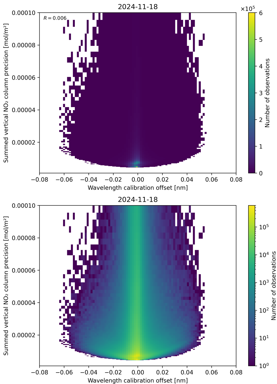
Figure 178: Scatter density plot of “Wavelength calibration offset” against “Summed vertical NO 2 column precision” for 2024-11-17 to 2024-11-19.
