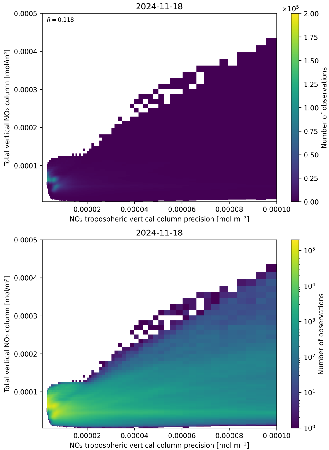
Figure 138: Scatter density plot of “NO 2 tropospheric vertical column precision” against “Total vertical NO 2 column” for 2024-11-17 to 2024-11-19.
