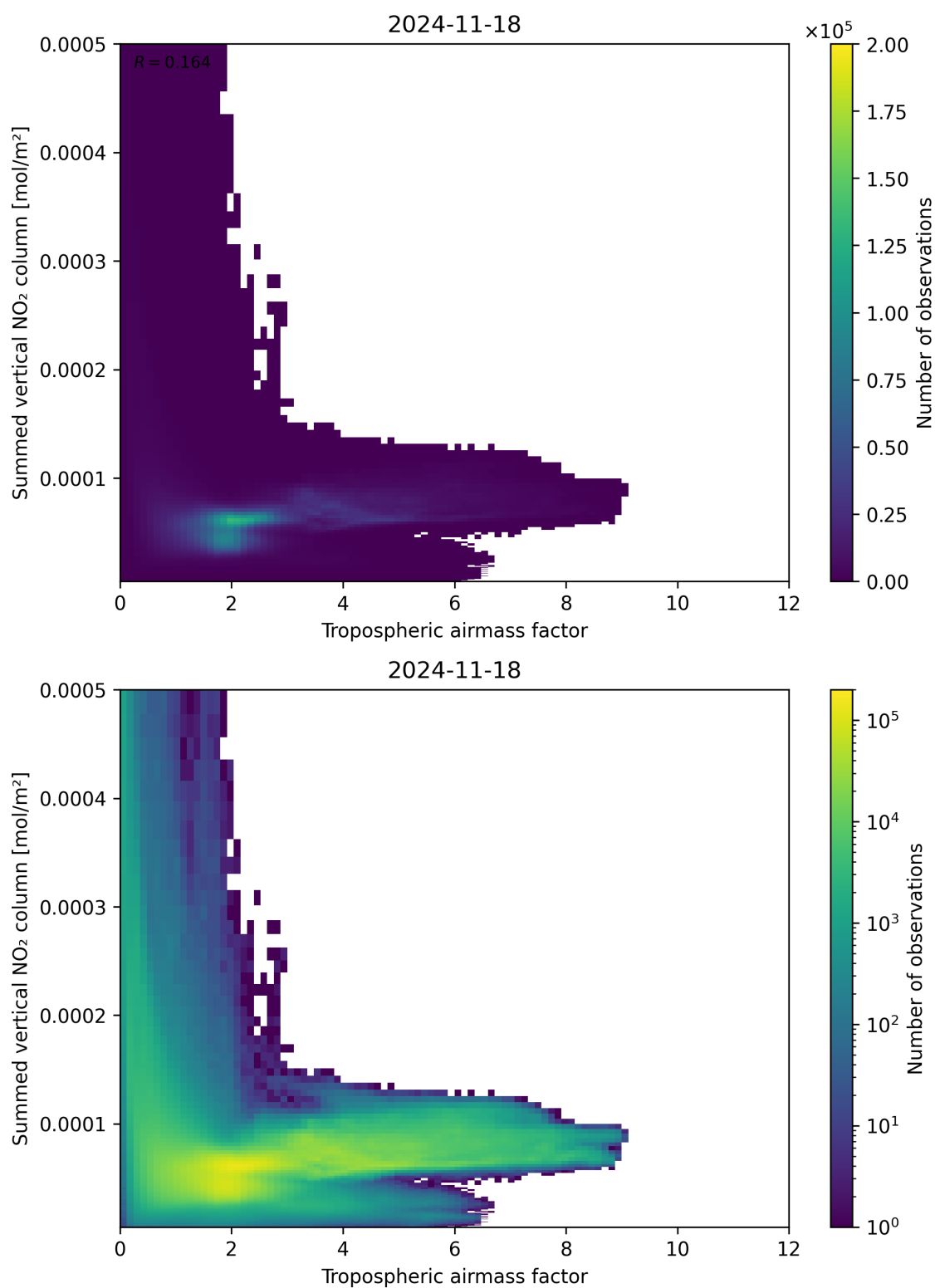
Figure 75: Scatter density plot of “Tropospheric airmass factor” against “Summed vertical NO 2 column” for 2024-11-17 to 2024-11-19.
