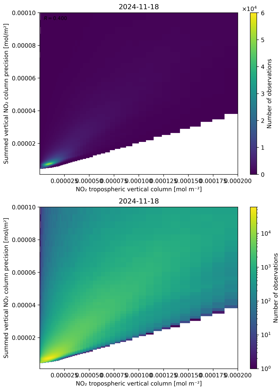
Figure 127: Scatter density plot of “NO 2 tropospheric vertical column” against “Summed vertical NO 2 column precision” for 2024-11-17 to 2024-11-19.
