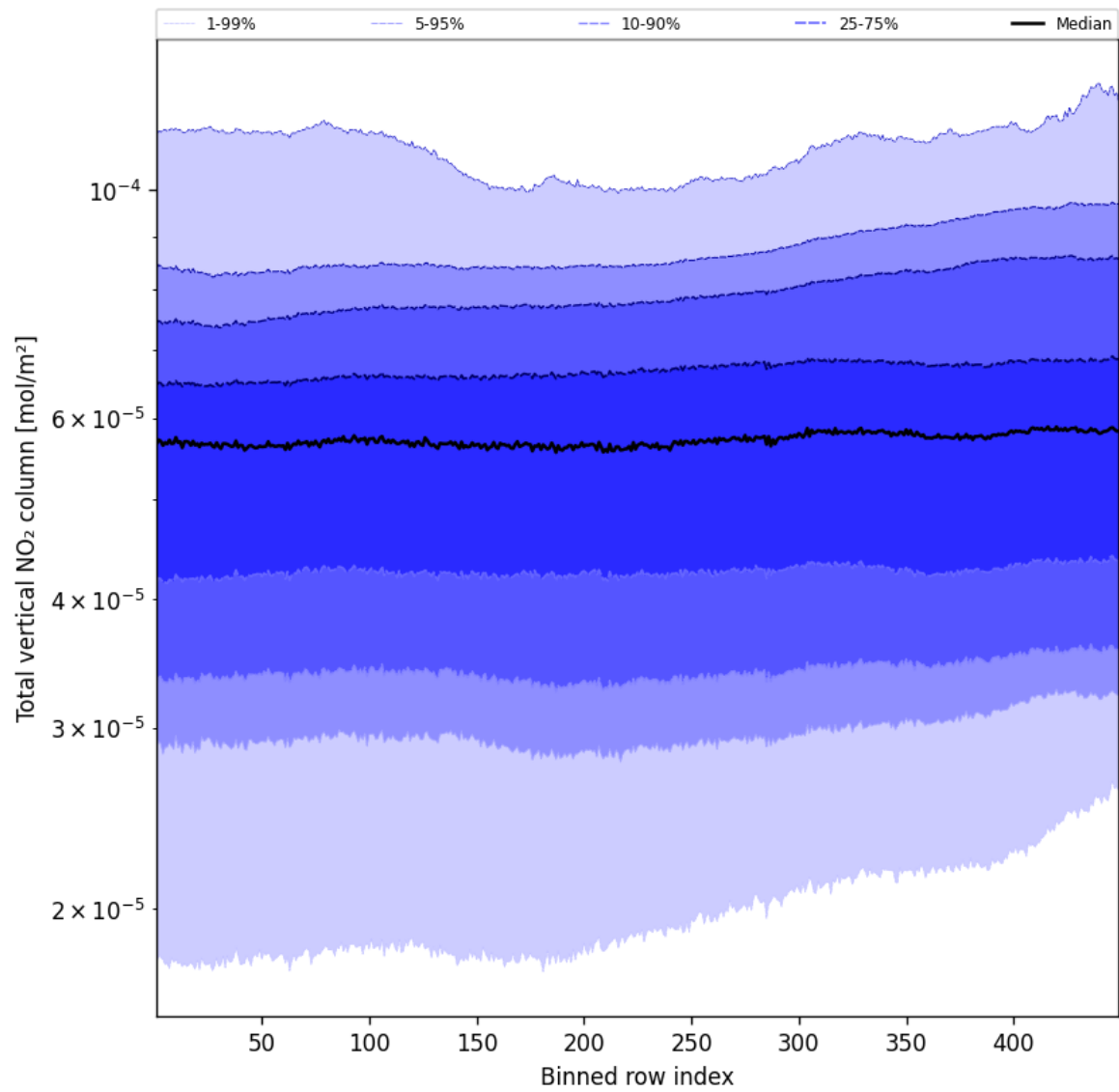
Figure 55: Along track statistics of “Total vertical NO 2 column” for 2024-11-17 to 2024-11-19
