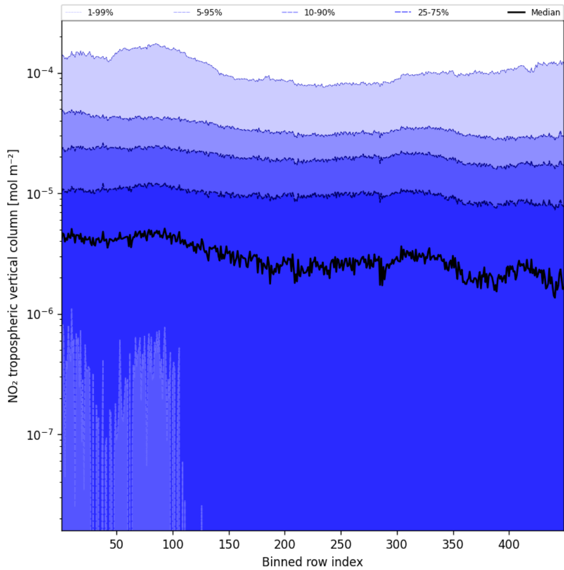
Figure 46: Along track statistics of “NO 2 tropospheric vertical column” for 2024-11-17 to 2024-11-19
