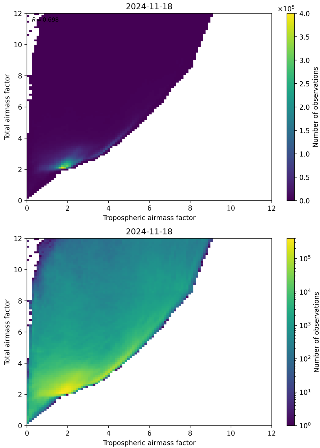
Figure 72: Scatter density plot of “Tropospheric airmass factor” against “Total airmass factor” for 2024-11-17 to 2024-11-19.
