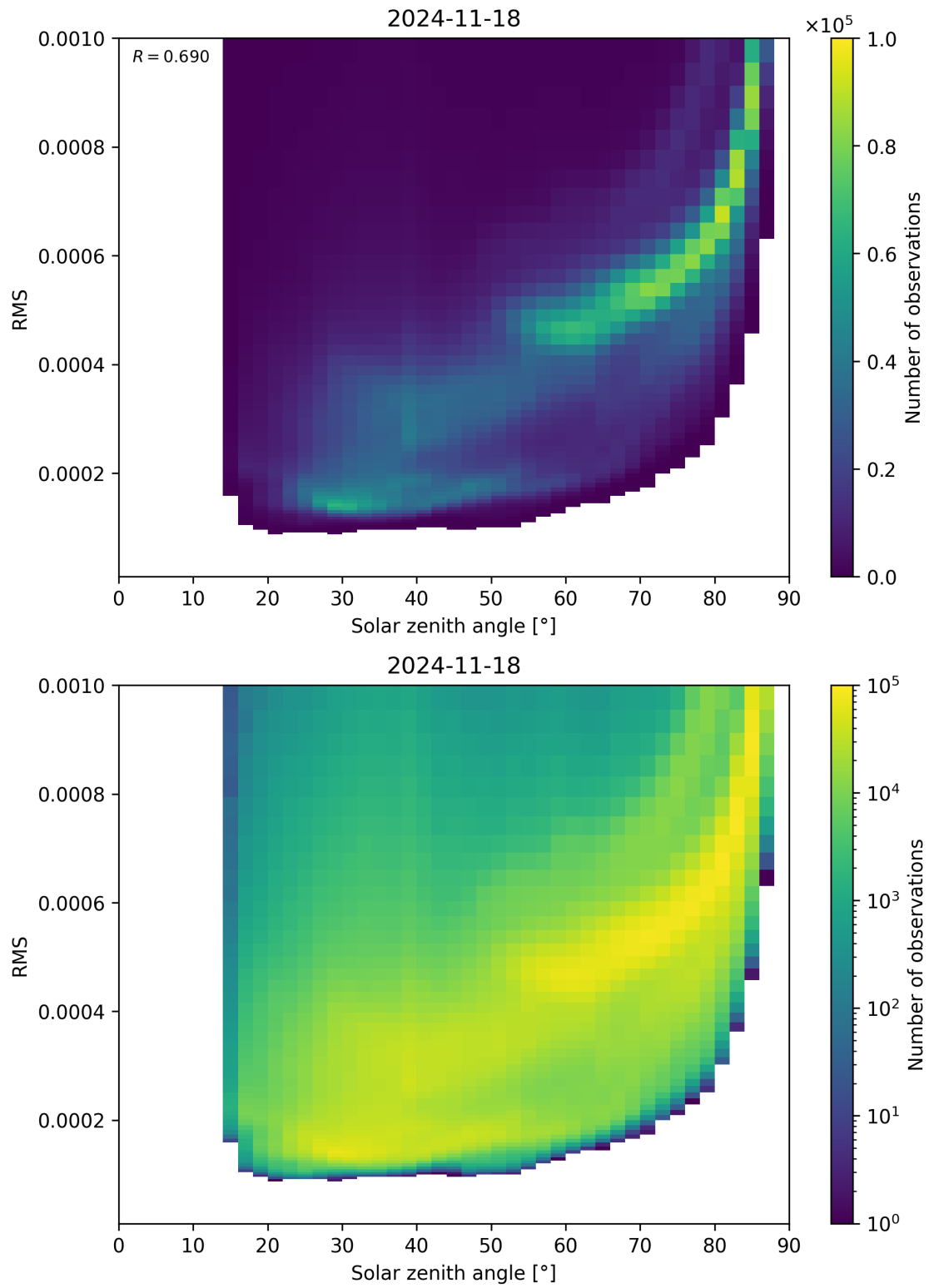
Figure 157: Scatter density plot of “Solar zenith angle” against “RMS” for 2024-11-17 to 2024-11-19.
