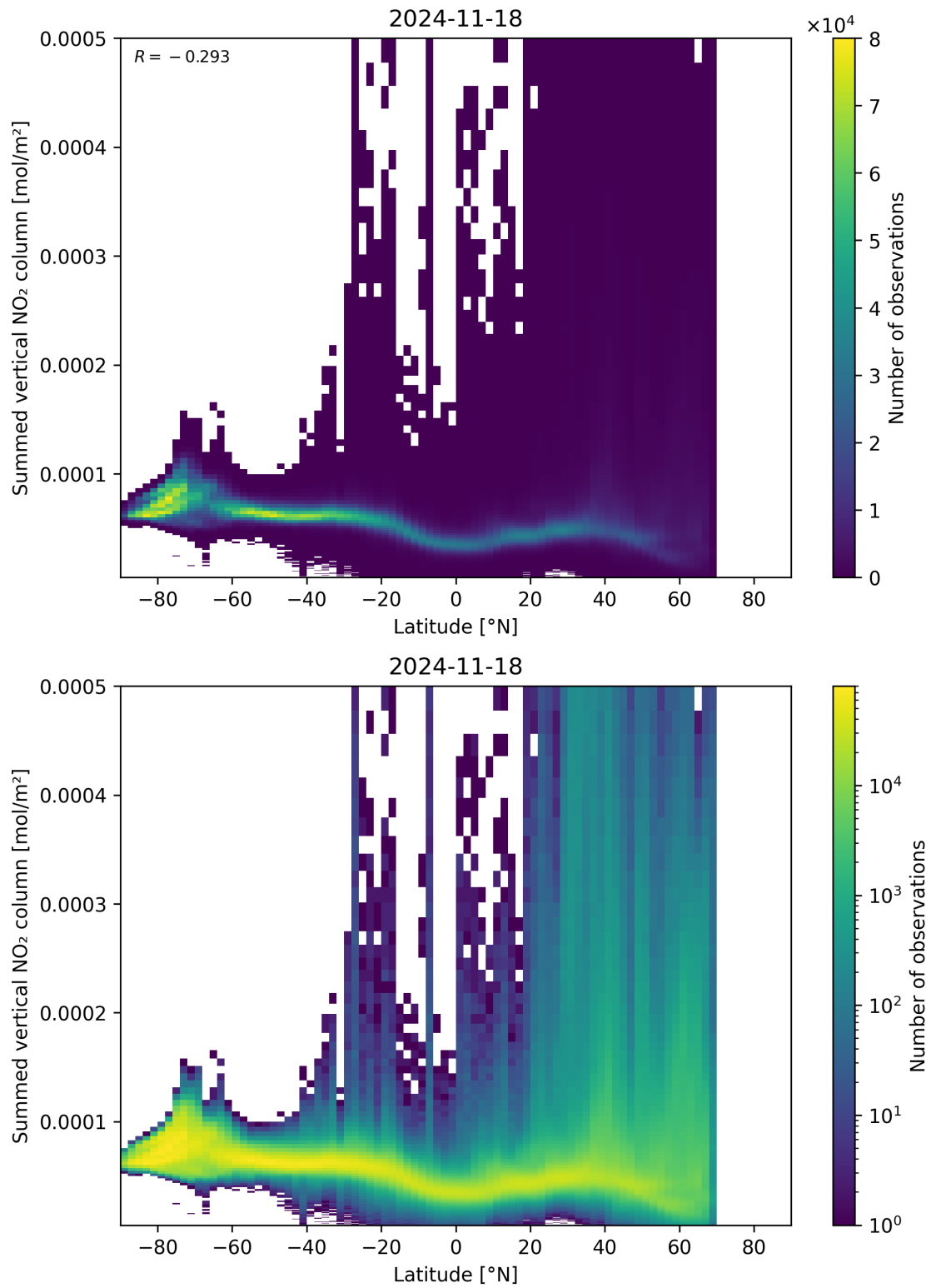
Figure 88: Scatter density plot of “Latitude” against “Summed vertical NO 2 column” for 2024-11-17 to 2024-11-19.
