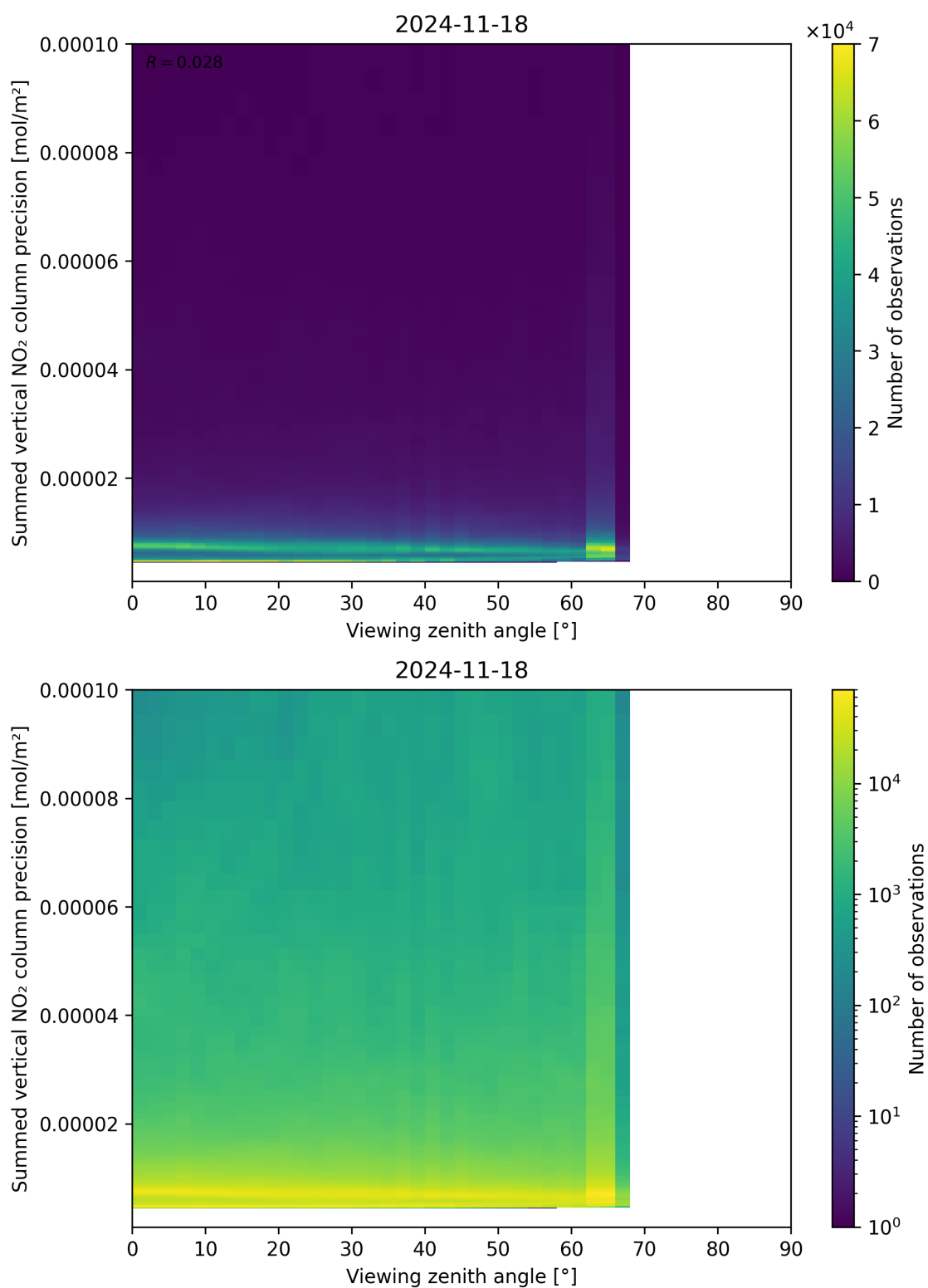
Figure 166: Scatter density plot of “Viewing zenith angle” against “Summed vertical NO 2 column precision” for 2024-11-17 to 2024-11-19.
