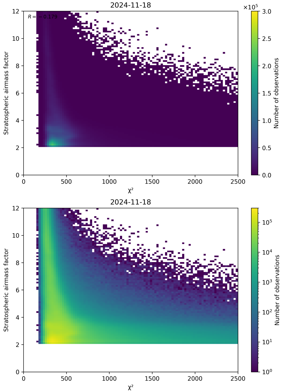
Figure 81: Scatter density plot of “ \chi^2 ” against “Stratospheric airmass factor” for 2024-11-17 to 2024-11-19.
