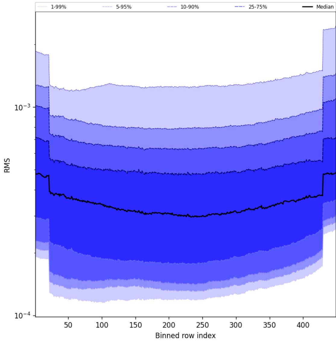
Figure 60: Along track statistics of “RMS” for 2024-11-17 to 2024-11-19
