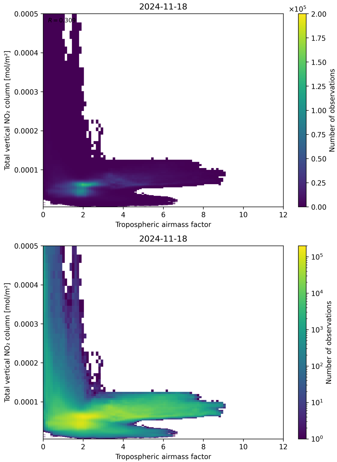
Figure 77: Scatter density plot of “Tropospheric airmass factor” against “Total vertical NO 2 column” for 2024-11-17 to 2024-11-19.
