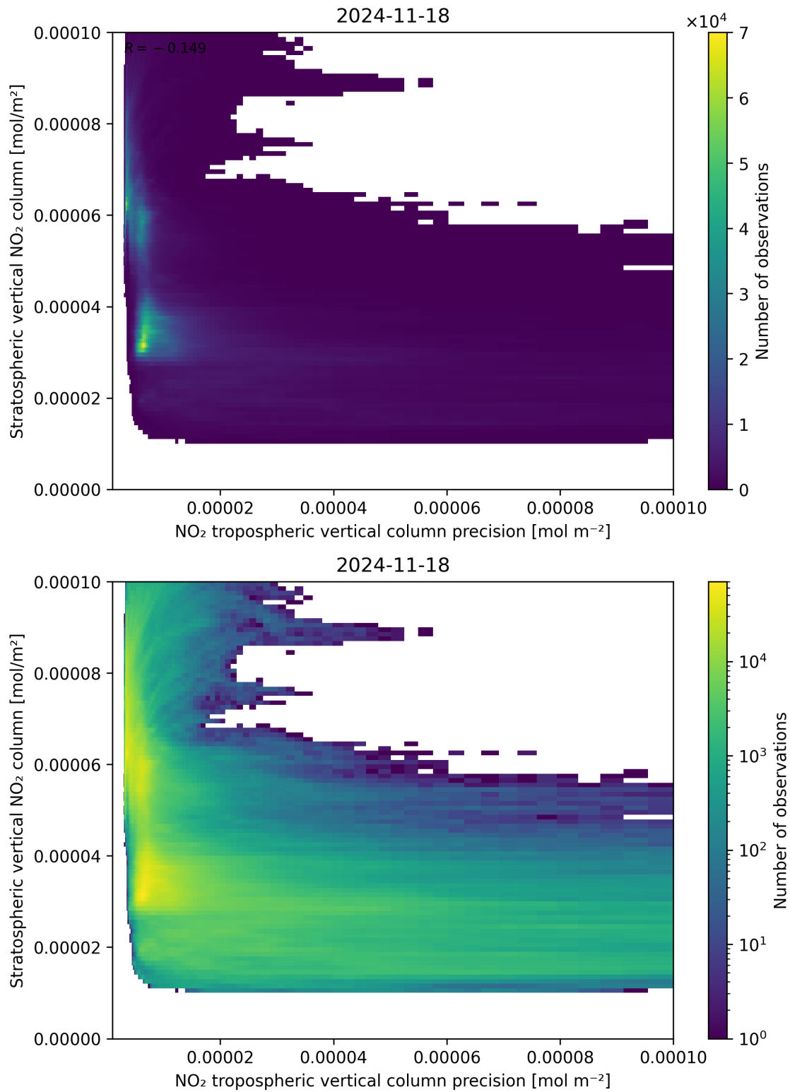
Figure 135: Scatter density plot of “NO 2 tropospheric vertical column precision” against “Stratospheric vertical NO 2 column” for 2024-11-17 to 2024-11-19.
