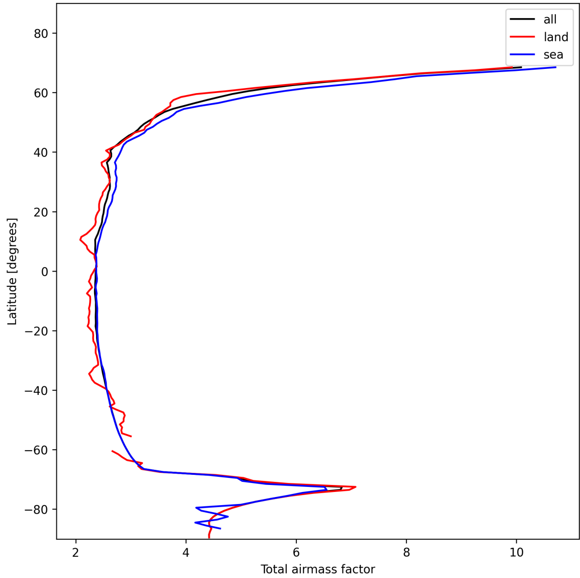
Figure 15: Zonal average of “Total airmass factor” for 2024-11-17 to 2024-11-19.
