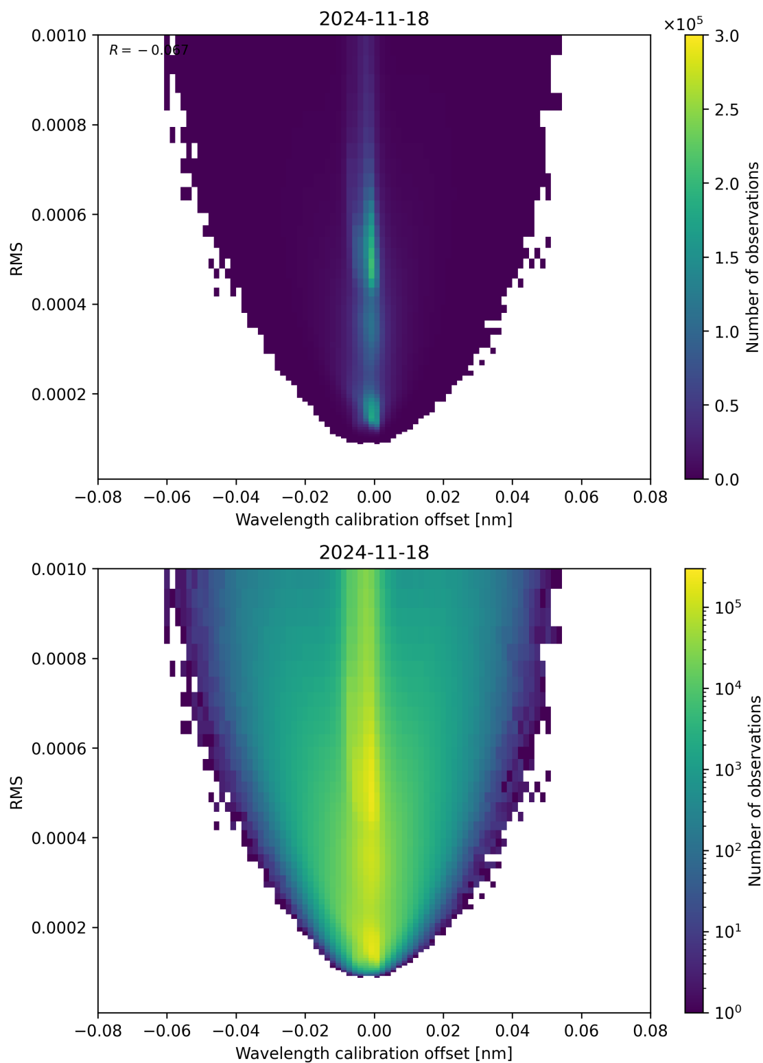
Figure 181: Scatter density plot of “Wavelength calibration offset” against “RMS” for 2024-11-17 to 2024-11-19.
