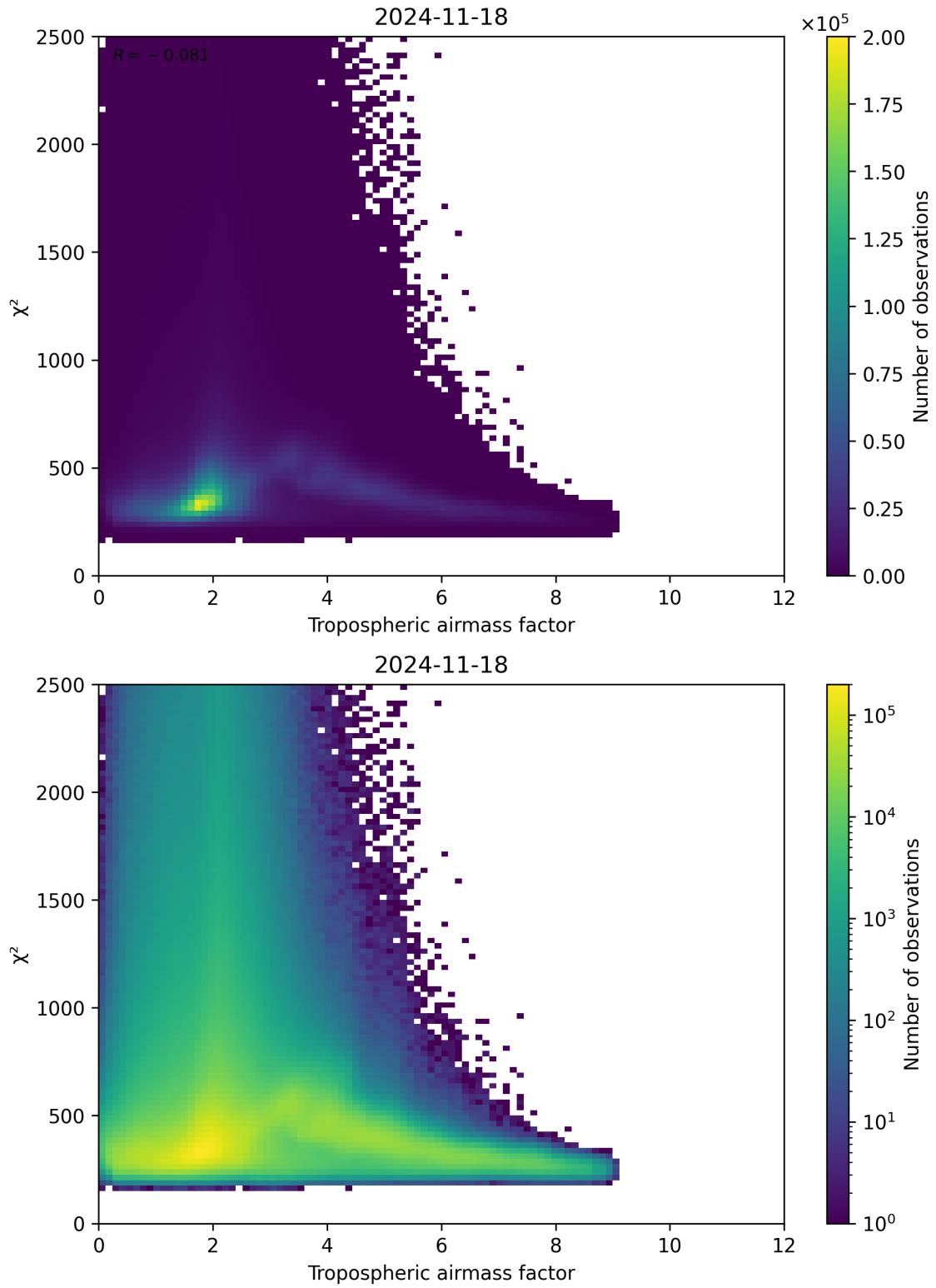
Figure 73: Scatter density plot of “Tropospheric airmass factor” against “ \chi^2 ” for 2024-11-17 to 2024-11-19.
