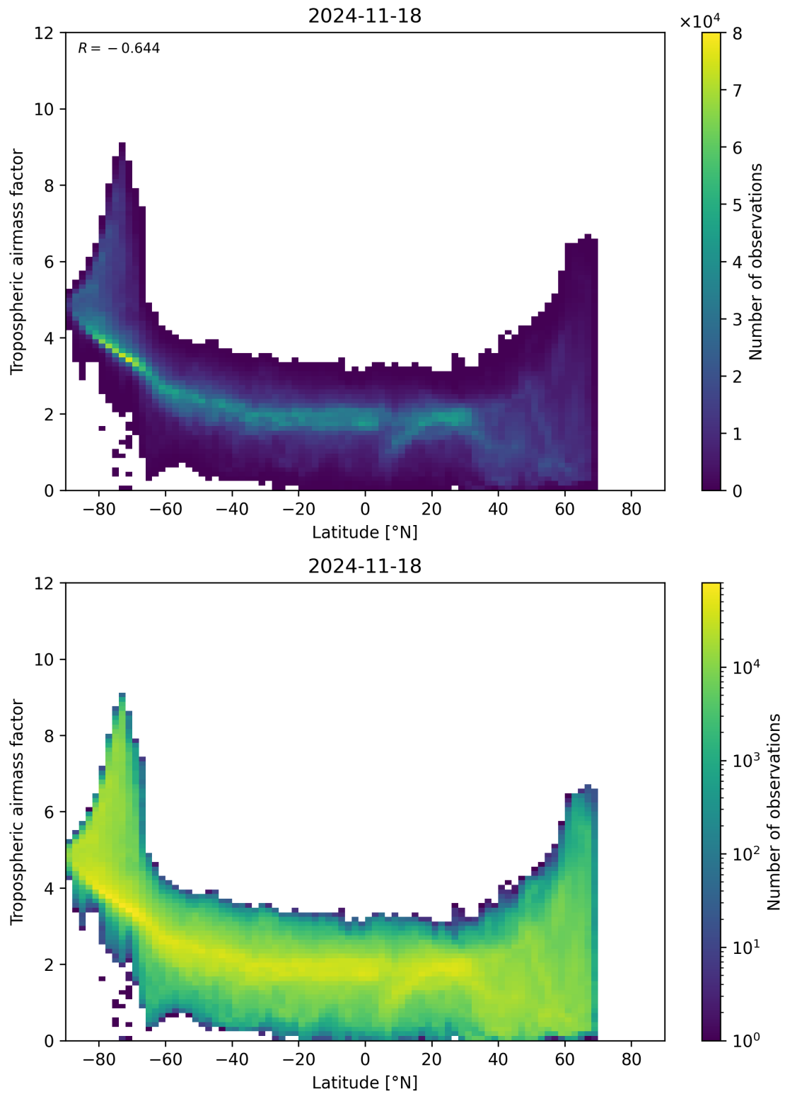
Figure 85: Scatter density plot of “Latitude” against “Tropospheric airmass factor” for 2024-11-17 to 2024-11-19.
