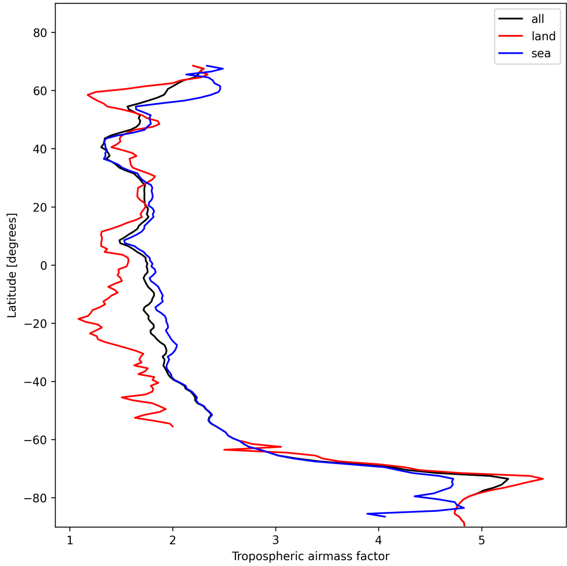
Figure 14: Zonal average of “Tropospheric airmass factor” for 2024-11-17 to 2024-11-19.
