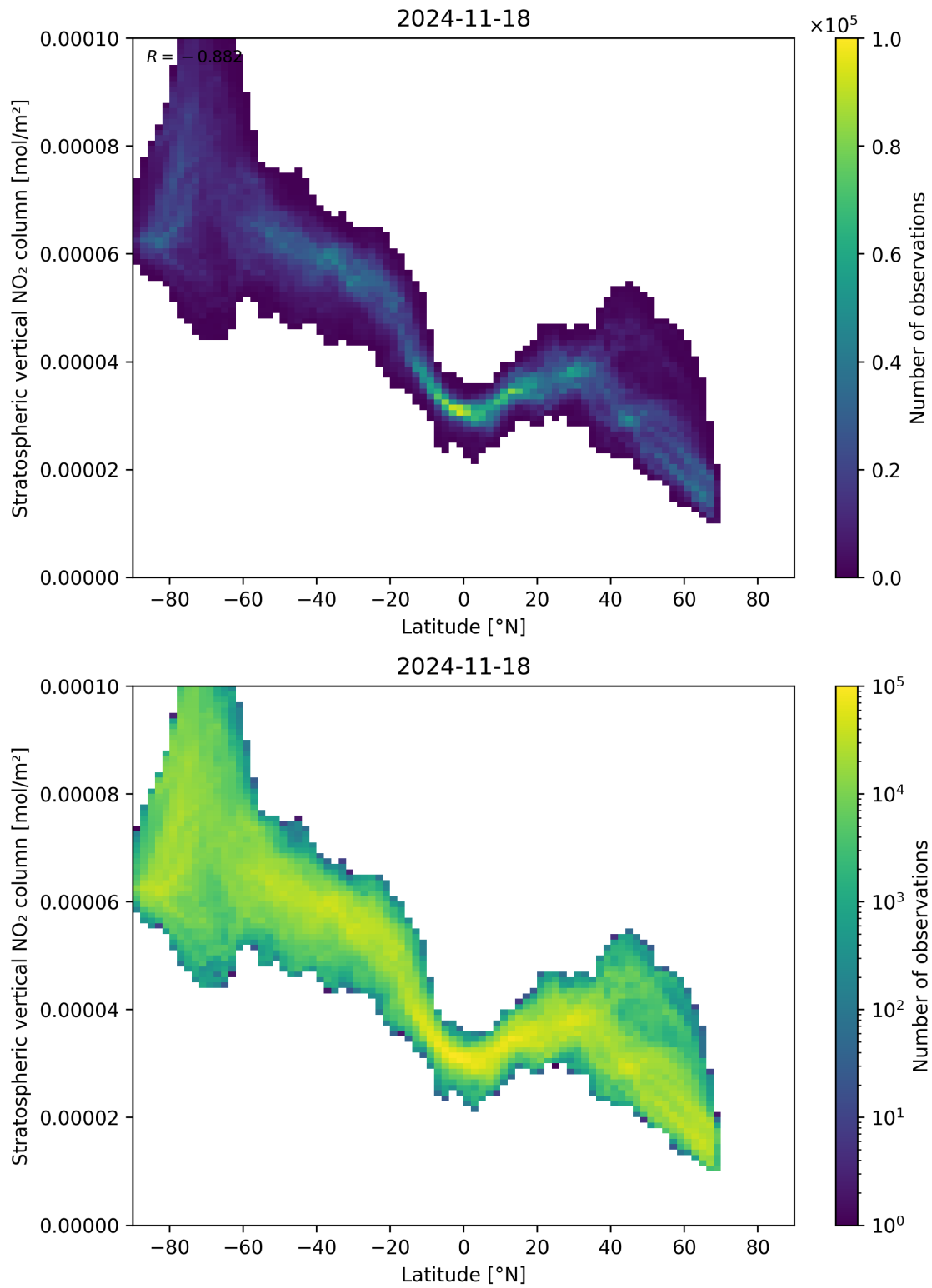
Figure 87: Scatter density plot of “Latitude” against “Stratospheric vertical NO 2 column” for 2024-11-17 to 2024-11-19.
