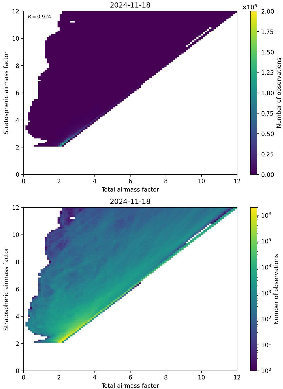
Figure 62: Scatter density plot of “Total airmass factor” against “Stratospheric airmass factor” for 2024-11-17 to 2024-11-19.
