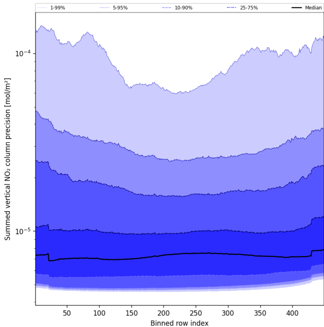
Figure 58: Along track statistics of “Summed vertical NO 2 column precision” for 2024-11-17 to 2024-11-19
