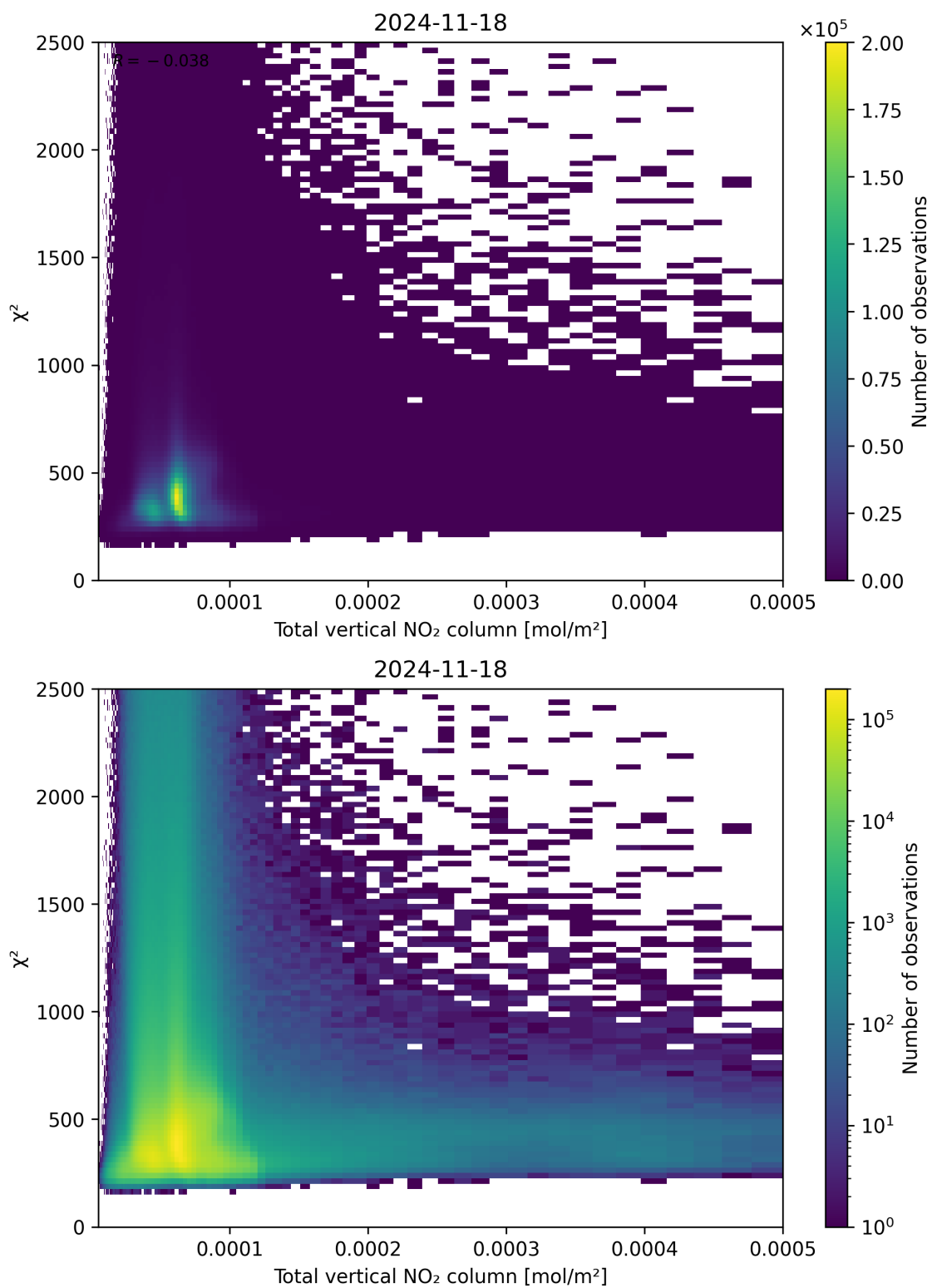
Figure 111: Scatter density plot of “Total vertical NO 2 column” against “ \chi^2 ” for 2024-11-17 to 2024-11-19.
