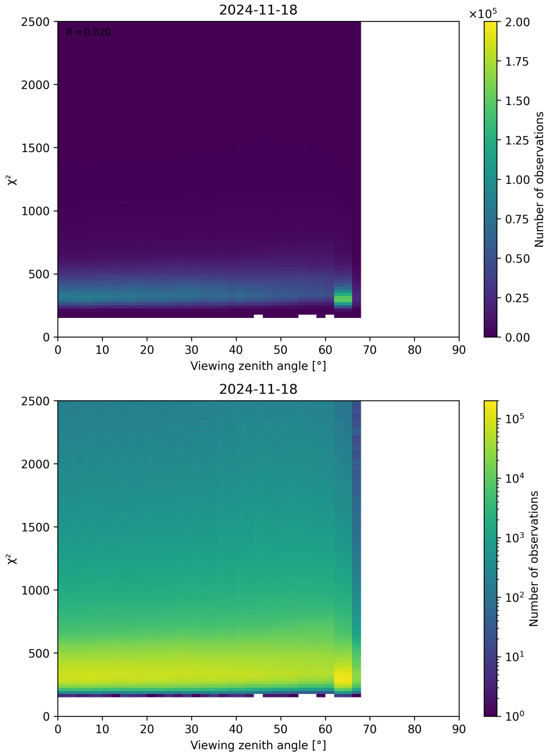
Figure 162: Scatter density plot of “Viewing zenith angle” against “ \chi^2 ” for 2024-11-17 to 2024-11-19.
