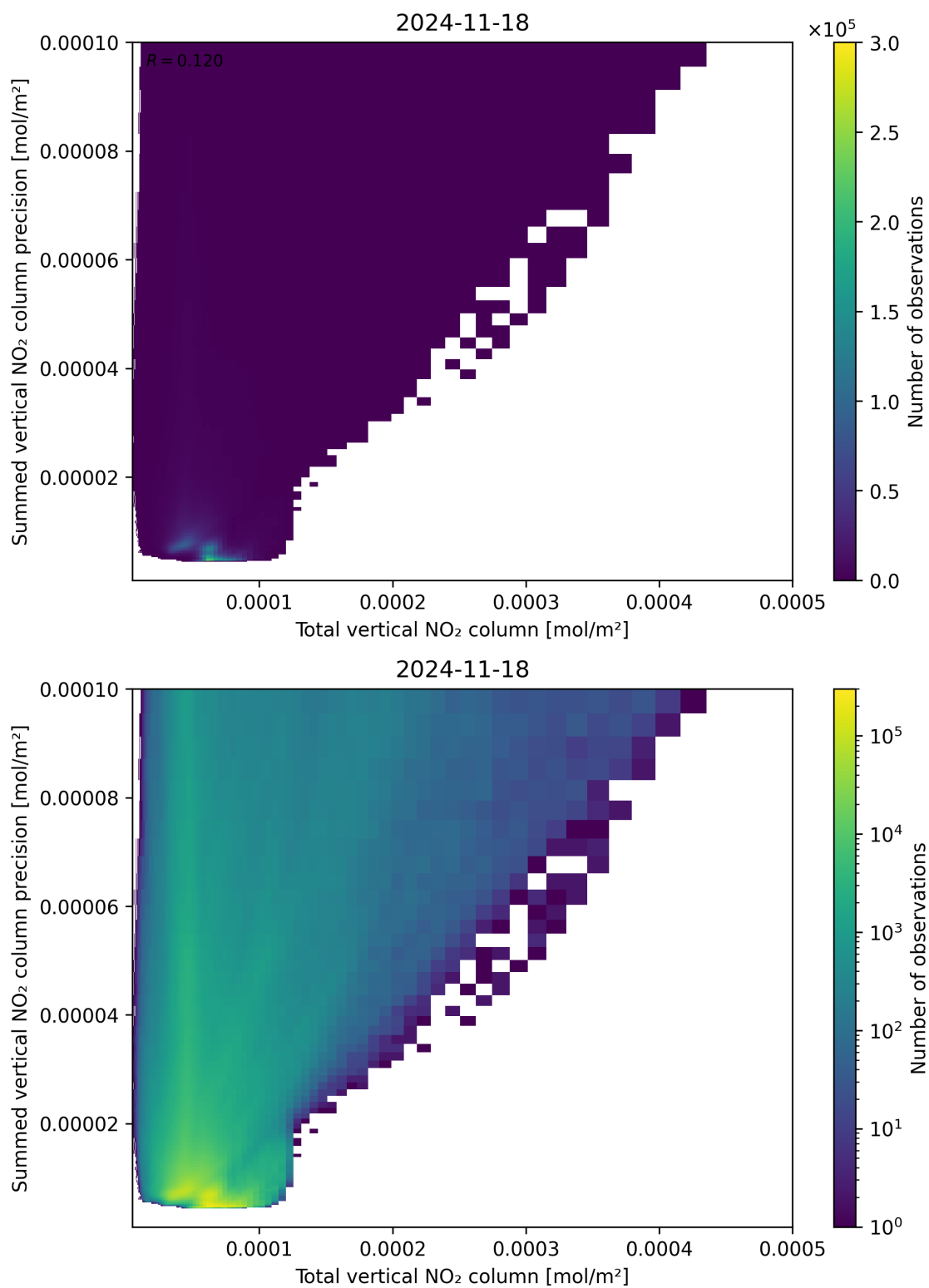
Figure 113: Scatter density plot of “Total vertical NO 2 column” against “Summed vertical NO 2 column precision” for 2024-11-17 to 2024-11-19.
