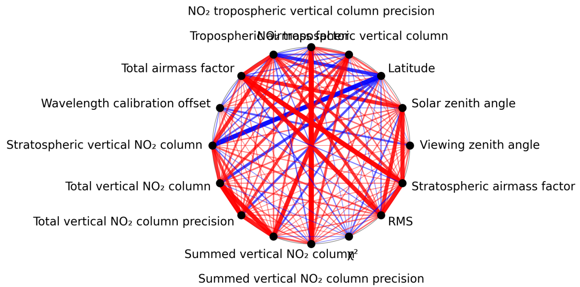
Figure 1: Map of correlation graph for 2024-11-17 to 2024-11-19.
