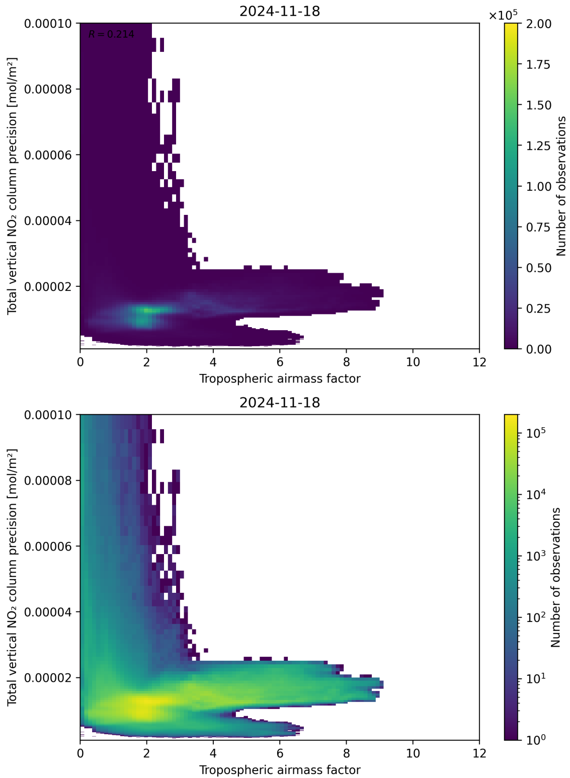
Figure 78: Scatter density plot of “Tropospheric air mass factor” against “Total vertical NO 2 column precision” for 2024-11-17 to 2024-11-19.
