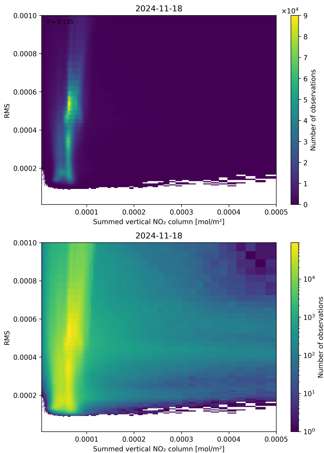
Figure 109: Scatter density plot of “Summed vertical NO 2 column” against “RMS” for 2024-11-17 to 2024-11-19.
