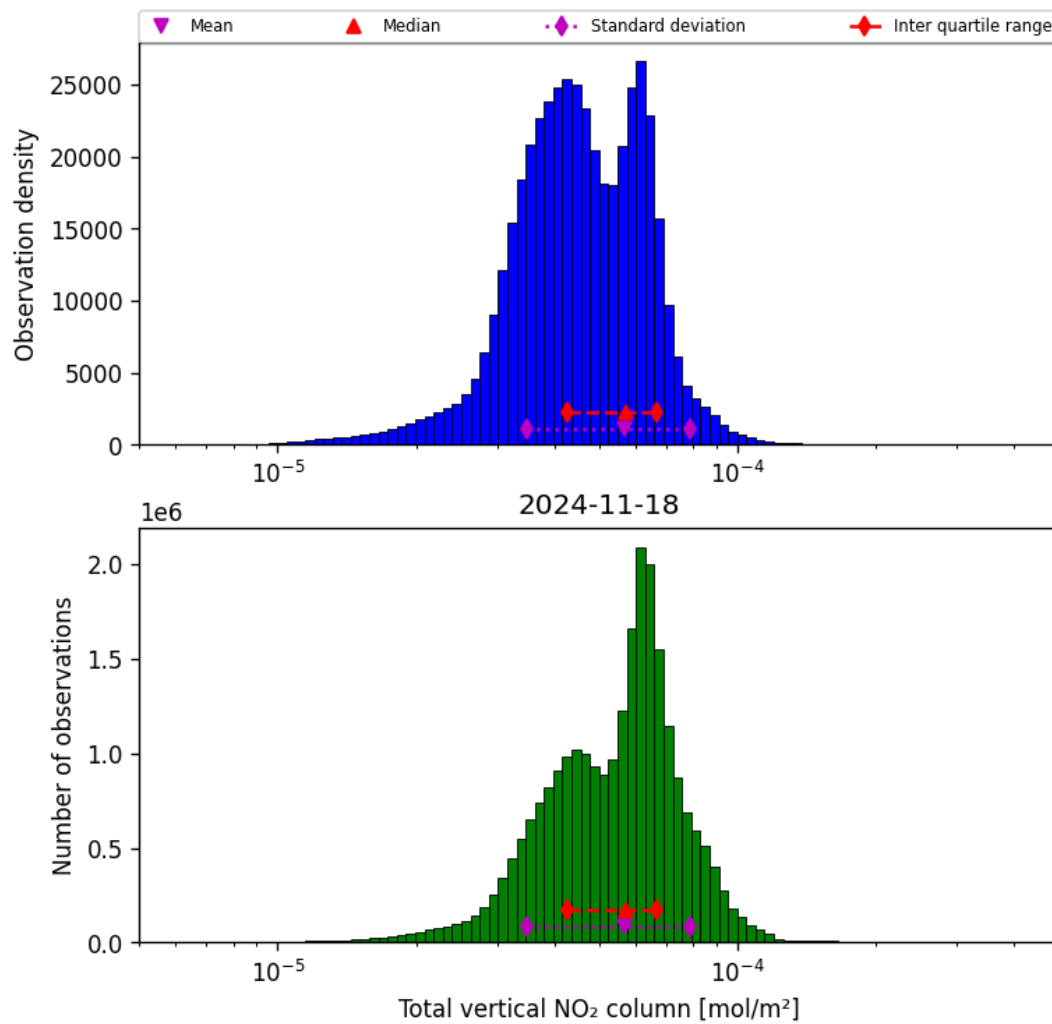
Figure 38: Histogram of “Total vertical NO 2 column” for 2024-11-17 to 2024-11-19
