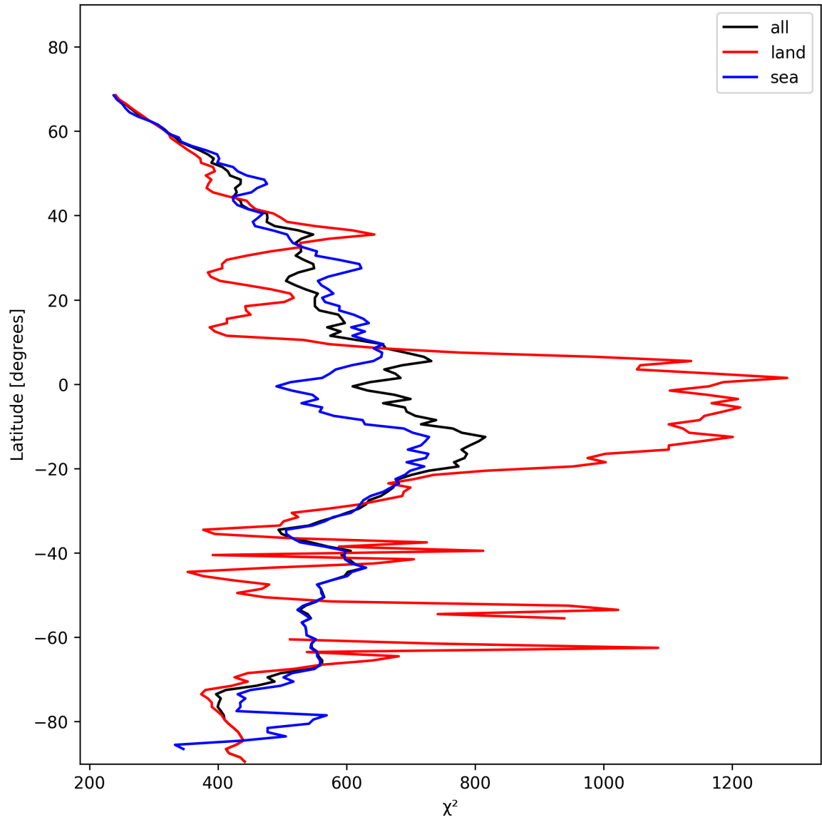
Figure 25: Zonal average of “ \chi^2 ” for 2024-11-17 to 2024-11-19.
