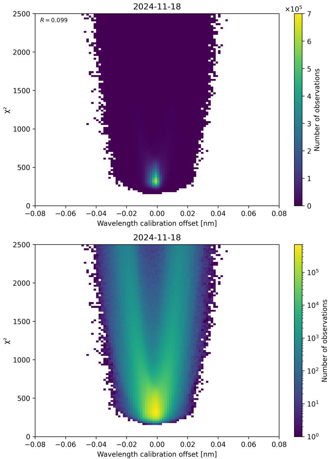
Figure 175: Scatter density plot of “Wavelength calibration offset” against “ \chi^2 ” for 2024-11-17 to 2024-11-19.
