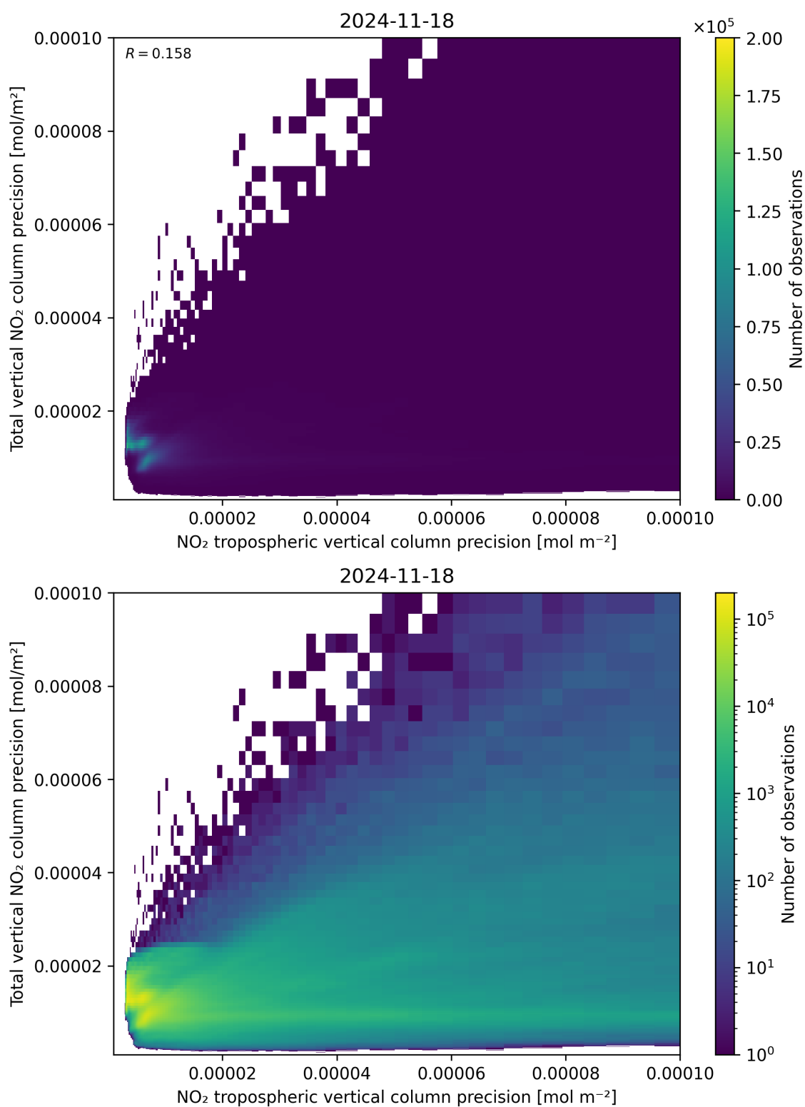
Figure 139: Scatter density plot of “NO 2 tropospheric vertical column precision” against “Total vertical NO 2 column precision” for 2024-11-17 to 2024-11-19.
