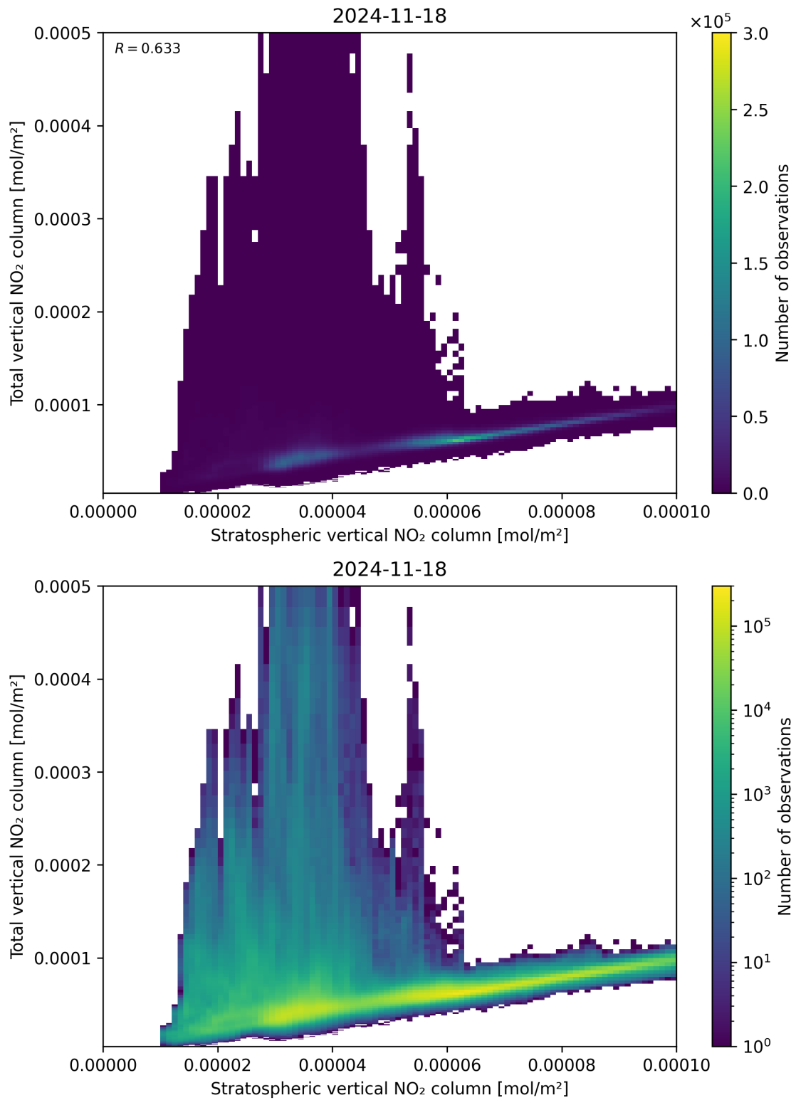
Figure 100: Scatter density plot of “Stratospheric vertical NO 2 column” against “Total vertical NO 2 column” for 2024-11-17 to 2024-11-19.
