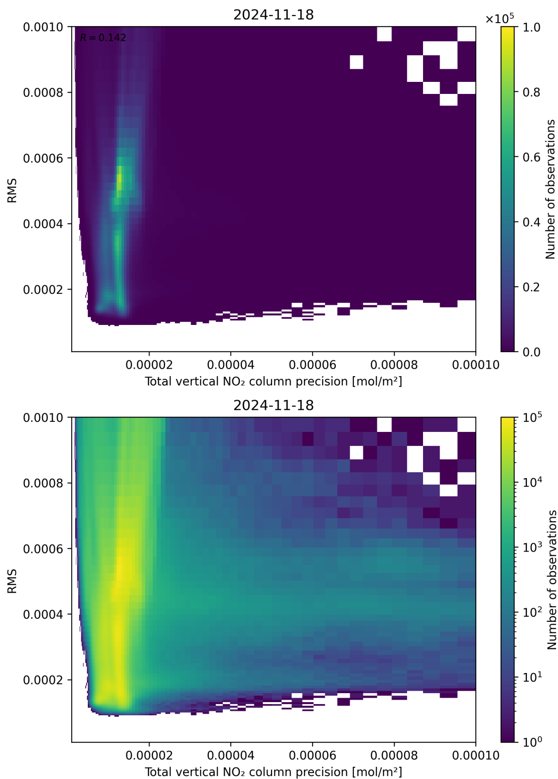
Figure 119: Scatter density plot of “Total vertical NO 2 column precision” against “RMS” for 2024-11-17 to 2024-11-19.
