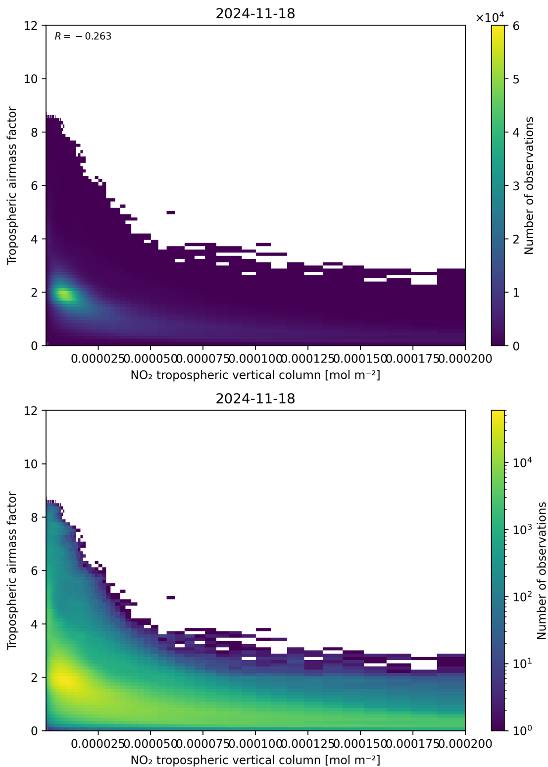
Figure 123: Scatter density plot of “NO 2 tropospheric vertical column” against “Tropospheric air mass factor” for 2024-11-17 to 2024-11-19.
