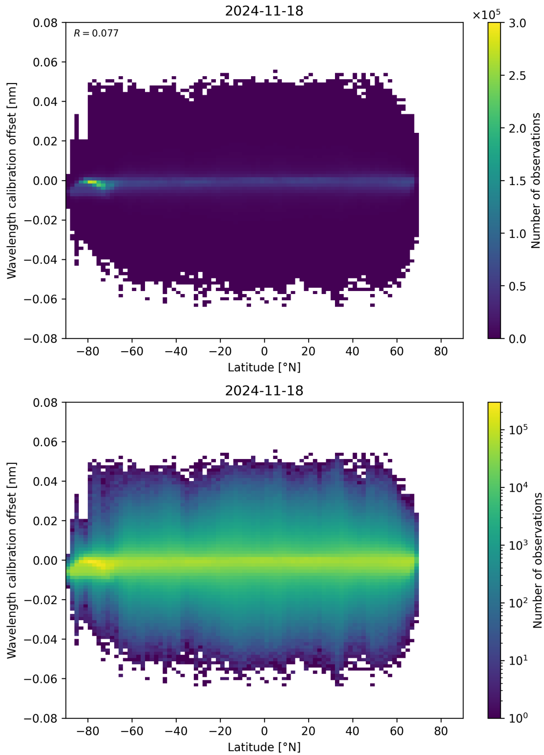
Figure 95: Scatter density plot of “Latitude” against “Wavelength calibration offset” for 2024-11-17 to 2024-11-19.
