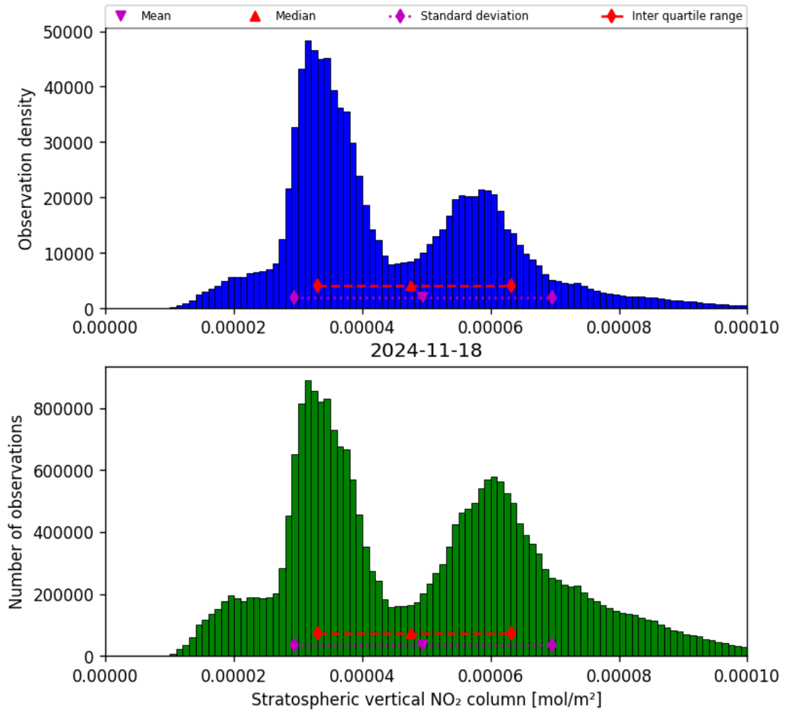
Figure 36: Histogram of “Stratospheric vertical NO 2 column” for 2024-11-17 to 2024-11-19
