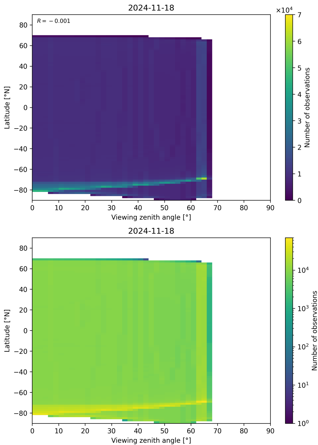
Figure 163: Scatter density plot of “Viewing zenith angle” against “Latitude” for 2024-11-17 to 2024-11-19.
