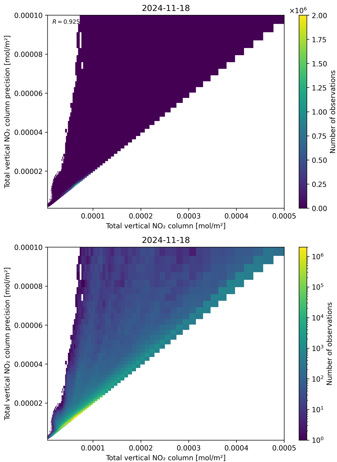
Figure 114: Scatter density plot of “Total vertical NO 2 column” against “Total vertical NO 2 column precision” for 2024-11-17 to 2024-11-19.
