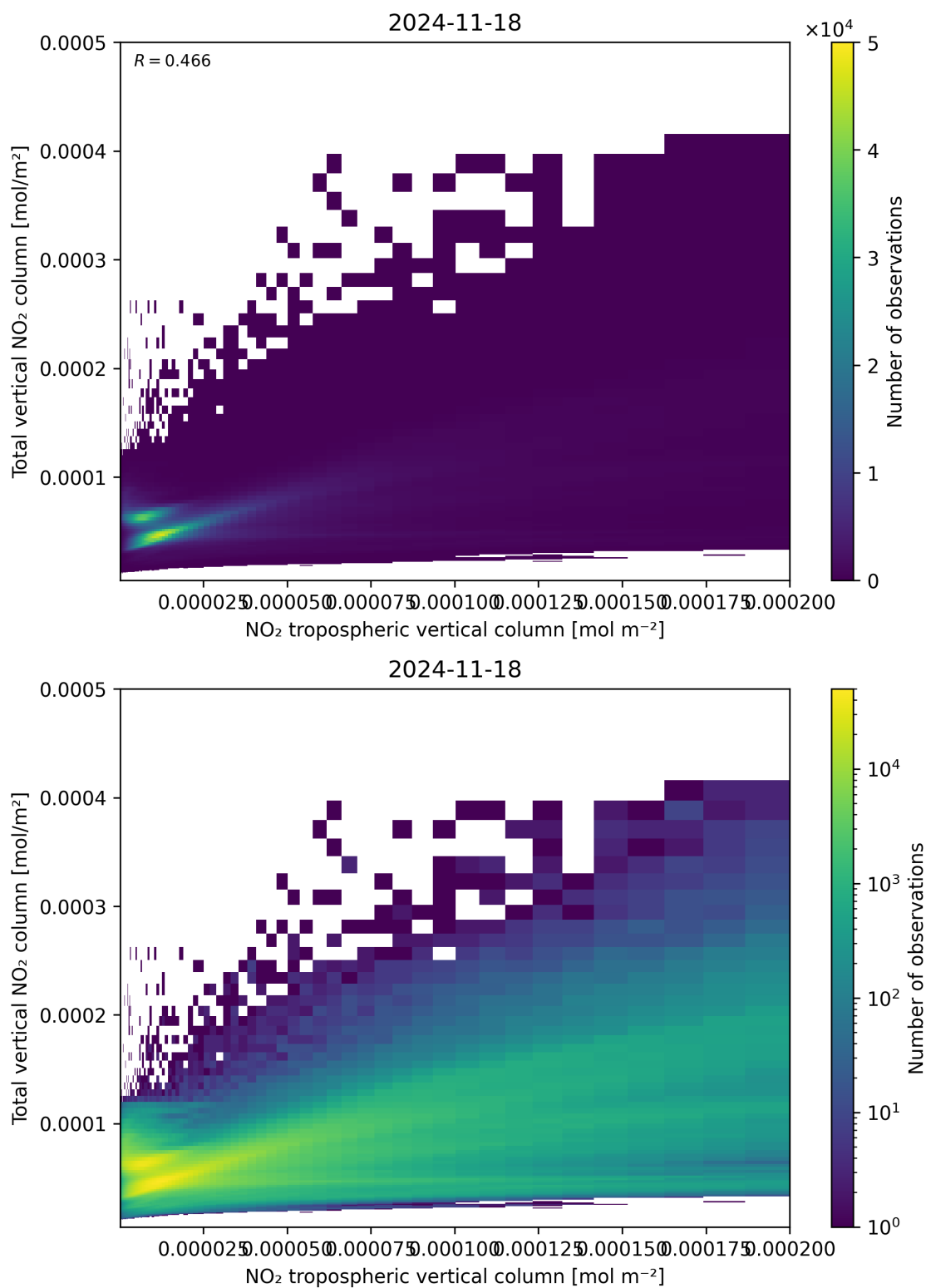
Figure 128: Scatter density plot of “NO 2 tropospheric vertical column” against “Total vertical NO 2 column” for 2024-11-17 to 2024-11-19.
