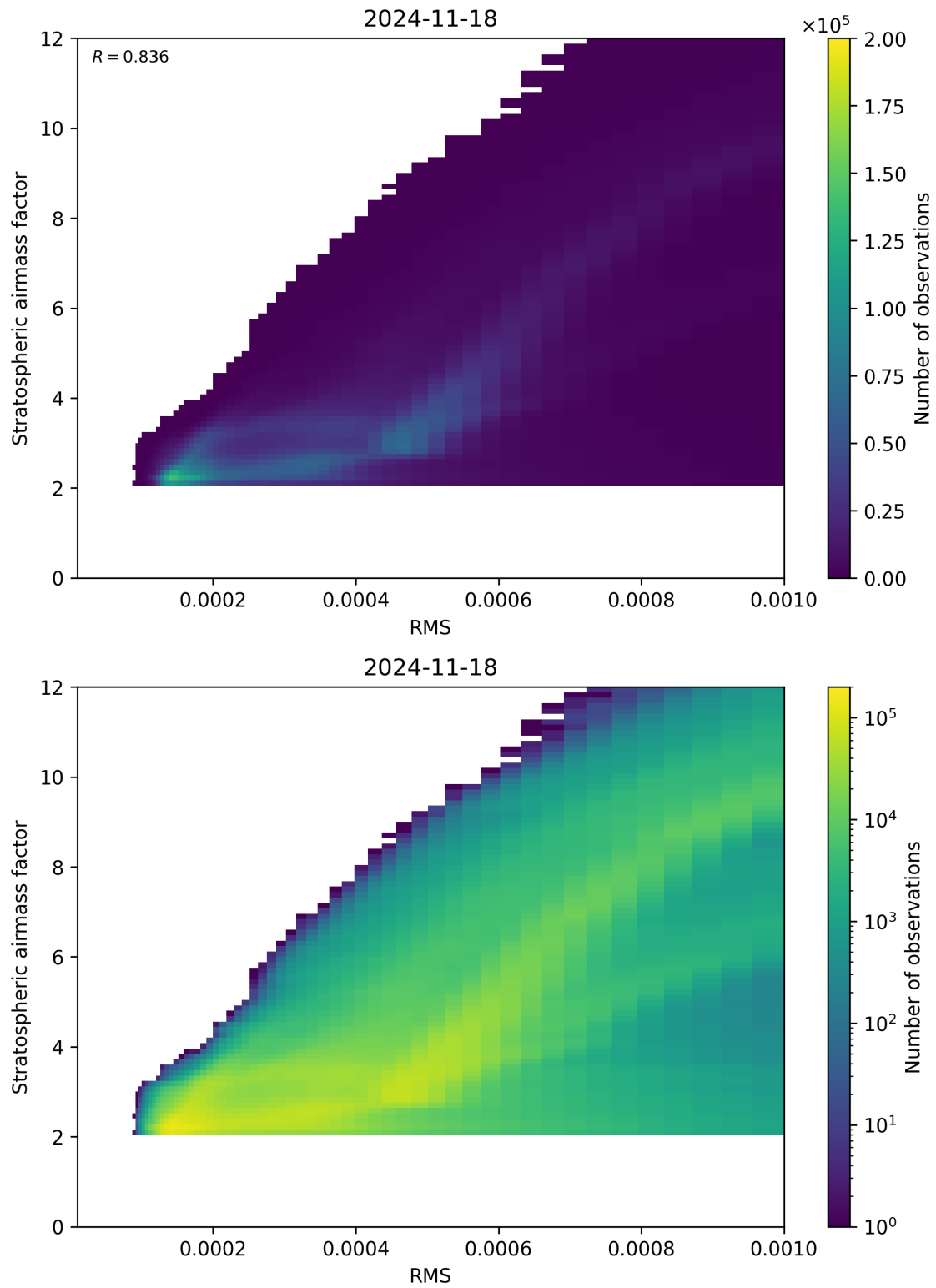
Figure 144: Scatter density plot of “RMS” against “Stratospheric airmass factor” for 2024-11-17 to 2024-11-19.
