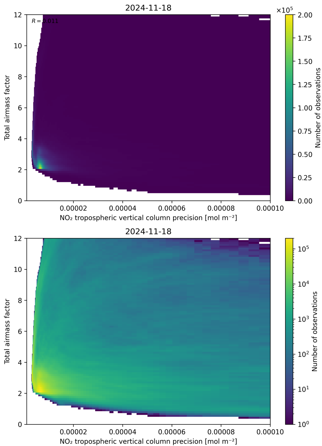
Figure 132: Scatter density plot of “NO 2 tropospheric vertical column precision” against “Total air mass factor” for 2024-11-17 to 2024-11-19.
