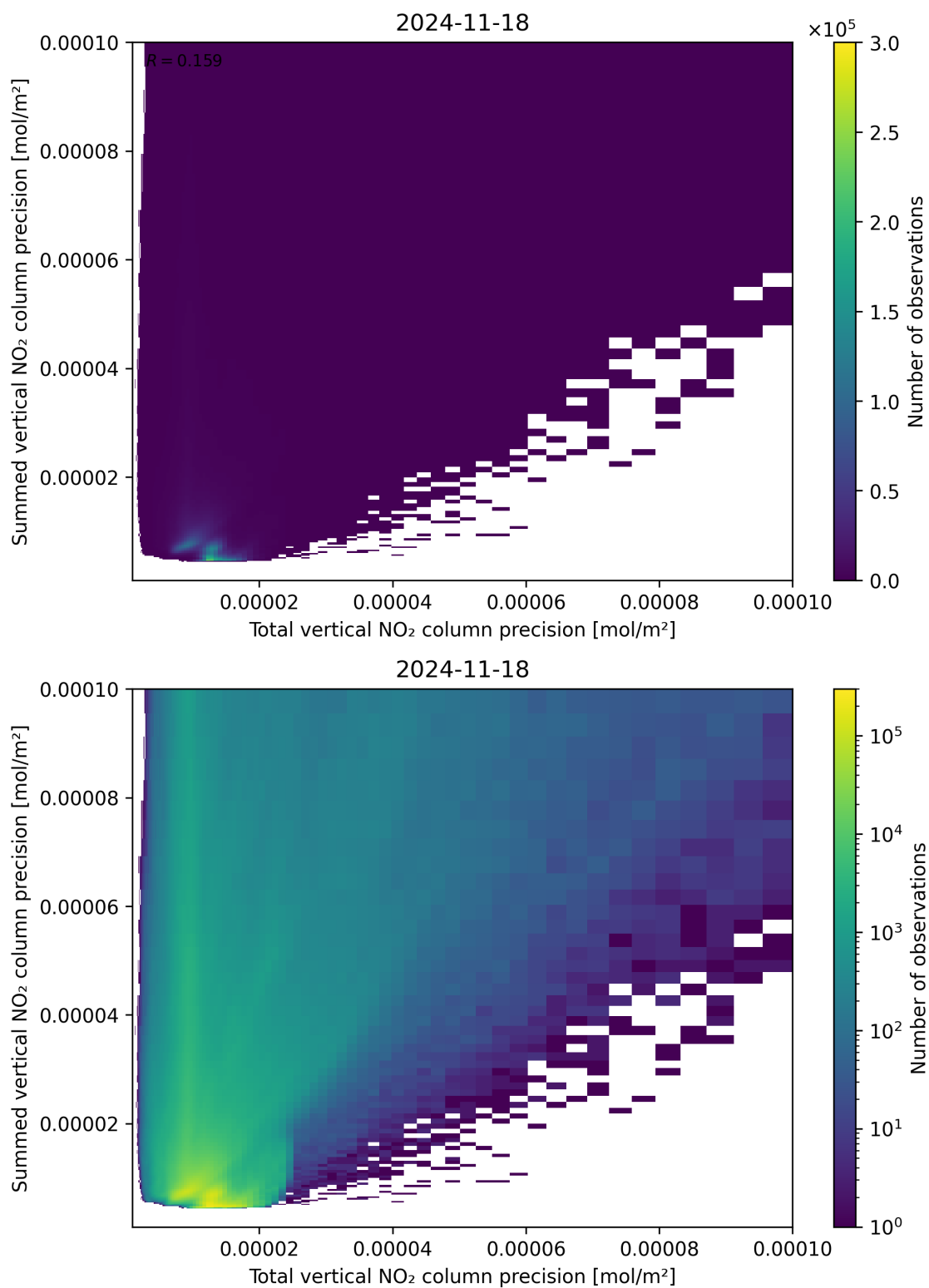
Figure 118: Scatter density plot of “Total vertical NO 2 column precision” against “Summed vertical NO 2 column precision” for 2024-11-17 to 2024-11-19.
