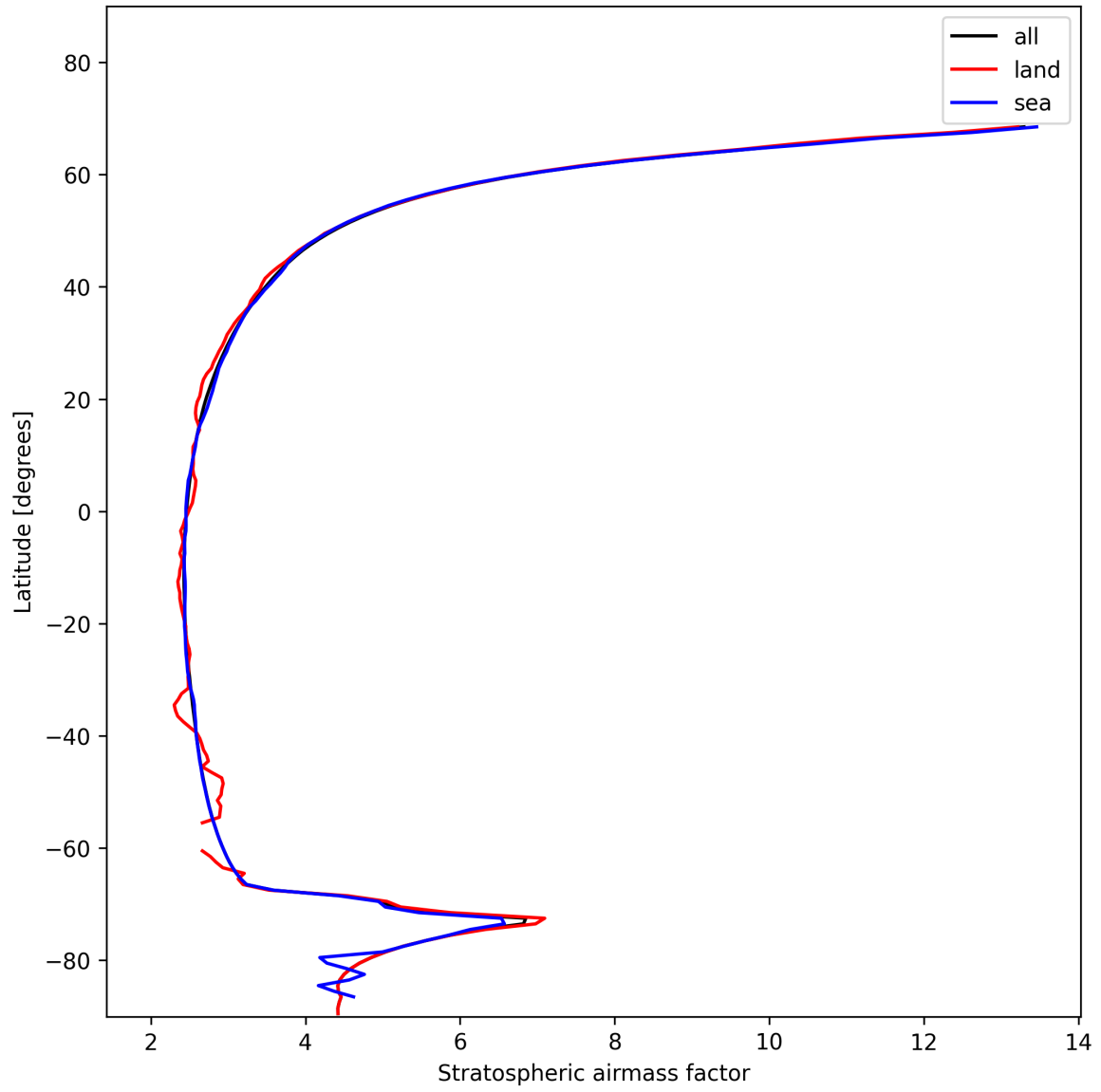
Figure 27: Zonal average of “Stratospheric airmass factor” for 2024-11-17 to 2024-11-19.
