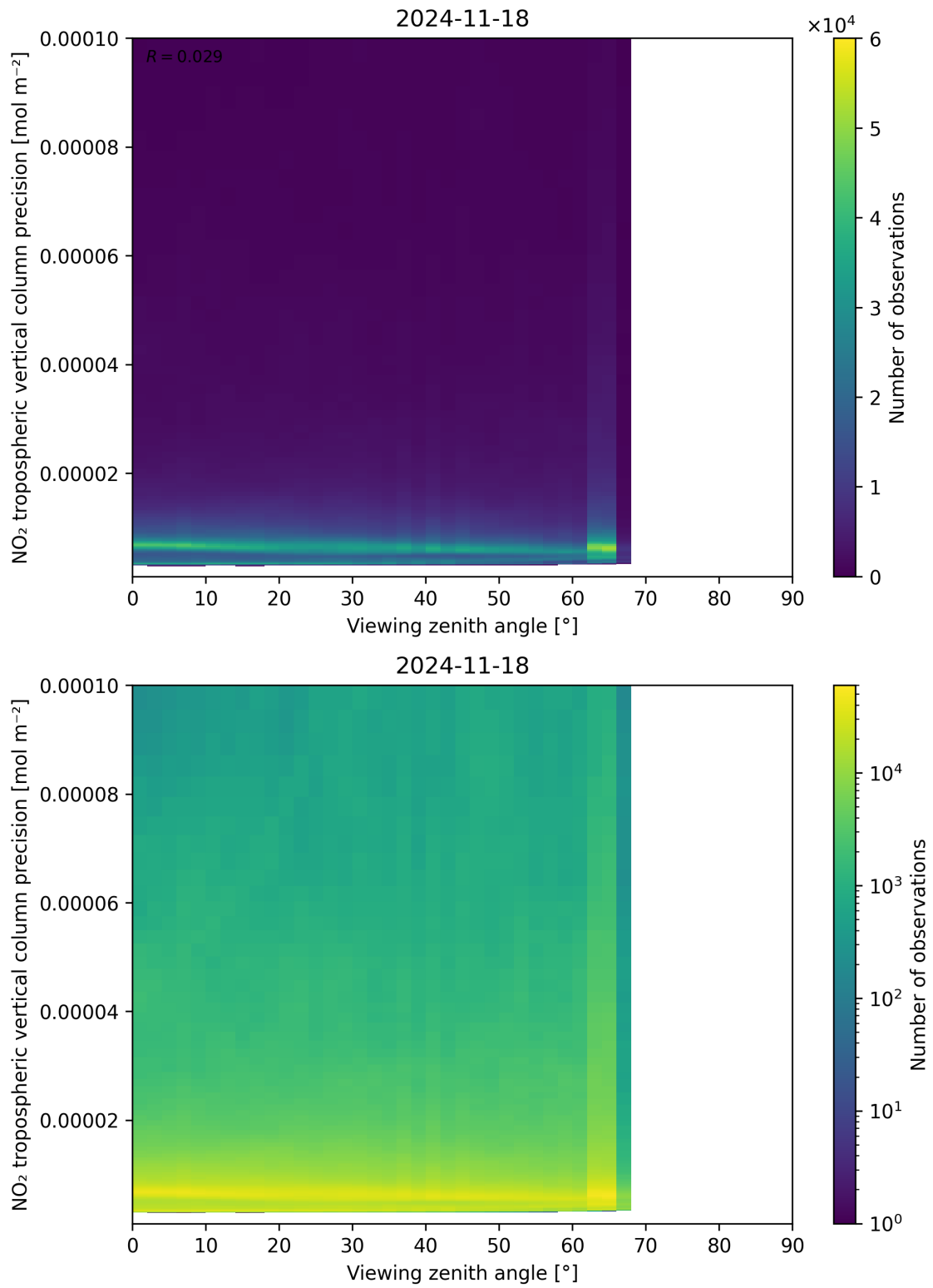
Figure 170: Scatter density plot of “Viewing zenith angle” against “NO 2 tropospheric vertical column precision” for 2024-11-17 to 2024-11-19.
