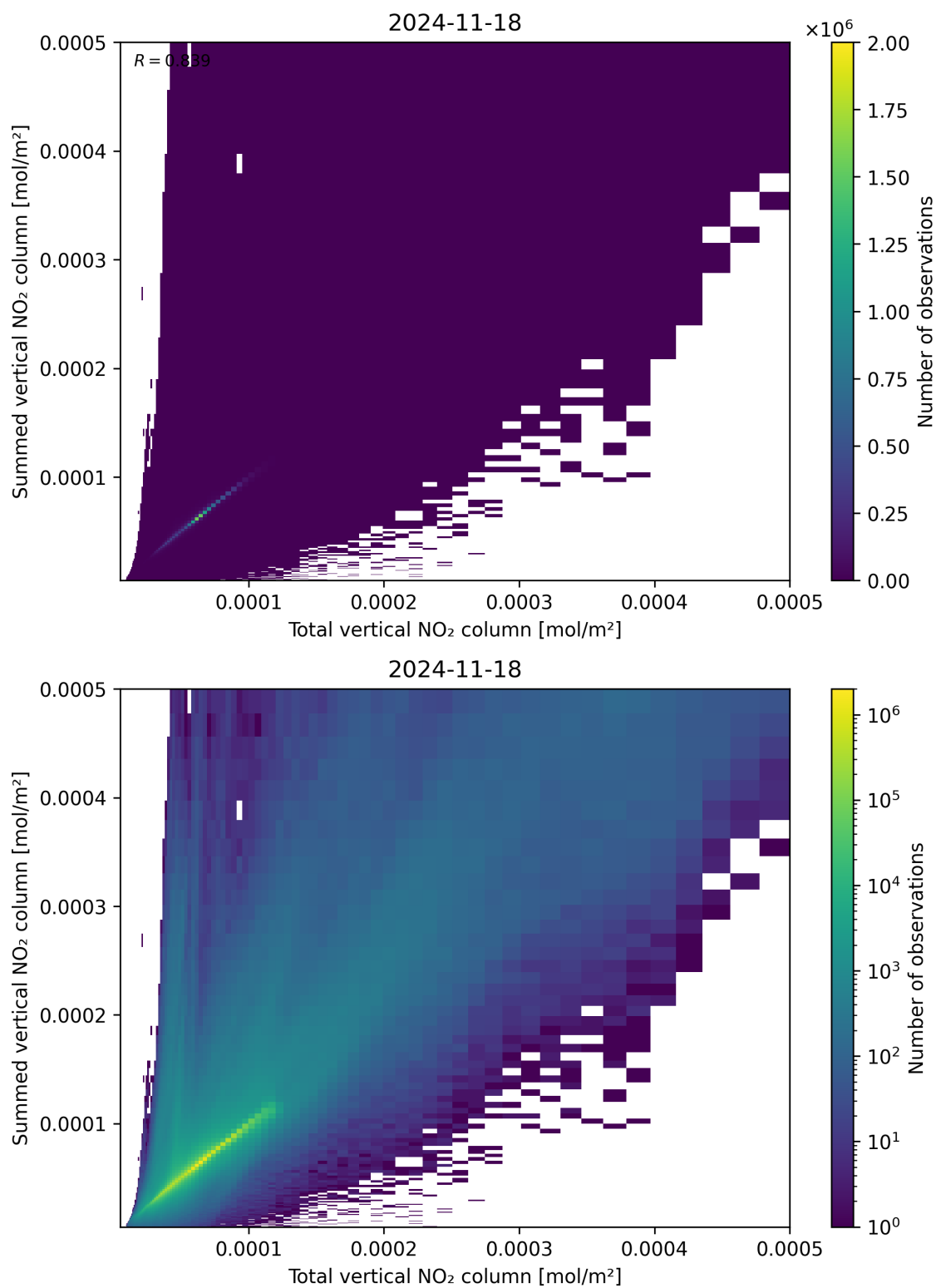
Figure 112: Scatter density plot of “Total vertical NO 2 column” against “Summed vertical NO 2 column” for 2024-11-17 to 2024-11-19.
