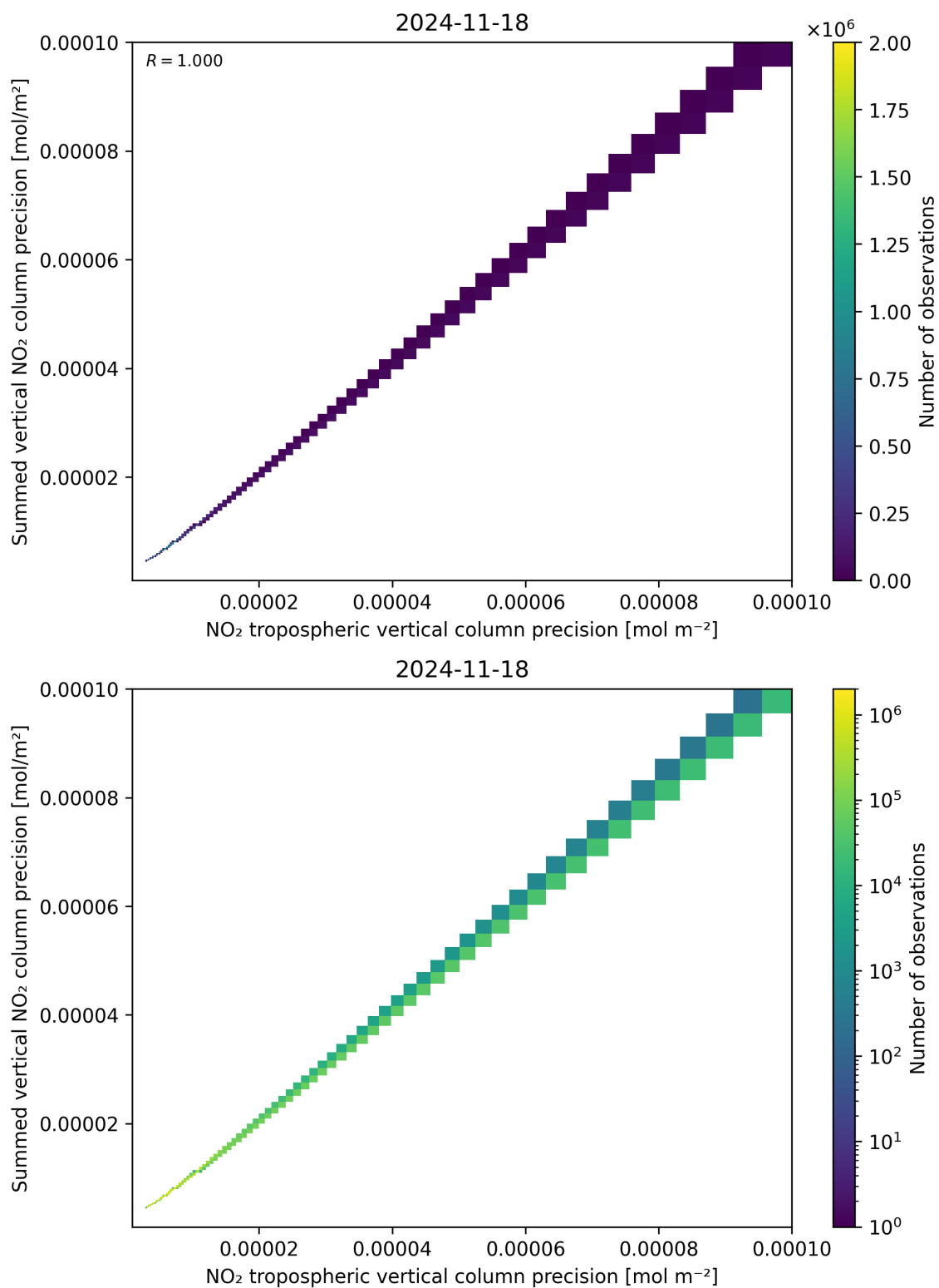
Figure 137: Scatter density plot of “NO 2 tropospheric vertical column precision” against “Summed vertical NO 2 column precision” for 2024-11-17 to 2024-11-19.
