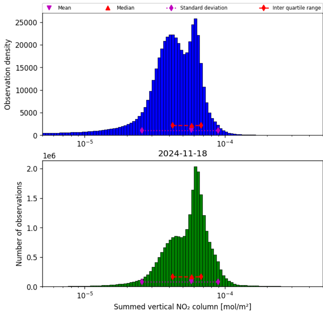
Figure 40: Histogram of “Summed vertical NO 2 column” for 2024-11-17 to 2024-11-19
