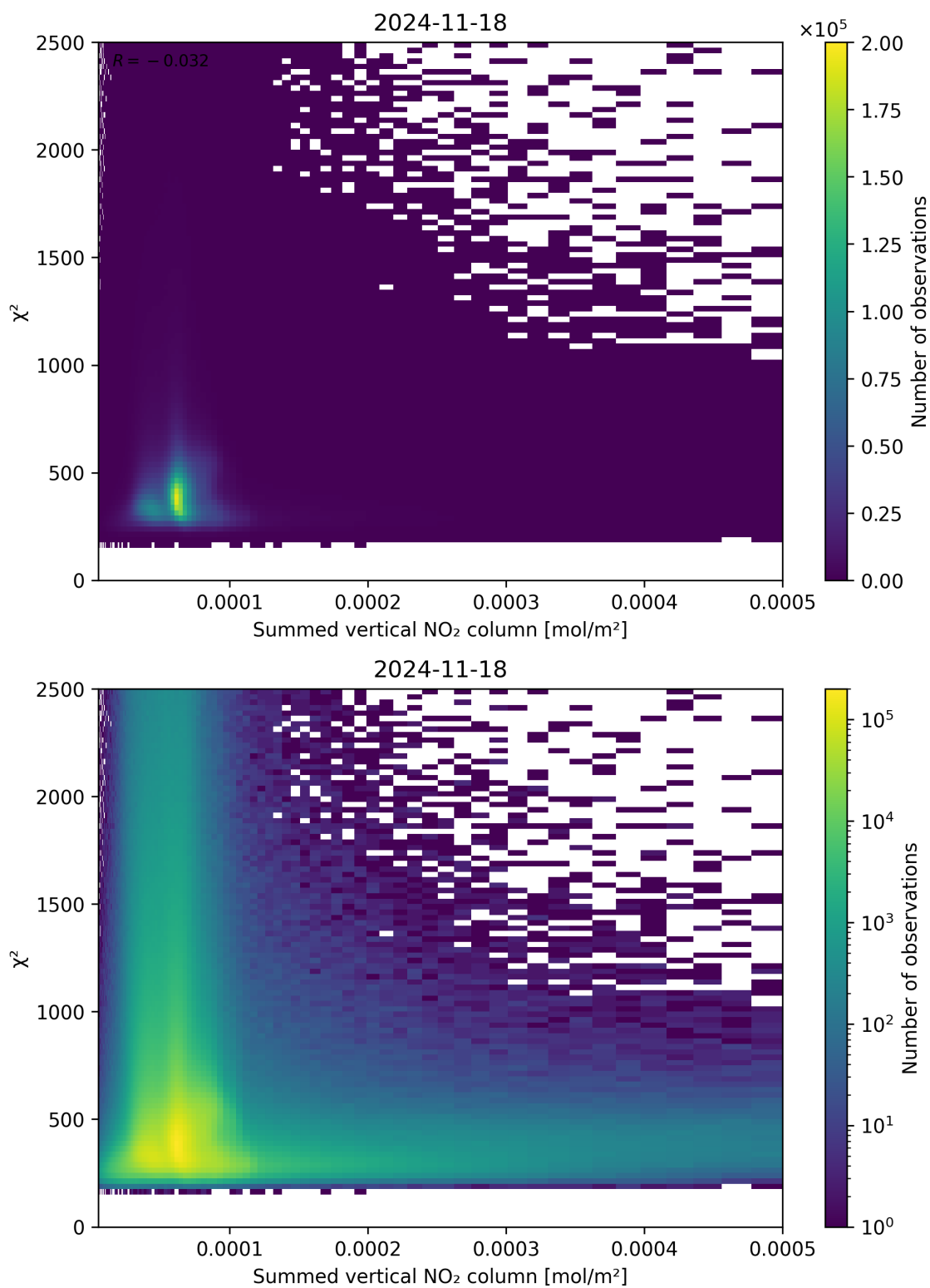
Figure 104: Scatter density plot of “Summed vertical NO 2 column” against “ \chi^2 ” for 2024-11-17 to 2024-11-19.
