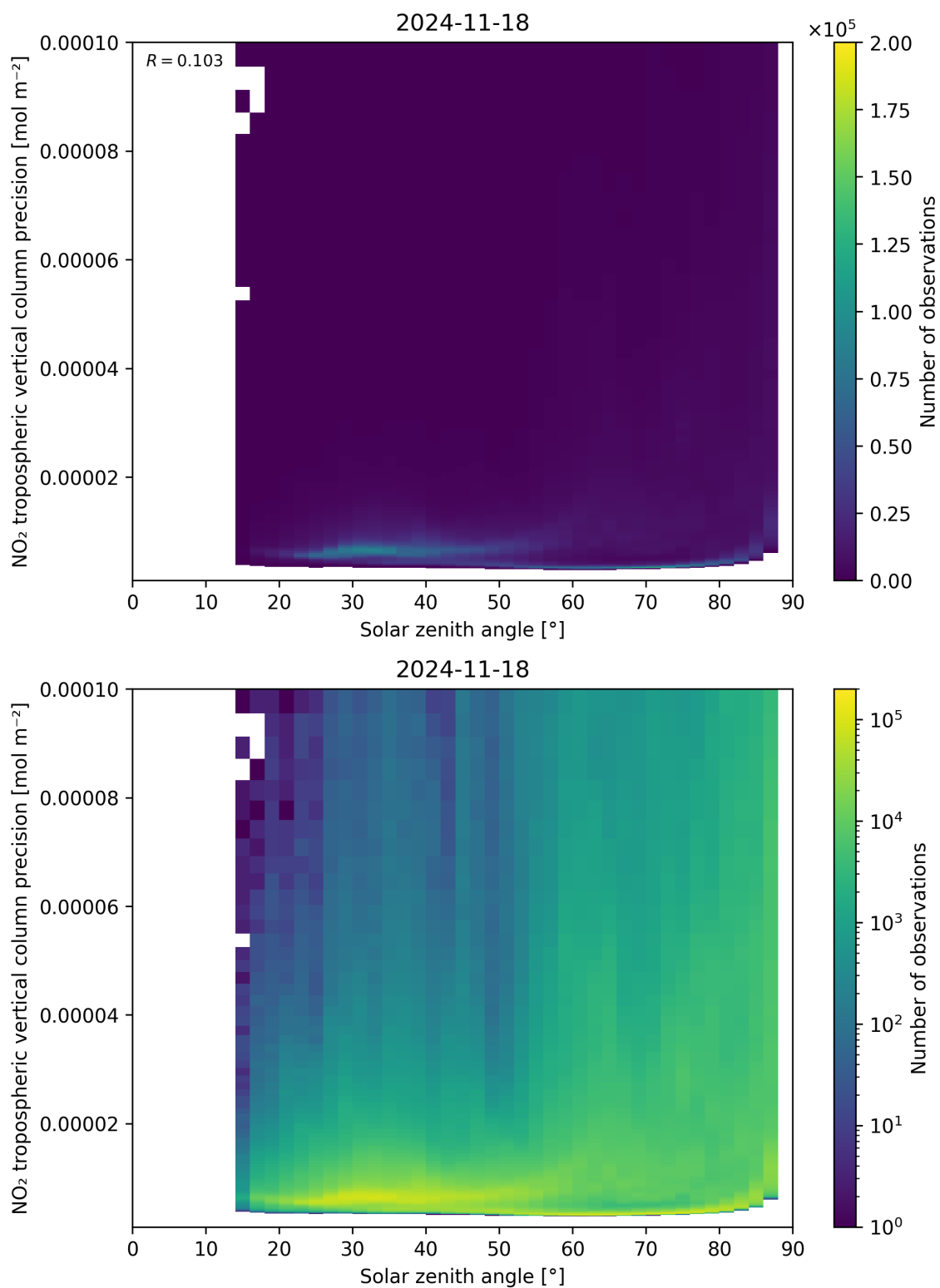
Figure 156: Scatter density plot of “Solar zenith angle” against “NO 2 tropospheric vertical column precision” for 2024-11-17 to 2024-11-19.
