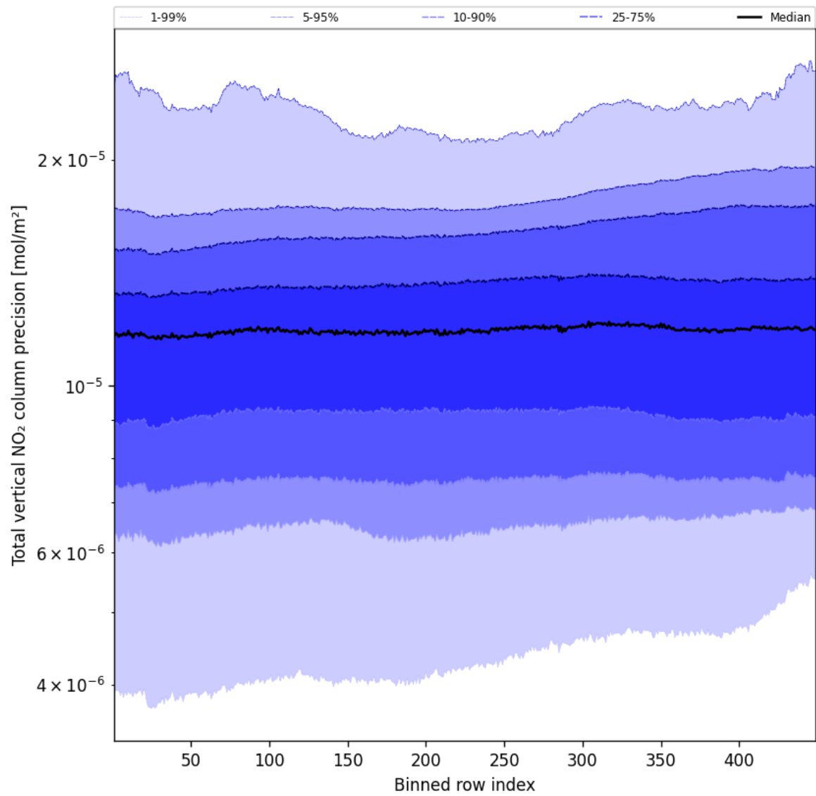
Figure 56: Along track statistics of “Total vertical NO 2 column precision” for 2024-11-17 to 2024-11-19
