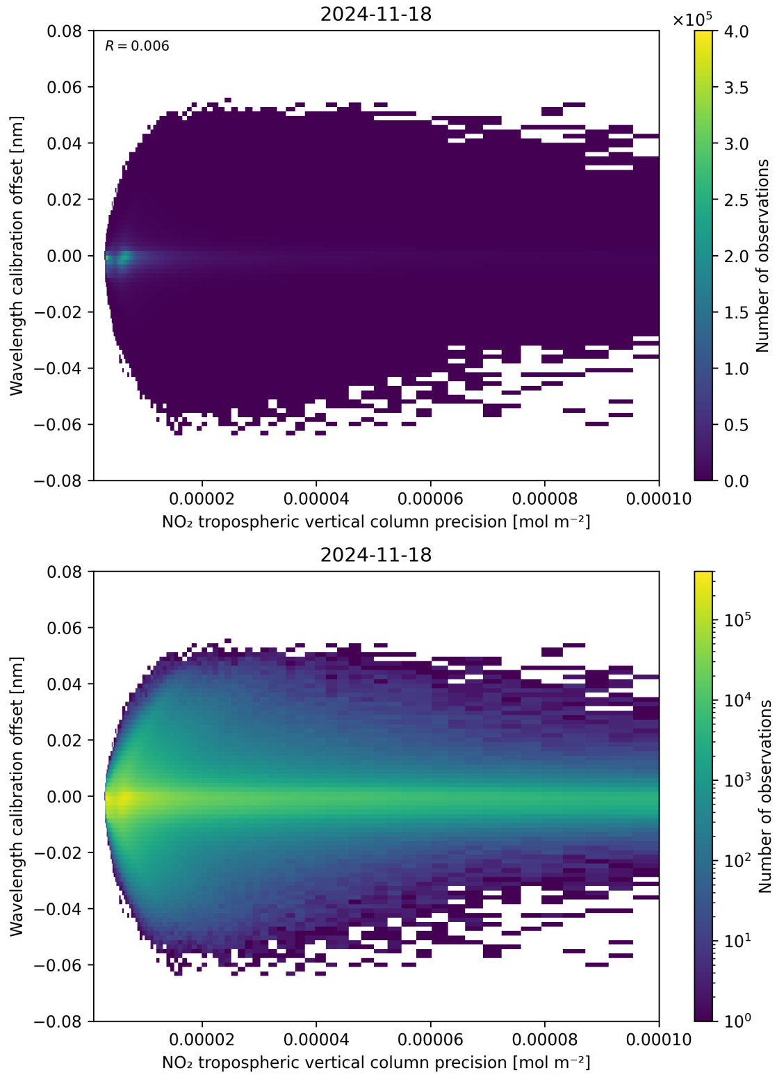
Figure 141: Scatter density plot of “NO 2 tropospheric vertical column precision” against “Wavelength calibration offset” for 2024-11-17 to 2024-11-19.
