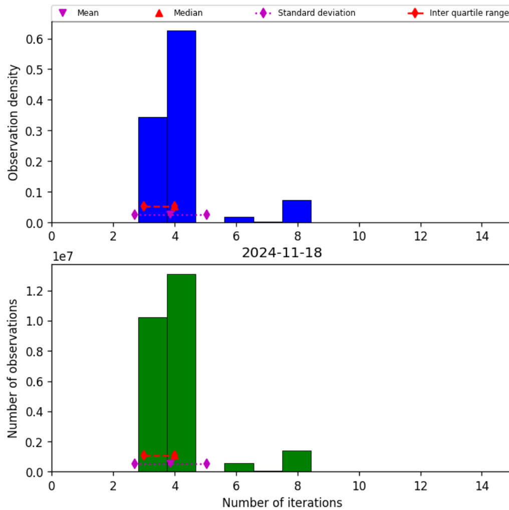
Figure 34: Histogram of “Number of iterations” for 2024-11-17 to 2024-11-19
