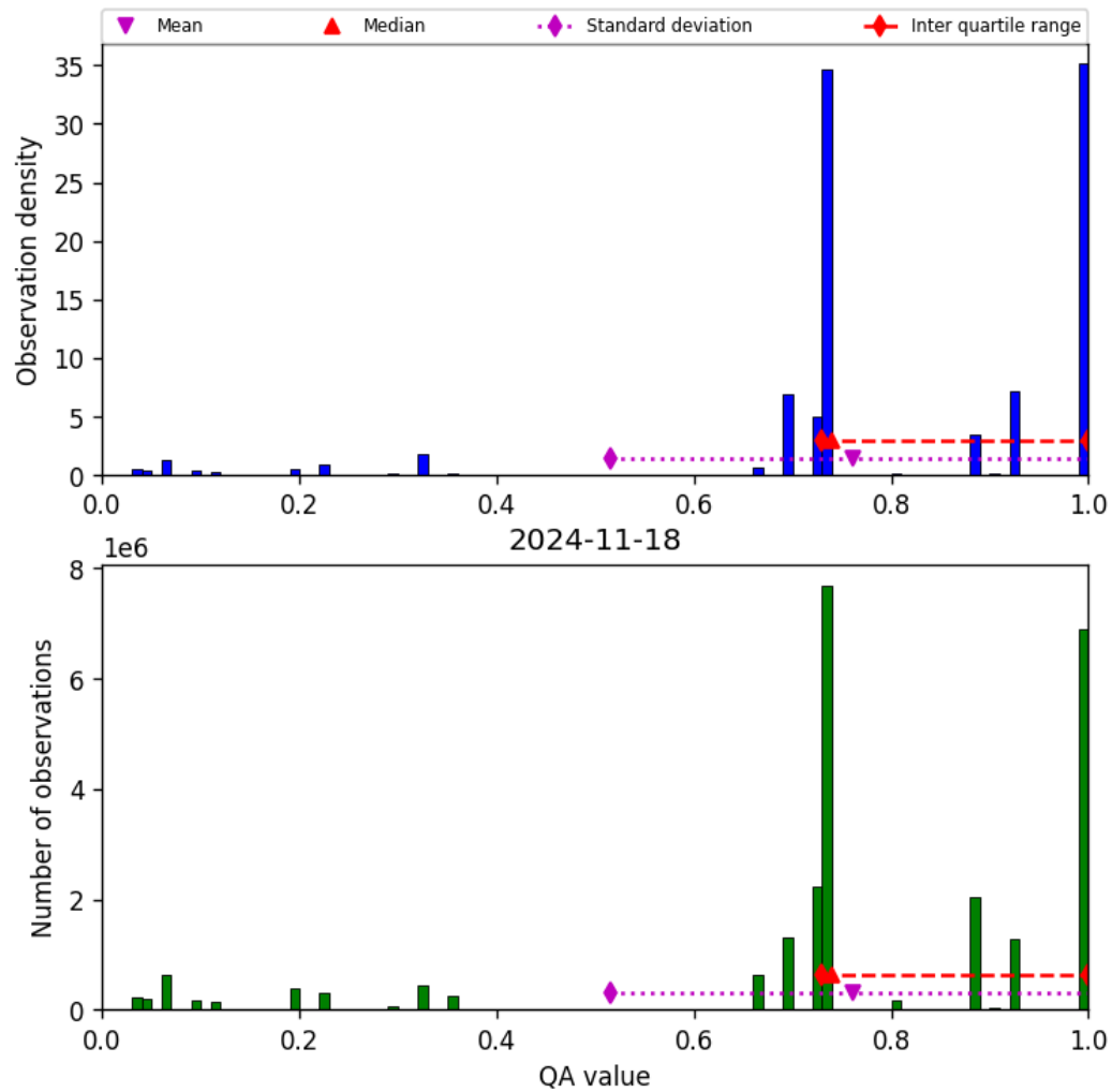
Figure 28: Histogram of “QA value” for 2024-11-17 to 2024-11-19
