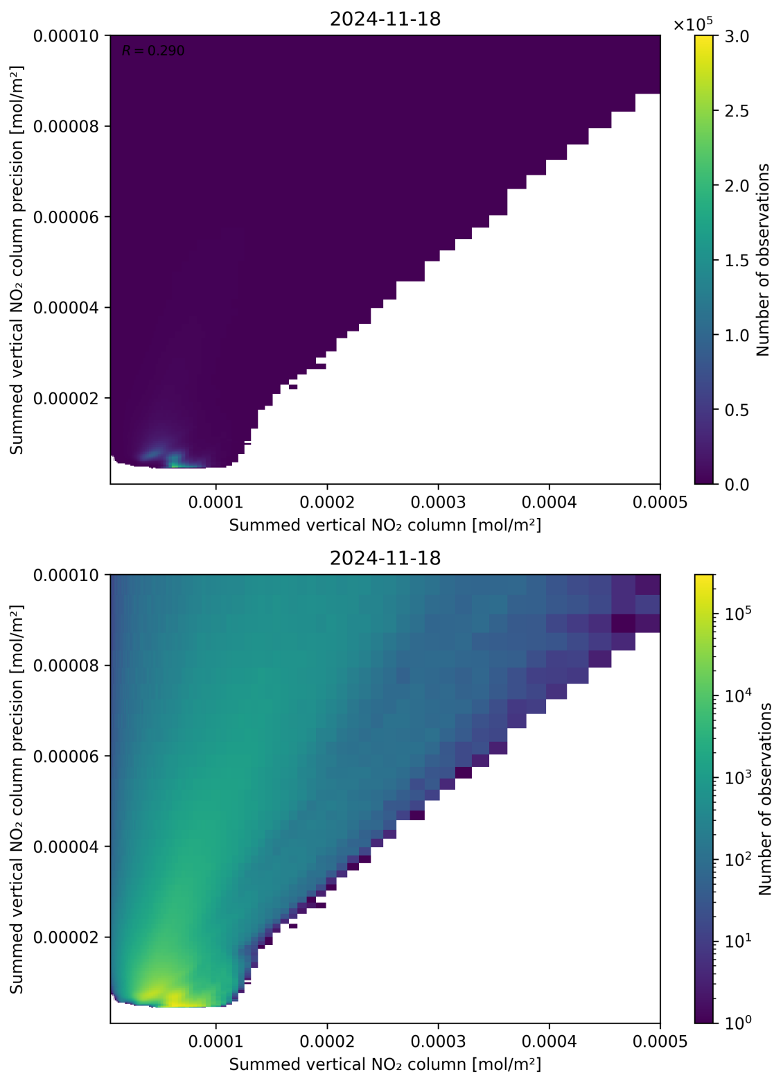
Figure 105: Scatter density plot of “Summed vertical NO 2 column” against “Summed vertical NO 2 column precision” for 2024-11-17 to 2024-11-19.
