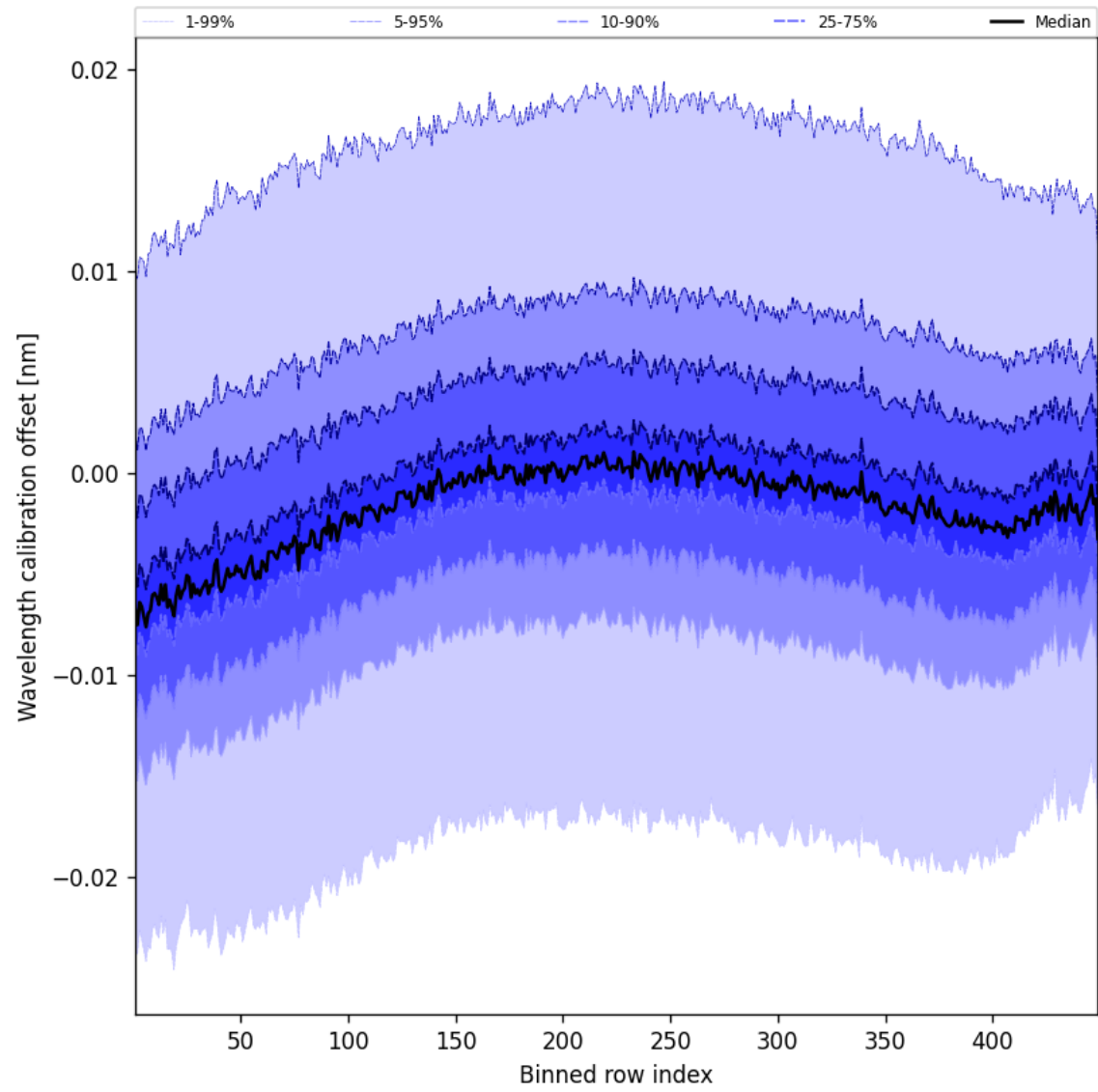
Figure 52: Along track statistics of “Wavelength calibration offset” for 2024-11-17 to 2024-11-19
