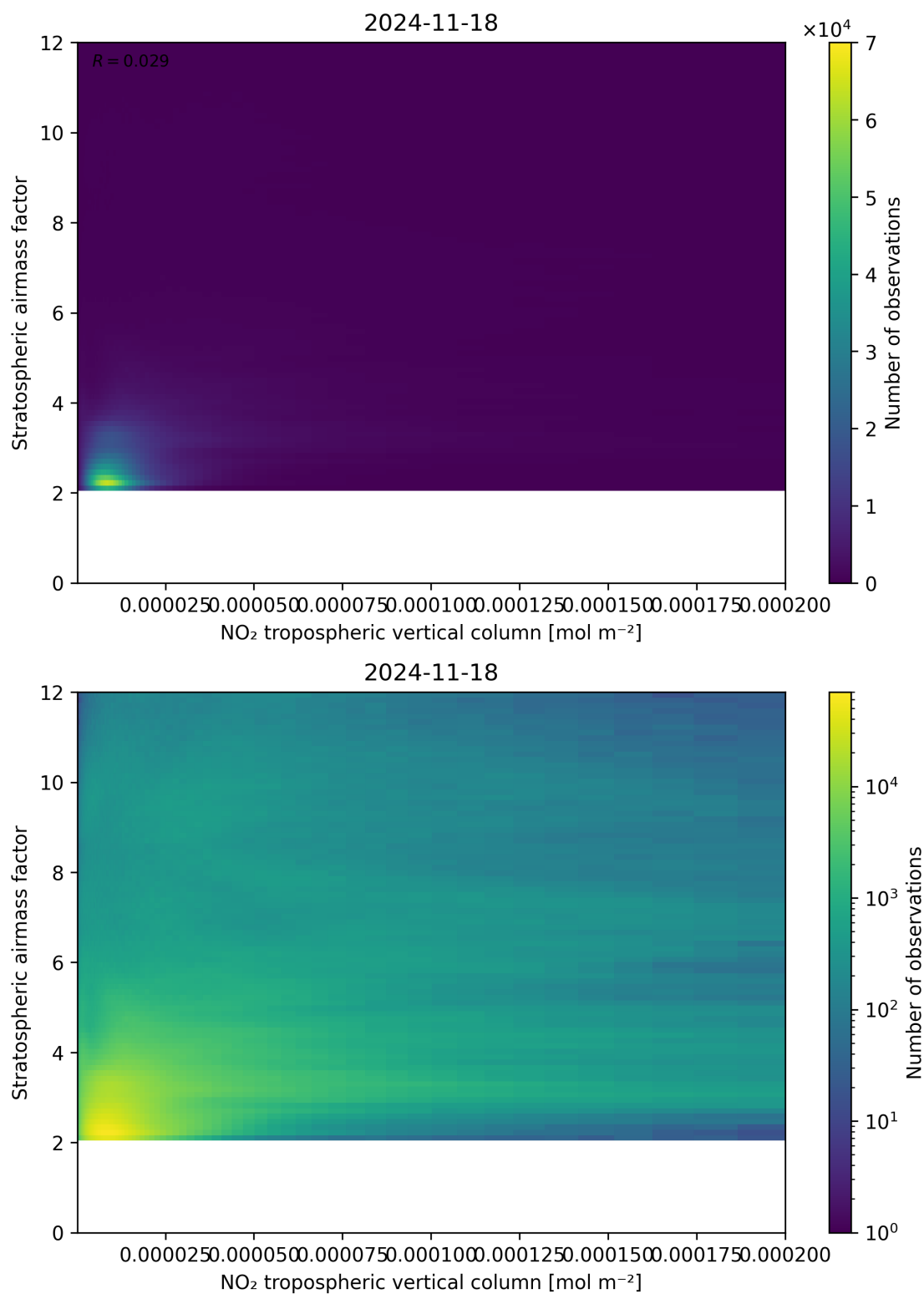
Figure 121: Scatter density plot of “NO 2 tropospheric vertical column” against “Stratospheric air mass factor” for 2024-11-17 to 2024-11-19.
