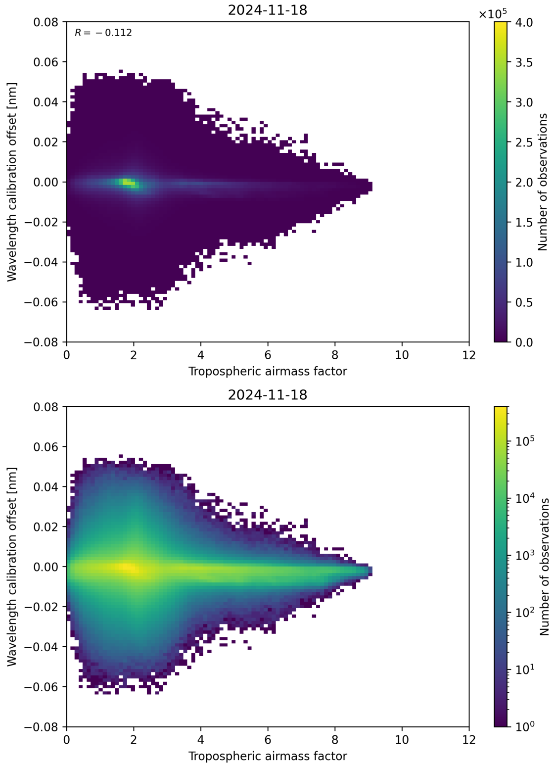
Figure 80: Scatter density plot of “Tropospheric airmass factor” against “Wavelength calibration offset” for 2024-11-17 to 2024-11-19.
