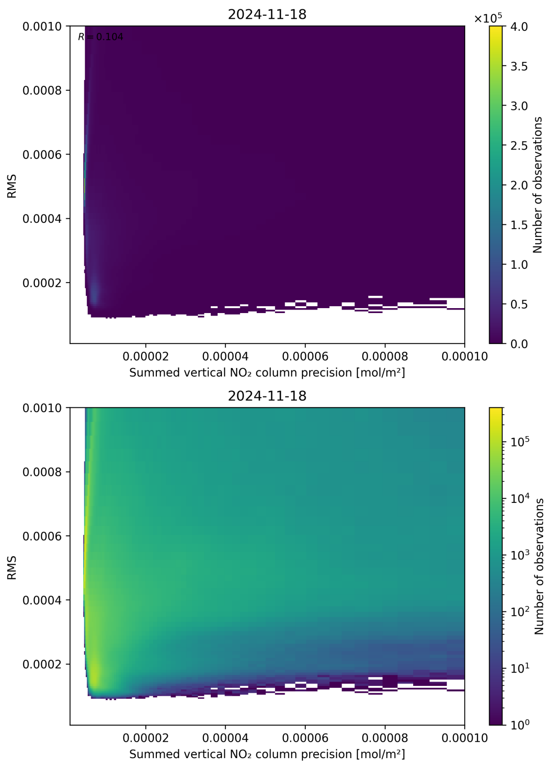
Figure 108: Scatter density plot of “Summed vertical NO 2 column precision” against “RMS” for 2024-11-17 to 2024-11-19.
