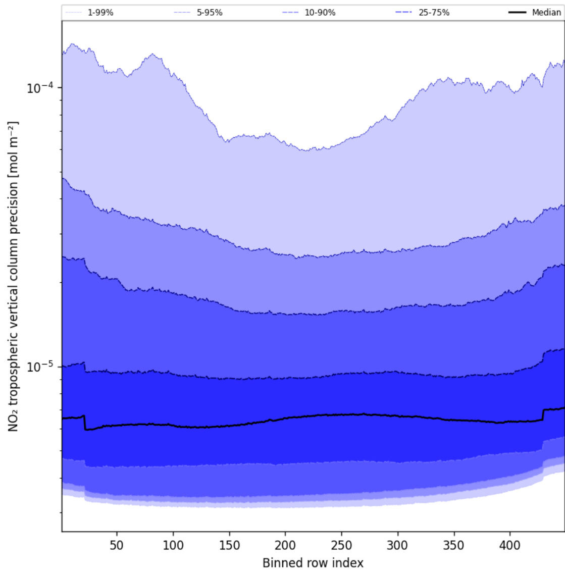
Figure 47: Along track statistics of “NO 2 tropospheric vertical column precision” for 2024-11-17 to 2024-11-19
