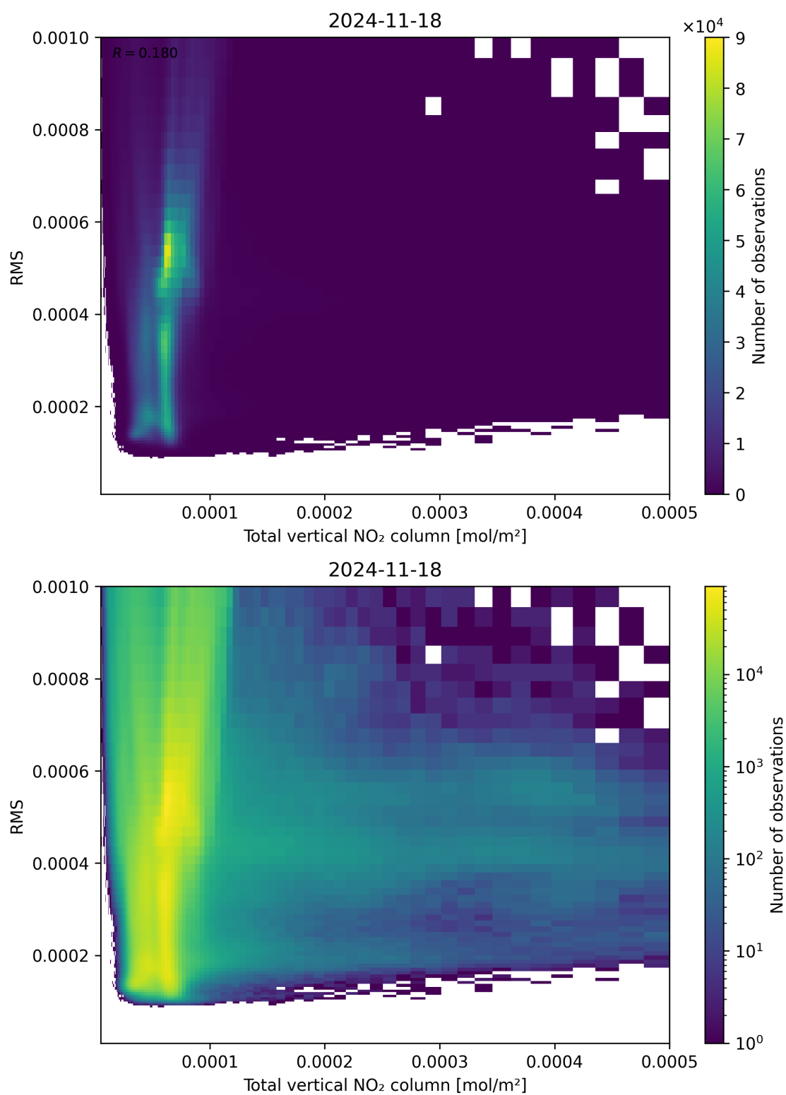
Figure 120: Scatter density plot of “Total vertical NO 2 column” against “RMS” for 2024-11-17 to 2024-11-19.
