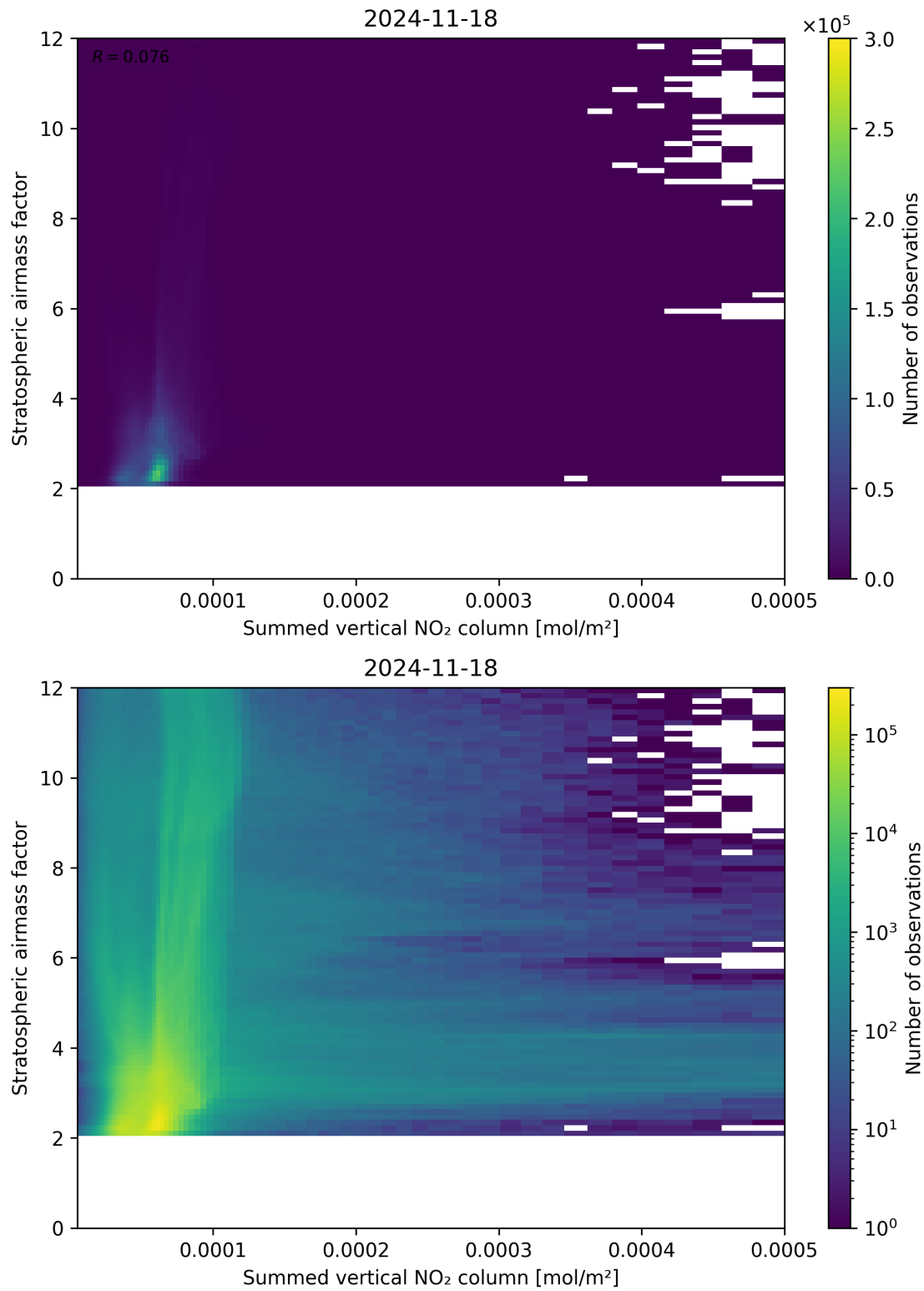
Figure 103: Scatter density plot of “Summed vertical NO 2 column” against “Stratospheric airmass factor” for 2024-11-17 to 2024-11-19.
