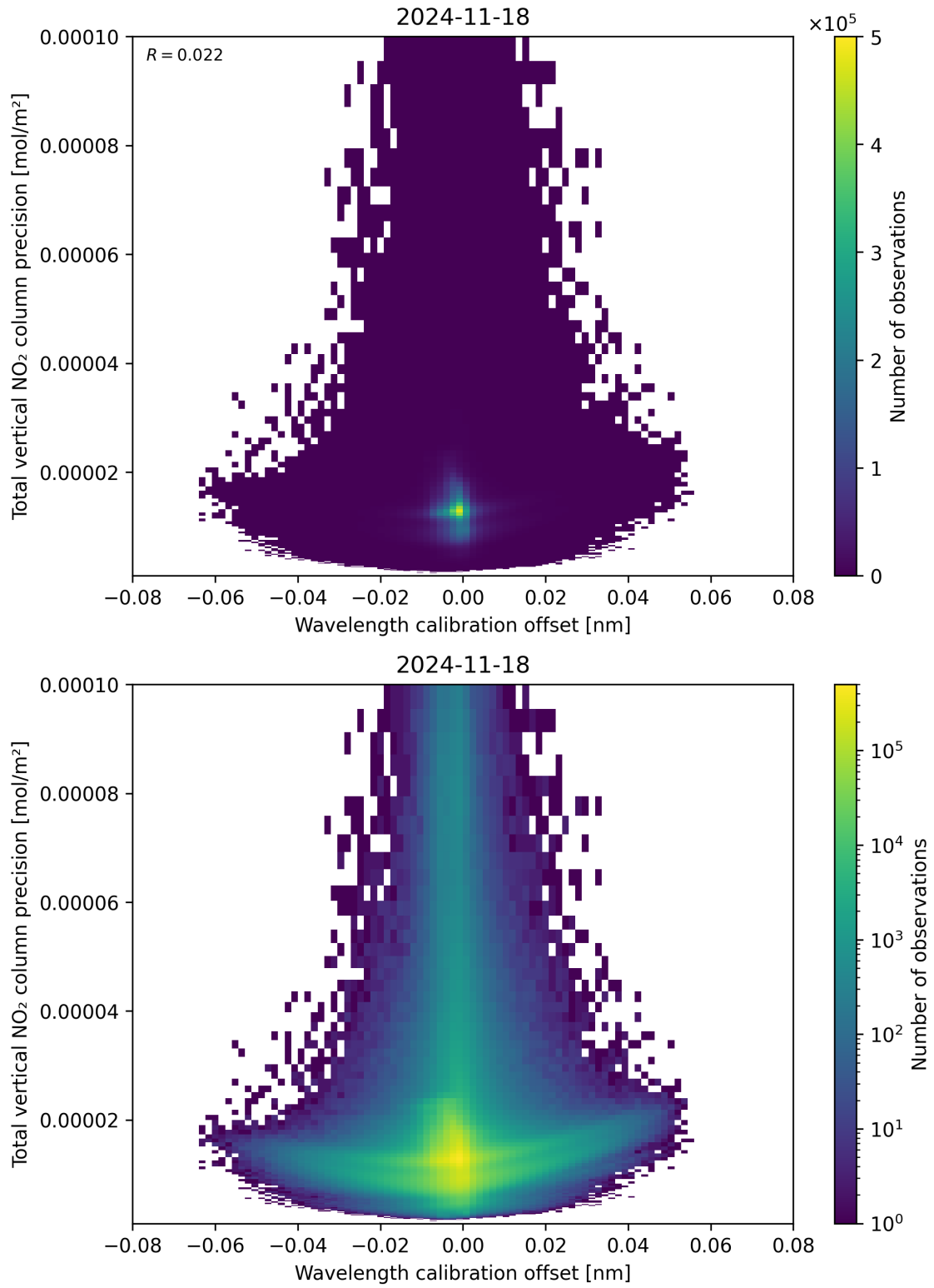
Figure 180: Scatter density plot of “Wavelength calibration offset” against “Total vertical NO 2 column precision” for 2024-11-17 to 2024-11-19.
