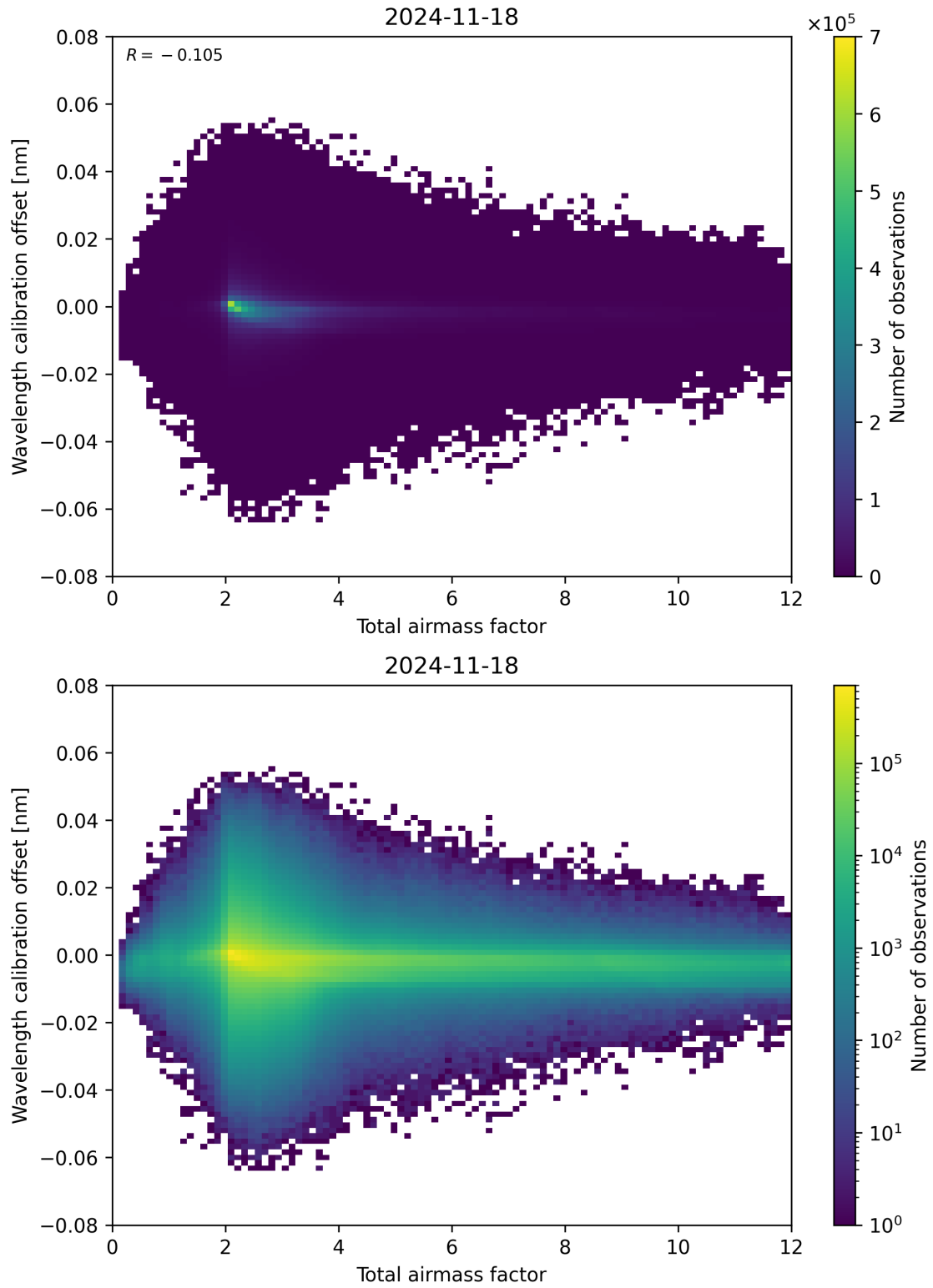
Figure 70: Scatter density plot of “Total airmass factor” against “Wavelength calibration offset” for 2024-11-17 to 2024-11-19.
