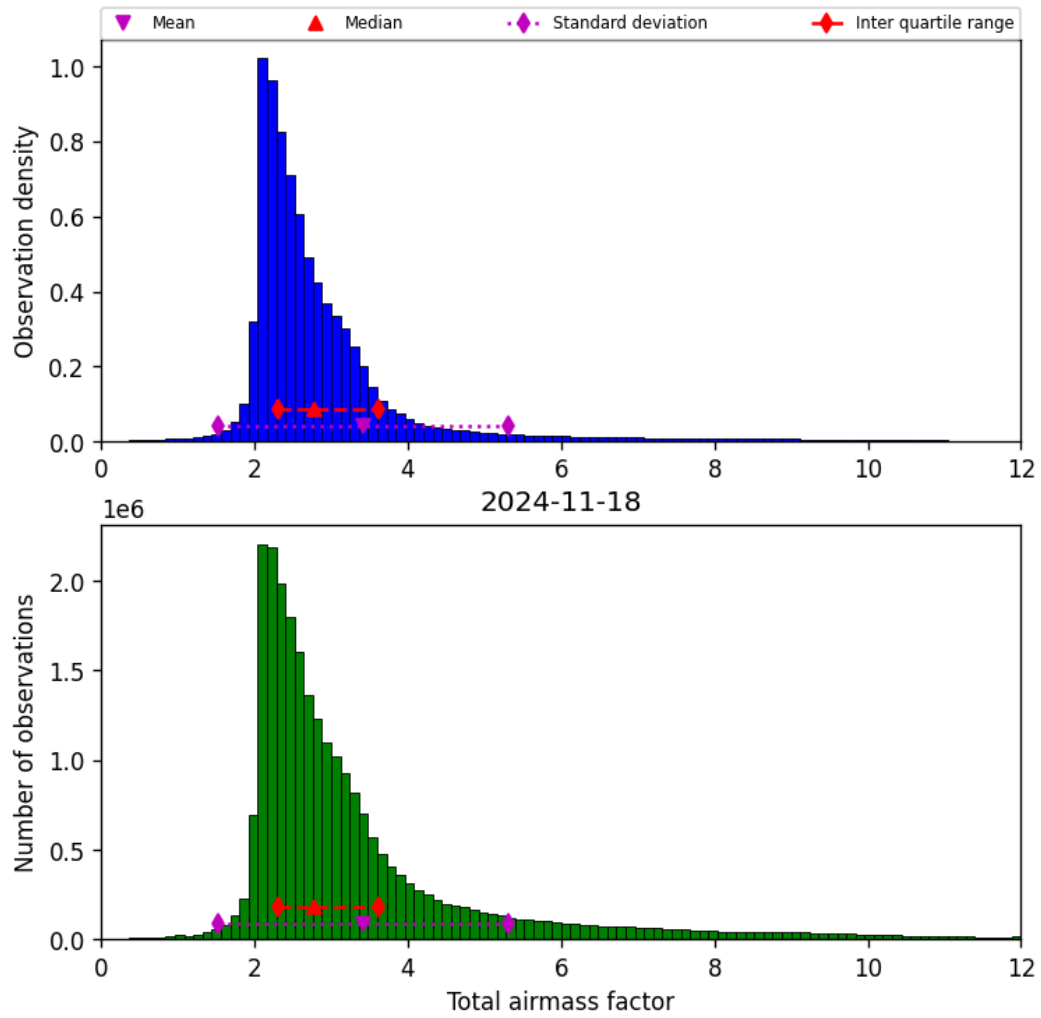
Figure 32: Histogram of “Total airmass factor” for 2024-11-17 to 2024-11-19
