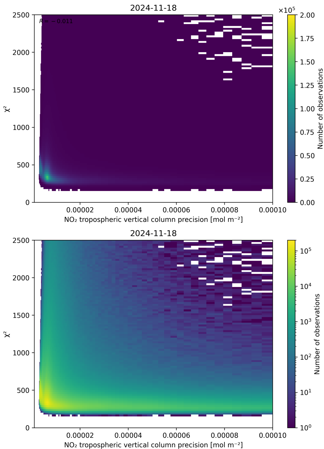
Figure 134: Scatter density plot of “NO 2 tropospheric vertical column precision” against “ \chi^2 ” for 2024-11-17 to 2024-11-19.
