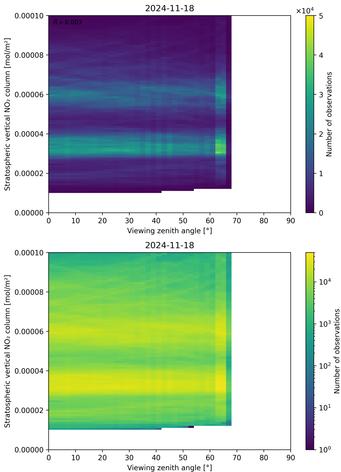
Figure 164: Scatter density plot of “Viewing zenith angle” against “Stratospheric vertical NO 2 column” for 2024-11-17 to 2024-11-19.
