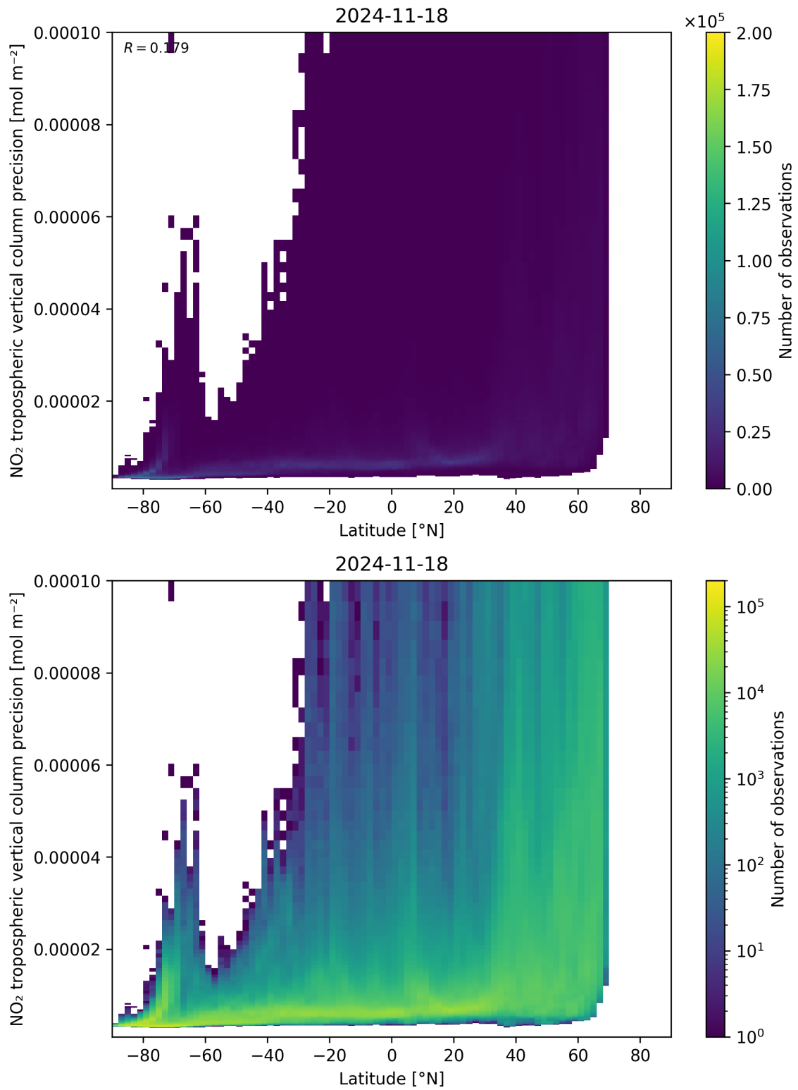
Figure 93: Scatter density plot of “Latitude” against “NO 2 tropospheric vertical column precision” for 2024-11-17 to 2024-11-19.
