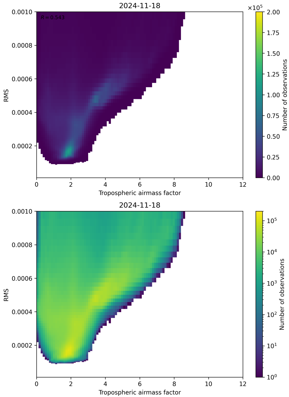
Figure 79: Scatter density plot of “Tropospheric airmass factor” against “RMS” for 2024-11-17 to 2024-11-19.
