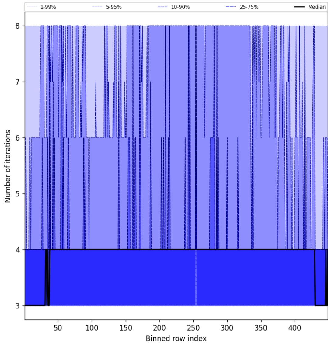
Figure 51: Along track statistics of “Number of iterations” for 2024-11-17 to 2024-11-19
