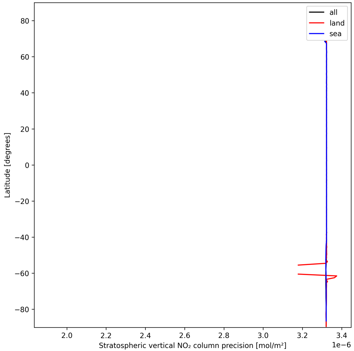
Figure 20: Zonal average of “Stratospheric vertical NO 2 column precision” for 2024-11-17 to 2024-11-19.
