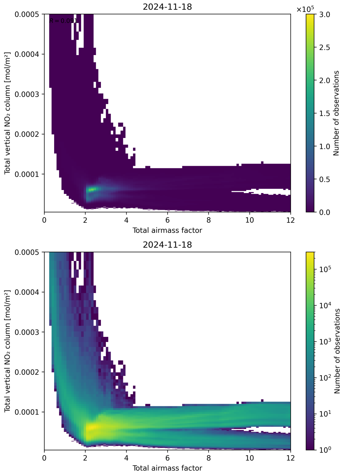
Figure 67: Scatter density plot of “Total air mass factor” against “Total vertical NO 2 column” for 2024-11-17 to 2024-11-19.
