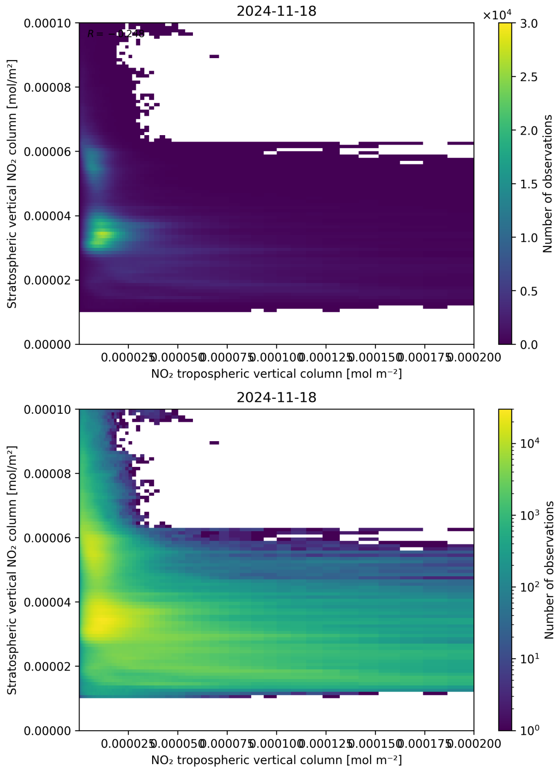
Figure 125: Scatter density plot of “NO 2 tropospheric vertical column” against “Stratospheric vertical NO 2 column” for 2024-11-17 to 2024-11-19.
