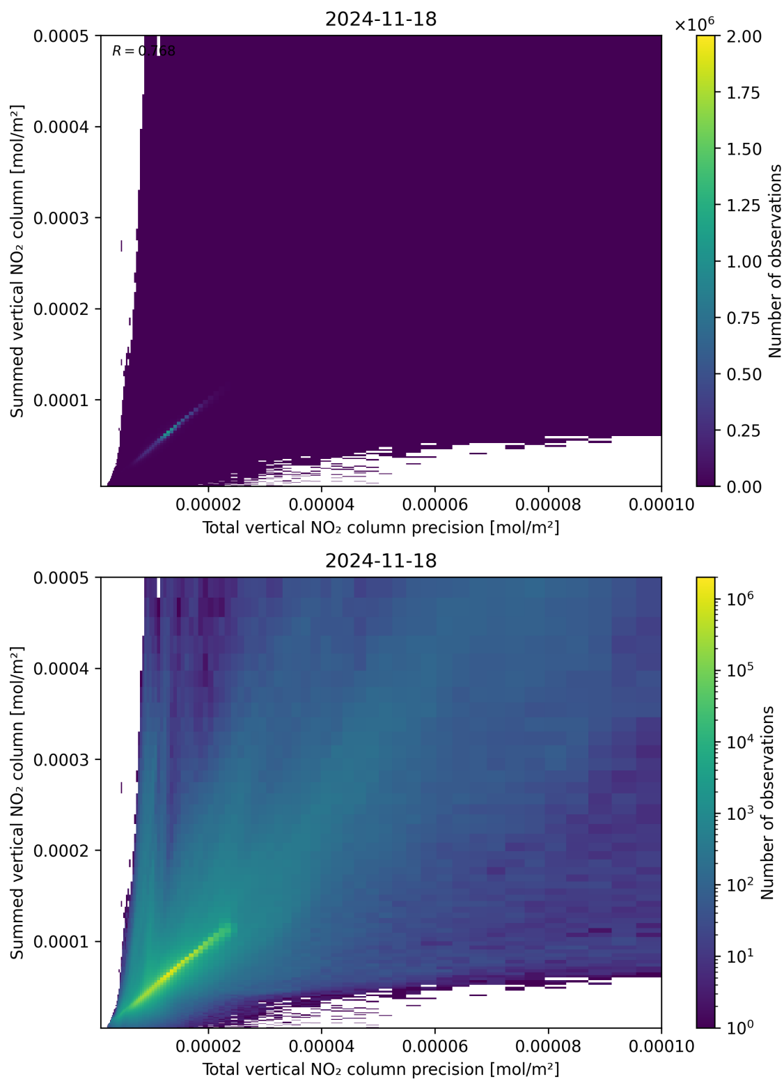
Figure 117: Scatter density plot of “Total vertical NO 2 column precision” against “Summed vertical NO 2 column” for 2024-11-17 to 2024-11-19.
