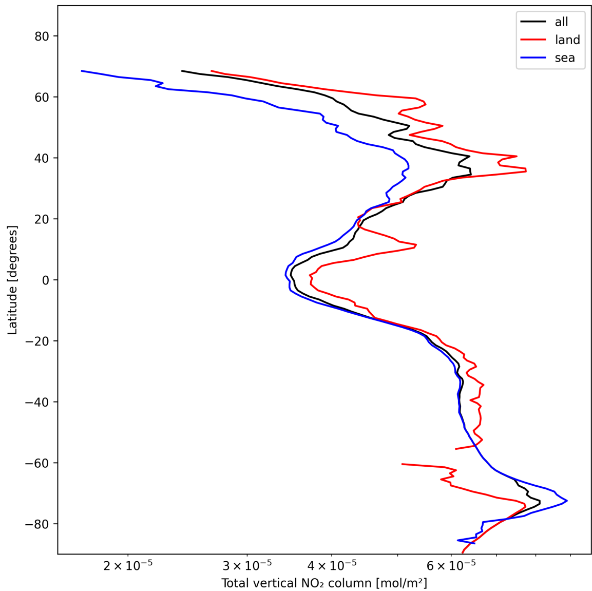
Figure 21: Zonal average of “Total vertical NO 2 column” for 2024-11-17 to 2024-11-19.
