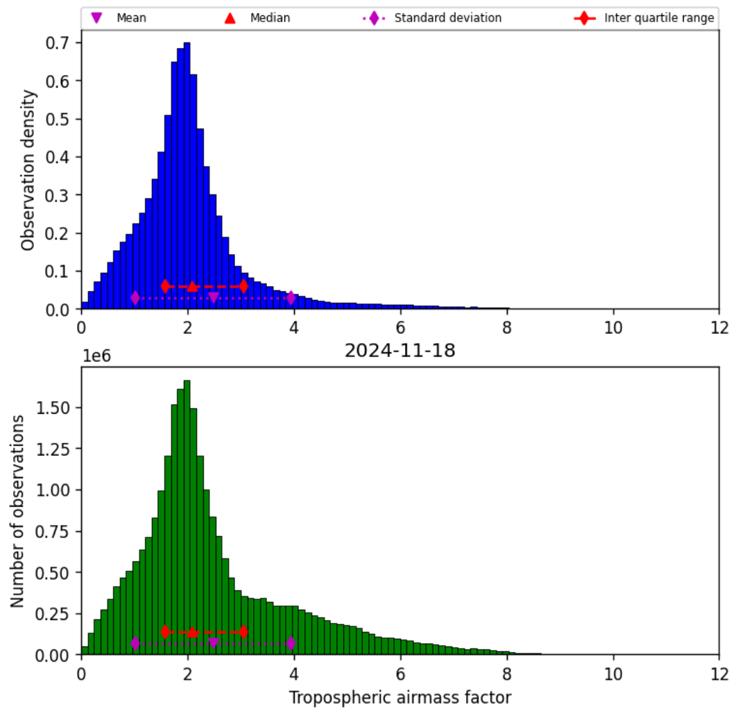
Figure 31: Histogram of “Tropospheric airmass factor” for 2024-11-17 to 2024-11-19
