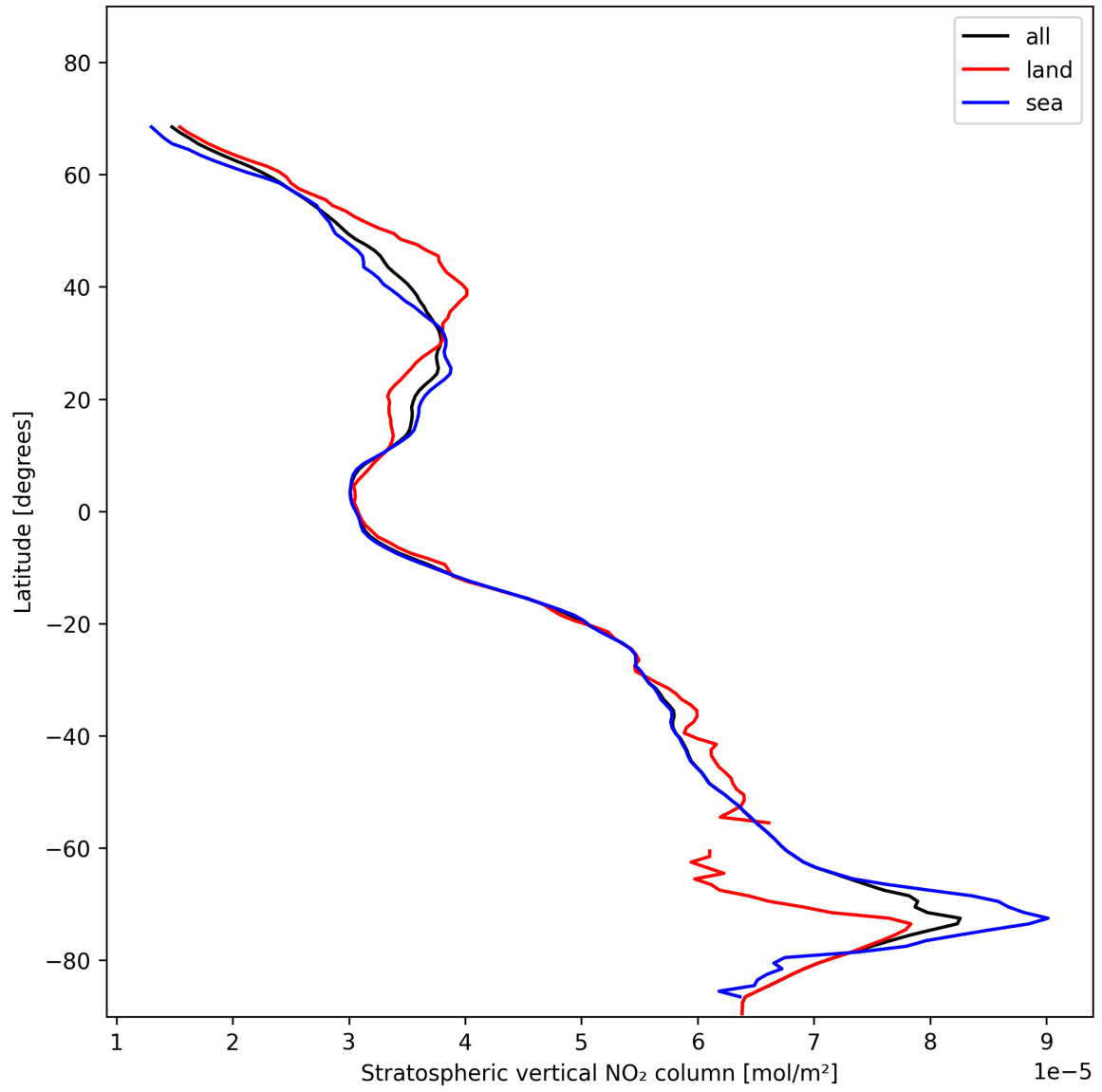
Figure 19: Zonal average of “Stratospheric vertical NO 2 column” for 2024-11-17 to 2024-11-19.
