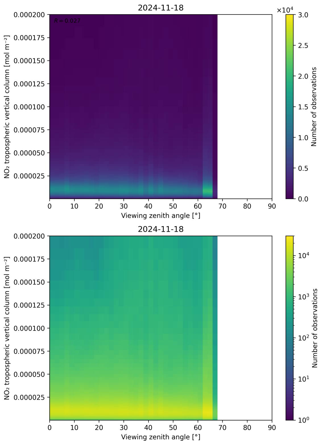
Figure 169: Scatter density plot of “Viewing zenith angle” against “NO 2 tropospheric vertical column” for 2024-11-17 to 2024-11-19.
