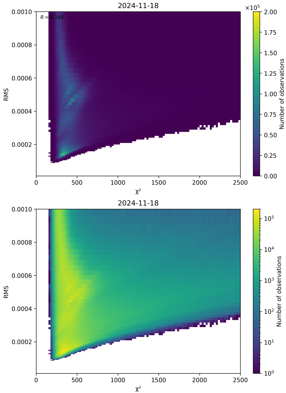
Figure 82: Scatter density plot of “ \chi^2 ” against “RMS” for 2024-11-17 to 2024-11-19.
