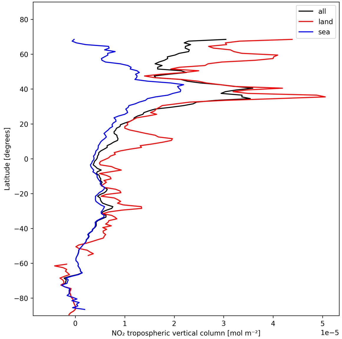
Figure 12: Zonal average of “NO 2 tropospheric vertical column” for 2024-11-17 to 2024-11-19.
