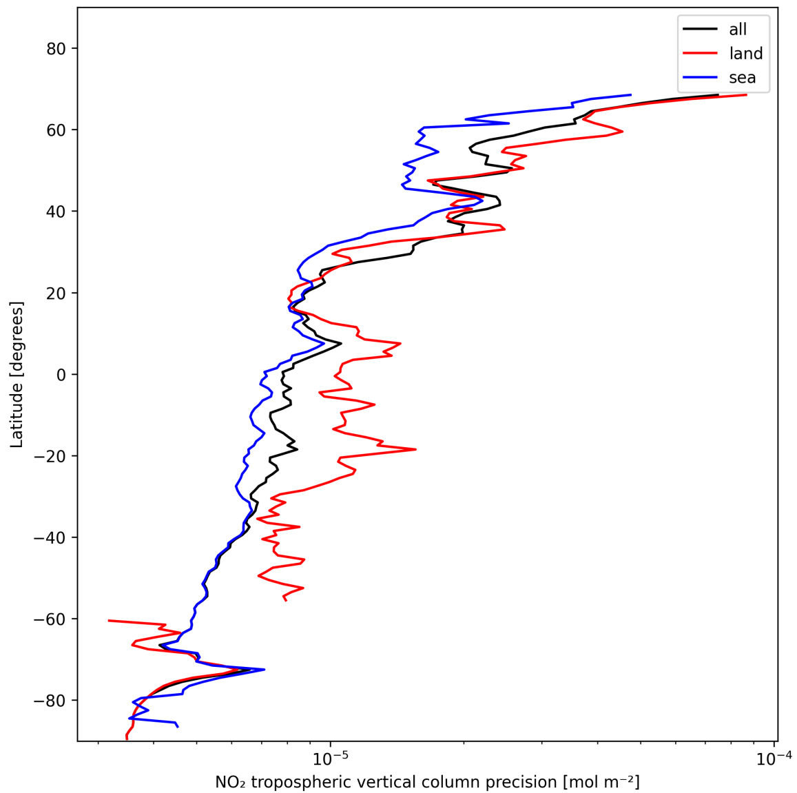
Figure 13: Zonal average of “NO 2 tropospheric vertical column precision” for 2024-11-17 to 2024-11-19.
