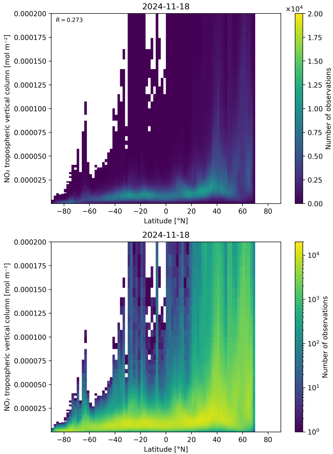
Figure 92: Scatter density plot of “Latitude” against “NO 2 tropospheric vertical column” for 2024-11-17 to 2024-11-19.
