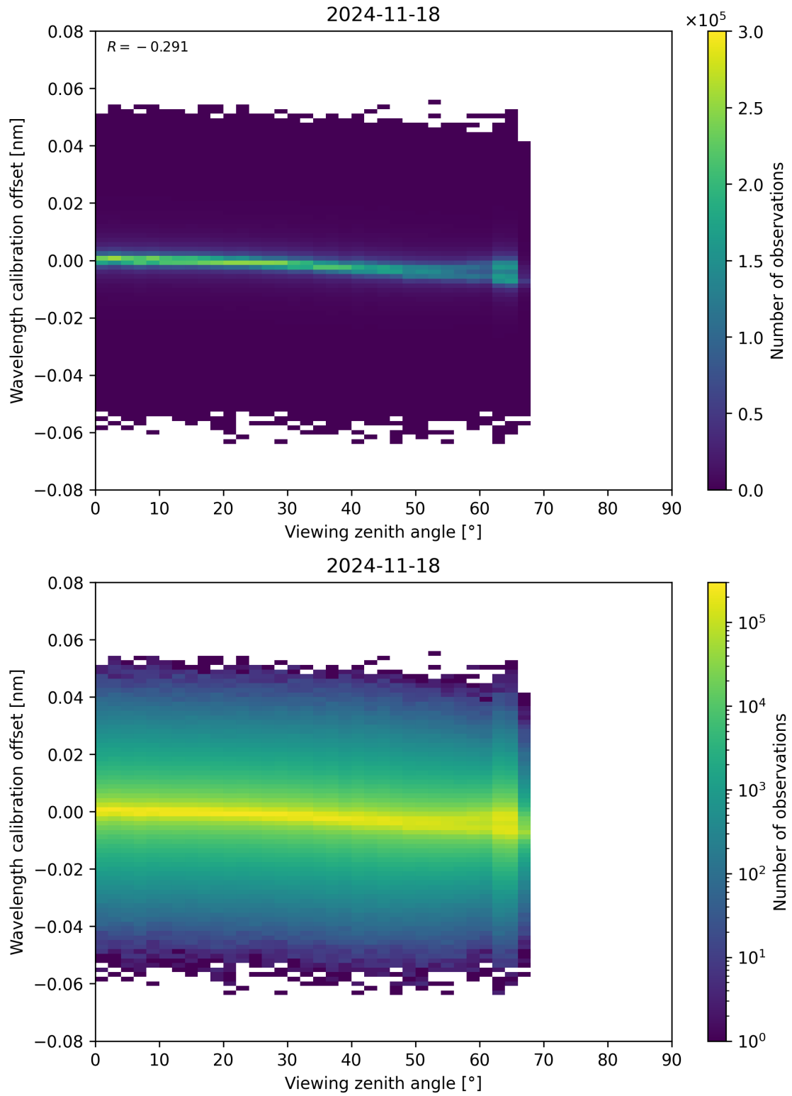
Figure 173: Scatter density plot of “Viewing zenith angle” against “Wavelength calibration offset” for 2024-11-17 to 2024-11-19.
