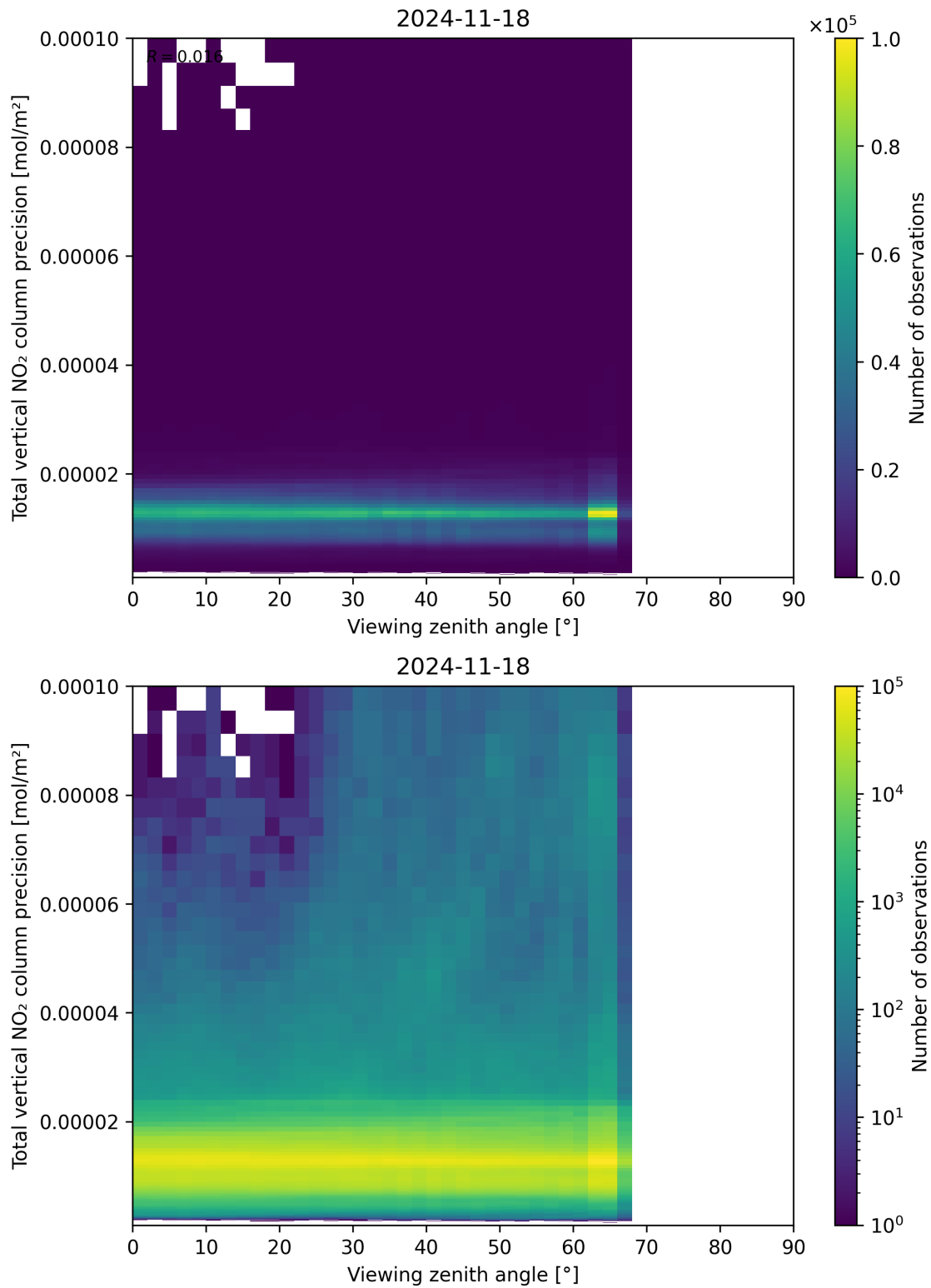
Figure 168: Scatter density plot of “Viewing zenith angle” against “Total vertical NO 2 column precision” for 2024-11-17 to 2024-11-19.
