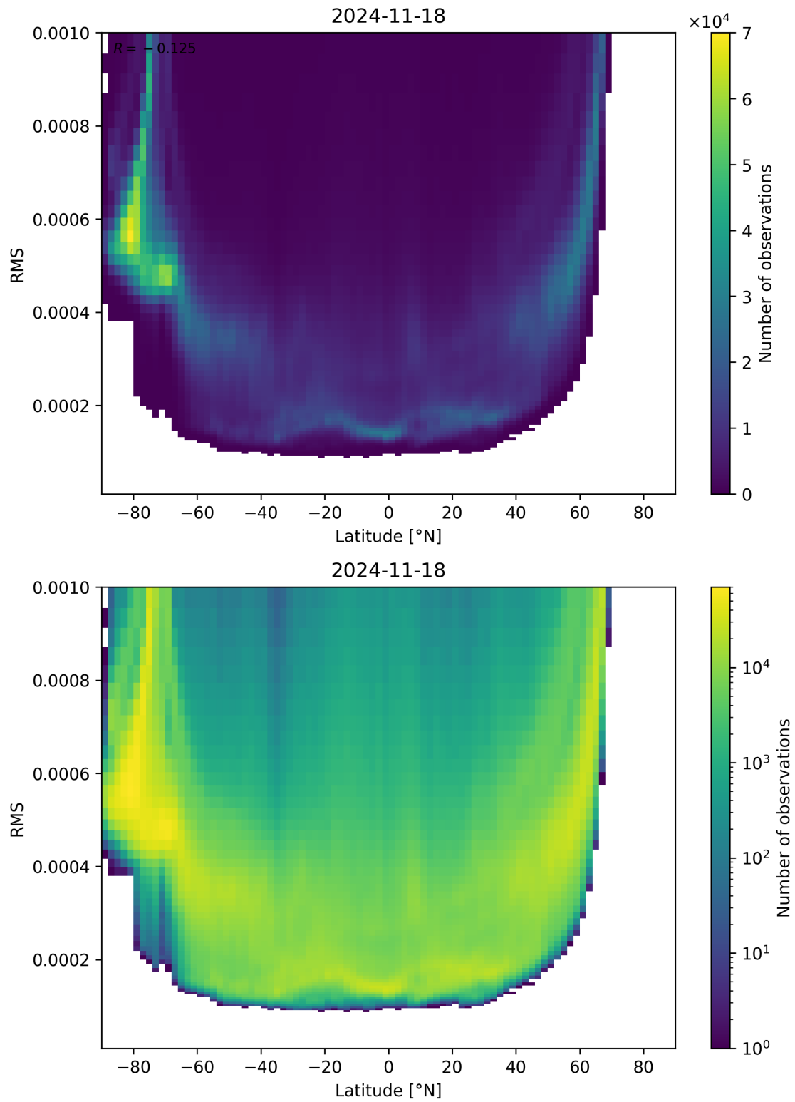
Figure 94: Scatter density plot of “Latitude” against “RMS” for 2024-11-17 to 2024-11-19.
