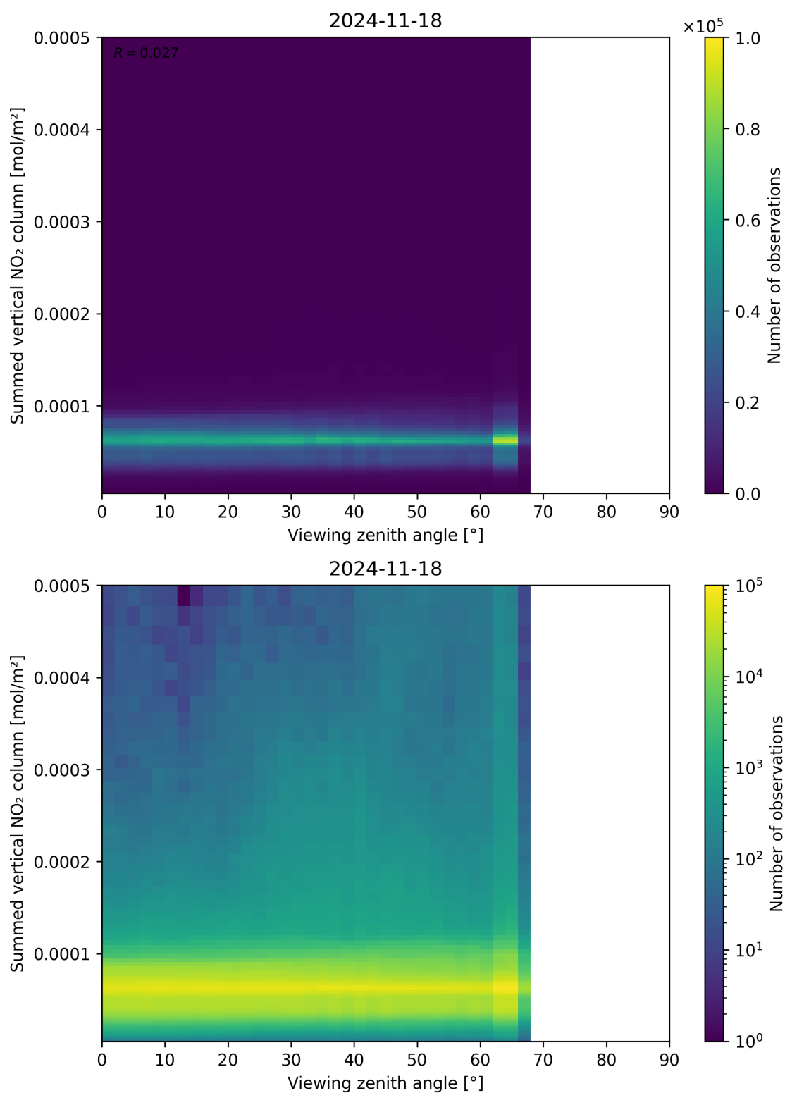
Figure 165: Scatter density plot of “Viewing zenith angle” against “Summed vertical NO 2 column” for 2024-11-17 to 2024-11-19.
