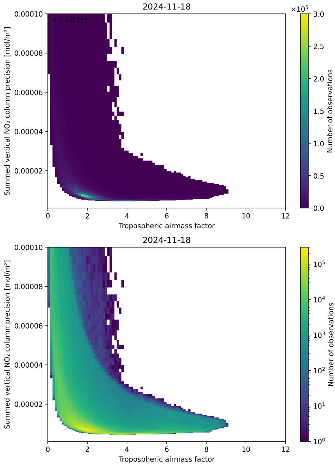
Figure 76: Scatter density plot of “Tropospheric air mass factor” against “Summed vertical NO 2 column precision” for 2024-11-17 to 2024-11-19.
