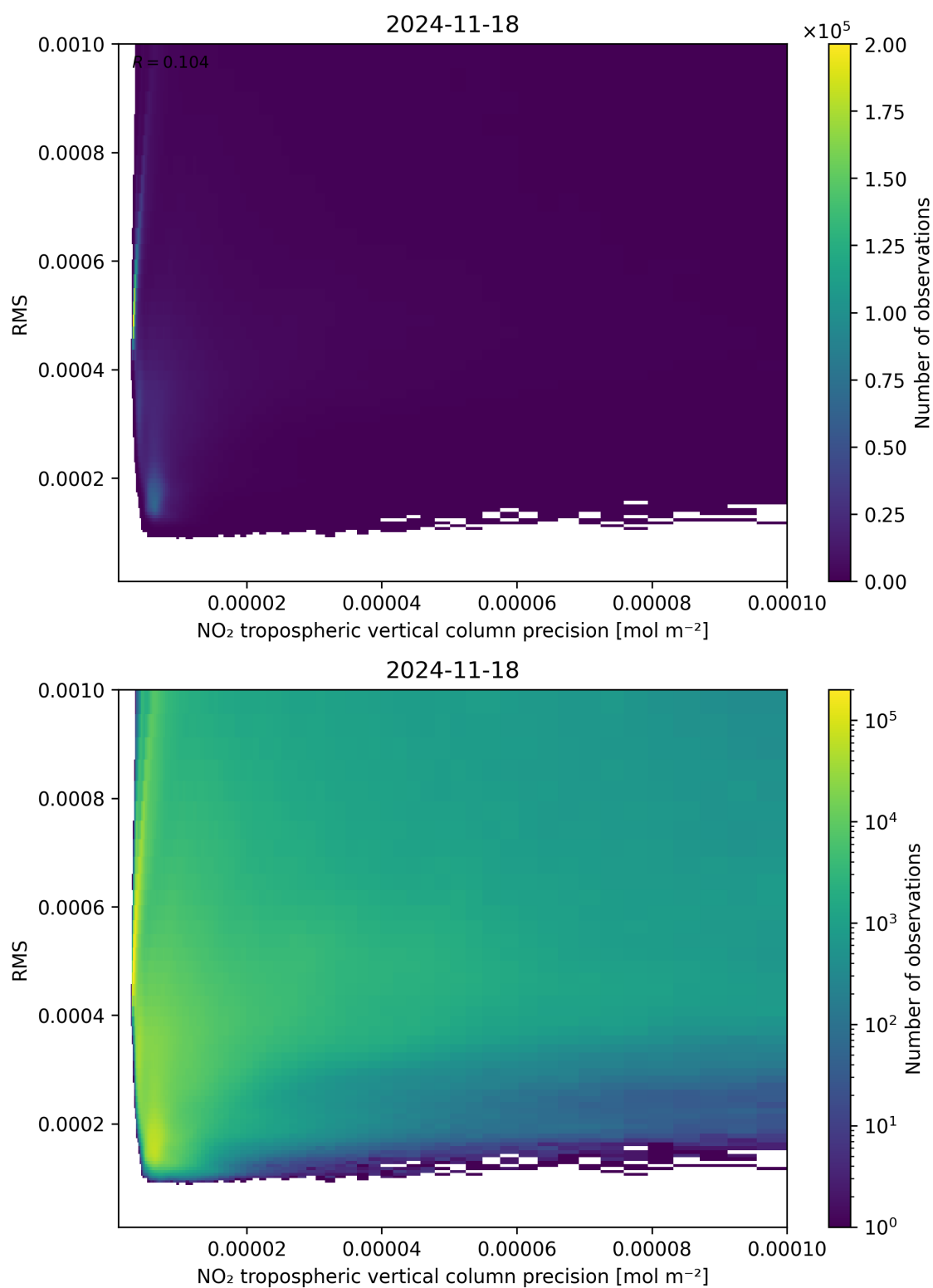
Figure 140: Scatter density plot of “NO 2 tropospheric vertical column precision” against “RMS” for 2024-11-17 to 2024-11-19.
