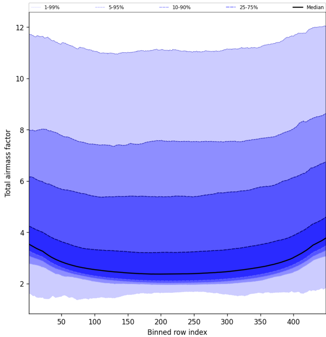
Figure 49: Along track statistics of “Total airmass factor” for 2024-11-17 to 2024-11-19
