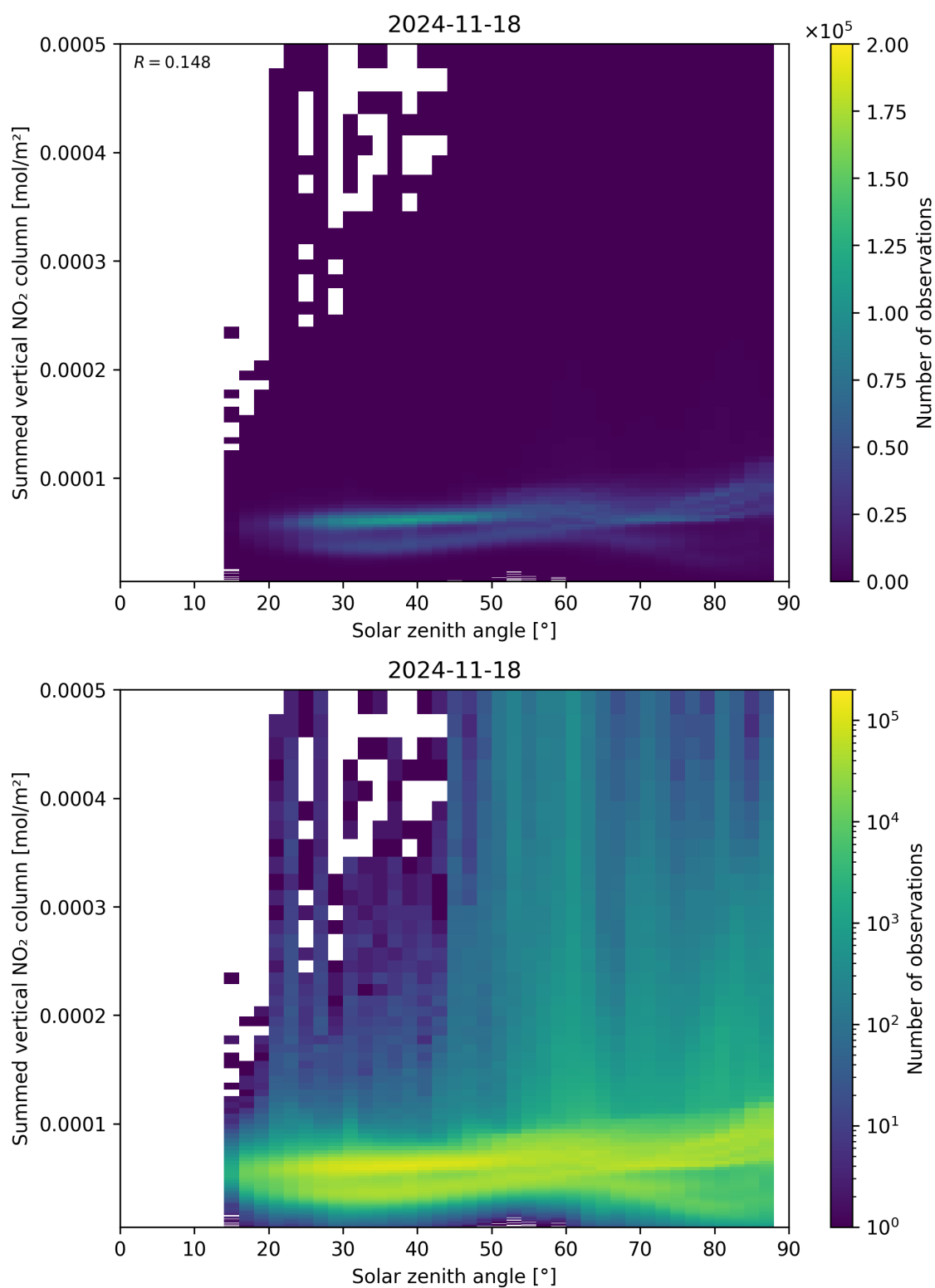
Figure 151: Scatter density plot of “Solar zenith angle” against “Summed vertical NO 2 column” for 2024-11-17 to 2024-11-19.
