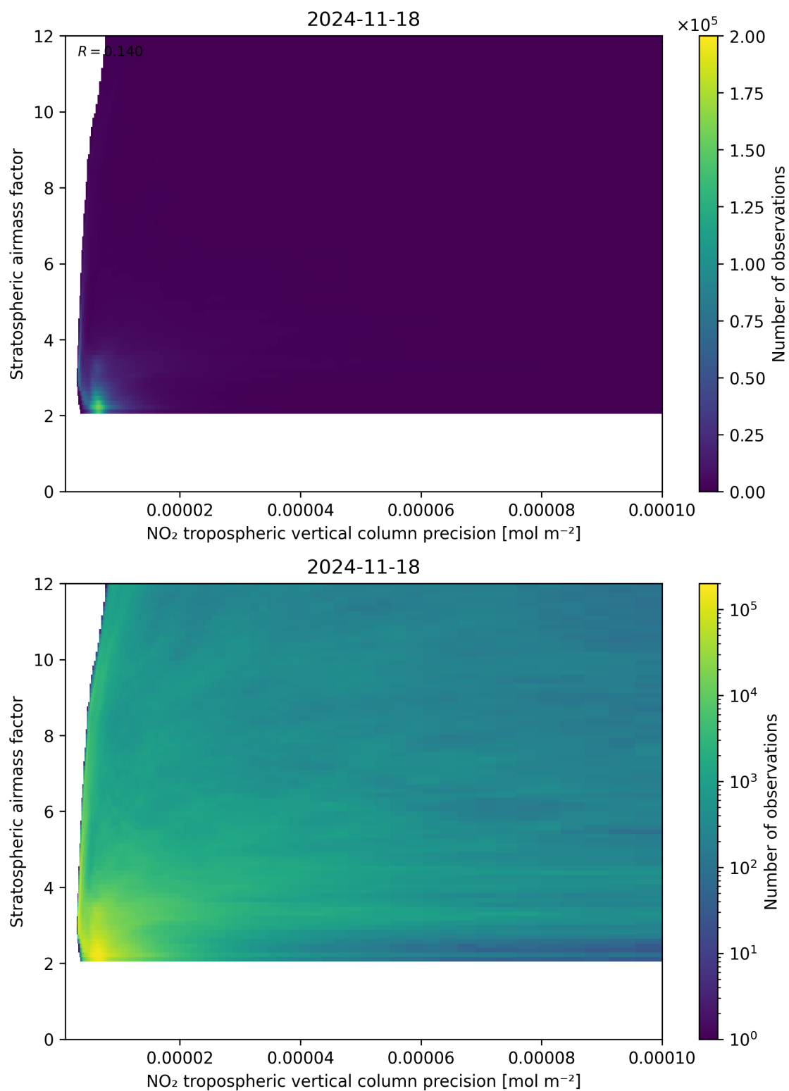
Figure 131: Scatter density plot of “NO 2 tropospheric vertical column precision” against “Stratospheric airmass factor” for 2024-11-17 to 2024-11-19.
