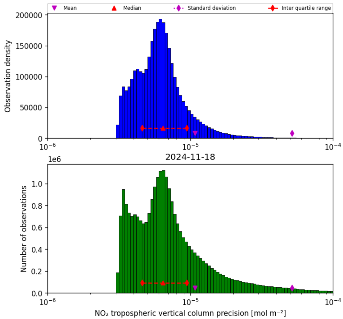
Figure 30: Histogram of “NO 2 tropospheric vertical column precision” for 2024-11-17 to 2024-11-19
