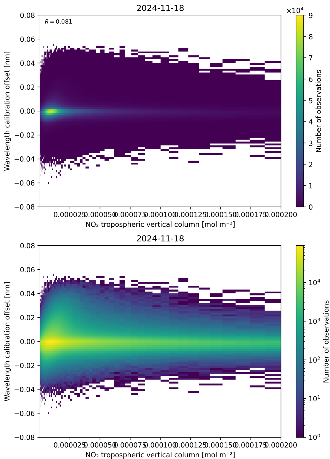
Figure 143: Scatter density plot of “NO 2 tropospheric vertical column” against “Wavelength calibration offset” for 2024-11-17 to 2024-11-19.
