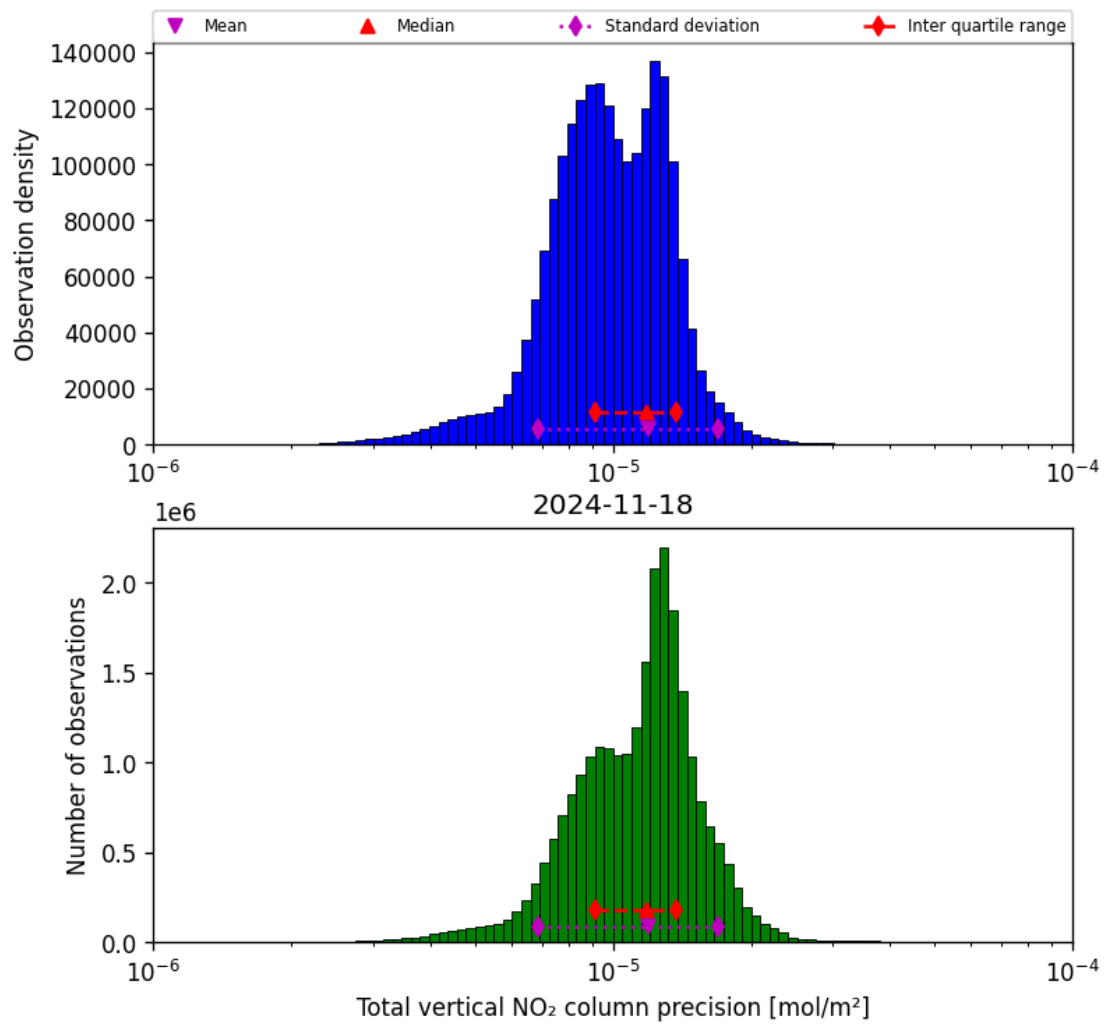
Figure 39: Histogram of “Total vertical NO 2 column precision” for 2024-11-17 to 2024-11-19
