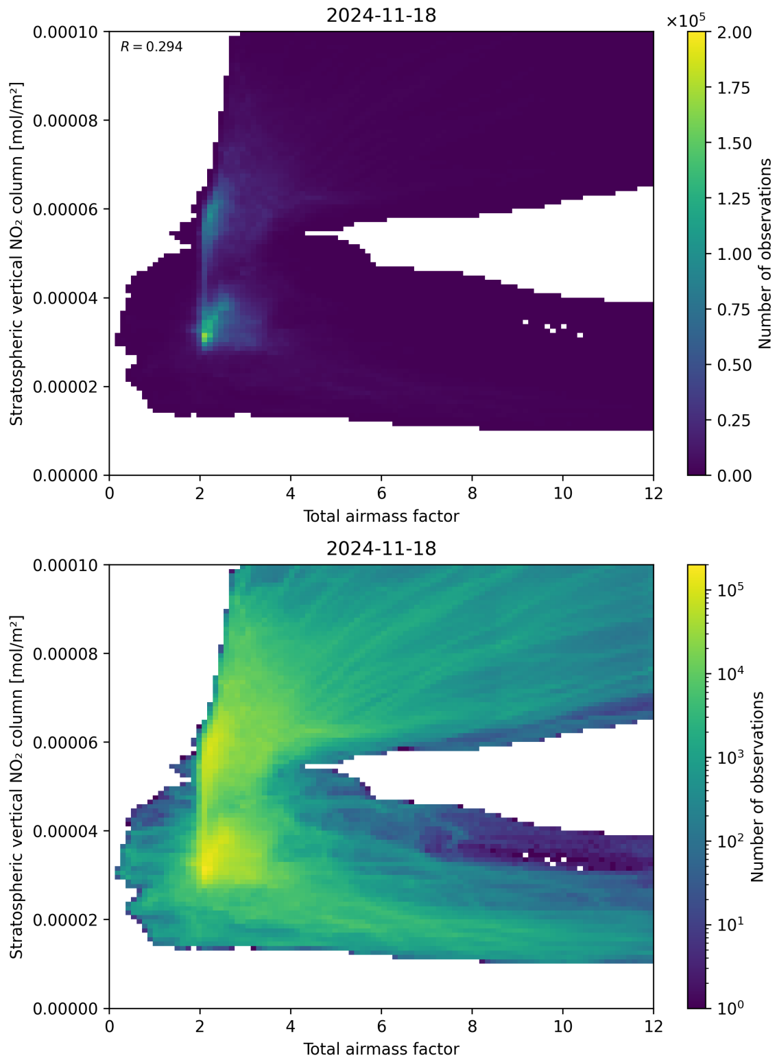
Figure 64: Scatter density plot of “Total airmass factor” against “Stratospheric vertical \text{NO}_2 column” for 2024-11-17 to 2024-11-19.
