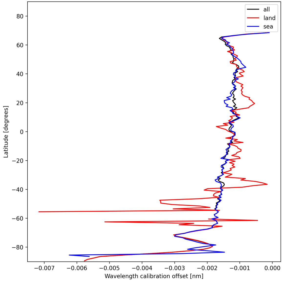
Figure 18: Zonal average of “Wavelength calibration offset” for 2024-11-17 to 2024-11-19.
