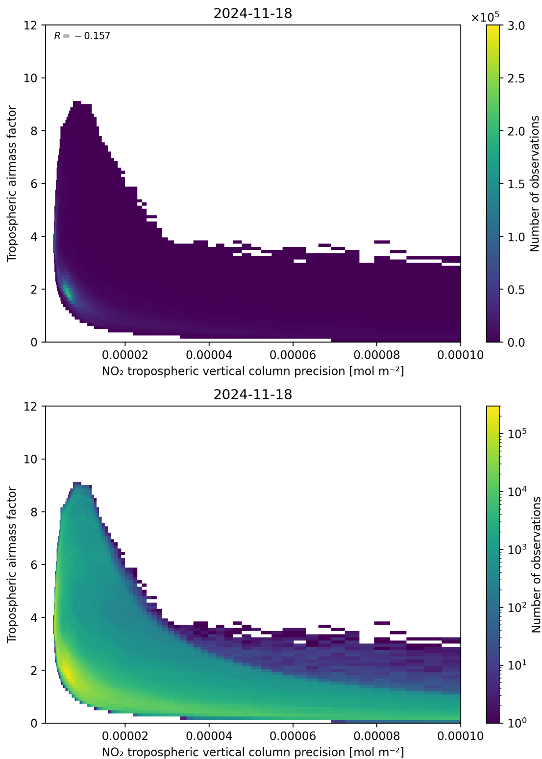
Figure 133: Scatter density plot of “NO 2 tropospheric vertical column precision” against “Tropospheric airmass factor” for 2024-11-17 to 2024-11-19.
