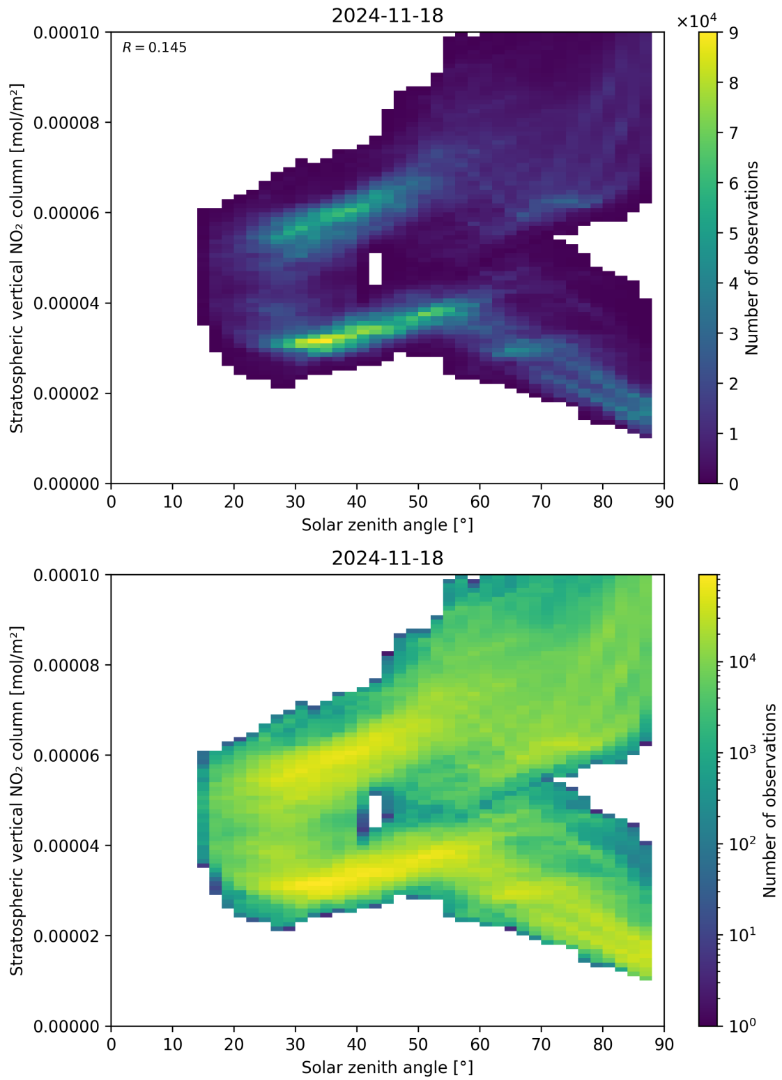
Figure 150: Scatter density plot of “Solar zenith angle” against “Stratospheric vertical NO 2 column” for 2024-11-17 to 2024-11-19.
