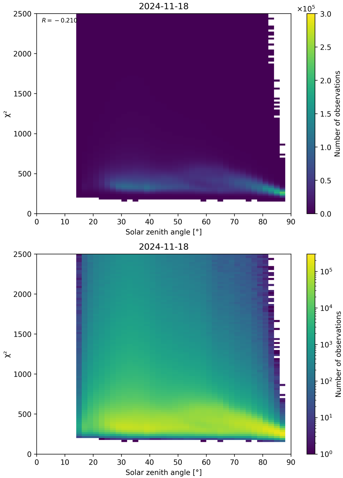
Figure 148: Scatter density plot of “Solar zenith angle” against “ \chi^2 ” for 2024-11-17 to 2024-11-19.
