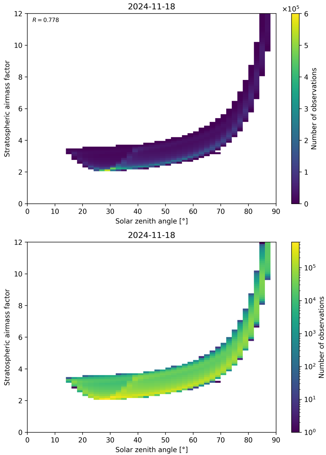
Figure 145: Scatter density plot of “Solar zenith angle” against “Stratospheric airmass factor” for 2024-11-17 to 2024-11-19.
