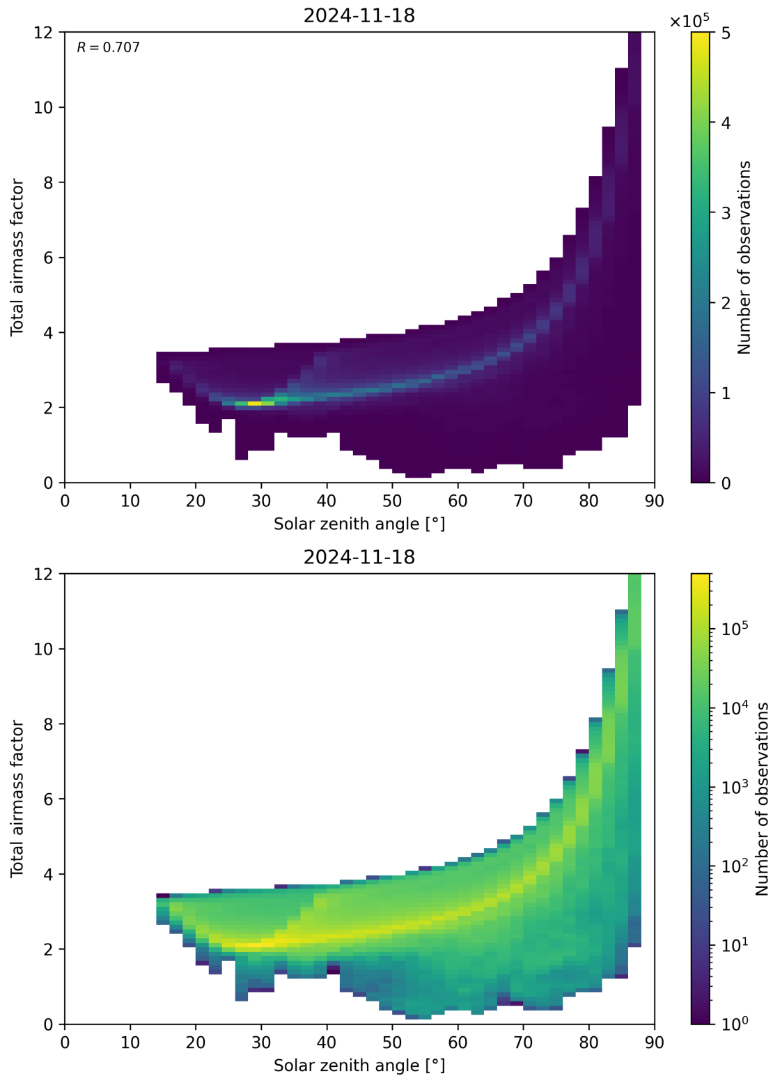
Figure 146: Scatter density plot of “Solar zenith angle” against “Total air mass factor” for 2024-11-17 to 2024-11-19.
