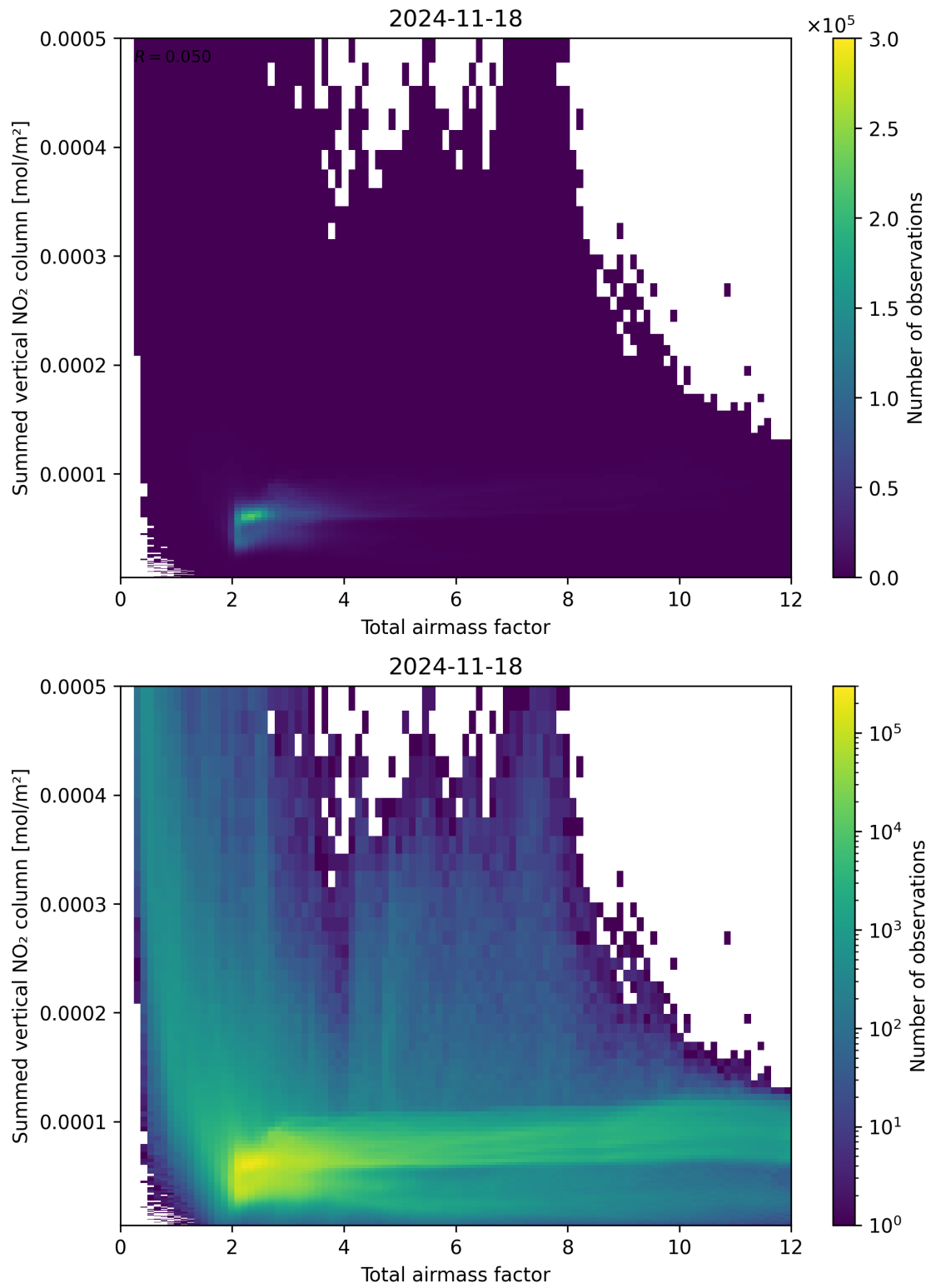
Figure 65: Scatter density plot of “Total airmass factor” against “Summed vertical NO 2 column” for 2024-11-17 to 2024-11-19.
