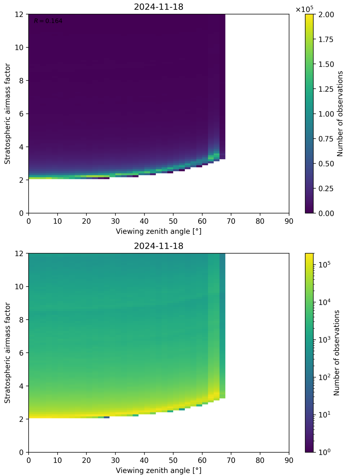
Figure 159: Scatter density plot of “Viewing zenith angle” against “Stratospheric airmass factor” for 2024-11-17 to 2024-11-19.
