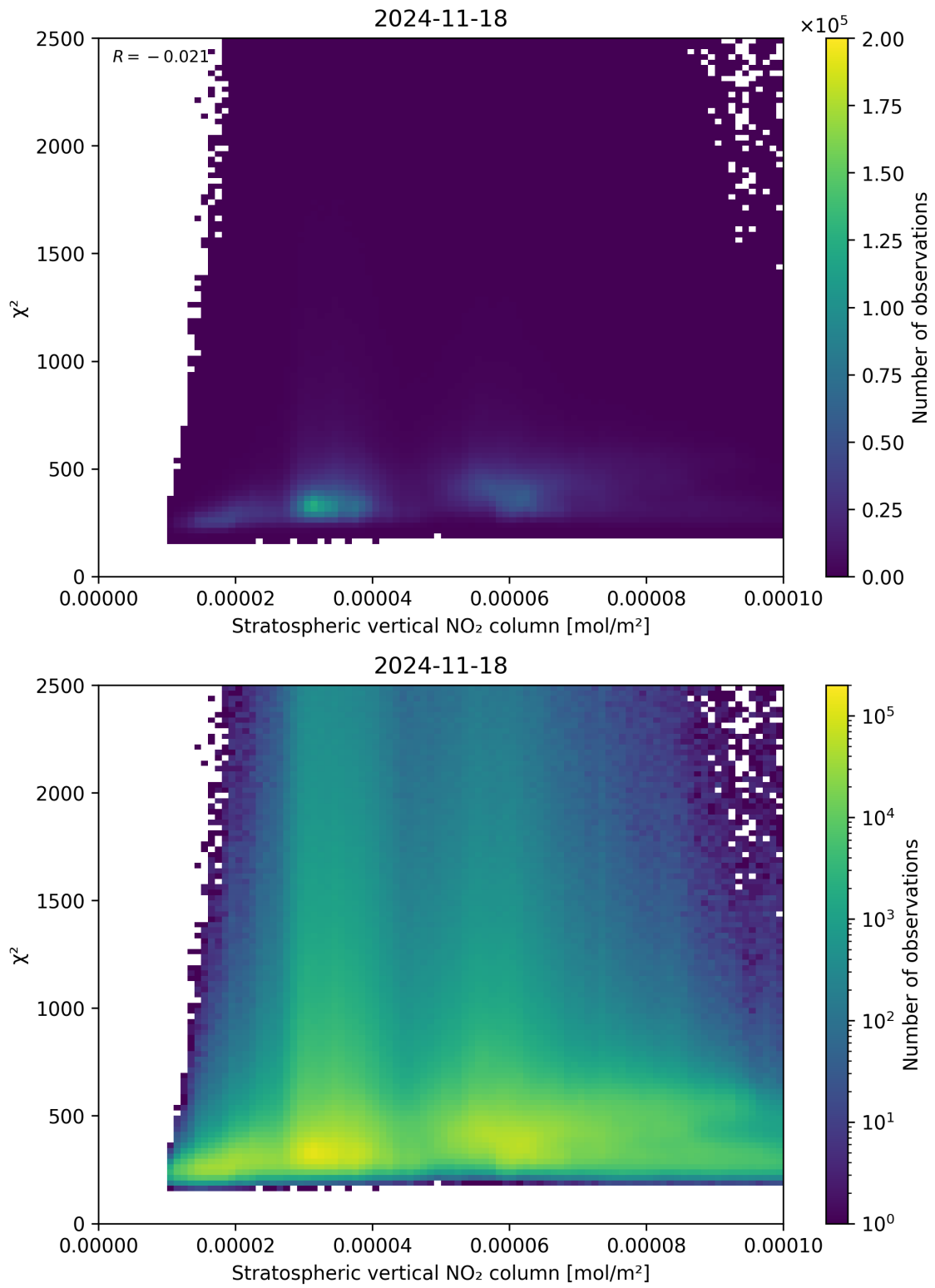
Figure 97: Scatter density plot of “Stratospheric vertical NO 2 column” against “ \chi^2 ” for 2024-11-17 to 2024-11-19.
