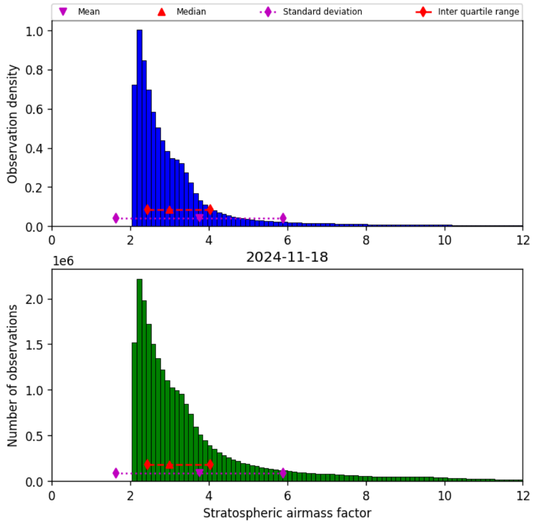
Figure 44: Histogram of “Stratospheric airmass factor” for 2024-11-17 to 2024-11-19
