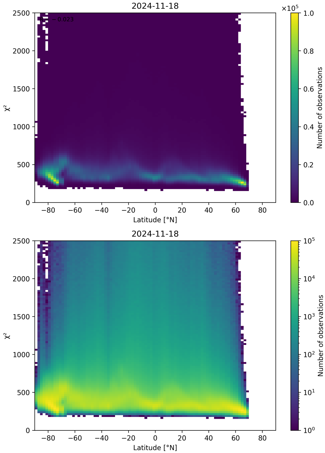
Figure 86: Scatter density plot of “Latitude” against “ \chi^2 ” for 2024-11-17 to 2024-11-19.
