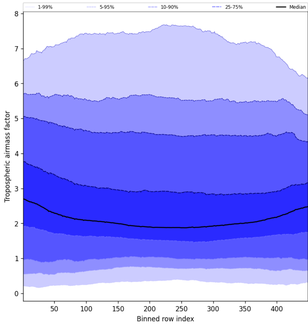
Figure 48: Along track statistics of “Tropospheric airmass factor” for 2024-11-17 to 2024-11-19
