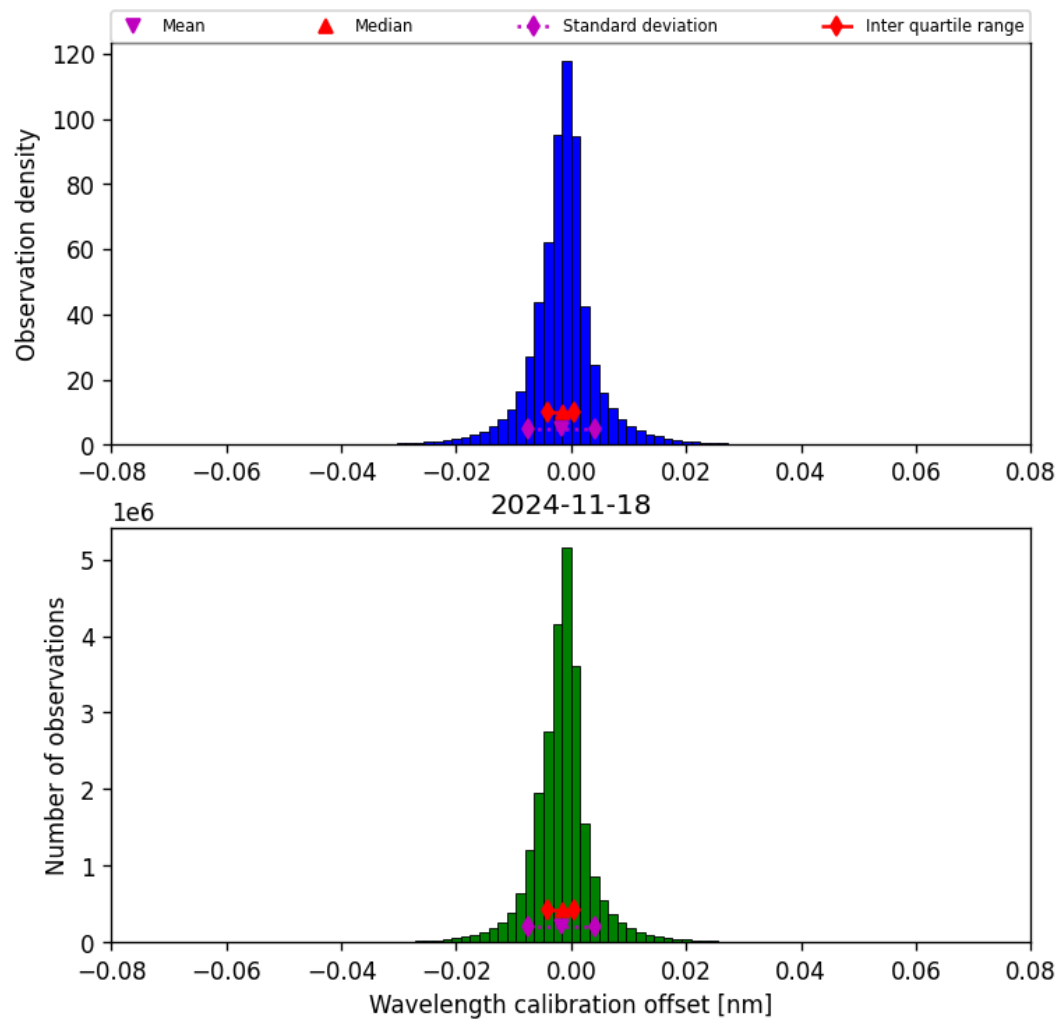
Figure 35: Histogram of “Wavelength calibration offset” for 2024-11-17 to 2024-11-19
