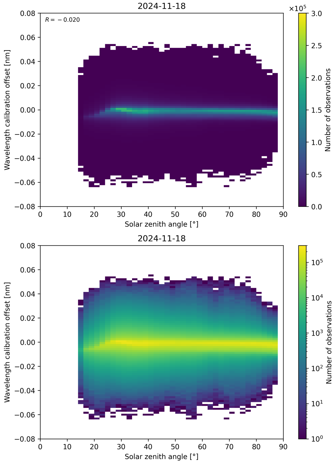
Figure 158: Scatter density plot of “Solar zenith angle” against “Wavelength calibration offset” for 2024-11-17 to 2024-11-19.
