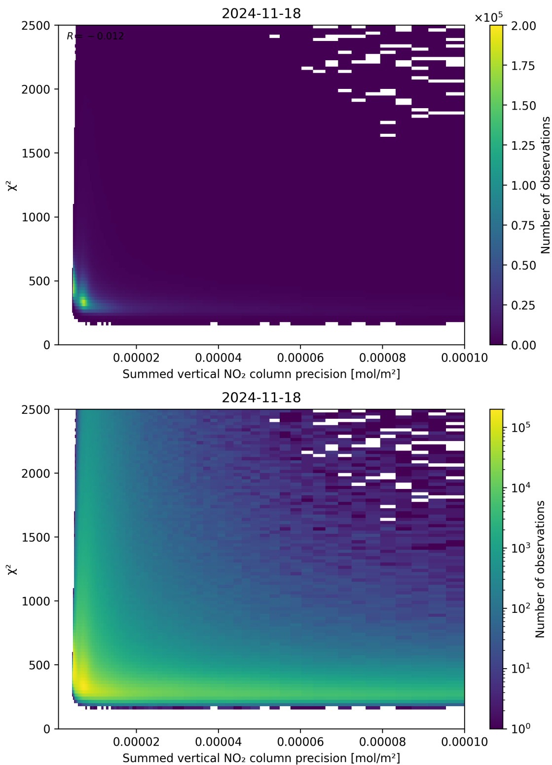
Figure 107: Scatter density plot of “Summed vertical NO 2 column precision” against “ \chi^2 ” for 2024-11-17 to 2024-11-19.
