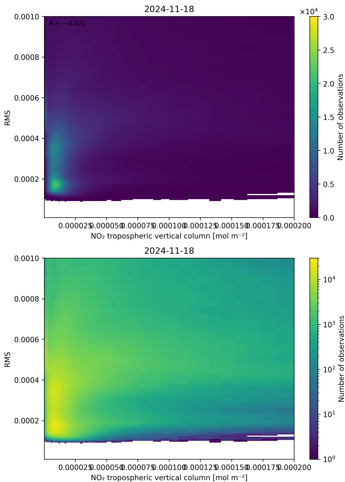
Figure 142: Scatter density plot of “NO 2 tropospheric vertical column” against “RMS” for 2024-11-17 to 2024-11-19.
