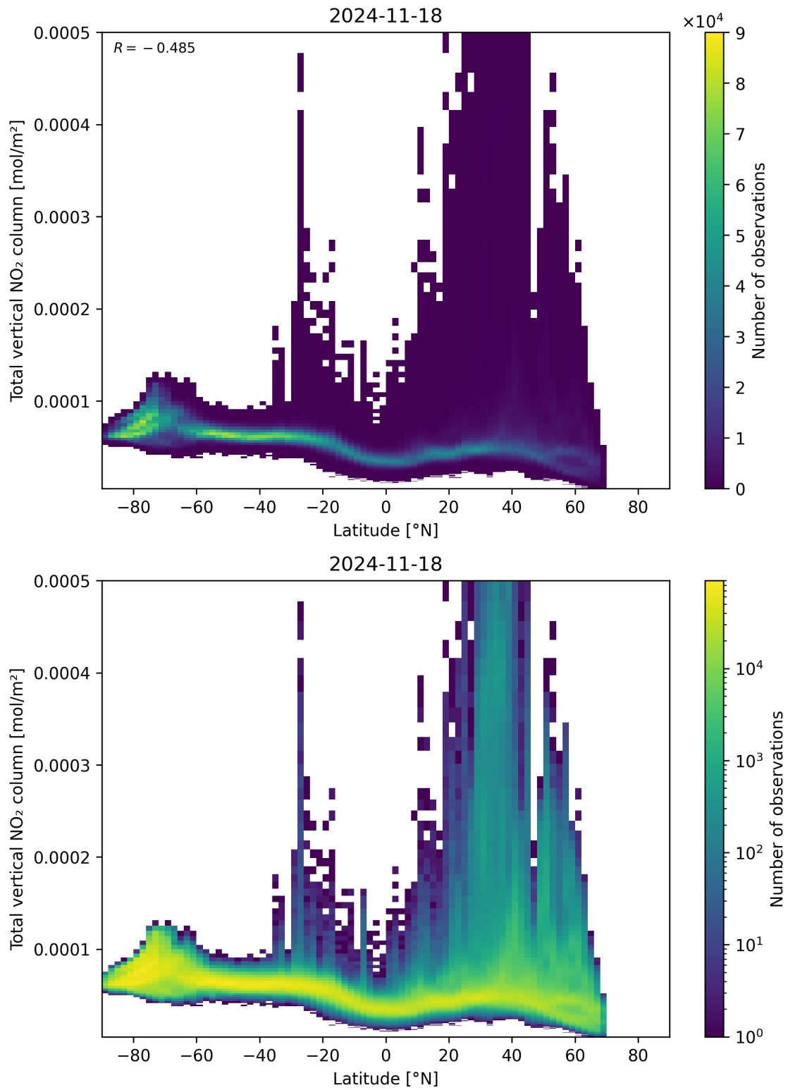
Figure 90: Scatter density plot of “Latitude” against “Total vertical NO 2 column” for 2024-11-17 to 2024-11-19.
