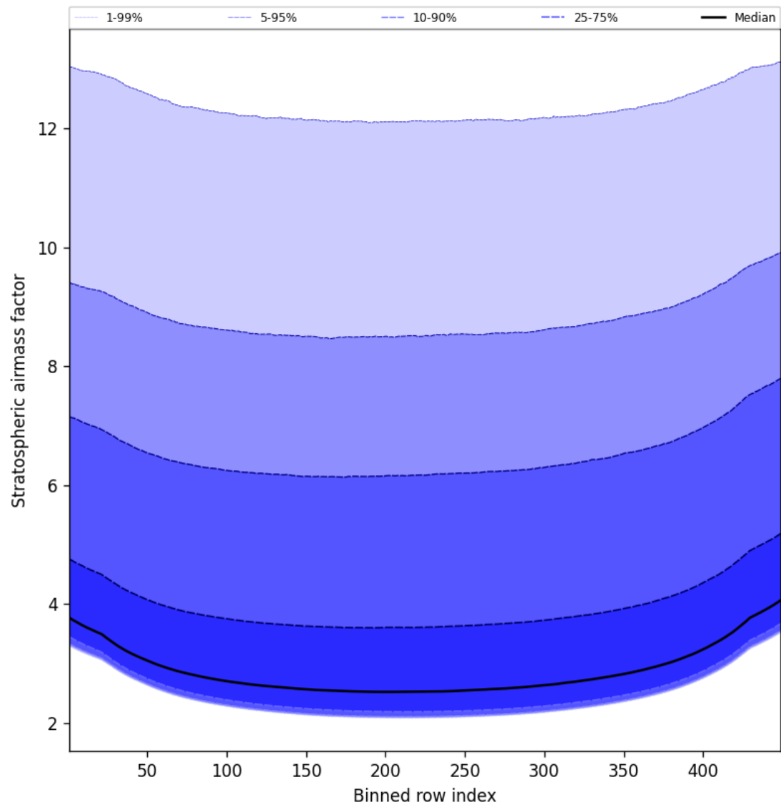
Figure 61: Along track statistics of “Stratospheric air mass factor” for 2024-11-17 to 2024-11-19
