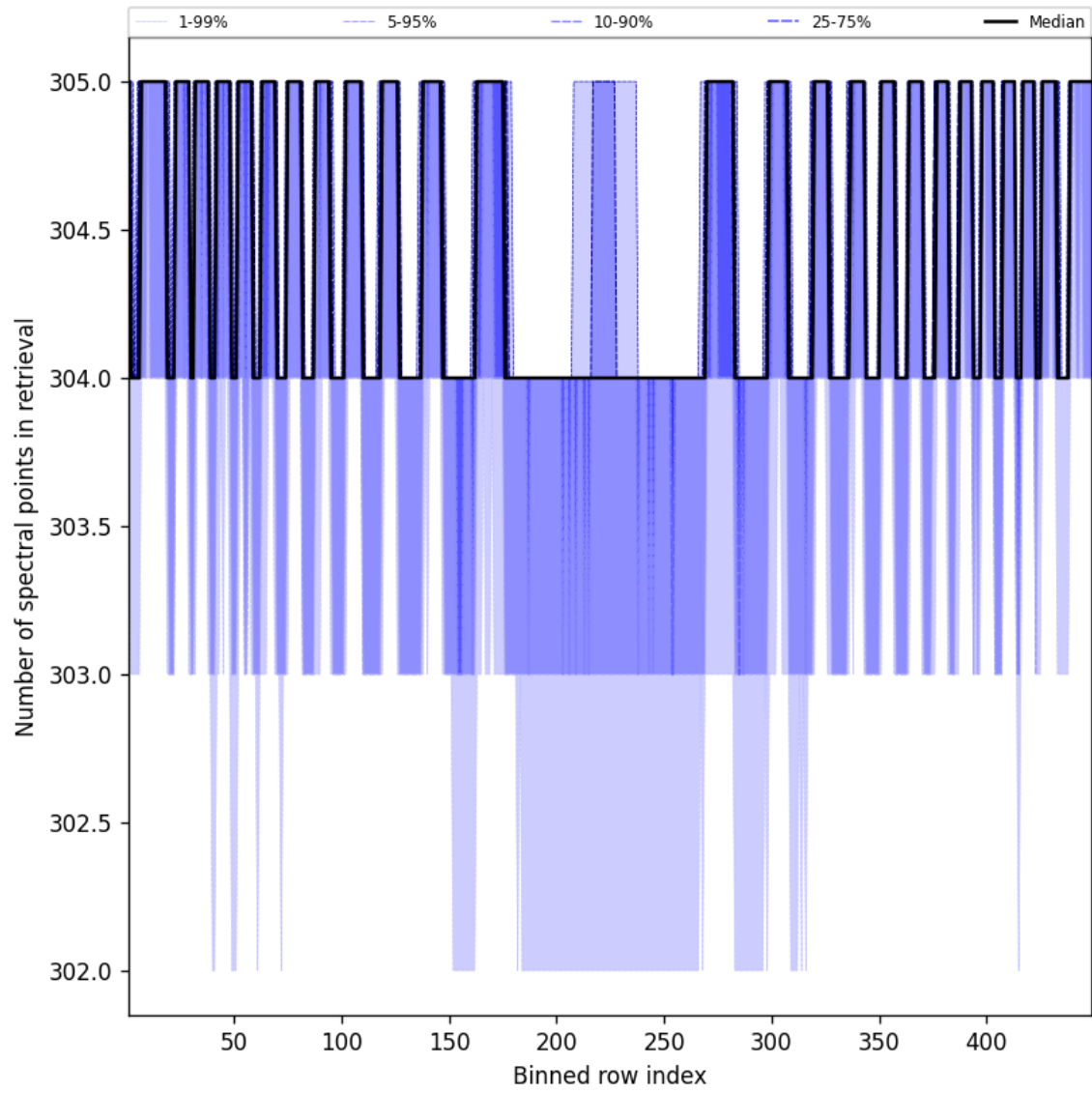
Figure 50: Along track statistics of “Number of spectral points in retrieval” for 2024-11-17 to 2024-11-19
