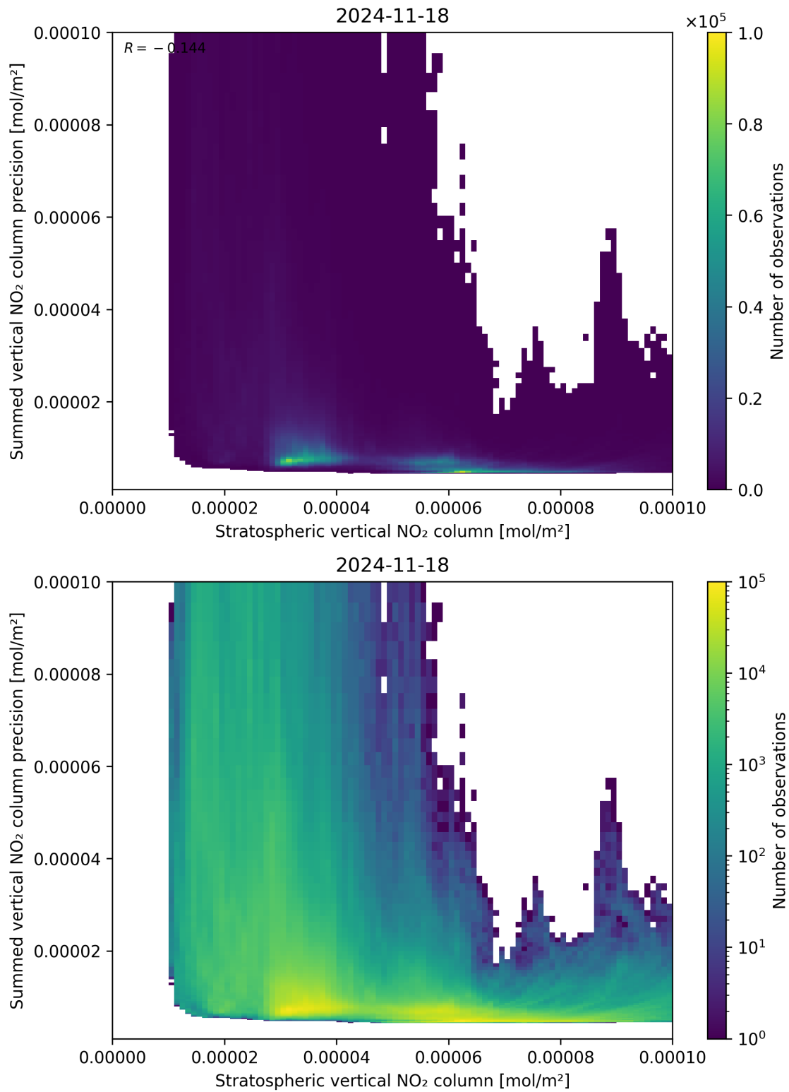
Figure 99: Scatter density plot of “Stratospheric vertical NO 2 column” against “Summed vertical NO 2 column precision” for 2024-11-17 to 2024-11-19.
