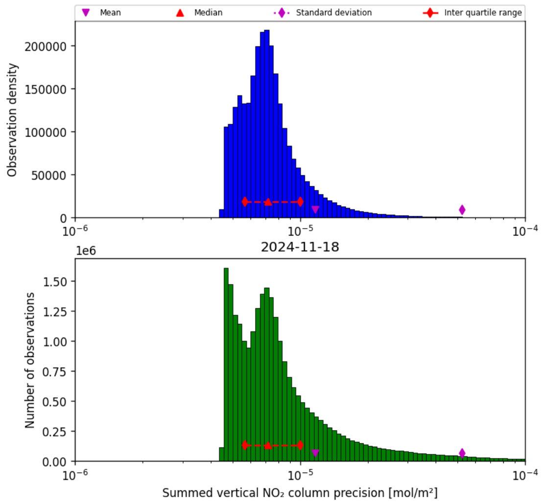
Figure 41: Histogram of “Summed vertical NO 2 column precision” for 2024-11-17 to 2024-11-19
