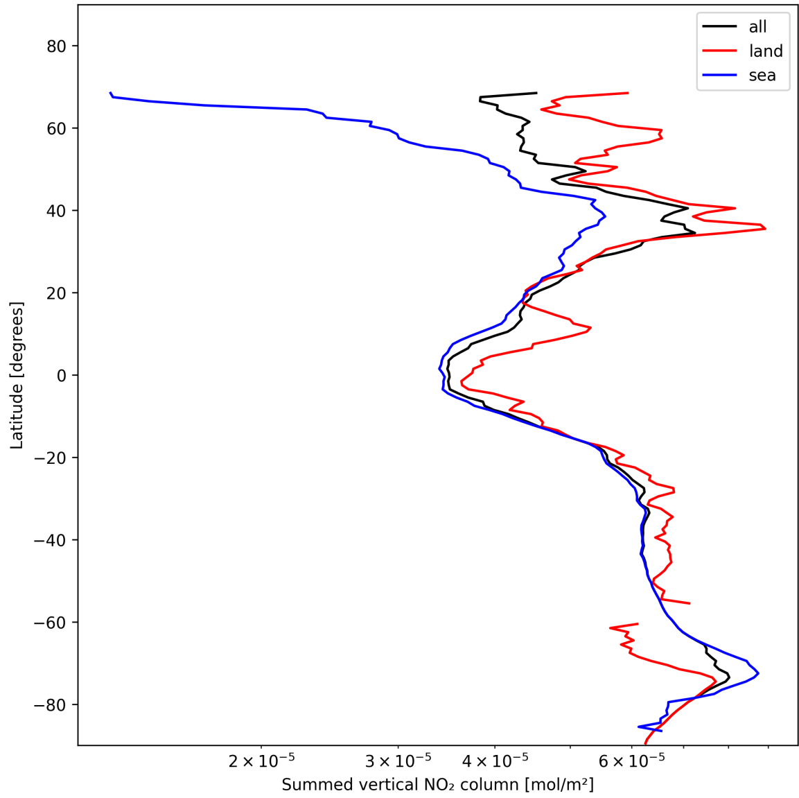
Figure 23: Zonal average of “Summed vertical NO 2 column” for 2024-11-17 to 2024-11-19.
