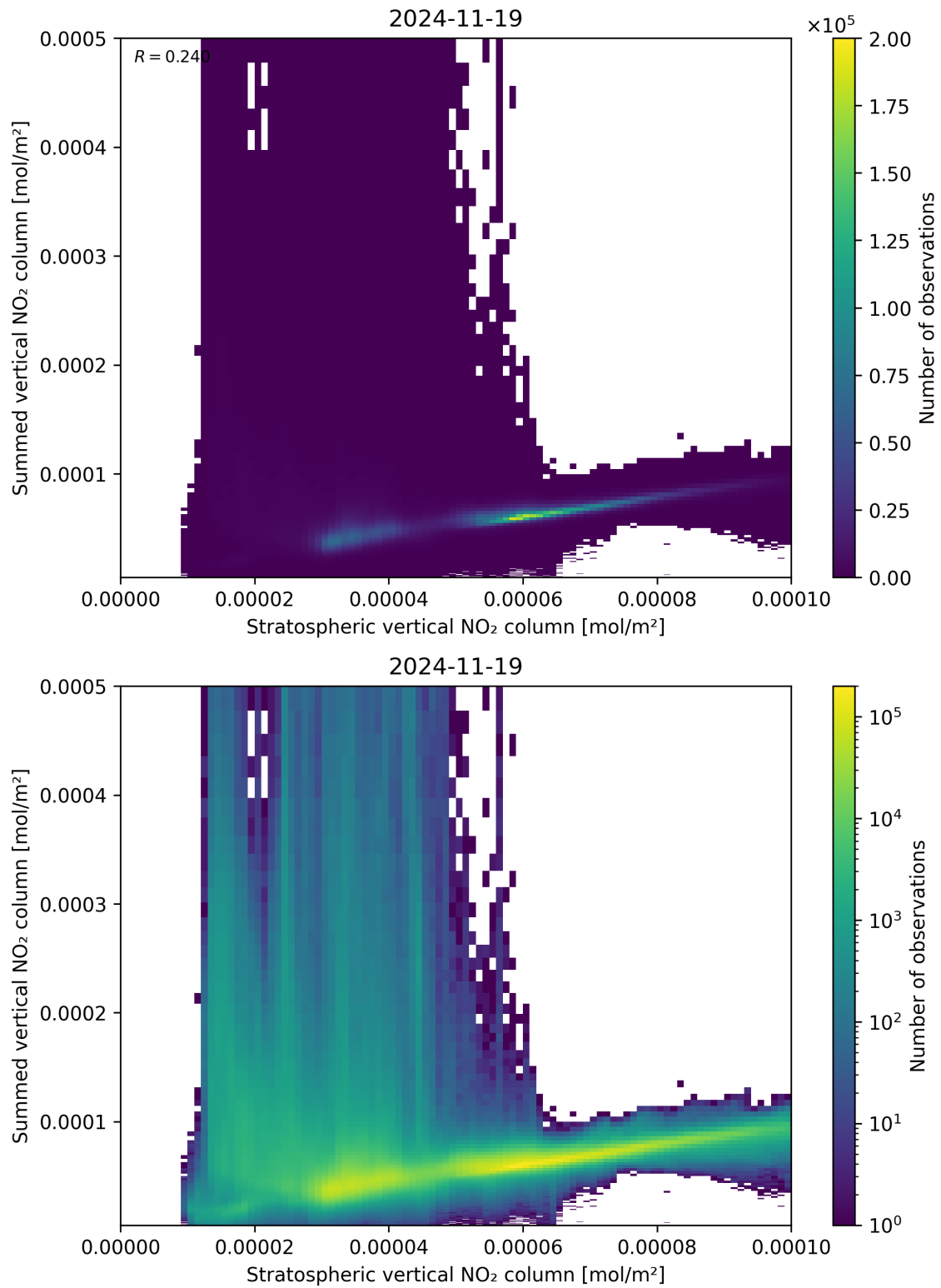
Figure 98: Scatter density plot of “Stratospheric vertical NO 2 column” against “Summed vertical NO 2 column” for 2024-11-18 to 2024-11-20.
