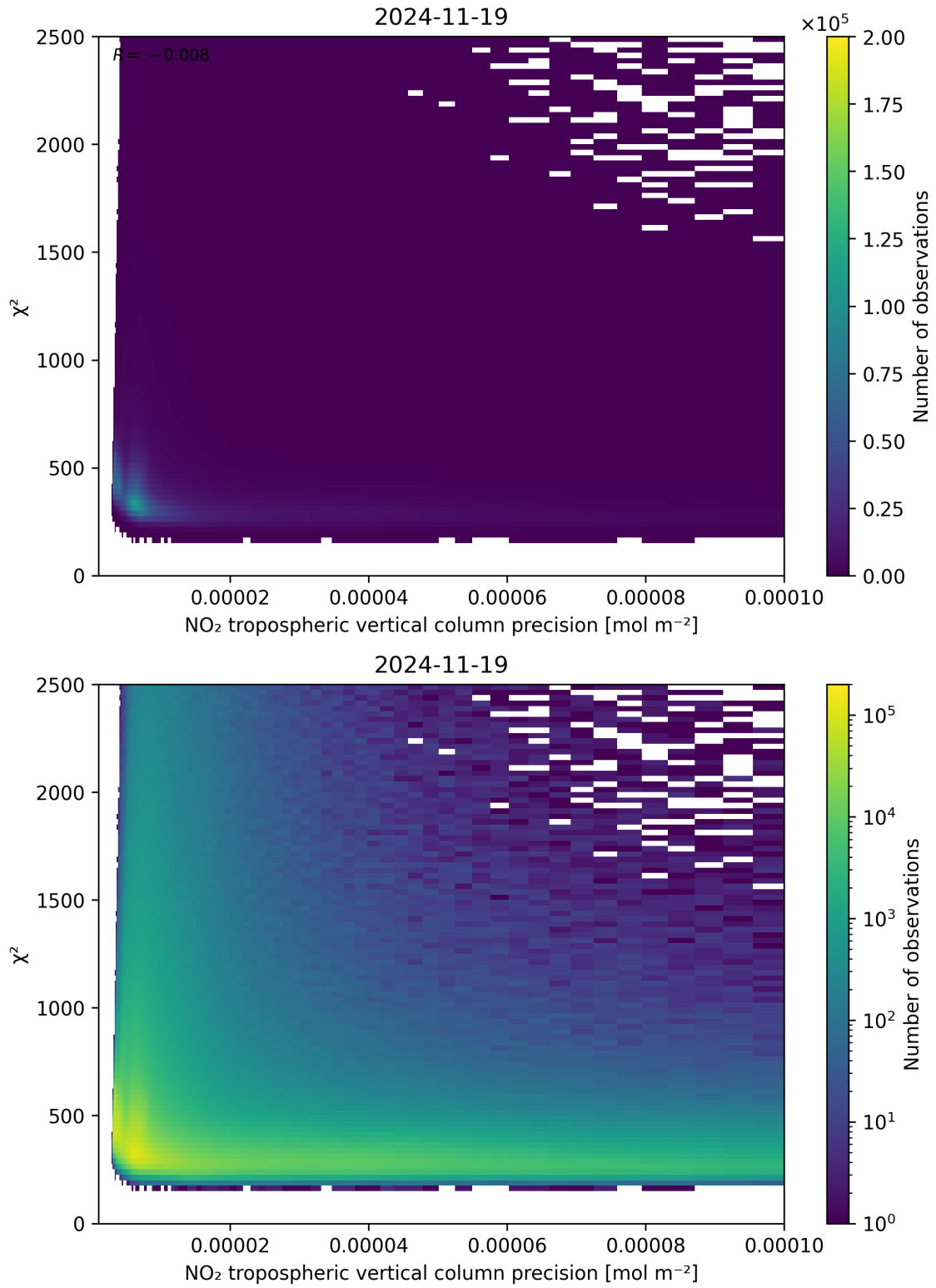
Figure 134: Scatter density plot of “NO 2 tropospheric vertical column precision” against “ \chi^2 ” for 2024-11-18 to 2024-11-20.
