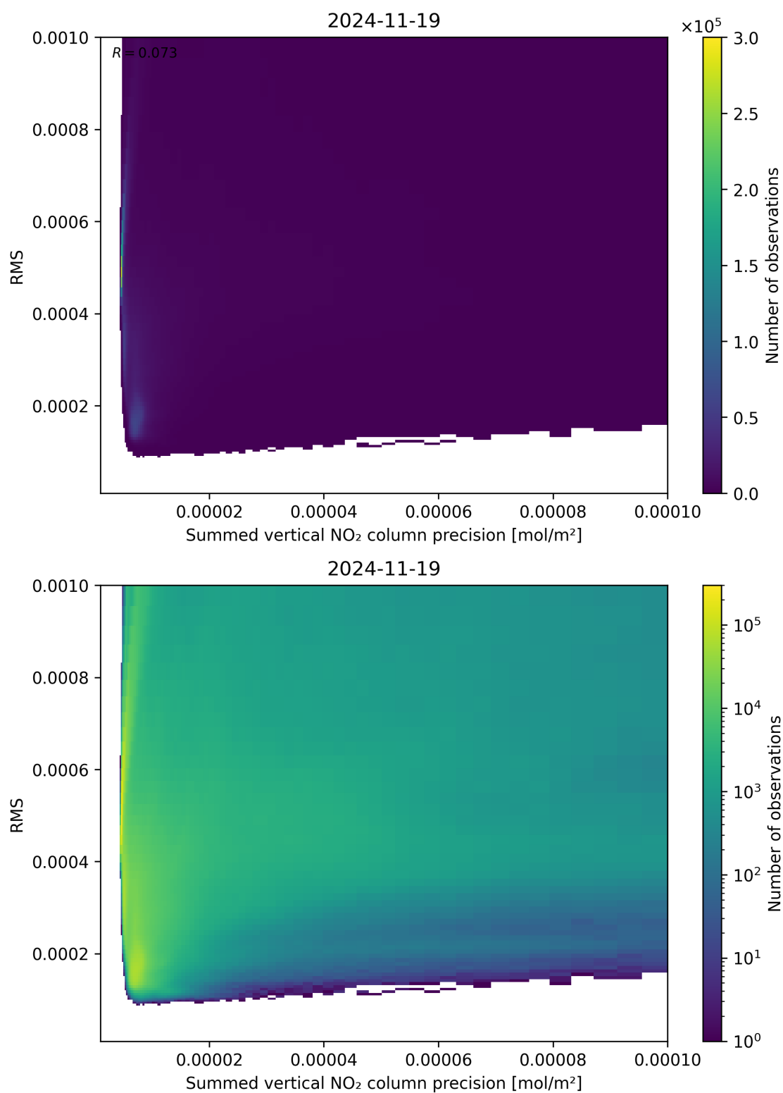
Figure 108: Scatter density plot of “Summed vertical NO 2 column precision” against “RMS” for 2024-11-18 to 2024-11-20.
