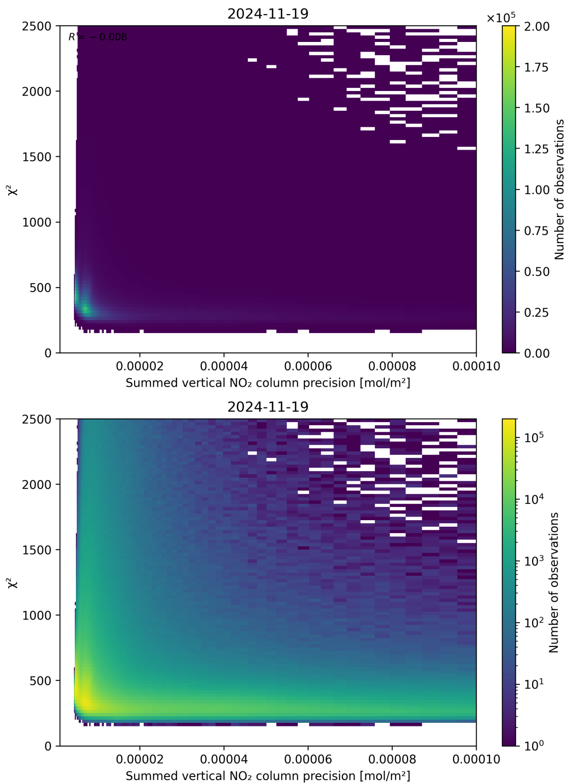
Figure 107: Scatter density plot of “Summed vertical NO 2 column precision” against “ \chi^2 ” for 2024-11-18 to 2024-11-20.
