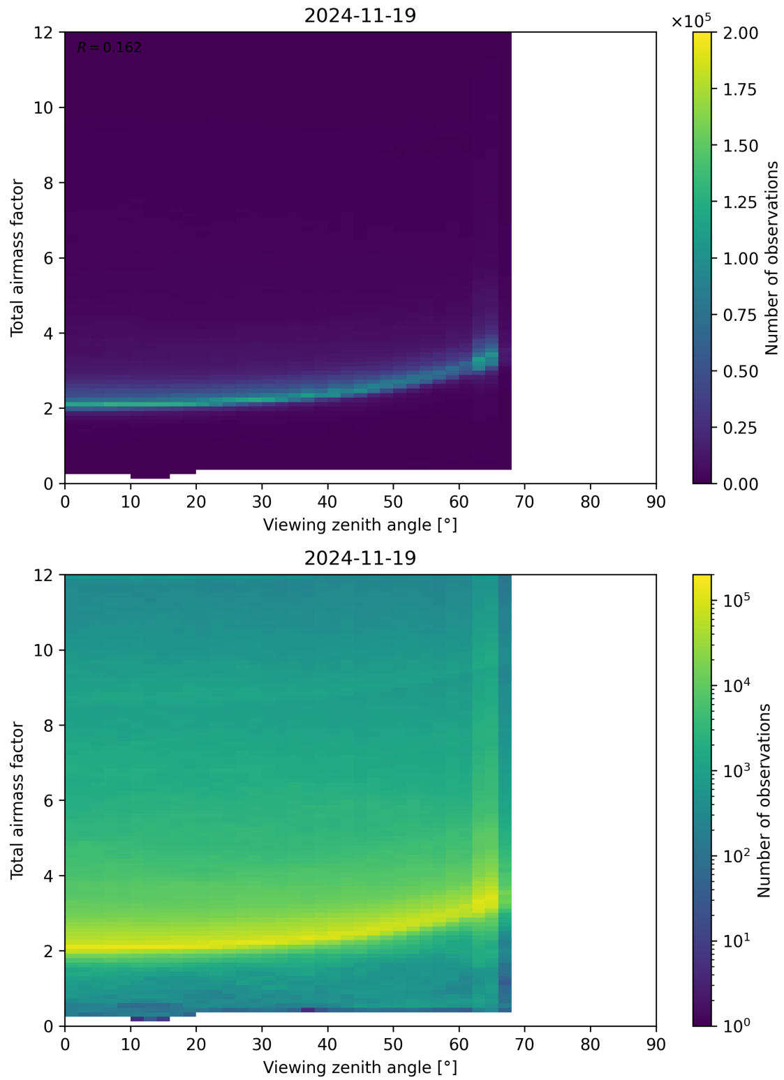
Figure 160: Scatter density plot of “Viewing zenith angle” against “Total airmass factor” for 2024-11-18 to 2024-11-20.
