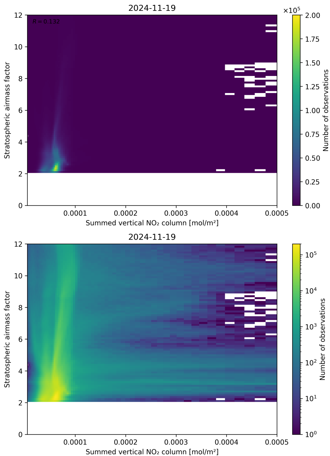
Figure 103: Scatter density plot of “Summed vertical NO 2 column” against “Stratospheric airmass factor” for 2024-11-18 to 2024-11-20.
