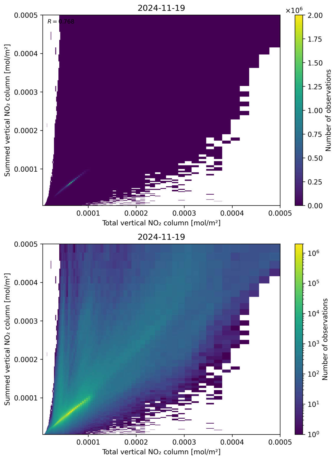
Figure 112: Scatter density plot of “Total vertical NO 2 column” against “Summed vertical NO 2 column” for 2024-11-18 to 2024-11-20.
