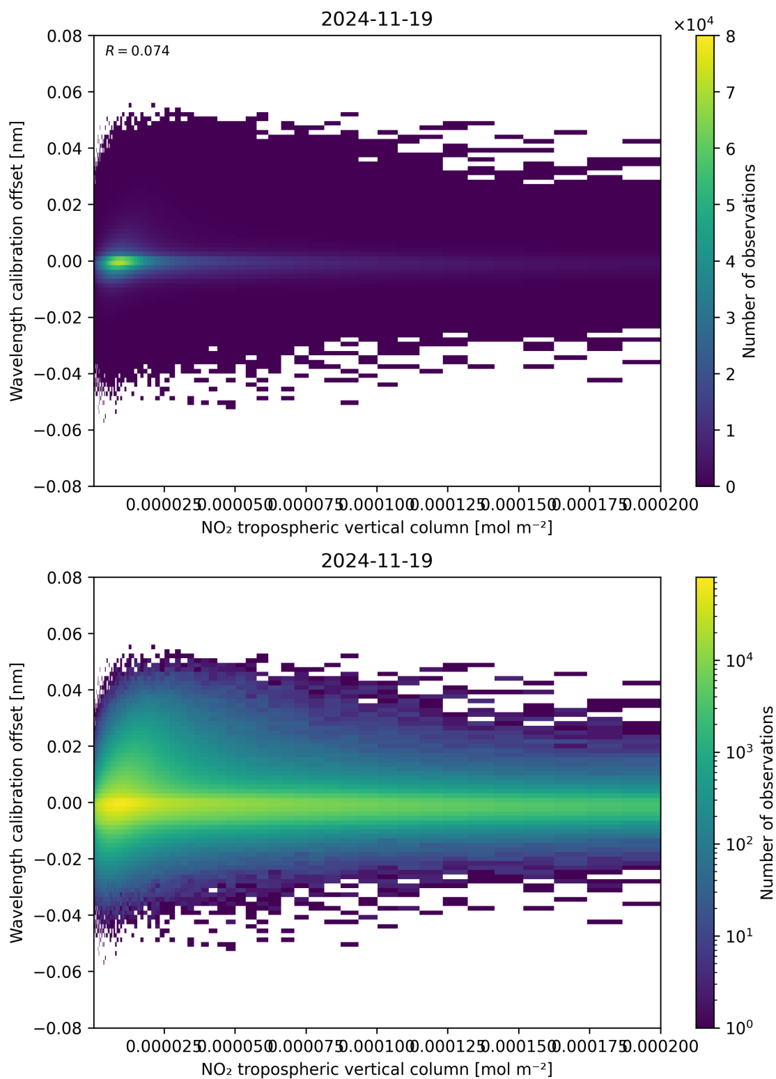
Figure 143: Scatter density plot of “NO 2 tropospheric vertical column” against “Wavelength calibration offset” for 2024-11-18 to 2024-11-20.
