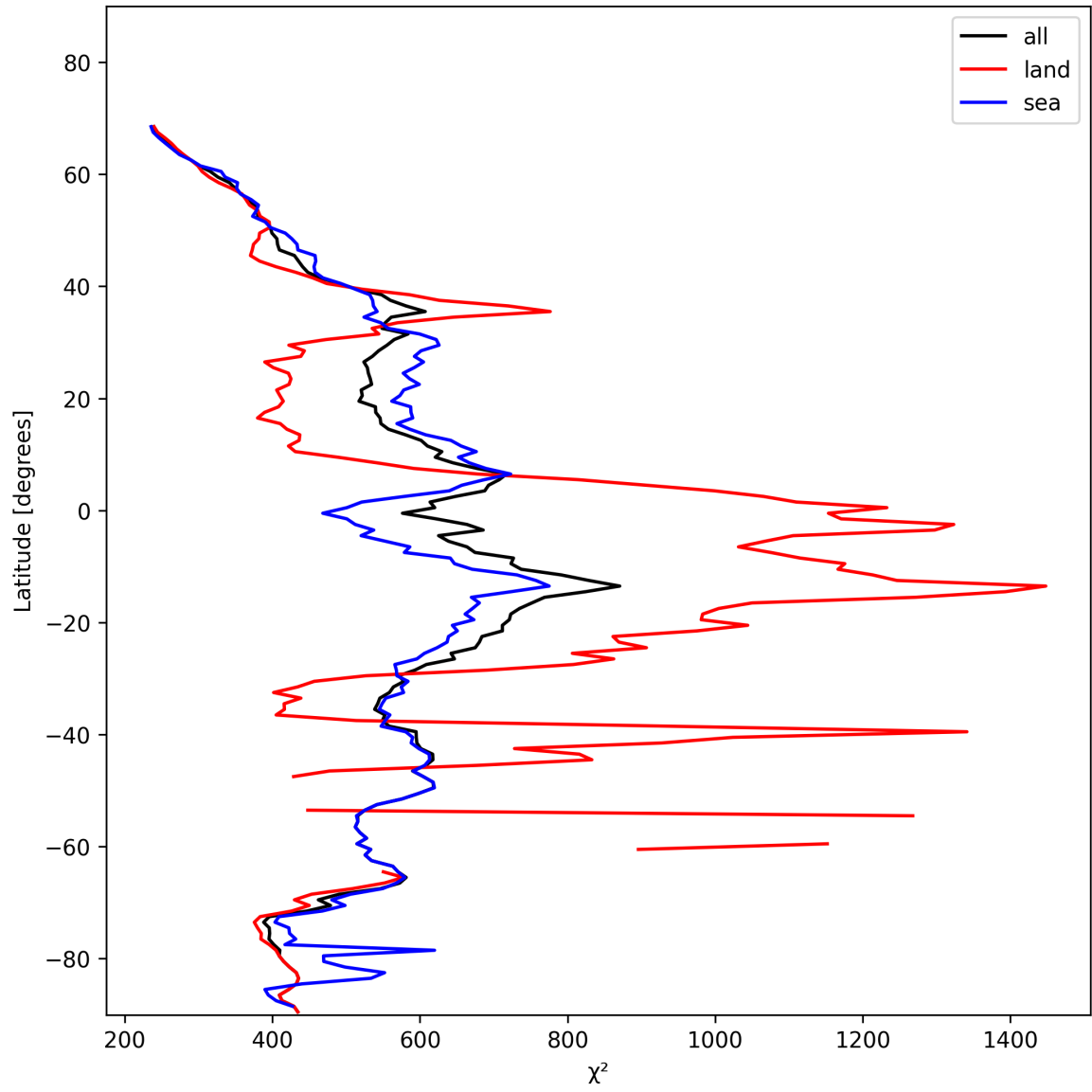
Figure 25: Zonal average of “ \chi^2 ” for 2024-11-18 to 2024-11-20.
