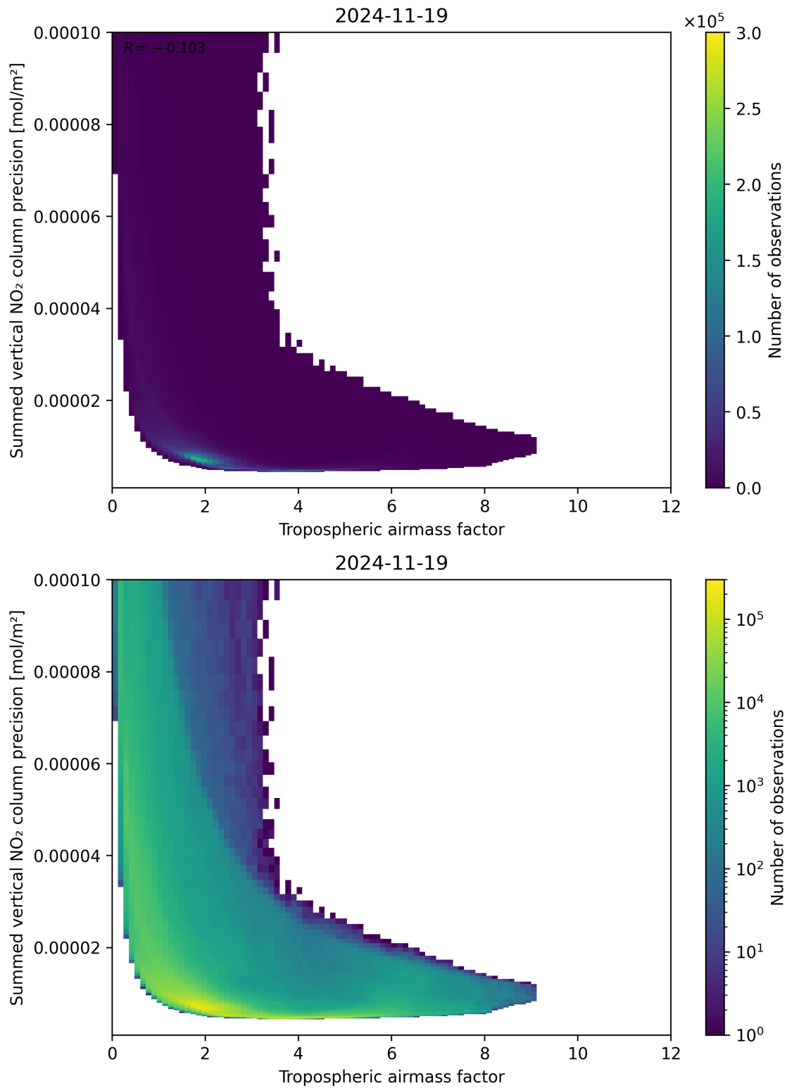
Figure 76: Scatter density plot of “Tropospheric air mass factor” against “Summed vertical NO 2 column precision” for 2024-11-18 to 2024-11-20.
