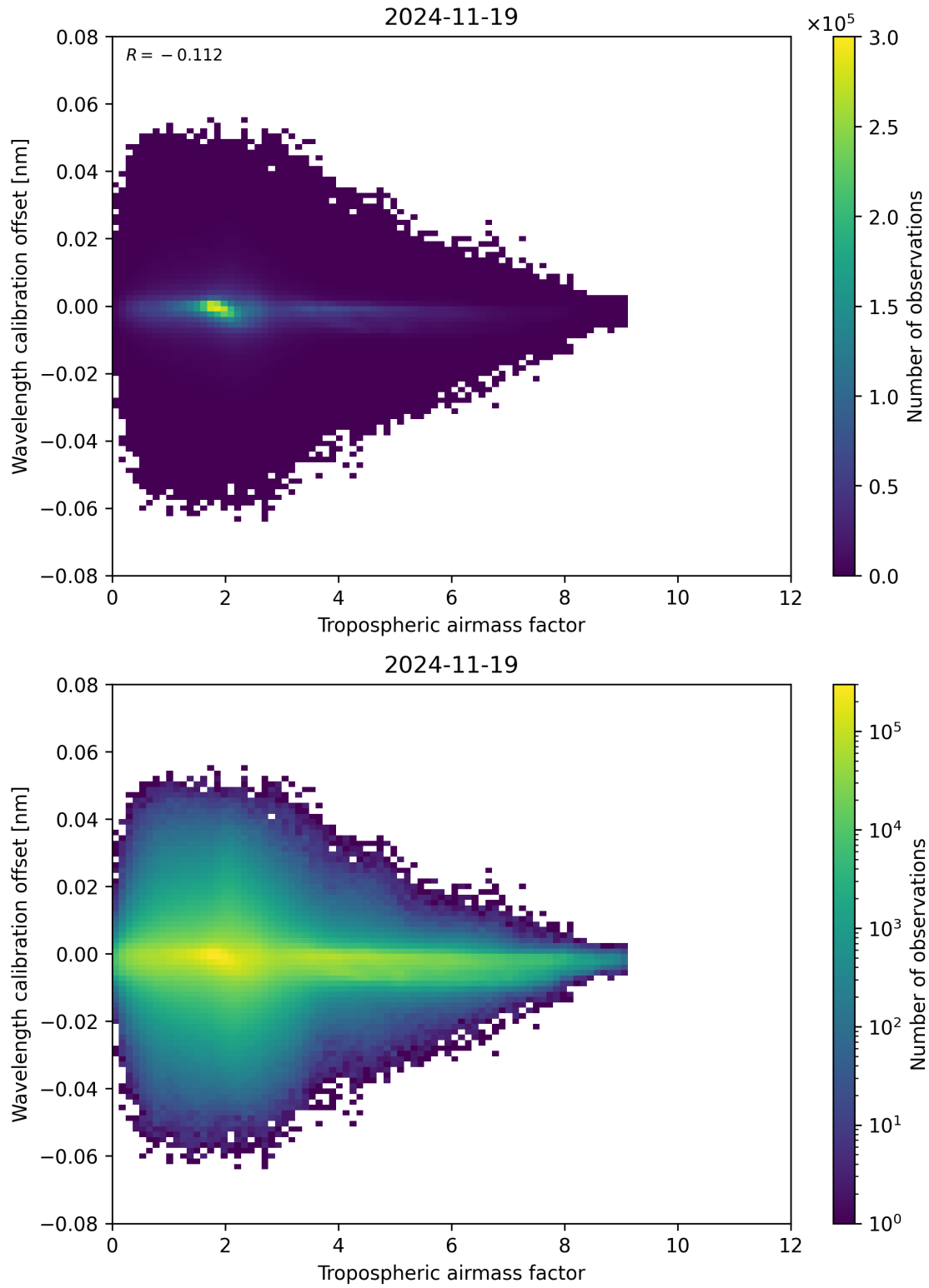
Figure 80: Scatter density plot of “Tropospheric airmass factor” against “Wavelength calibration offset” for 2024-11-18 to 2024-11-20.
