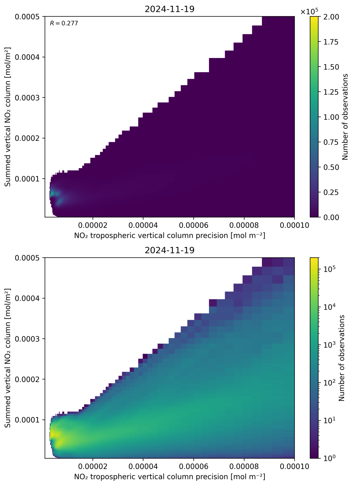
Figure 136: Scatter density plot of “NO 2 tropospheric vertical column precision” against “Summed vertical NO 2 column” for 2024-11-18 to 2024-11-20.
