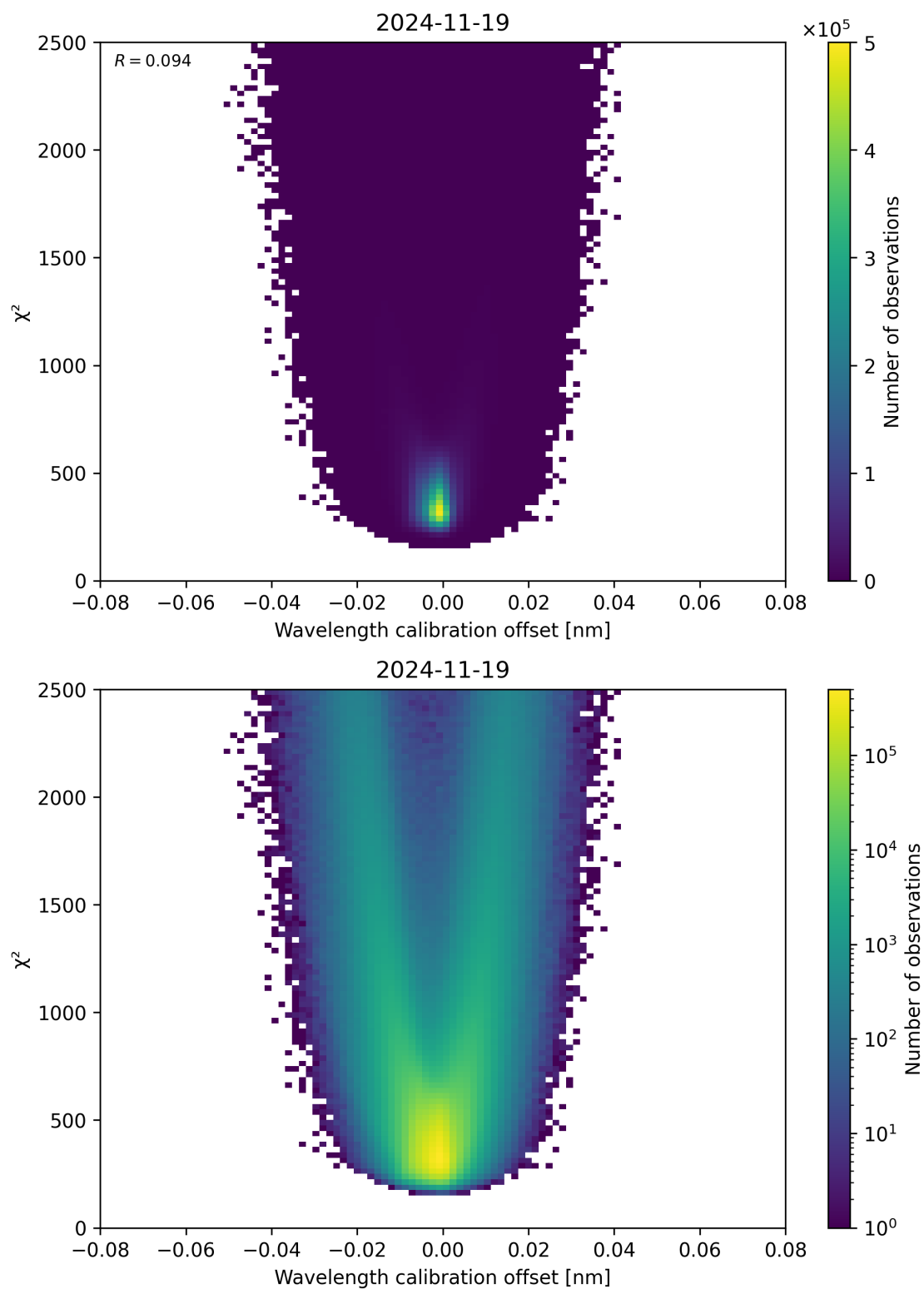
Figure 175: Scatter density plot of “Wavelength calibration offset” against “ \chi^2 ” for 2024-11-18 to 2024-11-20.
