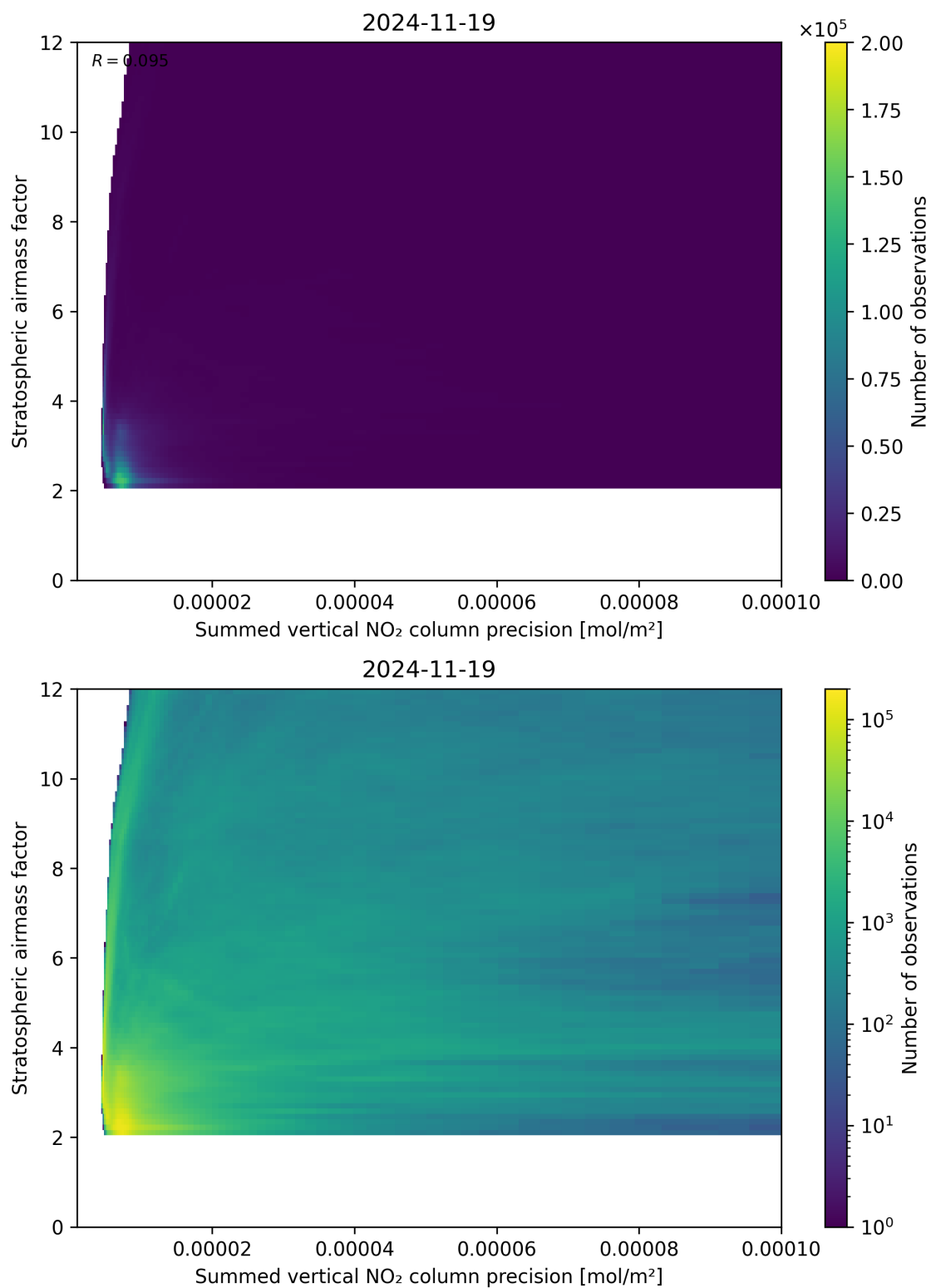
Figure 106: Scatter density plot of “Summed vertical NO 2 column precision” against “Stratospheric airmass factor” for 2024-11-18 to 2024-11-20.
