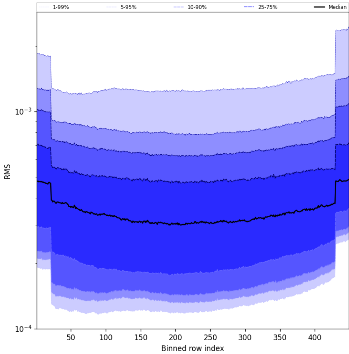
Figure 60: Along track statistics of “RMS” for 2024-11-18 to 2024-11-20
