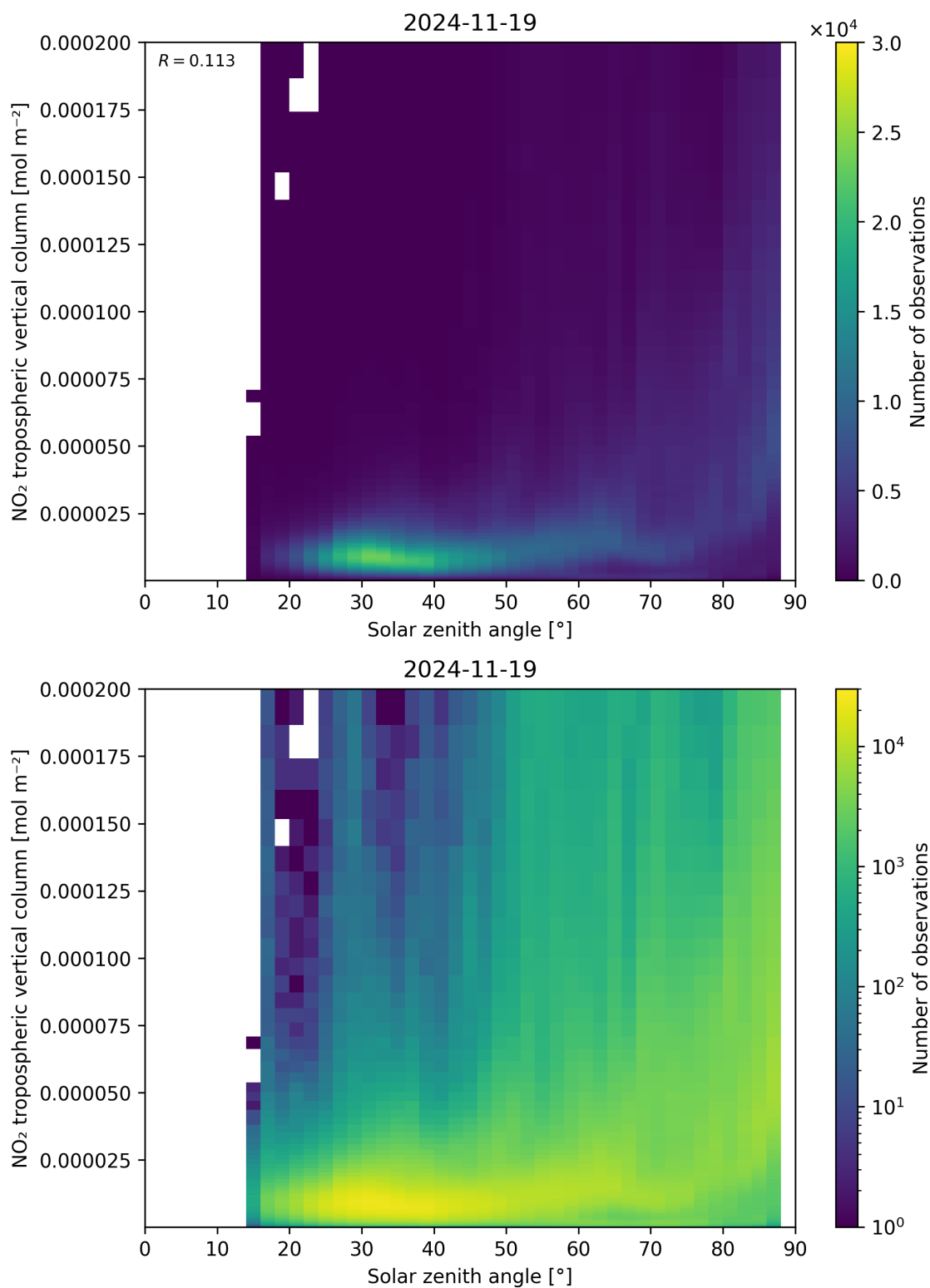
Figure 155: Scatter density plot of “Solar zenith angle” against “NO 2 tropospheric vertical column” for 2024-11-18 to 2024-11-20.
