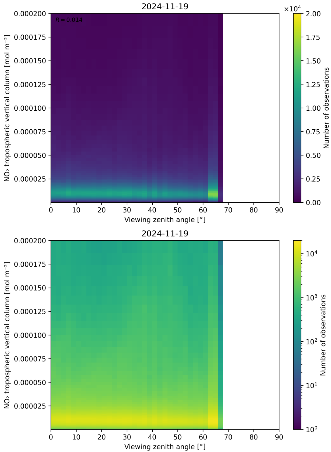
Figure 169: Scatter density plot of “Viewing zenith angle” against “NO 2 tropospheric vertical column” for 2024-11-18 to 2024-11-20.
