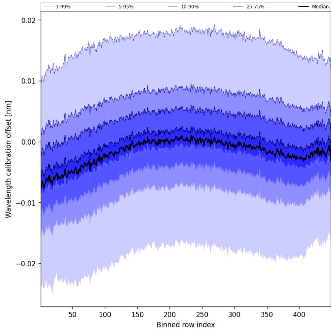
Figure 52: Along track statistics of “Wavelength calibration offset” for 2024-11-18 to 2024-11-20
