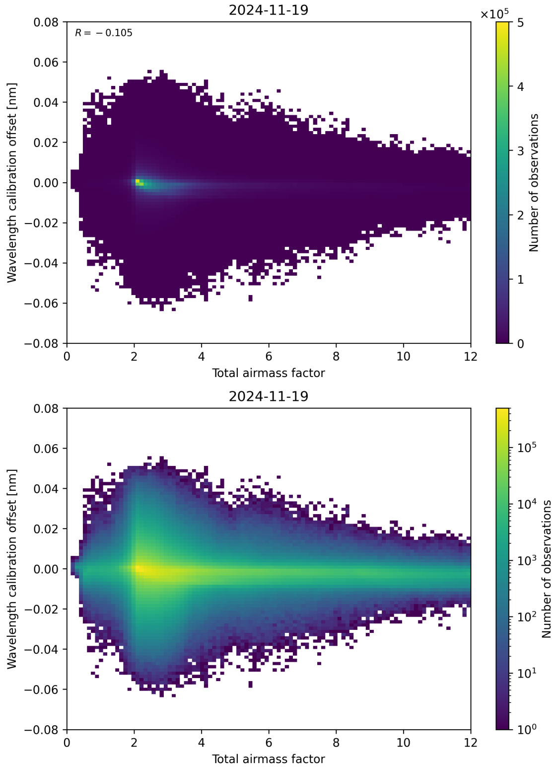
Figure 70: Scatter density plot of “Total airmass factor” against “Wavelength calibration offset” for 2024-11-18 to 2024-11-20.
