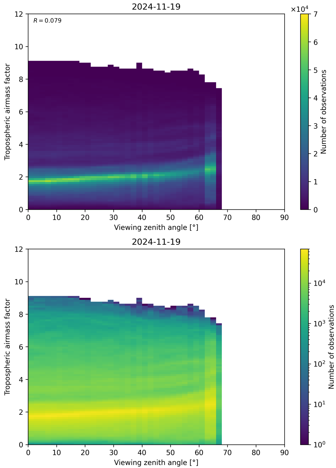
Figure 161: Scatter density plot of “Viewing zenith angle” against “Tropospheric airmass factor” for 2024-11-18 to 2024-11-20.
