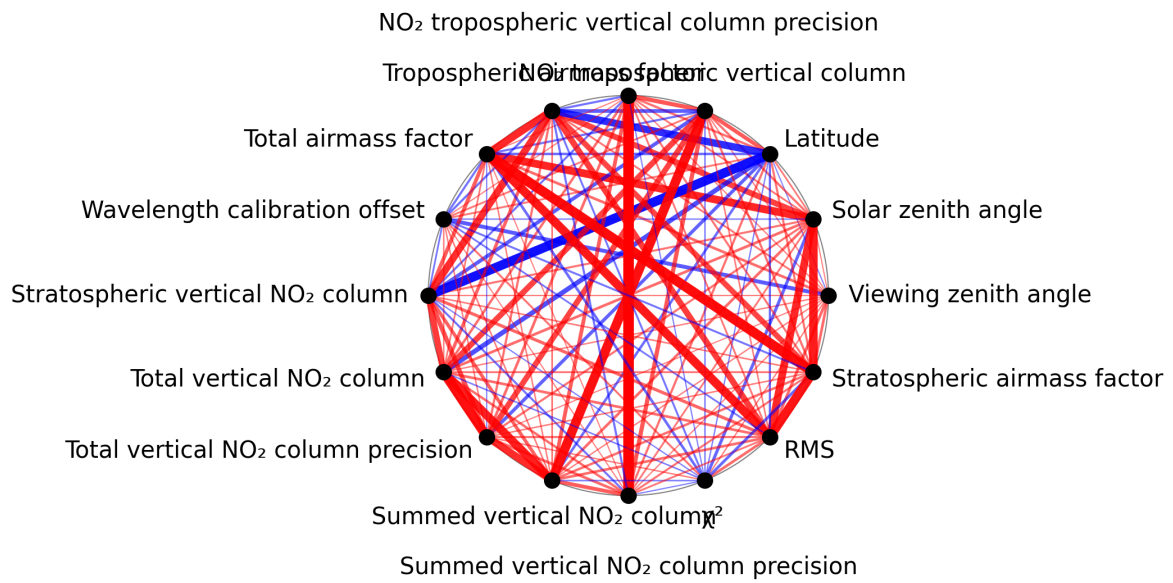
Figure 1: Map of correlation graph for 2024-11-18 to 2024-11-20.
