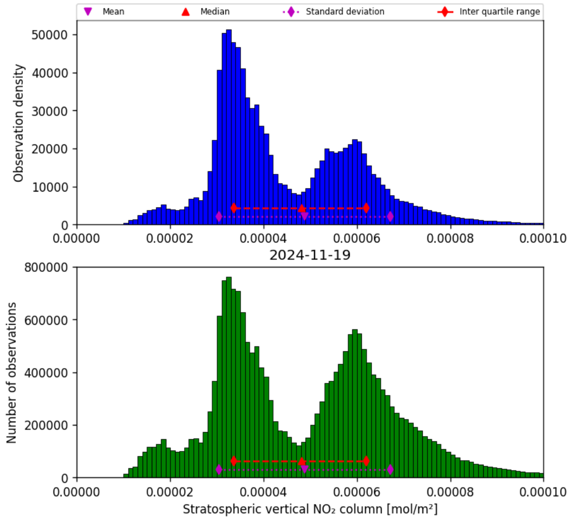
Figure 36: Histogram of “Stratospheric vertical NO 2 column” for 2024-11-18 to 2024-11-20
