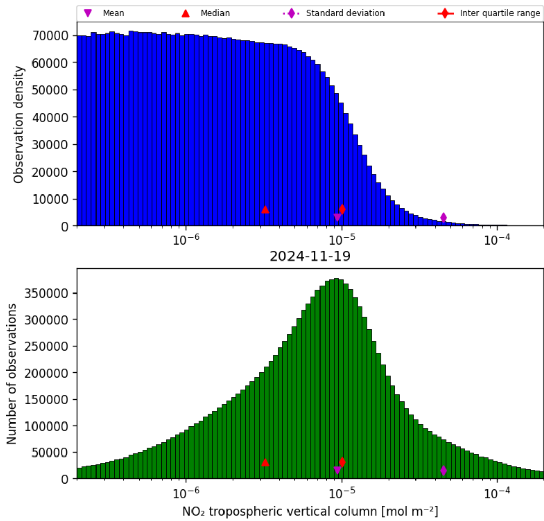
Figure 29: Histogram of “NO 2 tropospheric vertical column” for 2024-11-18 to 2024-11-20
