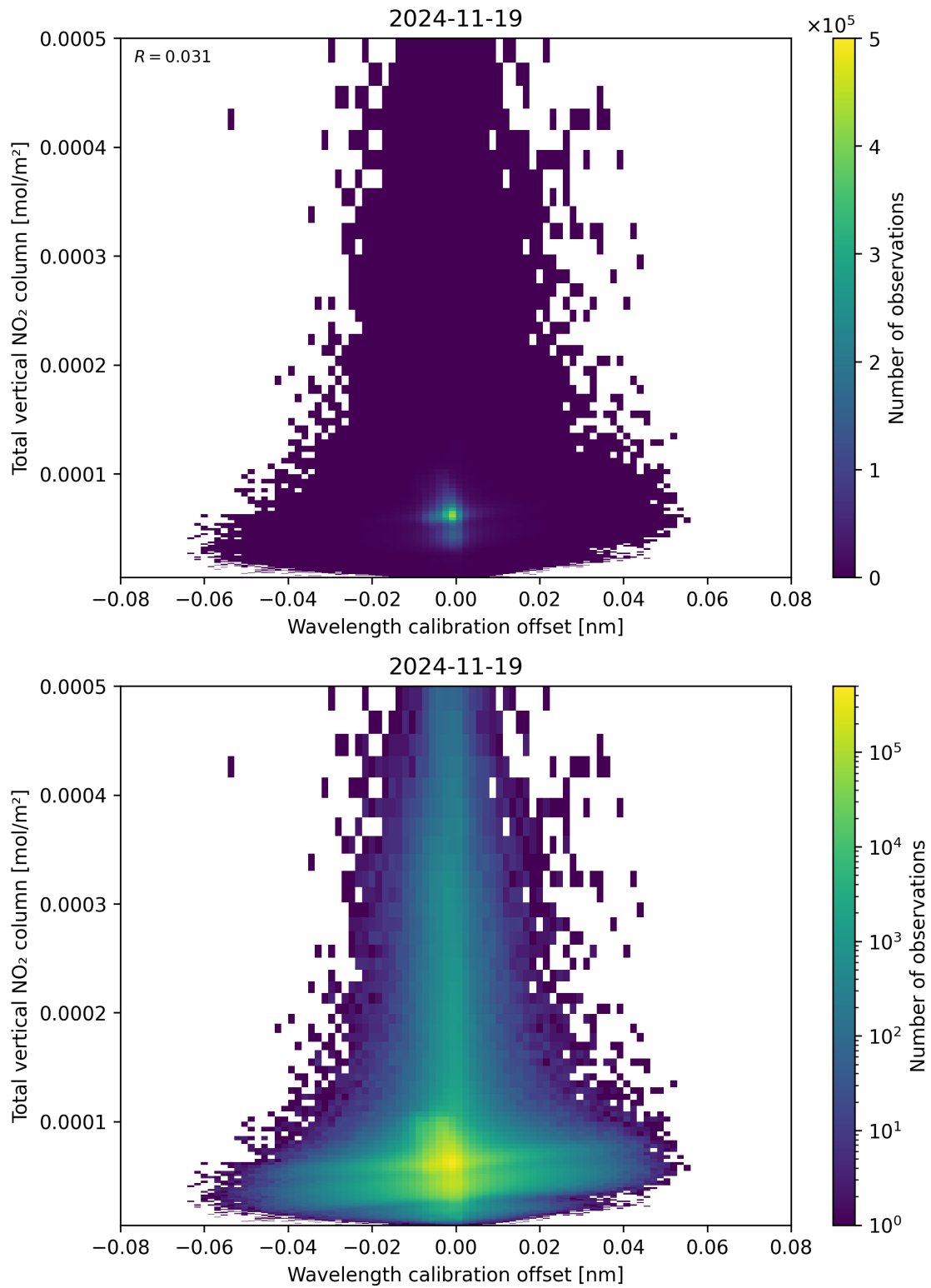
Figure 179: Scatter density plot of “Wavelength calibration offset” against “Total vertical NO 2 column” for 2024-11-18 to 2024-11-20.
