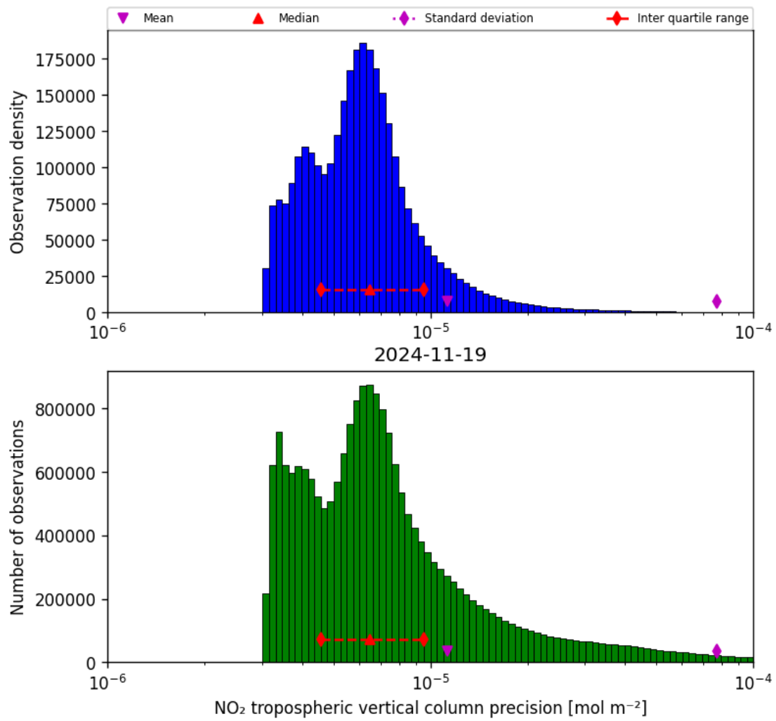
Figure 30: Histogram of “NO 2 tropospheric vertical column precision” for 2024-11-18 to 2024-11-20
