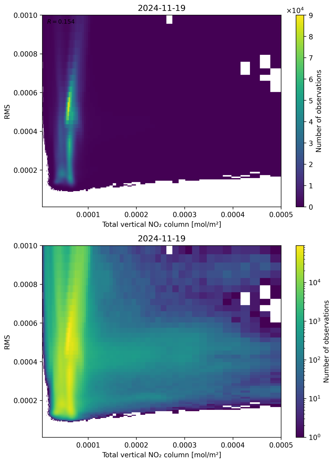
Figure 120: Scatter density plot of “Total vertical NO 2 column” against “RMS” for 2024-11-18 to 2024-11-20.
