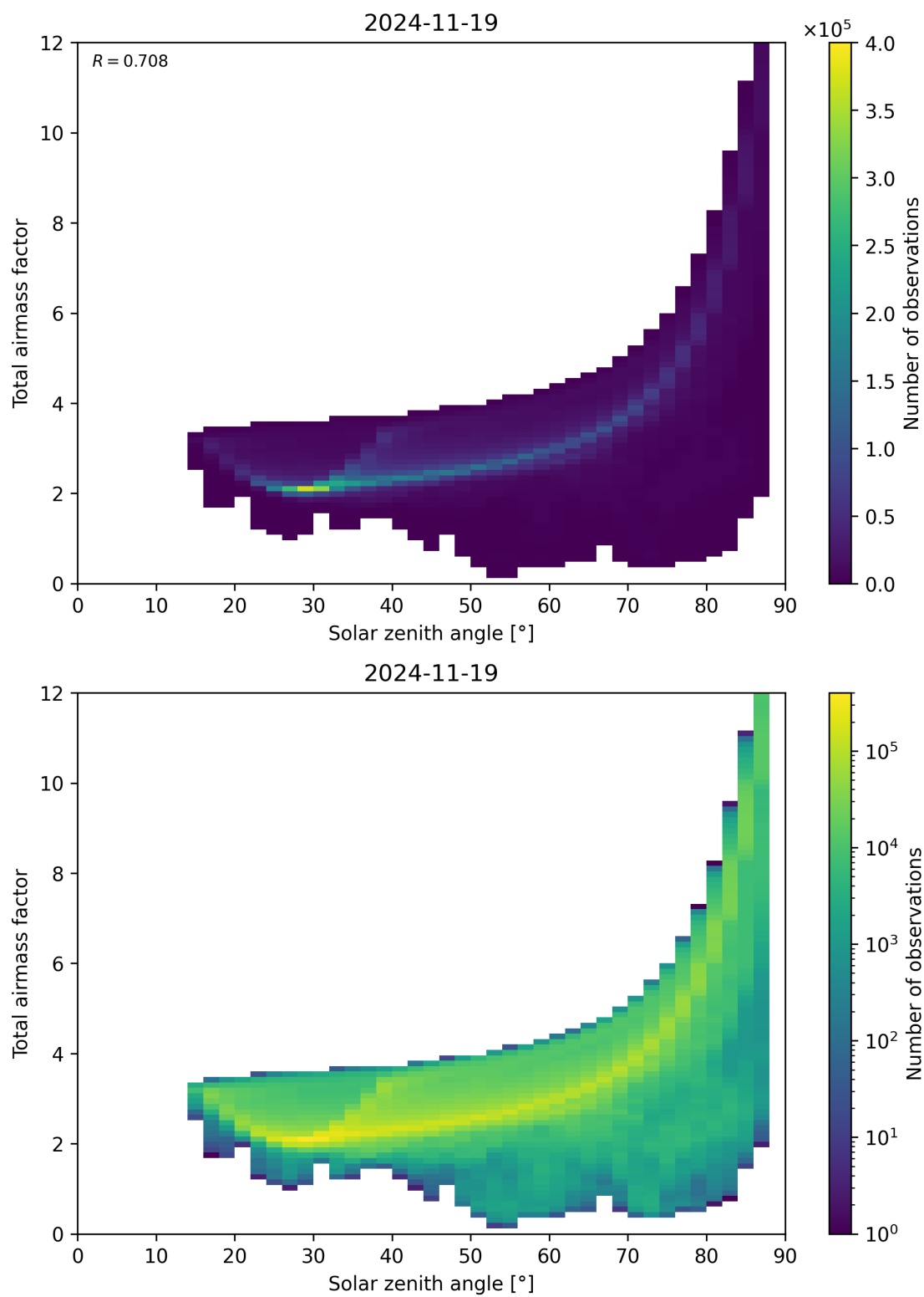
Figure 146: Scatter density plot of “Solar zenith angle” against “Total airmass factor” for 2024-11-18 to 2024-11-20.
