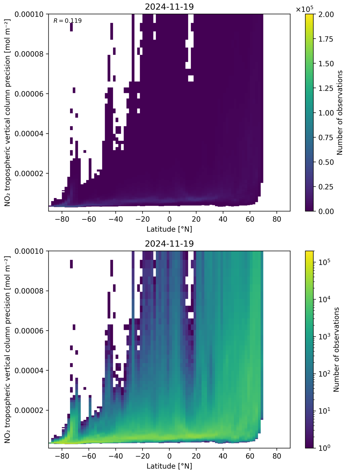
Figure 93: Scatter density plot of “Latitude” against “NO 2 tropospheric vertical column precision” for 2024-11-18 to 2024-11-20.
