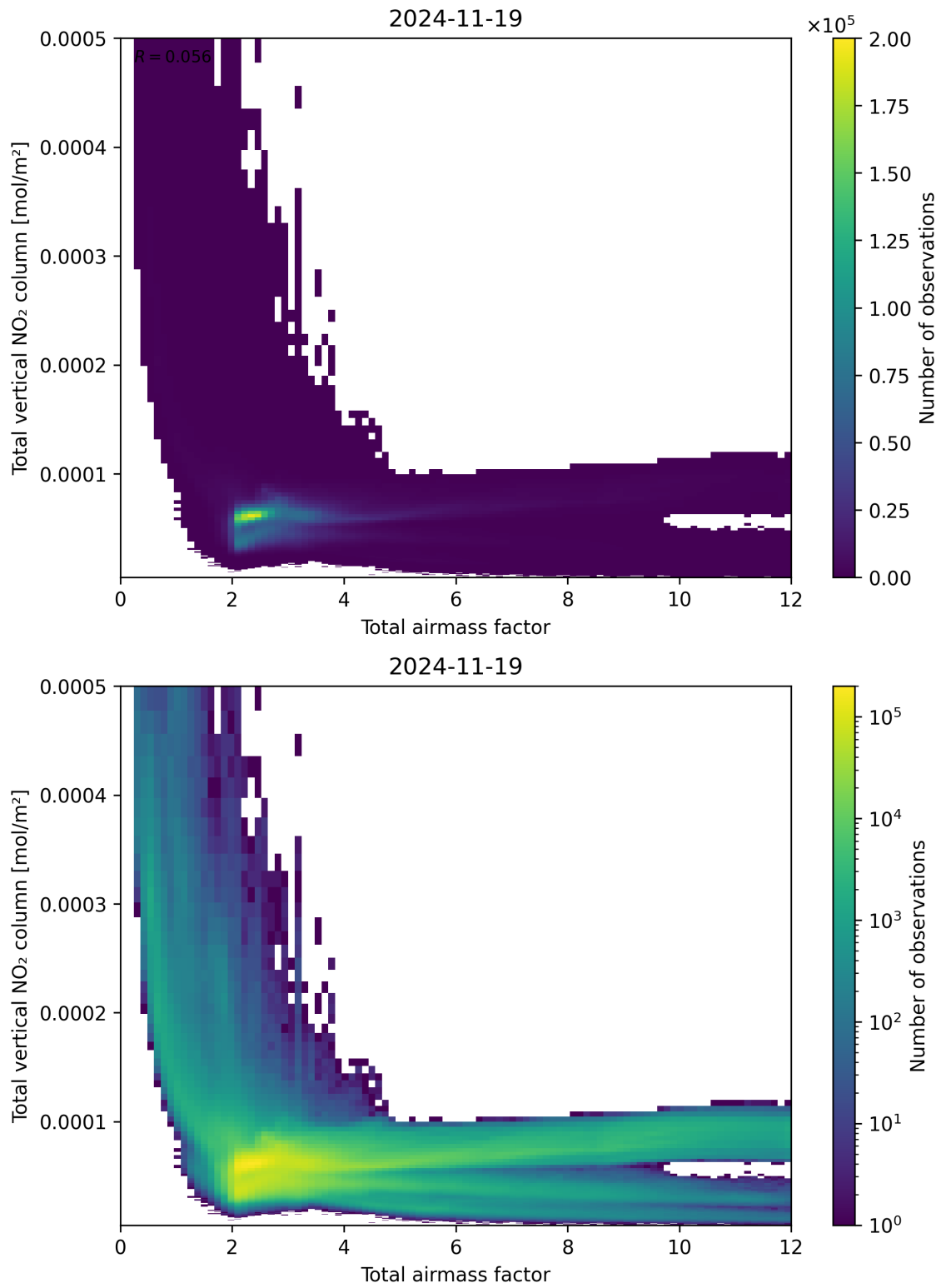
Figure 67: Scatter density plot of “Total airmass factor” against “Total vertical NO 2 column” for 2024-11-18 to 2024-11-20.
