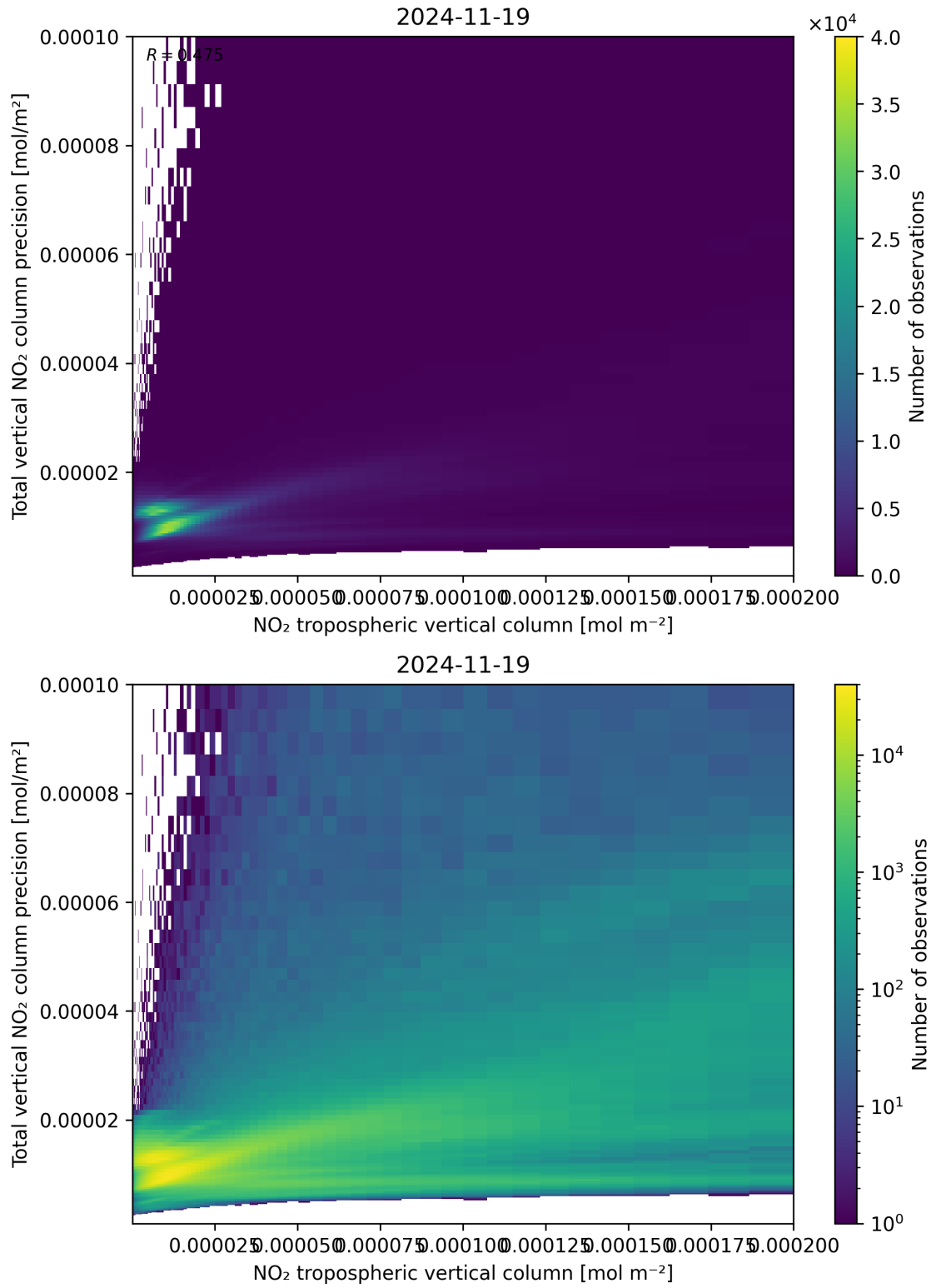
Figure 129: Scatter density plot of “NO 2 tropospheric vertical column” against “Total vertical NO 2 column precision” for 2024-11-18 to 2024-11-20.
