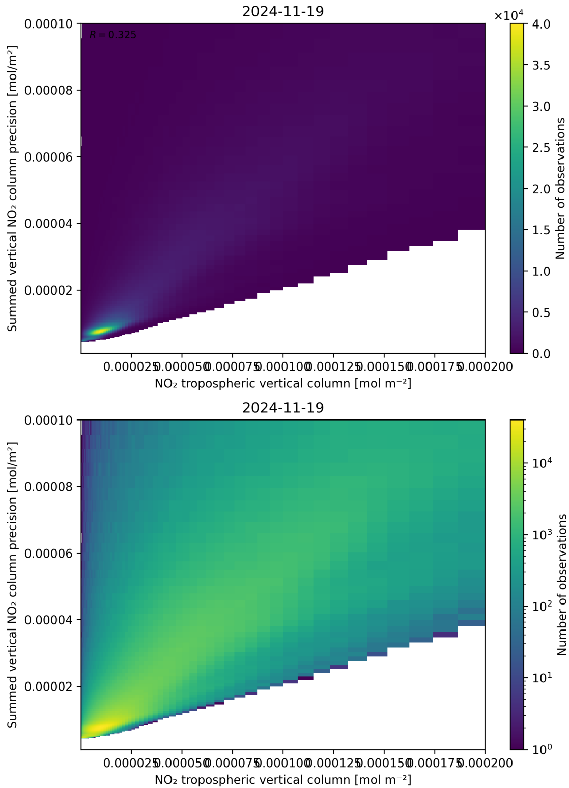
Figure 127: Scatter density plot of “NO 2 tropospheric vertical column” against “Summed vertical NO 2 column precision” for 2024-11-18 to 2024-11-20.
