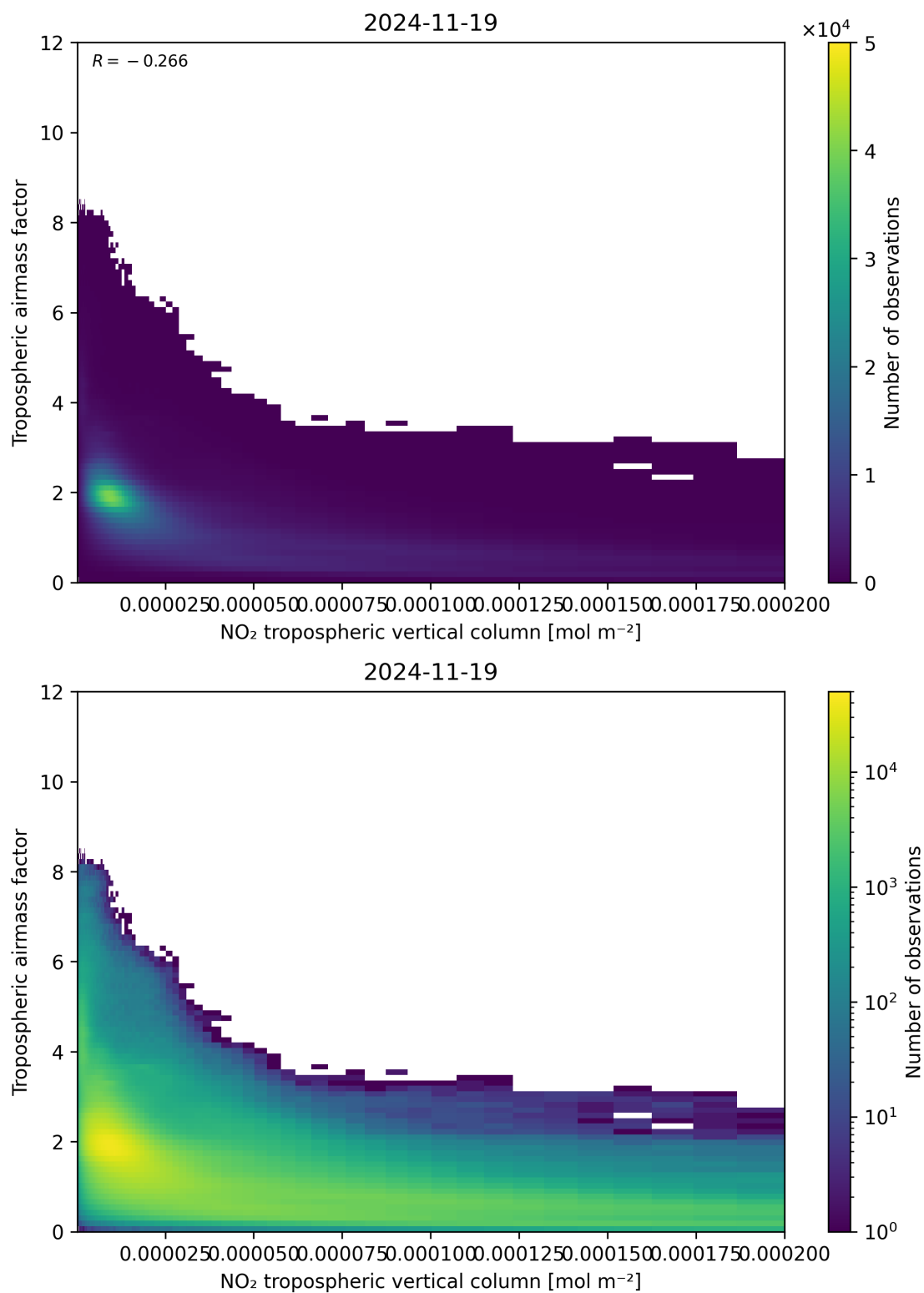
Figure 123: Scatter density plot of “NO 2 tropospheric vertical column” against “Tropospheric air mass factor” for 2024-11-18 to 2024-11-20.
