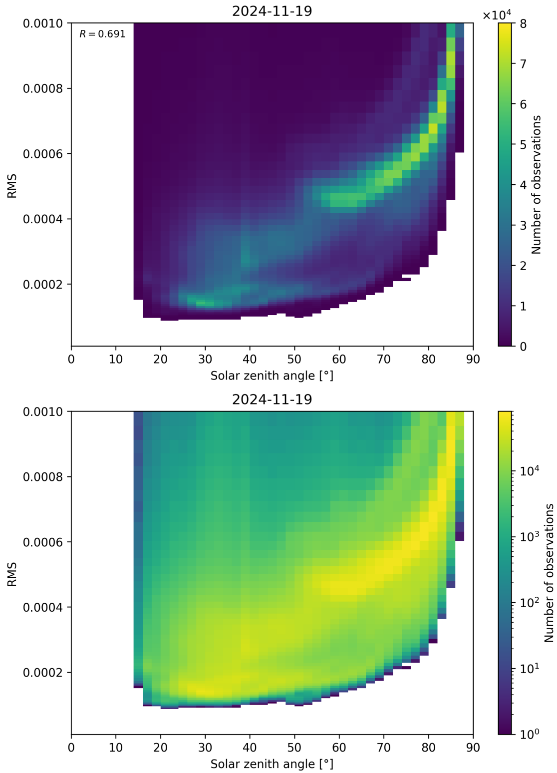
Figure 157: Scatter density plot of “Solar zenith angle” against “RMS” for 2024-11-18 to 2024-11-20.
