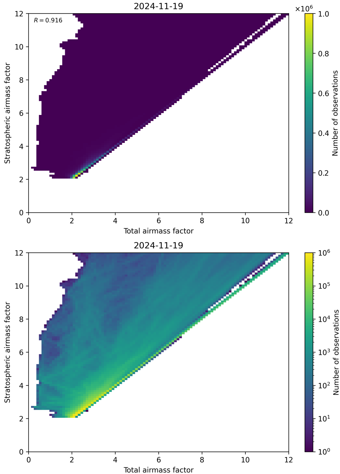
Figure 62: Scatter density plot of “Total airmass factor” against “Stratospheric airmass factor” for 2024-11-18 to 2024-11-20.
