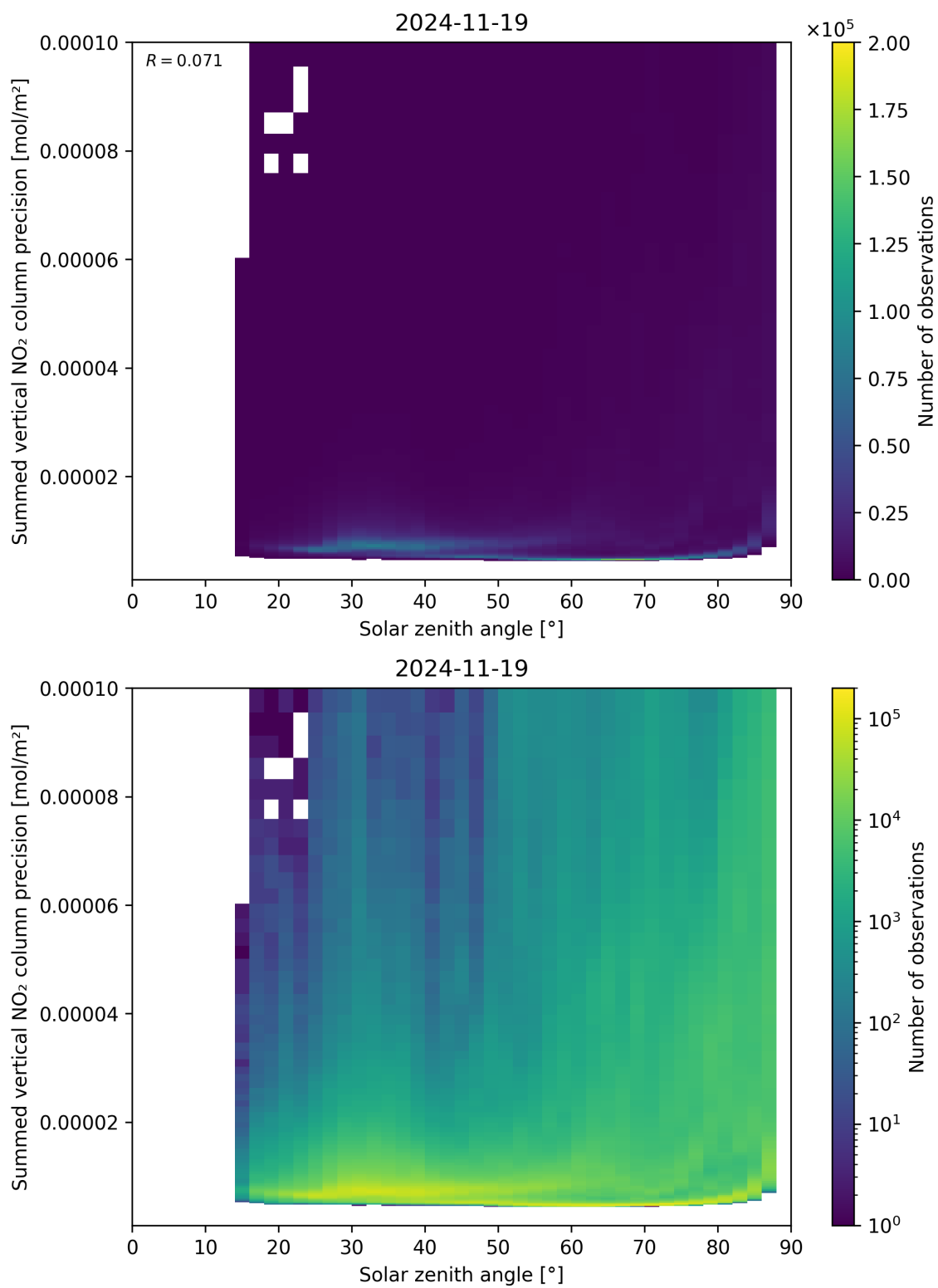
Figure 152: Scatter density plot of “Solar zenith angle” against “Summed vertical NO 2 column precision” for 2024-11-18 to 2024-11-20.
