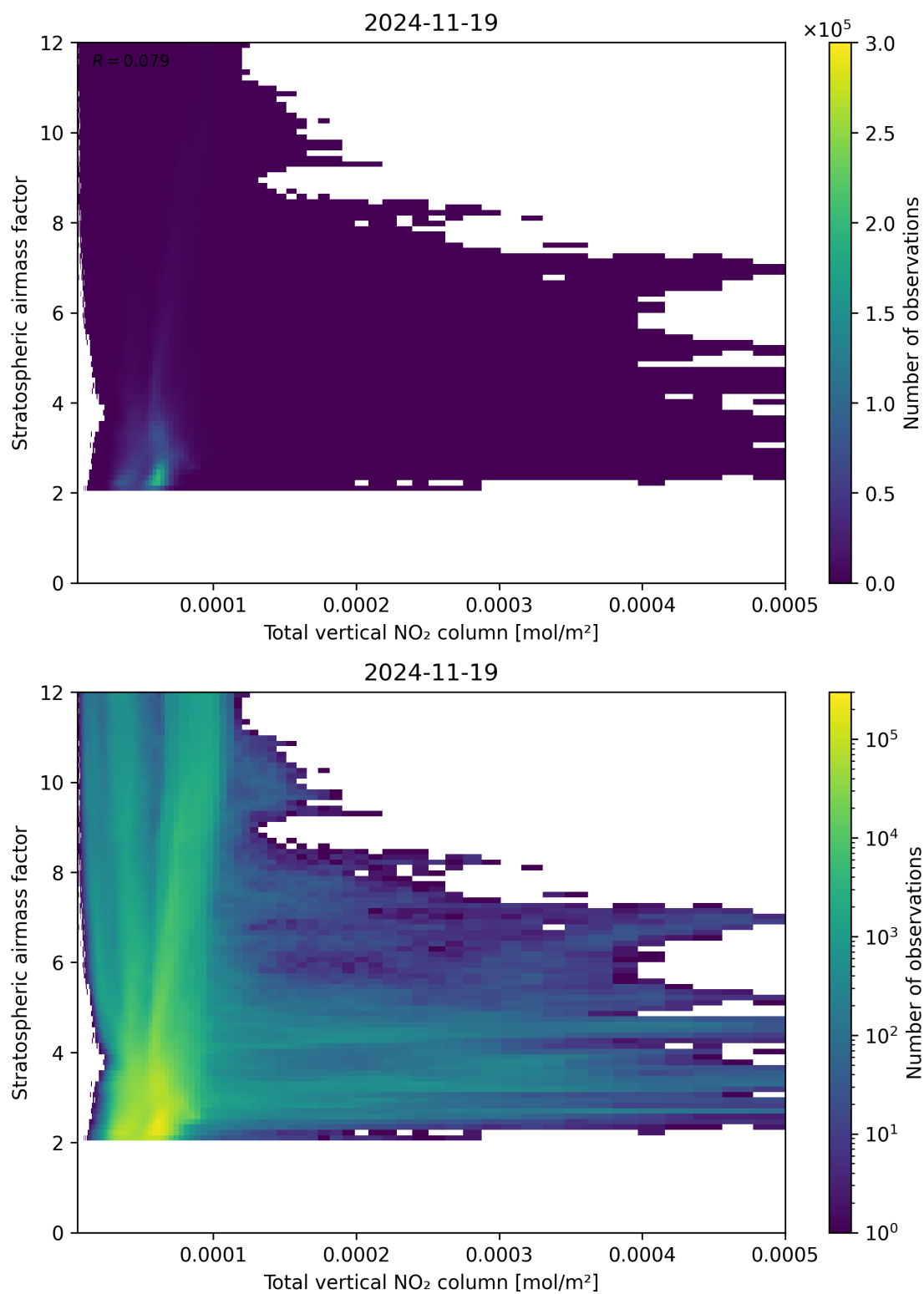
Figure 110: Scatter density plot of “Total vertical NO 2 column” against “Stratospheric airmass factor” for 2024-11-18 to 2024-11-20.
