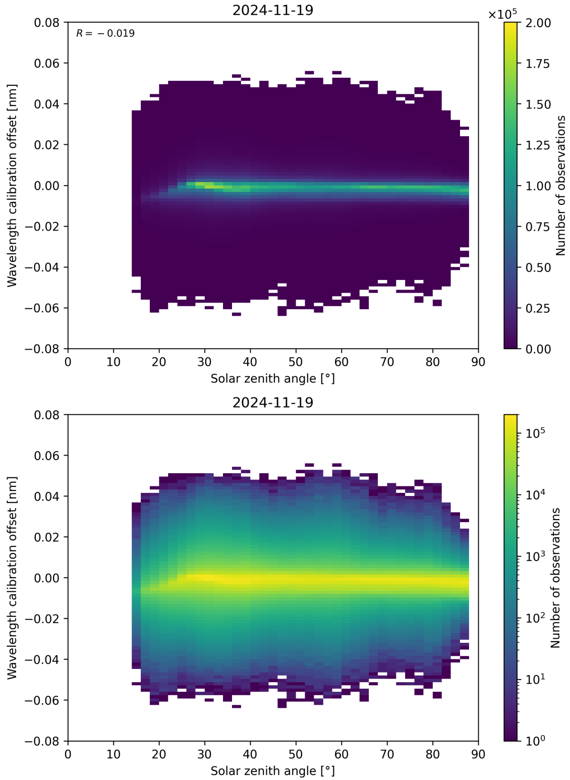
Figure 158: Scatter density plot of “Solar zenith angle” against “Wavelength calibration offset” for 2024-11-18 to 2024-11-20.
