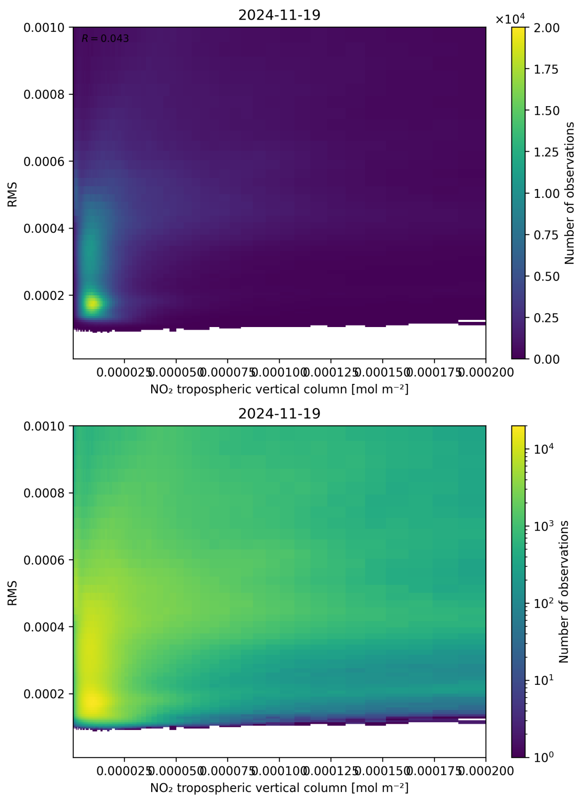
Figure 142: Scatter density plot of “NO 2 tropospheric vertical column” against “RMS” for 2024-11-18 to 2024-11-20.
