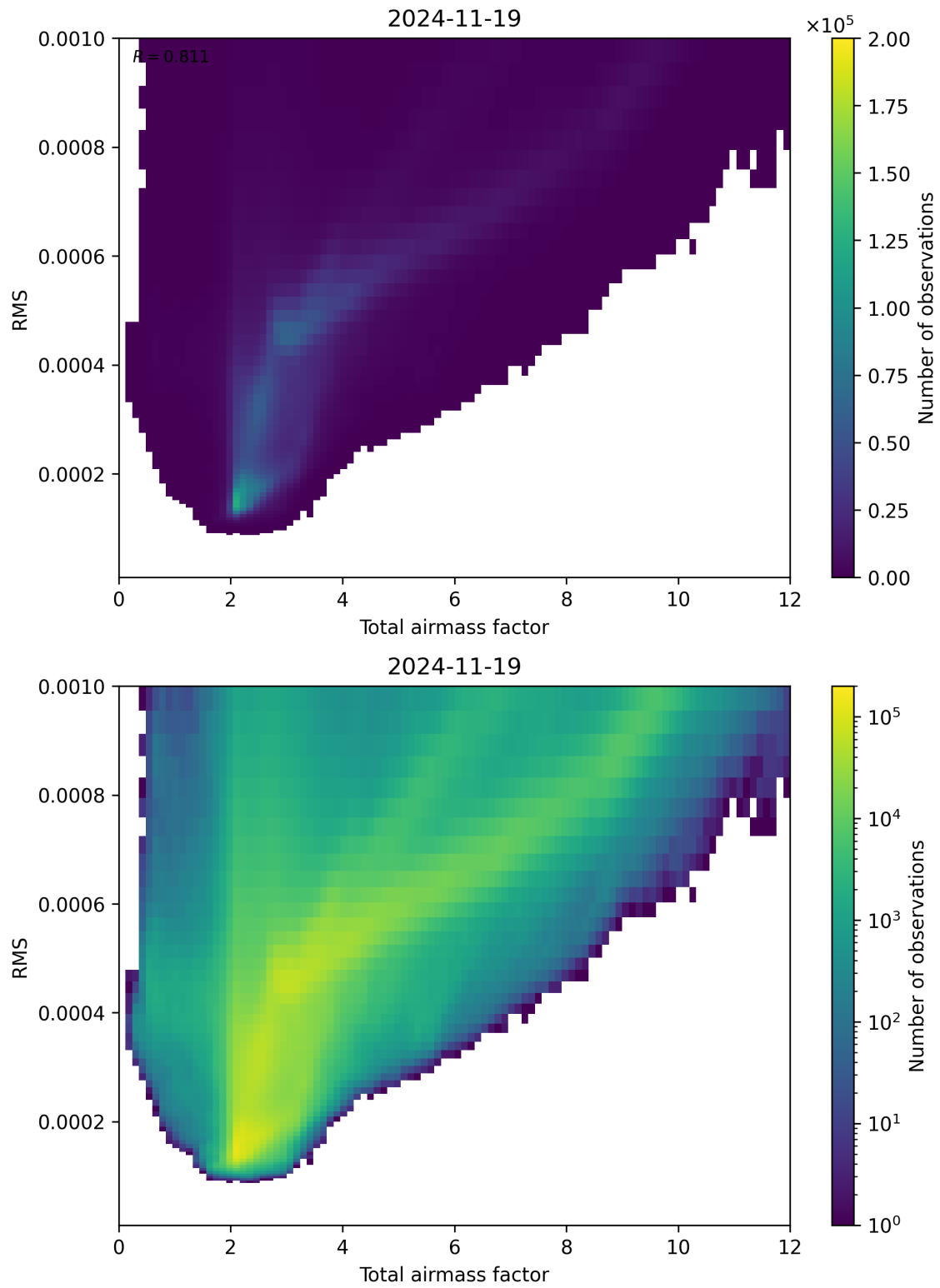
Figure 69: Scatter density plot of “Total airmass factor” against “RMS” for 2024-11-18 to 2024-11-20.
