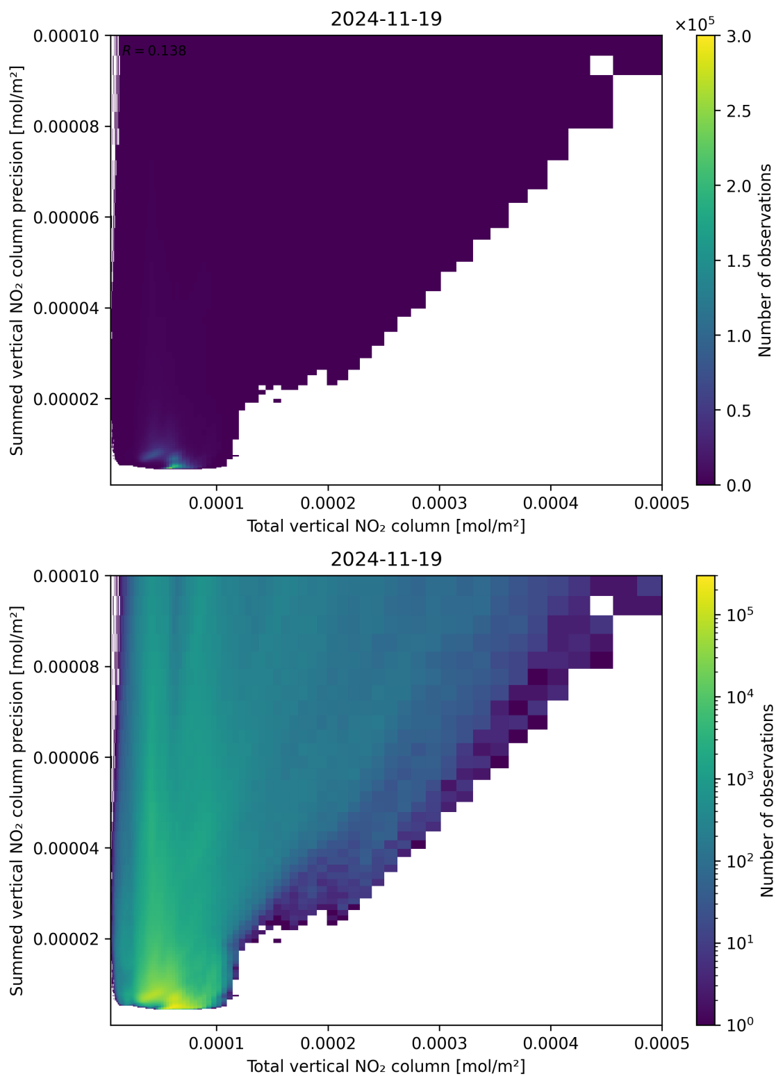
Figure 113: Scatter density plot of “Total vertical NO 2 column” against “Summed vertical NO 2 column precision” for 2024-11-18 to 2024-11-20.
