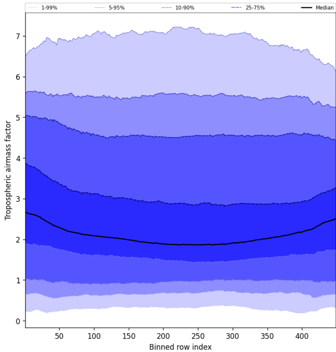
Figure 48: Along track statistics of “Tropospheric air mass factor” for 2024-11-18 to 2024-11-20
