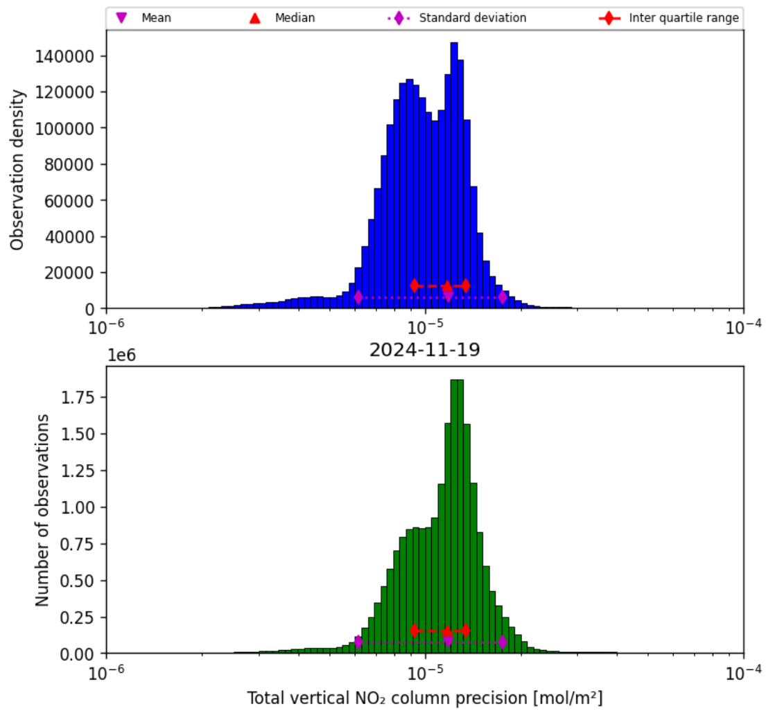
Figure 39: Histogram of “Total vertical NO 2 column precision” for 2024-11-18 to 2024-11-20
