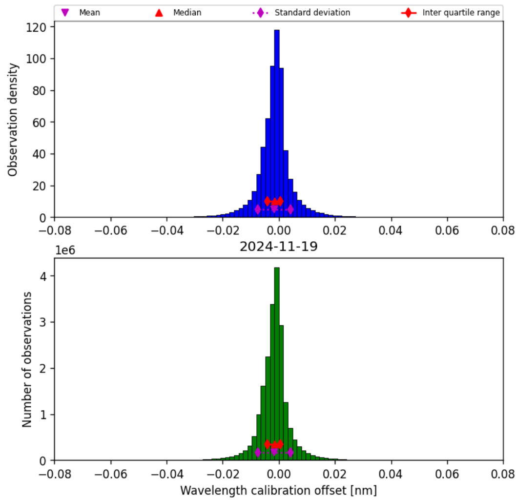
Figure 35: Histogram of “Wavelength calibration offset” for 2024-11-18 to 2024-11-20
