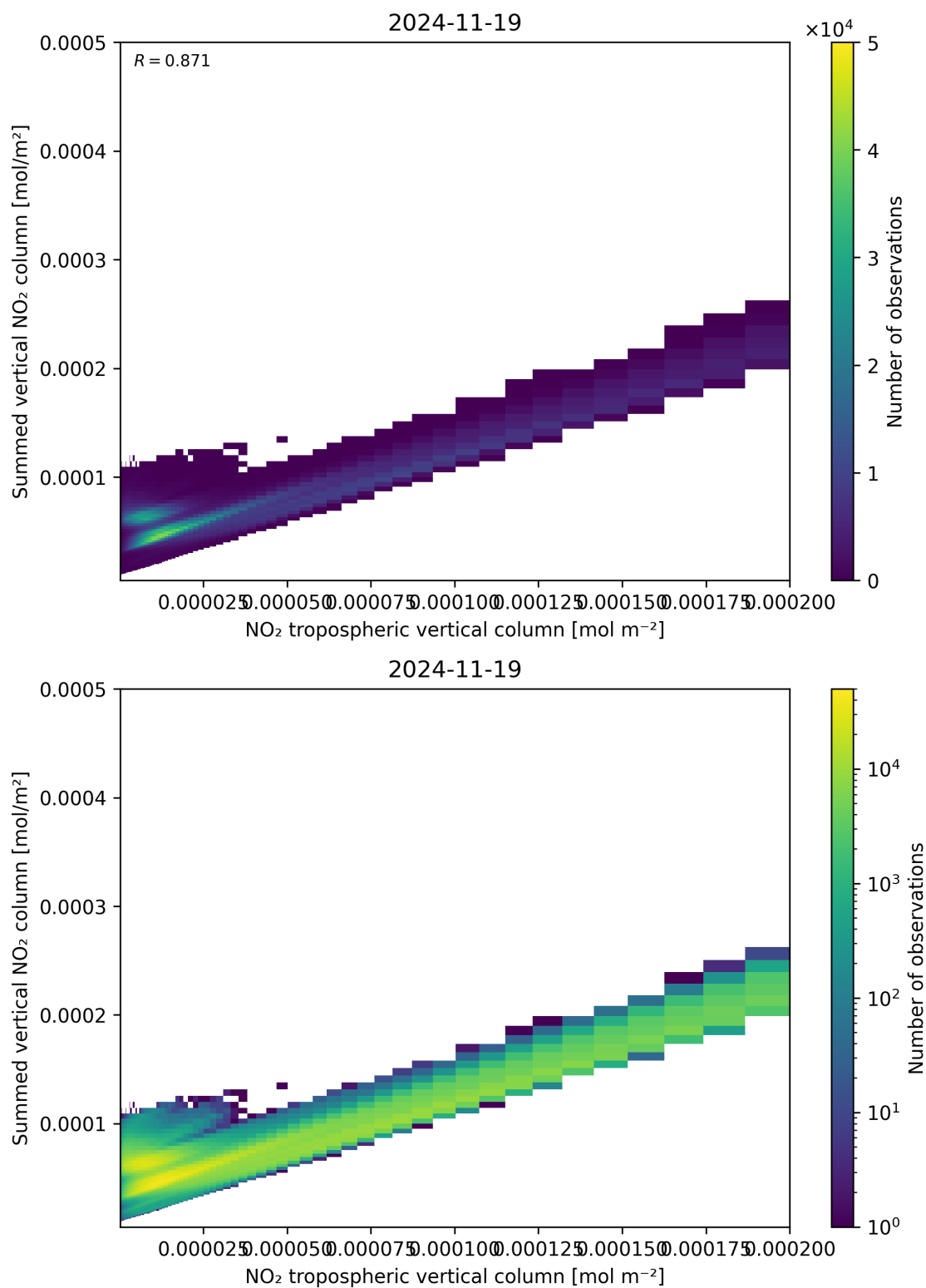
Figure 126: Scatter density plot of “NO 2 tropospheric vertical column” against “Summed vertical NO 2 column” for 2024-11-18 to 2024-11-20.
