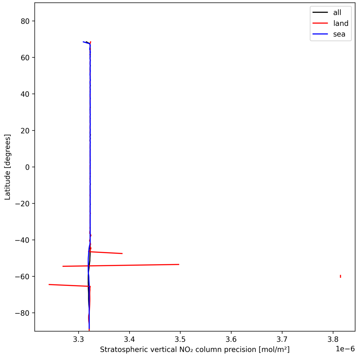
Figure 20: Zonal average of “Stratospheric vertical NO 2 column precision” for 2024-11-18 to 2024-11-20.
