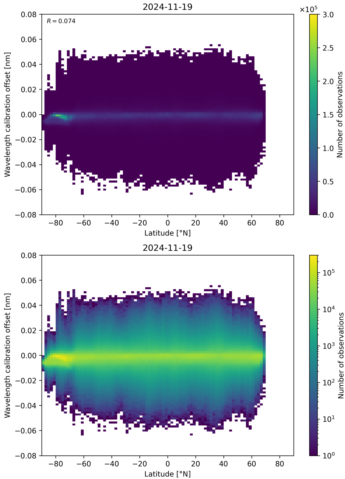
Figure 95: Scatter density plot of “Latitude” against “Wavelength calibration offset” for 2024-11-18 to 2024-11-20.
