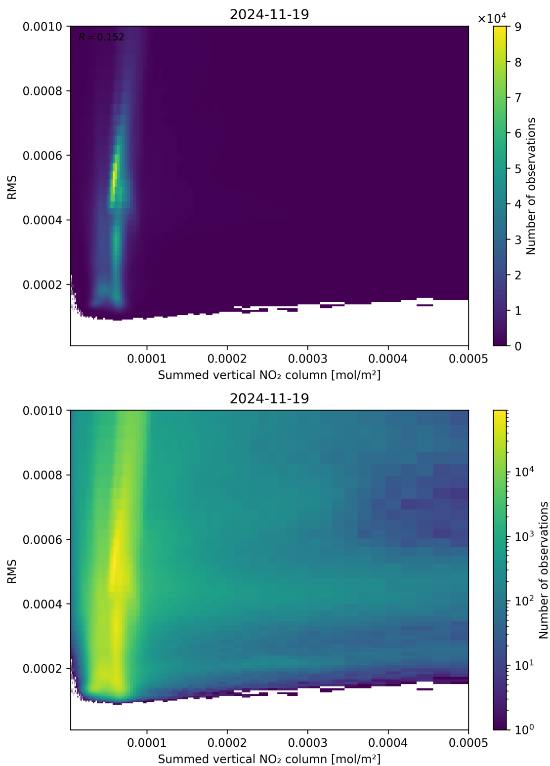
Figure 109: Scatter density plot of “Summed vertical NO 2 column” against “RMS” for 2024-11-18 to 2024-11-20.
