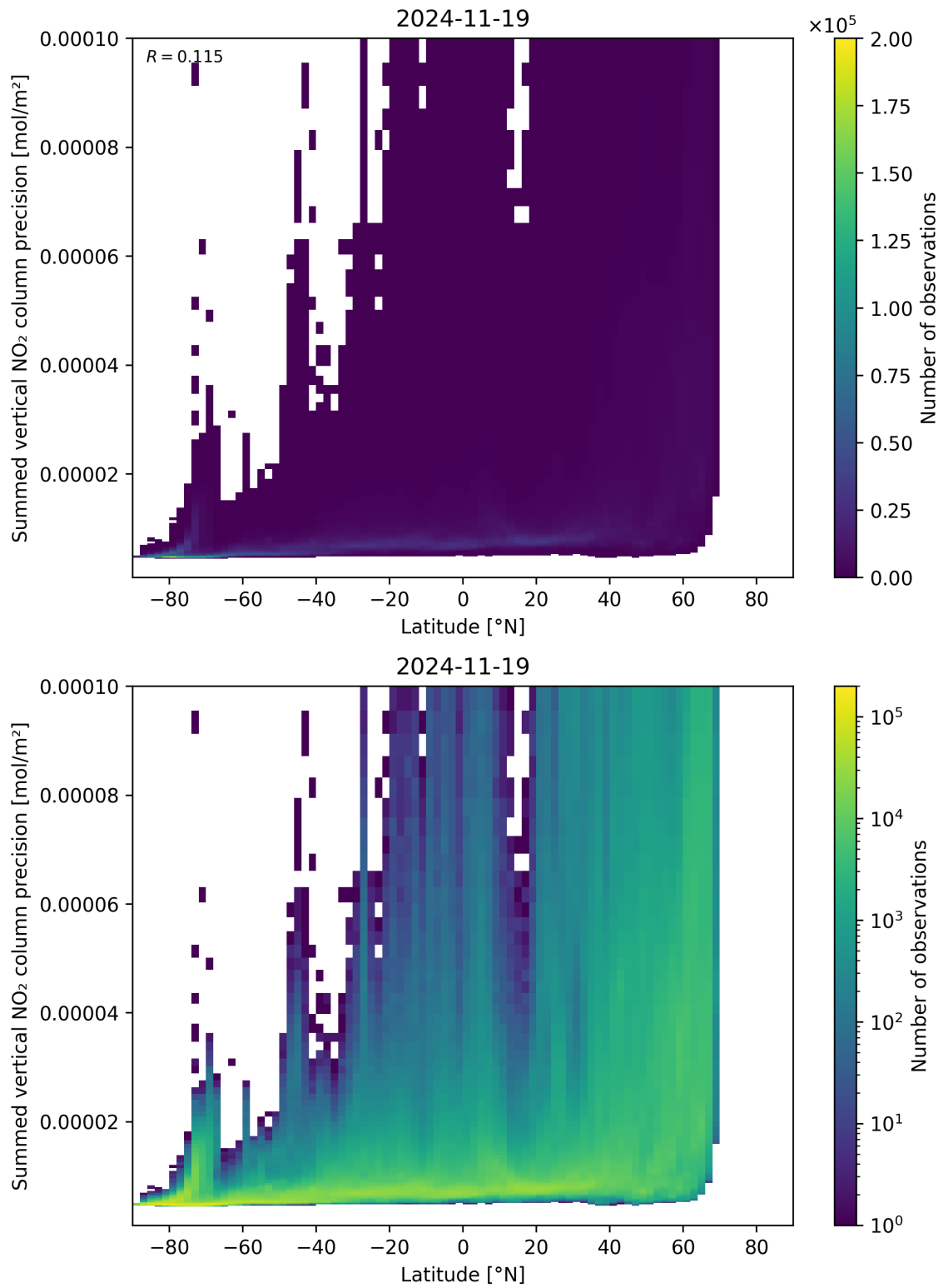
Figure 89: Scatter density plot of “Latitude” against “Summed vertical NO 2 column precision” for 2024-11-18 to 2024-11-20.
