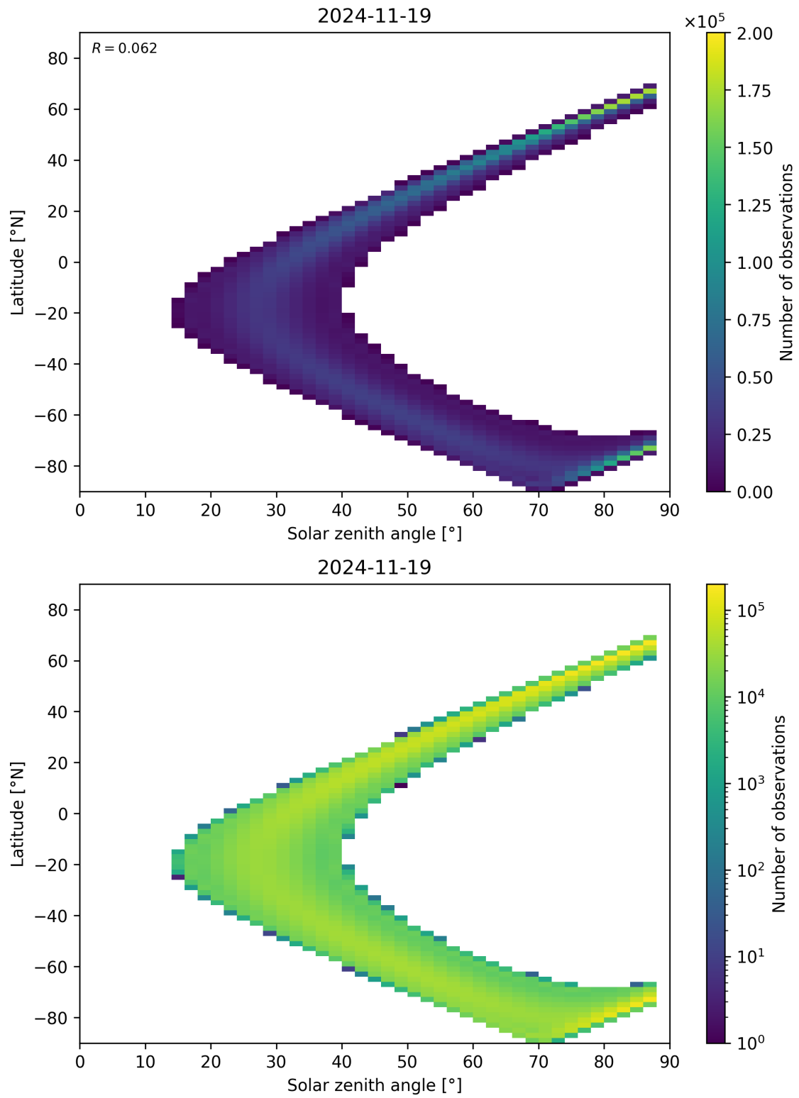
Figure 149: Scatter density plot of “Solar zenith angle” against “Latitude” for 2024-11-18 to 2024-11-20.
