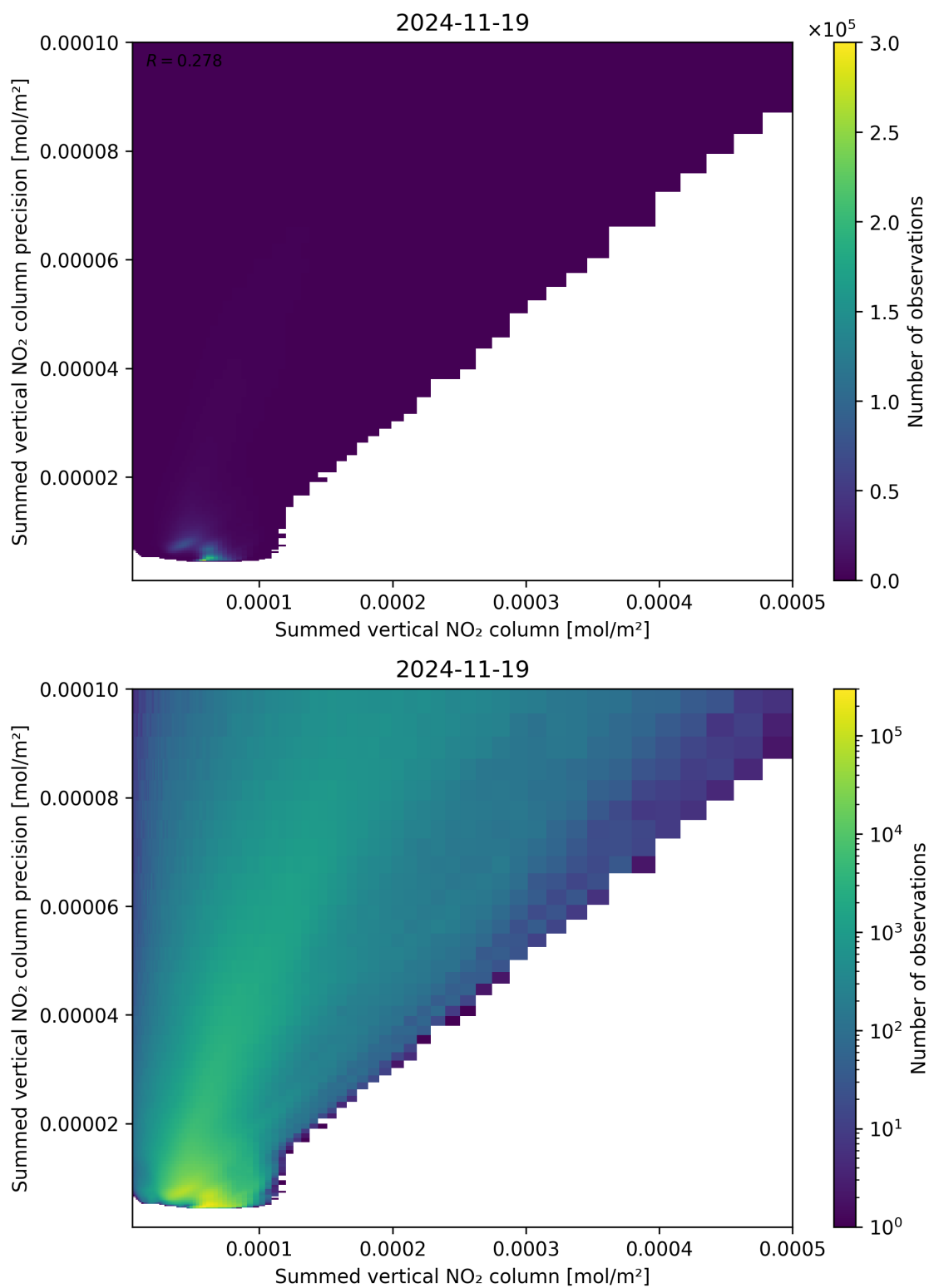
Figure 105: Scatter density plot of “Summed vertical NO 2 column” against “Summed vertical NO 2 column precision” for 2024-11-18 to 2024-11-20.
