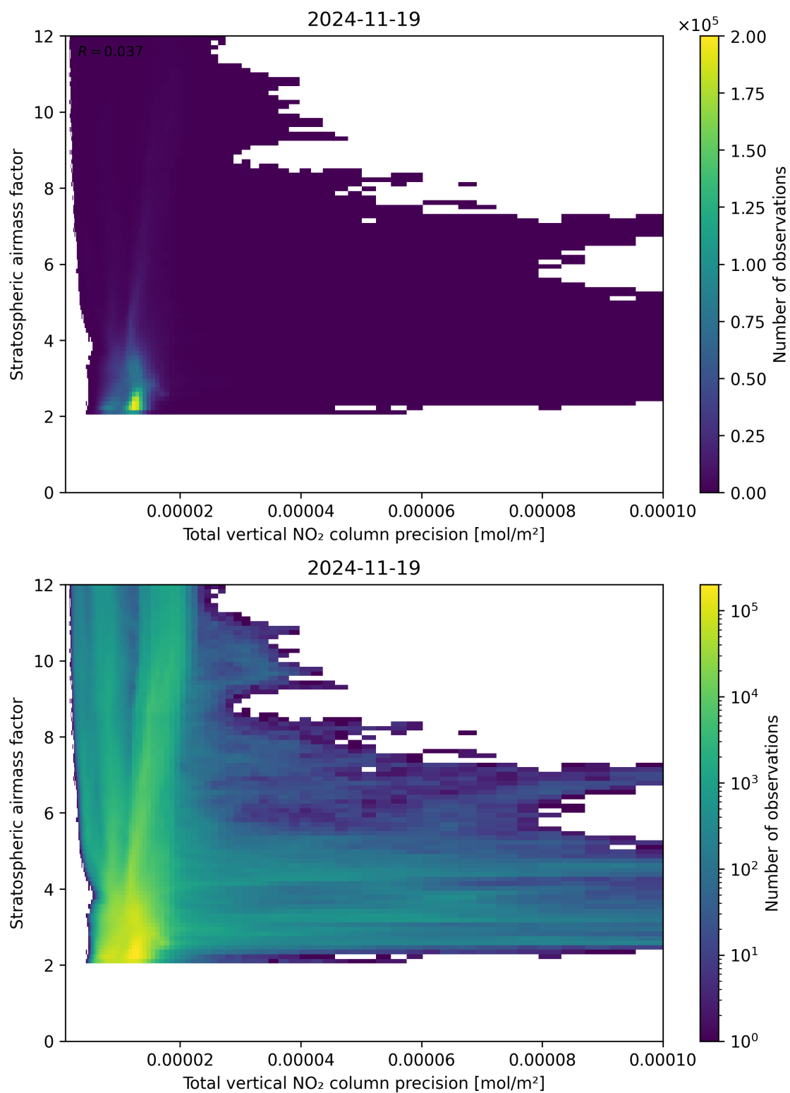
Figure 115: Scatter density plot of “Total vertical NO 2 column precision” against “Stratospheric air mass factor” for 2024-11-18 to 2024-11-20.
