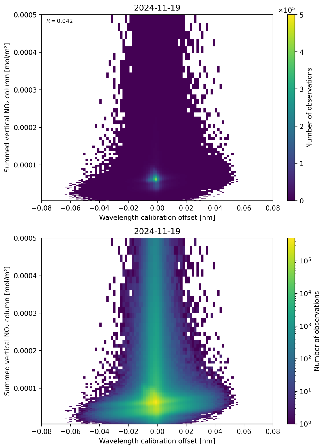
Figure 177: Scatter density plot of “Wavelength calibration offset” against “Summed vertical NO 2 column” for 2024-11-18 to 2024-11-20.
