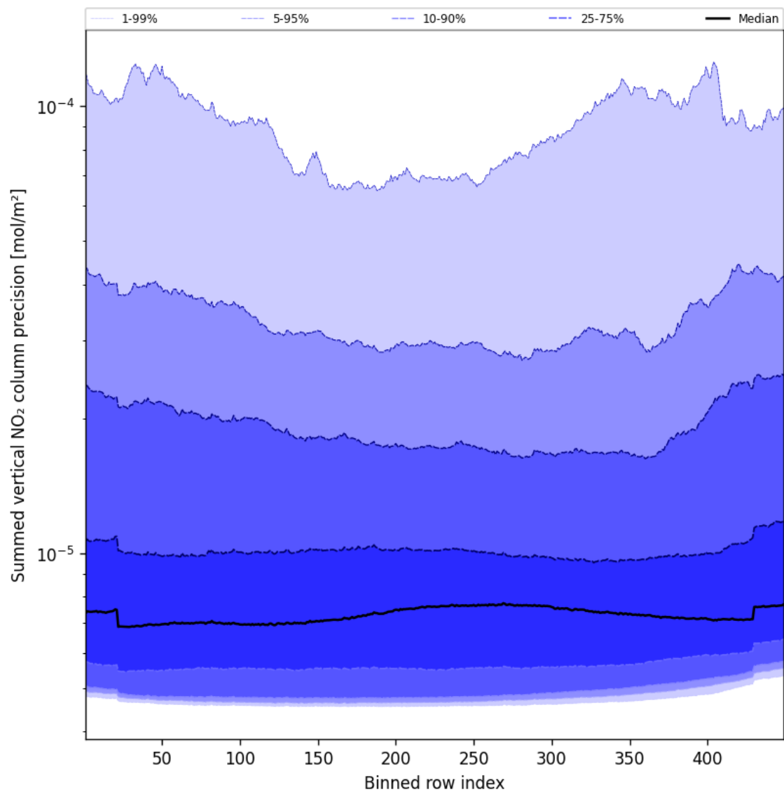
Figure 58: Along track statistics of “Summed vertical NO 2 column precision” for 2024-11-18 to 2024-11-20
