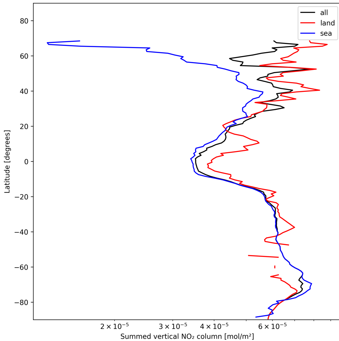
Figure 23: Zonal average of “Summed vertical NO 2 column” for 2024-11-18 to 2024-11-20.
