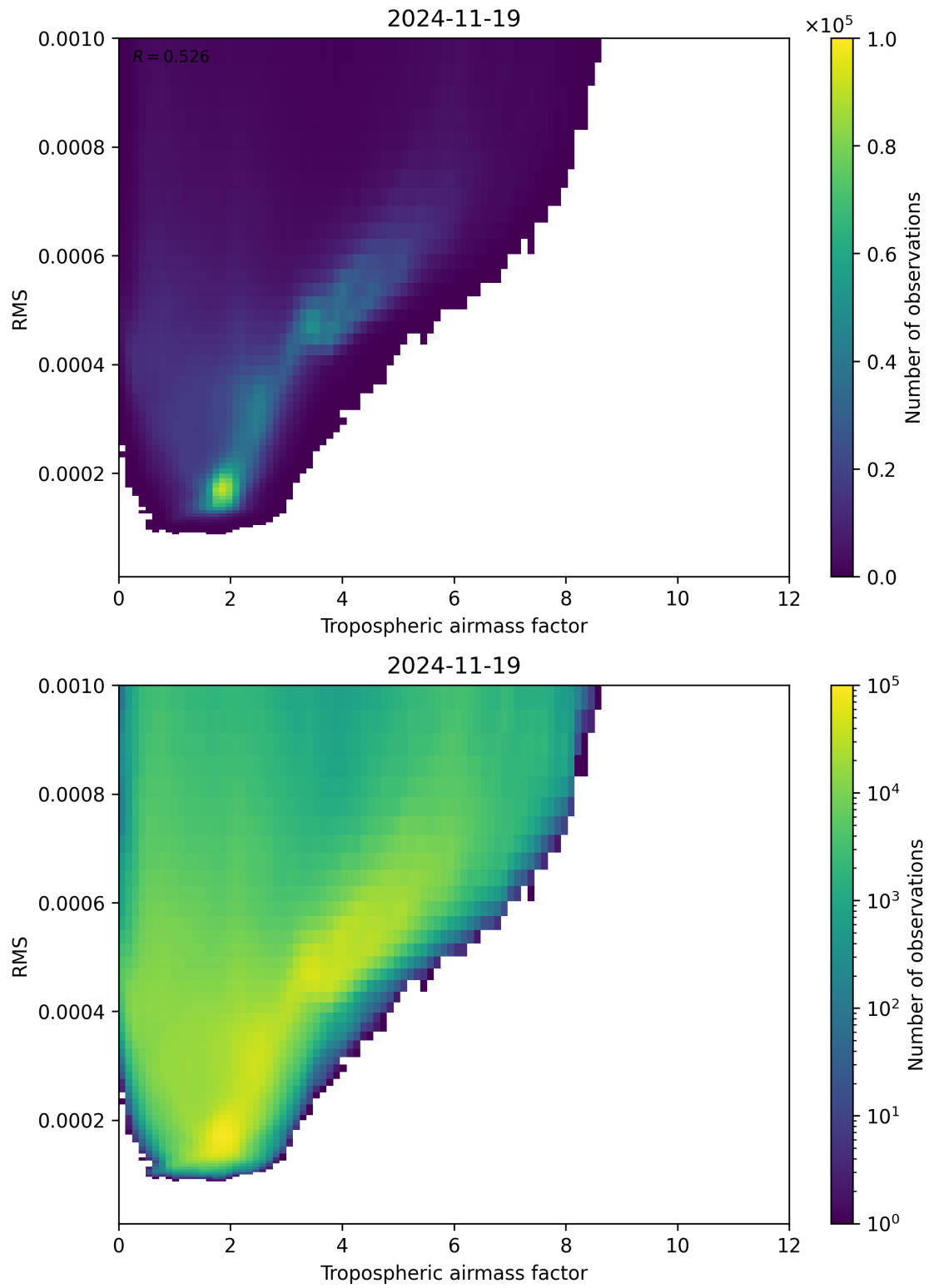
Figure 79: Scatter density plot of “Tropospheric airmass factor” against “RMS” for 2024-11-18 to 2024-11-20.
