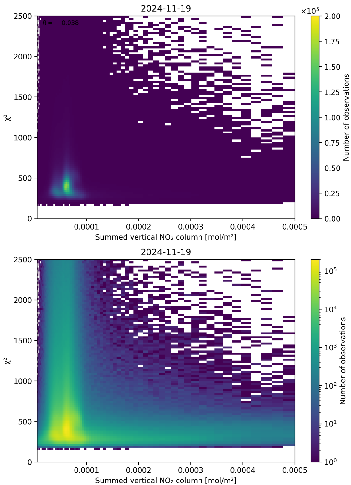
Figure 104: Scatter density plot of “Summed vertical NO 2 column” against “ \chi^2 ” for 2024-11-18 to 2024-11-20.
