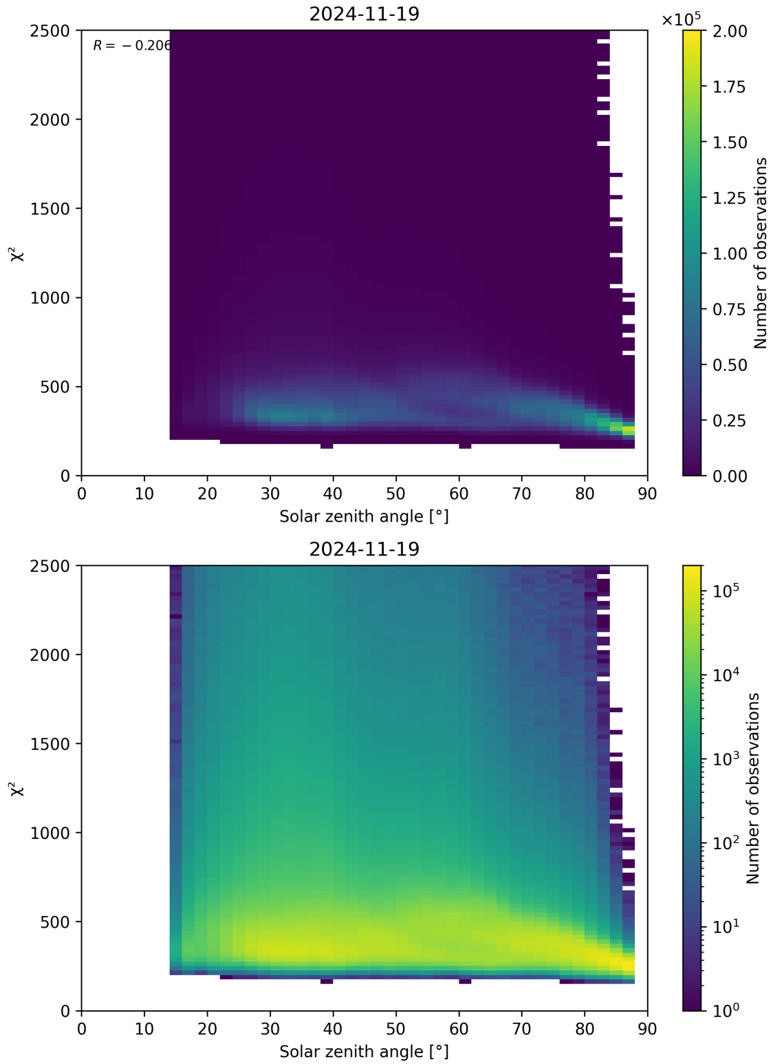
Figure 148: Scatter density plot of “Solar zenith angle” against “ \chi^2 ” for 2024-11-18 to 2024-11-20.
