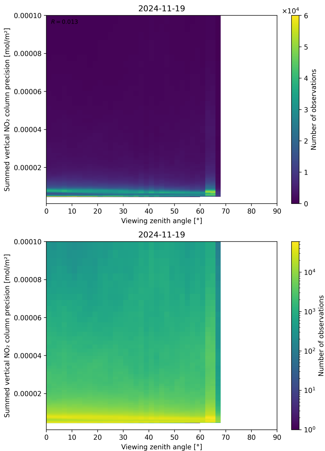
Figure 166: Scatter density plot of “Viewing zenith angle” against “Summed vertical NO 2 column precision” for 2024-11-18 to 2024-11-20.
