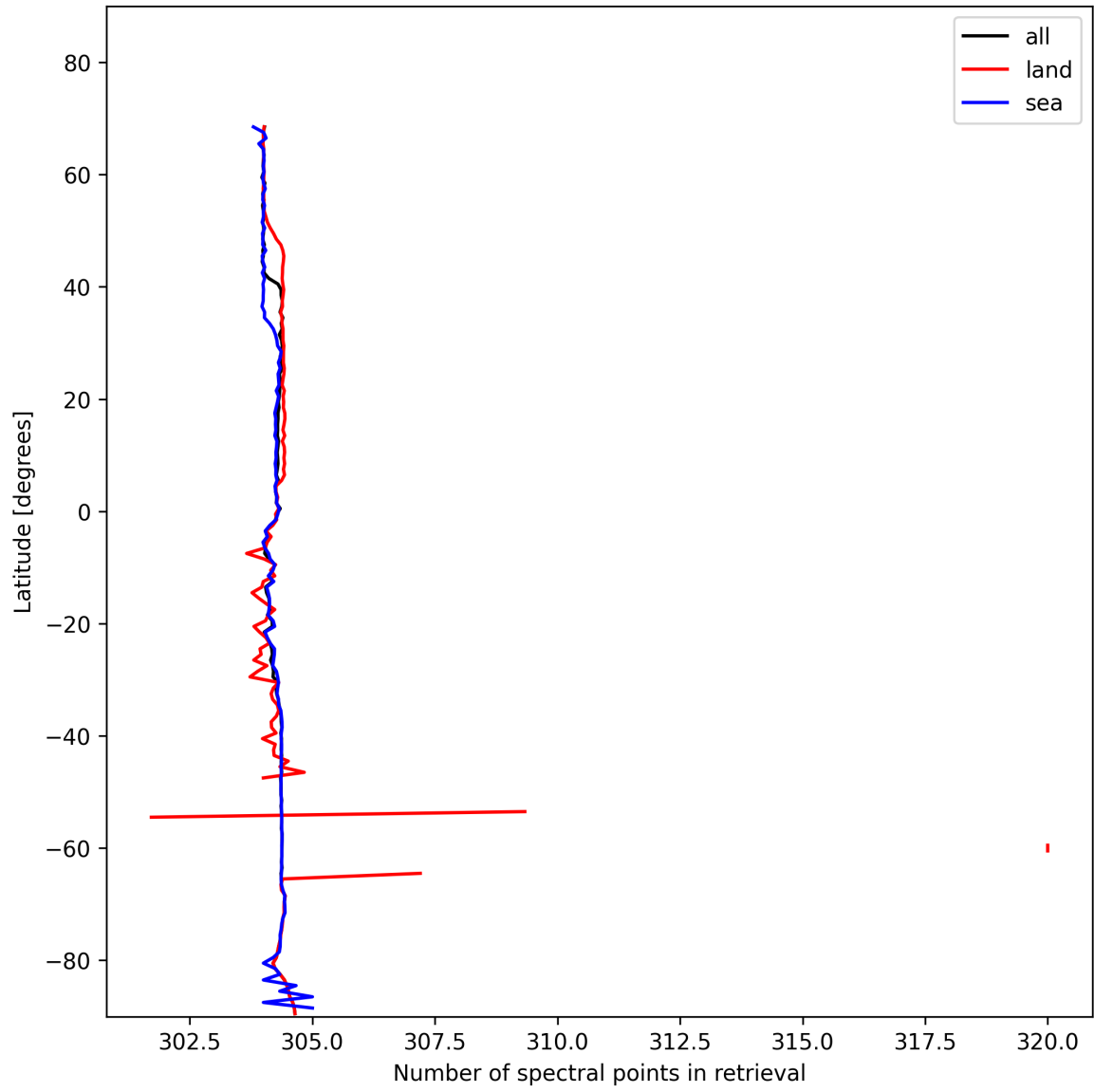
Figure 16: Zonal average of “Number of spectral points in retrieval” for 2024-11-18 to 2024-11-20.
