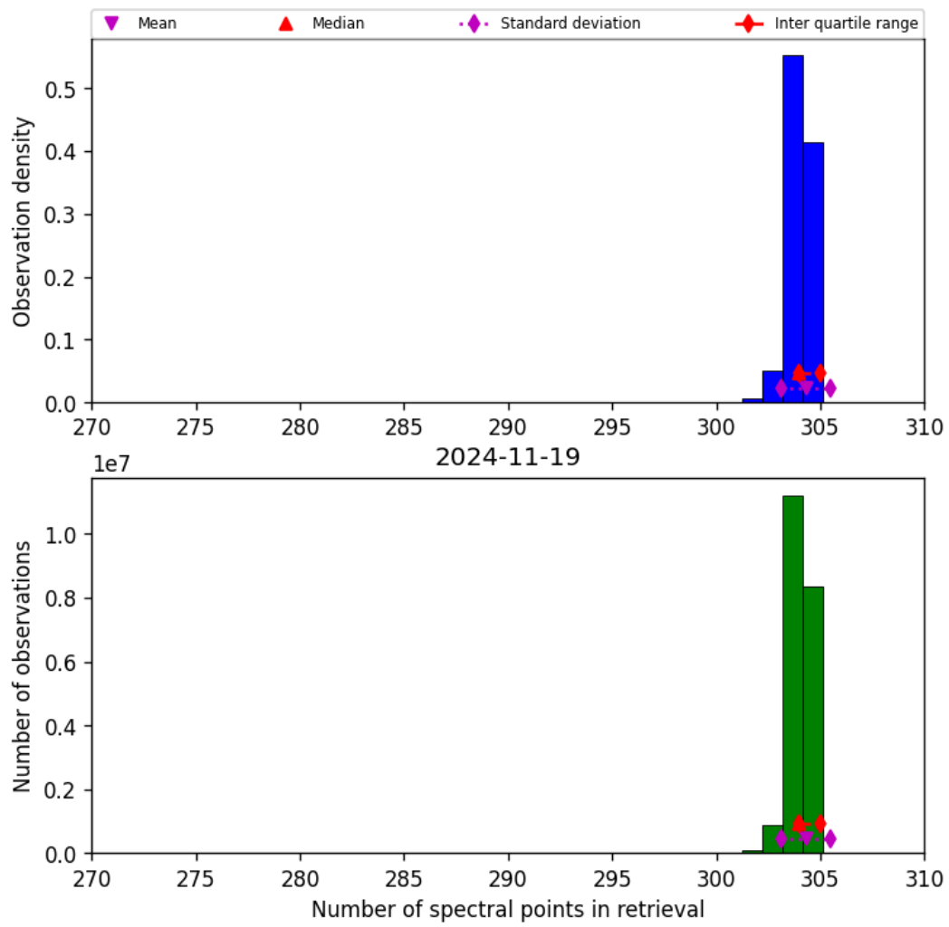
Figure 33: Histogram of “Number of spectral points in retrieval” for 2024-11-18 to 2024-11-20
