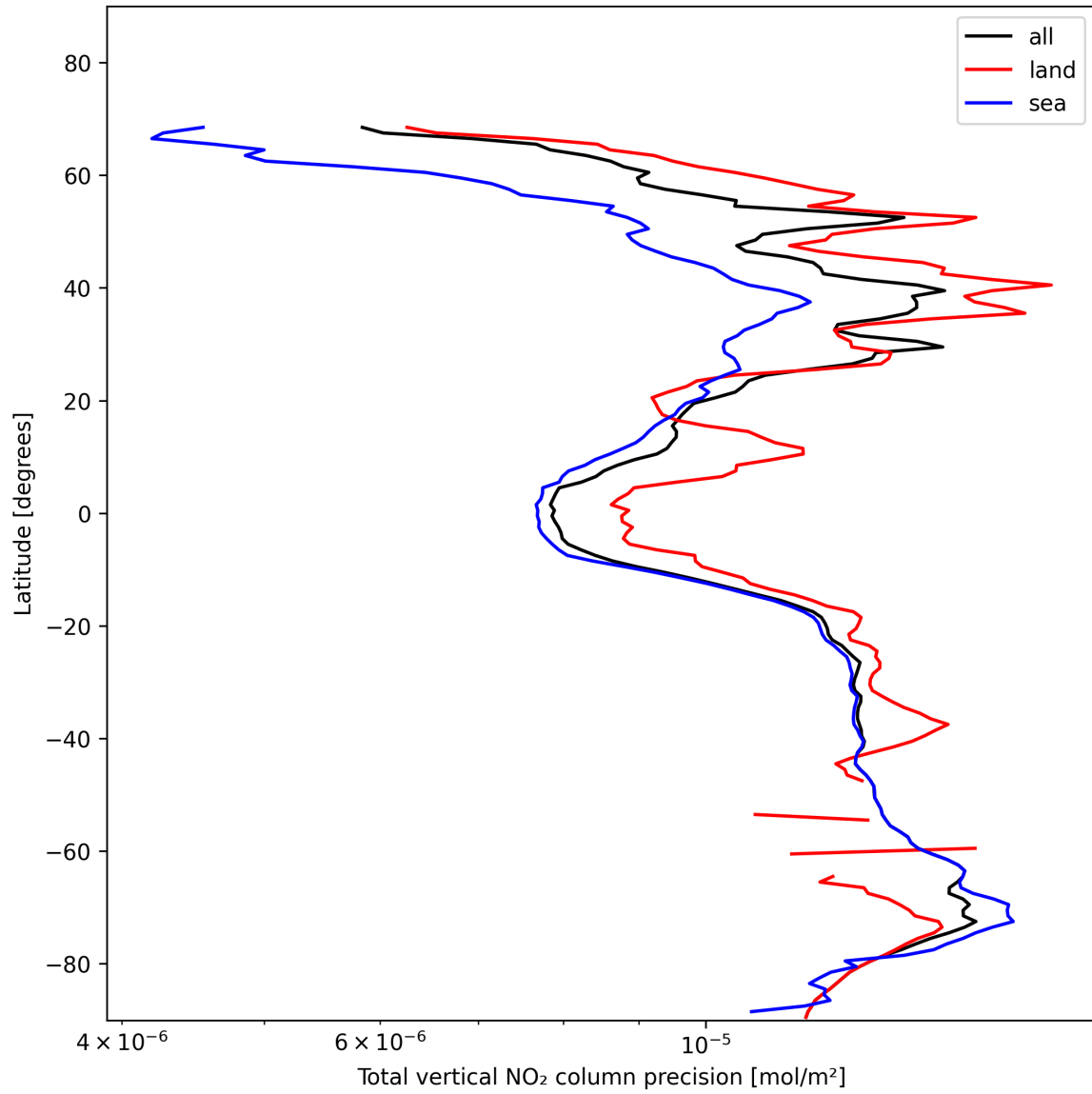
Figure 22: Zonal average of “Total vertical NO 2 column precision” for 2024-11-18 to 2024-11-20.
