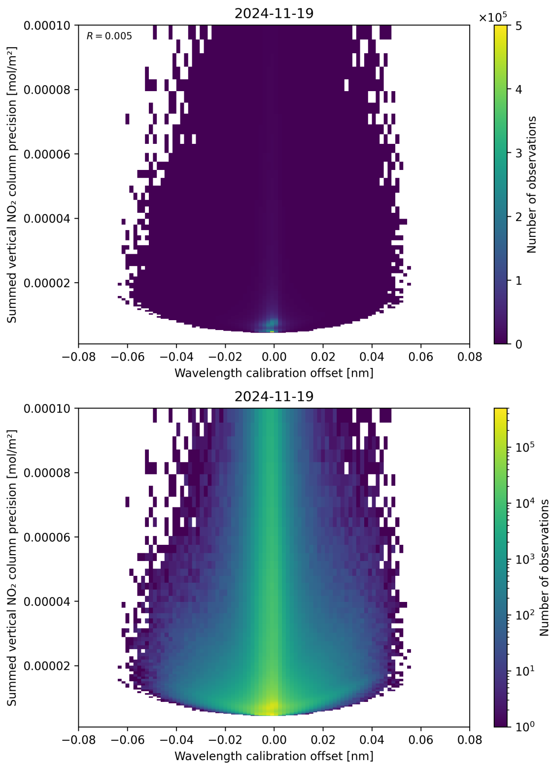
Figure 178: Scatter density plot of “Wavelength calibration offset” against “Summed vertical NO 2 column precision” for 2024-11-18 to 2024-11-20.
