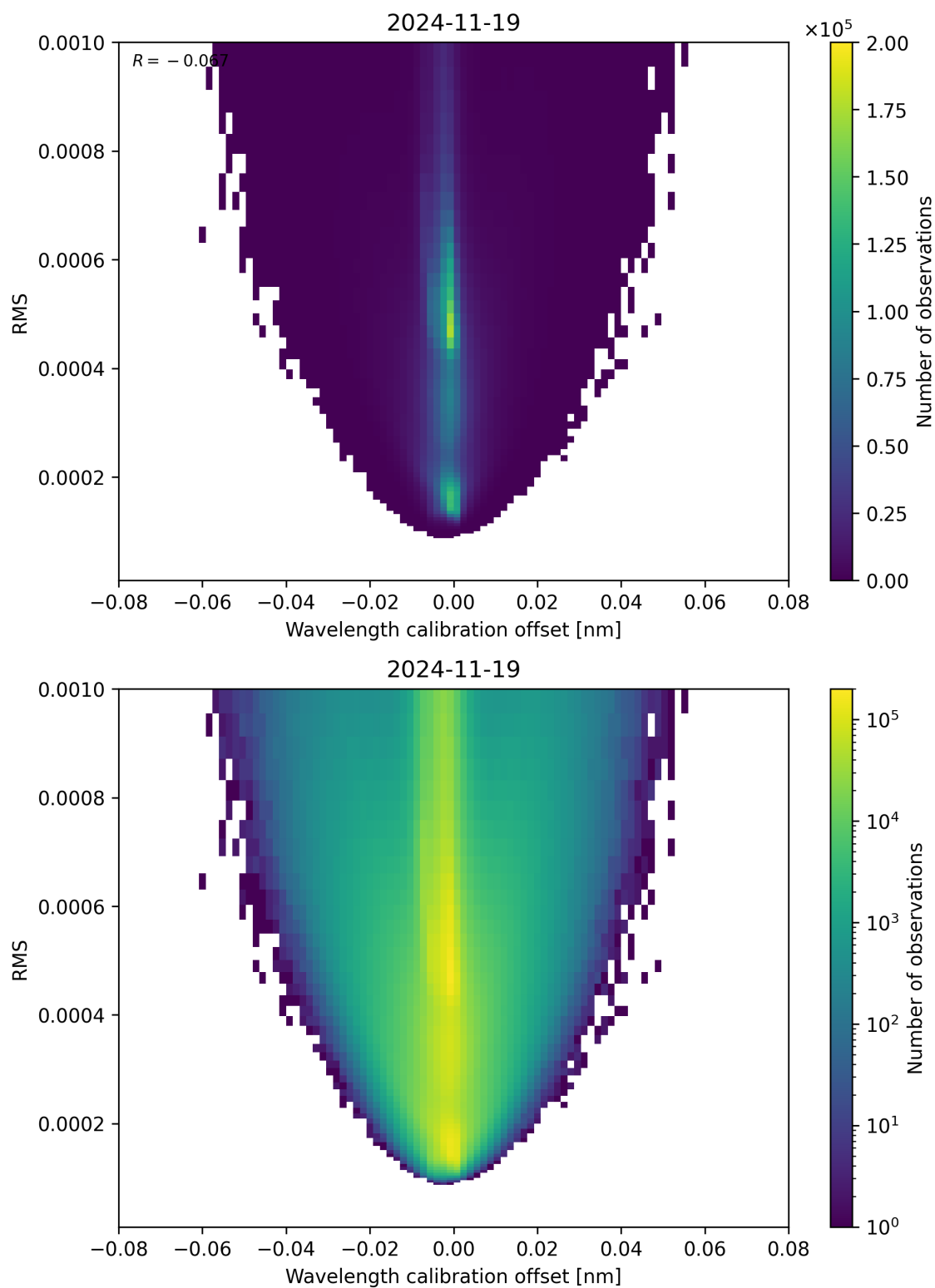
Figure 181: Scatter density plot of “Wavelength calibration offset” against “RMS” for 2024-11-18 to 2024-11-20.
