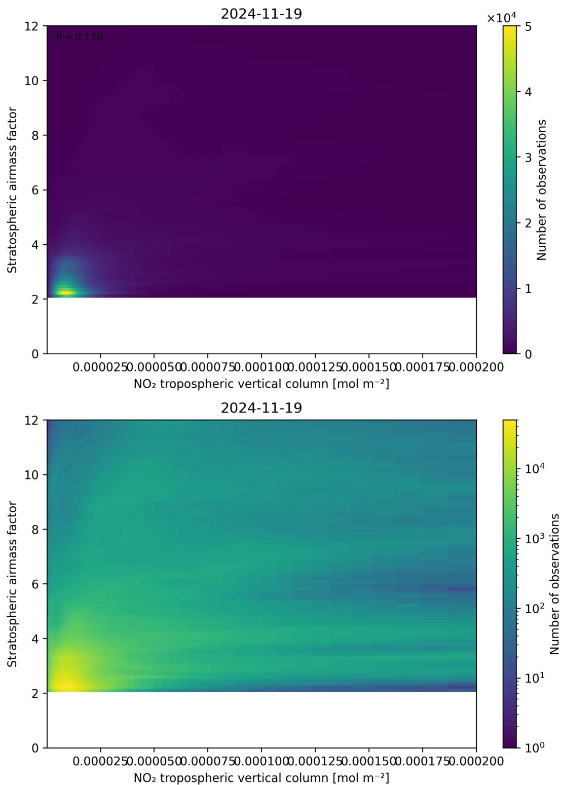
Figure 121: Scatter density plot of “NO 2 tropospheric vertical column” against “Stratospheric air mass factor” for 2024-11-18 to 2024-11-20.
