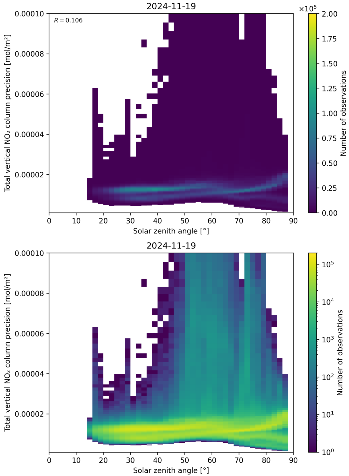
Figure 154: Scatter density plot of “Solar zenith angle” against “Total vertical NO 2 column precision” for 2024-11-18 to 2024-11-20.
