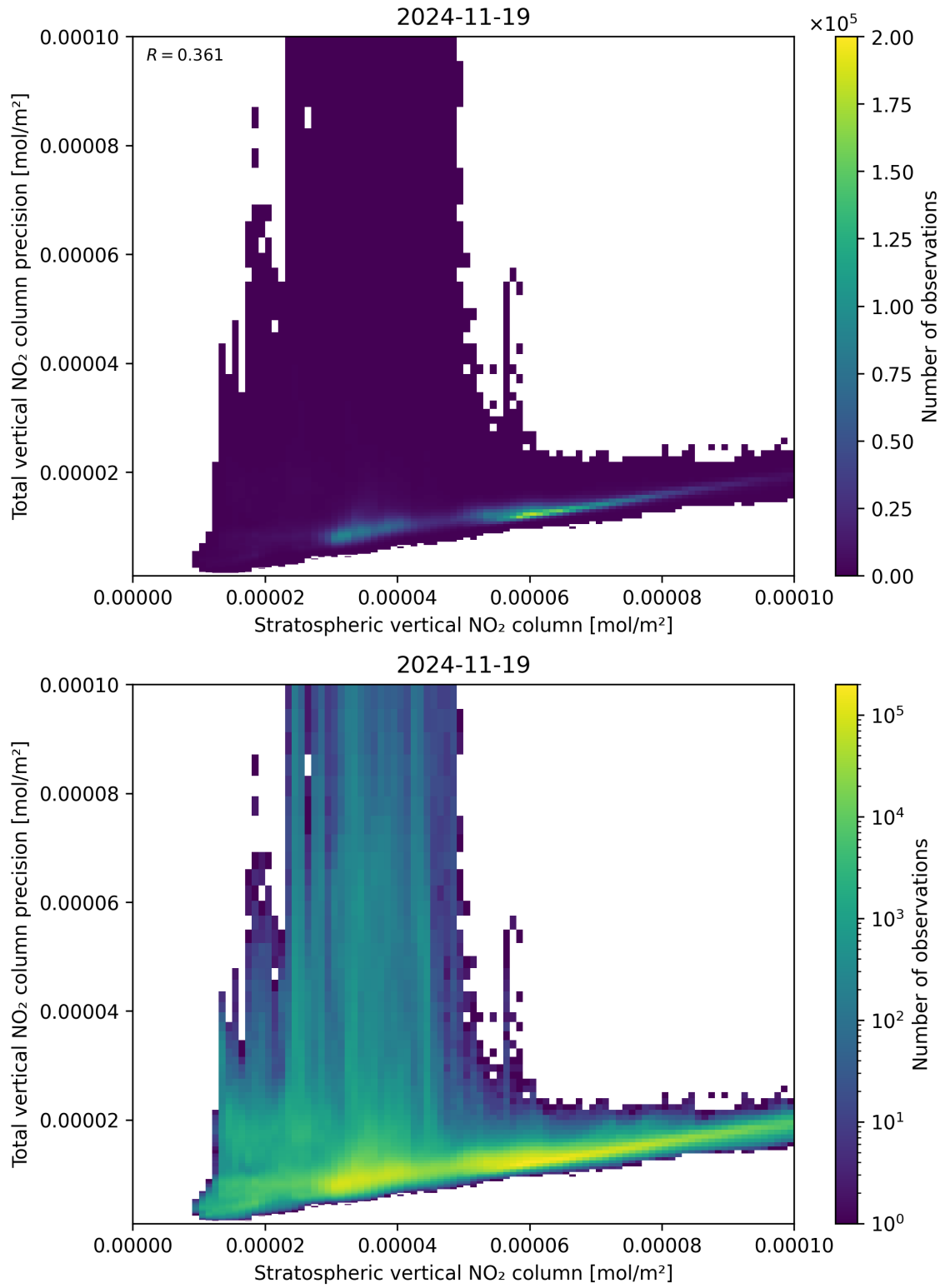
Figure 101: Scatter density plot of “Stratospheric vertical NO 2 column” against “Total vertical NO 2 column precision” for 2024-11-18 to 2024-11-20.
