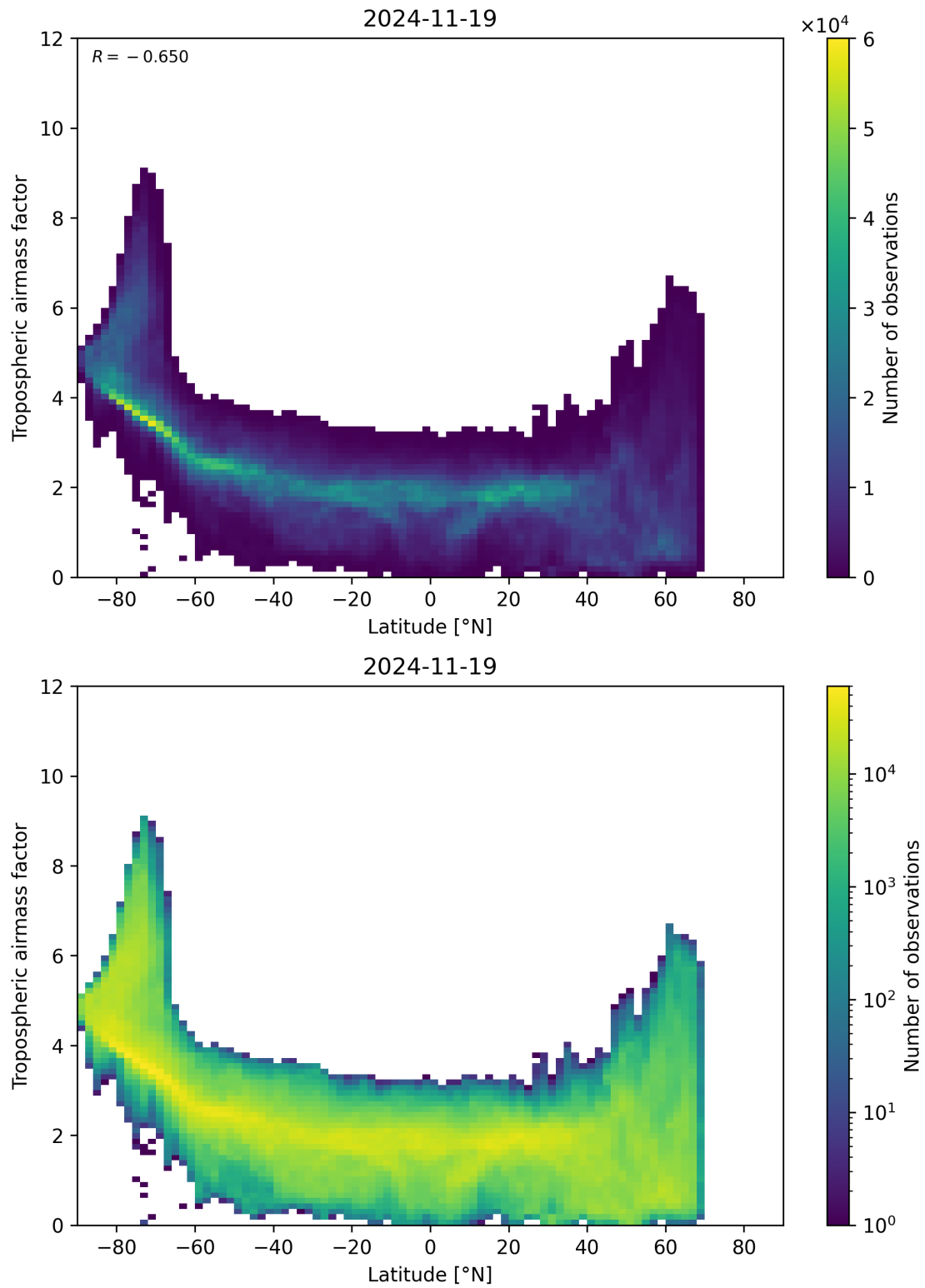
Figure 85: Scatter density plot of “Latitude” against “Tropospheric air mass factor” for 2024-11-18 to 2024-11-20.
