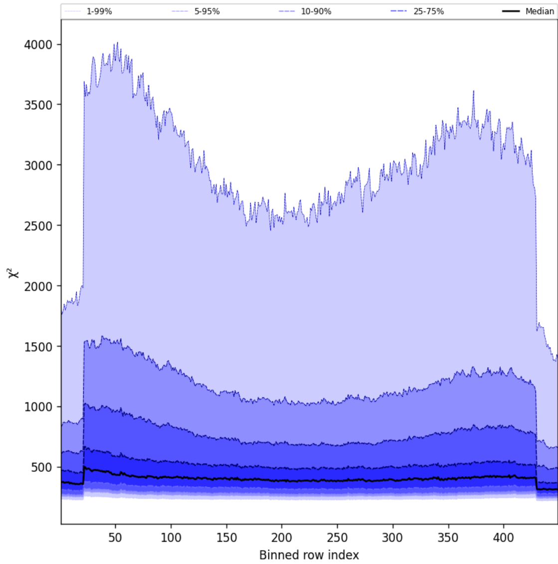
Figure 59: Along track statistics of “ \chi^2 ” for 2024-11-18 to 2024-11-20
