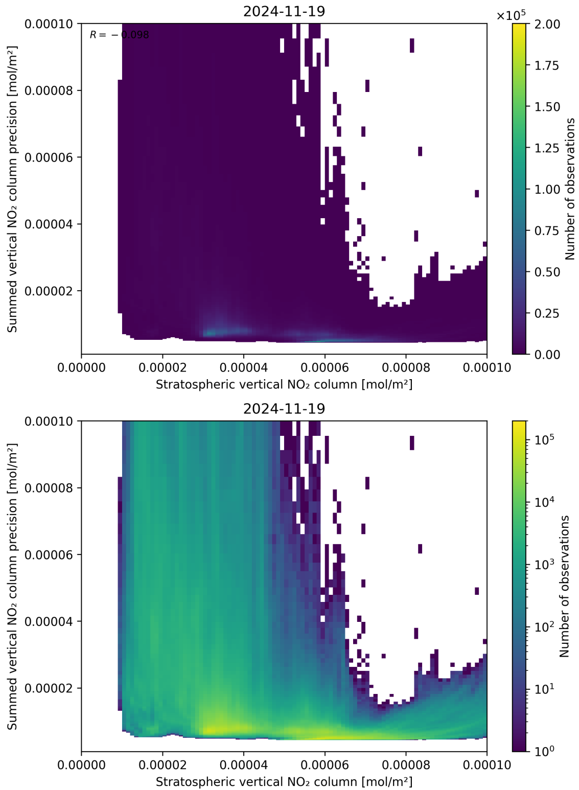
Figure 99: Scatter density plot of “Stratospheric vertical NO 2 column” against “Summed vertical NO 2 column precision” for 2024-11-18 to 2024-11-20.
