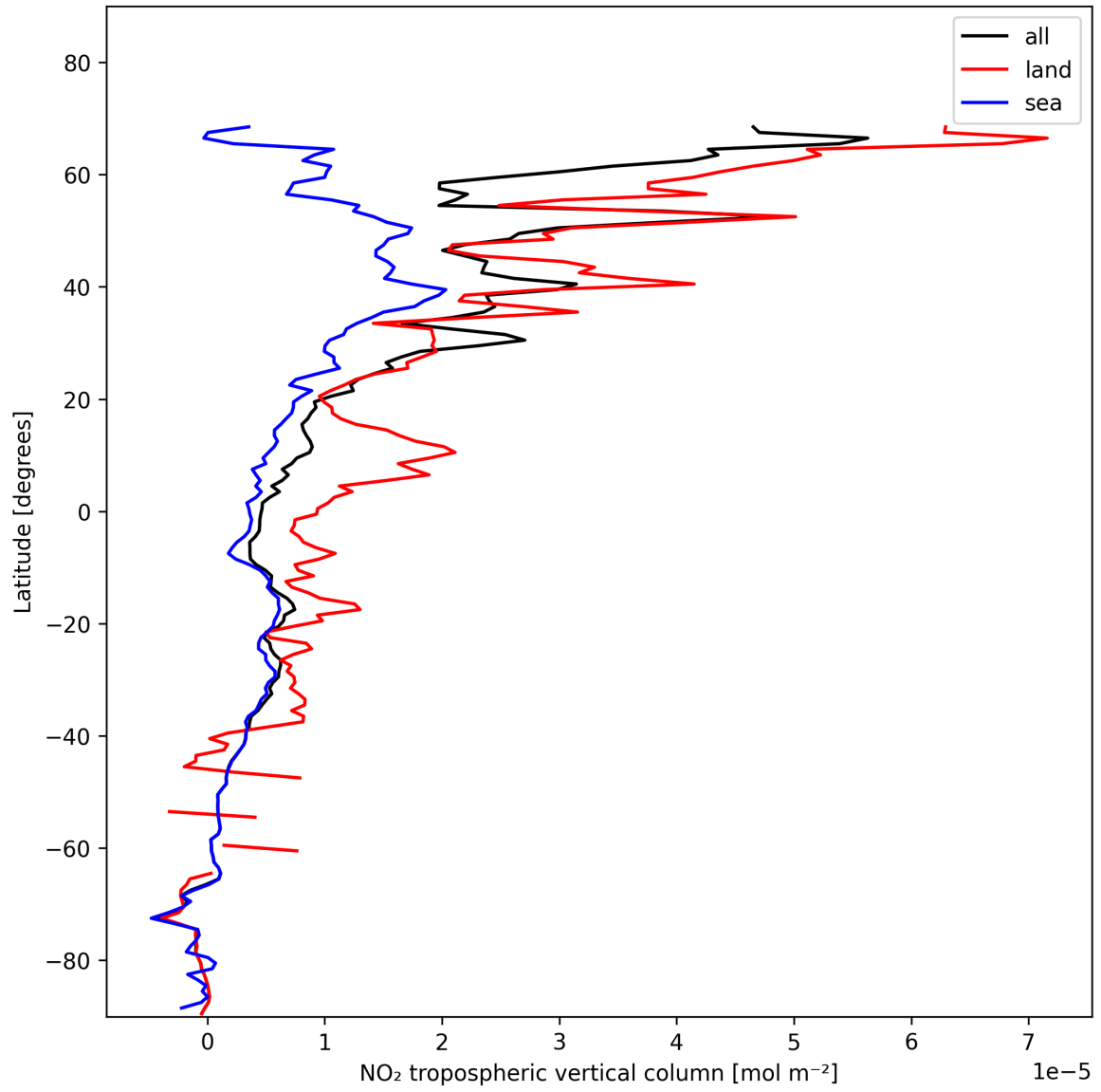
Figure 12: Zonal average of “NO 2 tropospheric vertical column” for 2024-11-18 to 2024-11-20.
