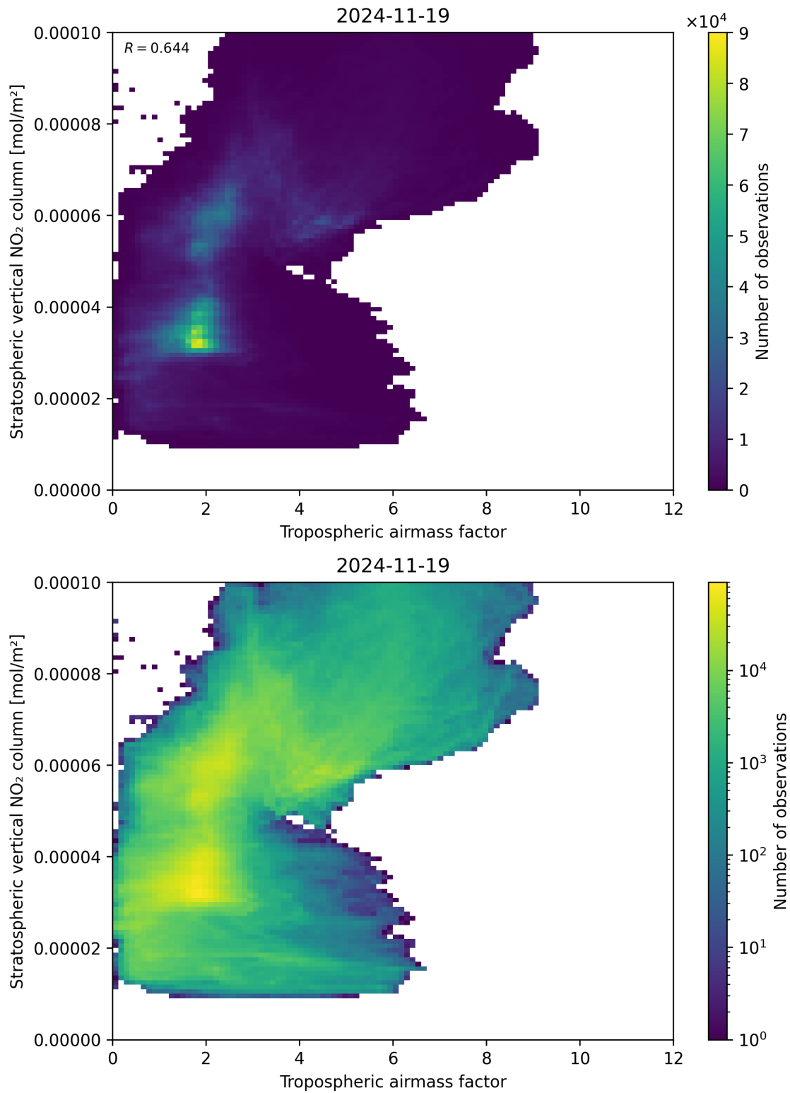
Figure 74: Scatter density plot of “Tropospheric air mass factor” against “Stratospheric vertical NO 2 column” for 2024-11-18 to 2024-11-20.
