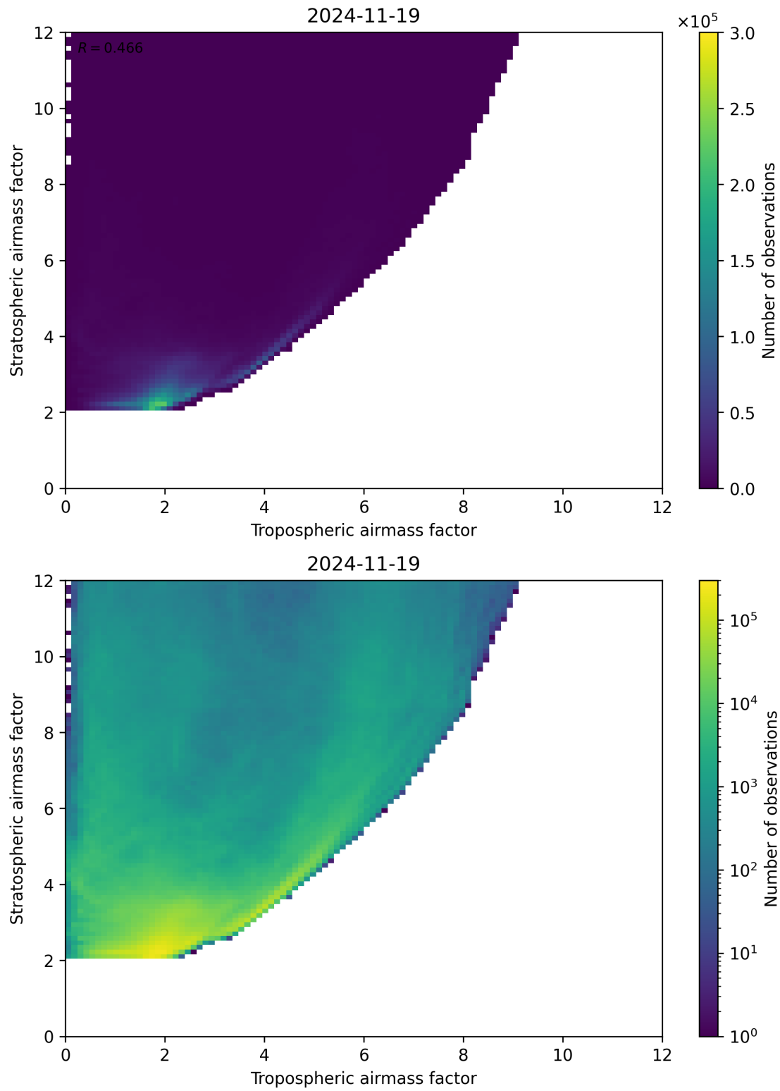
Figure 71: Scatter density plot of “Tropospheric airmass factor” against “Stratospheric airmass factor” for 2024-11-18 to 2024-11-20.
