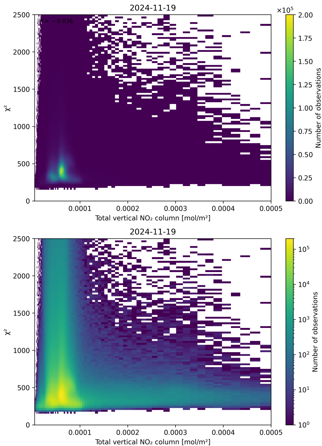
Figure 111: Scatter density plot of “Total vertical NO 2 column” against “ \chi^2 ” for 2024-11-18 to 2024-11-20.
