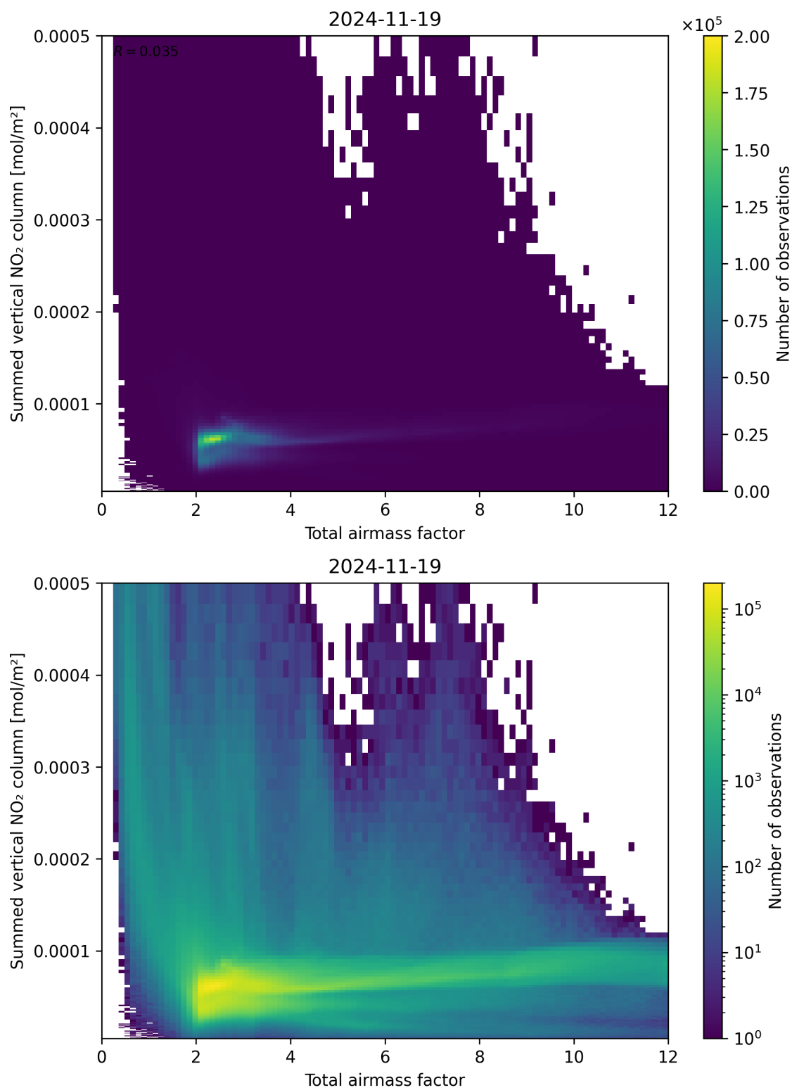
Figure 65: Scatter density plot of “Total airmass factor” against “Summed vertical NO 2 column” for 2024-11-18 to 2024-11-20.
