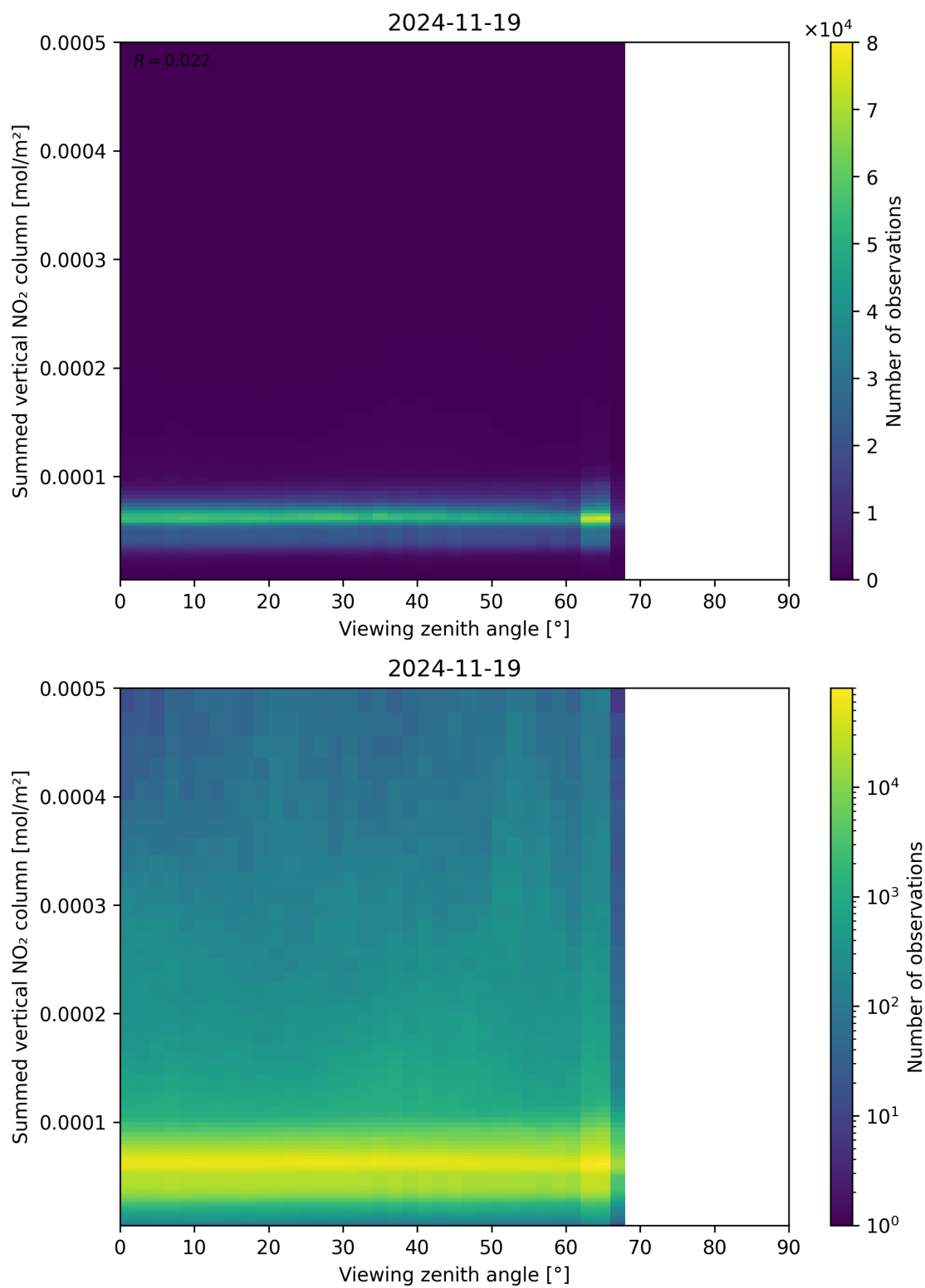
Figure 165: Scatter density plot of “Viewing zenith angle” against “Summed vertical NO 2 column” for 2024-11-18 to 2024-11-20.
