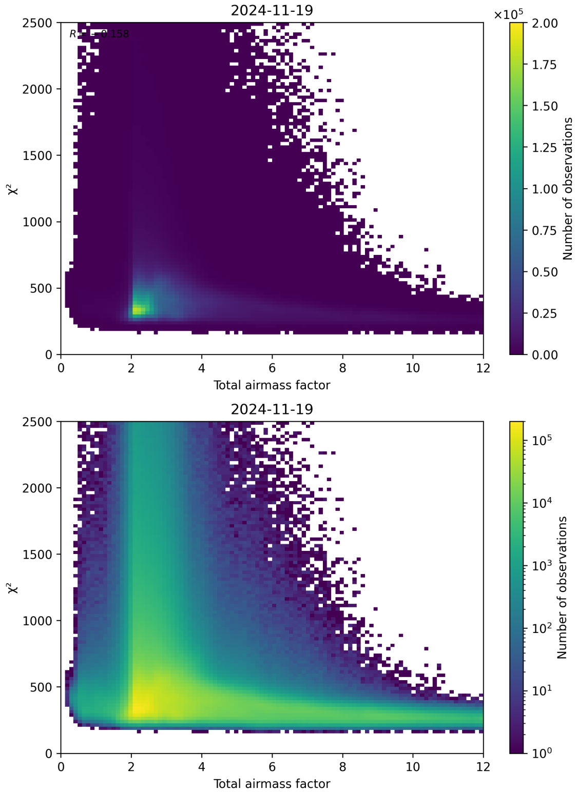
Figure 63: Scatter density plot of “Total airmass factor” against “ \chi^2 ” for 2024-11-18 to 2024-11-20.
