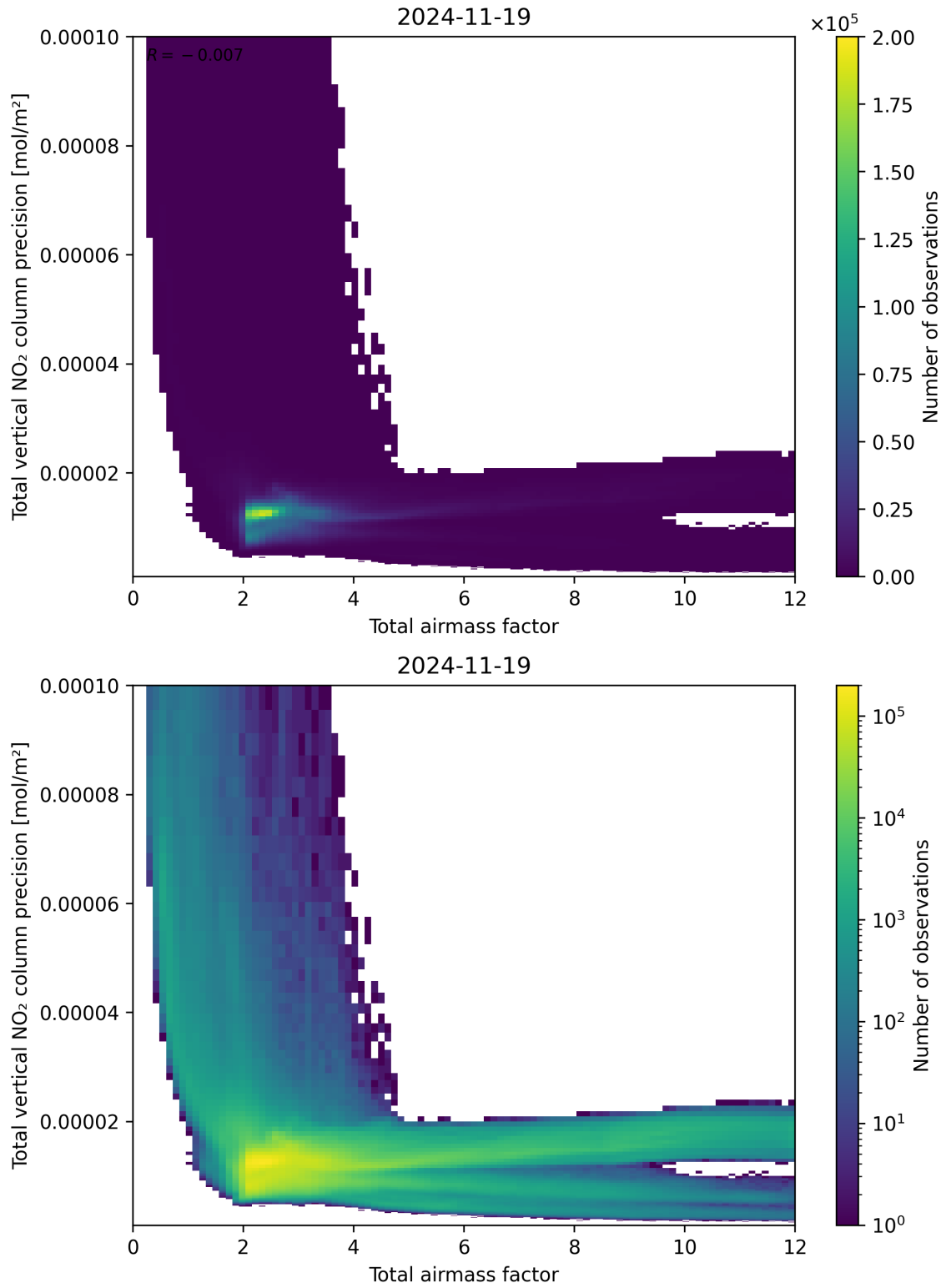
Figure 68: Scatter density plot of “Total airmass factor” against “Total vertical NO 2 column precision” for 2024-11-18 to 2024-11-20.
