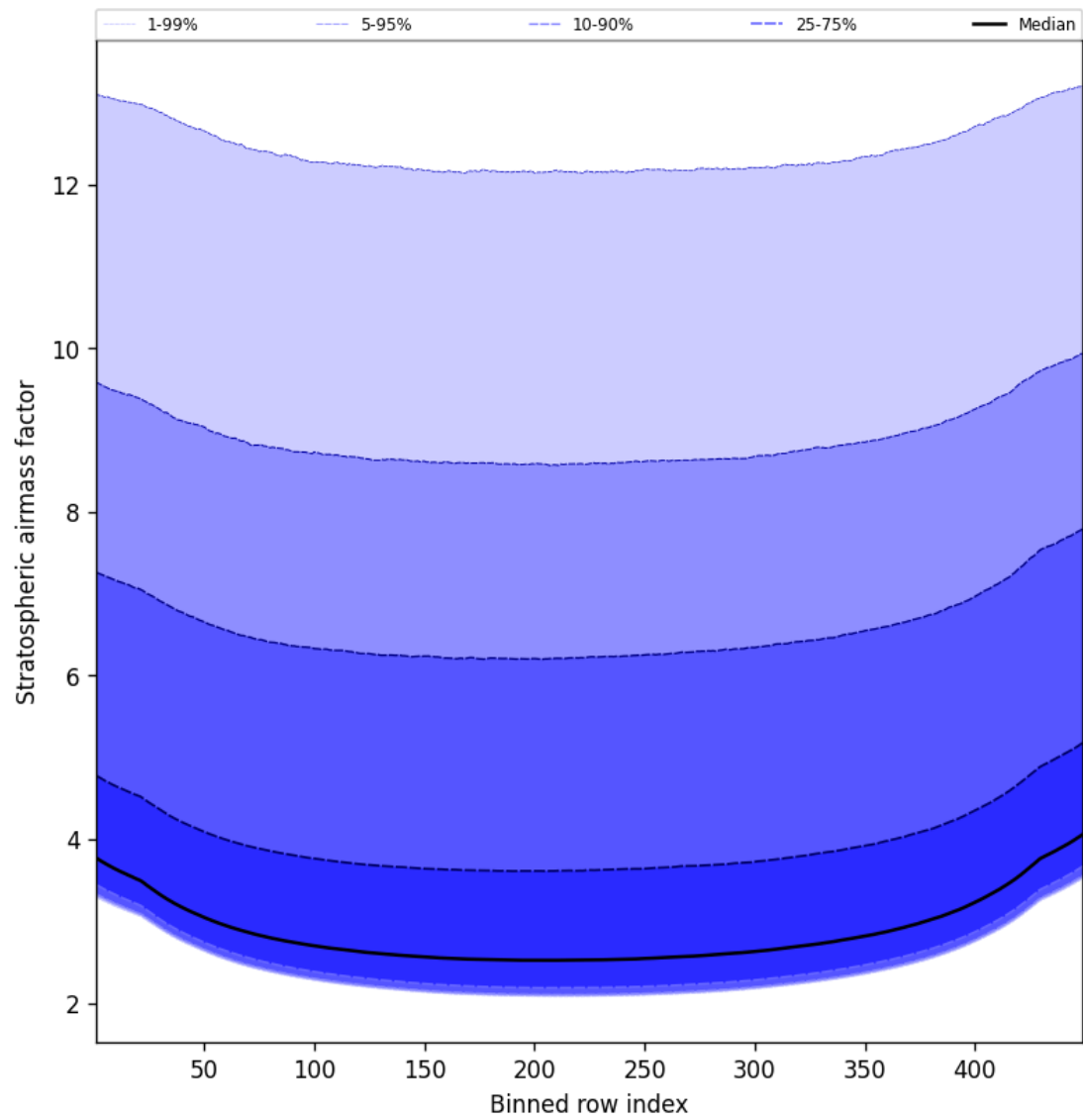
Figure 61: Along track statistics of “Stratospheric airmass factor” for 2024-11-18 to 2024-11-20
