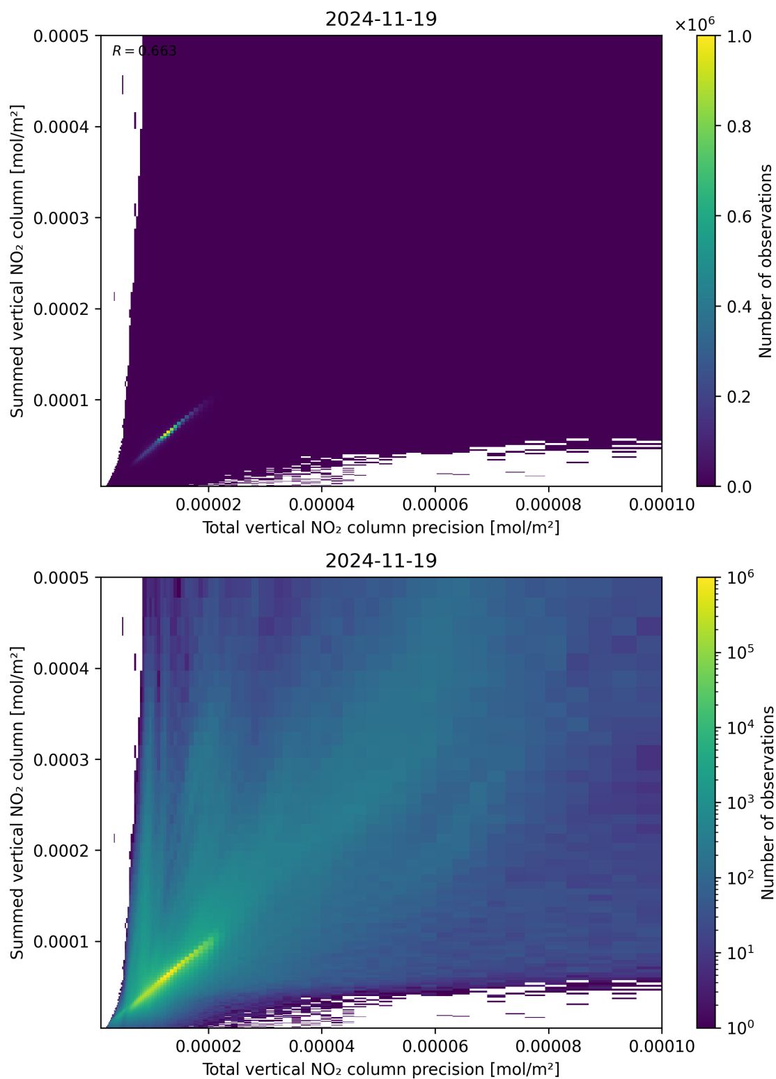
Figure 117: Scatter density plot of “Total vertical NO 2 column precision” against “Summed vertical NO 2 column” for 2024-11-18 to 2024-11-20.
