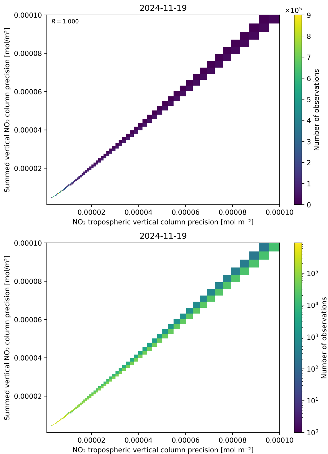
Figure 137: Scatter density plot of “NO 2 tropospheric vertical column precision” against “Summed vertical NO 2 column precision” for 2024-11-18 to 2024-11-20.
