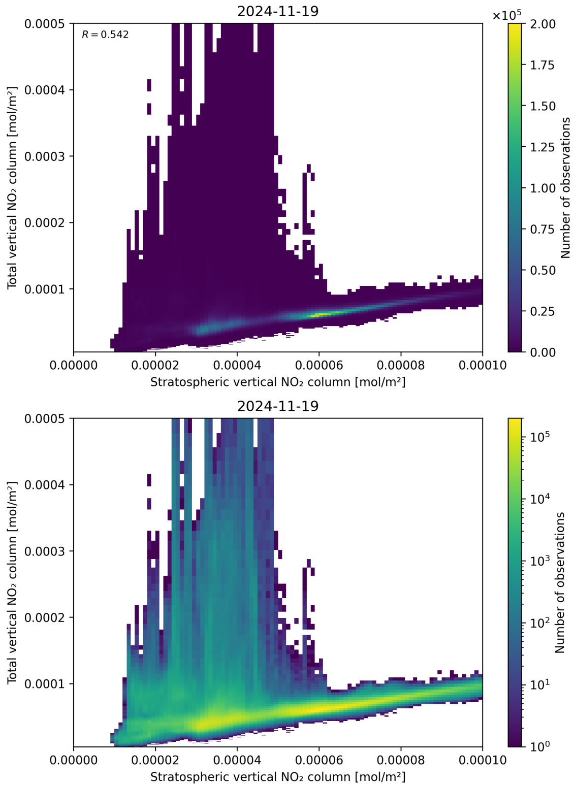
Figure 100: Scatter density plot of “Stratospheric vertical NO 2 column” against “Total vertical NO 2 column” for 2024-11-18 to 2024-11-20.
