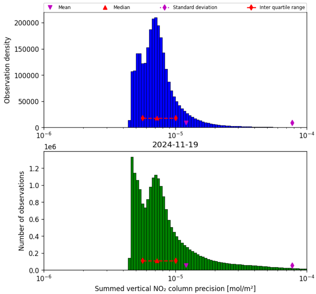
Figure 41: Histogram of "Summed vertical NO 2 column precision" for 2024-11-18 to 2024-11-20
