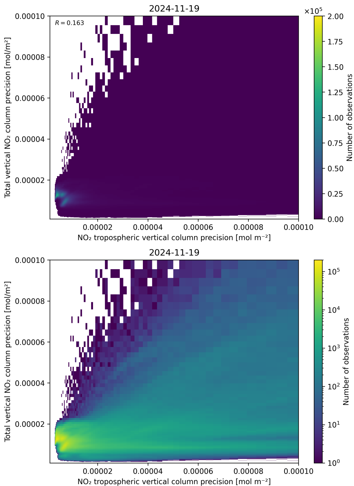
Figure 139: Scatter density plot of “NO 2 tropospheric vertical column precision” against “Total vertical NO 2 column precision” for 2024-11-18 to 2024-11-20.
