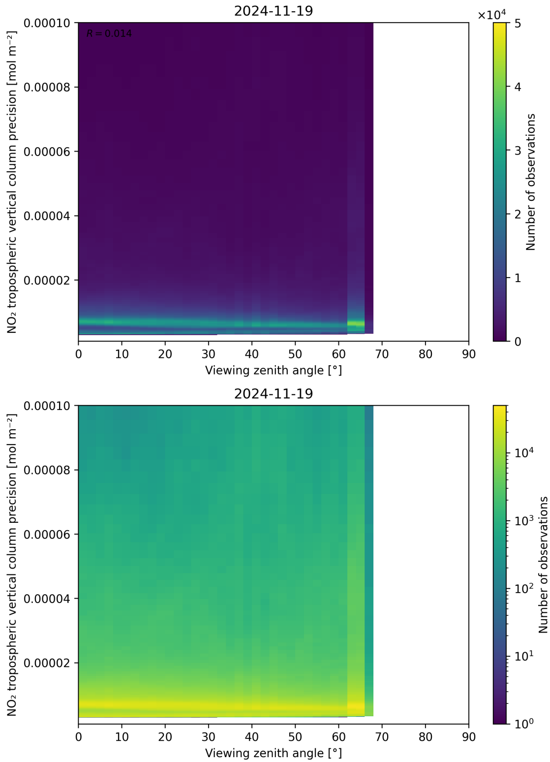
Figure 170: Scatter density plot of “Viewing zenith angle” against “NO 2 tropospheric vertical column precision” for 2024-11-18 to 2024-11-20.
