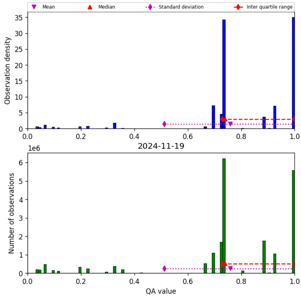
Figure 28: Histogram of “QA value” for 2024-11-18 to 2024-11-20
