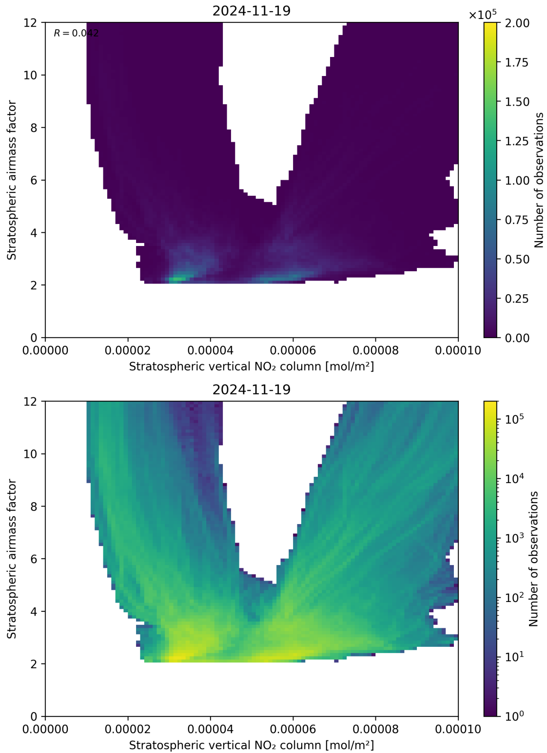
Figure 96: Scatter density plot of “Stratospheric vertical NO 2 column” against “Stratospheric airmass factor” for 2024-11-18 to 2024-11-20.
