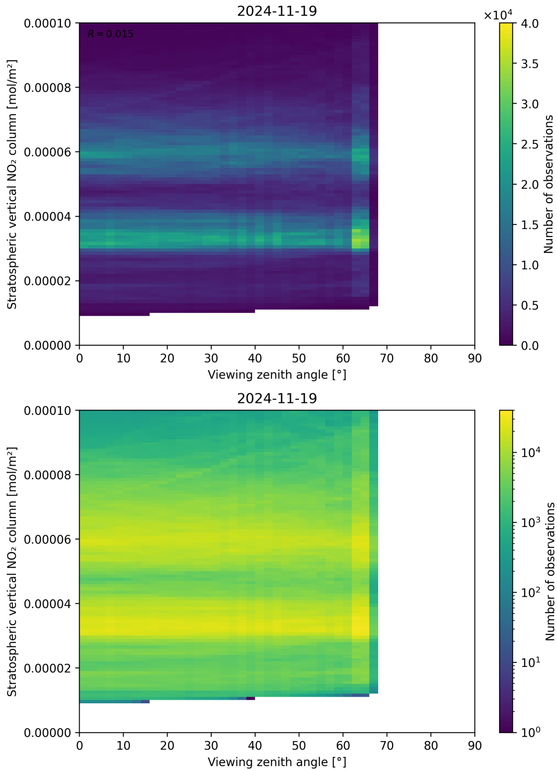
Figure 164: Scatter density plot of “Viewing zenith angle” against “Stratospheric vertical NO 2 column” for 2024-11-18 to 2024-11-20.
