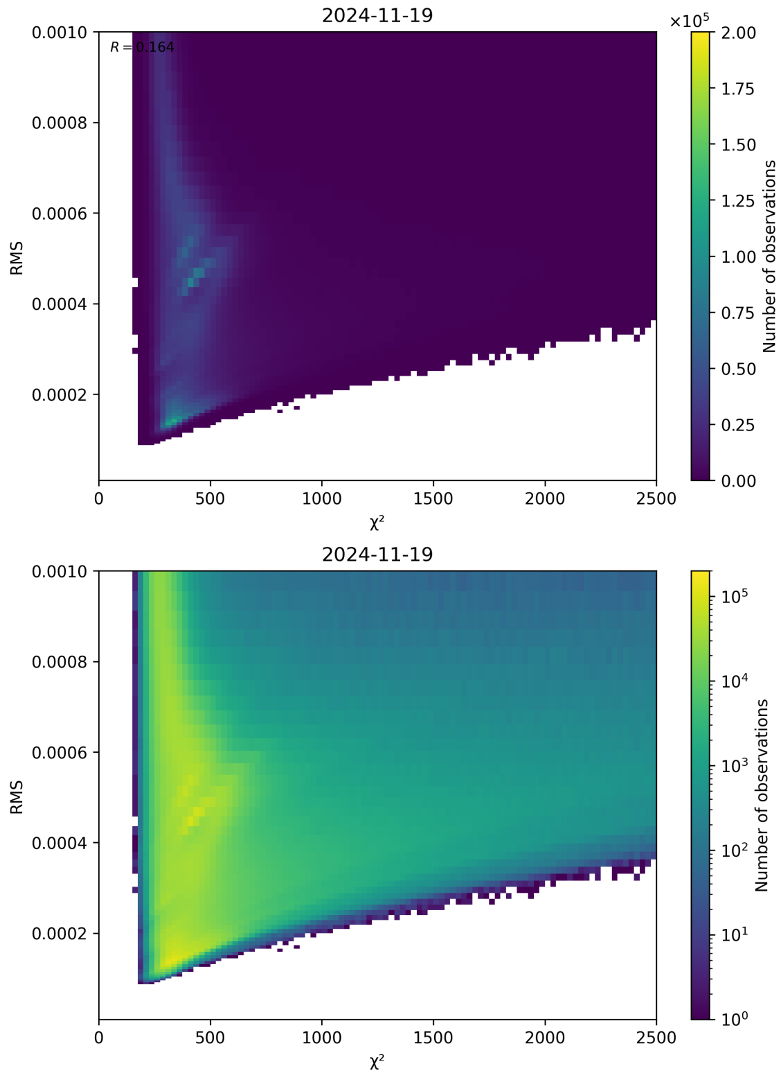
Figure 82: Scatter density plot of “ \chi^2 ” against “RMS” for 2024-11-18 to 2024-11-20.
