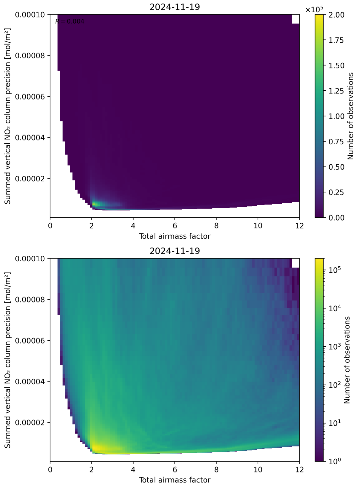
Figure 66: Scatter density plot of “Total airmass factor” against “Summed vertical NO 2 column precision” for 2024-11-18 to 2024-11-20.
