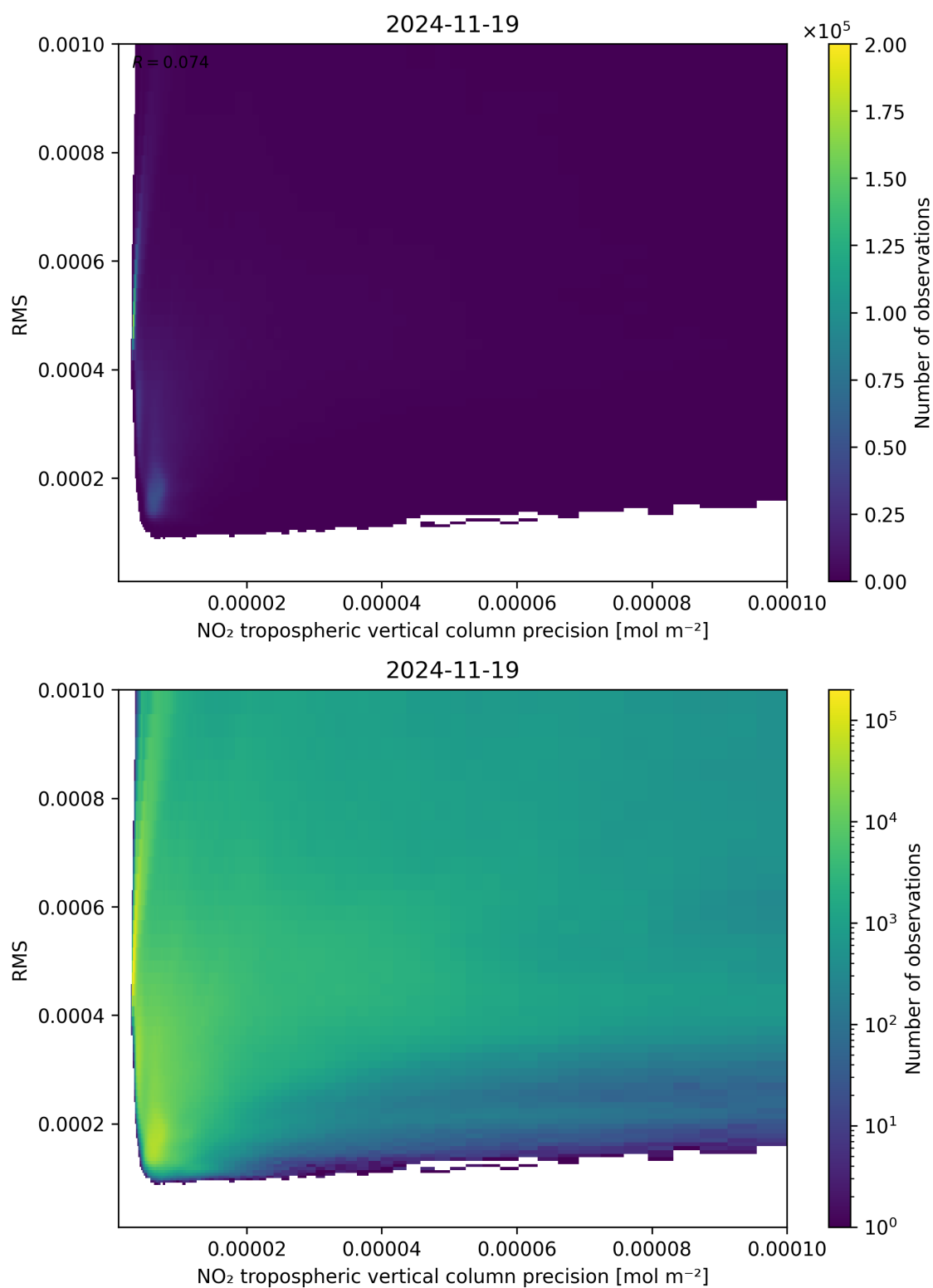
Figure 140: Scatter density plot of “NO 2 tropospheric vertical column precision” against “RMS” for 2024-11-18 to 2024-11-20.
