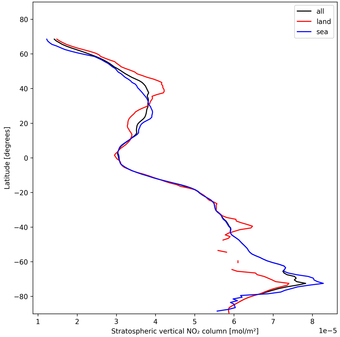
Figure 19: Zonal average of “Stratospheric vertical NO 2 column” for 2024-11-18 to 2024-11-20.
