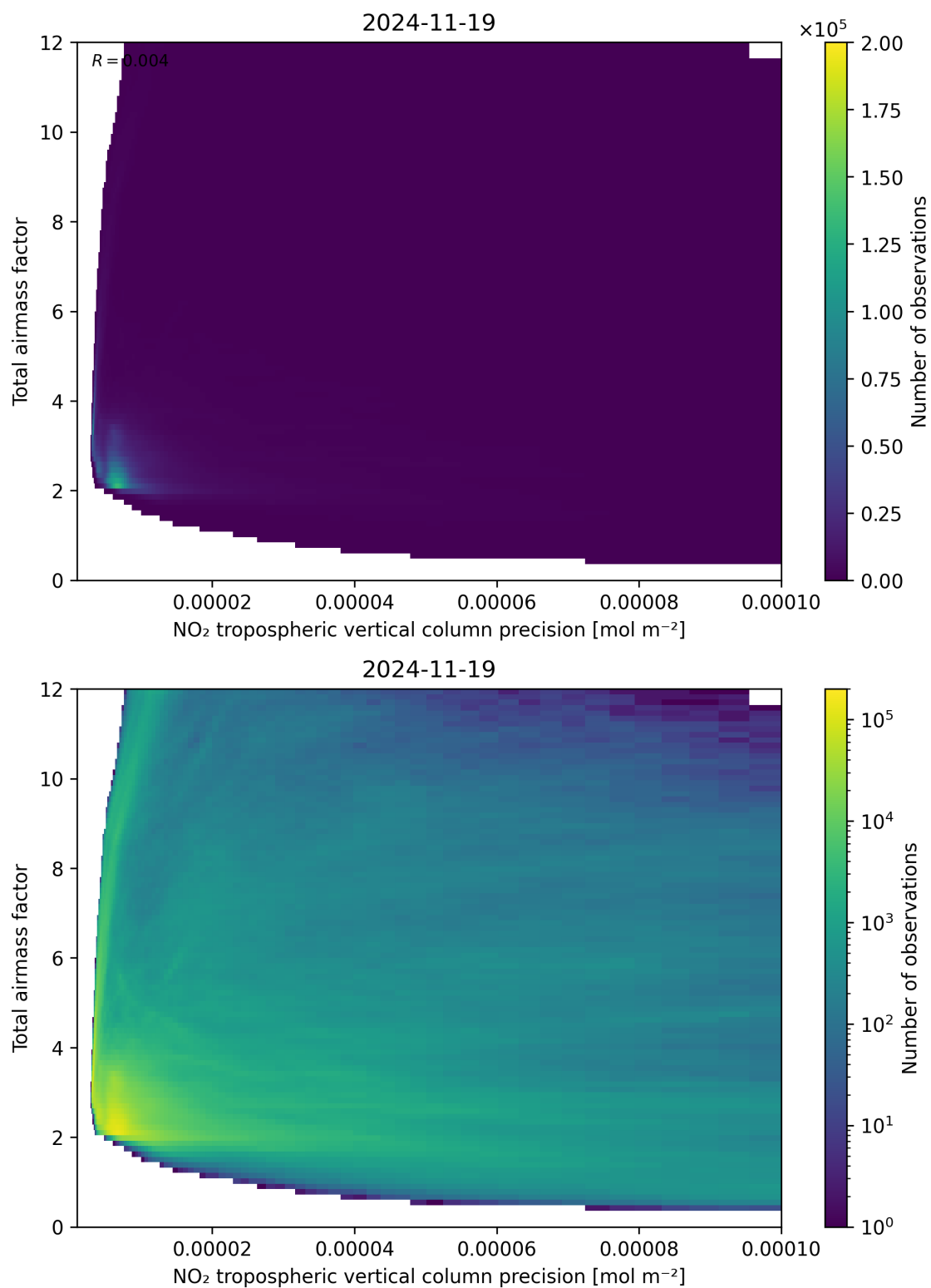
Figure 132: Scatter density plot of “NO 2 tropospheric vertical column precision” against “Total air mass factor” for 2024-11-18 to 2024-11-20.
