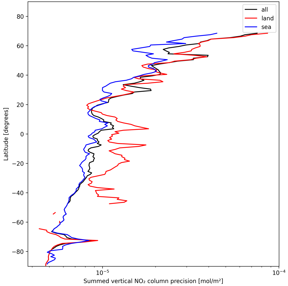
Figure 24: Zonal average of “Summed vertical NO 2 column precision” for 2024-11-18 to 2024-11-20.
