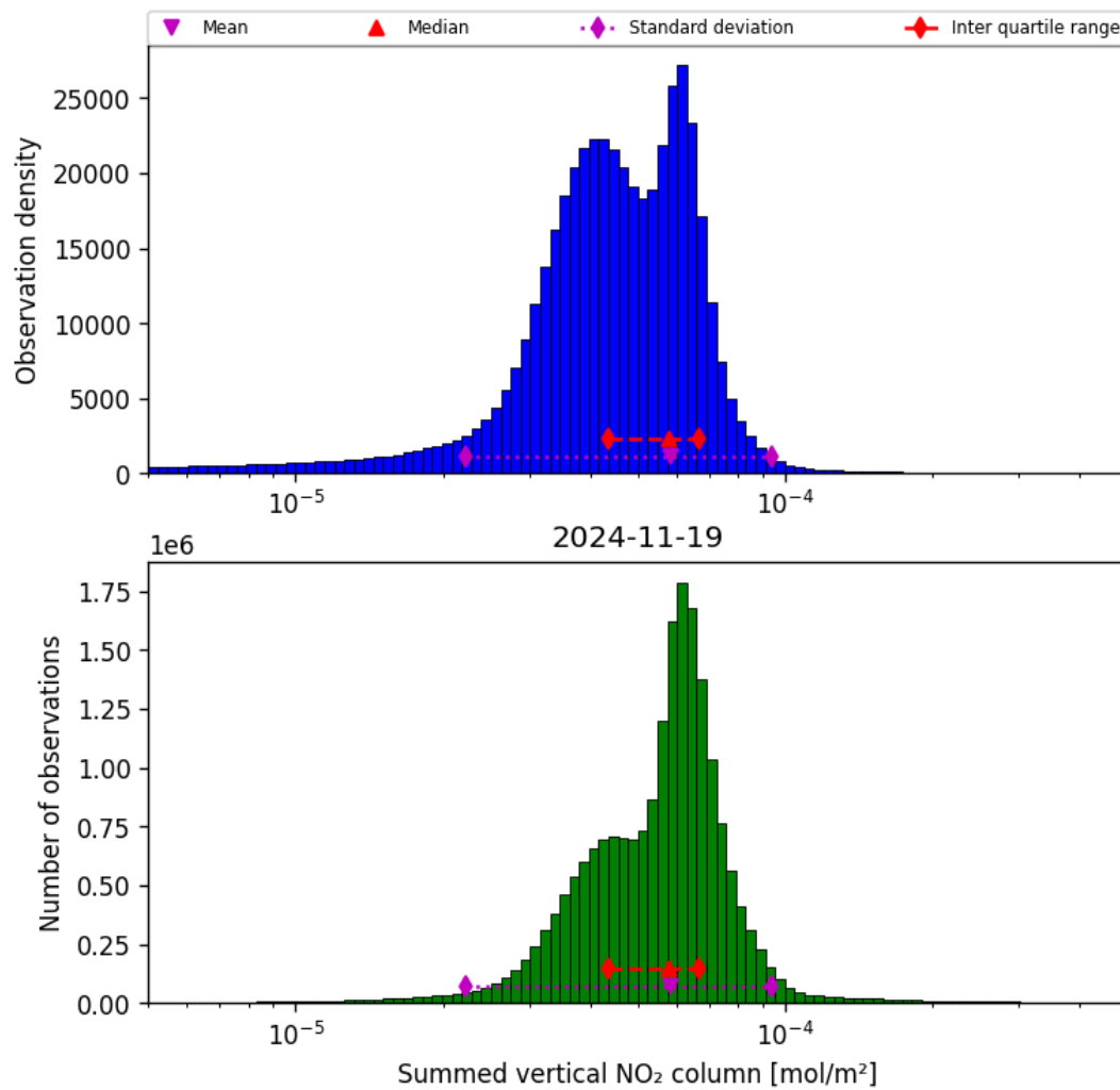
Figure 40: Histogram of “Summed vertical NO 2 column” for 2024-11-18 to 2024-11-20
