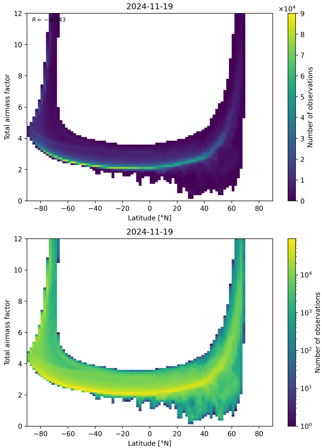
Figure 84: Scatter density plot of “Latitude” against “Total airmass factor” for 2024-11-18 to 2024-11-20.
