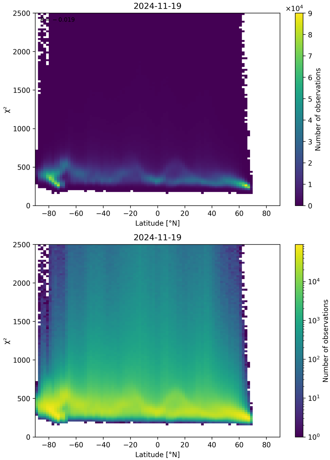
Figure 86: Scatter density plot of “Latitude” against “ \chi^2 ” for 2024-11-18 to 2024-11-20.
