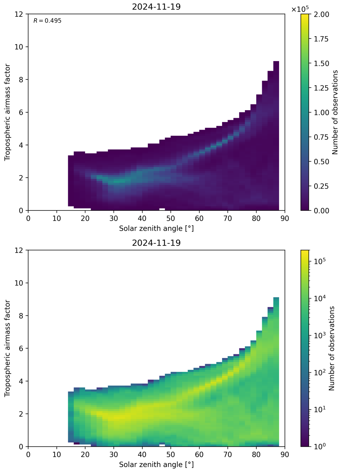
Figure 147: Scatter density plot of “Solar zenith angle” against “Tropospheric airmass factor” for 2024-11-18 to 2024-11-20.
