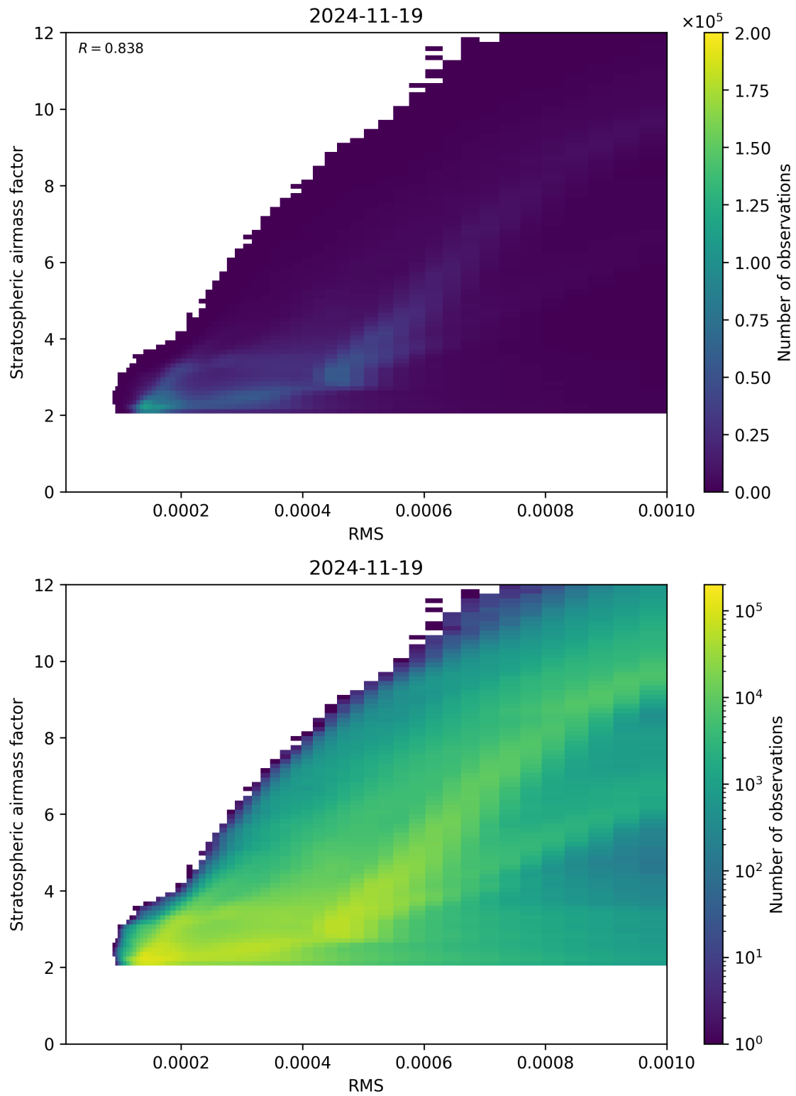
Figure 144: Scatter density plot of “RMS” against “Stratospheric airmass factor” for 2024-11-18 to 2024-11-20.
