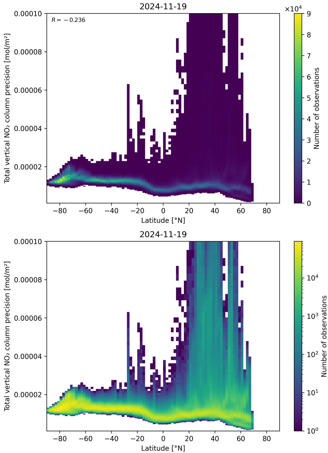
Figure 91: Scatter density plot of “Latitude” against “Total vertical NO 2 column precision” for 2024-11-18 to 2024-11-20.
