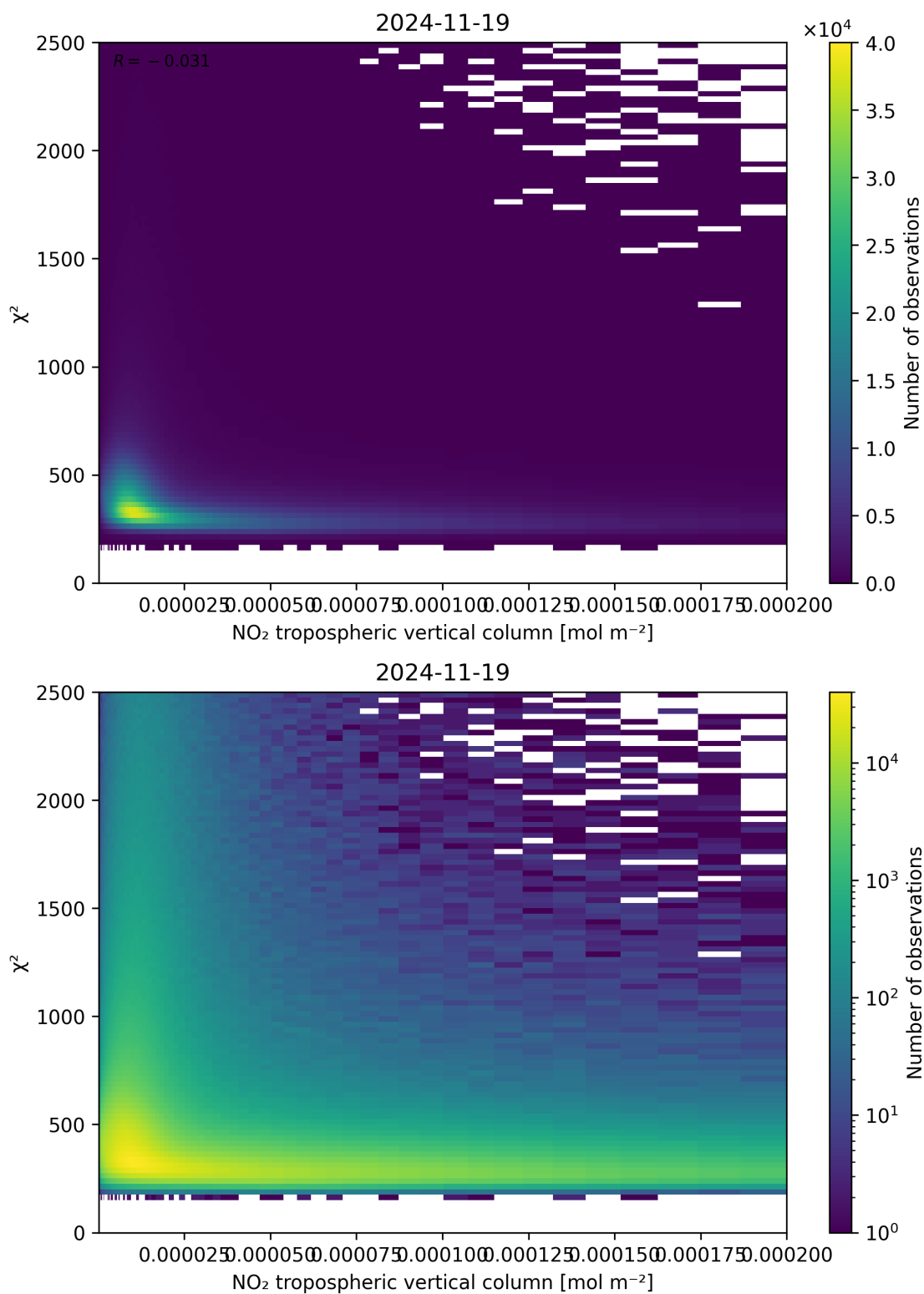
Figure 124: Scatter density plot of “NO 2 tropospheric vertical column” against “ \chi^2 ” for 2024-11-18 to 2024-11-20.
