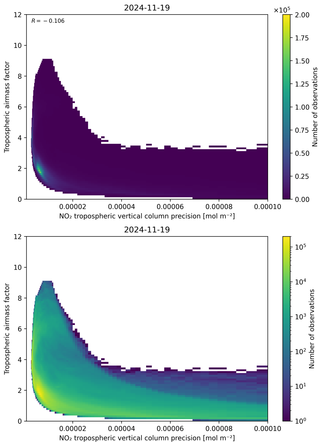
Figure 133: Scatter density plot of “NO 2 tropospheric vertical column precision” against “Tropospheric airmass factor” for 2024-11-18 to 2024-11-20.
