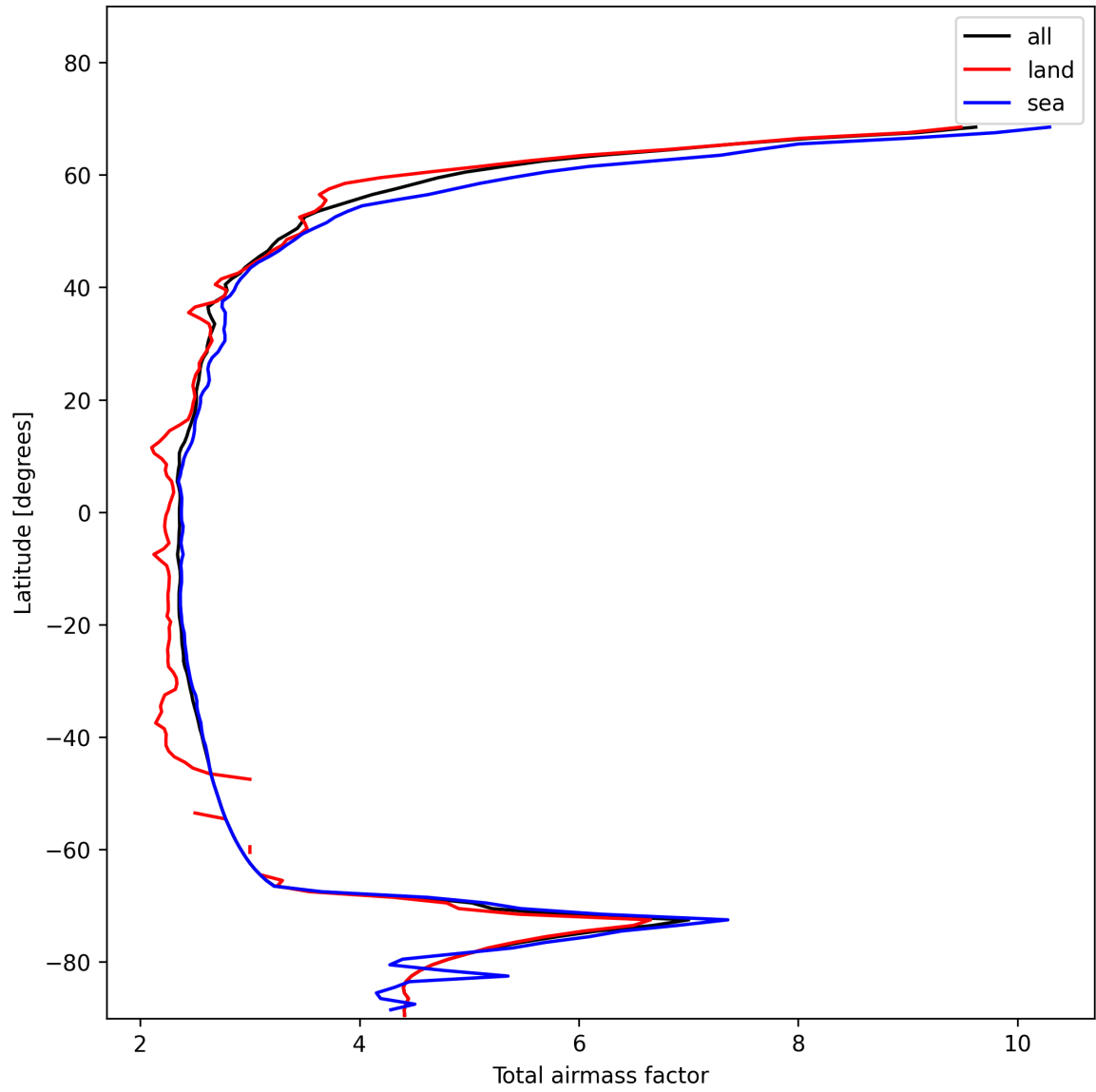
Figure 15: Zonal average of “Total airmass factor” for 2024-11-18 to 2024-11-20.
