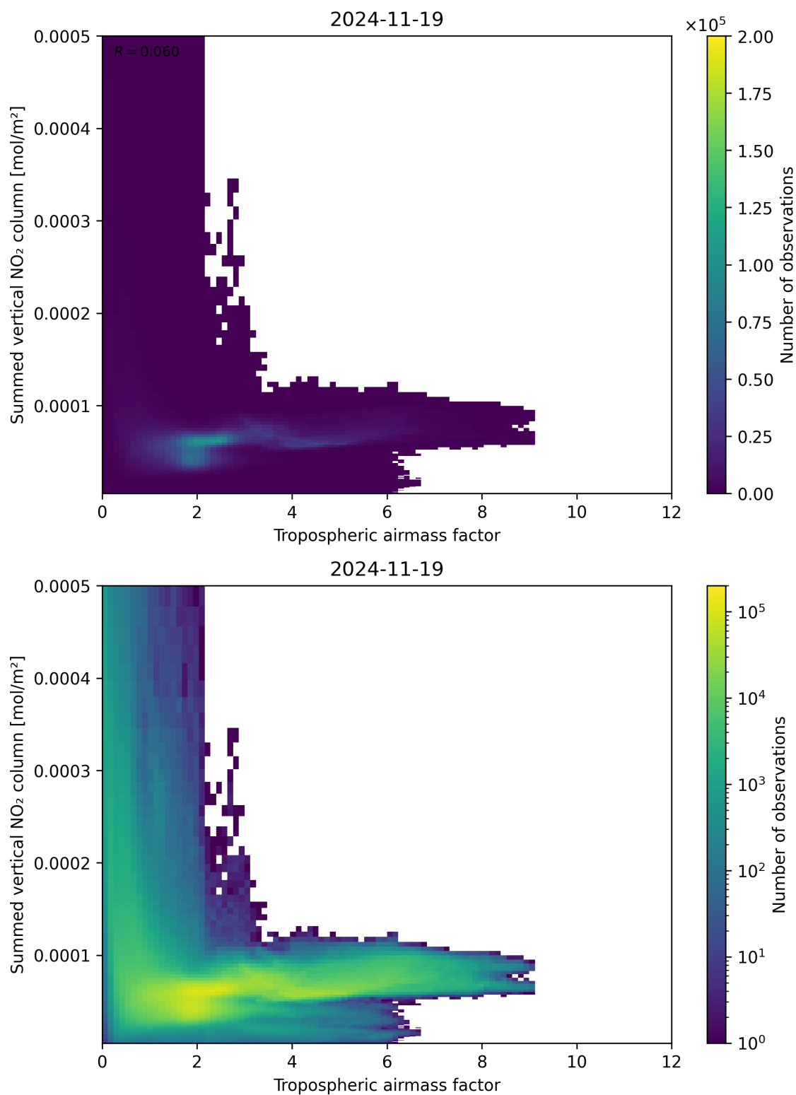
Figure 75: Scatter density plot of “Tropospheric air mass factor” against “Summed vertical NO 2 column” for 2024-11-18 to 2024-11-20.
