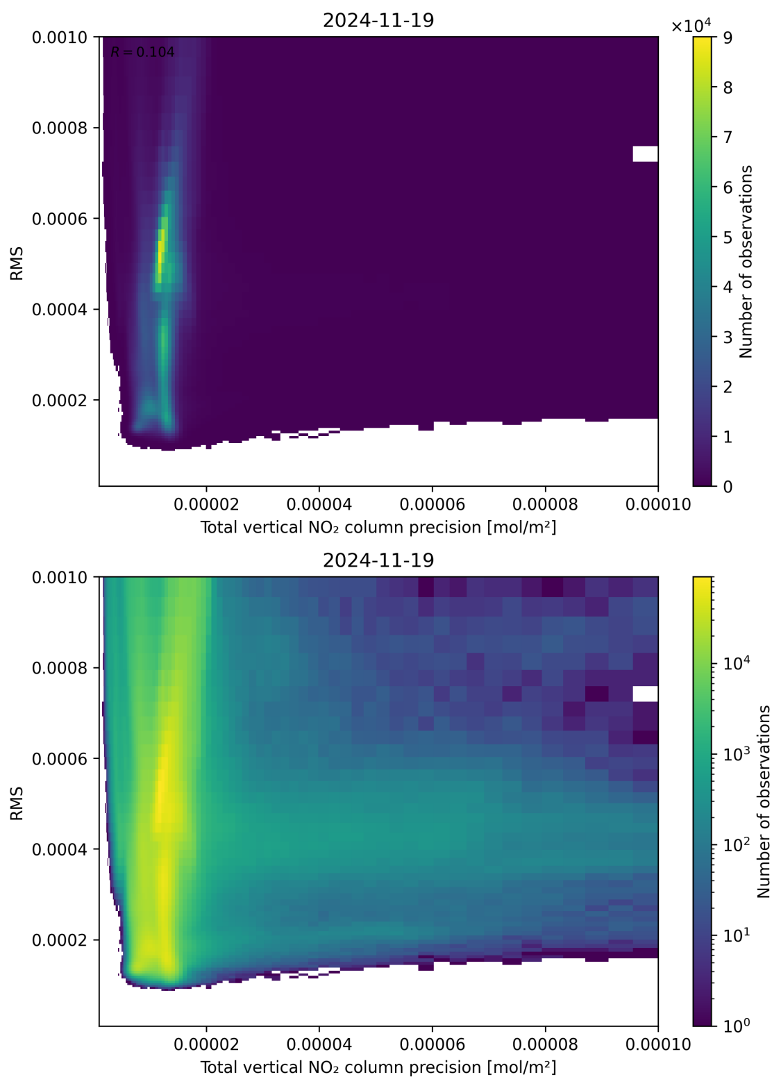
Figure 119: Scatter density plot of “Total vertical NO 2 column precision” against “RMS” for 2024-11-18 to 2024-11-20.
