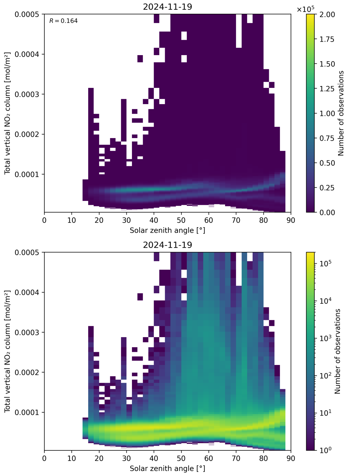
Figure 153: Scatter density plot of “Solar zenith angle” against “Total vertical NO 2 column” for 2024-11-18 to 2024-11-20.
