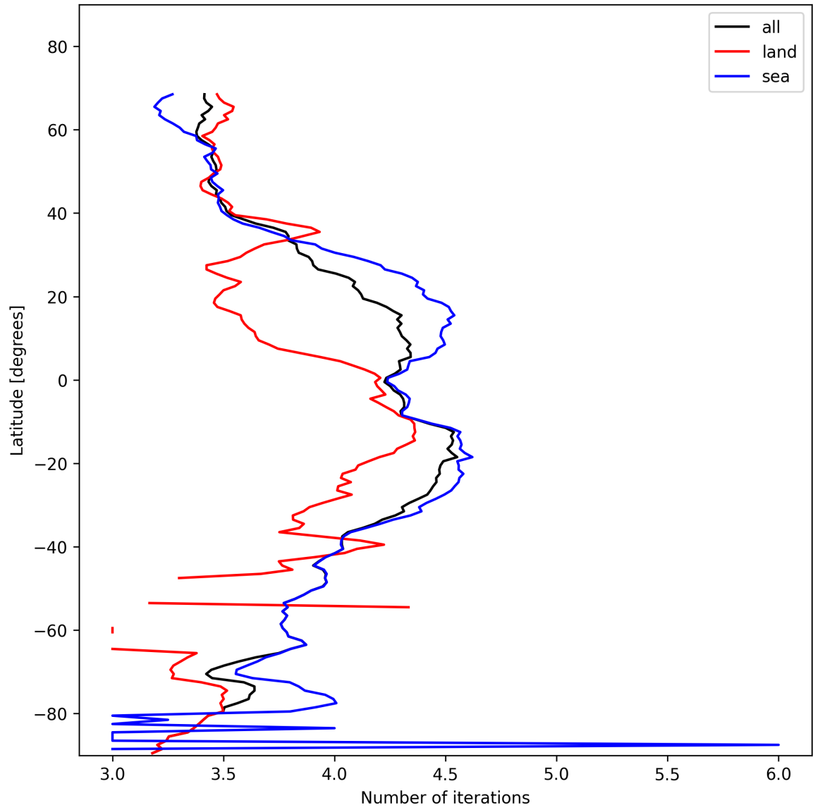
Figure 17: Zonal average of “Number of iterations” for 2024-11-18 to 2024-11-20.
