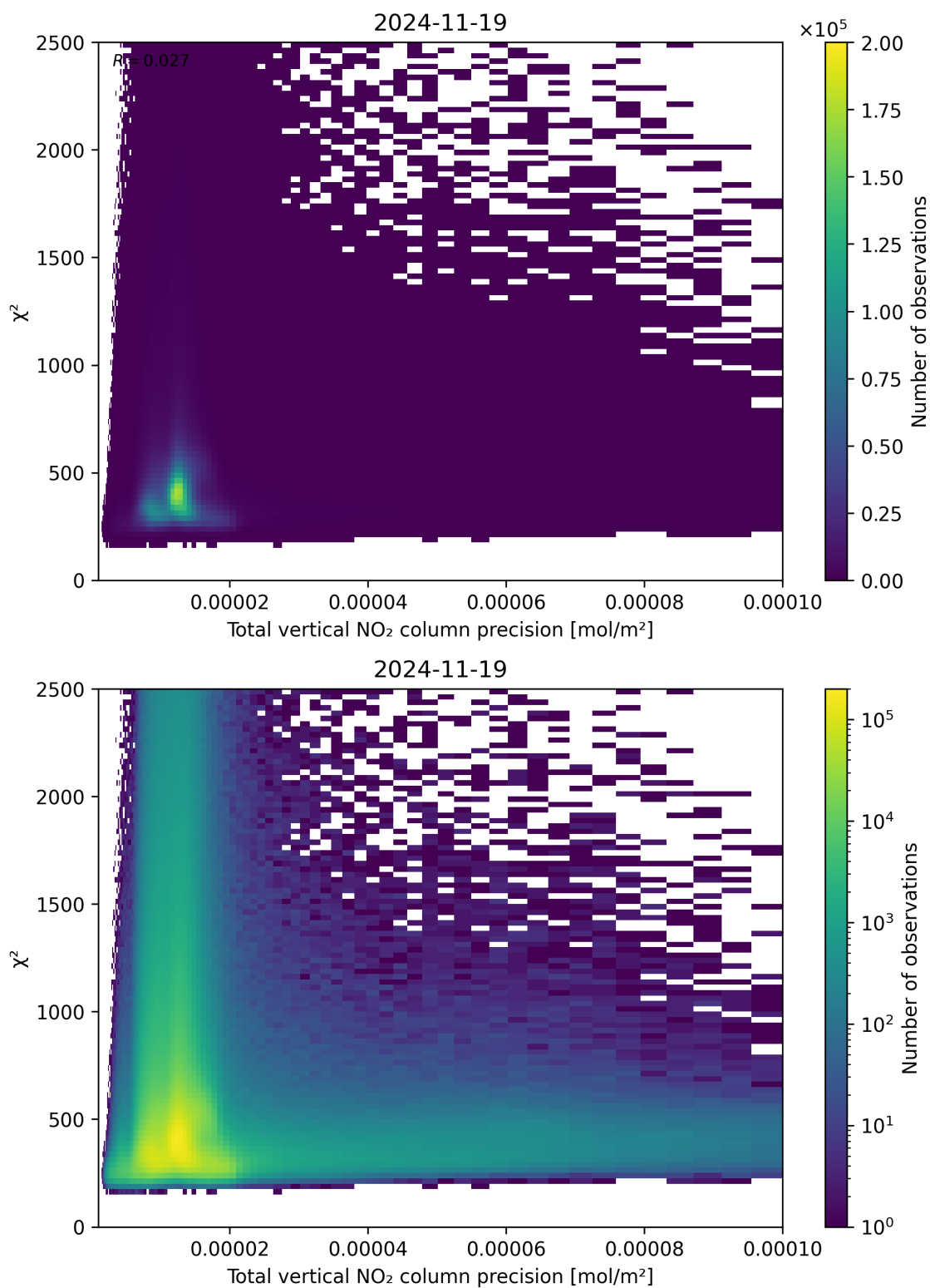
Figure 116: Scatter density plot of “Total vertical NO 2 column precision” against “ \chi^2 ” for 2024-11-18 to 2024-11-20.
