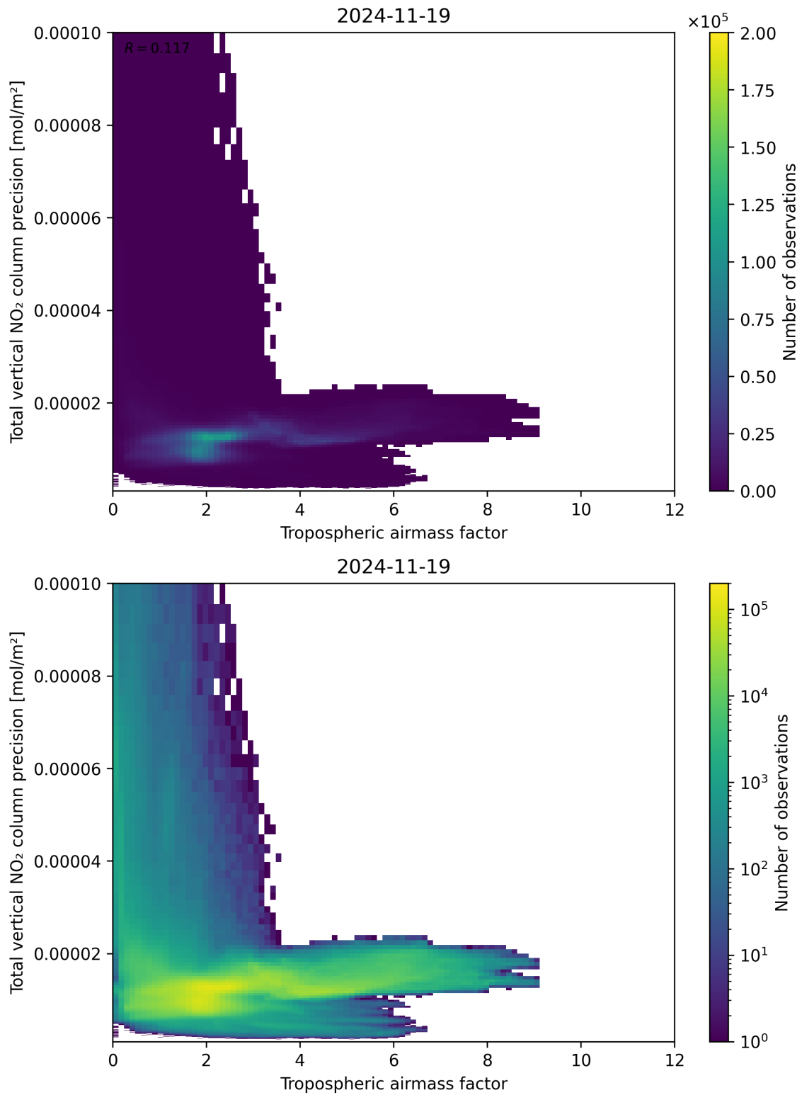
Figure 78: Scatter density plot of “Tropospheric air mass factor” against “Total vertical NO 2 column precision” for 2024-11-18 to 2024-11-20.
