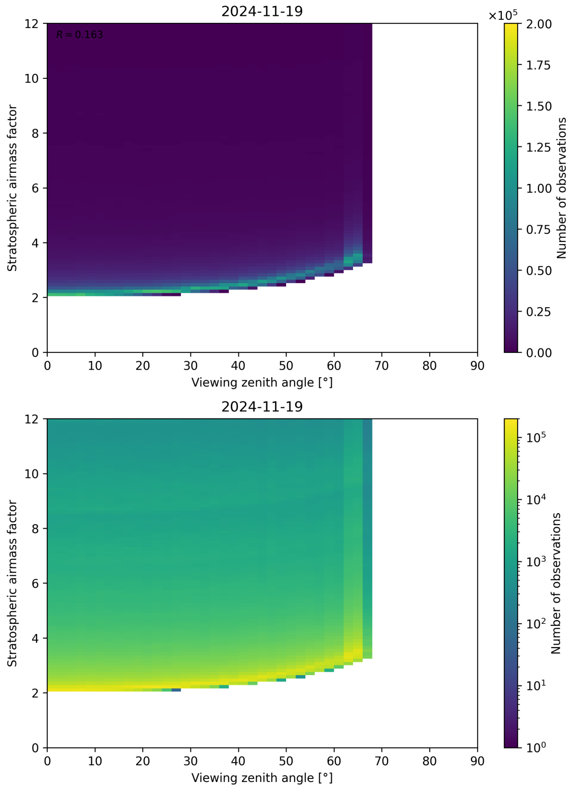
Figure 159: Scatter density plot of “Viewing zenith angle” against “Stratospheric airmass factor” for 2024-11-18 to 2024-11-20.
