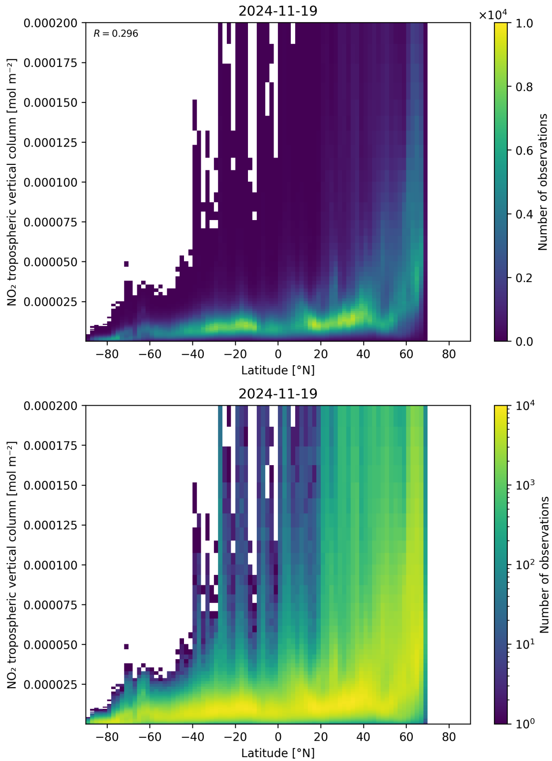
Figure 92: Scatter density plot of “Latitude” against “NO 2 tropospheric vertical column” for 2024-11-18 to 2024-11-20.
