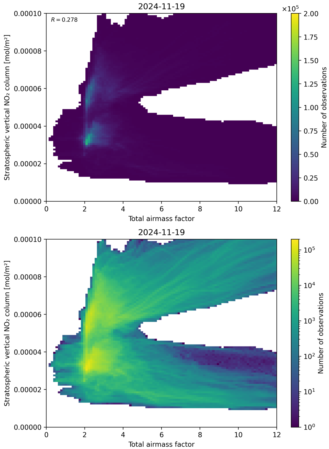
Figure 64: Scatter density plot of “Total airmass factor” against “Stratospheric vertical NO 2 column” for 2024-11-18 to 2024-11-20.
