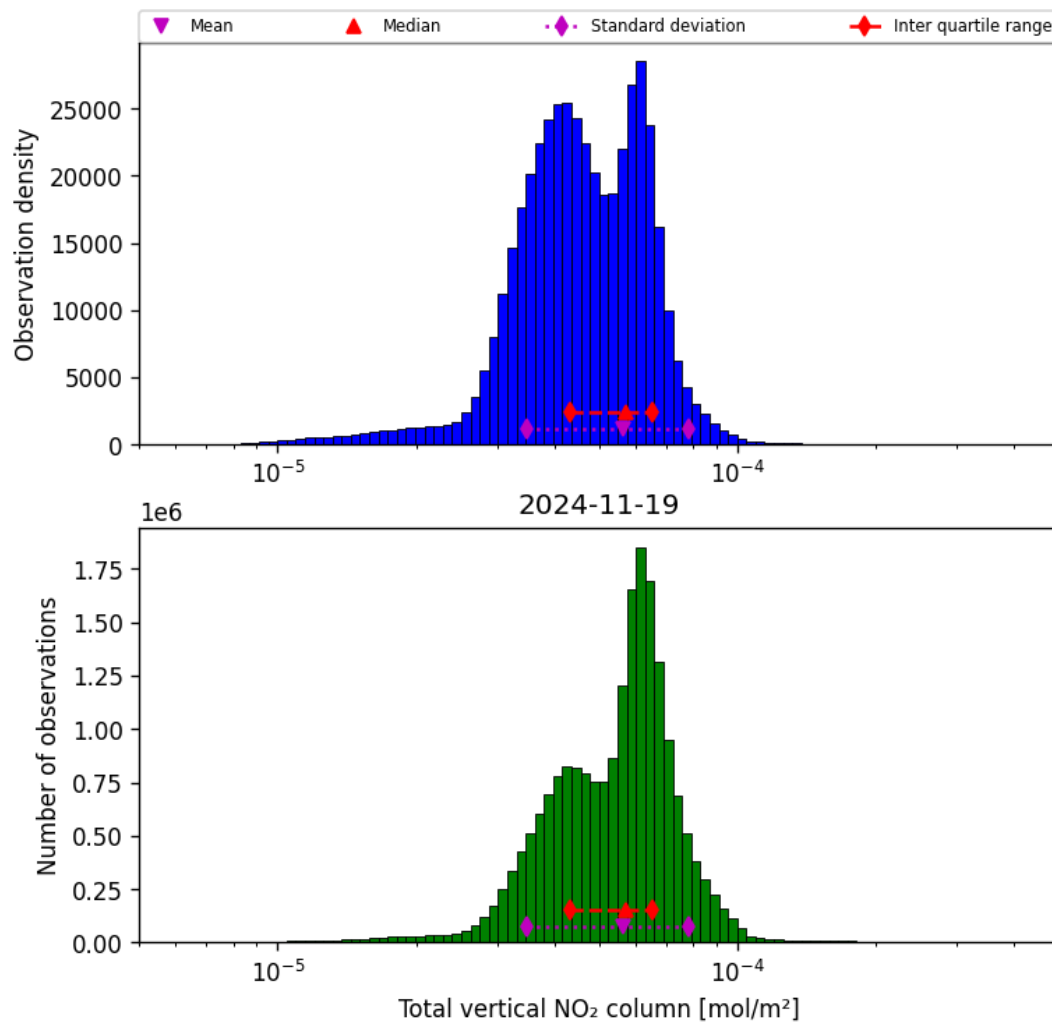
Figure 38: Histogram of “Total vertical NO 2 column” for 2024-11-18 to 2024-11-20
