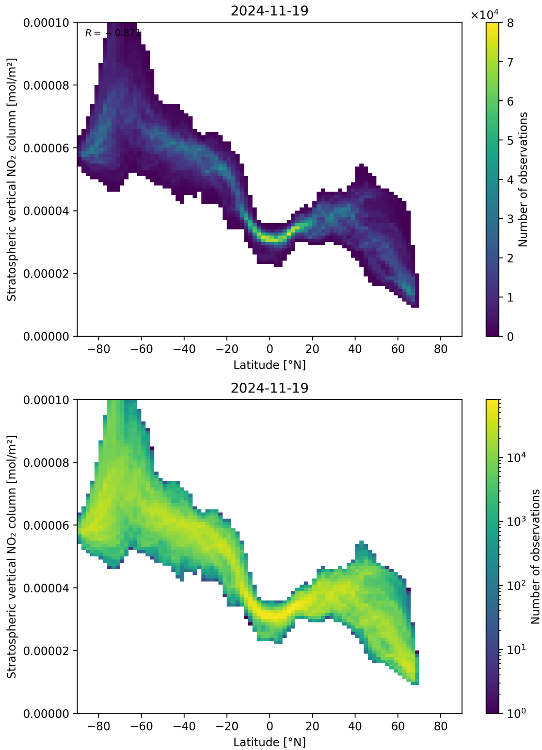
Figure 87: Scatter density plot of “Latitude” against “Stratospheric vertical NO 2 column” for 2024-11-18 to 2024-11-20.
