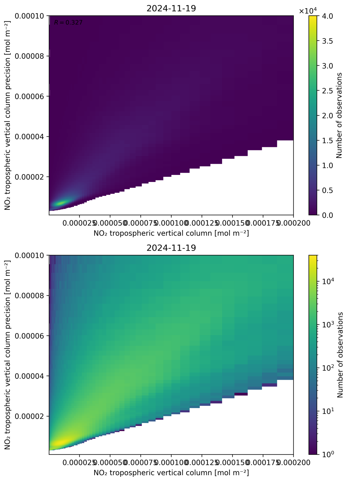
Figure 130: Scatter density plot of “NO 2 tropospheric vertical column” against “NO 2 tropospheric vertical column precision” for 2024-11-18 to 2024-11-20.
