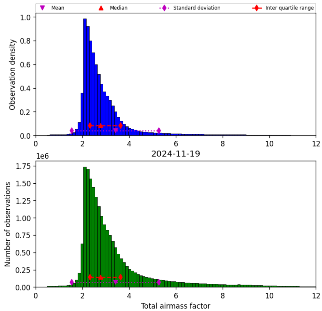
Figure 32: Histogram of “Total airmass factor” for 2024-11-18 to 2024-11-20
