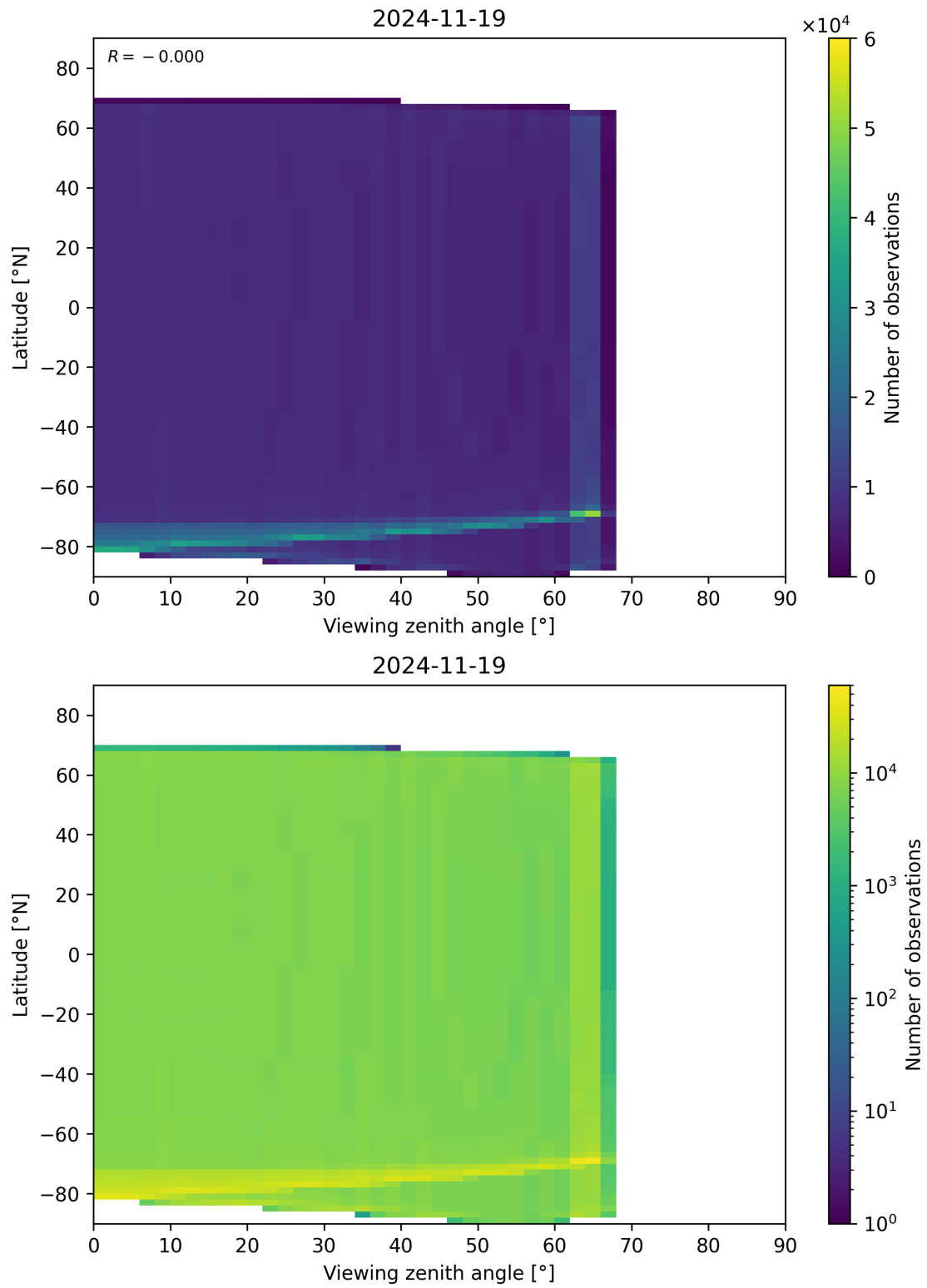
Figure 163: Scatter density plot of “Viewing zenith angle” against “Latitude” for 2024-11-18 to 2024-11-20.
