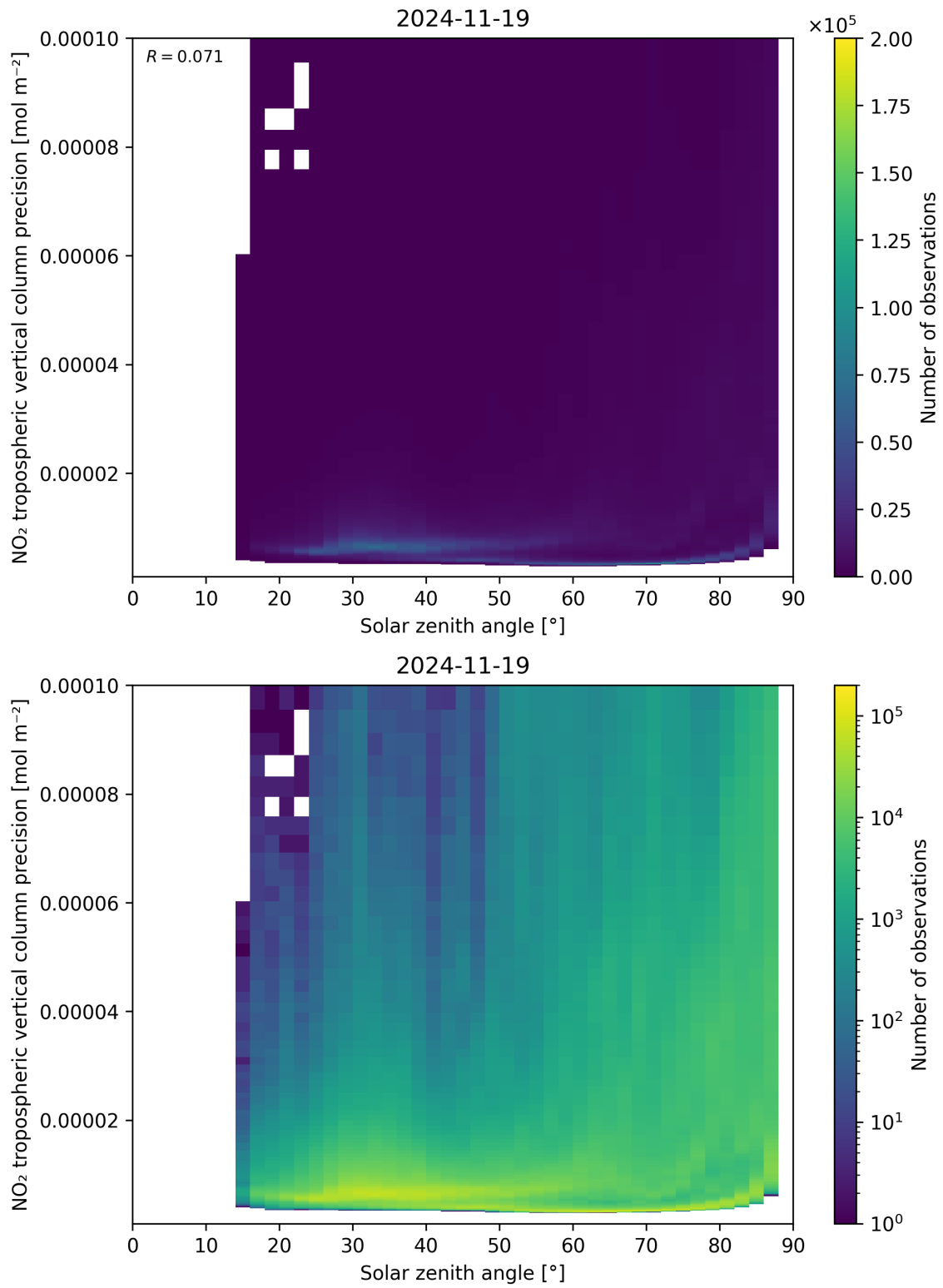
Figure 156: Scatter density plot of “Solar zenith angle” against “NO 2 tropospheric vertical column precision” for 2024-11-18 to 2024-11-20.
