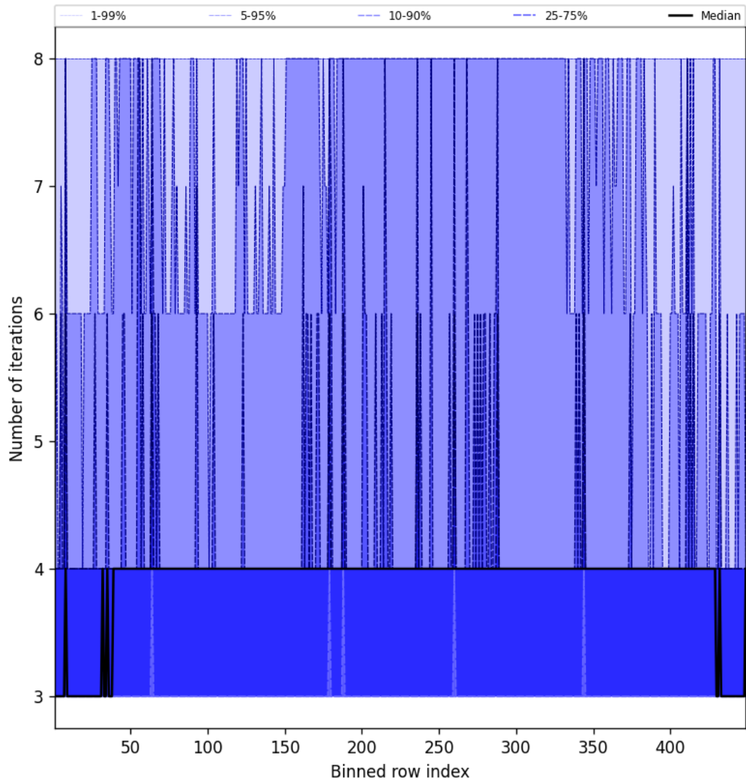
Figure 51: Along track statistics of “Number of iterations” for 2024-11-18 to 2024-11-20
