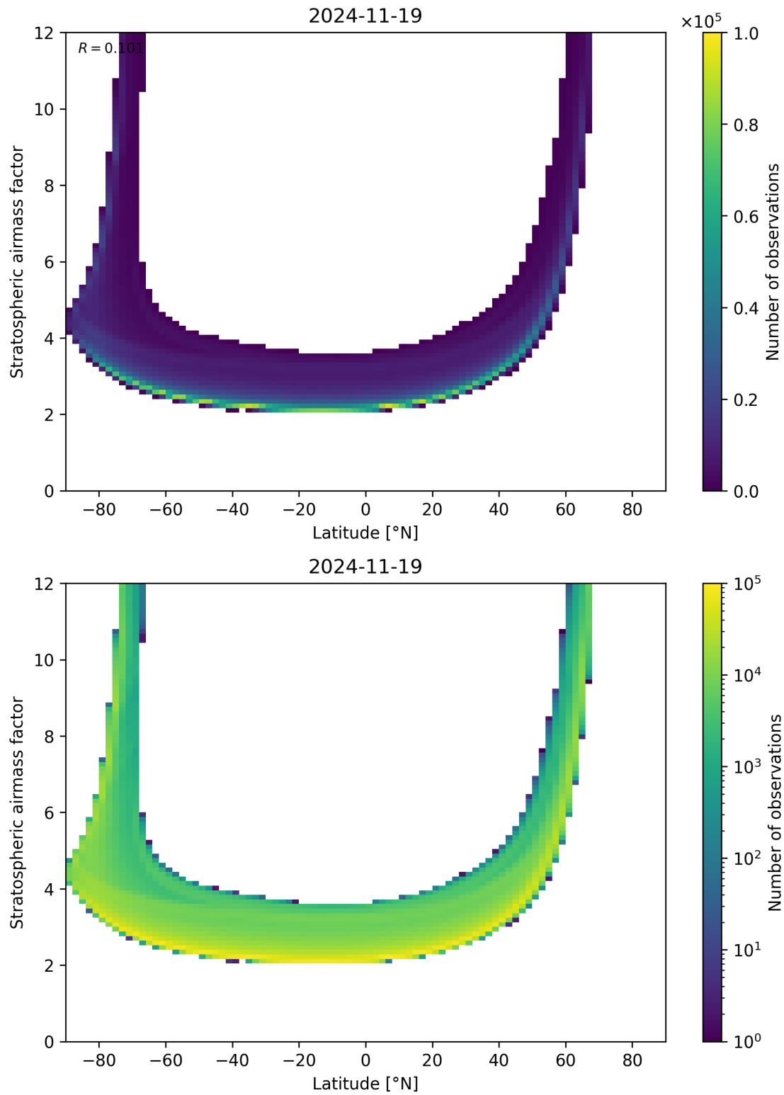
Figure 83: Scatter density plot of “Latitude” against “Stratospheric air mass factor” for 2024-11-18 to 2024-11-20.
