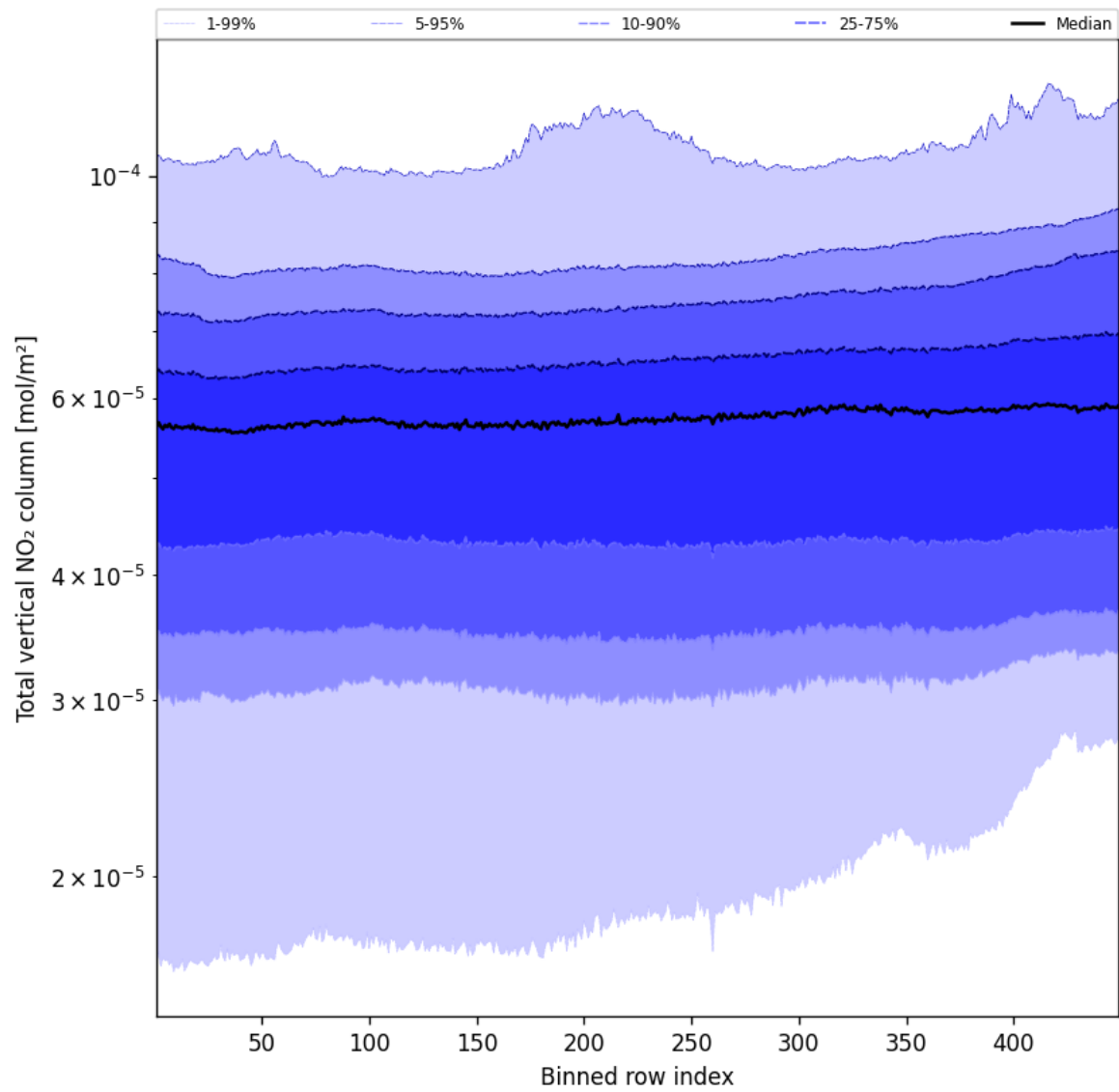
Figure 55: Along track statistics of “Total vertical NO 2 column” for 2024-11-18 to 2024-11-20
