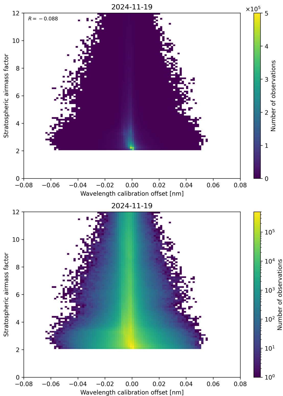
Figure 174: Scatter density plot of “Wavelength calibration offset” against “Stratospheric airmass factor” for 2024-11-18 to 2024-11-20.
