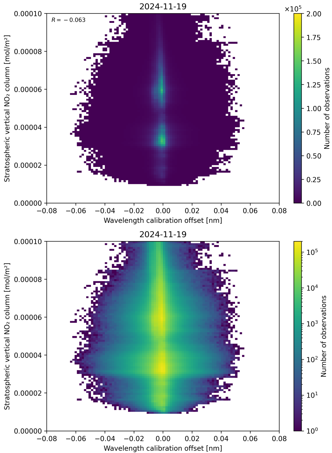
Figure 176: Scatter density plot of “Wavelength calibration offset” against “Stratospheric vertical NO 2 column” for 2024-11-18 to 2024-11-20.
