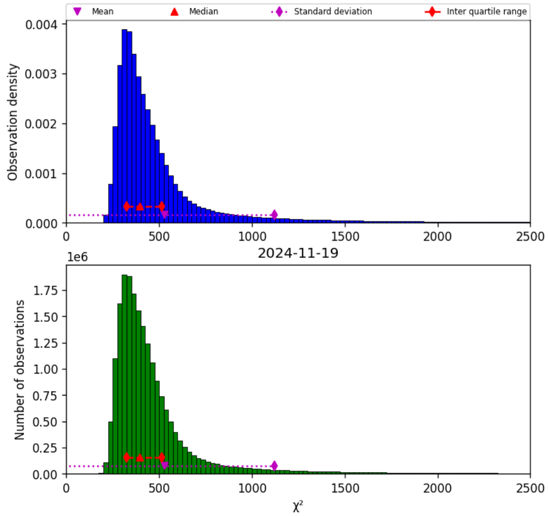
Figure 42: Histogram of " \chi^2 " for 2024-11-18 to 2024-11-20
