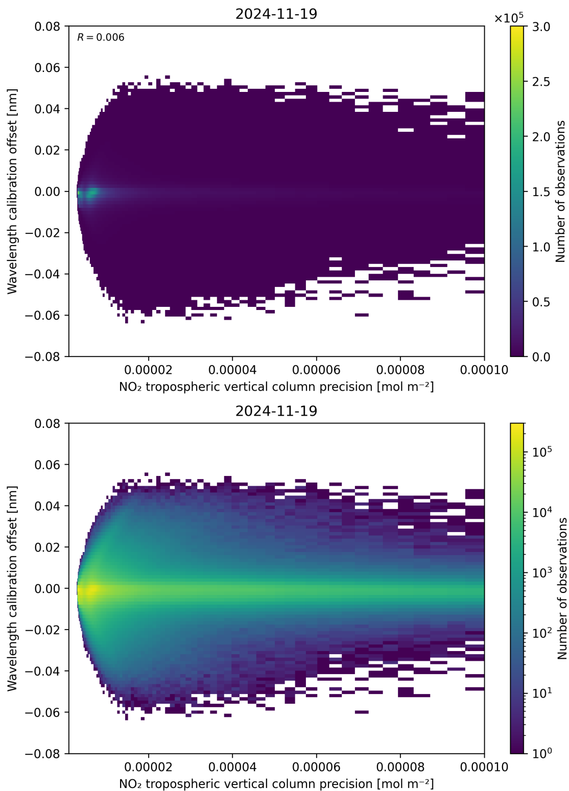
Figure 141: Scatter density plot of “NO 2 tropospheric vertical column precision” against “Wavelength calibration offset” for 2024-11-18 to 2024-11-20.
