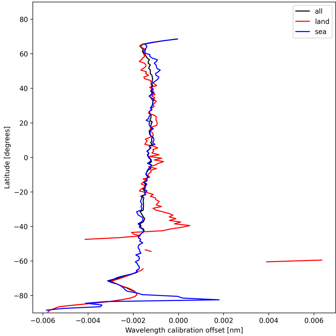
Figure 18: Zonal average of “Wavelength calibration offset” for 2024-11-18 to 2024-11-20.
