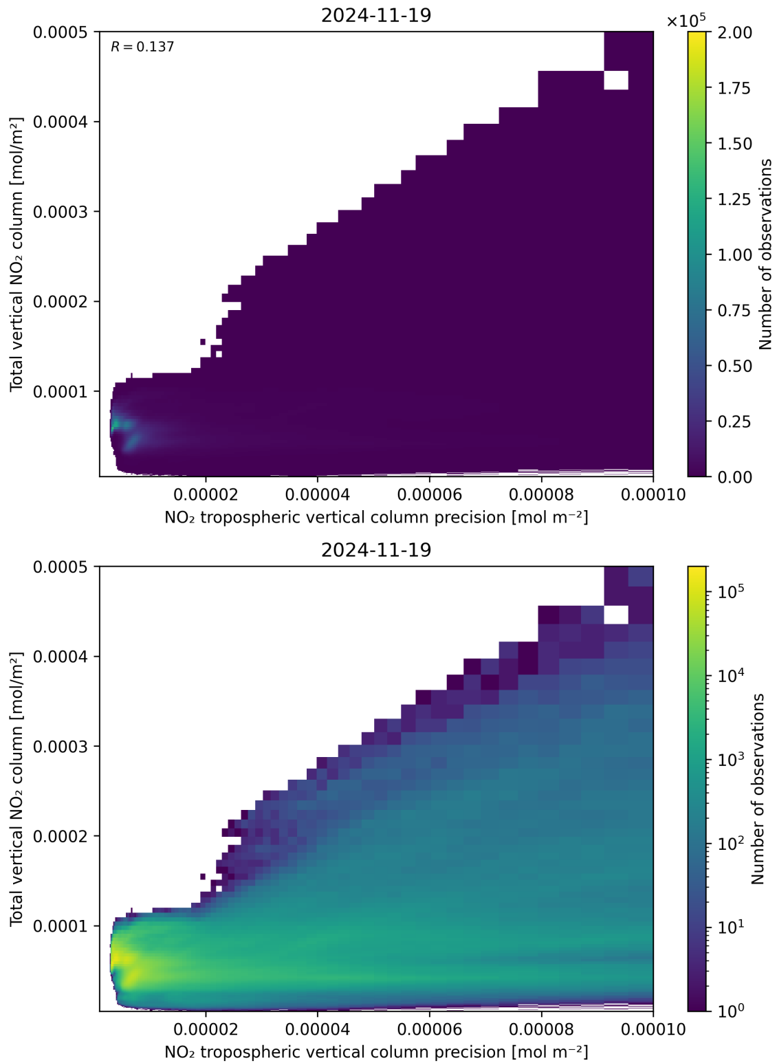
Figure 138: Scatter density plot of “NO 2 tropospheric vertical column precision” against “Total vertical NO 2 column” for 2024-11-18 to 2024-11-20.
