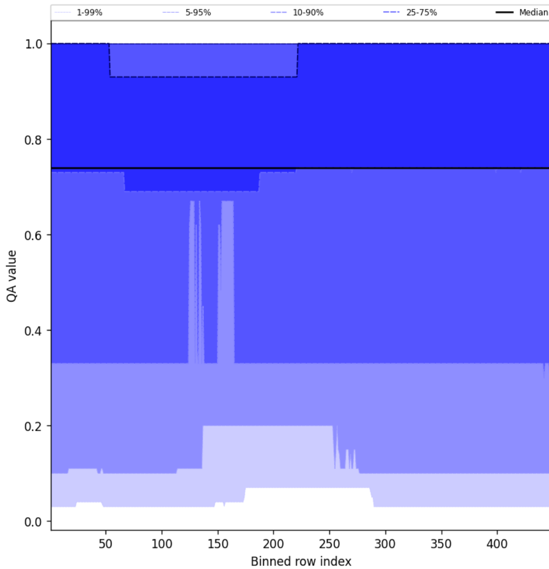
Figure 45: Along track statistics of “QA value” for 2024-11-18 to 2024-11-20
