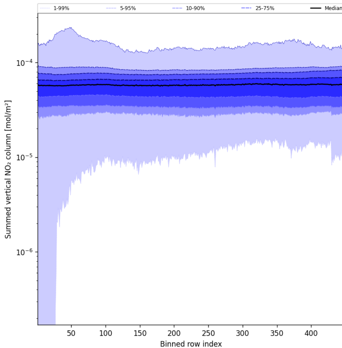
Figure 57: Along track statistics of “Summed vertical NO 2 column” for 2024-11-18 to 2024-11-20
