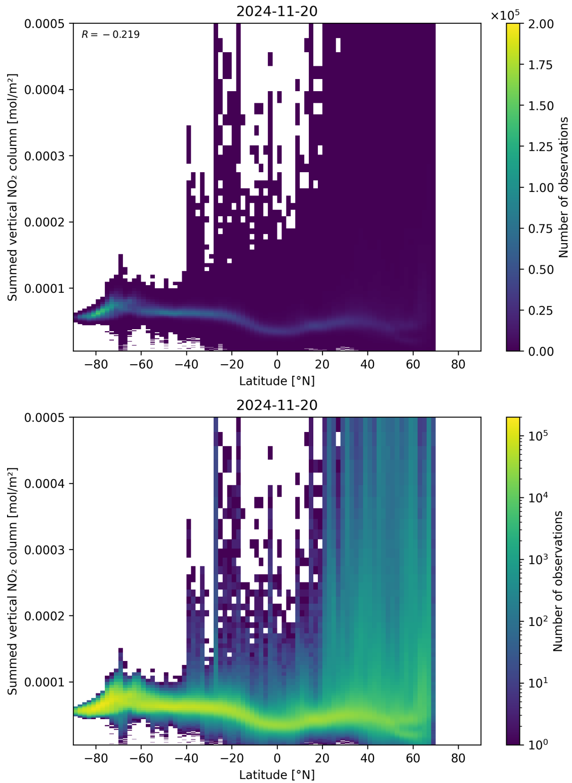
Figure 88: Scatter density plot of “Latitude” against “Summed vertical NO 2 column” for 2024-11-20 to 2024-11-21.
