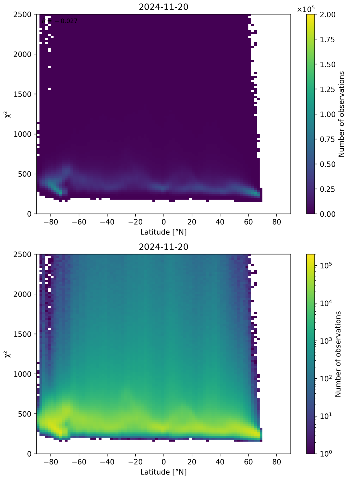
Figure 86: Scatter density plot of “Latitude” against “ \chi^2 ” for 2024-11-20 to 2024-11-21.
