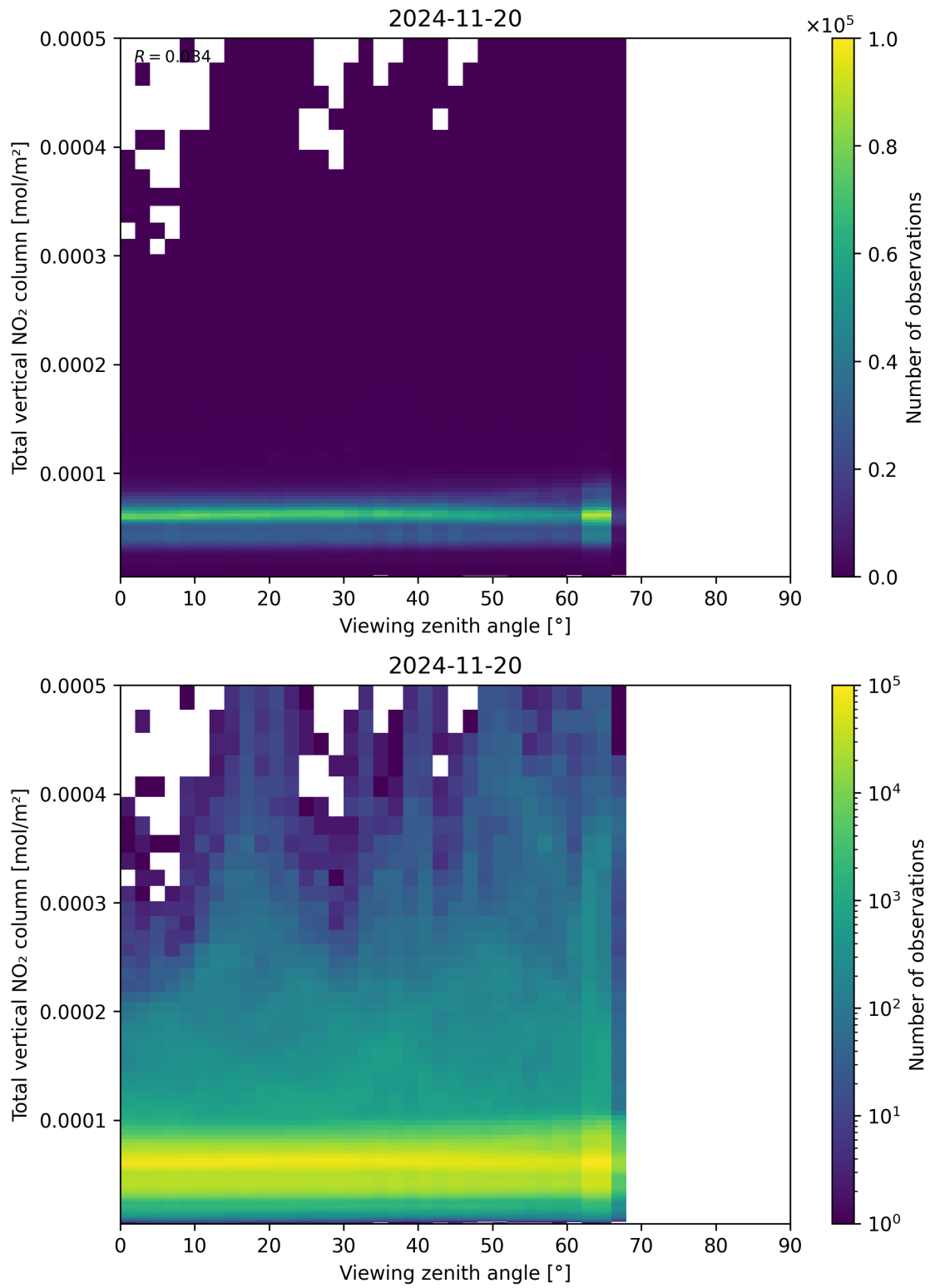
Figure 167: Scatter density plot of “Viewing zenith angle” against “Total vertical NO 2 column” for 2024-11-20 to 2024-11-21.
