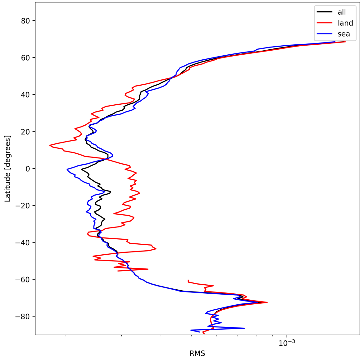
Figure 26: Zonal average of “RMS” for 2024-11-20 to 2024-11-21.
