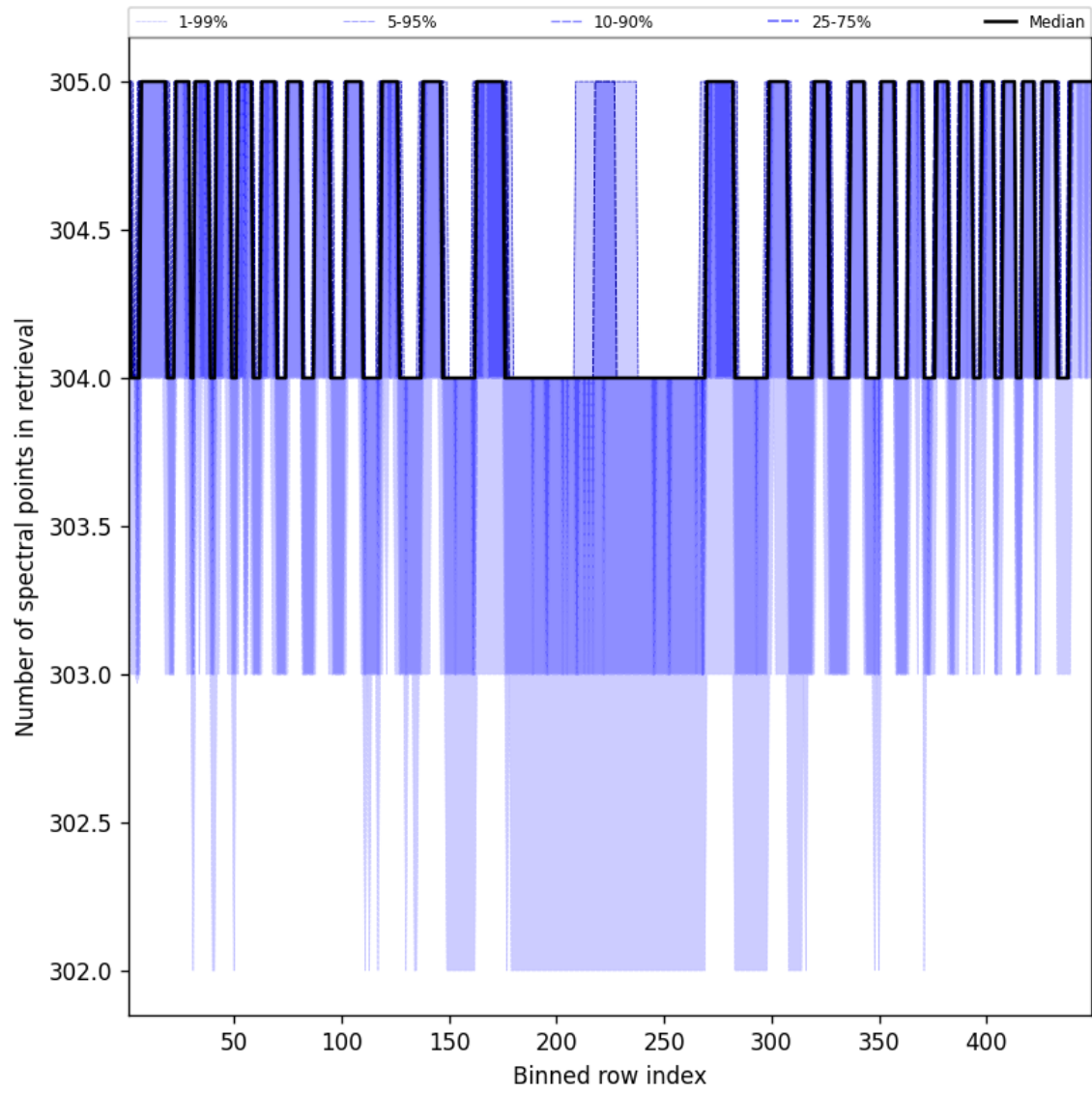
Figure 50: Along track statistics of “Number of spectral points in retrieval” for 2024-11-20 to 2024-11-21
