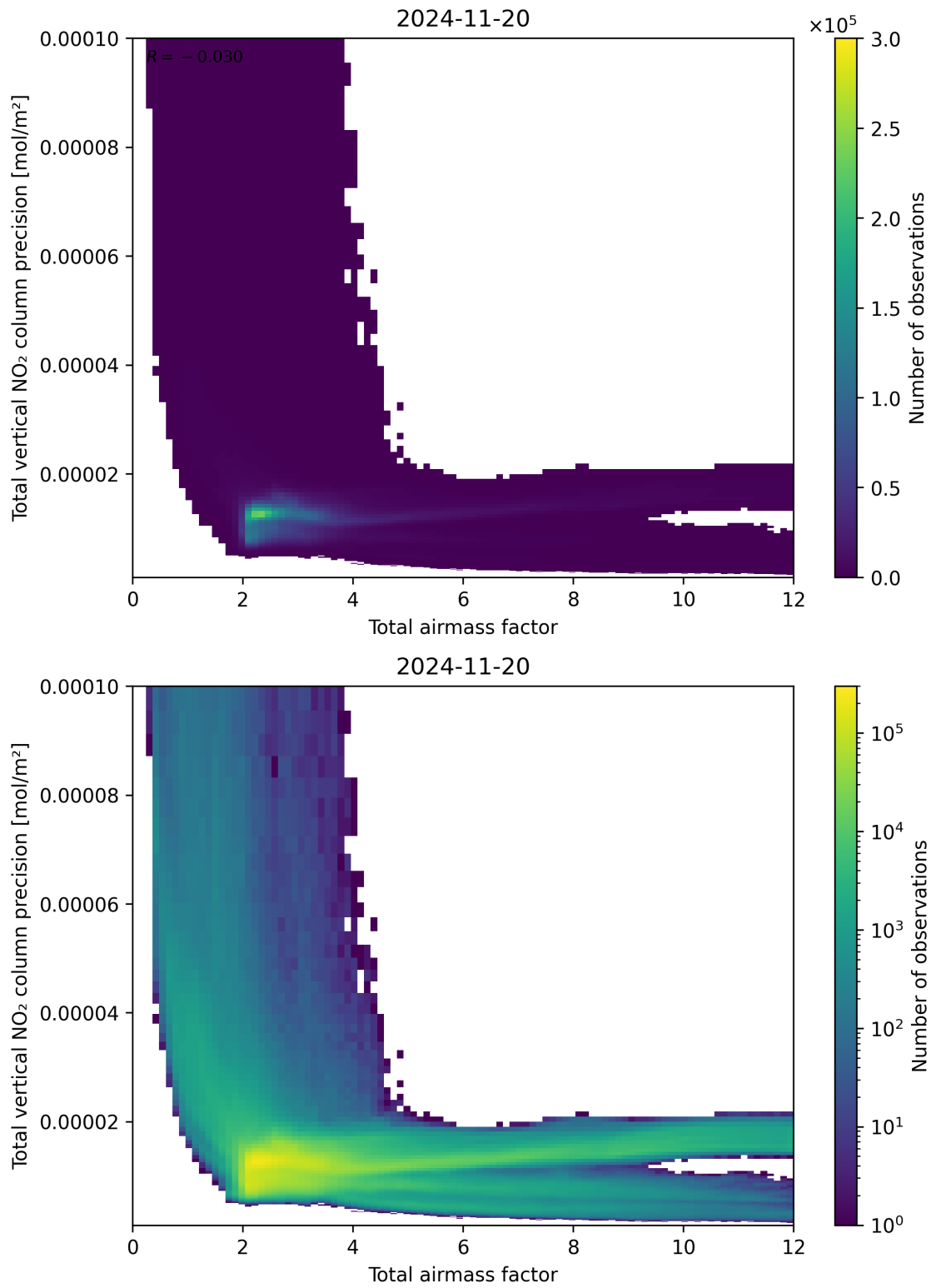
Figure 68: Scatter density plot of “Total airmass factor” against “Total vertical NO 2 column precision” for 2024-11-20 to 2024-11-21.
