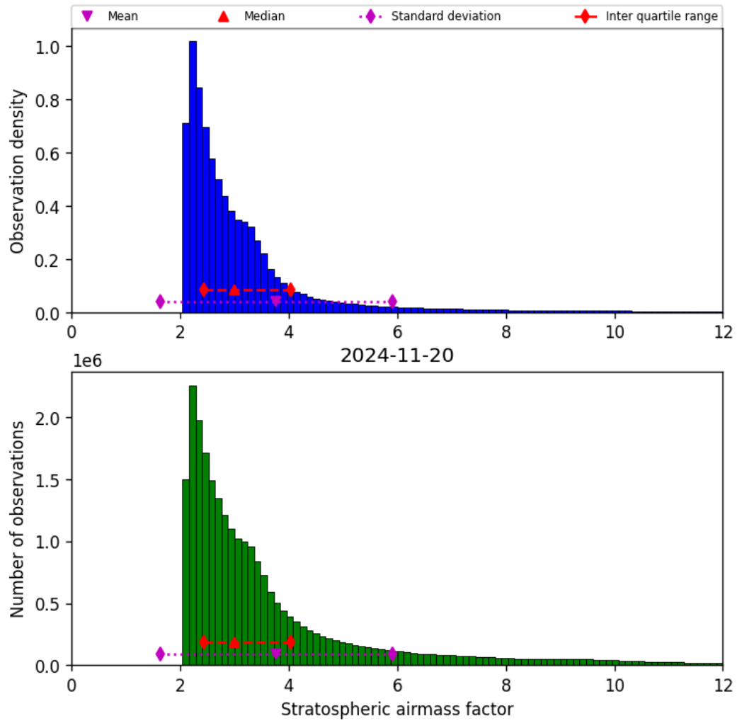
Figure 44: Histogram of “Stratospheric airmass factor” for 2024-11-20 to 2024-11-21
