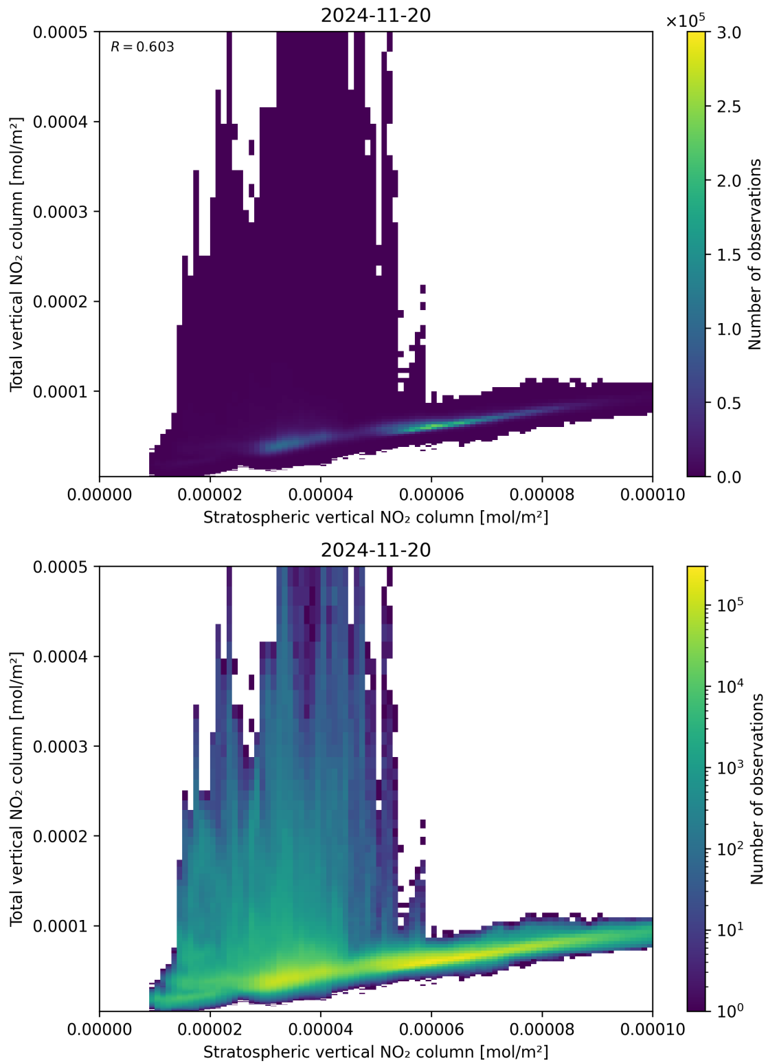
Figure 100: Scatter density plot of “Stratospheric vertical NO 2 column” against “Total vertical NO 2 column” for 2024-11-20 to 2024-11-21.
