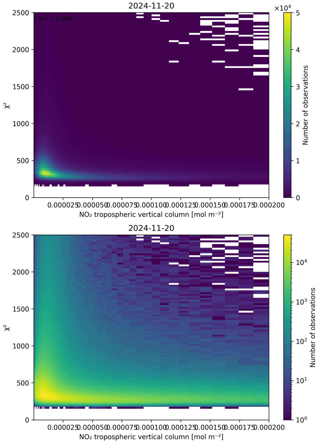
Figure 124: Scatter density plot of “NO 2 tropospheric vertical column” against “ \chi^2 ” for 2024-11-20 to 2024-11-21.
