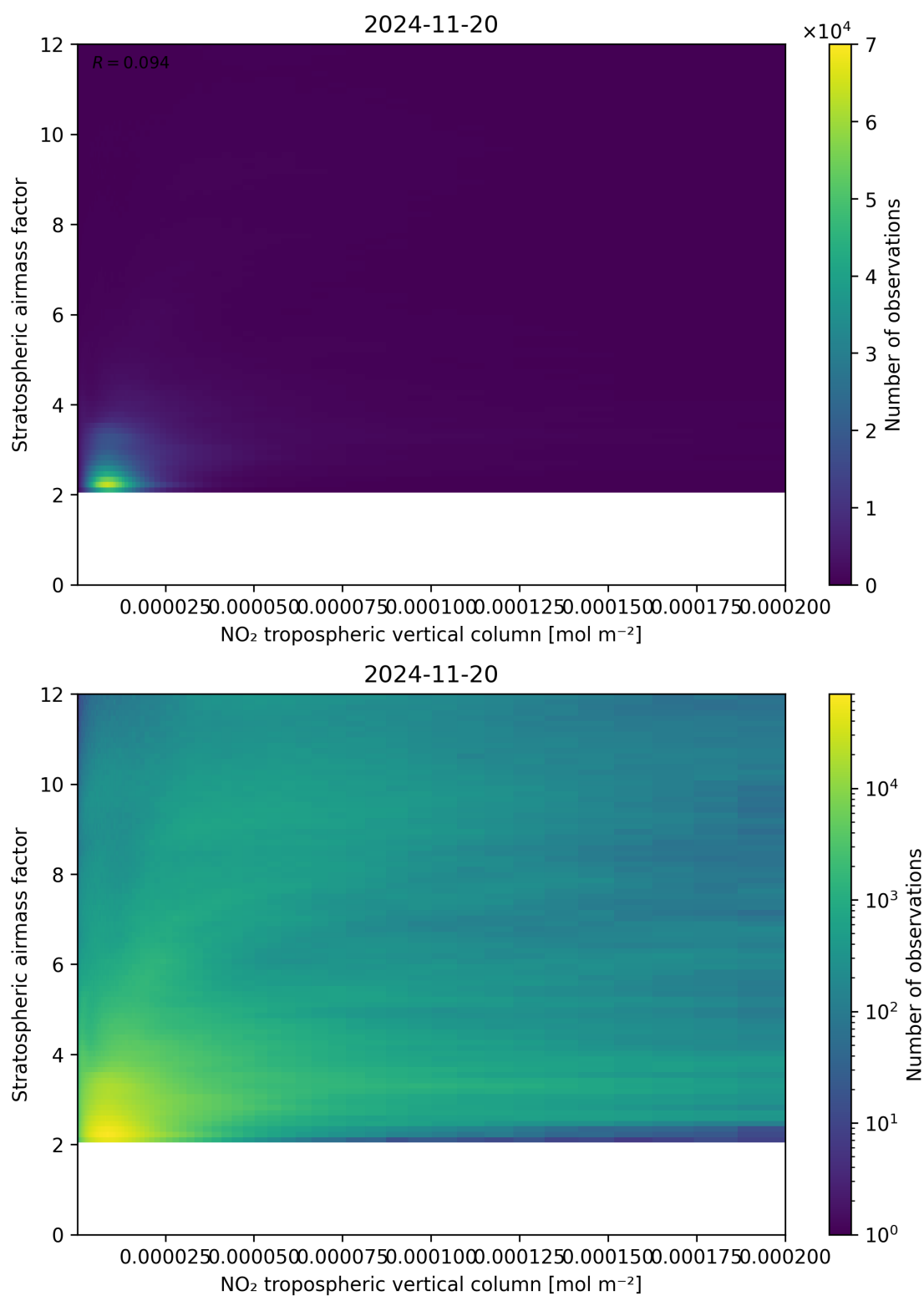
Figure 121: Scatter density plot of “NO 2 tropospheric vertical column” against “Stratospheric airmass factor” for 2024-11-20 to 2024-11-21.
