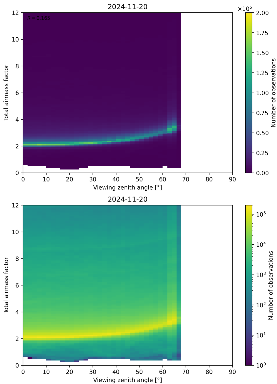
Figure 160: Scatter density plot of “Viewing zenith angle” against “Total airmass factor” for 2024-11-20 to 2024-11-21.
