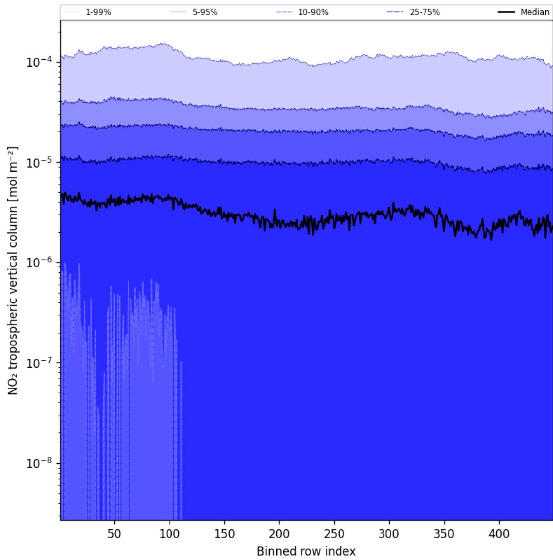
Figure 46: Along track statistics of “NO 2 tropospheric vertical column” for 2024-11-20 to 2024-11-21
