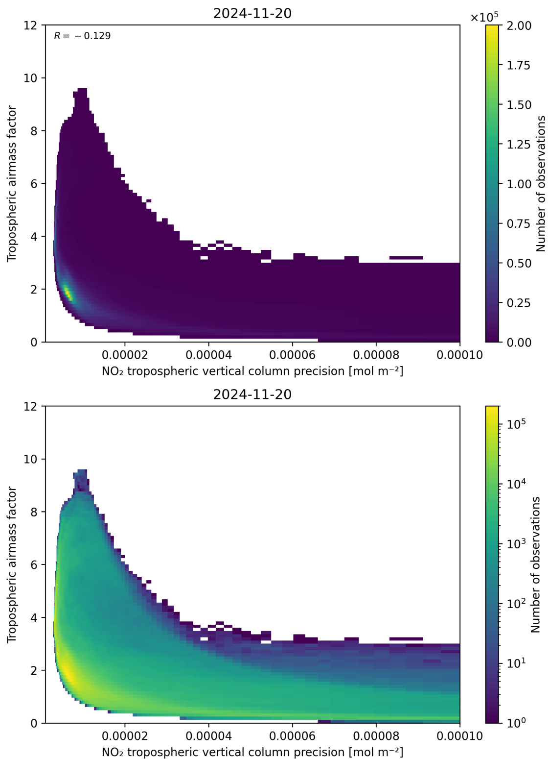
Figure 133: Scatter density plot of “NO 2 tropospheric vertical column precision” against “Tropospheric airmass factor” for 2024-11-20 to 2024-11-21.
