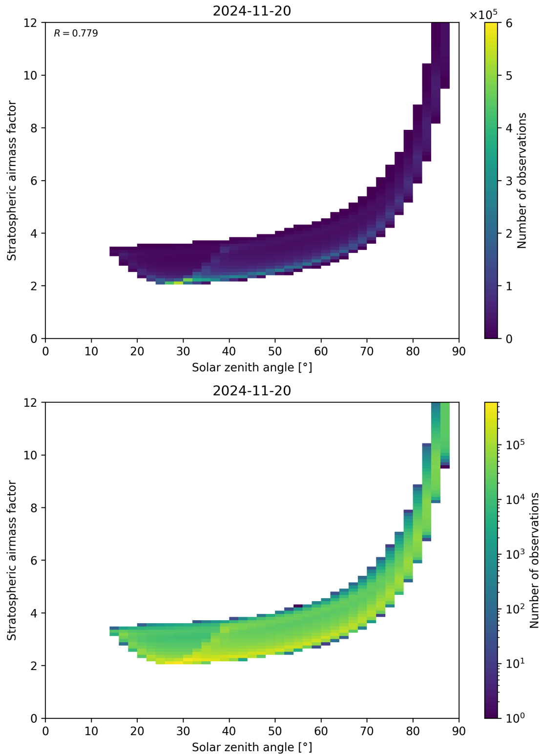
Figure 145: Scatter density plot of “Solar zenith angle” against “Stratospheric airmass factor” for 2024-11-20 to 2024-11-21.
