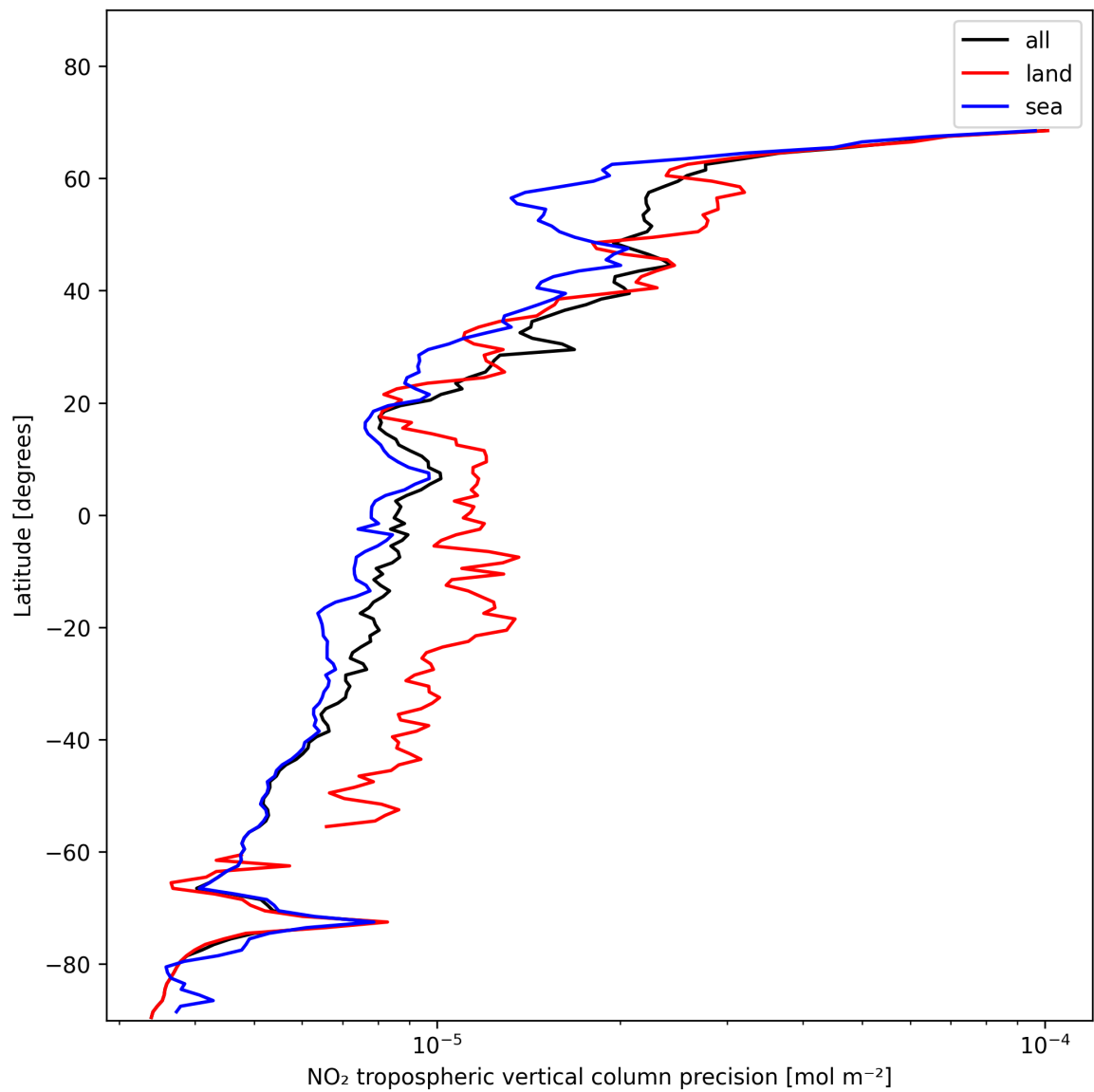
Figure 13: Zonal average of “NO 2 tropospheric vertical column precision” for 2024-11-20 to 2024-11-21.
