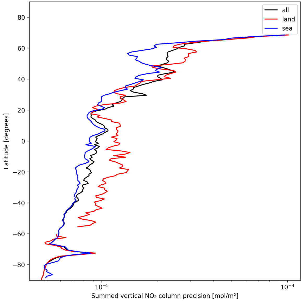
Figure 24: Zonal average of “Summed vertical NO 2 column precision” for 2024-11-20 to 2024-11-21.
