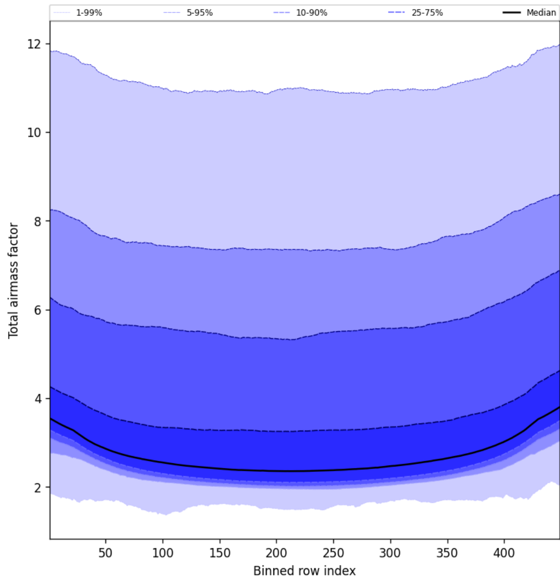
Figure 49: Along track statistics of “Total airmass factor” for 2024-11-20 to 2024-11-21
