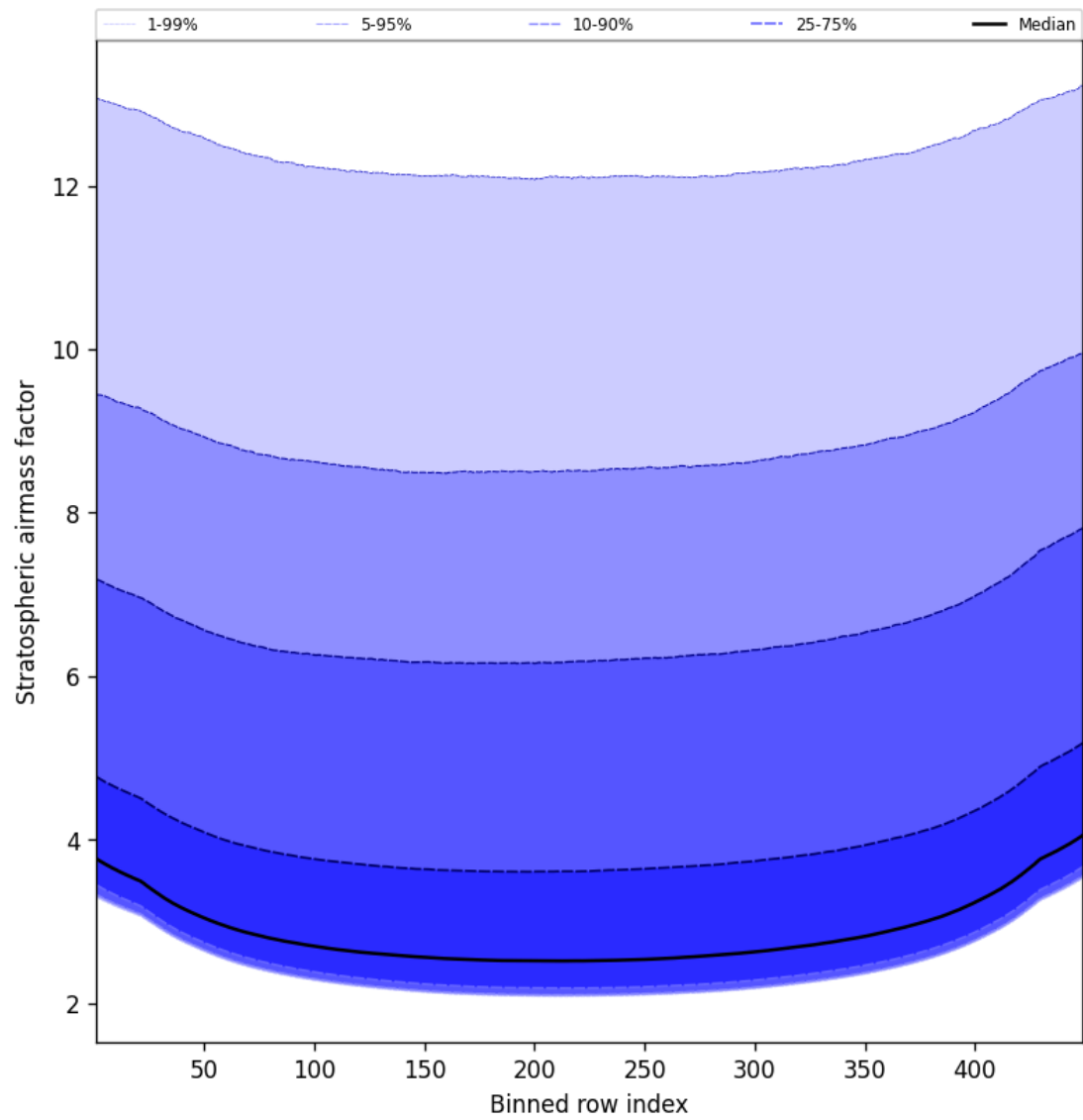
Figure 61: Along track statistics of “Stratospheric airmass factor” for 2024-11-20 to 2024-11-21
