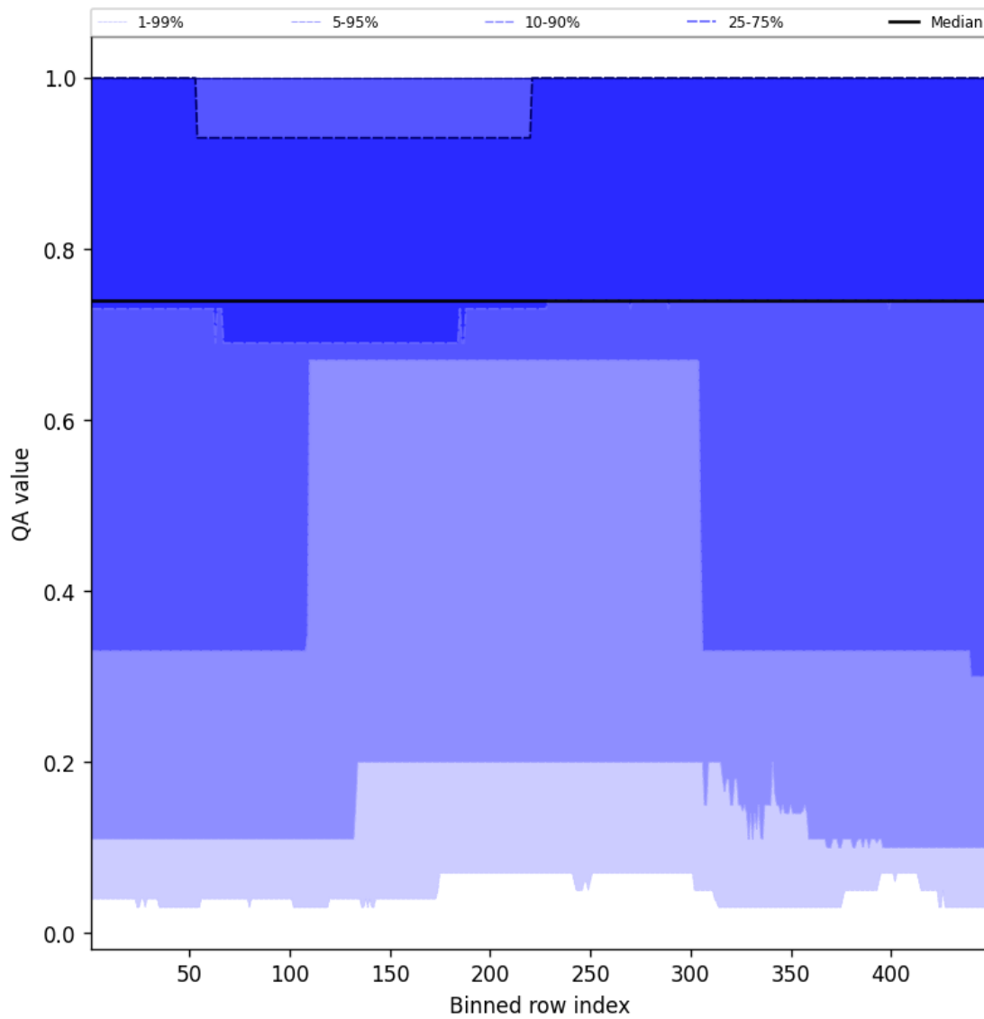
Figure 45: Along track statistics of “QA value” for 2024-11-20 to 2024-11-21
