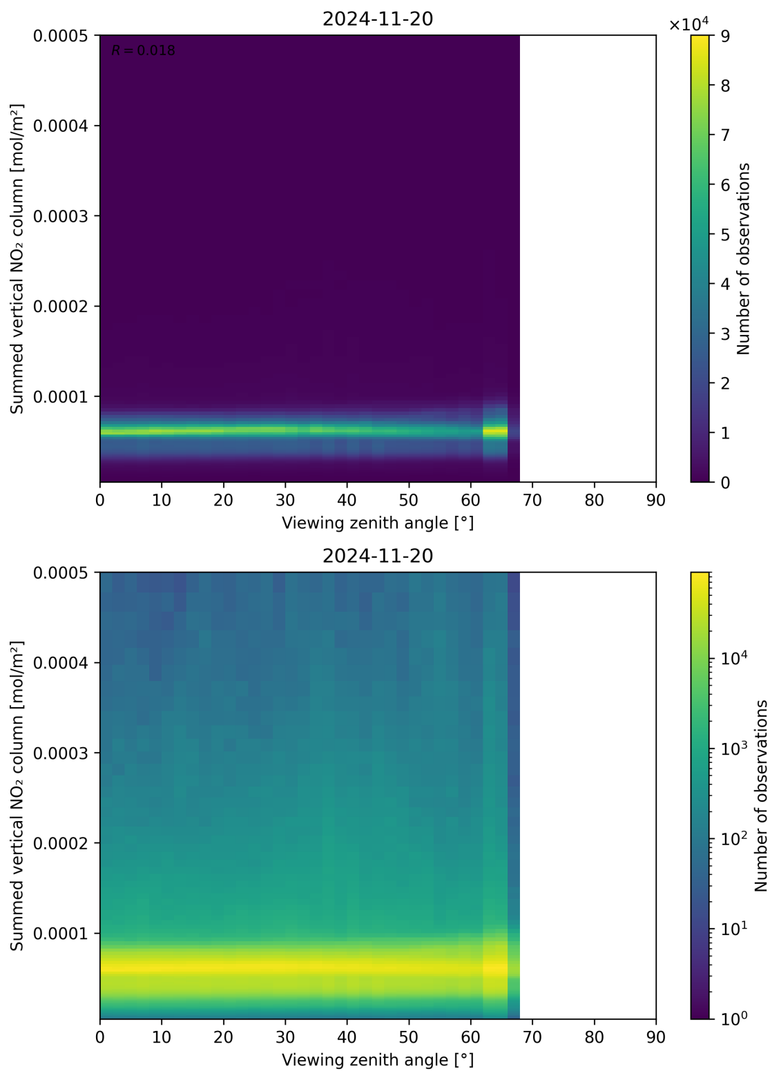
Figure 165: Scatter density plot of “Viewing zenith angle” against “Summed vertical NO 2 column” for 2024-11-20 to 2024-11-21.
