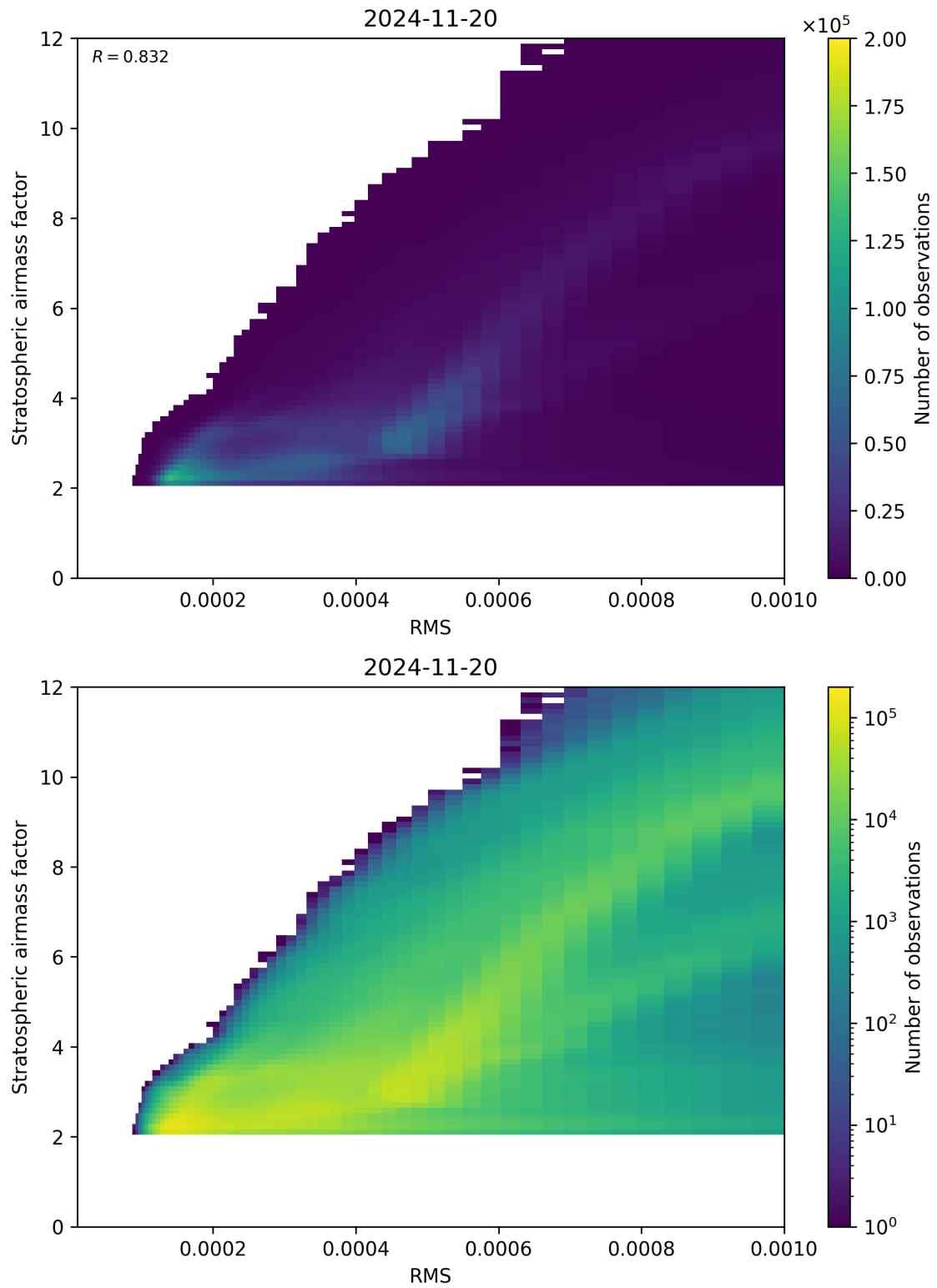
Figure 144: Scatter density plot of “RMS” against “Stratospheric airmass factor” for 2024-11-20 to 2024-11-21.
