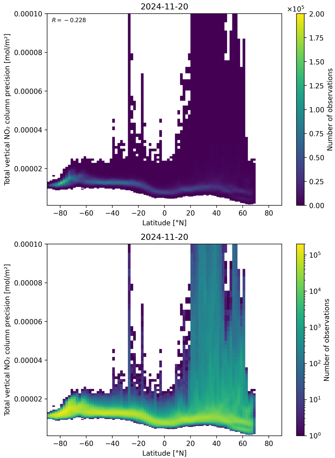
Figure 91: Scatter density plot of “Latitude” against “Total vertical NO 2 column precision” for 2024-11-20 to 2024-11-21.
