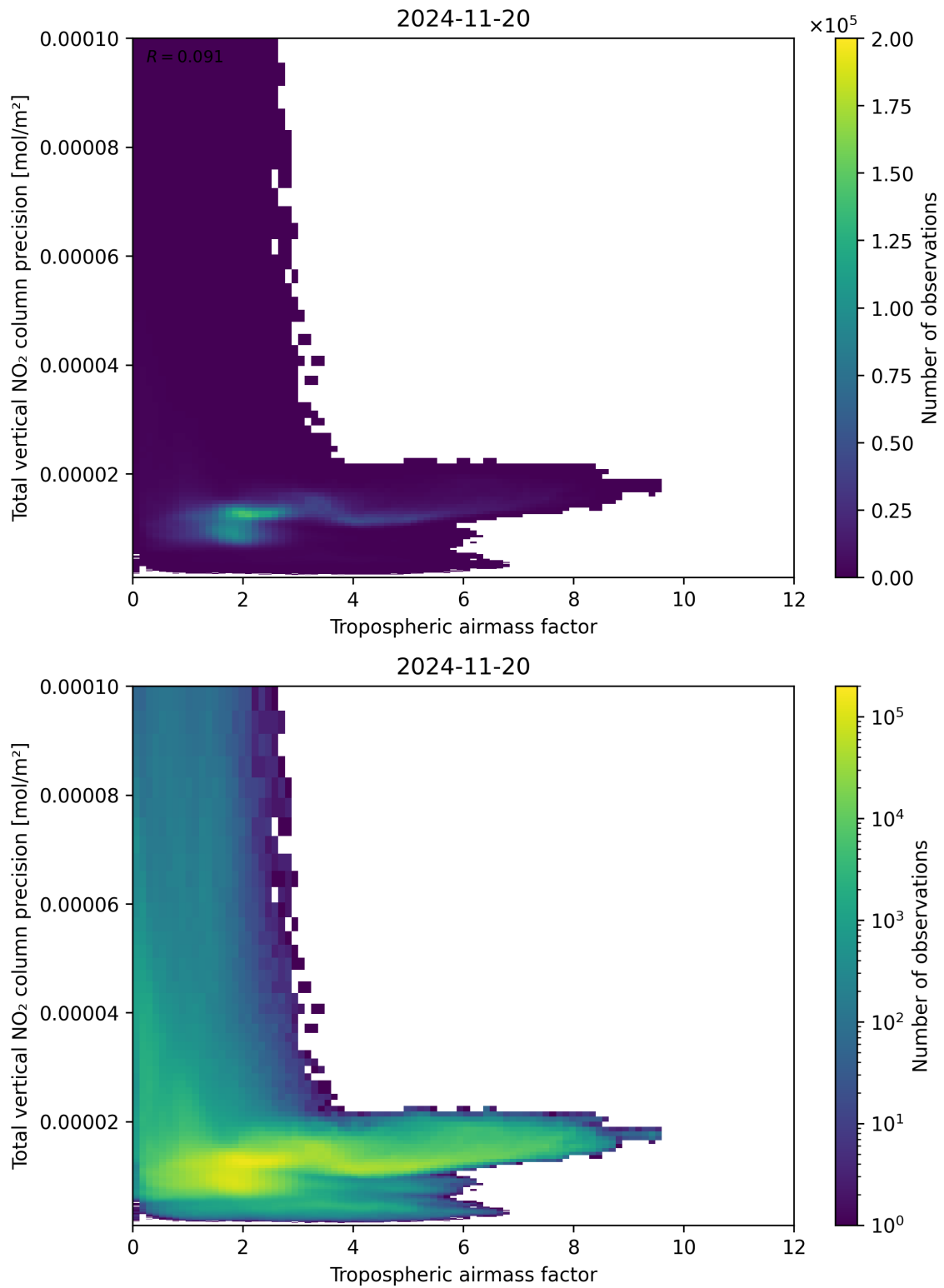
Figure 78: Scatter density plot of “Tropospheric air mass factor” against “Total vertical NO 2 column precision” for 2024-11-20 to 2024-11-21.
