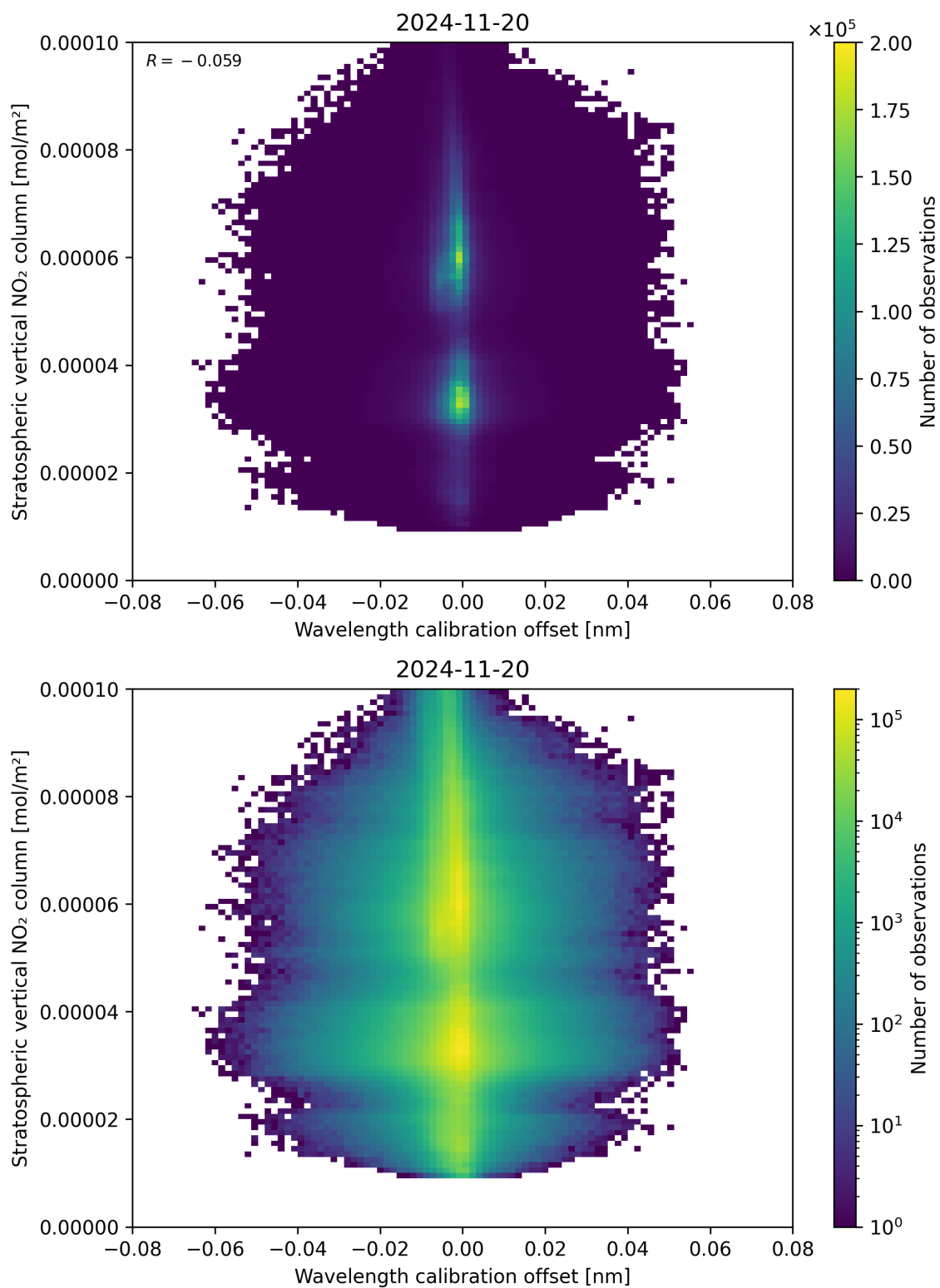
Figure 176: Scatter density plot of “Wavelength calibration offset” against “Stratospheric vertical NO 2 column” for 2024-11-20 to 2024-11-21.
