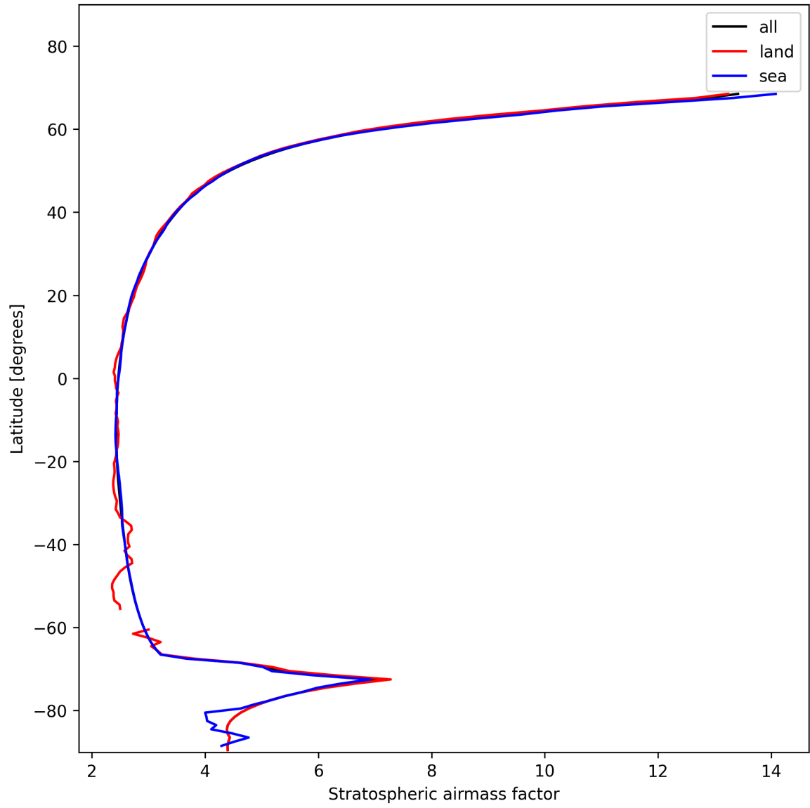
Figure 27: Zonal average of “Stratospheric air mass factor” for 2024-11-20 to 2024-11-21.
