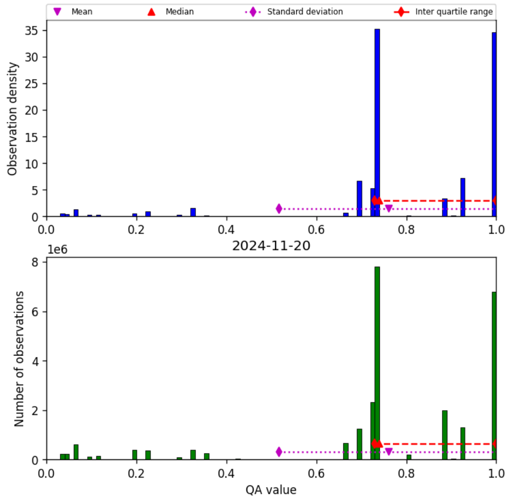
Figure 28: Histogram of “QA value” for 2024-11-20 to 2024-11-21
