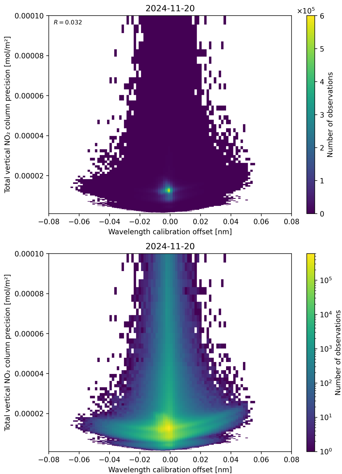
Figure 180: Scatter density plot of “Wavelength calibration offset” against “Total vertical NO 2 column precision” for 2024-11-20 to 2024-11-21.
