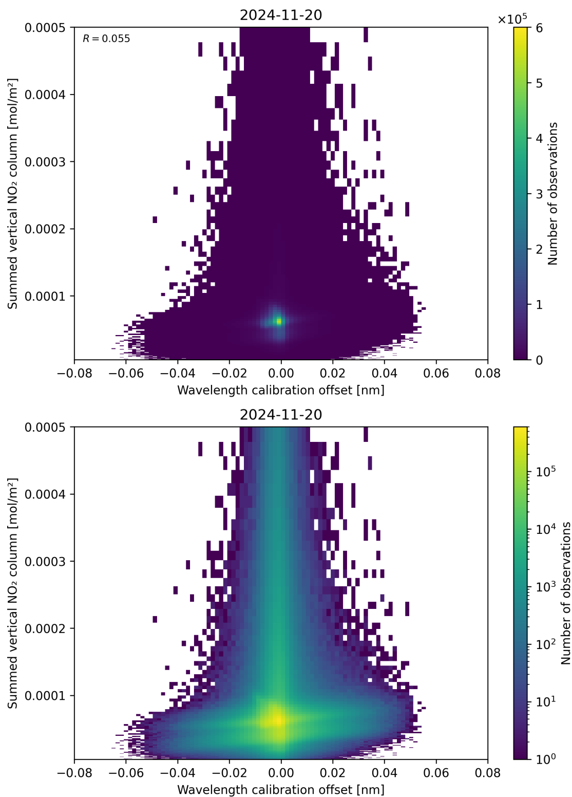
Figure 177: Scatter density plot of “Wavelength calibration offset” against “Summed vertical NO 2 column” for 2024-11-20 to 2024-11-21.
