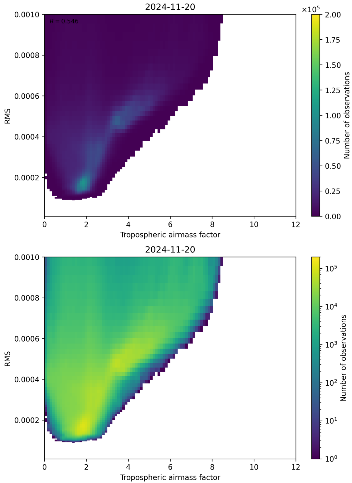
Figure 79: Scatter density plot of “Tropospheric airmass factor” against “RMS” for 2024-11-20 to 2024-11-21.
