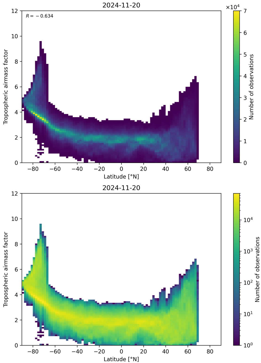
Figure 85: Scatter density plot of “Latitude” against “Tropospheric air mass factor” for 2024-11-20 to 2024-11-21.
