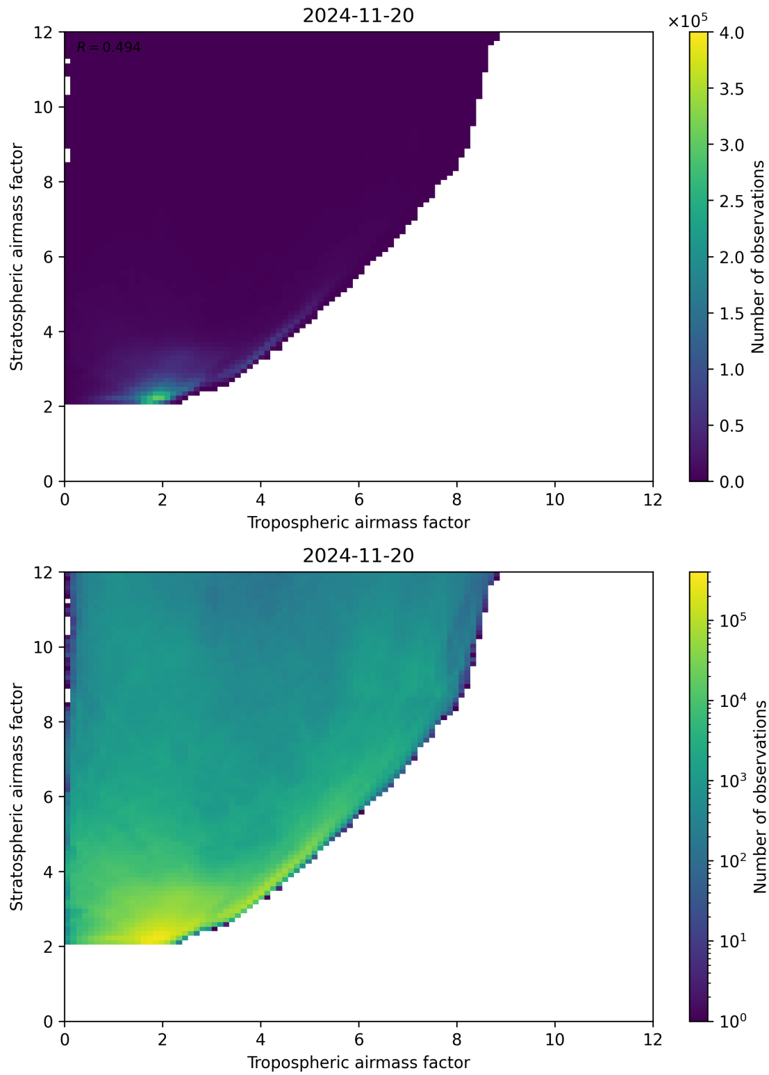
Figure 71: Scatter density plot of “Tropospheric airmass factor” against “Stratospheric airmass factor” for 2024-11-20 to 2024-11-21.
