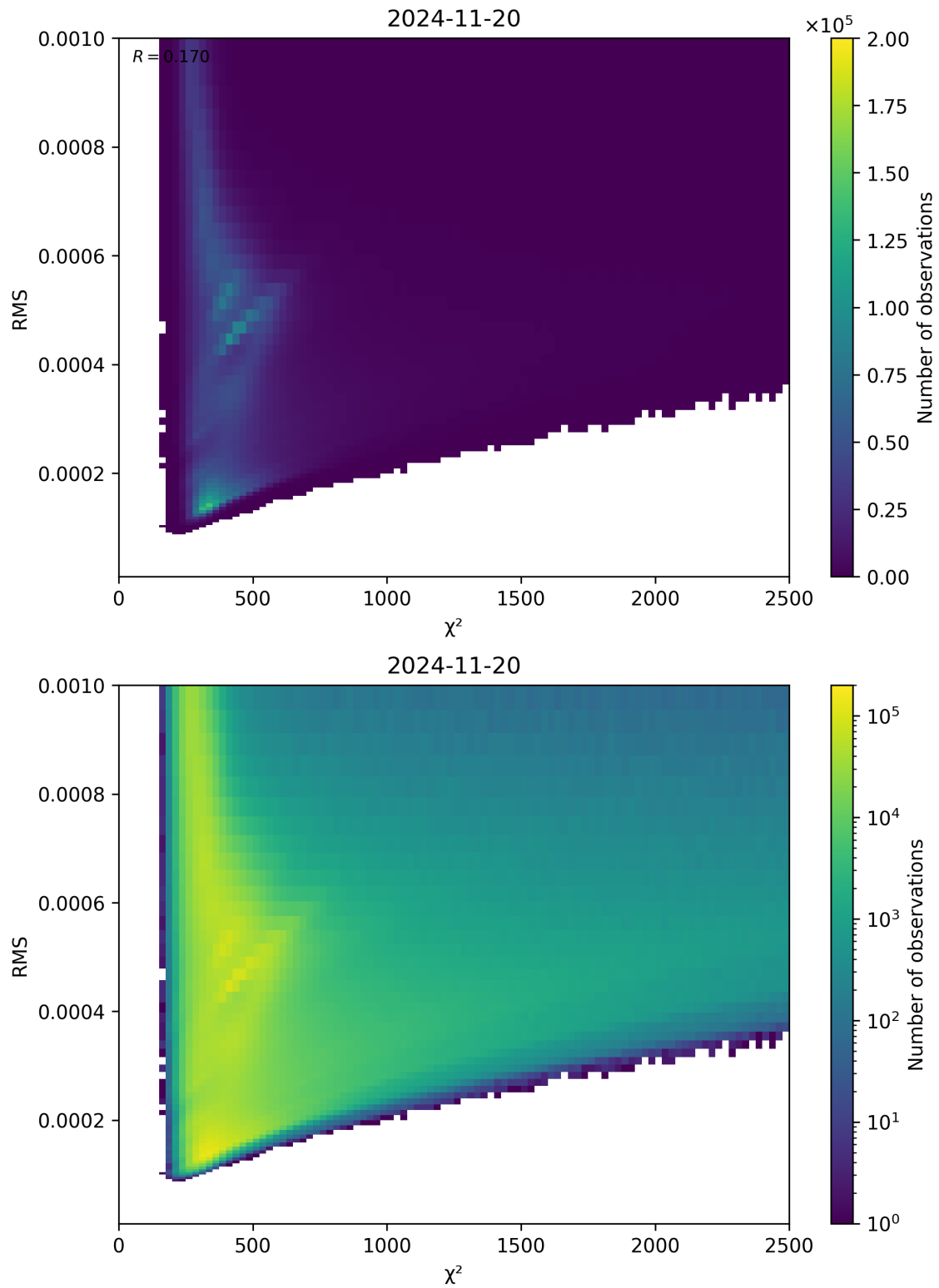
Figure 82: Scatter density plot of “ \chi^2 ” against “RMS” for 2024-11-20 to 2024-11-21.
