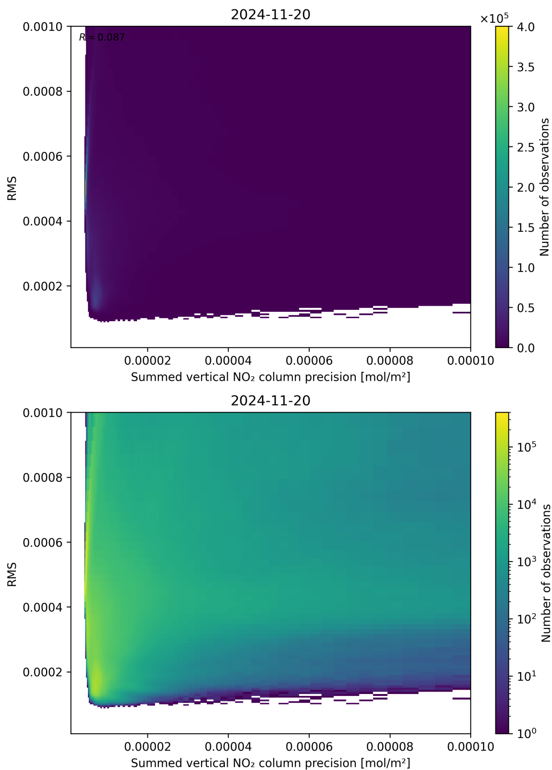
Figure 108: Scatter density plot of “Summed vertical NO 2 column precision” against “RMS” for 2024-11-20 to 2024-11-21.
