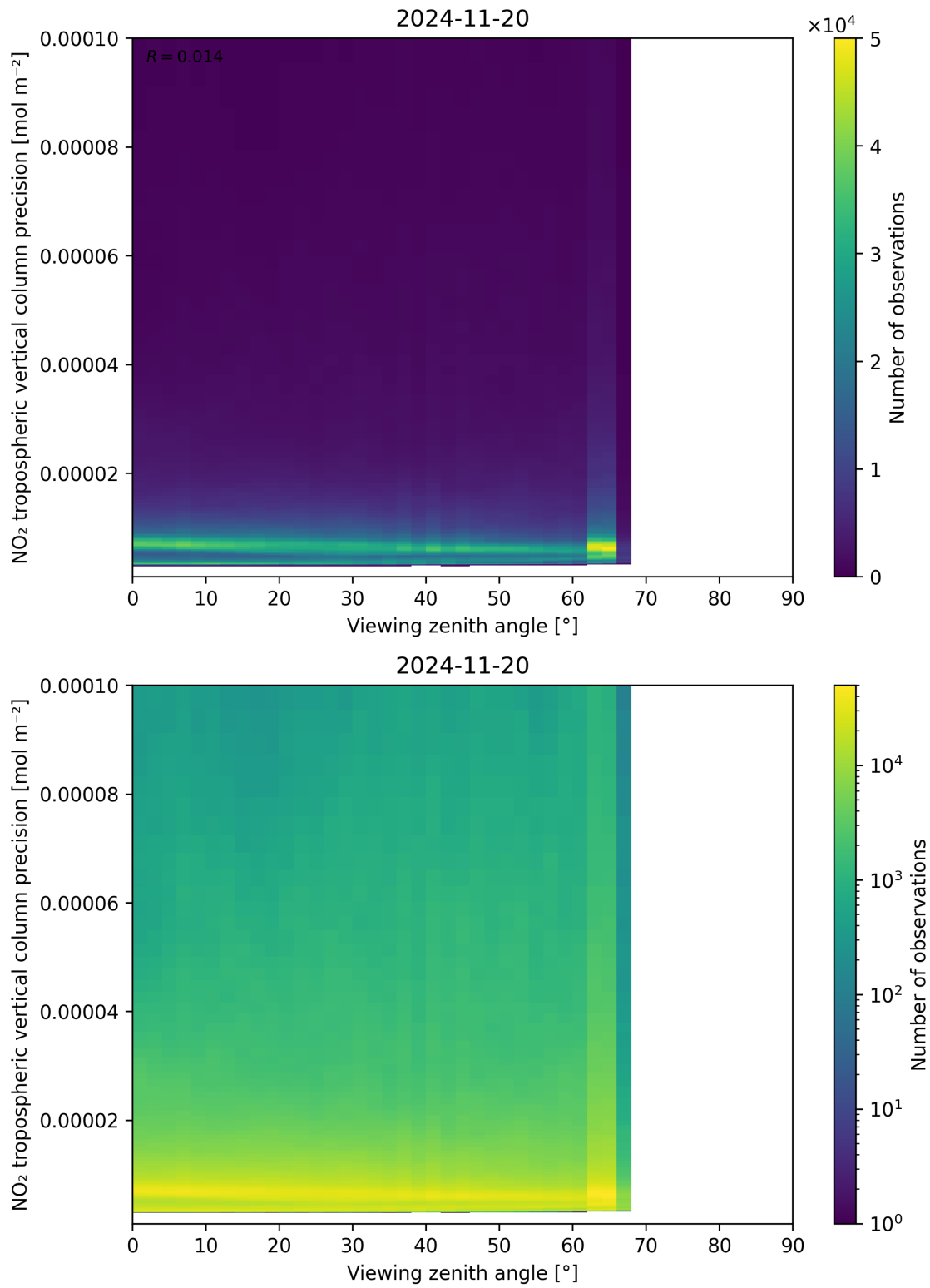
Figure 170: Scatter density plot of “Viewing zenith angle” against “NO 2 tropospheric vertical column precision” for 2024-11-20 to 2024-11-21.
