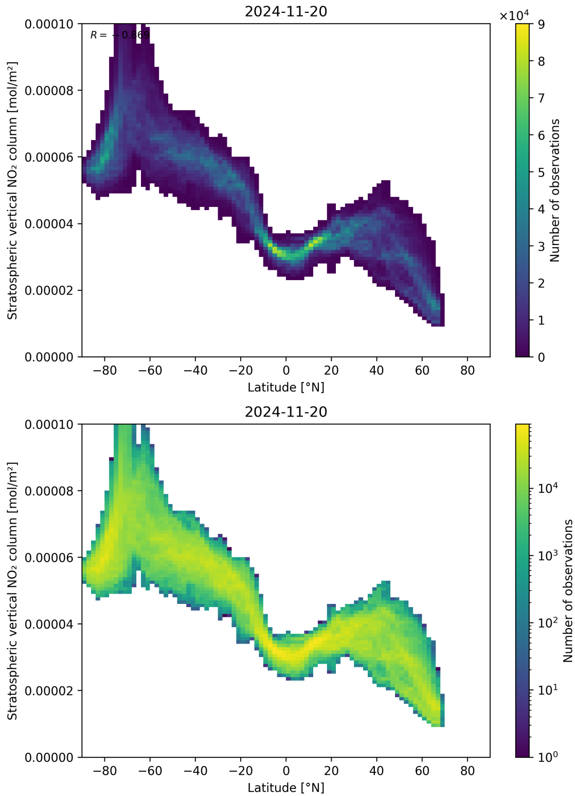
Figure 87: Scatter density plot of “Latitude” against “Stratospheric vertical NO 2 column” for 2024-11-20 to 2024-11-21.
