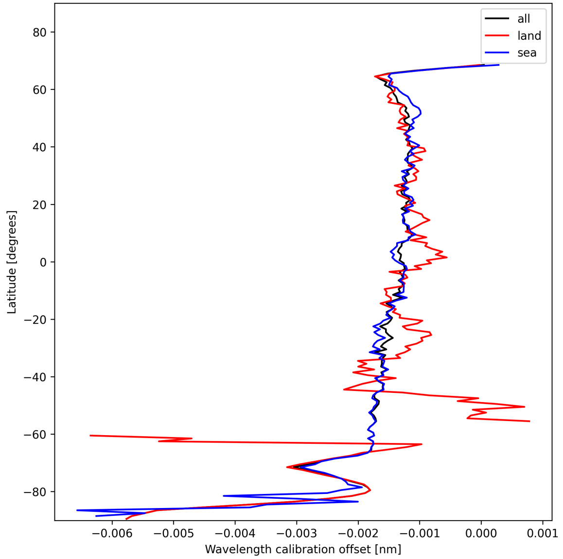
Figure 18: Zonal average of “Wavelength calibration offset” for 2024-11-20 to 2024-11-21.
