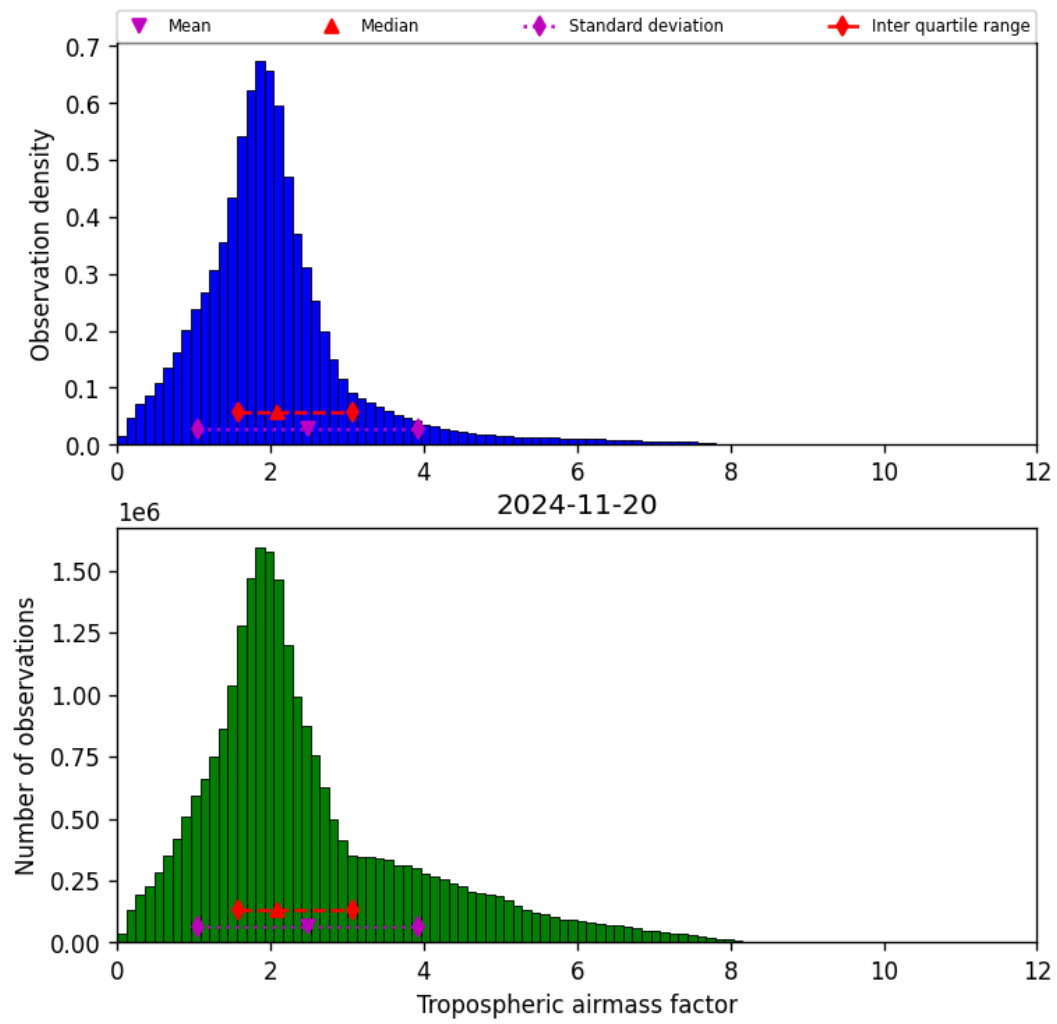
Figure 31: Histogram of “Tropospheric airmass factor” for 2024-11-20 to 2024-11-21
