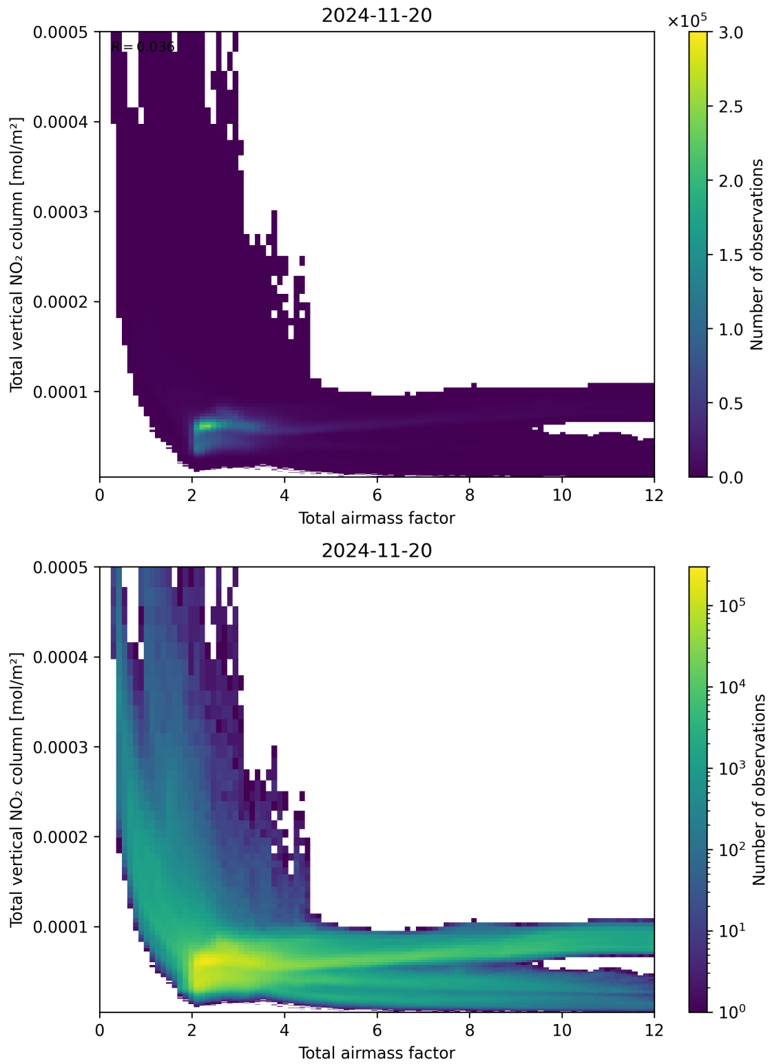
Figure 67: Scatter density plot of “Total airmass factor” against “Total vertical NO 2 column” for 2024-11-20 to 2024-11-21.
