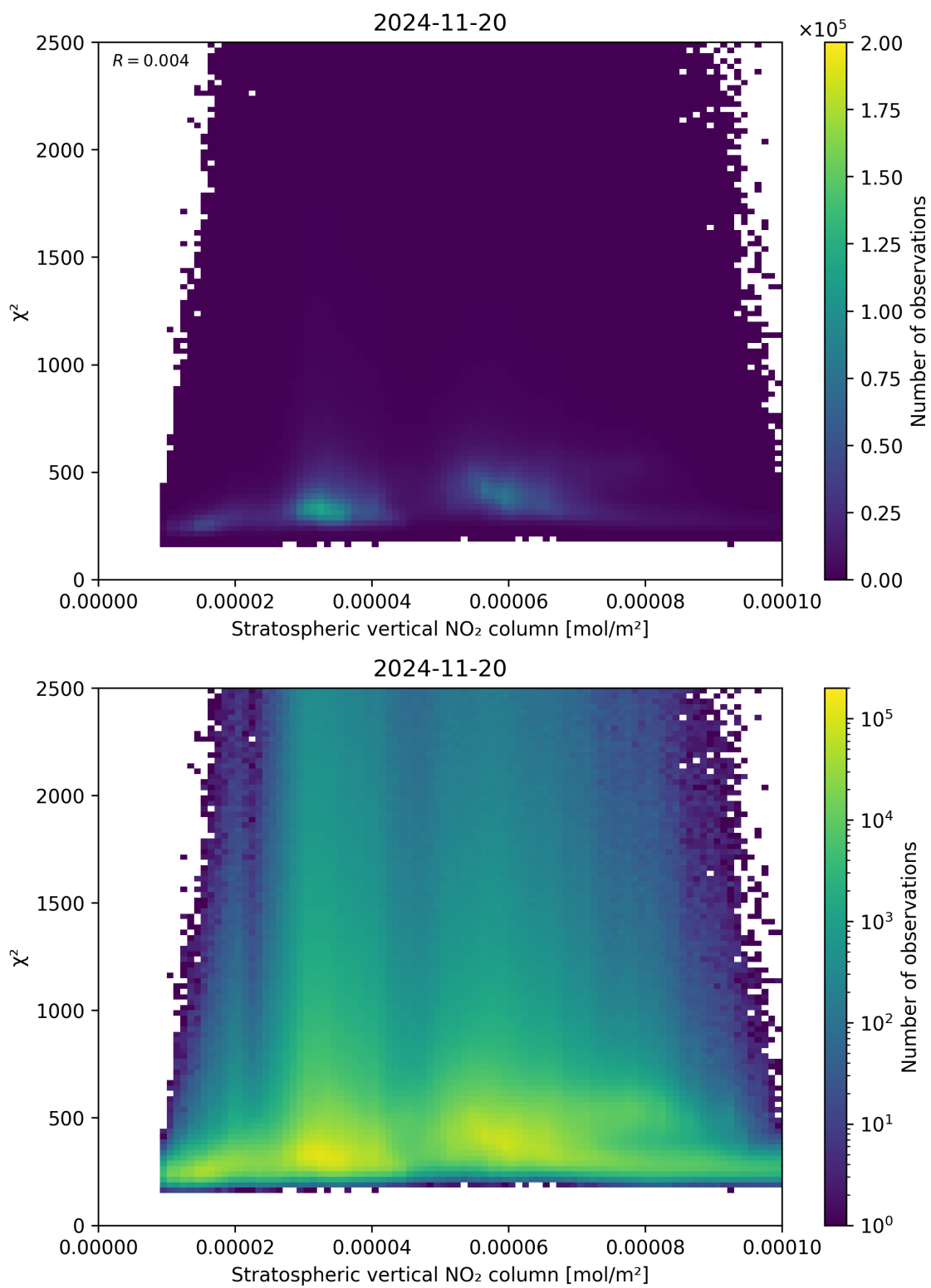
Figure 97: Scatter density plot of “Stratospheric vertical NO 2 column” against “ \chi^2 ” for 2024-11-20 to 2024-11-21.
