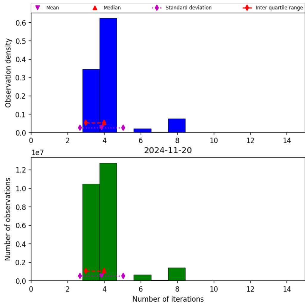
Figure 34: Histogram of “Number of iterations” for 2024-11-20 to 2024-11-21
