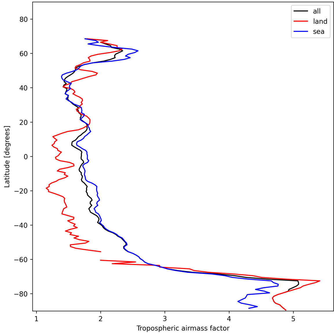
Figure 14: Zonal average of “Tropospheric airmass factor” for 2024-11-20 to 2024-11-21.
