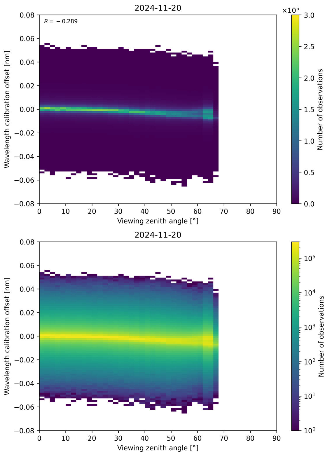
Figure 173: Scatter density plot of “Viewing zenith angle” against “Wavelength calibration offset” for 2024-11-20 to 2024-11-21.
