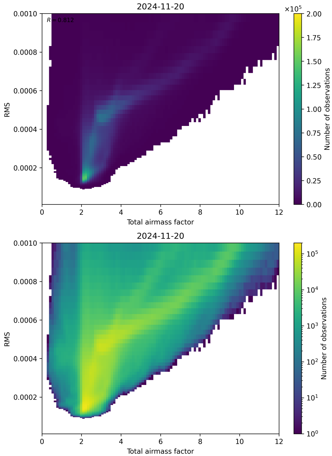
Figure 69: Scatter density plot of “Total airmass factor” against “RMS” for 2024-11-20 to 2024-11-21.
