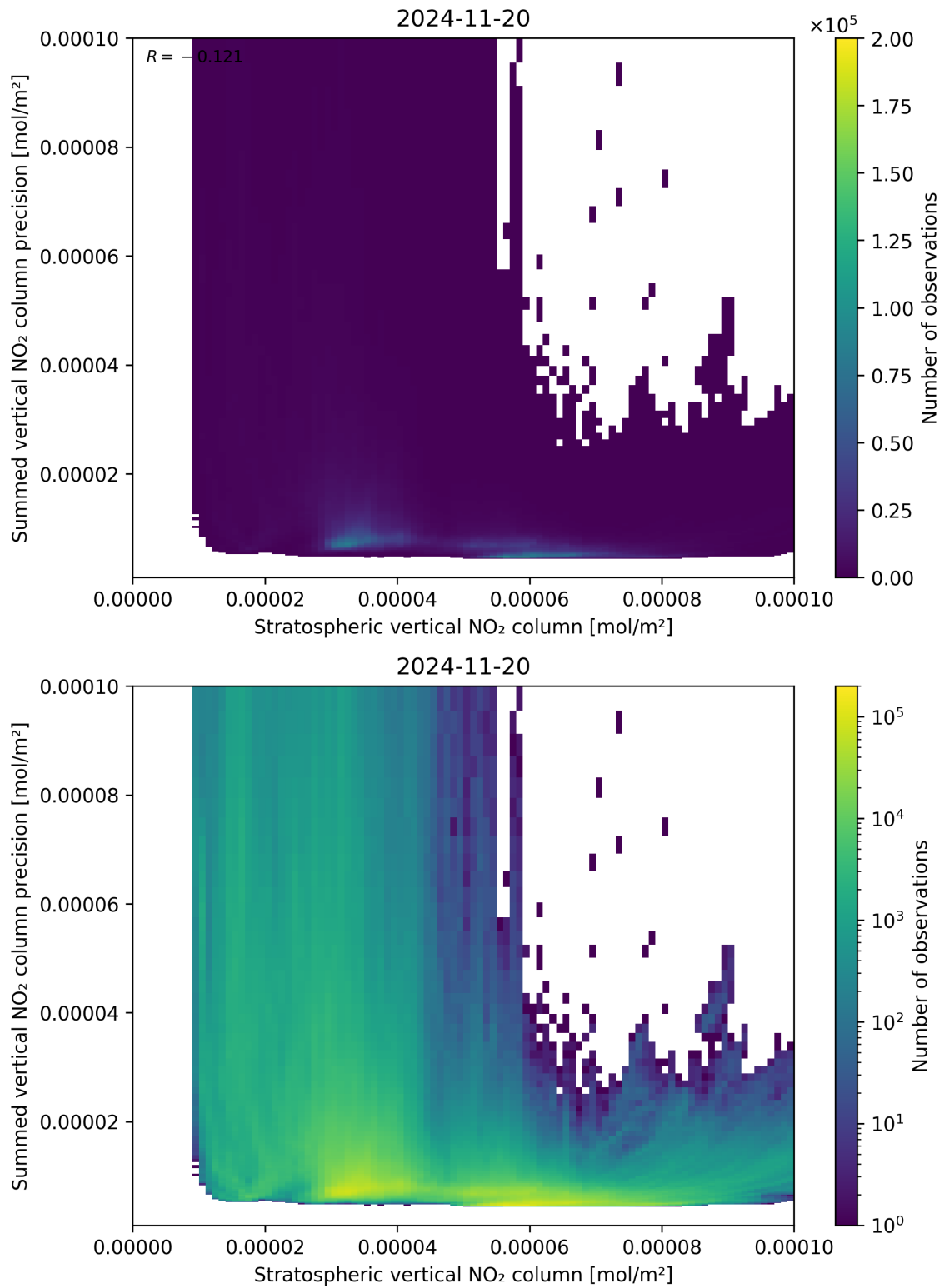
Figure 99: Scatter density plot of “Stratospheric vertical NO 2 column” against “Summed vertical NO 2 column precision” for 2024-11-20 to 2024-11-21.
