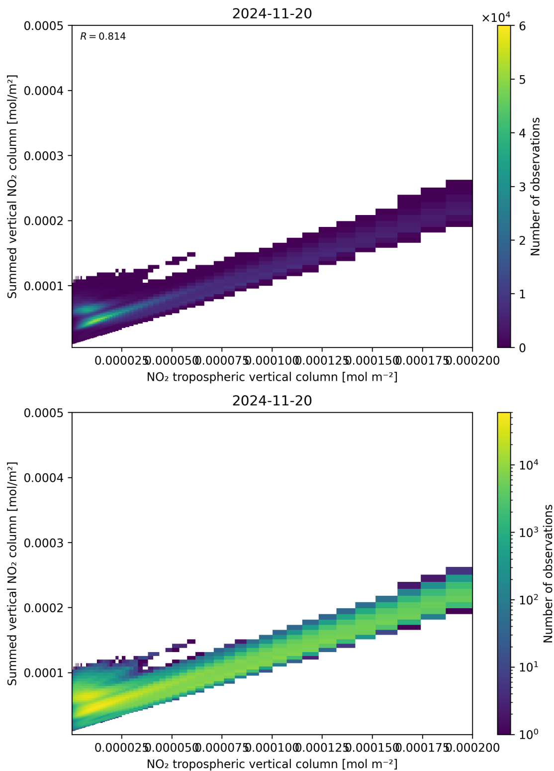
Figure 126: Scatter density plot of “NO 2 tropospheric vertical column” against “Summed vertical NO 2 column” for 2024-11-20 to 2024-11-21.
