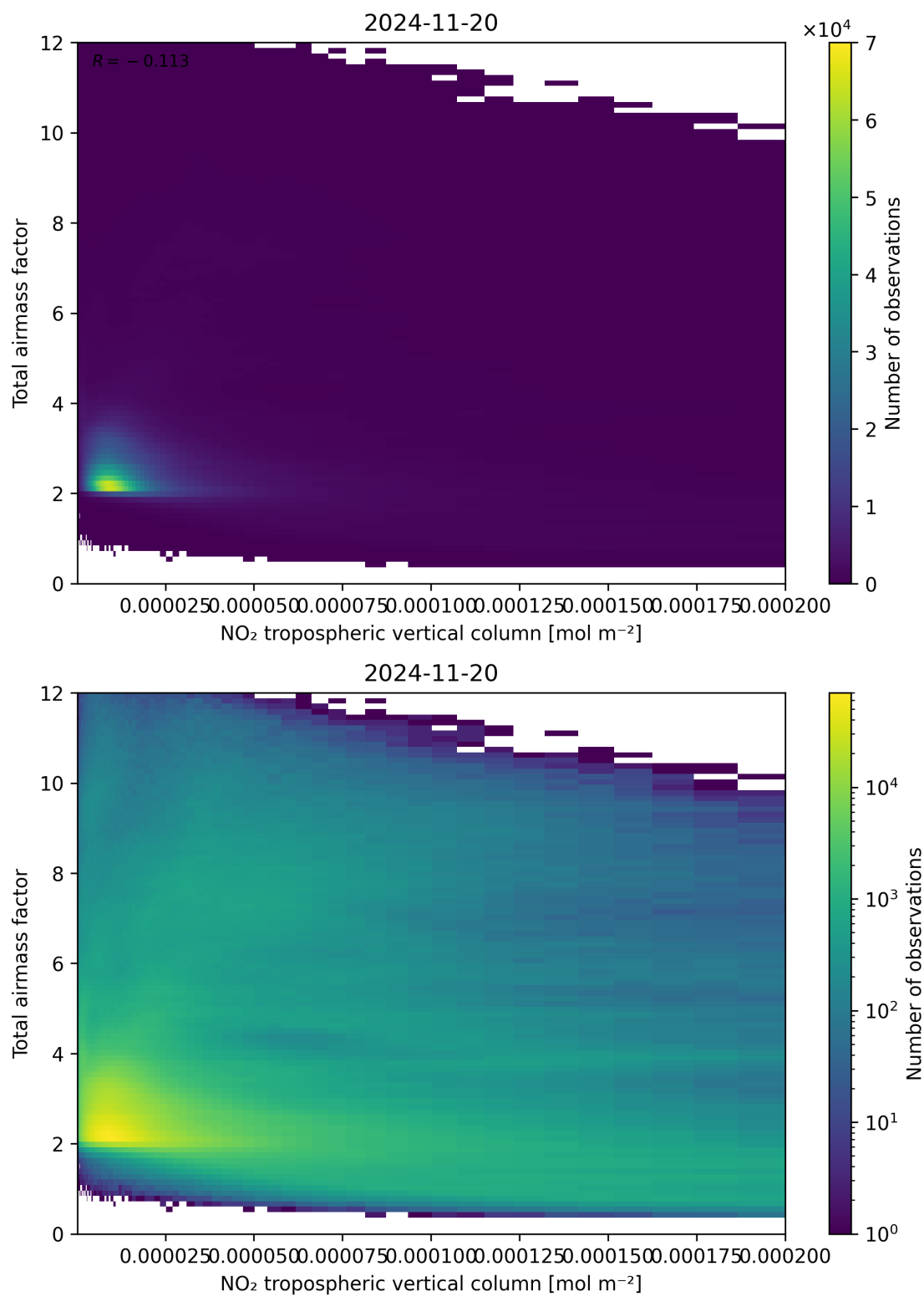
Figure 122: Scatter density plot of “NO 2 tropospheric vertical column” against “Total air mass factor” for 2024-11-20 to 2024-11-21.
