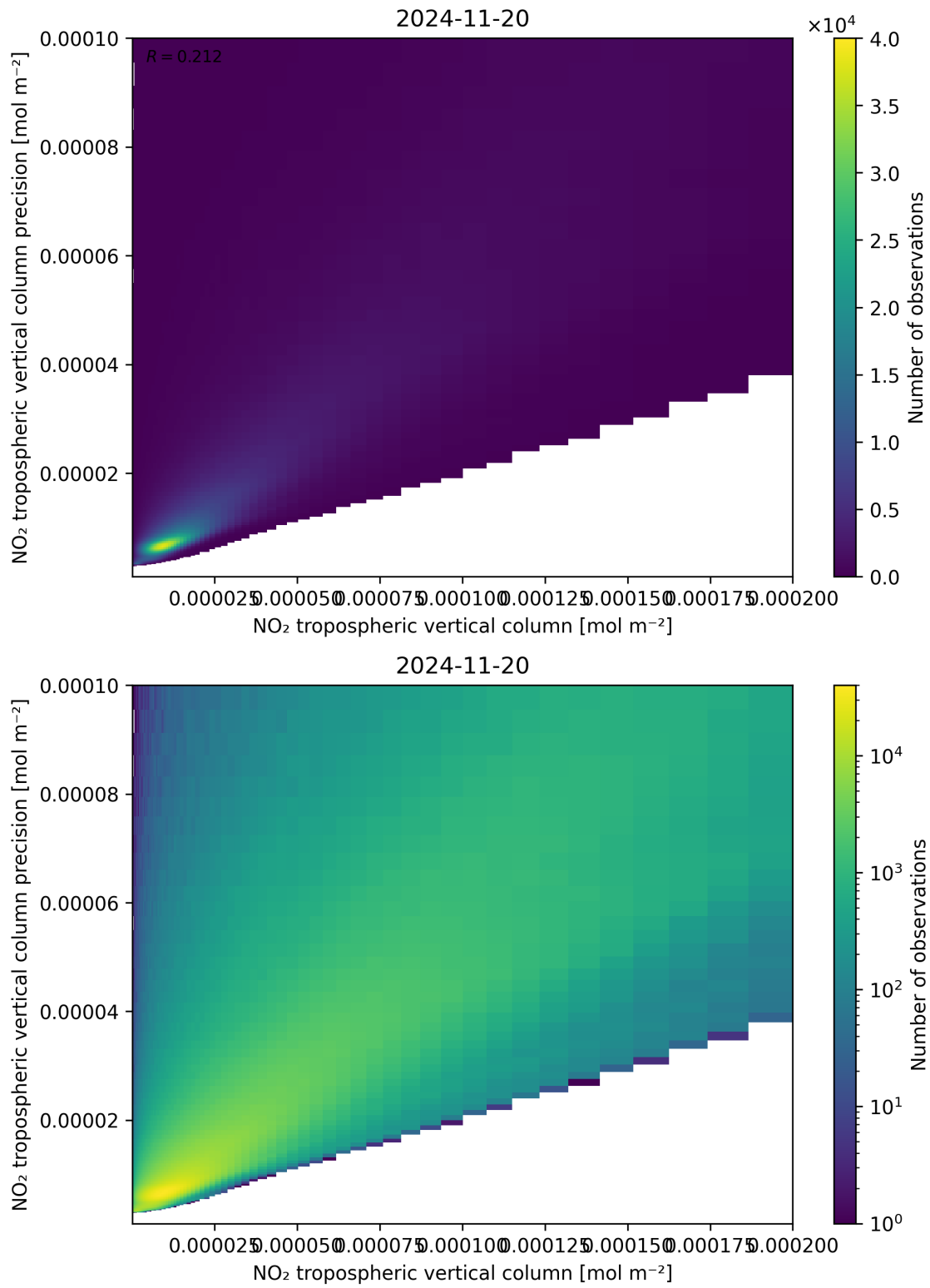
Figure 130: Scatter density plot of “NO 2 tropospheric vertical column” against “NO 2 tropospheric vertical column precision” for 2024-11-20 to 2024-11-21.
