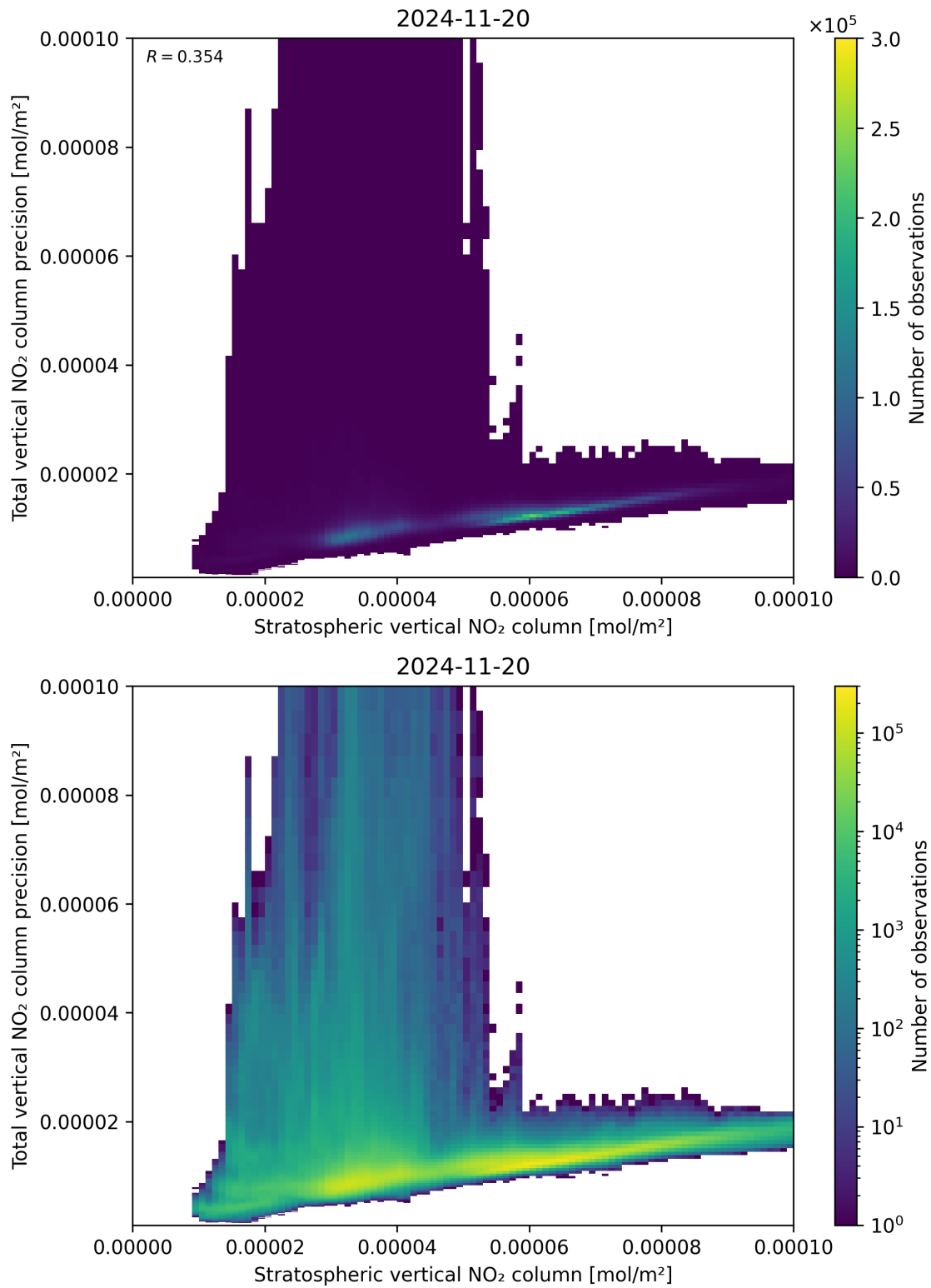
Figure 101: Scatter density plot of “Stratospheric vertical NO 2 column” against “Total vertical NO 2 column precision” for 2024-11-20 to 2024-11-21.
