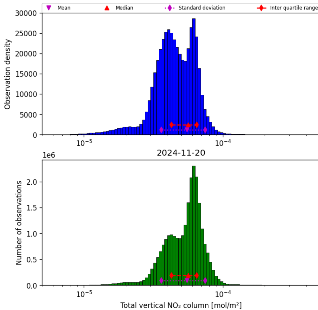
Figure 38: Histogram of "Total vertical NO 2 column" for 2024-11-20 to 2024-11-21
