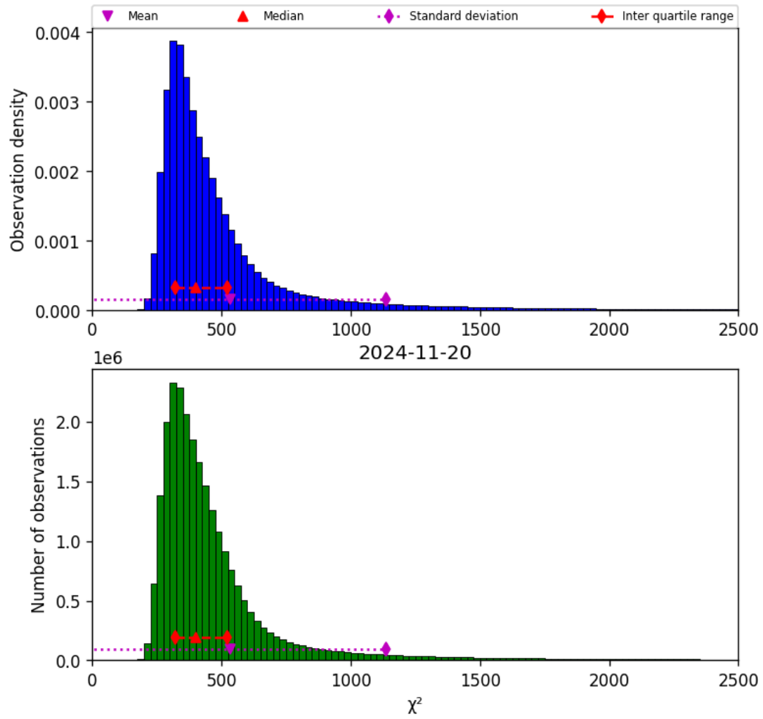
Figure 42: Histogram of “ \chi^2 ” for 2024-11-20 to 2024-11-21
