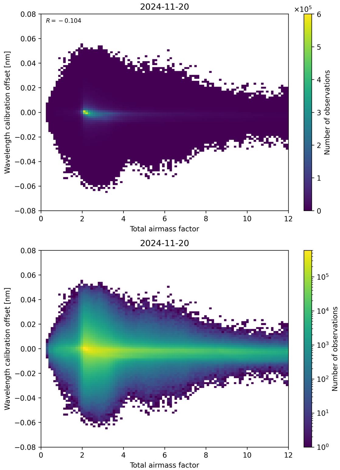
Figure 70: Scatter density plot of “Total airmass factor” against “Wavelength calibration offset” for 2024-11-20 to 2024-11-21.
