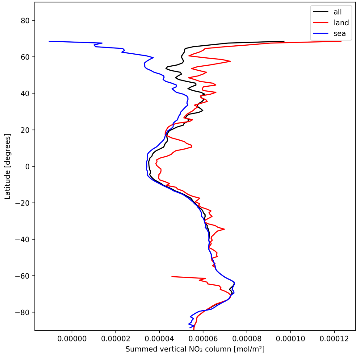
Figure 23: Zonal average of “Summed vertical NO 2 column” for 2024-11-20 to 2024-11-21.
