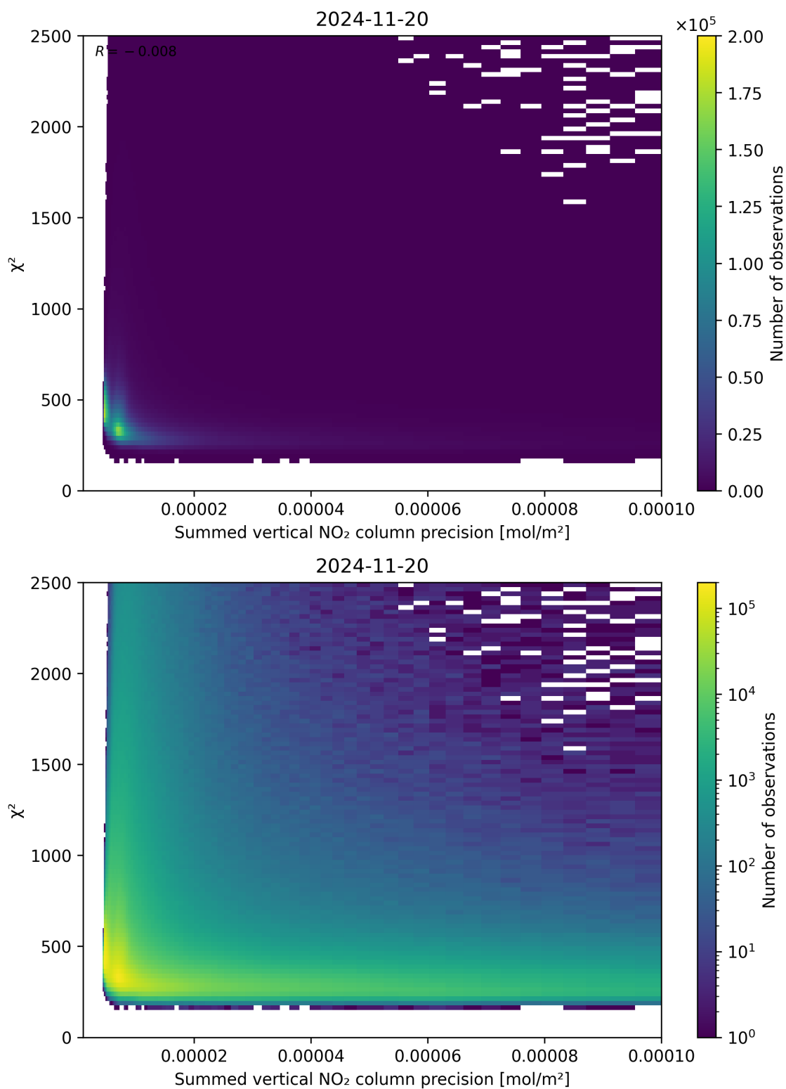
Figure 107: Scatter density plot of “Summed vertical NO 2 column precision” against “ \chi^2 ” for 2024-11-20 to 2024-11-21.
