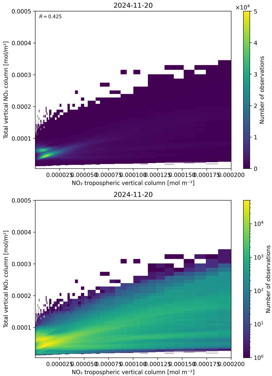
Figure 128: Scatter density plot of “NO 2 tropospheric vertical column” against “Total vertical NO 2 column” for 2024-11-20 to 2024-11-21.
