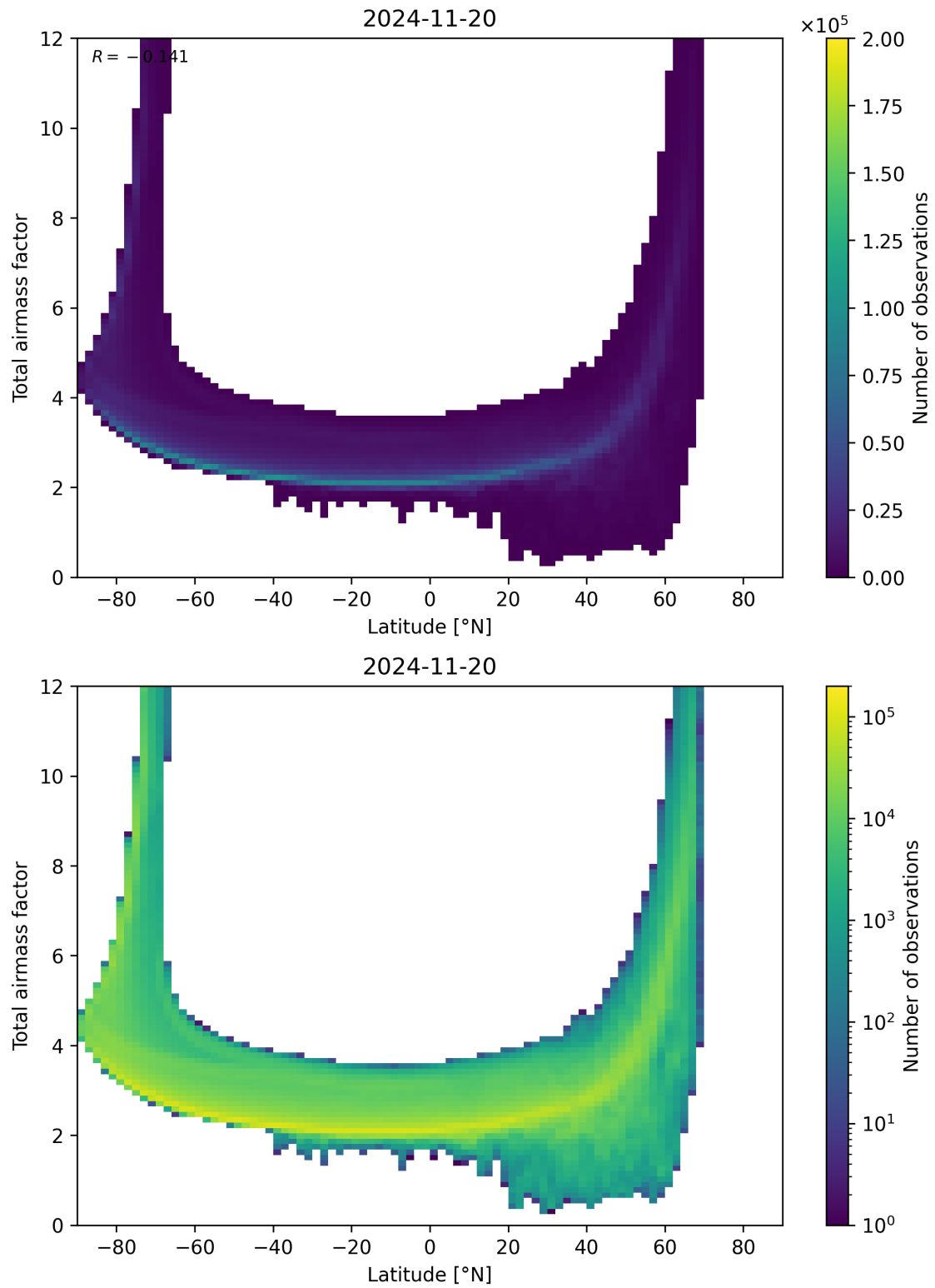
Figure 84: Scatter density plot of “Latitude” against “Total airmass factor” for 2024-11-20 to 2024-11-21.
