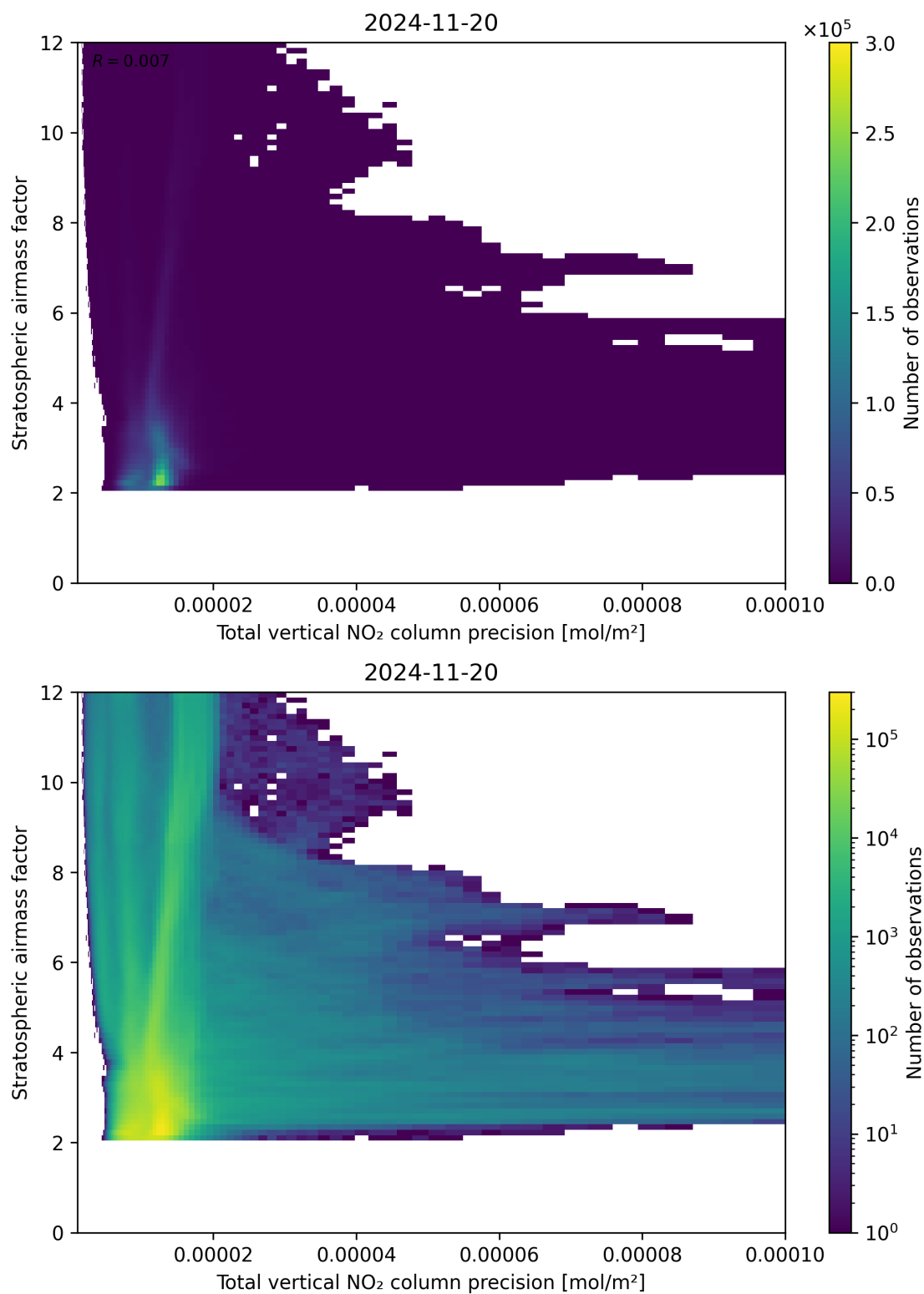
Figure 115: Scatter density plot of “Total vertical NO 2 column precision” against “Stratospheric air mass factor” for 2024-11-20 to 2024-11-21.
