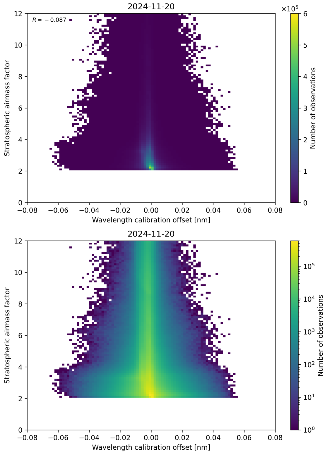
Figure 174: Scatter density plot of “Wavelength calibration offset” against “Stratospheric airmass factor” for 2024-11-20 to 2024-11-21.
