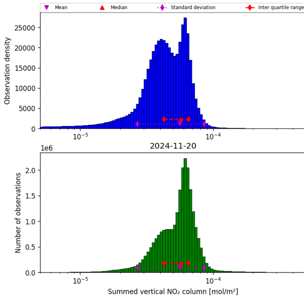
Figure 40: Histogram of “Summed vertical NO 2 column” for 2024-11-20 to 2024-11-21
