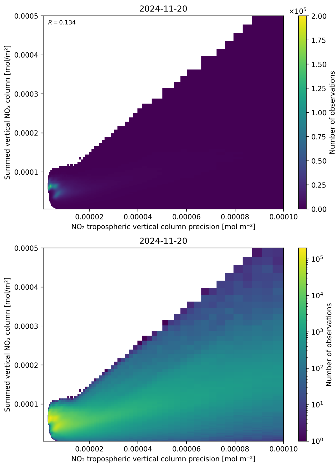
Figure 136: Scatter density plot of “NO 2 tropospheric vertical column precision” against “Summed vertical NO 2 column” for 2024-11-20 to 2024-11-21.
