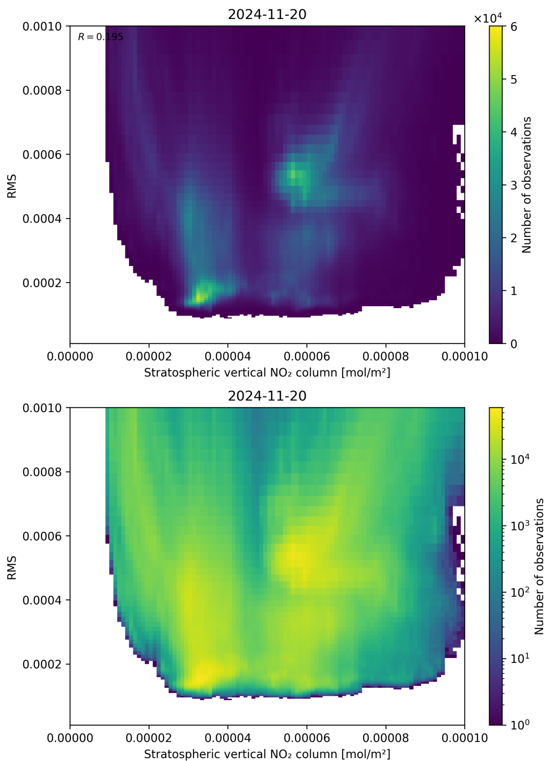
Figure 102: Scatter density plot of “Stratospheric vertical NO 2 column” against “RMS” for 2024-11-20 to 2024-11-21.
