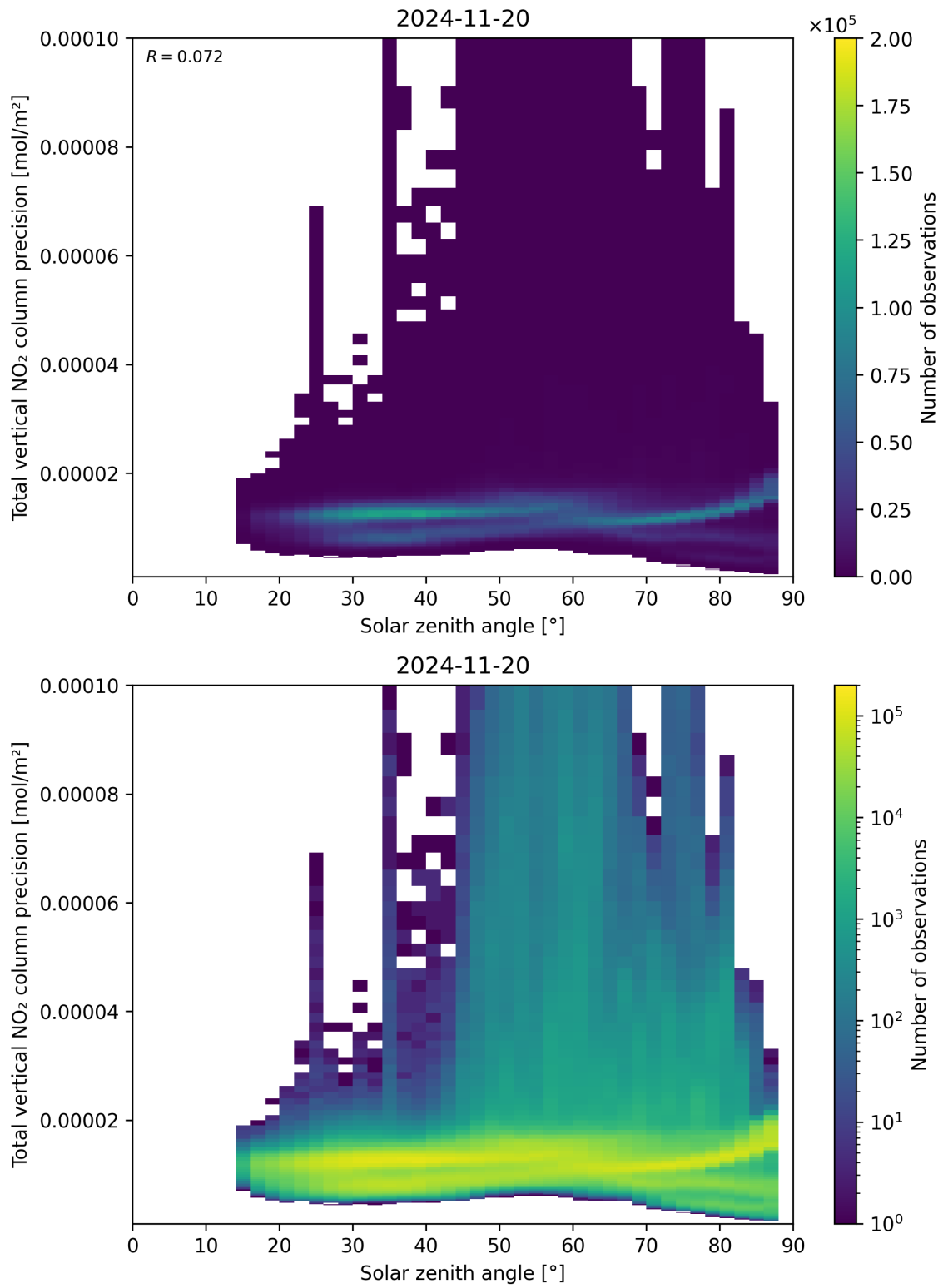
Figure 154: Scatter density plot of “Solar zenith angle” against “Total vertical NO 2 column precision” for 2024-11-20 to 2024-11-21.
