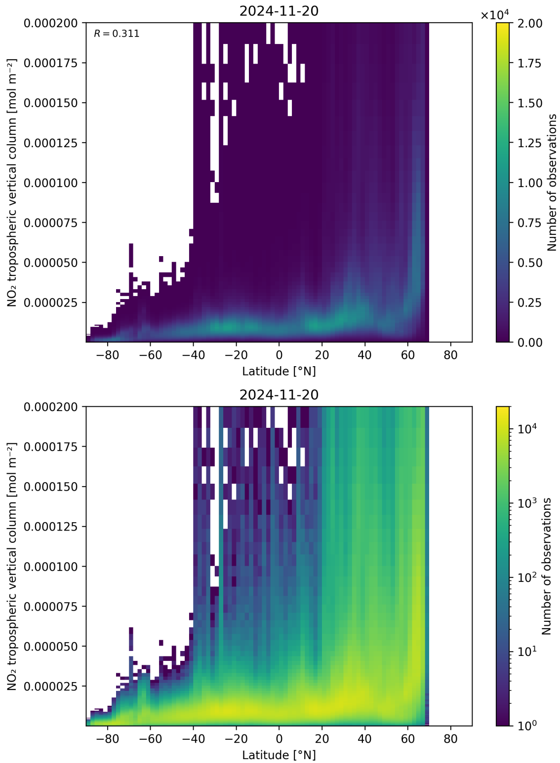
Figure 92: Scatter density plot of “Latitude” against “NO 2 tropospheric vertical column” for 2024-11-20 to 2024-11-21.
