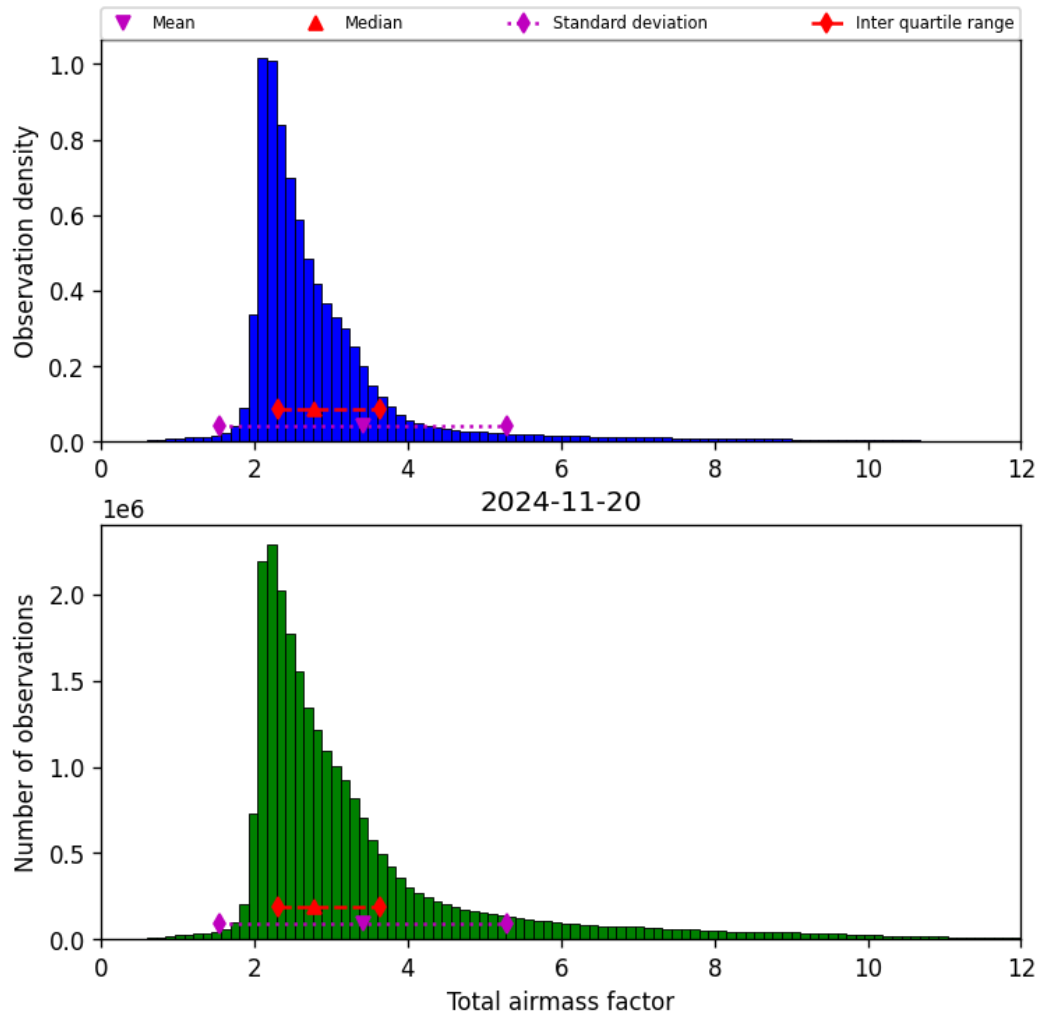
Figure 32: Histogram of “Total airmass factor” for 2024-11-20 to 2024-11-21
