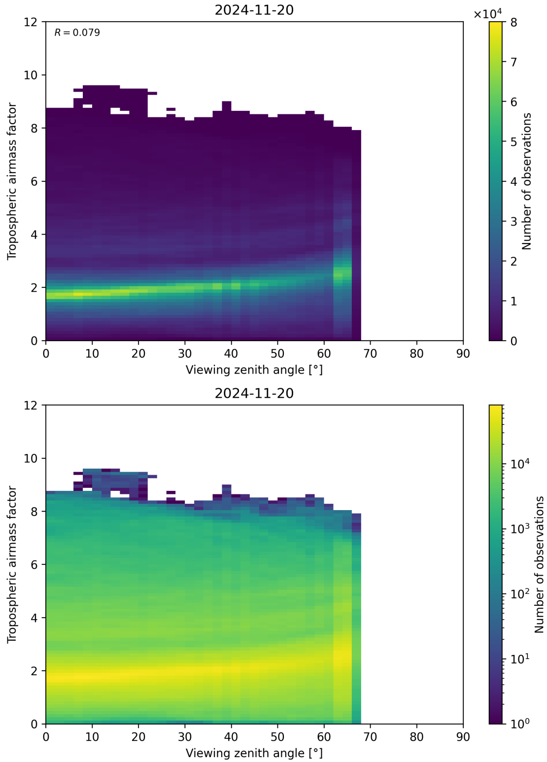
Figure 161: Scatter density plot of “Viewing zenith angle” against “Tropospheric airmass factor” for 2024-11-20 to 2024-11-21.
