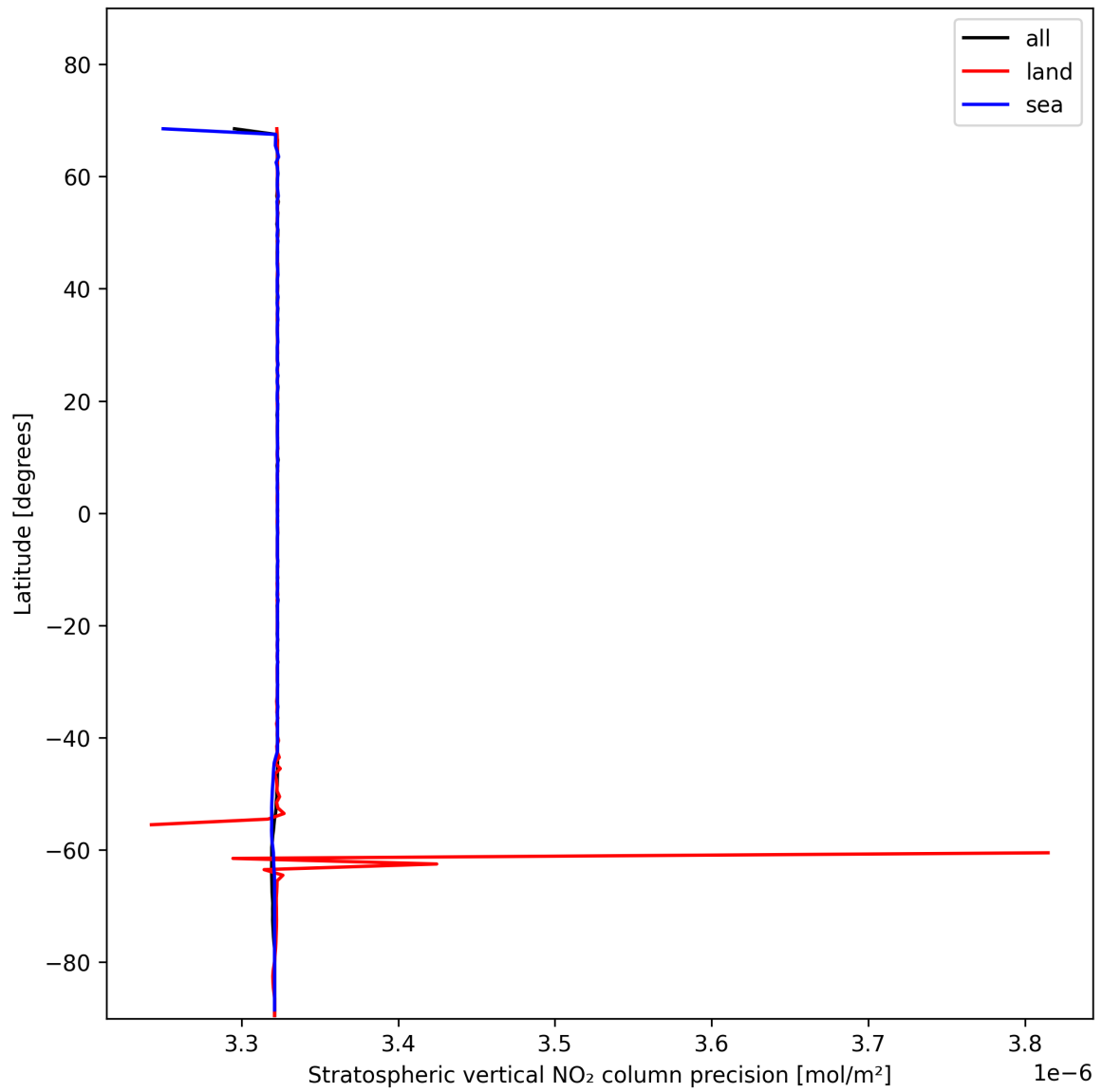
Figure 20: Zonal average of “Stratospheric vertical NO 2 column precision” for 2024-11-20 to 2024-11-21.
