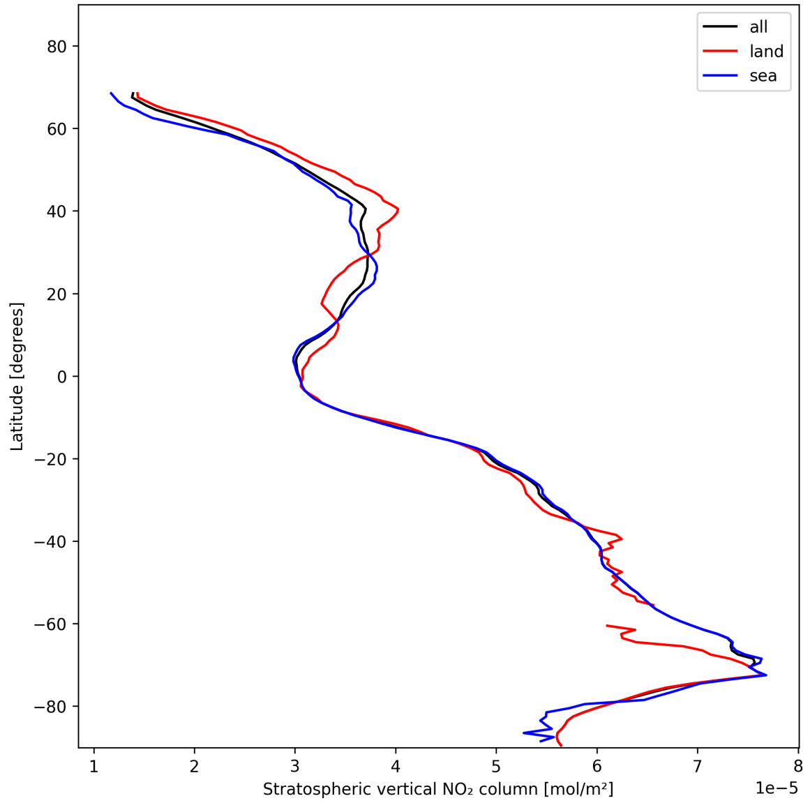
Figure 19: Zonal average of “Stratospheric vertical NO 2 column” for 2024-11-20 to 2024-11-21.
