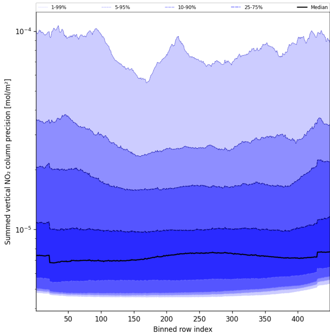
Figure 58: Along track statistics of “Summed vertical NO 2 column precision” for 2024-11-20 to 2024-11-21
