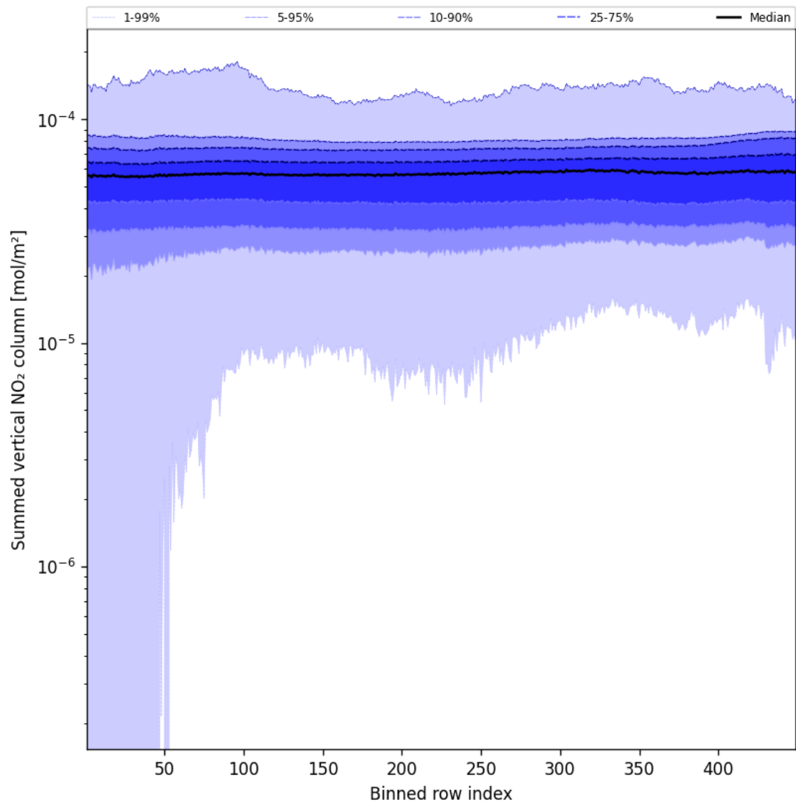
Figure 57: Along track statistics of “Summed vertical NO 2 column” for 2024-11-20 to 2024-11-21
