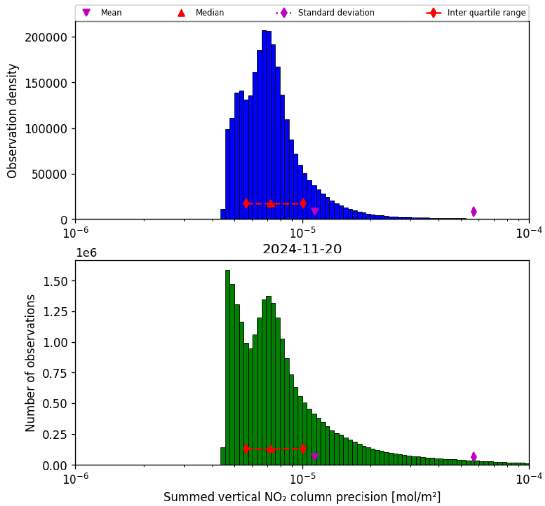
Figure 41: Histogram of “Summed vertical NO 2 column precision” for 2024-11-20 to 2024-11-21
