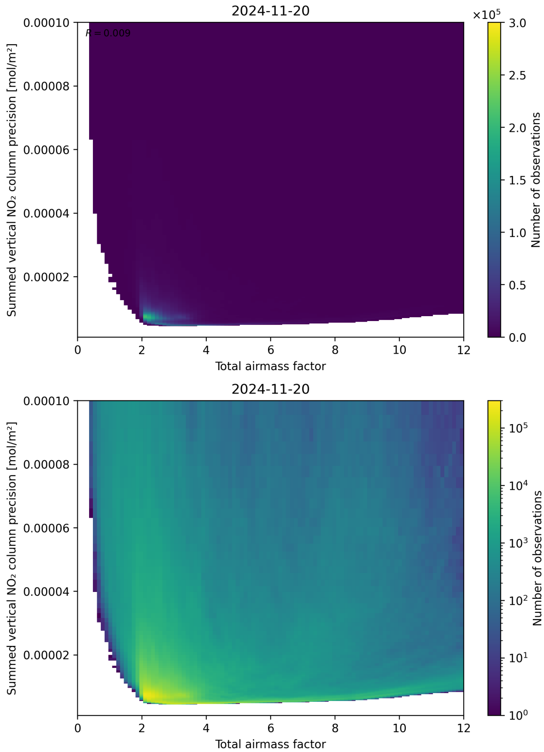
Figure 66: Scatter density plot of “Total airmass factor” against “Summed vertical NO 2 column precision” for 2024-11-20 to 2024-11-21.
