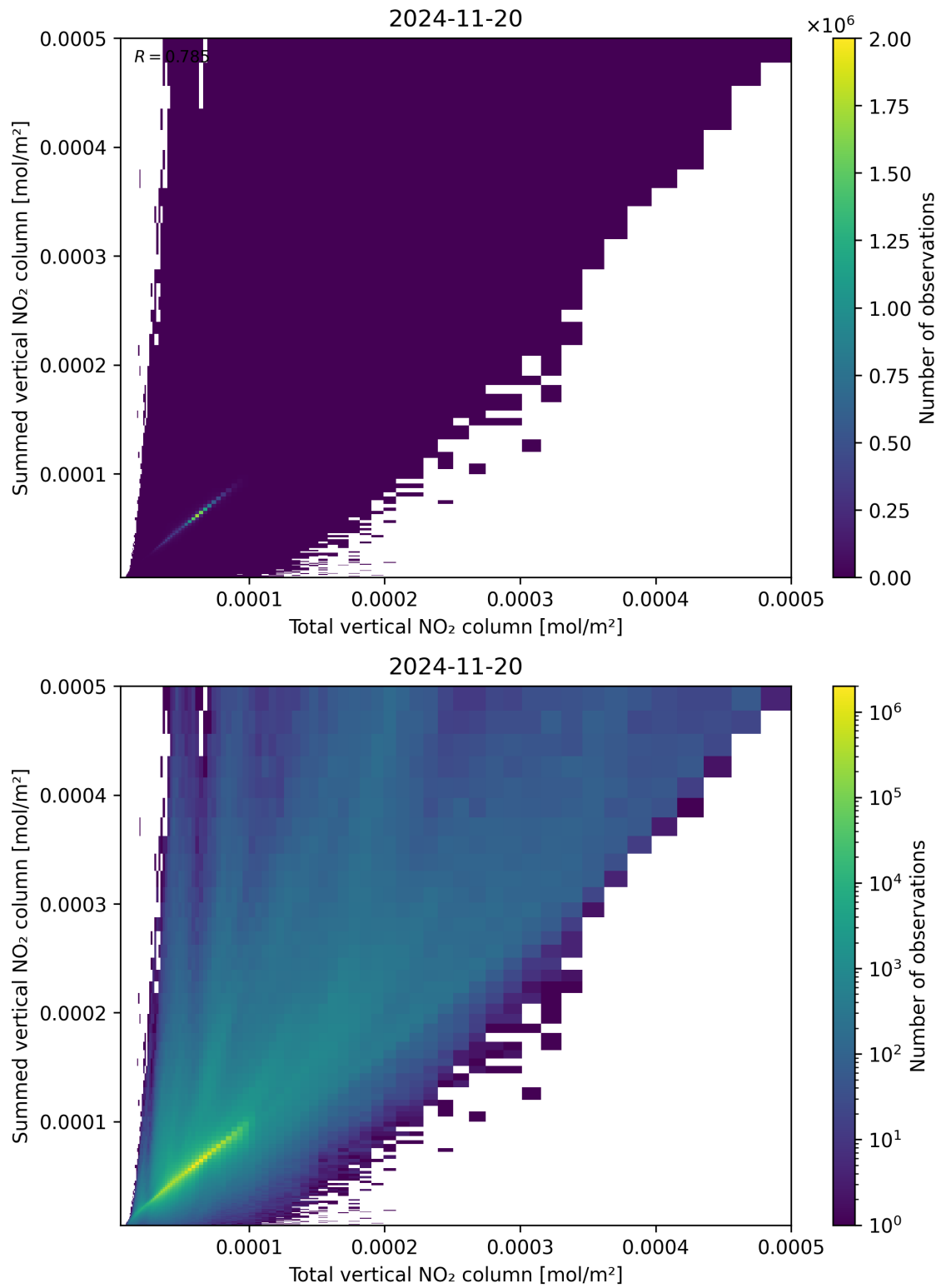
Figure 112: Scatter density plot of “Total vertical NO 2 column” against “Summed vertical NO 2 column” for 2024-11-20 to 2024-11-21.
