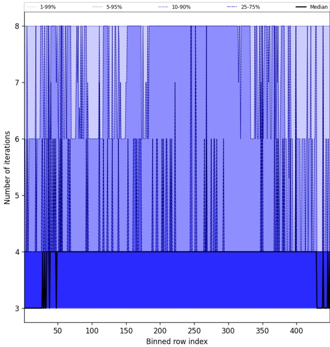
Figure 51: Along track statistics of “Number of iterations” for 2024-11-20 to 2024-11-21
