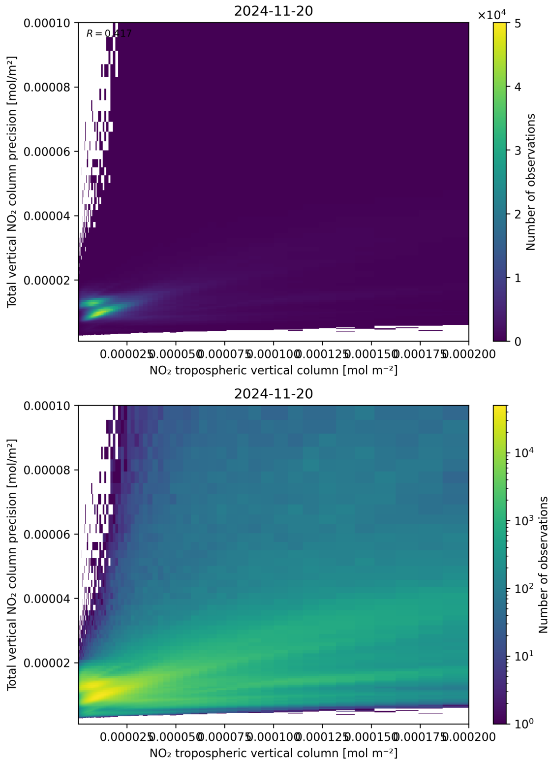
Figure 129: Scatter density plot of “NO 2 tropospheric vertical column” against “Total vertical NO 2 column precision” for 2024-11-20 to 2024-11-21.
