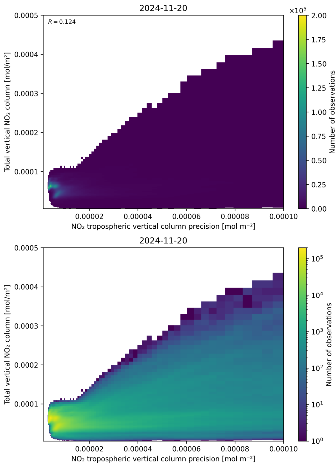
Figure 138: Scatter density plot of “NO 2 tropospheric vertical column precision” against “Total vertical NO 2 column” for 2024-11-20 to 2024-11-21.
