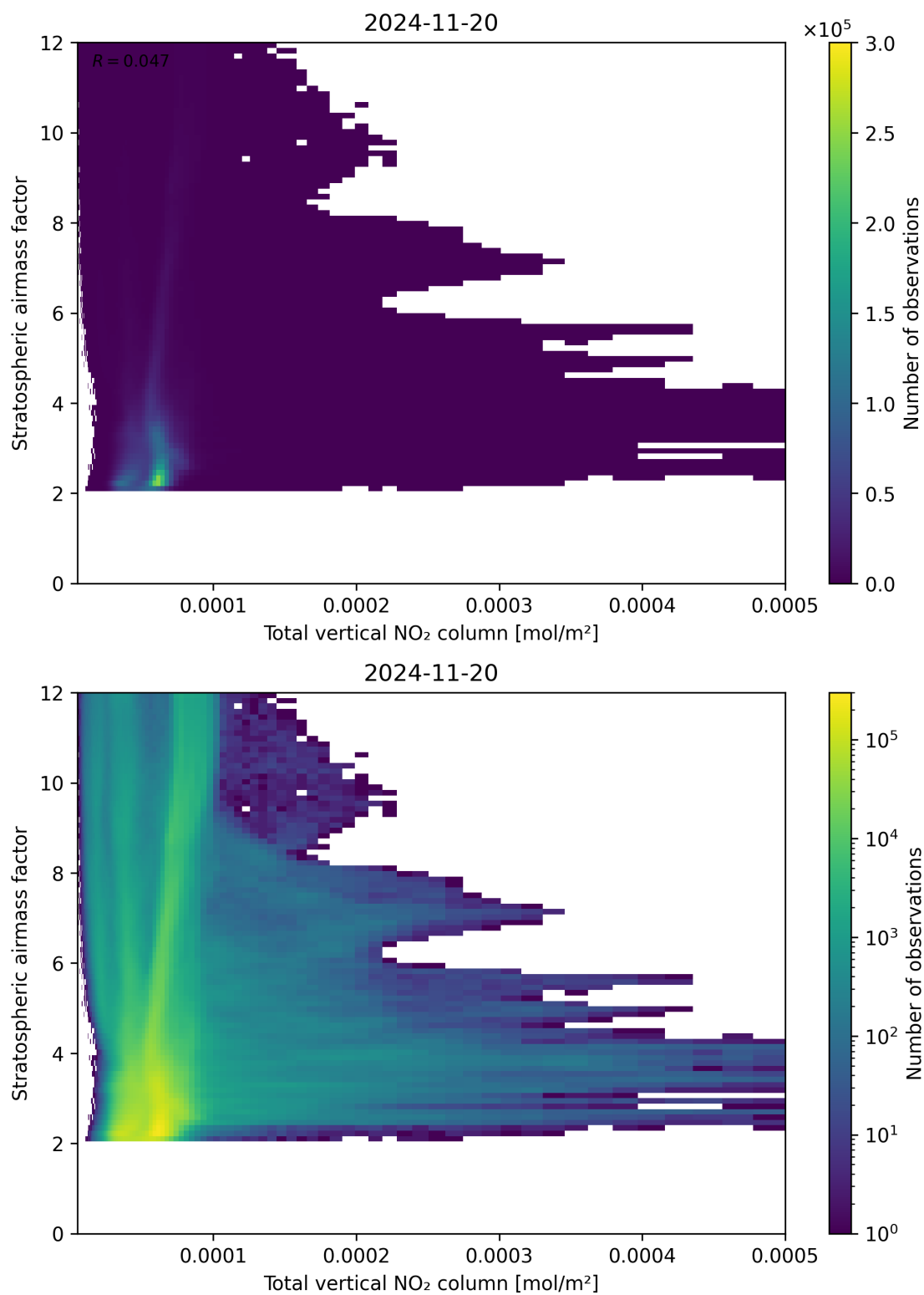
Figure 110: Scatter density plot of “Total vertical NO 2 column” against “Stratospheric airmass factor” for 2024-11-20 to 2024-11-21.
