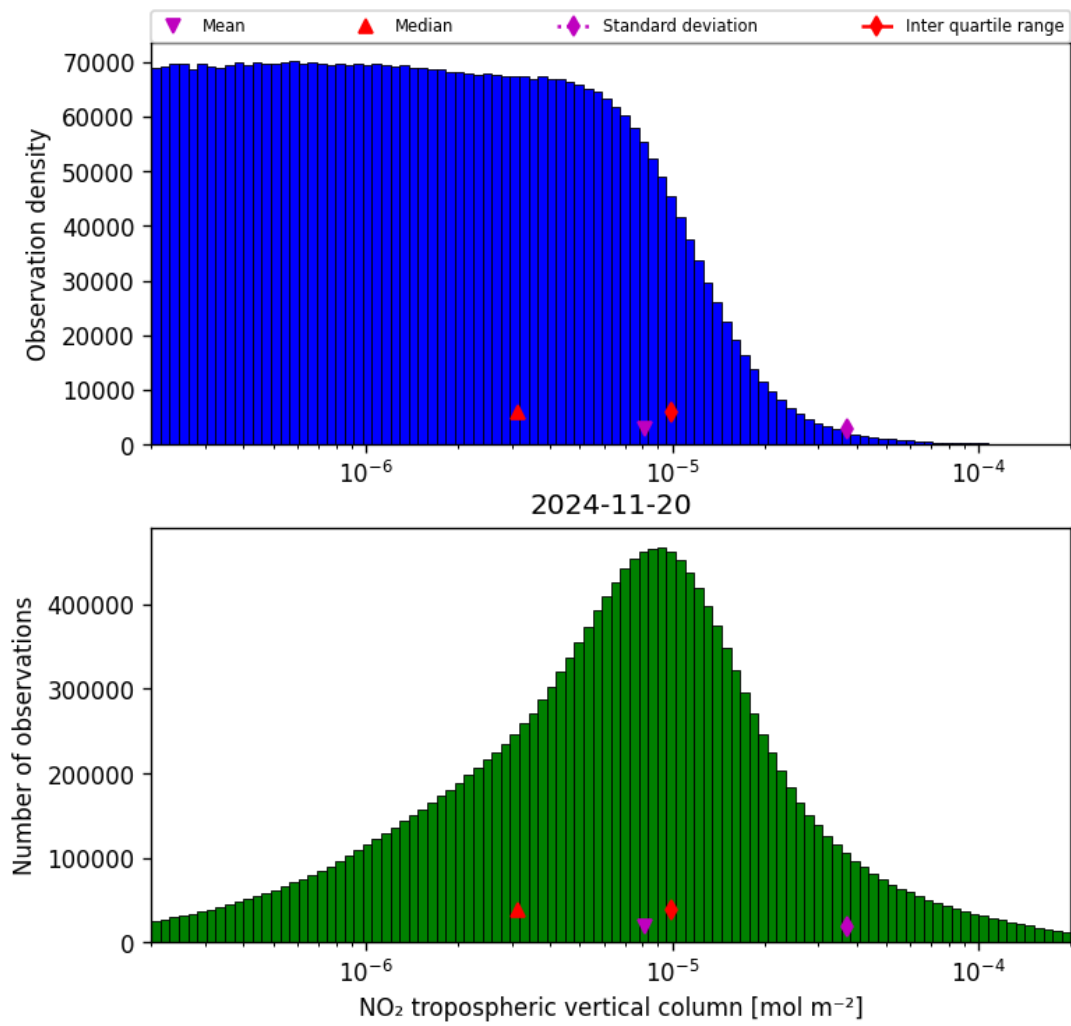
Figure 29: Histogram of “NO 2 tropospheric vertical column” for 2024-11-20 to 2024-11-21
