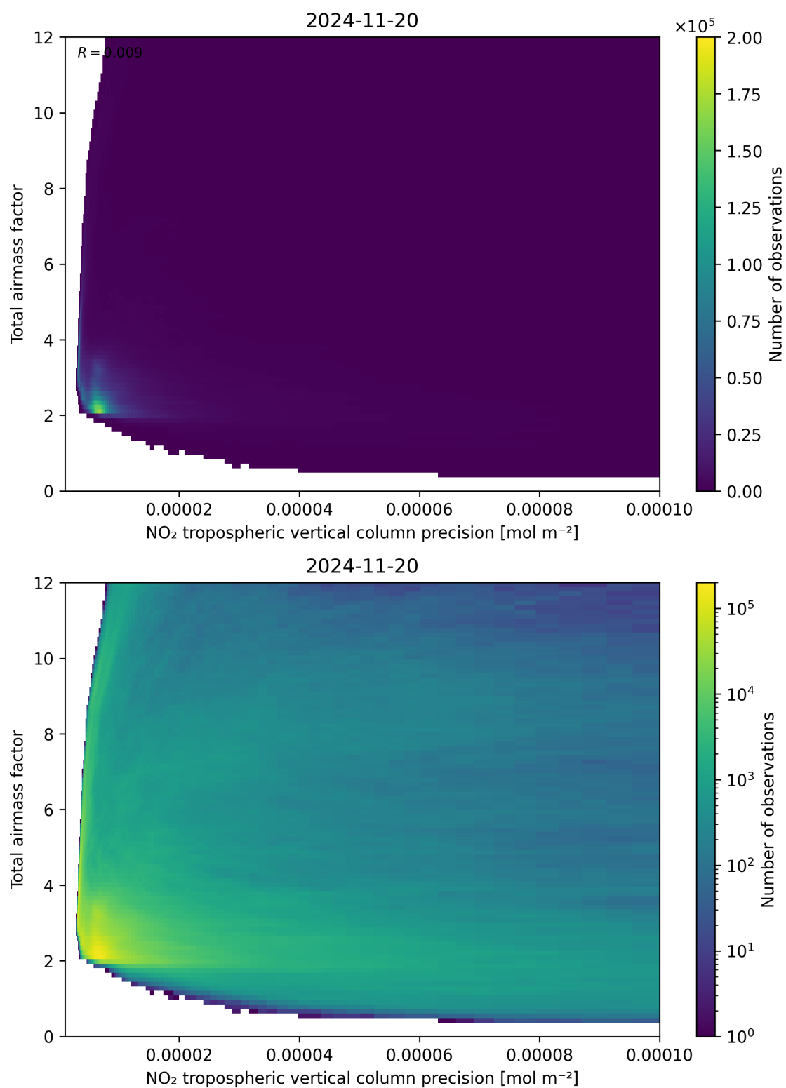
Figure 132: Scatter density plot of “NO 2 tropospheric vertical column precision” against “Total air mass factor” for 2024-11-20 to 2024-11-21.
