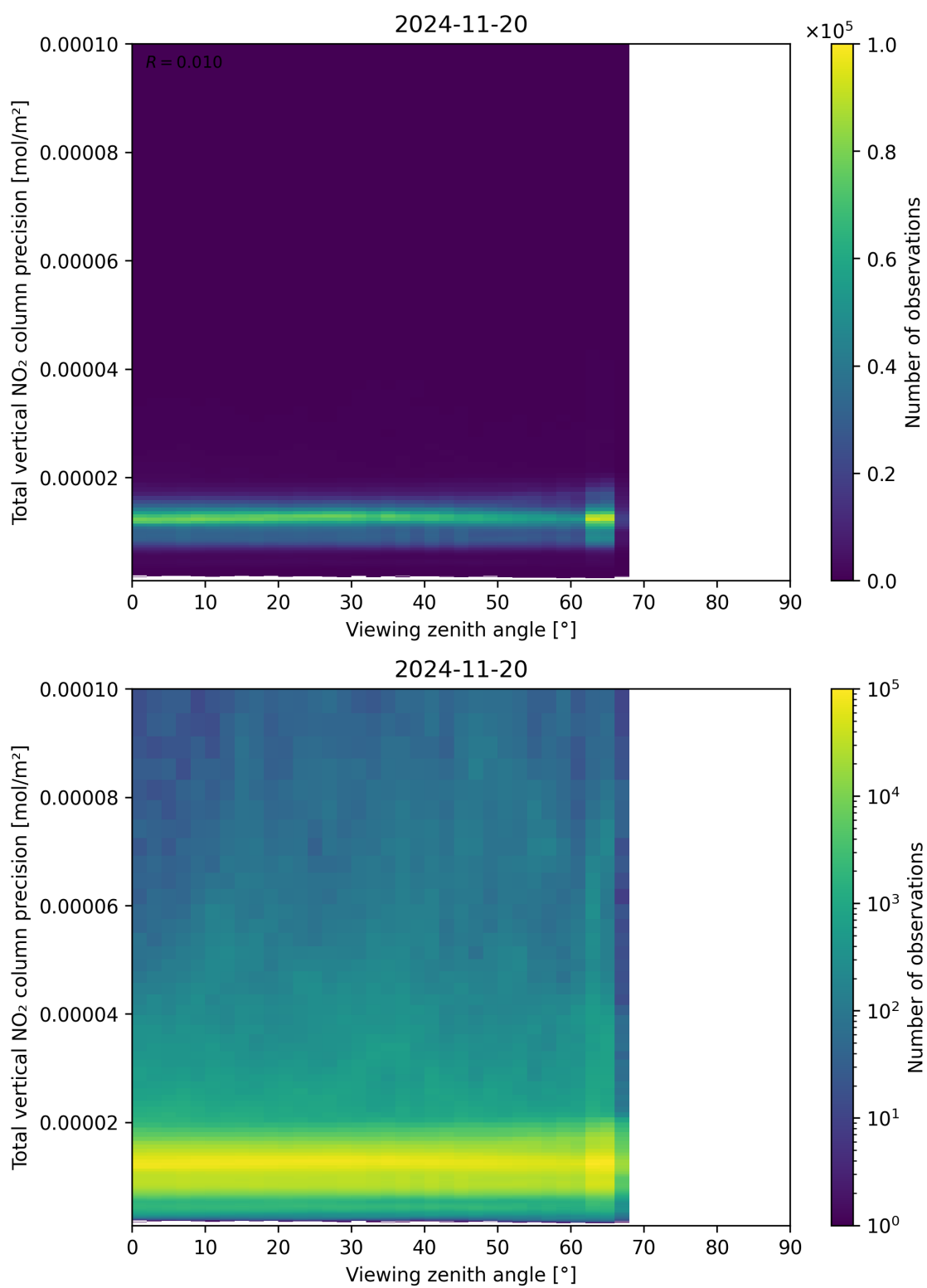
Figure 168: Scatter density plot of “Viewing zenith angle” against “Total vertical NO 2 column precision” for 2024-11-20 to 2024-11-21.
