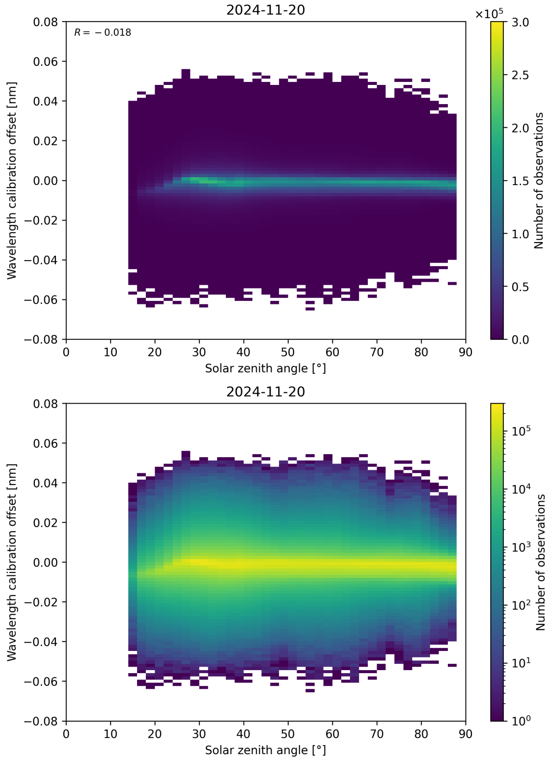
Figure 158: Scatter density plot of “Solar zenith angle” against “Wavelength calibration offset” for 2024-11-20 to 2024-11-21.
