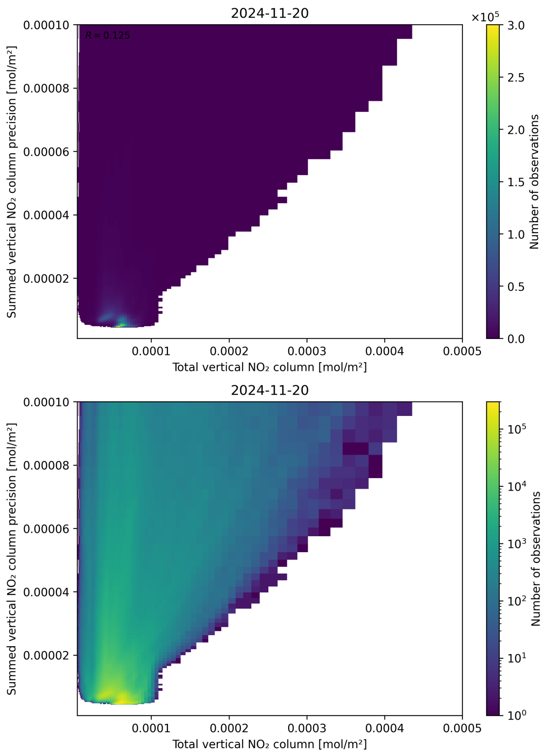
Figure 113: Scatter density plot of “Total vertical NO 2 column” against “Summed vertical NO 2 column precision” for 2024-11-20 to 2024-11-21.
