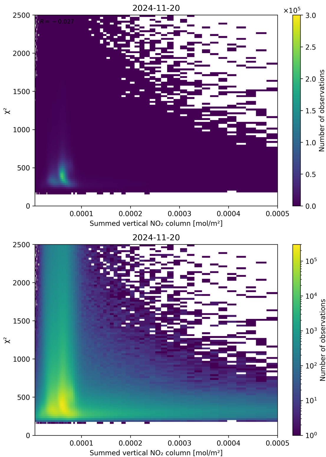
Figure 104: Scatter density plot of “Summed vertical NO 2 column” against “ \chi^2 ” for 2024-11-20 to 2024-11-21.
