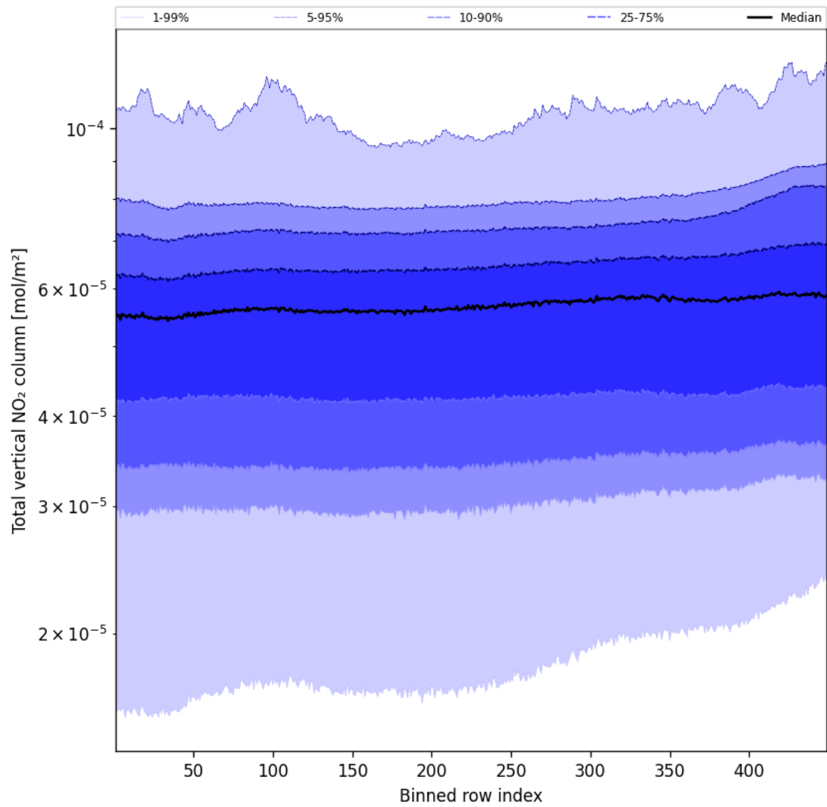
Figure 55: Along track statistics of “Total vertical NO 2 column” for 2024-11-20 to 2024-11-21
