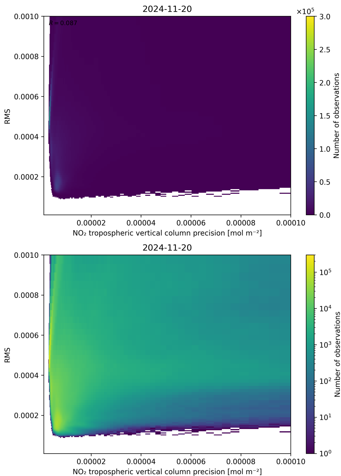
Figure 140: Scatter density plot of “NO 2 tropospheric vertical column precision” against “RMS” for 2024-11-20 to 2024-11-21.
