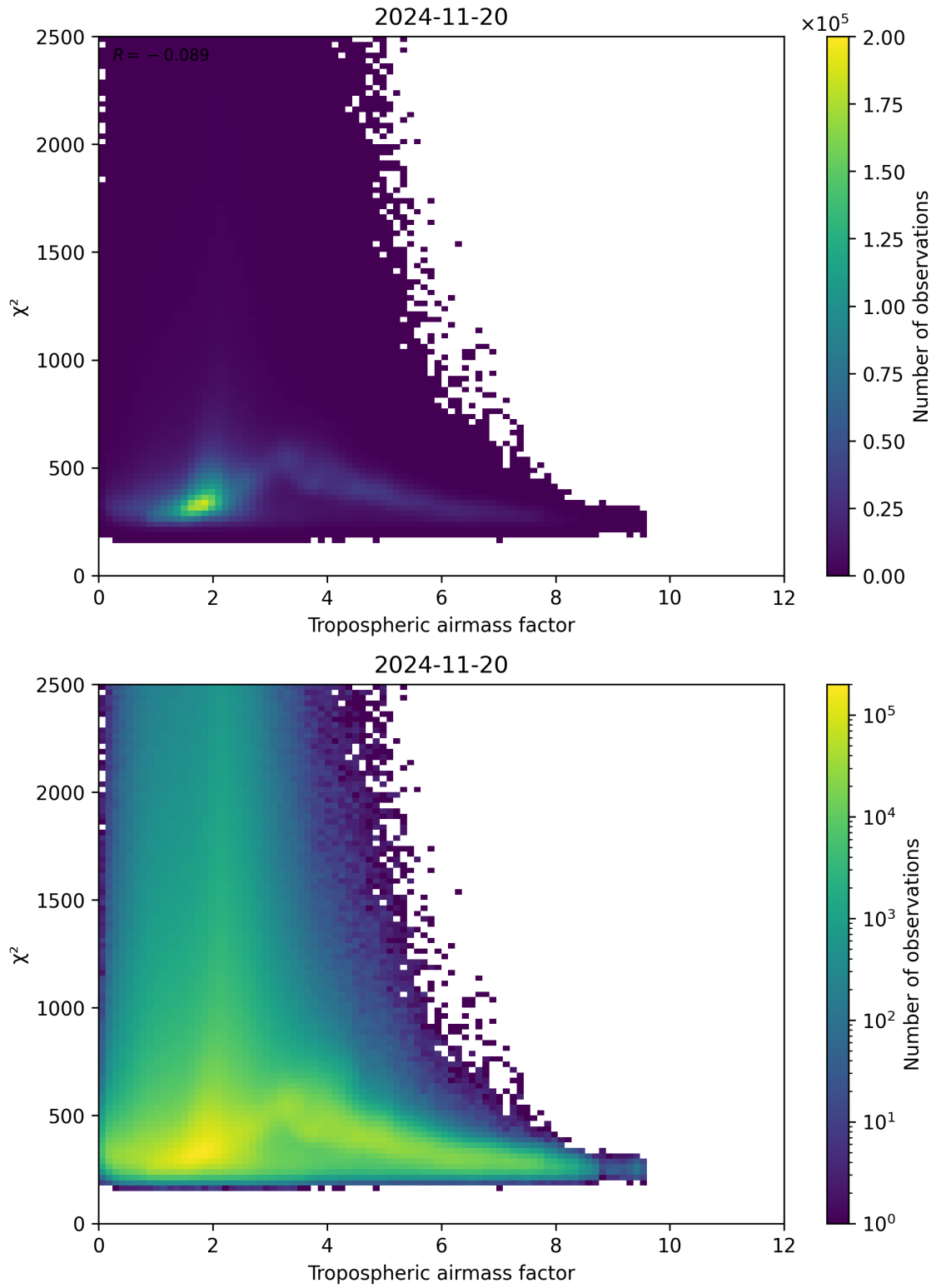
Figure 73: Scatter density plot of “Tropospheric airmass factor” against “ \chi^2 ” for 2024-11-20 to 2024-11-21.
