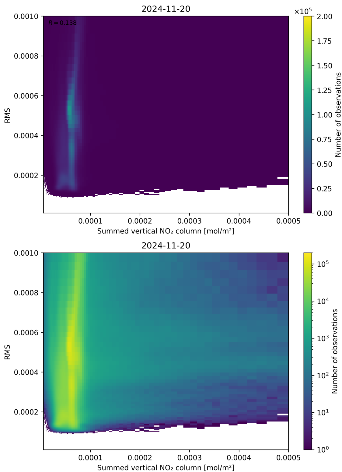
Figure 109: Scatter density plot of “Summed vertical NO 2 column” against “RMS” for 2024-11-20 to 2024-11-21.
