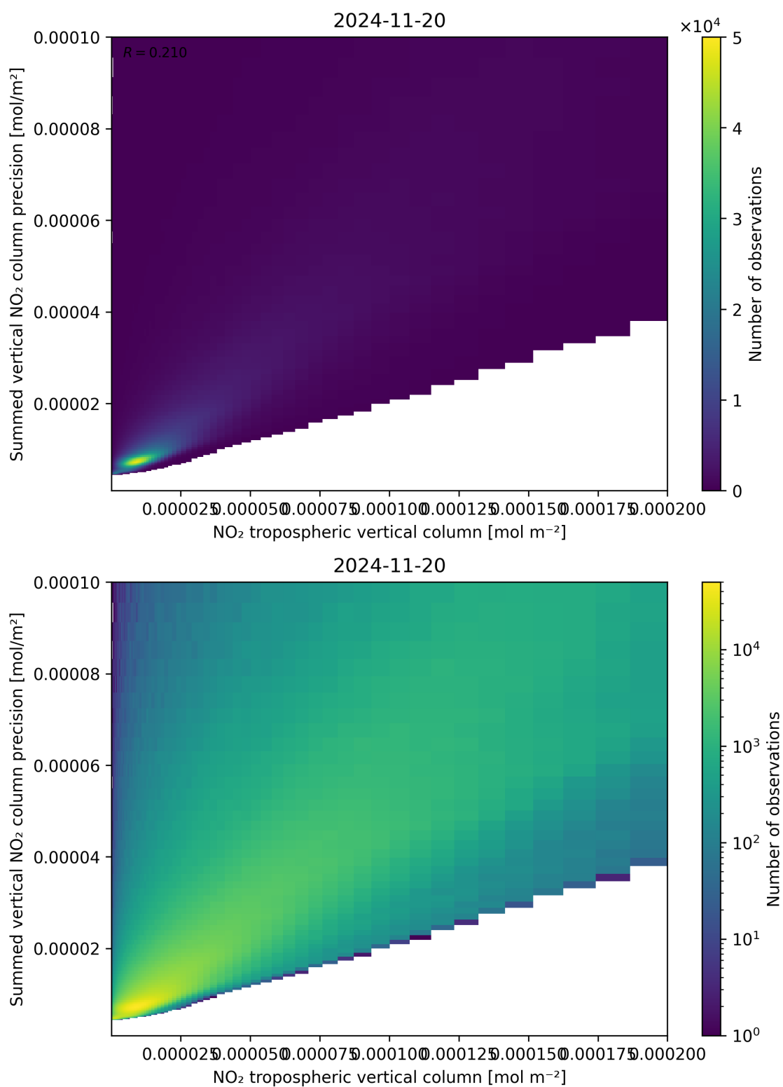
Figure 127: Scatter density plot of “NO 2 tropospheric vertical column” against “Summed vertical NO 2 column precision” for 2024-11-20 to 2024-11-21.
