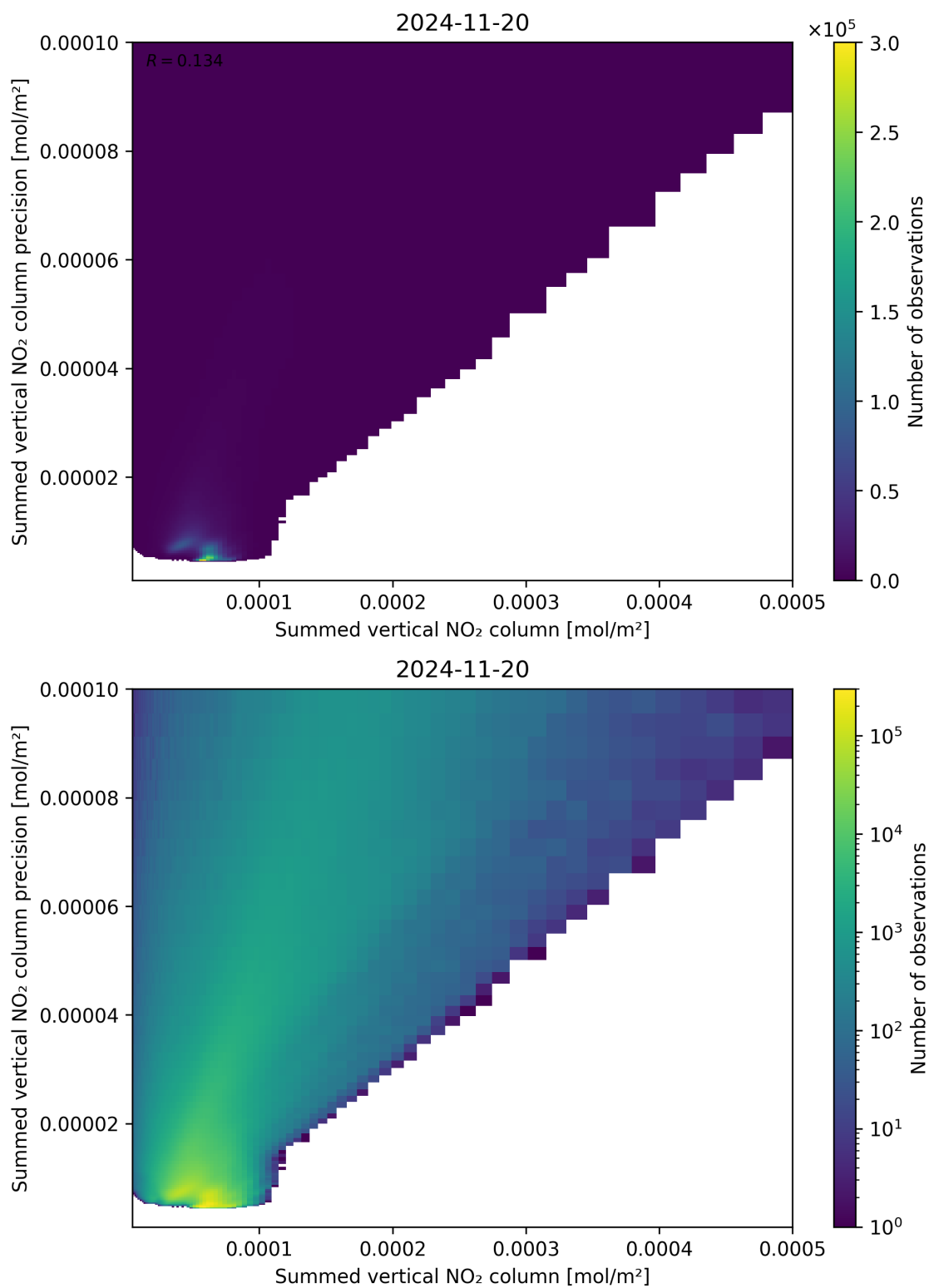
Figure 105: Scatter density plot of “Summed vertical NO 2 column” against “Summed vertical NO 2 column precision” for 2024-11-20 to 2024-11-21.
