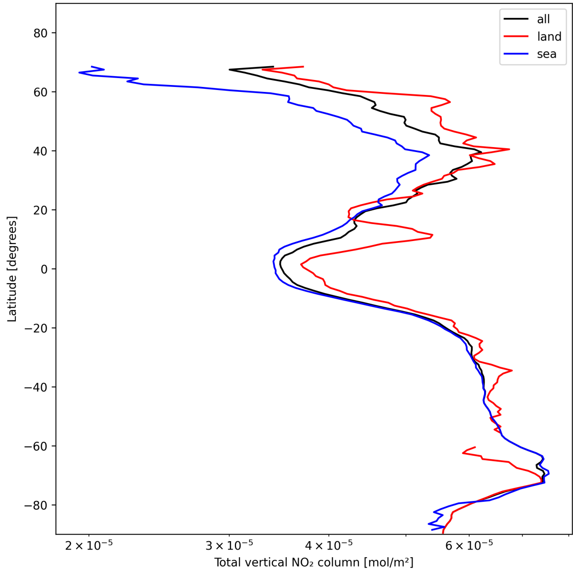
Figure 21: Zonal average of “Total vertical NO 2 column” for 2024-11-20 to 2024-11-21.
