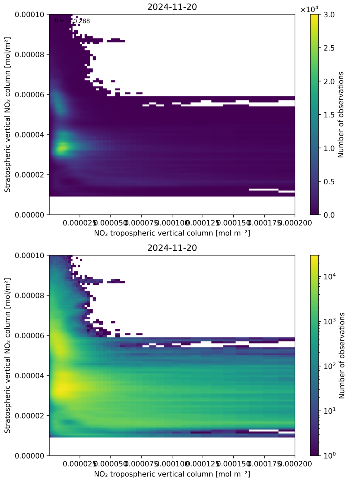
Figure 125: Scatter density plot of “NO 2 tropospheric vertical column” against “Stratospheric vertical NO 2 column” for 2024-11-20 to 2024-11-21.
