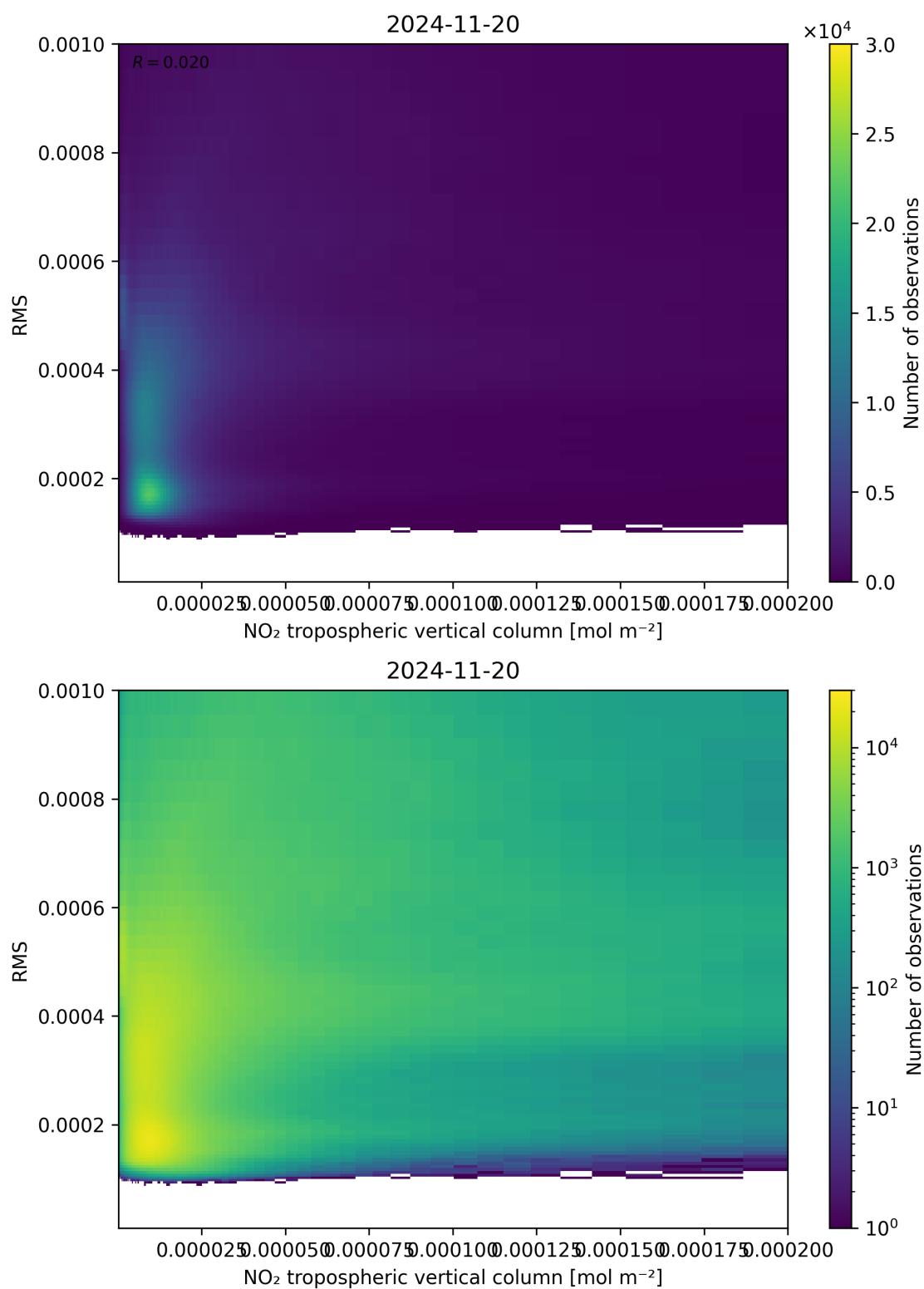
Figure 142: Scatter density plot of “NO 2 tropospheric vertical column” against “RMS” for 2024-11-20 to 2024-11-21.
