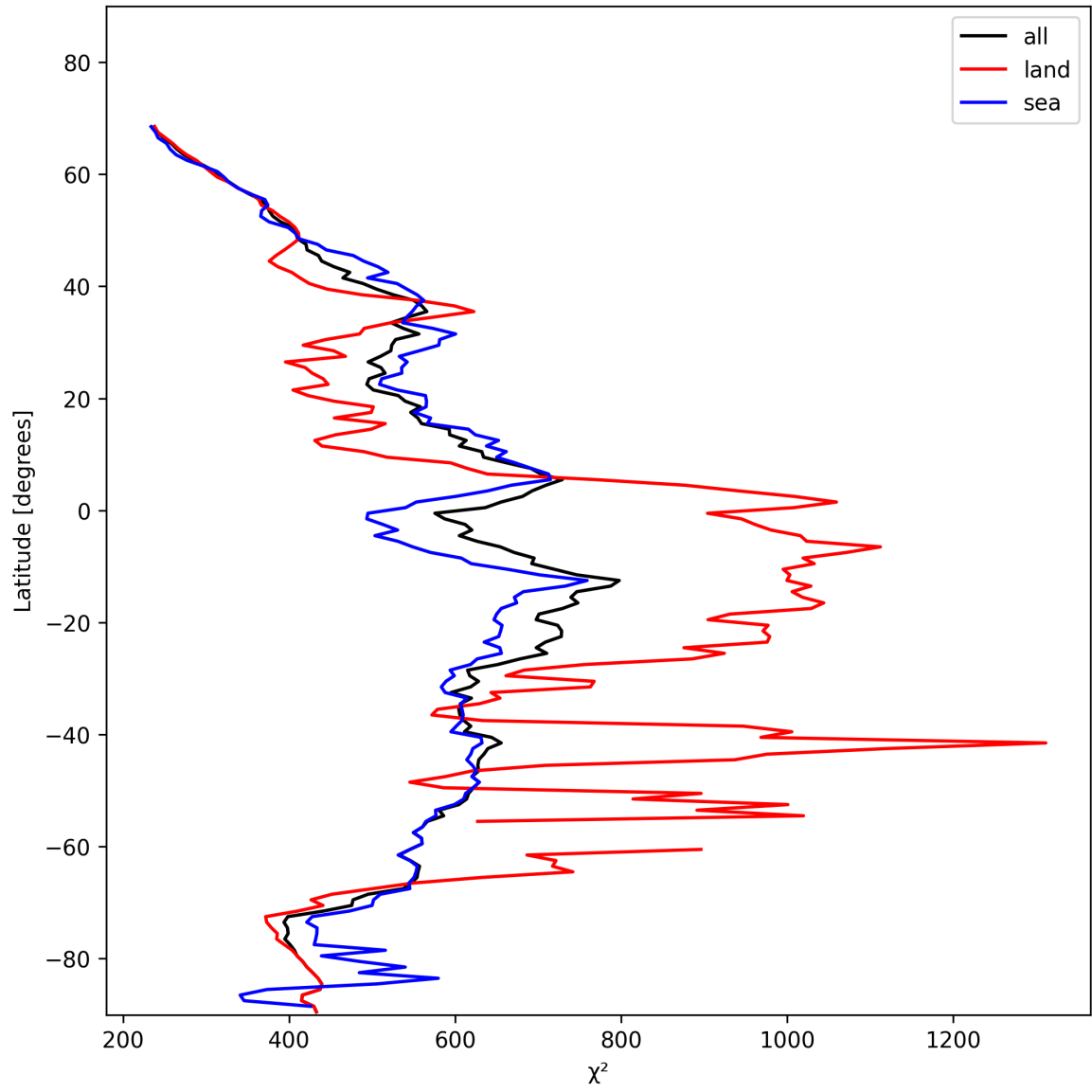
Figure 25: Zonal average of “ \chi^2 ” for 2024-11-20 to 2024-11-21.
