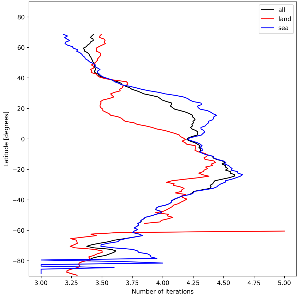
Figure 17: Zonal average of “Number of iterations” for 2024-11-20 to 2024-11-21.
