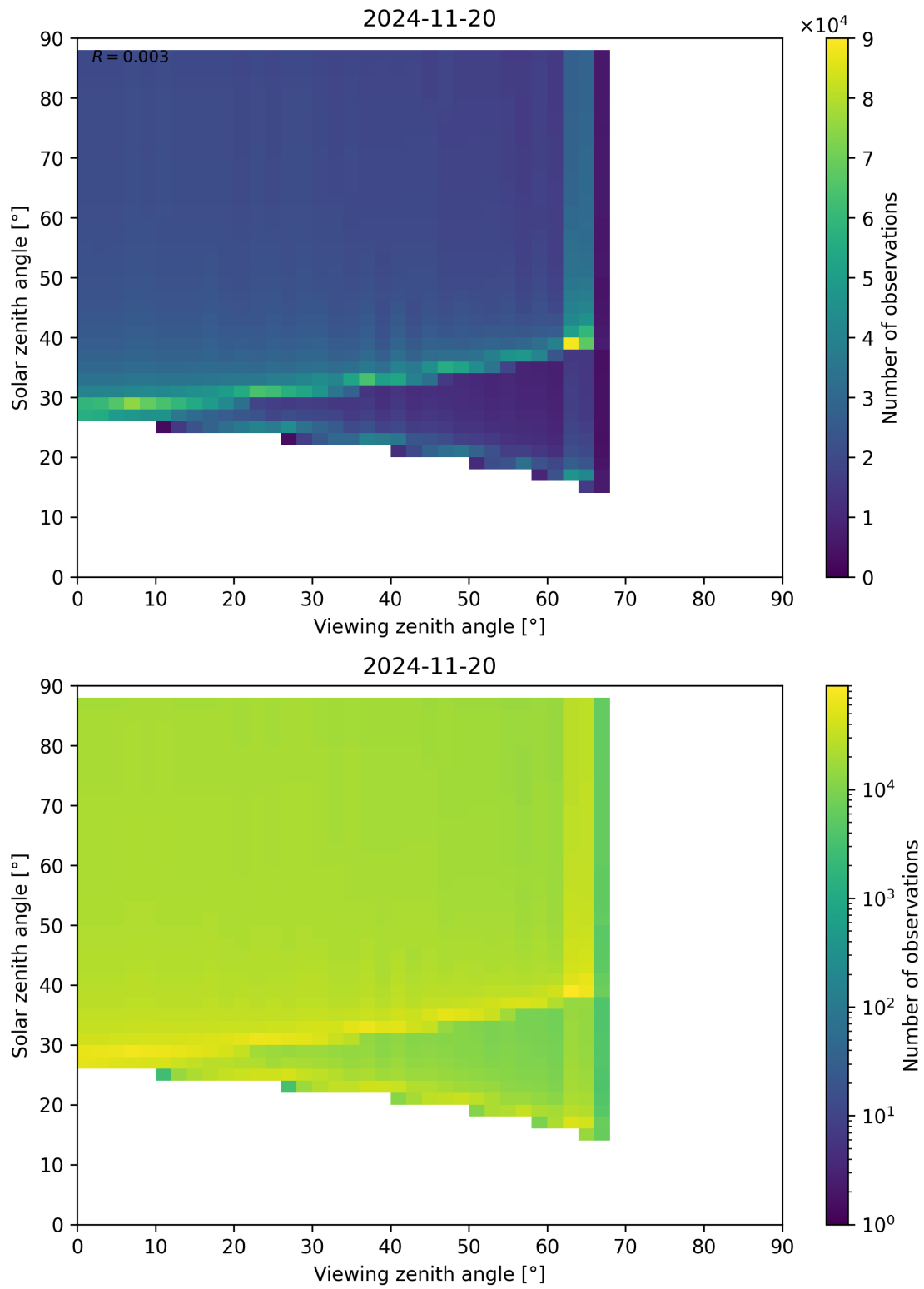
Figure 172: Scatter density plot of “Viewing zenith angle” against “Solar zenith angle” for 2024-11-20 to 2024-11-21.
