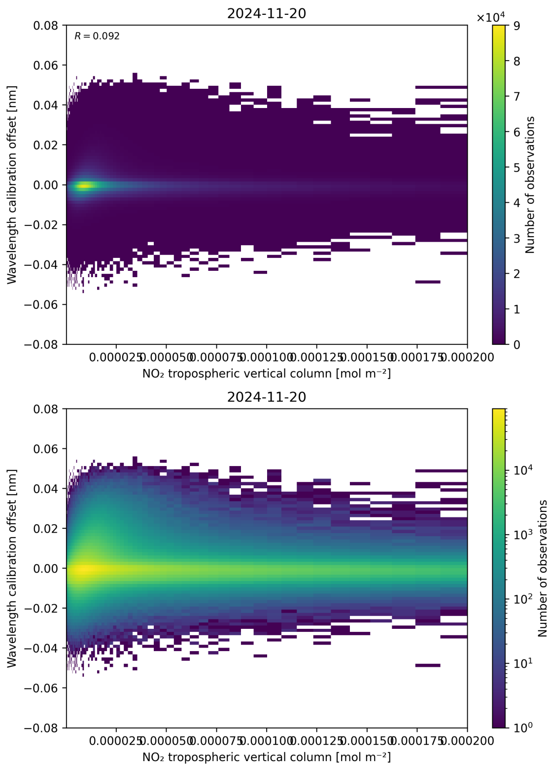
Figure 143: Scatter density plot of “NO 2 tropospheric vertical column” against “Wavelength calibration offset” for 2024-11-20 to 2024-11-21.
