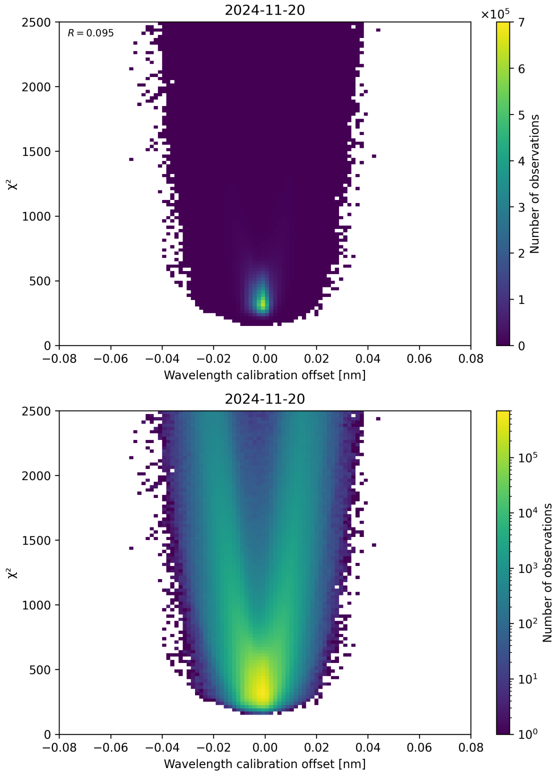
Figure 175: Scatter density plot of “Wavelength calibration offset” against “ \chi^2 ” for 2024-11-20 to 2024-11-21.
