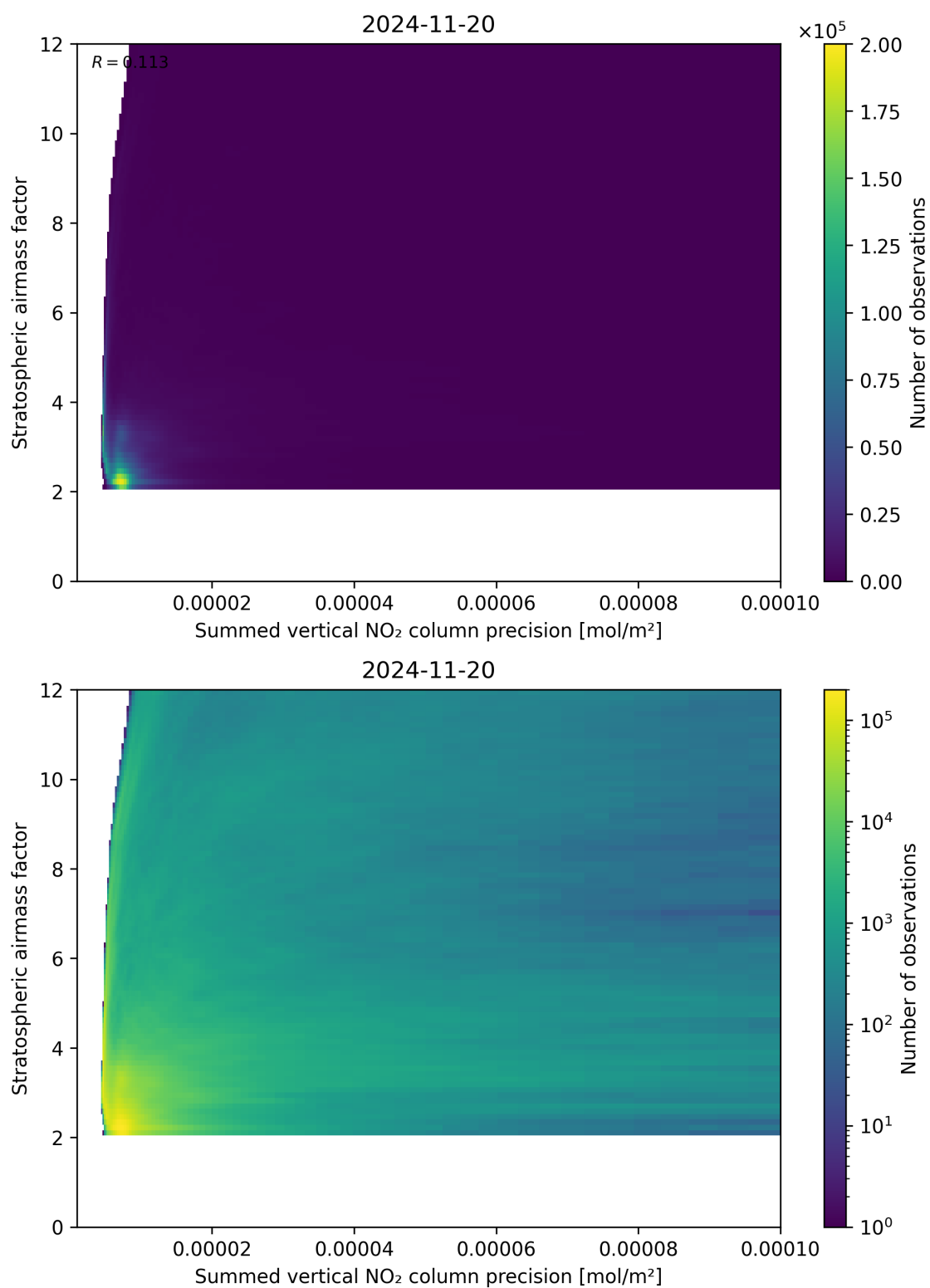
Figure 106: Scatter density plot of “Summed vertical NO 2 column precision” against “Stratospheric airmass factor” for 2024-11-20 to 2024-11-21.
