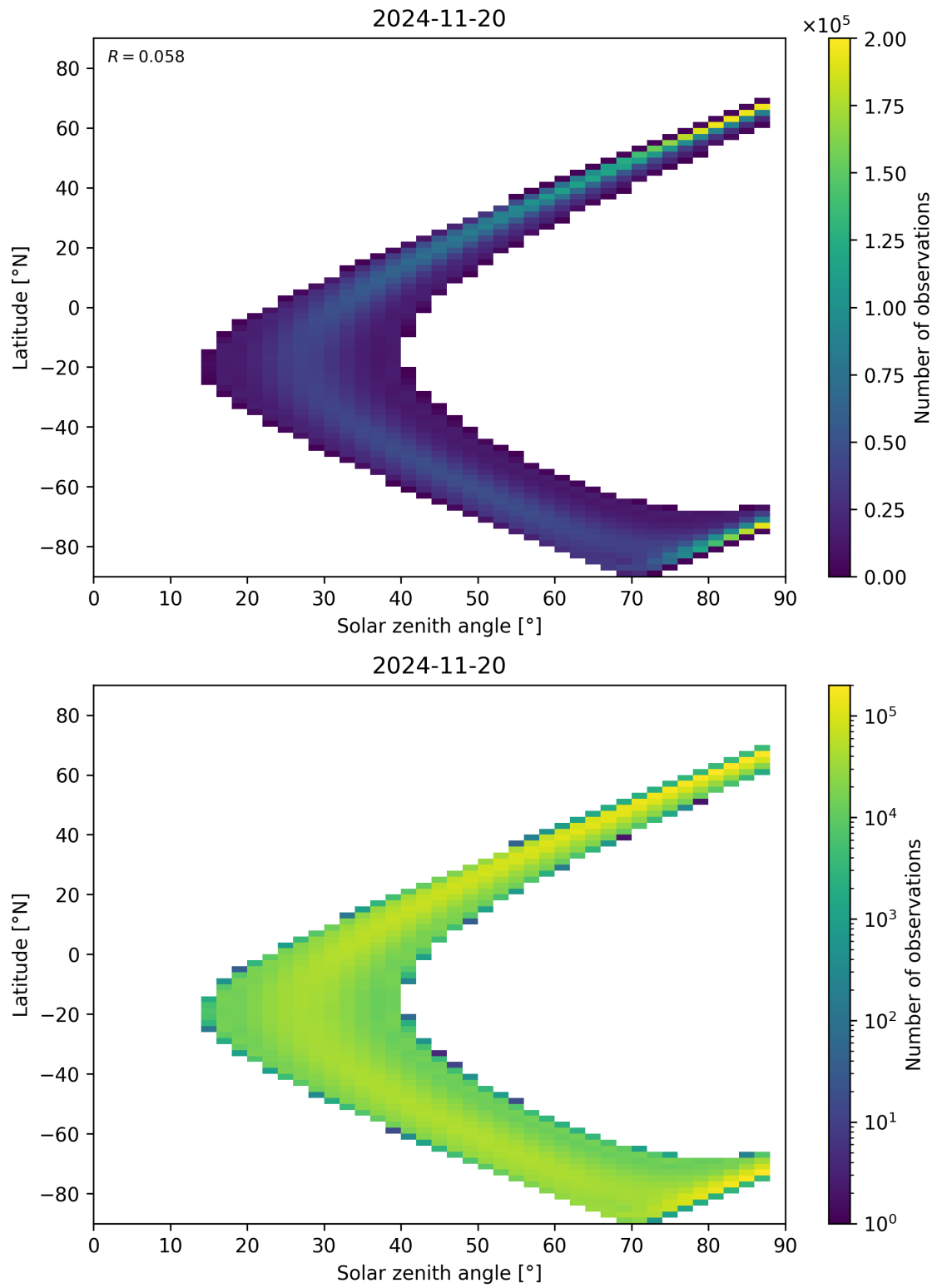
Figure 149: Scatter density plot of “Solar zenith angle” against “Latitude” for 2024-11-20 to 2024-11-21.
