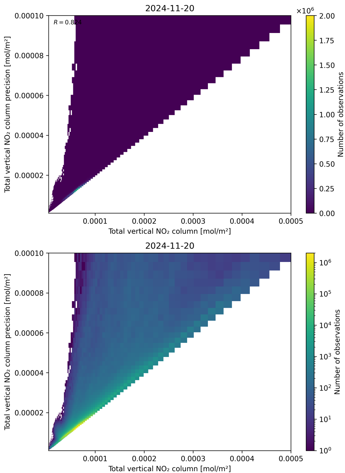
Figure 114: Scatter density plot of “Total vertical NO 2 column” against “Total vertical NO 2 column precision” for 2024-11-20 to 2024-11-21.
