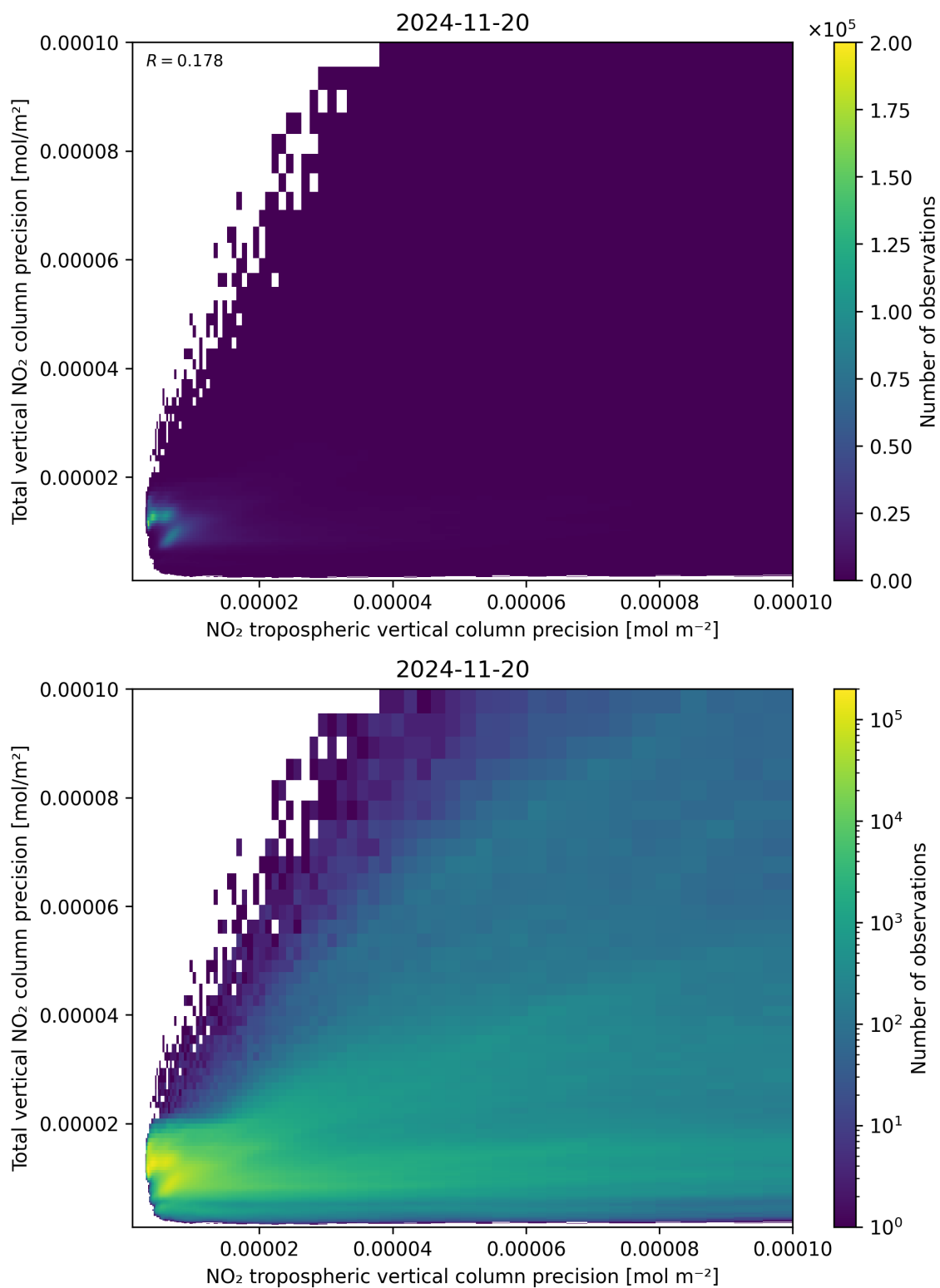
Figure 139: Scatter density plot of “NO 2 tropospheric vertical column precision” against “Total vertical NO 2 column precision” for 2024-11-20 to 2024-11-21.
