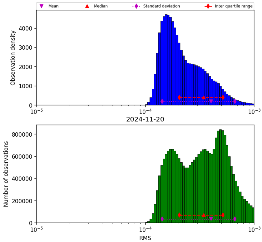
Figure 43: Histogram of “RMS” for 2024-11-20 to 2024-11-21
