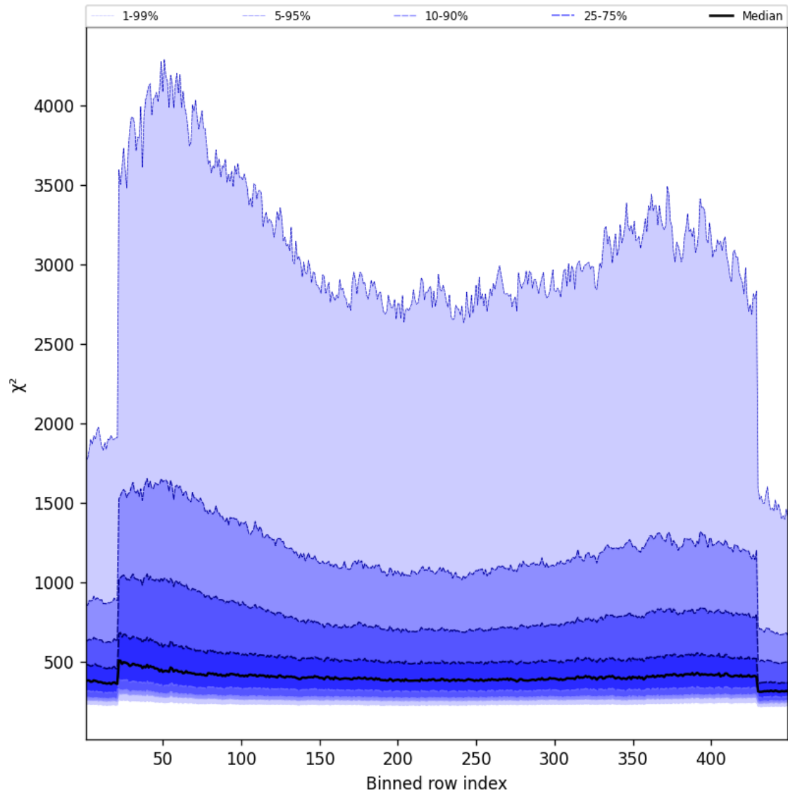
Figure 59: Along track statistics of “ \chi^2 ” for 2024-11-20 to 2024-11-21
