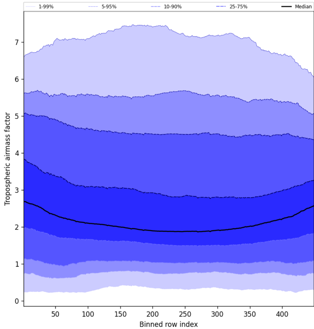
Figure 48: Along track statistics of “Tropospheric airmass factor” for 2024-11-20 to 2024-11-21
