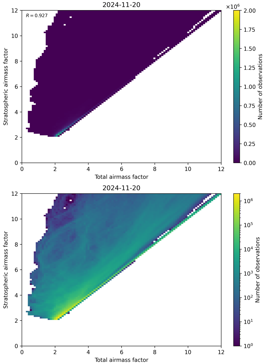
Figure 62: Scatter density plot of “Total airmass factor” against “Stratospheric airmass factor” for 2024-11-20 to 2024-11-21.
