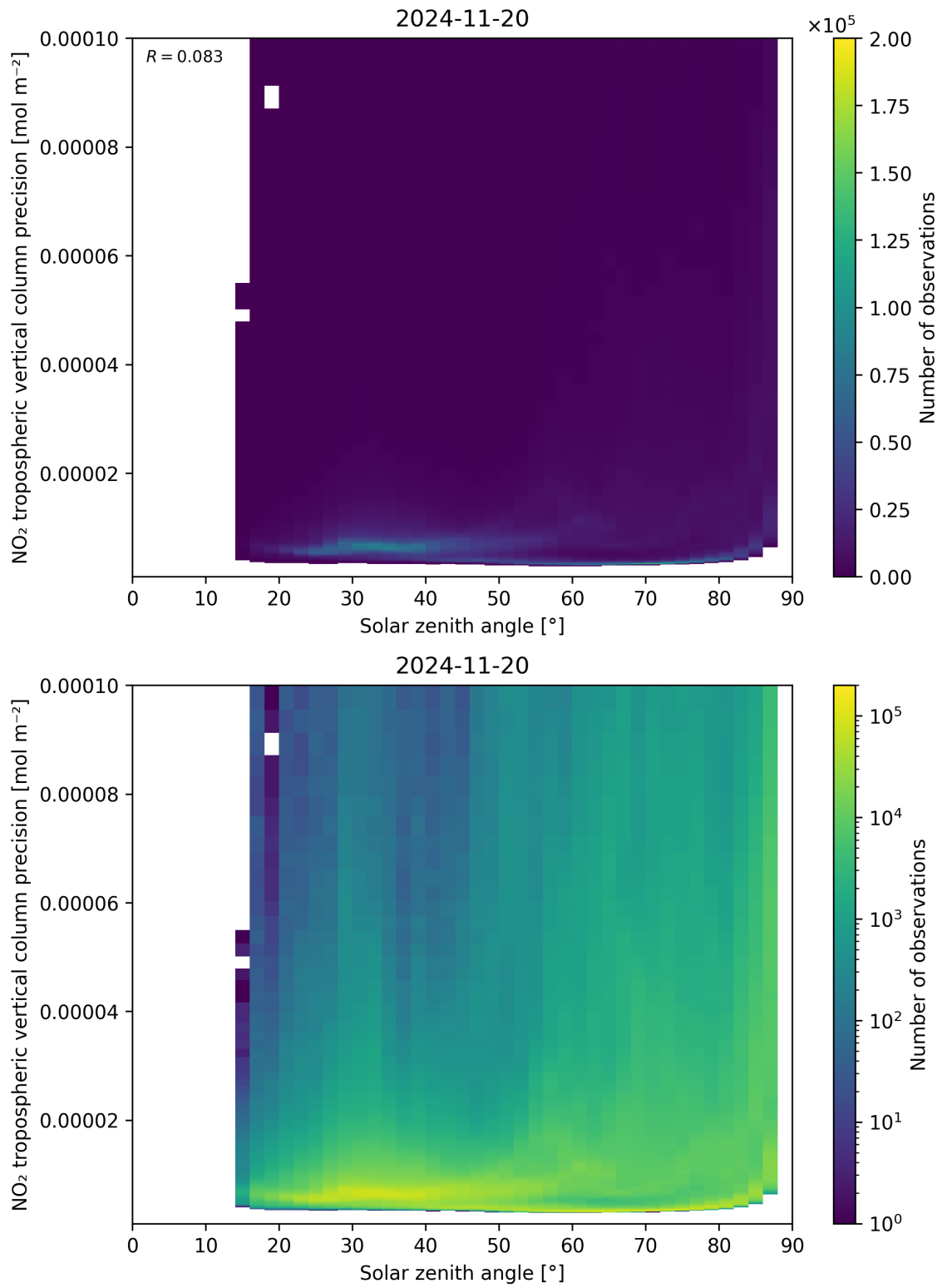
Figure 156: Scatter density plot of “Solar zenith angle” against “NO 2 tropospheric vertical column precision” for 2024-11-20 to 2024-11-21.
