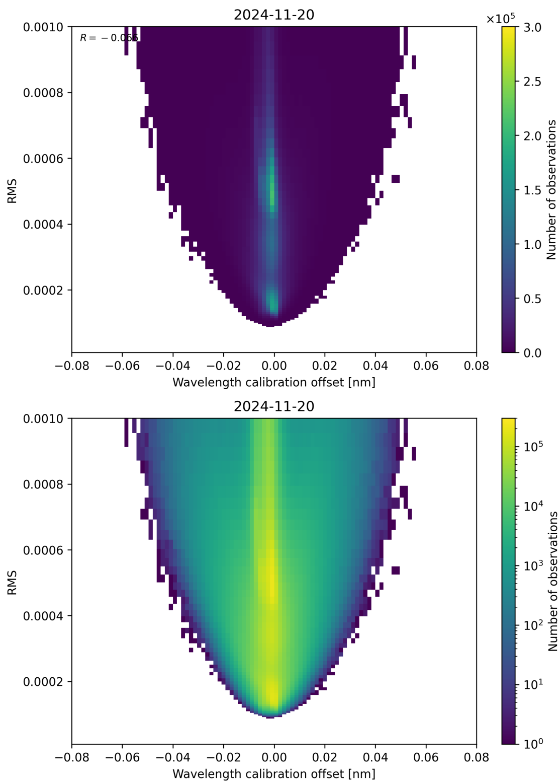
Figure 181: Scatter density plot of “Wavelength calibration offset” against “RMS” for 2024-11-20 to 2024-11-21.
