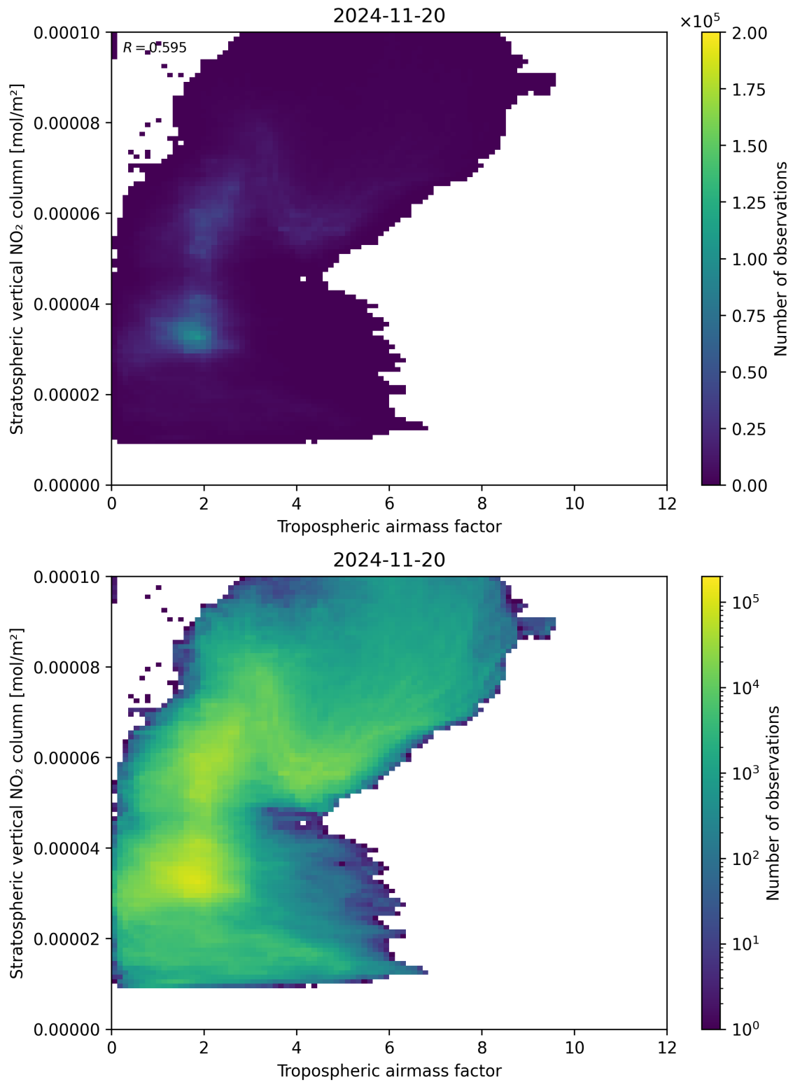
Figure 74: Scatter density plot of “Tropospheric airmass factor” against “Stratospheric vertical NO 2 column” for 2024-11-20 to 2024-11-21.
