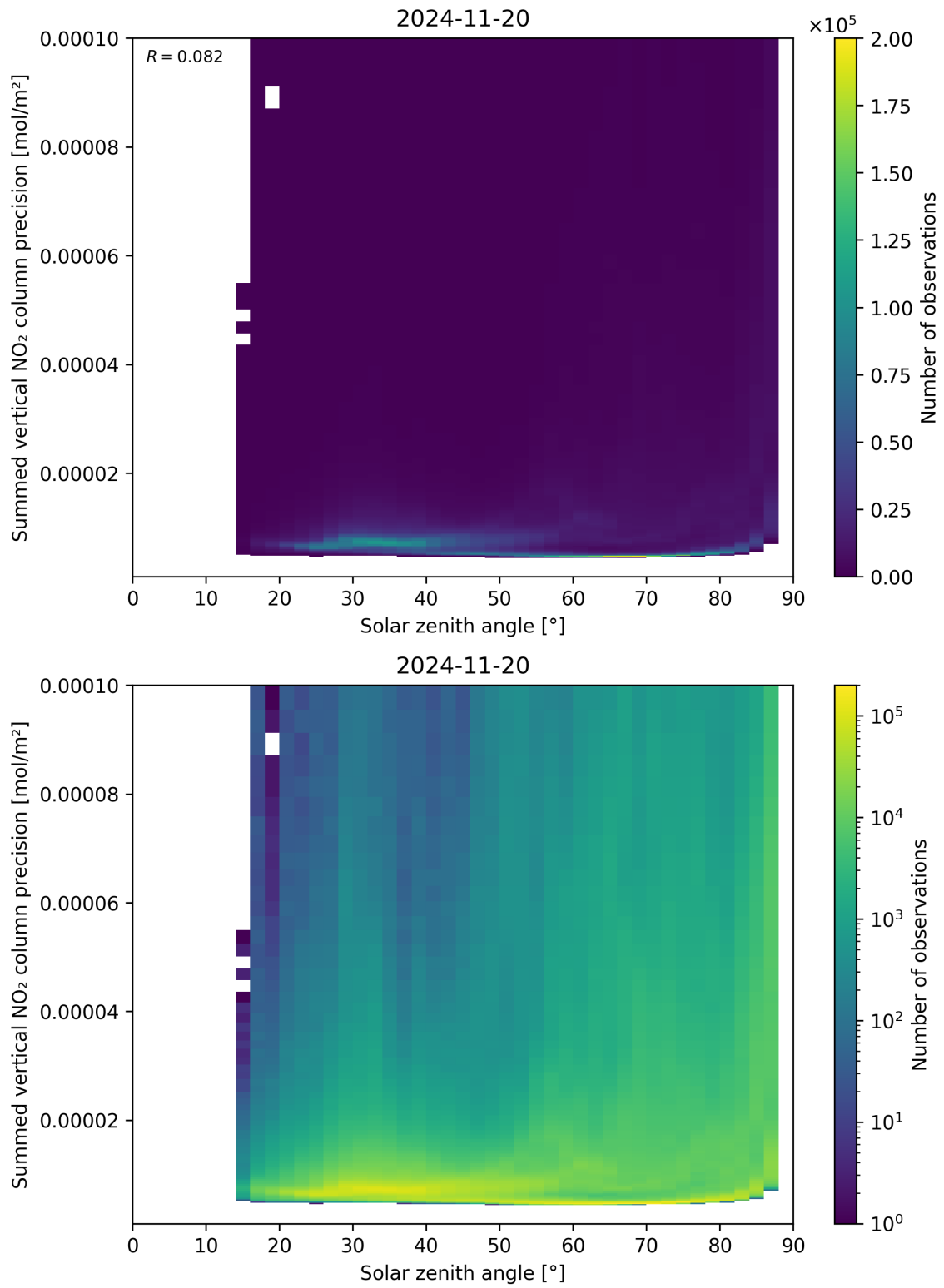
Figure 152: Scatter density plot of “Solar zenith angle” against “Summed vertical NO 2 column precision” for 2024-11-20 to 2024-11-21.
