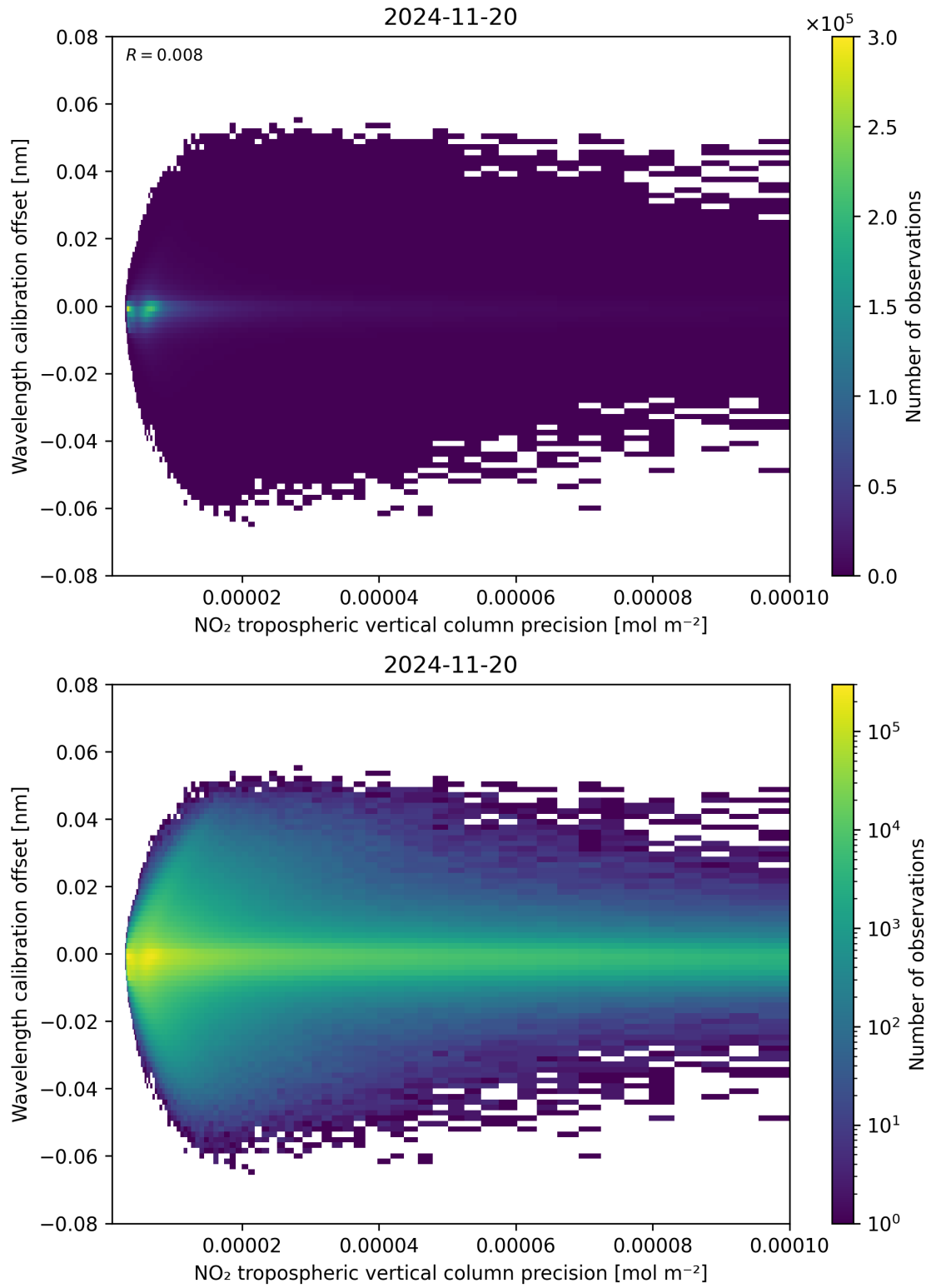
Figure 141: Scatter density plot of “NO 2 tropospheric vertical column precision” against “Wavelength calibration offset” for 2024-11-20 to 2024-11-21.
