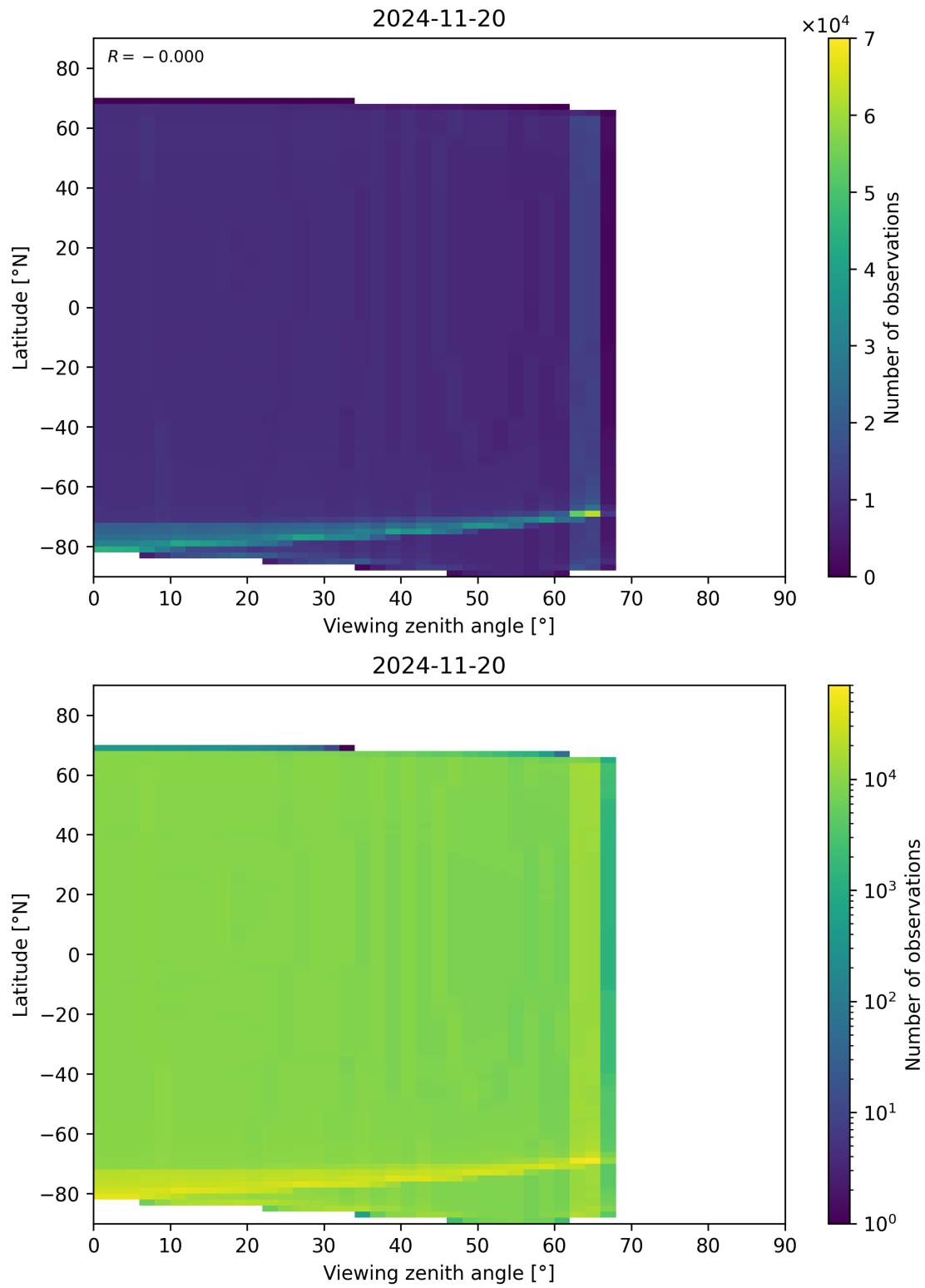
Figure 163: Scatter density plot of “Viewing zenith angle” against “Latitude” for 2024-11-20 to 2024-11-21.
