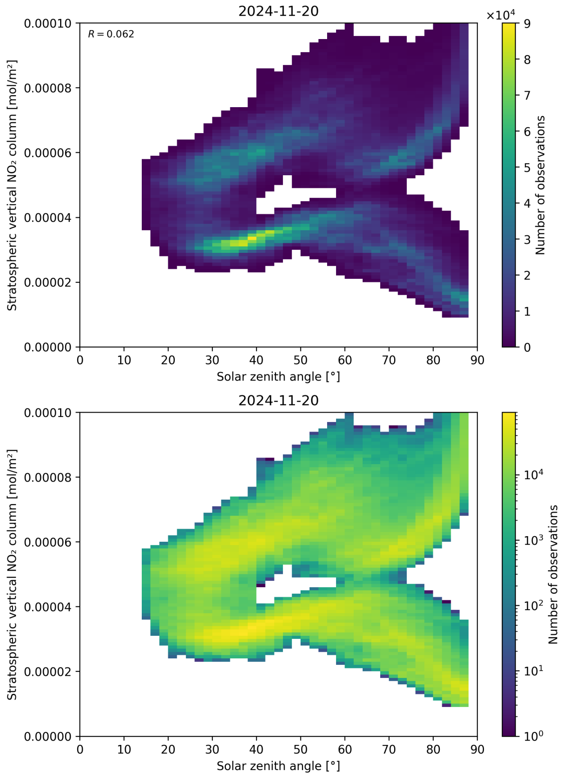
Figure 150: Scatter density plot of “Solar zenith angle” against “Stratospheric vertical NO 2 column” for 2024-11-20 to 2024-11-21.
