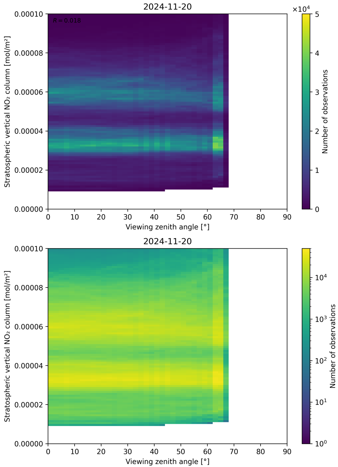
Figure 164: Scatter density plot of “Viewing zenith angle” against “Stratospheric vertical NO 2 column” for 2024-11-20 to 2024-11-21.
