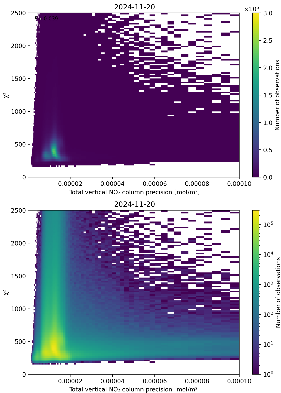
Figure 116: Scatter density plot of “Total vertical NO 2 column precision” against “ \chi^2 ” for 2024-11-20 to 2024-11-21.
