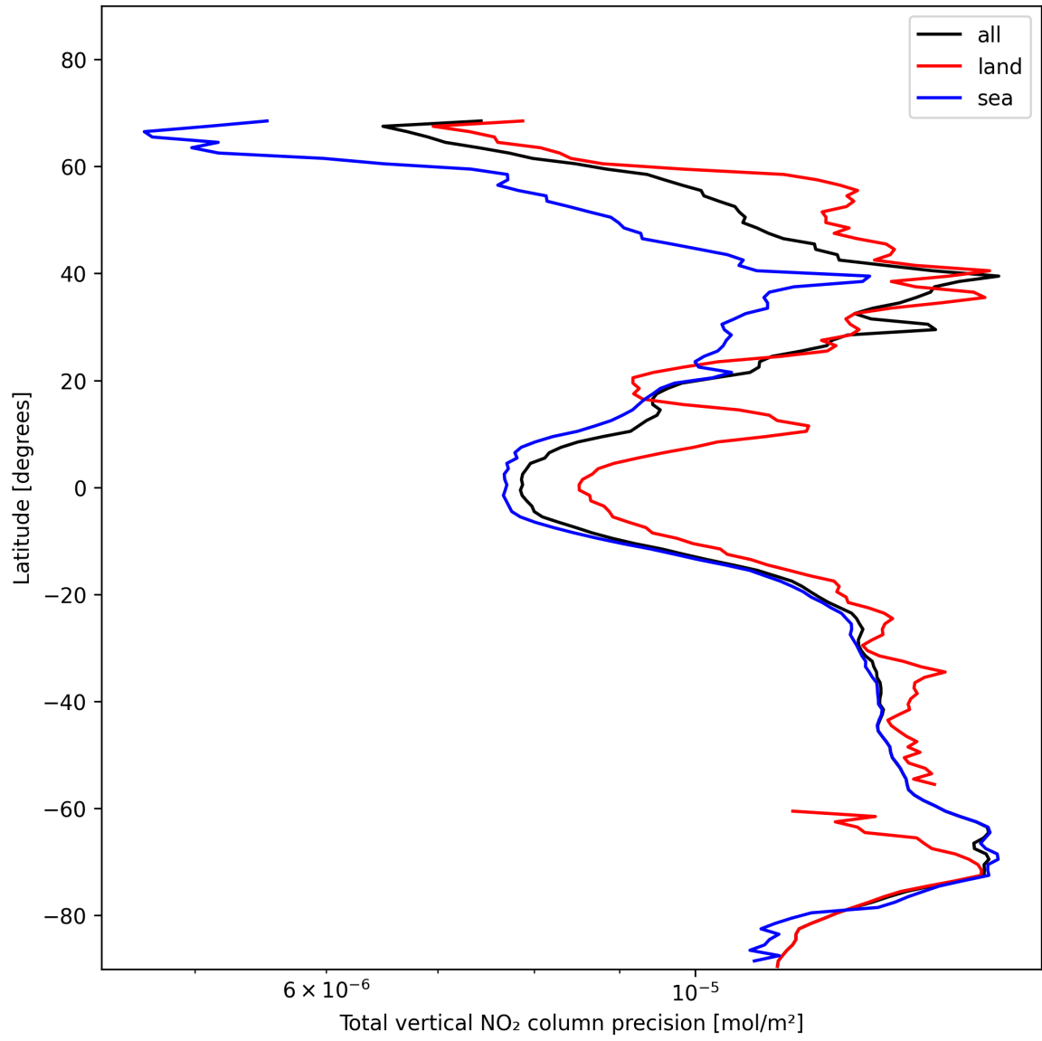
Figure 22: Zonal average of “Total vertical NO 2 column precision” for 2024-11-20 to 2024-11-21.
