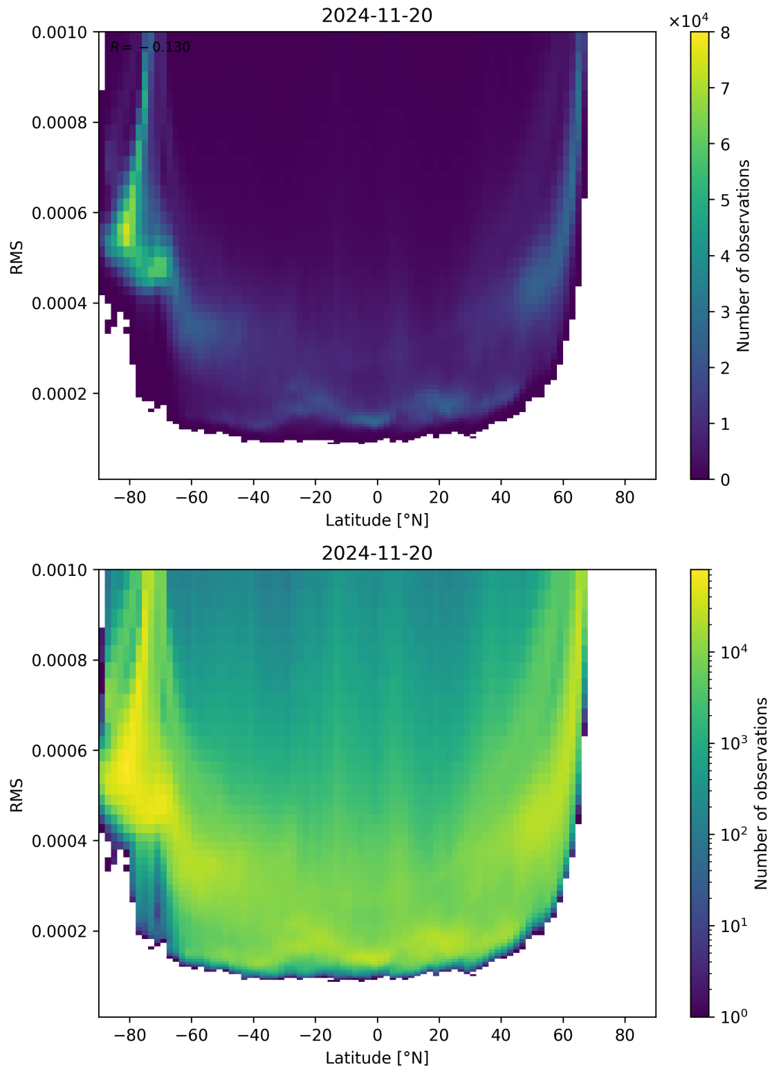
Figure 94: Scatter density plot of “Latitude” against “RMS” for 2024-11-20 to 2024-11-21.
