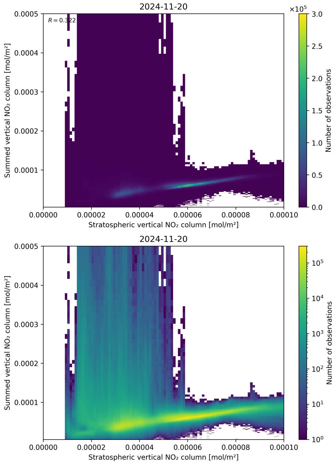
Figure 98: Scatter density plot of “Stratospheric vertical NO 2 column” against “Summed vertical NO 2 column” for 2024-11-20 to 2024-11-21.
