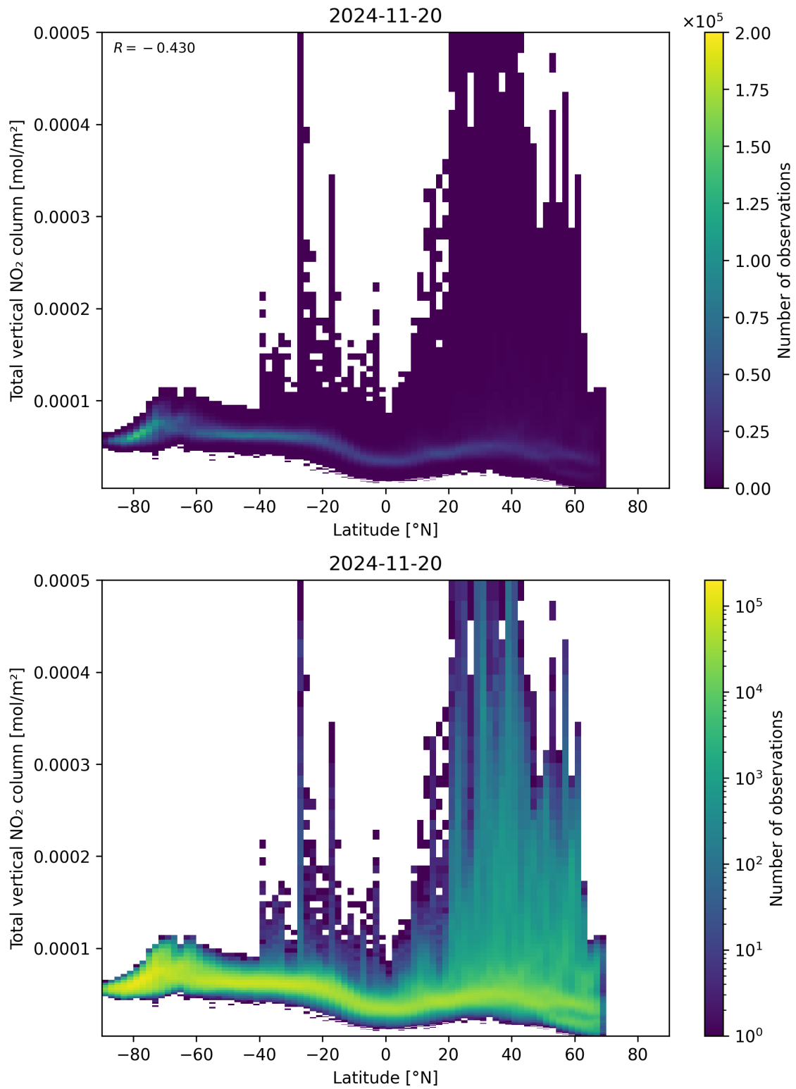
Figure 90: Scatter density plot of “Latitude” against “Total vertical NO 2 column” for 2024-11-20 to 2024-11-21.
