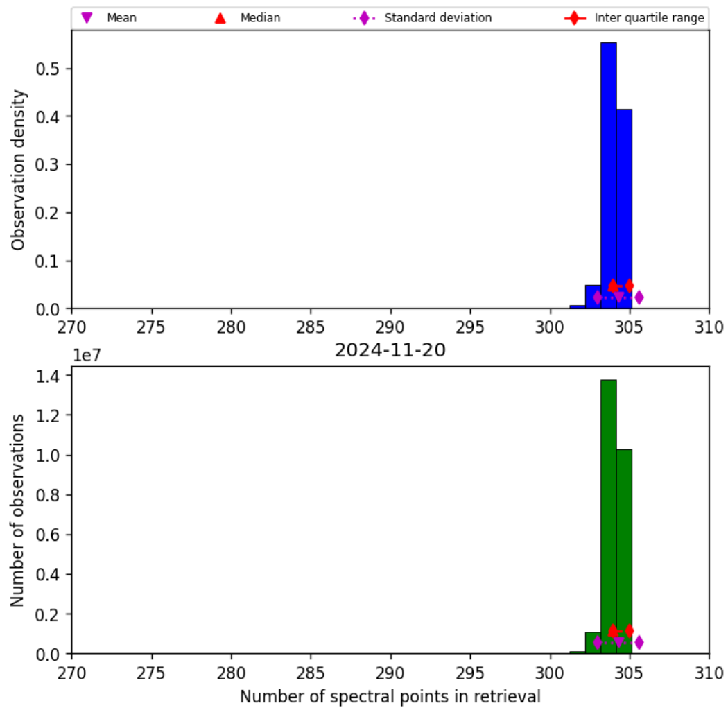
Figure 33: Histogram of “Number of spectral points in retrieval” for 2024-11-20 to 2024-11-21
