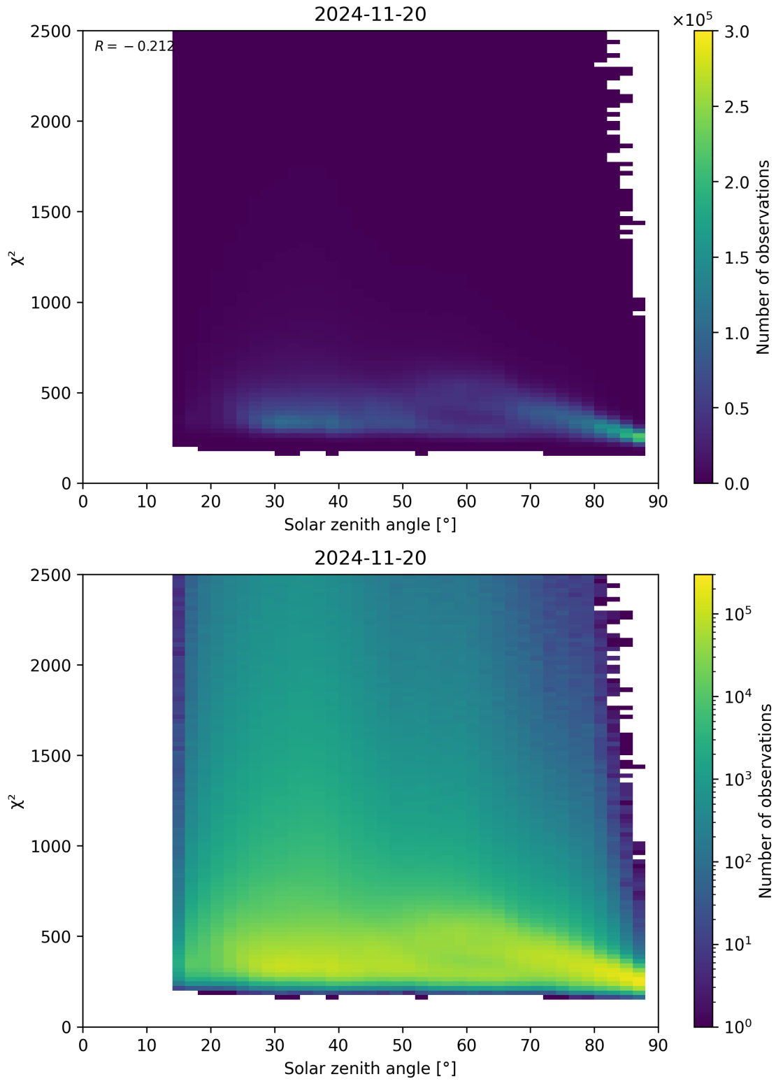
Figure 148: Scatter density plot of “Solar zenith angle” against “ \chi^2 ” for 2024-11-20 to 2024-11-21.
