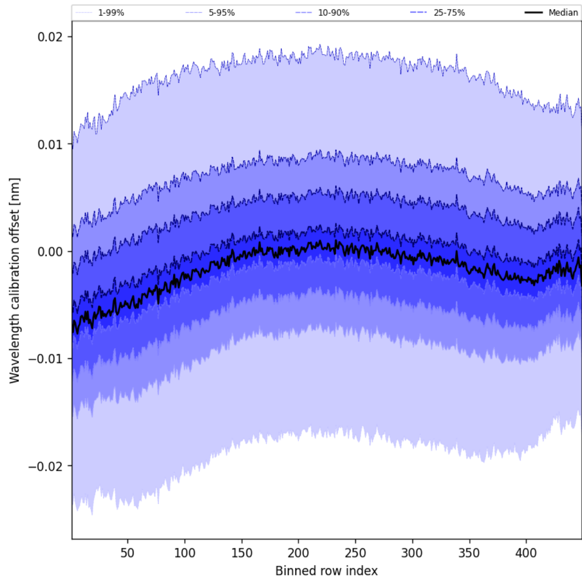
Figure 52: Along track statistics of “Wavelength calibration offset” for 2024-11-20 to 2024-11-21
