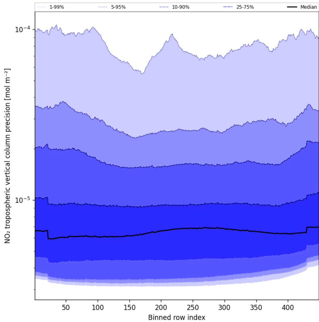
Figure 47: Along track statistics of “NO 2 tropospheric vertical column precision” for 2024-11-20 to 2024-11-21
