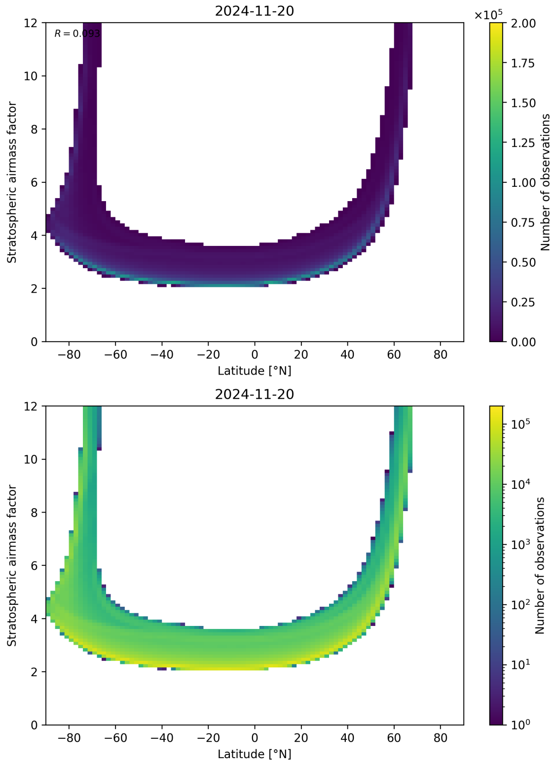
Figure 83: Scatter density plot of “Latitude” against “Stratospheric airmass factor” for 2024-11-20 to 2024-11-21.
