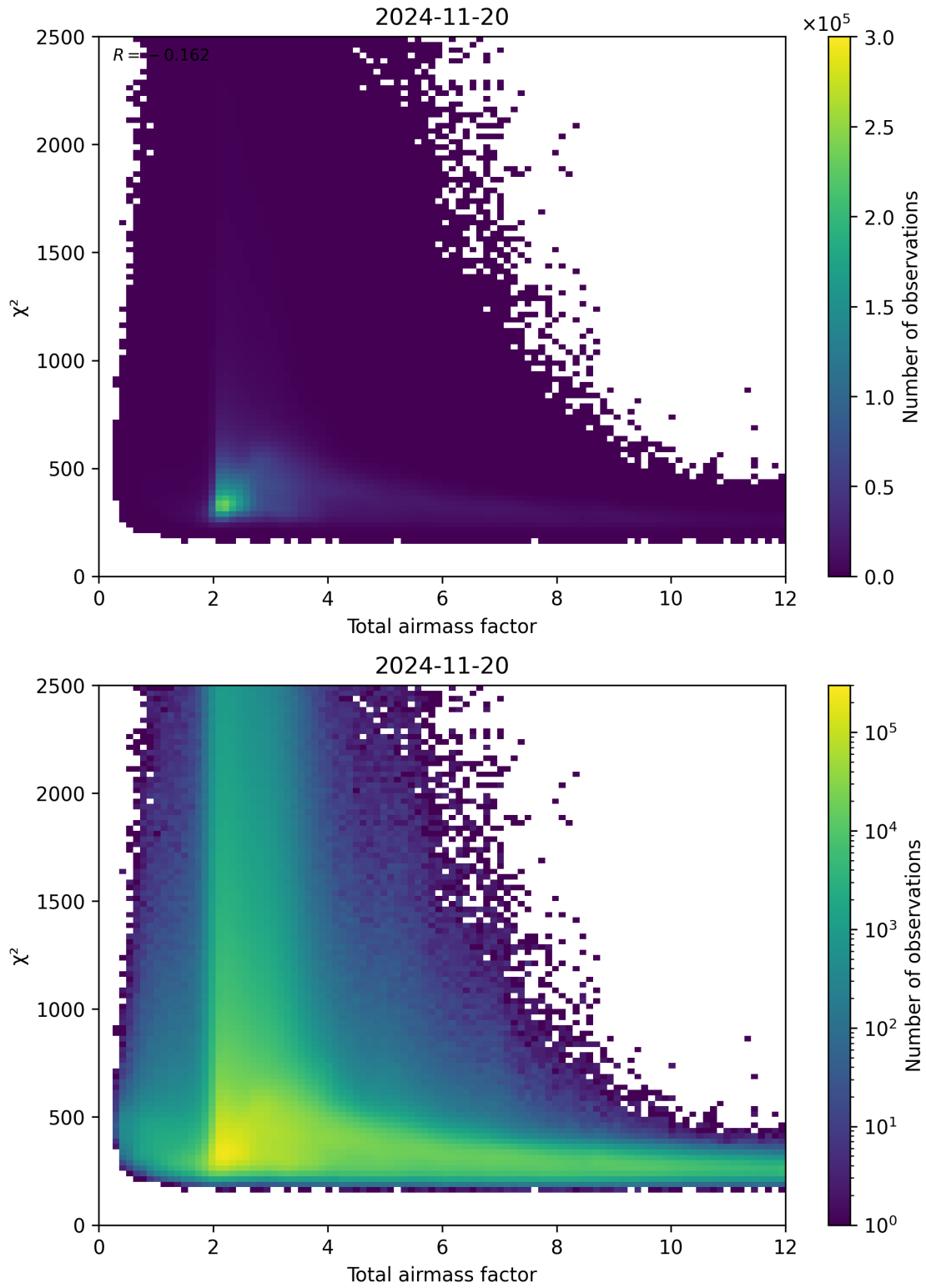
Figure 63: Scatter density plot of “Total airmass factor” against “ \chi^2 ” for 2024-11-20 to 2024-11-21.
