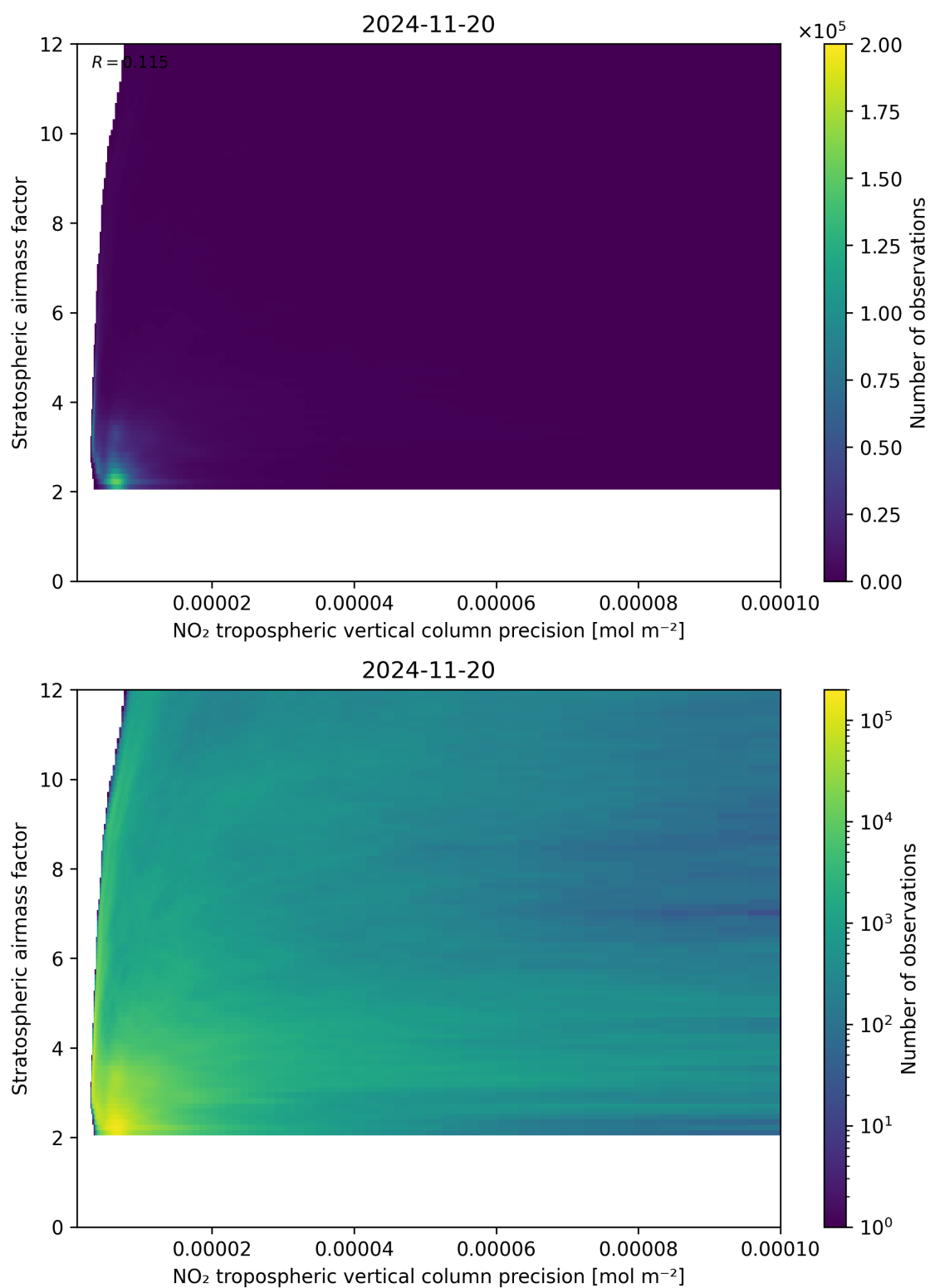
Figure 131: Scatter density plot of “NO 2 tropospheric vertical column precision” against “Stratospheric airmass factor” for 2024-11-20 to 2024-11-21.
