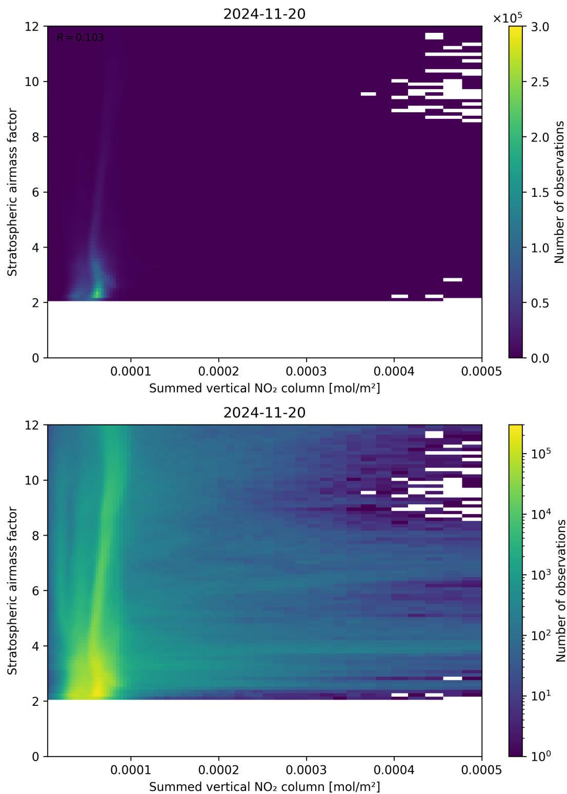
Figure 103: Scatter density plot of “Summed vertical NO 2 column” against “Stratospheric airmass factor” for 2024-11-20 to 2024-11-21.
