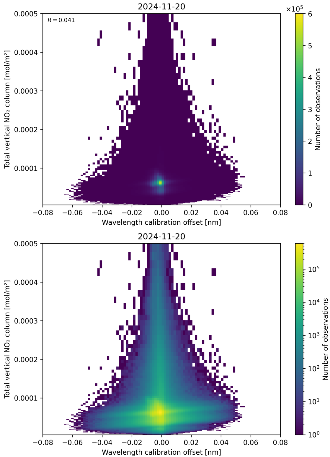
Figure 179: Scatter density plot of “Wavelength calibration offset” against “Total vertical NO 2 column” for 2024-11-20 to 2024-11-21.
