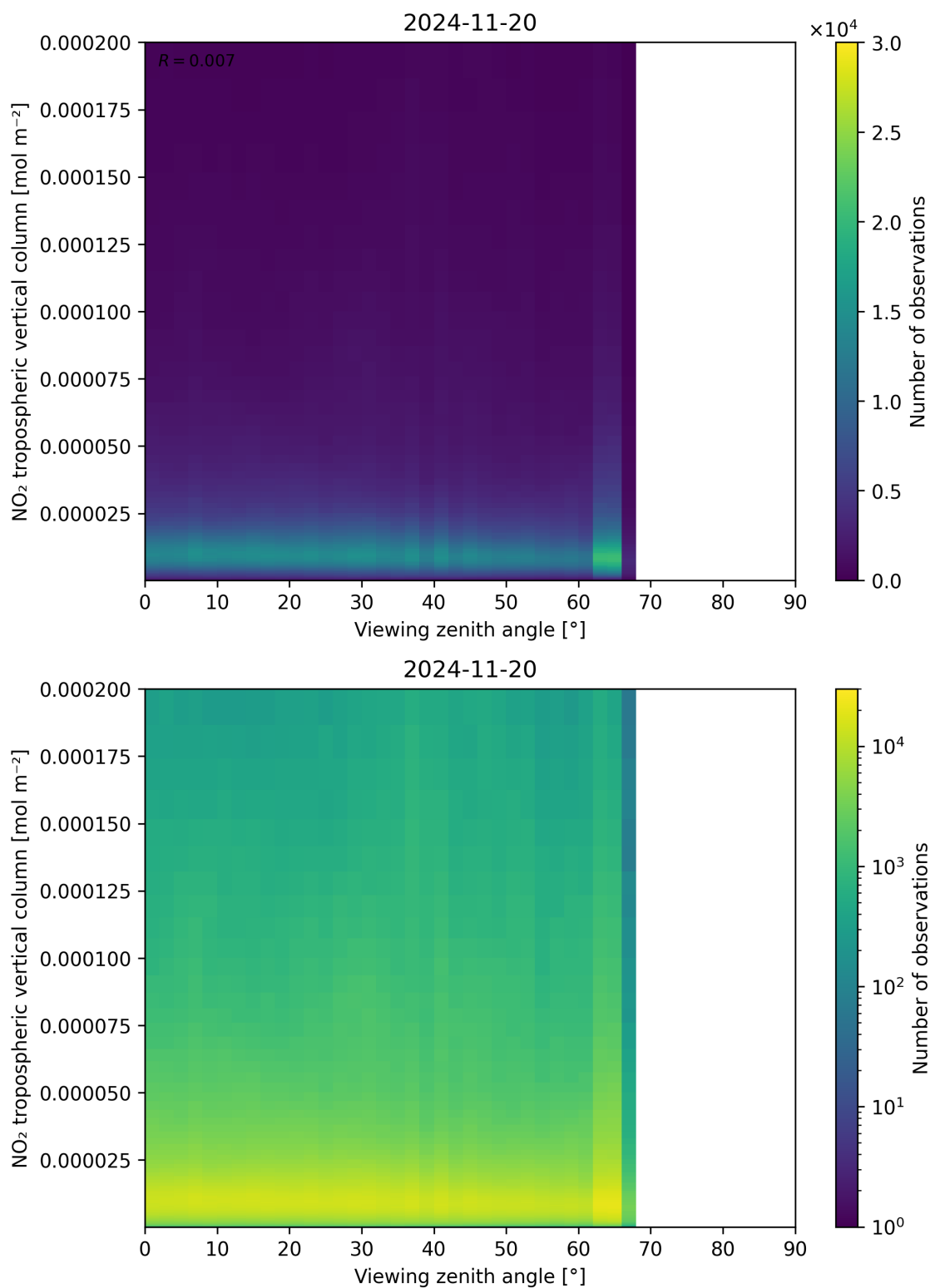
Figure 169: Scatter density plot of “Viewing zenith angle” against “NO 2 tropospheric vertical column” for 2024-11-20 to 2024-11-21.
