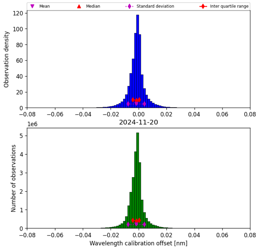
Figure 35: Histogram of “Wavelength calibration offset” for 2024-11-20 to 2024-11-21
