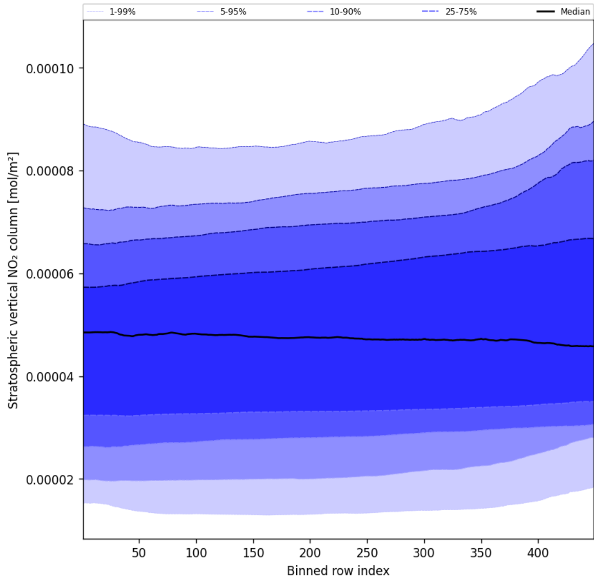
Figure 53: Along track statistics of “Stratospheric vertical NO 2 column” for 2024-11-20 to 2024-11-21
