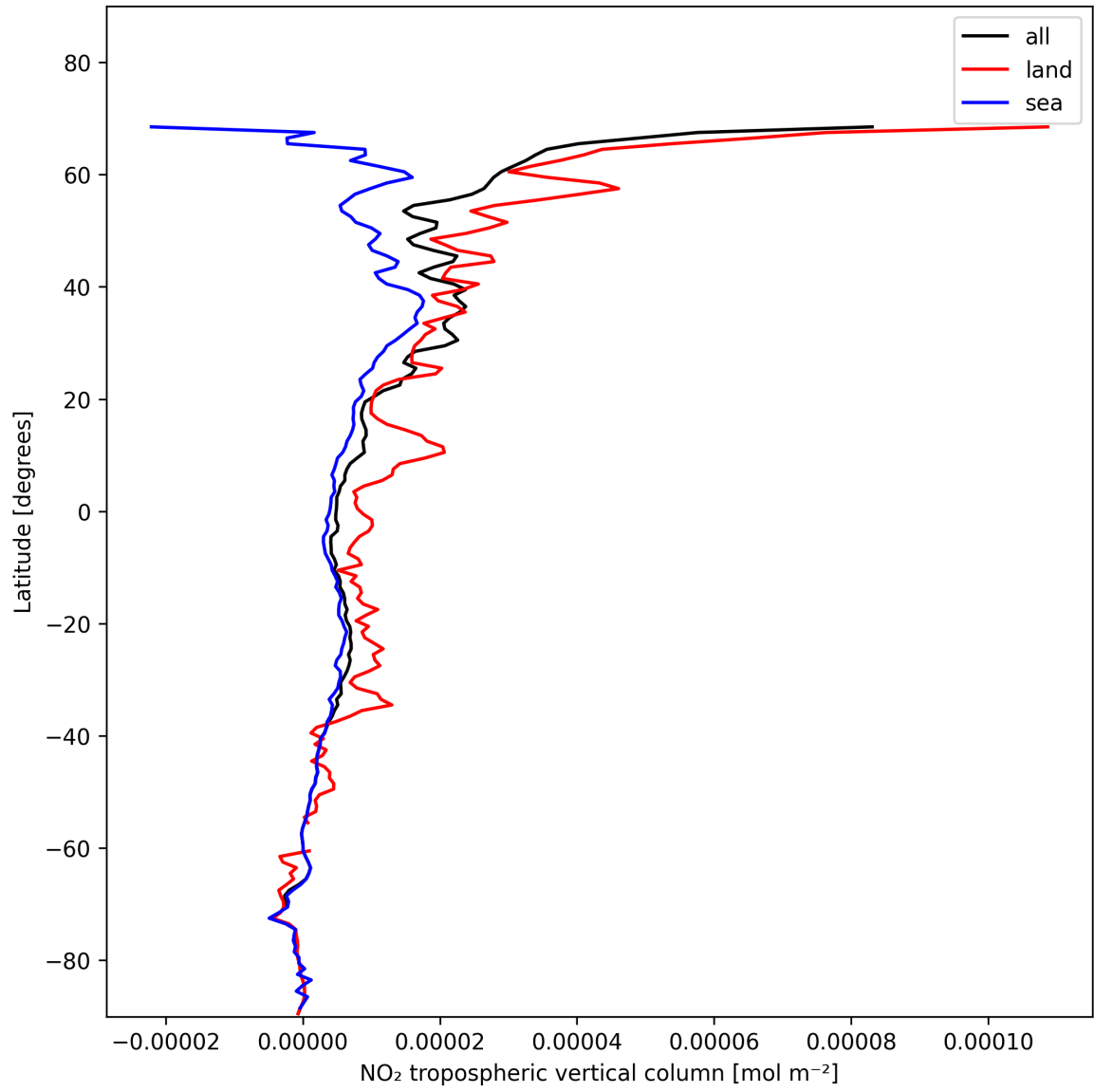
Figure 12: Zonal average of “NO 2 tropospheric vertical column” for 2024-11-20 to 2024-11-21.
