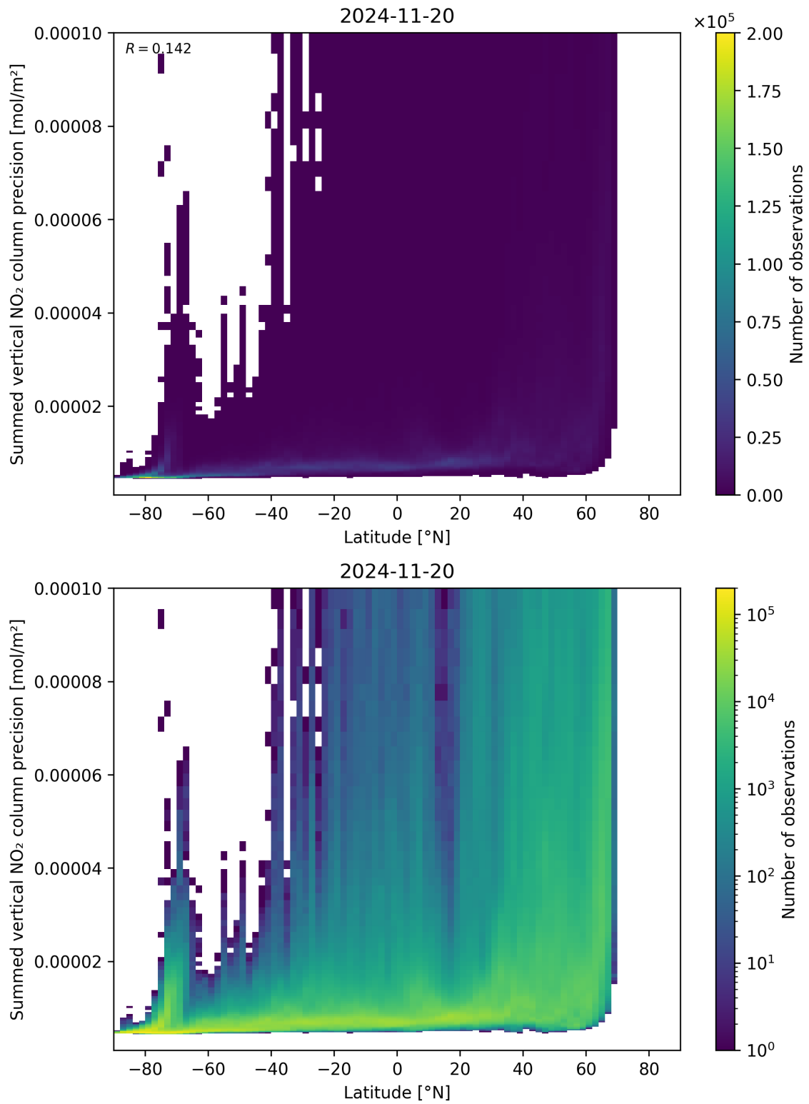
Figure 89: Scatter density plot of “Latitude” against “Summed vertical NO 2 column precision” for 2024-11-20 to 2024-11-21.
