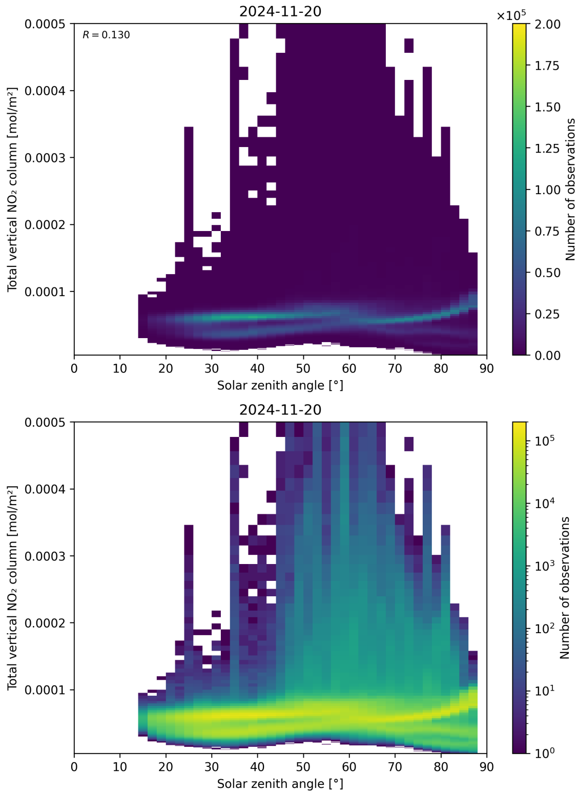
Figure 153: Scatter density plot of “Solar zenith angle” against “Total vertical NO 2 column” for 2024-11-20 to 2024-11-21.
