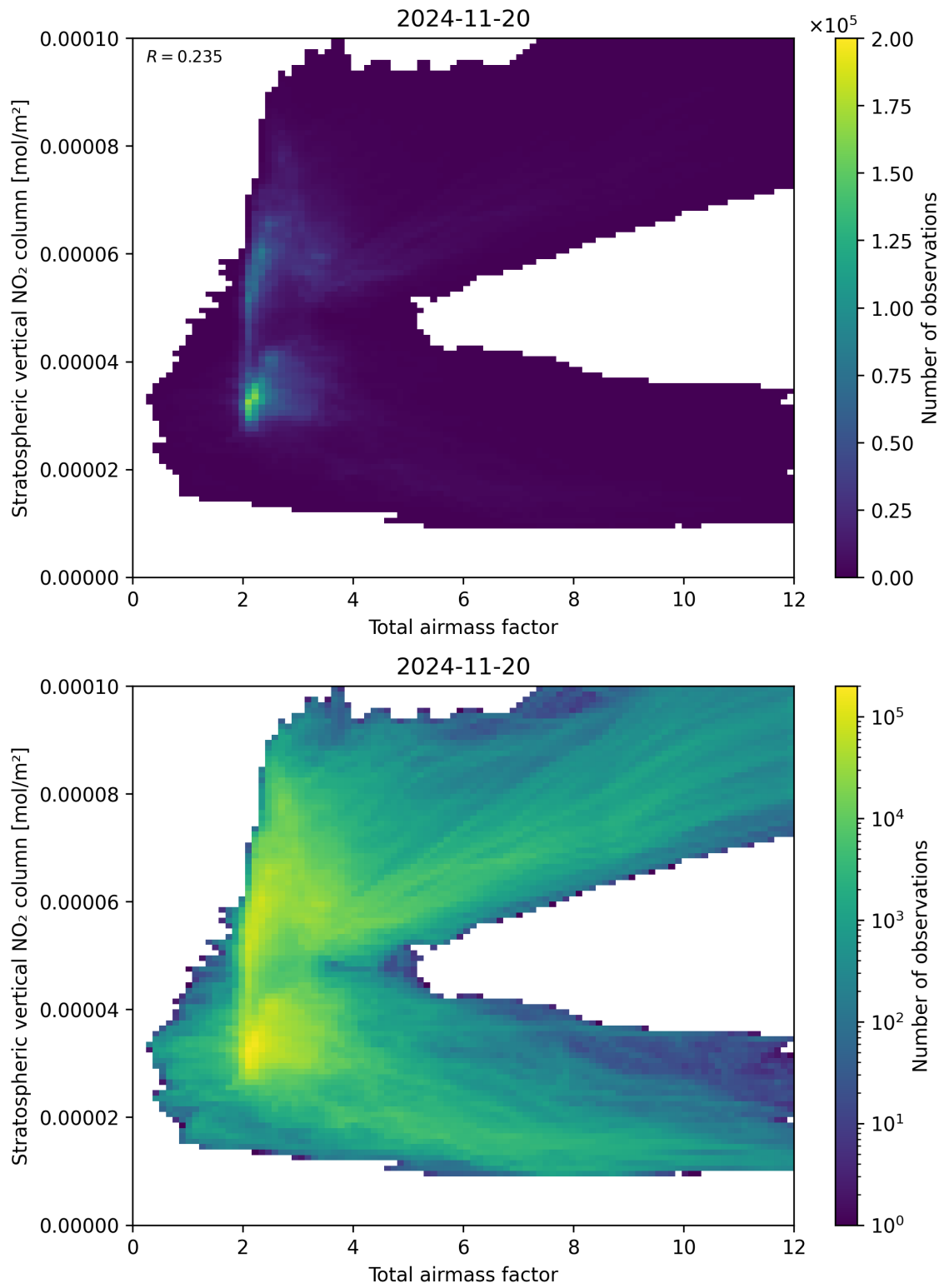
Figure 64: Scatter density plot of “Total airmass factor” against “Stratospheric vertical NO 2 column” for 2024-11-20 to 2024-11-21.
