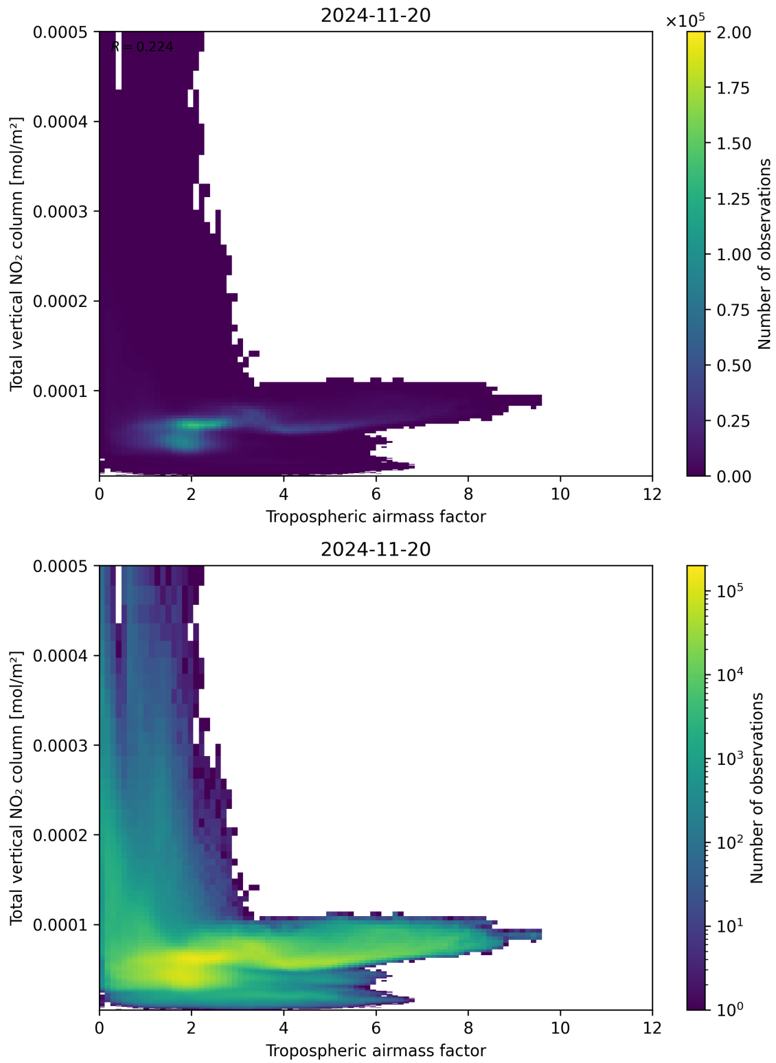
Figure 77: Scatter density plot of “Tropospheric airmass factor” against “Total vertical NO 2 column” for 2024-11-20 to 2024-11-21.
