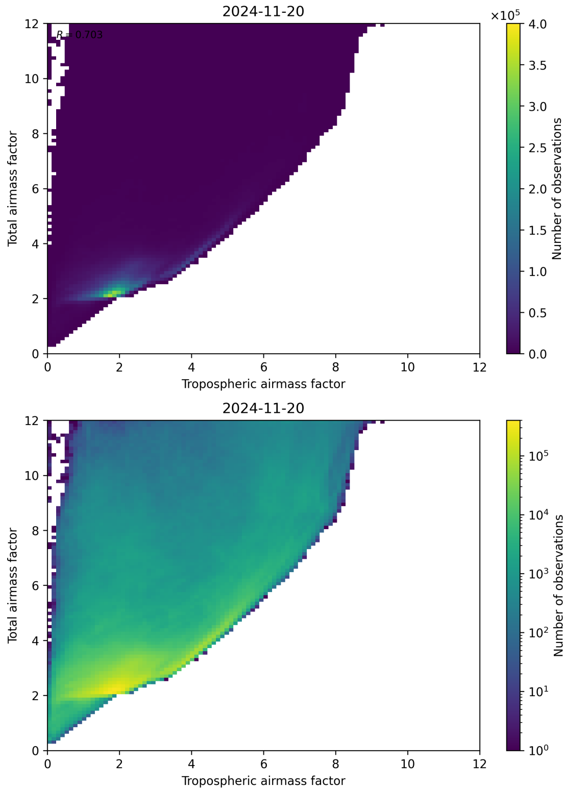
Figure 72: Scatter density plot of “Tropospheric airmass factor” against “Total airmass factor” for 2024-11-20 to 2024-11-21.
