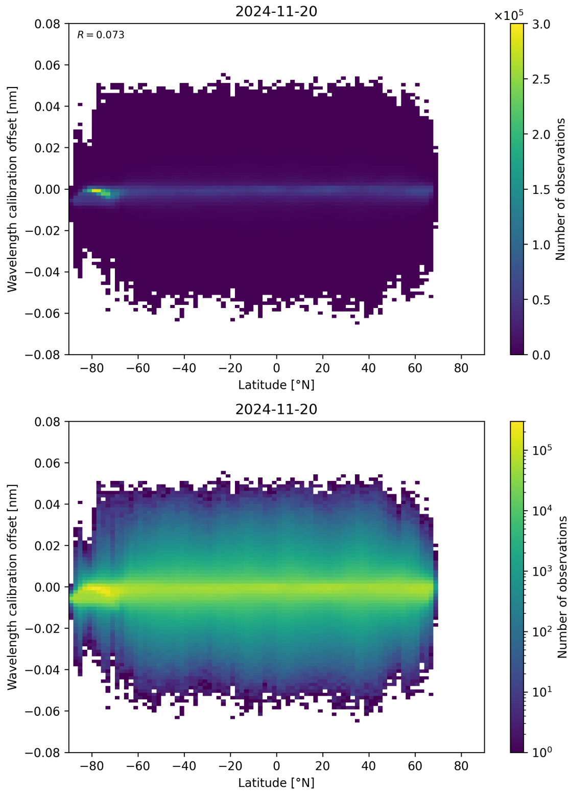
Figure 95: Scatter density plot of “Latitude” against “Wavelength calibration offset” for 2024-11-20 to 2024-11-21.
