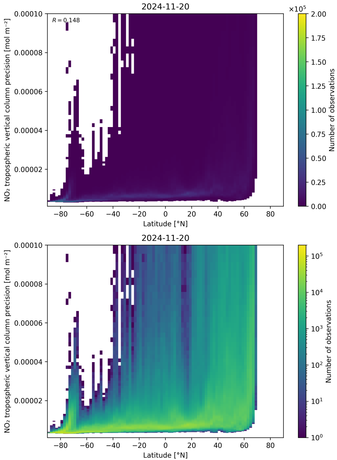
Figure 93: Scatter density plot of “Latitude” against “NO 2 tropospheric vertical column precision” for 2024-11-20 to 2024-11-21.
