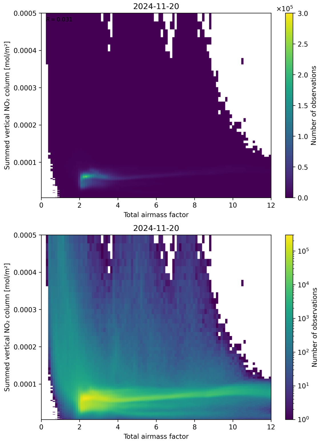
Figure 65: Scatter density plot of “Total air mass factor” against “Summed vertical NO 2 column” for 2024-11-20 to 2024-11-21.
