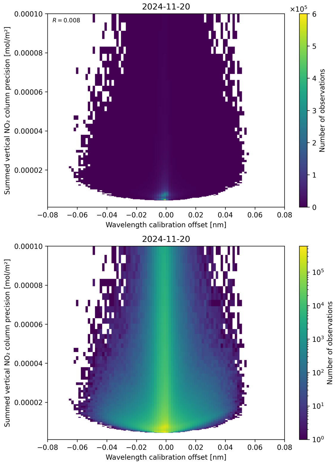
Figure 178: Scatter density plot of “Wavelength calibration offset” against “Summed vertical NO 2 column precision” for 2024-11-20 to 2024-11-21.
