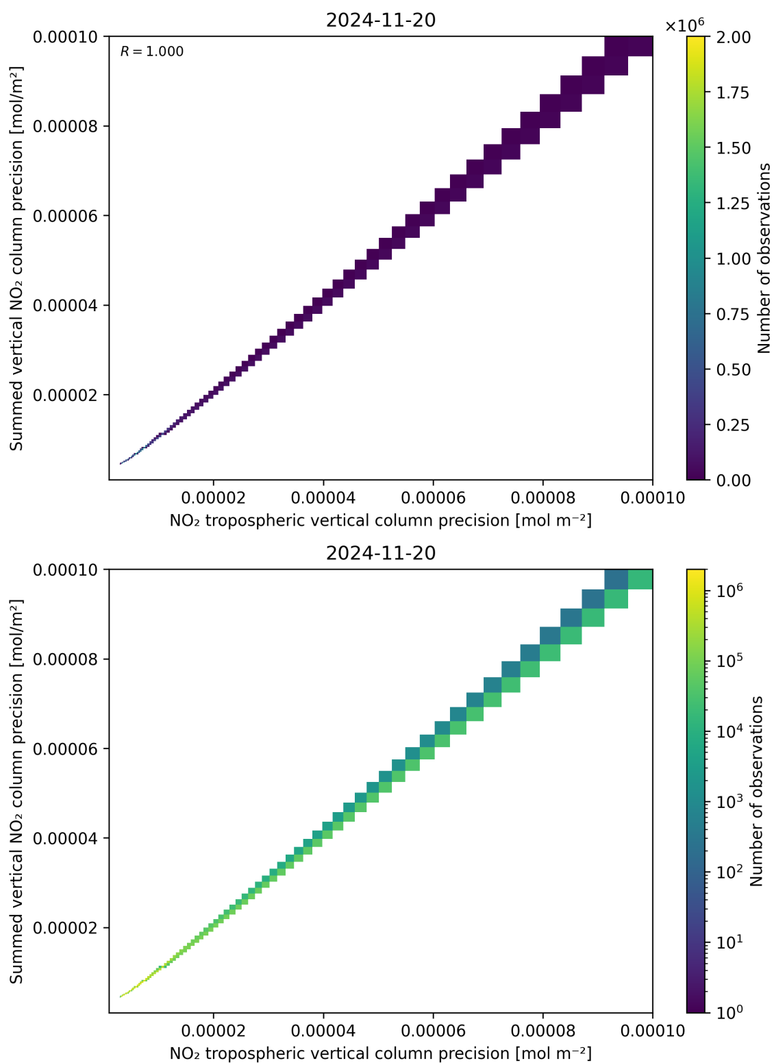
Figure 137: Scatter density plot of “NO 2 tropospheric vertical column precision” against “Summed vertical NO 2 column precision” for 2024-11-20 to 2024-11-21.
