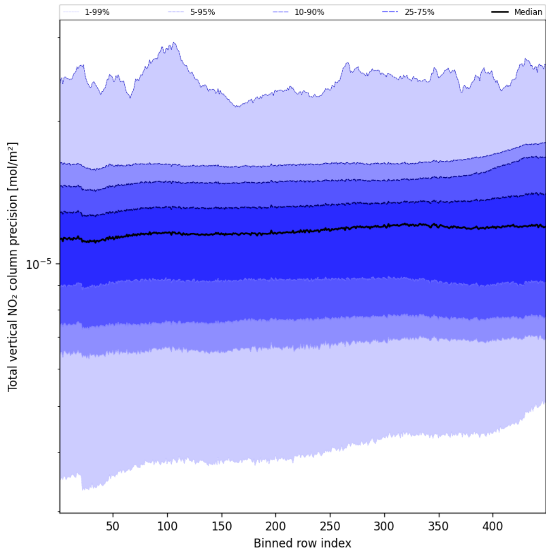
Figure 56: Along track statistics of “Total vertical NO 2 column precision” for 2024-11-20 to 2024-11-21
