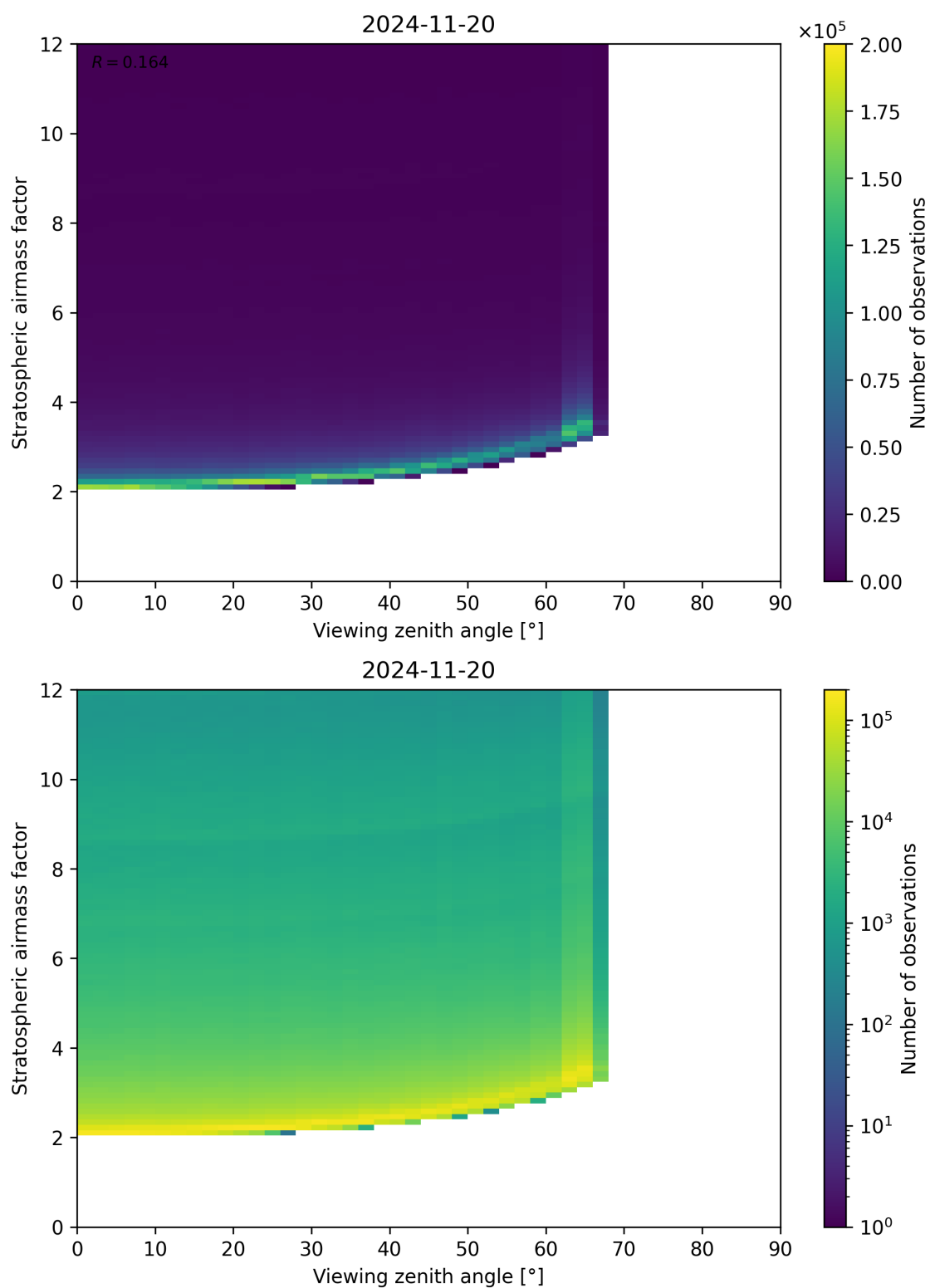
Figure 159: Scatter density plot of “Viewing zenith angle” against “Stratospheric airmass factor” for 2024-11-20 to 2024-11-21.
