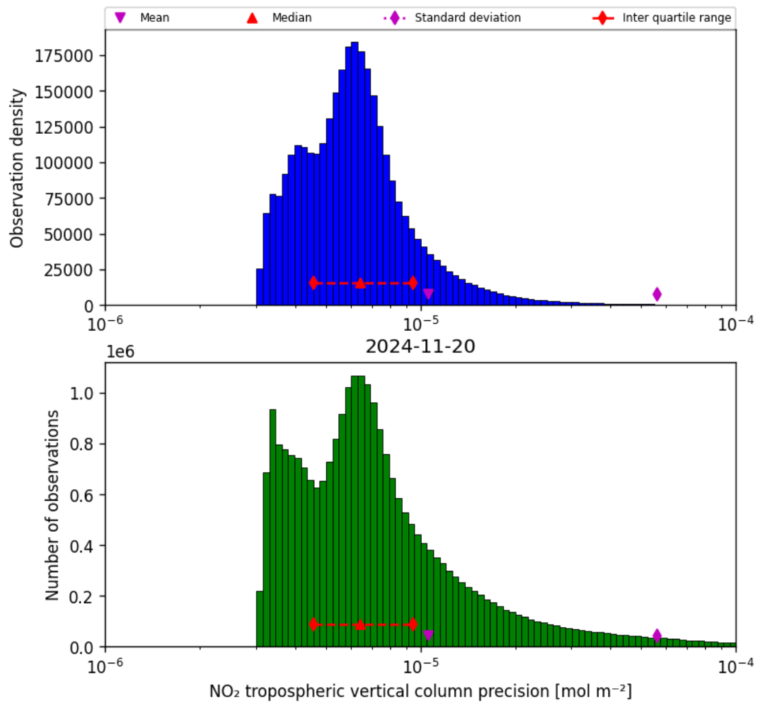
Figure 30: Histogram of “NO 2 tropospheric vertical column precision” for 2024-11-20 to 2024-11-21
