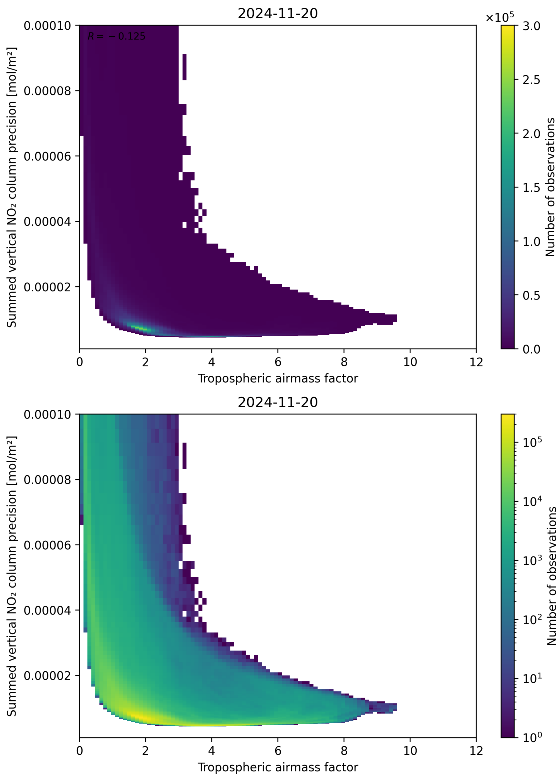
Figure 76: Scatter density plot of “Tropospheric air mass factor” against “Summed vertical NO 2 column precision” for 2024-11-20 to 2024-11-21.
