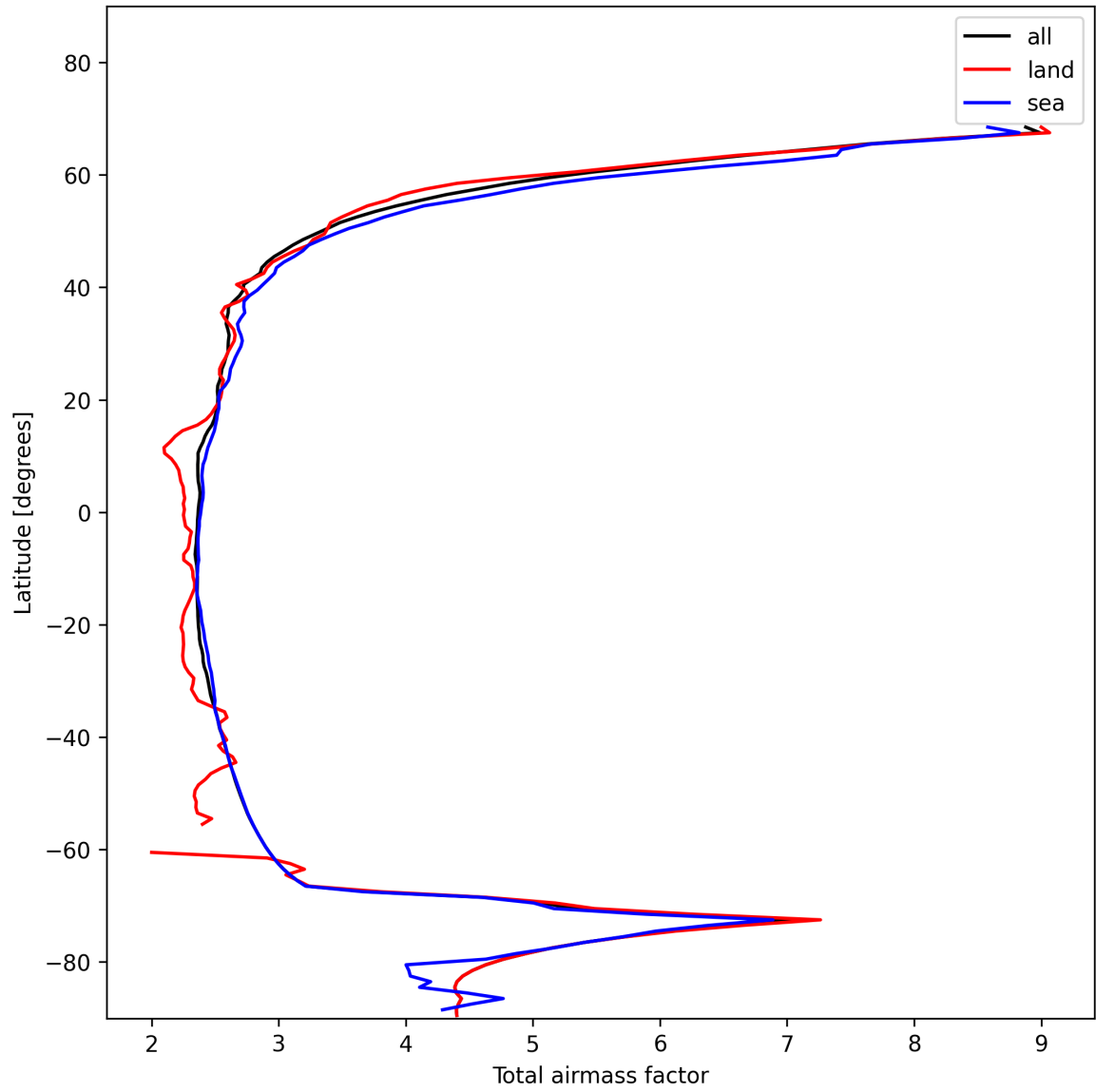
Figure 15: Zonal average of “Total airmass factor” for 2024-11-20 to 2024-11-21.
