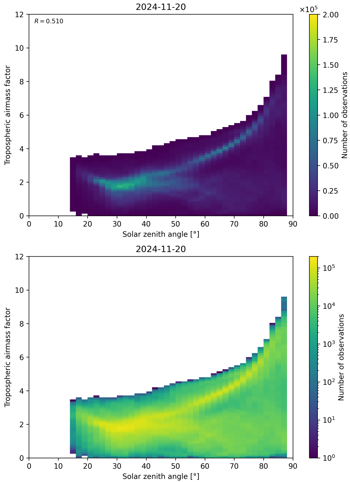
Figure 147: Scatter density plot of “Solar zenith angle” against “Tropospheric airmass factor” for 2024-11-20 to 2024-11-21.
