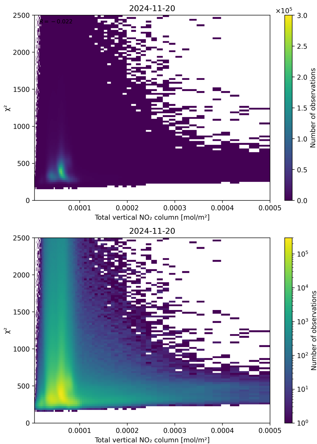
Figure 111: Scatter density plot of “Total vertical NO 2 column” against “ \chi^2 ” for 2024-11-20 to 2024-11-21.
