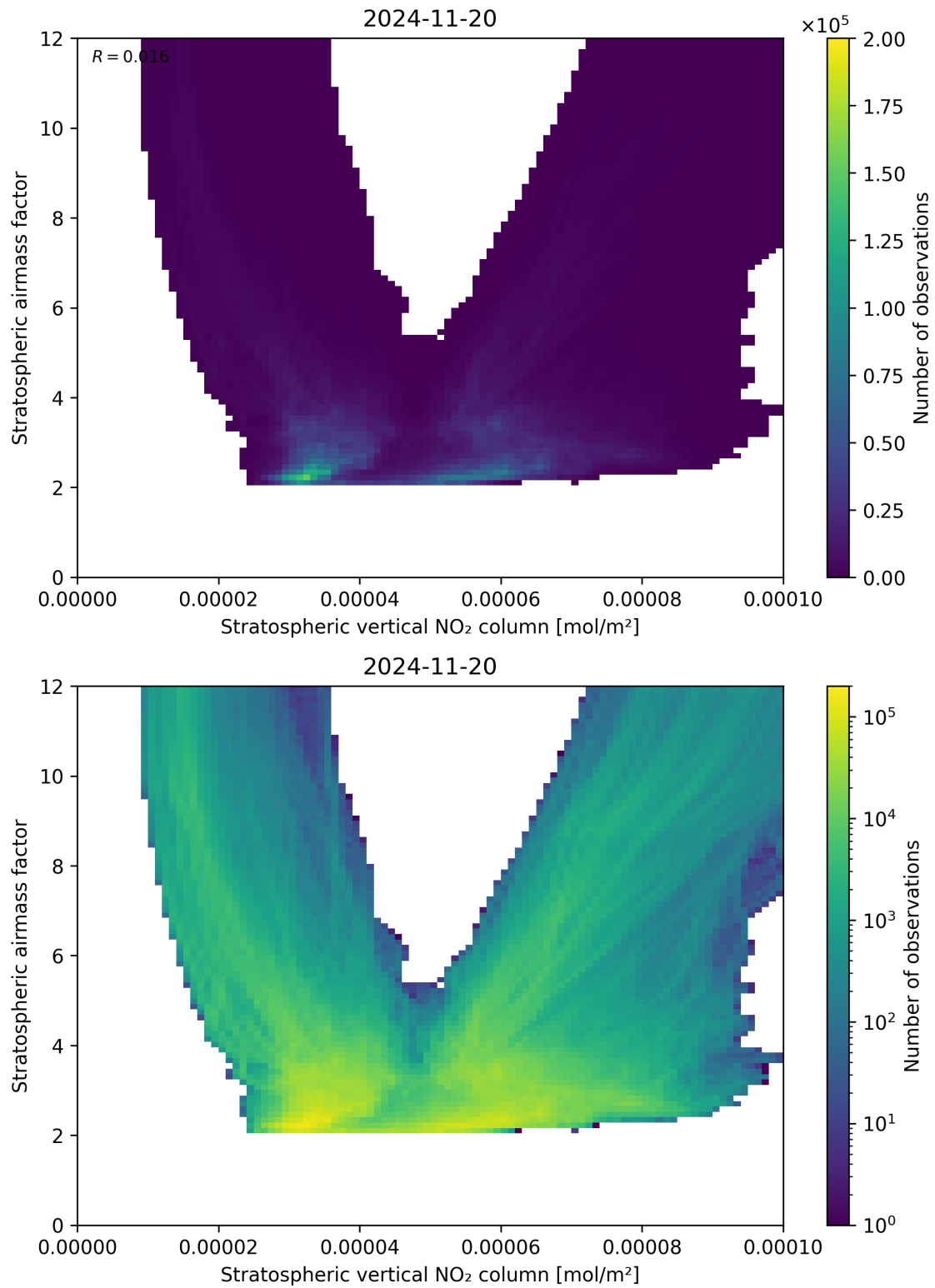
Figure 96: Scatter density plot of “Stratospheric vertical NO 2 column” against “Stratospheric airmass factor” for 2024-11-20 to 2024-11-21.
