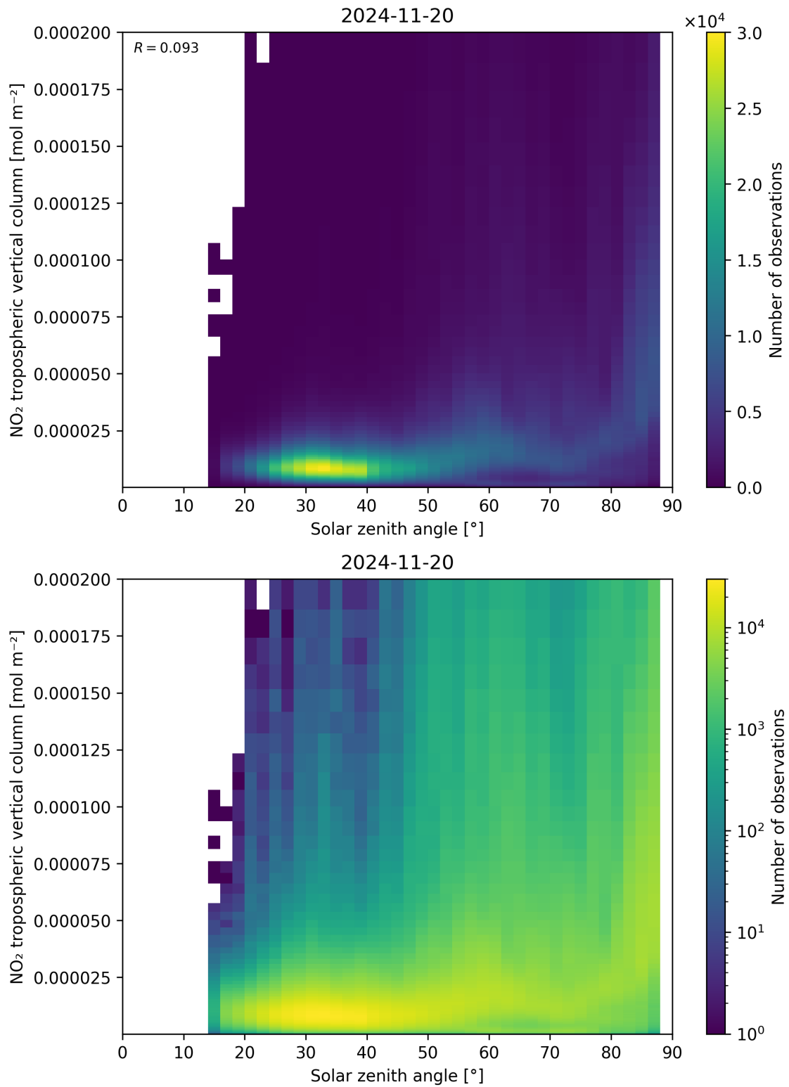
Figure 155: Scatter density plot of “Solar zenith angle” against “NO 2 tropospheric vertical column” for 2024-11-20 to 2024-11-21.
