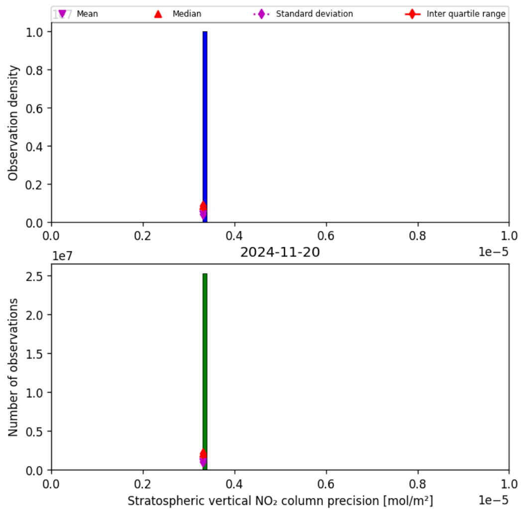
Figure 37: Histogram of “Stratospheric vertical NO 2 column precision” for 2024-11-20 to 2024-11-21
