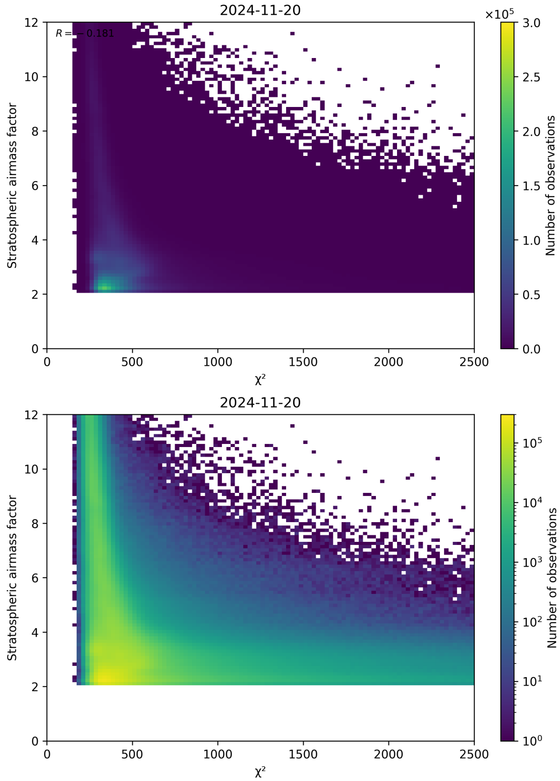
Figure 81: Scatter density plot of “ \chi^2 ” against “Stratospheric airmass factor” for 2024-11-20 to 2024-11-21.
