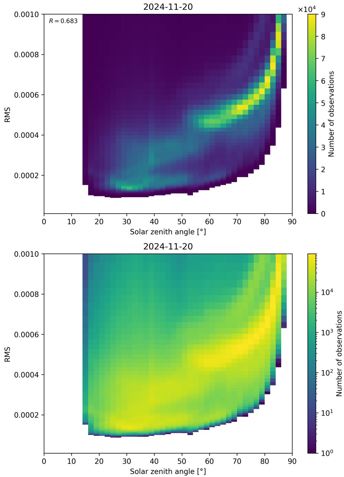
Figure 157: Scatter density plot of “Solar zenith angle” against “RMS” for 2024-11-20 to 2024-11-21.
