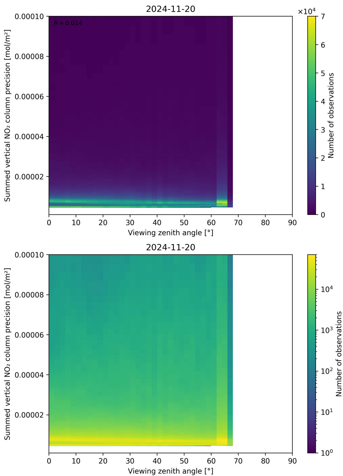
Figure 166: Scatter density plot of “Viewing zenith angle” against “Summed vertical NO 2 column precision” for 2024-11-20 to 2024-11-21.
