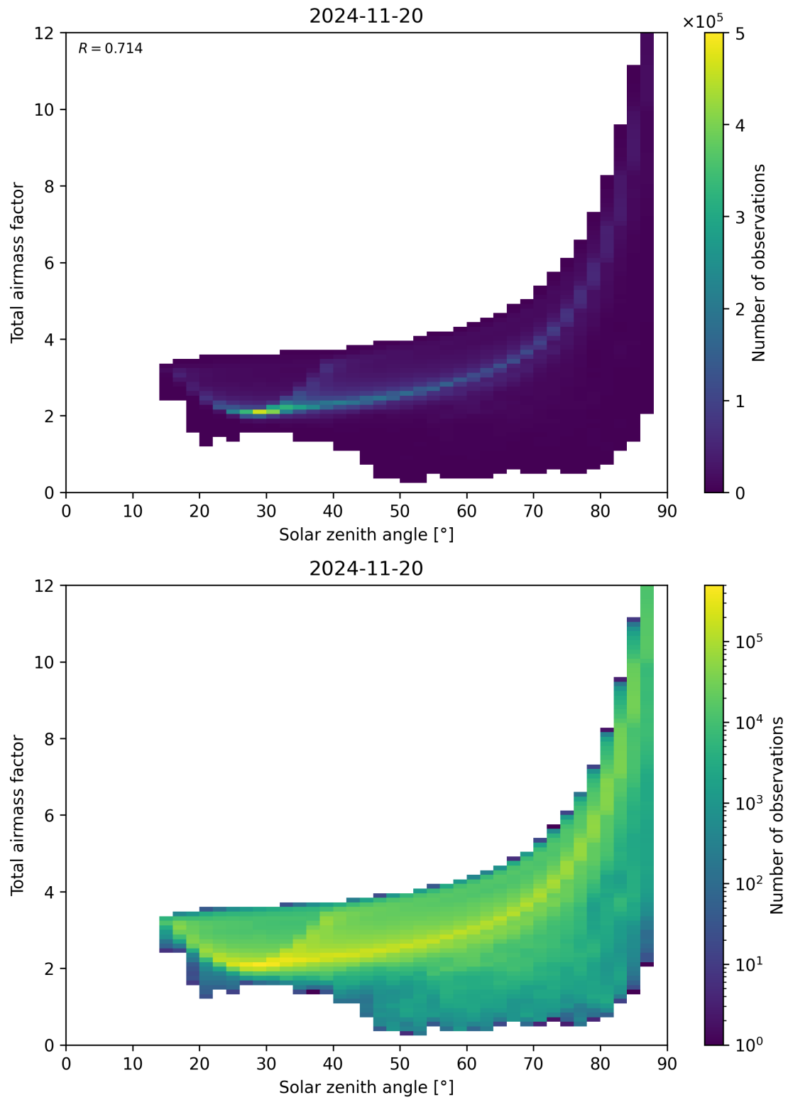
Figure 146: Scatter density plot of “Solar zenith angle” against “Total airmass factor” for 2024-11-20 to 2024-11-21.
