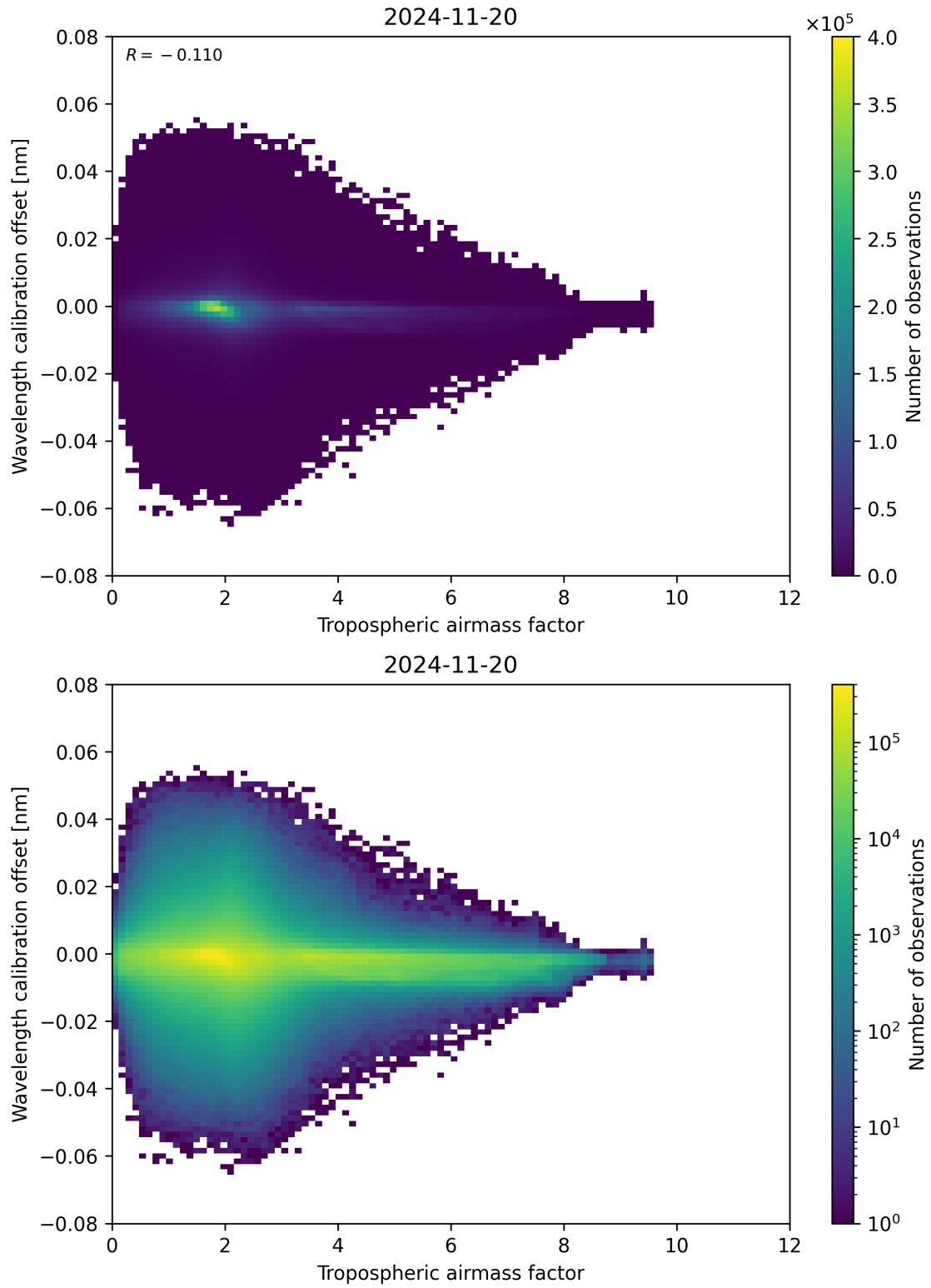
Figure 80: Scatter density plot of “Tropospheric airmass factor” against “Wavelength calibration offset” for 2024-11-20 to 2024-11-21.
