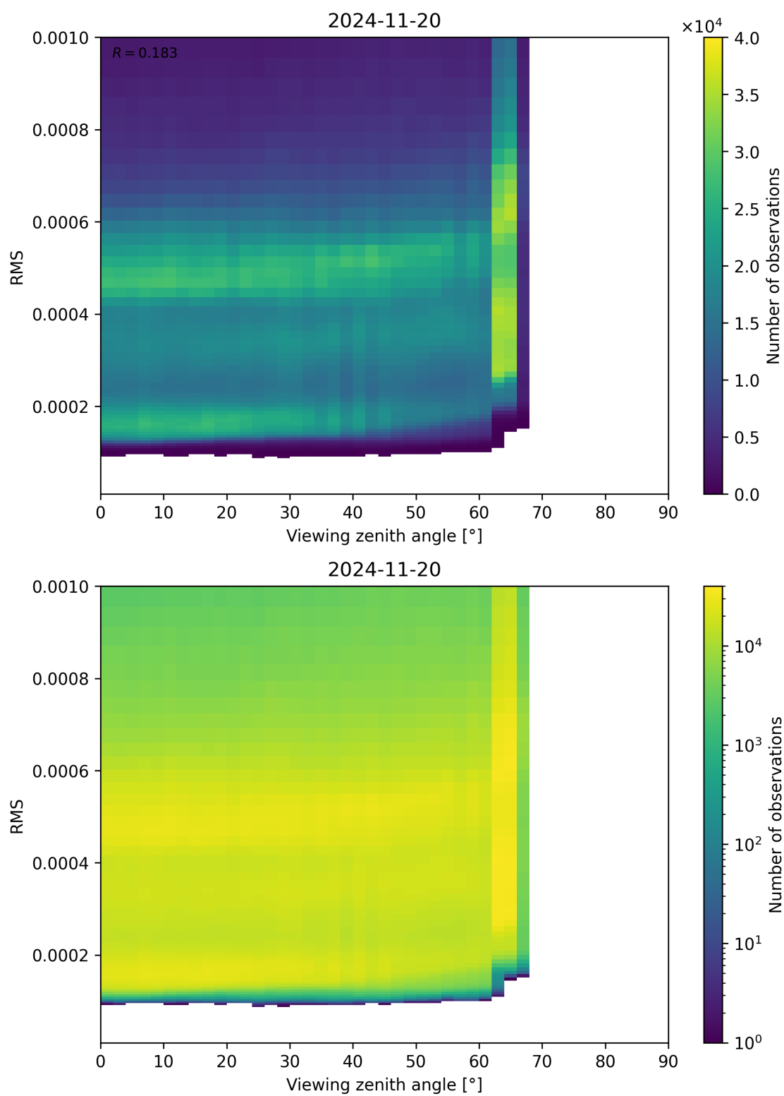
Figure 171: Scatter density plot of “Viewing zenith angle” against “RMS” for 2024-11-20 to 2024-11-21.
