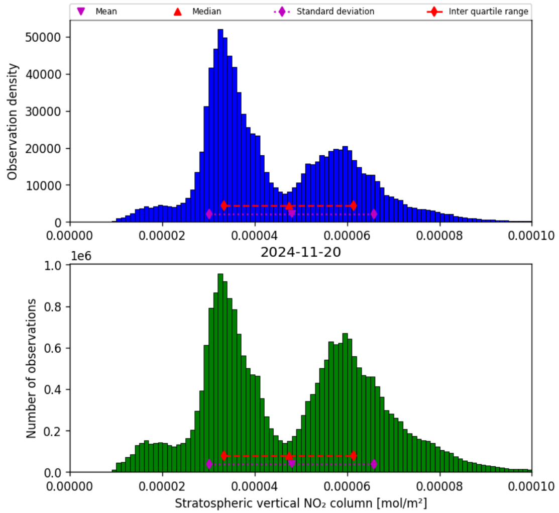
Figure 36: Histogram of “Stratospheric vertical NO 2 column” for 2024-11-20 to 2024-11-21
