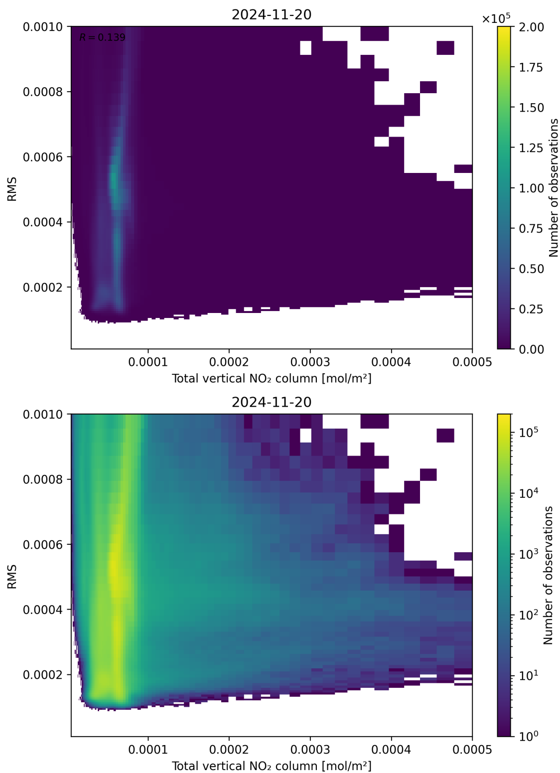
Figure 120: Scatter density plot of “Total vertical NO 2 column” against “RMS” for 2024-11-20 to 2024-11-21.
