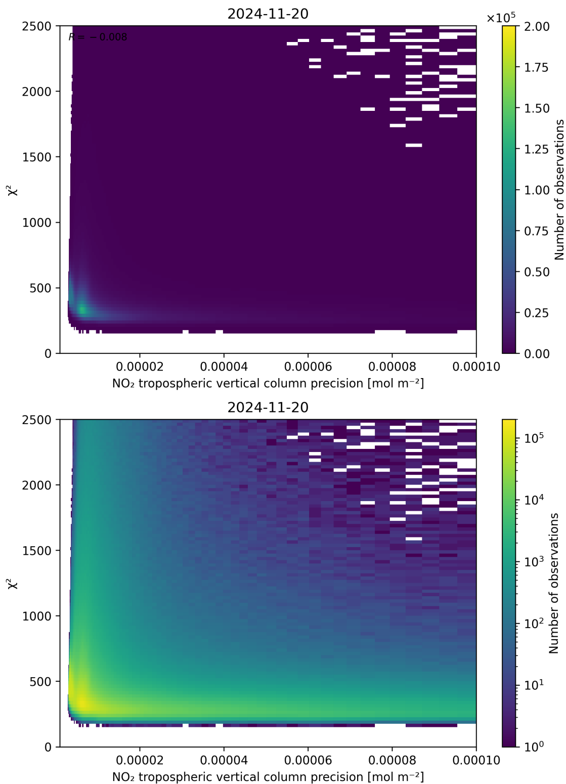
Figure 134: Scatter density plot of “NO 2 tropospheric vertical column precision” against “ \chi^2 ” for 2024-11-20 to 2024-11-21.
