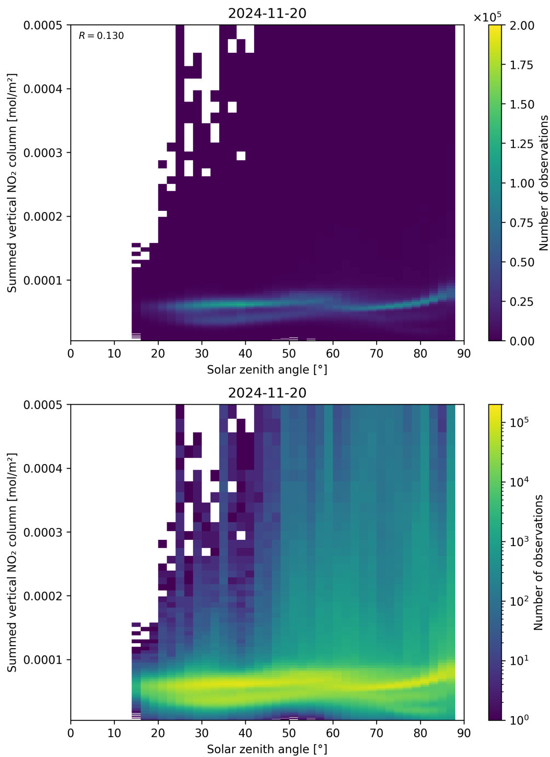
Figure 151: Scatter density plot of “Solar zenith angle” against “Summed vertical NO 2 column” for 2024-11-20 to 2024-11-21.
