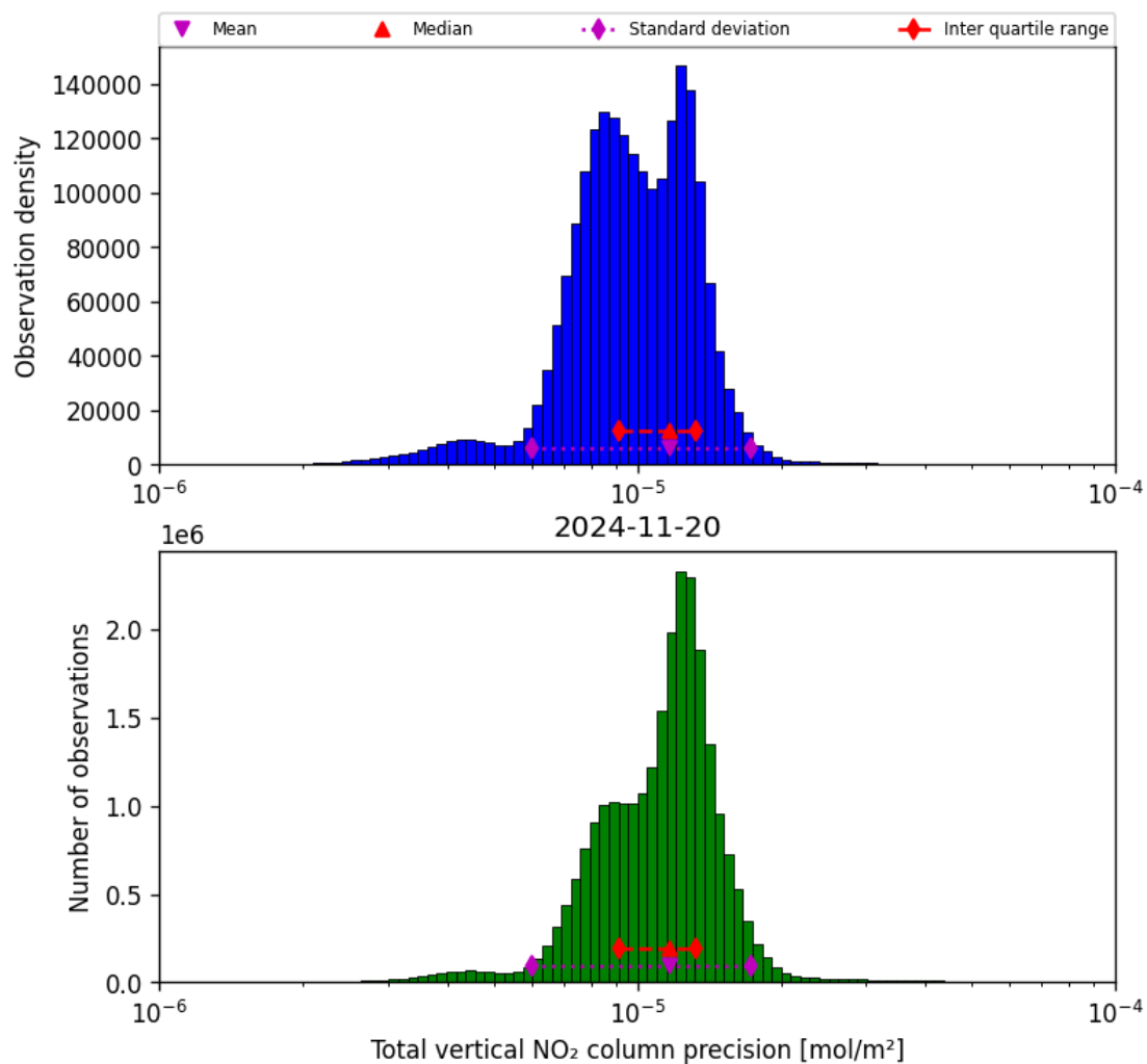
Figure 39: Histogram of “Total vertical NO 2 column precision” for 2024-11-20 to 2024-11-21
