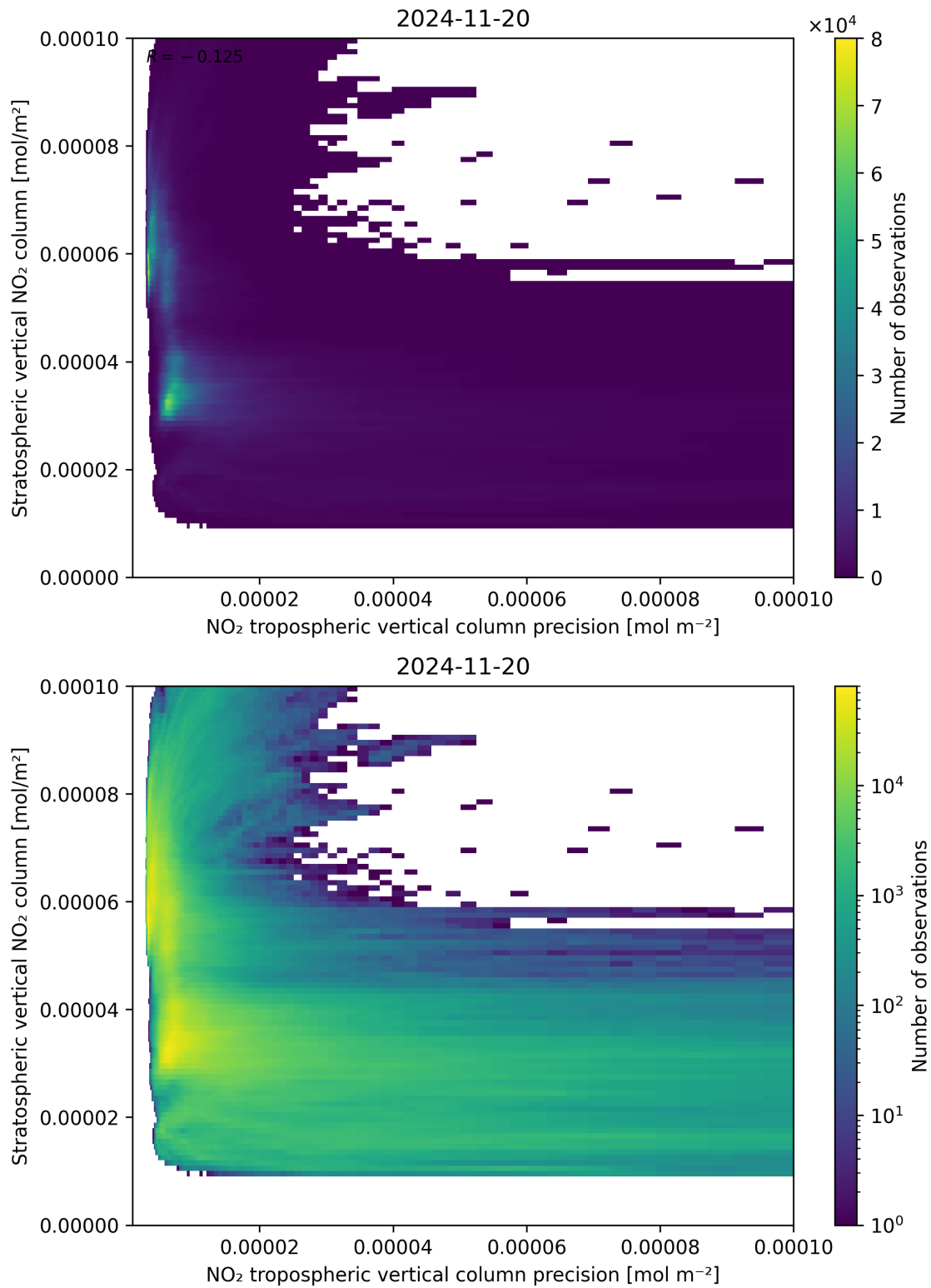
Figure 135: Scatter density plot of “NO 2 tropospheric vertical column precision” against “Stratospheric vertical NO 2 column” for 2024-11-20 to 2024-11-21.
