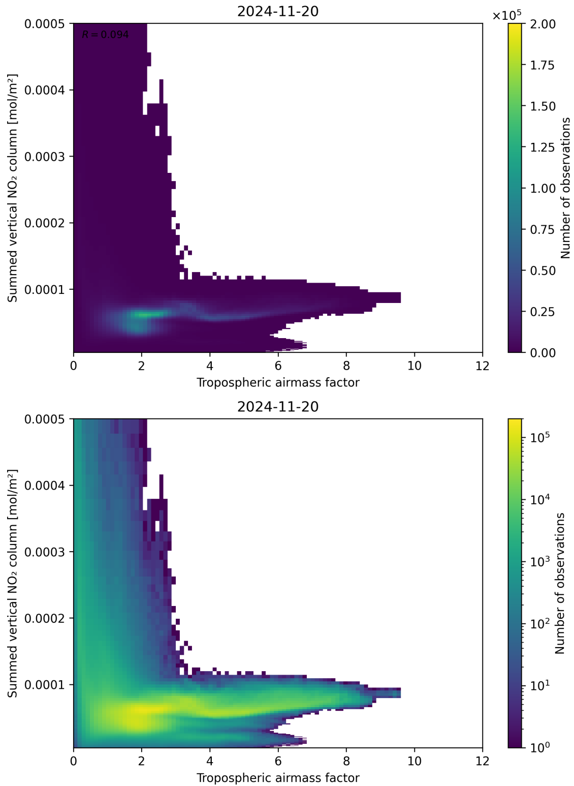
Figure 75: Scatter density plot of “Tropospheric air mass factor” against “Summed vertical NO 2 column” for 2024-11-20 to 2024-11-21.
