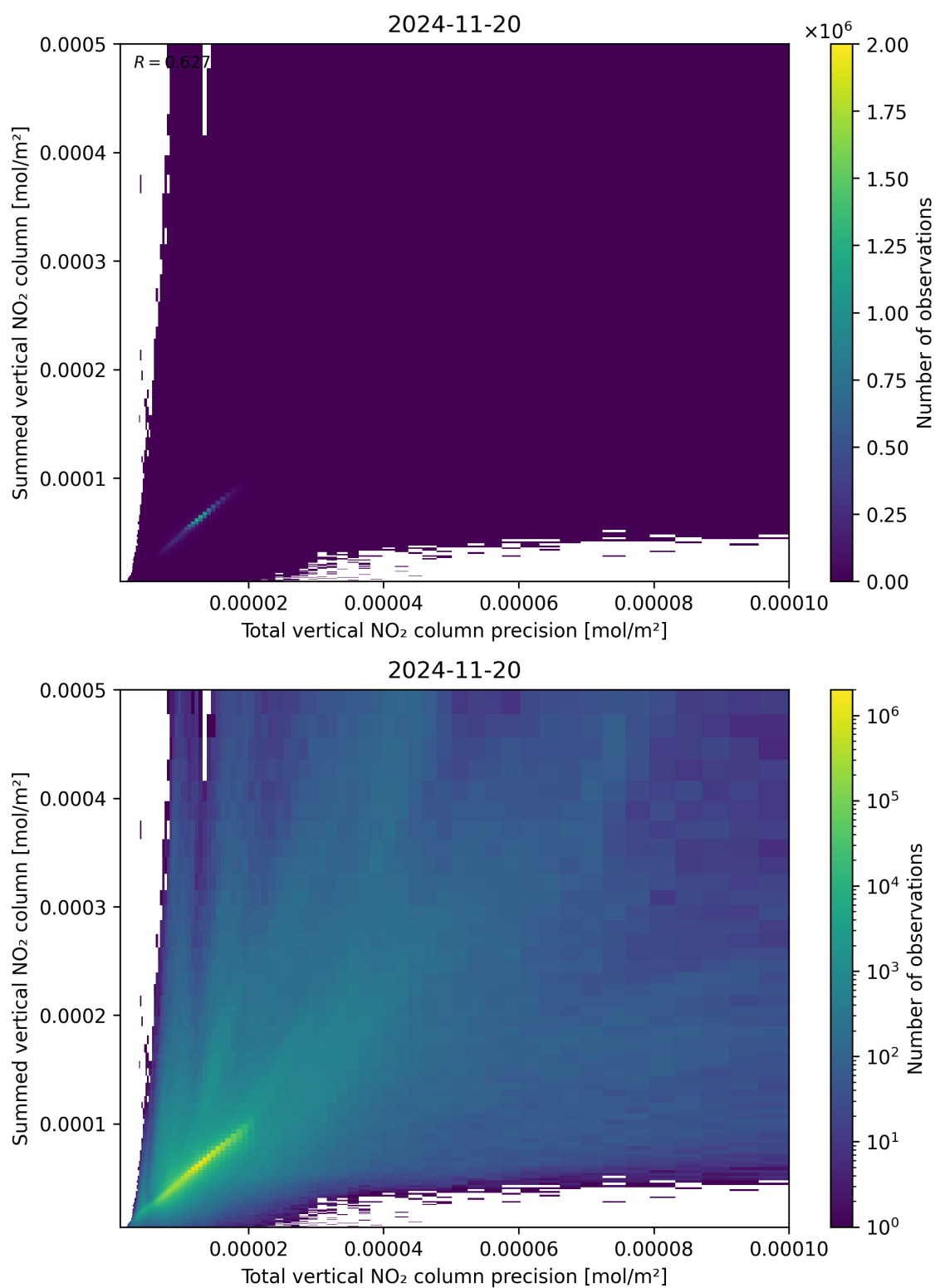
Figure 117: Scatter density plot of “Total vertical NO 2 column precision” against “Summed vertical NO 2 column” for 2024-11-20 to 2024-11-21.
