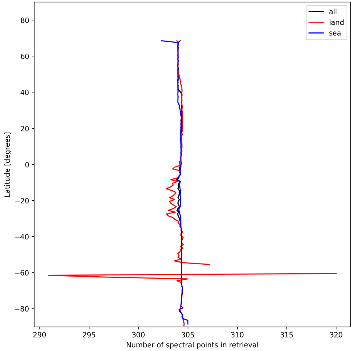
Figure 16: Zonal average of “Number of spectral points in retrieval” for 2024-11-20 to 2024-11-21.
