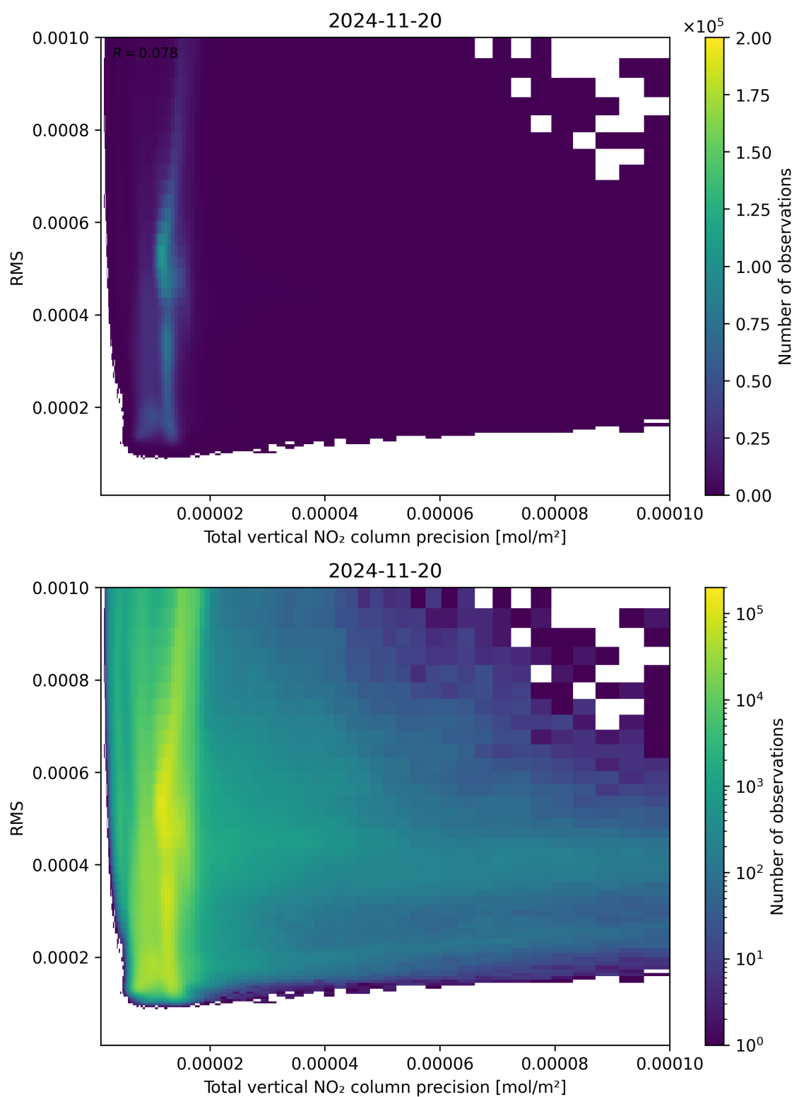
Figure 119: Scatter density plot of “Total vertical NO 2 column precision” against “RMS” for 2024-11-20 to 2024-11-21.
