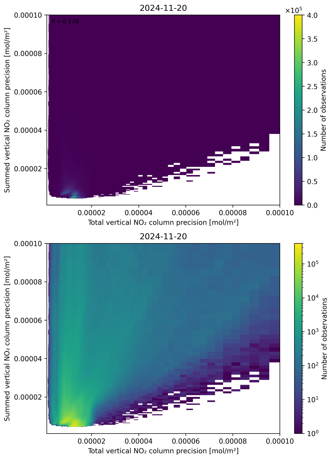
Figure 118: Scatter density plot of “Total vertical NO 2 column precision” against “Summed vertical NO 2 column precision” for 2024-11-20 to 2024-11-21.
