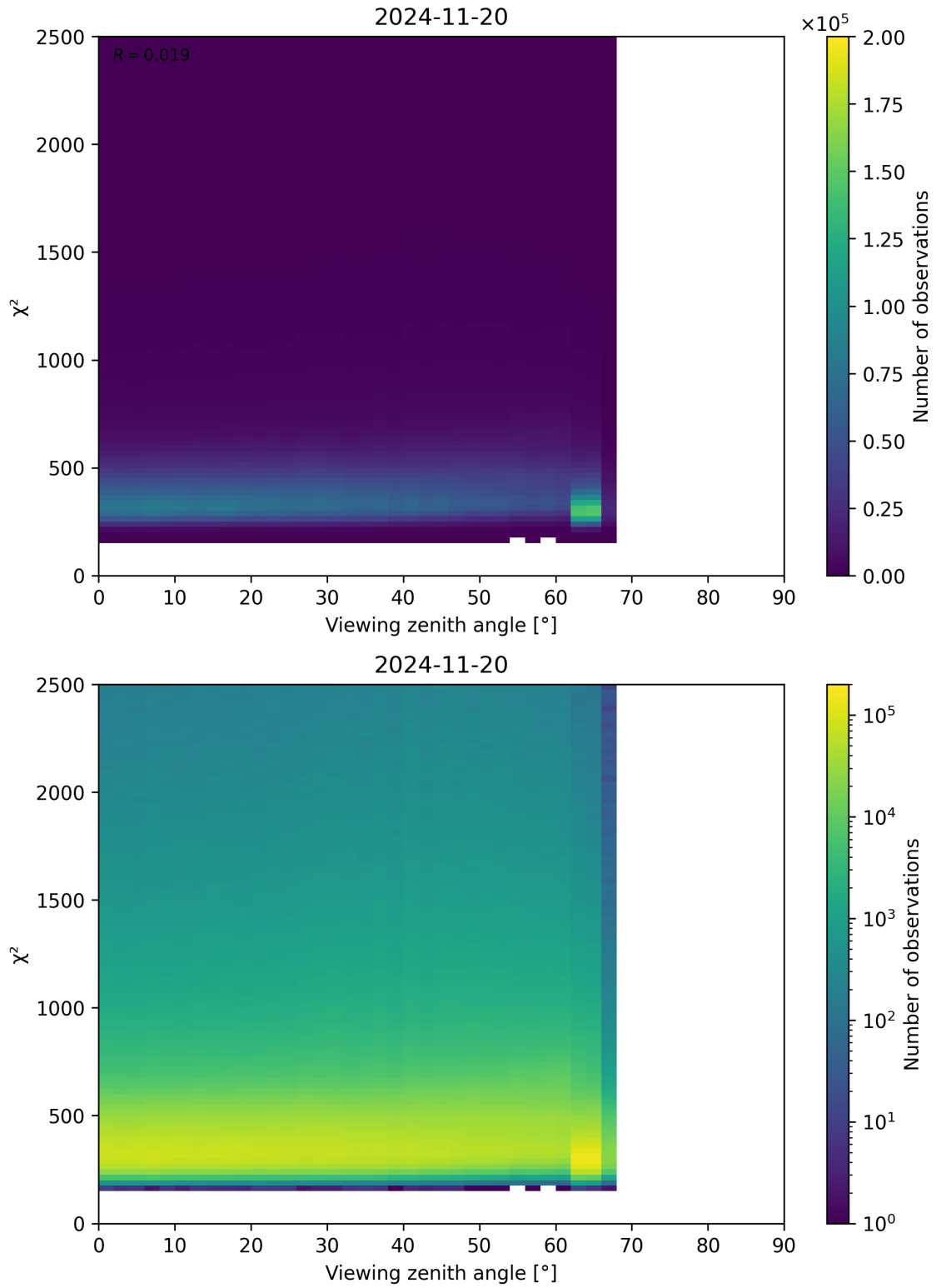
Figure 162: Scatter density plot of “Viewing zenith angle” against “ \chi^2 ” for 2024-11-20 to 2024-11-21.
