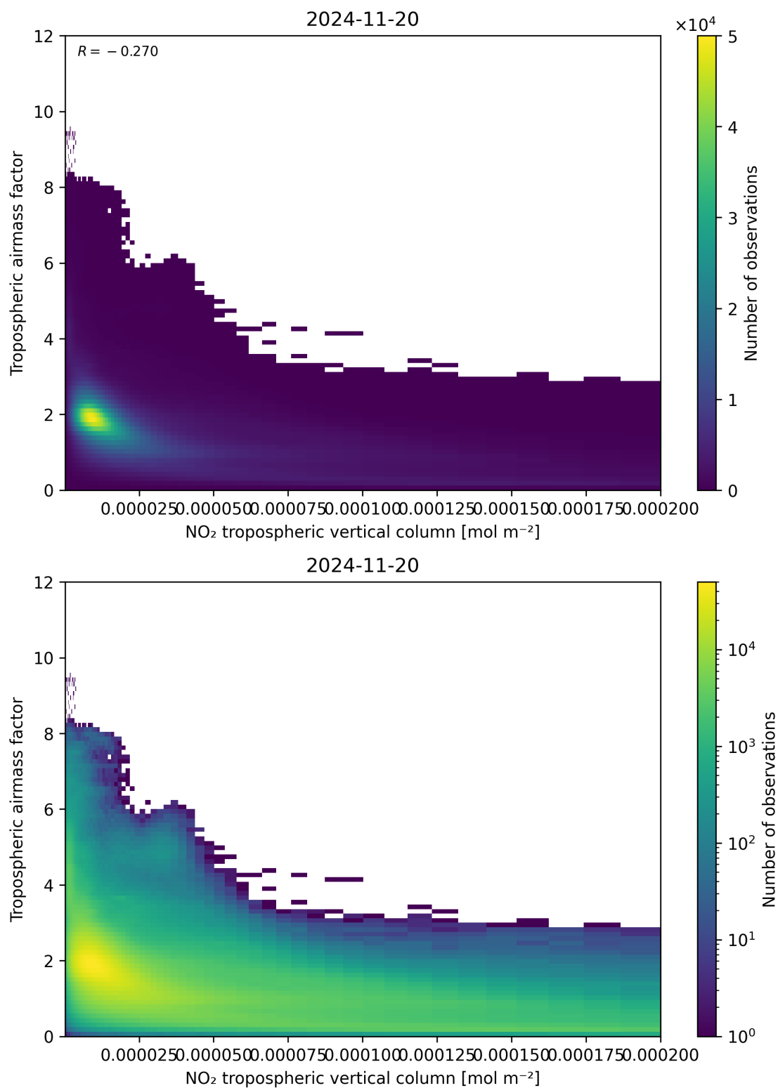
Figure 123: Scatter density plot of “NO 2 tropospheric vertical column” against “Tropospheric air mass factor” for 2024-11-20 to 2024-11-21.
