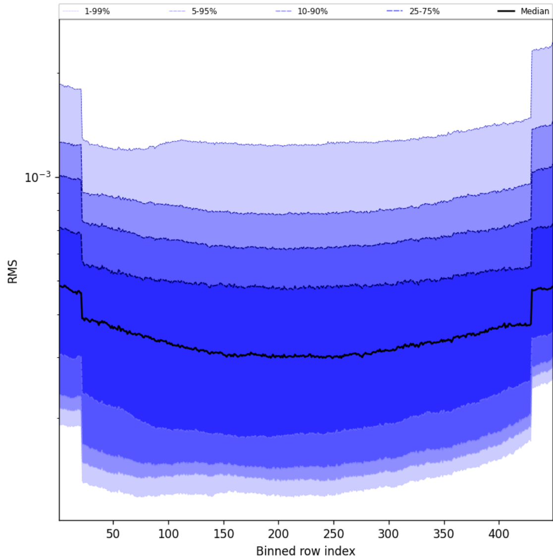
Figure 60: Along track statistics of “RMS” for 2024-11-20 to 2024-11-21
