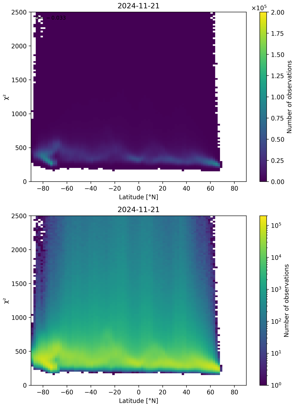
Figure 86: Scatter density plot of “Latitude” against “ \chi^2 ” for 2024-11-20 to 2024-11-22.
