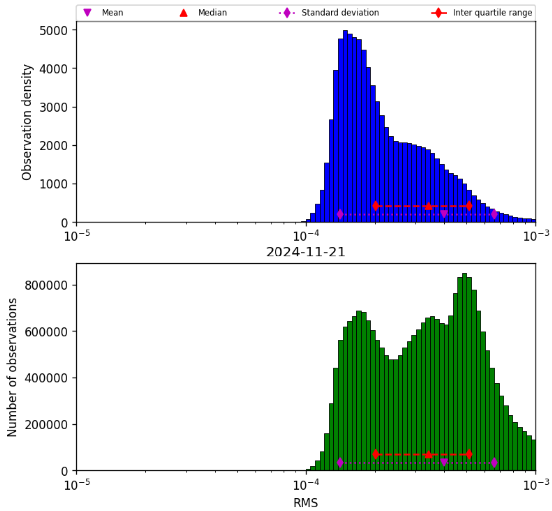
Figure 43: Histogram of “RMS” for 2024-11-20 to 2024-11-22
