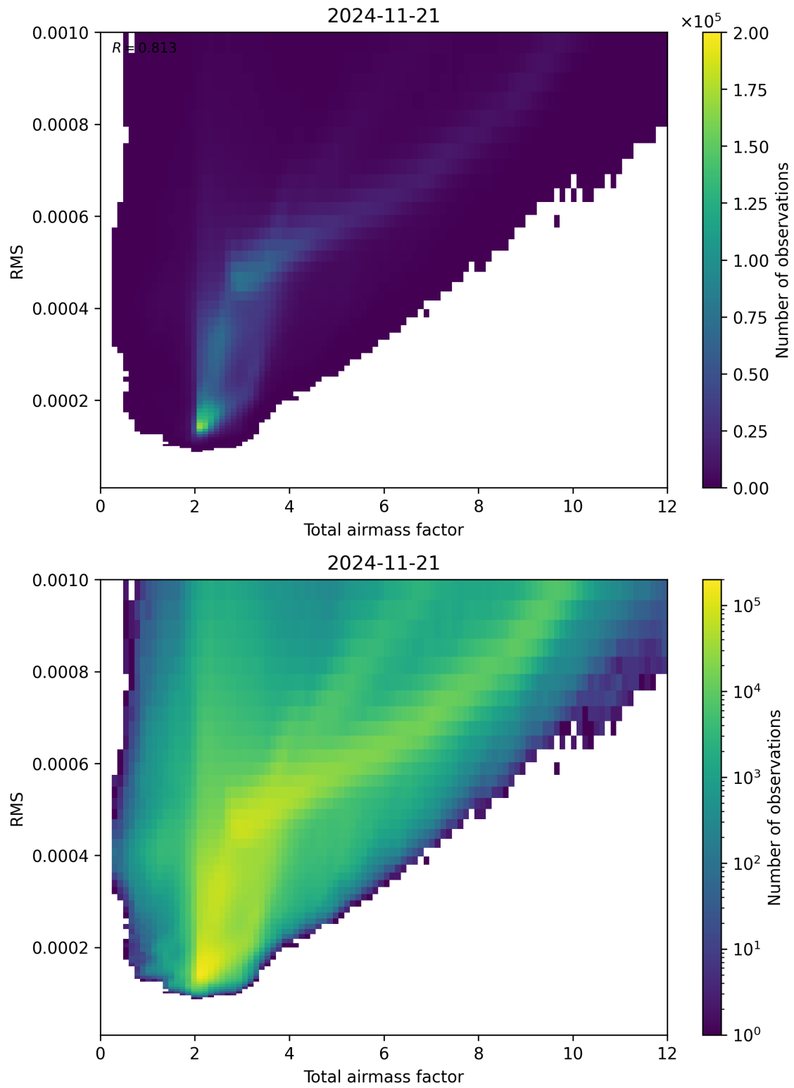
Figure 69: Scatter density plot of “Total airmass factor” against “RMS” for 2024-11-20 to 2024-11-22.
