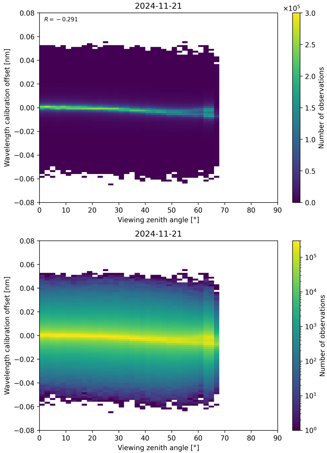
Figure 173: Scatter density plot of “Viewing zenith angle” against “Wavelength calibration offset” for 2024-11-20 to 2024-11-22.
