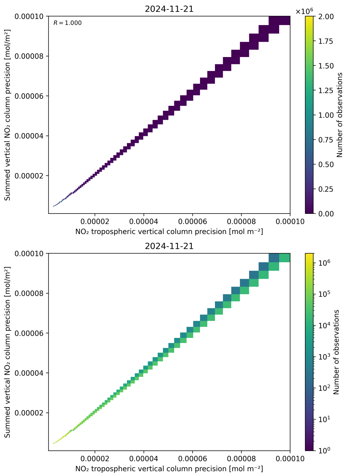
Figure 137: Scatter density plot of “NO 2 tropospheric vertical column precision” against “Summed vertical NO 2 column precision” for 2024-11-20 to 2024-11-22.
