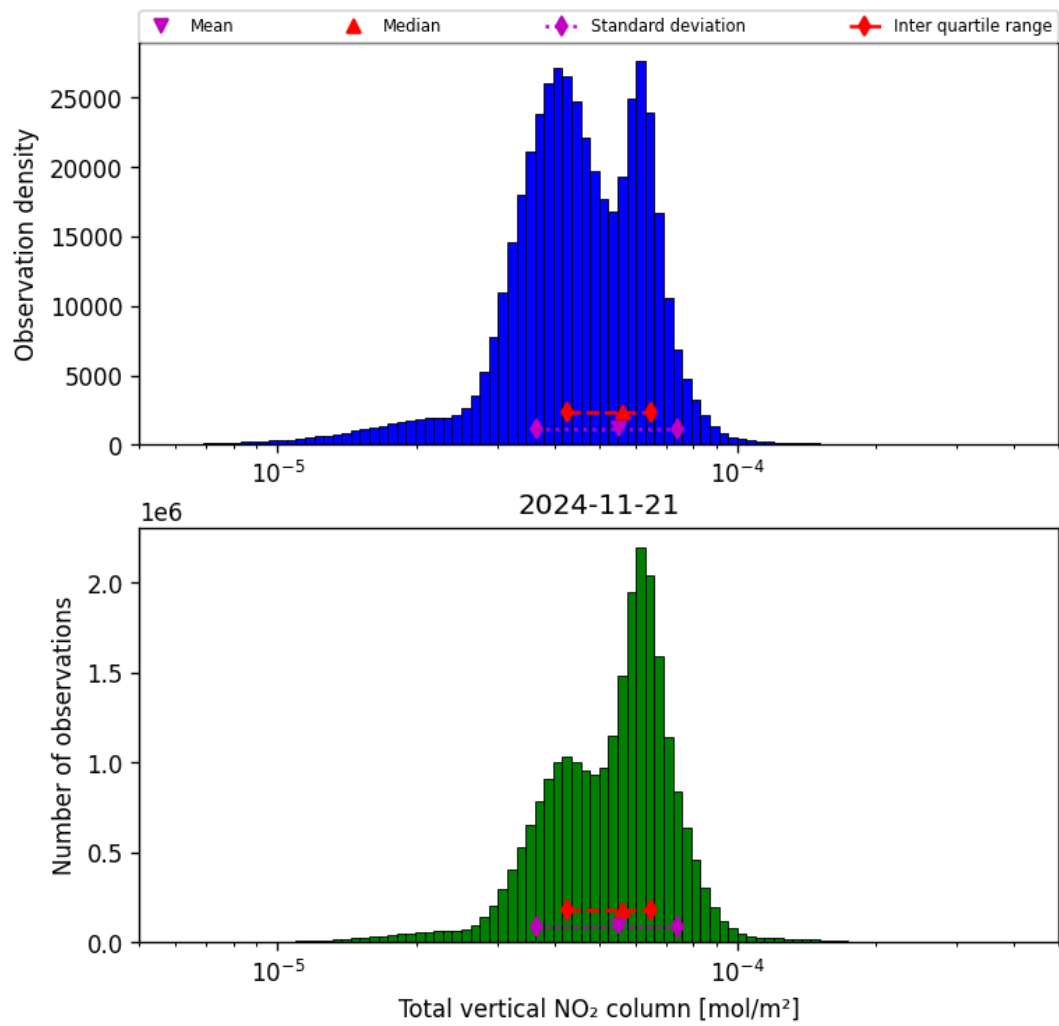
Figure 38: Histogram of “Total vertical NO 2 column” for 2024-11-20 to 2024-11-22
