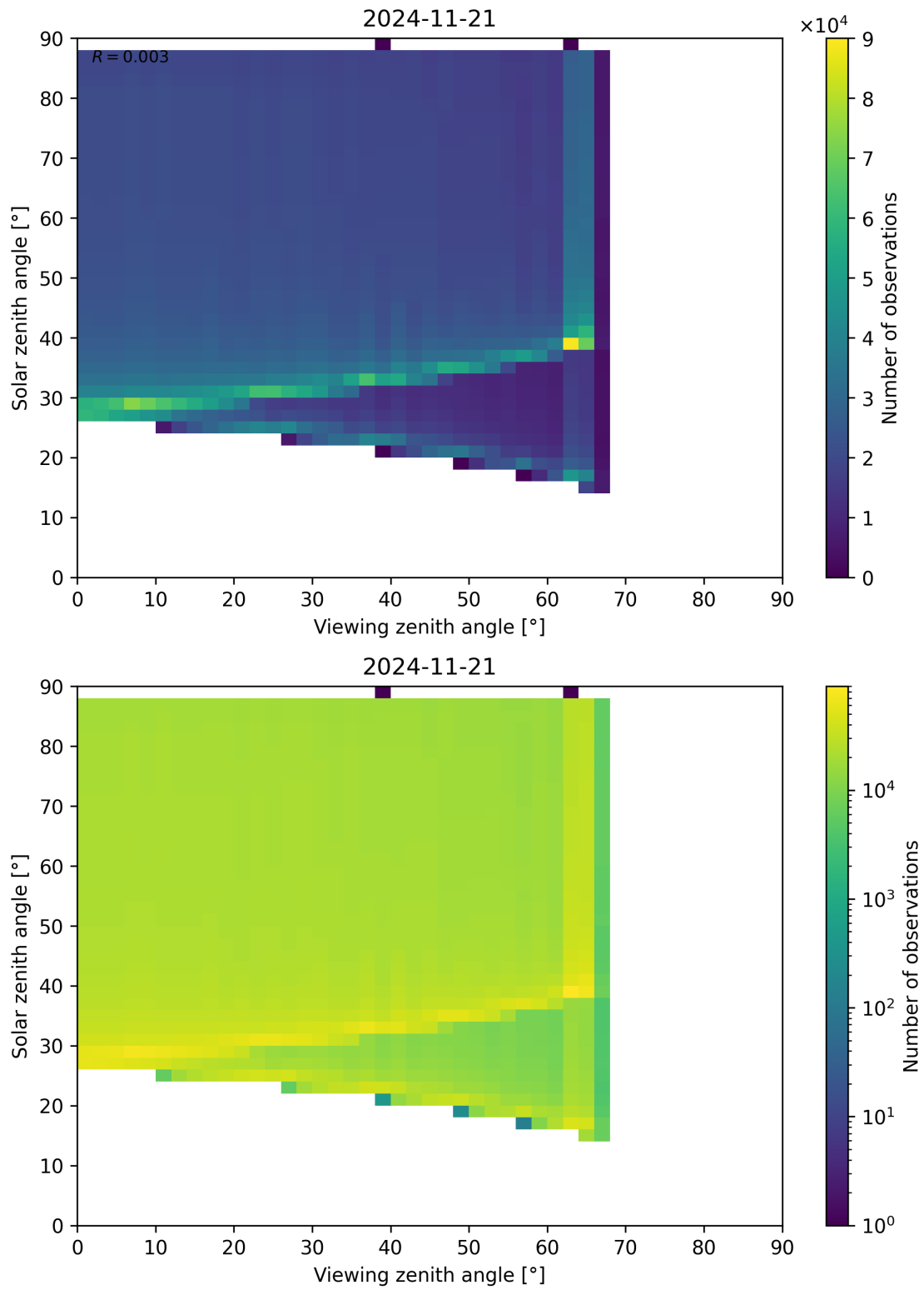
Figure 172: Scatter density plot of “Viewing zenith angle” against “Solar zenith angle” for 2024-11-20 to 2024-11-22.
