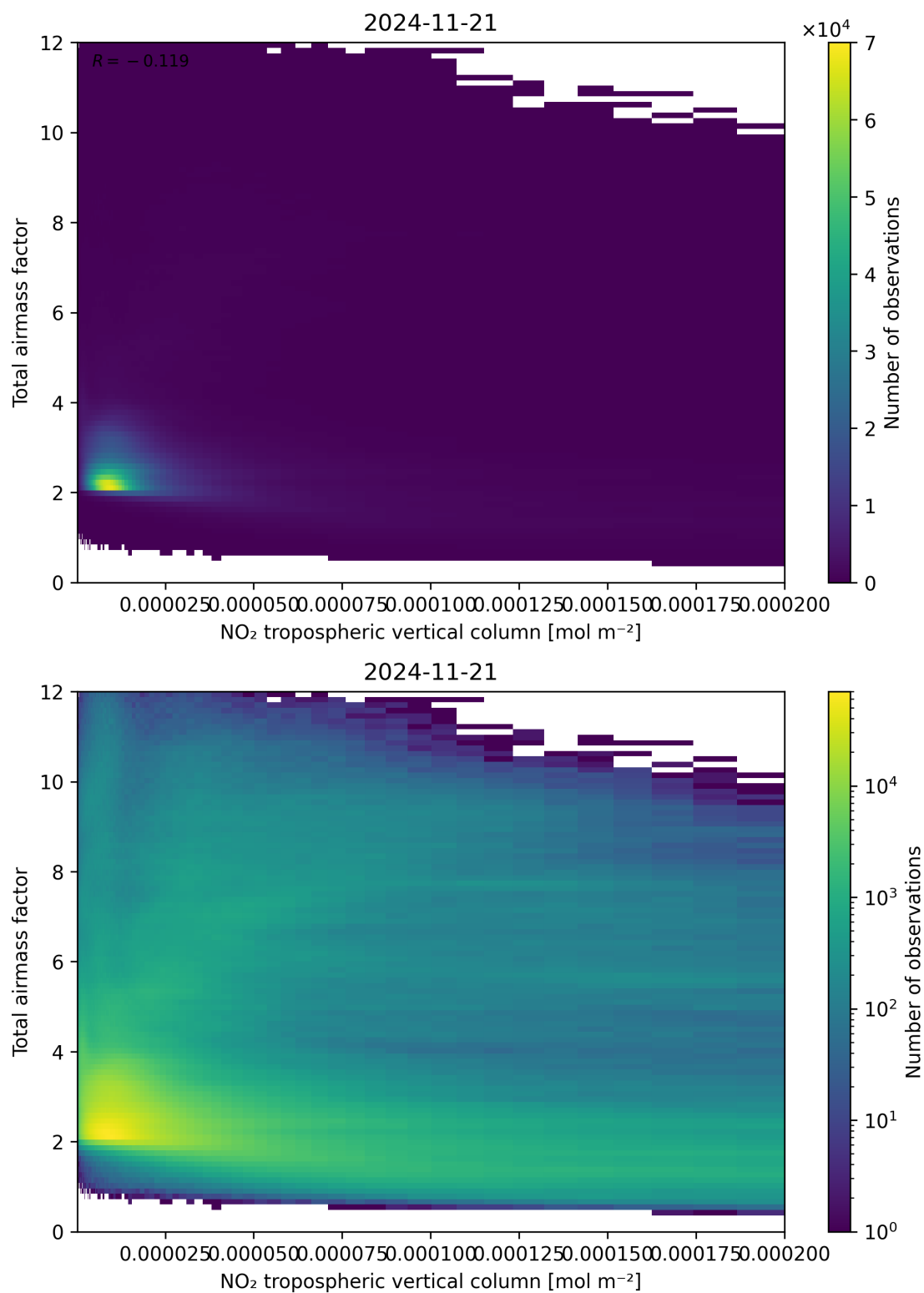
Figure 122: Scatter density plot of “NO 2 tropospheric vertical column” against “Total airmass factor” for 2024-11-20 to 2024-11-22.
