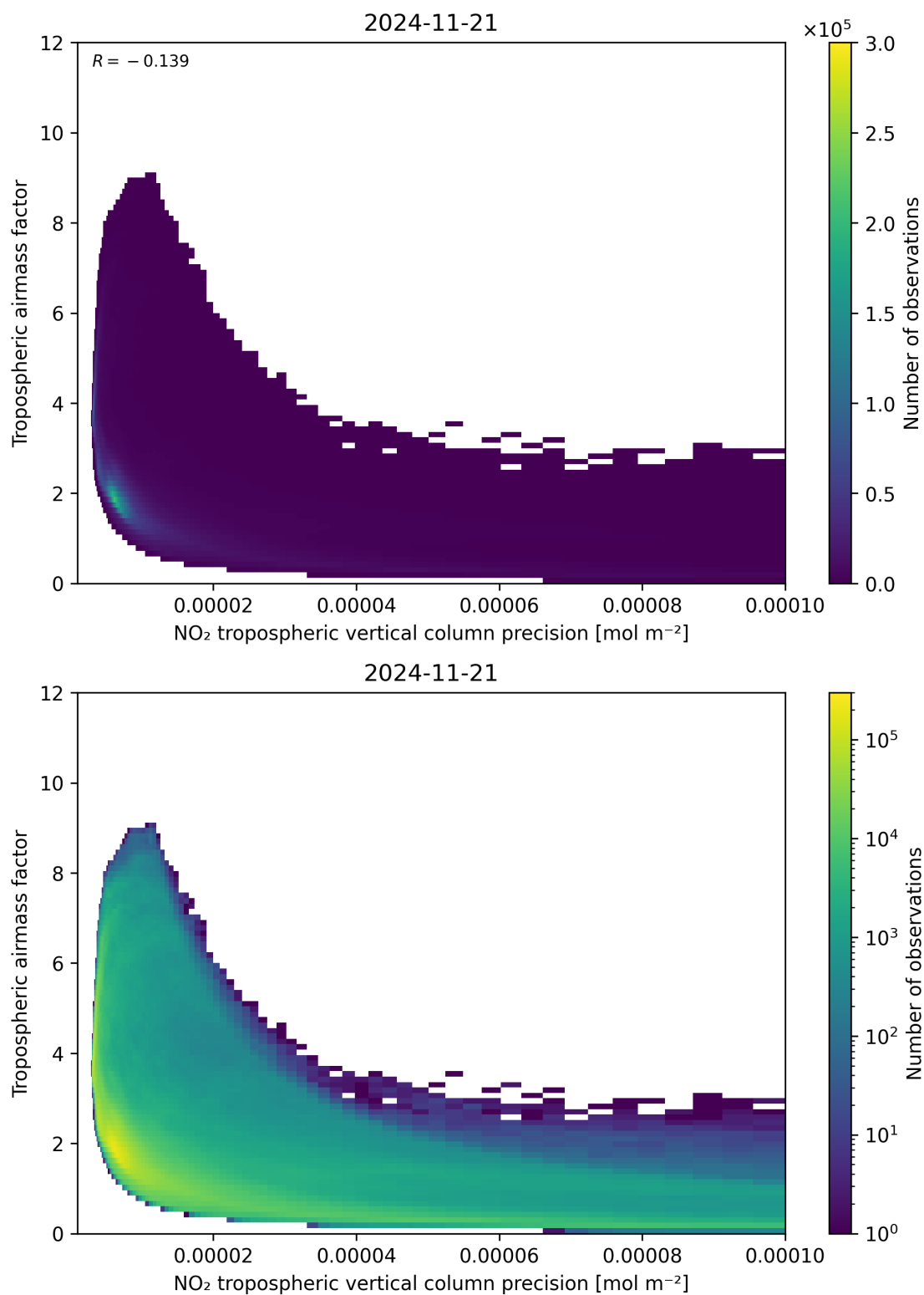
Figure 133: Scatter density plot of “NO 2 tropospheric vertical column precision” against “Tropospheric airmass factor” for 2024-11-20 to 2024-11-22.
