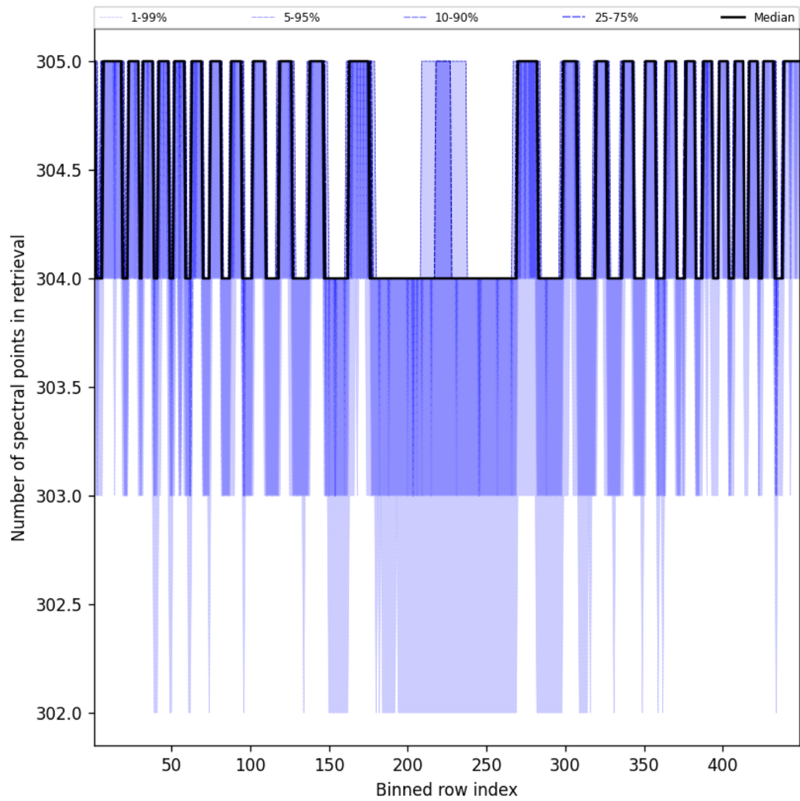
Figure 50: Along track statistics of “Number of spectral points in retrieval” for 2024-11-20 to 2024-11-22
