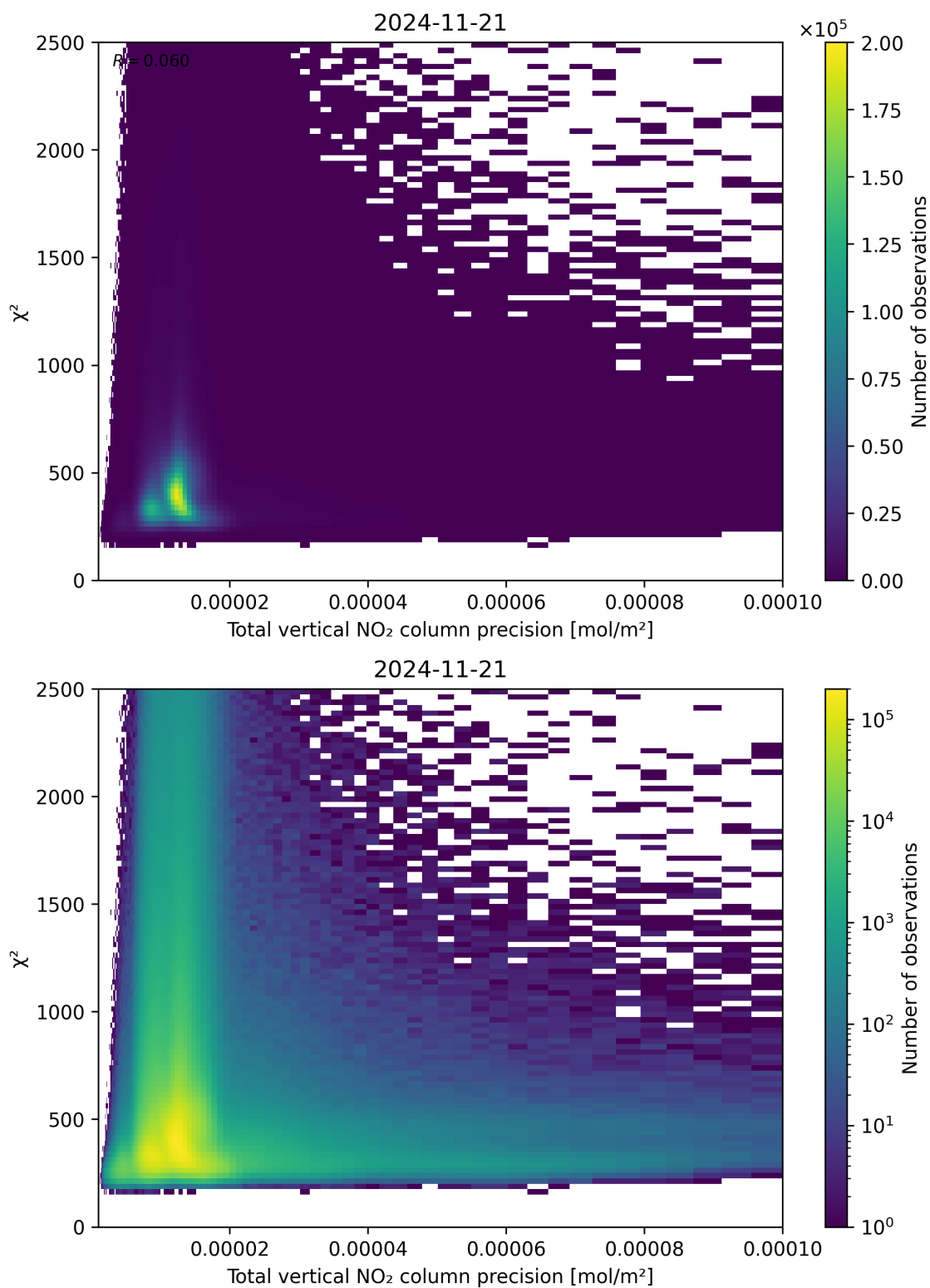
Figure 116: Scatter density plot of “Total vertical NO 2 column precision” against “ \chi^2 ” for 2024-11-20 to 2024-11-22.
