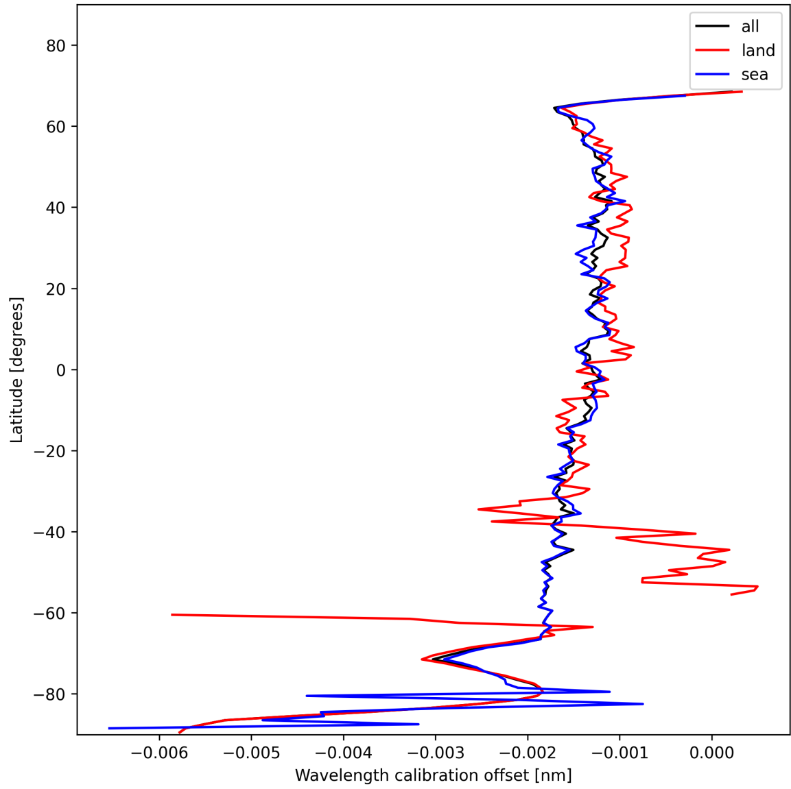
Figure 18: Zonal average of “Wavelength calibration offset” for 2024-11-20 to 2024-11-22.
