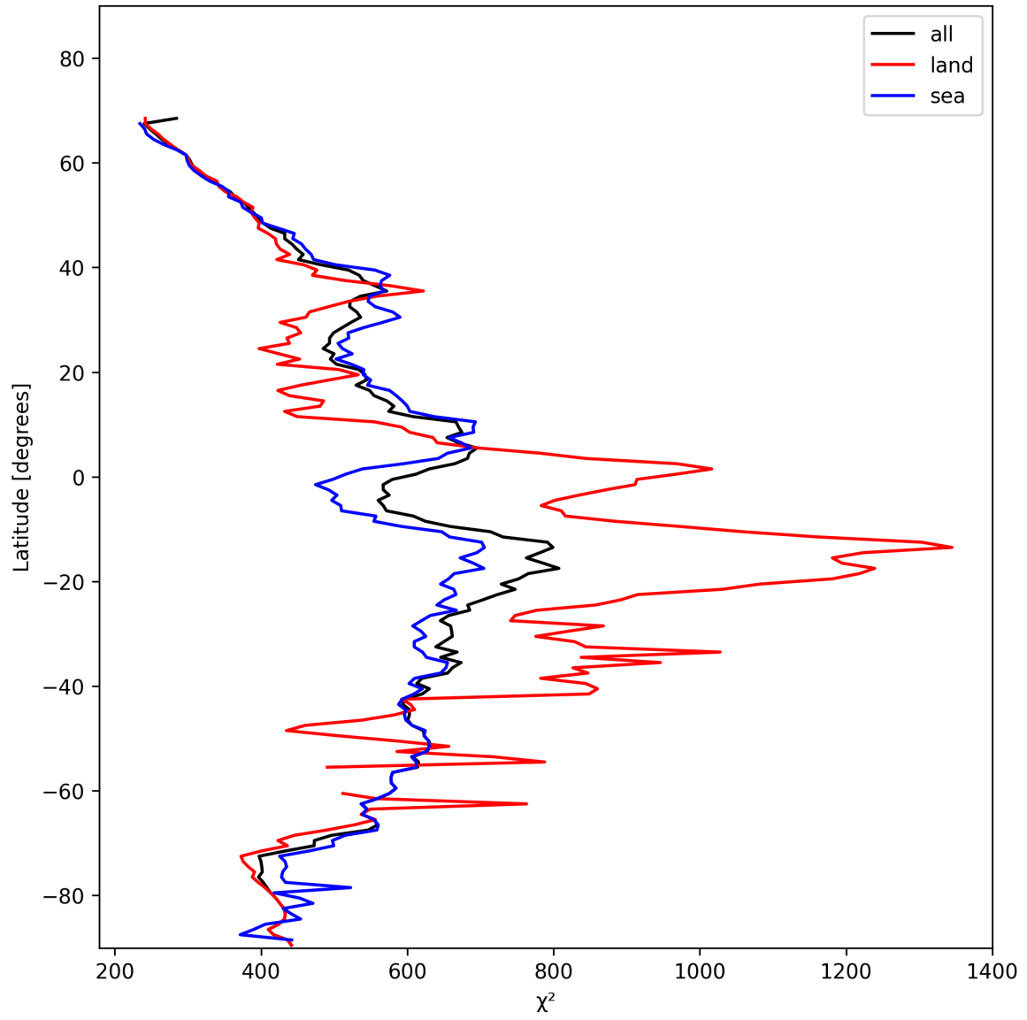
Figure 25: Zonal average of “ \chi^2 ” for 2024-11-20 to 2024-11-22.
