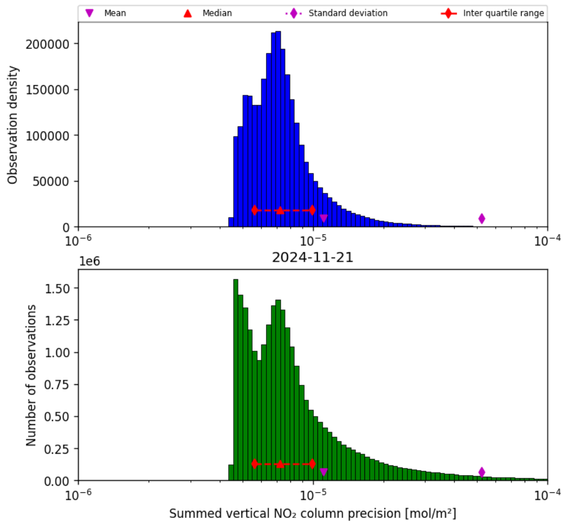
Figure 41: Histogram of "Summed vertical NO 2 column precision" for 2024-11-20 to 2024-11-22
