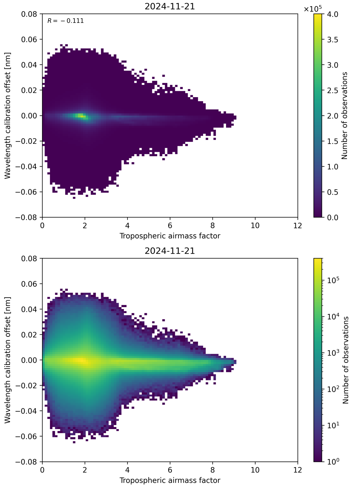
Figure 80: Scatter density plot of “Tropospheric airmass factor” against “Wavelength calibration offset” for 2024-11-20 to 2024-11-22.
