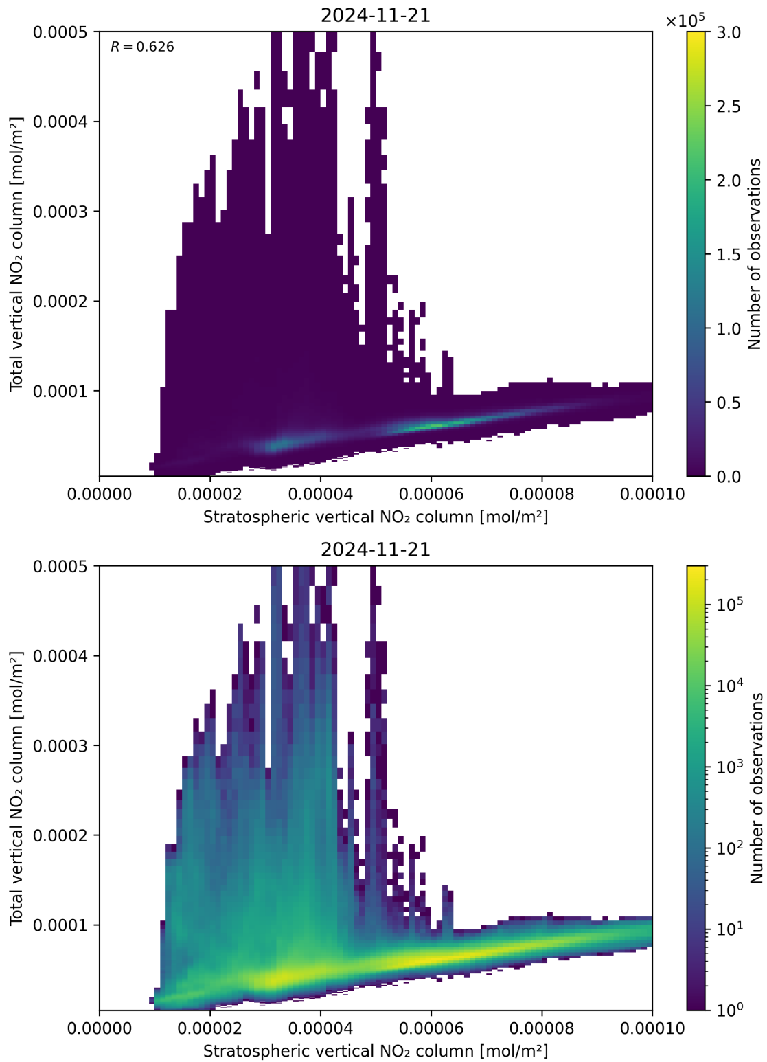
Figure 100: Scatter density plot of “Stratospheric vertical NO 2 column” against “Total vertical NO 2 column” for 2024-11-20 to 2024-11-22.
