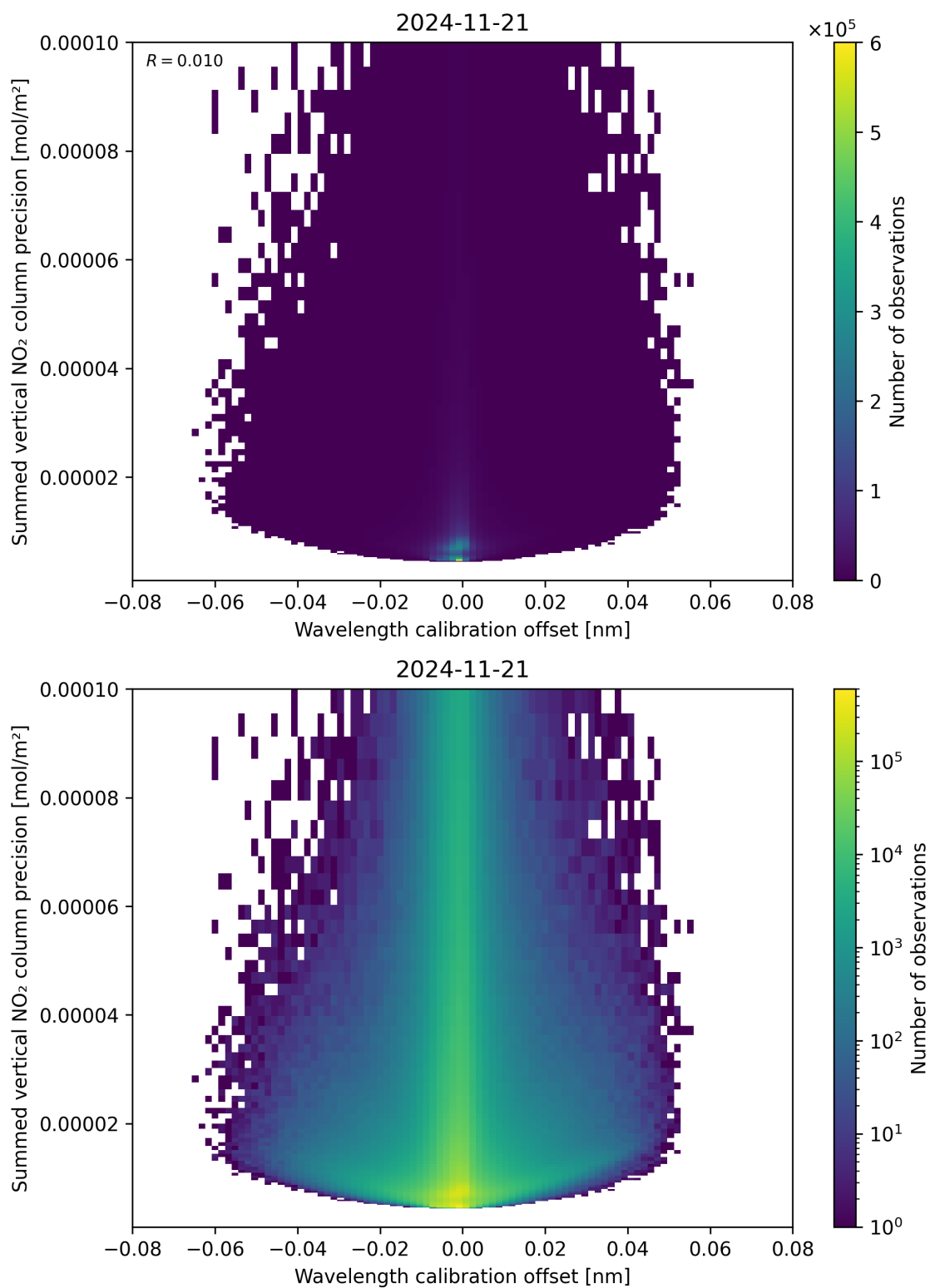
Figure 178: Scatter density plot of “Wavelength calibration offset” against “Summed vertical NO 2 column precision” for 2024-11-20 to 2024-11-22.
