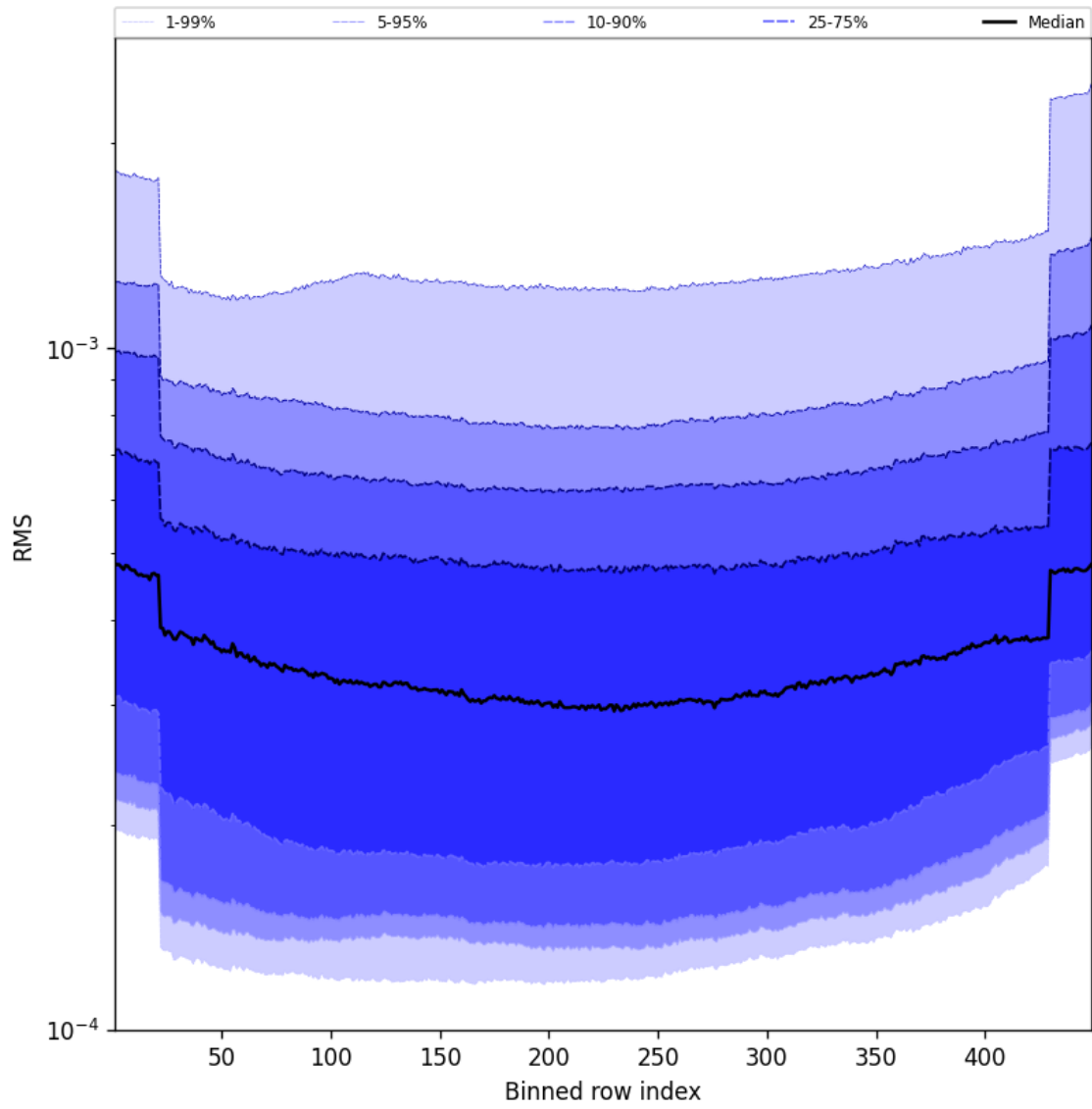
Figure 60: Along track statistics of “RMS” for 2024-11-20 to 2024-11-22
