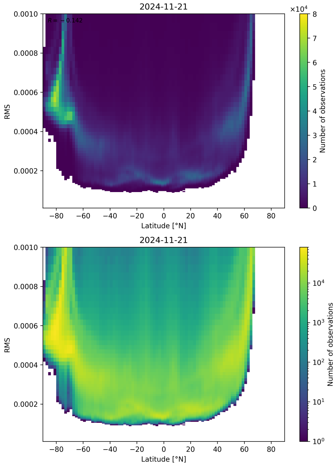
Figure 94: Scatter density plot of “Latitude” against “RMS” for 2024-11-20 to 2024-11-22.
