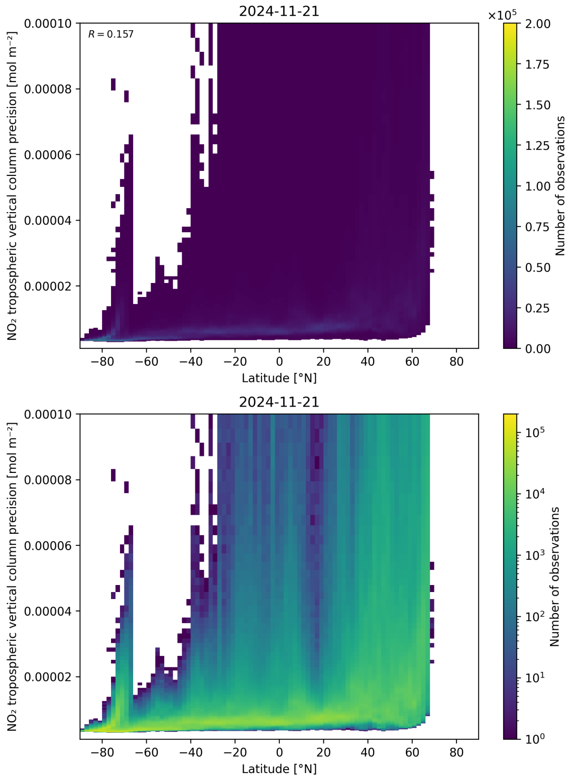
Figure 93: Scatter density plot of “Latitude” against “NO 2 tropospheric vertical column precision” for 2024-11-20 to 2024-11-22.
