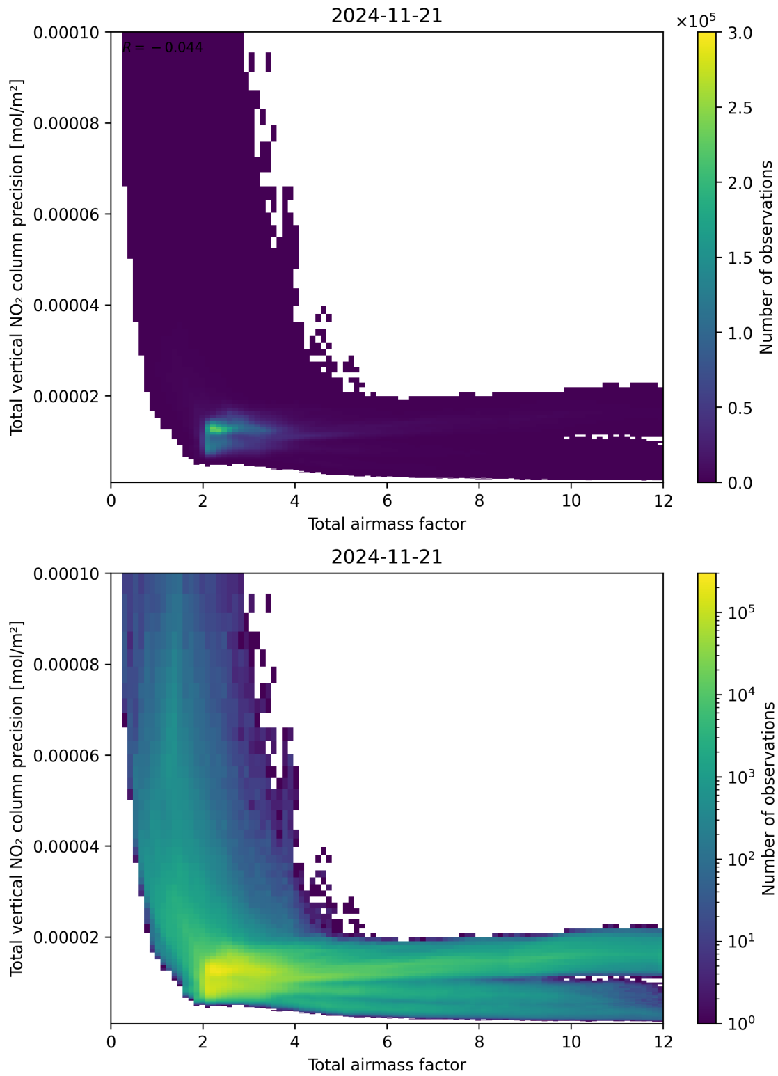
Figure 68: Scatter density plot of “Total airmass factor” against “Total vertical NO 2 column precision” for 2024-11-20 to 2024-11-22.
