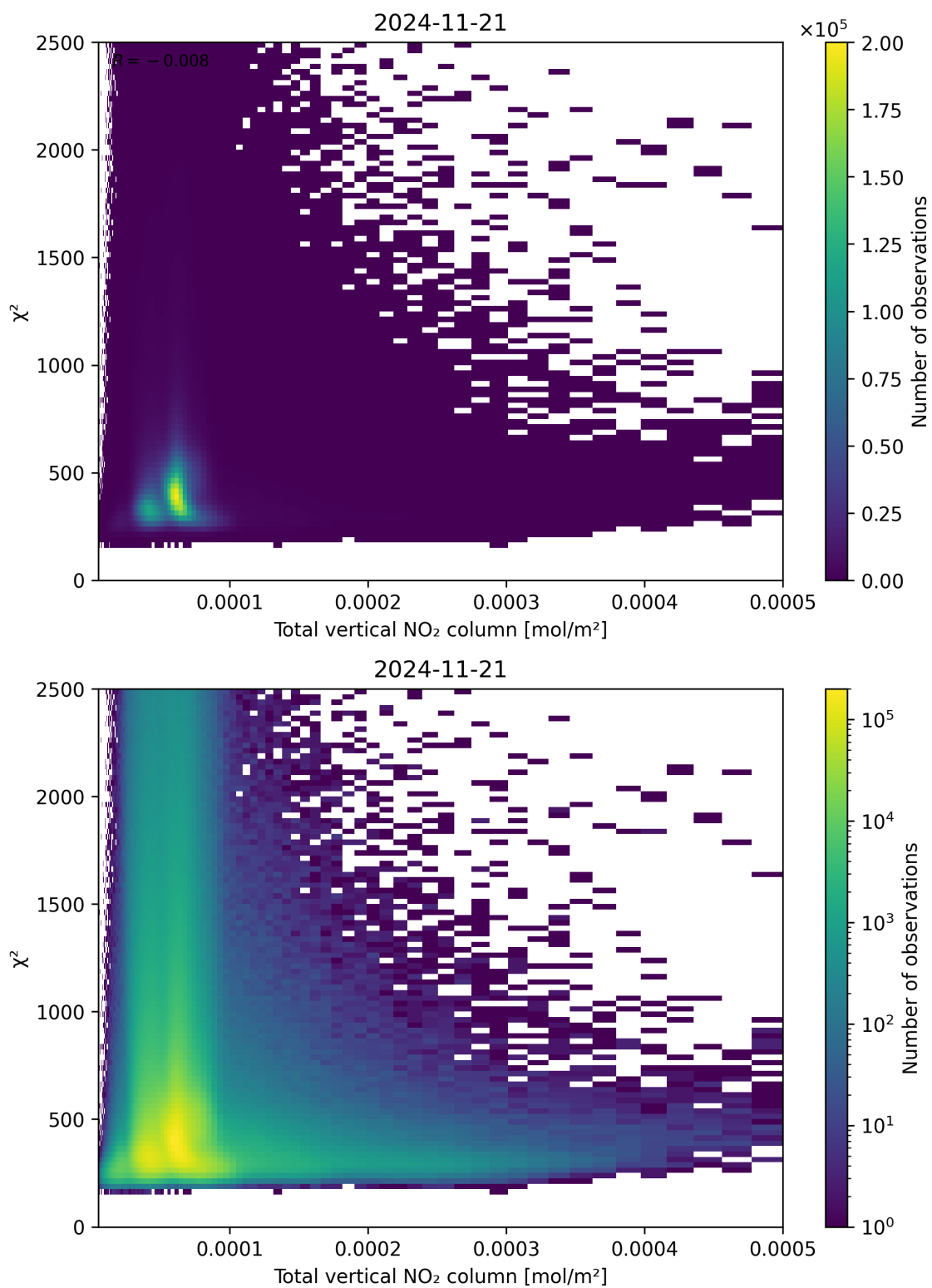
Figure 111: Scatter density plot of “Total vertical NO 2 column” against “ \chi^2 ” for 2024-11-20 to 2024-11-22.
