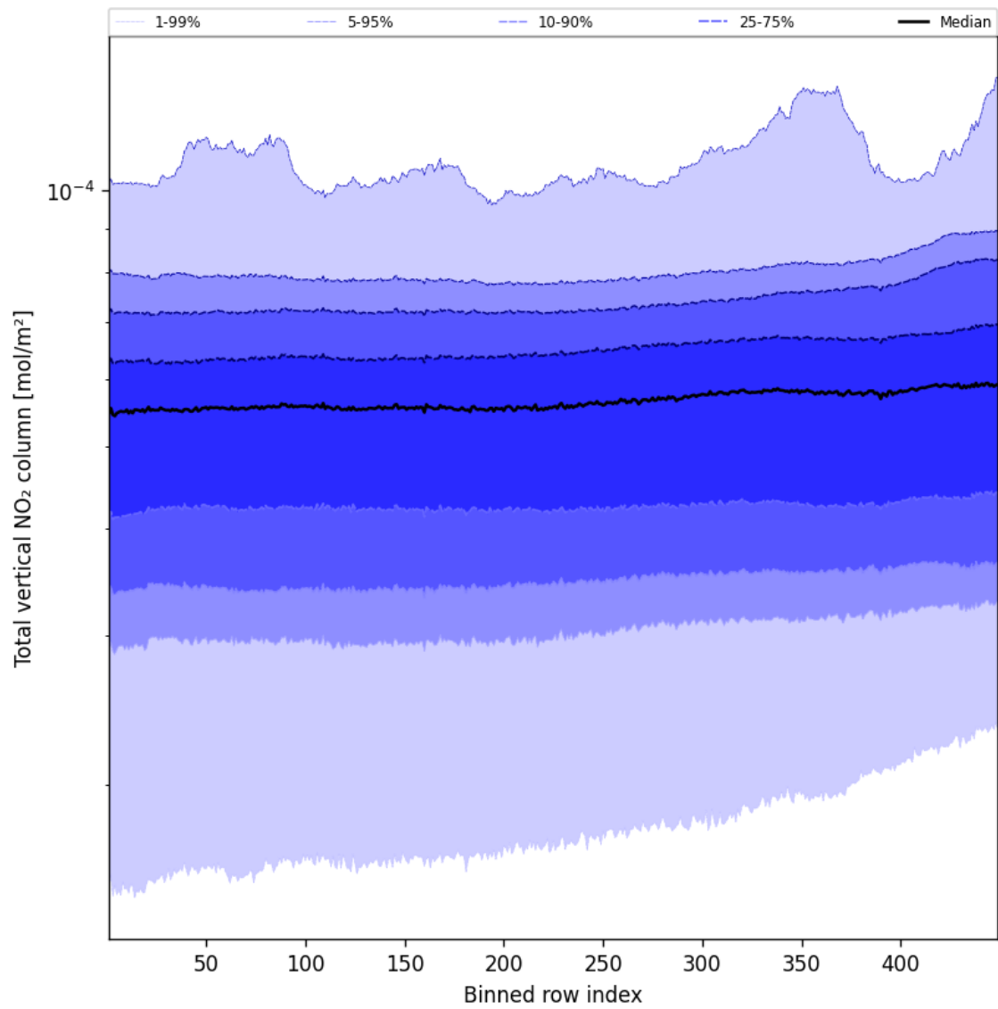
Figure 55: Along track statistics of “Total vertical NO 2 column” for 2024-11-20 to 2024-11-22
