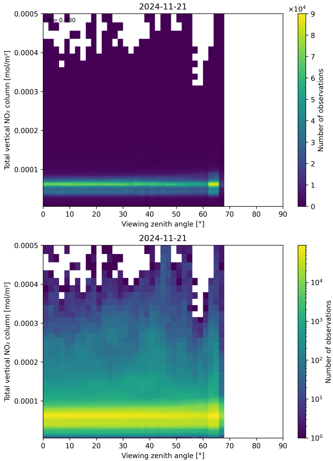
Figure 167: Scatter density plot of “Viewing zenith angle” against “Total vertical NO 2 column” for 2024-11-20 to 2024-11-22.
