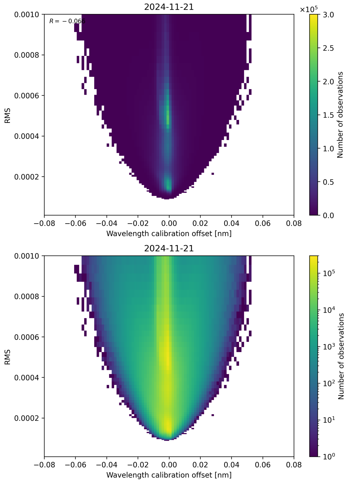
Figure 181: Scatter density plot of “Wavelength calibration offset” against “RMS” for 2024-11-20 to 2024-11-22.
