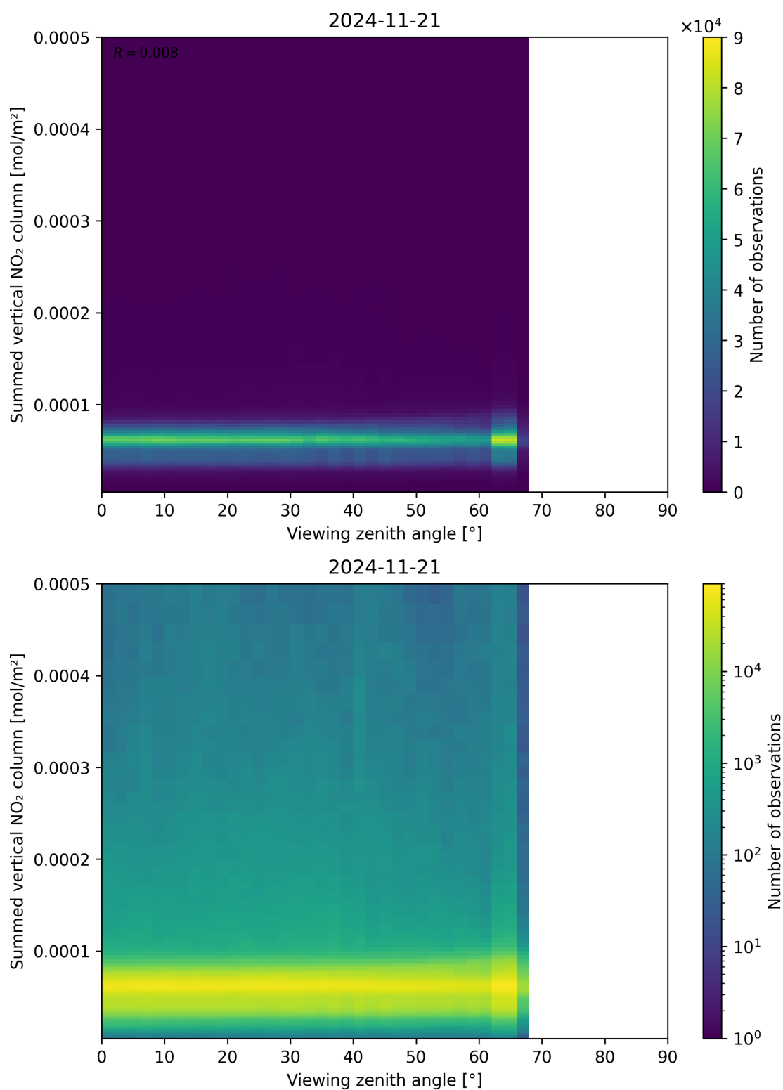
Figure 165: Scatter density plot of “Viewing zenith angle” against “Summed vertical NO 2 column” for 2024-11-20 to 2024-11-22.
