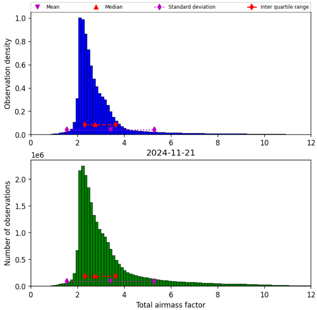
Figure 32: Histogram of “Total airmass factor” for 2024-11-20 to 2024-11-22
