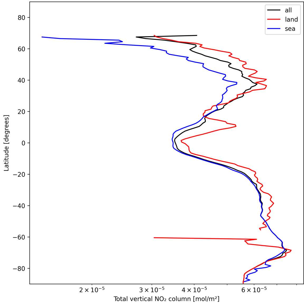
Figure 21: Zonal average of “Total vertical NO 2 column” for 2024-11-20 to 2024-11-22.
