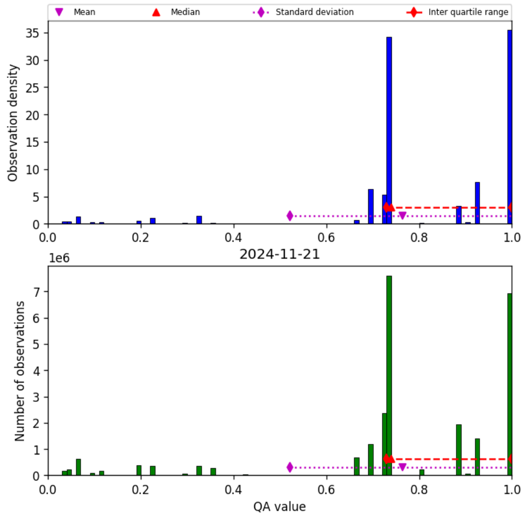
Figure 28: Histogram of “QA value” for 2024-11-20 to 2024-11-22
