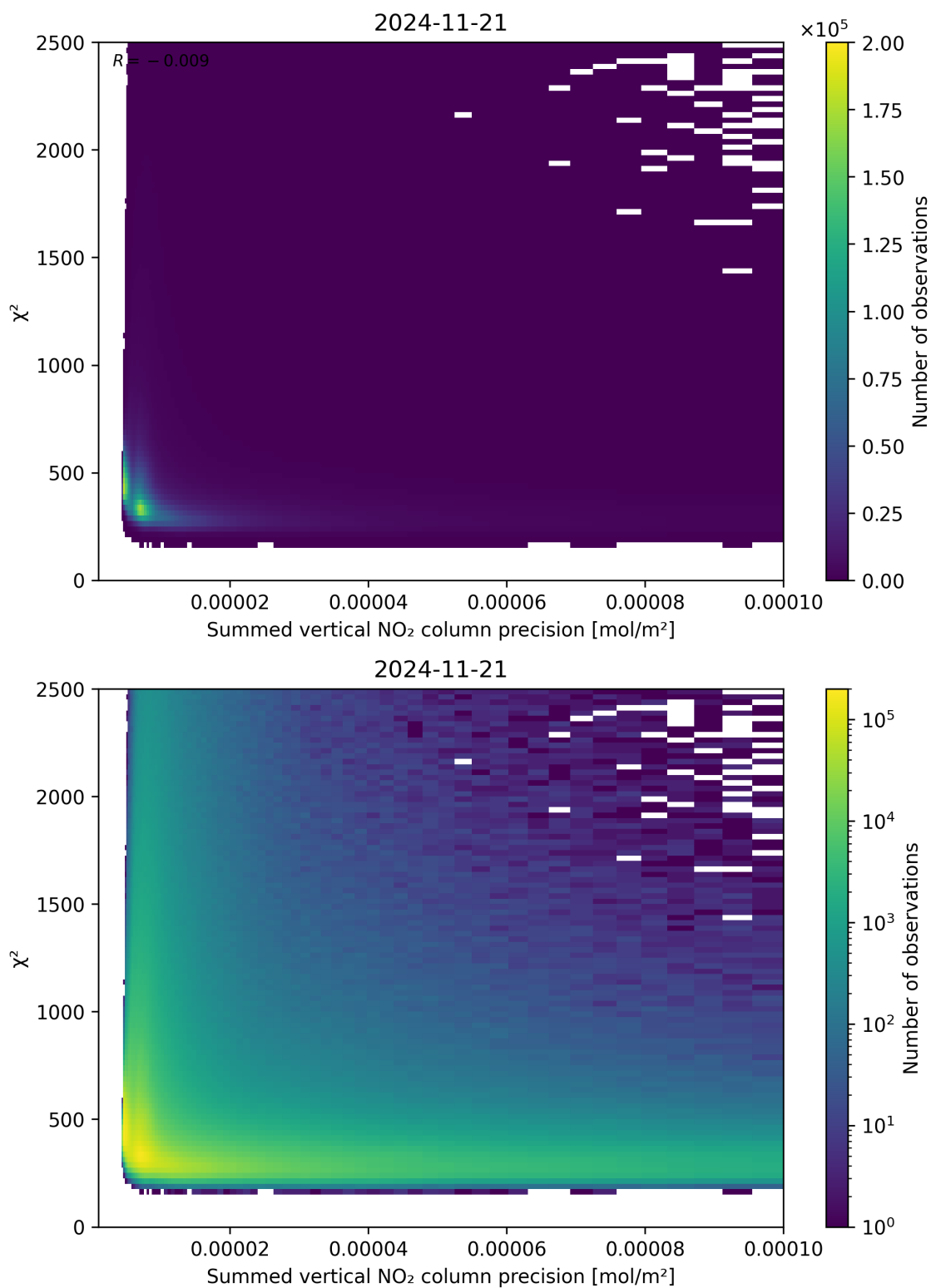
Figure 107: Scatter density plot of “Summed vertical NO 2 column precision” against “ \chi^2 ” for 2024-11-20 to 2024-11-22.
