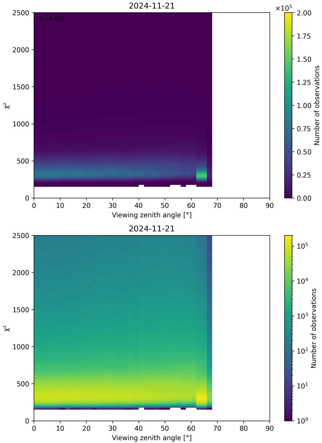
Figure 162: Scatter density plot of “Viewing zenith angle” against “ \chi^2 ” for 2024-11-20 to 2024-11-22.
