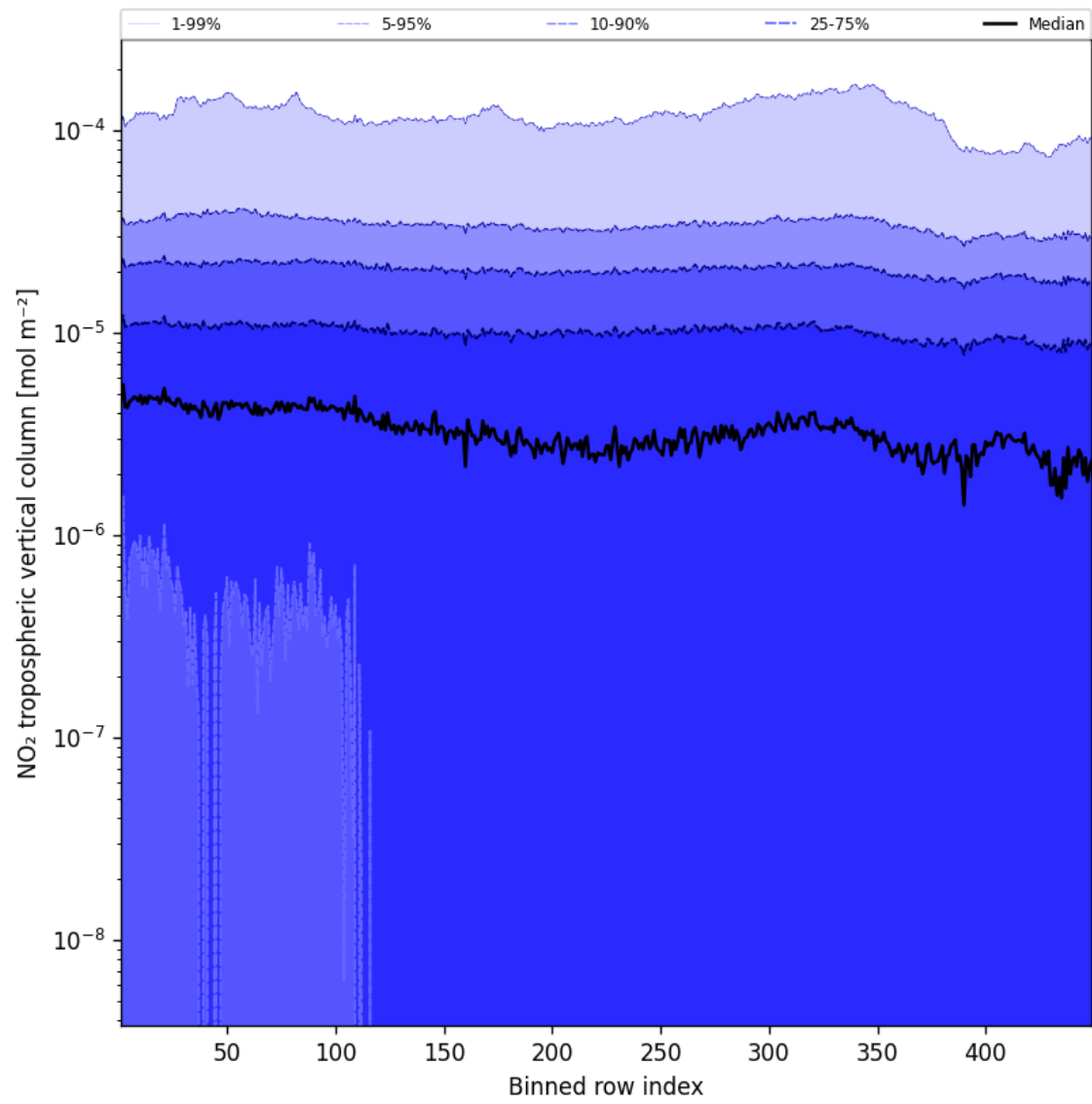
Figure 46: Along track statistics of “NO 2 tropospheric vertical column” for 2024-11-20 to 2024-11-22
