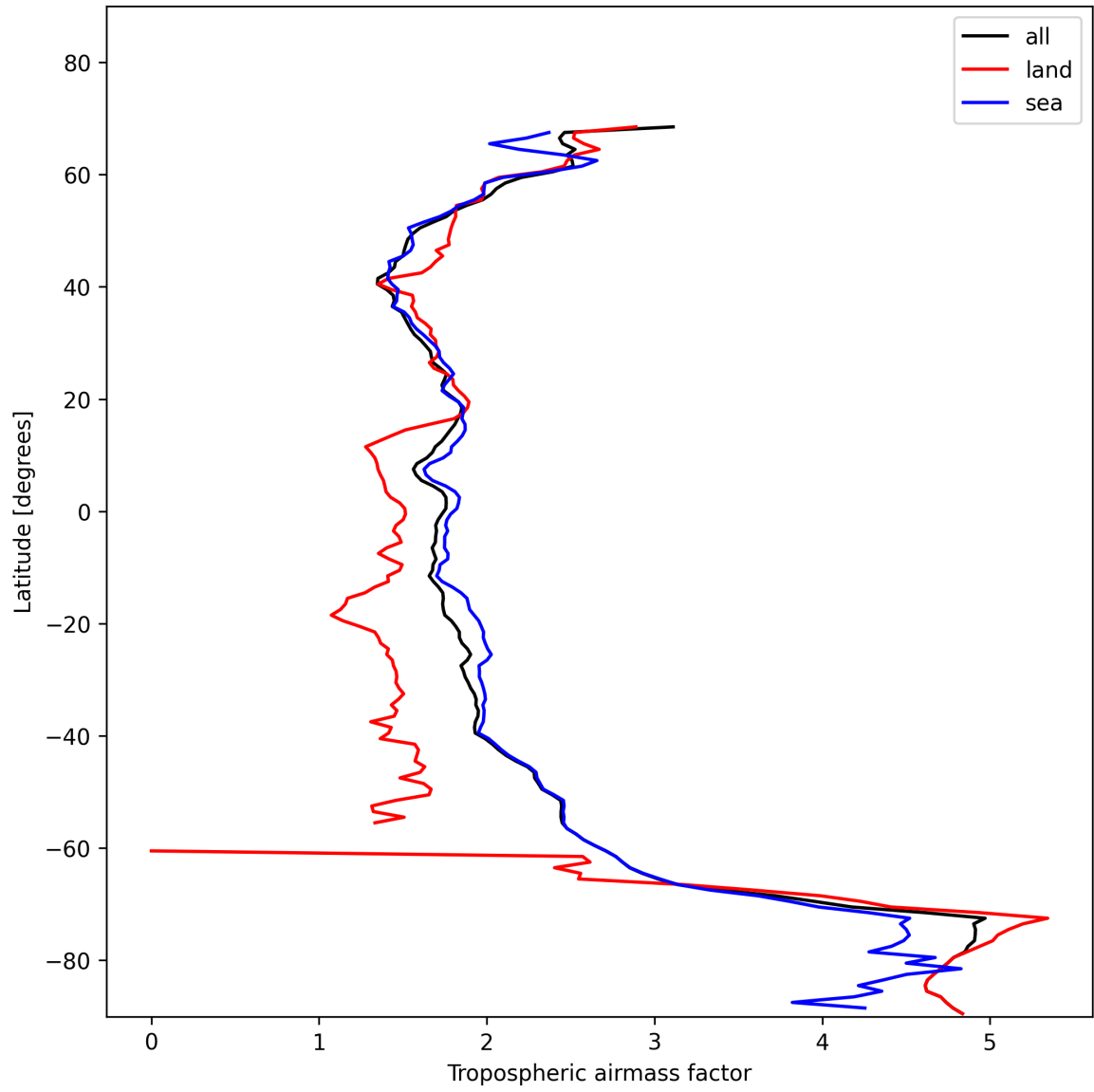
Figure 14: Zonal average of “Tropospheric airmass factor” for 2024-11-20 to 2024-11-22.
