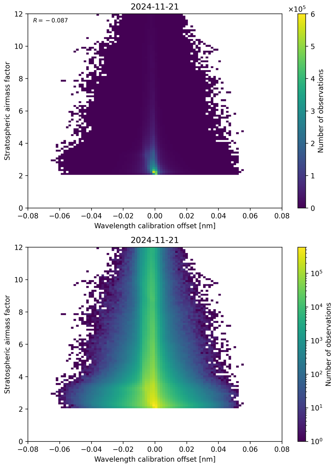
Figure 174: Scatter density plot of “Wavelength calibration offset” against “Stratospheric airmass factor” for 2024-11-20 to 2024-11-22.
