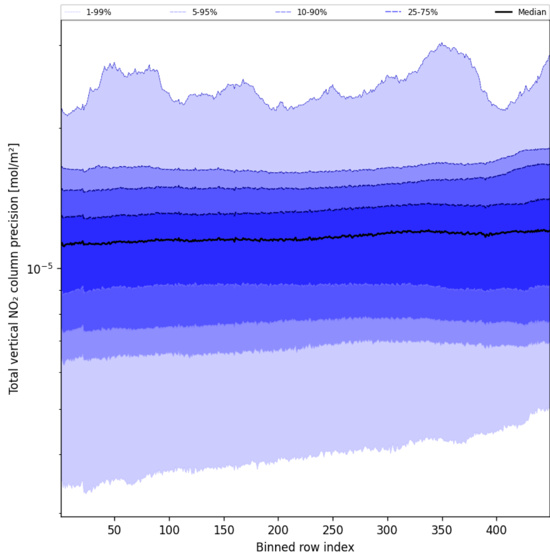
Figure 56: Along track statistics of “Total vertical NO 2 column precision” for 2024-11-20 to 2024-11-22
