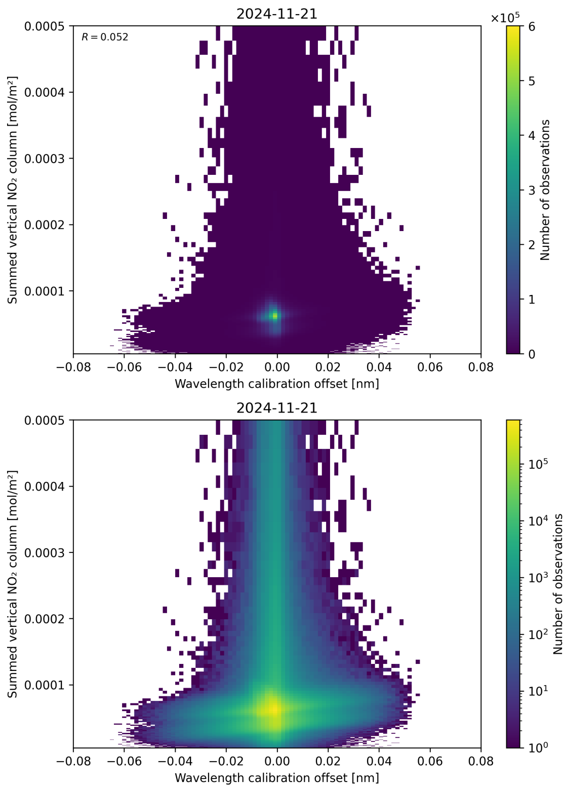
Figure 177: Scatter density plot of “Wavelength calibration offset” against “Summed vertical NO 2 column” for 2024-11-20 to 2024-11-22.
