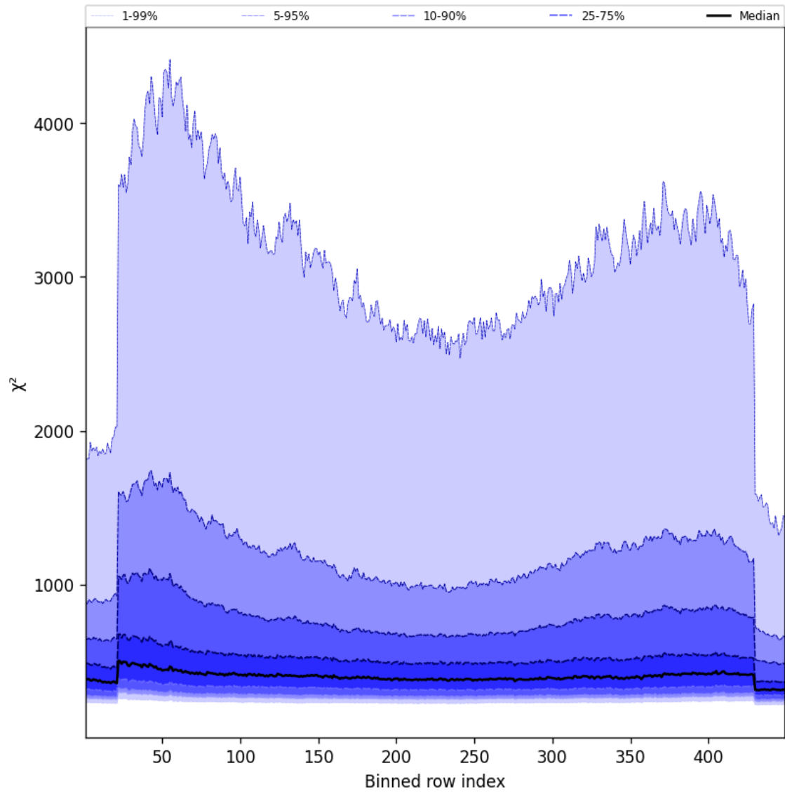
Figure 59: Along track statistics of “ \chi^2 ” for 2024-11-20 to 2024-11-22
