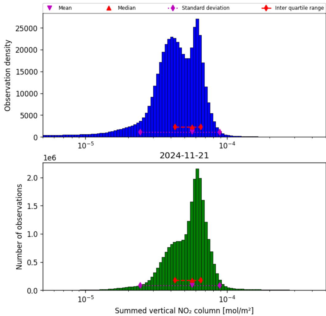
Figure 40: Histogram of “Summed vertical NO 2 column” for 2024-11-20 to 2024-11-22
