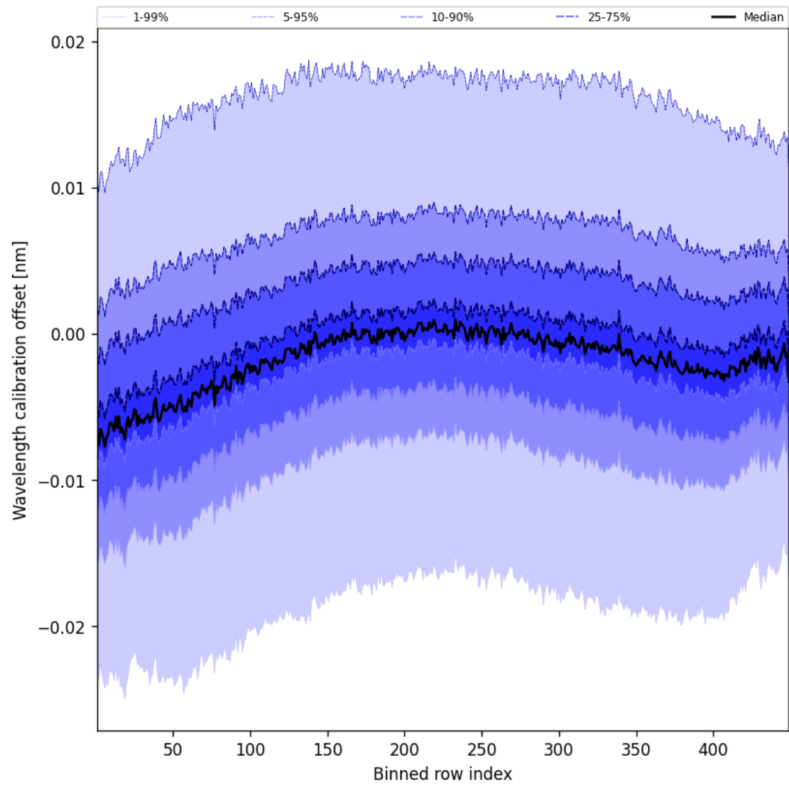
Figure 52: Along track statistics of “Wavelength calibration offset” for 2024-11-20 to 2024-11-22
