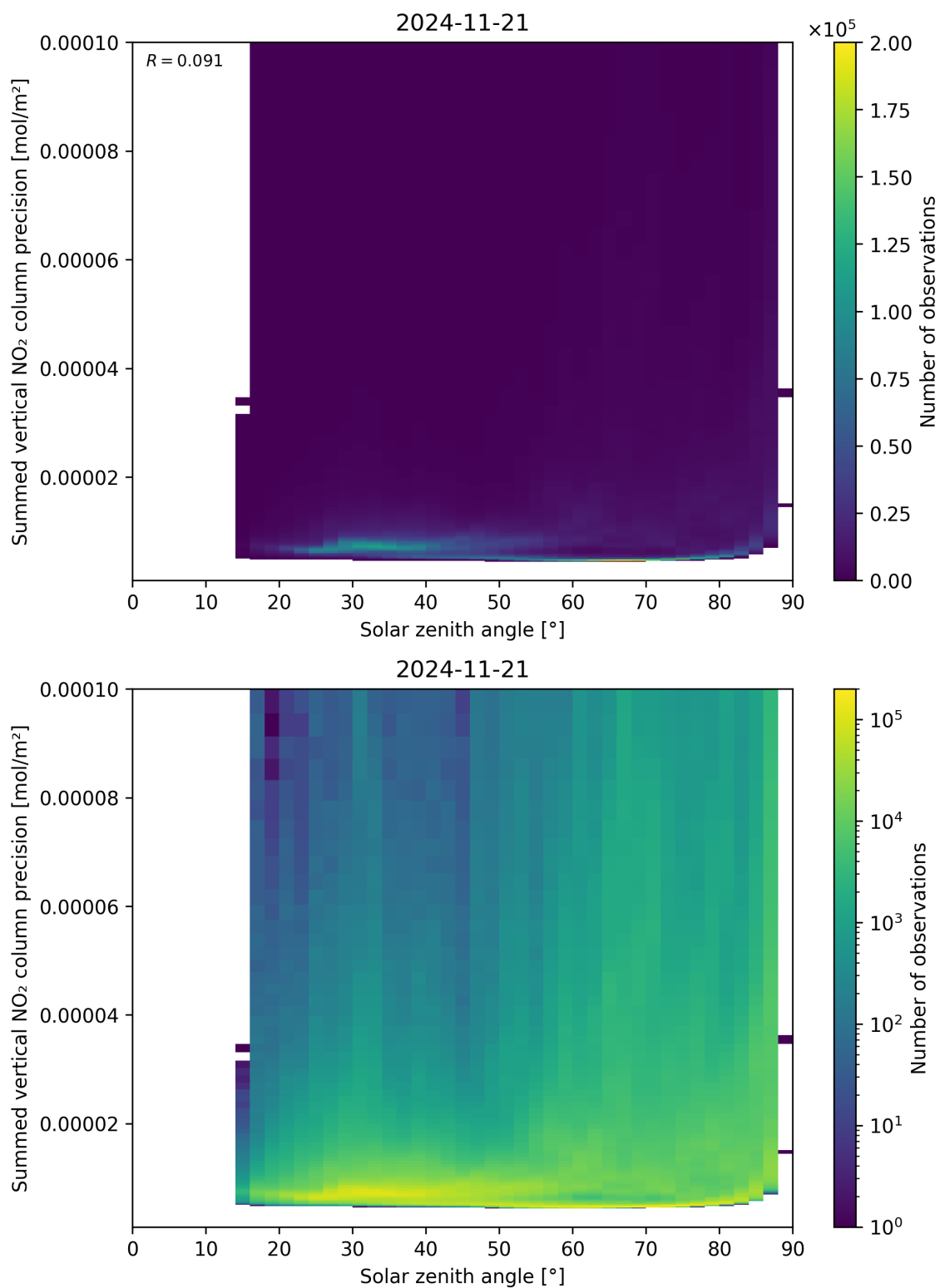
Figure 152: Scatter density plot of “Solar zenith angle” against “Summed vertical NO 2 column precision” for 2024-11-20 to 2024-11-22.
