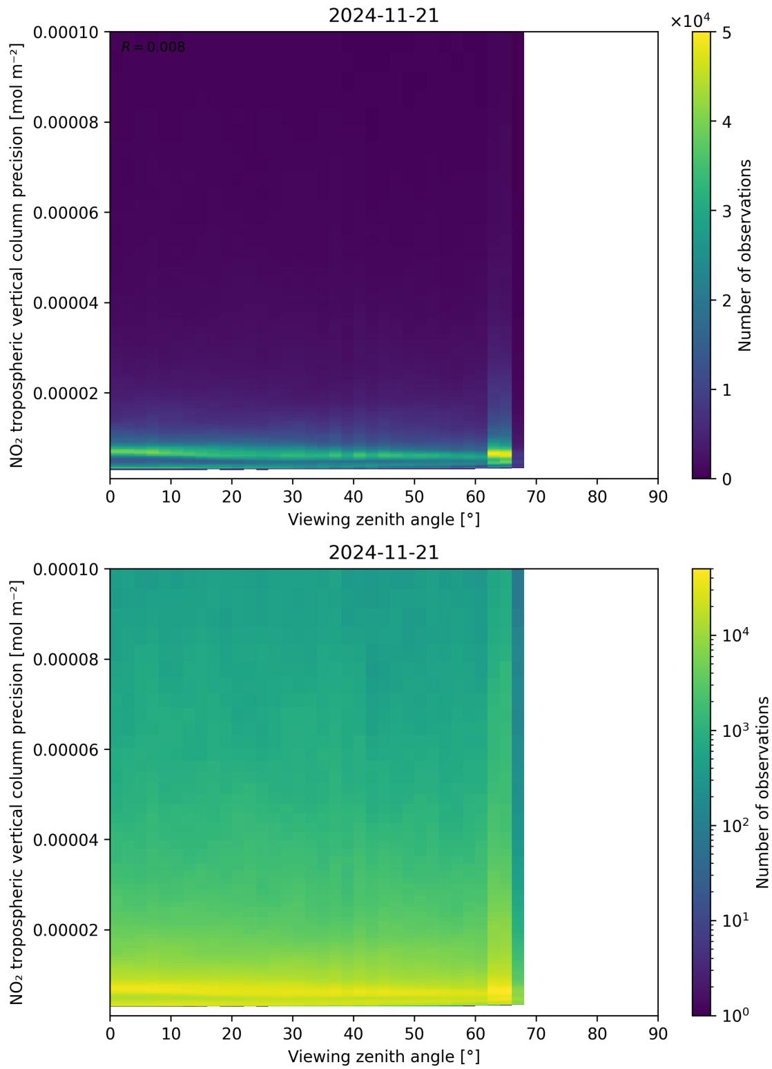
Figure 170: Scatter density plot of “Viewing zenith angle” against “NO 2 tropospheric vertical column precision” for 2024-11-20 to 2024-11-22.
