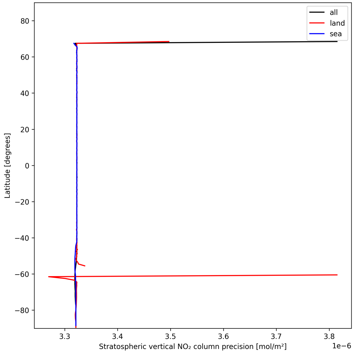
Figure 20: Zonal average of “Stratospheric vertical NO 2 column precision” for 2024-11-20 to 2024-11-22.
