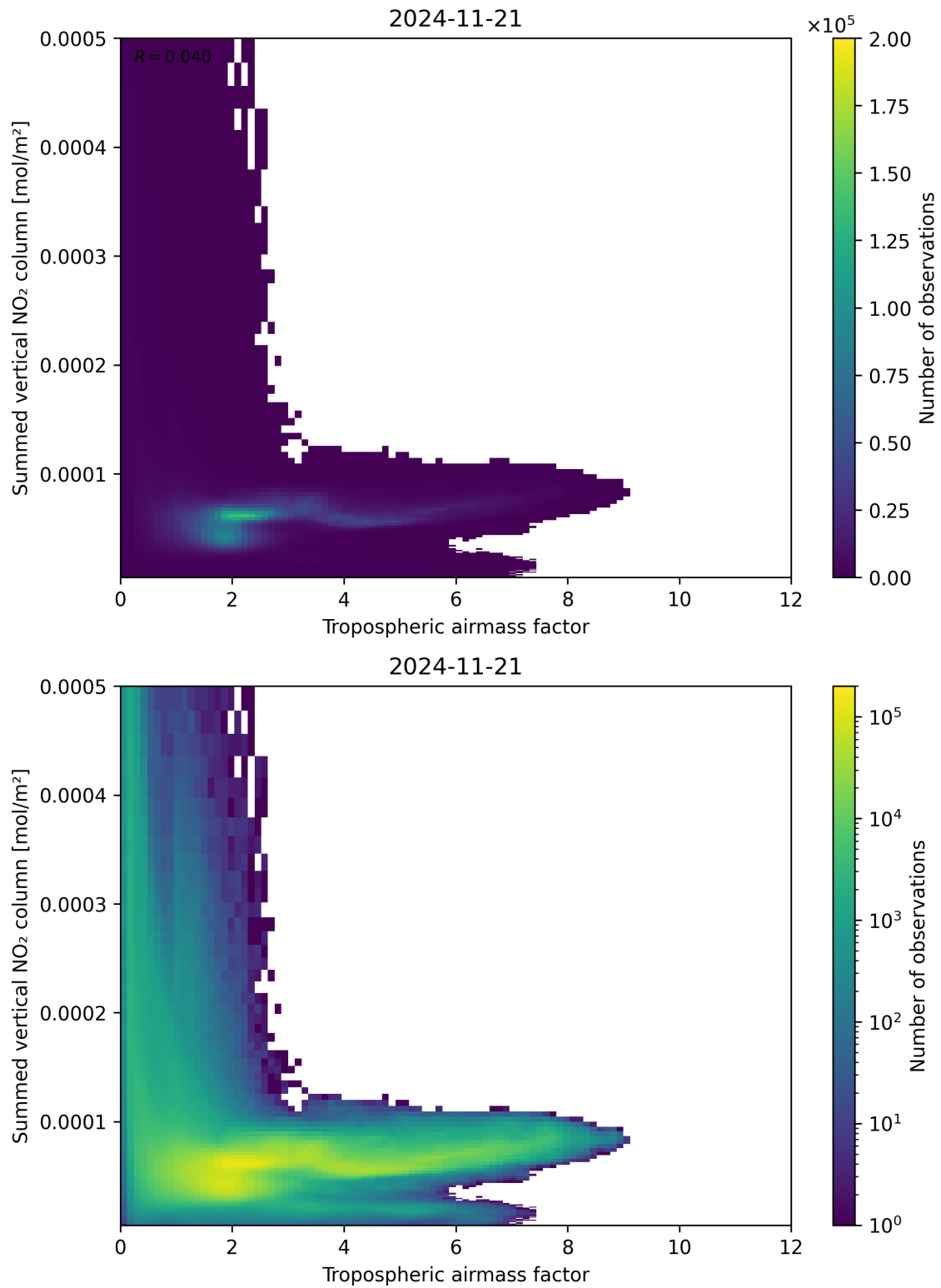
Figure 75: Scatter density plot of “Tropospheric air mass factor” against “Summed vertical NO 2 column” for 2024-11-20 to 2024-11-22.
