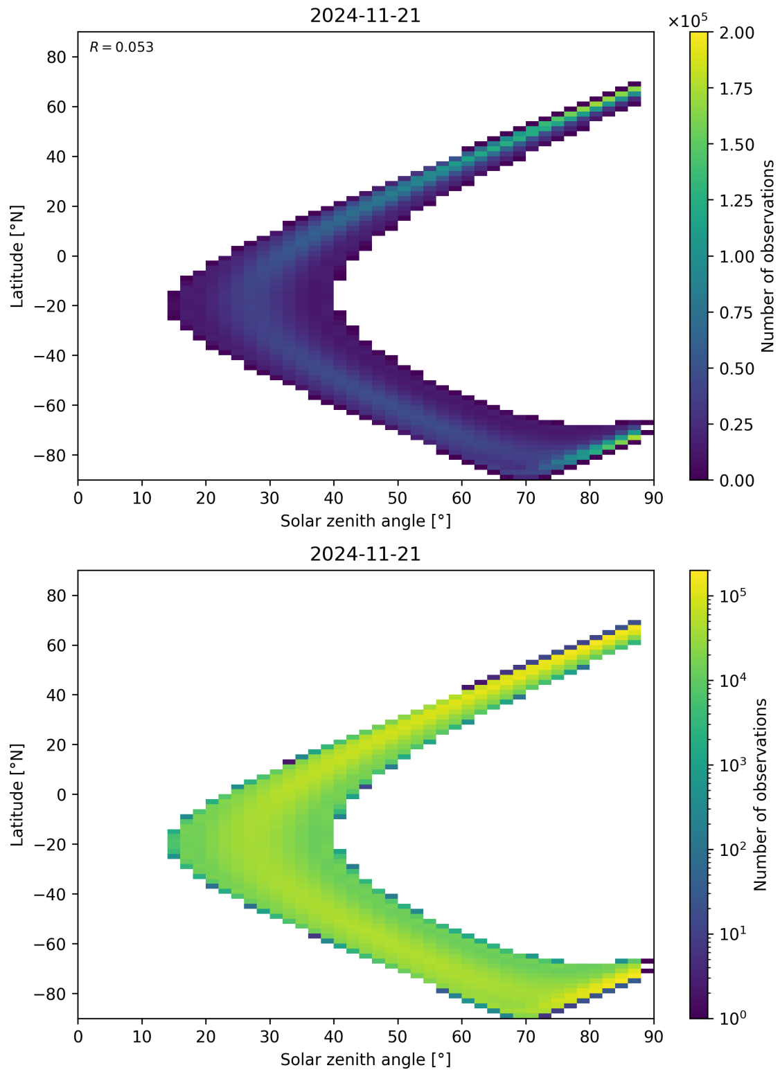
Figure 149: Scatter density plot of “Solar zenith angle” against “Latitude” for 2024-11-20 to 2024-11-22.
