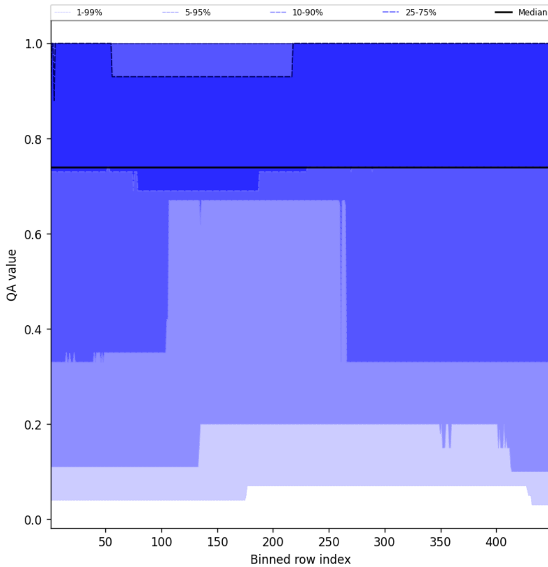
Figure 45: Along track statistics of “QA value” for 2024-11-20 to 2024-11-22
