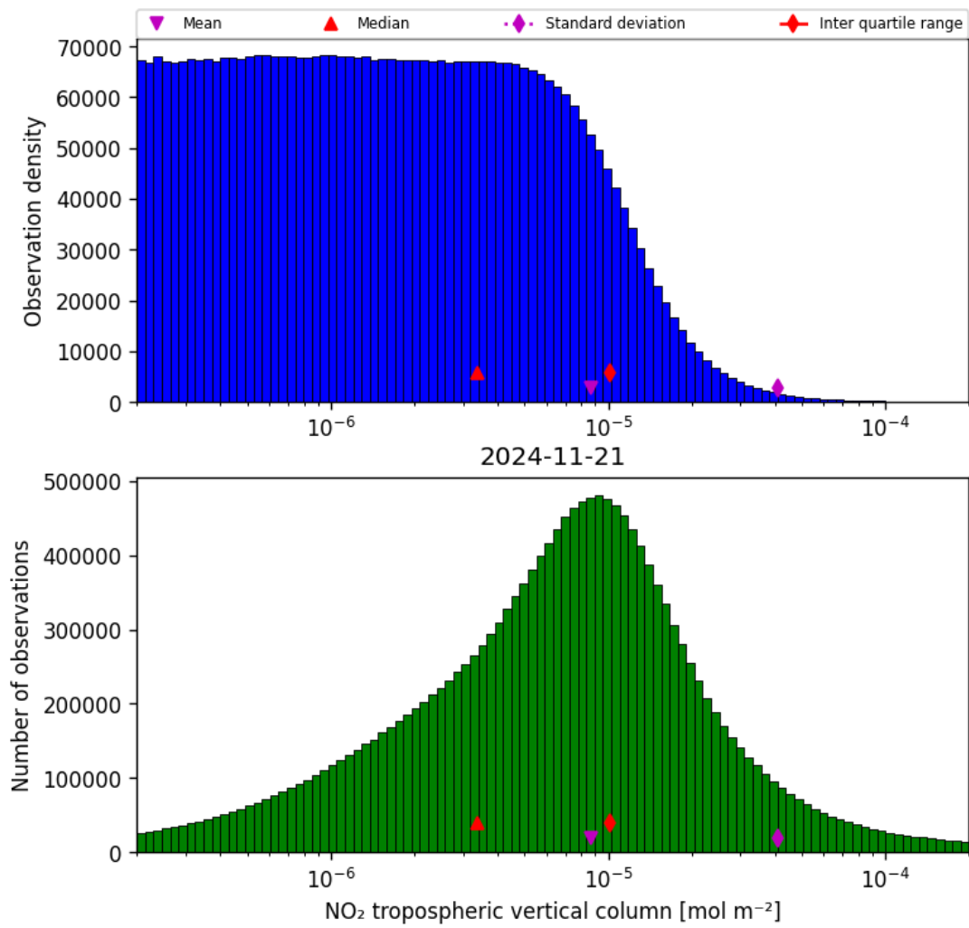
Figure 29: Histogram of “NO 2 tropospheric vertical column” for 2024-11-20 to 2024-11-22
