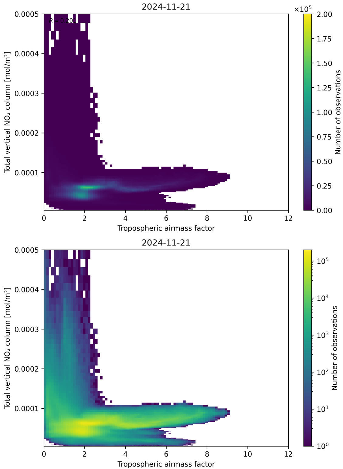
Figure 77: Scatter density plot of “Tropospheric airmass factor” against “Total vertical NO 2 column” for 2024-11-20 to 2024-11-22.
