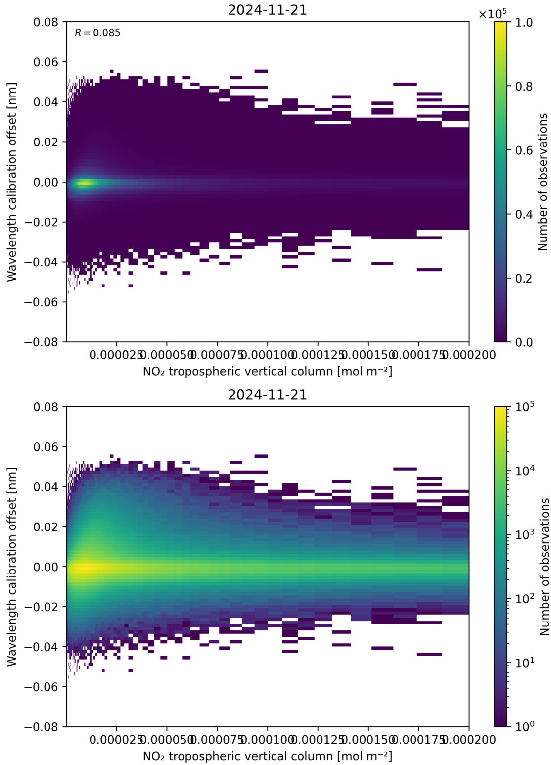
Figure 143: Scatter density plot of “NO 2 tropospheric vertical column” against “Wavelength calibration offset” for 2024-11-20 to 2024-11-22.
