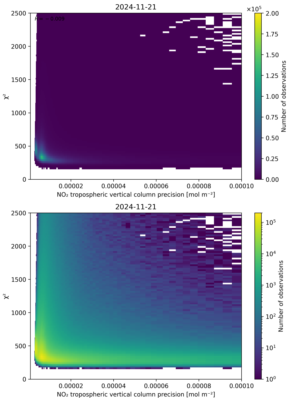
Figure 134: Scatter density plot of “NO 2 tropospheric vertical column precision” against “ \chi^2 ” for 2024-11-20 to 2024-11-22.
