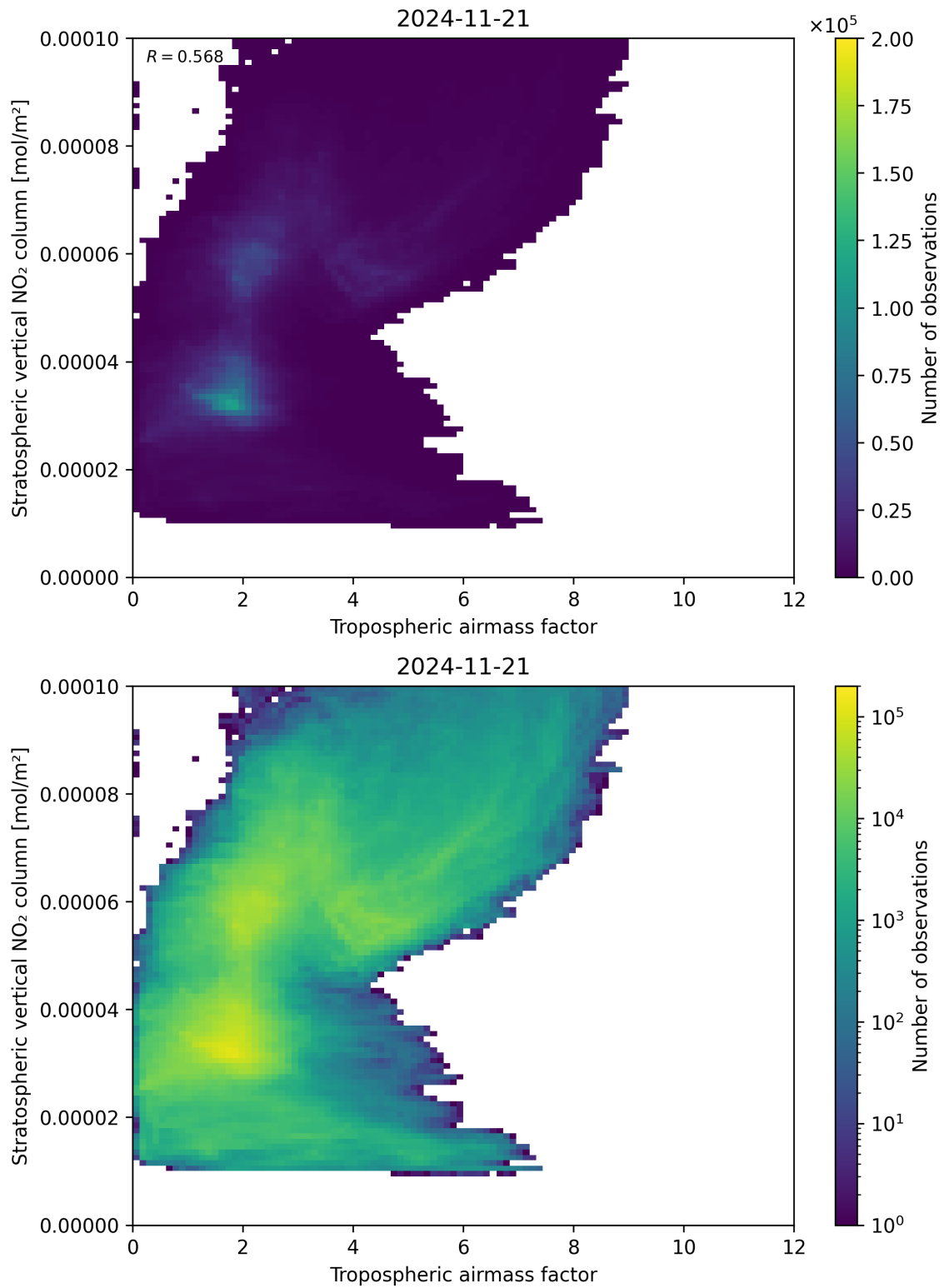
Figure 74: Scatter density plot of “Tropospheric air mass factor” against “Stratospheric vertical NO 2 column” for 2024-11-20 to 2024-11-22.
