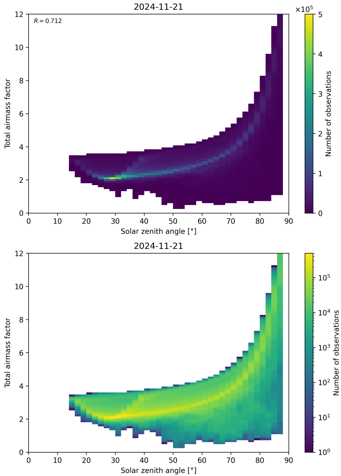
Figure 146: Scatter density plot of “Solar zenith angle” against “Total air mass factor” for 2024-11-20 to 2024-11-22.
