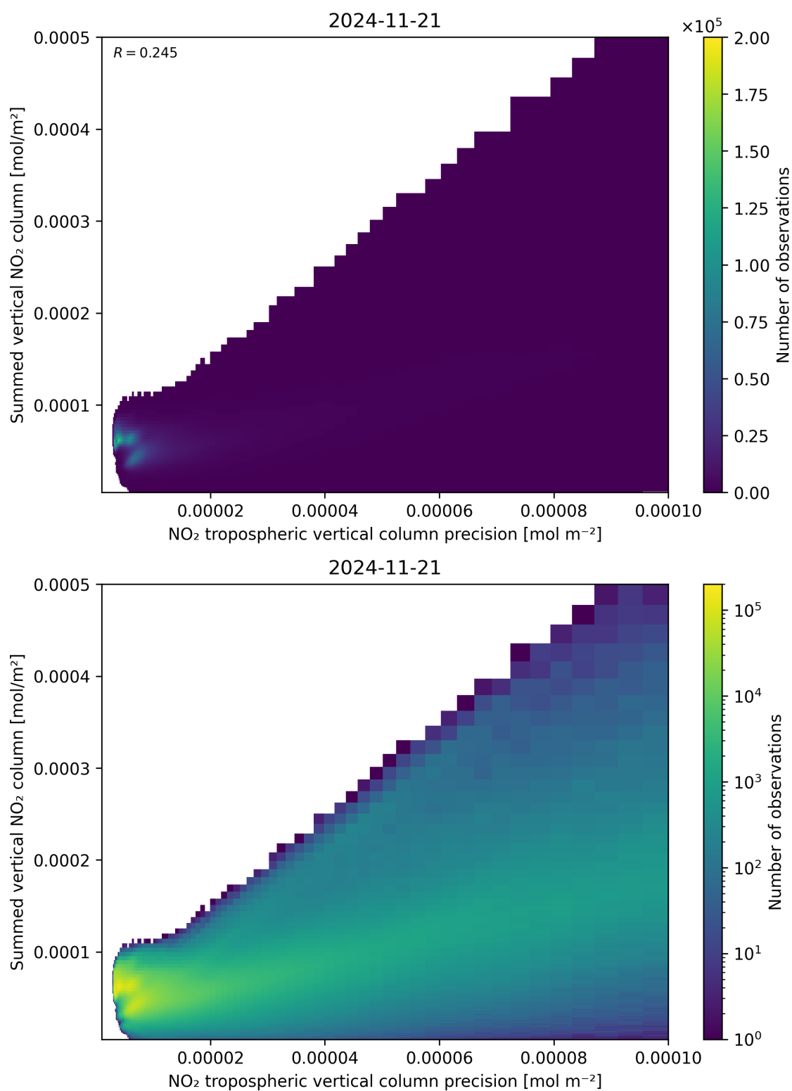
Figure 136: Scatter density plot of “NO 2 tropospheric vertical column precision” against “Summed vertical NO 2 column” for 2024-11-20 to 2024-11-22.
