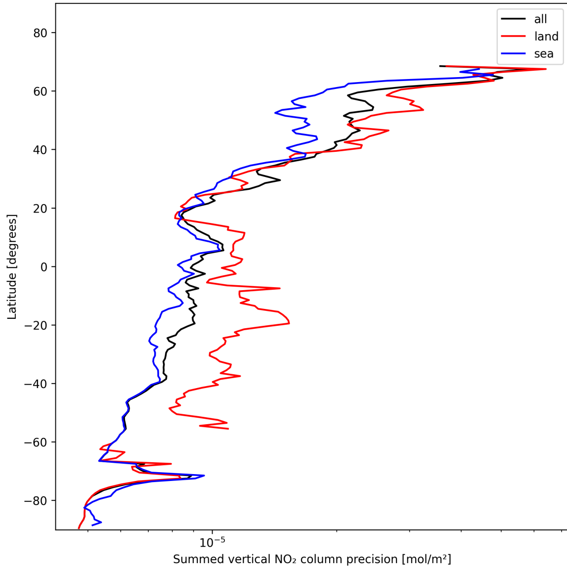
Figure 24: Zonal average of “Summed vertical NO 2 column precision” for 2024-11-20 to 2024-11-22.
