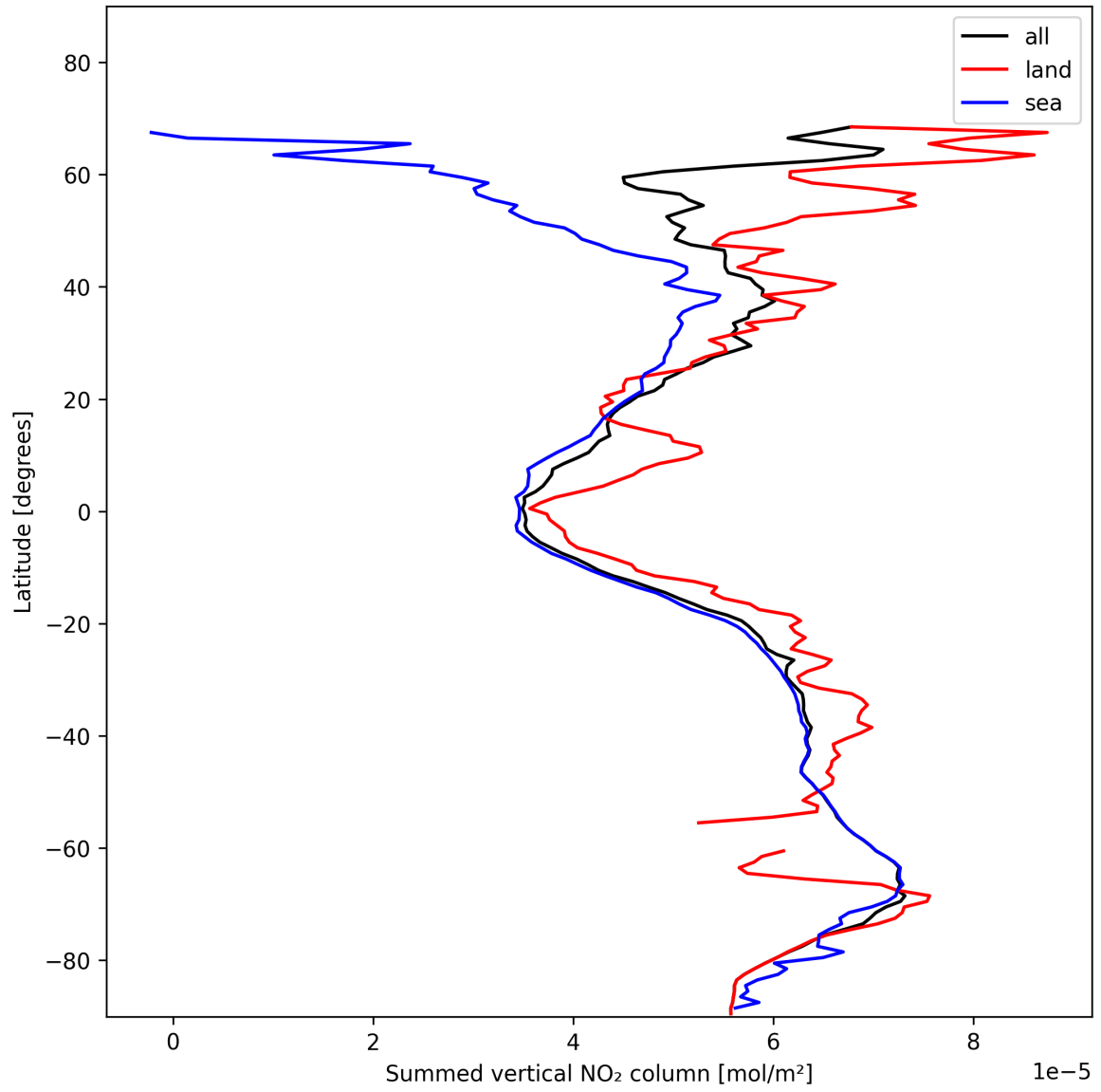
Figure 23: Zonal average of “Summed vertical NO 2 column” for 2024-11-20 to 2024-11-22.
