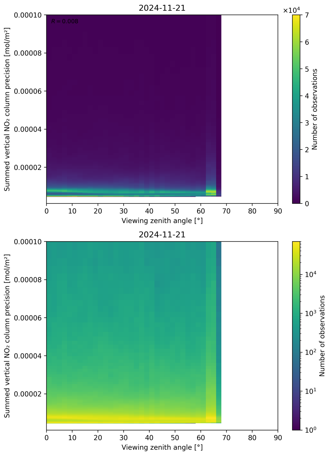
Figure 166: Scatter density plot of “Viewing zenith angle” against “Summed vertical NO 2 column precision” for 2024-11-20 to 2024-11-22.
