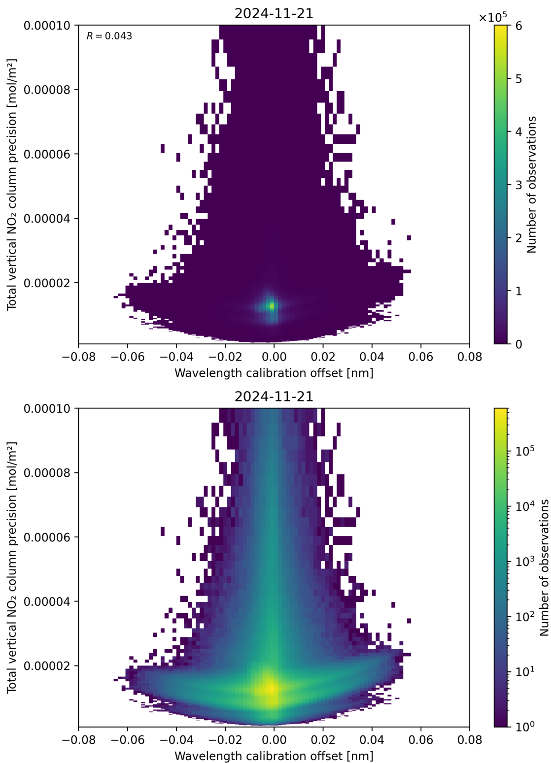
Figure 180: Scatter density plot of “Wavelength calibration offset” against “Total vertical NO 2 column precision” for 2024-11-20 to 2024-11-22.
