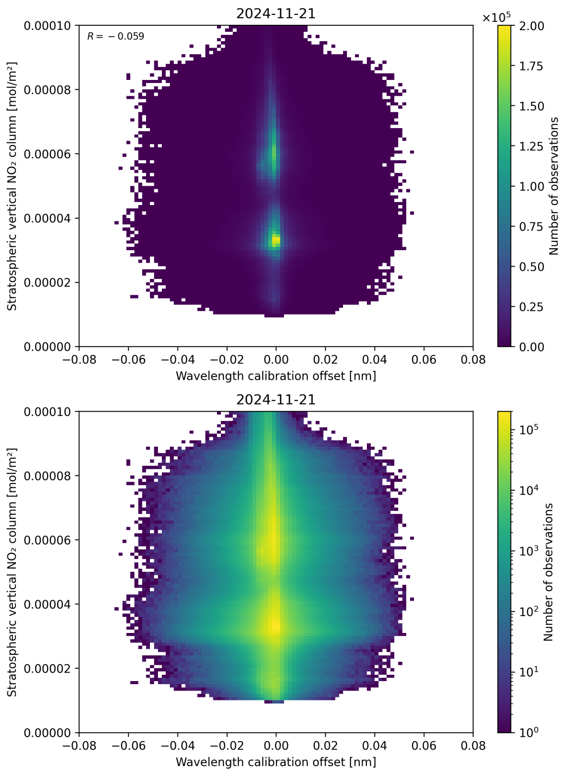
Figure 176: Scatter density plot of “Wavelength calibration offset” against “Stratospheric vertical NO 2 column” for 2024-11-20 to 2024-11-22.
