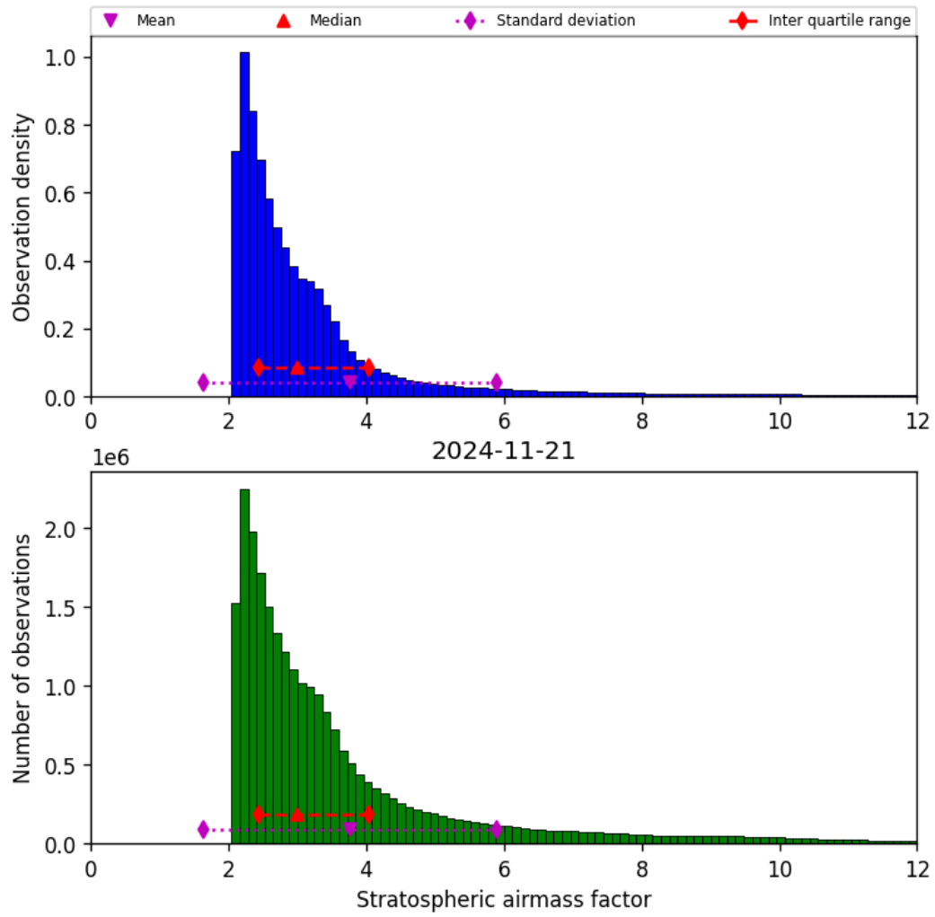
Figure 44: Histogram of “Stratospheric airmass factor” for 2024-11-20 to 2024-11-22
