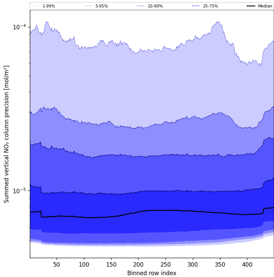
Figure 58: Along track statistics of “Summed vertical NO 2 column precision” for 2024-11-20 to 2024-11-22
