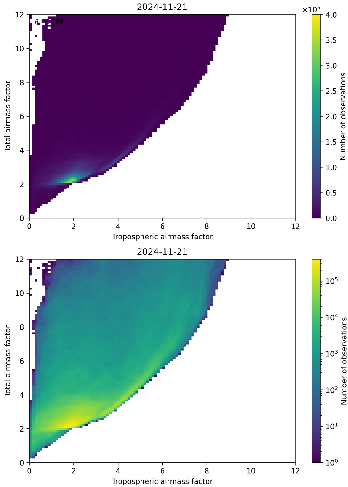
Figure 72: Scatter density plot of “Tropospheric airmass factor” against “Total airmass factor” for 2024-11-20 to 2024-11-22.
