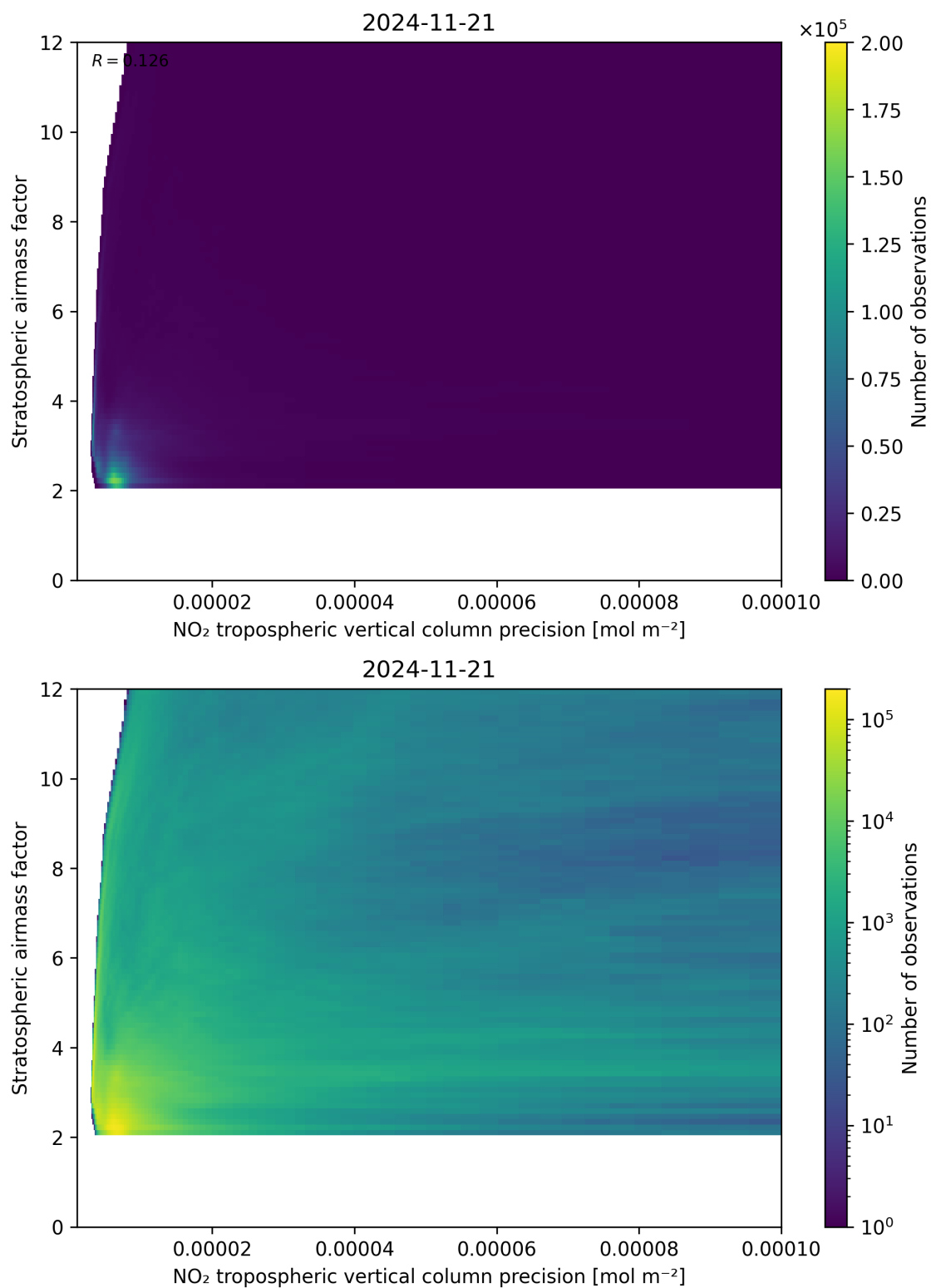
Figure 131: Scatter density plot of “NO 2 tropospheric vertical column precision” against “Stratospheric airmass factor” for 2024-11-20 to 2024-11-22.
