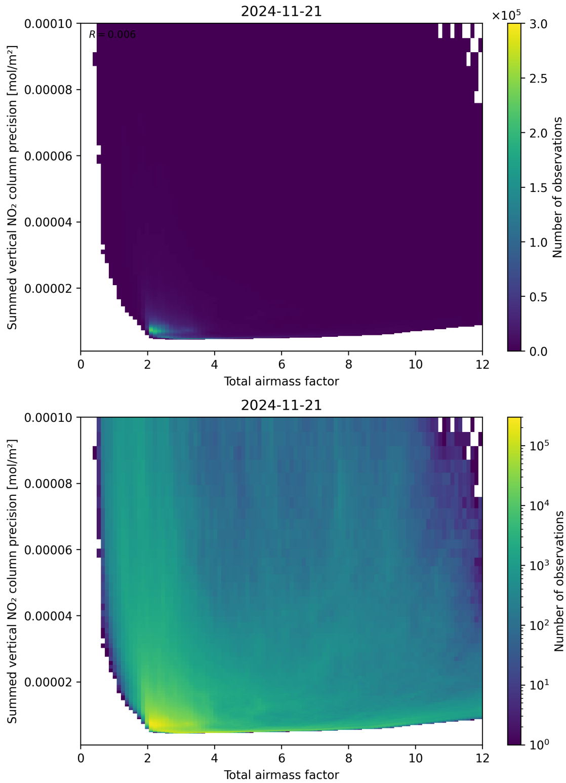
Figure 66: Scatter density plot of “Total airmass factor” against “Summed vertical NO 2 column precision” for 2024-11-20 to 2024-11-22.
