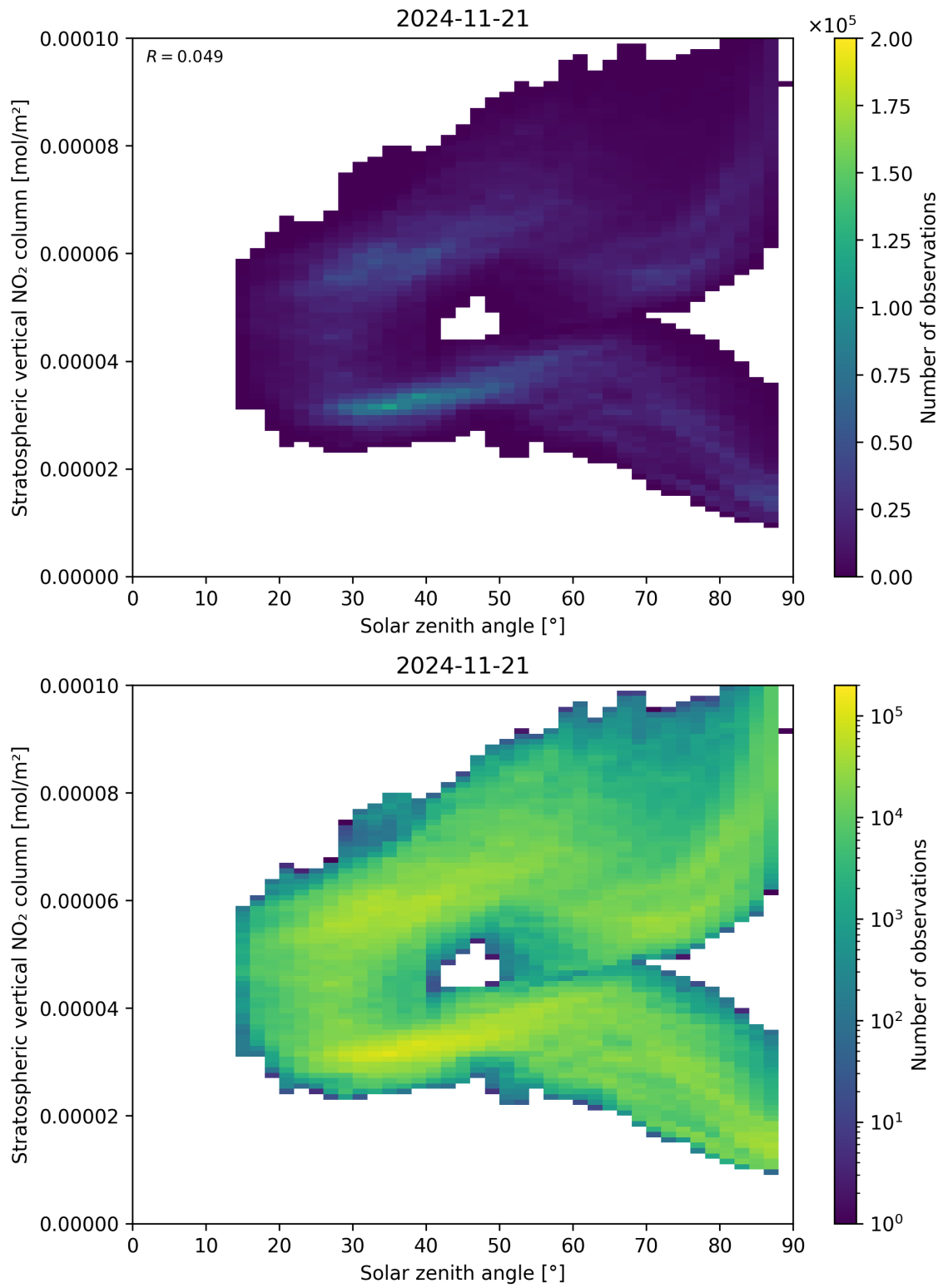
Figure 150: Scatter density plot of “Solar zenith angle” against “Stratospheric vertical NO 2 column” for 2024-11-20 to 2024-11-22.
