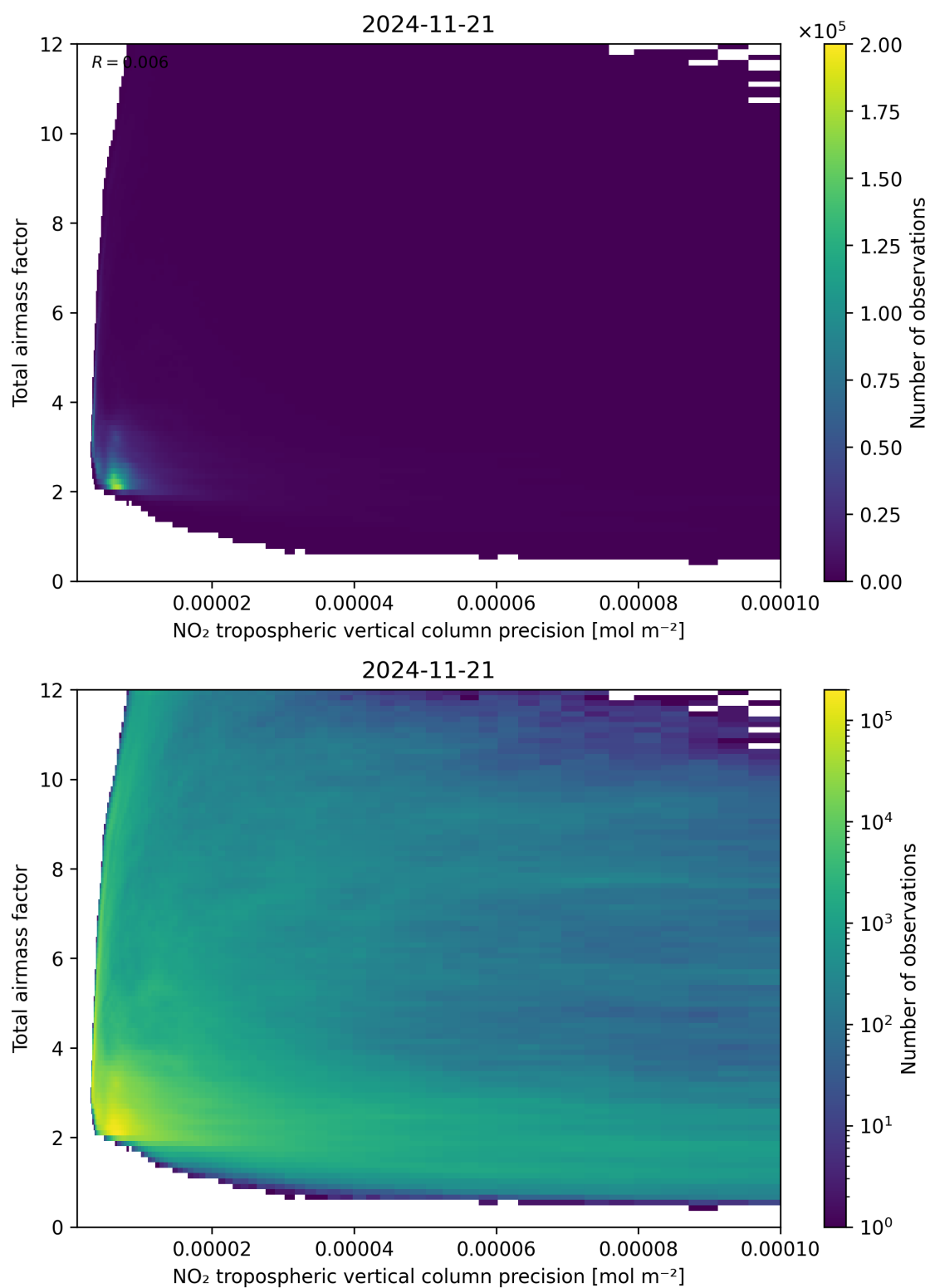
Figure 132: Scatter density plot of “NO 2 tropospheric vertical column precision” against “Total air mass factor” for 2024-11-20 to 2024-11-22.
