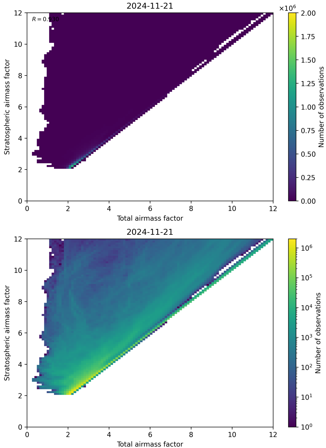
Figure 62: Scatter density plot of “Total airmass factor” against “Stratospheric airmass factor” for 2024-11-20 to 2024-11-22.
