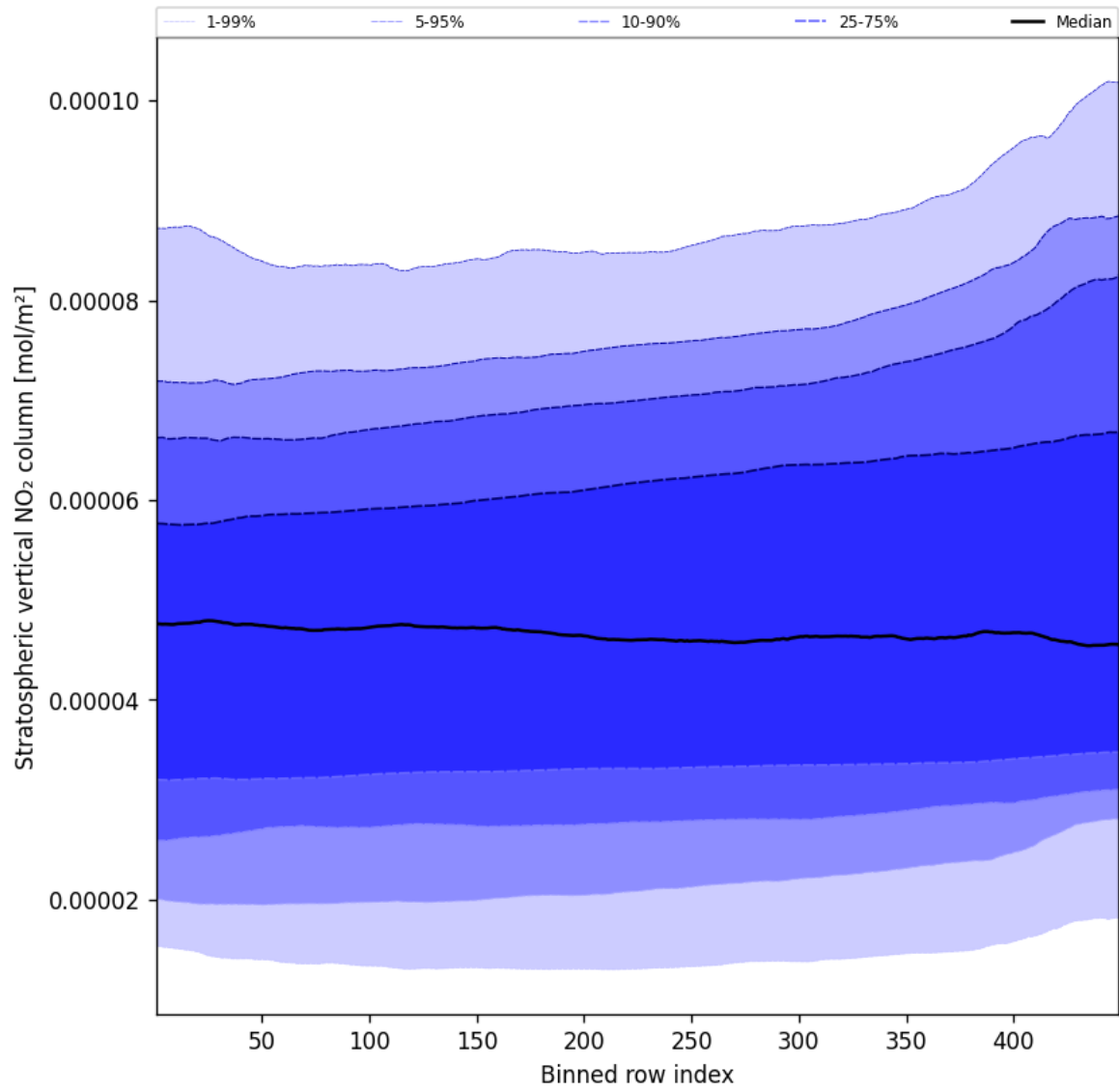
Figure 53: Along track statistics of “Stratospheric vertical NO 2 column” for 2024-11-20 to 2024-11-22
