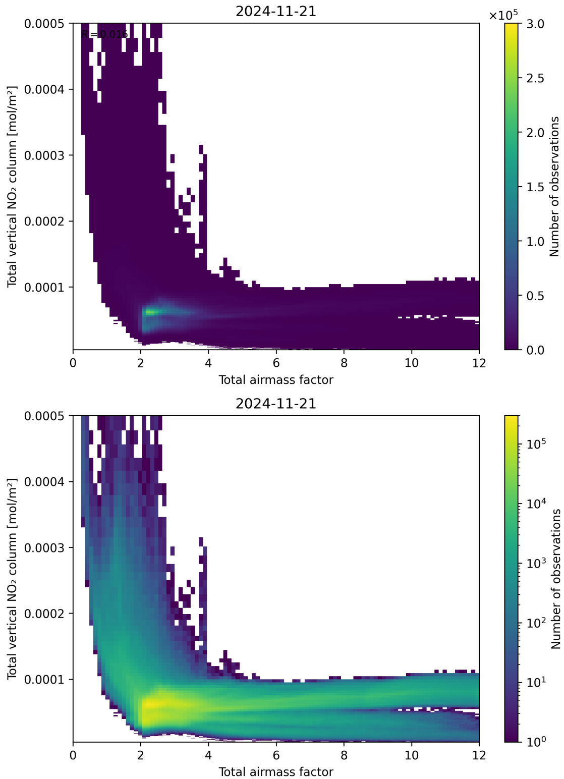
Figure 67: Scatter density plot of “Total air mass factor” against “Total vertical NO 2 column” for 2024-11-20 to 2024-11-22.
