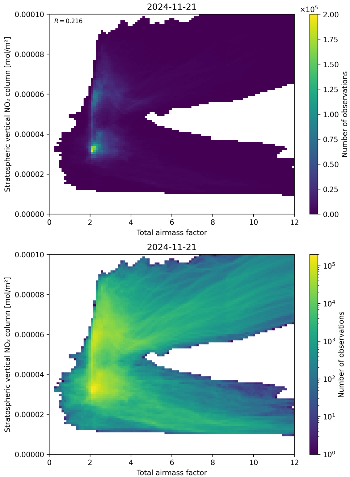
Figure 64: Scatter density plot of “Total airmass factor” against “Stratospheric vertical NO 2 column” for 2024-11-20 to 2024-11-22.
