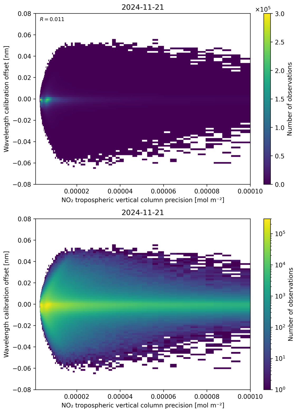
Figure 141: Scatter density plot of “NO 2 tropospheric vertical column precision” against “Wavelength calibration offset” for 2024-11-20 to 2024-11-22.
