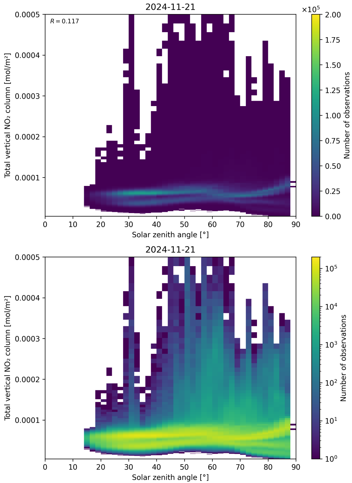
Figure 153: Scatter density plot of “Solar zenith angle” against “Total vertical NO 2 column” for 2024-11-20 to 2024-11-22.
