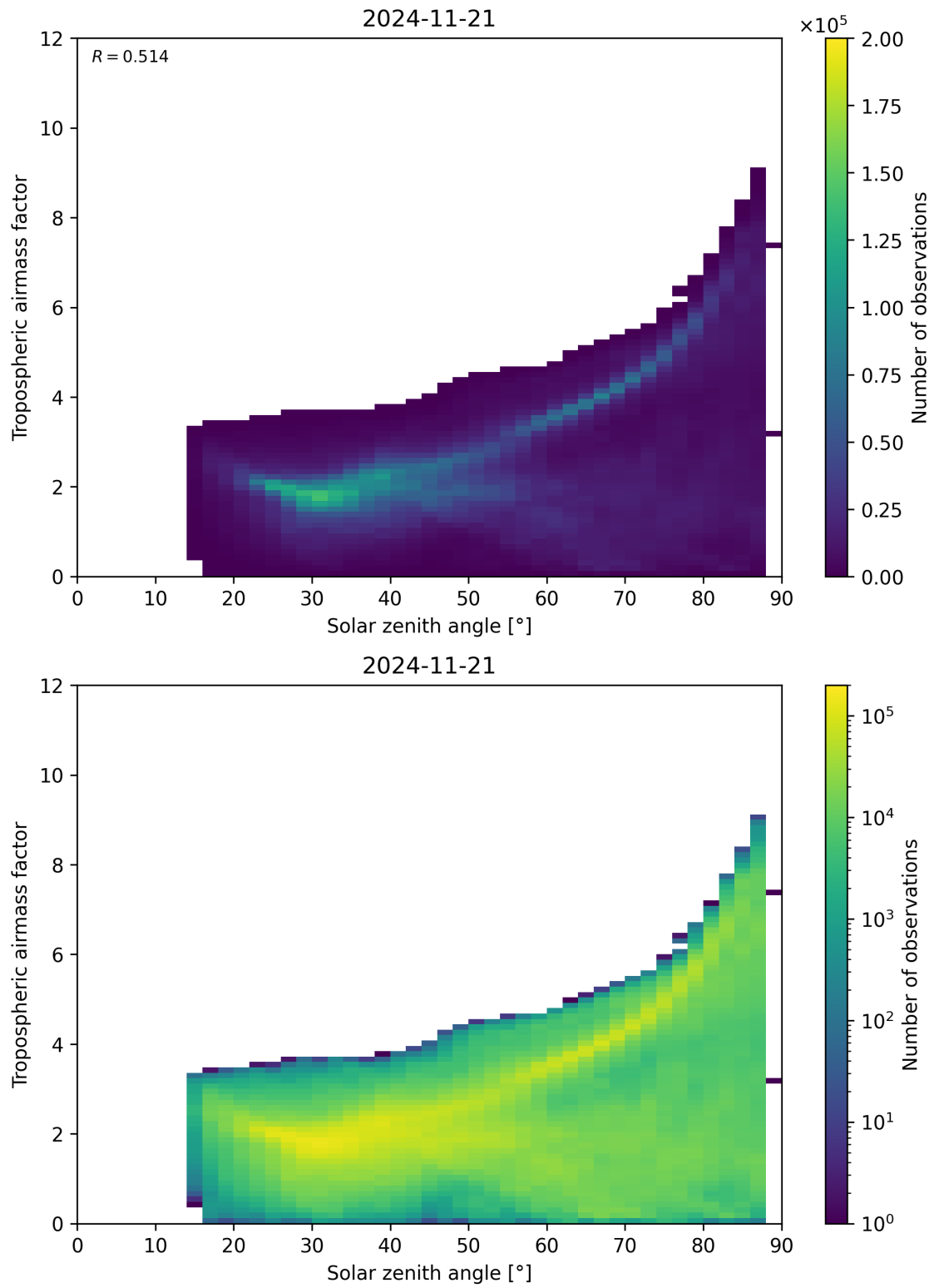
Figure 147: Scatter density plot of “Solar zenith angle” against “Tropospheric airmass factor” for 2024-11-20 to 2024-11-22.
