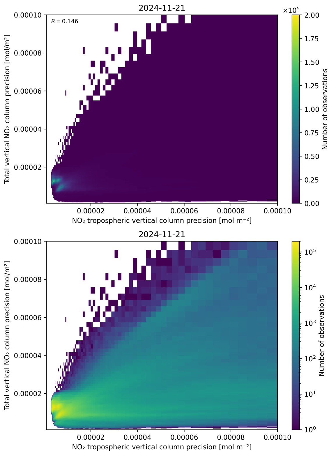
Figure 139: Scatter density plot of “NO 2 tropospheric vertical column precision” against “Total vertical NO 2 column precision” for 2024-11-20 to 2024-11-22.
