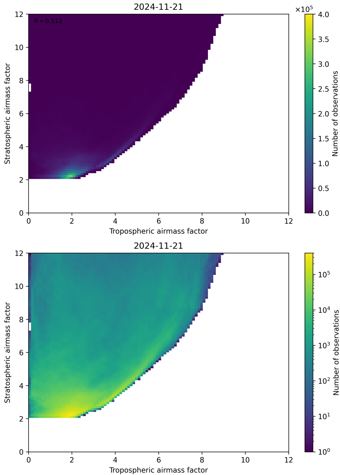
Figure 71: Scatter density plot of “Tropospheric airmass factor” against “Stratospheric airmass factor” for 2024-11-20 to 2024-11-22.
