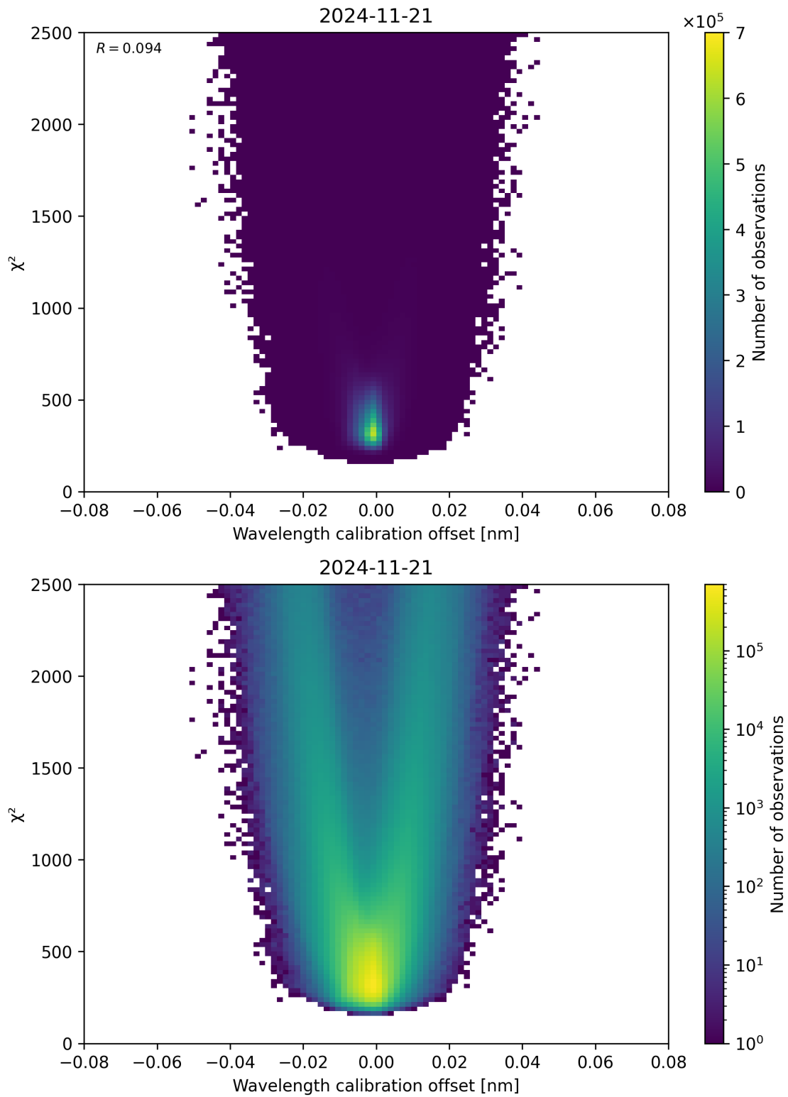
Figure 175: Scatter density plot of “Wavelength calibration offset” against “ \chi^2 ” for 2024-11-20 to 2024-11-22.
