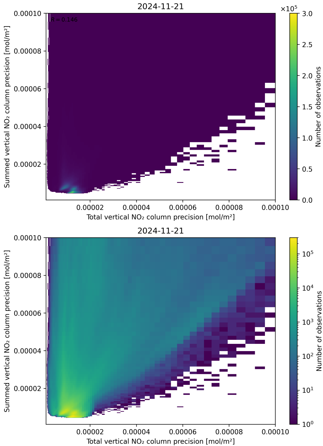
Figure 118: Scatter density plot of “Total vertical NO 2 column precision” against “Summed vertical NO 2 column precision” for 2024-11-20 to 2024-11-22.
