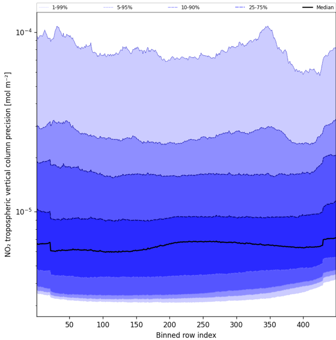
Figure 47: Along track statistics of “NO 2 tropospheric vertical column precision” for 2024-11-20 to 2024-11-22
