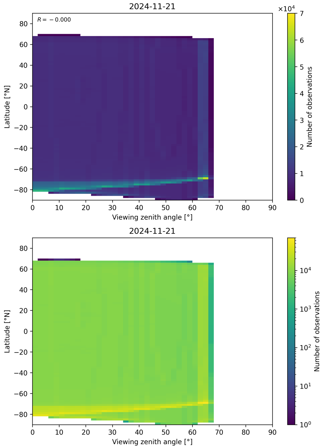
Figure 163: Scatter density plot of “Viewing zenith angle” against “Latitude” for 2024-11-20 to 2024-11-22.
