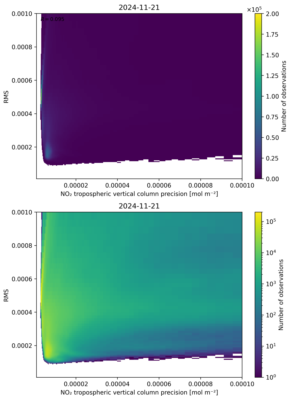
Figure 140: Scatter density plot of “NO 2 tropospheric vertical column precision” against “RMS” for 2024-11-20 to 2024-11-22.
