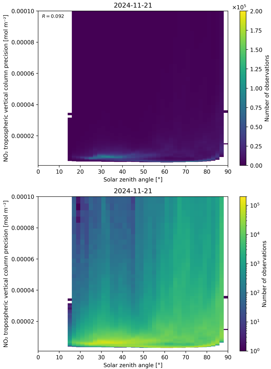
Figure 156: Scatter density plot of “Solar zenith angle” against “NO 2 tropospheric vertical column precision” for 2024-11-20 to 2024-11-22.
