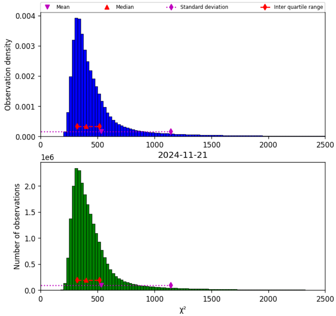
Figure 42: Histogram of “ \chi^2 ” for 2024-11-20 to 2024-11-22
