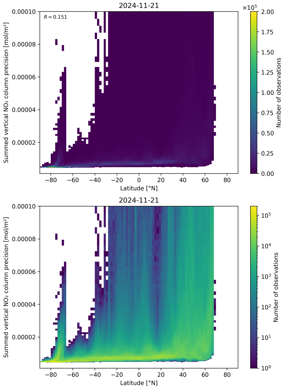
Figure 89: Scatter density plot of “Latitude” against “Summed vertical NO 2 column precision” for 2024-11-20 to 2024-11-22.
