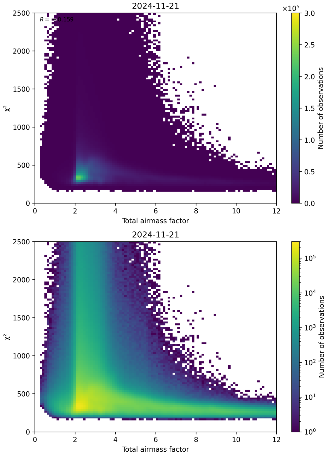
Figure 63: Scatter density plot of “Total airmass factor” against “ \chi^2 ” for 2024-11-20 to 2024-11-22.
