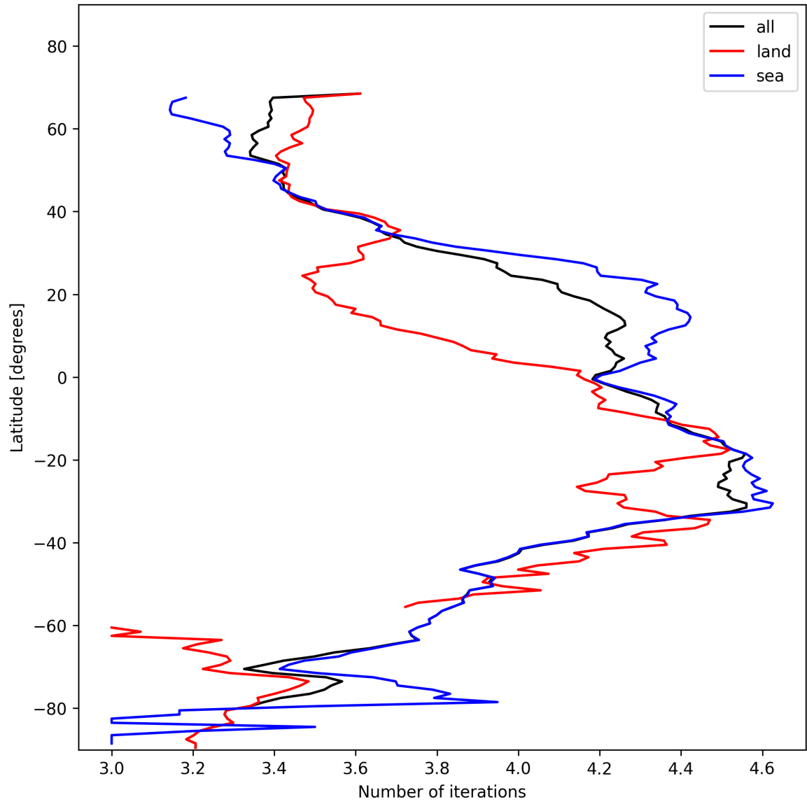
Figure 17: Zonal average of “Number of iterations” for 2024-11-20 to 2024-11-22.
