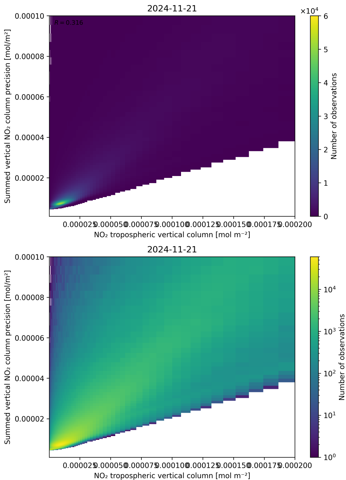
Figure 127: Scatter density plot of “NO 2 tropospheric vertical column” against “Summed vertical NO 2 column precision” for 2024-11-20 to 2024-11-22.
