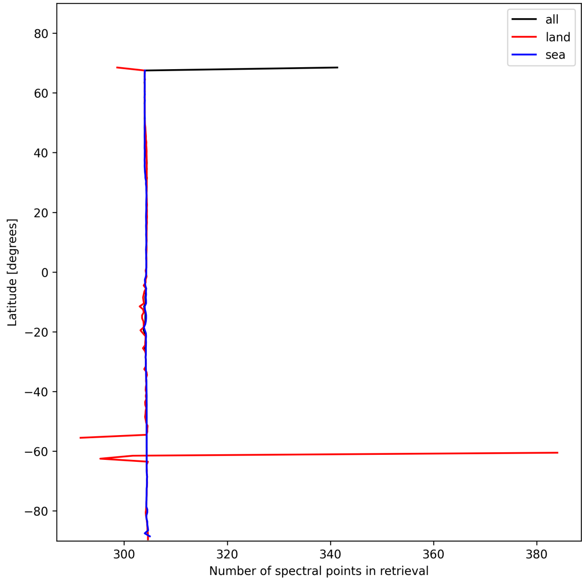
Figure 16: Zonal average of “Number of spectral points in retrieval” for 2024-11-20 to 2024-11-22.
