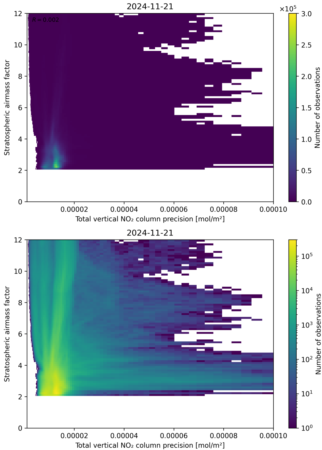
Figure 115: Scatter density plot of “Total vertical NO 2 column precision” against “Stratospheric air mass factor” for 2024-11-20 to 2024-11-22.
