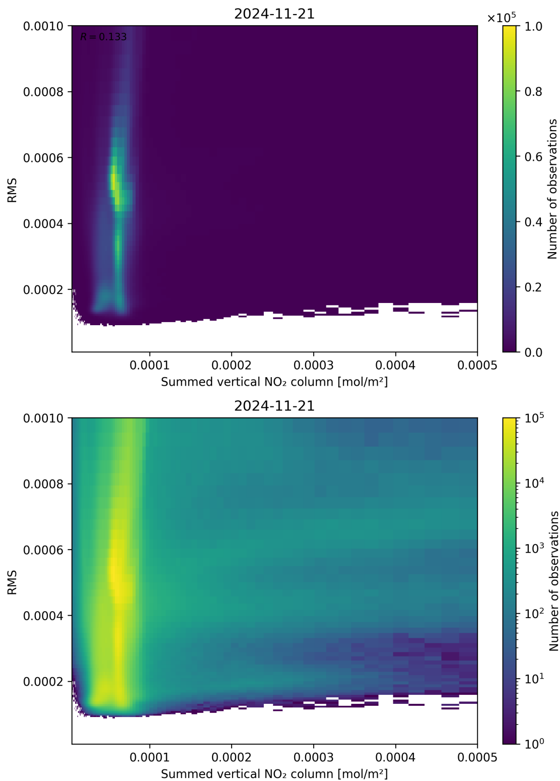
Figure 109: Scatter density plot of “Summed vertical NO 2 column” against “RMS” for 2024-11-20 to 2024-11-22.
