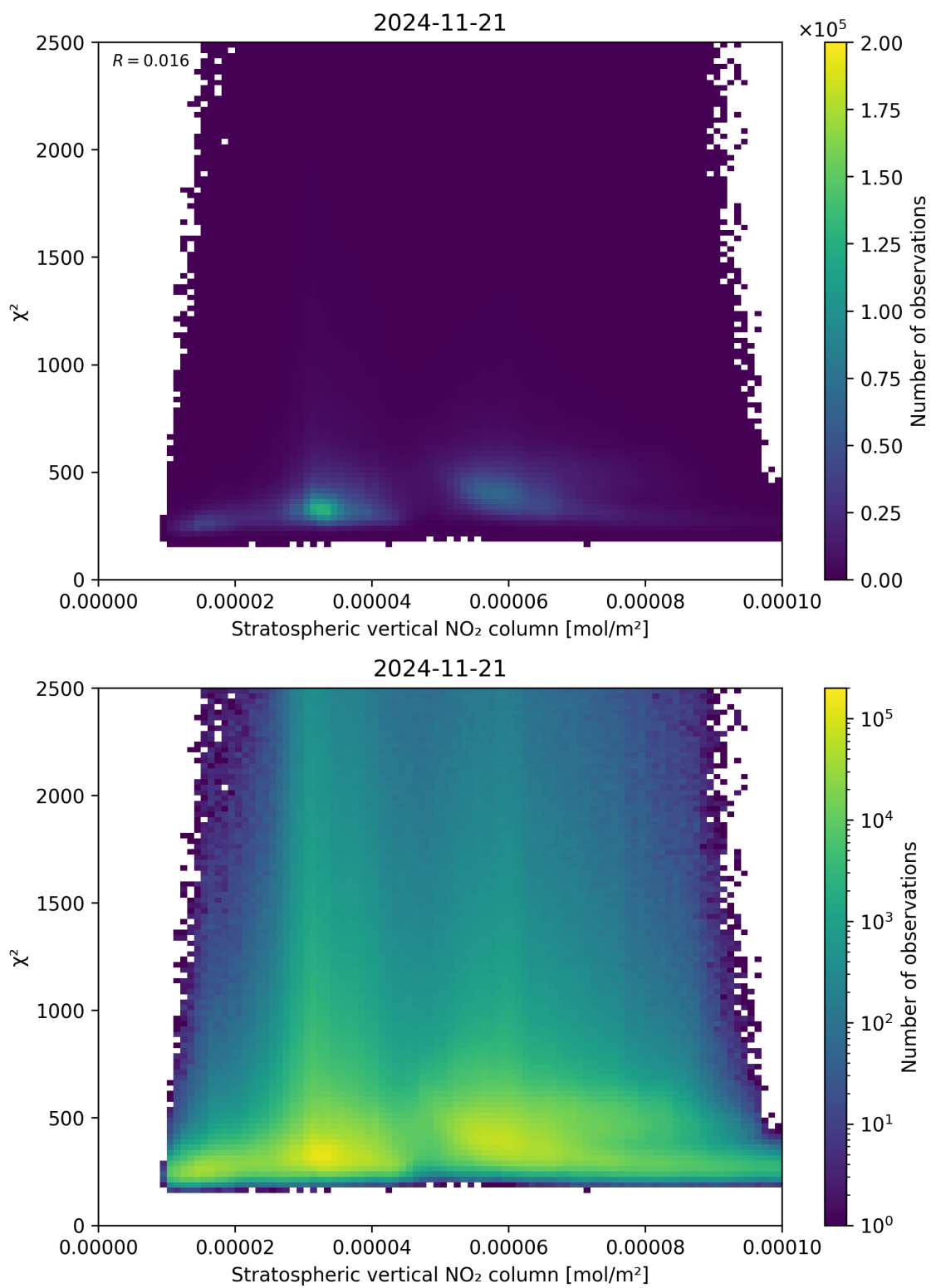
Figure 97: Scatter density plot of “Stratospheric vertical NO 2 column” against “ \chi^2 ” for 2024-11-20 to 2024-11-22.
