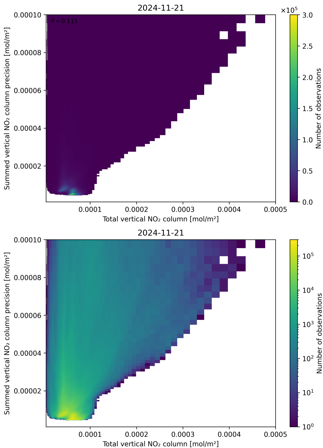
Figure 113: Scatter density plot of “Total vertical NO 2 column” against “Summed vertical NO 2 column precision” for 2024-11-20 to 2024-11-22.
