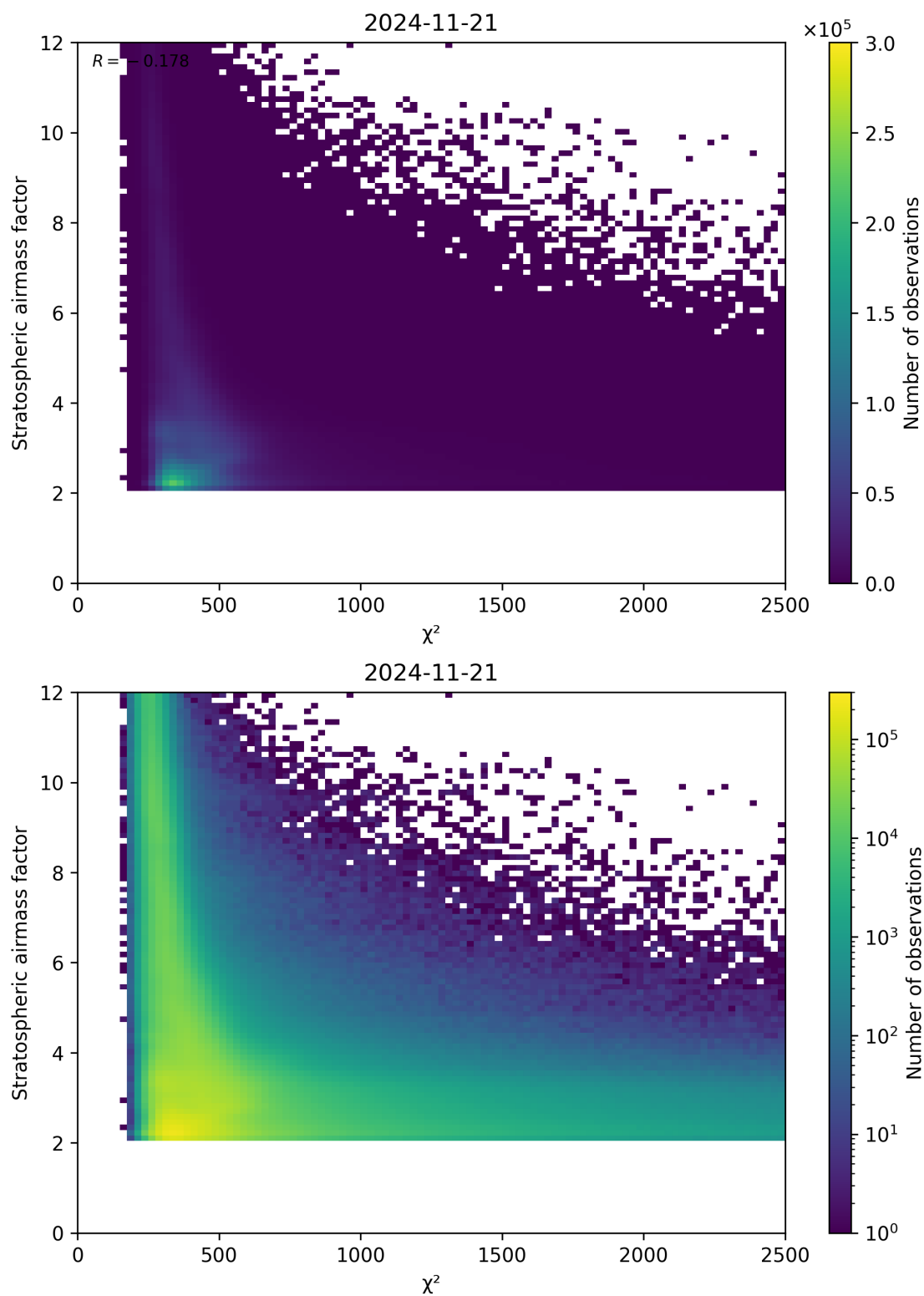
Figure 81: Scatter density plot of “ \chi^2 ” against “Stratospheric airmass factor” for 2024-11-20 to 2024-11-22.
