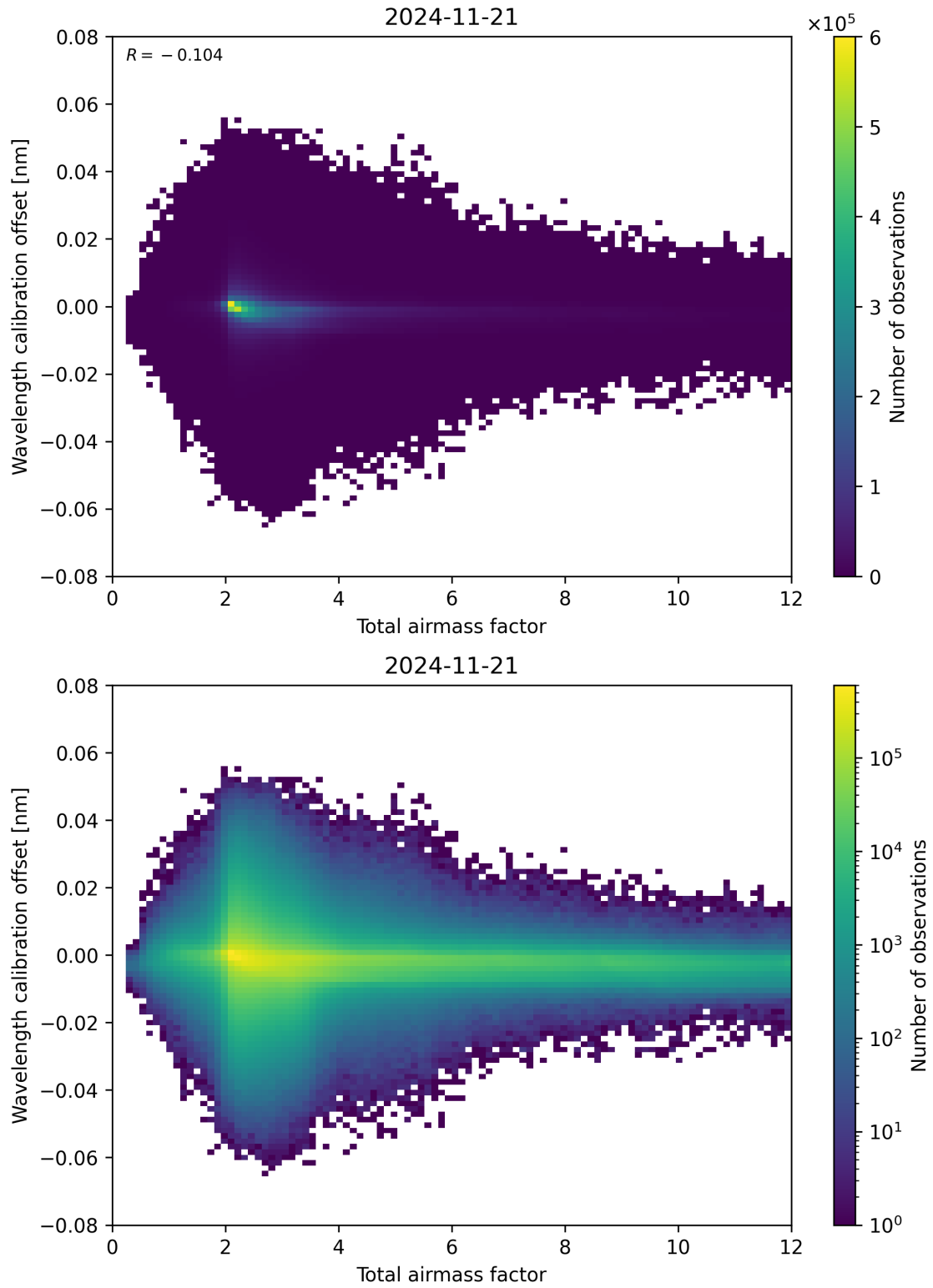
Figure 70: Scatter density plot of “Total airmass factor” against “Wavelength calibration offset” for 2024-11-20 to 2024-11-22.
