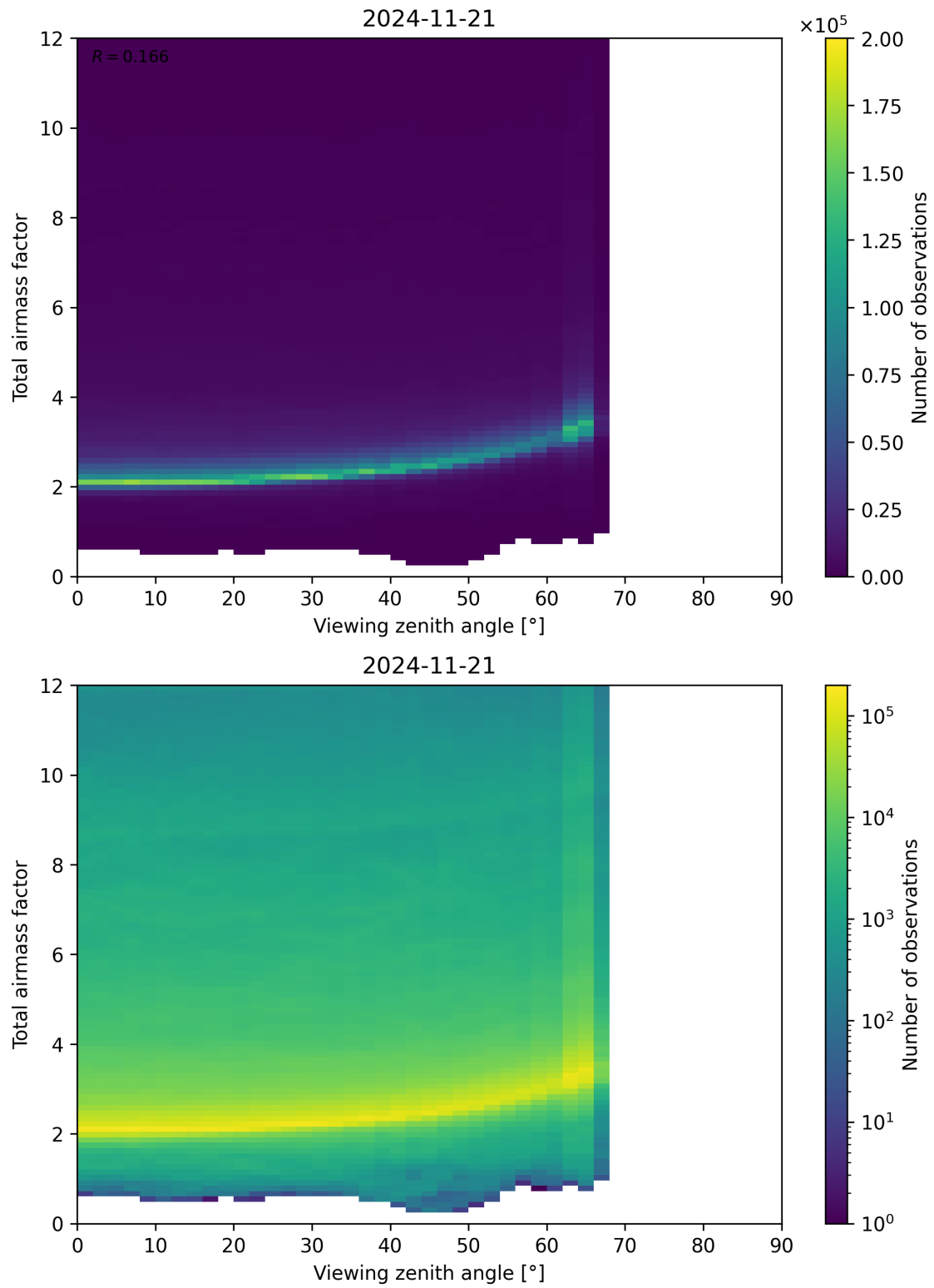
Figure 160: Scatter density plot of “Viewing zenith angle” against “Total airmass factor” for 2024-11-20 to 2024-11-22.
