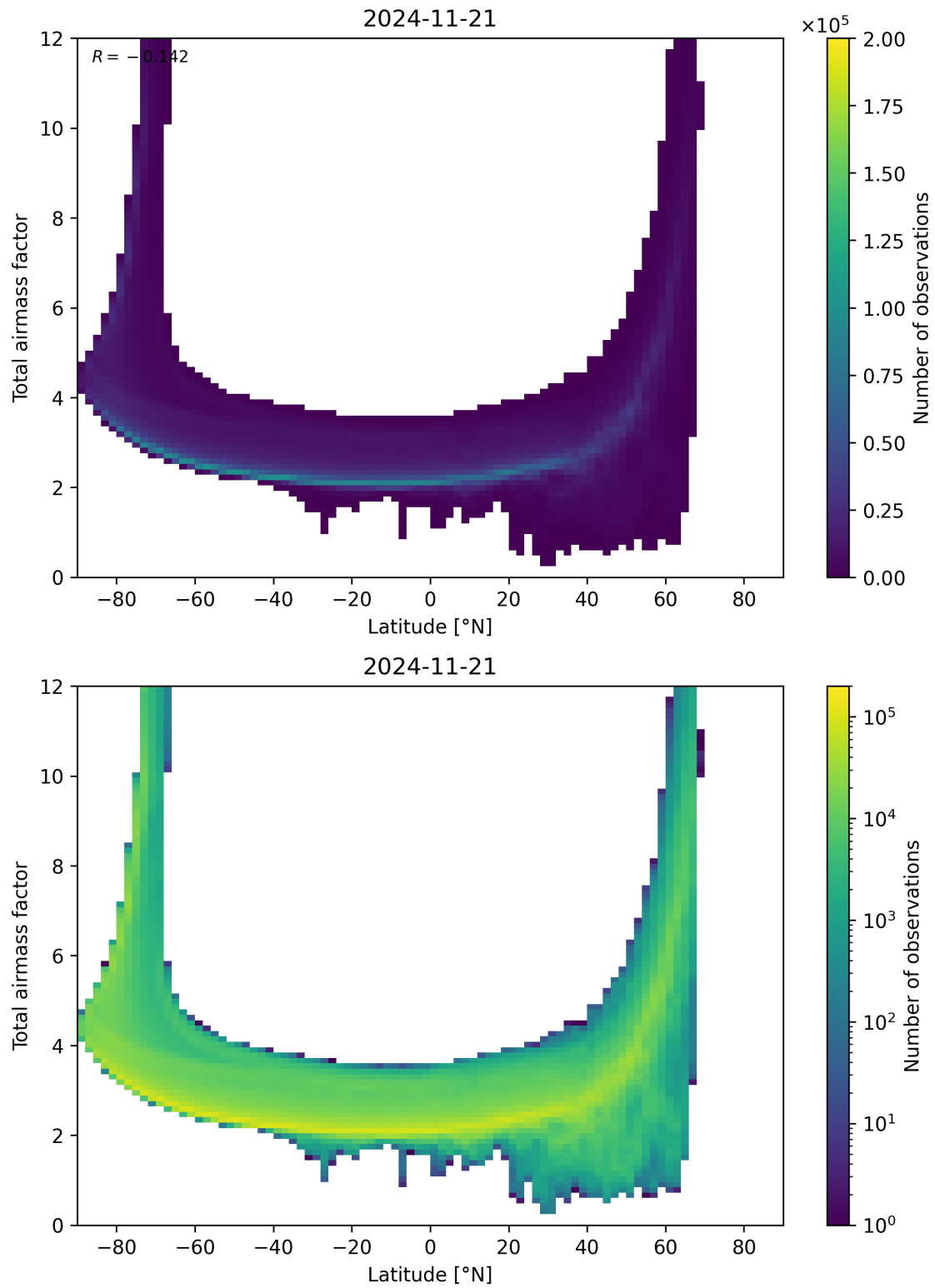
Figure 84: Scatter density plot of “Latitude” against “Total airmass factor” for 2024-11-20 to 2024-11-22.
