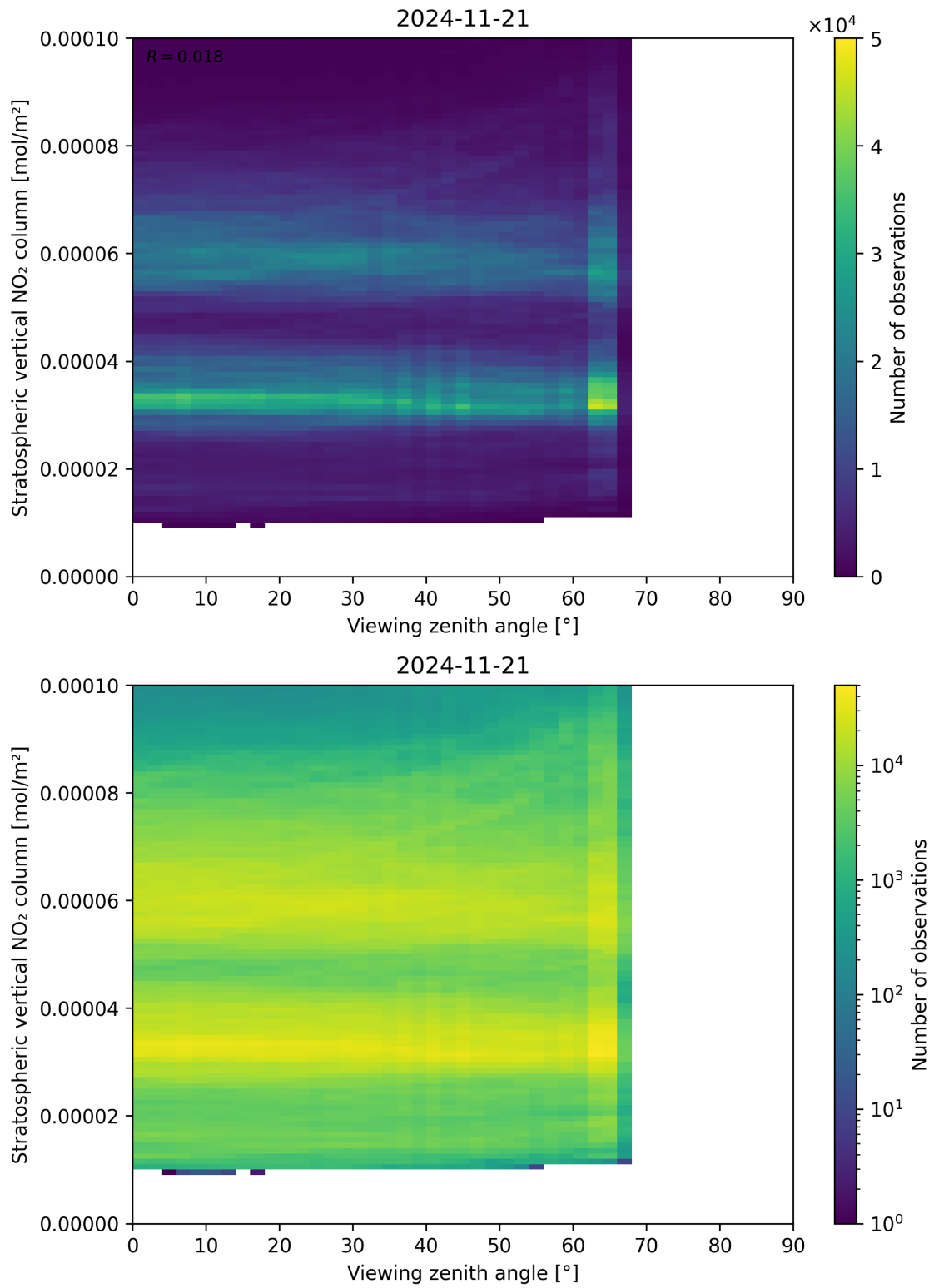
Figure 164: Scatter density plot of “Viewing zenith angle” against “Stratospheric vertical NO 2 column” for 2024-11-20 to 2024-11-22.
