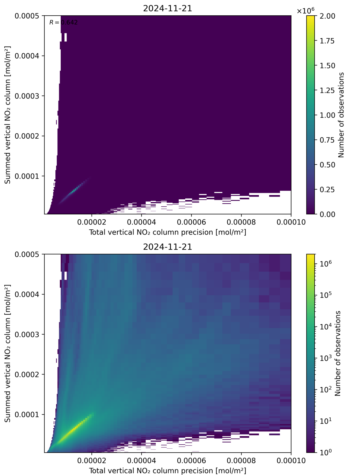
Figure 117: Scatter density plot of “Total vertical NO 2 column precision” against “Summed vertical NO 2 column” for 2024-11-20 to 2024-11-22.
