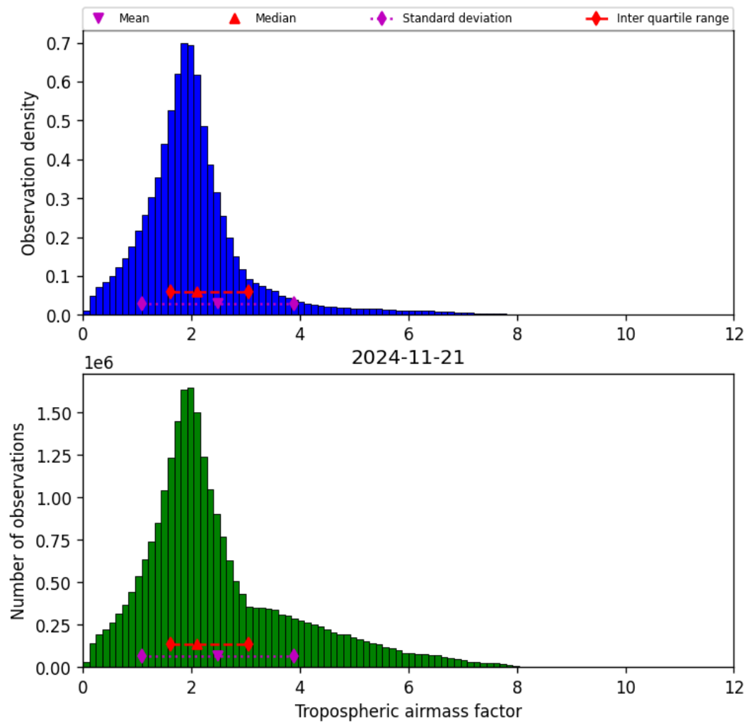
Figure 31: Histogram of “Tropospheric airmass factor” for 2024-11-20 to 2024-11-22
