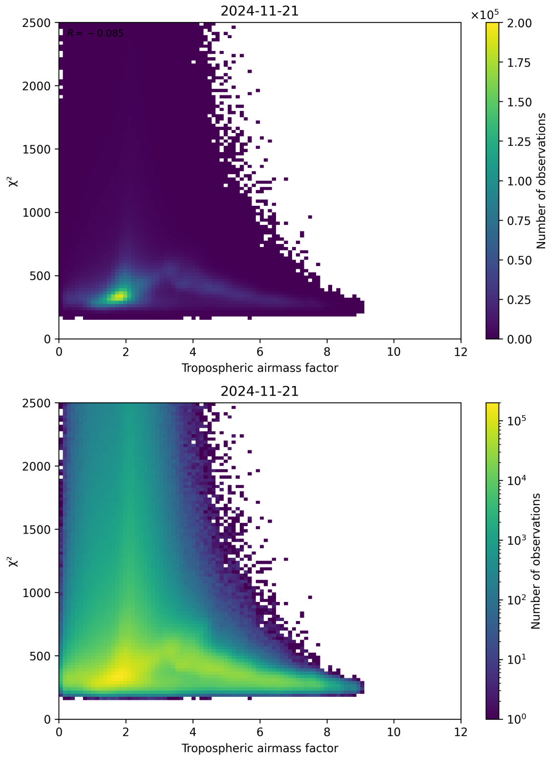
Figure 73: Scatter density plot of “Tropospheric airmass factor” against “ \chi^2 ” for 2024-11-20 to 2024-11-22.
