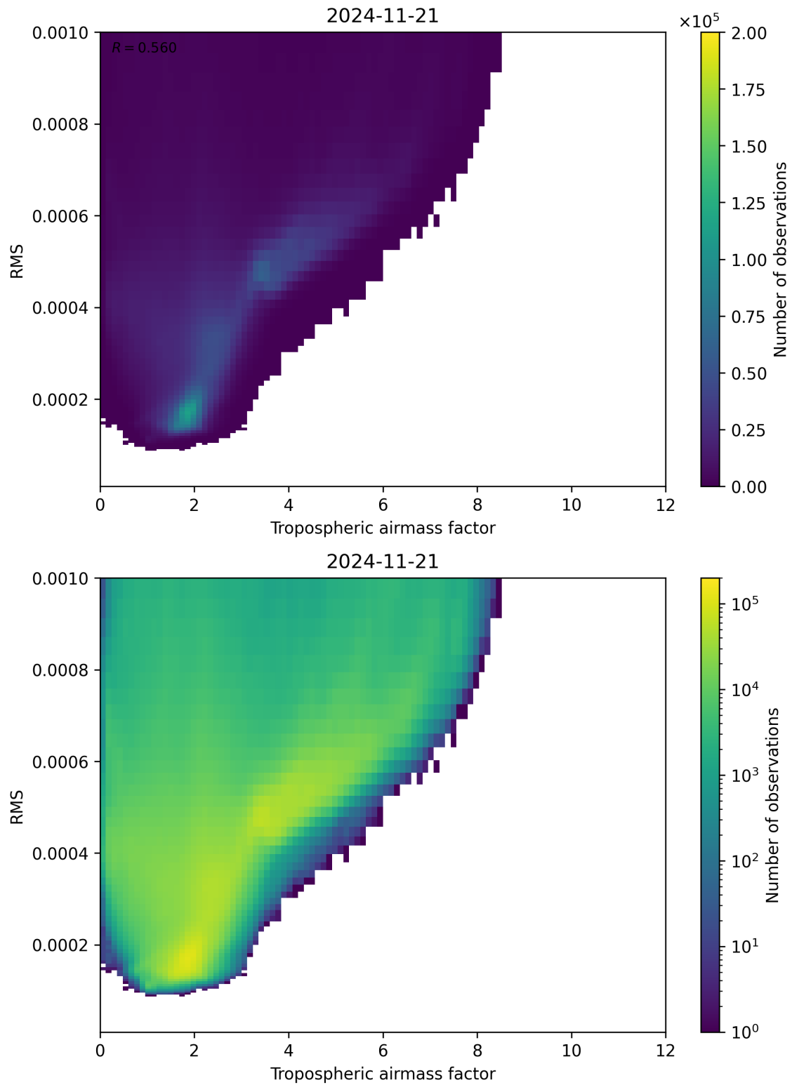
Figure 79: Scatter density plot of “Tropospheric airmass factor” against “RMS” for 2024-11-20 to 2024-11-22.
