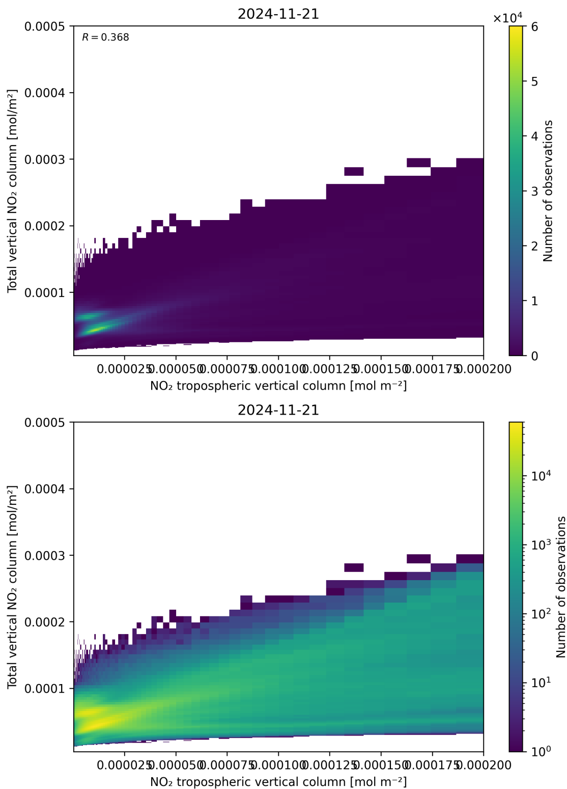
Figure 128: Scatter density plot of “NO 2 tropospheric vertical column” against “Total vertical NO 2 column” for 2024-11-20 to 2024-11-22.
