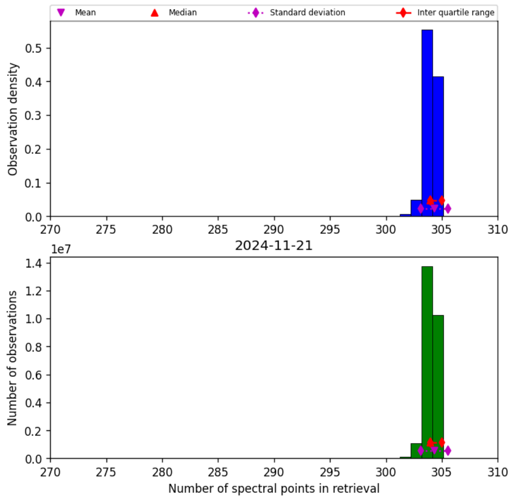
Figure 33: Histogram of “Number of spectral points in retrieval” for 2024-11-20 to 2024-11-22
