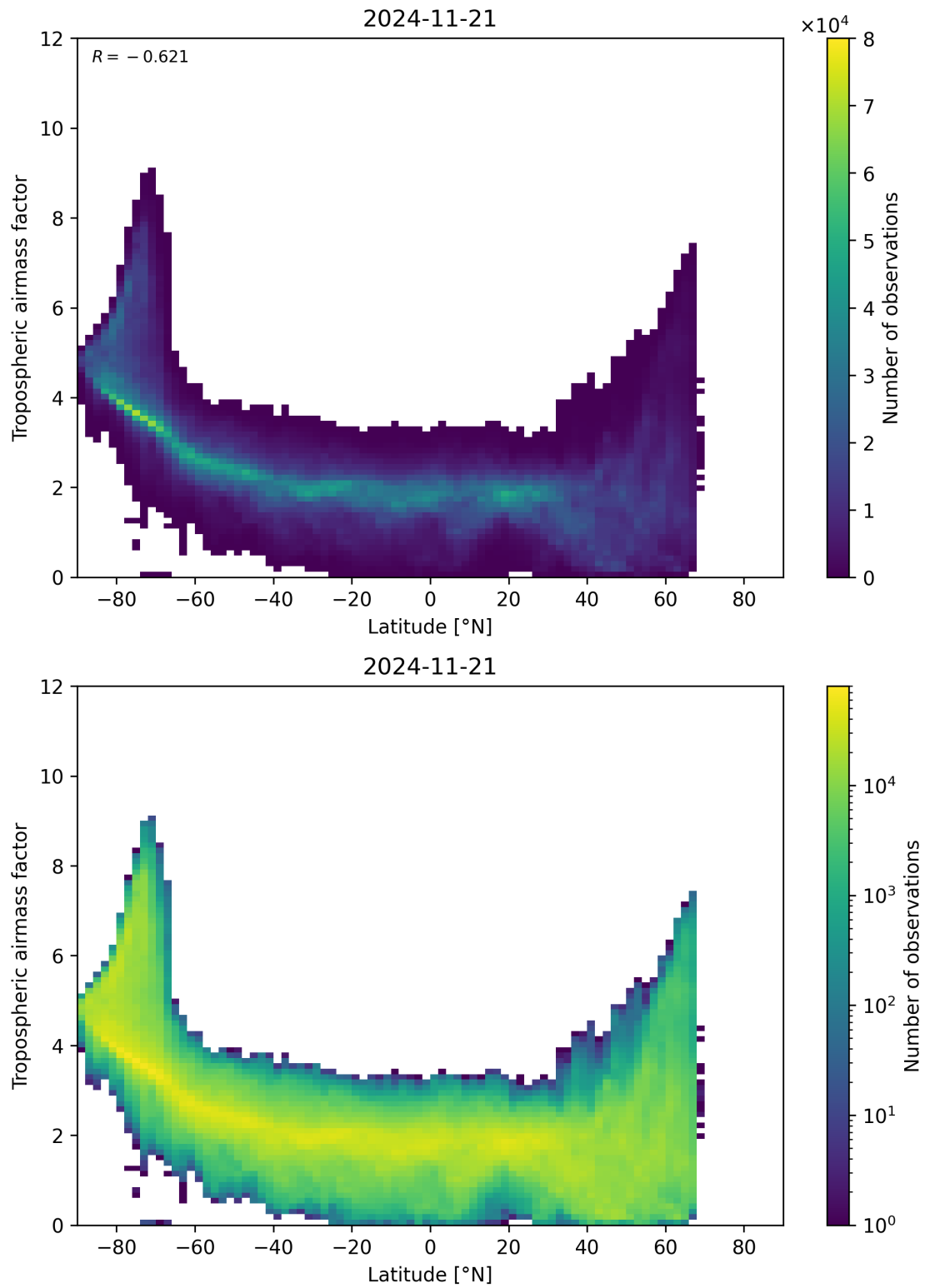
Figure 85: Scatter density plot of “Latitude” against “Tropospheric airmass factor” for 2024-11-20 to 2024-11-22.
