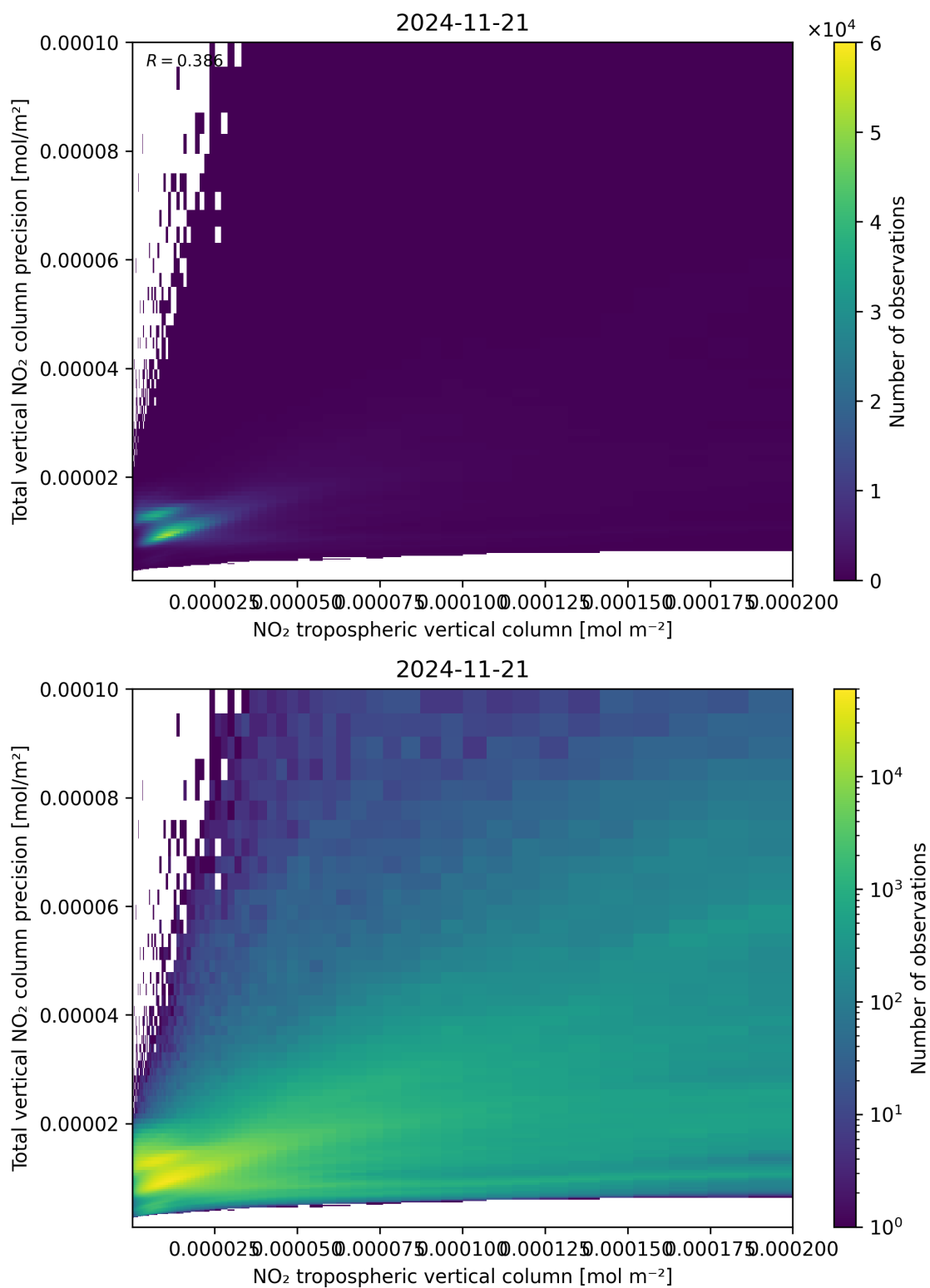
Figure 129: Scatter density plot of “NO 2 tropospheric vertical column” against “Total vertical NO 2 column precision” for 2024-11-20 to 2024-11-22.
