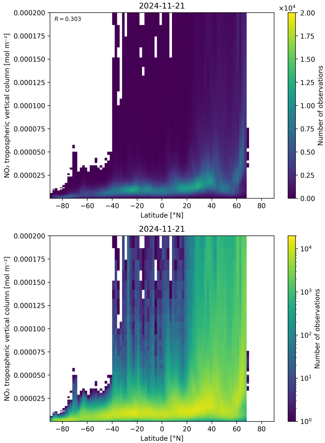
Figure 92: Scatter density plot of “Latitude” against “NO 2 tropospheric vertical column” for 2024-11-20 to 2024-11-22.
