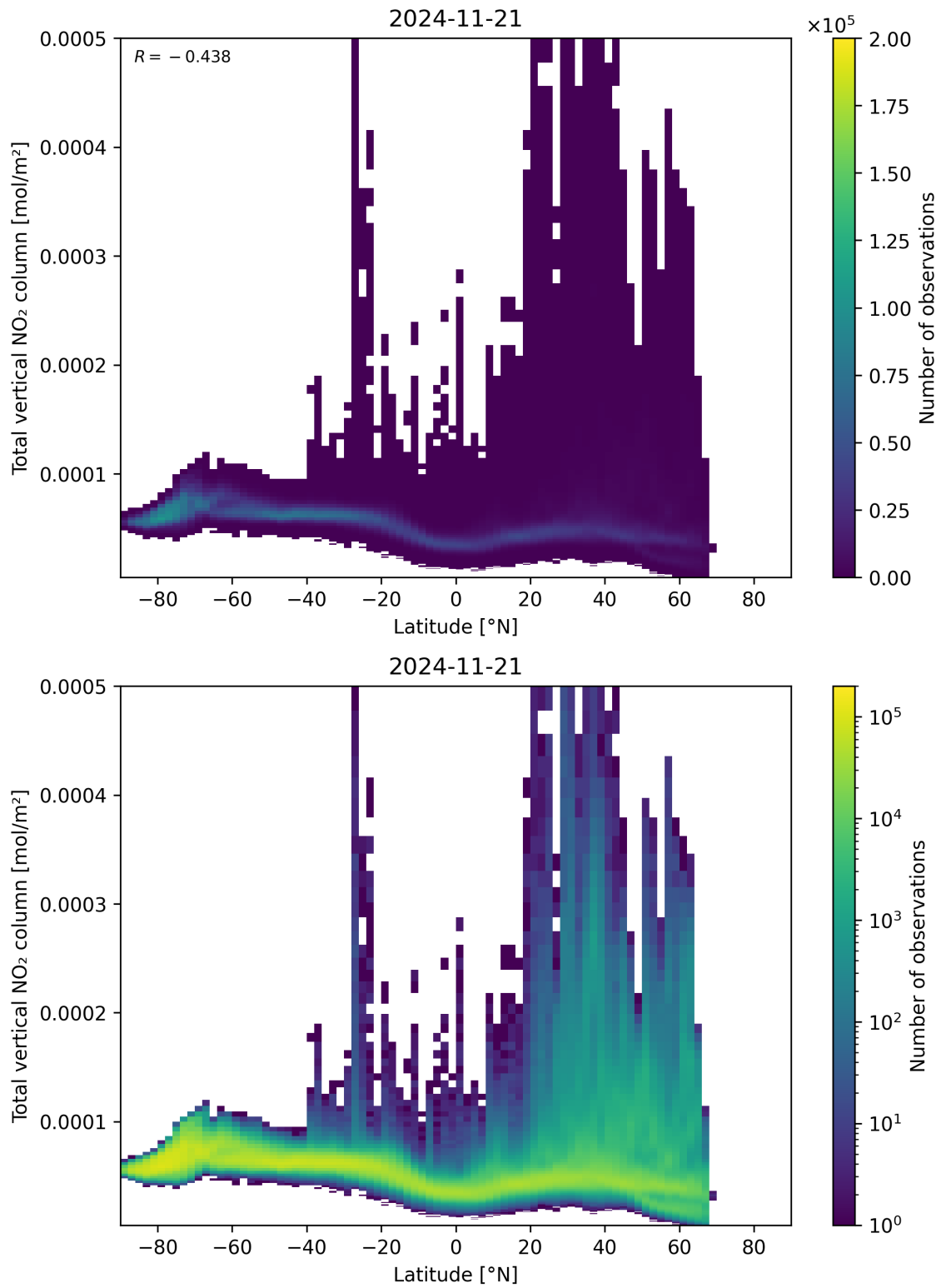
Figure 90: Scatter density plot of “Latitude” against “Total vertical NO 2 column” for 2024-11-20 to 2024-11-22.
