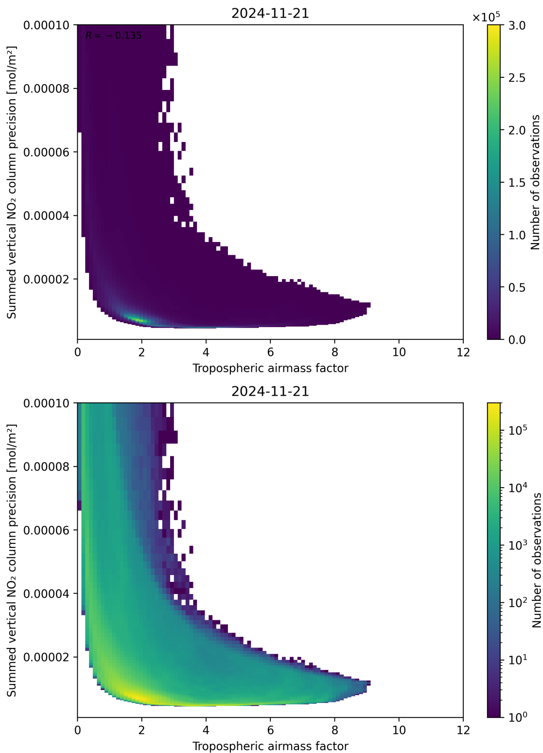
Figure 76: Scatter density plot of “Tropospheric air mass factor” against “Summed vertical NO 2 column precision” for 2024-11-20 to 2024-11-22.
