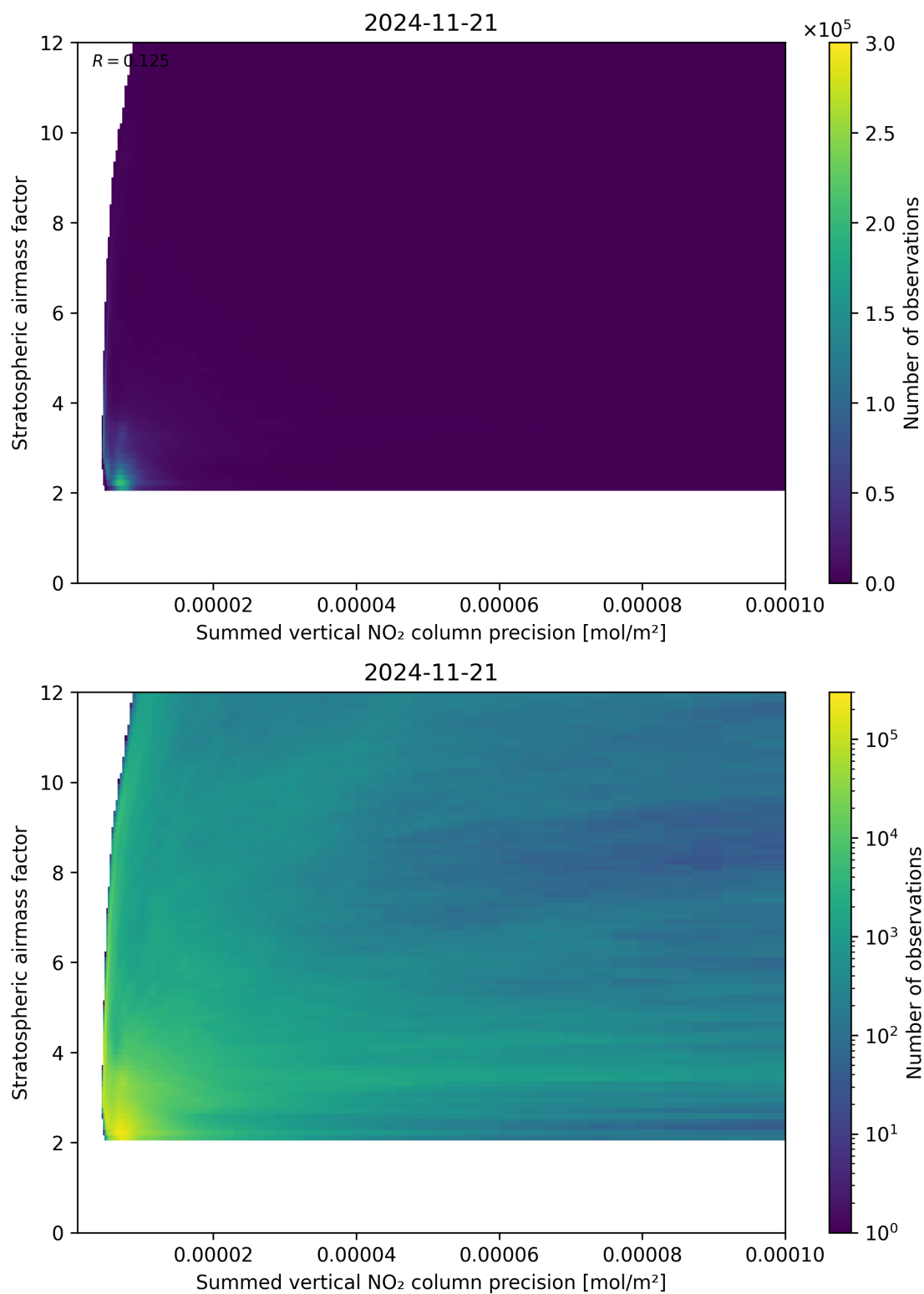
Figure 106: Scatter density plot of “Summed vertical NO 2 column precision” against “Stratospheric airmass factor” for 2024-11-20 to 2024-11-22.
