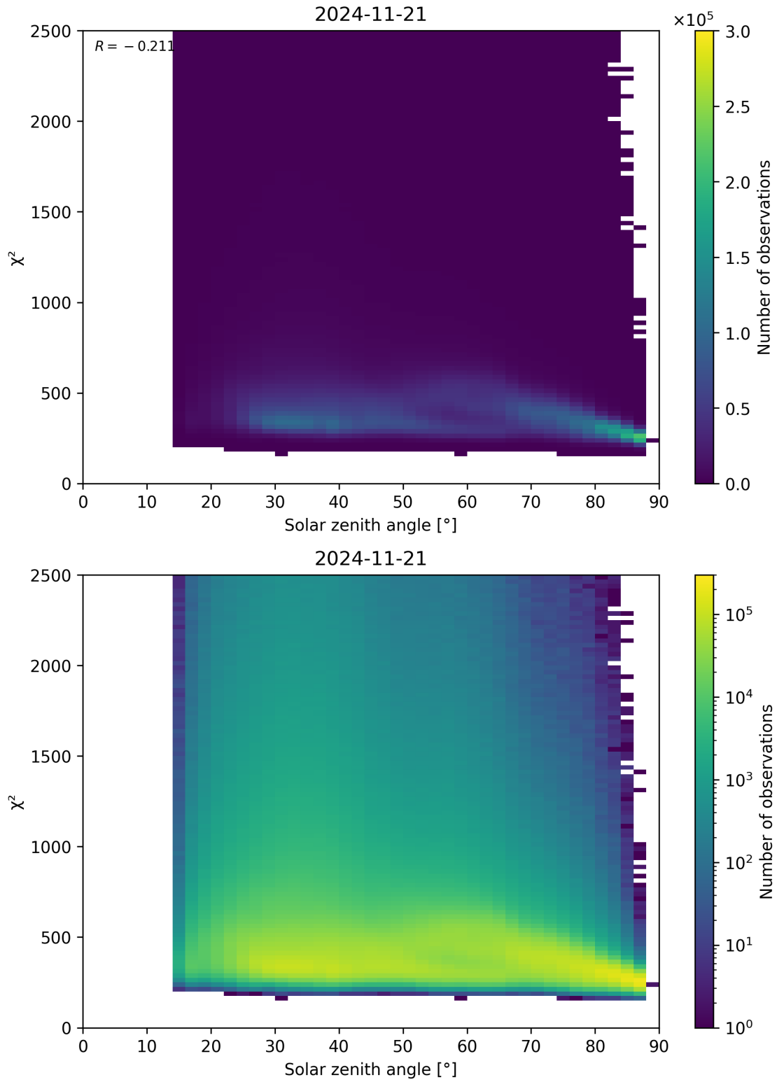
Figure 148: Scatter density plot of “Solar zenith angle” against “ \chi^2 ” for 2024-11-20 to 2024-11-22.
