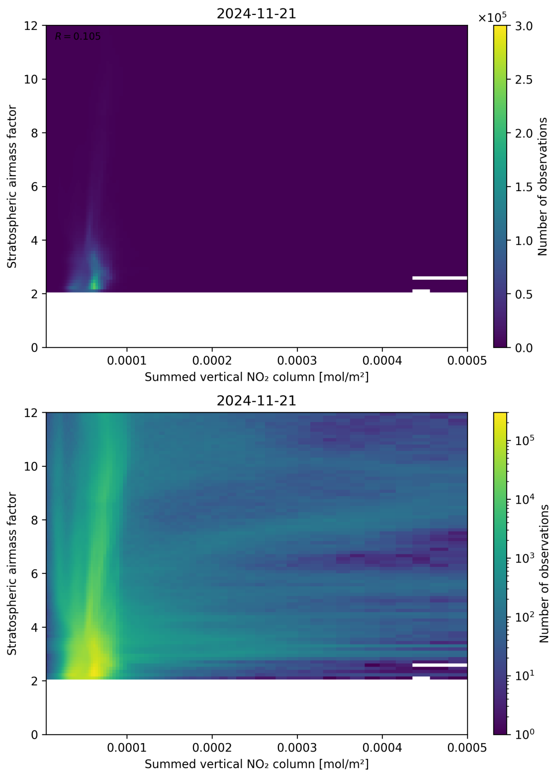
Figure 103: Scatter density plot of “Summed vertical NO 2 column” against “Stratospheric airmass factor” for 2024-11-20 to 2024-11-22.
