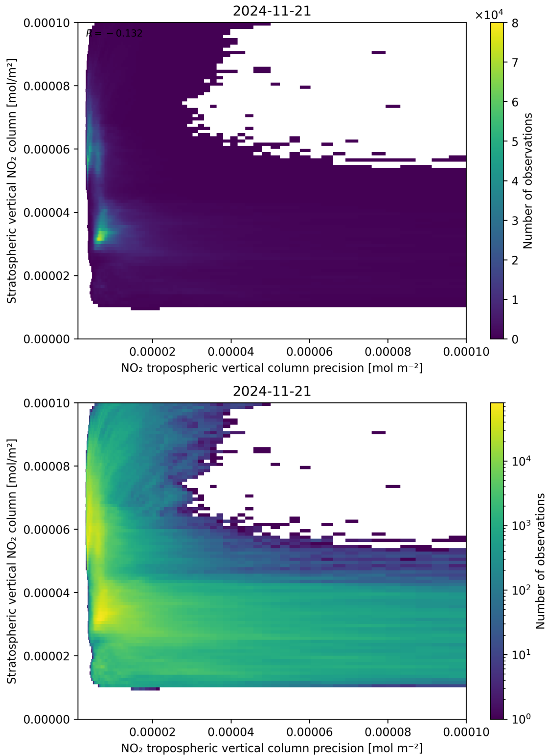
Figure 135: Scatter density plot of “NO 2 tropospheric vertical column precision” against “Stratospheric vertical NO 2 column” for 2024-11-20 to 2024-11-22.
