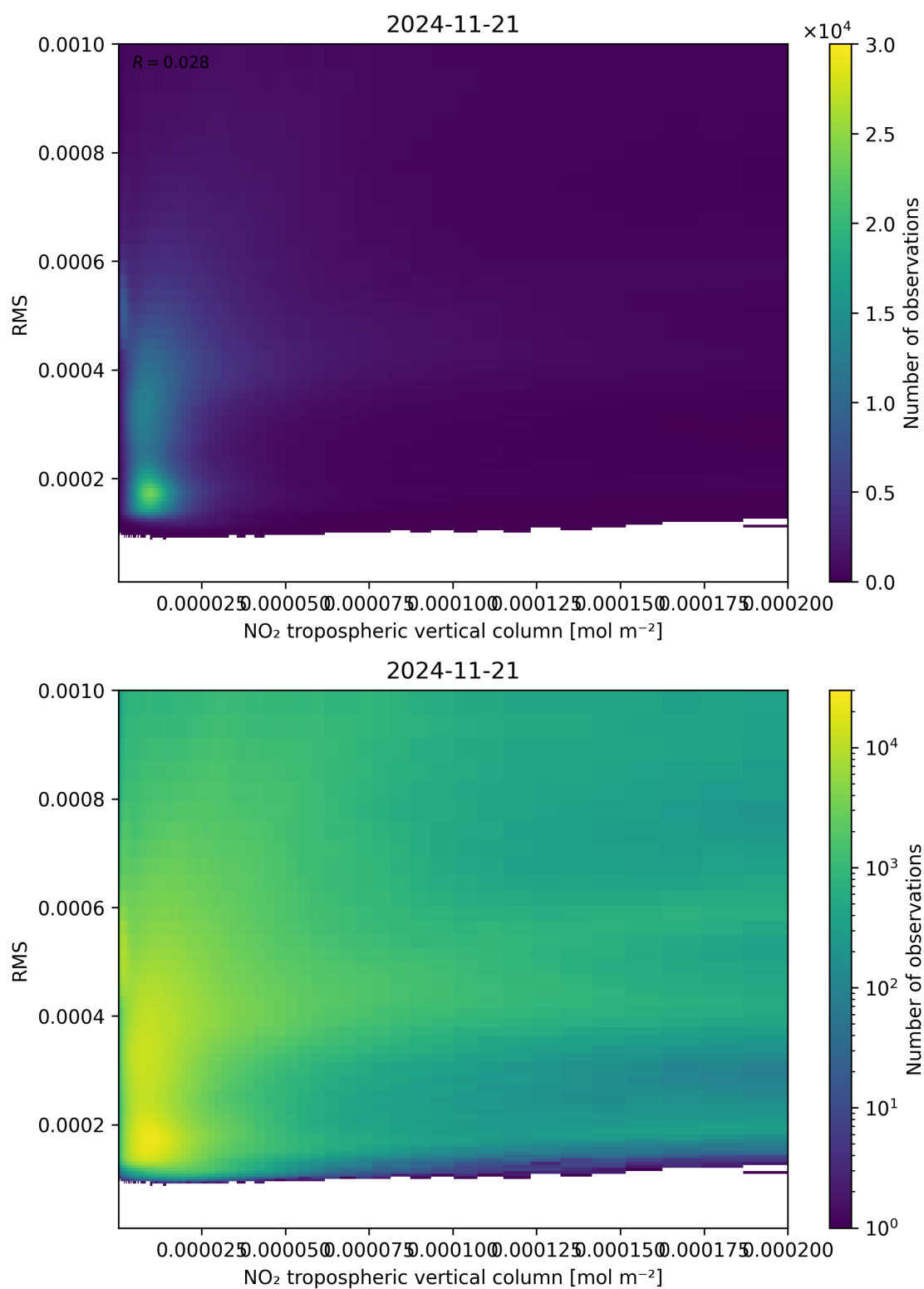
Figure 142: Scatter density plot of “NO 2 tropospheric vertical column” against “RMS” for 2024-11-20 to 2024-11-22.
