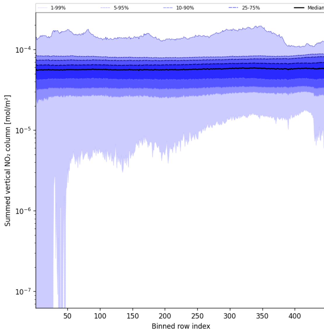
Figure 57: Along track statistics of “Summed vertical NO 2 column” for 2024-11-20 to 2024-11-22
