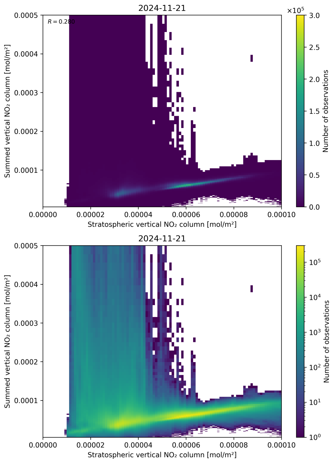
Figure 98: Scatter density plot of “Stratospheric vertical NO 2 column” against “Summed vertical NO 2 column” for 2024-11-20 to 2024-11-22.
