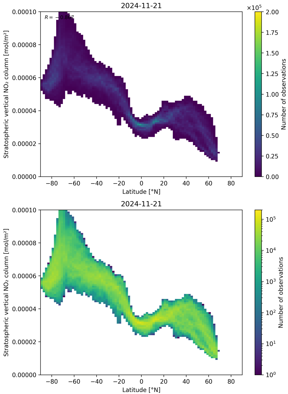
Figure 87: Scatter density plot of “Latitude” against “Stratospheric vertical NO 2 column” for 2024-11-20 to 2024-11-22.
