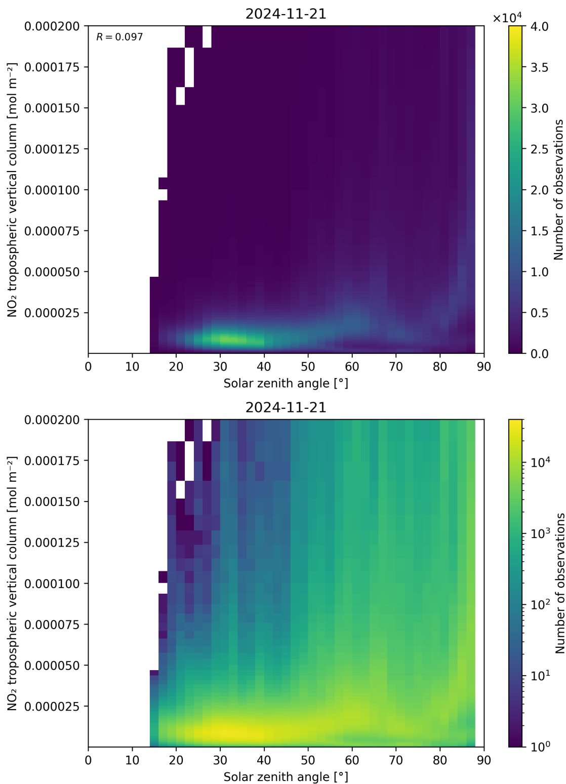
Figure 155: Scatter density plot of “Solar zenith angle” against “NO 2 tropospheric vertical column” for 2024-11-20 to 2024-11-22.
