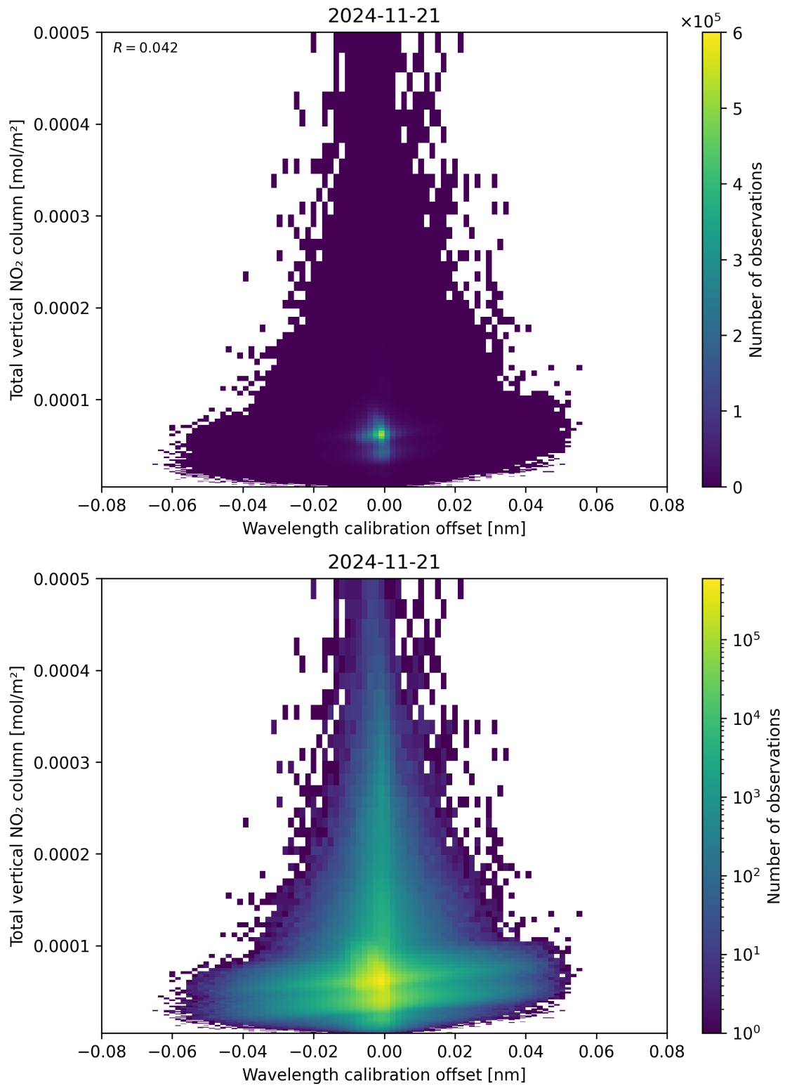
Figure 179: Scatter density plot of “Wavelength calibration offset” against “Total vertical NO 2 column” for 2024-11-20 to 2024-11-22.
