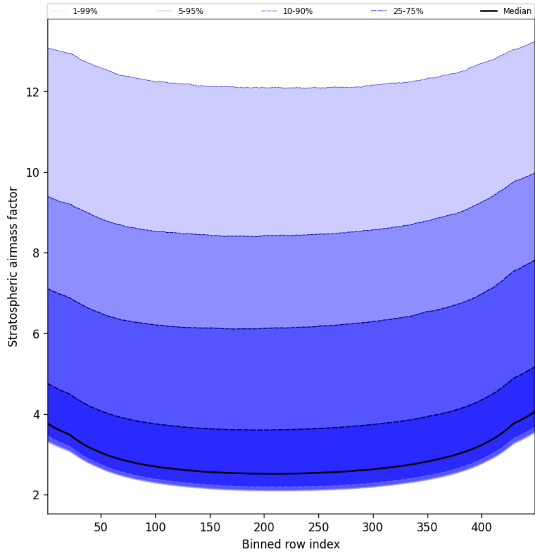
Figure 61: Along track statistics of “Stratospheric air mass factor” for 2024-11-20 to 2024-11-22
