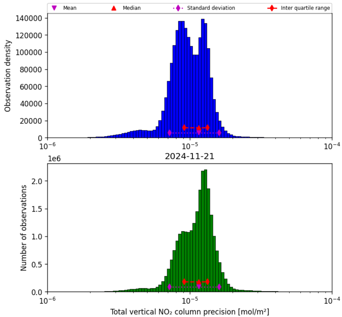
Figure 39: Histogram of “Total vertical NO 2 column precision” for 2024-11-20 to 2024-11-22
