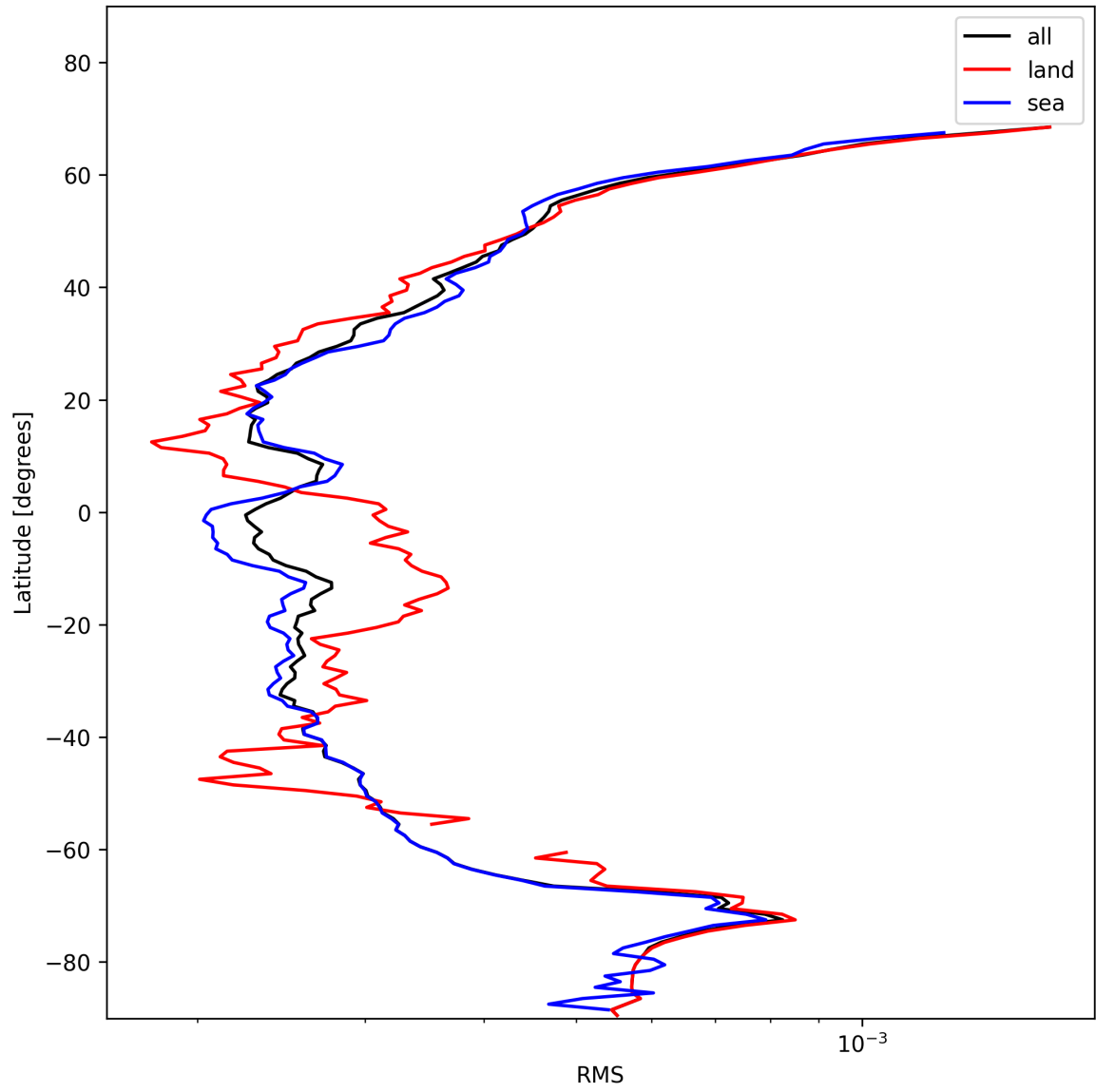
Figure 26: Zonal average of “RMS” for 2024-11-20 to 2024-11-22.
