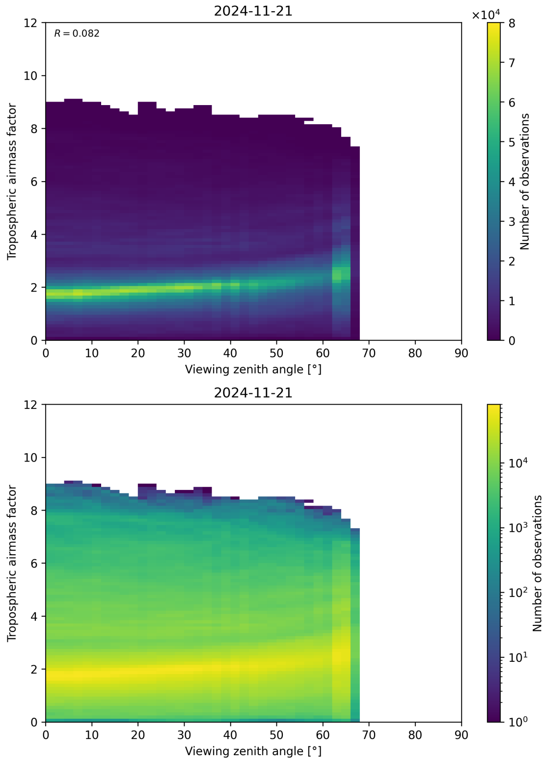
Figure 161: Scatter density plot of “Viewing zenith angle” against “Tropospheric airmass factor” for 2024-11-20 to 2024-11-22.
