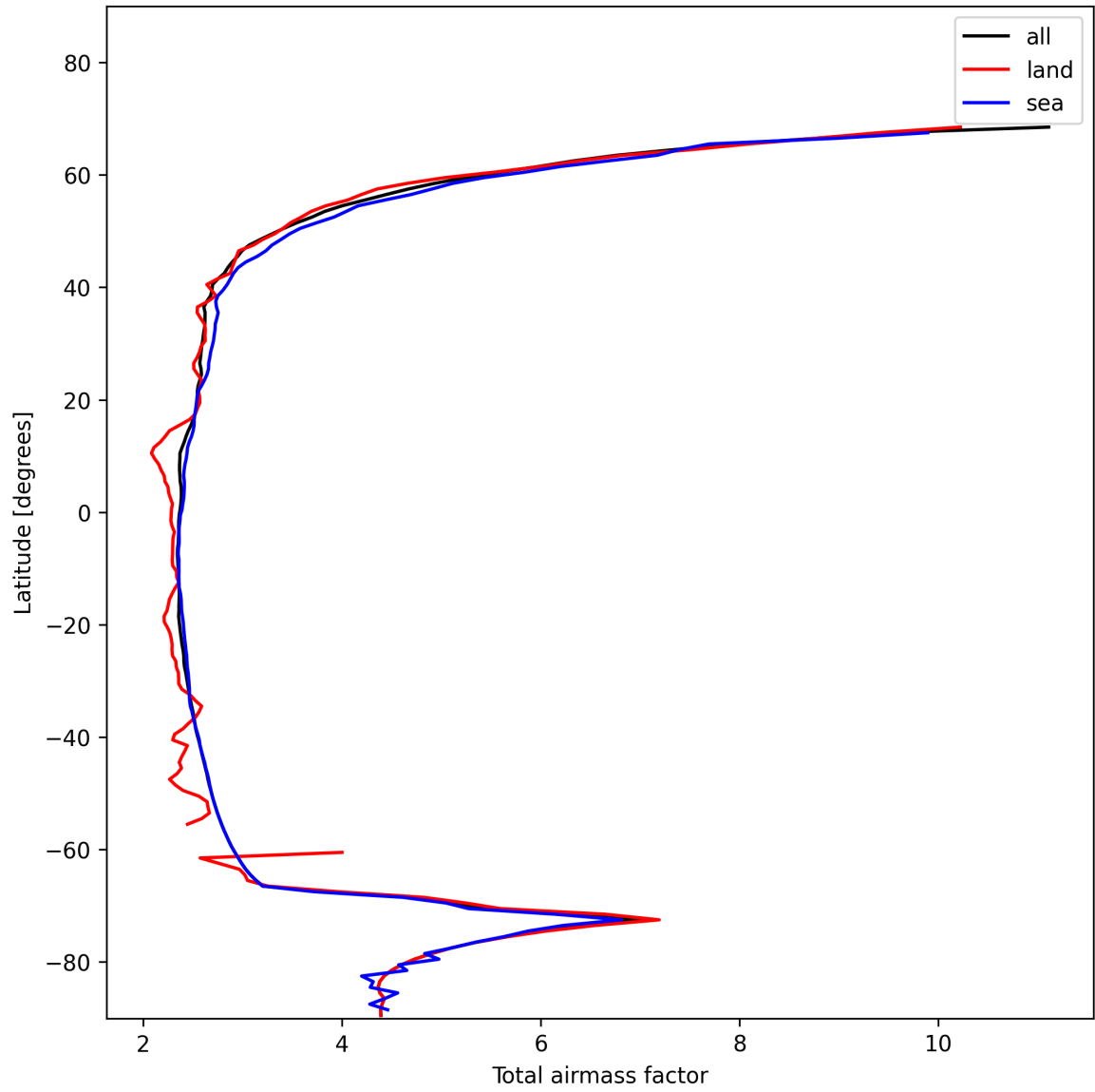
Figure 15: Zonal average of “Total airmass factor” for 2024-11-20 to 2024-11-22.
