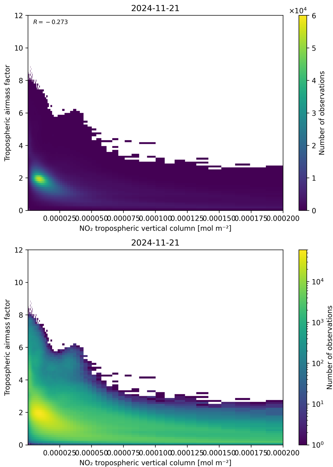
Figure 123: Scatter density plot of “NO 2 tropospheric vertical column” against “Tropospheric airmass factor” for 2024-11-20 to 2024-11-22.
