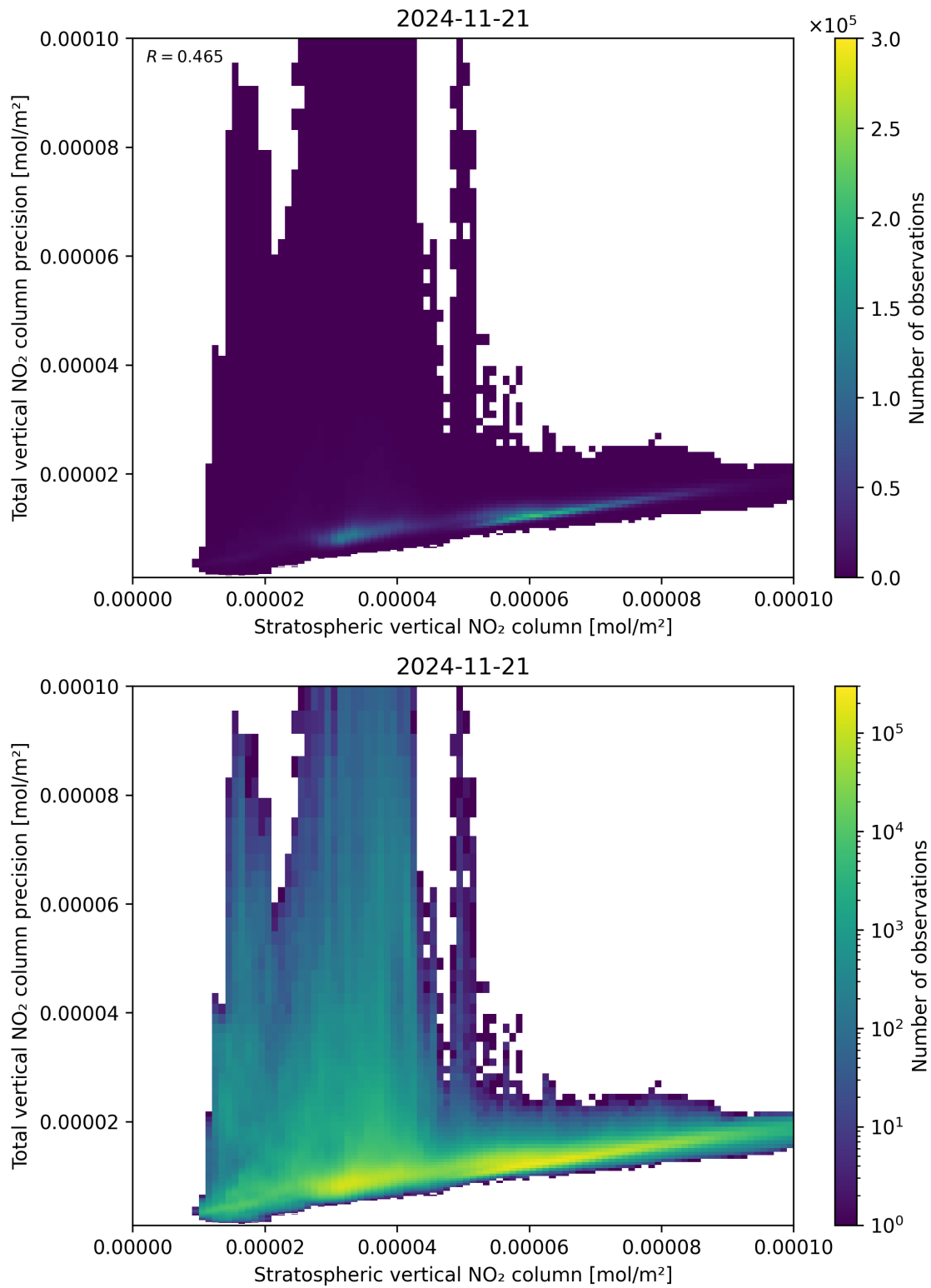
Figure 101: Scatter density plot of “Stratospheric vertical NO 2 column” against “Total vertical NO 2 column precision” for 2024-11-20 to 2024-11-22.
