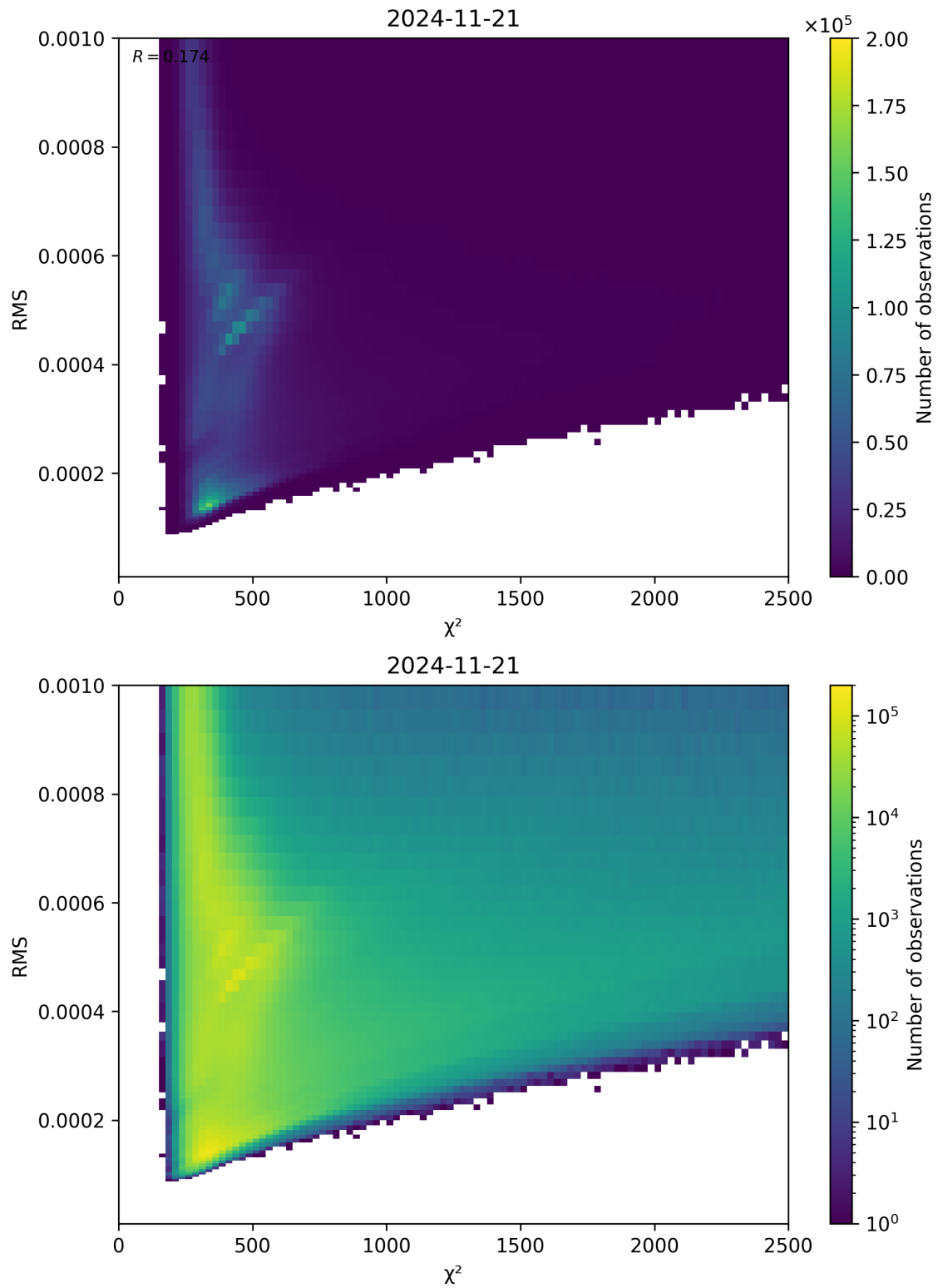
Figure 82: Scatter density plot of “ \chi^2 ” against “RMS” for 2024-11-20 to 2024-11-22.
