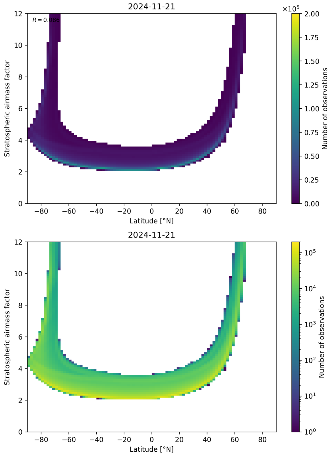
Figure 83: Scatter density plot of “Latitude” against “Stratospheric airmass factor” for 2024-11-20 to 2024-11-22.
