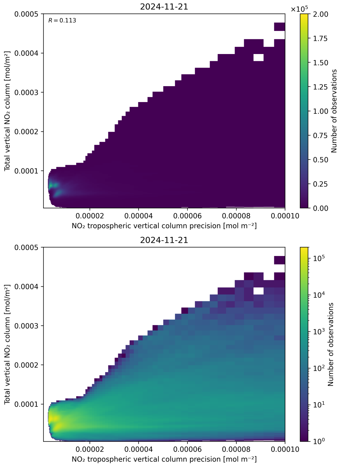
Figure 138: Scatter density plot of “NO 2 tropospheric vertical column precision” against “Total vertical NO 2 column” for 2024-11-20 to 2024-11-22.
