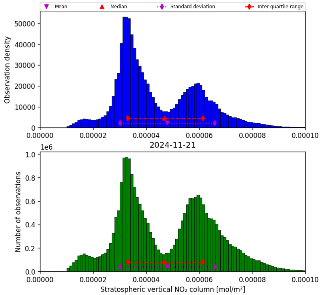
Figure 36: Histogram of “Stratospheric vertical NO 2 column” for 2024-11-20 to 2024-11-22
