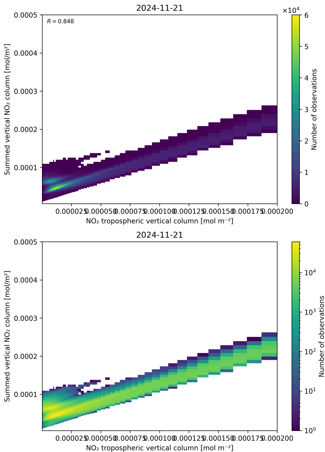
Figure 126: Scatter density plot of “NO 2 tropospheric vertical column” against “Summed vertical NO 2 column” for 2024-11-20 to 2024-11-22.
