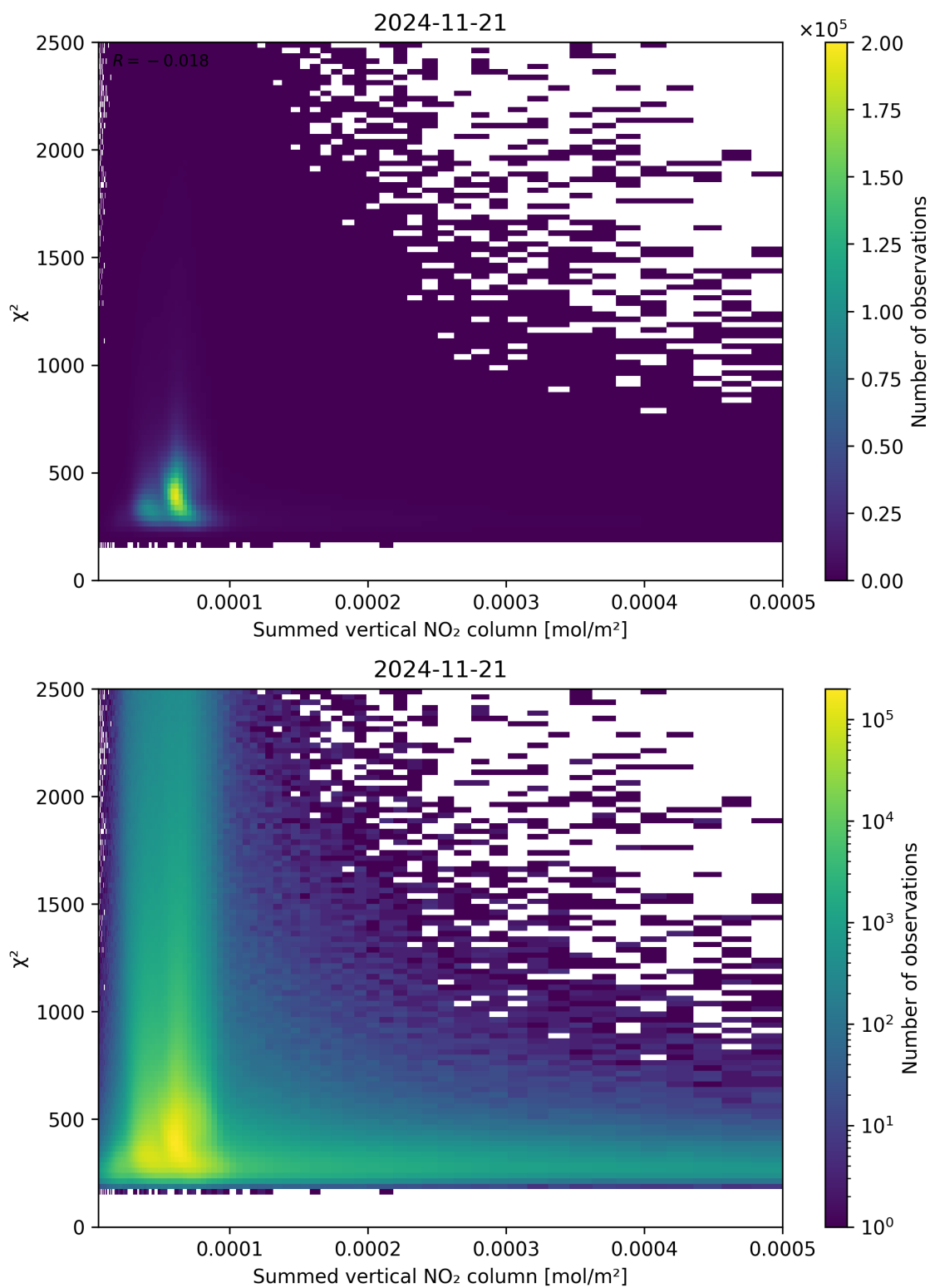
Figure 104: Scatter density plot of “Summed vertical NO 2 column” against “ \chi^2 ” for 2024-11-20 to 2024-11-22.
