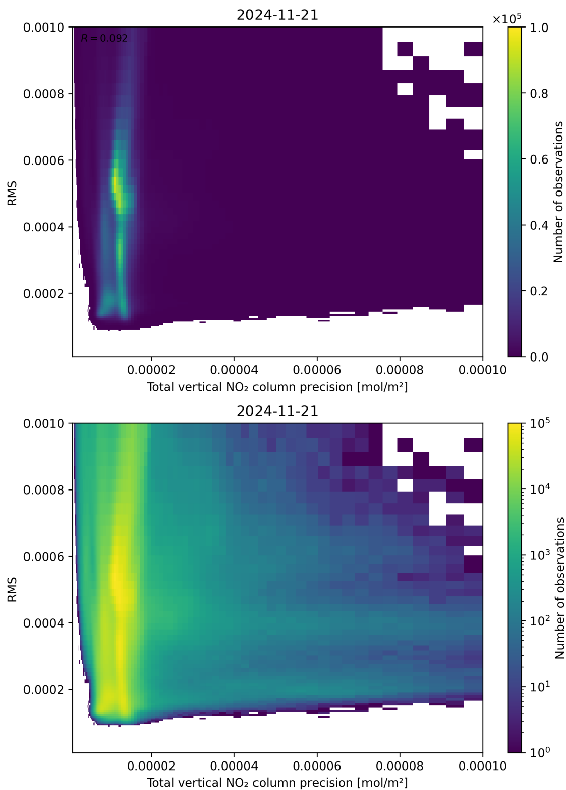
Figure 119: Scatter density plot of “Total vertical NO 2 column precision” against “RMS” for 2024-11-20 to 2024-11-22.
