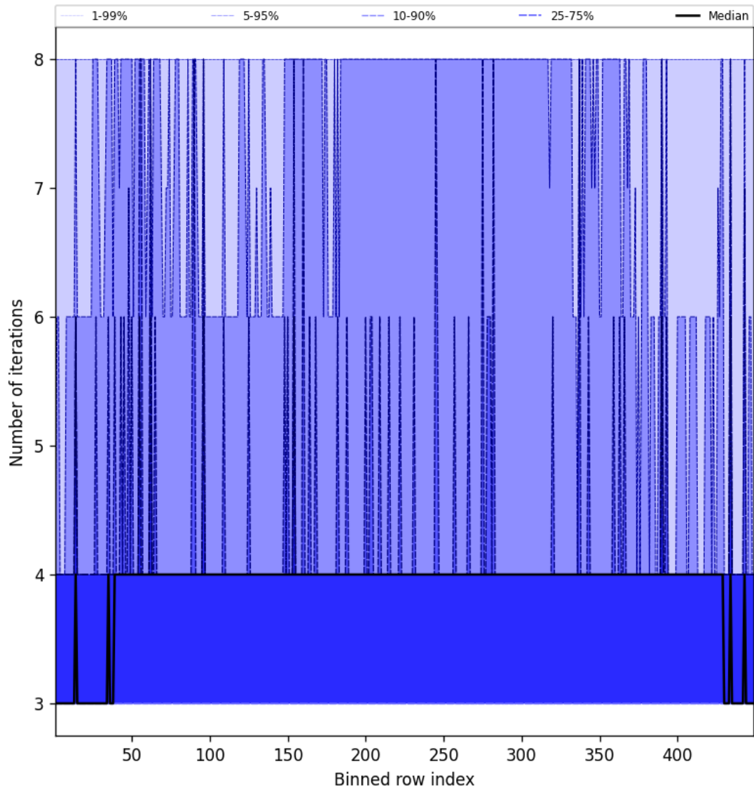
Figure 51: Along track statistics of “Number of iterations” for 2024-11-20 to 2024-11-22
