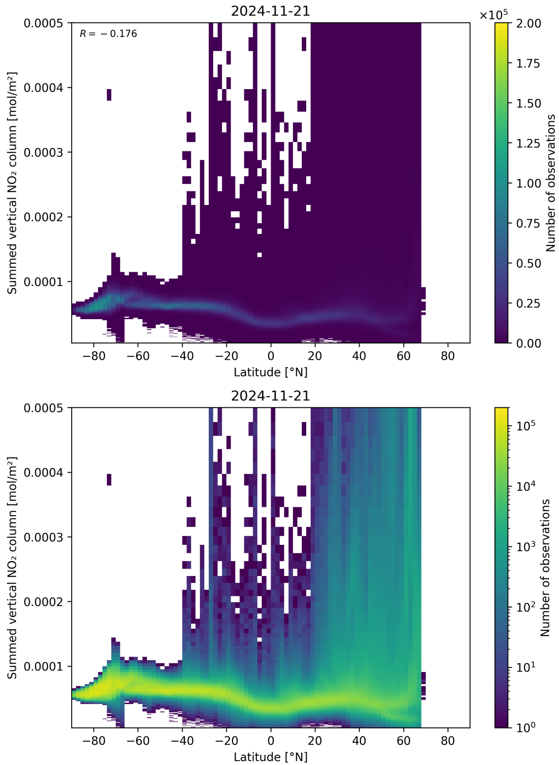
Figure 88: Scatter density plot of “Latitude” against “Summed vertical NO 2 column” for 2024-11-20 to 2024-11-22.
