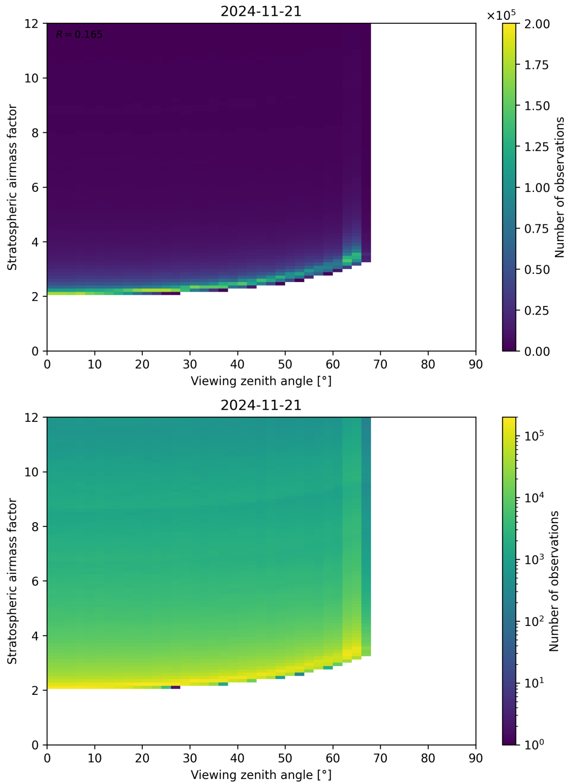
Figure 159: Scatter density plot of “Viewing zenith angle” against “Stratospheric airmass factor” for 2024-11-20 to 2024-11-22.
