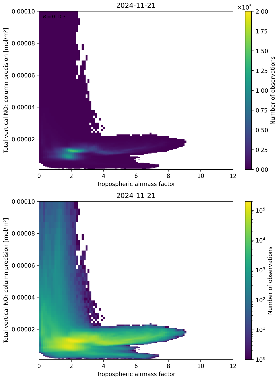
Figure 78: Scatter density plot of “Tropospheric air mass factor” against “Total vertical NO 2 column precision” for 2024-11-20 to 2024-11-22.
