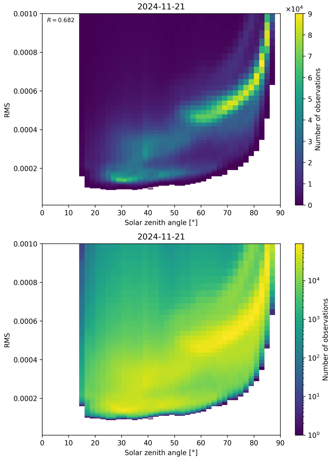
Figure 157: Scatter density plot of “Solar zenith angle” against “RMS” for 2024-11-20 to 2024-11-22.
