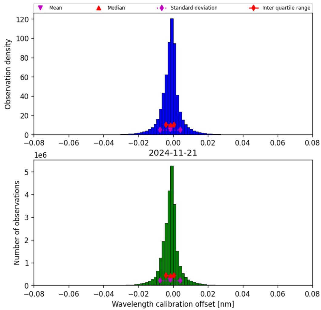
Figure 35: Histogram of “Wavelength calibration offset” for 2024-11-20 to 2024-11-22
