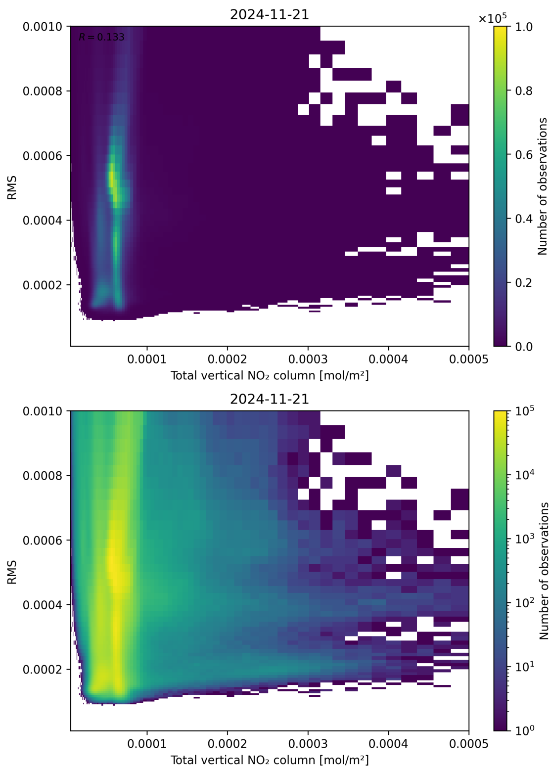
Figure 120: Scatter density plot of “Total vertical NO 2 column” against “RMS” for 2024-11-20 to 2024-11-22.
