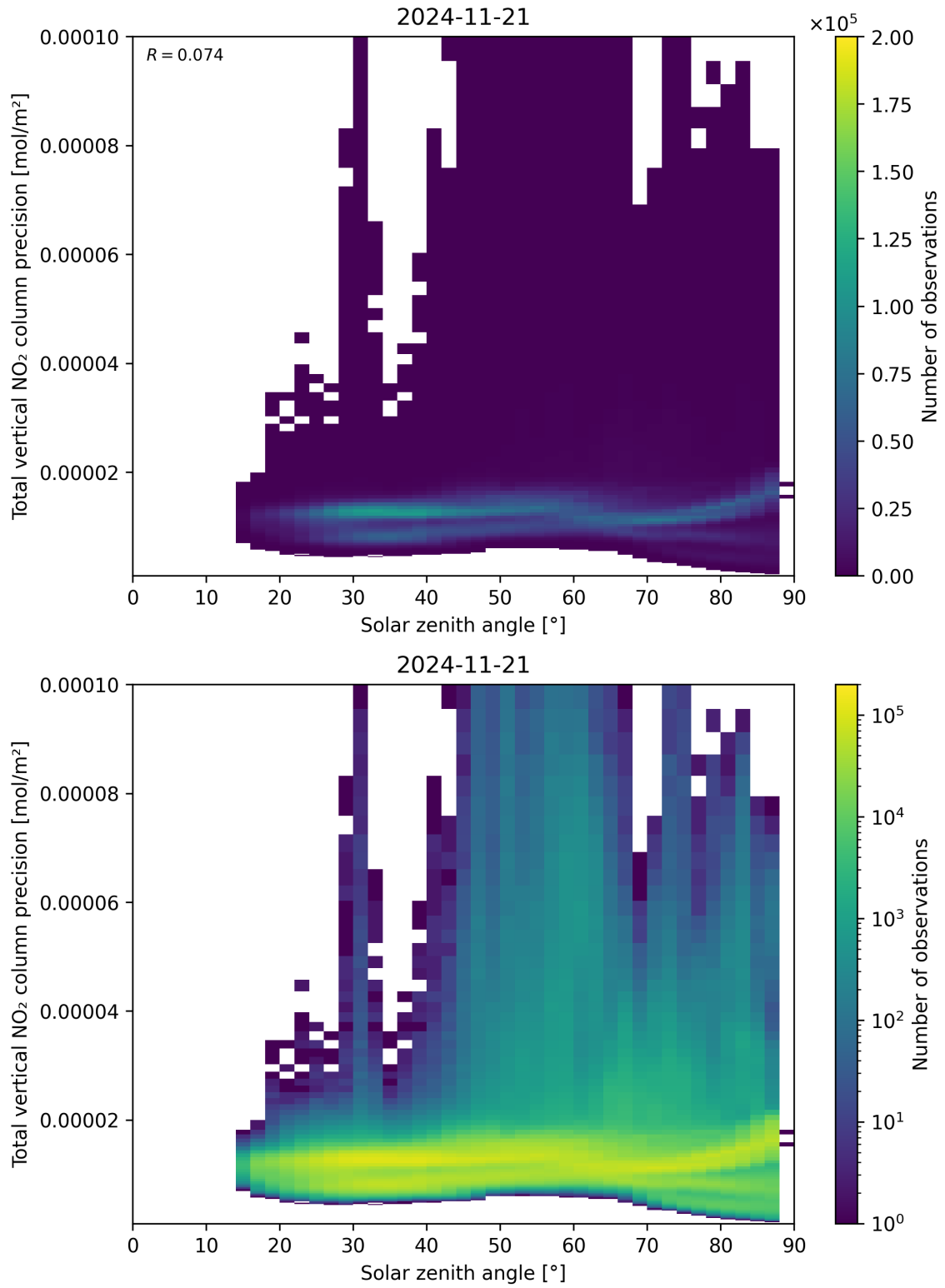
Figure 154: Scatter density plot of “Solar zenith angle” against “Total vertical NO 2 column precision” for 2024-11-20 to 2024-11-22.
