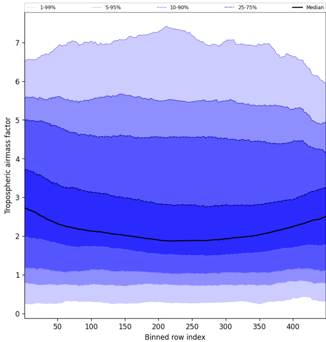
Figure 48: Along track statistics of “Tropospheric air mass factor” for 2024-11-20 to 2024-11-22
