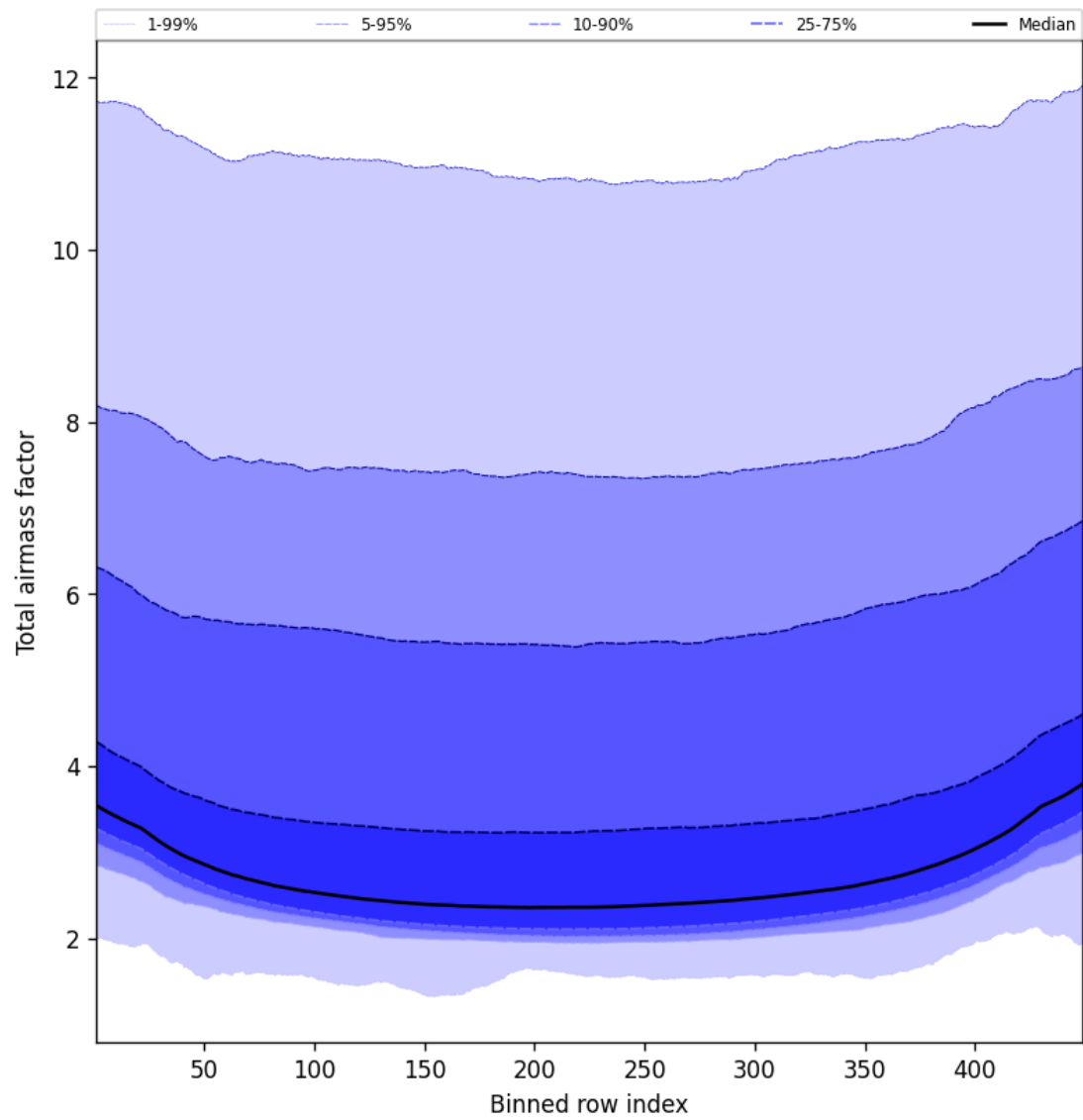
Figure 49: Along track statistics of “Total airmass factor” for 2024-11-20 to 2024-11-22
