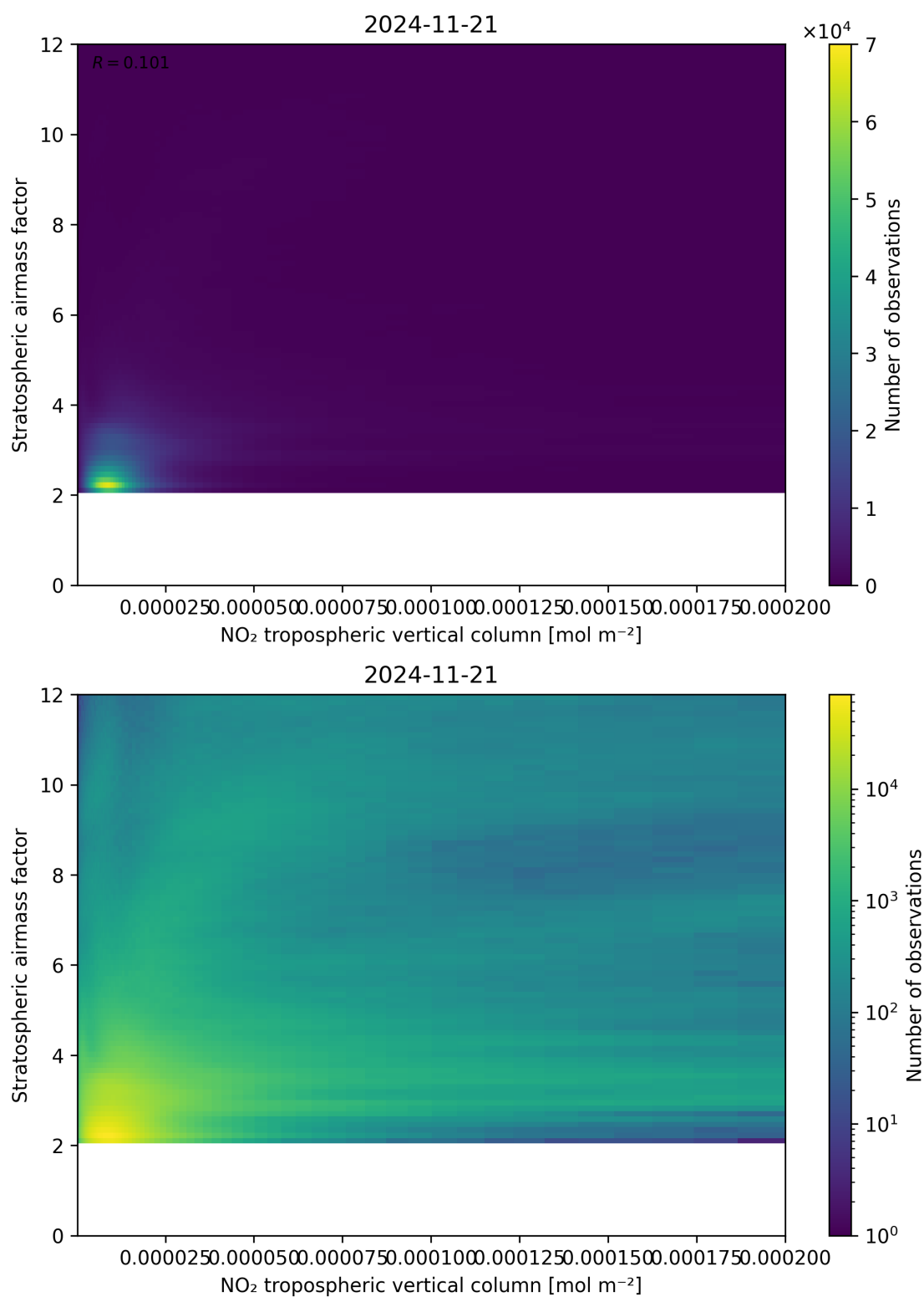
Figure 121: Scatter density plot of “NO 2 tropospheric vertical column” against “Stratospheric airmass factor” for 2024-11-20 to 2024-11-22.
