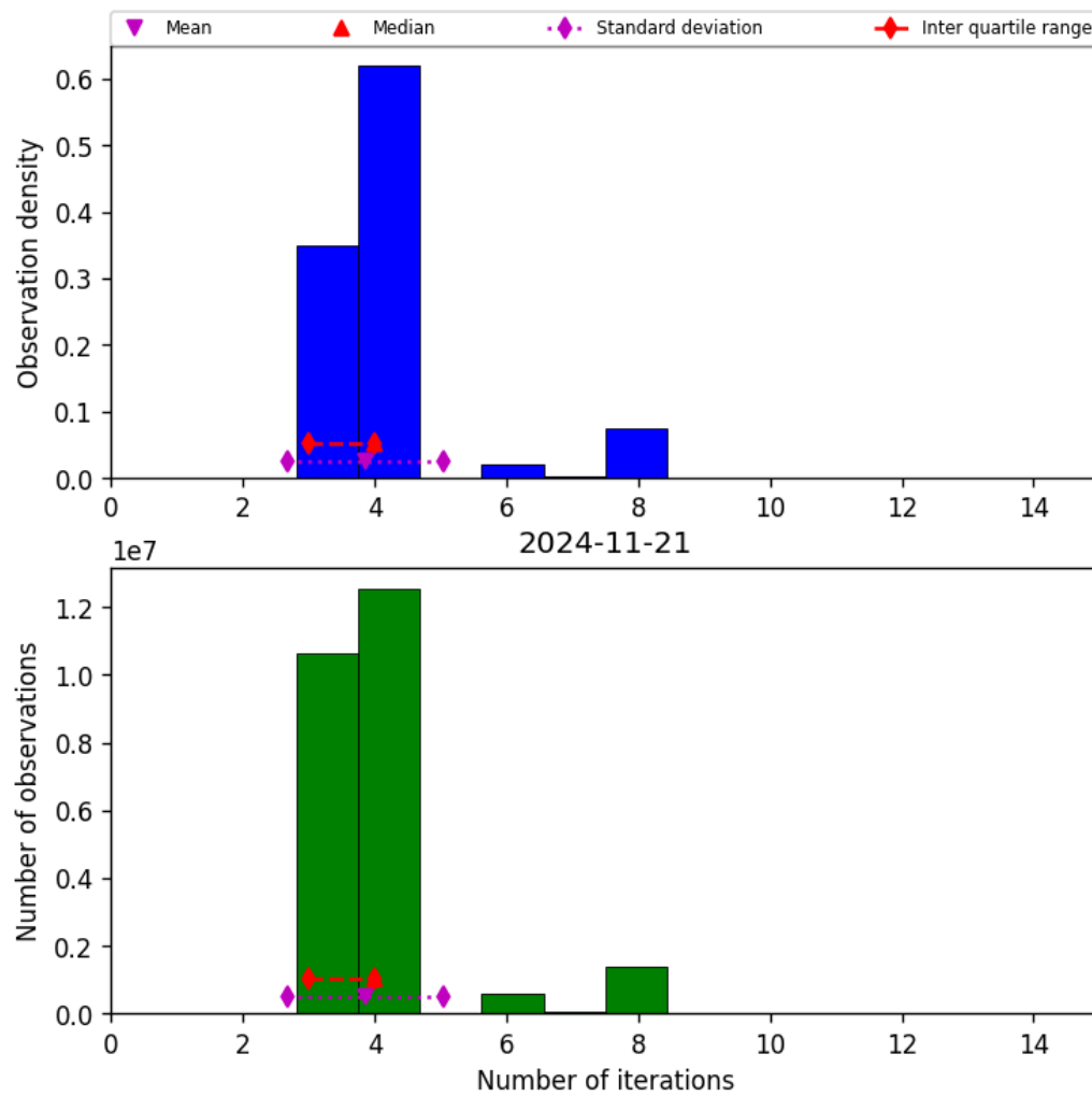
Figure 34: Histogram of “Number of iterations” for 2024-11-20 to 2024-11-22
