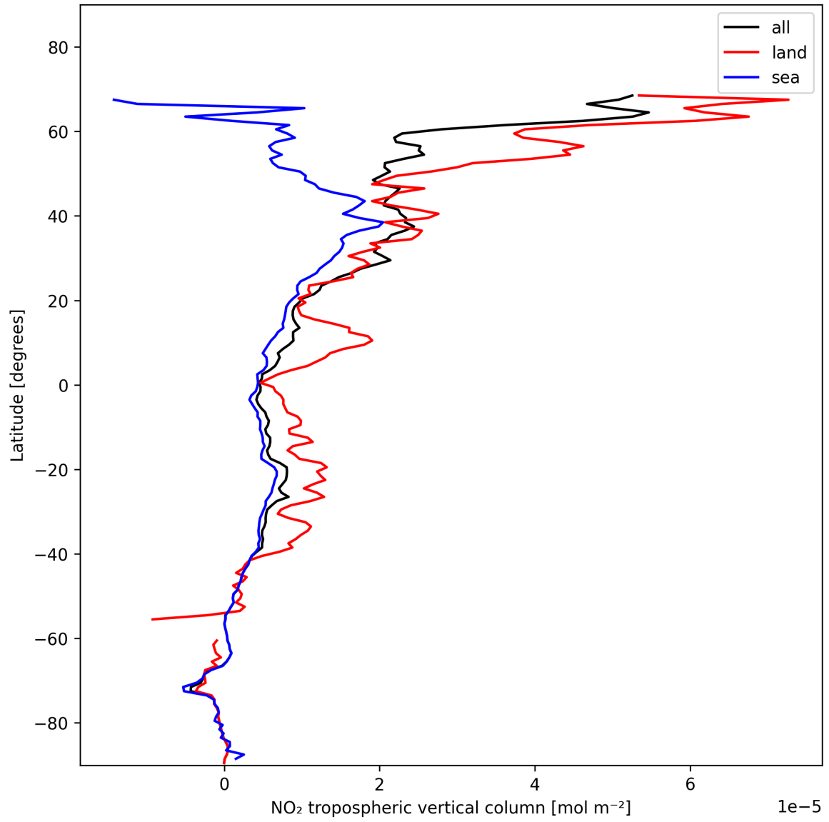
Figure 12: Zonal average of “NO 2 tropospheric vertical column” for 2024-11-20 to 2024-11-22.
