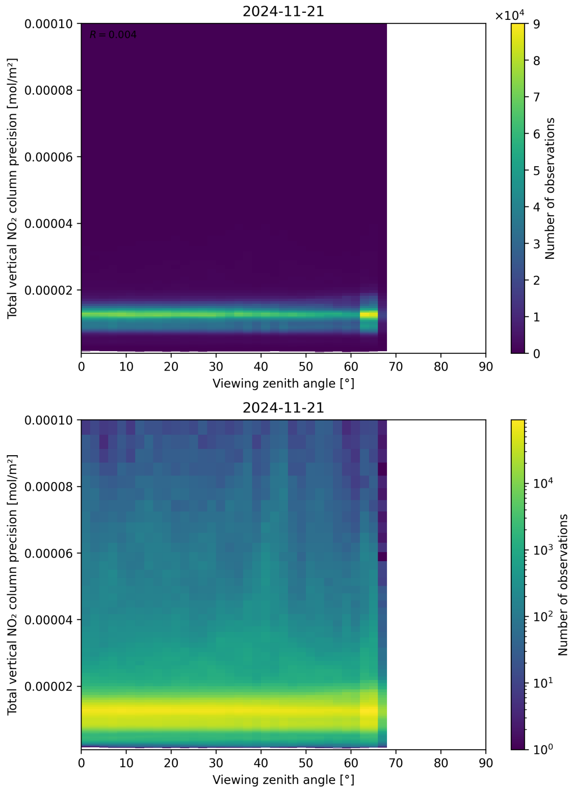
Figure 168: Scatter density plot of “Viewing zenith angle” against “Total vertical NO 2 column precision” for 2024-11-20 to 2024-11-22.
