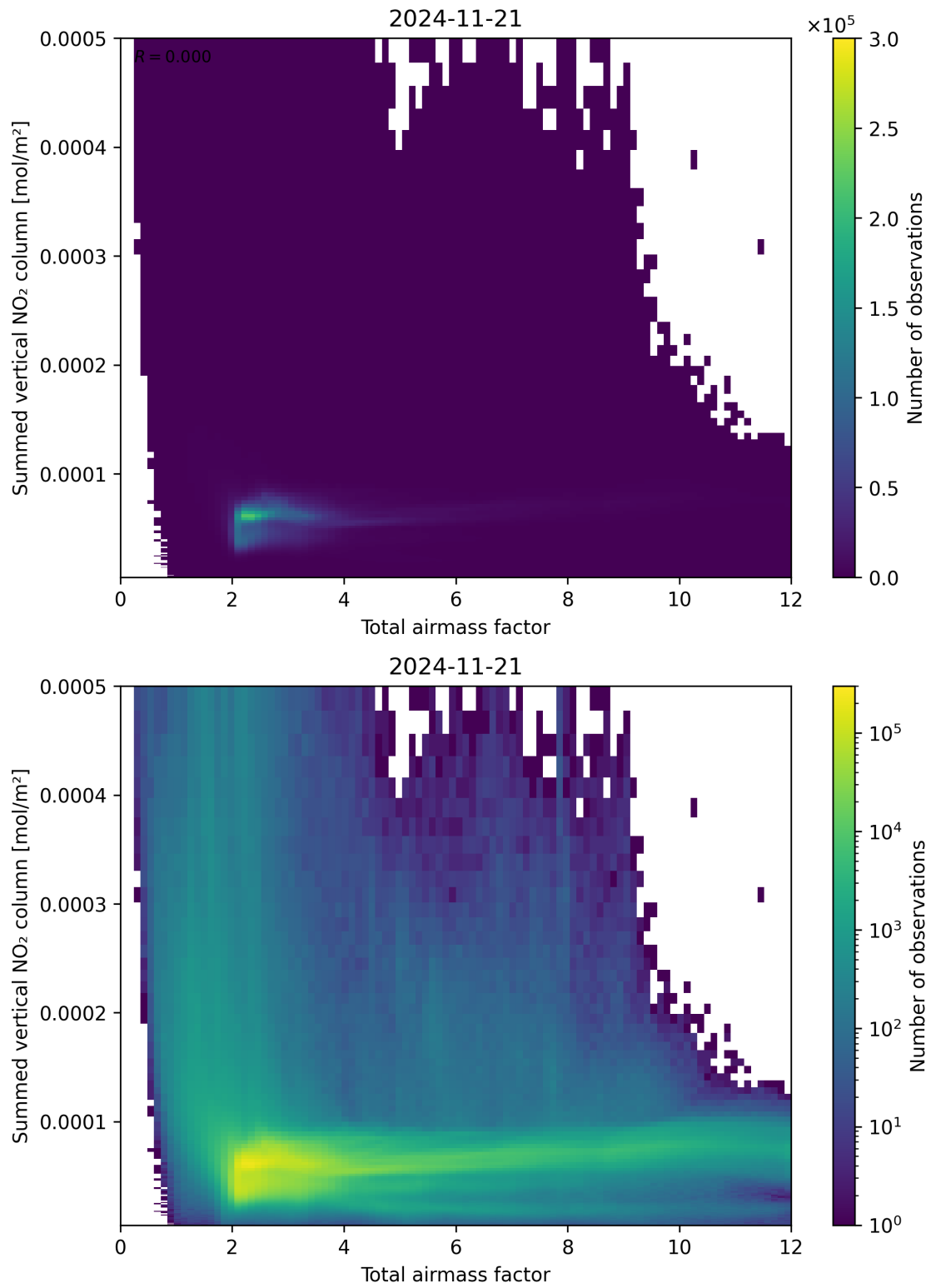
Figure 65: Scatter density plot of “Total airmass factor” against “Summed vertical NO 2 column” for 2024-11-20 to 2024-11-22.
