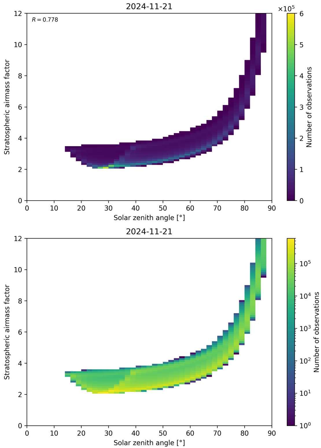
Figure 145: Scatter density plot of “Solar zenith angle” against “Stratospheric airmass factor” for 2024-11-20 to 2024-11-22.
