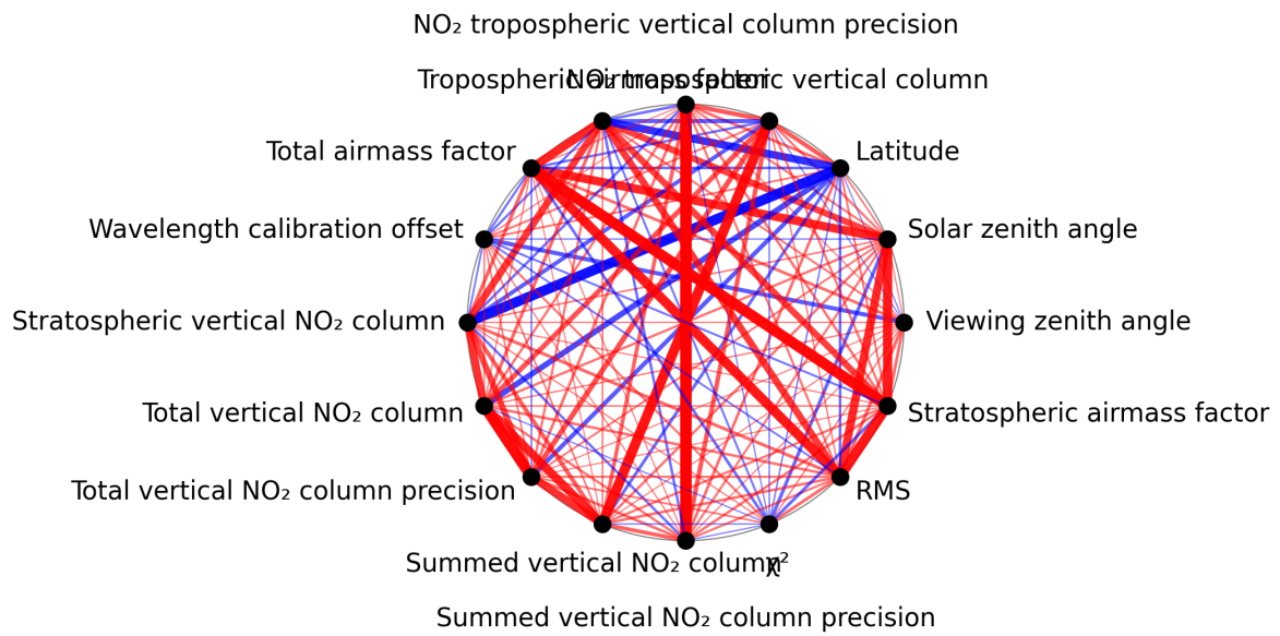
Figure 1: Map of correlation graph for 2024-11-20 to 2024-11-22.
