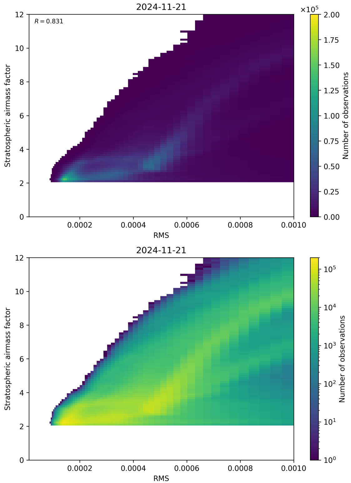
Figure 144: Scatter density plot of “RMS” against “Stratospheric airmass factor” for 2024-11-20 to 2024-11-22.
