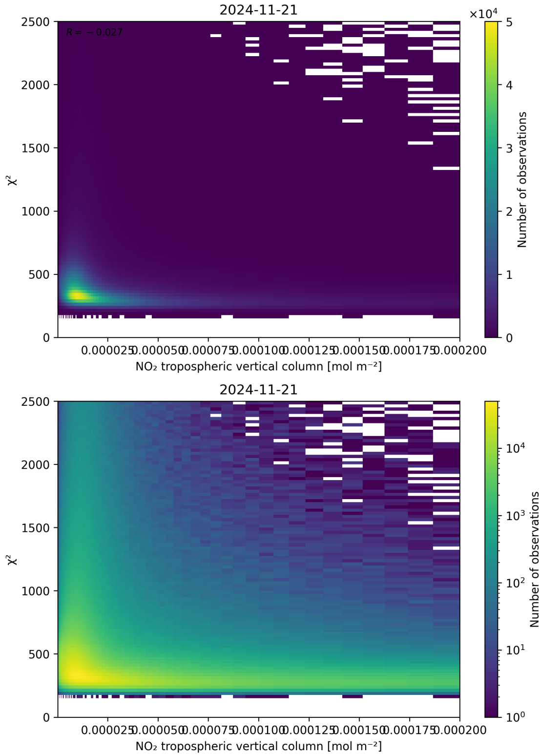
Figure 124: Scatter density plot of “NO 2 tropospheric vertical column” against “ \chi^2 ” for 2024-11-20 to 2024-11-22.
