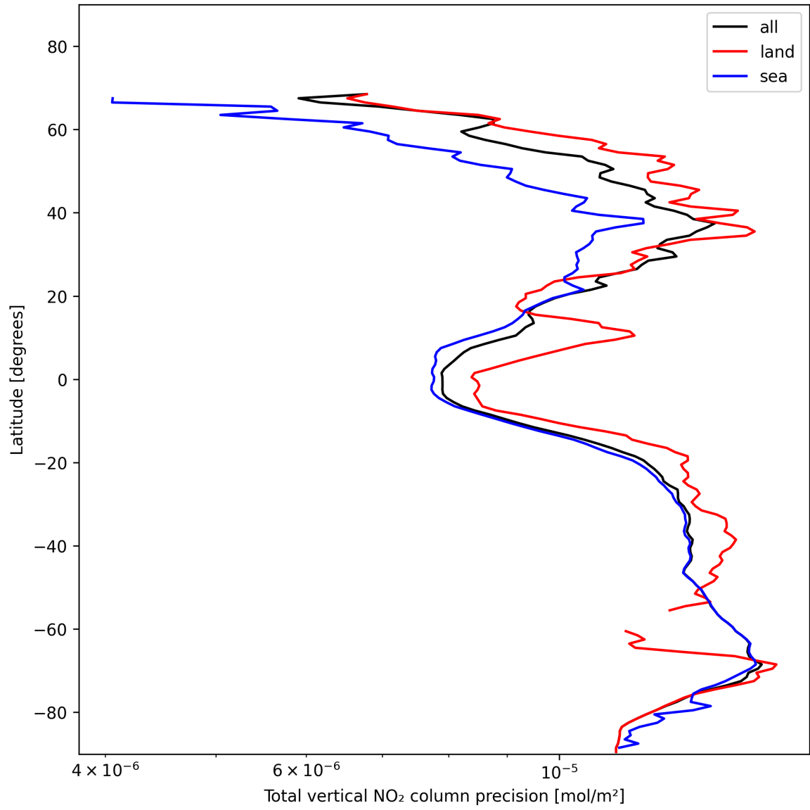
Figure 22: Zonal average of “Total vertical NO 2 column precision” for 2024-11-20 to 2024-11-22.
