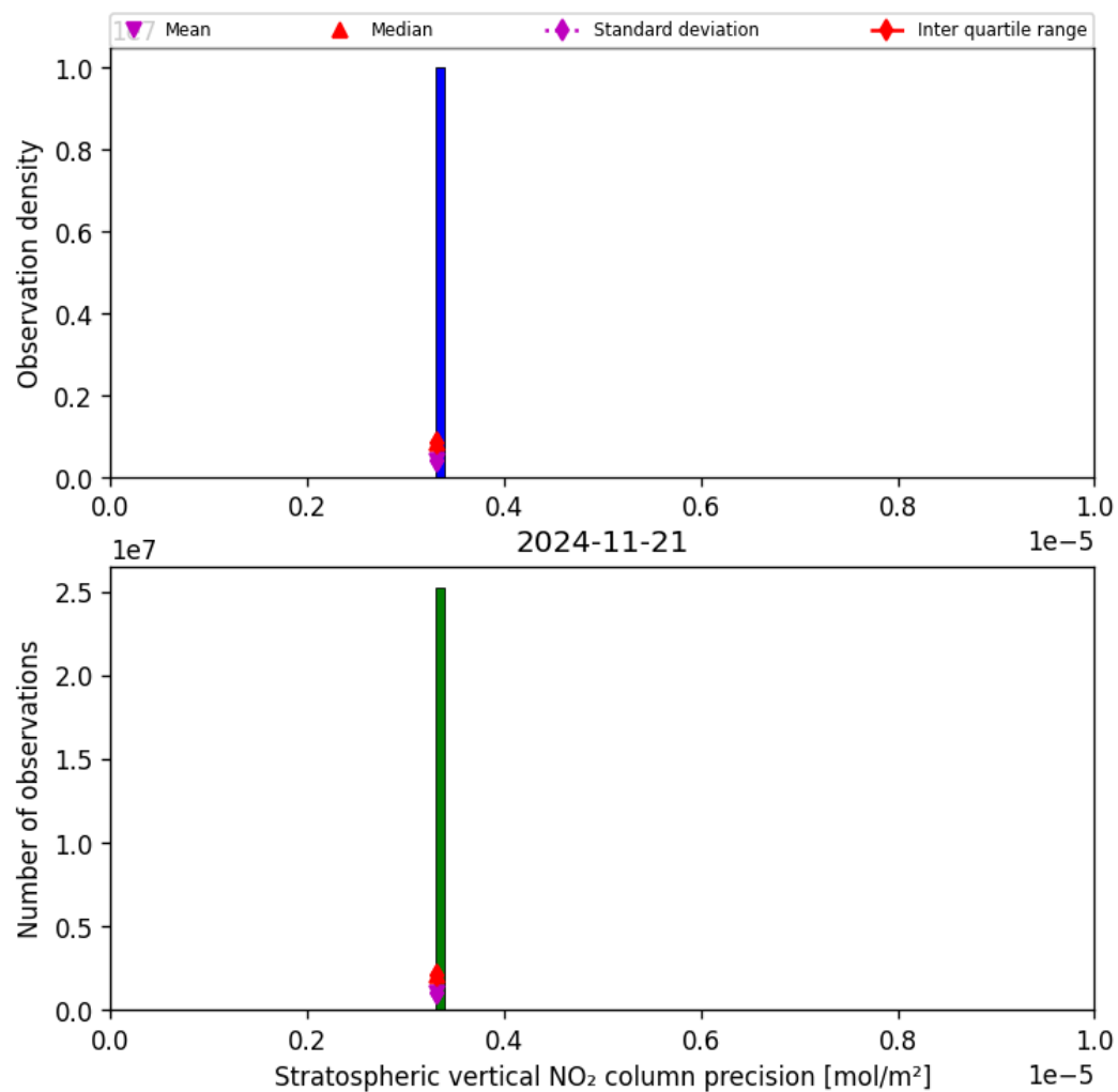
Figure 37: Histogram of “Stratospheric vertical NO 2 column precision” for 2024-11-20 to 2024-11-22
