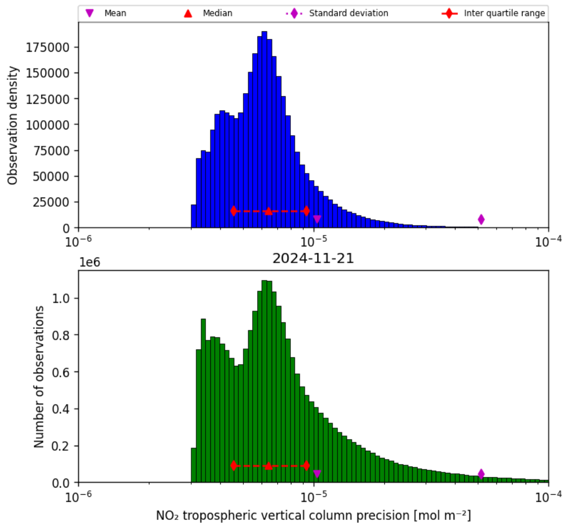
Figure 30: Histogram of “NO 2 tropospheric vertical column precision” for 2024-11-20 to 2024-11-22
