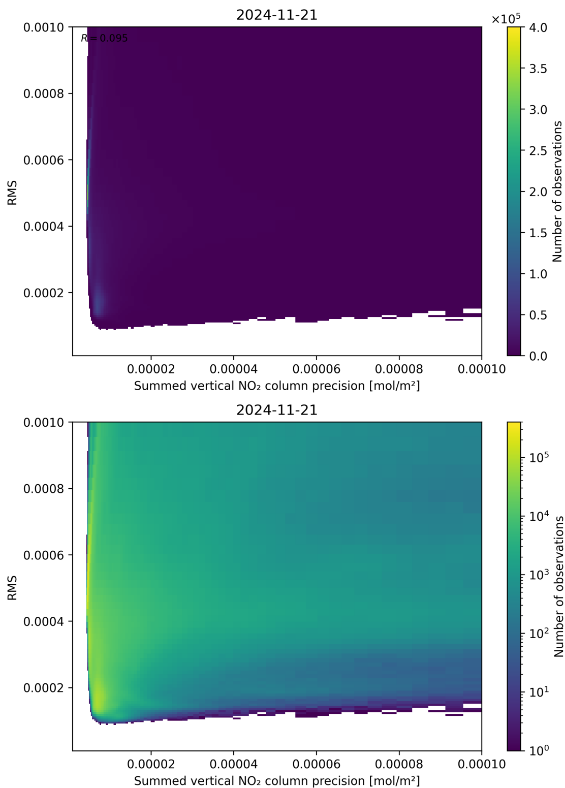
Figure 108: Scatter density plot of “Summed vertical NO 2 column precision” against “RMS” for 2024-11-20 to 2024-11-22.
