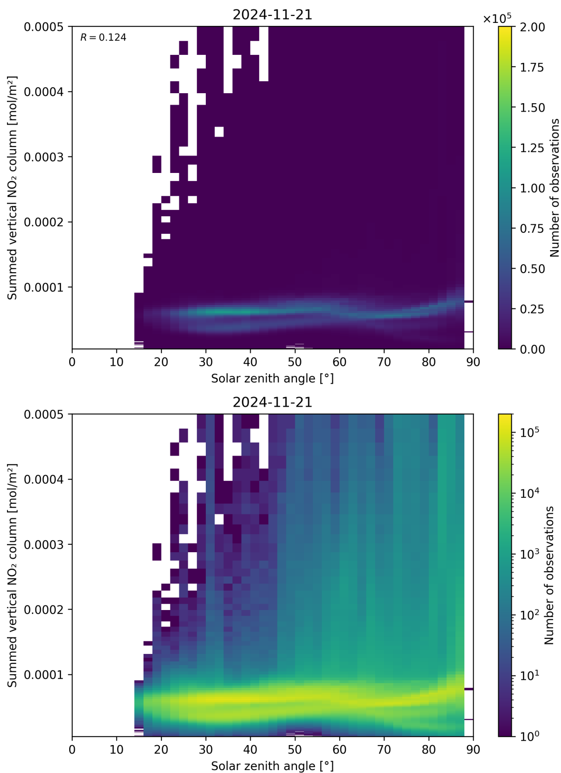
Figure 151: Scatter density plot of “Solar zenith angle” against “Summed vertical NO 2 column” for 2024-11-20 to 2024-11-22.
