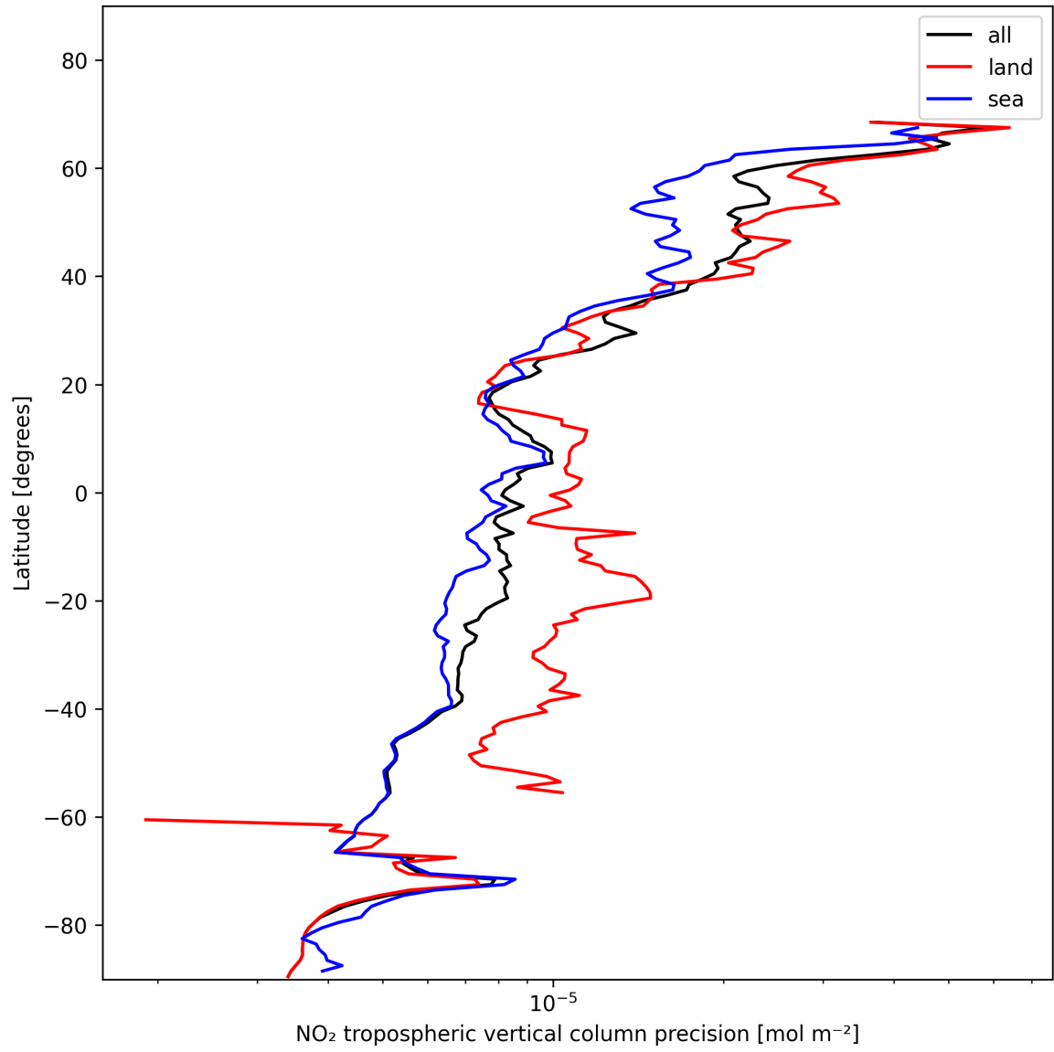
Figure 13: Zonal average of “NO 2 tropospheric vertical column precision” for 2024-11-20 to 2024-11-22.
