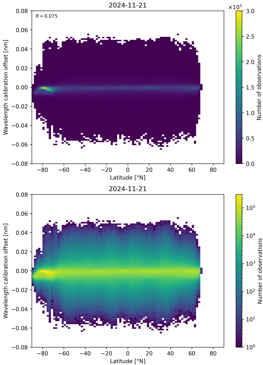
Figure 95: Scatter density plot of “Latitude” against “Wavelength calibration offset” for 2024-11-20 to 2024-11-22.
