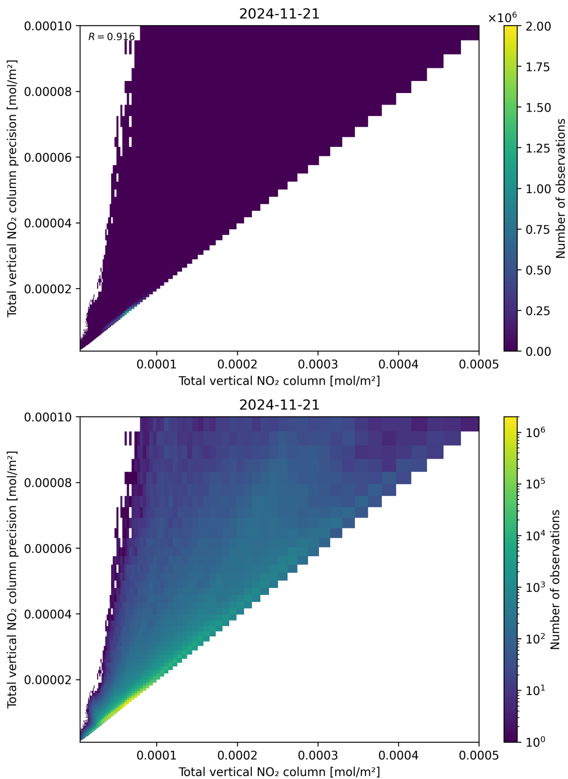
Figure 114: Scatter density plot of “Total vertical NO 2 column” against “Total vertical NO 2 column precision” for 2024-11-20 to 2024-11-22.
