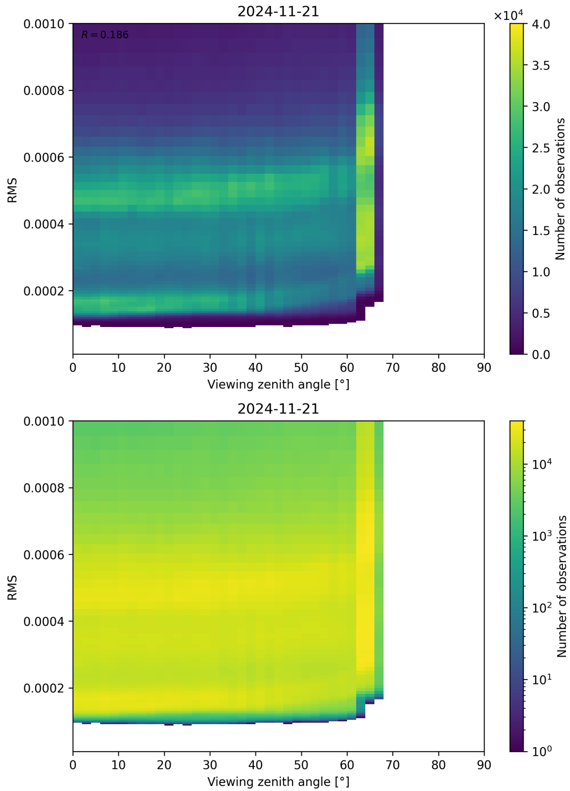
Figure 171: Scatter density plot of “Viewing zenith angle” against “RMS” for 2024-11-20 to 2024-11-22.
