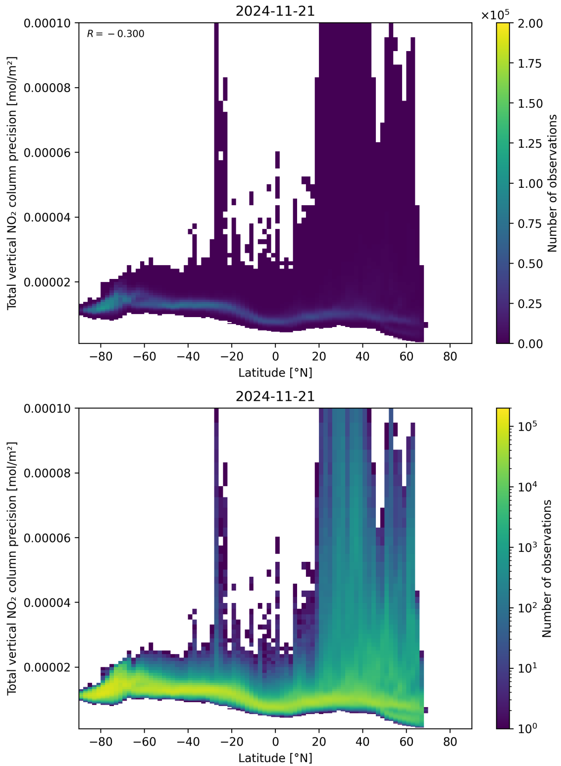
Figure 91: Scatter density plot of “Latitude” against “Total vertical NO 2 column precision” for 2024-11-20 to 2024-11-22.
