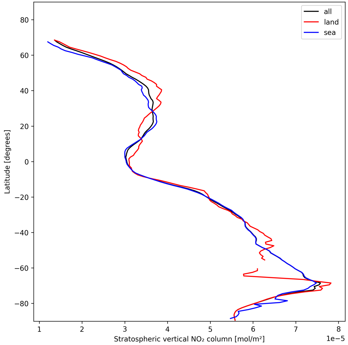
Figure 19: Zonal average of “Stratospheric vertical NO 2 column” for 2024-11-20 to 2024-11-22.
