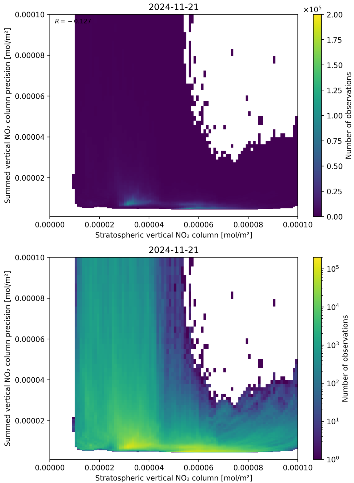
Figure 99: Scatter density plot of “Stratospheric vertical NO 2 column” against “Summed vertical NO 2 column precision” for 2024-11-20 to 2024-11-22.
