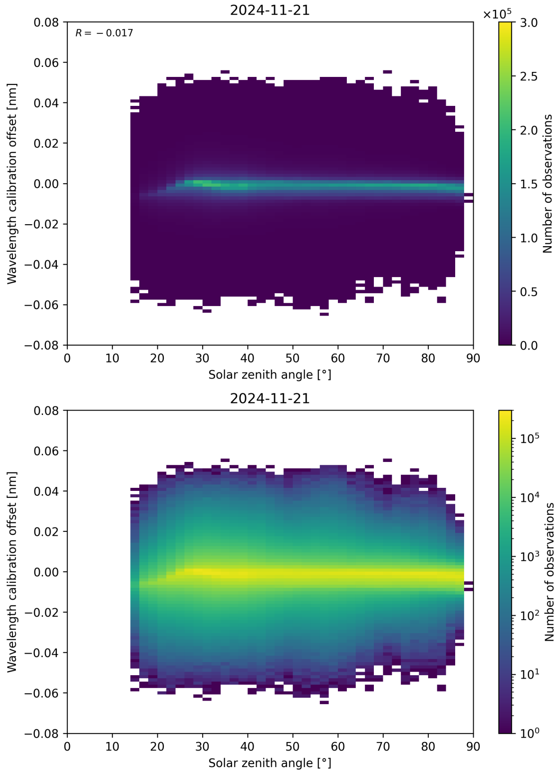
Figure 158: Scatter density plot of “Solar zenith angle” against “Wavelength calibration offset” for 2024-11-20 to 2024-11-22.
