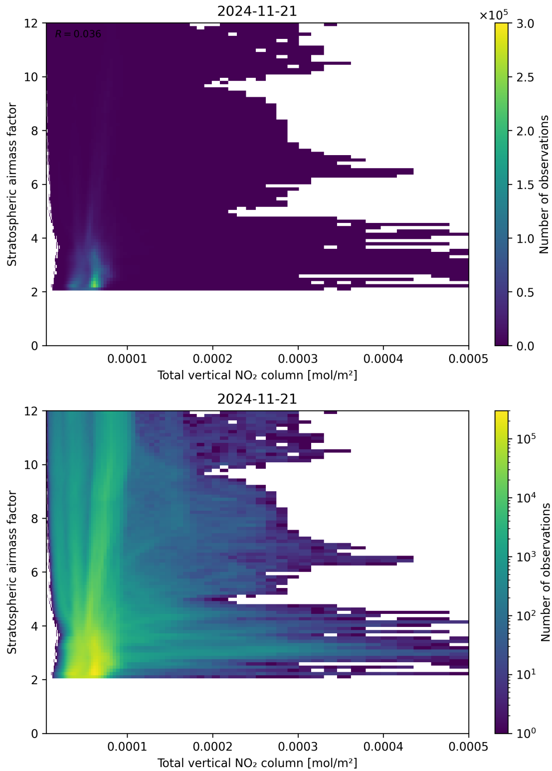
Figure 110: Scatter density plot of “Total vertical NO 2 column” against “Stratospheric airmass factor” for 2024-11-20 to 2024-11-22.
