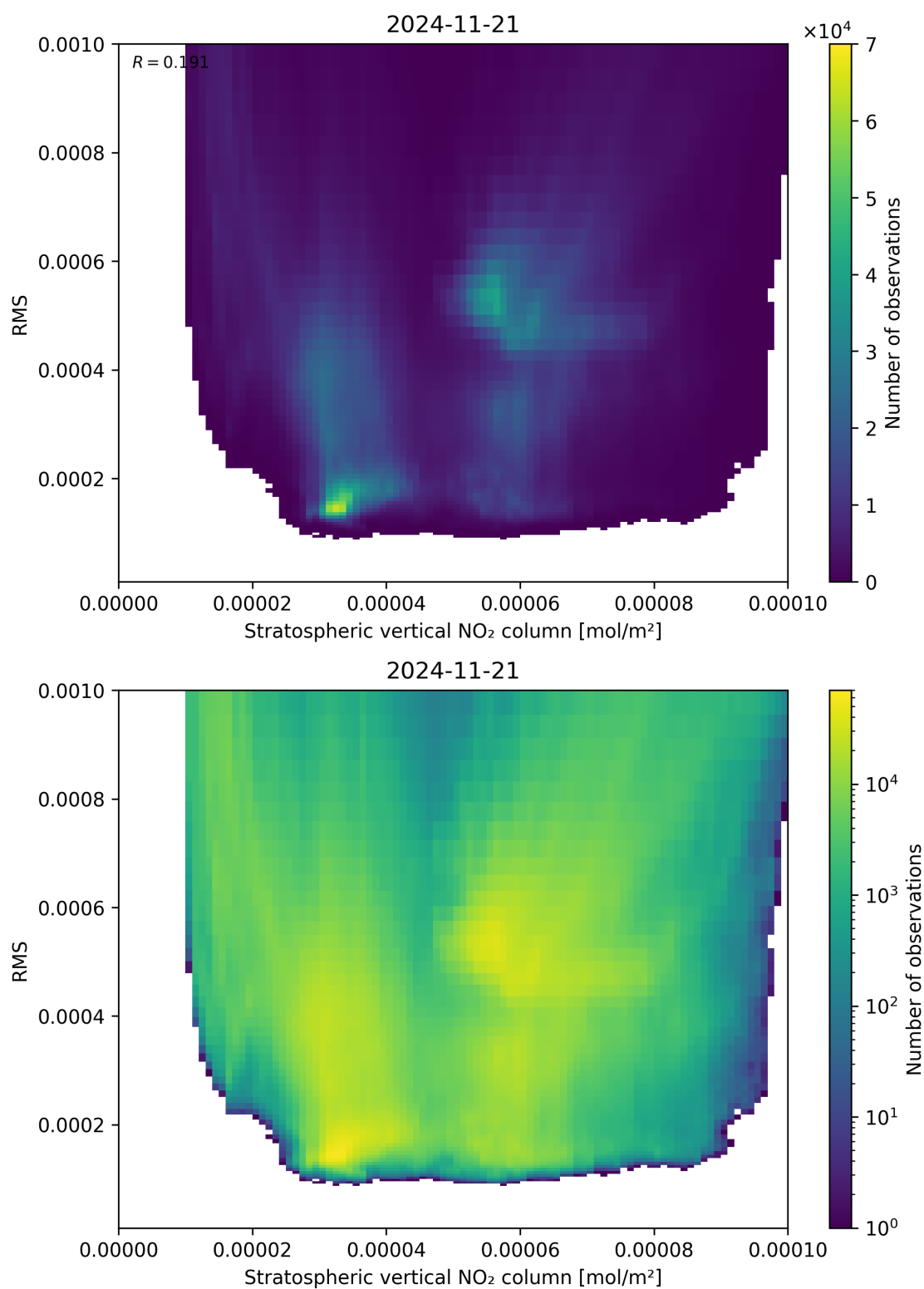
Figure 102: Scatter density plot of “Stratospheric vertical NO 2 column” against “RMS” for 2024-11-20 to 2024-11-22.
