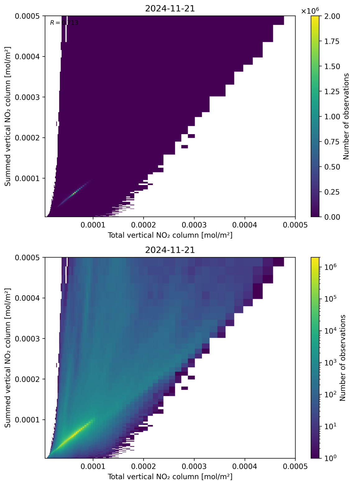
Figure 112: Scatter density plot of “Total vertical NO 2 column” against “Summed vertical NO 2 column” for 2024-11-20 to 2024-11-22.
