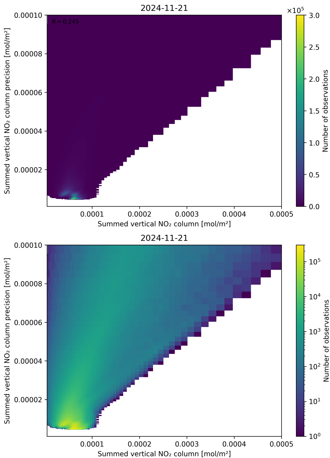
Figure 105: Scatter density plot of “Summed vertical NO 2 column” against “Summed vertical NO 2 column precision” for 2024-11-20 to 2024-11-22.
