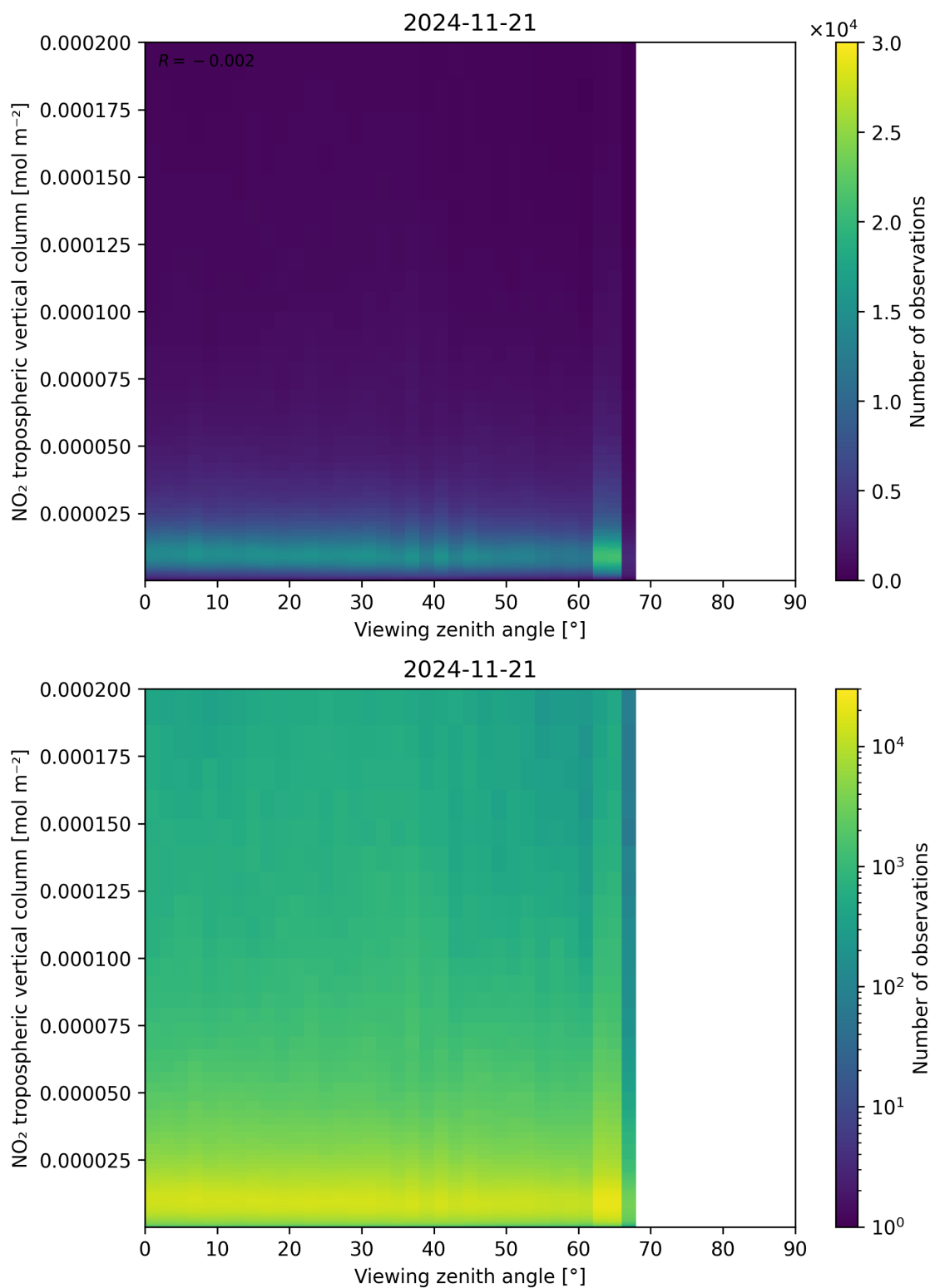
Figure 169: Scatter density plot of “Viewing zenith angle” against “NO 2 tropospheric vertical column” for 2024-11-20 to 2024-11-22.
