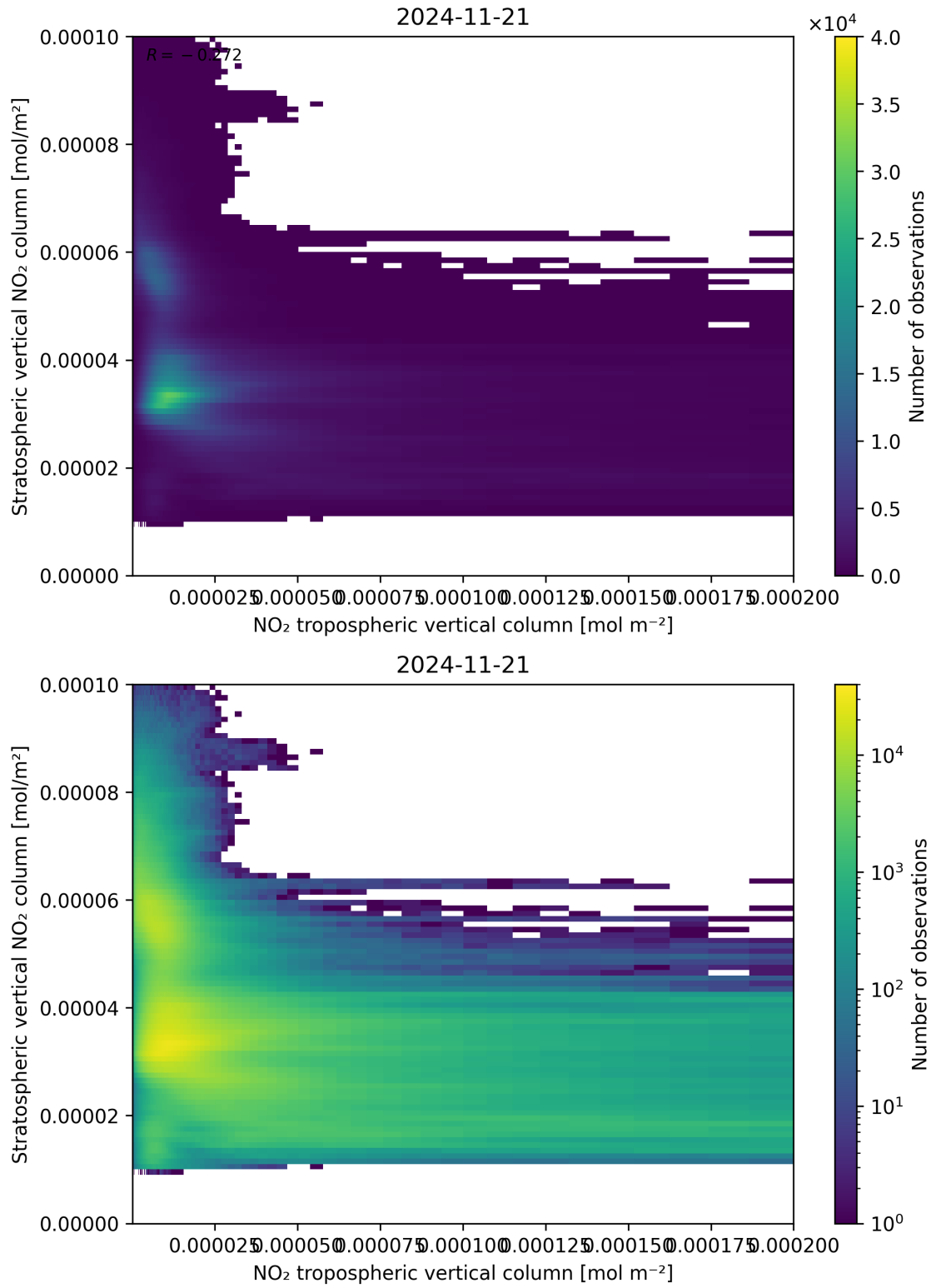
Figure 125: Scatter density plot of “NO 2 tropospheric vertical column” against “Stratospheric vertical NO 2 column” for 2024-11-20 to 2024-11-22.
