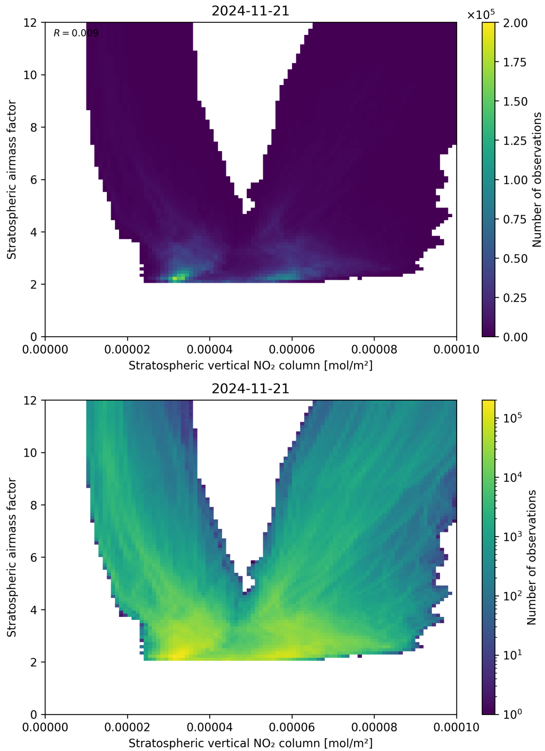
Figure 96: Scatter density plot of “Stratospheric vertical NO 2 column” against “Stratospheric airmass factor” for 2024-11-20 to 2024-11-22.
