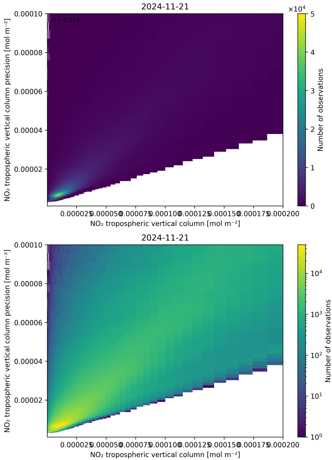
Figure 130: Scatter density plot of “NO 2 tropospheric vertical column” against “NO 2 tropospheric vertical column precision” for 2024-11-20 to 2024-11-22.
