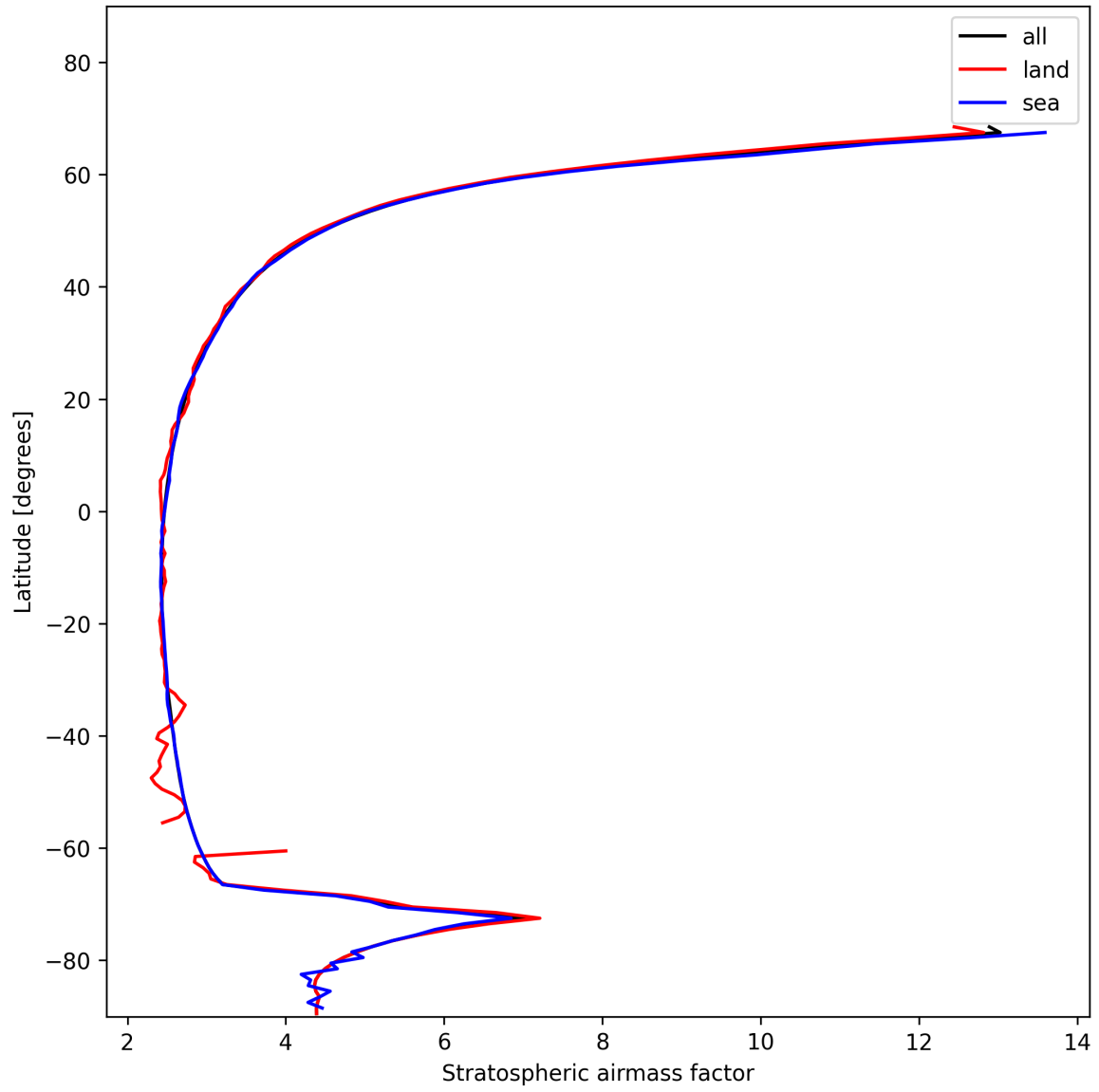
Figure 27: Zonal average of “Stratospheric airmass factor” for 2024-11-20 to 2024-11-22.
