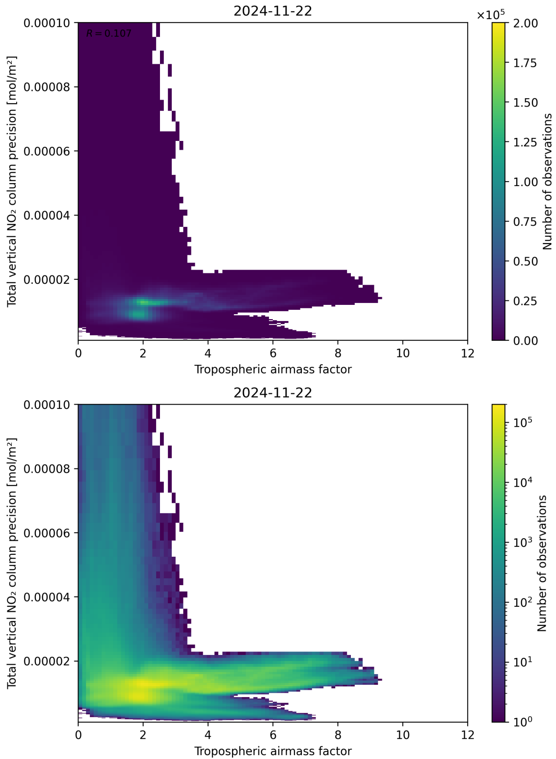
Figure 78: Scatter density plot of “Tropospheric air mass factor” against “Total vertical NO 2 column precision” for 2024-11-21 to 2024-11-23.
