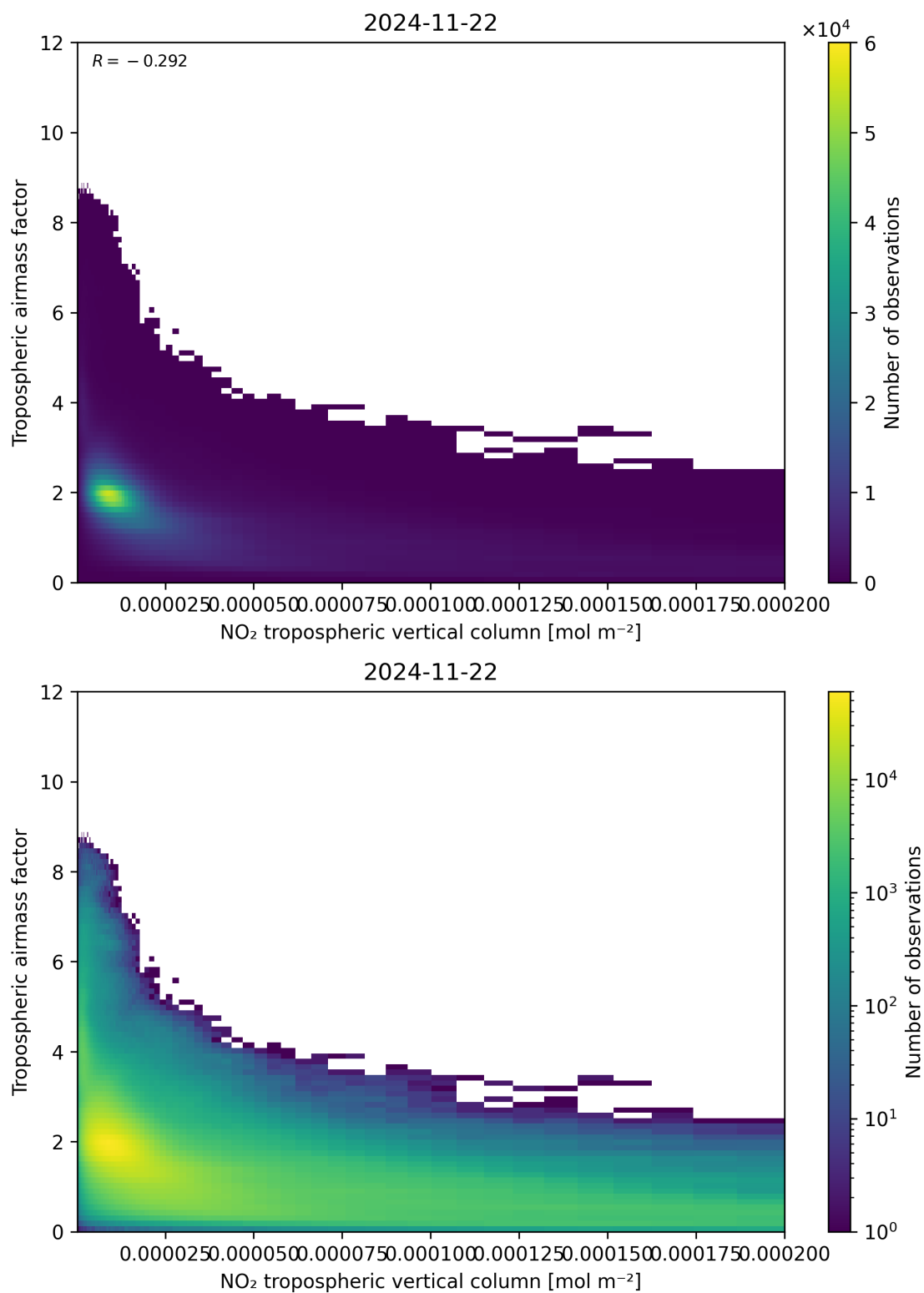
Figure 123: Scatter density plot of “NO 2 tropospheric vertical column” against “Tropospheric air mass factor” for 2024-11-21 to 2024-11-23.
