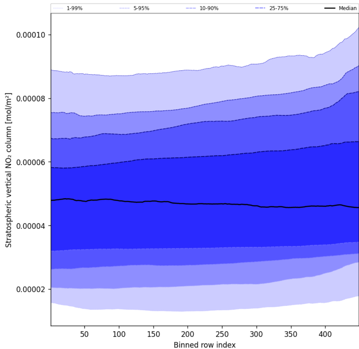
Figure 53: Along track statistics of “Stratospheric vertical NO 2 column” for 2024-11-21 to 2024-11-23
