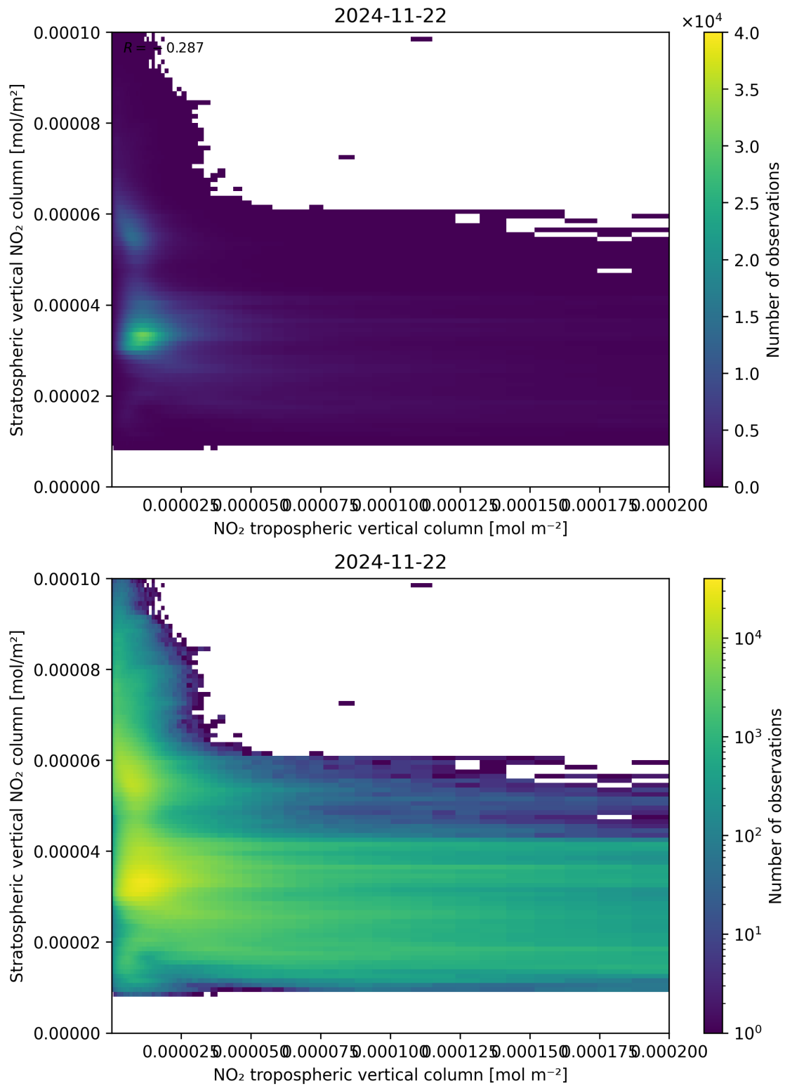
Figure 125: Scatter density plot of “NO 2 tropospheric vertical column” against “Stratospheric vertical NO 2 column” for 2024-11-21 to 2024-11-23.
