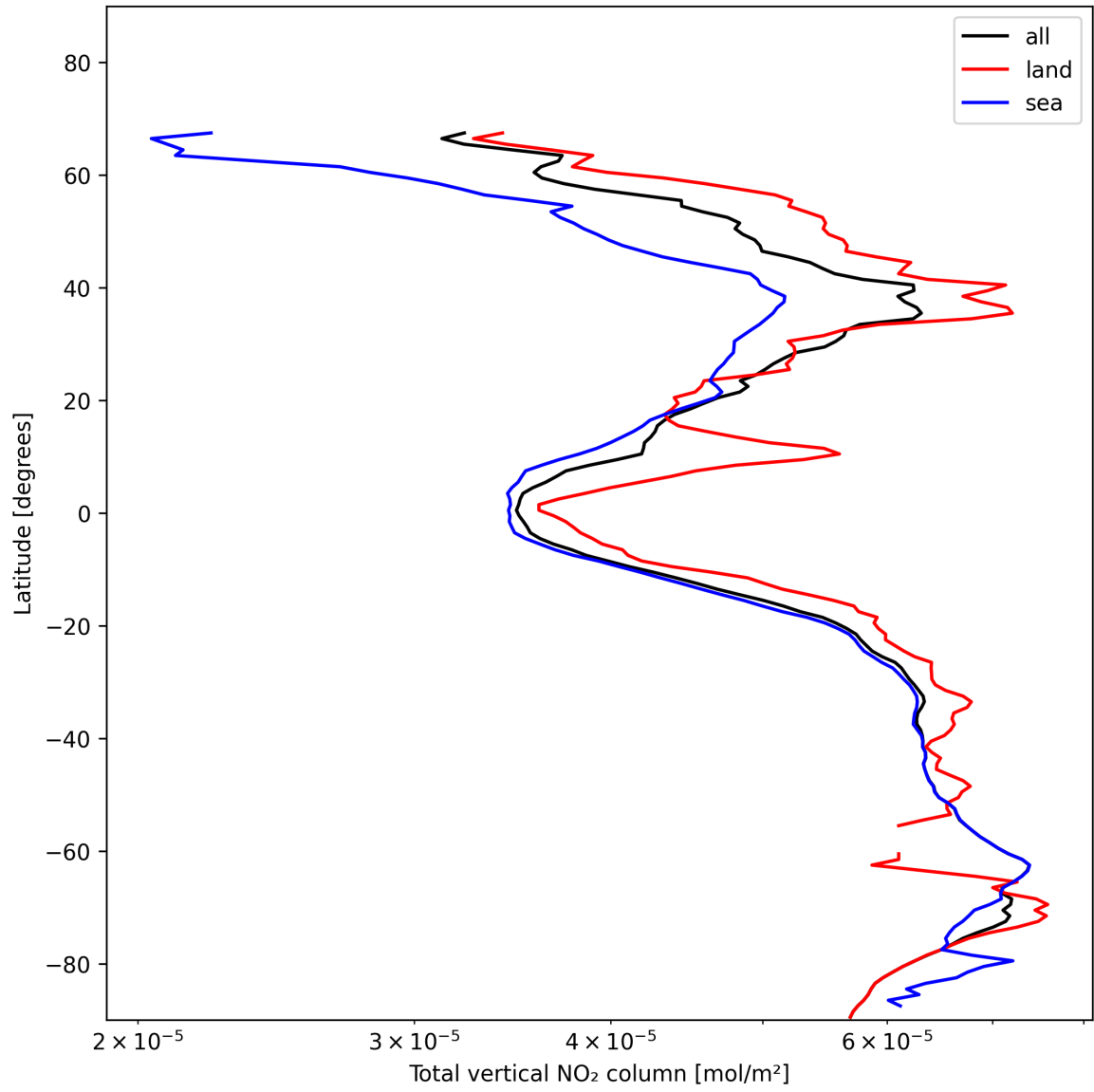
Figure 21: Zonal average of “Total vertical NO 2 column” for 2024-11-21 to 2024-11-23.
