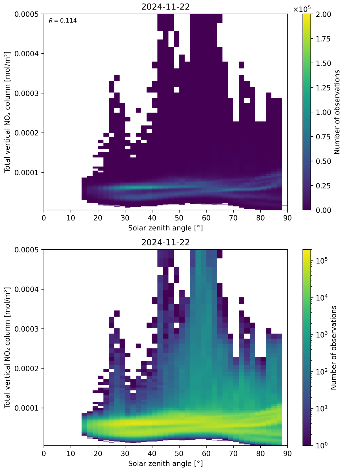
Figure 153: Scatter density plot of “Solar zenith angle” against “Total vertical NO 2 column” for 2024-11-21 to 2024-11-23.
