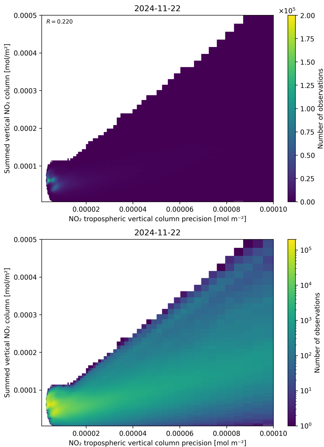
Figure 136: Scatter density plot of “NO 2 tropospheric vertical column precision” against “Summed vertical NO 2 column” for 2024-11-21 to 2024-11-23.
