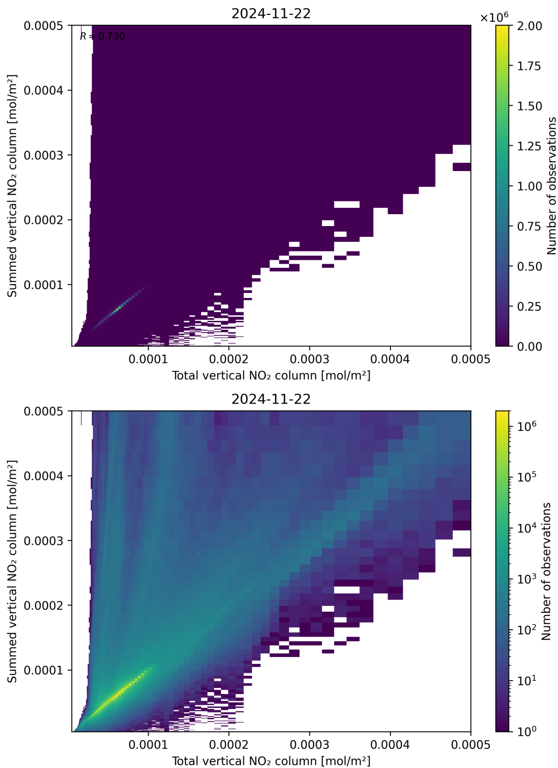
Figure 112: Scatter density plot of “Total vertical NO 2 column” against “Summed vertical NO 2 column” for 2024-11-21 to 2024-11-23.
