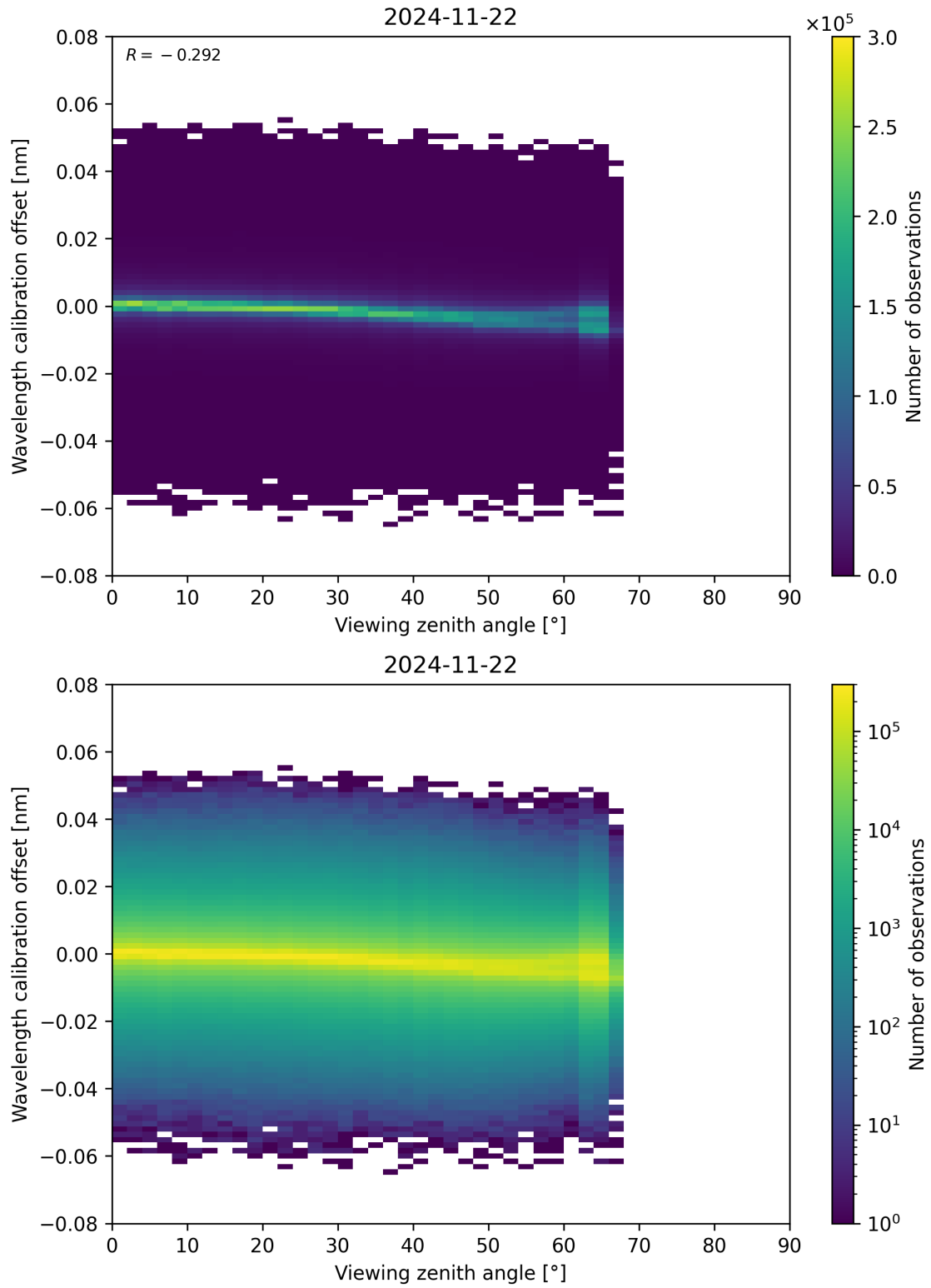
Figure 173: Scatter density plot of “Viewing zenith angle” against “Wavelength calibration offset” for 2024-11-21 to 2024-11-23.
