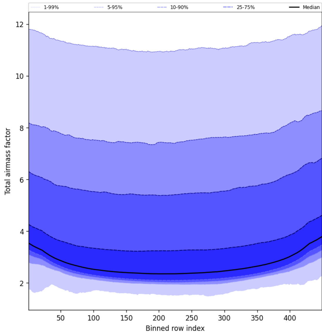
Figure 49: Along track statistics of “Total airmass factor” for 2024-11-21 to 2024-11-23
