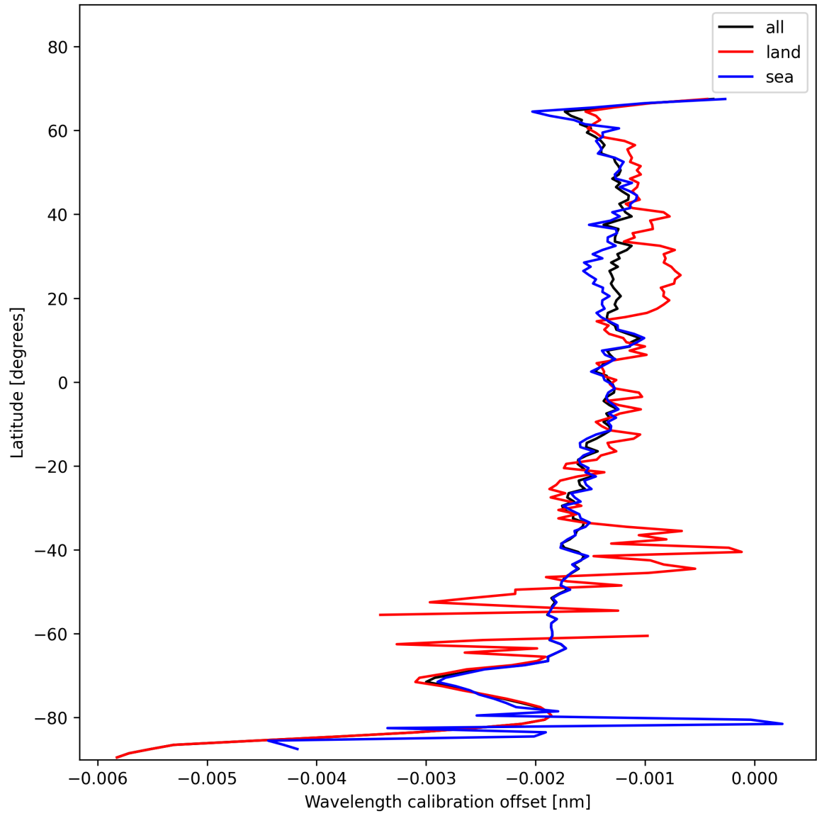
Figure 18: Zonal average of “Wavelength calibration offset” for 2024-11-21 to 2024-11-23.
