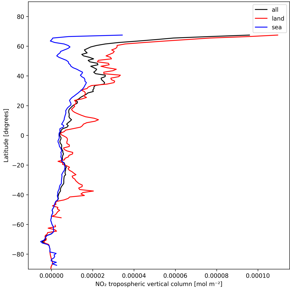
Figure 12: Zonal average of “NO 2 tropospheric vertical column” for 2024-11-21 to 2024-11-23.
