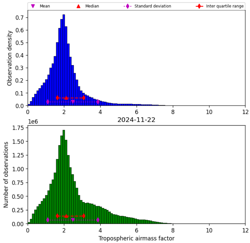
Figure 31: Histogram of “Tropospheric airmass factor” for 2024-11-21 to 2024-11-23
