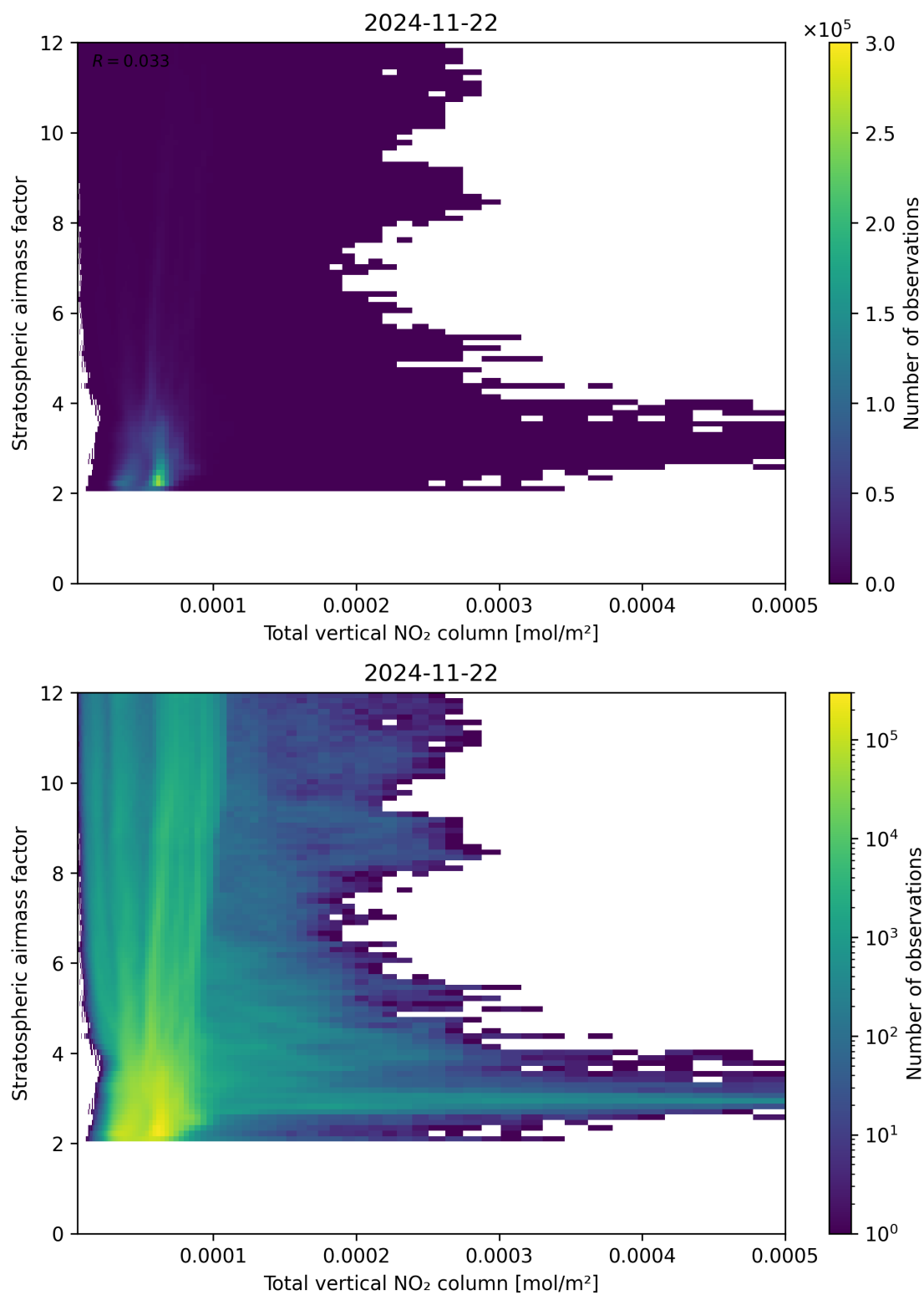
Figure 110: Scatter density plot of “Total vertical NO 2 column” against “Stratospheric airmass factor” for 2024-11-21 to 2024-11-23.
