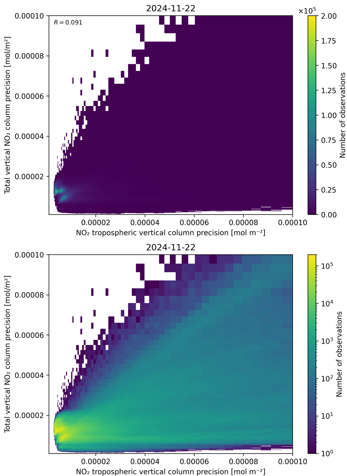
Figure 139: Scatter density plot of “NO 2 tropospheric vertical column precision” against “Total vertical NO 2 column precision” for 2024-11-21 to 2024-11-23.
