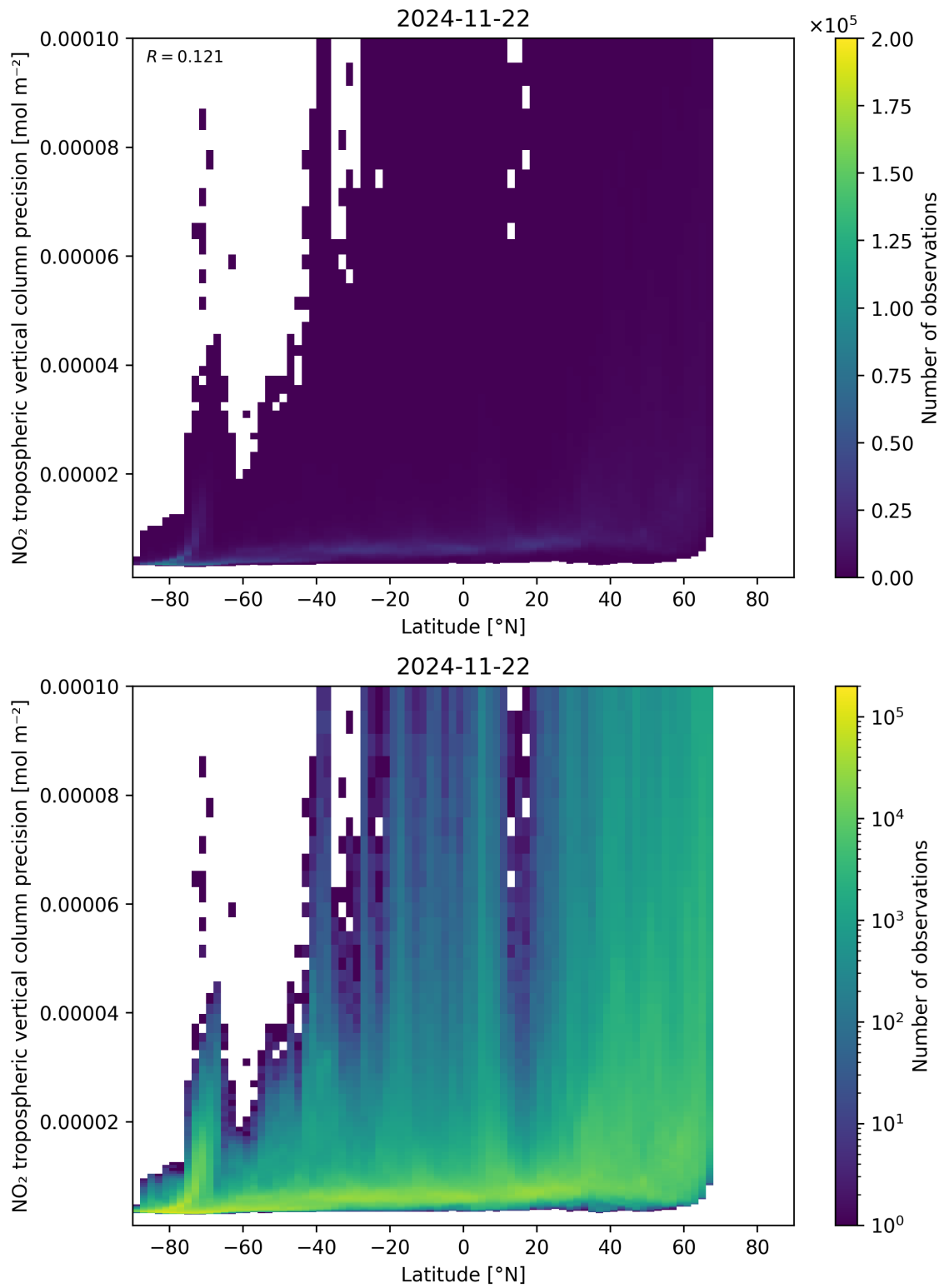
Figure 93: Scatter density plot of “Latitude” against “NO 2 tropospheric vertical column precision” for 2024-11-21 to 2024-11-23.
