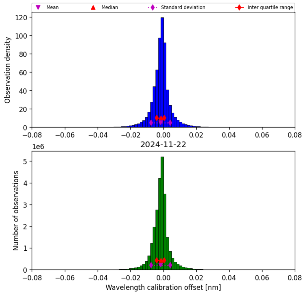
Figure 35: Histogram of “Wavelength calibration offset” for 2024-11-21 to 2024-11-23
