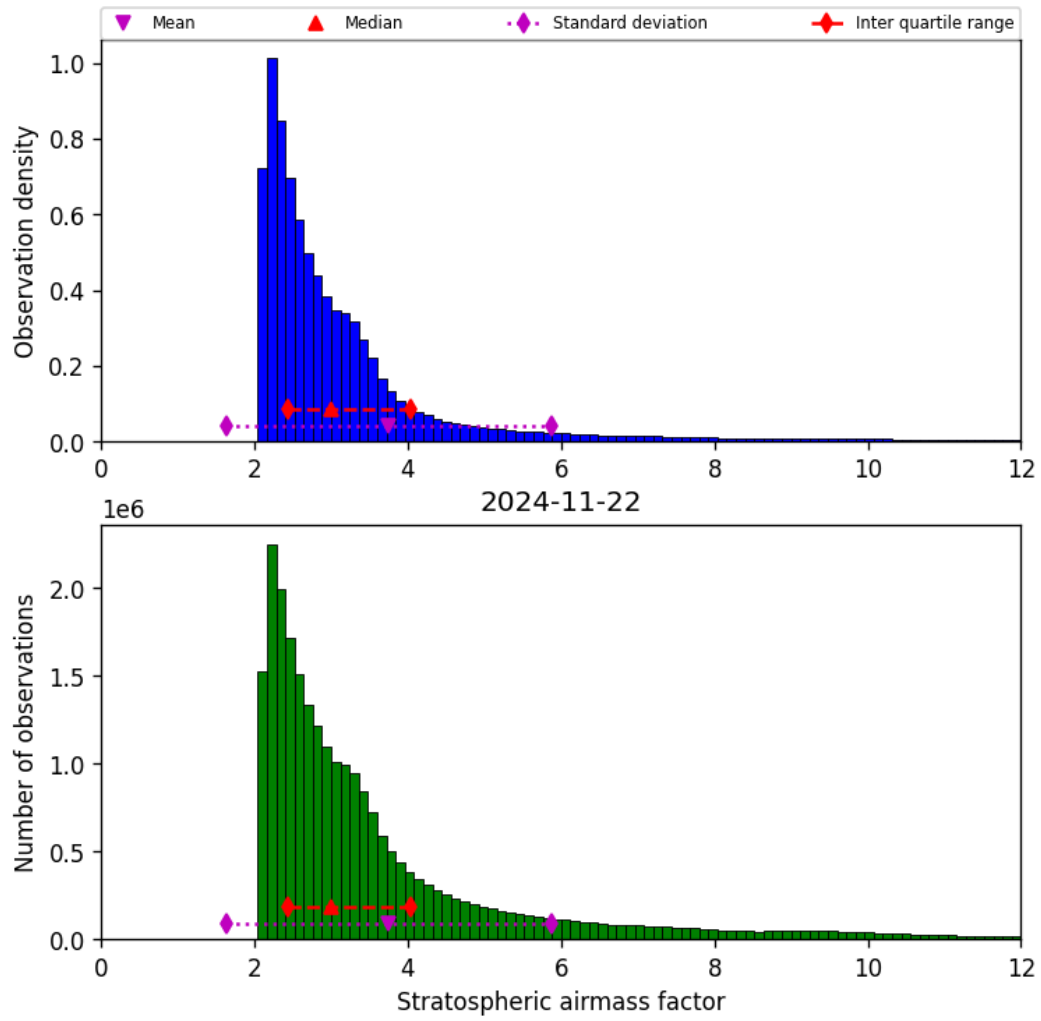
Figure 44: Histogram of “Stratospheric airmass factor” for 2024-11-21 to 2024-11-23
