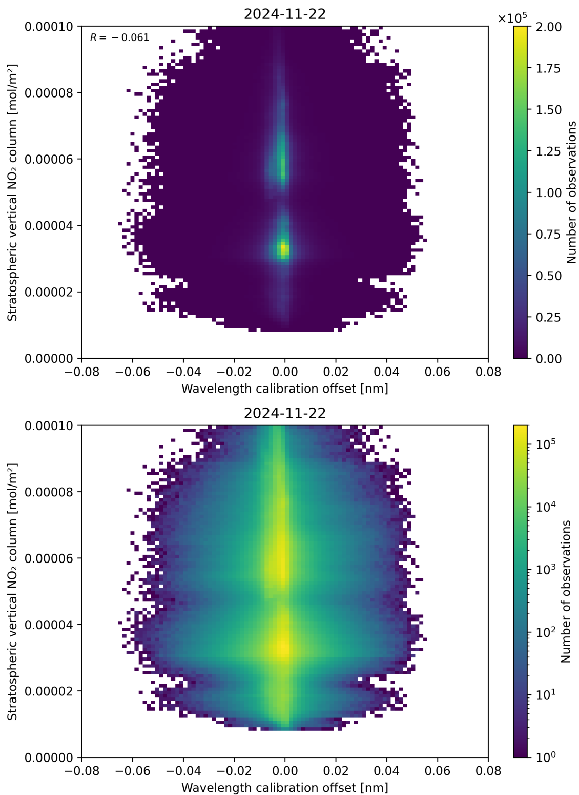
Figure 176: Scatter density plot of “Wavelength calibration offset” against “Stratospheric vertical NO 2 column” for 2024-11-21 to 2024-11-23.
