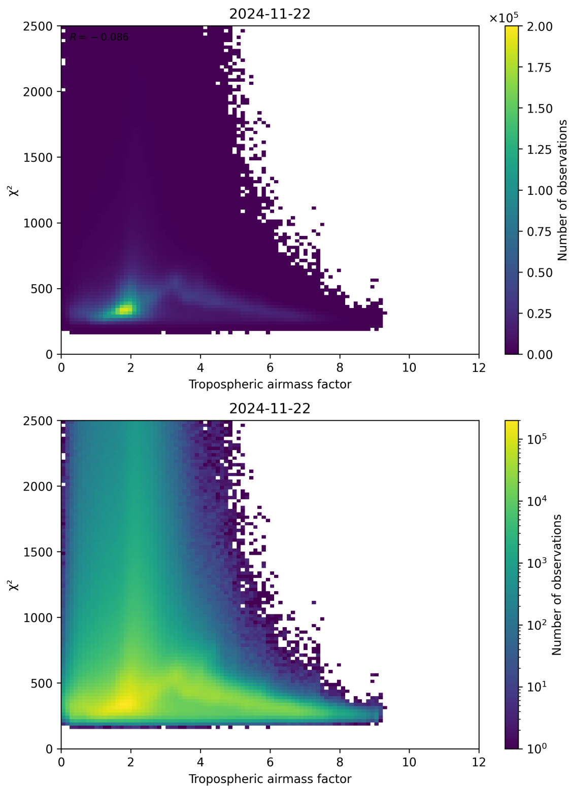
Figure 73: Scatter density plot of “Tropospheric airmass factor” against “ \chi^2 ” for 2024-11-21 to 2024-11-23.
