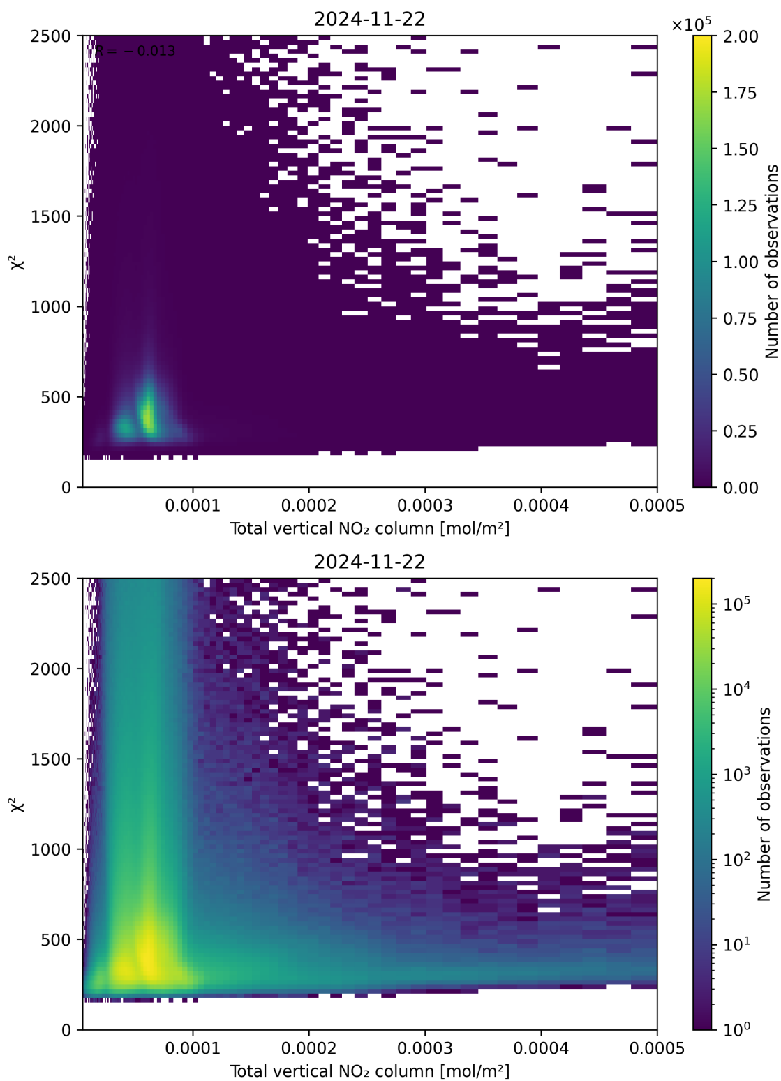
Figure 111: Scatter density plot of “Total vertical NO 2 column” against “ \chi^2 ” for 2024-11-21 to 2024-11-23.
