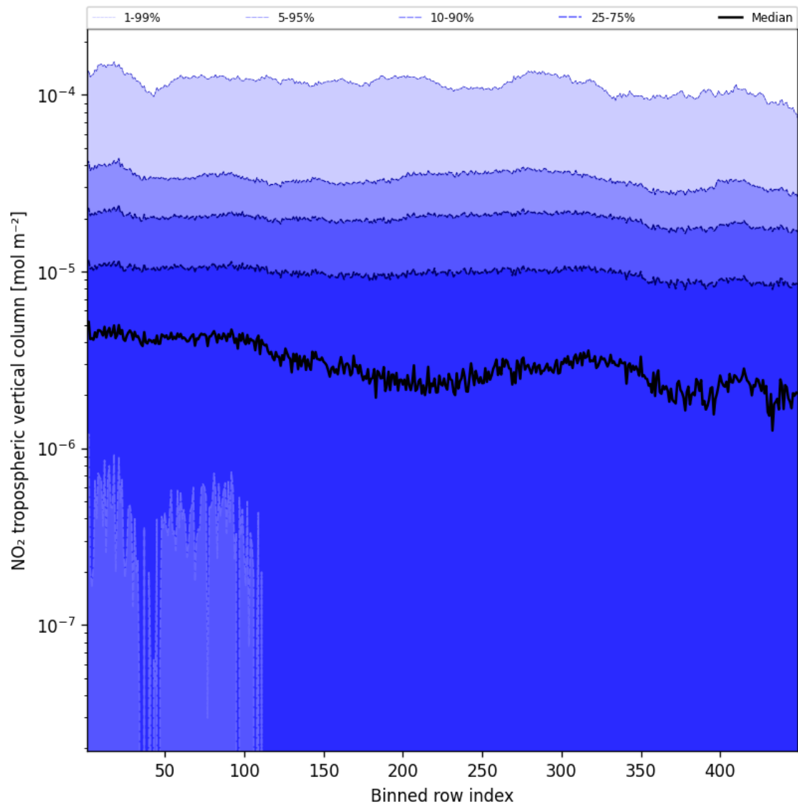
Figure 46: Along track statistics of “NO 2 tropospheric vertical column” for 2024-11-21 to 2024-11-23
