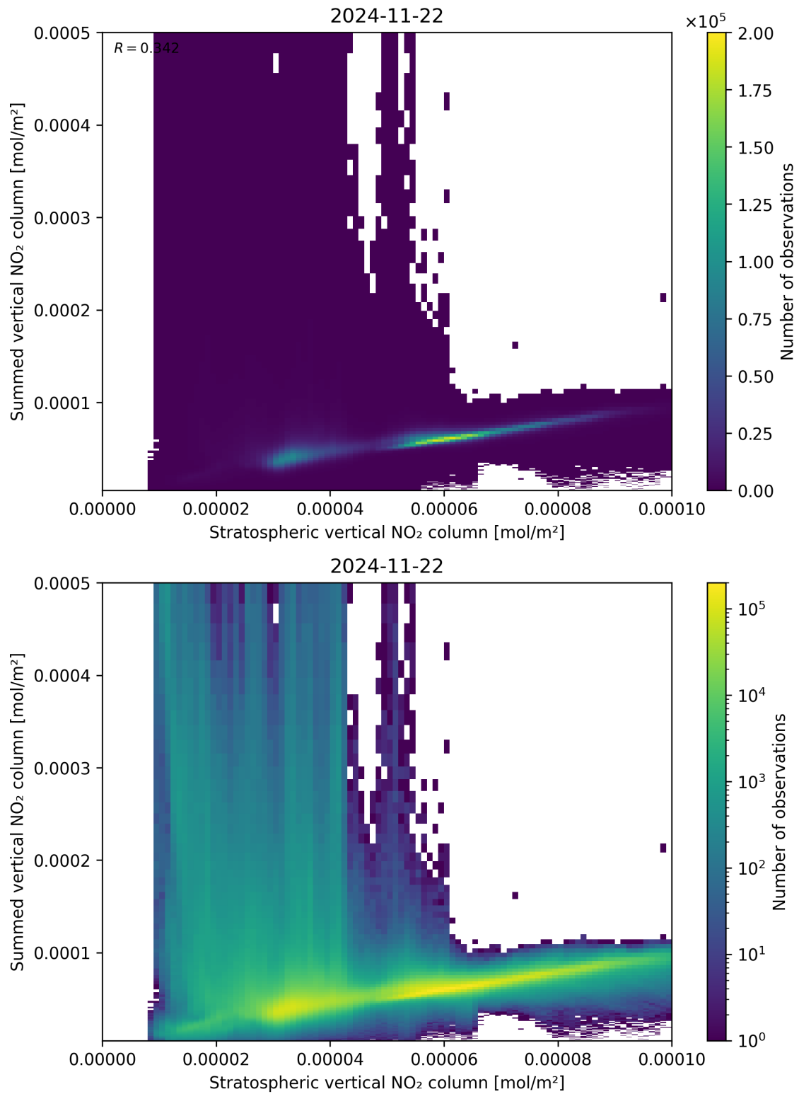
Figure 98: Scatter density plot of “Stratospheric vertical NO 2 column” against “Summed vertical NO 2 column” for 2024-11-21 to 2024-11-23.
