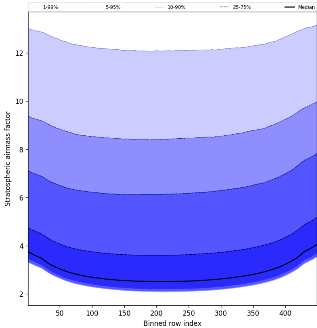
Figure 61: Along track statistics of “Stratospheric airmass factor” for 2024-11-21 to 2024-11-23
