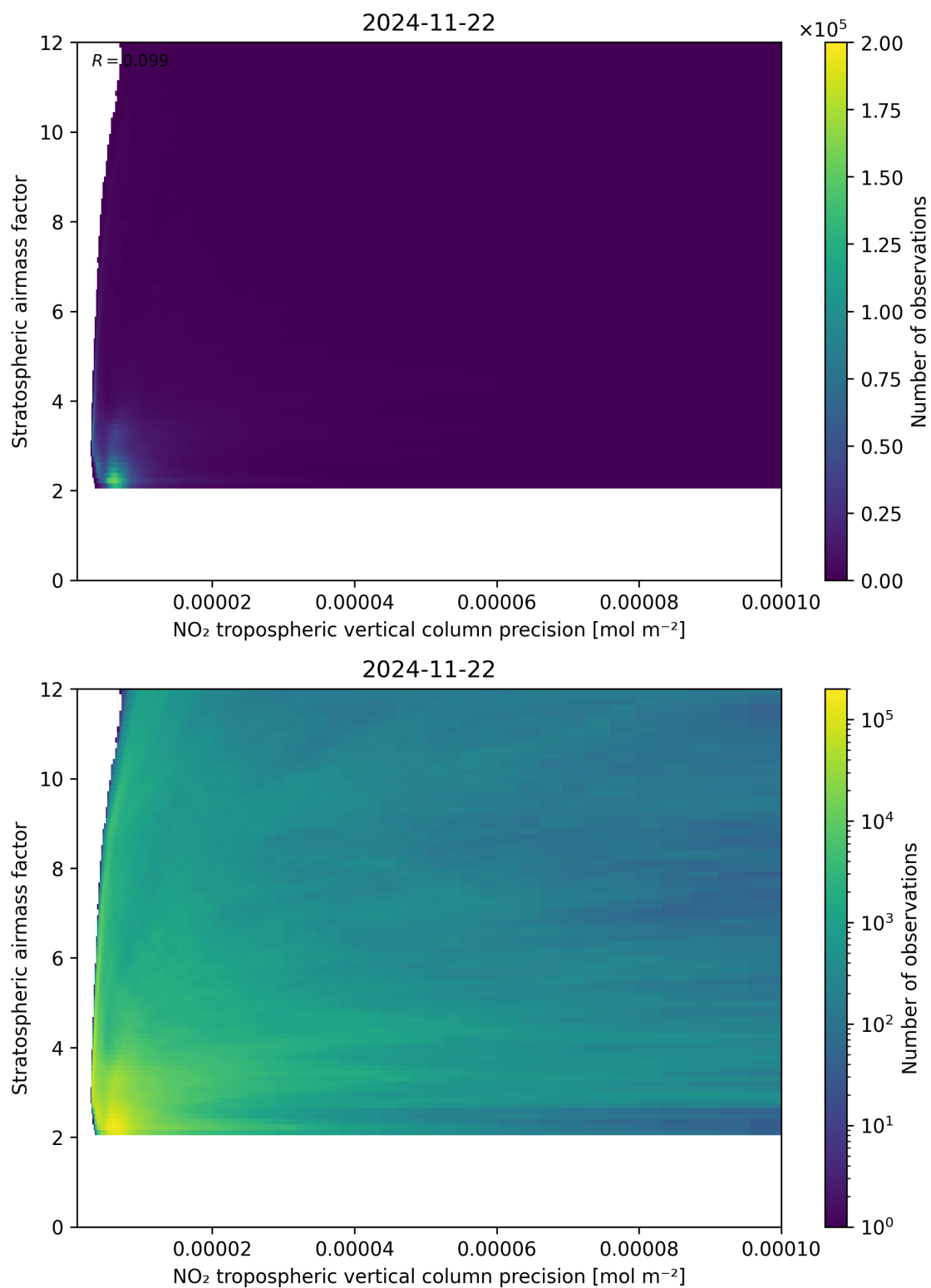
Figure 131: Scatter density plot of “NO 2 tropospheric vertical column precision” against “Stratospheric airmass factor” for 2024-11-21 to 2024-11-23.
