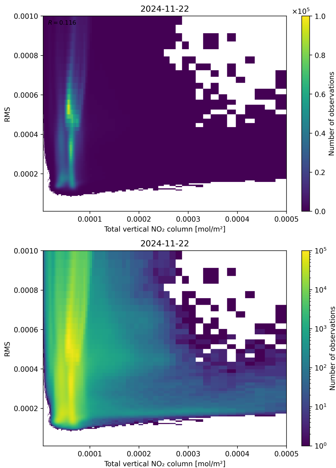
Figure 120: Scatter density plot of “Total vertical NO 2 column” against “RMS” for 2024-11-21 to 2024-11-23.
