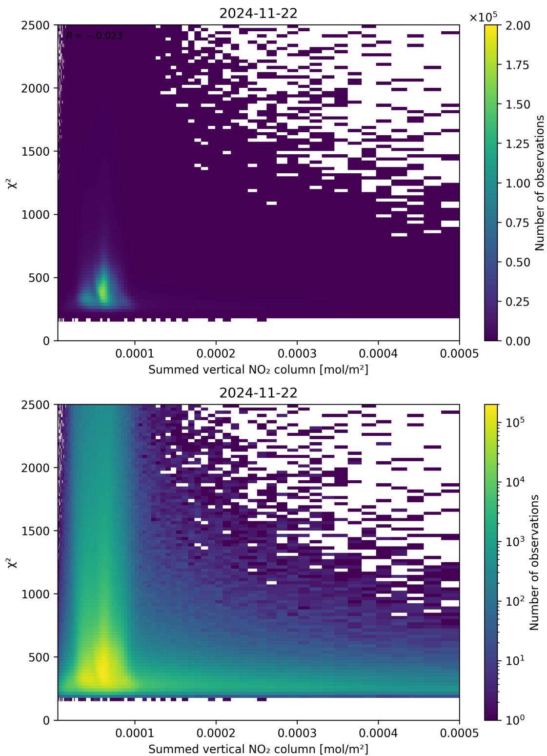
Figure 104: Scatter density plot of “Summed vertical NO 2 column” against “ \chi^2 ” for 2024-11-21 to 2024-11-23.
