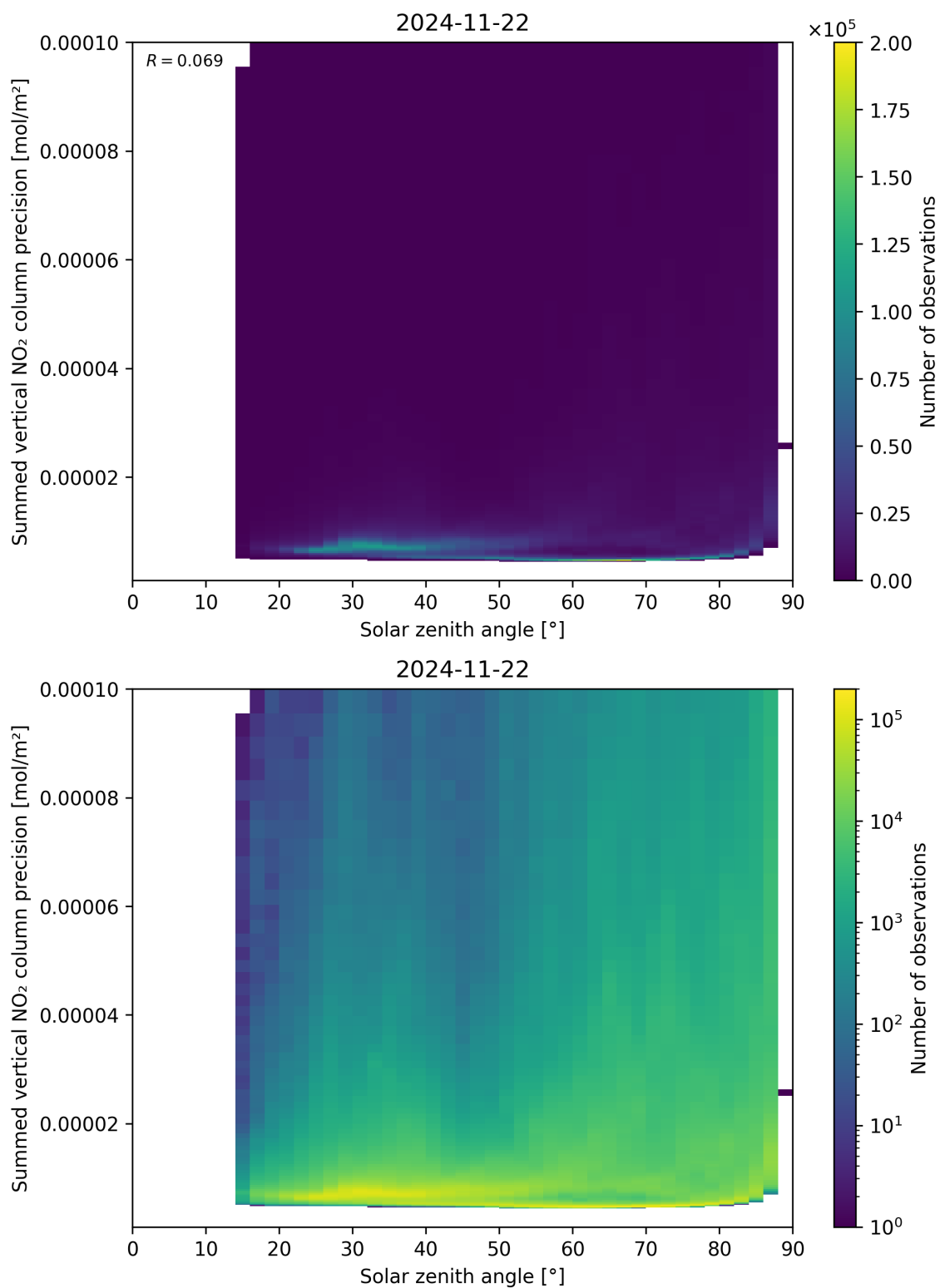
Figure 152: Scatter density plot of “Solar zenith angle” against “Summed vertical NO 2 column precision” for 2024-11-21 to 2024-11-23.
