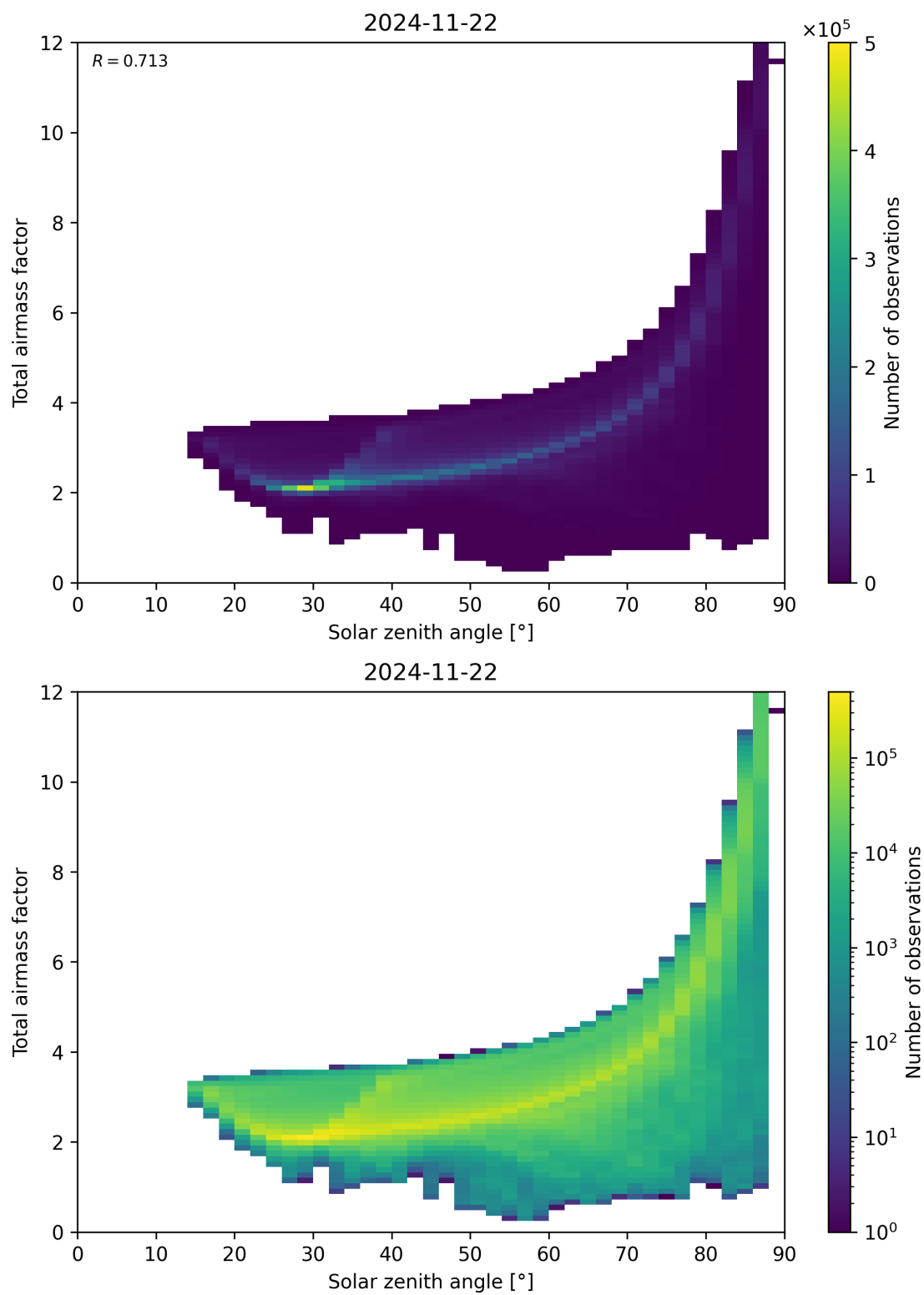
Figure 146: Scatter density plot of “Solar zenith angle” against “Total air mass factor” for 2024-11-21 to 2024-11-23.
