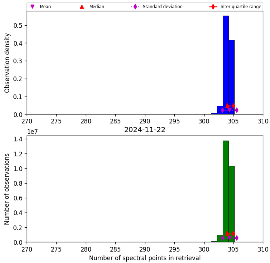
Figure 33: Histogram of “Number of spectral points in retrieval” for 2024-11-21 to 2024-11-23
