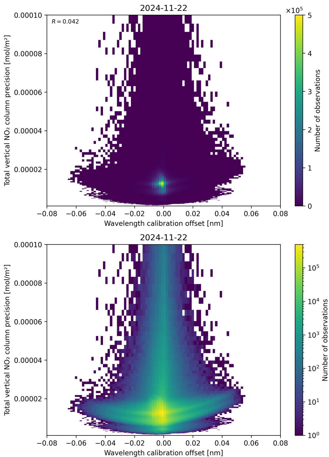
Figure 180: Scatter density plot of “Wavelength calibration offset” against “Total vertical NO 2 column precision” for 2024-11-21 to 2024-11-23.
