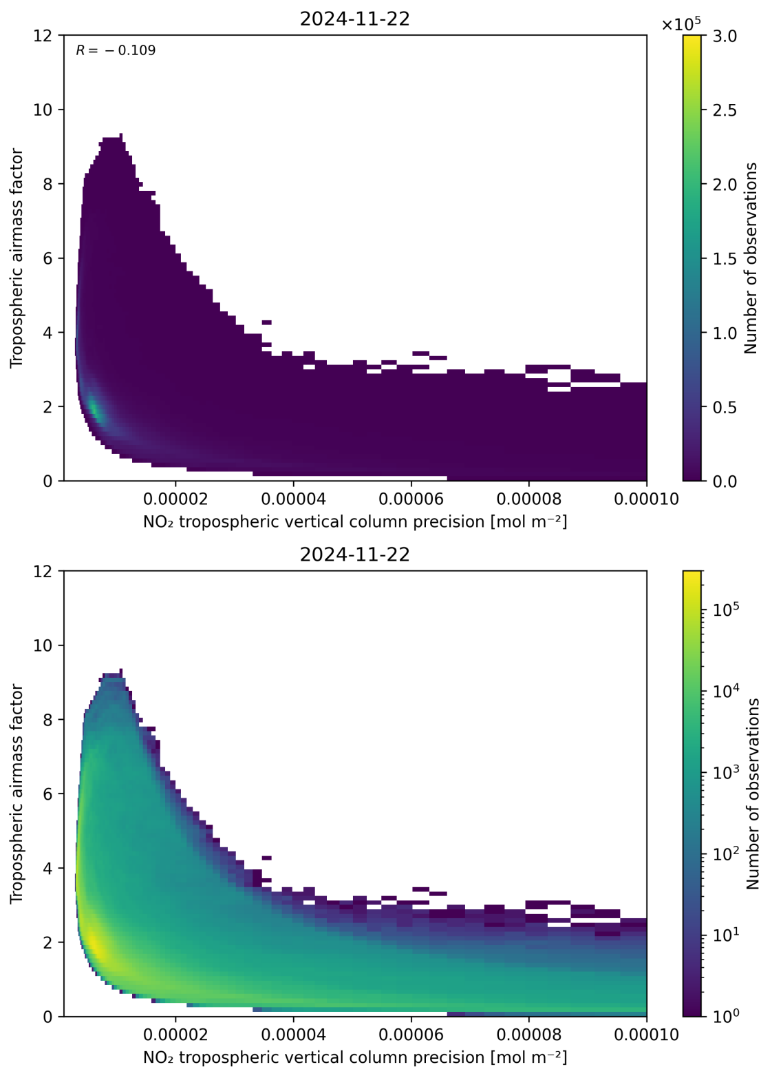
Figure 133: Scatter density plot of “NO 2 tropospheric vertical column precision” against “Tropospheric air mass factor” for 2024-11-21 to 2024-11-23.
