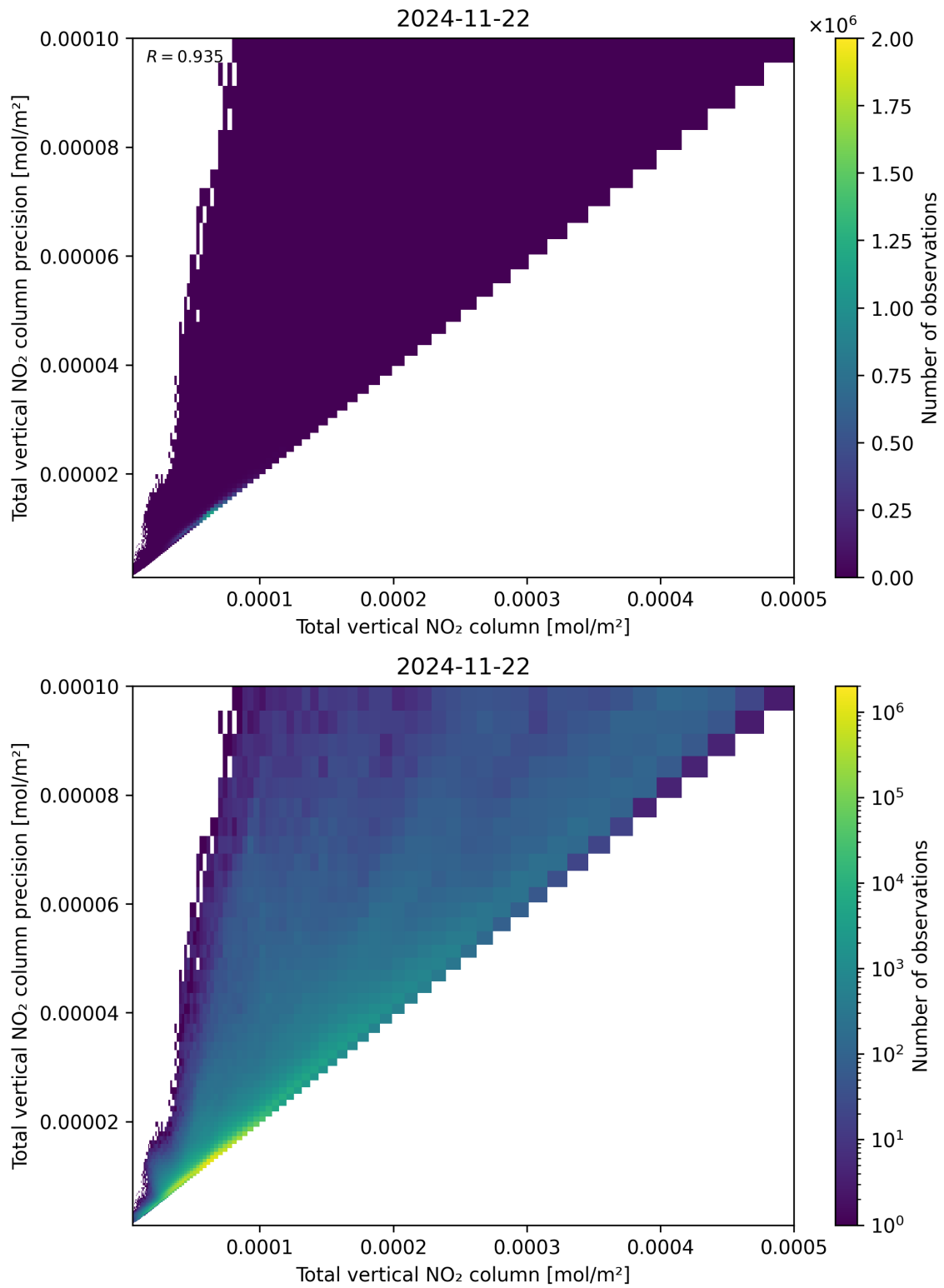
Figure 114: Scatter density plot of “Total vertical NO 2 column” against “Total vertical NO 2 column precision” for 2024-11-21 to 2024-11-23.
