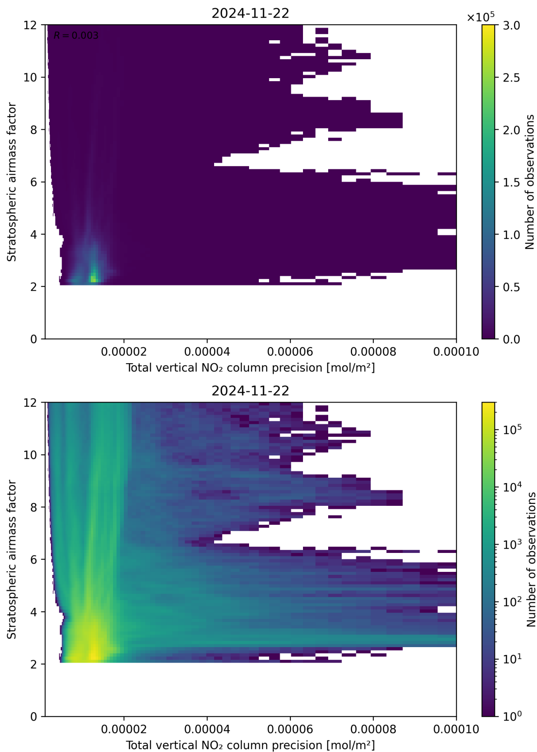
Figure 115: Scatter density plot of “Total vertical NO 2 column precision” against “Stratospheric air mass factor” for 2024-11-21 to 2024-11-23.
