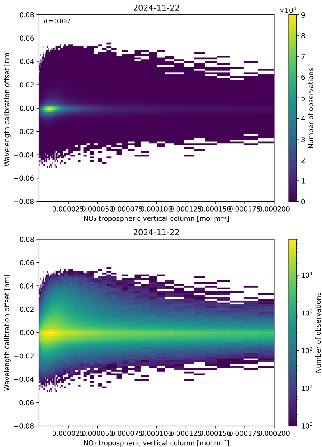
Figure 143: Scatter density plot of “NO 2 tropospheric vertical column” against “Wavelength calibration offset” for 2024-11-21 to 2024-11-23.
