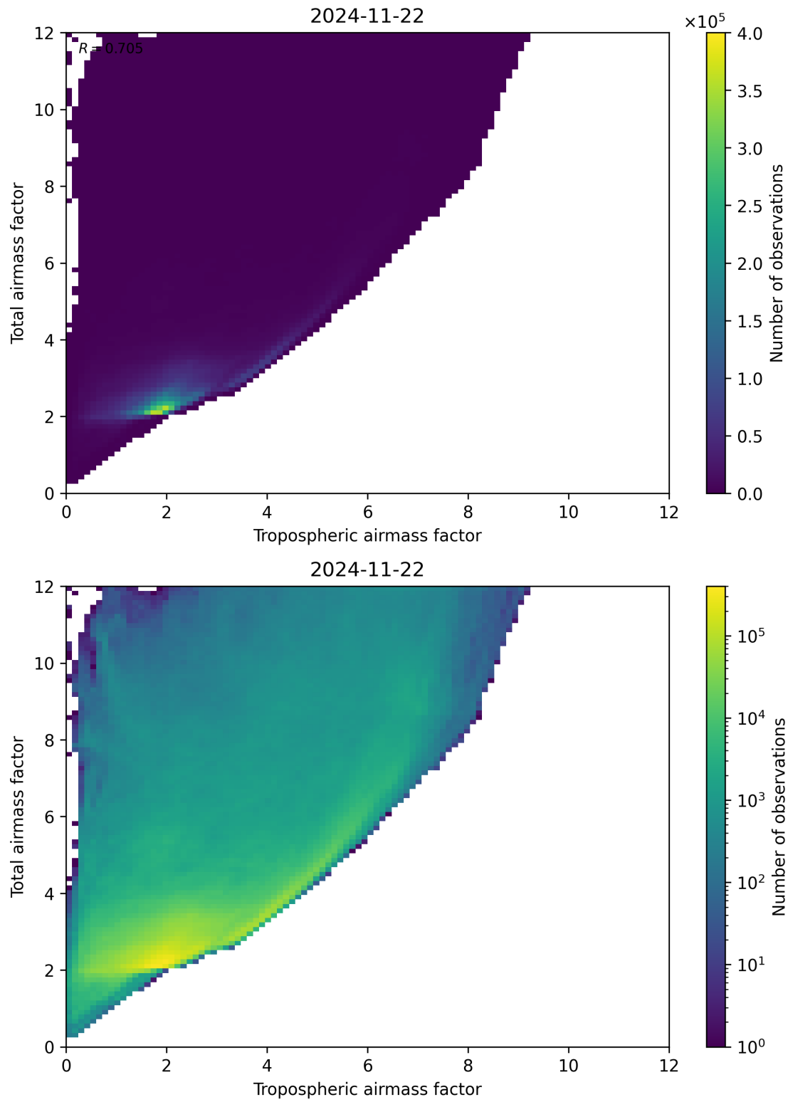
Figure 72: Scatter density plot of “Tropospheric airmass factor” against “Total airmass factor” for 2024-11-21 to 2024-11-23.
