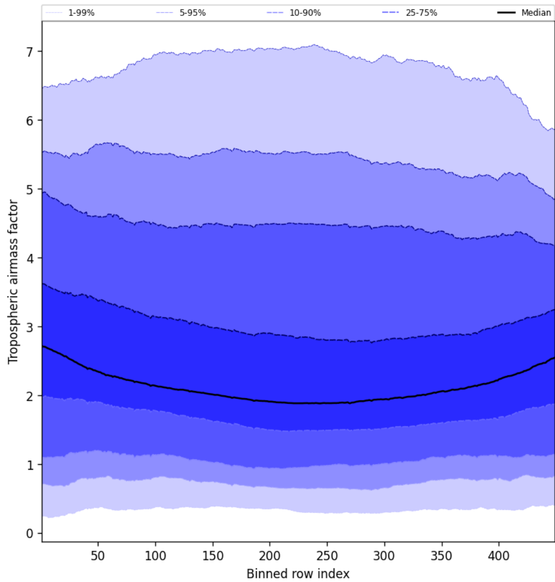
Figure 48: Along track statistics of “Tropospheric airmass factor” for 2024-11-21 to 2024-11-23
