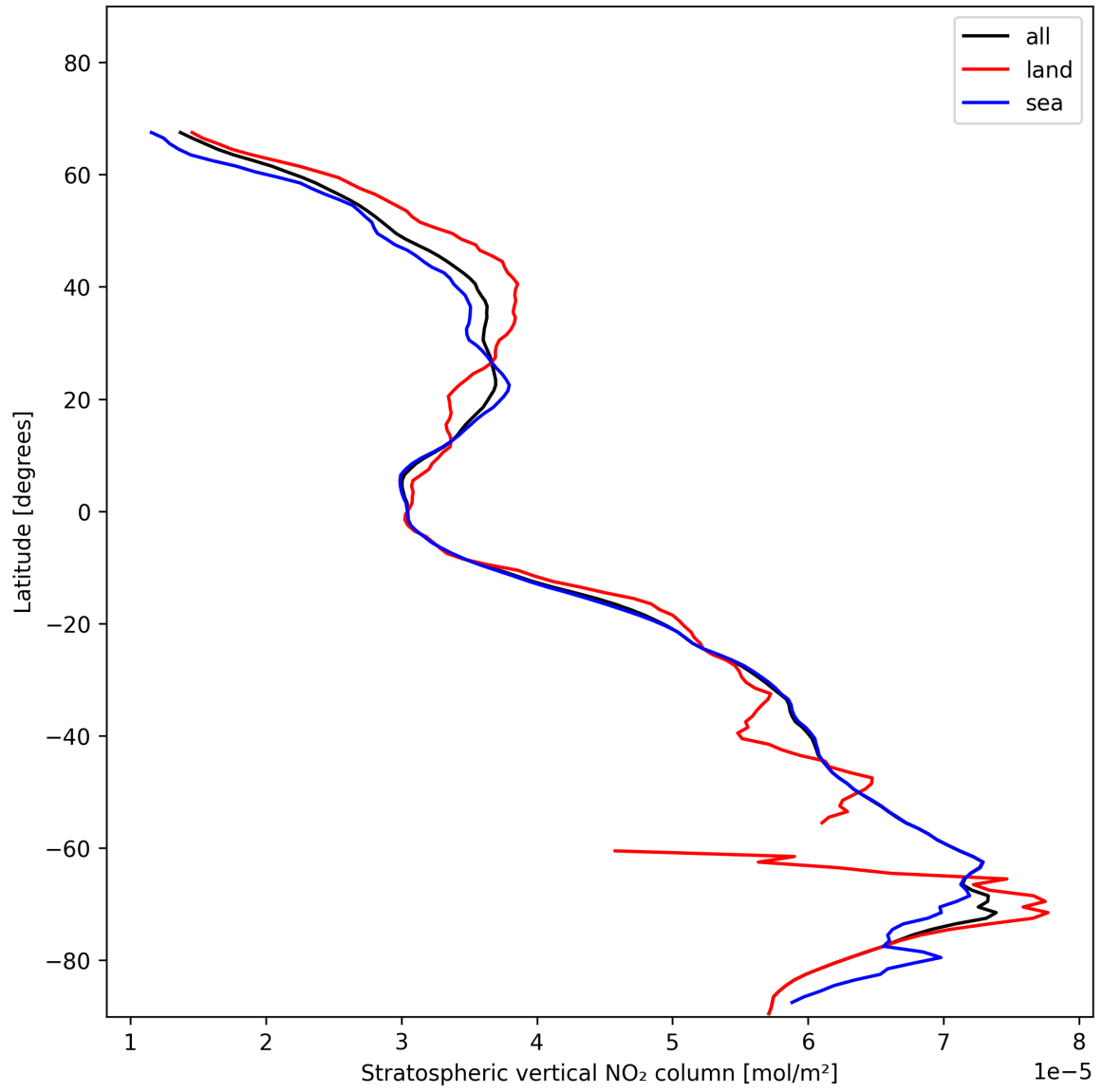
Figure 19: Zonal average of “Stratospheric vertical NO 2 column” for 2024-11-21 to 2024-11-23.
