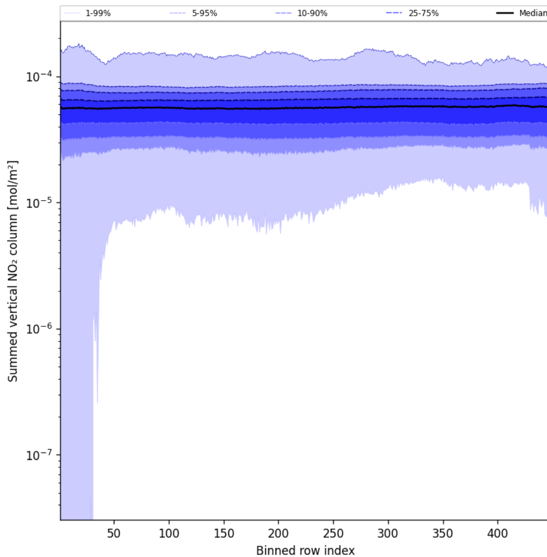
Figure 57: Along track statistics of “Summed vertical NO 2 column” for 2024-11-21 to 2024-11-23
