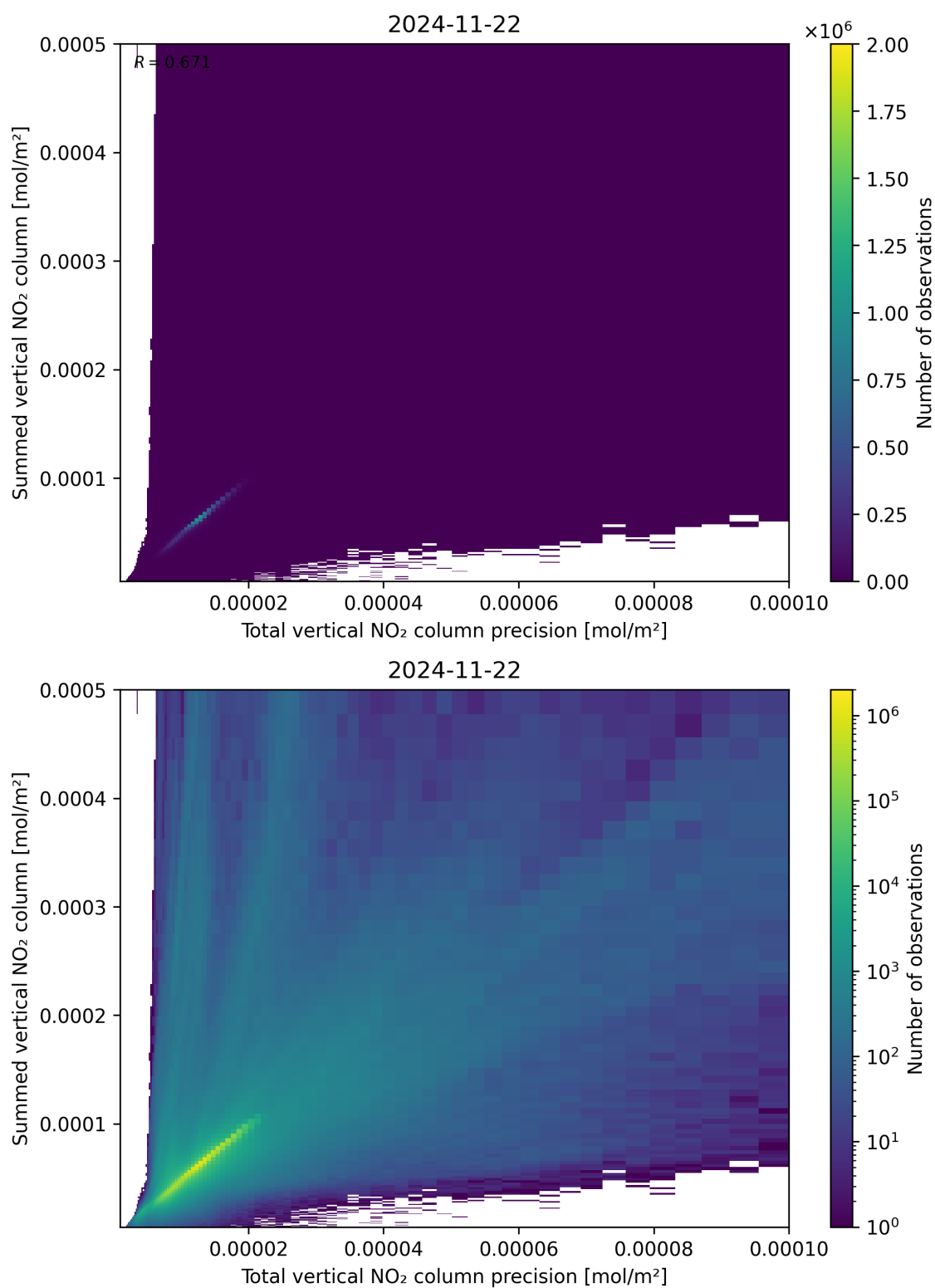
Figure 117: Scatter density plot of “Total vertical NO 2 column precision” against “Summed vertical NO 2 column” for 2024-11-21 to 2024-11-23.
