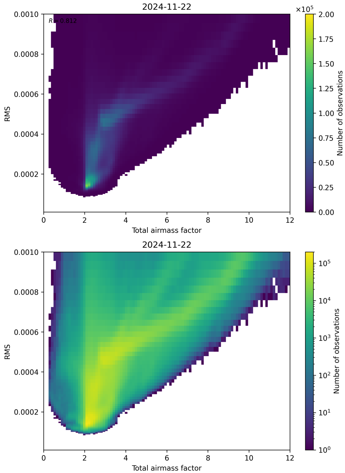
Figure 69: Scatter density plot of “Total airmass factor” against “RMS” for 2024-11-21 to 2024-11-23.
