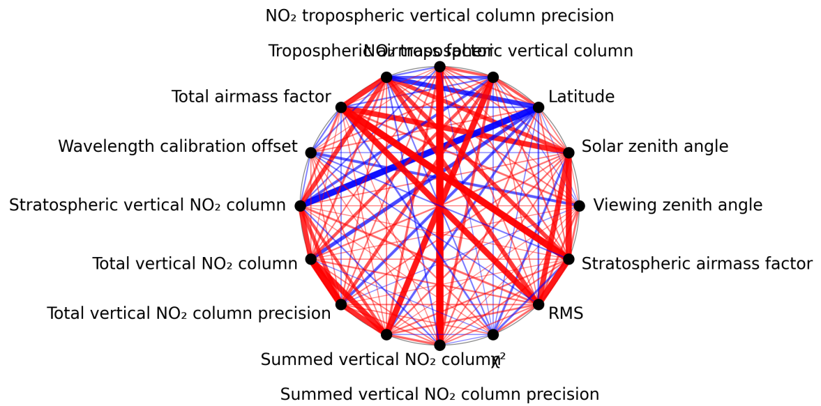
Figure 1: Map of correlation graph for 2024-11-21 to 2024-11-23.
