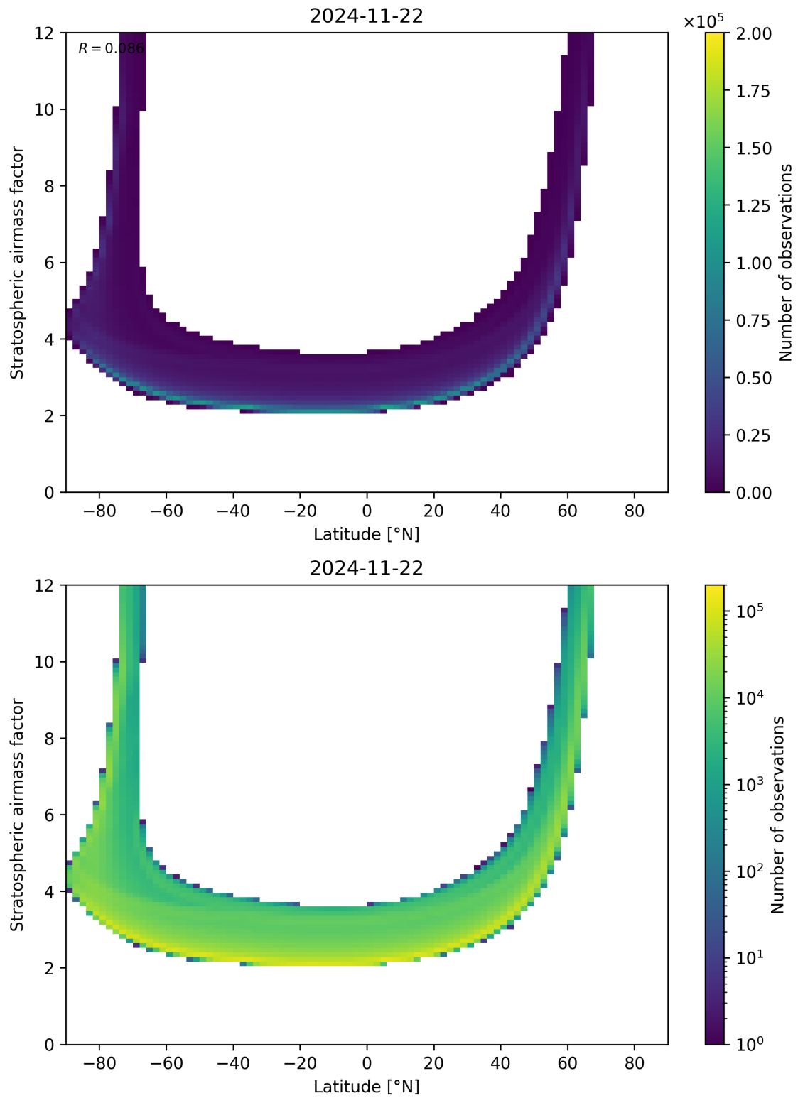
Figure 83: Scatter density plot of “Latitude” against “Stratospheric air mass factor” for 2024-11-21 to 2024-11-23.
