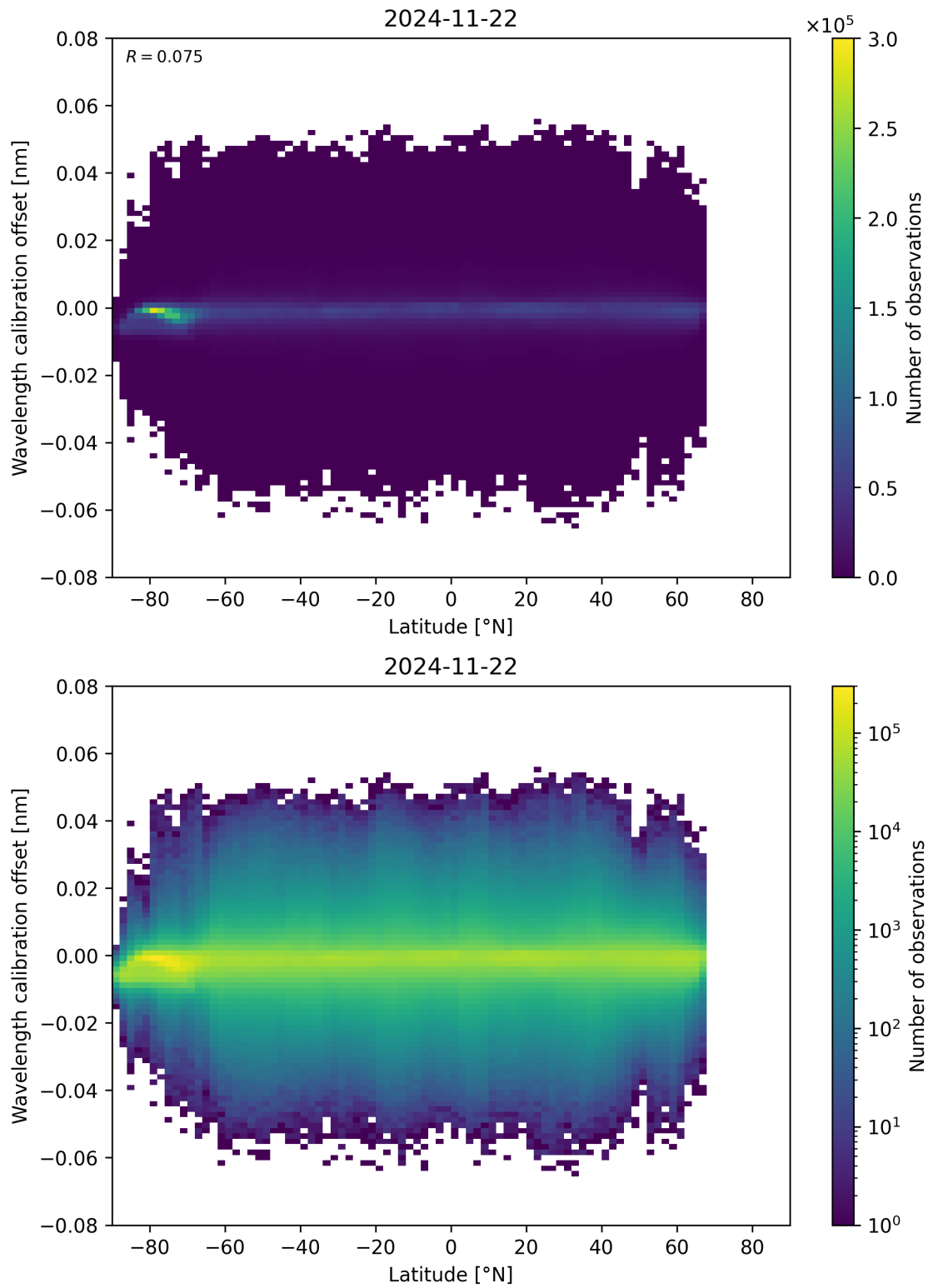
Figure 95: Scatter density plot of “Latitude” against “Wavelength calibration offset” for 2024-11-21 to 2024-11-23.
