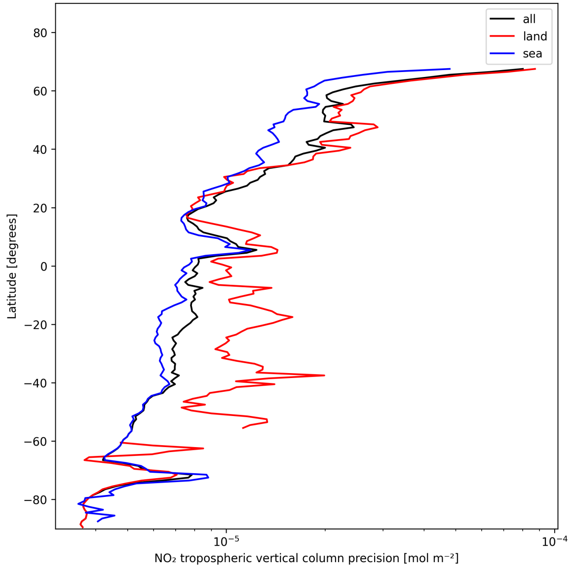
Figure 13: Zonal average of “NO 2 tropospheric vertical column precision” for 2024-11-21 to 2024-11-23.
