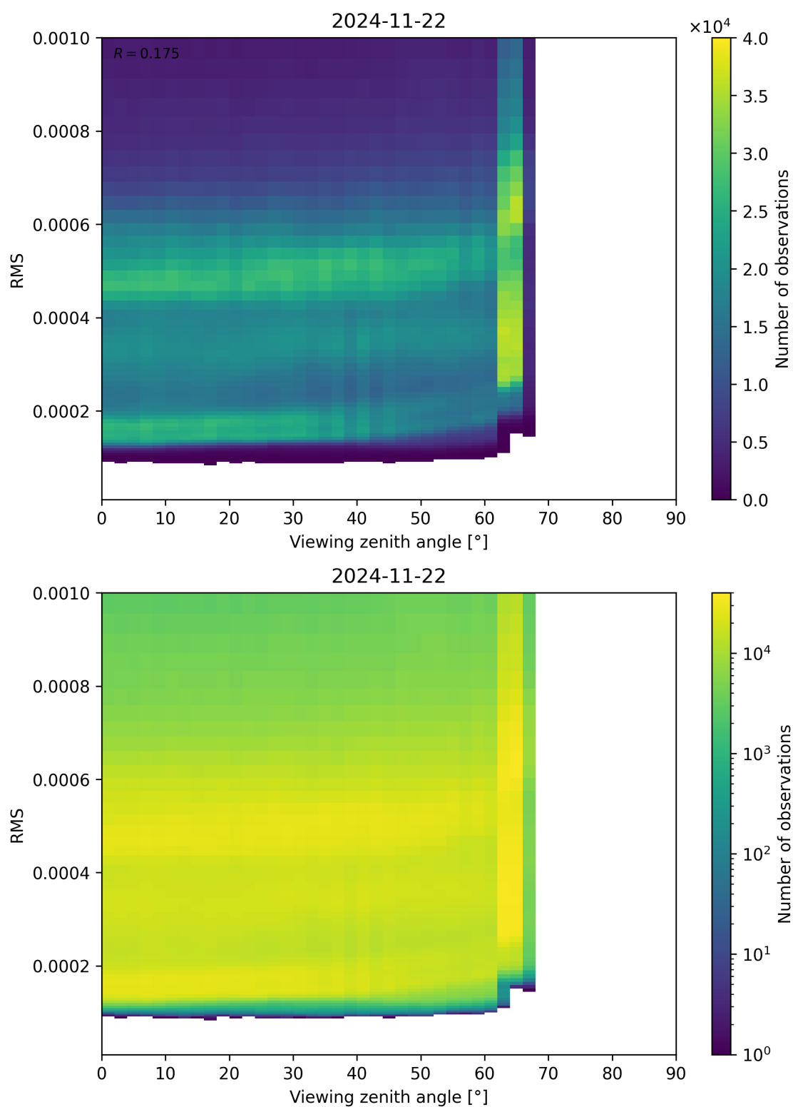
Figure 171: Scatter density plot of “Viewing zenith angle” against “RMS” for 2024-11-21 to 2024-11-23.
