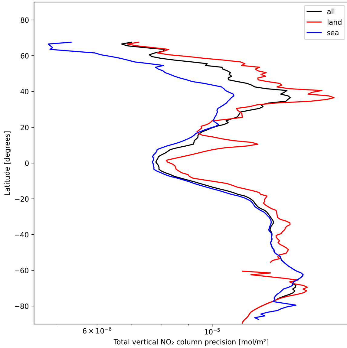
Figure 22: Zonal average of “Total vertical NO 2 column precision” for 2024-11-21 to 2024-11-23.
