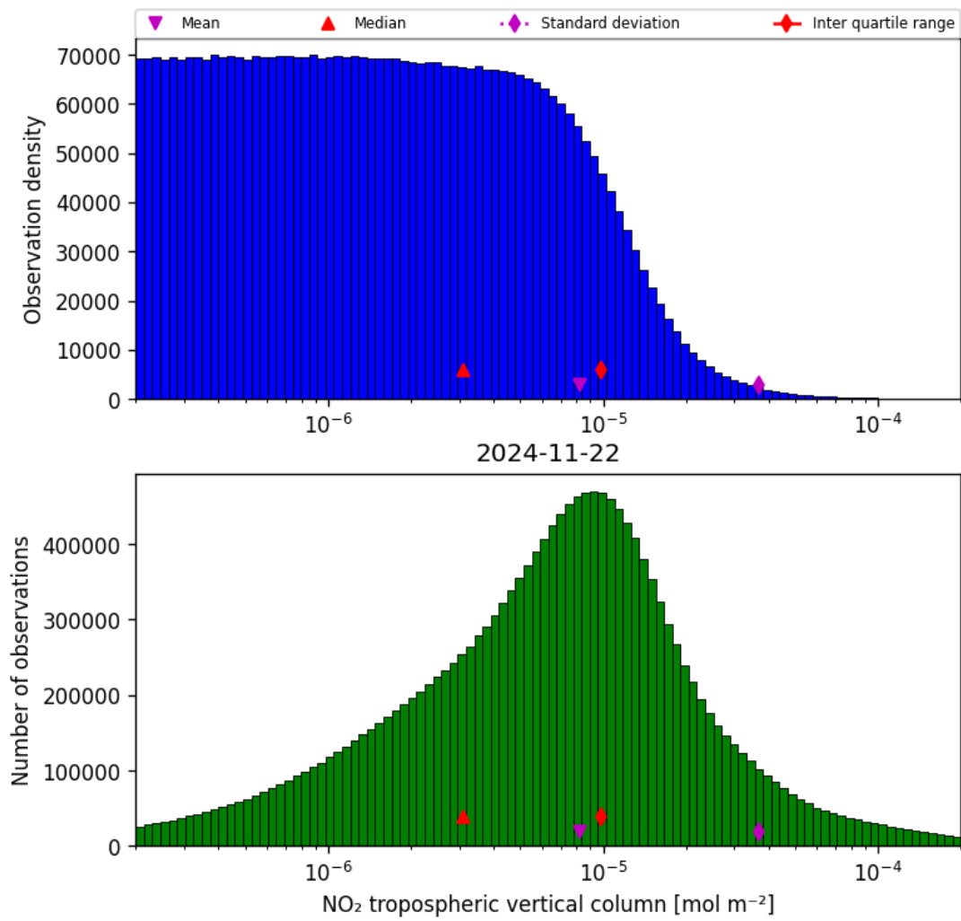
Figure 29: Histogram of “NO 2 tropospheric vertical column” for 2024-11-21 to 2024-11-23
