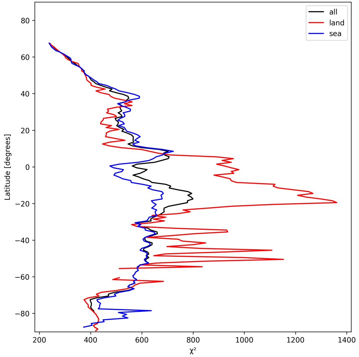
Figure 25: Zonal average of “ \chi^2 ” for 2024-11-21 to 2024-11-23.
