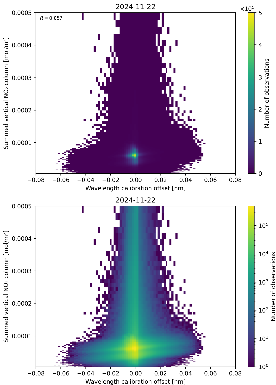
Figure 177: Scatter density plot of “Wavelength calibration offset” against “Summed vertical NO 2 column” for 2024-11-21 to 2024-11-23.
