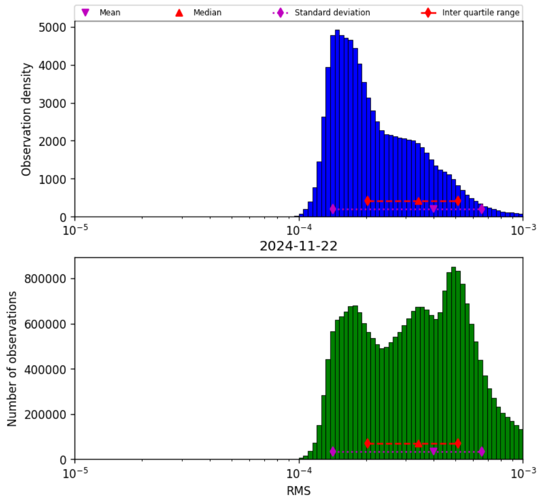
Figure 43: Histogram of “RMS” for 2024-11-21 to 2024-11-23
