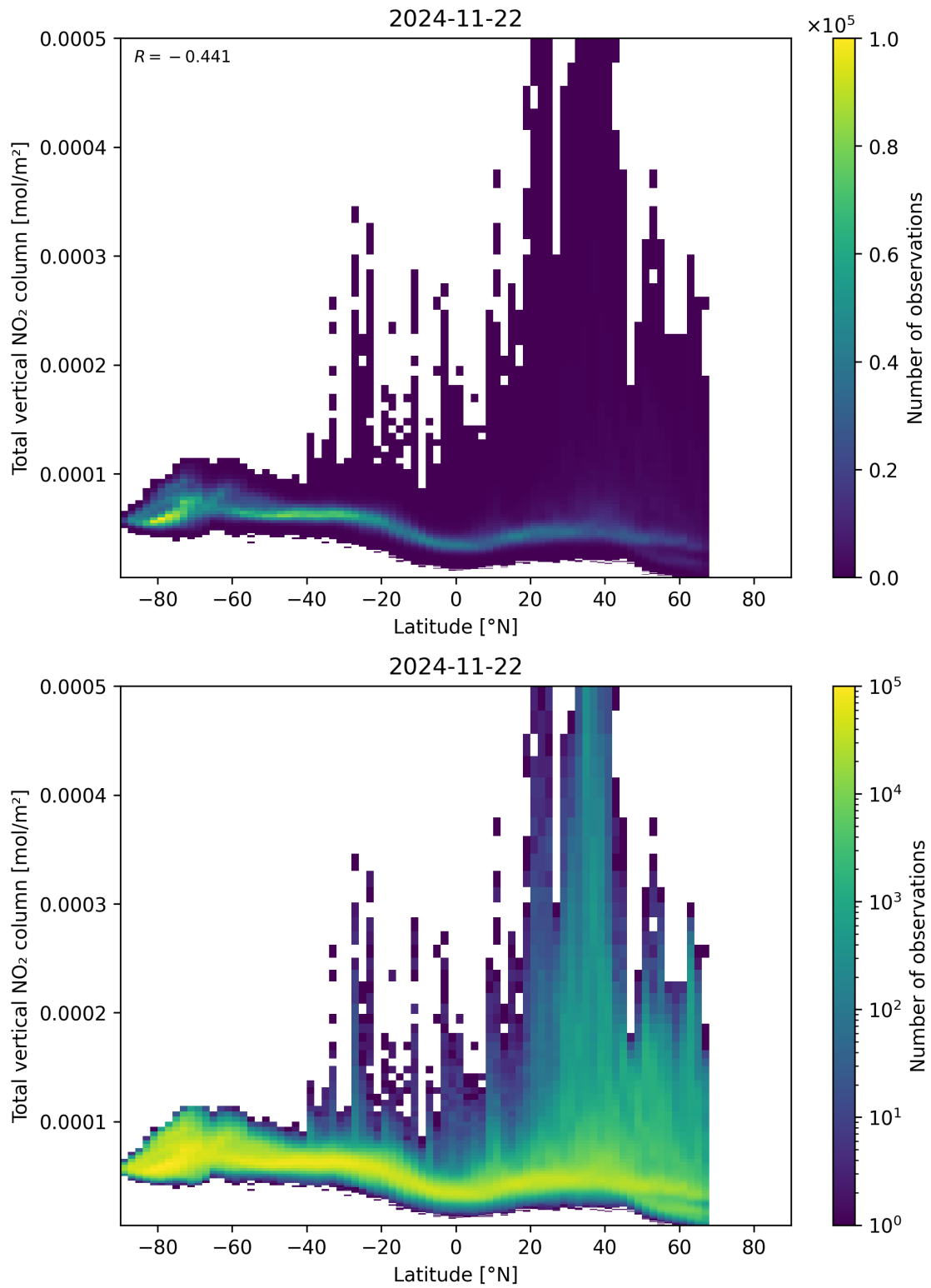
Figure 90: Scatter density plot of “Latitude” against “Total vertical NO 2 column” for 2024-11-21 to 2024-11-23.
