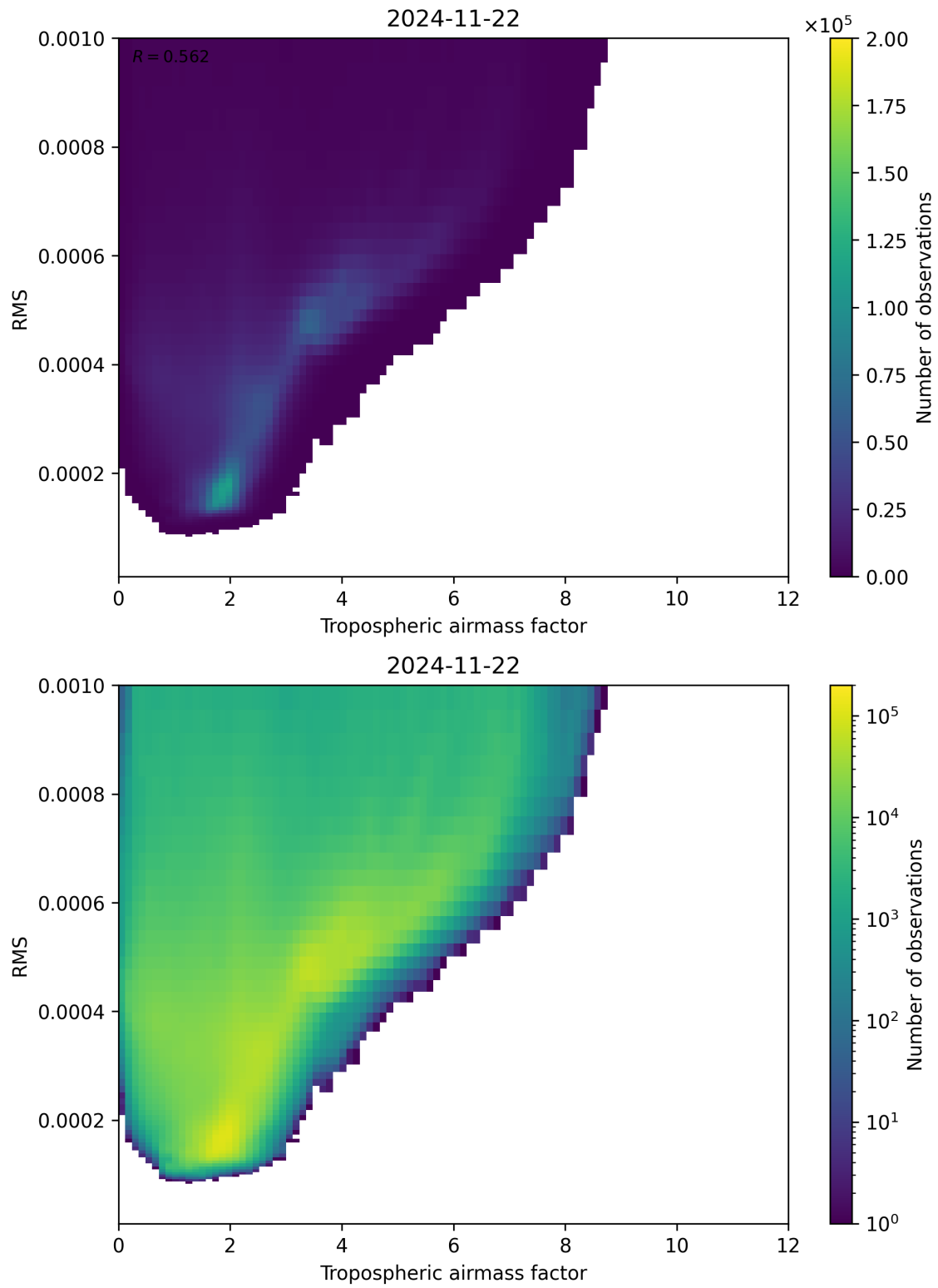
Figure 79: Scatter density plot of “Tropospheric airmass factor” against “RMS” for 2024-11-21 to 2024-11-23.
