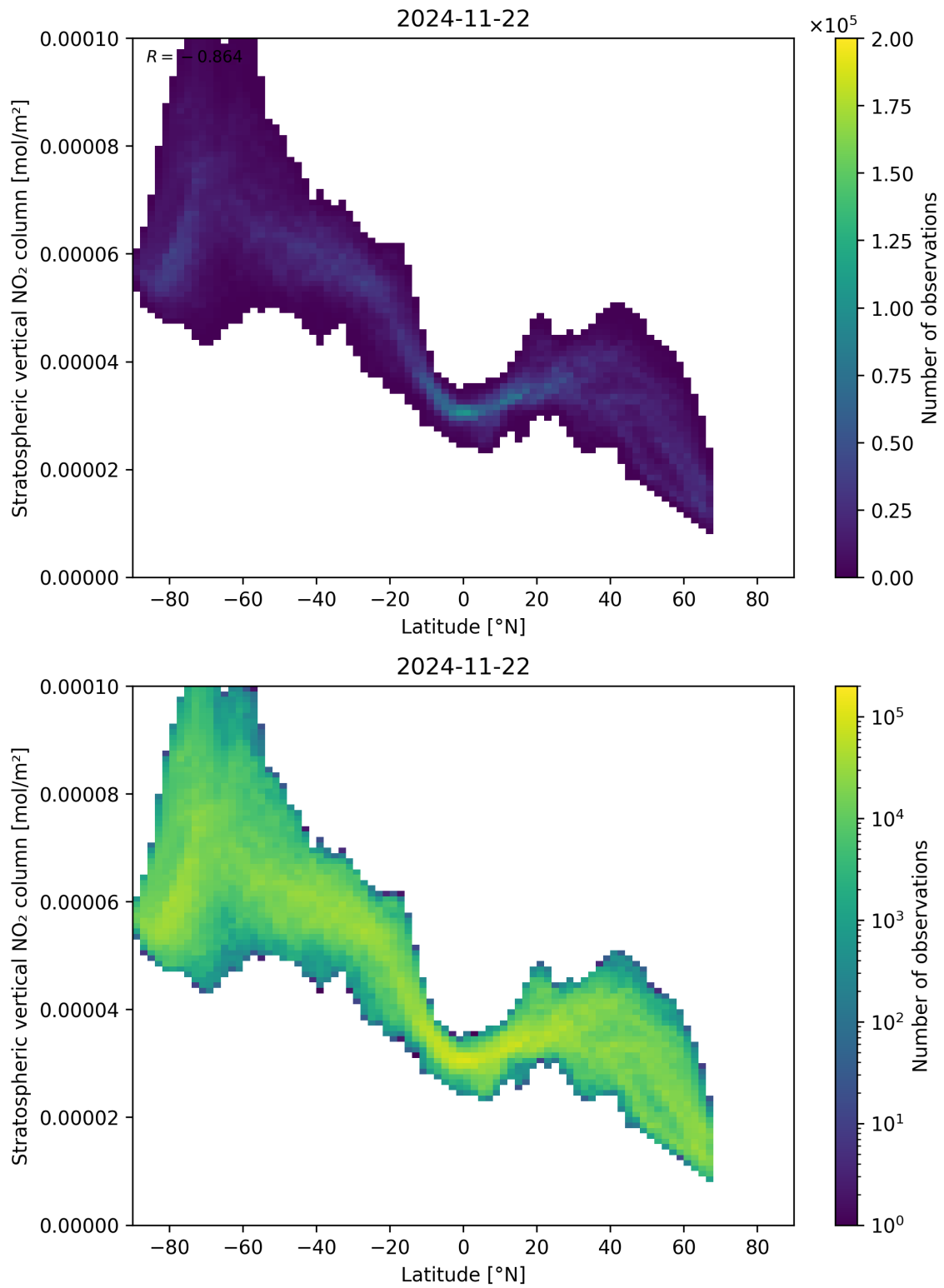
Figure 87: Scatter density plot of “Latitude” against “Stratospheric vertical NO 2 column” for 2024-11-21 to 2024-11-23.
