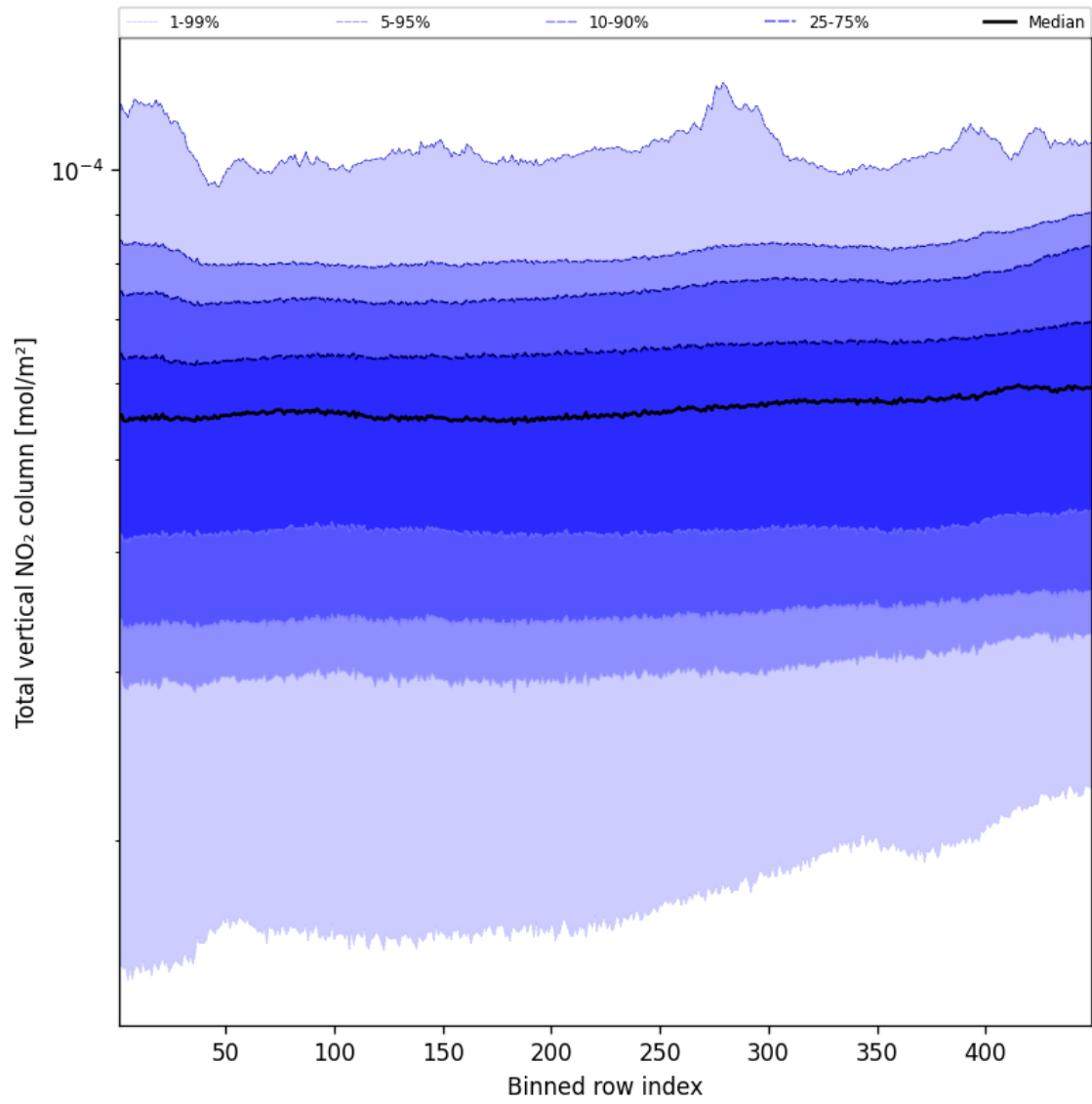
Figure 55: Along track statistics of “Total vertical NO 2 column” for 2024-11-21 to 2024-11-23
