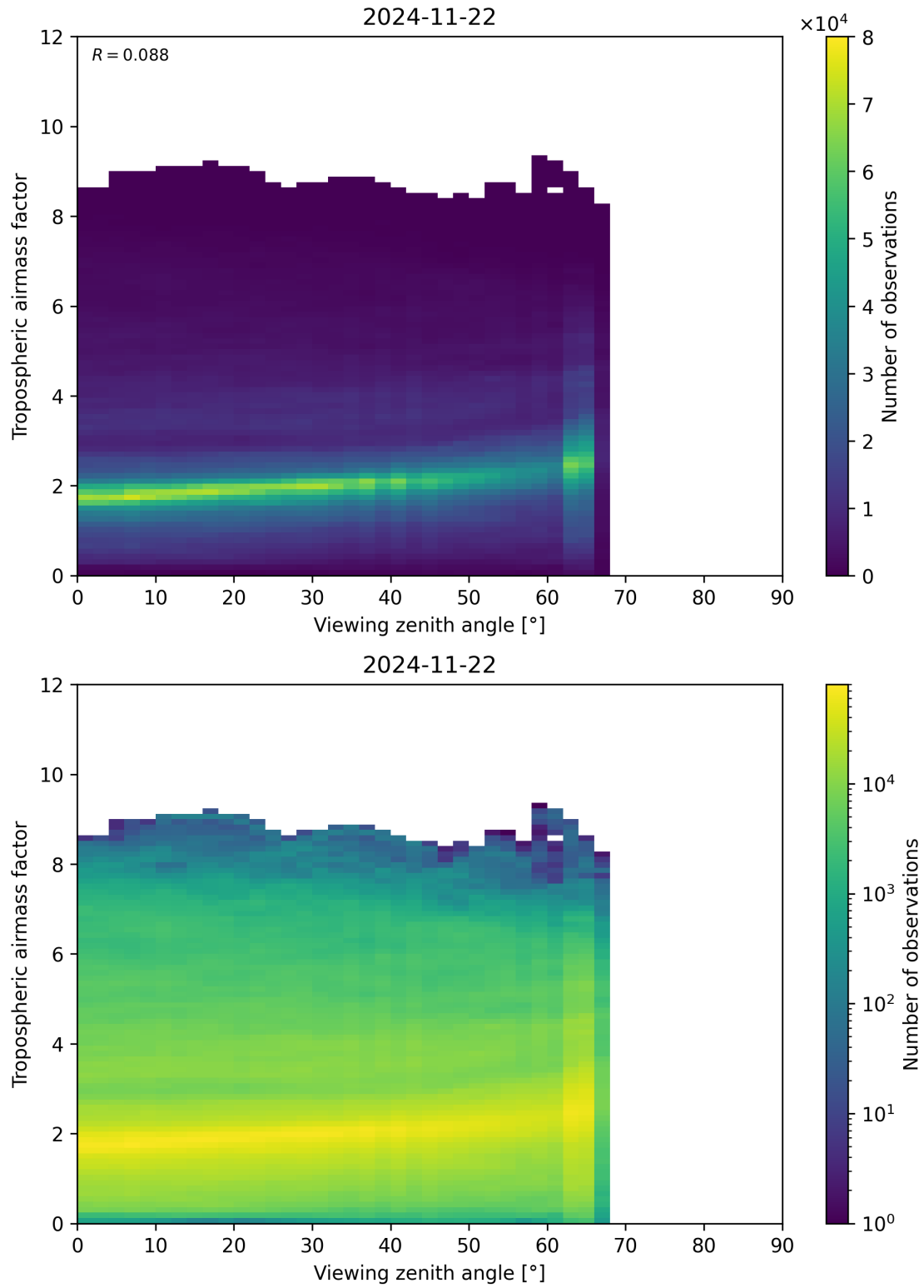
Figure 161: Scatter density plot of “Viewing zenith angle” against “Tropospheric airmass factor” for 2024-11-21 to 2024-11-23.
