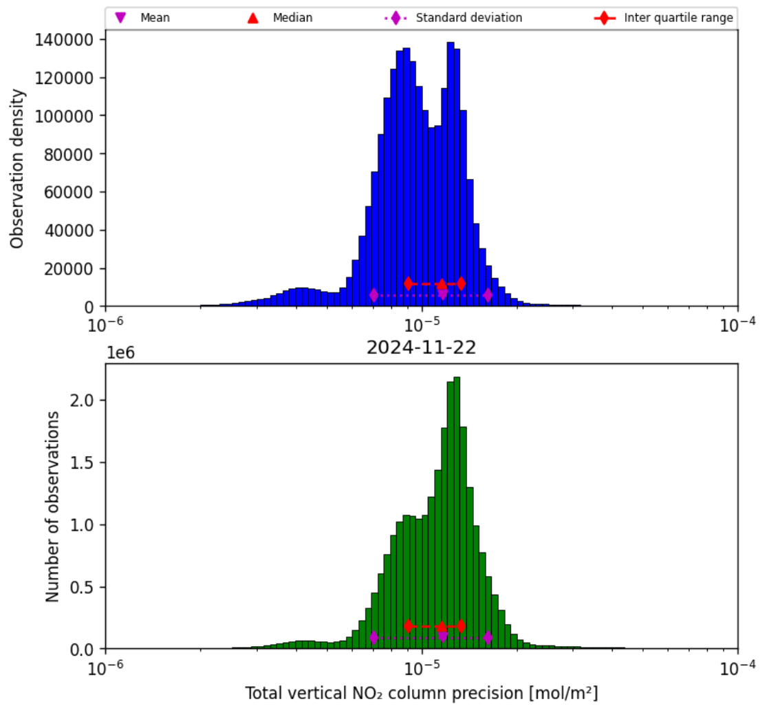
Figure 39: Histogram of “Total vertical NO 2 column precision” for 2024-11-21 to 2024-11-23
