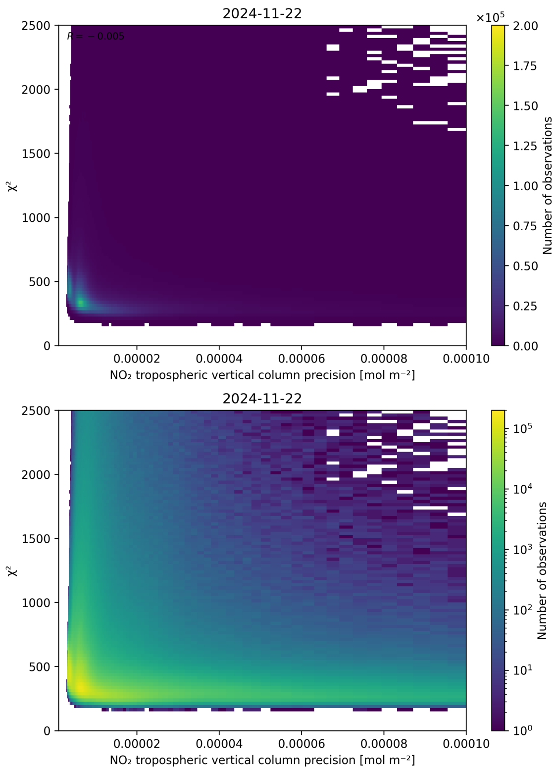
Figure 134: Scatter density plot of “NO 2 tropospheric vertical column precision” against “ \chi^2 ” for 2024-11-21 to 2024-11-23.
