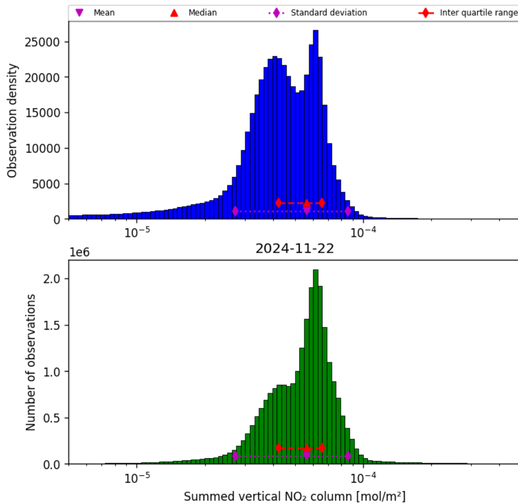
Figure 40: Histogram of “Summed vertical NO 2 column” for 2024-11-21 to 2024-11-23
