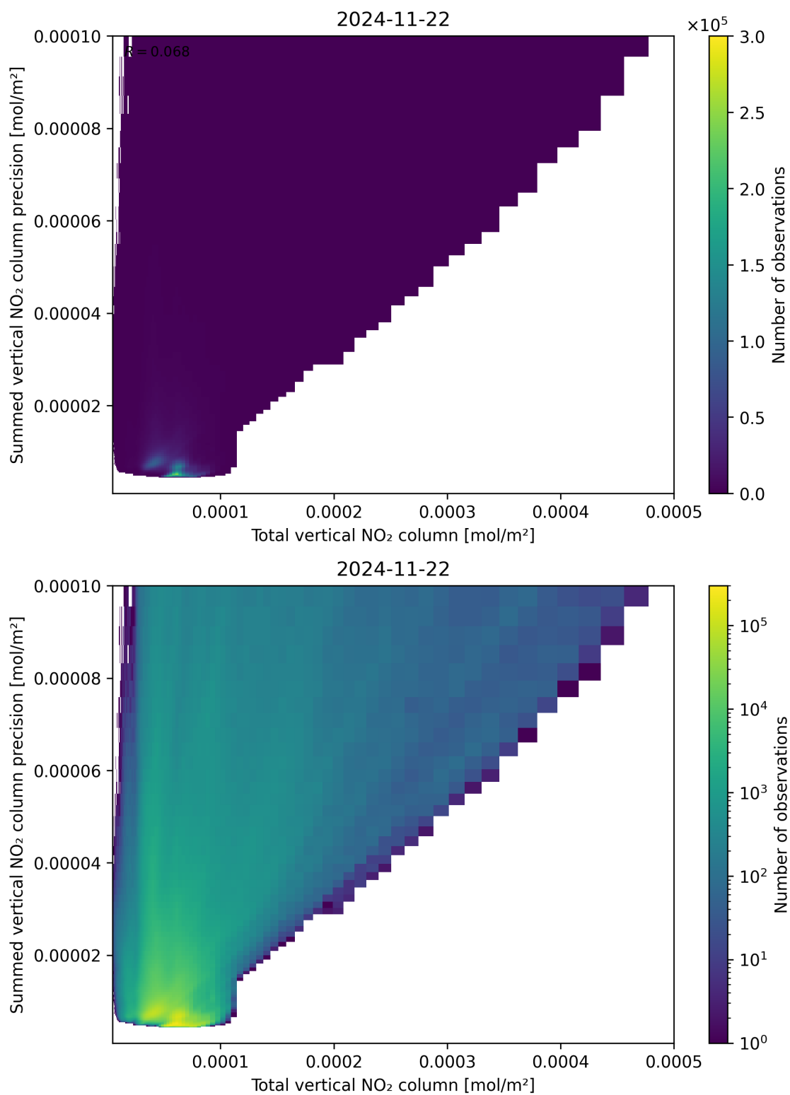
Figure 113: Scatter density plot of “Total vertical NO 2 column” against “Summed vertical NO 2 column precision” for 2024-11-21 to 2024-11-23.
