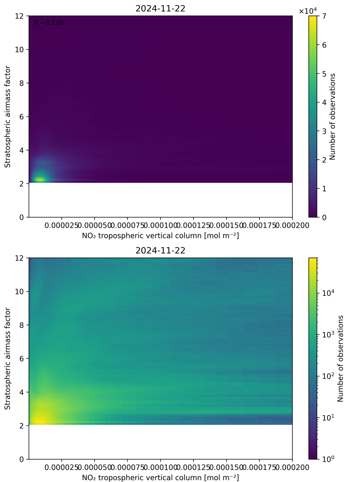
Figure 121: Scatter density plot of “NO 2 tropospheric vertical column” against “Stratospheric airmass factor” for 2024-11-21 to 2024-11-23.
