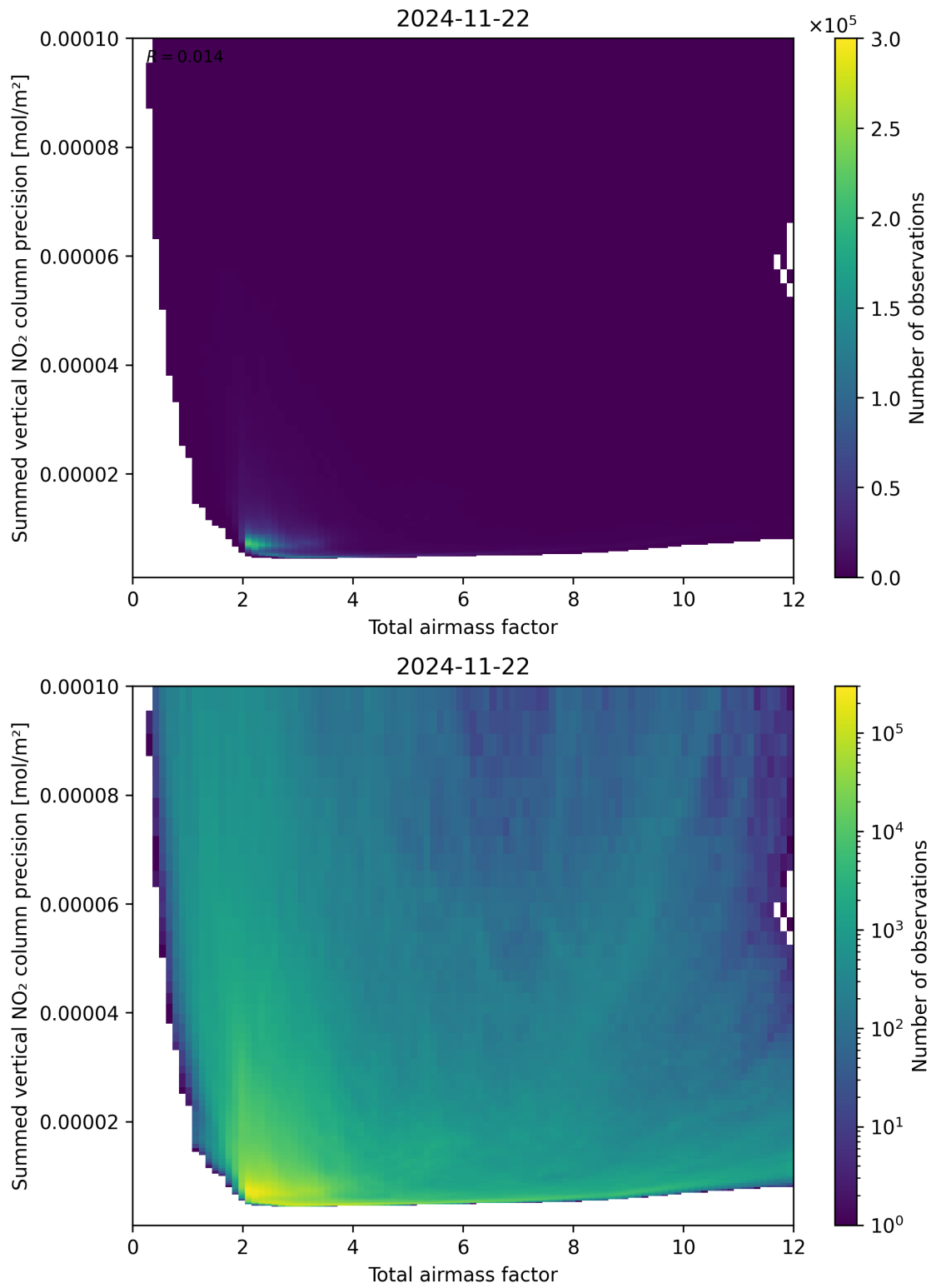
Figure 66: Scatter density plot of “Total airmass factor” against “Summed vertical NO 2 column precision” for 2024-11-21 to 2024-11-23.
