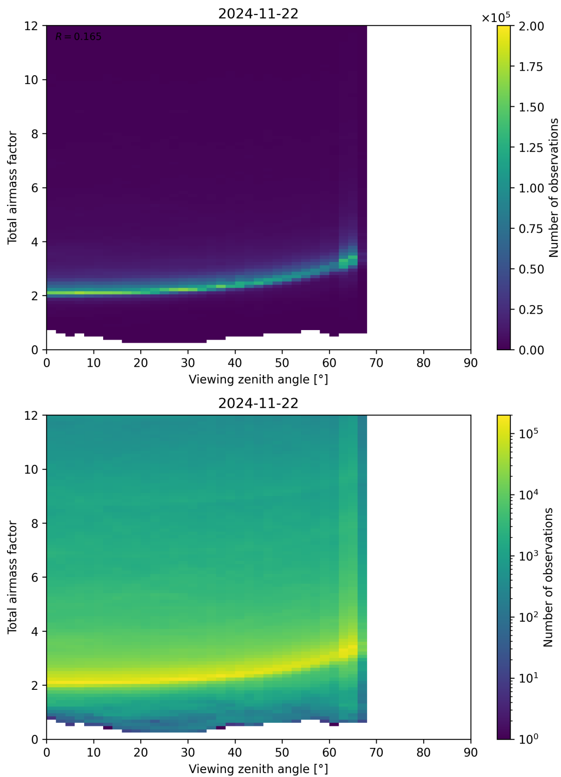
Figure 160: Scatter density plot of “Viewing zenith angle” against “Total airmass factor” for 2024-11-21 to 2024-11-23.
