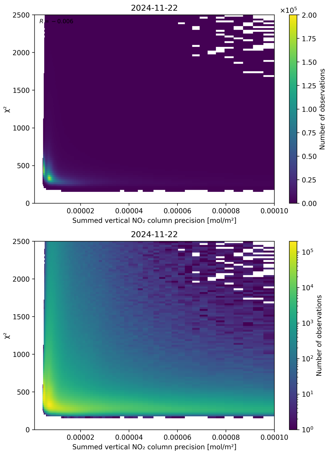
Figure 107: Scatter density plot of “Summed vertical NO 2 column precision” against “ \chi^2 ” for 2024-11-21 to 2024-11-23.
