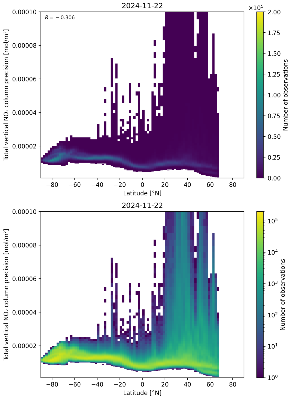
Figure 91: Scatter density plot of “Latitude” against “Total vertical NO 2 column precision” for 2024-11-21 to 2024-11-23.
