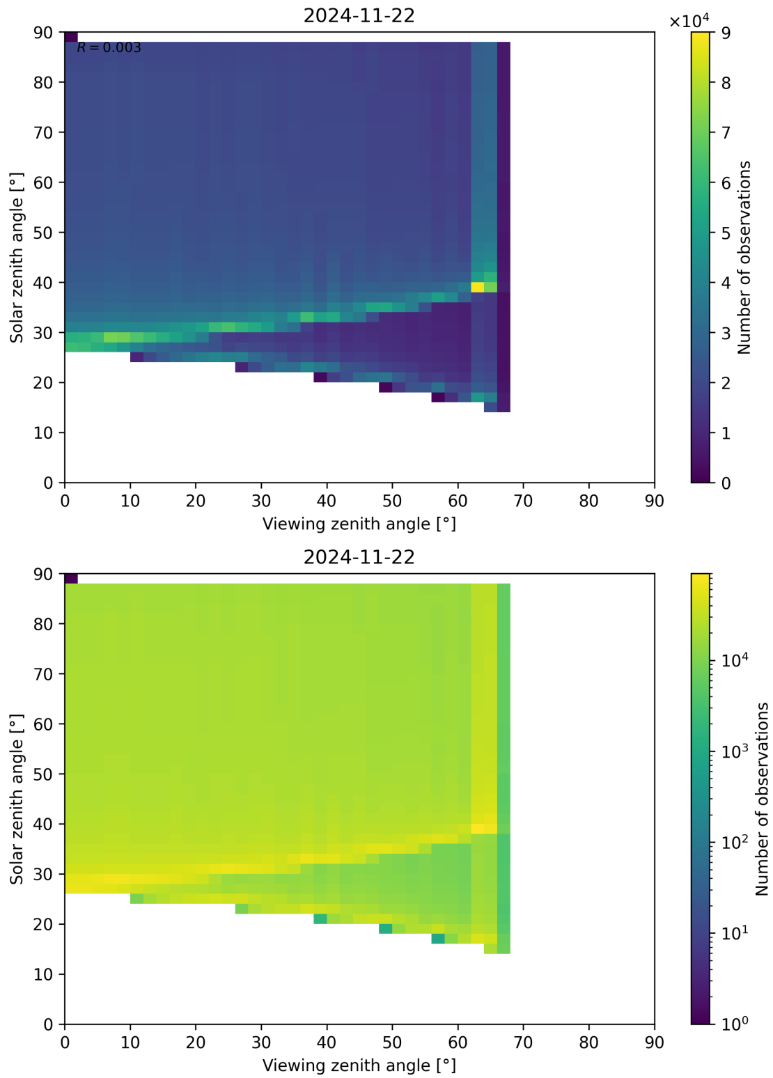
Figure 172: Scatter density plot of “Viewing zenith angle” against “Solar zenith angle” for 2024-11-21 to 2024-11-23.
