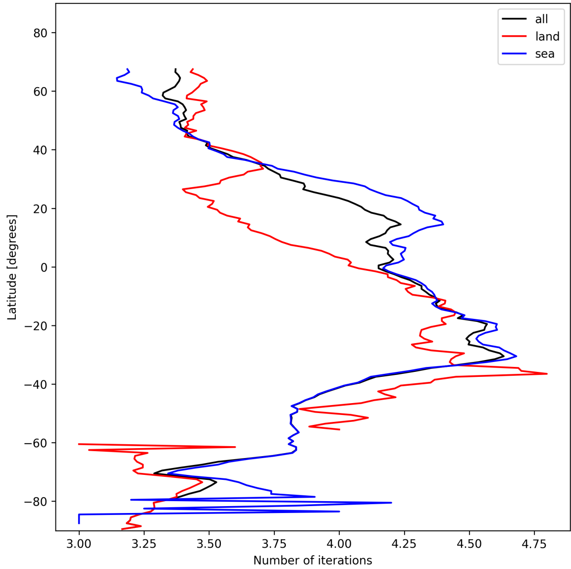
Figure 17: Zonal average of “Number of iterations” for 2024-11-21 to 2024-11-23.
