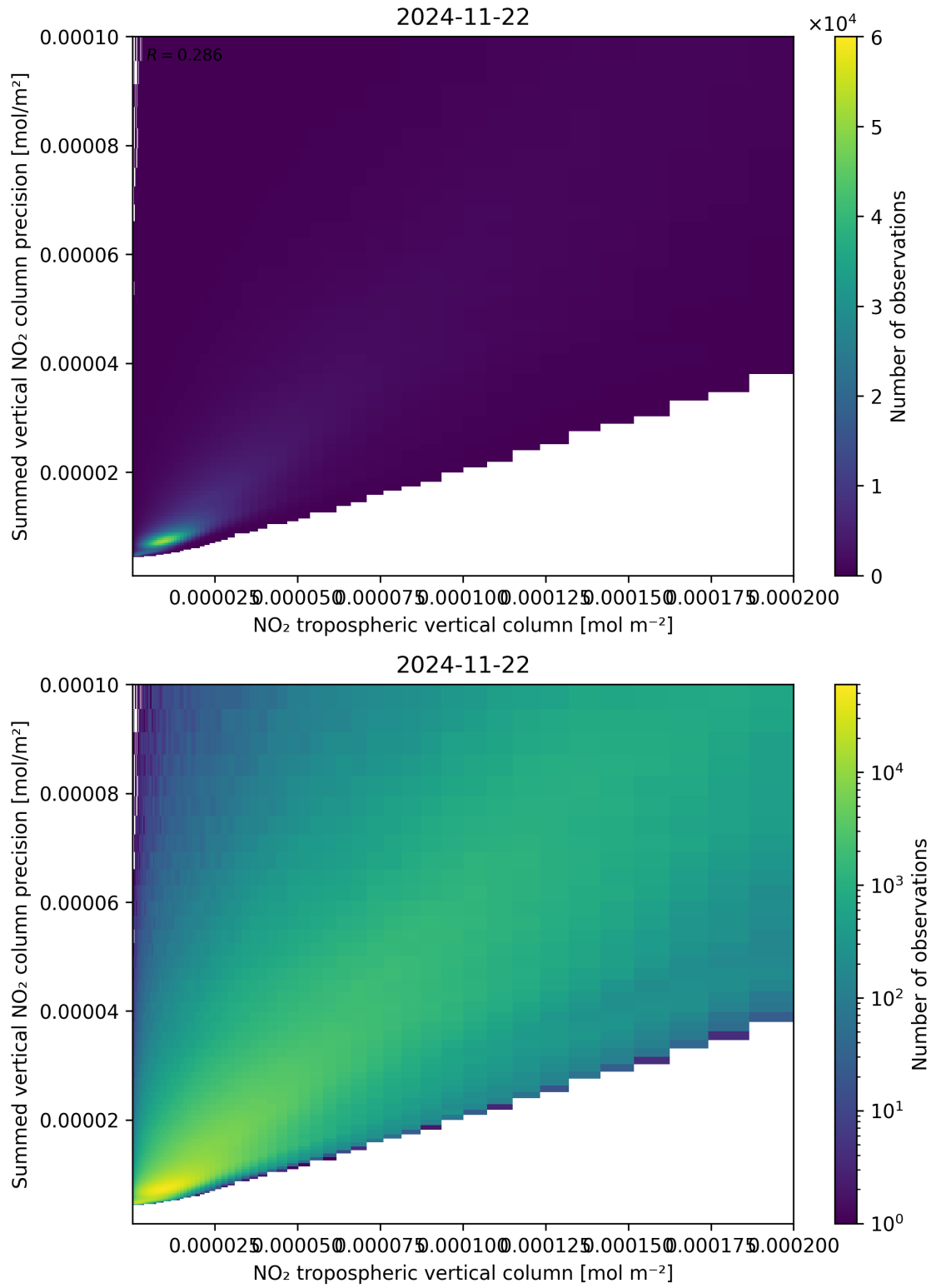
Figure 127: Scatter density plot of “NO 2 tropospheric vertical column” against “Summed vertical NO 2 column precision” for 2024-11-21 to 2024-11-23.
