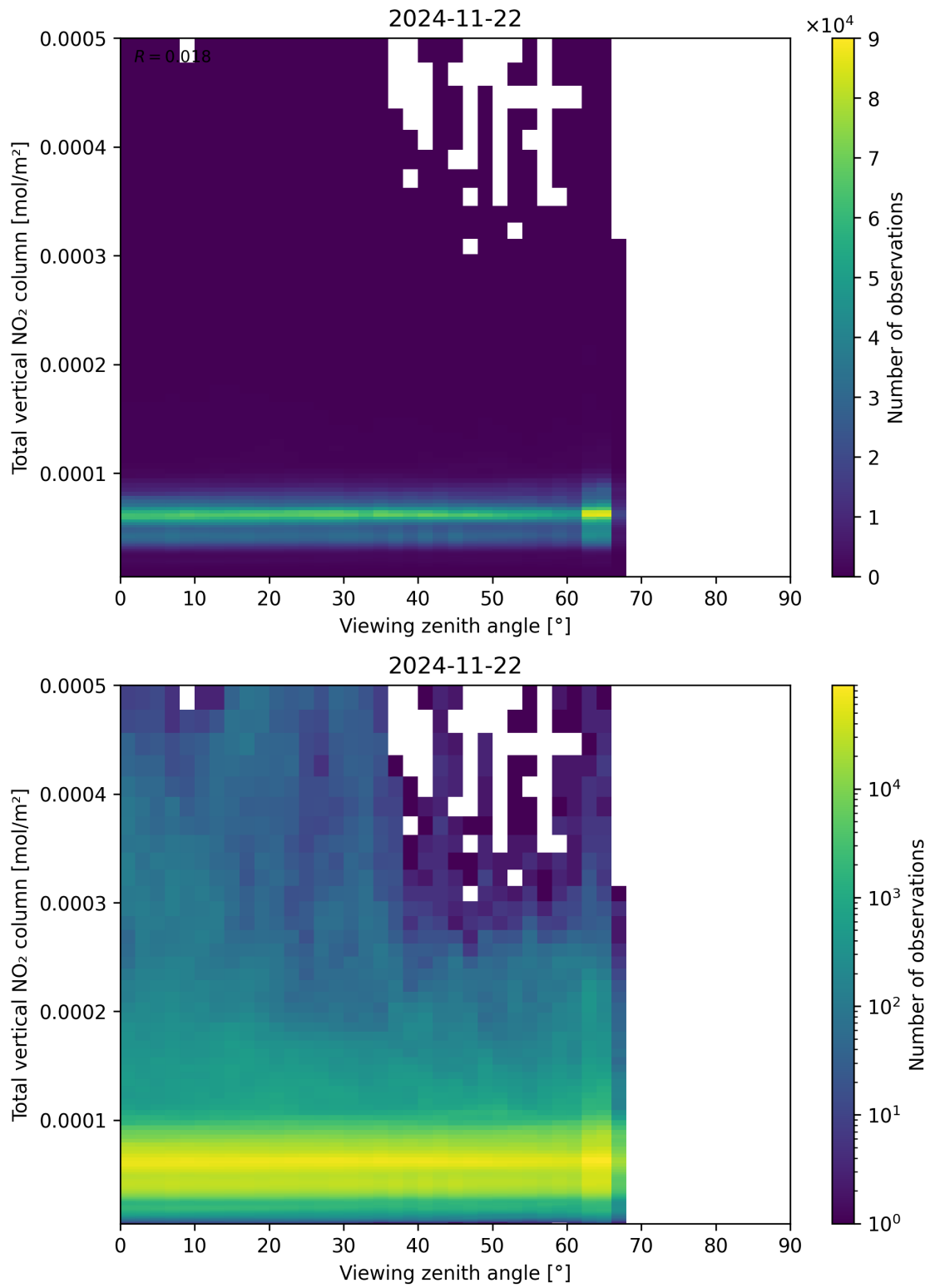
Figure 167: Scatter density plot of “Viewing zenith angle” against “Total vertical NO 2 column” for 2024-11-21 to 2024-11-23.
