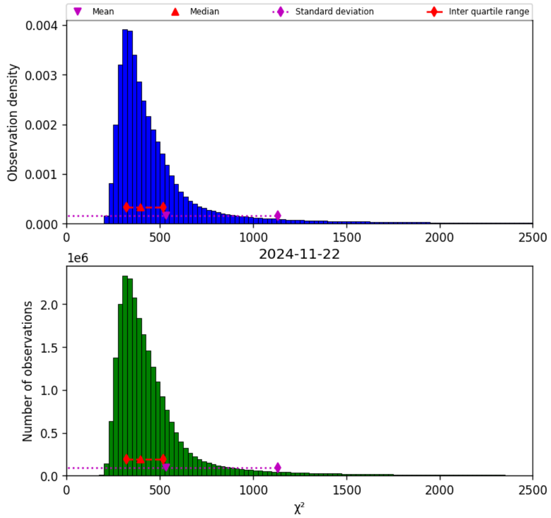
Figure 42: Histogram of “ \chi^2 ” for 2024-11-21 to 2024-11-23
