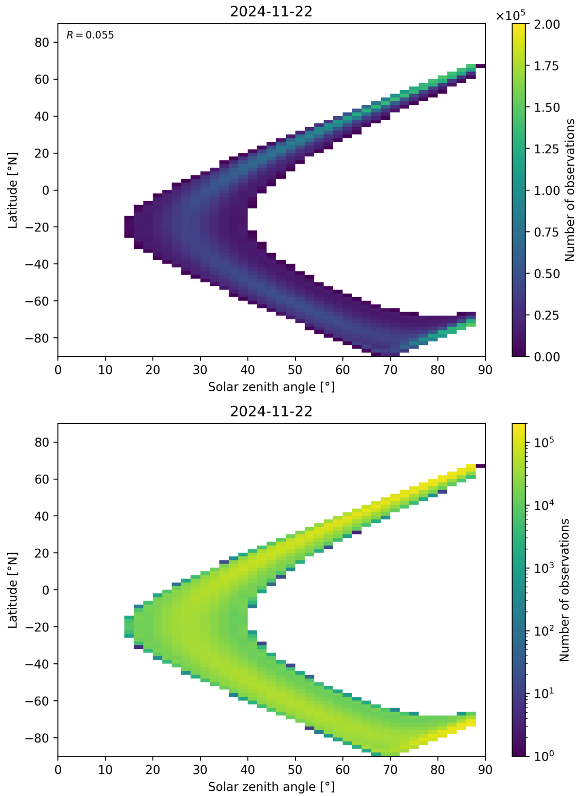
Figure 149: Scatter density plot of “Solar zenith angle” against “Latitude” for 2024-11-21 to 2024-11-23.
