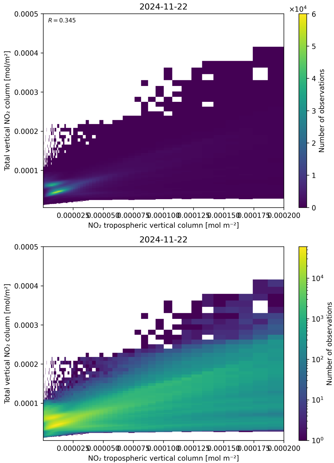
Figure 128: Scatter density plot of “NO 2 tropospheric vertical column” against “Total vertical NO 2 column” for 2024-11-21 to 2024-11-23.
