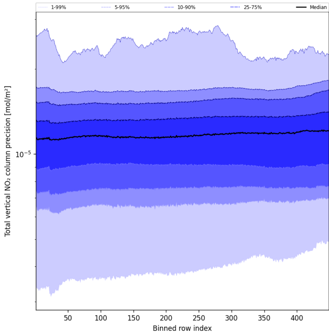
Figure 56: Along track statistics of “Total vertical NO 2 column precision” for 2024-11-21 to 2024-11-23
