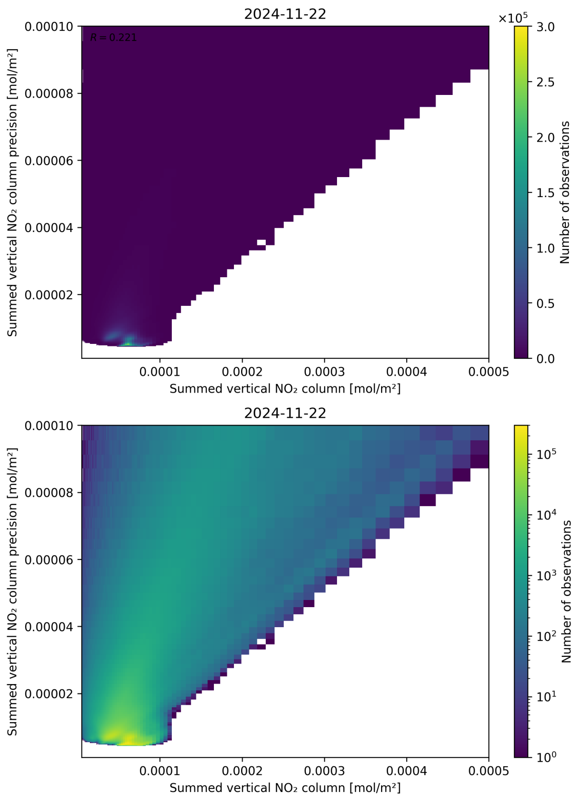
Figure 105: Scatter density plot of “Summed vertical NO 2 column” against “Summed vertical NO 2 column precision” for 2024-11-21 to 2024-11-23.
