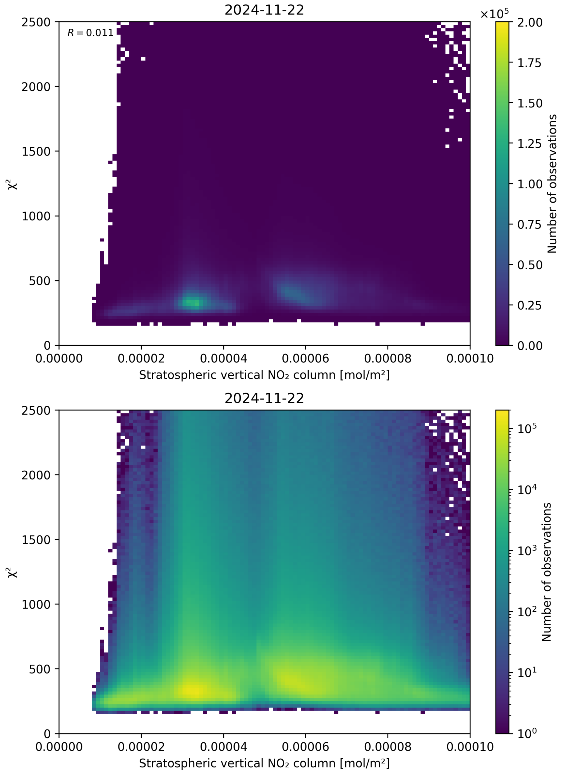
Figure 97: Scatter density plot of “Stratospheric vertical NO 2 column” against “ \chi^2 ” for 2024-11-21 to 2024-11-23.
