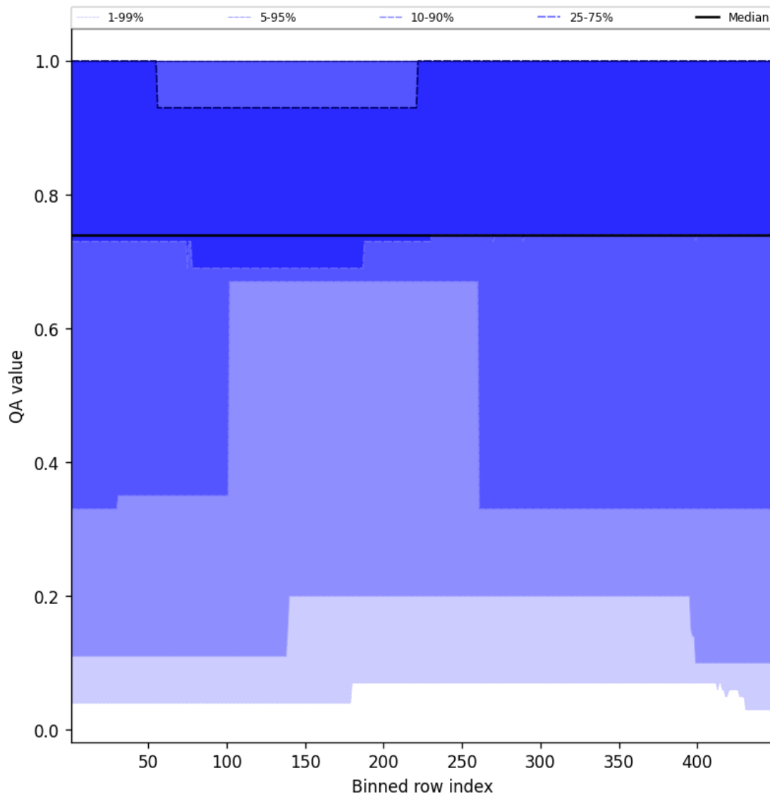
Figure 45: Along track statistics of “QA value” for 2024-11-21 to 2024-11-23
