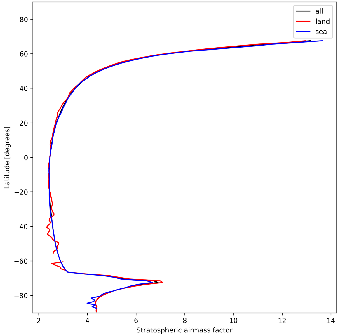
Figure 27: Zonal average of “Stratospheric airmass factor” for 2024-11-21 to 2024-11-23.
