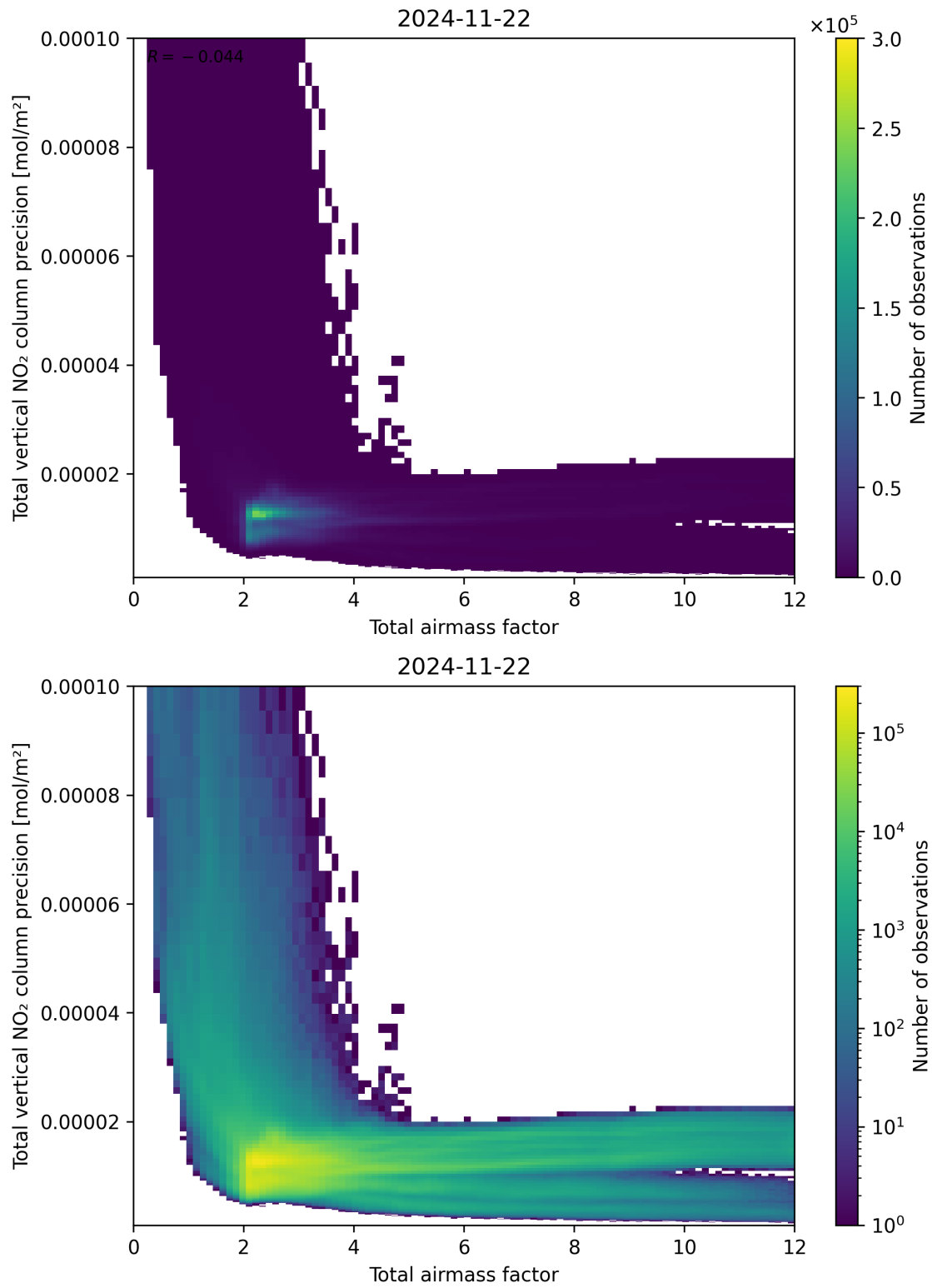
Figure 68: Scatter density plot of “Total airmass factor” against “Total vertical NO 2 column precision” for 2024-11-21 to 2024-11-23.
