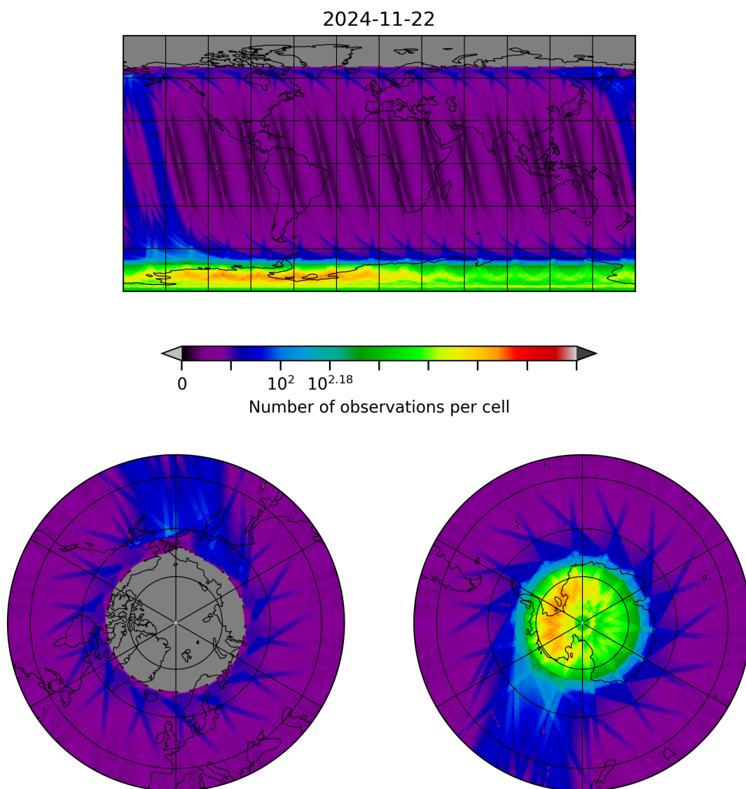
Figure 10: Map of the number of observations for 2024-11-21 to 2024-11-23
