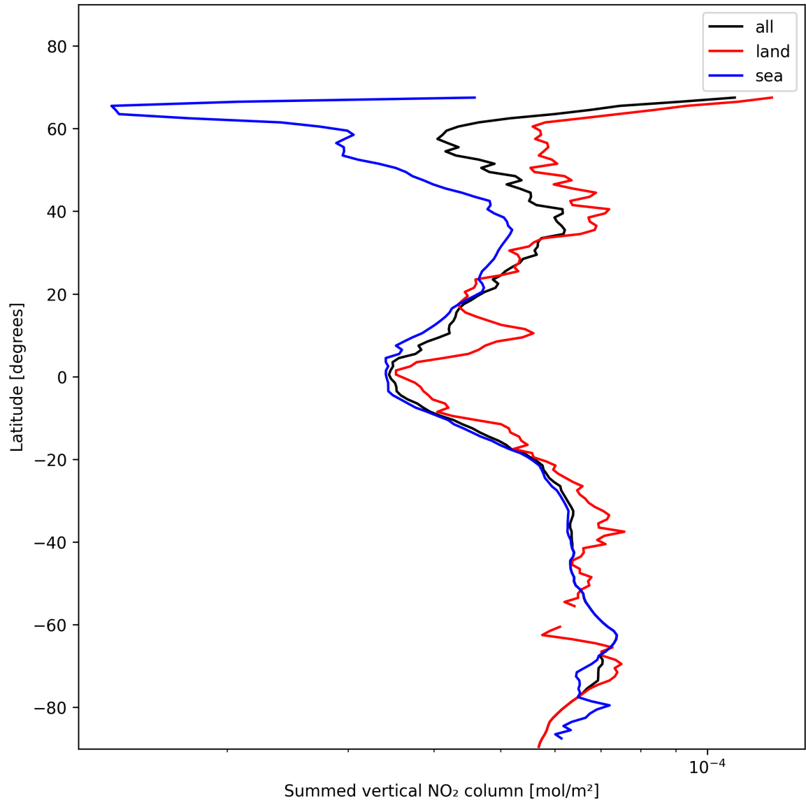
Figure 23: Zonal average of “Summed vertical NO 2 column” for 2024-11-21 to 2024-11-23.
