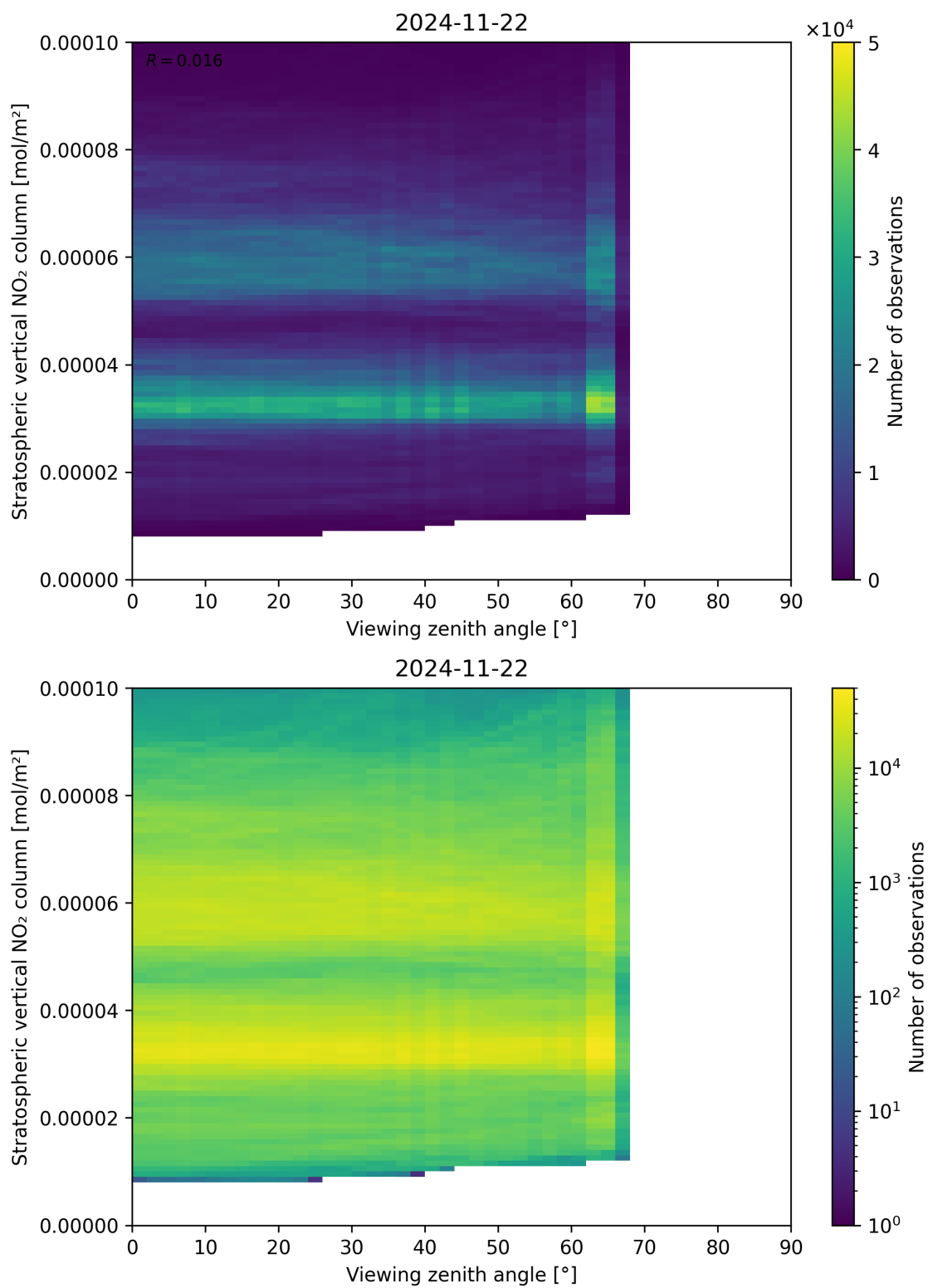
Figure 164: Scatter density plot of “Viewing zenith angle” against “Stratospheric vertical NO 2 column” for 2024-11-21 to 2024-11-23.
