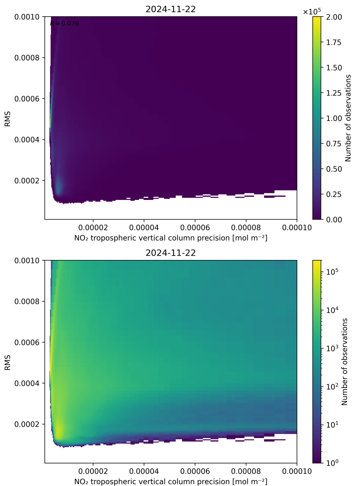
Figure 140: Scatter density plot of “NO 2 tropospheric vertical column precision” against “RMS” for 2024-11-21 to 2024-11-23.
