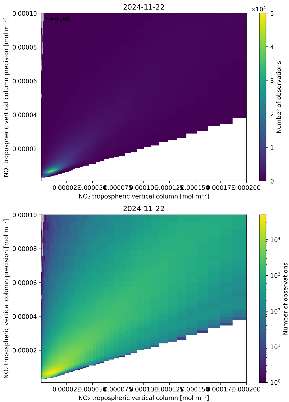
Figure 130: Scatter density plot of “NO 2 tropospheric vertical column” against “NO 2 tropospheric vertical column precision” for 2024-11-21 to 2024-11-23.
