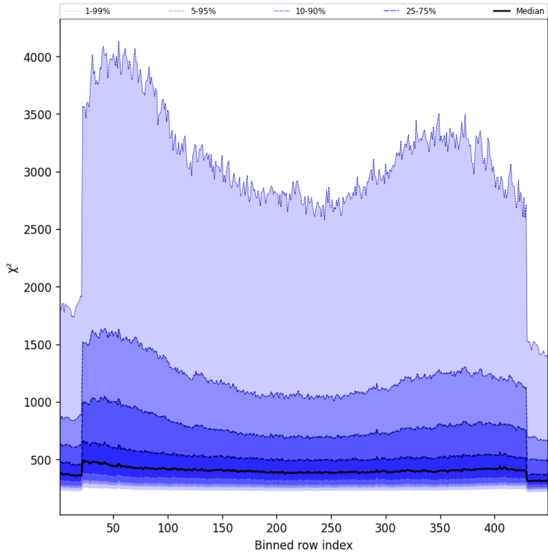
Figure 59: Along track statistics of “ \chi^2 ” for 2024-11-21 to 2024-11-23
