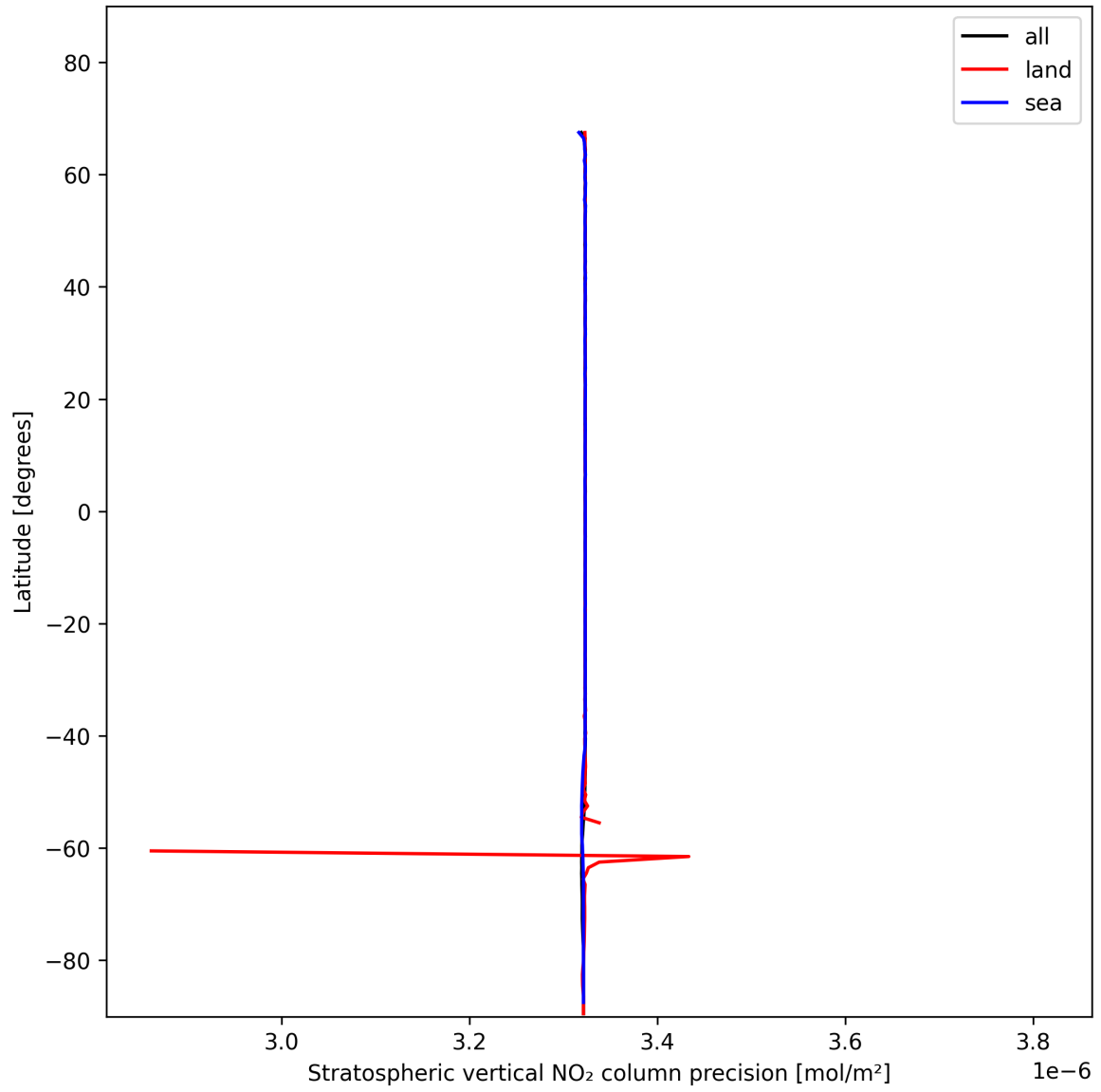
Figure 20: Zonal average of “Stratospheric vertical NO 2 column precision” for 2024-11-21 to 2024-11-23.
