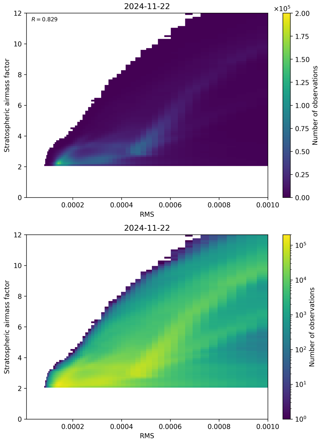
Figure 144: Scatter density plot of “RMS” against “Stratospheric airmass factor” for 2024-11-21 to 2024-11-23.
