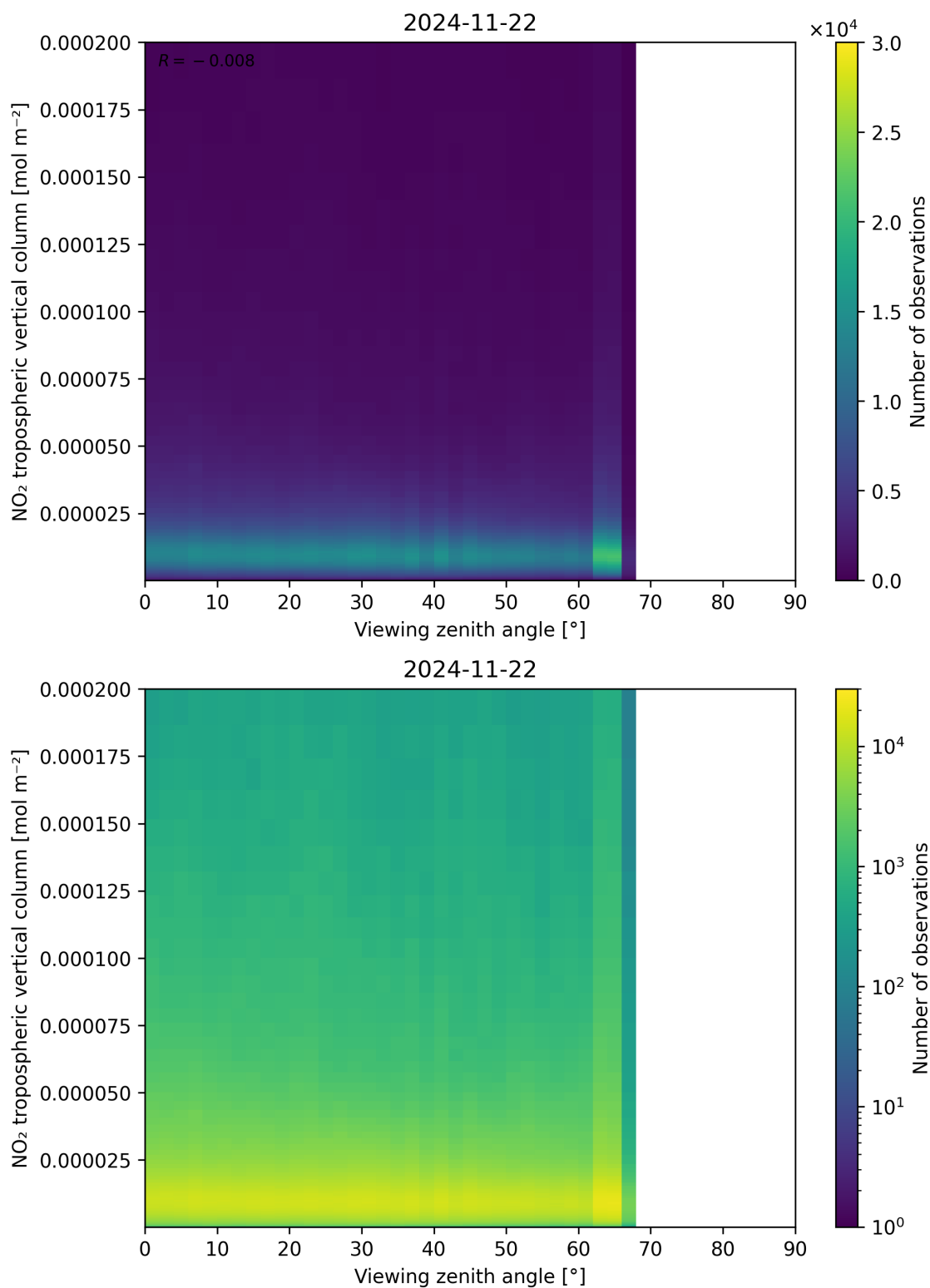
Figure 169: Scatter density plot of “Viewing zenith angle” against “NO 2 tropospheric vertical column” for 2024-11-21 to 2024-11-23.
