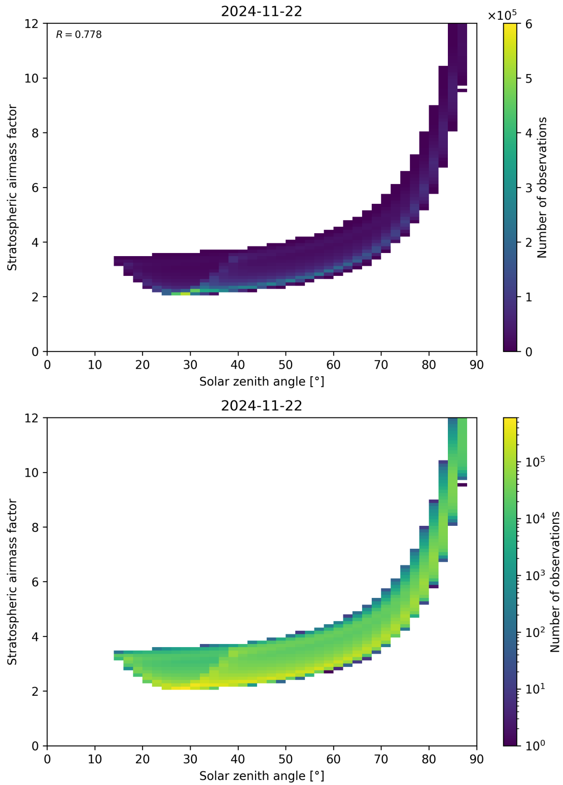
Figure 145: Scatter density plot of “Solar zenith angle” against “Stratospheric airmass factor” for 2024-11-21 to 2024-11-23.
