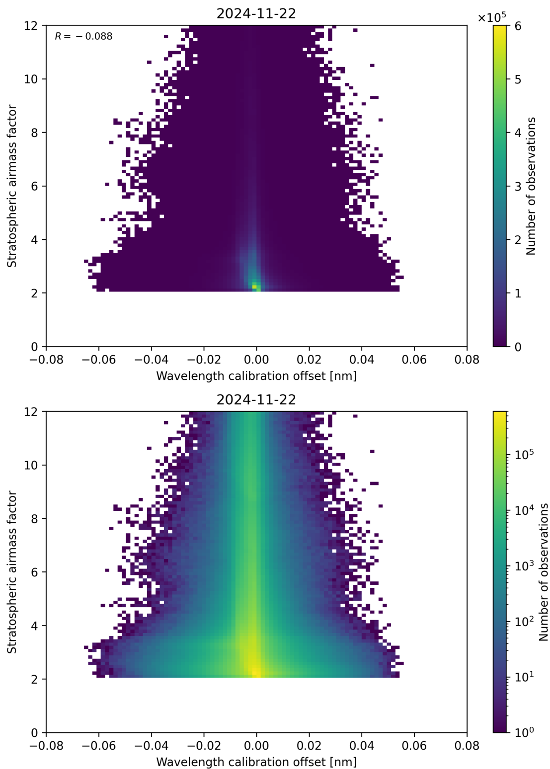
Figure 174: Scatter density plot of “Wavelength calibration offset” against “Stratospheric airmass factor” for 2024-11-21 to 2024-11-23.
