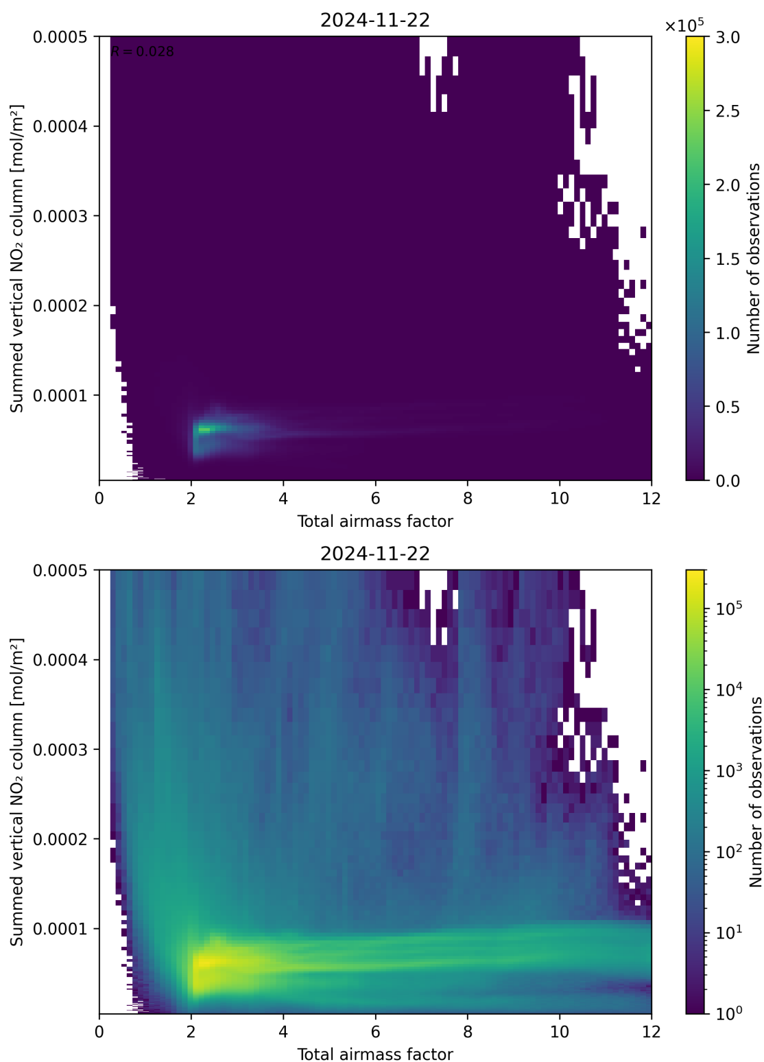
Figure 65: Scatter density plot of “Total airmass factor” against “Summed vertical NO 2 column” for 2024-11-21 to 2024-11-23.
