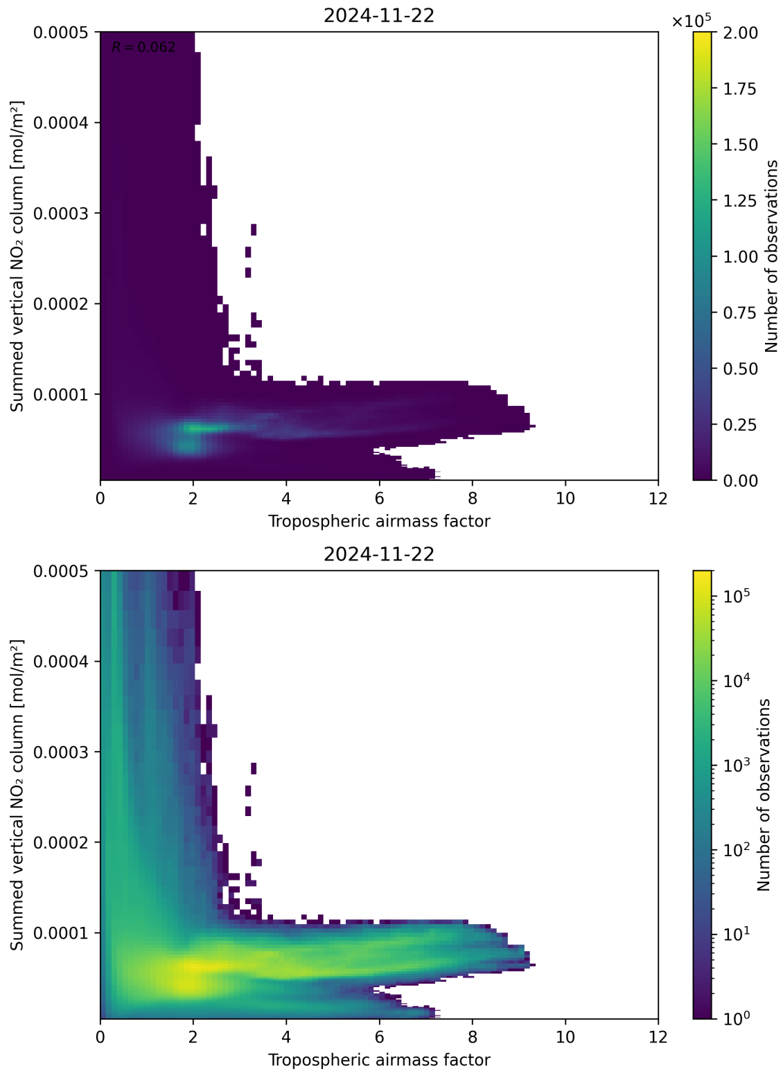
Figure 75: Scatter density plot of “Tropospheric air mass factor” against “Summed vertical NO 2 column” for 2024-11-21 to 2024-11-23.
