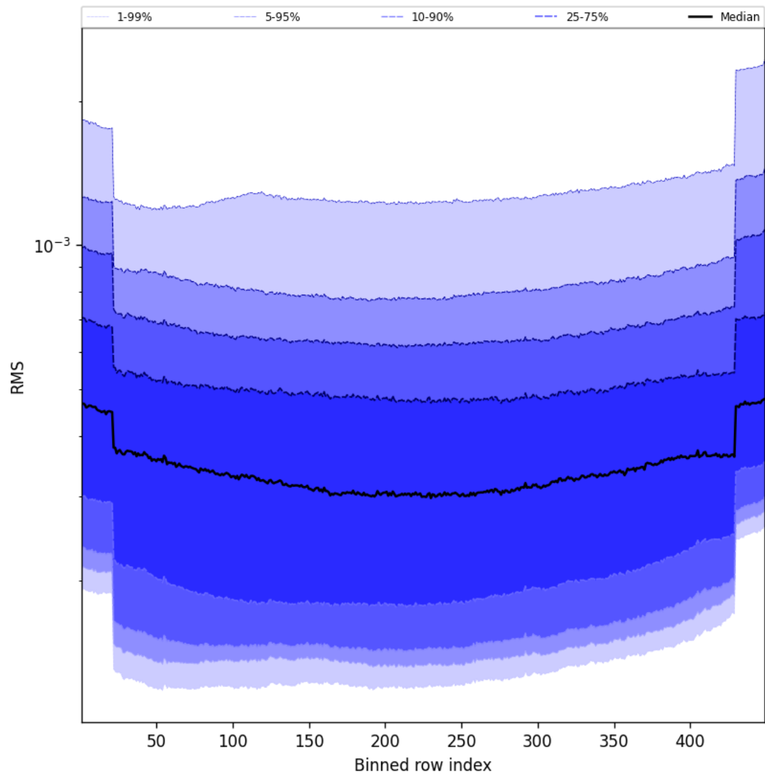
Figure 60: Along track statistics of “RMS” for 2024-11-21 to 2024-11-23
