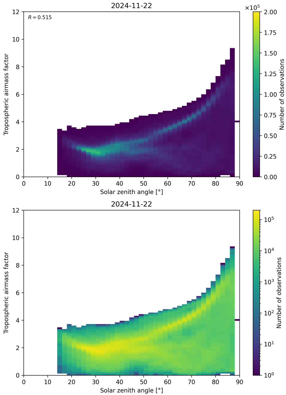
Figure 147: Scatter density plot of “Solar zenith angle” against “Tropospheric airmass factor” for 2024-11-21 to 2024-11-23.
