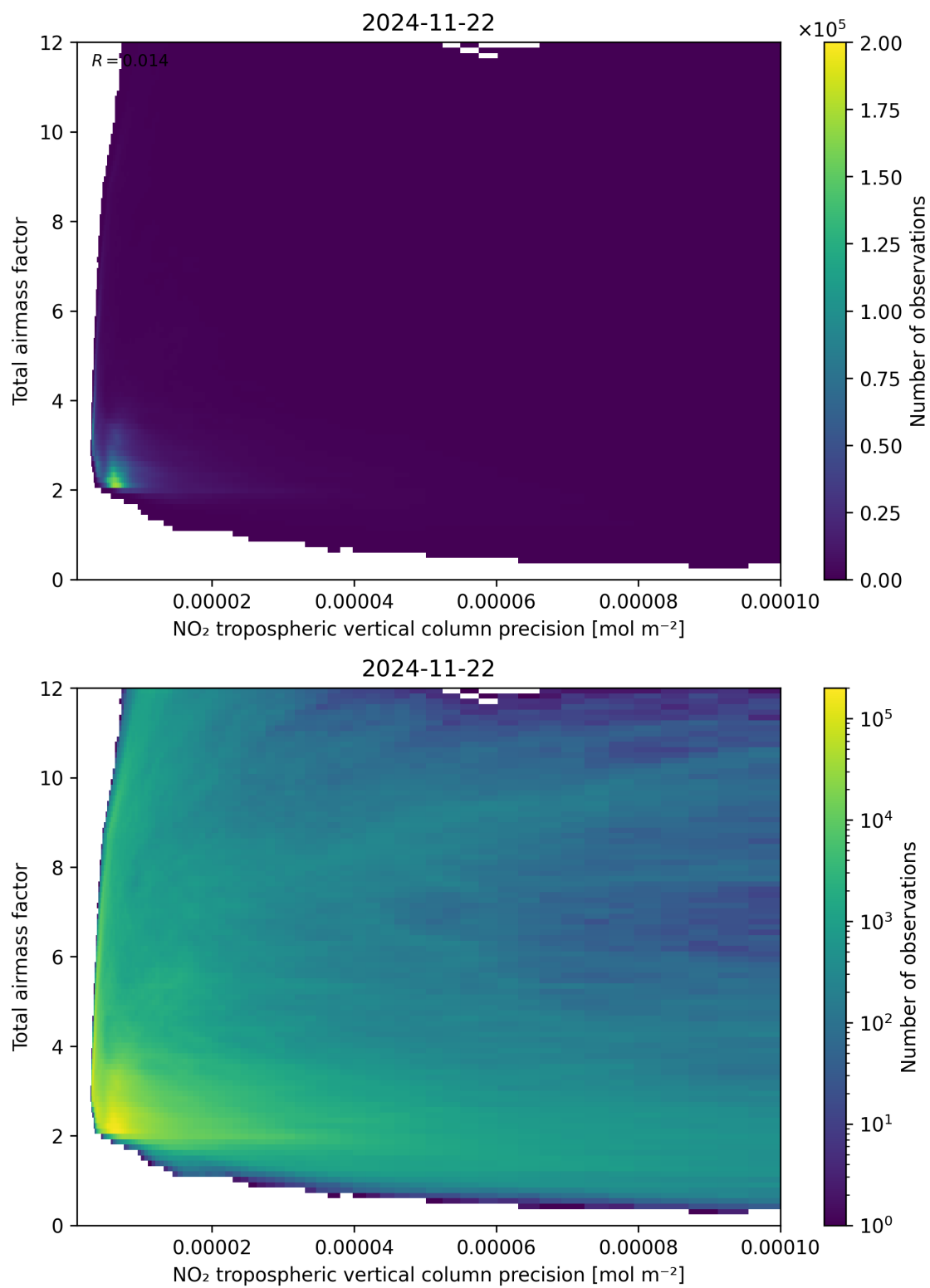
Figure 132: Scatter density plot of “NO 2 tropospheric vertical column precision” against “Total air mass factor” for 2024-11-21 to 2024-11-23.
