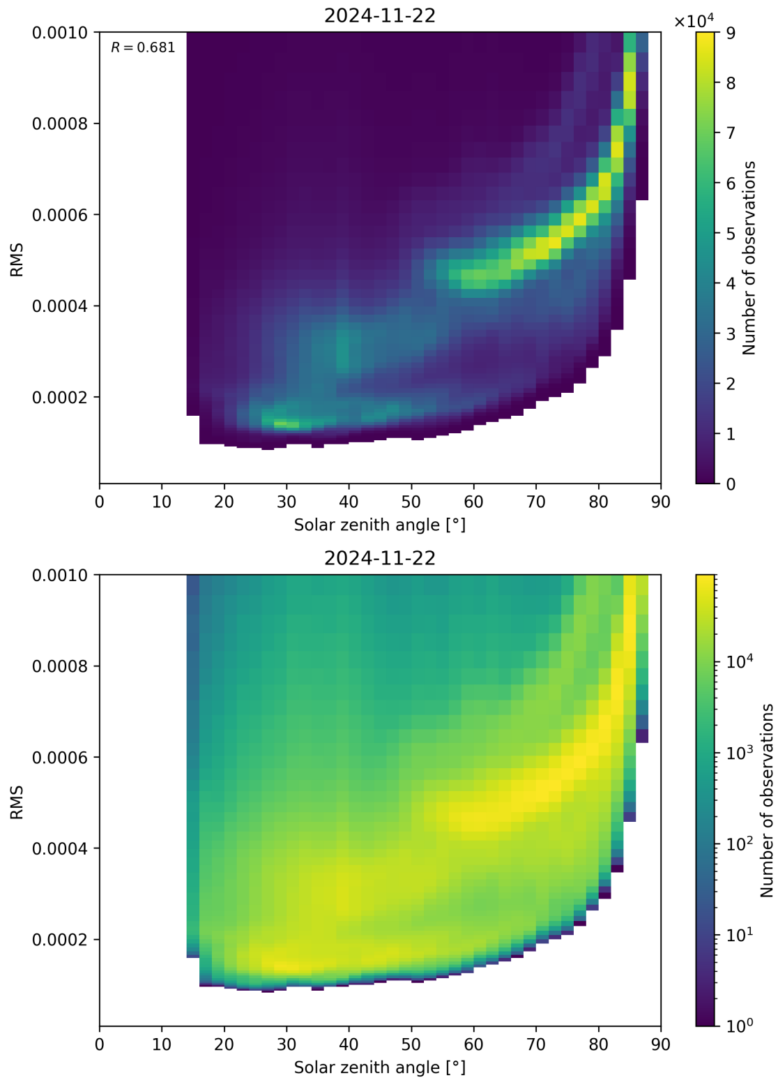
Figure 157: Scatter density plot of “Solar zenith angle” against “RMS” for 2024-11-21 to 2024-11-23.
