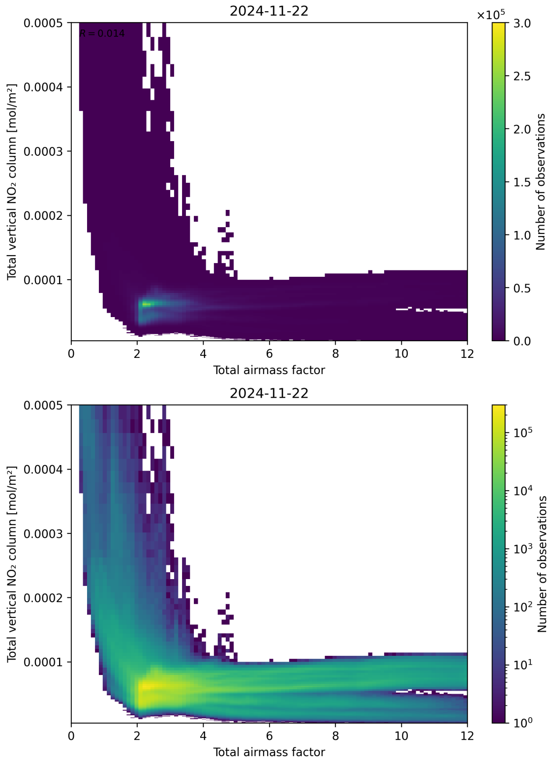
Figure 67: Scatter density plot of “Total air mass factor” against “Total vertical \text{NO}_2 column” for 2024-11-21 to 2024-11-23.
