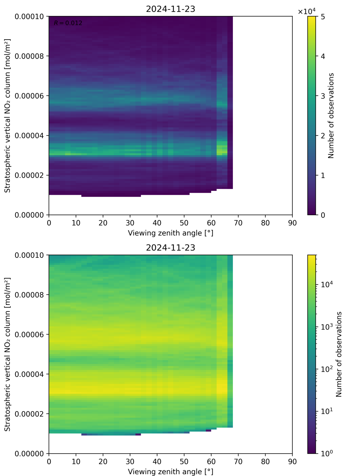
Figure 164: Scatter density plot of “Viewing zenith angle” against “Stratospheric vertical NO 2 column” for 2024-11-22 to 2024-11-24.
