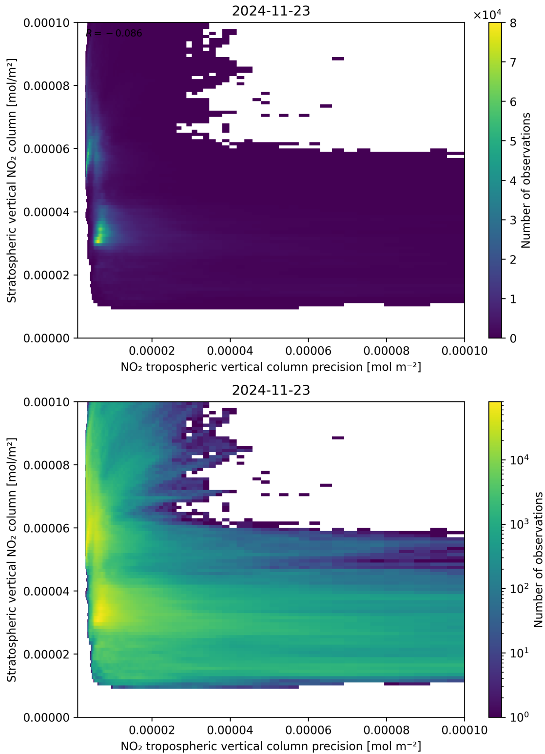
Figure 135: Scatter density plot of “NO 2 tropospheric vertical column precision” against “Stratospheric vertical NO 2 column” for 2024-11-22 to 2024-11-24.
