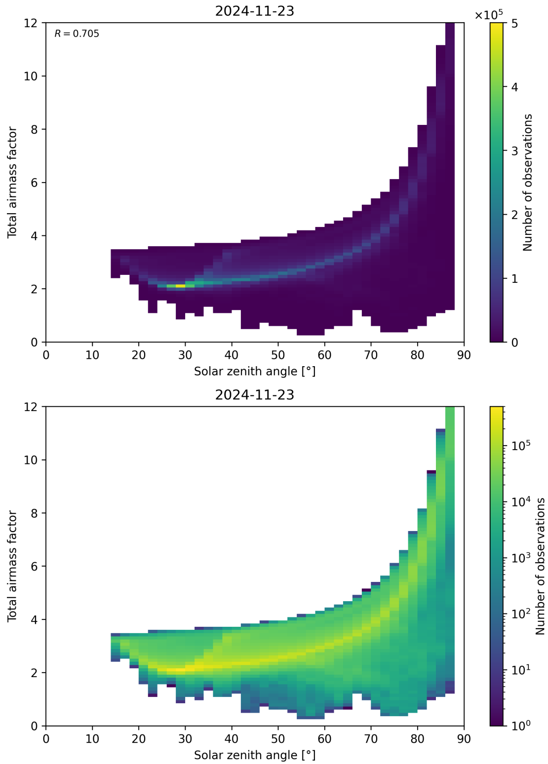
Figure 146: Scatter density plot of “Solar zenith angle” against “Total airmass factor” for 2024-11-22 to 2024-11-24.
