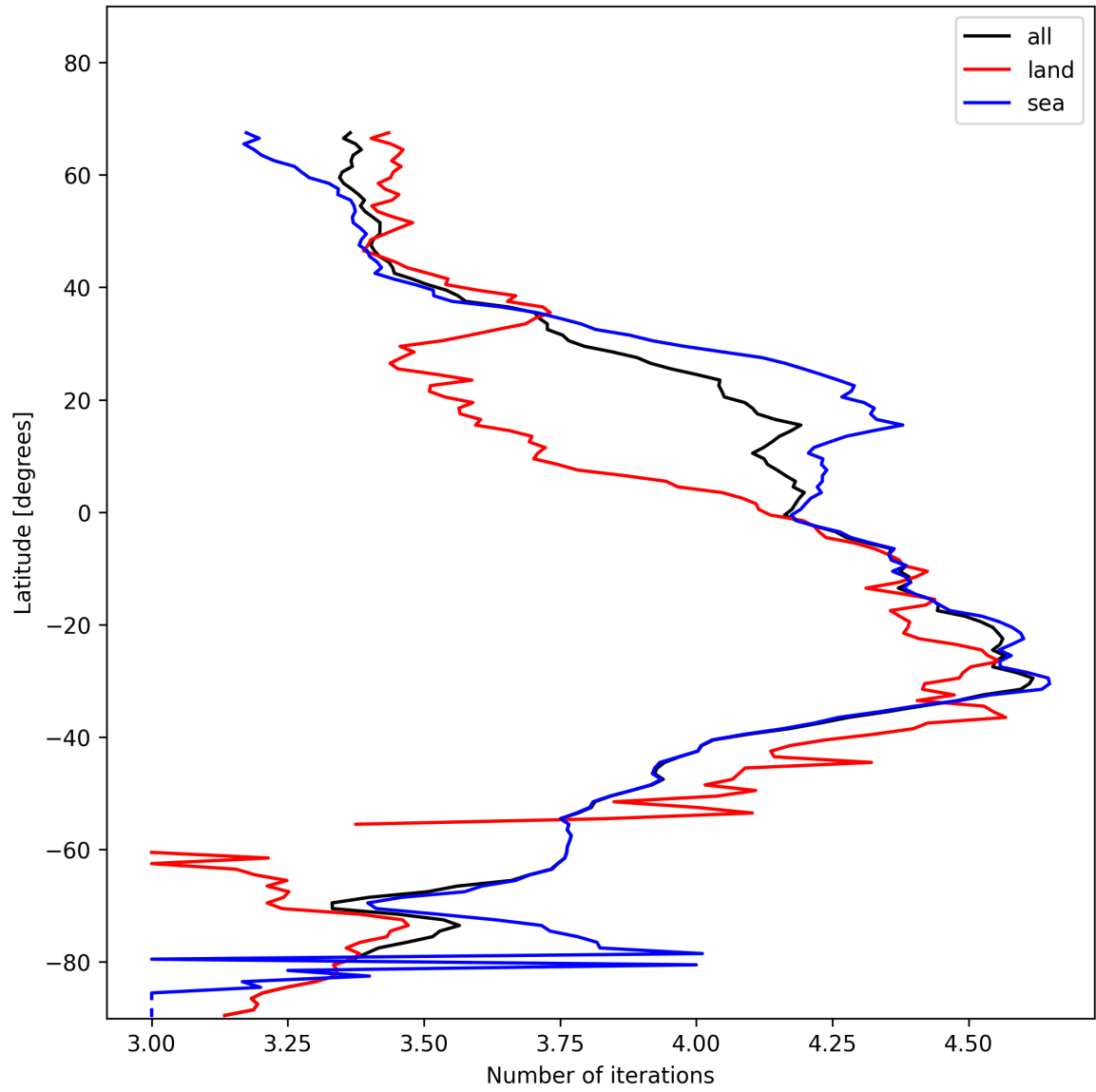
Figure 17: Zonal average of “Number of iterations” for 2024-11-22 to 2024-11-24.
