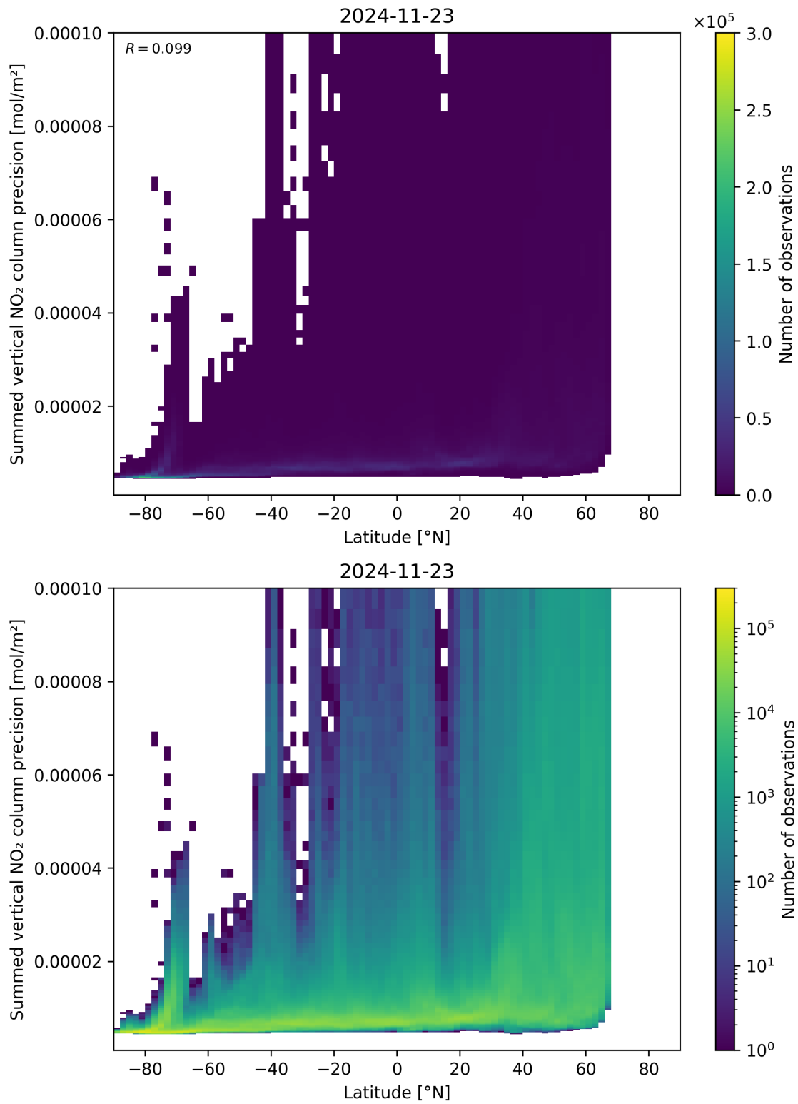
Figure 89: Scatter density plot of “Latitude” against “Summed vertical NO 2 column precision” for 2024-11-22 to 2024-11-24.
