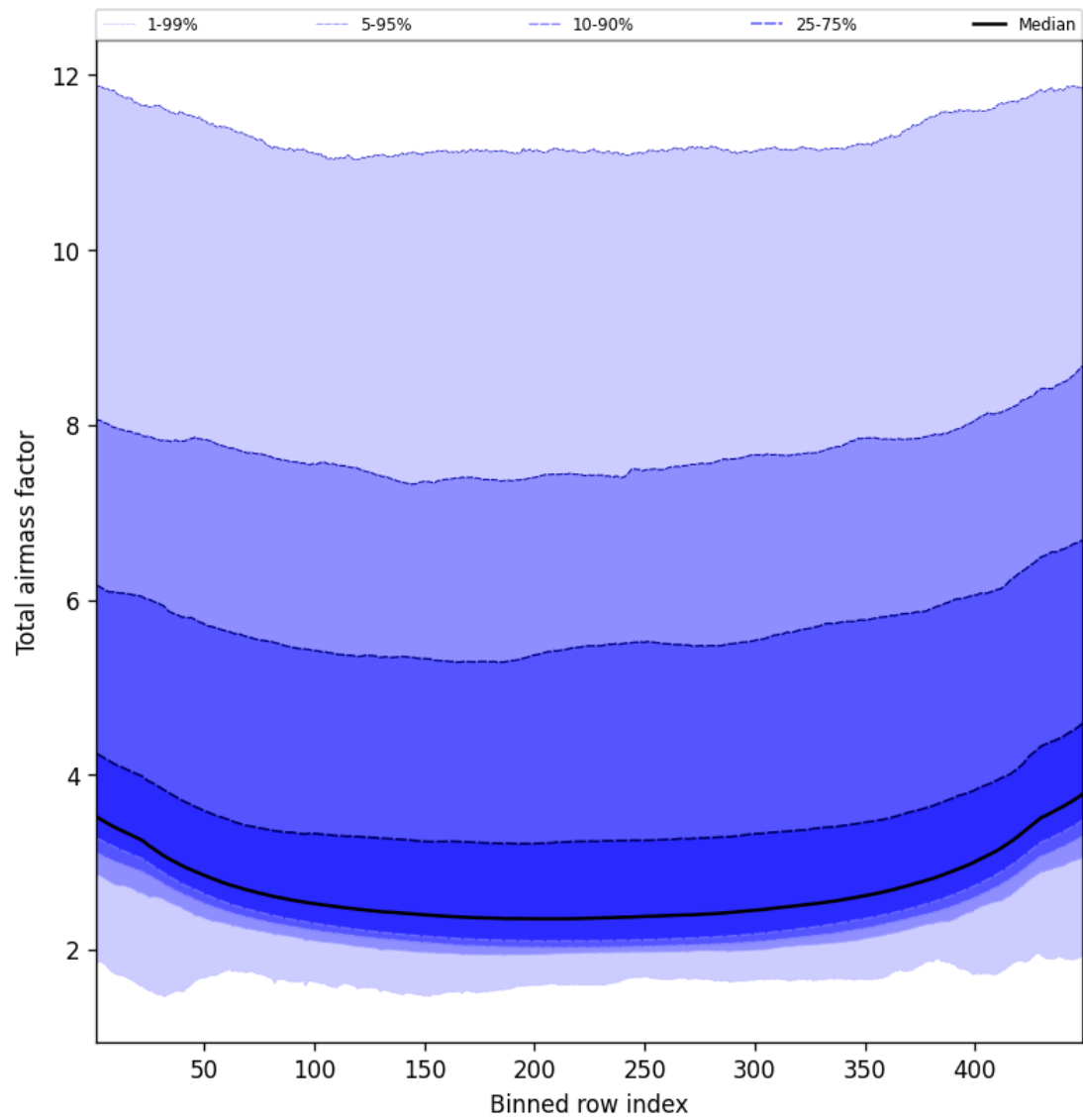
Figure 49: Along track statistics of “Total airmass factor” for 2024-11-22 to 2024-11-24
