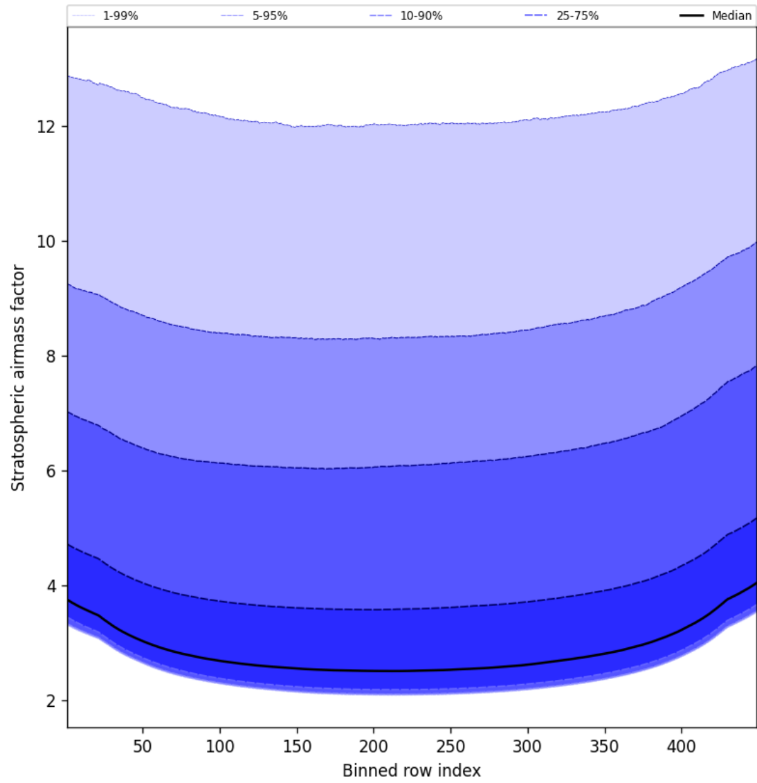
Figure 61: Along track statistics of “Stratospheric airmass factor” for 2024-11-22 to 2024-11-24
