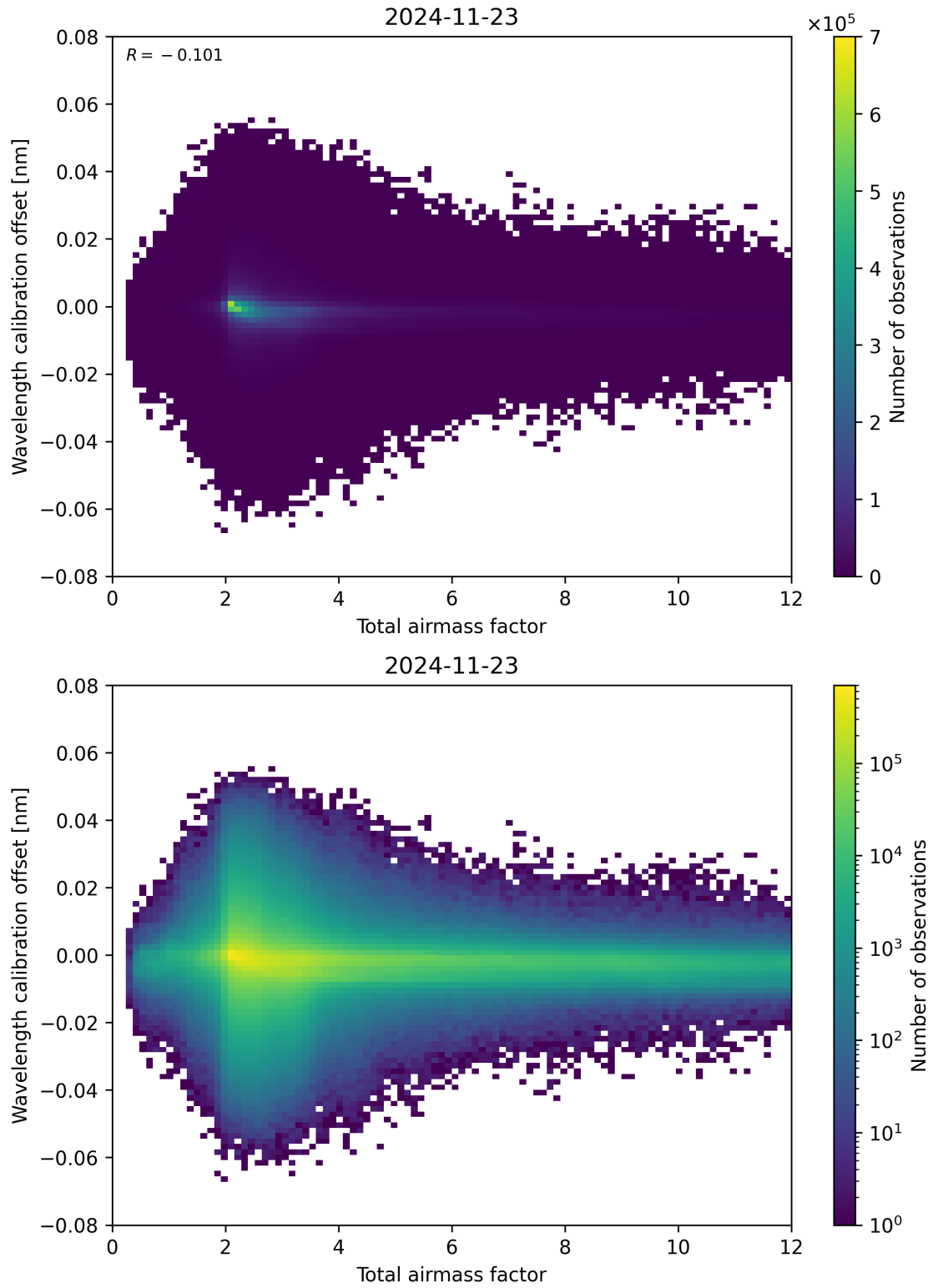
Figure 70: Scatter density plot of “Total airmass factor” against “Wavelength calibration offset” for 2024-11-22 to 2024-11-24.
