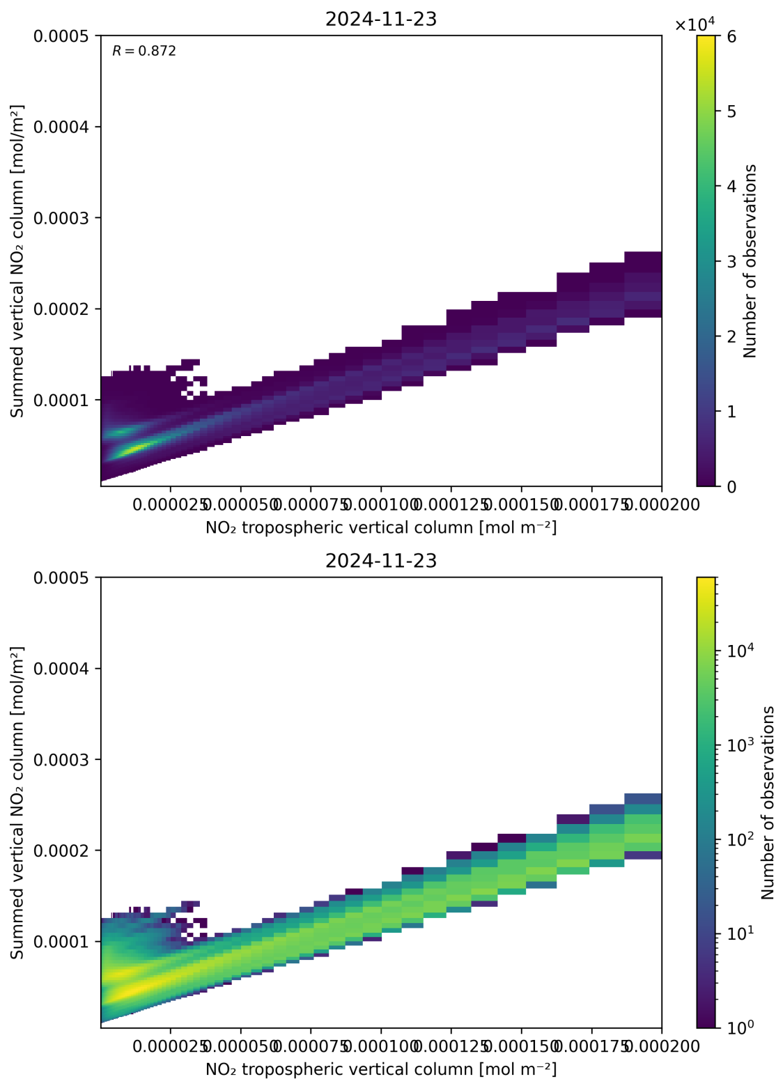
Figure 126: Scatter density plot of “NO 2 tropospheric vertical column” against “Summed vertical NO 2 column” for 2024-11-22 to 2024-11-24.
