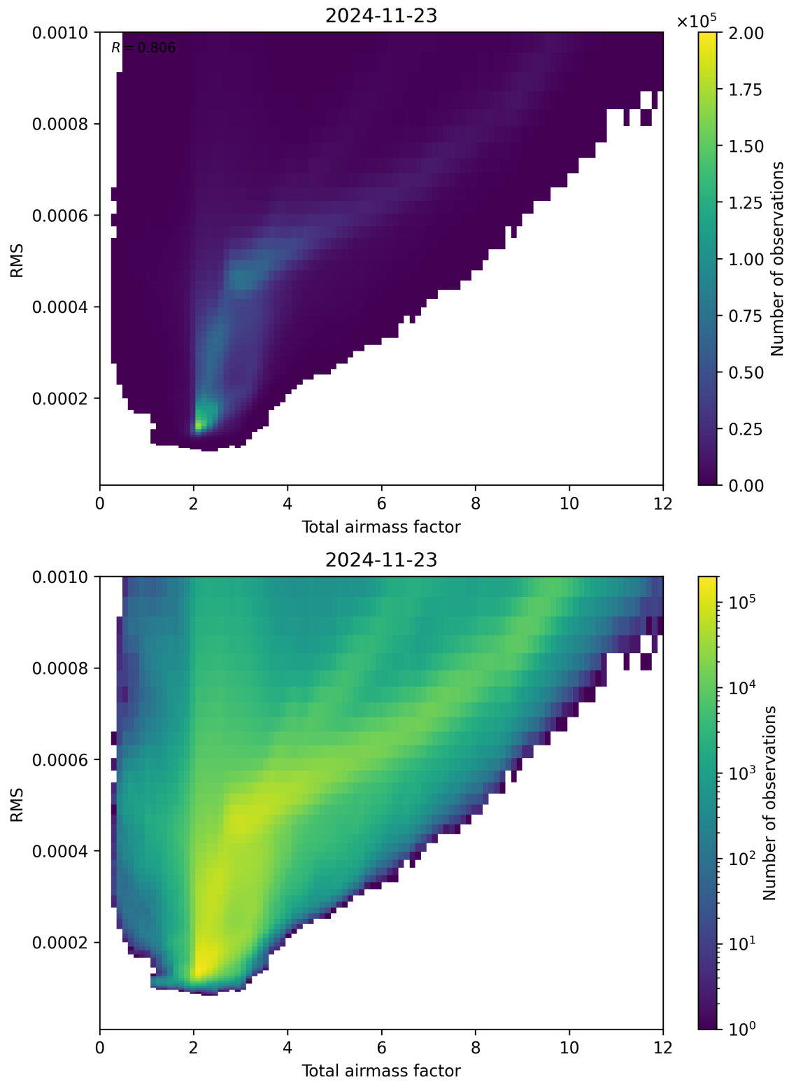
Figure 69: Scatter density plot of “Total airmass factor” against “RMS” for 2024-11-22 to 2024-11-24.
