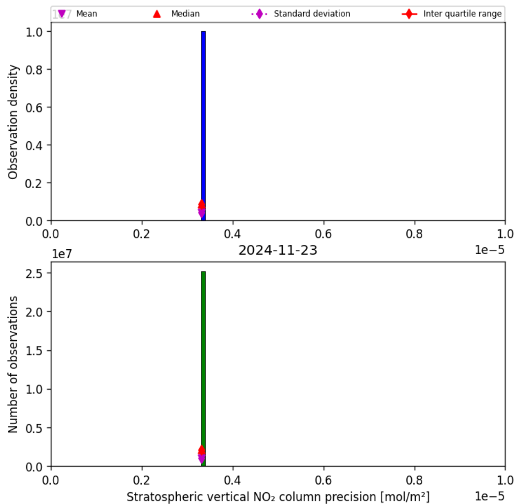
Figure 37: Histogram of “Stratospheric vertical NO 2 column precision” for 2024-11-22 to 2024-11-24
