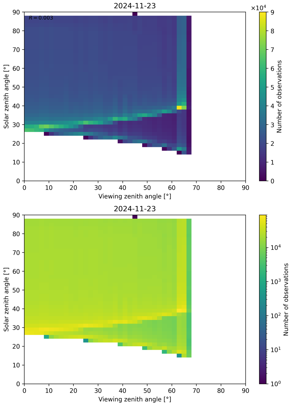
Figure 172: Scatter density plot of “Viewing zenith angle” against “Solar zenith angle” for 2024-11-22 to 2024-11-24.
