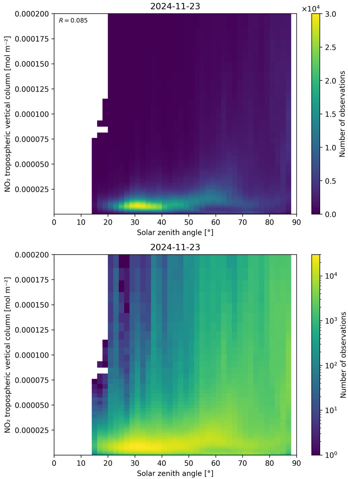
Figure 155: Scatter density plot of “Solar zenith angle” against “NO 2 tropospheric vertical column” for 2024-11-22 to 2024-11-24.
