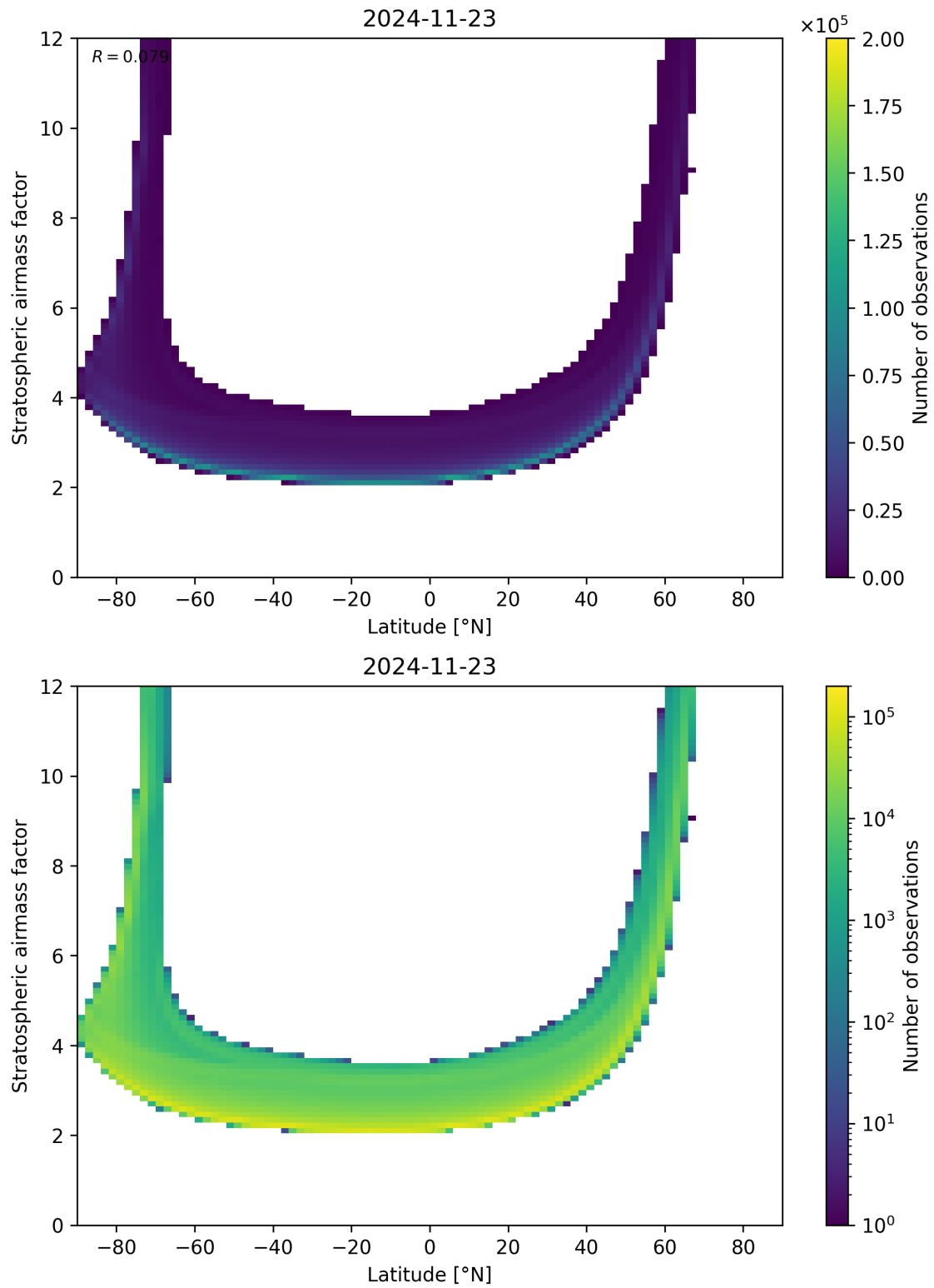
Figure 83: Scatter density plot of “Latitude” against “Stratospheric air mass factor” for 2024-11-22 to 2024-11-24.
