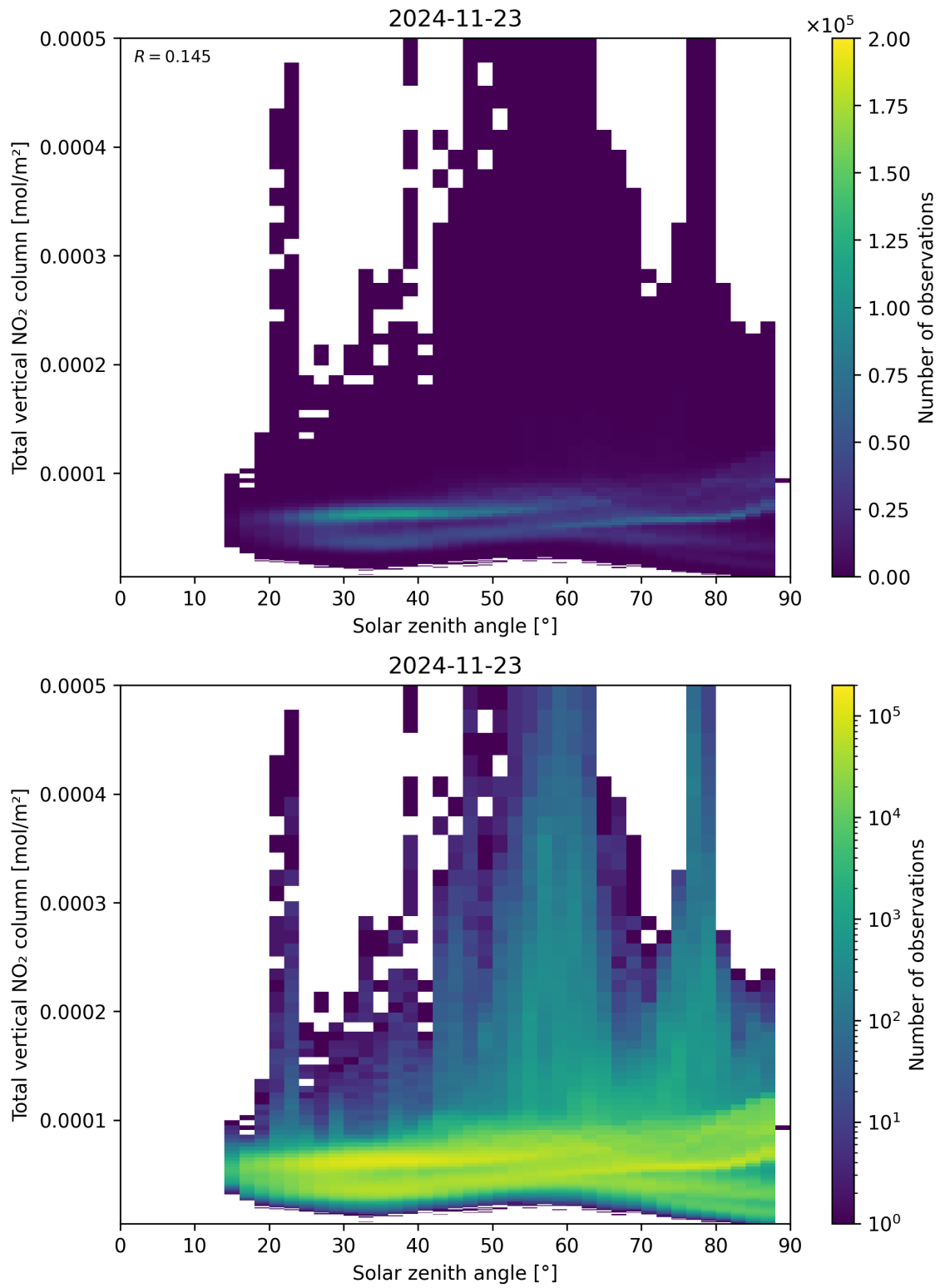
Figure 153: Scatter density plot of “Solar zenith angle” against “Total vertical NO 2 column” for 2024-11-22 to 2024-11-24.
