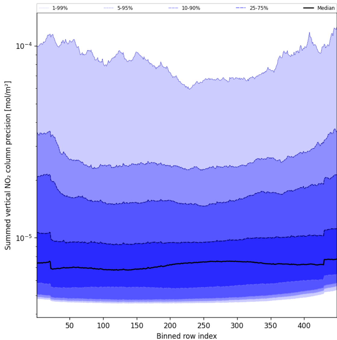
Figure 58: Along track statistics of “Summed vertical NO 2 column precision” for 2024-11-22 to 2024-11-24
