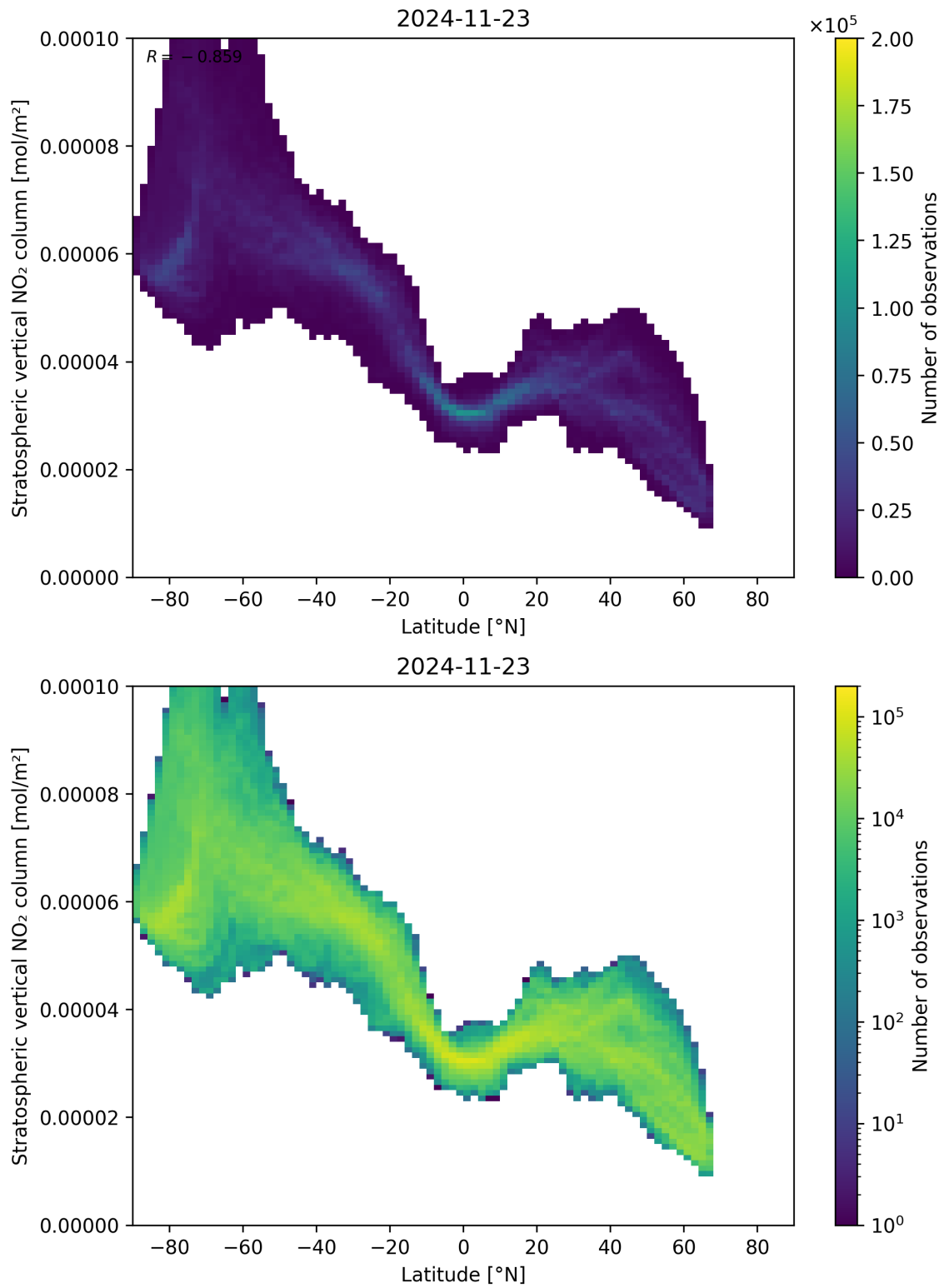
Figure 87: Scatter density plot of “Latitude” against “Stratospheric vertical NO 2 column” for 2024-11-22 to 2024-11-24.
