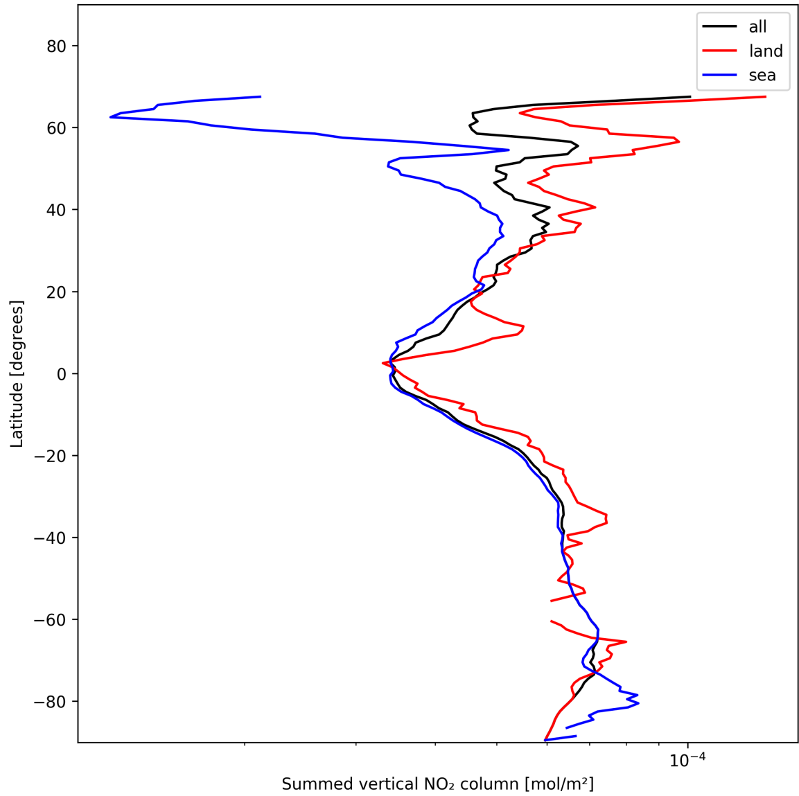
Figure 23: Zonal average of “Summed vertical NO 2 column” for 2024-11-22 to 2024-11-24.
