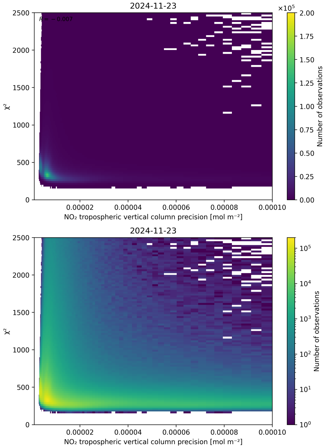
Figure 134: Scatter density plot of “NO 2 tropospheric vertical column precision” against “ \chi^2 ” for 2024-11-22 to 2024-11-24.
