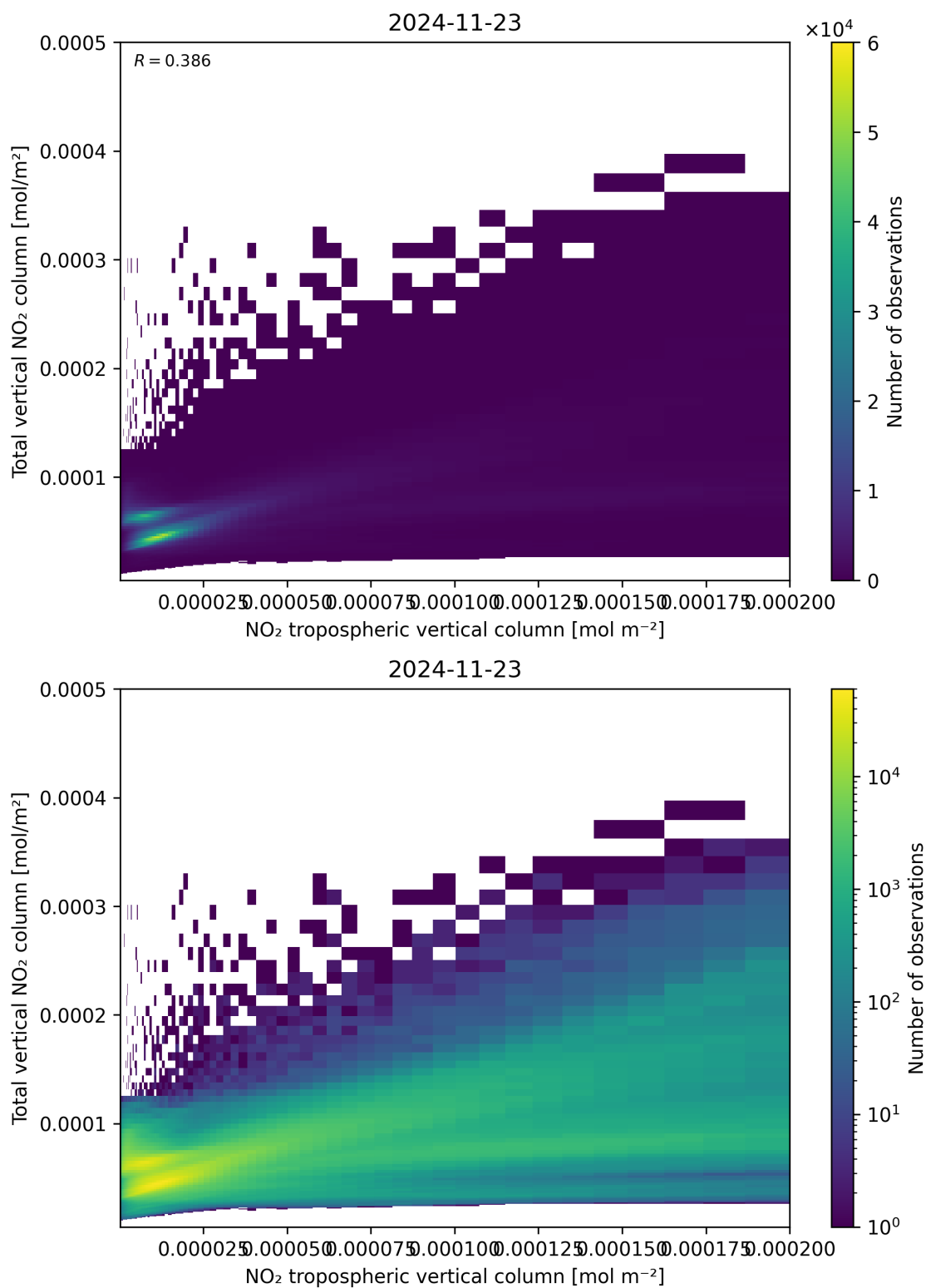
Figure 128: Scatter density plot of “NO 2 tropospheric vertical column” against “Total vertical NO 2 column” for 2024-11-22 to 2024-11-24.
