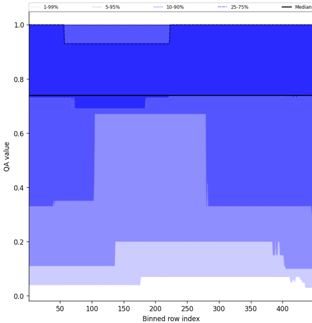
Figure 45: Along track statistics of “QA value” for 2024-11-22 to 2024-11-24
