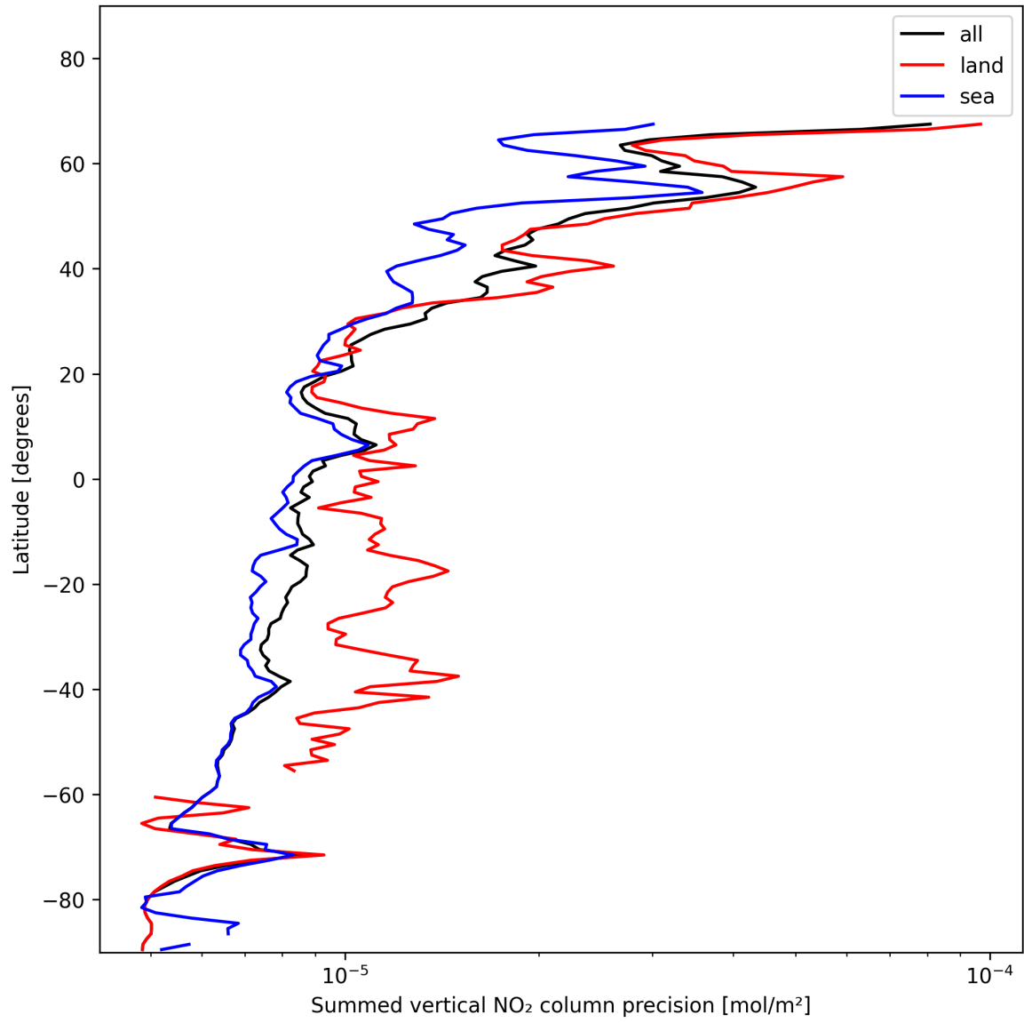
Figure 24: Zonal average of “Summed vertical NO 2 column precision” for 2024-11-22 to 2024-11-24.
