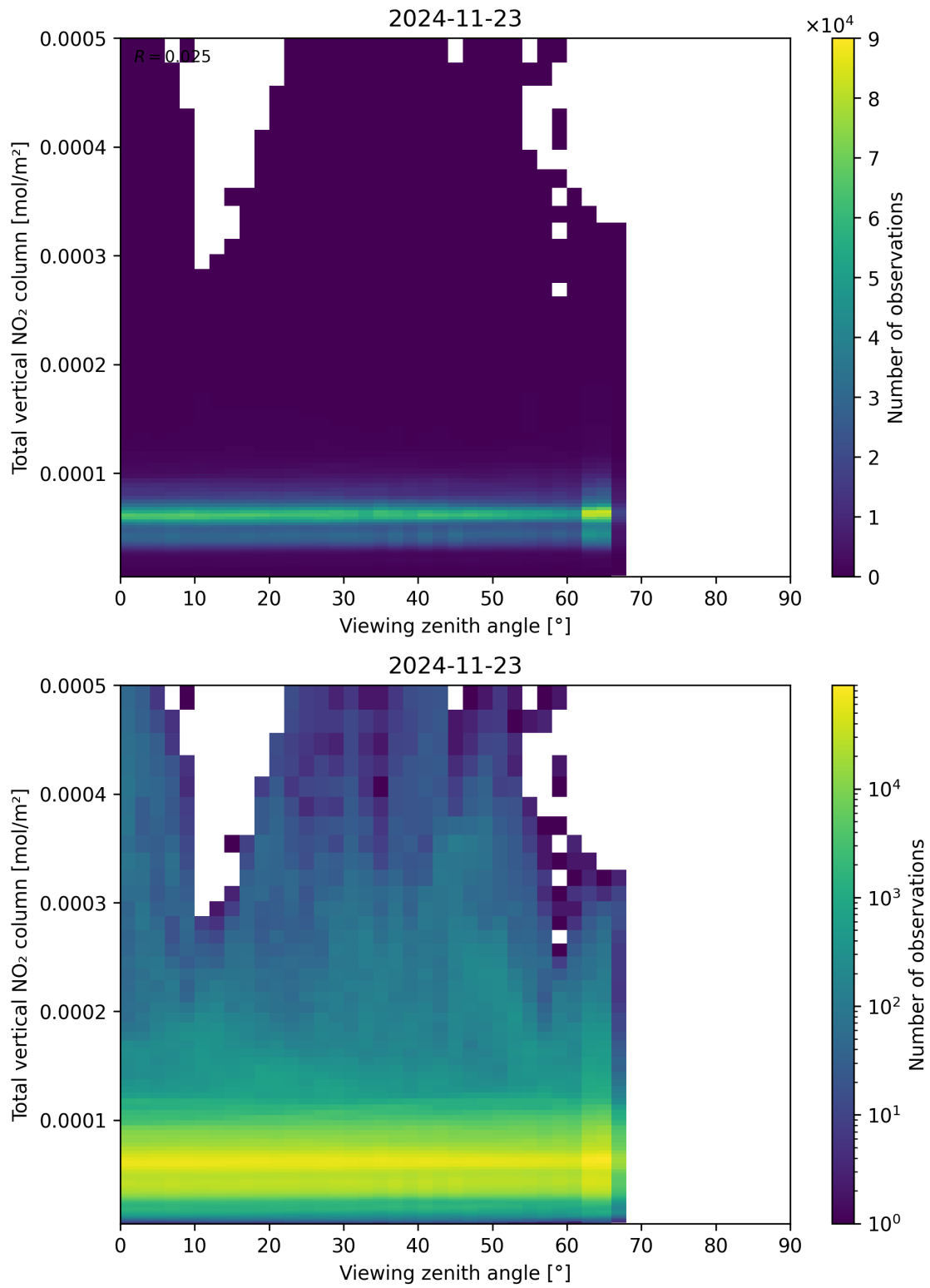
Figure 167: Scatter density plot of “Viewing zenith angle” against “Total vertical NO 2 column” for 2024-11-22 to 2024-11-24.
