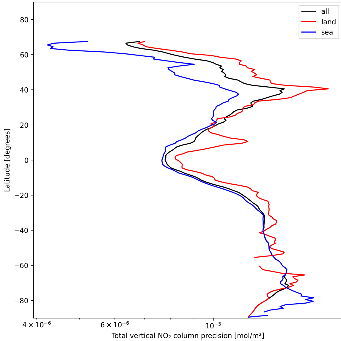
Figure 22: Zonal average of "Total vertical NO 2 column precision" for 2024-11-22 to 2024-11-24.
