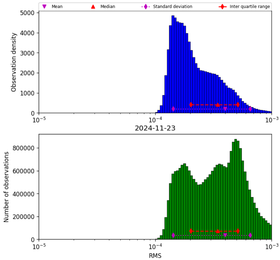
Figure 43: Histogram of “RMS” for 2024-11-22 to 2024-11-24
