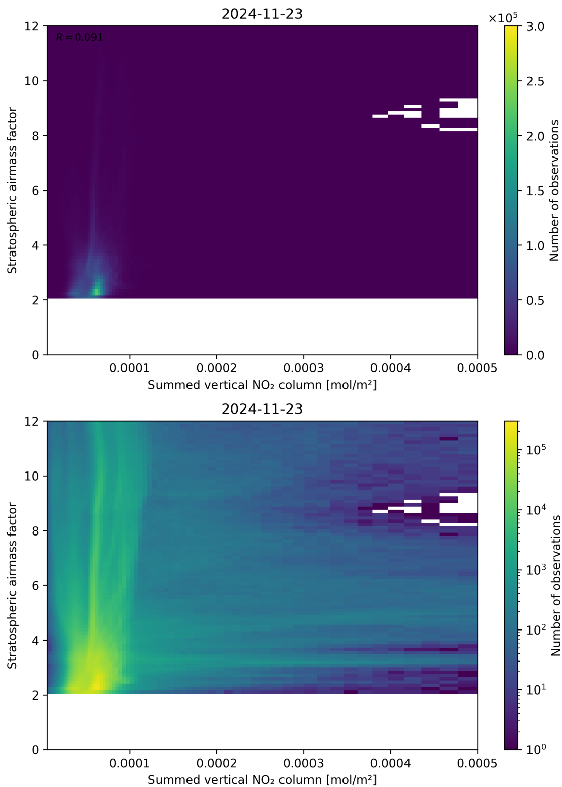
Figure 103: Scatter density plot of “Summed vertical NO 2 column” against “Stratospheric airmass factor” for 2024-11-22 to 2024-11-24.
