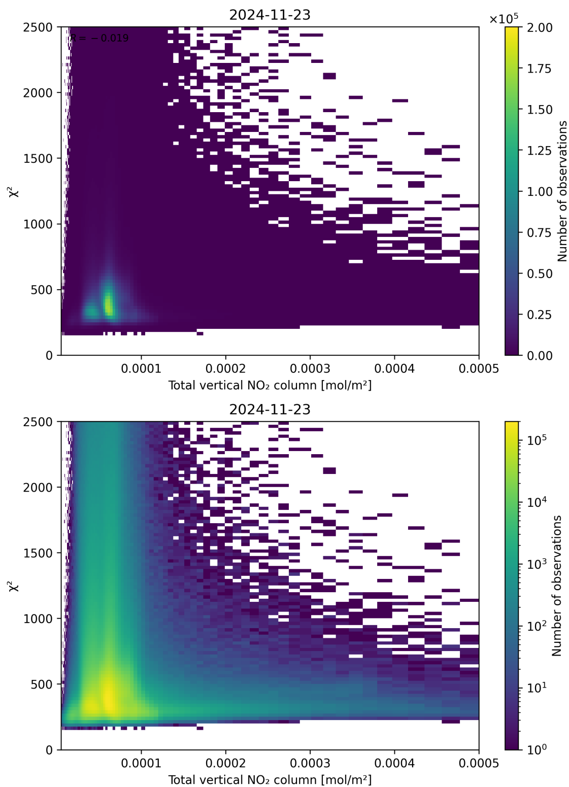
Figure 111: Scatter density plot of “Total vertical NO 2 column” against “ \chi^2 ” for 2024-11-22 to 2024-11-24.
