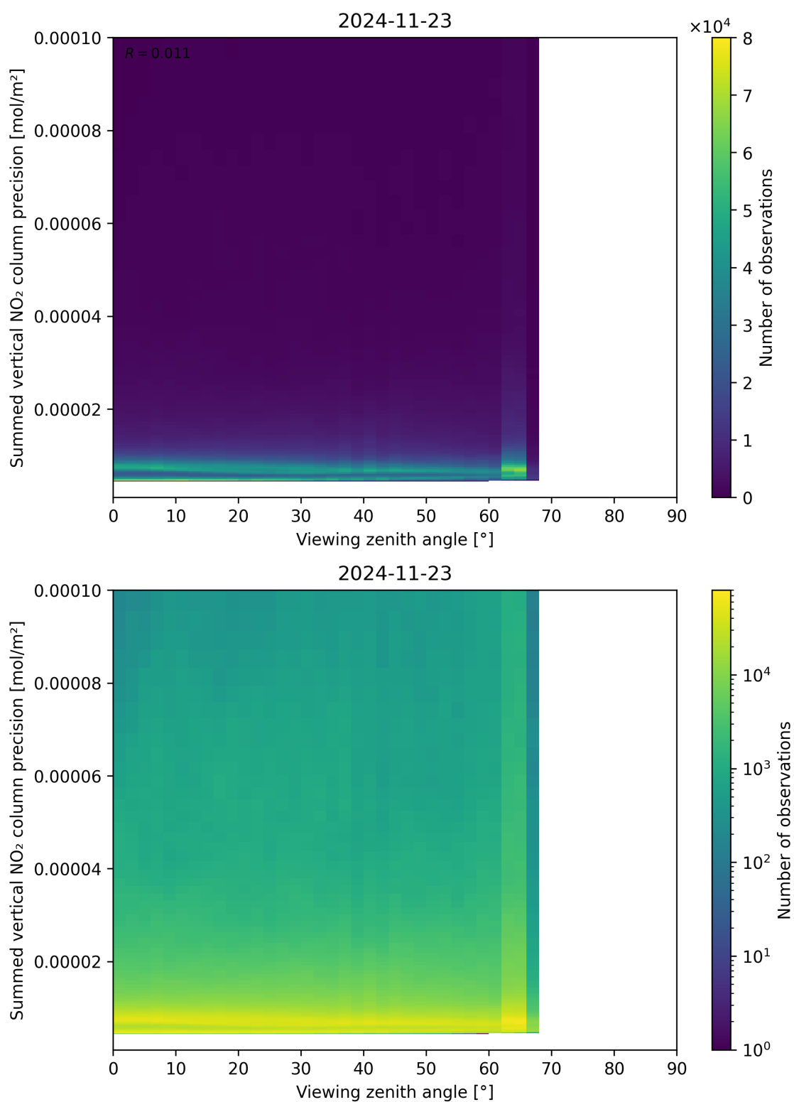
Figure 166: Scatter density plot of “Viewing zenith angle” against “Summed vertical NO 2 column precision” for 2024-11-22 to 2024-11-24.
