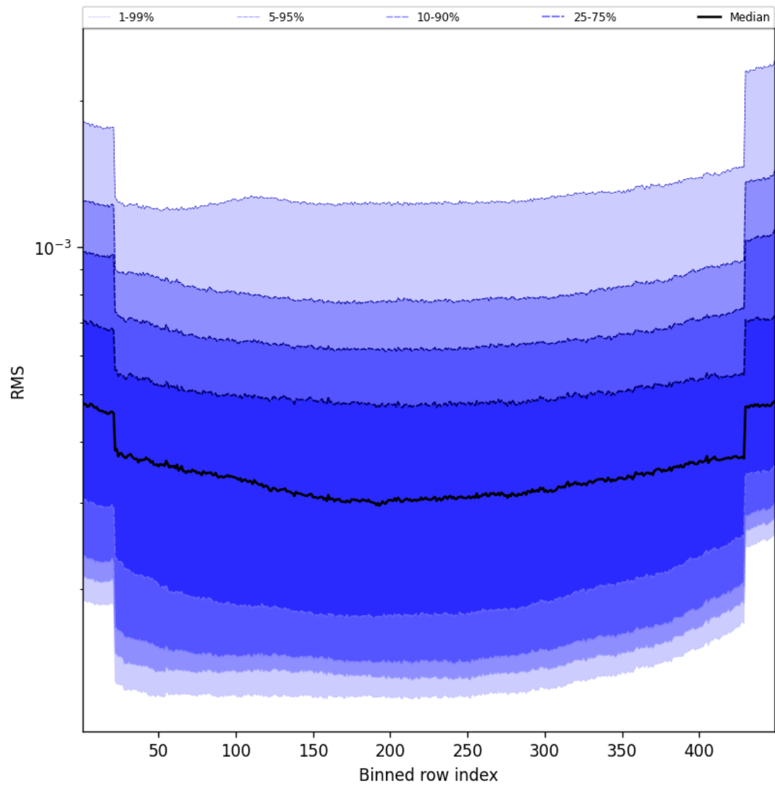
Figure 60: Along track statistics of “RMS” for 2024-11-22 to 2024-11-24
