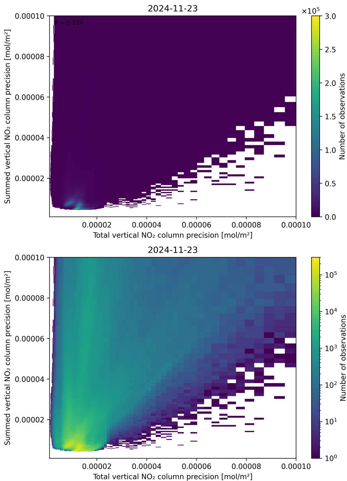
Figure 118: Scatter density plot of “Total vertical NO 2 column precision” against “Summed vertical NO 2 column precision” for 2024-11-22 to 2024-11-24.
