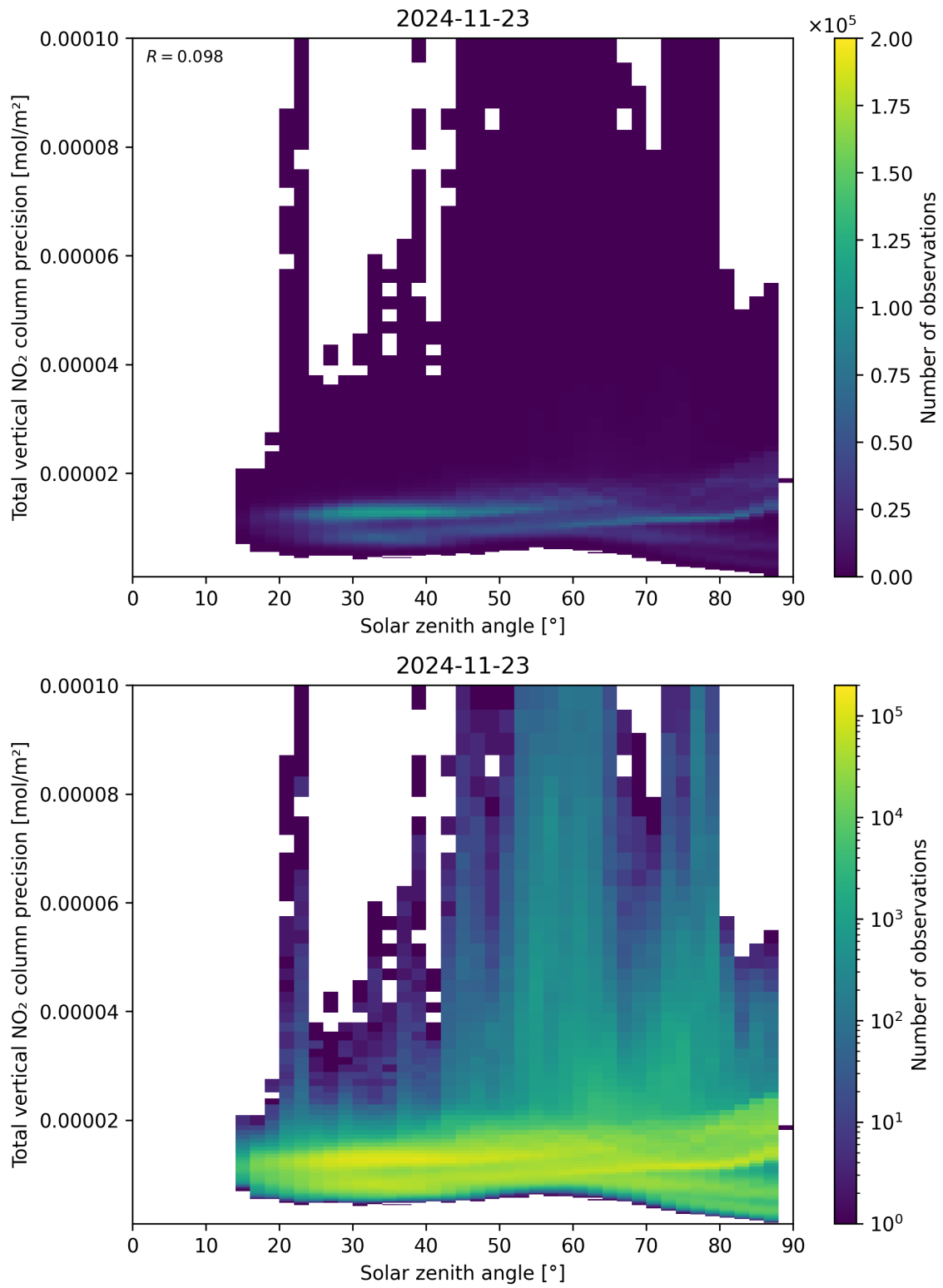
Figure 154: Scatter density plot of “Solar zenith angle” against “Total vertical NO 2 column precision” for 2024-11-22 to 2024-11-24.
