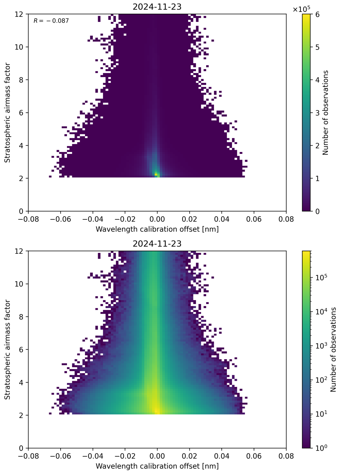
Figure 174: Scatter density plot of “Wavelength calibration offset” against “Stratospheric airmass factor” for 2024-11-22 to 2024-11-24.
