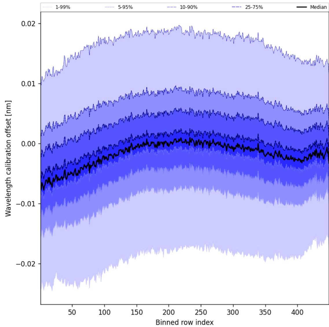
Figure 52: Along track statistics of “Wavelength calibration offset” for 2024-11-22 to 2024-11-24
