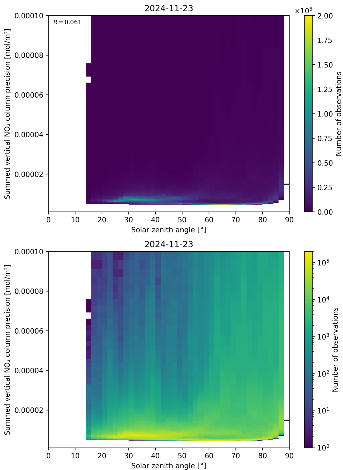
Figure 152: Scatter density plot of “Solar zenith angle” against “Summed vertical NO 2 column precision” for 2024-11-22 to 2024-11-24.
