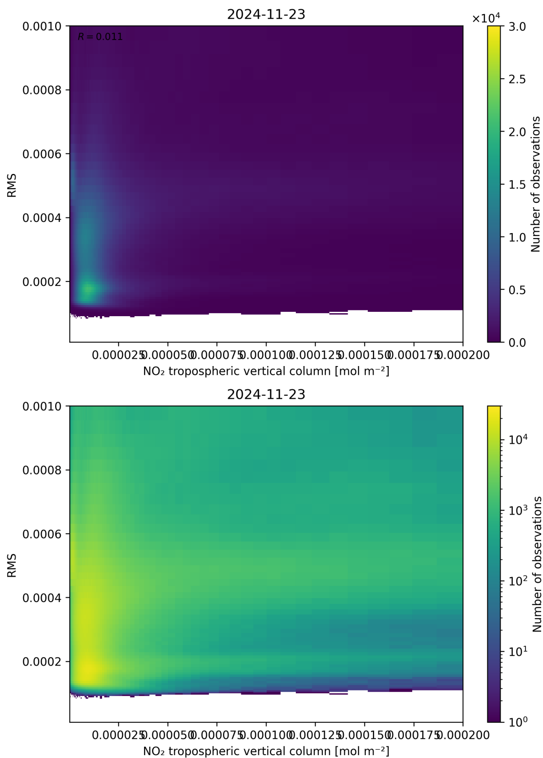
Figure 142: Scatter density plot of “NO 2 tropospheric vertical column” against “RMS” for 2024-11-22 to 2024-11-24.
