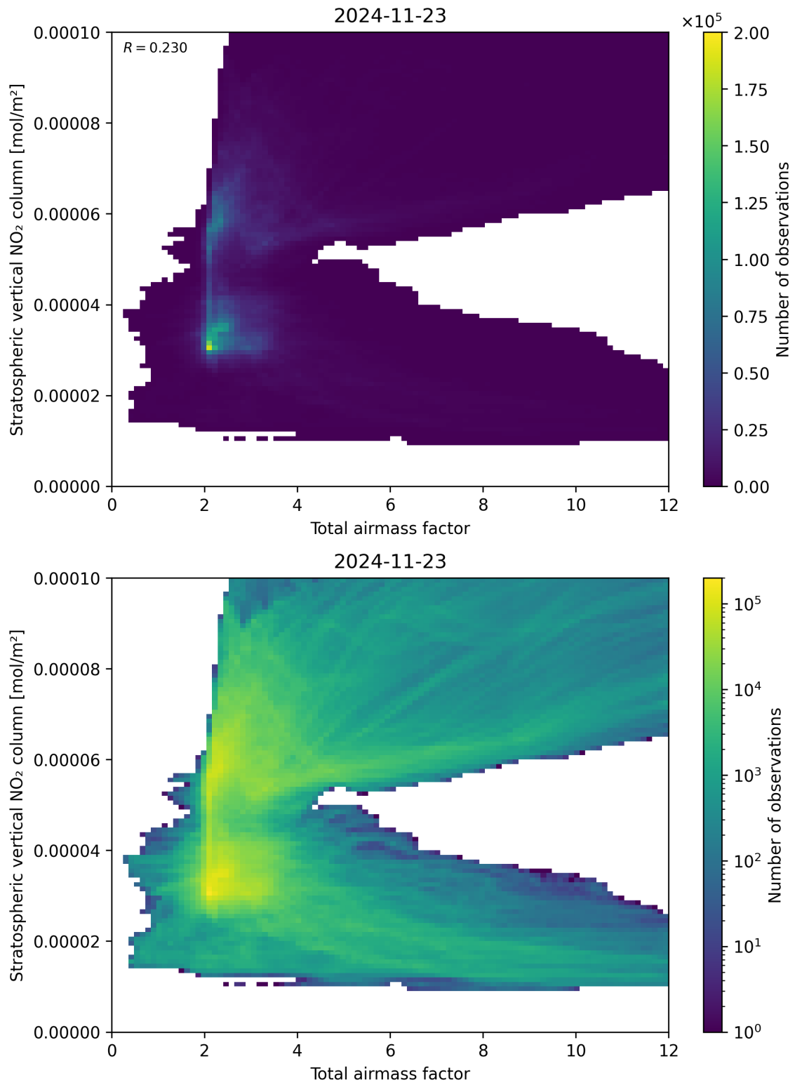
Figure 64: Scatter density plot of “Total airmass factor” against “Stratospheric vertical \text{NO}_2 column” for 2024-11-22 to 2024-11-24.
