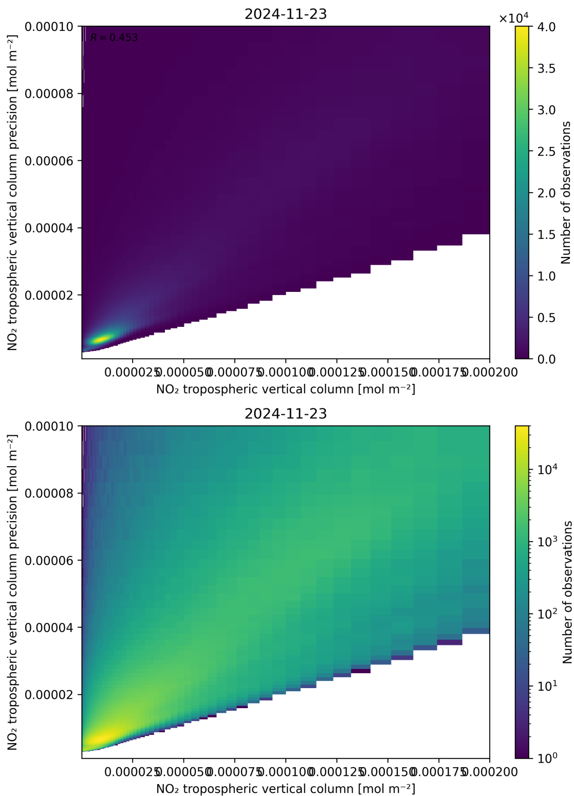
Figure 130: Scatter density plot of “NO 2 tropospheric vertical column” against “NO 2 tropospheric vertical column precision” for 2024-11-22 to 2024-11-24.
