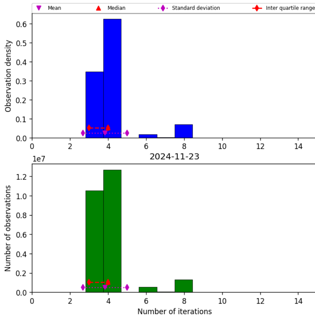
Figure 34: Histogram of “Number of iterations” for 2024-11-22 to 2024-11-24
