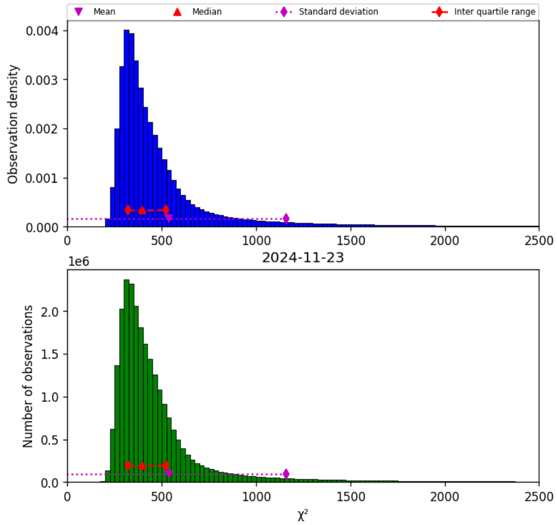
Figure 42: Histogram of " \chi^2 " for 2024-11-22 to 2024-11-24
