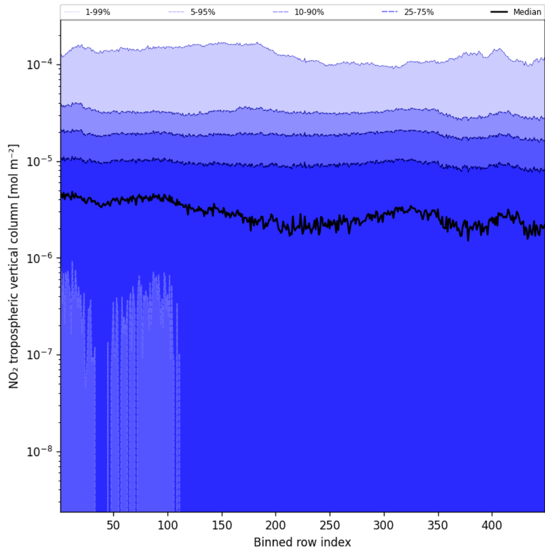
Figure 46: Along track statistics of “NO 2 tropospheric vertical column” for 2024-11-22 to 2024-11-24
