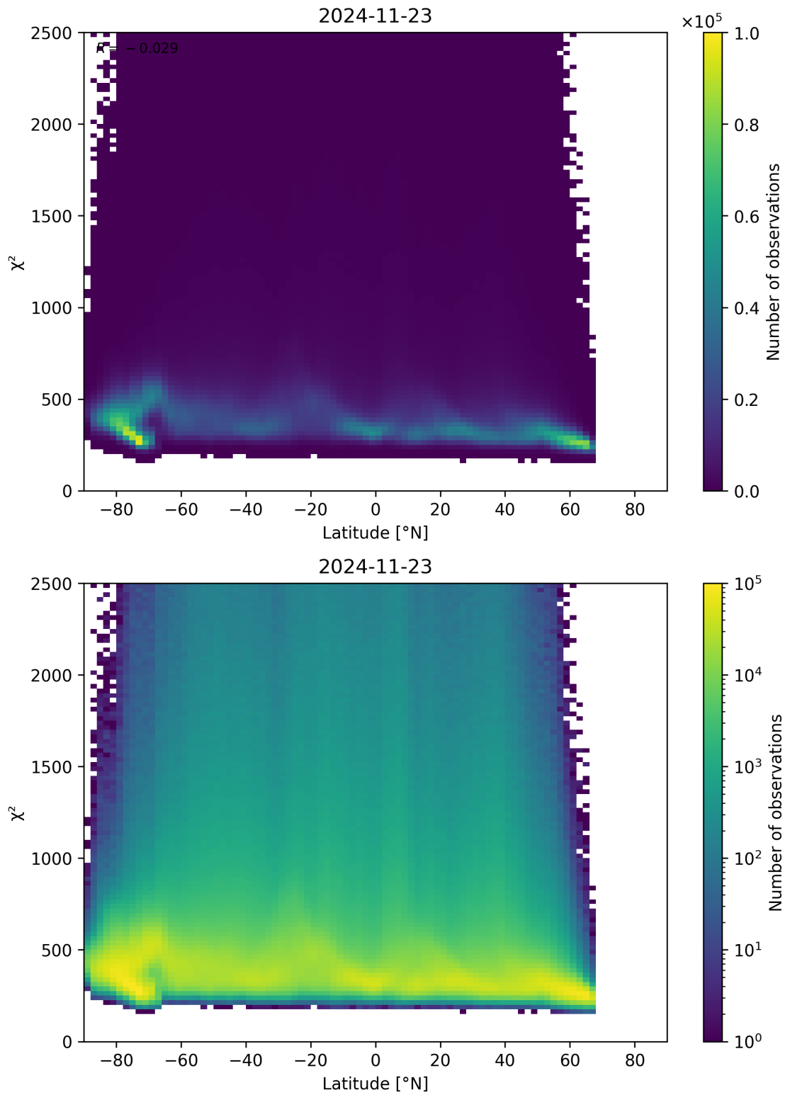
Figure 86: Scatter density plot of “Latitude” against “ \chi^2 ” for 2024-11-22 to 2024-11-24.
