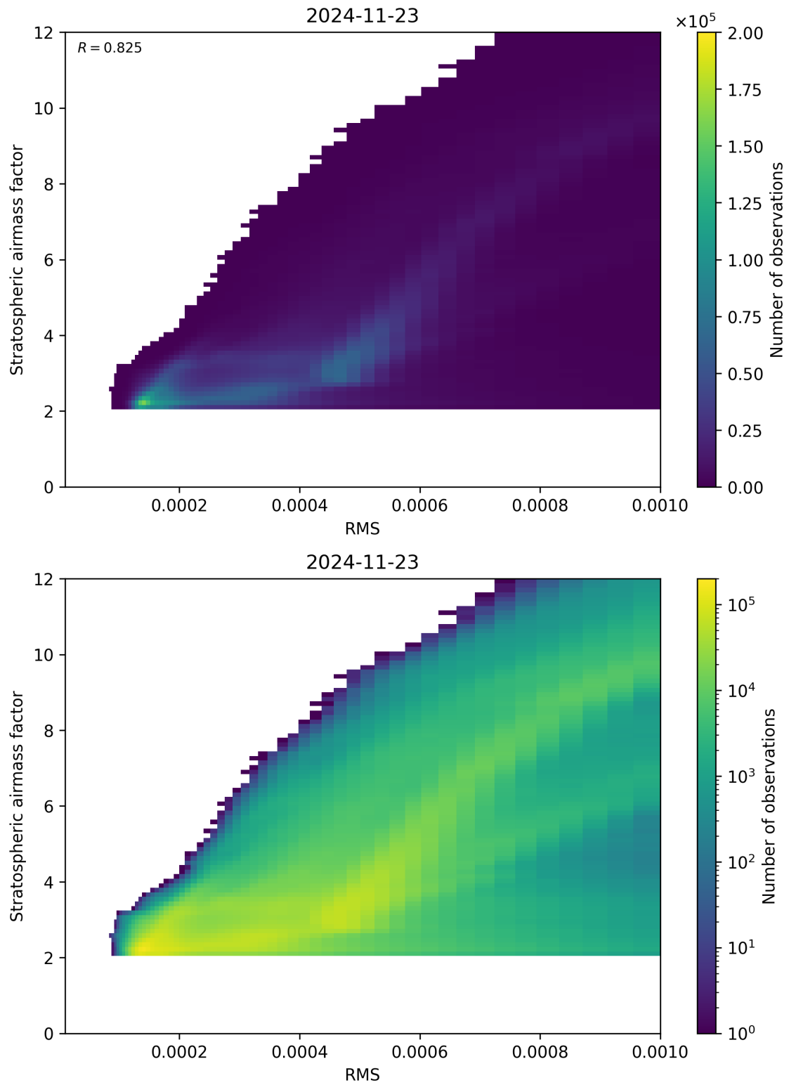
Figure 144: Scatter density plot of “RMS” against “Stratospheric airmass factor” for 2024-11-22 to 2024-11-24.
