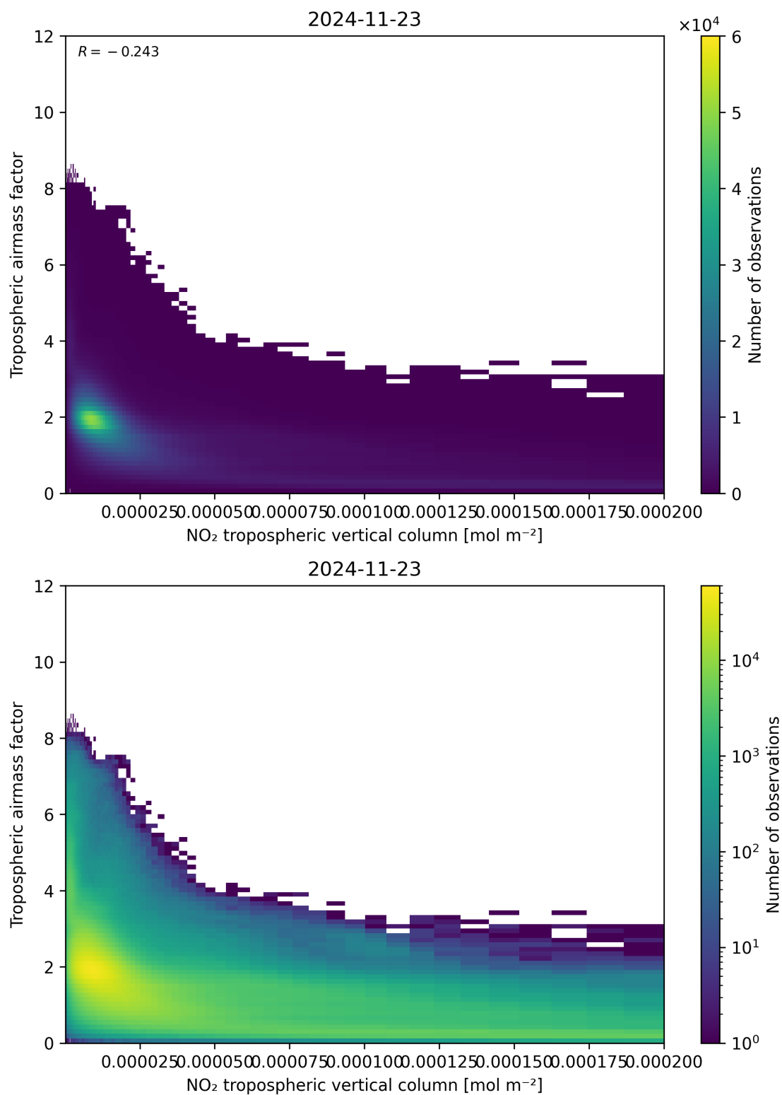
Figure 123: Scatter density plot of “NO 2 tropospheric vertical column” against “Tropospheric air mass factor” for 2024-11-22 to 2024-11-24.
