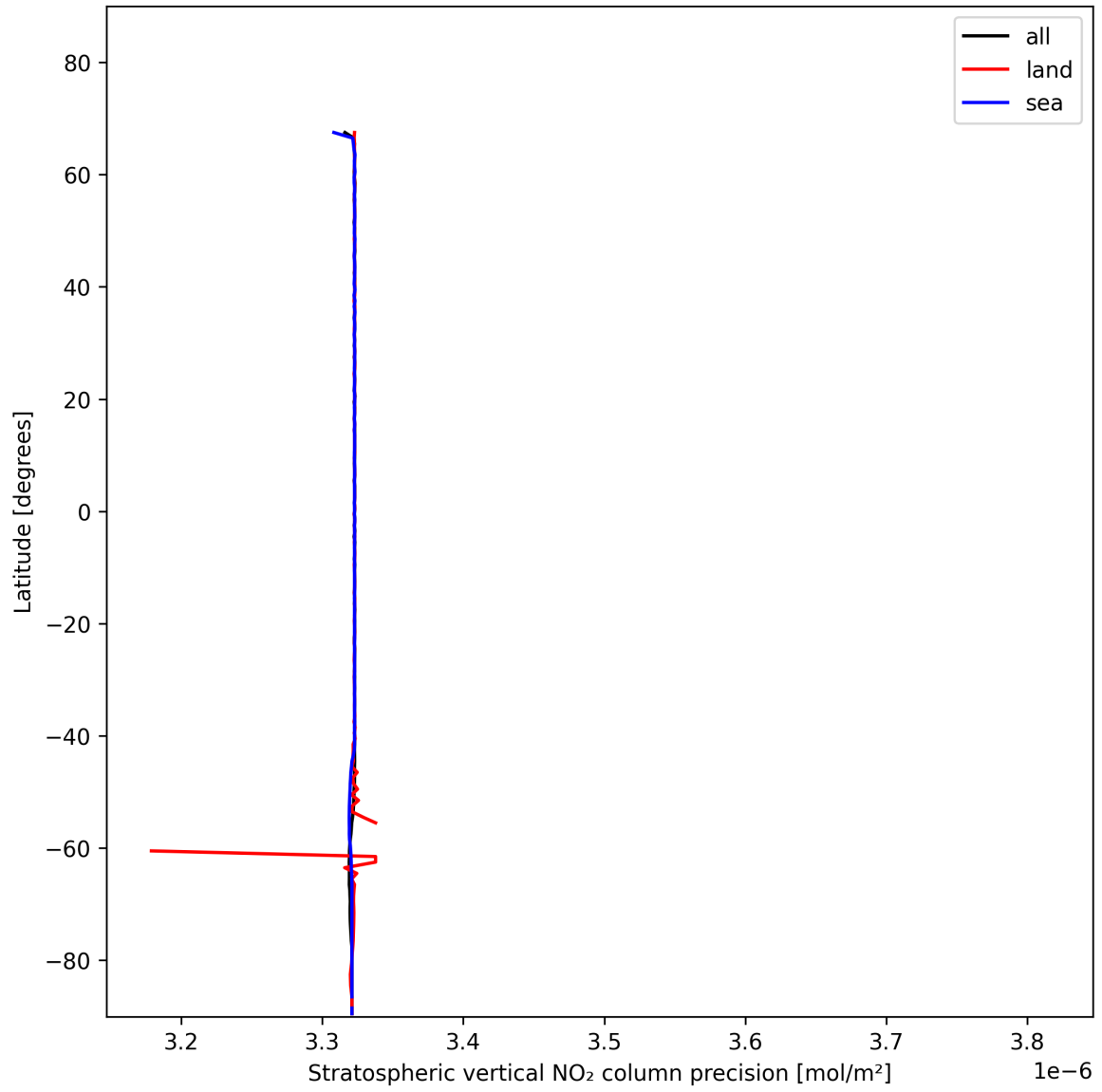
Figure 20: Zonal average of “Stratospheric vertical NO 2 column precision” for 2024-11-22 to 2024-11-24.
