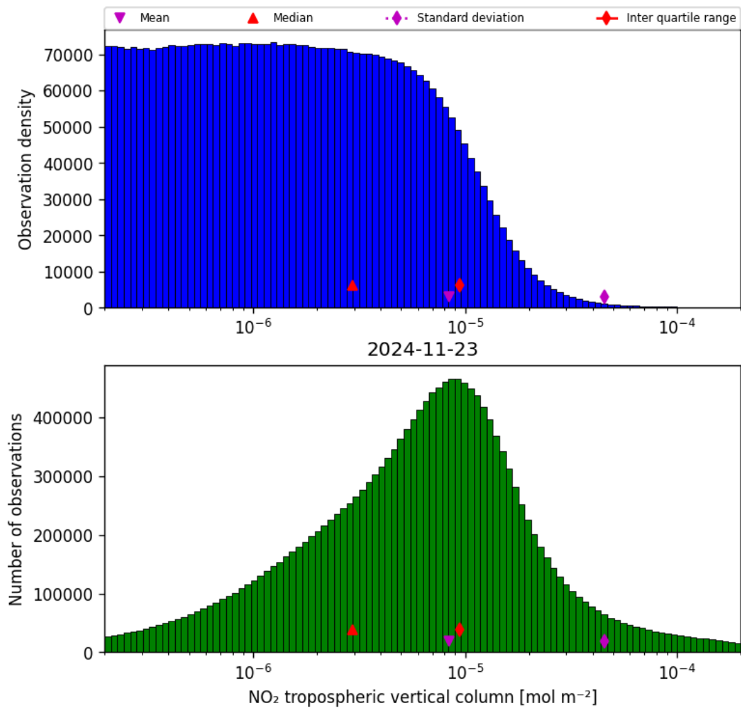
Figure 29: Histogram of “NO 2 tropospheric vertical column” for 2024-11-22 to 2024-11-24
