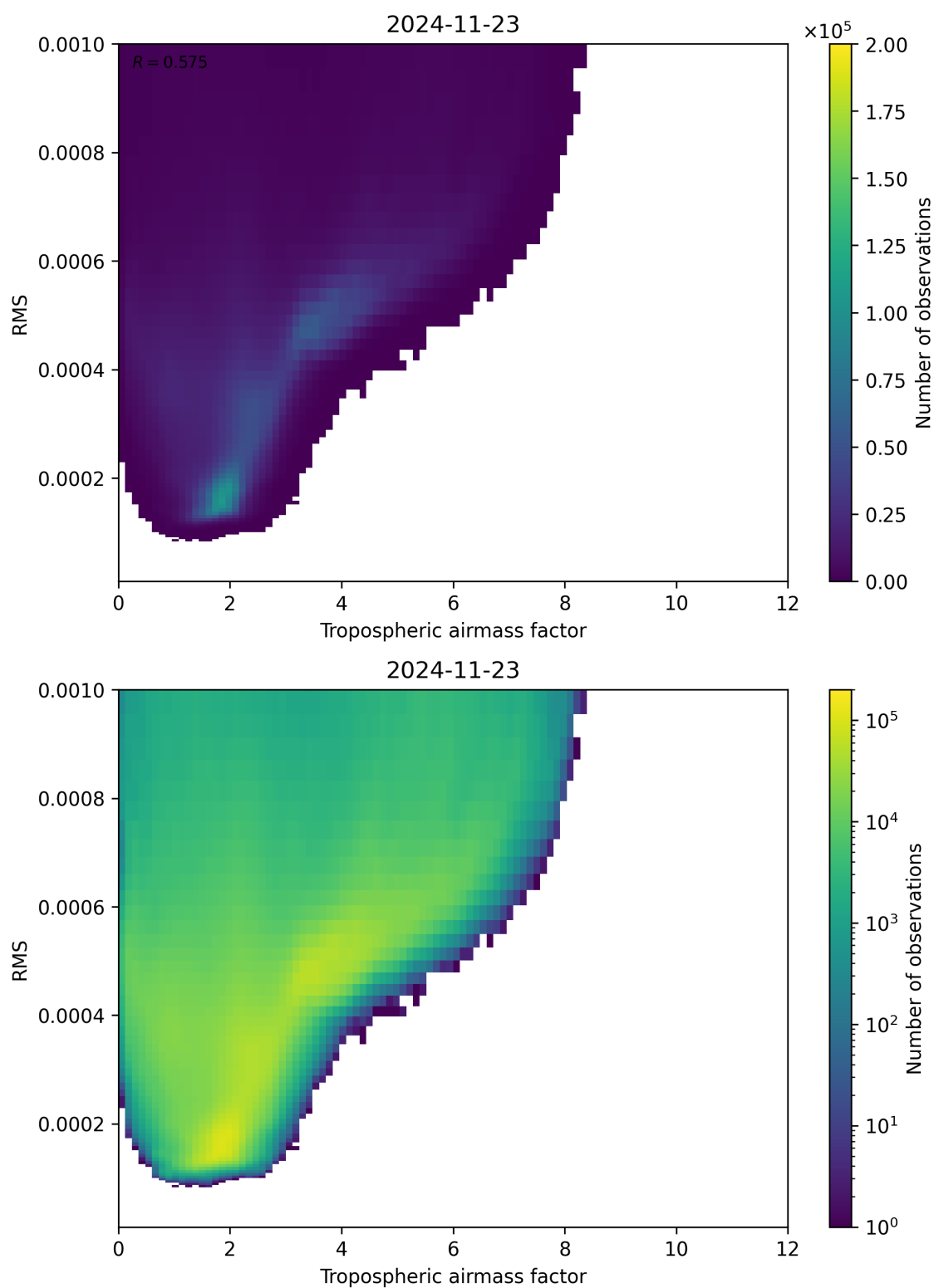
Figure 79: Scatter density plot of “Tropospheric airmass factor” against “RMS” for 2024-11-22 to 2024-11-24.
