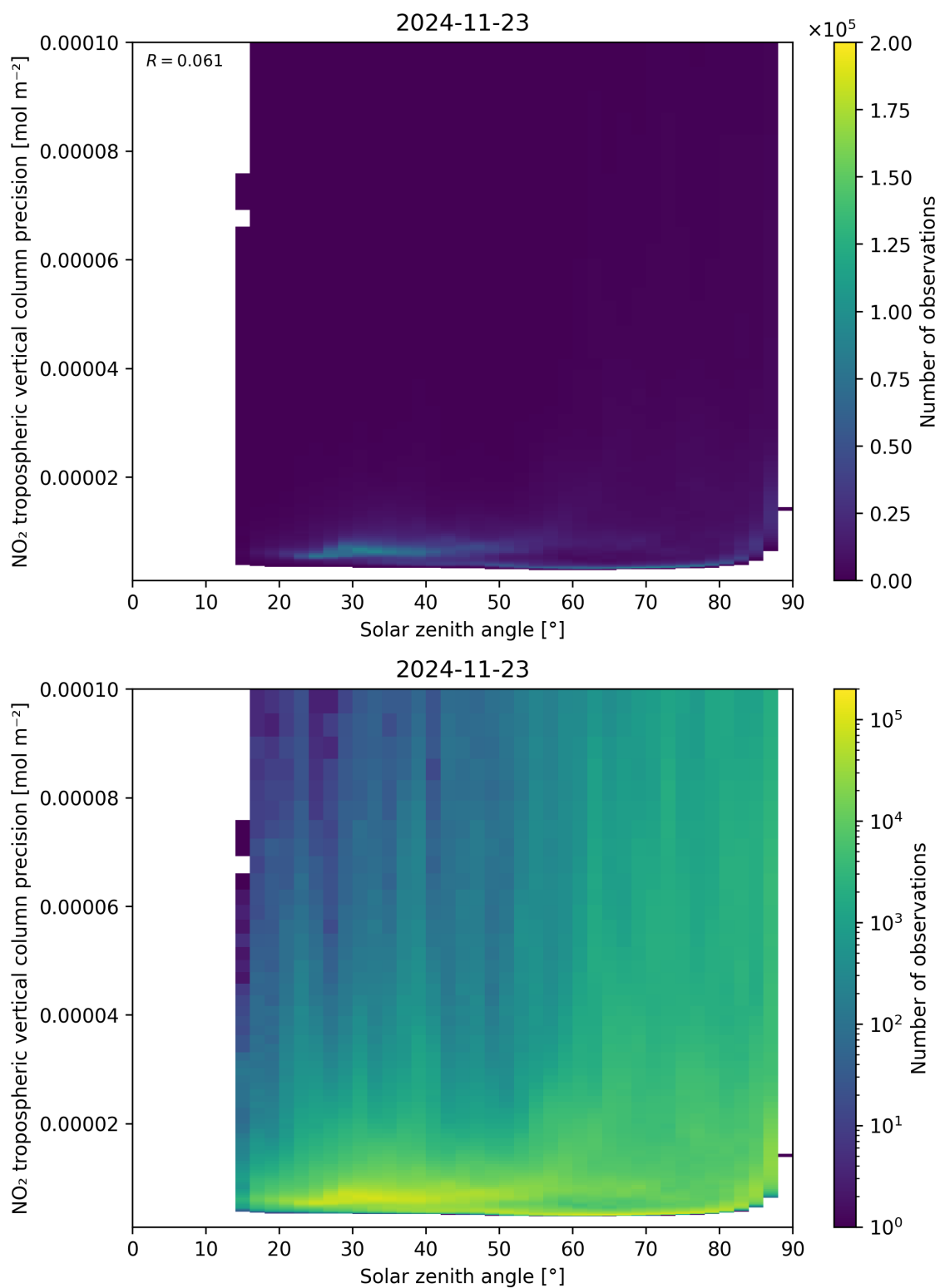
Figure 156: Scatter density plot of “Solar zenith angle” against “NO 2 tropospheric vertical column precision” for 2024-11-22 to 2024-11-24.
