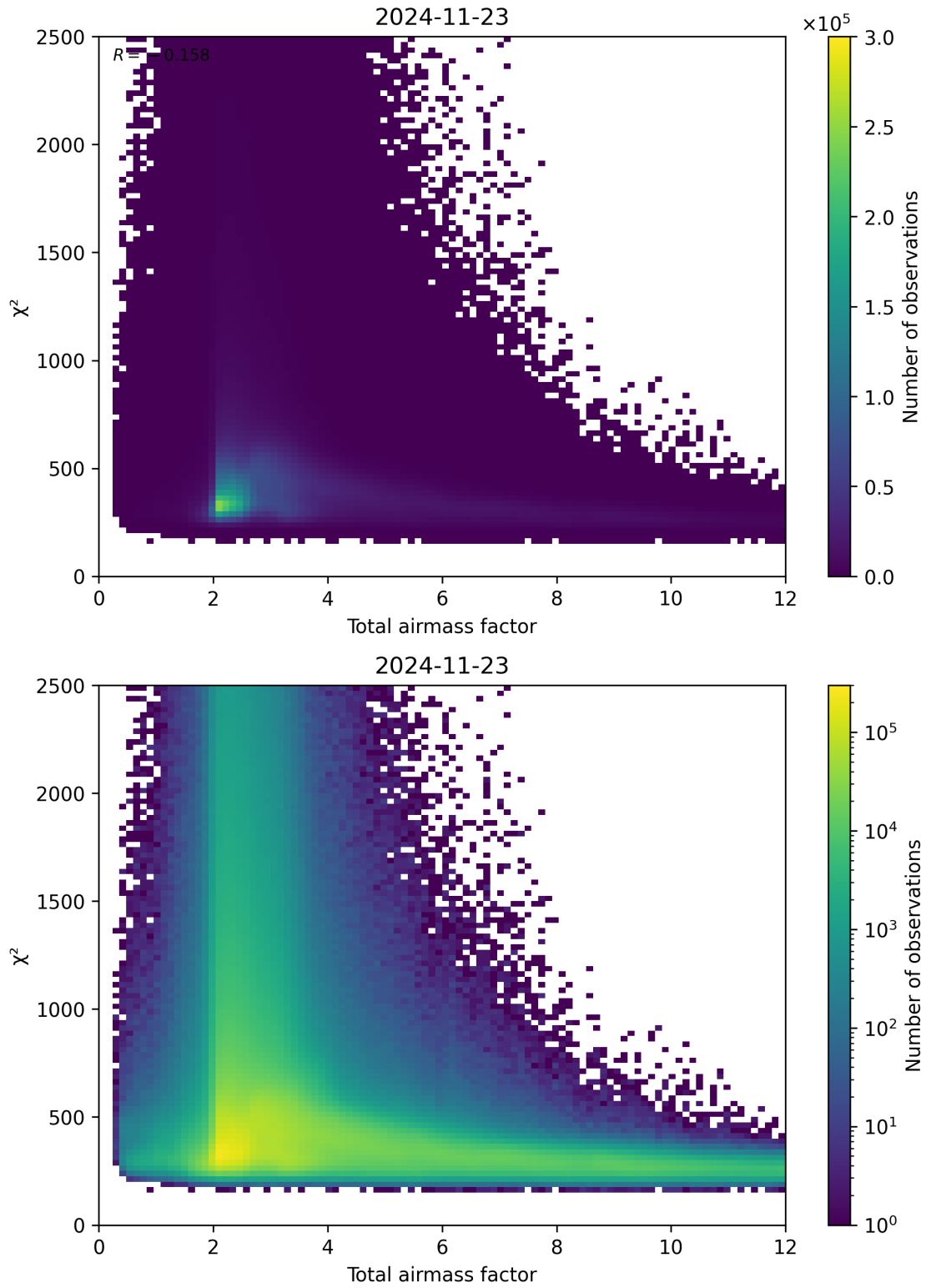
Figure 63: Scatter density plot of “Total airmass factor” against “ \chi^2 ” for 2024-11-22 to 2024-11-24.
