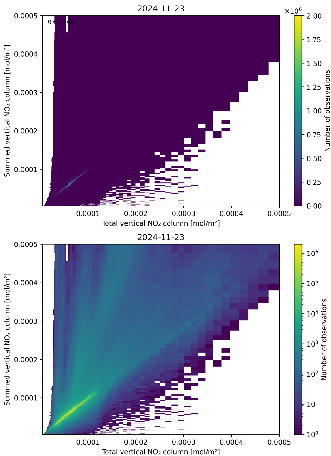
Figure 112: Scatter density plot of “Total vertical NO 2 column” against “Summed vertical NO 2 column” for 2024-11-22 to 2024-11-24.
