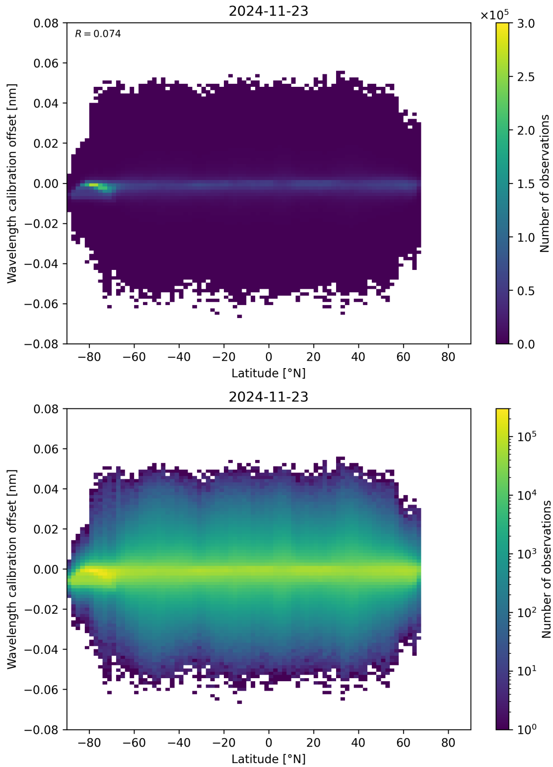
Figure 95: Scatter density plot of “Latitude” against “Wavelength calibration offset” for 2024-11-22 to 2024-11-24.
