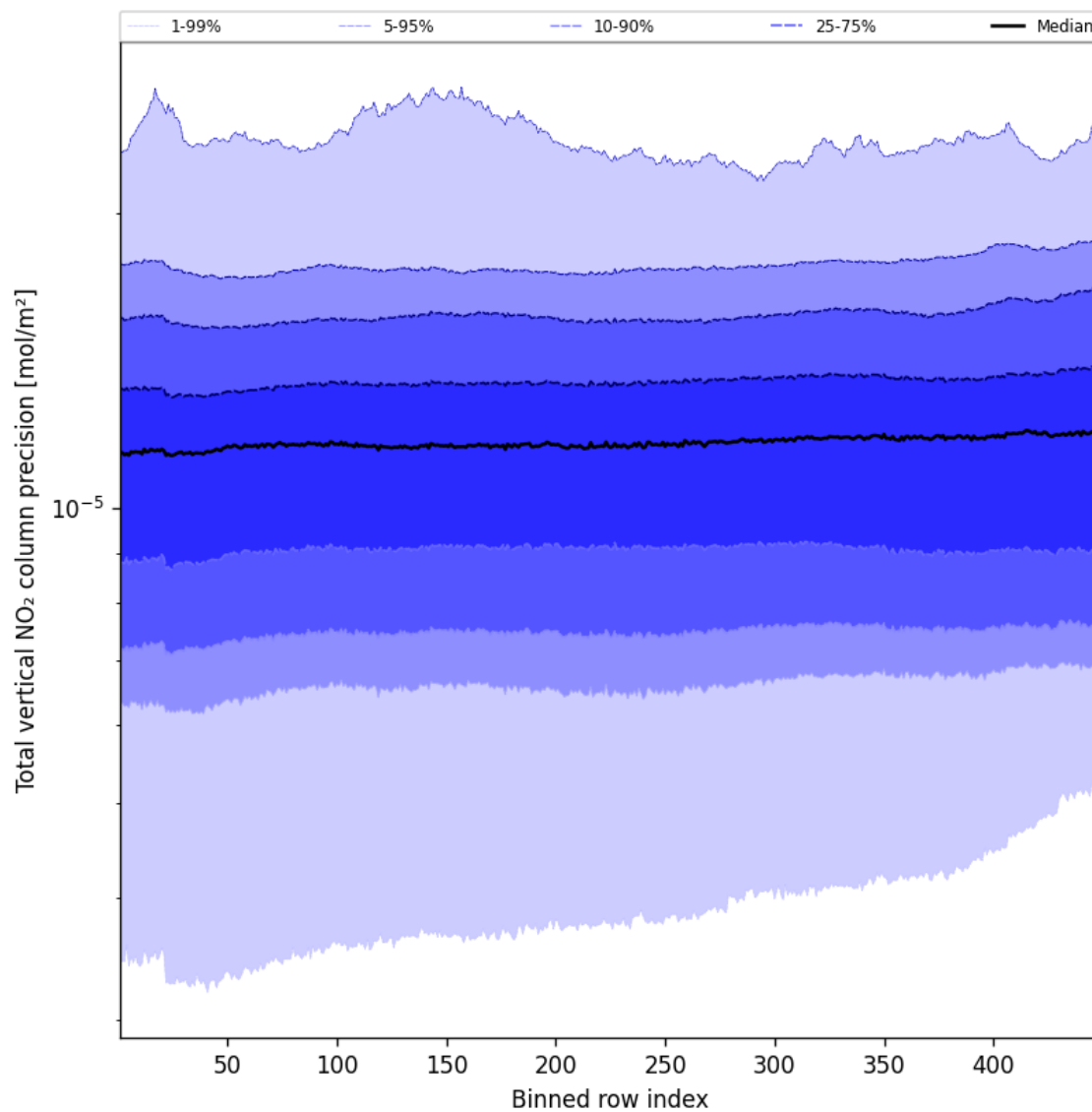
Figure 56: Along track statistics of “Total vertical NO 2 column precision” for 2024-11-22 to 2024-11-24
