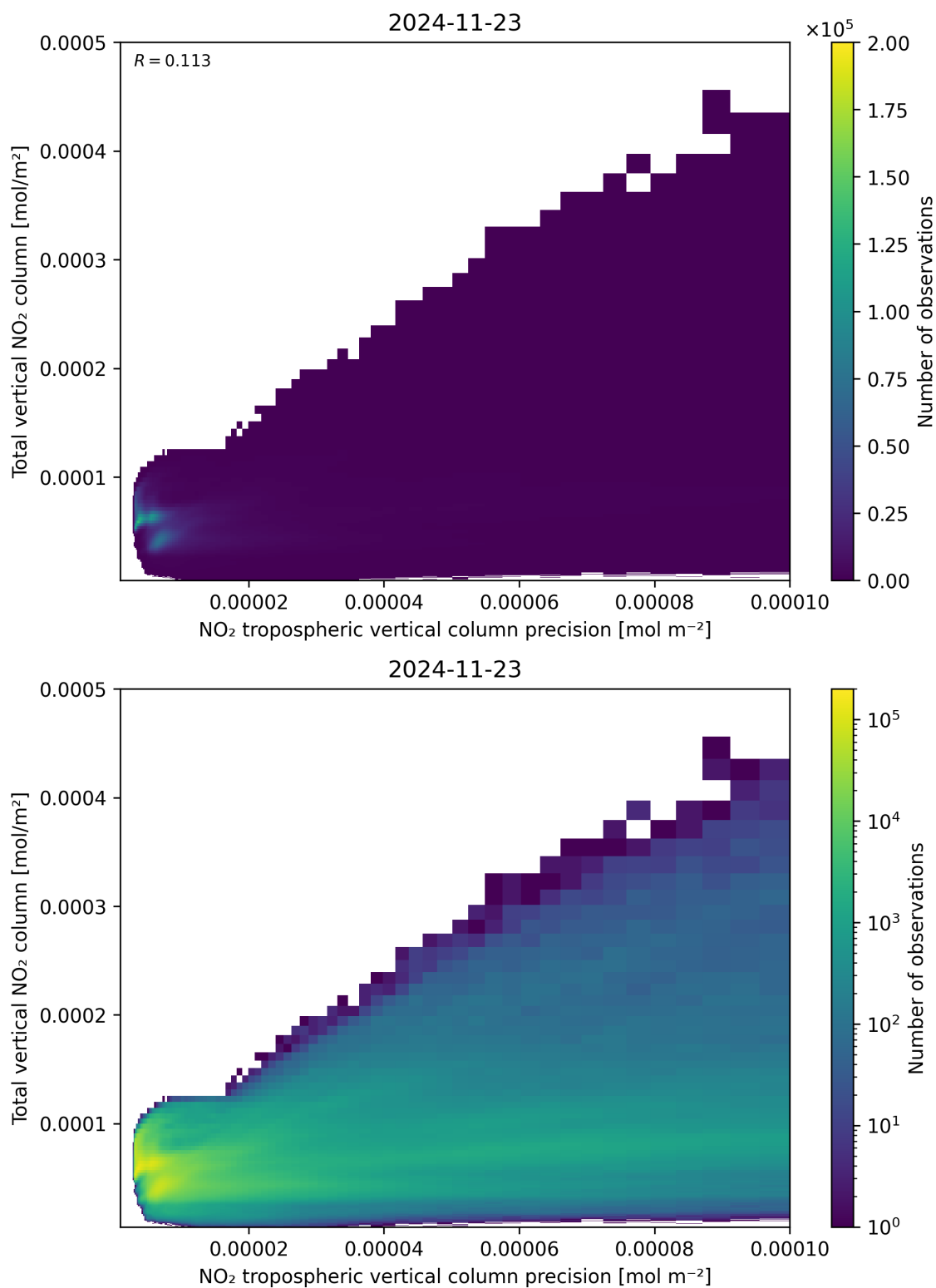
Figure 138: Scatter density plot of “NO 2 tropospheric vertical column precision” against “Total vertical NO 2 column” for 2024-11-22 to 2024-11-24.
