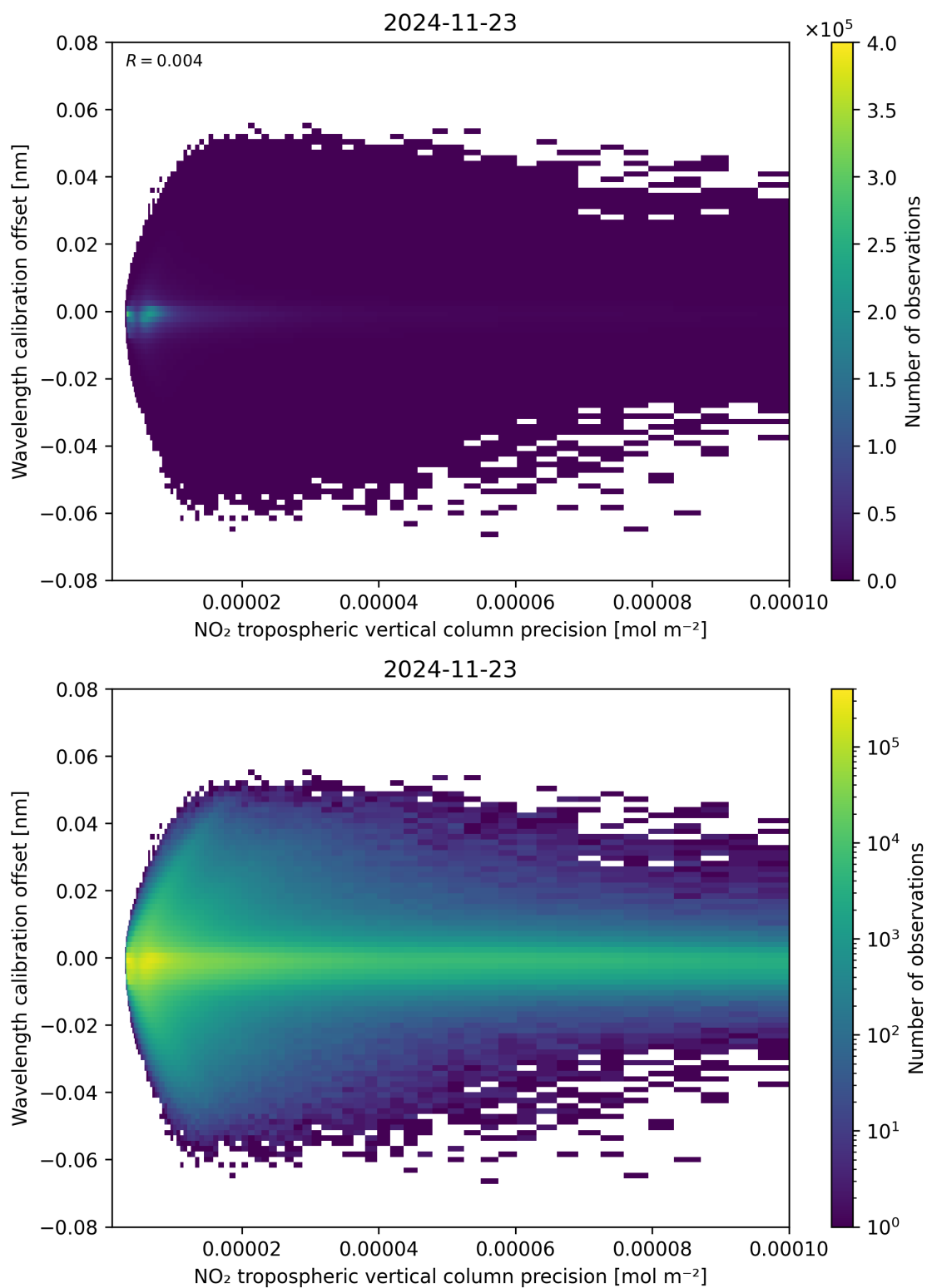
Figure 141: Scatter density plot of “NO 2 tropospheric vertical column precision” against “Wavelength calibration offset” for 2024-11-22 to 2024-11-24.
