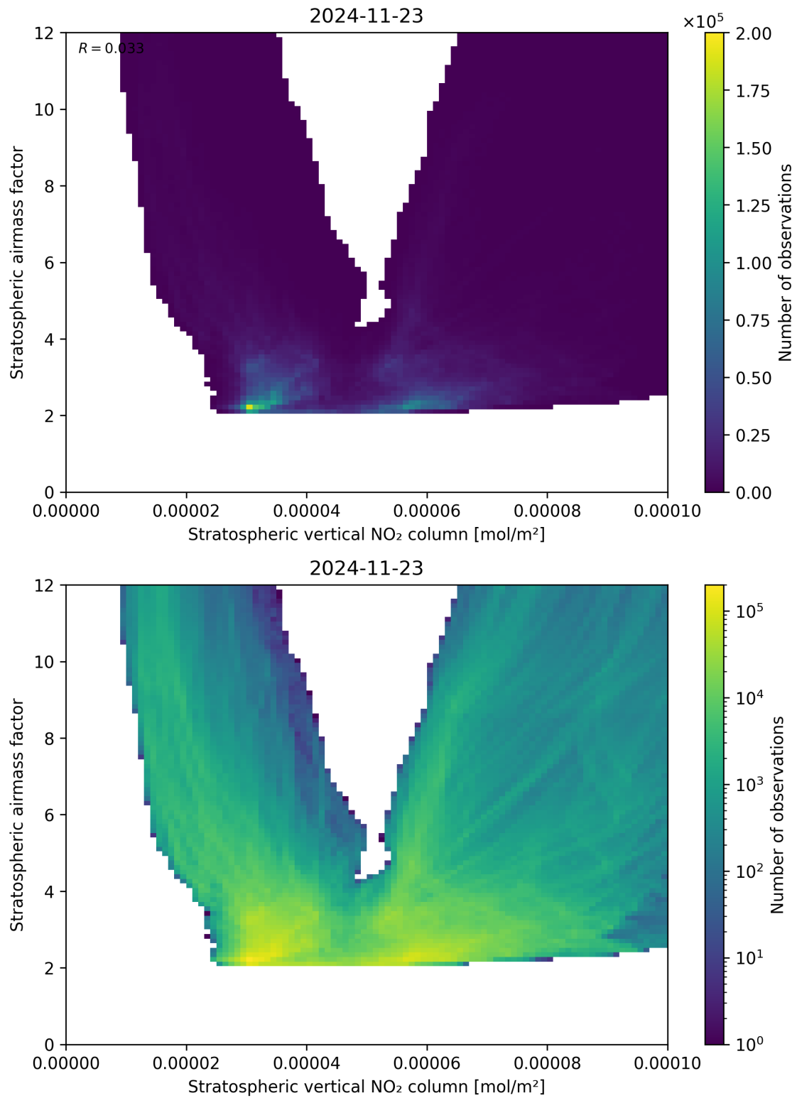
Figure 96: Scatter density plot of “Stratospheric vertical NO 2 column” against “Stratospheric airmass factor” for 2024-11-22 to 2024-11-24.
