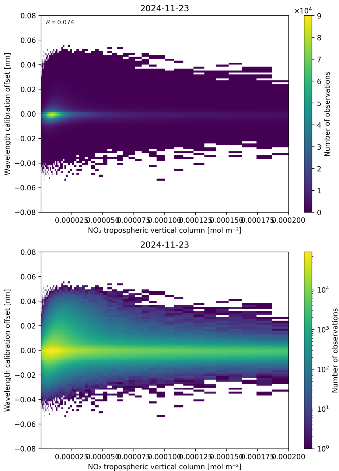
Figure 143: Scatter density plot of “NO 2 tropospheric vertical column” against “Wavelength calibration offset” for 2024-11-22 to 2024-11-24.
