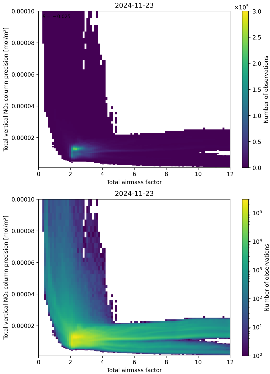
Figure 68: Scatter density plot of “Total airmass factor” against “Total vertical NO 2 column precision” for 2024-11-22 to 2024-11-24.
