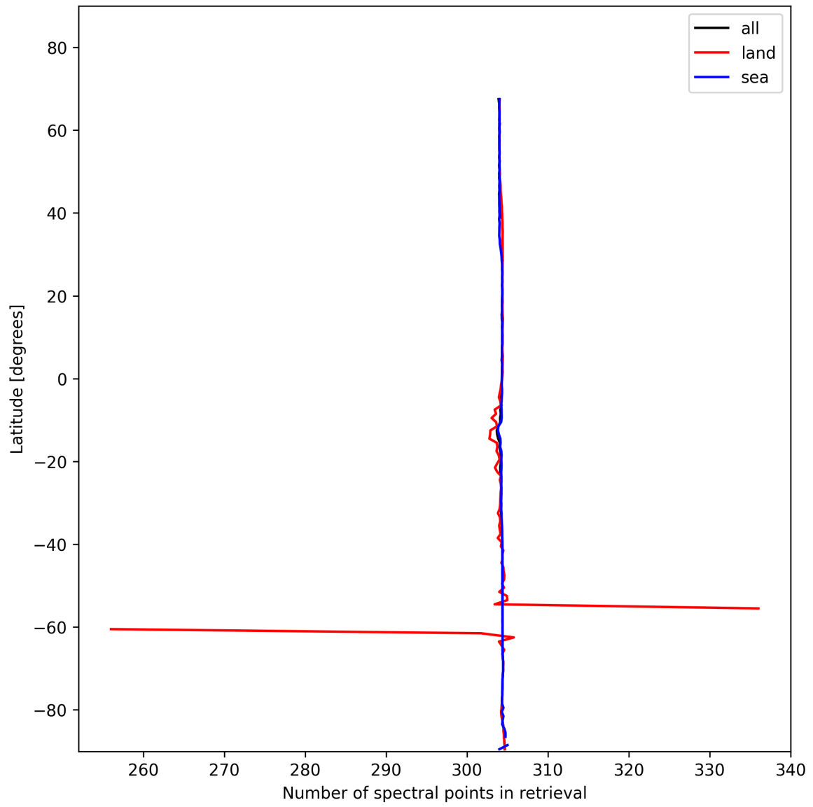
Figure 16: Zonal average of “Number of spectral points in retrieval” for 2024-11-22 to 2024-11-24.
