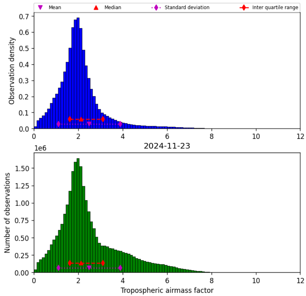
Figure 31: Histogram of “Tropospheric airmass factor” for 2024-11-22 to 2024-11-24
