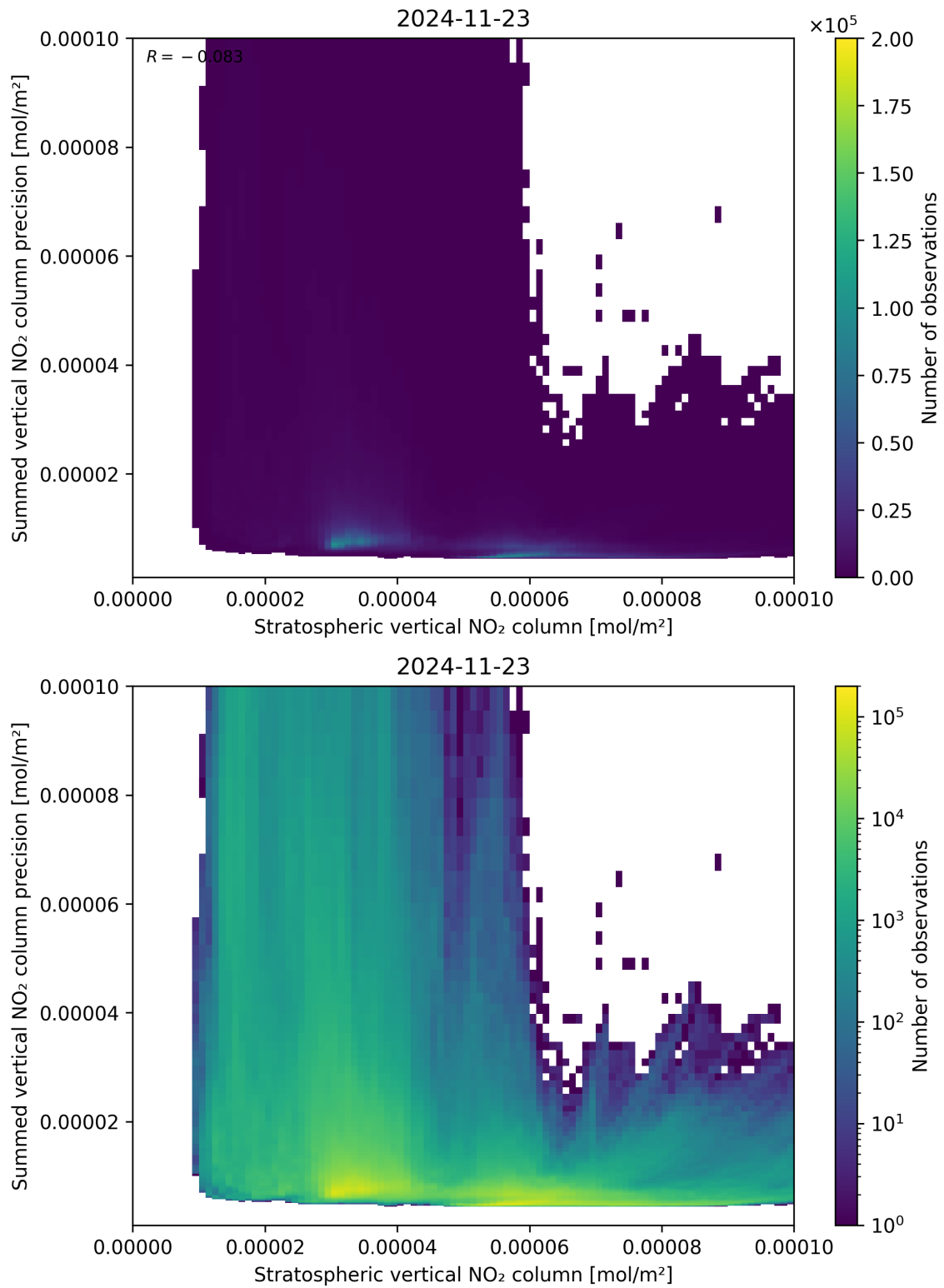
Figure 99: Scatter density plot of “Stratospheric vertical NO 2 column” against “Summed vertical NO 2 column precision” for 2024-11-22 to 2024-11-24.
