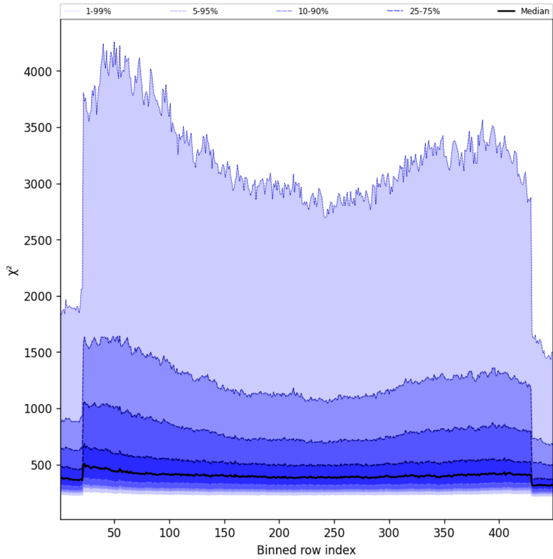
Figure 59: Along track statistics of “ \chi^2 ” for 2024-11-22 to 2024-11-24
