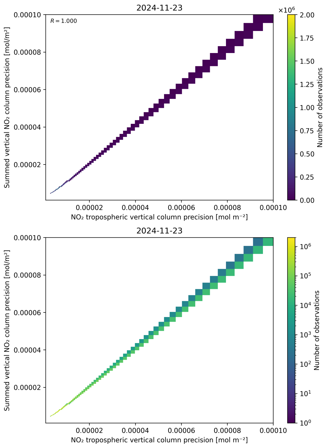
Figure 137: Scatter density plot of “NO 2 tropospheric vertical column precision” against “Summed vertical NO 2 column precision” for 2024-11-22 to 2024-11-24.
