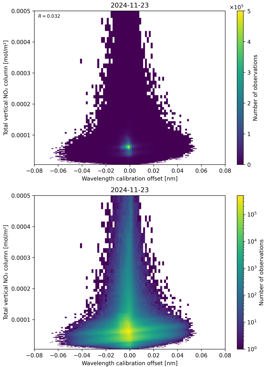
Figure 179: Scatter density plot of “Wavelength calibration offset” against “Total vertical NO 2 column” for 2024-11-22 to 2024-11-24.
