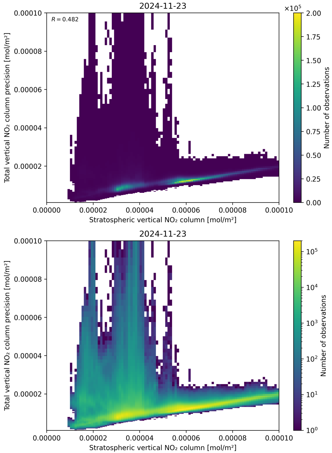
Figure 101: Scatter density plot of “Stratospheric vertical NO 2 column” against “Total vertical NO 2 column precision” for 2024-11-22 to 2024-11-24.
