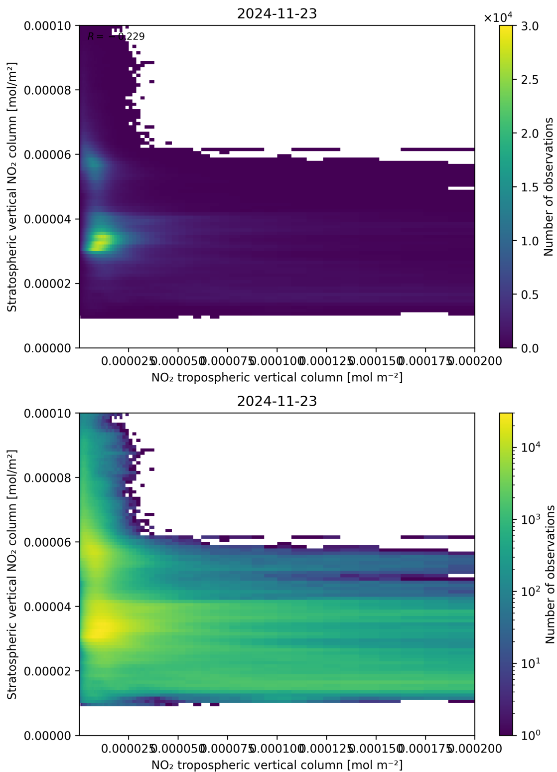
Figure 125: Scatter density plot of “NO 2 tropospheric vertical column” against “Stratospheric vertical NO 2 column” for 2024-11-22 to 2024-11-24.
