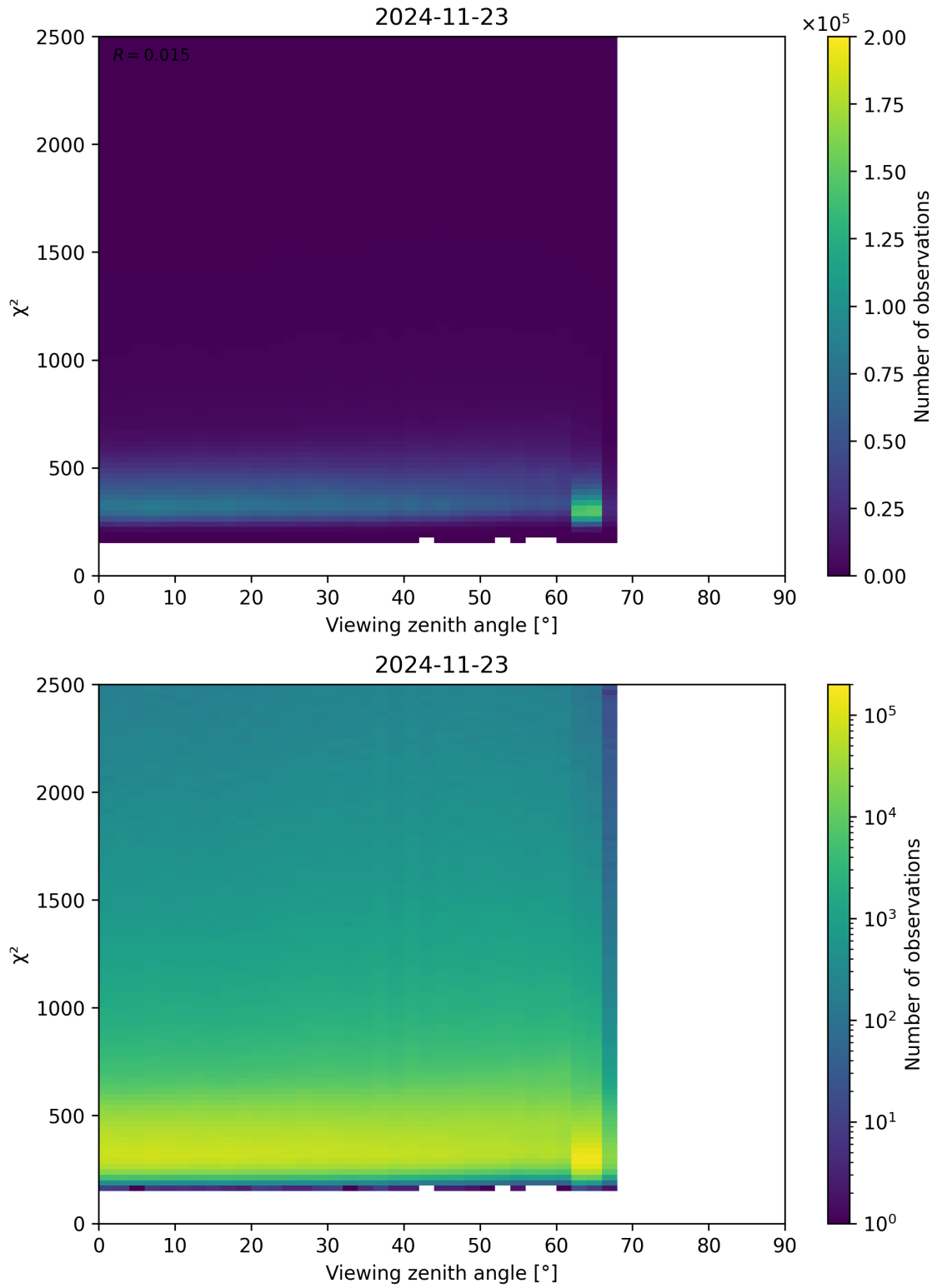
Figure 162: Scatter density plot of “Viewing zenith angle” against “ \chi^2 ” for 2024-11-22 to 2024-11-24.
