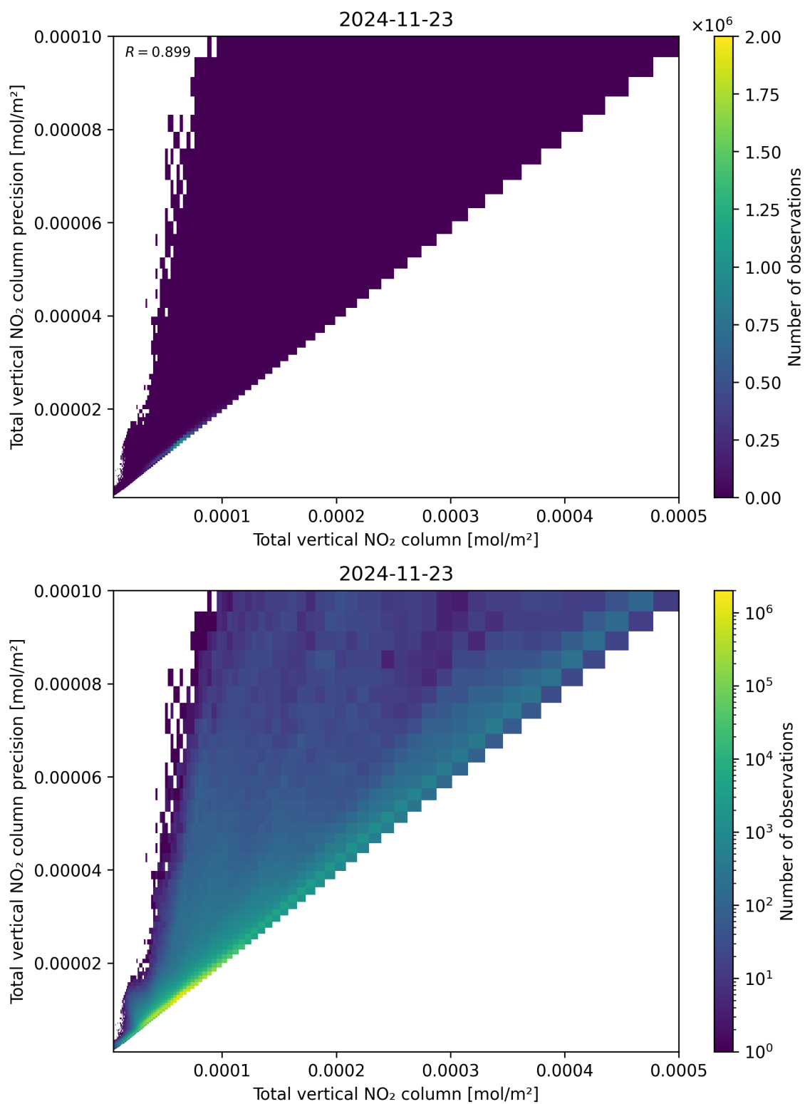
Figure 114: Scatter density plot of “Total vertical NO 2 column” against “Total vertical NO 2 column precision” for 2024-11-22 to 2024-11-24.
