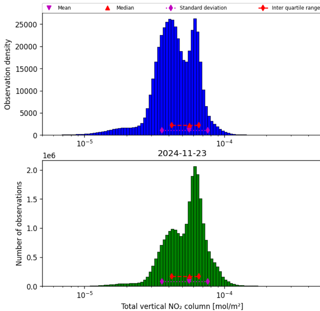
Figure 38: Histogram of “Total vertical NO 2 column” for 2024-11-22 to 2024-11-24
