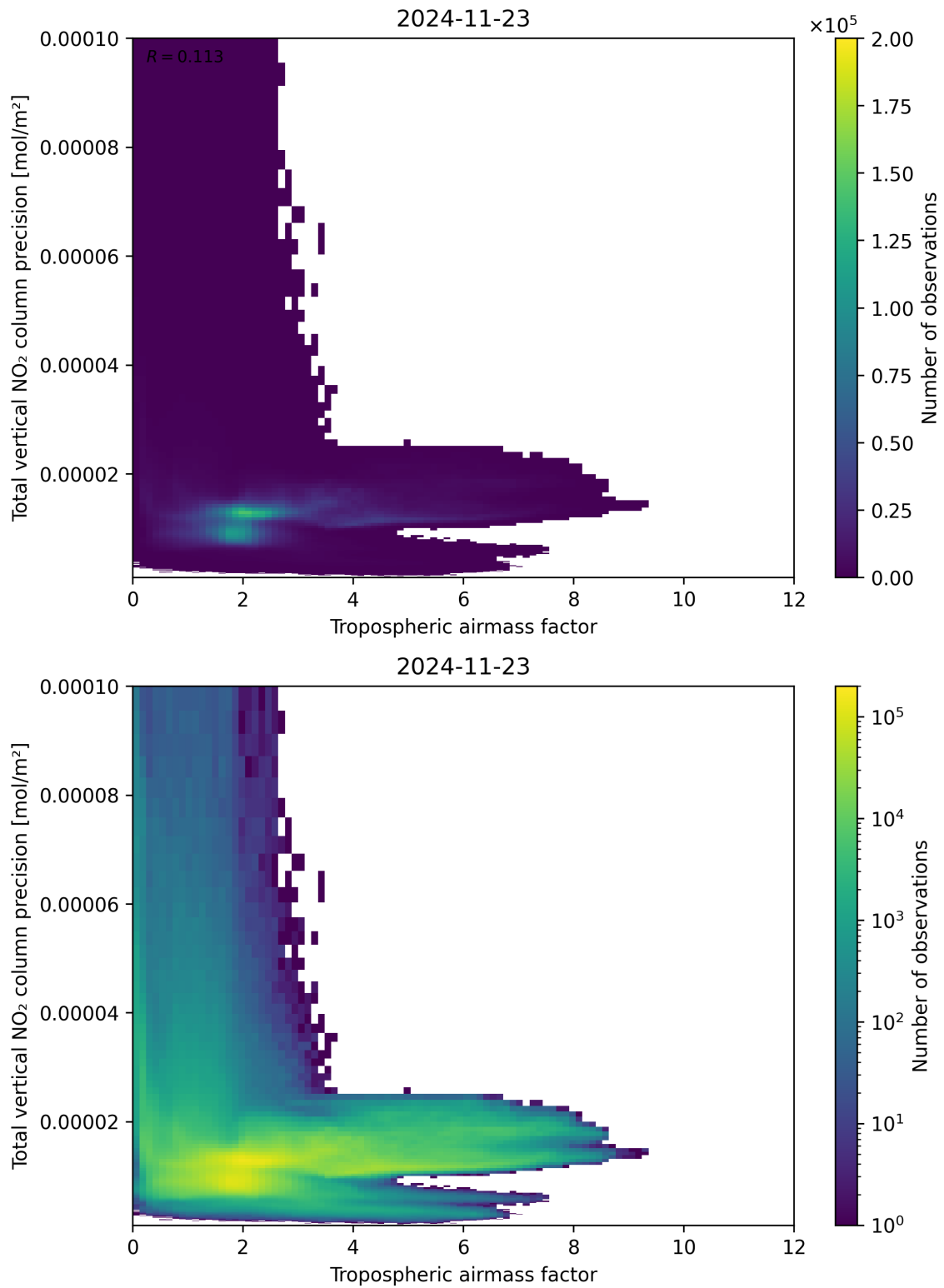
Figure 78: Scatter density plot of “Tropospheric air mass factor” against “Total vertical NO 2 column precision” for 2024-11-22 to 2024-11-24.
