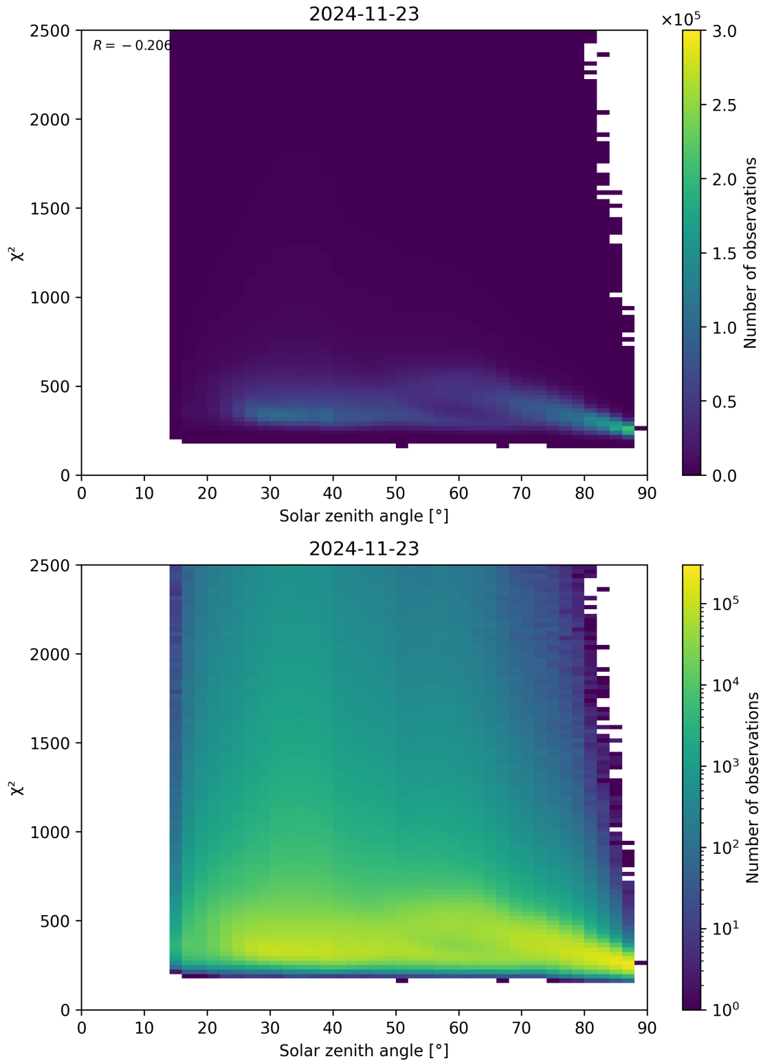
Figure 148: Scatter density plot of “Solar zenith angle” against “ \chi^2 ” for 2024-11-22 to 2024-11-24.
