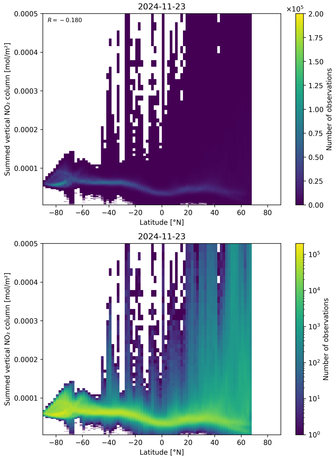
Figure 88: Scatter density plot of “Latitude” against “Summed vertical NO 2 column” for 2024-11-22 to 2024-11-24.
