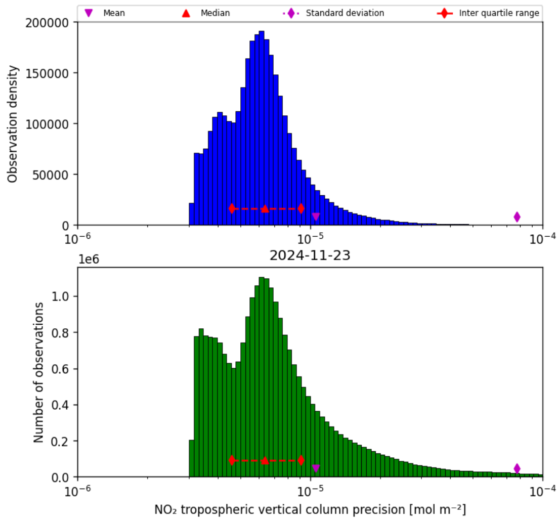
Figure 30: Histogram of “NO 2 tropospheric vertical column precision” for 2024-11-22 to 2024-11-24
