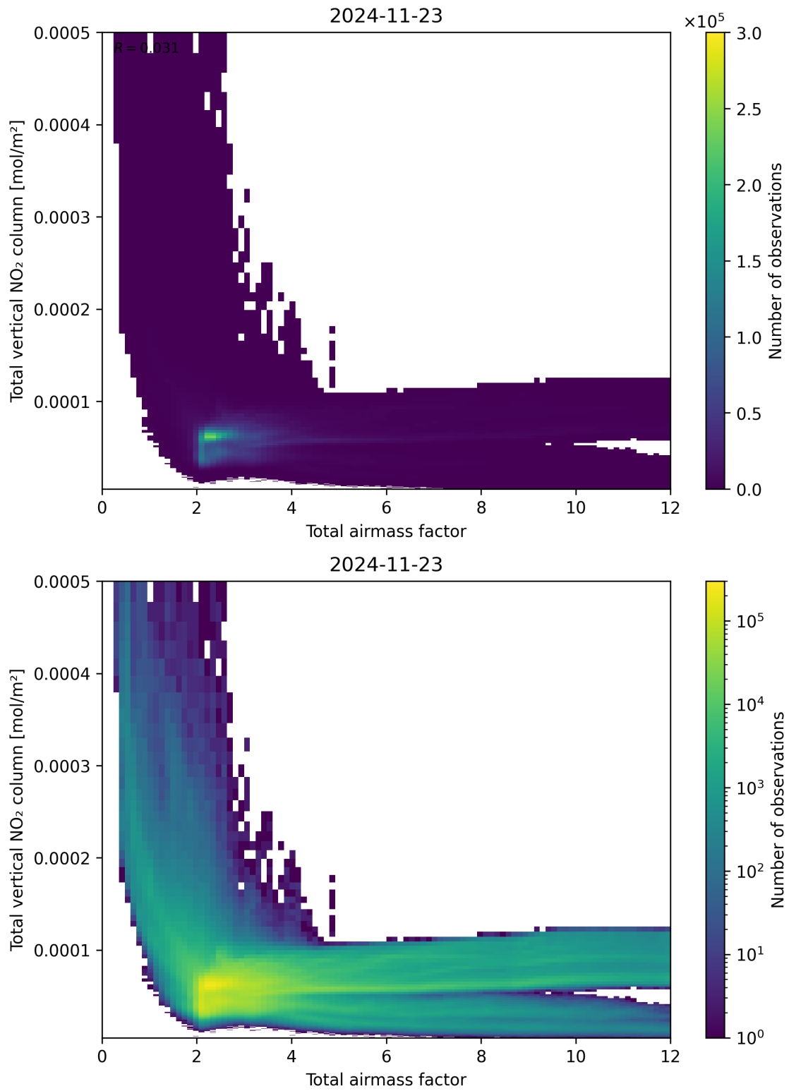
Figure 67: Scatter density plot of “Total airmass factor” against “Total vertical NO 2 column” for 2024-11-22 to 2024-11-24.
