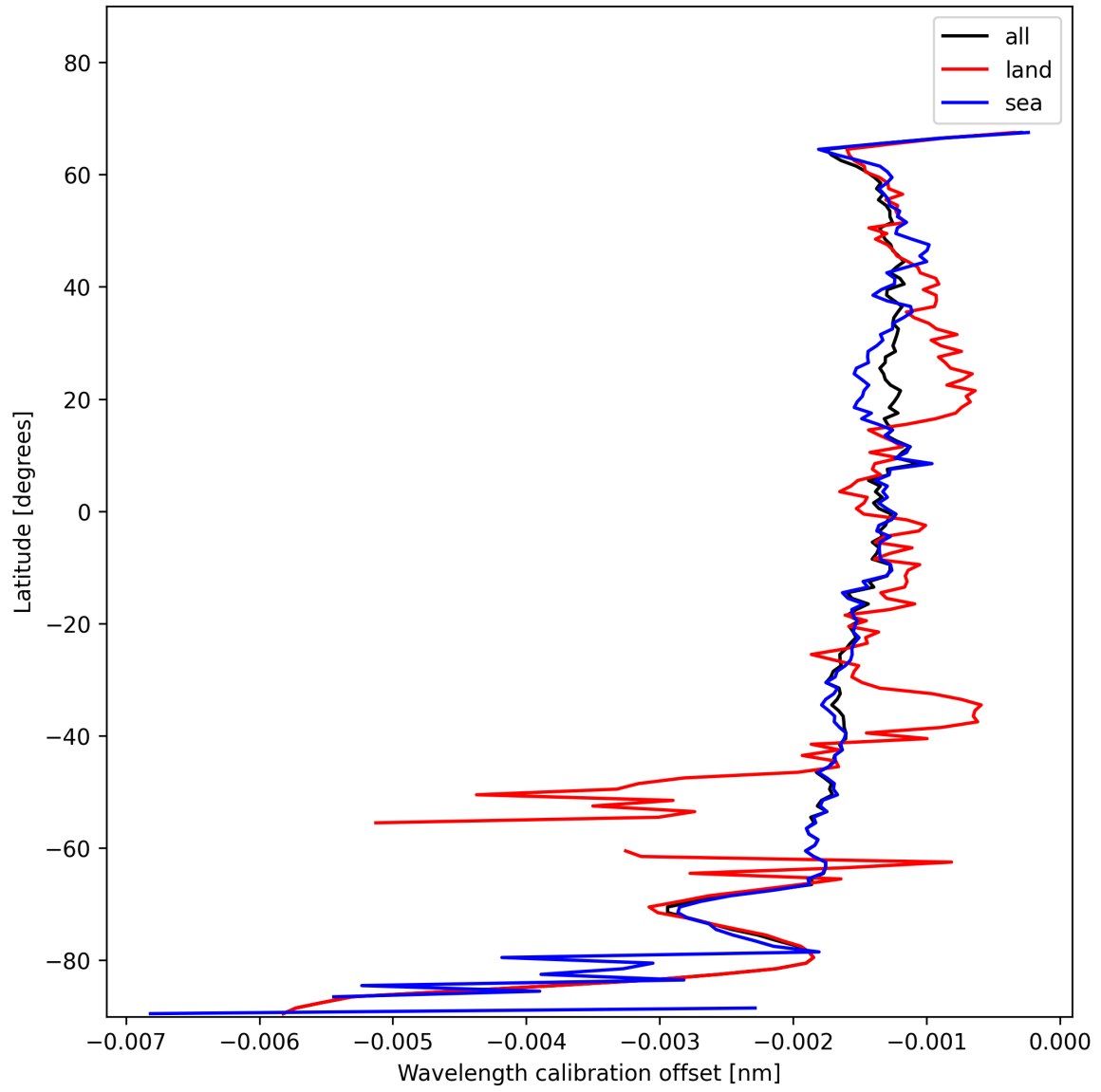
Figure 18: Zonal average of “Wavelength calibration offset” for 2024-11-22 to 2024-11-24.
