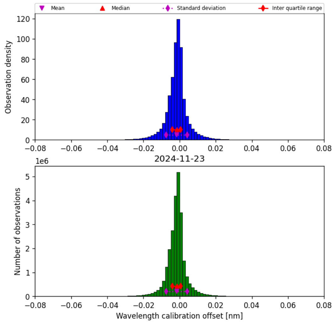
Figure 35: Histogram of “Wavelength calibration offset” for 2024-11-22 to 2024-11-24
