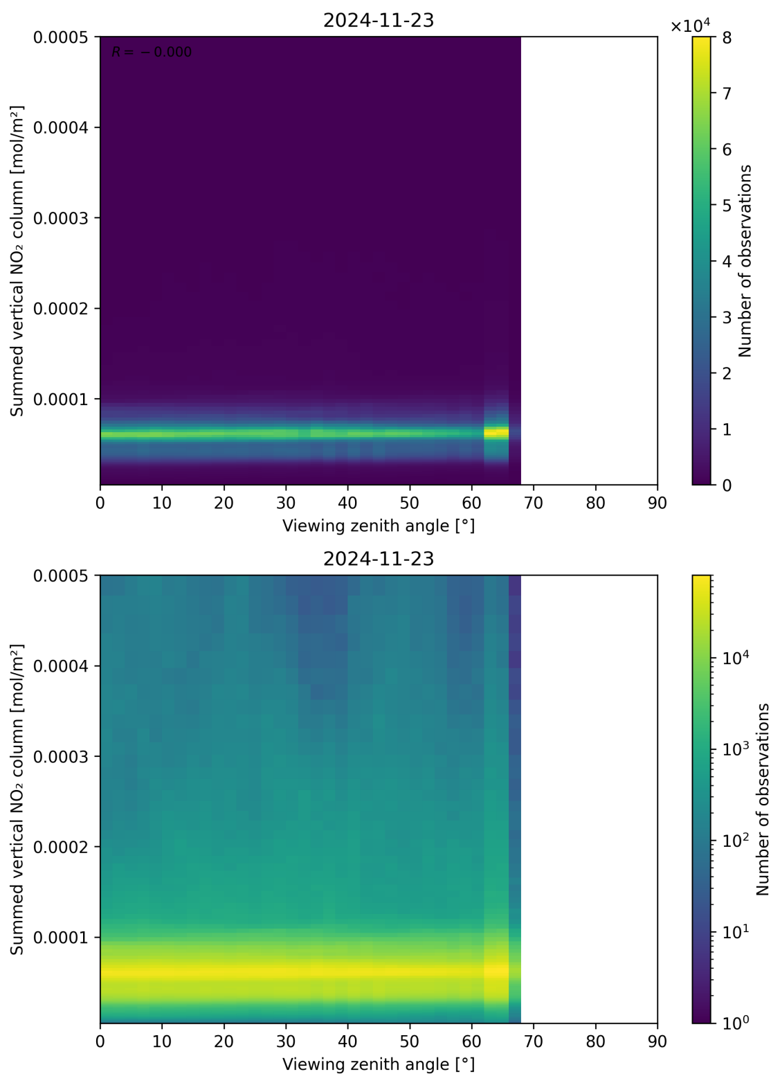
Figure 165: Scatter density plot of “Viewing zenith angle” against “Summed vertical NO 2 column” for 2024-11-22 to 2024-11-24.
