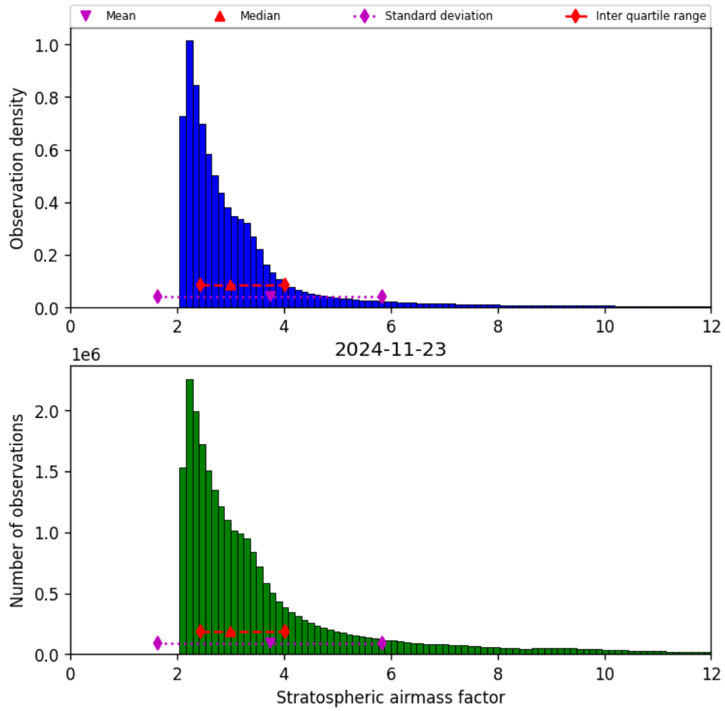
Figure 44: Histogram of “Stratospheric airmass factor” for 2024-11-22 to 2024-11-24
