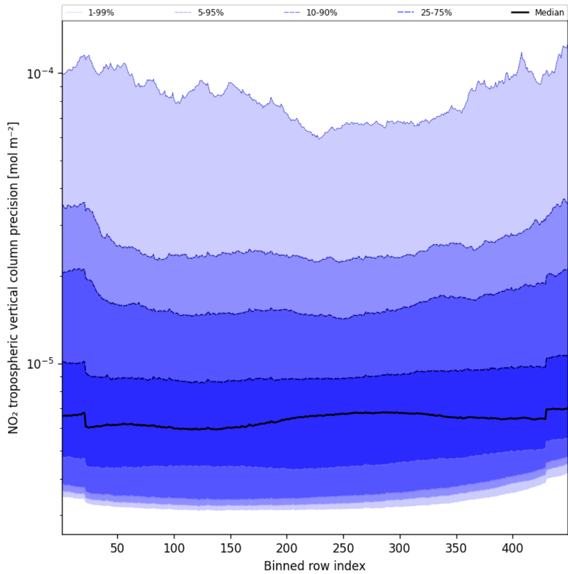
Figure 47: Along track statistics of “NO 2 tropospheric vertical column precision” for 2024-11-22 to 2024-11-24
