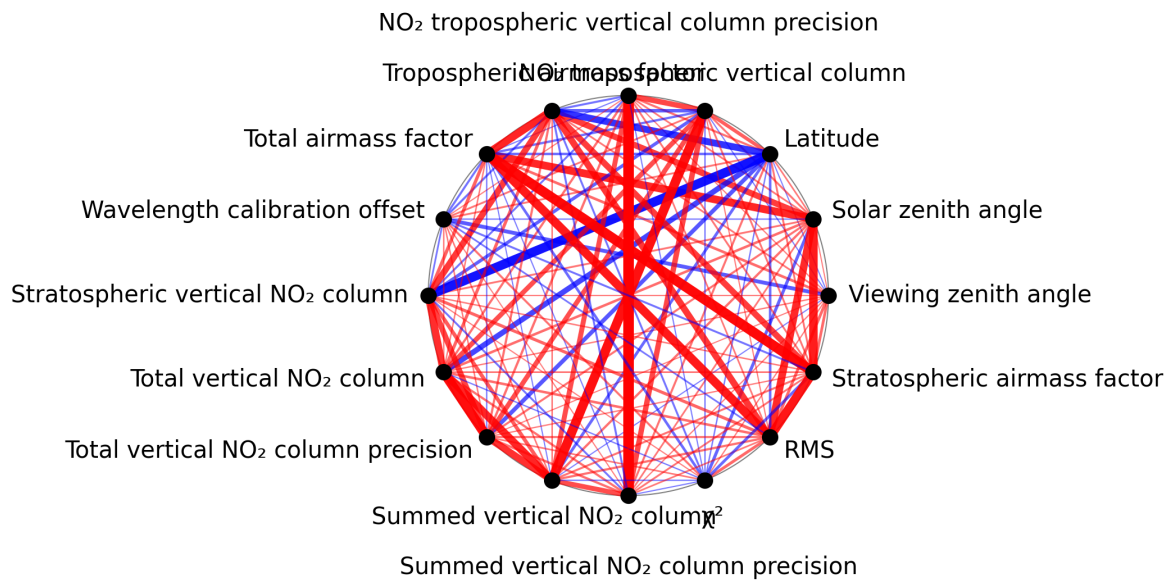
Figure 1: Map of correlation graph for 2024-11-22 to 2024-11-24.
