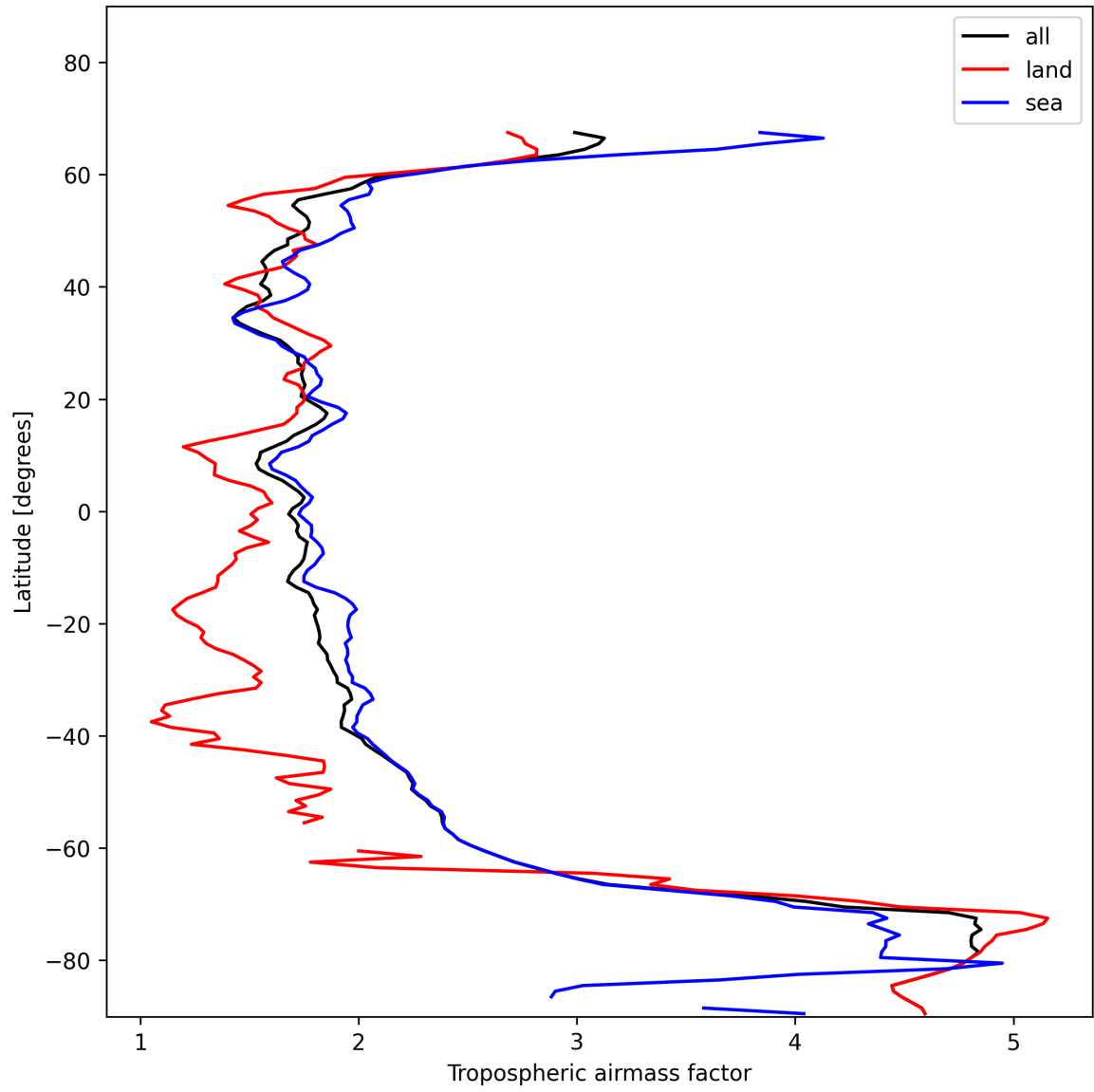
Figure 14: Zonal average of “Tropospheric airmass factor” for 2024-11-22 to 2024-11-24.
