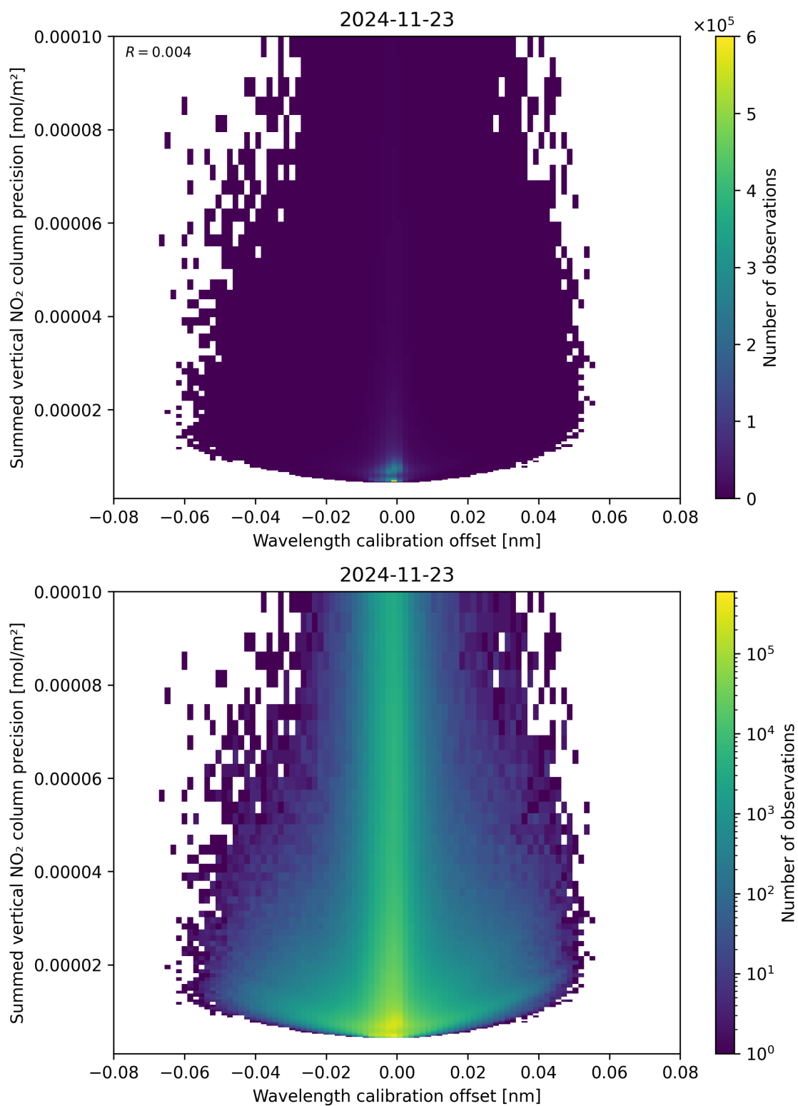
Figure 178: Scatter density plot of “Wavelength calibration offset” against “Summed vertical NO 2 column precision” for 2024-11-22 to 2024-11-24.
