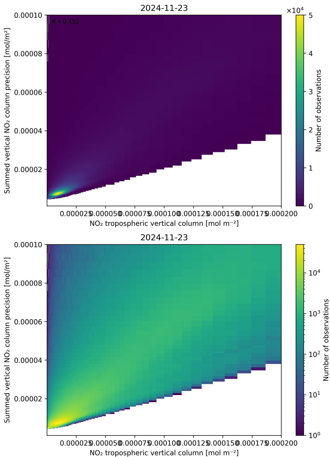
Figure 127: Scatter density plot of “NO 2 tropospheric vertical column” against “Summed vertical NO 2 column precision” for 2024-11-22 to 2024-11-24.
