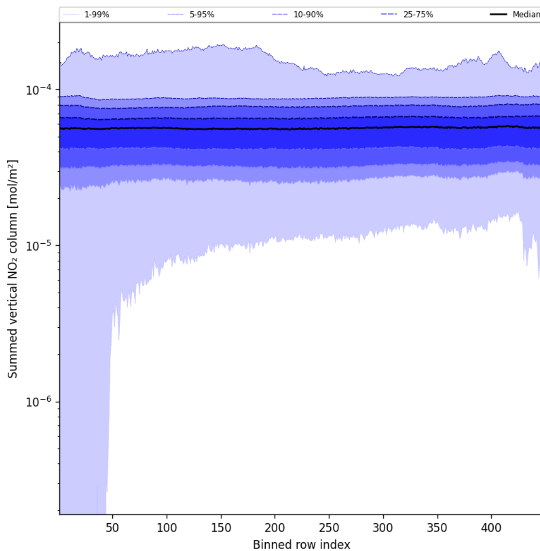
Figure 57: Along track statistics of “Summed vertical NO 2 column” for 2024-11-22 to 2024-11-24
