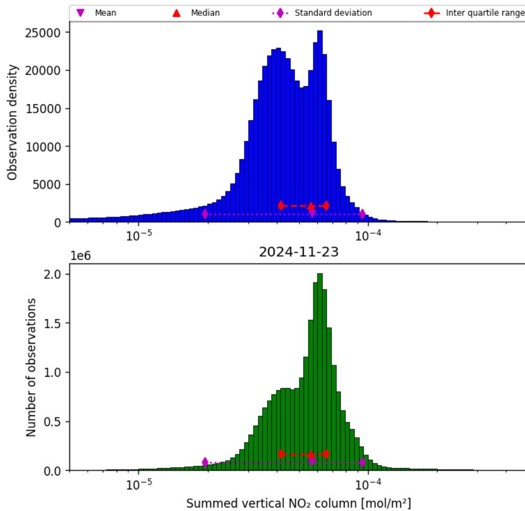
Figure 40: Histogram of “Summed vertical NO 2 column” for 2024-11-22 to 2024-11-24
