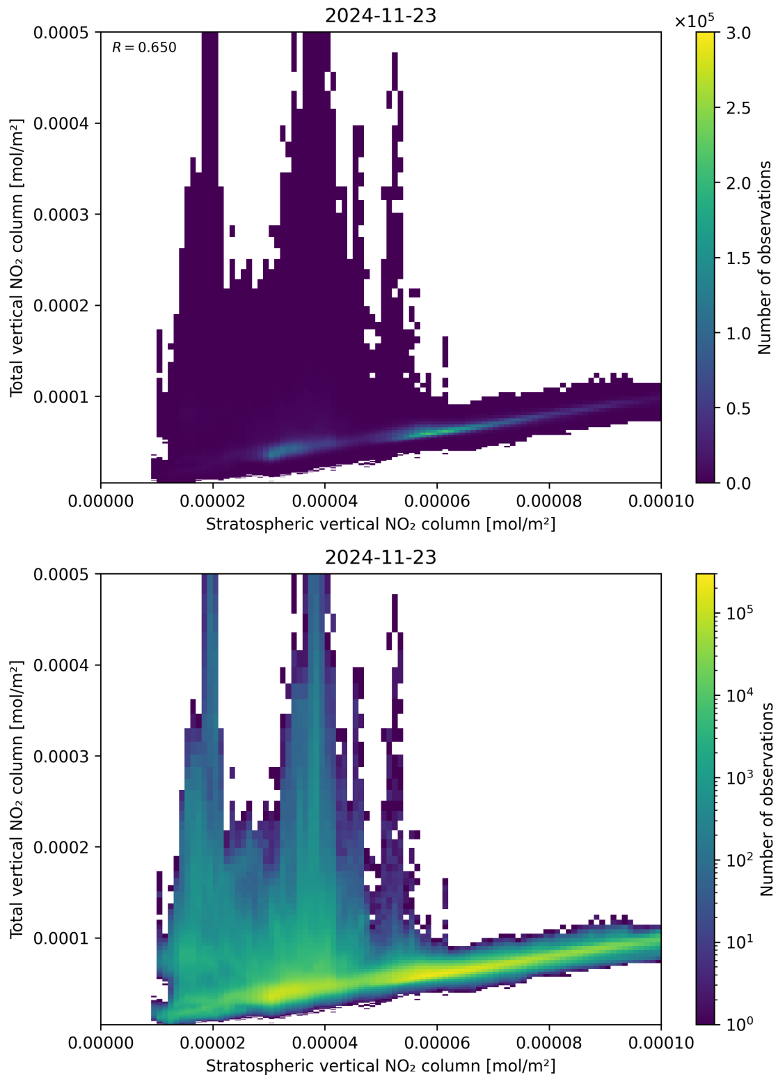
Figure 100: Scatter density plot of “Stratospheric vertical NO 2 column” against “Total vertical NO 2 column” for 2024-11-22 to 2024-11-24.
