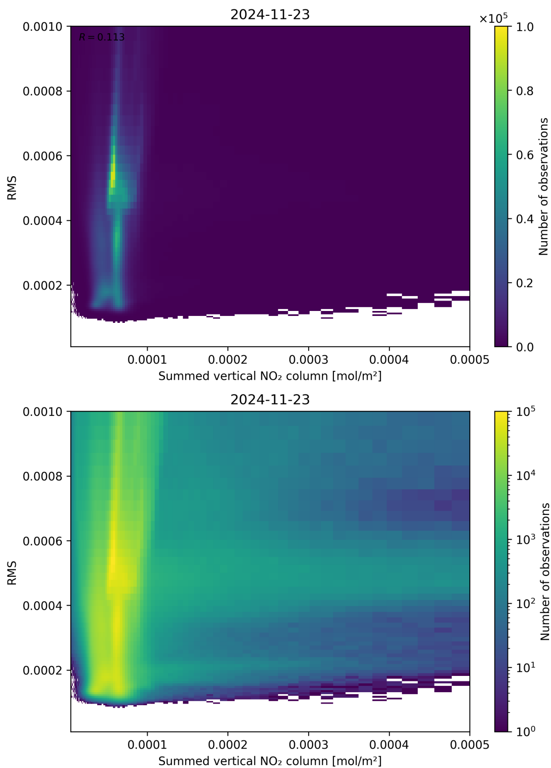
Figure 109: Scatter density plot of “Summed vertical NO 2 column” against “RMS” for 2024-11-22 to 2024-11-24.
