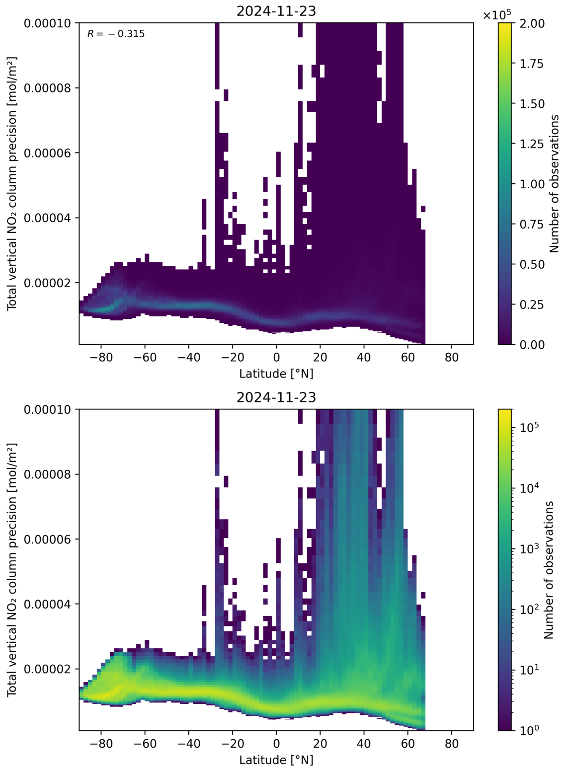
Figure 91: Scatter density plot of “Latitude” against “Total vertical NO 2 column precision” for 2024-11-22 to 2024-11-24.
