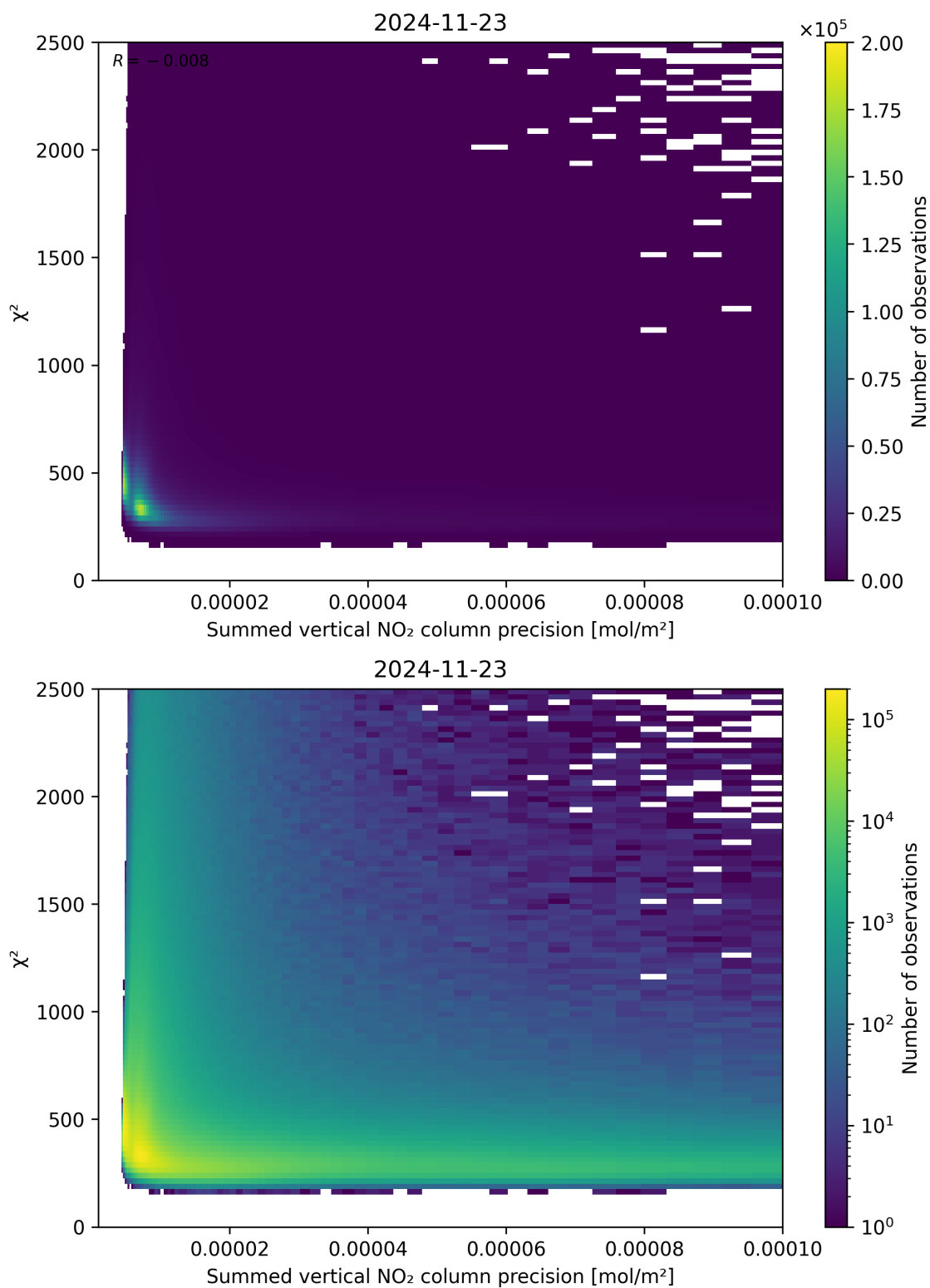
Figure 107: Scatter density plot of “Summed vertical NO 2 column precision” against “ \chi^2 ” for 2024-11-22 to 2024-11-24.
