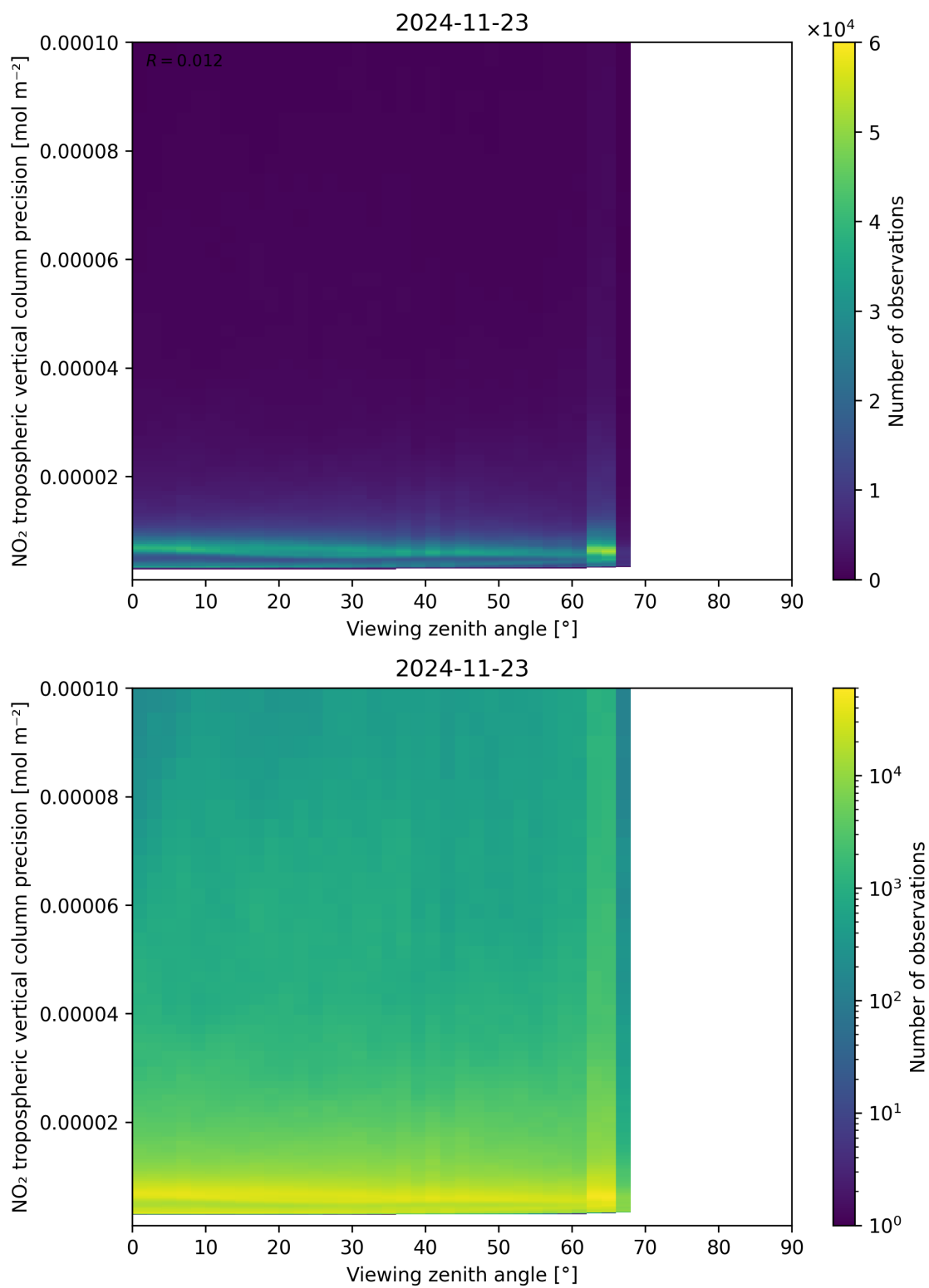
Figure 170: Scatter density plot of “Viewing zenith angle” against “NO 2 tropospheric vertical column precision” for 2024-11-22 to 2024-11-24.
