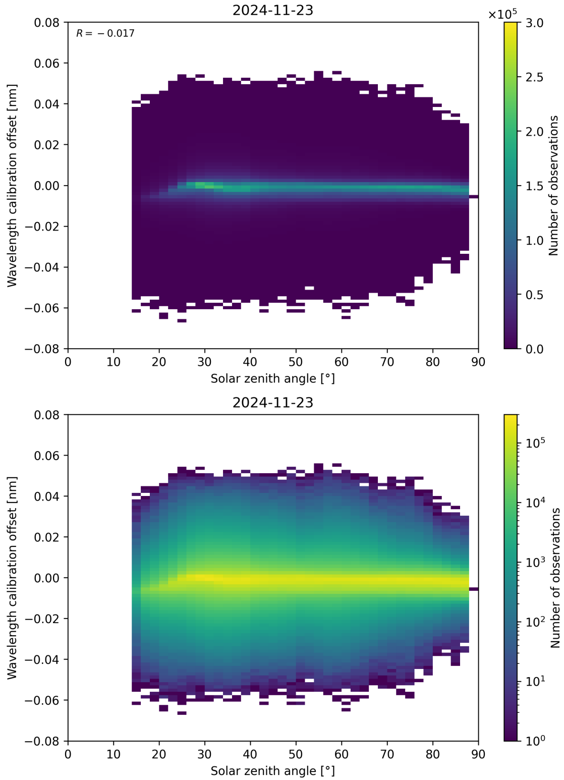
Figure 158: Scatter density plot of “Solar zenith angle” against “Wavelength calibration offset” for 2024-11-22 to 2024-11-24.
