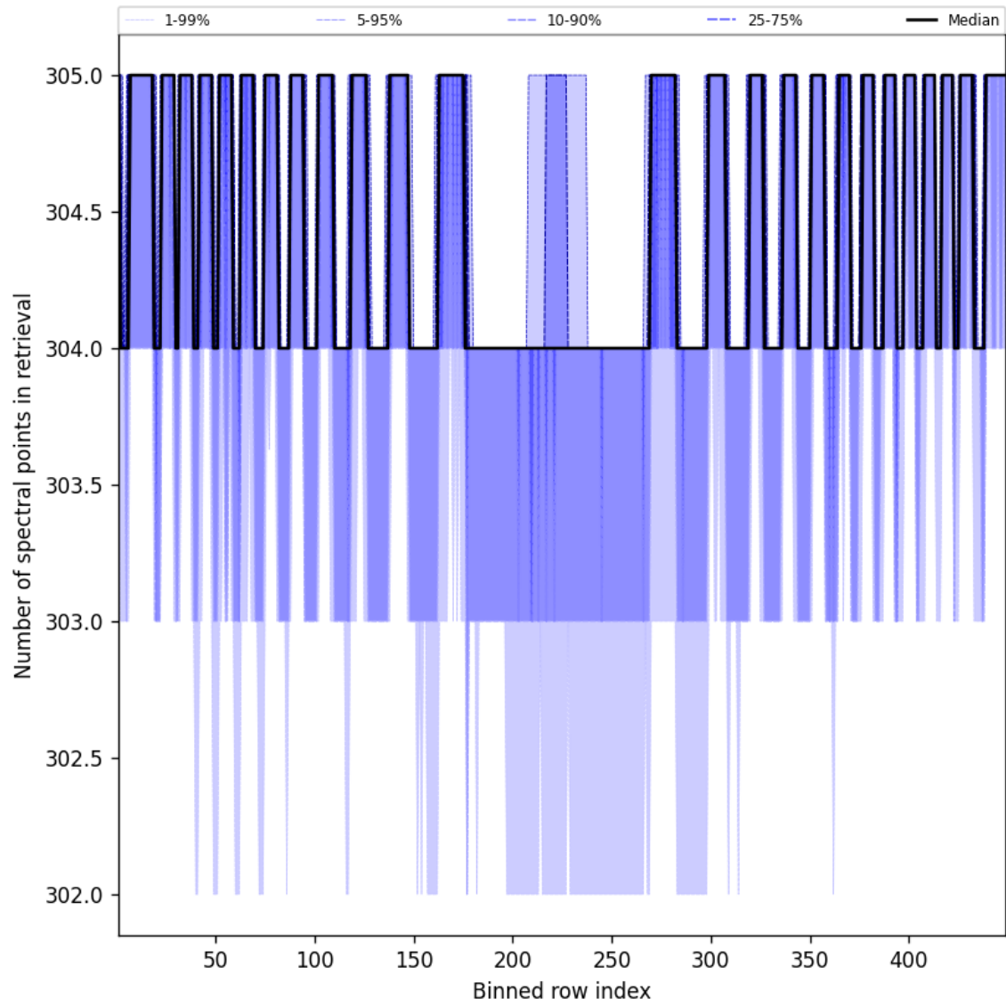
Figure 50: Along track statistics of “Number of spectral points in retrieval” for 2024-11-22 to 2024-11-24
