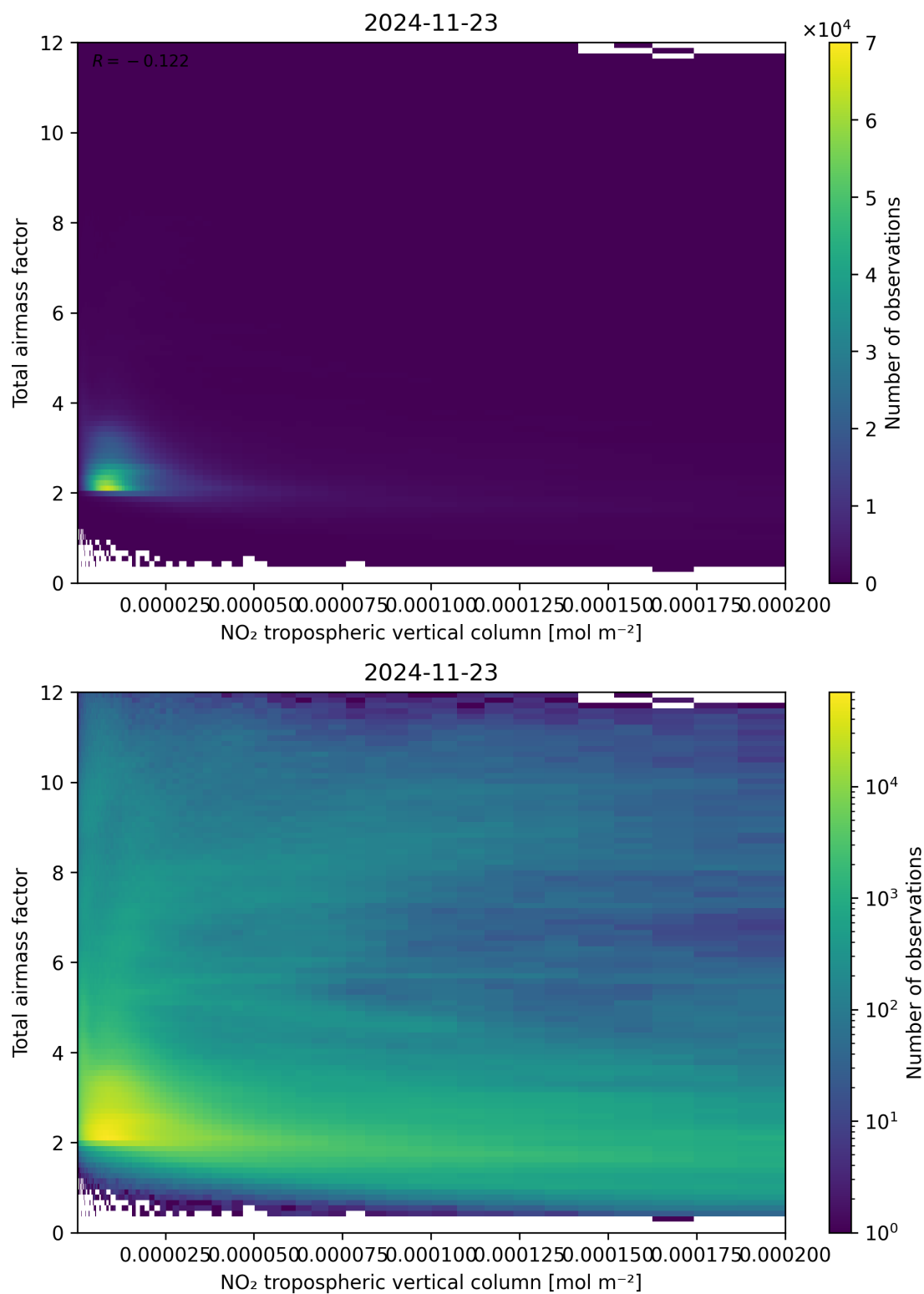
Figure 122: Scatter density plot of “NO 2 tropospheric vertical column” against “Total airmass factor” for 2024-11-22 to 2024-11-24.
