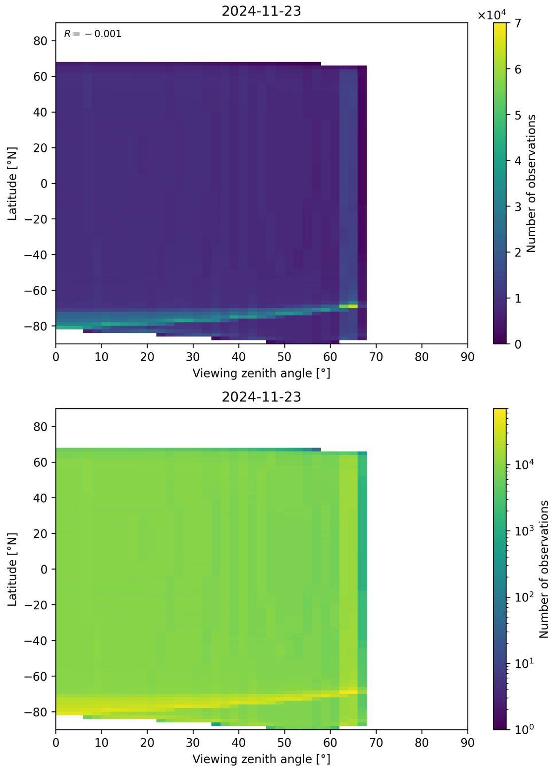
Figure 163: Scatter density plot of “Viewing zenith angle” against “Latitude” for 2024-11-22 to 2024-11-24.
