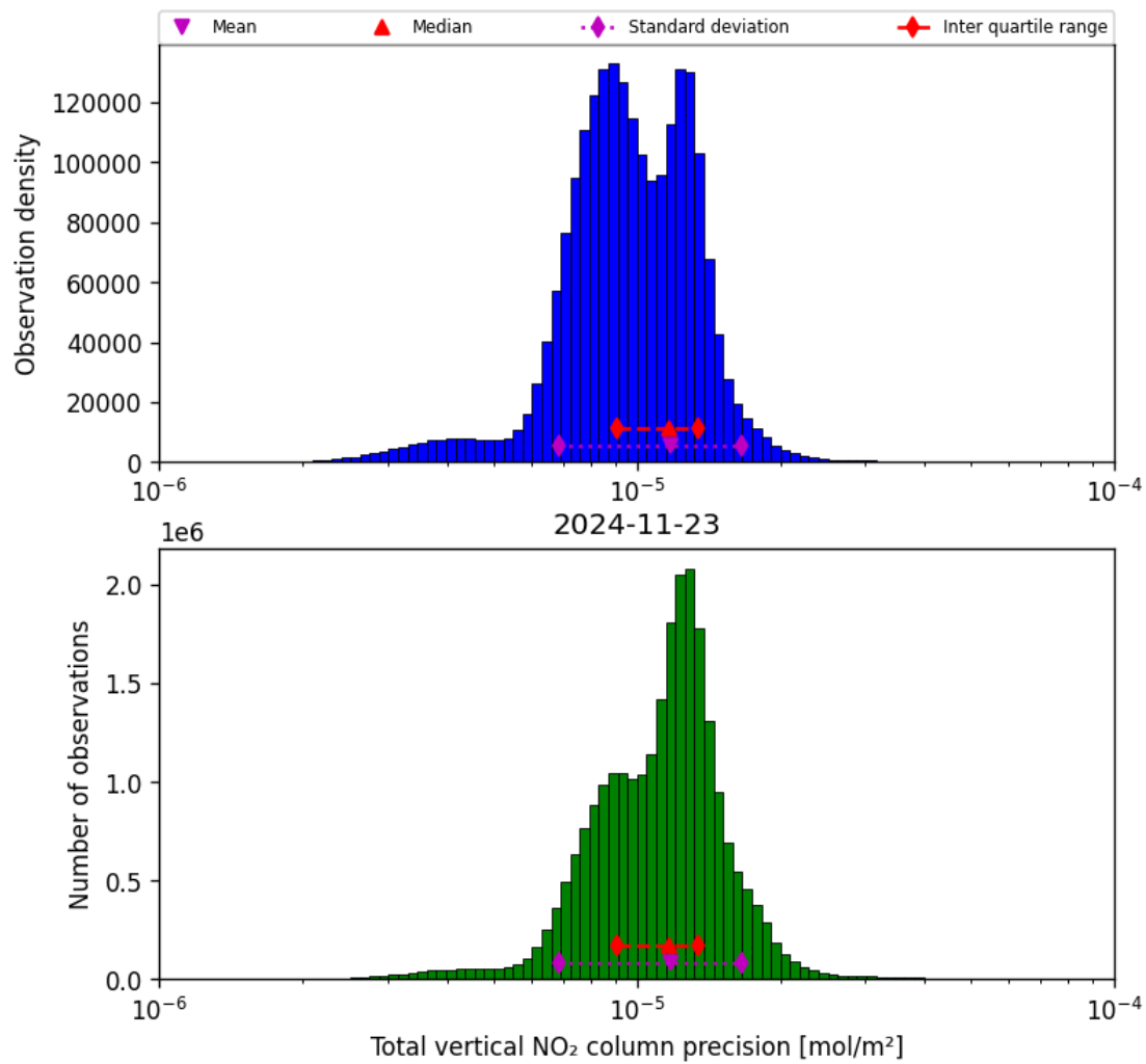
Figure 39: Histogram of “Total vertical NO 2 column precision” for 2024-11-22 to 2024-11-24
