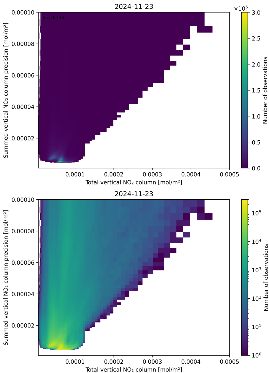
Figure 113: Scatter density plot of “Total vertical NO 2 column” against “Summed vertical NO 2 column precision” for 2024-11-22 to 2024-11-24.
