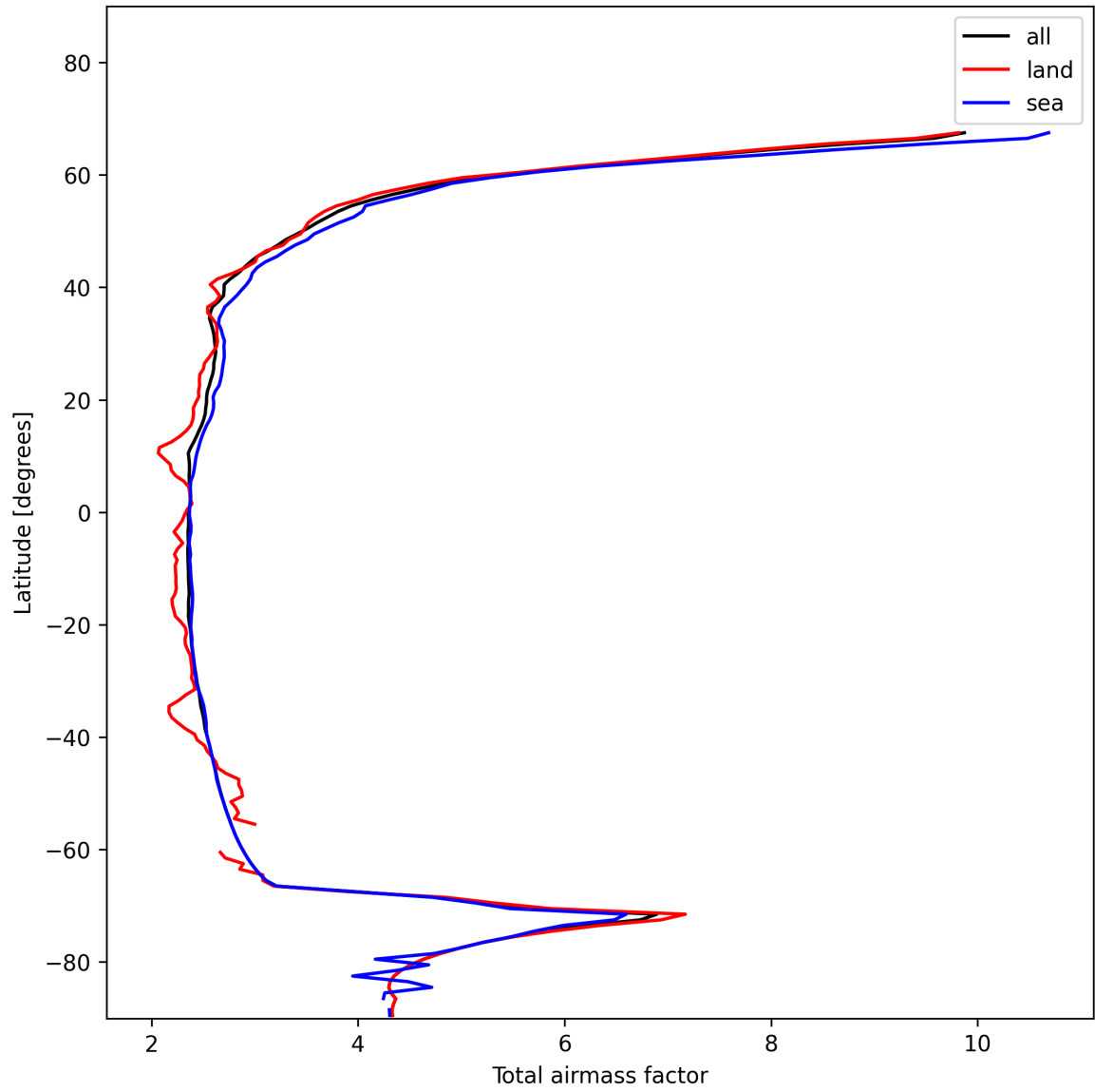
Figure 15: Zonal average of “Total airmass factor” for 2024-11-22 to 2024-11-24.
