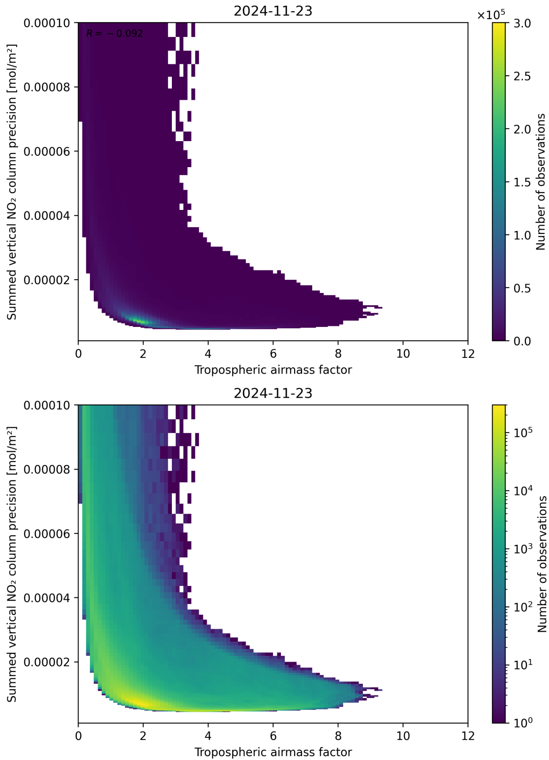
Figure 76: Scatter density plot of “Tropospheric air mass factor” against “Summed vertical NO 2 column precision” for 2024-11-22 to 2024-11-24.
