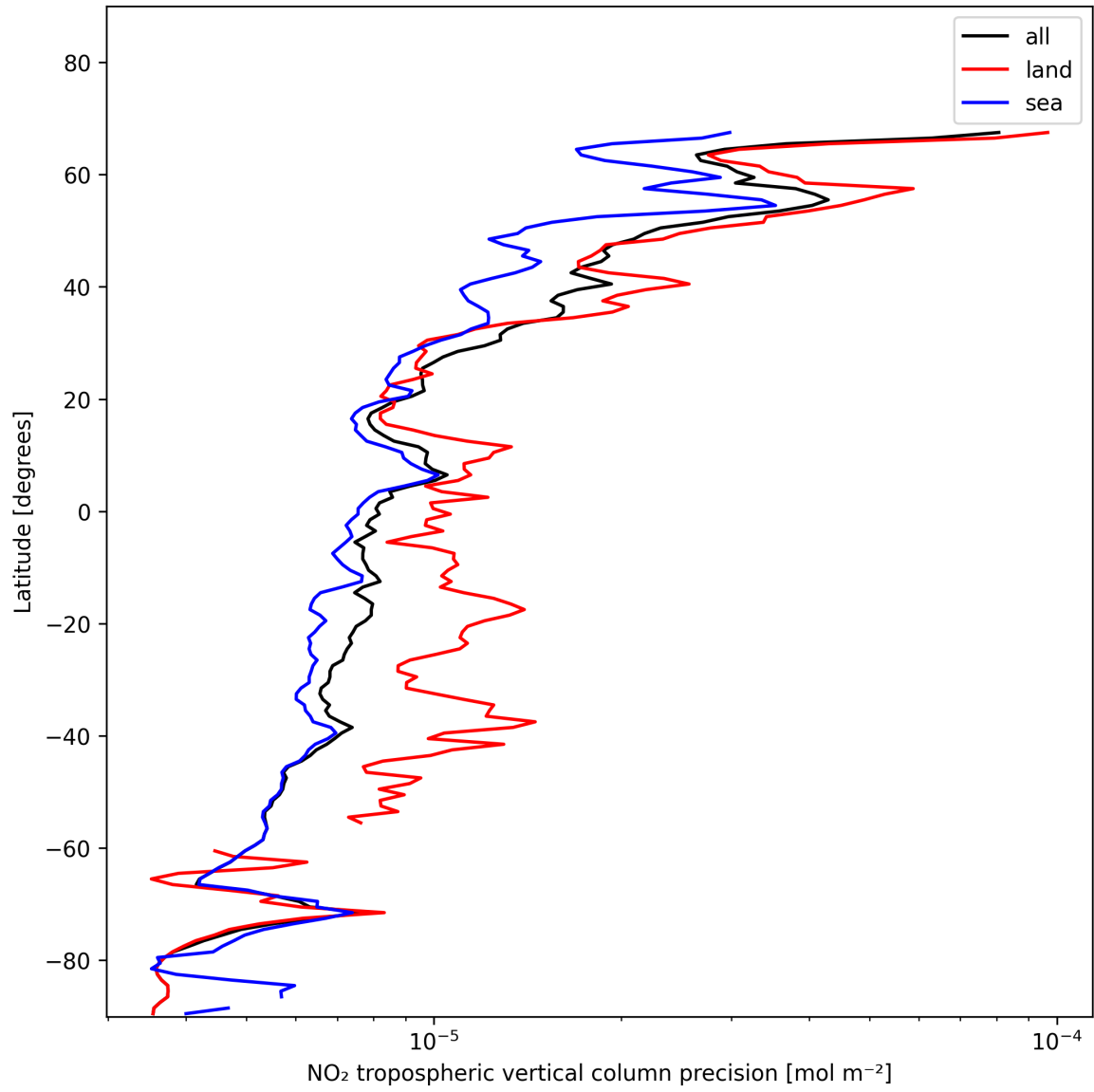
Figure 13: Zonal average of “NO 2 tropospheric vertical column precision” for 2024-11-22 to 2024-11-24.
