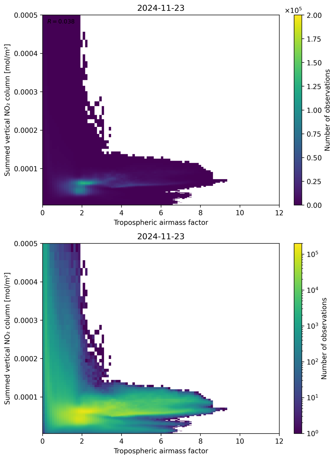
Figure 75: Scatter density plot of “Tropospheric airmass factor” against “Summed vertical NO 2 column” for 2024-11-22 to 2024-11-24.
