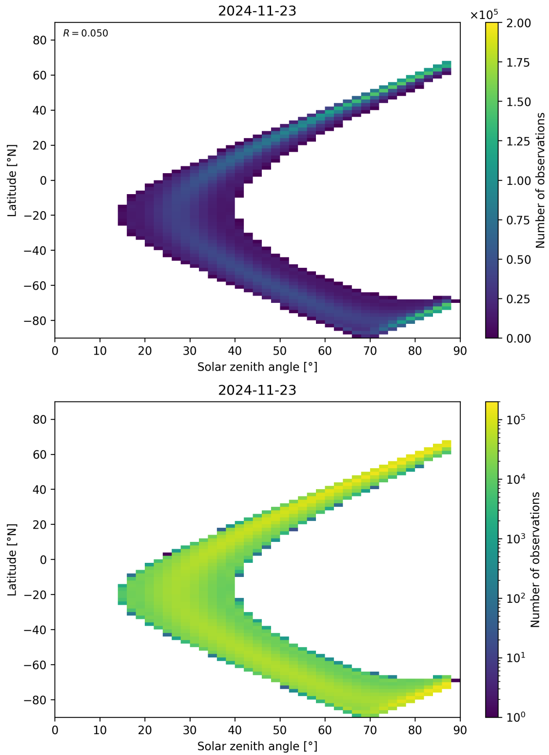
Figure 149: Scatter density plot of “Solar zenith angle” against “Latitude” for 2024-11-22 to 2024-11-24.
