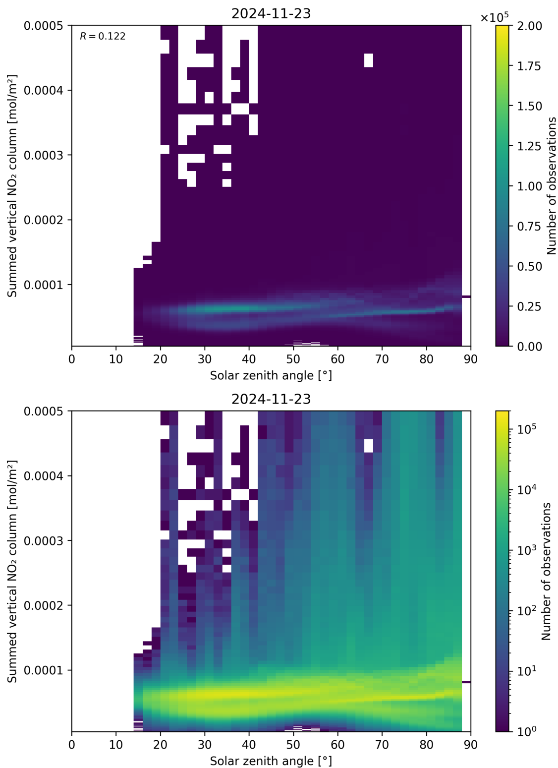
Figure 151: Scatter density plot of “Solar zenith angle” against “Summed vertical NO 2 column” for 2024-11-22 to 2024-11-24.
