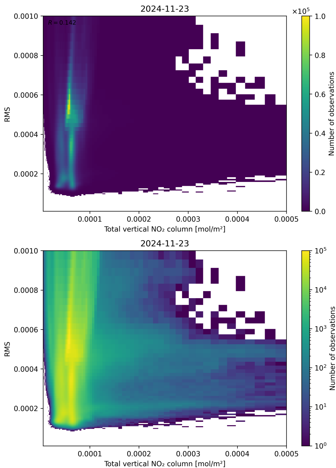
Figure 120: Scatter density plot of “Total vertical NO 2 column” against “RMS” for 2024-11-22 to 2024-11-24.
