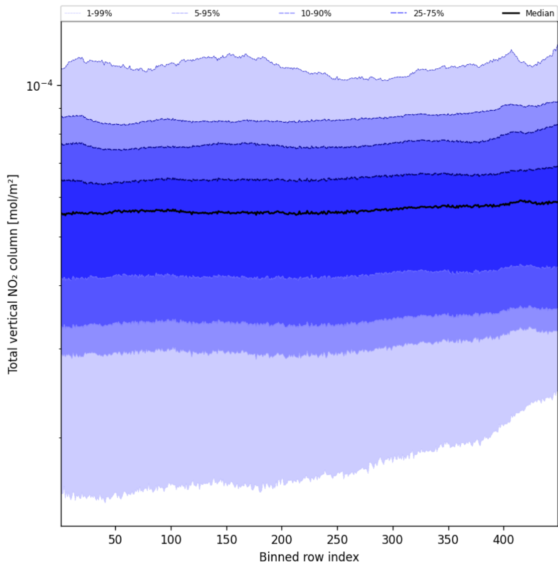
Figure 55: Along track statistics of “Total vertical NO 2 column” for 2024-11-22 to 2024-11-24
