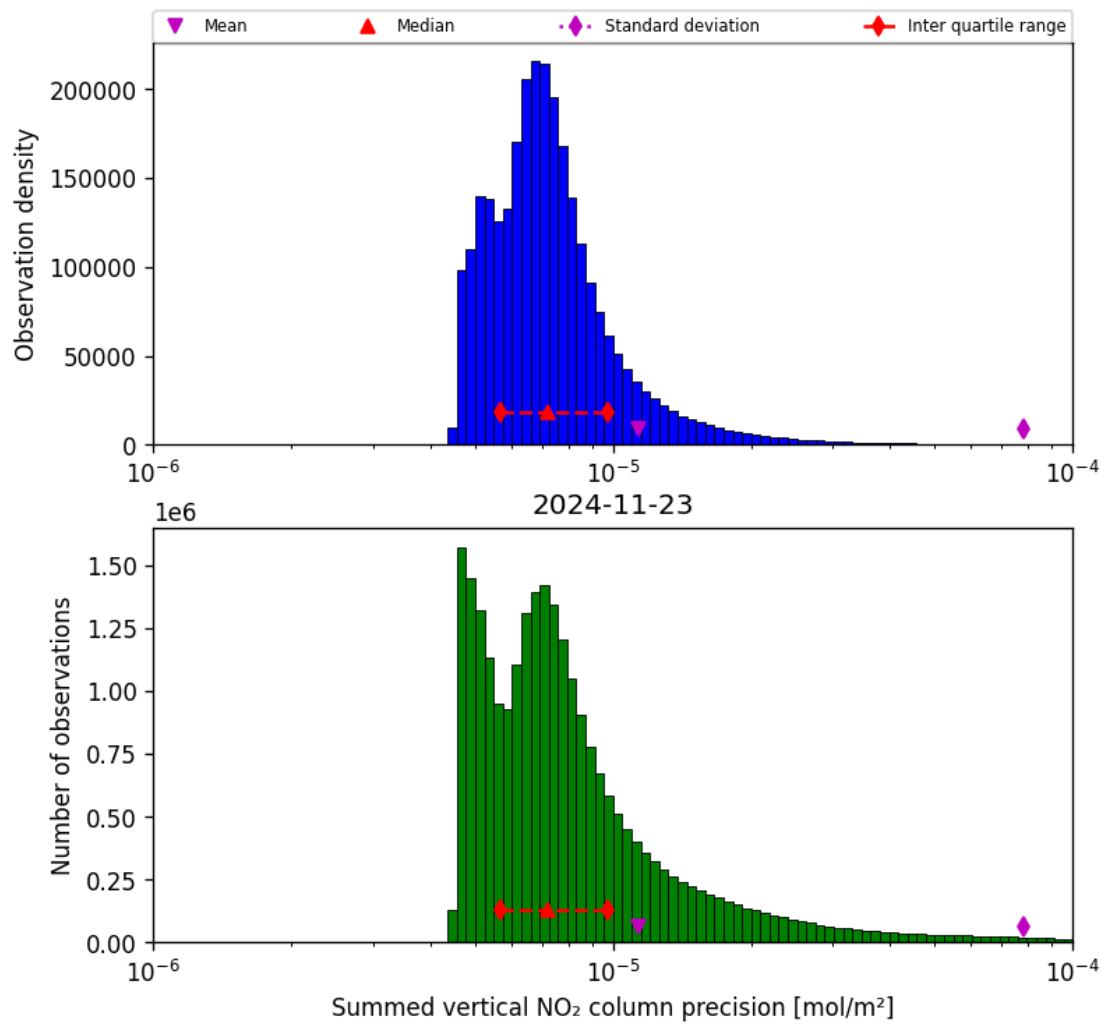
Figure 41: Histogram of "Summed vertical NO 2 column precision" for 2024-11-22 to 2024-11-24
