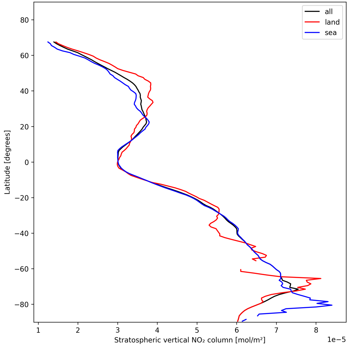
Figure 19: Zonal average of “Stratospheric vertical NO 2 column” for 2024-11-22 to 2024-11-24.
