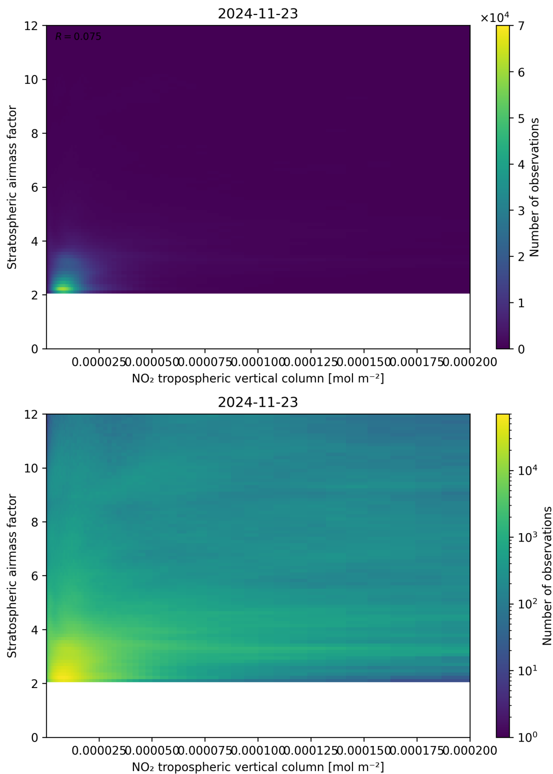
Figure 121: Scatter density plot of “NO 2 tropospheric vertical column” against “Stratospheric airmass factor” for 2024-11-22 to 2024-11-24.
