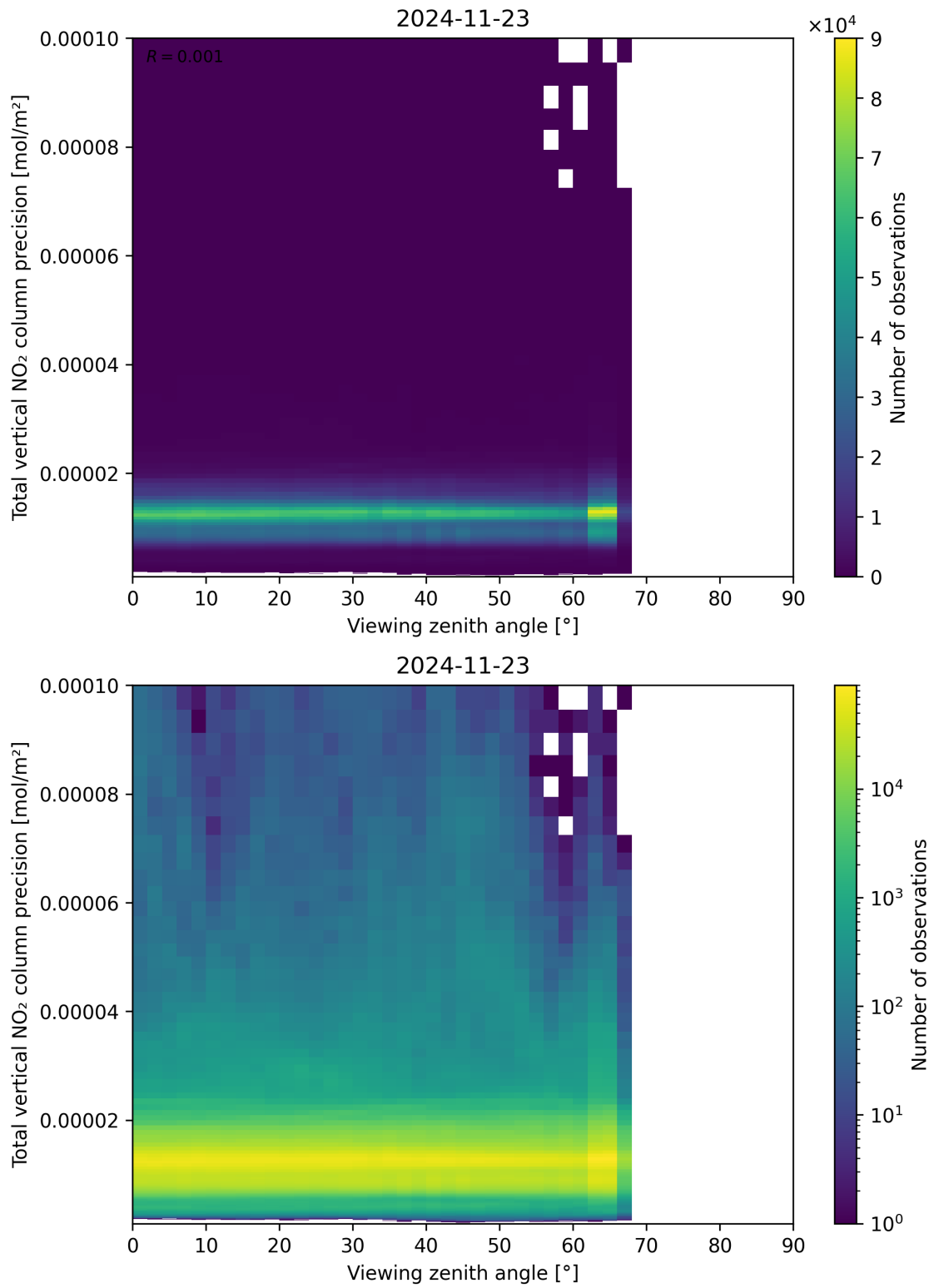
Figure 168: Scatter density plot of “Viewing zenith angle” against “Total vertical NO 2 column precision” for 2024-11-22 to 2024-11-24.
