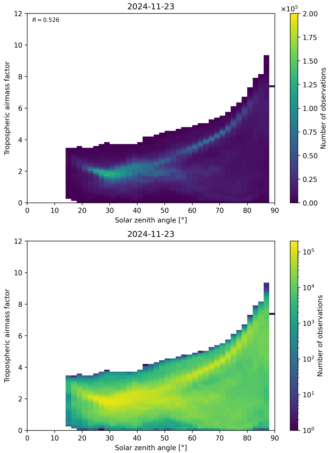
Figure 147: Scatter density plot of “Solar zenith angle” against “Tropospheric airmass factor” for 2024-11-22 to 2024-11-24.
