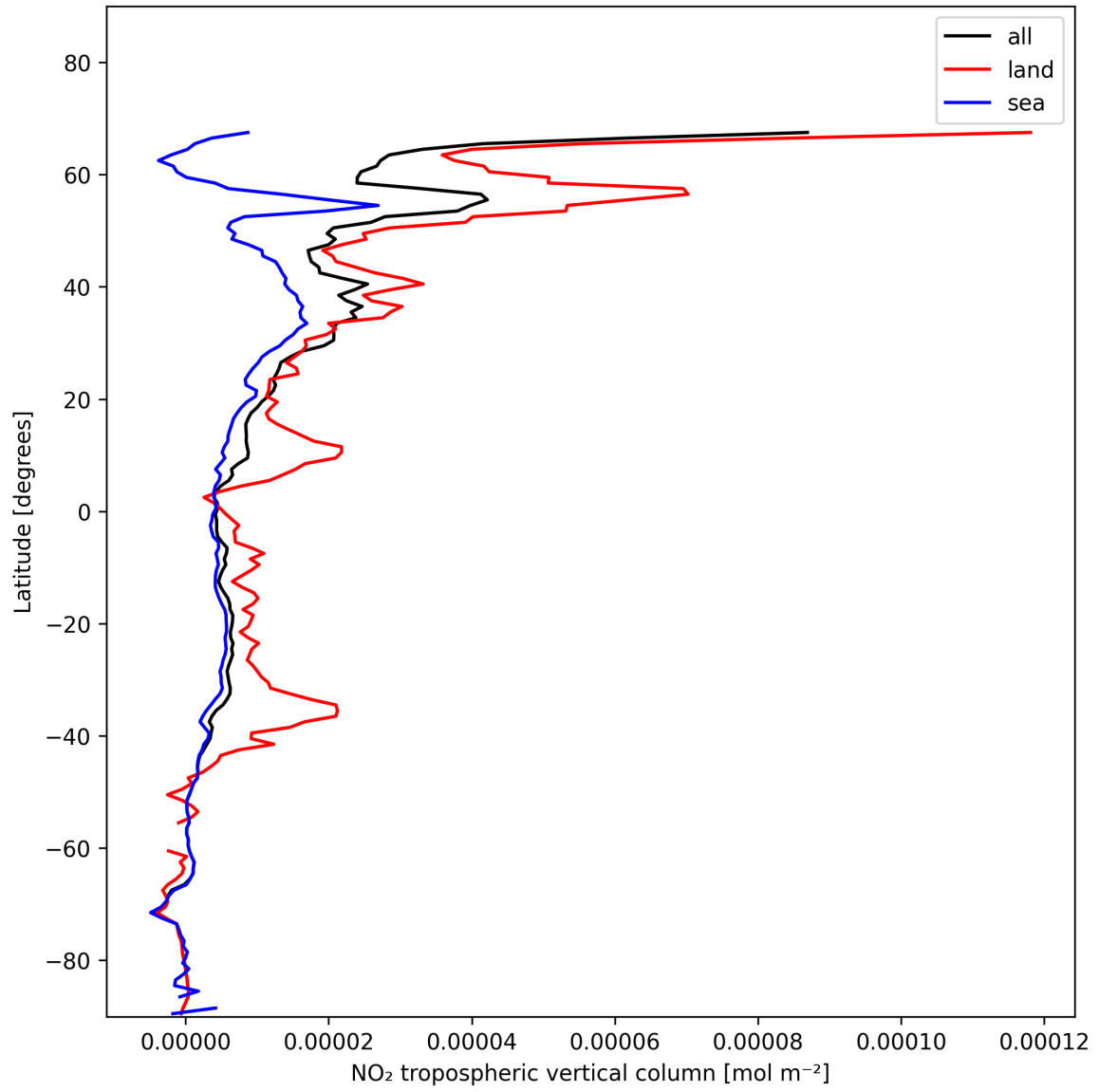
Figure 12: Zonal average of “NO 2 tropospheric vertical column” for 2024-11-22 to 2024-11-24.
