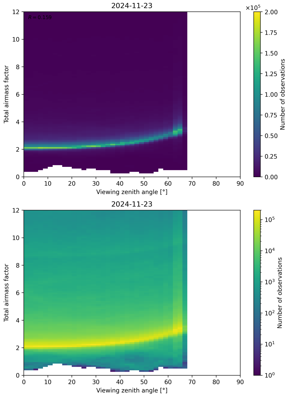
Figure 160: Scatter density plot of “Viewing zenith angle” against “Total airmass factor” for 2024-11-22 to 2024-11-24.
