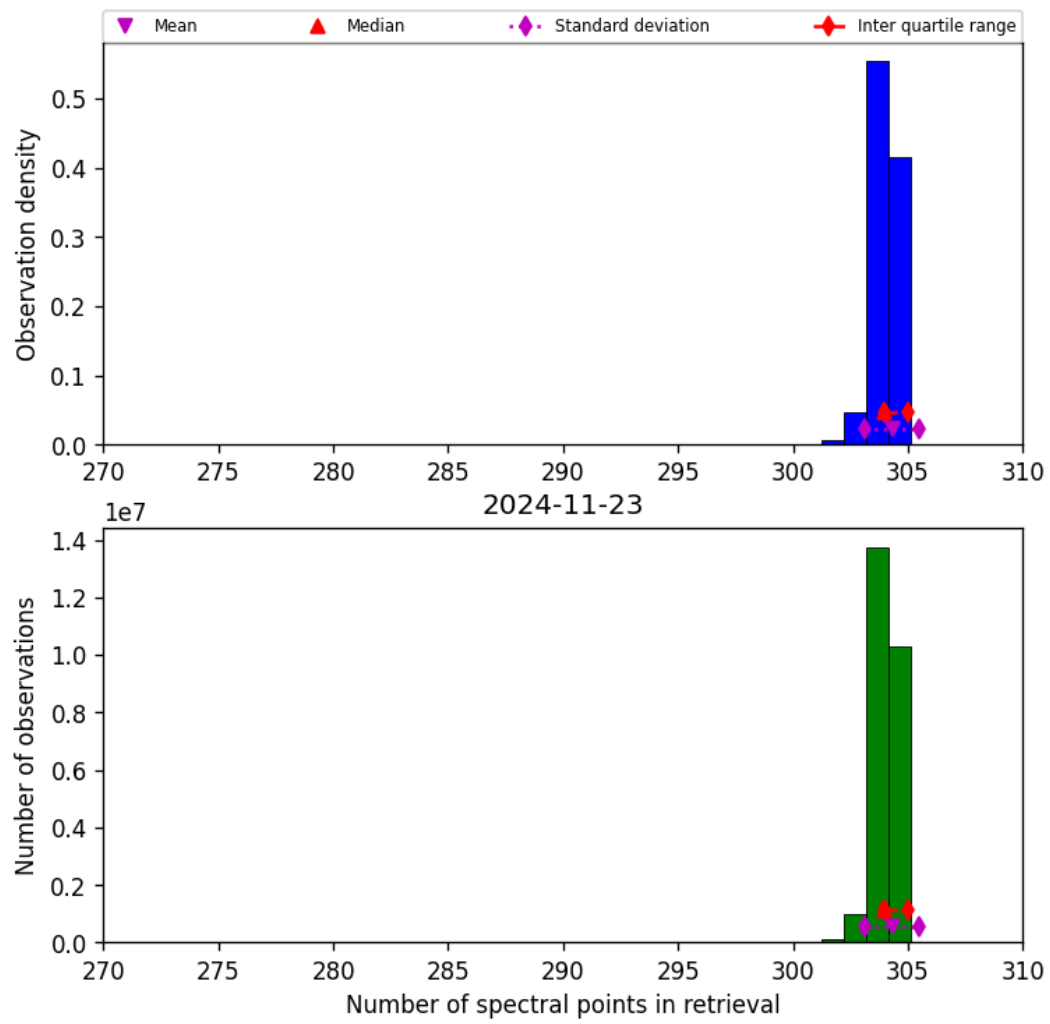
Figure 33: Histogram of “Number of spectral points in retrieval” for 2024-11-22 to 2024-11-24
