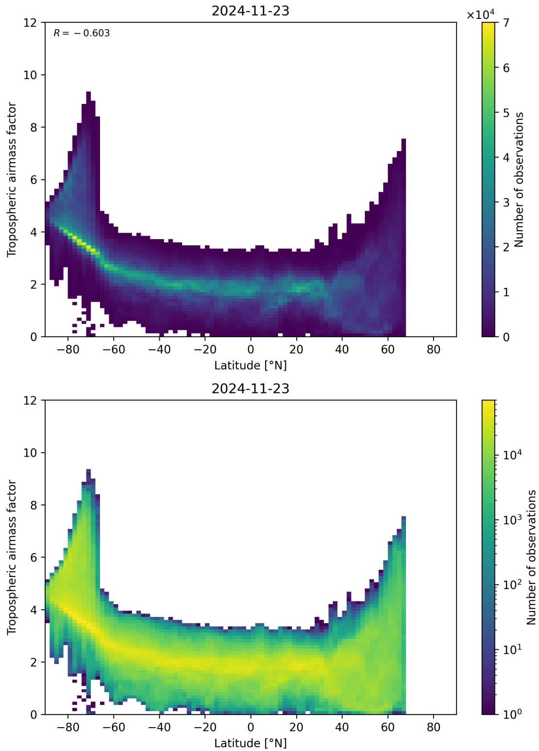
Figure 85: Scatter density plot of “Latitude” against “Tropospheric air mass factor” for 2024-11-22 to 2024-11-24.
