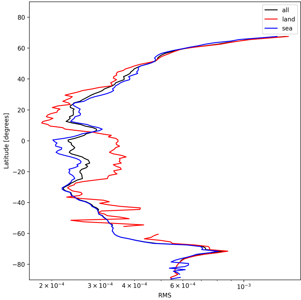
Figure 26: Zonal average of “RMS” for 2024-11-22 to 2024-11-24.
