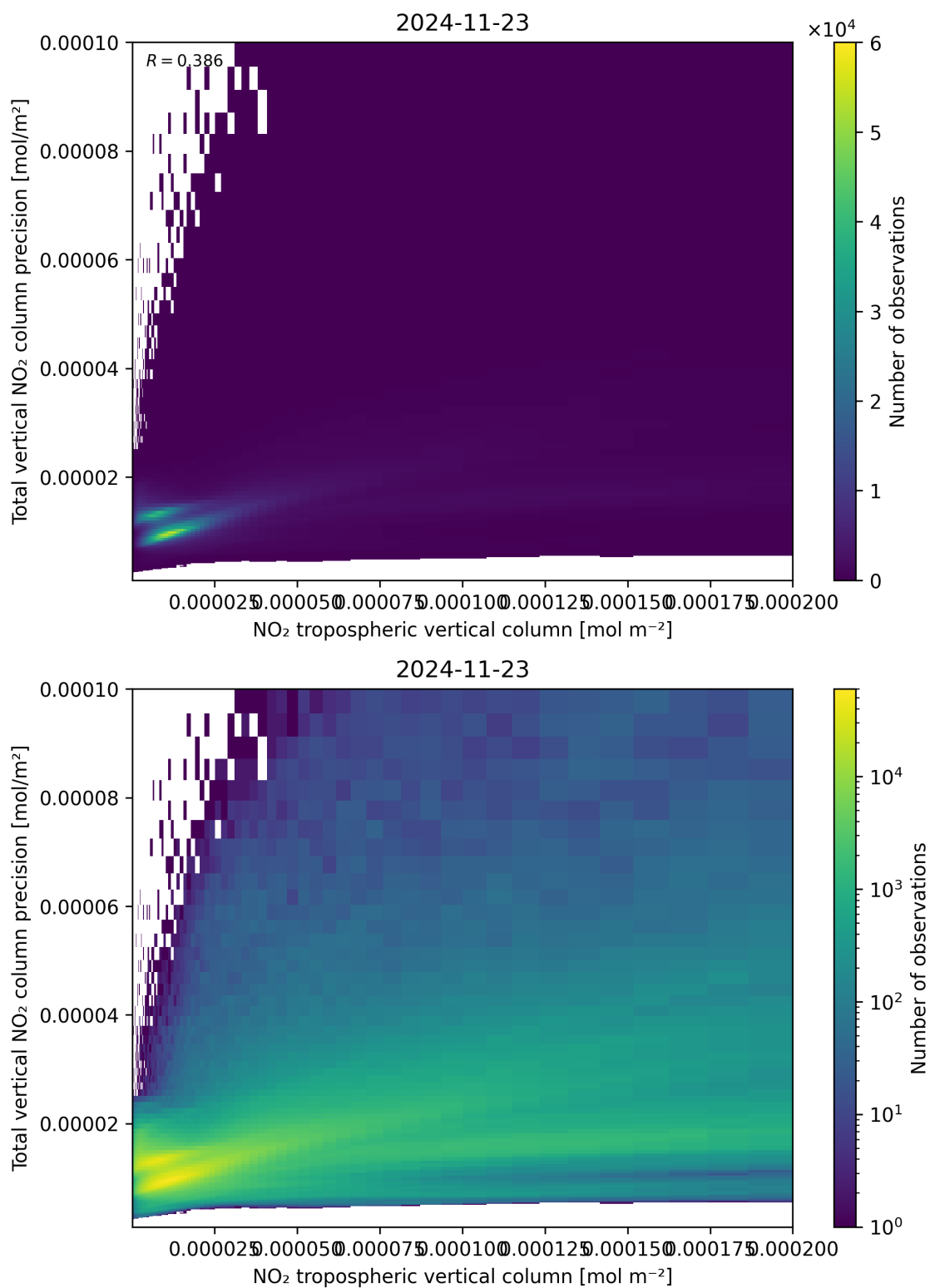
Figure 129: Scatter density plot of “NO 2 tropospheric vertical column” against “Total vertical NO 2 column precision” for 2024-11-22 to 2024-11-24.
