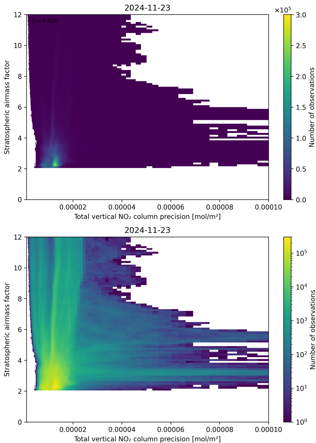
Figure 115: Scatter density plot of “Total vertical NO 2 column precision” against “Stratospheric air mass factor” for 2024-11-22 to 2024-11-24.
