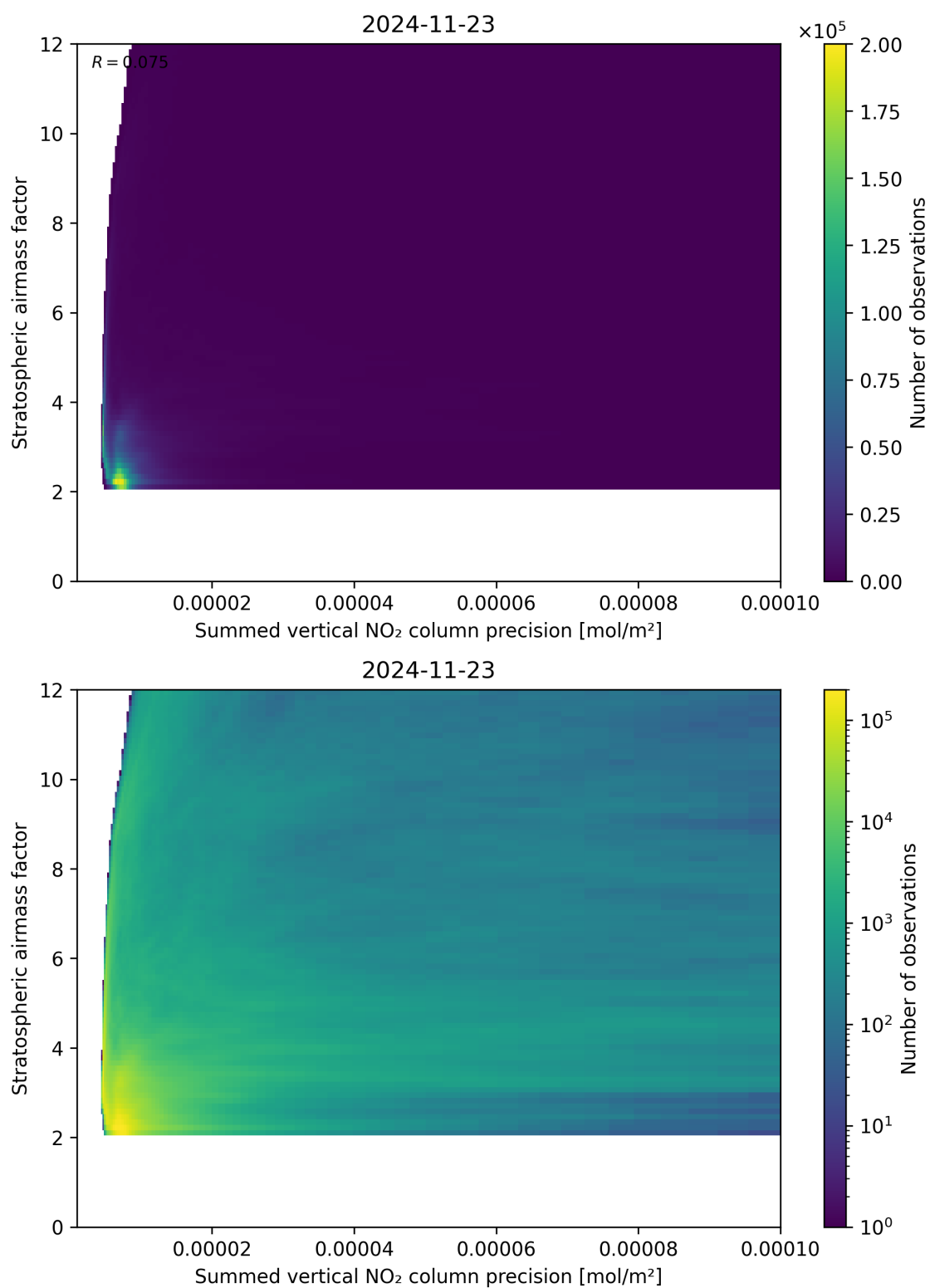
Figure 106: Scatter density plot of “Summed vertical NO 2 column precision” against “Stratospheric airmass factor” for 2024-11-22 to 2024-11-24.
