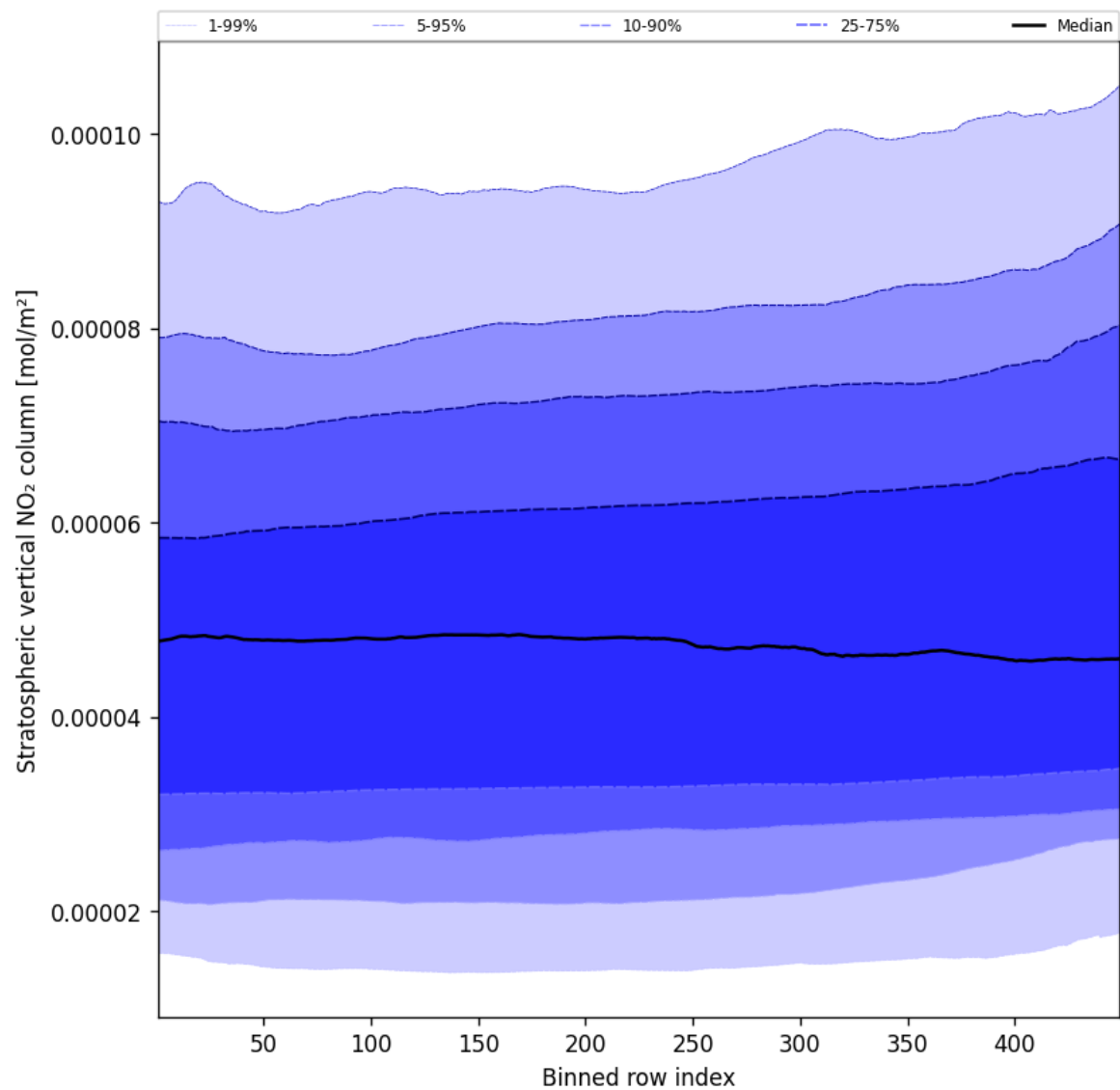
Figure 53: Along track statistics of “Stratospheric vertical NO 2 column” for 2024-11-22 to 2024-11-24
