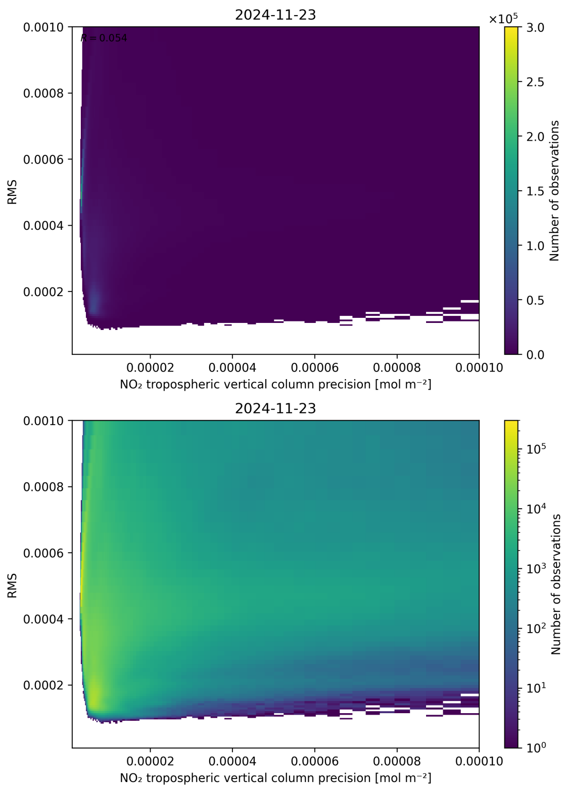
Figure 140: Scatter density plot of “NO 2 tropospheric vertical column precision” against “RMS” for 2024-11-22 to 2024-11-24.
