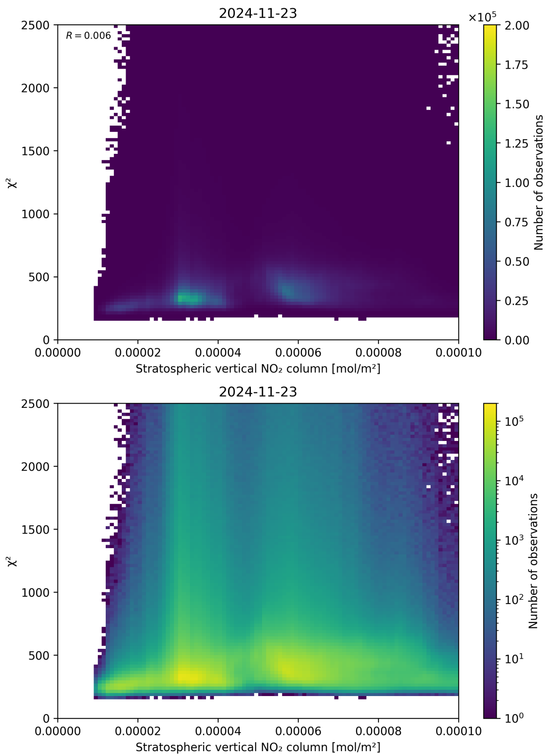
Figure 97: Scatter density plot of “Stratospheric vertical NO 2 column” against “ \chi^2 ” for 2024-11-22 to 2024-11-24.
