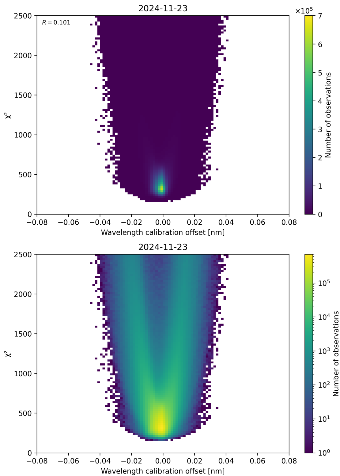
Figure 175: Scatter density plot of “Wavelength calibration offset” against “ \chi^2 ” for 2024-11-22 to 2024-11-24.
