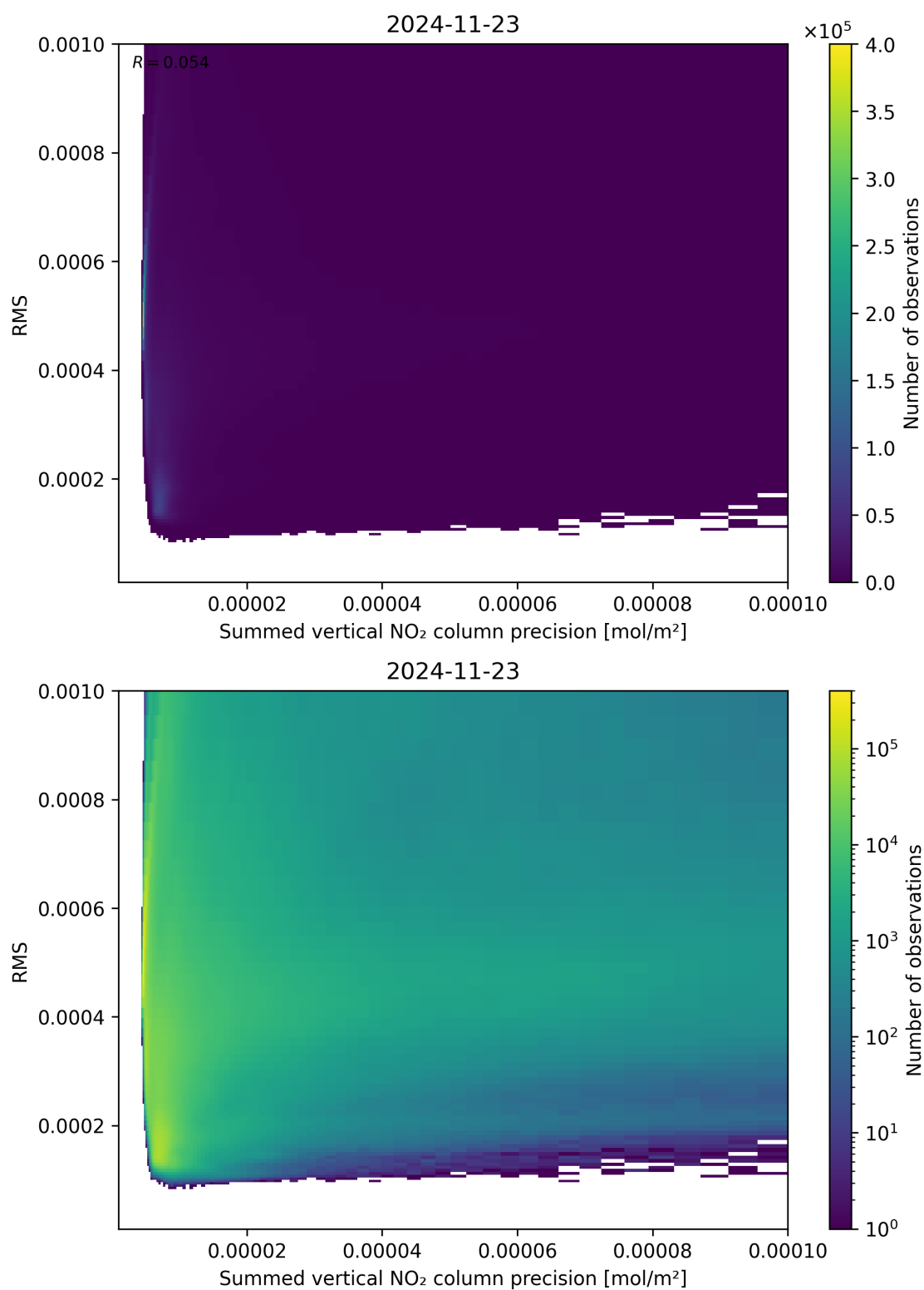
Figure 108: Scatter density plot of “Summed vertical NO 2 column precision” against “RMS” for 2024-11-22 to 2024-11-24.
