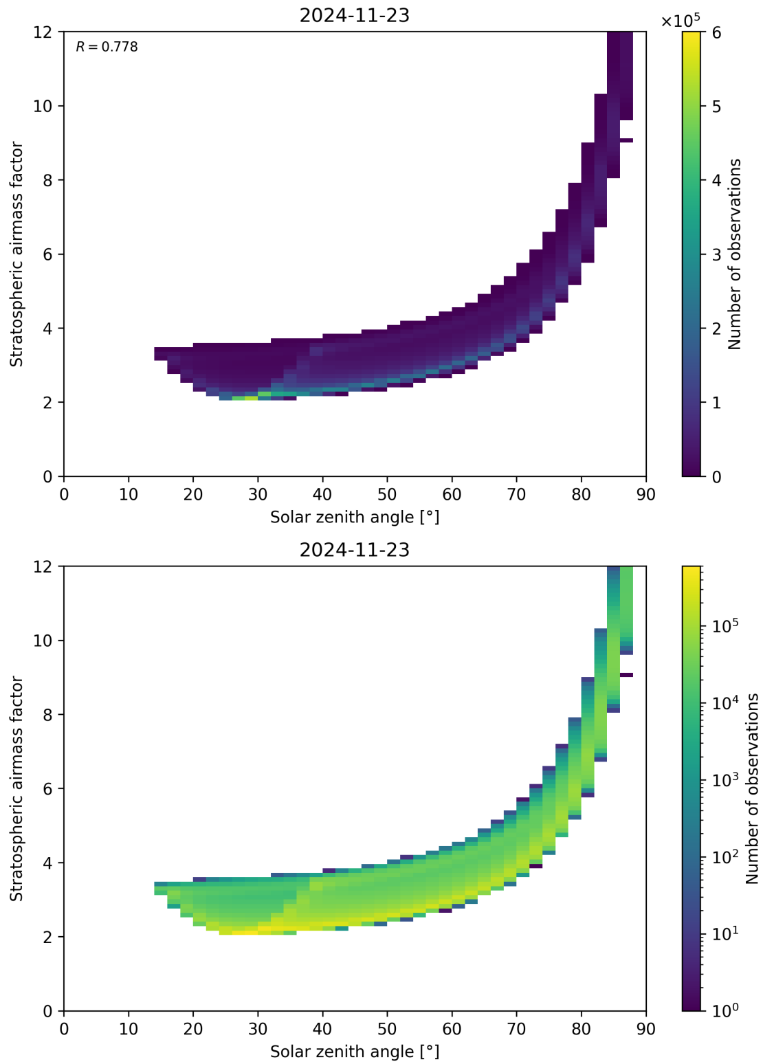
Figure 145: Scatter density plot of “Solar zenith angle” against “Stratospheric airmass factor” for 2024-11-22 to 2024-11-24.
