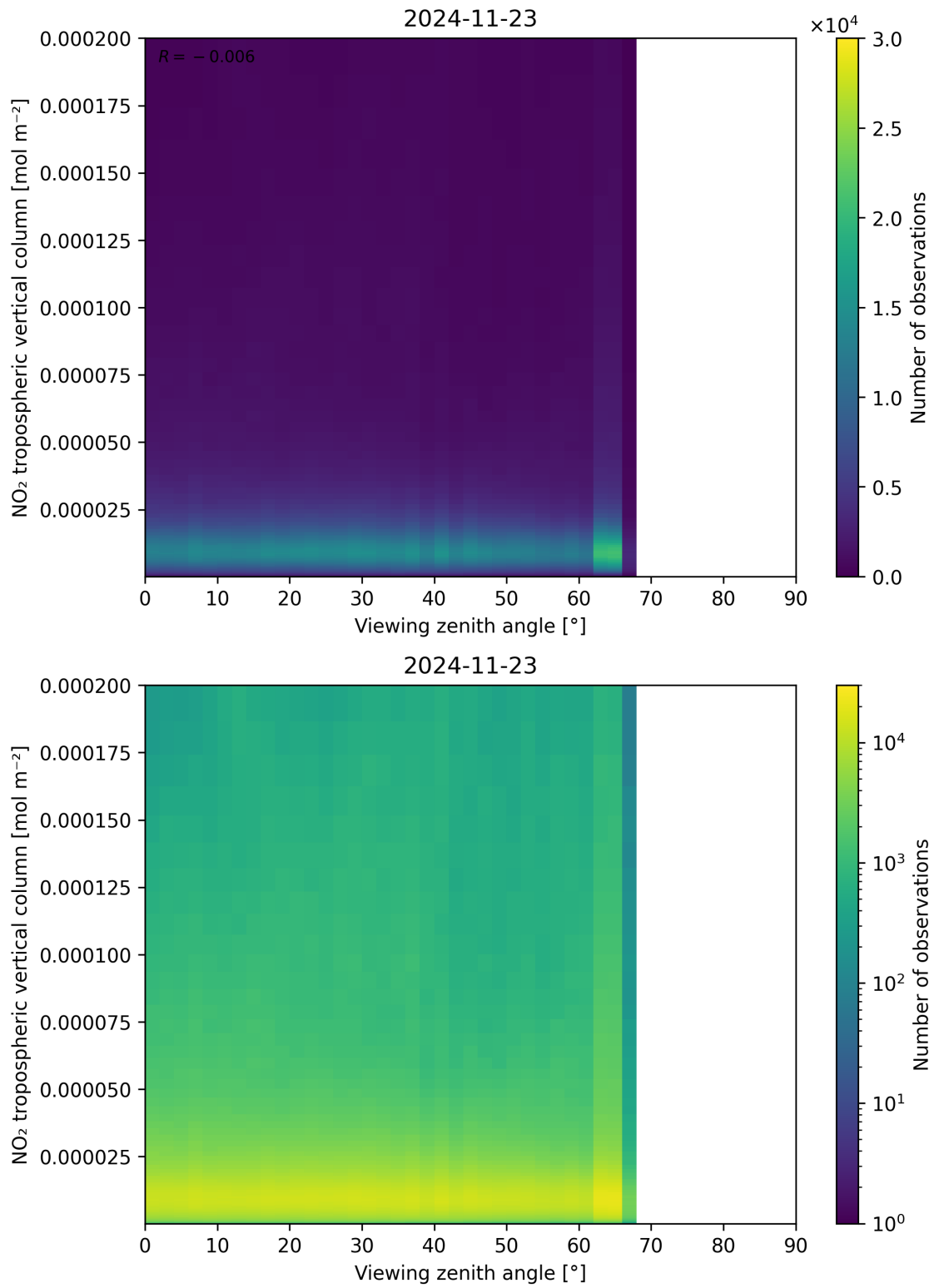
Figure 169: Scatter density plot of “Viewing zenith angle” against “NO 2 tropospheric vertical column” for 2024-11-22 to 2024-11-24.
