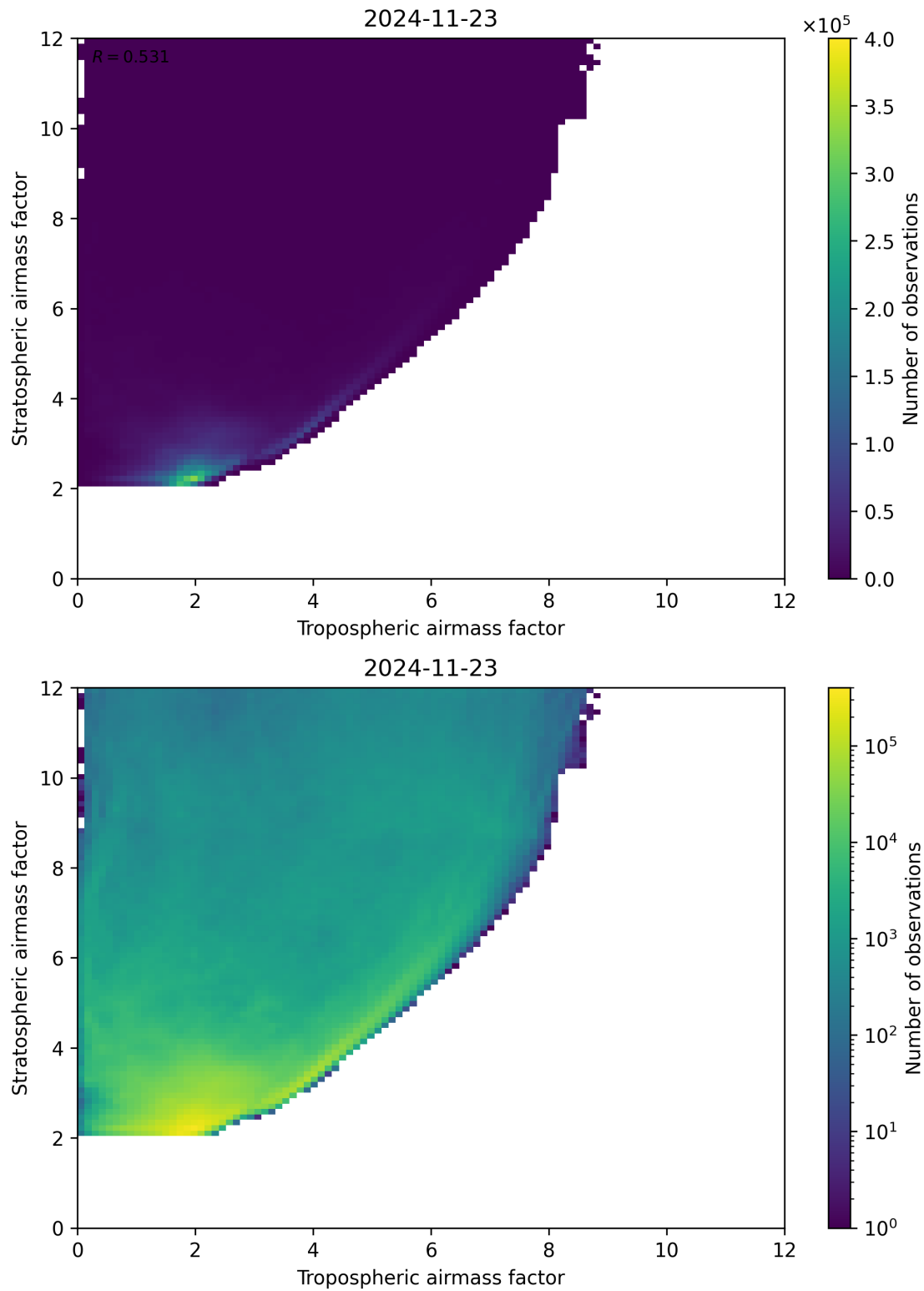
Figure 71: Scatter density plot of “Tropospheric airmass factor” against “Stratospheric airmass factor” for 2024-11-22 to 2024-11-24.
