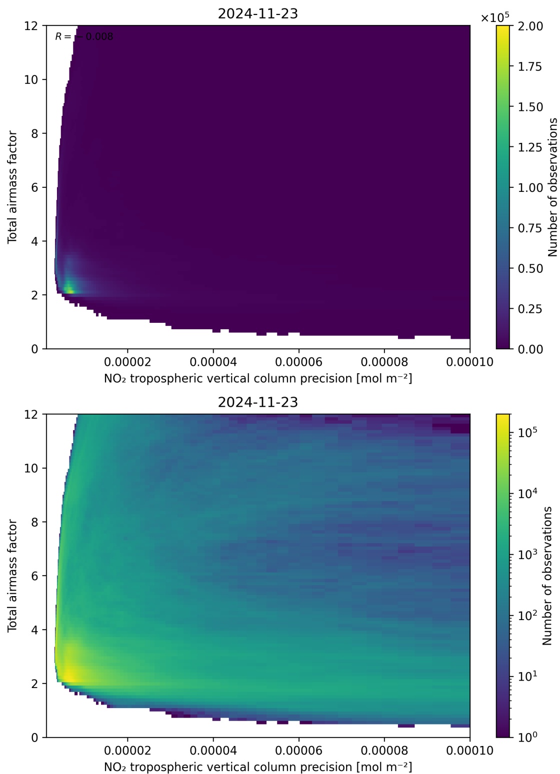
Figure 132: Scatter density plot of “NO 2 tropospheric vertical column precision” against “Total air mass factor” for 2024-11-22 to 2024-11-24.
