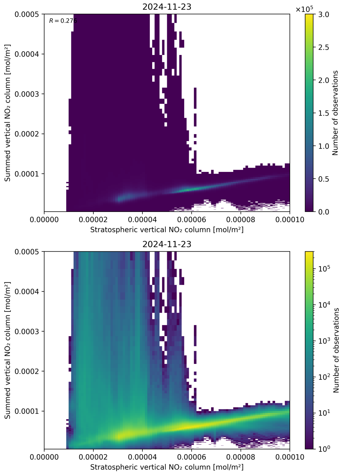
Figure 98: Scatter density plot of “Stratospheric vertical NO 2 column” against “Summed vertical NO 2 column” for 2024-11-22 to 2024-11-24.
