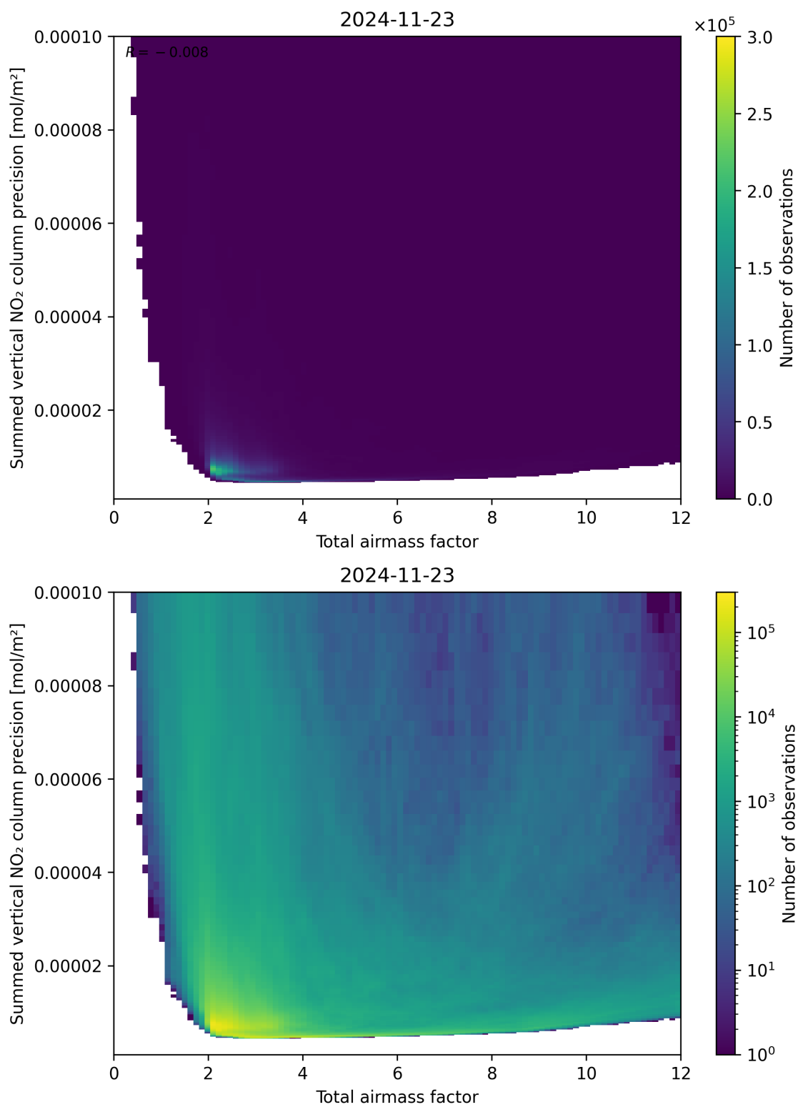
Figure 66: Scatter density plot of “Total airmass factor” against “Summed vertical NO 2 column precision” for 2024-11-22 to 2024-11-24.
