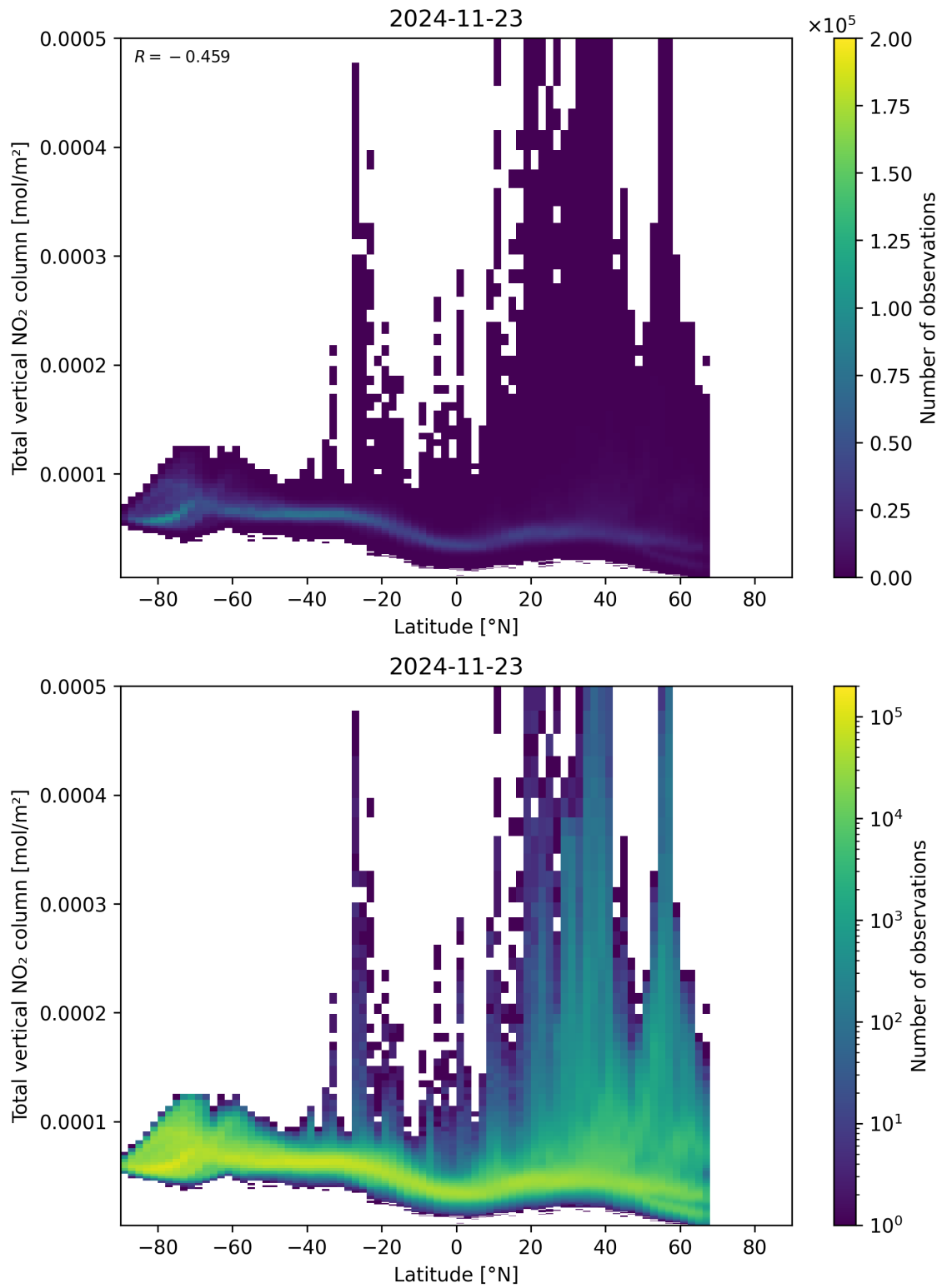
Figure 90: Scatter density plot of “Latitude” against “Total vertical NO 2 column” for 2024-11-22 to 2024-11-24.
