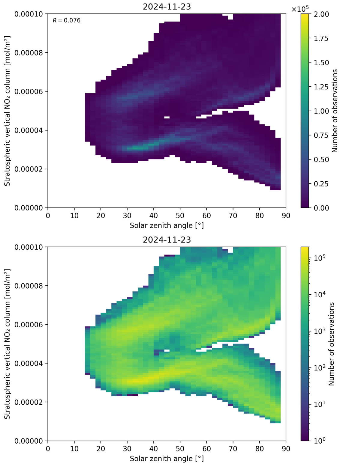
Figure 150: Scatter density plot of “Solar zenith angle” against “Stratospheric vertical NO 2 column” for 2024-11-22 to 2024-11-24.
