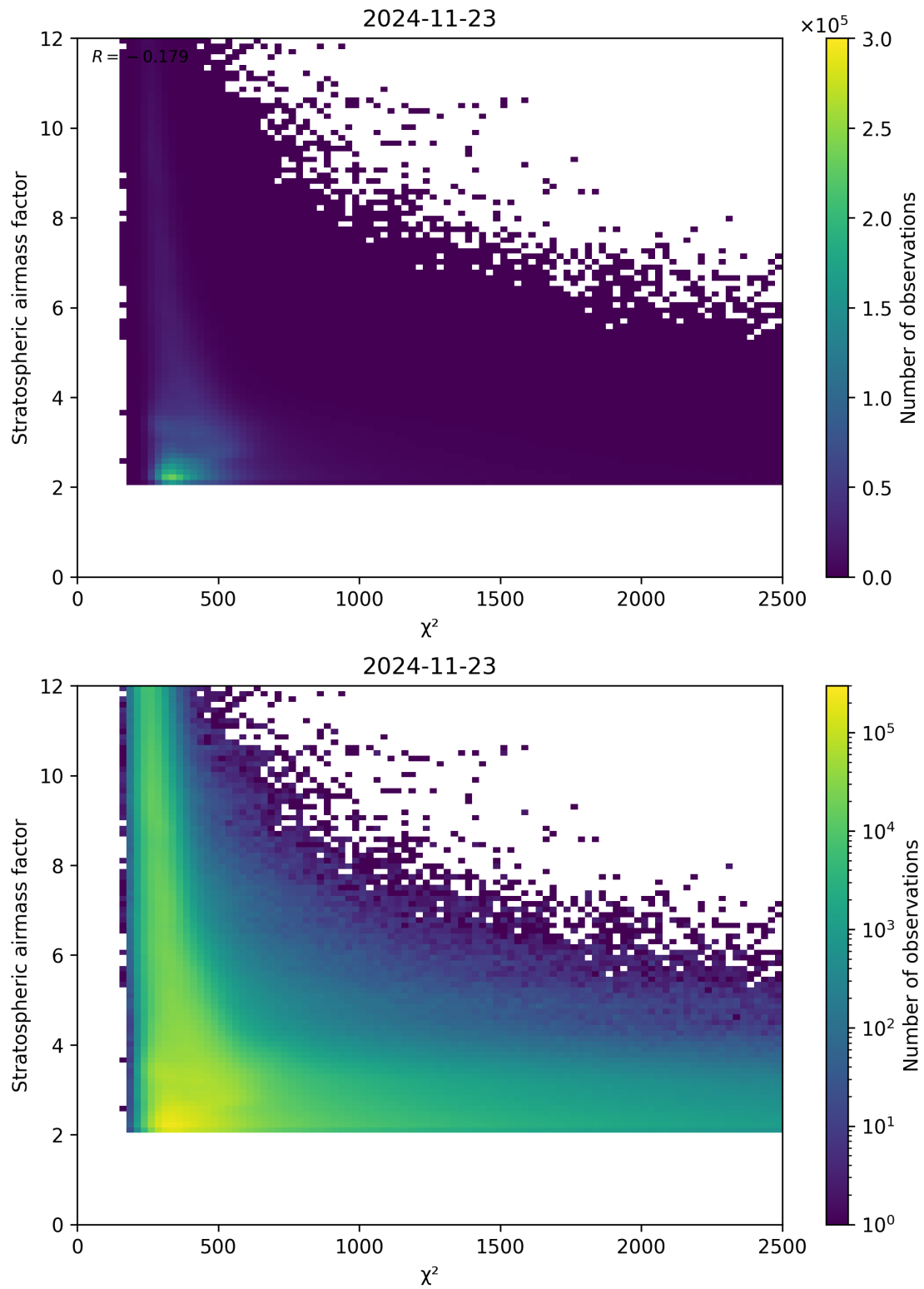
Figure 81: Scatter density plot of “ \chi^2 ” against “Stratospheric airmass factor” for 2024-11-22 to 2024-11-24.
