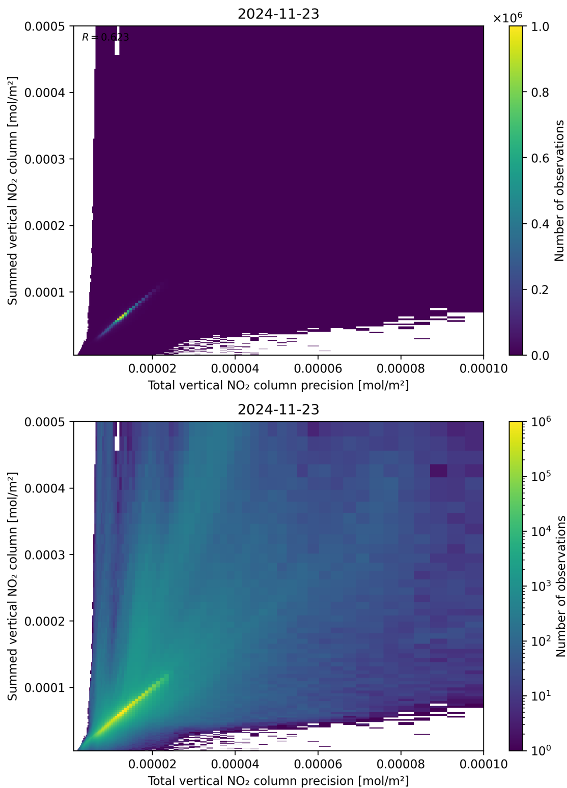
Figure 117: Scatter density plot of “Total vertical NO 2 column precision” against “Summed vertical NO 2 column” for 2024-11-22 to 2024-11-24.
