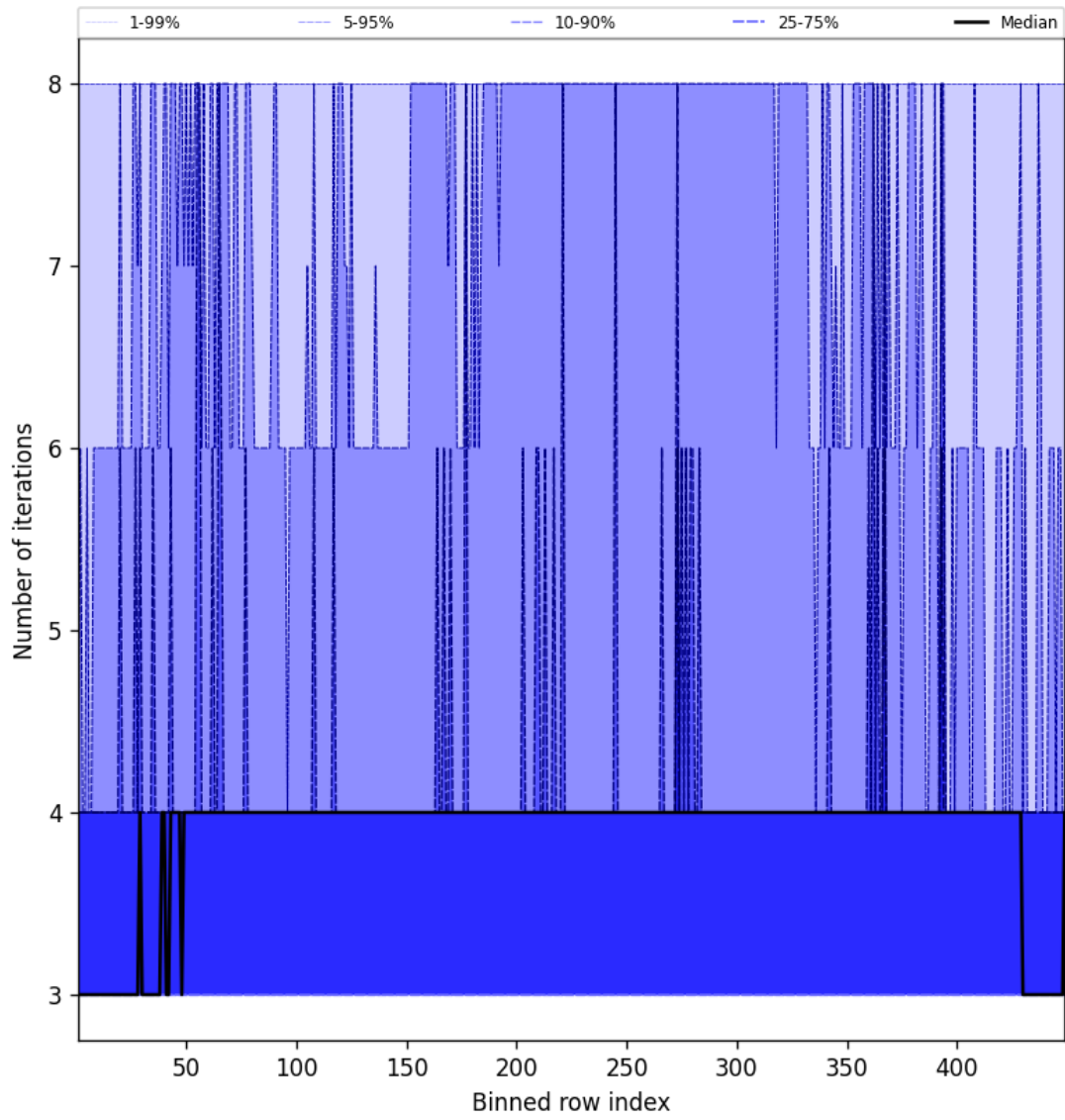
Figure 51: Along track statistics of “Number of iterations” for 2024-11-22 to 2024-11-24
