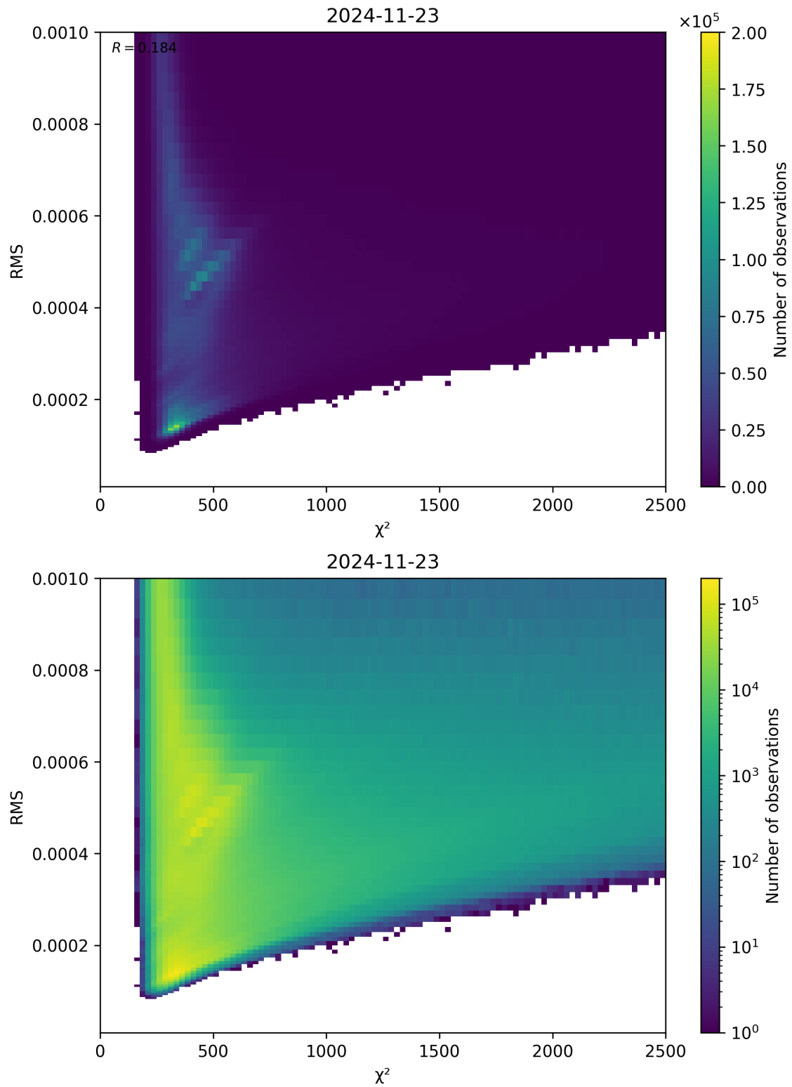
Figure 82: Scatter density plot of “ \chi^2 ” against “RMS” for 2024-11-22 to 2024-11-24.
