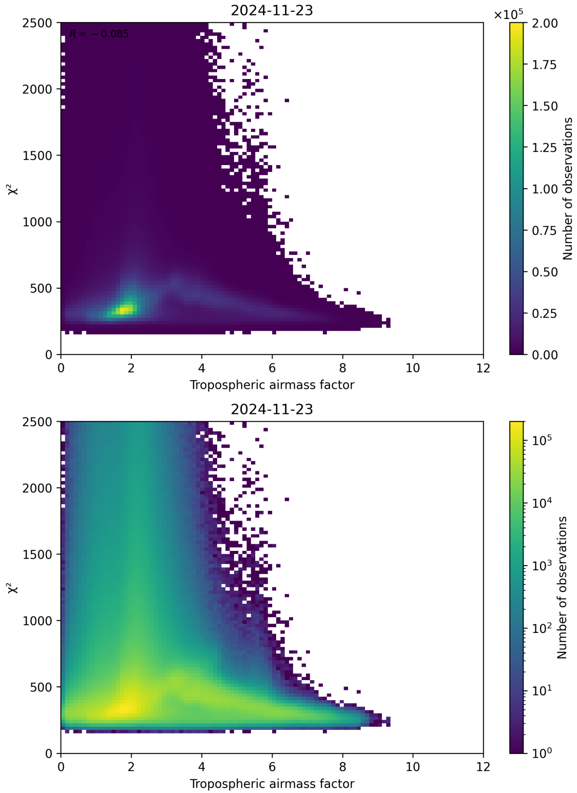
Figure 73: Scatter density plot of “Tropospheric airmass factor” against “ \chi^2 ” for 2024-11-22 to 2024-11-24.
