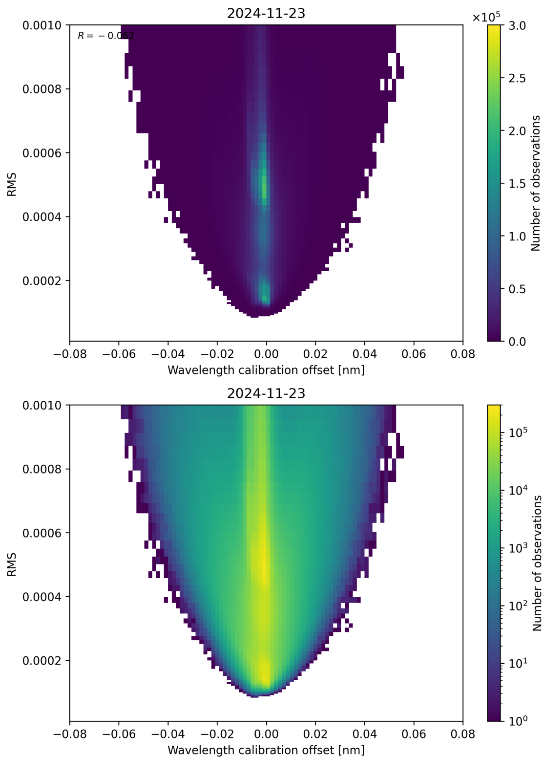
Figure 181: Scatter density plot of “Wavelength calibration offset” against “RMS” for 2024-11-22 to 2024-11-24.
