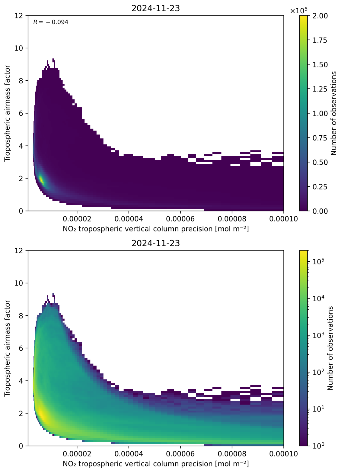
Figure 133: Scatter density plot of “NO 2 tropospheric vertical column precision” against “Tropospheric airmass factor” for 2024-11-22 to 2024-11-24.
