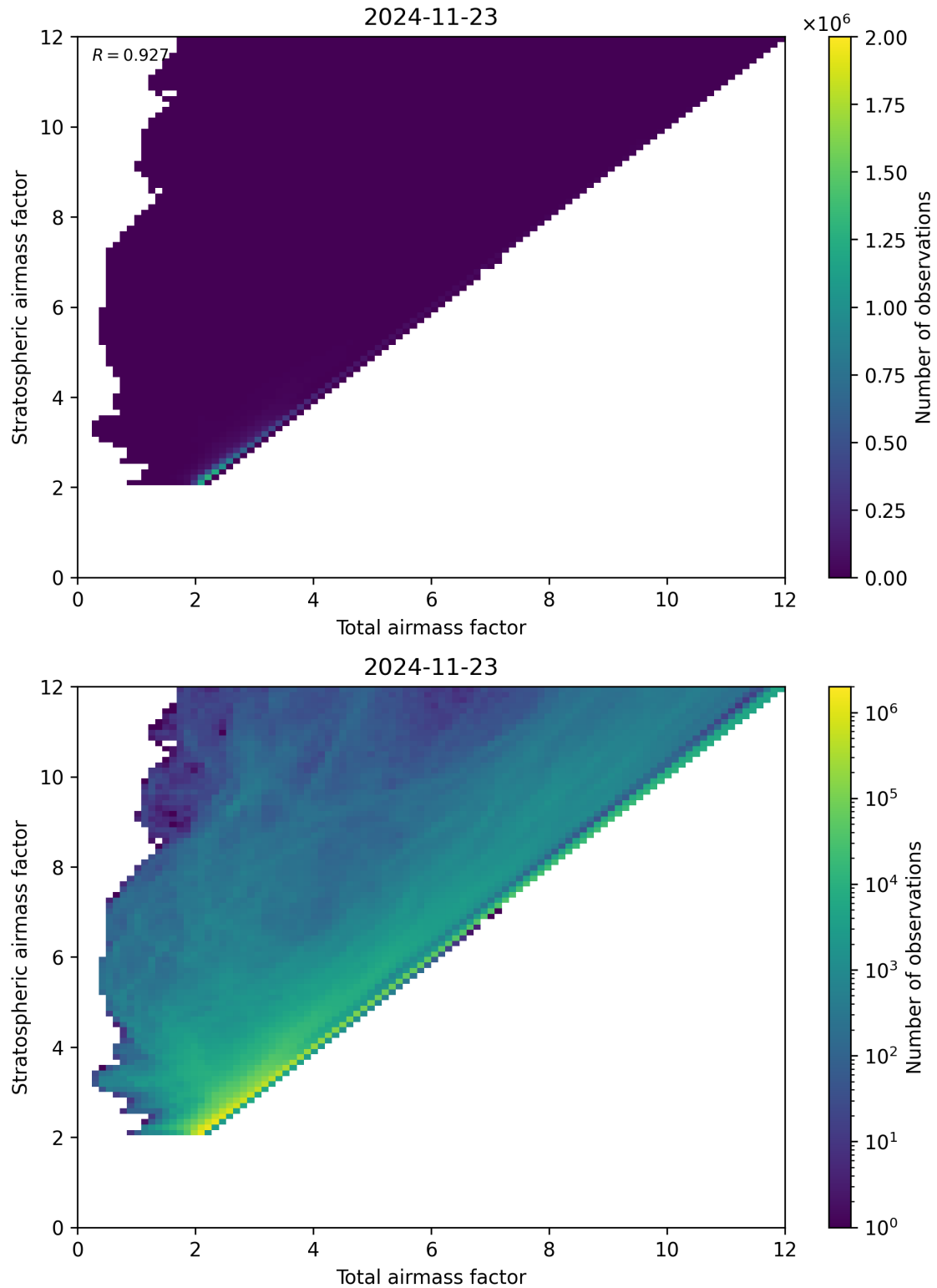
Figure 62: Scatter density plot of “Total airmass factor” against “Stratospheric airmass factor” for 2024-11-22 to 2024-11-24.
