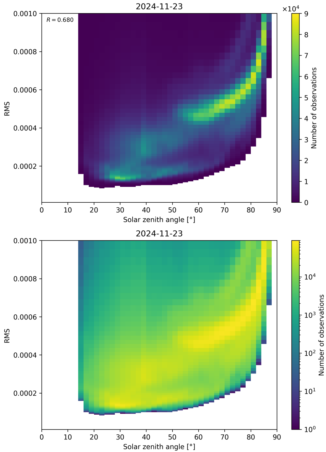
Figure 157: Scatter density plot of “Solar zenith angle” against “RMS” for 2024-11-22 to 2024-11-24.
