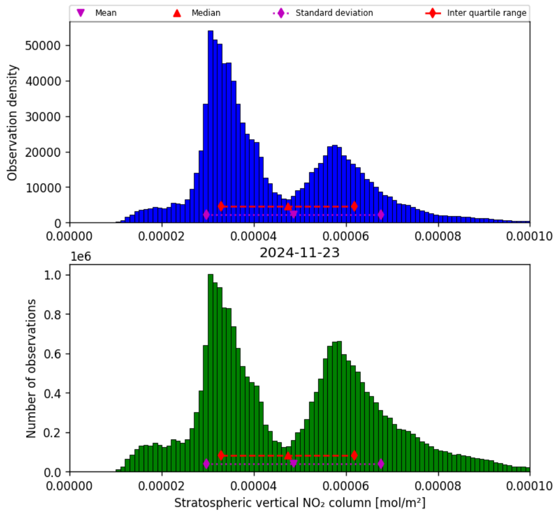
Figure 36: Histogram of “Stratospheric vertical NO 2 column” for 2024-11-22 to 2024-11-24
