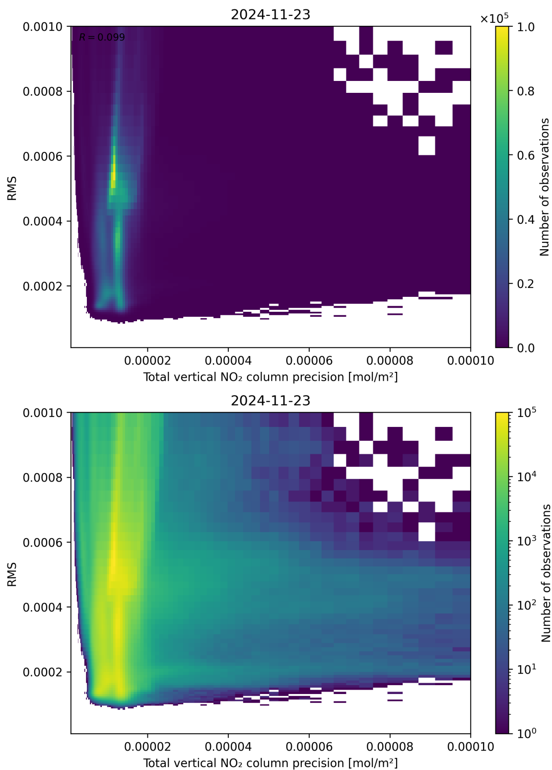
Figure 119: Scatter density plot of “Total vertical NO 2 column precision” against “RMS” for 2024-11-22 to 2024-11-24.
