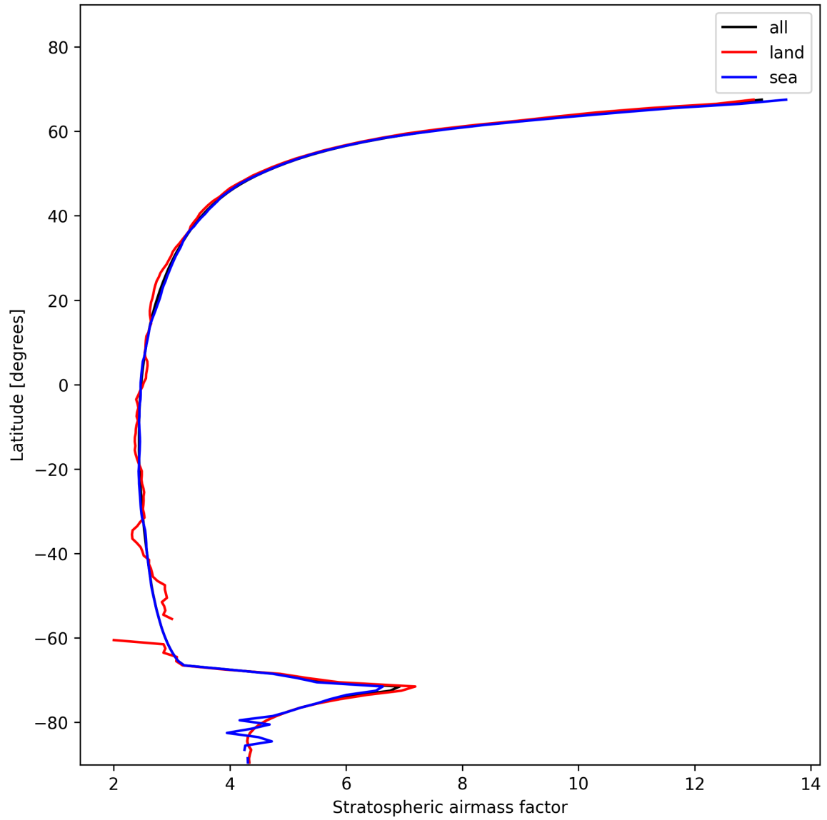
Figure 27: Zonal average of “Stratospheric airmass factor” for 2024-11-22 to 2024-11-24.
