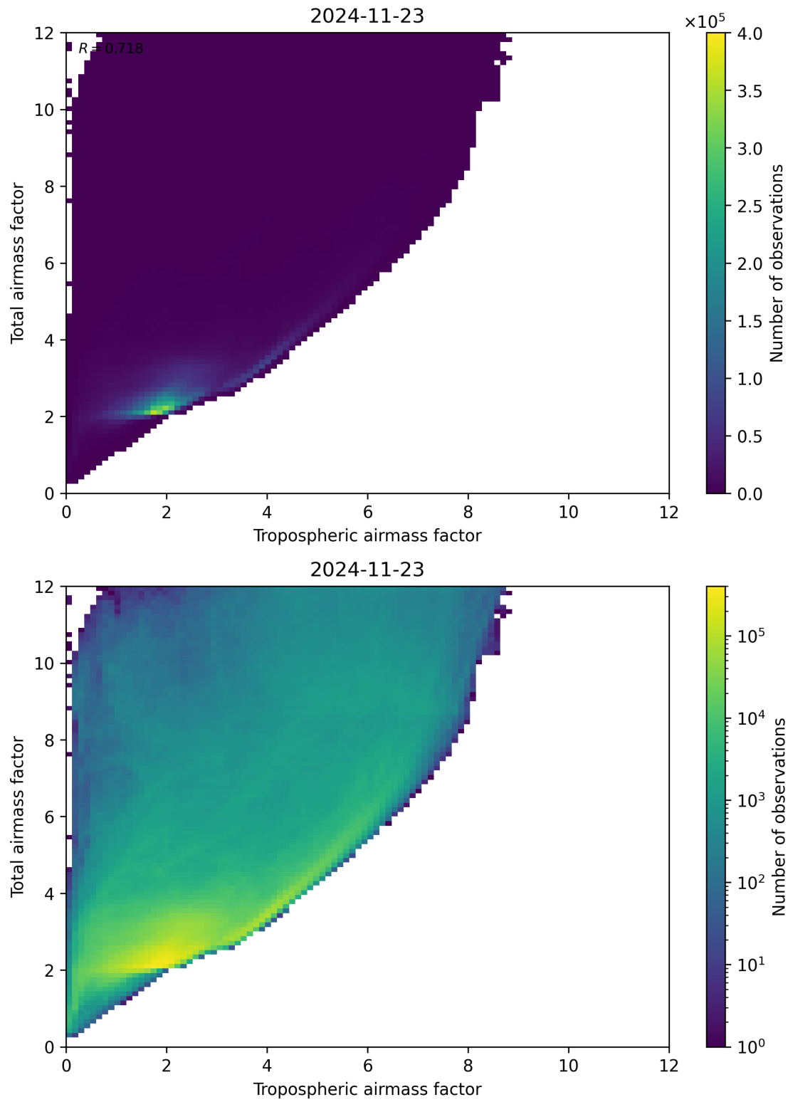
Figure 72: Scatter density plot of “Tropospheric airmass factor” against “Total airmass factor” for 2024-11-22 to 2024-11-24.
