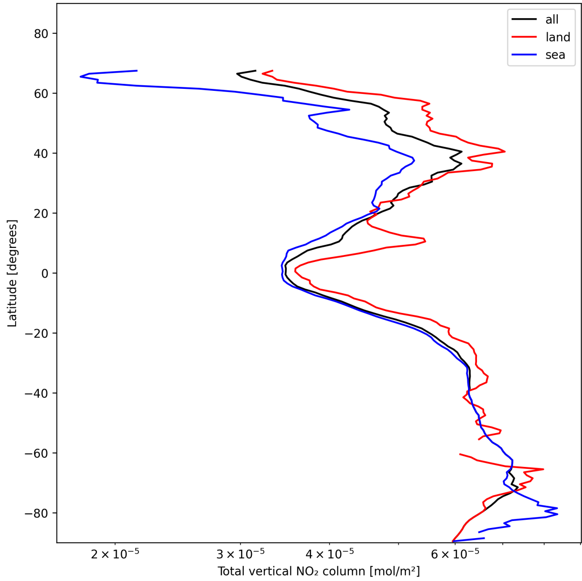
Figure 21: Zonal average of “Total vertical NO 2 column” for 2024-11-22 to 2024-11-24.
