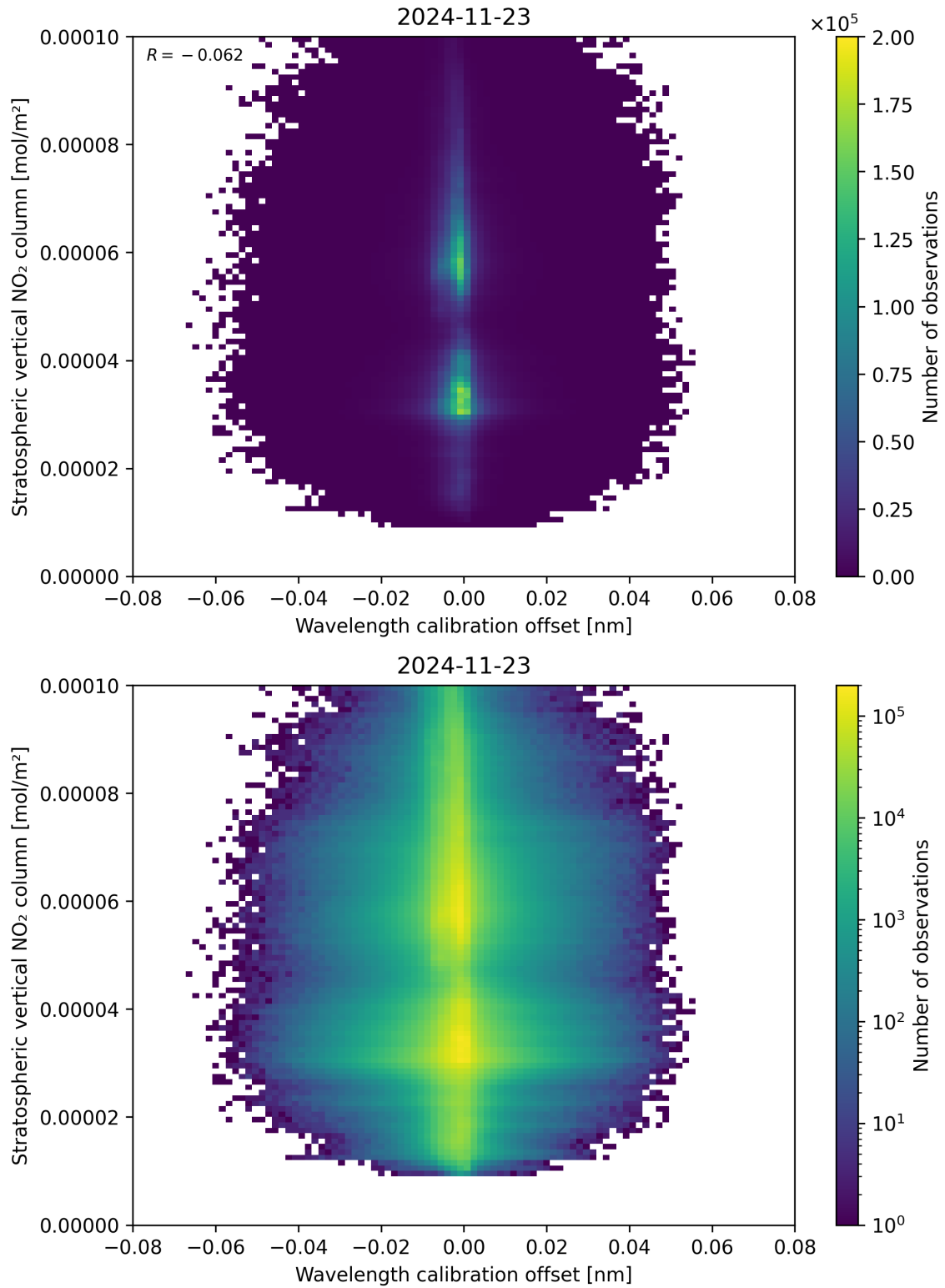
Figure 176: Scatter density plot of “Wavelength calibration offset” against “Stratospheric vertical NO 2 column” for 2024-11-22 to 2024-11-24.
