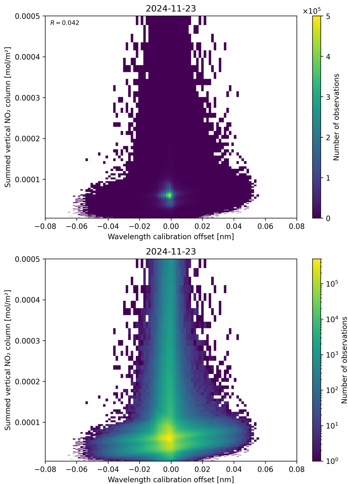
Figure 177: Scatter density plot of “Wavelength calibration offset” against “Summed vertical NO 2 column” for 2024-11-22 to 2024-11-24.
