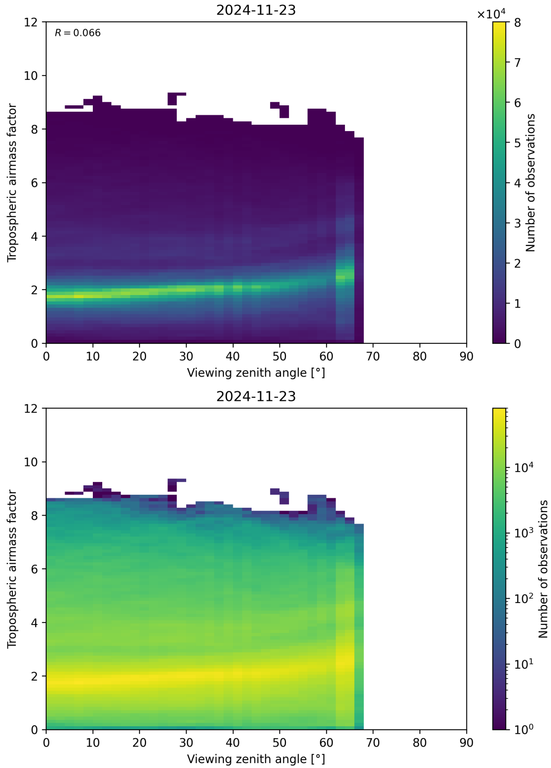
Figure 161: Scatter density plot of “Viewing zenith angle” against “Tropospheric airmass factor” for 2024-11-22 to 2024-11-24.
