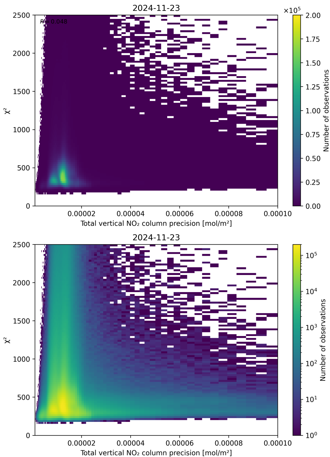
Figure 116: Scatter density plot of “Total vertical NO 2 column precision” against “ \chi^2 ” for 2024-11-22 to 2024-11-24.
