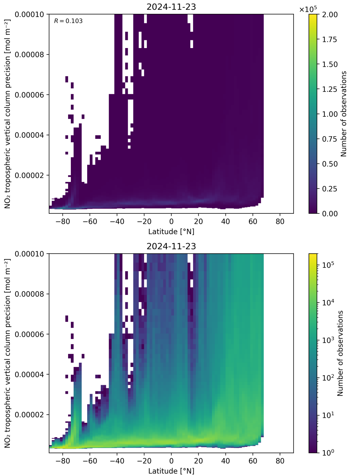
Figure 93: Scatter density plot of “Latitude” against “NO 2 tropospheric vertical column precision” for 2024-11-22 to 2024-11-24.
