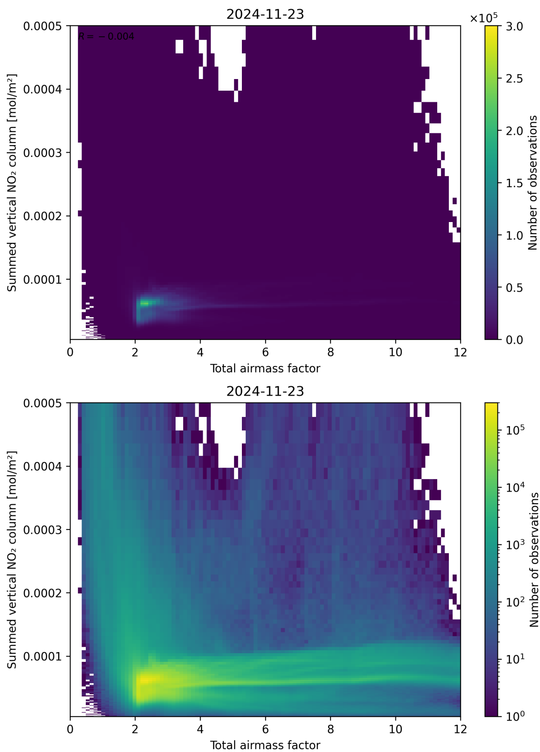
Figure 65: Scatter density plot of “Total airmass factor” against “Summed vertical NO 2 column” for 2024-11-22 to 2024-11-24.
