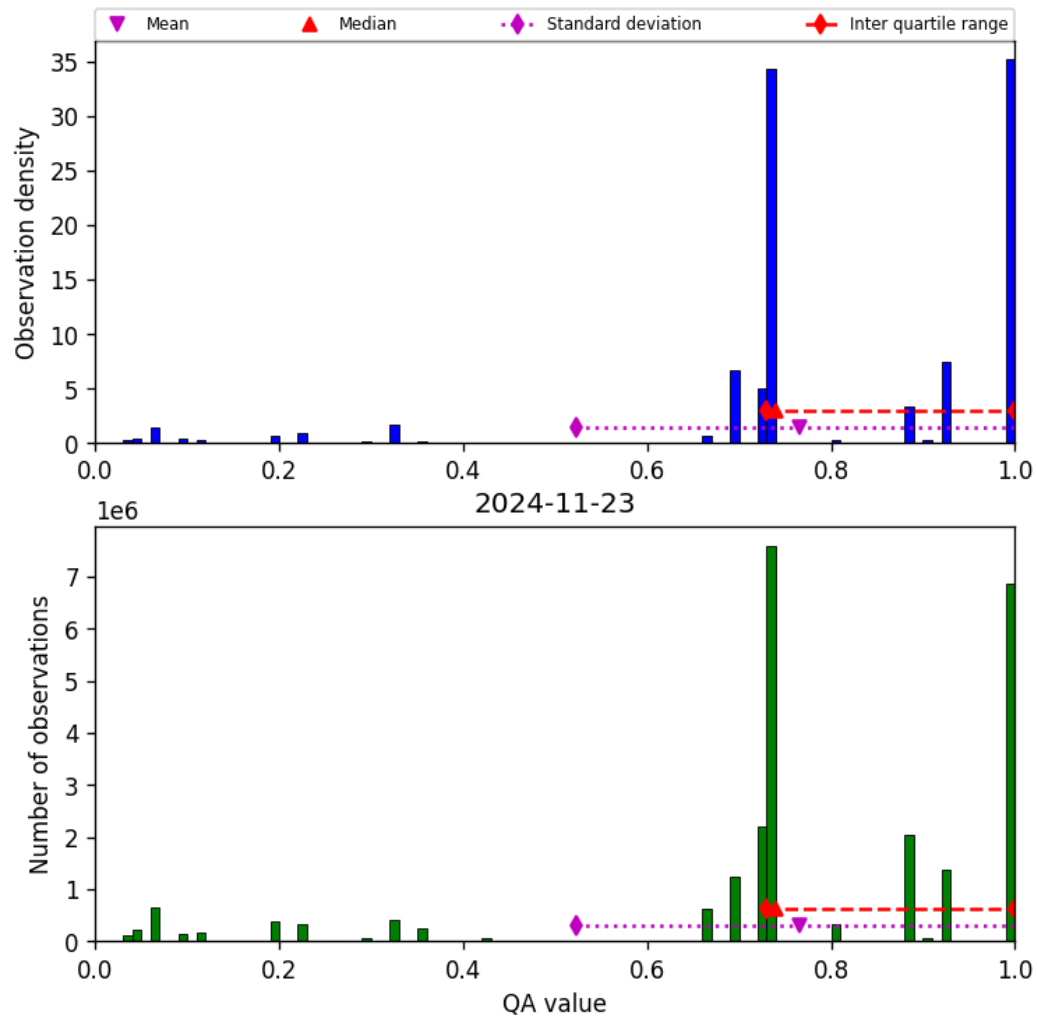
Figure 28: Histogram of “QA value” for 2024-11-22 to 2024-11-24
