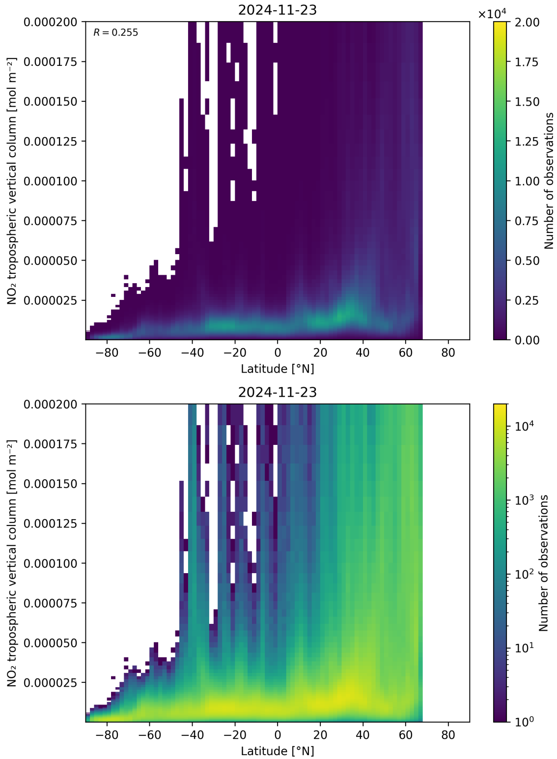
Figure 92: Scatter density plot of “Latitude” against “NO 2 tropospheric vertical column” for 2024-11-22 to 2024-11-24.
