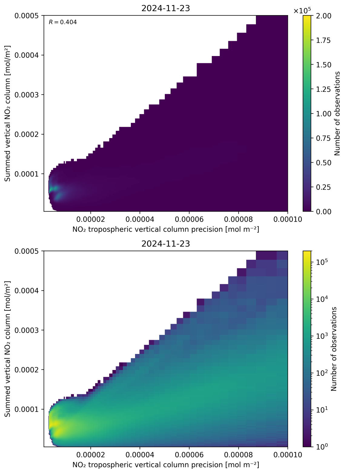
Figure 136: Scatter density plot of “NO 2 tropospheric vertical column precision” against “Summed vertical NO 2 column” for 2024-11-22 to 2024-11-24.
