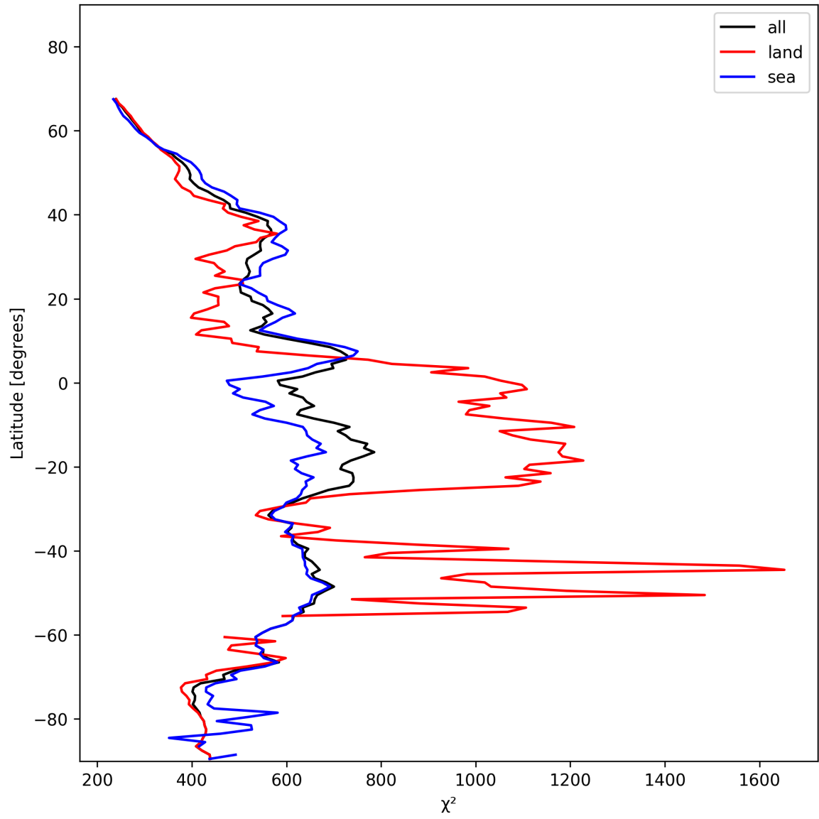
Figure 25: Zonal average of “ \chi^2 ” for 2024-11-22 to 2024-11-24.
