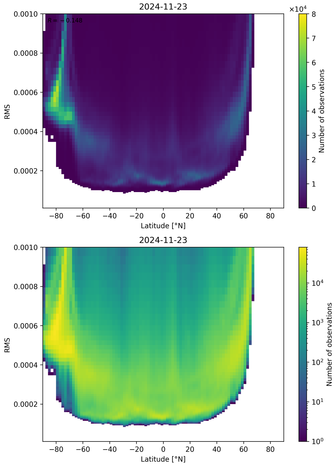
Figure 94: Scatter density plot of “Latitude” against “RMS” for 2024-11-22 to 2024-11-24.
