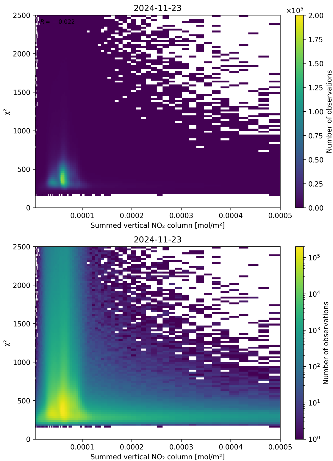
Figure 104: Scatter density plot of “Summed vertical NO 2 column” against “ \chi^2 ” for 2024-11-22 to 2024-11-24.
