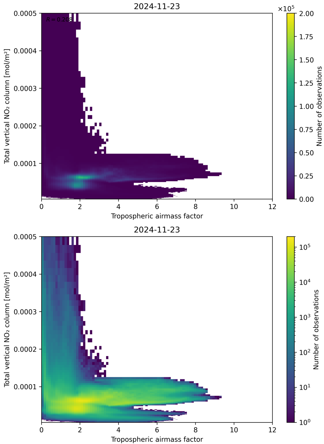
Figure 77: Scatter density plot of “Tropospheric airmass factor” against “Total vertical NO 2 column” for 2024-11-22 to 2024-11-24.
