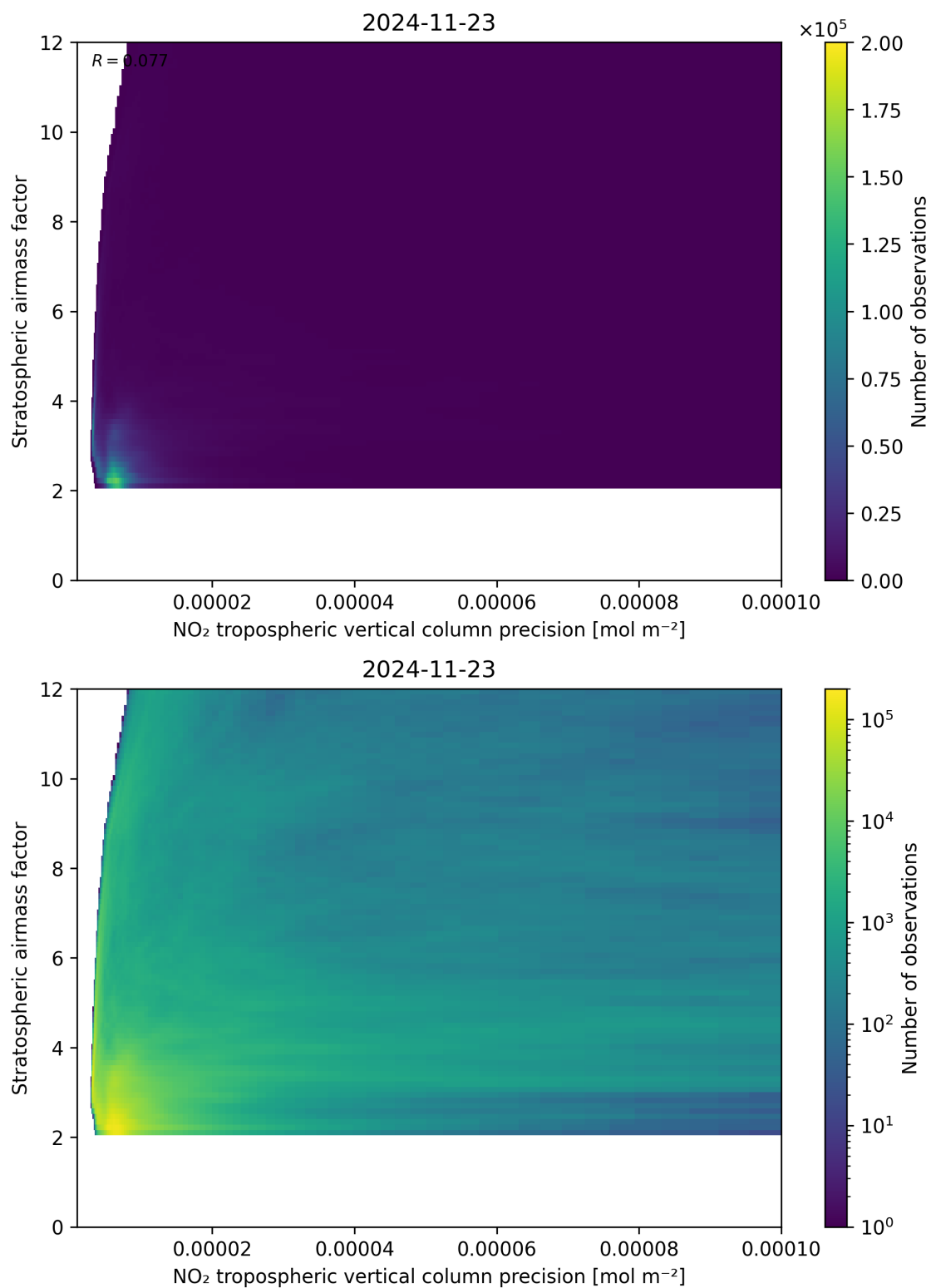
Figure 131: Scatter density plot of “NO 2 tropospheric vertical column precision” against “Stratospheric airmass factor” for 2024-11-22 to 2024-11-24.
