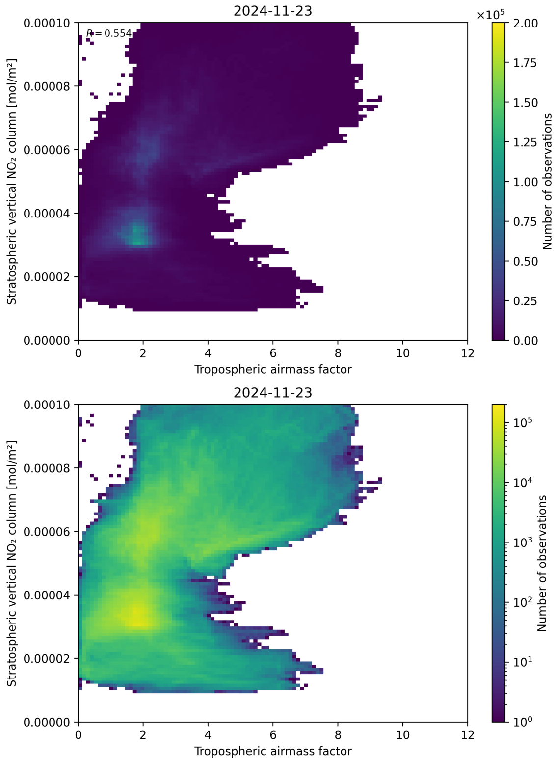
Figure 74: Scatter density plot of “Tropospheric air mass factor” against “Stratospheric vertical NO 2 column” for 2024-11-22 to 2024-11-24.
