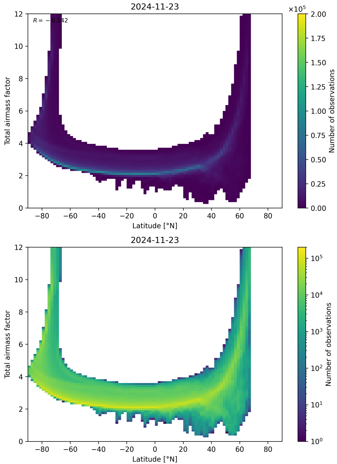
Figure 84: Scatter density plot of “Latitude” against “Total airmass factor” for 2024-11-22 to 2024-11-24.
