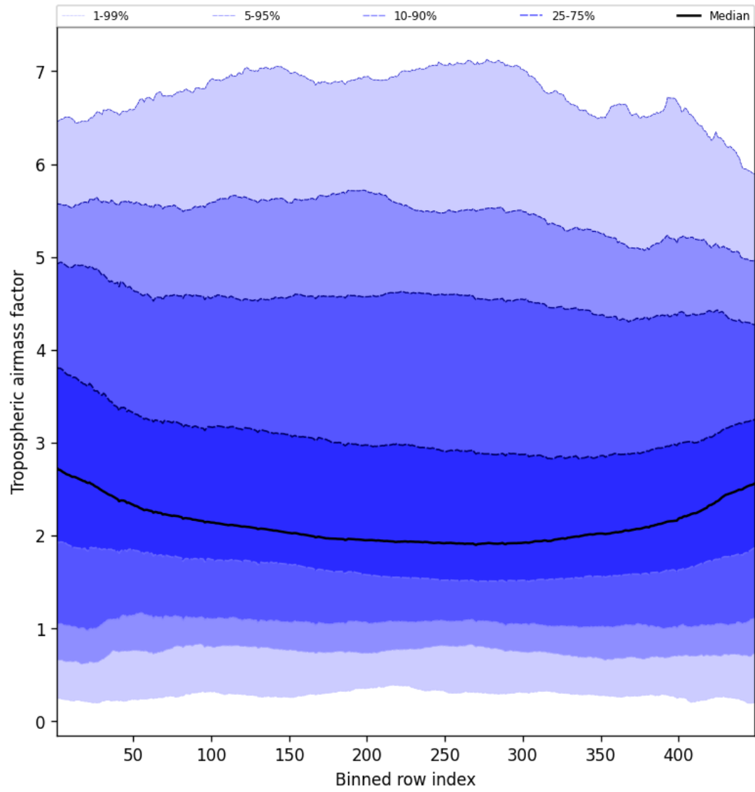
Figure 48: Along track statistics of “Tropospheric airmass factor” for 2024-11-22 to 2024-11-24
