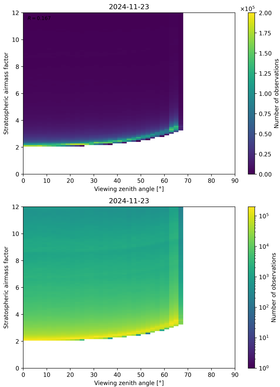
Figure 159: Scatter density plot of “Viewing zenith angle” against “Stratospheric airmass factor” for 2024-11-22 to 2024-11-24.
