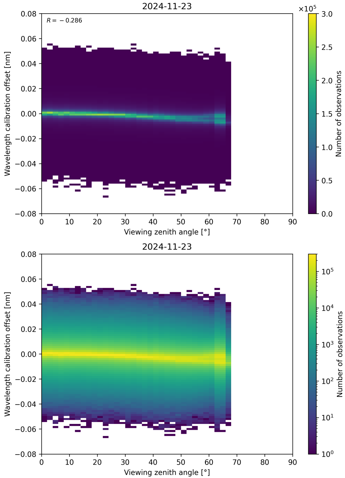
Figure 173: Scatter density plot of “Viewing zenith angle” against “Wavelength calibration offset” for 2024-11-22 to 2024-11-24.
