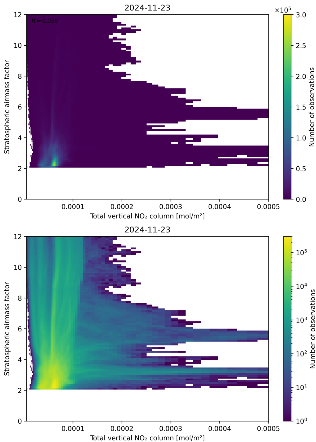
Figure 110: Scatter density plot of “Total vertical NO 2 column” against “Stratospheric airmass factor” for 2024-11-22 to 2024-11-24.
