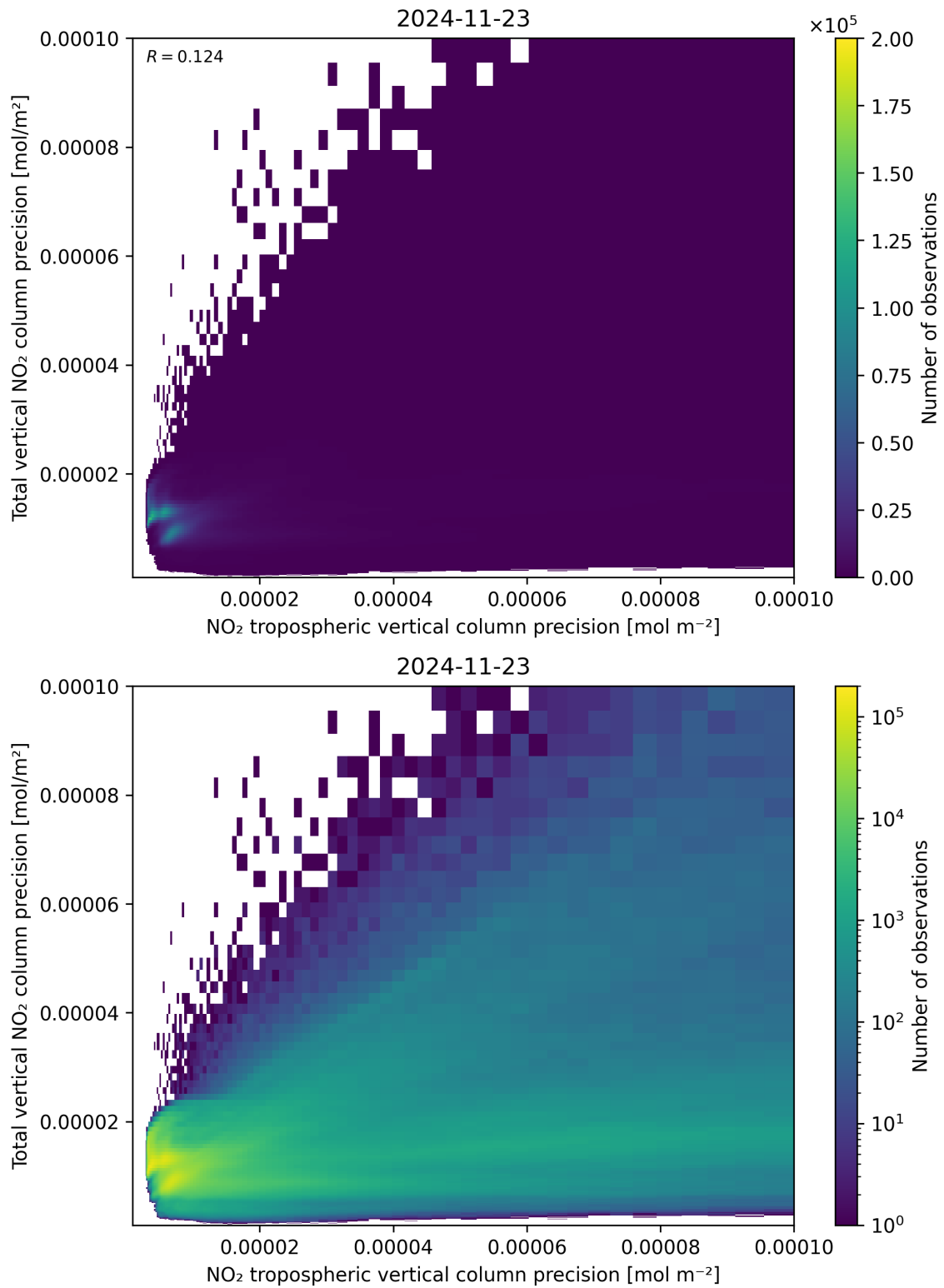
Figure 139: Scatter density plot of “NO 2 tropospheric vertical column precision” against “Total vertical NO 2 column precision” for 2024-11-22 to 2024-11-24.
