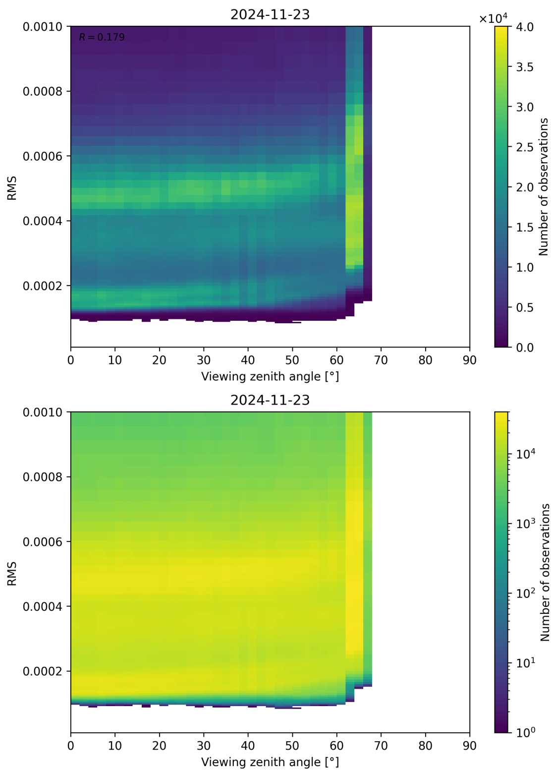
Figure 171: Scatter density plot of “Viewing zenith angle” against “RMS” for 2024-11-22 to 2024-11-24.
