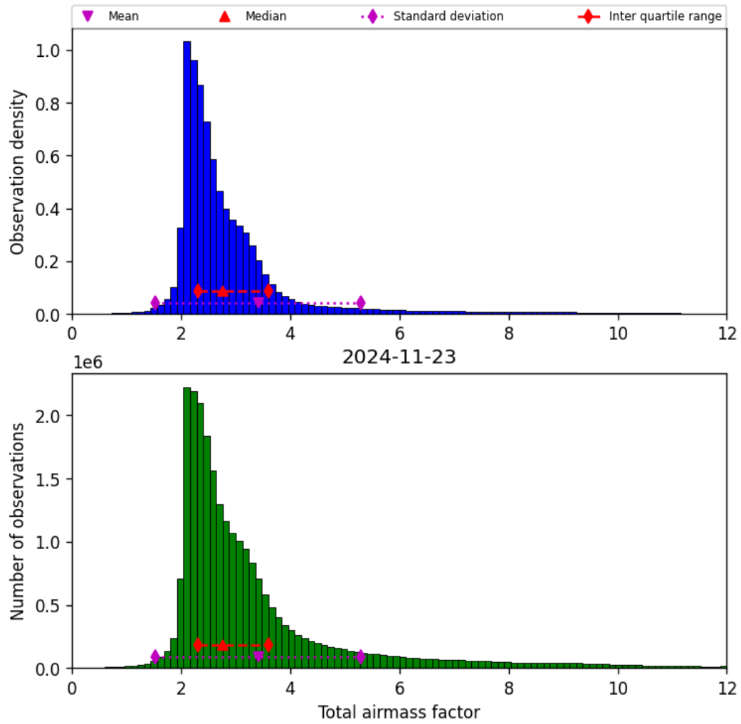
Figure 32: Histogram of “Total airmass factor” for 2024-11-22 to 2024-11-24
