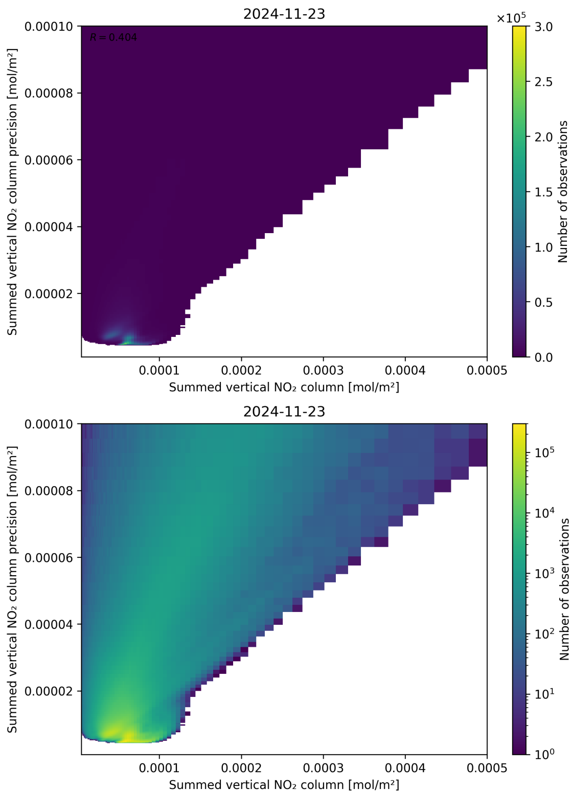
Figure 105: Scatter density plot of “Summed vertical NO 2 column” against “Summed vertical NO 2 column precision” for 2024-11-22 to 2024-11-24.
