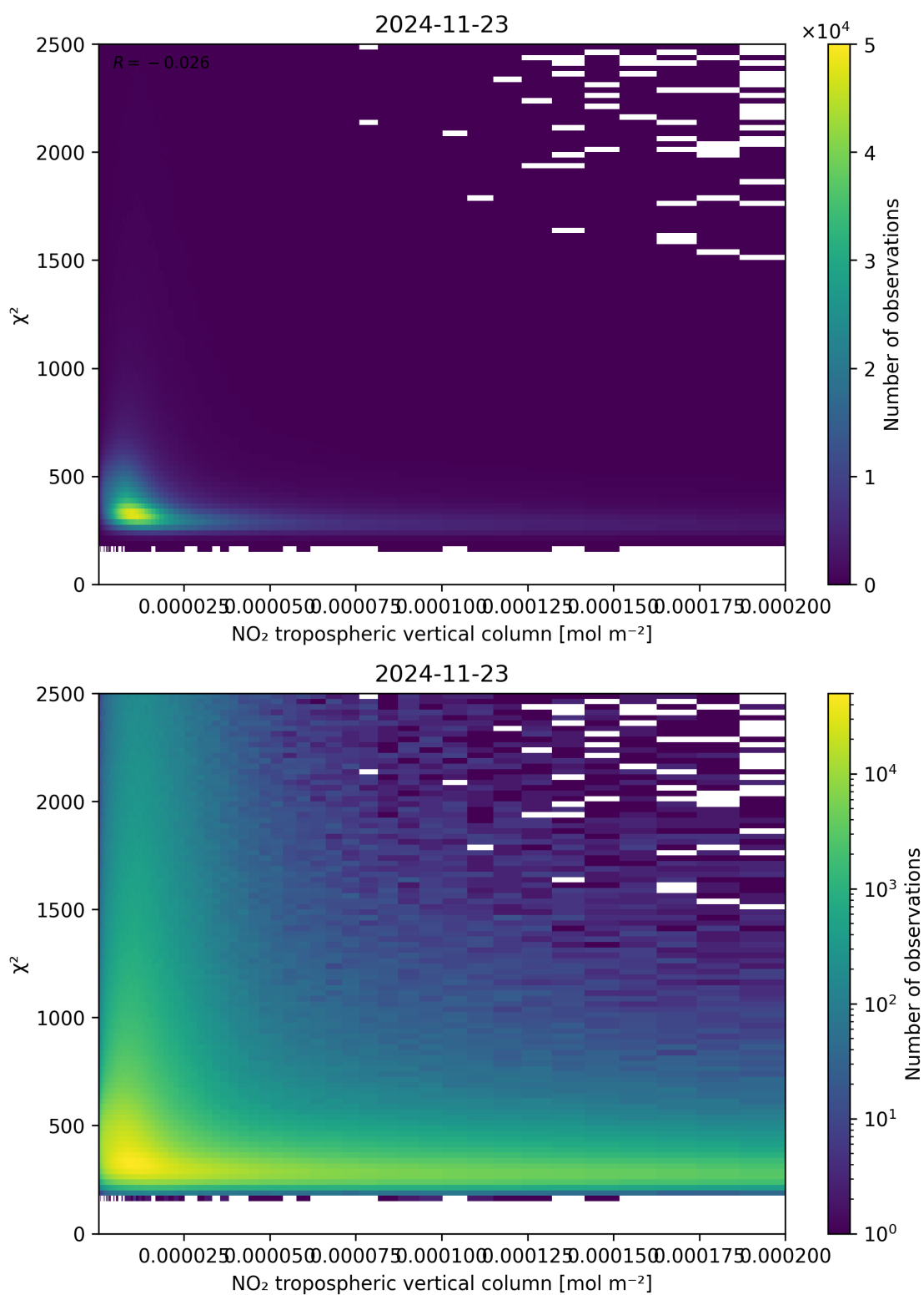
Figure 124: Scatter density plot of “NO 2 tropospheric vertical column” against “ \chi^2 ” for 2024-11-22 to 2024-11-24.
