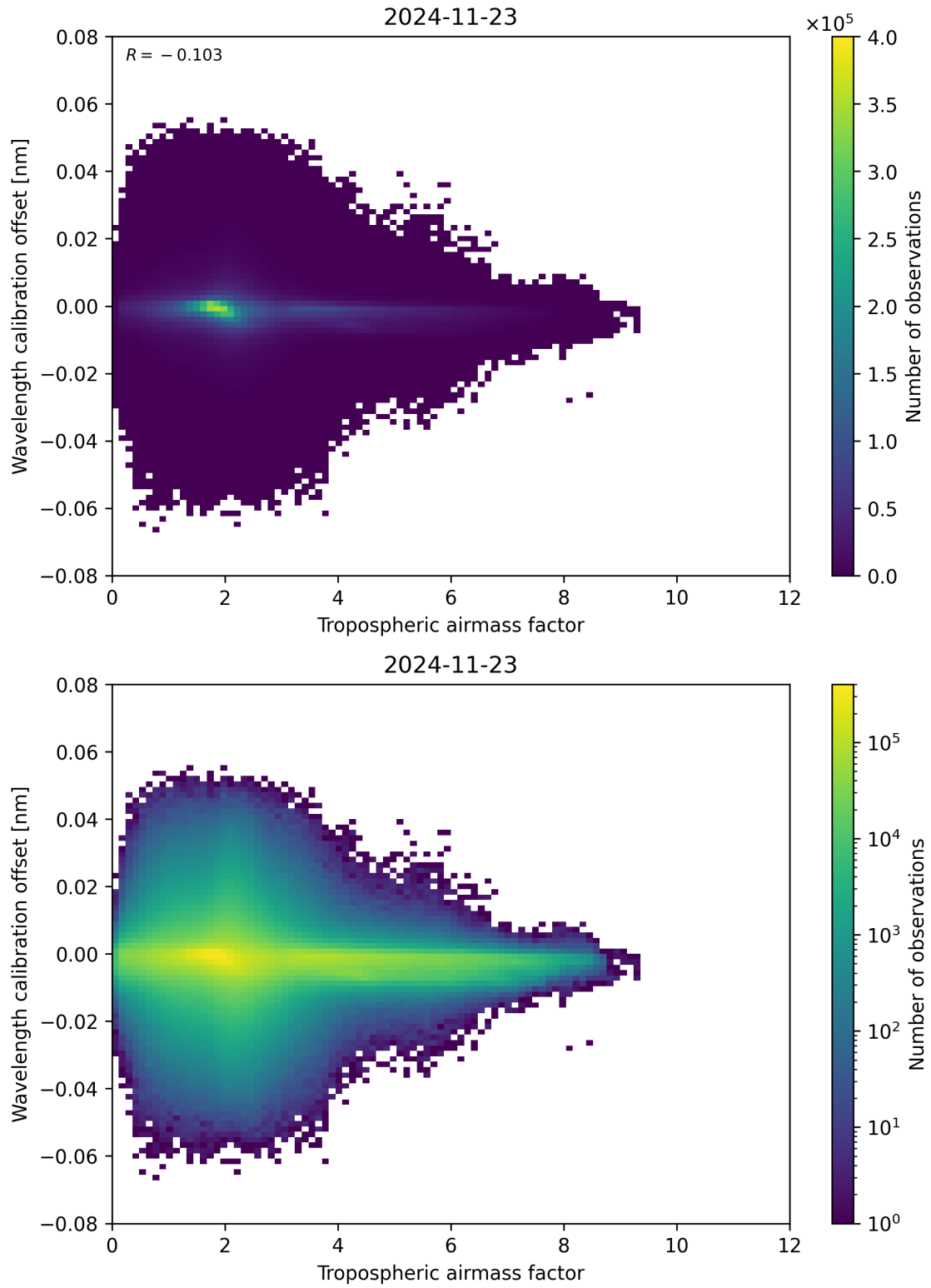
Figure 80: Scatter density plot of “Tropospheric airmass factor” against “Wavelength calibration offset” for 2024-11-22 to 2024-11-24.
