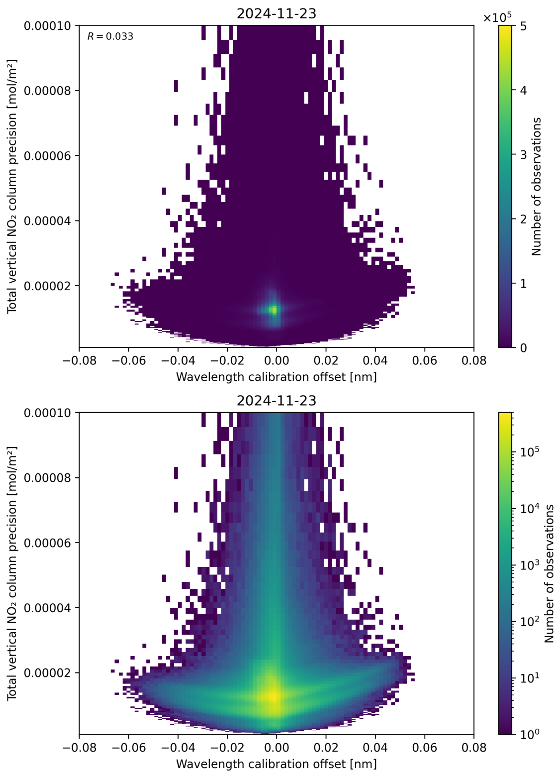
Figure 180: Scatter density plot of “Wavelength calibration offset” against “Total vertical NO 2 column precision” for 2024-11-22 to 2024-11-24.
