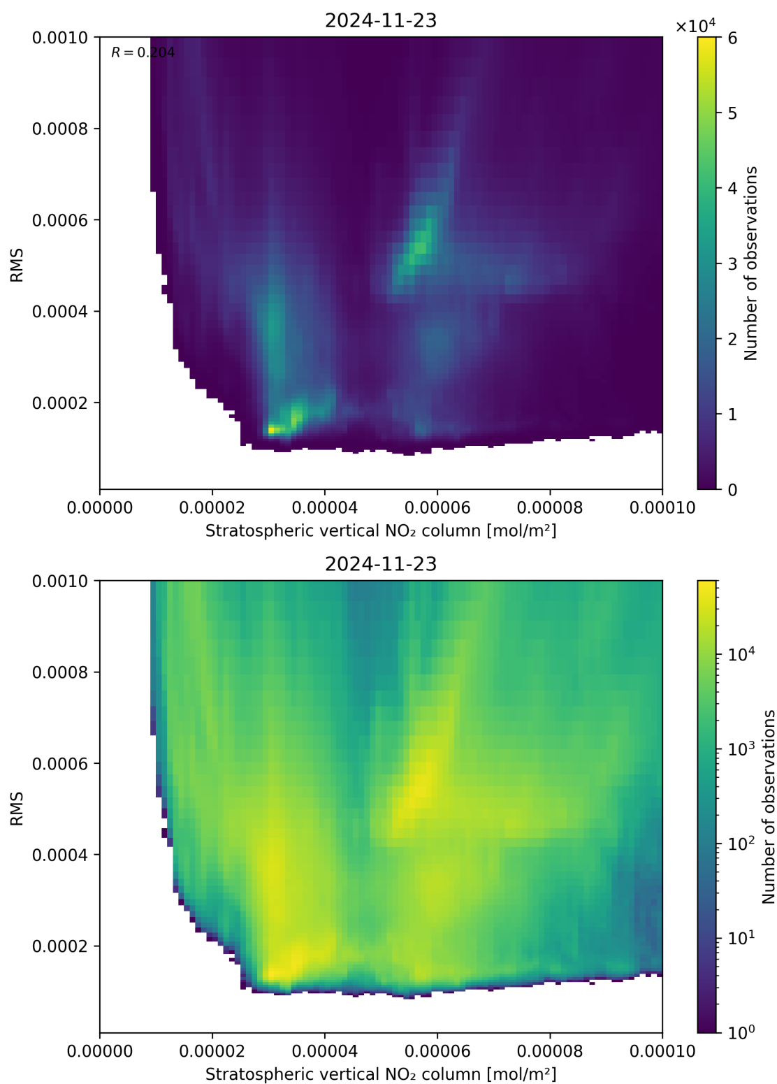
Figure 102: Scatter density plot of “Stratospheric vertical NO 2 column” against “RMS” for 2024-11-22 to 2024-11-24.
