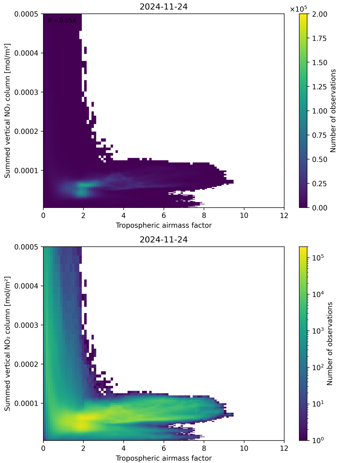
Figure 75: Scatter density plot of “Tropospheric airmass factor” against “Summed vertical NO 2 column” for 2024-11-23 to 2024-11-25.
