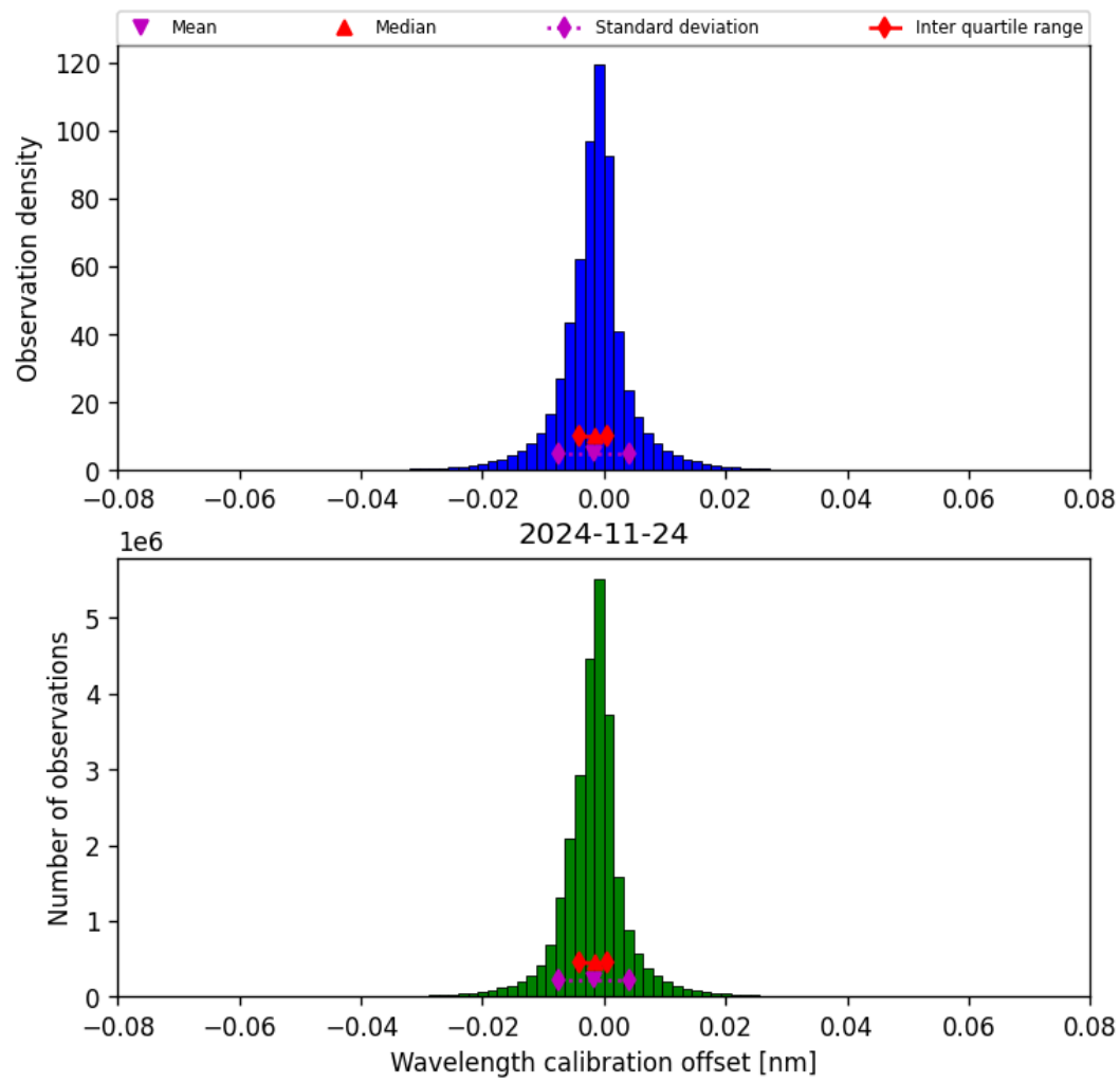
Figure 35: Histogram of “Wavelength calibration offset” for 2024-11-23 to 2024-11-25
