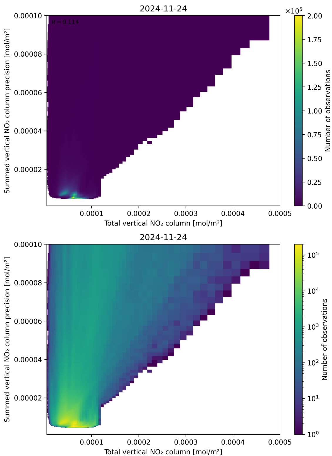
Figure 113: Scatter density plot of “Total vertical NO 2 column” against “Summed vertical NO 2 column precision” for 2024-11-23 to 2024-11-25.
