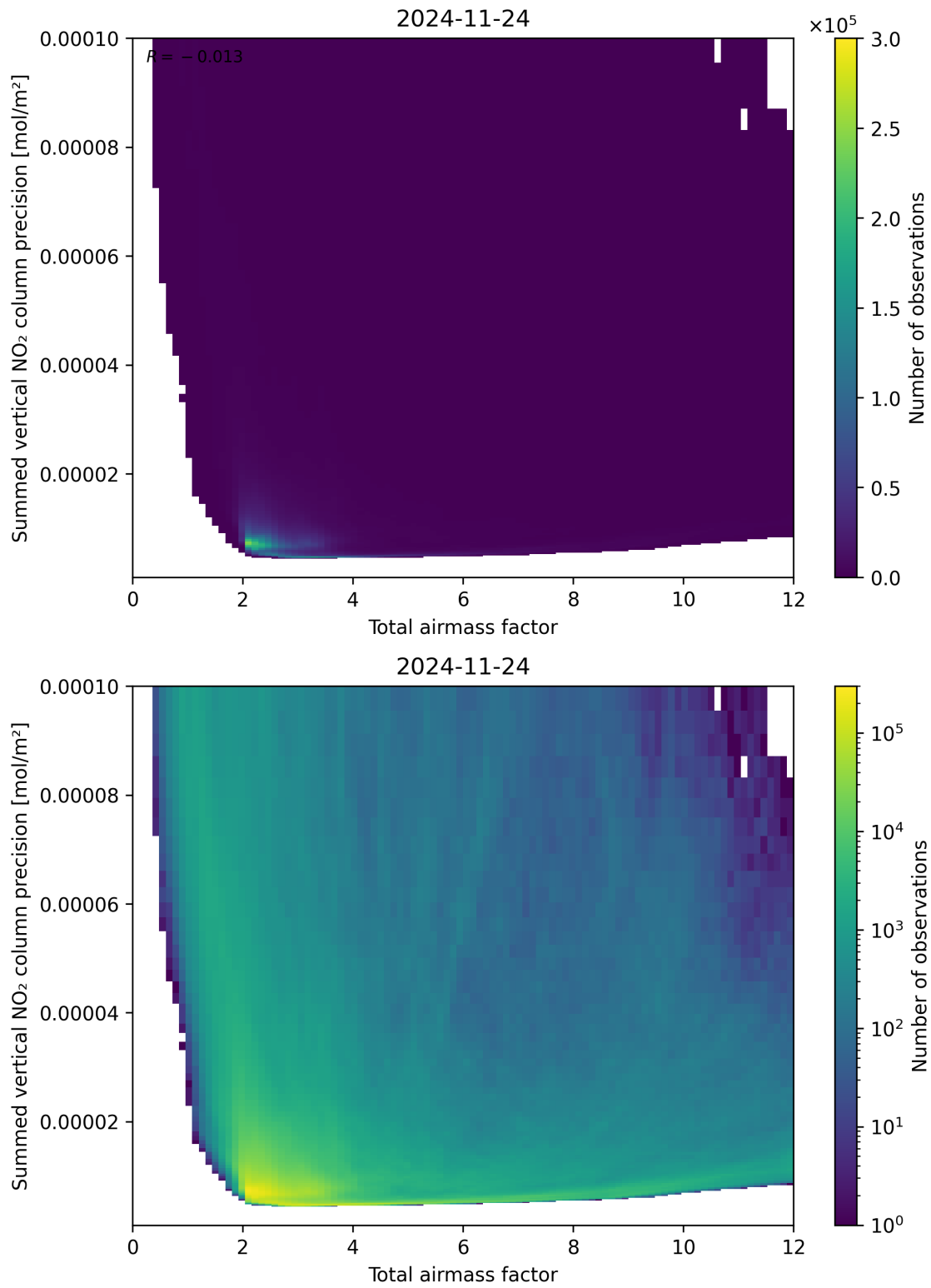
Figure 66: Scatter density plot of “Total airmass factor” against “Summed vertical NO 2 column precision” for 2024-11-23 to 2024-11-25.
