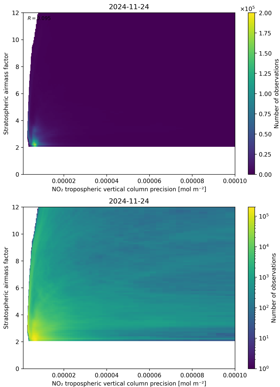
Figure 131: Scatter density plot of “NO 2 tropospheric vertical column precision” against “Stratospheric airmass factor” for 2024-11-23 to 2024-11-25.
