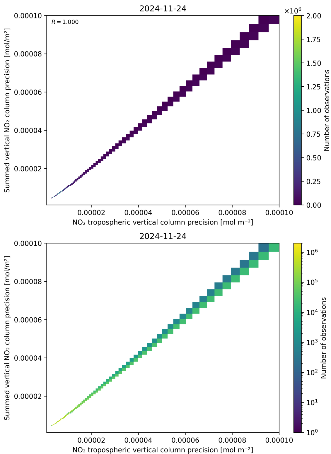
Figure 137: Scatter density plot of “NO 2 tropospheric vertical column precision” against “Summed vertical NO 2 column precision” for 2024-11-23 to 2024-11-25.
