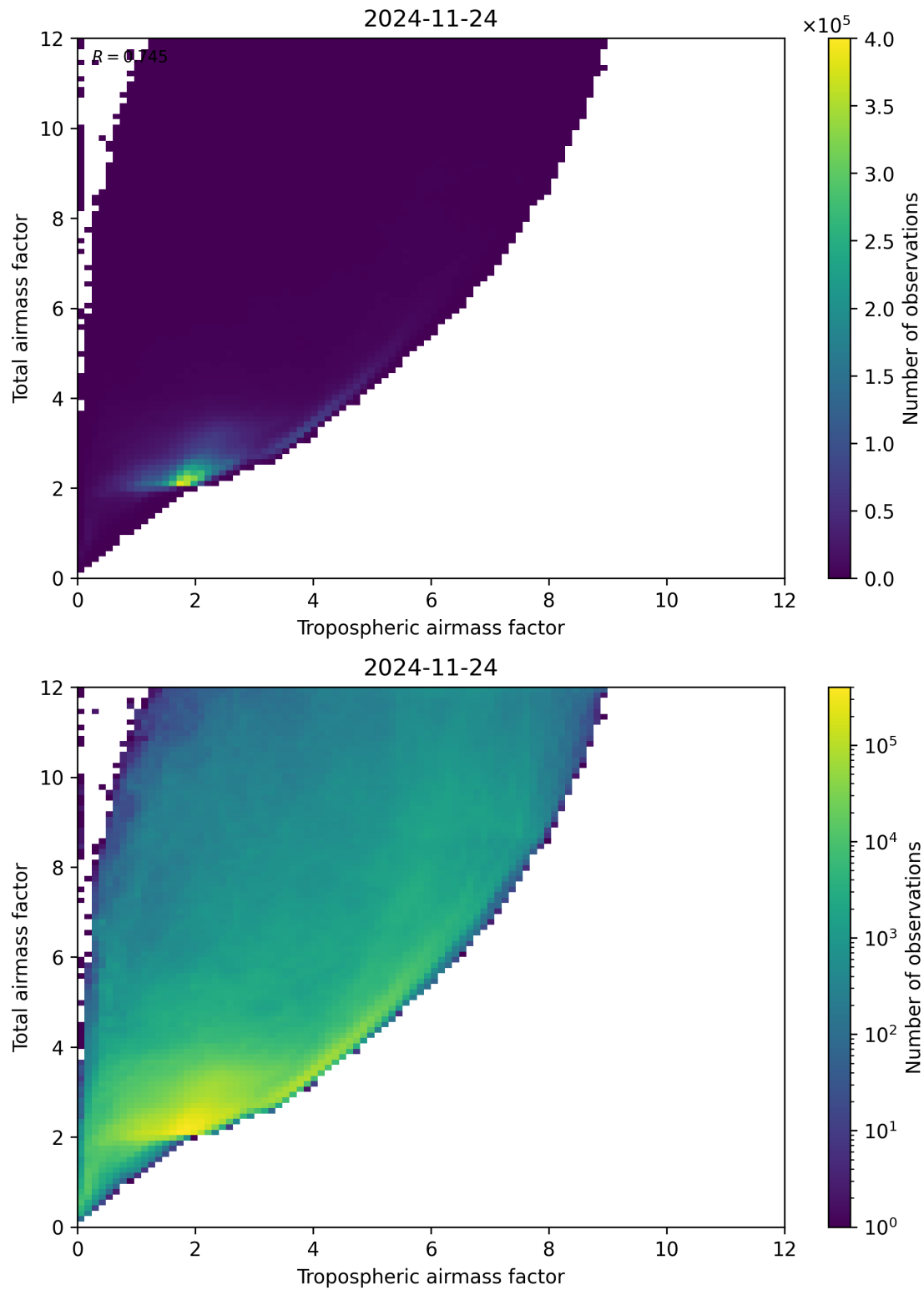
Figure 72: Scatter density plot of “Tropospheric airmass factor” against “Total airmass factor” for 2024-11-23 to 2024-11-25.
