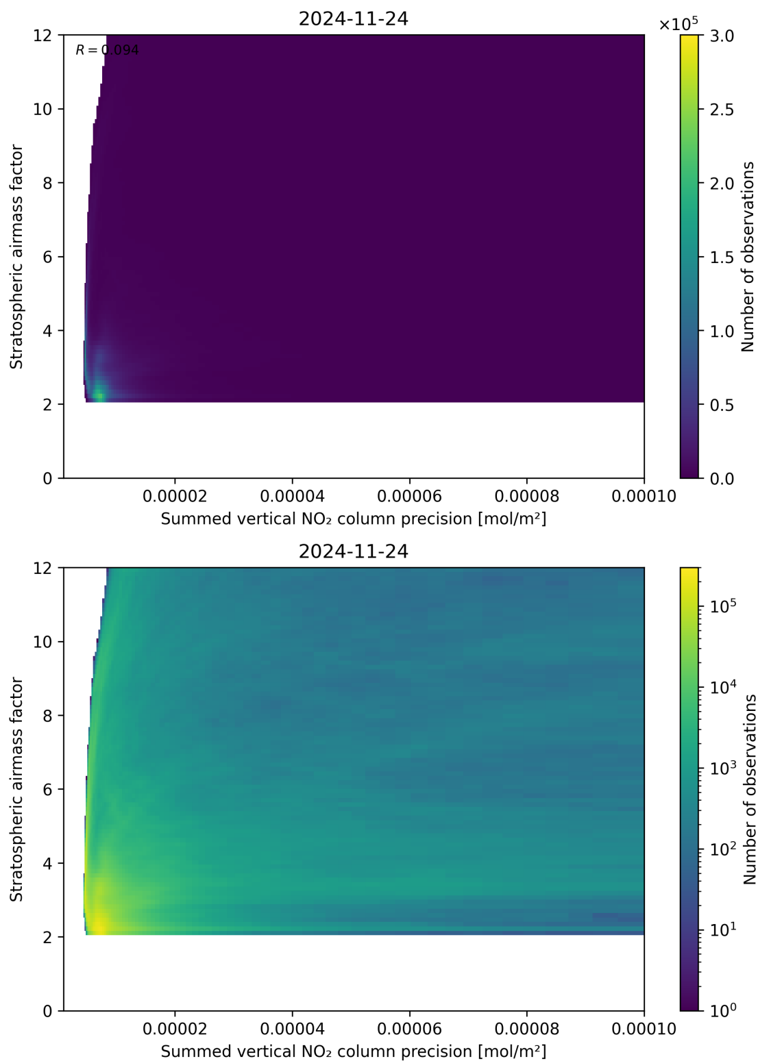
Figure 106: Scatter density plot of “Summed vertical NO 2 column precision” against “Stratospheric airmass factor” for 2024-11-23 to 2024-11-25.
