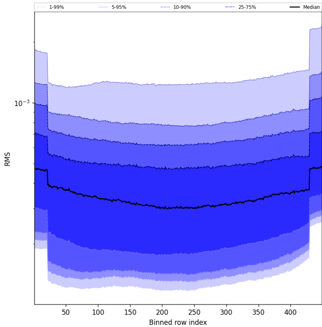
Figure 60: Along track statistics of “RMS” for 2024-11-23 to 2024-11-25
