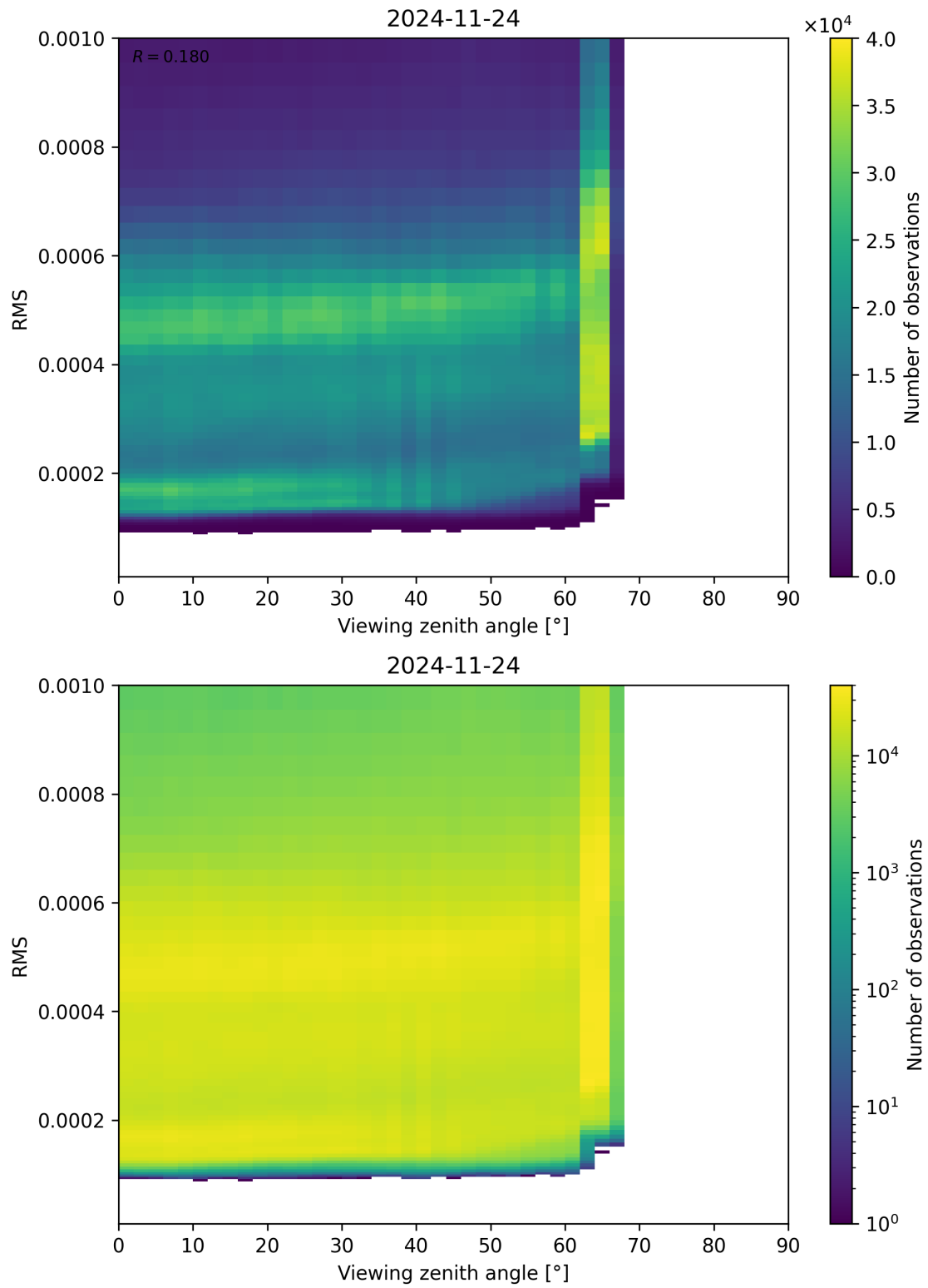
Figure 171: Scatter density plot of “Viewing zenith angle” against “RMS” for 2024-11-23 to 2024-11-25.
