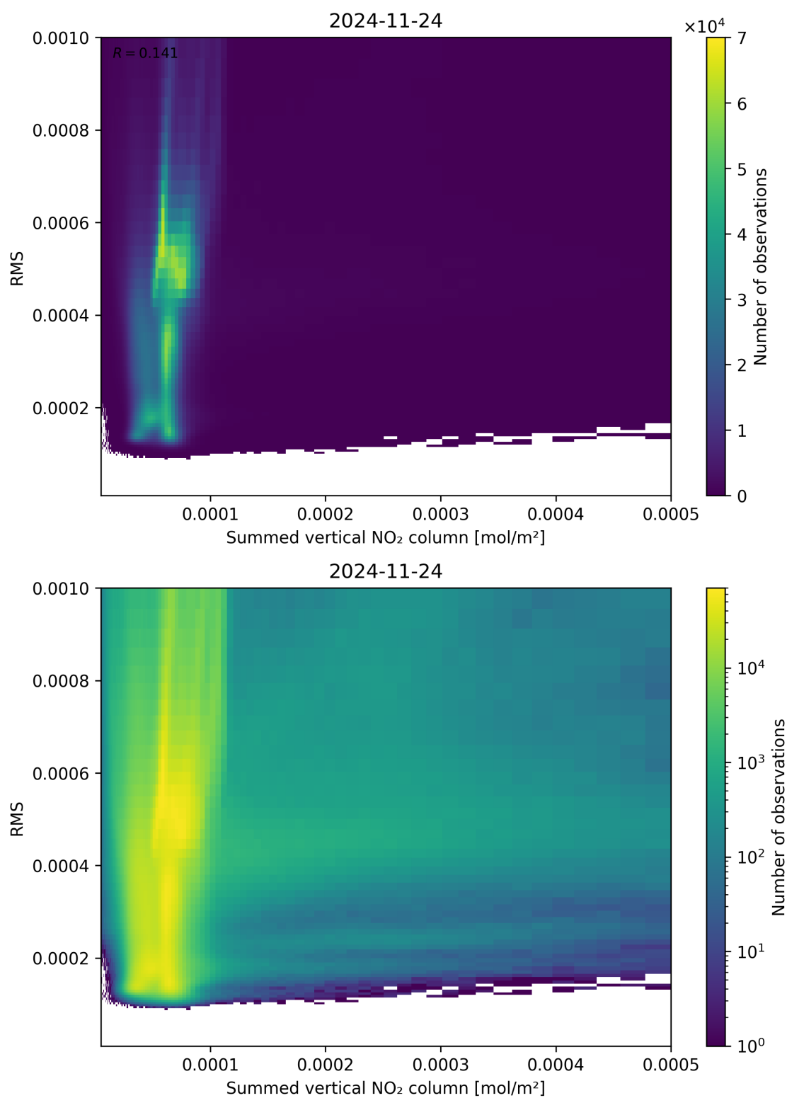
Figure 109: Scatter density plot of “Summed vertical NO 2 column” against “RMS” for 2024-11-23 to 2024-11-25.
