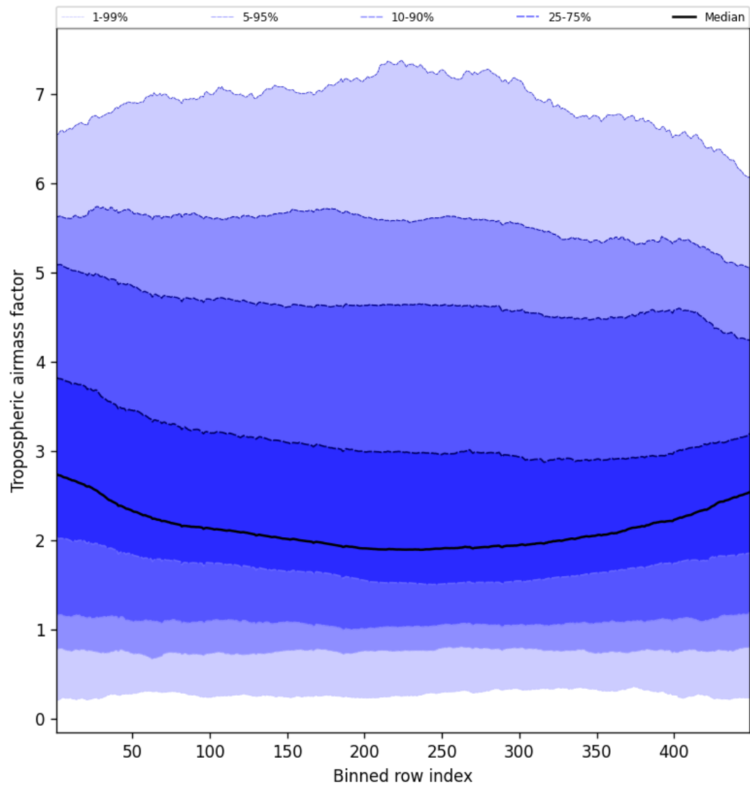
Figure 48: Along track statistics of “Tropospheric air mass factor” for 2024-11-23 to 2024-11-25
