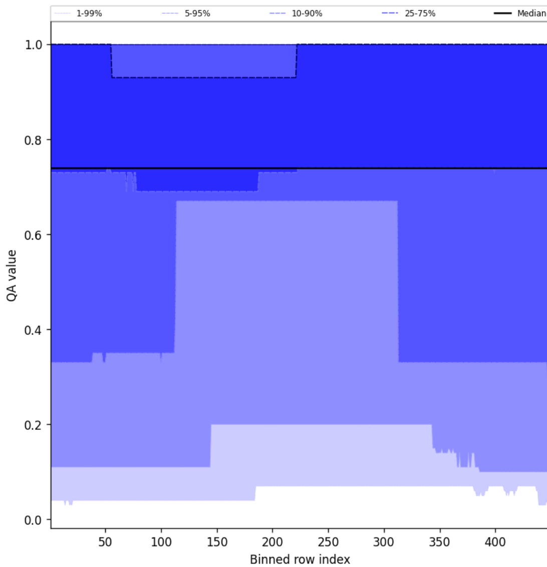
Figure 45: Along track statistics of “QA value” for 2024-11-23 to 2024-11-25
