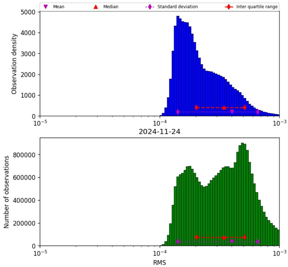
Figure 43: Histogram of “RMS” for 2024-11-23 to 2024-11-25
