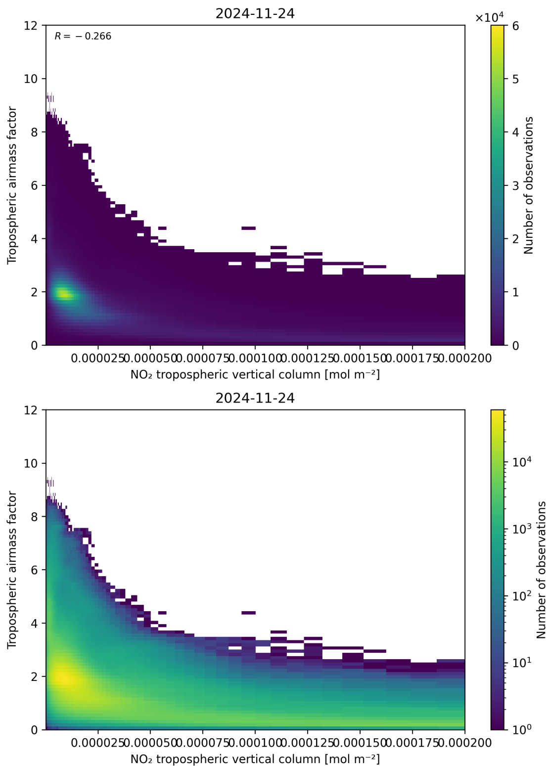
Figure 123: Scatter density plot of “NO 2 tropospheric vertical column” against “Tropospheric air mass factor” for 2024-11-23 to 2024-11-25.
