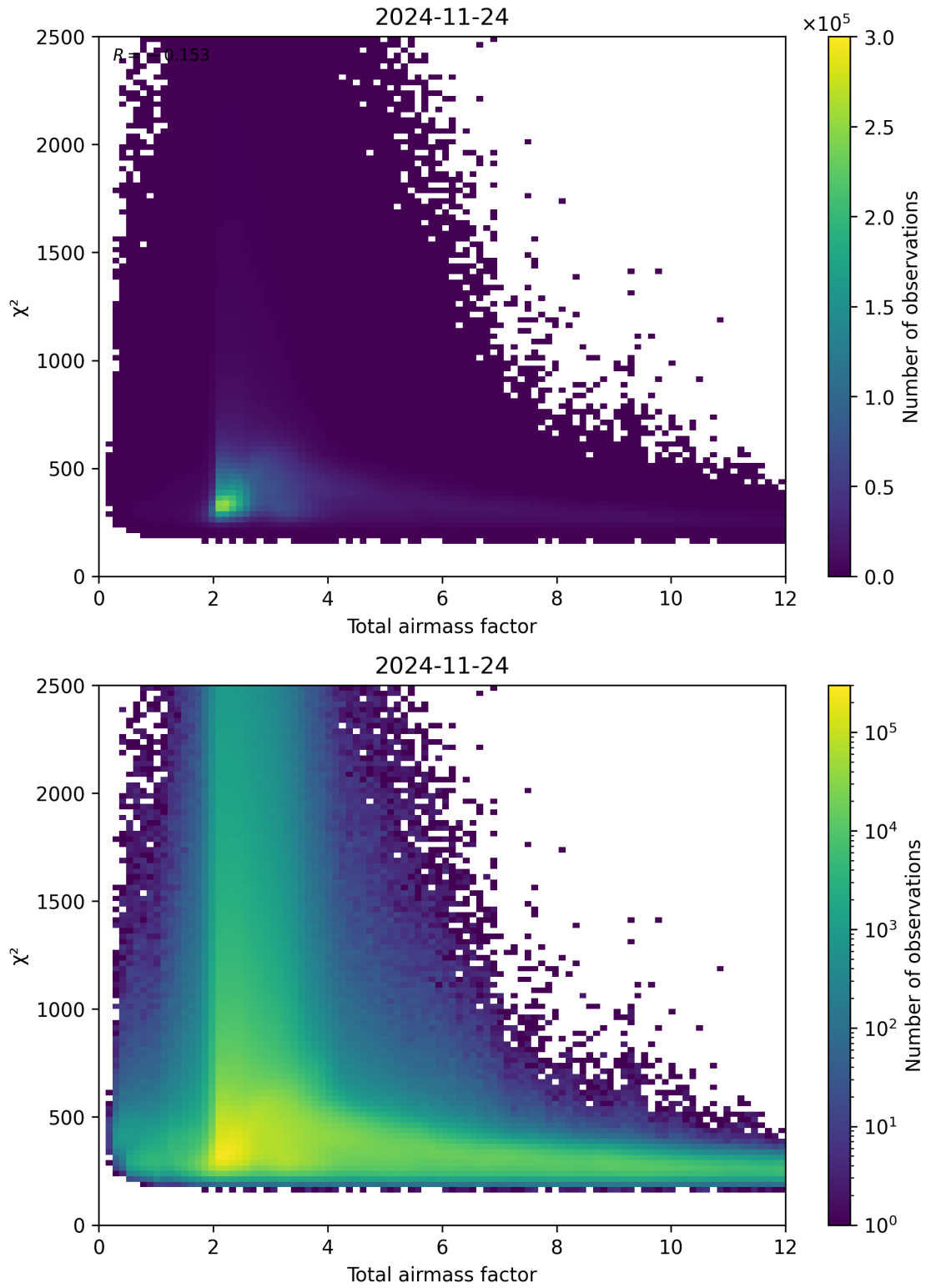
Figure 63: Scatter density plot of “Total airmass factor” against “ \chi^2 ” for 2024-11-23 to 2024-11-25.
