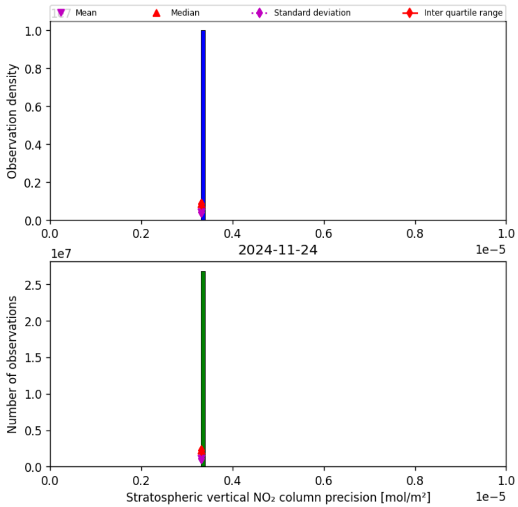
Figure 37: Histogram of “Stratospheric vertical NO 2 column precision” for 2024-11-23 to 2024-11-25
