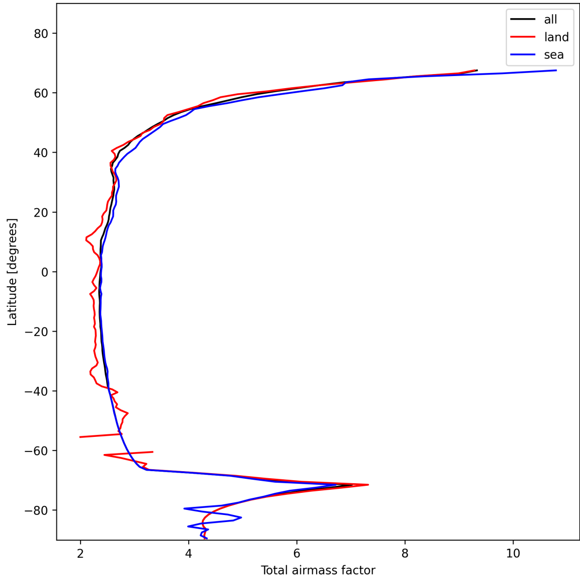
Figure 15: Zonal average of “Total airmass factor” for 2024-11-23 to 2024-11-25.
