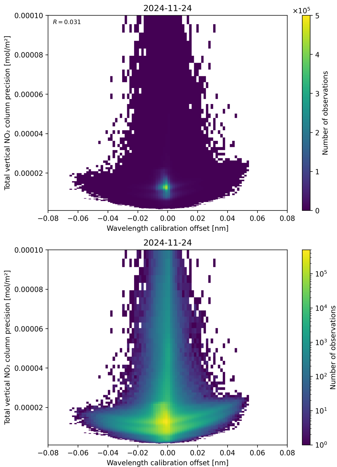
Figure 180: Scatter density plot of “Wavelength calibration offset” against “Total vertical NO 2 column precision” for 2024-11-23 to 2024-11-25.
