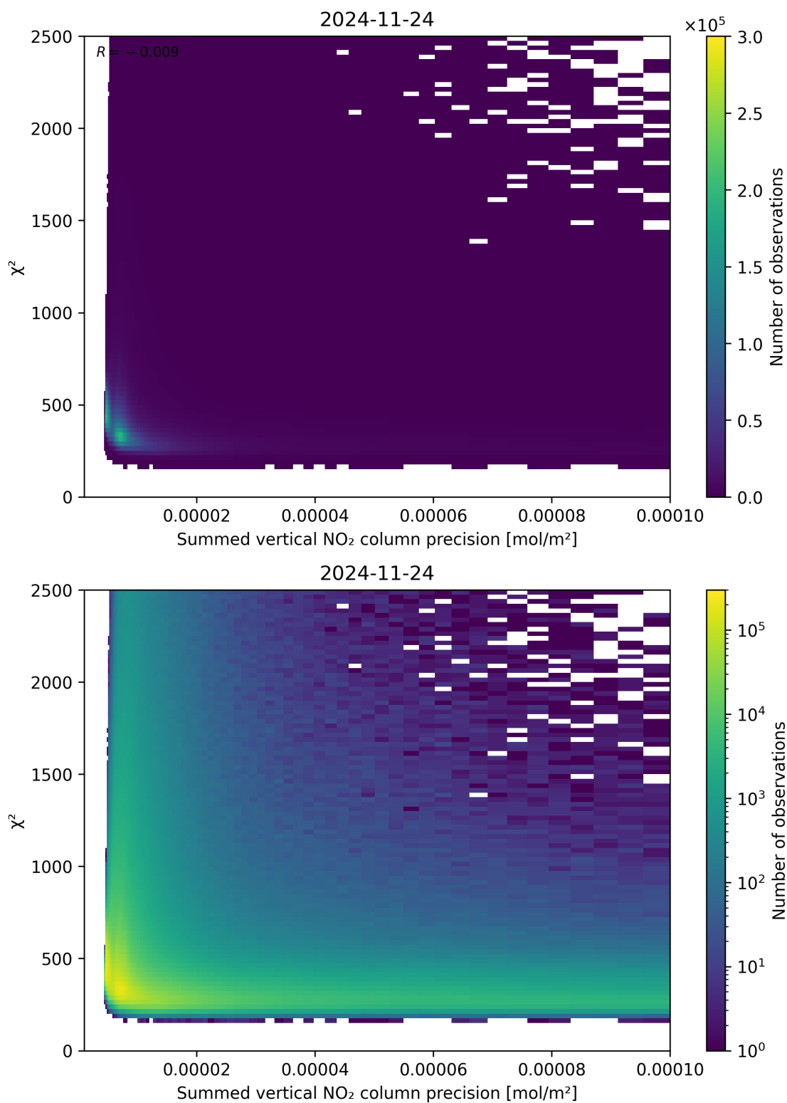
Figure 107: Scatter density plot of “Summed vertical NO 2 column precision” against “ \chi^2 ” for 2024-11-23 to 2024-11-25.
