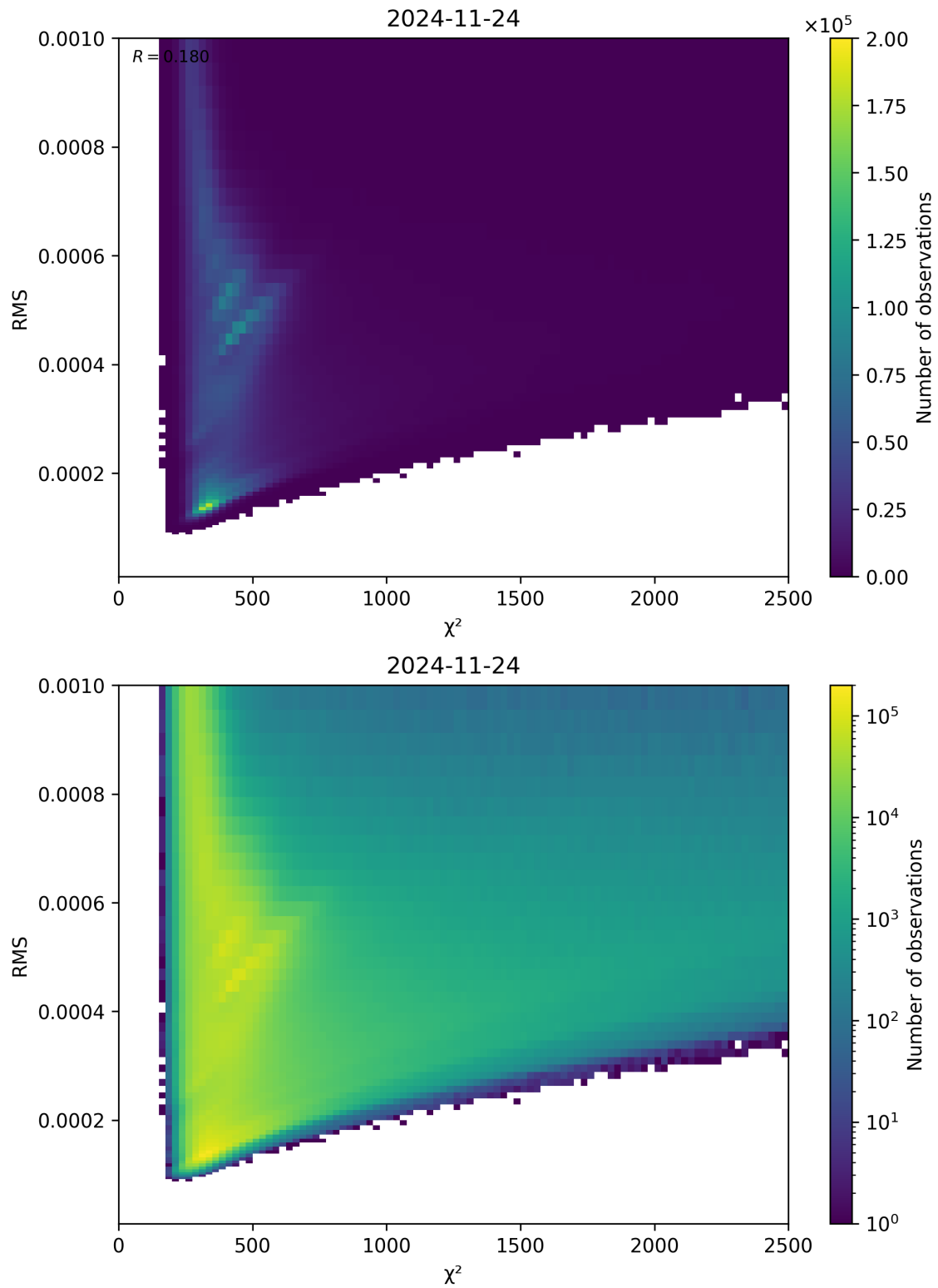
Figure 82: Scatter density plot of “ \chi^2 ” against “RMS” for 2024-11-23 to 2024-11-25.
