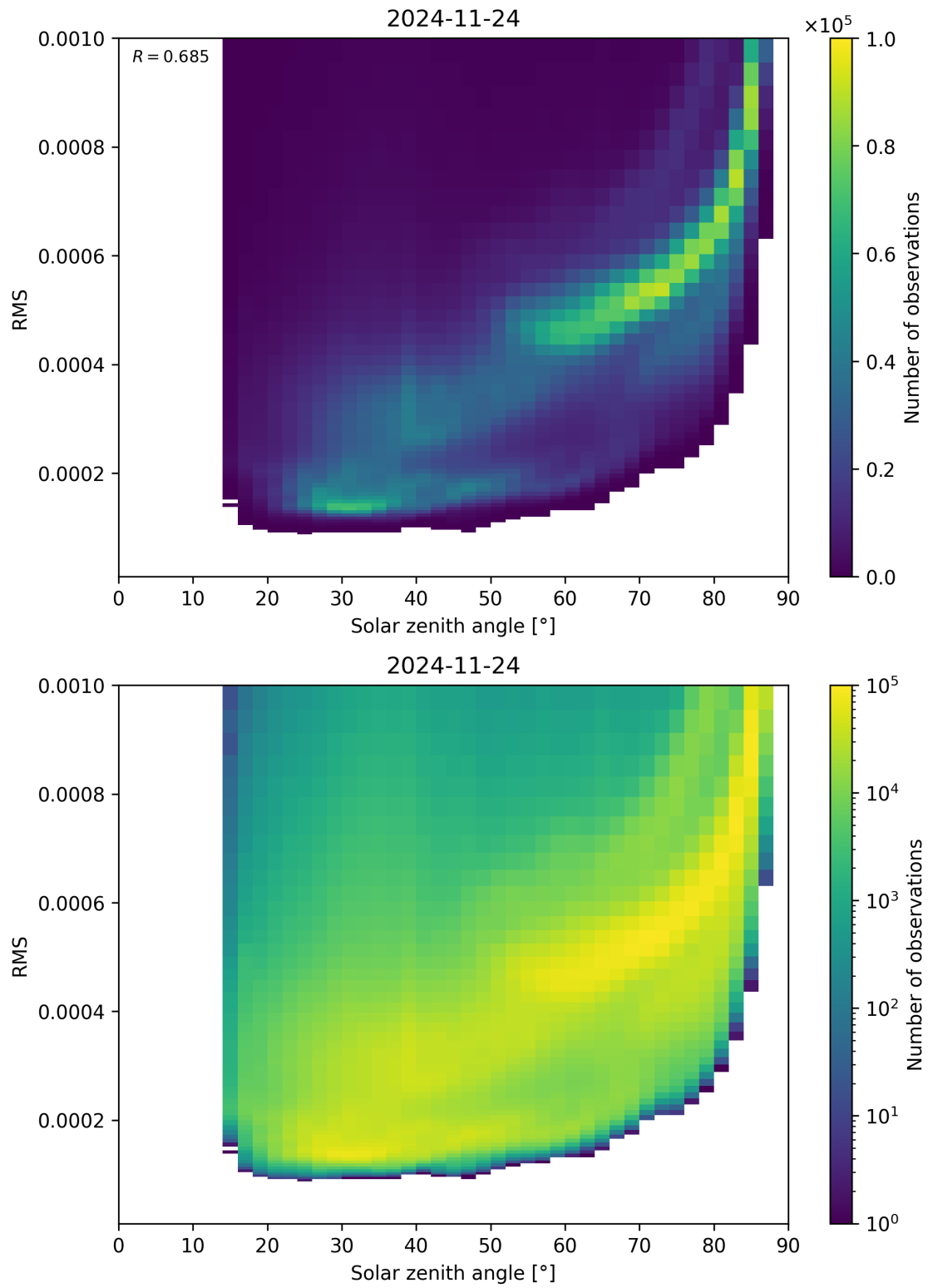
Figure 157: Scatter density plot of “Solar zenith angle” against “RMS” for 2024-11-23 to 2024-11-25.
