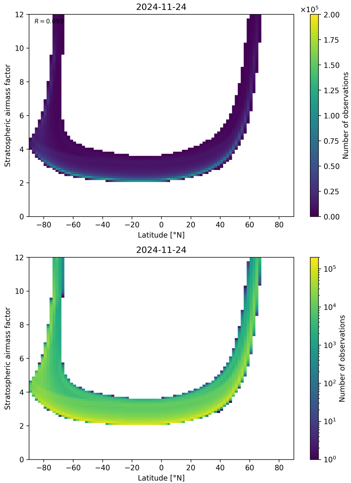
Figure 83: Scatter density plot of “Latitude” against “Stratospheric airmass factor” for 2024-11-23 to 2024-11-25.
