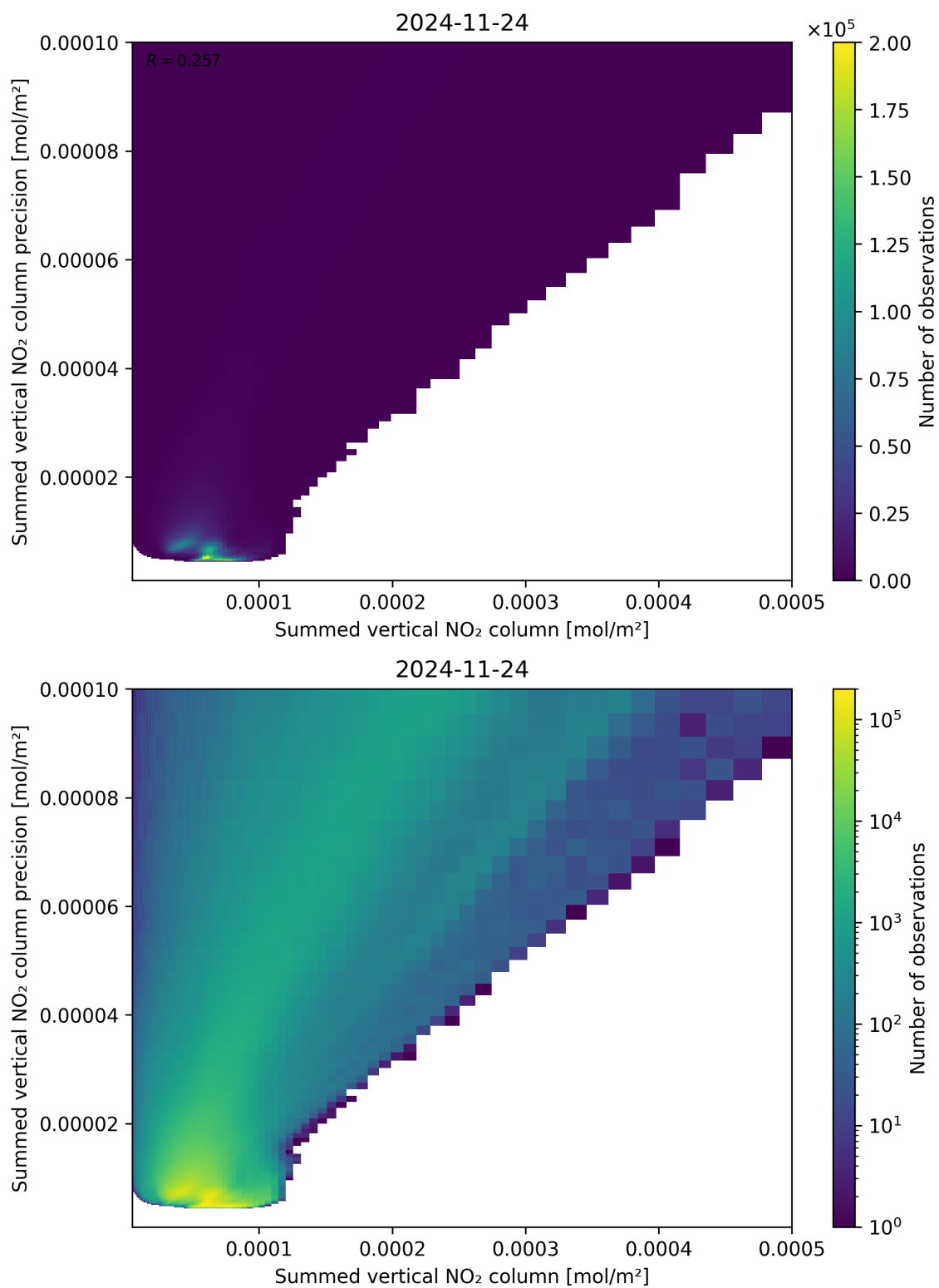
Figure 105: Scatter density plot of “Summed vertical NO 2 column” against “Summed vertical NO 2 column precision” for 2024-11-23 to 2024-11-25.
