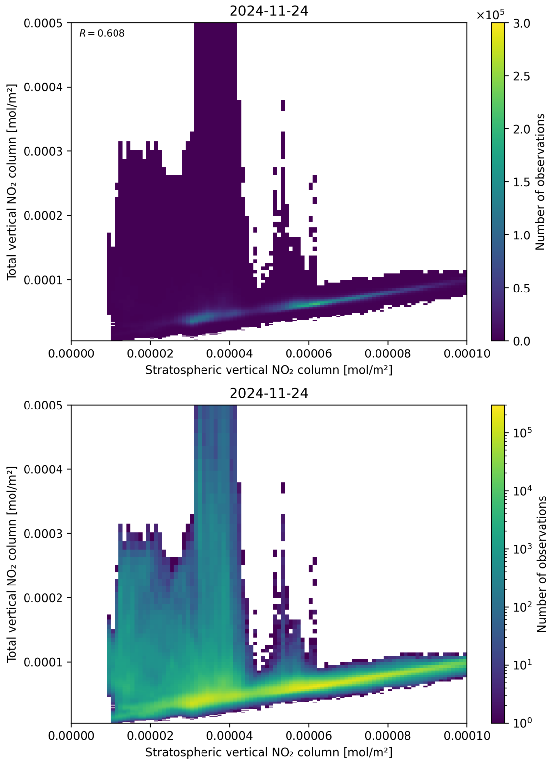
Figure 100: Scatter density plot of “Stratospheric vertical NO 2 column” against “Total vertical NO 2 column” for 2024-11-23 to 2024-11-25.
