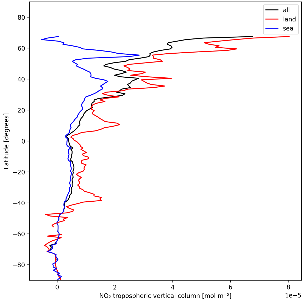
Figure 12: Zonal average of “NO 2 tropospheric vertical column” for 2024-11-23 to 2024-11-25.
