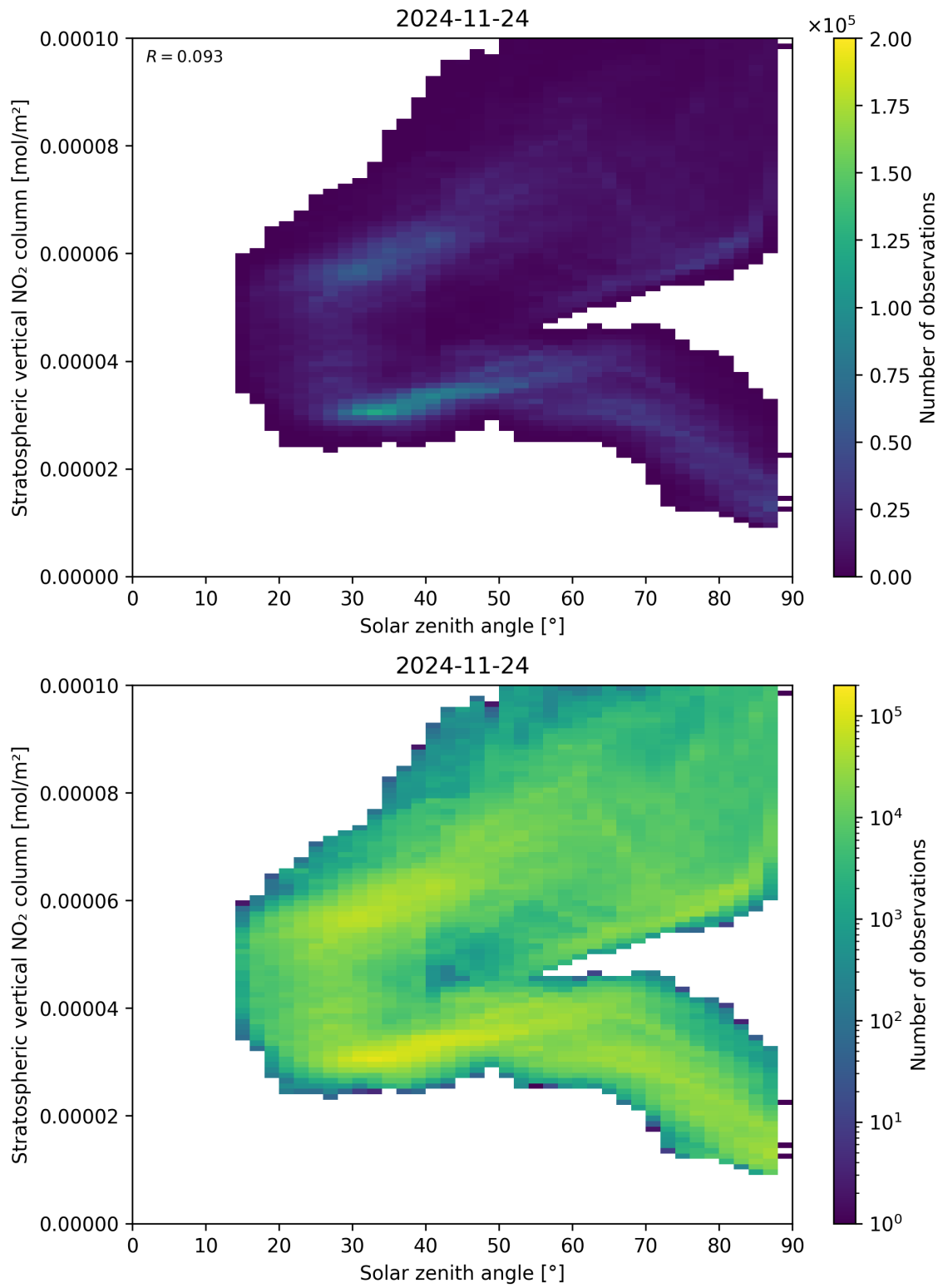
Figure 150: Scatter density plot of “Solar zenith angle” against “Stratospheric vertical NO 2 column” for 2024-11-23 to 2024-11-25.
