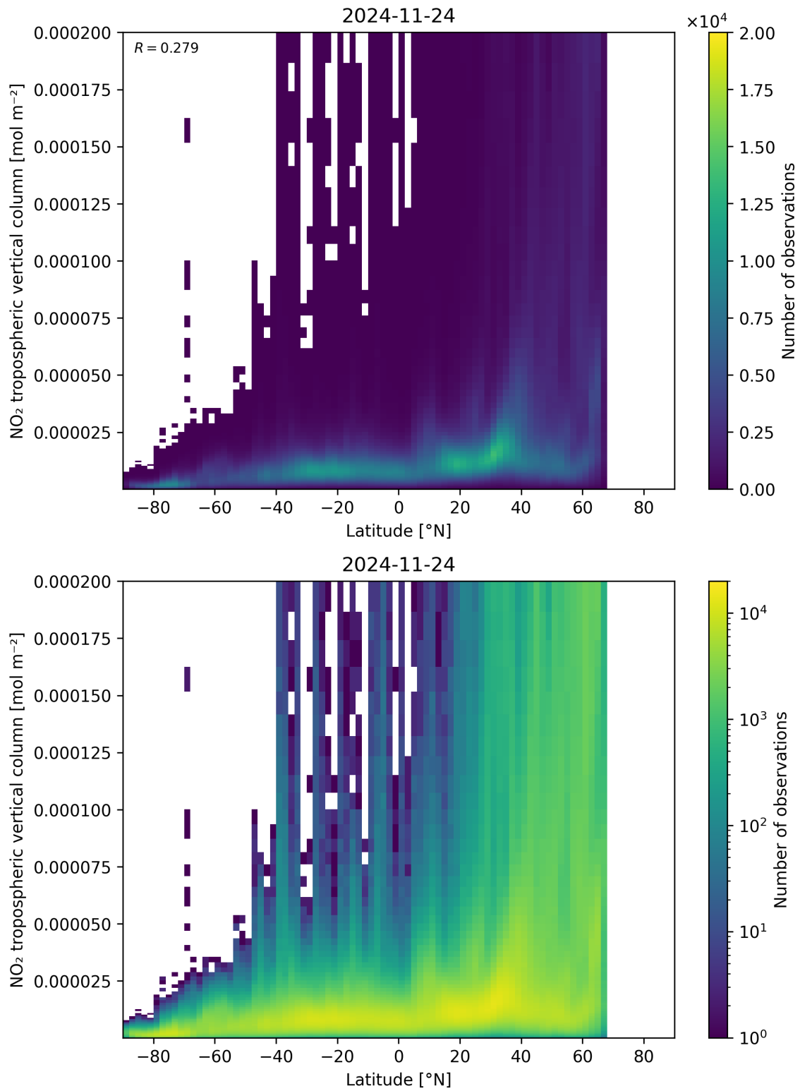
Figure 92: Scatter density plot of “Latitude” against “NO 2 tropospheric vertical column” for 2024-11-23 to 2024-11-25.
