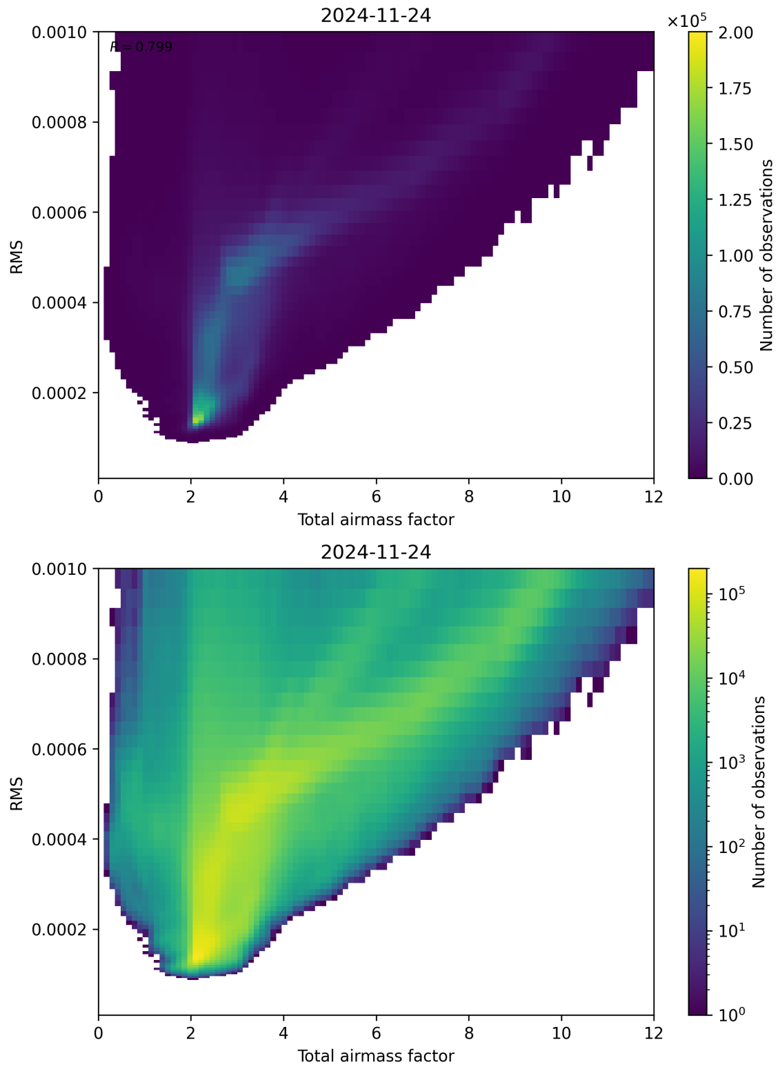
Figure 69: Scatter density plot of “Total airmass factor” against “RMS” for 2024-11-23 to 2024-11-25.
