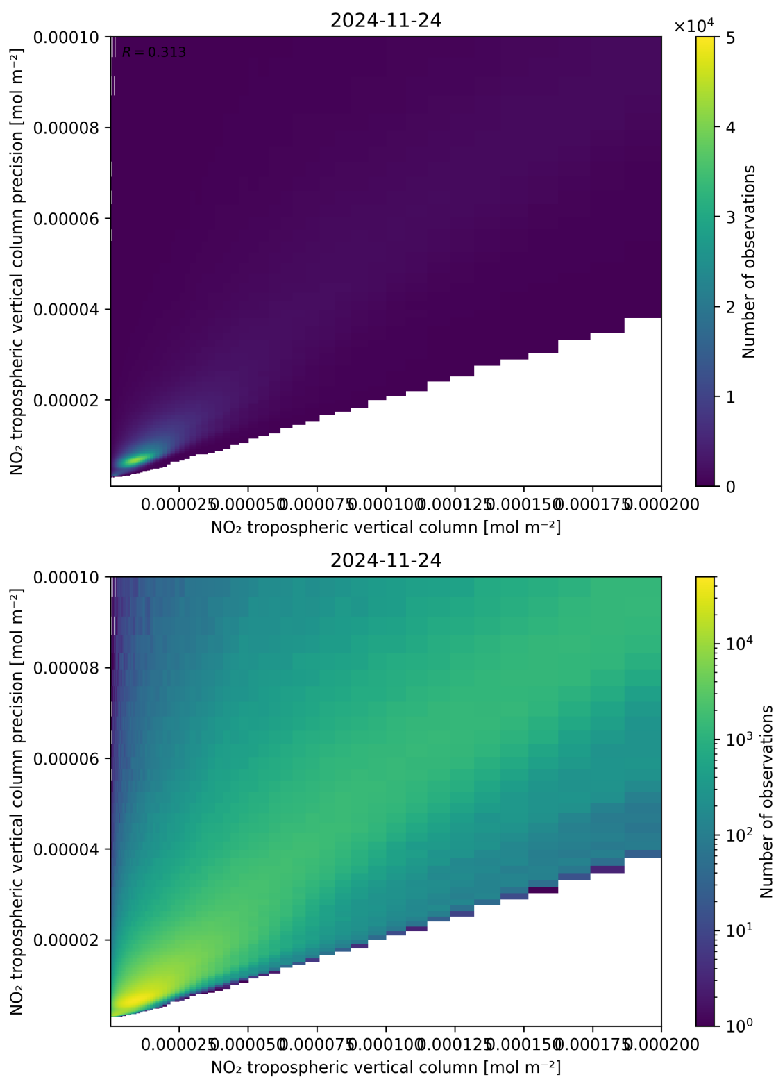
Figure 130: Scatter density plot of “NO 2 tropospheric vertical column” against “NO 2 tropospheric vertical column precision” for 2024-11-23 to 2024-11-25.
