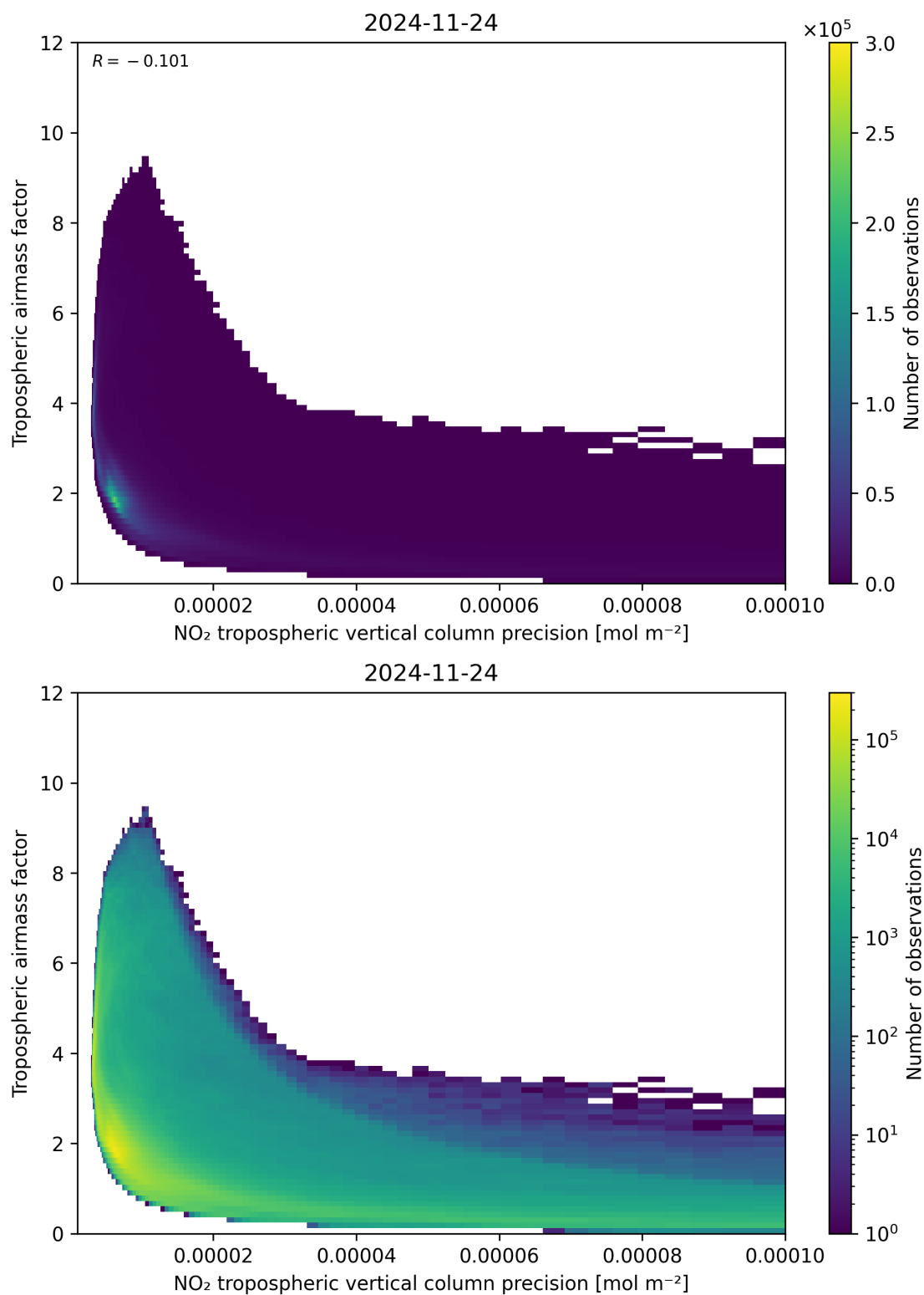
Figure 133: Scatter density plot of “NO 2 tropospheric vertical column precision” against “Tropospheric airmass factor” for 2024-11-23 to 2024-11-25.
