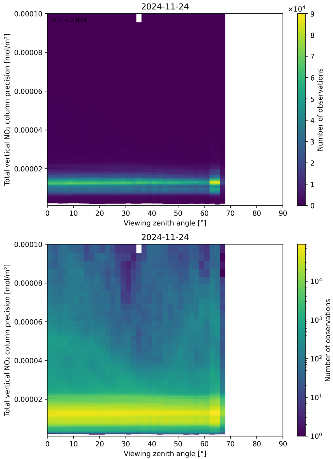
Figure 168: Scatter density plot of “Viewing zenith angle” against “Total vertical NO 2 column precision” for 2024-11-23 to 2024-11-25.
