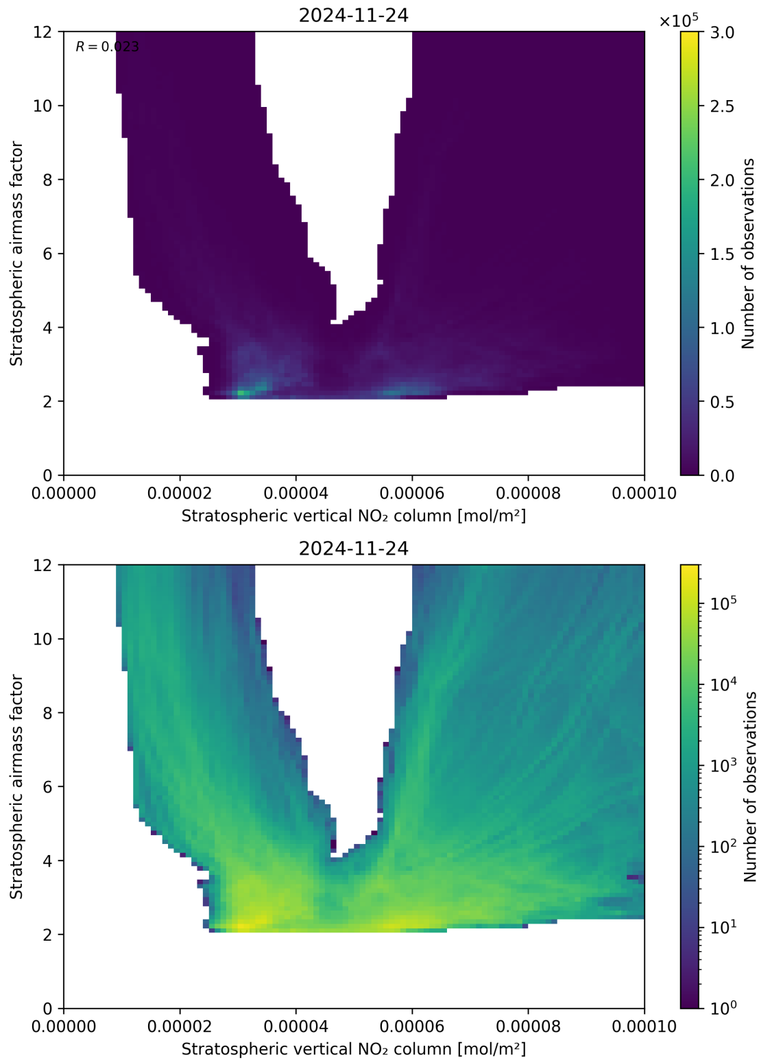
Figure 96: Scatter density plot of “Stratospheric vertical NO 2 column” against “Stratospheric airmass factor” for 2024-11-23 to 2024-11-25.
