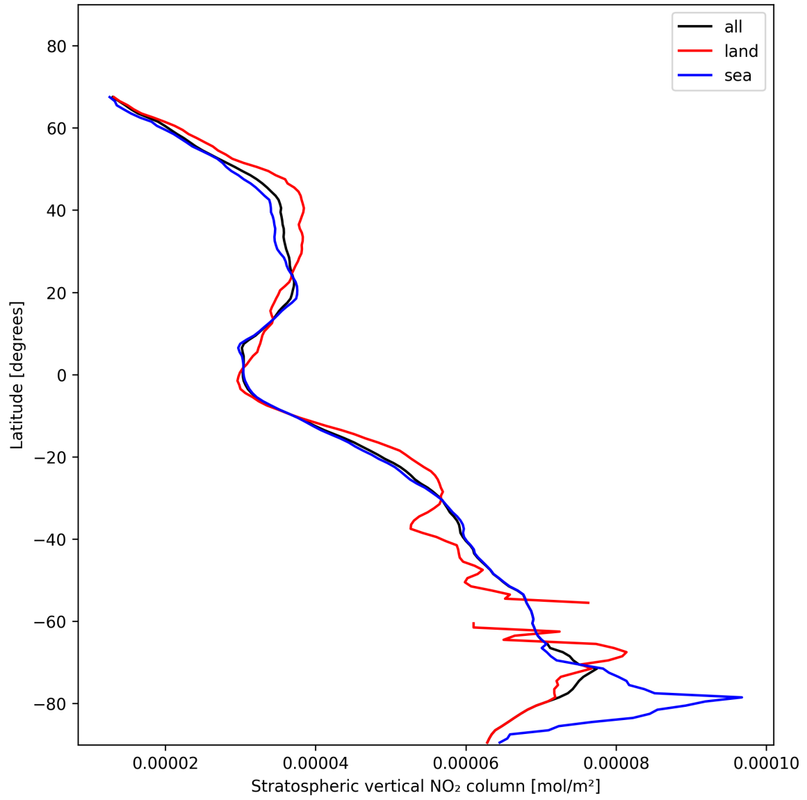
Figure 19: Zonal average of “Stratospheric vertical NO 2 column” for 2024-11-23 to 2024-11-25.
