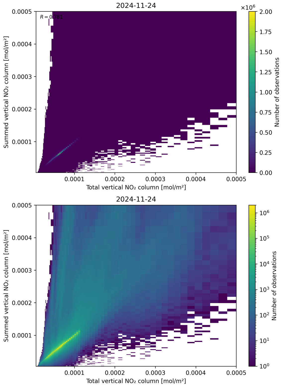
Figure 112: Scatter density plot of “Total vertical NO 2 column” against “Summed vertical NO 2 column” for 2024-11-23 to 2024-11-25.
