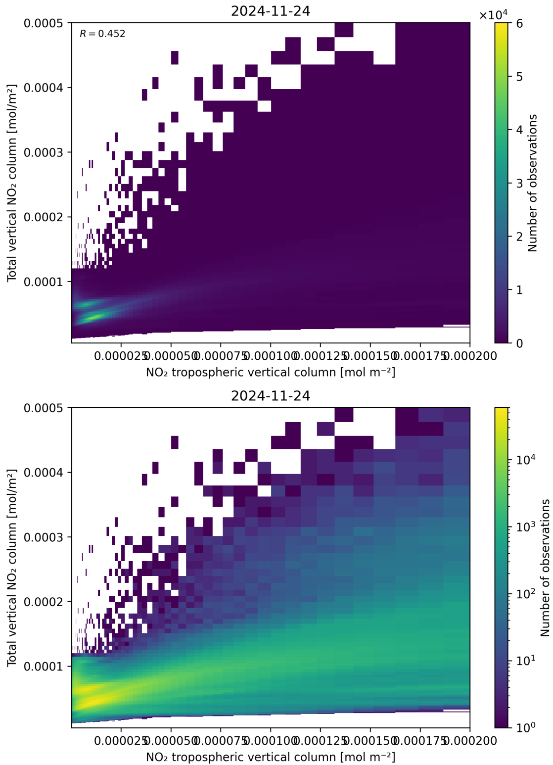
Figure 128: Scatter density plot of “NO 2 tropospheric vertical column” against “Total vertical NO 2 column” for 2024-11-23 to 2024-11-25.
