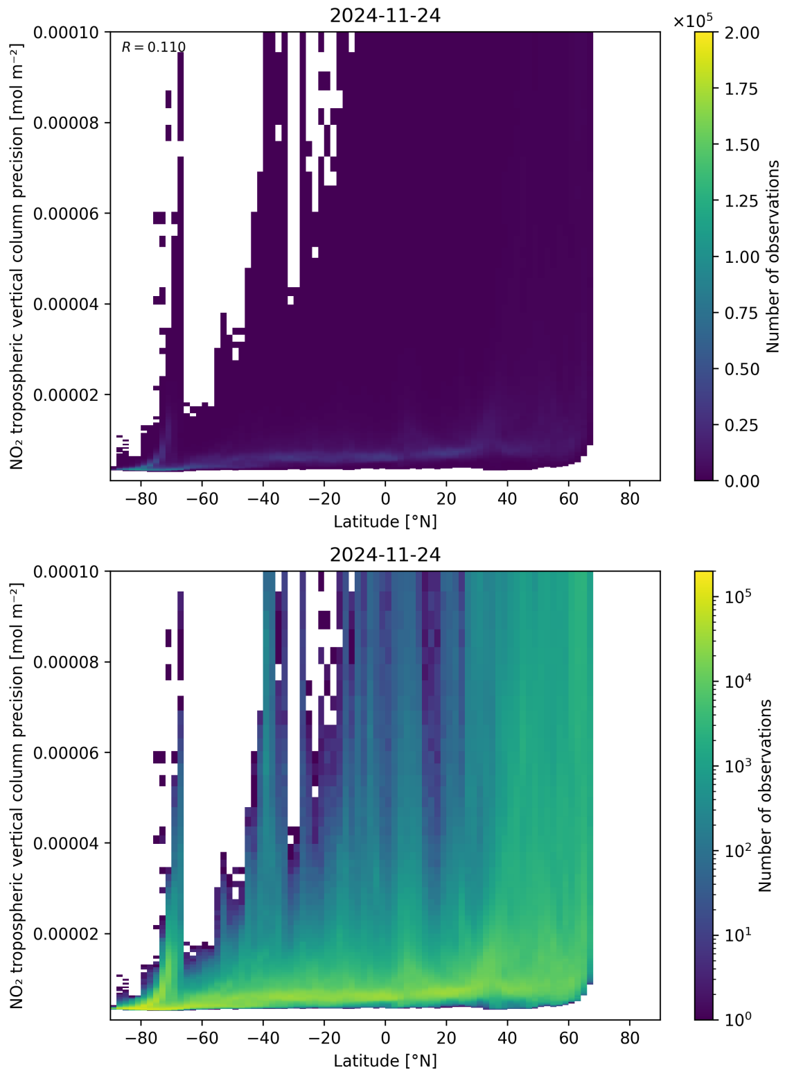
Figure 93: Scatter density plot of “Latitude” against “NO 2 tropospheric vertical column precision” for 2024-11-23 to 2024-11-25.
