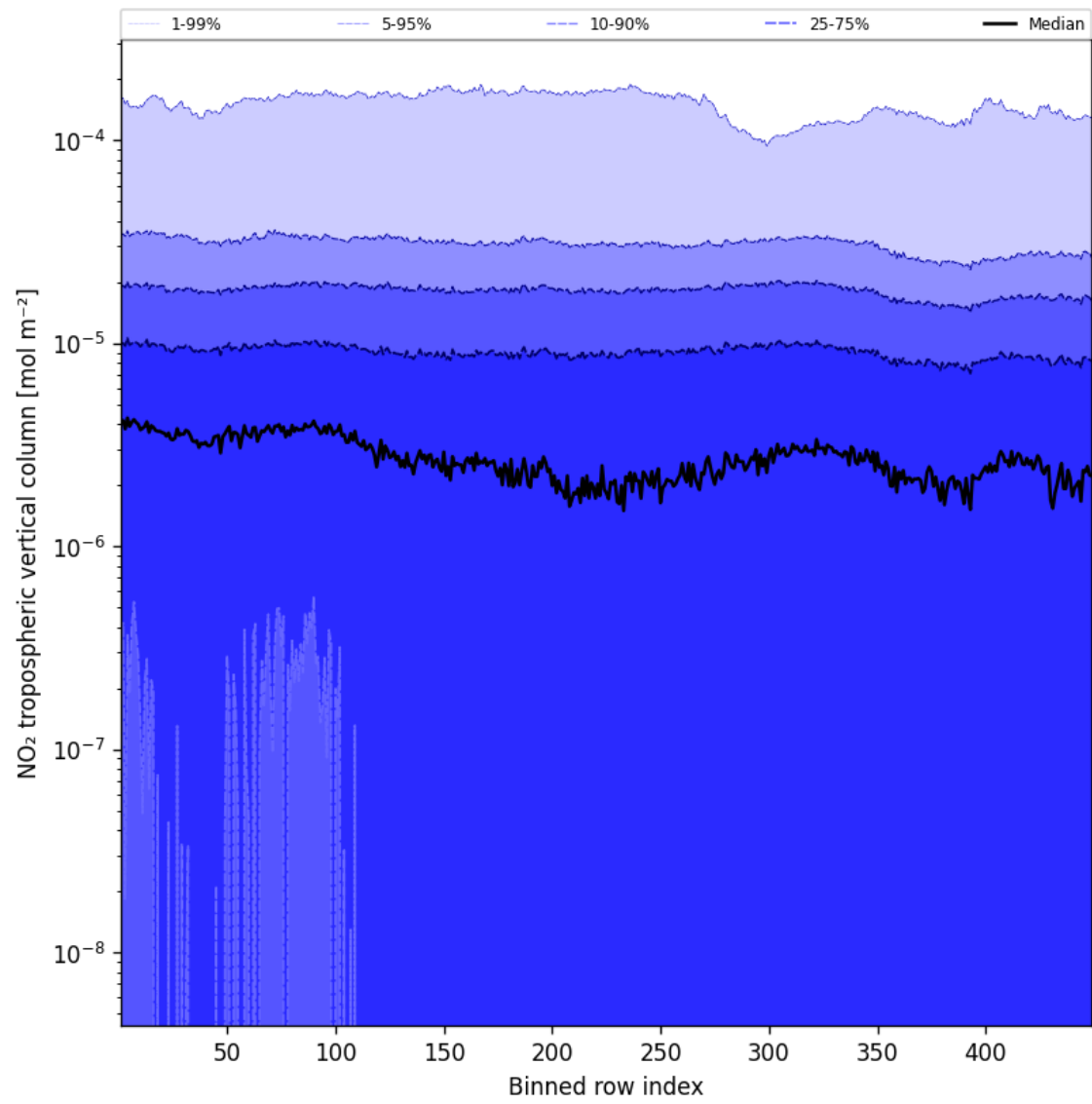
Figure 46: Along track statistics of “NO 2 tropospheric vertical column” for 2024-11-23 to 2024-11-25
