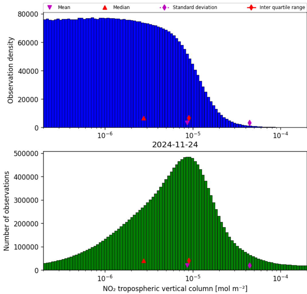
Figure 29: Histogram of “NO 2 tropospheric vertical column” for 2024-11-23 to 2024-11-25
