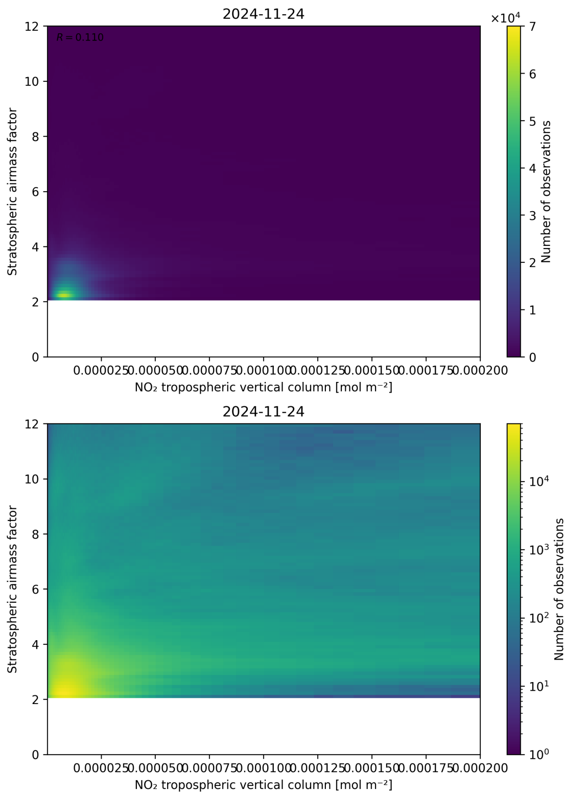
Figure 121: Scatter density plot of “NO 2 tropospheric vertical column” against “Stratospheric airmass factor” for 2024-11-23 to 2024-11-25.
