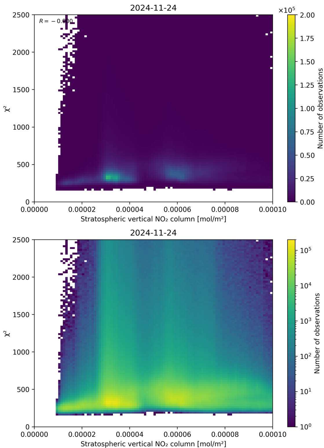
Figure 97: Scatter density plot of “Stratospheric vertical NO 2 column” against “ \chi^2 ” for 2024-11-23 to 2024-11-25.
