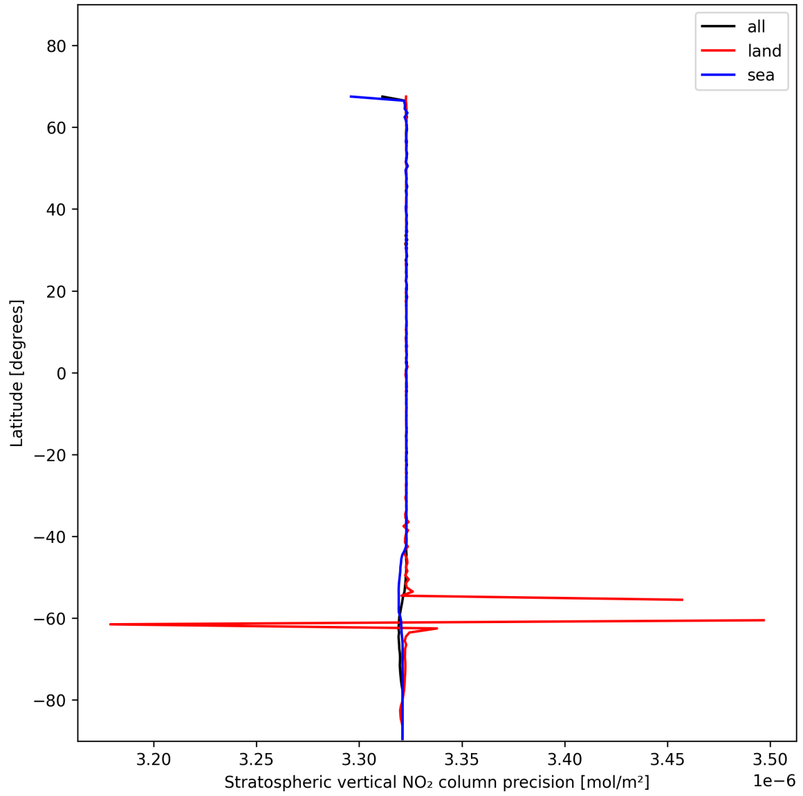
Figure 20: Zonal average of “Stratospheric vertical NO 2 column precision” for 2024-11-23 to 2024-11-25.
