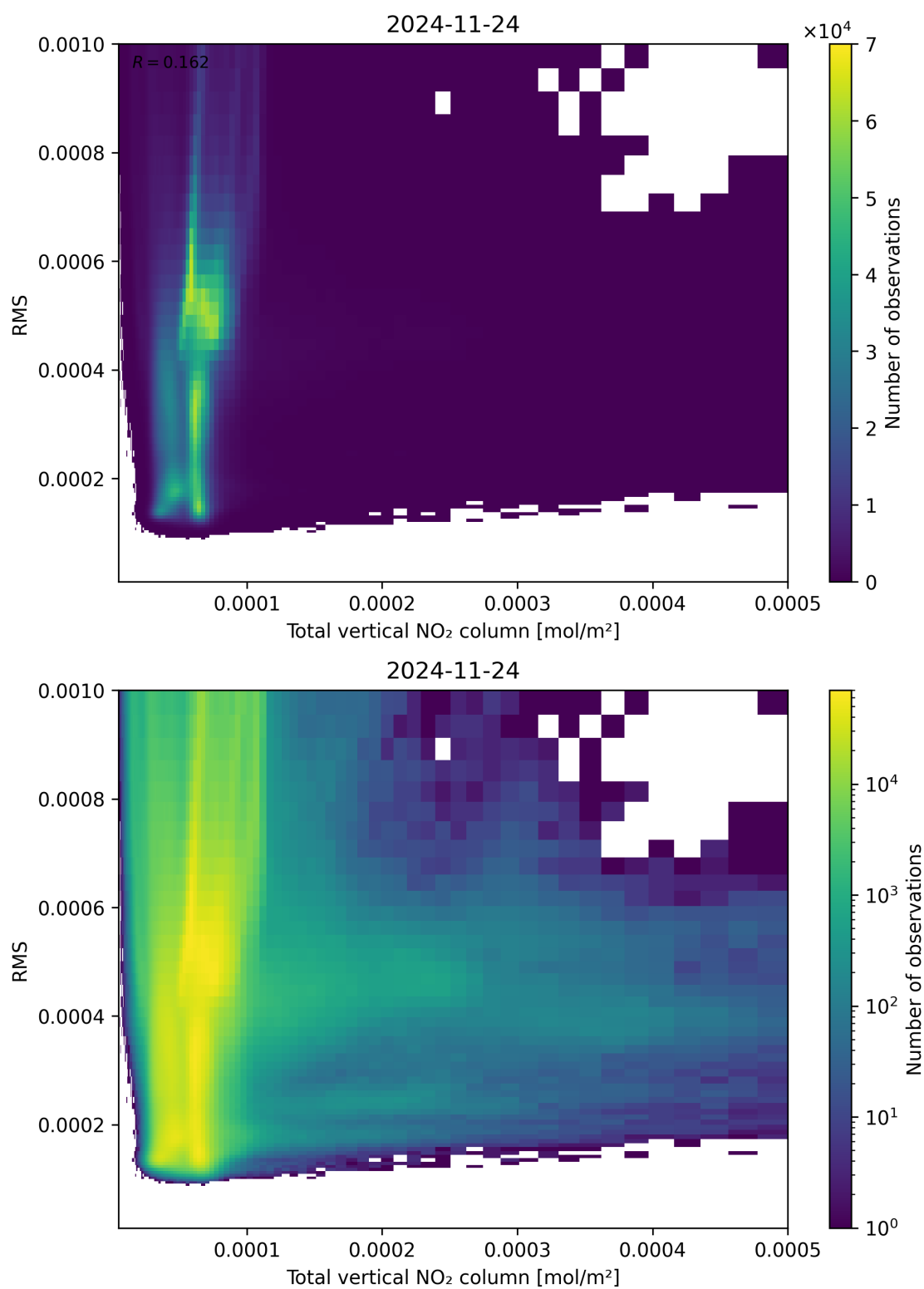
Figure 120: Scatter density plot of “Total vertical NO 2 column” against “RMS” for 2024-11-23 to 2024-11-25.
