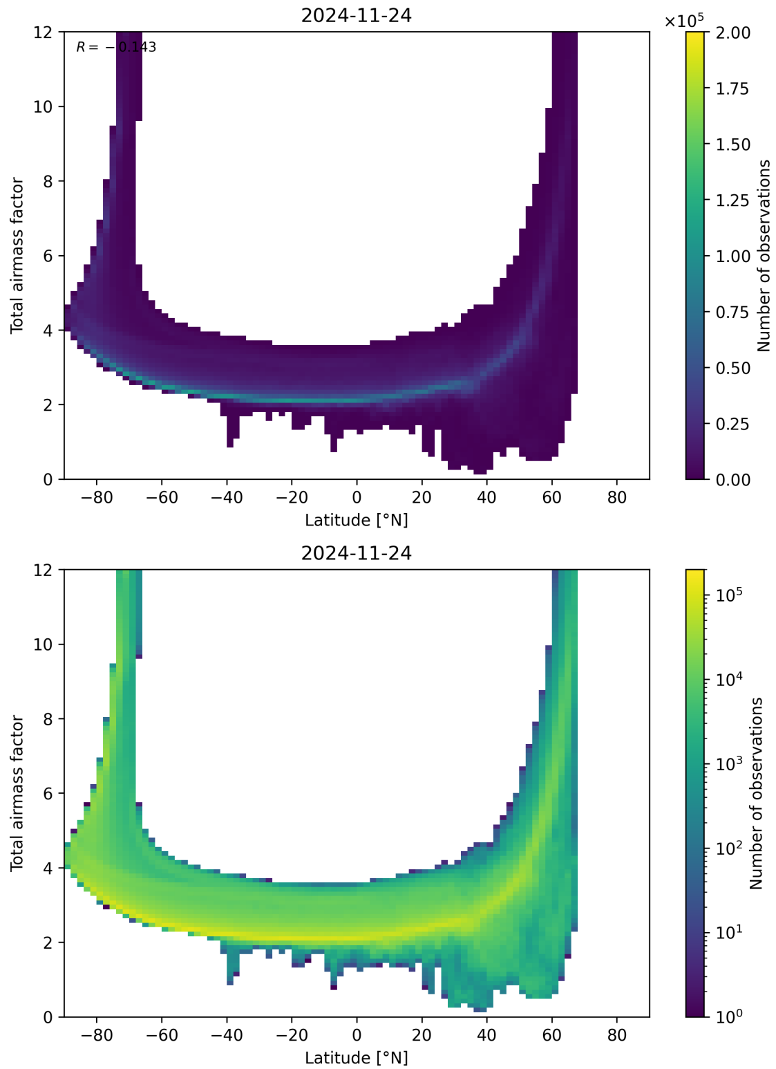
Figure 84: Scatter density plot of “Latitude” against “Total airmass factor” for 2024-11-23 to 2024-11-25.
