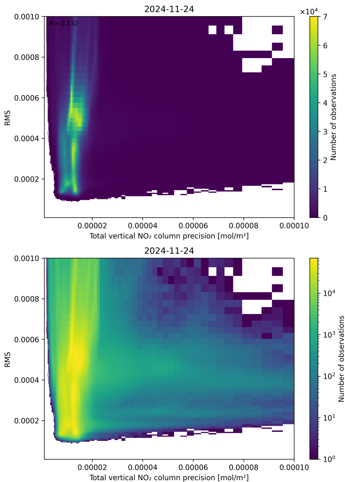
Figure 119: Scatter density plot of “Total vertical NO 2 column precision” against “RMS” for 2024-11-23 to 2024-11-25.
