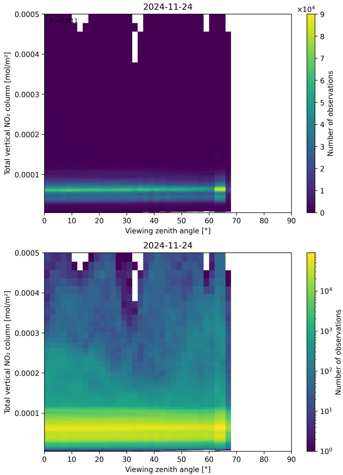
Figure 167: Scatter density plot of “Viewing zenith angle” against “Total vertical NO 2 column” for 2024-11-23 to 2024-11-25.
