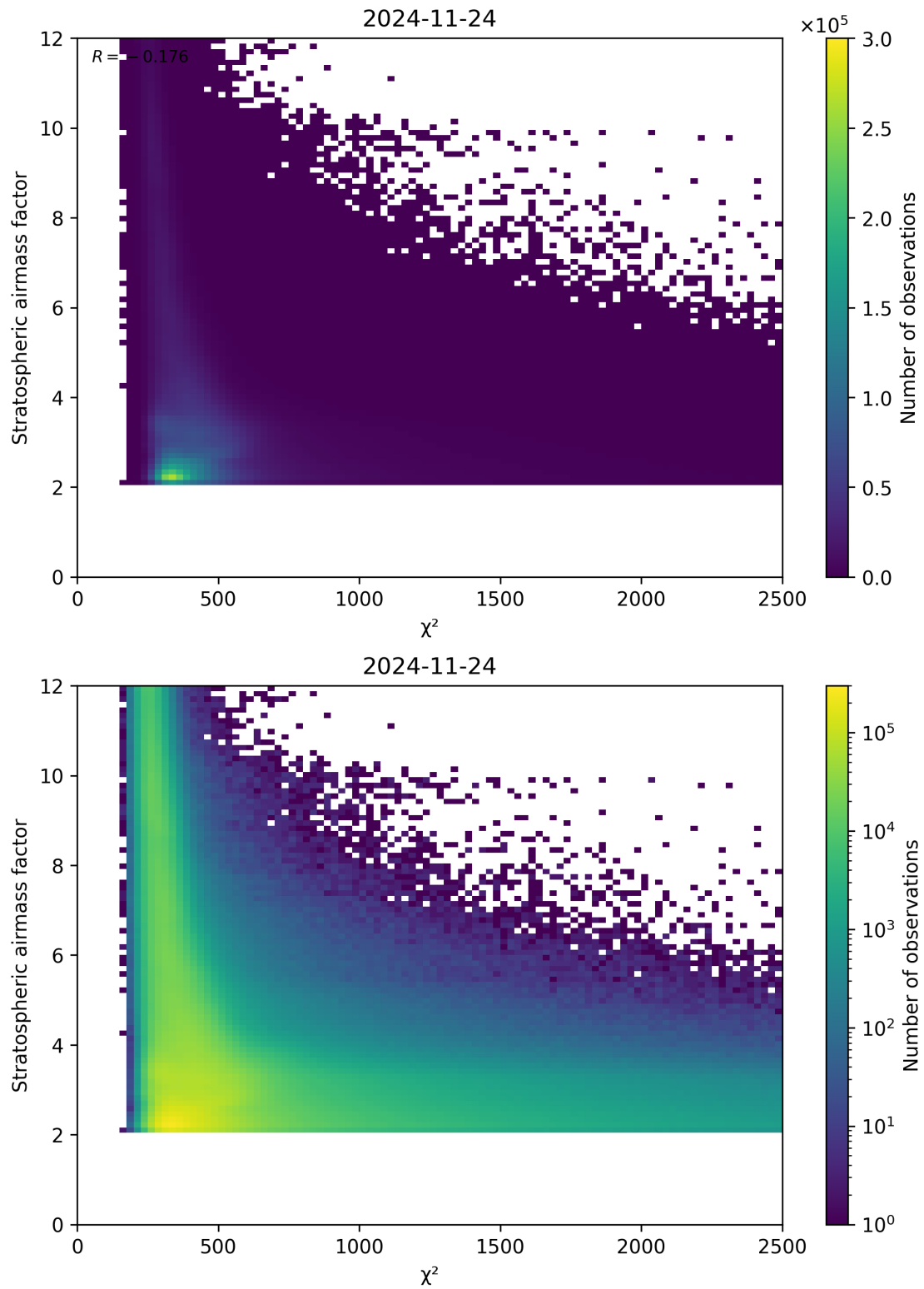
Figure 81: Scatter density plot of “ \chi^2 ” against “Stratospheric airmass factor” for 2024-11-23 to 2024-11-25.
