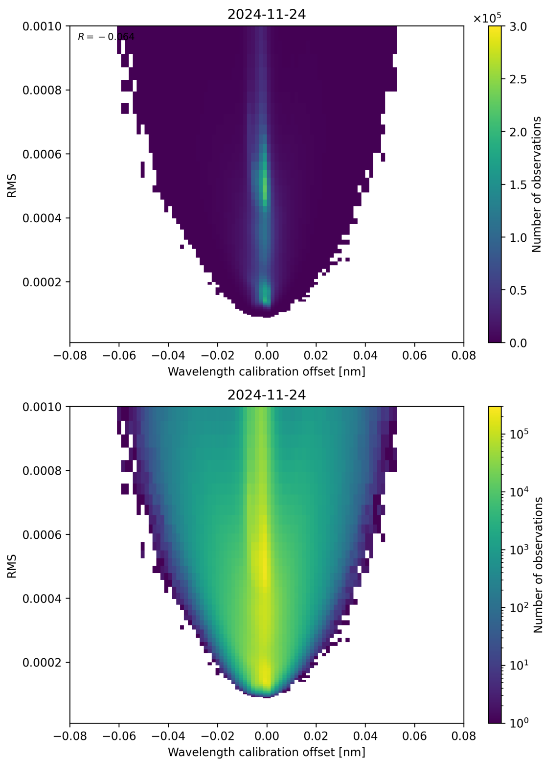
Figure 181: Scatter density plot of “Wavelength calibration offset” against “RMS” for 2024-11-23 to 2024-11-25.
