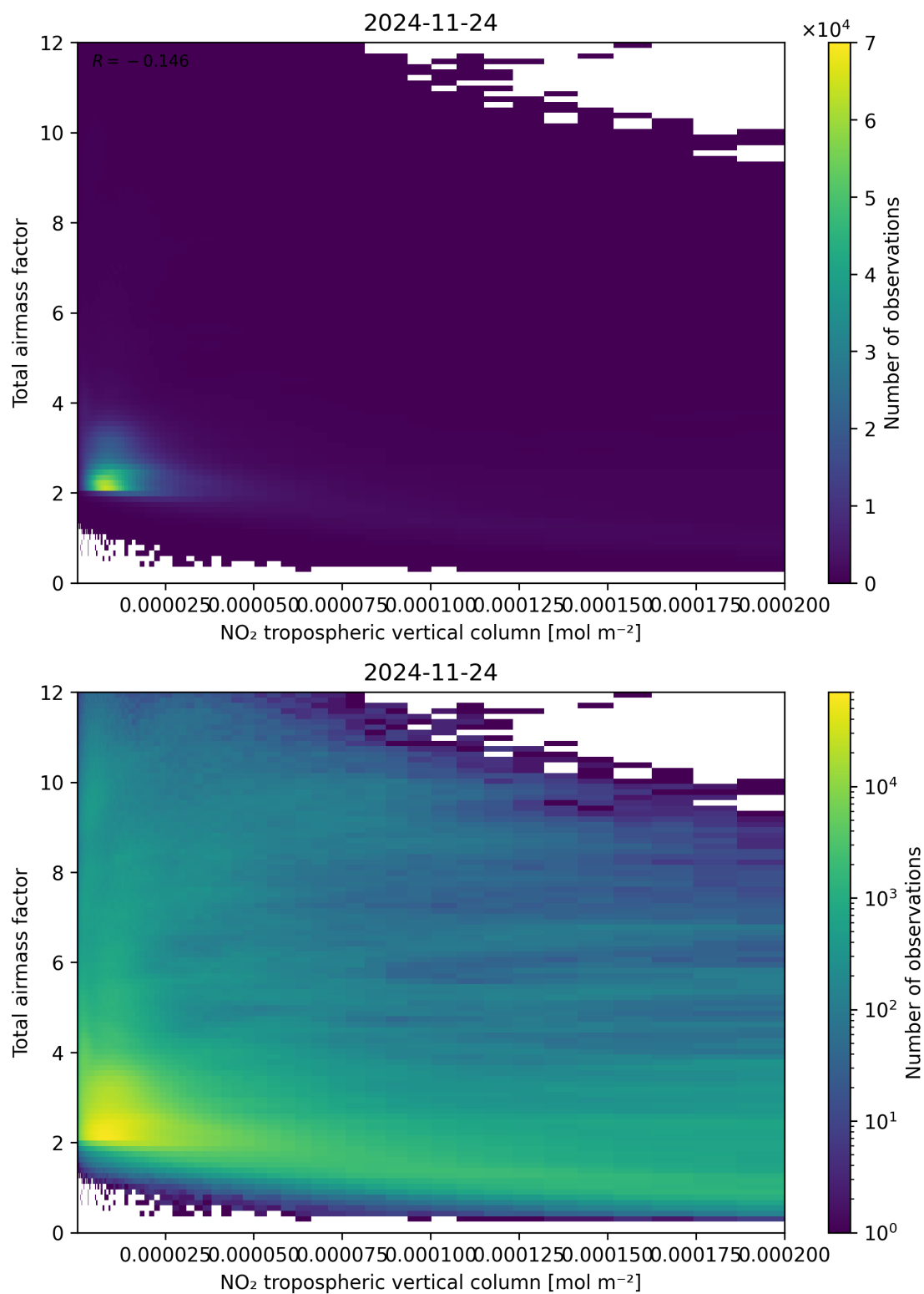
Figure 122: Scatter density plot of “NO 2 tropospheric vertical column” against “Total air mass factor” for 2024-11-23 to 2024-11-25.
