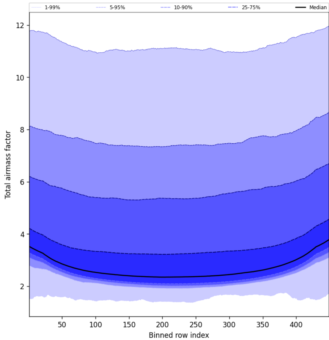
Figure 49: Along track statistics of “Total airmass factor” for 2024-11-23 to 2024-11-25
