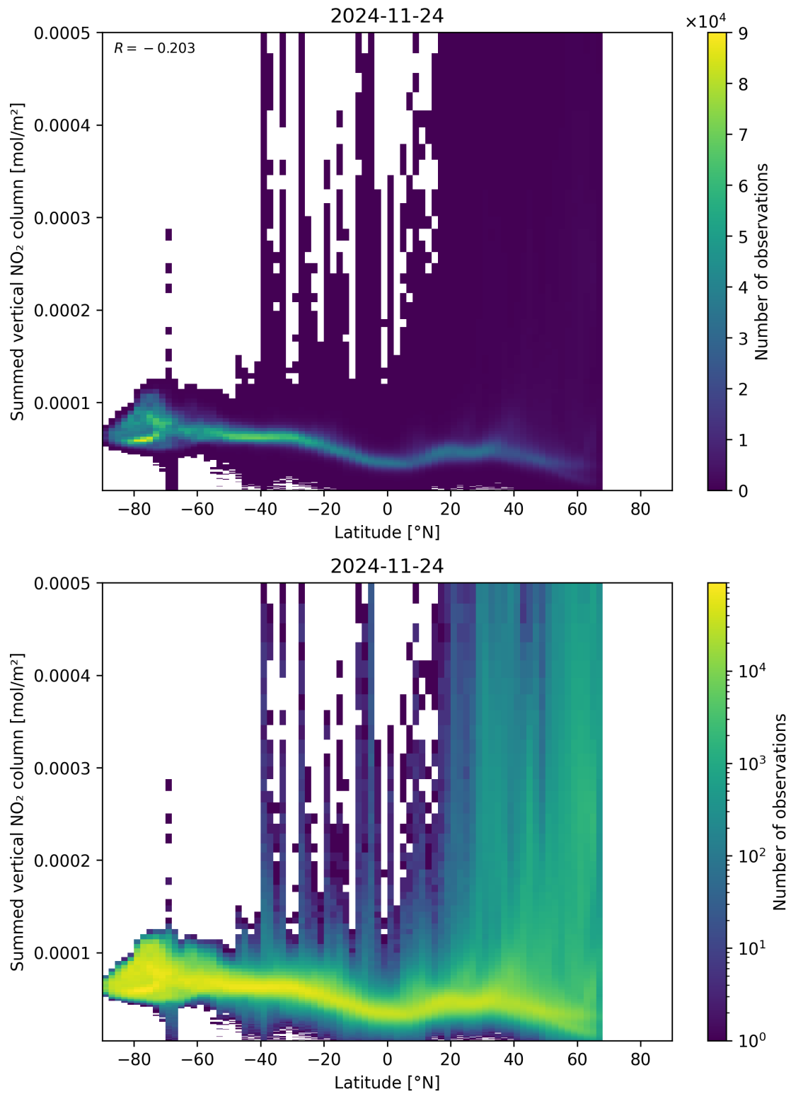
Figure 88: Scatter density plot of “Latitude” against “Summed vertical NO 2 column” for 2024-11-23 to 2024-11-25.
