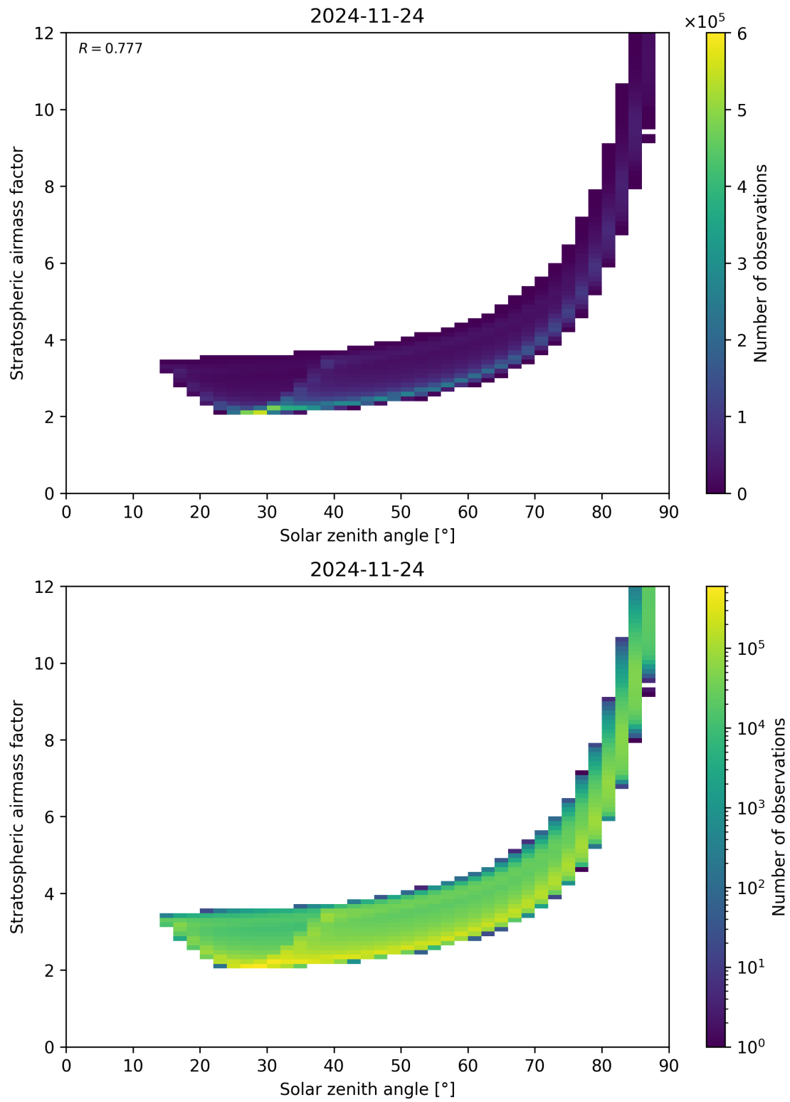
Figure 145: Scatter density plot of “Solar zenith angle” against “Stratospheric airmass factor” for 2024-11-23 to 2024-11-25.
