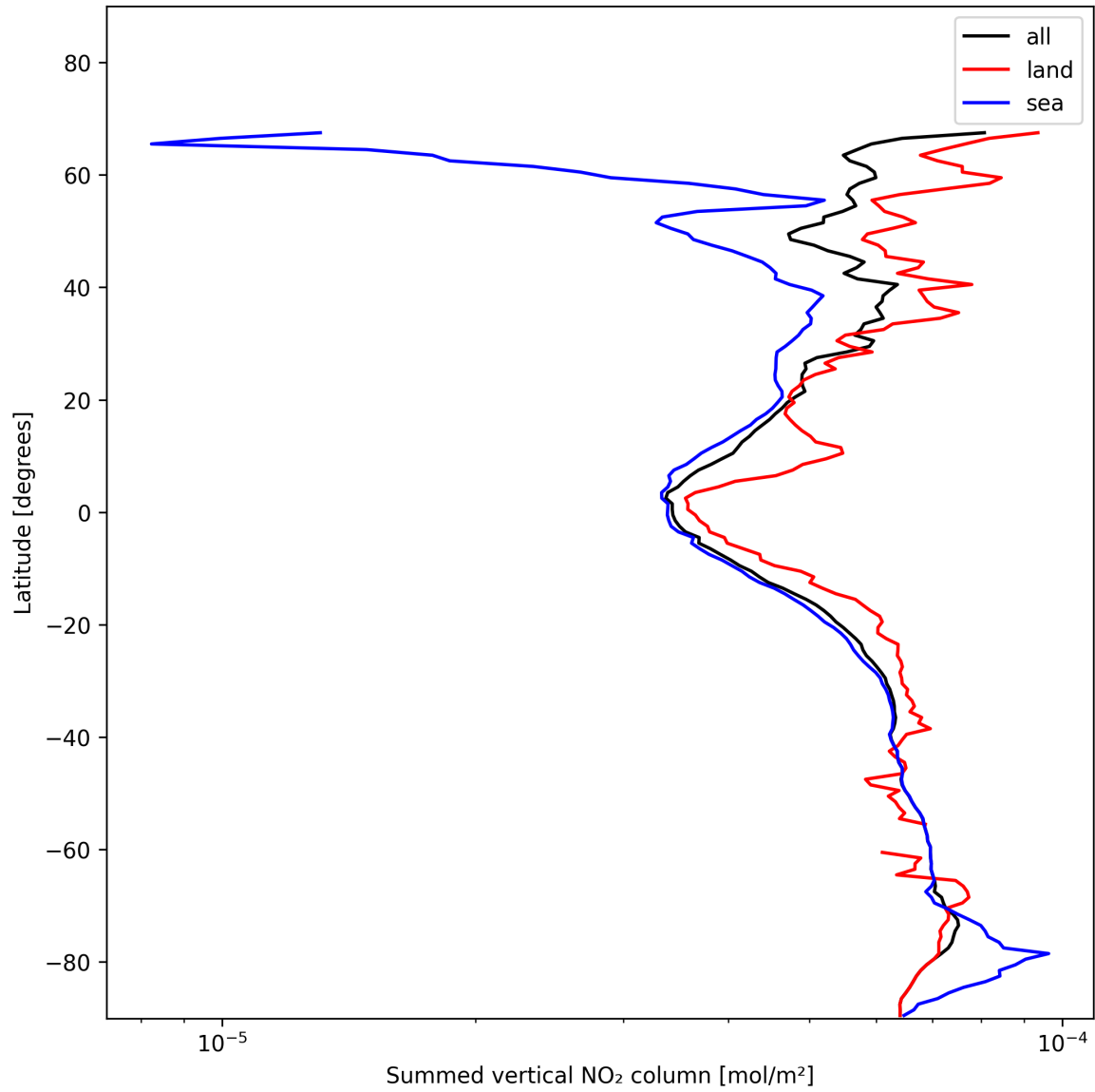
Figure 23: Zonal average of “Summed vertical NO 2 column” for 2024-11-23 to 2024-11-25.
