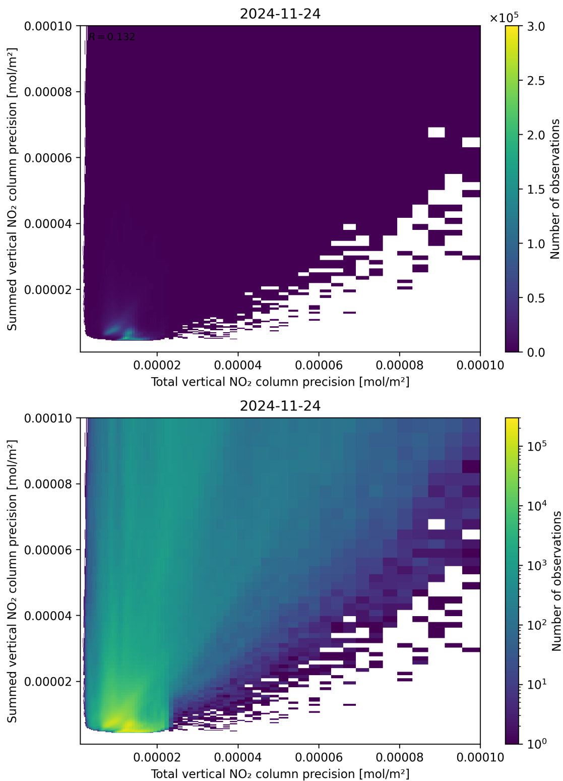
Figure 118: Scatter density plot of “Total vertical NO 2 column precision” against “Summed vertical NO 2 column precision” for 2024-11-23 to 2024-11-25.
