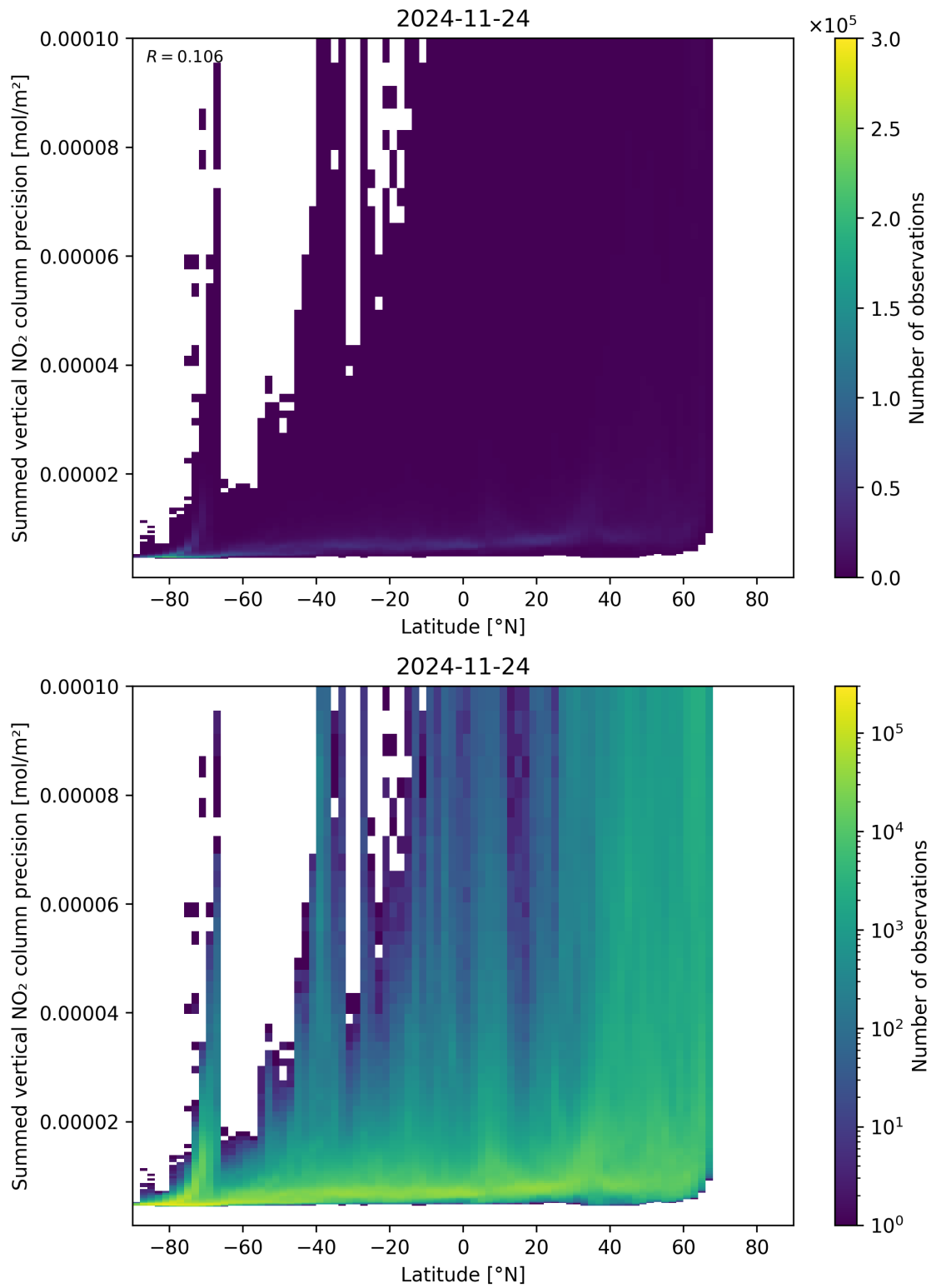
Figure 89: Scatter density plot of “Latitude” against “Summed vertical NO 2 column precision” for 2024-11-23 to 2024-11-25.
