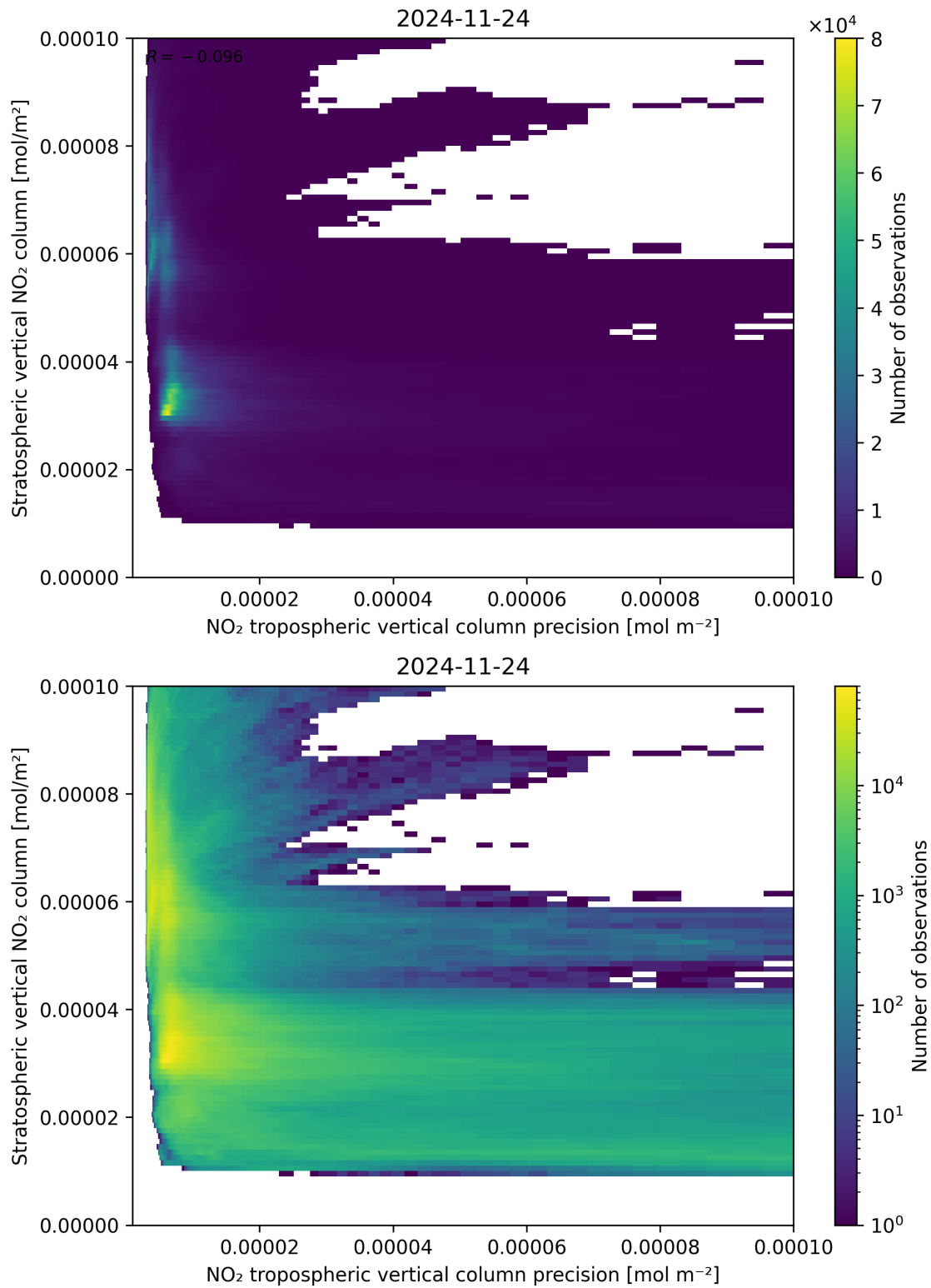
Figure 135: Scatter density plot of “NO 2 tropospheric vertical column precision” against “Stratospheric vertical NO 2 column” for 2024-11-23 to 2024-11-25.
