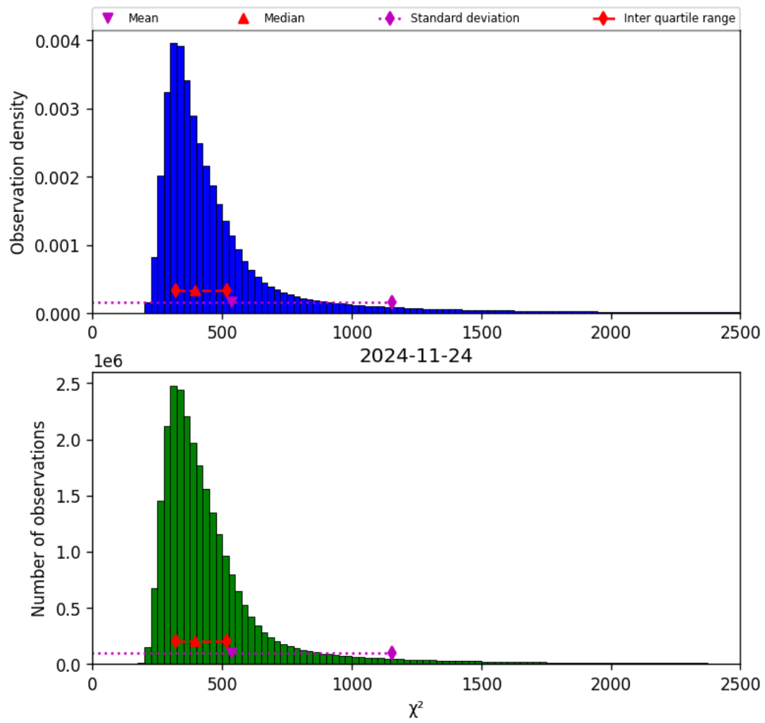
Figure 42: Histogram of “ \chi^2 ” for 2024-11-23 to 2024-11-25
