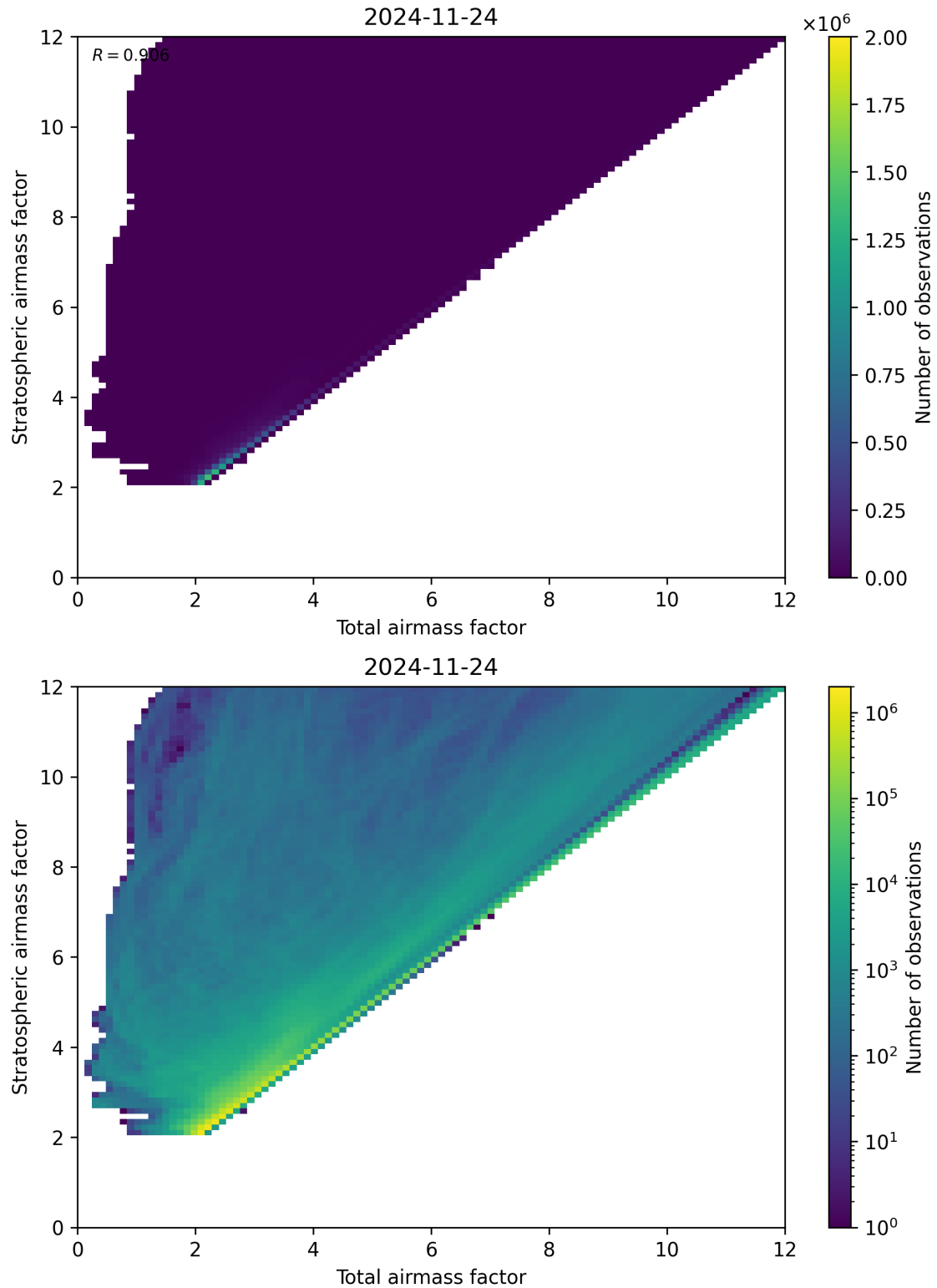
Figure 62: Scatter density plot of “Total airmass factor” against “Stratospheric airmass factor” for 2024-11-23 to 2024-11-25.
