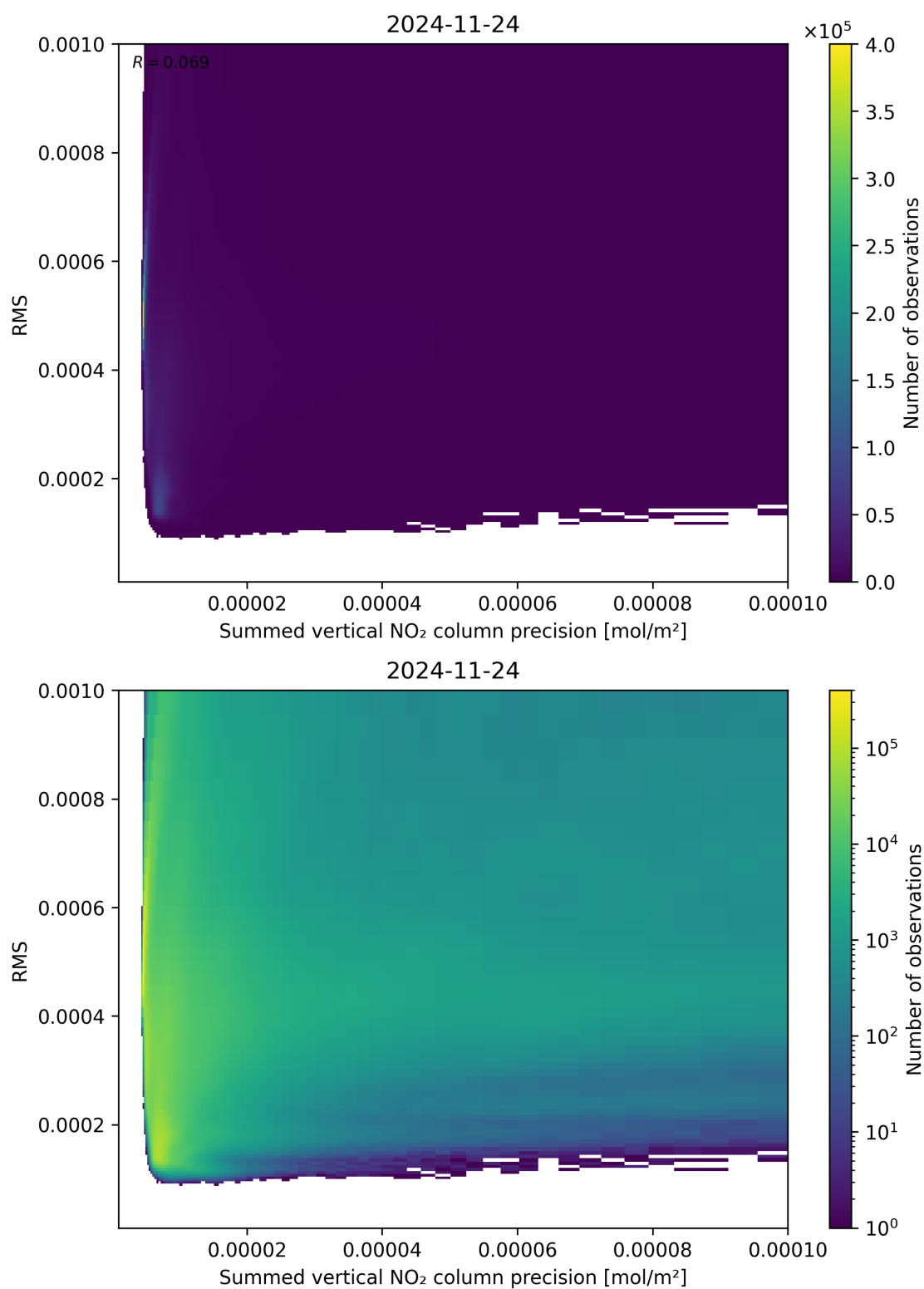
Figure 108: Scatter density plot of “Summed vertical NO 2 column precision” against “RMS” for 2024-11-23 to 2024-11-25.
