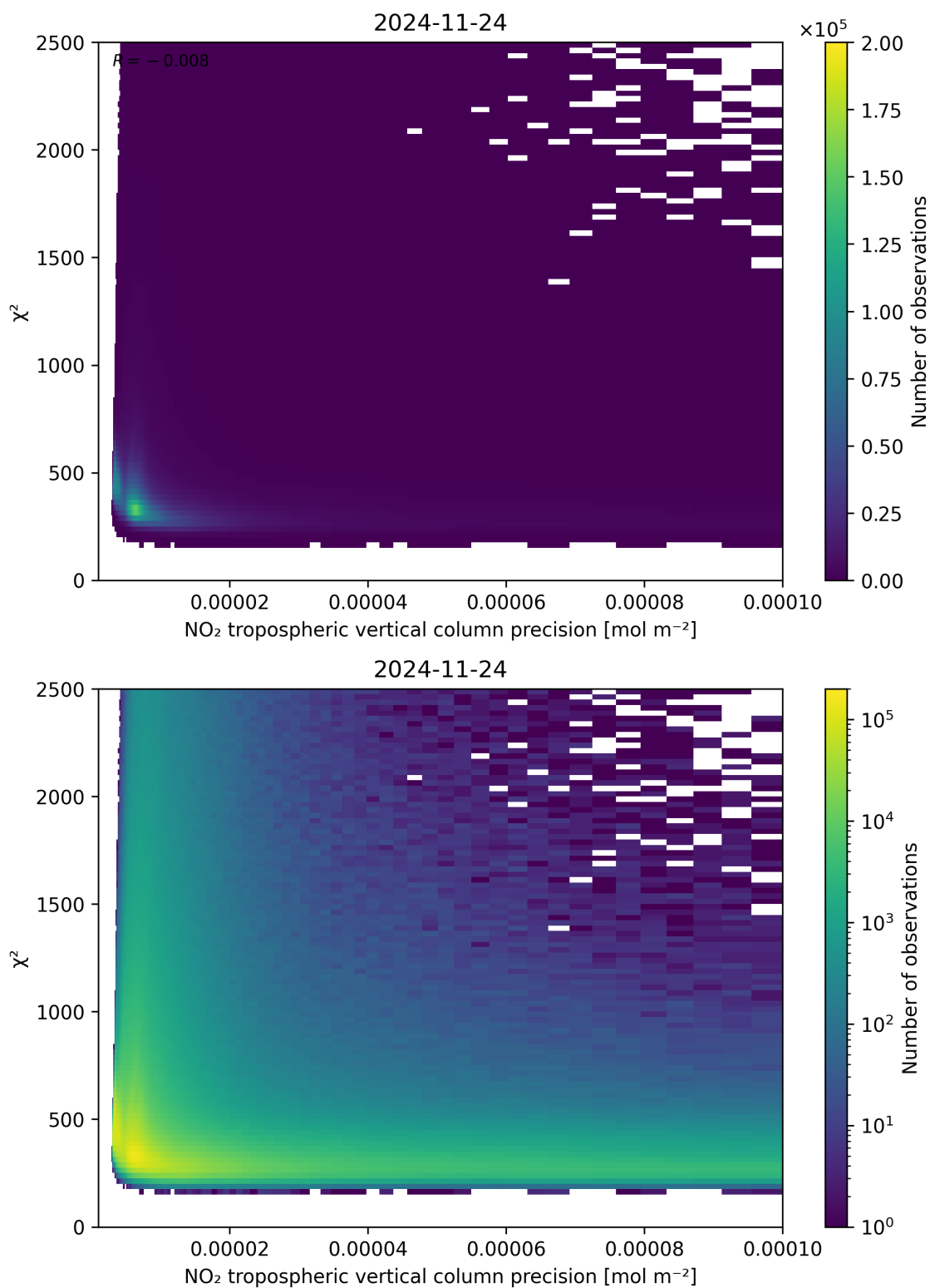
Figure 134: Scatter density plot of “NO 2 tropospheric vertical column precision” against “ \chi^2 ” for 2024-11-23 to 2024-11-25.
