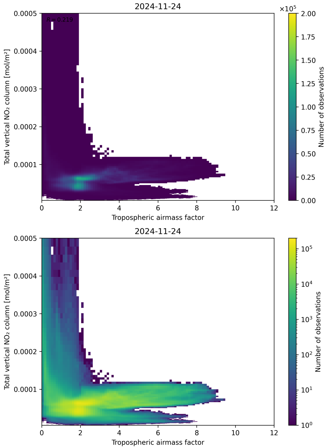
Figure 77: Scatter density plot of “Tropospheric airmass factor” against “Total vertical NO 2 column” for 2024-11-23 to 2024-11-25.
