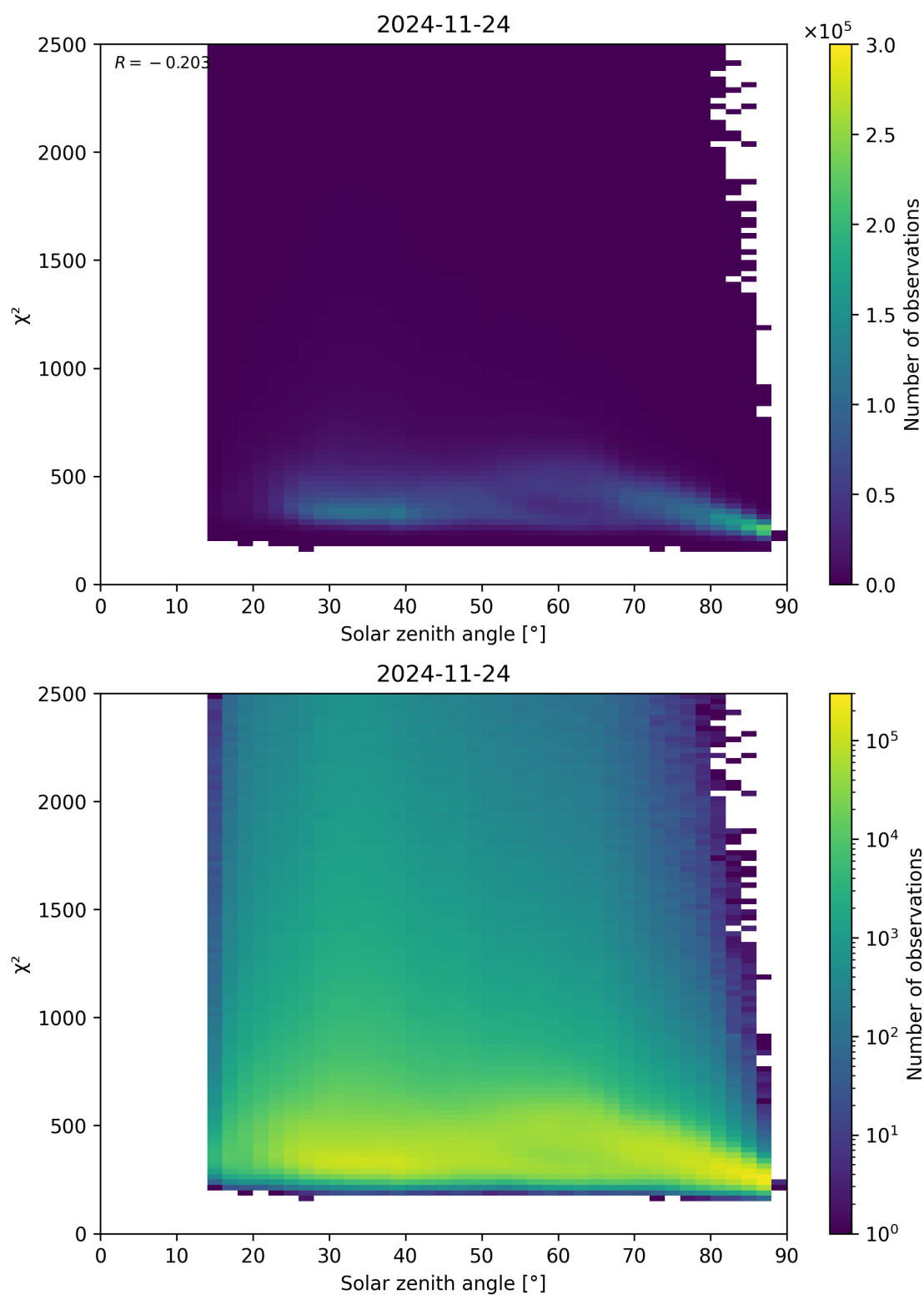
Figure 148: Scatter density plot of “Solar zenith angle” against “ \chi^2 ” for 2024-11-23 to 2024-11-25.
