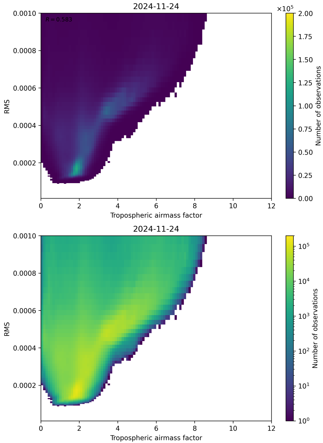
Figure 79: Scatter density plot of “Tropospheric airmass factor” against “RMS” for 2024-11-23 to 2024-11-25.
