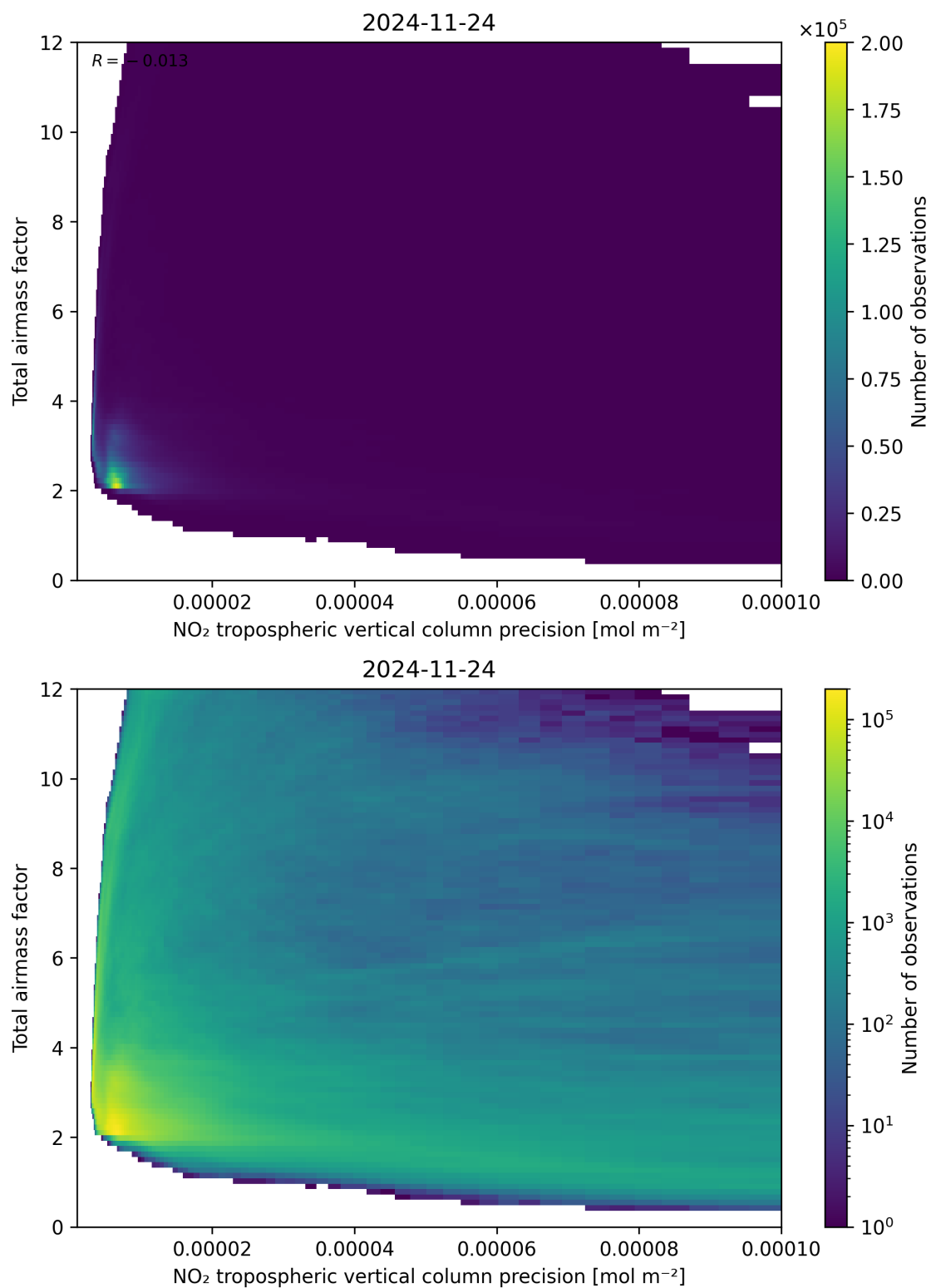
Figure 132: Scatter density plot of “NO 2 tropospheric vertical column precision” against “Total air mass factor” for 2024-11-23 to 2024-11-25.
