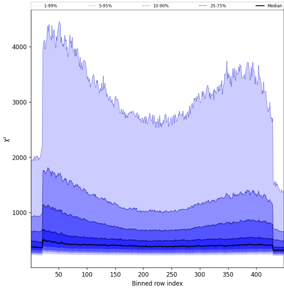
Figure 59: Along track statistics of “ \chi^2 ” for 2024-11-23 to 2024-11-25
