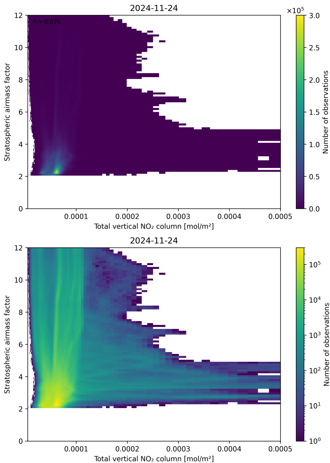
Figure 110: Scatter density plot of “Total vertical NO 2 column” against “Stratospheric air mass factor” for 2024-11-23 to 2024-11-25.
