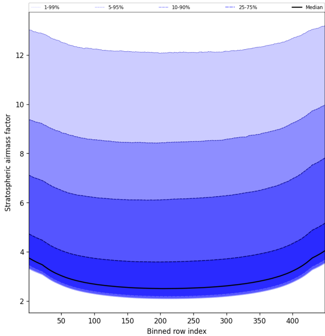
Figure 61: Along track statistics of “Stratospheric airmass factor” for 2024-11-23 to 2024-11-25
