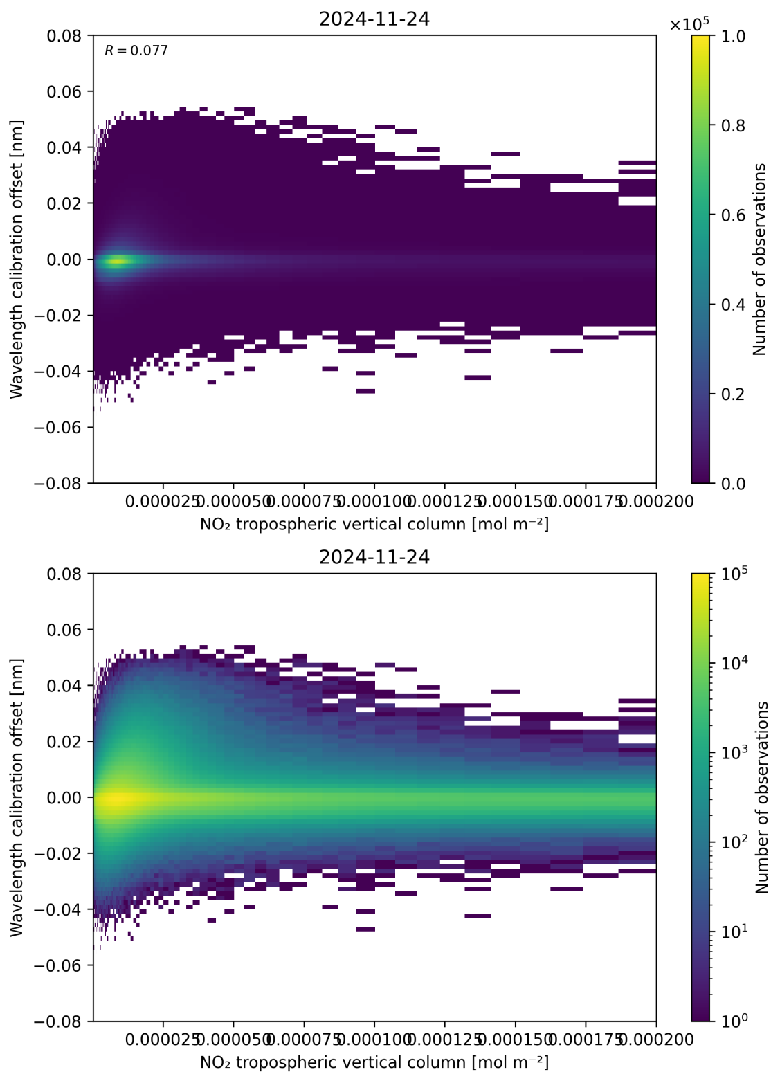
Figure 143: Scatter density plot of “NO 2 tropospheric vertical column” against “Wavelength calibration offset” for 2024-11-23 to 2024-11-25.
