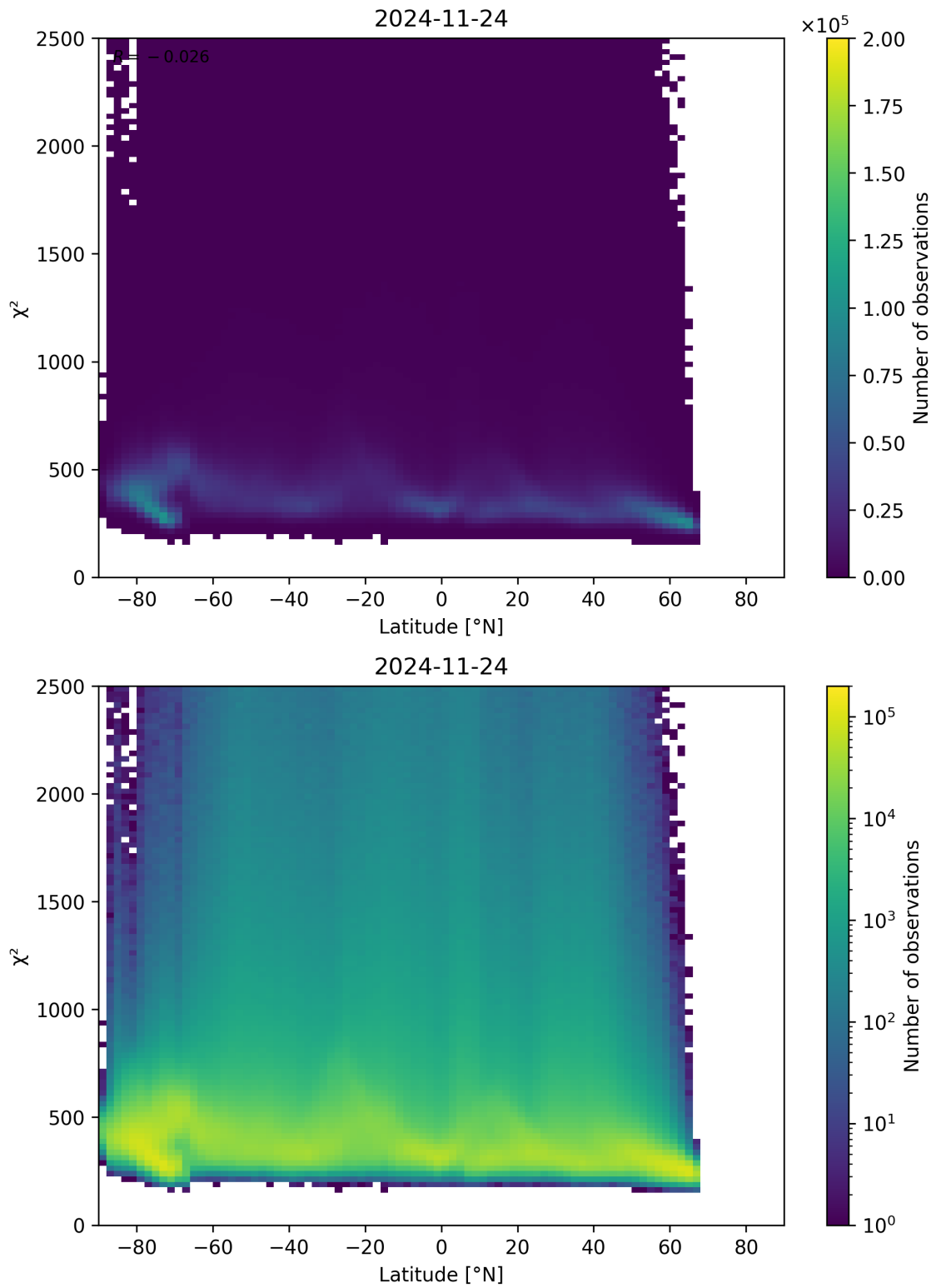
Figure 86: Scatter density plot of “Latitude” against “ \chi^2 ” for 2024-11-23 to 2024-11-25.
