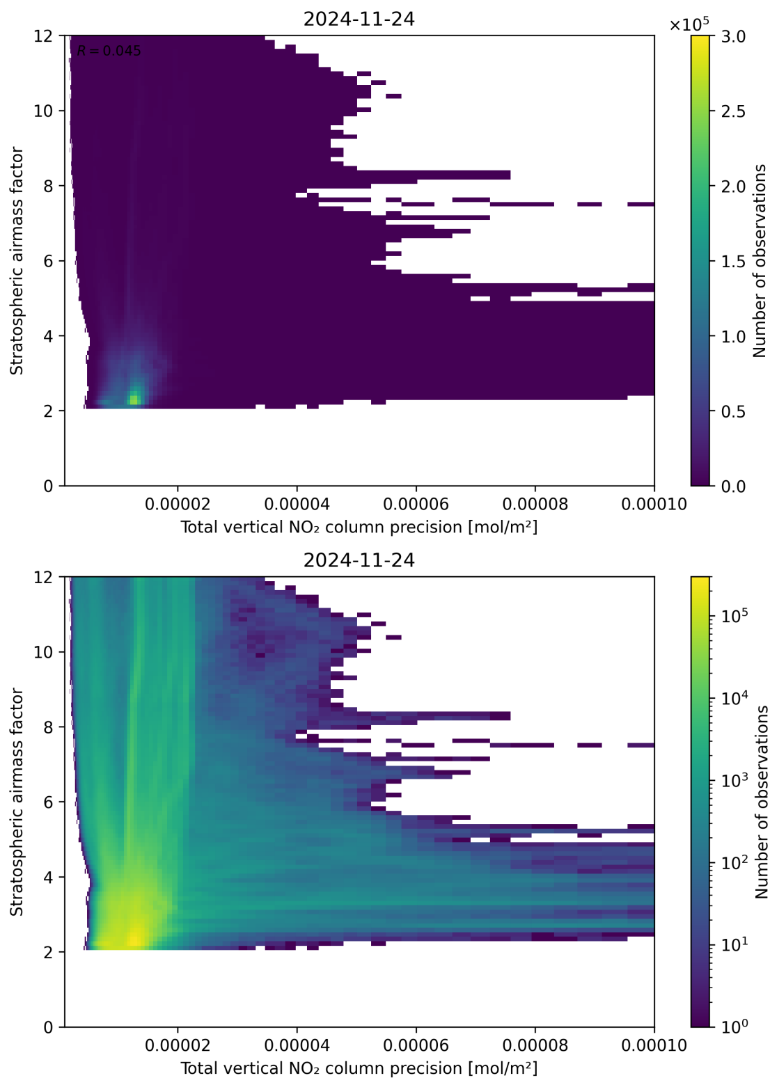
Figure 115: Scatter density plot of “Total vertical NO 2 column precision” against “Stratospheric air mass factor” for 2024-11-23 to 2024-11-25.
