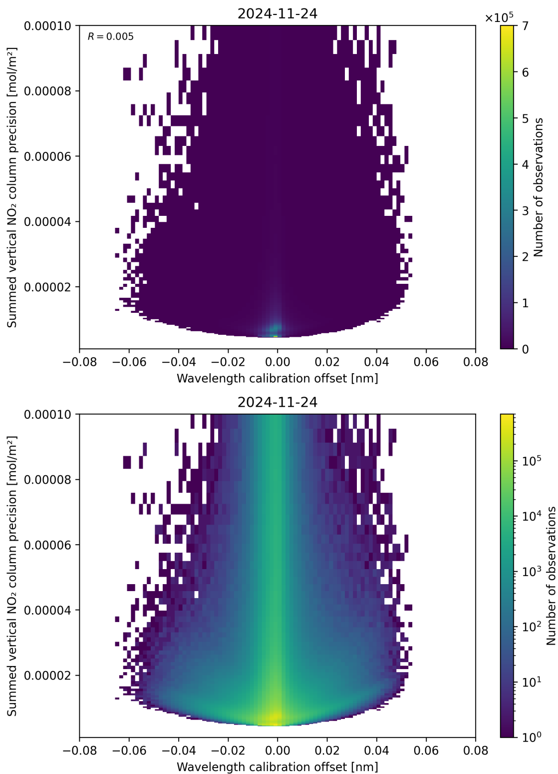
Figure 178: Scatter density plot of “Wavelength calibration offset” against “Summed vertical NO 2 column precision” for 2024-11-23 to 2024-11-25.
