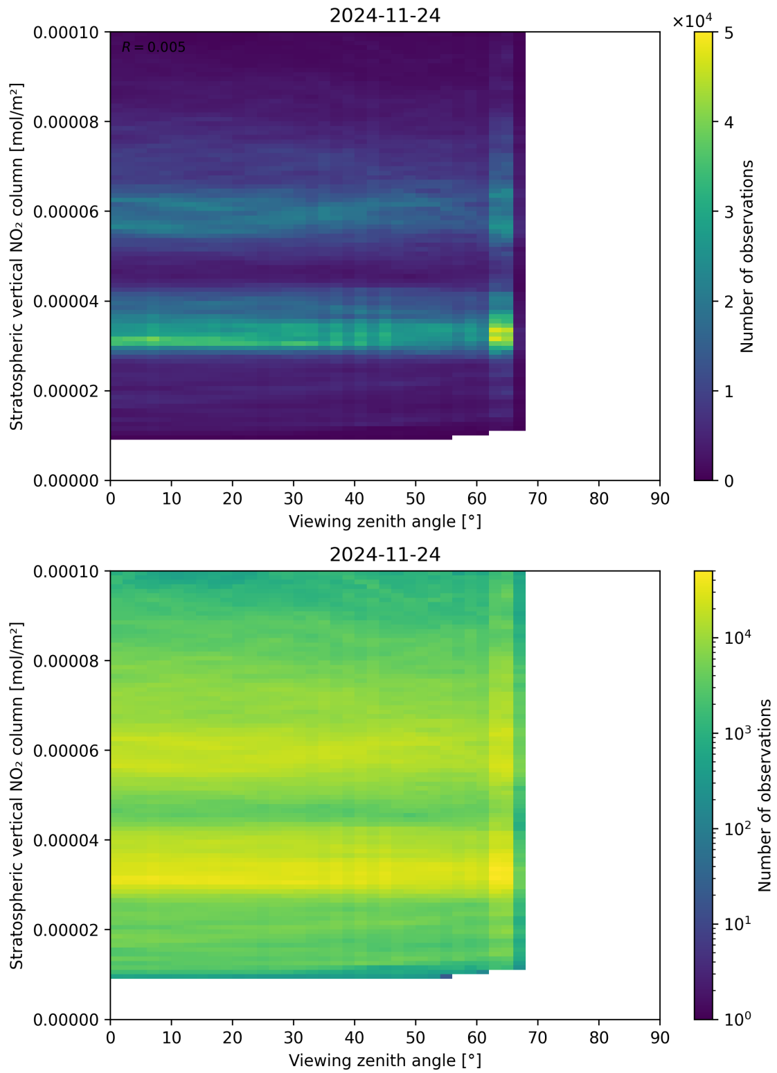
Figure 164: Scatter density plot of “Viewing zenith angle” against “Stratospheric vertical NO 2 column” for 2024-11-23 to 2024-11-25.
