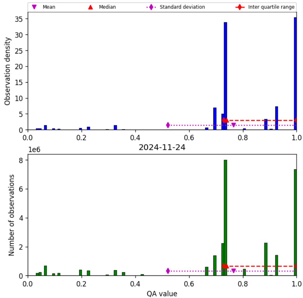
Figure 28: Histogram of “QA value” for 2024-11-23 to 2024-11-25
