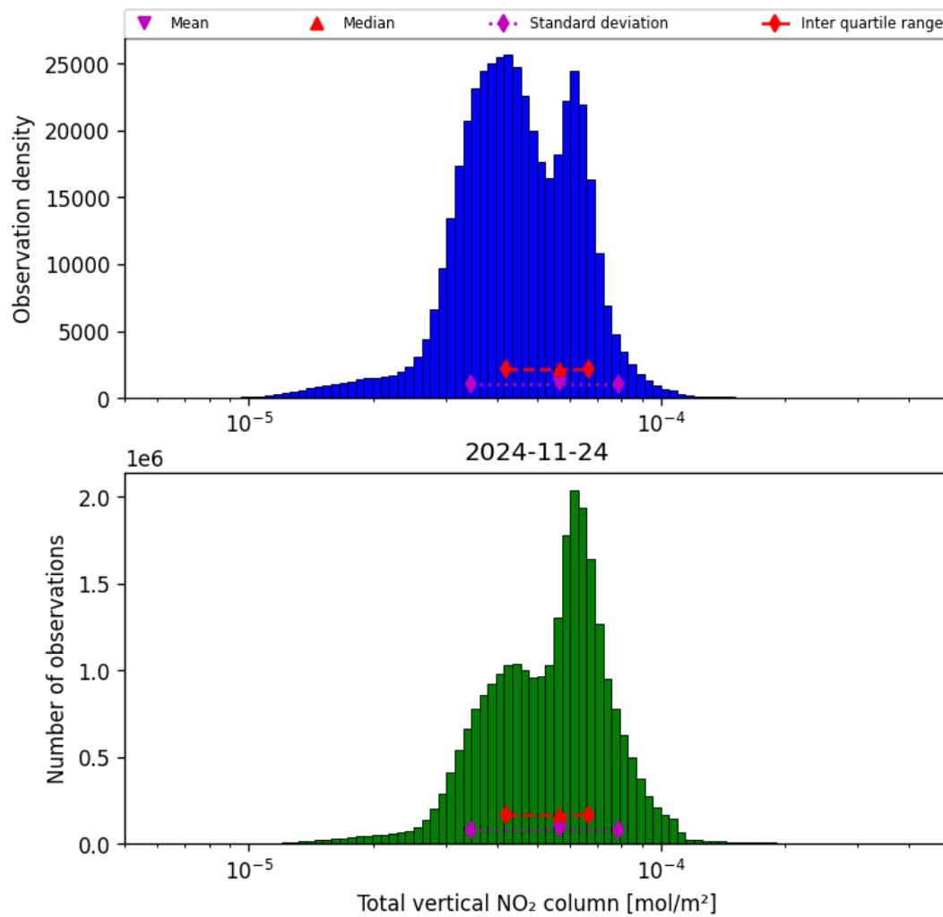
Figure 38: Histogram of “Total vertical NO 2 column” for 2024-11-23 to 2024-11-25
