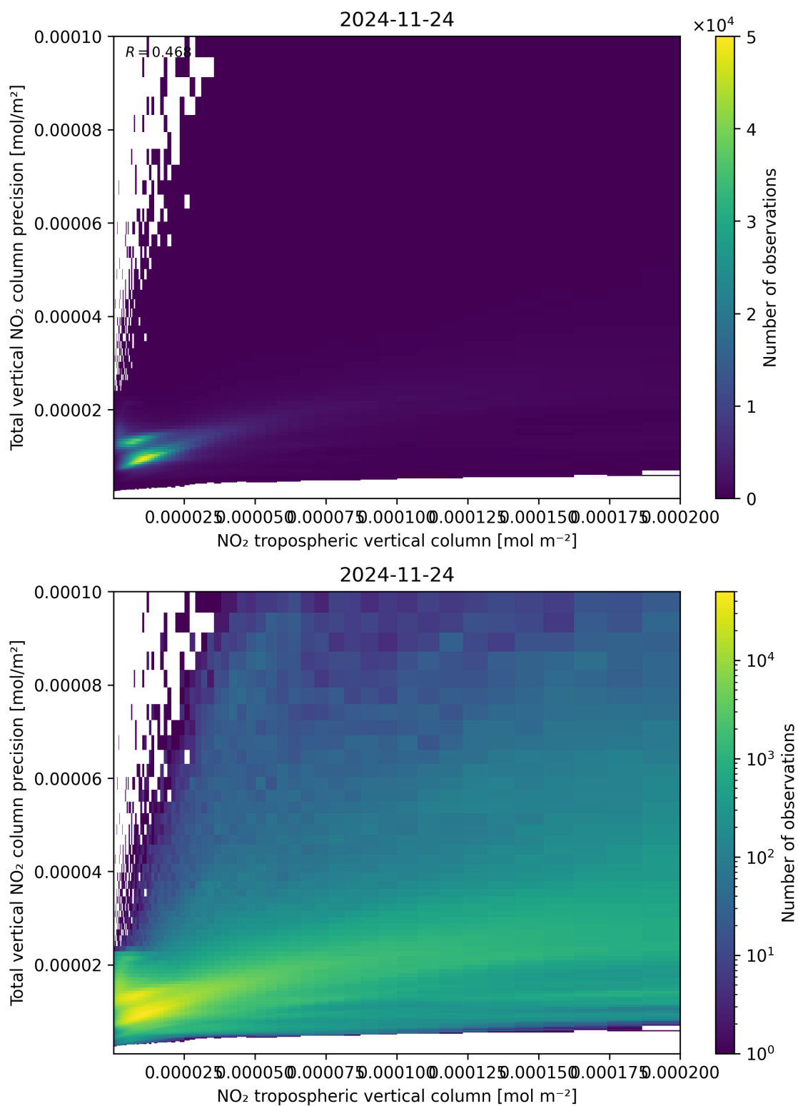
Figure 129: Scatter density plot of “NO 2 tropospheric vertical column” against “Total vertical NO 2 column precision” for 2024-11-23 to 2024-11-25.
