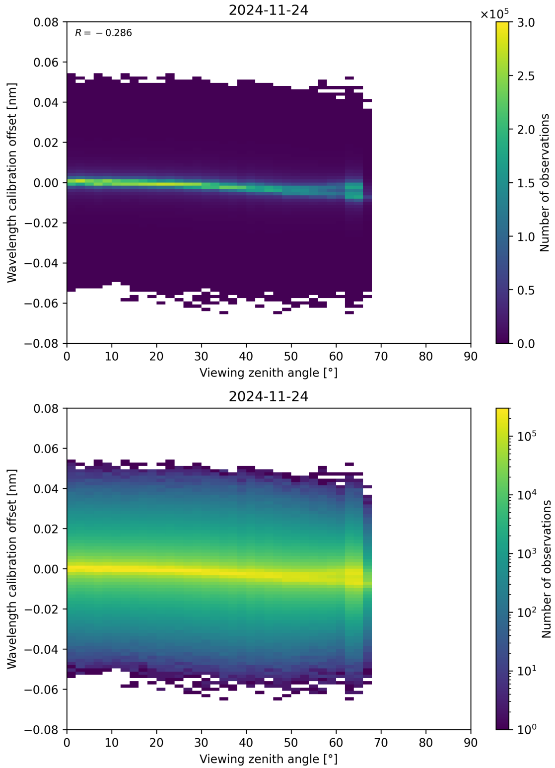
Figure 173: Scatter density plot of “Viewing zenith angle” against “Wavelength calibration offset” for 2024-11-23 to 2024-11-25.
