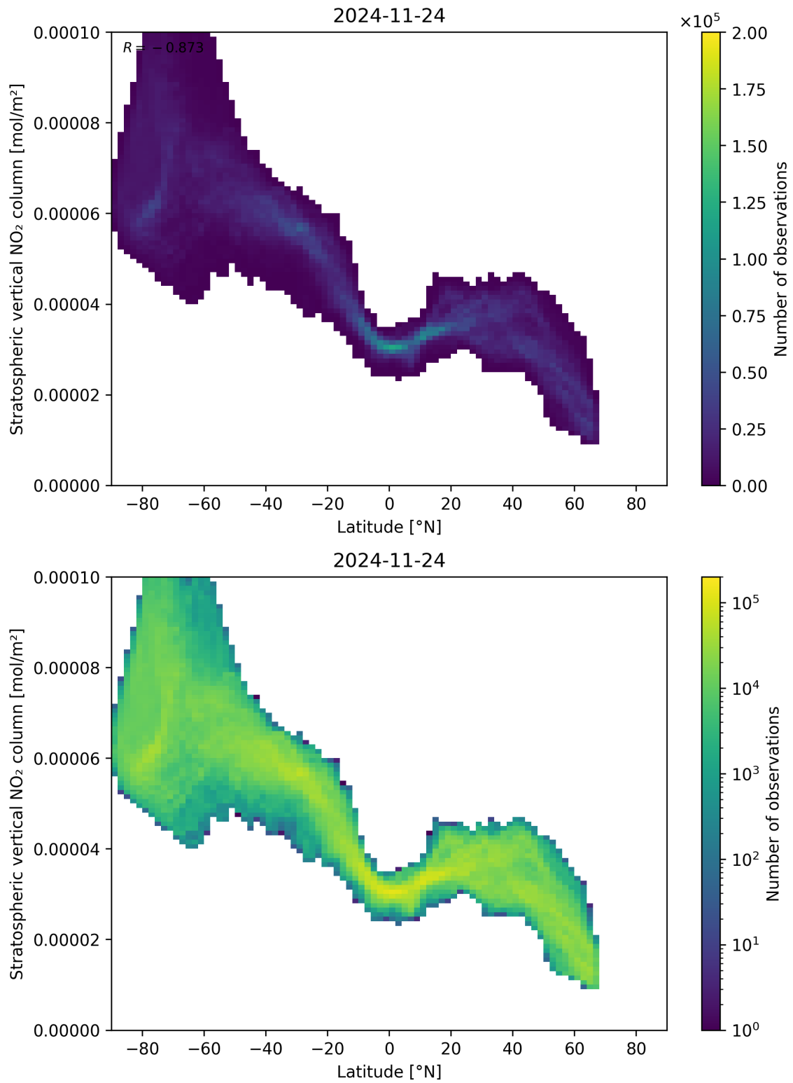
Figure 87: Scatter density plot of “Latitude” against “Stratospheric vertical NO 2 column” for 2024-11-23 to 2024-11-25.
