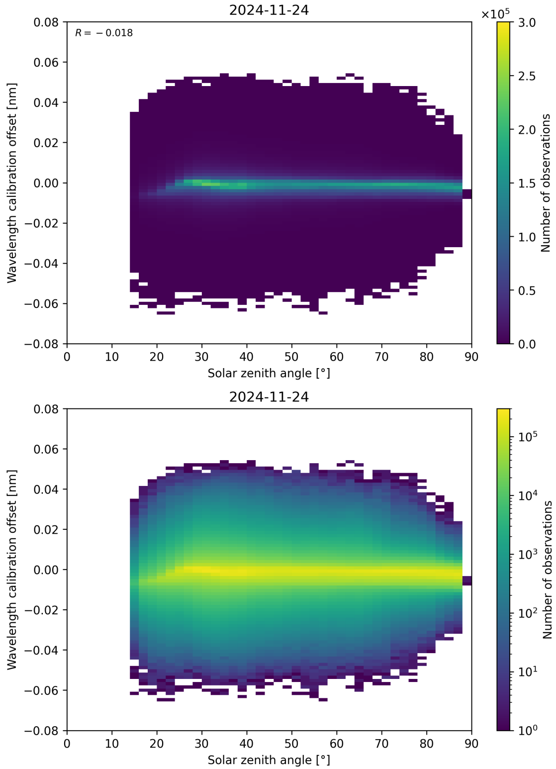
Figure 158: Scatter density plot of “Solar zenith angle” against “Wavelength calibration offset” for 2024-11-23 to 2024-11-25.
