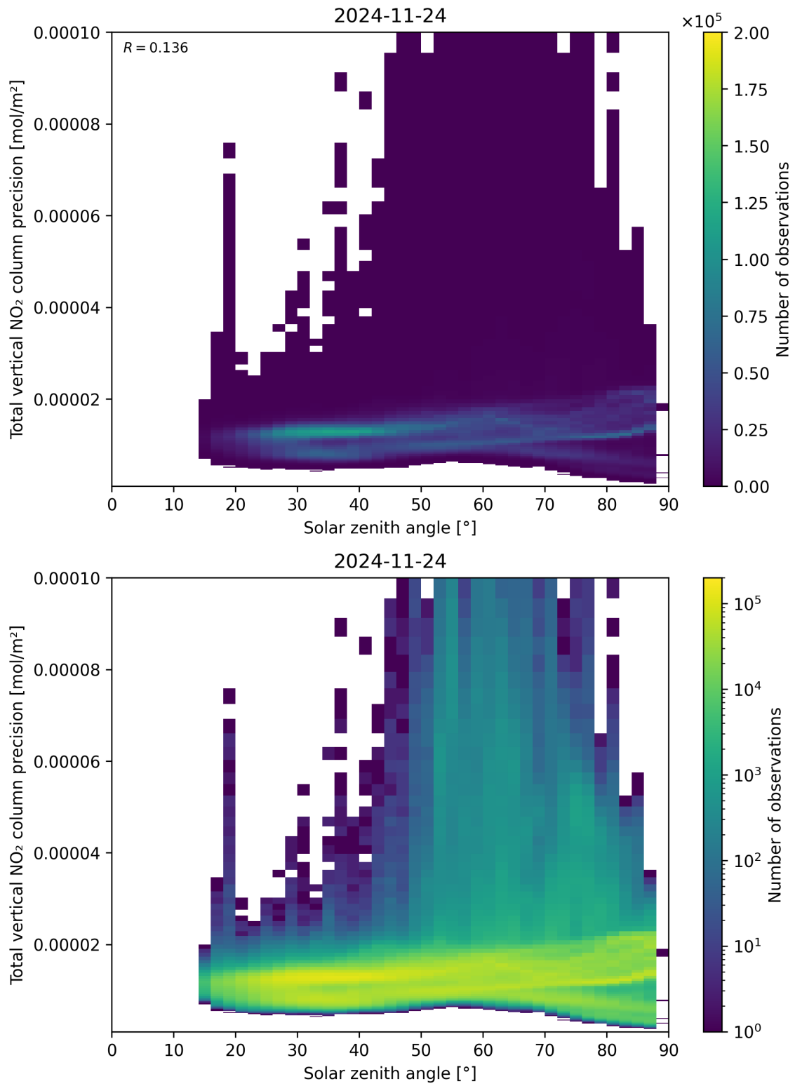
Figure 154: Scatter density plot of “Solar zenith angle” against “Total vertical NO 2 column precision” for 2024-11-23 to 2024-11-25.
