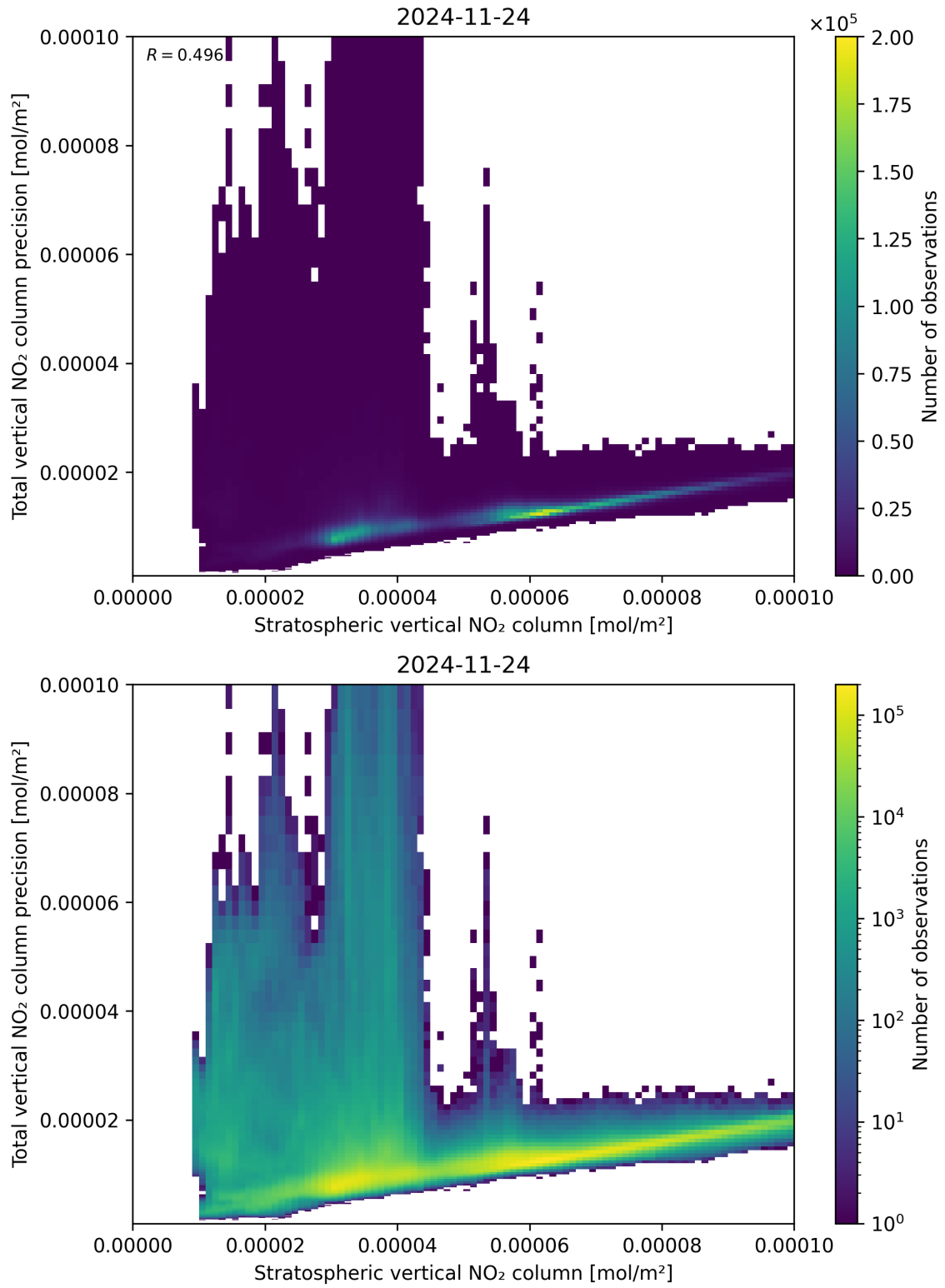
Figure 101: Scatter density plot of “Stratospheric vertical NO 2 column” against “Total vertical NO 2 column precision” for 2024-11-23 to 2024-11-25.
