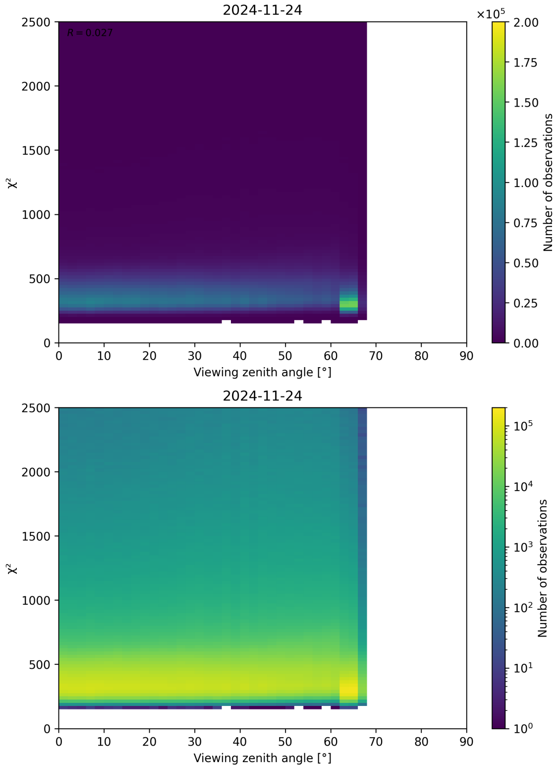
Figure 162: Scatter density plot of “Viewing zenith angle” against “ \chi^2 ” for 2024-11-23 to 2024-11-25.
