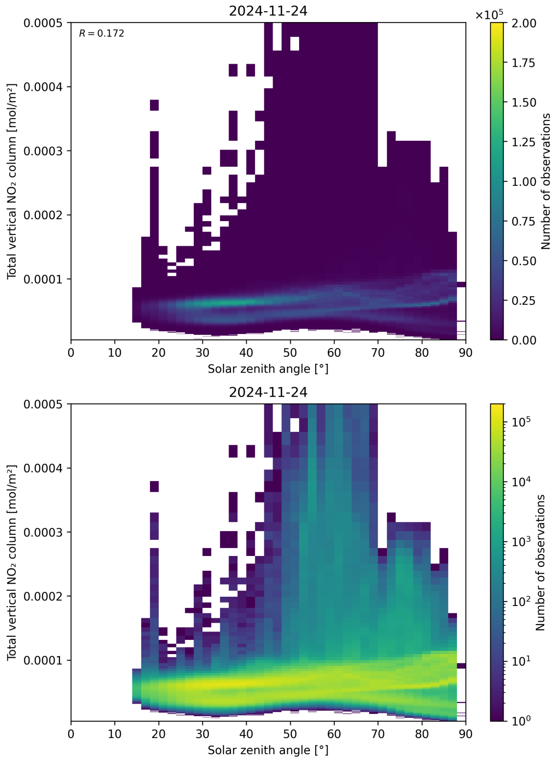
Figure 153: Scatter density plot of “Solar zenith angle” against “Total vertical NO 2 column” for 2024-11-23 to 2024-11-25.
