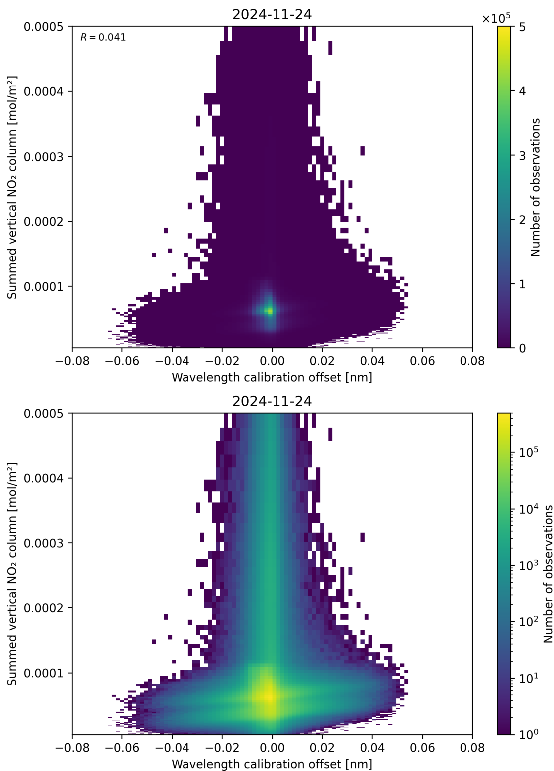
Figure 177: Scatter density plot of “Wavelength calibration offset” against “Summed vertical NO 2 column” for 2024-11-23 to 2024-11-25.
