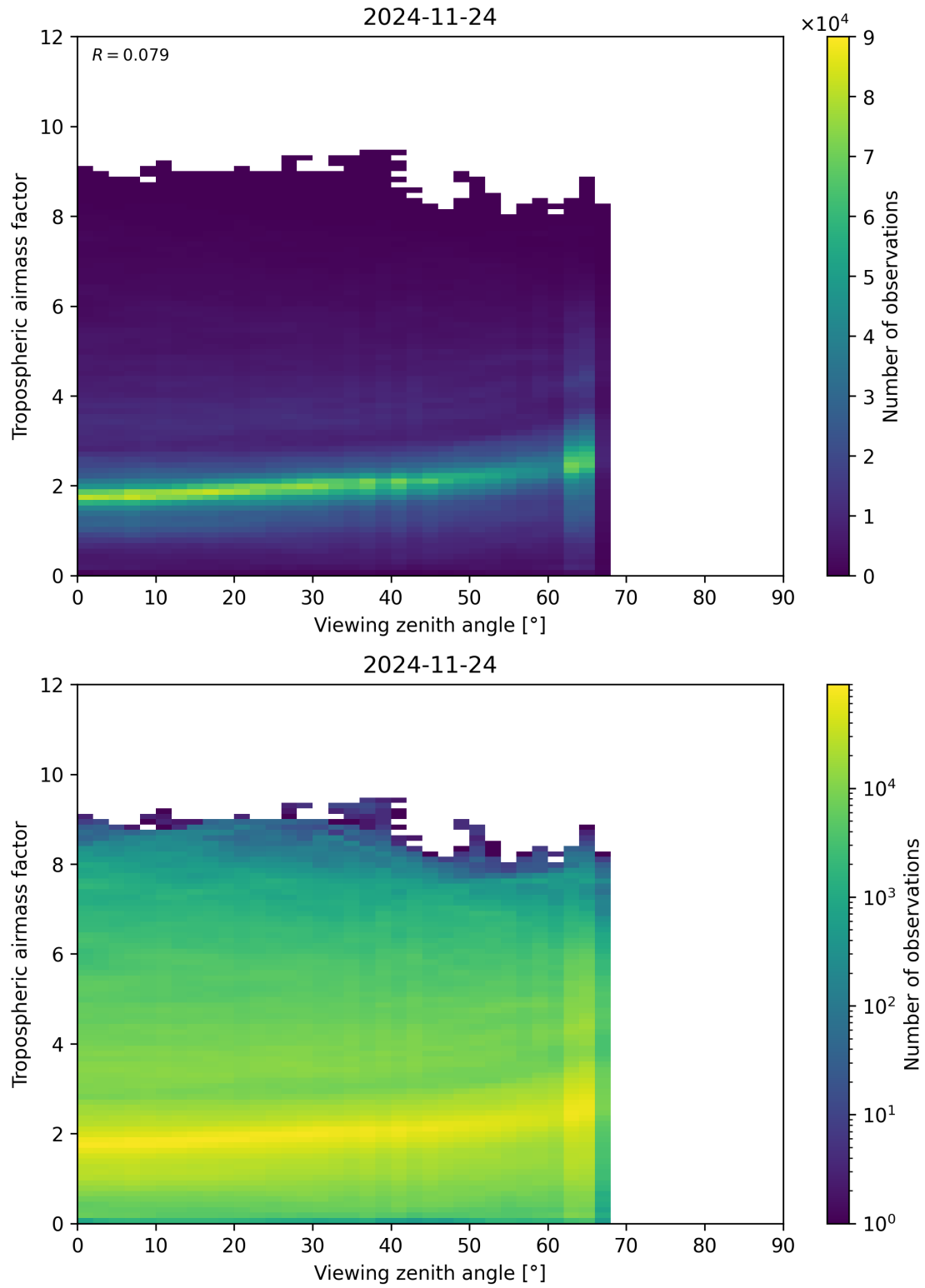
Figure 161: Scatter density plot of “Viewing zenith angle” against “Tropospheric airmass factor” for 2024-11-23 to 2024-11-25.
