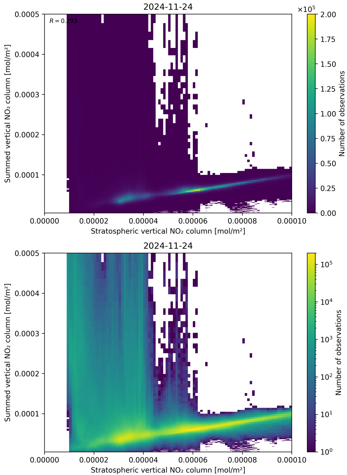
Figure 98: Scatter density plot of “Stratospheric vertical NO 2 column” against “Summed vertical NO 2 column” for 2024-11-23 to 2024-11-25.
