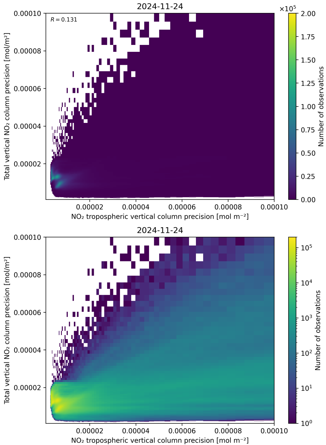
Figure 139: Scatter density plot of “NO 2 tropospheric vertical column precision” against “Total vertical NO 2 column precision” for 2024-11-23 to 2024-11-25.
