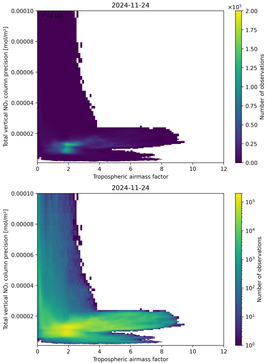
Figure 78: Scatter density plot of “Tropospheric air mass factor” against “Total vertical NO 2 column precision” for 2024-11-23 to 2024-11-25.
