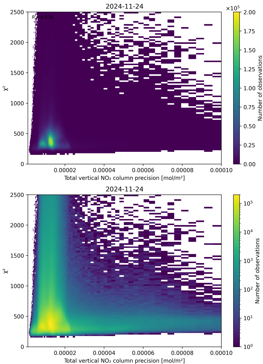
Figure 116: Scatter density plot of “Total vertical NO 2 column precision” against “ \chi^2 ” for 2024-11-23 to 2024-11-25.
