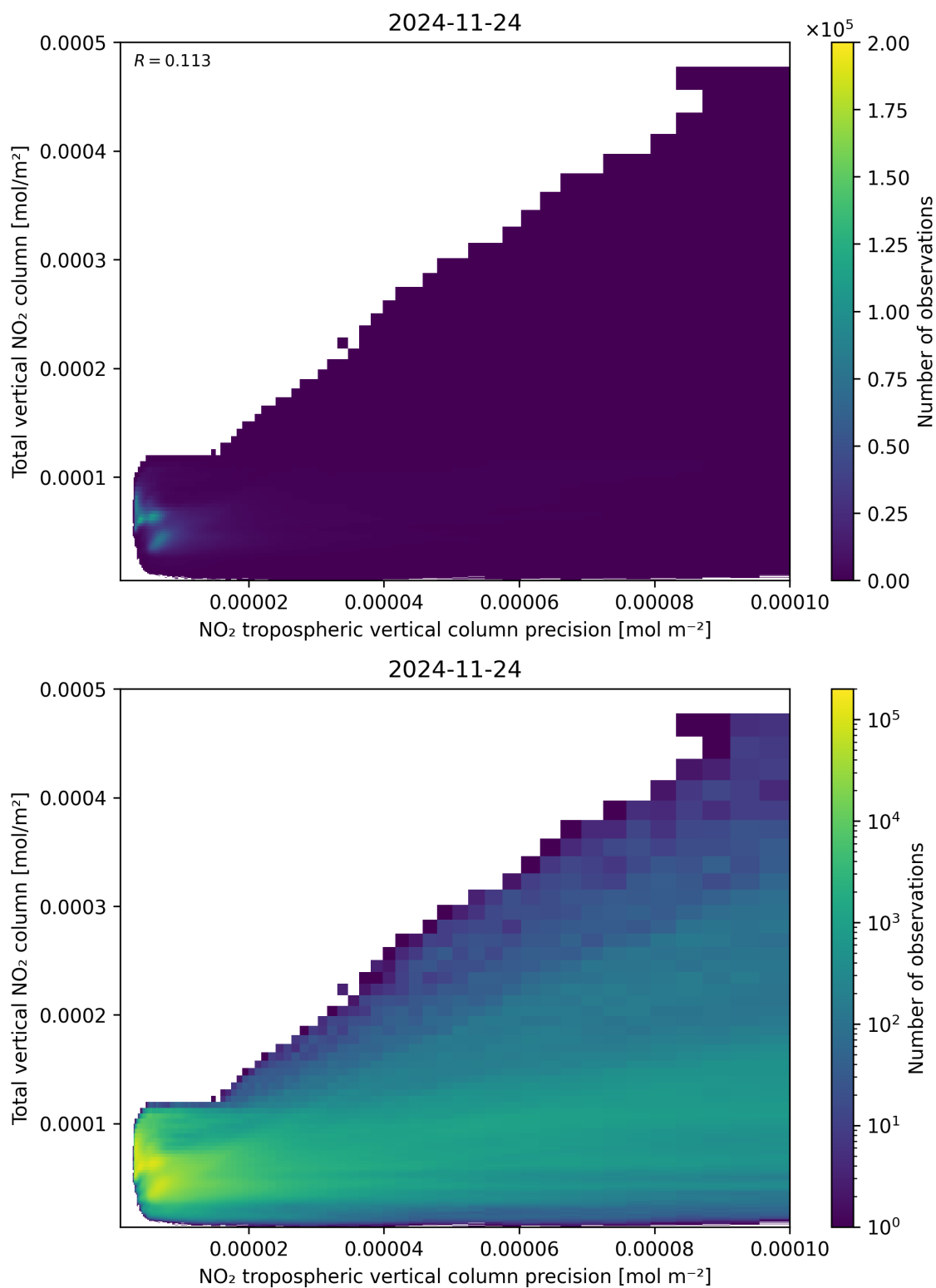
Figure 138: Scatter density plot of “NO 2 tropospheric vertical column precision” against “Total vertical NO 2 column” for 2024-11-23 to 2024-11-25.
