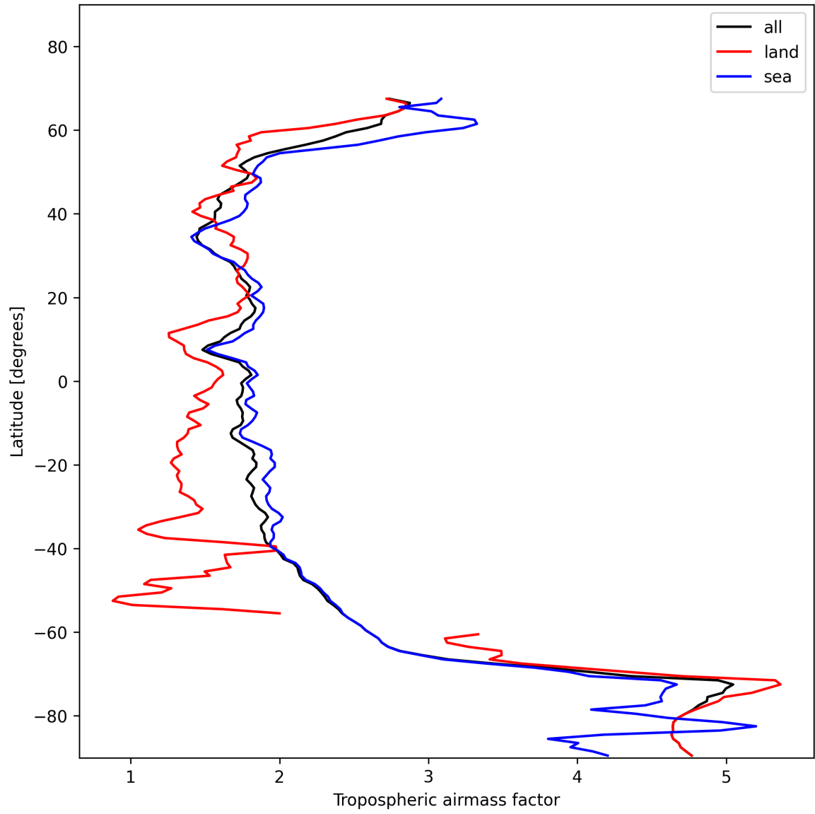
Figure 14: Zonal average of “Tropospheric airmass factor” for 2024-11-23 to 2024-11-25.
