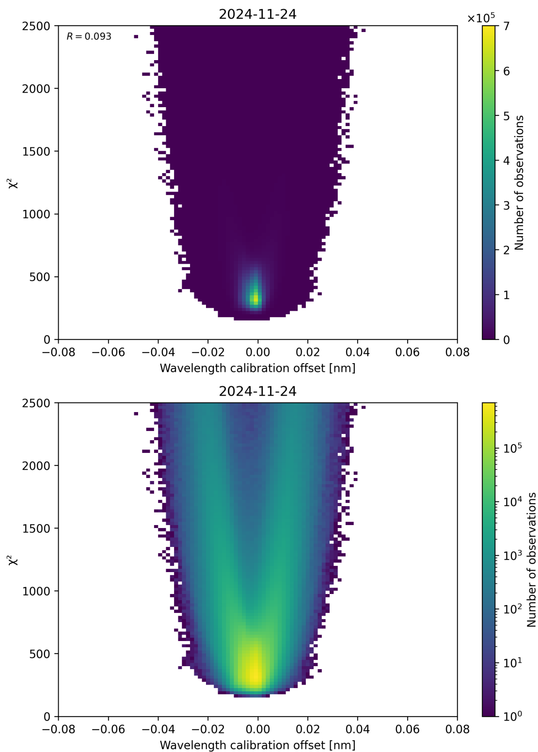
Figure 175: Scatter density plot of “Wavelength calibration offset” against “ \chi^2 ” for 2024-11-23 to 2024-11-25.
