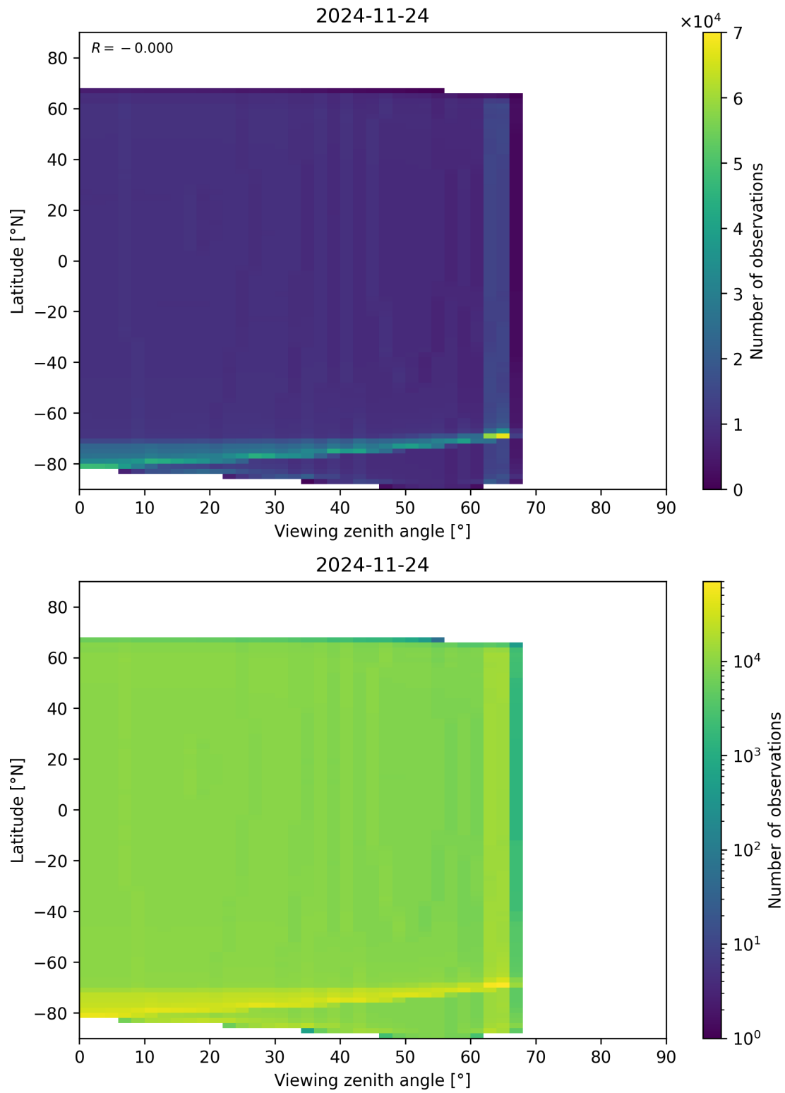
Figure 163: Scatter density plot of “Viewing zenith angle” against “Latitude” for 2024-11-23 to 2024-11-25.
