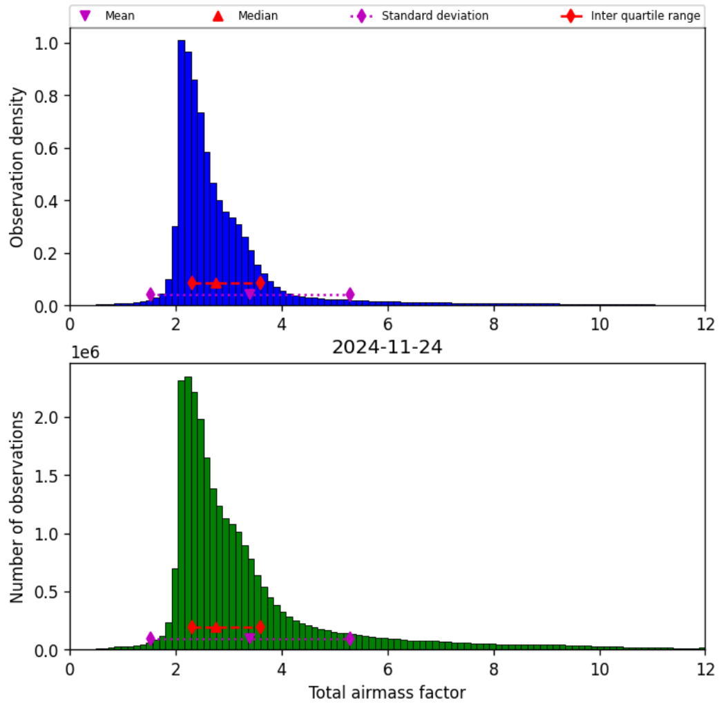
Figure 32: Histogram of “Total airmass factor” for 2024-11-23 to 2024-11-25
