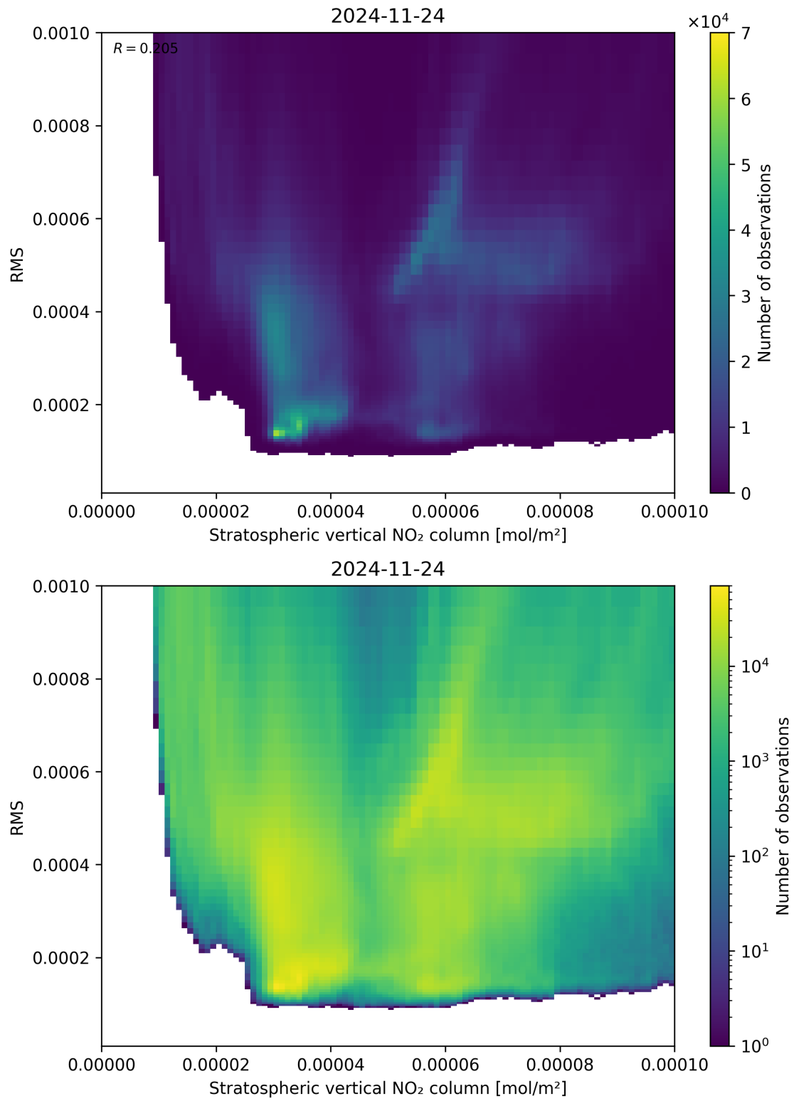
Figure 102: Scatter density plot of “Stratospheric vertical NO 2 column” against “RMS” for 2024-11-23 to 2024-11-25.
