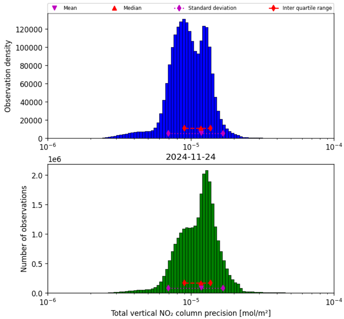
Figure 39: Histogram of “Total vertical NO 2 column precision” for 2024-11-23 to 2024-11-25
