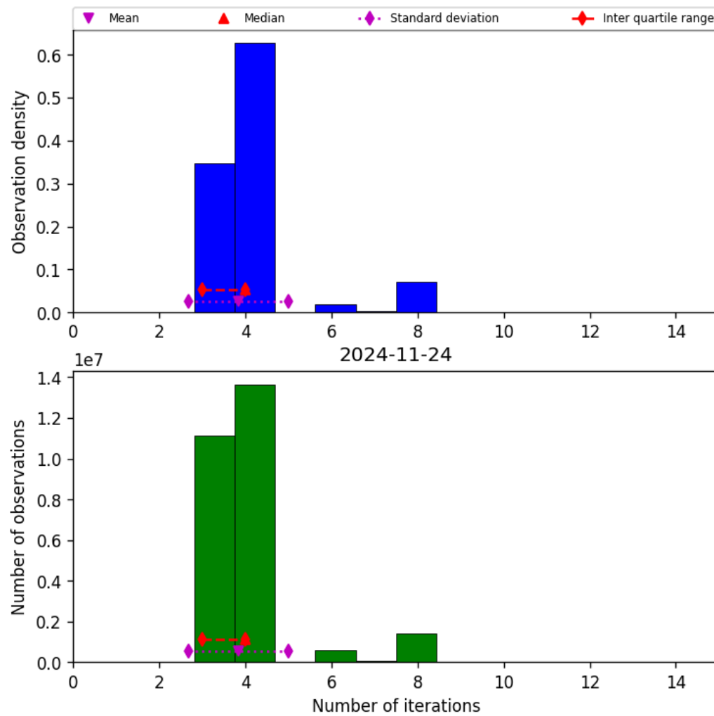
Figure 34: Histogram of “Number of iterations” for 2024-11-23 to 2024-11-25
