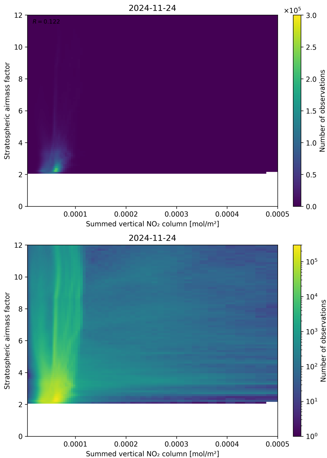
Figure 103: Scatter density plot of “Summed vertical NO 2 column” against “Stratospheric airmass factor” for 2024-11-23 to 2024-11-25.
