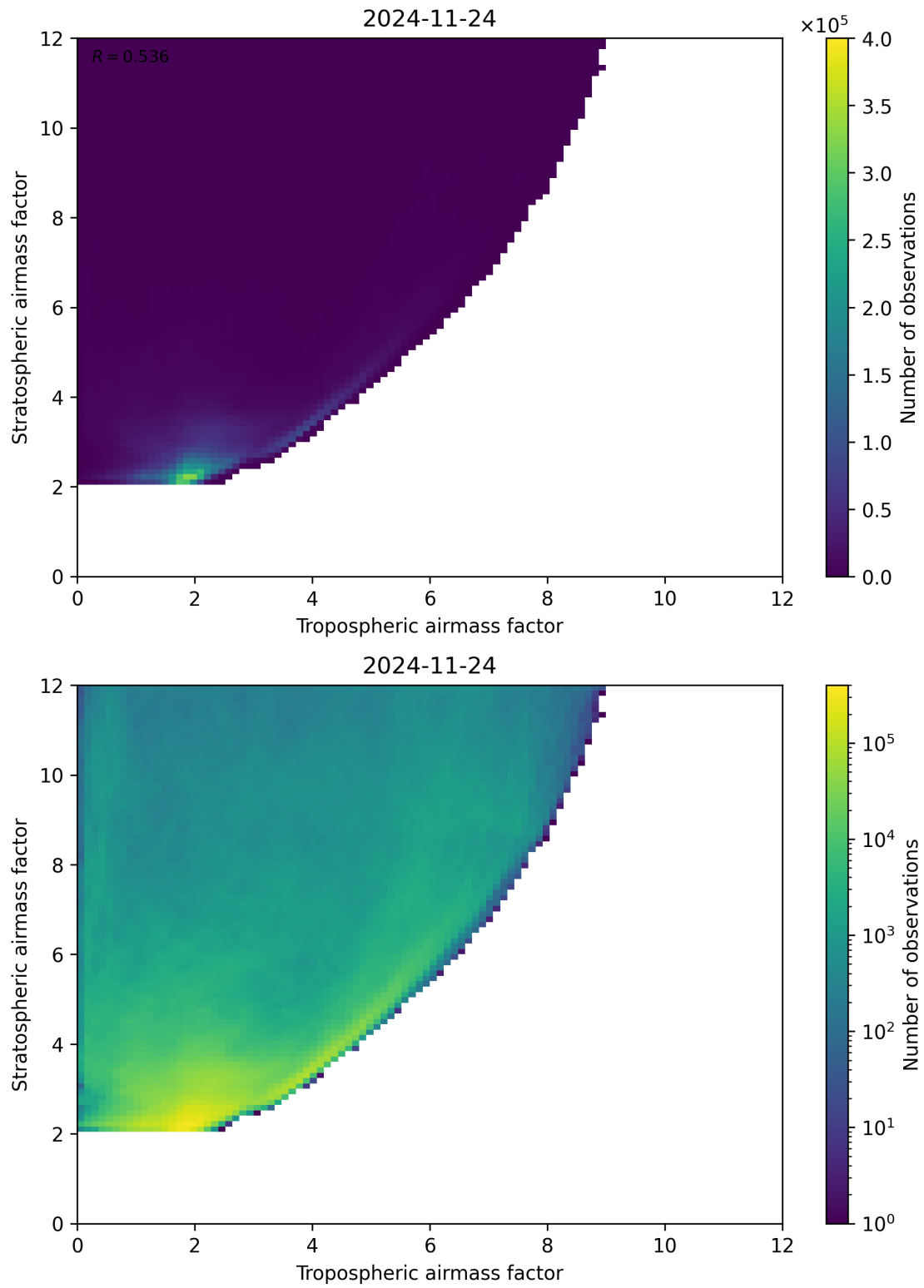
Figure 71: Scatter density plot of “Tropospheric airmass factor” against “Stratospheric airmass factor” for 2024-11-23 to 2024-11-25.
