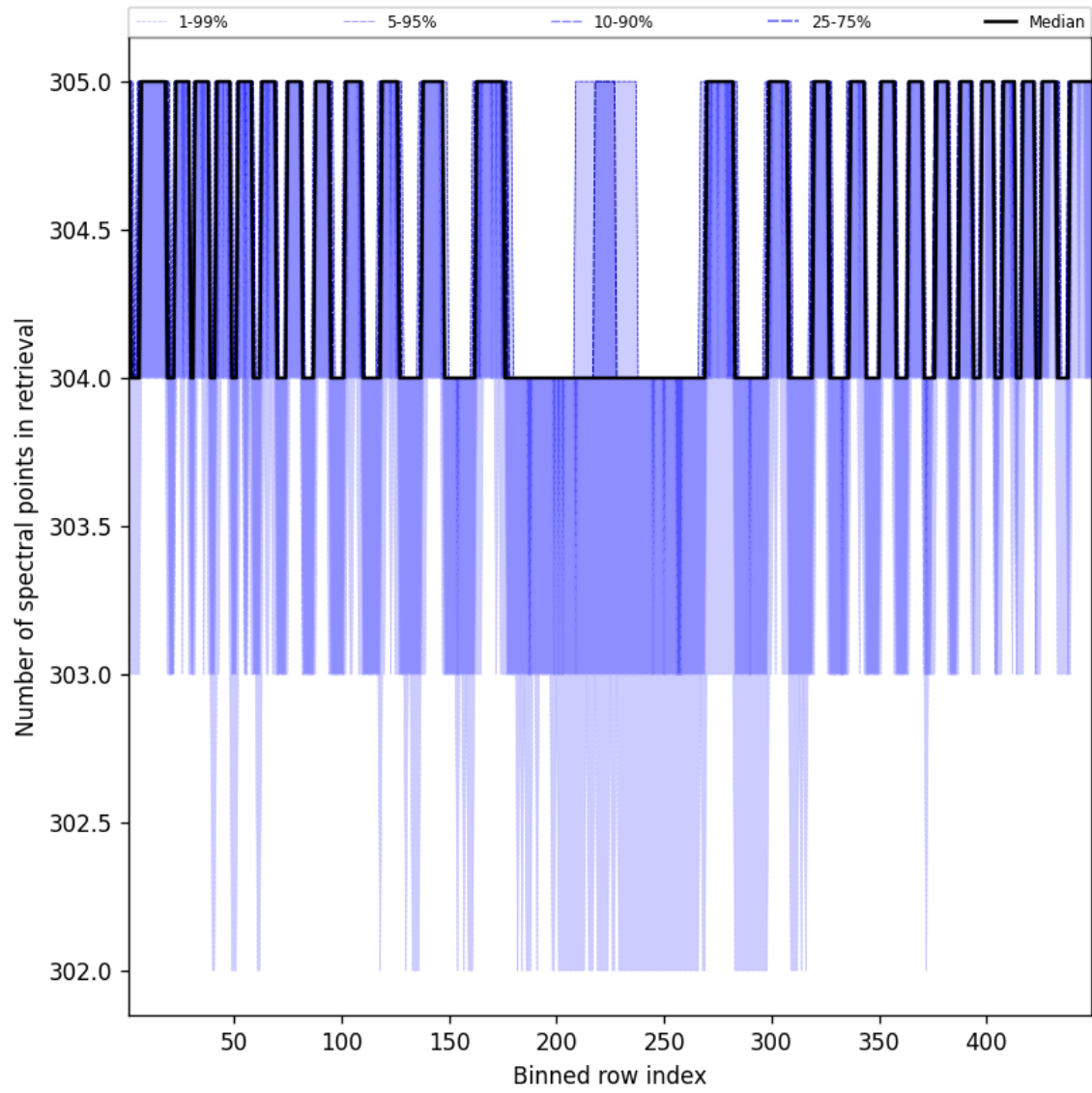
Figure 50: Along track statistics of “Number of spectral points in retrieval” for 2024-11-23 to 2024-11-25
