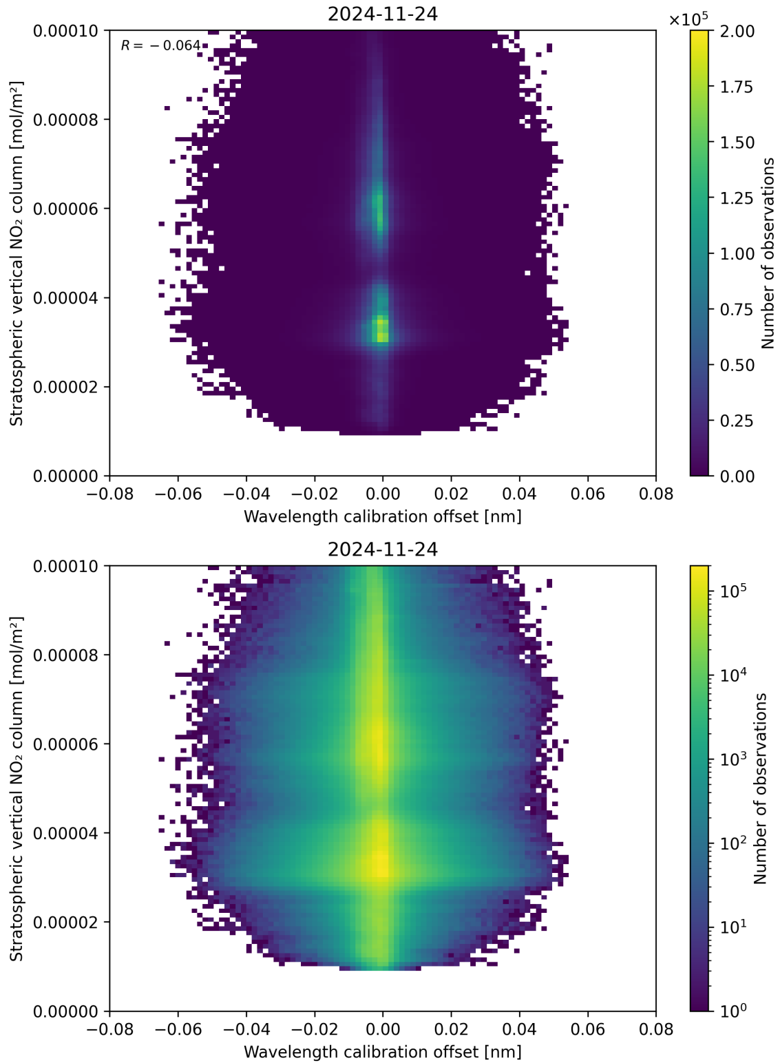
Figure 176: Scatter density plot of “Wavelength calibration offset” against “Stratospheric vertical NO 2 column” for 2024-11-23 to 2024-11-25.
