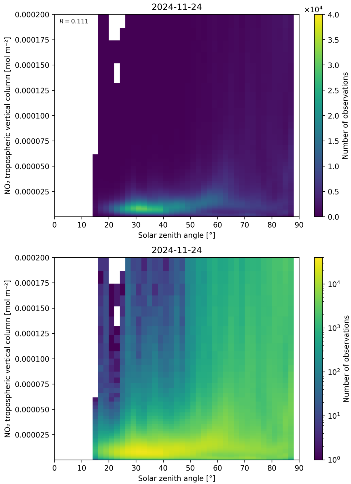
Figure 155: Scatter density plot of “Solar zenith angle” against “NO 2 tropospheric vertical column” for 2024-11-23 to 2024-11-25.
