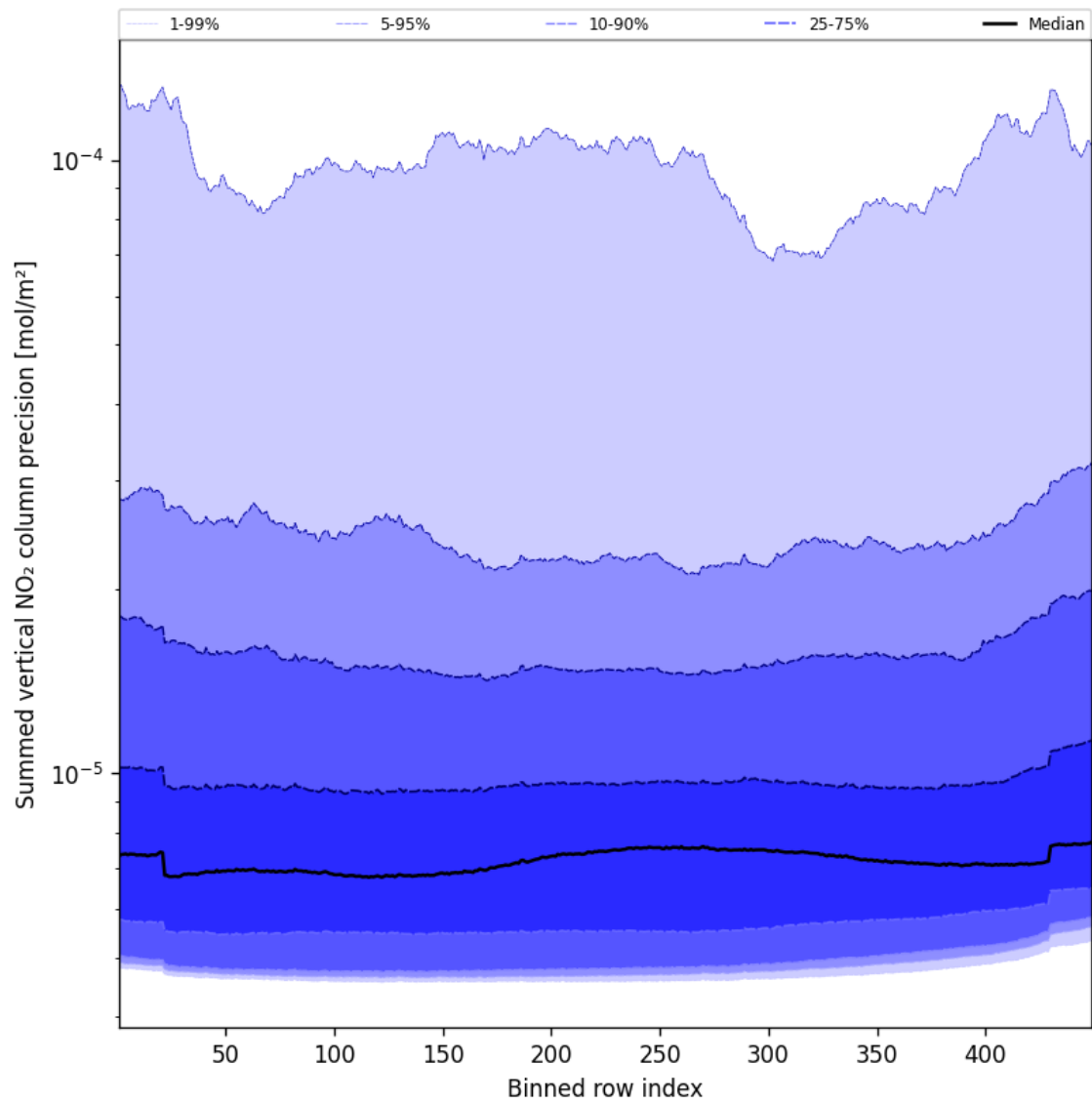
Figure 58: Along track statistics of “Summed vertical NO 2 column precision” for 2024-11-23 to 2024-11-25
