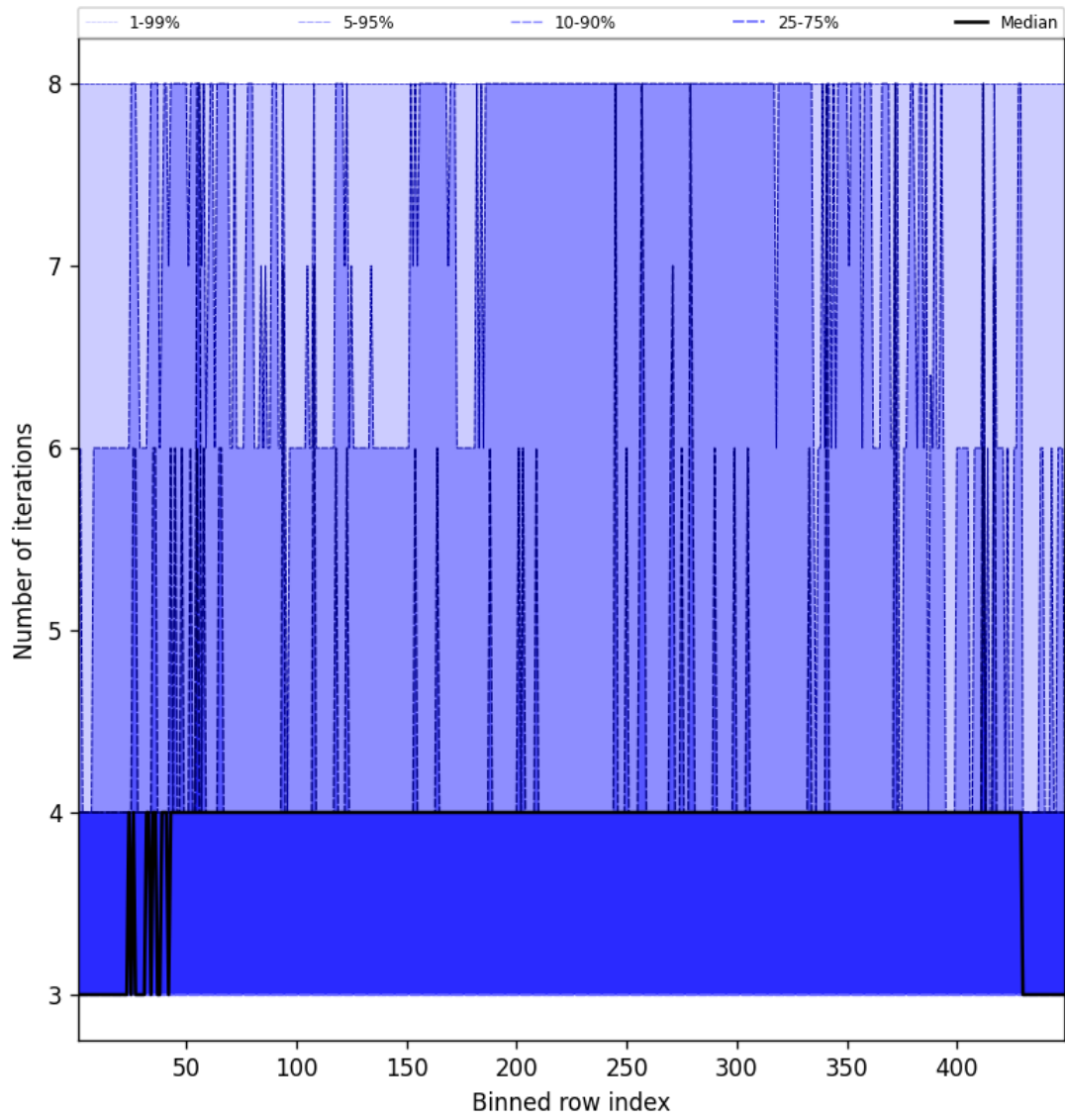
Figure 51: Along track statistics of “Number of iterations” for 2024-11-23 to 2024-11-25
