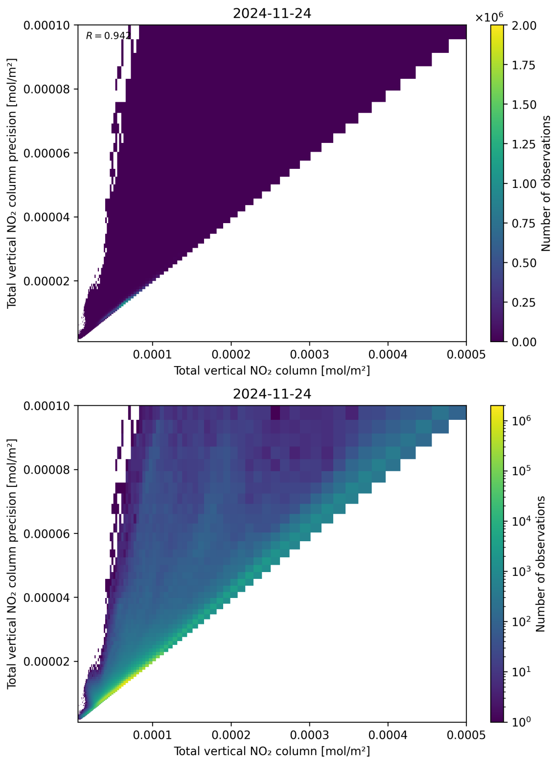
Figure 114: Scatter density plot of “Total vertical NO 2 column” against “Total vertical NO 2 column precision” for 2024-11-23 to 2024-11-25.
