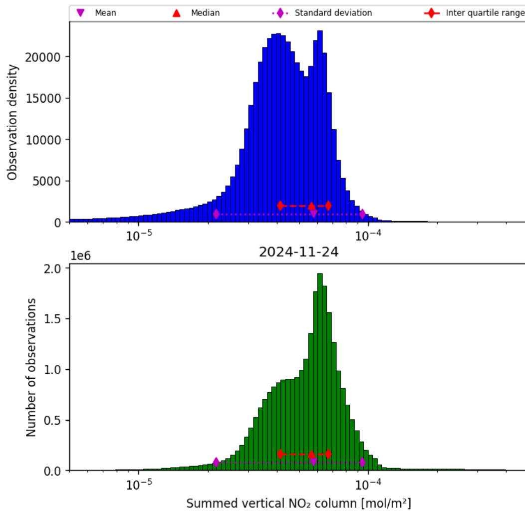
Figure 40: Histogram of “Summed vertical NO 2 column” for 2024-11-23 to 2024-11-25
