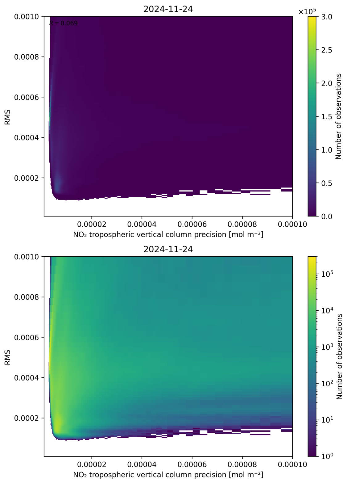
Figure 140: Scatter density plot of “NO 2 tropospheric vertical column precision” against “RMS” for 2024-11-23 to 2024-11-25.
