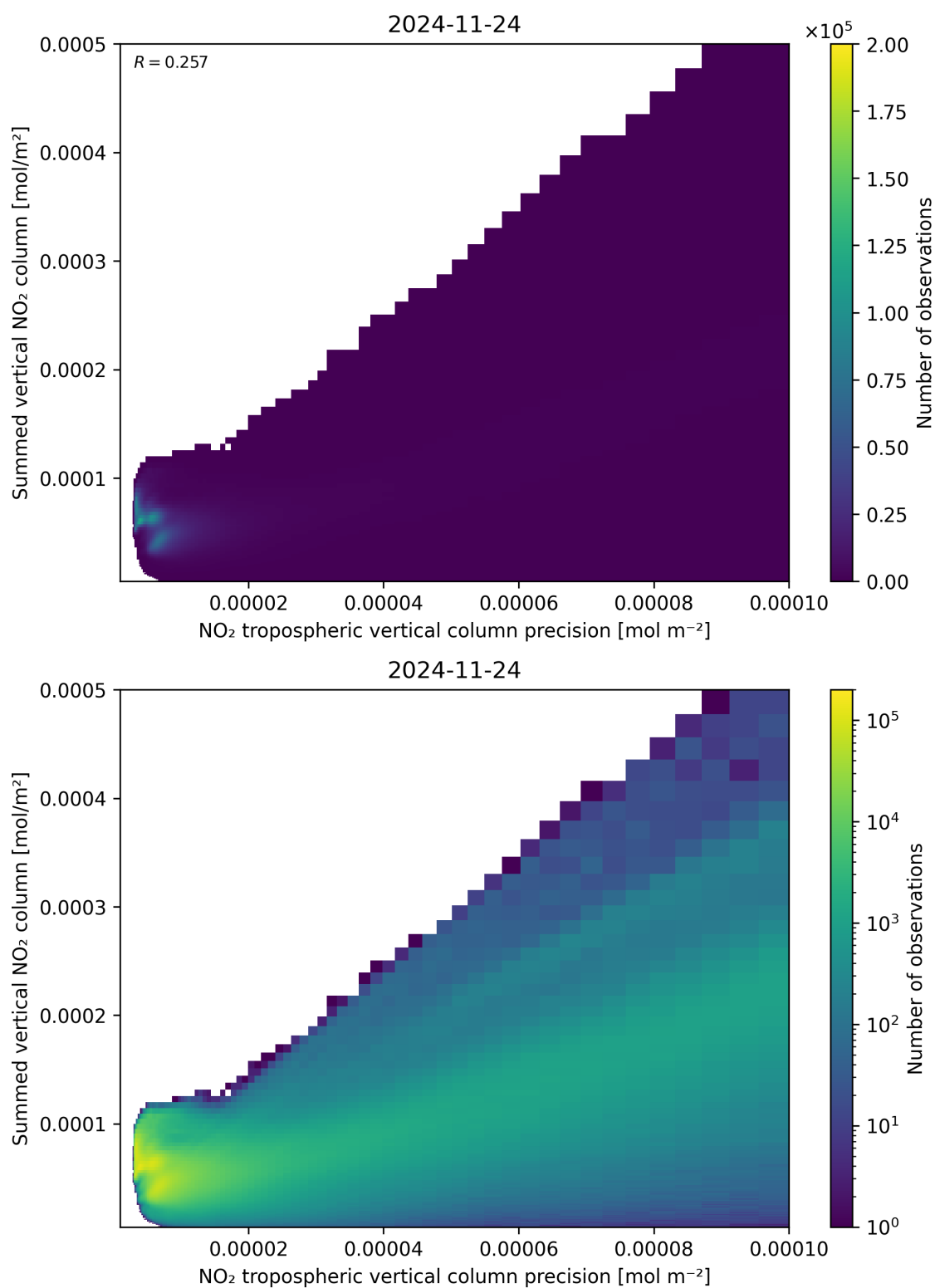
Figure 136: Scatter density plot of “NO 2 tropospheric vertical column precision” against “Summed vertical NO 2 column” for 2024-11-23 to 2024-11-25.
