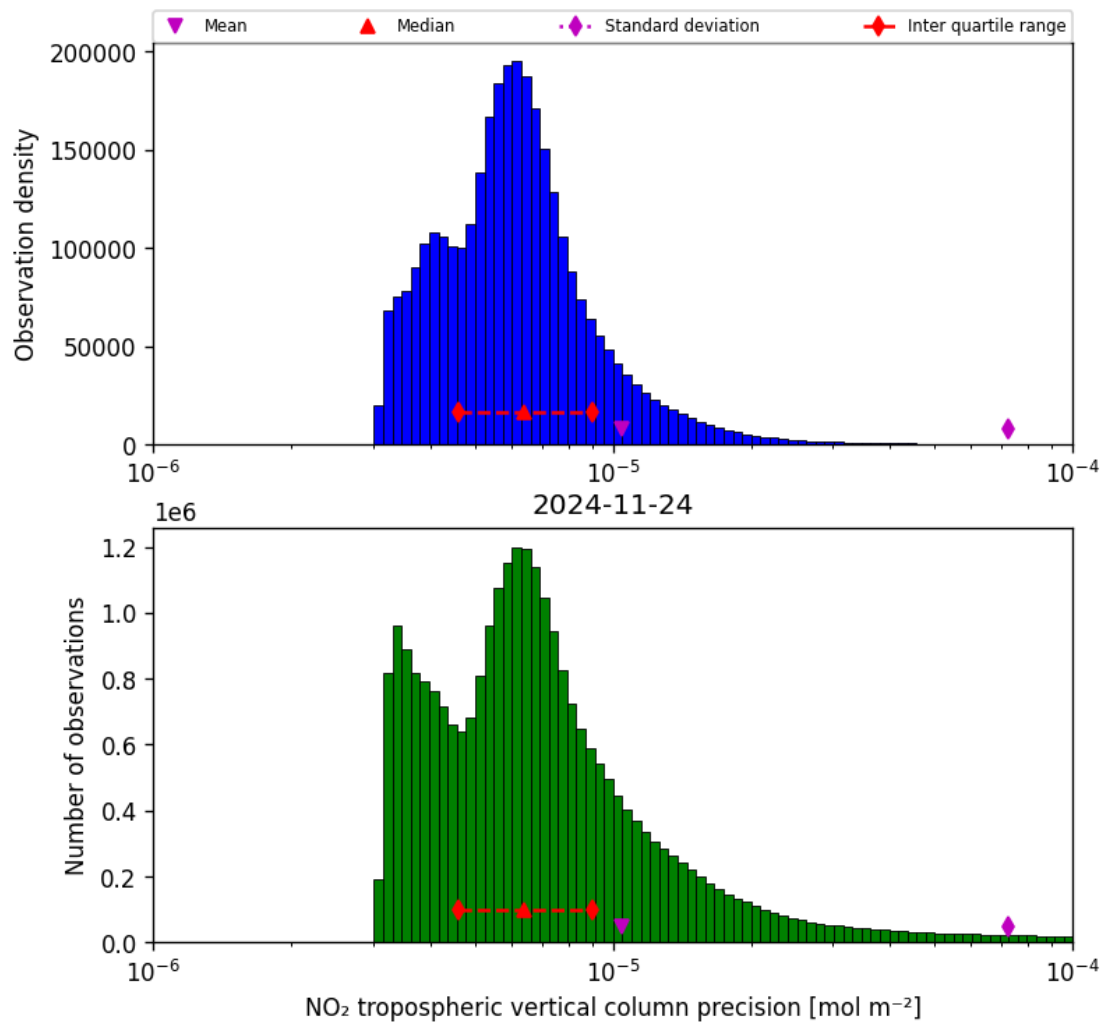
Figure 30: Histogram of “NO 2 tropospheric vertical column precision” for 2024-11-23 to 2024-11-25
