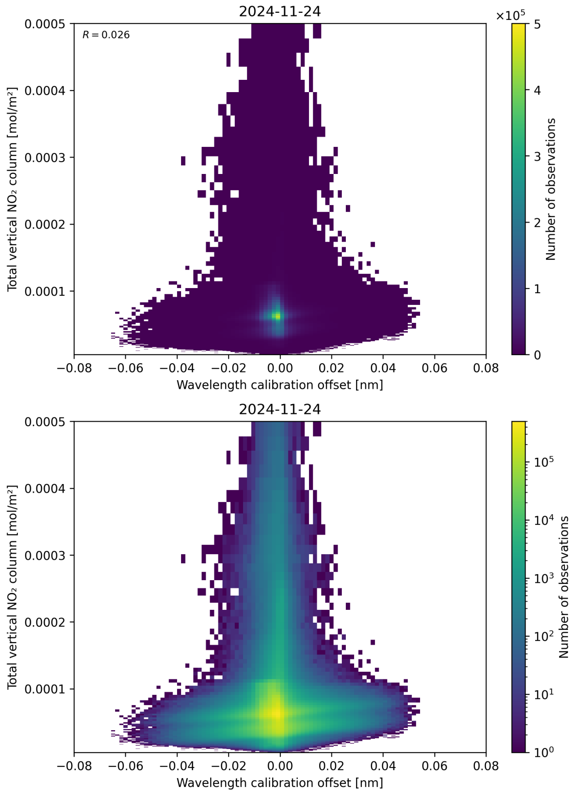
Figure 179: Scatter density plot of “Wavelength calibration offset” against “Total vertical NO 2 column” for 2024-11-23 to 2024-11-25.
