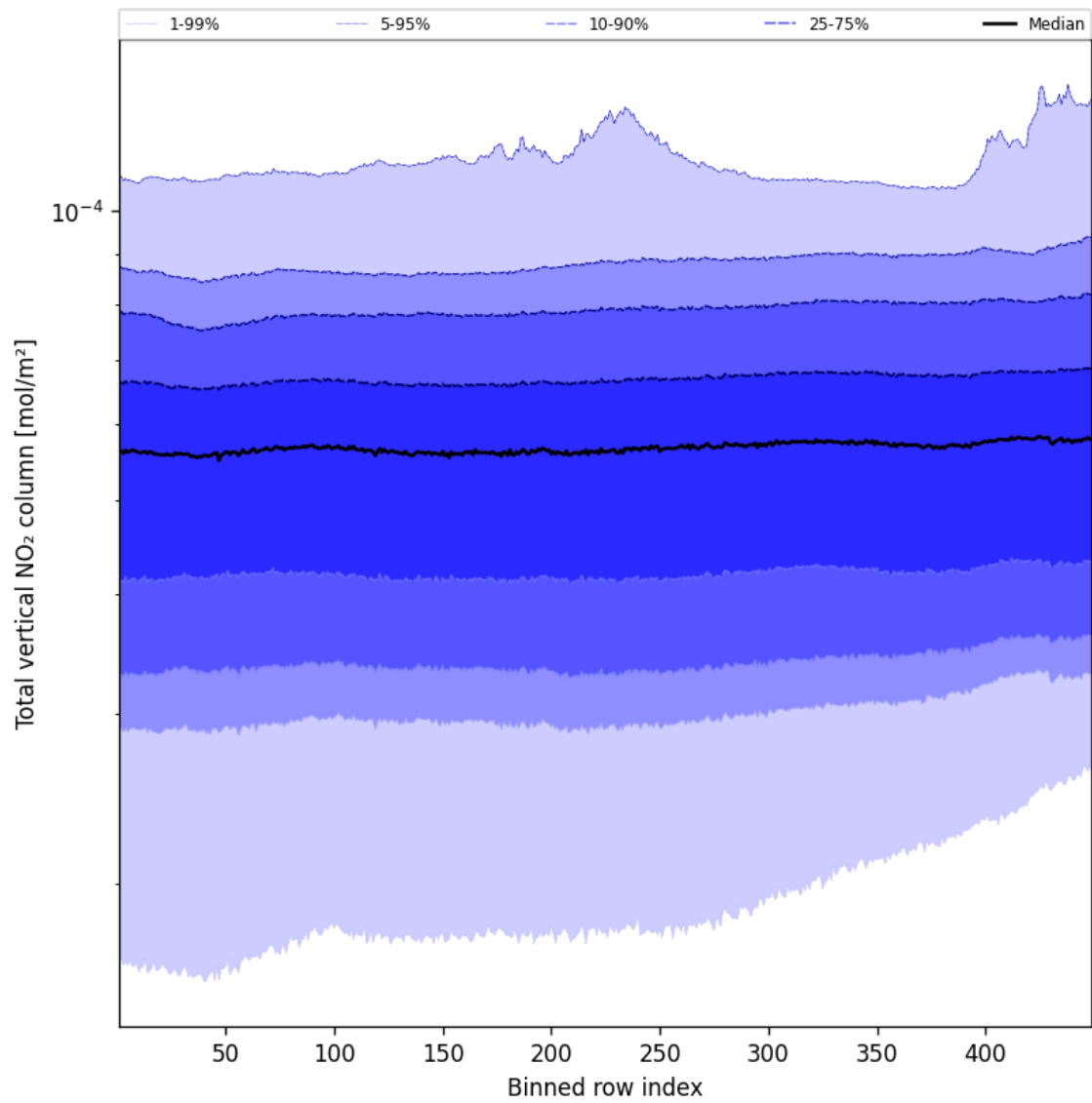
Figure 55: Along track statistics of “Total vertical NO 2 column” for 2024-11-23 to 2024-11-25
