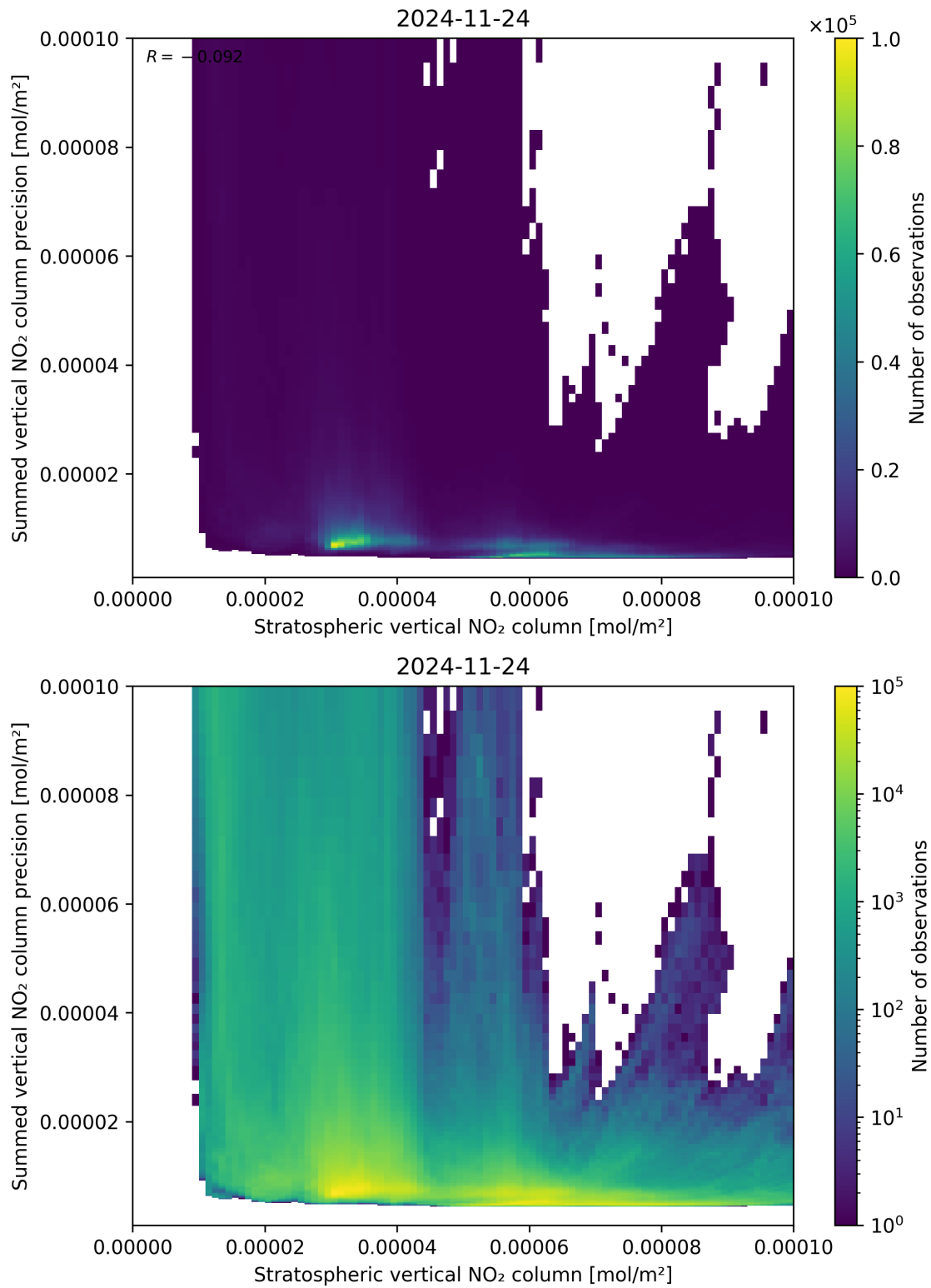
Figure 99: Scatter density plot of “Stratospheric vertical NO 2 column” against “Summed vertical NO 2 column precision” for 2024-11-23 to 2024-11-25.
