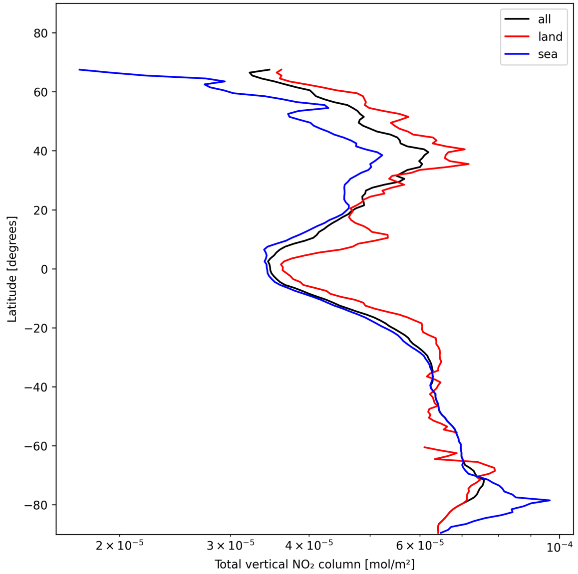
Figure 21: Zonal average of “Total vertical NO 2 column” for 2024-11-23 to 2024-11-25.
