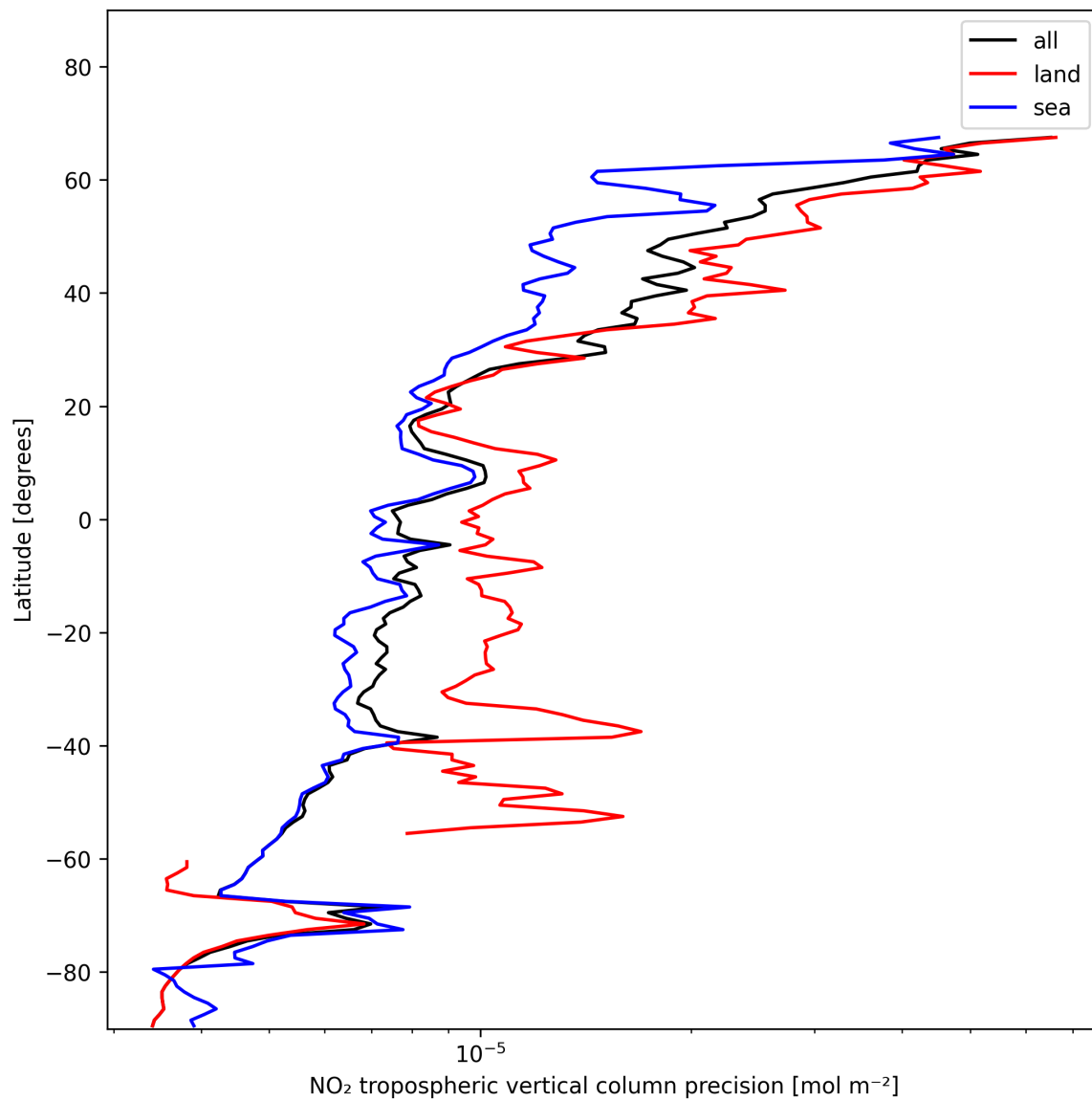
Figure 13: Zonal average of “NO 2 tropospheric vertical column precision” for 2024-11-23 to 2024-11-25.
