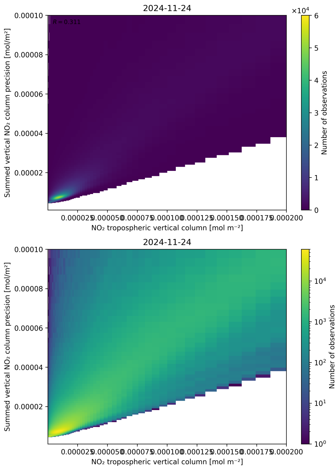
Figure 127: Scatter density plot of “NO 2 tropospheric vertical column” against “Summed vertical NO 2 column precision” for 2024-11-23 to 2024-11-25.
