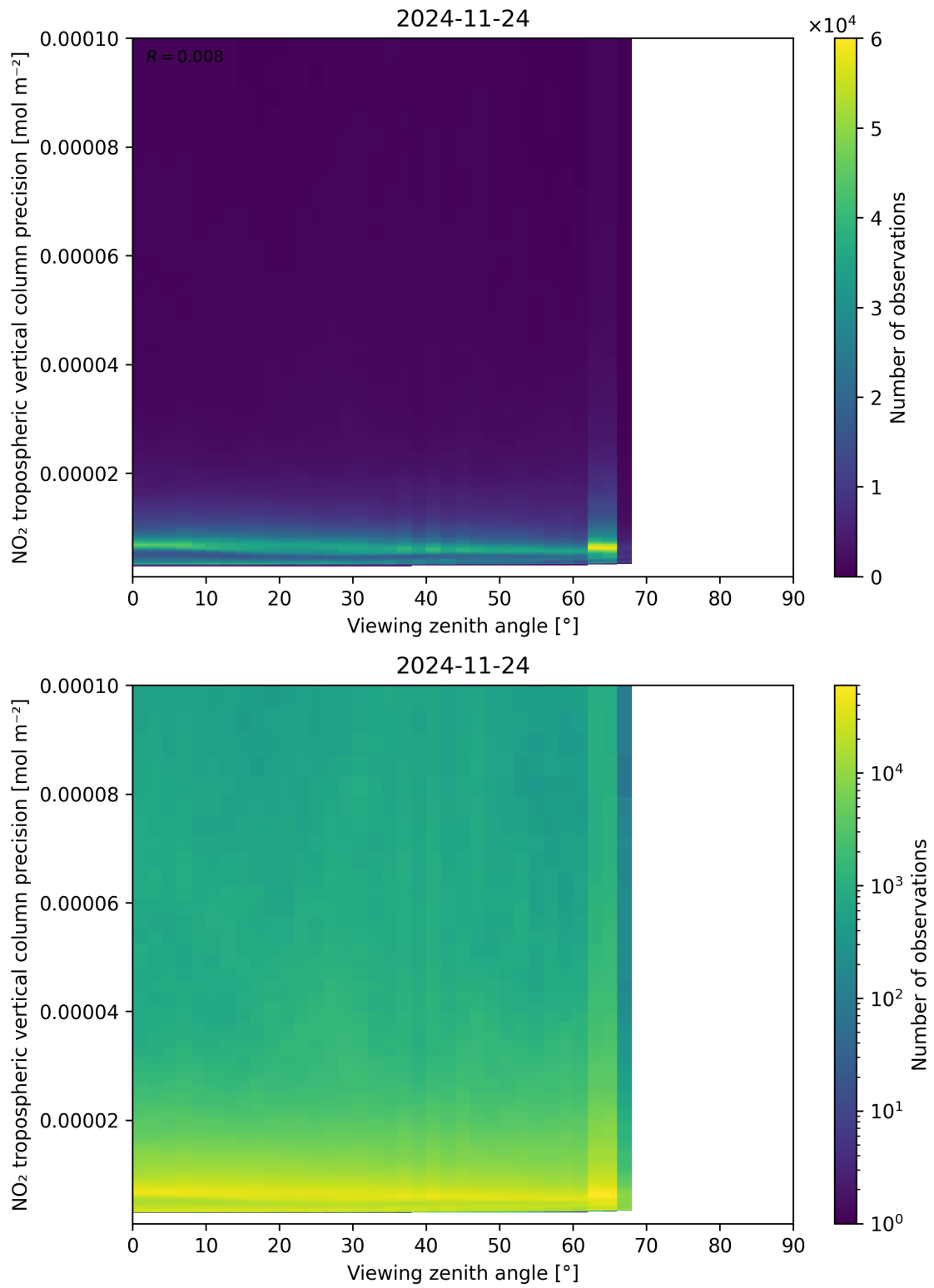
Figure 170: Scatter density plot of “Viewing zenith angle” against “NO 2 tropospheric vertical column precision” for 2024-11-23 to 2024-11-25.
