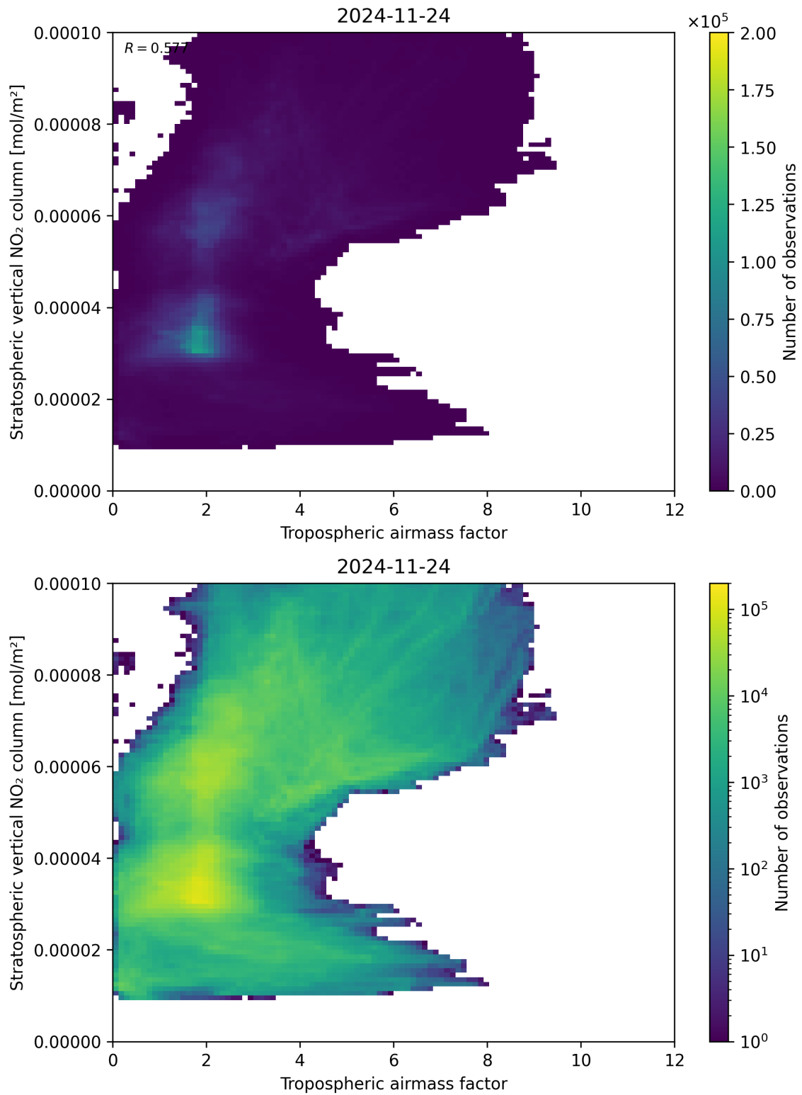
Figure 74: Scatter density plot of “Tropospheric air mass factor” against “Stratospheric vertical NO 2 column” for 2024-11-23 to 2024-11-25.
