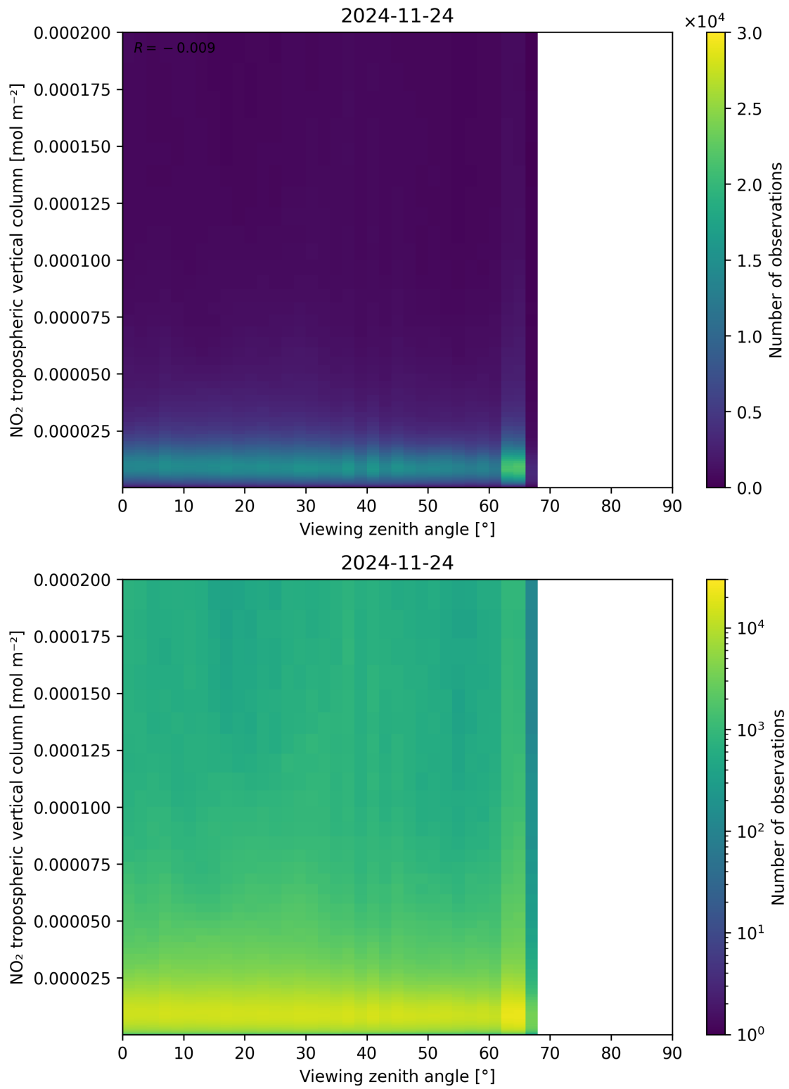
Figure 169: Scatter density plot of “Viewing zenith angle” against “NO 2 tropospheric vertical column” for 2024-11-23 to 2024-11-25.
