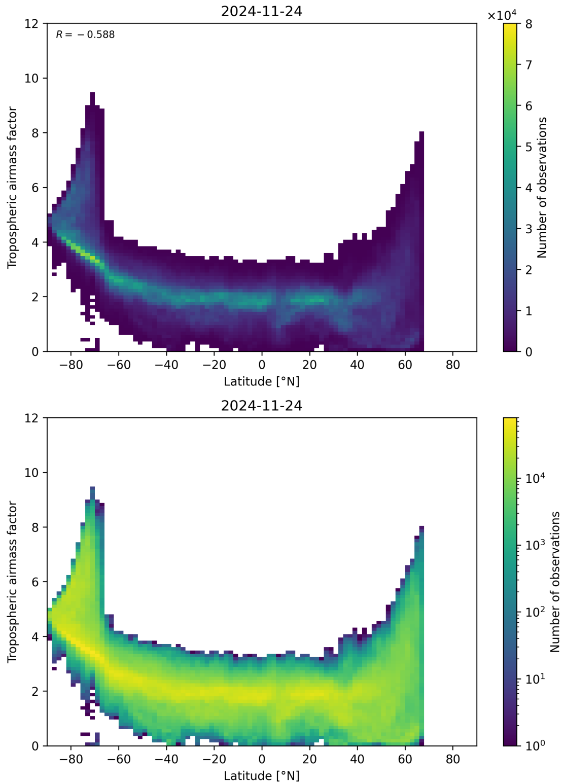
Figure 85: Scatter density plot of “Latitude” against “Tropospheric airmass factor” for 2024-11-23 to 2024-11-25.
