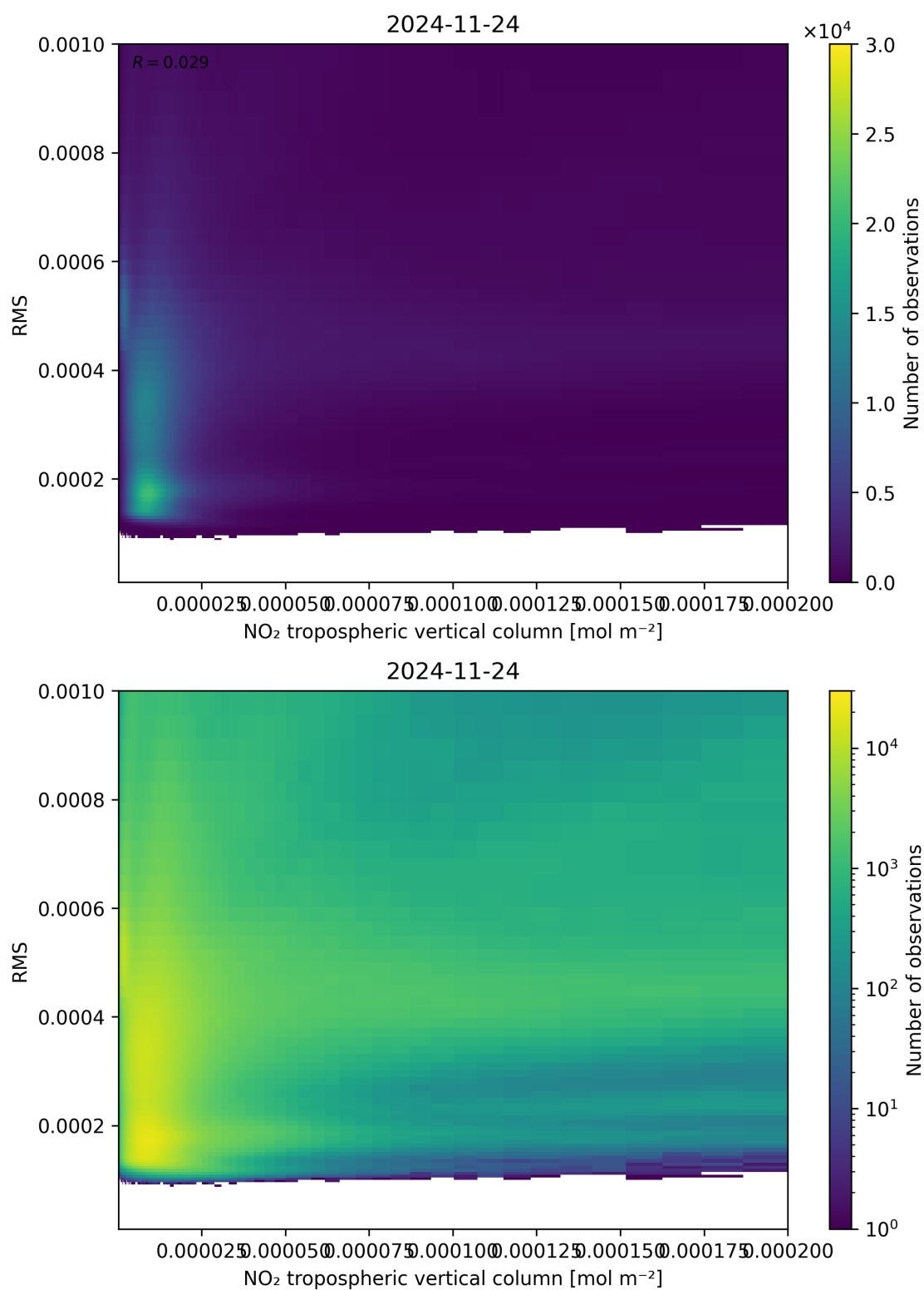
Figure 142: Scatter density plot of “NO 2 tropospheric vertical column” against “RMS” for 2024-11-23 to 2024-11-25.
