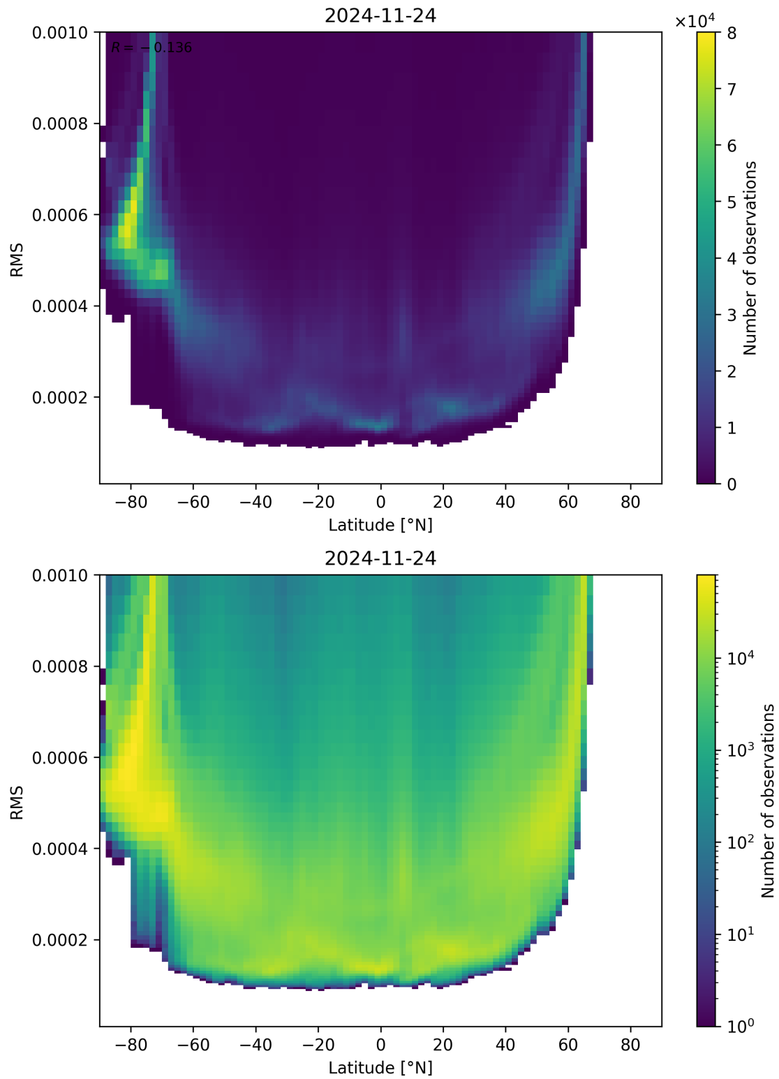
Figure 94: Scatter density plot of “Latitude” against “RMS” for 2024-11-23 to 2024-11-25.
