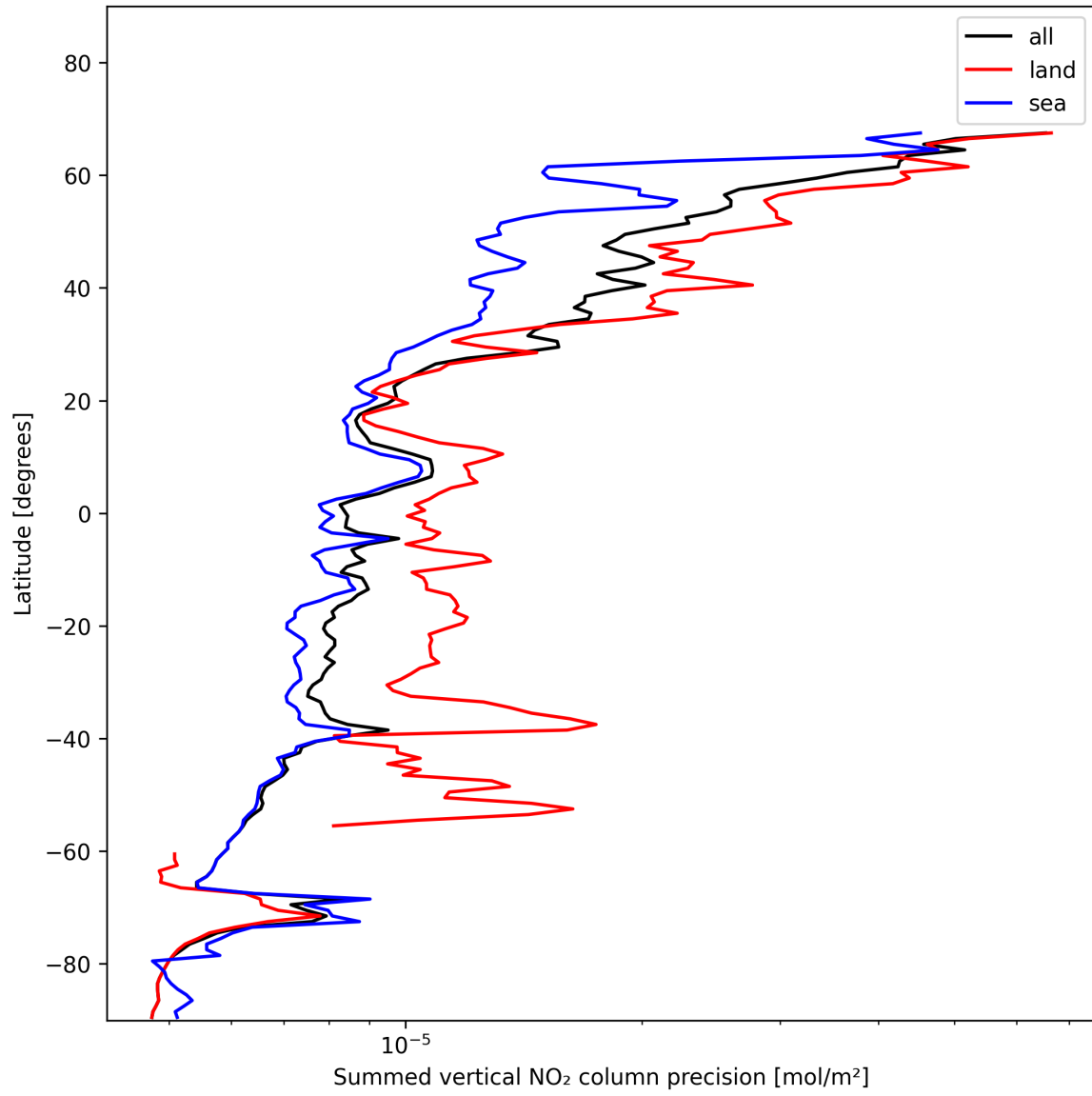
Figure 24: Zonal average of “Summed vertical NO 2 column precision” for 2024-11-23 to 2024-11-25.
