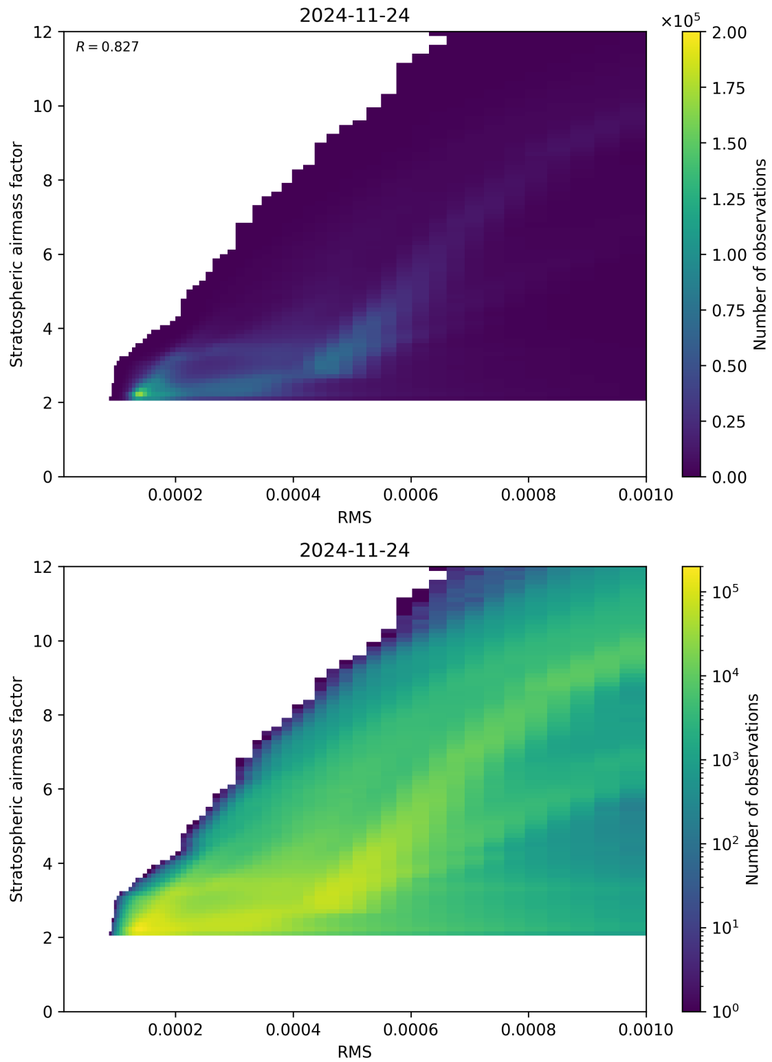
Figure 144: Scatter density plot of “RMS” against “Stratospheric airmass factor” for 2024-11-23 to 2024-11-25.
