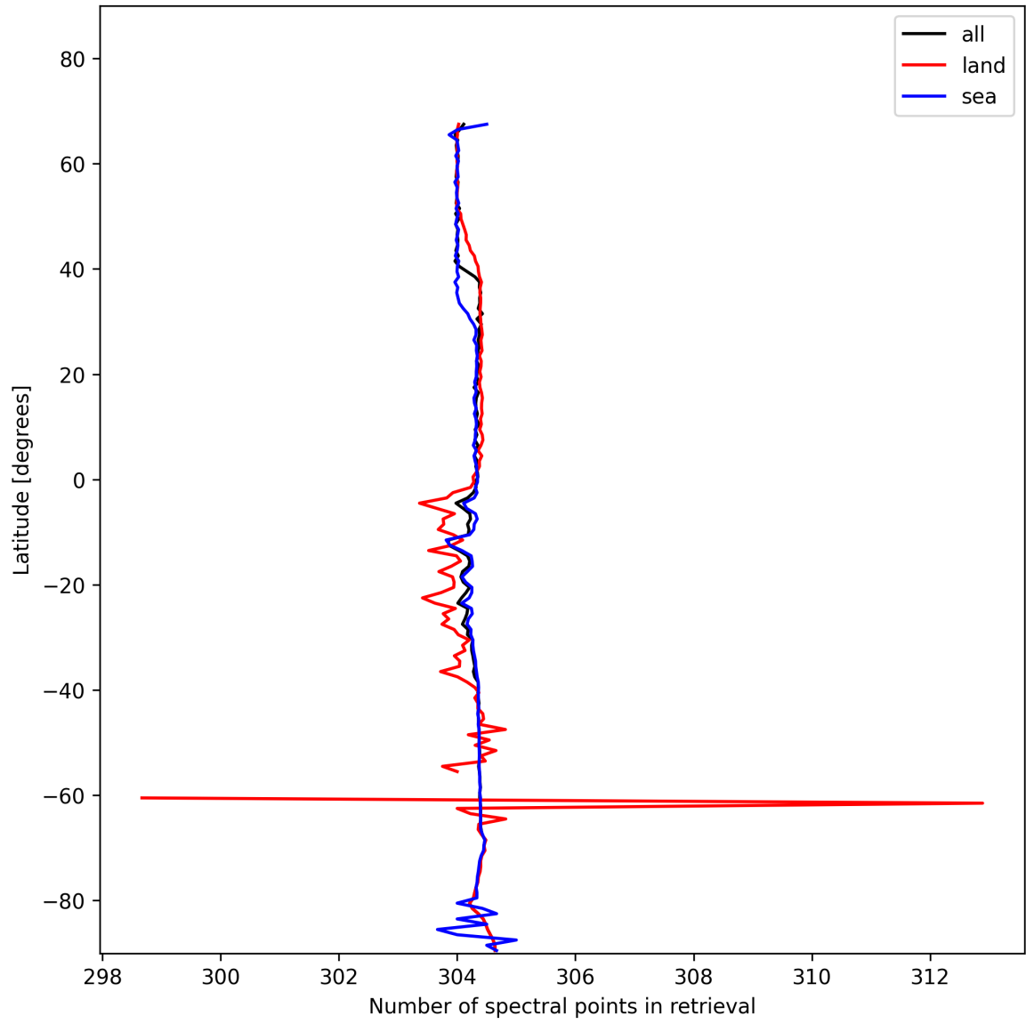
Figure 16: Zonal average of “Number of spectral points in retrieval” for 2024-11-23 to 2024-11-25.
