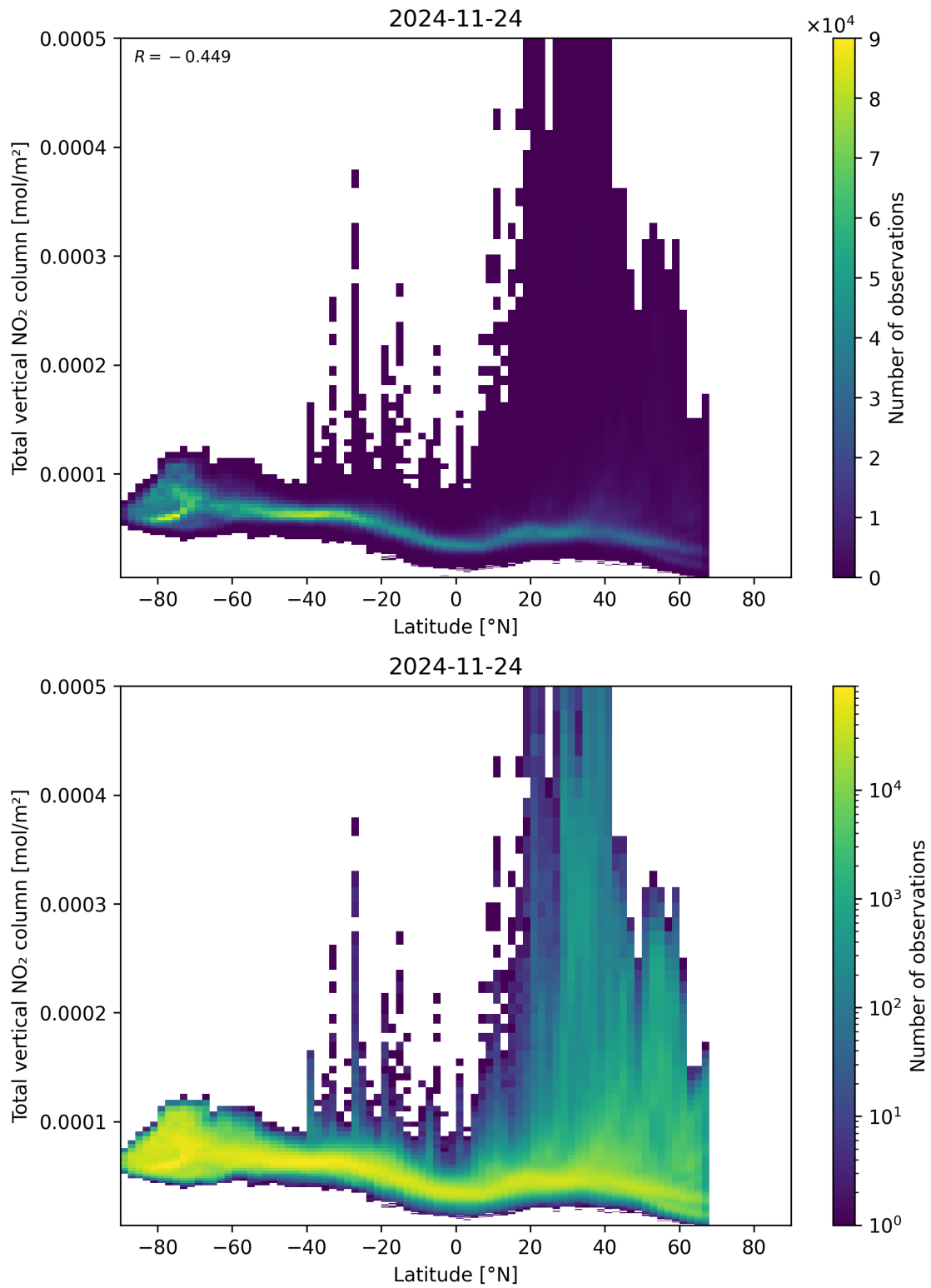
Figure 90: Scatter density plot of “Latitude” against “Total vertical NO 2 column” for 2024-11-23 to 2024-11-25.
