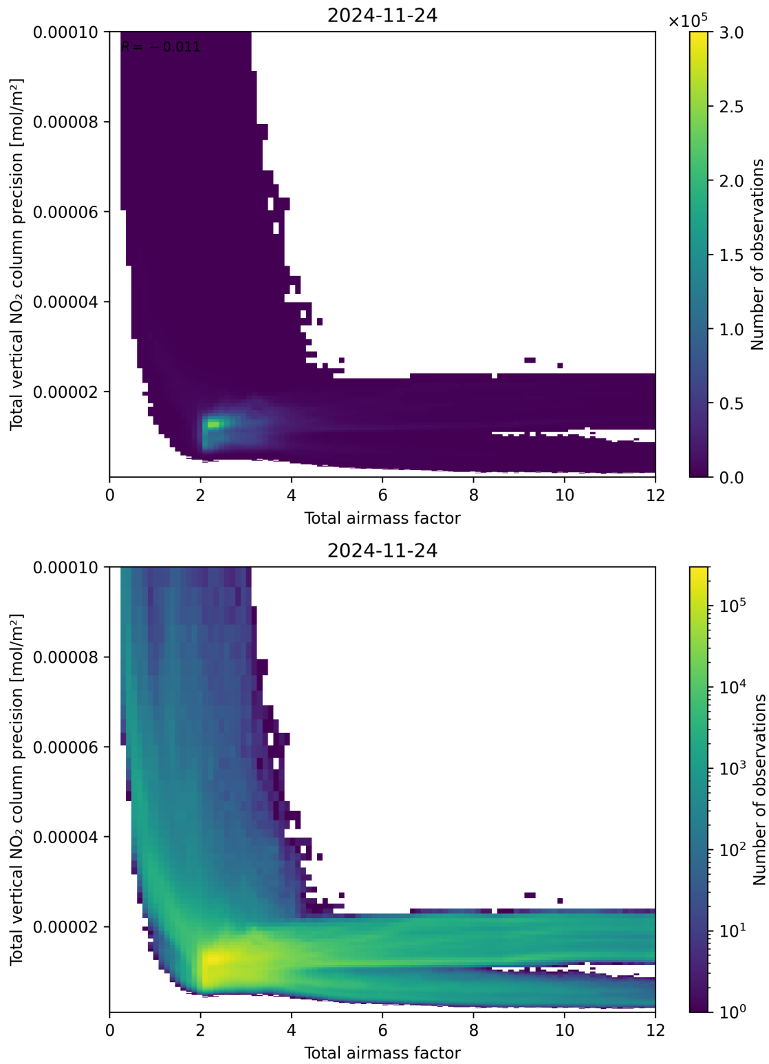
Figure 68: Scatter density plot of “Total airmass factor” against “Total vertical NO 2 column precision” for 2024-11-23 to 2024-11-25.
