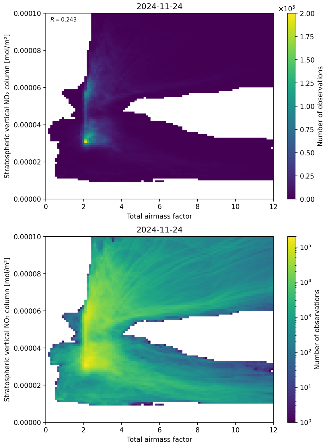
Figure 64: Scatter density plot of “Total airmass factor” against “Stratospheric vertical NO 2 column” for 2024-11-23 to 2024-11-25.
