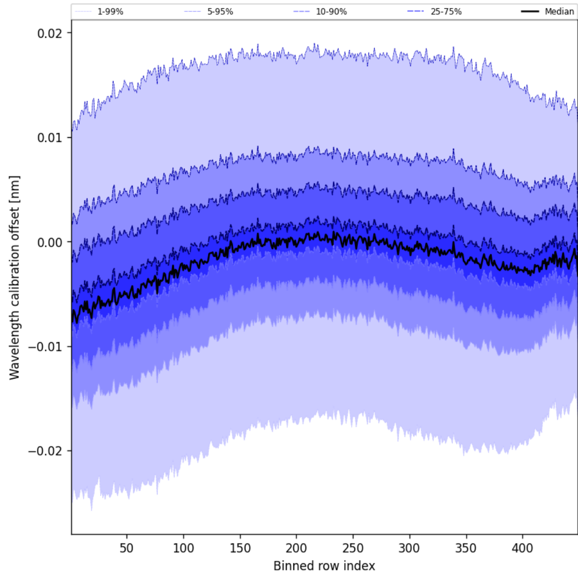
Figure 52: Along track statistics of “Wavelength calibration offset” for 2024-11-23 to 2024-11-25
