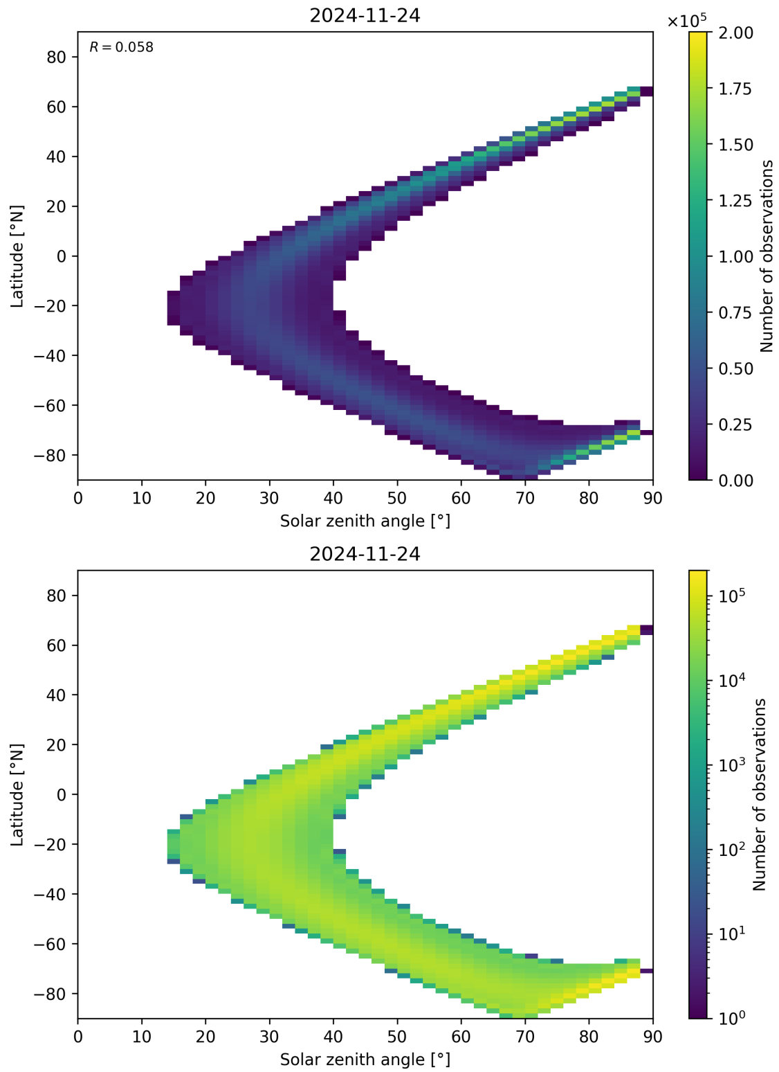
Figure 149: Scatter density plot of “Solar zenith angle” against “Latitude” for 2024-11-23 to 2024-11-25.
