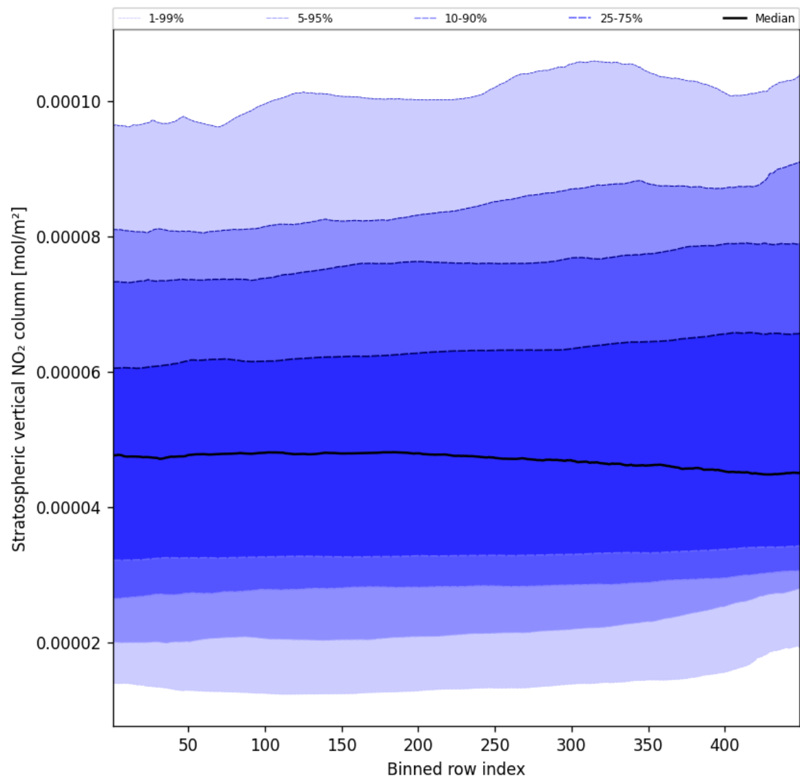
Figure 53: Along track statistics of “Stratospheric vertical NO 2 column” for 2024-11-23 to 2024-11-25
