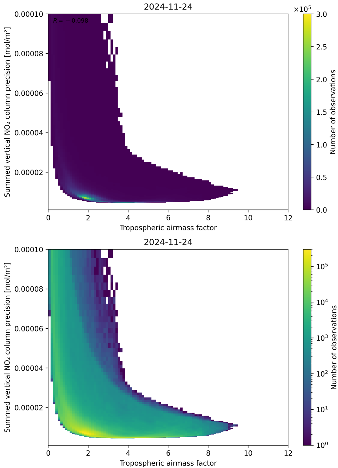
Figure 76: Scatter density plot of “Tropospheric air mass factor” against “Summed vertical NO 2 column precision” for 2024-11-23 to 2024-11-25.
