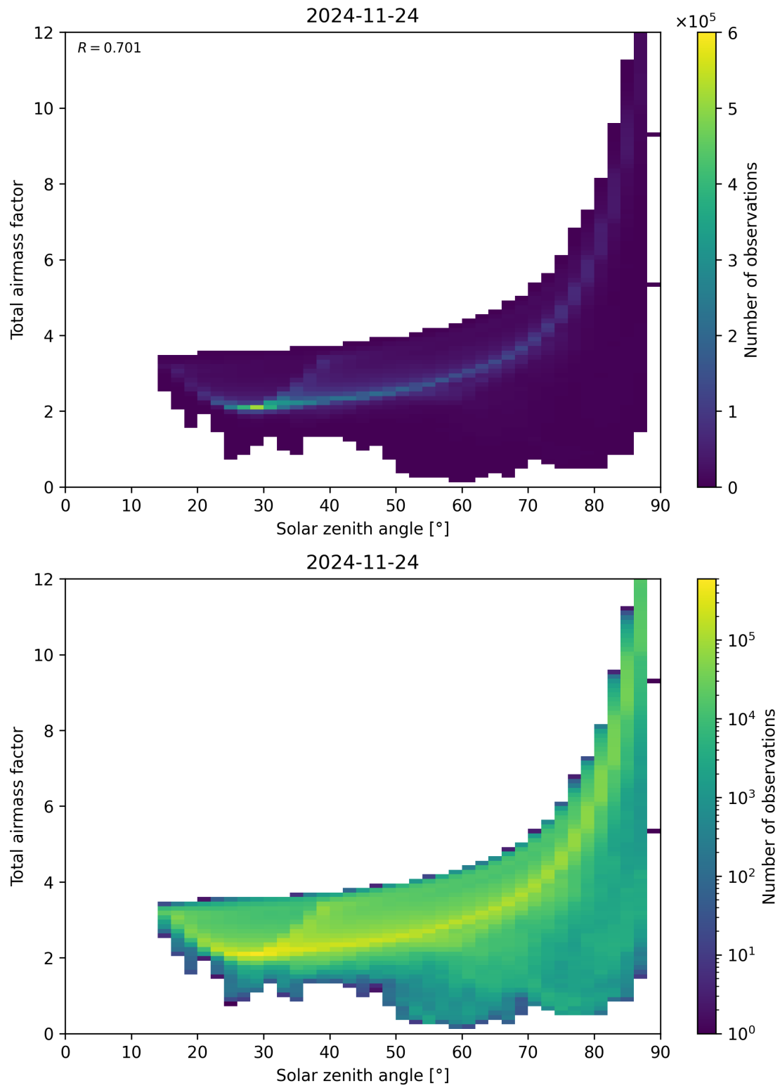
Figure 146: Scatter density plot of “Solar zenith angle” against “Total airmass factor” for 2024-11-23 to 2024-11-25.
