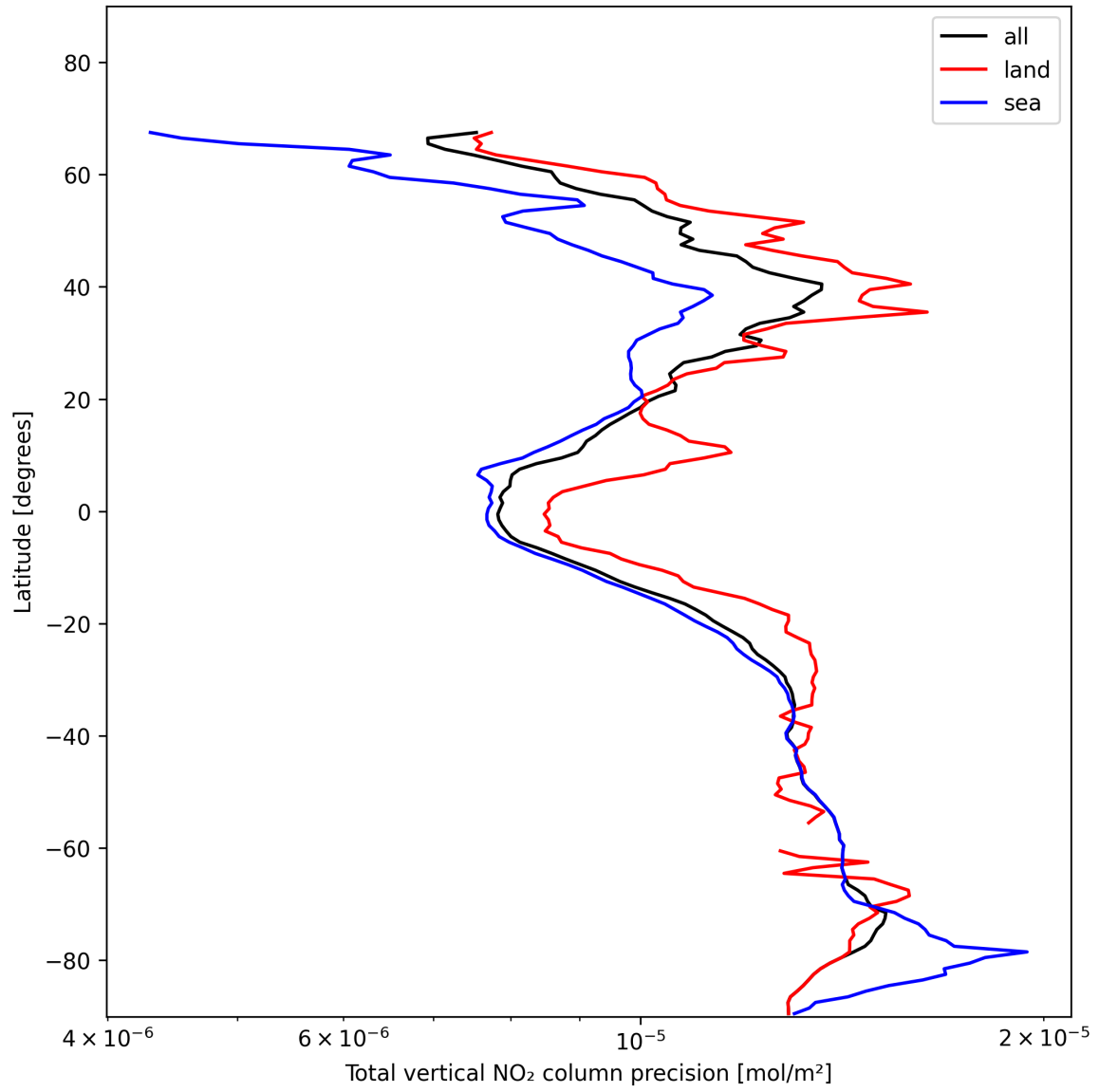
Figure 22: Zonal average of “Total vertical NO 2 column precision” for 2024-11-23 to 2024-11-25.
