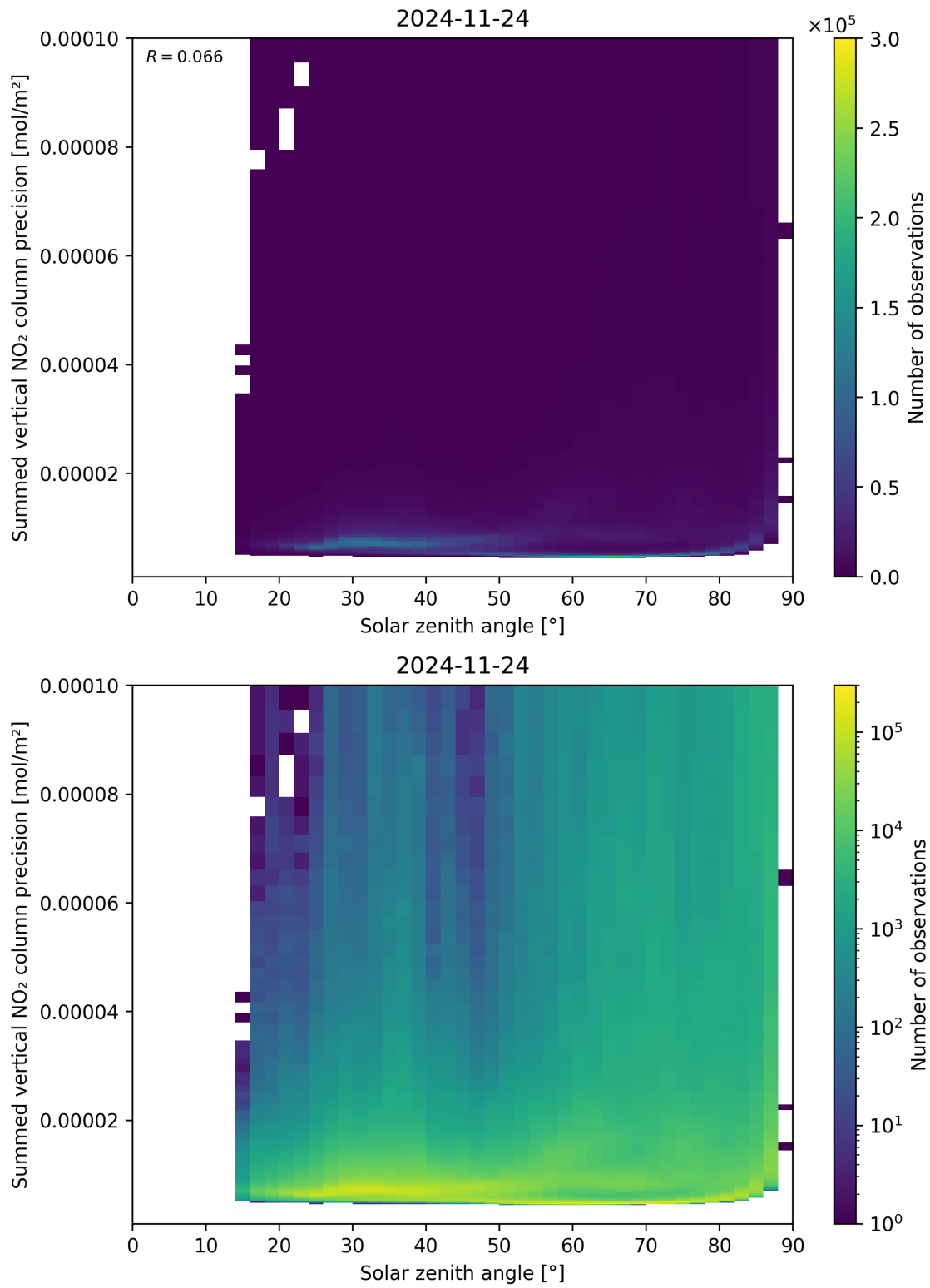
Figure 152: Scatter density plot of “Solar zenith angle” against “Summed vertical NO 2 column precision” for 2024-11-23 to 2024-11-25.
