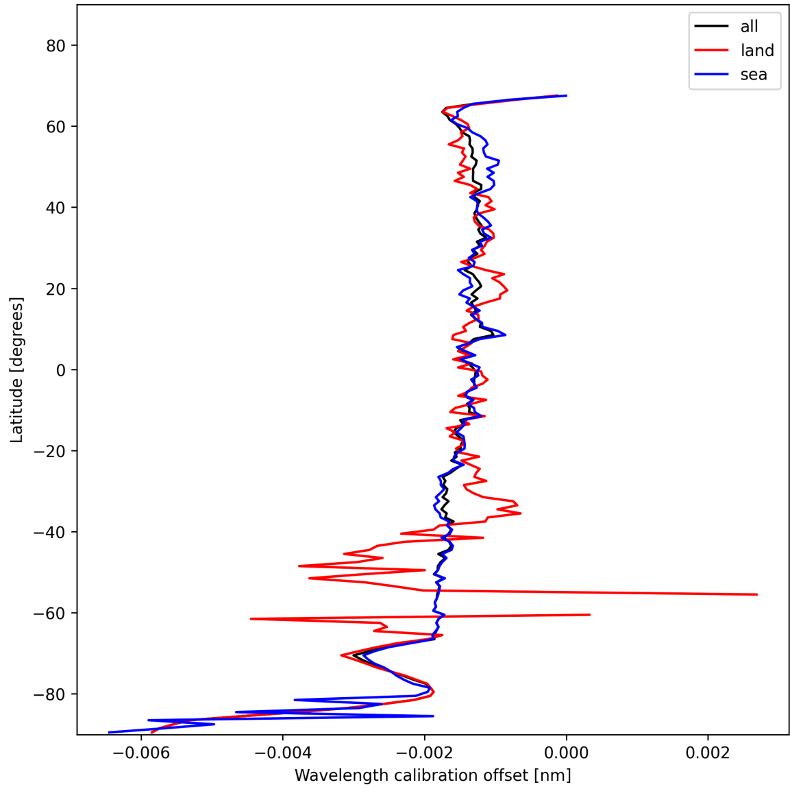
Figure 18: Zonal average of “Wavelength calibration offset” for 2024-11-23 to 2024-11-25.
