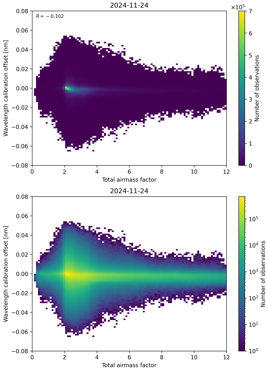
Figure 70: Scatter density plot of “Total airmass factor” against “Wavelength calibration offset” for 2024-11-23 to 2024-11-25.
