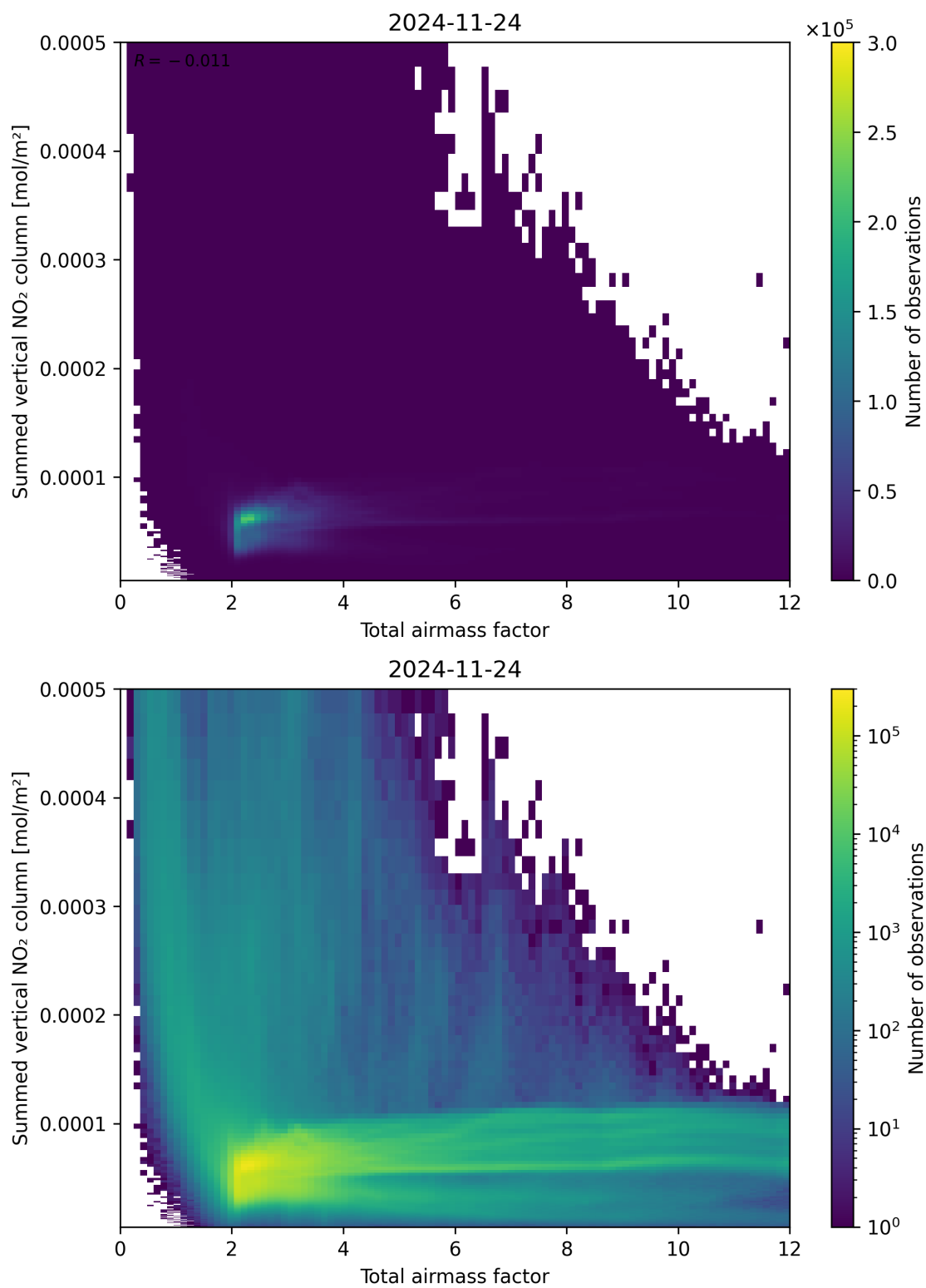
Figure 65: Scatter density plot of “Total airmass factor” against “Summed vertical NO 2 column” for 2024-11-23 to 2024-11-25.
