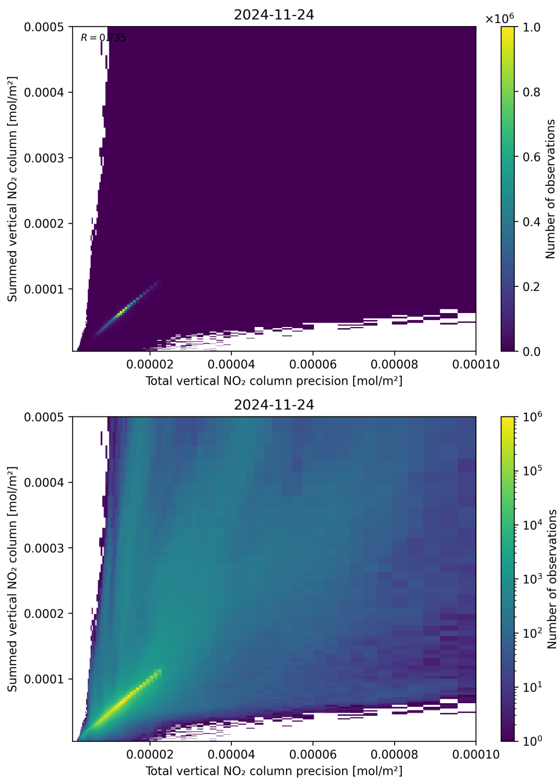
Figure 117: Scatter density plot of “Total vertical NO 2 column precision” against “Summed vertical NO 2 column” for 2024-11-23 to 2024-11-25.
