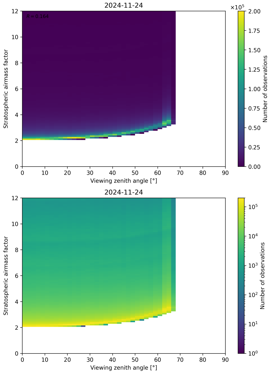
Figure 159: Scatter density plot of “Viewing zenith angle” against “Stratospheric airmass factor” for 2024-11-23 to 2024-11-25.
