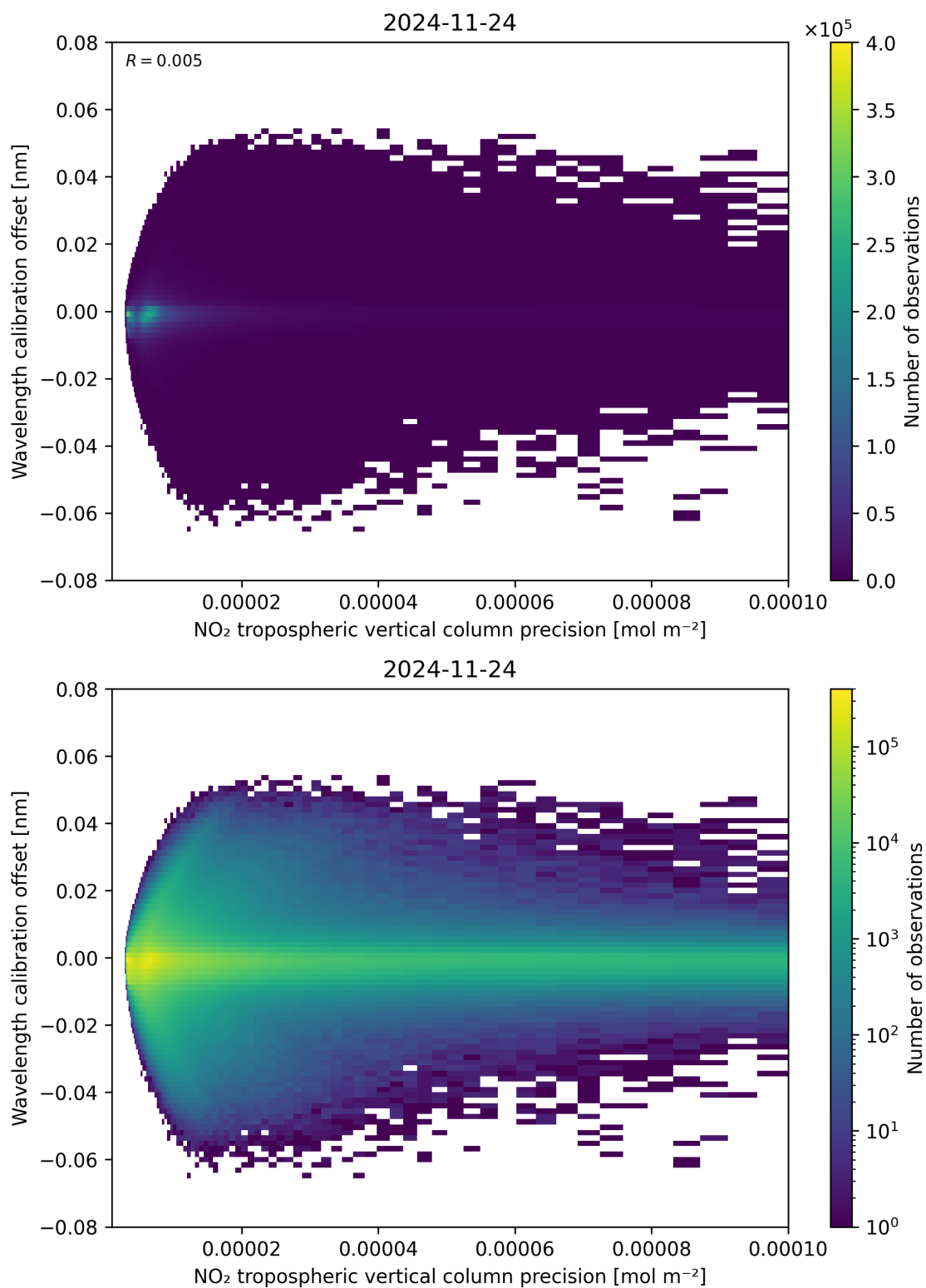
Figure 141: Scatter density plot of “NO 2 tropospheric vertical column precision” against “Wavelength calibration offset” for 2024-11-23 to 2024-11-25.
