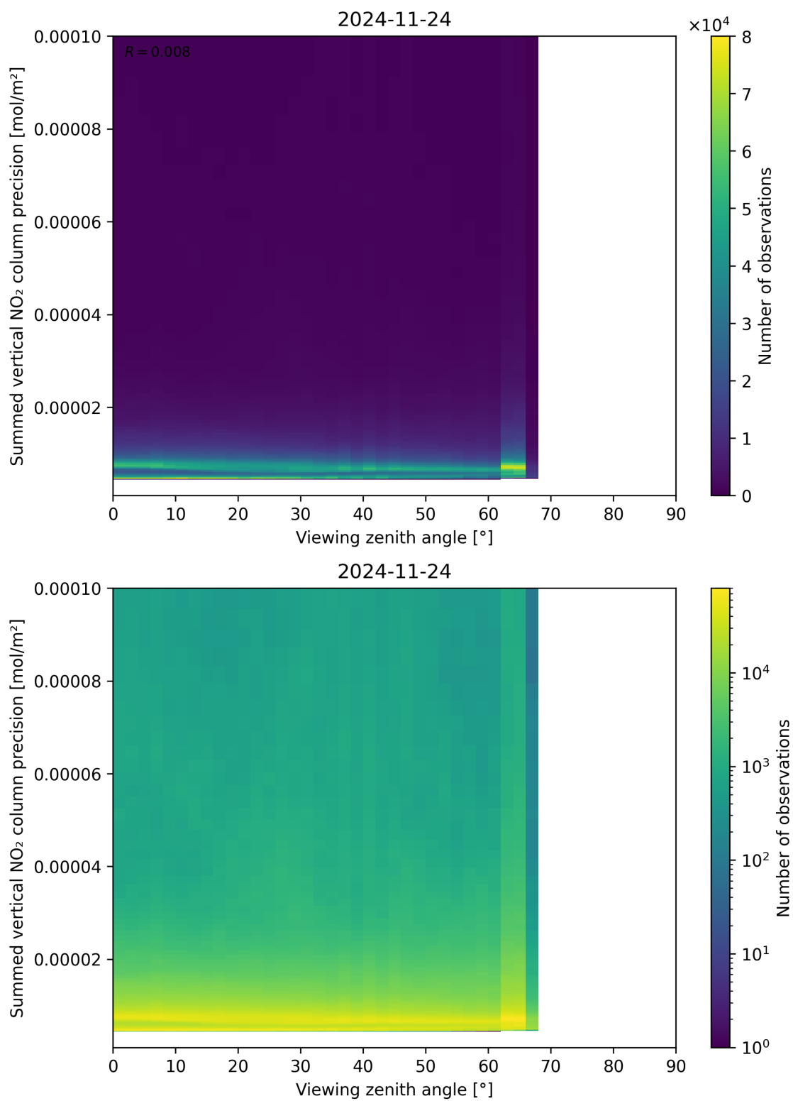
Figure 166: Scatter density plot of “Viewing zenith angle” against “Summed vertical NO 2 column precision” for 2024-11-23 to 2024-11-25.
