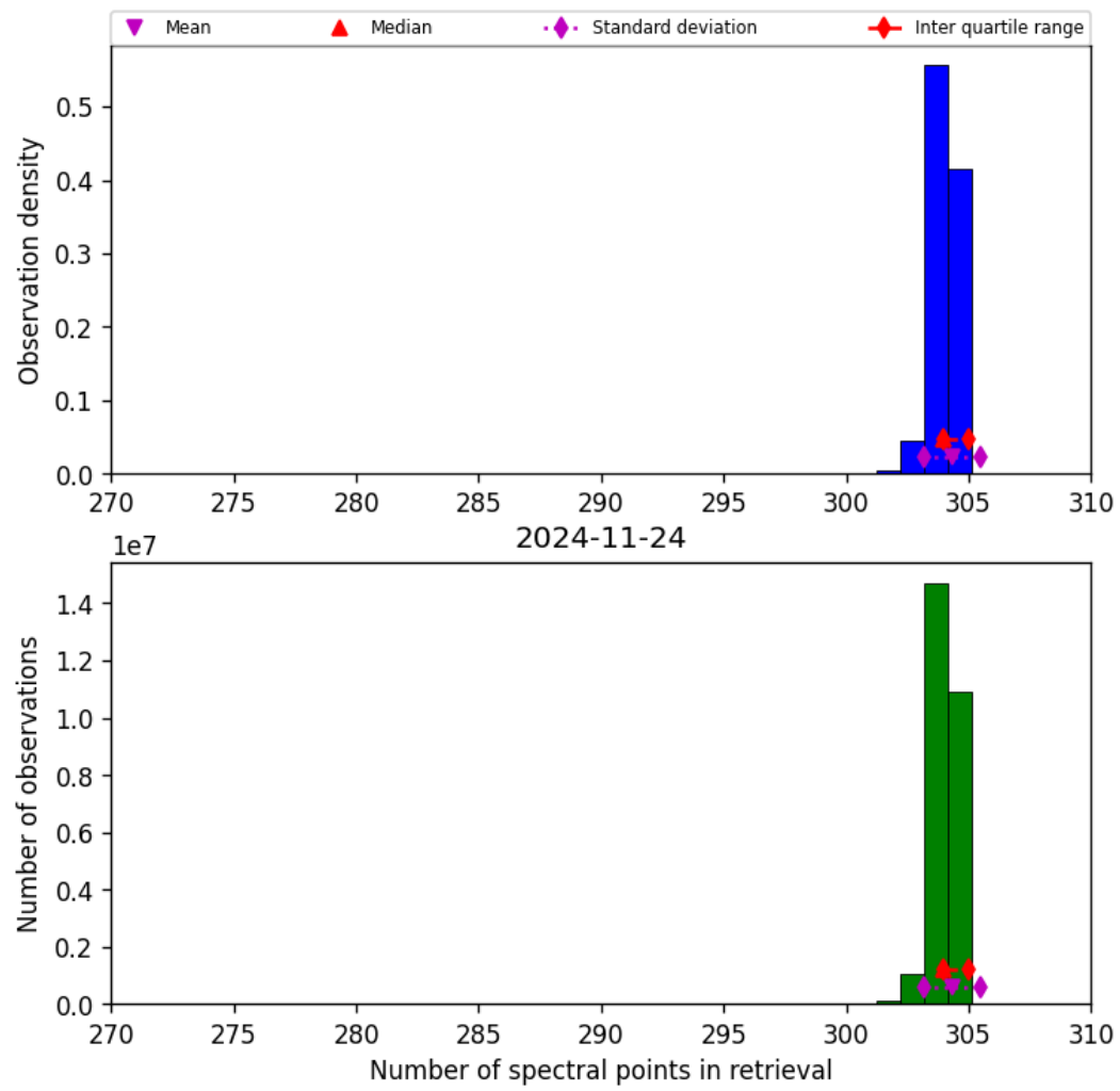
Figure 33: Histogram of “Number of spectral points in retrieval” for 2024-11-23 to 2024-11-25
