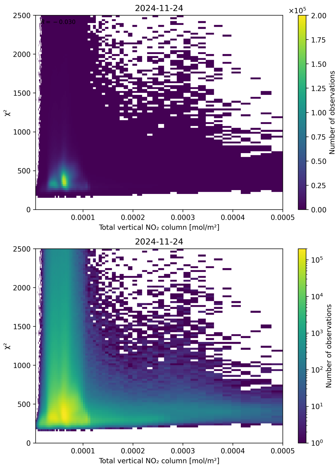
Figure 111: Scatter density plot of “Total vertical NO 2 column” against “ \chi^2 ” for 2024-11-23 to 2024-11-25.
