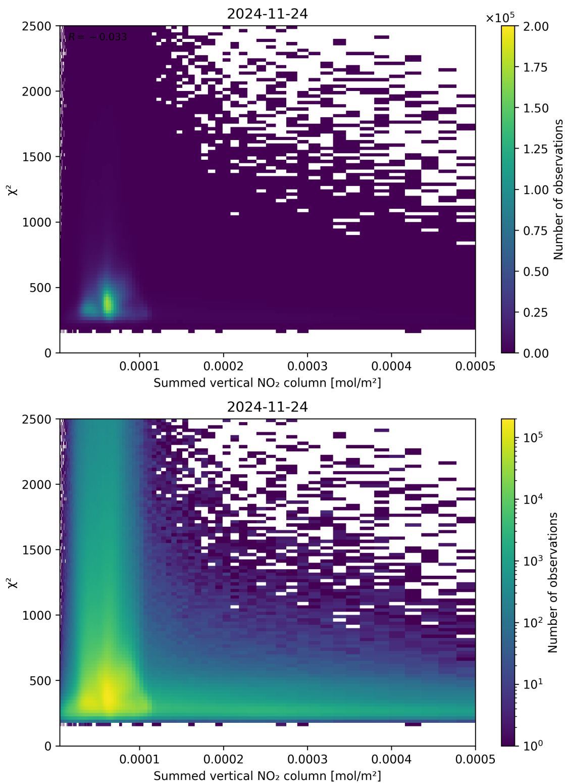
Figure 104: Scatter density plot of “Summed vertical NO 2 column” against “ \chi^2 ” for 2024-11-23 to 2024-11-25.
