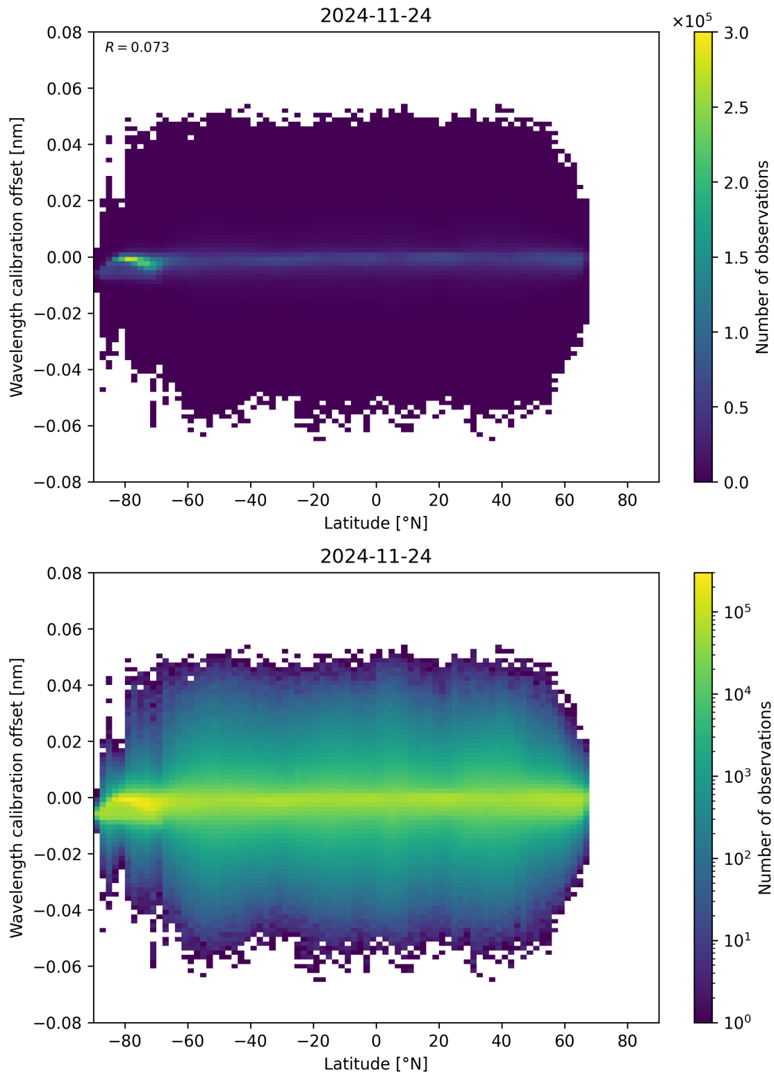
Figure 95: Scatter density plot of “Latitude” against “Wavelength calibration offset” for 2024-11-23 to 2024-11-25.
