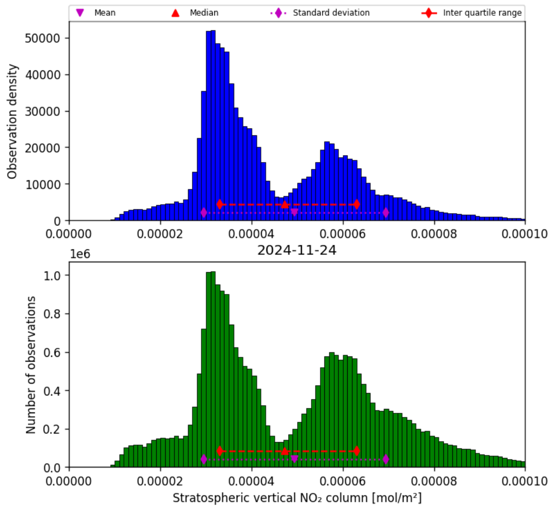
Figure 36: Histogram of “Stratospheric vertical NO 2 column” for 2024-11-23 to 2024-11-25
