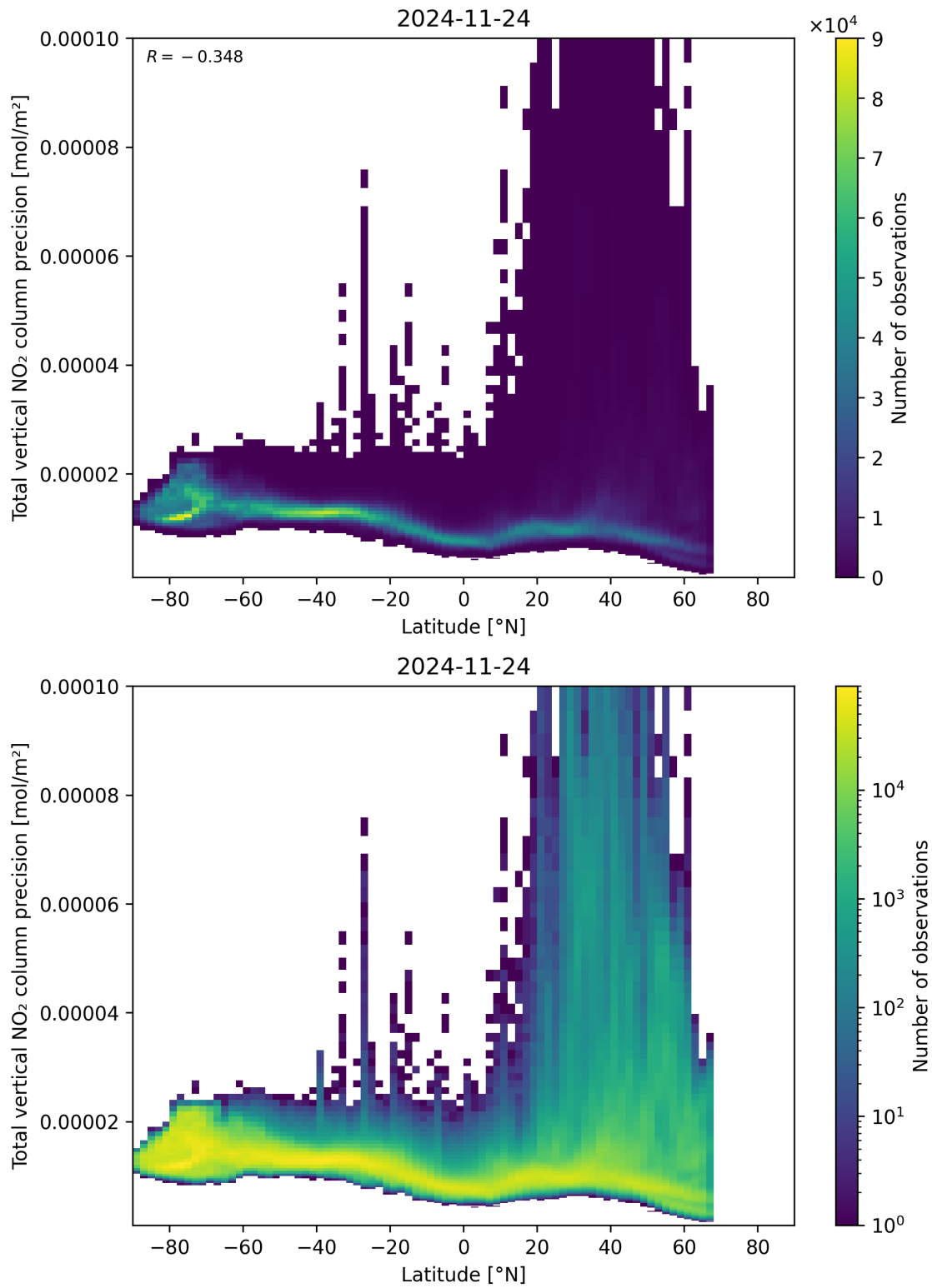
Figure 91: Scatter density plot of “Latitude” against “Total vertical NO 2 column precision” for 2024-11-23 to 2024-11-25.
