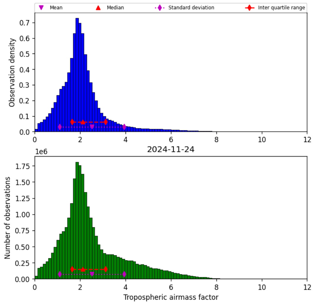
Figure 31: Histogram of “Tropospheric airmass factor” for 2024-11-23 to 2024-11-25
