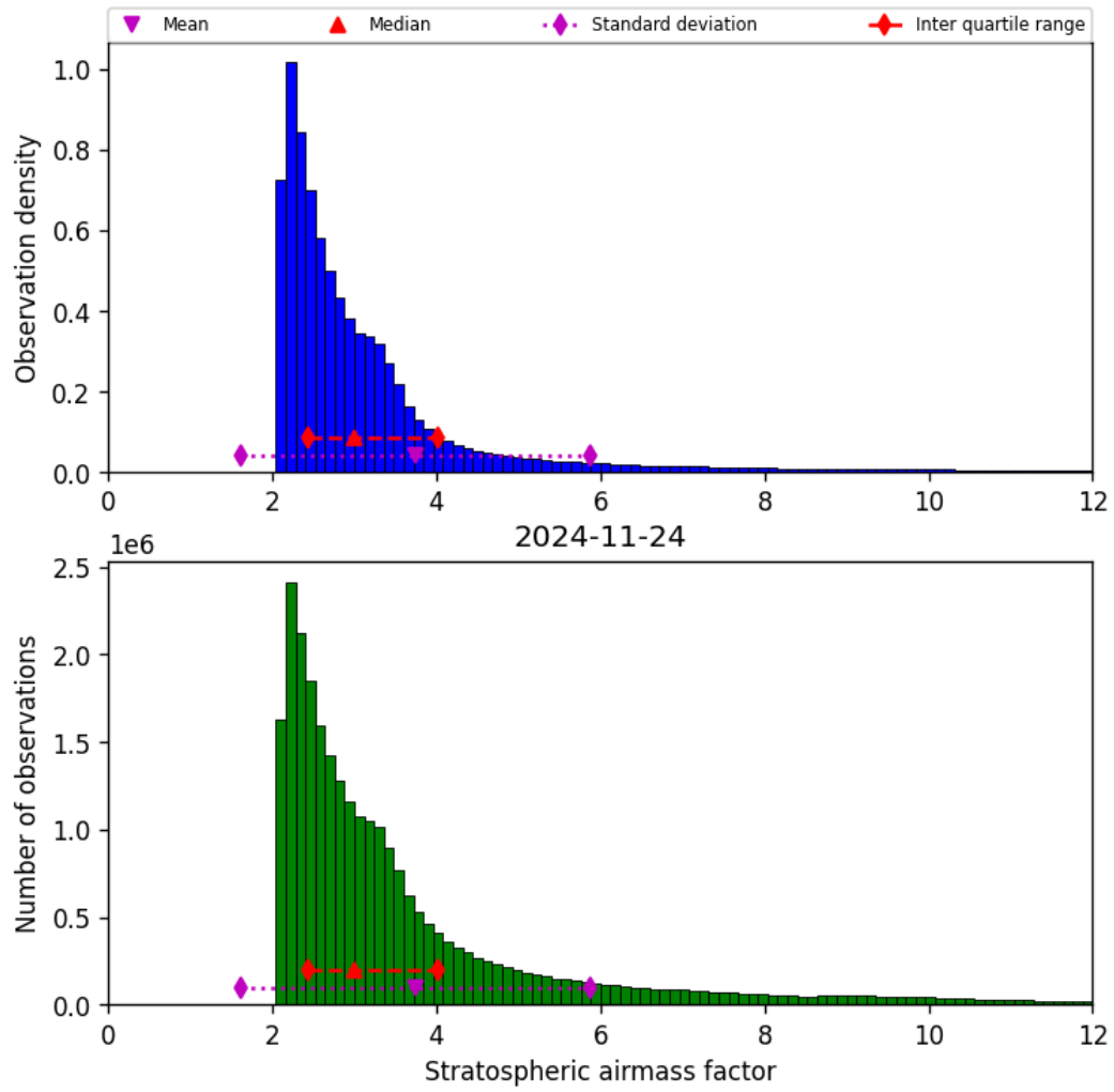
Figure 44: Histogram of “Stratospheric airmass factor” for 2024-11-23 to 2024-11-25
