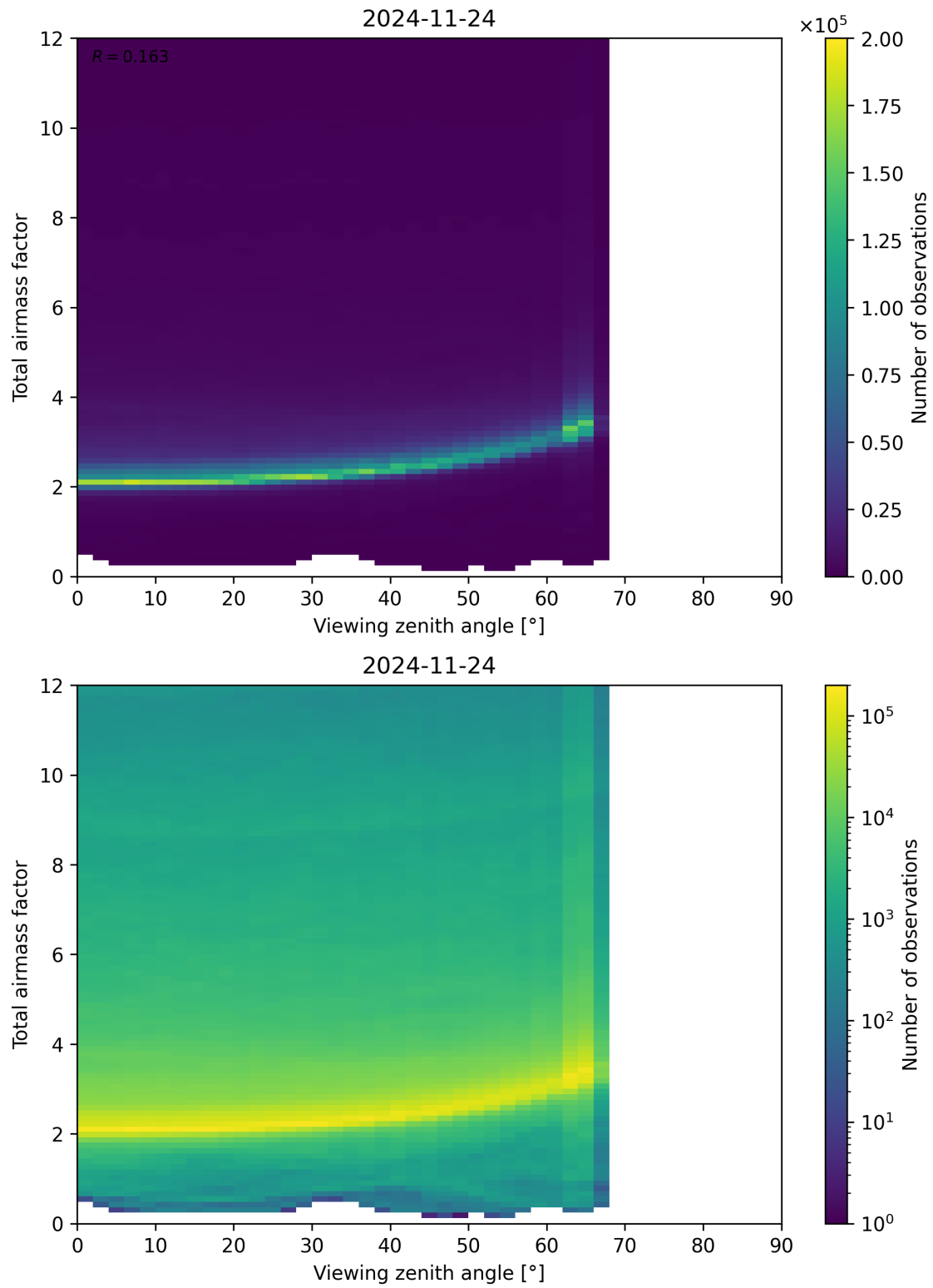
Figure 160: Scatter density plot of “Viewing zenith angle” against “Total airmass factor” for 2024-11-23 to 2024-11-25.
