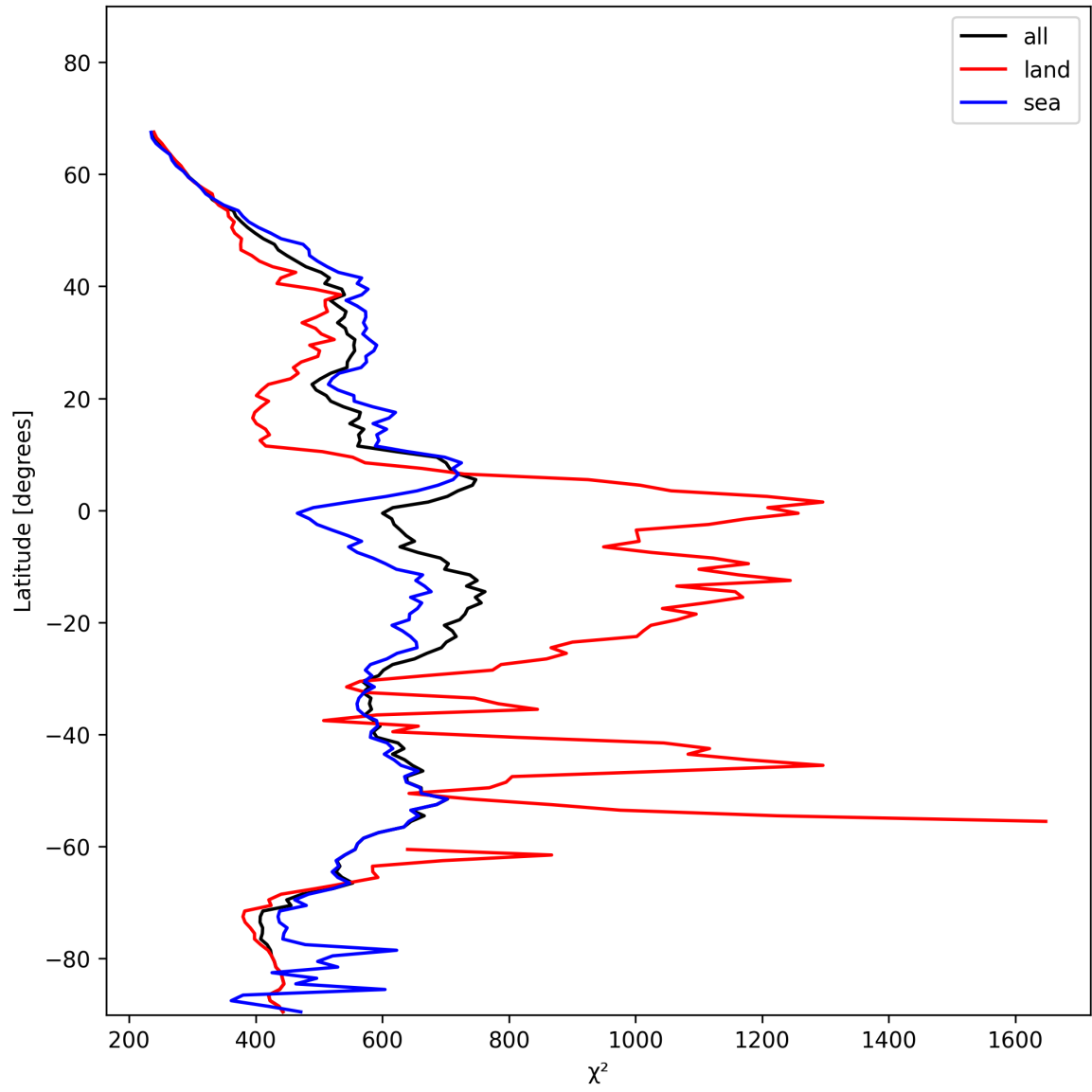
Figure 25: Zonal average of “ \chi^2 ” for 2024-11-23 to 2024-11-25.
