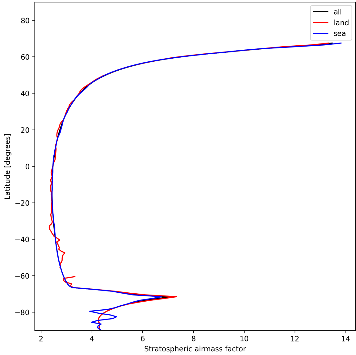
Figure 27: Zonal average of “Stratospheric airmass factor” for 2024-11-23 to 2024-11-25.
