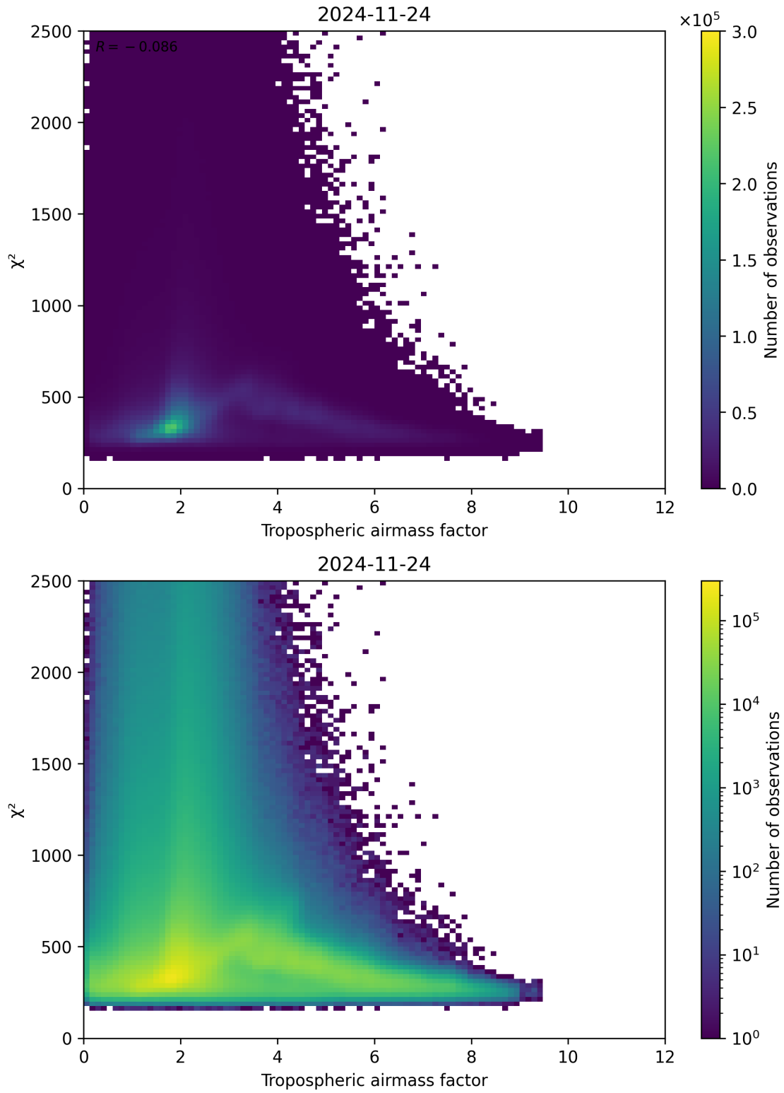
Figure 73: Scatter density plot of “Tropospheric airmass factor” against “ \chi^2 ” for 2024-11-23 to 2024-11-25.
