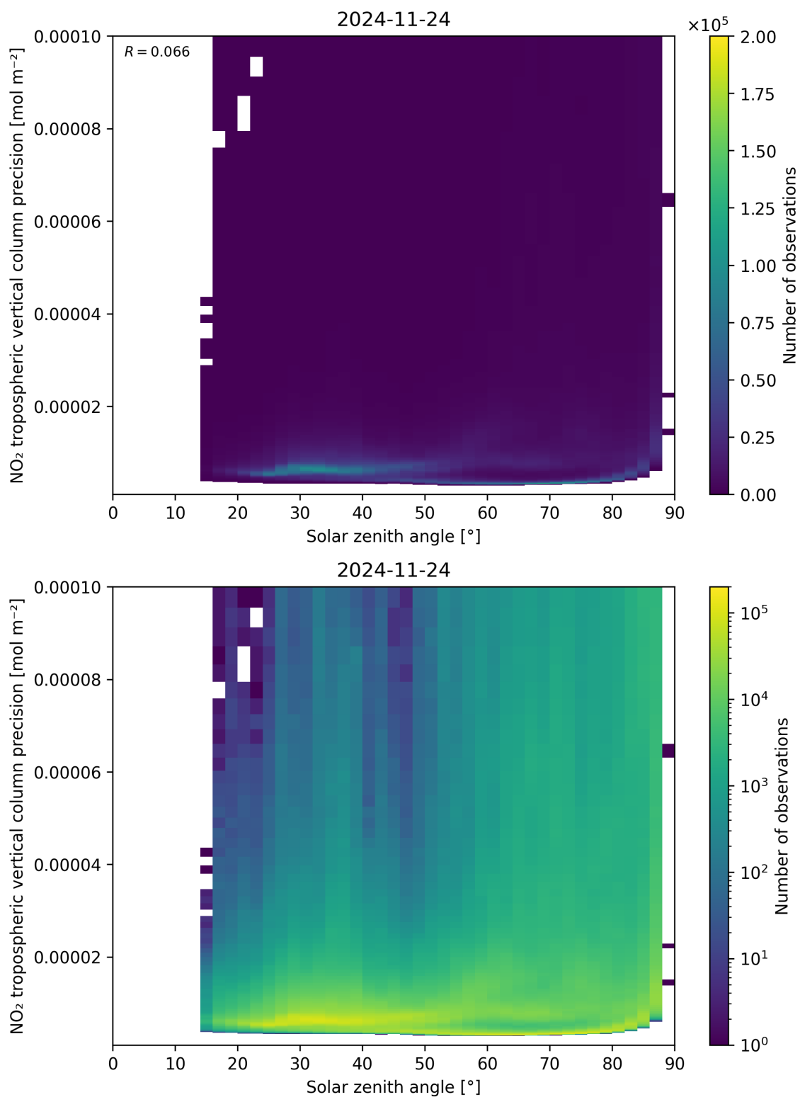
Figure 156: Scatter density plot of “Solar zenith angle” against “NO 2 tropospheric vertical column precision” for 2024-11-23 to 2024-11-25.
