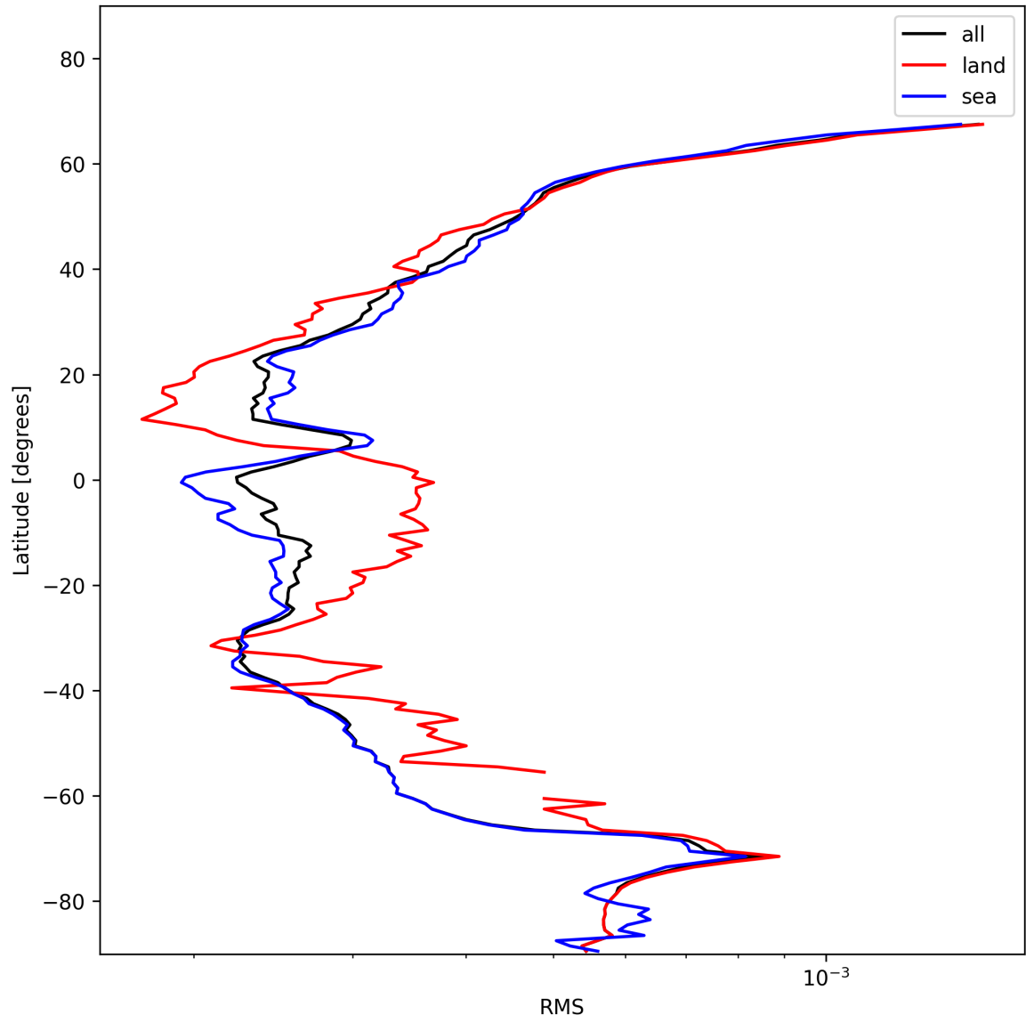
Figure 26: Zonal average of “RMS” for 2024-11-23 to 2024-11-25.
