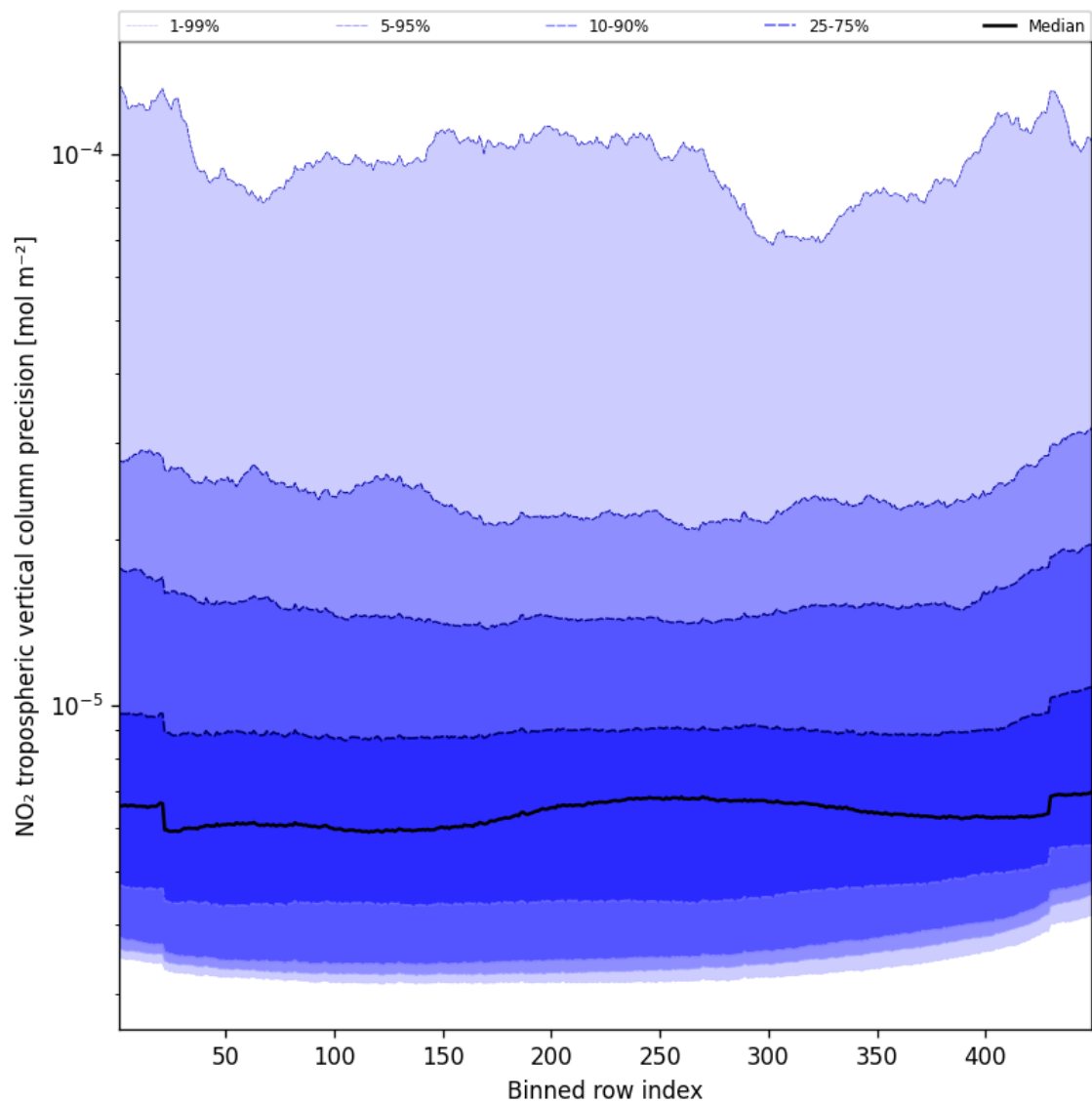
Figure 47: Along track statistics of “NO 2 tropospheric vertical column precision” for 2024-11-23 to 2024-11-25
