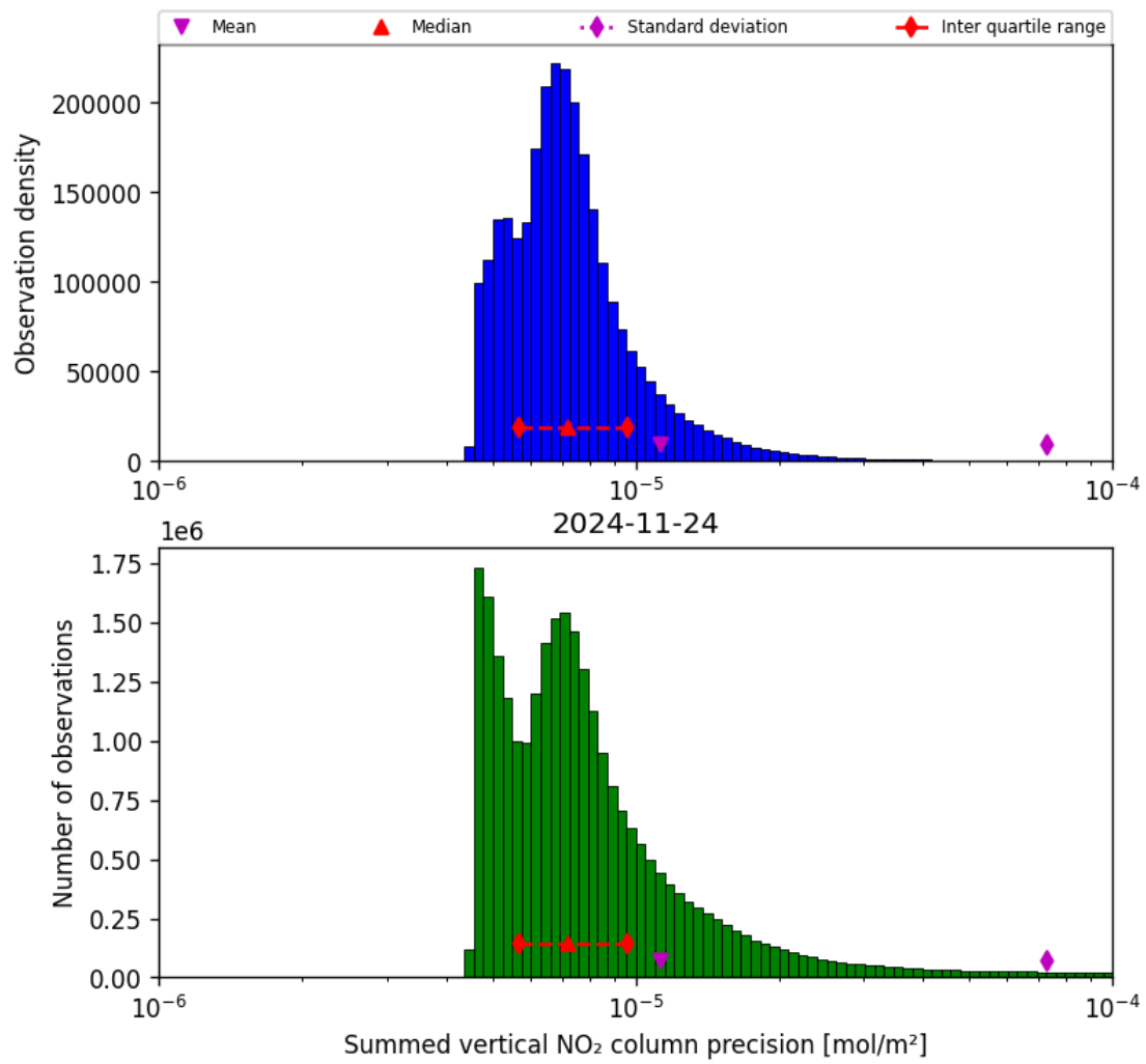
Figure 41: Histogram of "Summed vertical NO 2 column precision" for 2024-11-23 to 2024-11-25
