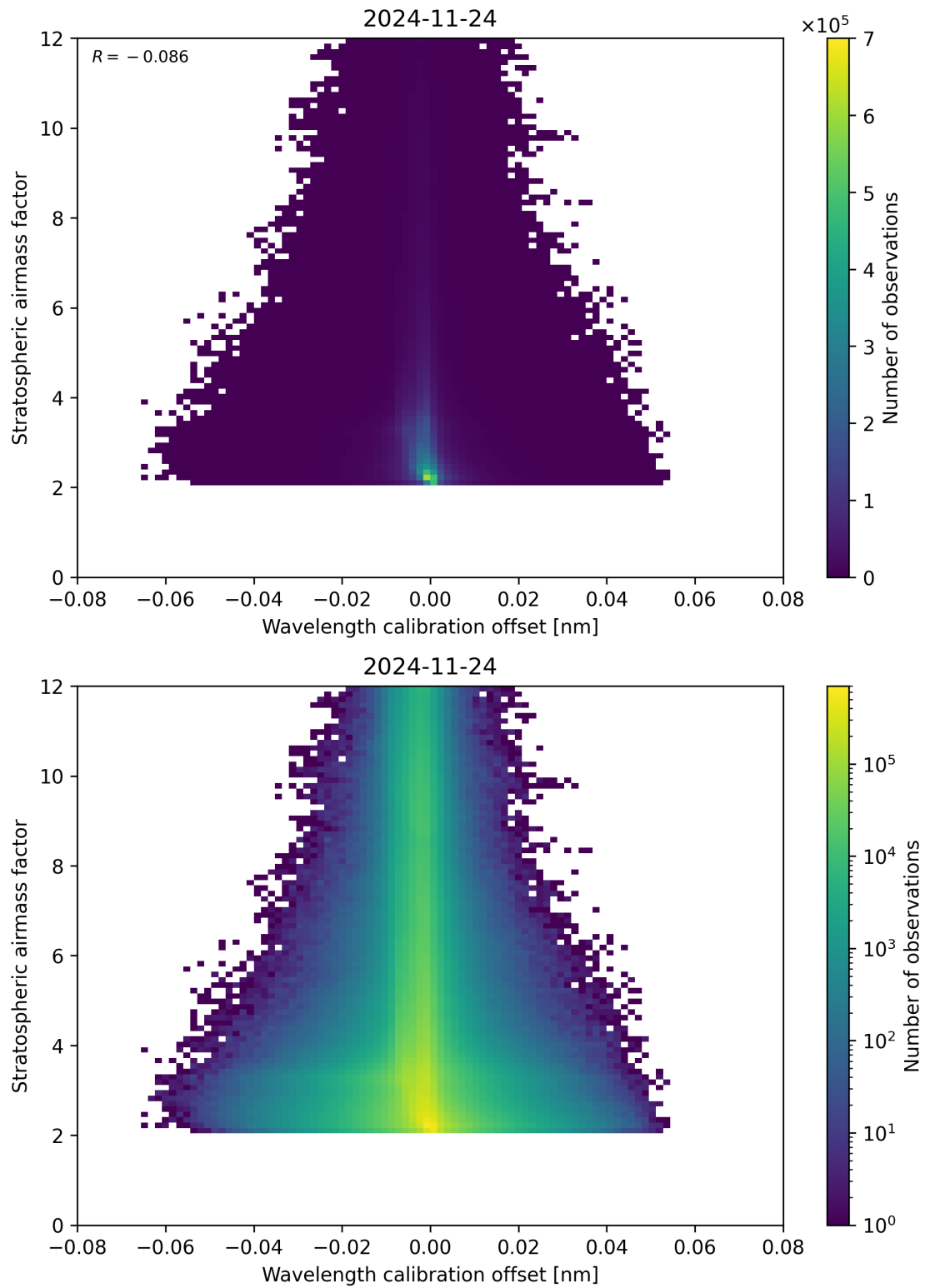
Figure 174: Scatter density plot of “Wavelength calibration offset” against “Stratospheric airmass factor” for 2024-11-23 to 2024-11-25.
