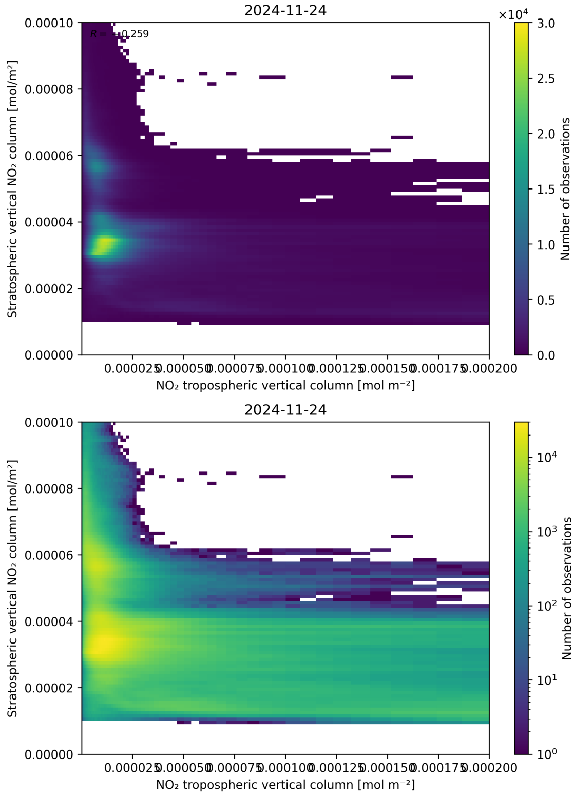
Figure 125: Scatter density plot of “NO 2 tropospheric vertical column” against “Stratospheric vertical NO 2 column” for 2024-11-23 to 2024-11-25.
