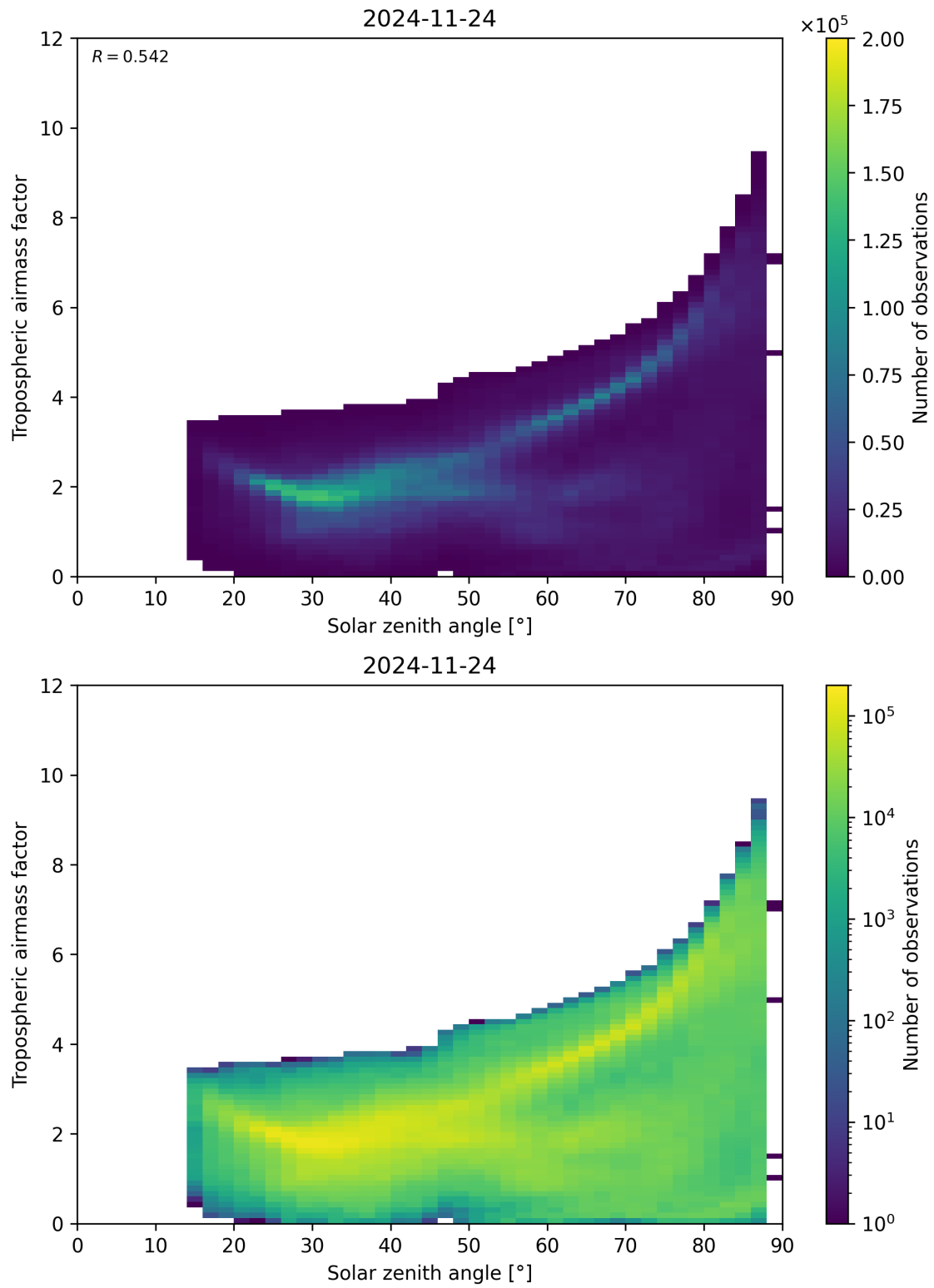
Figure 147: Scatter density plot of “Solar zenith angle” against “Tropospheric airmass factor” for 2024-11-23 to 2024-11-25.
