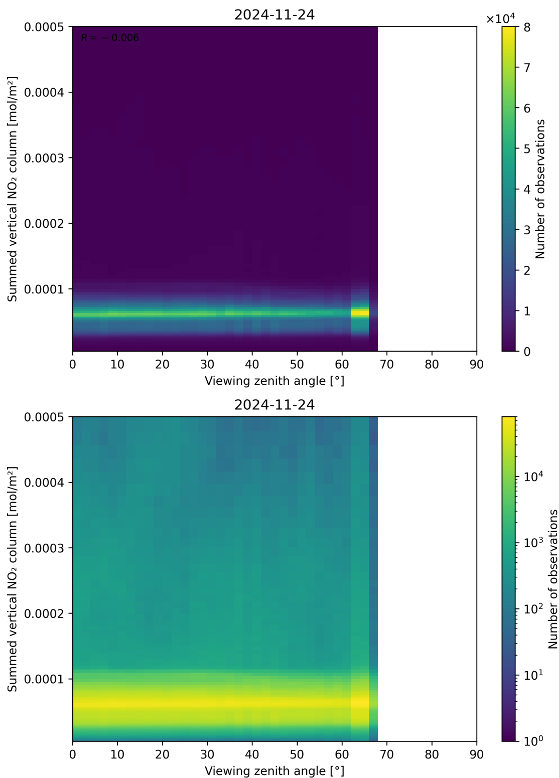
Figure 165: Scatter density plot of “Viewing zenith angle” against “Summed vertical NO 2 column” for 2024-11-23 to 2024-11-25.
