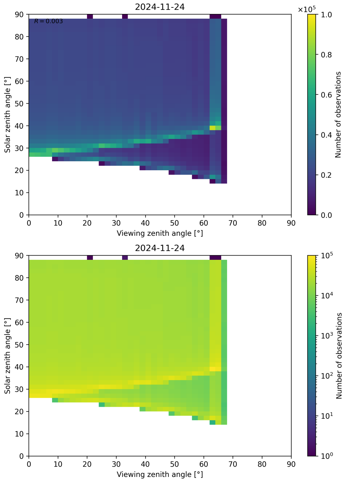
Figure 172: Scatter density plot of “Viewing zenith angle” against “Solar zenith angle” for 2024-11-23 to 2024-11-25.
