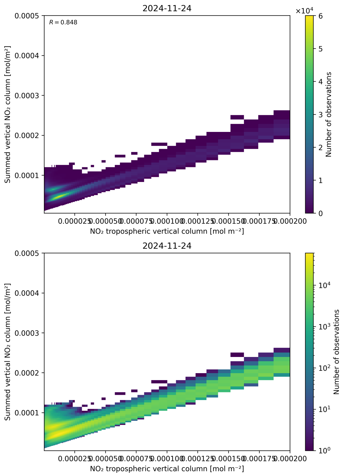
Figure 126: Scatter density plot of “NO 2 tropospheric vertical column” against “Summed vertical NO 2 column” for 2024-11-23 to 2024-11-25.
