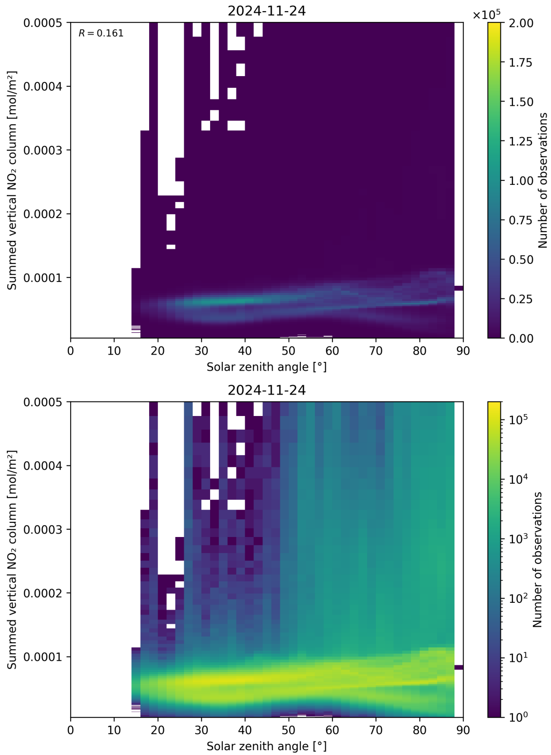
Figure 151: Scatter density plot of “Solar zenith angle” against “Summed vertical NO 2 column” for 2024-11-23 to 2024-11-25.
