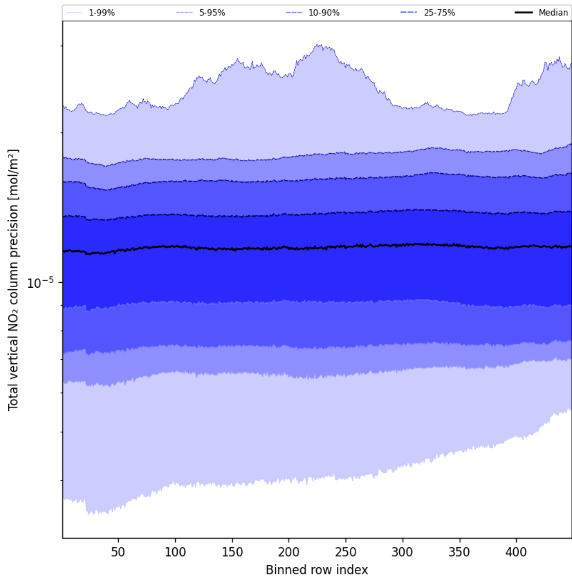
Figure 56: Along track statistics of “Total vertical NO 2 column precision” for 2024-11-23 to 2024-11-25
