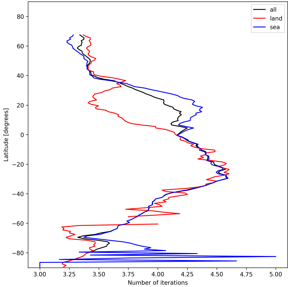
Figure 17: Zonal average of “Number of iterations” for 2024-11-23 to 2024-11-25.
