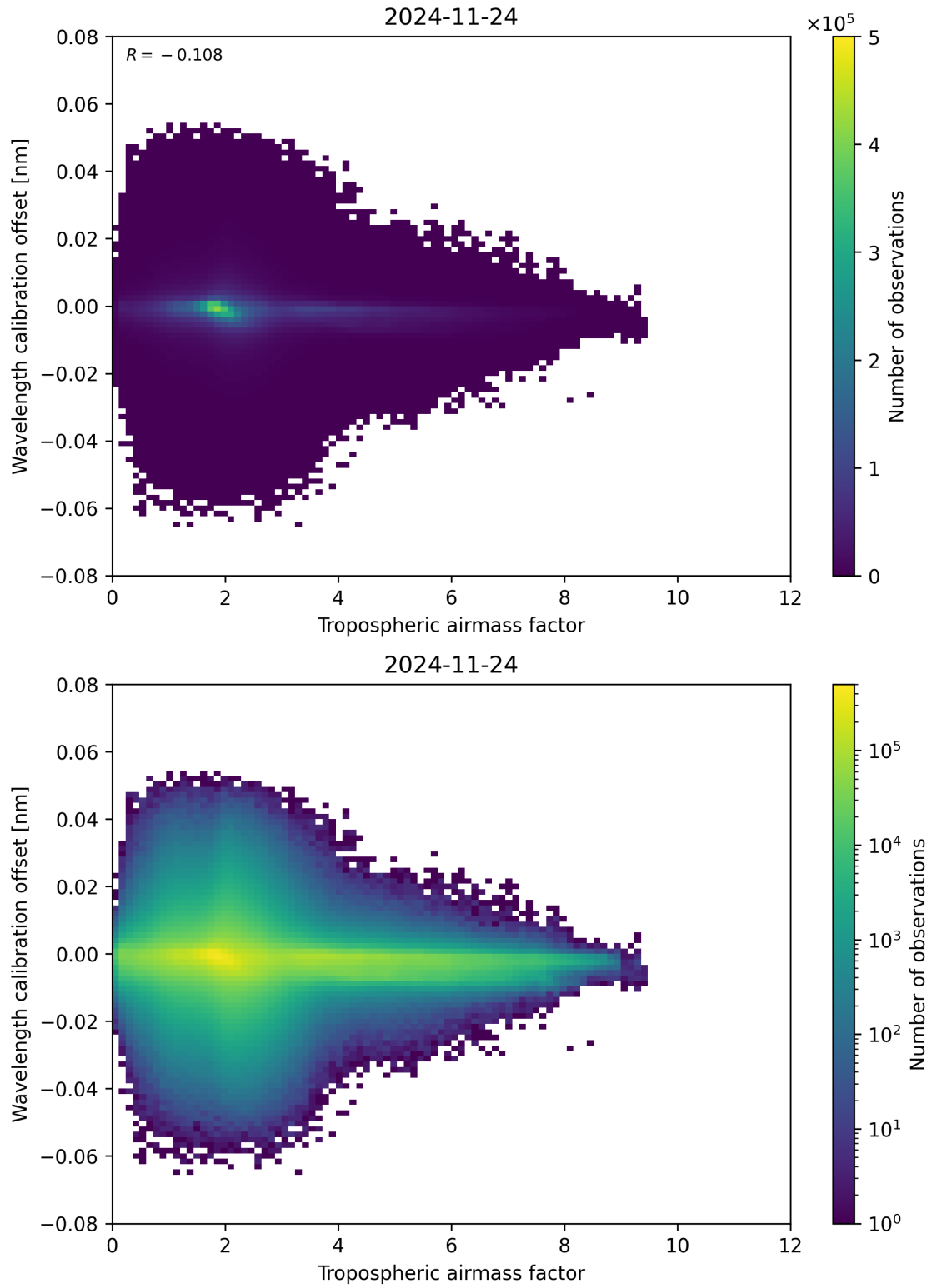
Figure 80: Scatter density plot of “Tropospheric airmass factor” against “Wavelength calibration offset” for 2024-11-23 to 2024-11-25.
