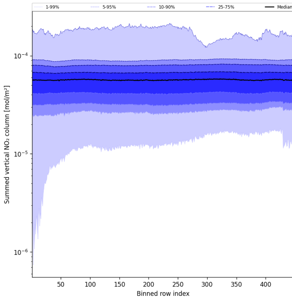
Figure 57: Along track statistics of “Summed vertical NO 2 column” for 2024-11-23 to 2024-11-25
