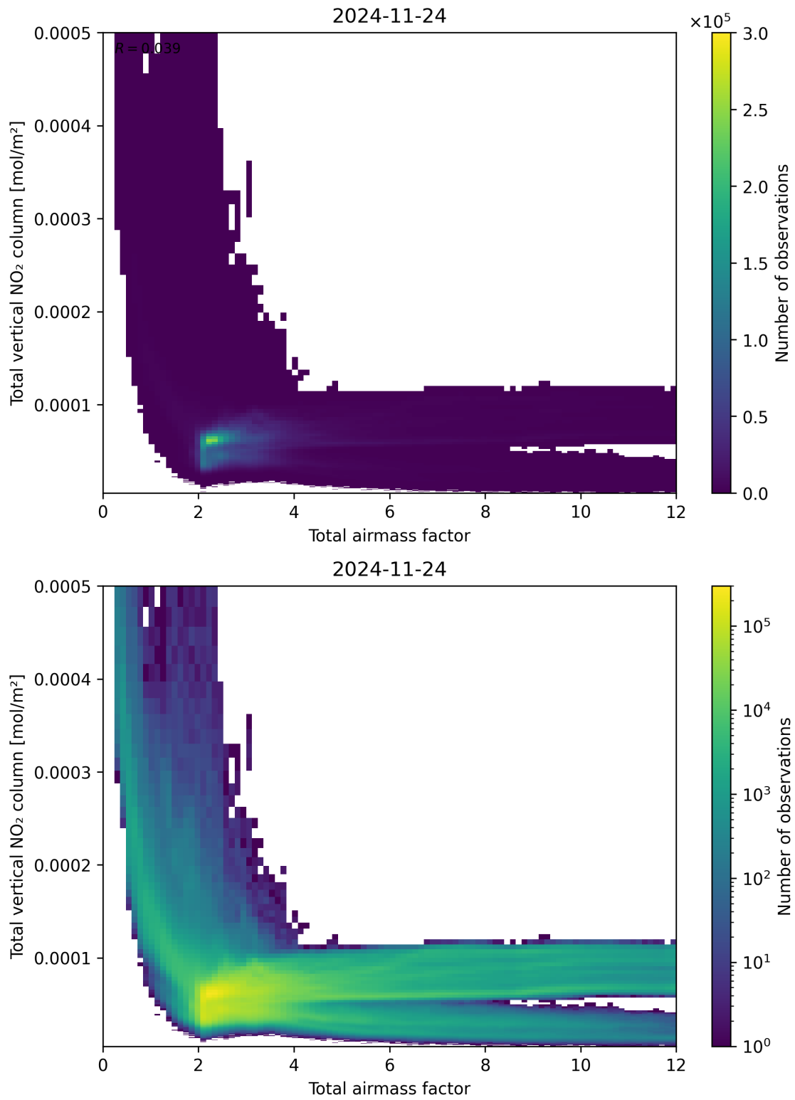
Figure 67: Scatter density plot of “Total airmass factor” against “Total vertical NO 2 column” for 2024-11-23 to 2024-11-25.
