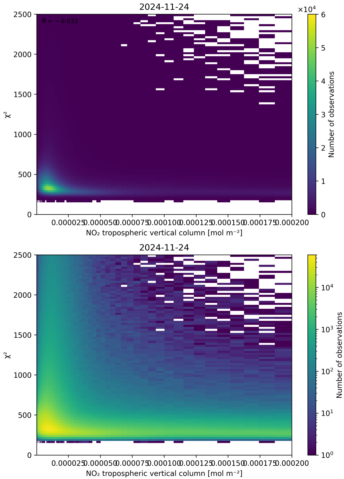
Figure 124: Scatter density plot of “NO 2 tropospheric vertical column” against “ \chi^2 ” for 2024-11-23 to 2024-11-25.
