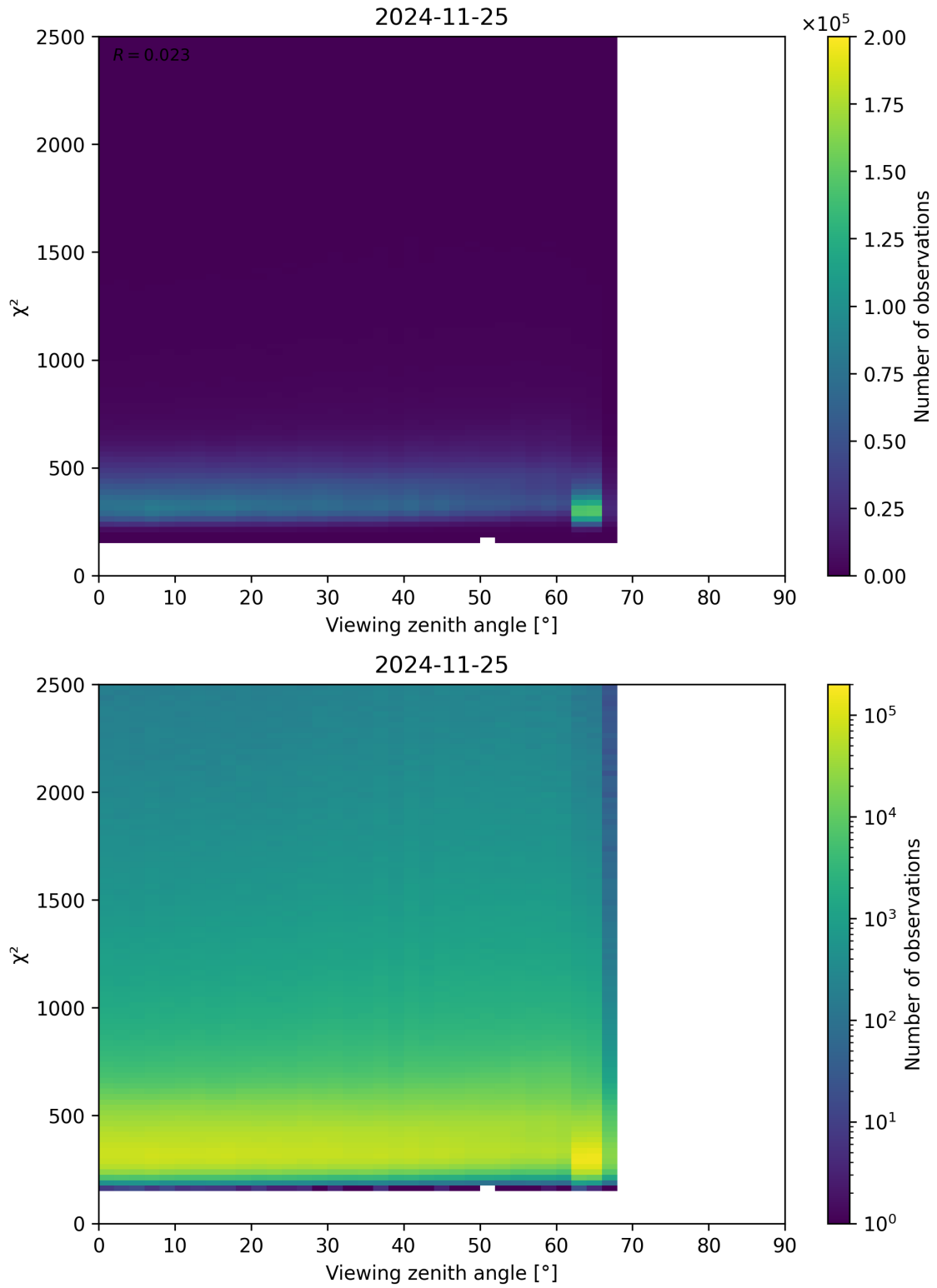
Figure 162: Scatter density plot of “Viewing zenith angle” against “ \chi^2 ” for 2024-11-25 to 2024-11-26.
