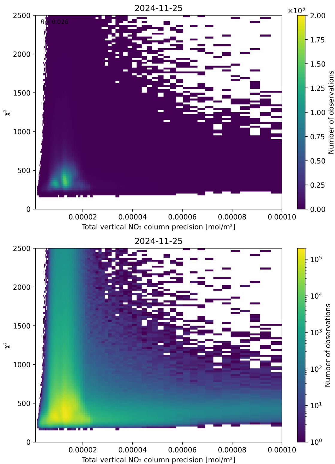
Figure 116: Scatter density plot of “Total vertical NO 2 column precision” against “ \chi^2 ” for 2024-11-25 to 2024-11-26.
