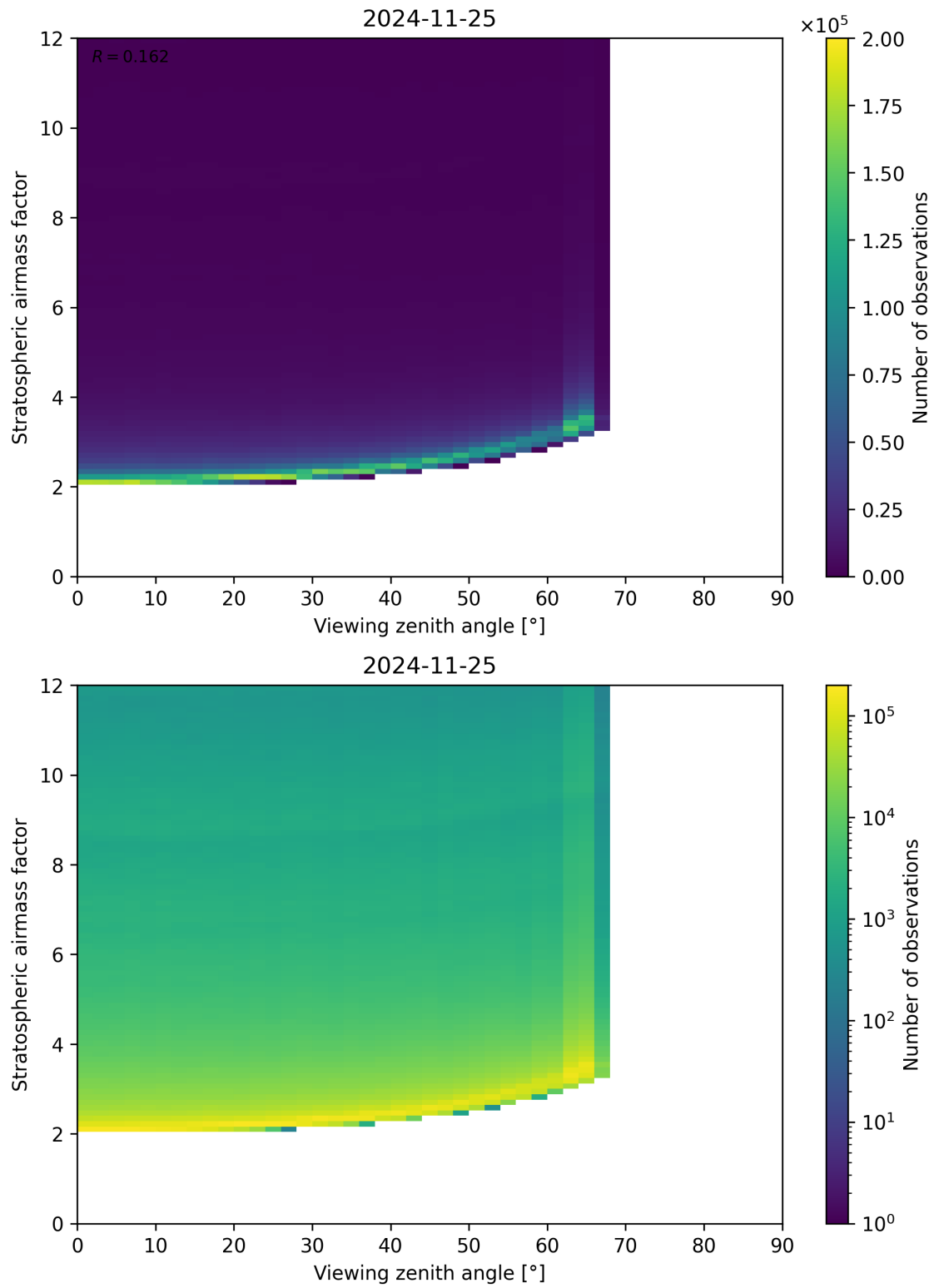
Figure 159: Scatter density plot of “Viewing zenith angle” against “Stratospheric airmass factor” for 2024-11-25 to 2024-11-26.
