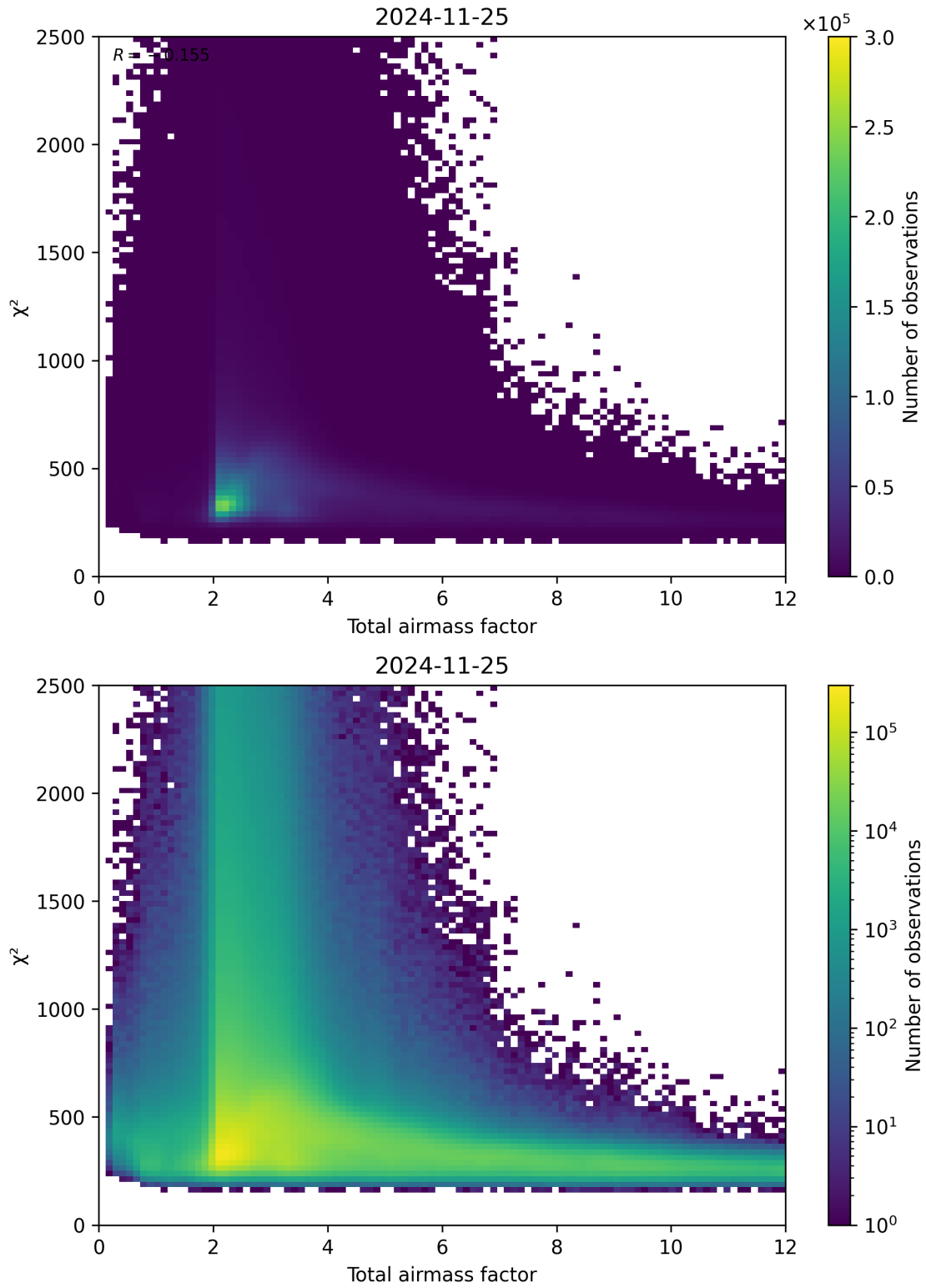
Figure 63: Scatter density plot of “Total airmass factor” against “ \chi^2 ” for 2024-11-25 to 2024-11-26.
