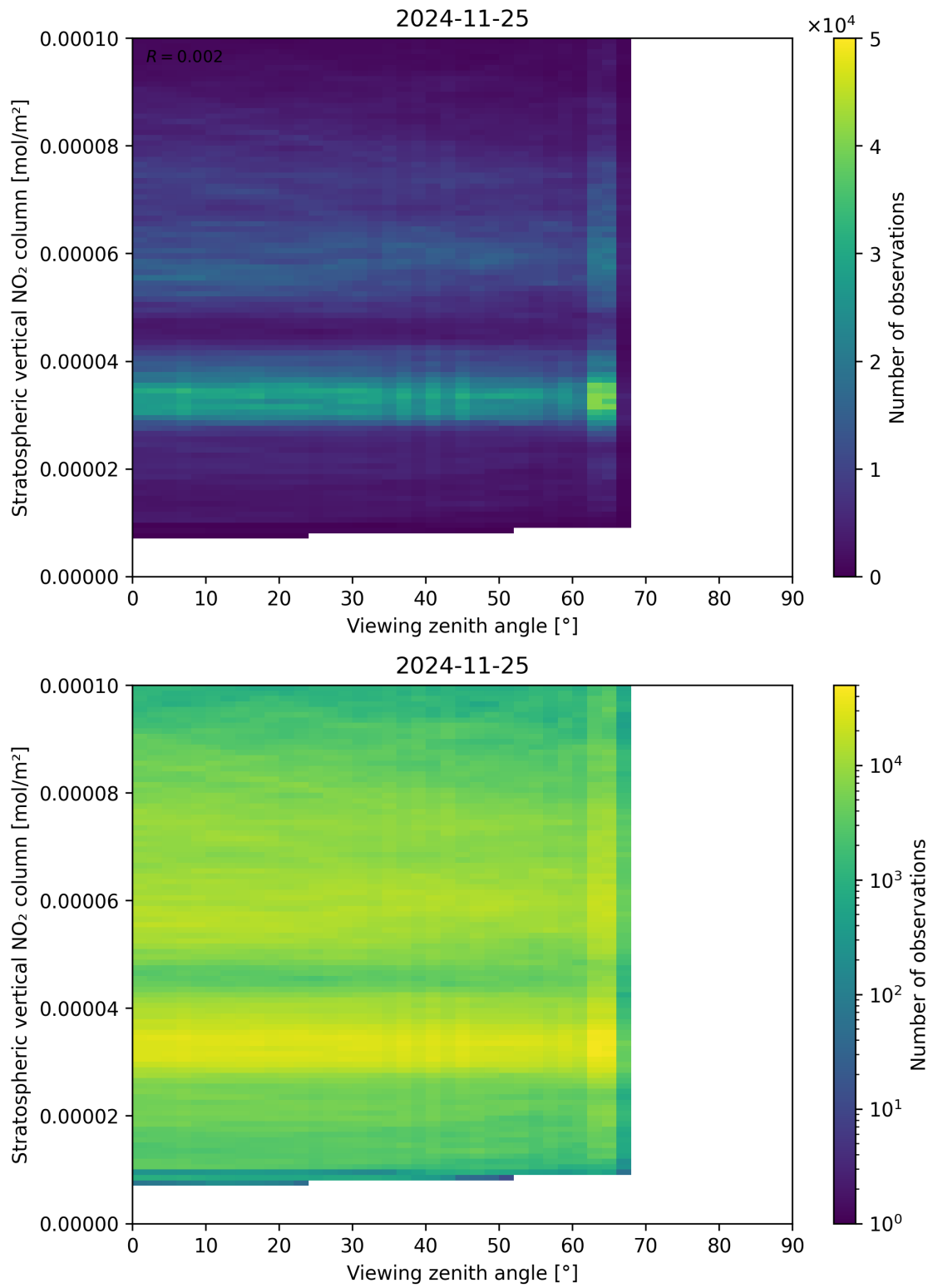
Figure 164: Scatter density plot of “Viewing zenith angle” against “Stratospheric vertical NO 2 column” for 2024-11-25 to 2024-11-26.
