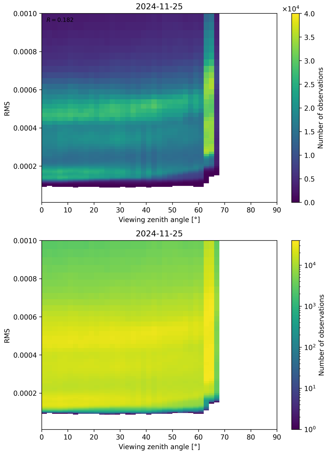
Figure 171: Scatter density plot of “Viewing zenith angle” against “RMS” for 2024-11-25 to 2024-11-26.
