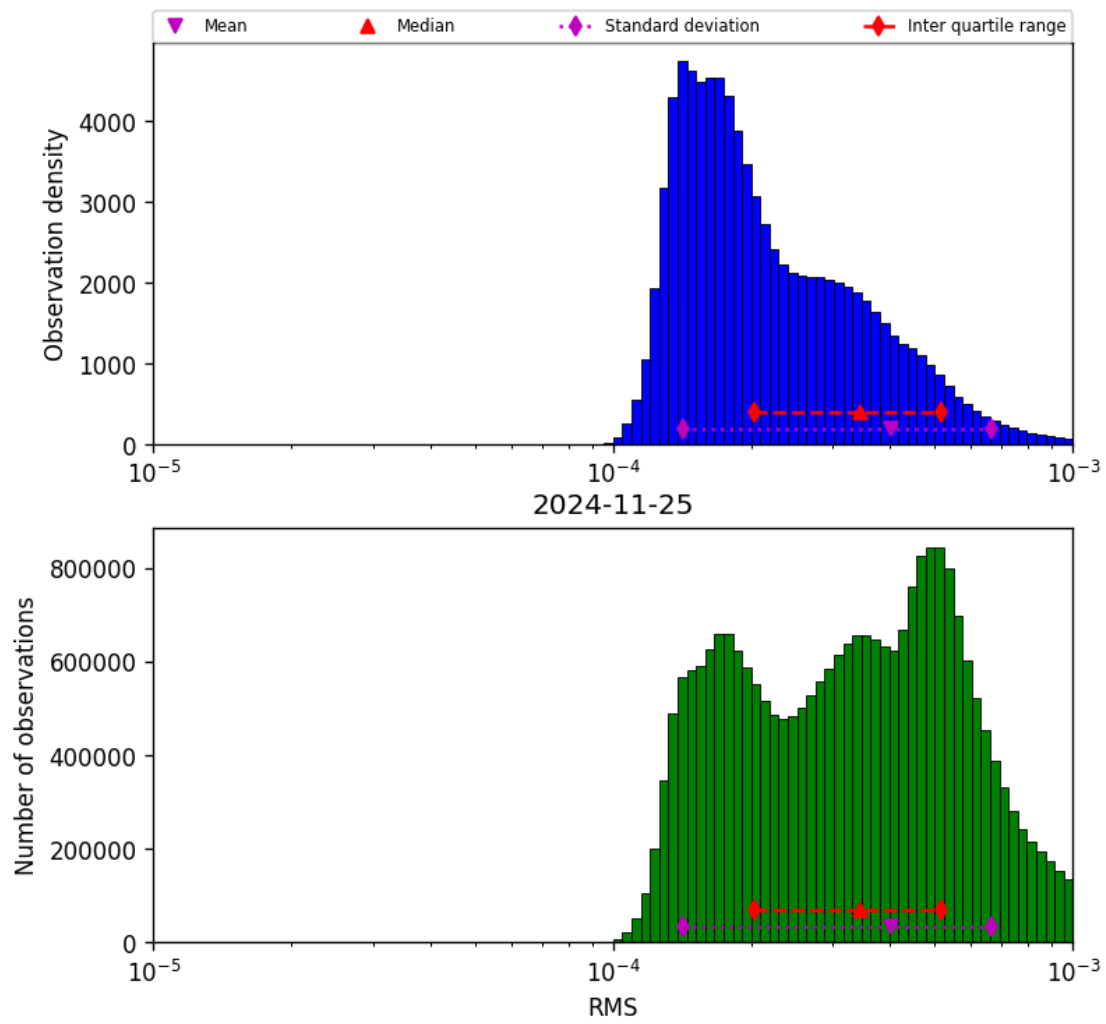
Figure 43: Histogram of “RMS” for 2024-11-25 to 2024-11-26
