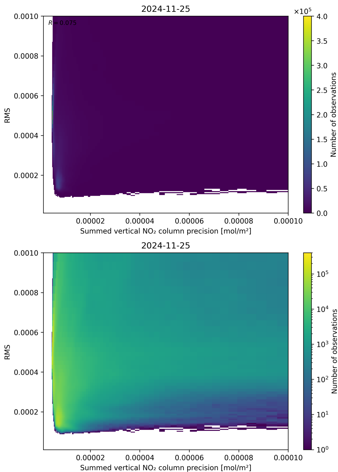
Figure 108: Scatter density plot of “Summed vertical NO 2 column precision” against “RMS” for 2024-11-25 to 2024-11-26.
