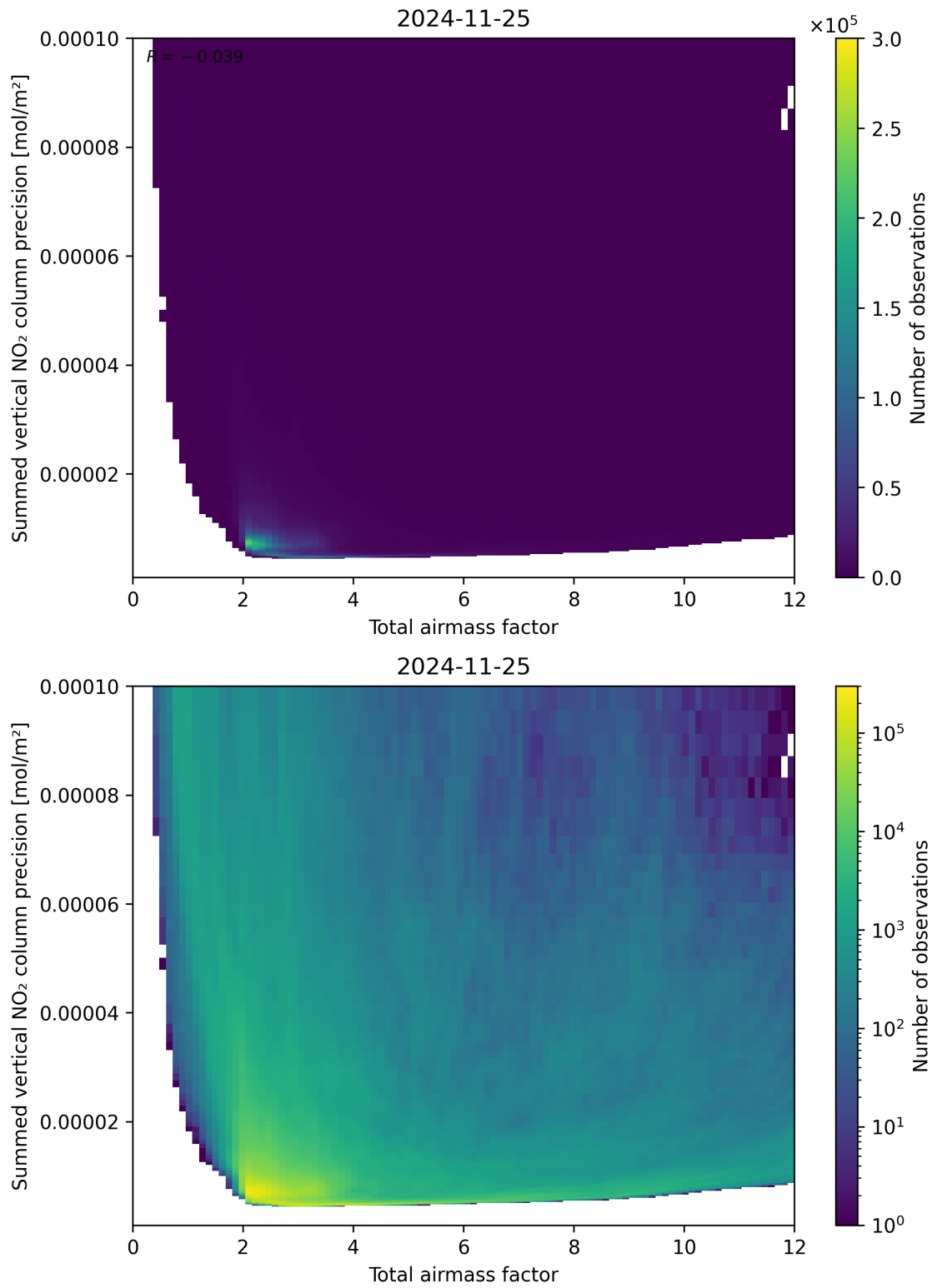
Figure 66: Scatter density plot of “Total airmass factor” against “Summed vertical NO 2 column precision” for 2024-11-25 to 2024-11-26.
