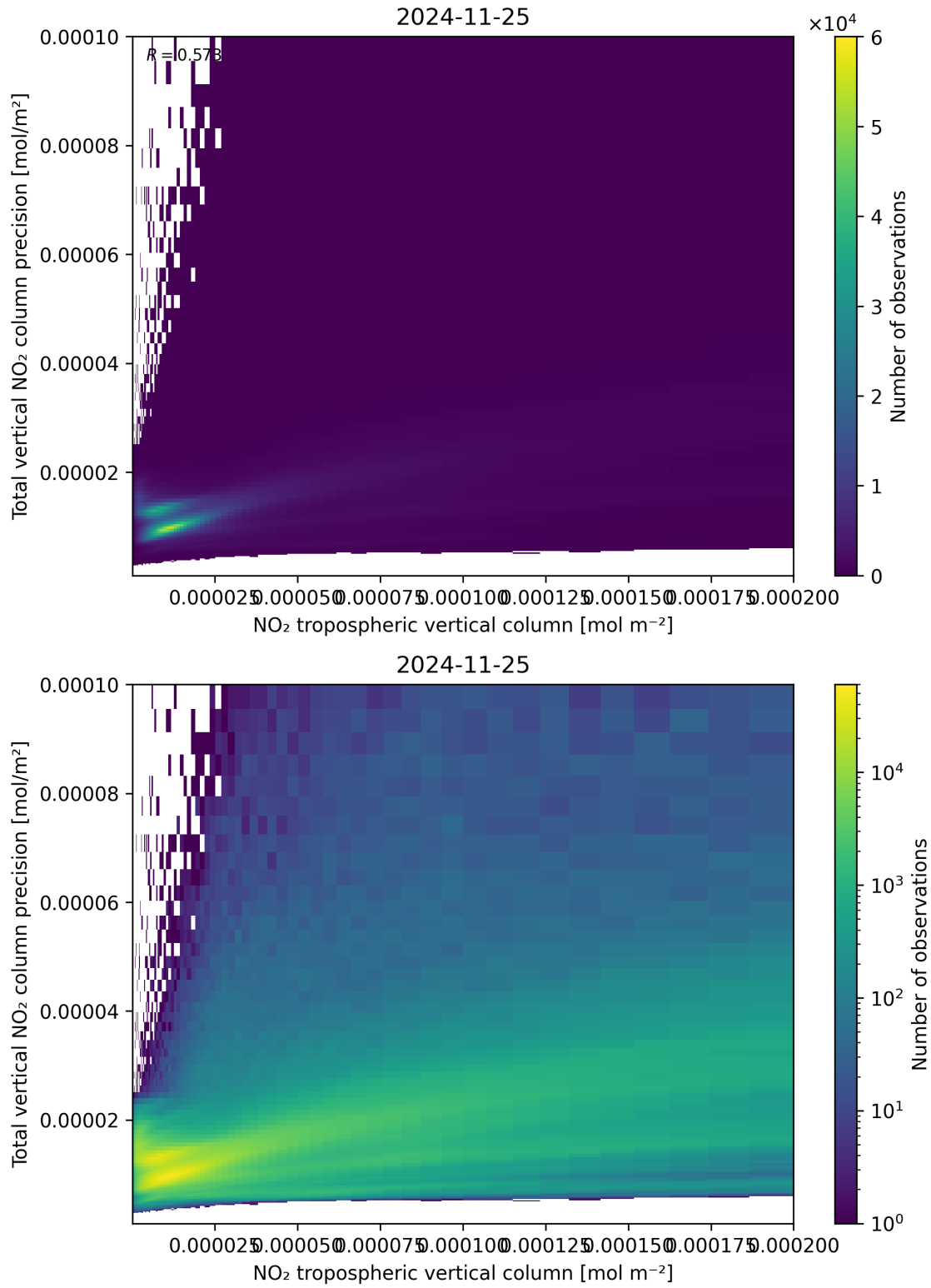
Figure 129: Scatter density plot of “NO 2 tropospheric vertical column” against “Total vertical NO 2 column precision” for 2024-11-25 to 2024-11-26.
