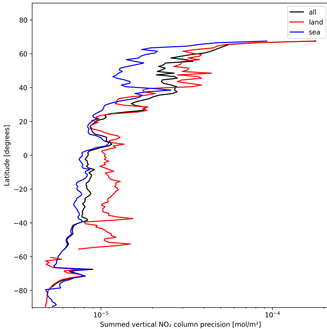
Figure 24: Zonal average of “Summed vertical NO 2 column precision” for 2024-11-25 to 2024-11-26.
