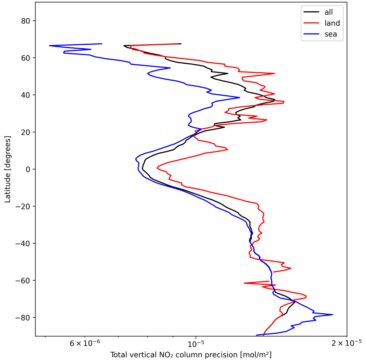
Figure 22: Zonal average of “Total vertical NO 2 column precision” for 2024-11-25 to 2024-11-26.
