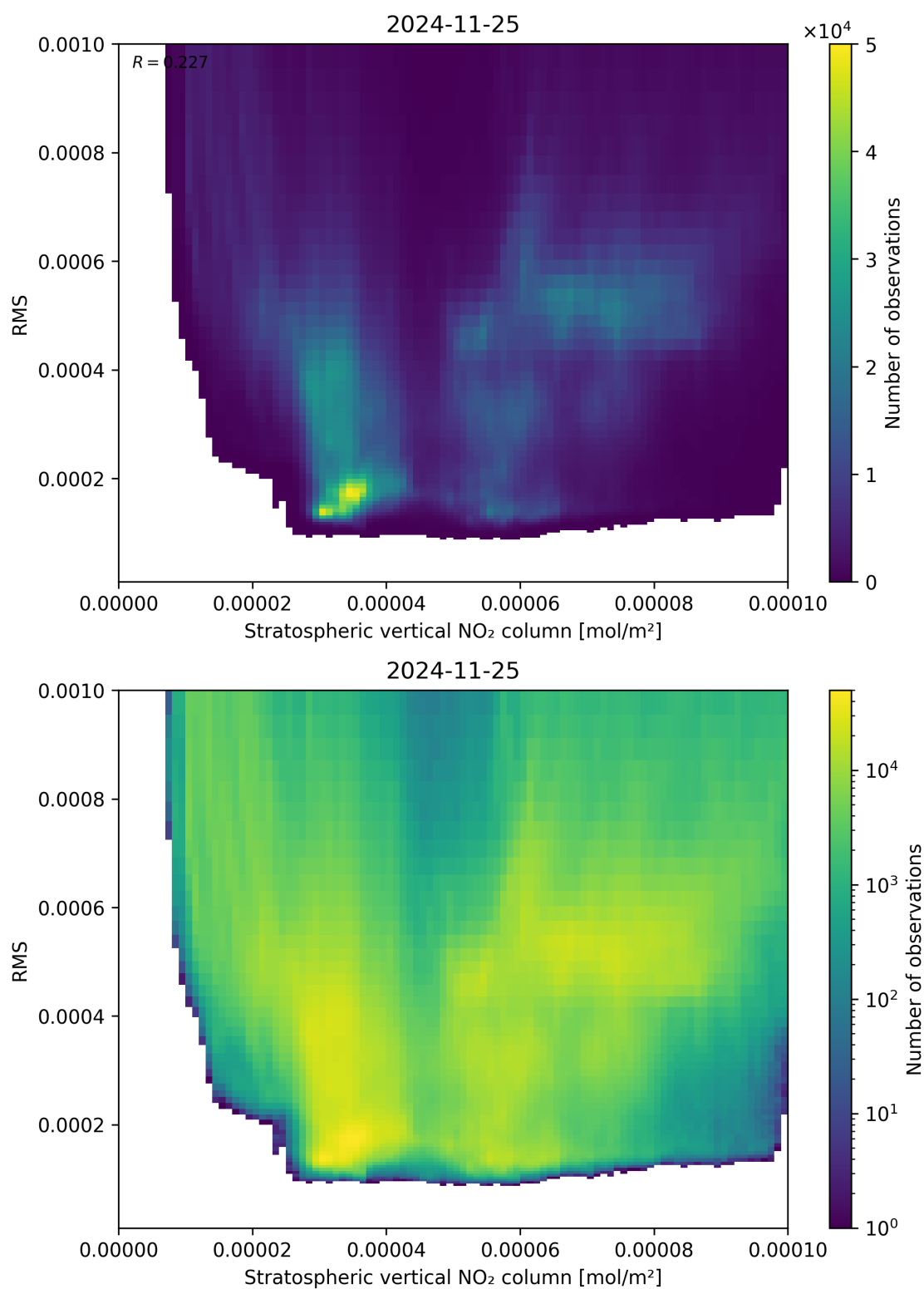
Figure 102: Scatter density plot of “Stratospheric vertical NO 2 column” against “RMS” for 2024-11-25 to 2024-11-26.
