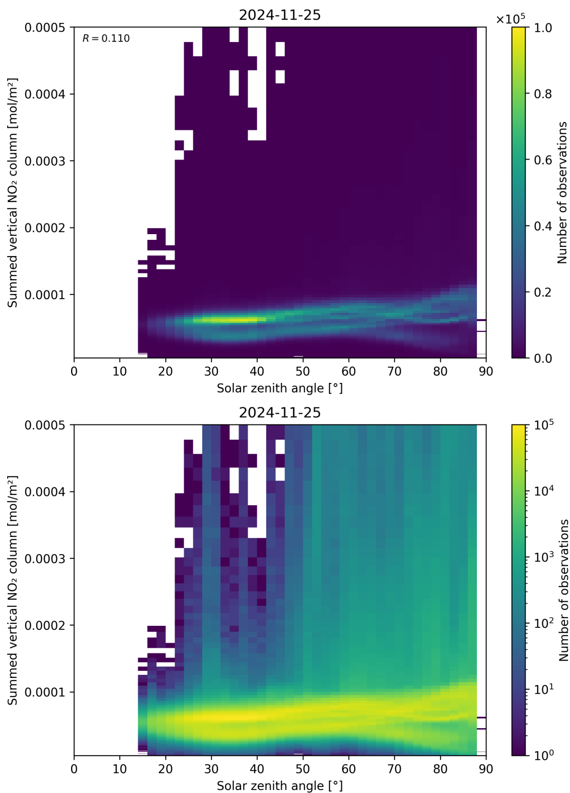
Figure 151: Scatter density plot of “Solar zenith angle” against “Summed vertical NO 2 column” for 2024-11-25 to 2024-11-26.
