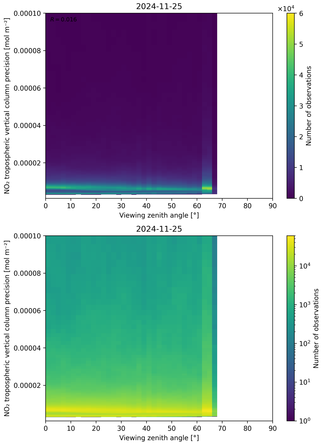
Figure 170: Scatter density plot of “Viewing zenith angle” against “NO 2 tropospheric vertical column precision” for 2024-11-25 to 2024-11-26.
