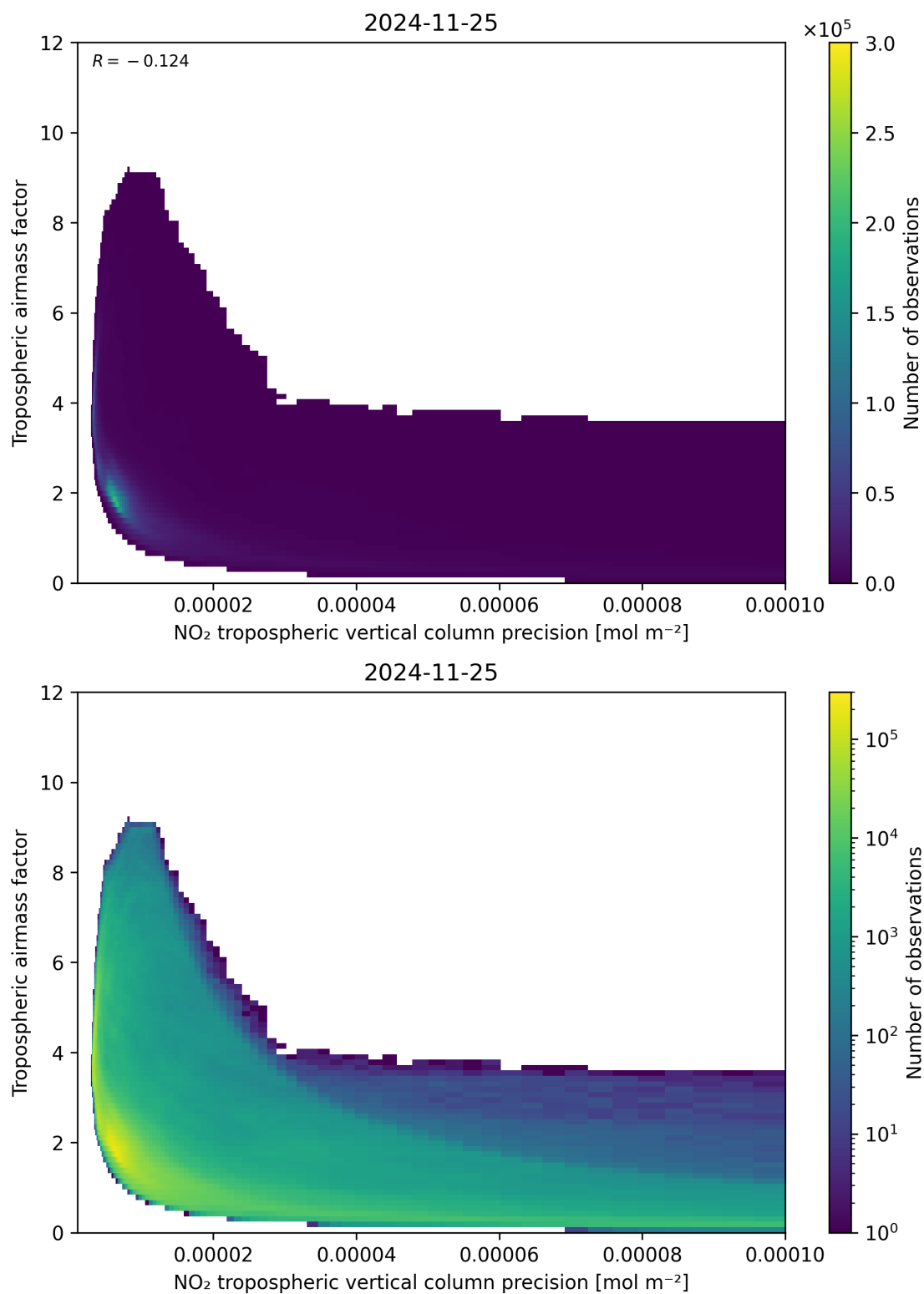
Figure 133: Scatter density plot of “NO 2 tropospheric vertical column precision” against “Tropospheric airmass factor” for 2024-11-25 to 2024-11-26.
