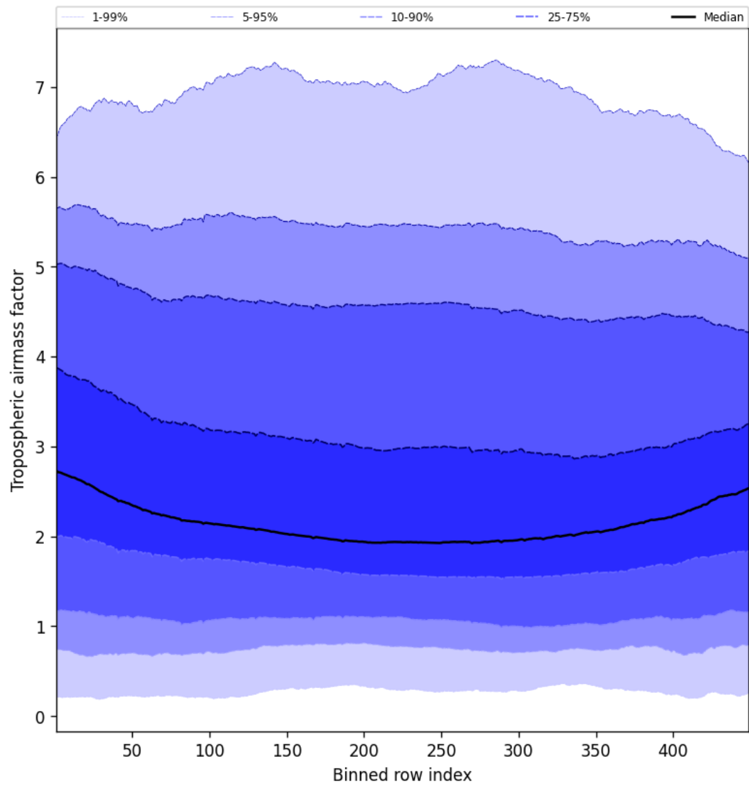
Figure 48: Along track statistics of “Tropospheric airmass factor” for 2024-11-25 to 2024-11-26
