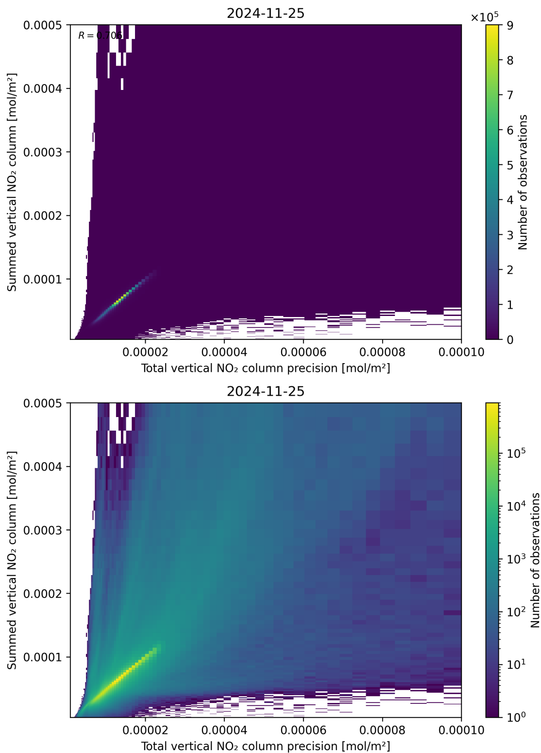
Figure 117: Scatter density plot of “Total vertical NO 2 column precision” against “Summed vertical NO 2 column” for 2024-11-25 to 2024-11-26.
