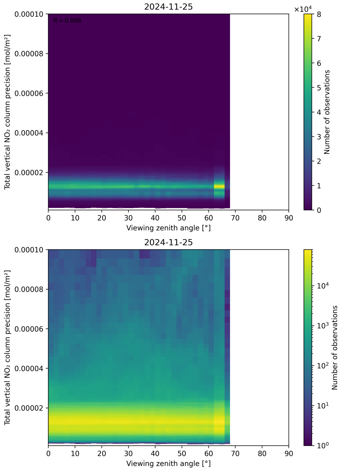
Figure 168: Scatter density plot of “Viewing zenith angle” against “Total vertical NO 2 column precision” for 2024-11-25 to 2024-11-26.
