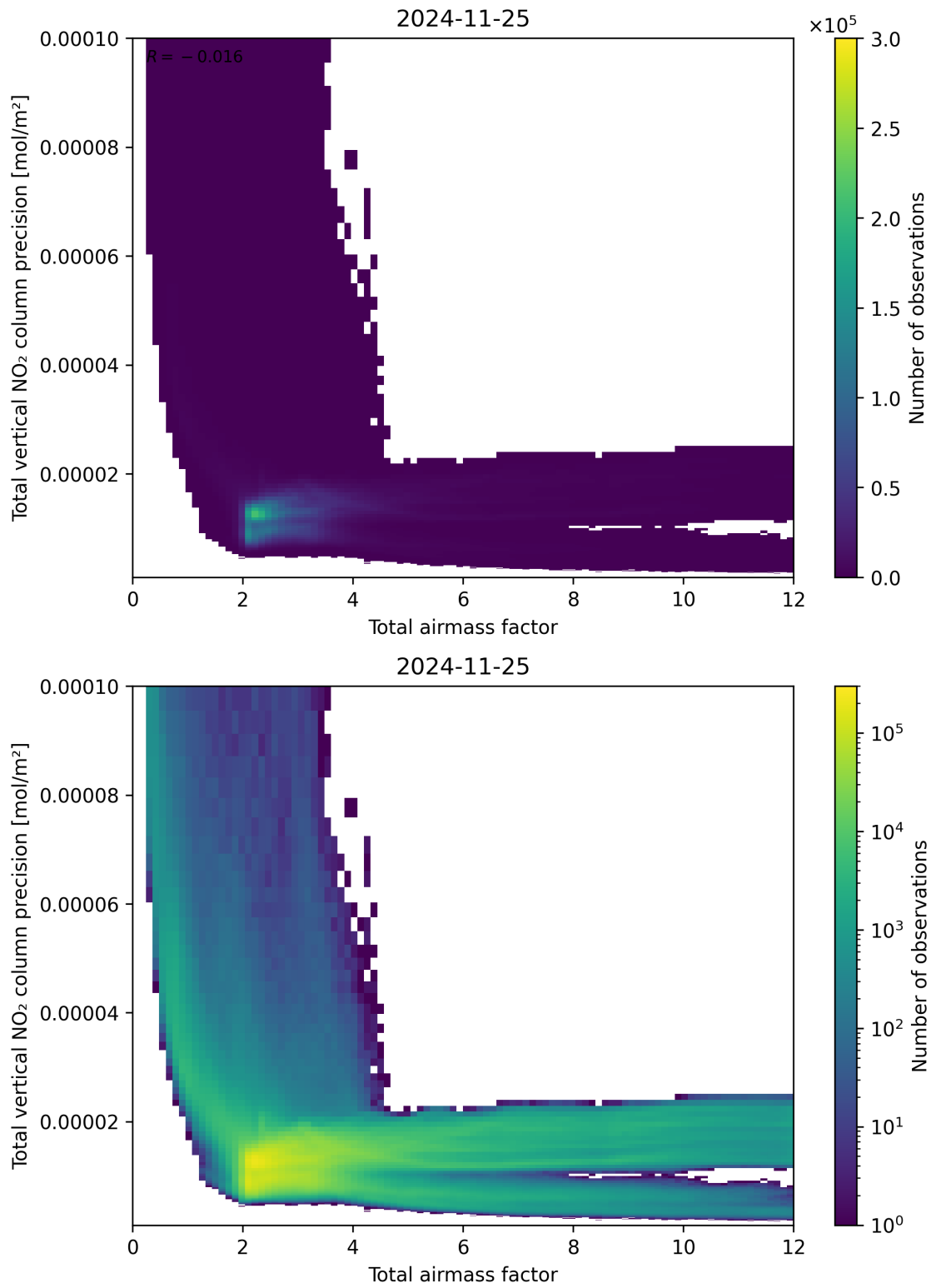
Figure 68: Scatter density plot of “Total airmass factor” against “Total vertical NO 2 column precision” for 2024-11-25 to 2024-11-26.
