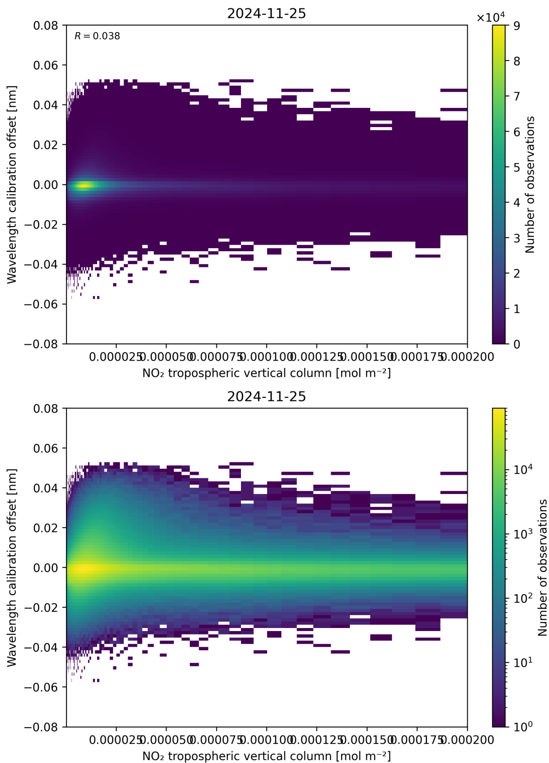
Figure 143: Scatter density plot of “NO 2 tropospheric vertical column” against “Wavelength calibration offset” for 2024-11-25 to 2024-11-26.
