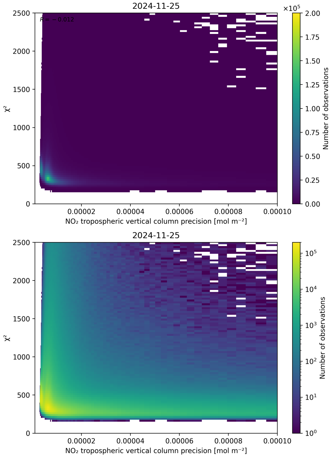
Figure 134: Scatter density plot of “NO 2 tropospheric vertical column precision” against “ \chi^2 ” for 2024-11-25 to 2024-11-26.
