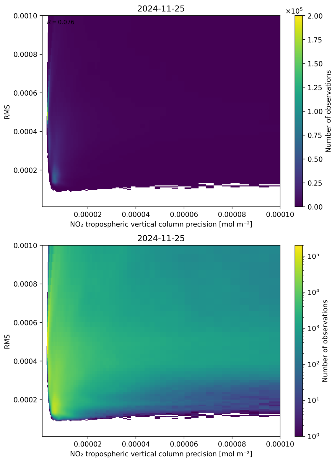
Figure 140: Scatter density plot of “NO 2 tropospheric vertical column precision” against “RMS” for 2024-11-25 to 2024-11-26.
