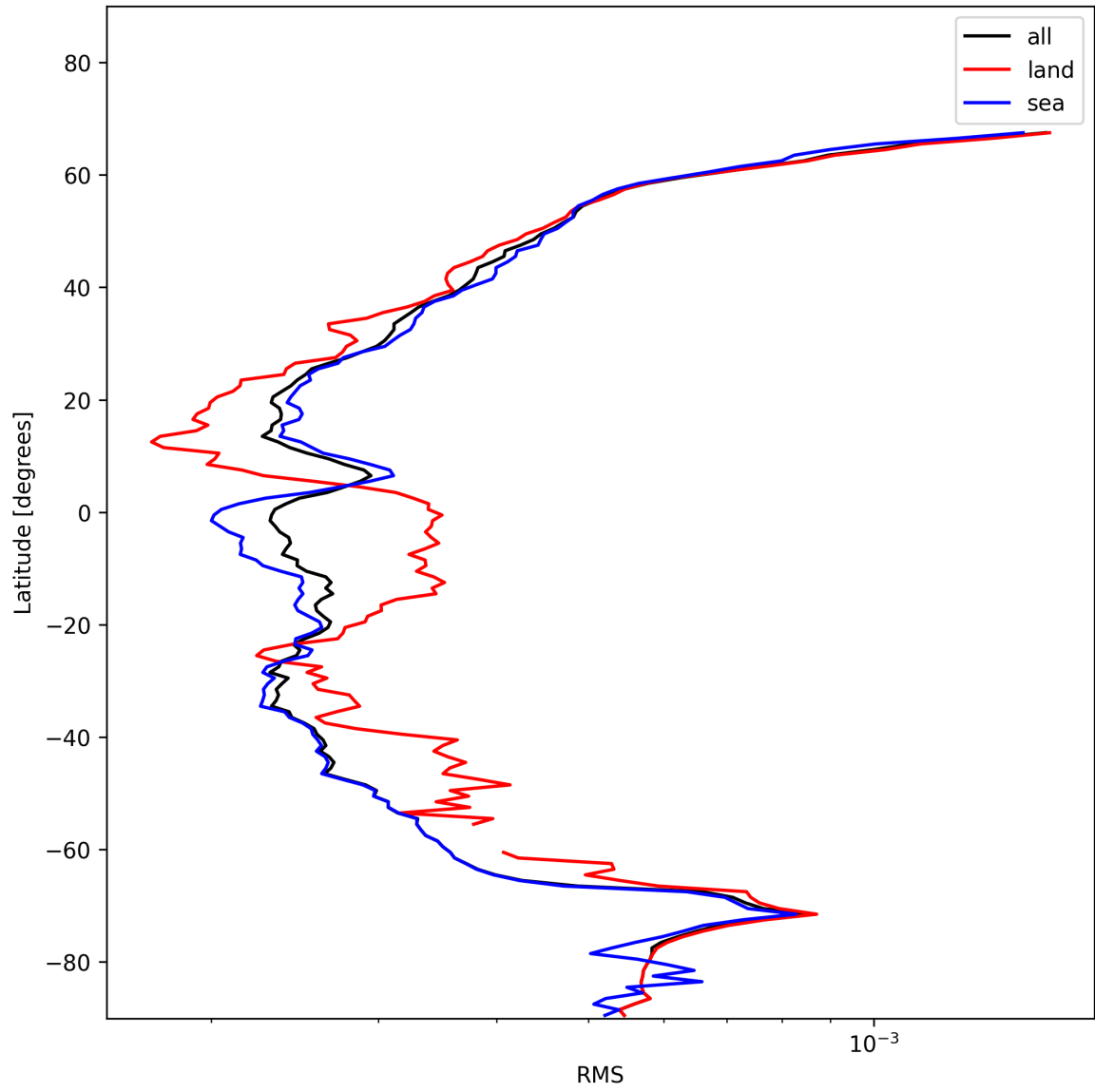
Figure 26: Zonal average of “RMS” for 2024-11-25 to 2024-11-26.
