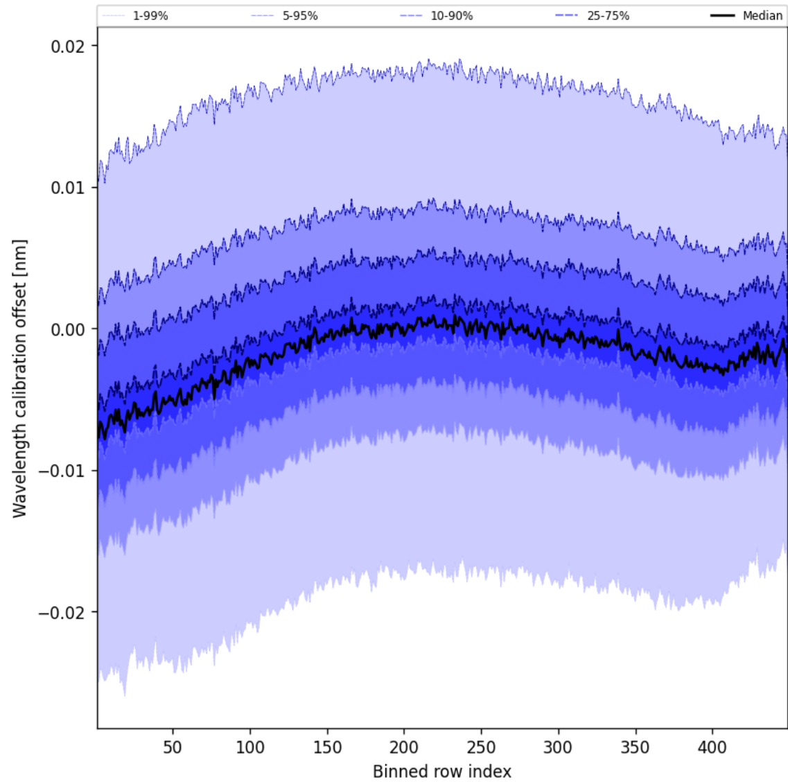
Figure 52: Along track statistics of “Wavelength calibration offset” for 2024-11-25 to 2024-11-26
