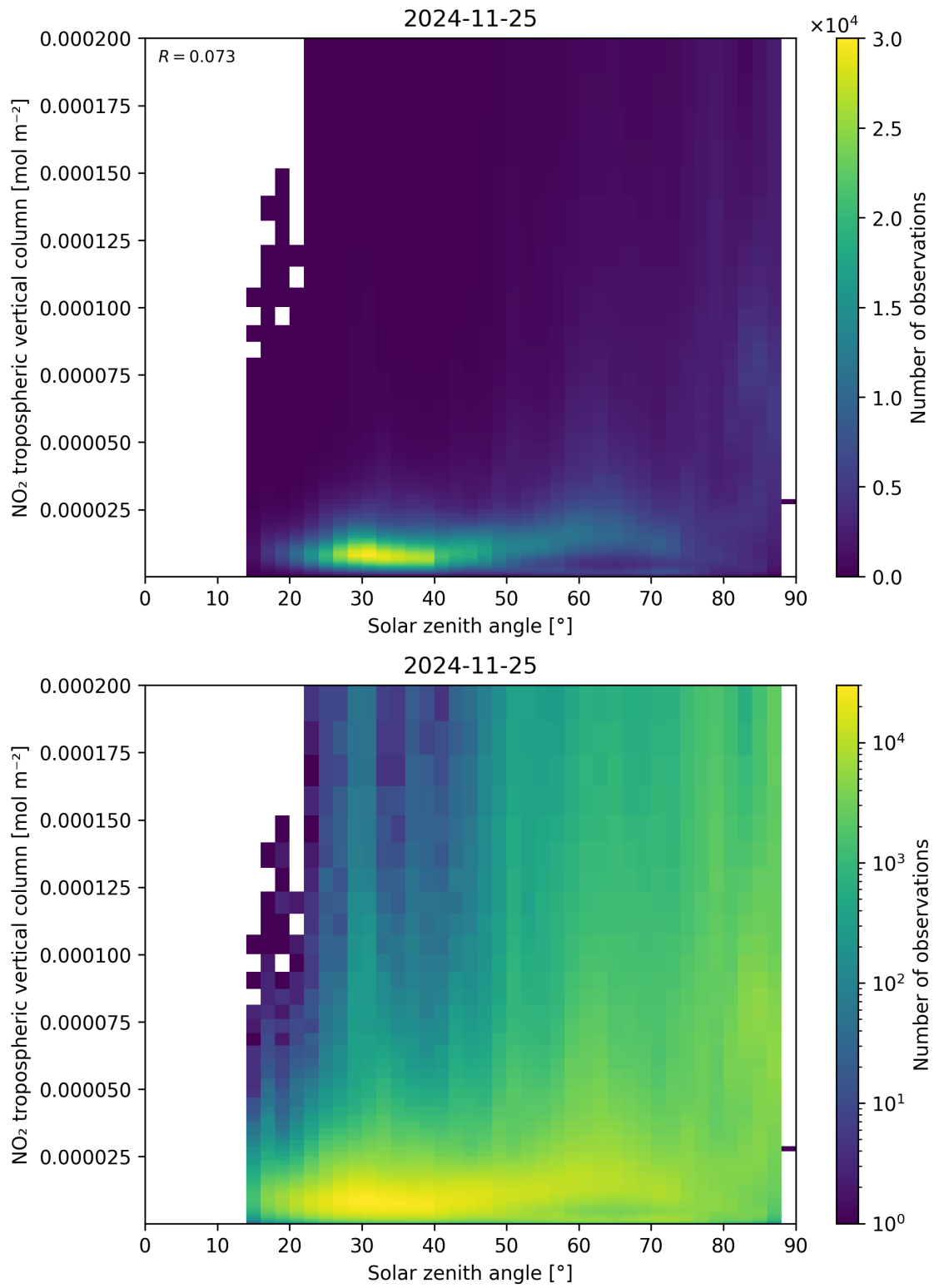
Figure 155: Scatter density plot of “Solar zenith angle” against “NO 2 tropospheric vertical column” for 2024-11-25 to 2024-11-26.
