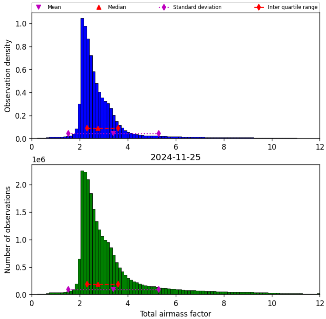
Figure 32: Histogram of “Total airmass factor” for 2024-11-25 to 2024-11-26
