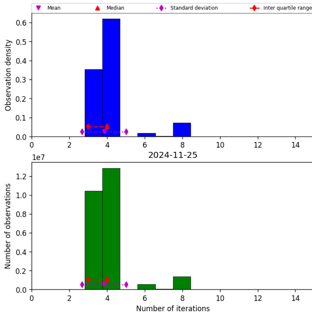
Figure 34: Histogram of “Number of iterations” for 2024-11-25 to 2024-11-26
