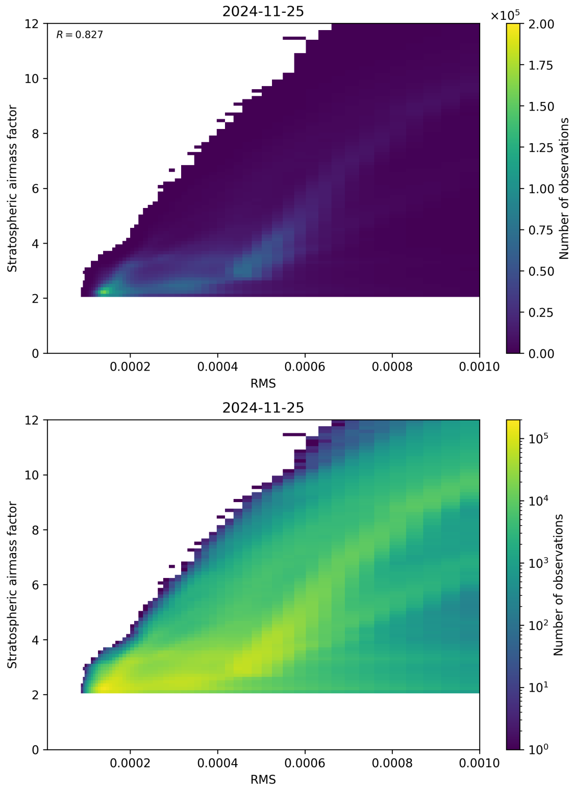
Figure 144: Scatter density plot of “RMS” against “Stratospheric airmass factor” for 2024-11-25 to 2024-11-26.
