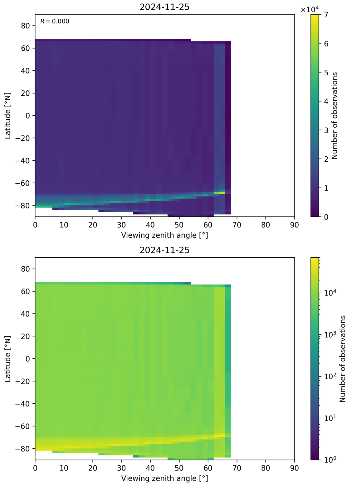
Figure 163: Scatter density plot of “Viewing zenith angle” against “Latitude” for 2024-11-25 to 2024-11-26.
