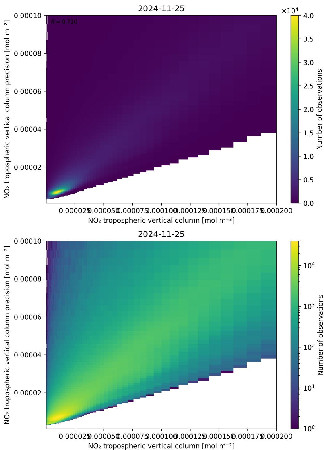
Figure 130: Scatter density plot of “NO 2 tropospheric vertical column” against “NO 2 tropospheric vertical column precision” for 2024-11-25 to 2024-11-26.
