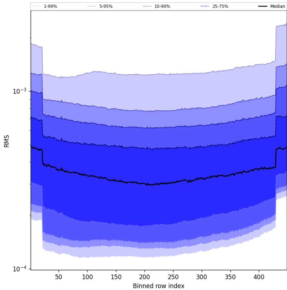
Figure 60: Along track statistics of “RMS” for 2024-11-25 to 2024-11-26
