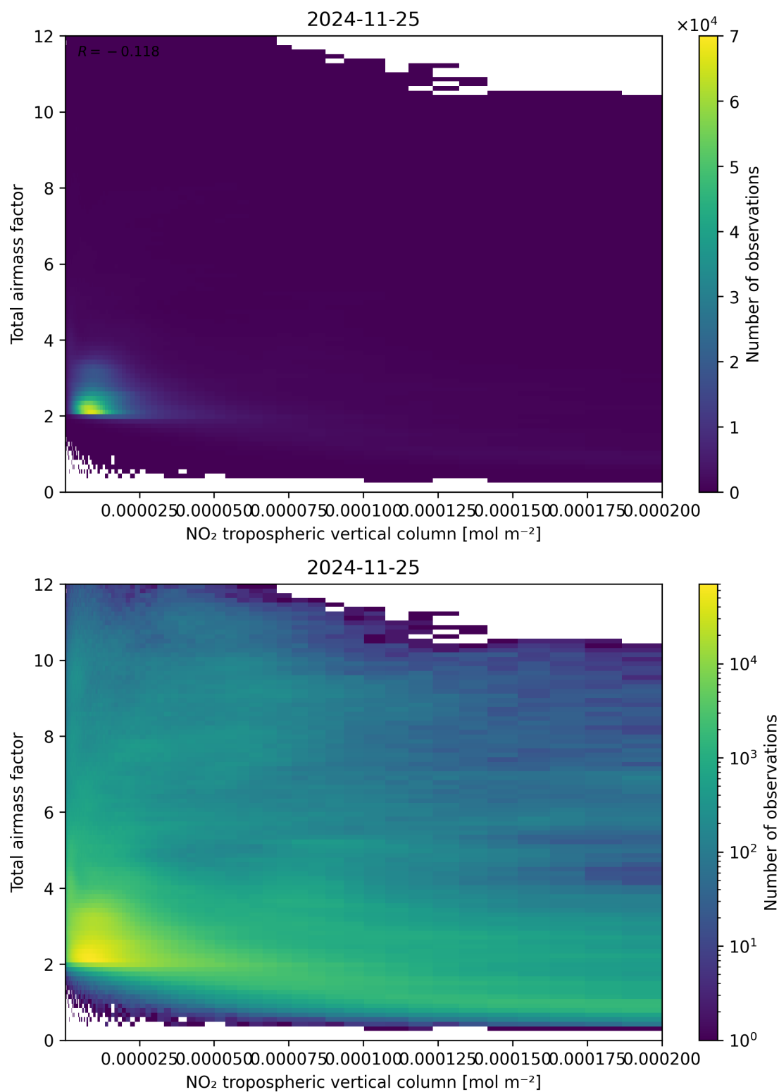
Figure 122: Scatter density plot of “NO 2 tropospheric vertical column” against “Total airmass factor” for 2024-11-25 to 2024-11-26.
