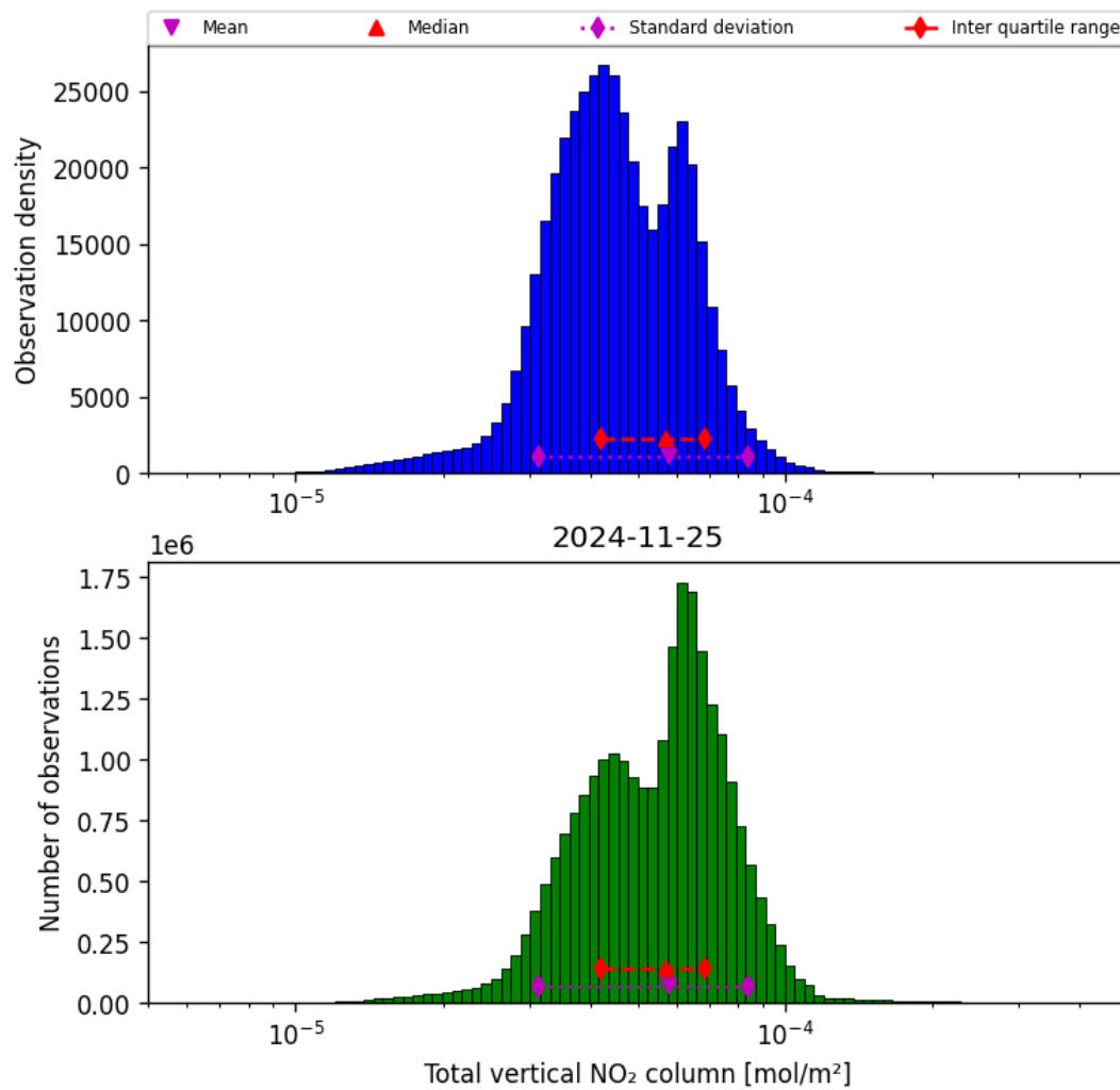
Figure 38: Histogram of "Total vertical NO 2 column" for 2024-11-25 to 2024-11-26
