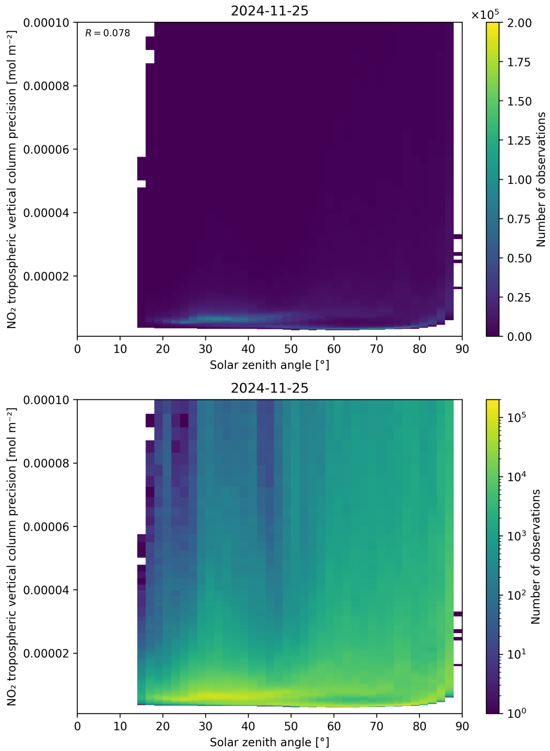
Figure 156: Scatter density plot of “Solar zenith angle” against “NO 2 tropospheric vertical column precision” for 2024-11-25 to 2024-11-26.
