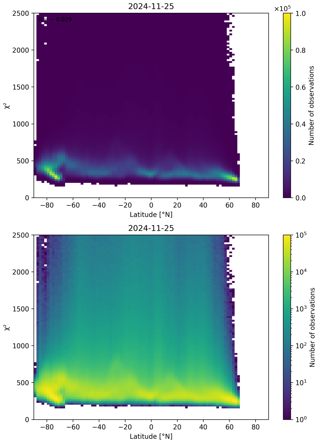
Figure 86: Scatter density plot of “Latitude” against “ \chi^2 ” for 2024-11-25 to 2024-11-26.
