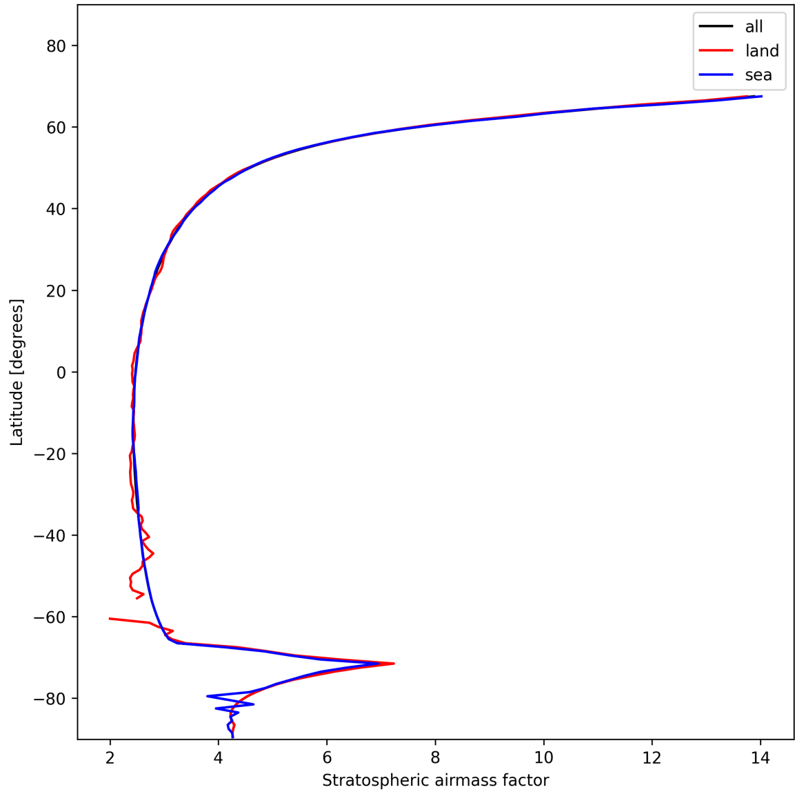
Figure 27: Zonal average of “Stratospheric airmass factor” for 2024-11-25 to 2024-11-26.
