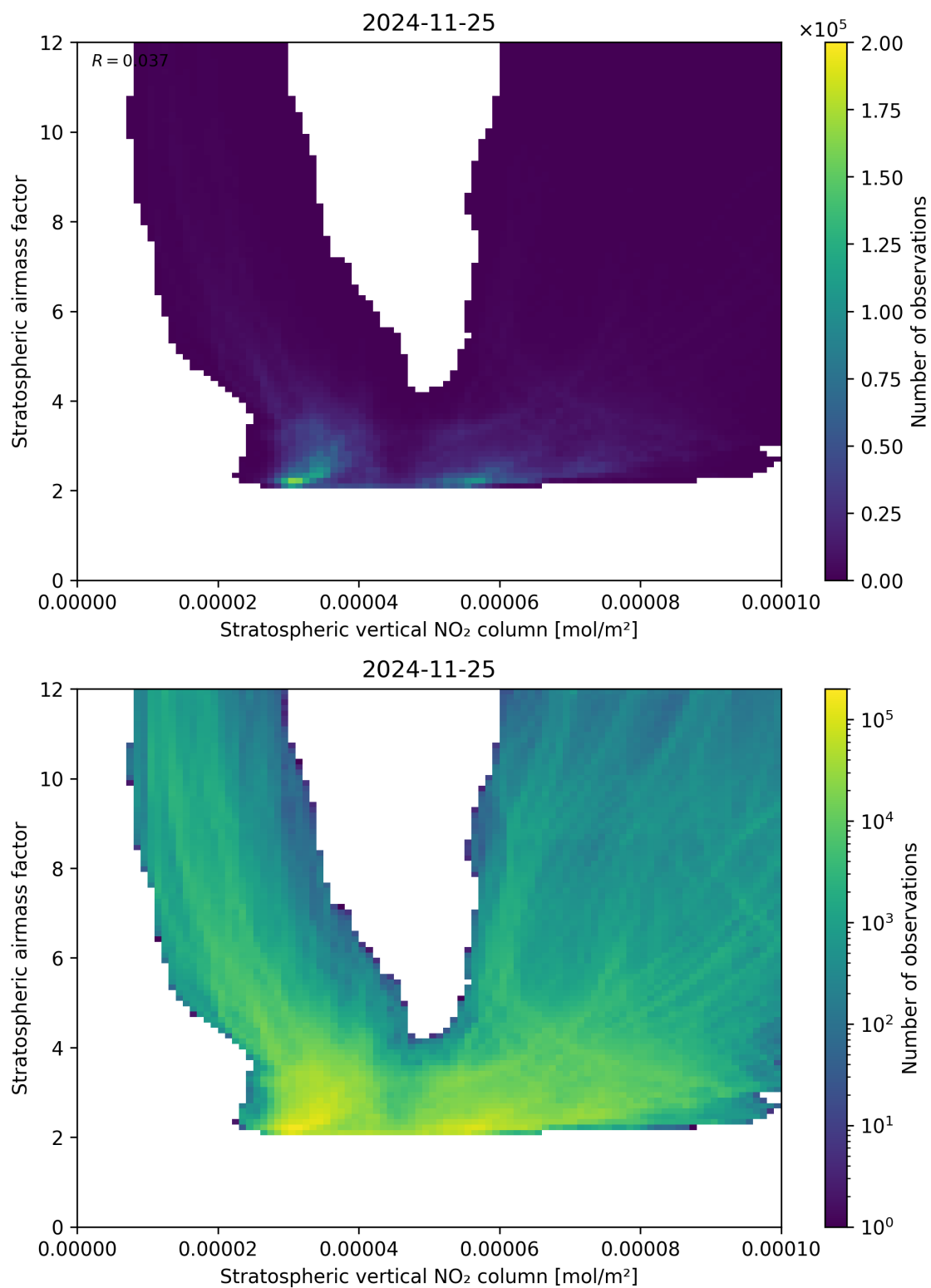
Figure 96: Scatter density plot of “Stratospheric vertical NO 2 column” against “Stratospheric airmass factor” for 2024-11-25 to 2024-11-26.
