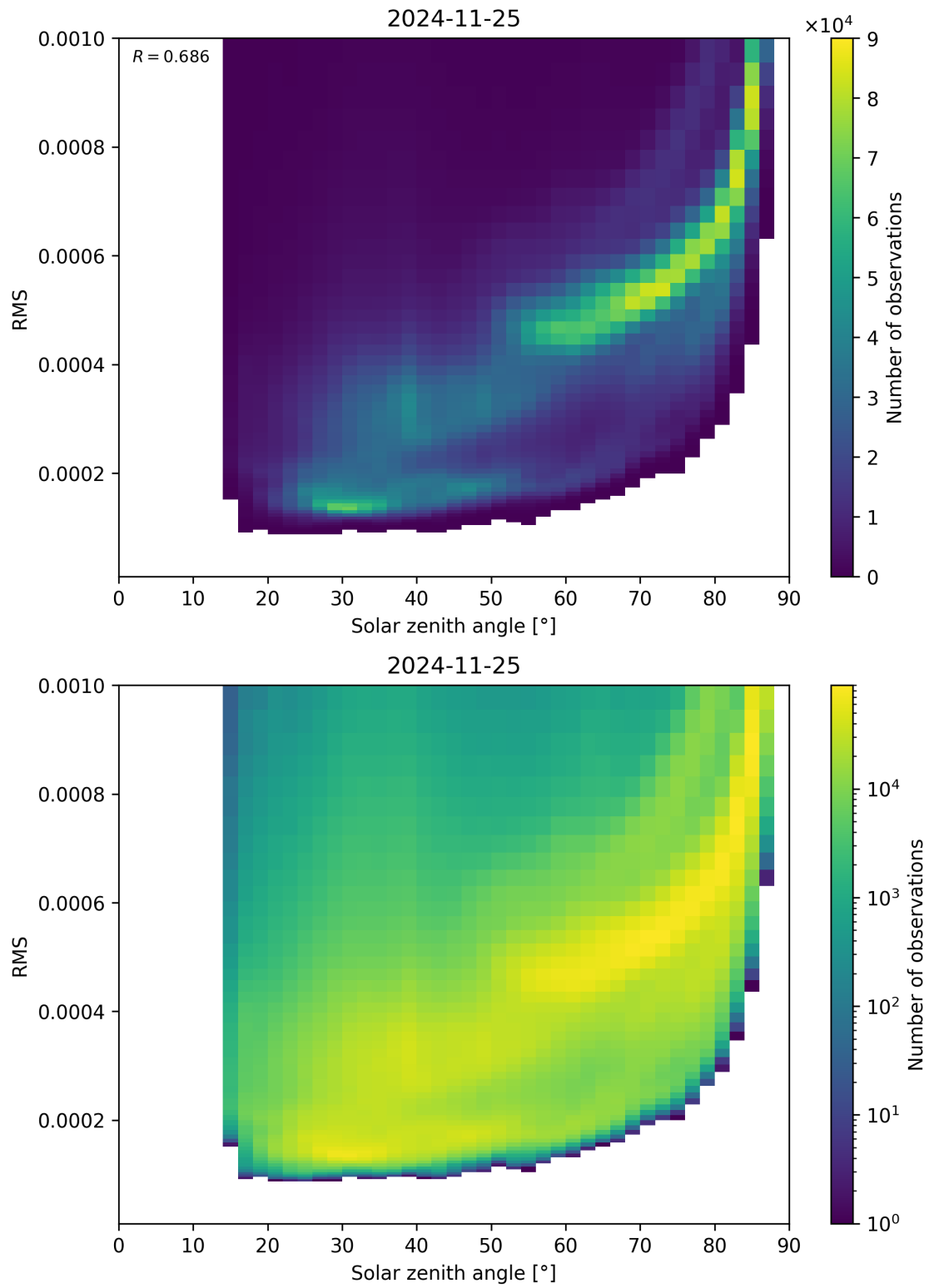
Figure 157: Scatter density plot of “Solar zenith angle” against “RMS” for 2024-11-25 to 2024-11-26.
