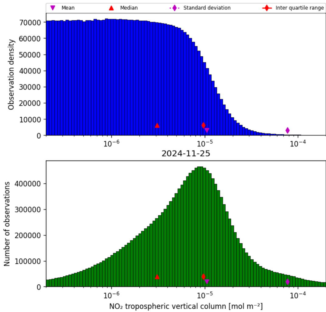
Figure 29: Histogram of “NO 2 tropospheric vertical column” for 2024-11-25 to 2024-11-26
