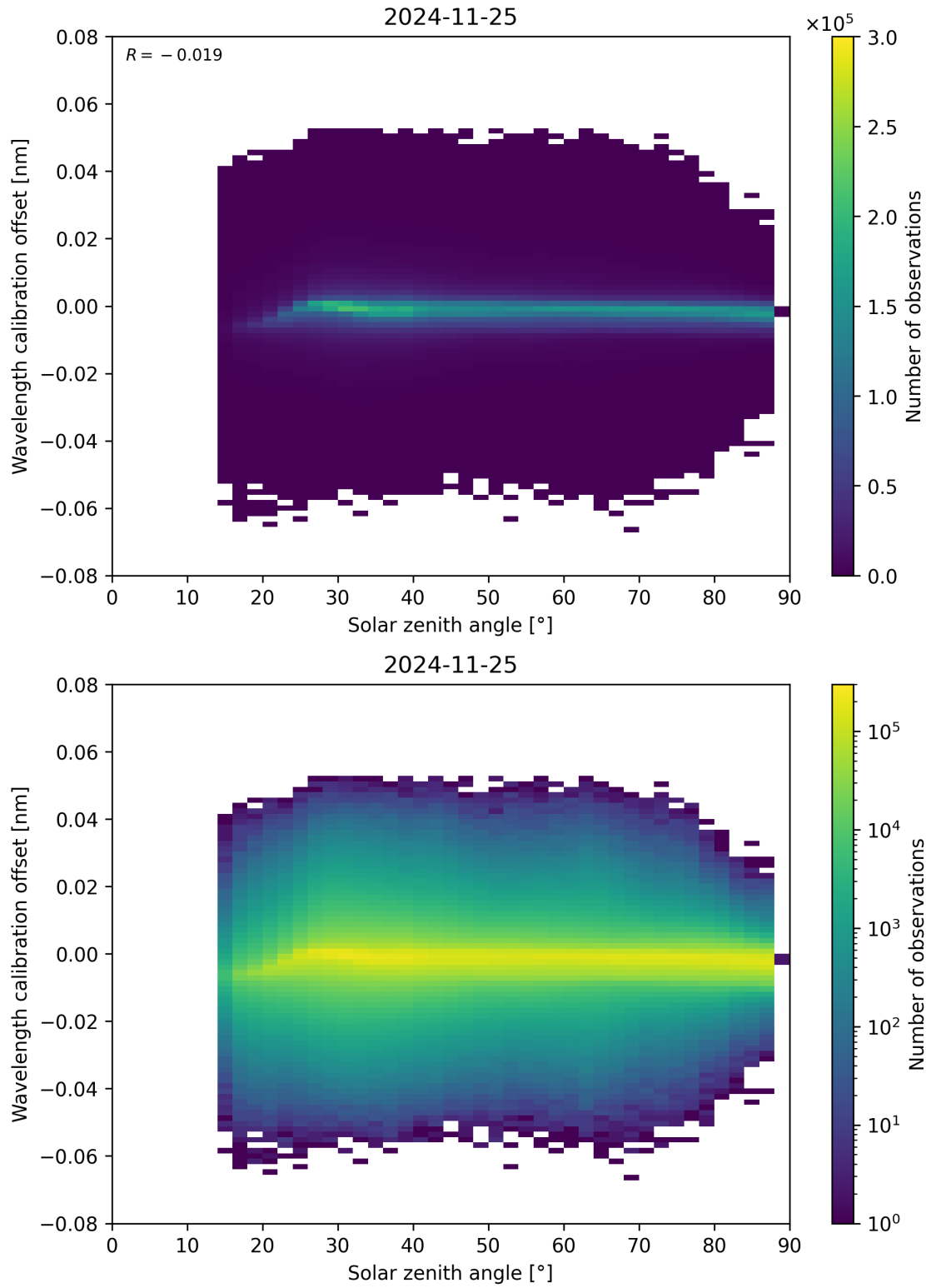
Figure 158: Scatter density plot of “Solar zenith angle” against “Wavelength calibration offset” for 2024-11-25 to 2024-11-26.
