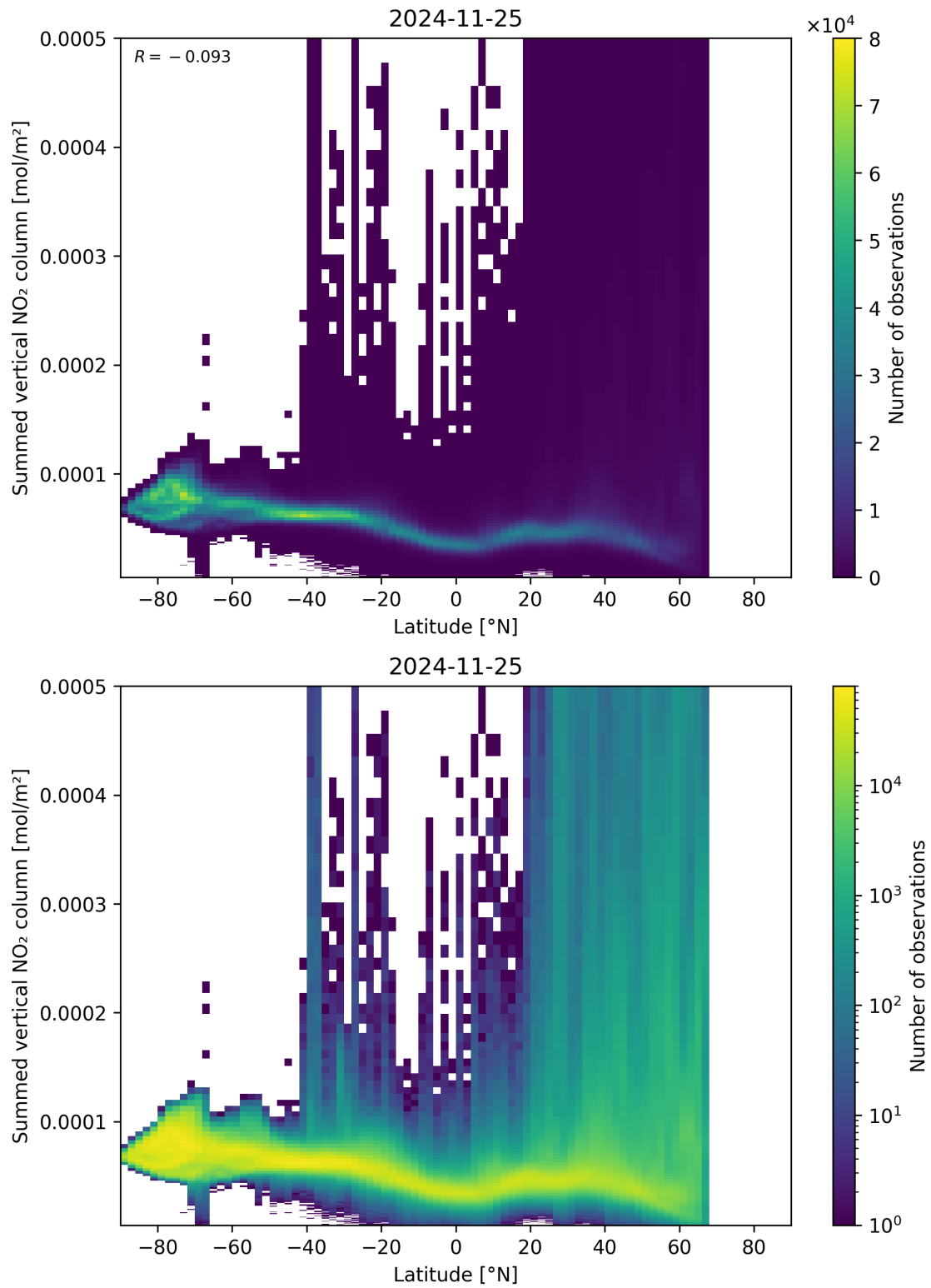
Figure 88: Scatter density plot of “Latitude” against “Summed vertical NO 2 column” for 2024-11-25 to 2024-11-26.
