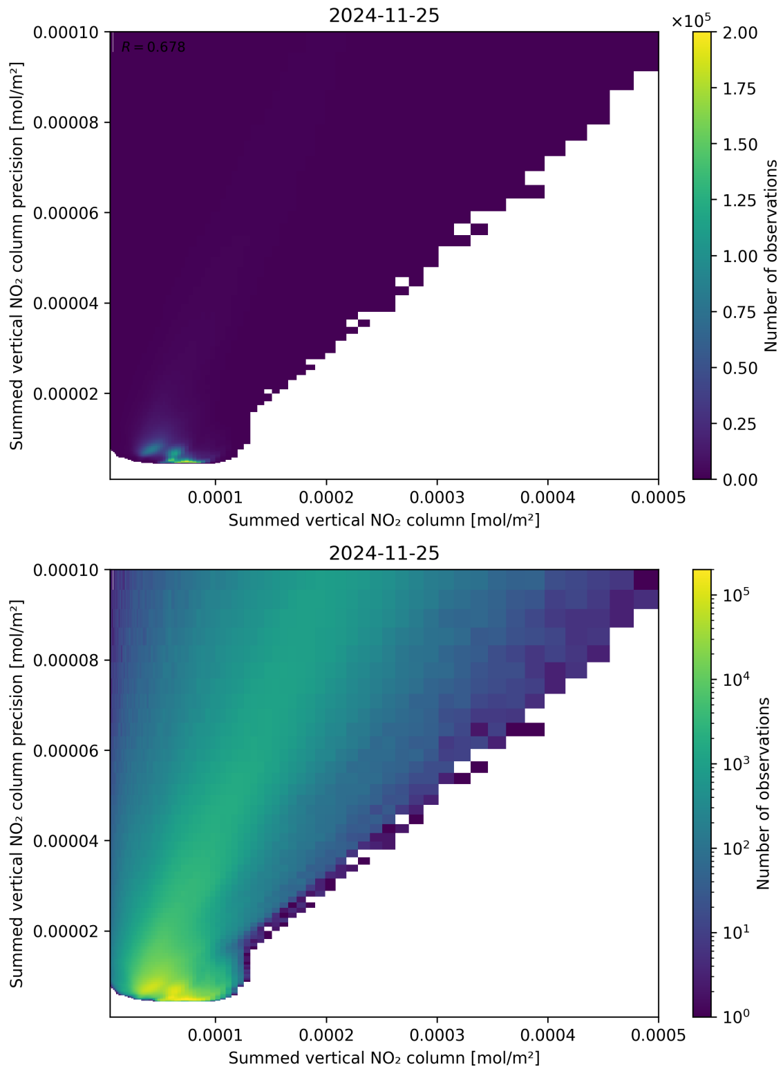
Figure 105: Scatter density plot of “Summed vertical NO 2 column” against “Summed vertical NO 2 column precision” for 2024-11-25 to 2024-11-26.
