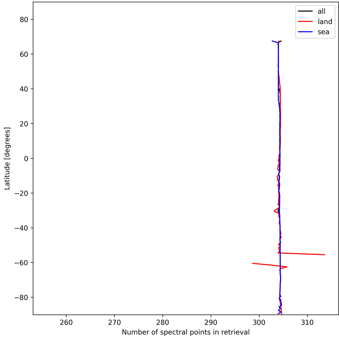
Figure 16: Zonal average of “Number of spectral points in retrieval” for 2024-11-25 to 2024-11-26.
