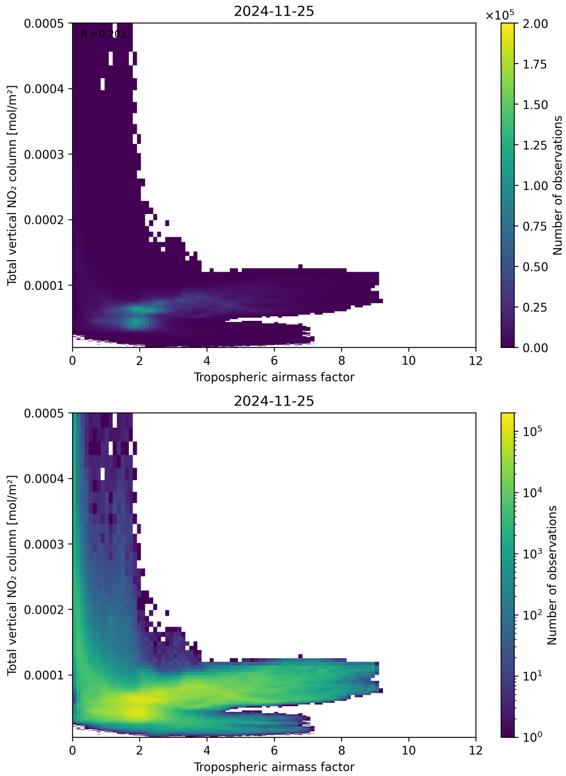
Figure 77: Scatter density plot of “Tropospheric airmass factor” against “Total vertical NO 2 column” for 2024-11-25 to 2024-11-26.
