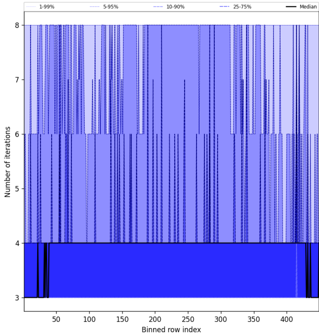
Figure 51: Along track statistics of “Number of iterations” for 2024-11-25 to 2024-11-26
