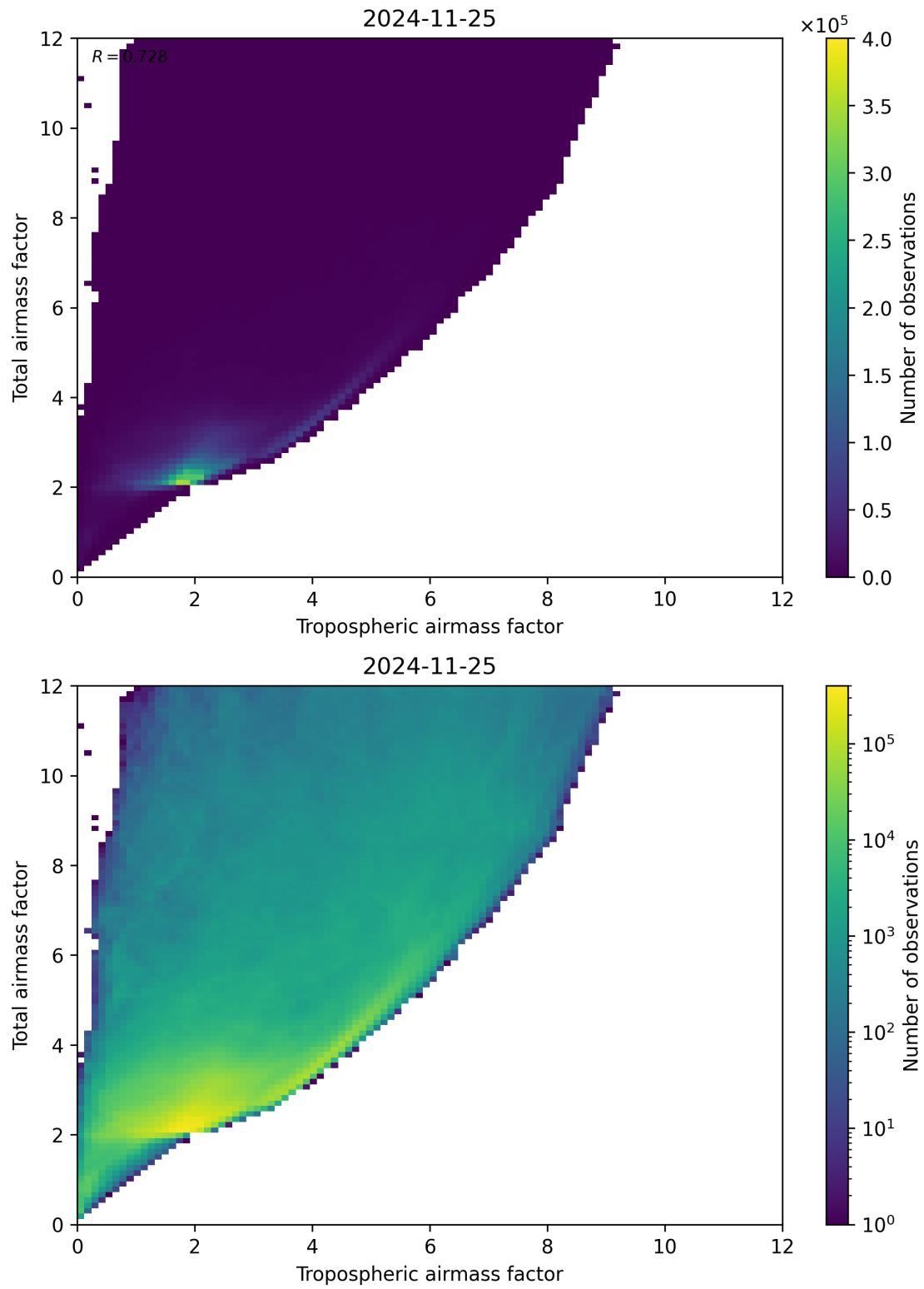
Figure 72: Scatter density plot of “Tropospheric airmass factor” against “Total airmass factor” for 2024-11-25 to 2024-11-26.
