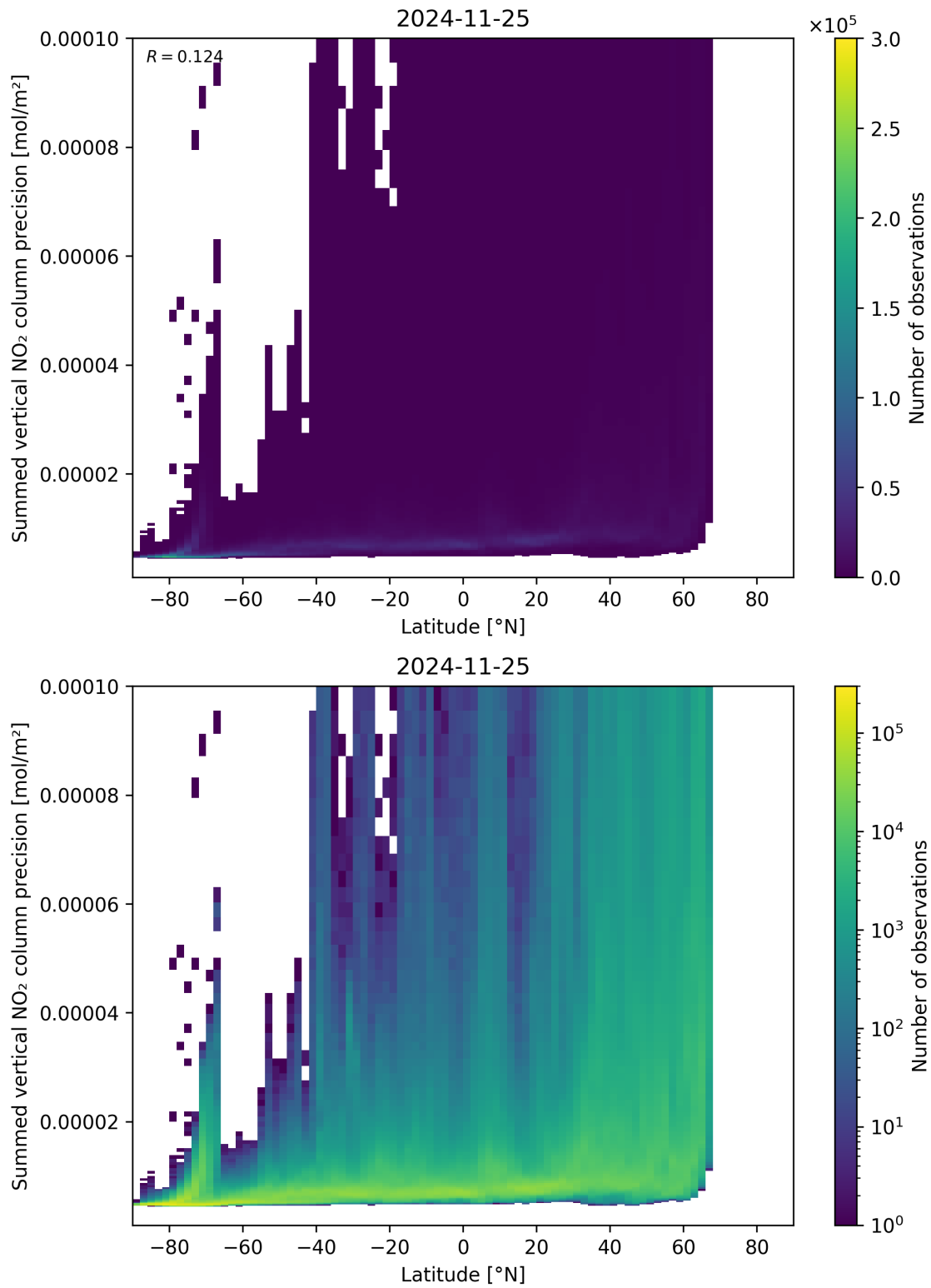
Figure 89: Scatter density plot of “Latitude” against “Summed vertical NO 2 column precision” for 2024-11-25 to 2024-11-26.
