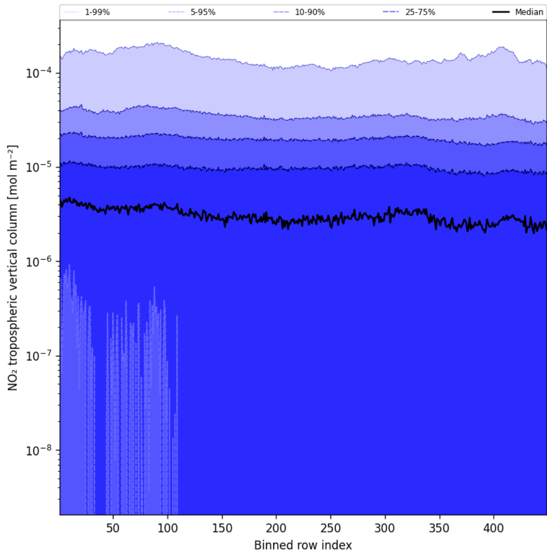
Figure 46: Along track statistics of “NO 2 tropospheric vertical column” for 2024-11-25 to 2024-11-26
