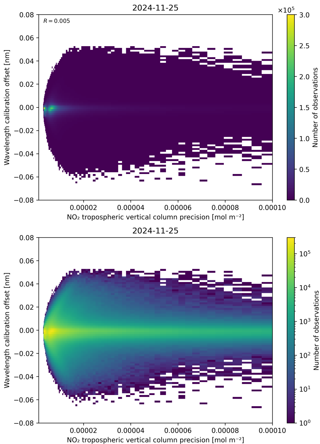
Figure 141: Scatter density plot of “NO 2 tropospheric vertical column precision” against “Wavelength calibration offset” for 2024-11-25 to 2024-11-26.
