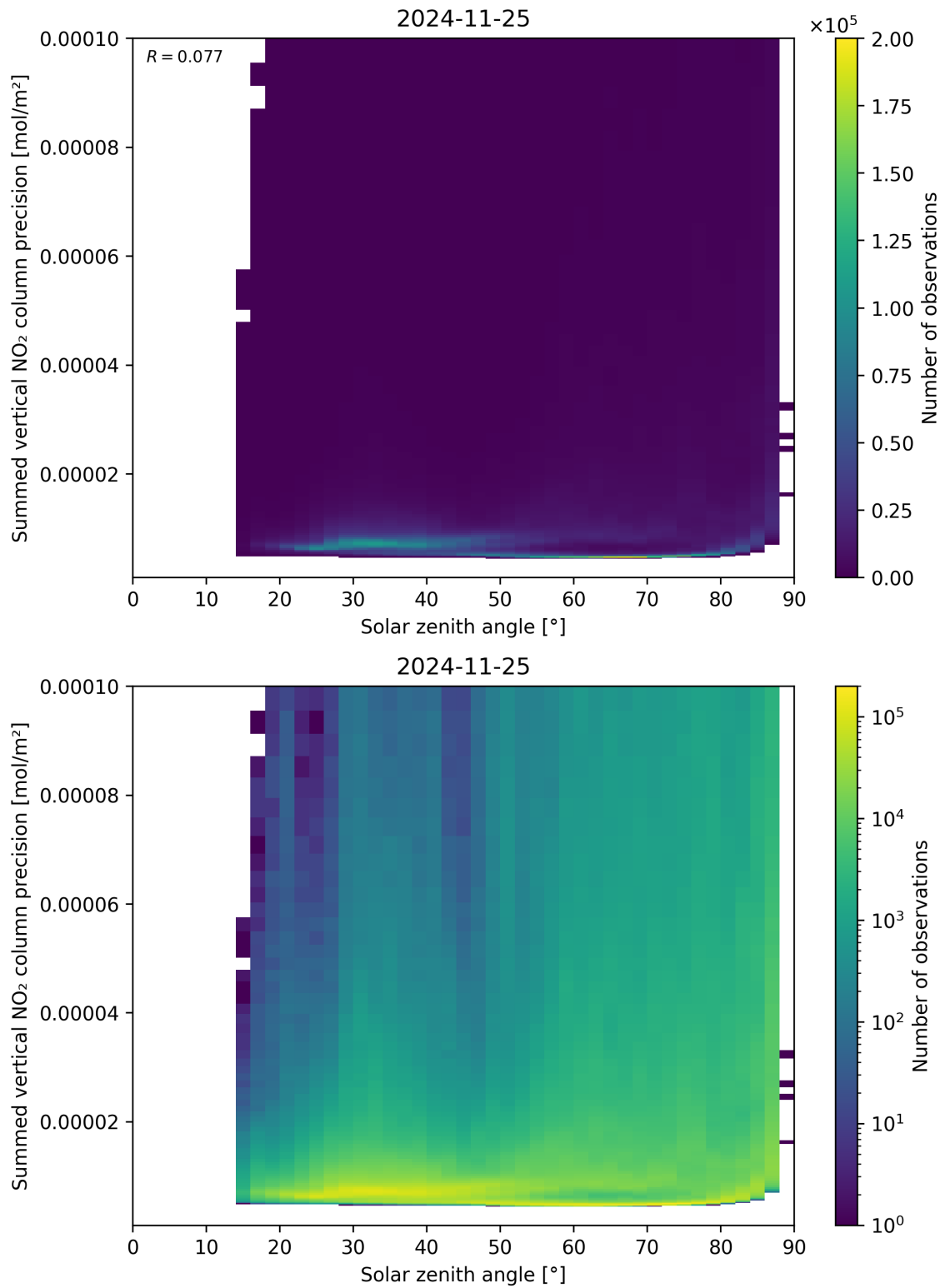
Figure 152: Scatter density plot of “Solar zenith angle” against “Summed vertical NO 2 column precision” for 2024-11-25 to 2024-11-26.
