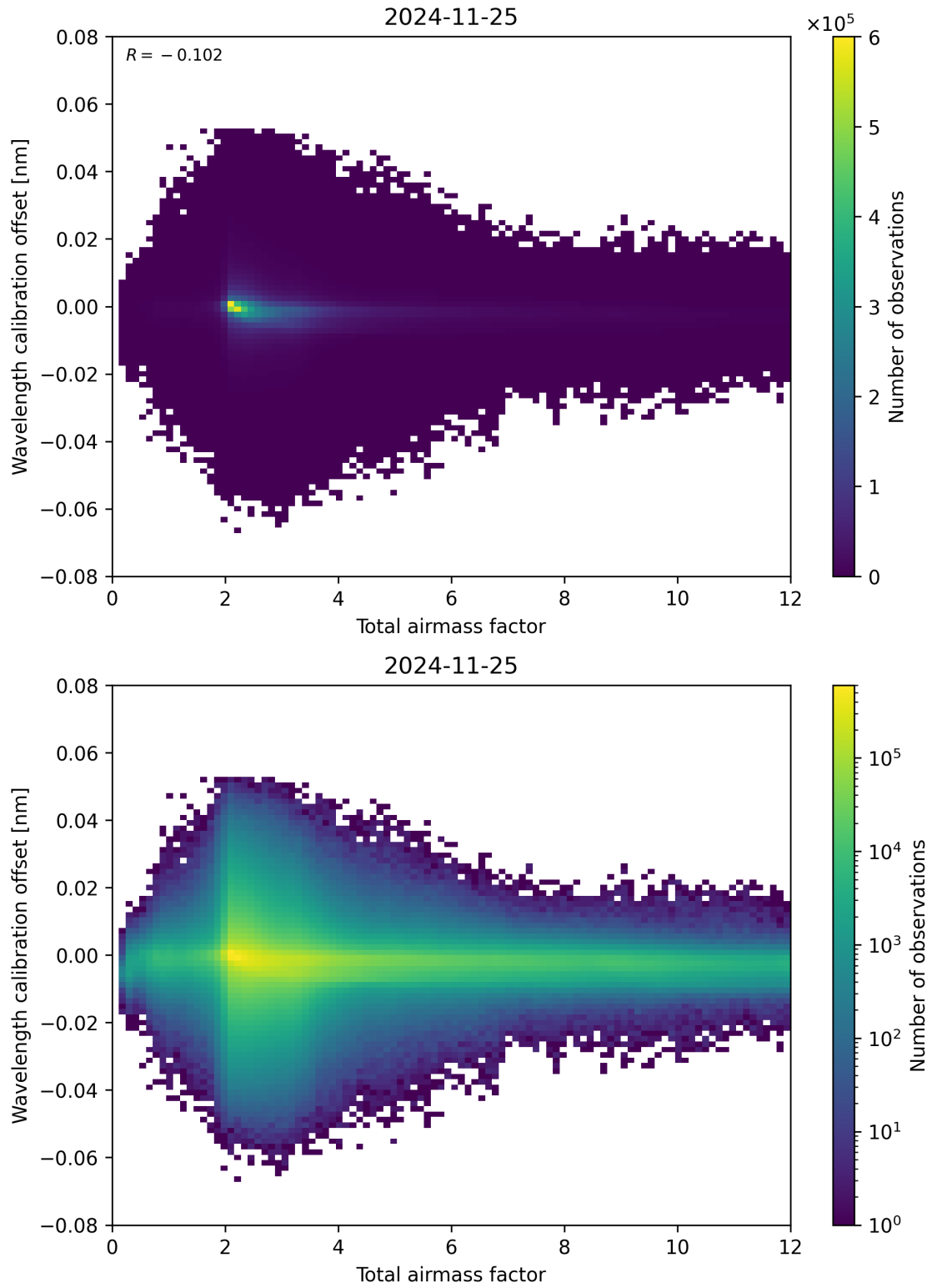
Figure 70: Scatter density plot of “Total airmass factor” against “Wavelength calibration offset” for 2024-11-25 to 2024-11-26.
