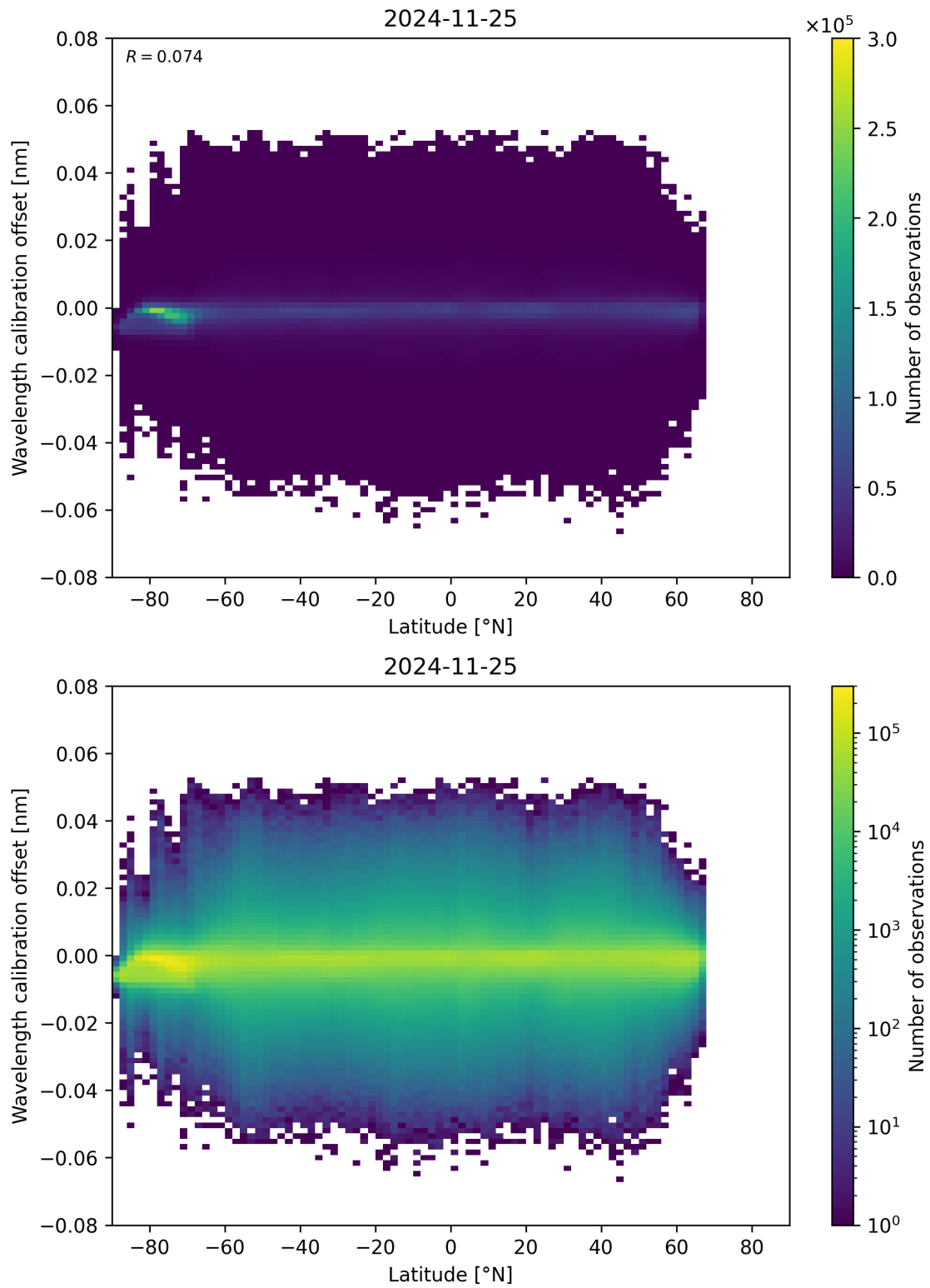
Figure 95: Scatter density plot of “Latitude” against “Wavelength calibration offset” for 2024-11-25 to 2024-11-26.
