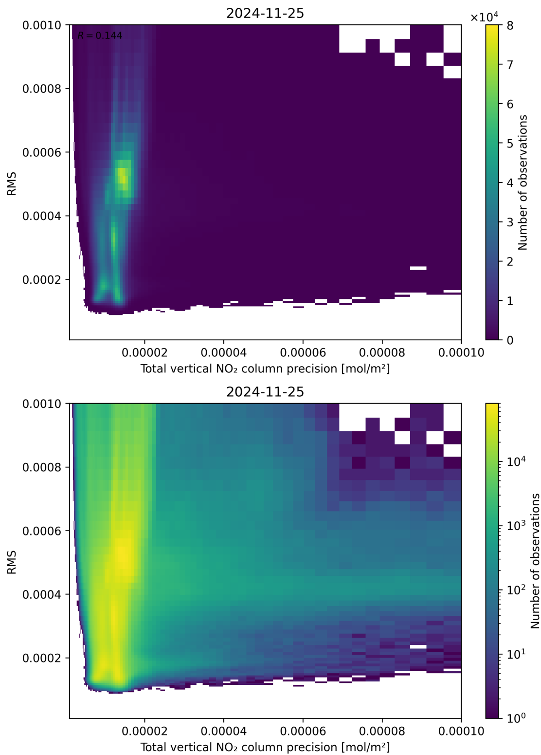
Figure 119: Scatter density plot of “Total vertical NO 2 column precision” against “RMS” for 2024-11-25 to 2024-11-26.
