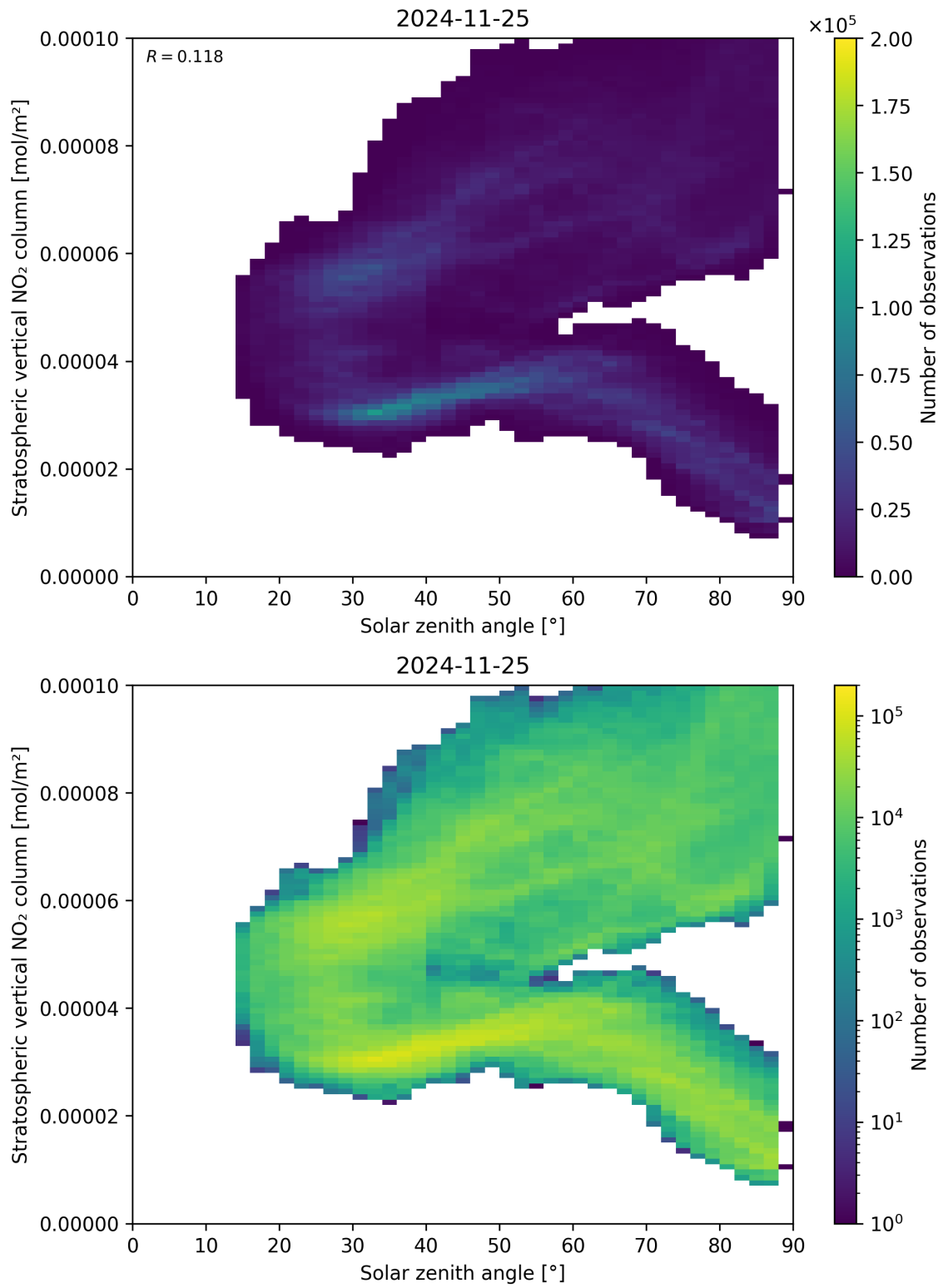
Figure 150: Scatter density plot of “Solar zenith angle” against “Stratospheric vertical NO 2 column” for 2024-11-25 to 2024-11-26.
