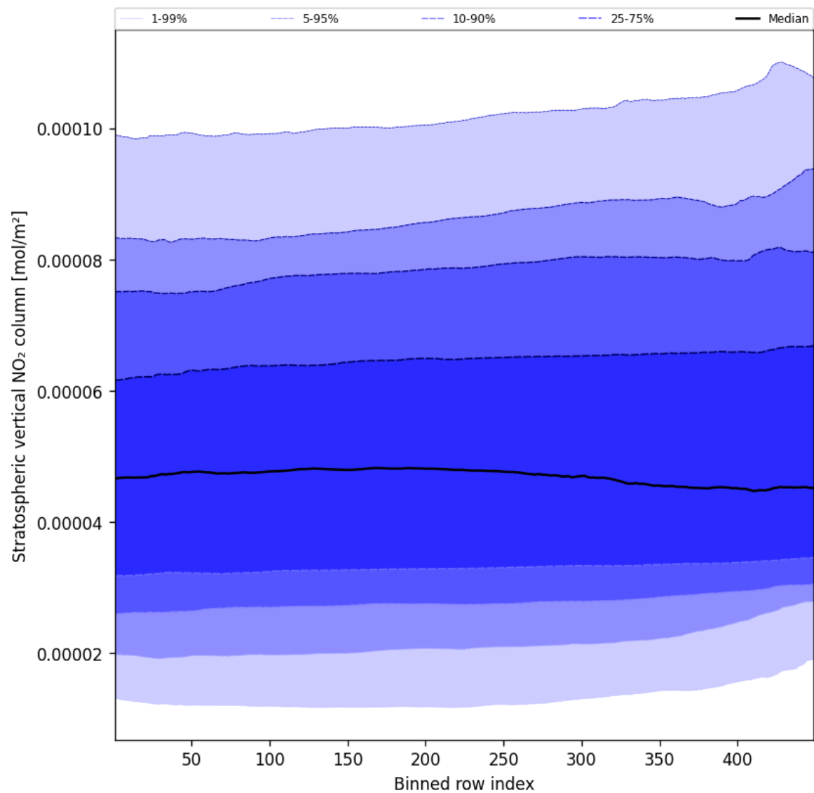
Figure 53: Along track statistics of “Stratospheric vertical NO 2 column” for 2024-11-25 to 2024-11-26
