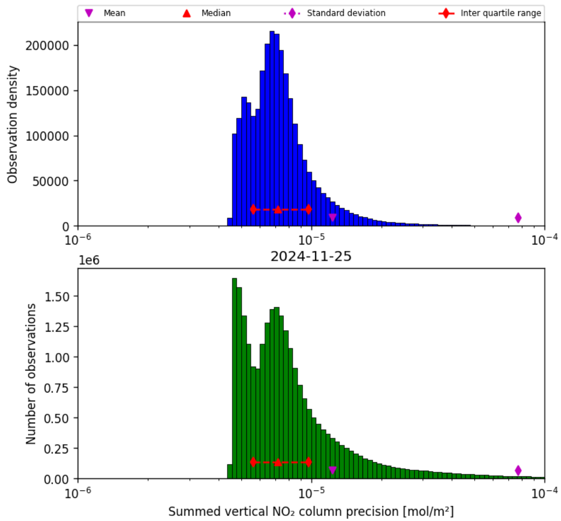
Figure 41: Histogram of “Summed vertical NO 2 column precision” for 2024-11-25 to 2024-11-26
