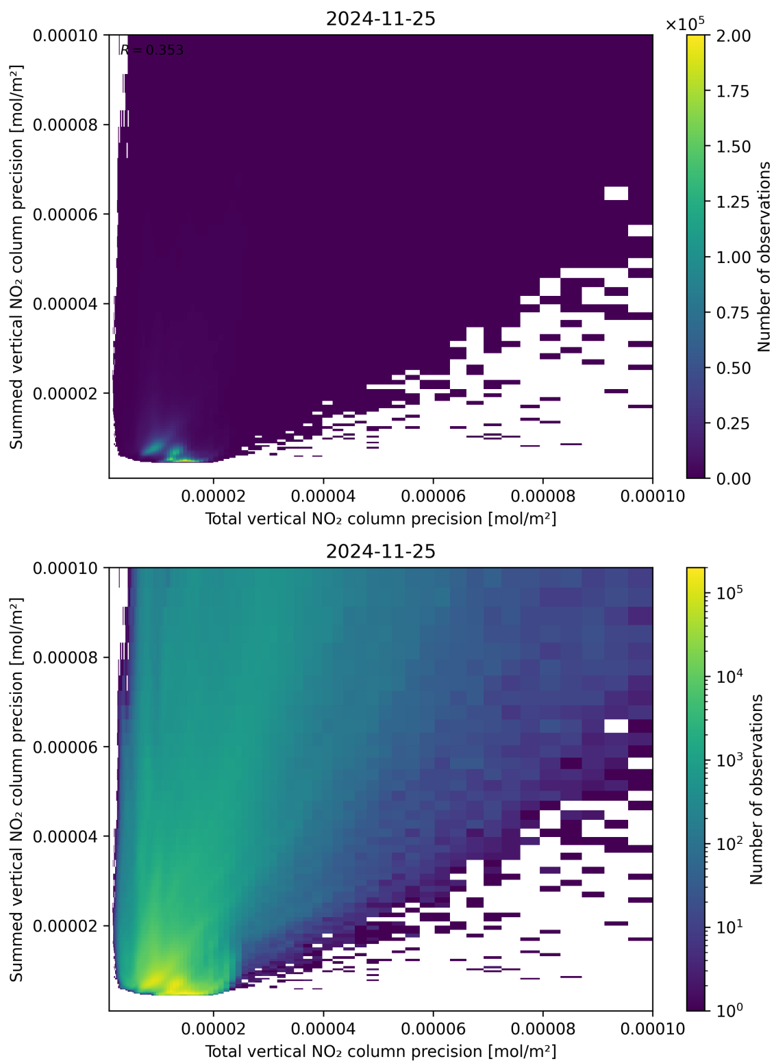
Figure 118: Scatter density plot of “Total vertical NO 2 column precision” against “Summed vertical NO 2 column precision” for 2024-11-25 to 2024-11-26.
