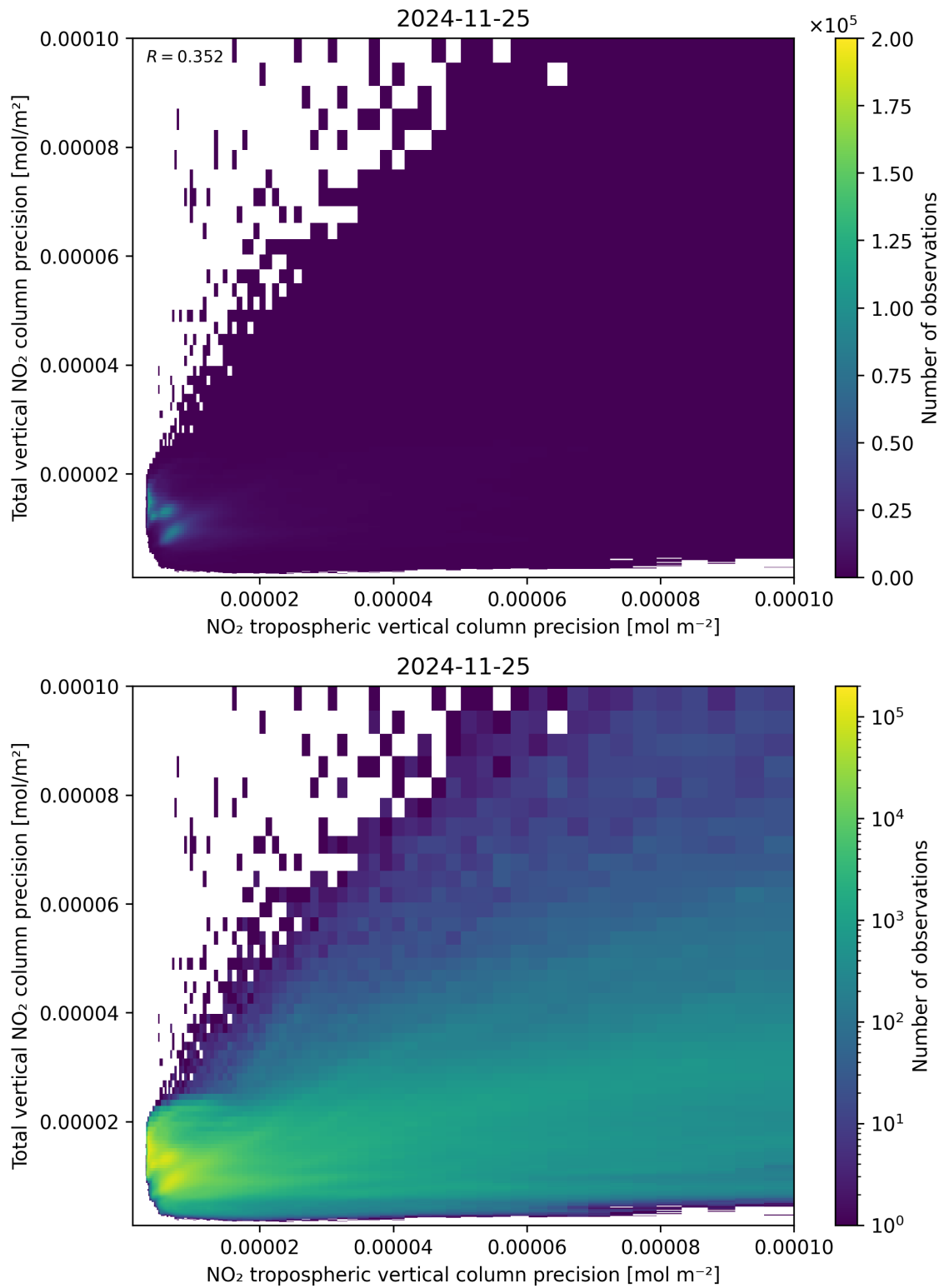
Figure 139: Scatter density plot of “NO 2 tropospheric vertical column precision” against “Total vertical NO 2 column precision” for 2024-11-25 to 2024-11-26.
