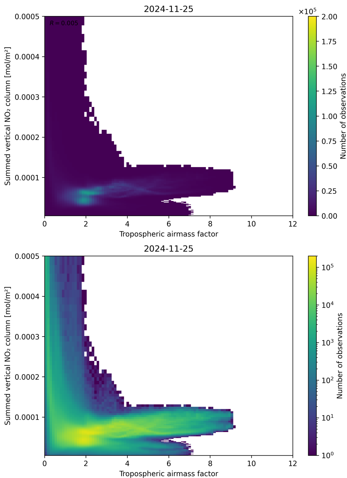
Figure 75: Scatter density plot of “Tropospheric air mass factor” against “Summed vertical NO 2 column” for 2024-11-25 to 2024-11-26.
