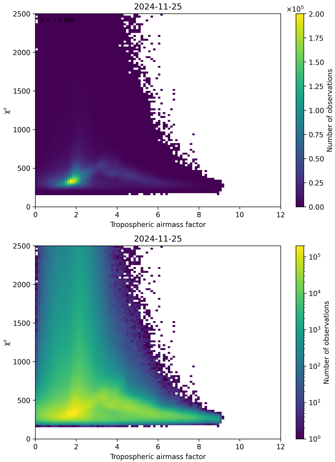
Figure 73: Scatter density plot of “Tropospheric airmass factor” against “ \chi^2 ” for 2024-11-25 to 2024-11-26.
