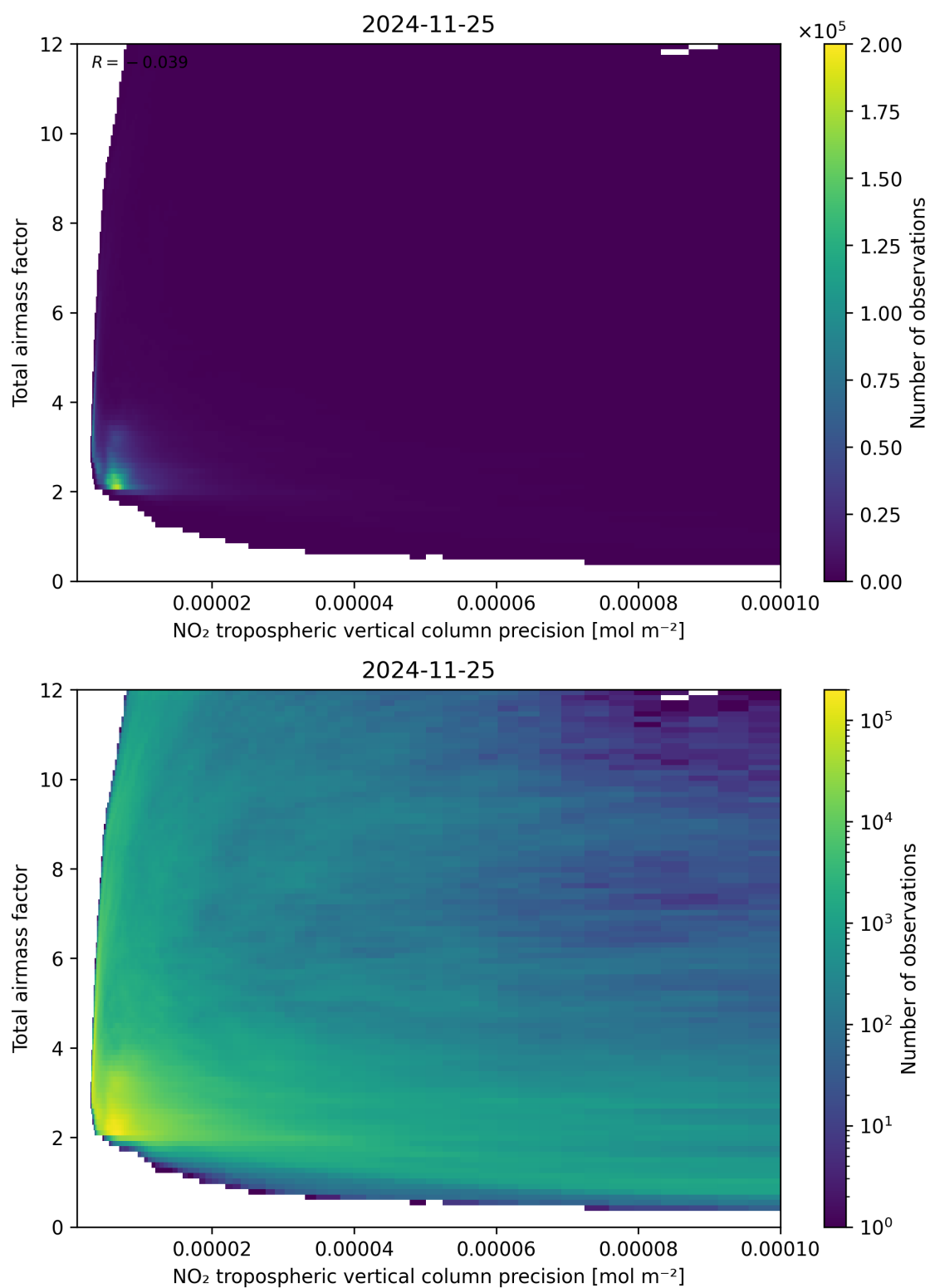
Figure 132: Scatter density plot of “NO 2 tropospheric vertical column precision” against “Total air mass factor” for 2024-11-25 to 2024-11-26.
