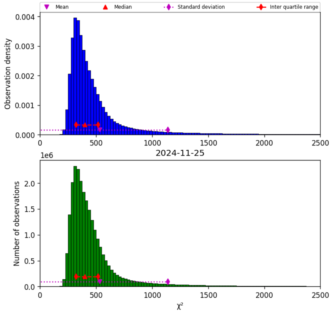
Figure 42: Histogram of “ \chi^2 ” for 2024-11-25 to 2024-11-26
