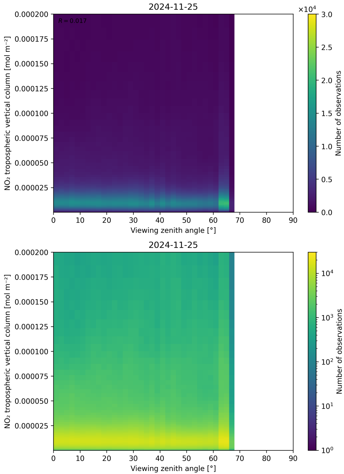
Figure 169: Scatter density plot of “Viewing zenith angle” against “NO 2 tropospheric vertical column” for 2024-11-25 to 2024-11-26.
