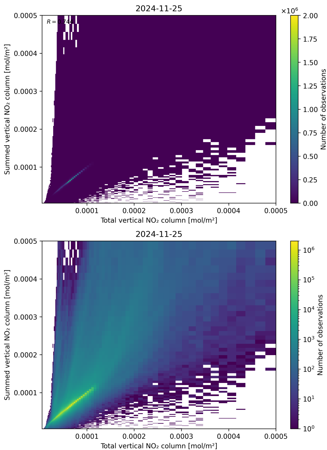
Figure 112: Scatter density plot of “Total vertical NO 2 column” against “Summed vertical NO 2 column” for 2024-11-25 to 2024-11-26.
