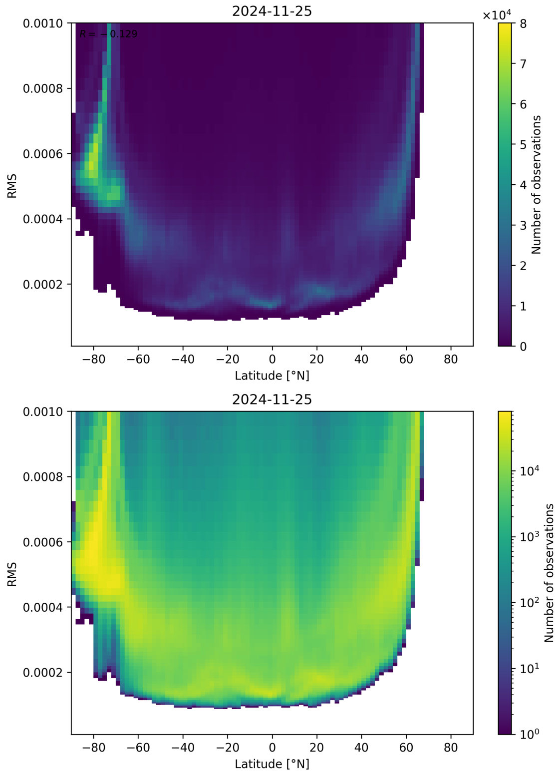
Figure 94: Scatter density plot of “Latitude” against “RMS” for 2024-11-25 to 2024-11-26.
