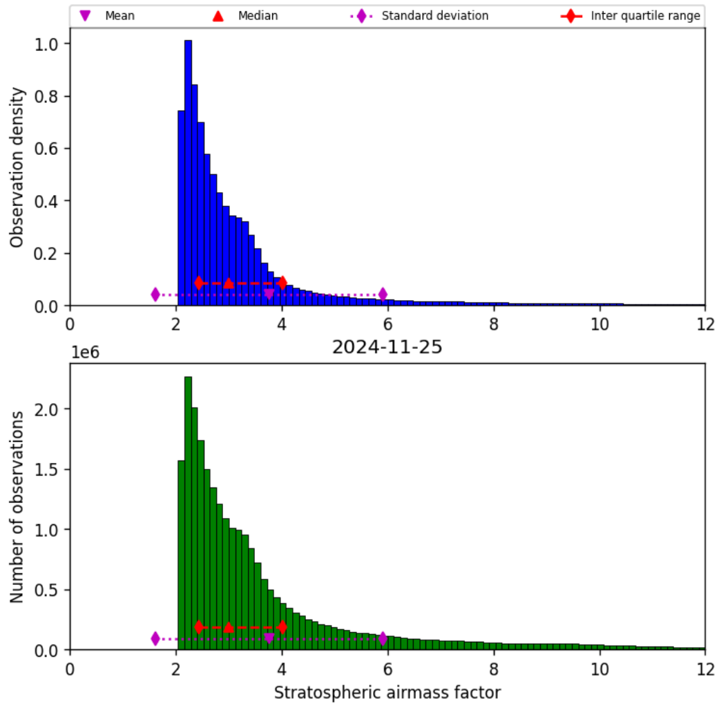
Figure 44: Histogram of “Stratospheric airmass factor” for 2024-11-25 to 2024-11-26
