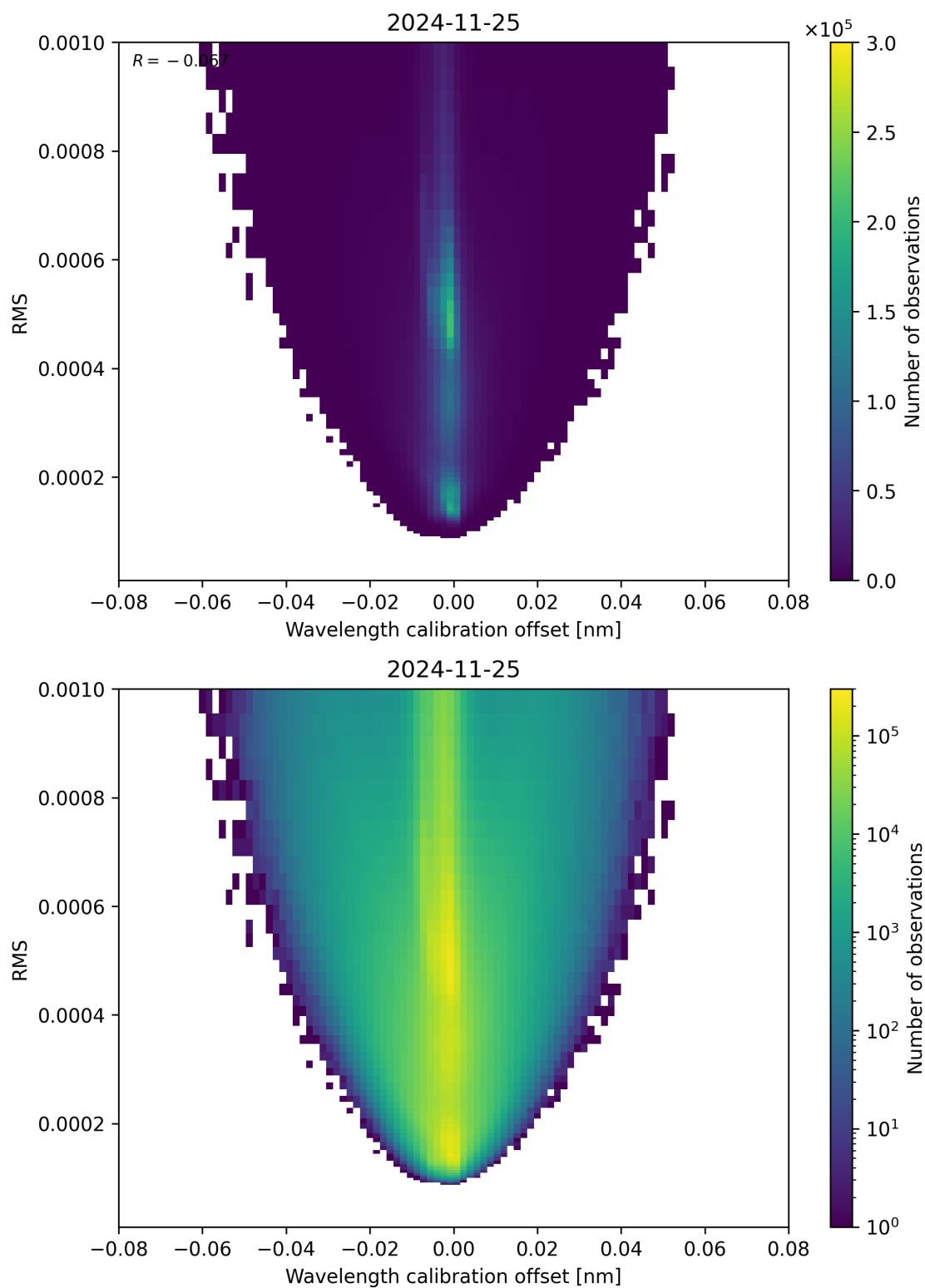
Figure 181: Scatter density plot of “Wavelength calibration offset” against “RMS” for 2024-11-25 to 2024-11-26.
