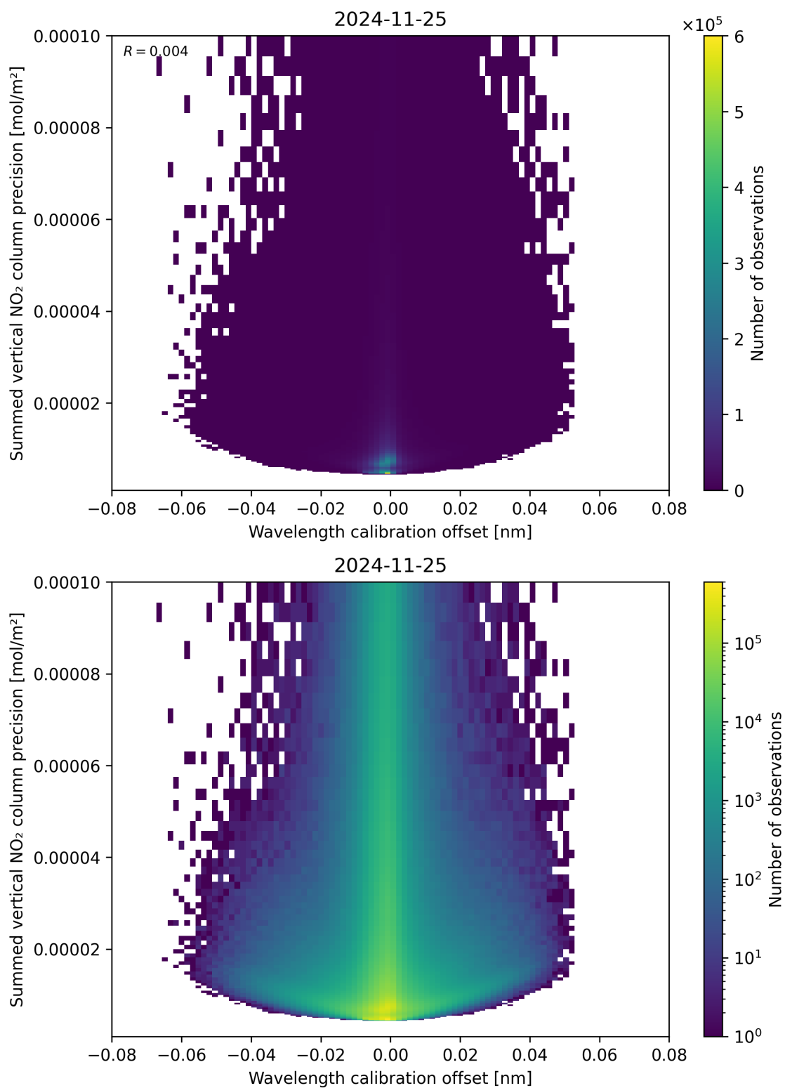
Figure 178: Scatter density plot of “Wavelength calibration offset” against “Summed vertical NO 2 column precision” for 2024-11-25 to 2024-11-26.
