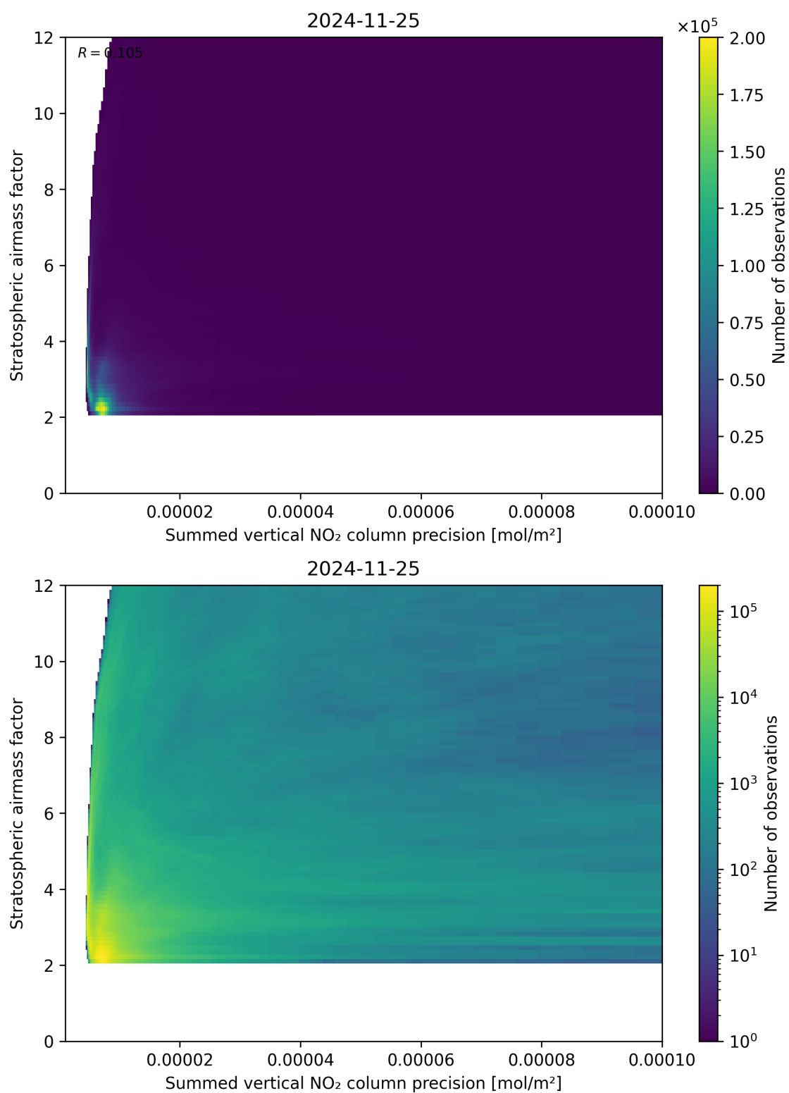
Figure 106: Scatter density plot of “Summed vertical NO 2 column precision” against “Stratospheric airmass factor” for 2024-11-25 to 2024-11-26.
