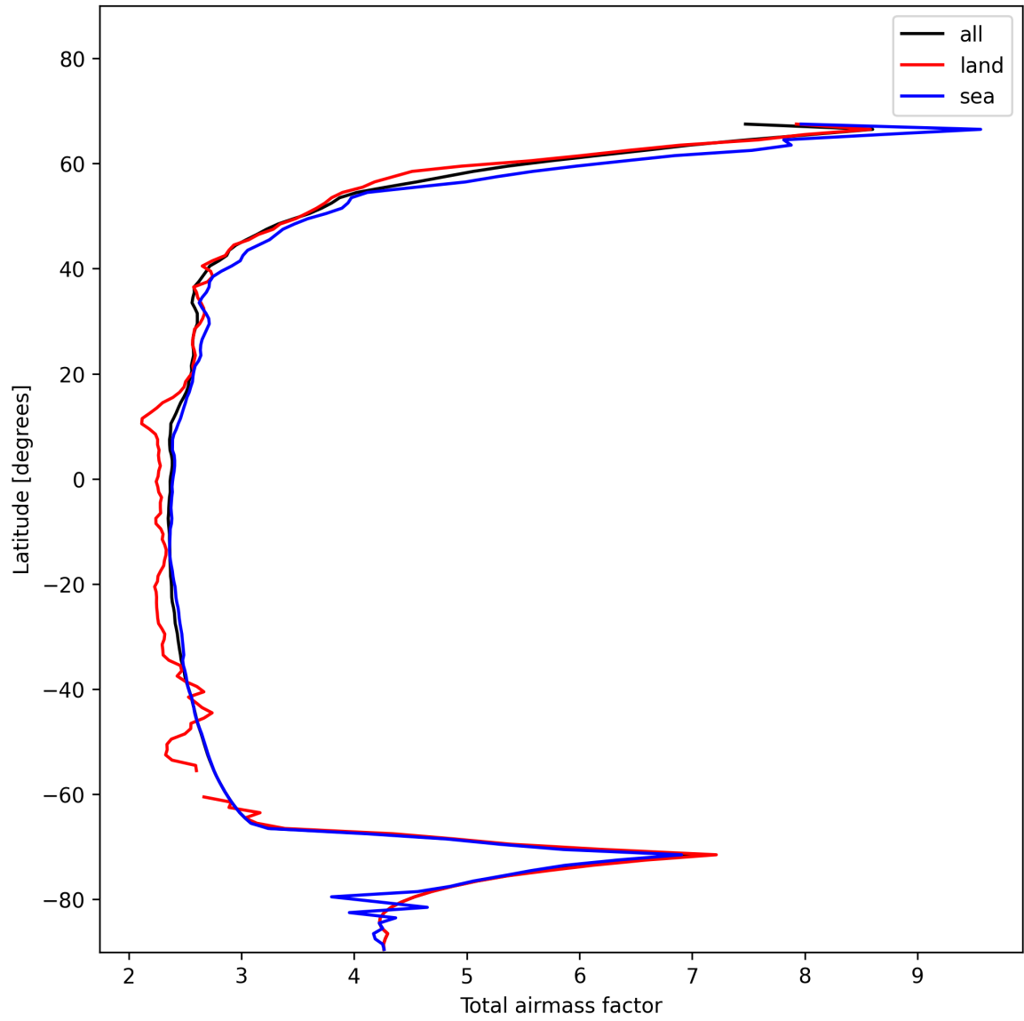
Figure 15: Zonal average of “Total airmass factor” for 2024-11-25 to 2024-11-26.
