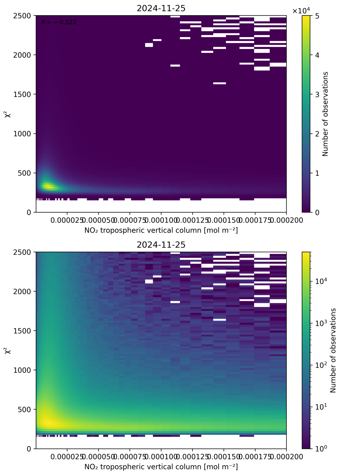
Figure 124: Scatter density plot of “NO 2 tropospheric vertical column” against “ \chi^2 ” for 2024-11-25 to 2024-11-26.
