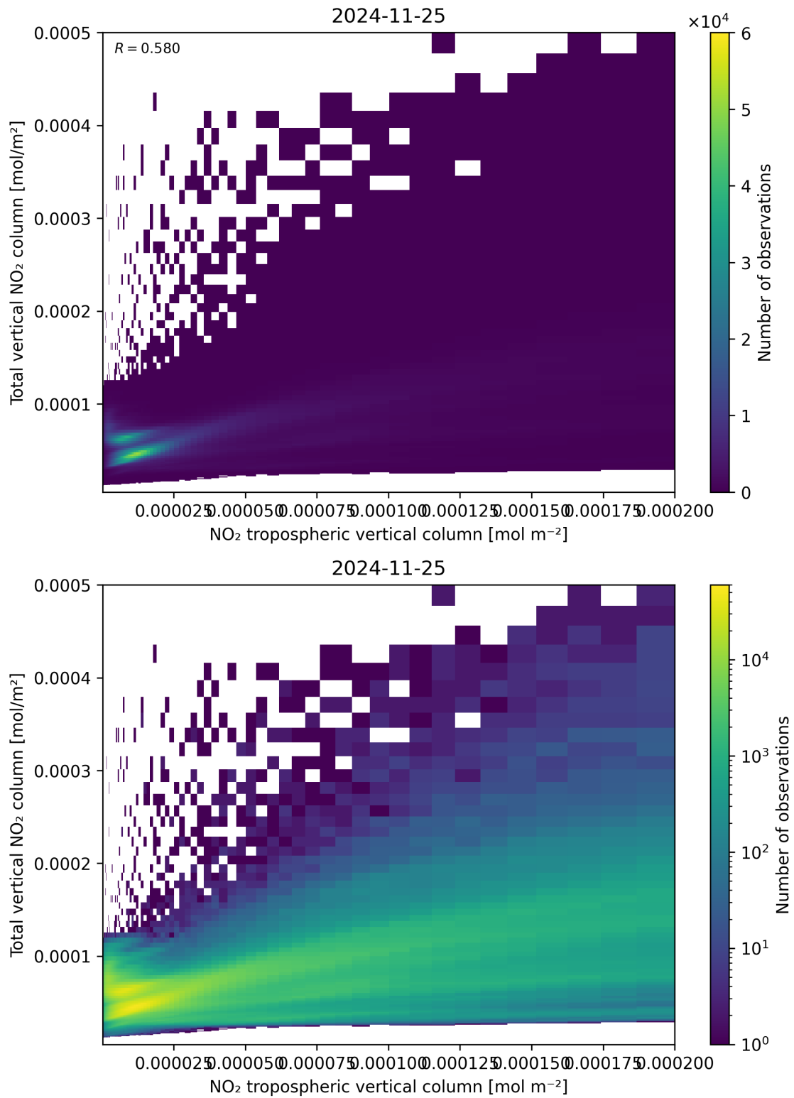
Figure 128: Scatter density plot of “NO 2 tropospheric vertical column” against “Total vertical NO 2 column” for 2024-11-25 to 2024-11-26.
