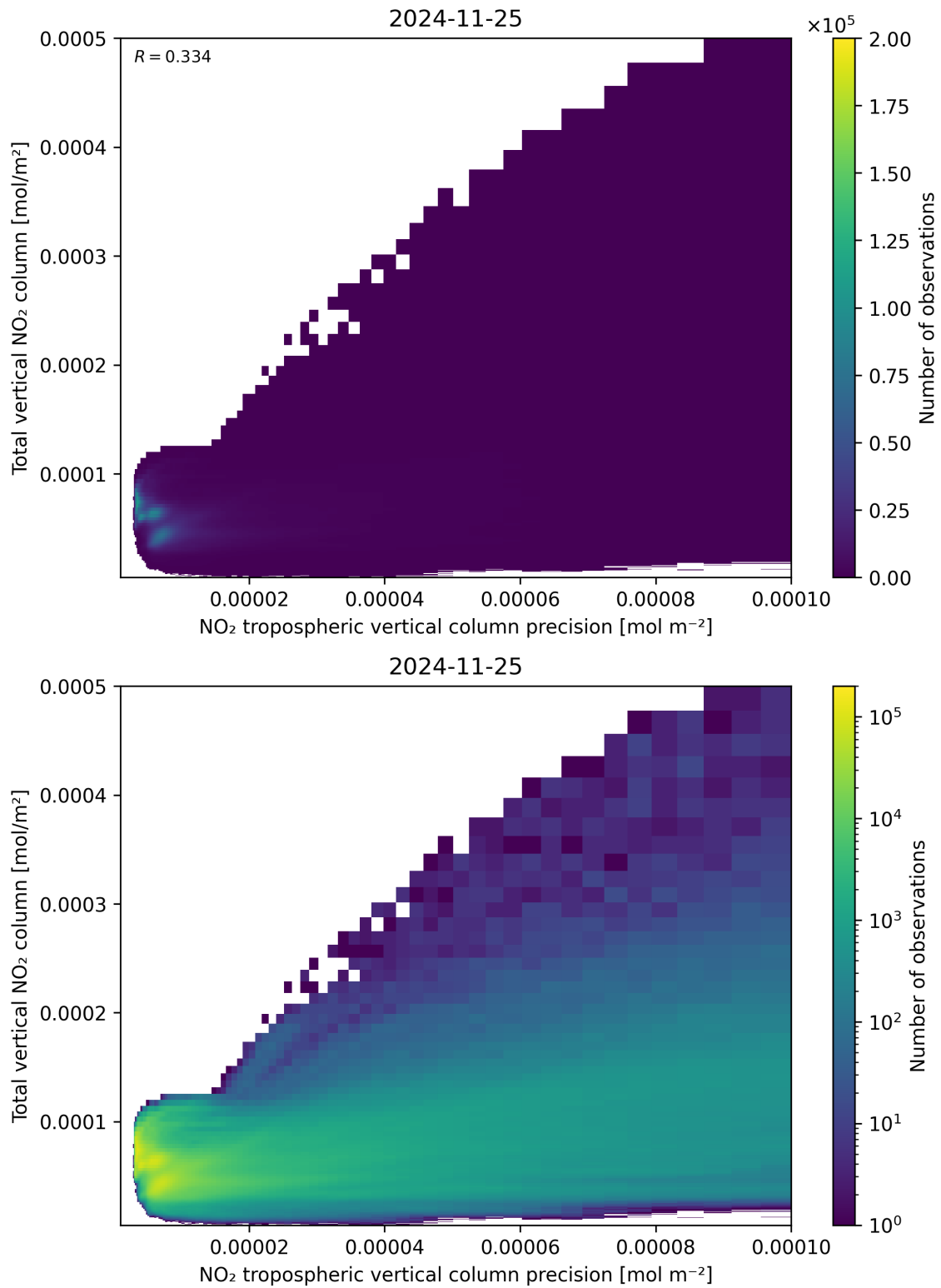
Figure 138: Scatter density plot of “NO 2 tropospheric vertical column precision” against “Total vertical NO 2 column” for 2024-11-25 to 2024-11-26.
