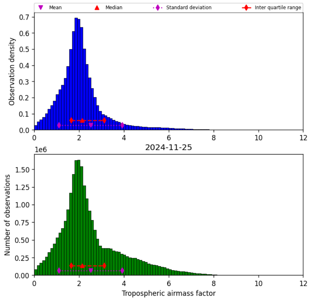
Figure 31: Histogram of “Tropospheric airmass factor” for 2024-11-25 to 2024-11-26
