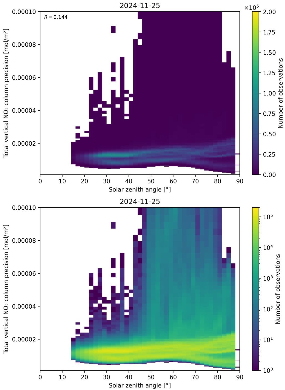
Figure 154: Scatter density plot of “Solar zenith angle” against “Total vertical NO 2 column precision” for 2024-11-25 to 2024-11-26.
