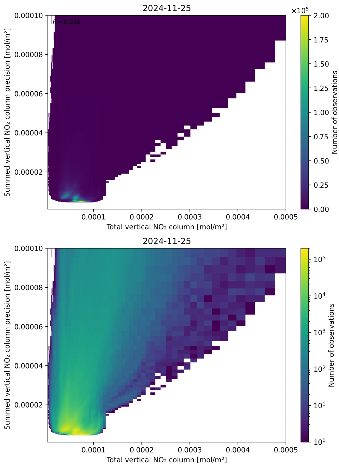
Figure 113: Scatter density plot of “Total vertical NO 2 column” against “Summed vertical NO 2 column precision” for 2024-11-25 to 2024-11-26.
