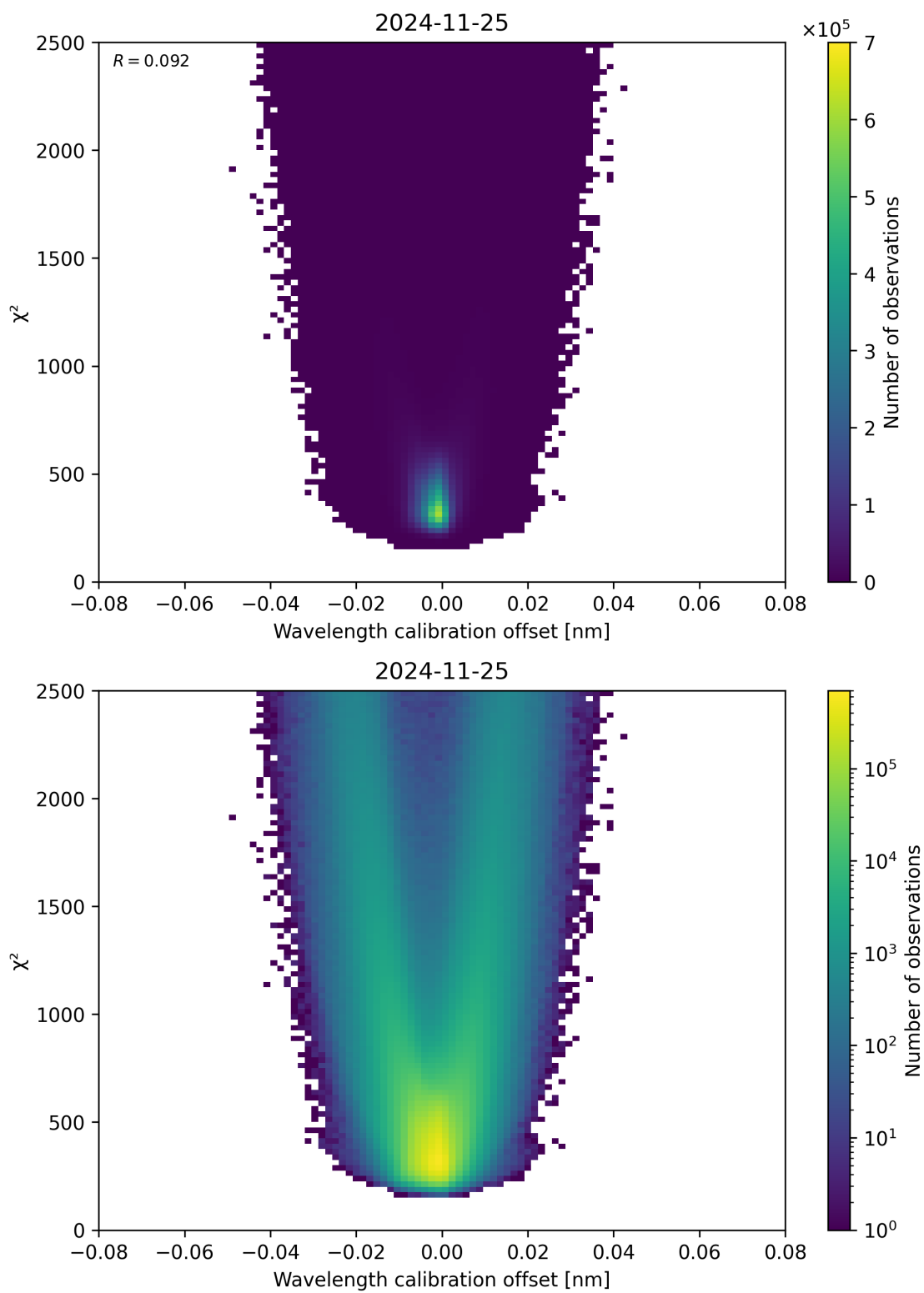
Figure 175: Scatter density plot of “Wavelength calibration offset” against “ \chi^2 ” for 2024-11-25 to 2024-11-26.
