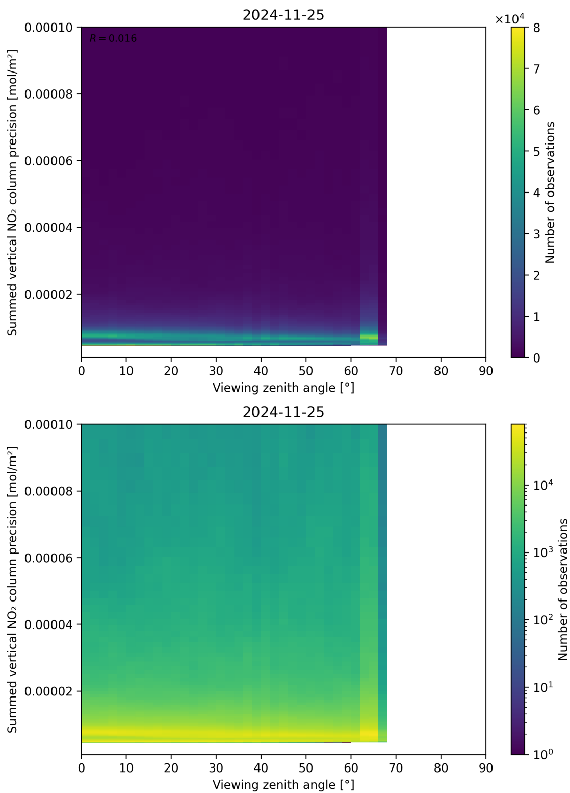
Figure 166: Scatter density plot of “Viewing zenith angle” against “Summed vertical NO 2 column precision” for 2024-11-25 to 2024-11-26.
