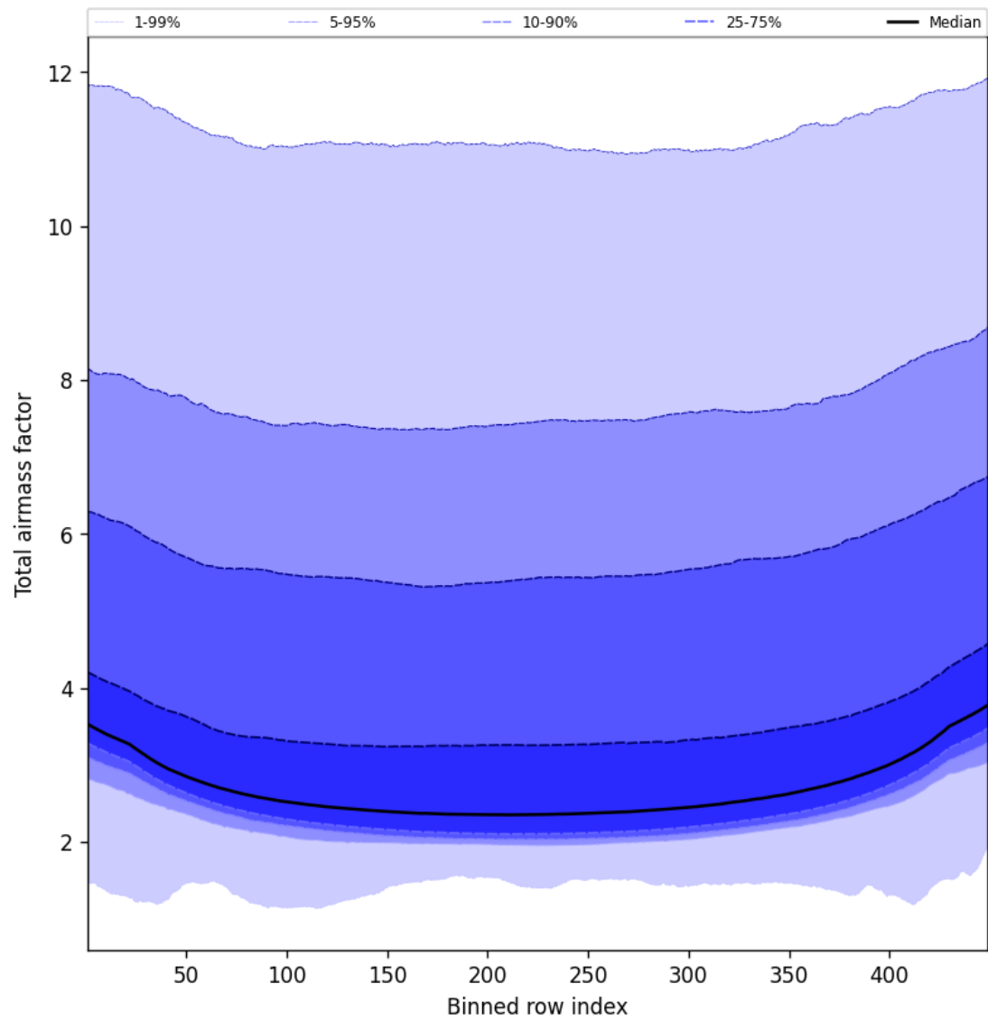
Figure 49: Along track statistics of “Total airmass factor” for 2024-11-25 to 2024-11-26
