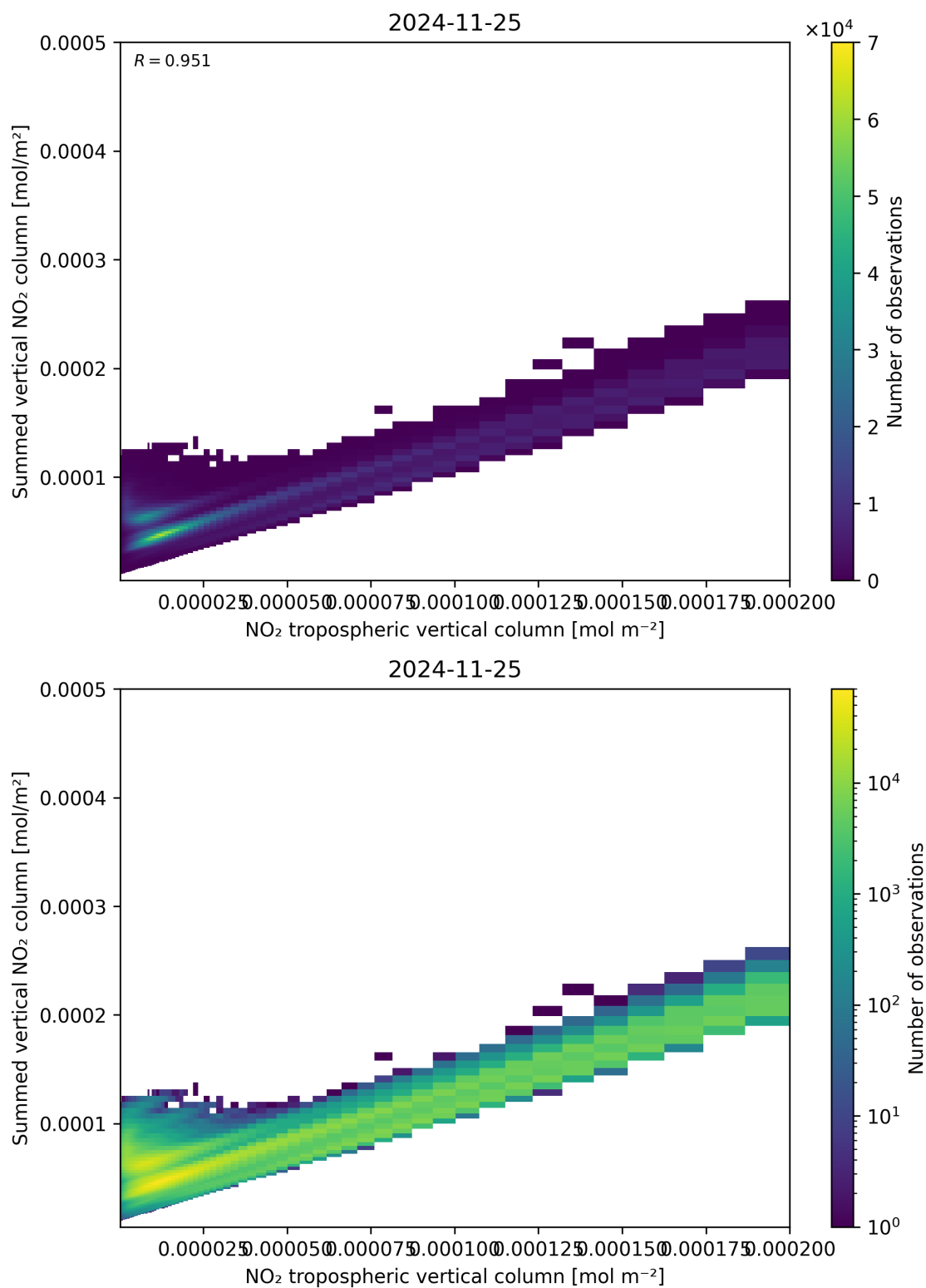
Figure 126: Scatter density plot of “NO 2 tropospheric vertical column” against “Summed vertical NO 2 column” for 2024-11-25 to 2024-11-26.
