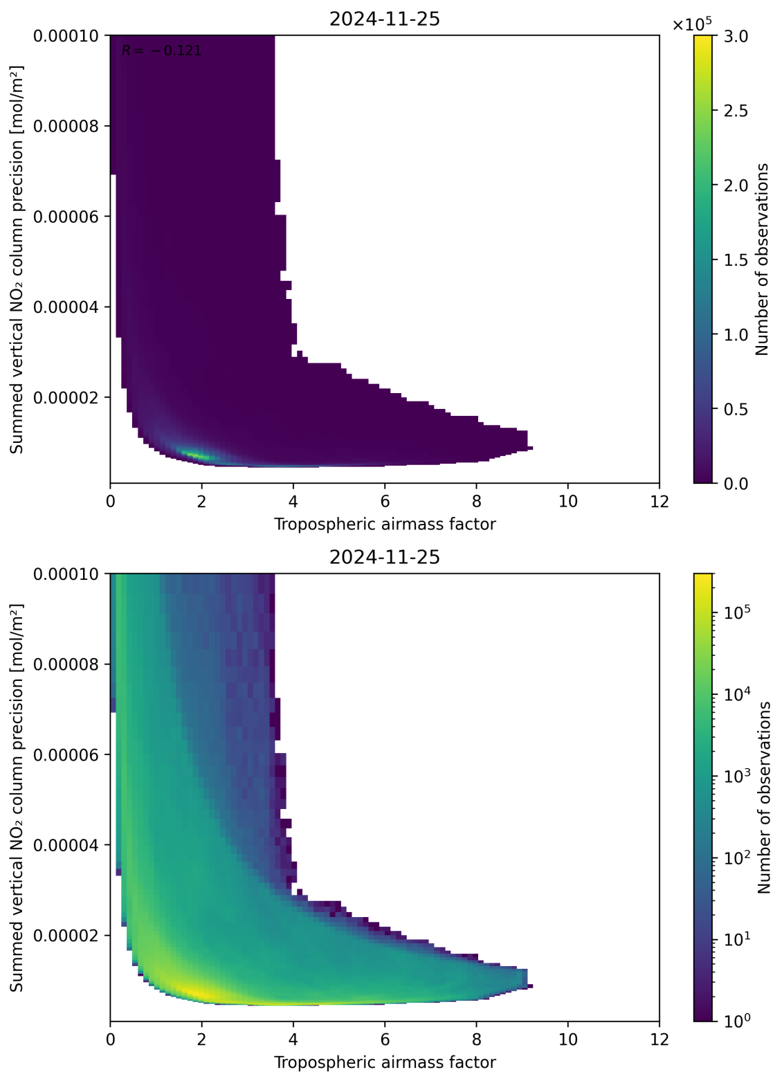
Figure 76: Scatter density plot of “Tropospheric air mass factor” against “Summed vertical NO 2 column precision” for 2024-11-25 to 2024-11-26.
