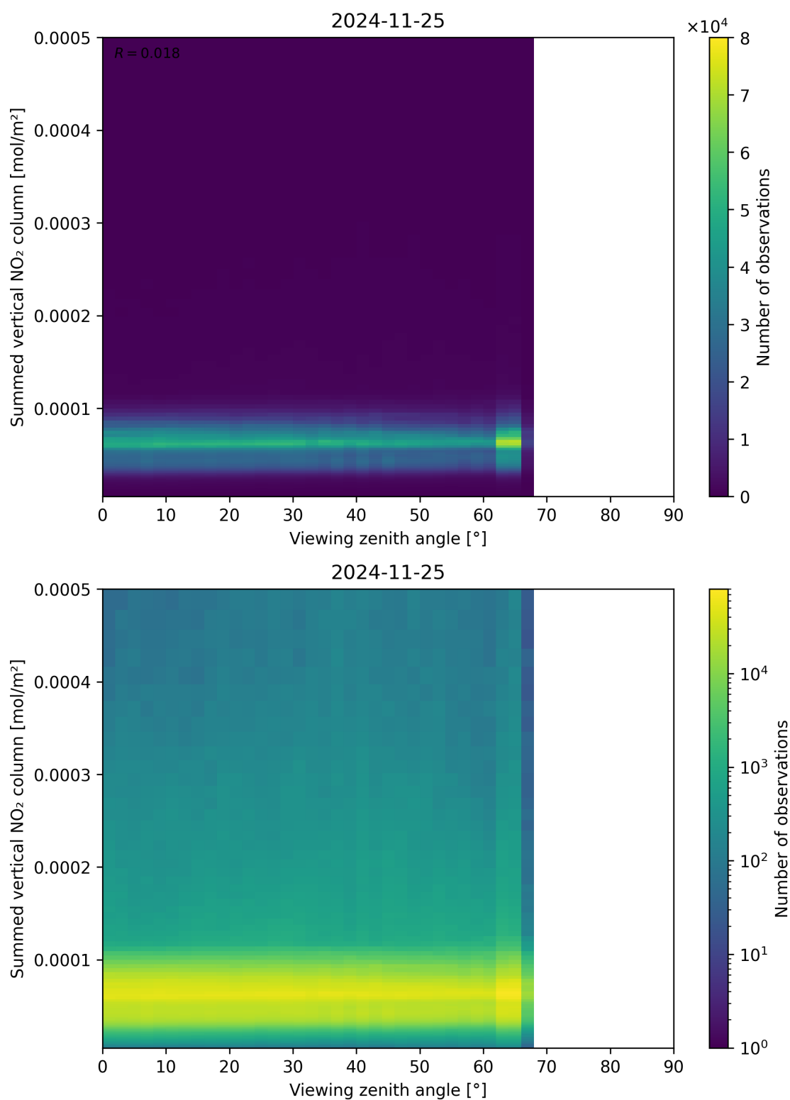
Figure 165: Scatter density plot of “Viewing zenith angle” against “Summed vertical NO 2 column” for 2024-11-25 to 2024-11-26.
