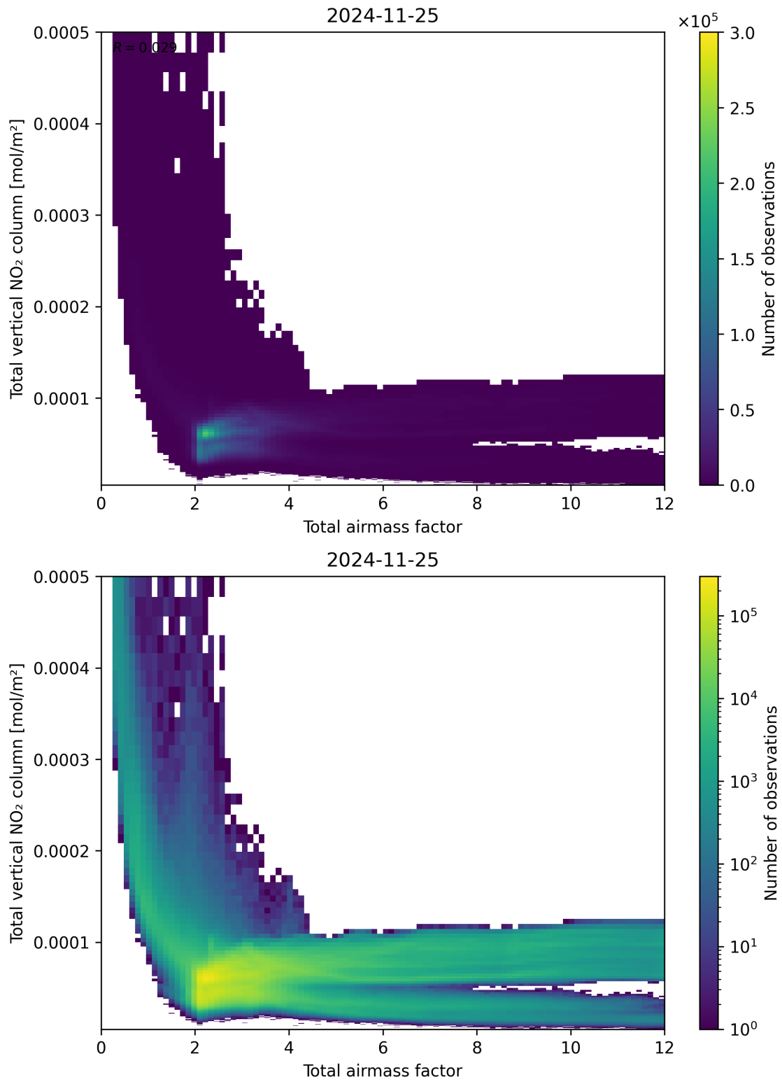
Figure 67: Scatter density plot of “Total airmass factor” against “Total vertical NO 2 column” for 2024-11-25 to 2024-11-26.
