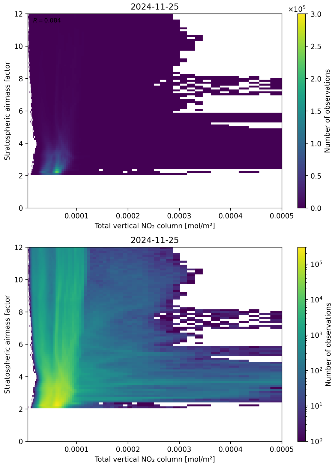
Figure 110: Scatter density plot of “Total vertical NO 2 column” against “Stratospheric airmass factor” for 2024-11-25 to 2024-11-26.
