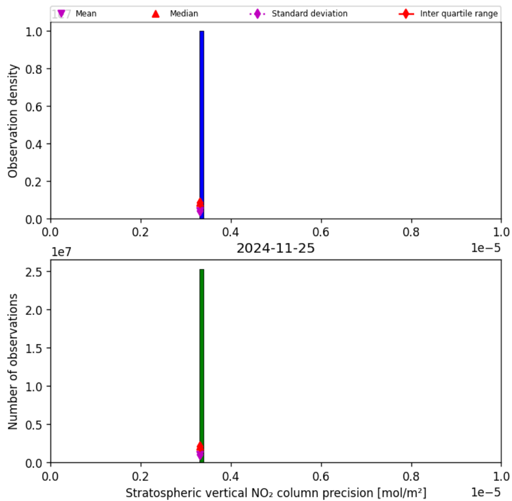
Figure 37: Histogram of “Stratospheric vertical NO 2 column precision” for 2024-11-25 to 2024-11-26
