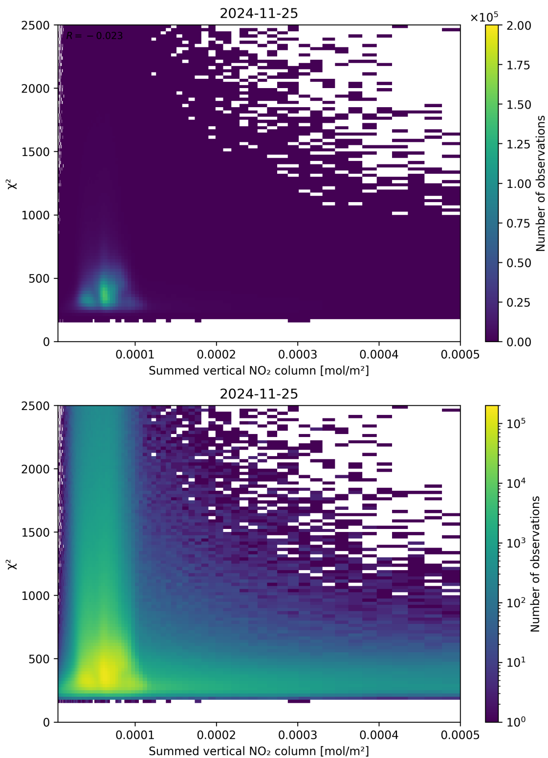
Figure 104: Scatter density plot of “Summed vertical NO 2 column” against “ \chi^2 ” for 2024-11-25 to 2024-11-26.
