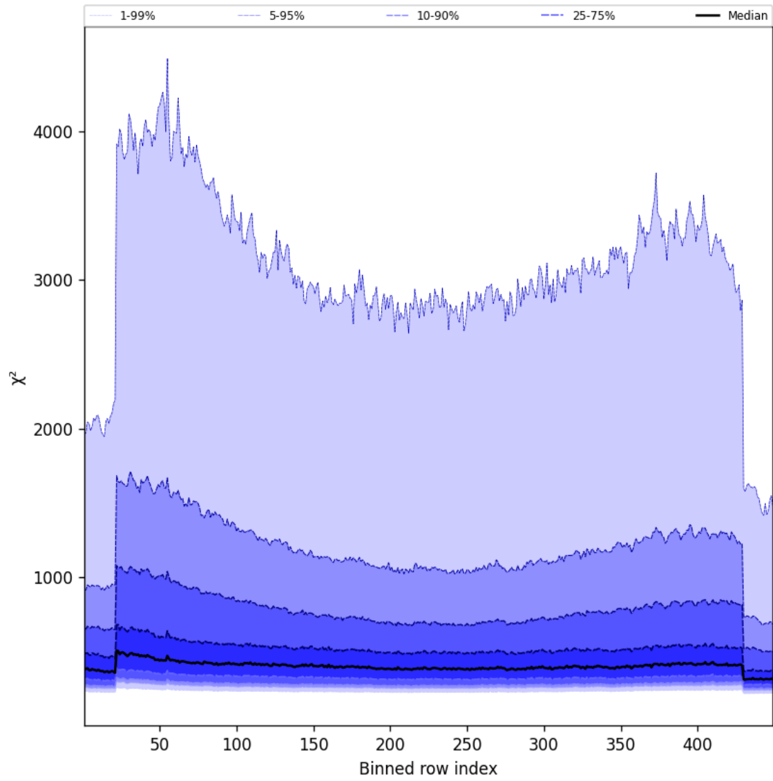
Figure 59: Along track statistics of “ \chi^2 ” for 2024-11-25 to 2024-11-26
