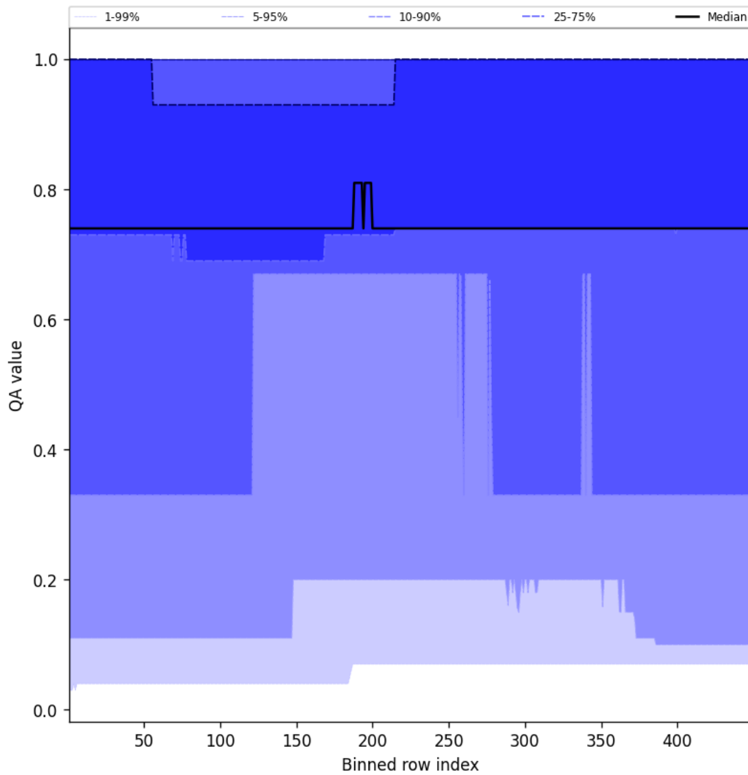
Figure 45: Along track statistics of “QA value” for 2024-11-25 to 2024-11-26
