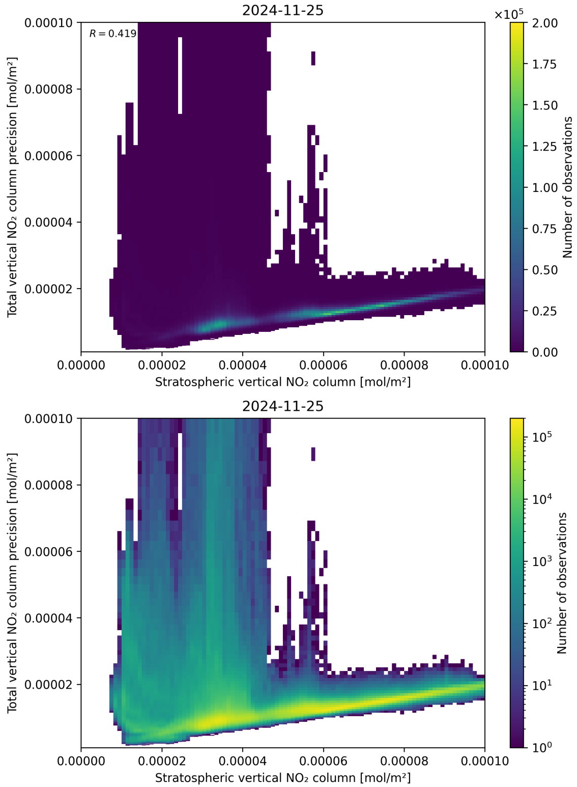
Figure 101: Scatter density plot of “Stratospheric vertical NO 2 column” against “Total vertical NO 2 column precision” for 2024-11-25 to 2024-11-26.
