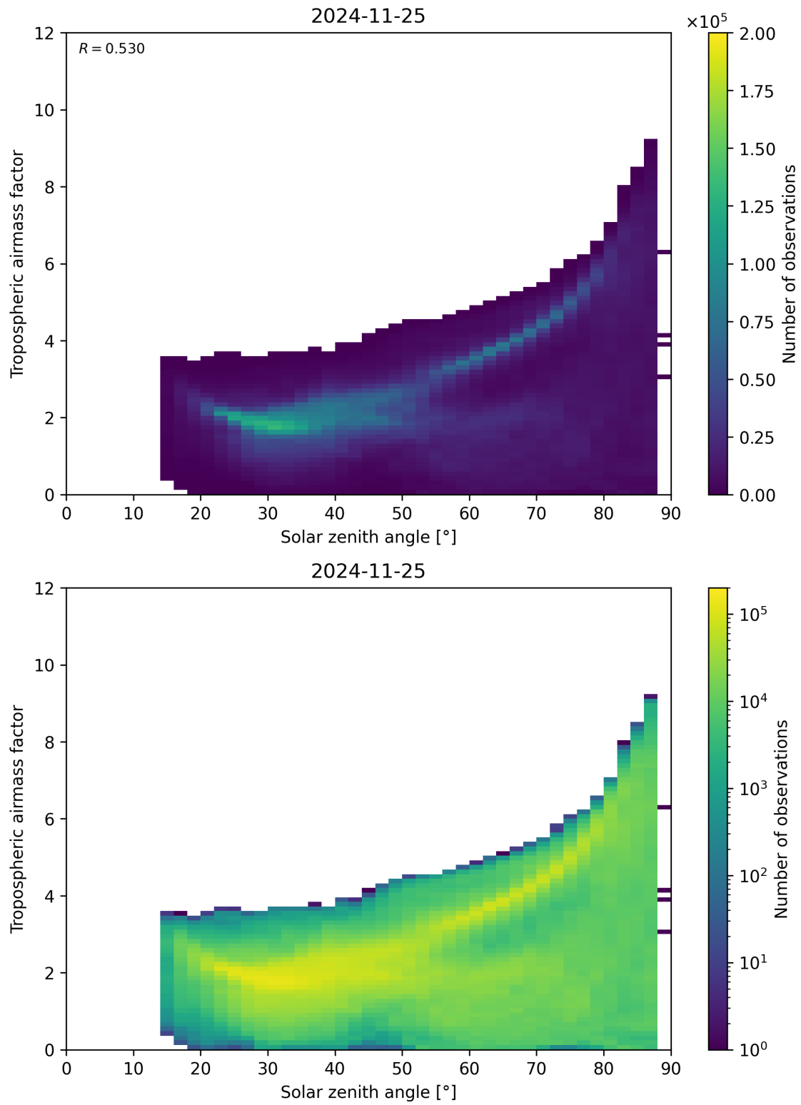
Figure 147: Scatter density plot of “Solar zenith angle” against “Tropospheric airmass factor” for 2024-11-25 to 2024-11-26.
