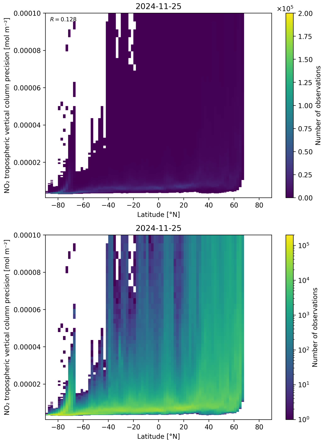
Figure 93: Scatter density plot of “Latitude” against “NO 2 tropospheric vertical column precision” for 2024-11-25 to 2024-11-26.
