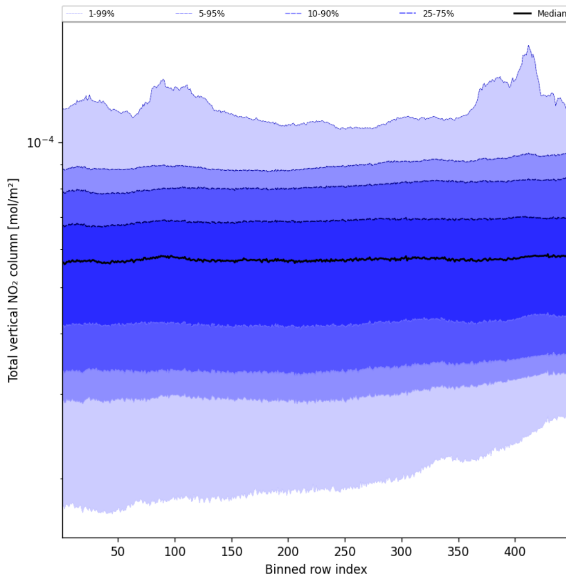
Figure 55: Along track statistics of “Total vertical NO 2 column” for 2024-11-25 to 2024-11-26
