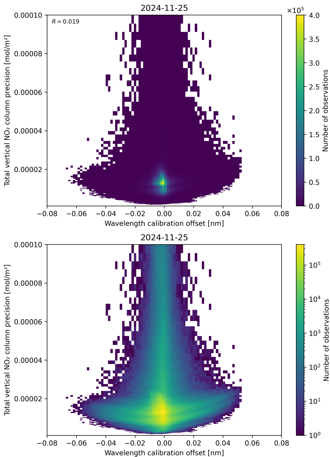
Figure 180: Scatter density plot of “Wavelength calibration offset” against “Total vertical NO 2 column precision” for 2024-11-25 to 2024-11-26.
