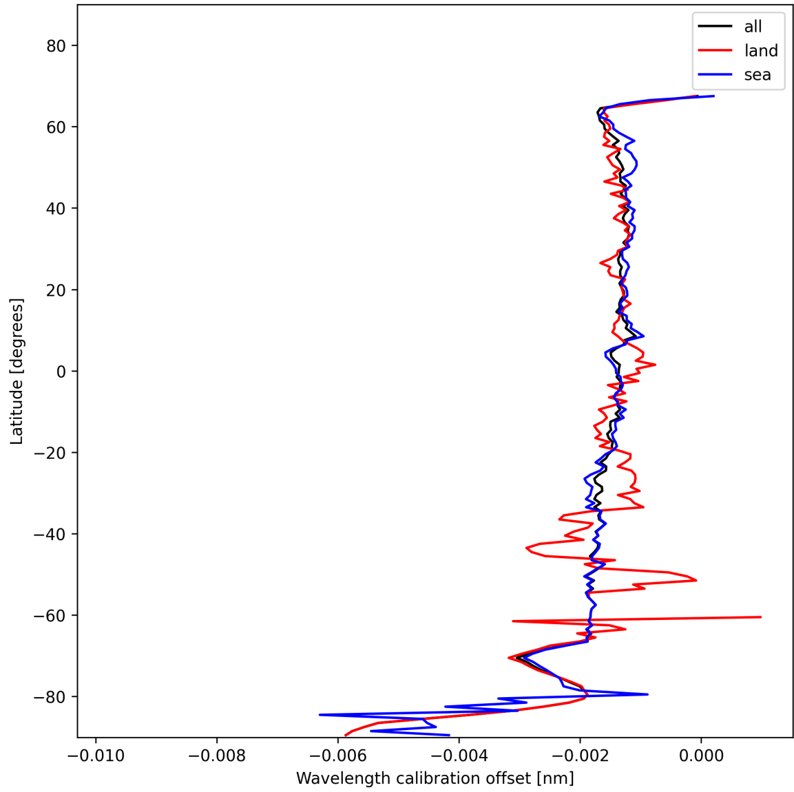
Figure 18: Zonal average of “Wavelength calibration offset” for 2024-11-25 to 2024-11-26.
