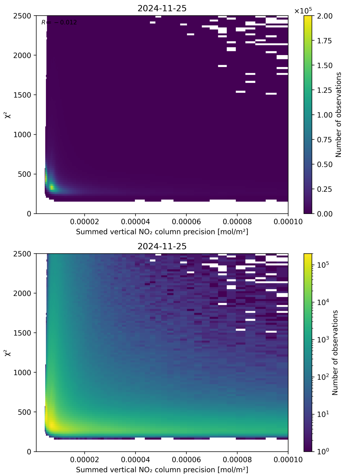
Figure 107: Scatter density plot of “Summed vertical NO 2 column precision” against “ \chi^2 ” for 2024-11-25 to 2024-11-26.
