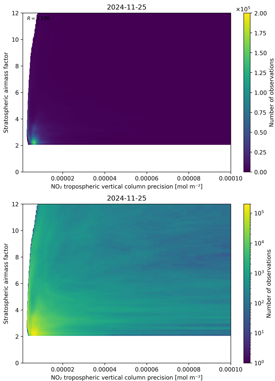
Figure 131: Scatter density plot of “NO 2 tropospheric vertical column precision” against “Stratospheric airmass factor” for 2024-11-25 to 2024-11-26.
