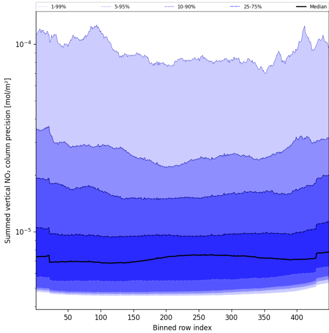
Figure 58: Along track statistics of “Summed vertical NO 2 column precision” for 2024-11-25 to 2024-11-26
