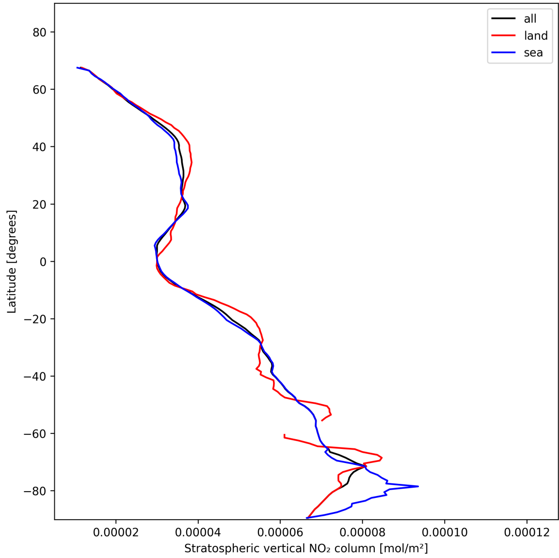
Figure 19: Zonal average of “Stratospheric vertical NO 2 column” for 2024-11-25 to 2024-11-26.
