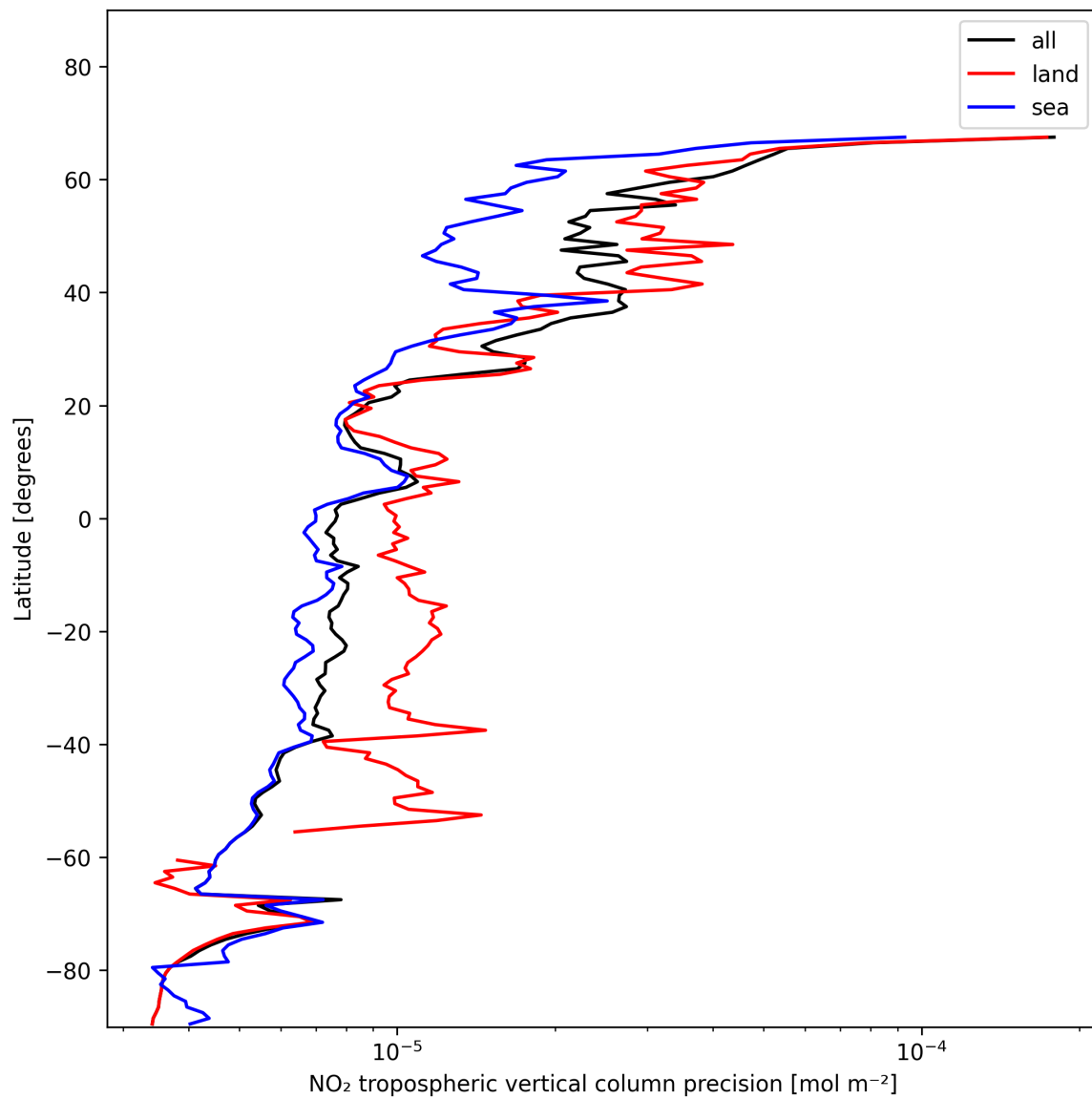
Figure 13: Zonal average of “NO 2 tropospheric vertical column precision” for 2024-11-25 to 2024-11-26.
