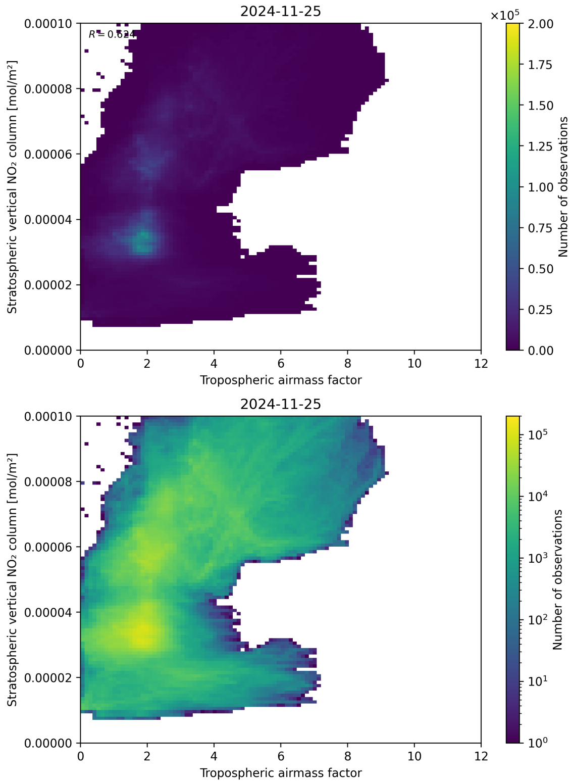
Figure 74: Scatter density plot of “Tropospheric air mass factor” against “Stratospheric vertical NO 2 column” for 2024-11-25 to 2024-11-26.
