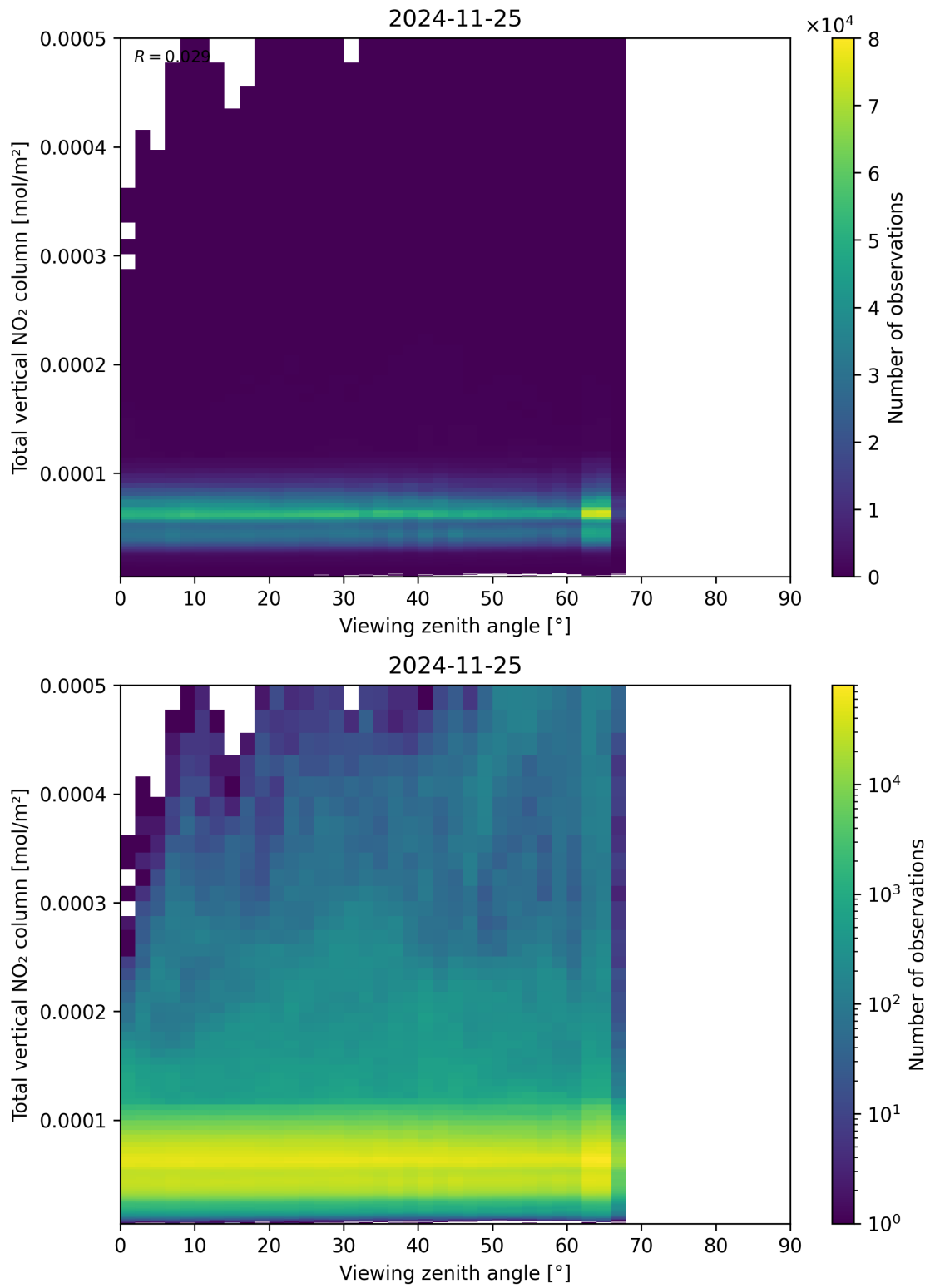
Figure 167: Scatter density plot of “Viewing zenith angle” against “Total vertical NO 2 column” for 2024-11-25 to 2024-11-26.
