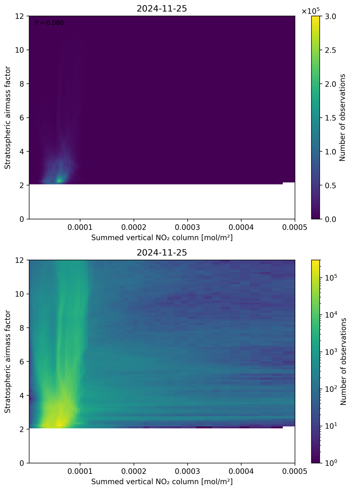
Figure 103: Scatter density plot of “Summed vertical NO 2 column” against “Stratospheric airmass factor” for 2024-11-25 to 2024-11-26.
