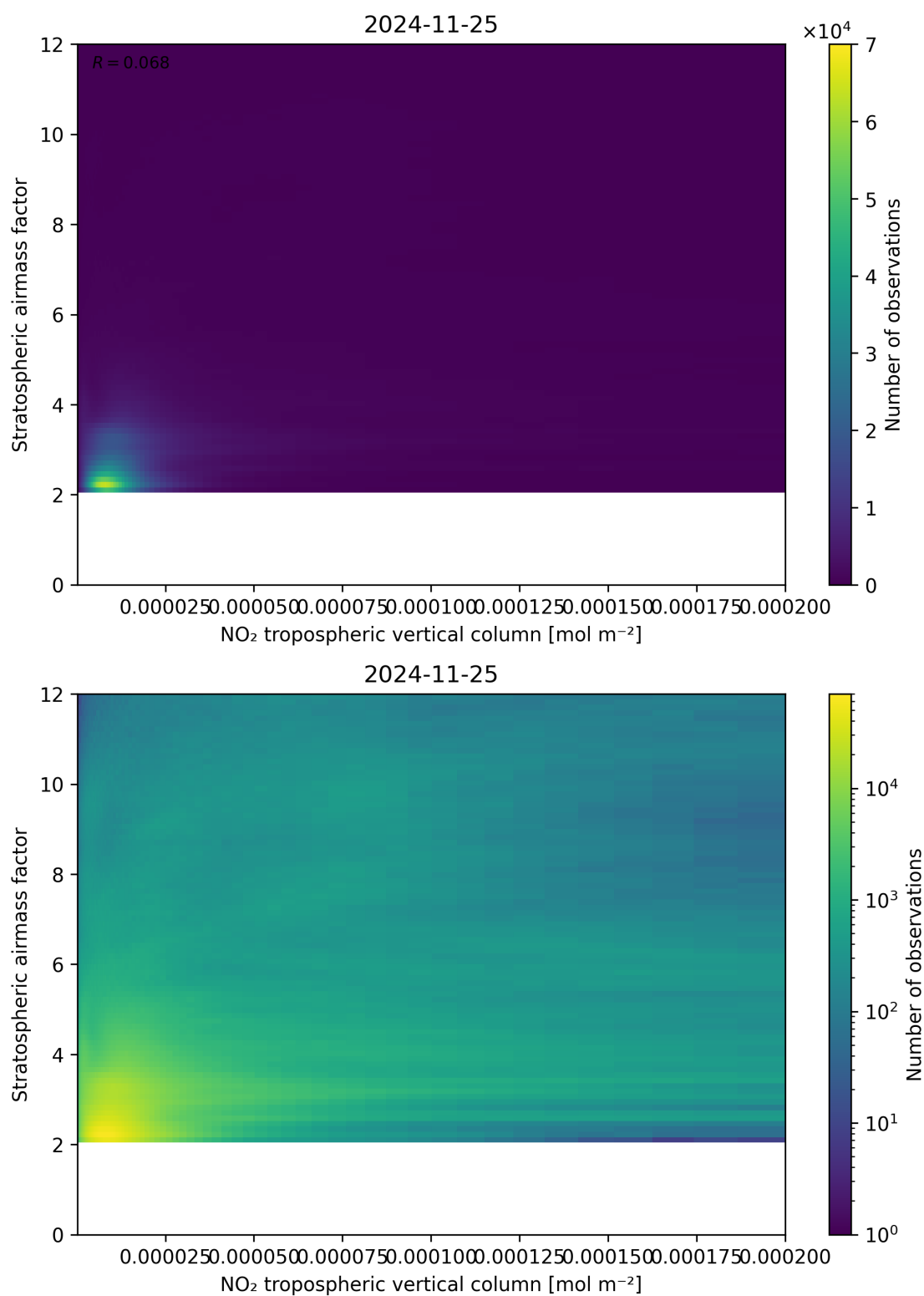
Figure 121: Scatter density plot of “NO 2 tropospheric vertical column” against “Stratospheric airmass factor” for 2024-11-25 to 2024-11-26.
