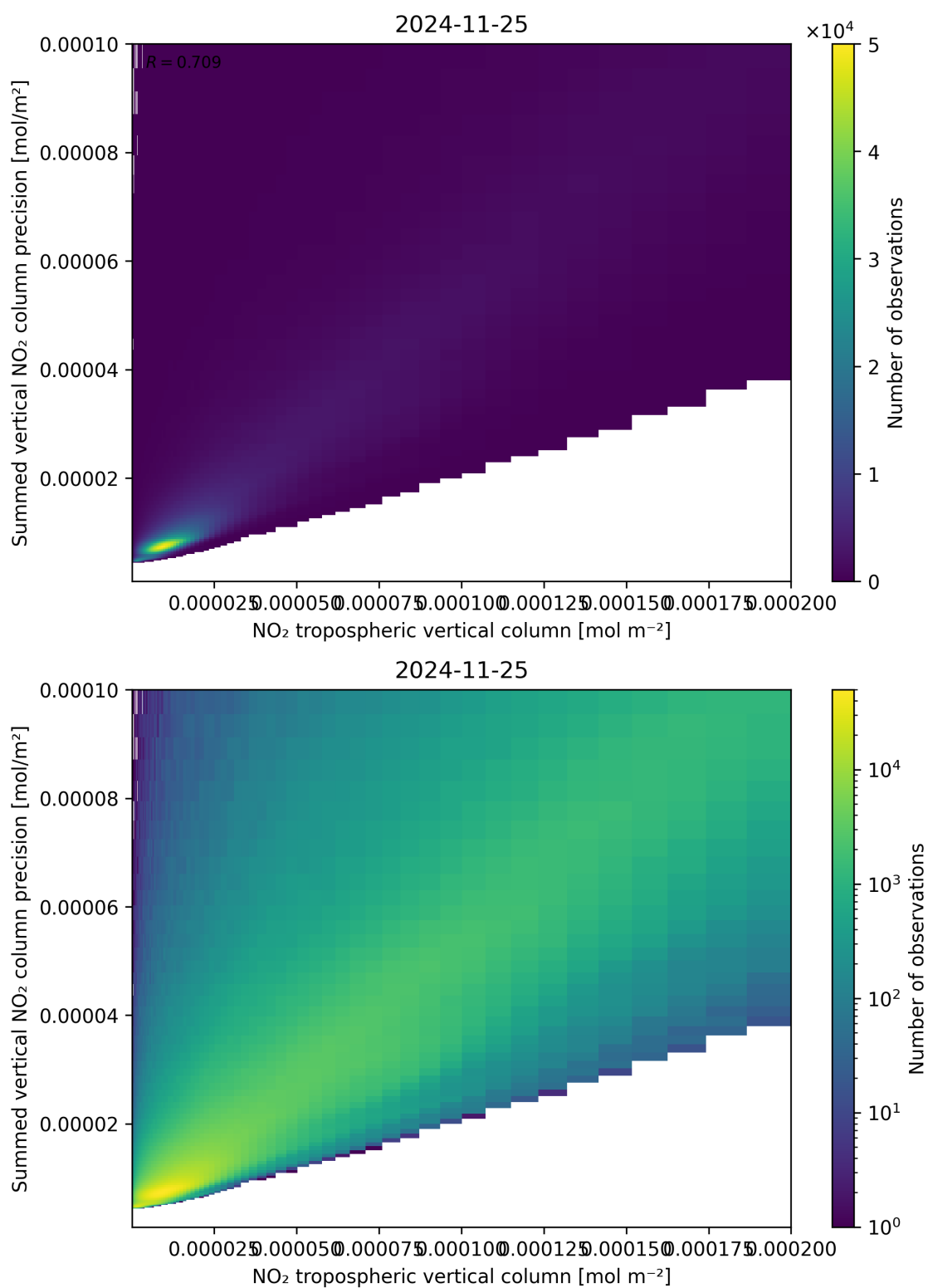
Figure 127: Scatter density plot of “NO 2 tropospheric vertical column” against “Summed vertical NO 2 column precision” for 2024-11-25 to 2024-11-26.
