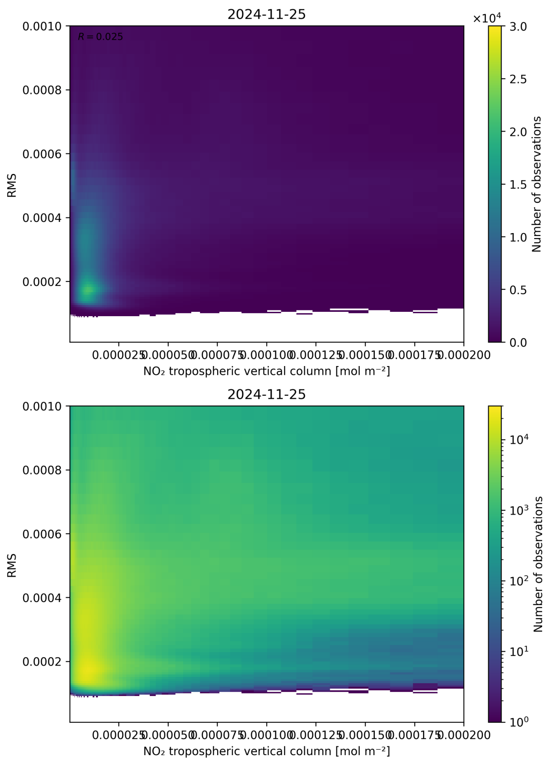
Figure 142: Scatter density plot of “NO 2 tropospheric vertical column” against “RMS” for 2024-11-25 to 2024-11-26.
