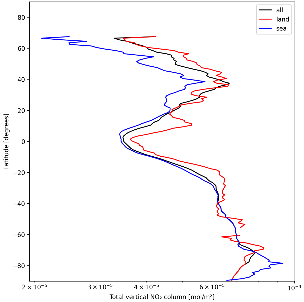
Figure 21: Zonal average of “Total vertical NO 2 column” for 2024-11-25 to 2024-11-26.
