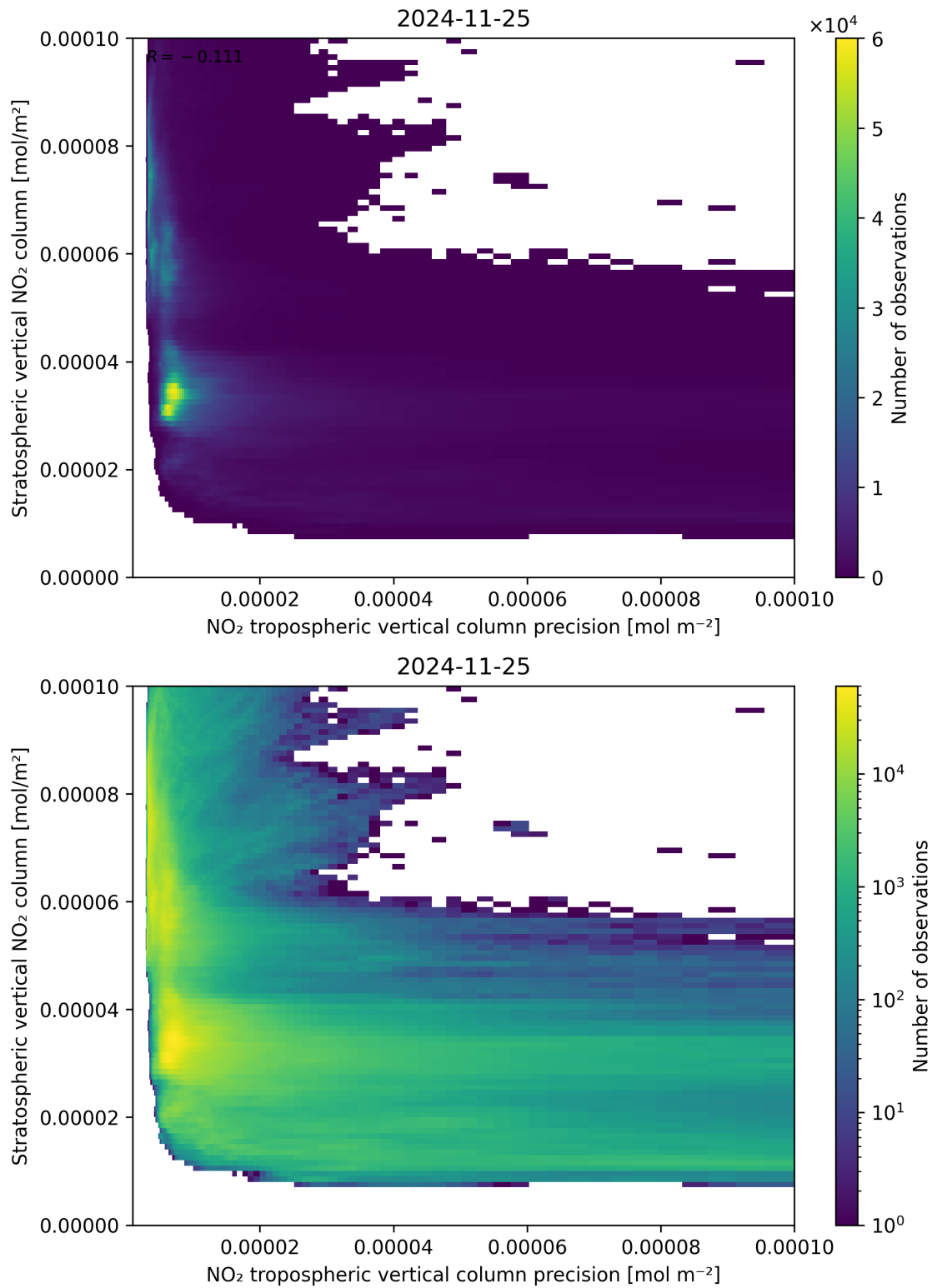
Figure 135: Scatter density plot of “NO 2 tropospheric vertical column precision” against “Stratospheric vertical NO 2 column” for 2024-11-25 to 2024-11-26.
