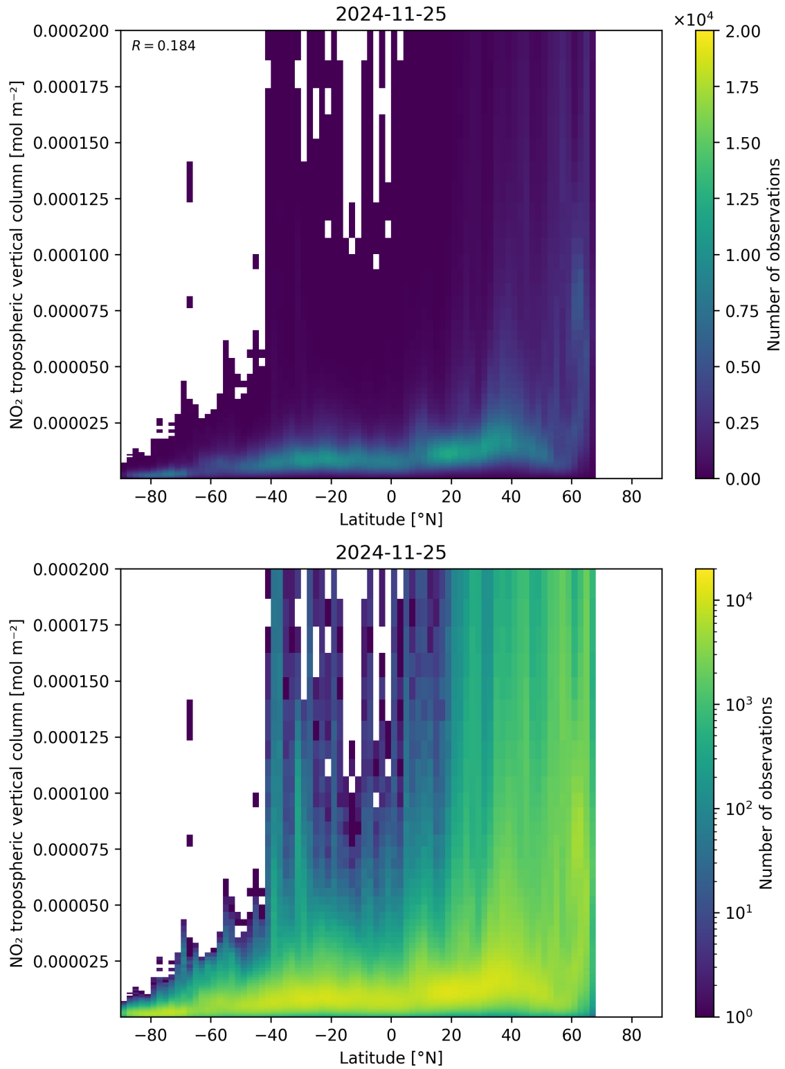
Figure 92: Scatter density plot of “Latitude” against “NO 2 tropospheric vertical column” for 2024-11-25 to 2024-11-26.
