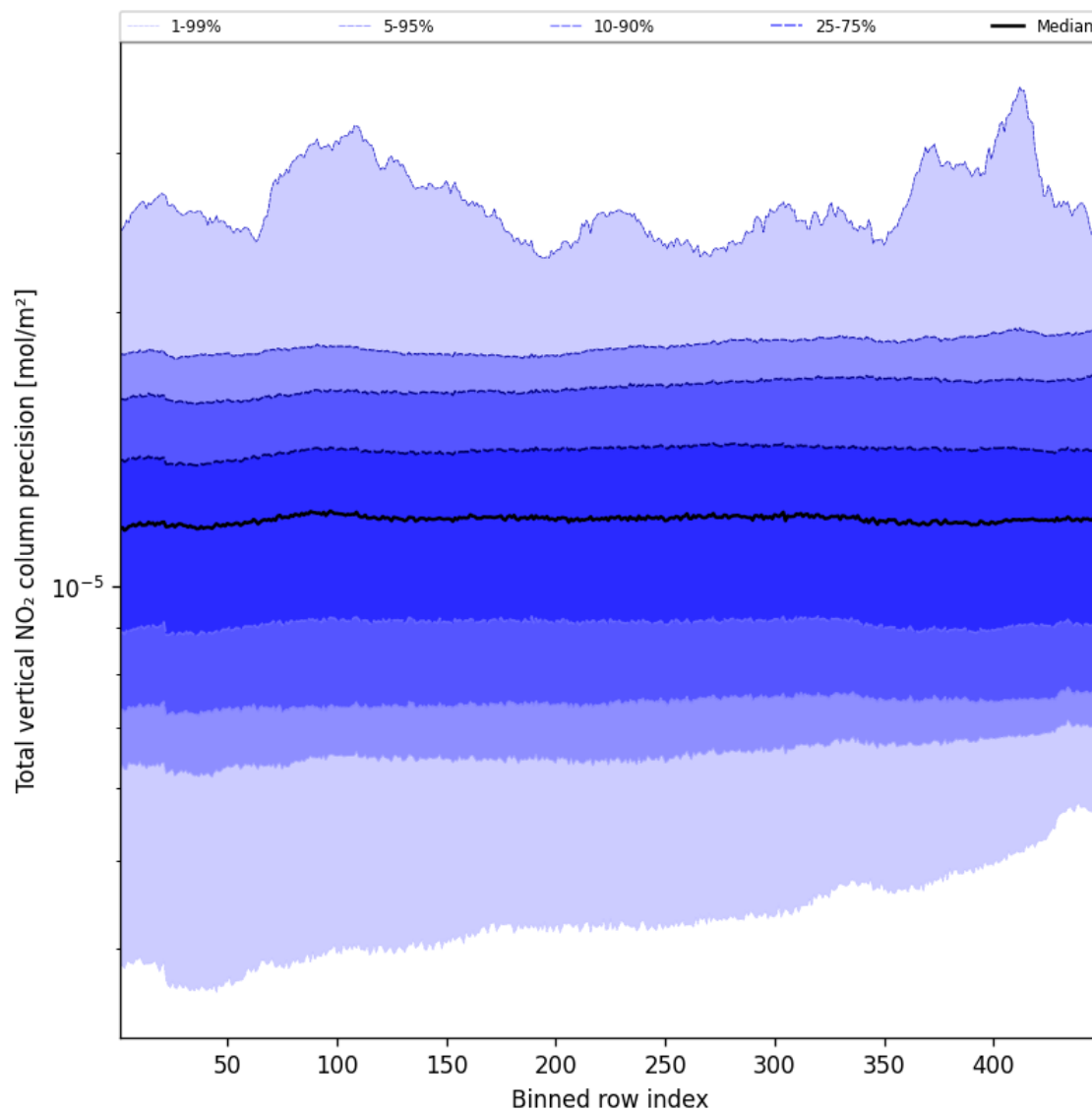
Figure 56: Along track statistics of “Total vertical NO 2 column precision” for 2024-11-25 to 2024-11-26
