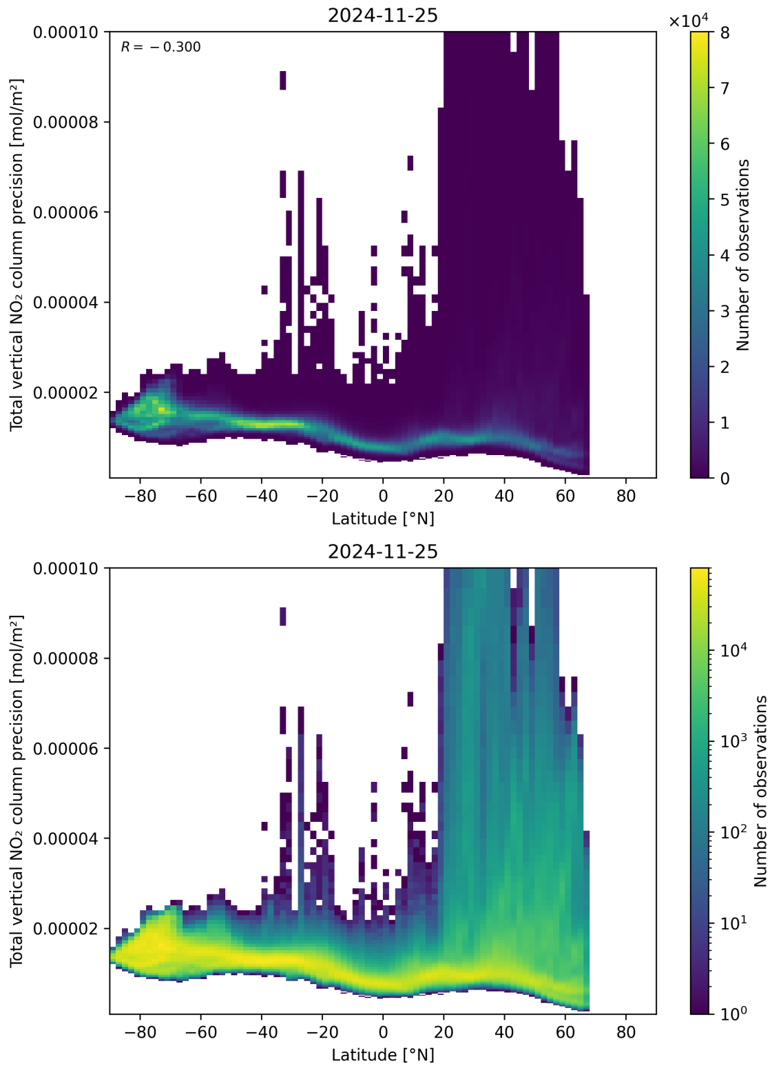
Figure 91: Scatter density plot of “Latitude” against “Total vertical NO 2 column precision” for 2024-11-25 to 2024-11-26.
