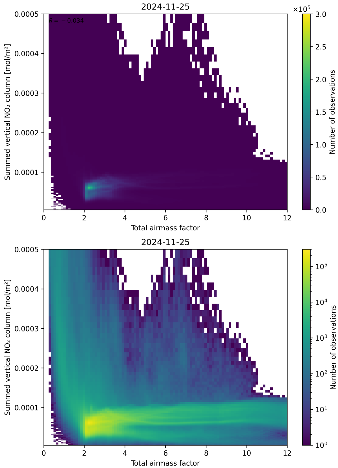
Figure 65: Scatter density plot of “Total airmass factor” against “Summed vertical NO 2 column” for 2024-11-25 to 2024-11-26.
