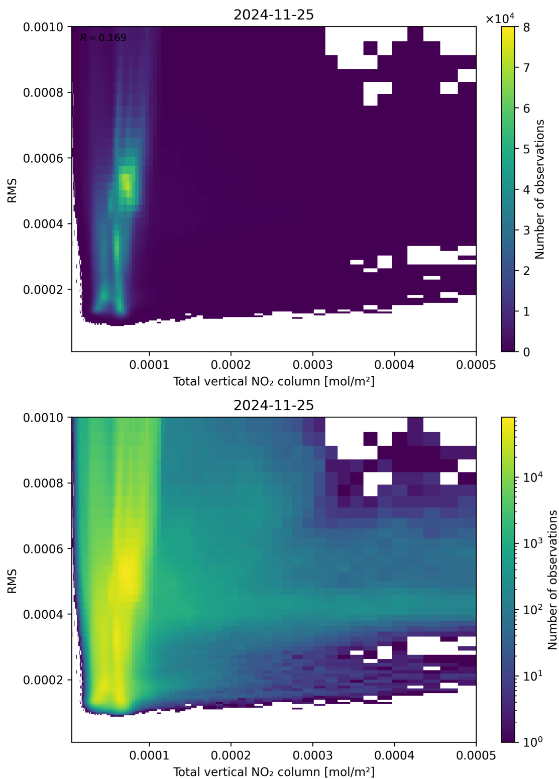
Figure 120: Scatter density plot of “Total vertical NO 2 column” against “RMS” for 2024-11-25 to 2024-11-26.
