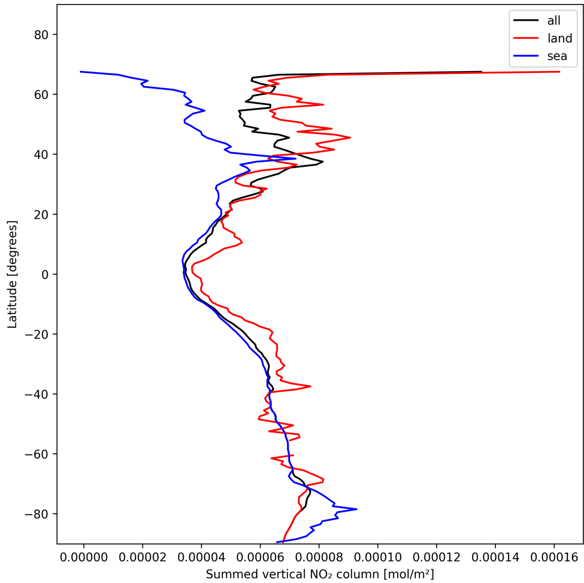
Figure 23: Zonal average of “Summed vertical NO 2 column” for 2024-11-25 to 2024-11-26.
