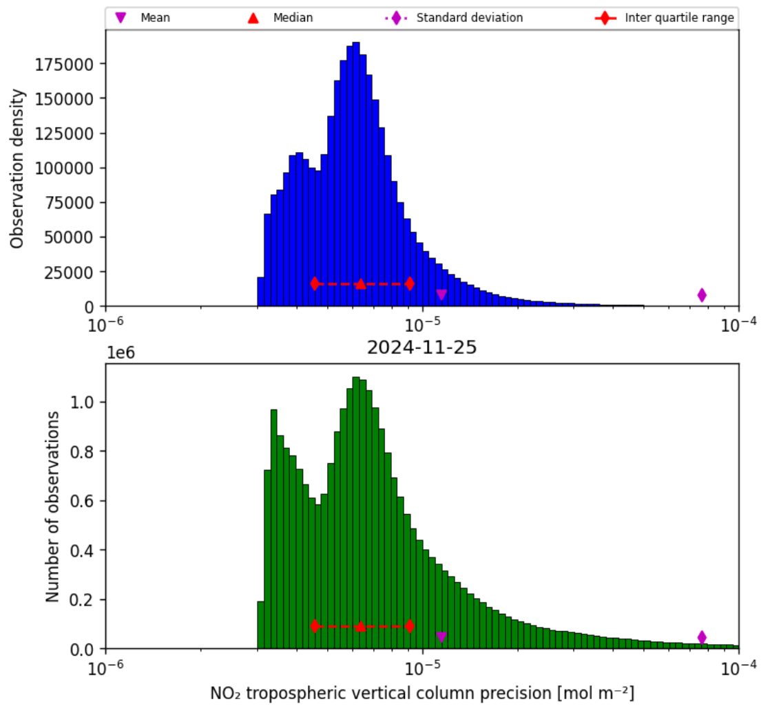
Figure 30: Histogram of “NO 2 tropospheric vertical column precision” for 2024-11-25 to 2024-11-26
