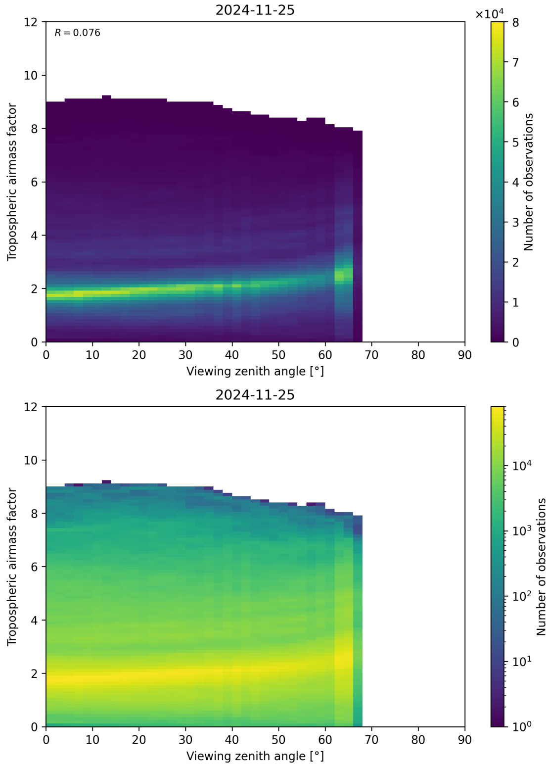
Figure 161: Scatter density plot of “Viewing zenith angle” against “Tropospheric airmass factor” for 2024-11-25 to 2024-11-26.
