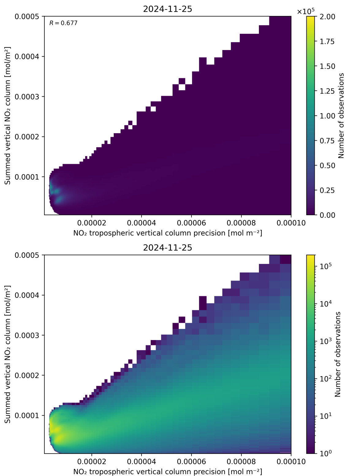
Figure 136: Scatter density plot of “NO 2 tropospheric vertical column precision” against “Summed vertical NO 2 column” for 2024-11-25 to 2024-11-26.
