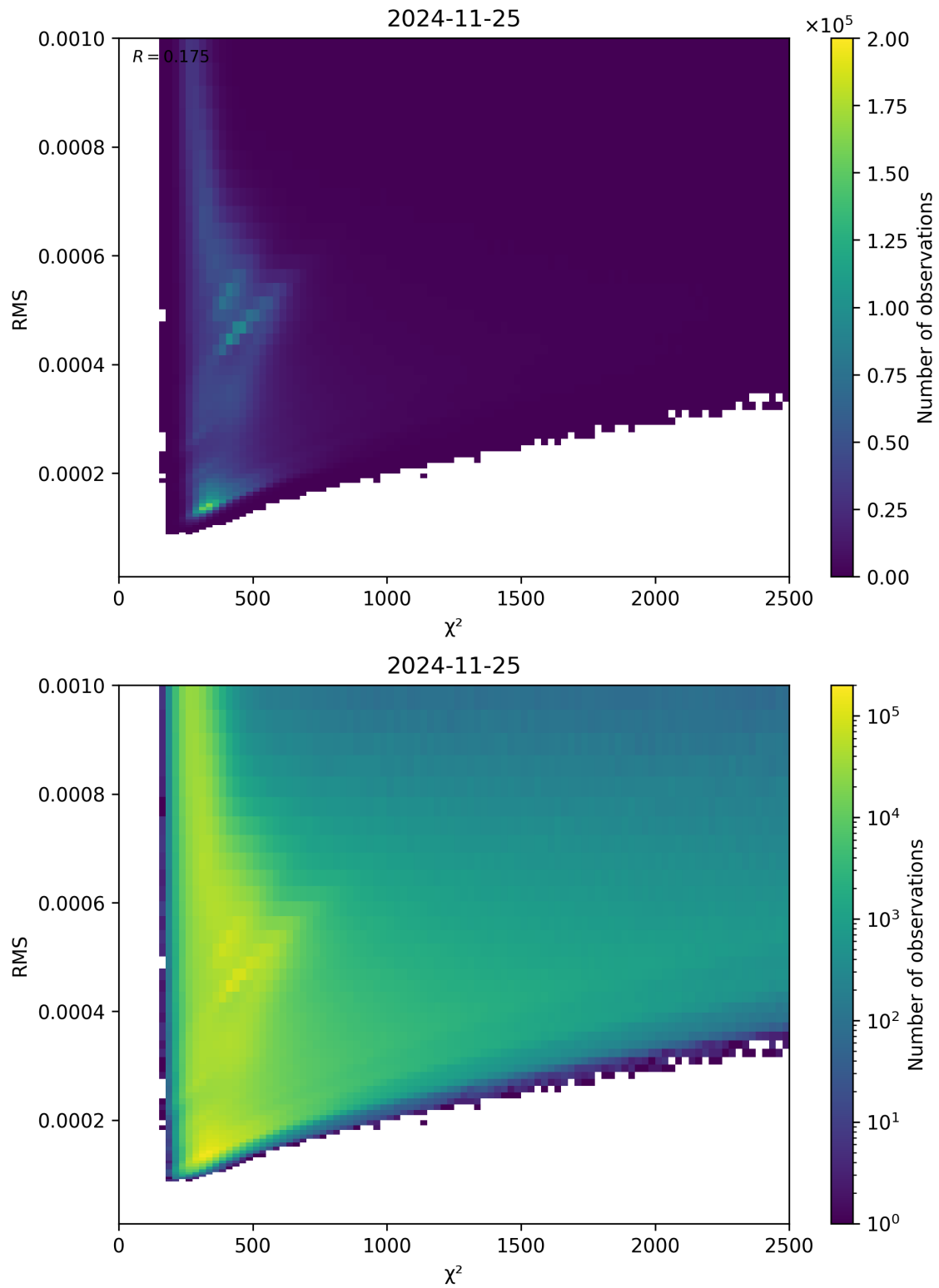
Figure 82: Scatter density plot of “ \chi^2 ” against “RMS” for 2024-11-25 to 2024-11-26.
