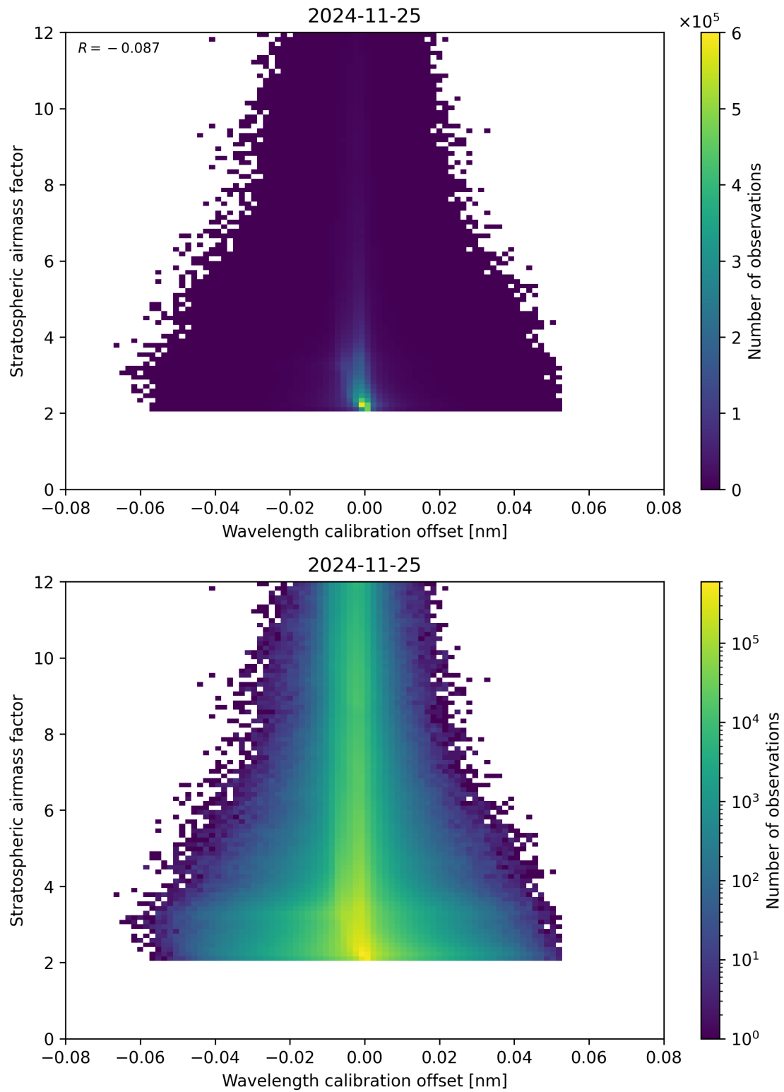
Figure 174: Scatter density plot of “Wavelength calibration offset” against “Stratospheric air mass factor” for 2024-11-25 to 2024-11-26.
