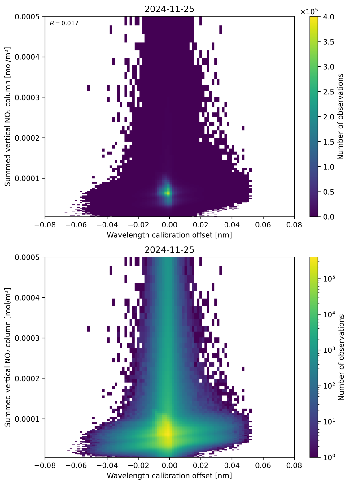
Figure 177: Scatter density plot of “Wavelength calibration offset” against “Summed vertical NO 2 column” for 2024-11-25 to 2024-11-26.
