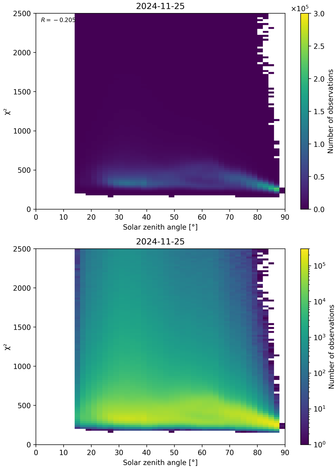
Figure 148: Scatter density plot of “Solar zenith angle” against “ \chi^2 ” for 2024-11-25 to 2024-11-26.
