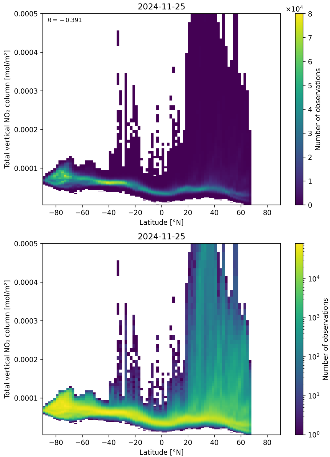
Figure 90: Scatter density plot of “Latitude” against “Total vertical NO 2 column” for 2024-11-25 to 2024-11-26.
