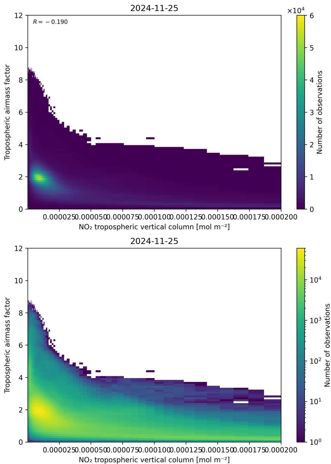
Figure 123: Scatter density plot of “NO 2 tropospheric vertical column” against “Tropospheric air mass factor” for 2024-11-25 to 2024-11-26.
