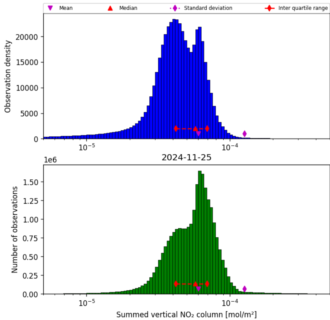
Figure 40: Histogram of “Summed vertical NO 2 column” for 2024-11-25 to 2024-11-26
