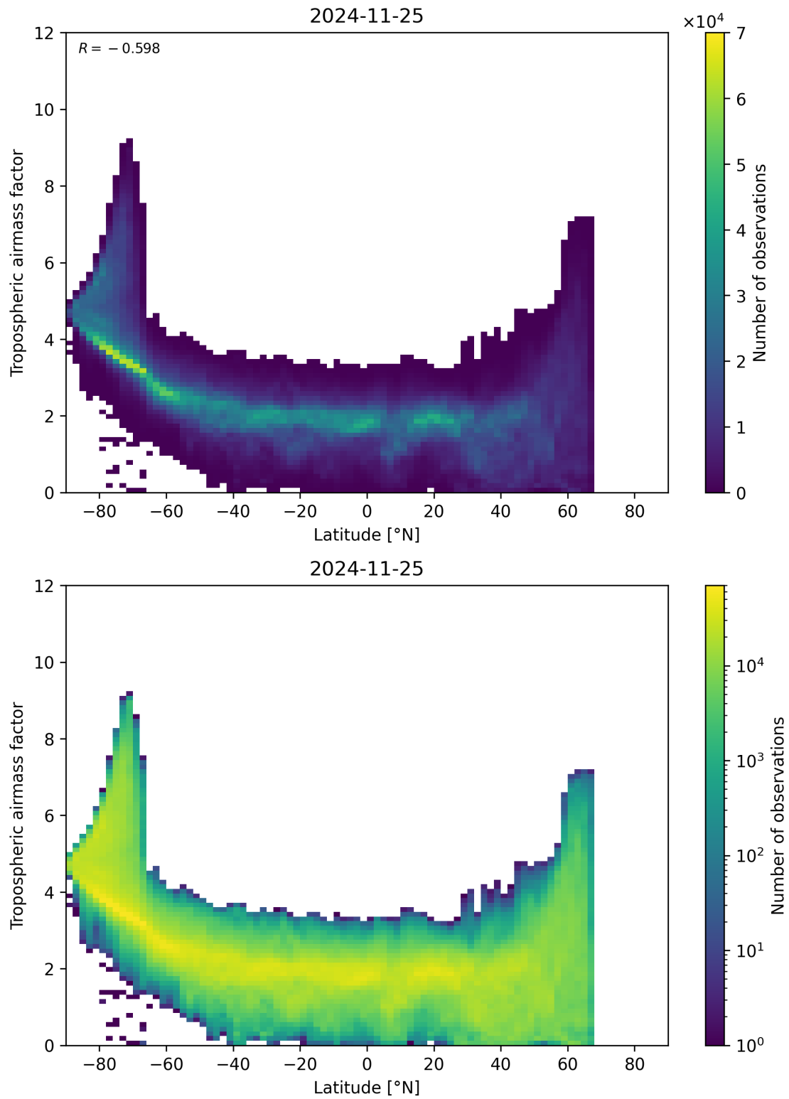
Figure 85: Scatter density plot of “Latitude” against “Tropospheric air mass factor” for 2024-11-25 to 2024-11-26.
