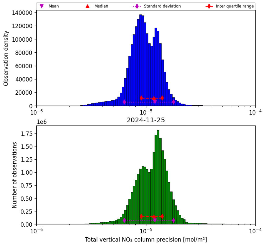
Figure 39: Histogram of "Total vertical NO 2 column precision" for 2024-11-25 to 2024-11-26
