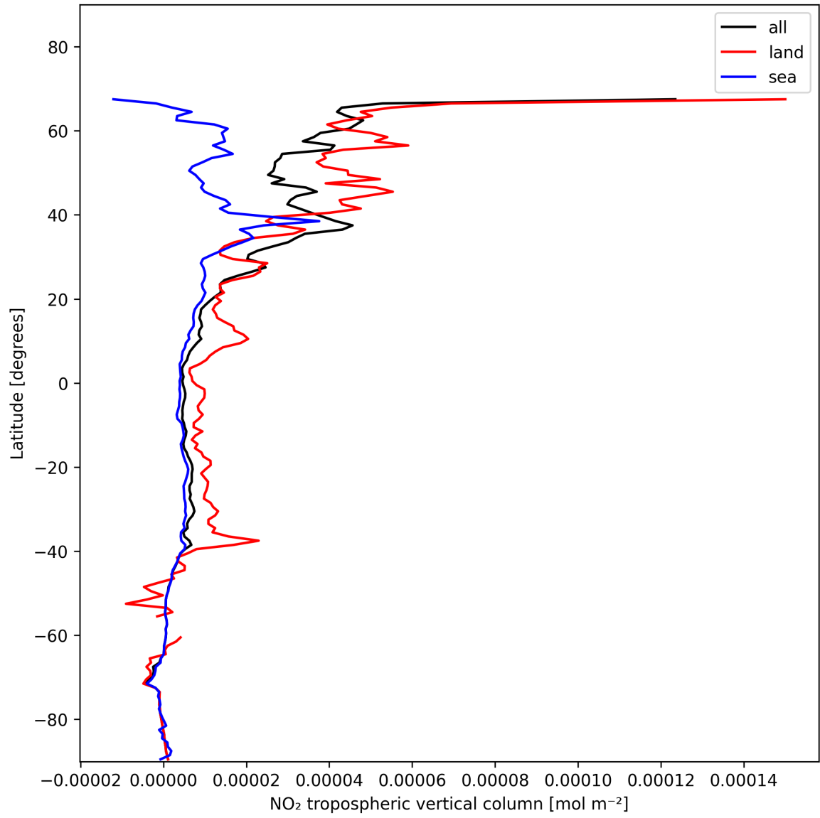
Figure 12: Zonal average of “NO 2 tropospheric vertical column” for 2024-11-25 to 2024-11-26.
