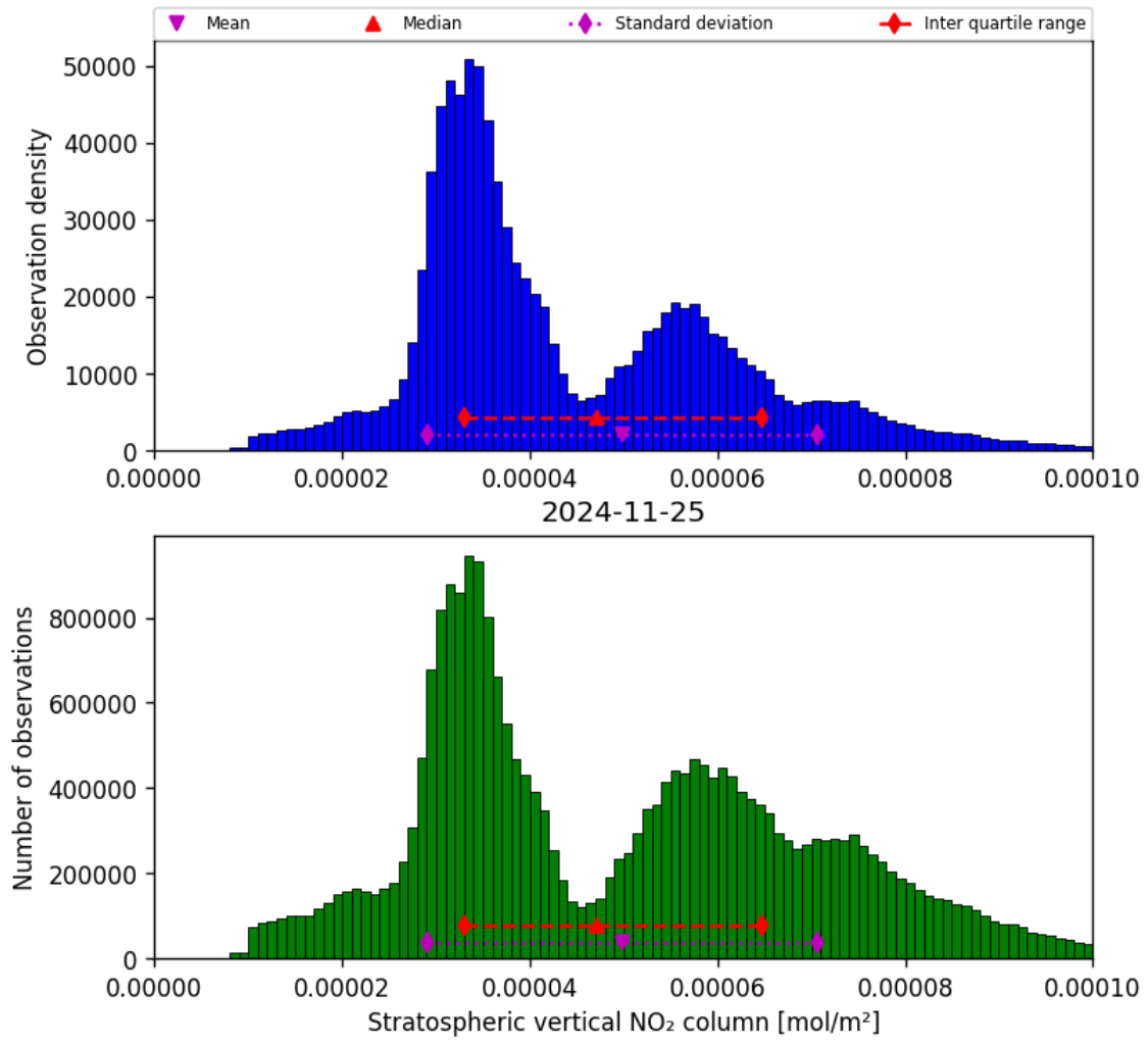
Figure 36: Histogram of “Stratospheric vertical NO 2 column” for 2024-11-25 to 2024-11-26
