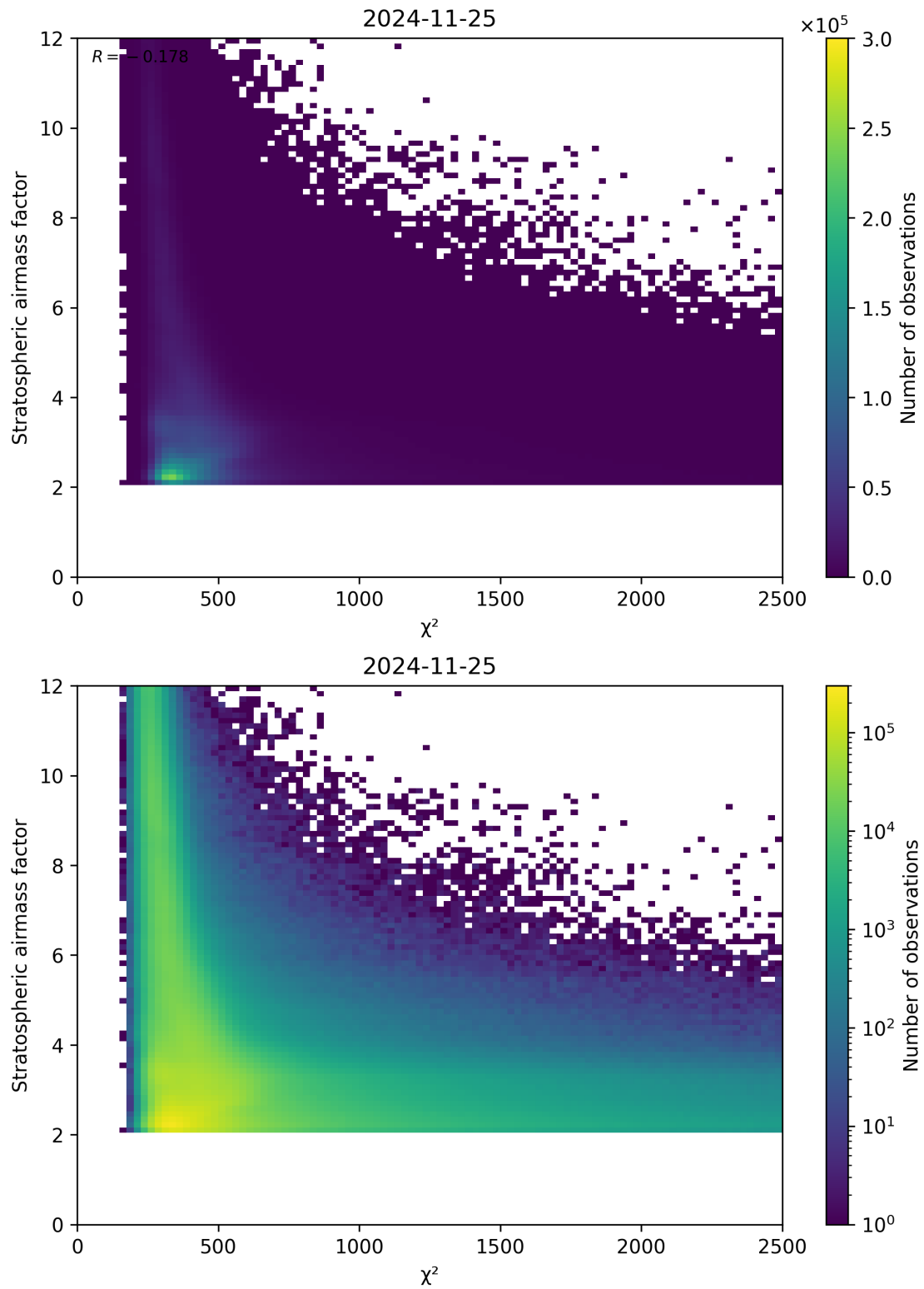
Figure 81: Scatter density plot of “ \chi^2 ” against “Stratospheric airmass factor” for 2024-11-25 to 2024-11-26.
