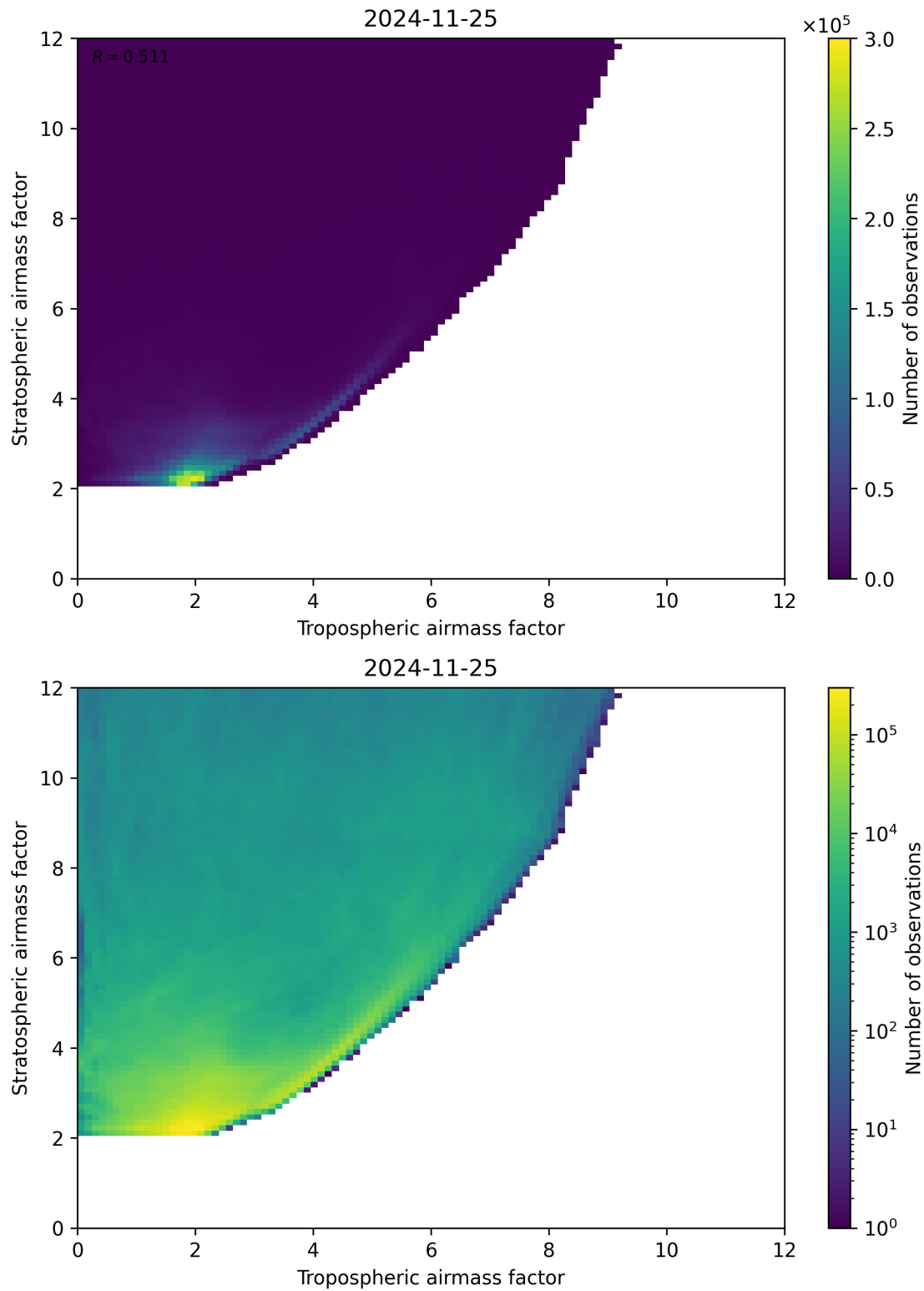
Figure 71: Scatter density plot of “Tropospheric airmass factor” against “Stratospheric airmass factor” for 2024-11-25 to 2024-11-26.
