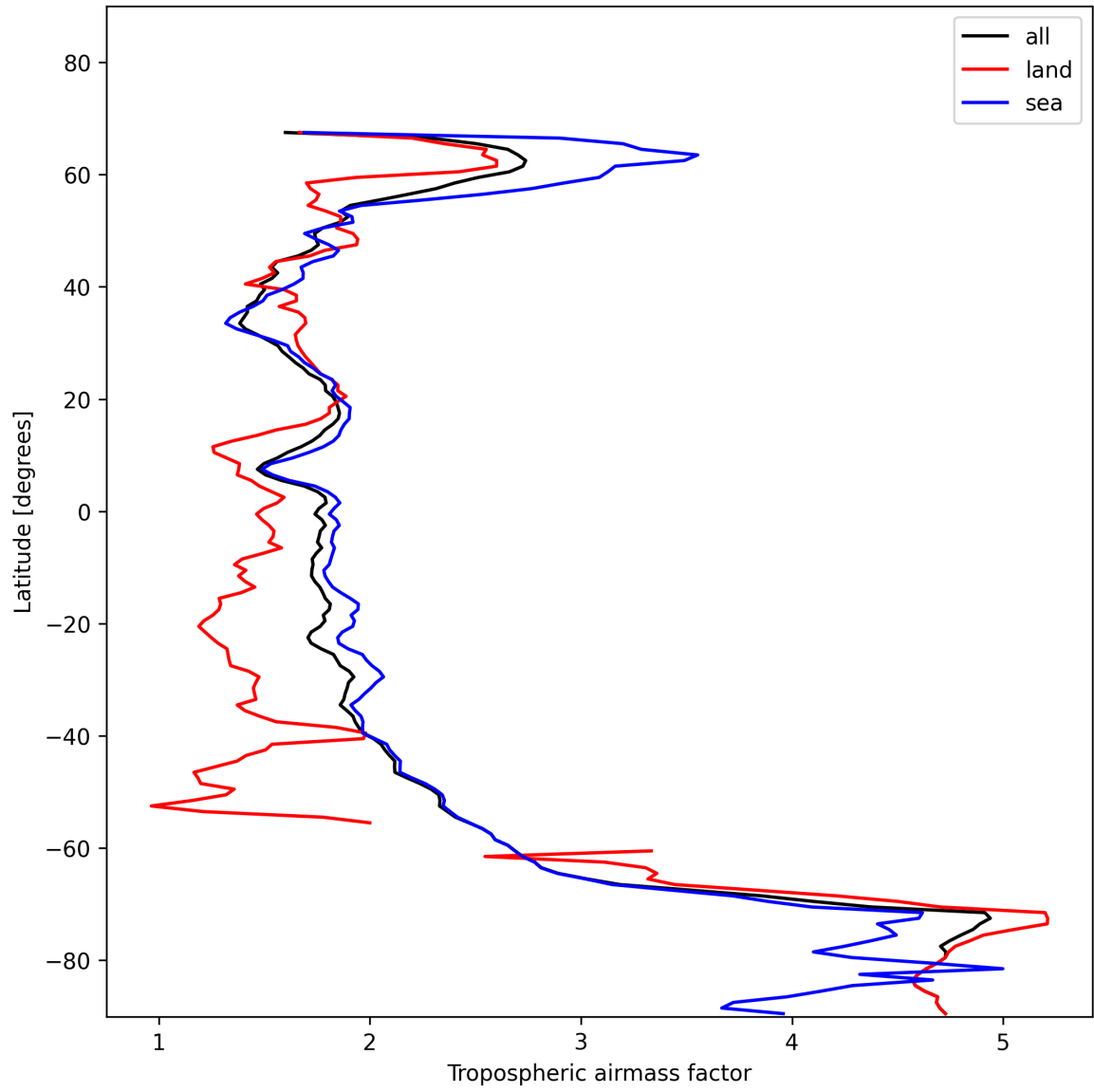
Figure 14: Zonal average of “Tropospheric airmass factor” for 2024-11-25 to 2024-11-26.
