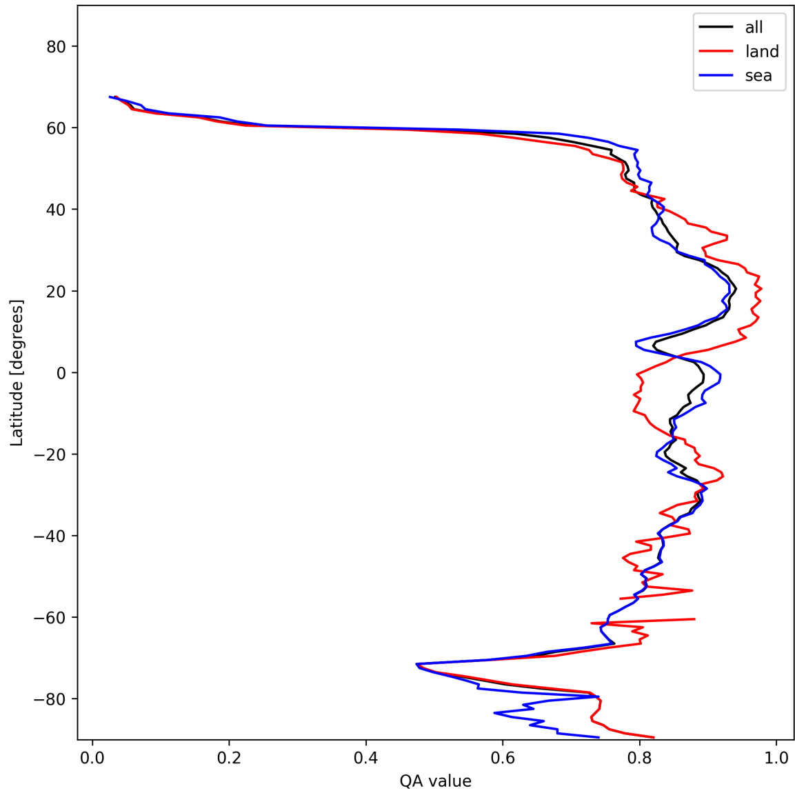
Figure 11: Zonal average of “QA value” for 2024-11-25 to 2024-11-26.
