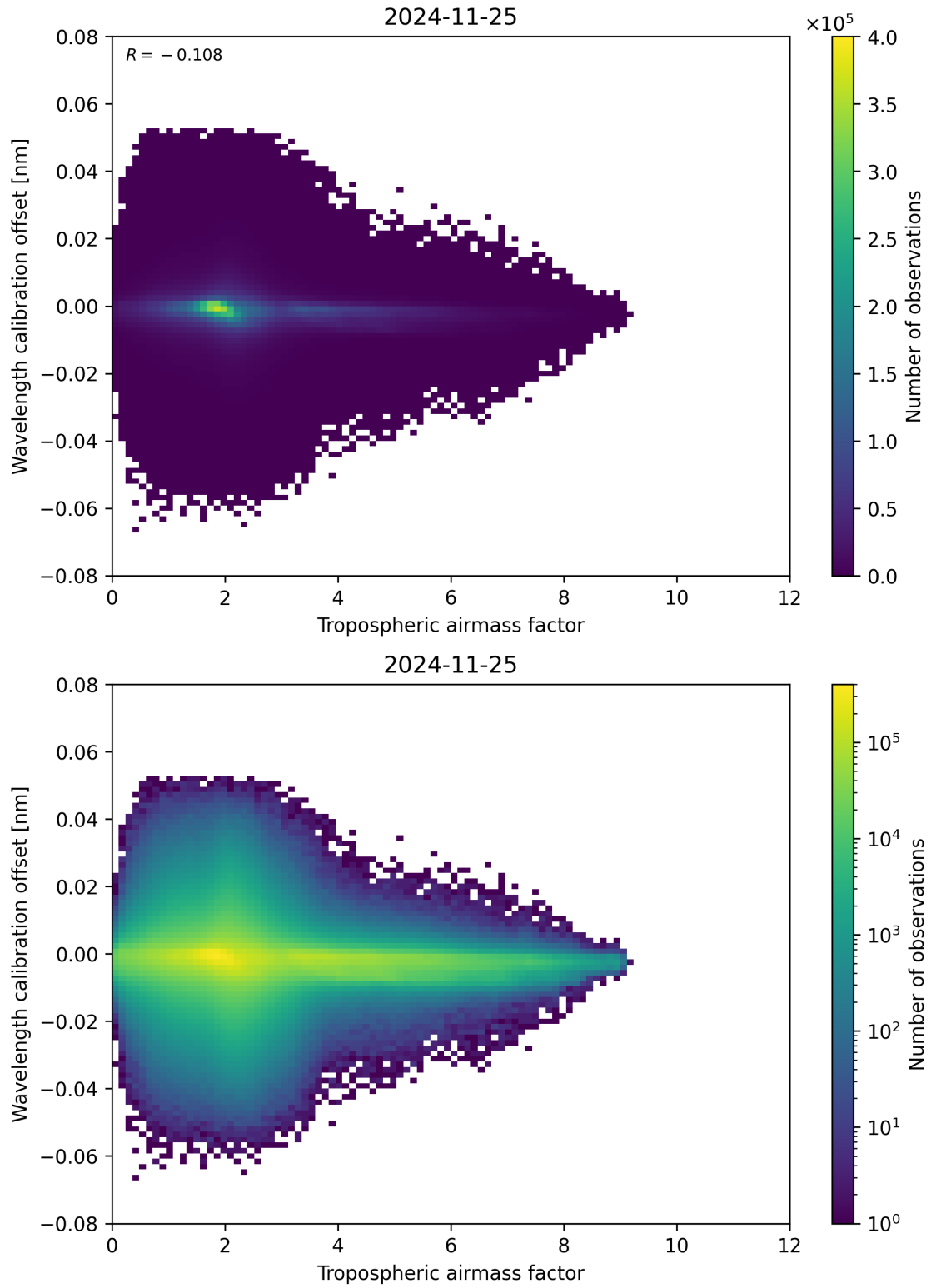
Figure 80: Scatter density plot of “Tropospheric airmass factor” against “Wavelength calibration offset” for 2024-11-25 to 2024-11-26.
