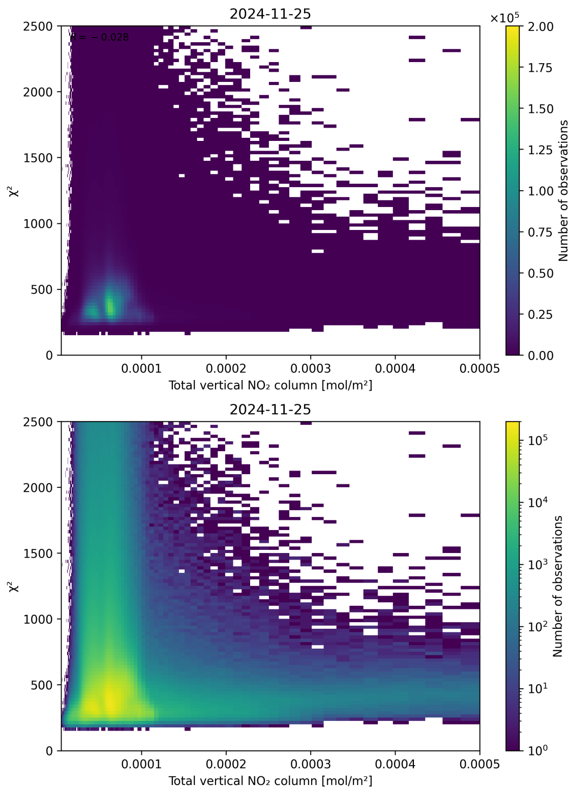
Figure 111: Scatter density plot of “Total vertical NO 2 column” against “ \chi^2 ” for 2024-11-25 to 2024-11-26.
