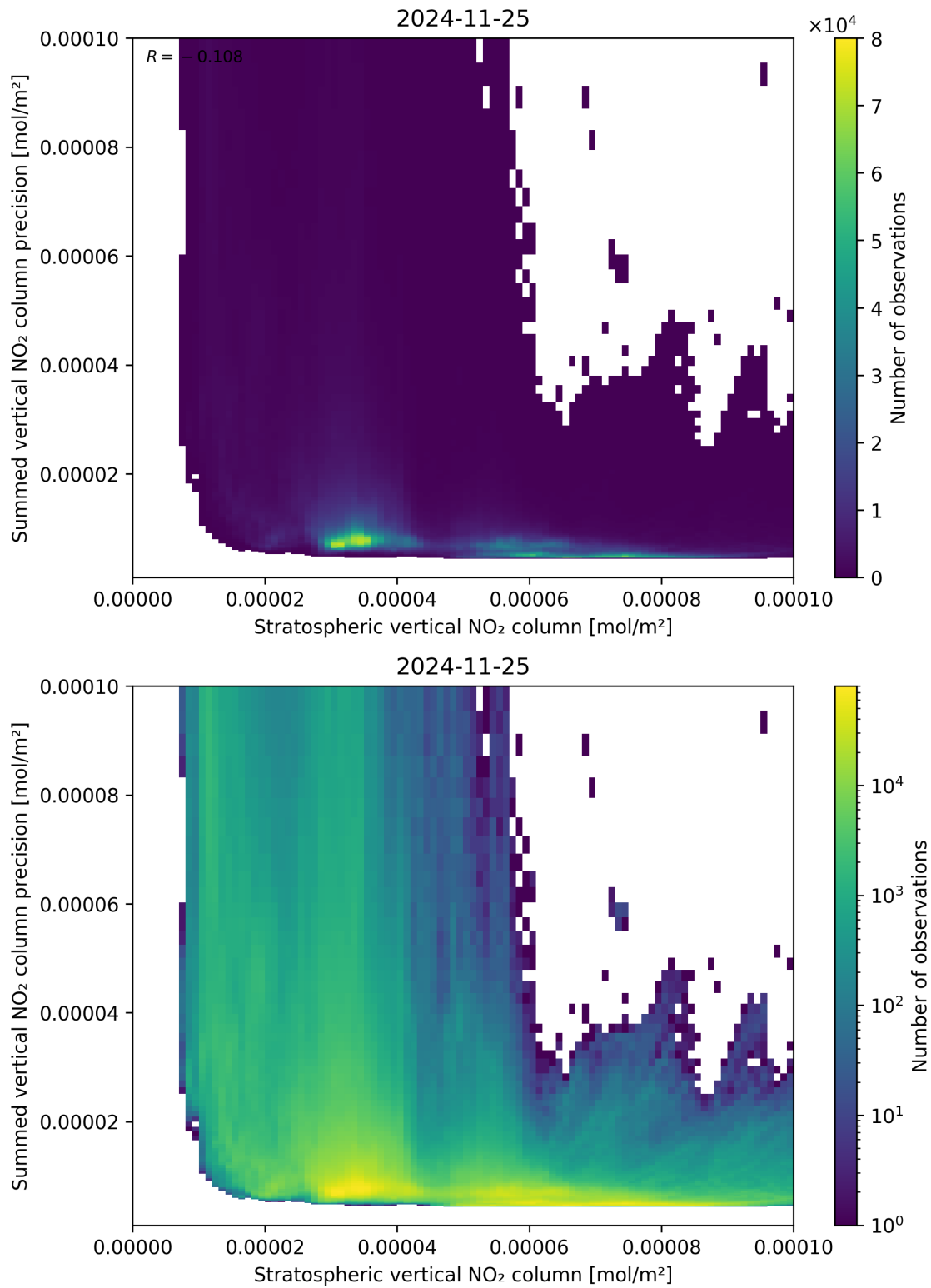
Figure 99: Scatter density plot of “Stratospheric vertical NO 2 column” against “Summed vertical NO 2 column precision” for 2024-11-25 to 2024-11-26.
