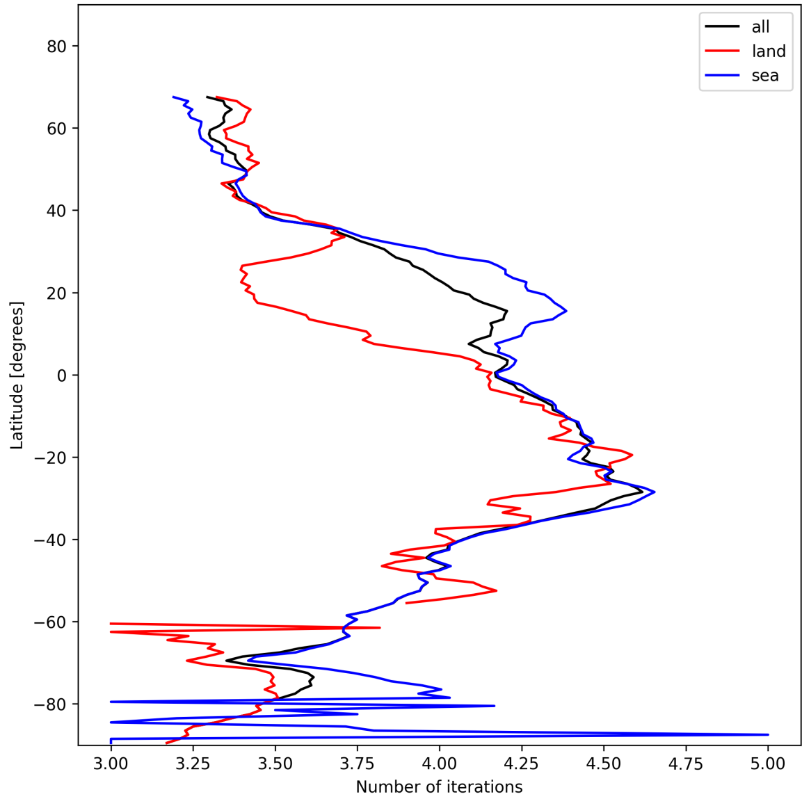
Figure 17: Zonal average of “Number of iterations” for 2024-11-25 to 2024-11-26.
