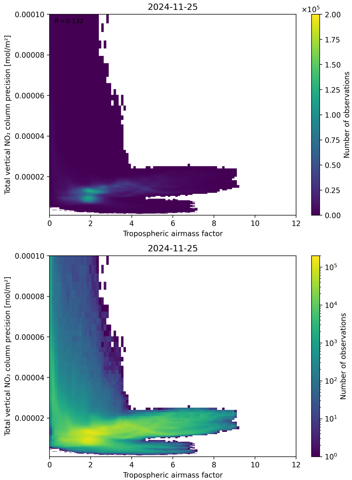
Figure 78: Scatter density plot of “Tropospheric air mass factor” against “Total vertical NO 2 column precision” for 2024-11-25 to 2024-11-26.
