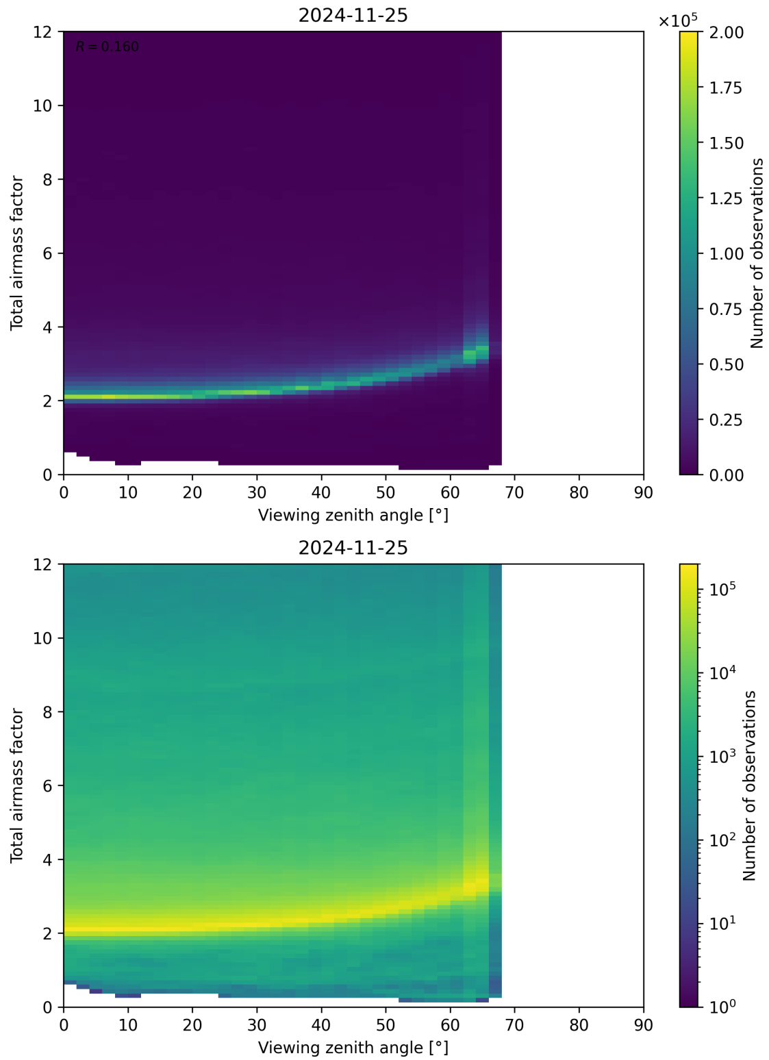
Figure 160: Scatter density plot of “Viewing zenith angle” against “Total airmass factor” for 2024-11-25 to 2024-11-26.
