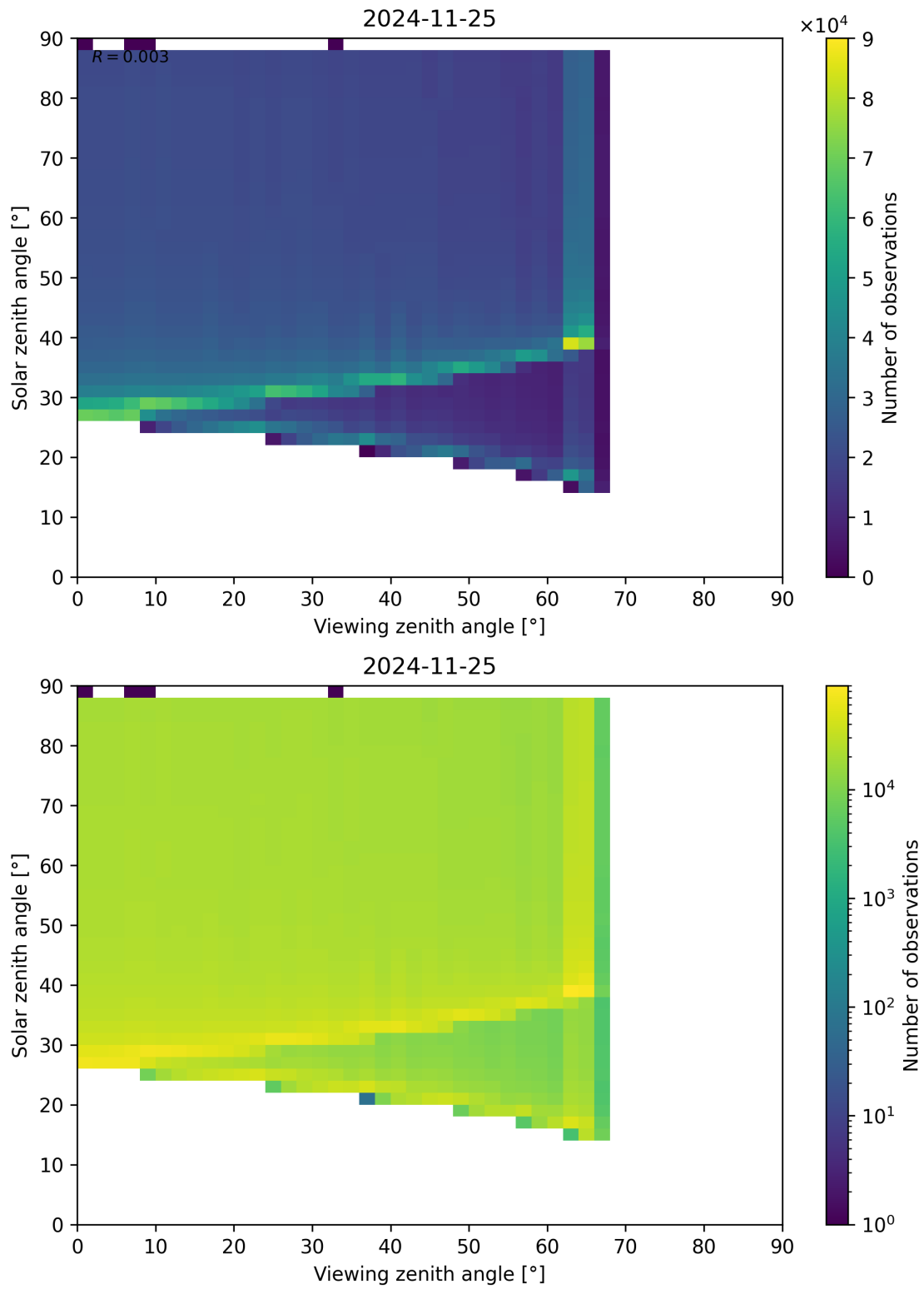
Figure 172: Scatter density plot of “Viewing zenith angle” against “Solar zenith angle” for 2024-11-25 to 2024-11-26.
