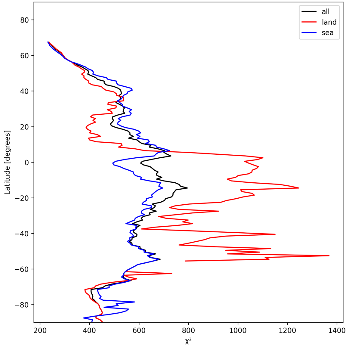
Figure 25: Zonal average of “ \chi^2 ” for 2024-11-25 to 2024-11-26.
