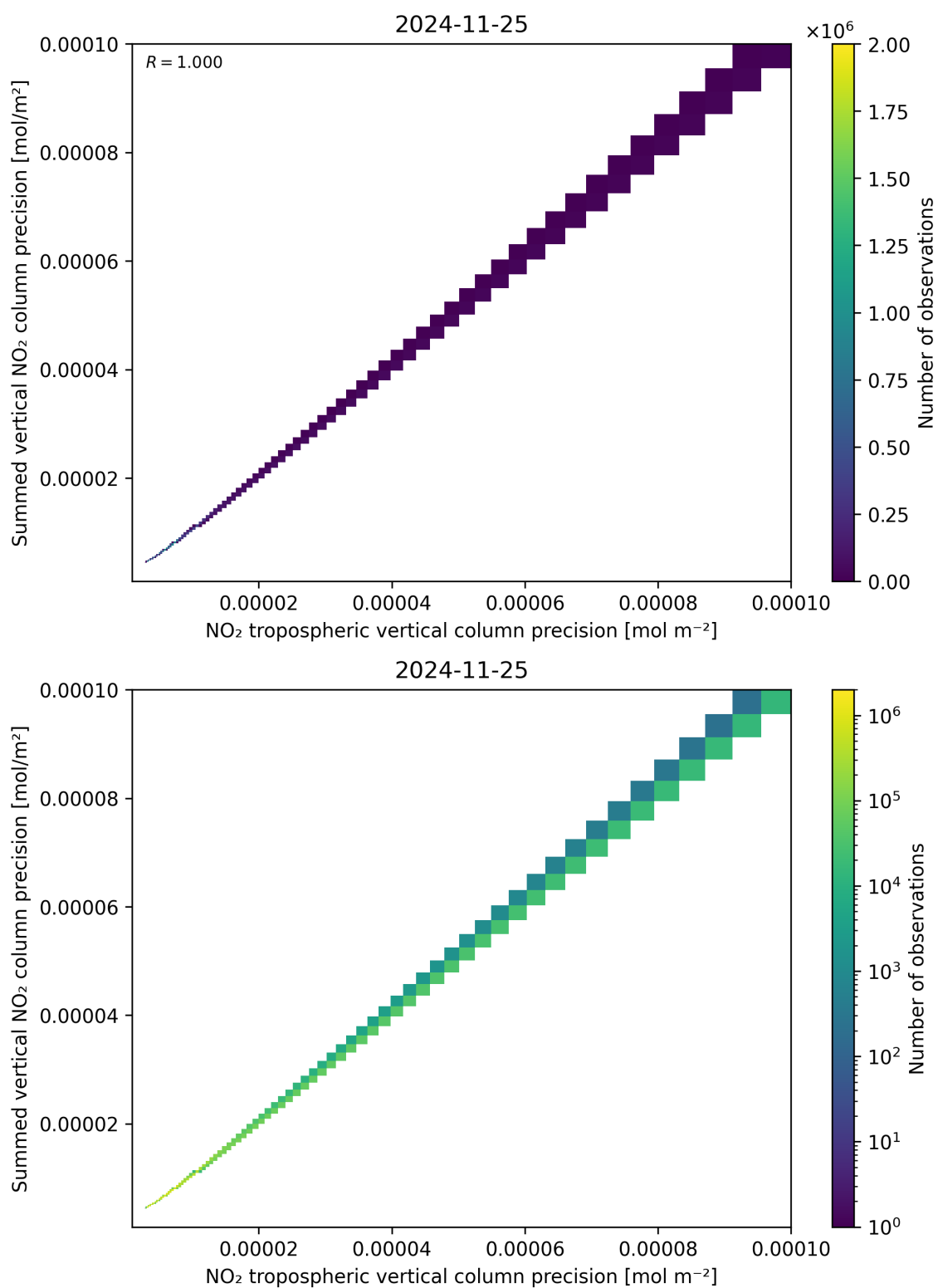
Figure 137: Scatter density plot of “NO 2 tropospheric vertical column precision” against “Summed vertical NO 2 column precision” for 2024-11-25 to 2024-11-26.
