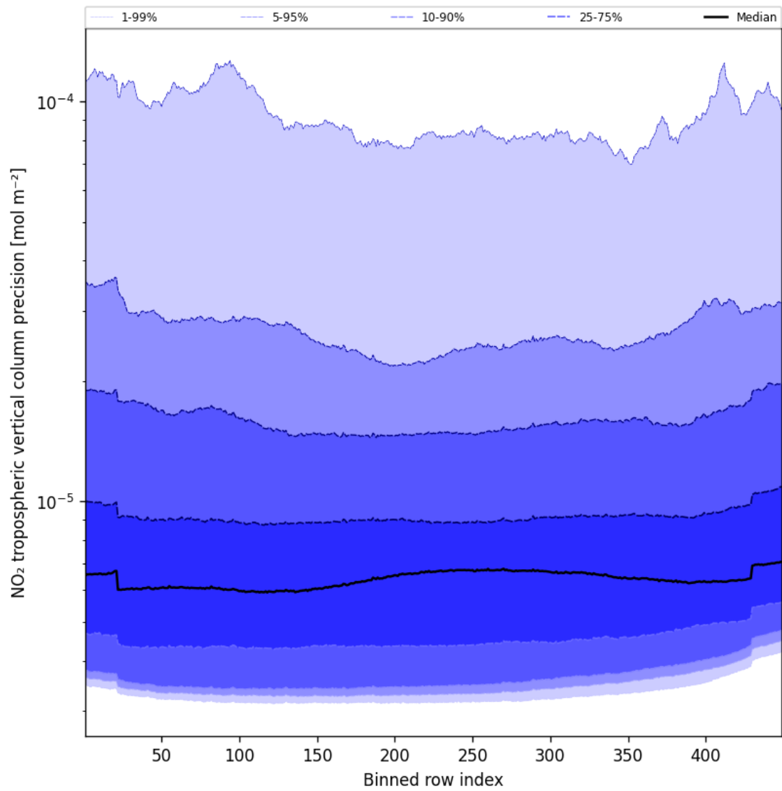
Figure 47: Along track statistics of “NO 2 tropospheric vertical column precision” for 2024-11-25 to 2024-11-26
