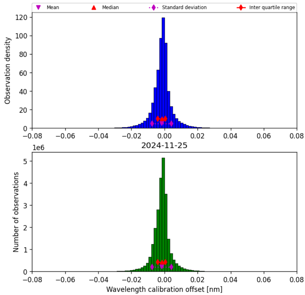
Figure 35: Histogram of “Wavelength calibration offset” for 2024-11-25 to 2024-11-26
