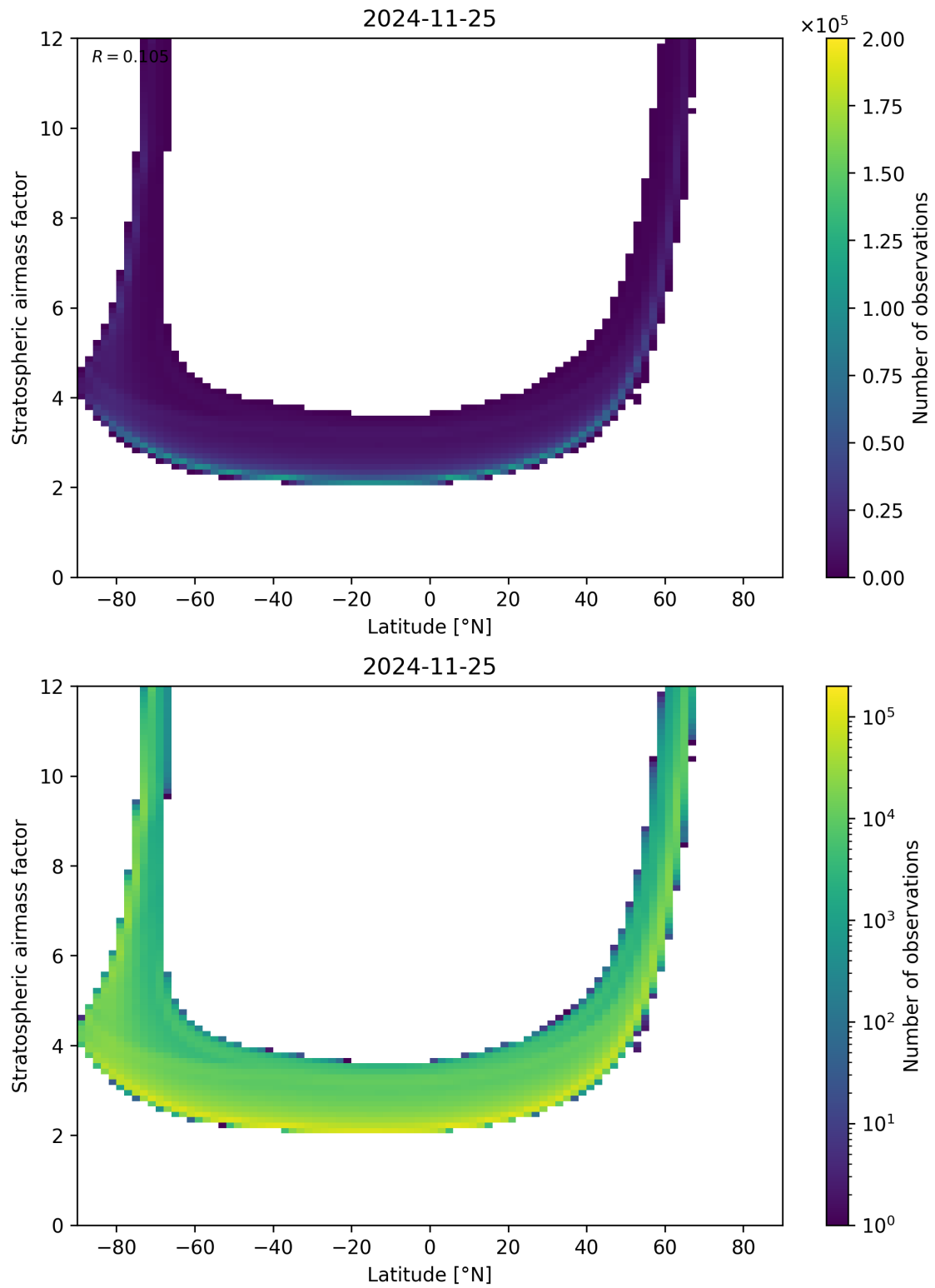
Figure 83: Scatter density plot of “Latitude” against “Stratospheric airmass factor” for 2024-11-25 to 2024-11-26.
