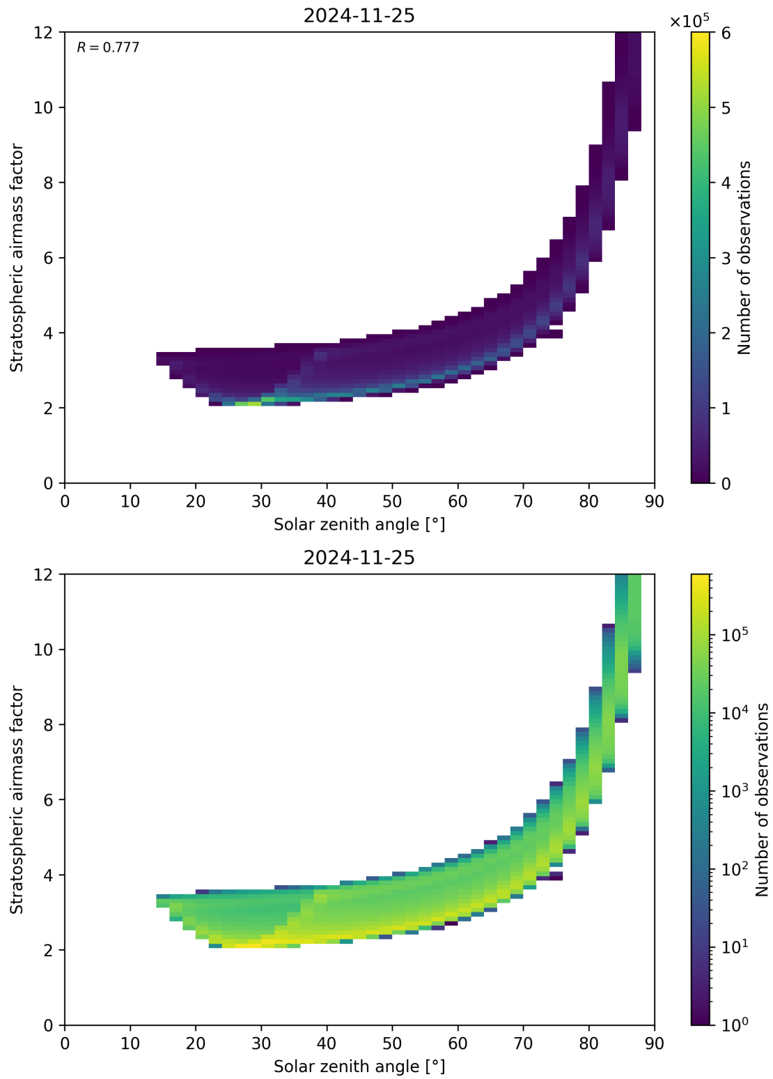
Figure 145: Scatter density plot of “Solar zenith angle” against “Stratospheric airmass factor” for 2024-11-25 to 2024-11-26.
