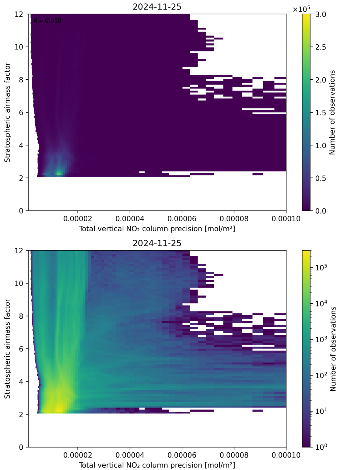
Figure 115: Scatter density plot of “Total vertical NO 2 column precision” against “Stratospheric airmass factor” for 2024-11-25 to 2024-11-26.
