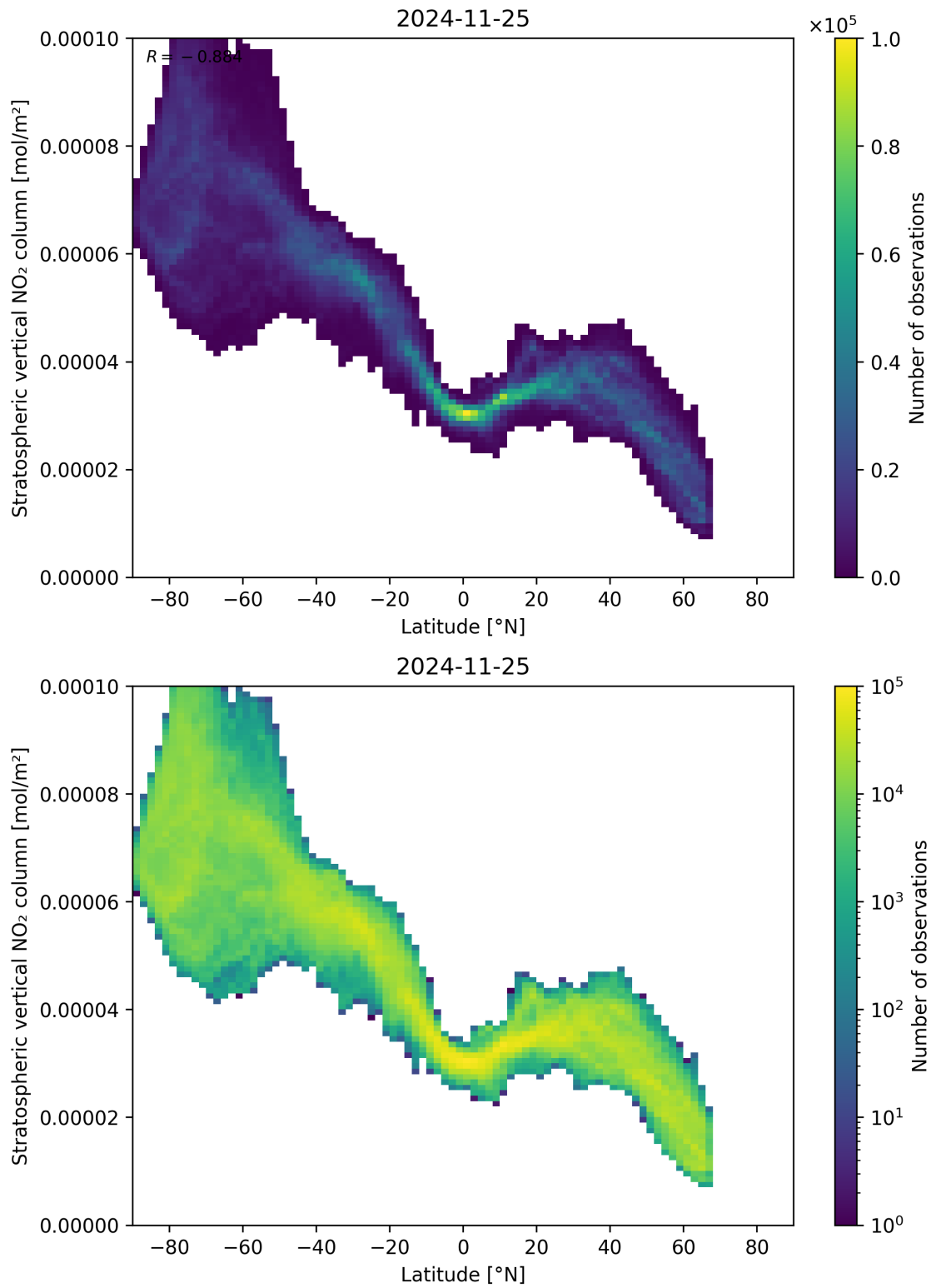
Figure 87: Scatter density plot of “Latitude” against “Stratospheric vertical NO 2 column” for 2024-11-25 to 2024-11-26.
