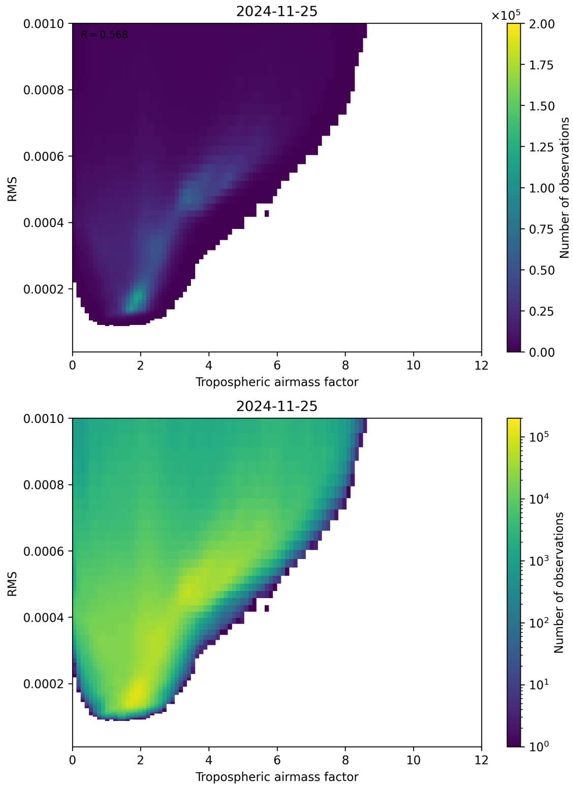
Figure 79: Scatter density plot of “Tropospheric airmass factor” against “RMS” for 2024-11-25 to 2024-11-26.
