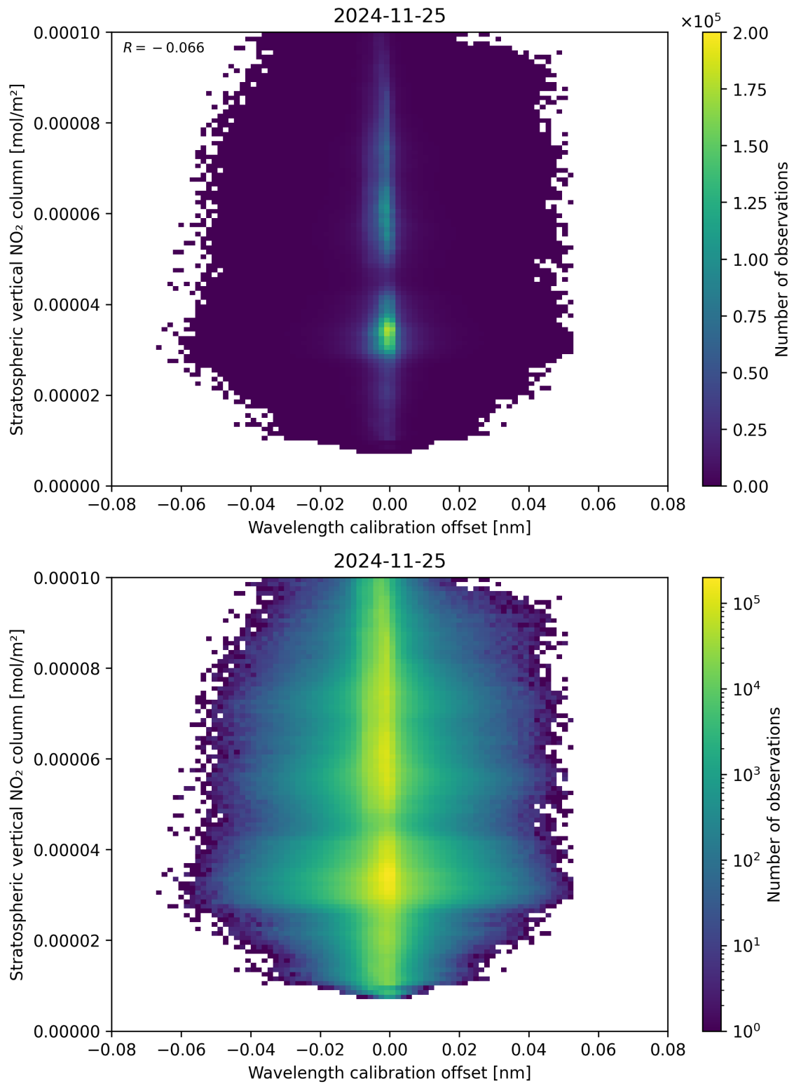
Figure 176: Scatter density plot of “Wavelength calibration offset” against “Stratospheric vertical NO 2 column” for 2024-11-25 to 2024-11-26.
