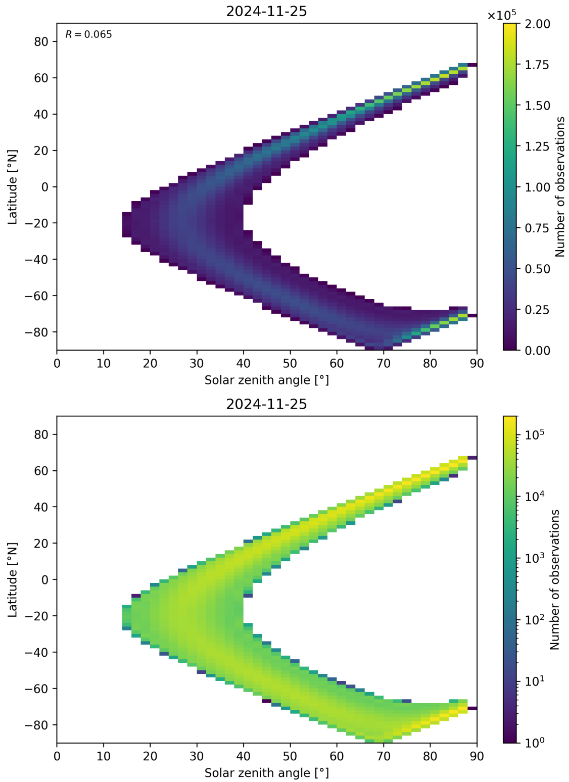
Figure 149: Scatter density plot of “Solar zenith angle” against “Latitude” for 2024-11-25 to 2024-11-26.
