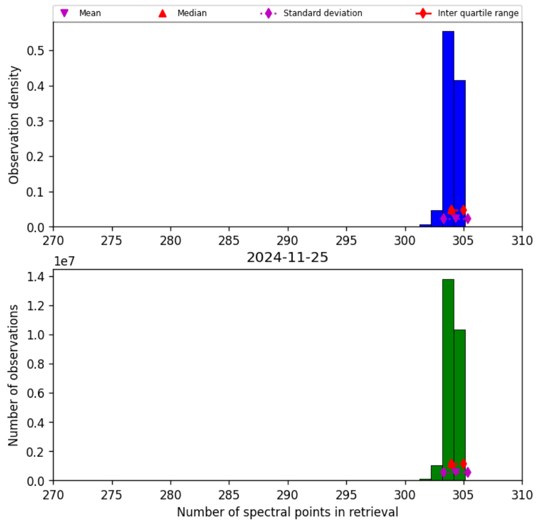
Figure 33: Histogram of “Number of spectral points in retrieval” for 2024-11-25 to 2024-11-26
