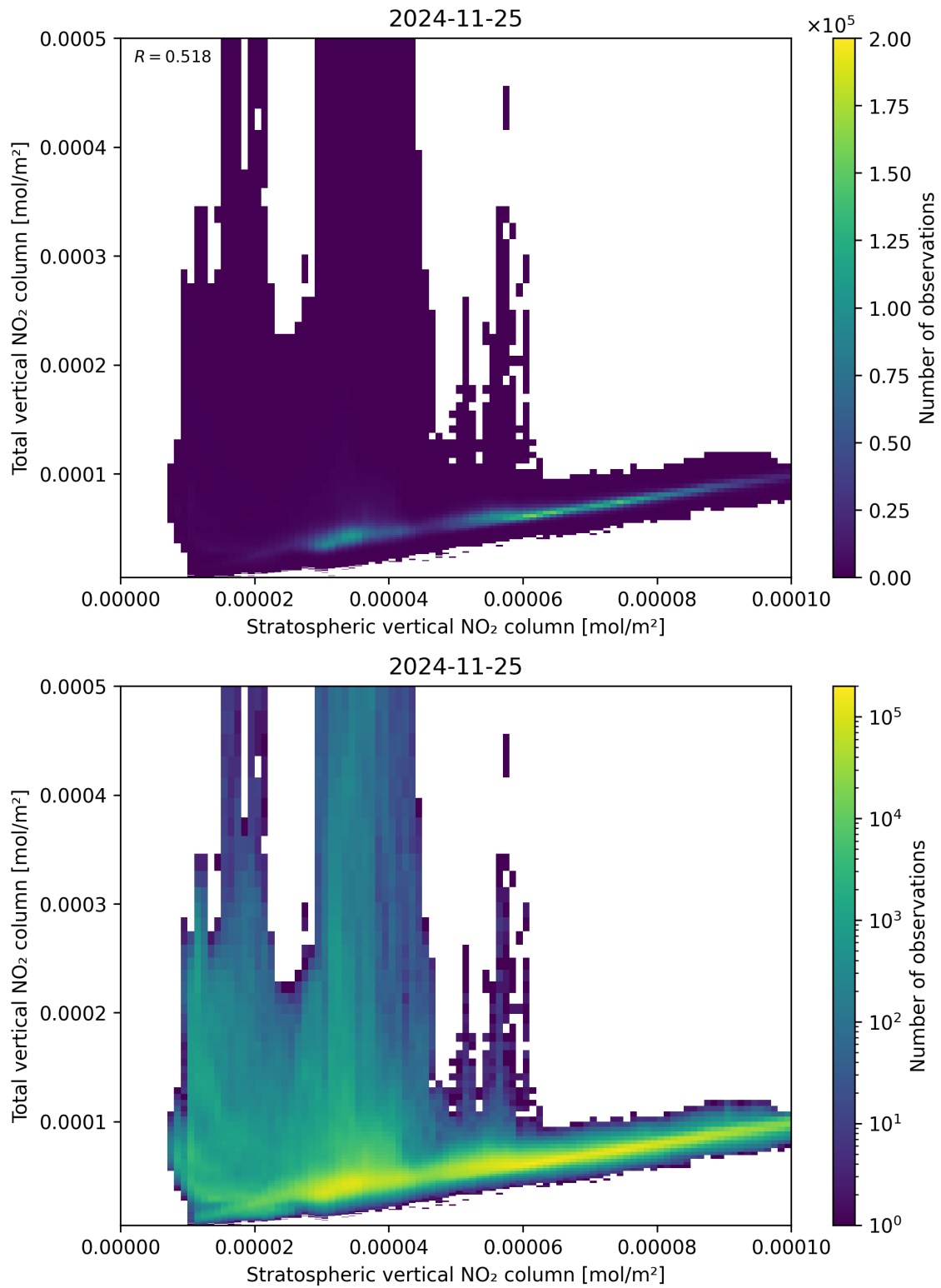
Figure 100: Scatter density plot of “Stratospheric vertical NO 2 column” against “Total vertical NO 2 column” for 2024-11-25 to 2024-11-26.
