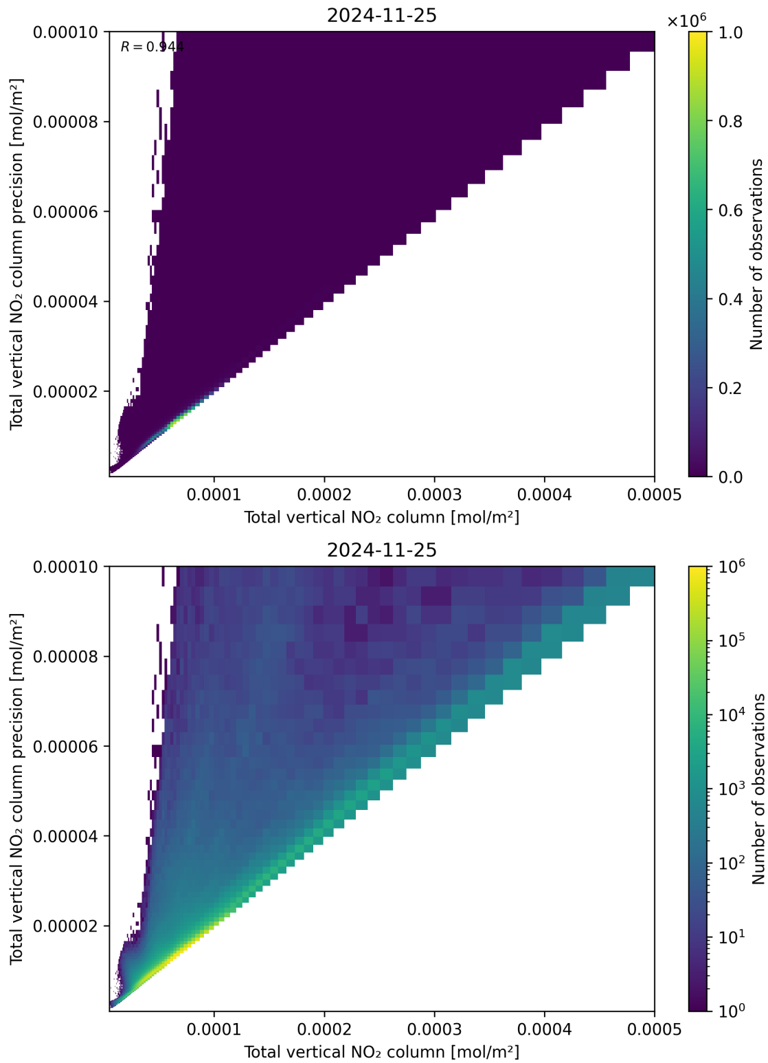
Figure 114: Scatter density plot of “Total vertical NO 2 column” against “Total vertical NO 2 column precision” for 2024-11-25 to 2024-11-26.
