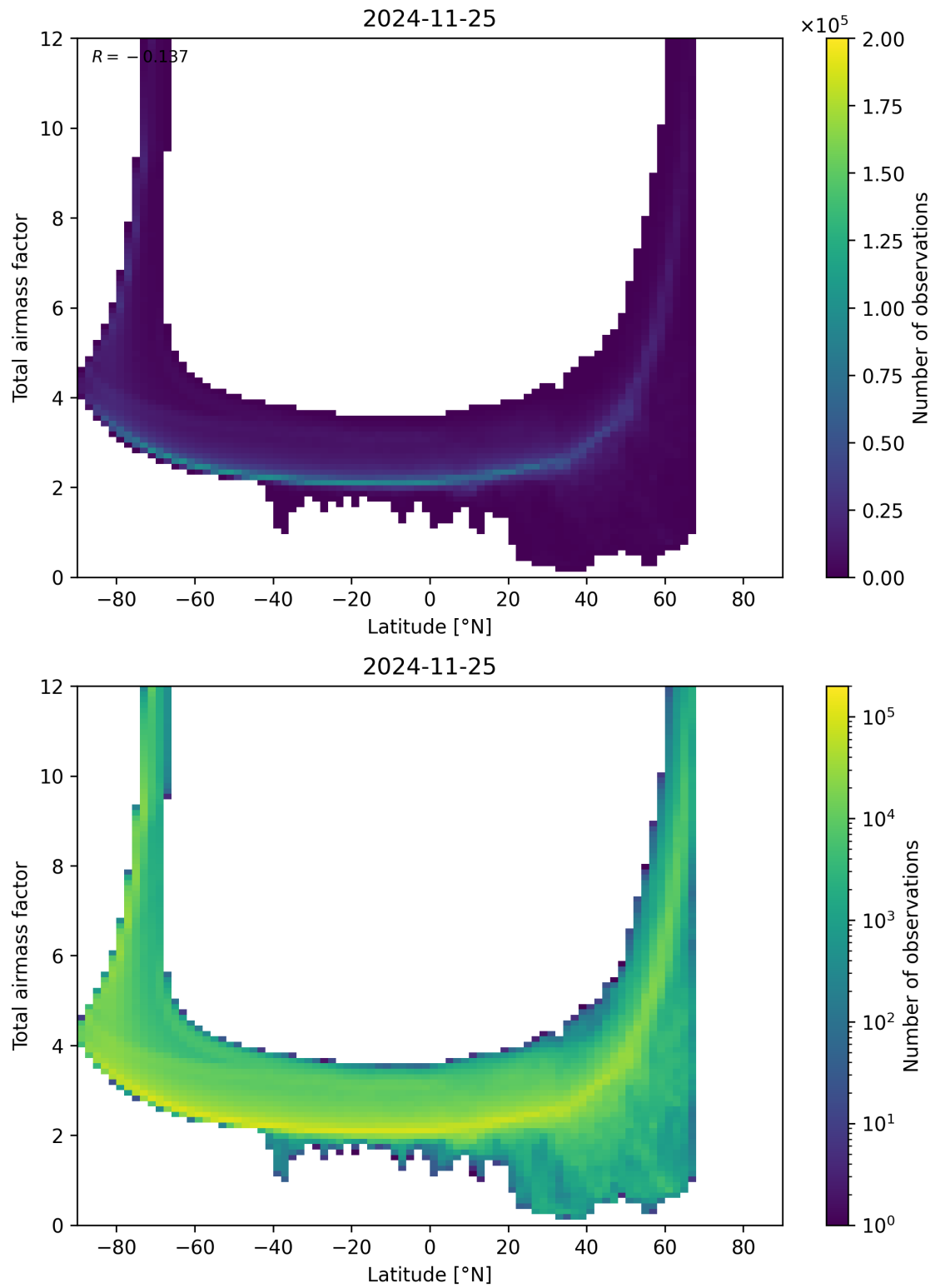
Figure 84: Scatter density plot of “Latitude” against “Total airmass factor” for 2024-11-25 to 2024-11-26.
