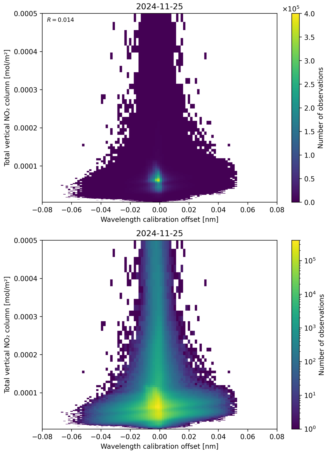
Figure 179: Scatter density plot of “Wavelength calibration offset” against “Total vertical NO 2 column” for 2024-11-25 to 2024-11-26.
