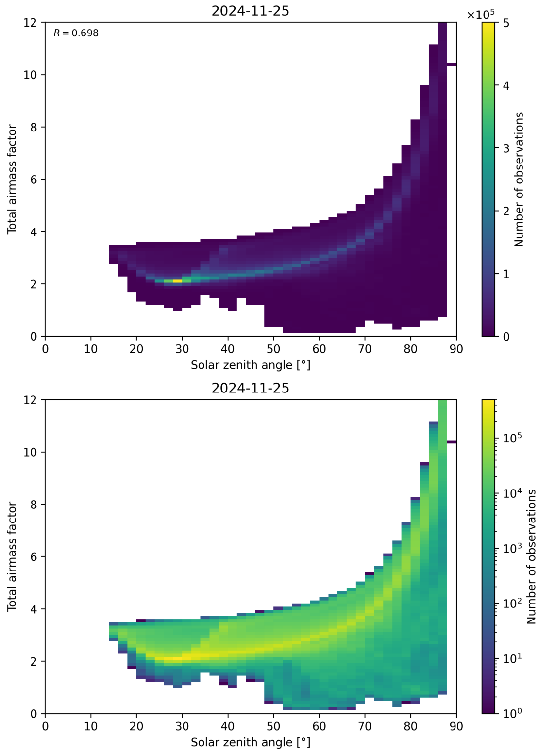
Figure 146: Scatter density plot of “Solar zenith angle” against “Total airmass factor” for 2024-11-25 to 2024-11-26.
