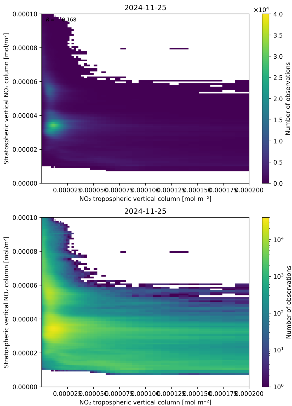
Figure 125: Scatter density plot of “NO 2 tropospheric vertical column” against “Stratospheric vertical NO 2 column” for 2024-11-25 to 2024-11-26.
