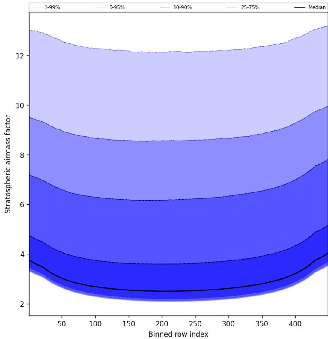
Figure 61: Along track statistics of “Stratospheric air mass factor” for 2024-11-25 to 2024-11-26
