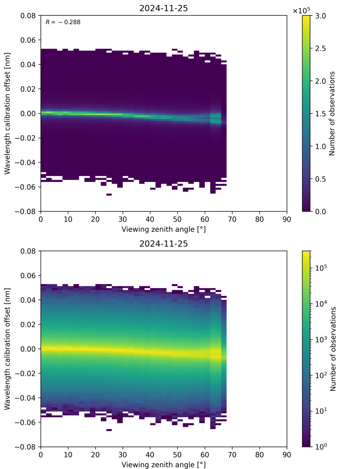
Figure 173: Scatter density plot of “Viewing zenith angle” against “Wavelength calibration offset” for 2024-11-25 to 2024-11-26.
