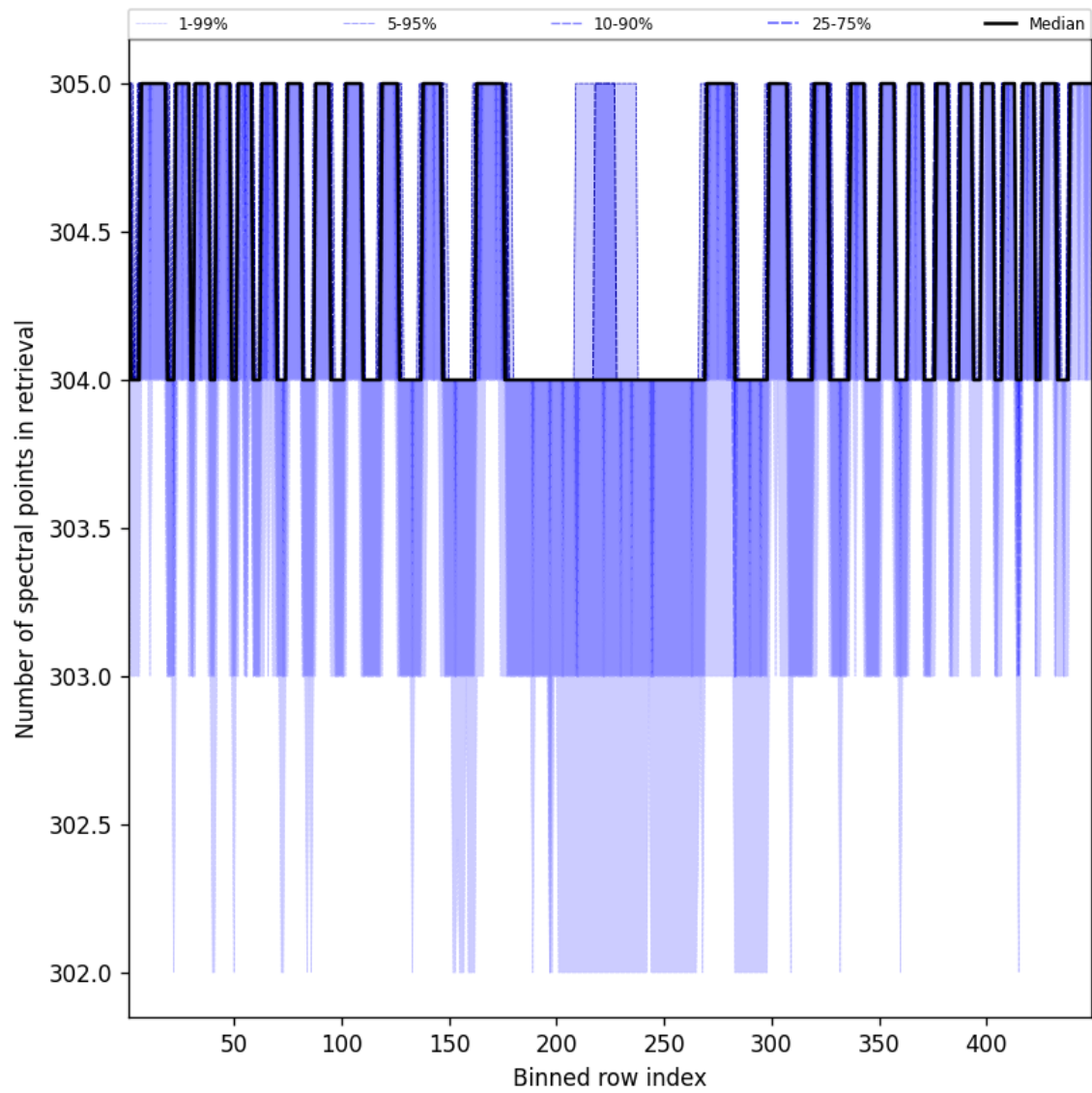
Figure 50: Along track statistics of “Number of spectral points in retrieval” for 2024-11-25 to 2024-11-26
