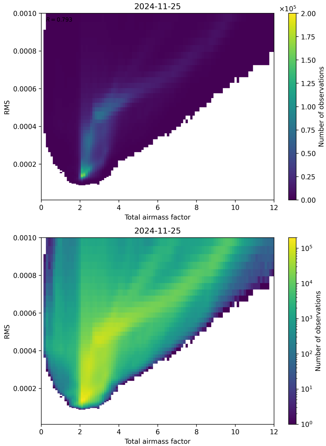
Figure 69: Scatter density plot of “Total airmass factor” against “RMS” for 2024-11-25 to 2024-11-26.
