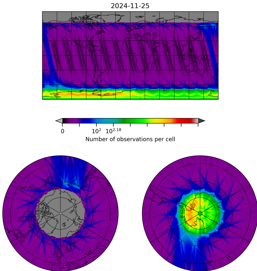
Figure 10: Map of the number of observations for 2024-11-25 to 2024-11-26
