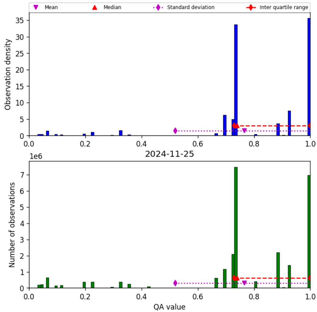
Figure 28: Histogram of “QA value” for 2024-11-25 to 2024-11-26
