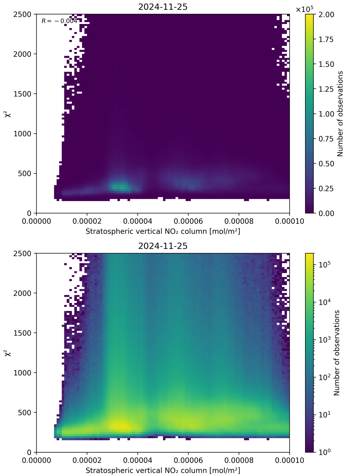
Figure 97: Scatter density plot of “Stratospheric vertical NO 2 column” against “ \chi^2 ” for 2024-11-25 to 2024-11-26.
