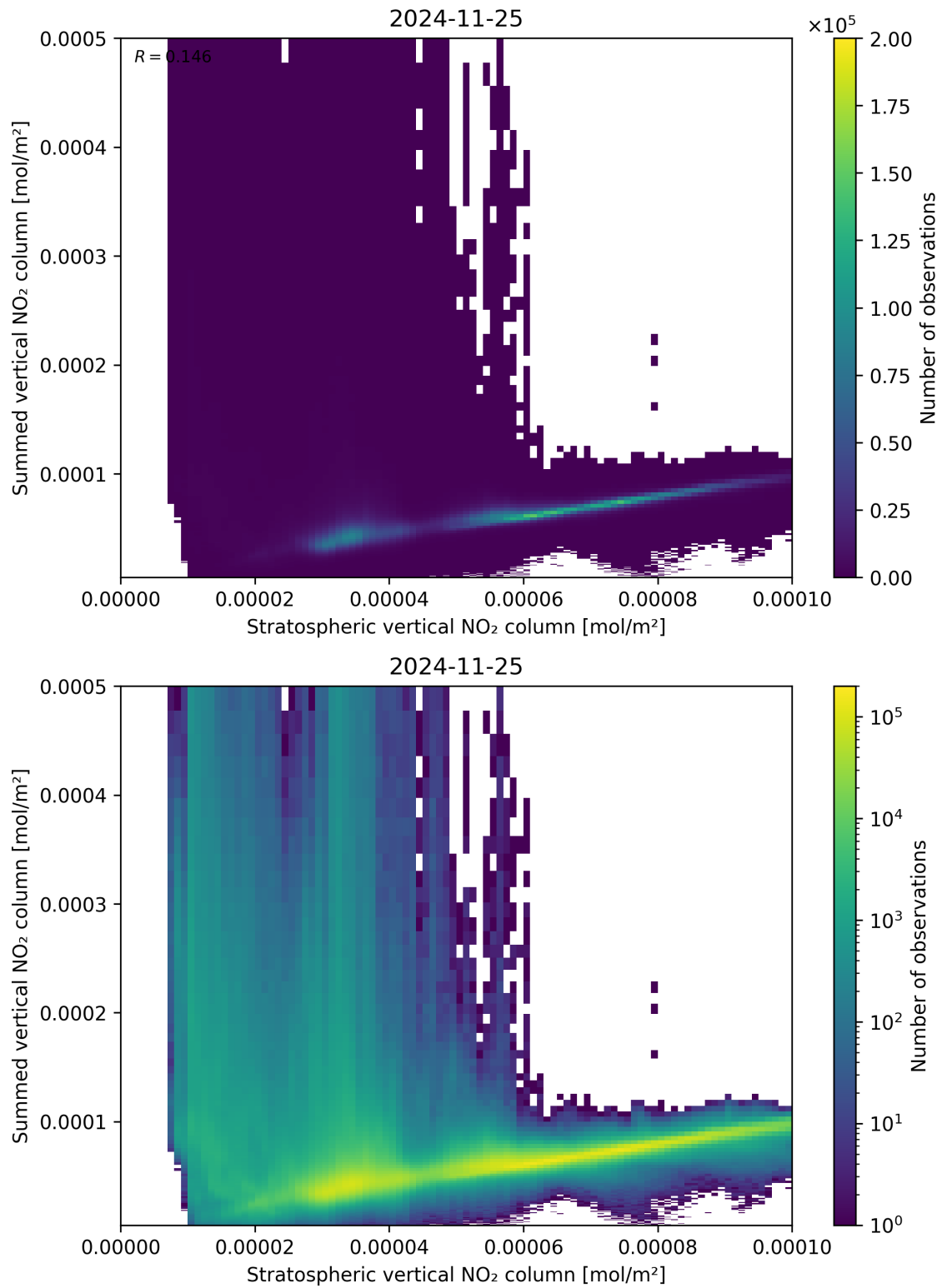
Figure 98: Scatter density plot of “Stratospheric vertical NO 2 column” against “Summed vertical NO 2 column” for 2024-11-25 to 2024-11-26.
