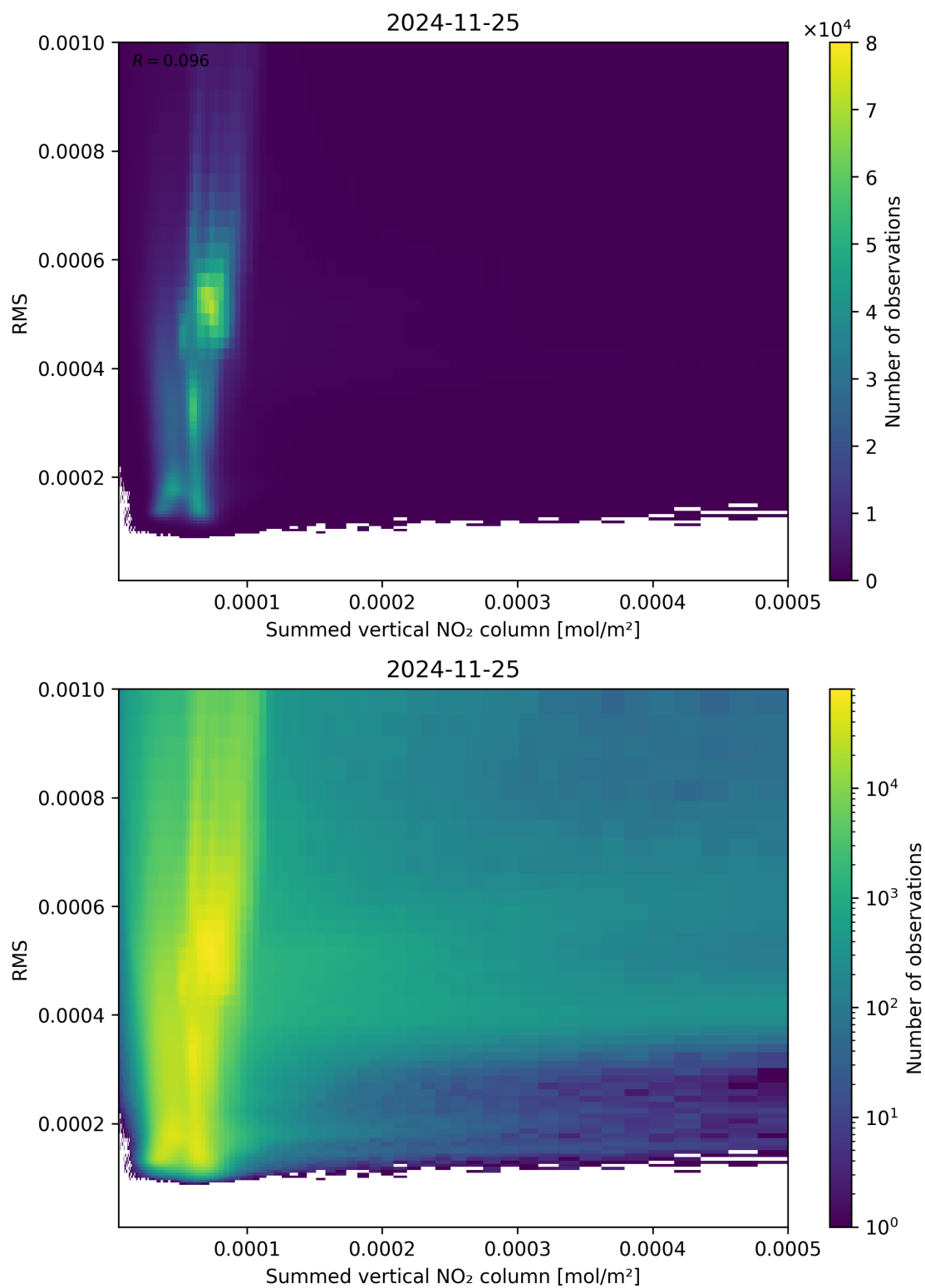
Figure 109: Scatter density plot of “Summed vertical NO 2 column” against “RMS” for 2024-11-25 to 2024-11-26.
