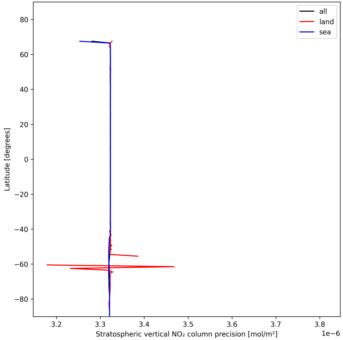
Figure 20: Zonal average of “Stratospheric vertical NO 2 column precision” for 2024-11-25 to 2024-11-26.
