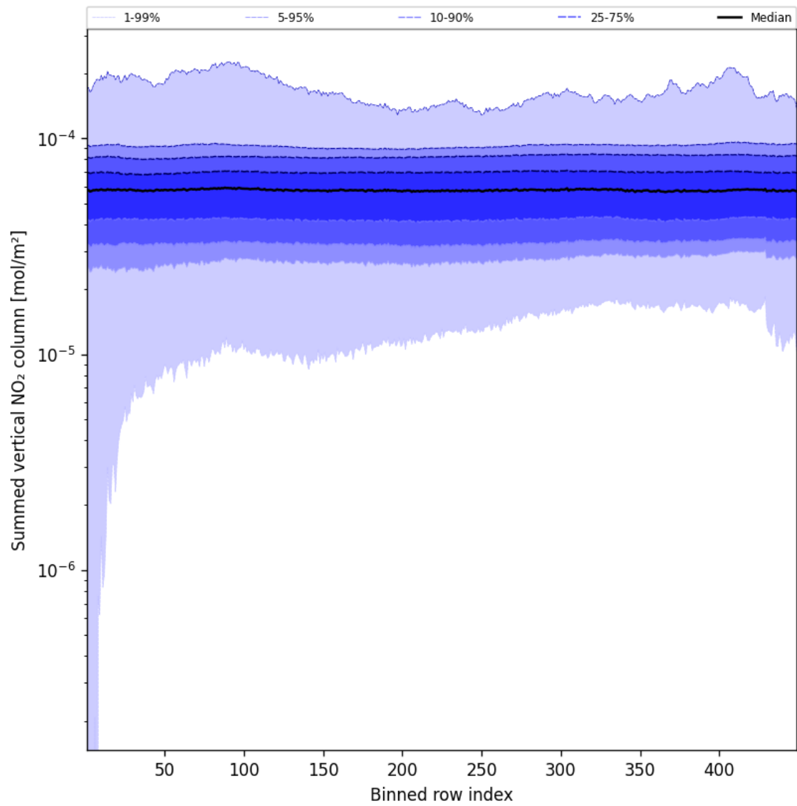
Figure 57: Along track statistics of “Summed vertical NO 2 column” for 2024-11-25 to 2024-11-26
