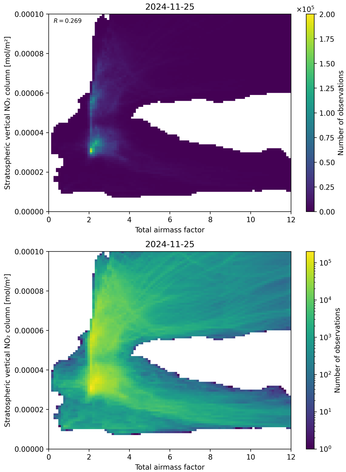
Figure 64: Scatter density plot of “Total airmass factor” against “Stratospheric vertical \text{NO}_2 column” for 2024-11-25 to 2024-11-26.
