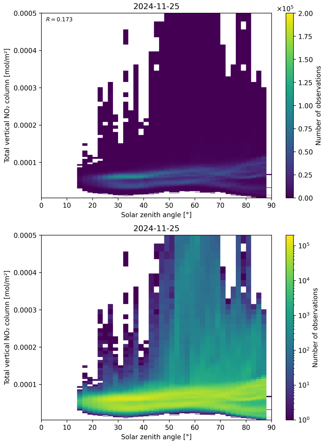
Figure 153: Scatter density plot of “Solar zenith angle” against “Total vertical NO 2 column” for 2024-11-25 to 2024-11-26.
