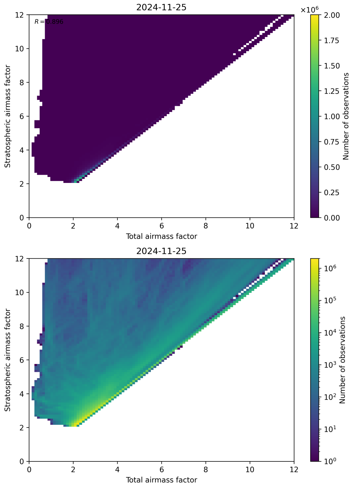
Figure 62: Scatter density plot of “Total airmass factor” against “Stratospheric airmass factor” for 2024-11-25 to 2024-11-26.
