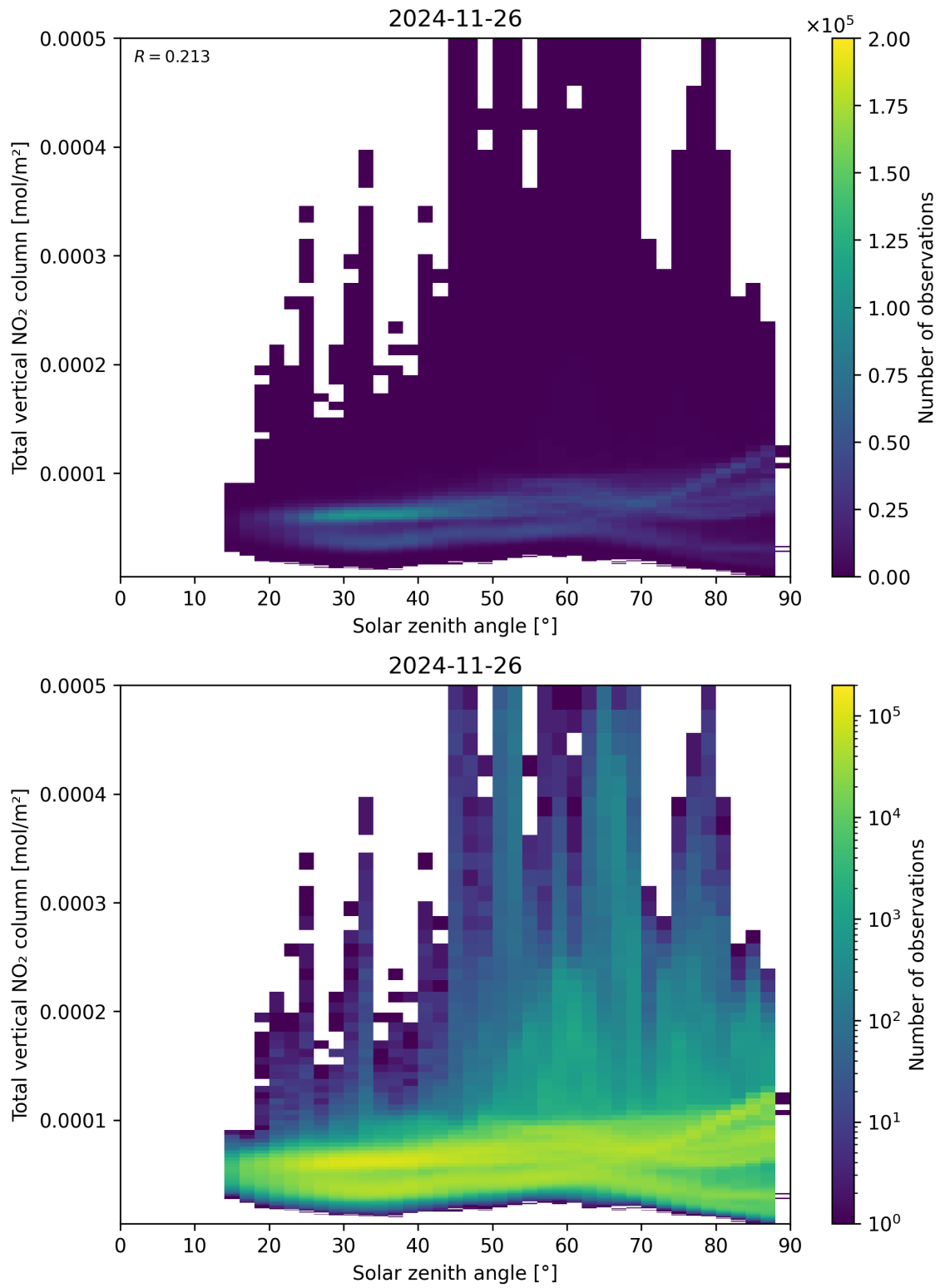
Figure 153: Scatter density plot of “Solar zenith angle” against “Total vertical NO 2 column” for 2024-11-25 to 2024-11-27.
