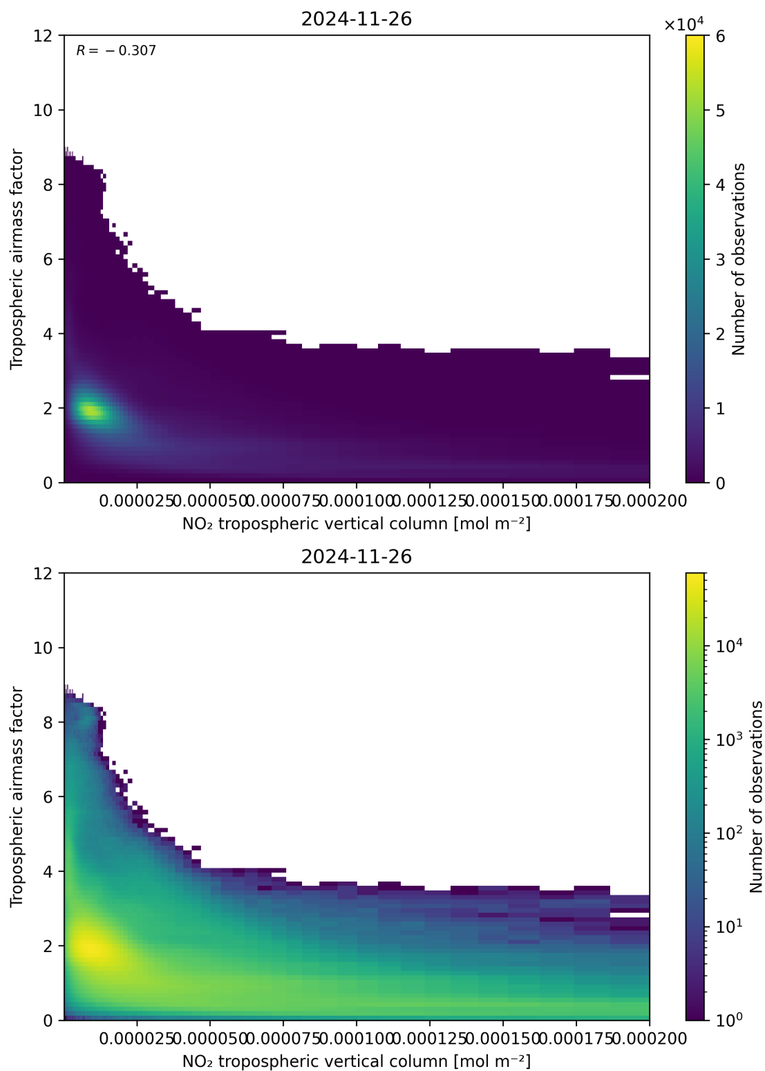
Figure 123: Scatter density plot of “NO 2 tropospheric vertical column” against “Tropospheric air mass factor” for 2024-11-25 to 2024-11-27.
