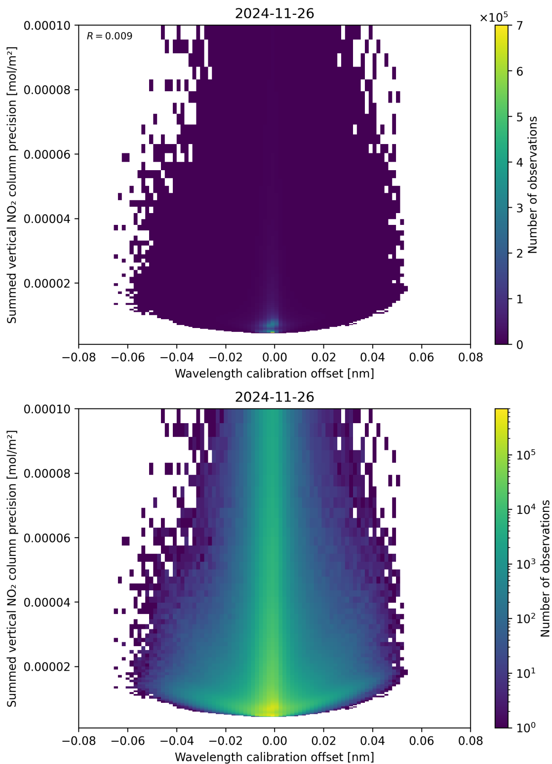
Figure 178: Scatter density plot of “Wavelength calibration offset” against “Summed vertical NO 2 column precision” for 2024-11-25 to 2024-11-27.
