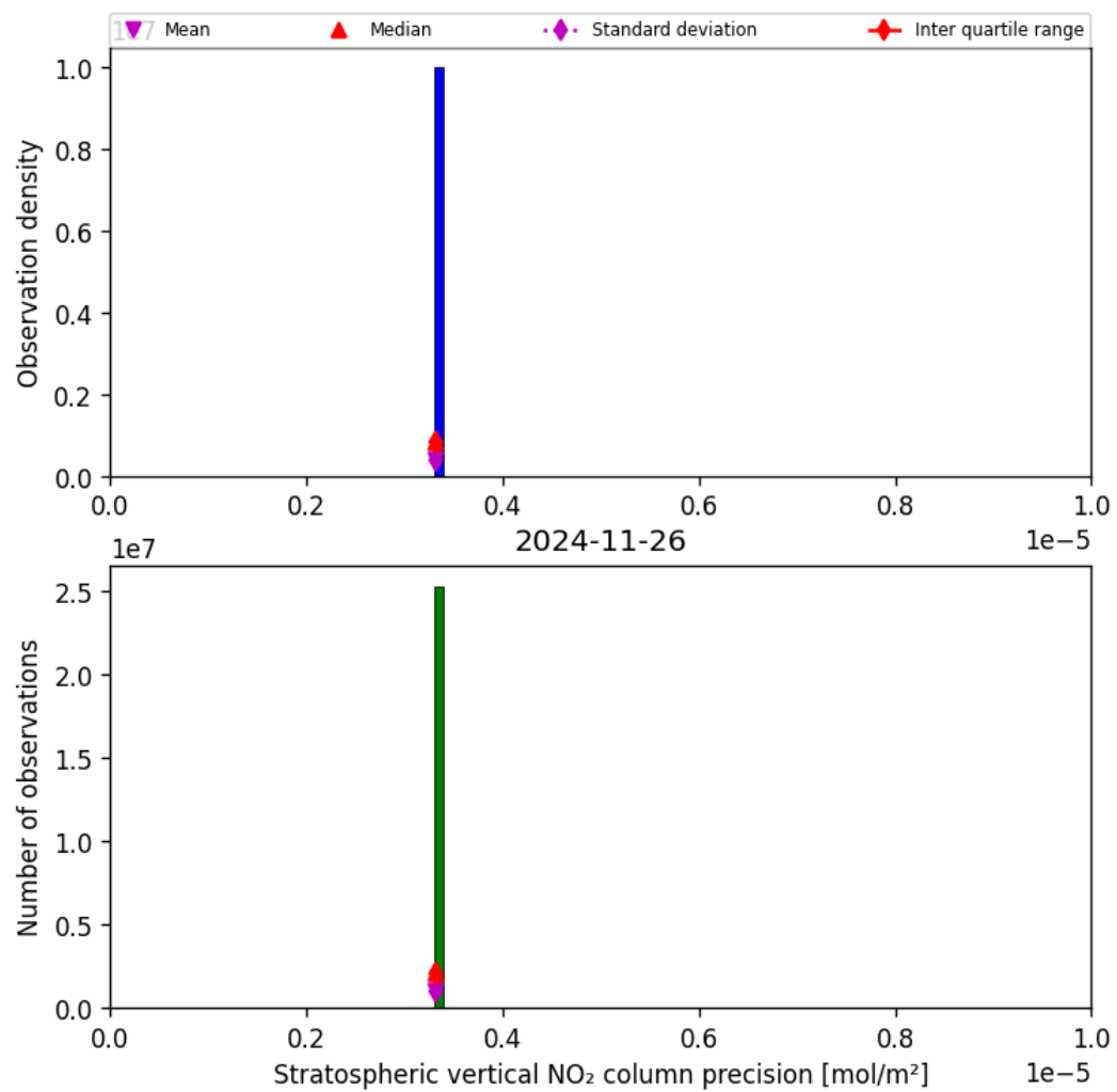
Figure 37: Histogram of “Stratospheric vertical NO 2 column precision” for 2024-11-25 to 2024-11-27
