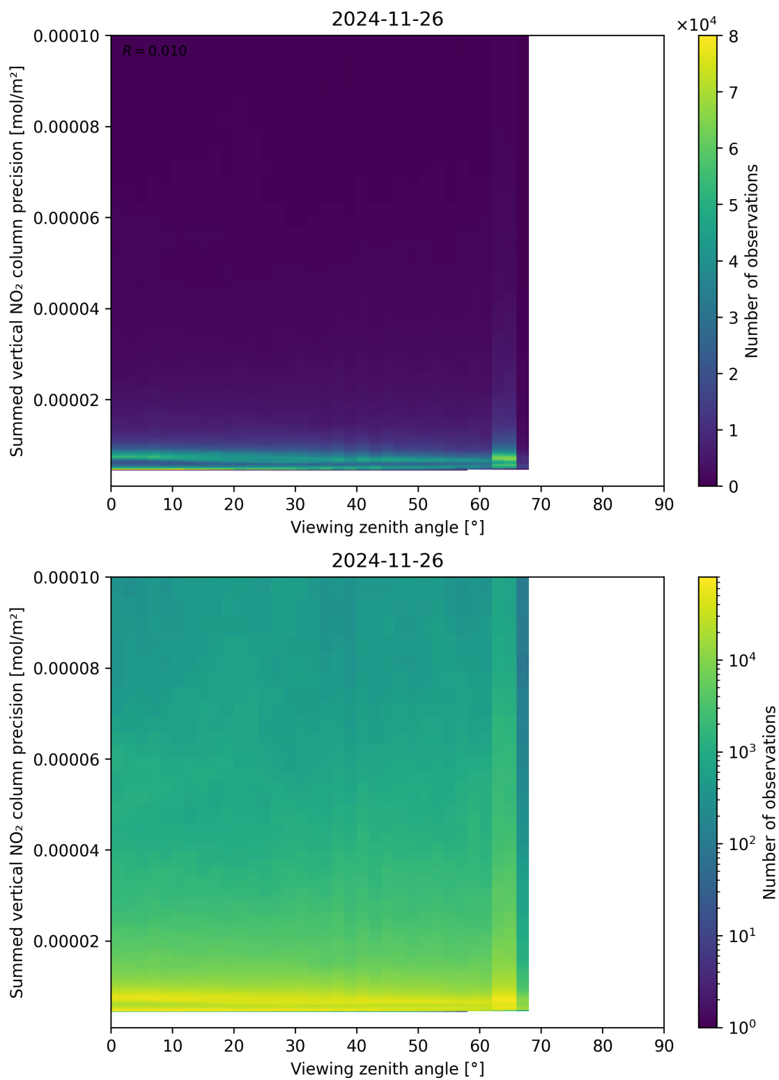
Figure 166: Scatter density plot of “Viewing zenith angle” against “Summed vertical NO 2 column precision” for 2024-11-25 to 2024-11-27.
