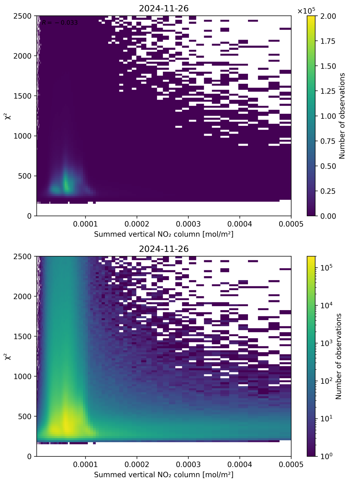
Figure 104: Scatter density plot of “Summed vertical NO 2 column” against “ \chi^2 ” for 2024-11-25 to 2024-11-27.
