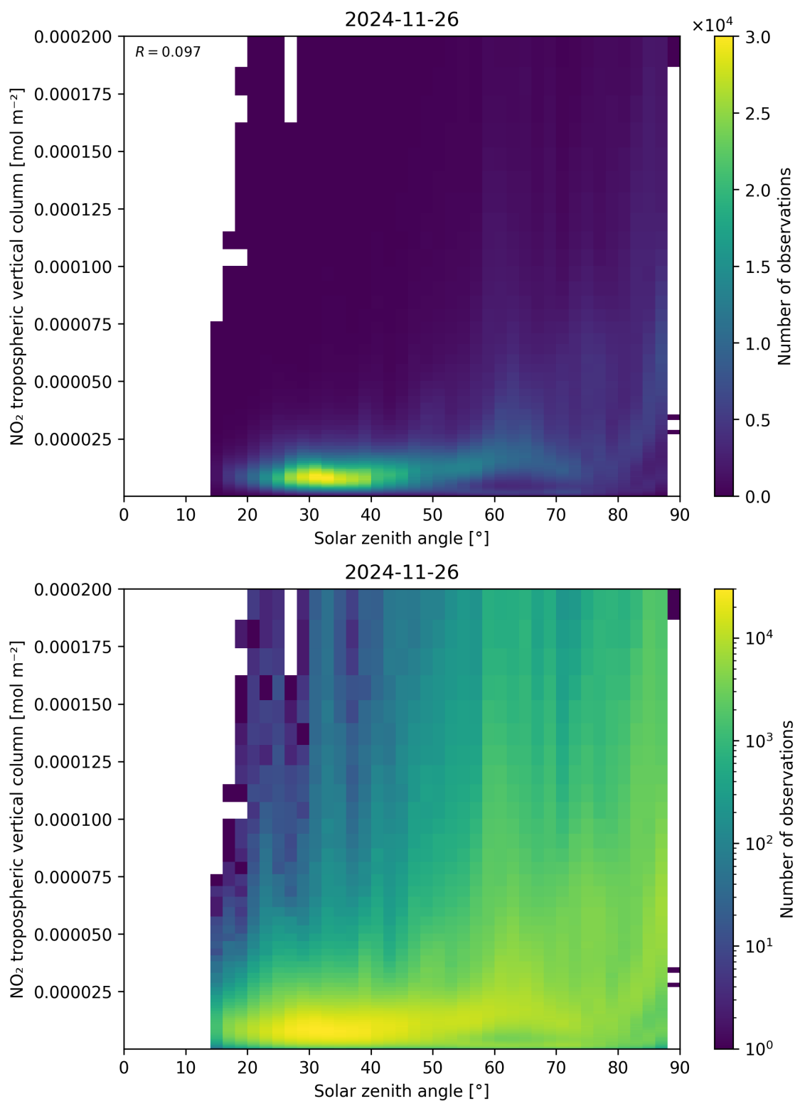
Figure 155: Scatter density plot of “Solar zenith angle” against “NO 2 tropospheric vertical column” for 2024-11-25 to 2024-11-27.
