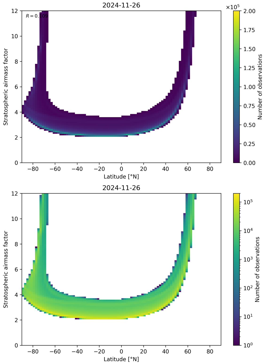
Figure 83: Scatter density plot of “Latitude” against “Stratospheric air mass factor” for 2024-11-25 to 2024-11-27.
