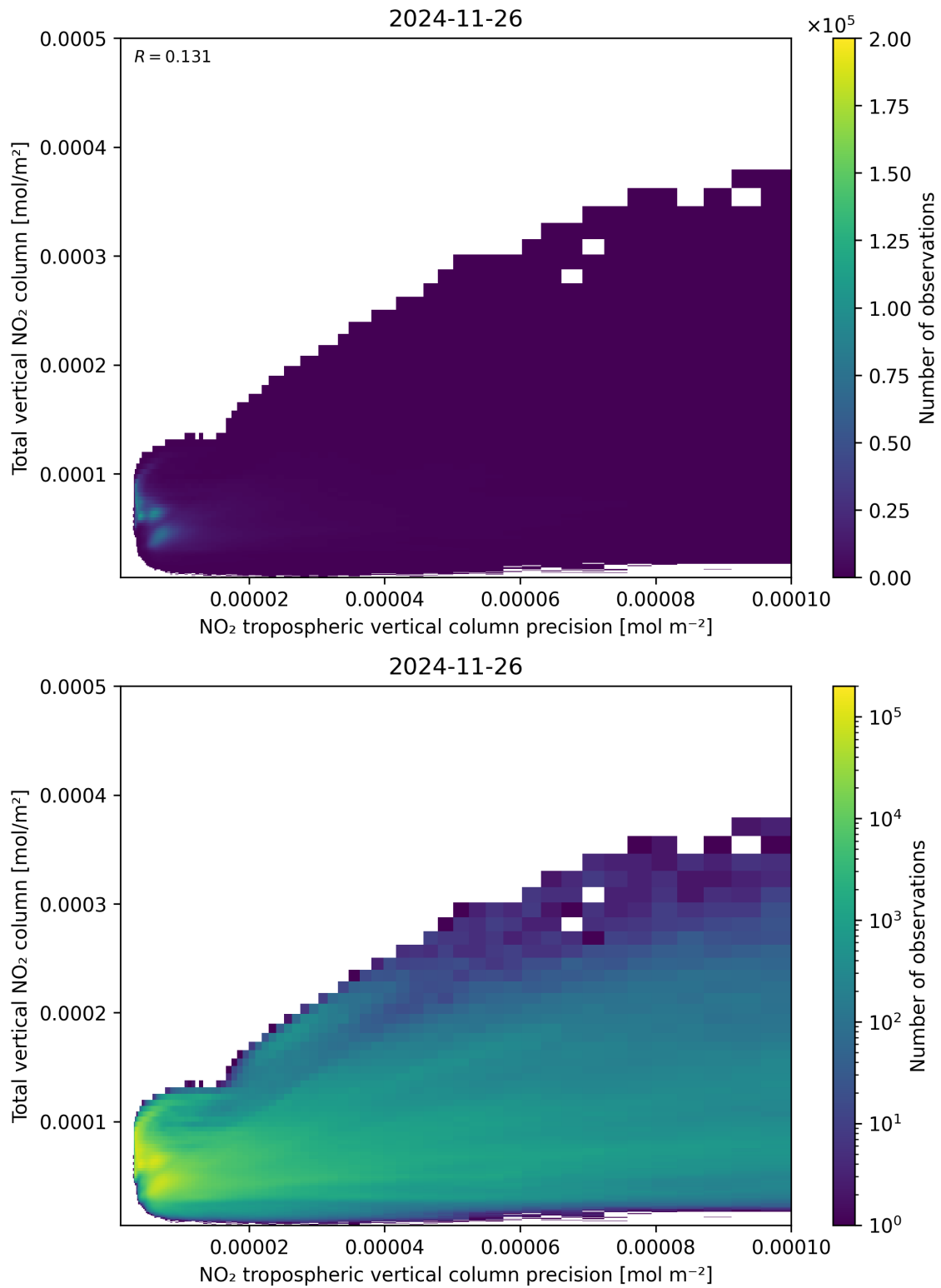
Figure 138: Scatter density plot of “NO 2 tropospheric vertical column precision” against “Total vertical NO 2 column” for 2024-11-25 to 2024-11-27.
