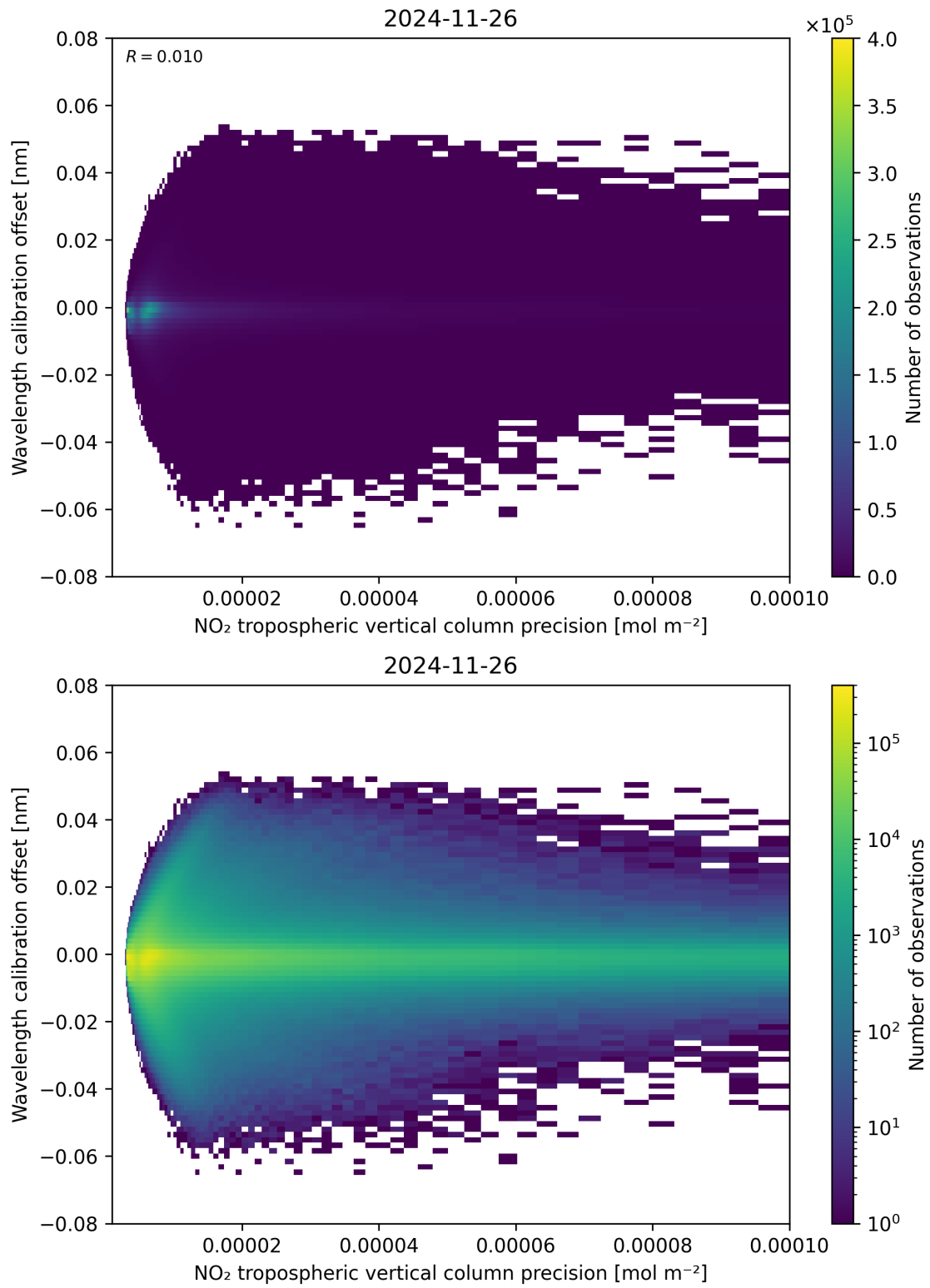
Figure 141: Scatter density plot of “NO 2 tropospheric vertical column precision” against “Wavelength calibration offset” for 2024-11-25 to 2024-11-27.
