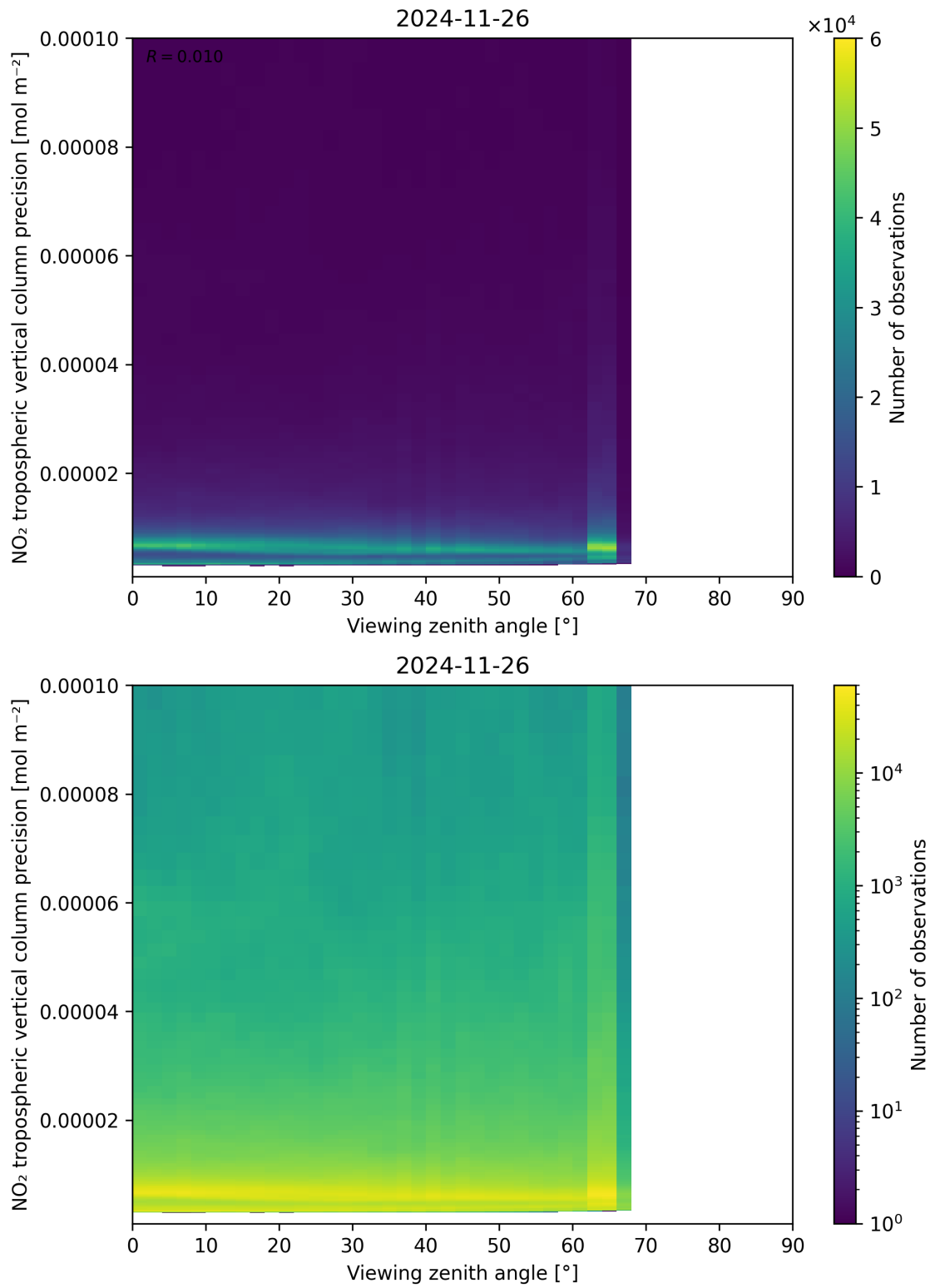
Figure 170: Scatter density plot of “Viewing zenith angle” against “NO 2 tropospheric vertical column precision” for 2024-11-25 to 2024-11-27.
