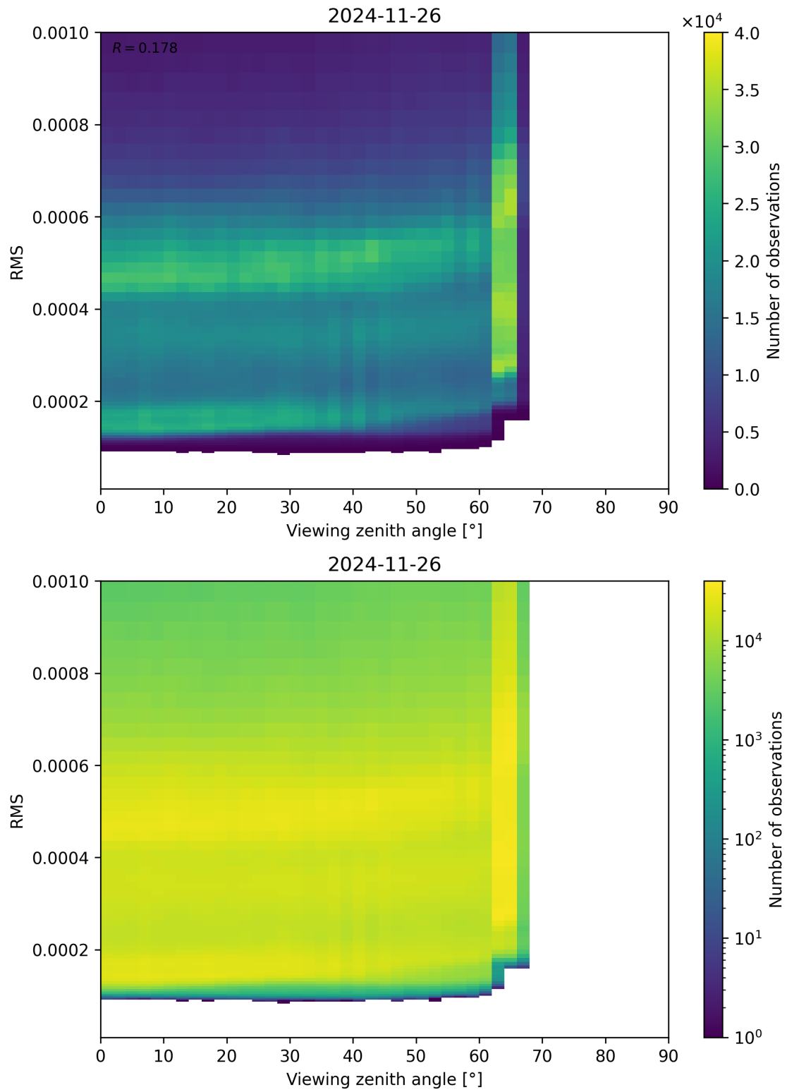
Figure 171: Scatter density plot of “Viewing zenith angle” against “RMS” for 2024-11-25 to 2024-11-27.
