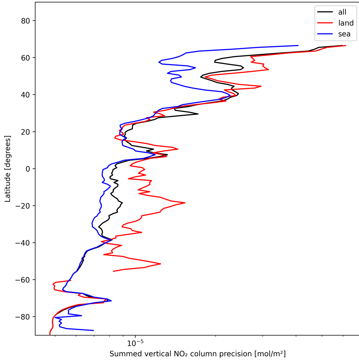
Figure 24: Zonal average of “Summed vertical NO 2 column precision” for 2024-11-25 to 2024-11-27.
