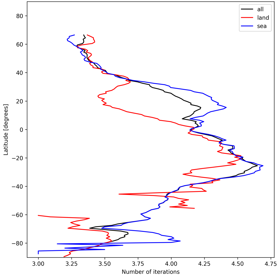
Figure 17: Zonal average of “Number of iterations” for 2024-11-25 to 2024-11-27.
