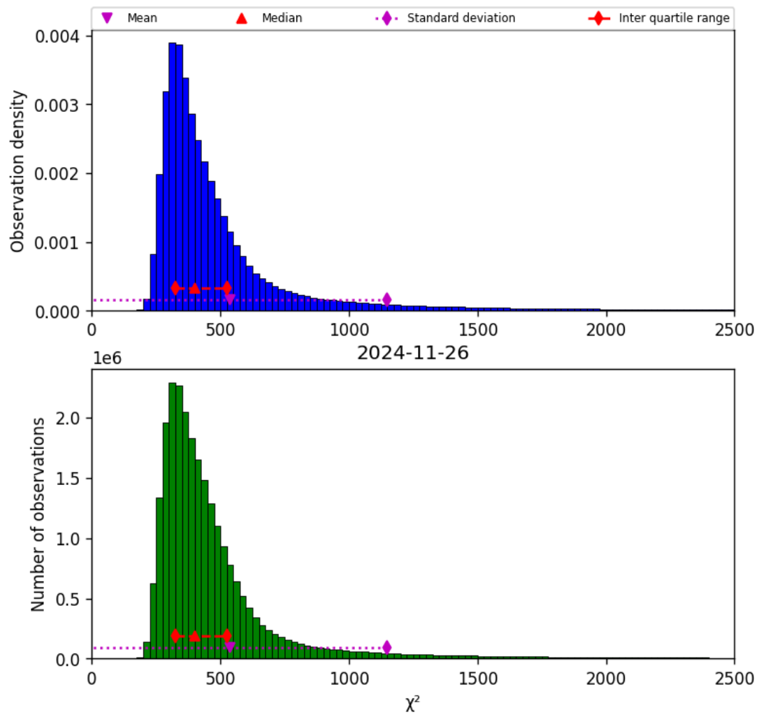
Figure 42: Histogram of " \chi^2 " for 2024-11-25 to 2024-11-27
