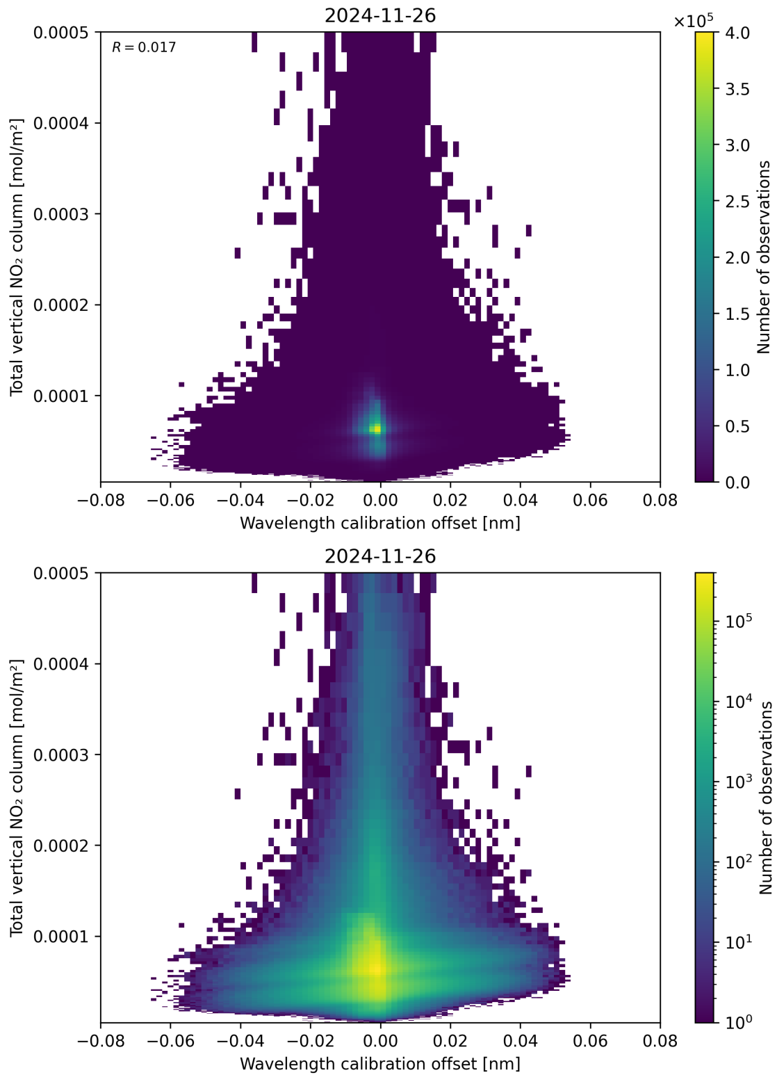
Figure 179: Scatter density plot of “Wavelength calibration offset” against “Total vertical NO 2 column” for 2024-11-25 to 2024-11-27.
