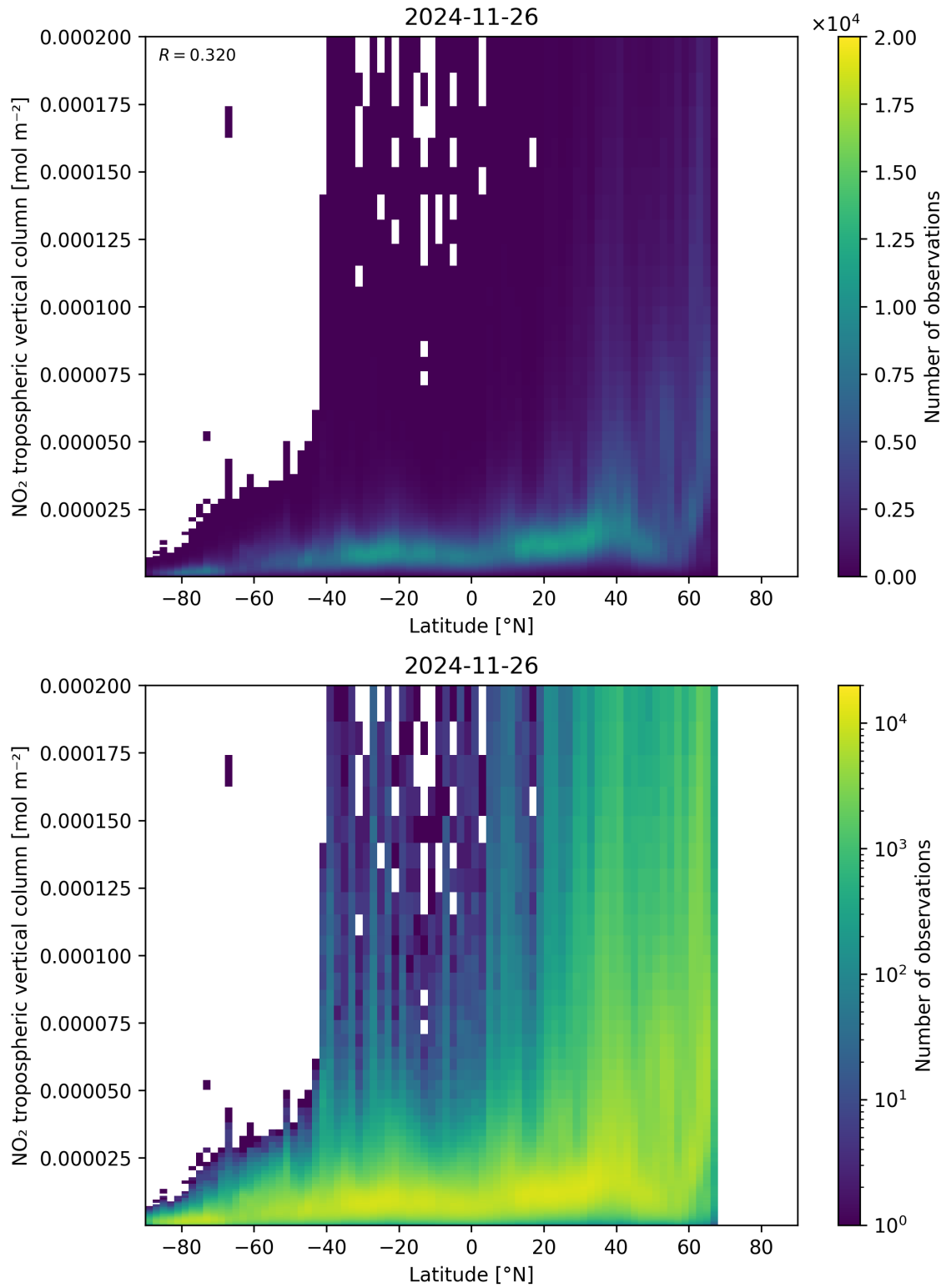
Figure 92: Scatter density plot of “Latitude” against “NO 2 tropospheric vertical column” for 2024-11-25 to 2024-11-27.
