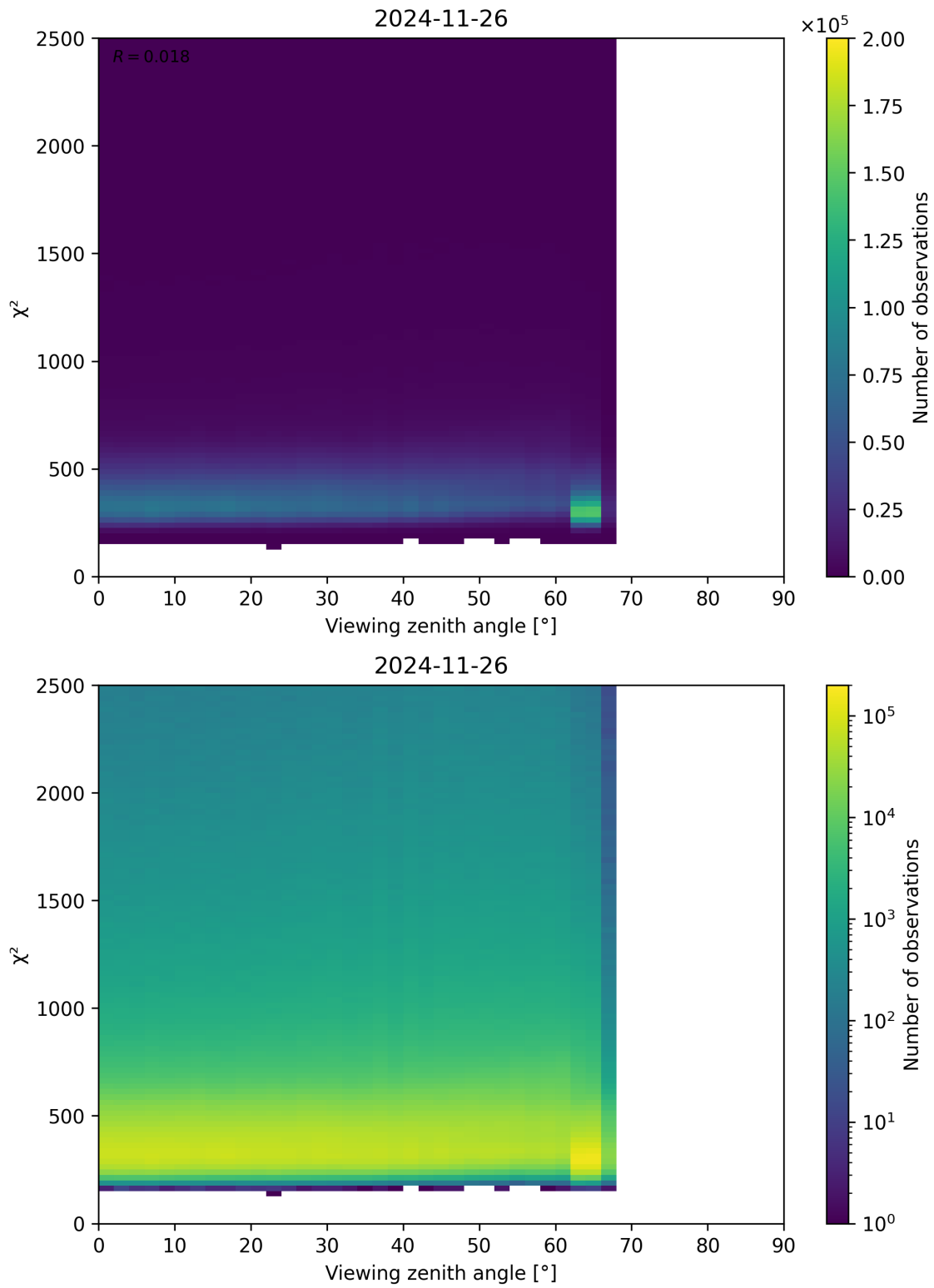
Figure 162: Scatter density plot of “Viewing zenith angle” against “ \chi^2 ” for 2024-11-25 to 2024-11-27.
