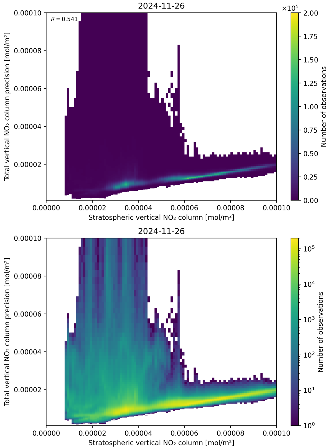
Figure 101: Scatter density plot of “Stratospheric vertical NO 2 column” against “Total vertical NO 2 column precision” for 2024-11-25 to 2024-11-27.
