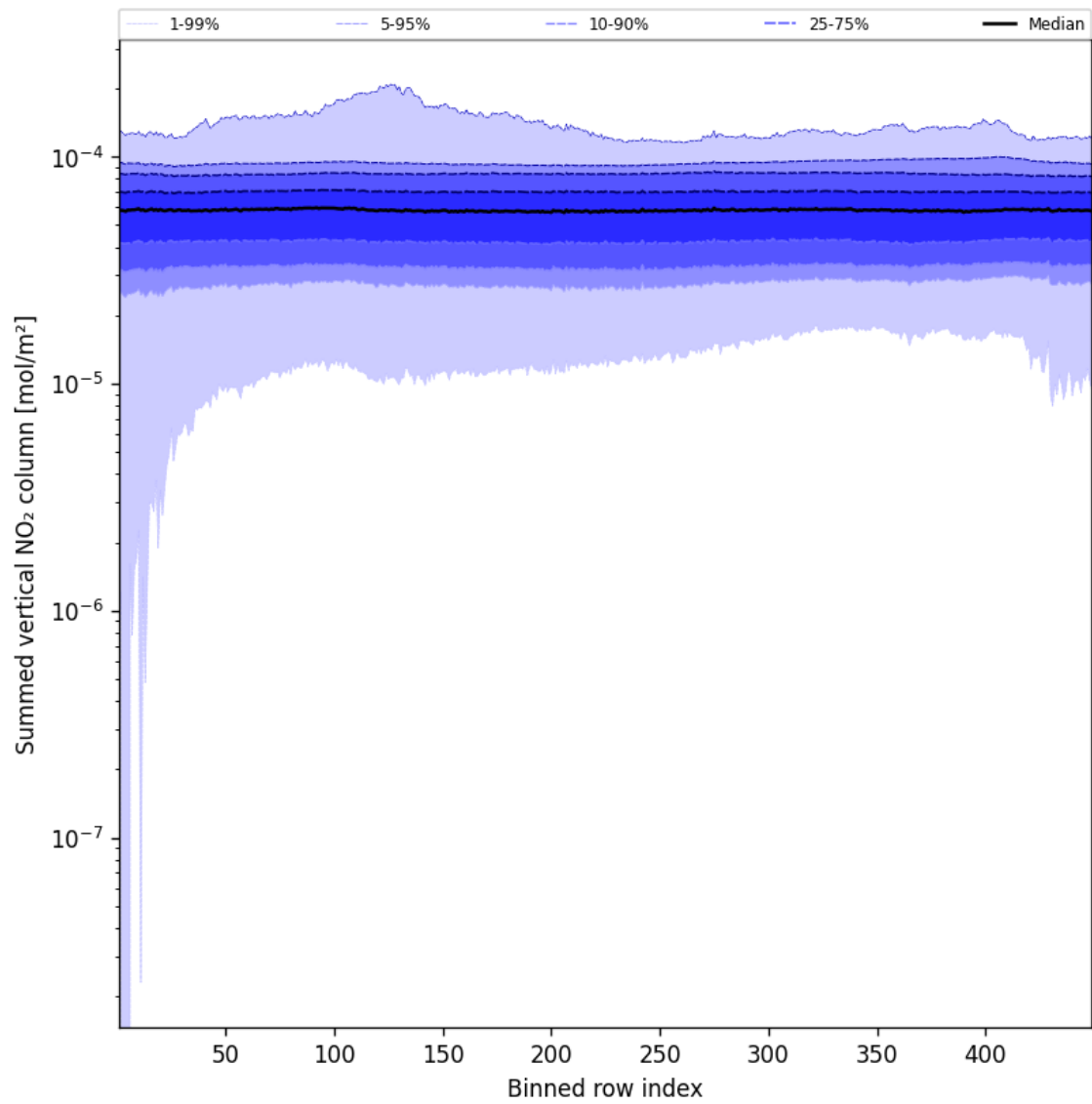
Figure 57: Along track statistics of “Summed vertical NO 2 column” for 2024-11-25 to 2024-11-27
