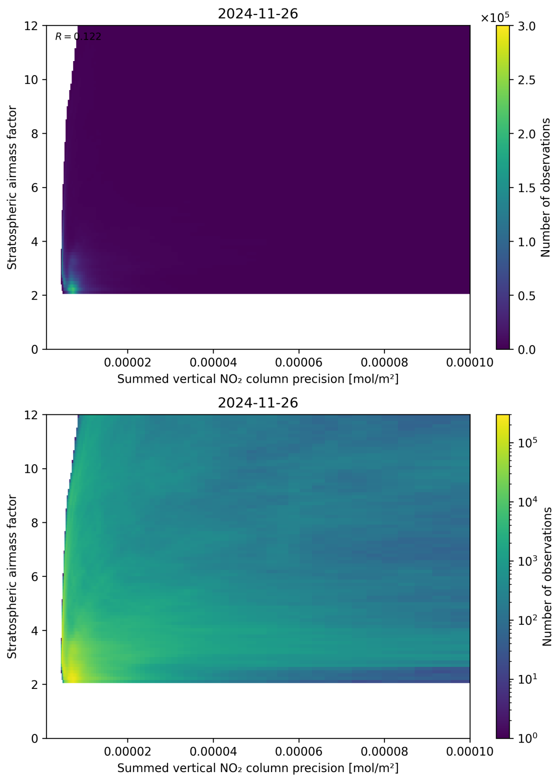
Figure 106: Scatter density plot of “Summed vertical NO 2 column precision” against “Stratospheric airmass factor” for 2024-11-25 to 2024-11-27.
