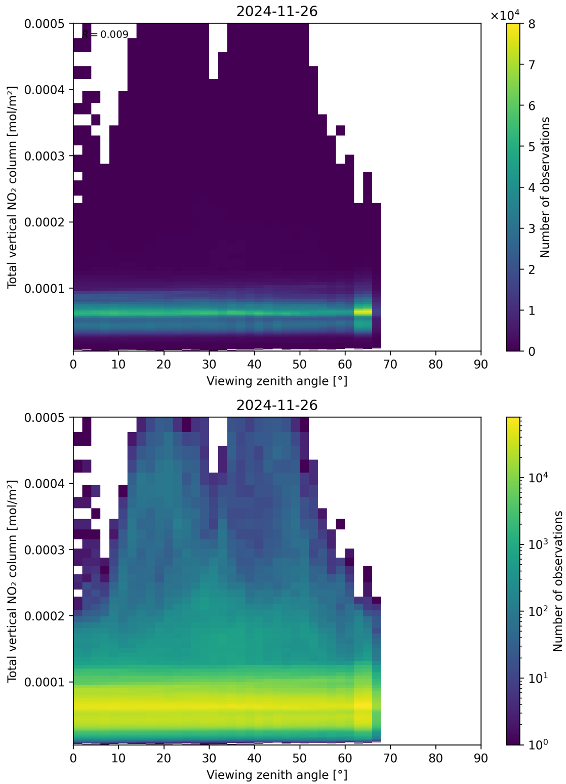
Figure 167: Scatter density plot of “Viewing zenith angle” against “Total vertical NO 2 column” for 2024-11-25 to 2024-11-27.
