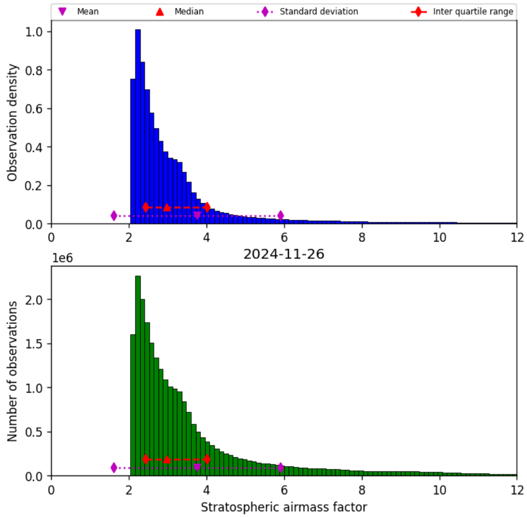
Figure 44: Histogram of “Stratospheric airmass factor” for 2024-11-25 to 2024-11-27
