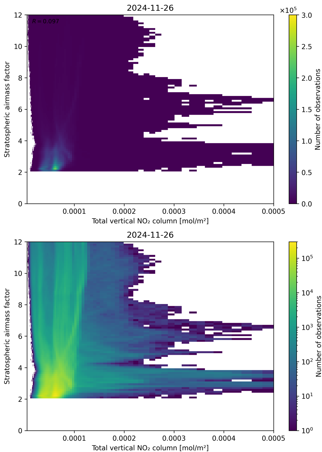
Figure 110: Scatter density plot of “Total vertical NO 2 column” against “Stratospheric air mass factor” for 2024-11-25 to 2024-11-27.
