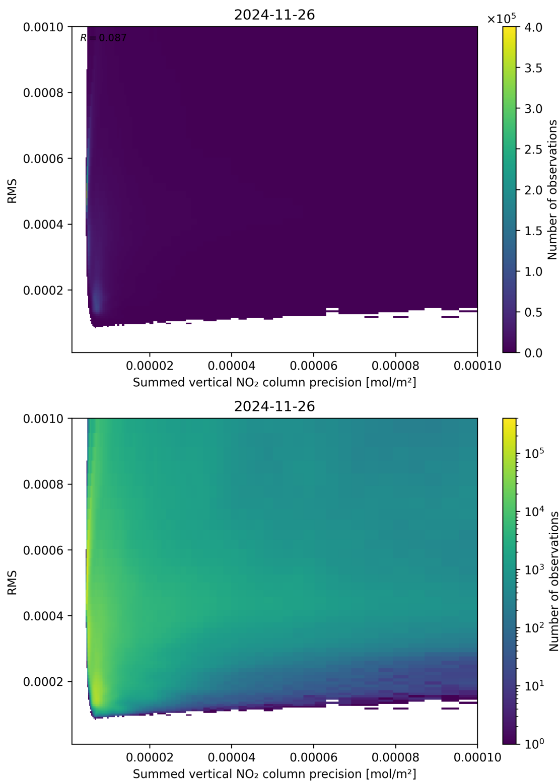
Figure 108: Scatter density plot of “Summed vertical NO 2 column precision” against “RMS” for 2024-11-25 to 2024-11-27.
