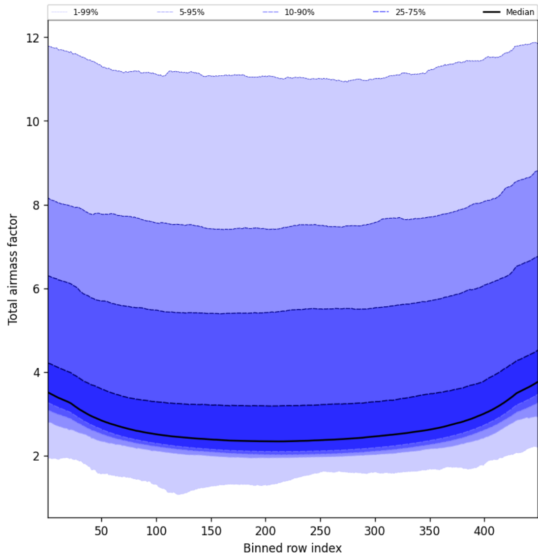
Figure 49: Along track statistics of “Total airmass factor” for 2024-11-25 to 2024-11-27
