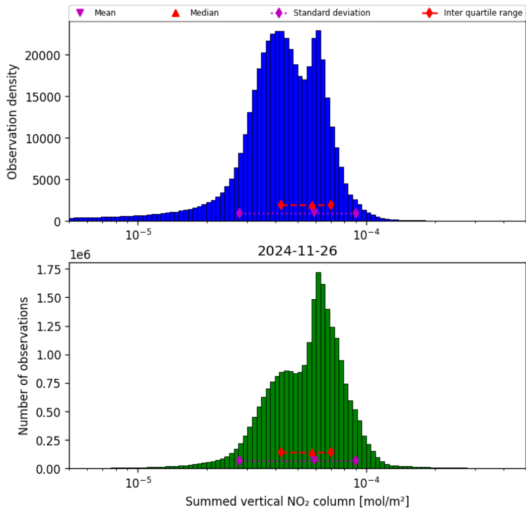
Figure 40: Histogram of “Summed vertical NO 2 column” for 2024-11-25 to 2024-11-27
