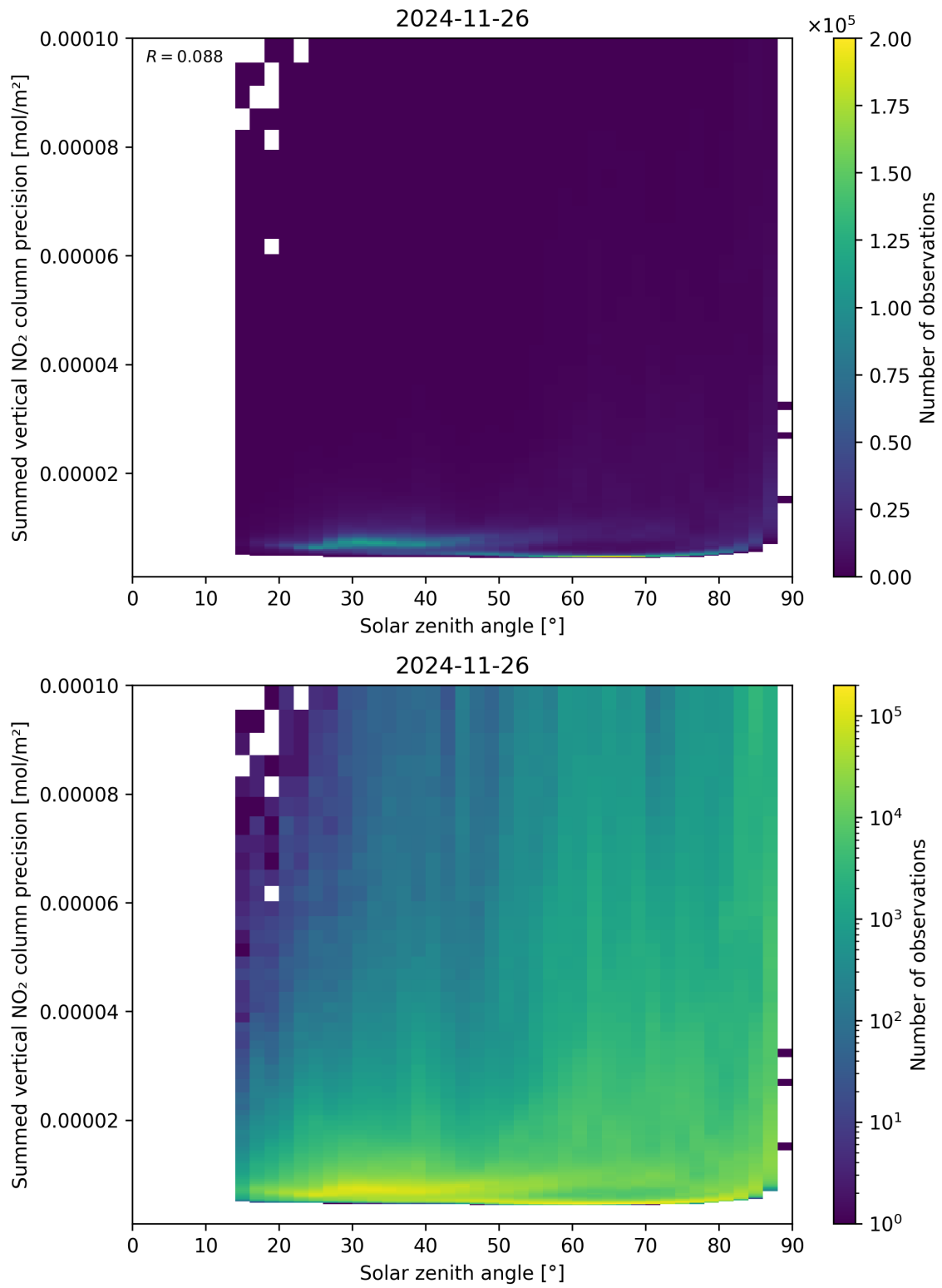
Figure 152: Scatter density plot of “Solar zenith angle” against “Summed vertical NO 2 column precision” for 2024-11-25 to 2024-11-27.
