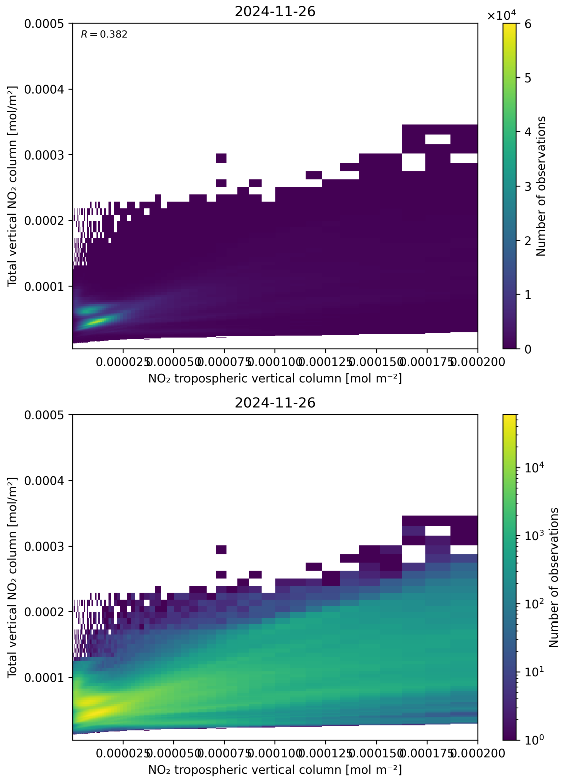
Figure 128: Scatter density plot of “NO 2 tropospheric vertical column” against “Total vertical NO 2 column” for 2024-11-25 to 2024-11-27.
