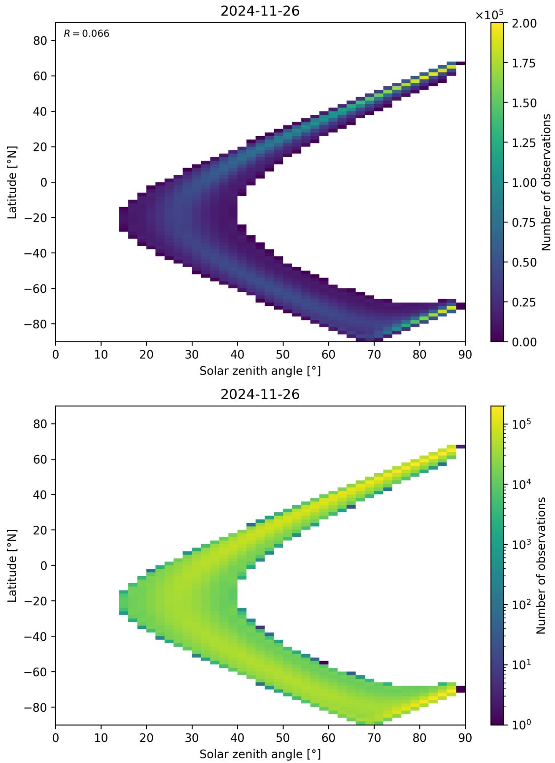
Figure 149: Scatter density plot of “Solar zenith angle” against “Latitude” for 2024-11-25 to 2024-11-27.
