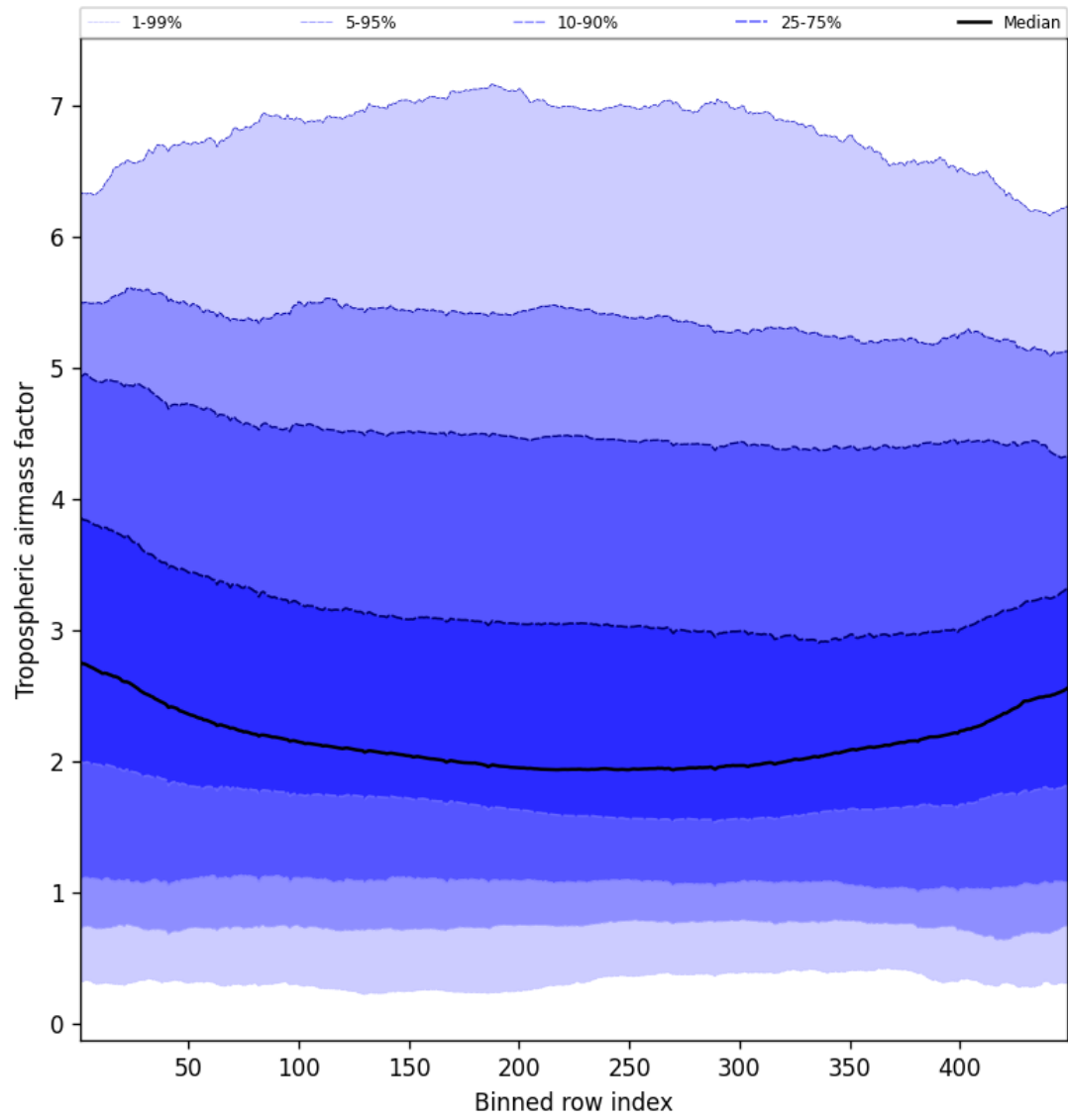
Figure 48: Along track statistics of “Tropospheric air mass factor” for 2024-11-25 to 2024-11-27
