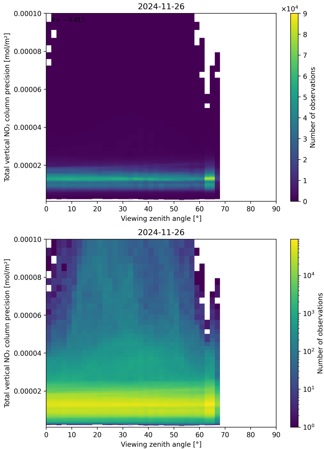
Figure 168: Scatter density plot of “Viewing zenith angle” against “Total vertical NO 2 column precision” for 2024-11-25 to 2024-11-27.
