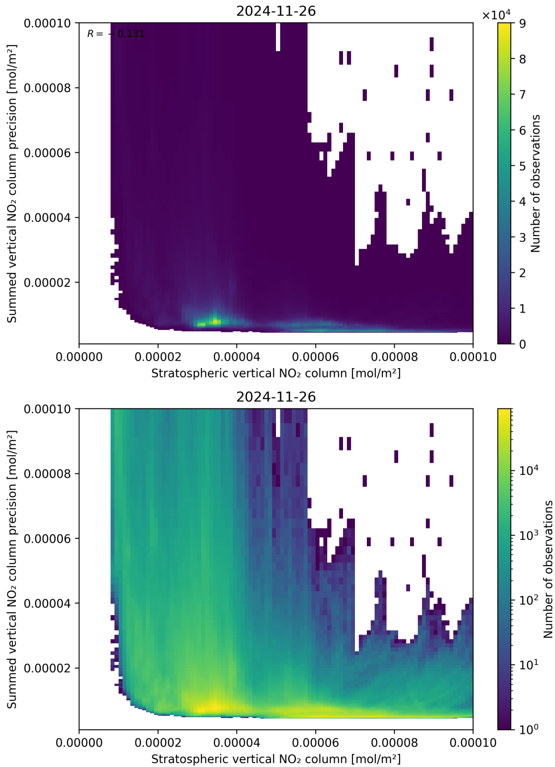
Figure 99: Scatter density plot of “Stratospheric vertical NO 2 column” against “Summed vertical NO 2 column precision” for 2024-11-25 to 2024-11-27.
