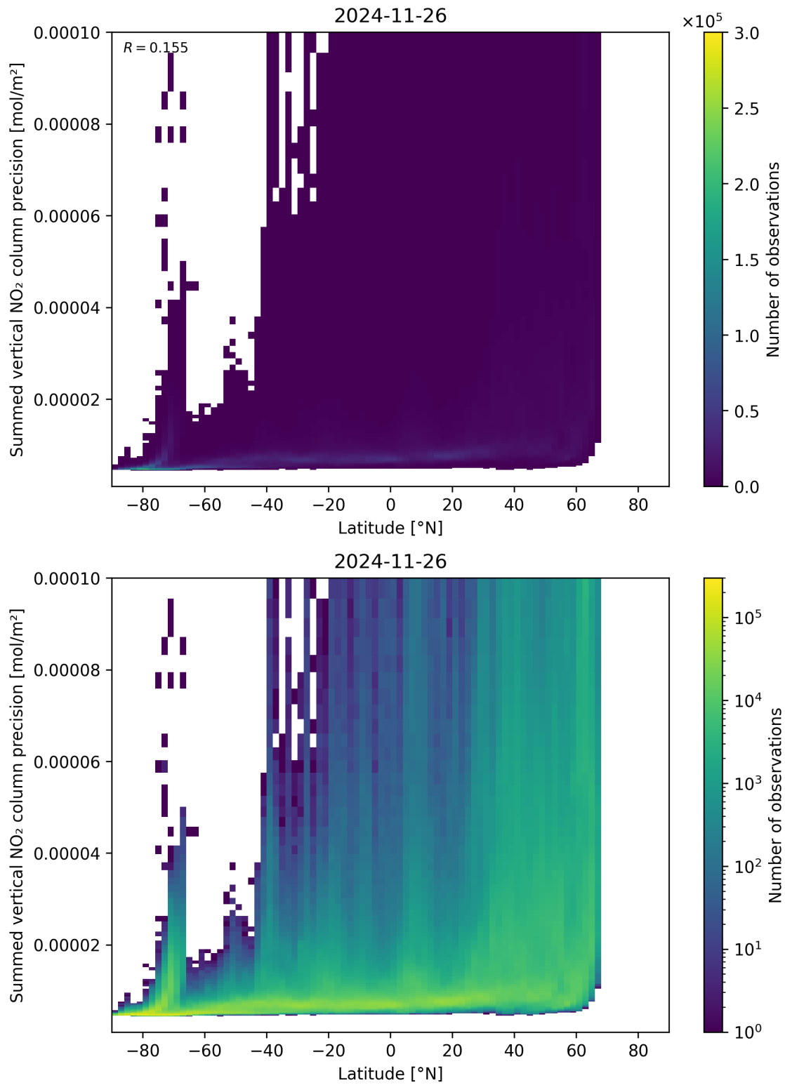
Figure 89: Scatter density plot of “Latitude” against “Summed vertical NO 2 column precision” for 2024-11-25 to 2024-11-27.
