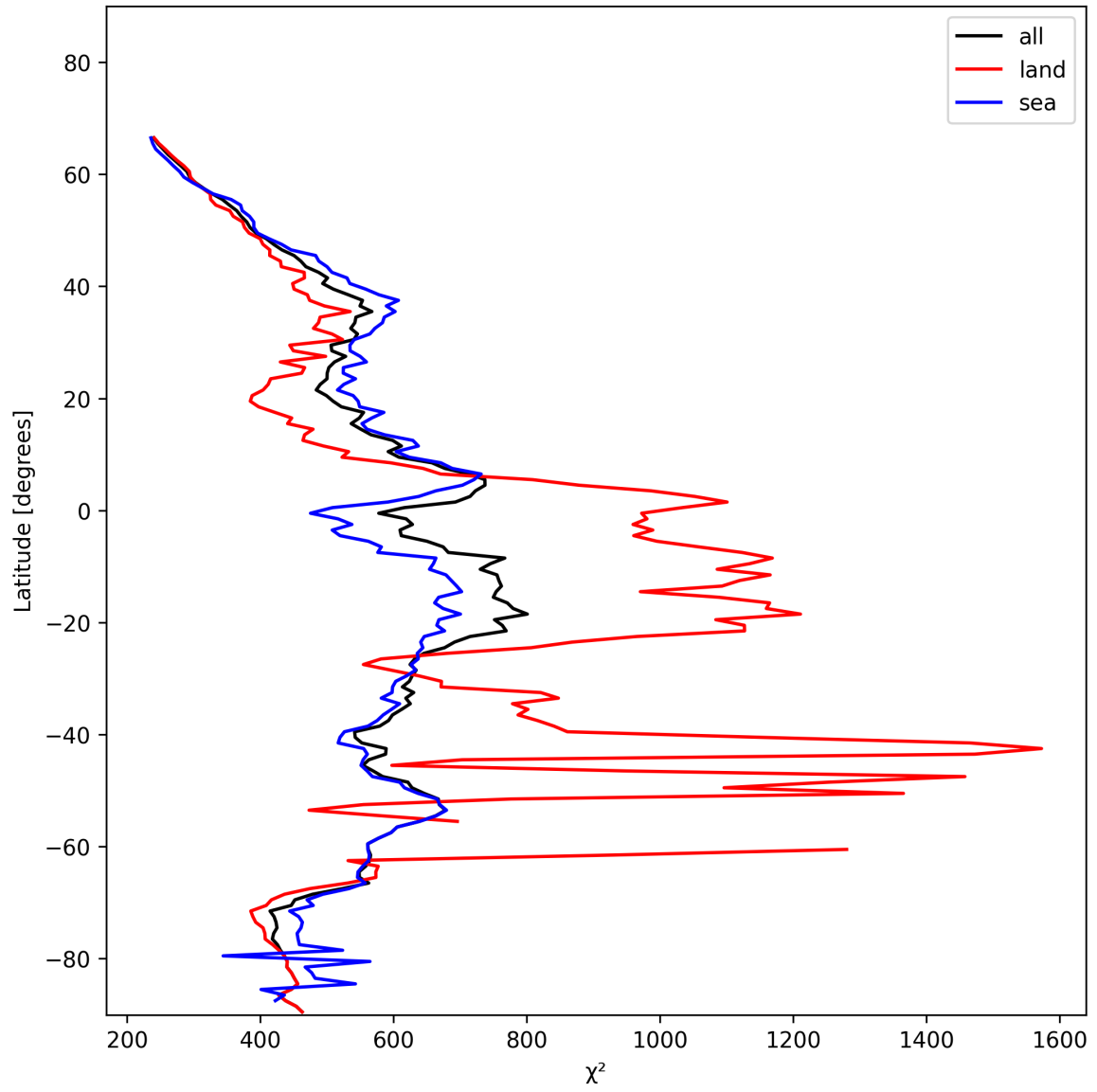
Figure 25: Zonal average of “ \chi^2 ” for 2024-11-25 to 2024-11-27.
