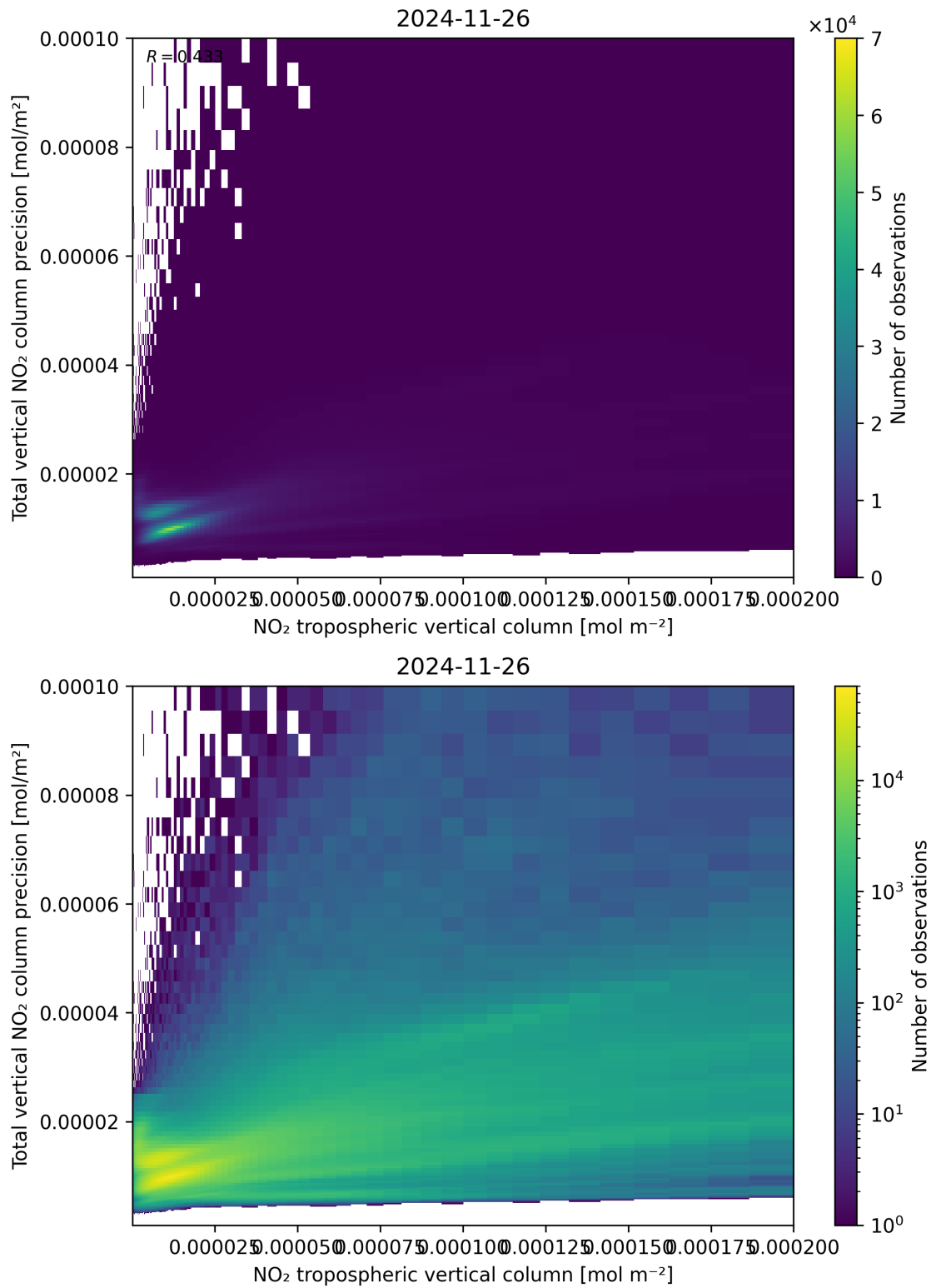
Figure 129: Scatter density plot of “NO 2 tropospheric vertical column” against “Total vertical NO 2 column precision” for 2024-11-25 to 2024-11-27.
