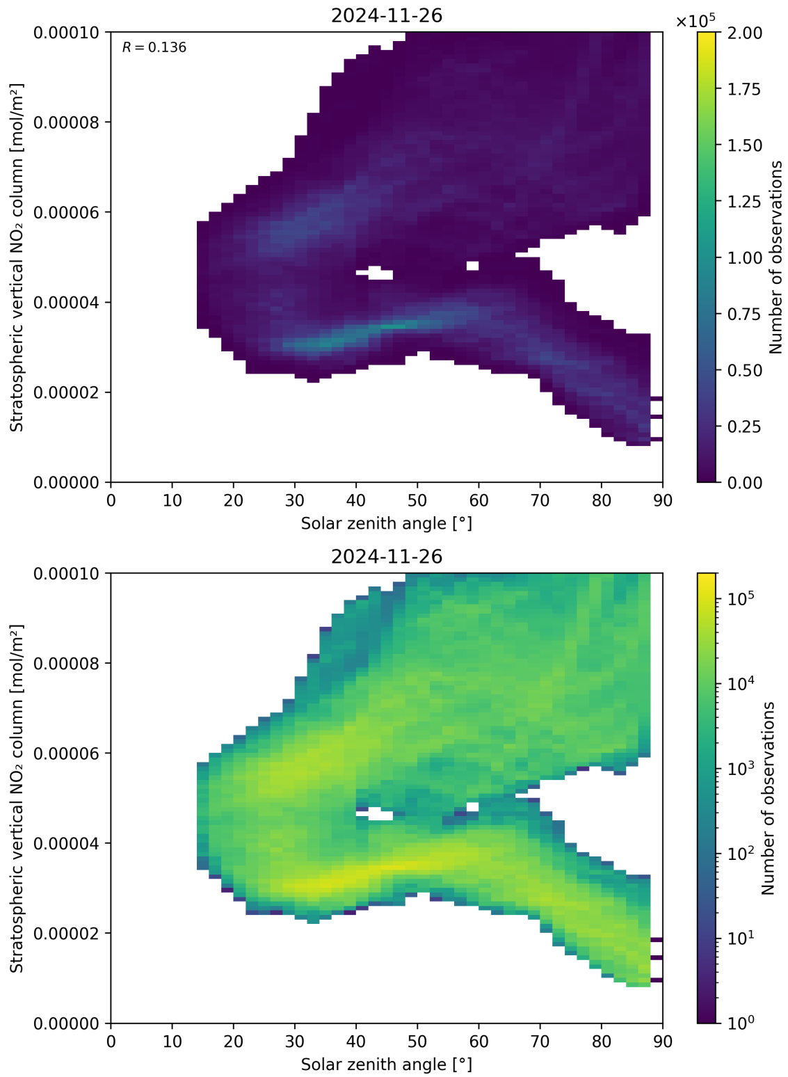
Figure 150: Scatter density plot of “Solar zenith angle” against “Stratospheric vertical NO 2 column” for 2024-11-25 to 2024-11-27.
