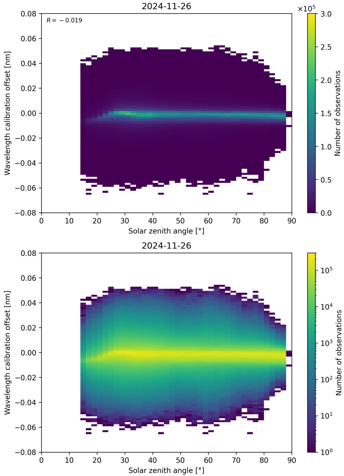
Figure 158: Scatter density plot of “Solar zenith angle” against “Wavelength calibration offset” for 2024-11-25 to 2024-11-27.
