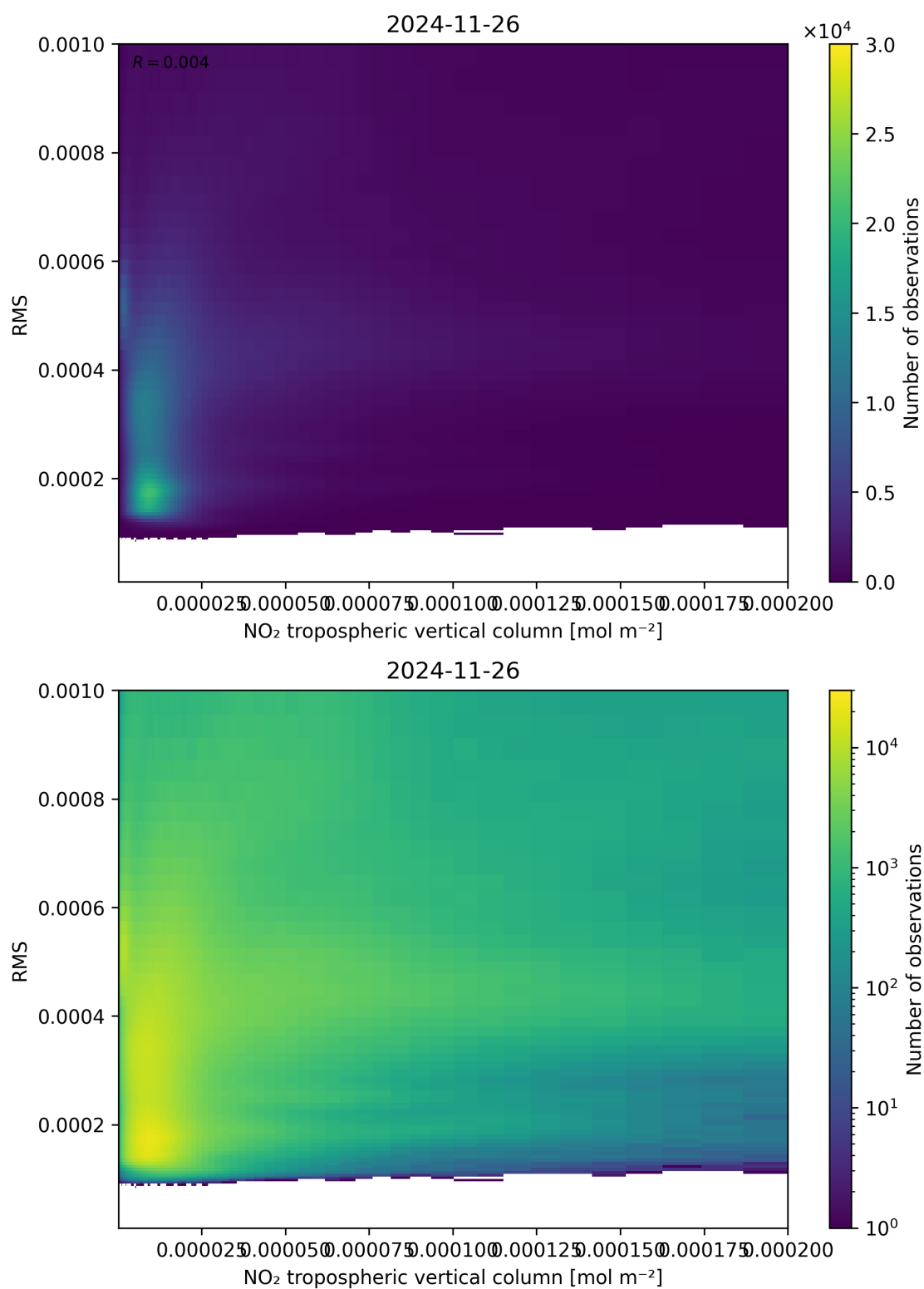
Figure 142: Scatter density plot of “NO 2 tropospheric vertical column” against “RMS” for 2024-11-25 to 2024-11-27.
