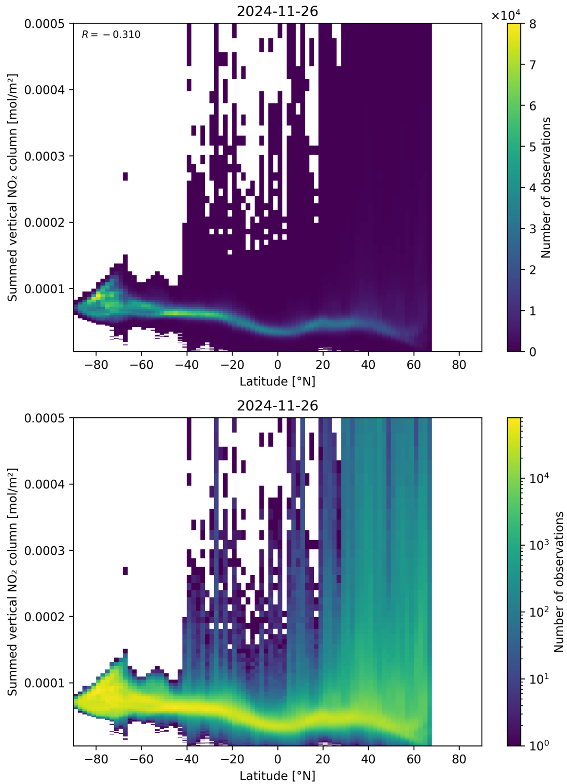
Figure 88: Scatter density plot of “Latitude” against “Summed vertical NO 2 column” for 2024-11-25 to 2024-11-27.
