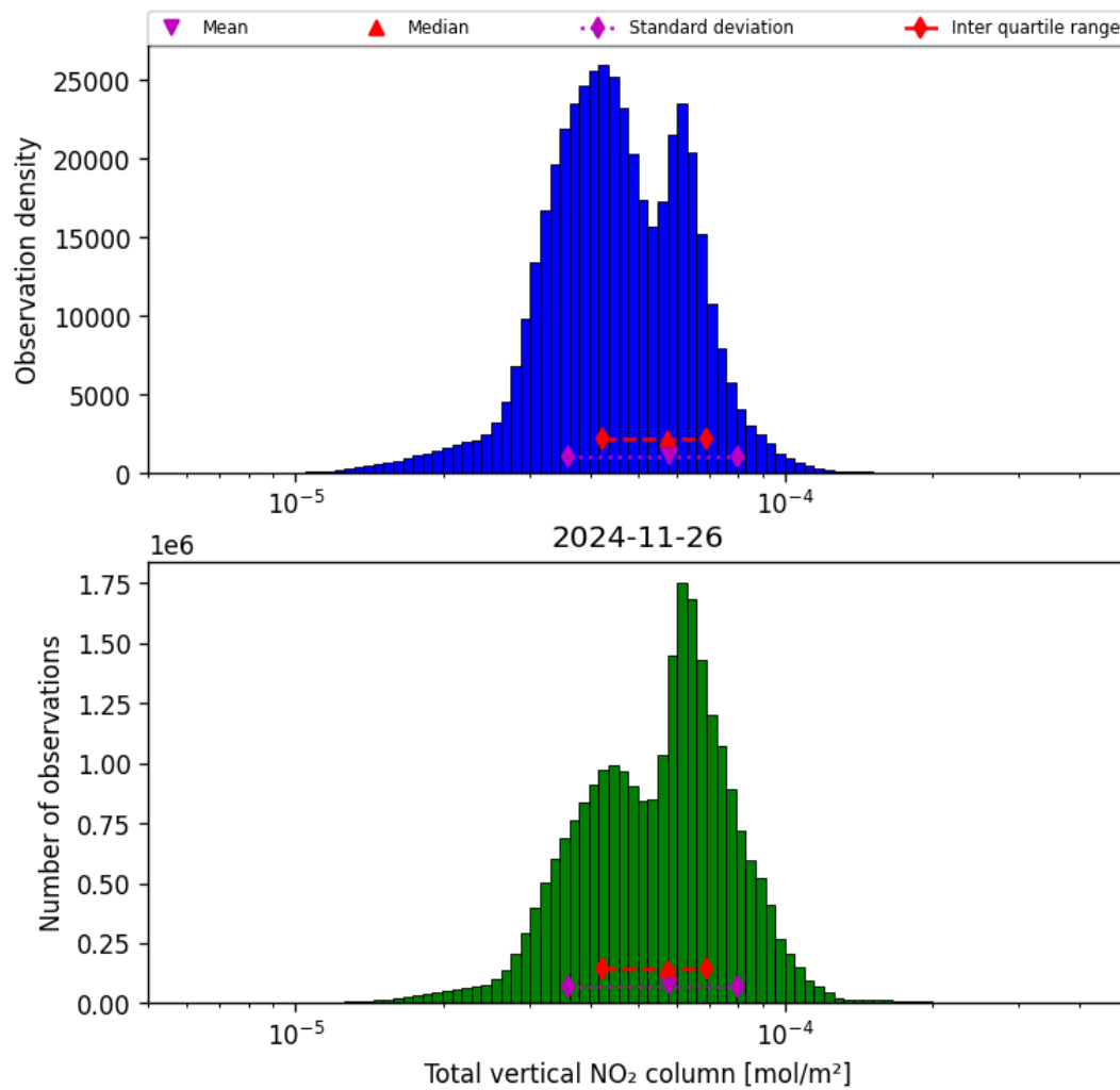
Figure 38: Histogram of “Total vertical NO 2 column” for 2024-11-25 to 2024-11-27
