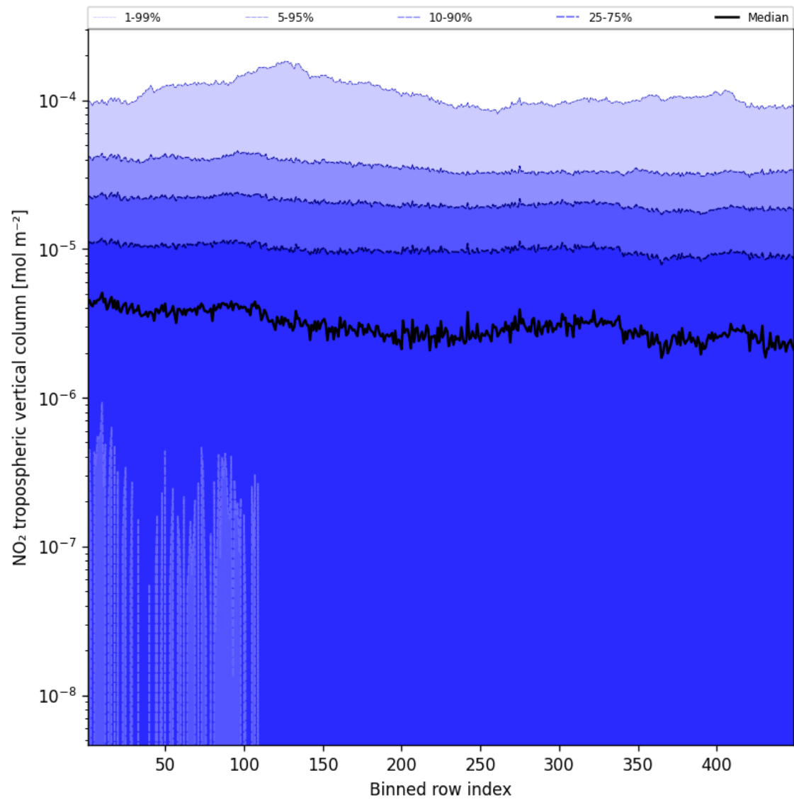
Figure 46: Along track statistics of “NO 2 tropospheric vertical column” for 2024-11-25 to 2024-11-27
