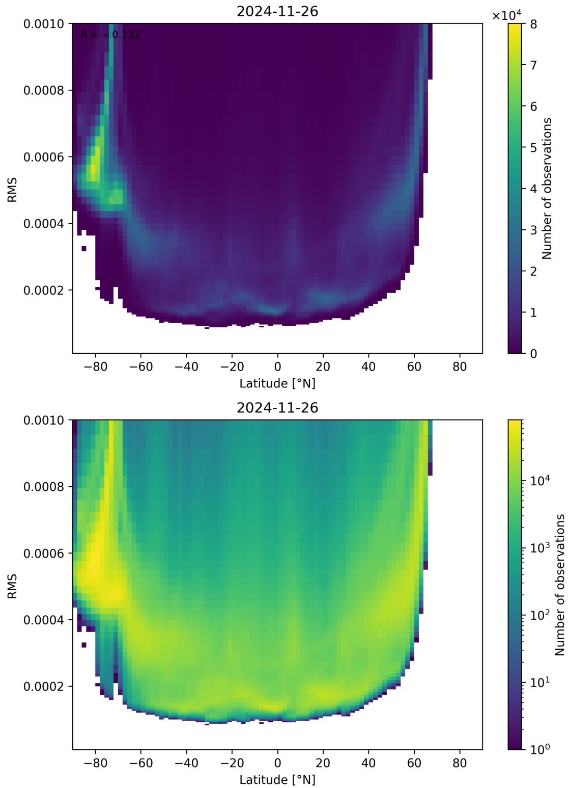
Figure 94: Scatter density plot of “Latitude” against “RMS” for 2024-11-25 to 2024-11-27.
