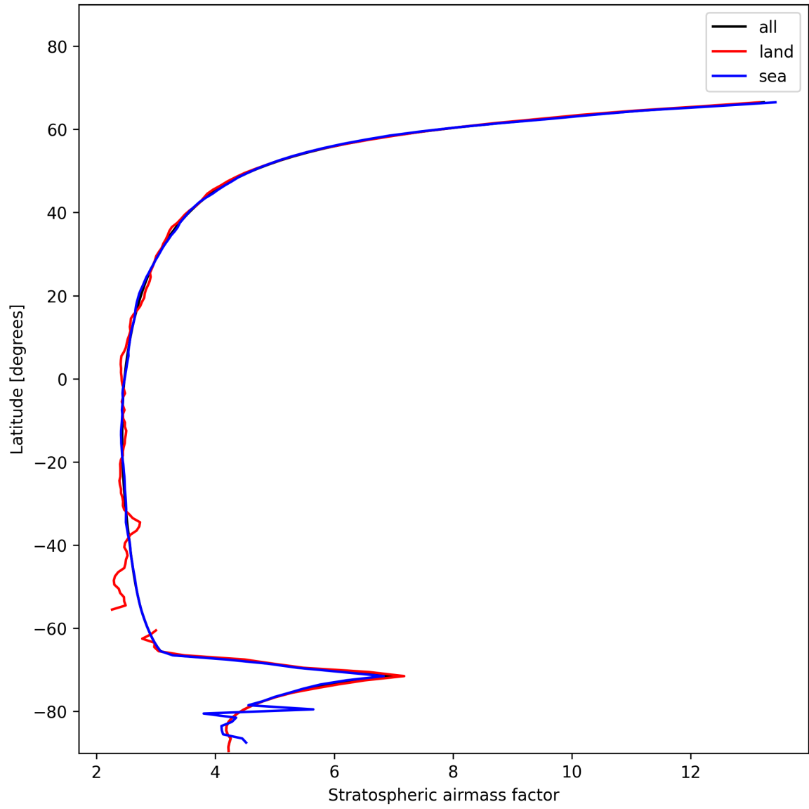
Figure 27: Zonal average of “Stratospheric air mass factor” for 2024-11-25 to 2024-11-27.
