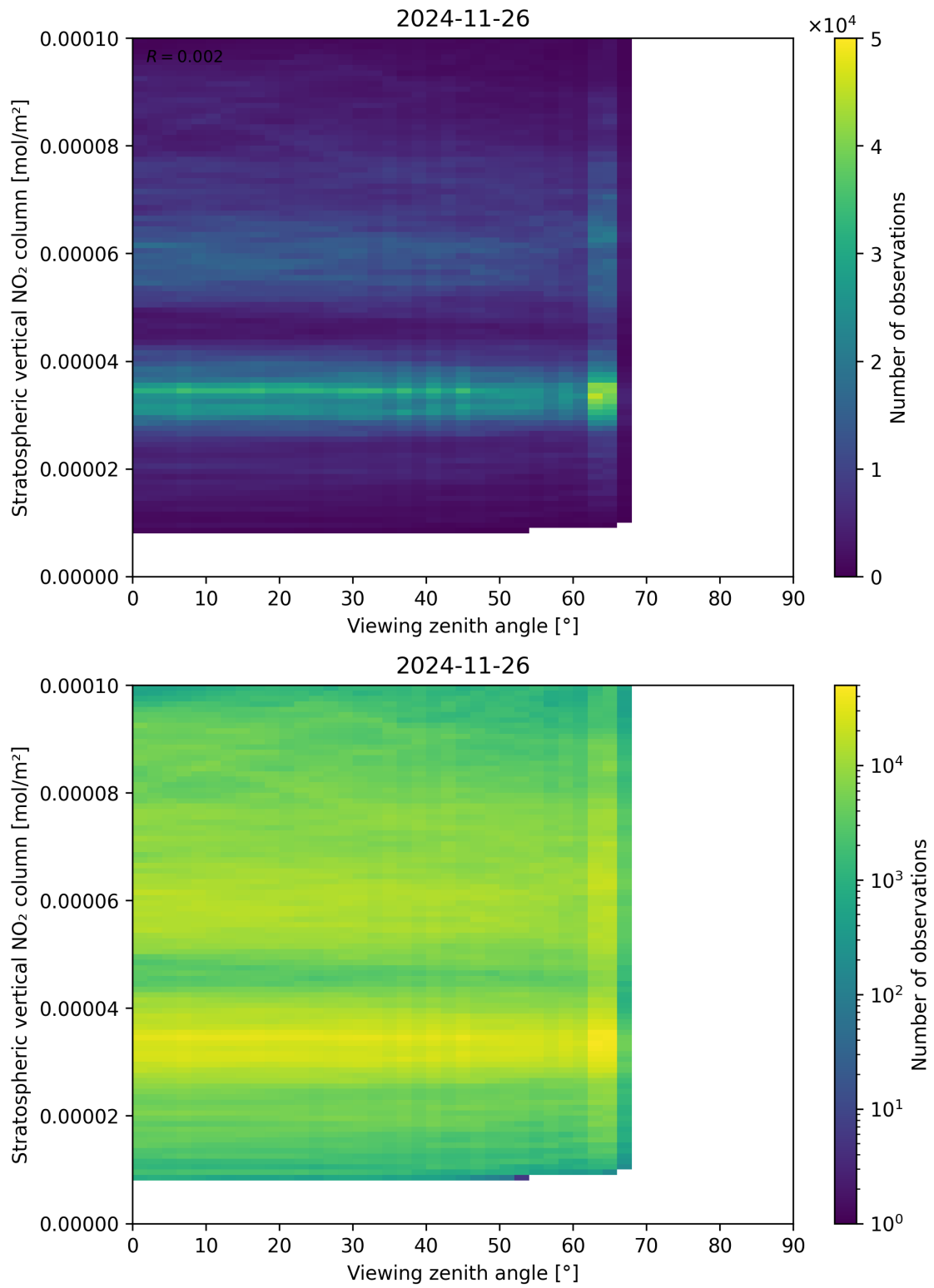
Figure 164: Scatter density plot of “Viewing zenith angle” against “Stratospheric vertical NO 2 column” for 2024-11-25 to 2024-11-27.
