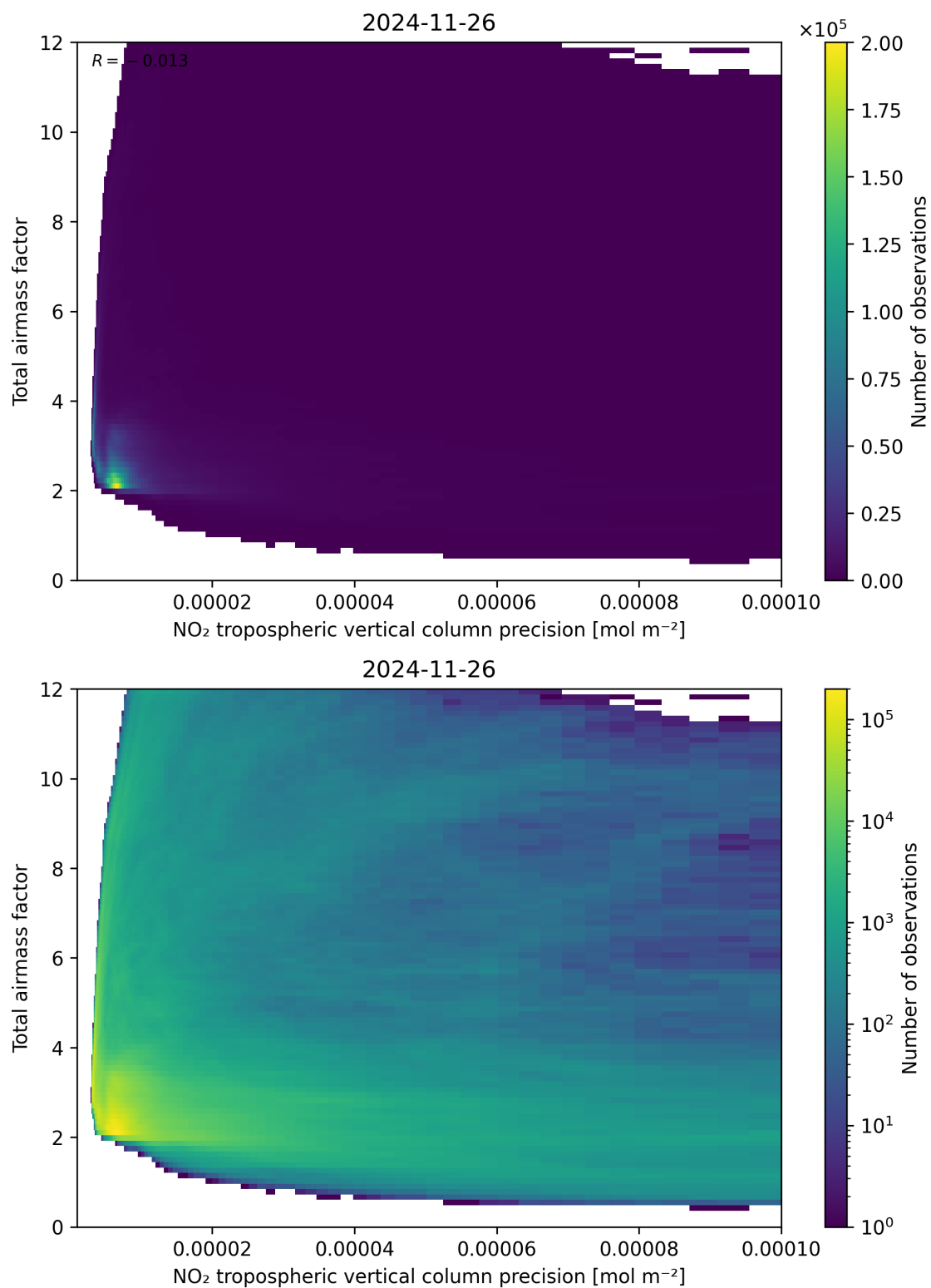
Figure 132: Scatter density plot of “NO 2 tropospheric vertical column precision” against “Total air mass factor” for 2024-11-25 to 2024-11-27.
