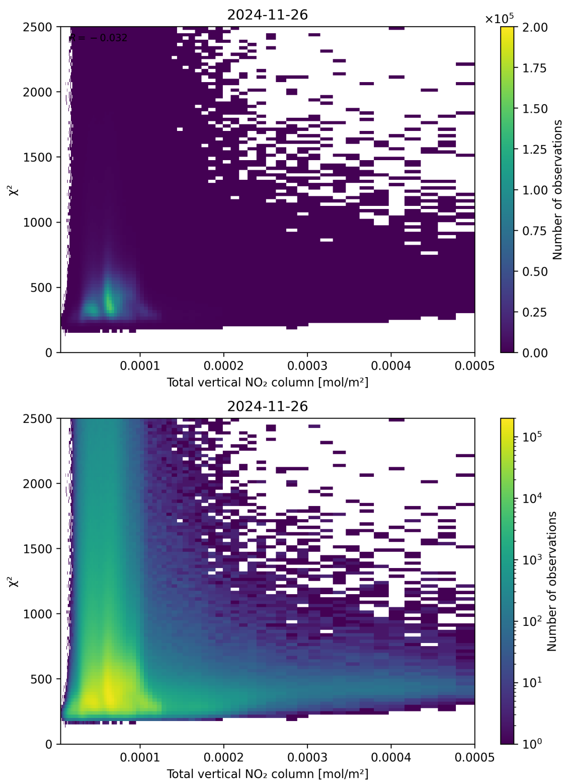
Figure 111: Scatter density plot of “Total vertical NO 2 column” against “ \chi^2 ” for 2024-11-25 to 2024-11-27.
