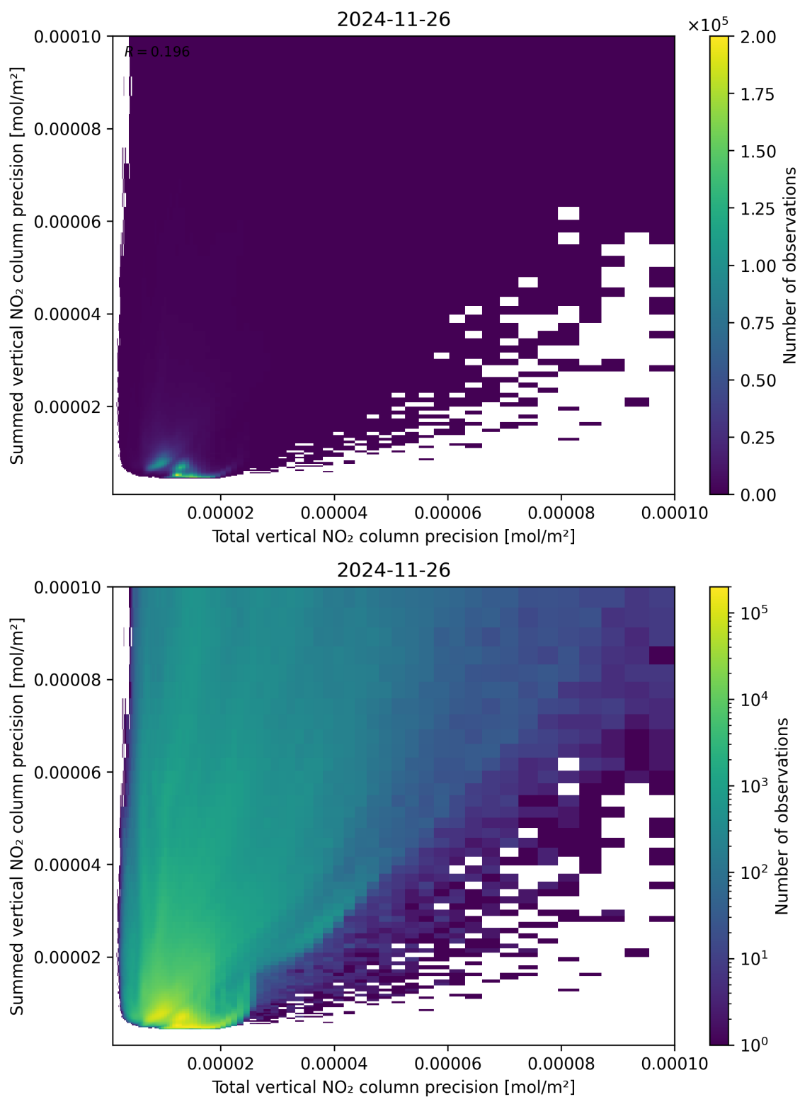
Figure 118: Scatter density plot of “Total vertical NO 2 column precision” against “Summed vertical NO 2 column precision” for 2024-11-25 to 2024-11-27.
