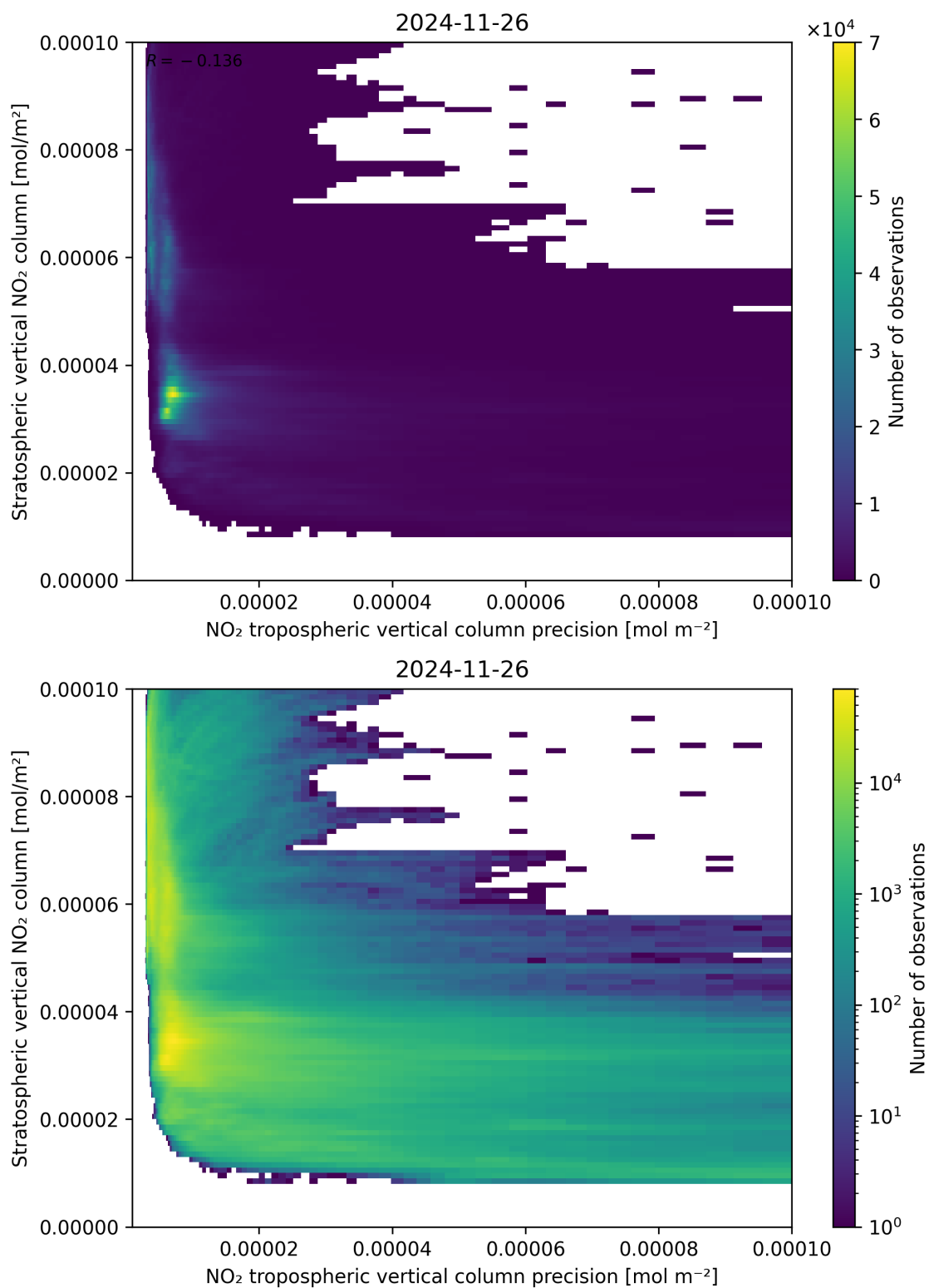
Figure 135: Scatter density plot of “NO 2 tropospheric vertical column precision” against “Stratospheric vertical NO 2 column” for 2024-11-25 to 2024-11-27.
