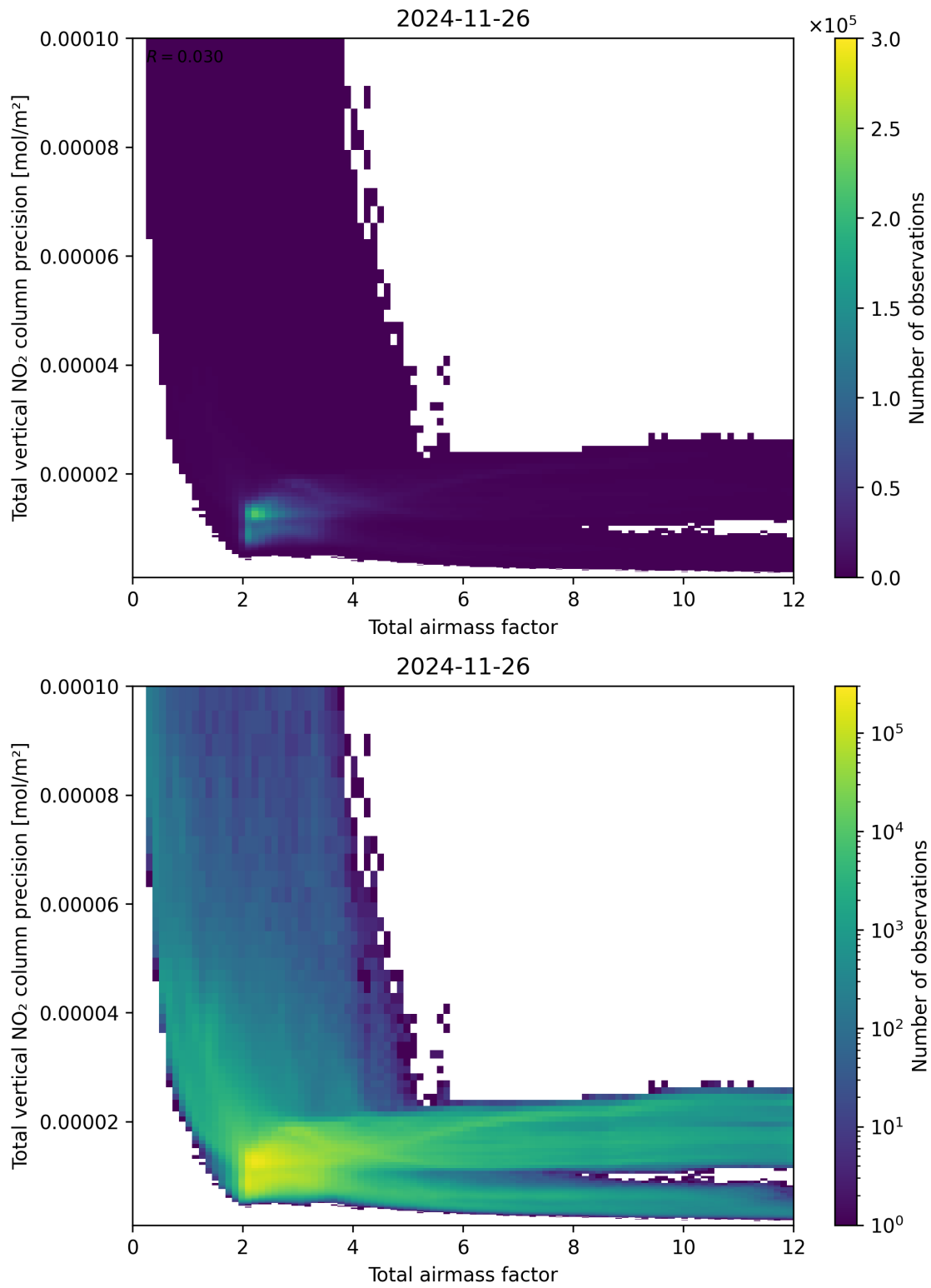
Figure 68: Scatter density plot of “Total airmass factor” against “Total vertical NO 2 column precision” for 2024-11-25 to 2024-11-27.
