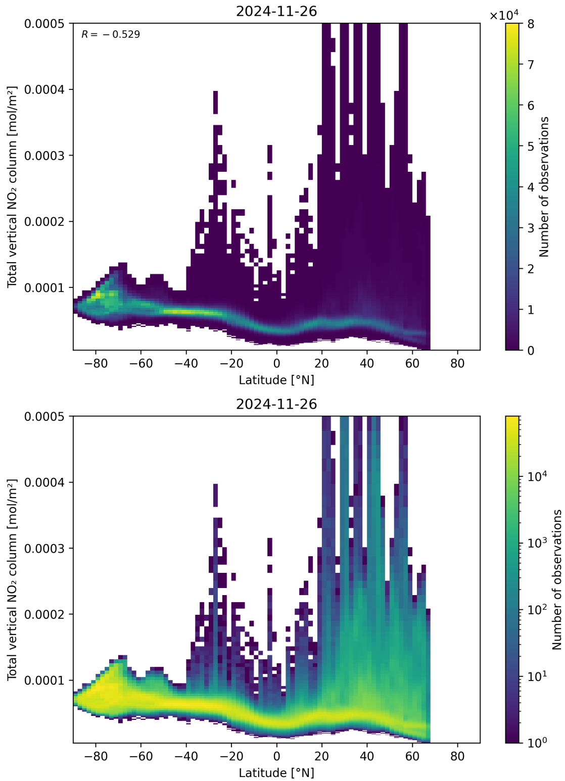
Figure 90: Scatter density plot of “Latitude” against “Total vertical NO 2 column” for 2024-11-25 to 2024-11-27.
