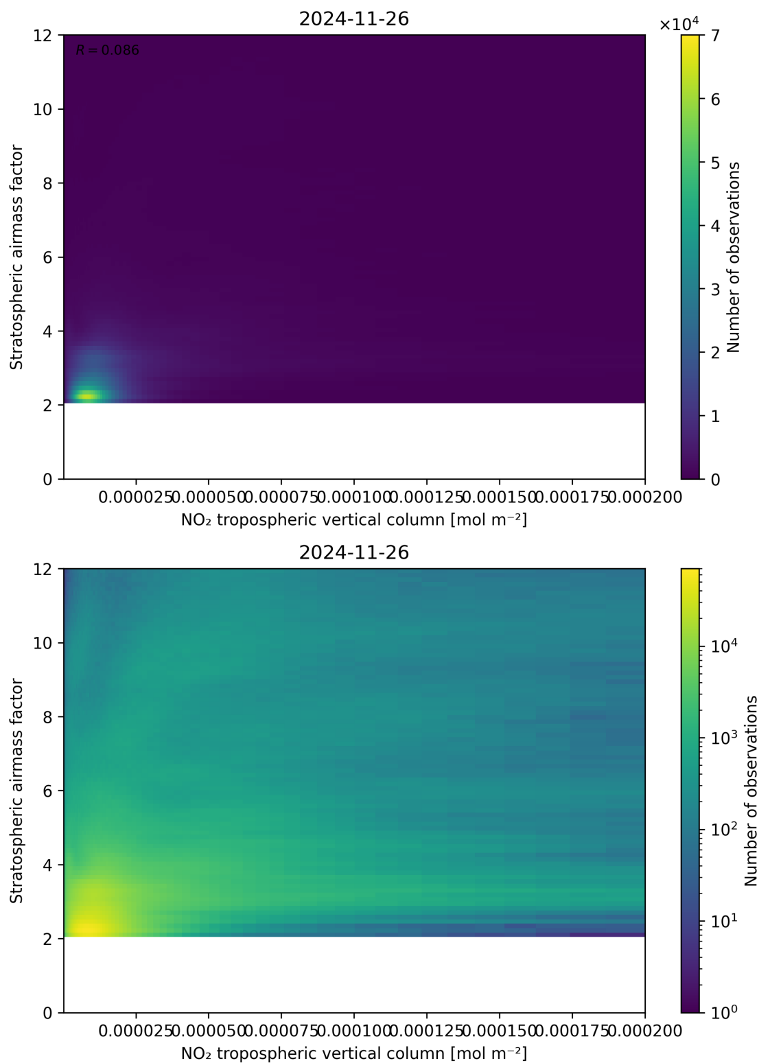
Figure 121: Scatter density plot of “NO 2 tropospheric vertical column” against “Stratospheric airmass factor” for 2024-11-25 to 2024-11-27.
