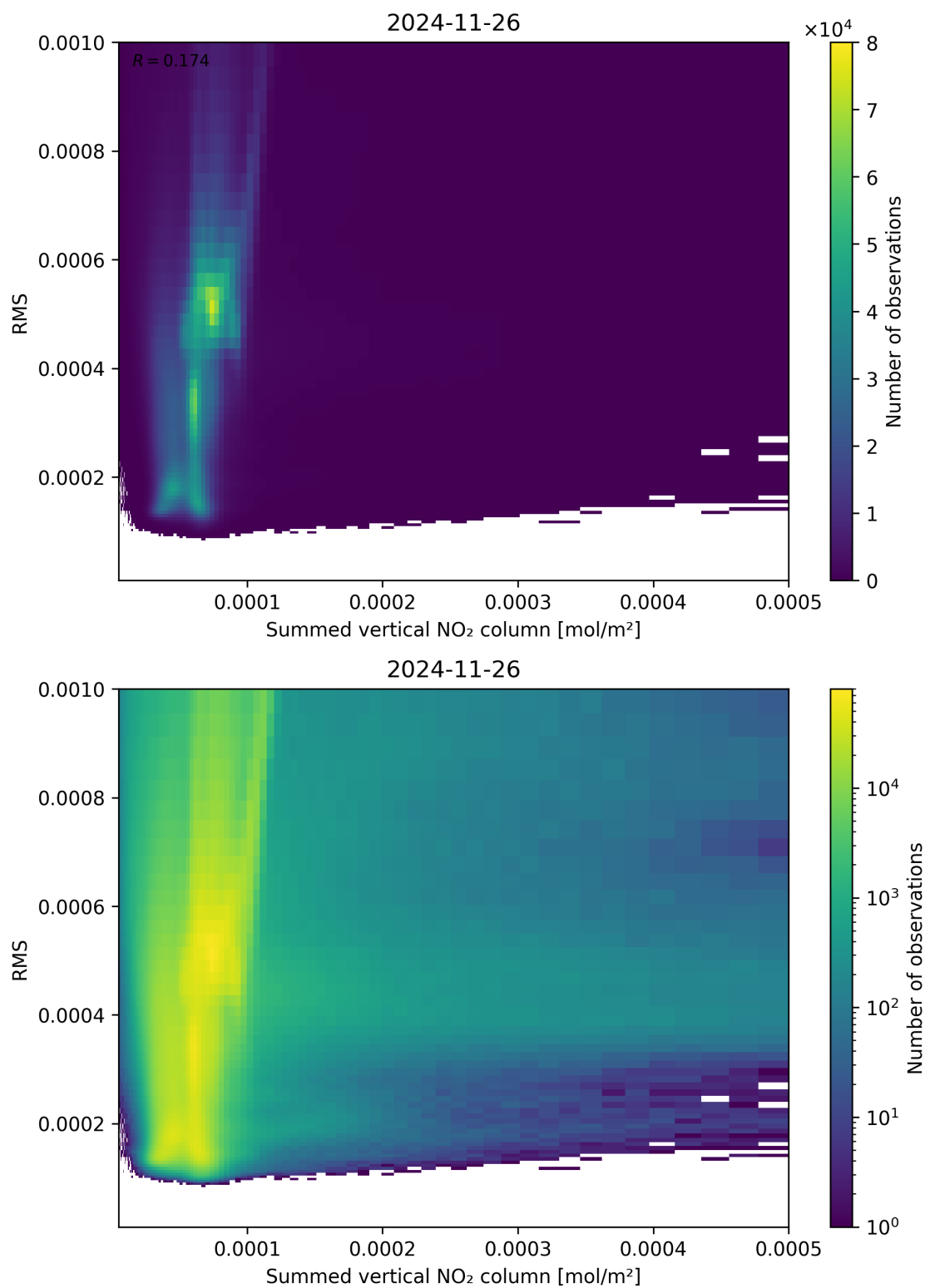
Figure 109: Scatter density plot of “Summed vertical NO 2 column” against “RMS” for 2024-11-25 to 2024-11-27.
