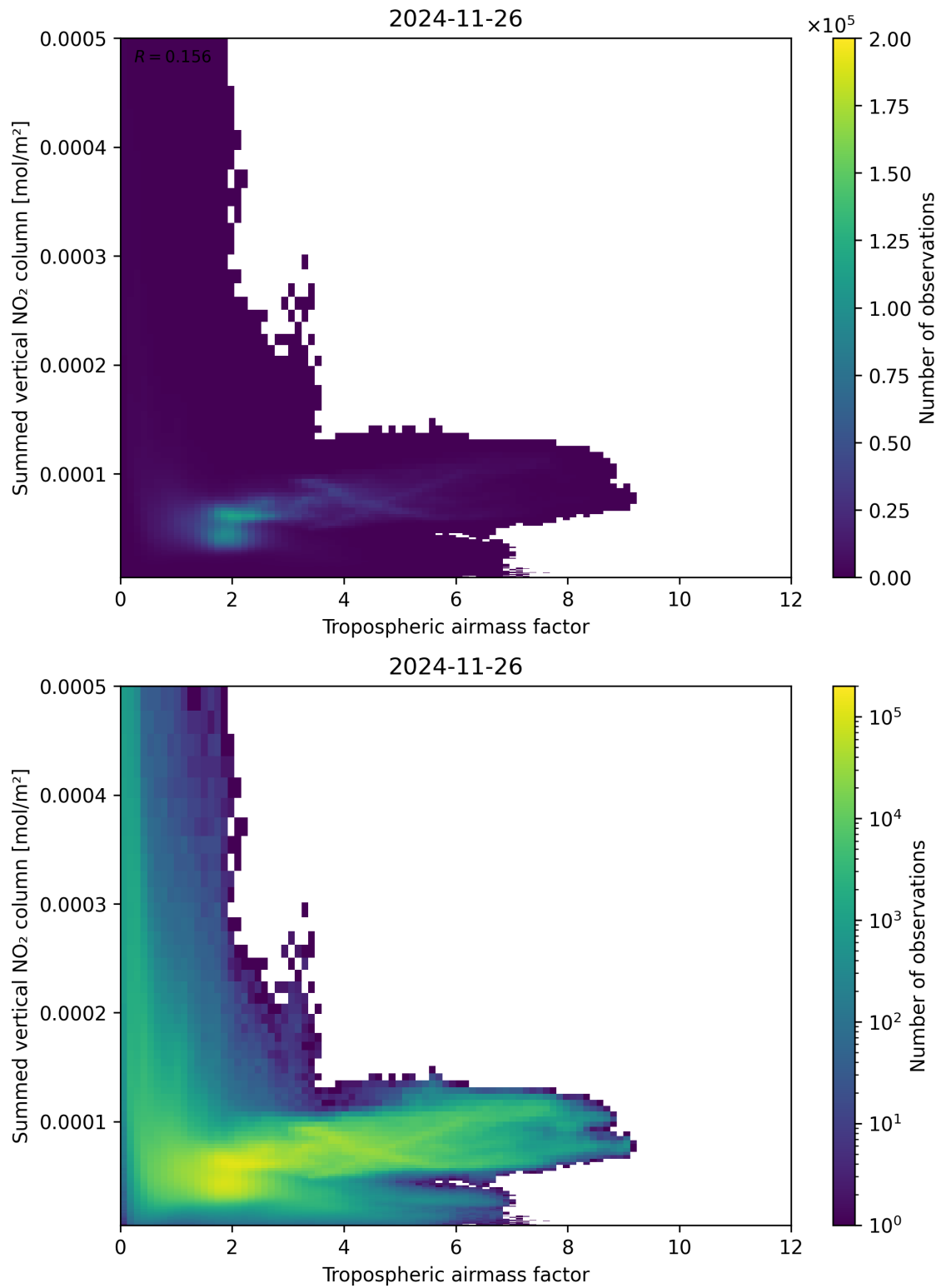
Figure 75: Scatter density plot of “Tropospheric airmass factor” against “Summed vertical NO 2 column” for 2024-11-25 to 2024-11-27.
