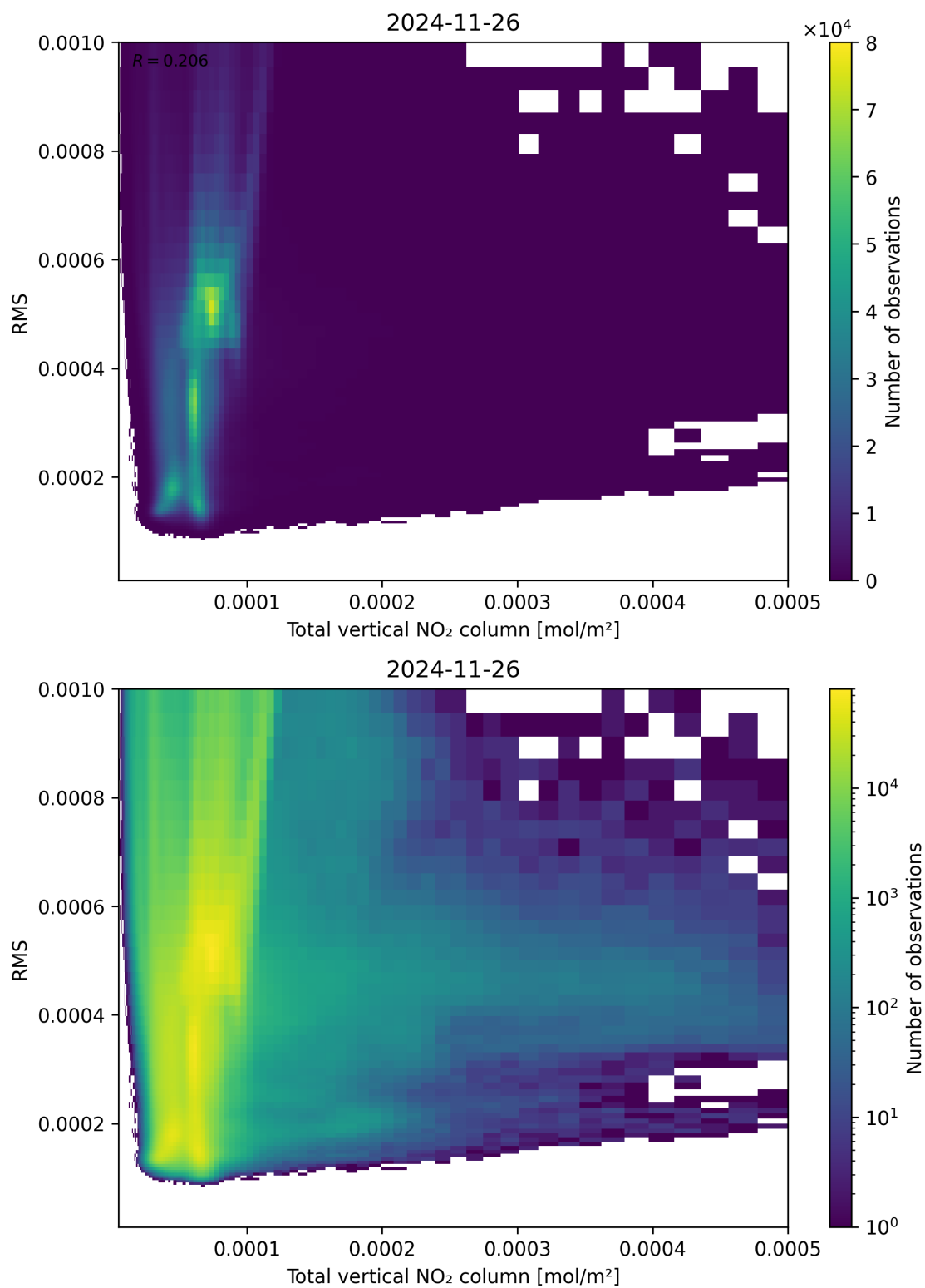
Figure 120: Scatter density plot of “Total vertical NO 2 column” against “RMS” for 2024-11-25 to 2024-11-27.
