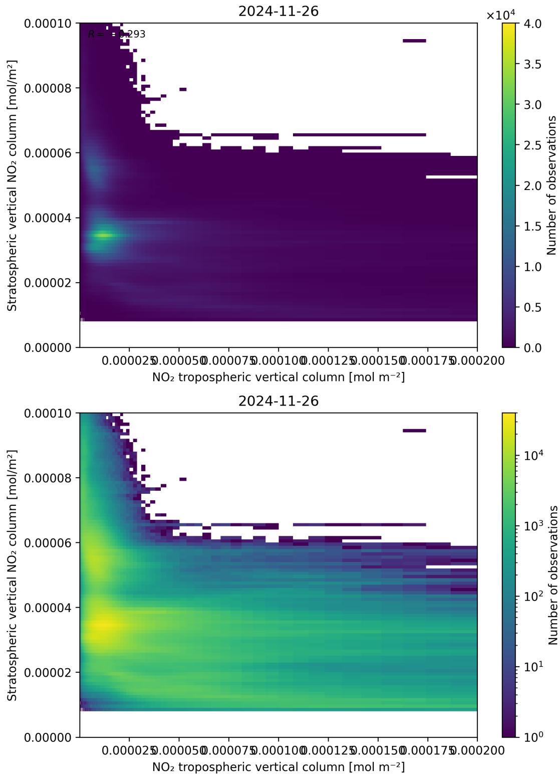
Figure 125: Scatter density plot of “NO 2 tropospheric vertical column” against “Stratospheric vertical NO 2 column” for 2024-11-25 to 2024-11-27.
