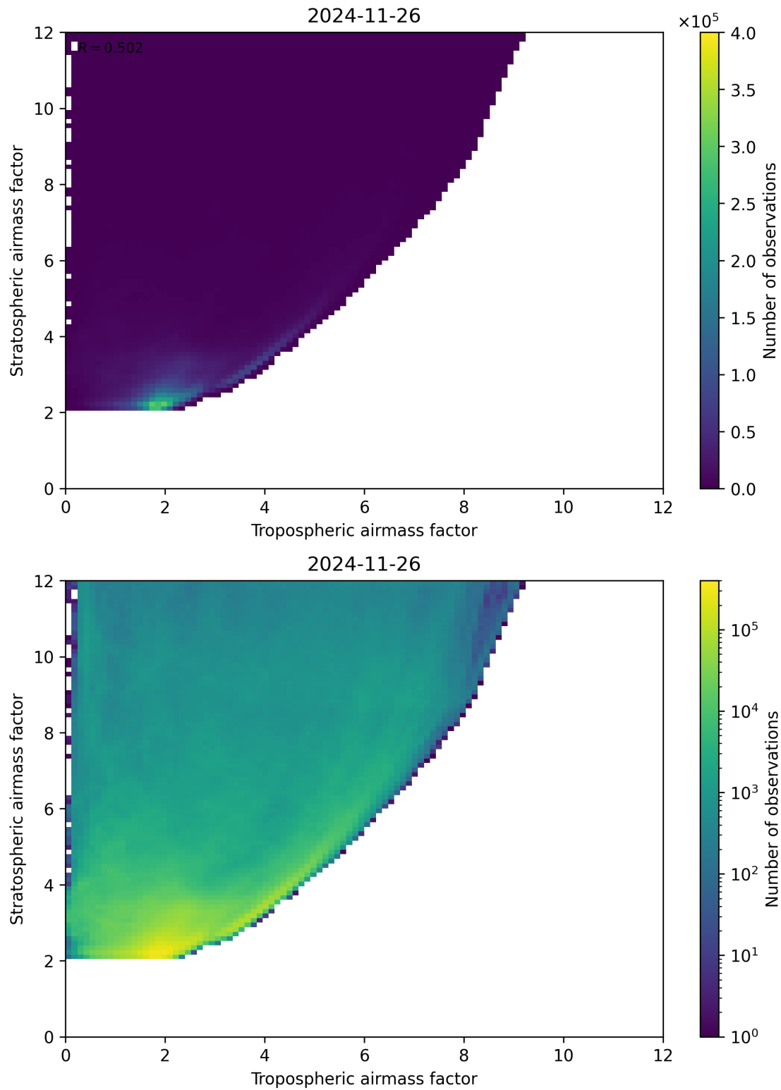
Figure 71: Scatter density plot of “Tropospheric airmass factor” against “Stratospheric airmass factor” for 2024-11-25 to 2024-11-27.
