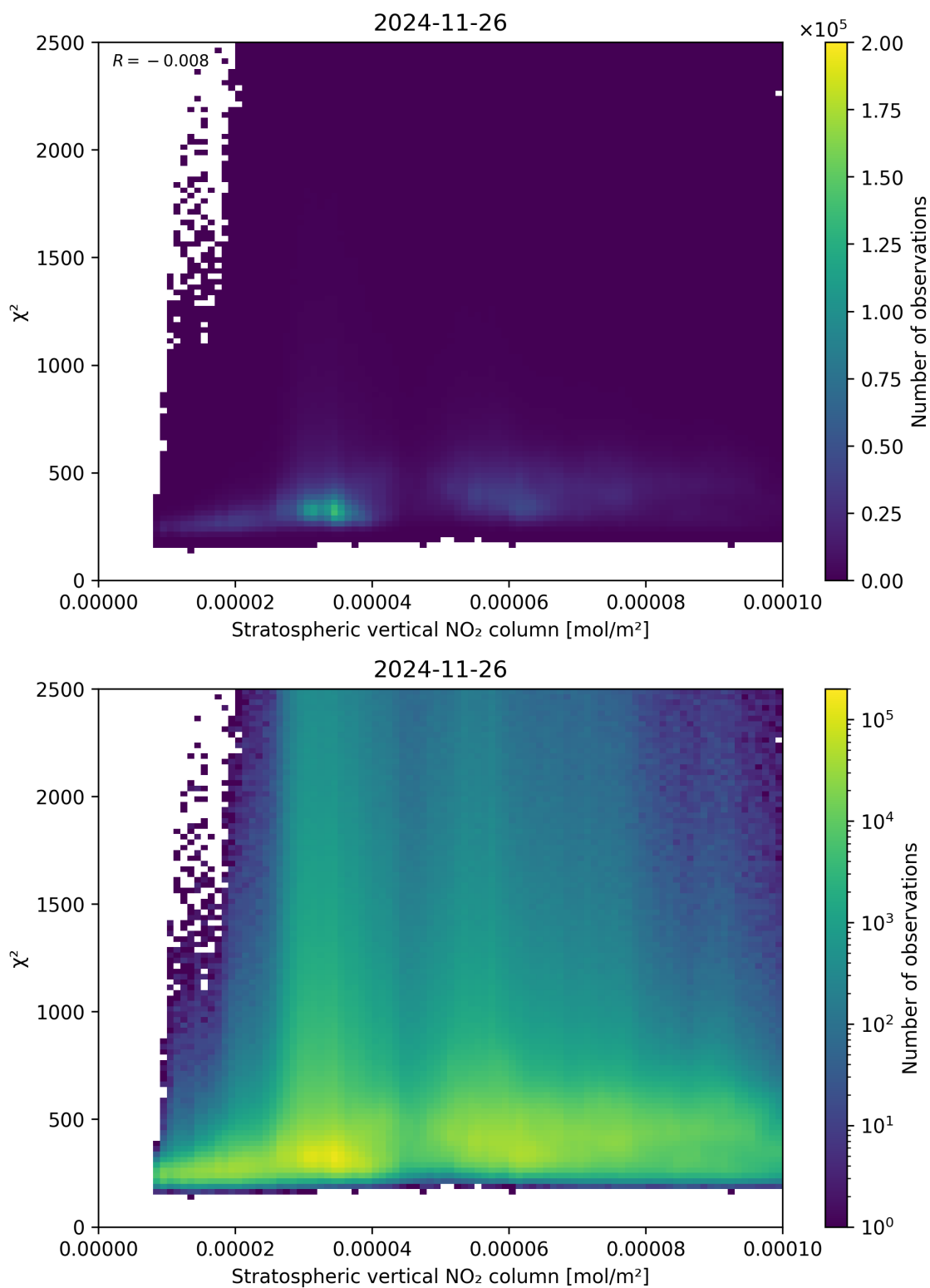
Figure 97: Scatter density plot of “Stratospheric vertical NO 2 column” against “ \chi^2 ” for 2024-11-25 to 2024-11-27.
