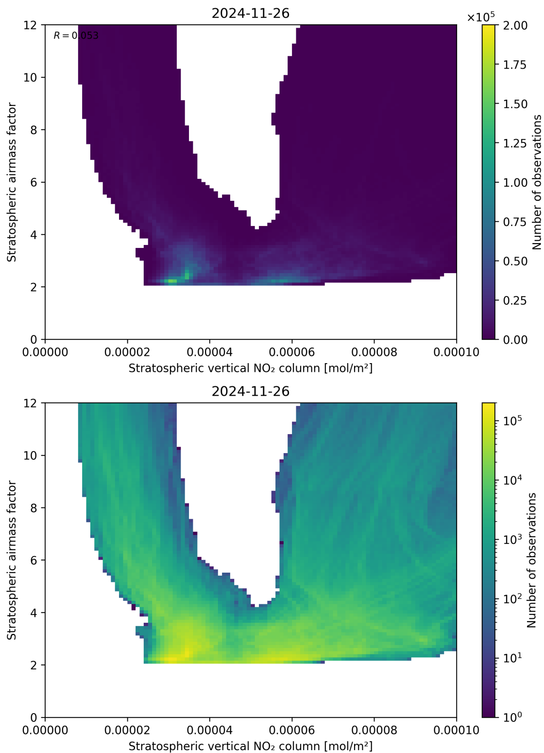
Figure 96: Scatter density plot of “Stratospheric vertical NO 2 column” against “Stratospheric airmass factor” for 2024-11-25 to 2024-11-27.
