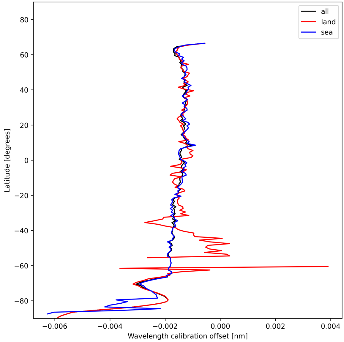
Figure 18: Zonal average of “Wavelength calibration offset” for 2024-11-25 to 2024-11-27.
