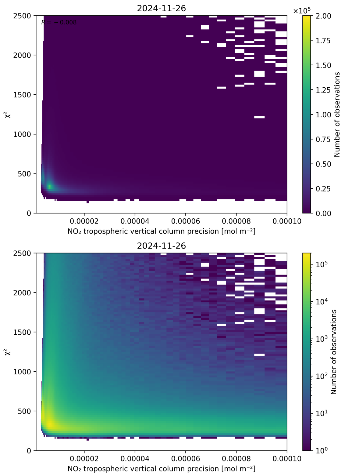
Figure 134: Scatter density plot of “NO 2 tropospheric vertical column precision” against “ \chi^2 ” for 2024-11-25 to 2024-11-27.
