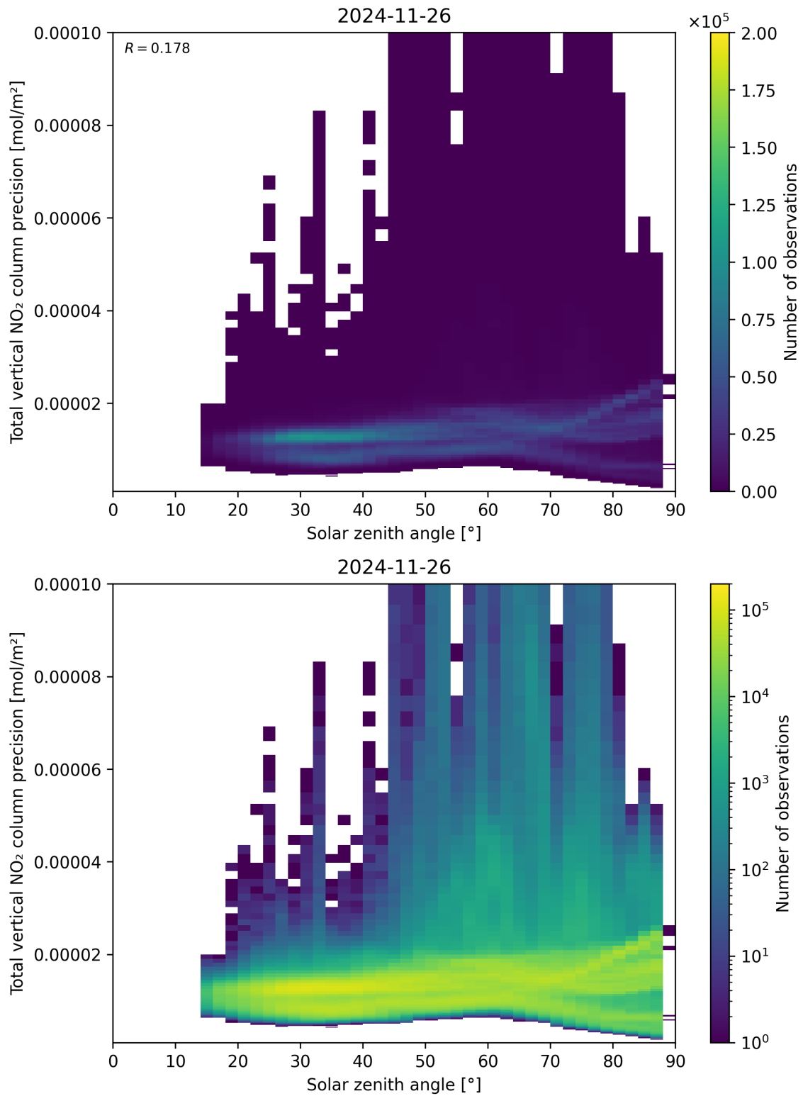
Figure 154: Scatter density plot of “Solar zenith angle” against “Total vertical NO 2 column precision” for 2024-11-25 to 2024-11-27.
