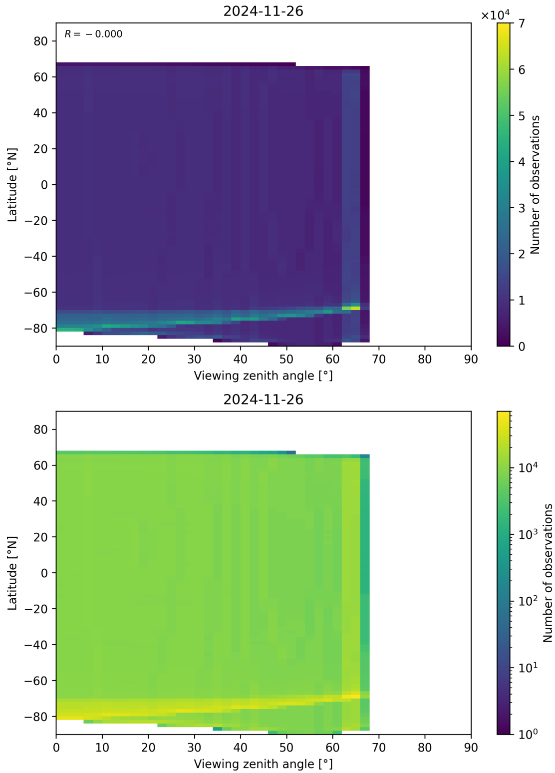
Figure 163: Scatter density plot of “Viewing zenith angle” against “Latitude” for 2024-11-25 to 2024-11-27.
