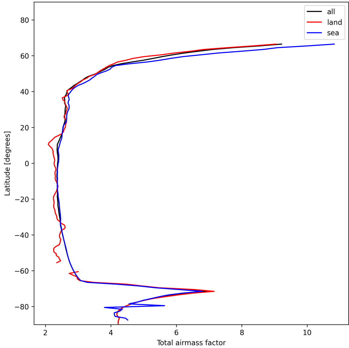
Figure 15: Zonal average of “Total airmass factor” for 2024-11-25 to 2024-11-27.
