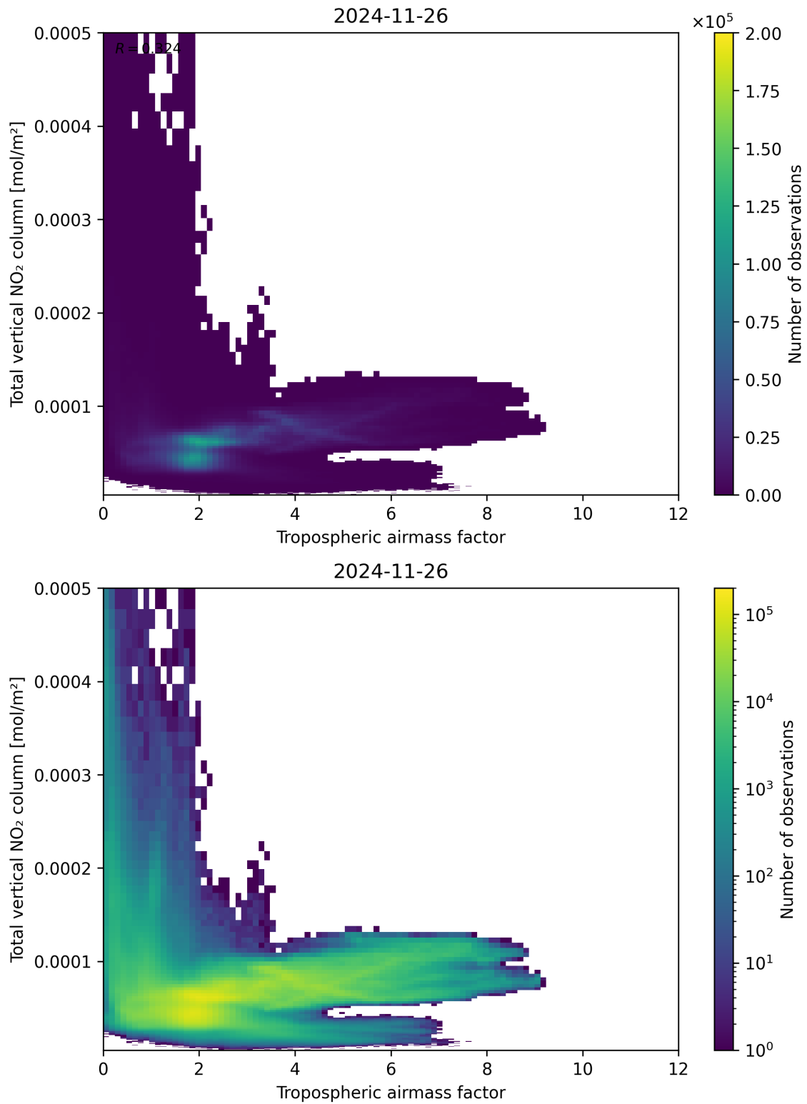
Figure 77: Scatter density plot of “Tropospheric airmass factor” against “Total vertical NO 2 column” for 2024-11-25 to 2024-11-27.
