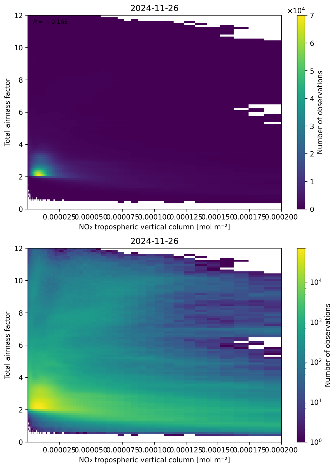
Figure 122: Scatter density plot of “NO 2 tropospheric vertical column” against “Total air mass factor” for 2024-11-25 to 2024-11-27.
