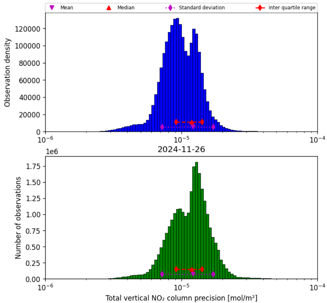
Figure 39: Histogram of “Total vertical NO 2 column precision” for 2024-11-25 to 2024-11-27
