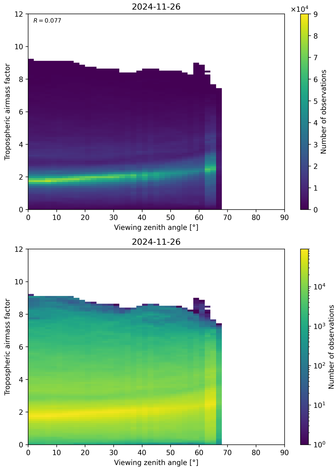
Figure 161: Scatter density plot of “Viewing zenith angle” against “Tropospheric airmass factor” for 2024-11-25 to 2024-11-27.
