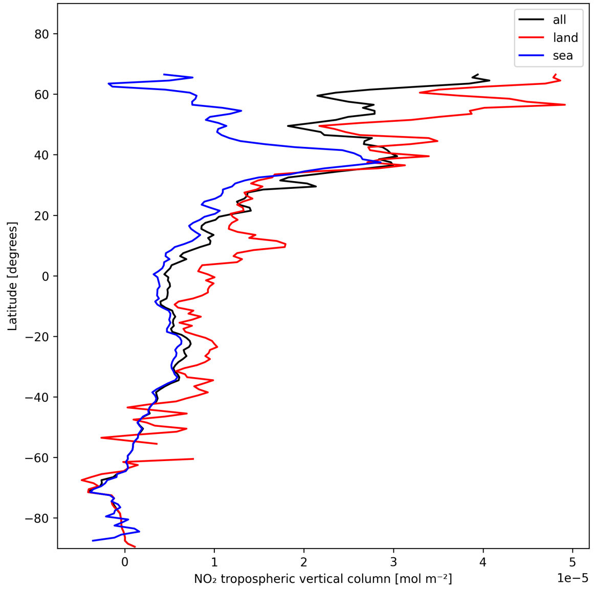
Figure 12: Zonal average of “NO 2 tropospheric vertical column” for 2024-11-25 to 2024-11-27.
