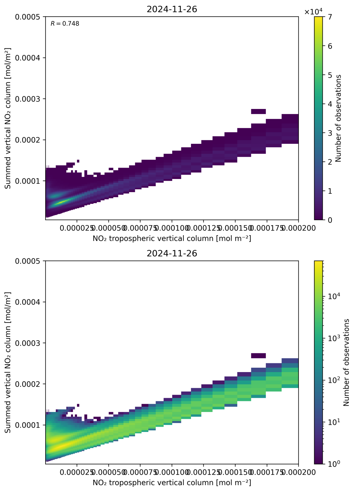
Figure 126: Scatter density plot of “NO 2 tropospheric vertical column” against “Summed vertical NO 2 column” for 2024-11-25 to 2024-11-27.
