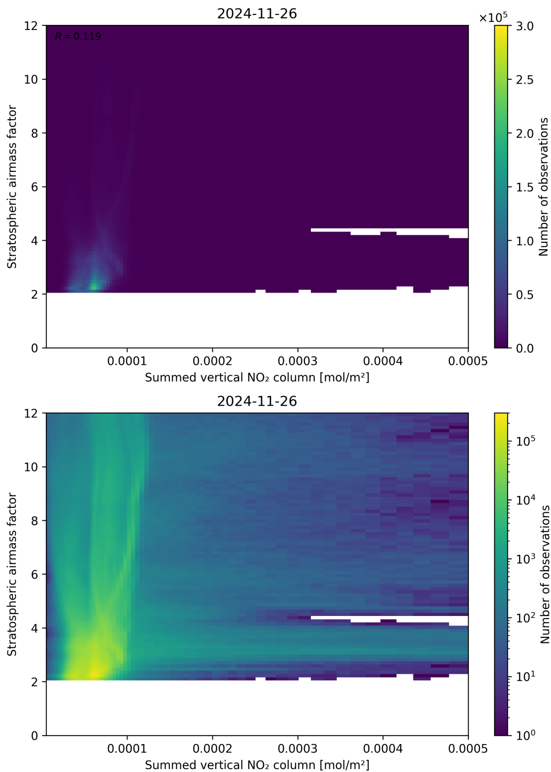
Figure 103: Scatter density plot of “Summed vertical NO 2 column” against “Stratospheric airmass factor” for 2024-11-25 to 2024-11-27.
