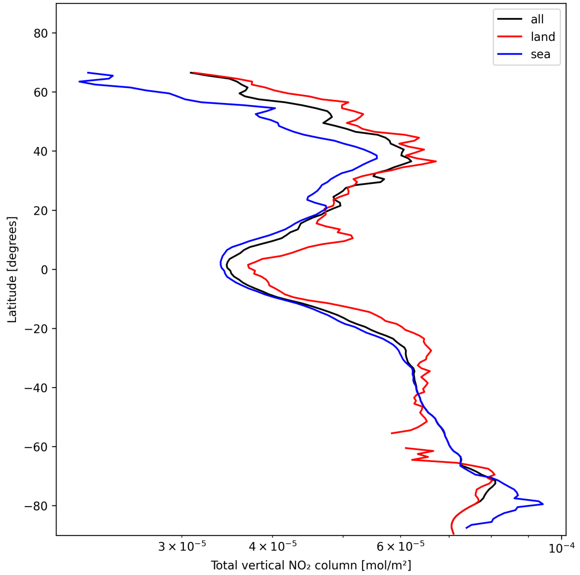
Figure 21: Zonal average of “Total vertical NO 2 column” for 2024-11-25 to 2024-11-27.
