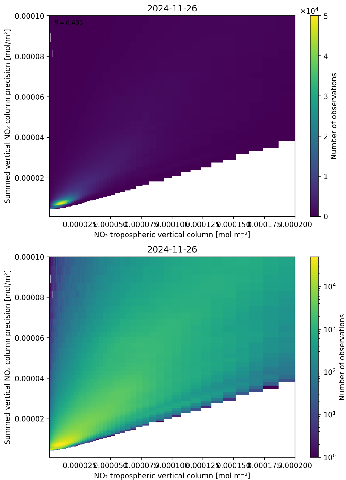
Figure 127: Scatter density plot of “NO 2 tropospheric vertical column” against “Summed vertical NO 2 column precision” for 2024-11-25 to 2024-11-27.
