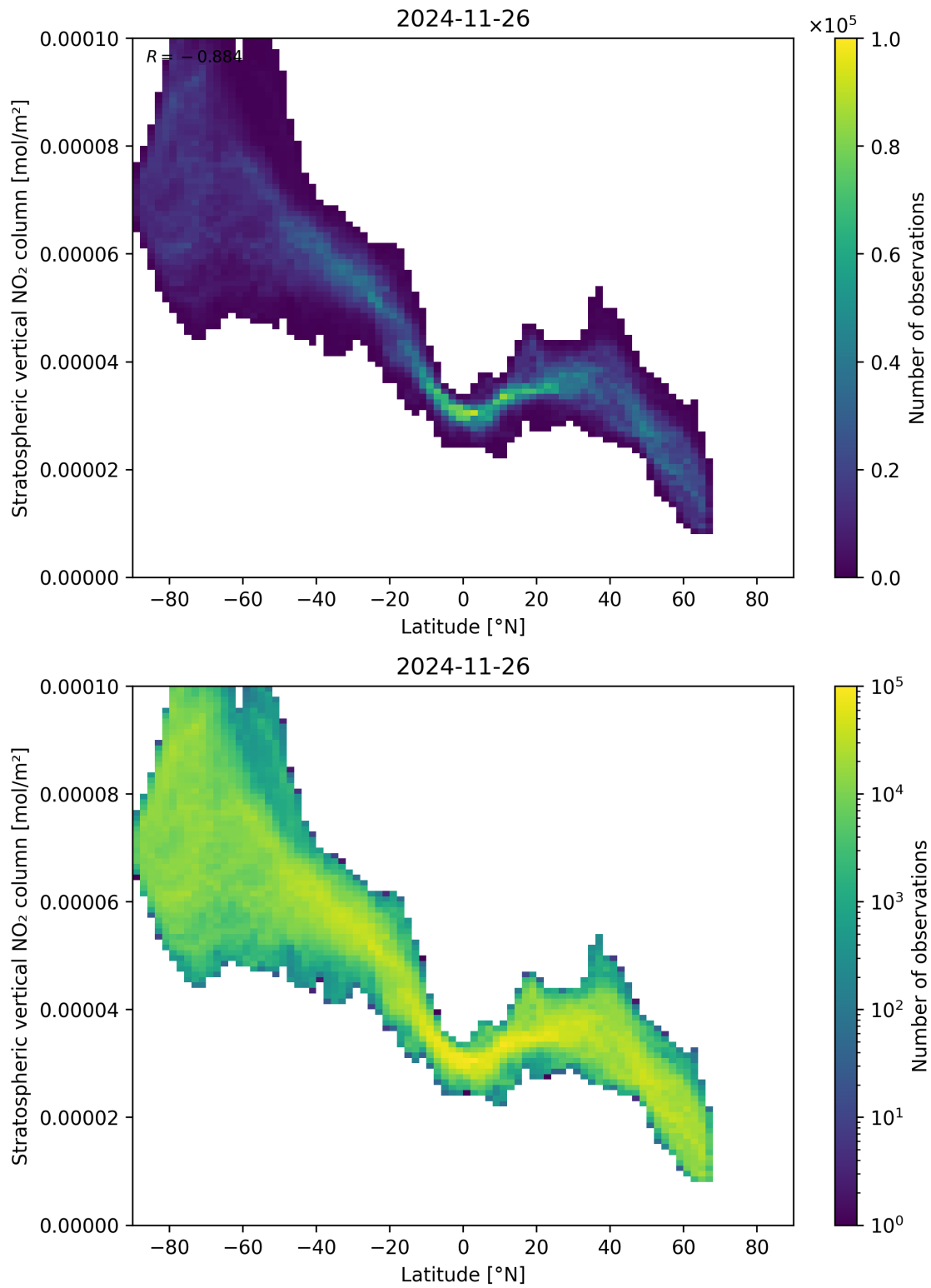
Figure 87: Scatter density plot of “Latitude” against “Stratospheric vertical NO 2 column” for 2024-11-25 to 2024-11-27.
