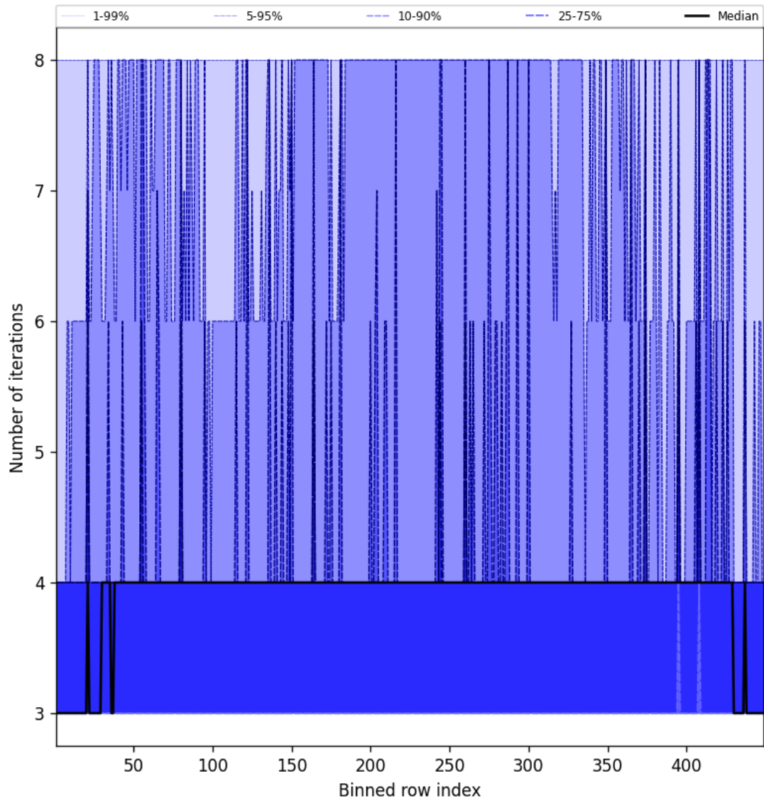
Figure 51: Along track statistics of “Number of iterations” for 2024-11-25 to 2024-11-27
