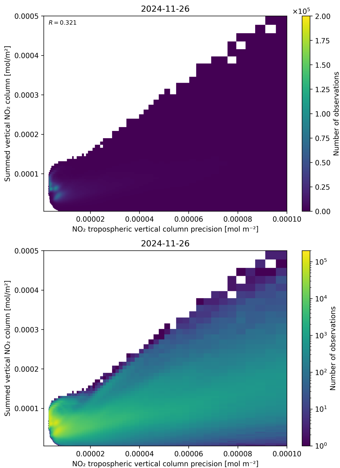
Figure 136: Scatter density plot of “NO 2 tropospheric vertical column precision” against “Summed vertical NO 2 column” for 2024-11-25 to 2024-11-27.
