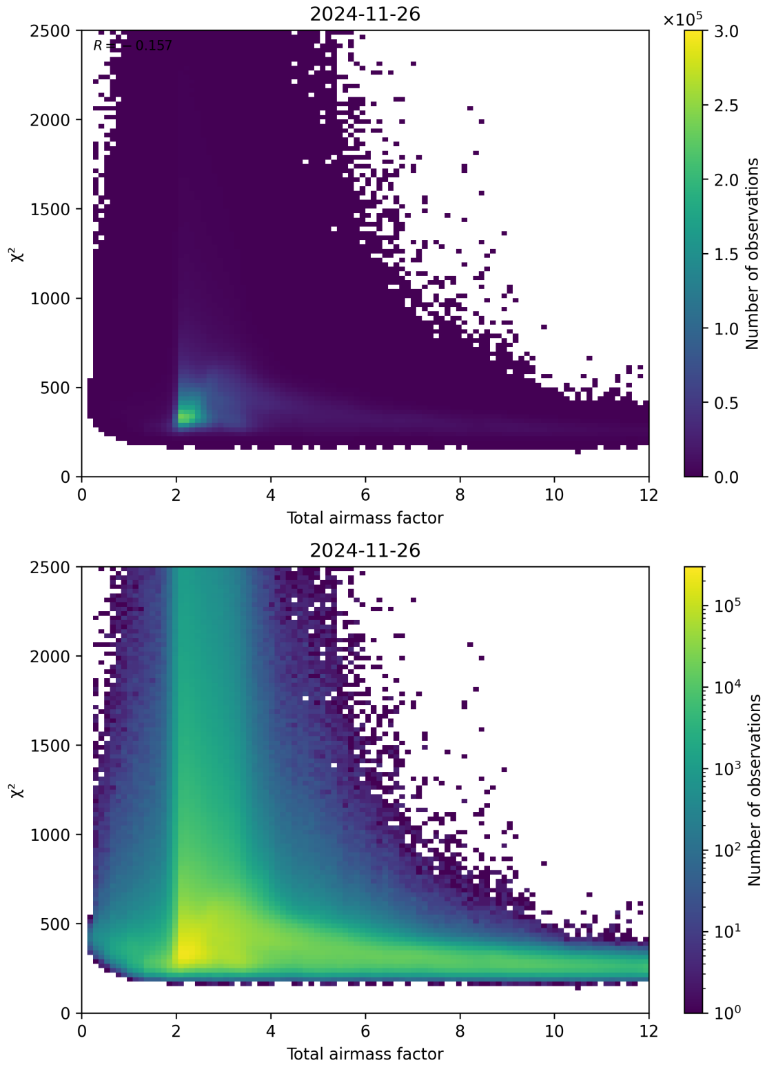
Figure 63: Scatter density plot of “Total airmass factor” against “ \chi^2 ” for 2024-11-25 to 2024-11-27.
