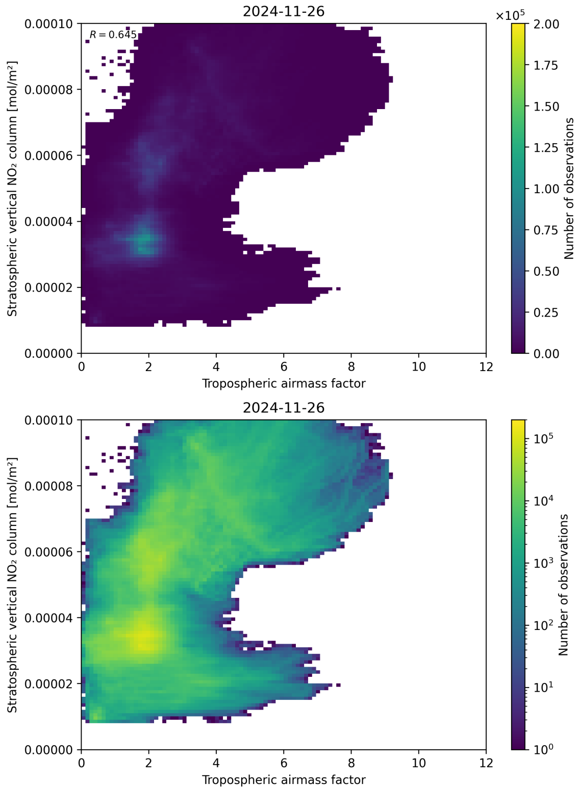
Figure 74: Scatter density plot of “Tropospheric air mass factor” against “Stratospheric vertical NO 2 column” for 2024-11-25 to 2024-11-27.
