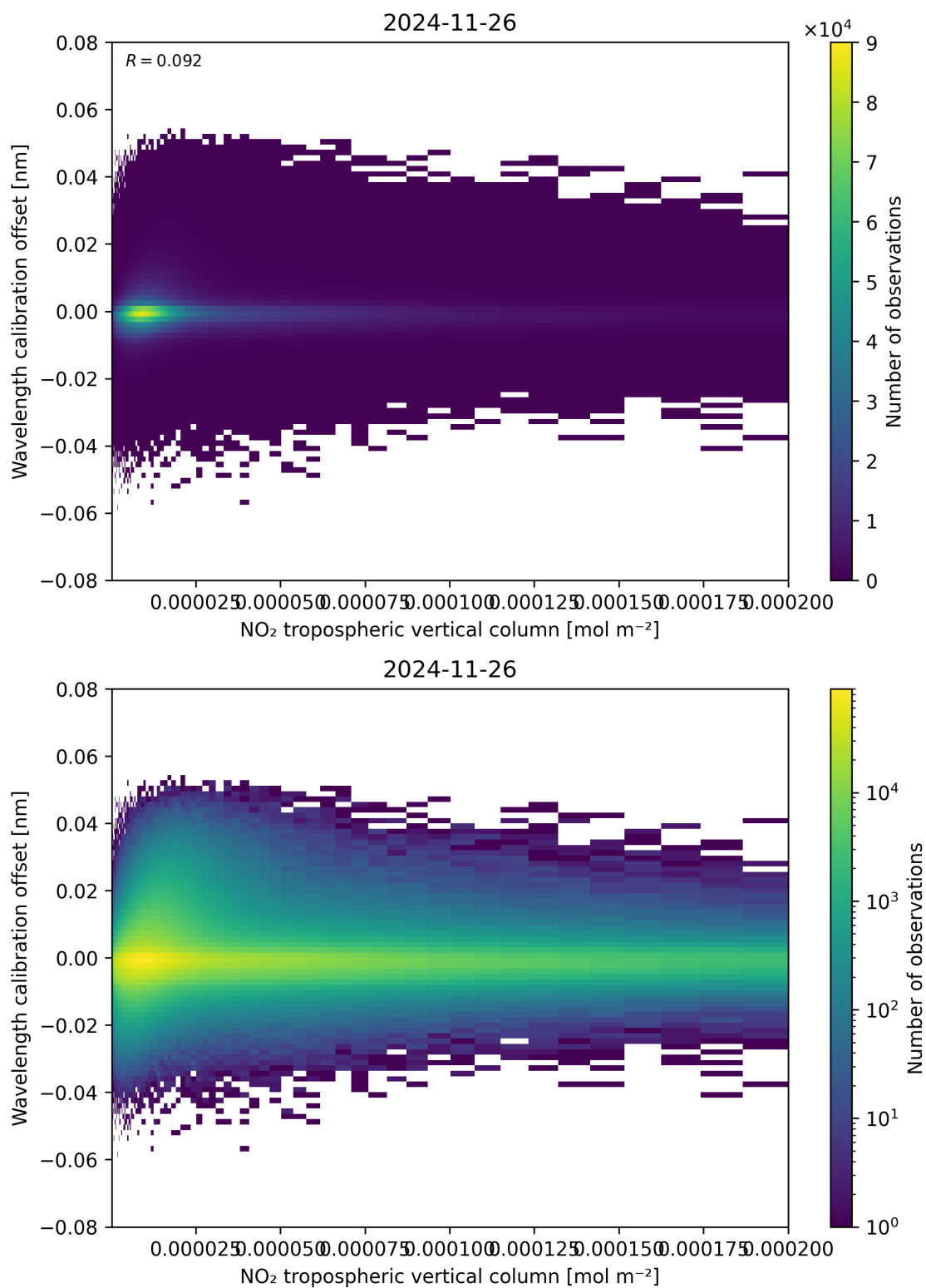
Figure 143: Scatter density plot of “NO 2 tropospheric vertical column” against “Wavelength calibration offset” for 2024-11-25 to 2024-11-27.
