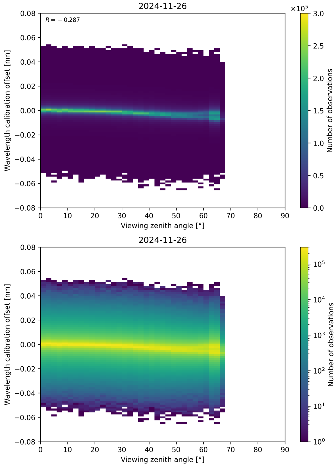
Figure 173: Scatter density plot of “Viewing zenith angle” against “Wavelength calibration offset” for 2024-11-25 to 2024-11-27.
