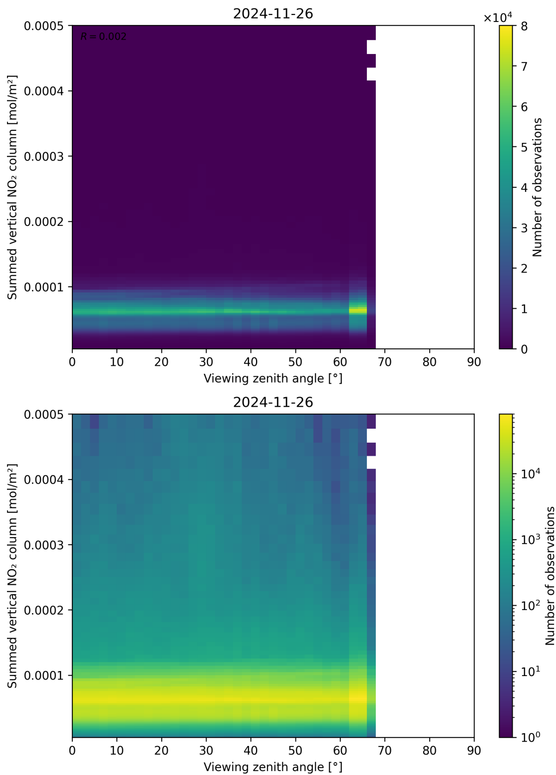
Figure 165: Scatter density plot of “Viewing zenith angle” against “Summed vertical NO 2 column” for 2024-11-25 to 2024-11-27.
