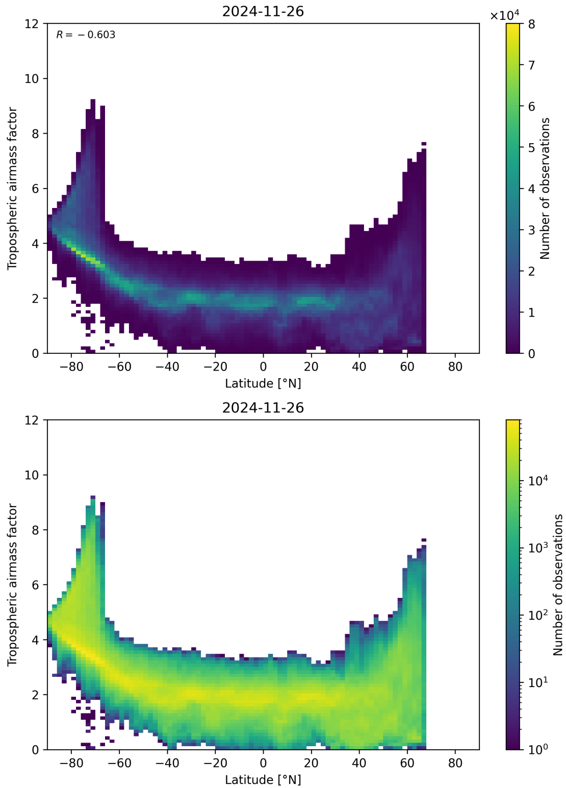
Figure 85: Scatter density plot of “Latitude” against “Tropospheric air mass factor” for 2024-11-25 to 2024-11-27.
