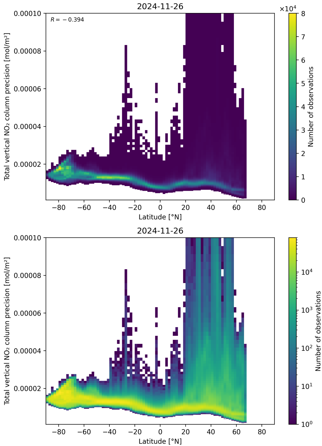
Figure 91: Scatter density plot of “Latitude” against “Total vertical NO 2 column precision” for 2024-11-25 to 2024-11-27.
