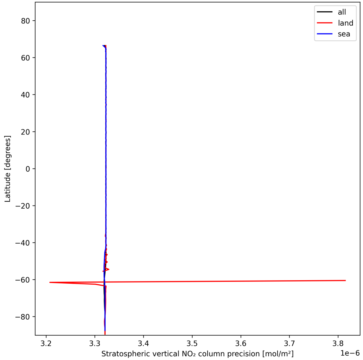
Figure 20: Zonal average of “Stratospheric vertical NO 2 column precision” for 2024-11-25 to 2024-11-27.
