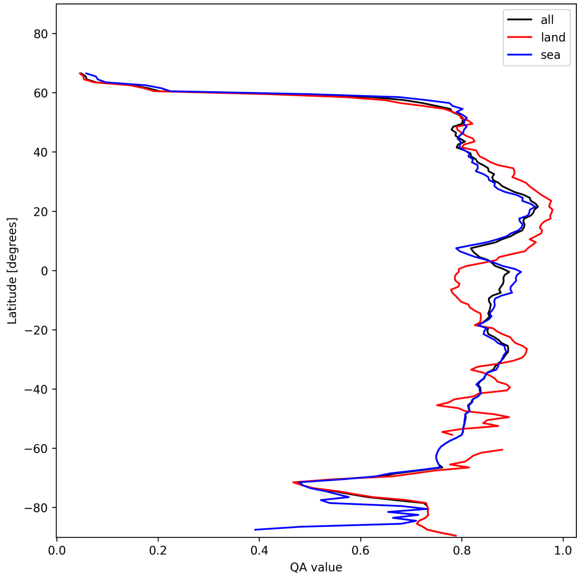
Figure 11: Zonal average of “QA value” for 2024-11-25 to 2024-11-27.
