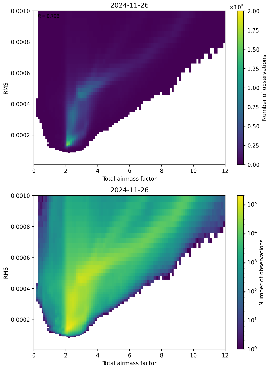
Figure 69: Scatter density plot of “Total airmass factor” against “RMS” for 2024-11-25 to 2024-11-27.
