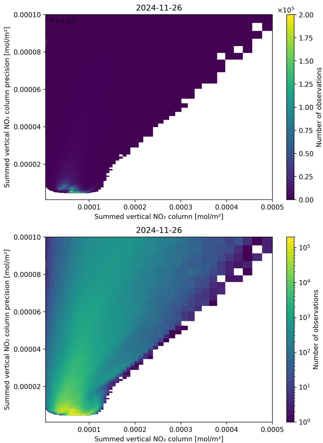
Figure 105: Scatter density plot of “Summed vertical NO 2 column” against “Summed vertical NO 2 column precision” for 2024-11-25 to 2024-11-27.
