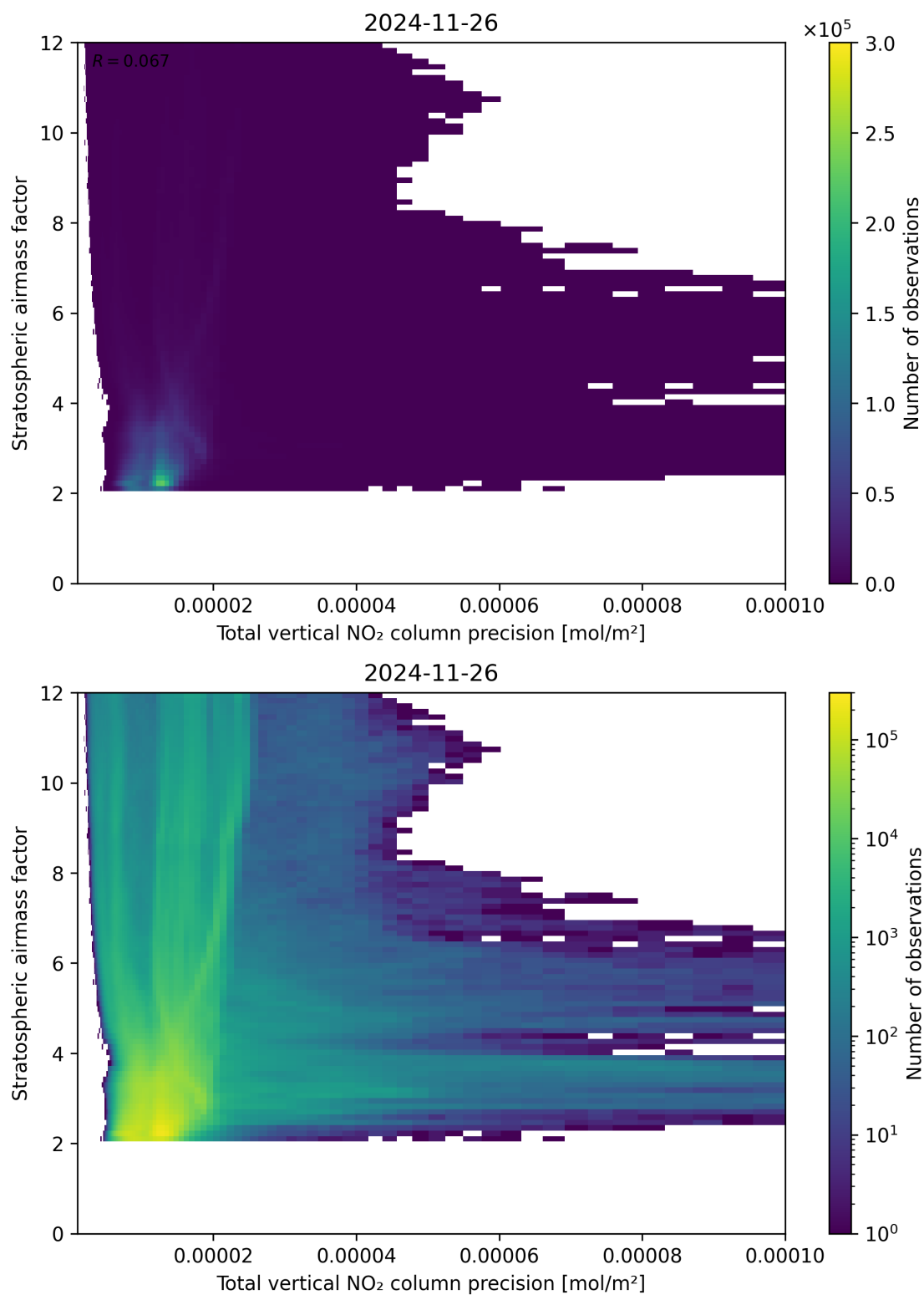
Figure 115: Scatter density plot of “Total vertical NO 2 column precision” against “Stratospheric air mass factor” for 2024-11-25 to 2024-11-27.
