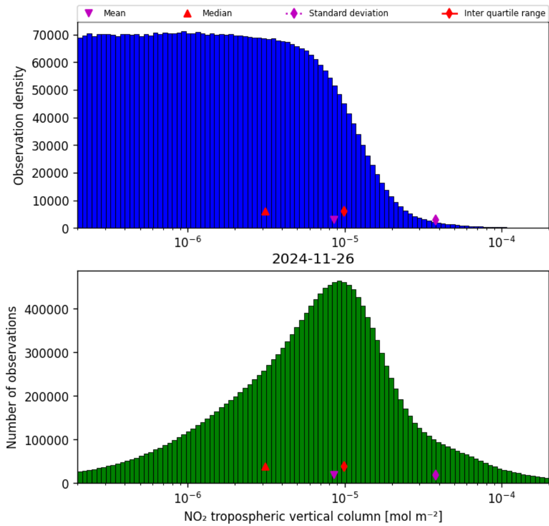
Figure 29: Histogram of “NO 2 tropospheric vertical column” for 2024-11-25 to 2024-11-27
