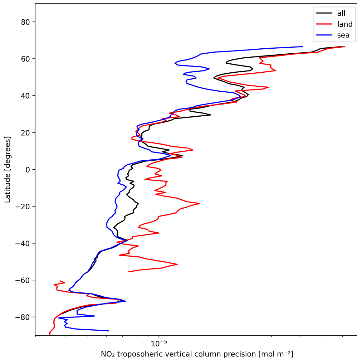
Figure 13: Zonal average of “NO 2 tropospheric vertical column precision” for 2024-11-25 to 2024-11-27.
