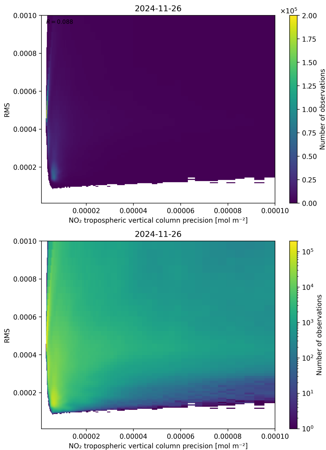
Figure 140: Scatter density plot of “NO 2 tropospheric vertical column precision” against “RMS” for 2024-11-25 to 2024-11-27.
