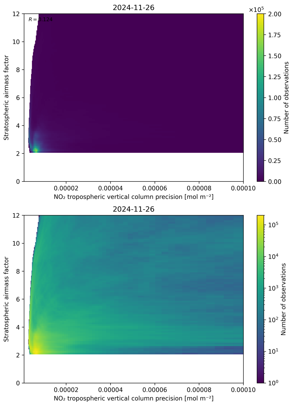
Figure 131: Scatter density plot of “NO 2 tropospheric vertical column precision” against “Stratospheric airmass factor” for 2024-11-25 to 2024-11-27.
