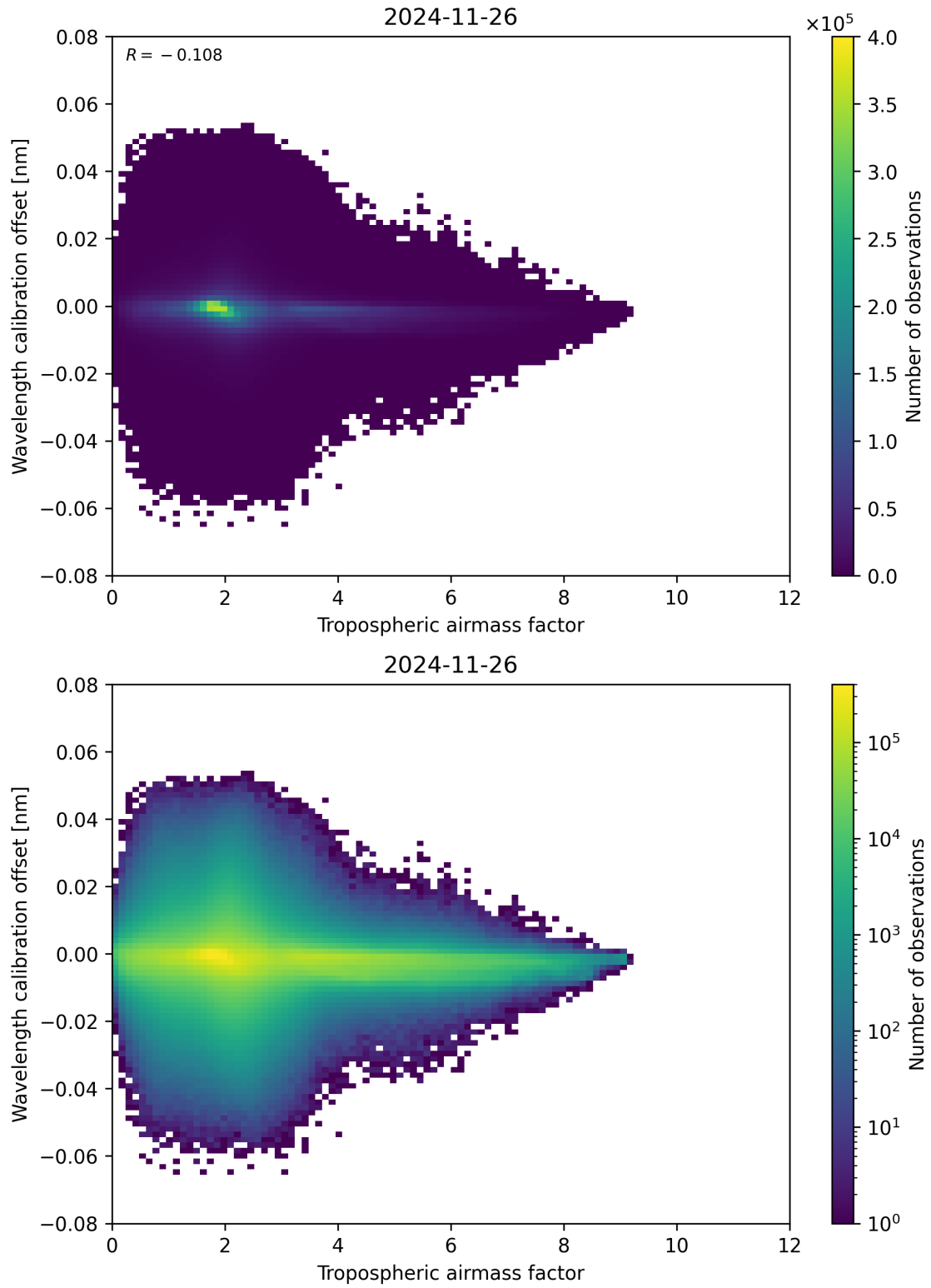
Figure 80: Scatter density plot of “Tropospheric airmass factor” against “Wavelength calibration offset” for 2024-11-25 to 2024-11-27.
