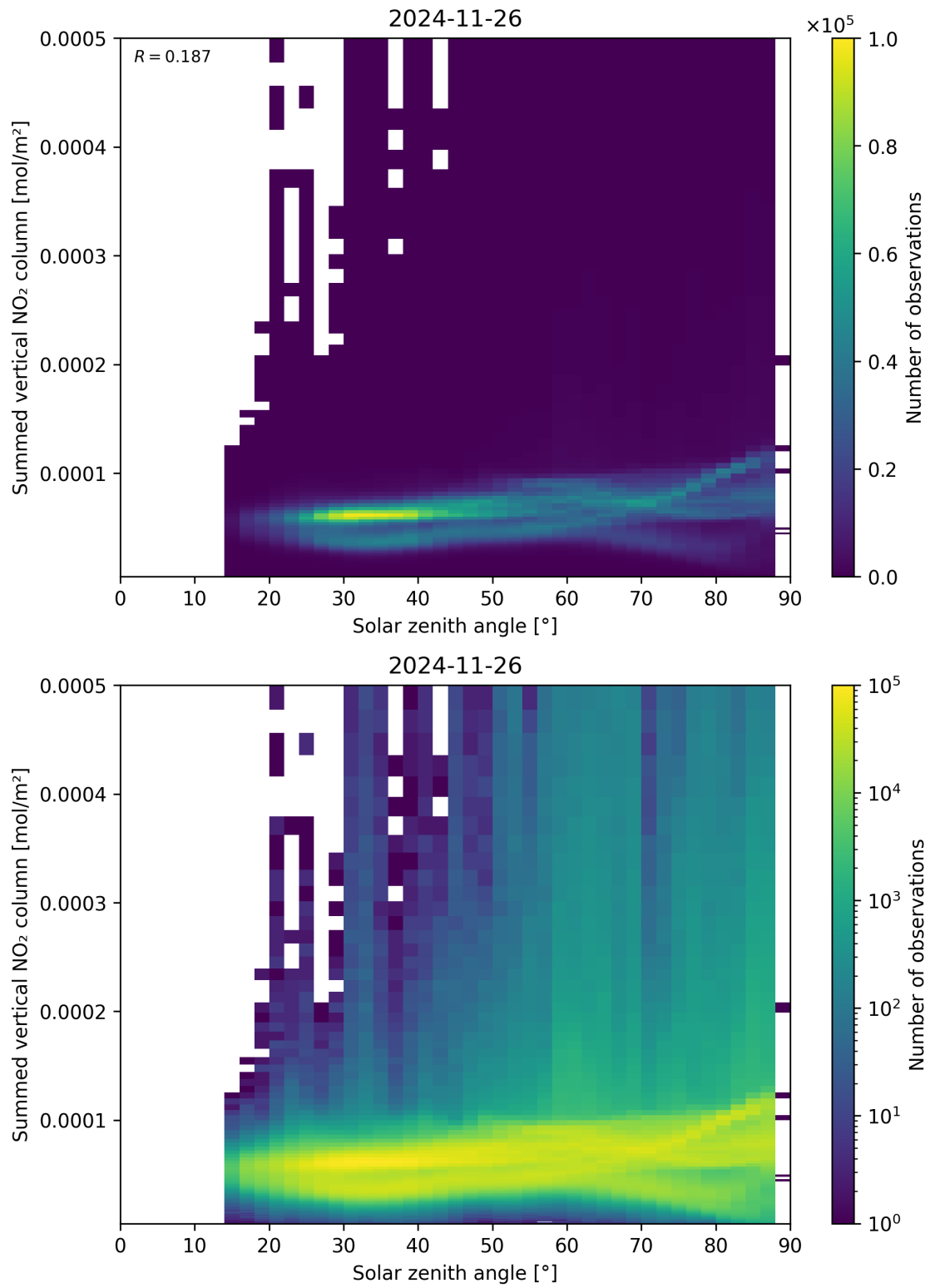
Figure 151: Scatter density plot of “Solar zenith angle” against “Summed vertical NO 2 column” for 2024-11-25 to 2024-11-27.
