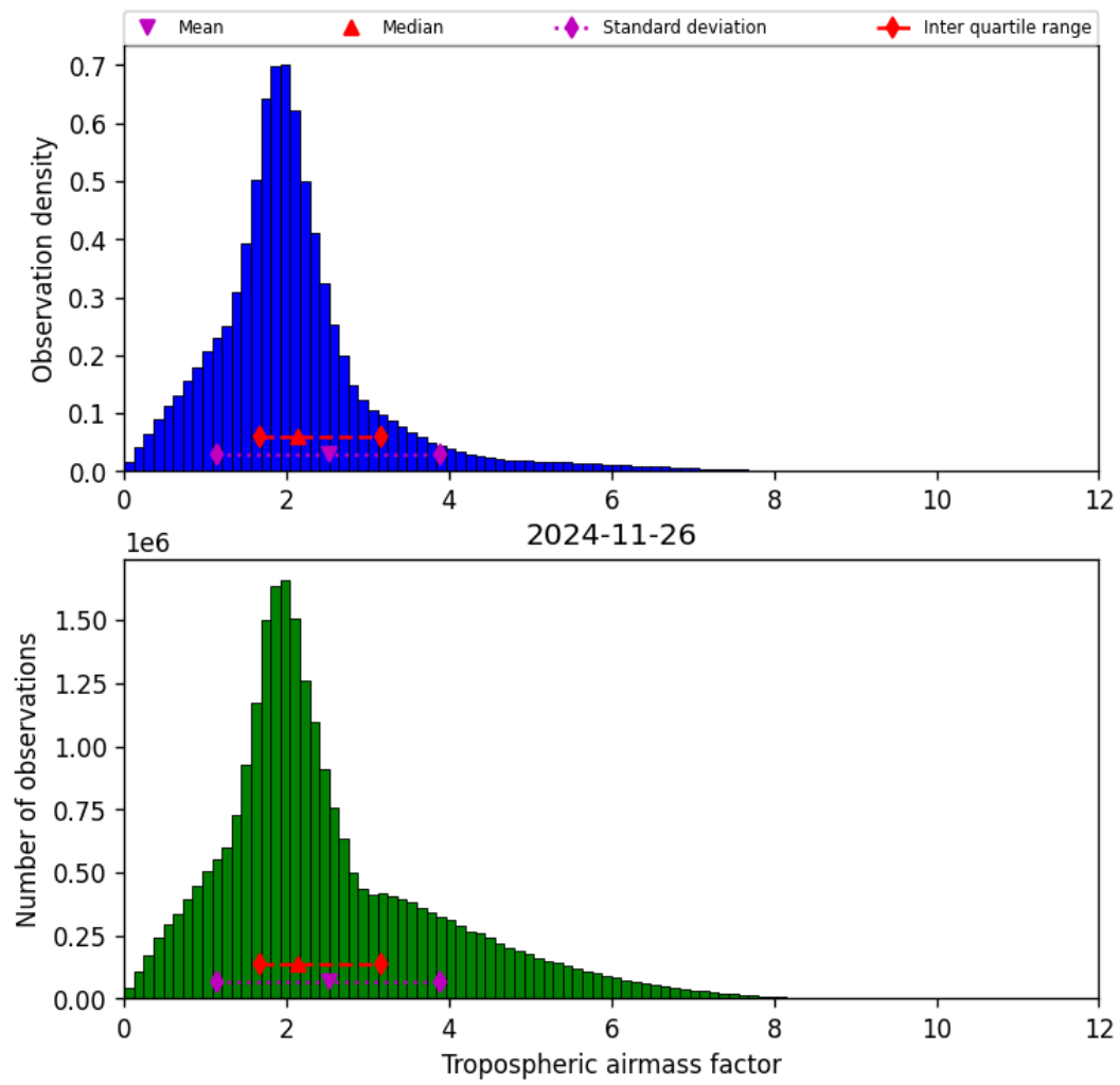
Figure 31: Histogram of “Tropospheric airmass factor” for 2024-11-25 to 2024-11-27
