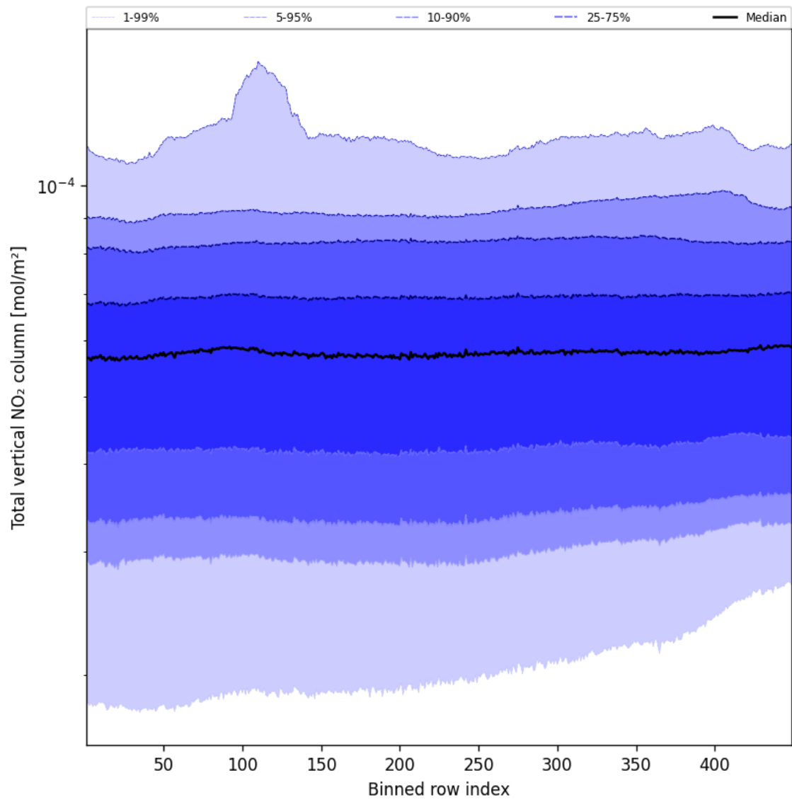
Figure 55: Along track statistics of “Total vertical NO 2 column” for 2024-11-25 to 2024-11-27
