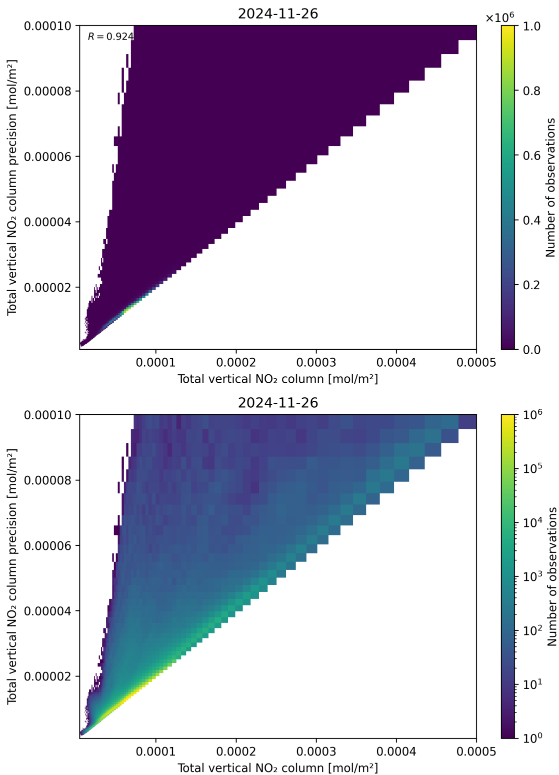
Figure 114: Scatter density plot of “Total vertical NO 2 column” against “Total vertical NO 2 column precision” for 2024-11-25 to 2024-11-27.
