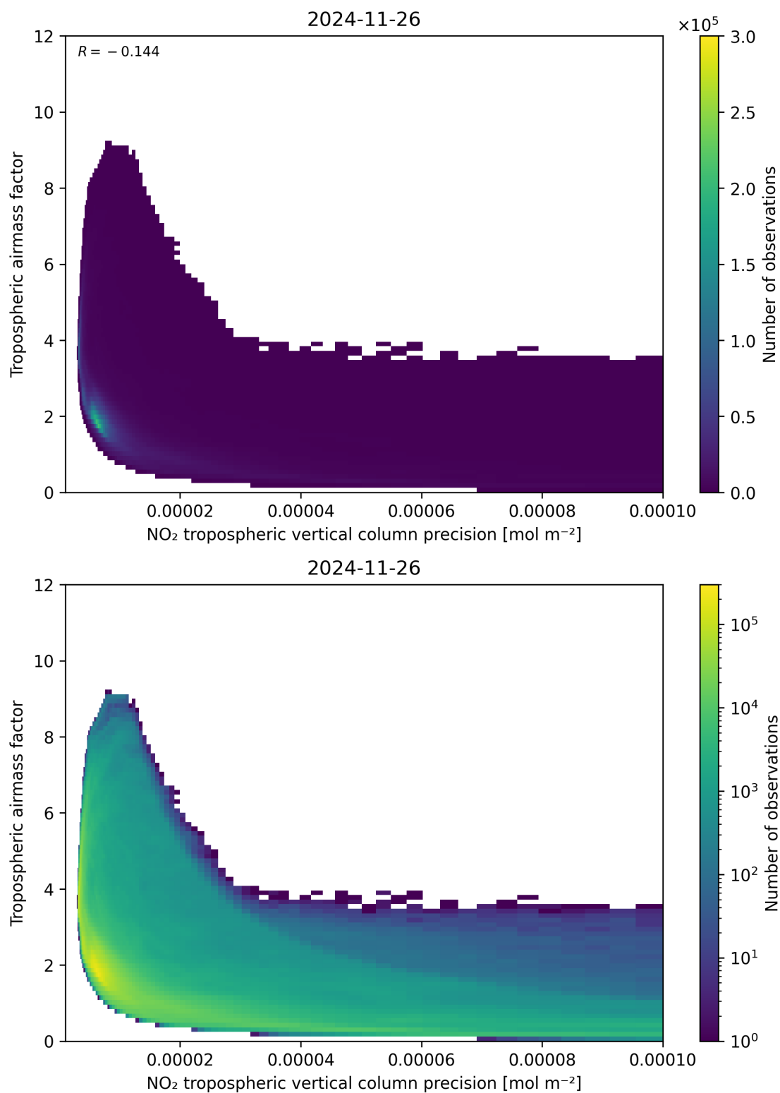
Figure 133: Scatter density plot of “NO 2 tropospheric vertical column precision” against “Tropospheric air mass factor” for 2024-11-25 to 2024-11-27.
