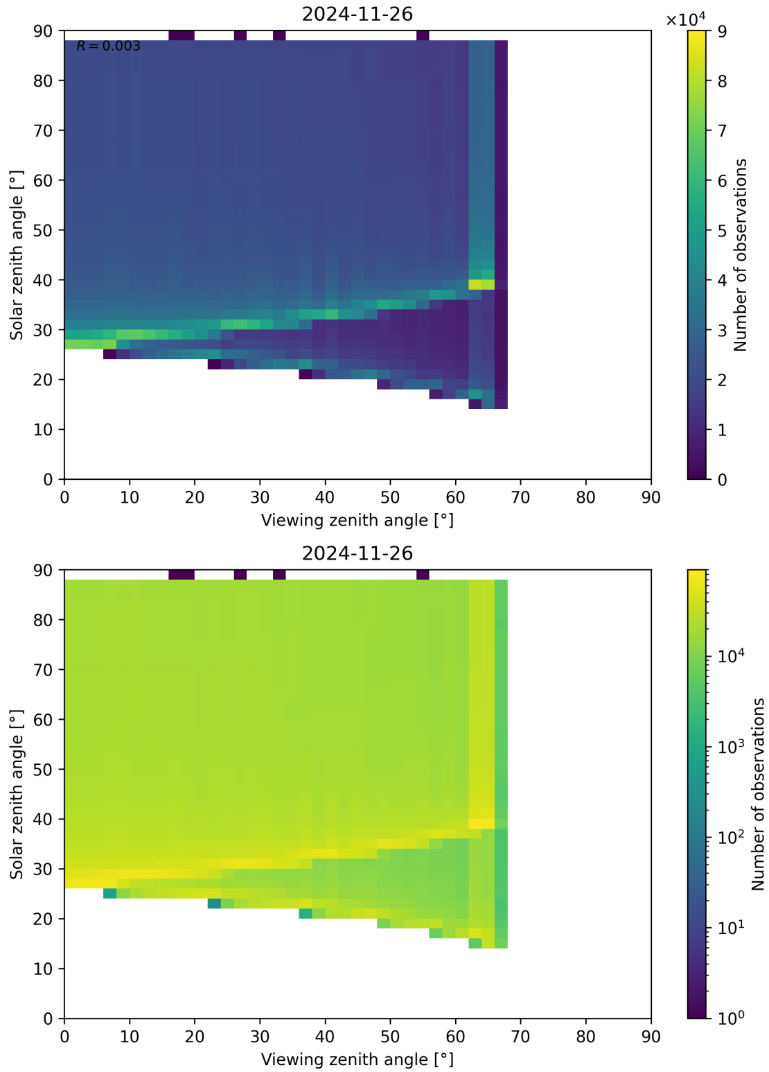
Figure 172: Scatter density plot of “Viewing zenith angle” against “Solar zenith angle” for 2024-11-25 to 2024-11-27.
