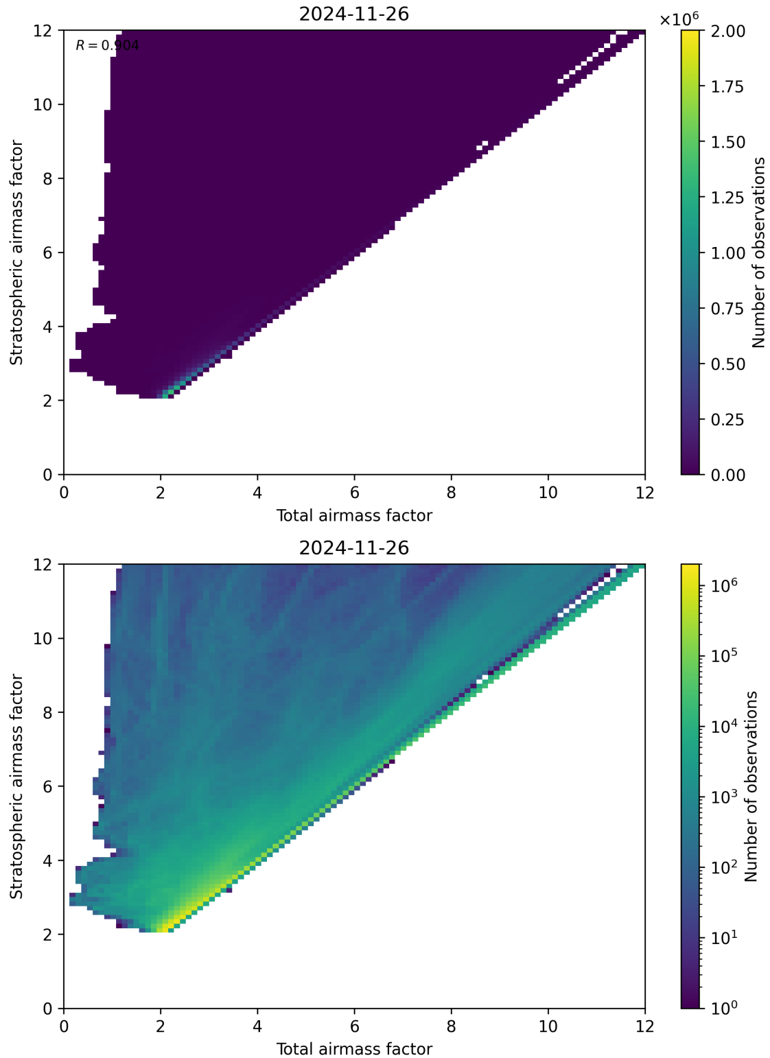
Figure 62: Scatter density plot of “Total airmass factor” against “Stratospheric airmass factor” for 2024-11-25 to 2024-11-27.
