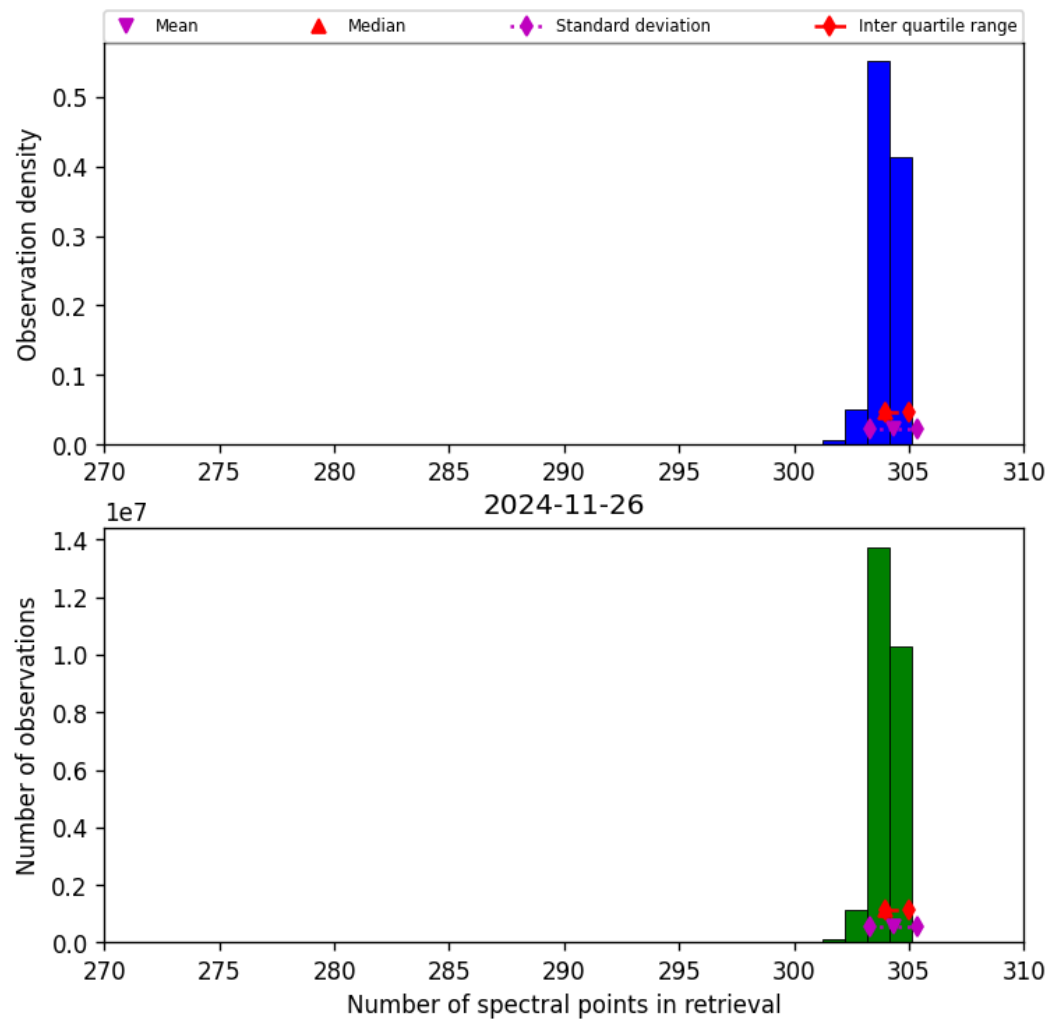
Figure 33: Histogram of “Number of spectral points in retrieval” for 2024-11-25 to 2024-11-27
