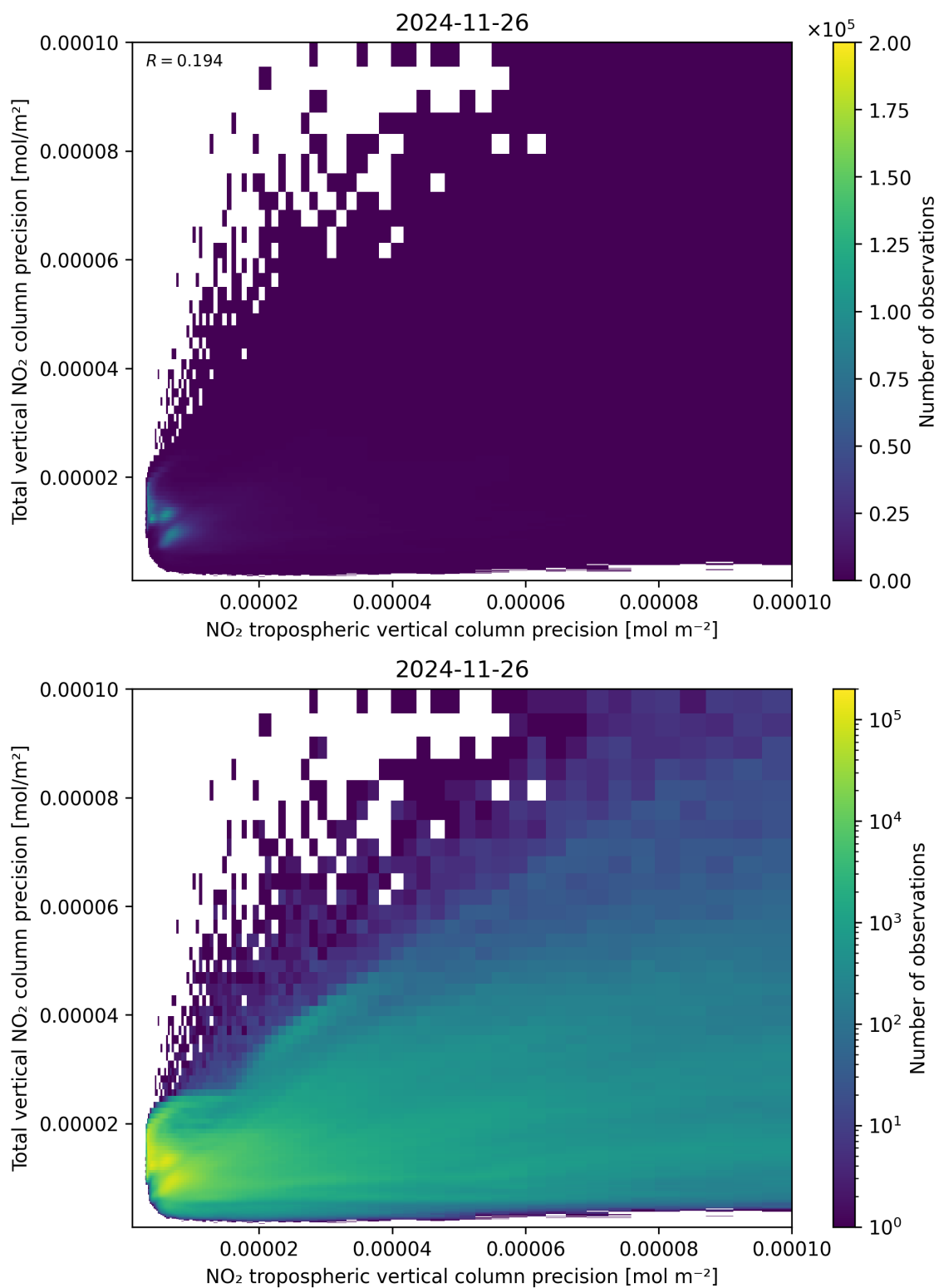
Figure 139: Scatter density plot of “NO 2 tropospheric vertical column precision” against “Total vertical NO 2 column precision” for 2024-11-25 to 2024-11-27.
