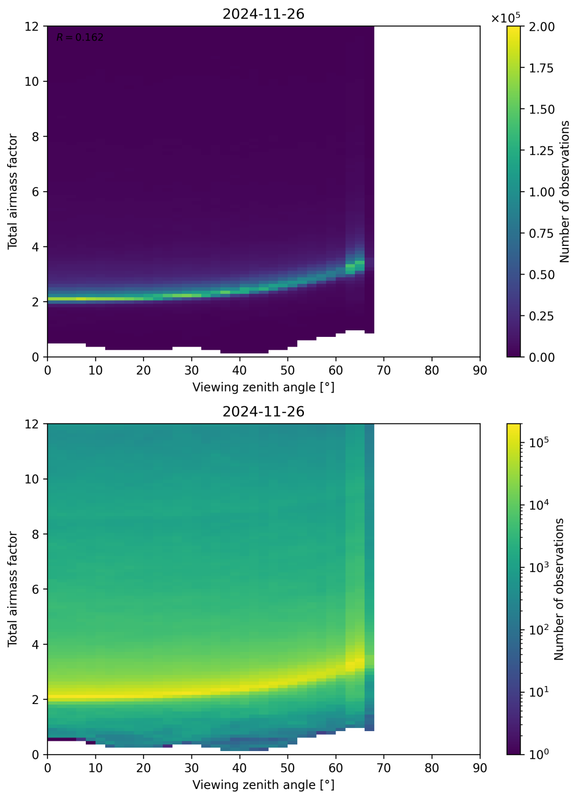
Figure 160: Scatter density plot of “Viewing zenith angle” against “Total airmass factor” for 2024-11-25 to 2024-11-27.
