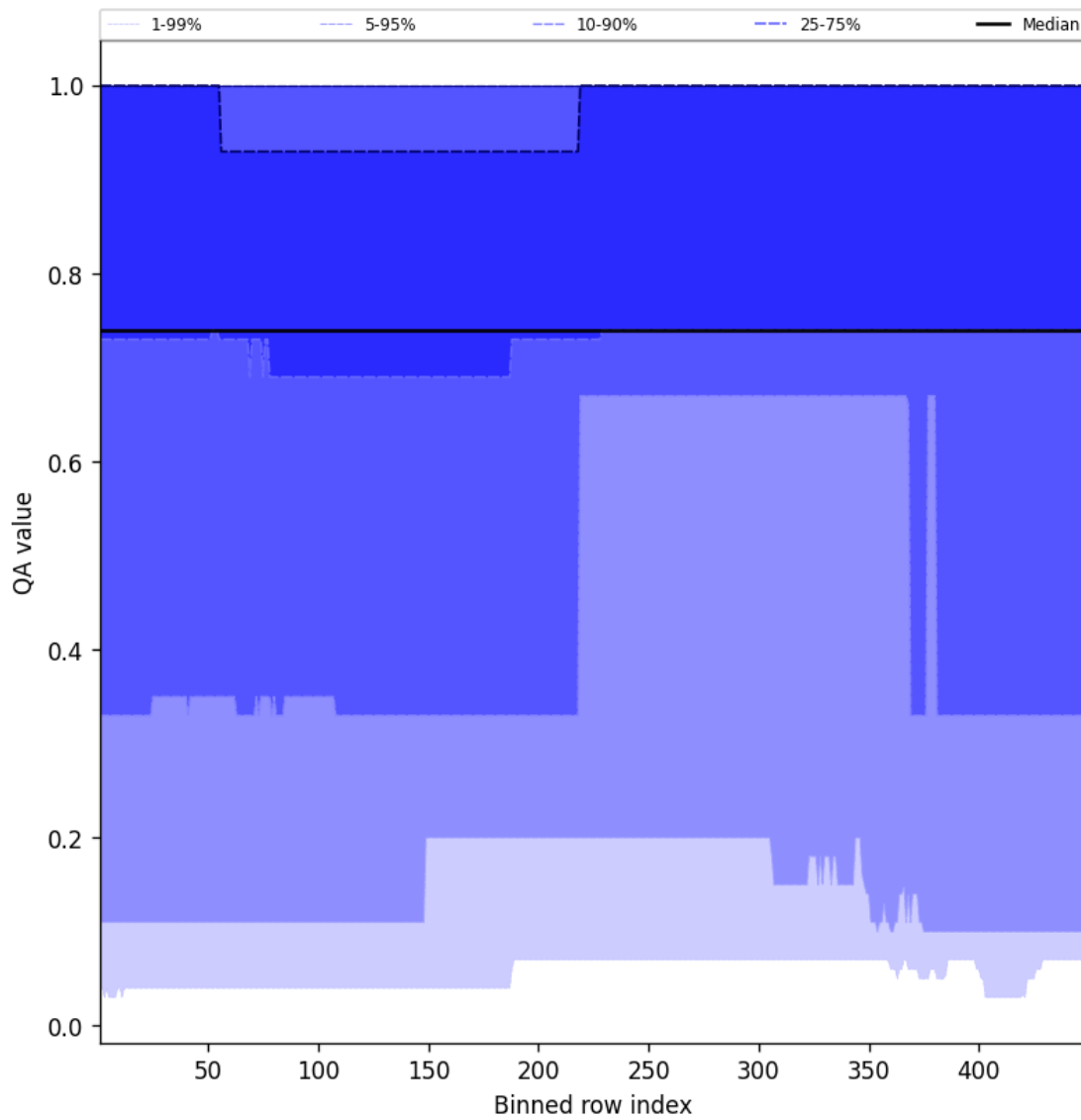
Figure 45: Along track statistics of “QA value” for 2024-11-25 to 2024-11-27
