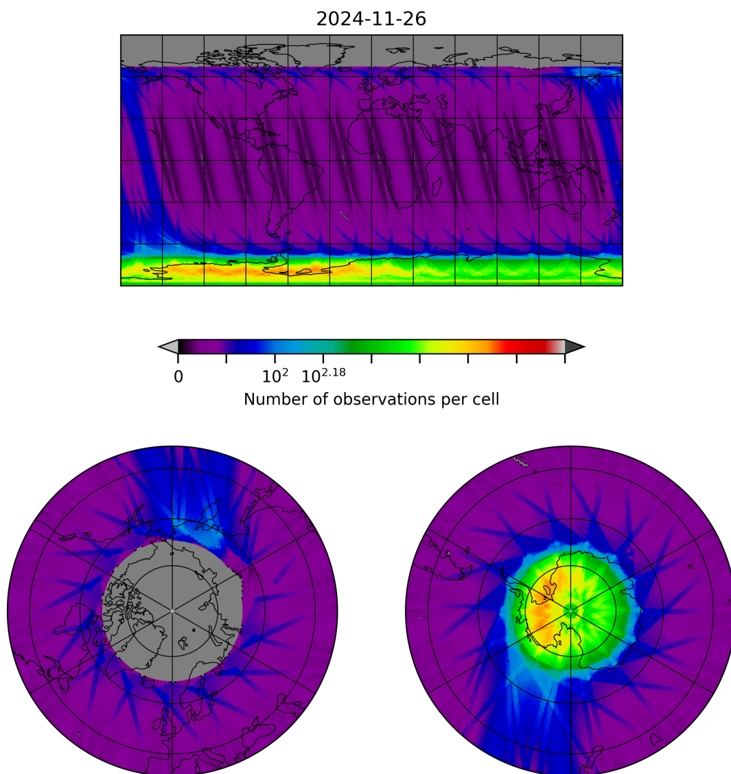
Figure 10: Map of the number of observations for 2024-11-25 to 2024-11-27
