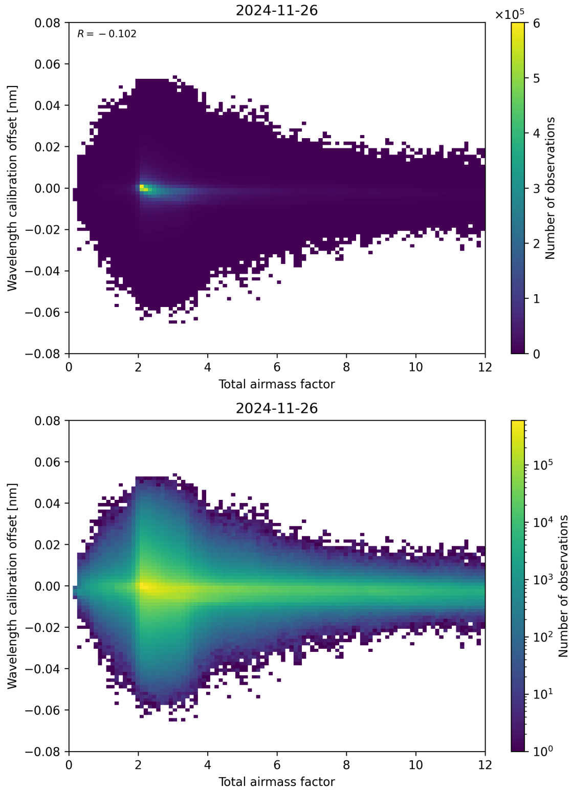
Figure 70: Scatter density plot of “Total airmass factor” against “Wavelength calibration offset” for 2024-11-25 to 2024-11-27.
