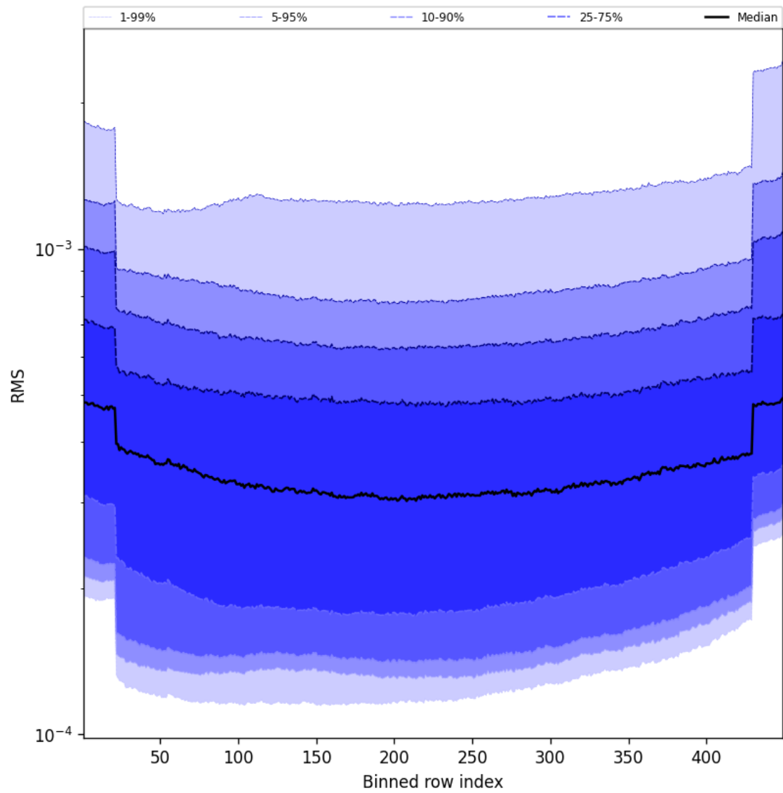
Figure 60: Along track statistics of “RMS” for 2024-11-25 to 2024-11-27
