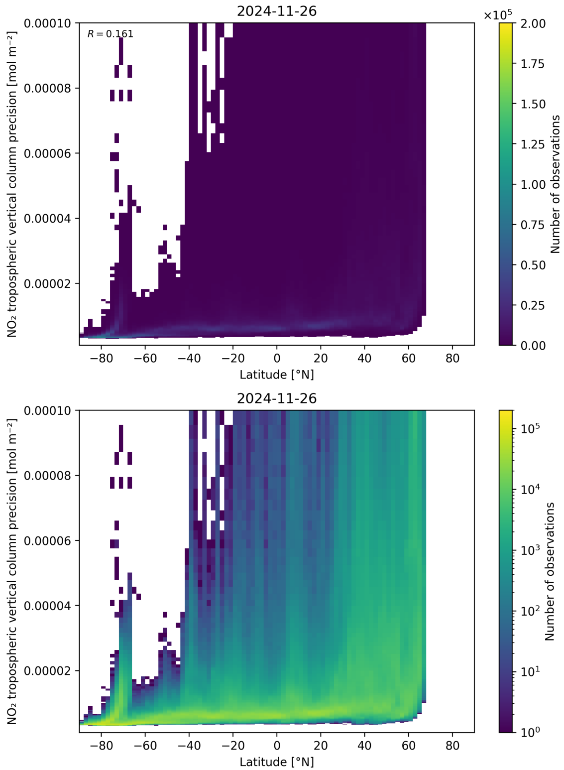
Figure 93: Scatter density plot of “Latitude” against “NO 2 tropospheric vertical column precision” for 2024-11-25 to 2024-11-27.
