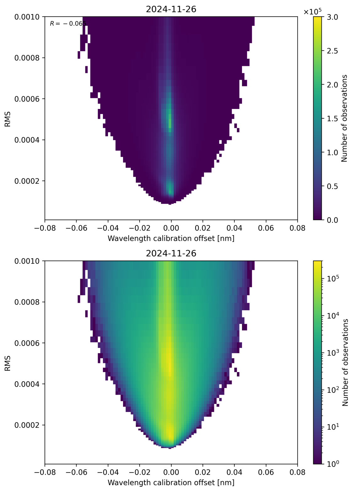
Figure 181: Scatter density plot of “Wavelength calibration offset” against “RMS” for 2024-11-25 to 2024-11-27.
