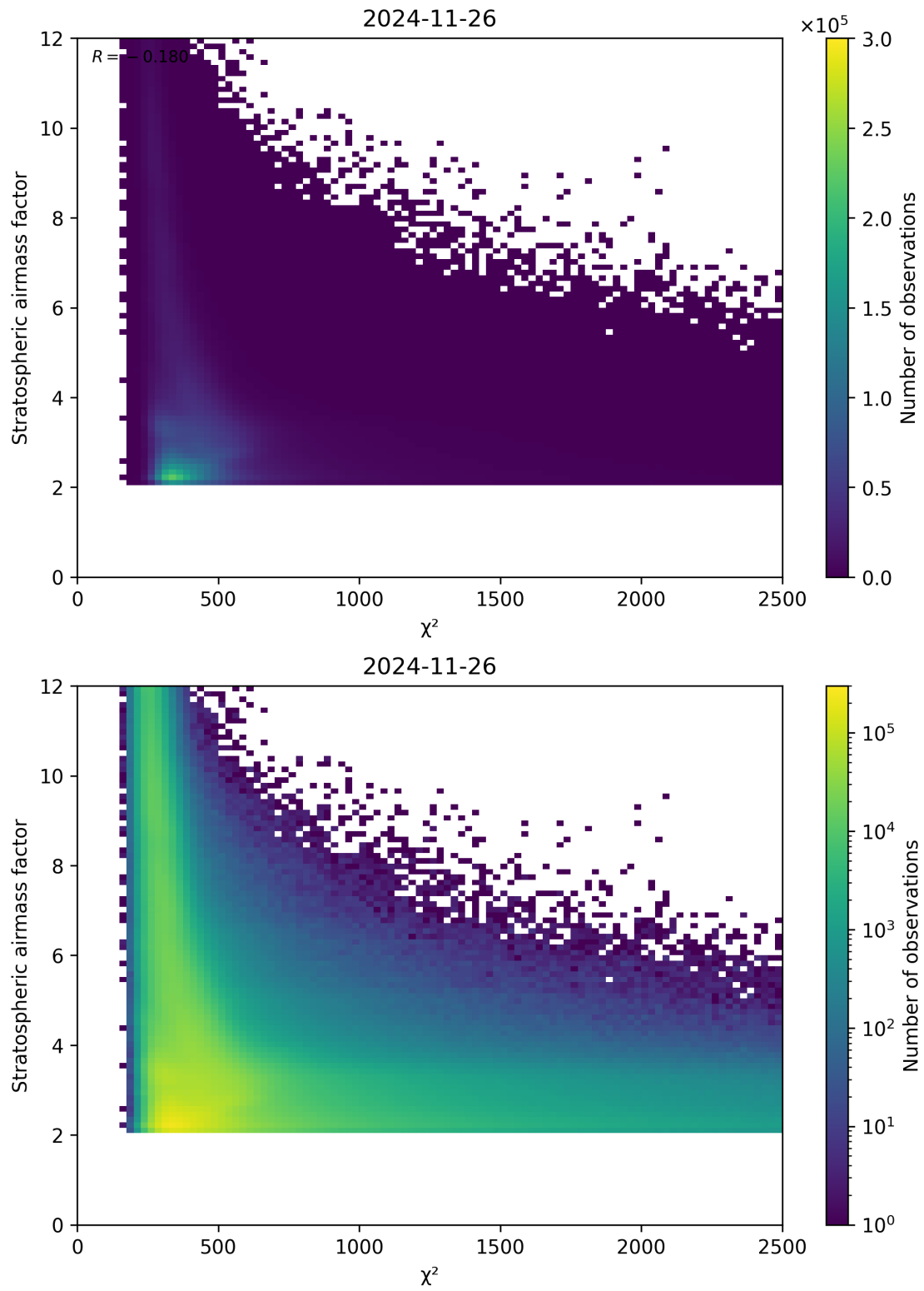
Figure 81: Scatter density plot of “ \chi^2 ” against “Stratospheric airmass factor” for 2024-11-25 to 2024-11-27.
