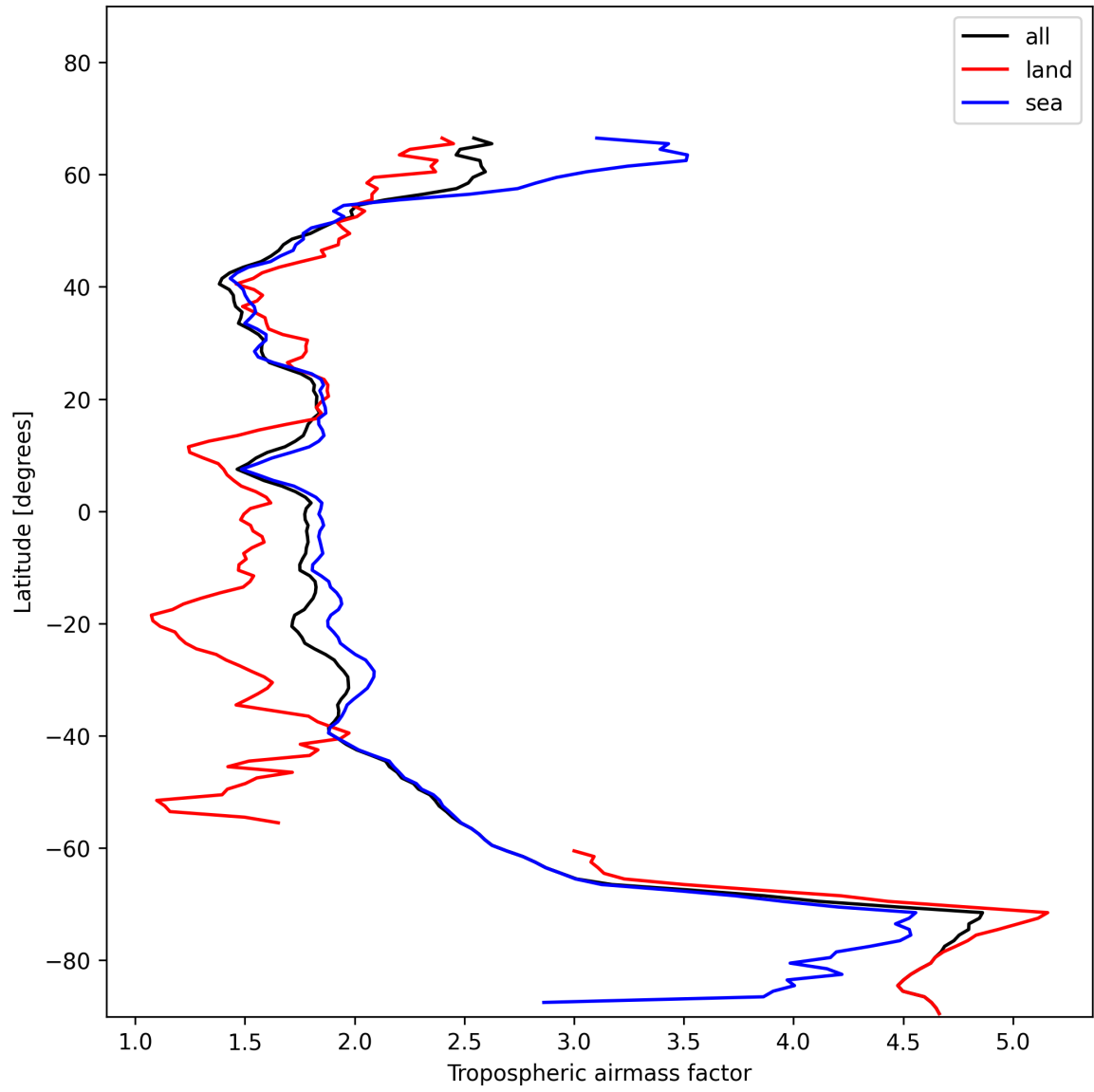
Figure 14: Zonal average of “Tropospheric airmass factor” for 2024-11-25 to 2024-11-27.
