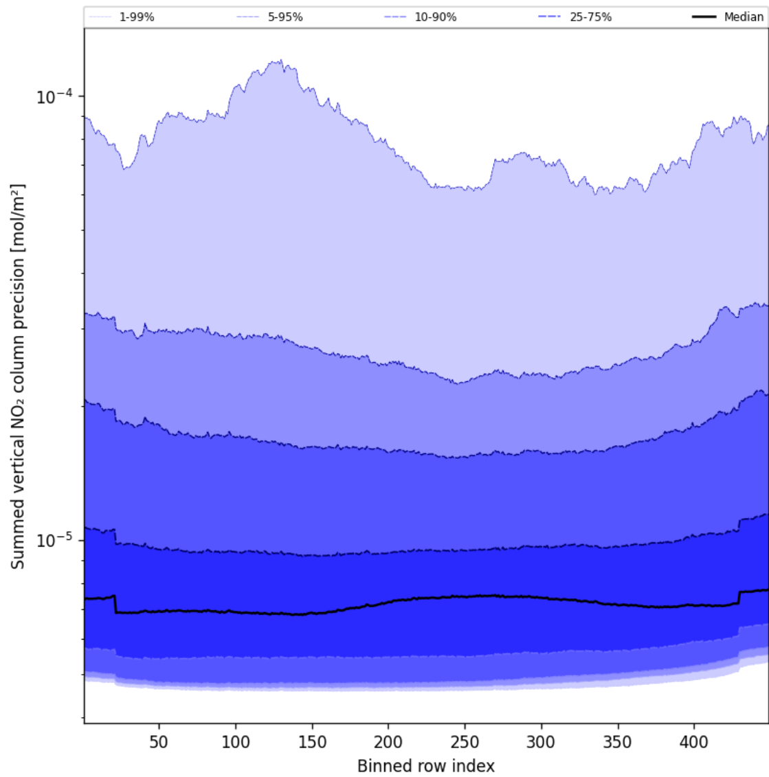
Figure 58: Along track statistics of “Summed vertical NO 2 column precision” for 2024-11-25 to 2024-11-27
