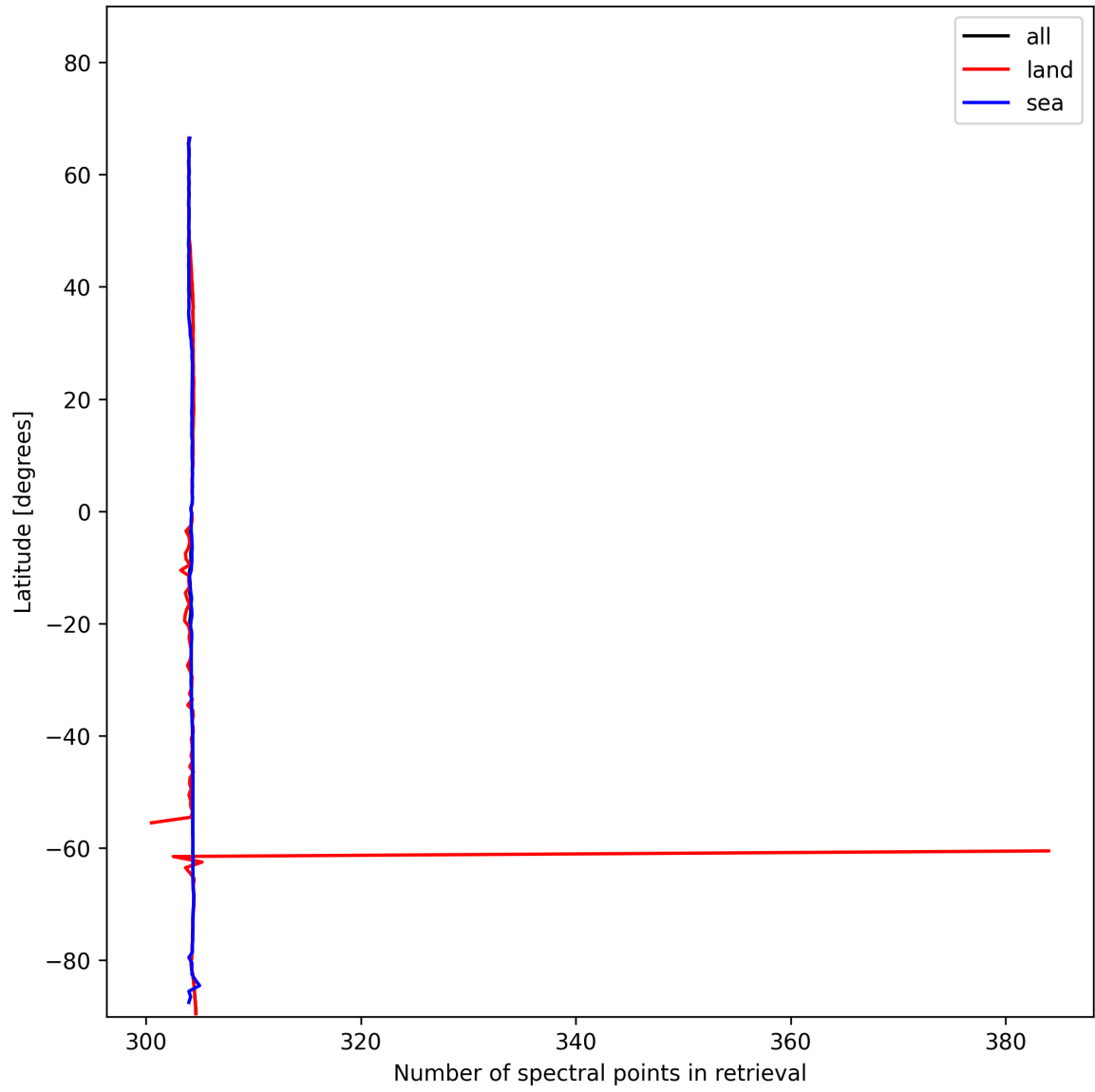
Figure 16: Zonal average of “Number of spectral points in retrieval” for 2024-11-25 to 2024-11-27.
