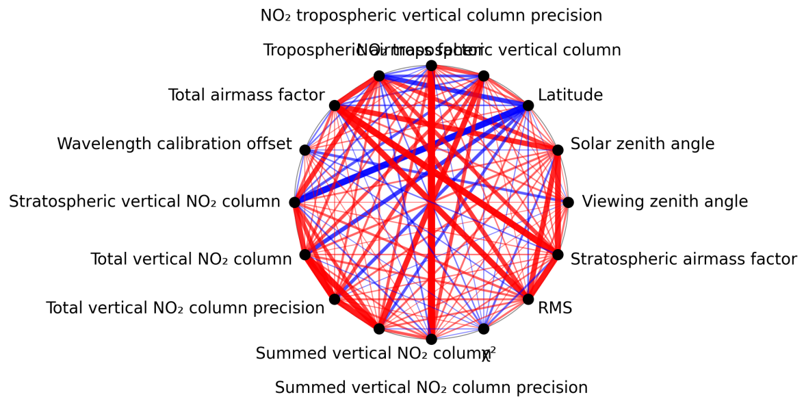
Figure 1: Map of correlation graph for 2024-11-25 to 2024-11-27.
