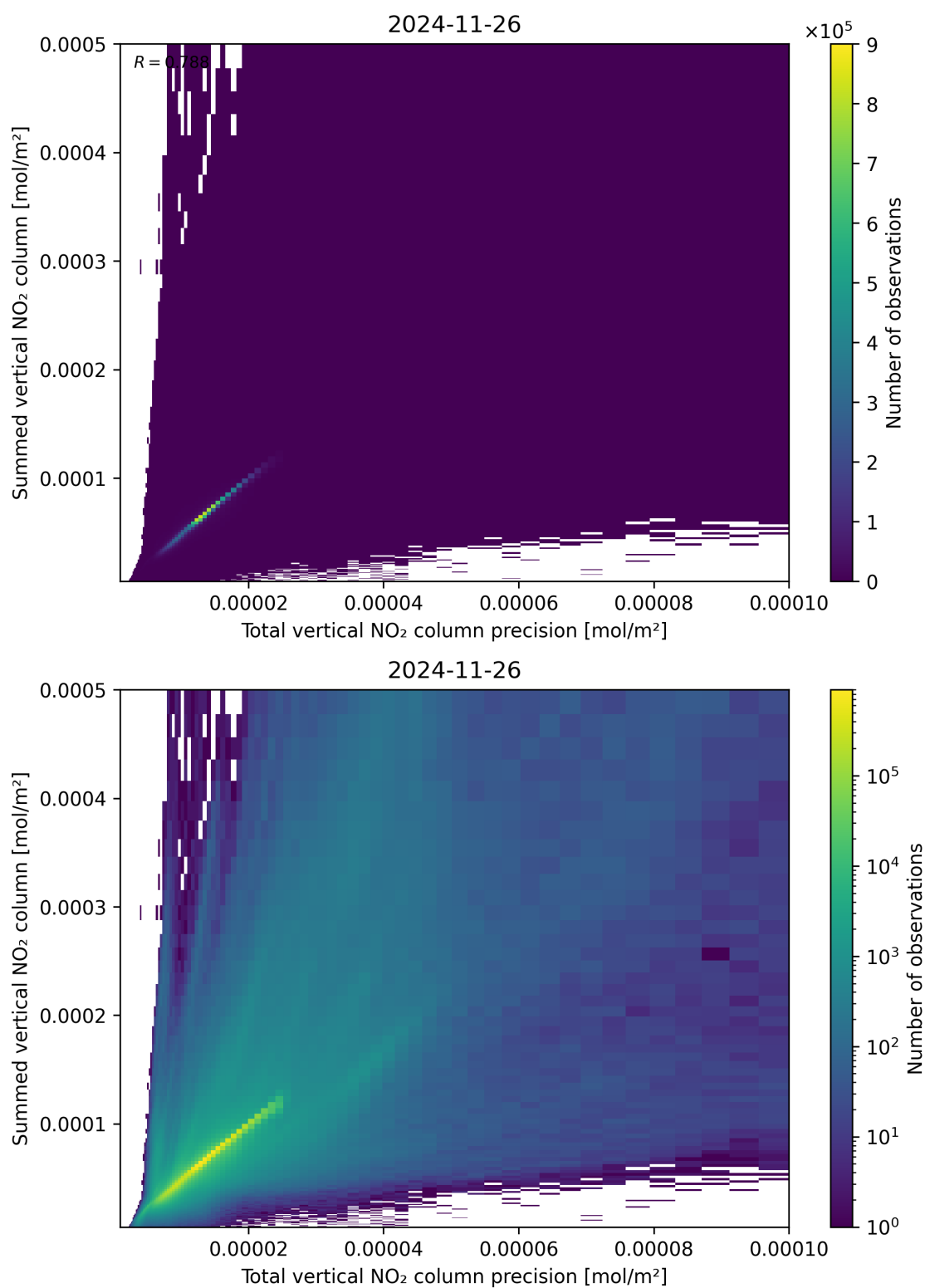
Figure 117: Scatter density plot of “Total vertical NO 2 column precision” against “Summed vertical NO 2 column” for 2024-11-25 to 2024-11-27.
