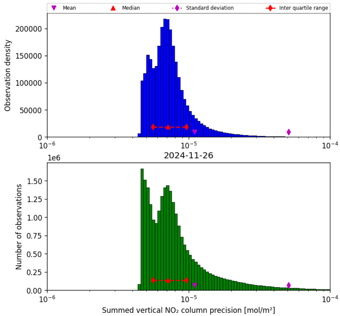
Figure 41: Histogram of "Summed vertical NO 2 column precision" for 2024-11-25 to 2024-11-27
