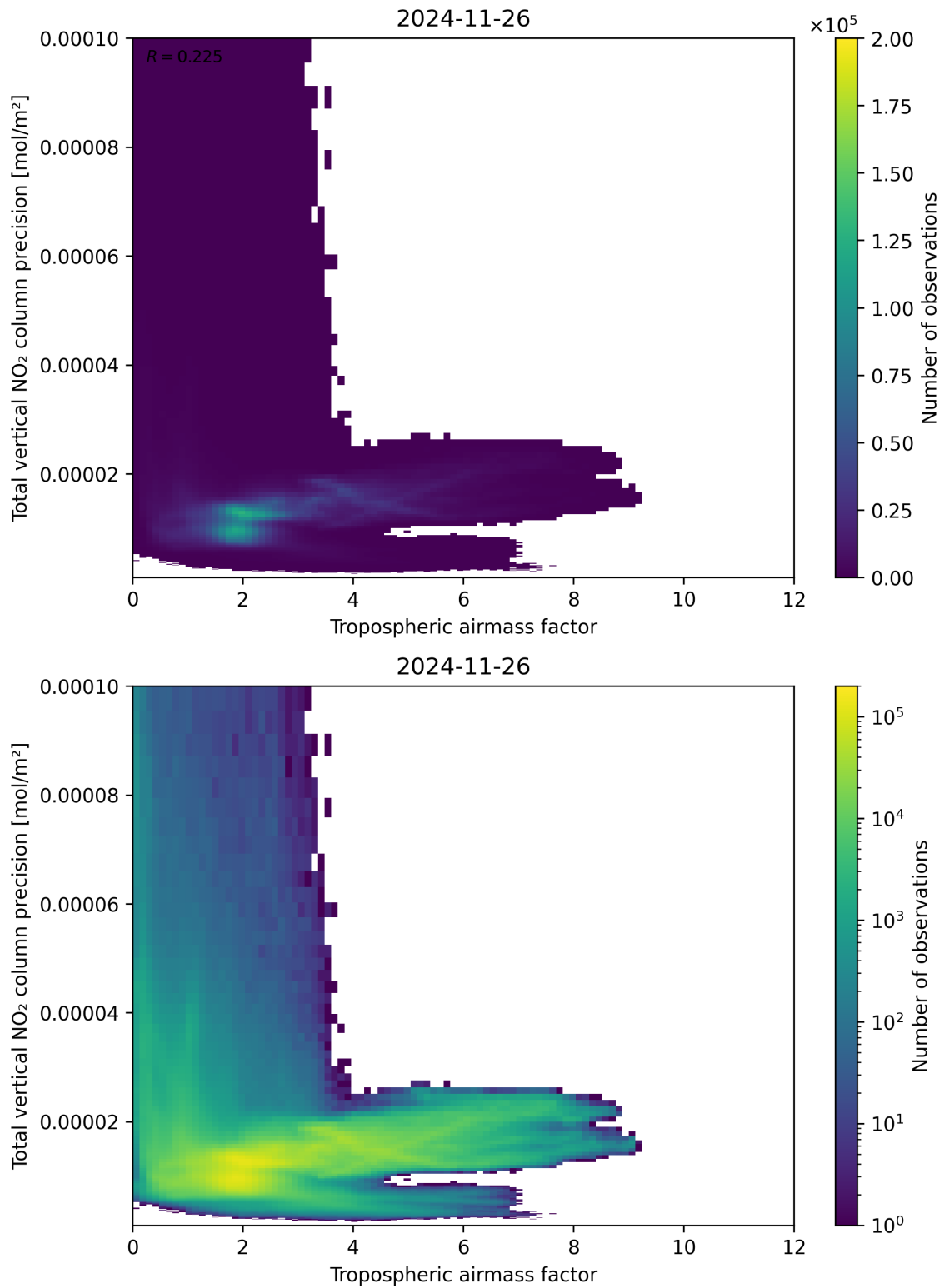
Figure 78: Scatter density plot of “Tropospheric air mass factor” against “Total vertical NO 2 column precision” for 2024-11-25 to 2024-11-27.
