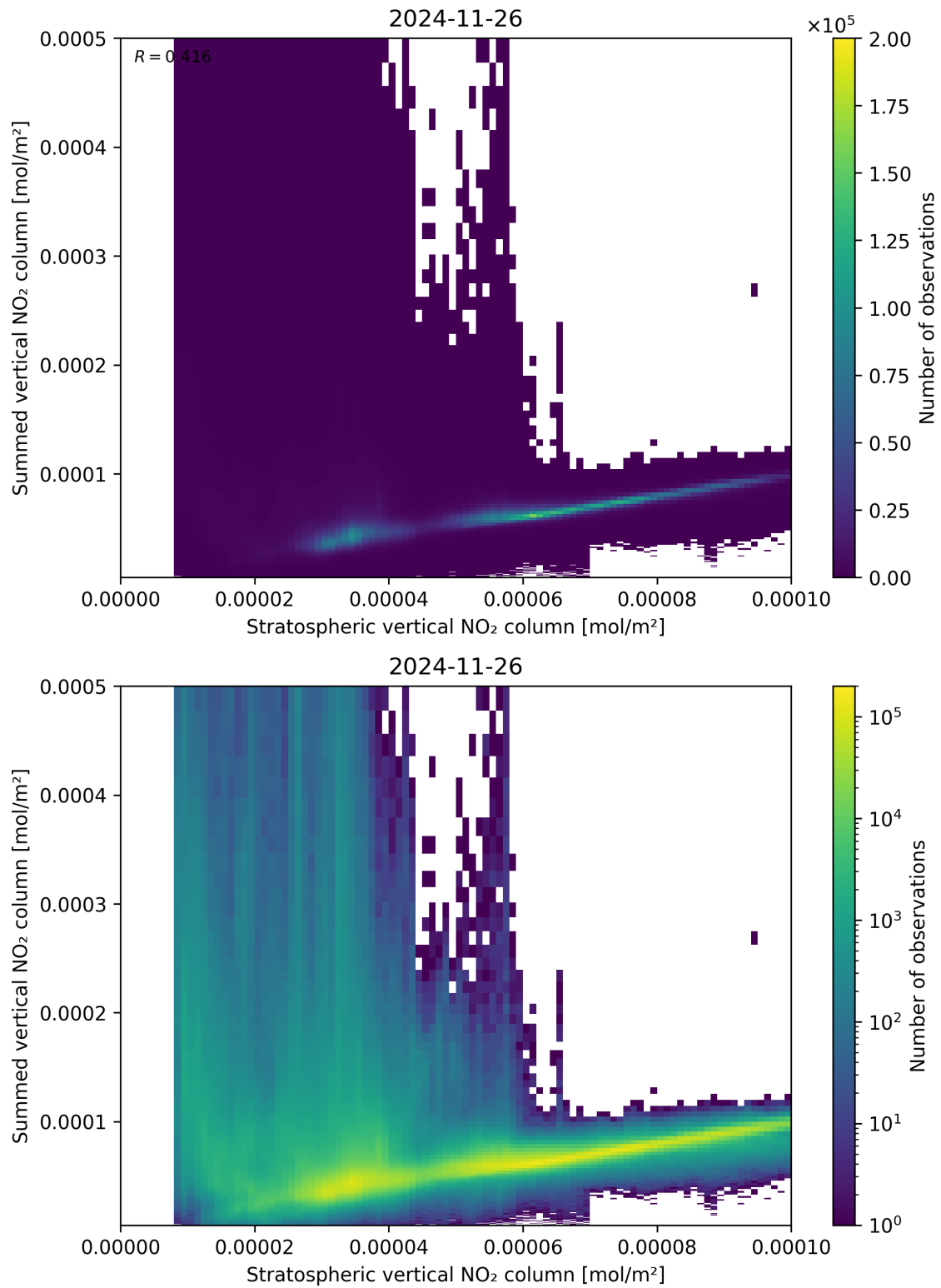
Figure 98: Scatter density plot of “Stratospheric vertical NO 2 column” against “Summed vertical NO 2 column” for 2024-11-25 to 2024-11-27.
