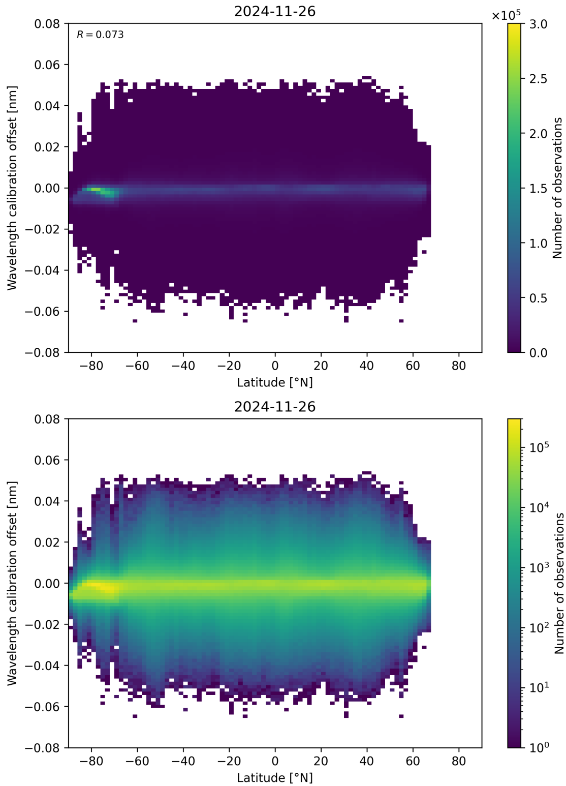
Figure 95: Scatter density plot of “Latitude” against “Wavelength calibration offset” for 2024-11-25 to 2024-11-27.
