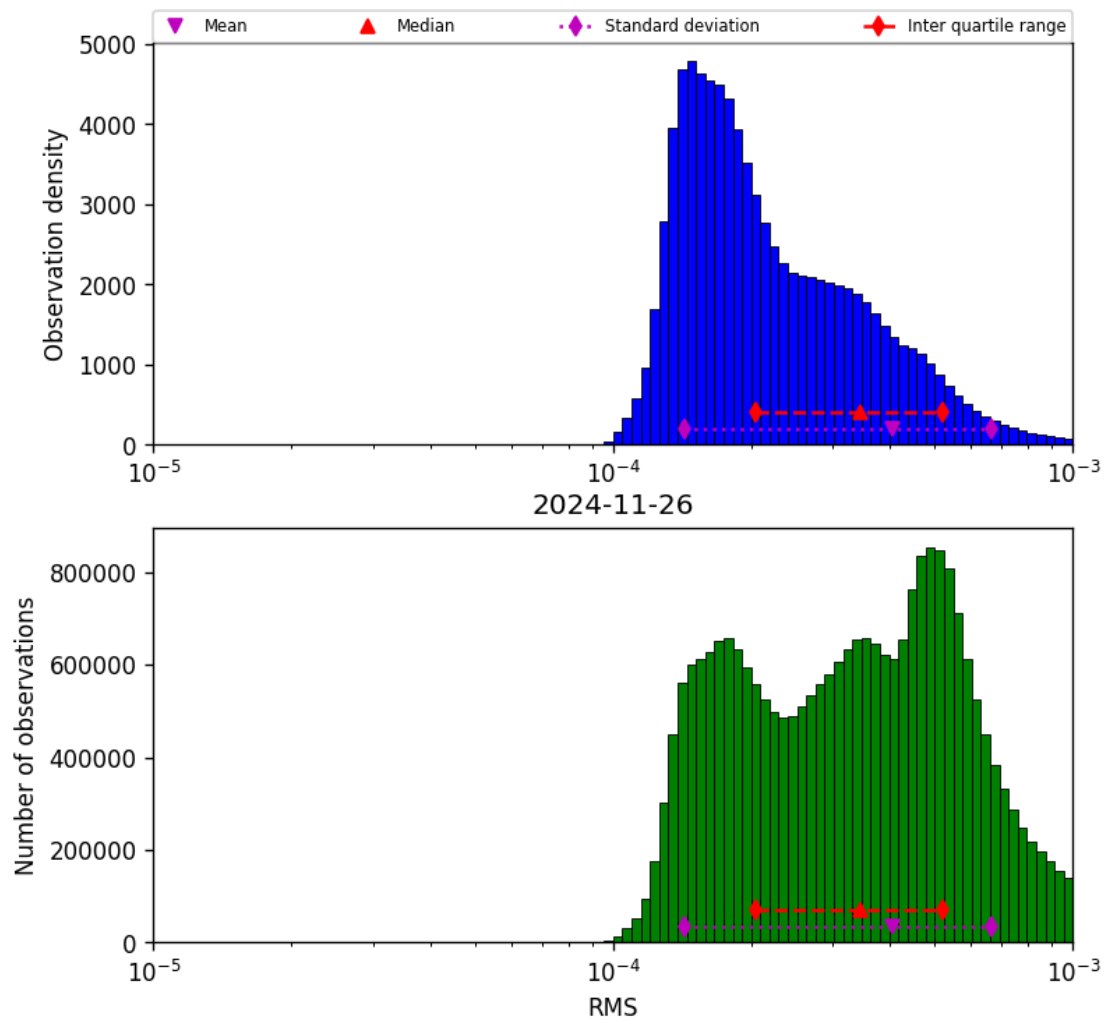
Figure 43: Histogram of “RMS” for 2024-11-25 to 2024-11-27
