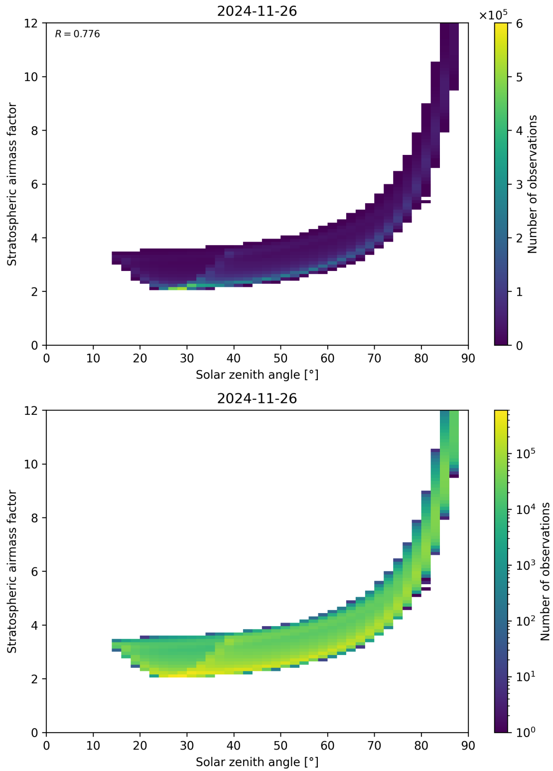
Figure 145: Scatter density plot of “Solar zenith angle” against “Stratospheric airmass factor” for 2024-11-25 to 2024-11-27.
