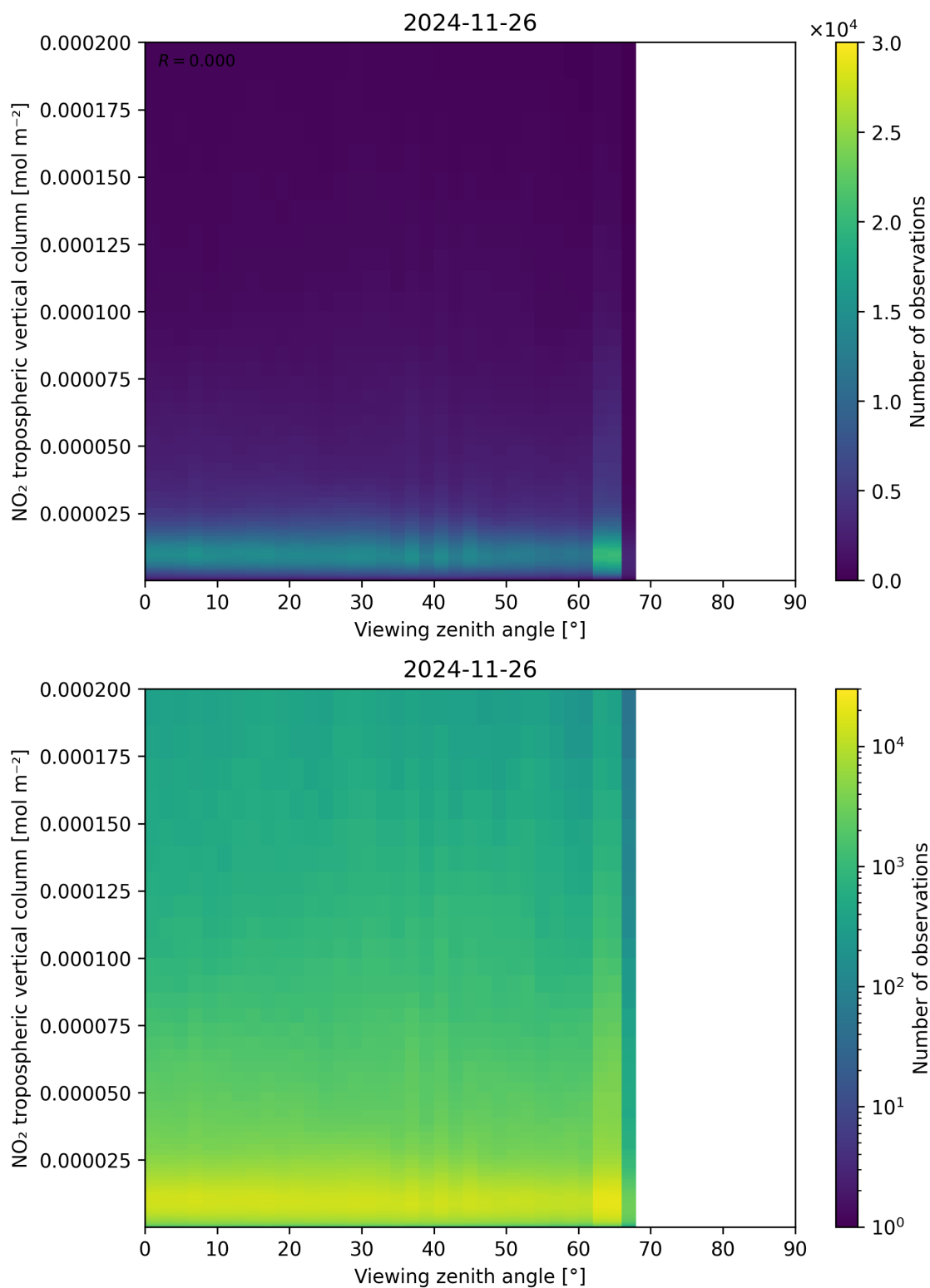
Figure 169: Scatter density plot of “Viewing zenith angle” against “NO 2 tropospheric vertical column” for 2024-11-25 to 2024-11-27.
