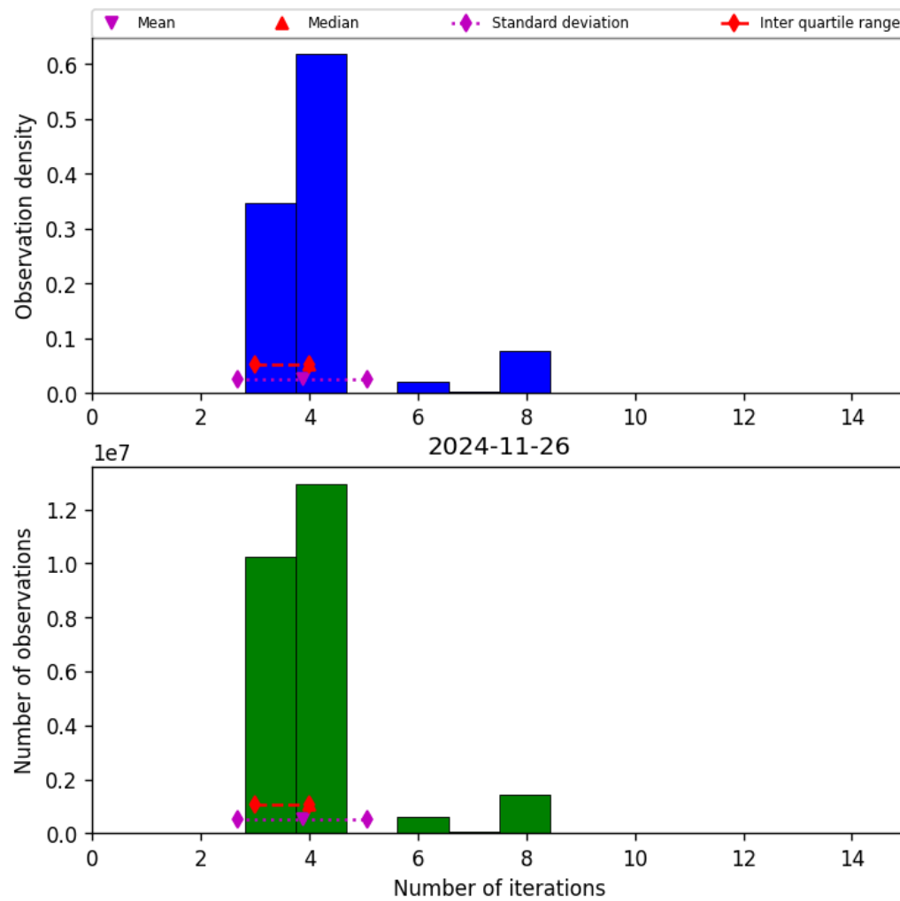
Figure 34: Histogram of “Number of iterations” for 2024-11-25 to 2024-11-27
