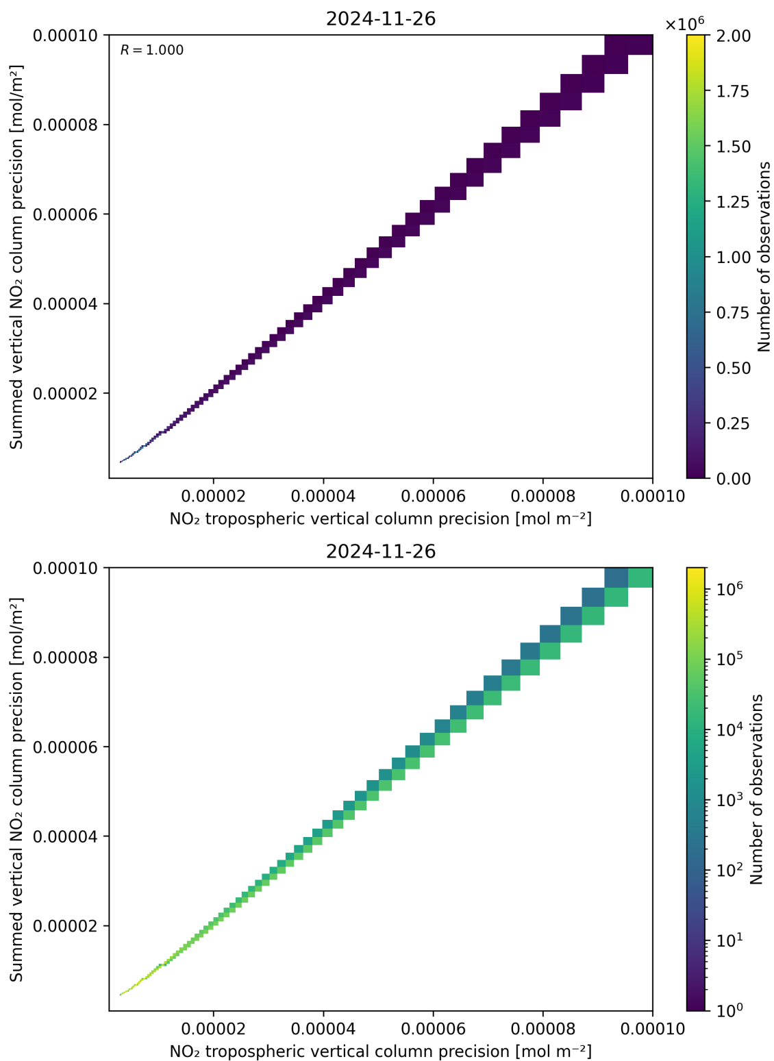
Figure 137: Scatter density plot of “NO 2 tropospheric vertical column precision” against “Summed vertical NO 2 column precision” for 2024-11-25 to 2024-11-27.
