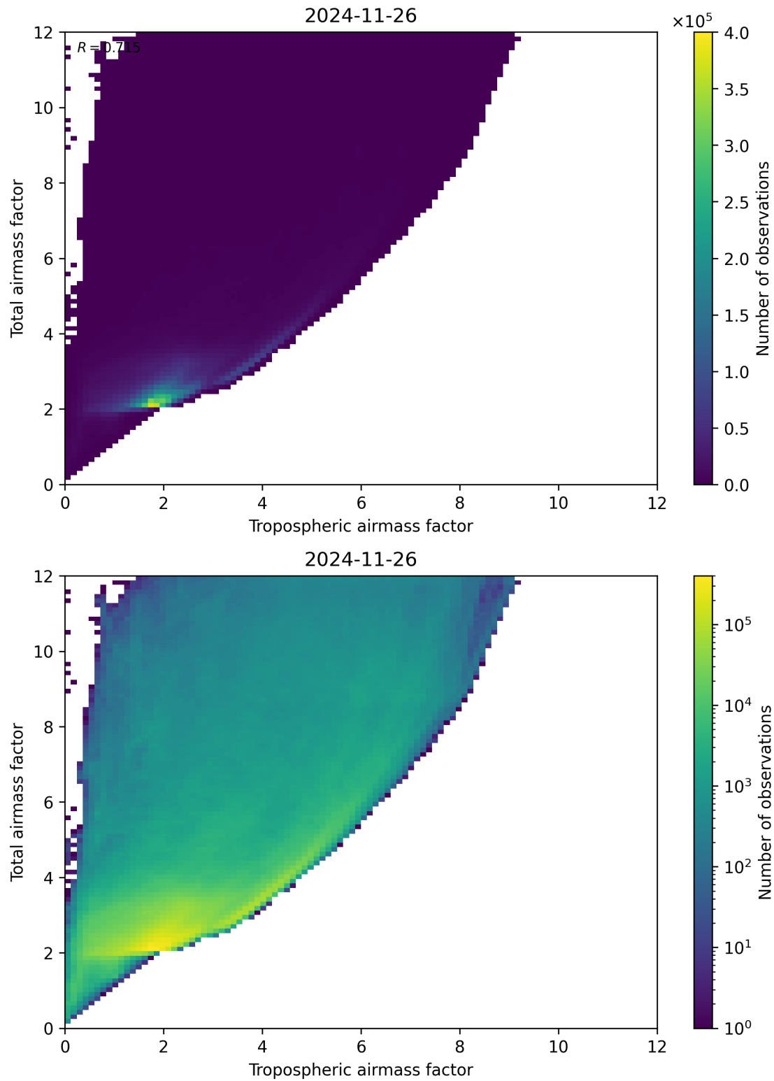
Figure 72: Scatter density plot of “Tropospheric airmass factor” against “Total airmass factor” for 2024-11-25 to 2024-11-27.
