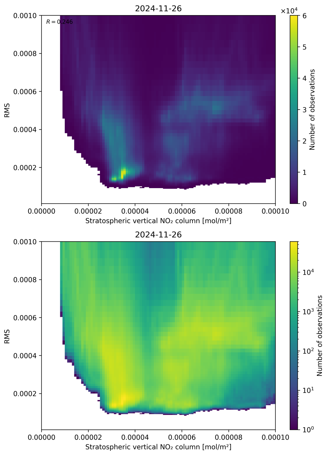
Figure 102: Scatter density plot of “Stratospheric vertical NO 2 column” against “RMS” for 2024-11-25 to 2024-11-27.
