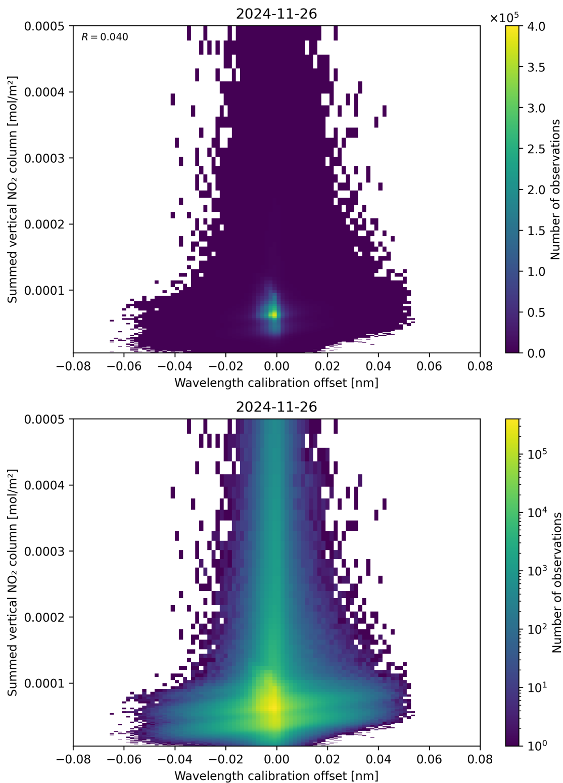
Figure 177: Scatter density plot of “Wavelength calibration offset” against “Summed vertical NO 2 column” for 2024-11-25 to 2024-11-27.
