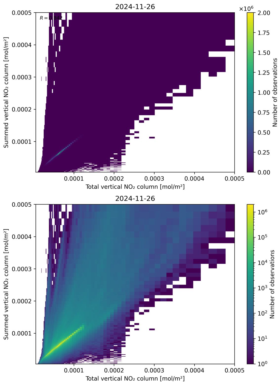
Figure 112: Scatter density plot of “Total vertical NO 2 column” against “Summed vertical NO 2 column” for 2024-11-25 to 2024-11-27.
