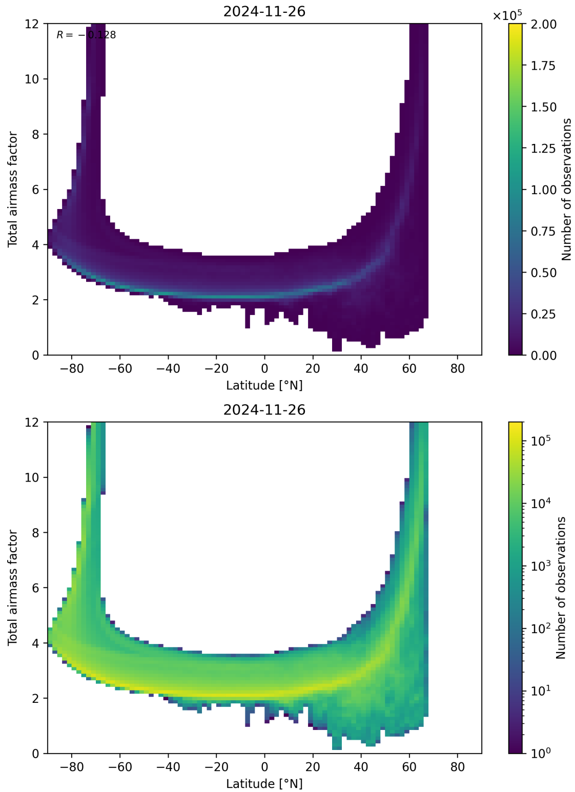
Figure 84: Scatter density plot of “Latitude” against “Total airmass factor” for 2024-11-25 to 2024-11-27.
