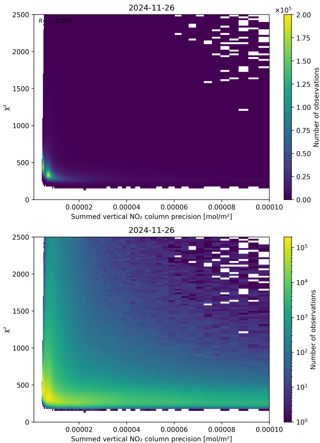
Figure 107: Scatter density plot of “Summed vertical NO 2 column precision” against “ \chi^2 ” for 2024-11-25 to 2024-11-27.
