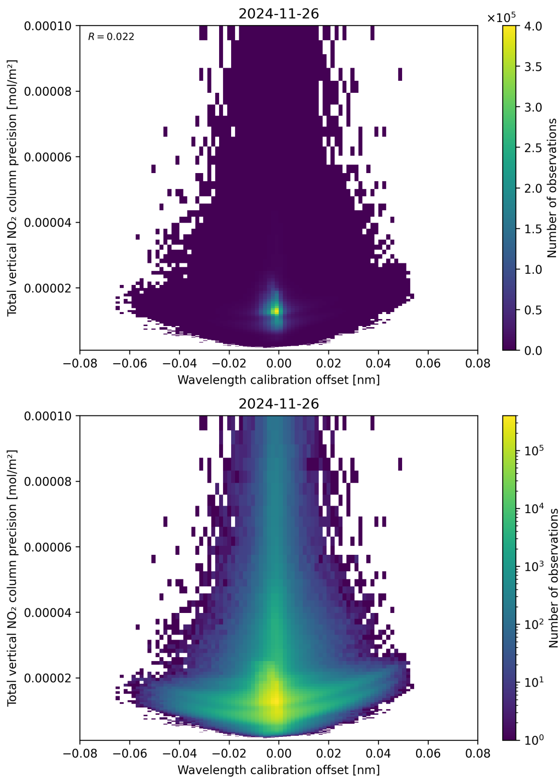
Figure 180: Scatter density plot of “Wavelength calibration offset” against “Total vertical NO 2 column precision” for 2024-11-25 to 2024-11-27.
