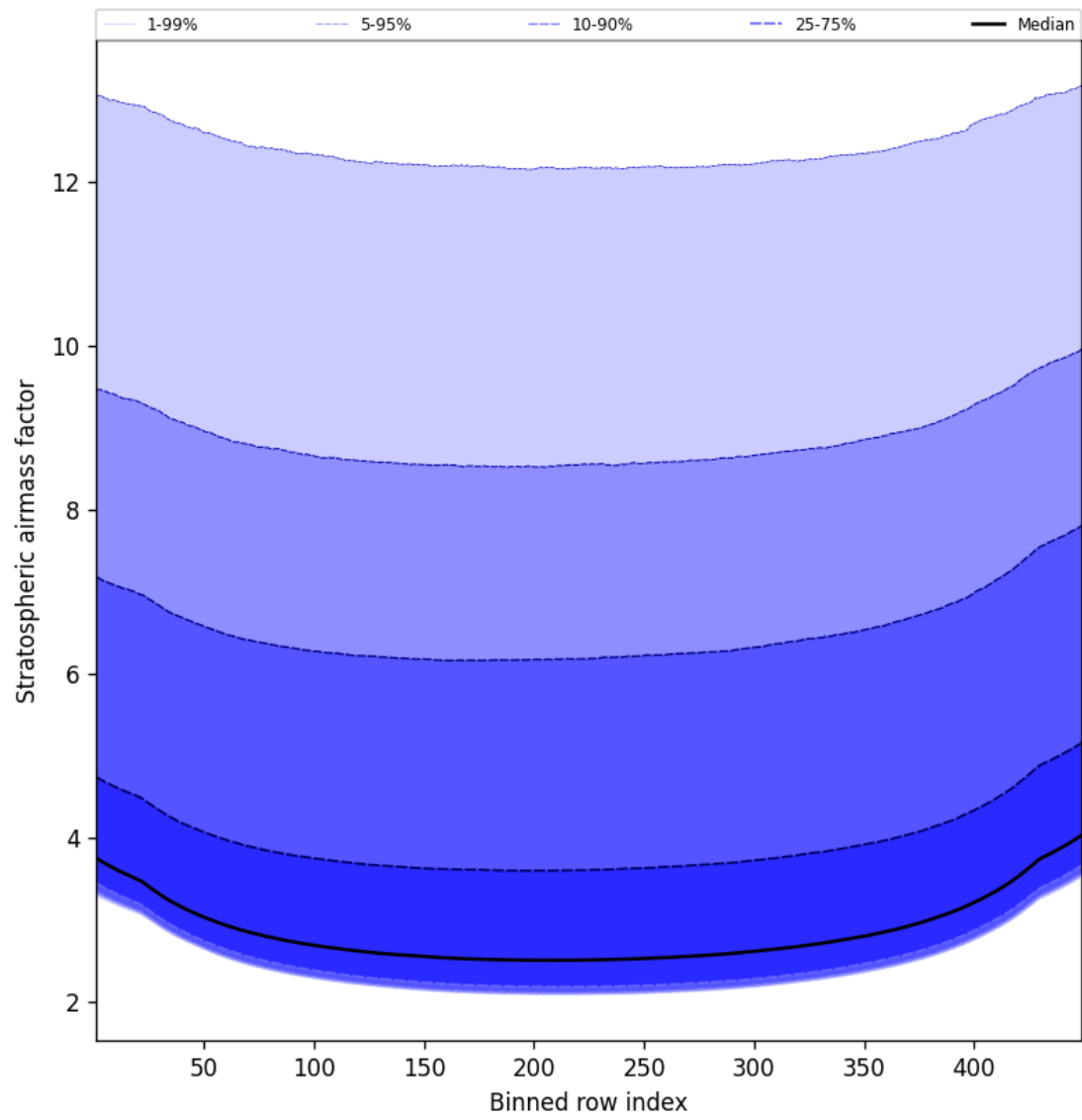
Figure 61: Along track statistics of “Stratospheric air mass factor” for 2024-11-25 to 2024-11-27
