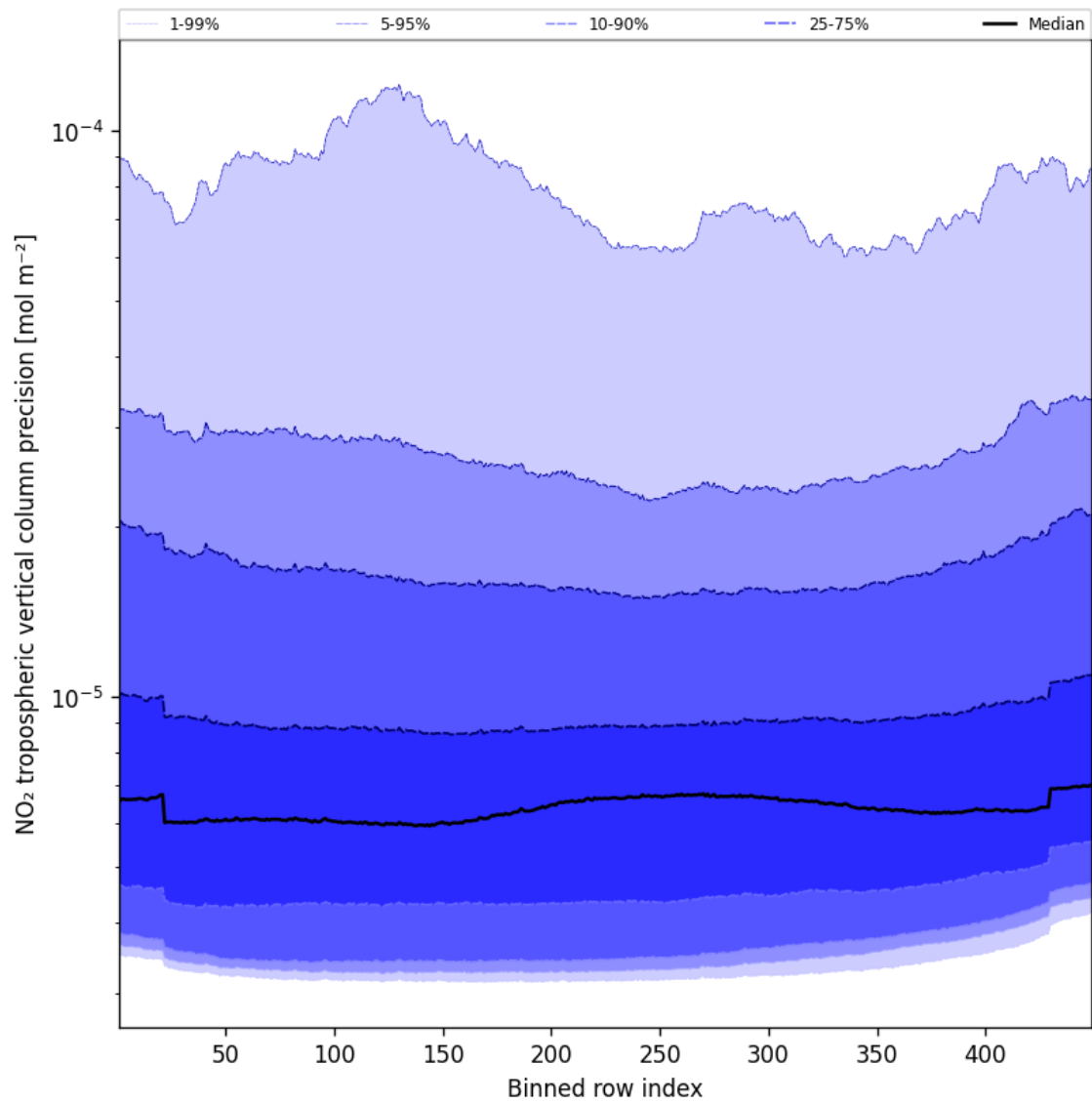
Figure 47: Along track statistics of “NO 2 tropospheric vertical column precision” for 2024-11-25 to 2024-11-27
