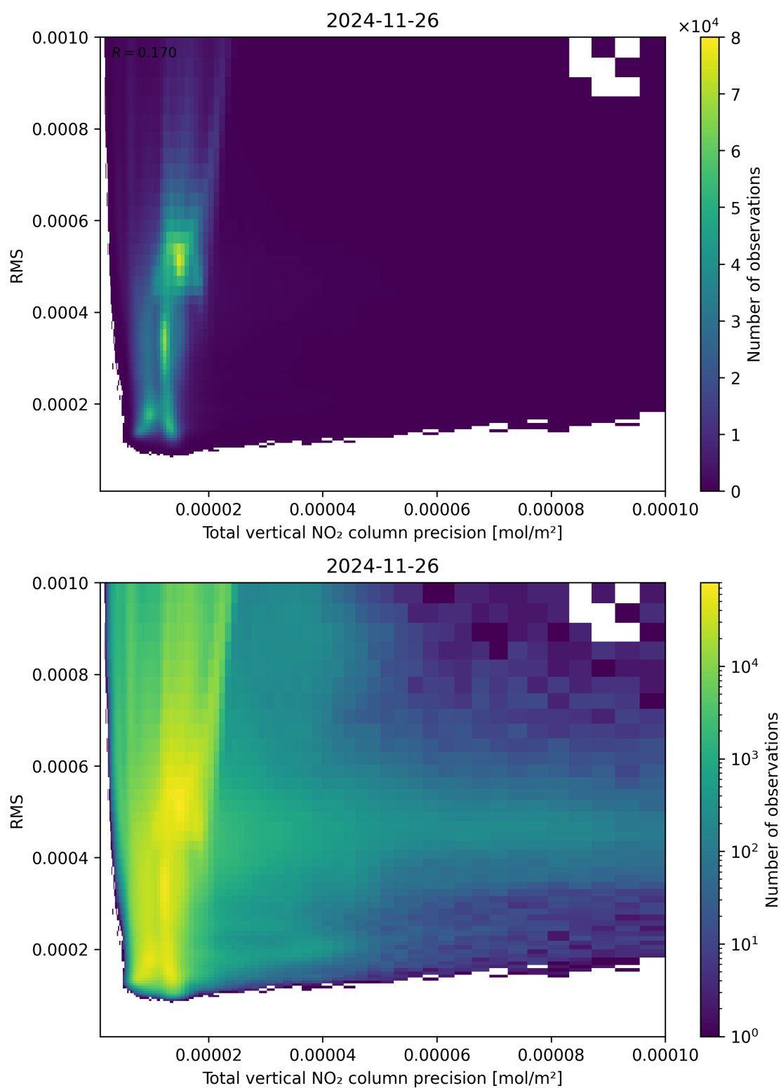
Figure 119: Scatter density plot of “Total vertical NO 2 column precision” against “RMS” for 2024-11-25 to 2024-11-27.
