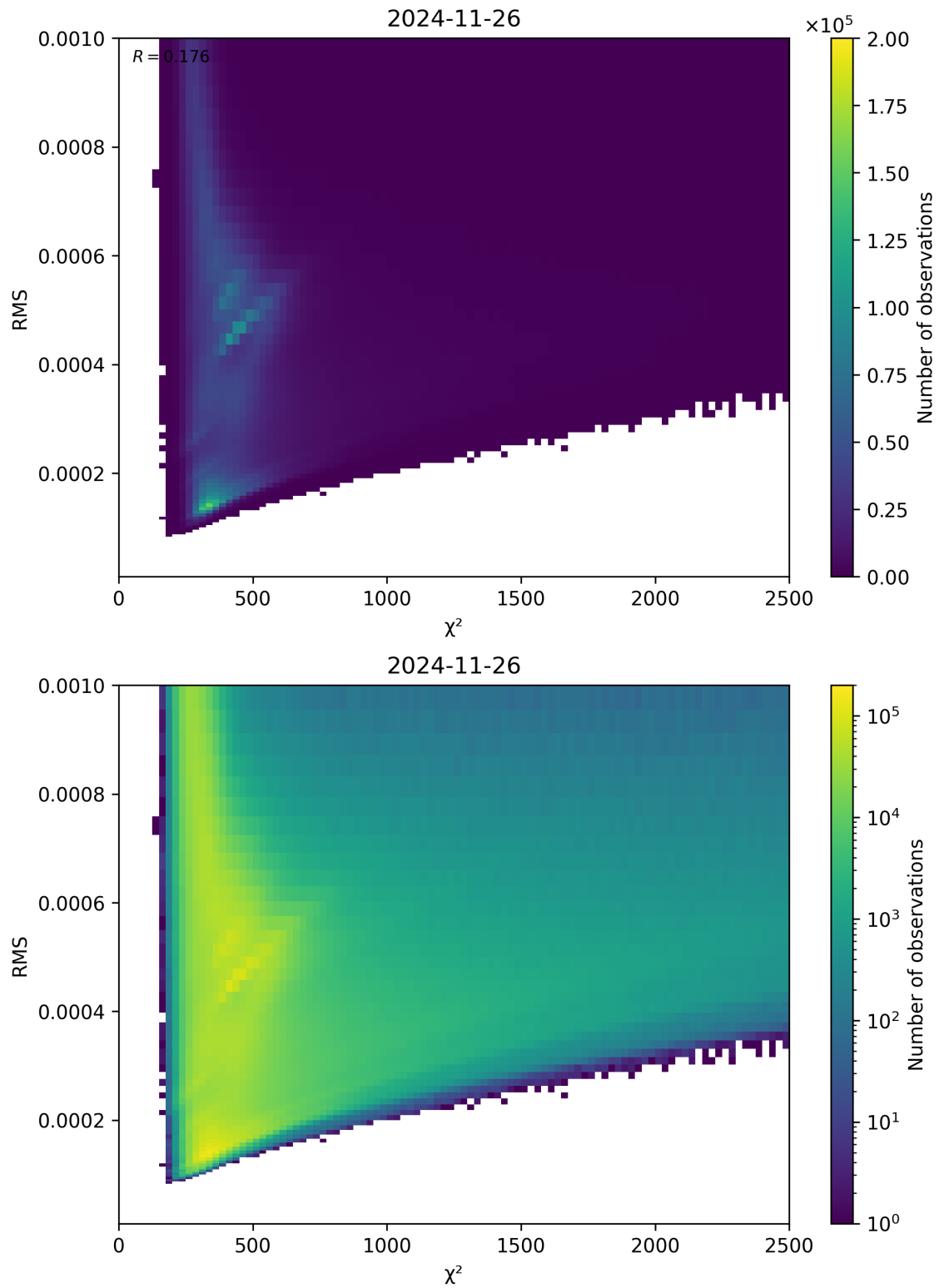
Figure 82: Scatter density plot of “ \chi^2 ” against “RMS” for 2024-11-25 to 2024-11-27.
