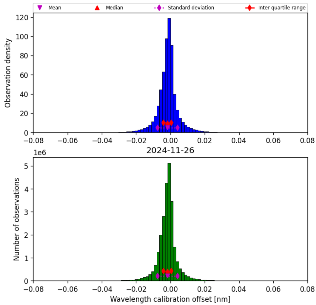
Figure 35: Histogram of “Wavelength calibration offset” for 2024-11-25 to 2024-11-27
