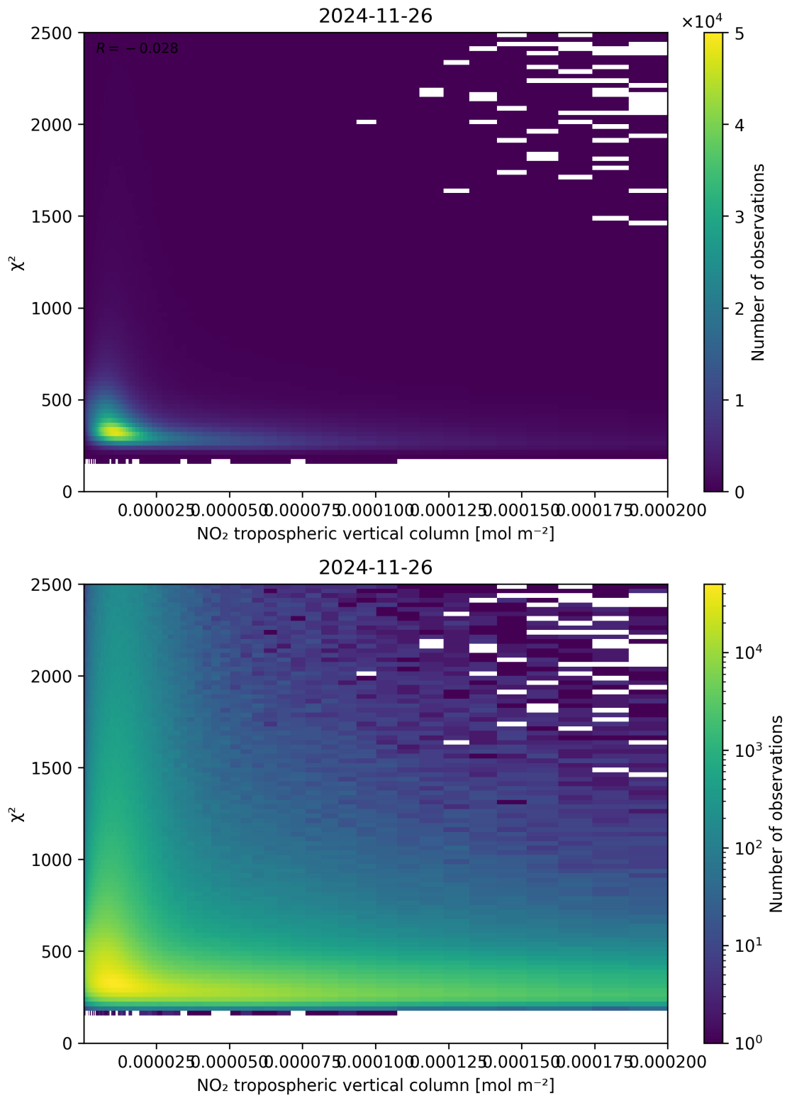
Figure 124: Scatter density plot of “NO 2 tropospheric vertical column” against “ \chi^2 ” for 2024-11-25 to 2024-11-27.
