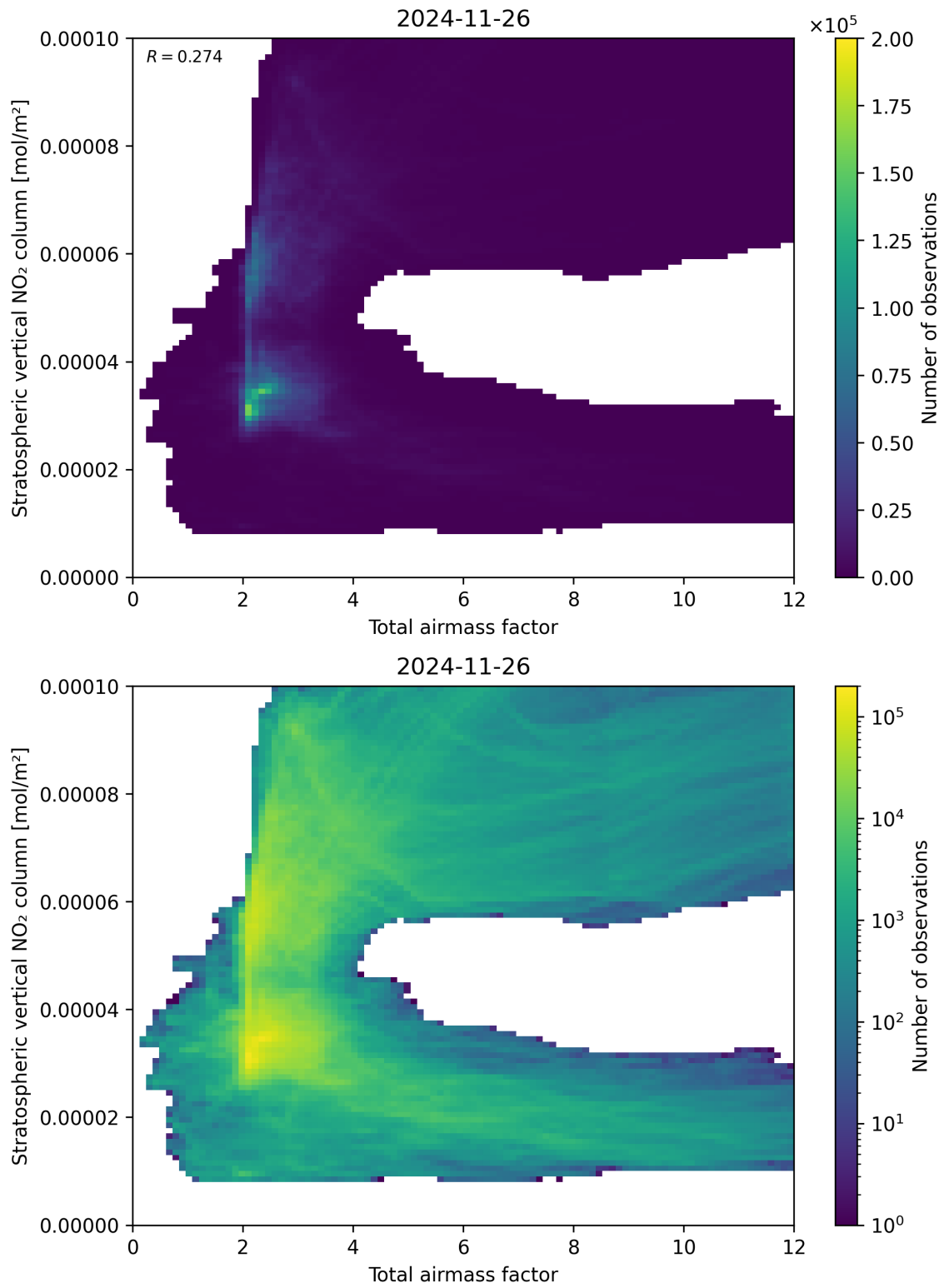
Figure 64: Scatter density plot of “Total airmass factor” against “Stratospheric vertical \text{NO}_2 column” for 2024-11-25 to 2024-11-27.
