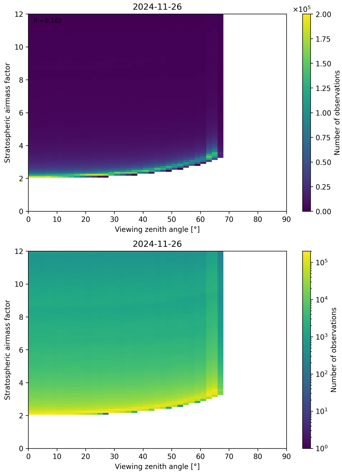
Figure 159: Scatter density plot of “Viewing zenith angle” against “Stratospheric airmass factor” for 2024-11-25 to 2024-11-27.
