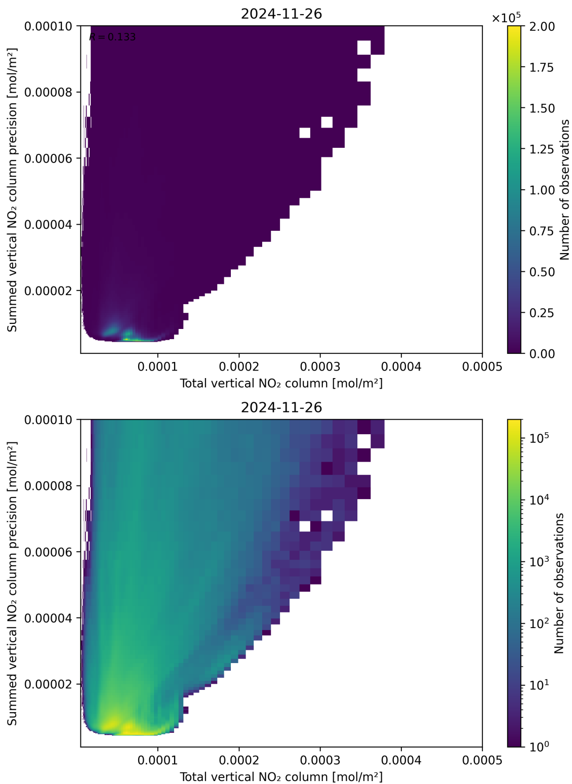
Figure 113: Scatter density plot of “Total vertical NO 2 column” against “Summed vertical NO 2 column precision” for 2024-11-25 to 2024-11-27.
