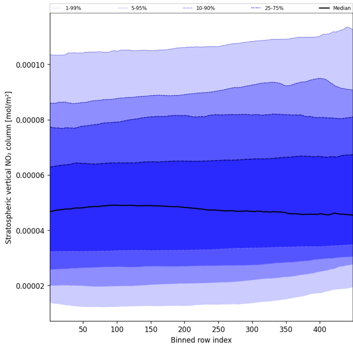
Figure 53: Along track statistics of “Stratospheric vertical NO 2 column” for 2024-11-25 to 2024-11-27
