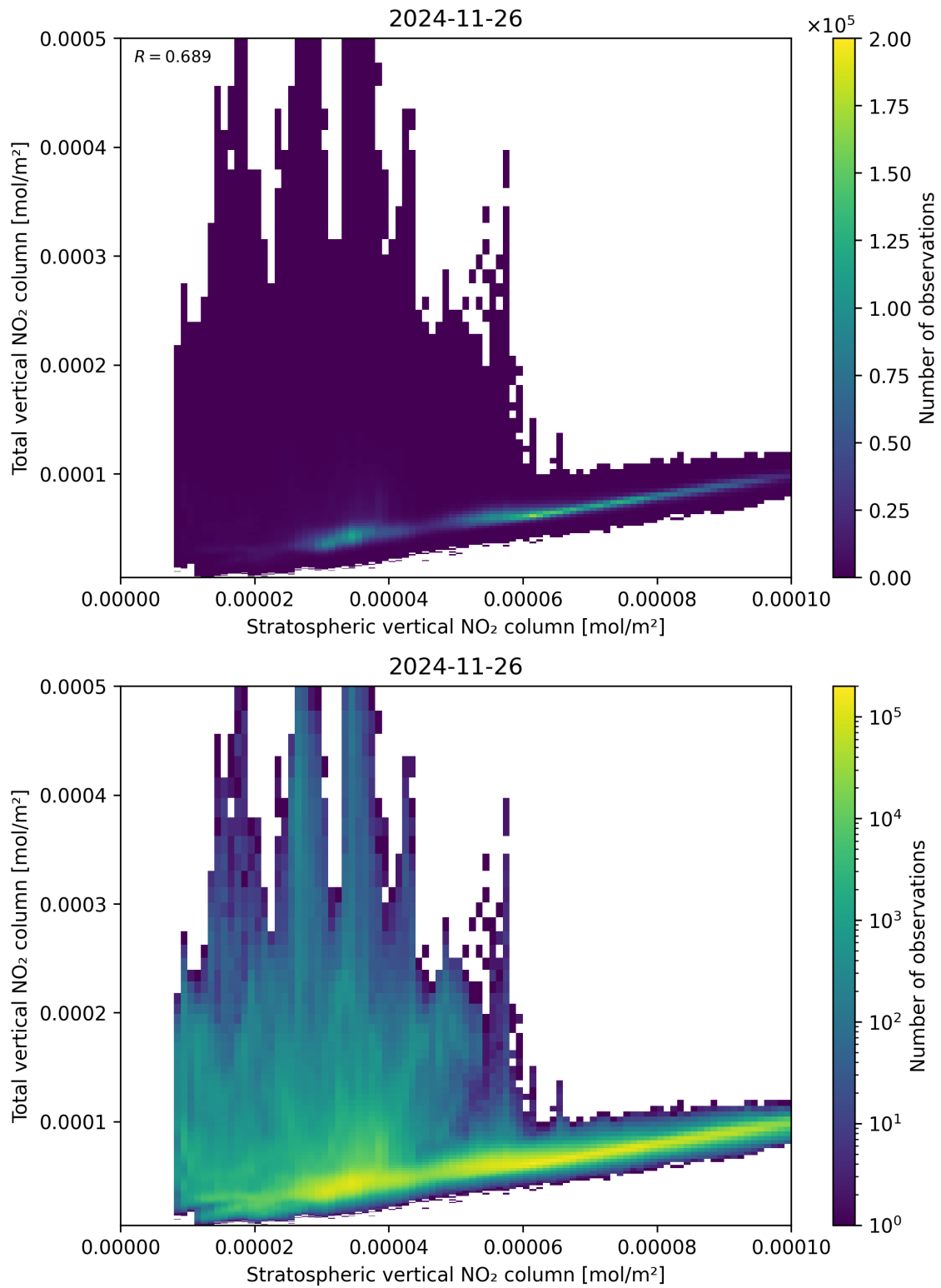
Figure 100: Scatter density plot of “Stratospheric vertical NO 2 column” against “Total vertical NO 2 column” for 2024-11-25 to 2024-11-27.
