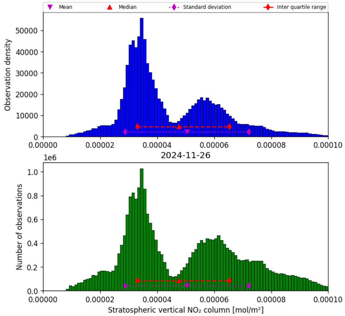
Figure 36: Histogram of “Stratospheric vertical NO 2 column” for 2024-11-25 to 2024-11-27
