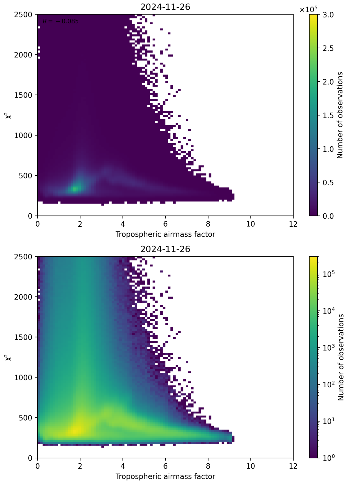
Figure 73: Scatter density plot of “Tropospheric airmass factor” against “ \chi^2 ” for 2024-11-25 to 2024-11-27.
