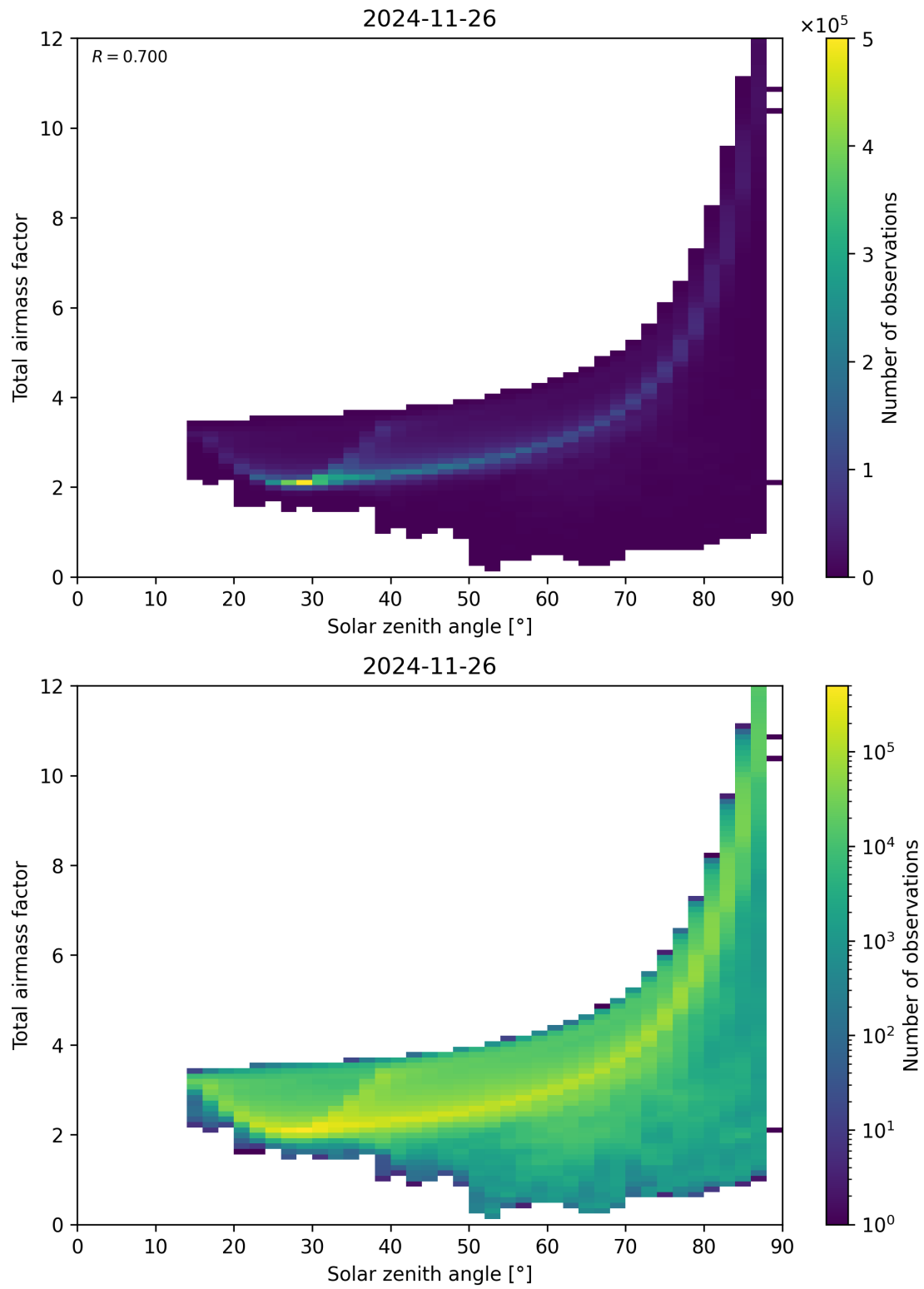
Figure 146: Scatter density plot of “Solar zenith angle” against “Total airmass factor” for 2024-11-25 to 2024-11-27.
