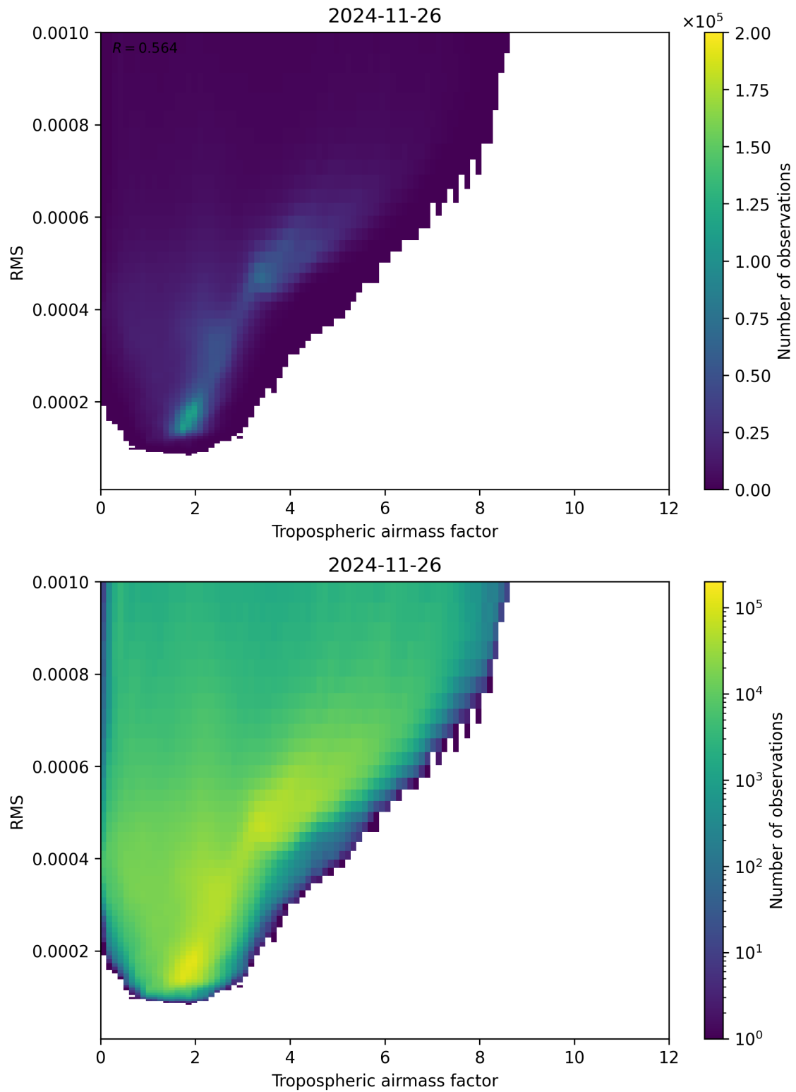
Figure 79: Scatter density plot of “Tropospheric airmass factor” against “RMS” for 2024-11-25 to 2024-11-27.
