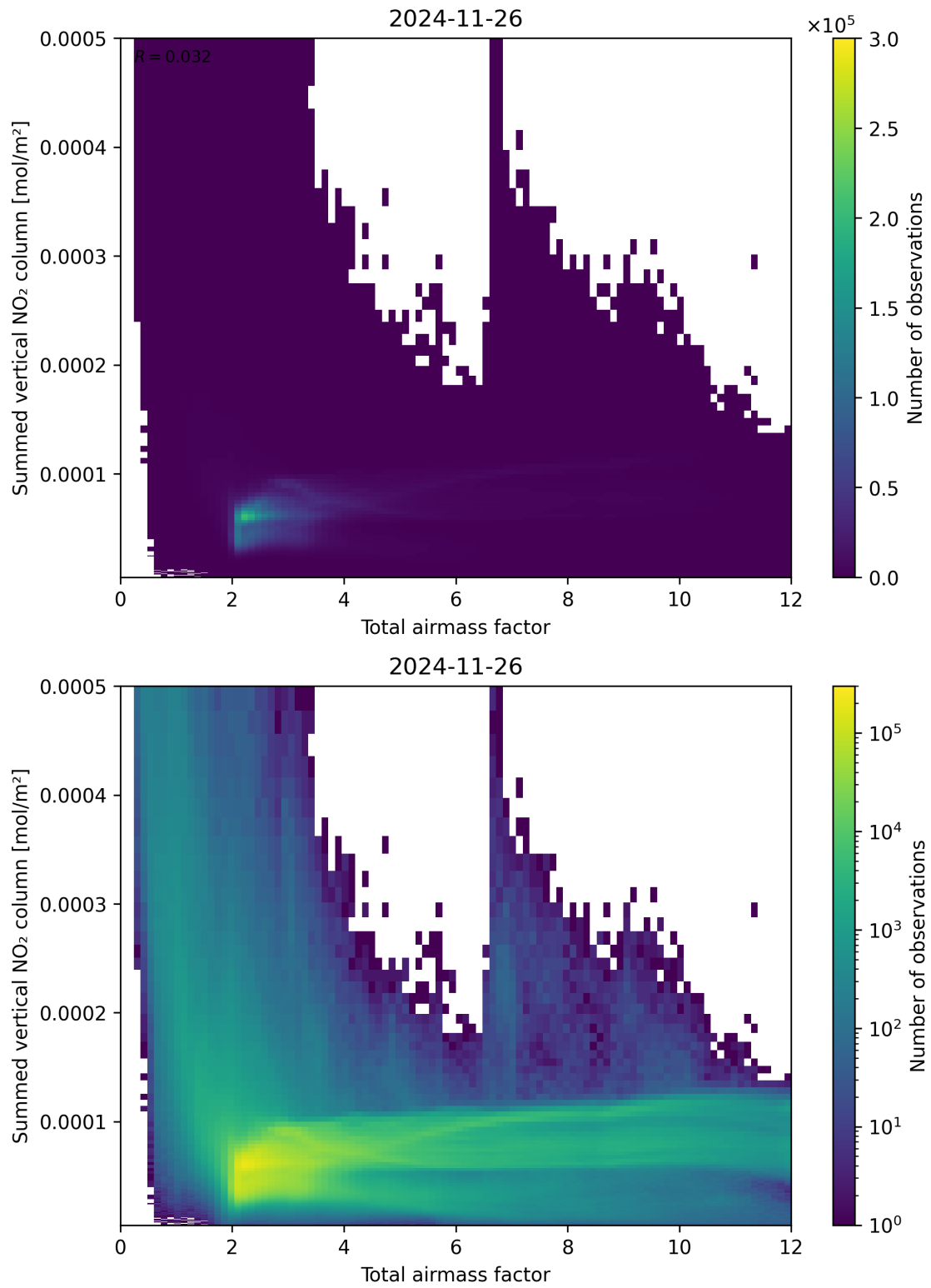
Figure 65: Scatter density plot of “Total airmass factor” against “Summed vertical NO 2 column” for 2024-11-25 to 2024-11-27.
