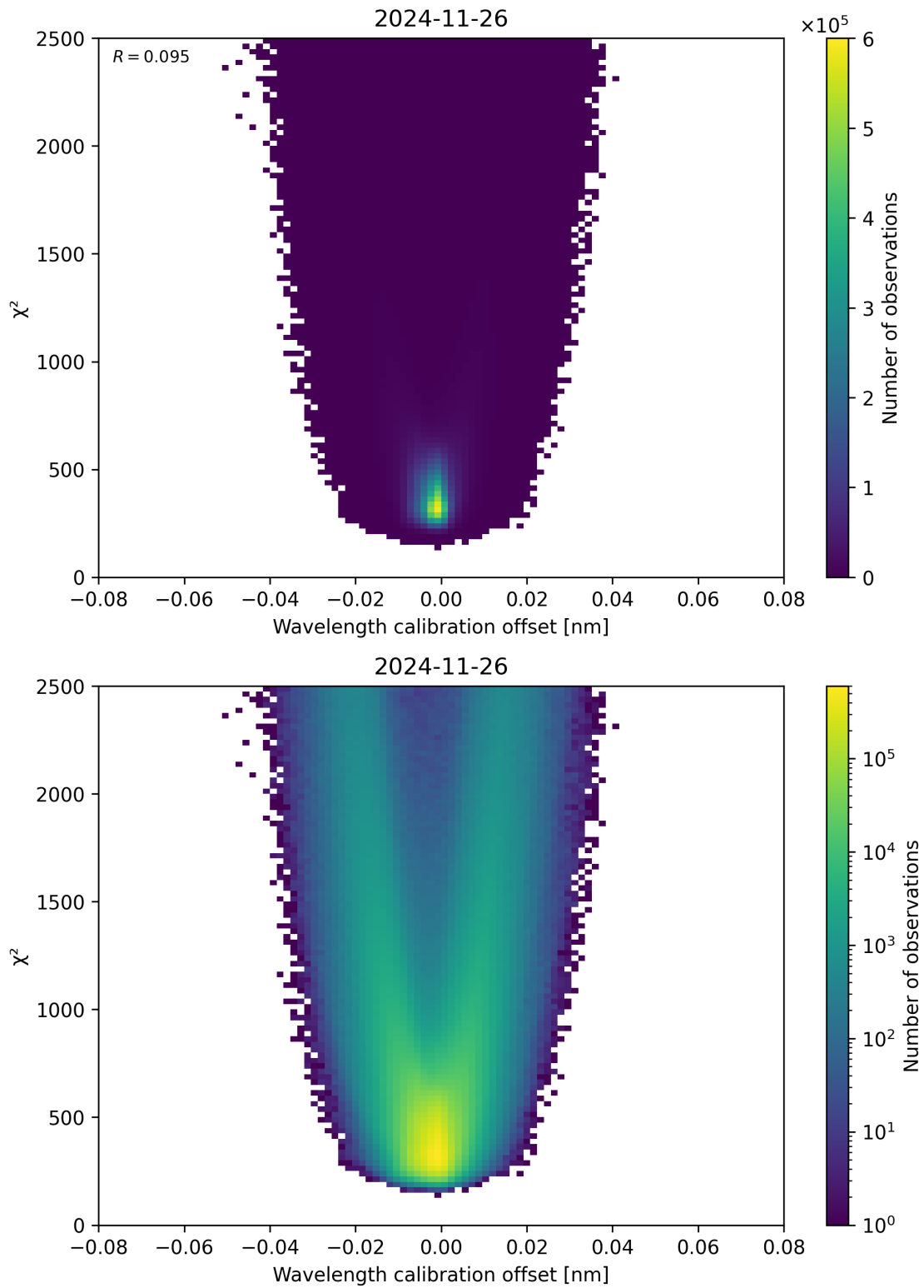
Figure 175: Scatter density plot of “Wavelength calibration offset” against “ \chi^2 ” for 2024-11-25 to 2024-11-27.
