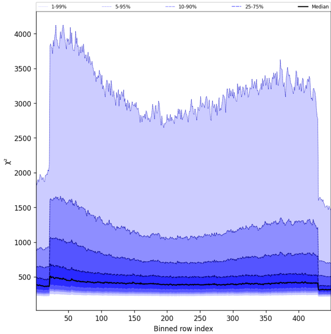
Figure 59: Along track statistics of “ \chi^2 ” for 2024-11-25 to 2024-11-27
