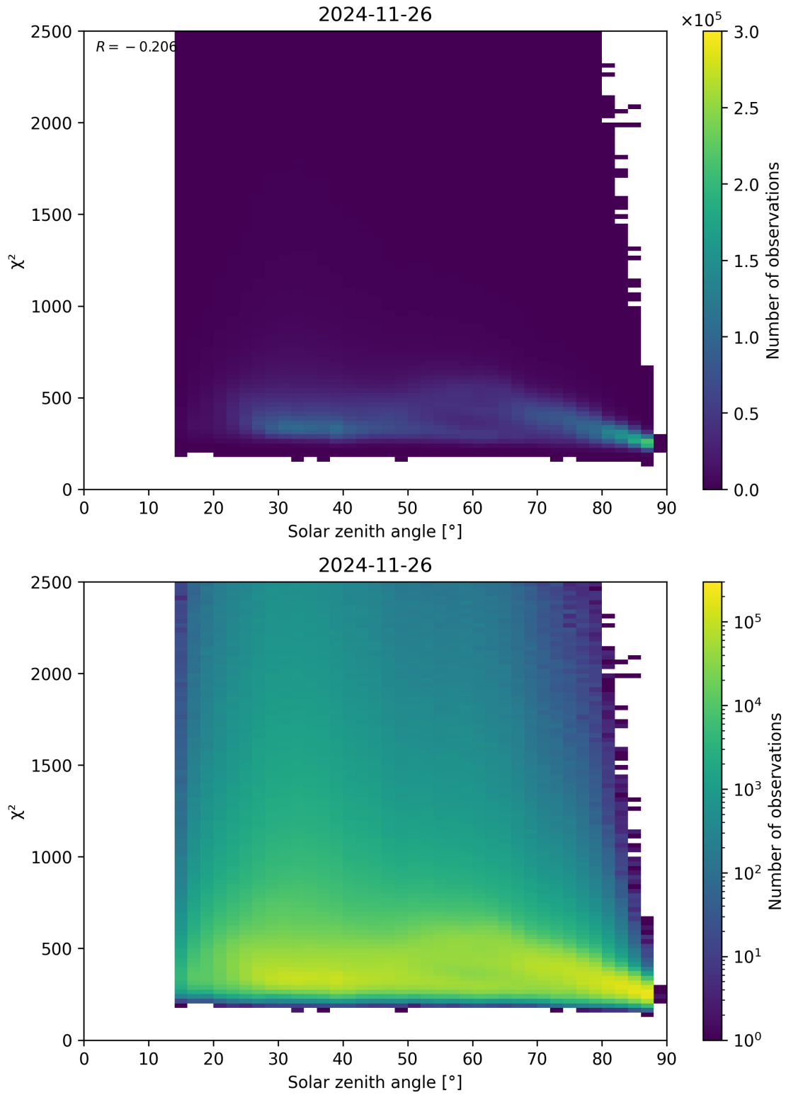
Figure 148: Scatter density plot of “Solar zenith angle” against “ \chi^2 ” for 2024-11-25 to 2024-11-27.
