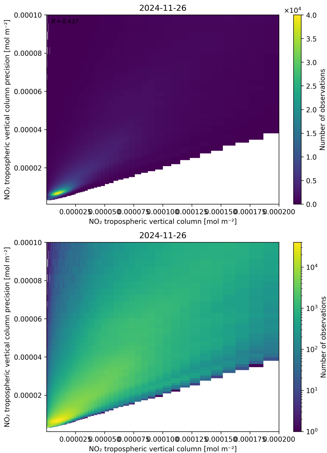
Figure 130: Scatter density plot of “NO 2 tropospheric vertical column” against “NO 2 tropospheric vertical column precision” for 2024-11-25 to 2024-11-27.
