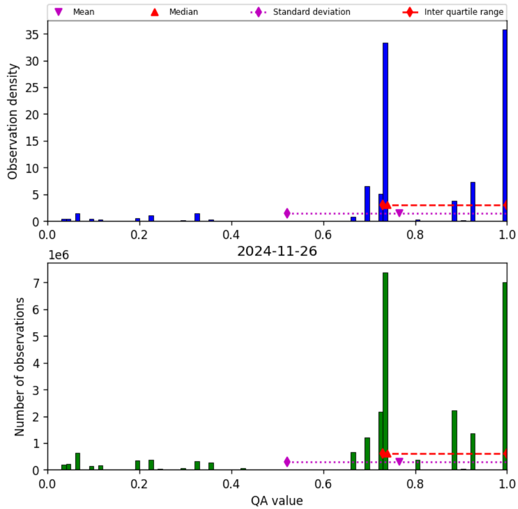
Figure 28: Histogram of “QA value” for 2024-11-25 to 2024-11-27
