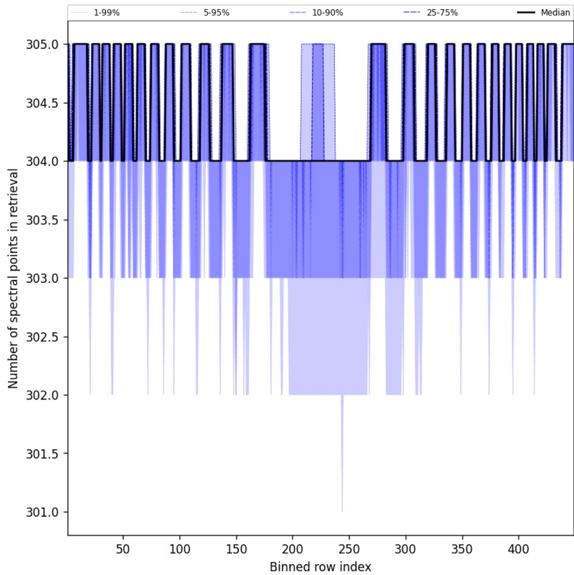
Figure 50: Along track statistics of “Number of spectral points in retrieval” for 2024-11-25 to 2024-11-27
