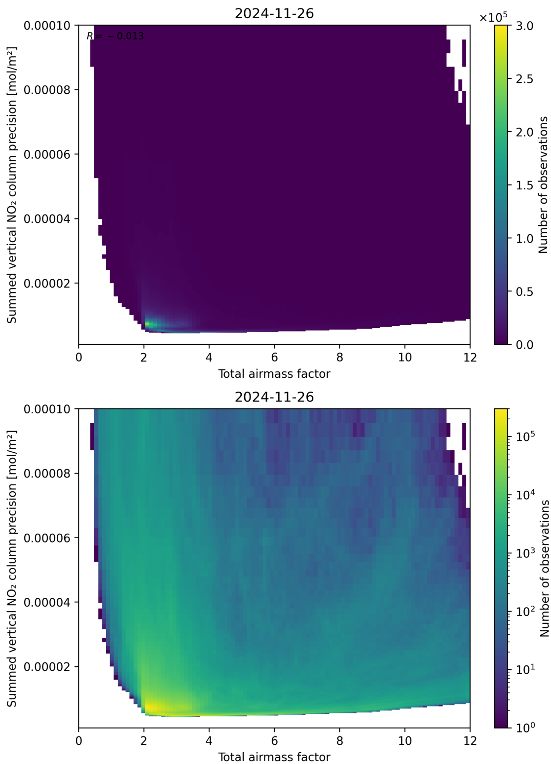
Figure 66: Scatter density plot of “Total airmass factor” against “Summed vertical NO 2 column precision” for 2024-11-25 to 2024-11-27.
