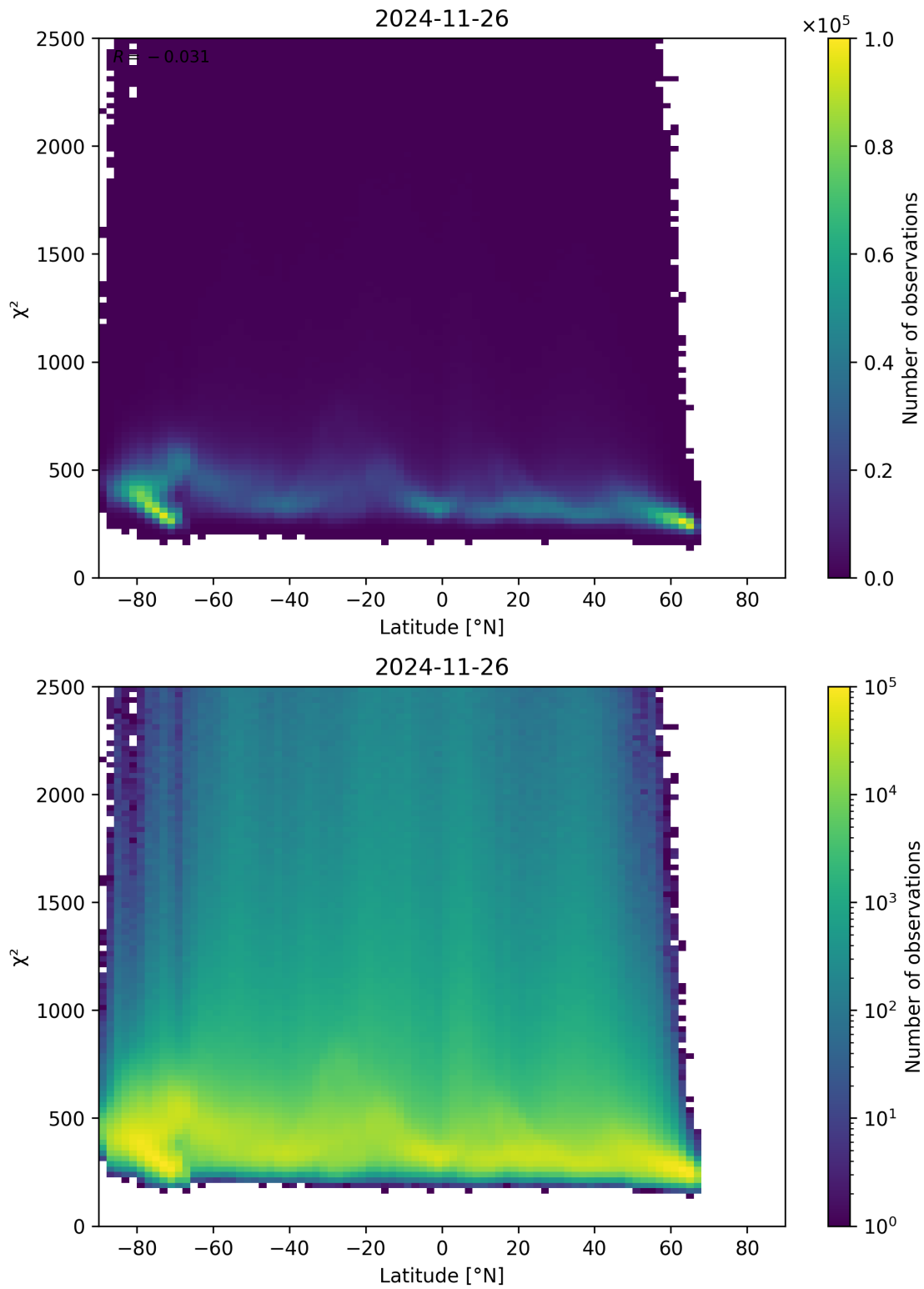
Figure 86: Scatter density plot of “Latitude” against “ \chi^2 ” for 2024-11-25 to 2024-11-27.
