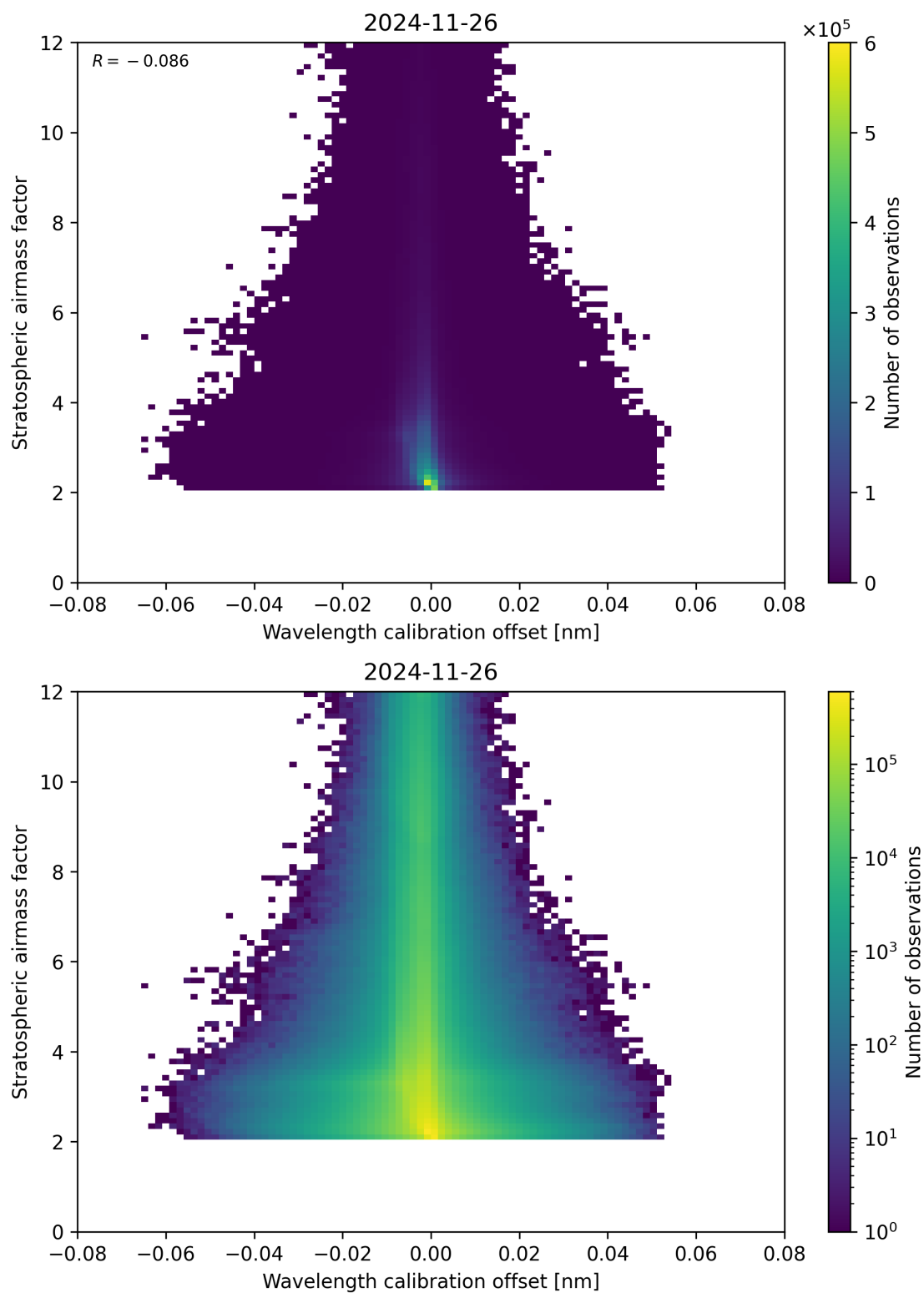
Figure 174: Scatter density plot of “Wavelength calibration offset” against “Stratospheric airmass factor” for 2024-11-25 to 2024-11-27.
