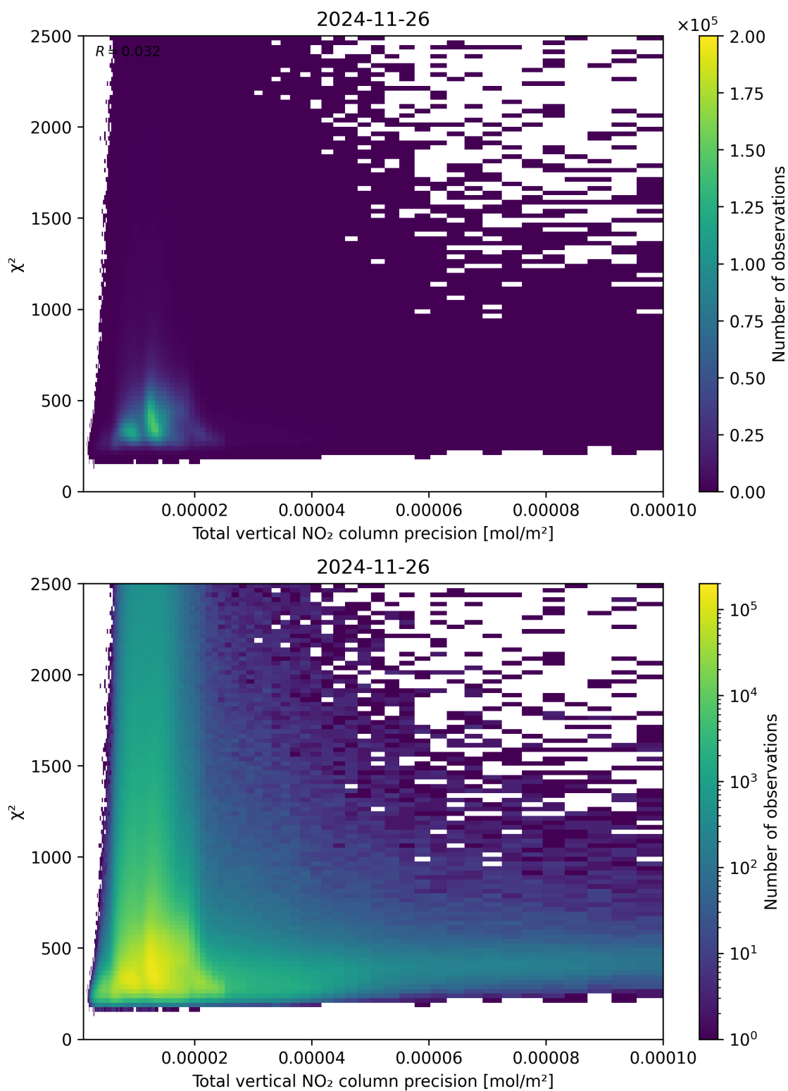
Figure 116: Scatter density plot of “Total vertical NO 2 column precision” against “ \chi^2 ” for 2024-11-25 to 2024-11-27.
