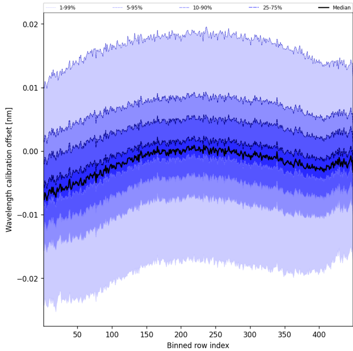
Figure 52: Along track statistics of “Wavelength calibration offset” for 2024-11-25 to 2024-11-27
