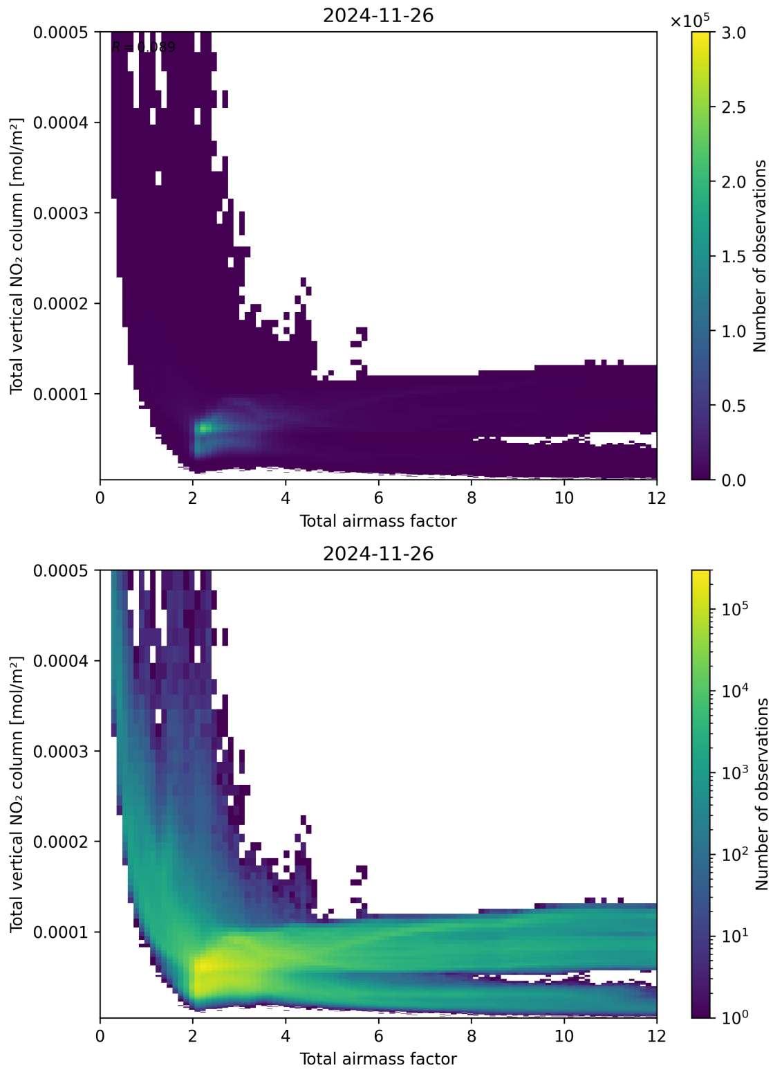
Figure 67: Scatter density plot of “Total airmass factor” against “Total vertical NO 2 column” for 2024-11-25 to 2024-11-27.
