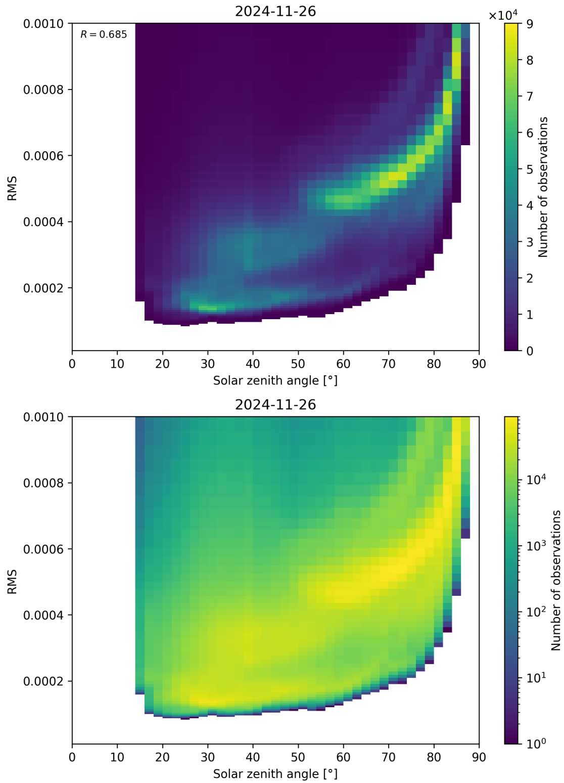
Figure 157: Scatter density plot of “Solar zenith angle” against “RMS” for 2024-11-25 to 2024-11-27.
