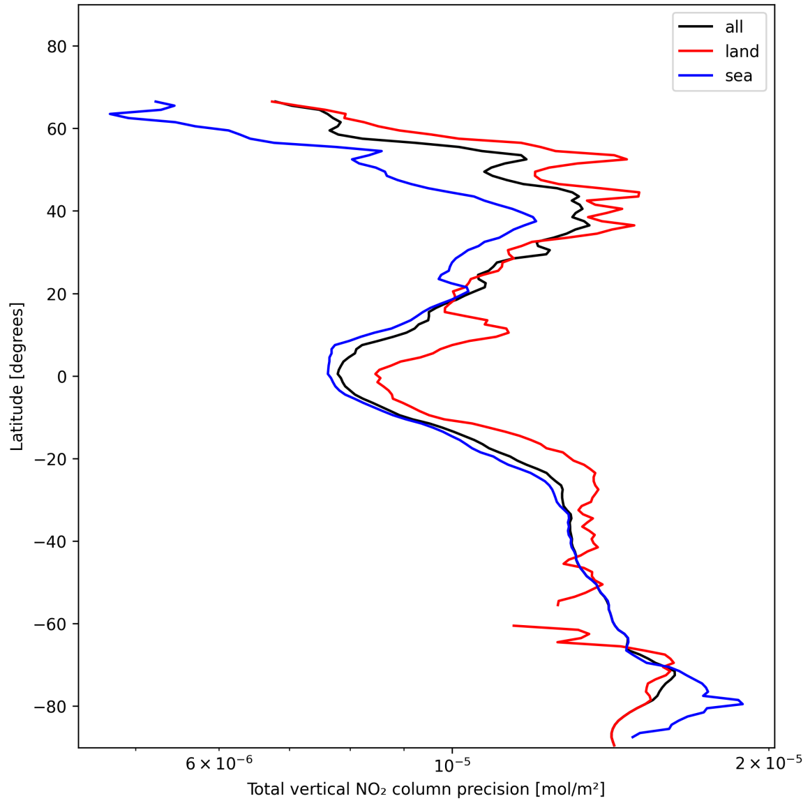
Figure 22: Zonal average of “Total vertical NO 2 column precision” for 2024-11-25 to 2024-11-27.
