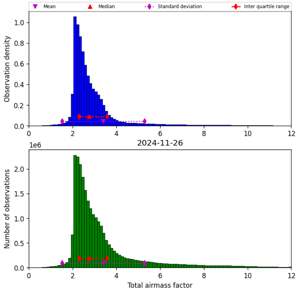
Figure 32: Histogram of “Total airmass factor” for 2024-11-25 to 2024-11-27
