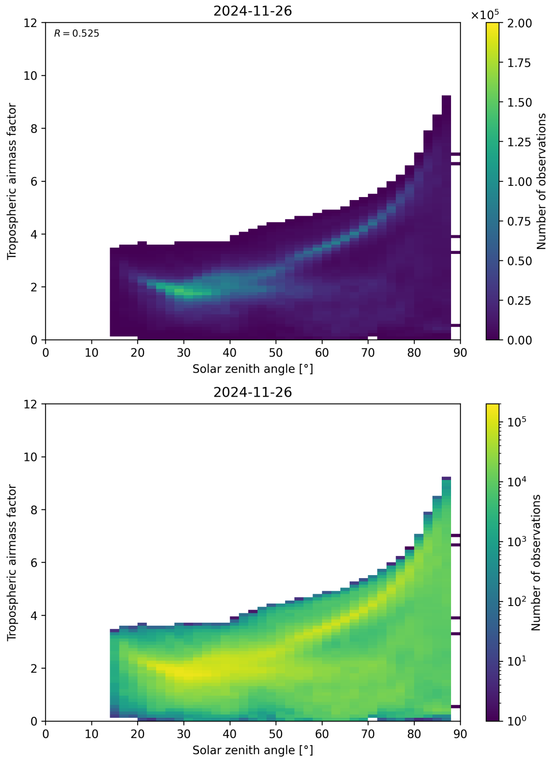
Figure 147: Scatter density plot of “Solar zenith angle” against “Tropospheric airmass factor” for 2024-11-25 to 2024-11-27.
