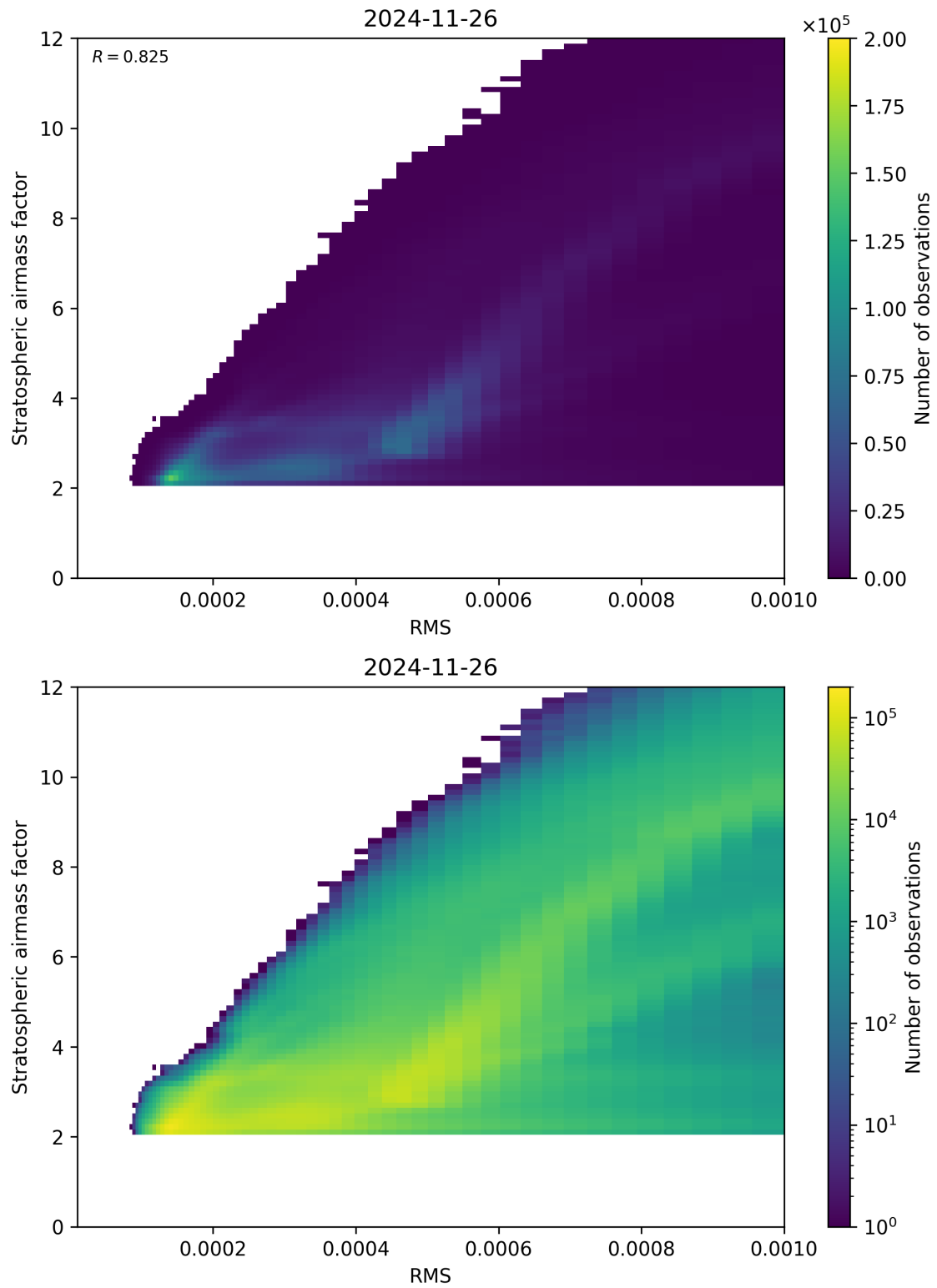
Figure 144: Scatter density plot of “RMS” against “Stratospheric airmass factor” for 2024-11-25 to 2024-11-27.
