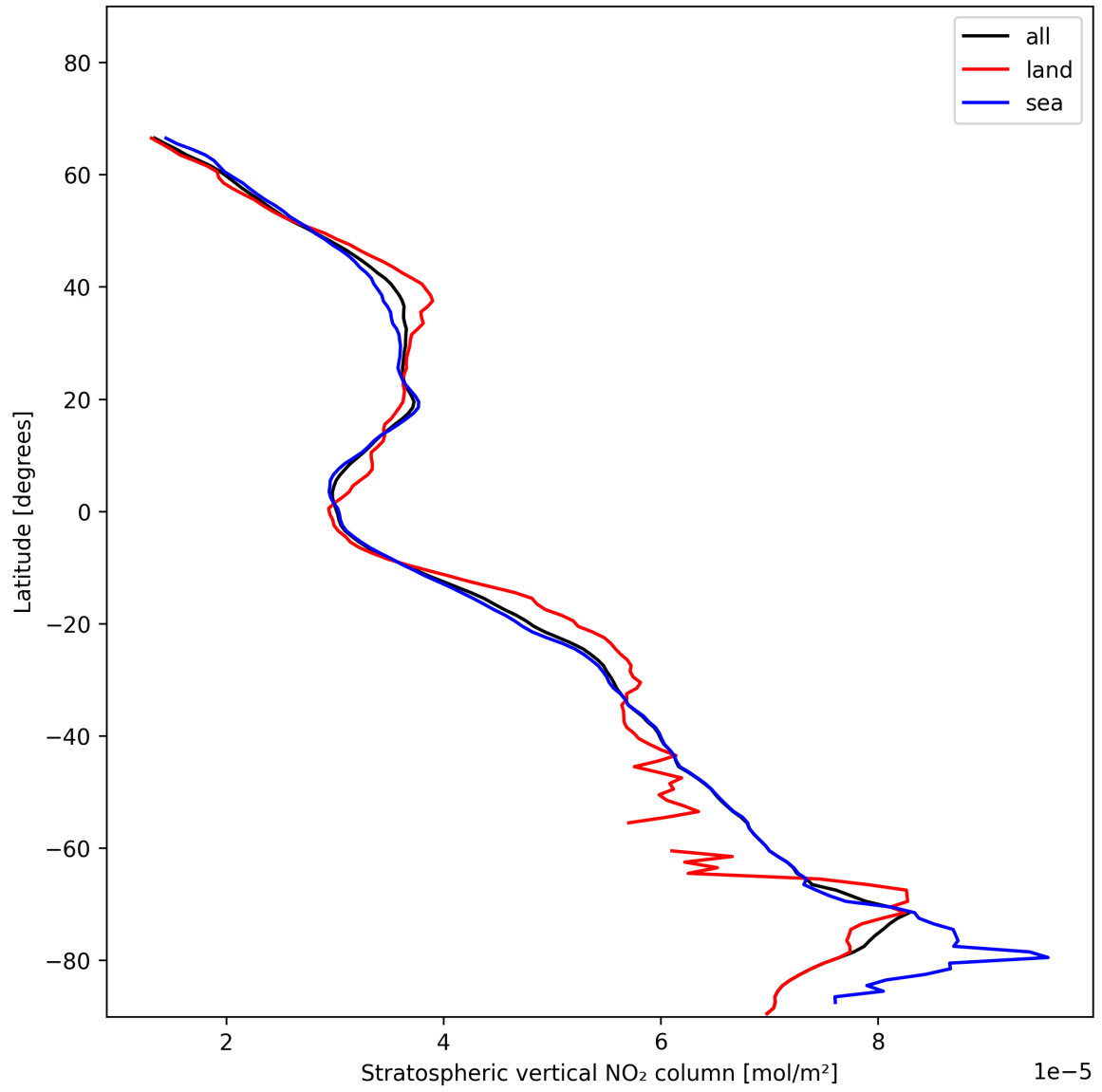
Figure 19: Zonal average of “Stratospheric vertical NO 2 column” for 2024-11-25 to 2024-11-27.
