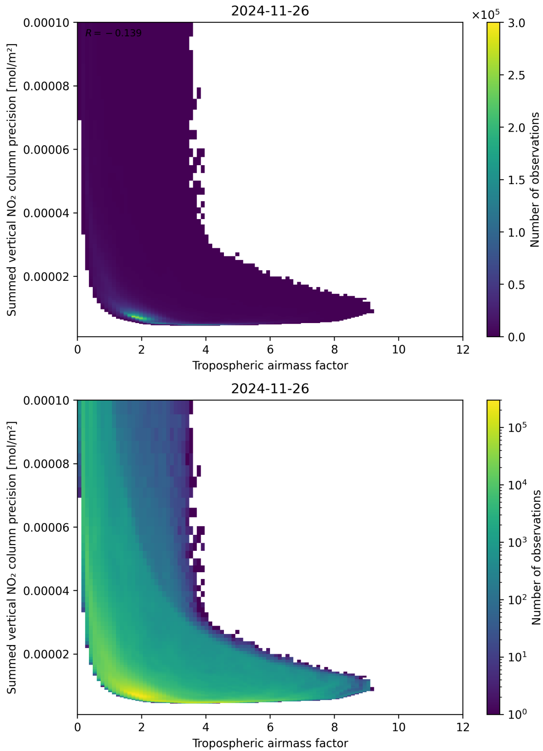
Figure 76: Scatter density plot of “Tropospheric air mass factor” against “Summed vertical NO 2 column precision” for 2024-11-25 to 2024-11-27.
