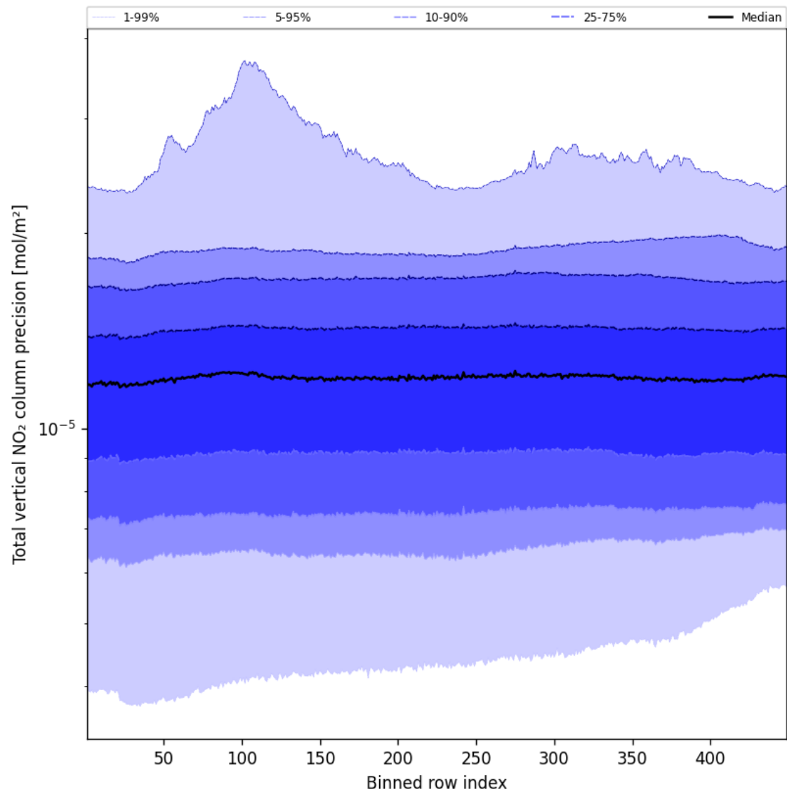
Figure 56: Along track statistics of "Total vertical NO 2 column precision" for 2024-11-25 to 2024-11-27
