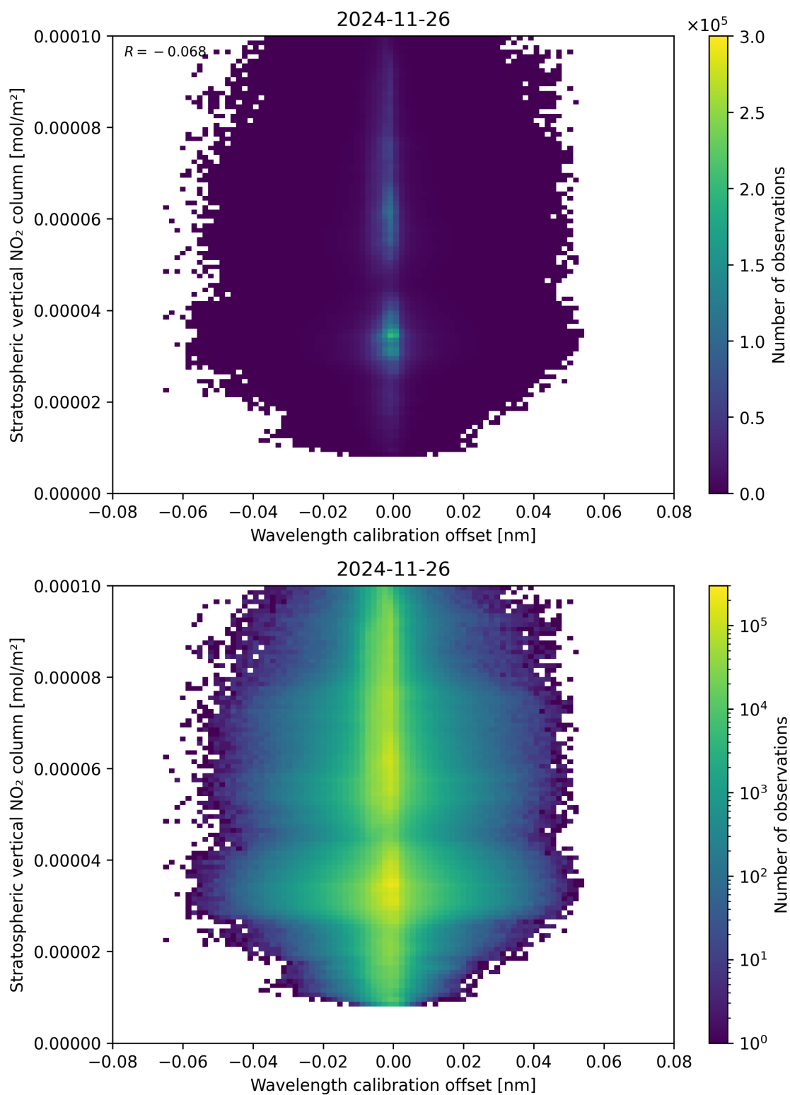
Figure 176: Scatter density plot of “Wavelength calibration offset” against “Stratospheric vertical NO 2 column” for 2024-11-25 to 2024-11-27.
