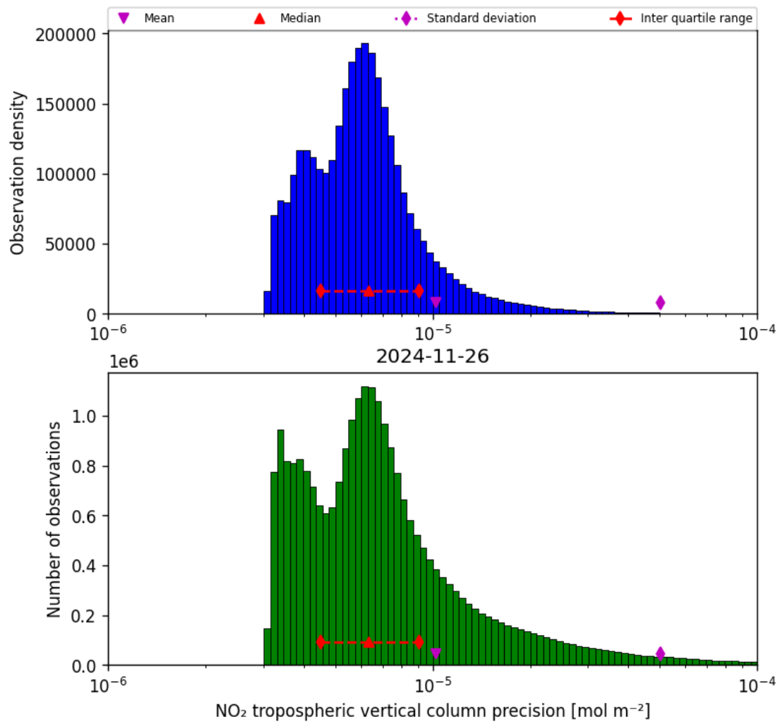
Figure 30: Histogram of “NO 2 tropospheric vertical column precision” for 2024-11-25 to 2024-11-27
