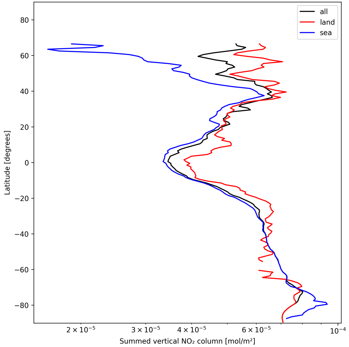
Figure 23: Zonal average of “Summed vertical NO 2 column” for 2024-11-25 to 2024-11-27.
