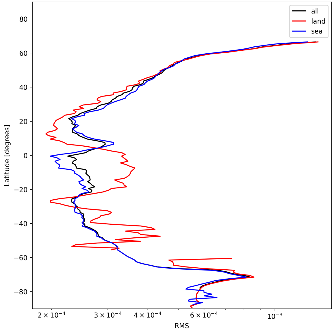
Figure 26: Zonal average of “RMS” for 2024-11-25 to 2024-11-27.
