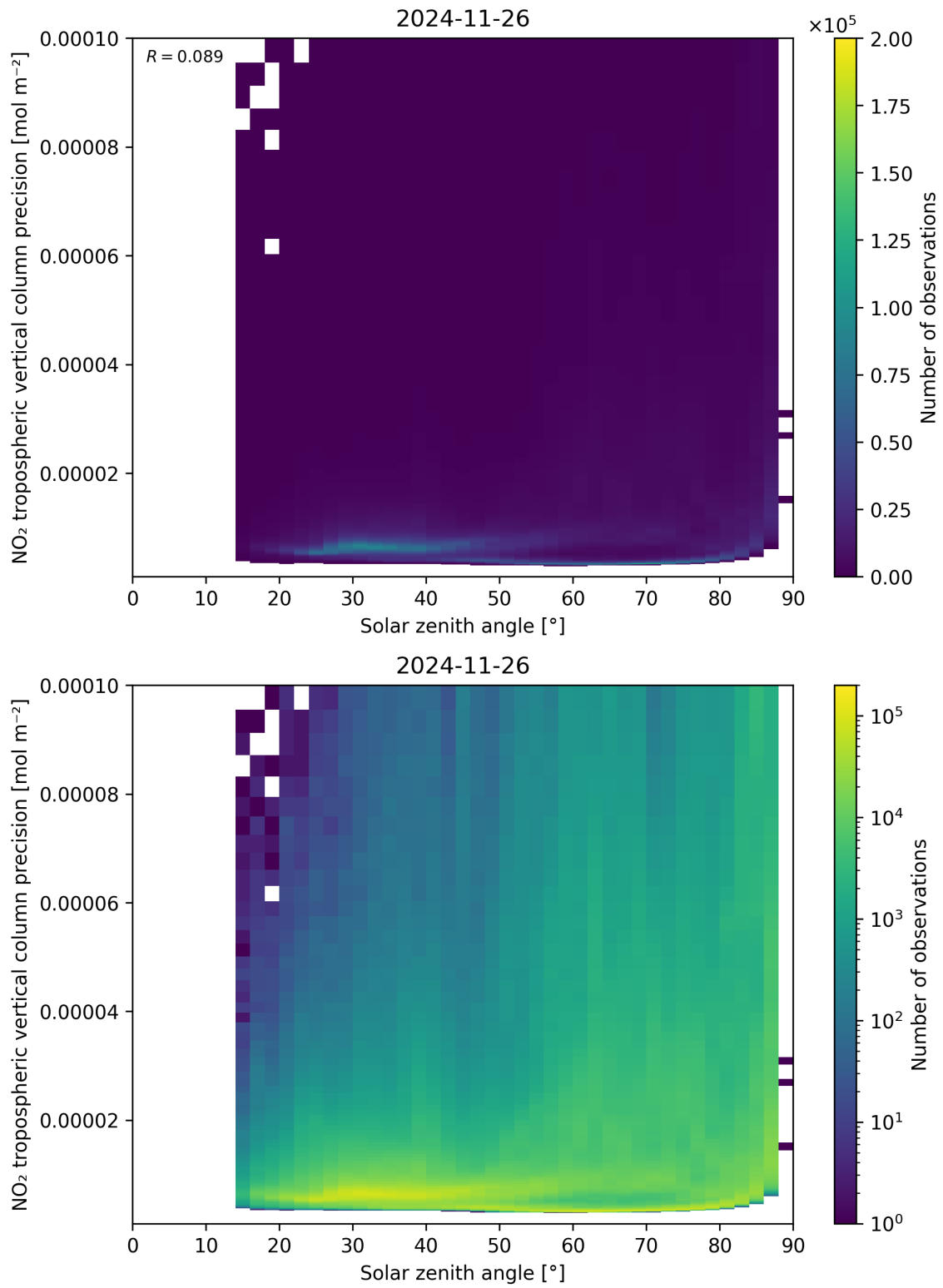
Figure 156: Scatter density plot of “Solar zenith angle” against “NO 2 tropospheric vertical column precision” for 2024-11-25 to 2024-11-27.
