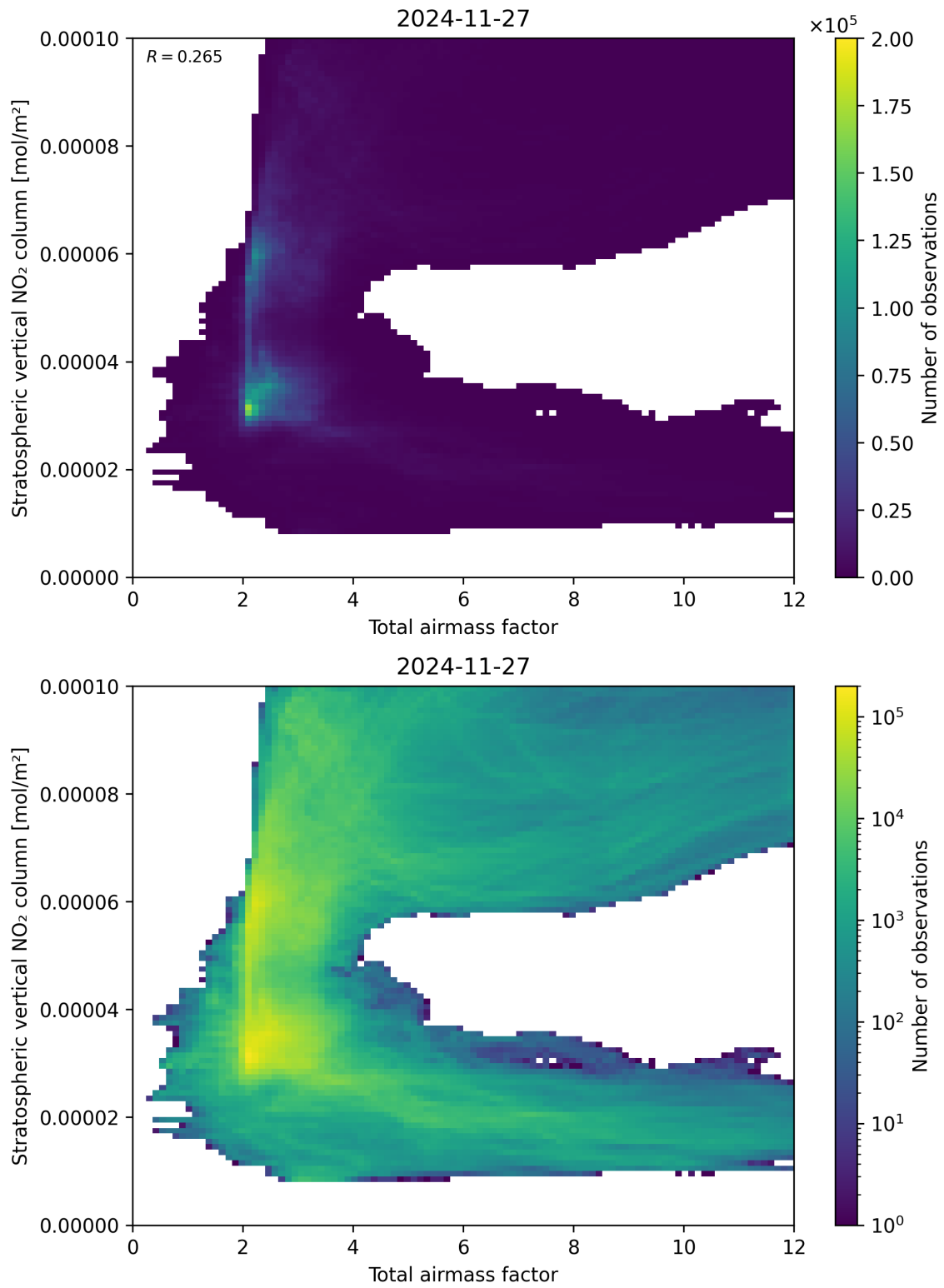
Figure 64: Scatter density plot of “Total airmass factor” against “Stratospheric vertical NO 2 column” for 2024-11-26 to 2024-11-28.
