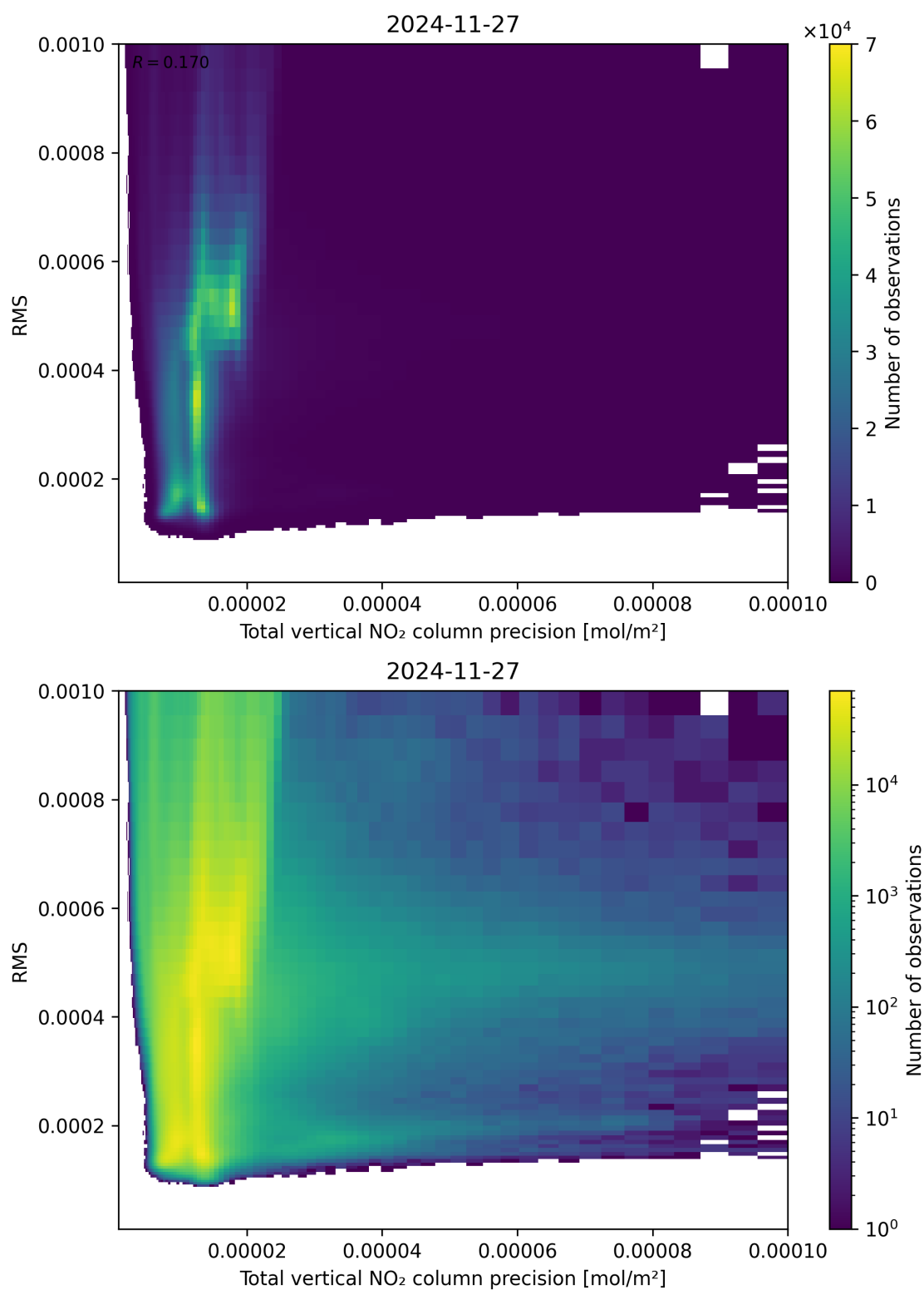
Figure 119: Scatter density plot of “Total vertical NO 2 column precision” against “RMS” for 2024-11-26 to 2024-11-28.
