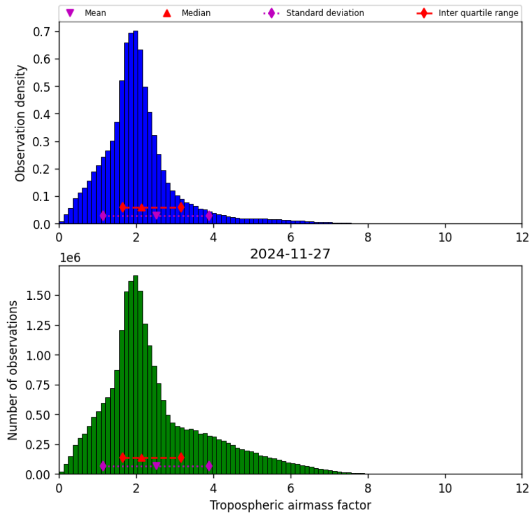
Figure 31: Histogram of “Tropospheric airmass factor” for 2024-11-26 to 2024-11-28
