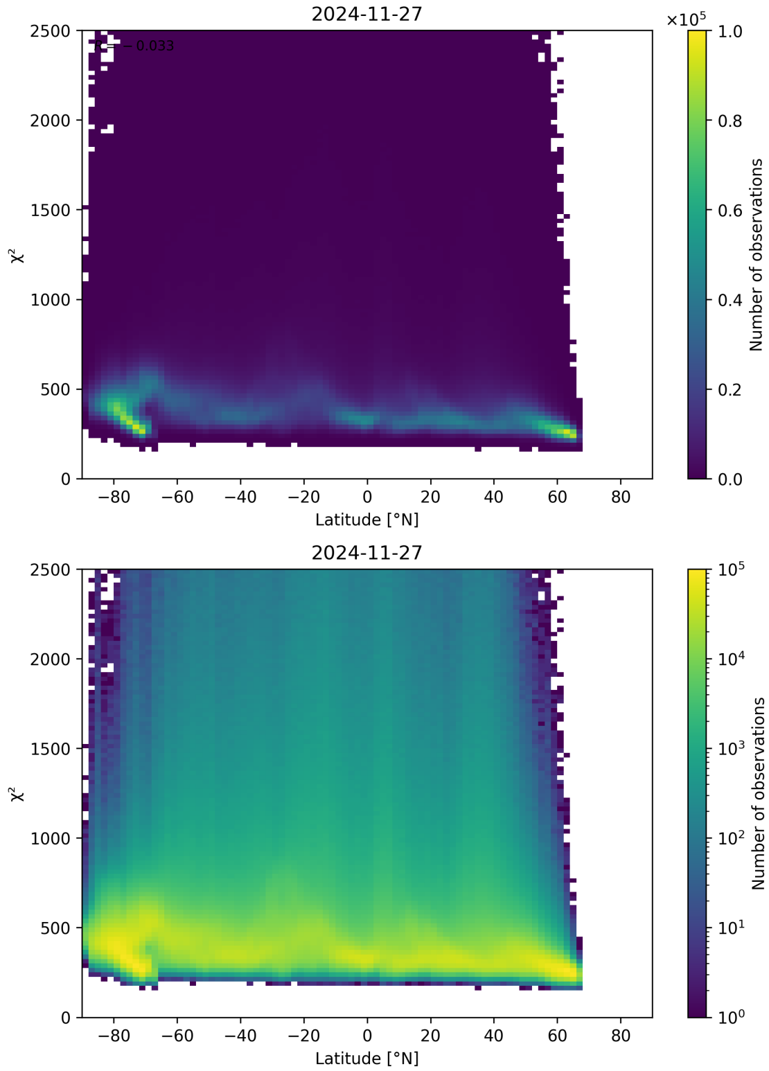
Figure 86: Scatter density plot of “Latitude” against “ \chi^2 ” for 2024-11-26 to 2024-11-28.
