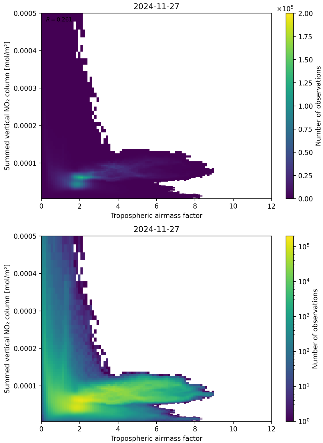
Figure 75: Scatter density plot of “Tropospheric air mass factor” against “Summed vertical NO 2 column” for 2024-11-26 to 2024-11-28.
