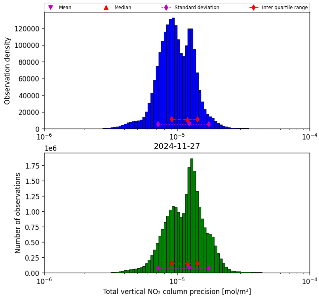
Figure 39: Histogram of “Total vertical NO 2 column precision” for 2024-11-26 to 2024-11-28
