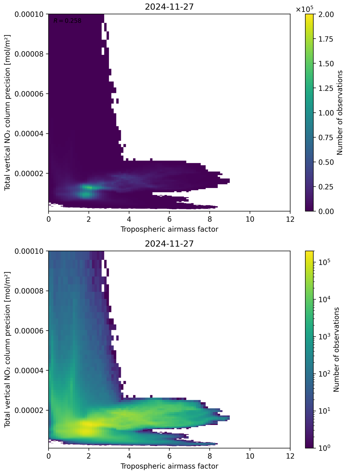
Figure 78: Scatter density plot of “Tropospheric air mass factor” against “Total vertical NO 2 column precision” for 2024-11-26 to 2024-11-28.
