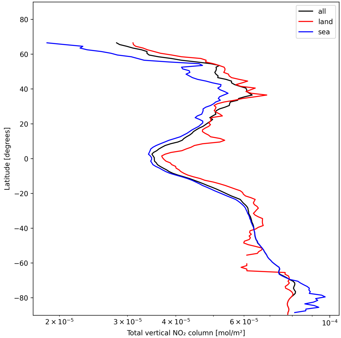
Figure 21: Zonal average of “Total vertical NO 2 column” for 2024-11-26 to 2024-11-28.
