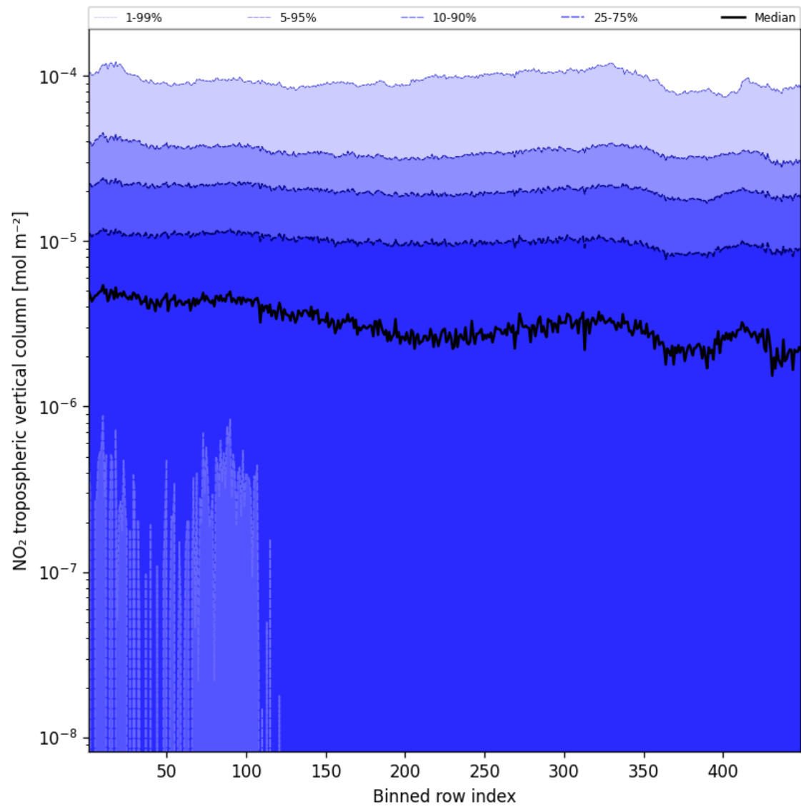
Figure 46: Along track statistics of “NO 2 tropospheric vertical column” for 2024-11-26 to 2024-11-28
