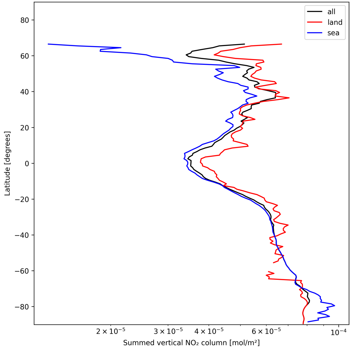
Figure 23: Zonal average of “Summed vertical NO 2 column” for 2024-11-26 to 2024-11-28.
