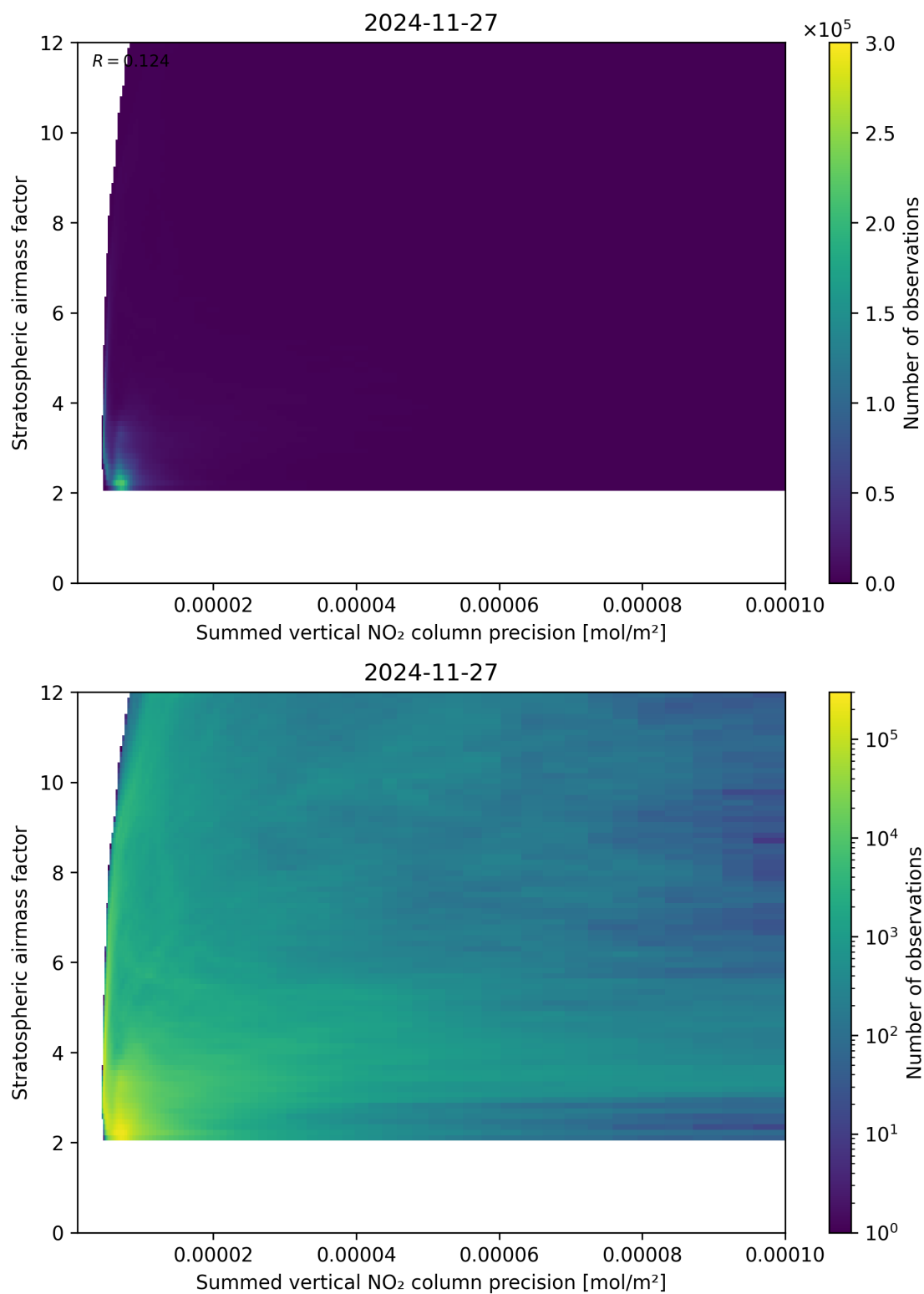
Figure 106: Scatter density plot of “Summed vertical NO 2 column precision” against “Stratospheric airmass factor” for 2024-11-26 to 2024-11-28.
