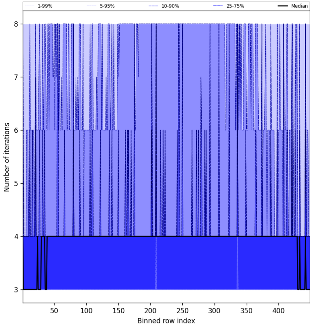
Figure 51: Along track statistics of “Number of iterations” for 2024-11-26 to 2024-11-28
