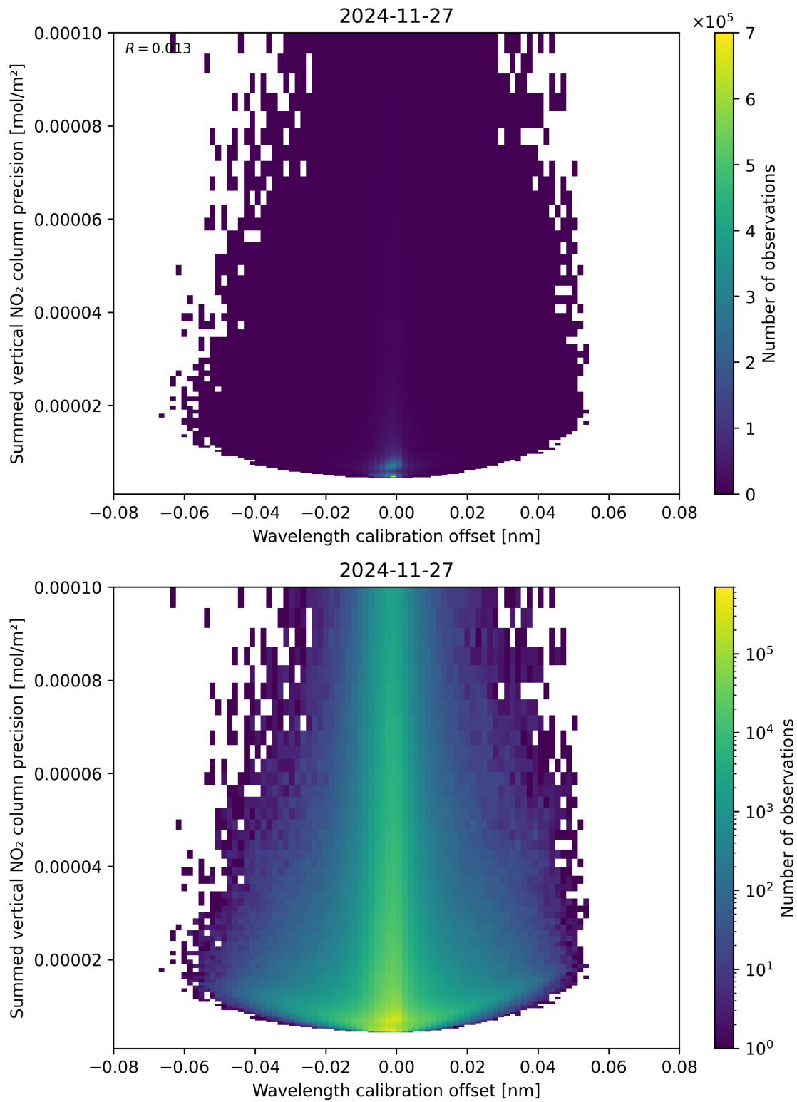
Figure 178: Scatter density plot of “Wavelength calibration offset” against “Summed vertical NO 2 column precision” for 2024-11-26 to 2024-11-28.
