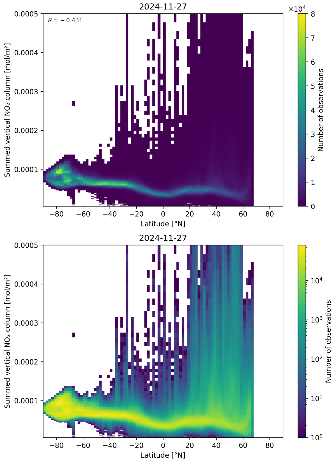
Figure 88: Scatter density plot of “Latitude” against “Summed vertical NO 2 column” for 2024-11-26 to 2024-11-28.
