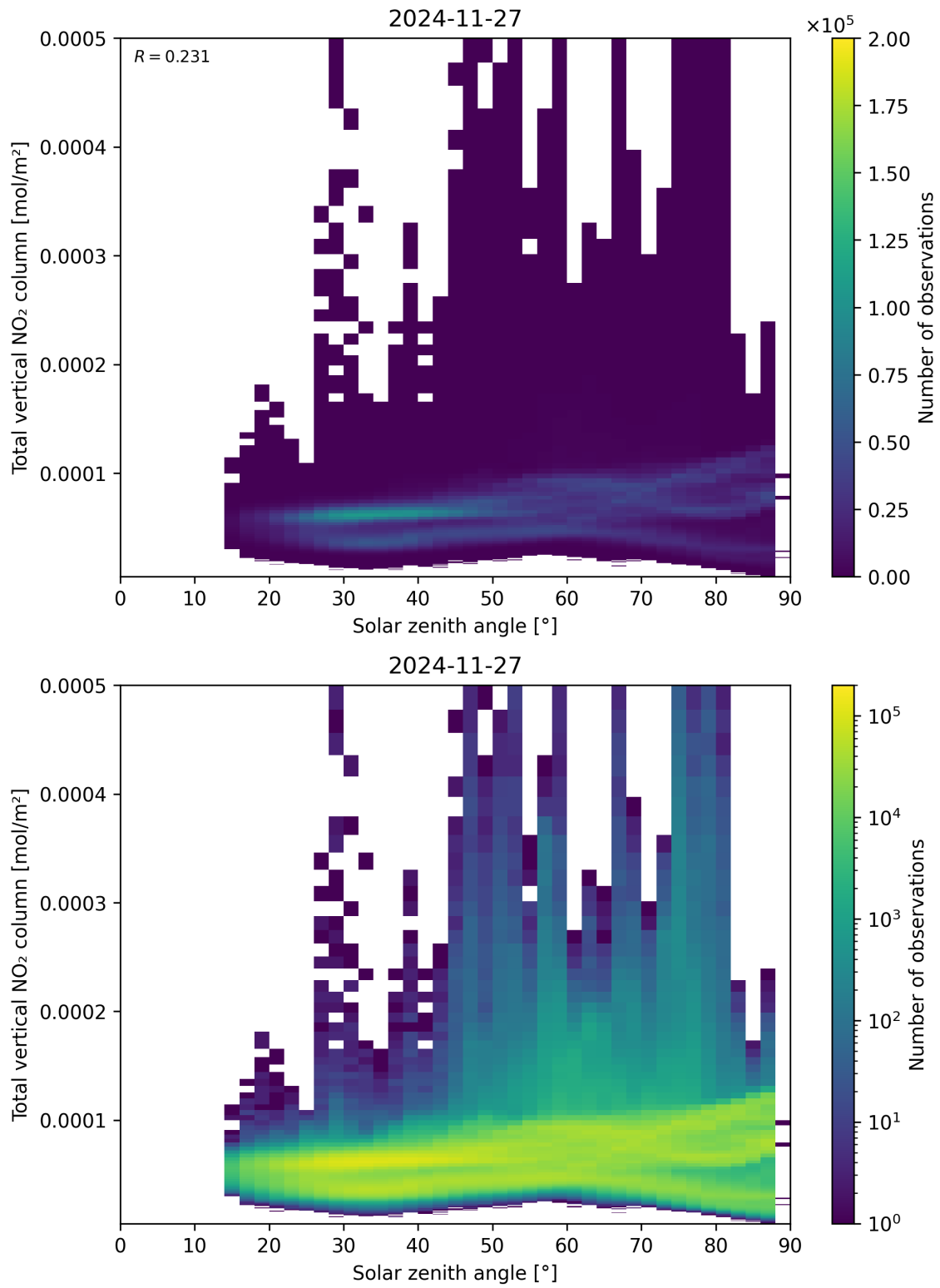
Figure 153: Scatter density plot of “Solar zenith angle” against “Total vertical NO 2 column” for 2024-11-26 to 2024-11-28.
