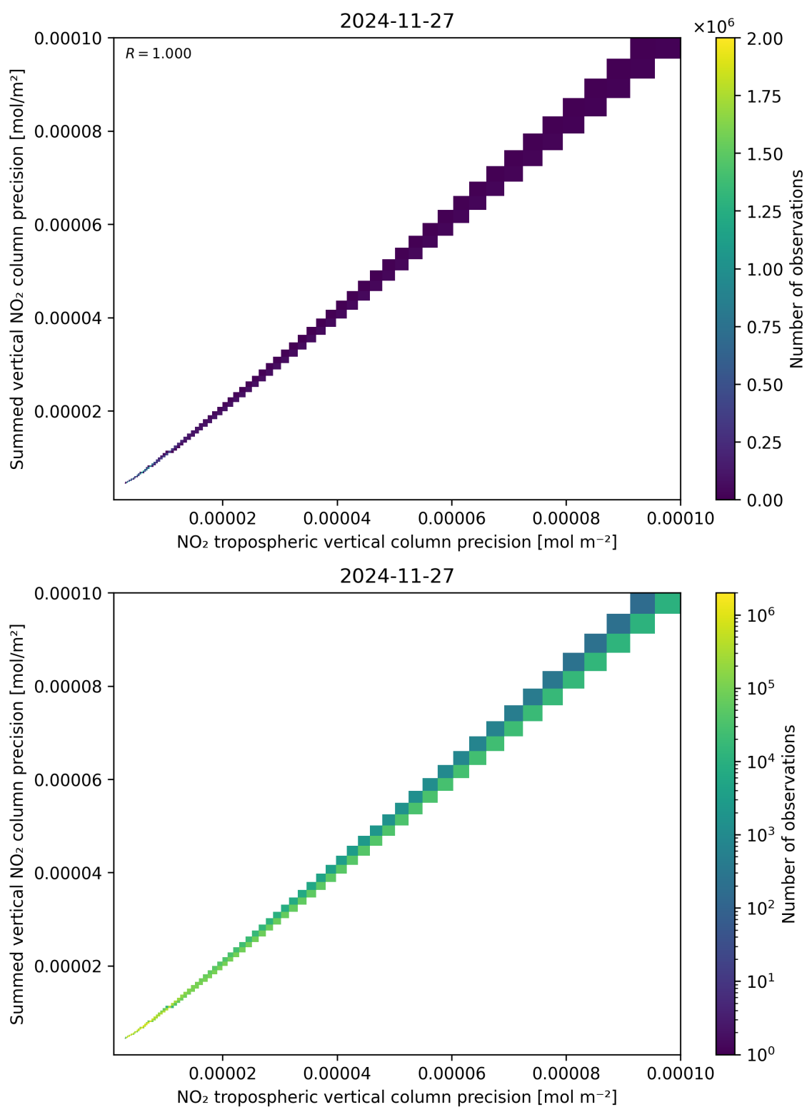
Figure 137: Scatter density plot of “NO 2 tropospheric vertical column precision” against “Summed vertical NO 2 column precision” for 2024-11-26 to 2024-11-28.
