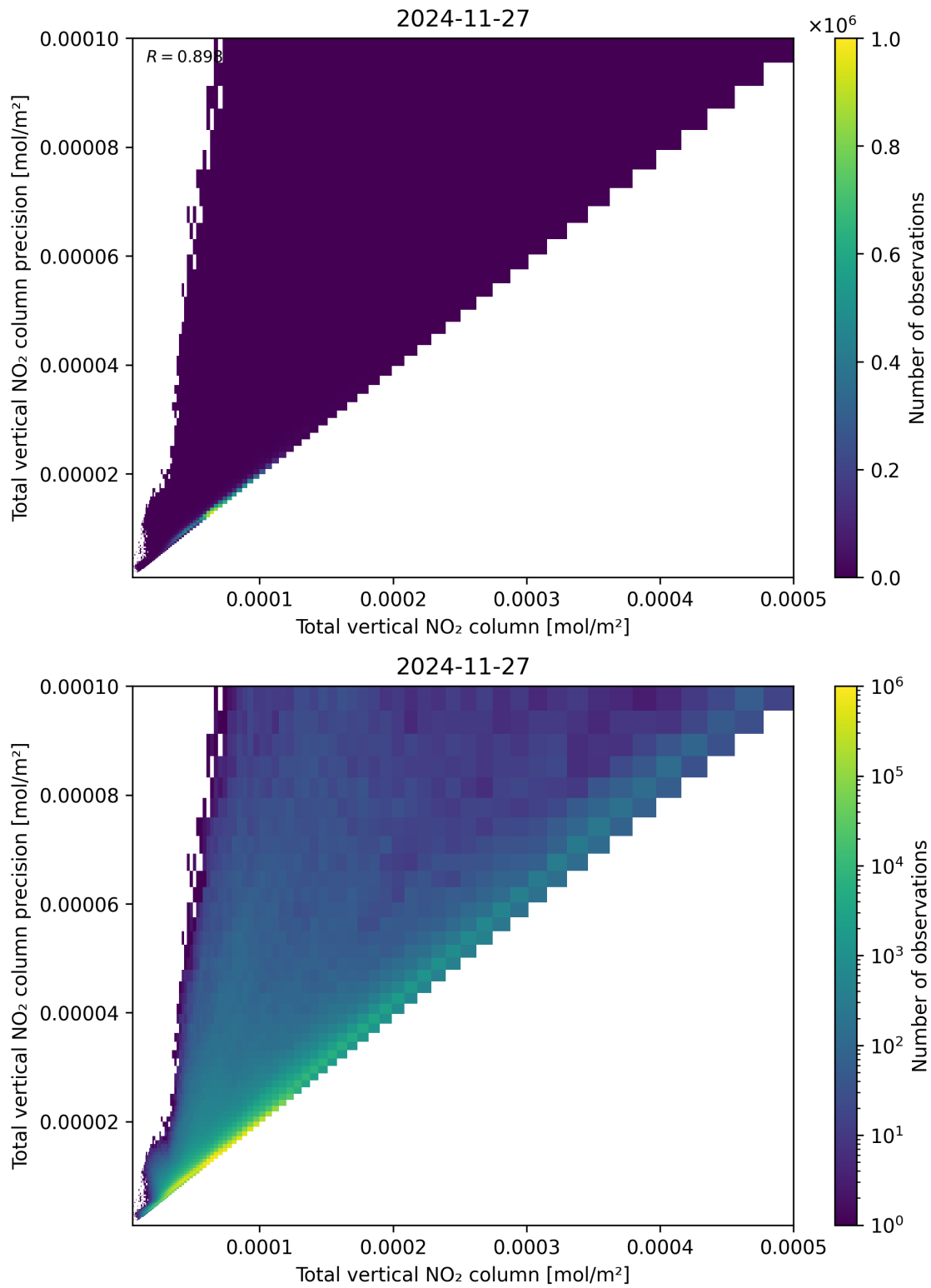
Figure 114: Scatter density plot of “Total vertical NO 2 column” against “Total vertical NO 2 column precision” for 2024-11-26 to 2024-11-28.
