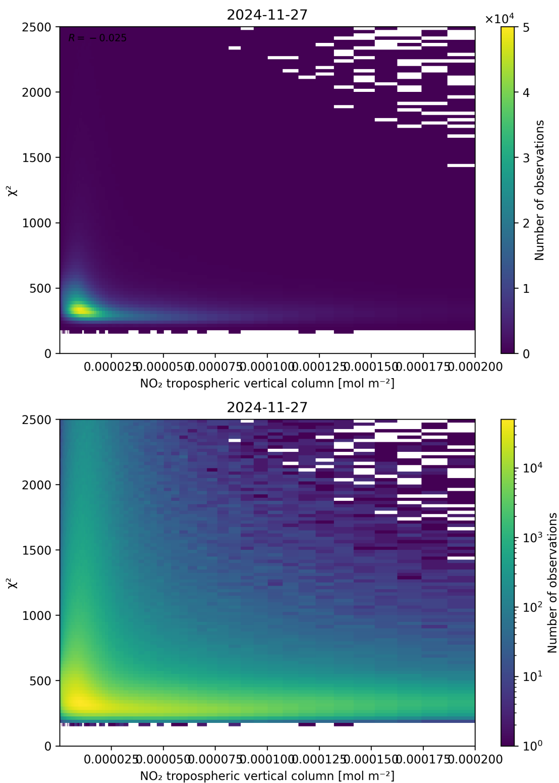
Figure 124: Scatter density plot of “NO 2 tropospheric vertical column” against “ \chi^2 ” for 2024-11-26 to 2024-11-28.
