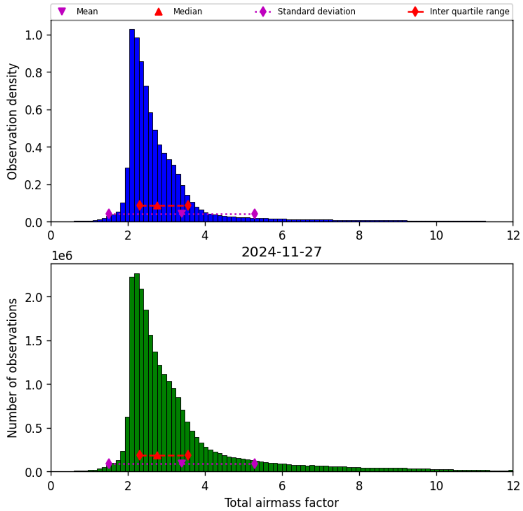
Figure 32: Histogram of “Total airmass factor” for 2024-11-26 to 2024-11-28
