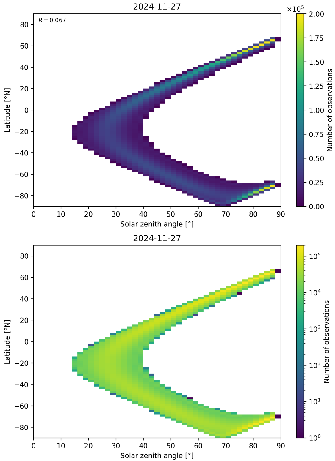
Figure 149: Scatter density plot of “Solar zenith angle” against “Latitude” for 2024-11-26 to 2024-11-28.
