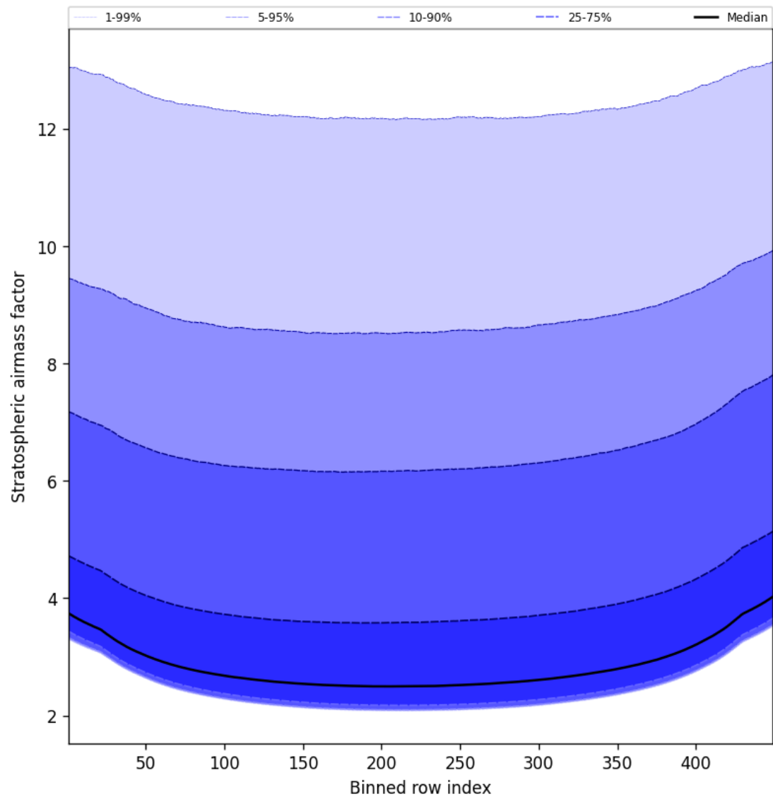
Figure 61: Along track statistics of “Stratospheric air mass factor” for 2024-11-26 to 2024-11-28
