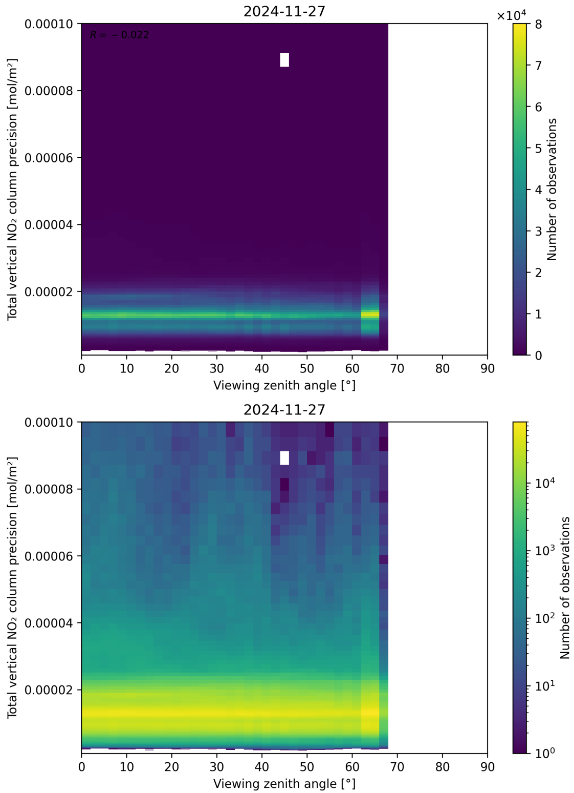
Figure 168: Scatter density plot of “Viewing zenith angle” against “Total vertical NO 2 column precision” for 2024-11-26 to 2024-11-28.
