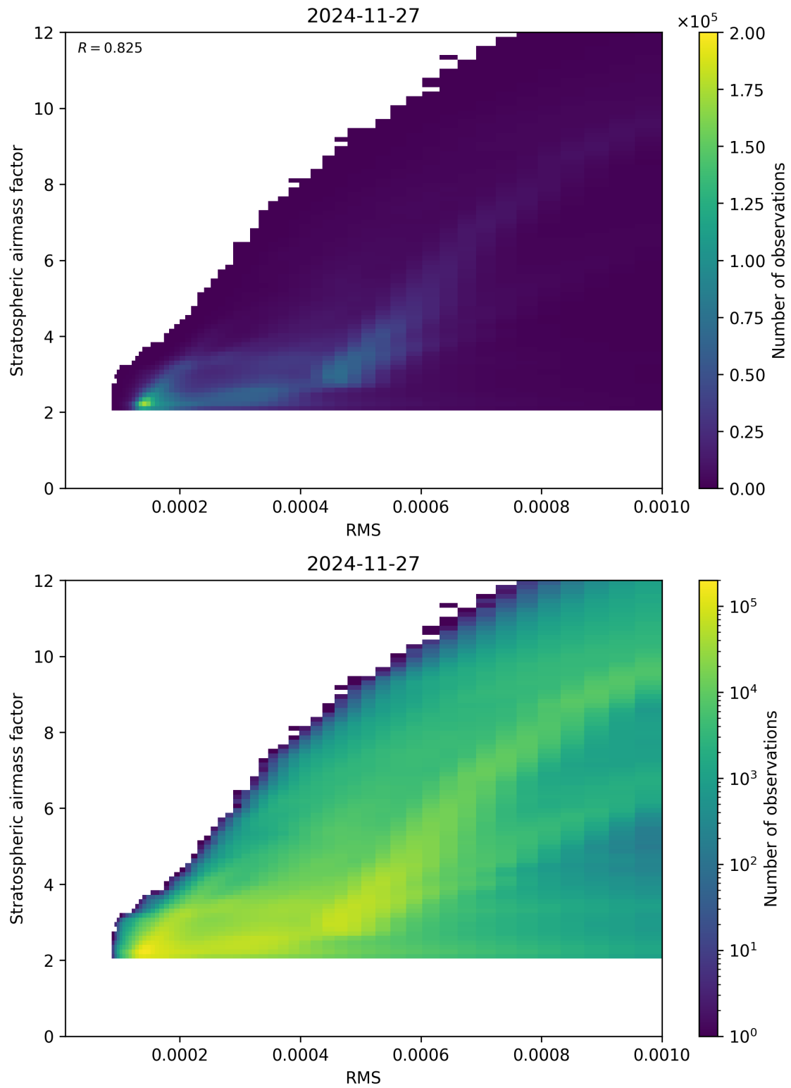
Figure 144: Scatter density plot of “RMS” against “Stratospheric airmass factor” for 2024-11-26 to 2024-11-28.
