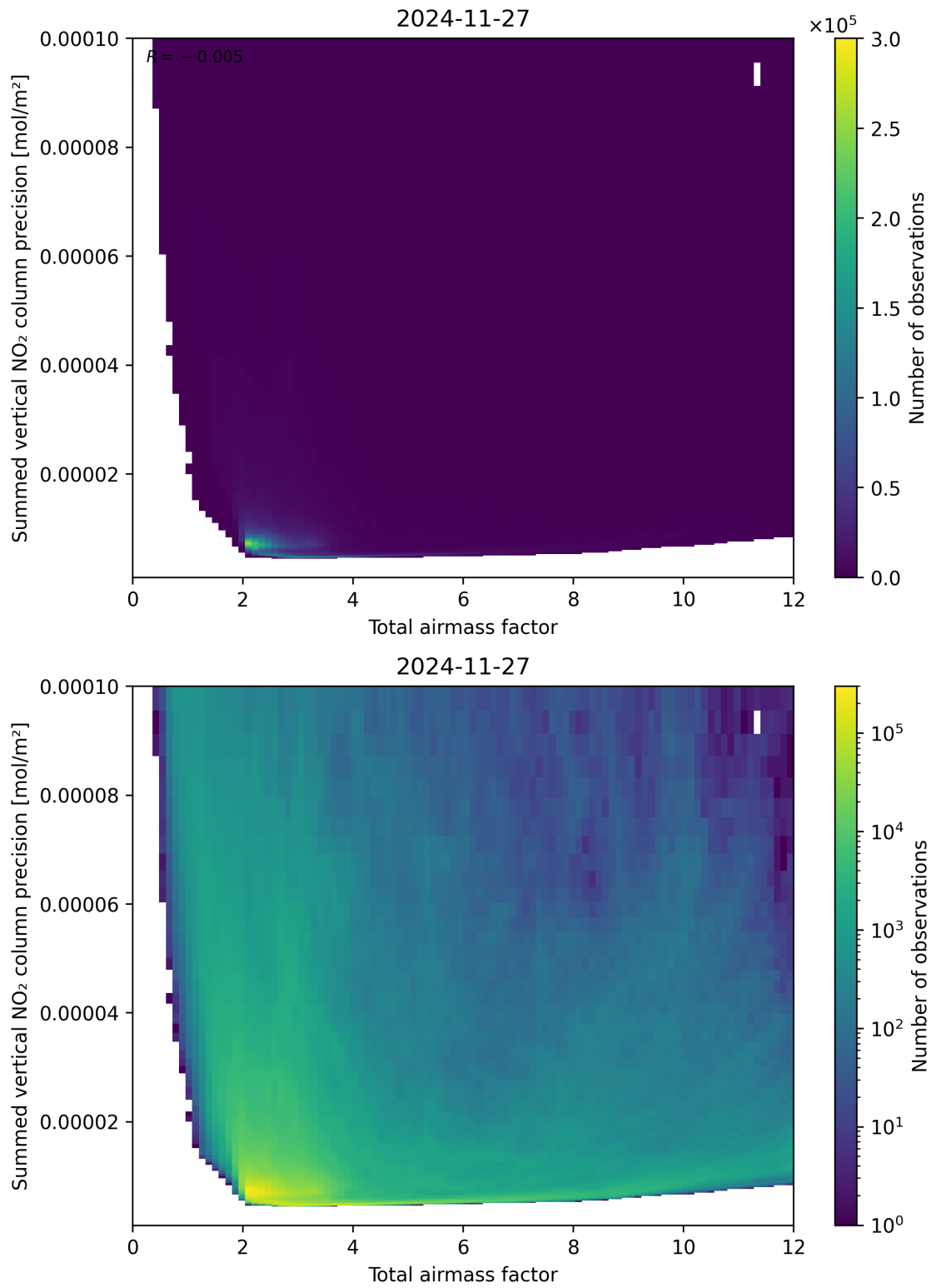
Figure 66: Scatter density plot of “Total airmass factor” against “Summed vertical NO 2 column precision” for 2024-11-26 to 2024-11-28.
