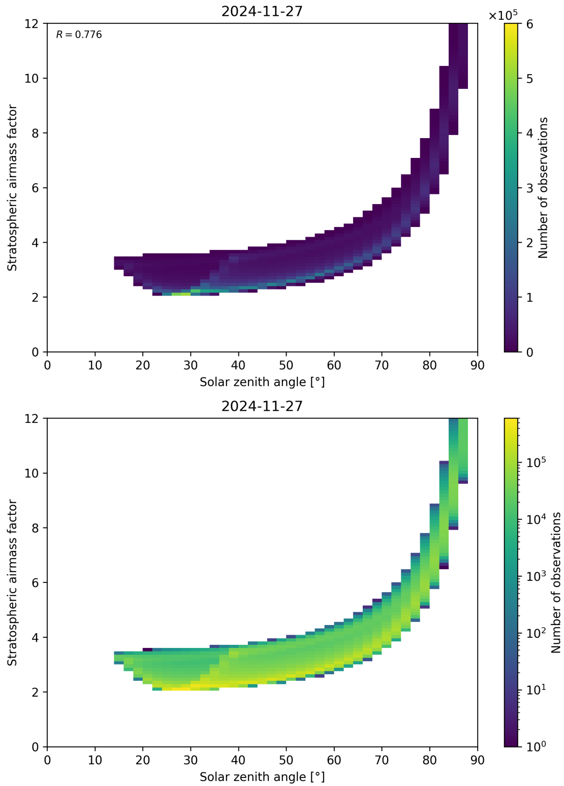
Figure 145: Scatter density plot of “Solar zenith angle” against “Stratospheric airmass factor” for 2024-11-26 to 2024-11-28.
