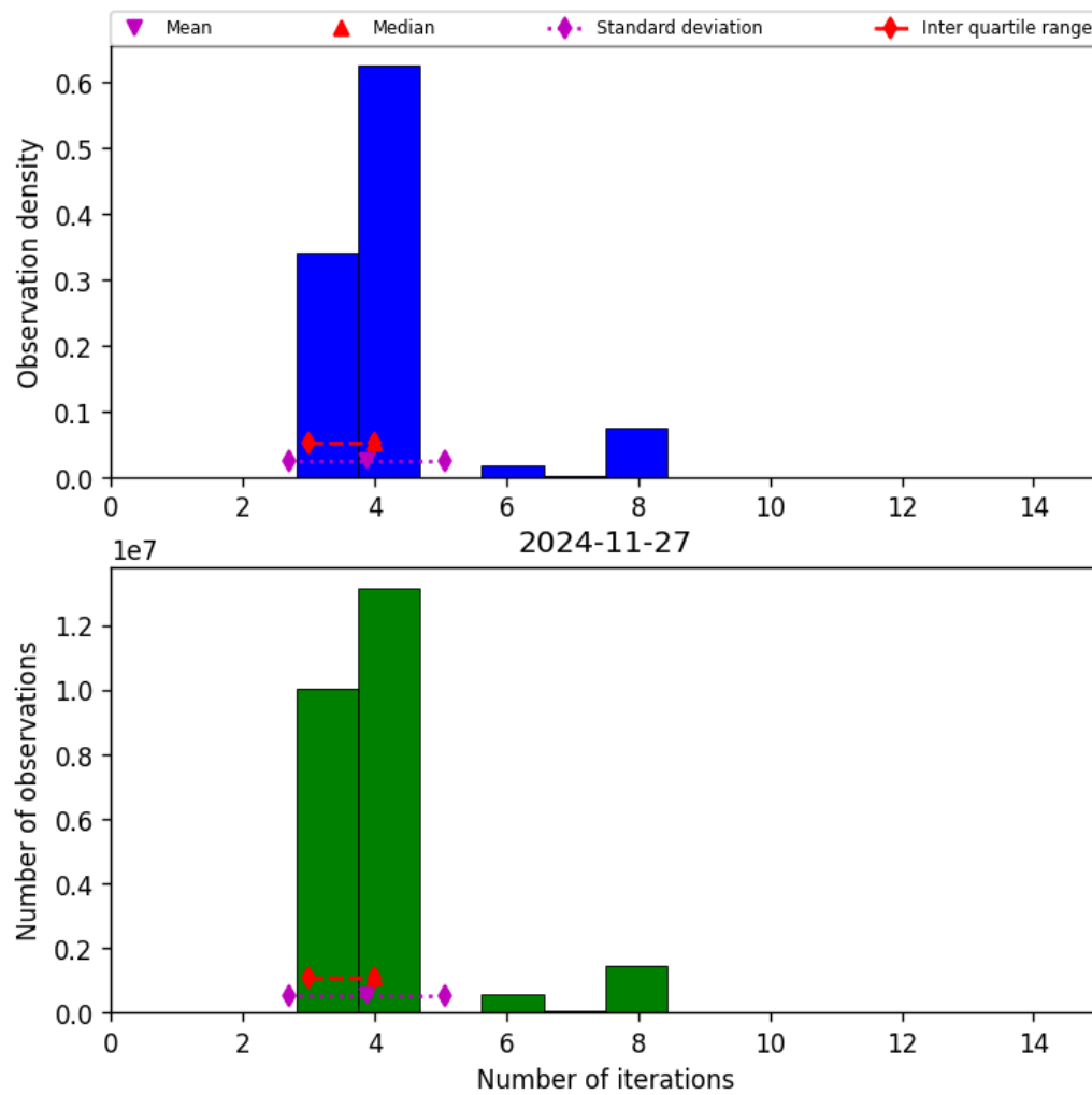
Figure 34: Histogram of “Number of iterations” for 2024-11-26 to 2024-11-28
