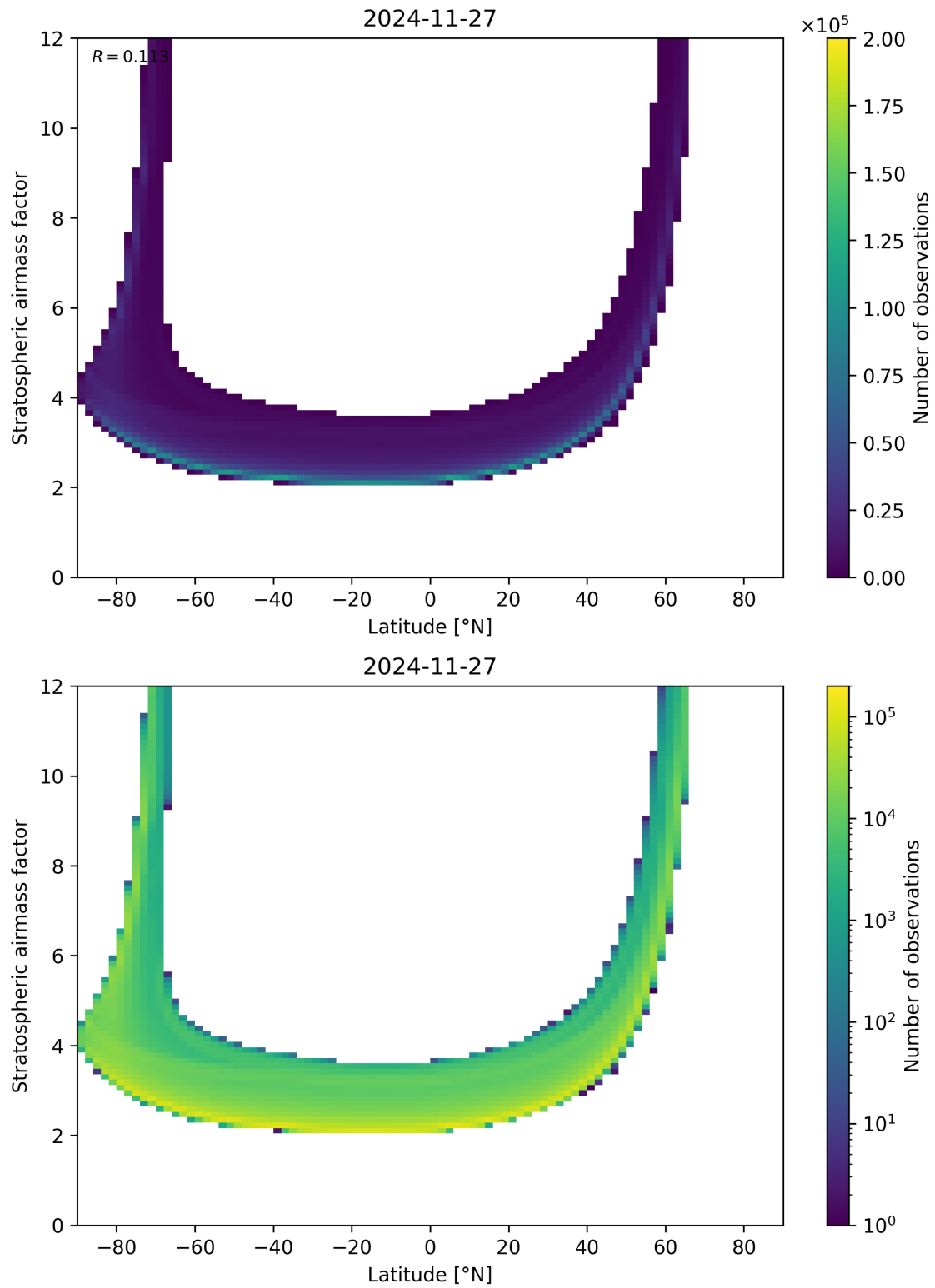
Figure 83: Scatter density plot of “Latitude” against “Stratospheric air mass factor” for 2024-11-26 to 2024-11-28.
