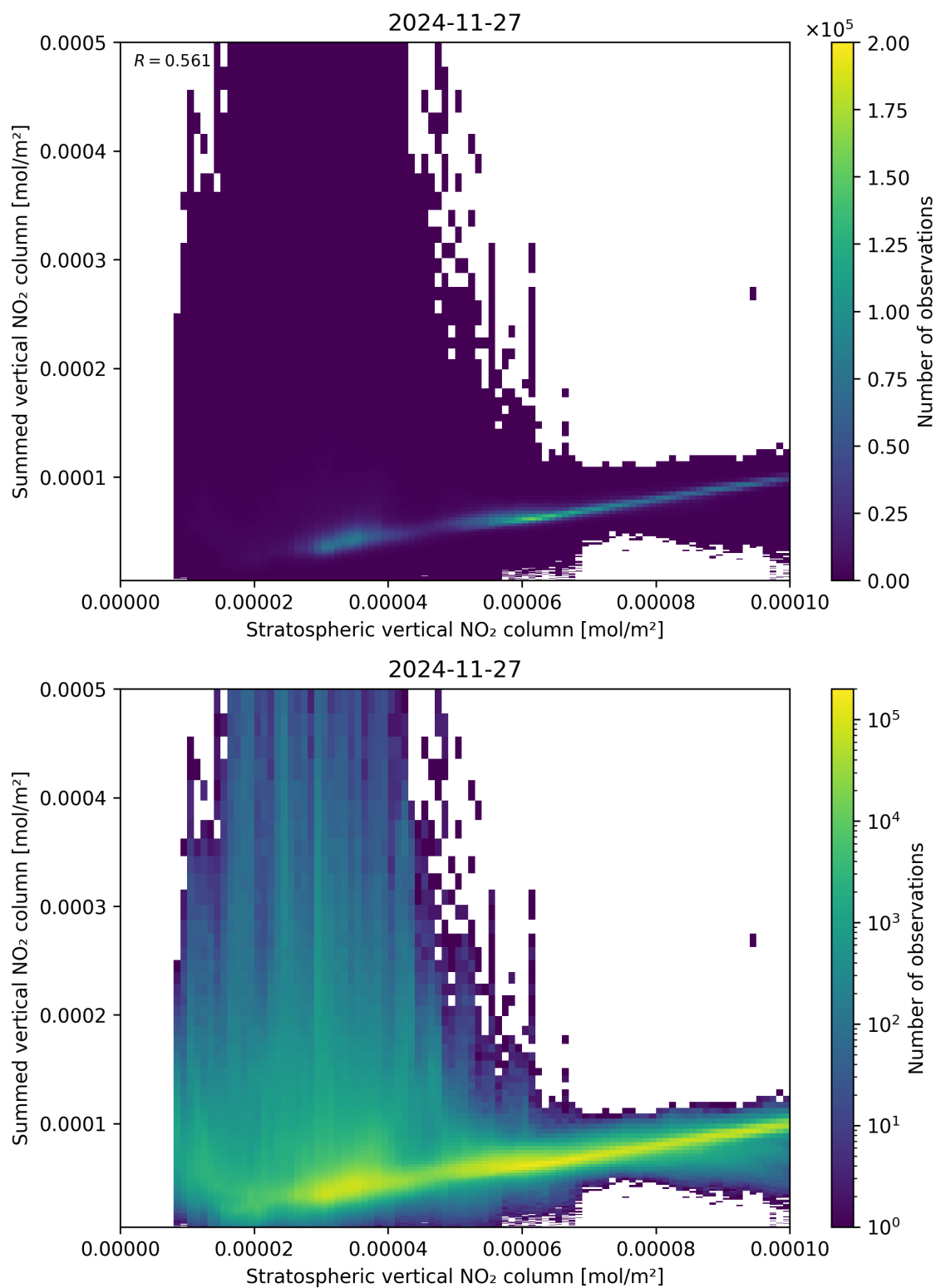
Figure 98: Scatter density plot of “Stratospheric vertical NO 2 column” against “Summed vertical NO 2 column” for 2024-11-26 to 2024-11-28.
