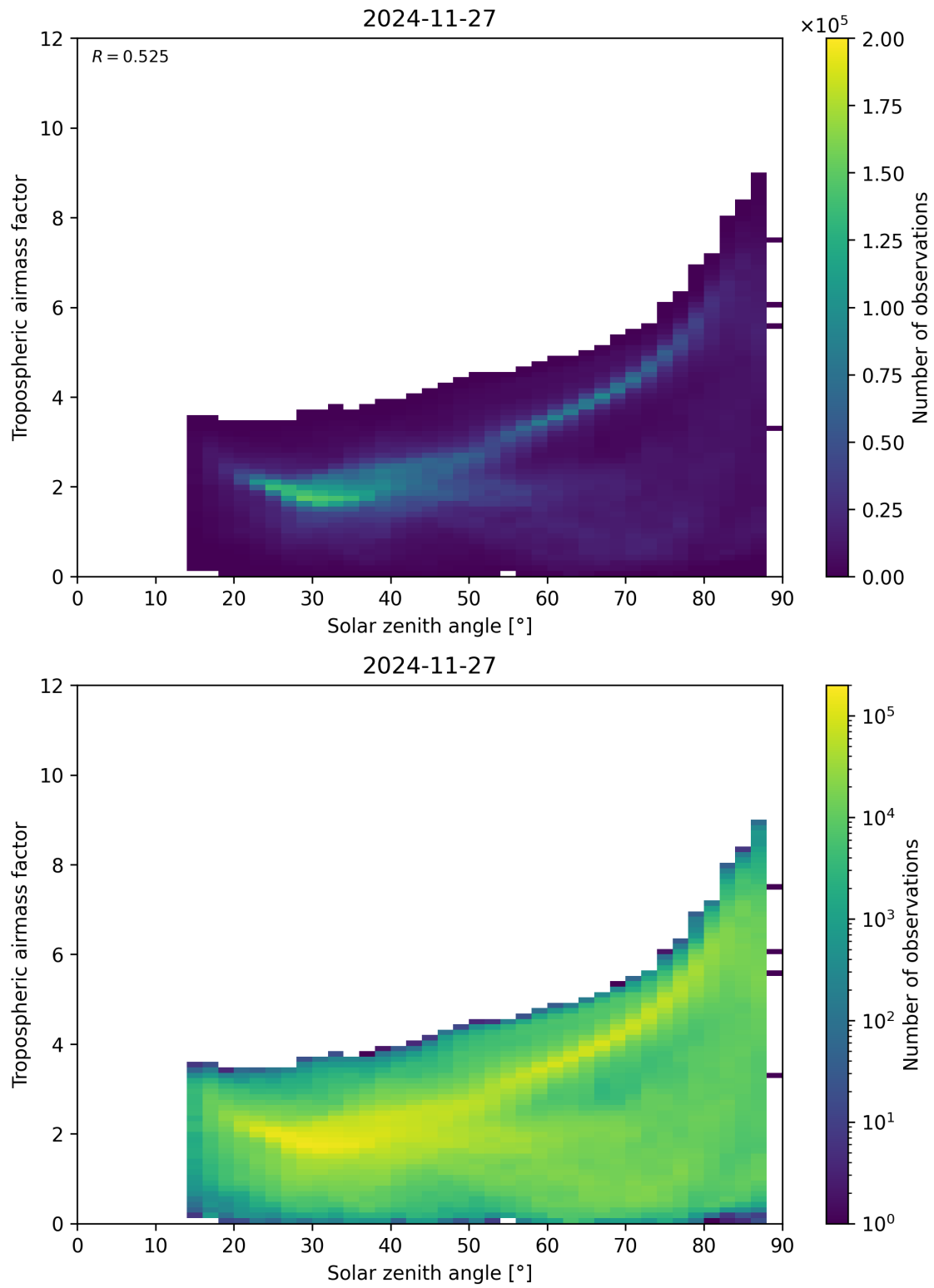
Figure 147: Scatter density plot of “Solar zenith angle” against “Tropospheric airmass factor” for 2024-11-26 to 2024-11-28.
