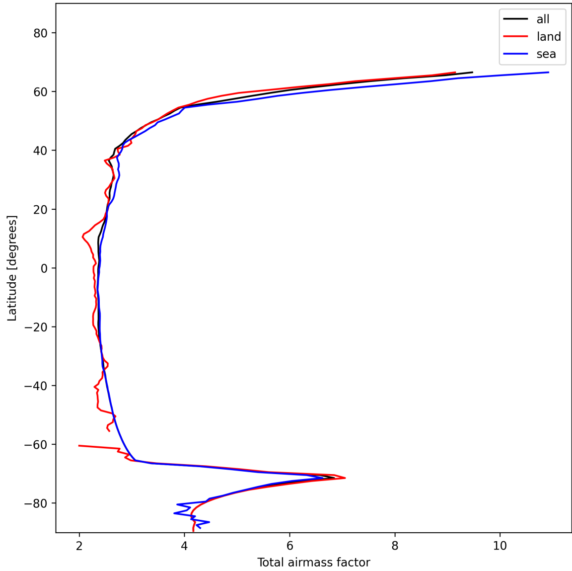
Figure 15: Zonal average of “Total airmass factor” for 2024-11-26 to 2024-11-28.
