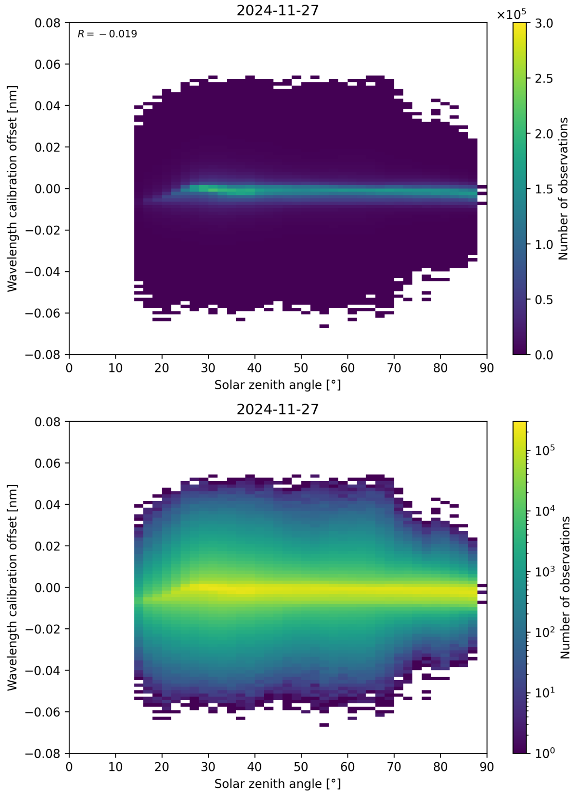
Figure 158: Scatter density plot of “Solar zenith angle” against “Wavelength calibration offset” for 2024-11-26 to 2024-11-28.
