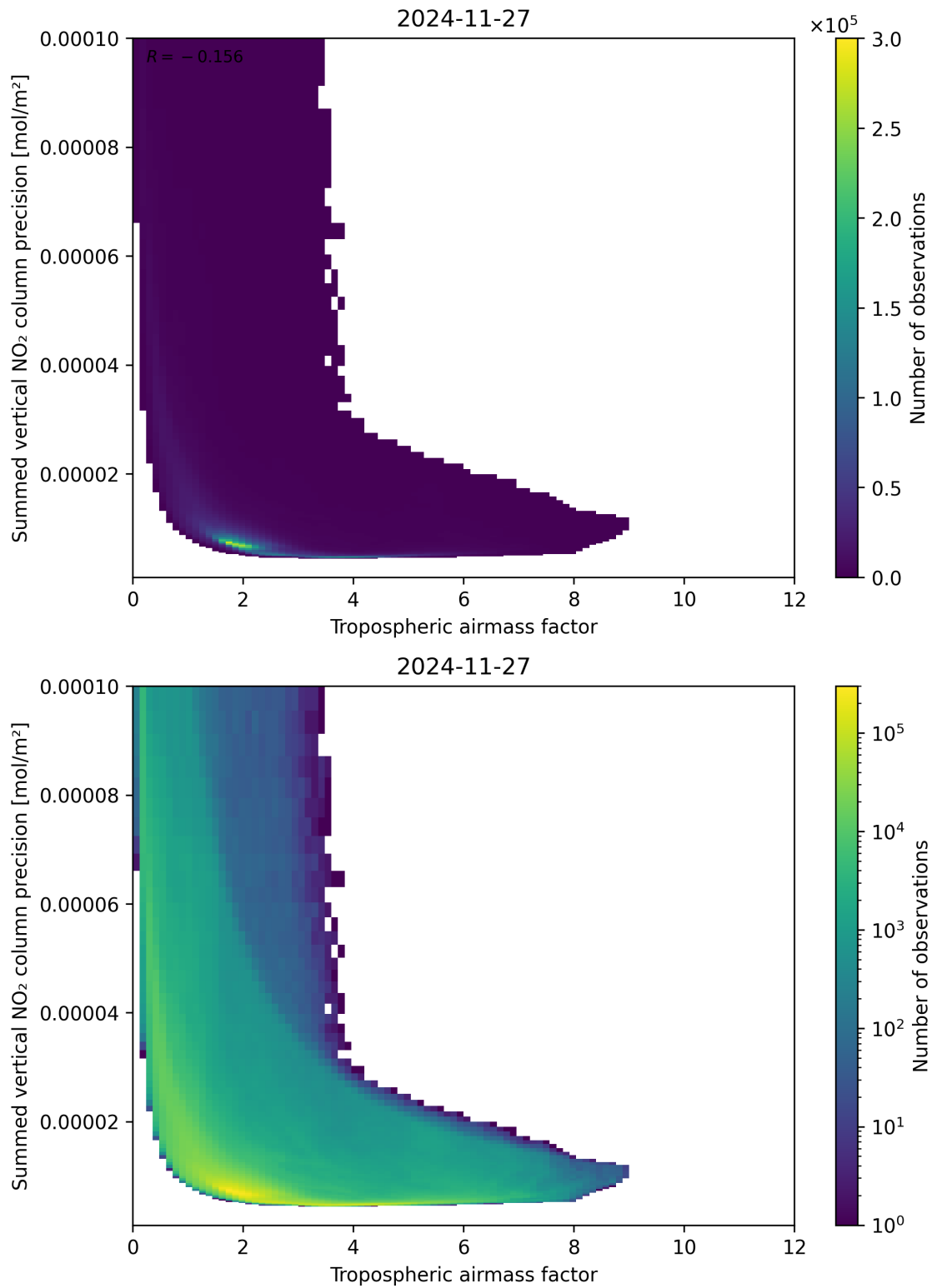
Figure 76: Scatter density plot of “Tropospheric air mass factor” against “Summed vertical NO 2 column precision” for 2024-11-26 to 2024-11-28.
