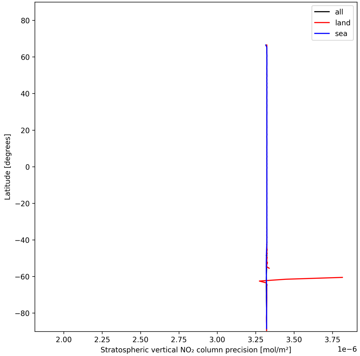
Figure 20: Zonal average of “Stratospheric vertical NO 2 column precision” for 2024-11-26 to 2024-11-28.
