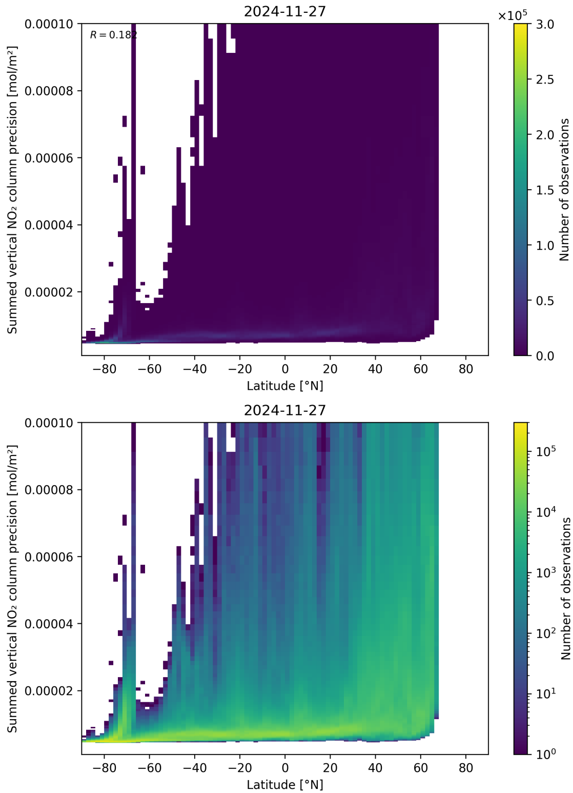
Figure 89: Scatter density plot of “Latitude” against “Summed vertical NO 2 column precision” for 2024-11-26 to 2024-11-28.
