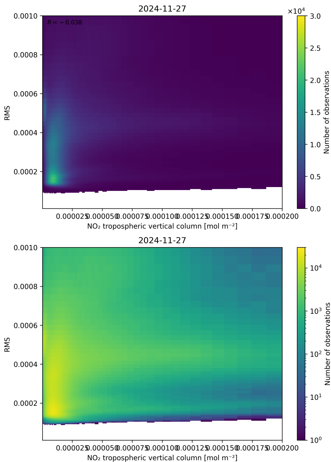
Figure 142: Scatter density plot of “NO 2 tropospheric vertical column” against “RMS” for 2024-11-26 to 2024-11-28.
