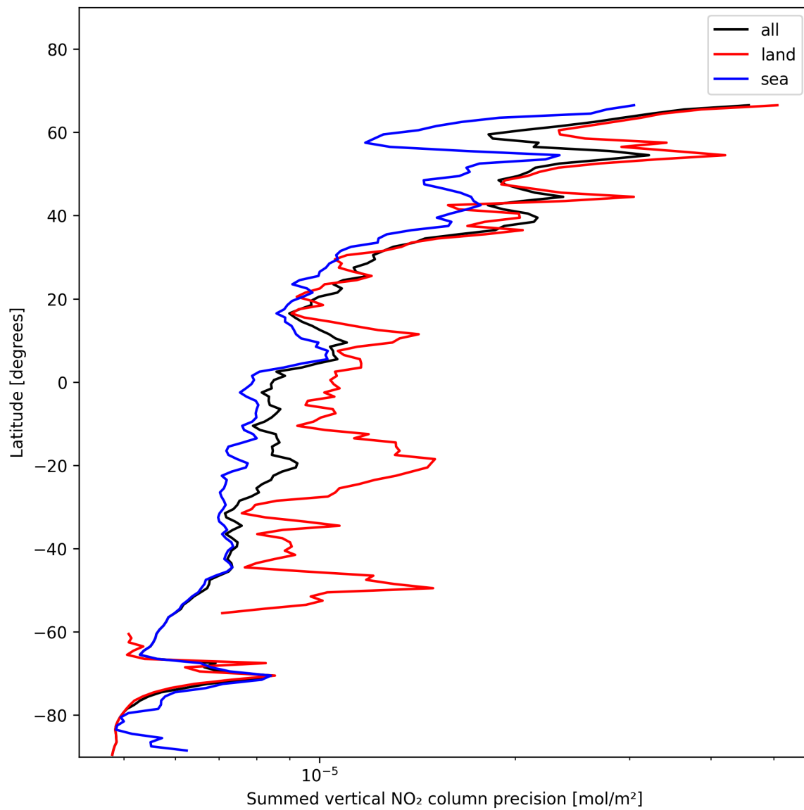
Figure 24: Zonal average of “Summed vertical NO 2 column precision” for 2024-11-26 to 2024-11-28.
