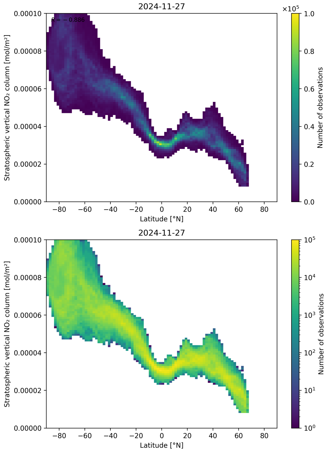
Figure 87: Scatter density plot of “Latitude” against “Stratospheric vertical NO 2 column” for 2024-11-26 to 2024-11-28.
