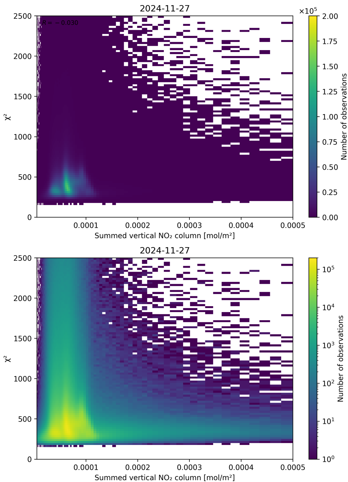
Figure 104: Scatter density plot of “Summed vertical NO 2 column” against “ \chi^2 ” for 2024-11-26 to 2024-11-28.
