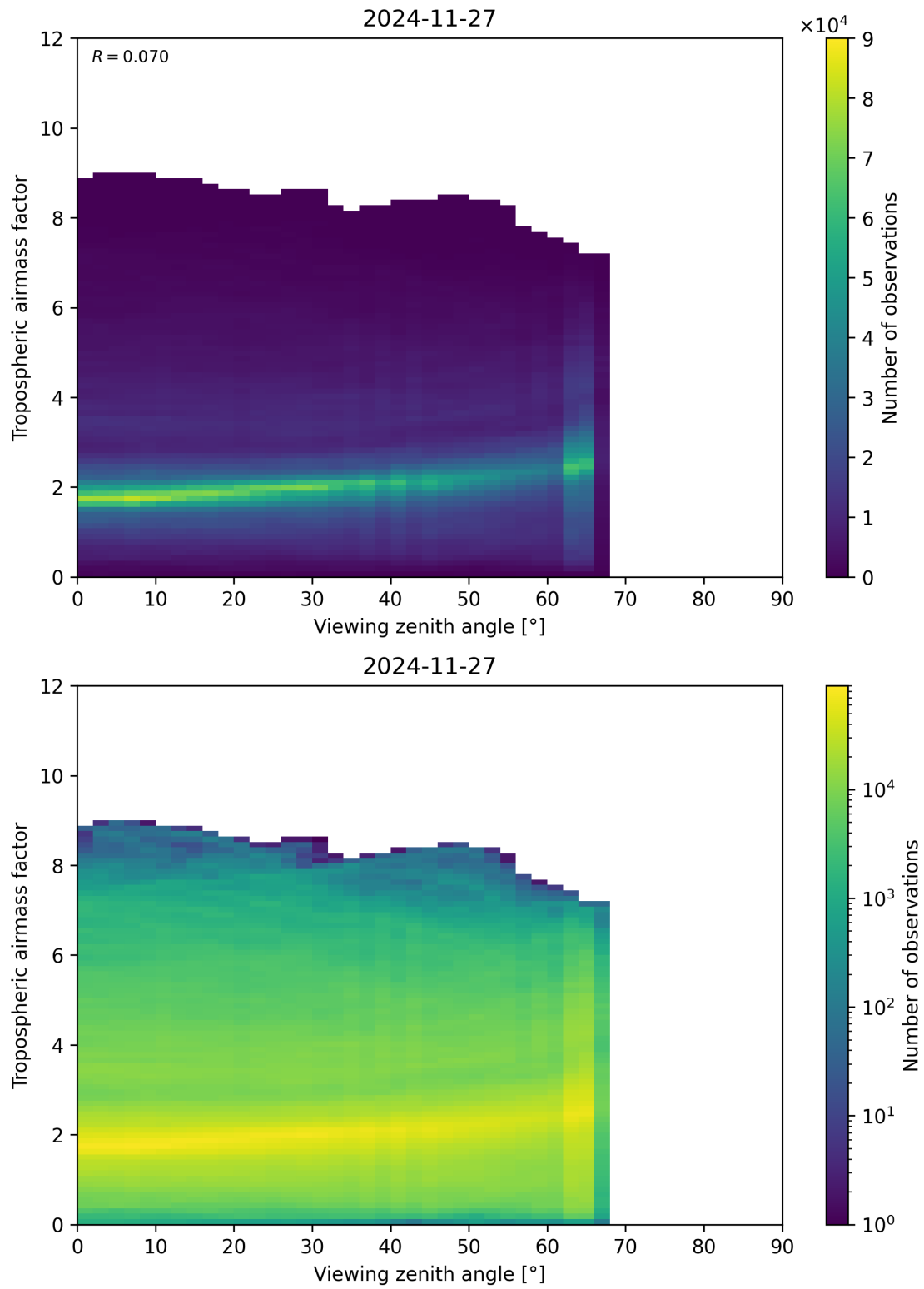
Figure 161: Scatter density plot of “Viewing zenith angle” against “Tropospheric airmass factor” for 2024-11-26 to 2024-11-28.
