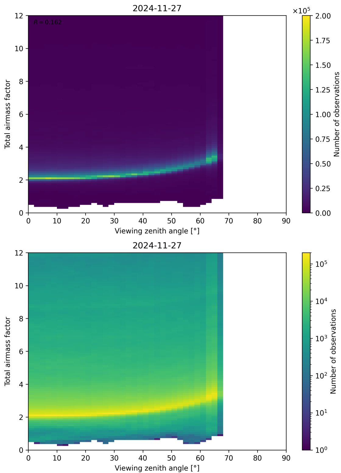
Figure 160: Scatter density plot of “Viewing zenith angle” against “Total airmass factor” for 2024-11-26 to 2024-11-28.
