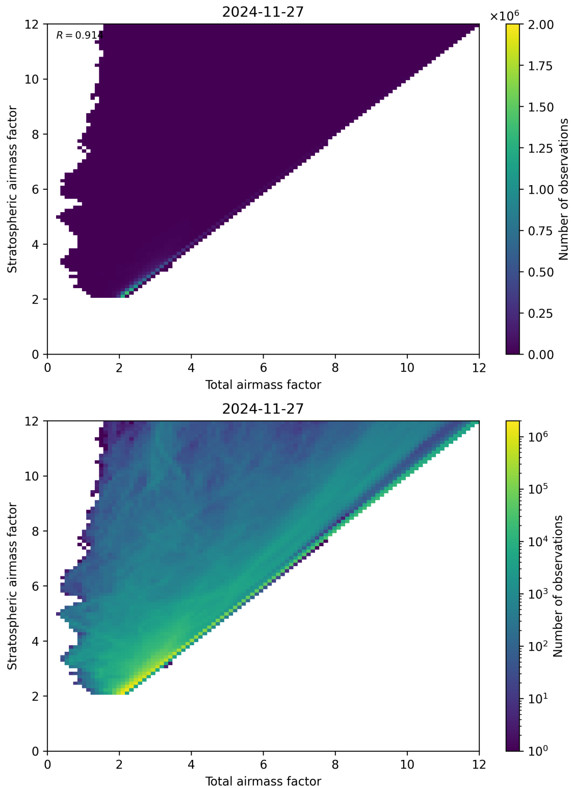
Figure 62: Scatter density plot of “Total airmass factor” against “Stratospheric airmass factor” for 2024-11-26 to 2024-11-28.
