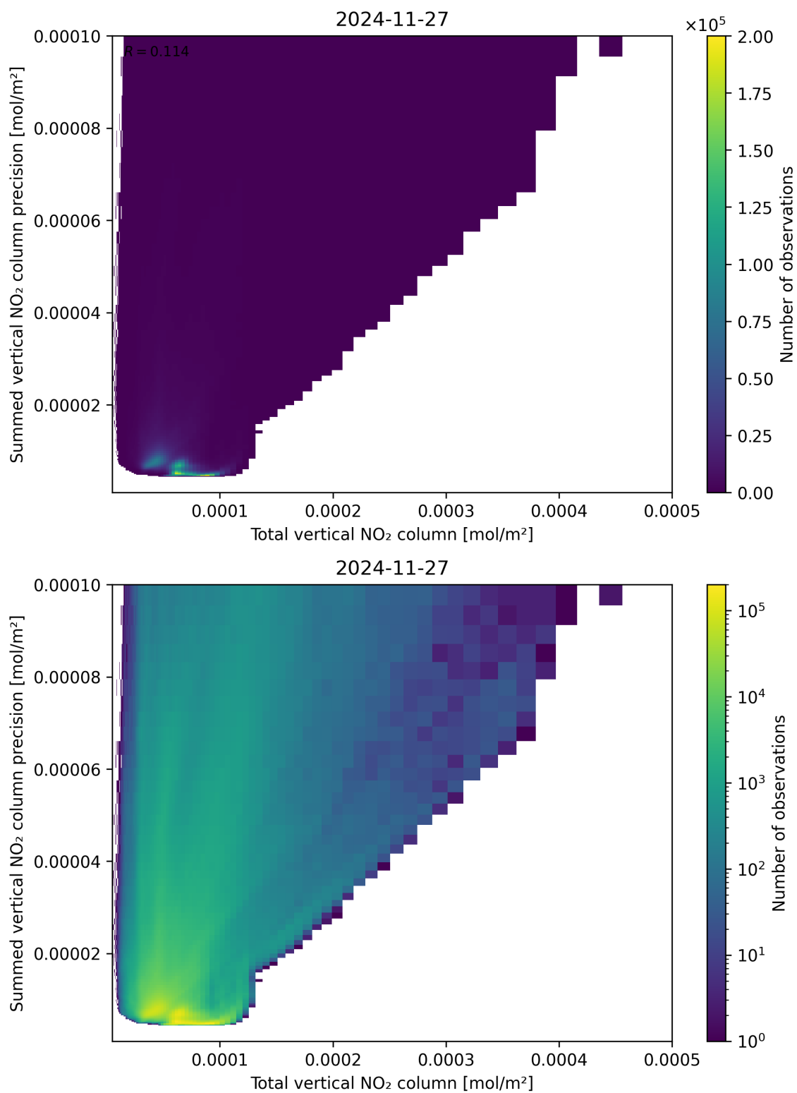
Figure 113: Scatter density plot of “Total vertical NO 2 column” against “Summed vertical NO 2 column precision” for 2024-11-26 to 2024-11-28.
