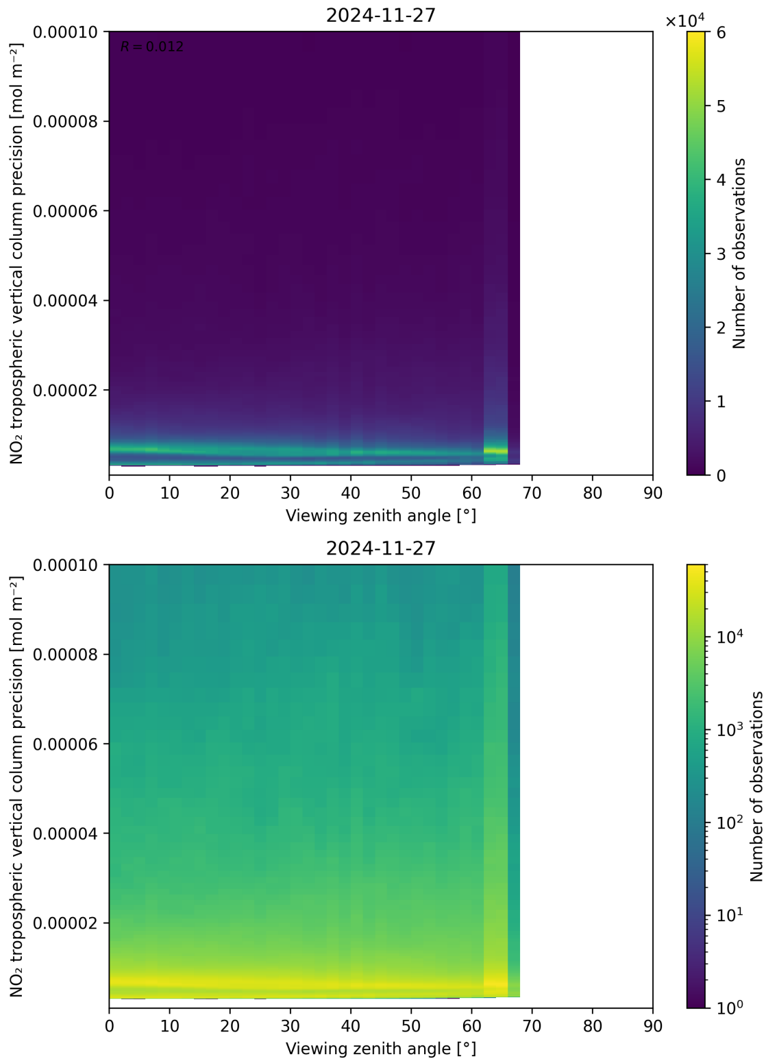
Figure 170: Scatter density plot of “Viewing zenith angle” against “NO 2 tropospheric vertical column precision” for 2024-11-26 to 2024-11-28.
