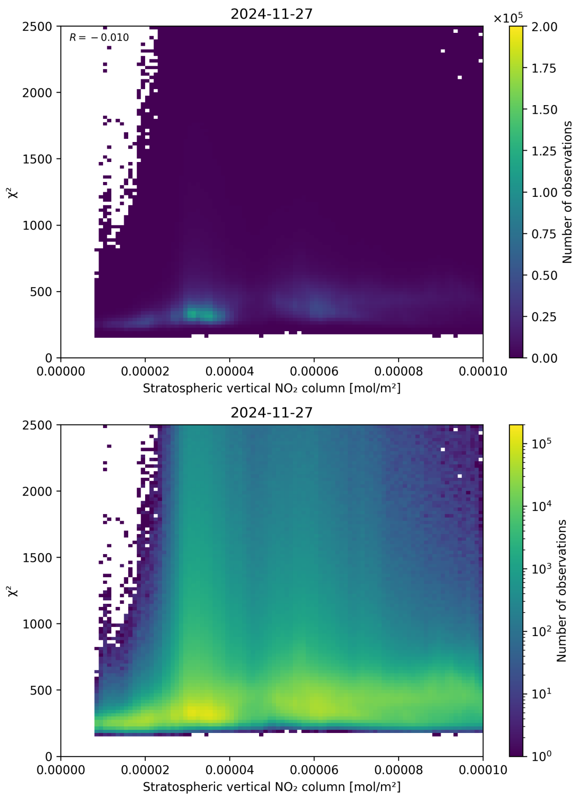
Figure 97: Scatter density plot of “Stratospheric vertical NO 2 column” against “ \chi^2 ” for 2024-11-26 to 2024-11-28.
