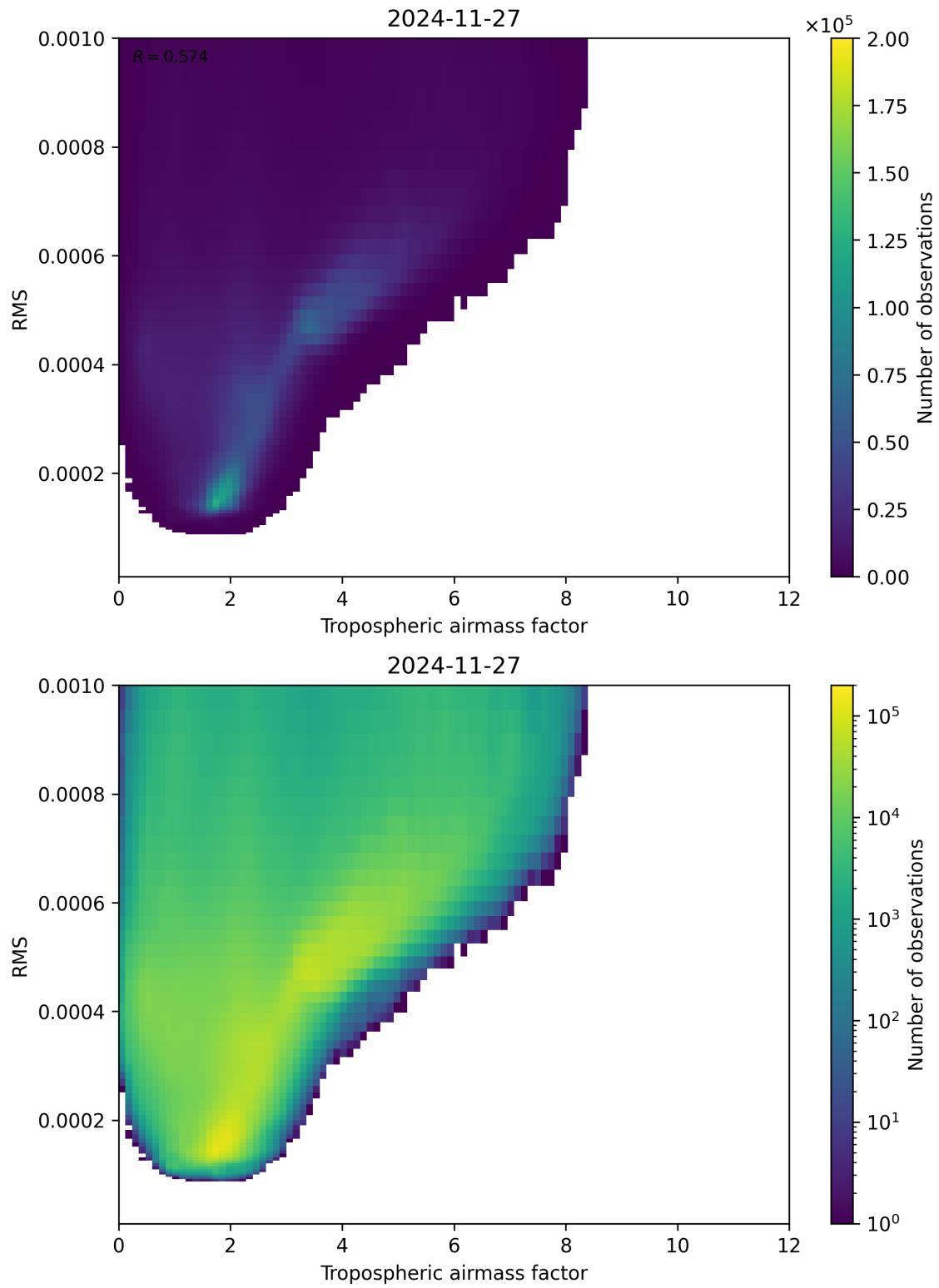
Figure 79: Scatter density plot of “Tropospheric airmass factor” against “RMS” for 2024-11-26 to 2024-11-28.
