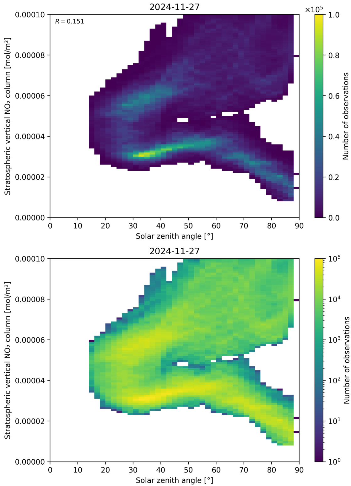
Figure 150: Scatter density plot of “Solar zenith angle” against “Stratospheric vertical NO 2 column” for 2024-11-26 to 2024-11-28.
