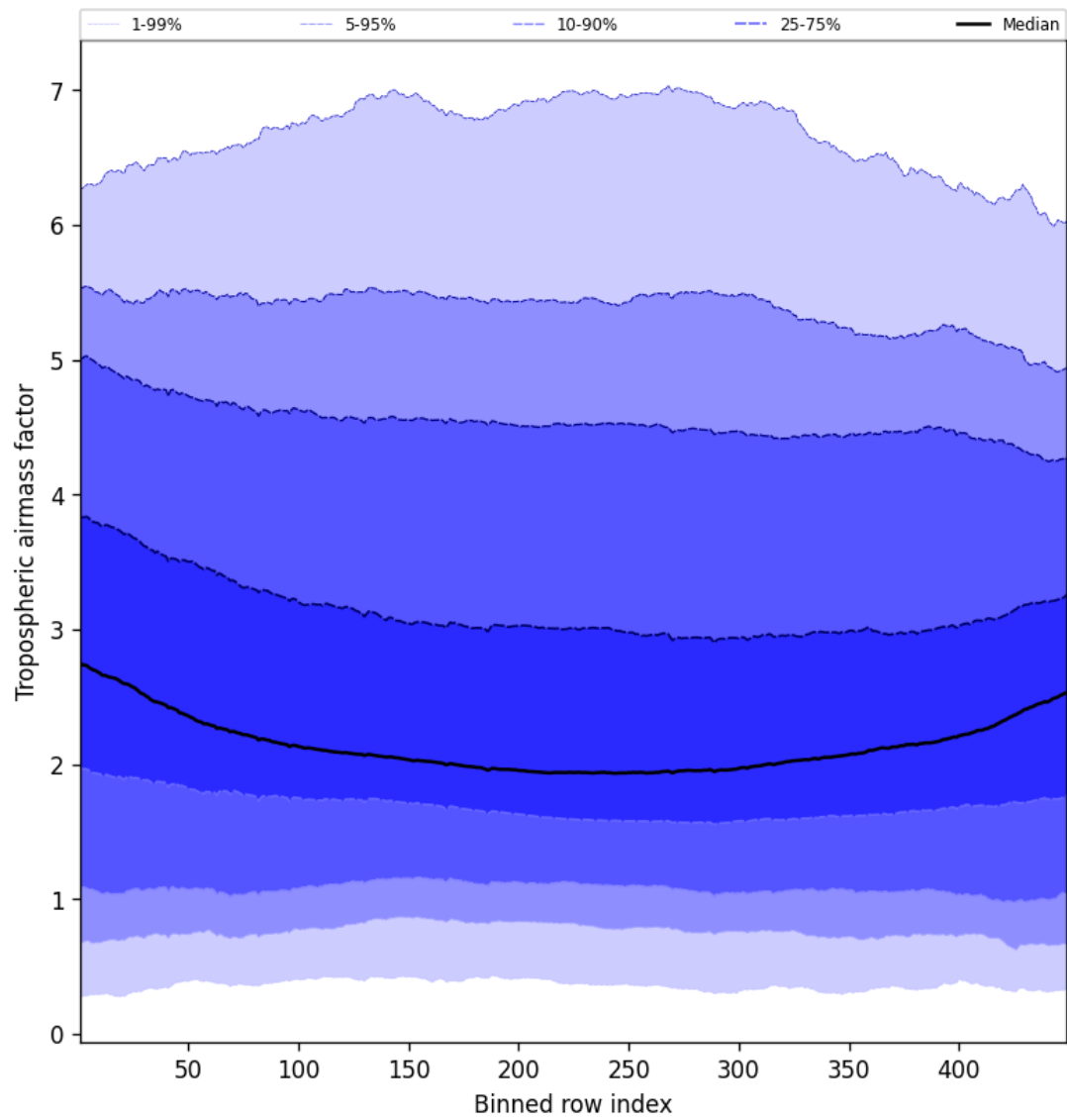
Figure 48: Along track statistics of “Tropospheric airmass factor” for 2024-11-26 to 2024-11-28
