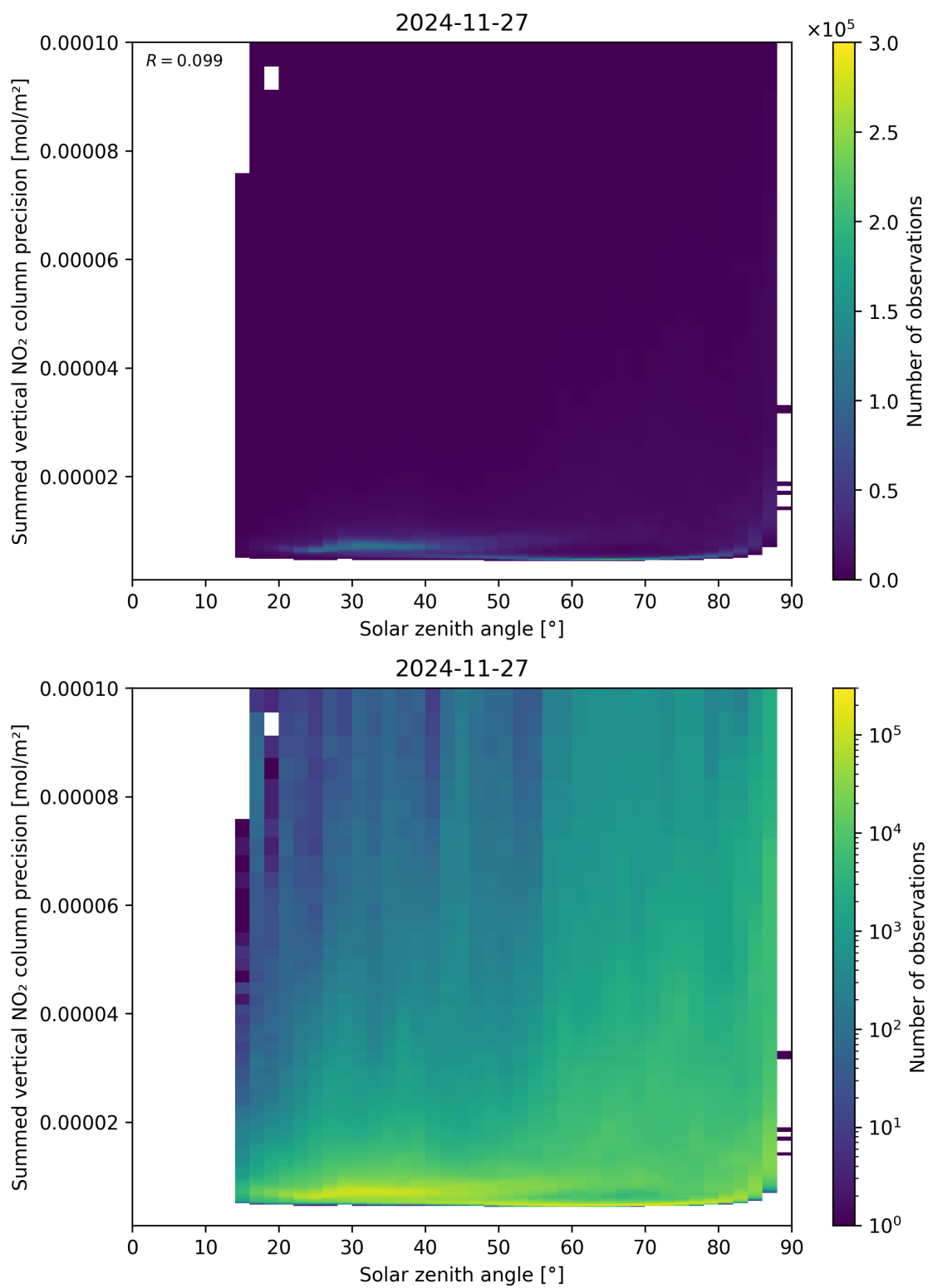
Figure 152: Scatter density plot of “Solar zenith angle” against “Summed vertical NO 2 column precision” for 2024-11-26 to 2024-11-28.
