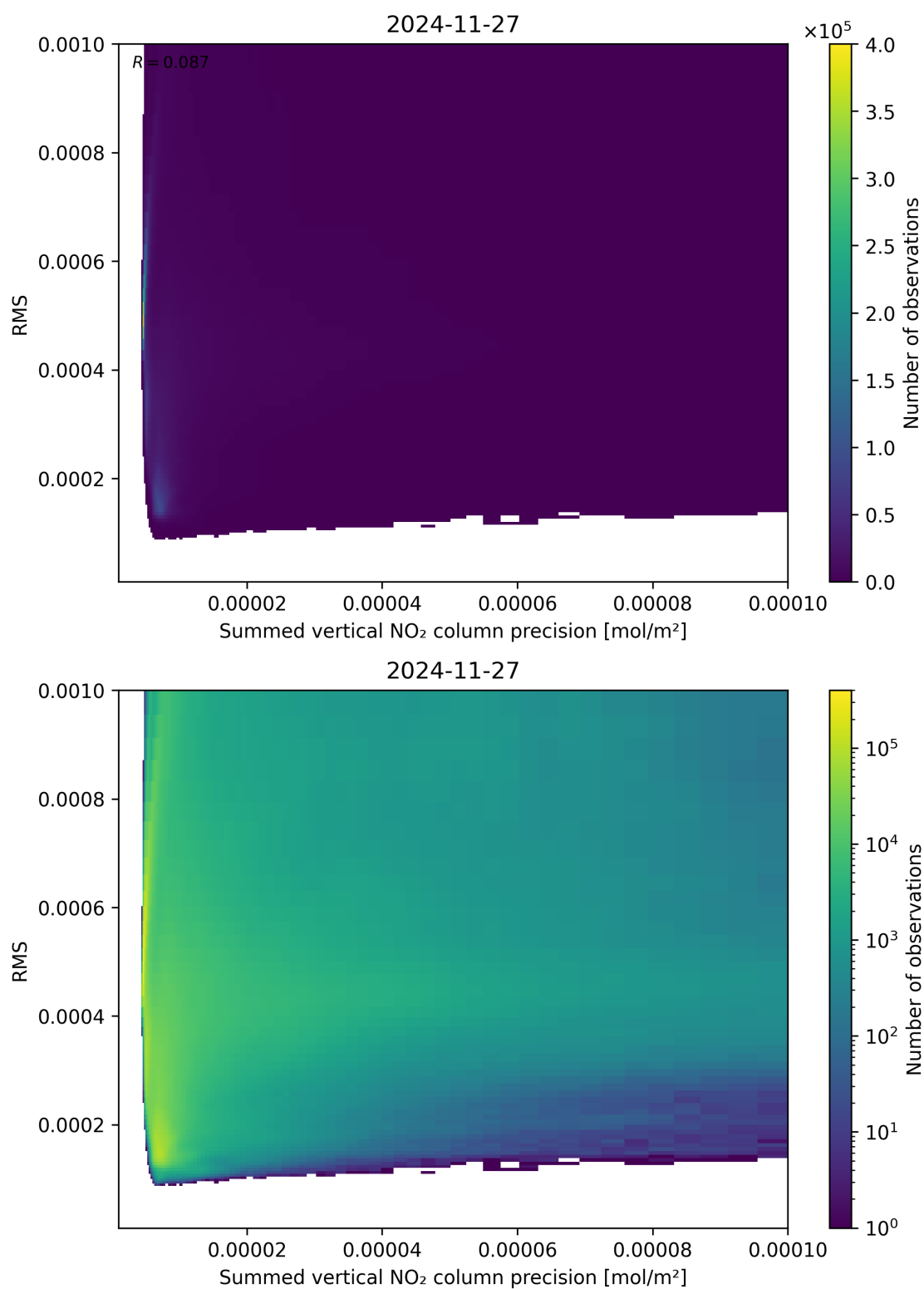
Figure 108: Scatter density plot of “Summed vertical NO 2 column precision” against “RMS” for 2024-11-26 to 2024-11-28.
