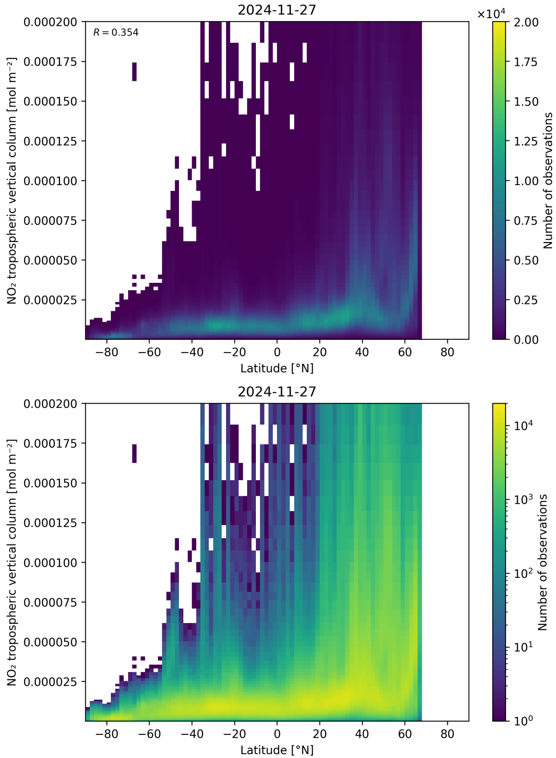
Figure 92: Scatter density plot of “Latitude” against “NO 2 tropospheric vertical column” for 2024-11-26 to 2024-11-28.
