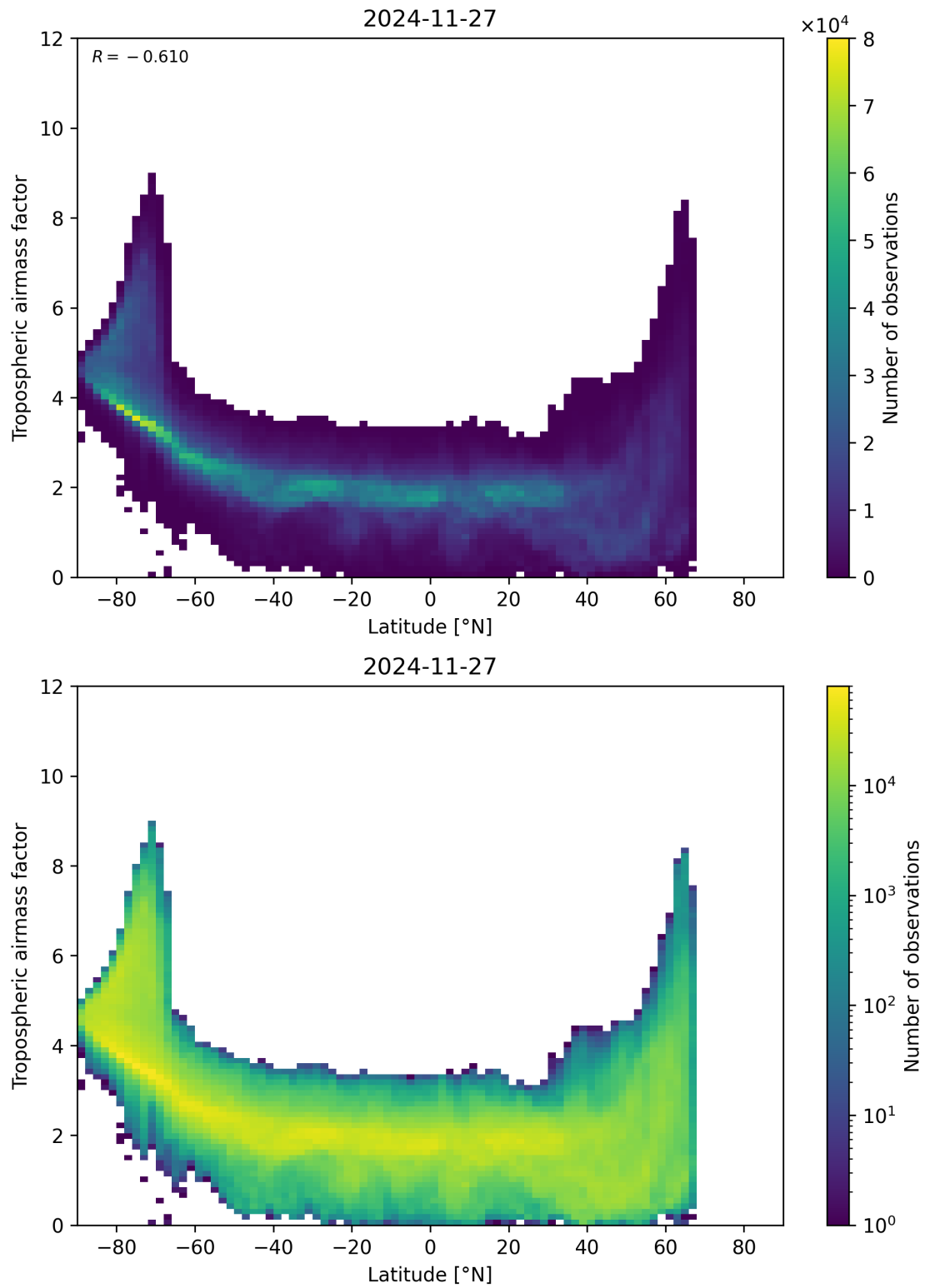
Figure 85: Scatter density plot of “Latitude” against “Tropospheric air mass factor” for 2024-11-26 to 2024-11-28.
