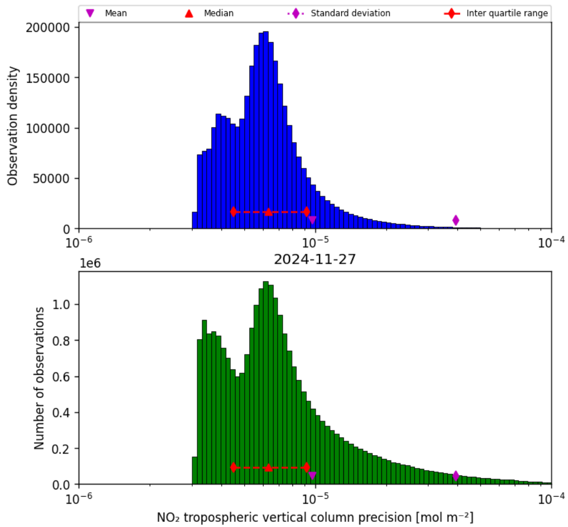
Figure 30: Histogram of “NO 2 tropospheric vertical column precision” for 2024-11-26 to 2024-11-28
