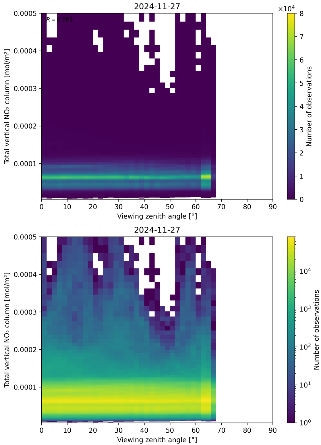
Figure 167: Scatter density plot of “Viewing zenith angle” against “Total vertical NO 2 column” for 2024-11-26 to 2024-11-28.
