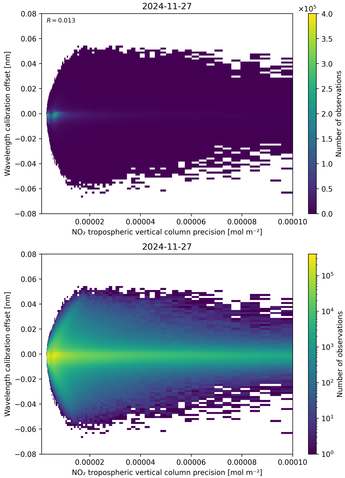
Figure 141: Scatter density plot of “NO 2 tropospheric vertical column precision” against “Wavelength calibration offset” for 2024-11-26 to 2024-11-28.
