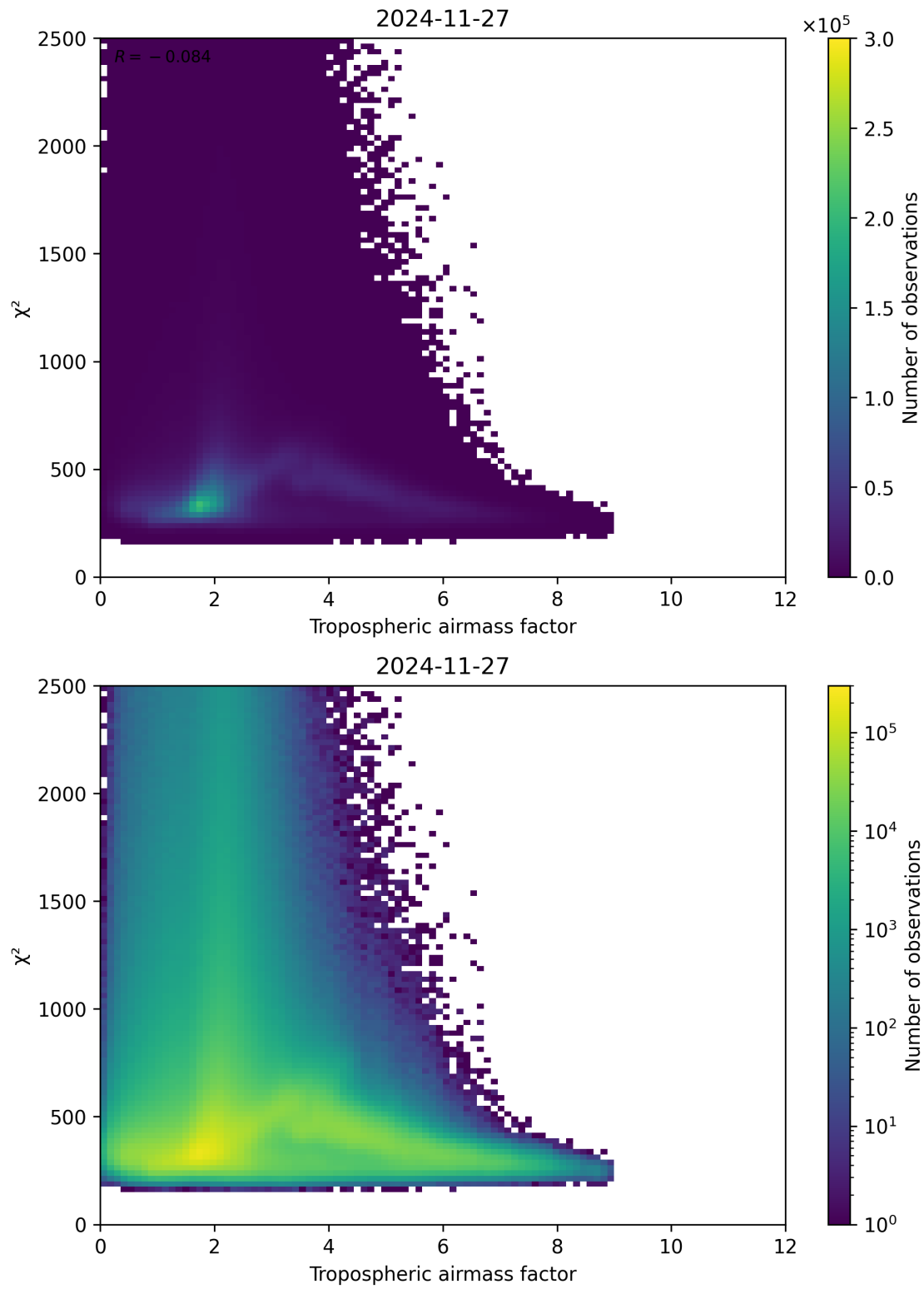
Figure 73: Scatter density plot of “Tropospheric airmass factor” against “ \chi^2 ” for 2024-11-26 to 2024-11-28.
