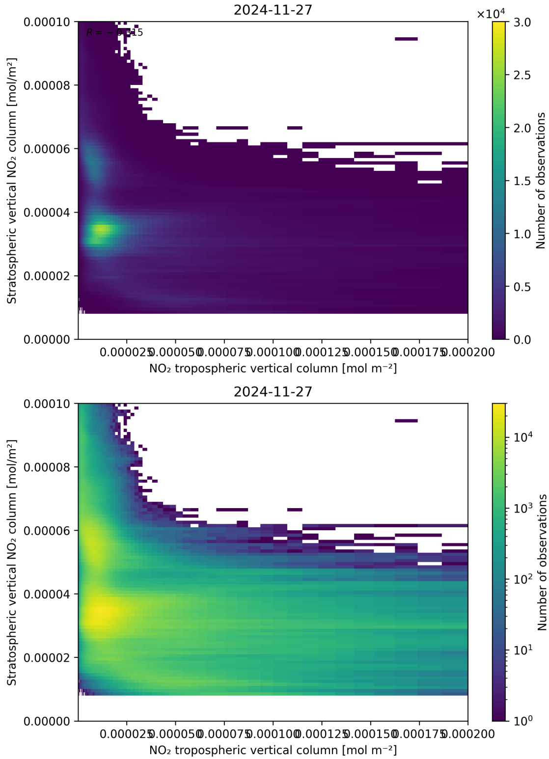
Figure 125: Scatter density plot of “NO 2 tropospheric vertical column” against “Stratospheric vertical NO 2 column” for 2024-11-26 to 2024-11-28.
