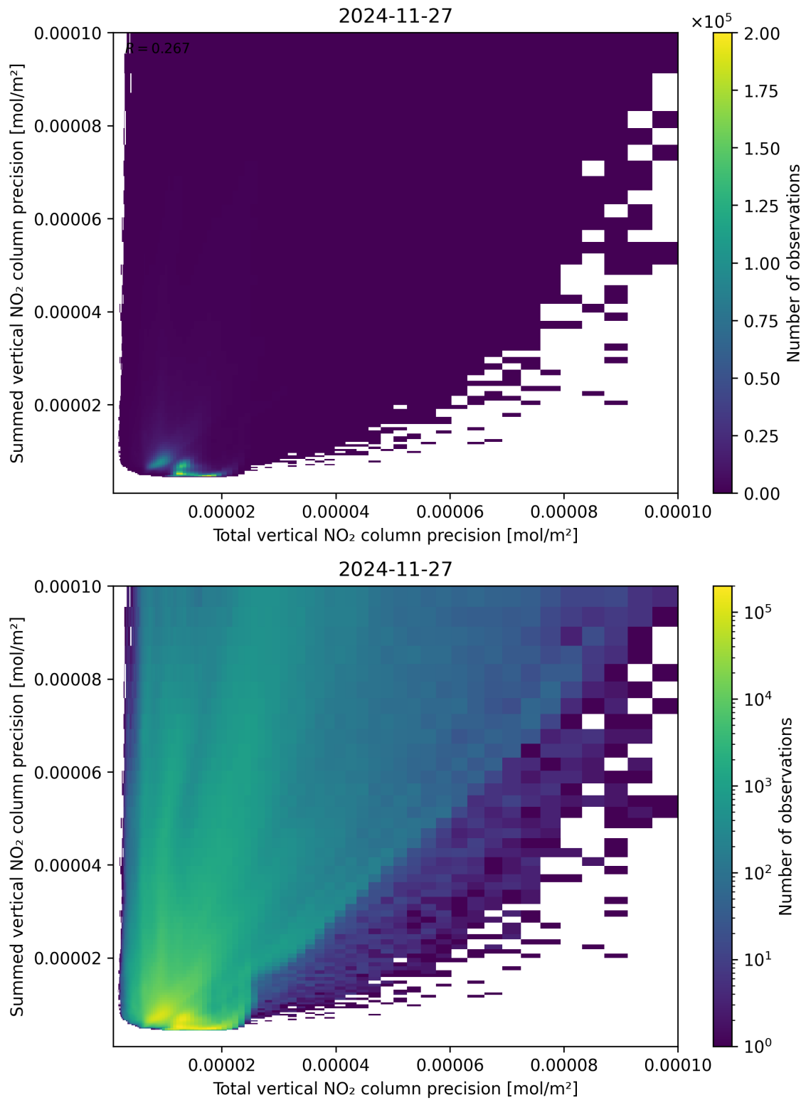
Figure 118: Scatter density plot of “Total vertical NO 2 column precision” against “Summed vertical NO 2 column precision” for 2024-11-26 to 2024-11-28.
