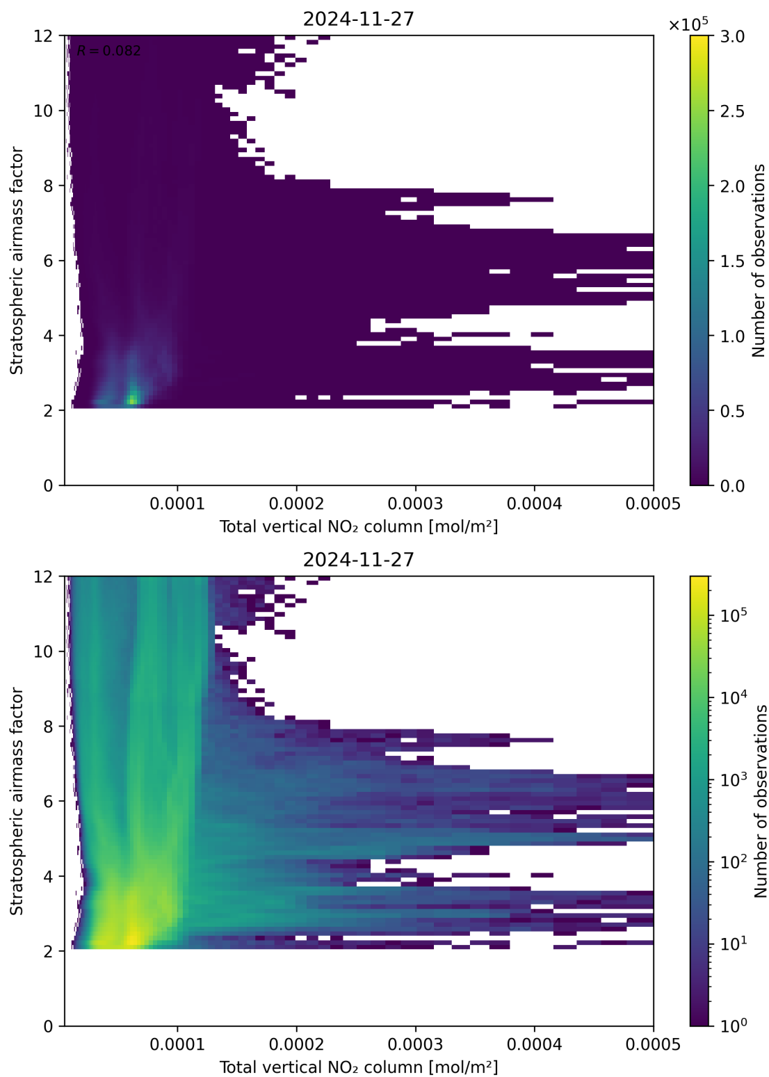
Figure 110: Scatter density plot of “Total vertical NO 2 column” against “Stratospheric airmass factor” for 2024-11-26 to 2024-11-28.
