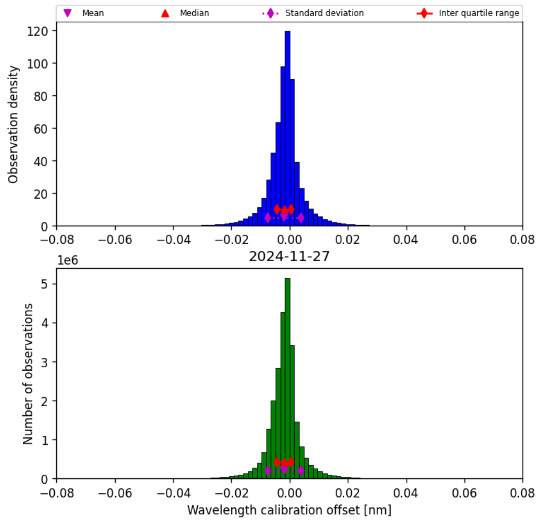
Figure 35: Histogram of “Wavelength calibration offset” for 2024-11-26 to 2024-11-28
