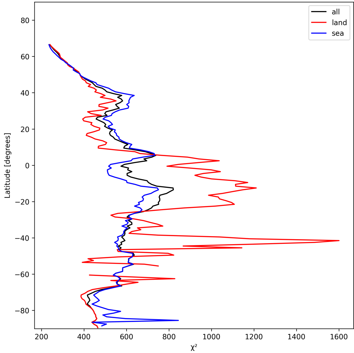
Figure 25: Zonal average of “ \chi^2 ” for 2024-11-26 to 2024-11-28.
