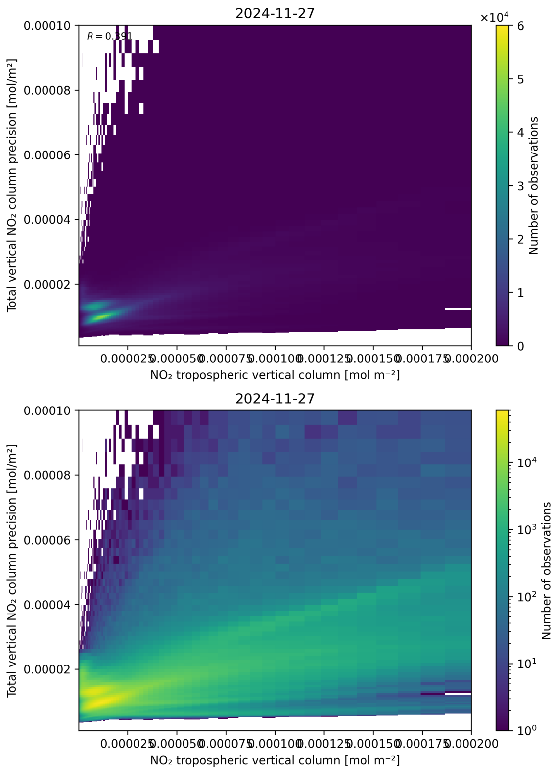
Figure 129: Scatter density plot of “NO 2 tropospheric vertical column” against “Total vertical NO 2 column precision” for 2024-11-26 to 2024-11-28.
