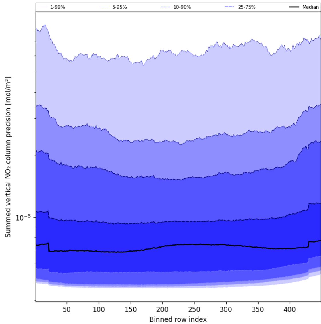
Figure 58: Along track statistics of “Summed vertical NO 2 column precision” for 2024-11-26 to 2024-11-28
