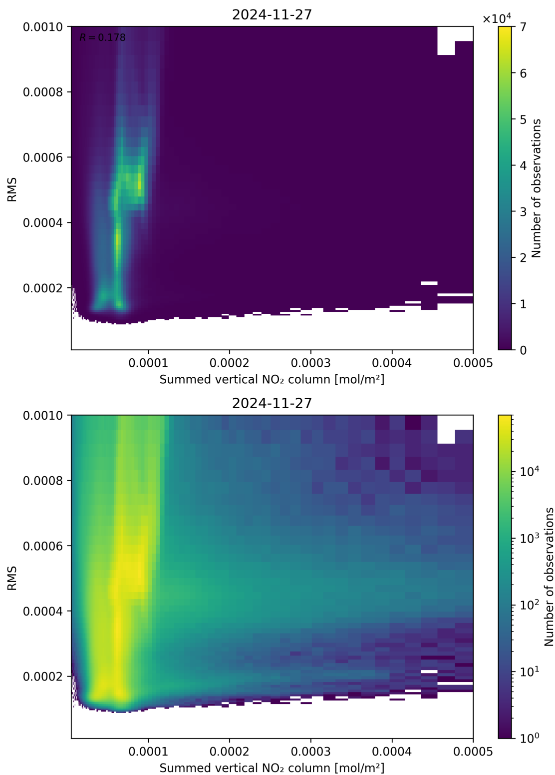
Figure 109: Scatter density plot of “Summed vertical NO 2 column” against “RMS” for 2024-11-26 to 2024-11-28.
