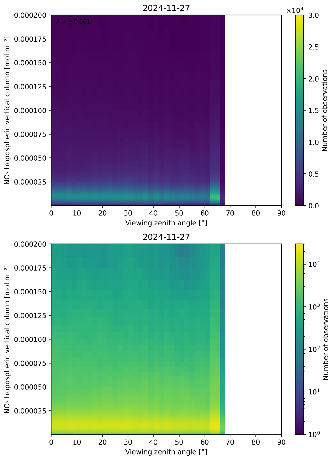
Figure 169: Scatter density plot of “Viewing zenith angle” against “NO 2 tropospheric vertical column” for 2024-11-26 to 2024-11-28.
