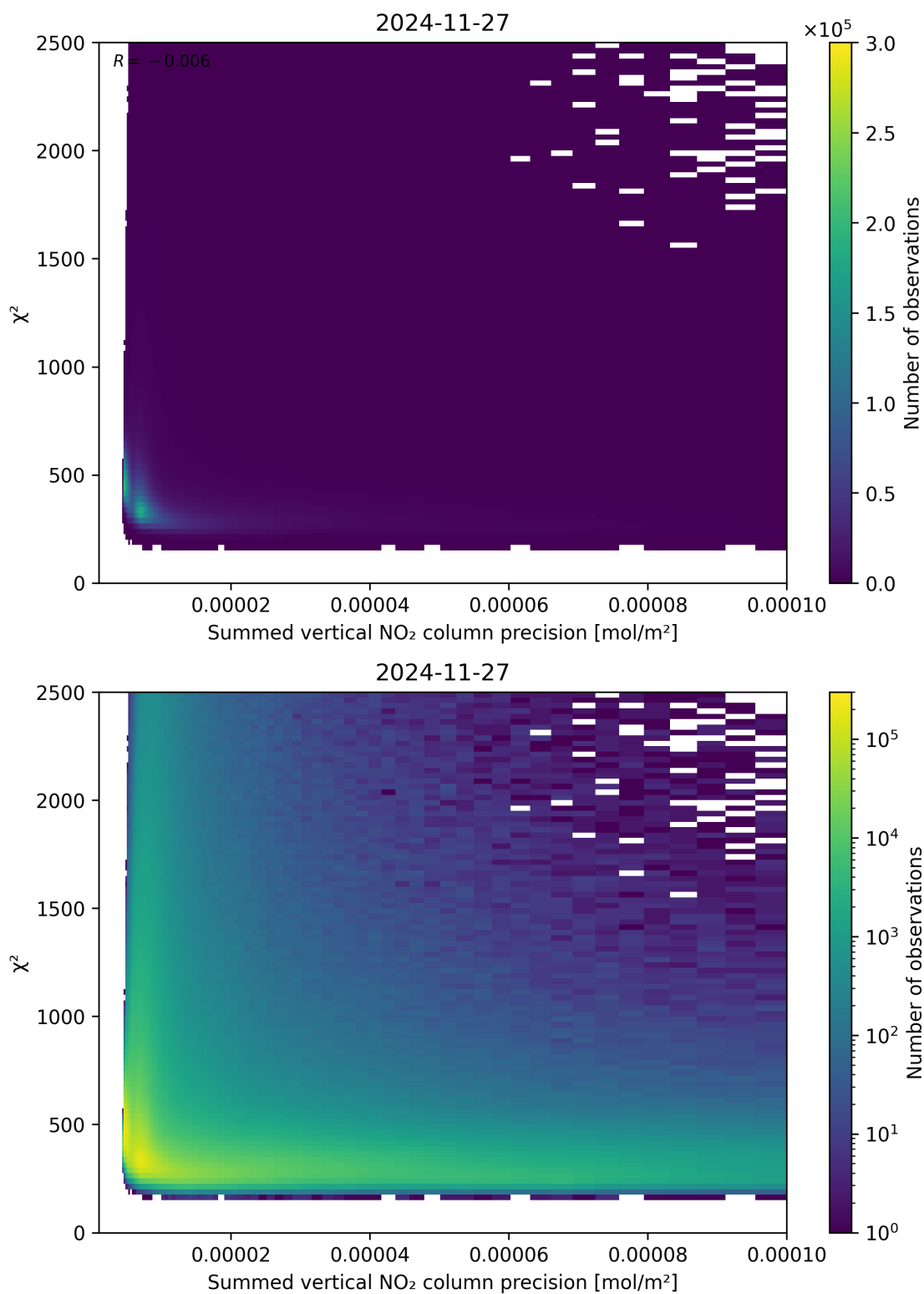
Figure 107: Scatter density plot of “Summed vertical NO 2 column precision” against “ \chi^2 ” for 2024-11-26 to 2024-11-28.
