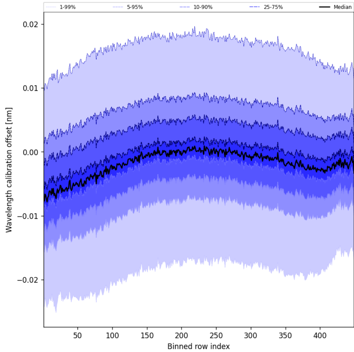
Figure 52: Along track statistics of “Wavelength calibration offset” for 2024-11-26 to 2024-11-28
