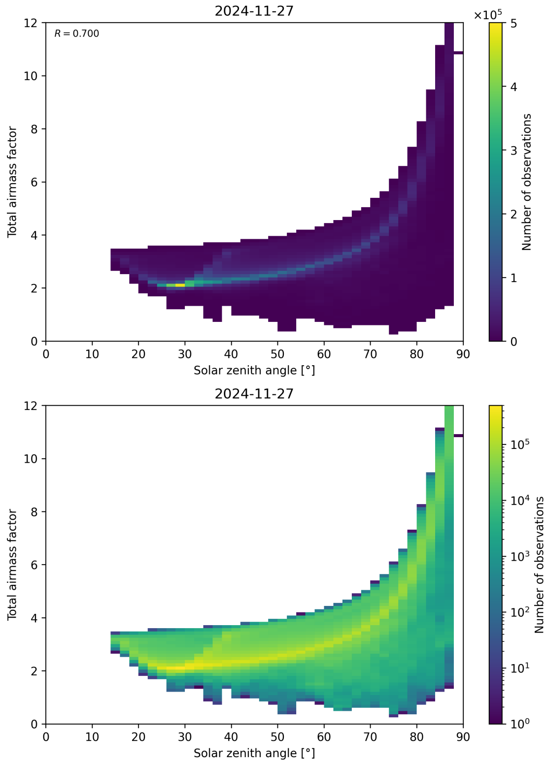
Figure 146: Scatter density plot of “Solar zenith angle” against “Total airmass factor” for 2024-11-26 to 2024-11-28.
