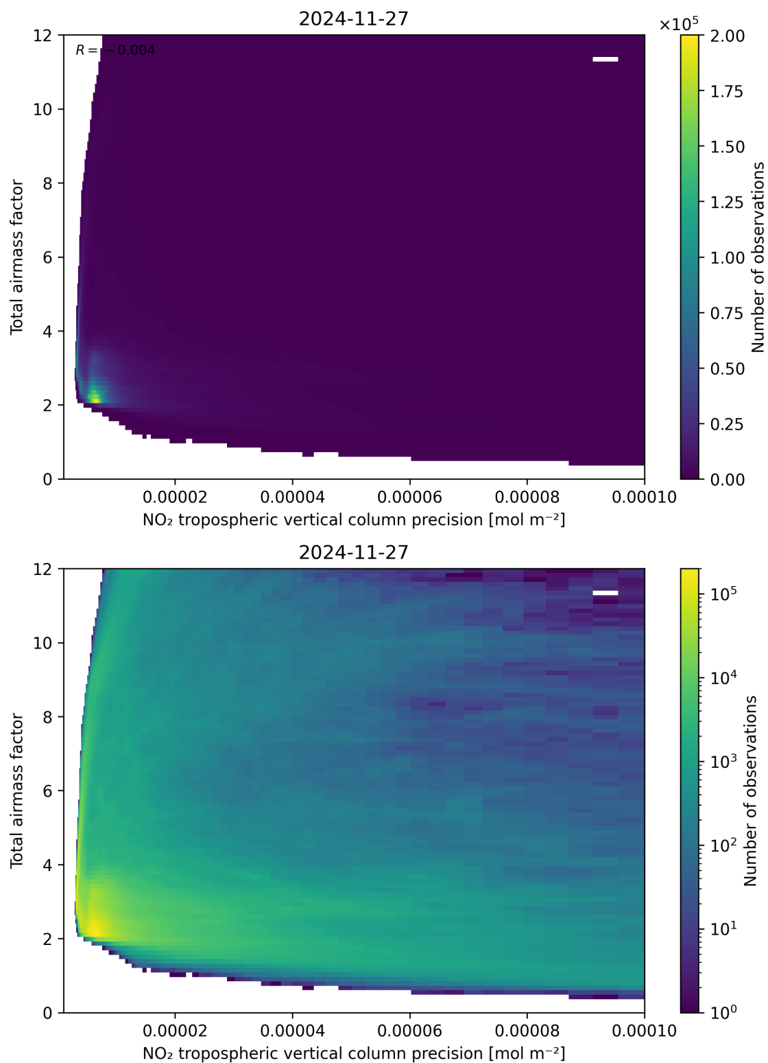
Figure 132: Scatter density plot of “NO 2 tropospheric vertical column precision” against “Total airmass factor” for 2024-11-26 to 2024-11-28.
