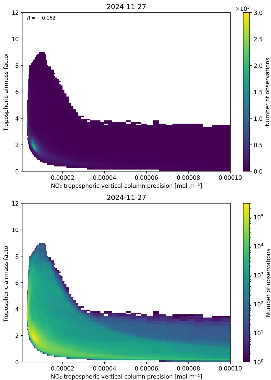
Figure 133: Scatter density plot of “NO 2 tropospheric vertical column precision” against “Tropospheric air mass factor” for 2024-11-26 to 2024-11-28.
