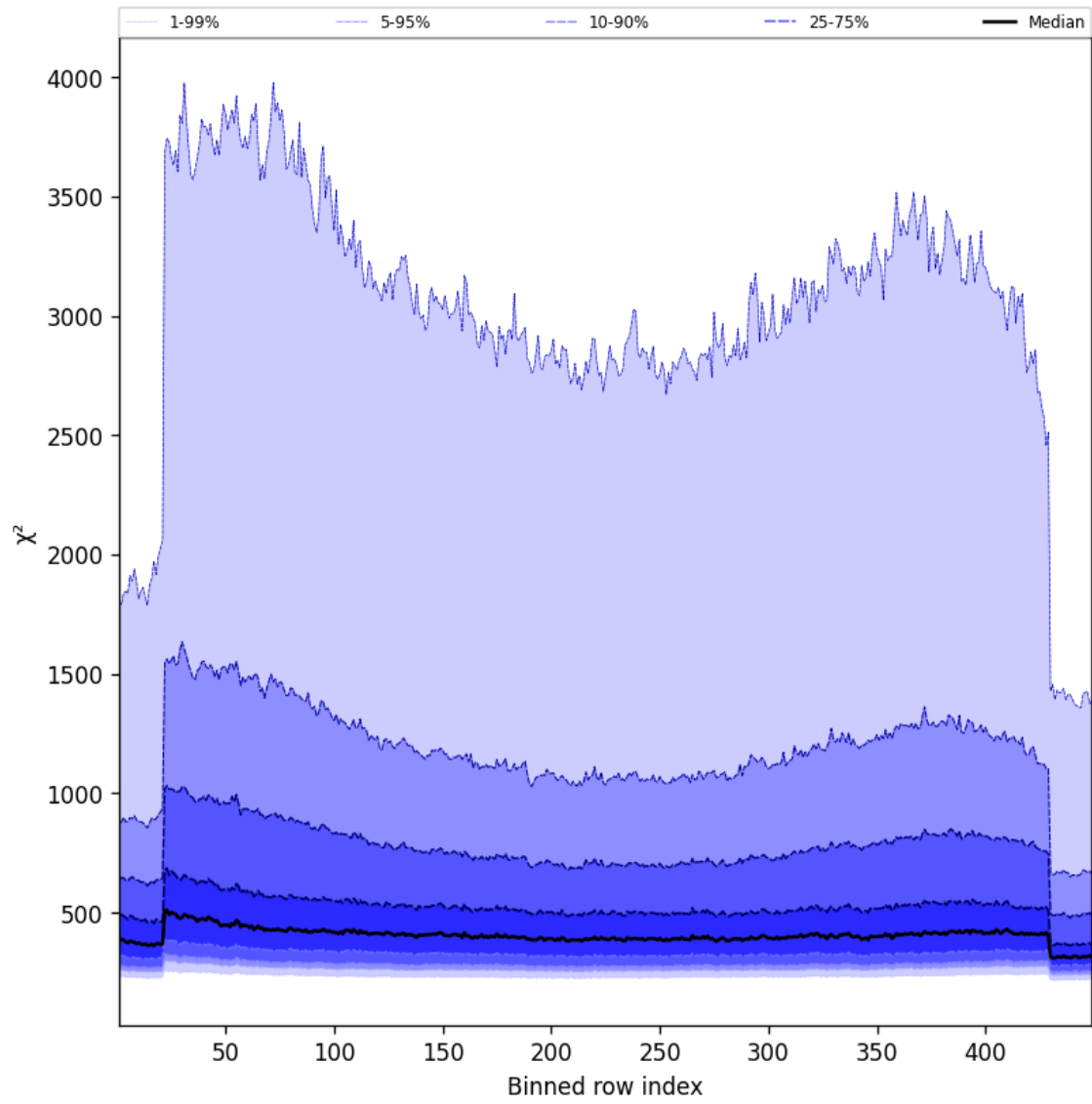
Figure 59: Along track statistics of “ \chi^2 ” for 2024-11-26 to 2024-11-28
