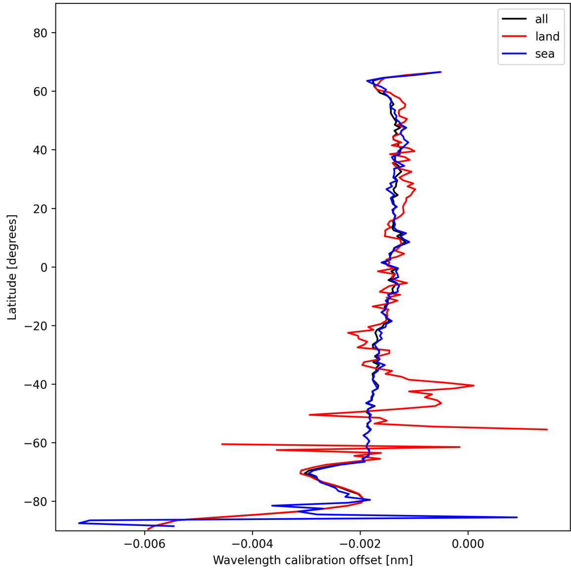
Figure 18: Zonal average of “Wavelength calibration offset” for 2024-11-26 to 2024-11-28.
