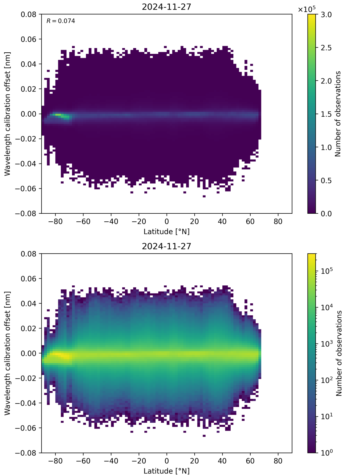
Figure 95: Scatter density plot of “Latitude” against “Wavelength calibration offset” for 2024-11-26 to 2024-11-28.
