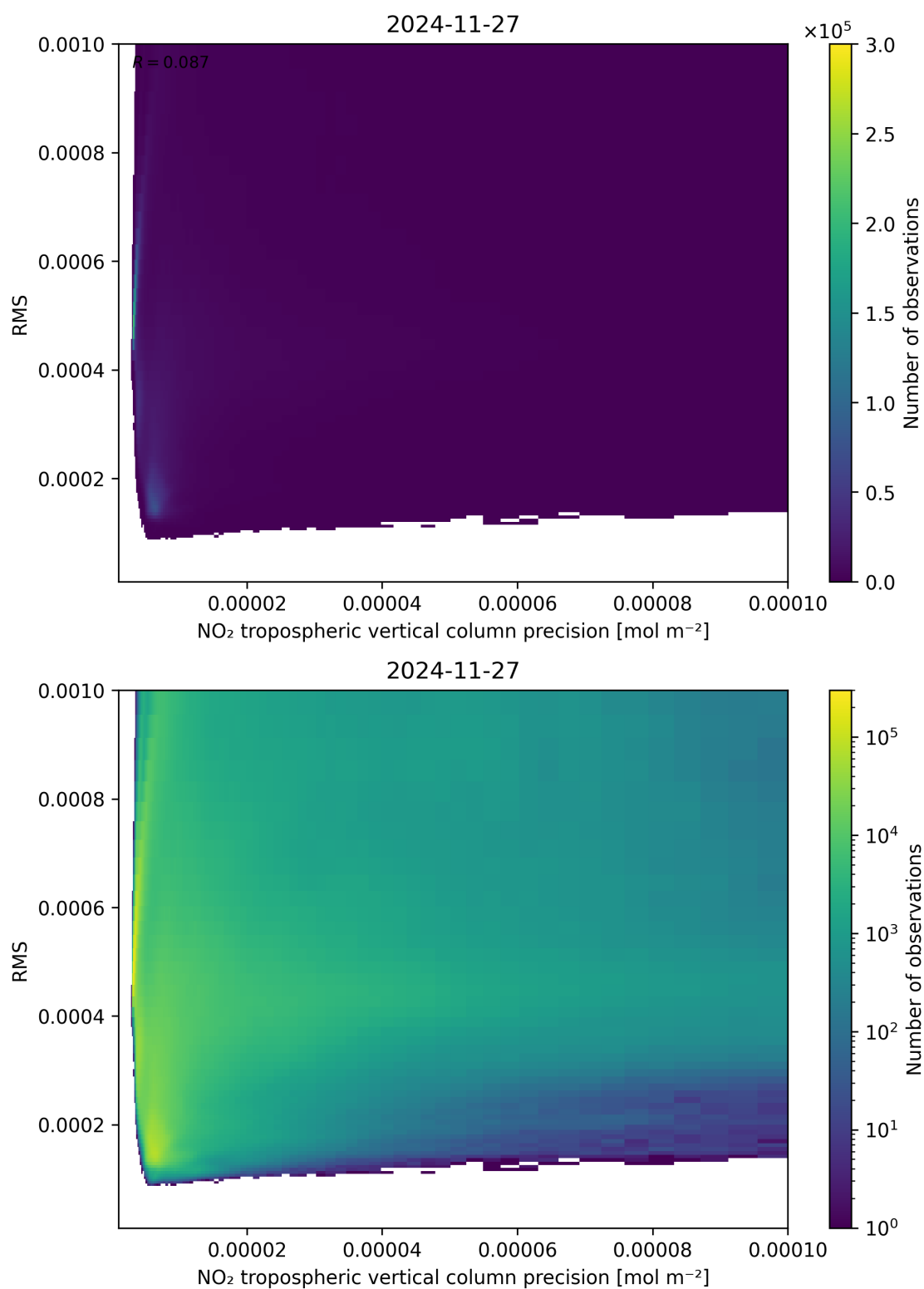
Figure 140: Scatter density plot of “NO 2 tropospheric vertical column precision” against “RMS” for 2024-11-26 to 2024-11-28.
