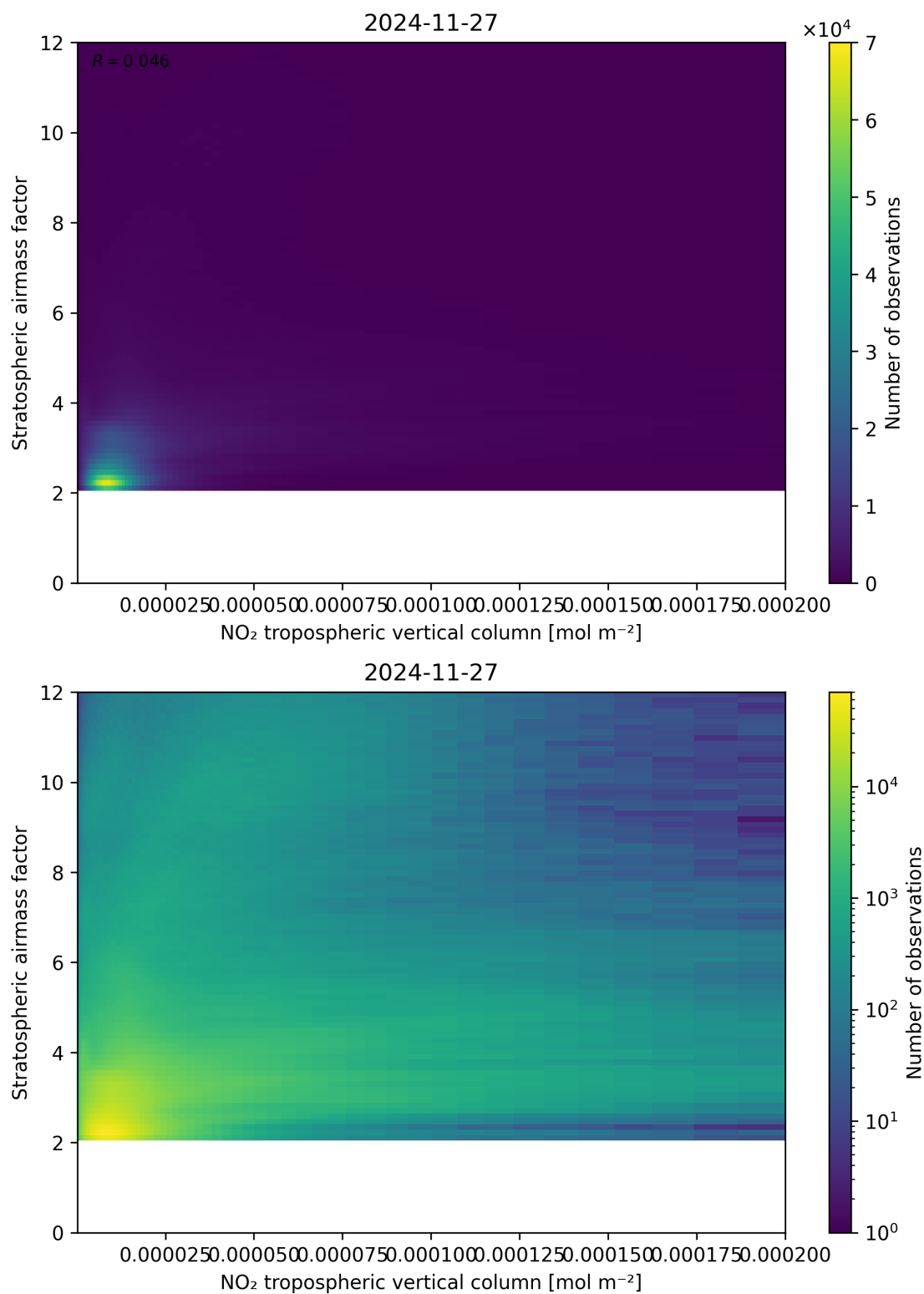
Figure 121: Scatter density plot of “NO 2 tropospheric vertical column” against “Stratospheric airmass factor” for 2024-11-26 to 2024-11-28.
