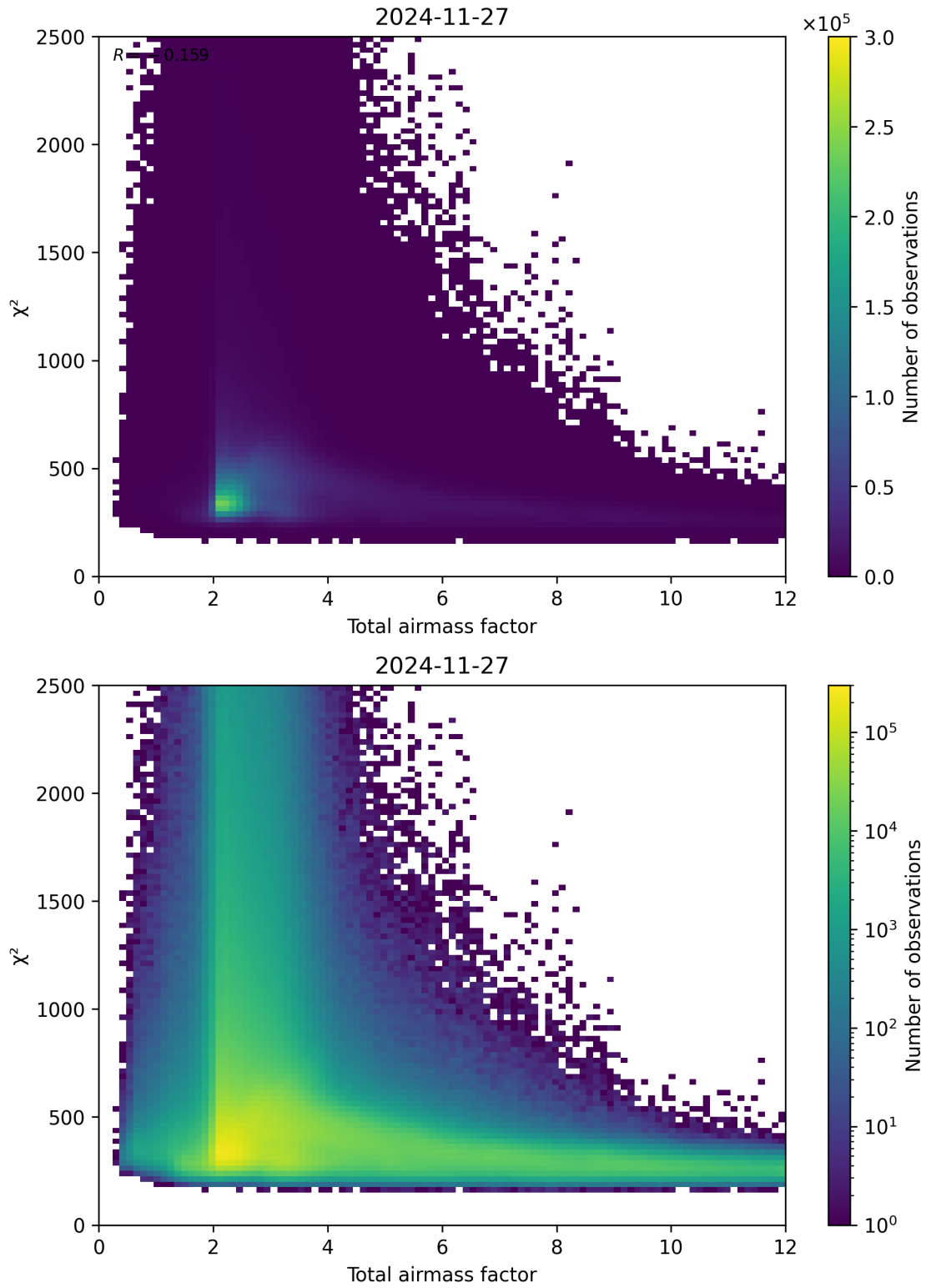
Figure 63: Scatter density plot of “Total airmass factor” against “ \chi^2 ” for 2024-11-26 to 2024-11-28.
