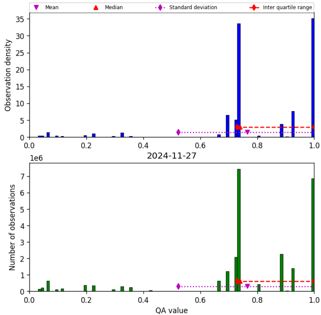
Figure 28: Histogram of “QA value” for 2024-11-26 to 2024-11-28
