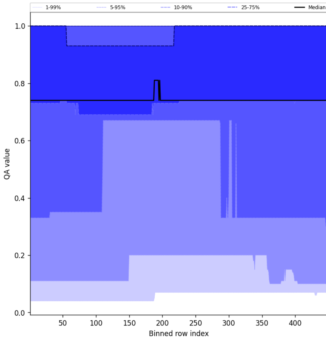
Figure 45: Along track statistics of “QA value” for 2024-11-26 to 2024-11-28
