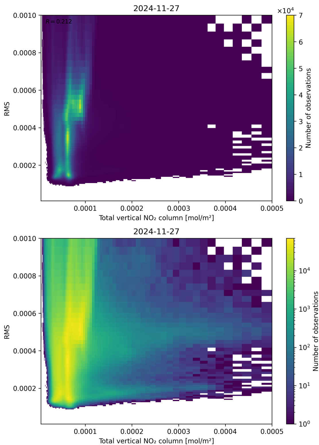
Figure 120: Scatter density plot of “Total vertical NO 2 column” against “RMS” for 2024-11-26 to 2024-11-28.
