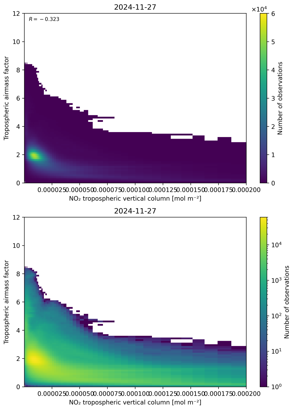
Figure 123: Scatter density plot of “NO 2 tropospheric vertical column” against “Tropospheric air mass factor” for 2024-11-26 to 2024-11-28.
