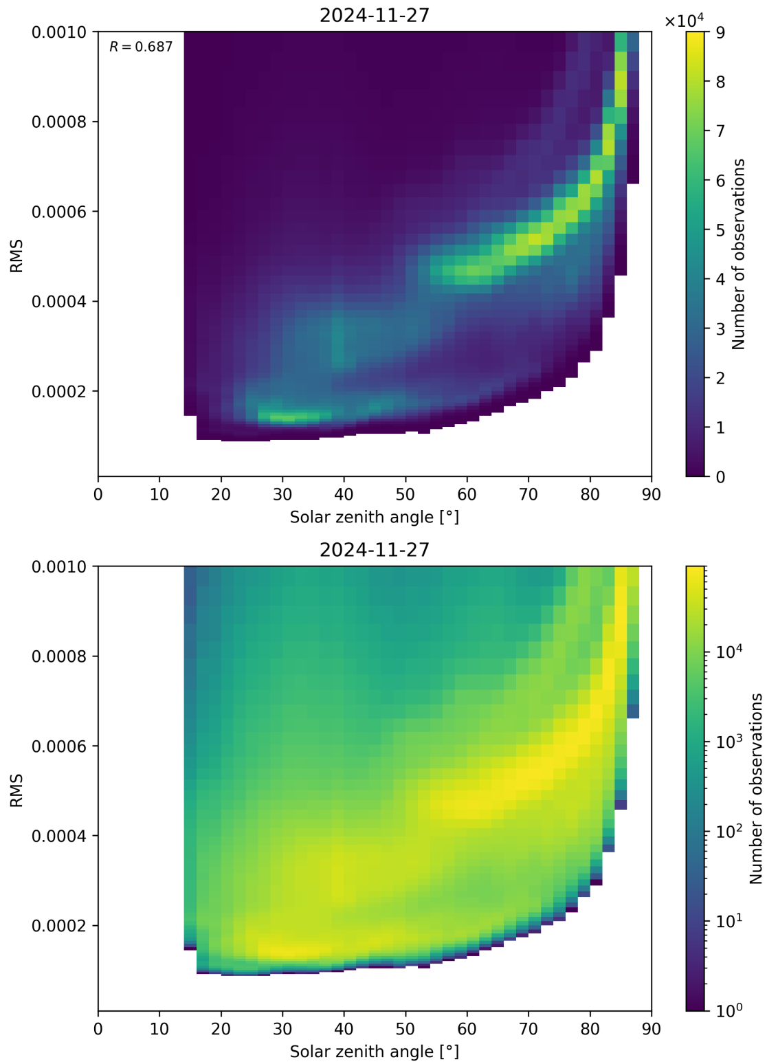
Figure 157: Scatter density plot of “Solar zenith angle” against “RMS” for 2024-11-26 to 2024-11-28.
