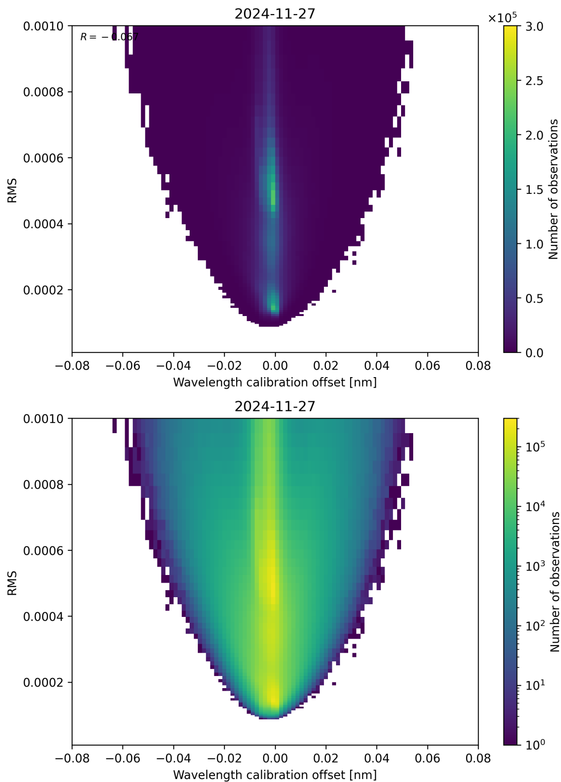
Figure 181: Scatter density plot of “Wavelength calibration offset” against “RMS” for 2024-11-26 to 2024-11-28.
