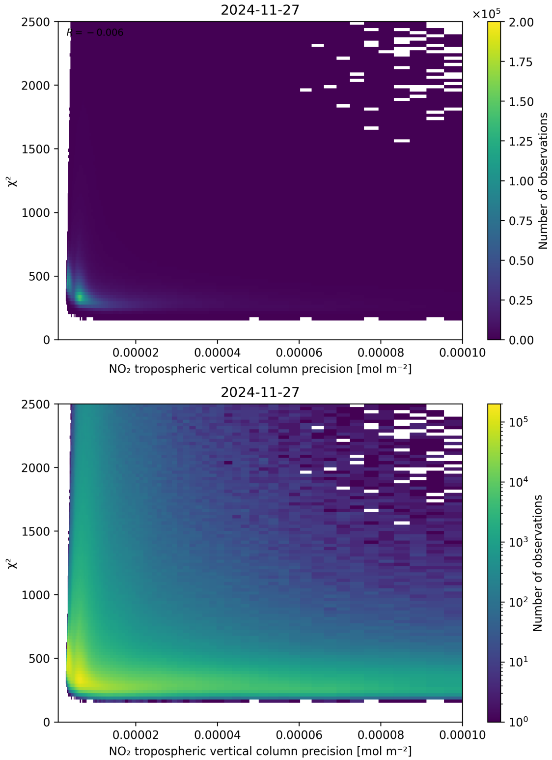
Figure 134: Scatter density plot of “NO 2 tropospheric vertical column precision” against “ \chi^2 ” for 2024-11-26 to 2024-11-28.
