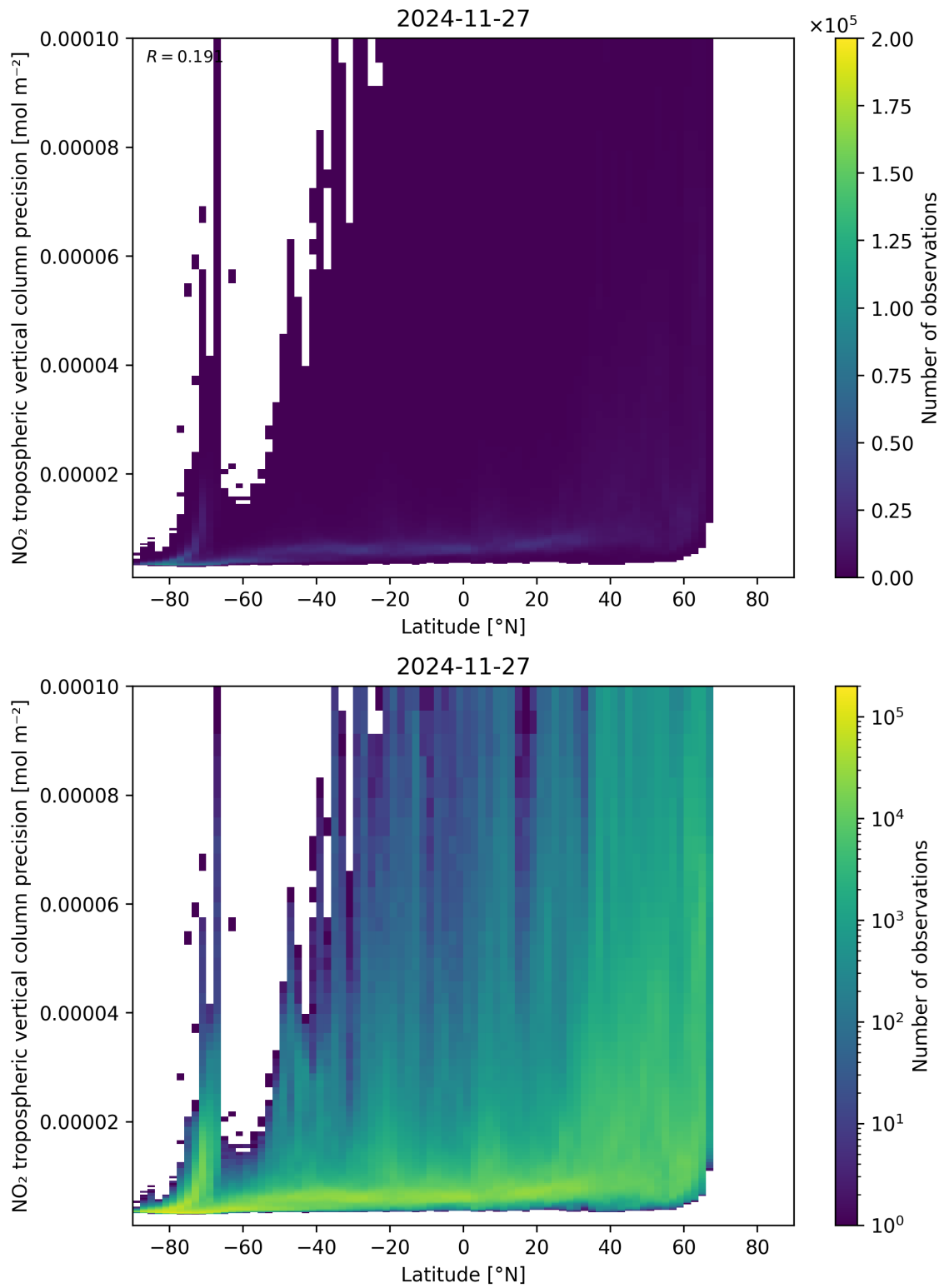
Figure 93: Scatter density plot of “Latitude” against “NO 2 tropospheric vertical column precision” for 2024-11-26 to 2024-11-28.
