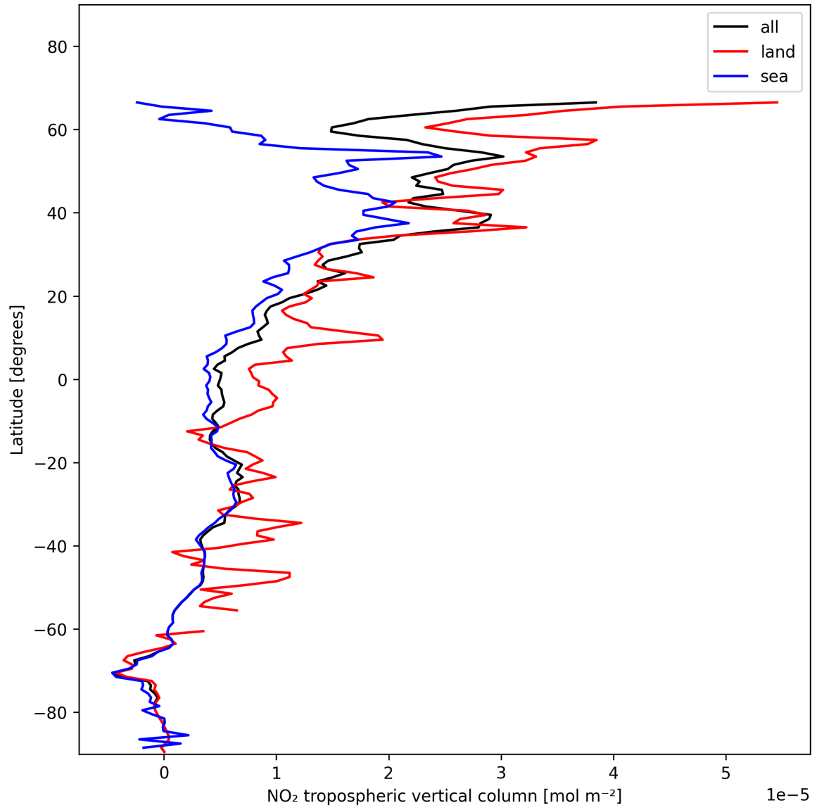
Figure 12: Zonal average of “NO 2 tropospheric vertical column” for 2024-11-26 to 2024-11-28.
