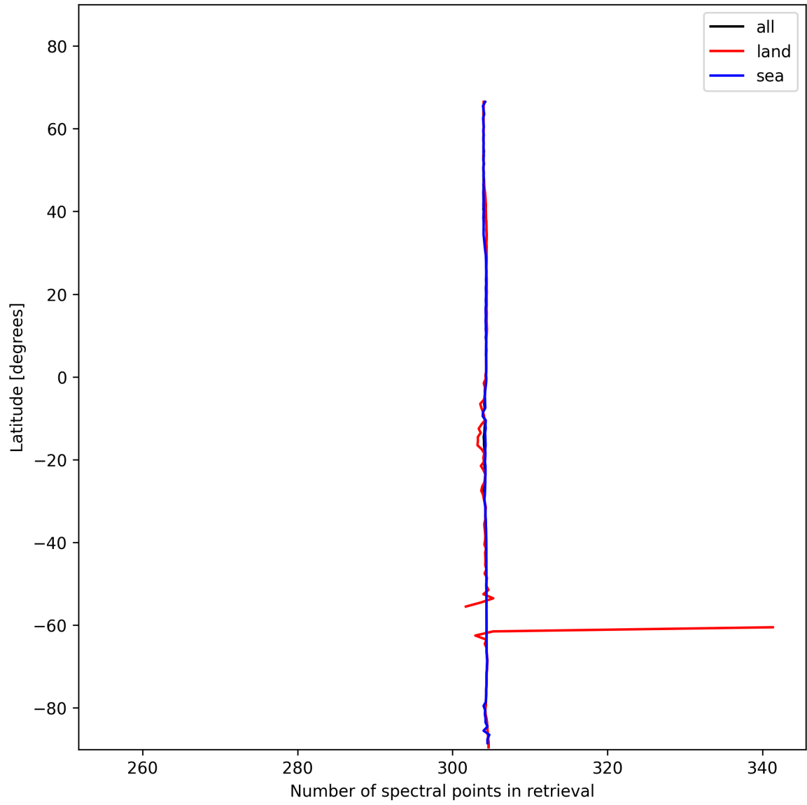
Figure 16: Zonal average of “Number of spectral points in retrieval” for 2024-11-26 to 2024-11-28.
