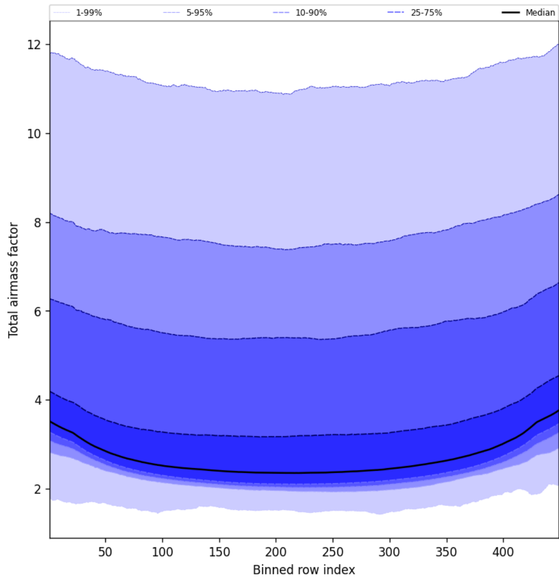
Figure 49: Along track statistics of “Total airmass factor” for 2024-11-26 to 2024-11-28
