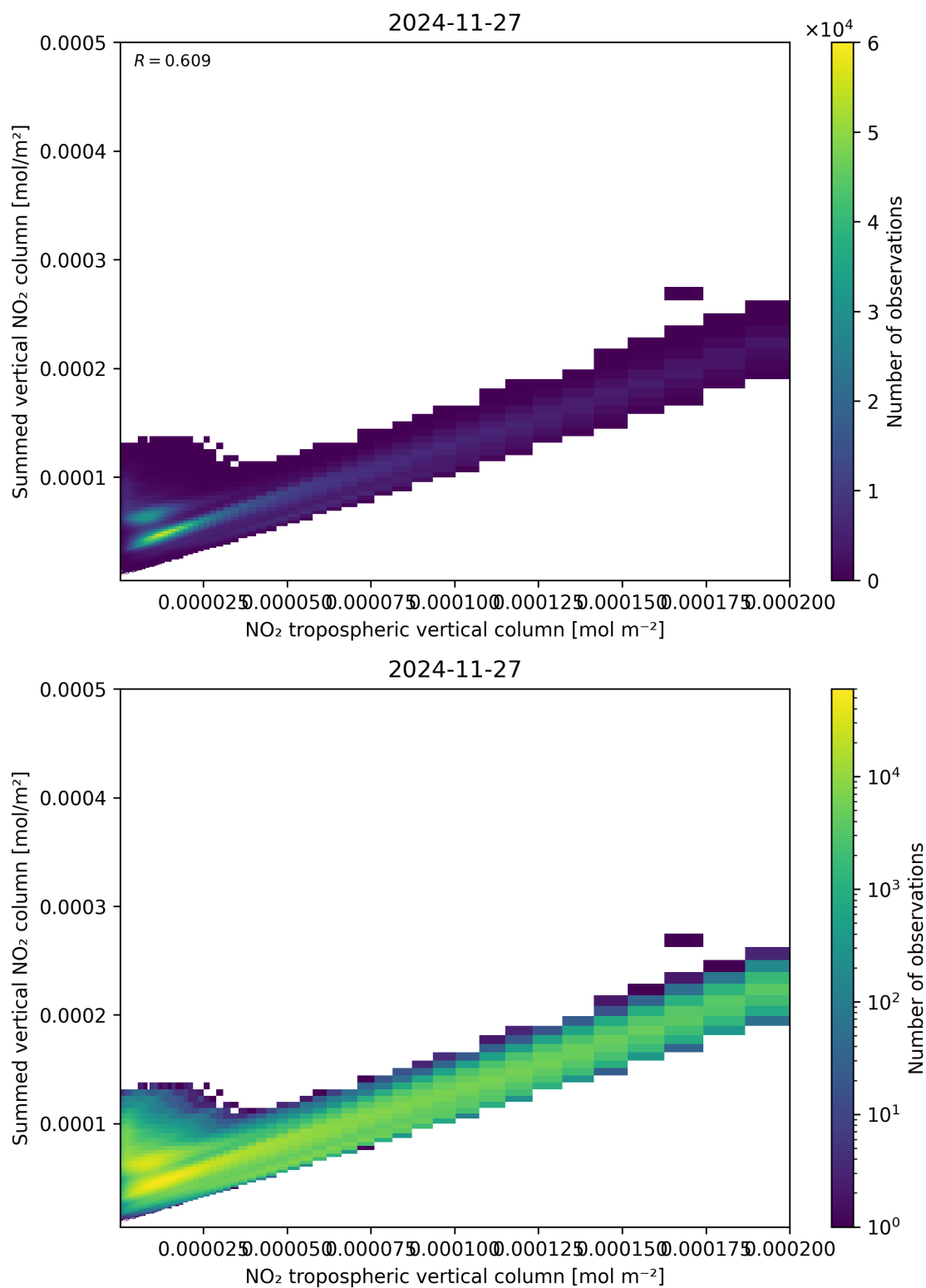
Figure 126: Scatter density plot of “NO 2 tropospheric vertical column” against “Summed vertical NO 2 column” for 2024-11-26 to 2024-11-28.
