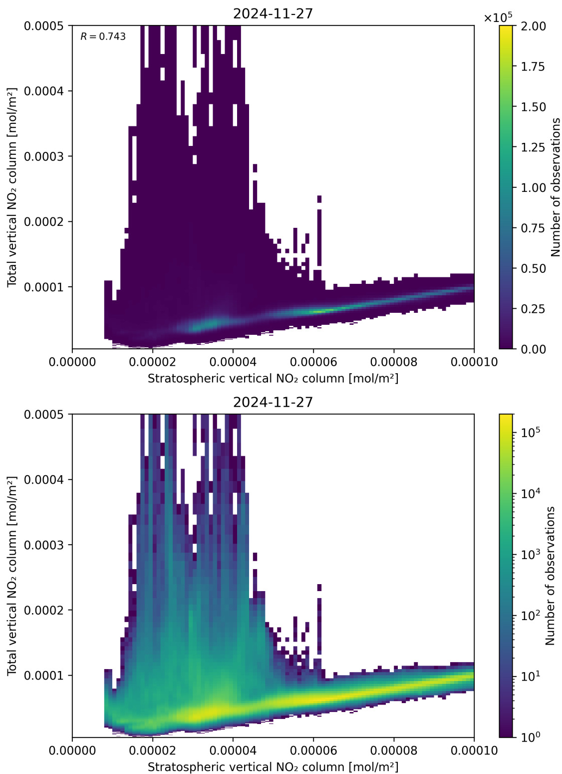
Figure 100: Scatter density plot of “Stratospheric vertical NO 2 column” against “Total vertical NO 2 column” for 2024-11-26 to 2024-11-28.
