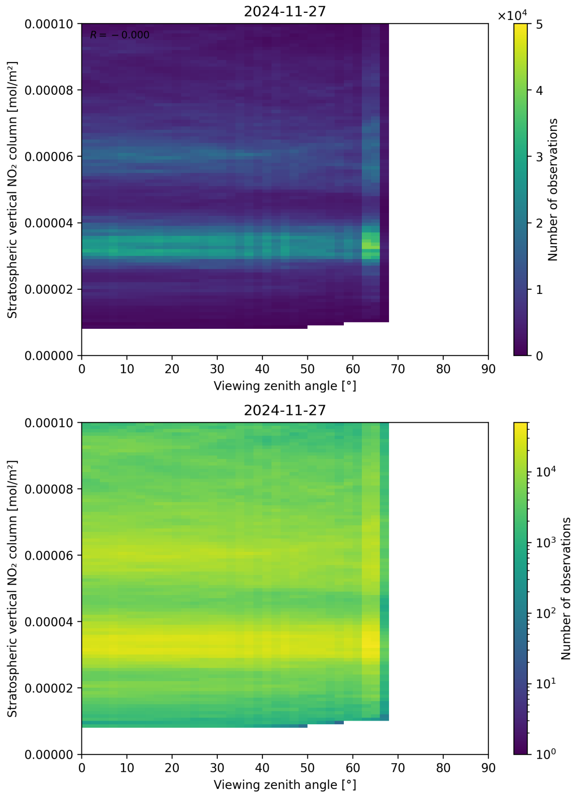
Figure 164: Scatter density plot of “Viewing zenith angle” against “Stratospheric vertical NO 2 column” for 2024-11-26 to 2024-11-28.
