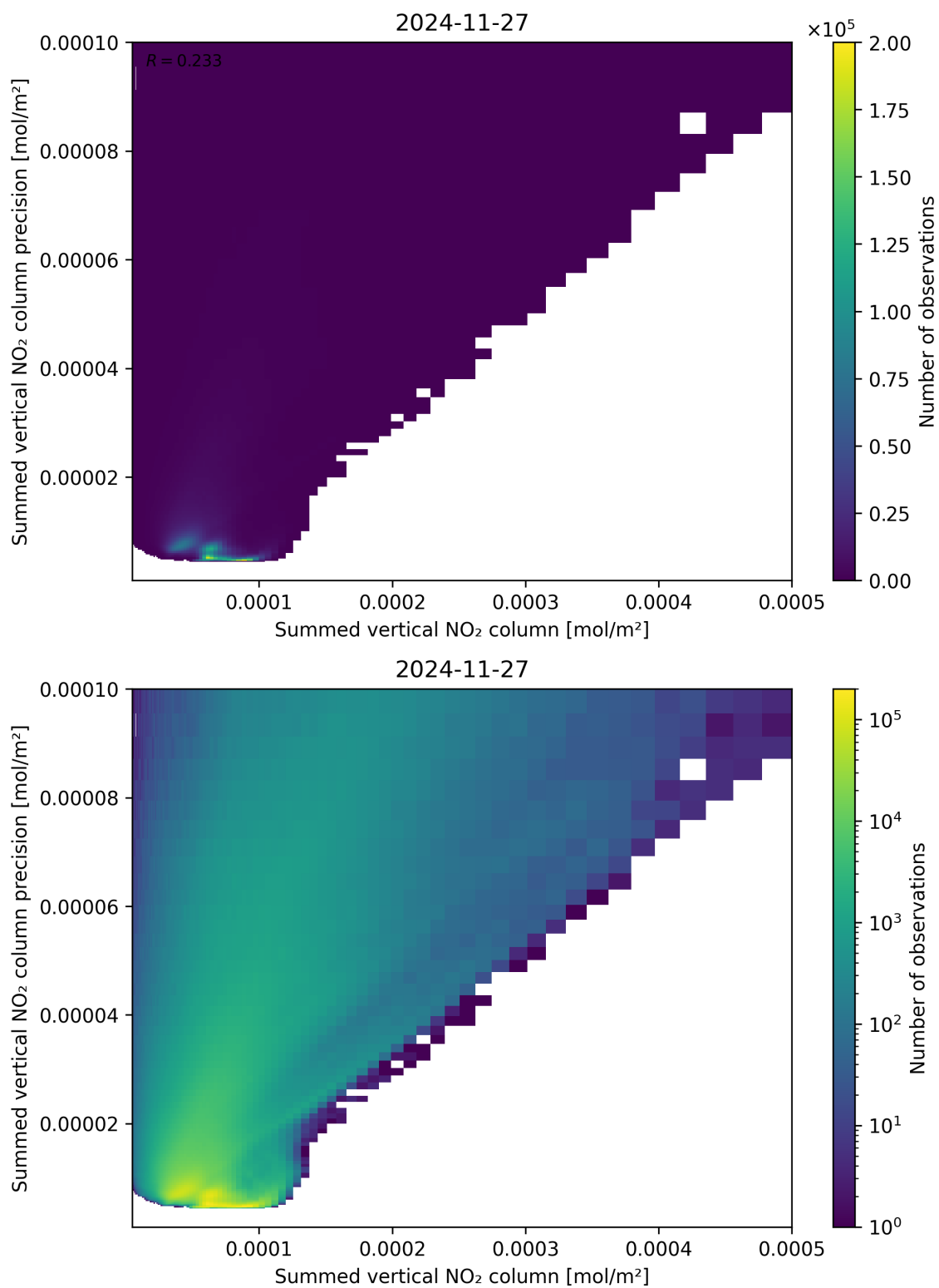
Figure 105: Scatter density plot of “Summed vertical NO 2 column” against “Summed vertical NO 2 column precision” for 2024-11-26 to 2024-11-28.
