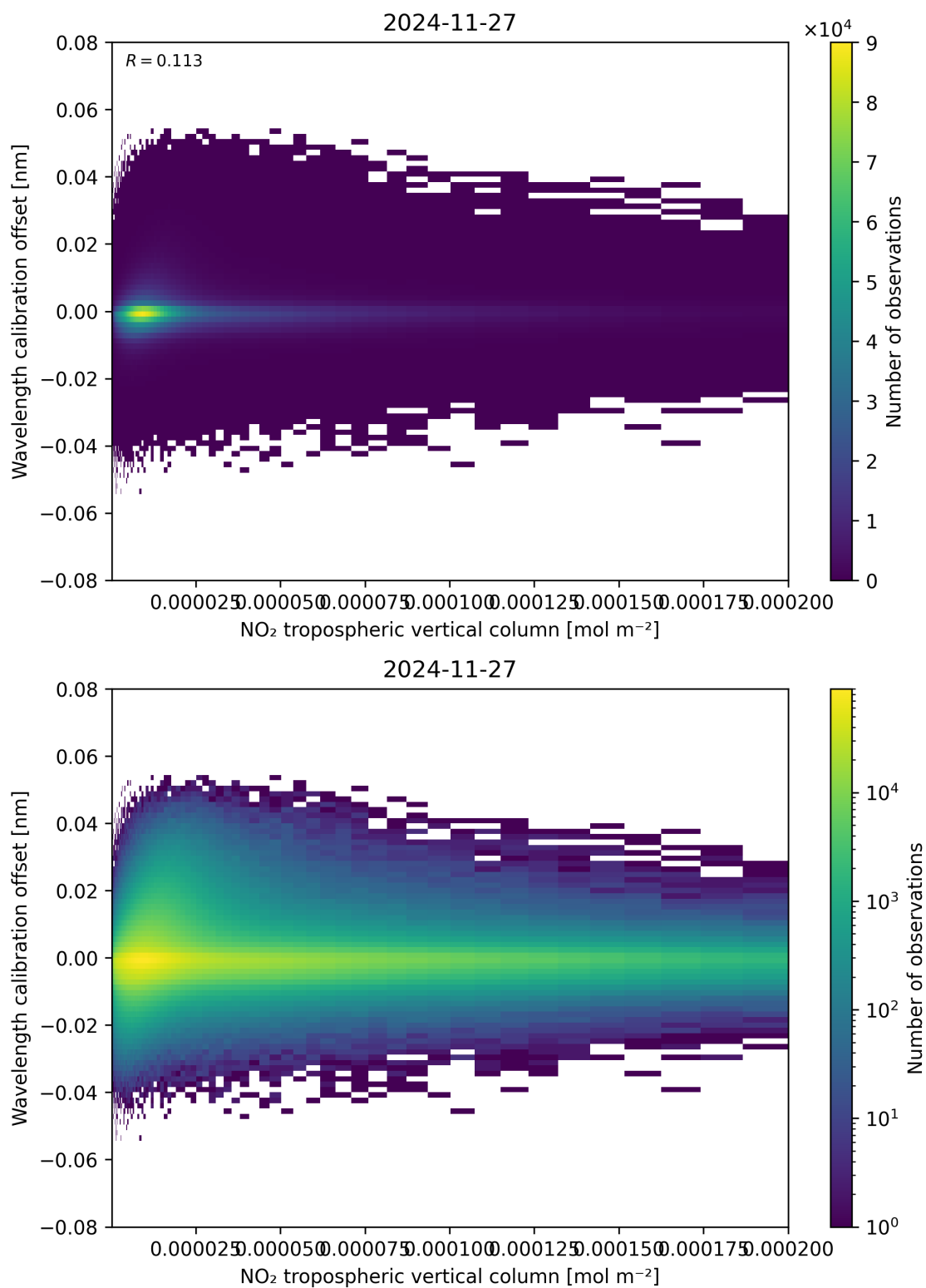
Figure 143: Scatter density plot of “NO 2 tropospheric vertical column” against “Wavelength calibration offset” for 2024-11-26 to 2024-11-28.
