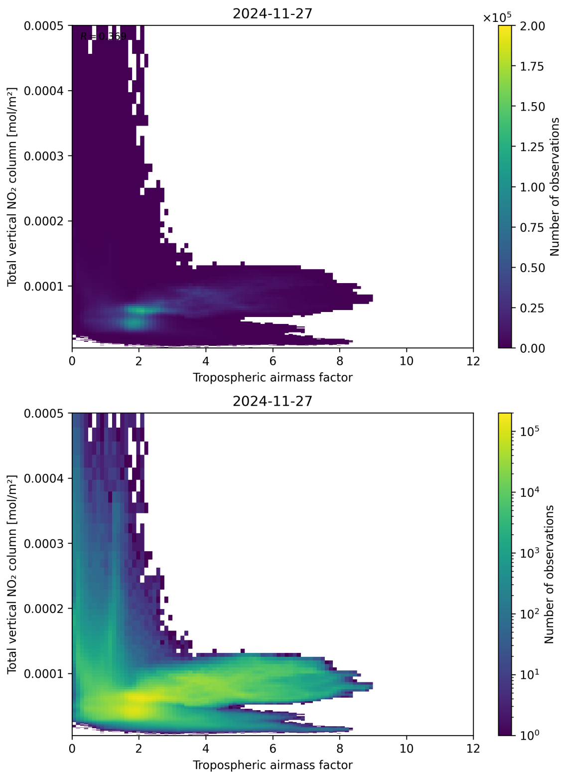
Figure 77: Scatter density plot of “Tropospheric airmass factor” against “Total vertical NO 2 column” for 2024-11-26 to 2024-11-28.
