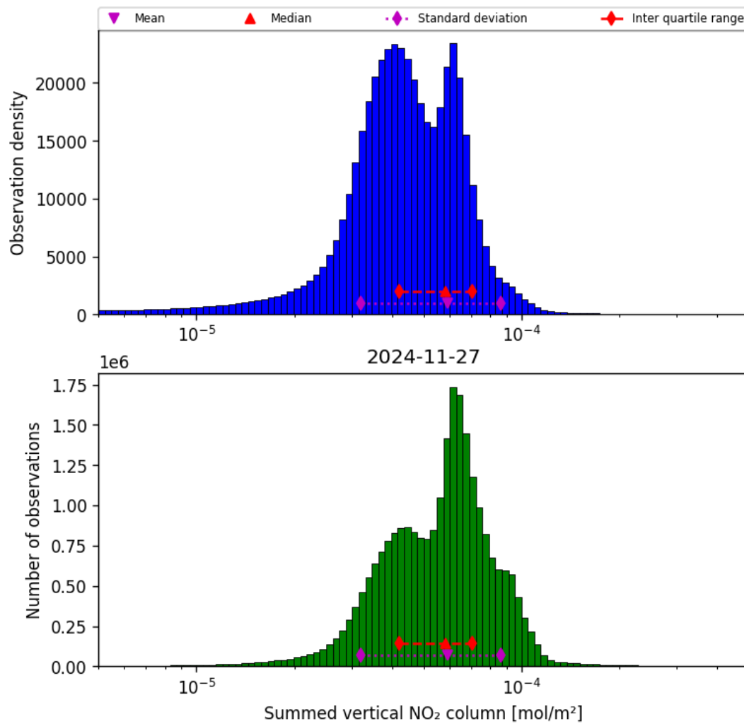
Figure 40: Histogram of “Summed vertical NO 2 column” for 2024-11-26 to 2024-11-28
