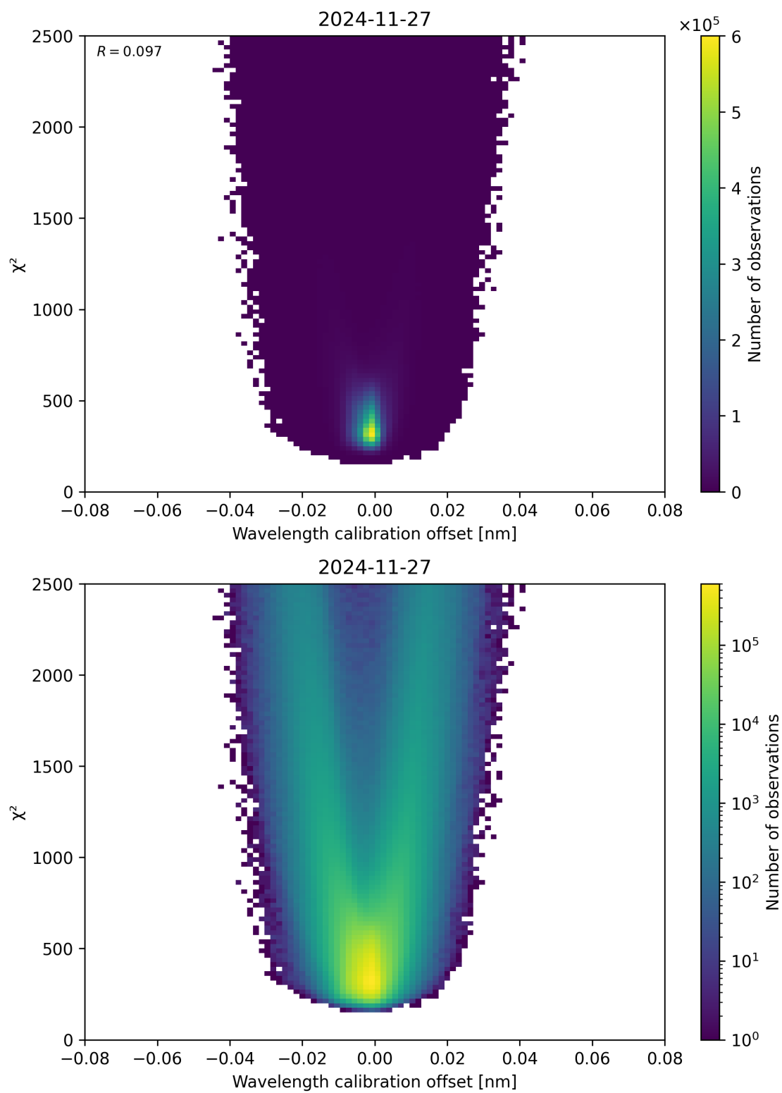
Figure 175: Scatter density plot of “Wavelength calibration offset” against “ \chi^2 ” for 2024-11-26 to 2024-11-28.
