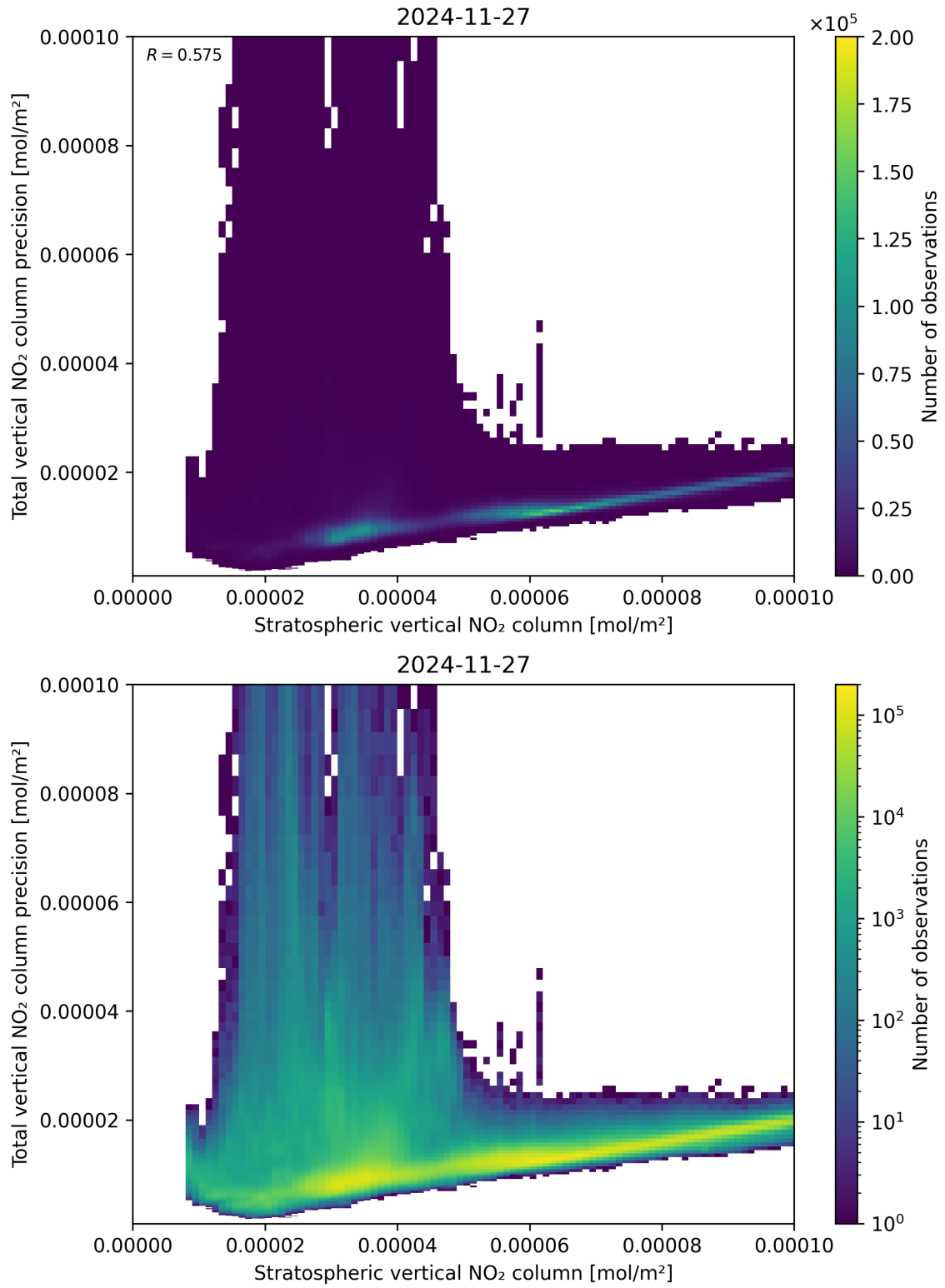
Figure 101: Scatter density plot of “Stratospheric vertical NO 2 column” against “Total vertical NO 2 column precision” for 2024-11-26 to 2024-11-28.
