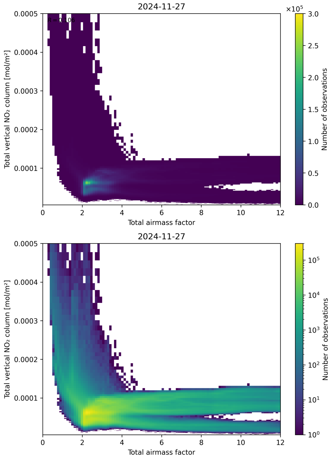
Figure 67: Scatter density plot of “Total airmass factor” against “Total vertical NO 2 column” for 2024-11-26 to 2024-11-28.
