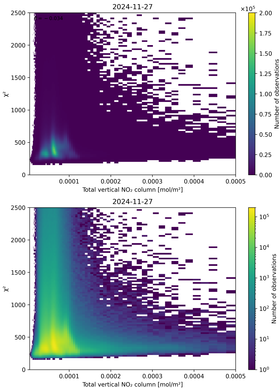
Figure 111: Scatter density plot of “Total vertical NO 2 column” against “ \chi^2 ” for 2024-11-26 to 2024-11-28.
