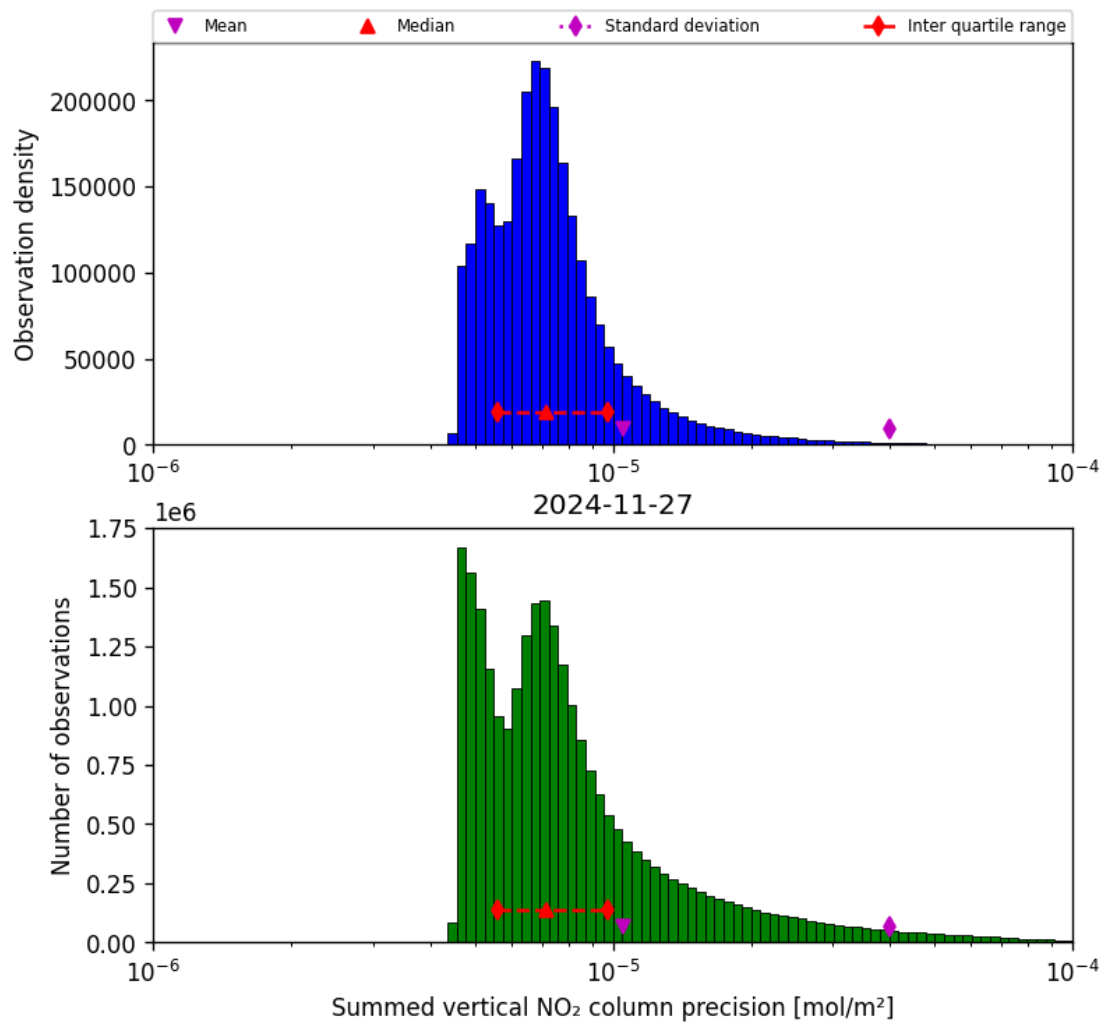
Figure 41: Histogram of “Summed vertical NO 2 column precision” for 2024-11-26 to 2024-11-28
