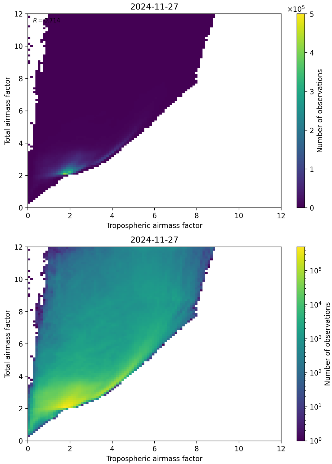
Figure 72: Scatter density plot of “Tropospheric airmass factor” against “Total airmass factor” for 2024-11-26 to 2024-11-28.
