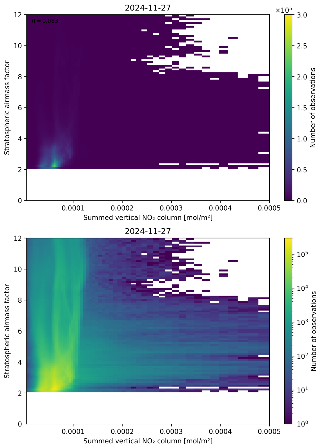
Figure 103: Scatter density plot of “Summed vertical NO 2 column” against “Stratospheric airmass factor” for 2024-11-26 to 2024-11-28.
