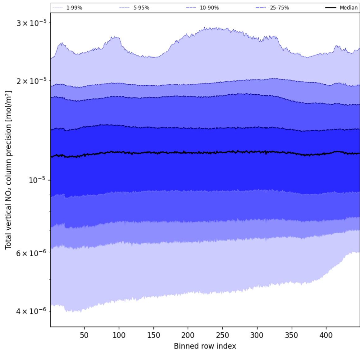
Figure 56: Along track statistics of “Total vertical NO 2 column precision” for 2024-11-26 to 2024-11-28
