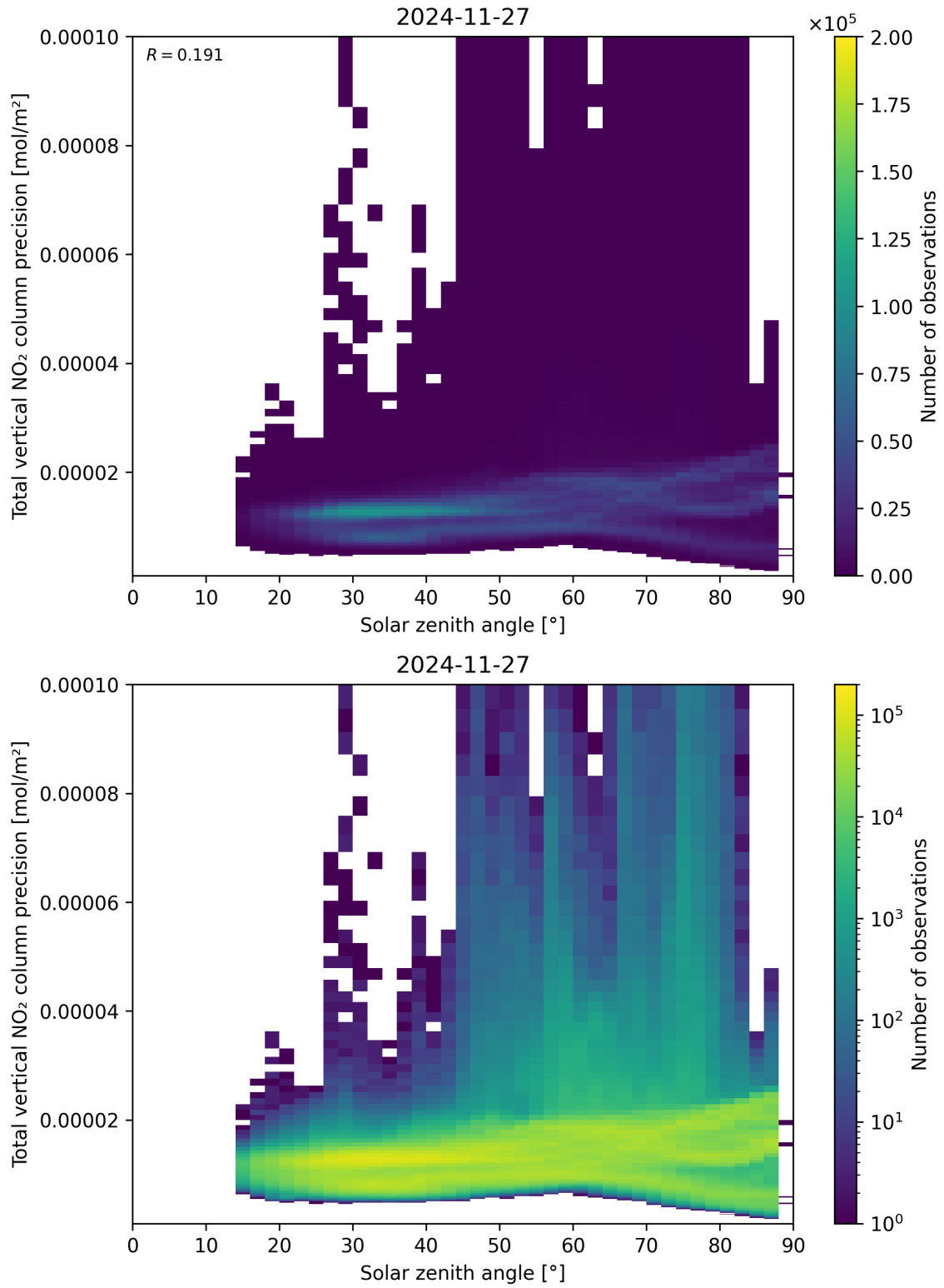
Figure 154: Scatter density plot of “Solar zenith angle” against “Total vertical NO 2 column precision” for 2024-11-26 to 2024-11-28.
