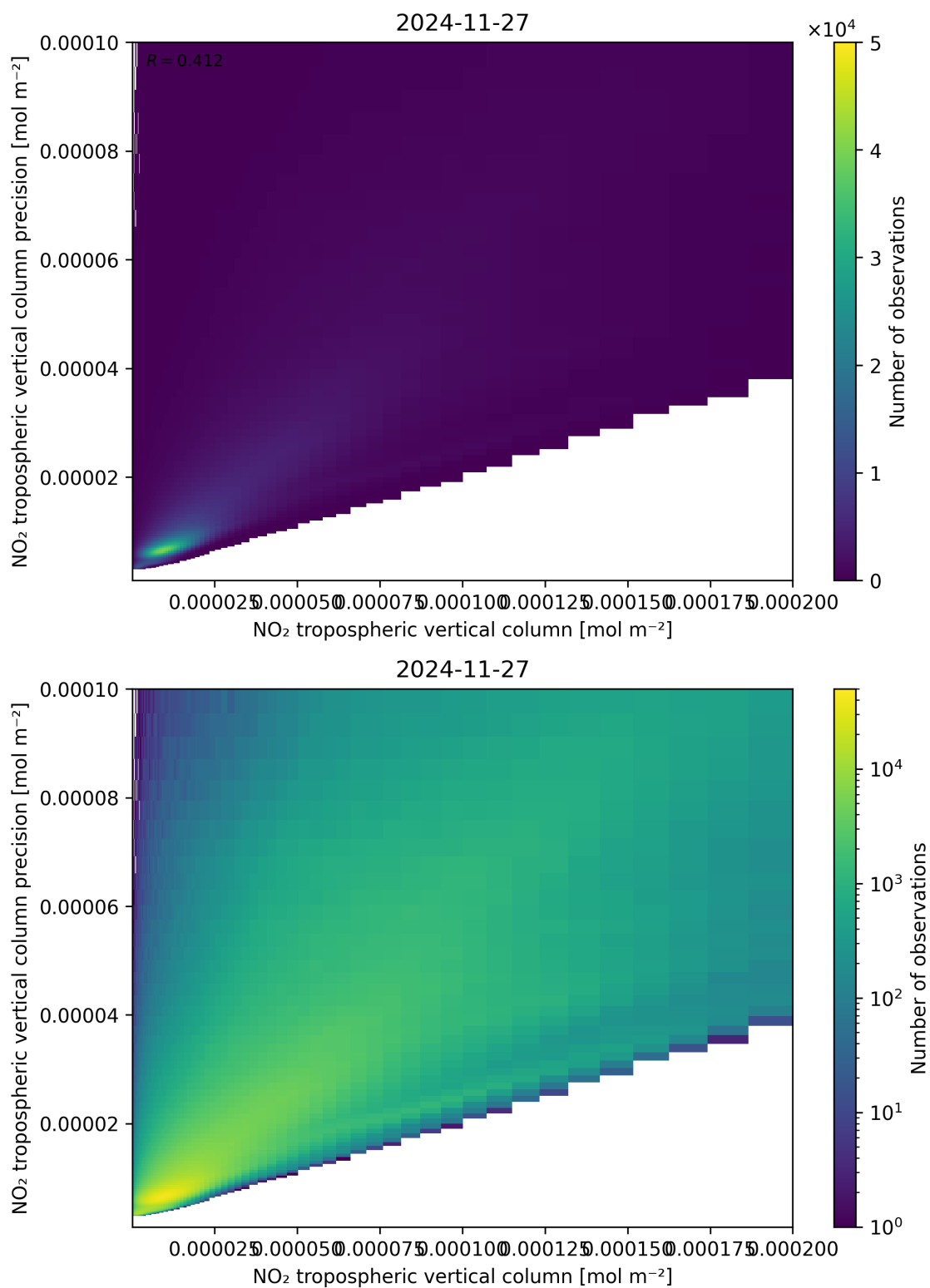
Figure 130: Scatter density plot of “NO 2 tropospheric vertical column” against “NO 2 tropospheric vertical column precision” for 2024-11-26 to 2024-11-28.
