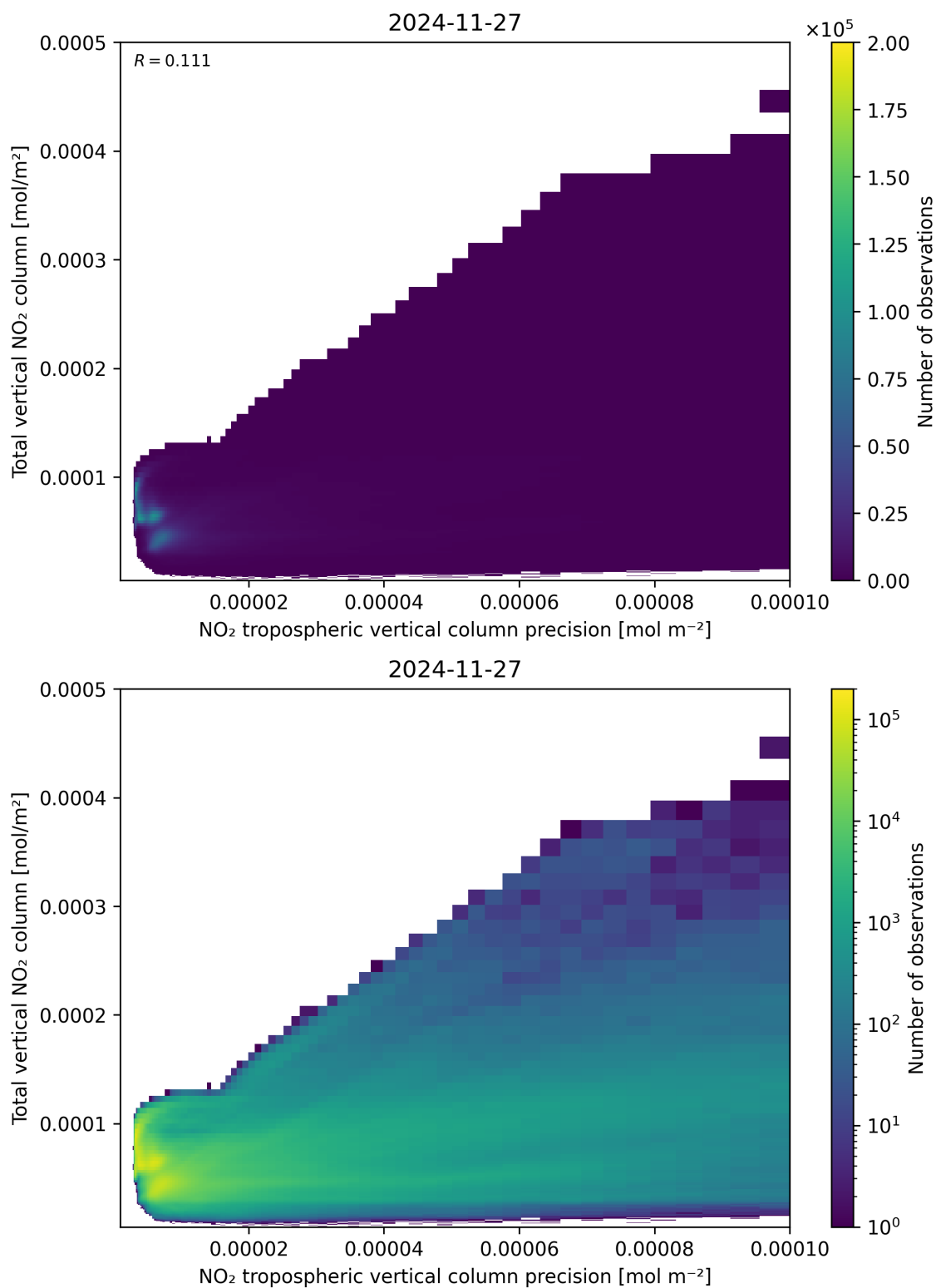
Figure 138: Scatter density plot of “NO 2 tropospheric vertical column precision” against “Total vertical NO 2 column” for 2024-11-26 to 2024-11-28.
