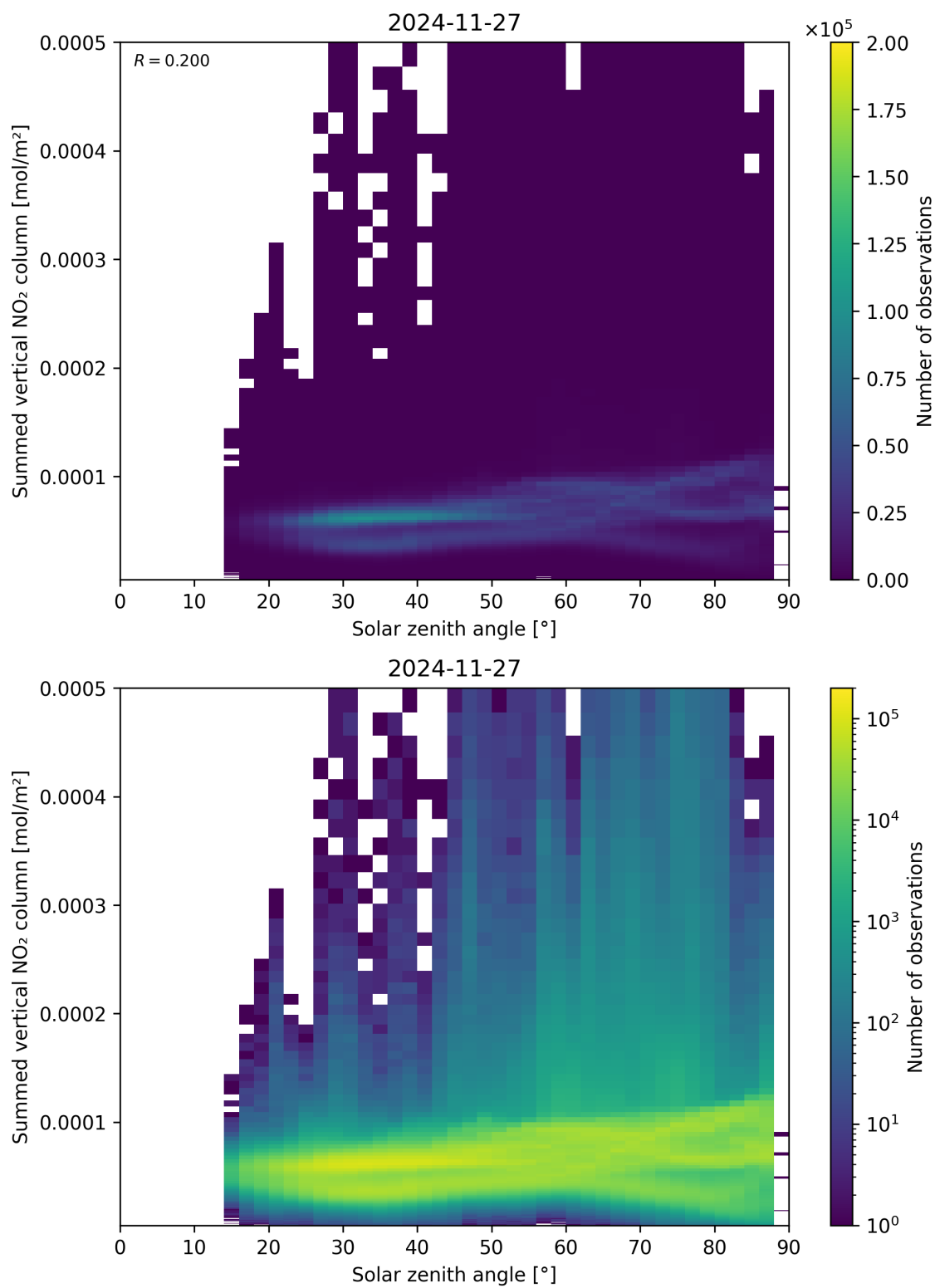
Figure 151: Scatter density plot of “Solar zenith angle” against “Summed vertical NO 2 column” for 2024-11-26 to 2024-11-28.
