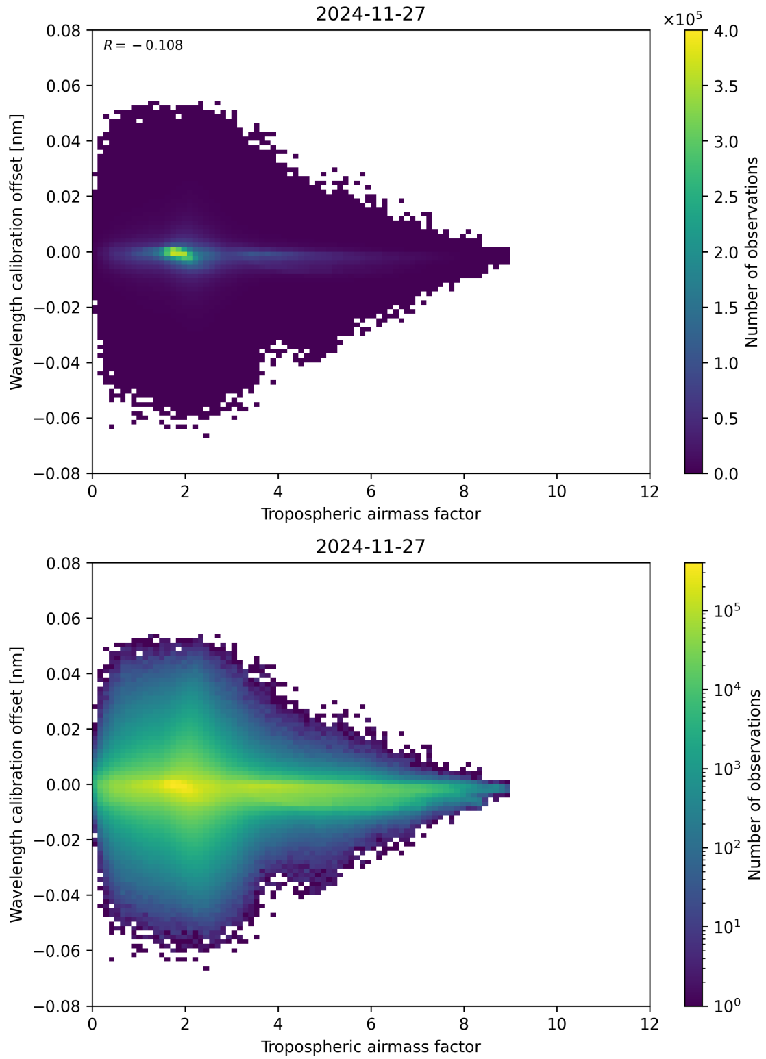
Figure 80: Scatter density plot of “Tropospheric airmass factor” against “Wavelength calibration offset” for 2024-11-26 to 2024-11-28.
