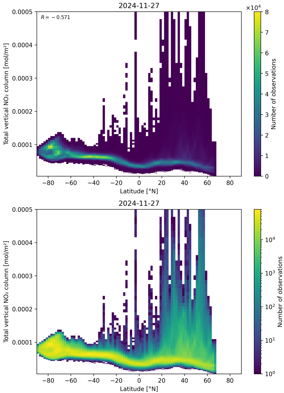
Figure 90: Scatter density plot of “Latitude” against “Total vertical NO 2 column” for 2024-11-26 to 2024-11-28.
