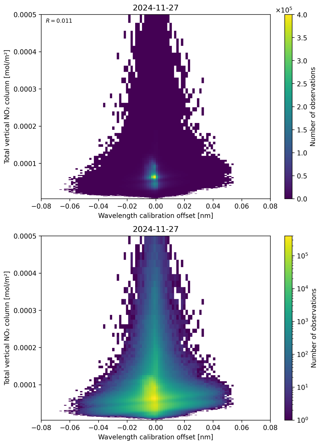
Figure 179: Scatter density plot of “Wavelength calibration offset” against “Total vertical NO 2 column” for 2024-11-26 to 2024-11-28.
