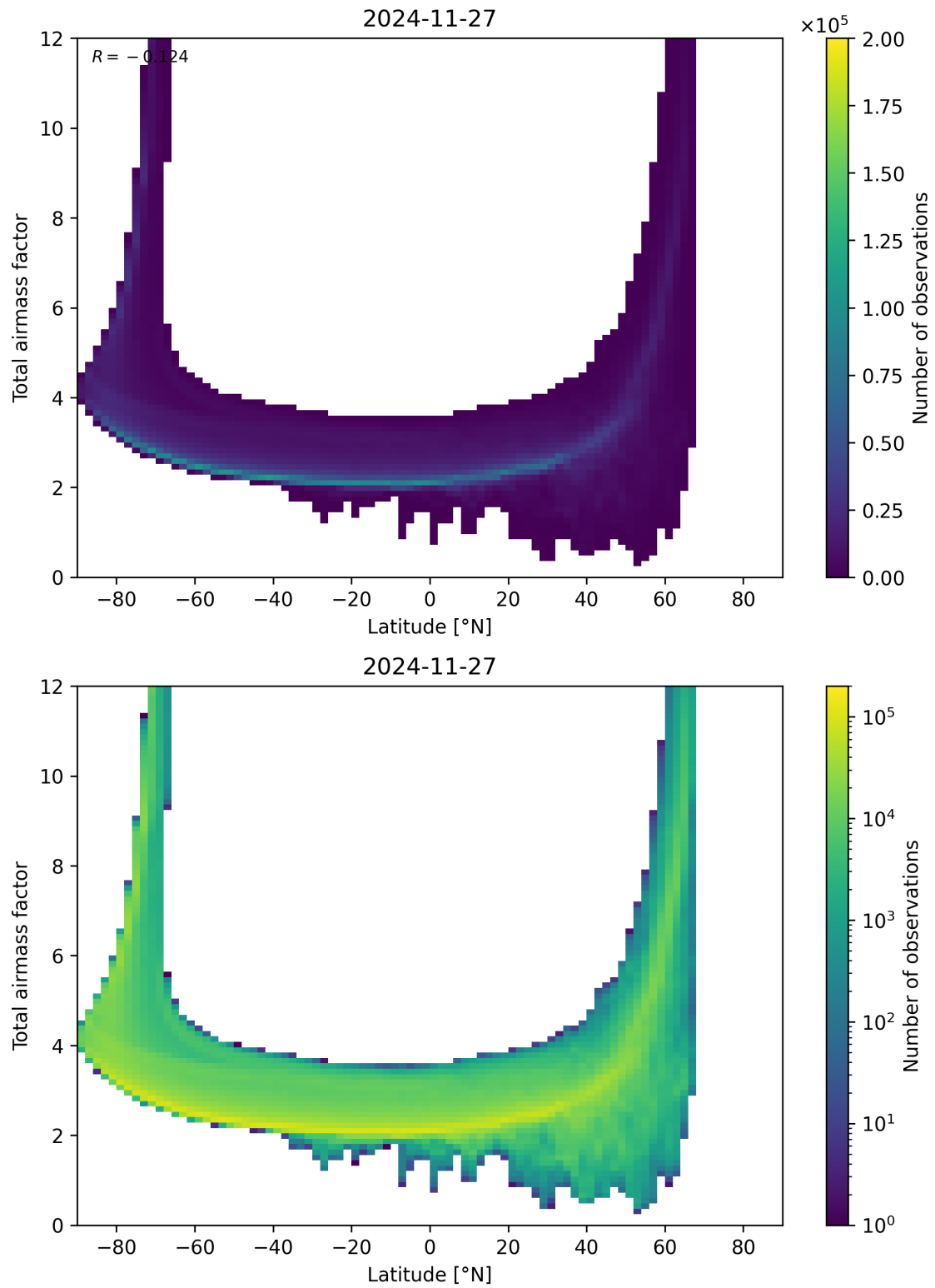
Figure 84: Scatter density plot of “Latitude” against “Total airmass factor” for 2024-11-26 to 2024-11-28.
