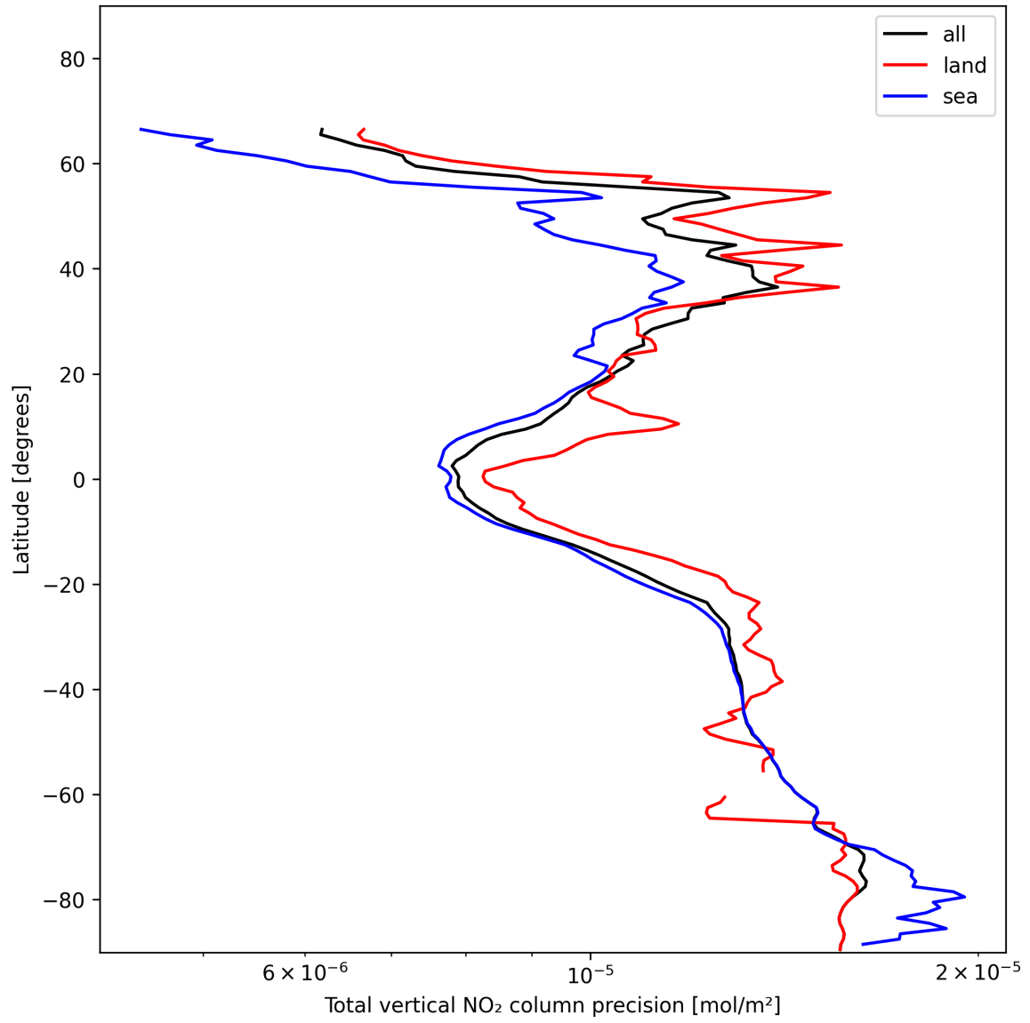
Figure 22: Zonal average of “Total vertical NO 2 column precision” for 2024-11-26 to 2024-11-28.
