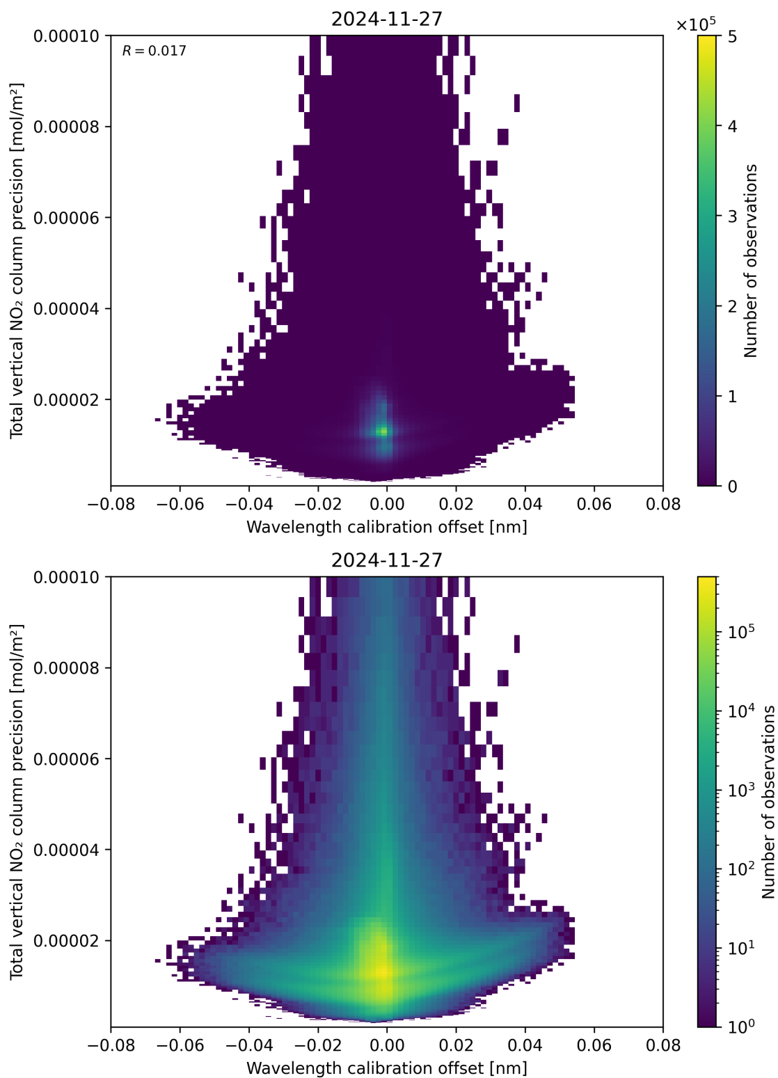
Figure 180: Scatter density plot of “Wavelength calibration offset” against “Total vertical NO 2 column precision” for 2024-11-26 to 2024-11-28.
