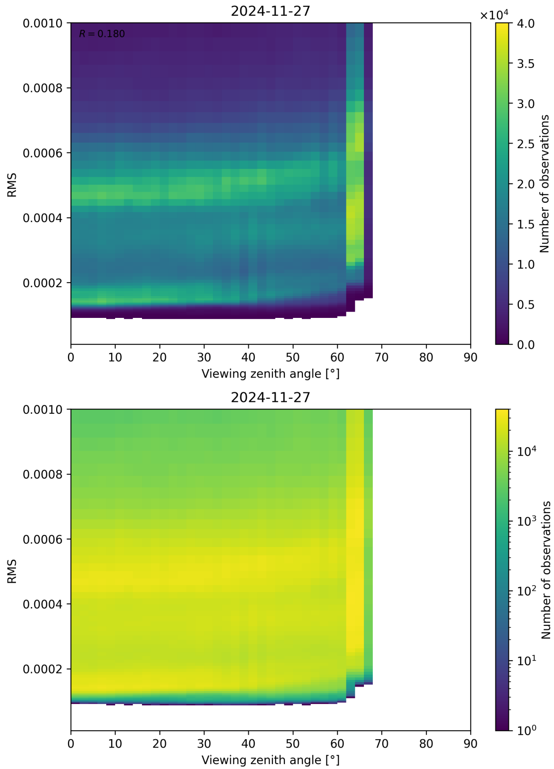
Figure 171: Scatter density plot of “Viewing zenith angle” against “RMS” for 2024-11-26 to 2024-11-28.
