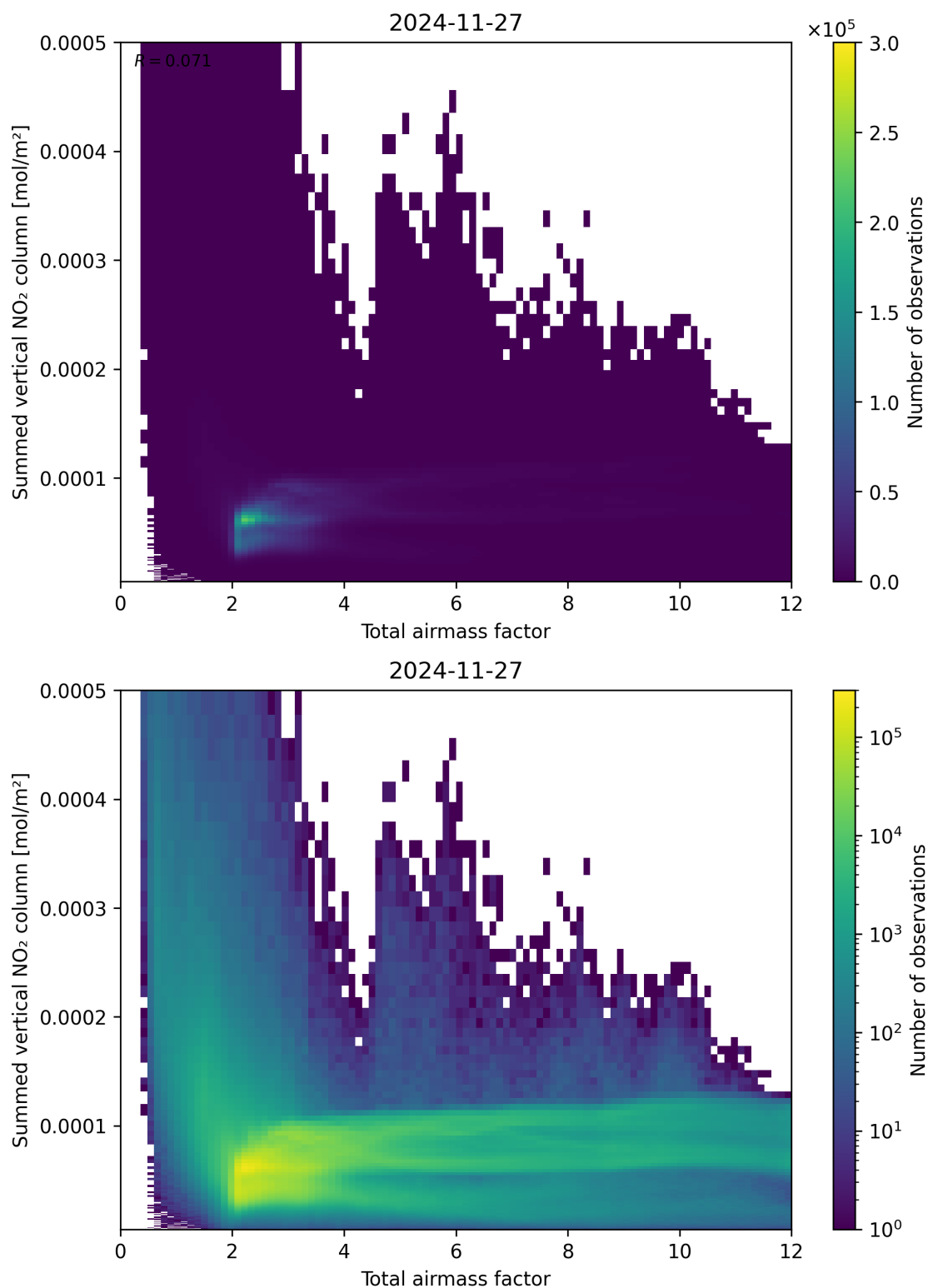
Figure 65: Scatter density plot of “Total airmass factor” against “Summed vertical NO 2 column” for 2024-11-26 to 2024-11-28.
