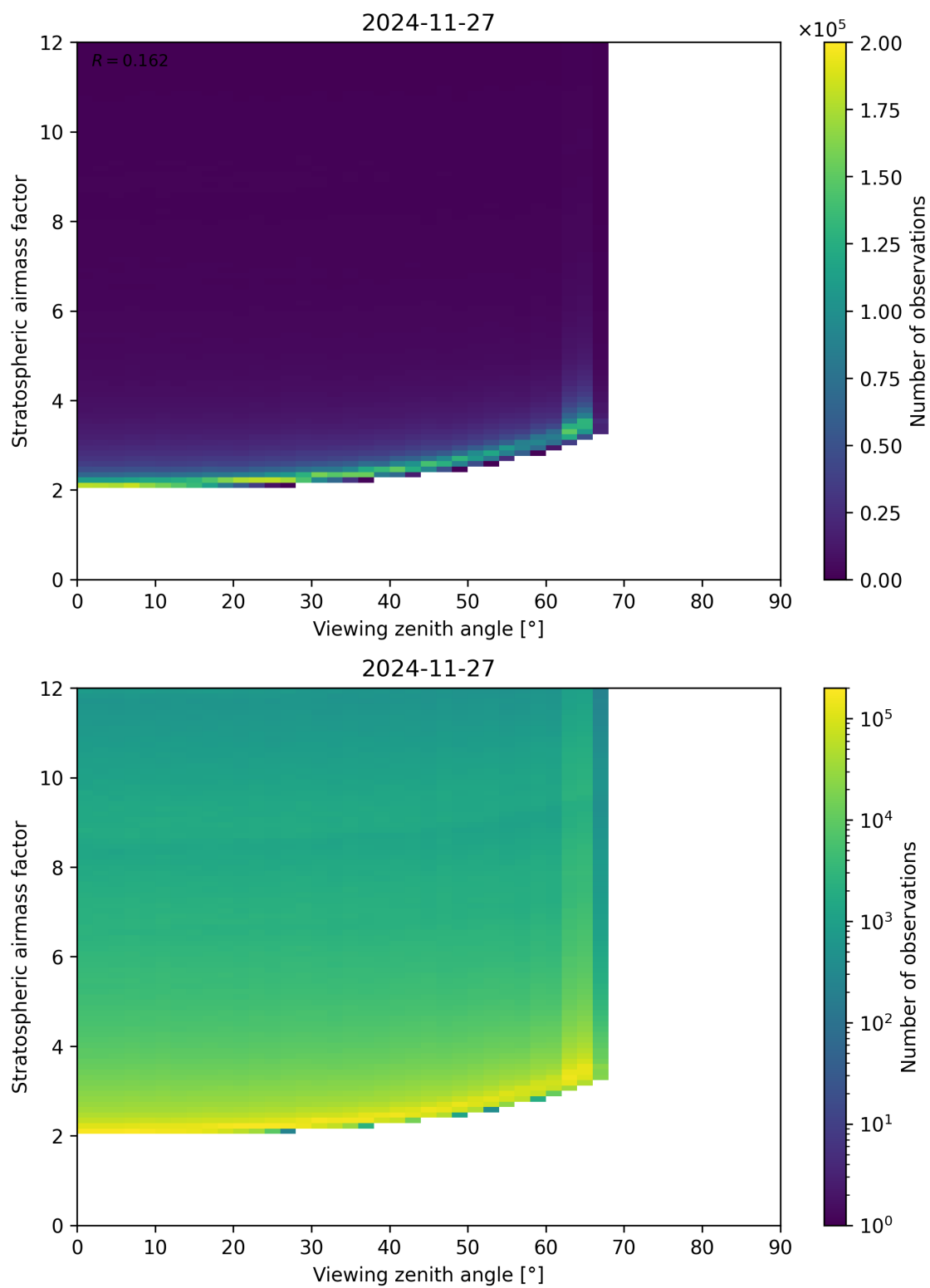
Figure 159: Scatter density plot of “Viewing zenith angle” against “Stratospheric airmass factor” for 2024-11-26 to 2024-11-28.
