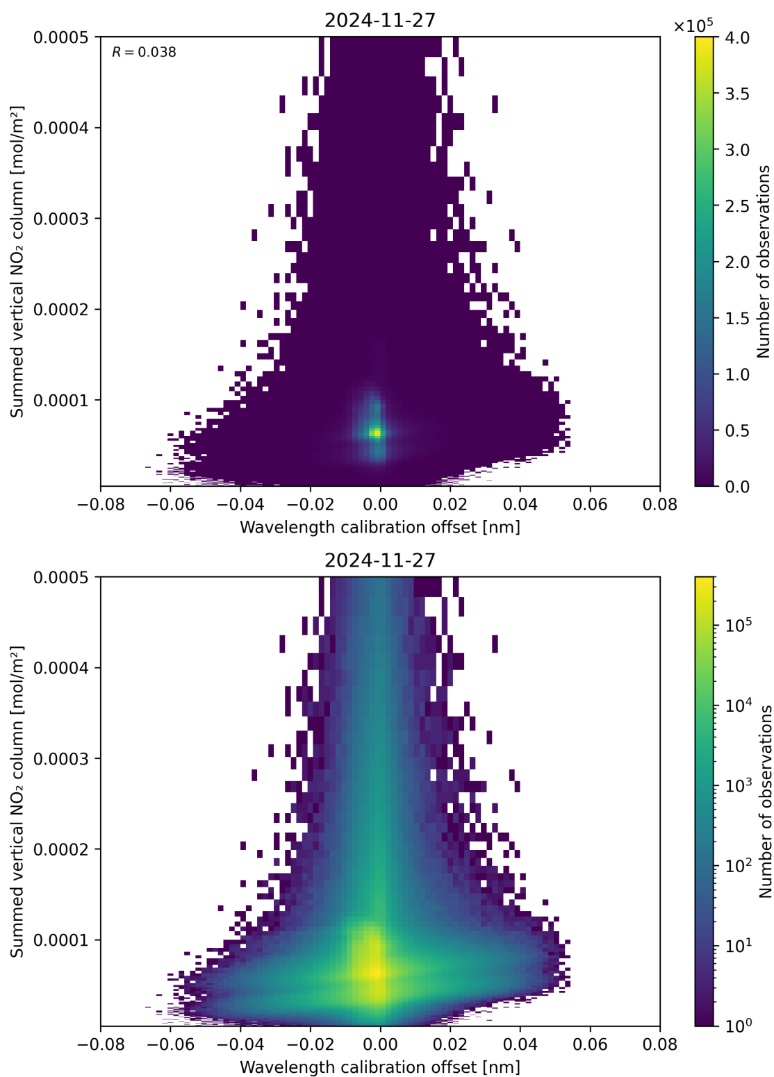
Figure 177: Scatter density plot of “Wavelength calibration offset” against “Summed vertical NO 2 column” for 2024-11-26 to 2024-11-28.
