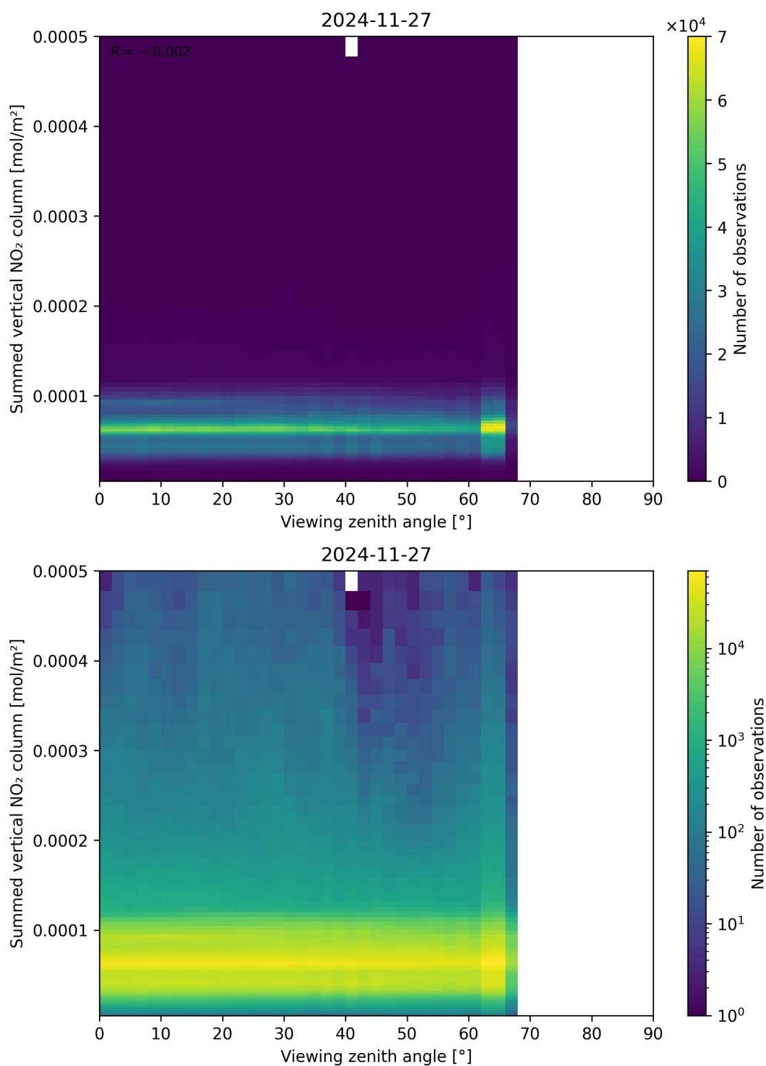
Figure 165: Scatter density plot of “Viewing zenith angle” against “Summed vertical NO 2 column” for 2024-11-26 to 2024-11-28.
