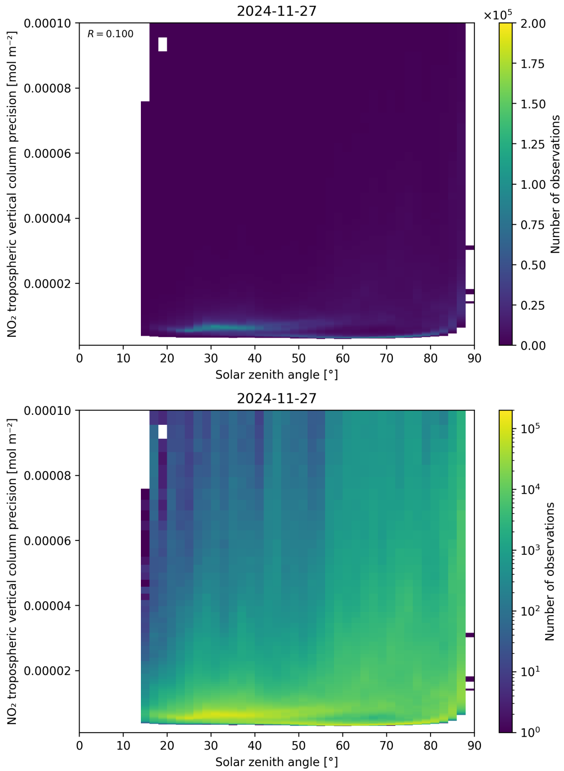
Figure 156: Scatter density plot of “Solar zenith angle” against “NO 2 tropospheric vertical column precision” for 2024-11-26 to 2024-11-28.
