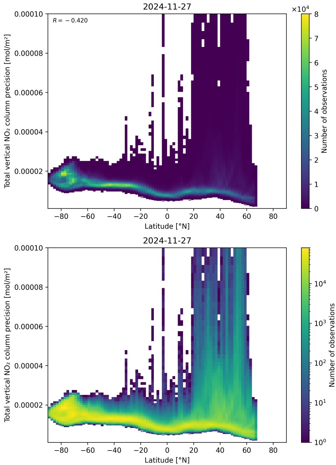
Figure 91: Scatter density plot of “Latitude” against “Total vertical NO 2 column precision” for 2024-11-26 to 2024-11-28.
