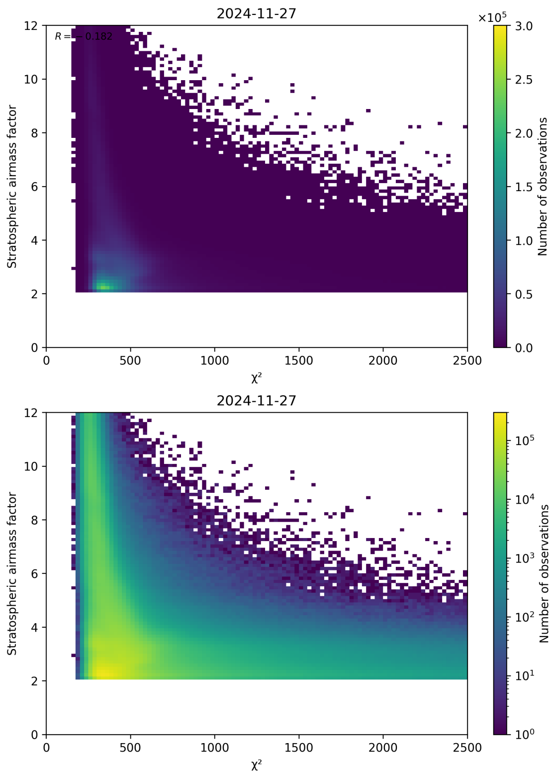
Figure 81: Scatter density plot of “ \chi^2 ” against “Stratospheric airmass factor” for 2024-11-26 to 2024-11-28.
