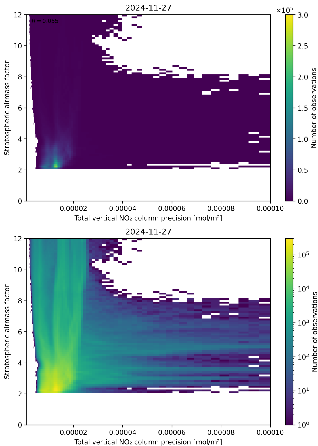
Figure 115: Scatter density plot of “Total vertical NO 2 column precision” against “Stratospheric air mass factor” for 2024-11-26 to 2024-11-28.
