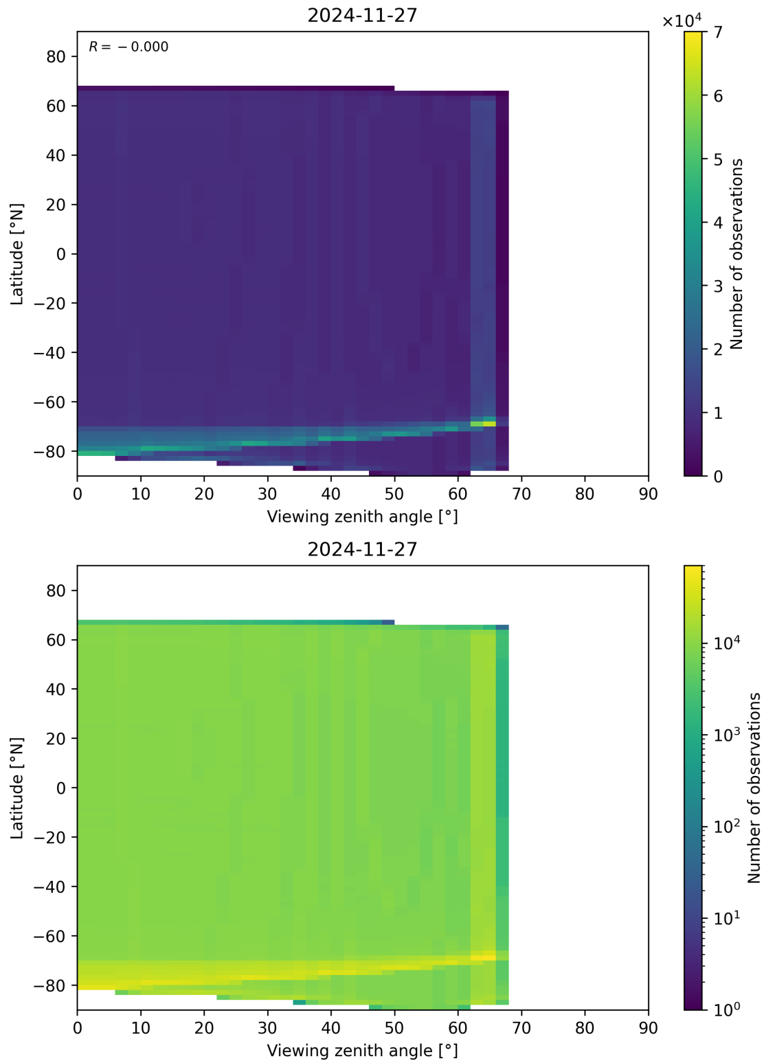
Figure 163: Scatter density plot of “Viewing zenith angle” against “Latitude” for 2024-11-26 to 2024-11-28.
