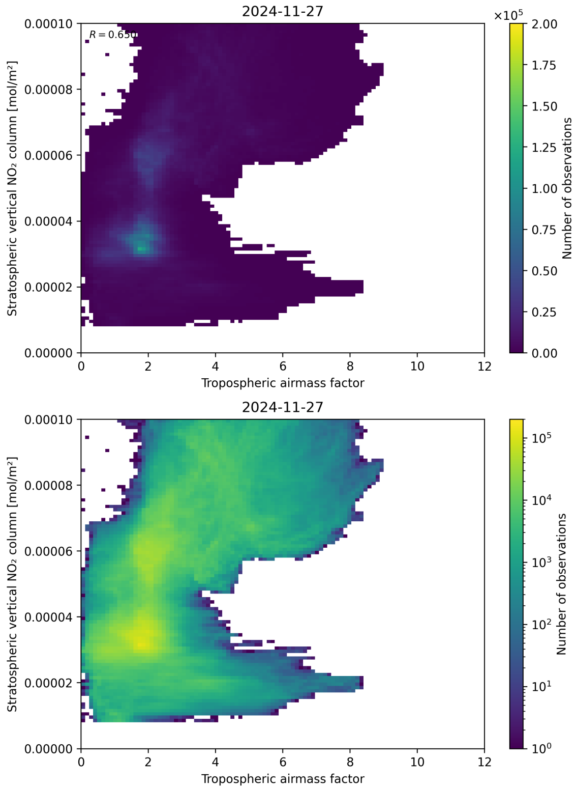
Figure 74: Scatter density plot of “Tropospheric air mass factor” against “Stratospheric vertical NO 2 column” for 2024-11-26 to 2024-11-28.
