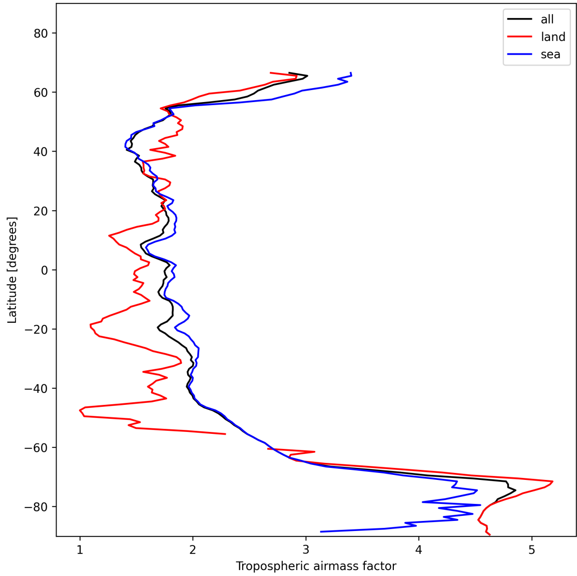
Figure 14: Zonal average of “Tropospheric airmass factor” for 2024-11-26 to 2024-11-28.
