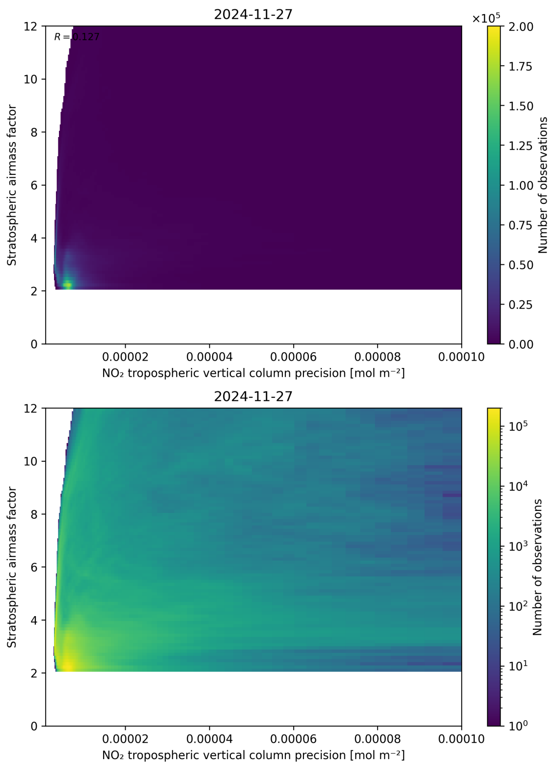
Figure 131: Scatter density plot of “NO 2 tropospheric vertical column precision” against “Stratospheric airmass factor” for 2024-11-26 to 2024-11-28.
