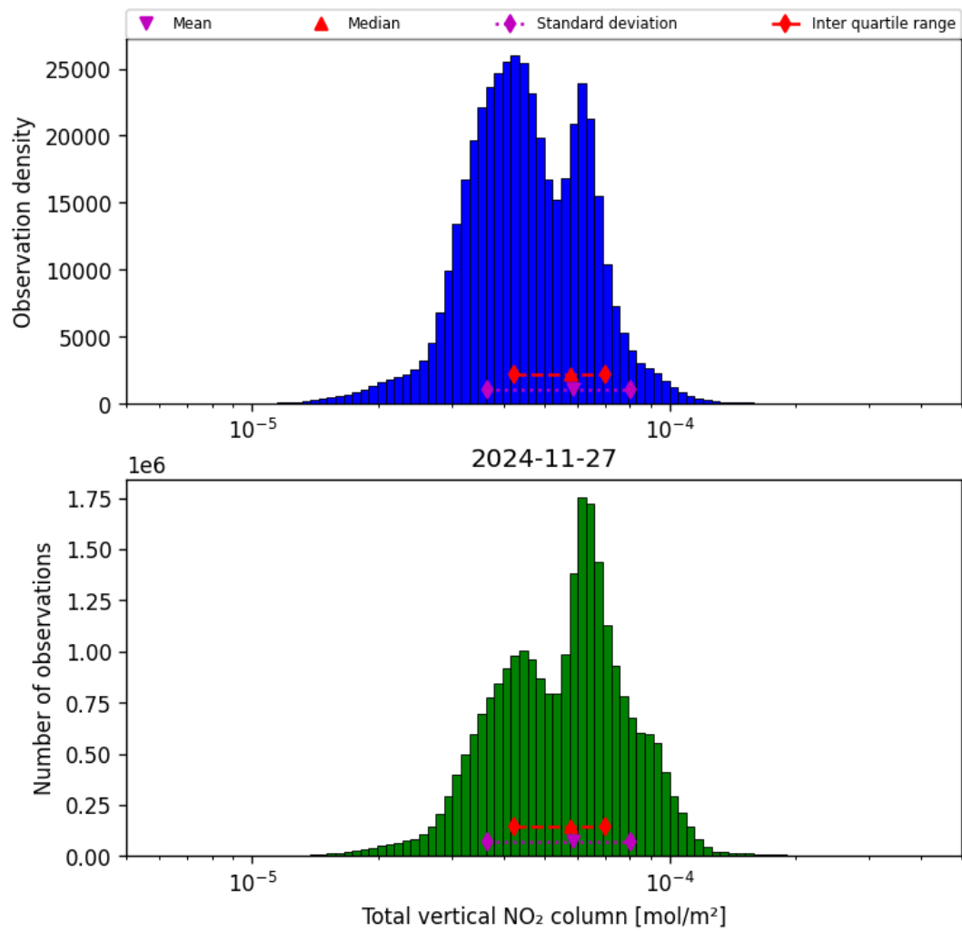
Figure 38: Histogram of “Total vertical NO 2 column” for 2024-11-26 to 2024-11-28
