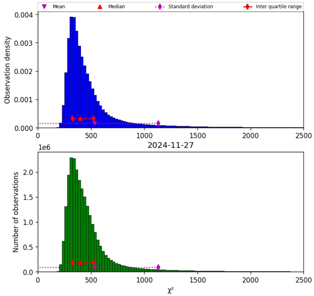
Figure 42: Histogram of “ \chi^2 ” for 2024-11-26 to 2024-11-28
