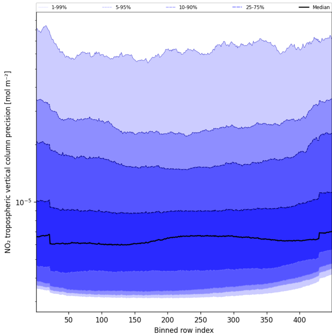
Figure 47: Along track statistics of “NO 2 tropospheric vertical column precision” for 2024-11-26 to 2024-11-28
