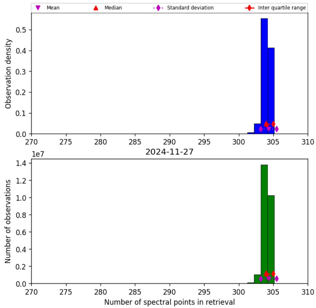
Figure 33: Histogram of “Number of spectral points in retrieval” for 2024-11-26 to 2024-11-28
