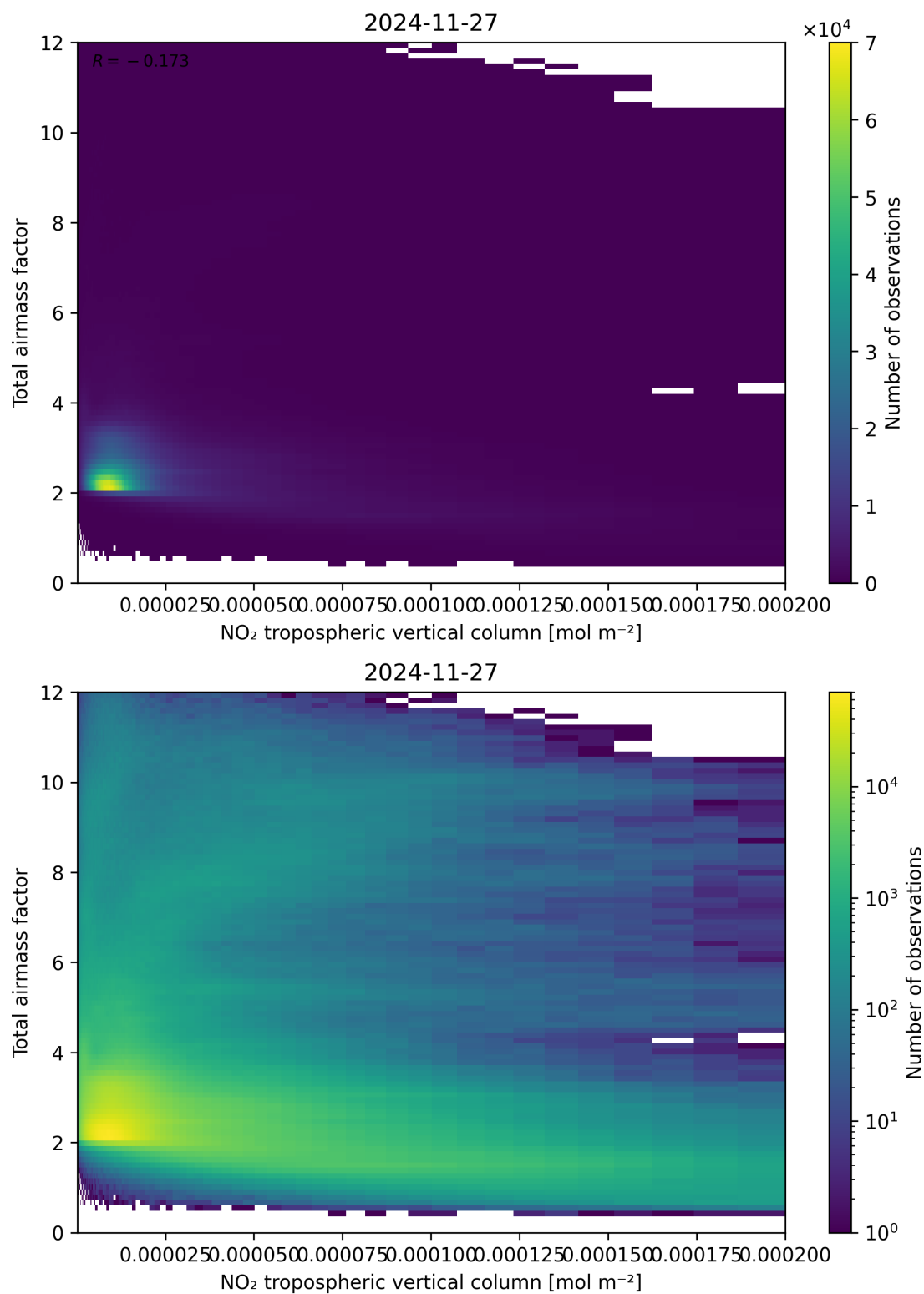
Figure 122: Scatter density plot of “NO 2 tropospheric vertical column” against “Total air mass factor” for 2024-11-26 to 2024-11-28.
