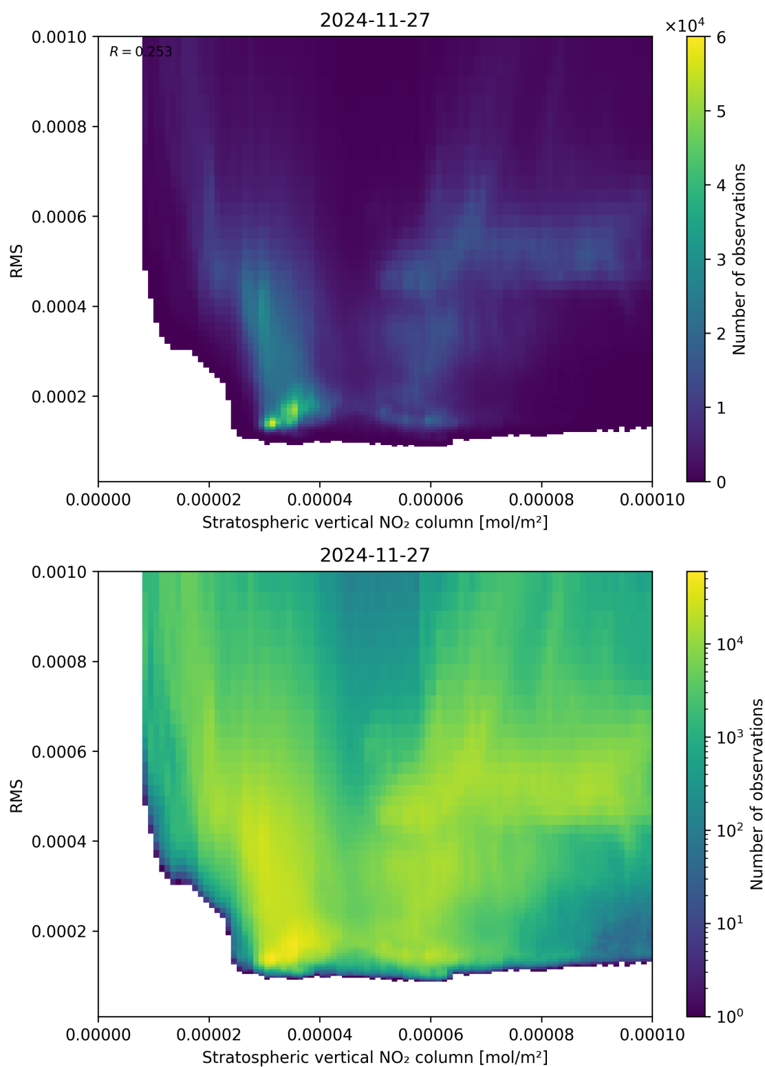
Figure 102: Scatter density plot of “Stratospheric vertical NO 2 column” against “RMS” for 2024-11-26 to 2024-11-28.
