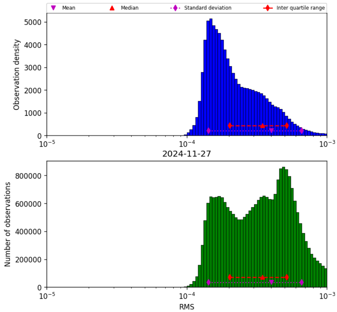
Figure 43: Histogram of “RMS” for 2024-11-26 to 2024-11-28
