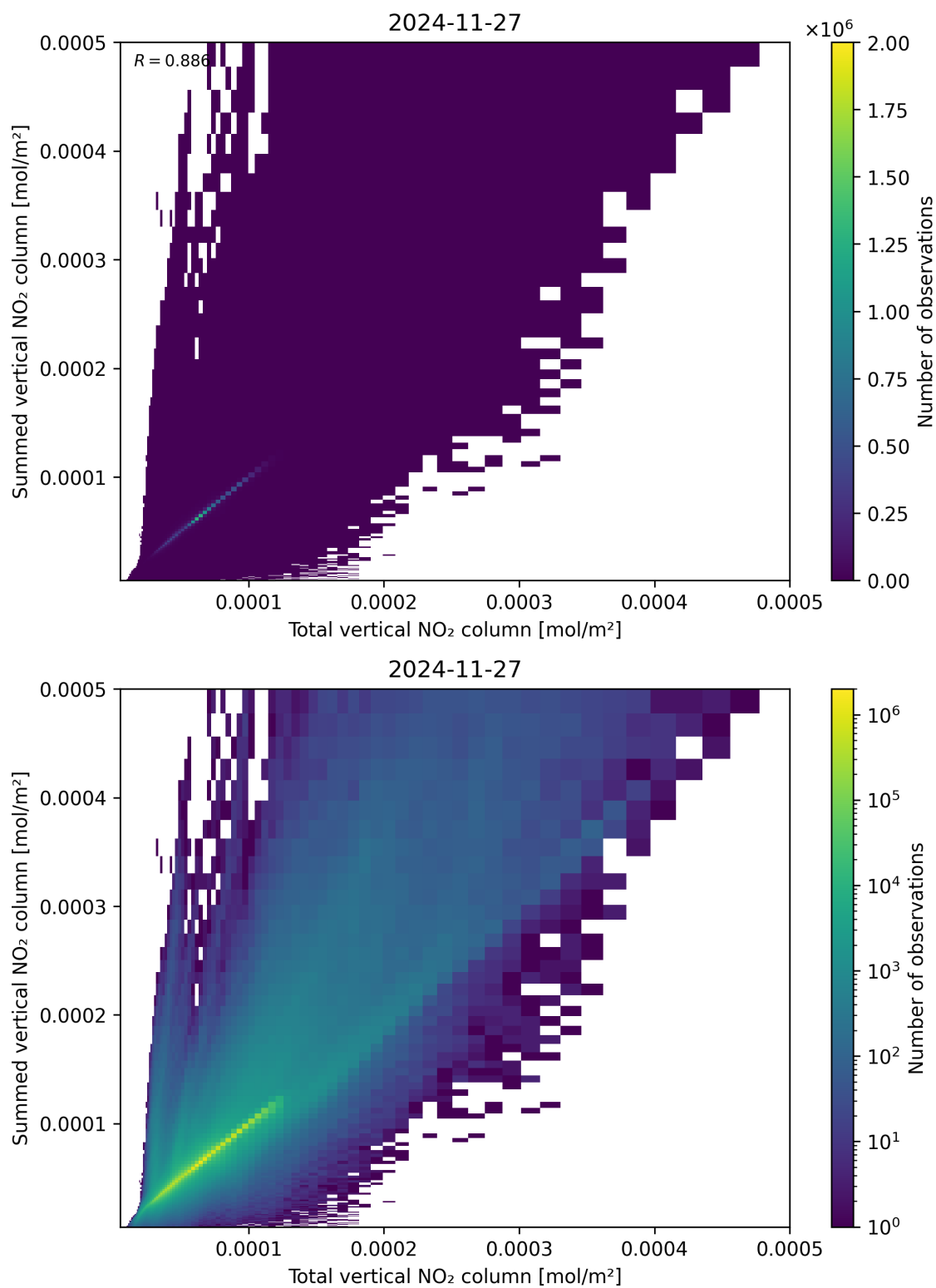
Figure 112: Scatter density plot of “Total vertical NO 2 column” against “Summed vertical NO 2 column” for 2024-11-26 to 2024-11-28.
