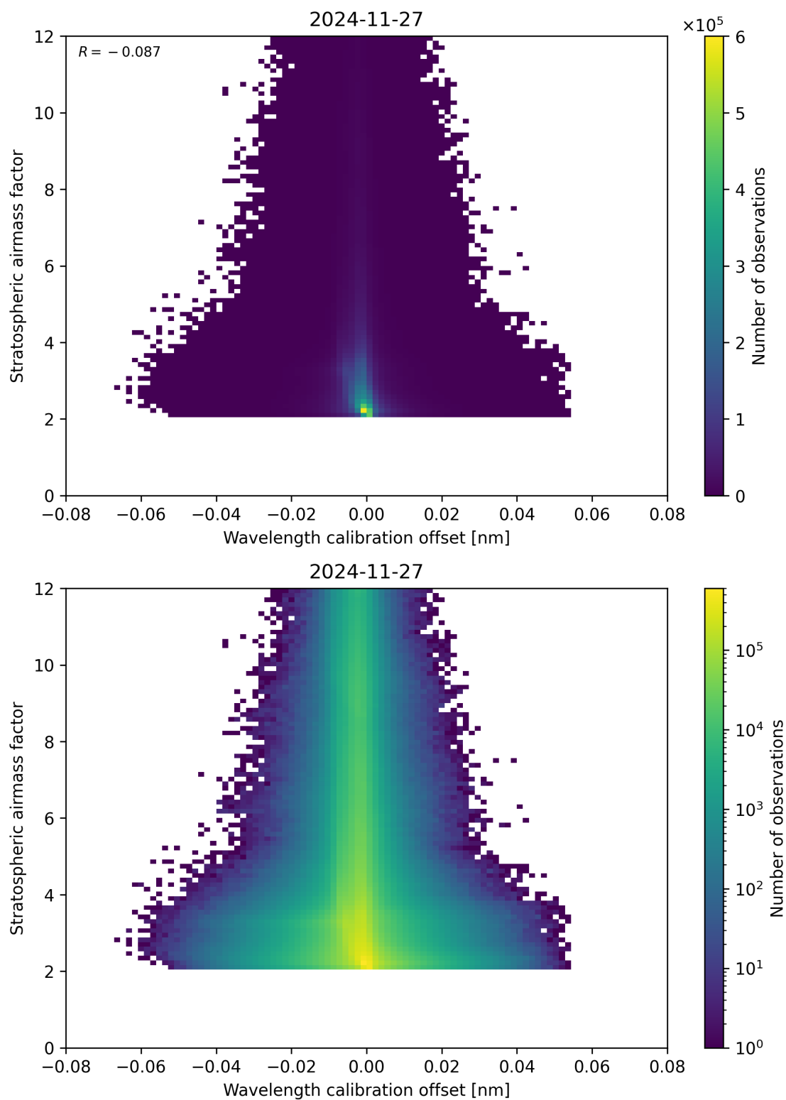
Figure 174: Scatter density plot of “Wavelength calibration offset” against “Stratospheric airmass factor” for 2024-11-26 to 2024-11-28.
