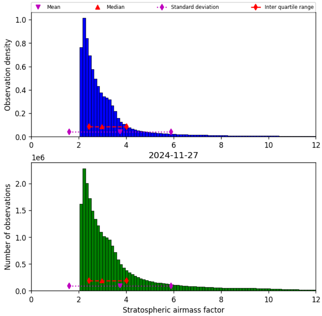
Figure 44: Histogram of “Stratospheric airmass factor” for 2024-11-26 to 2024-11-28
