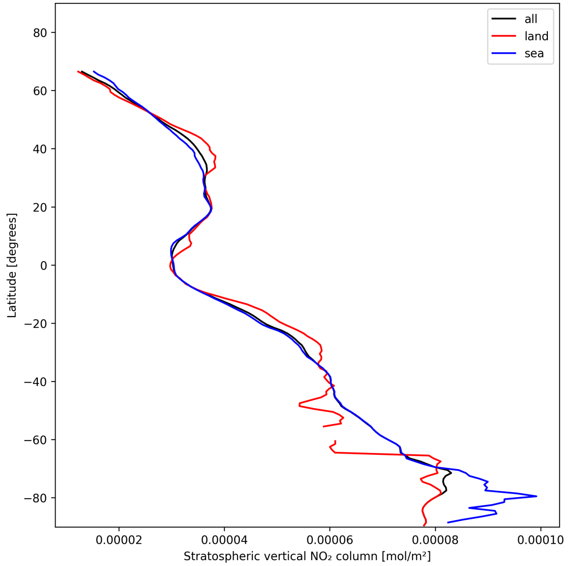
Figure 19: Zonal average of “Stratospheric vertical NO 2 column” for 2024-11-26 to 2024-11-28.
