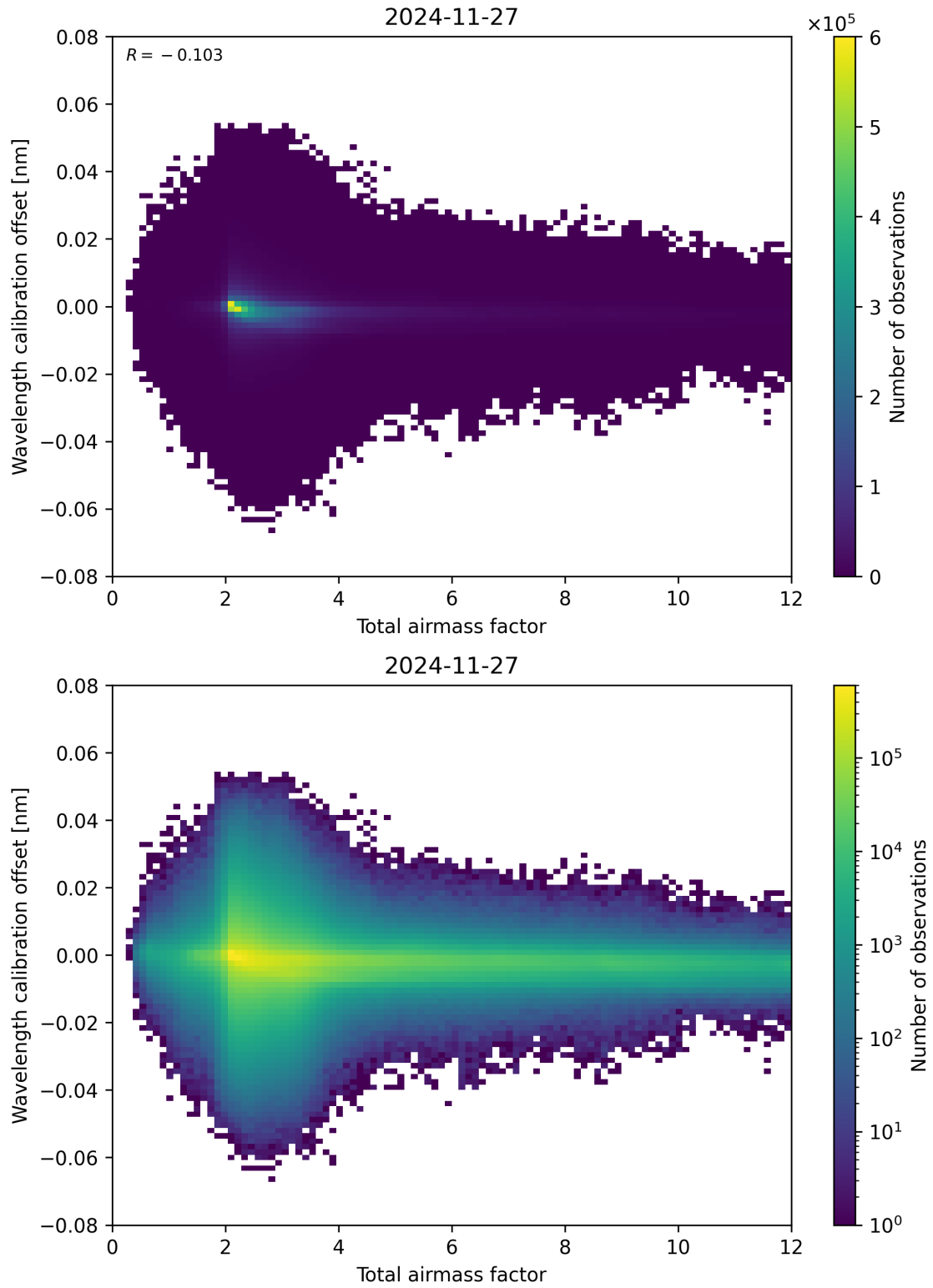
Figure 70: Scatter density plot of “Total airmass factor” against “Wavelength calibration offset” for 2024-11-26 to 2024-11-28.
