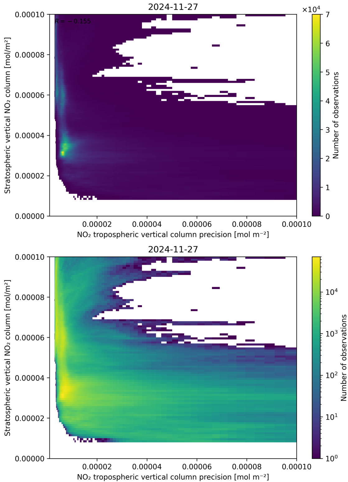
Figure 135: Scatter density plot of “NO 2 tropospheric vertical column precision” against “Stratospheric vertical NO 2 column” for 2024-11-26 to 2024-11-28.
