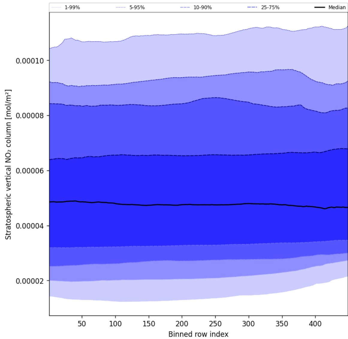
Figure 53: Along track statistics of “Stratospheric vertical NO 2 column” for 2024-11-26 to 2024-11-28
