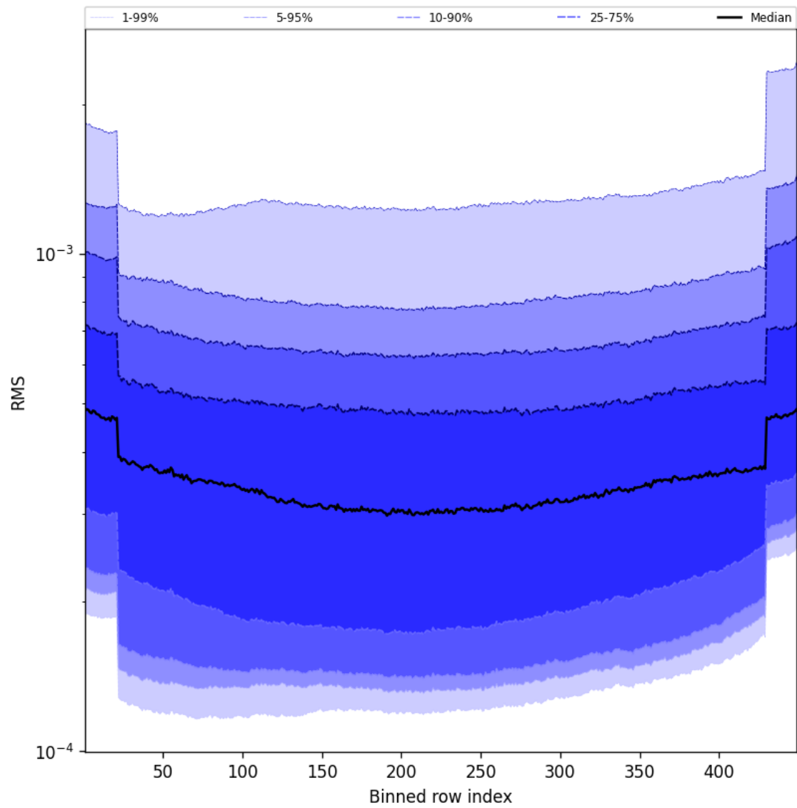
Figure 60: Along track statistics of “RMS” for 2024-11-26 to 2024-11-28
