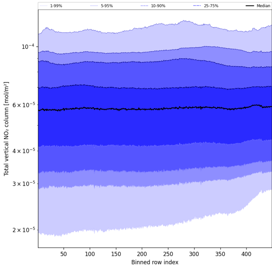
Figure 55: Along track statistics of “Total vertical NO 2 column” for 2024-11-26 to 2024-11-28
