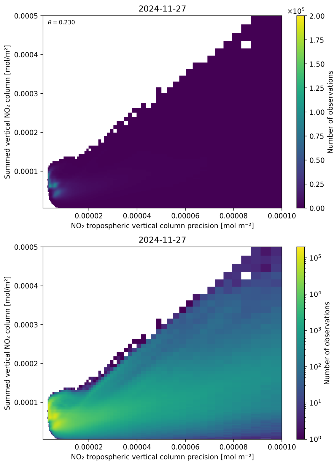
Figure 136: Scatter density plot of “NO 2 tropospheric vertical column precision” against “Summed vertical NO 2 column” for 2024-11-26 to 2024-11-28.
