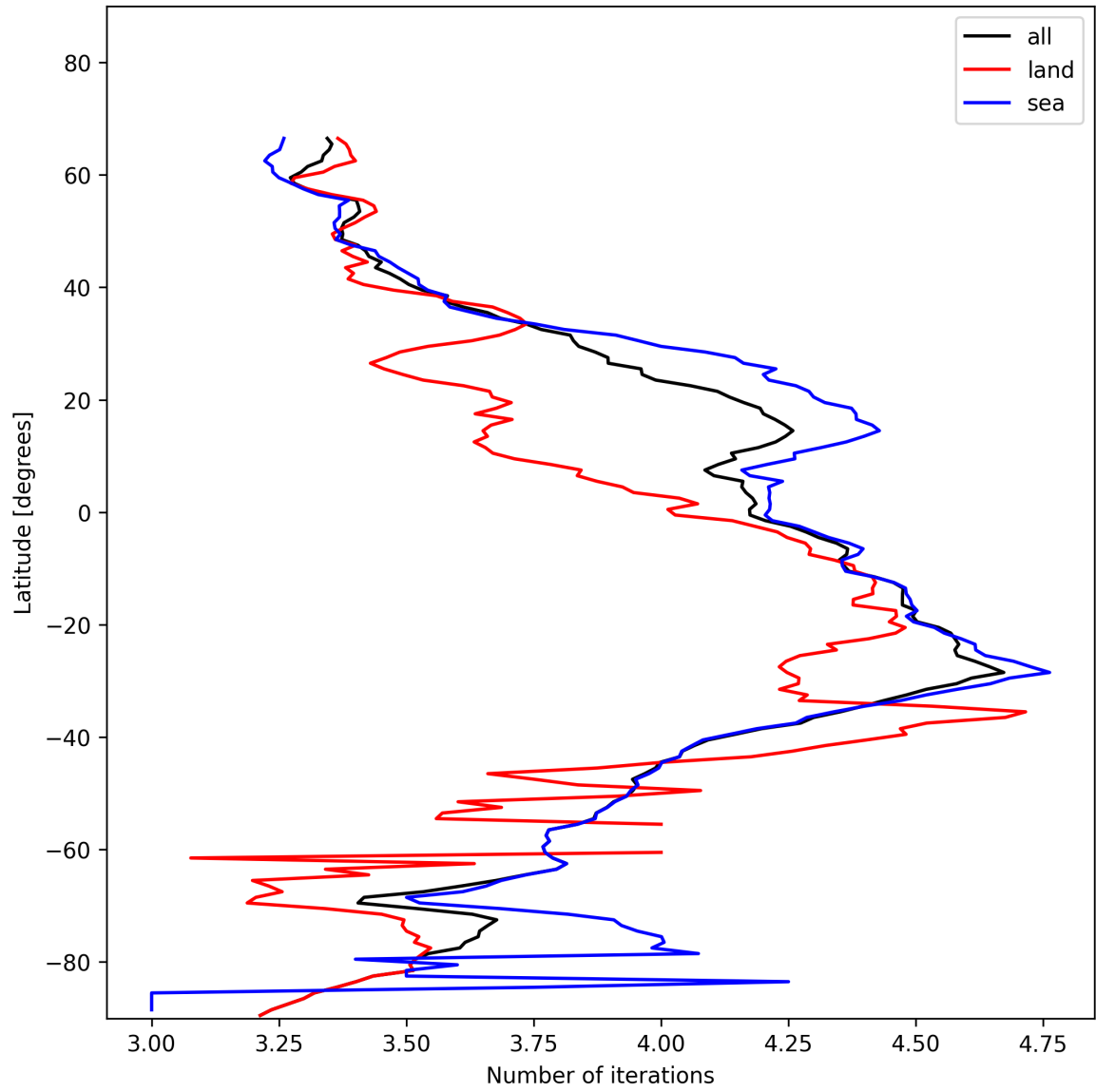
Figure 17: Zonal average of “Number of iterations” for 2024-11-26 to 2024-11-28.
