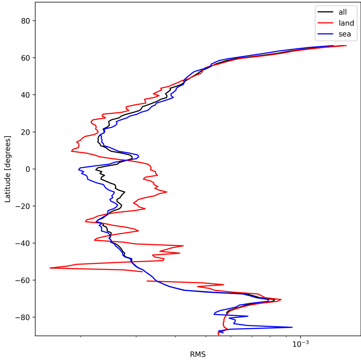
Figure 26: Zonal average of “RMS” for 2024-11-26 to 2024-11-28.
