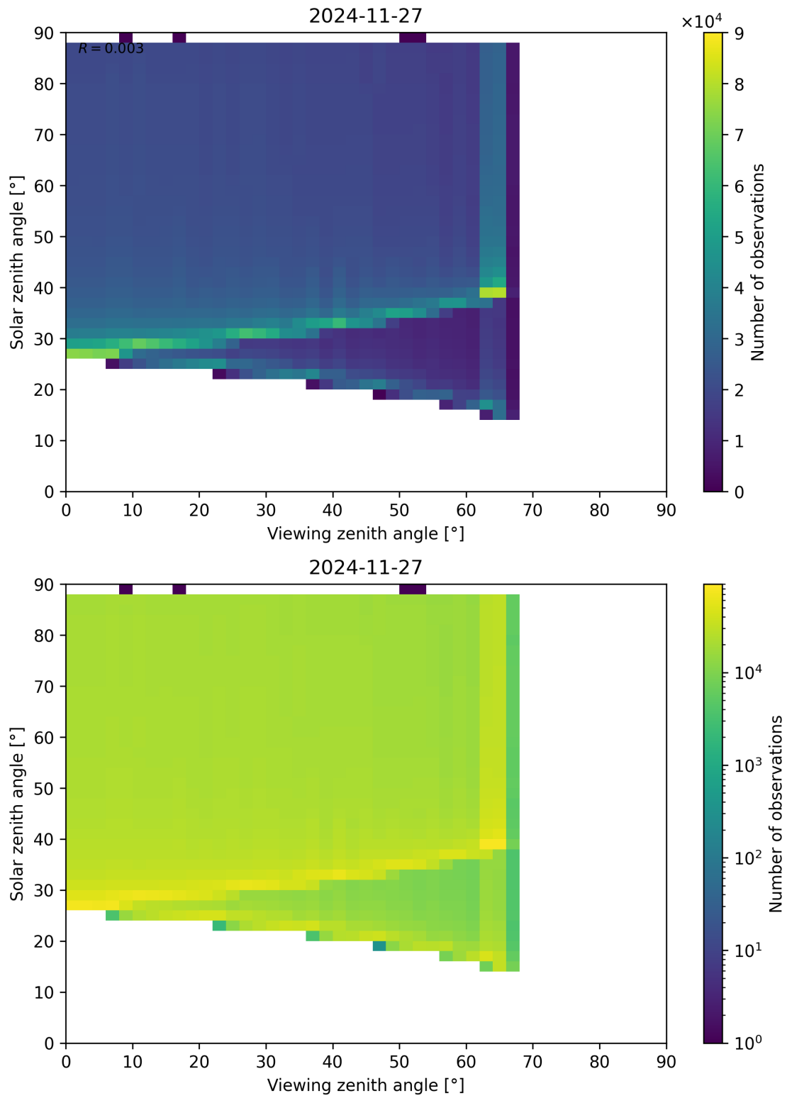
Figure 172: Scatter density plot of “Viewing zenith angle” against “Solar zenith angle” for 2024-11-26 to 2024-11-28.
