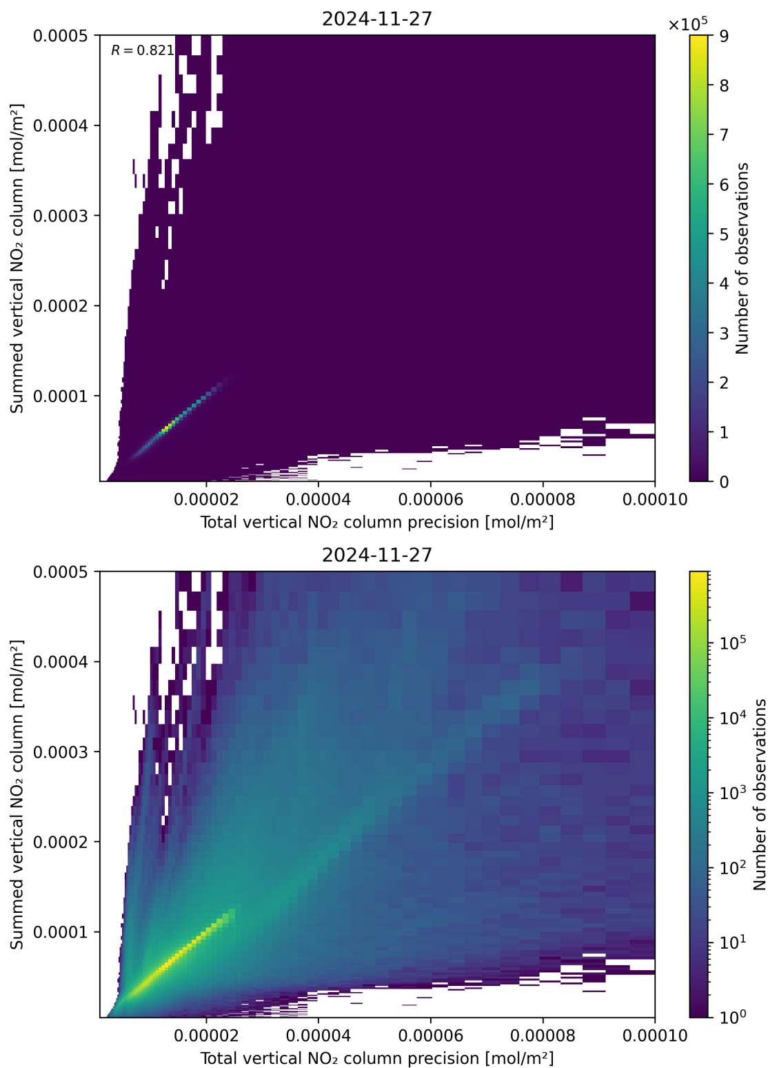
Figure 117: Scatter density plot of “Total vertical NO 2 column precision” against “Summed vertical NO 2 column” for 2024-11-26 to 2024-11-28.
