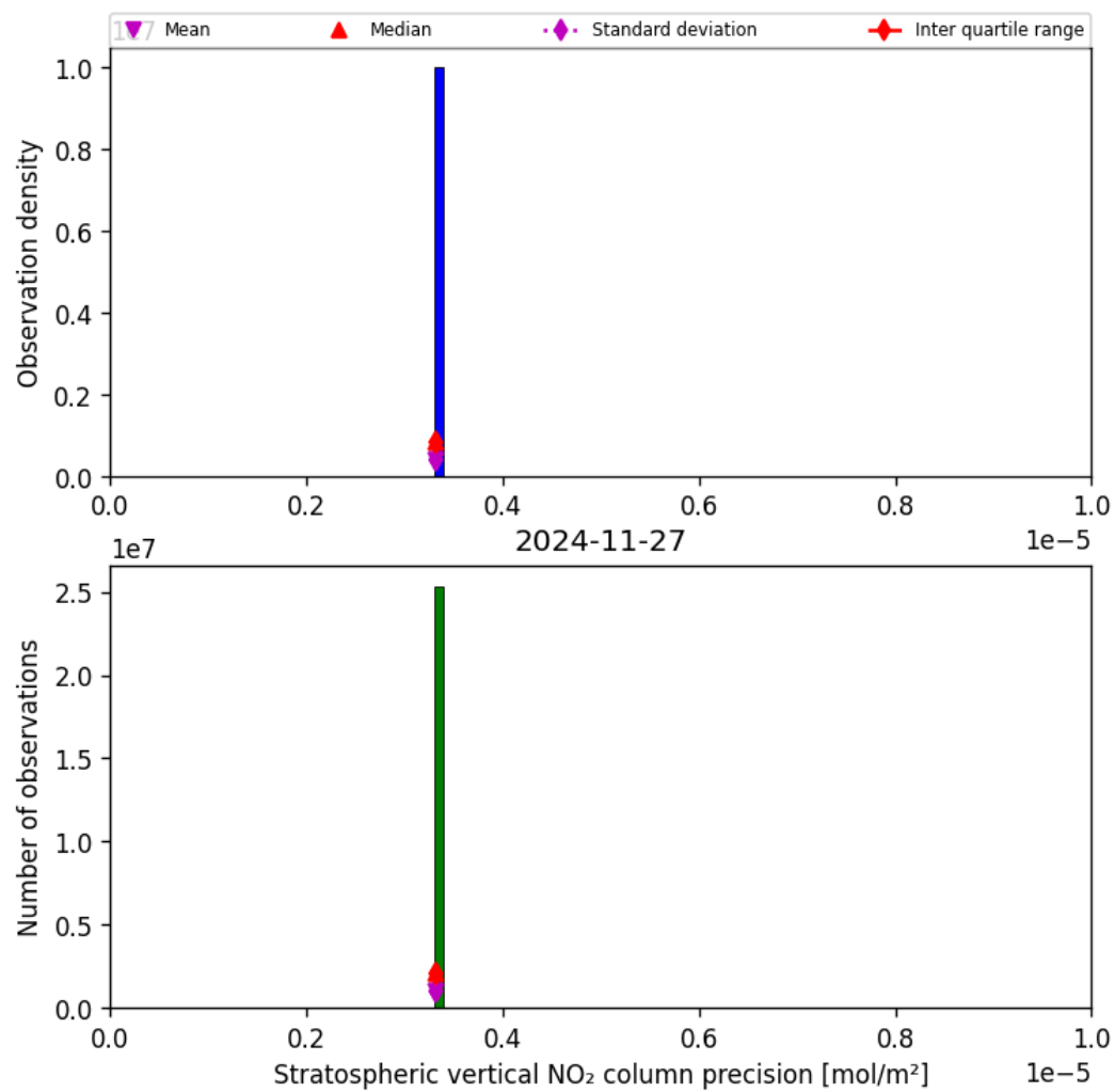
Figure 37: Histogram of “Stratospheric vertical NO 2 column precision” for 2024-11-26 to 2024-11-28
