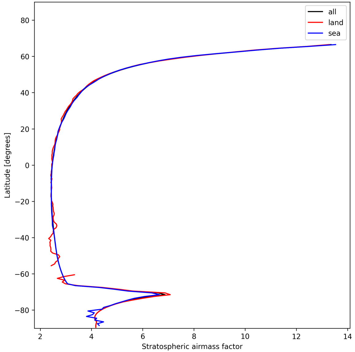
Figure 27: Zonal average of “Stratospheric air mass factor” for 2024-11-26 to 2024-11-28.
