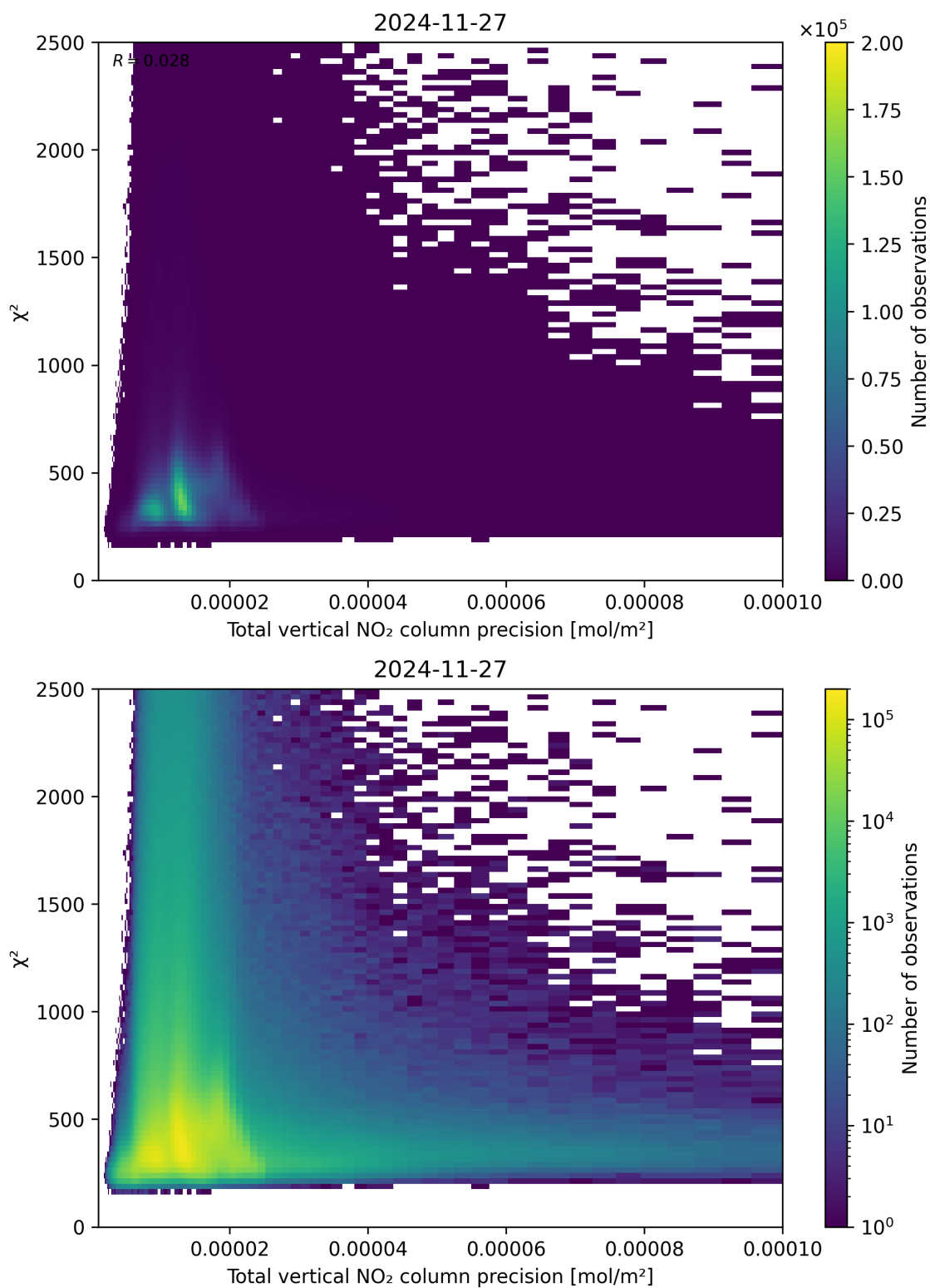
Figure 116: Scatter density plot of “Total vertical NO 2 column precision” against “ \chi^2 ” for 2024-11-26 to 2024-11-28.
