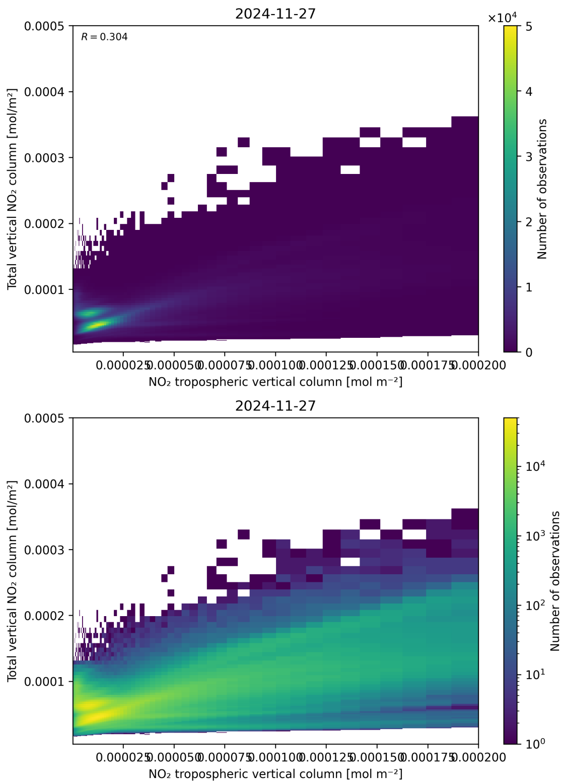
Figure 128: Scatter density plot of “NO 2 tropospheric vertical column” against “Total vertical NO 2 column” for 2024-11-26 to 2024-11-28.
