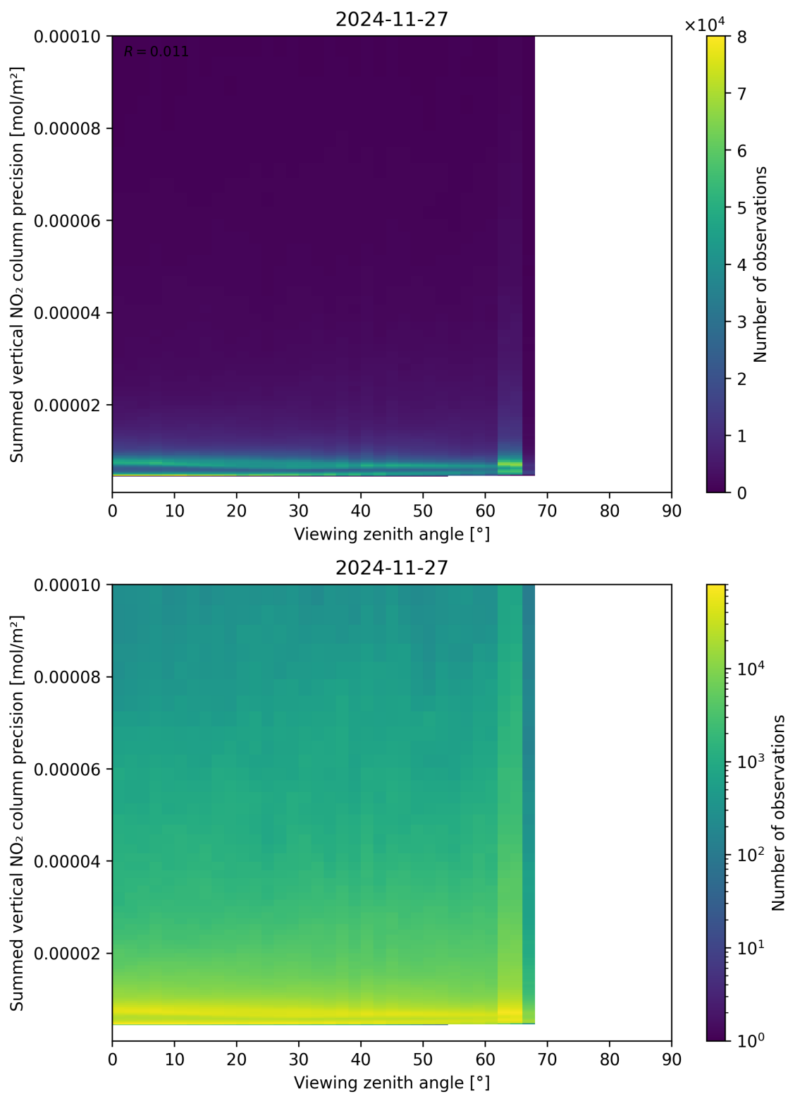
Figure 166: Scatter density plot of “Viewing zenith angle” against “Summed vertical NO 2 column precision” for 2024-11-26 to 2024-11-28.
