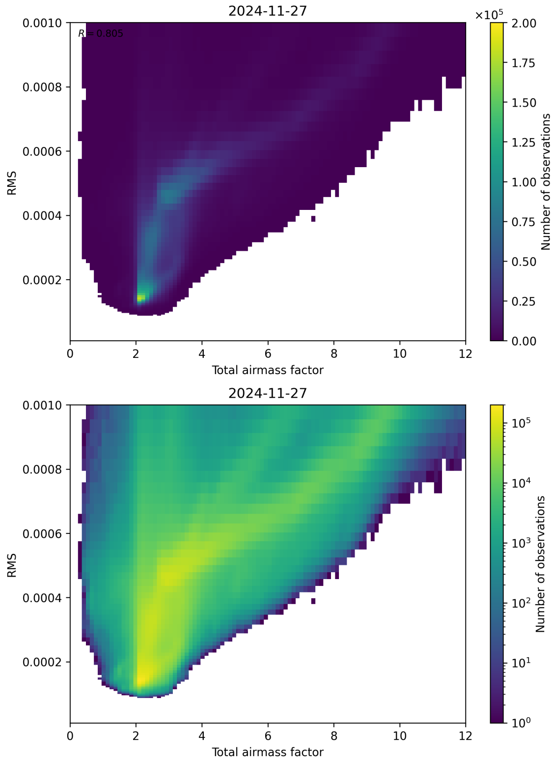
Figure 69: Scatter density plot of “Total airmass factor” against “RMS” for 2024-11-26 to 2024-11-28.
