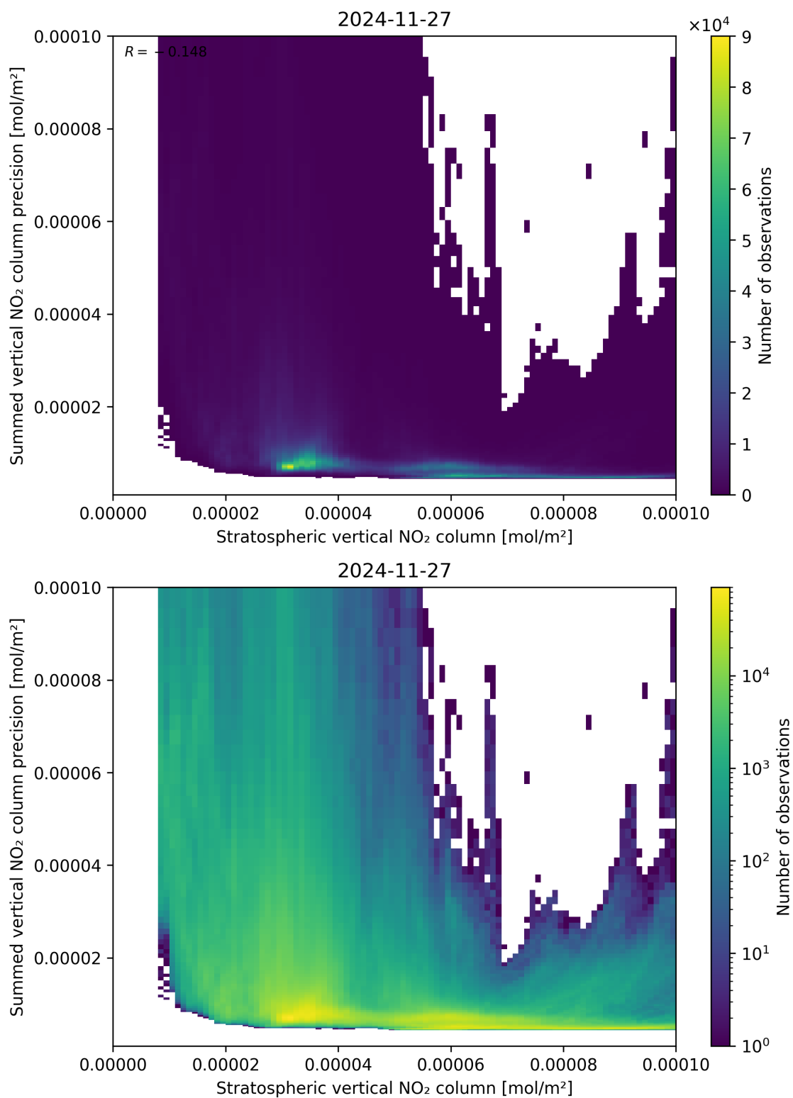
Figure 99: Scatter density plot of “Stratospheric vertical NO 2 column” against “Summed vertical NO 2 column precision” for 2024-11-26 to 2024-11-28.
