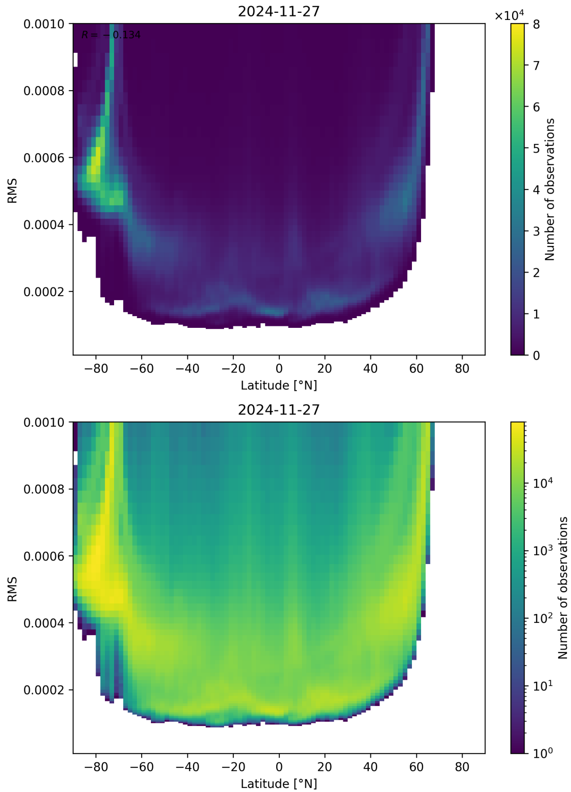
Figure 94: Scatter density plot of “Latitude” against “RMS” for 2024-11-26 to 2024-11-28.
