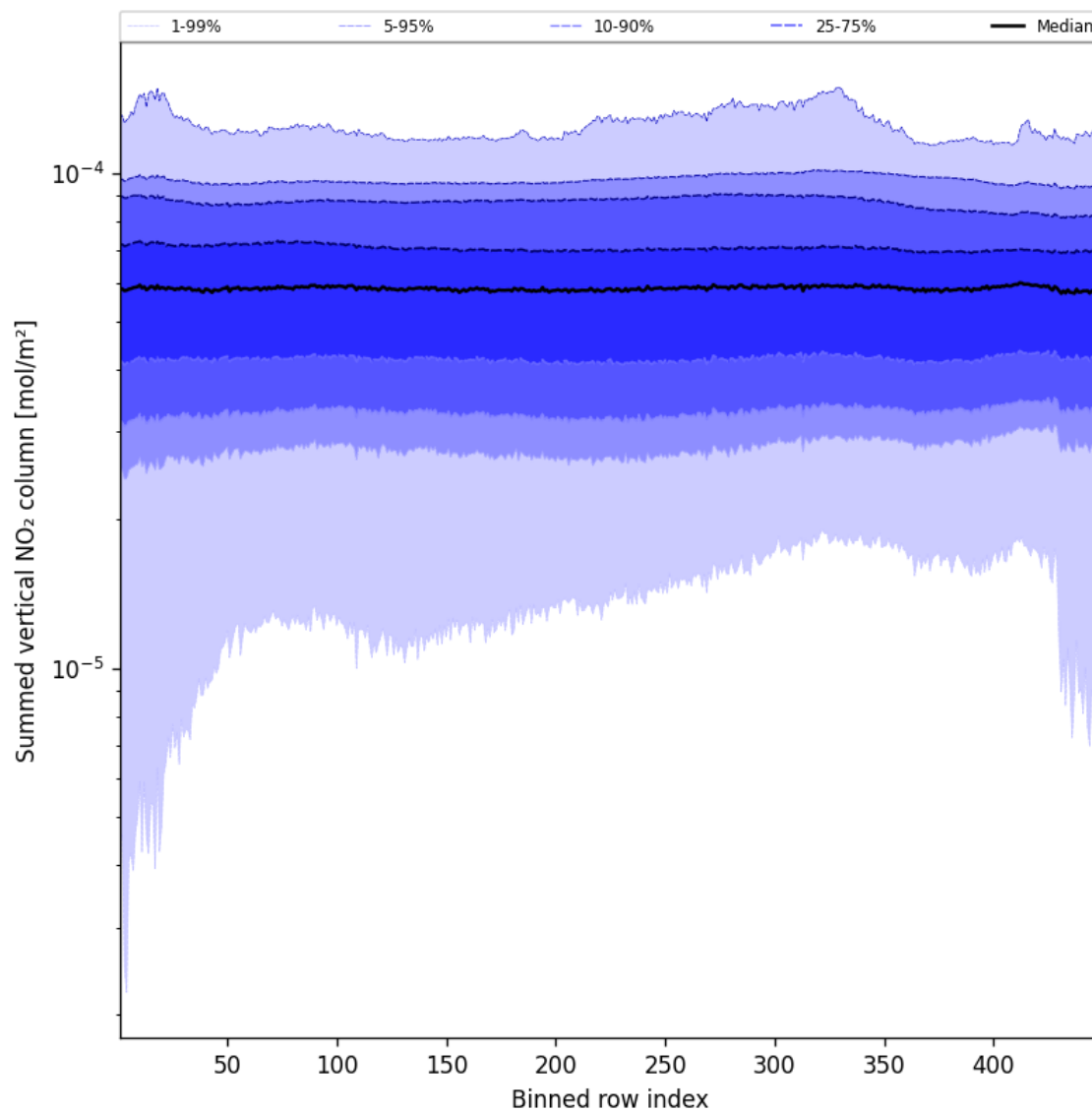
Figure 57: Along track statistics of “Summed vertical NO 2 column” for 2024-11-26 to 2024-11-28
