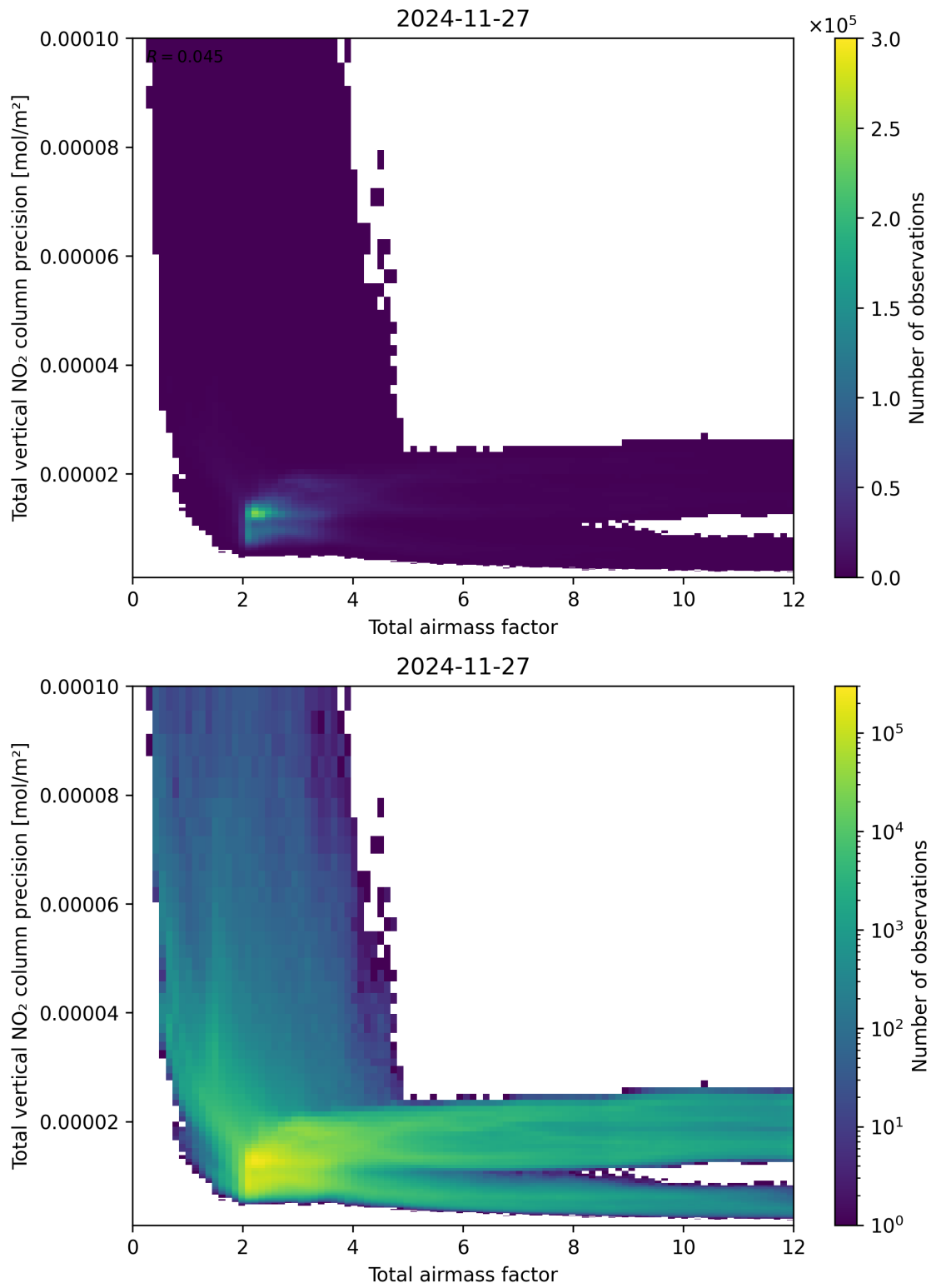
Figure 68: Scatter density plot of “Total airmass factor” against “Total vertical NO 2 column precision” for 2024-11-26 to 2024-11-28.
