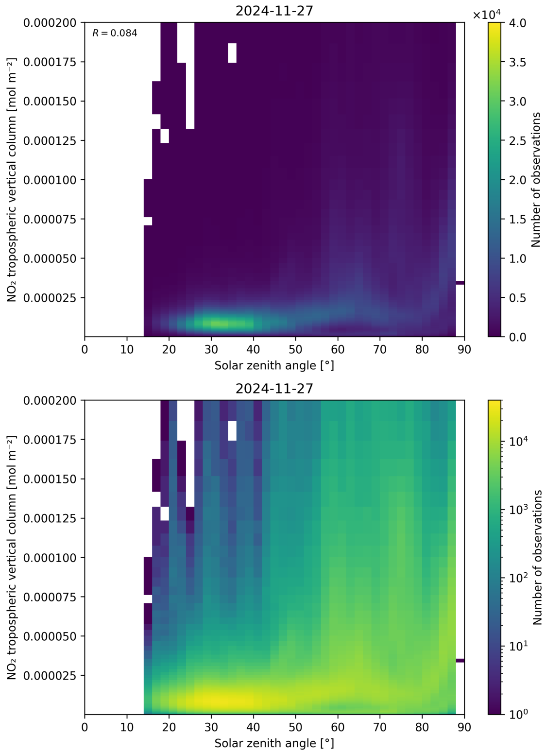
Figure 155: Scatter density plot of “Solar zenith angle” against “NO 2 tropospheric vertical column” for 2024-11-26 to 2024-11-28.
