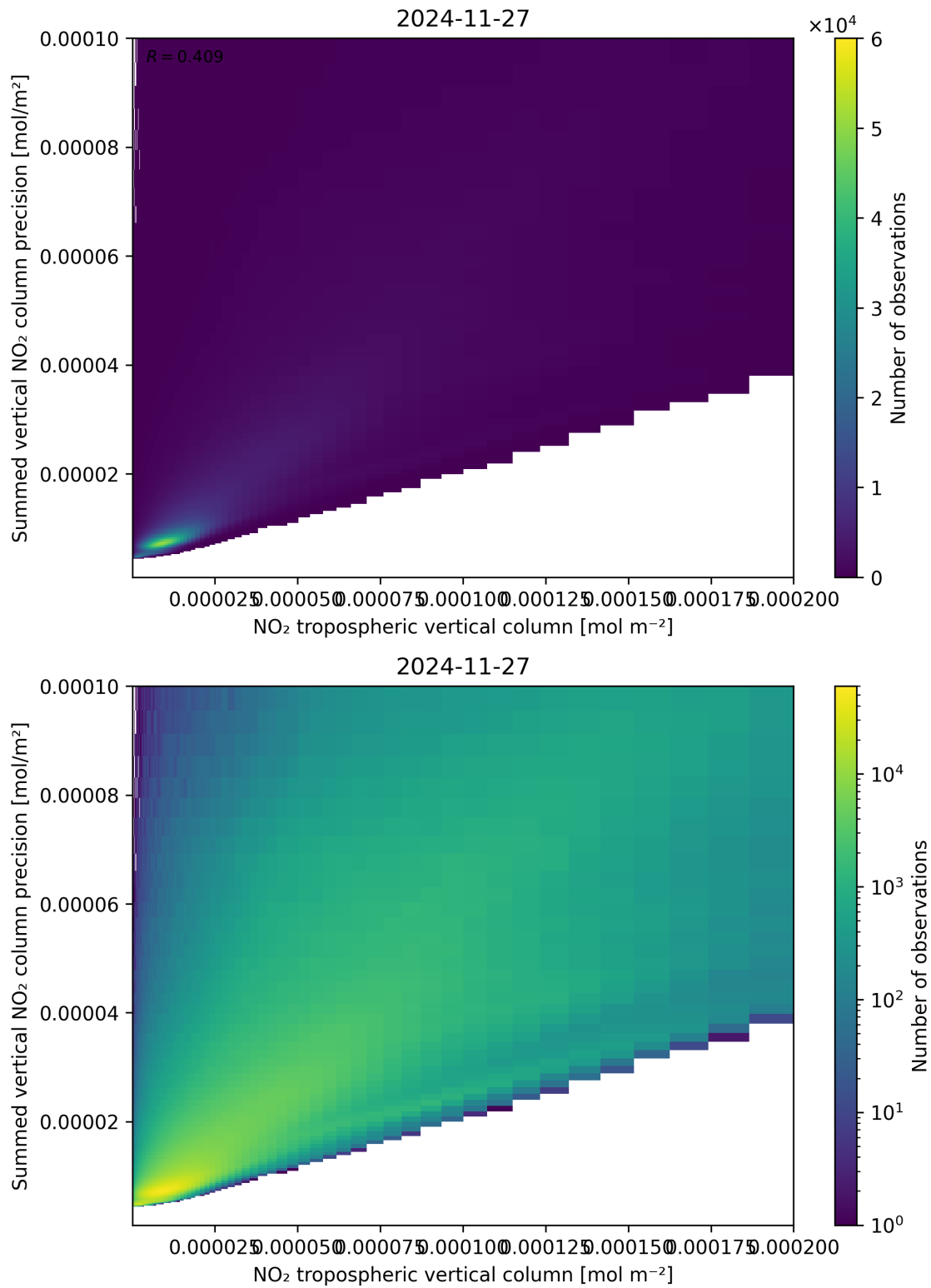
Figure 127: Scatter density plot of “NO 2 tropospheric vertical column” against “Summed vertical NO 2 column precision” for 2024-11-26 to 2024-11-28.
