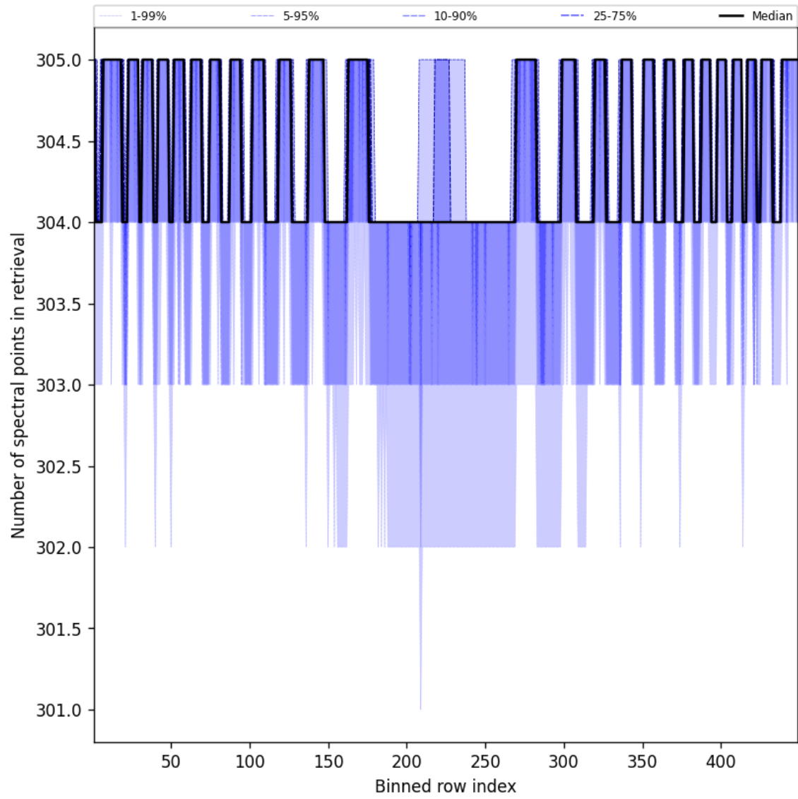
Figure 50: Along track statistics of “Number of spectral points in retrieval” for 2024-11-26 to 2024-11-28
