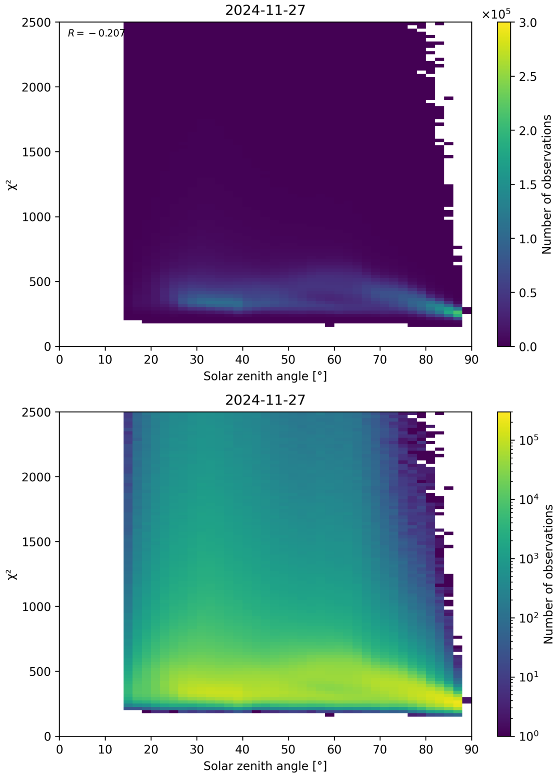
Figure 148: Scatter density plot of “Solar zenith angle” against “ \chi^2 ” for 2024-11-26 to 2024-11-28.
