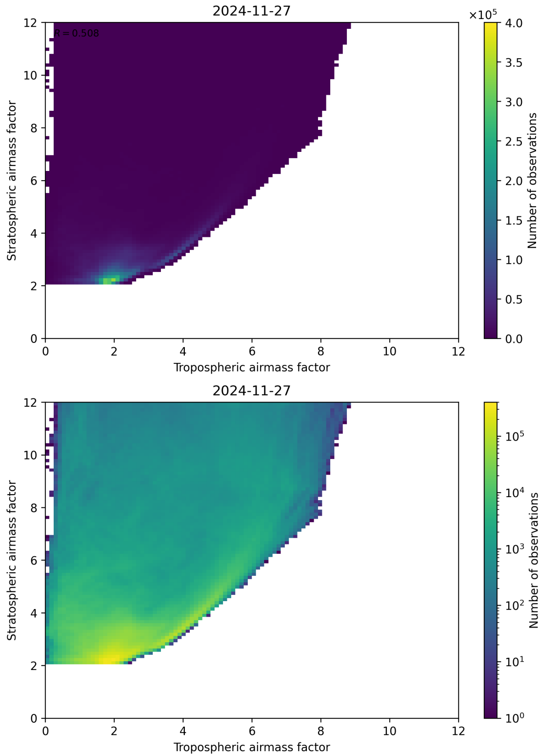
Figure 71: Scatter density plot of “Tropospheric airmass factor” against “Stratospheric airmass factor” for 2024-11-26 to 2024-11-28.
