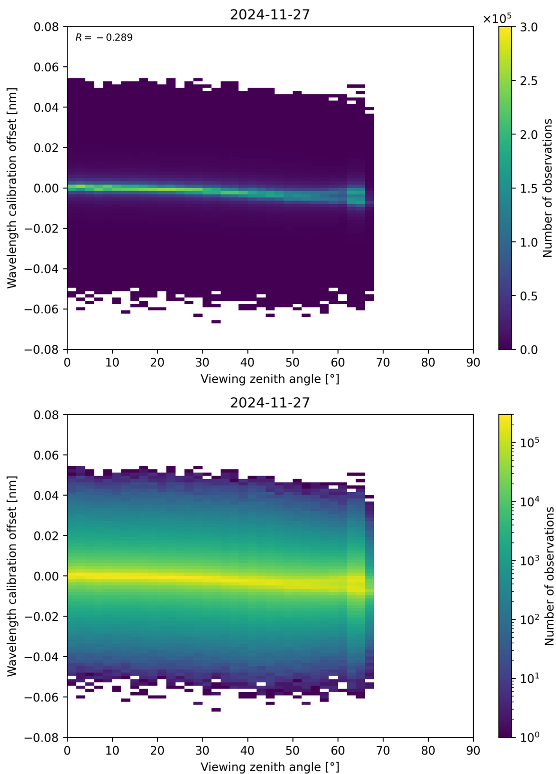
Figure 173: Scatter density plot of “Viewing zenith angle” against “Wavelength calibration offset” for 2024-11-26 to 2024-11-28.
