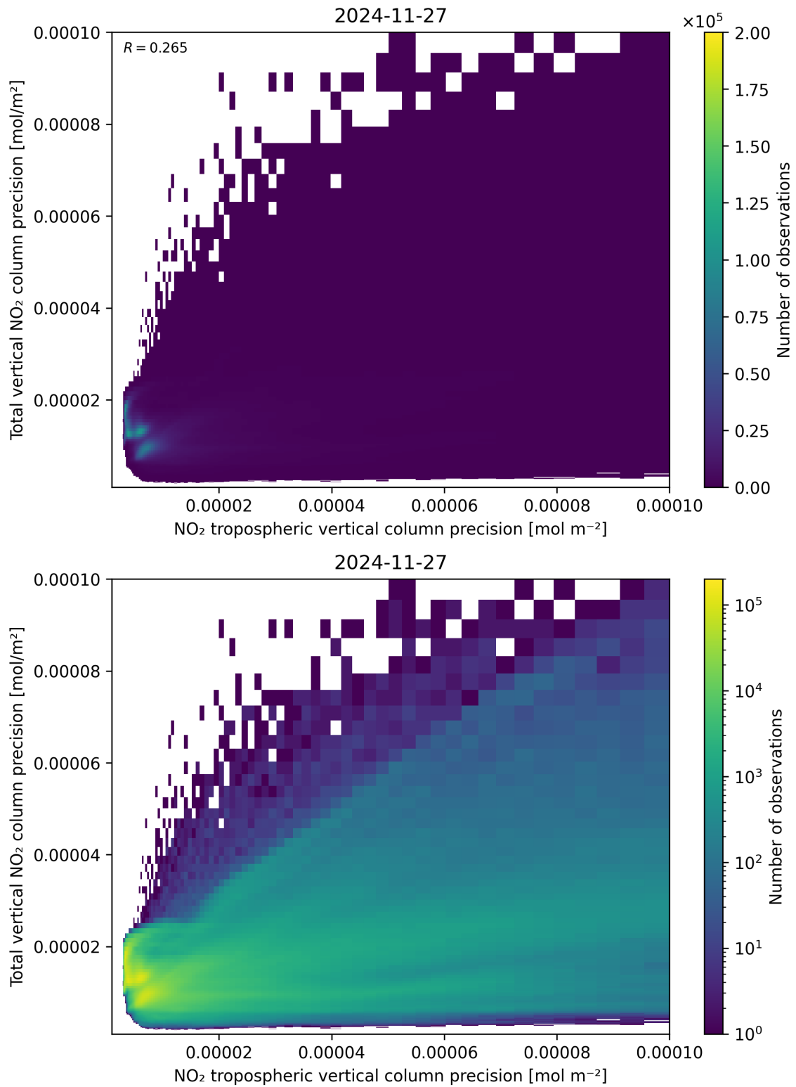
Figure 139: Scatter density plot of “NO 2 tropospheric vertical column precision” against “Total vertical NO 2 column precision” for 2024-11-26 to 2024-11-28.
