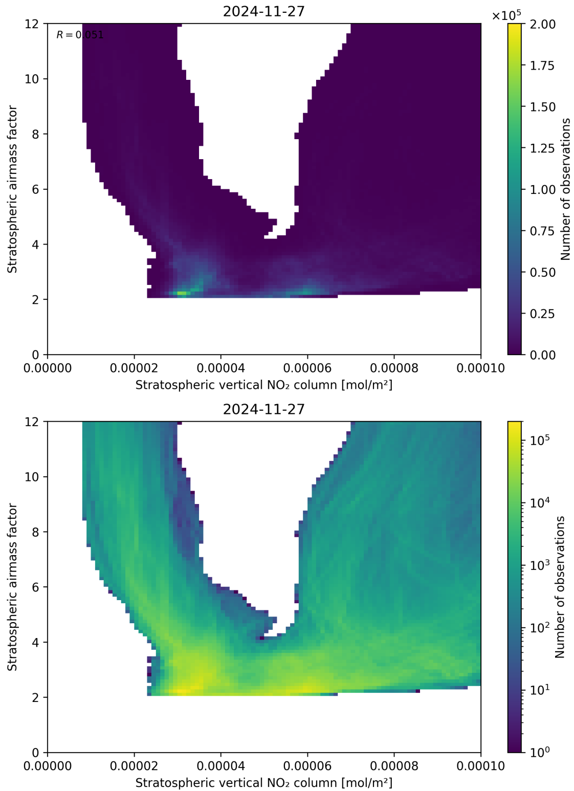
Figure 96: Scatter density plot of “Stratospheric vertical NO 2 column” against “Stratospheric airmass factor” for 2024-11-26 to 2024-11-28.
