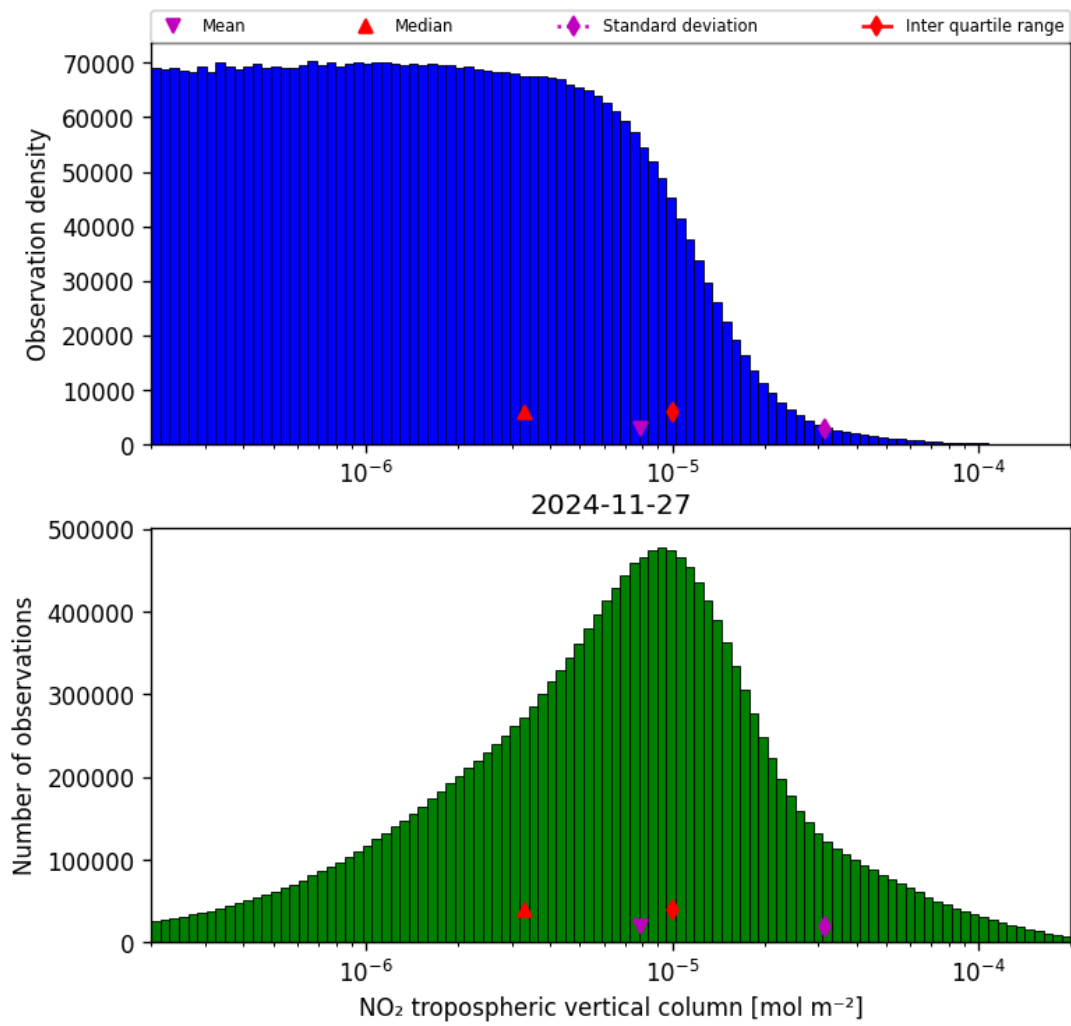
Figure 29: Histogram of “NO 2 tropospheric vertical column” for 2024-11-26 to 2024-11-28
