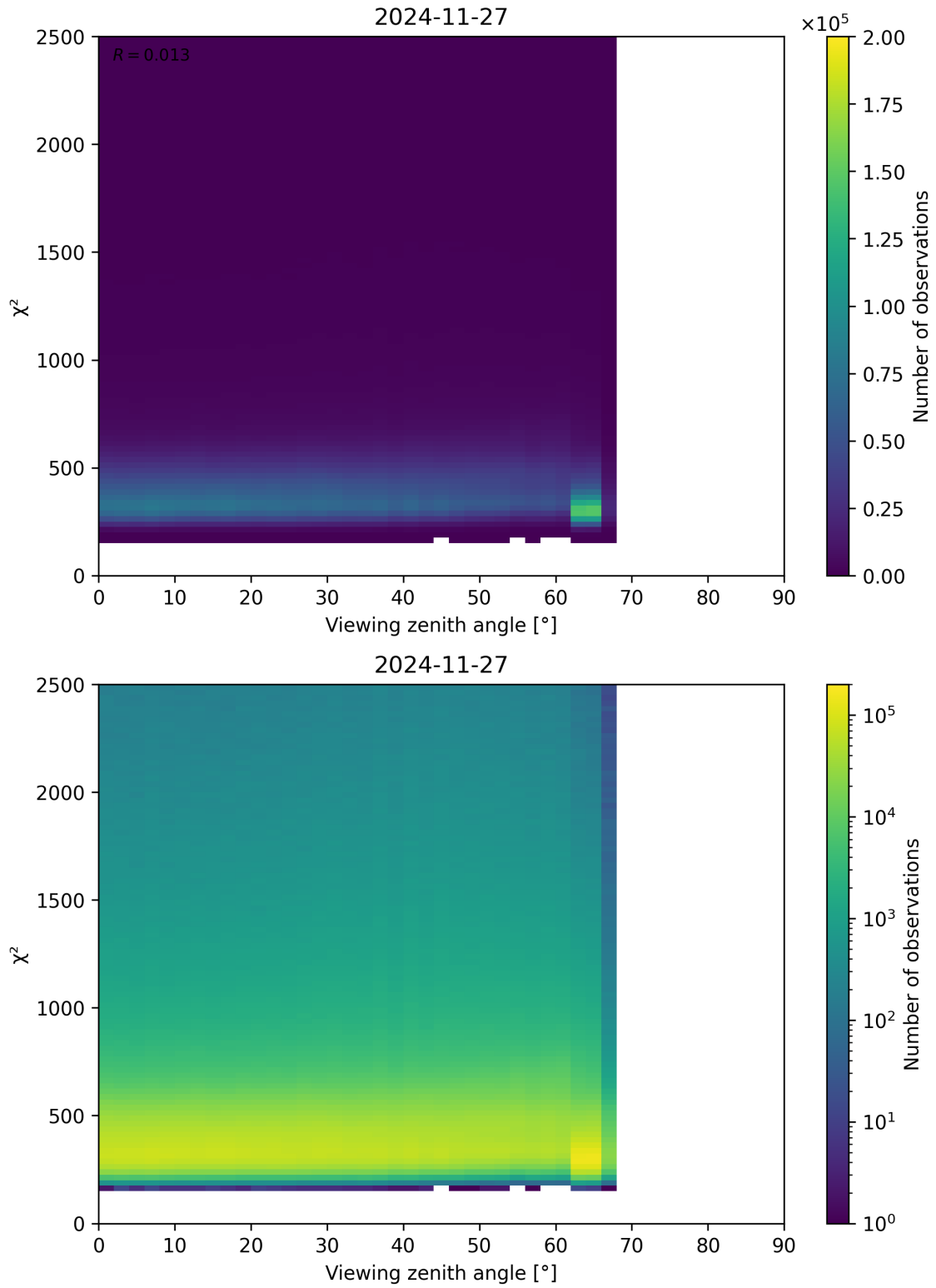
Figure 162: Scatter density plot of “Viewing zenith angle” against “ \chi^2 ” for 2024-11-26 to 2024-11-28.
