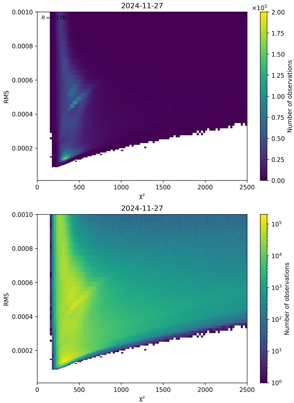
Figure 82: Scatter density plot of “ \chi^2 ” against “RMS” for 2024-11-26 to 2024-11-28.
