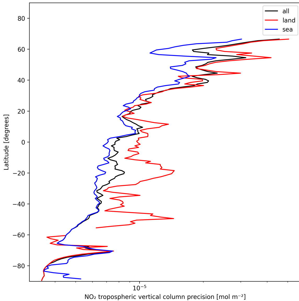
Figure 13: Zonal average of “NO 2 tropospheric vertical column precision” for 2024-11-26 to 2024-11-28.
