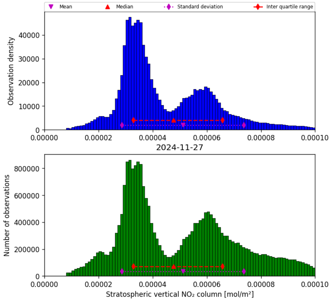
Figure 36: Histogram of “Stratospheric vertical NO 2 column” for 2024-11-26 to 2024-11-28
