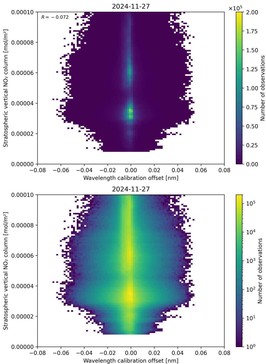
Figure 176: Scatter density plot of “Wavelength calibration offset” against “Stratospheric vertical NO 2 column” for 2024-11-26 to 2024-11-28.
