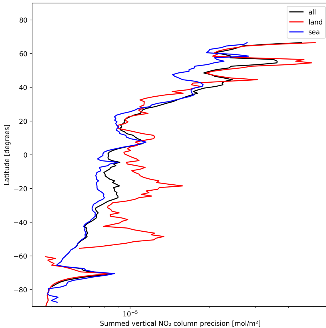
Figure 24: Zonal average of “Summed vertical NO 2 column precision” for 2024-11-27 to 2024-11-29.
