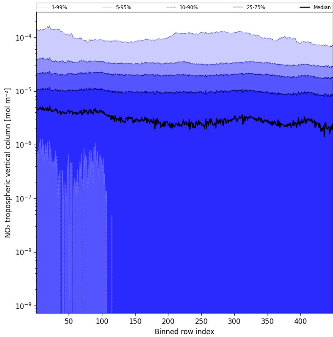
Figure 46: Along track statistics of “NO 2 tropospheric vertical column” for 2024-11-27 to 2024-11-29
