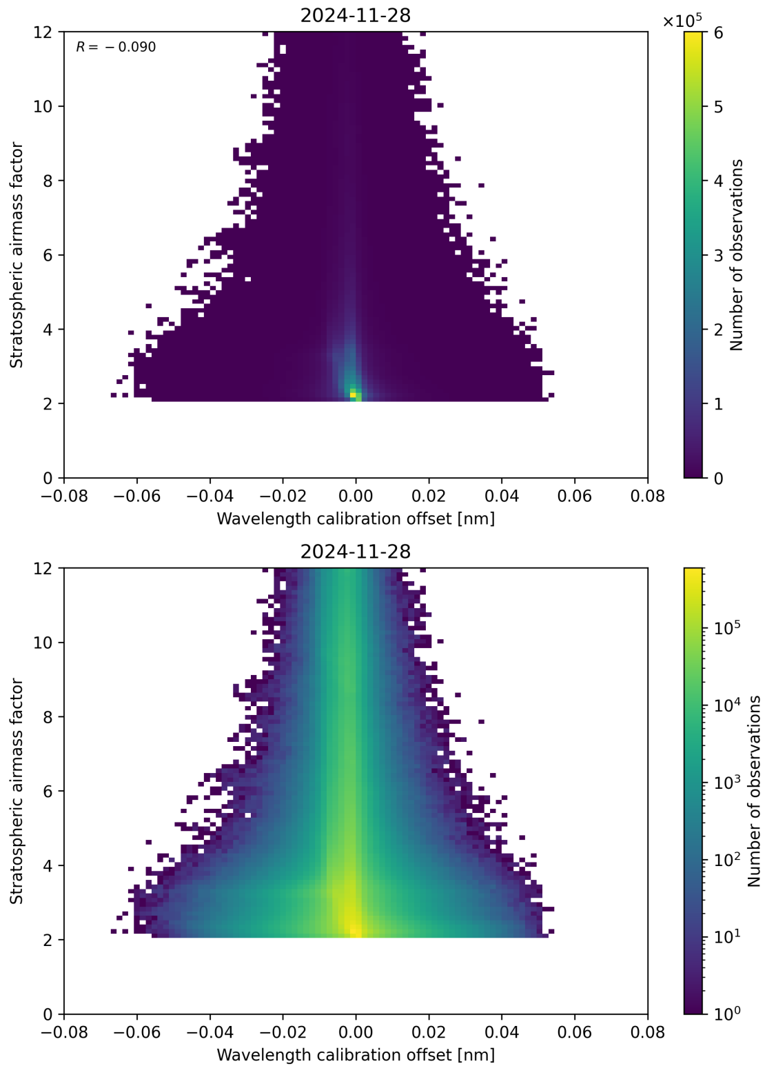
Figure 174: Scatter density plot of “Wavelength calibration offset” against “Stratospheric airmass factor” for 2024-11-27 to 2024-11-29.
