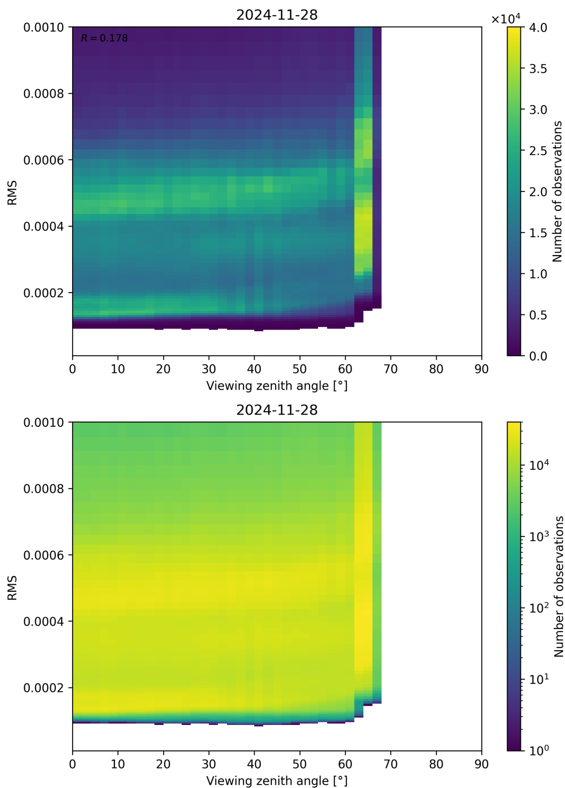
Figure 171: Scatter density plot of “Viewing zenith angle” against “RMS” for 2024-11-27 to 2024-11-29.
