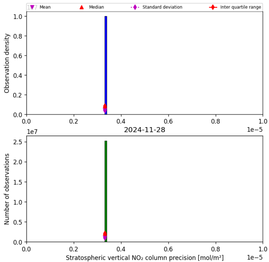
Figure 37: Histogram of “Stratospheric vertical NO 2 column precision” for 2024-11-27 to 2024-11-29
