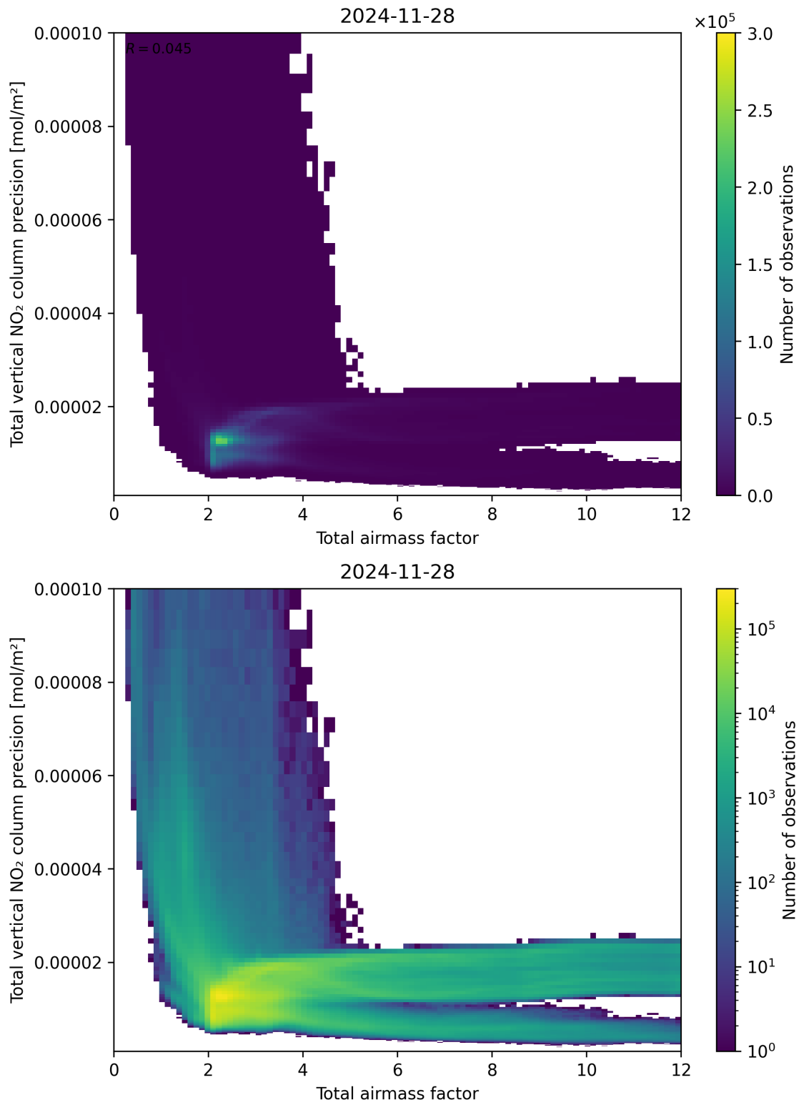
Figure 68: Scatter density plot of “Total airmass factor” against “Total vertical NO 2 column precision” for 2024-11-27 to 2024-11-29.
