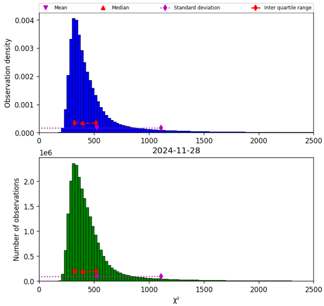
Figure 42: Histogram of " \chi^2 " for 2024-11-27 to 2024-11-29
