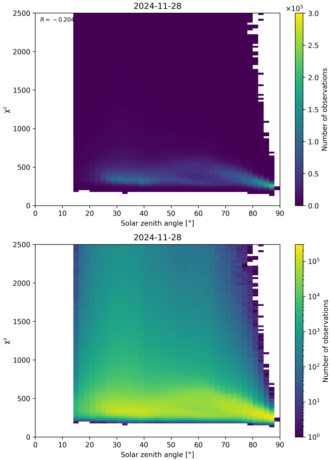
Figure 148: Scatter density plot of “Solar zenith angle” against “ \chi^2 ” for 2024-11-27 to 2024-11-29.
