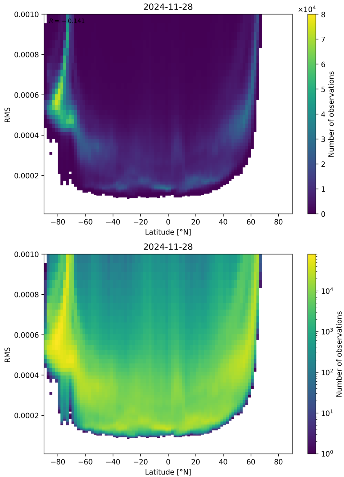
Figure 94: Scatter density plot of “Latitude” against “RMS” for 2024-11-27 to 2024-11-29.
