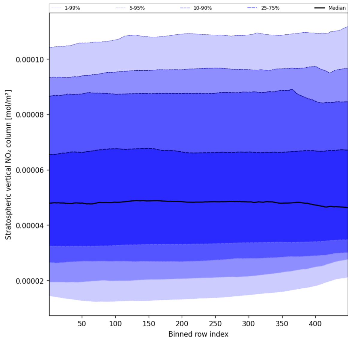
Figure 53: Along track statistics of “Stratospheric vertical NO 2 column” for 2024-11-27 to 2024-11-29
