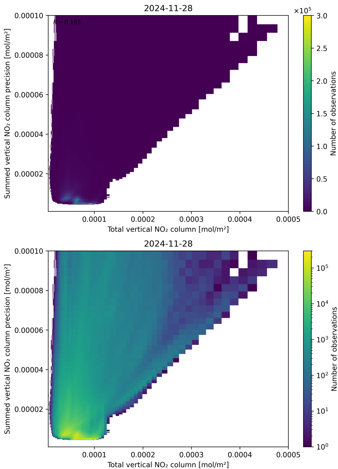
Figure 113: Scatter density plot of “Total vertical NO 2 column” against “Summed vertical NO 2 column precision” for 2024-11-27 to 2024-11-29.
