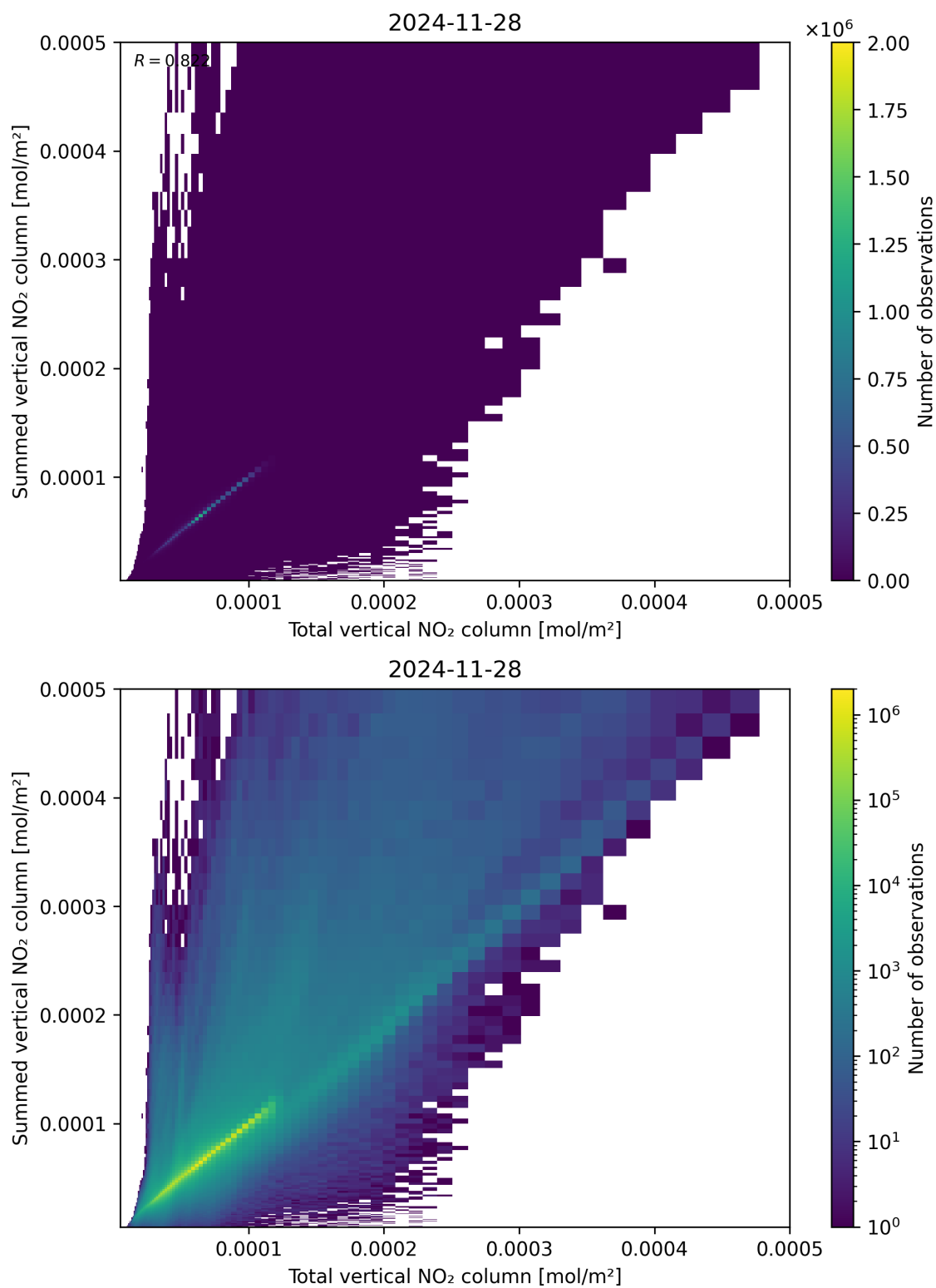
Figure 112: Scatter density plot of “Total vertical NO 2 column” against “Summed vertical NO 2 column” for 2024-11-27 to 2024-11-29.
