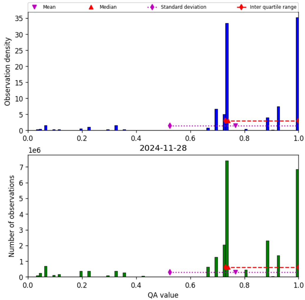
Figure 28: Histogram of “QA value” for 2024-11-27 to 2024-11-29
