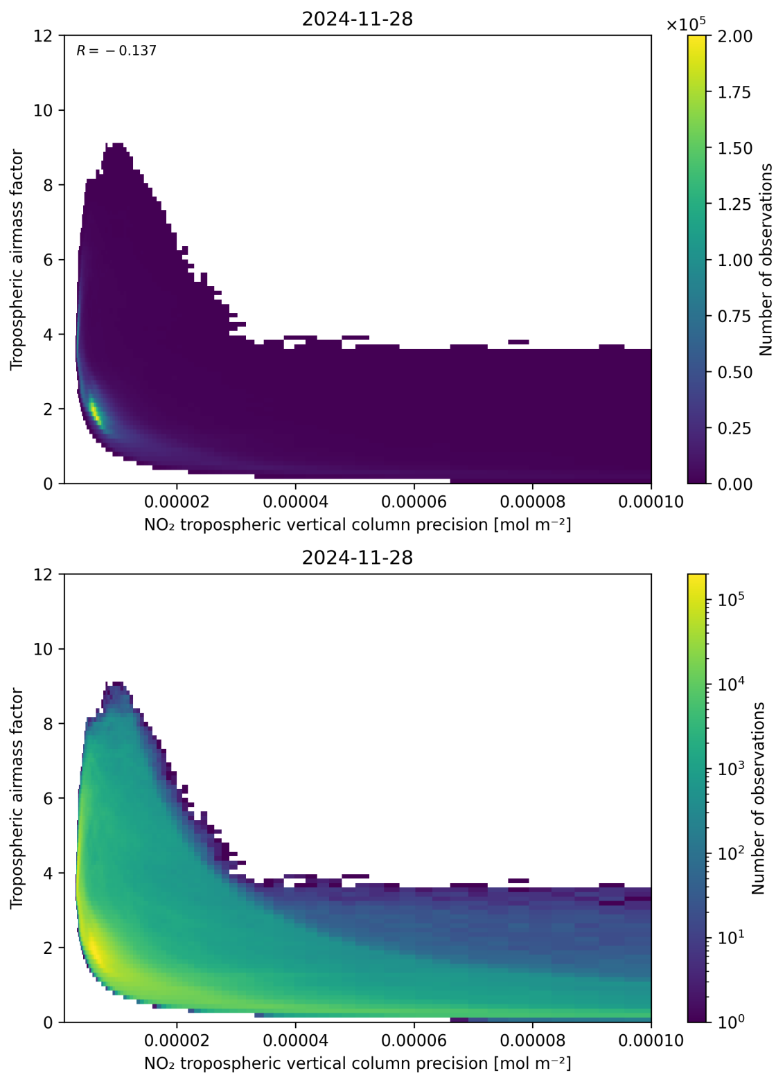
Figure 133: Scatter density plot of “NO 2 tropospheric vertical column precision” against “Tropospheric airmass factor” for 2024-11-27 to 2024-11-29.
