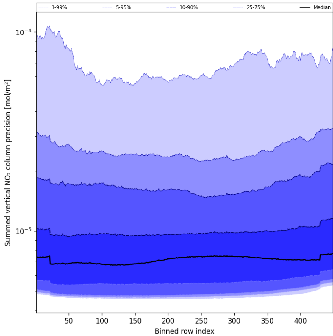
Figure 58: Along track statistics of “Summed vertical NO 2 column precision” for 2024-11-27 to 2024-11-29
