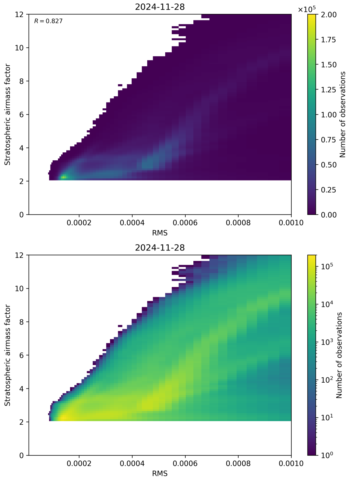
Figure 144: Scatter density plot of “RMS” against “Stratospheric airmass factor” for 2024-11-27 to 2024-11-29.
