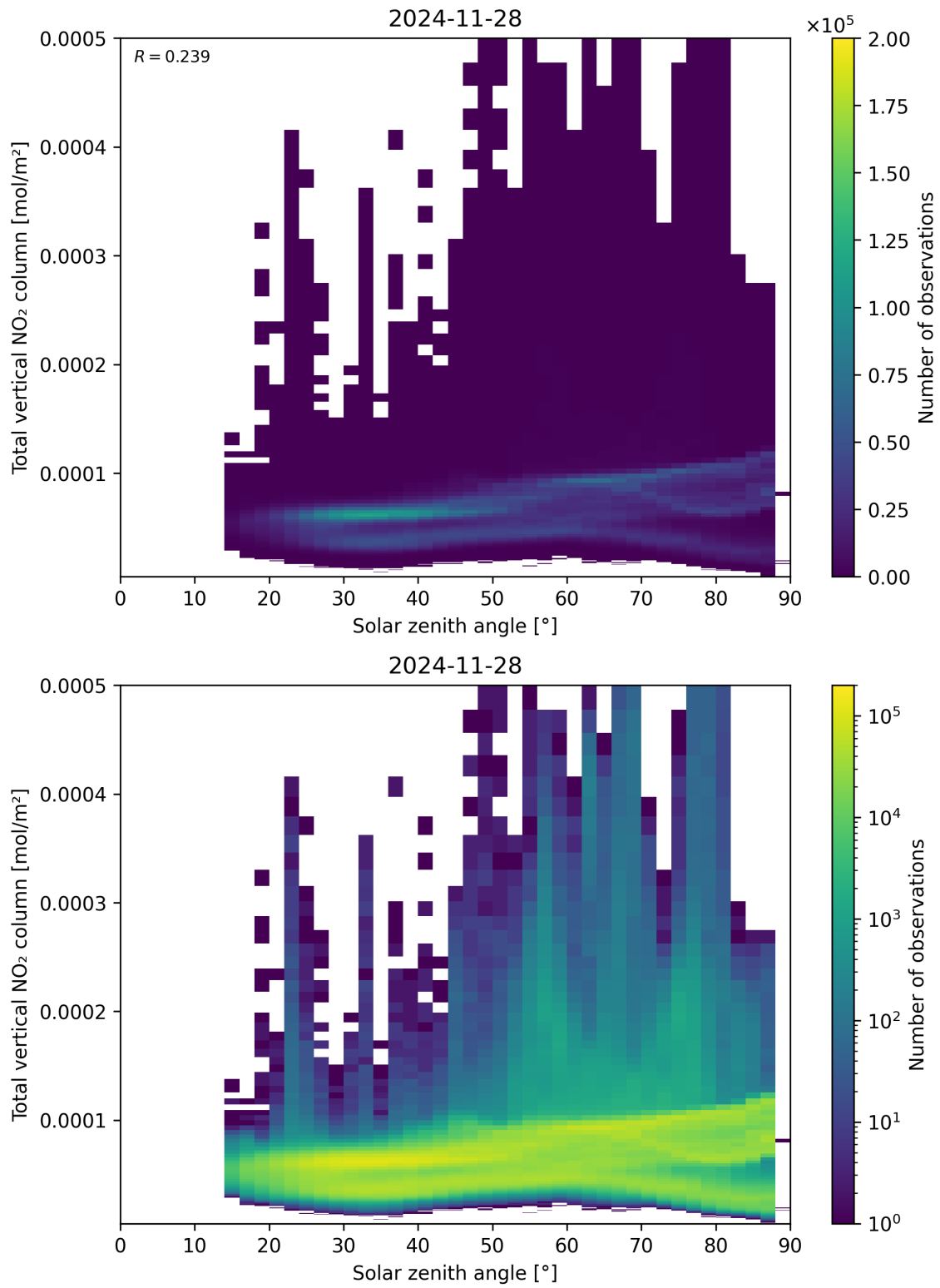
Figure 153: Scatter density plot of “Solar zenith angle” against “Total vertical \text{NO}_2 column” for 2024-11-27 to 2024-11-29.
