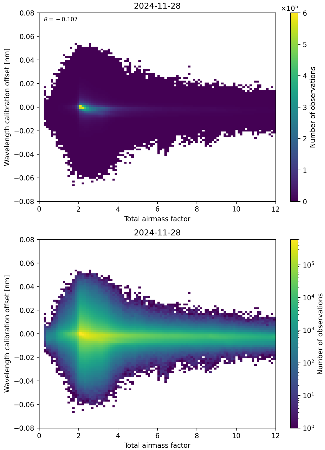
Figure 70: Scatter density plot of “Total airmass factor” against “Wavelength calibration offset” for 2024-11-27 to 2024-11-29.
