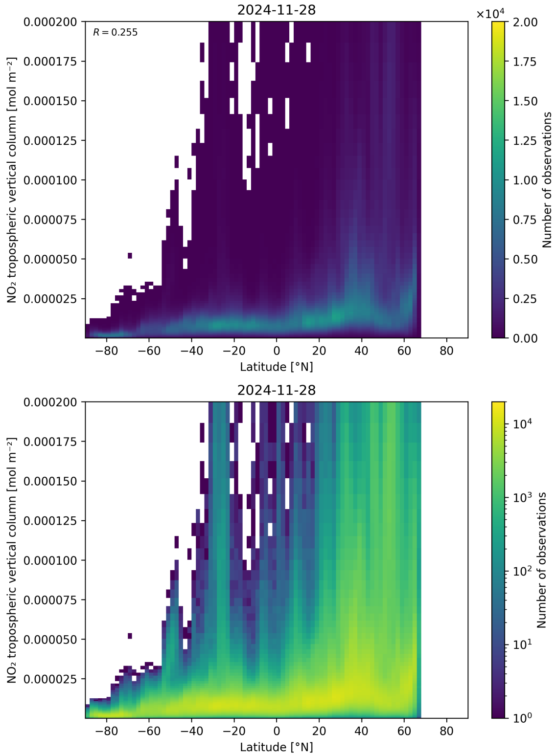
Figure 92: Scatter density plot of “Latitude” against “NO 2 tropospheric vertical column” for 2024-11-27 to 2024-11-29.
