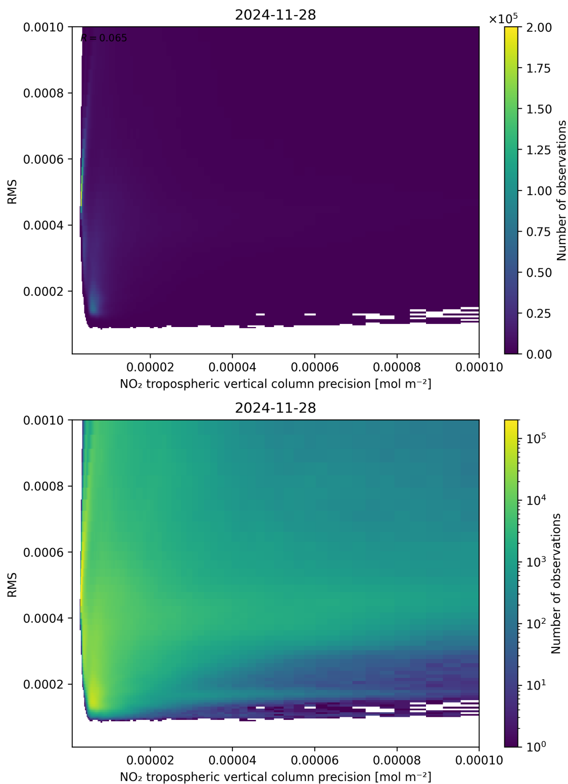
Figure 140: Scatter density plot of “NO 2 tropospheric vertical column precision” against “RMS” for 2024-11-27 to 2024-11-29.
