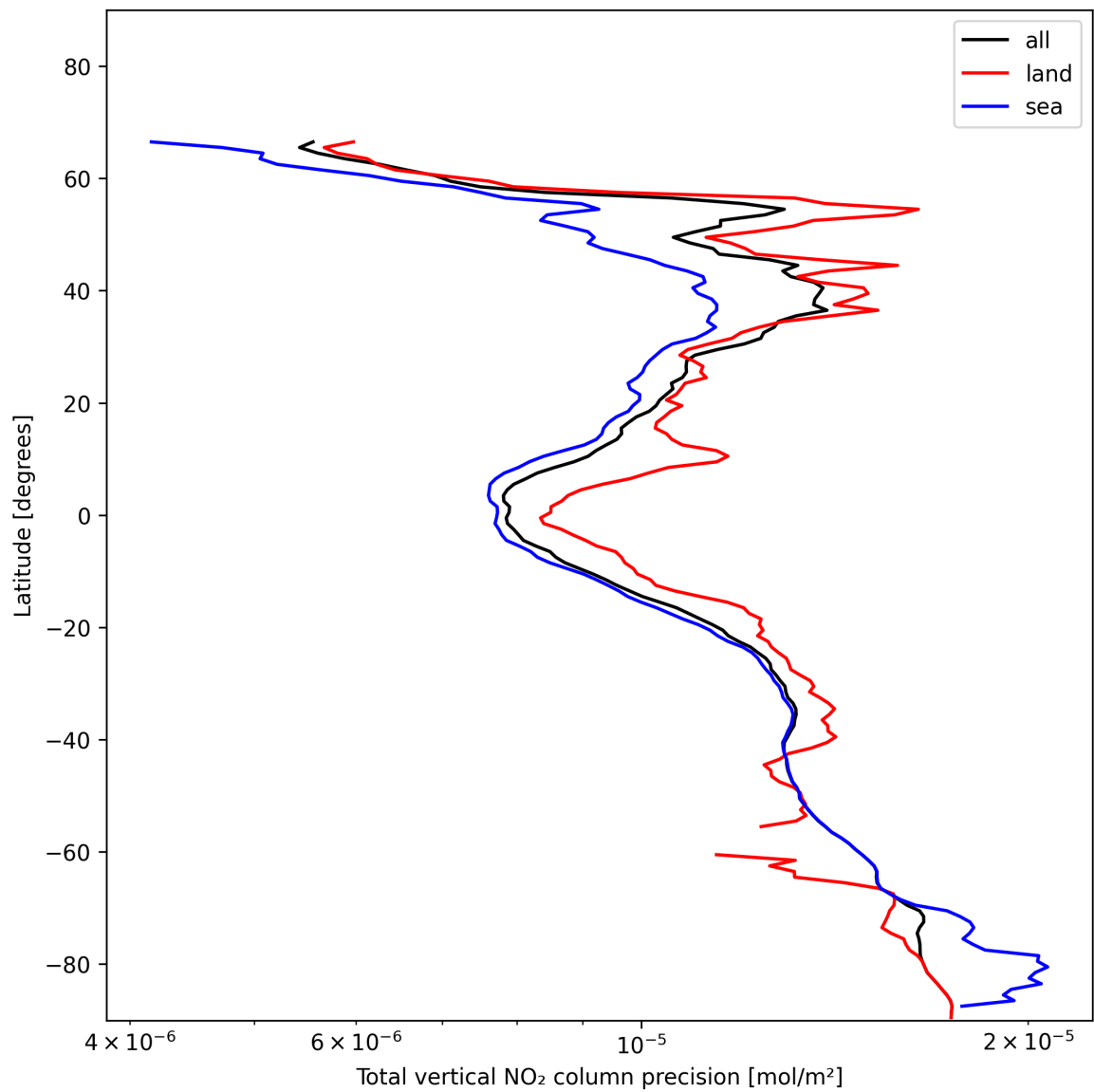
Figure 22: Zonal average of “Total vertical NO 2 column precision” for 2024-11-27 to 2024-11-29.
