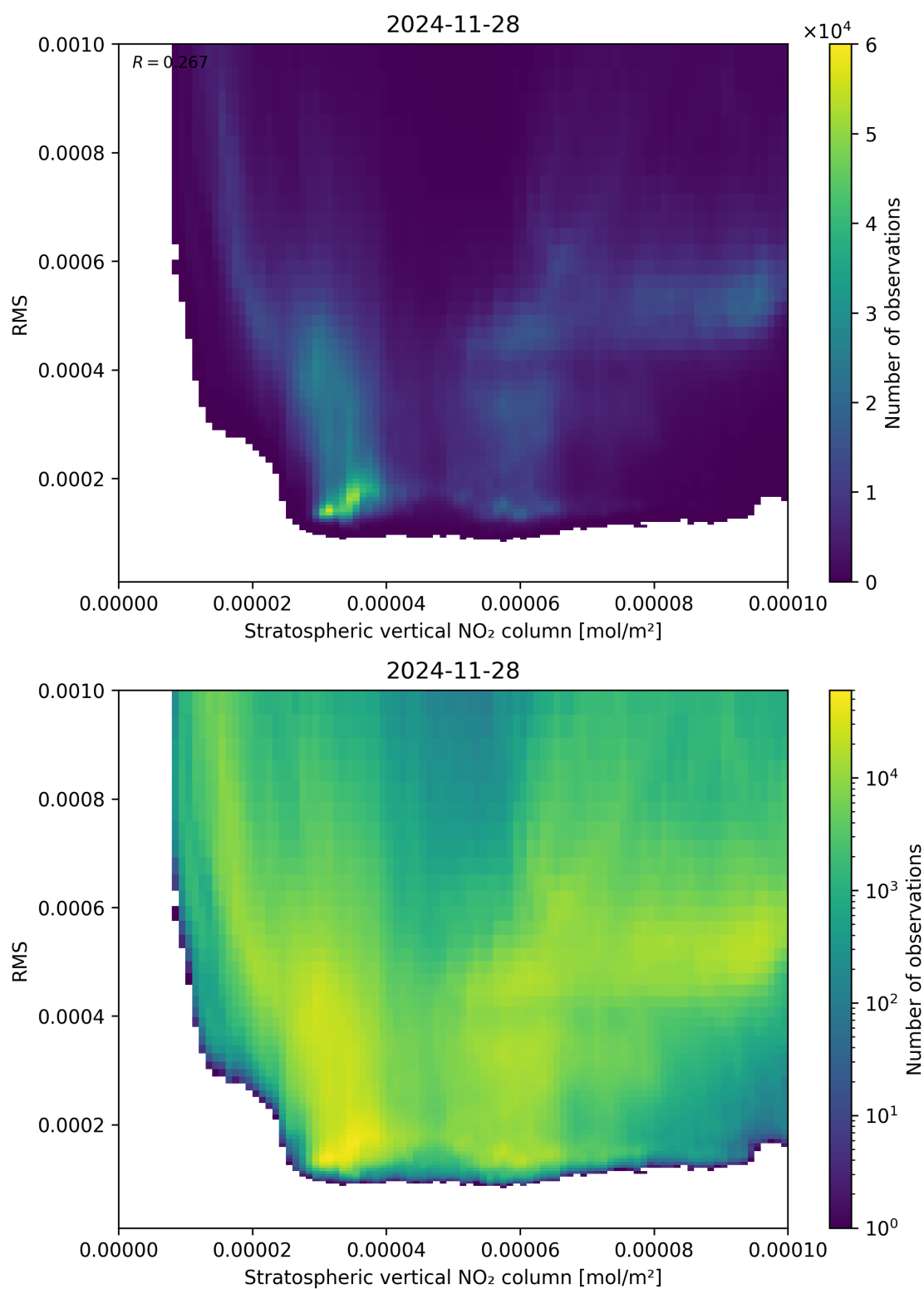
Figure 102: Scatter density plot of “Stratospheric vertical NO 2 column” against “RMS” for 2024-11-27 to 2024-11-29.
