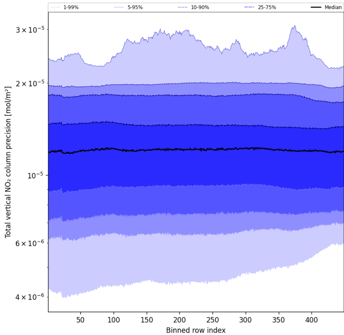
Figure 56: Along track statistics of “Total vertical NO 2 column precision” for 2024-11-27 to 2024-11-29
