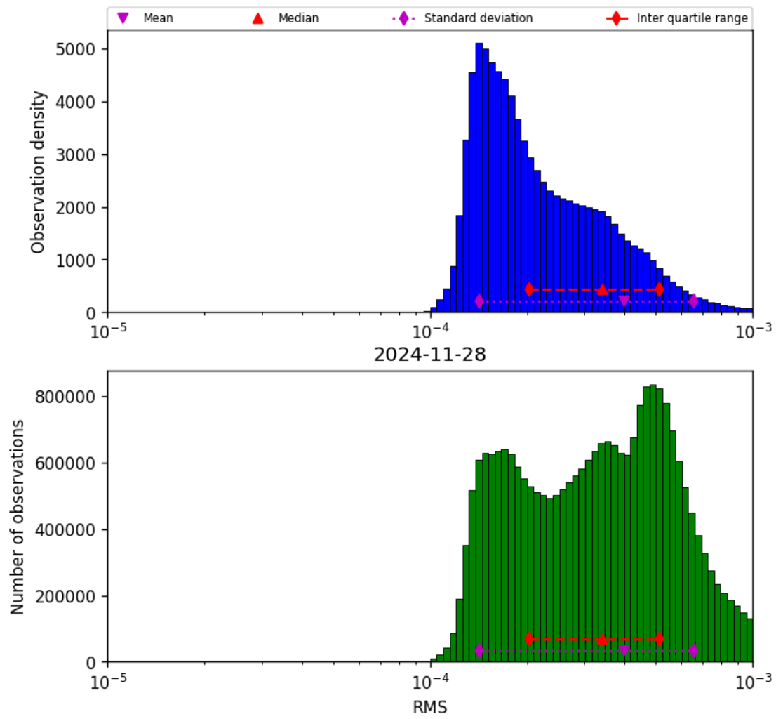
Figure 43: Histogram of “RMS” for 2024-11-27 to 2024-11-29
