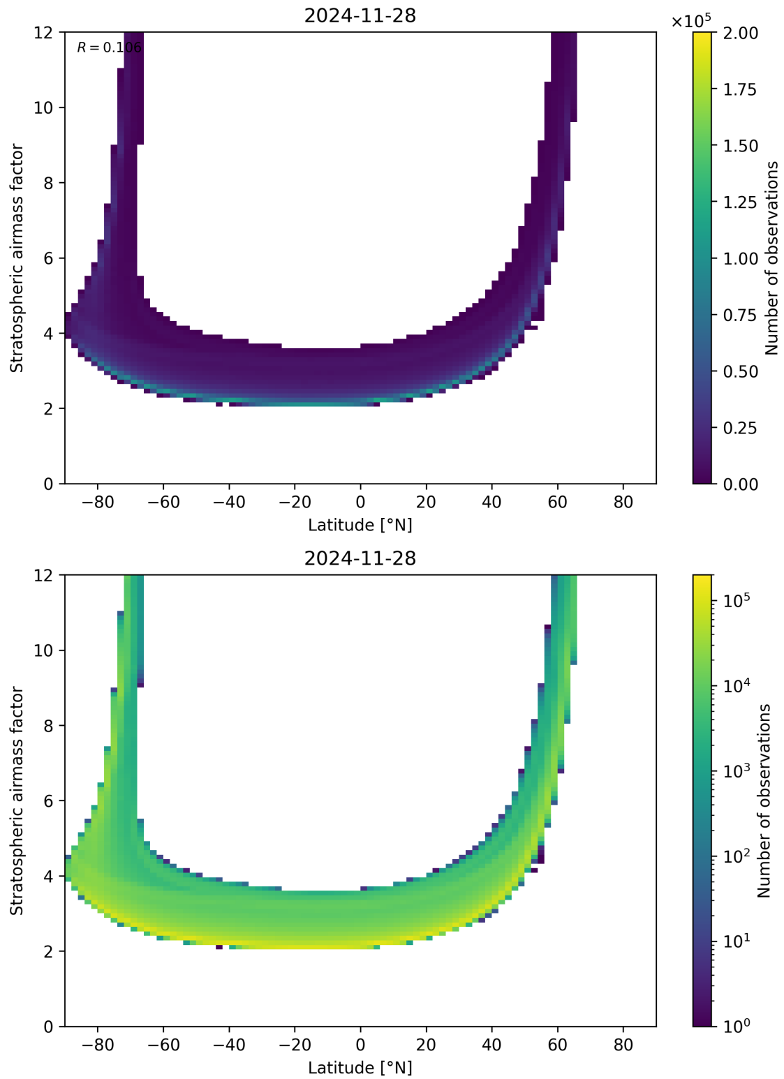
Figure 83: Scatter density plot of “Latitude” against “Stratospheric airmass factor” for 2024-11-27 to 2024-11-29.
