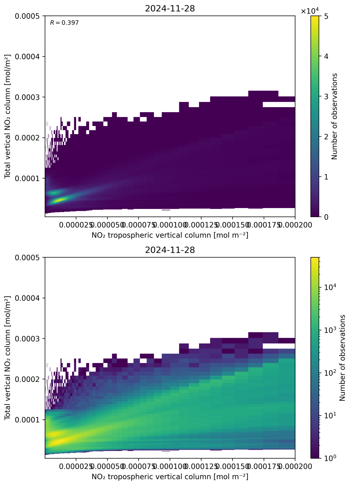
Figure 128: Scatter density plot of “NO 2 tropospheric vertical column” against “Total vertical NO 2 column” for 2024-11-27 to 2024-11-29.
