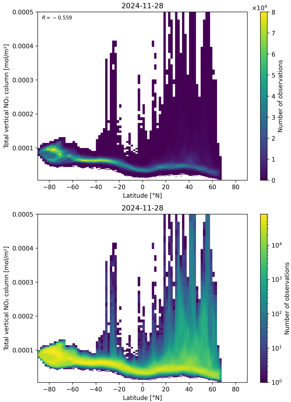
Figure 90: Scatter density plot of “Latitude” against “Total vertical NO 2 column” for 2024-11-27 to 2024-11-29.
