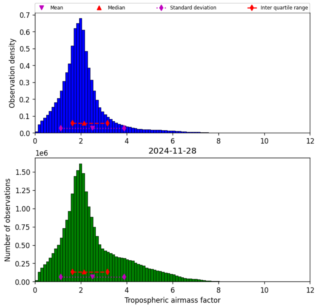
Figure 31: Histogram of “Tropospheric airmass factor” for 2024-11-27 to 2024-11-29
