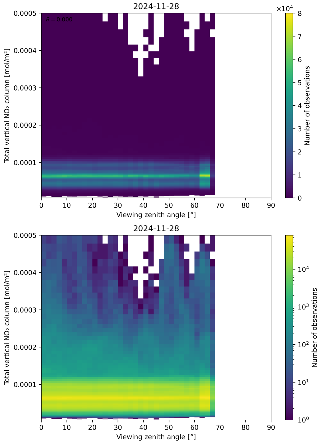
Figure 167: Scatter density plot of “Viewing zenith angle” against “Total vertical NO 2 column” for 2024-11-27 to 2024-11-29.
