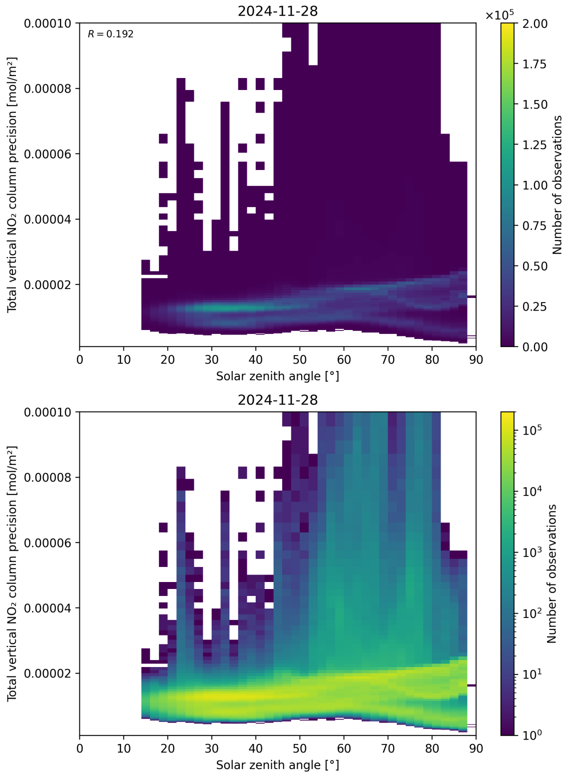
Figure 154: Scatter density plot of “Solar zenith angle” against “Total vertical NO 2 column precision” for 2024-11-27 to 2024-11-29.
