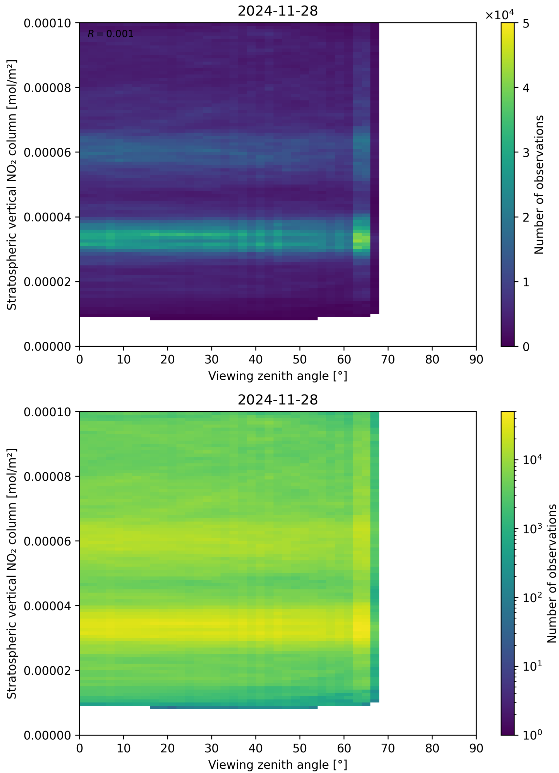
Figure 164: Scatter density plot of “Viewing zenith angle” against “Stratospheric vertical NO 2 column” for 2024-11-27 to 2024-11-29.
