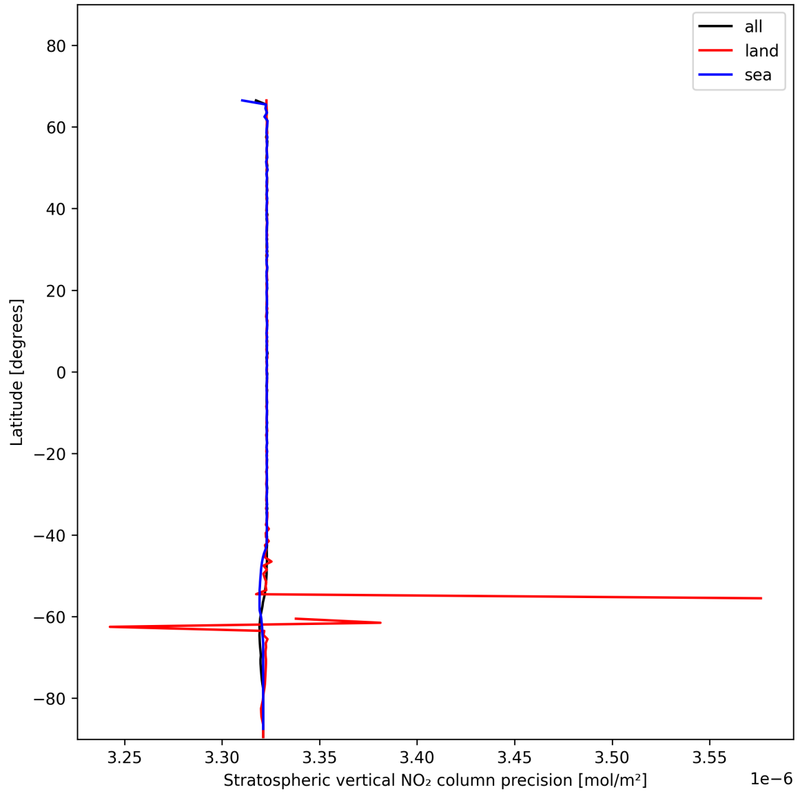
Figure 20: Zonal average of “Stratospheric vertical NO 2 column precision” for 2024-11-27 to 2024-11-29.
