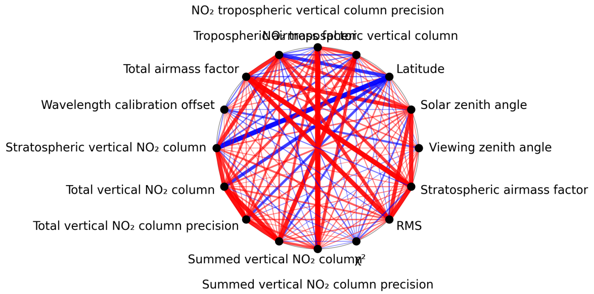
Figure 1: Map of correlation graph for 2024-11-27 to 2024-11-29.
