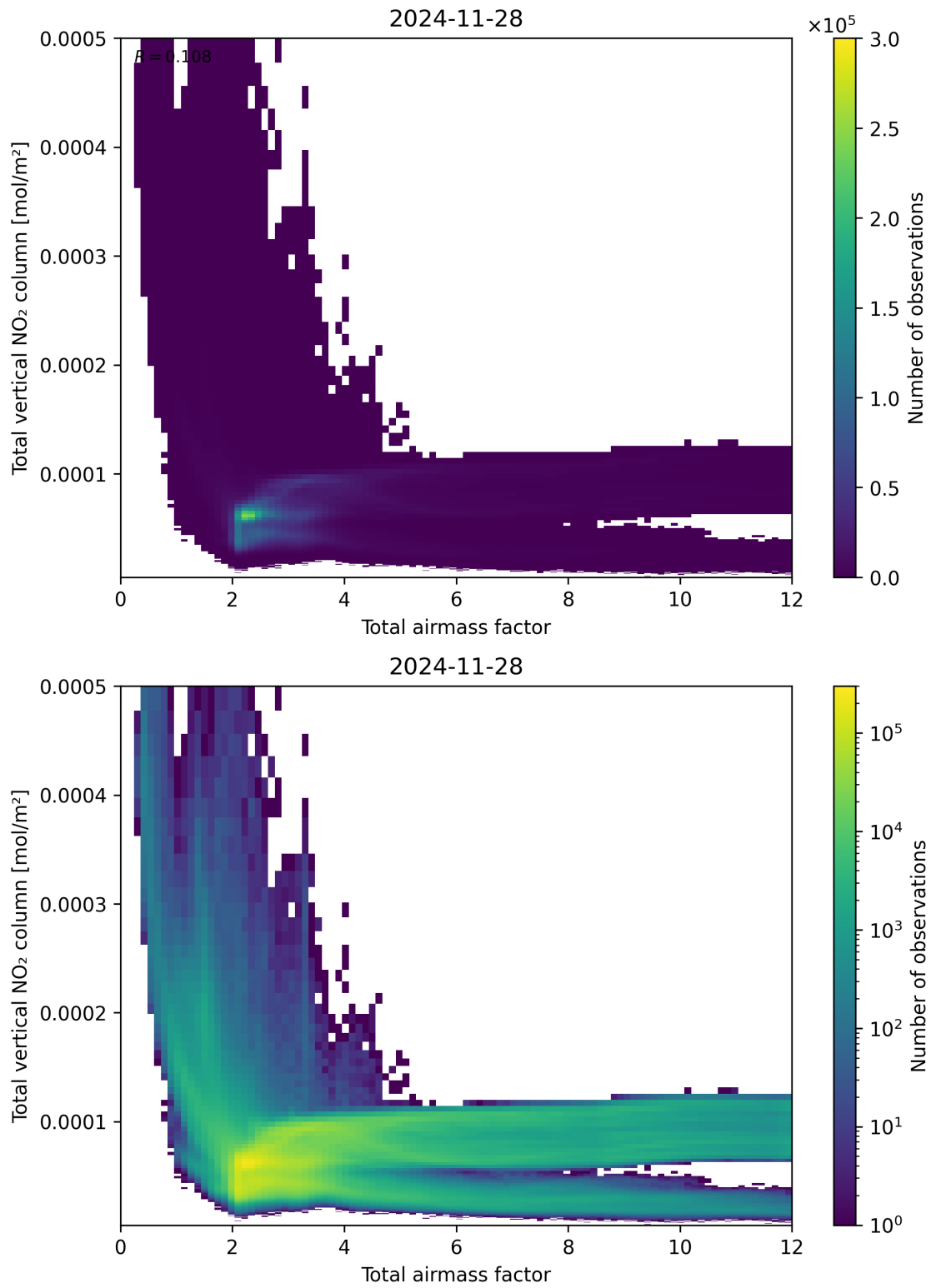
Figure 67: Scatter density plot of “Total airmass factor” against “Total vertical NO 2 column” for 2024-11-27 to 2024-11-29.
