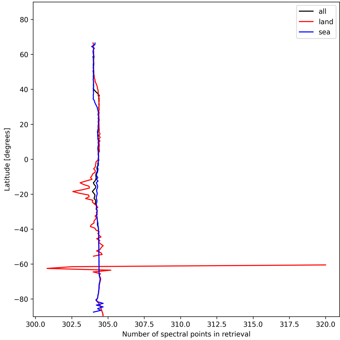
Figure 16: Zonal average of “Number of spectral points in retrieval” for 2024-11-27 to 2024-11-29.
