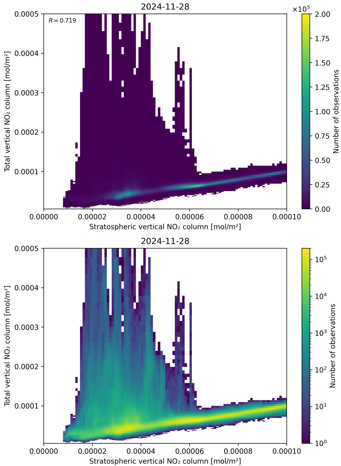
Figure 100: Scatter density plot of “Stratospheric vertical NO 2 column” against “Total vertical NO 2 column” for 2024-11-27 to 2024-11-29.
