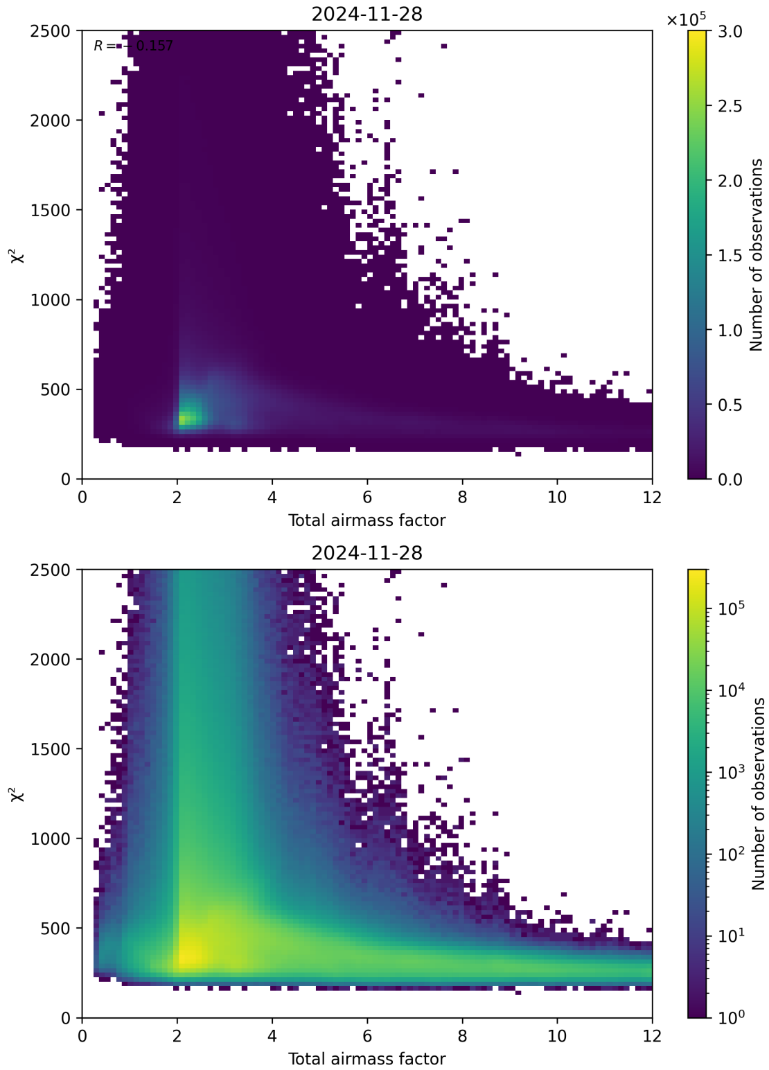
Figure 63: Scatter density plot of “Total airmass factor” against “ \chi^2 ” for 2024-11-27 to 2024-11-29.
