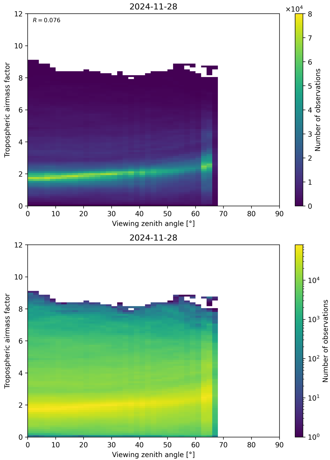
Figure 161: Scatter density plot of “Viewing zenith angle” against “Tropospheric airmass factor” for 2024-11-27 to 2024-11-29.
