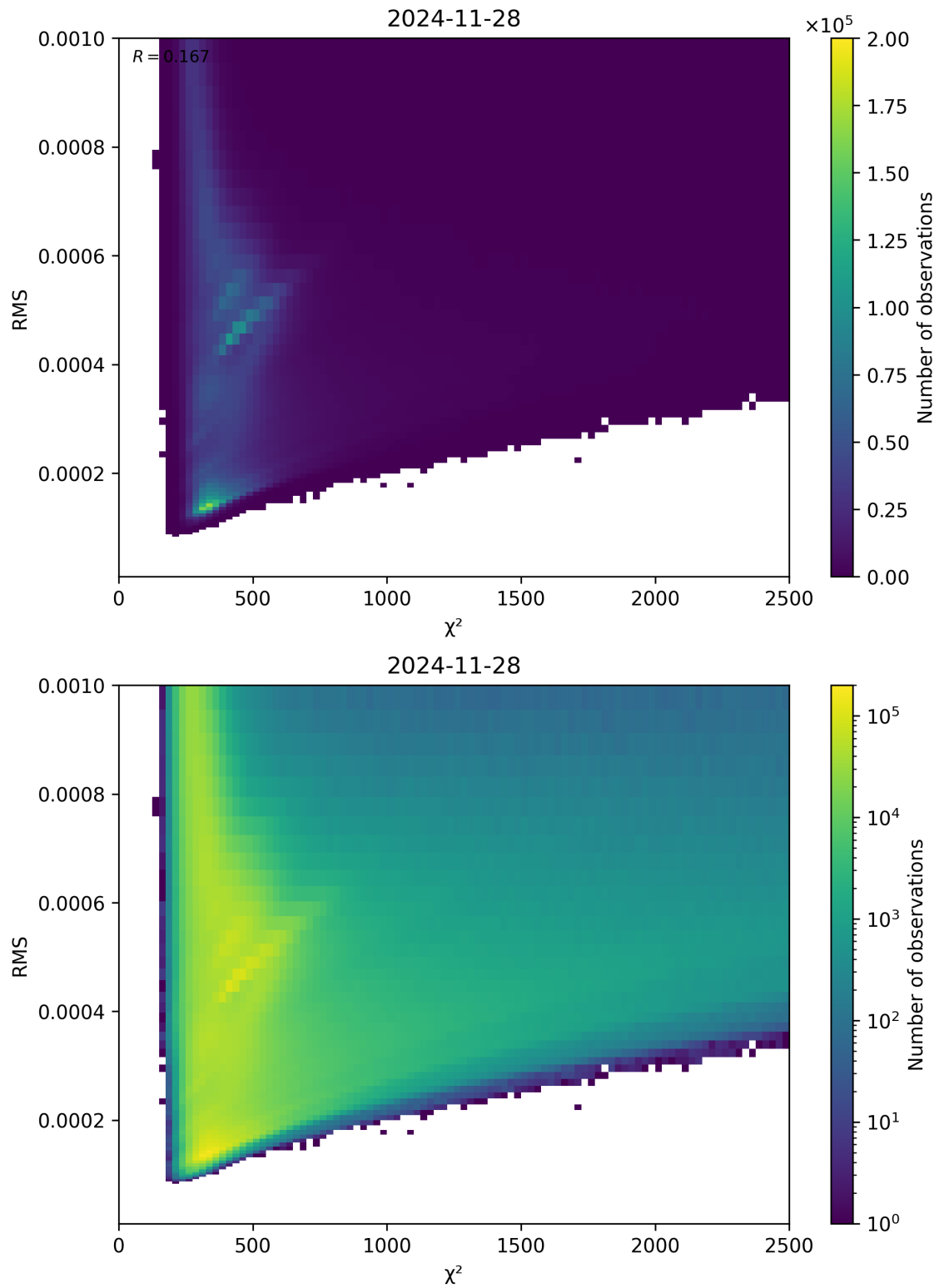
Figure 82: Scatter density plot of “ \chi^2 ” against “RMS” for 2024-11-27 to 2024-11-29.
