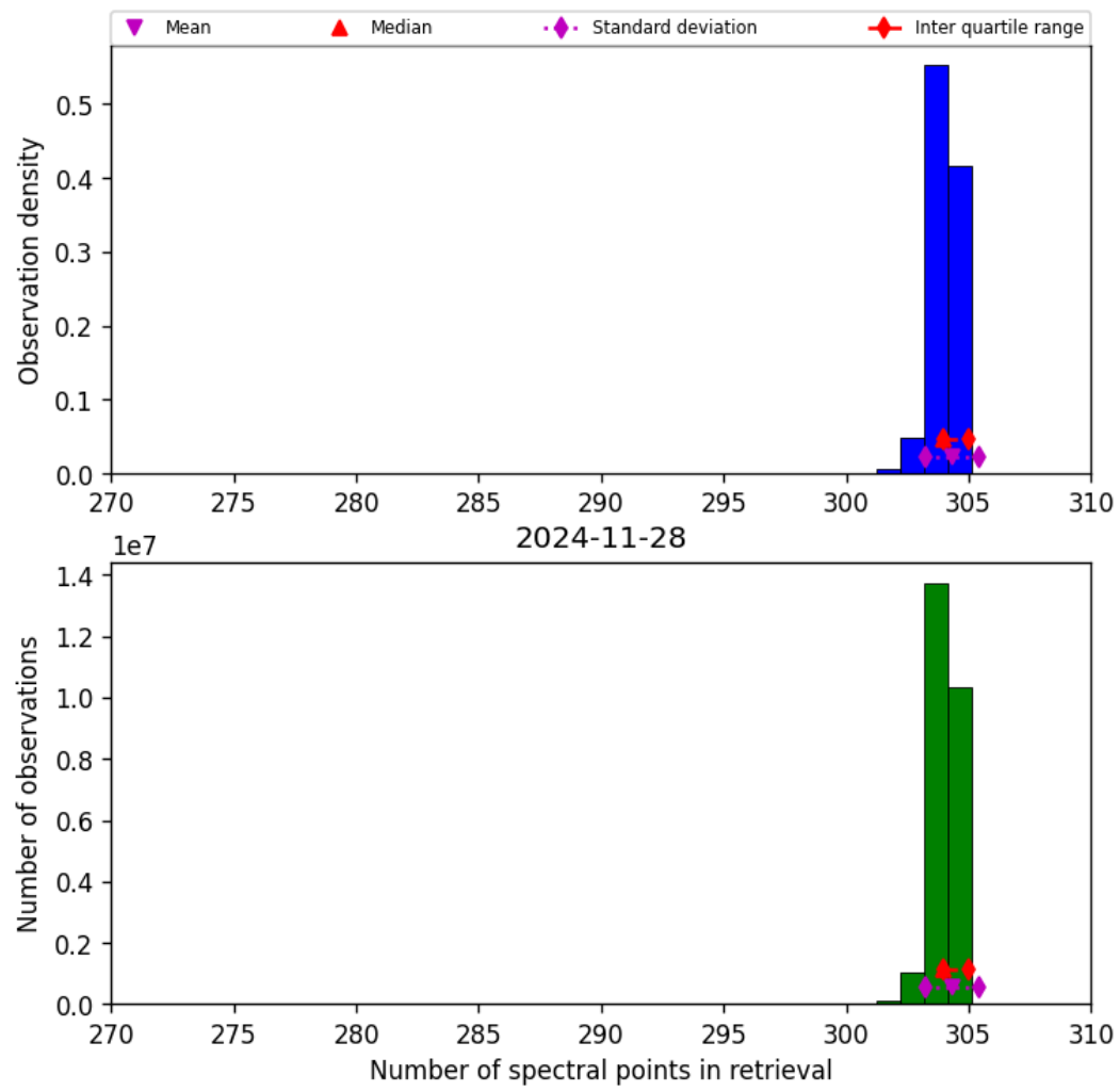
Figure 33: Histogram of “Number of spectral points in retrieval” for 2024-11-27 to 2024-11-29
