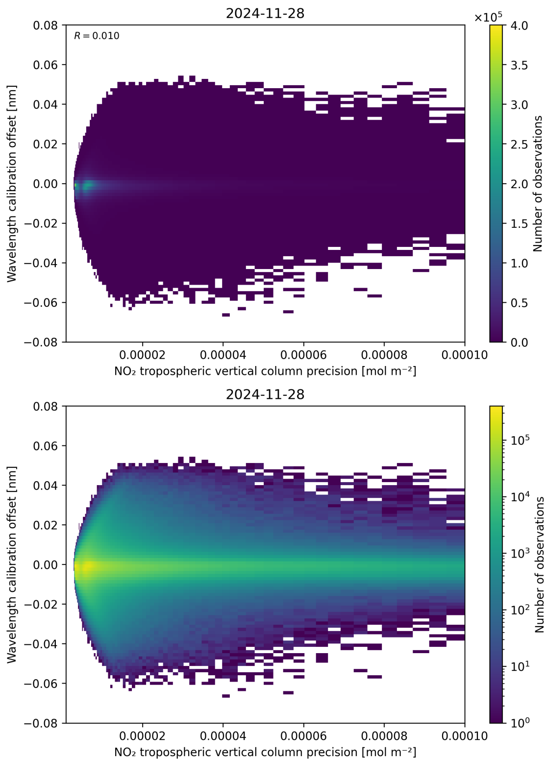
Figure 141: Scatter density plot of “NO 2 tropospheric vertical column precision” against “Wavelength calibration offset” for 2024-11-27 to 2024-11-29.
