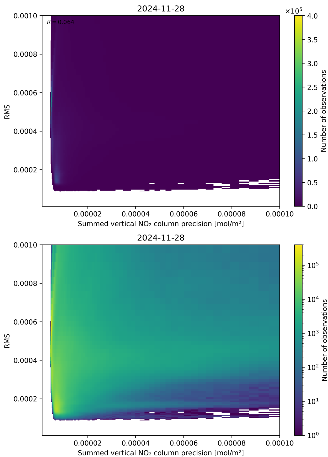
Figure 108: Scatter density plot of “Summed vertical NO 2 column precision” against “RMS” for 2024-11-27 to 2024-11-29.
