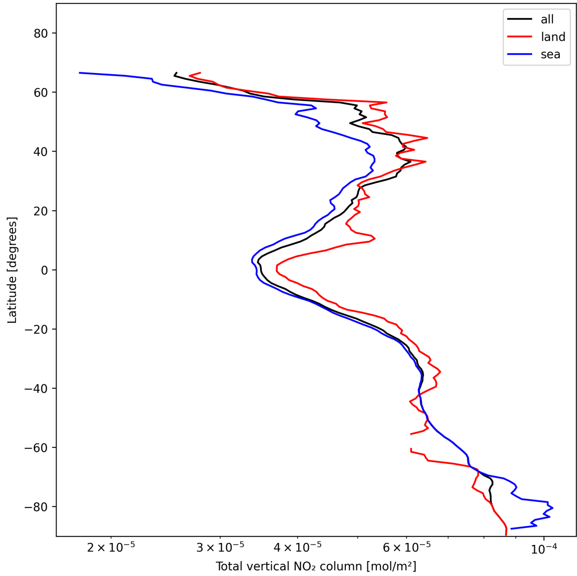
Figure 21: Zonal average of “Total vertical NO 2 column” for 2024-11-27 to 2024-11-29.
