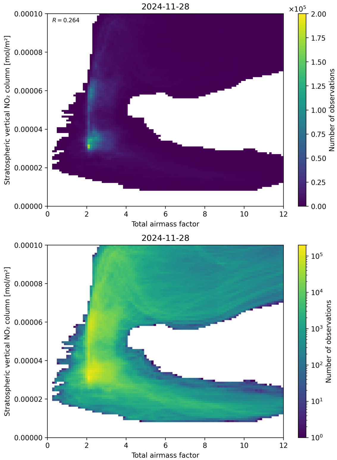
Figure 64: Scatter density plot of “Total airmass factor” against “Stratospheric vertical \text{NO}_2 column” for 2024-11-27 to 2024-11-29.
