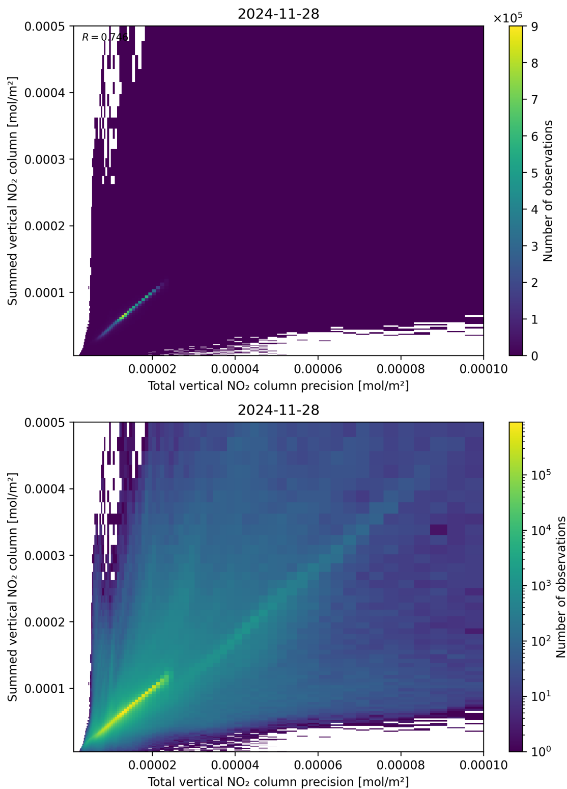
Figure 117: Scatter density plot of “Total vertical NO 2 column precision” against “Summed vertical NO 2 column” for 2024-11-27 to 2024-11-29.
