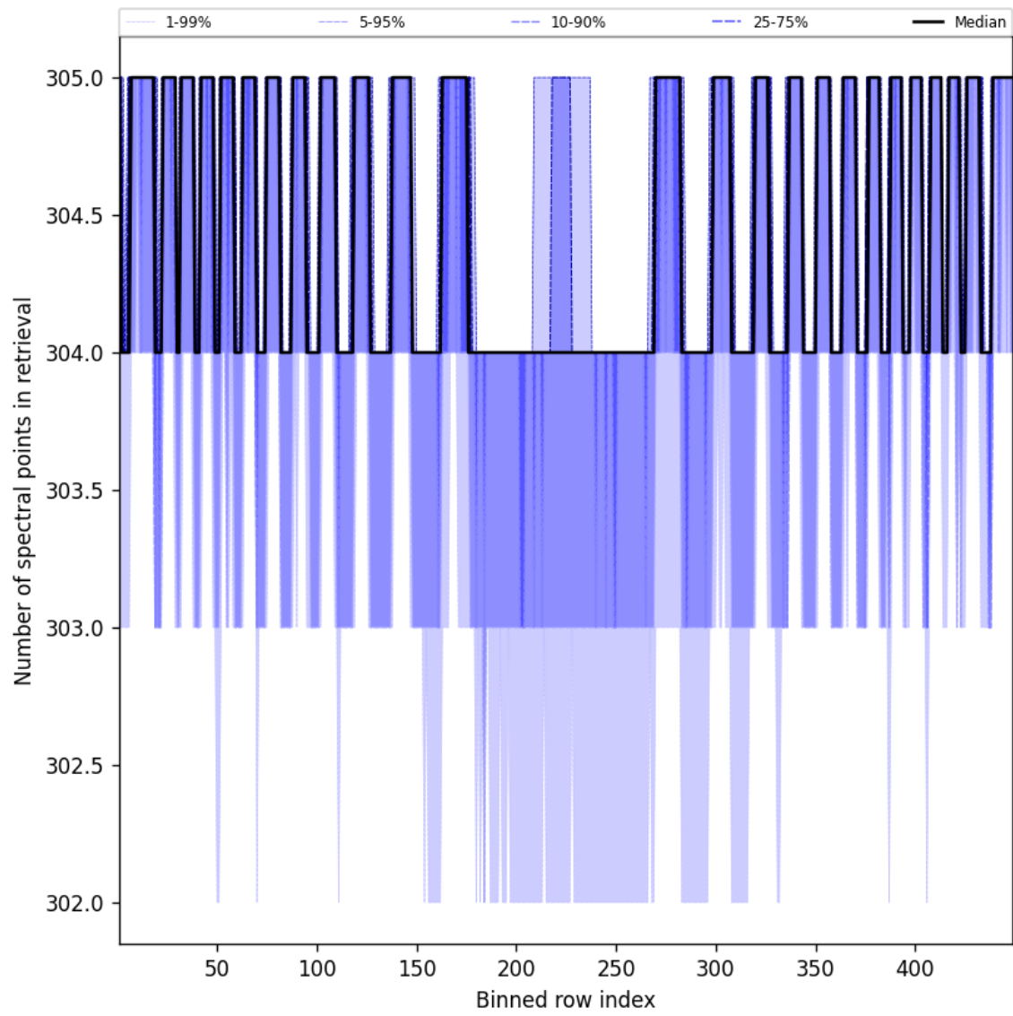
Figure 50: Along track statistics of “Number of spectral points in retrieval” for 2024-11-27 to 2024-11-29
