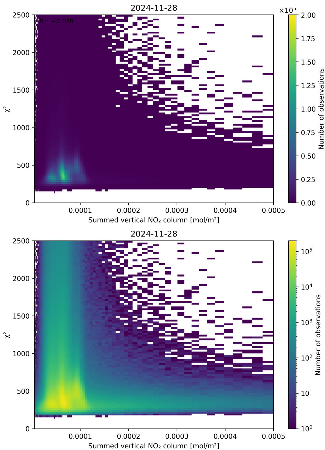
Figure 104: Scatter density plot of “Summed vertical NO 2 column” against “ \chi^2 ” for 2024-11-27 to 2024-11-29.
