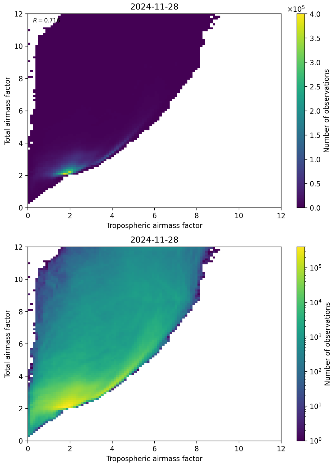
Figure 72: Scatter density plot of “Tropospheric airmass factor” against “Total airmass factor” for 2024-11-27 to 2024-11-29.
