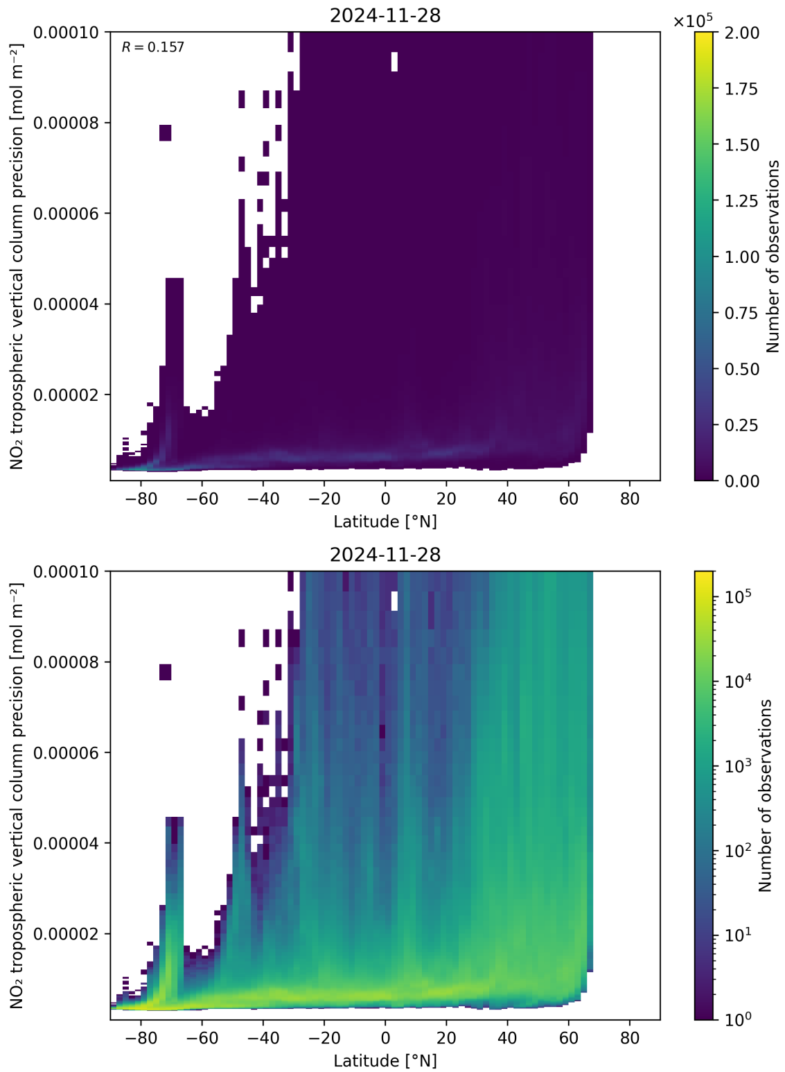
Figure 93: Scatter density plot of “Latitude” against “NO 2 tropospheric vertical column precision” for 2024-11-27 to 2024-11-29.
