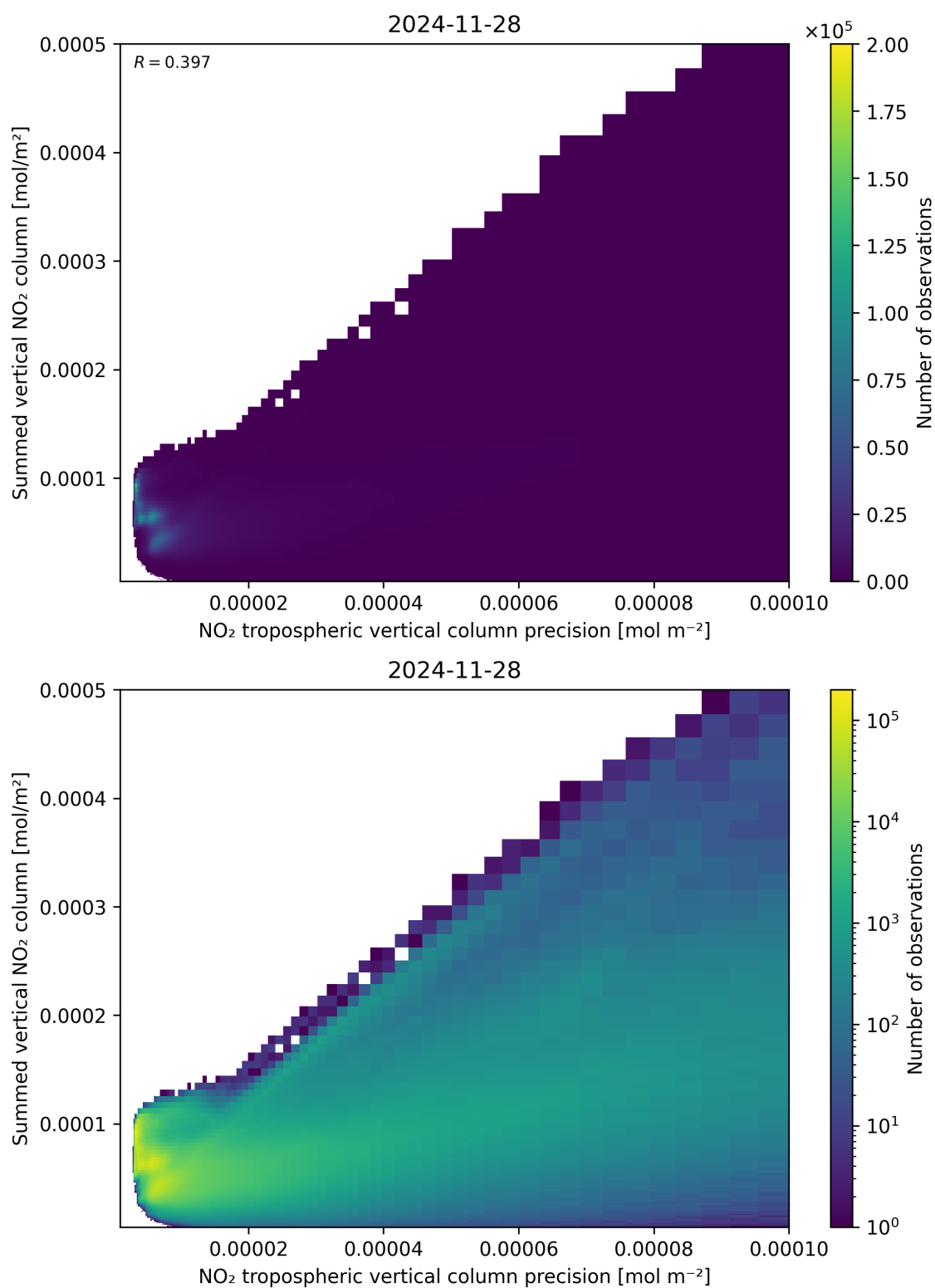
Figure 136: Scatter density plot of “NO 2 tropospheric vertical column precision” against “Summed vertical NO 2 column” for 2024-11-27 to 2024-11-29.
