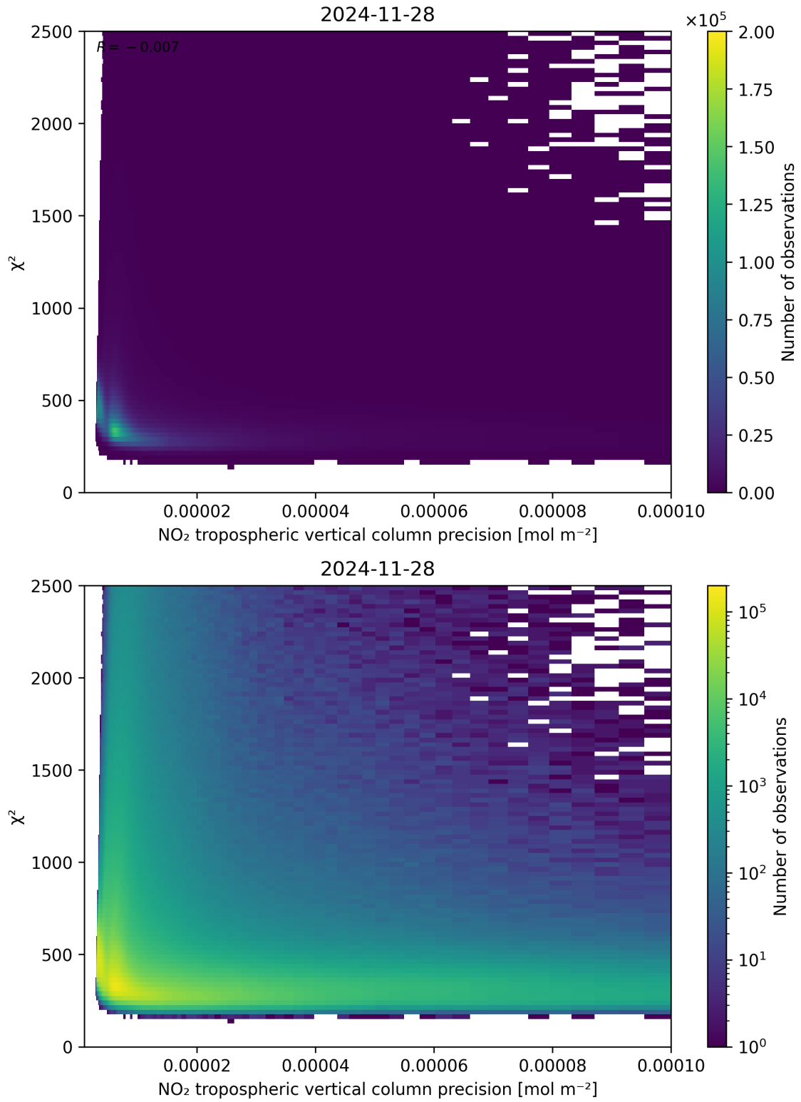
Figure 134: Scatter density plot of “NO 2 tropospheric vertical column precision” against “ \chi^2 ” for 2024-11-27 to 2024-11-29.
