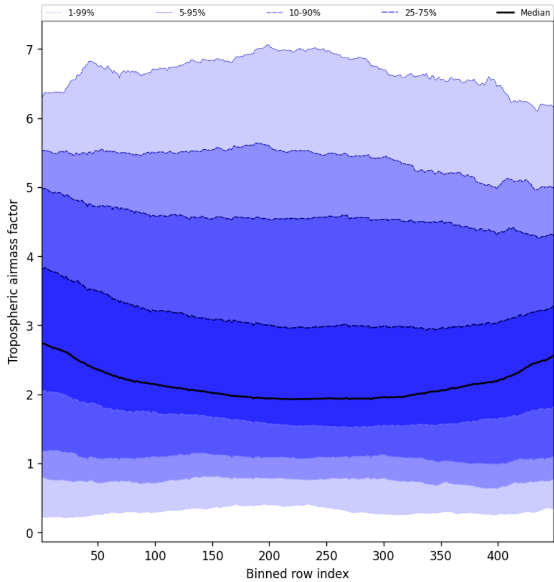
Figure 48: Along track statistics of “Tropospheric airmass factor” for 2024-11-27 to 2024-11-29
