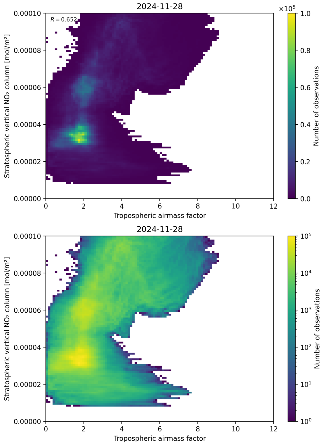
Figure 74: Scatter density plot of “Tropospheric air mass factor” against “Stratospheric vertical NO 2 column” for 2024-11-27 to 2024-11-29.
