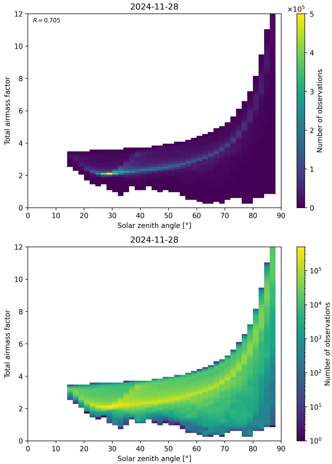
Figure 146: Scatter density plot of “Solar zenith angle” against “Total airmass factor” for 2024-11-27 to 2024-11-29.
