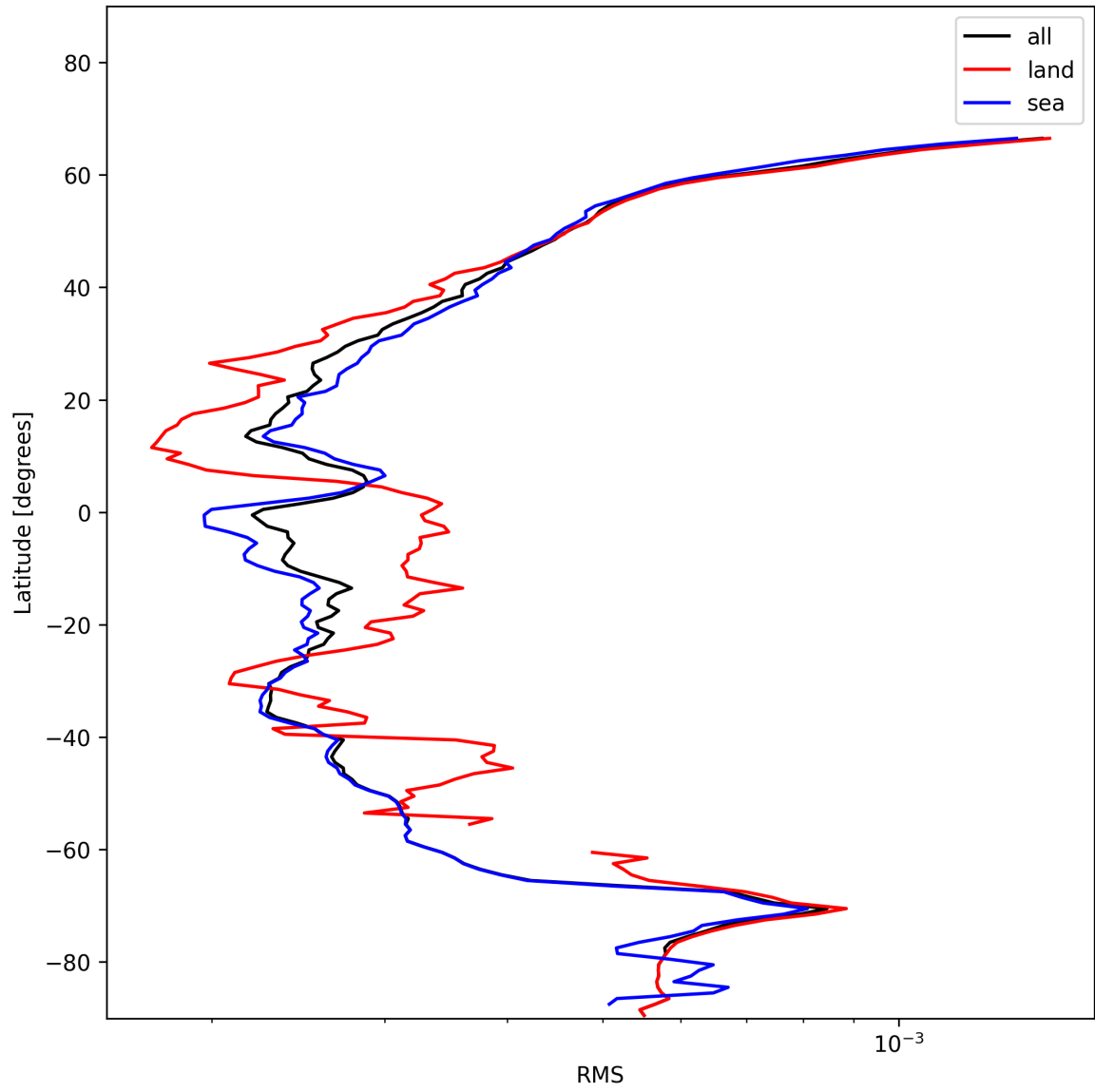
Figure 26: Zonal average of “RMS” for 2024-11-27 to 2024-11-29.
