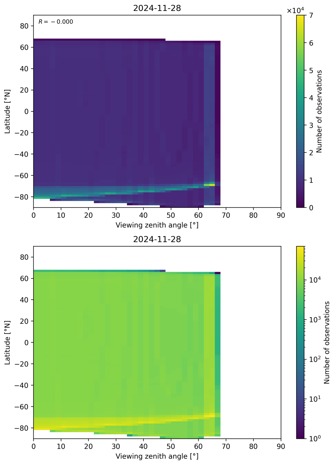
Figure 163: Scatter density plot of “Viewing zenith angle” against “Latitude” for 2024-11-27 to 2024-11-29.
