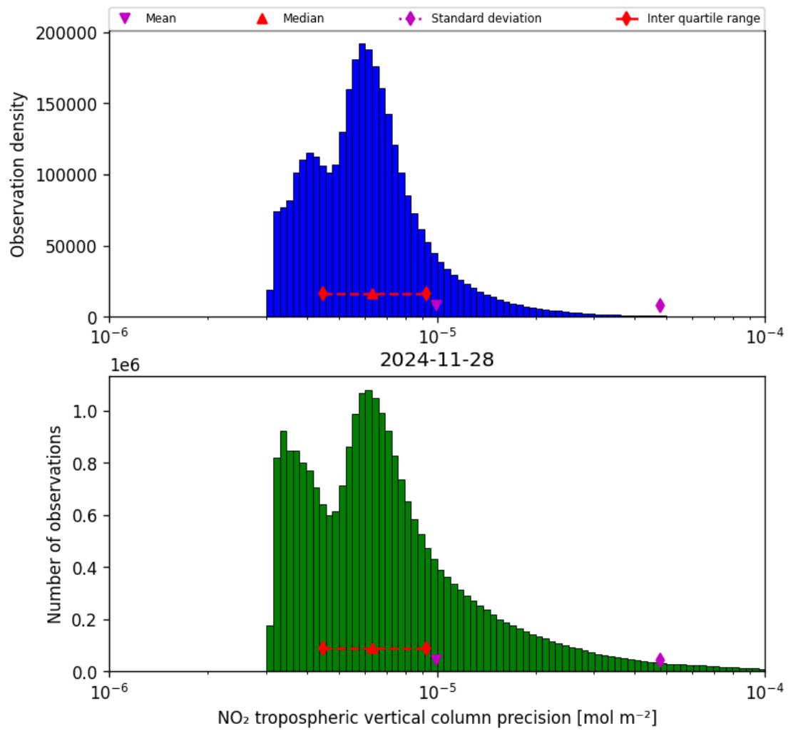
Figure 30: Histogram of “NO 2 tropospheric vertical column precision” for 2024-11-27 to 2024-11-29
