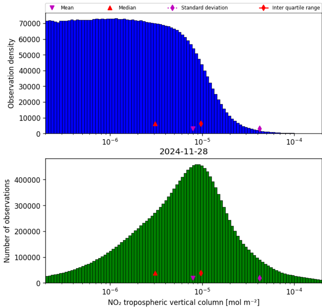
Figure 29: Histogram of “NO 2 tropospheric vertical column” for 2024-11-27 to 2024-11-29
