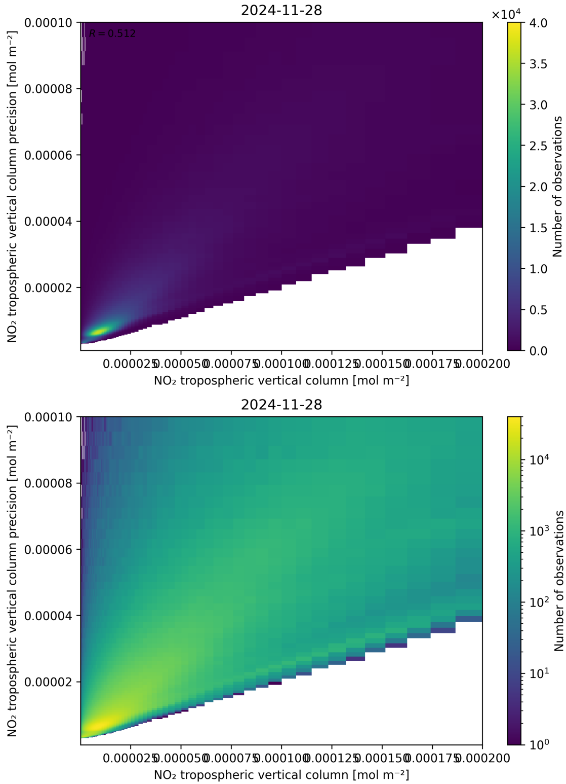
Figure 130: Scatter density plot of “NO 2 tropospheric vertical column” against “NO 2 tropospheric vertical column precision” for 2024-11-27 to 2024-11-29.
