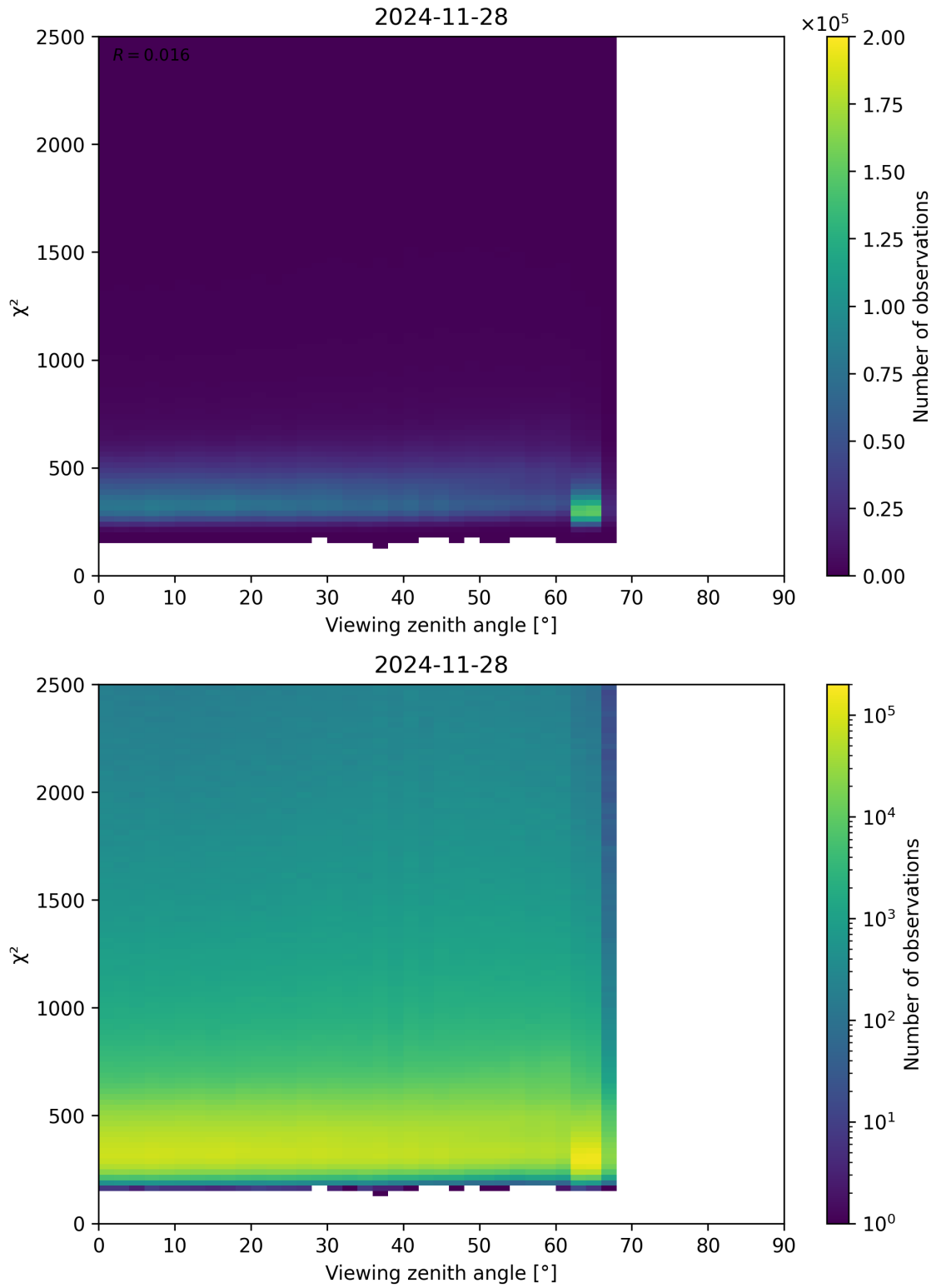
Figure 162: Scatter density plot of “Viewing zenith angle” against “ \chi^2 ” for 2024-11-27 to 2024-11-29.
