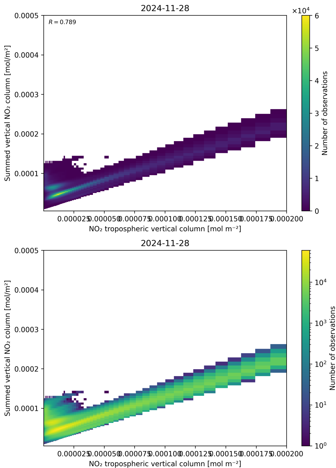
Figure 126: Scatter density plot of “NO 2 tropospheric vertical column” against “Summed vertical NO 2 column” for 2024-11-27 to 2024-11-29.
