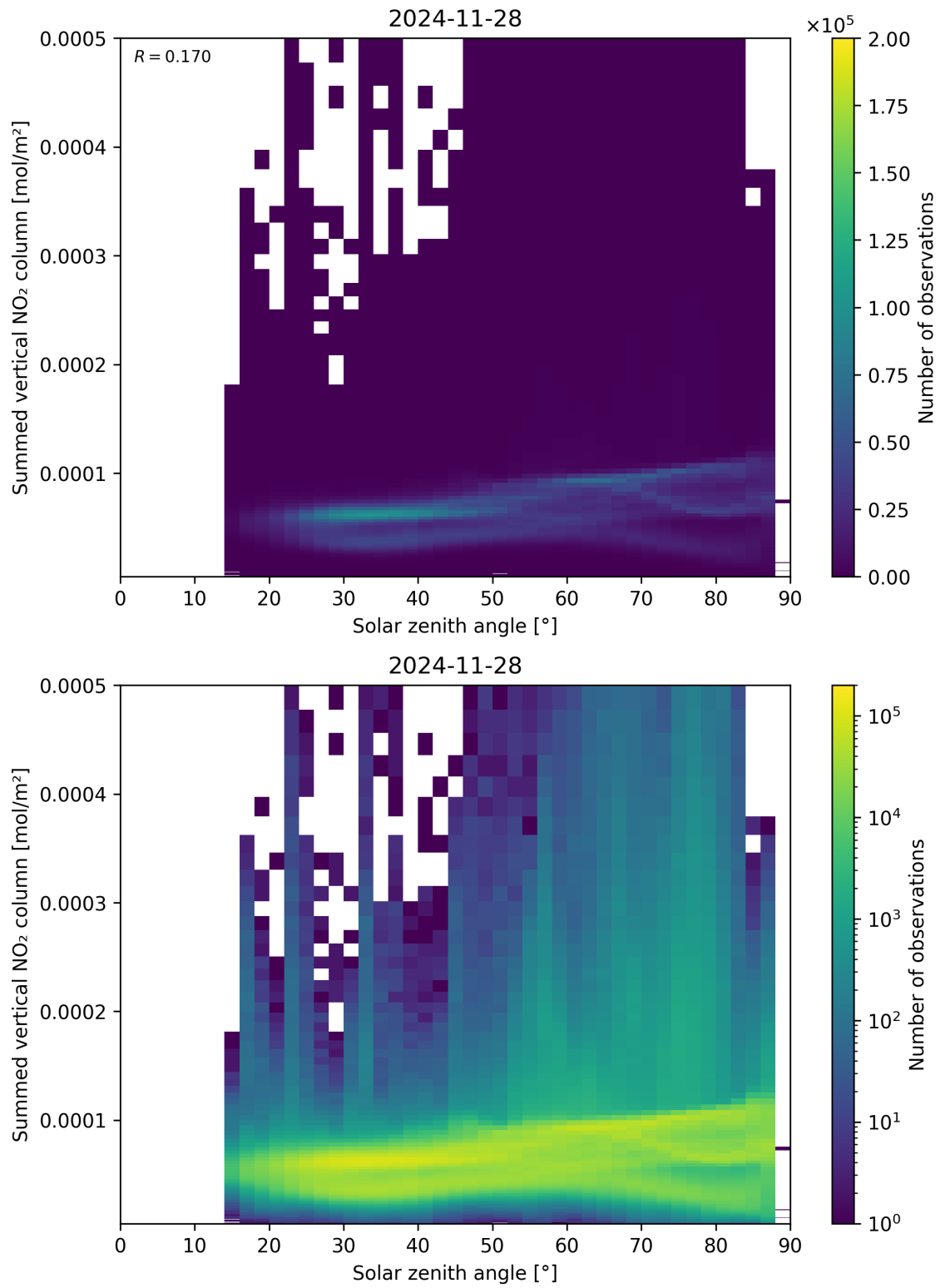
Figure 151: Scatter density plot of “Solar zenith angle” against “Summed vertical NO 2 column” for 2024-11-27 to 2024-11-29.
