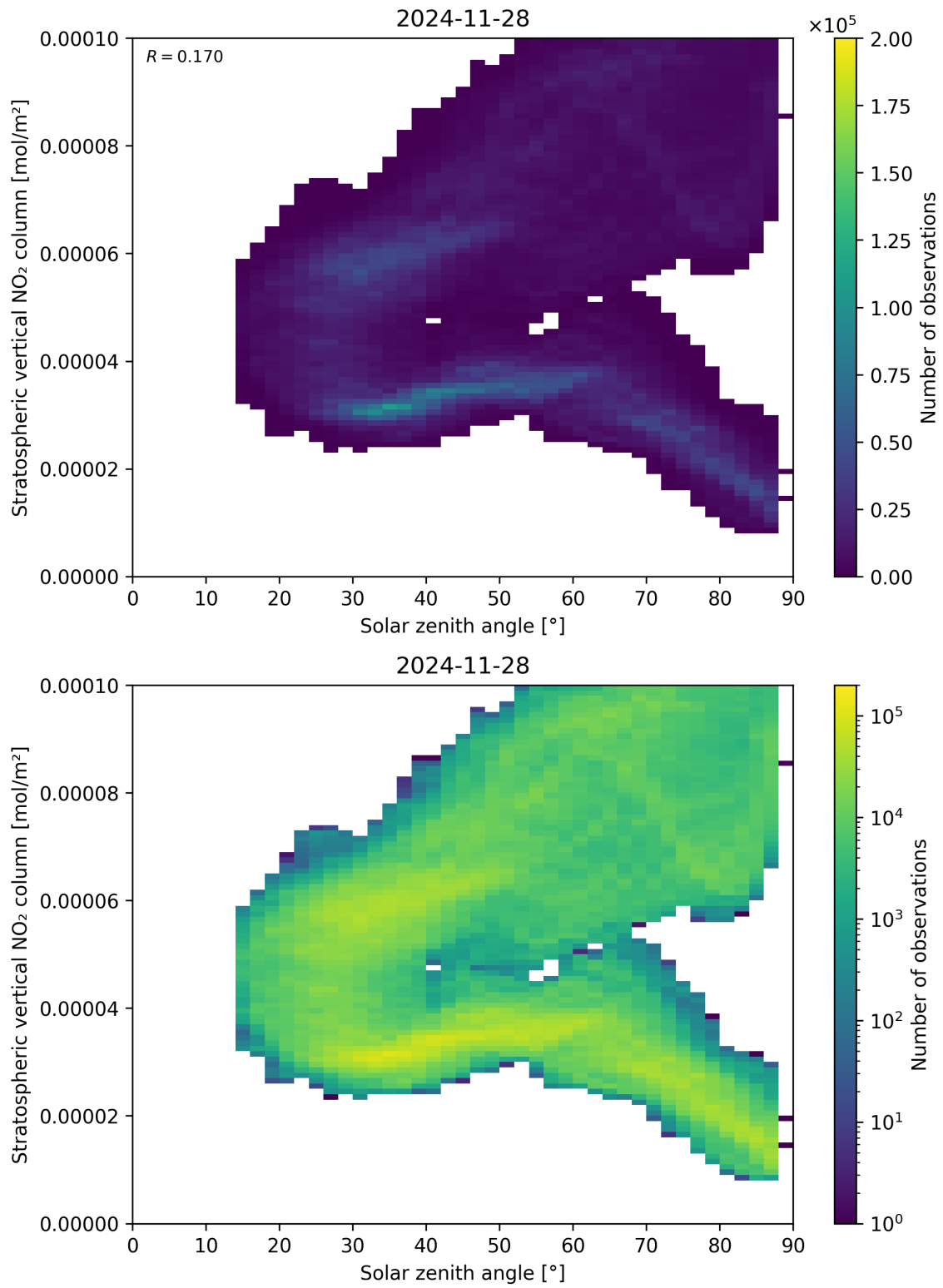
Figure 150: Scatter density plot of “Solar zenith angle” against “Stratospheric vertical NO 2 column” for 2024-11-27 to 2024-11-29.
