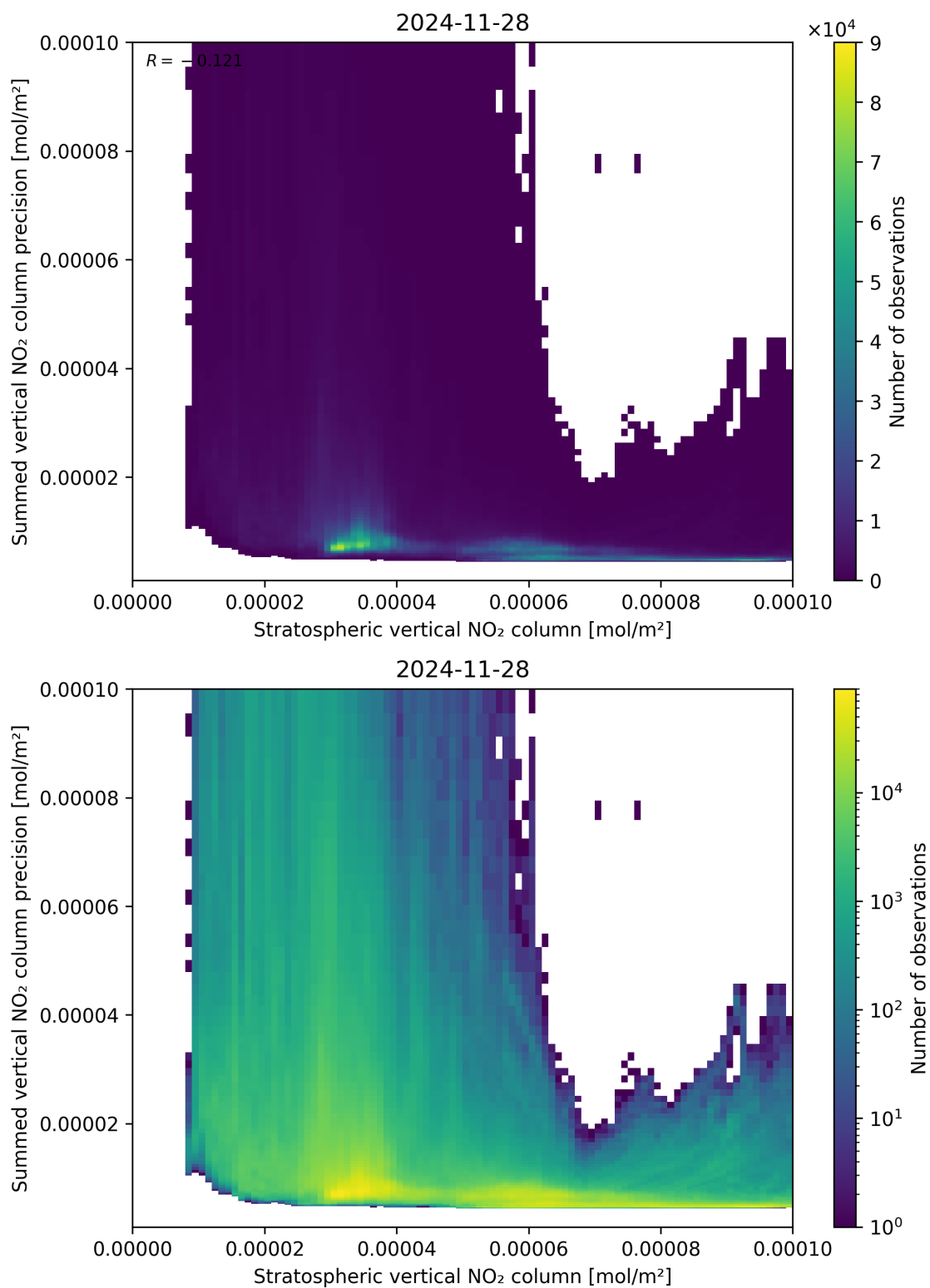
Figure 99: Scatter density plot of “Stratospheric vertical NO 2 column” against “Summed vertical NO 2 column precision” for 2024-11-27 to 2024-11-29.
