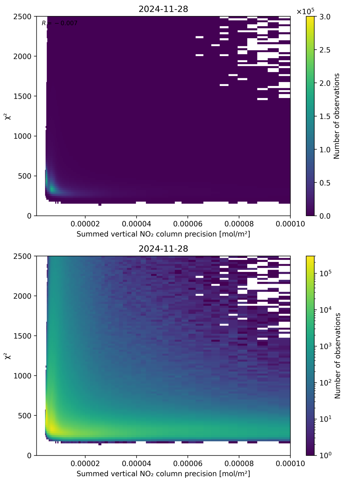
Figure 107: Scatter density plot of “Summed vertical NO 2 column precision” against “ \chi^2 ” for 2024-11-27 to 2024-11-29.
