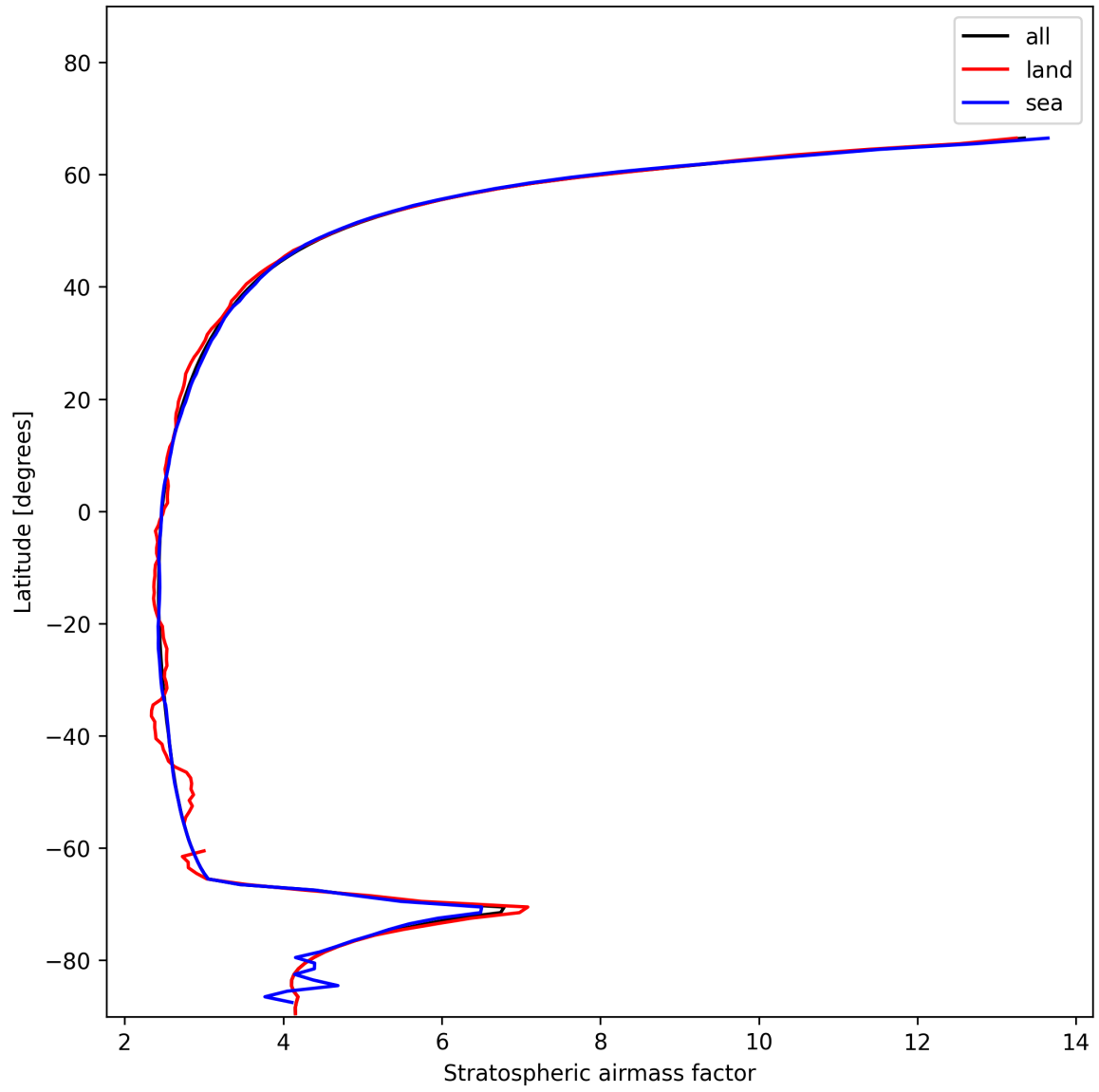
Figure 27: Zonal average of “Stratospheric airmass factor” for 2024-11-27 to 2024-11-29.
