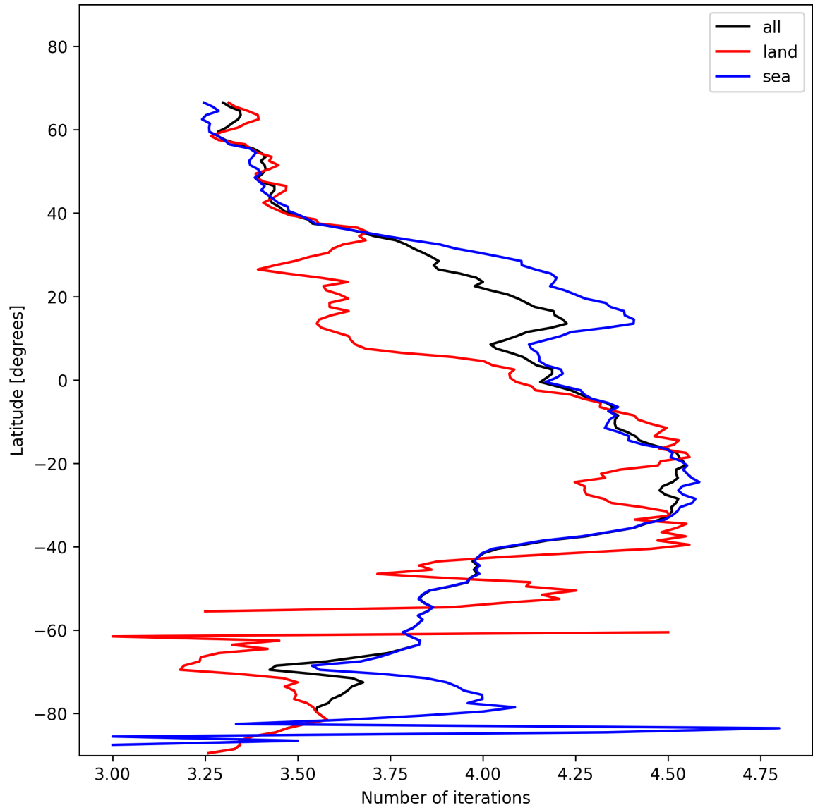
Figure 17: Zonal average of “Number of iterations” for 2024-11-27 to 2024-11-29.
