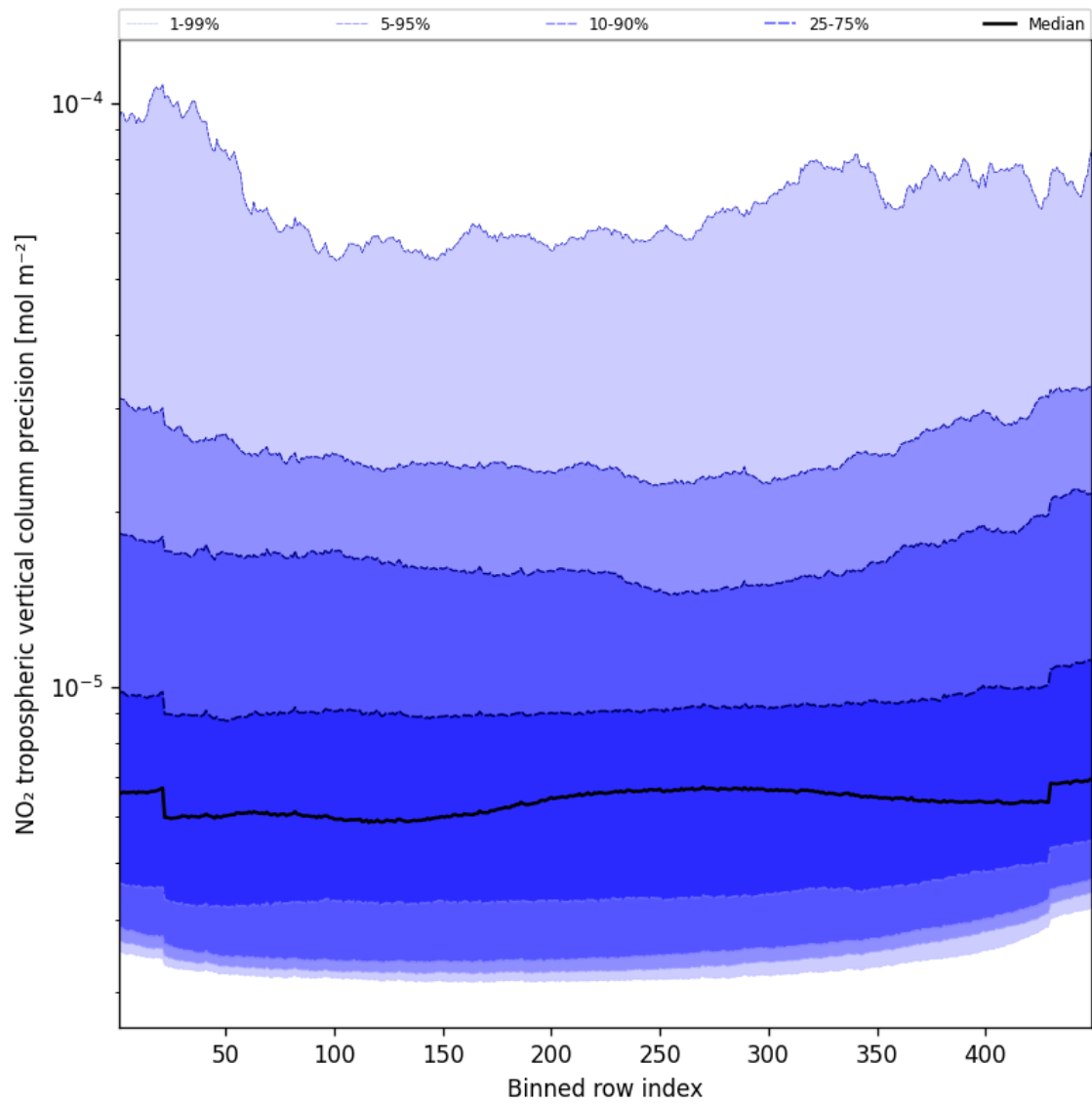
Figure 47: Along track statistics of “NO 2 tropospheric vertical column precision” for 2024-11-27 to 2024-11-29
