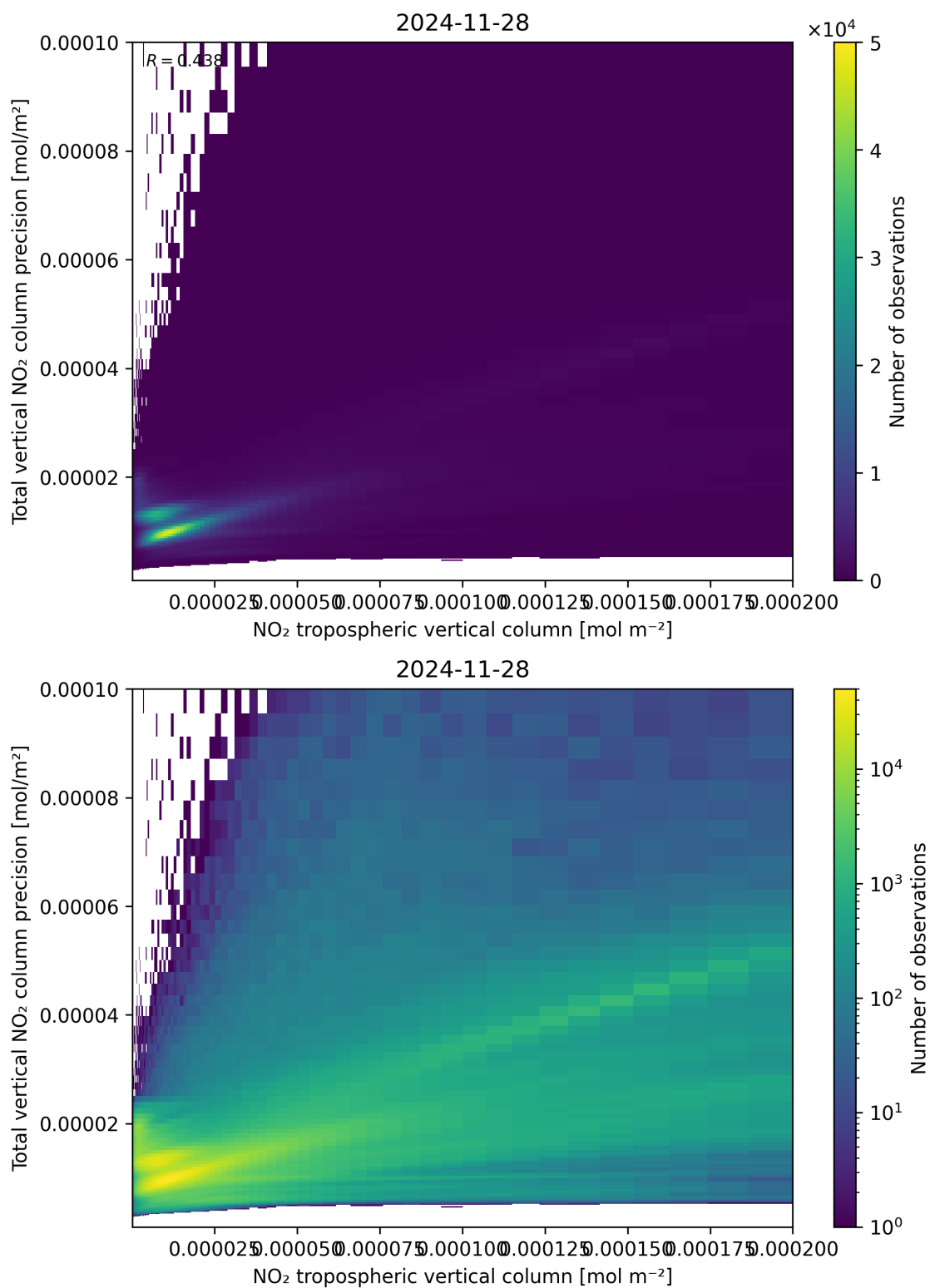
Figure 129: Scatter density plot of “NO 2 tropospheric vertical column” against “Total vertical NO 2 column precision” for 2024-11-27 to 2024-11-29.
