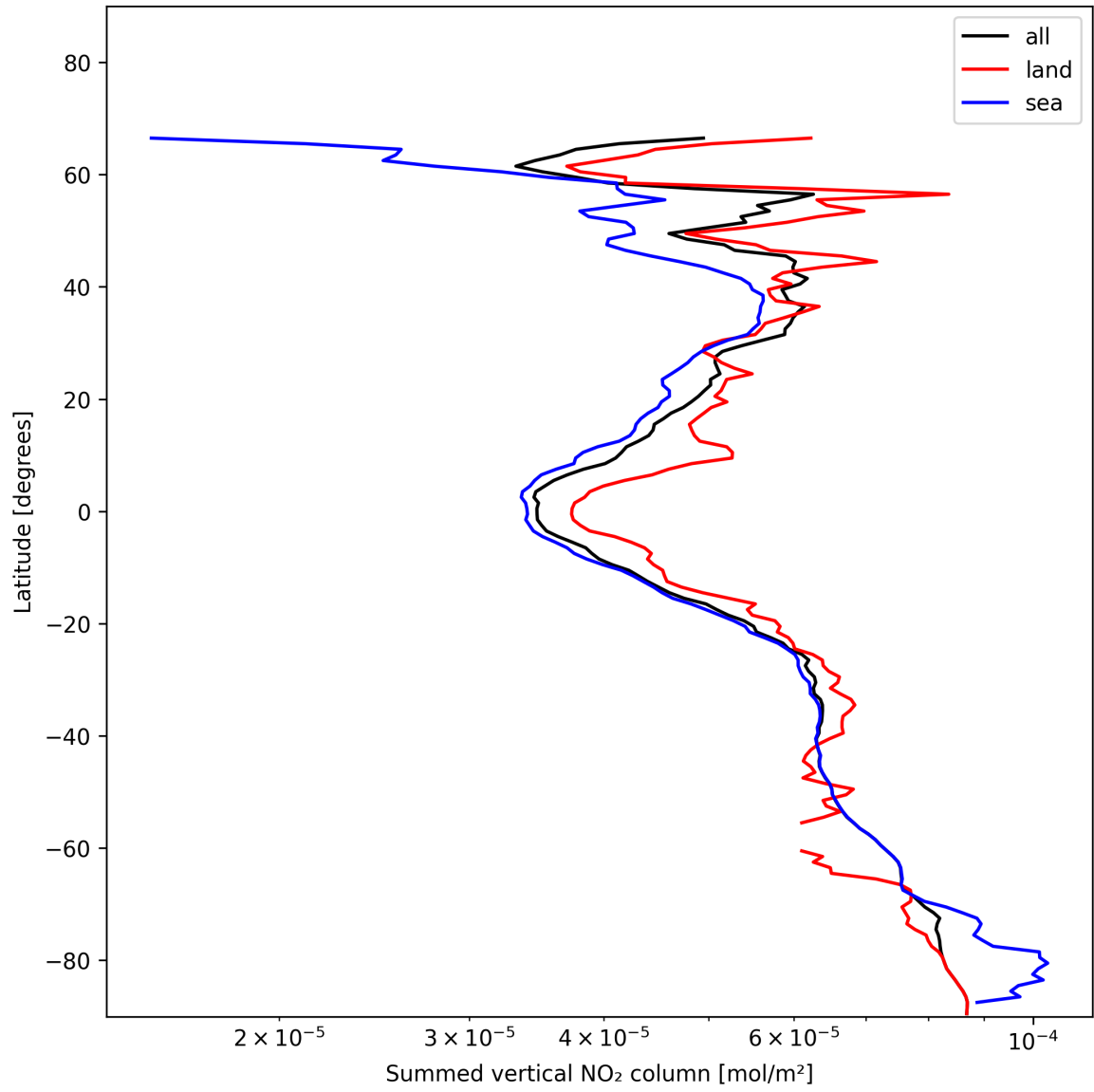
Figure 23: Zonal average of “Summed vertical NO 2 column” for 2024-11-27 to 2024-11-29.
