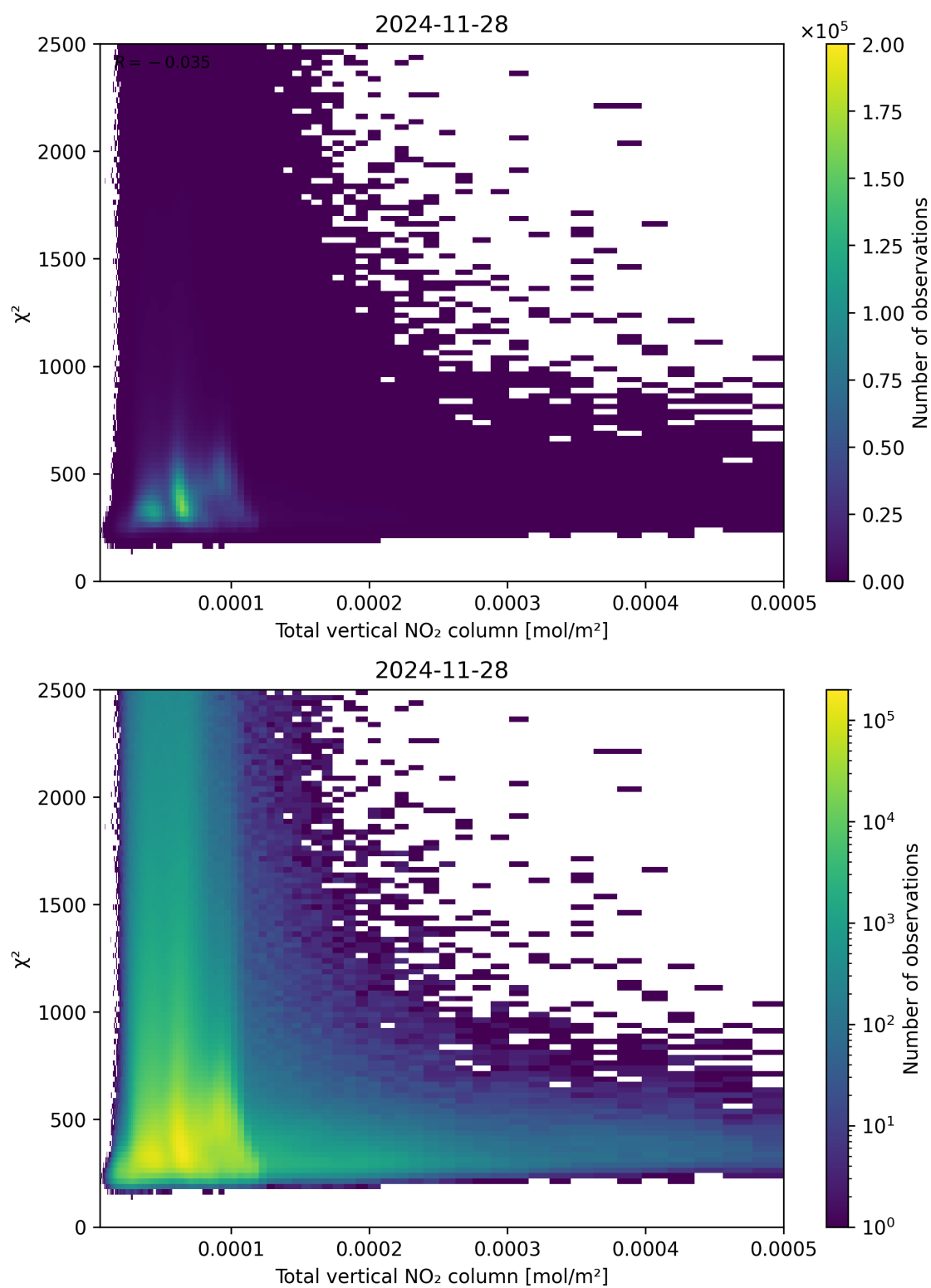
Figure 111: Scatter density plot of “Total vertical NO 2 column” against “ \chi^2 ” for 2024-11-27 to 2024-11-29.
