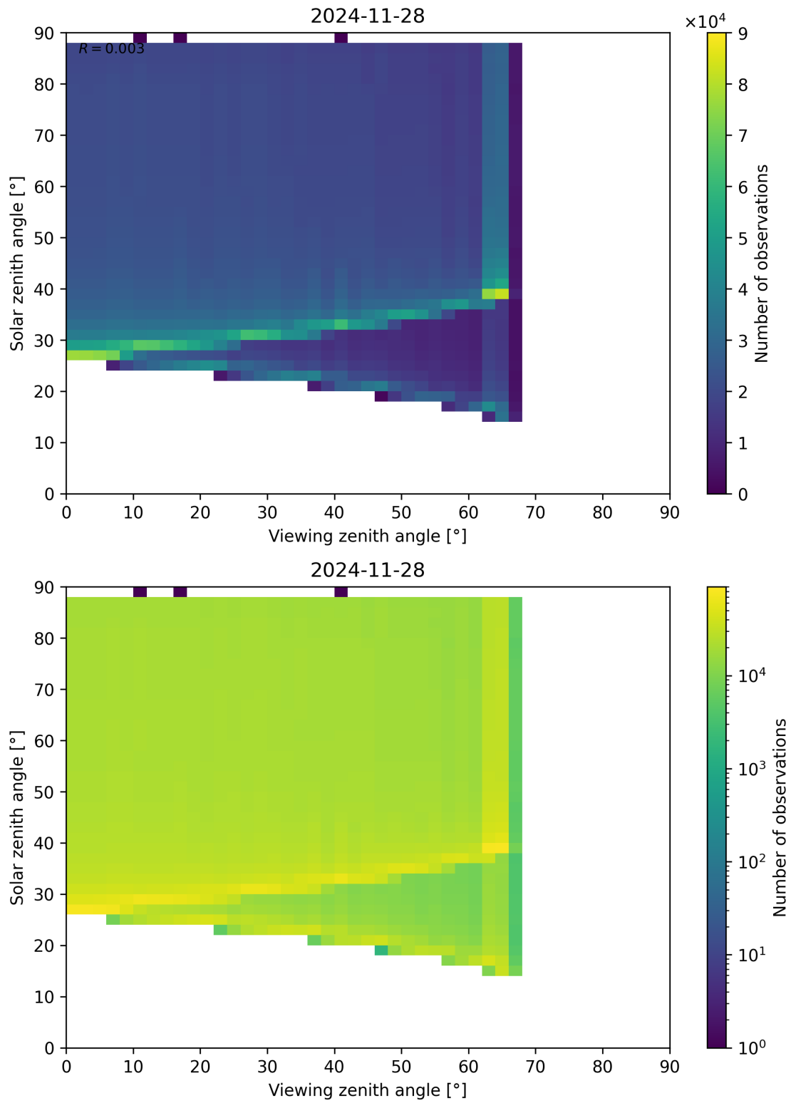
Figure 172: Scatter density plot of “Viewing zenith angle” against “Solar zenith angle” for 2024-11-27 to 2024-11-29.
