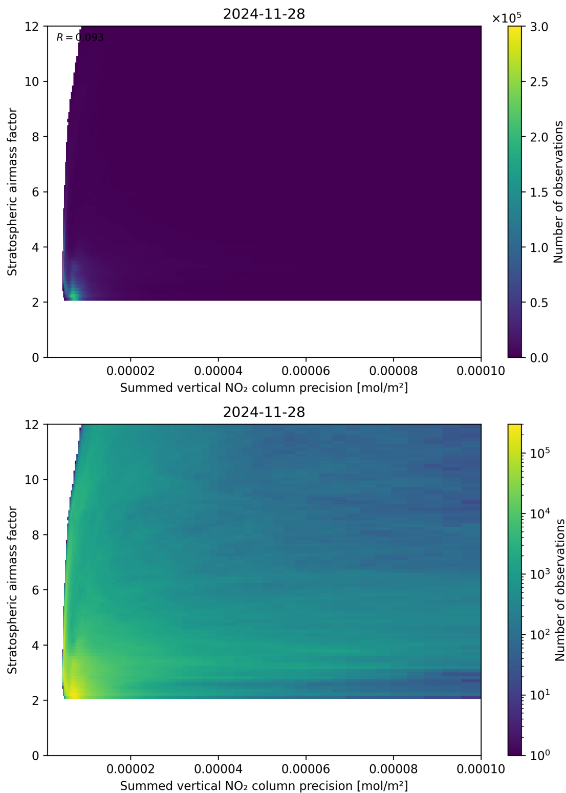
Figure 106: Scatter density plot of “Summed vertical NO 2 column precision” against “Stratospheric airmass factor” for 2024-11-27 to 2024-11-29.
