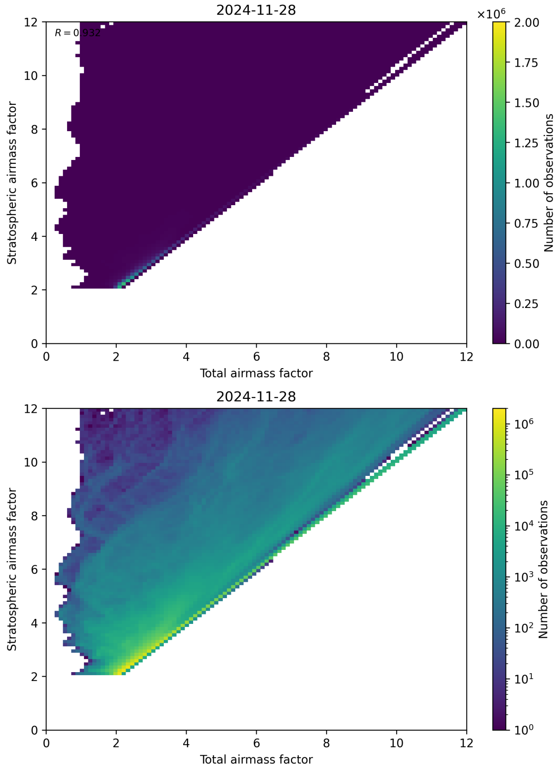
Figure 62: Scatter density plot of “Total airmass factor” against “Stratospheric airmass factor” for 2024-11-27 to 2024-11-29.
