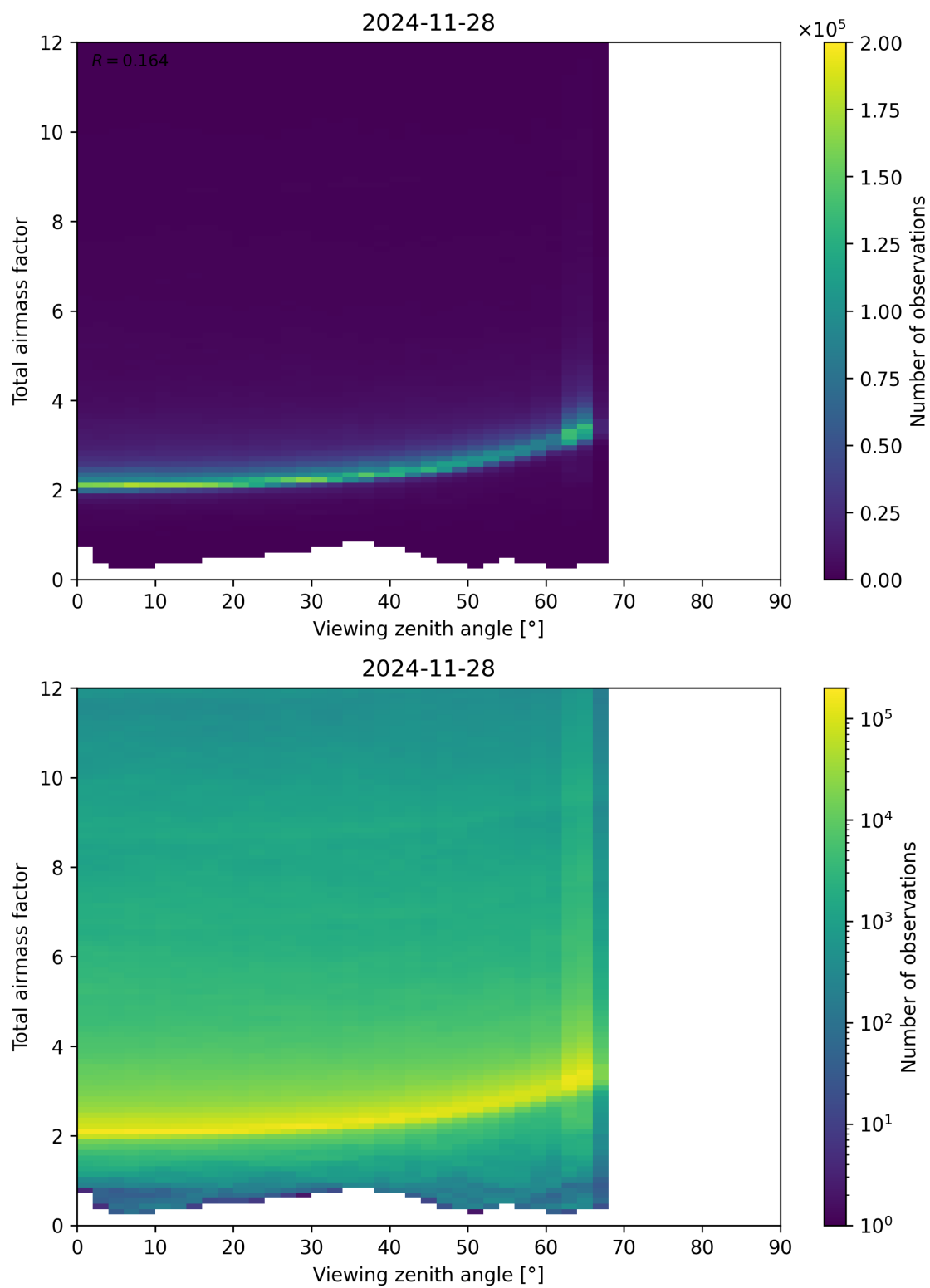
Figure 160: Scatter density plot of “Viewing zenith angle” against “Total airmass factor” for 2024-11-27 to 2024-11-29.
