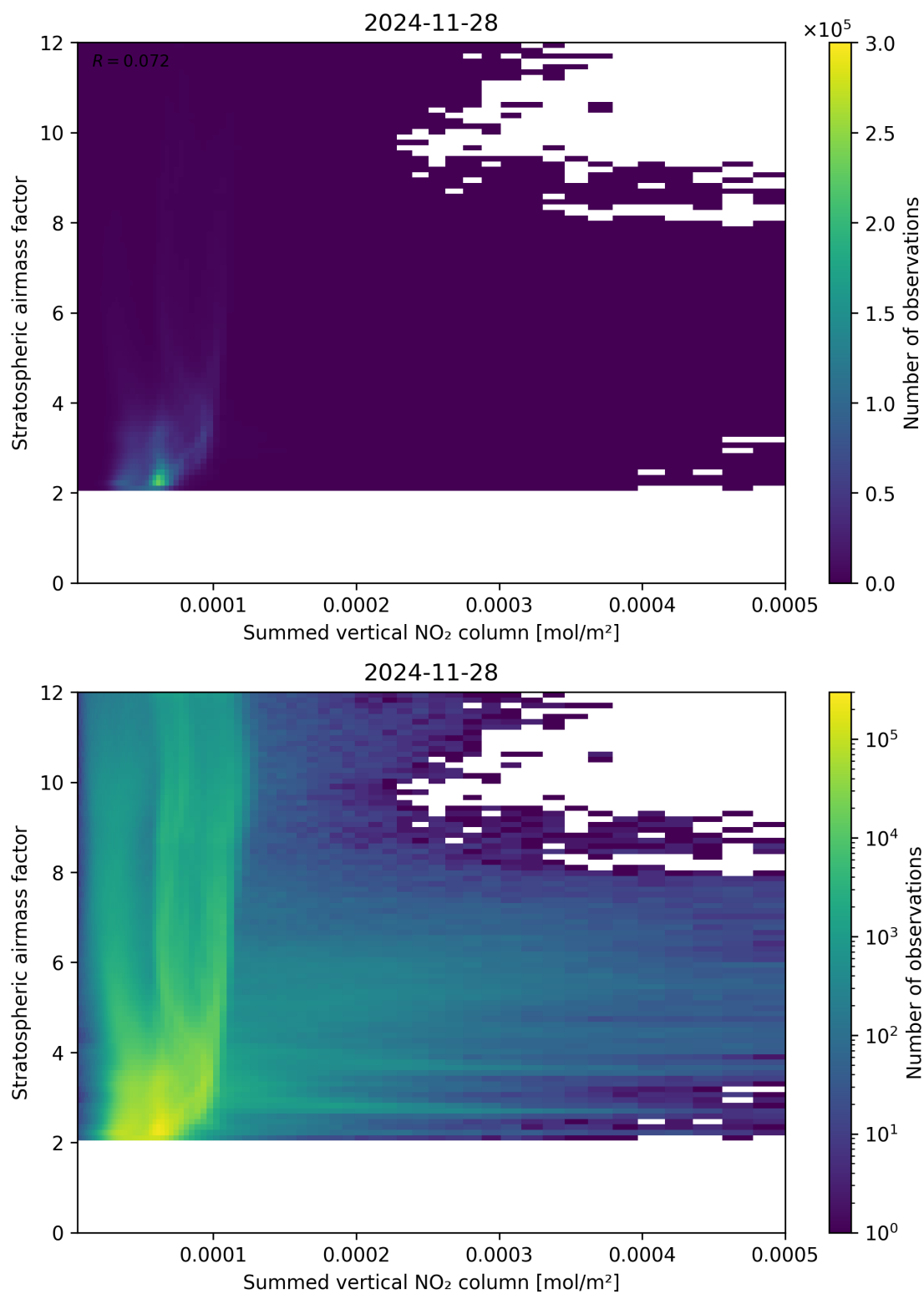
Figure 103: Scatter density plot of “Summed vertical NO 2 column” against “Stratospheric air mass factor” for 2024-11-27 to 2024-11-29.
