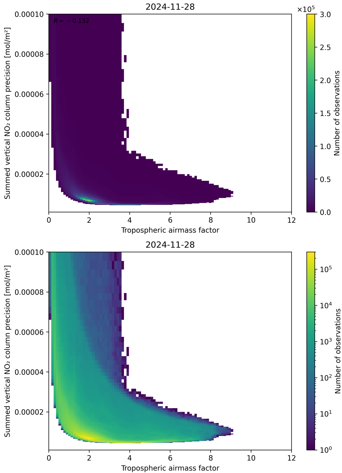
Figure 76: Scatter density plot of “Tropospheric air mass factor” against “Summed vertical NO 2 column precision” for 2024-11-27 to 2024-11-29.
