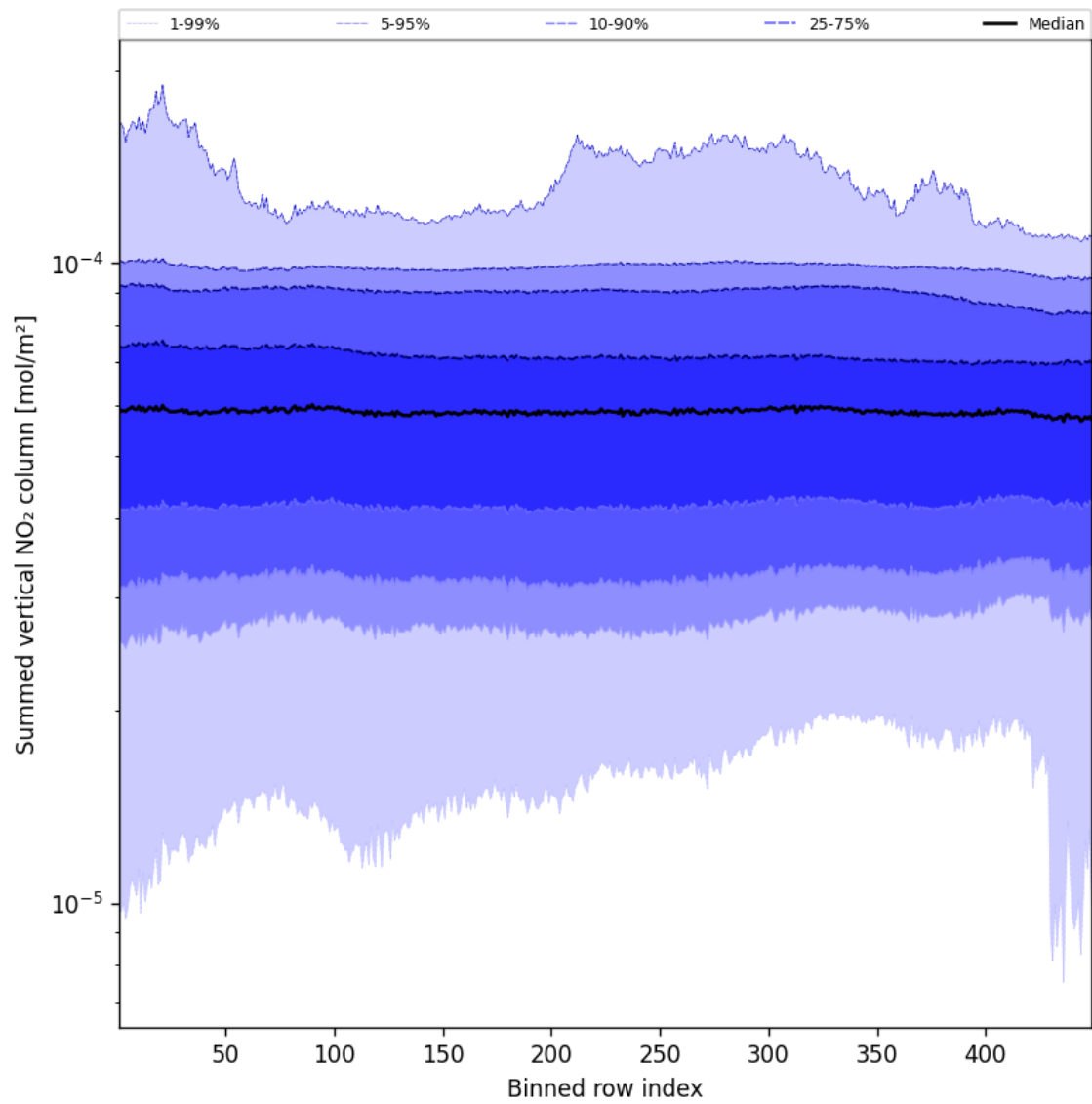
Figure 57: Along track statistics of “Summed vertical NO 2 column” for 2024-11-27 to 2024-11-29
