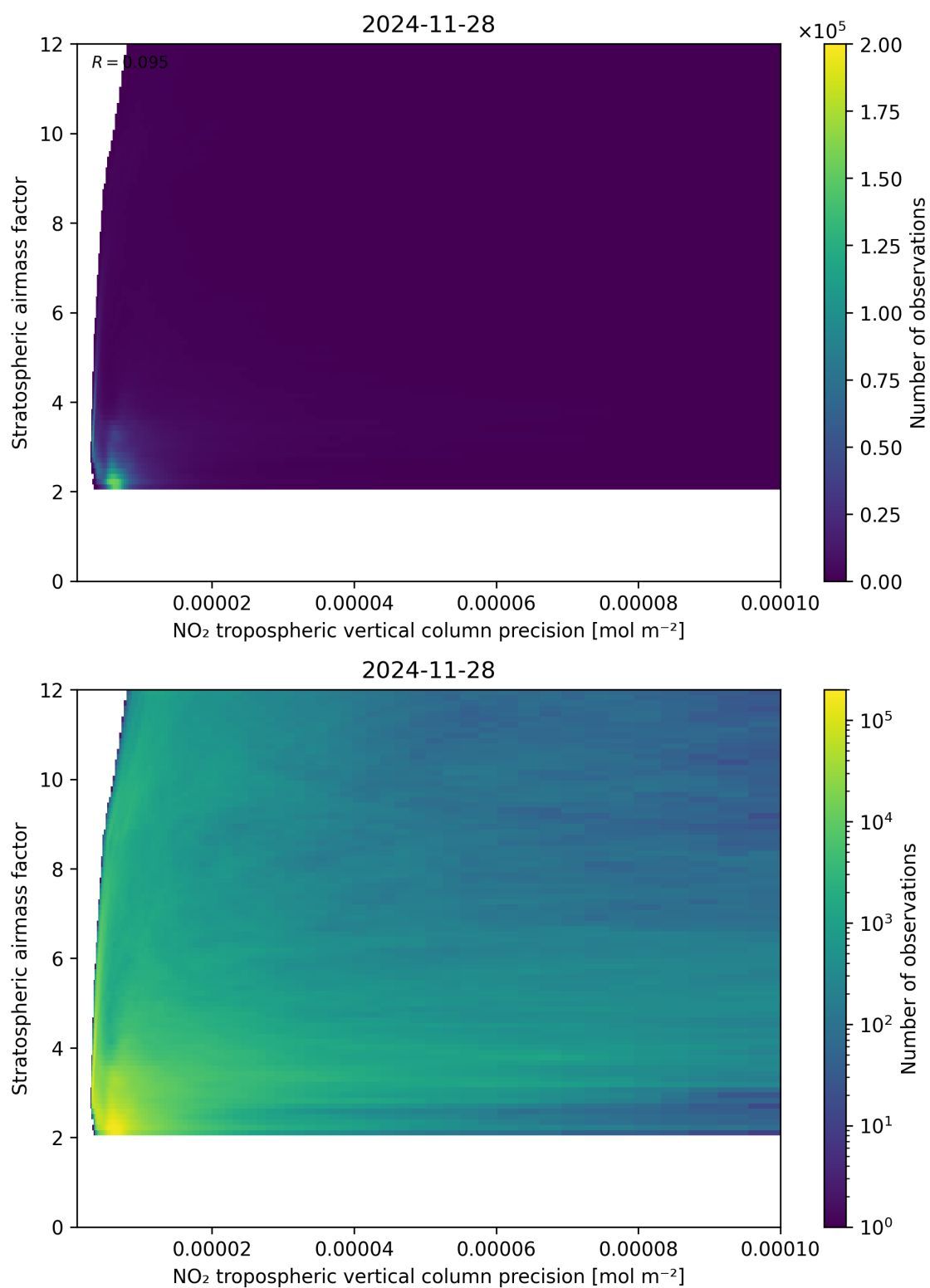
Figure 131: Scatter density plot of “NO 2 tropospheric vertical column precision” against “Stratospheric airmass factor” for 2024-11-27 to 2024-11-29.
