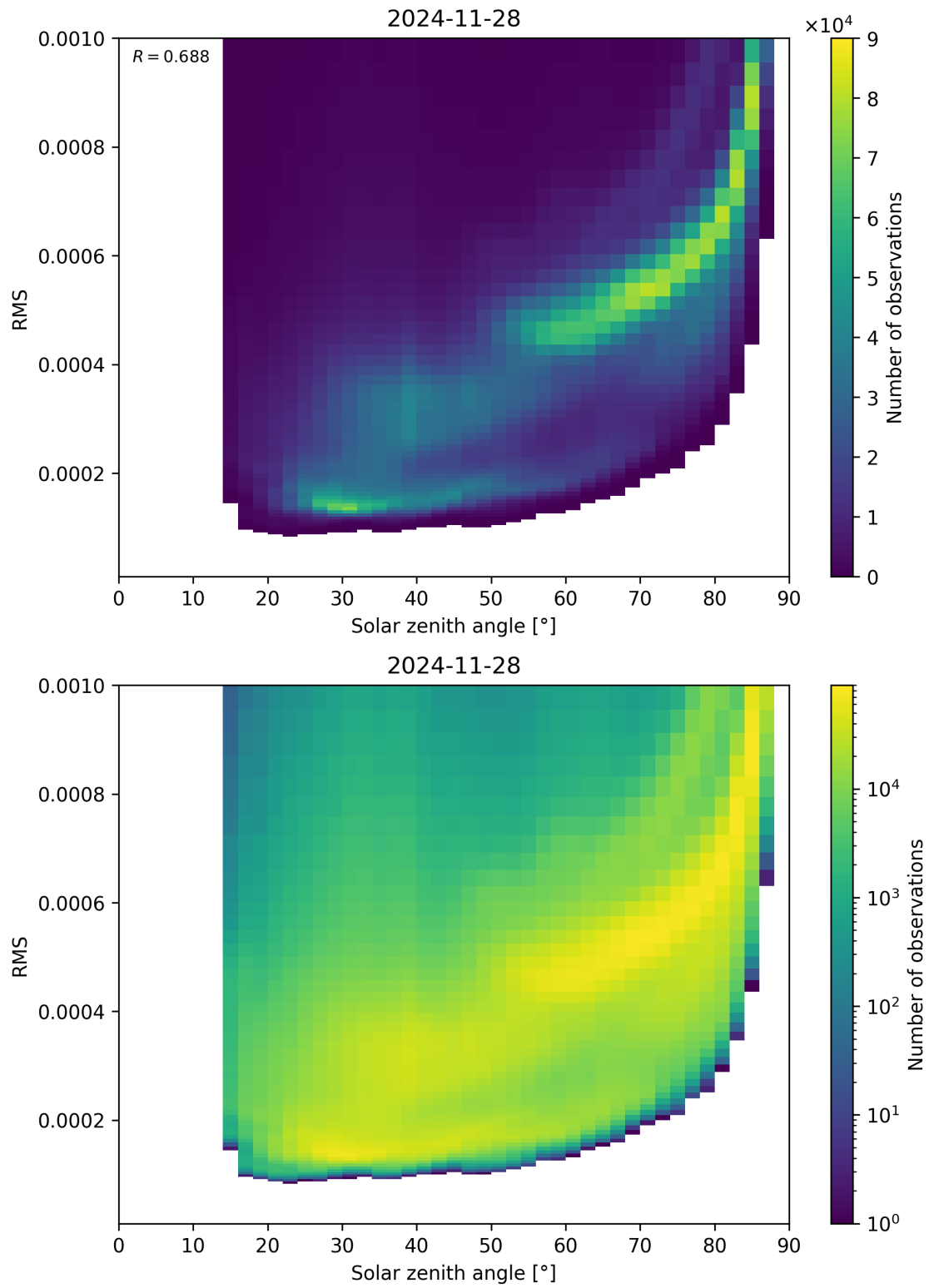
Figure 157: Scatter density plot of “Solar zenith angle” against “RMS” for 2024-11-27 to 2024-11-29.
