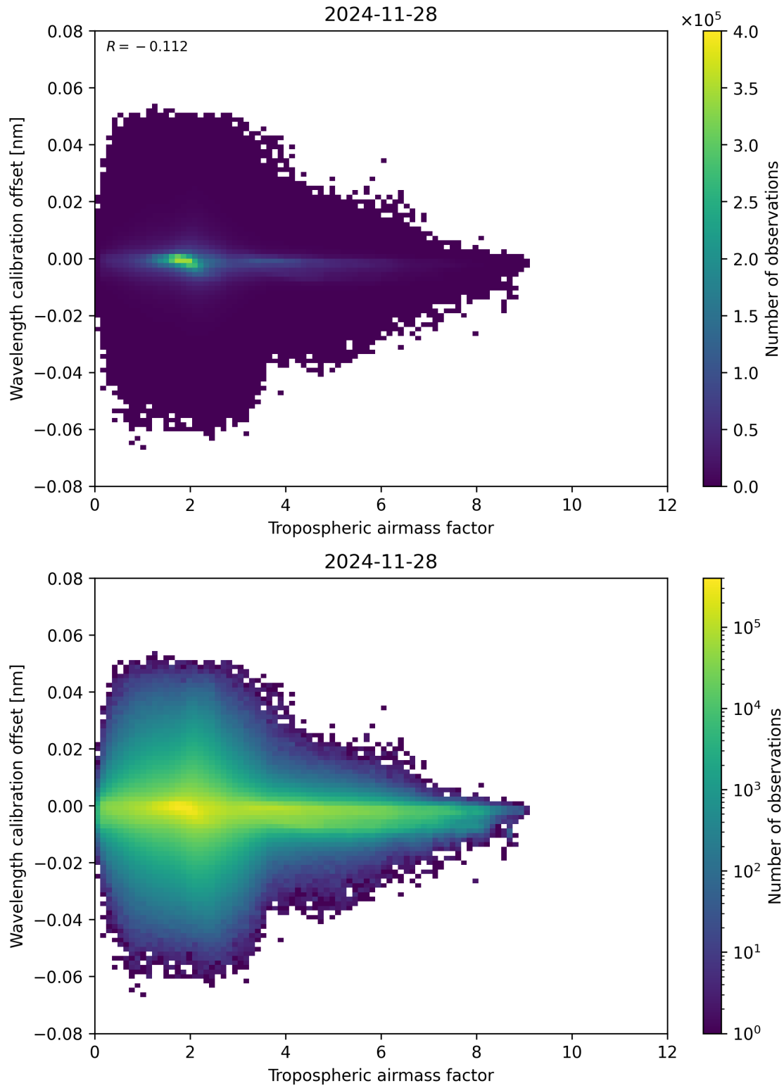
Figure 80: Scatter density plot of “Tropospheric airmass factor” against “Wavelength calibration offset” for 2024-11-27 to 2024-11-29.
