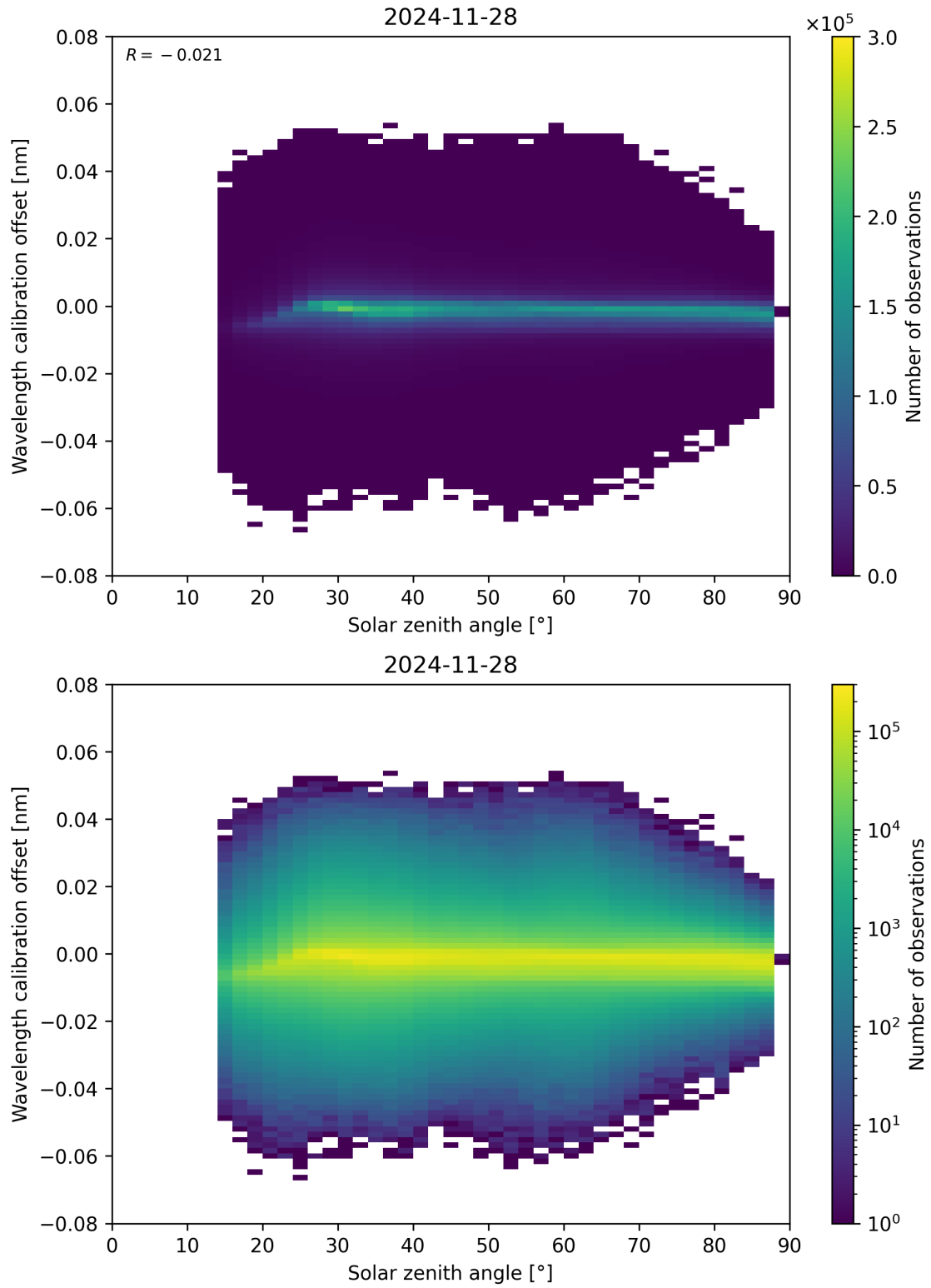
Figure 158: Scatter density plot of “Solar zenith angle” against “Wavelength calibration offset” for 2024-11-27 to 2024-11-29.
