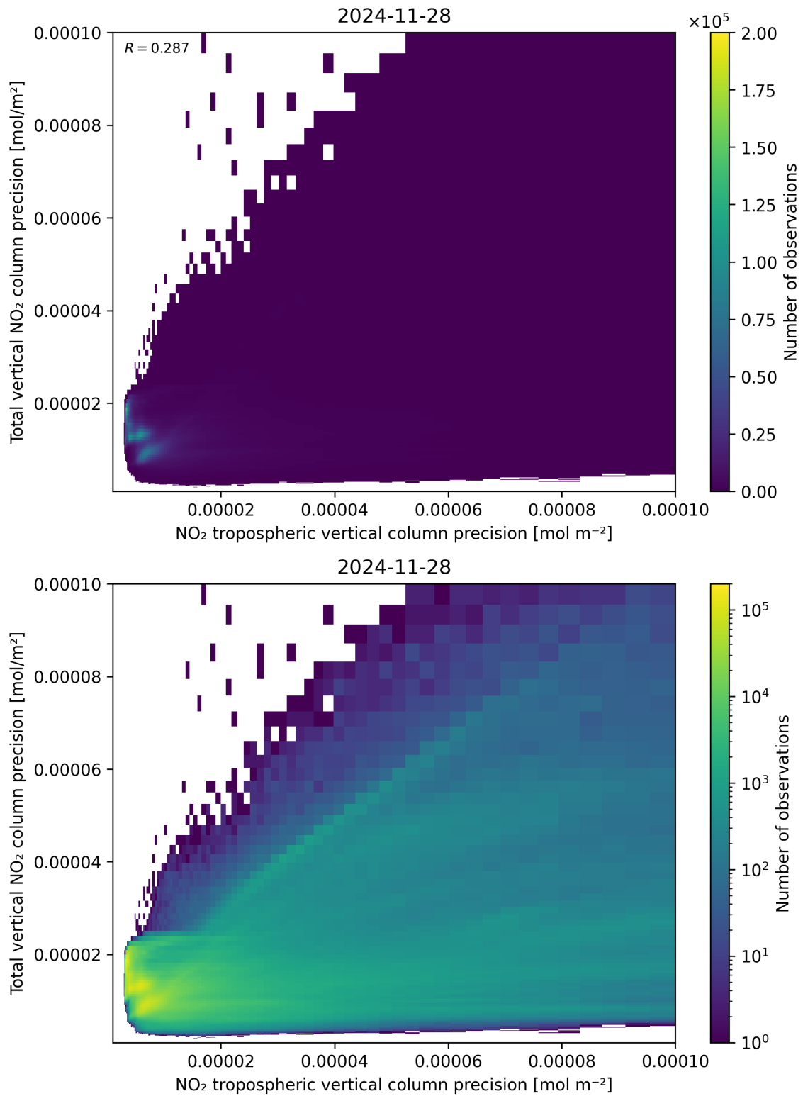
Figure 139: Scatter density plot of “NO 2 tropospheric vertical column precision” against “Total vertical NO 2 column precision” for 2024-11-27 to 2024-11-29.
