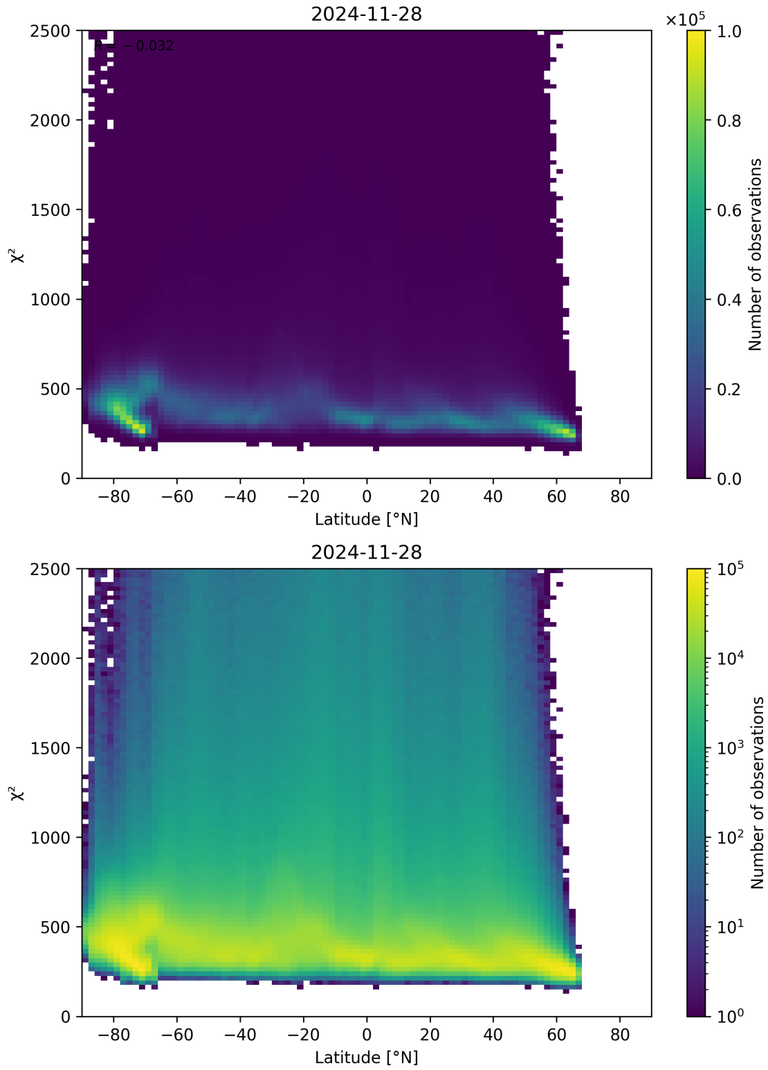
Figure 86: Scatter density plot of “Latitude” against “ \chi^2 ” for 2024-11-27 to 2024-11-29.
