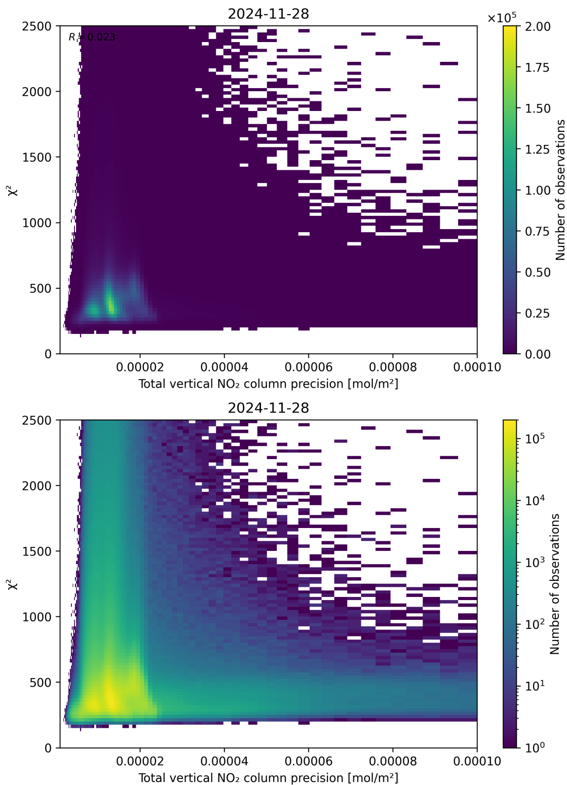
Figure 116: Scatter density plot of “Total vertical NO 2 column precision” against “ \chi^2 ” for 2024-11-27 to 2024-11-29.
