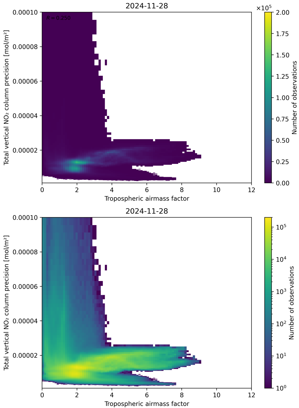
Figure 78: Scatter density plot of “Tropospheric air mass factor” against “Total vertical NO 2 column precision” for 2024-11-27 to 2024-11-29.
