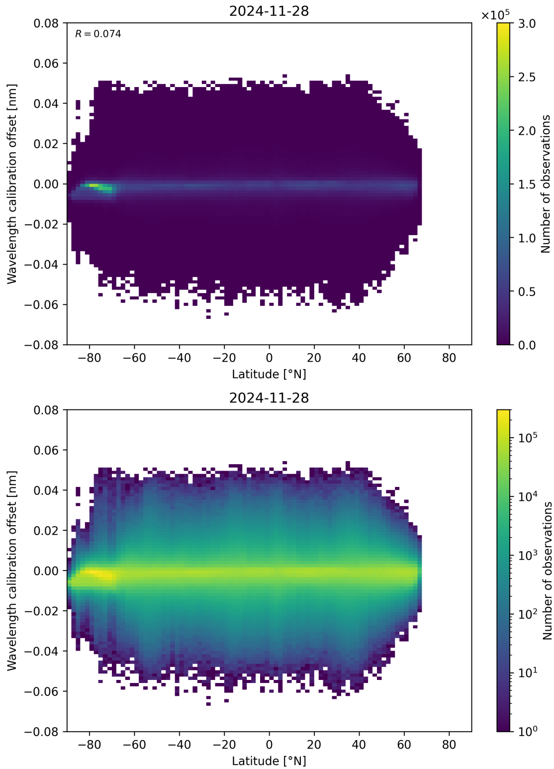
Figure 95: Scatter density plot of “Latitude” against “Wavelength calibration offset” for 2024-11-27 to 2024-11-29.
