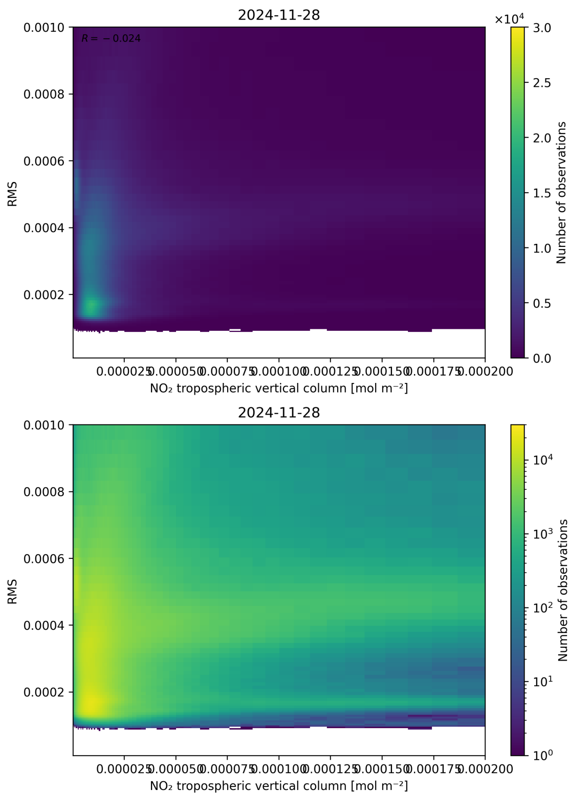
Figure 142: Scatter density plot of “NO 2 tropospheric vertical column” against “RMS” for 2024-11-27 to 2024-11-29.
