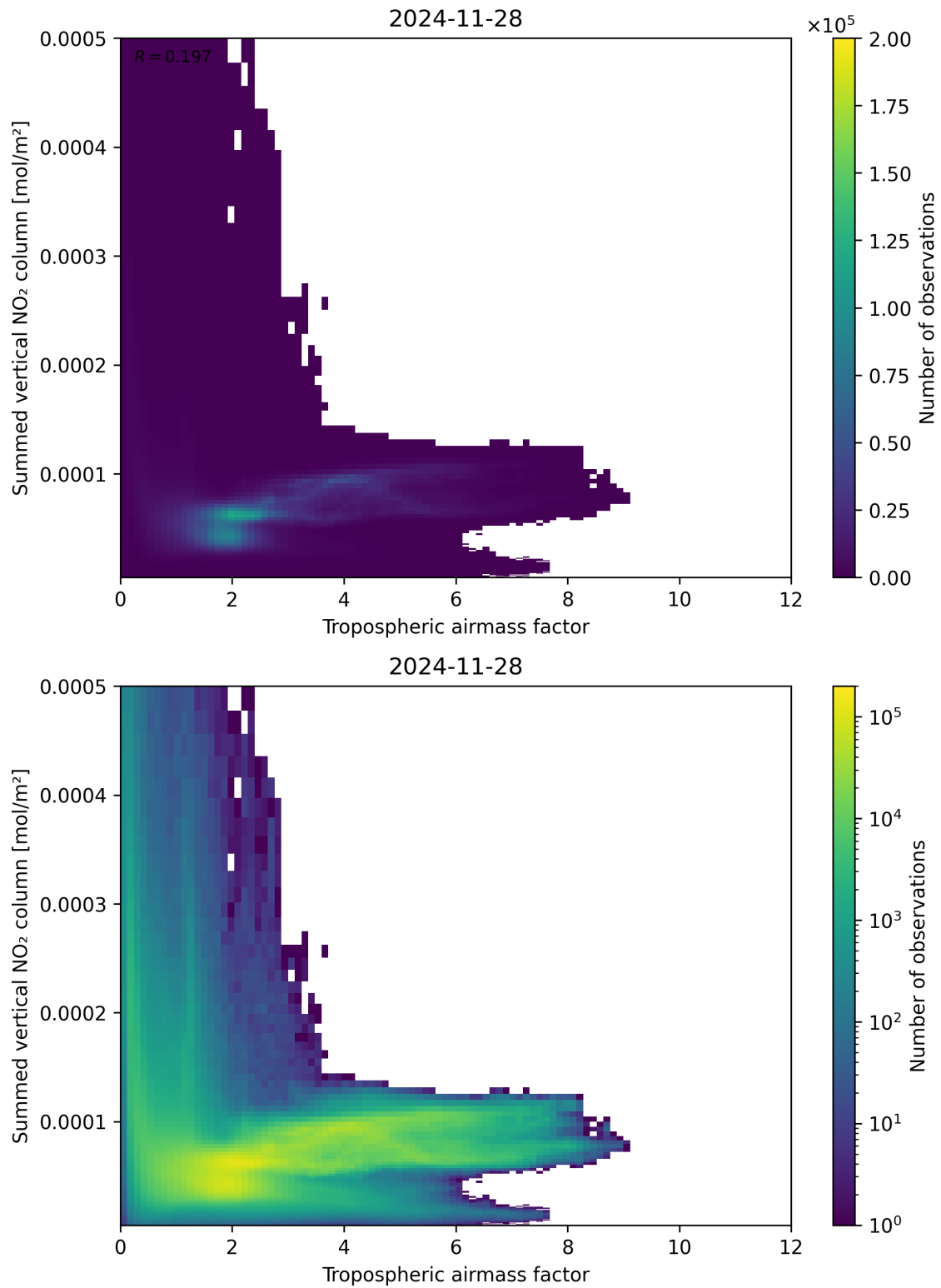
Figure 75: Scatter density plot of “Tropospheric airmass factor” against “Summed vertical NO 2 column” for 2024-11-27 to 2024-11-29.
