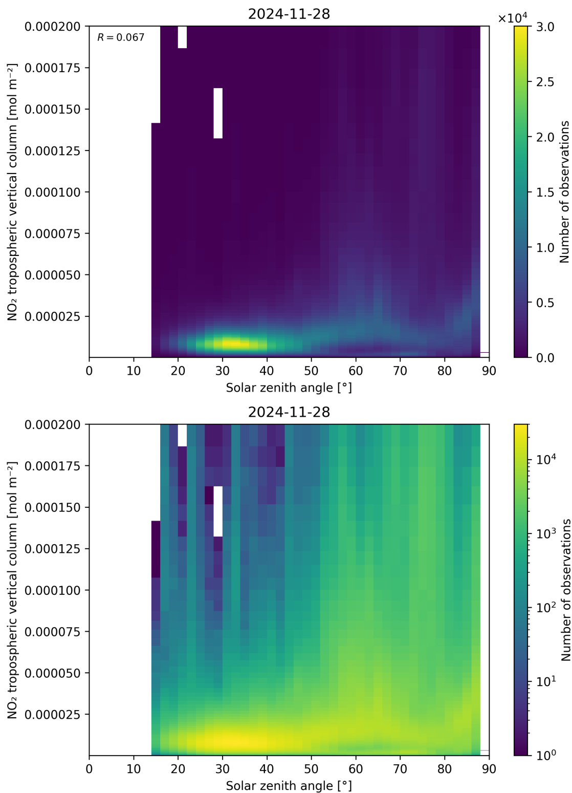
Figure 155: Scatter density plot of “Solar zenith angle” against “NO 2 tropospheric vertical column” for 2024-11-27 to 2024-11-29.
