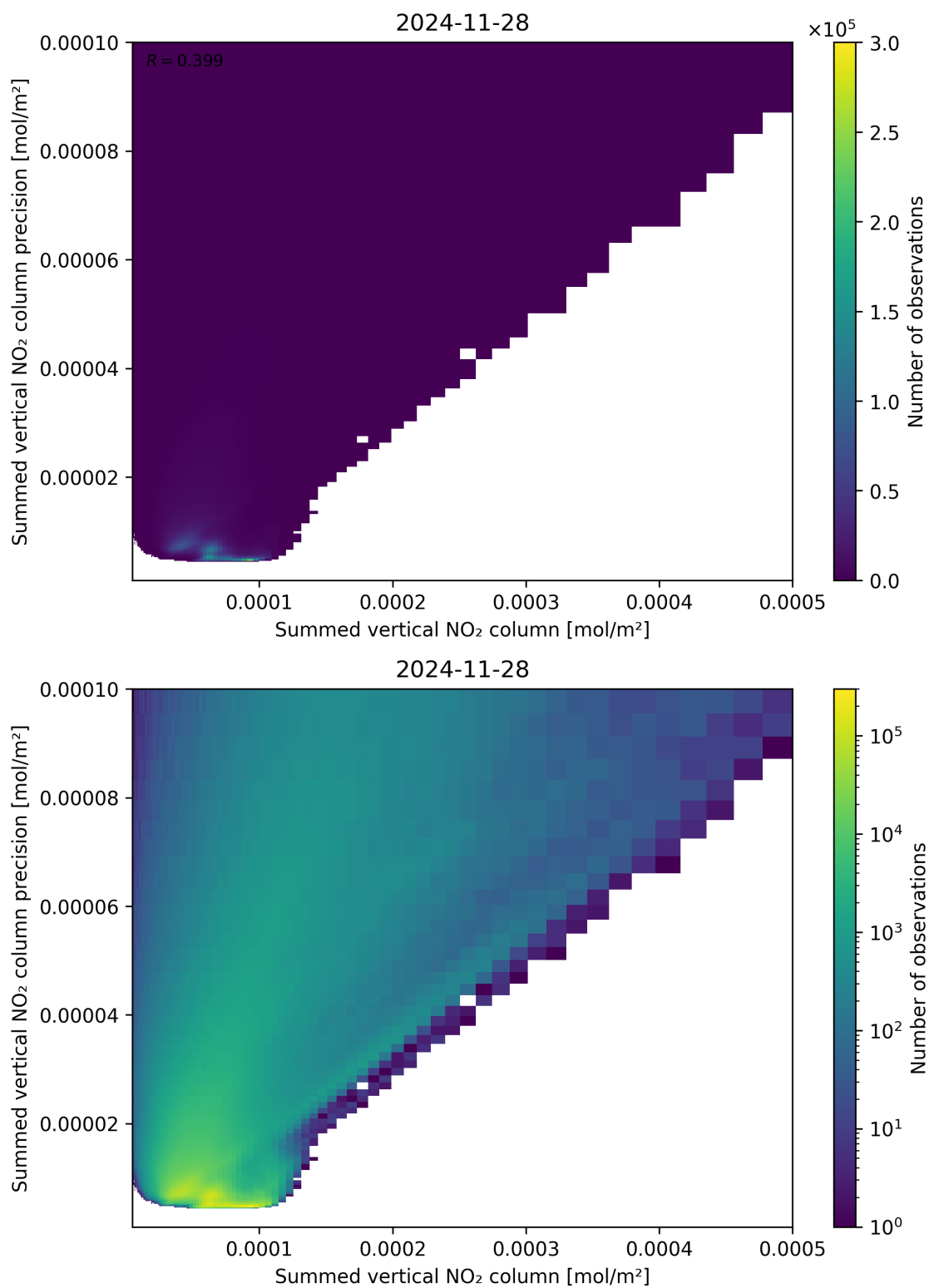
Figure 105: Scatter density plot of “Summed vertical NO 2 column” against “Summed vertical NO 2 column precision” for 2024-11-27 to 2024-11-29.
