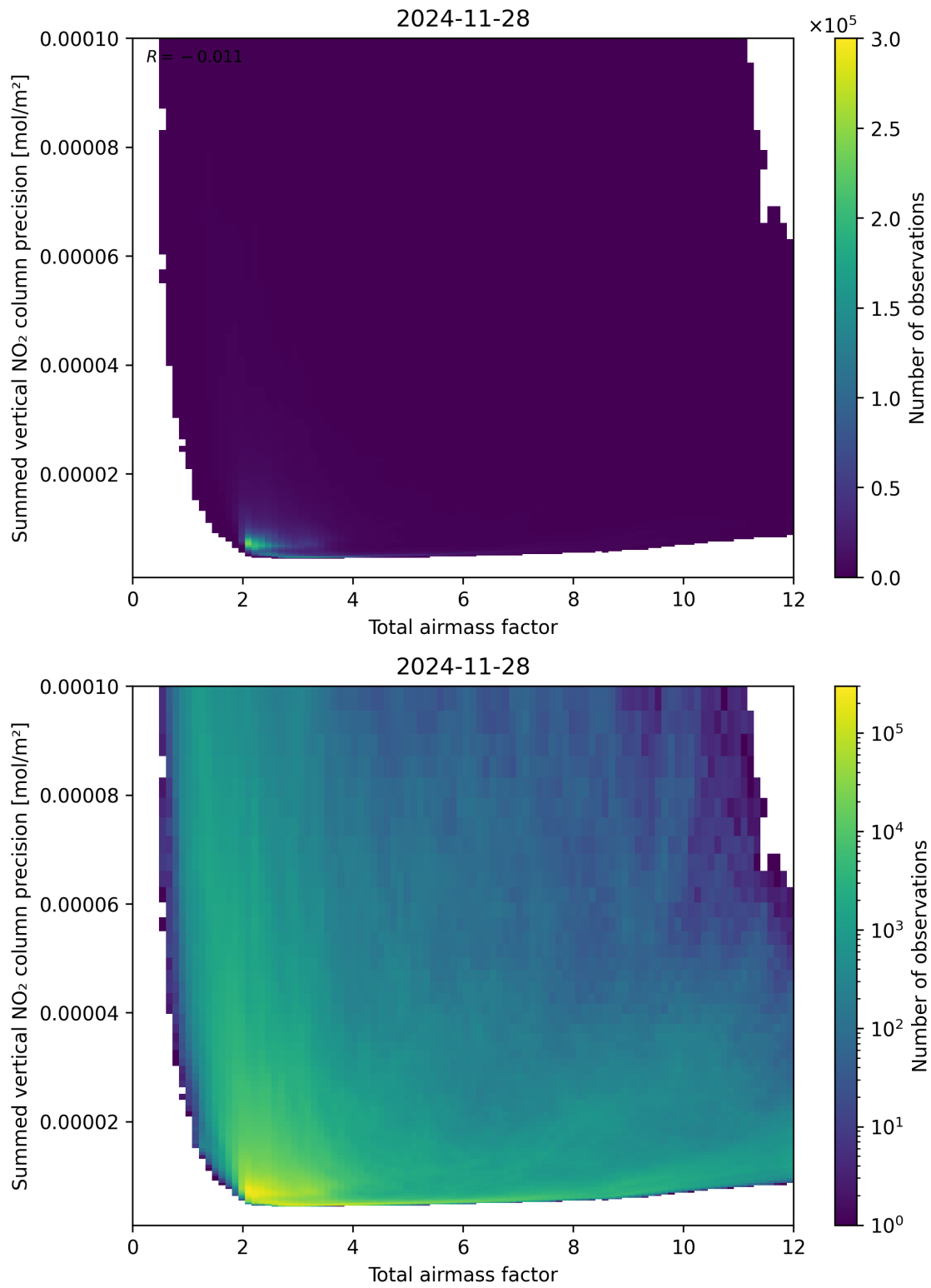
Figure 66: Scatter density plot of “Total airmass factor” against “Summed vertical NO 2 column precision” for 2024-11-27 to 2024-11-29.
