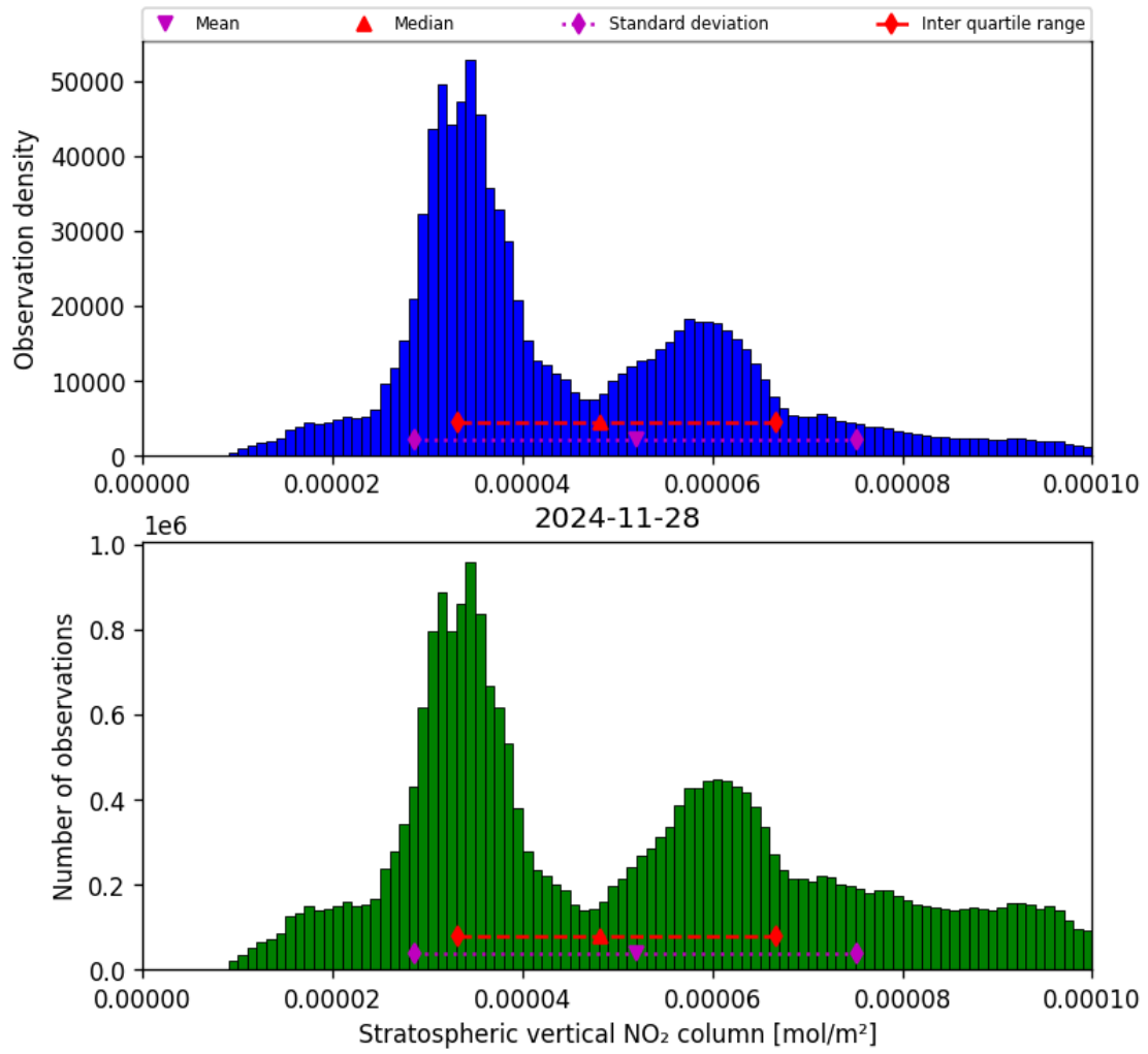
Figure 36: Histogram of “Stratospheric vertical NO 2 column” for 2024-11-27 to 2024-11-29
