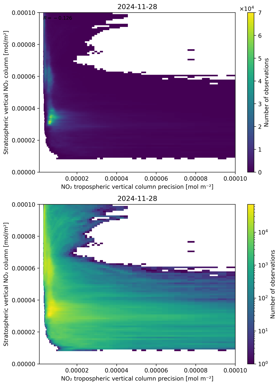
Figure 135: Scatter density plot of “NO 2 tropospheric vertical column precision” against “Stratospheric vertical NO 2 column” for 2024-11-27 to 2024-11-29.
