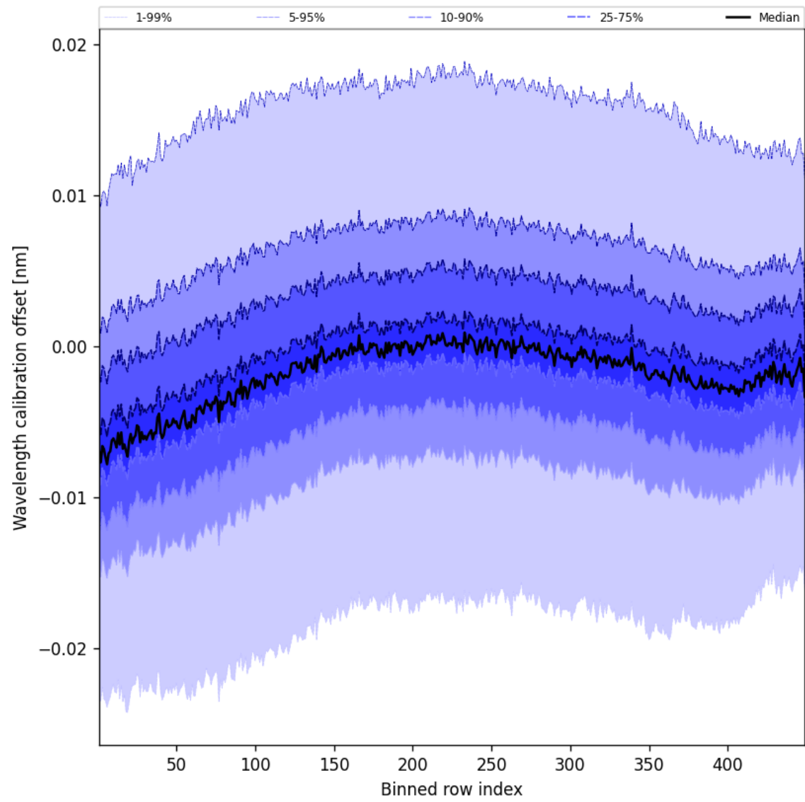
Figure 52: Along track statistics of “Wavelength calibration offset” for 2024-11-27 to 2024-11-29
