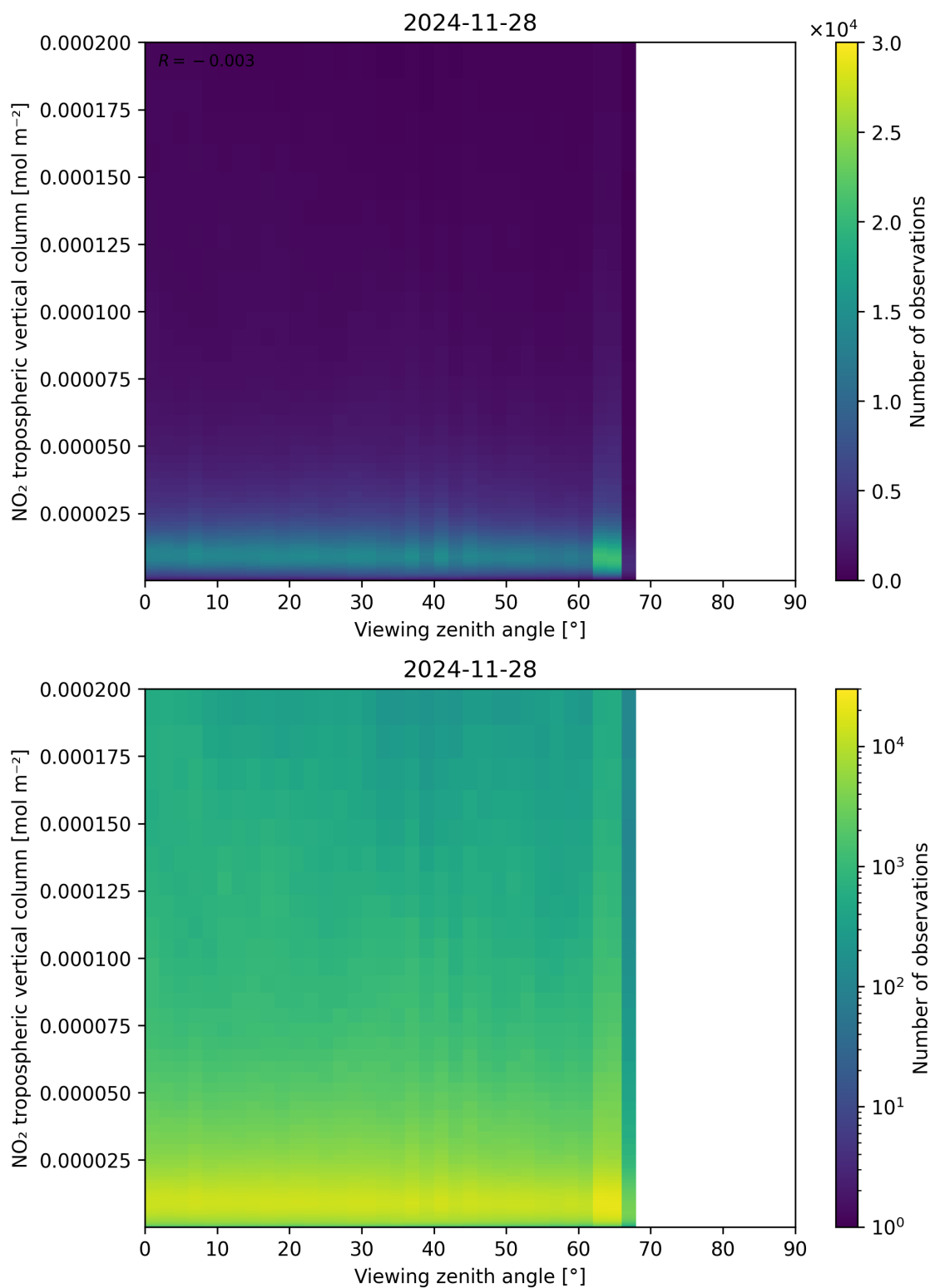
Figure 169: Scatter density plot of “Viewing zenith angle” against “NO 2 tropospheric vertical column” for 2024-11-27 to 2024-11-29.
