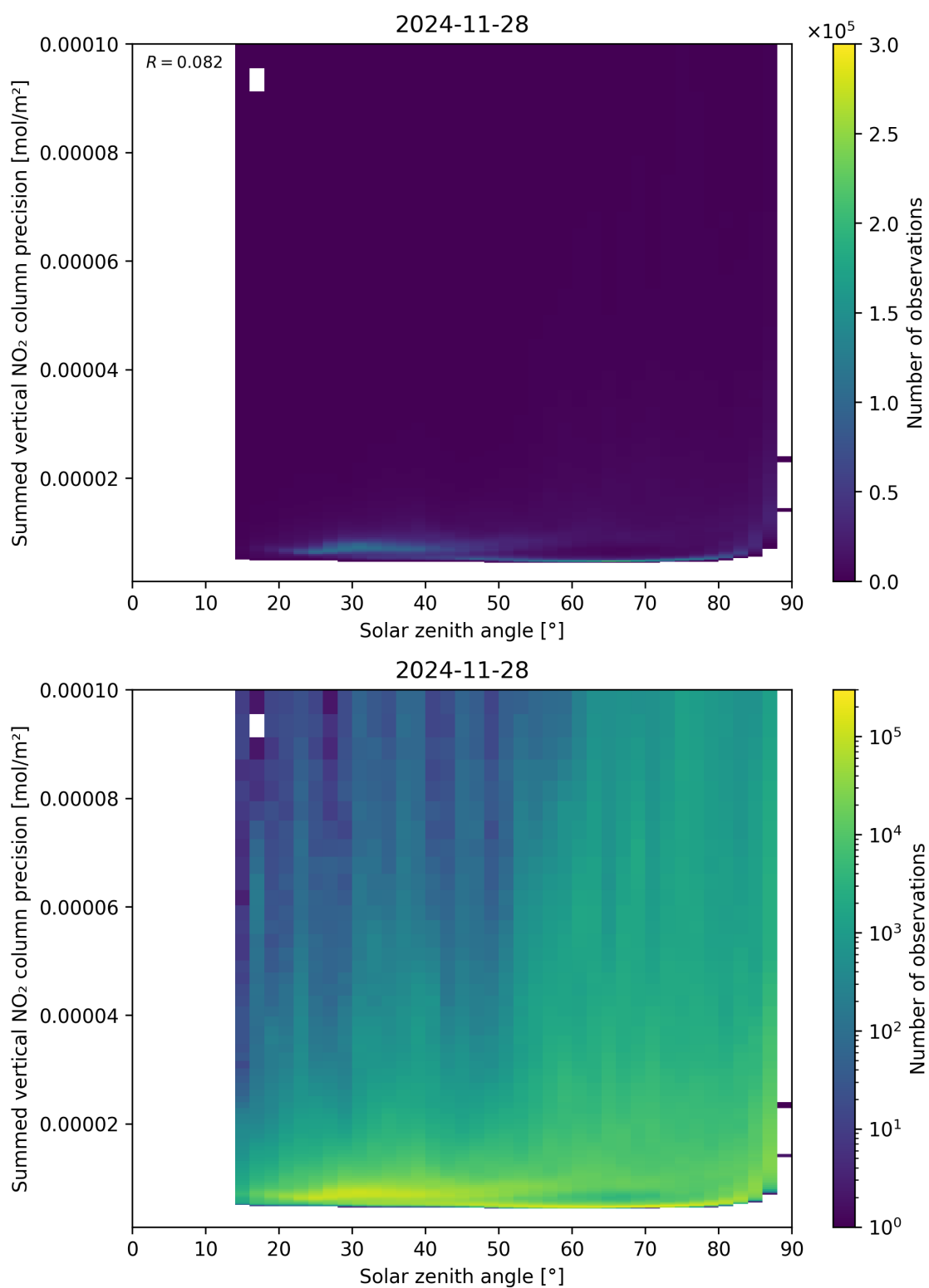
Figure 152: Scatter density plot of “Solar zenith angle” against “Summed vertical NO 2 column precision” for 2024-11-27 to 2024-11-29.
