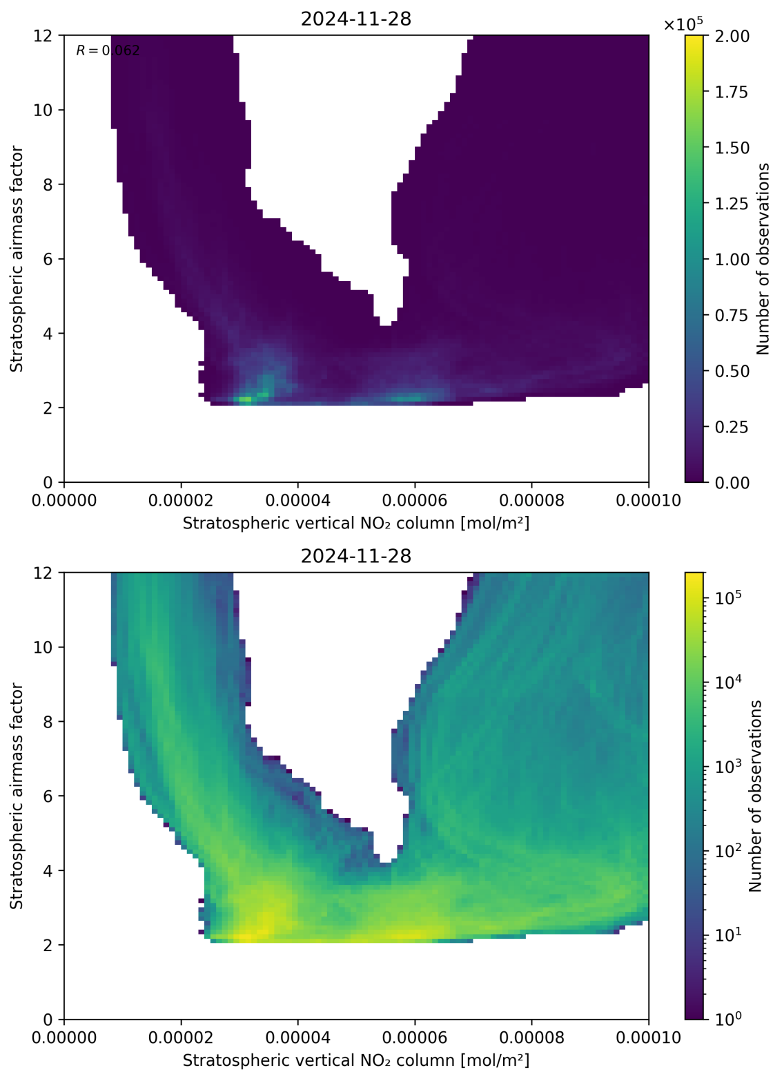
Figure 96: Scatter density plot of “Stratospheric vertical NO 2 column” against “Stratospheric airmass factor” for 2024-11-27 to 2024-11-29.
