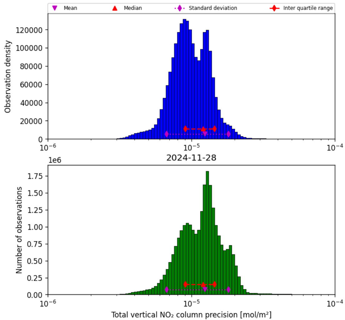
Figure 39: Histogram of “Total vertical NO 2 column precision” for 2024-11-27 to 2024-11-29
