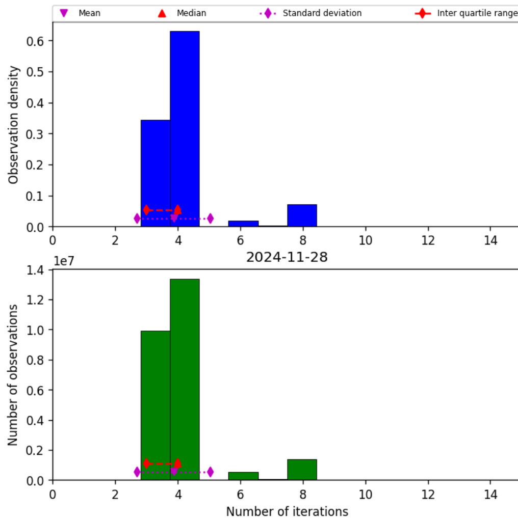
Figure 34: Histogram of “Number of iterations” for 2024-11-27 to 2024-11-29
