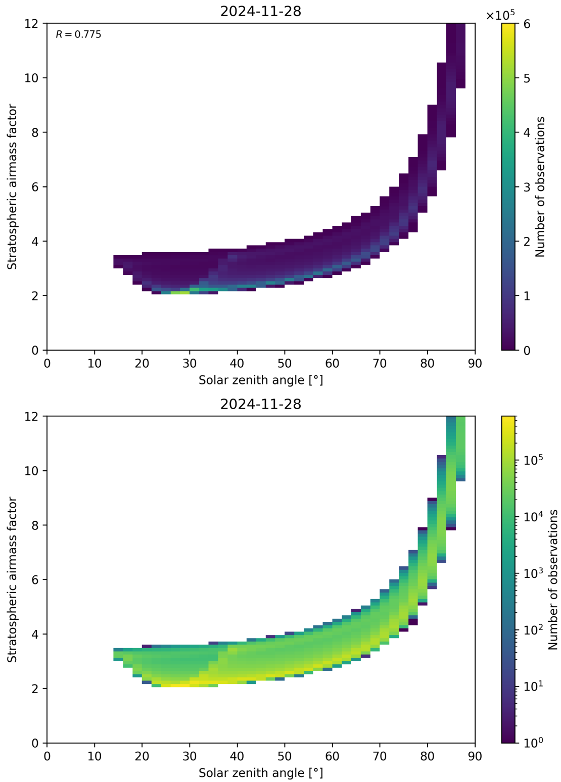
Figure 145: Scatter density plot of “Solar zenith angle” against “Stratospheric airmass factor” for 2024-11-27 to 2024-11-29.
