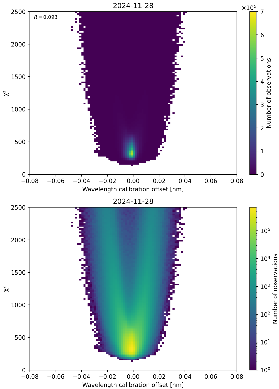
Figure 175: Scatter density plot of “Wavelength calibration offset” against “ \chi^2 ” for 2024-11-27 to 2024-11-29.
