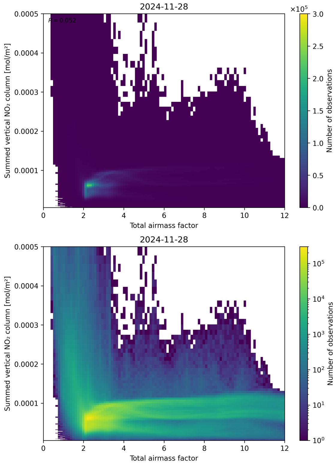
Figure 65: Scatter density plot of “Total airmass factor” against “Summed vertical NO 2 column” for 2024-11-27 to 2024-11-29.
