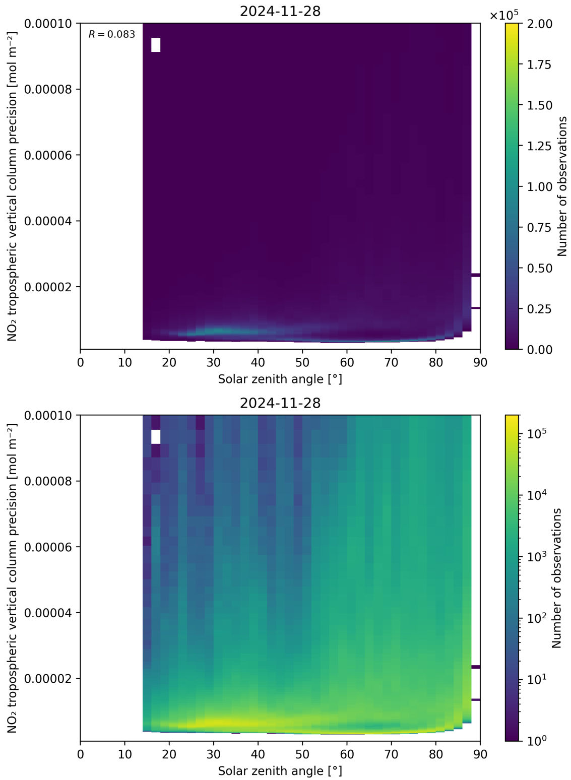
Figure 156: Scatter density plot of “Solar zenith angle” against “NO 2 tropospheric vertical column precision” for 2024-11-27 to 2024-11-29.
