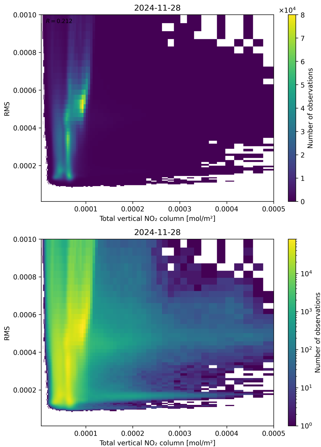
Figure 120: Scatter density plot of “Total vertical NO 2 column” against “RMS” for 2024-11-27 to 2024-11-29.
