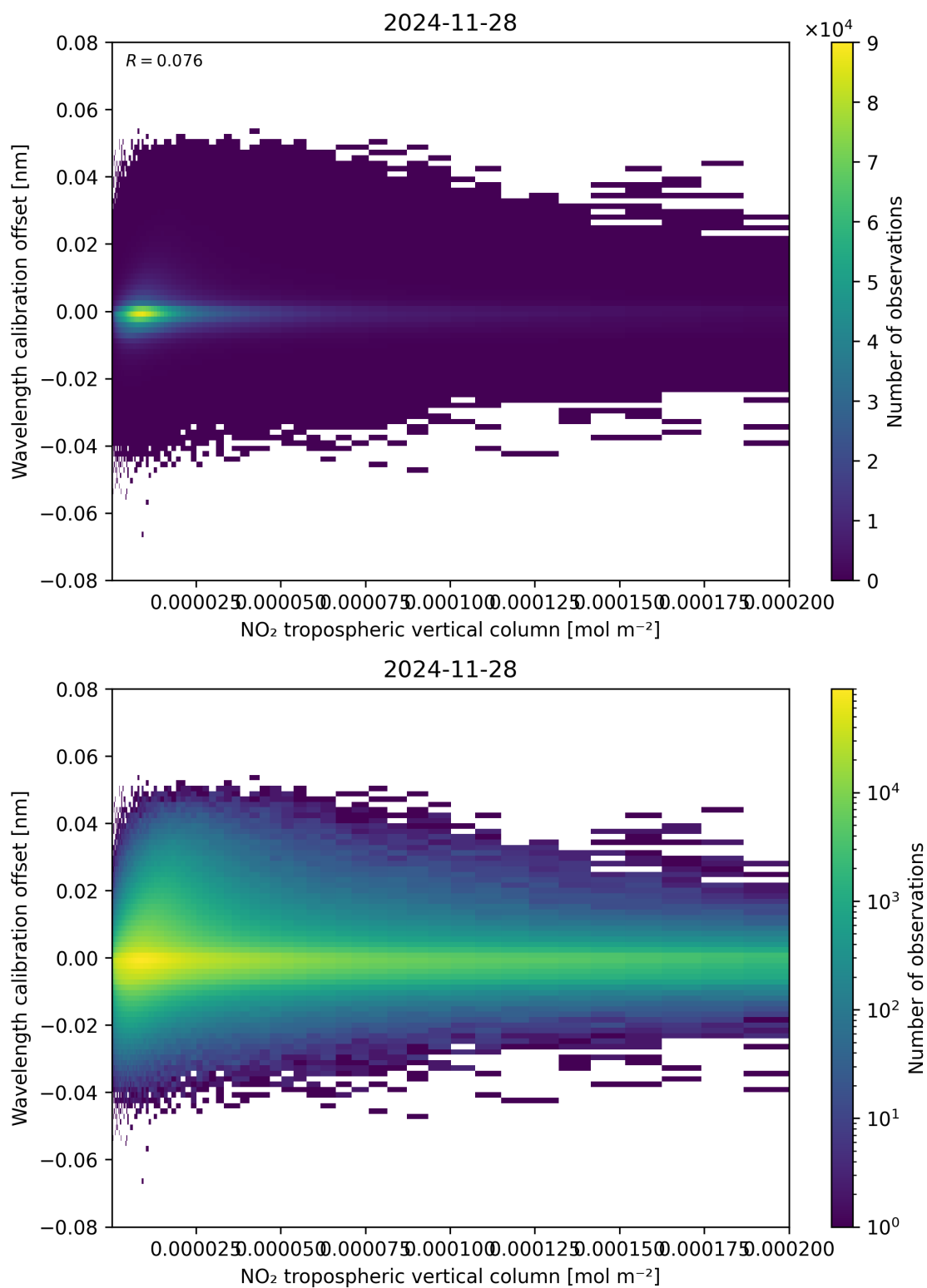
Figure 143: Scatter density plot of “NO 2 tropospheric vertical column” against “Wavelength calibration offset” for 2024-11-27 to 2024-11-29.
