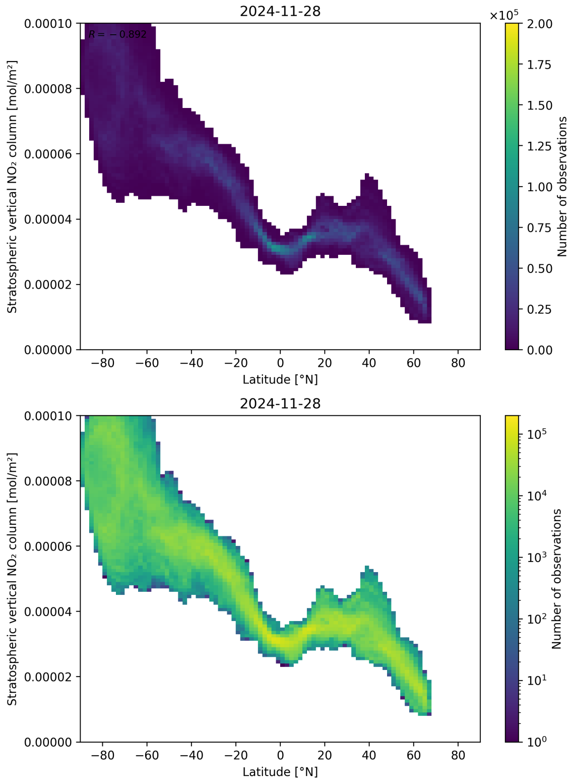
Figure 87: Scatter density plot of “Latitude” against “Stratospheric vertical NO 2 column” for 2024-11-27 to 2024-11-29.
