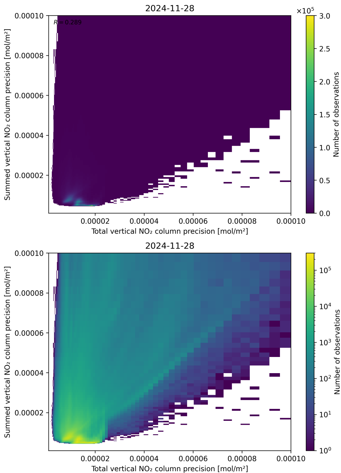
Figure 118: Scatter density plot of “Total vertical NO 2 column precision” against “Summed vertical NO 2 column precision” for 2024-11-27 to 2024-11-29.
