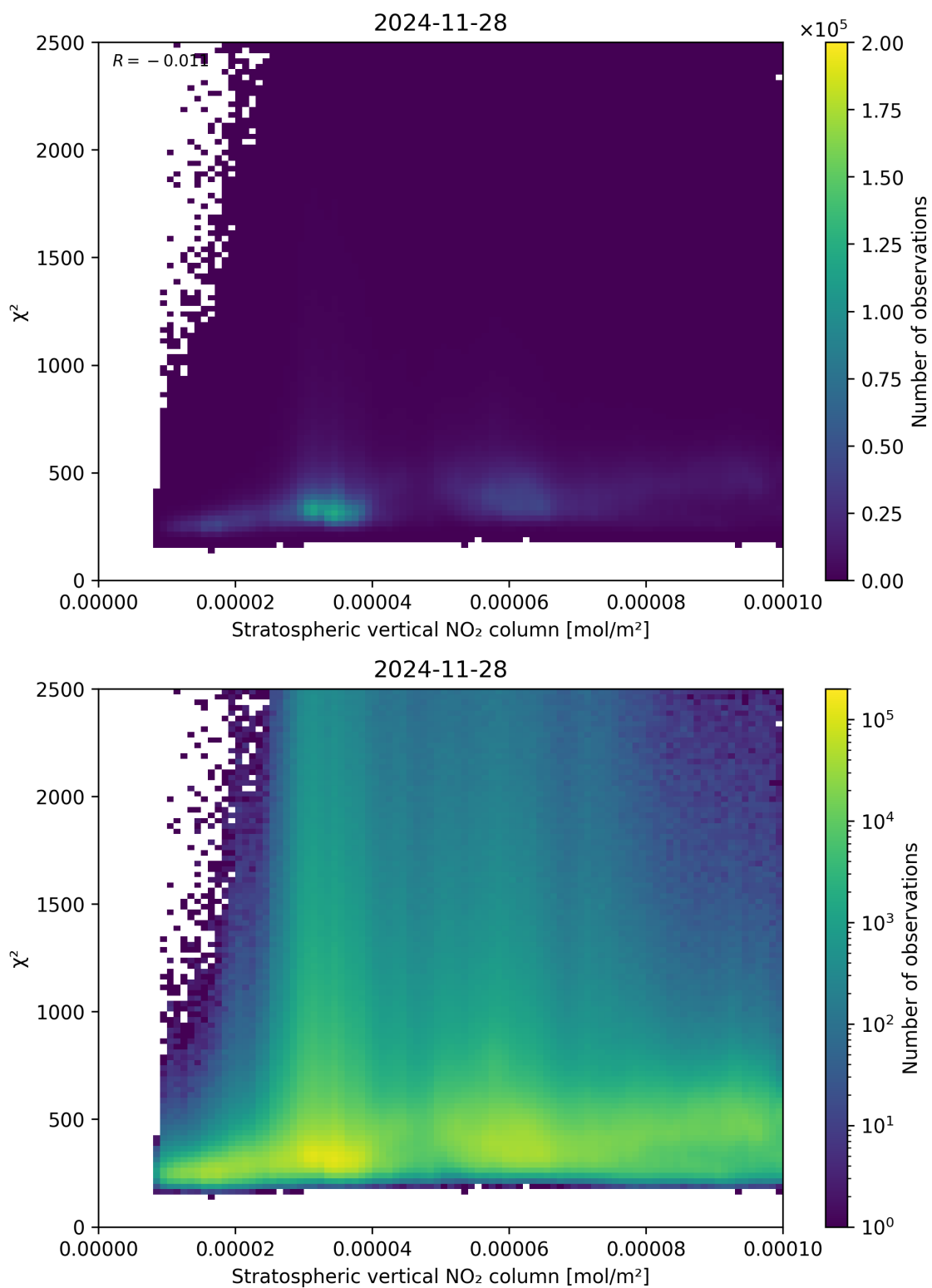
Figure 97: Scatter density plot of “Stratospheric vertical NO 2 column” against “ \chi^2 ” for 2024-11-27 to 2024-11-29.
