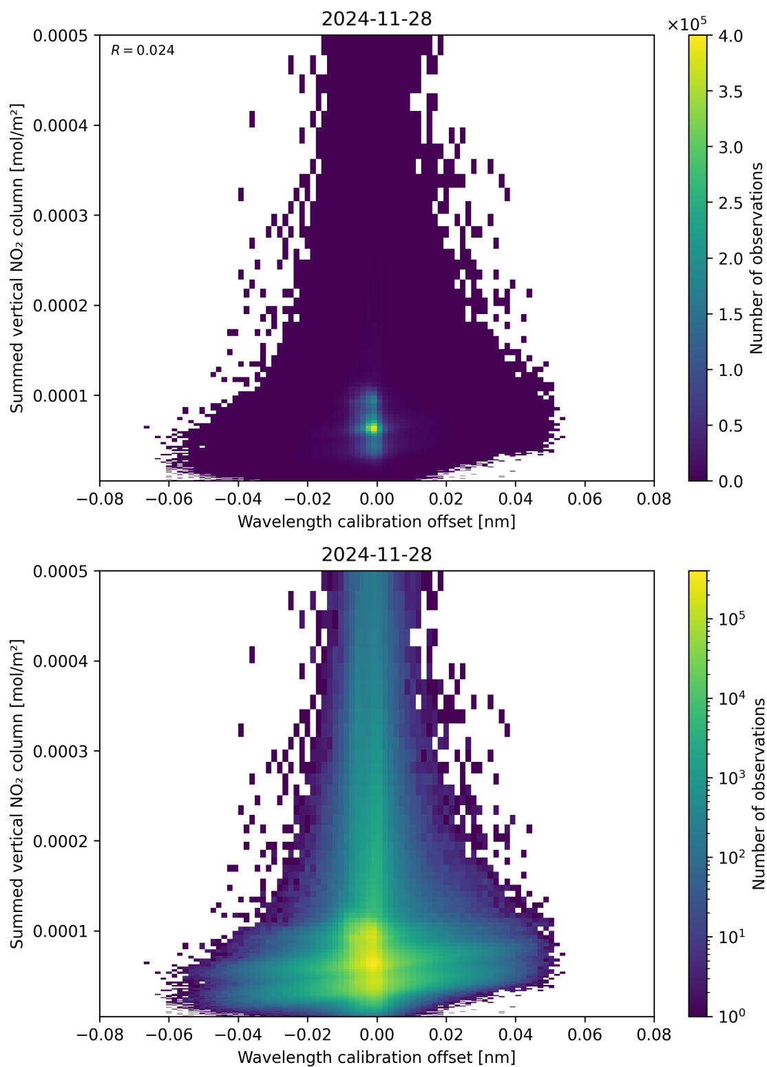
Figure 177: Scatter density plot of “Wavelength calibration offset” against “Summed vertical NO 2 column” for 2024-11-27 to 2024-11-29.
