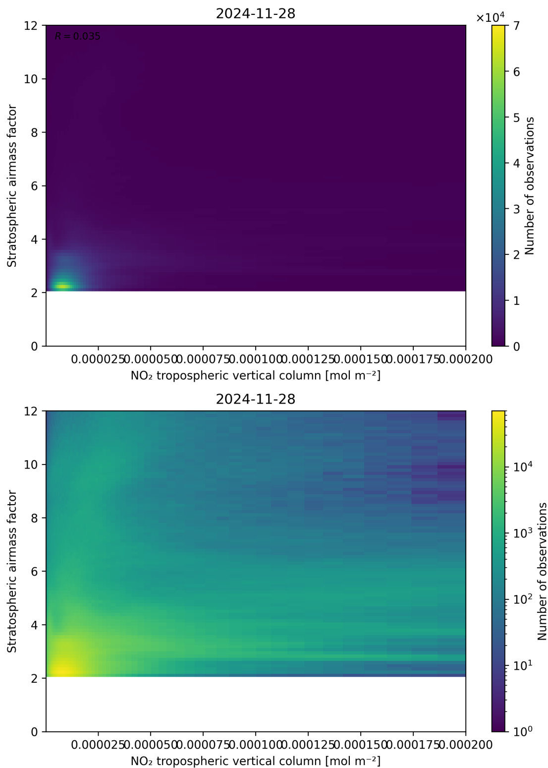
Figure 121: Scatter density plot of “NO 2 tropospheric vertical column” against “Stratospheric airmass factor” for 2024-11-27 to 2024-11-29.
