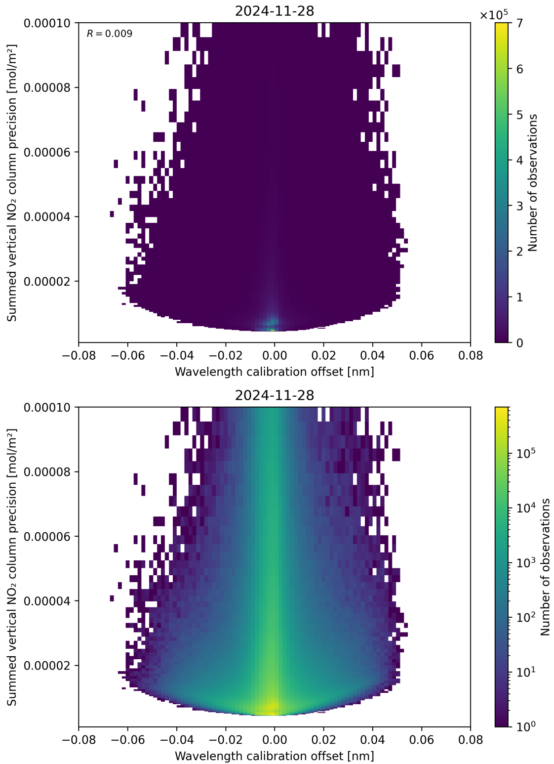
Figure 178: Scatter density plot of “Wavelength calibration offset” against “Summed vertical NO 2 column precision” for 2024-11-27 to 2024-11-29.
