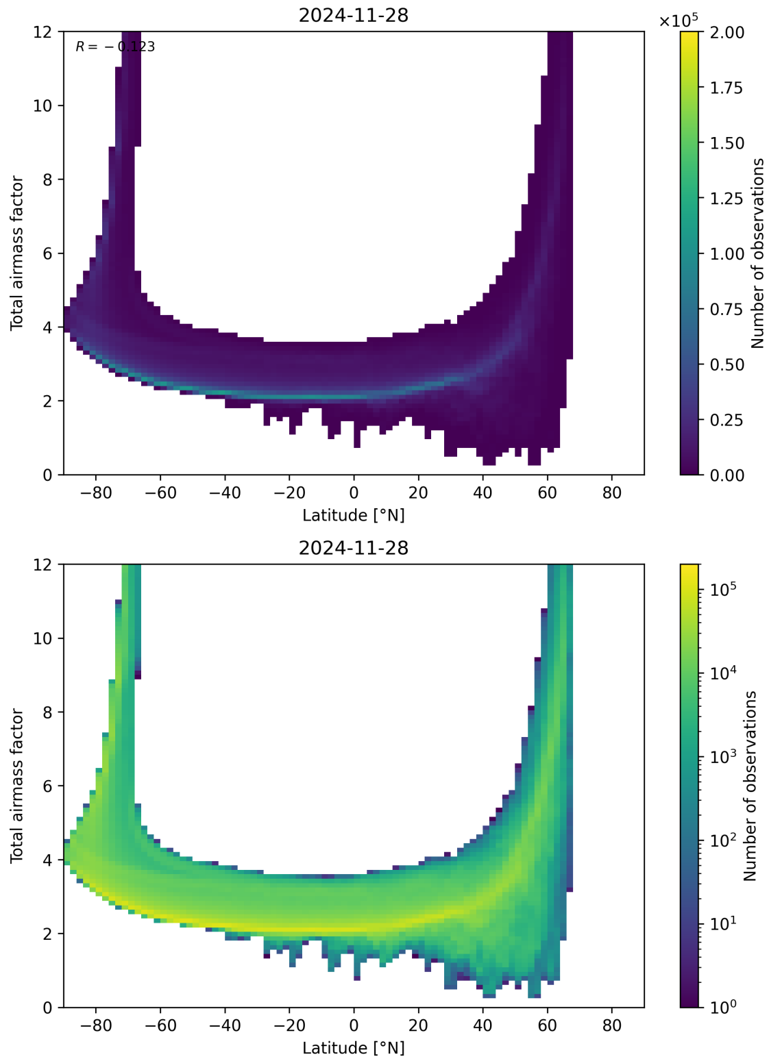
Figure 84: Scatter density plot of “Latitude” against “Total airmass factor” for 2024-11-27 to 2024-11-29.
