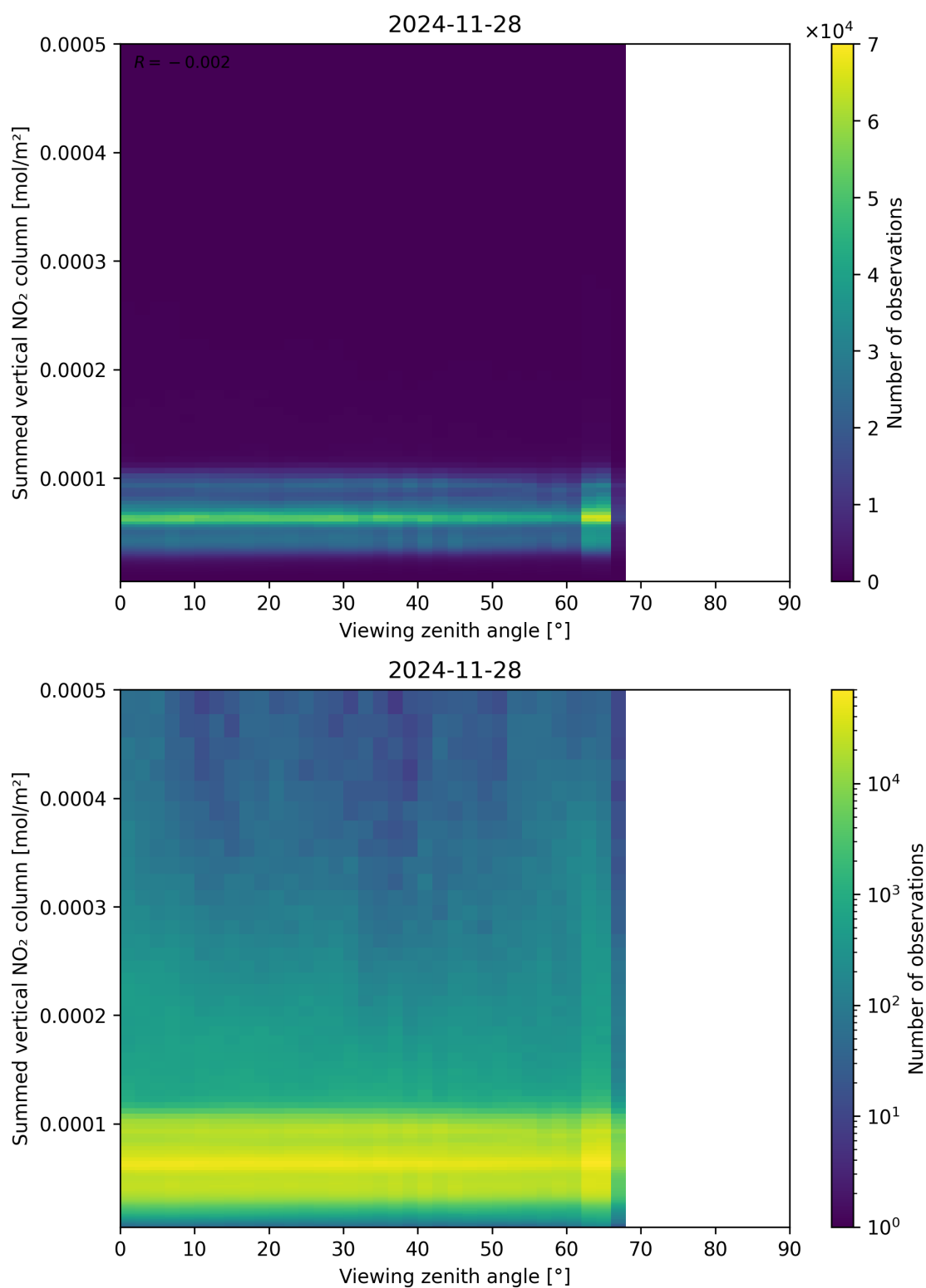
Figure 165: Scatter density plot of “Viewing zenith angle” against “Summed vertical NO 2 column” for 2024-11-27 to 2024-11-29.
