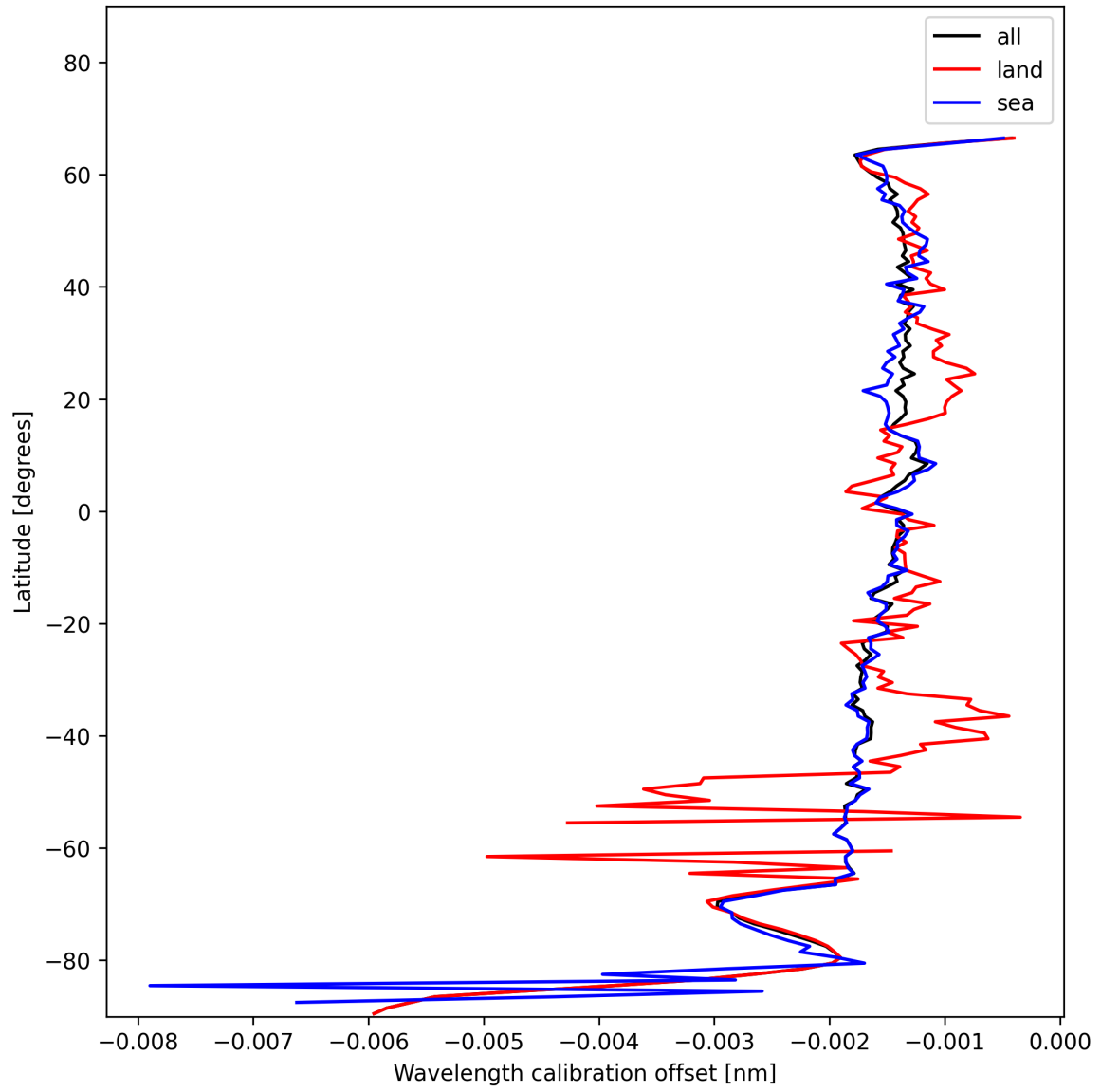
Figure 18: Zonal average of “Wavelength calibration offset” for 2024-11-27 to 2024-11-29.
