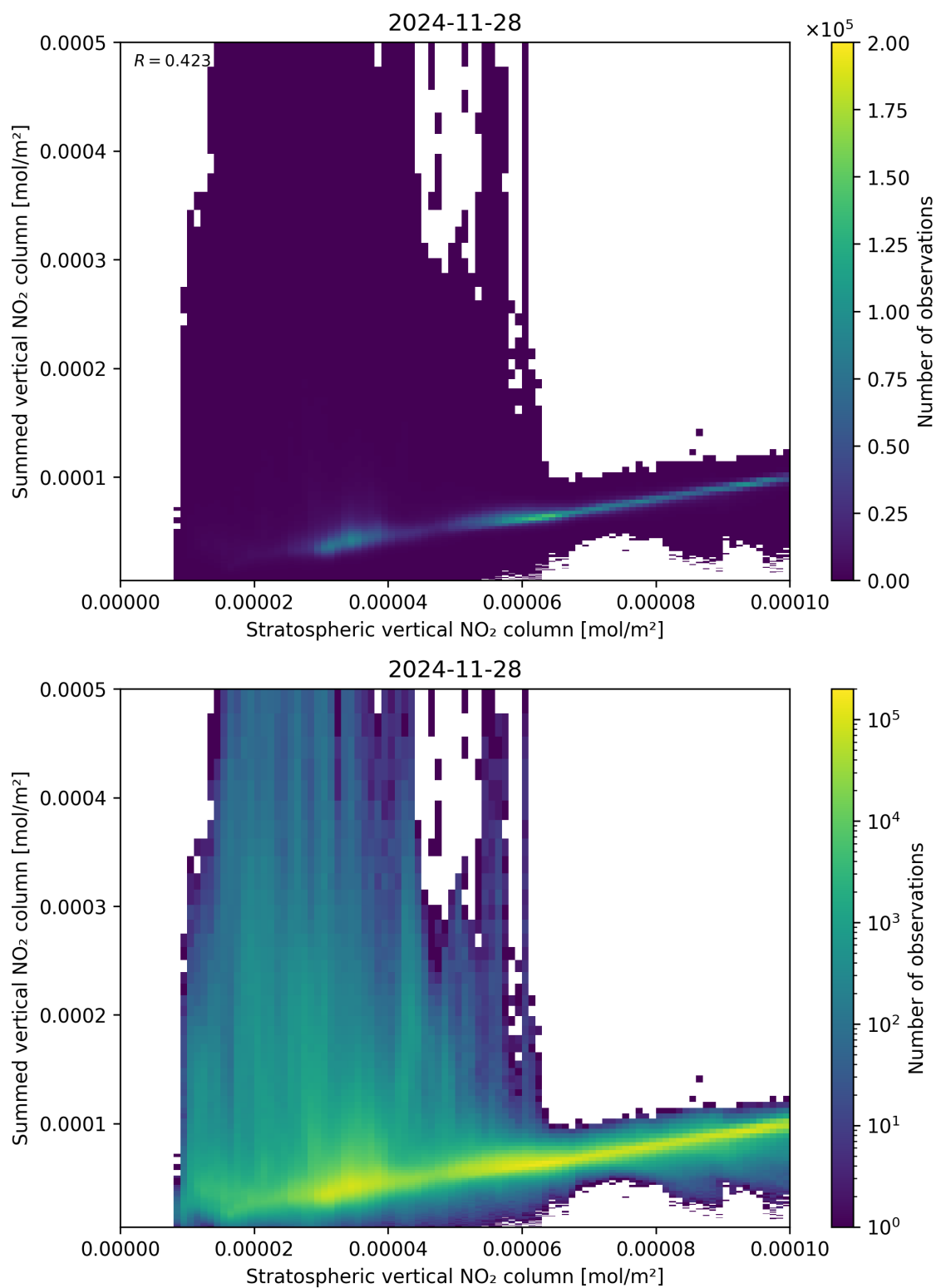
Figure 98: Scatter density plot of “Stratospheric vertical NO 2 column” against “Summed vertical NO 2 column” for 2024-11-27 to 2024-11-29.
