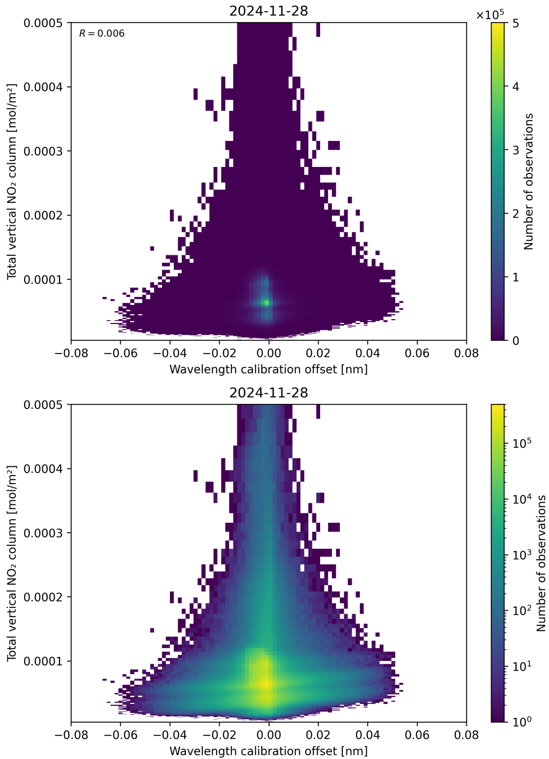
Figure 179: Scatter density plot of “Wavelength calibration offset” against “Total vertical NO 2 column” for 2024-11-27 to 2024-11-29.
