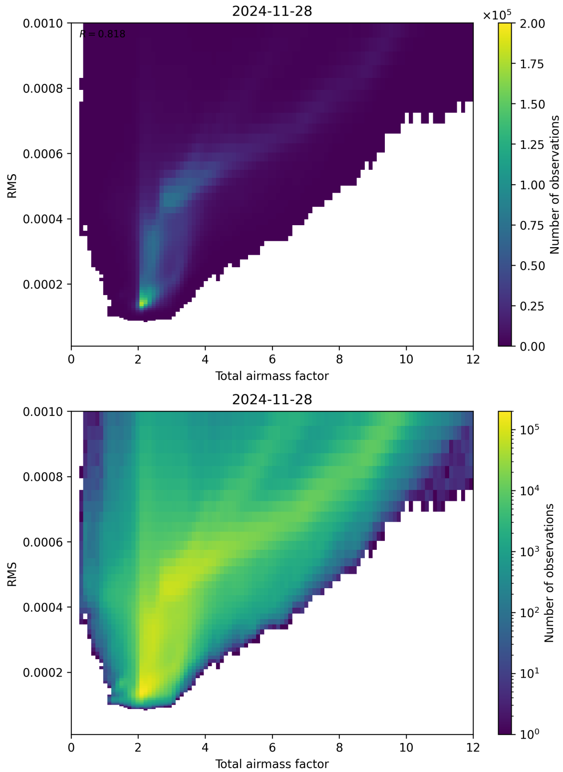
Figure 69: Scatter density plot of “Total airmass factor” against “RMS” for 2024-11-27 to 2024-11-29.
