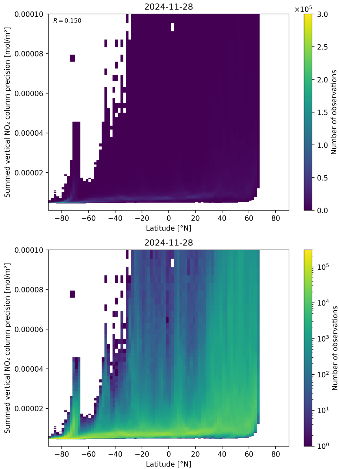
Figure 89: Scatter density plot of “Latitude” against “Summed vertical NO 2 column precision” for 2024-11-27 to 2024-11-29.
