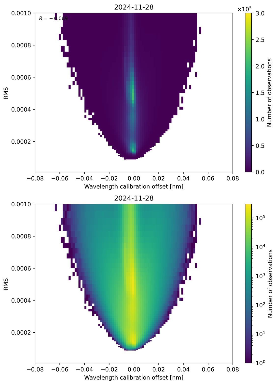
Figure 181: Scatter density plot of “Wavelength calibration offset” against “RMS” for 2024-11-27 to 2024-11-29.
