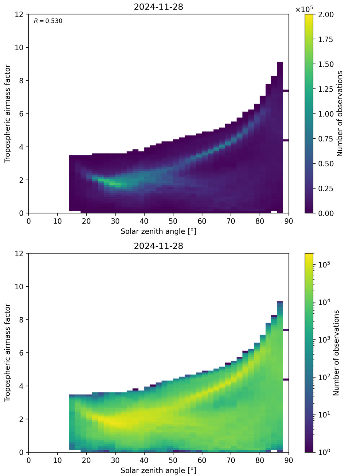
Figure 147: Scatter density plot of “Solar zenith angle” against “Tropospheric airmass factor” for 2024-11-27 to 2024-11-29.
