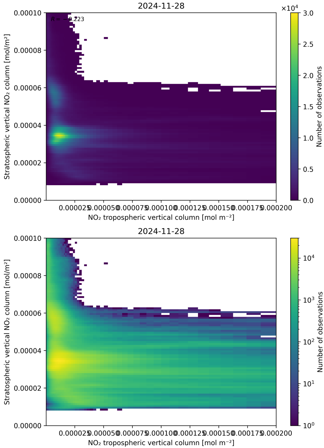
Figure 125: Scatter density plot of “NO 2 tropospheric vertical column” against “Stratospheric vertical NO 2 column” for 2024-11-27 to 2024-11-29.
