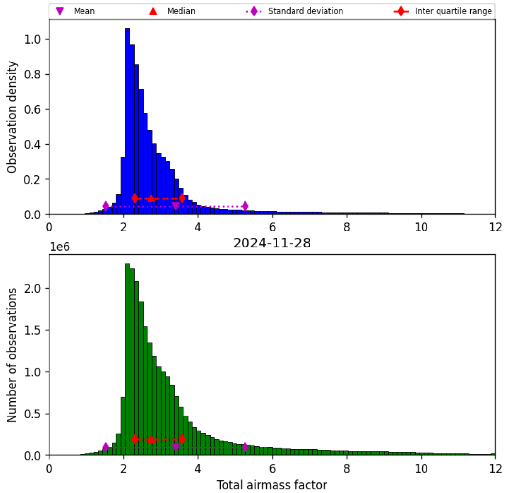
Figure 32: Histogram of “Total airmass factor” for 2024-11-27 to 2024-11-29
