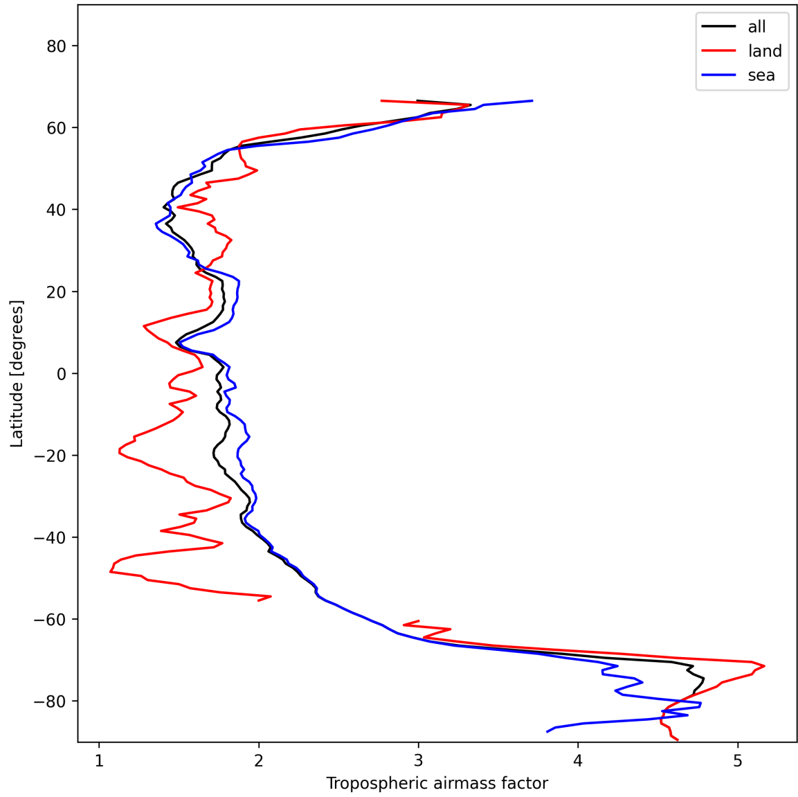
Figure 14: Zonal average of “Tropospheric airmass factor” for 2024-11-27 to 2024-11-29.
