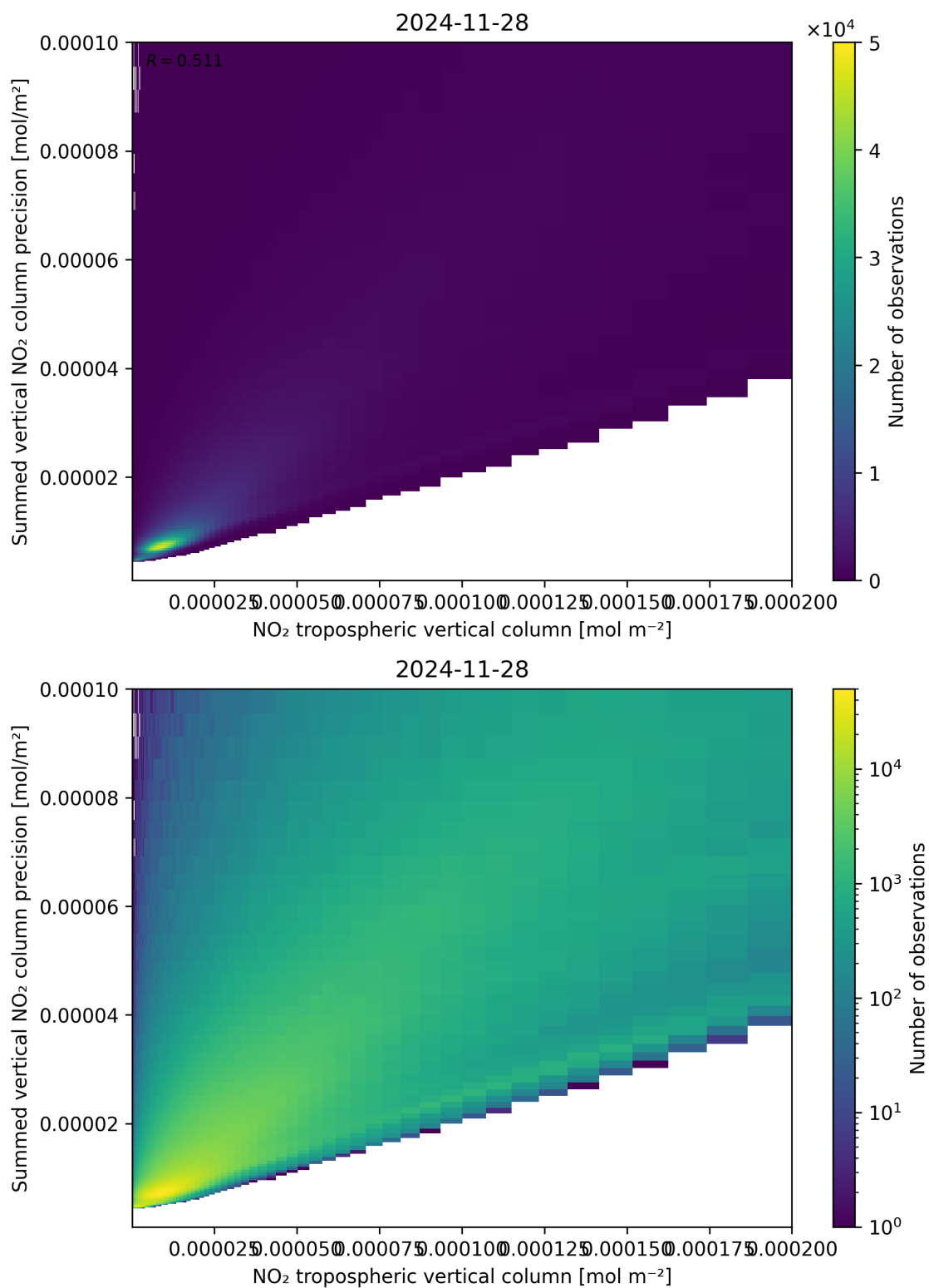
Figure 127: Scatter density plot of “NO 2 tropospheric vertical column” against “Summed vertical NO 2 column precision” for 2024-11-27 to 2024-11-29.
