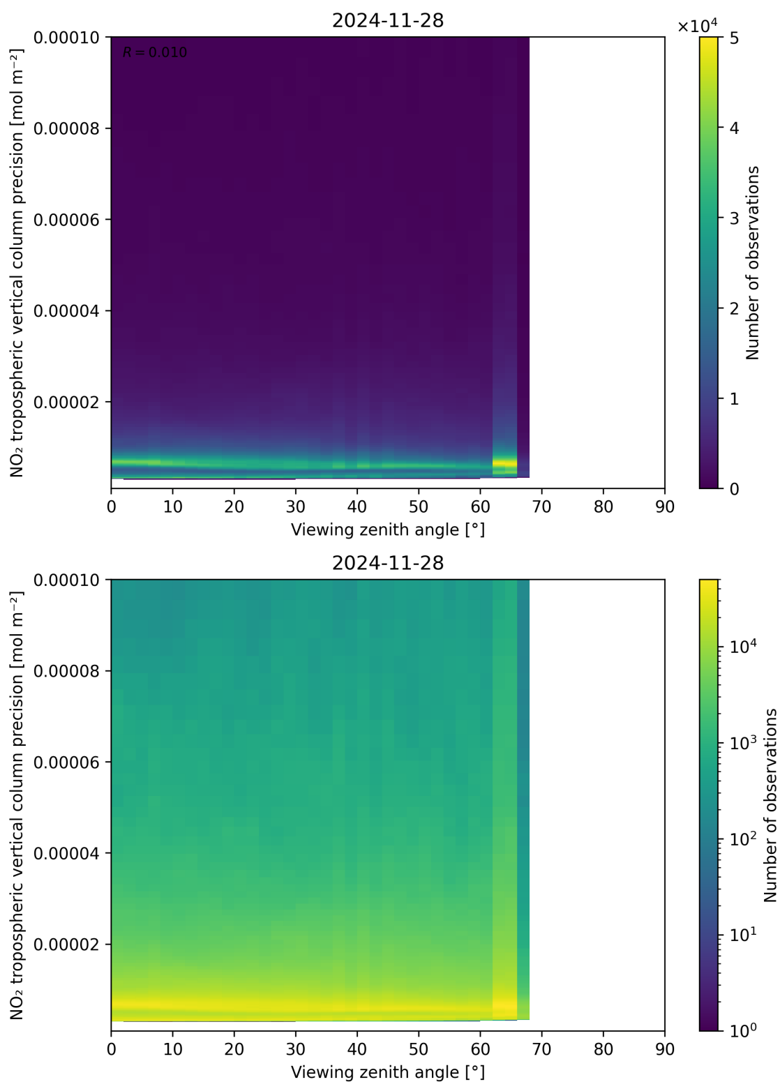
Figure 170: Scatter density plot of “Viewing zenith angle” against “NO 2 tropospheric vertical column precision” for 2024-11-27 to 2024-11-29.
