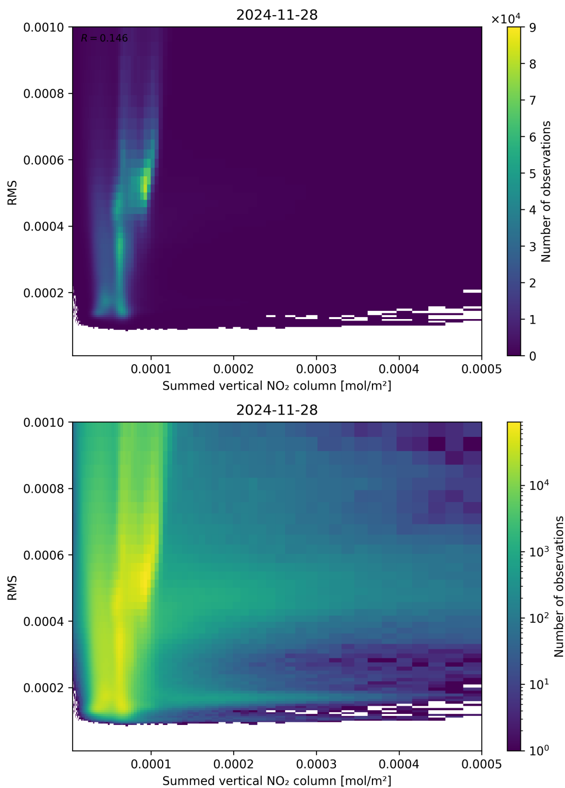
Figure 109: Scatter density plot of “Summed vertical NO 2 column” against “RMS” for 2024-11-27 to 2024-11-29.
