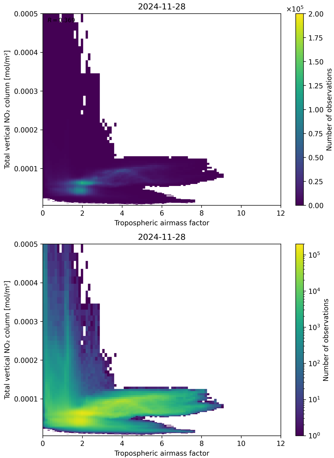
Figure 77: Scatter density plot of “Tropospheric airmass factor” against “Total vertical NO 2 column” for 2024-11-27 to 2024-11-29.
