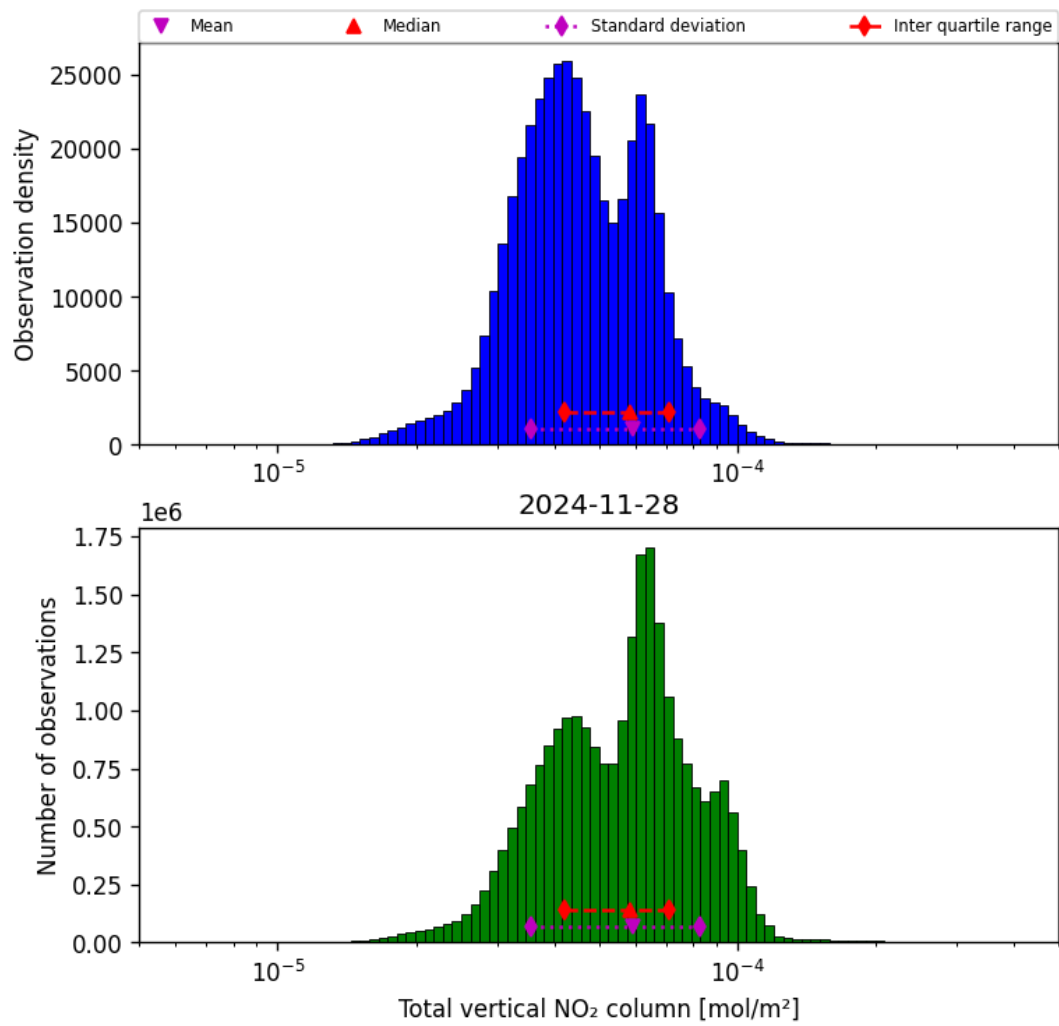
Figure 38: Histogram of “Total vertical NO 2 column” for 2024-11-27 to 2024-11-29
