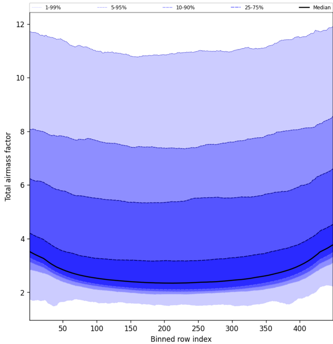
Figure 49: Along track statistics of “Total airmass factor” for 2024-11-27 to 2024-11-29
