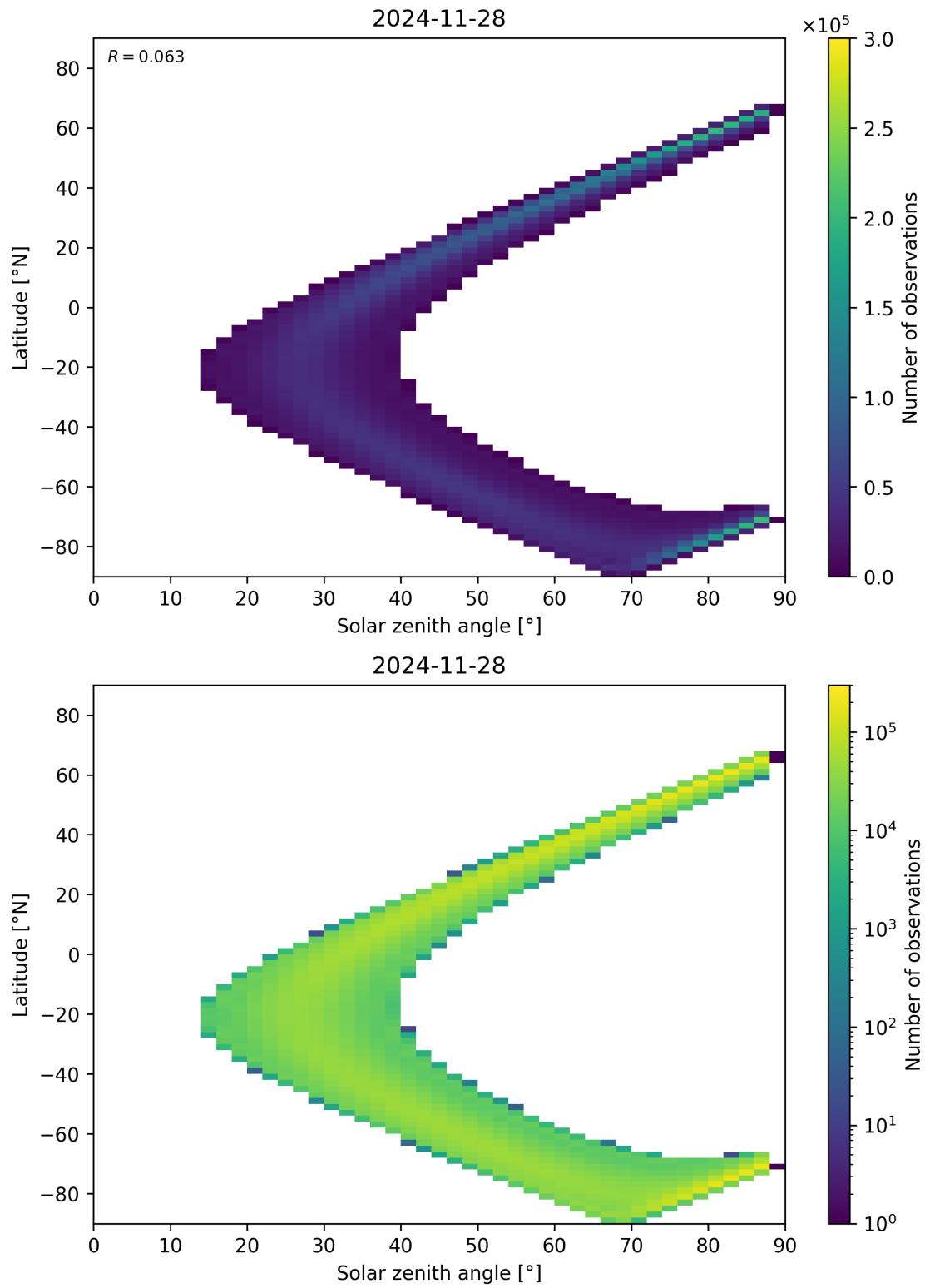
Figure 149: Scatter density plot of “Solar zenith angle” against “Latitude” for 2024-11-27 to 2024-11-29.
