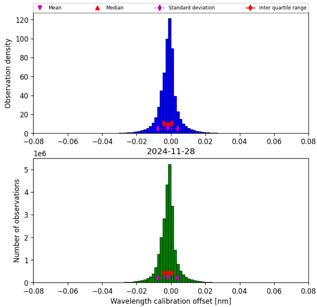
Figure 35: Histogram of “Wavelength calibration offset” for 2024-11-27 to 2024-11-29
