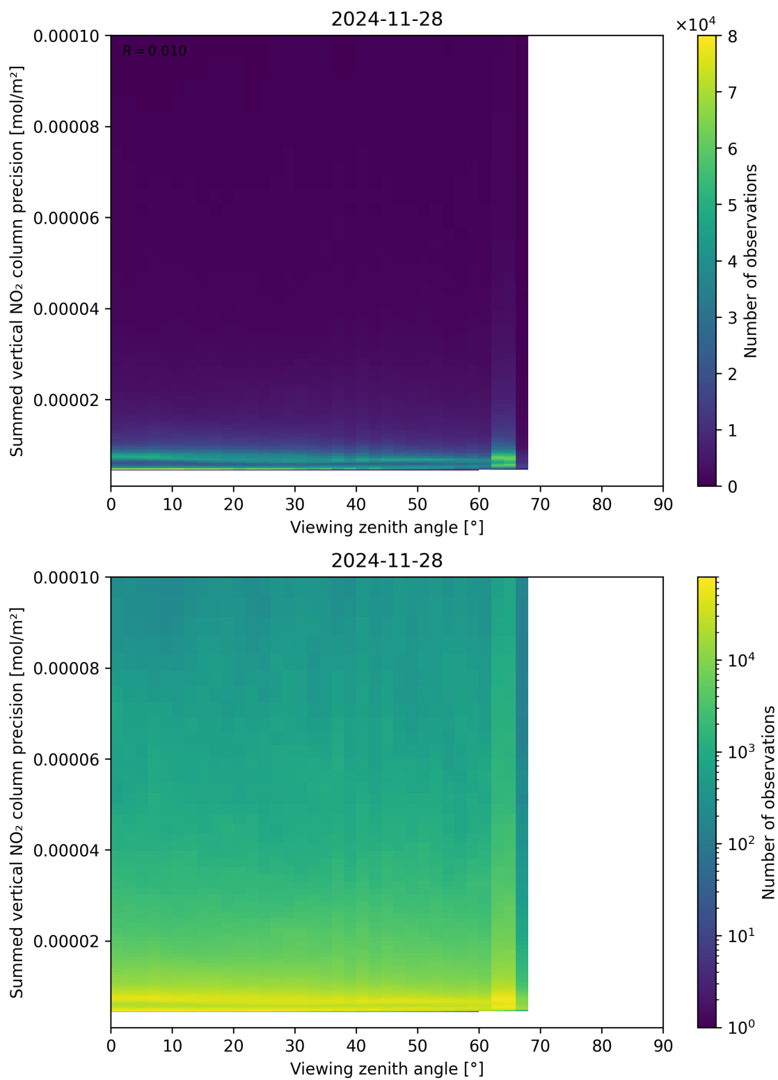
Figure 166: Scatter density plot of “Viewing zenith angle” against “Summed vertical NO 2 column precision” for 2024-11-27 to 2024-11-29.
