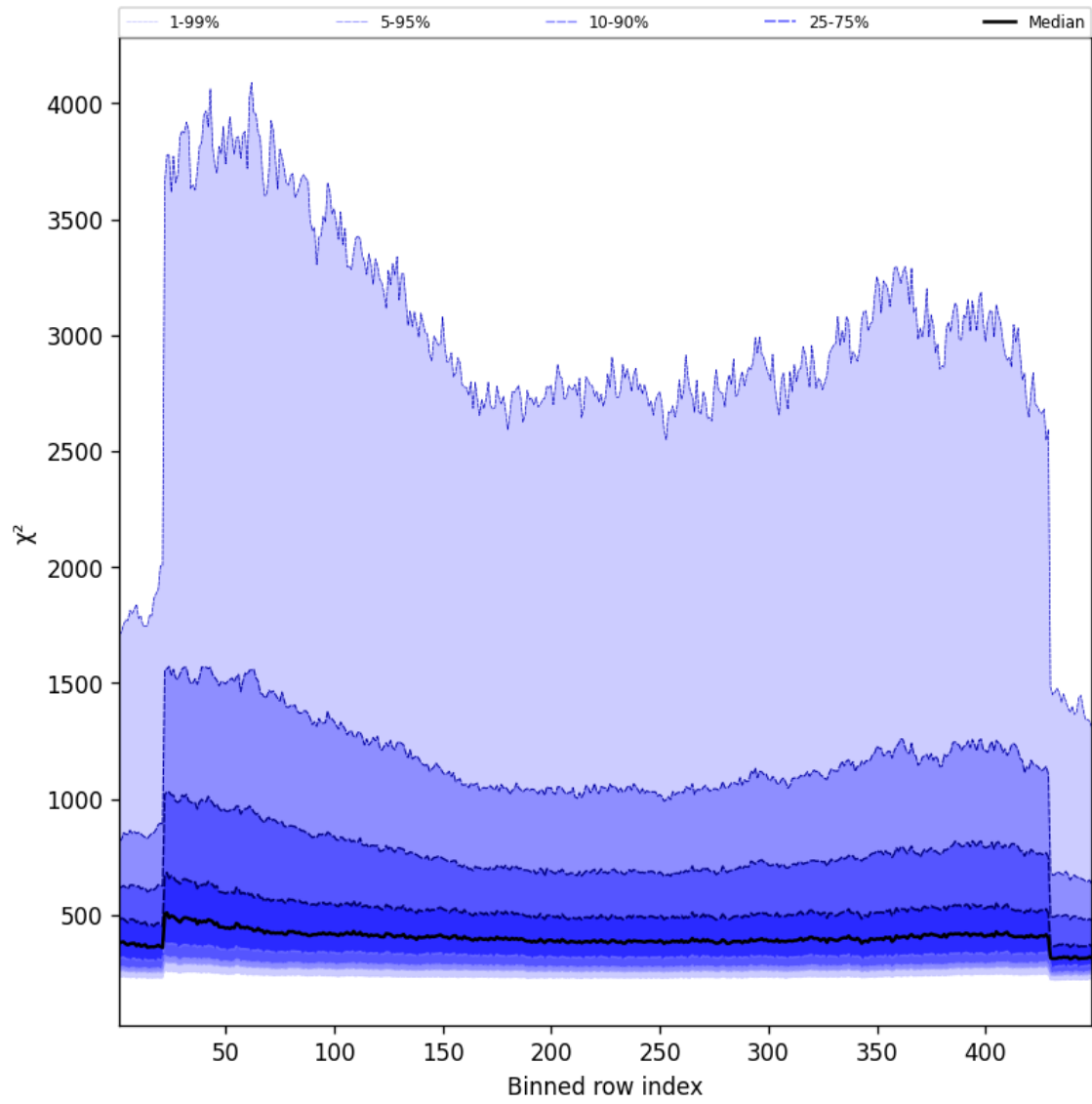
Figure 59: Along track statistics of “ \chi^2 ” for 2024-11-27 to 2024-11-29
