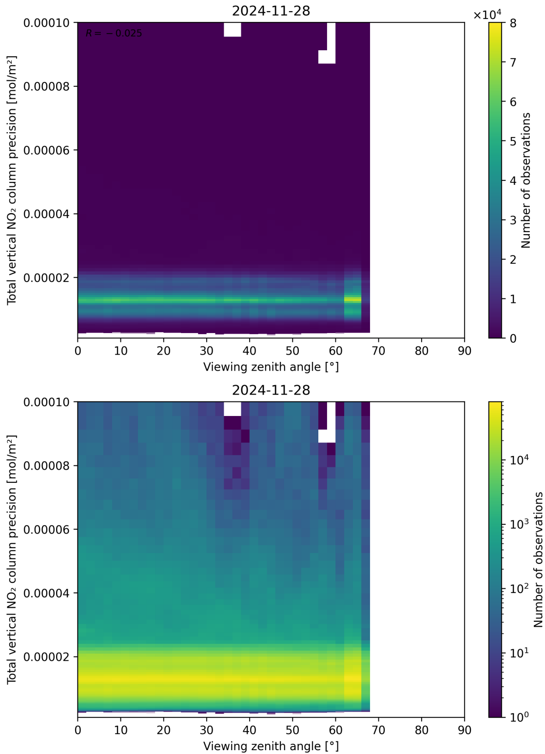
Figure 168: Scatter density plot of “Viewing zenith angle” against “Total vertical NO 2 column precision” for 2024-11-27 to 2024-11-29.
