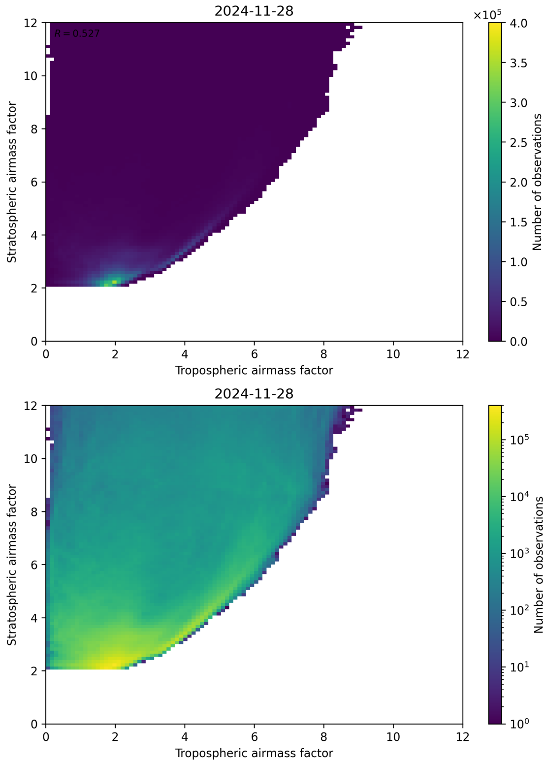
Figure 71: Scatter density plot of “Tropospheric airmass factor” against “Stratospheric airmass factor” for 2024-11-27 to 2024-11-29.
