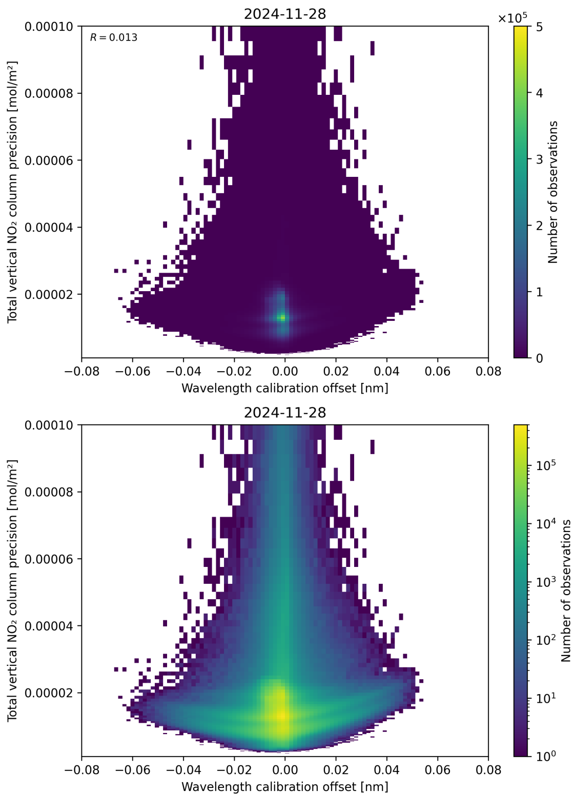
Figure 180: Scatter density plot of “Wavelength calibration offset” against “Total vertical NO 2 column precision” for 2024-11-27 to 2024-11-29.
