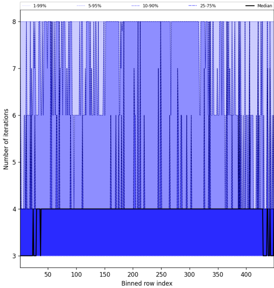
Figure 51: Along track statistics of “Number of iterations” for 2024-11-27 to 2024-11-29
