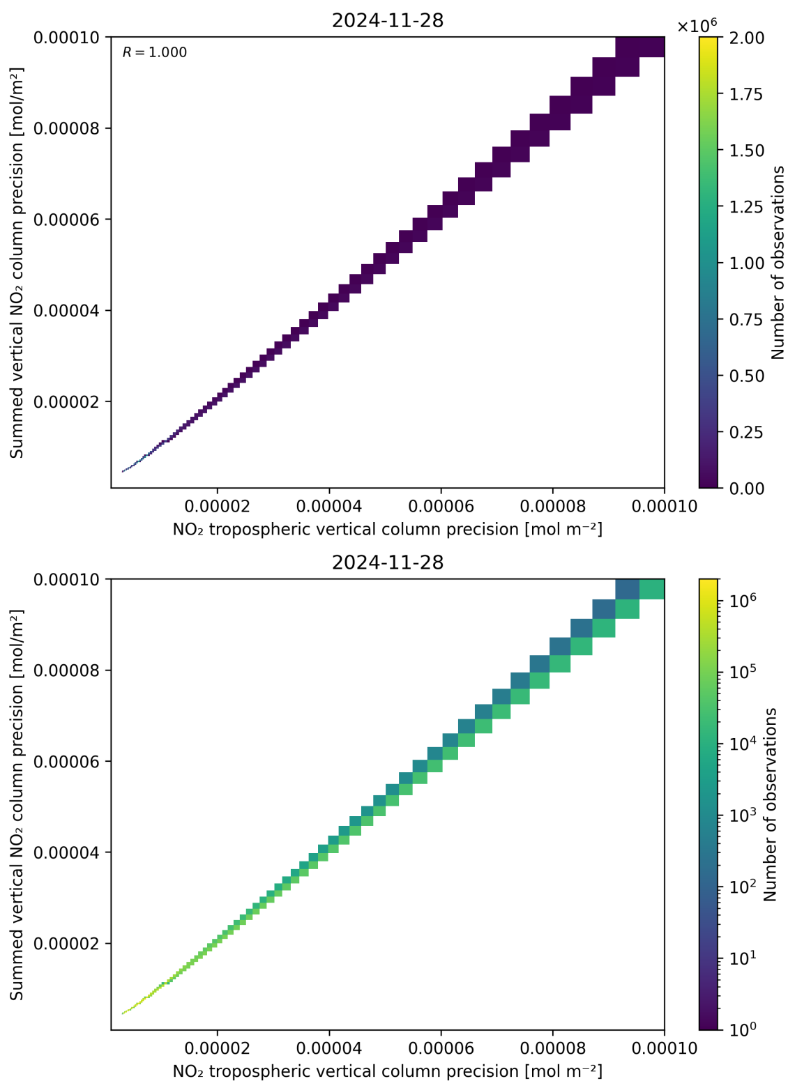
Figure 137: Scatter density plot of “NO 2 tropospheric vertical column precision” against “Summed vertical NO 2 column precision” for 2024-11-27 to 2024-11-29.
