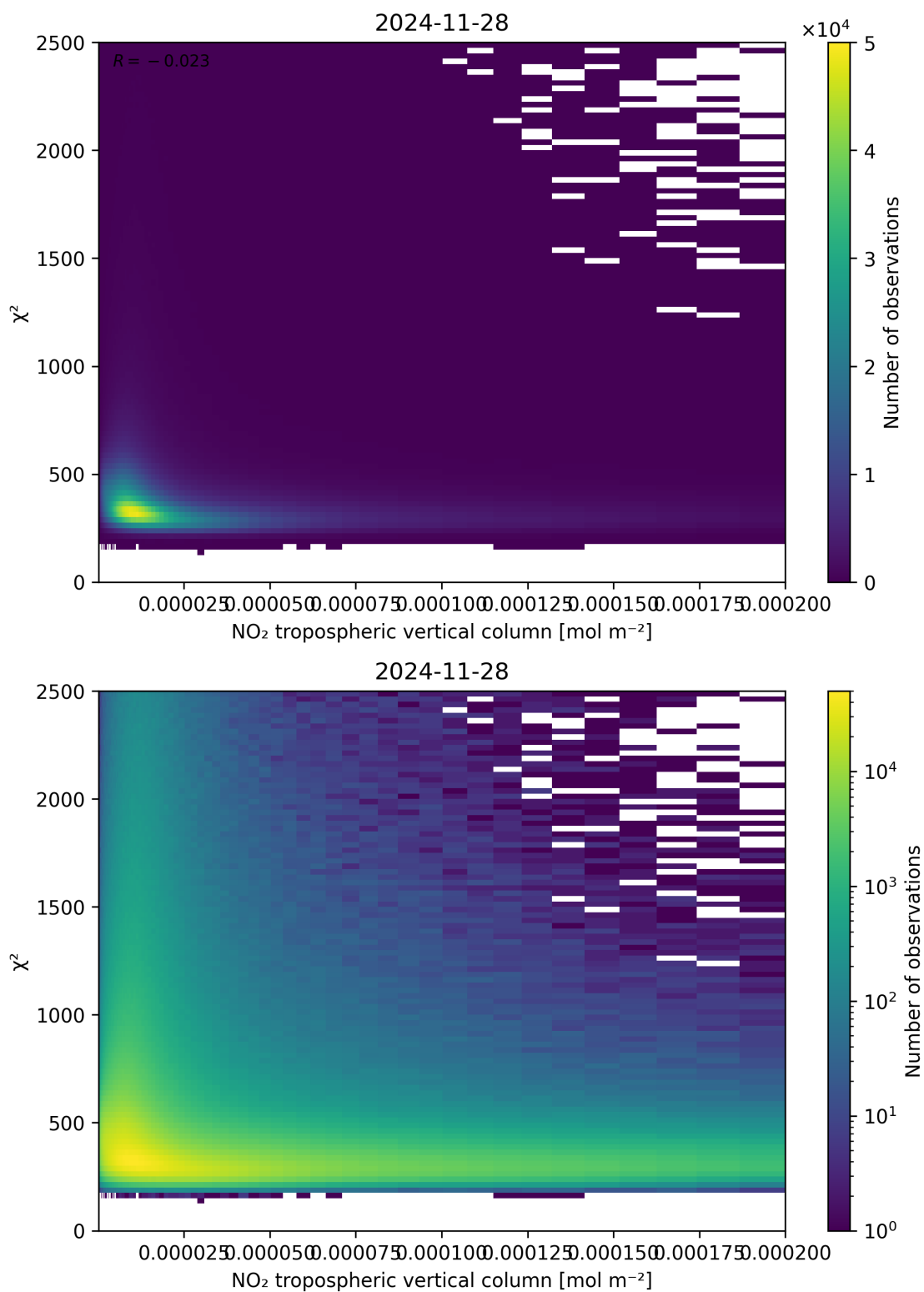
Figure 124: Scatter density plot of “NO 2 tropospheric vertical column” against “ \chi^2 ” for 2024-11-27 to 2024-11-29.
