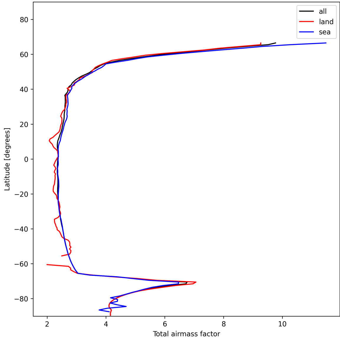
Figure 15: Zonal average of “Total airmass factor” for 2024-11-27 to 2024-11-29.
