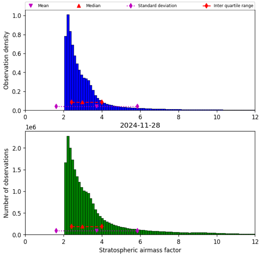
Figure 44: Histogram of “Stratospheric airmass factor” for 2024-11-27 to 2024-11-29
