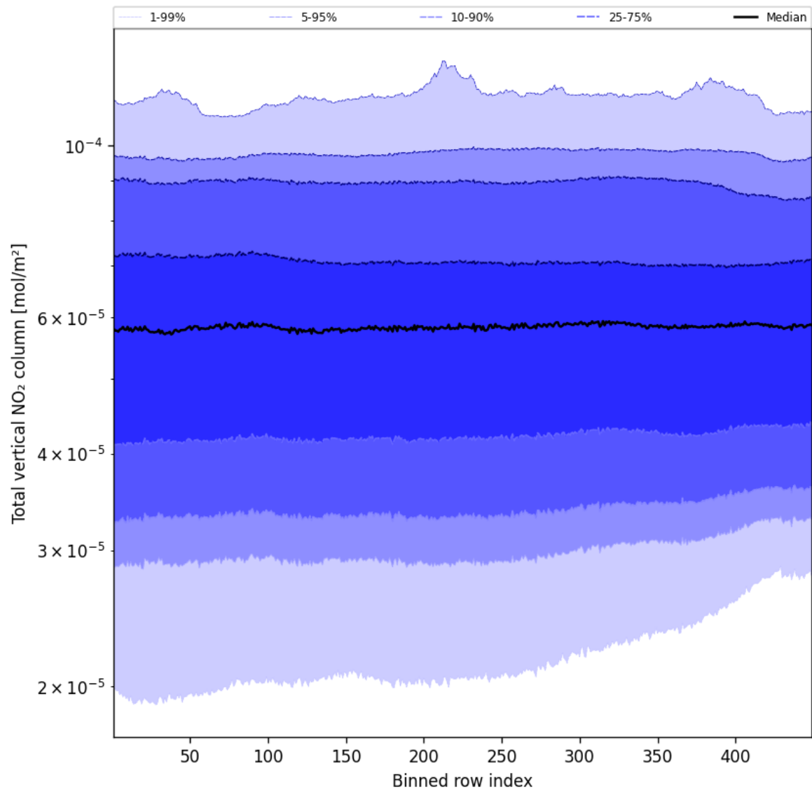
Figure 55: Along track statistics of “Total vertical NO 2 column” for 2024-11-27 to 2024-11-29
