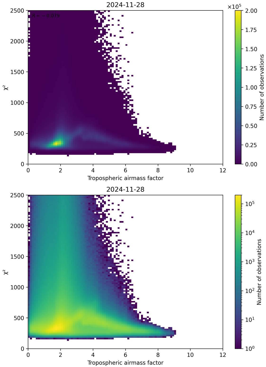
Figure 73: Scatter density plot of “Tropospheric airmass factor” against “ \chi^2 ” for 2024-11-27 to 2024-11-29.
