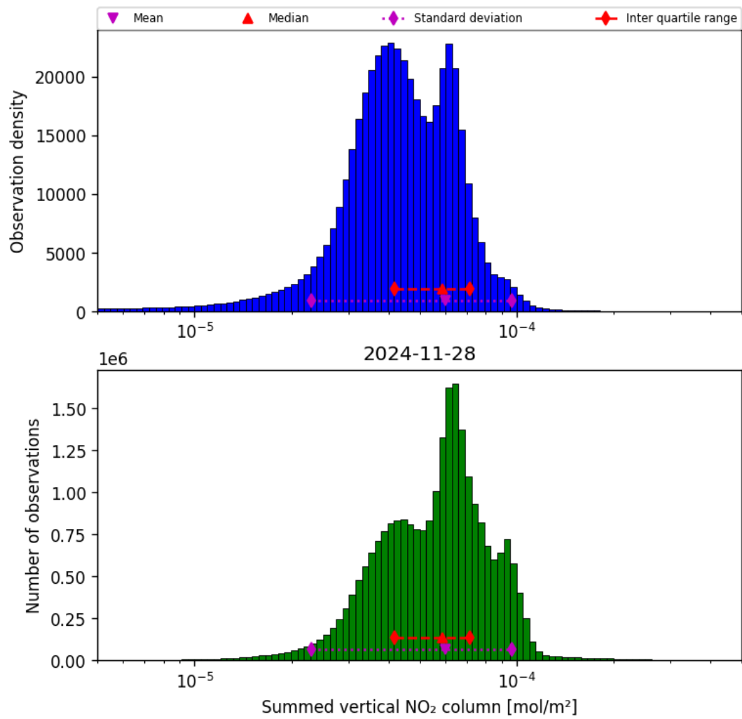
Figure 40: Histogram of “Summed vertical NO 2 column” for 2024-11-27 to 2024-11-29
