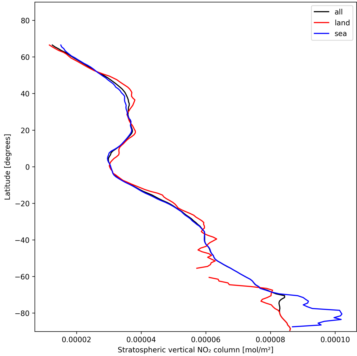
Figure 19: Zonal average of “Stratospheric vertical NO 2 column” for 2024-11-27 to 2024-11-29.
