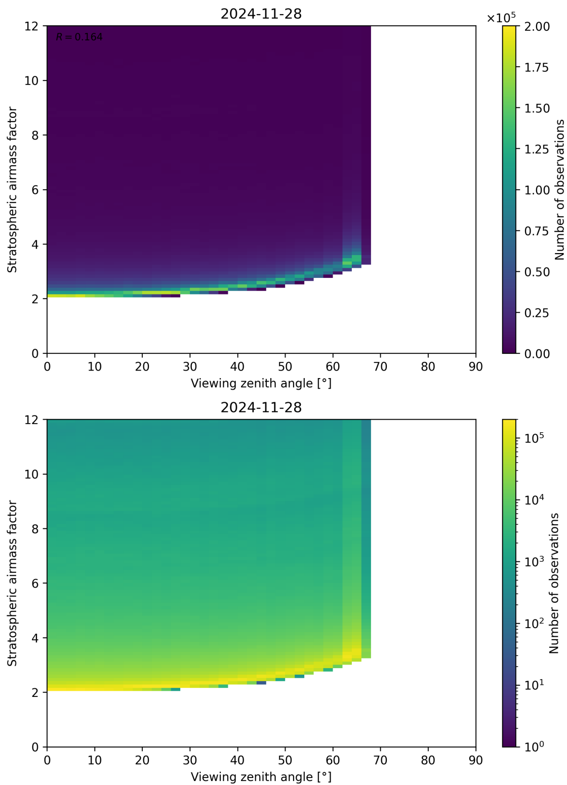
Figure 159: Scatter density plot of “Viewing zenith angle” against “Stratospheric airmass factor” for 2024-11-27 to 2024-11-29.
