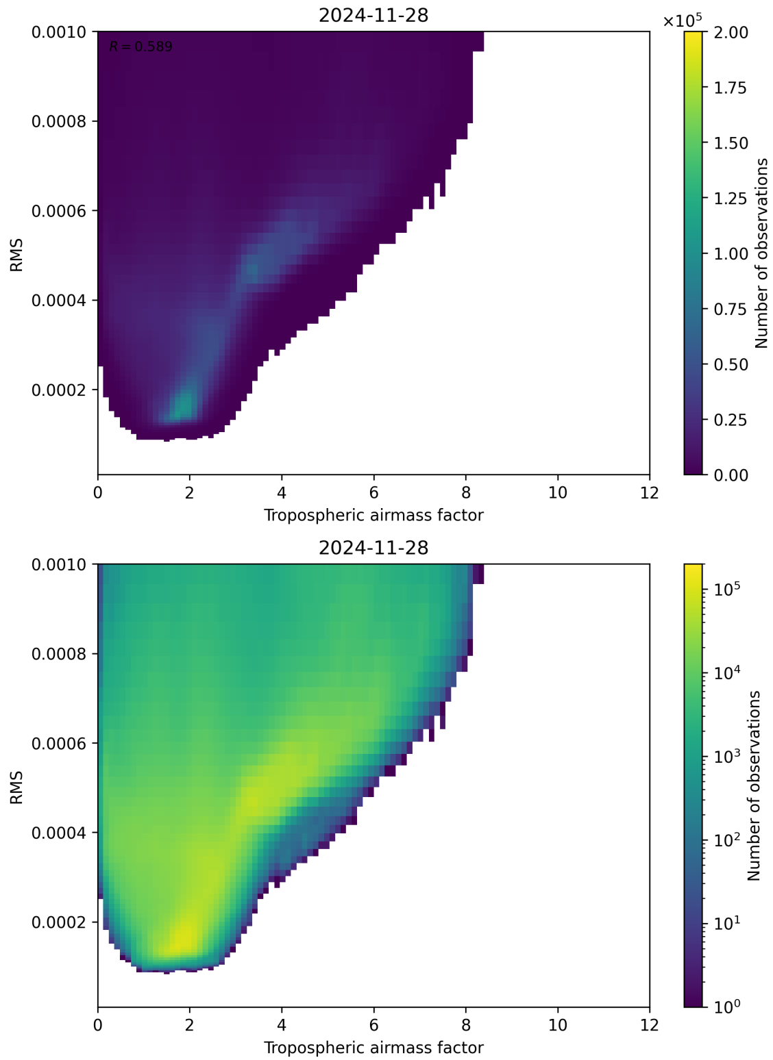
Figure 79: Scatter density plot of “Tropospheric airmass factor” against “RMS” for 2024-11-27 to 2024-11-29.
