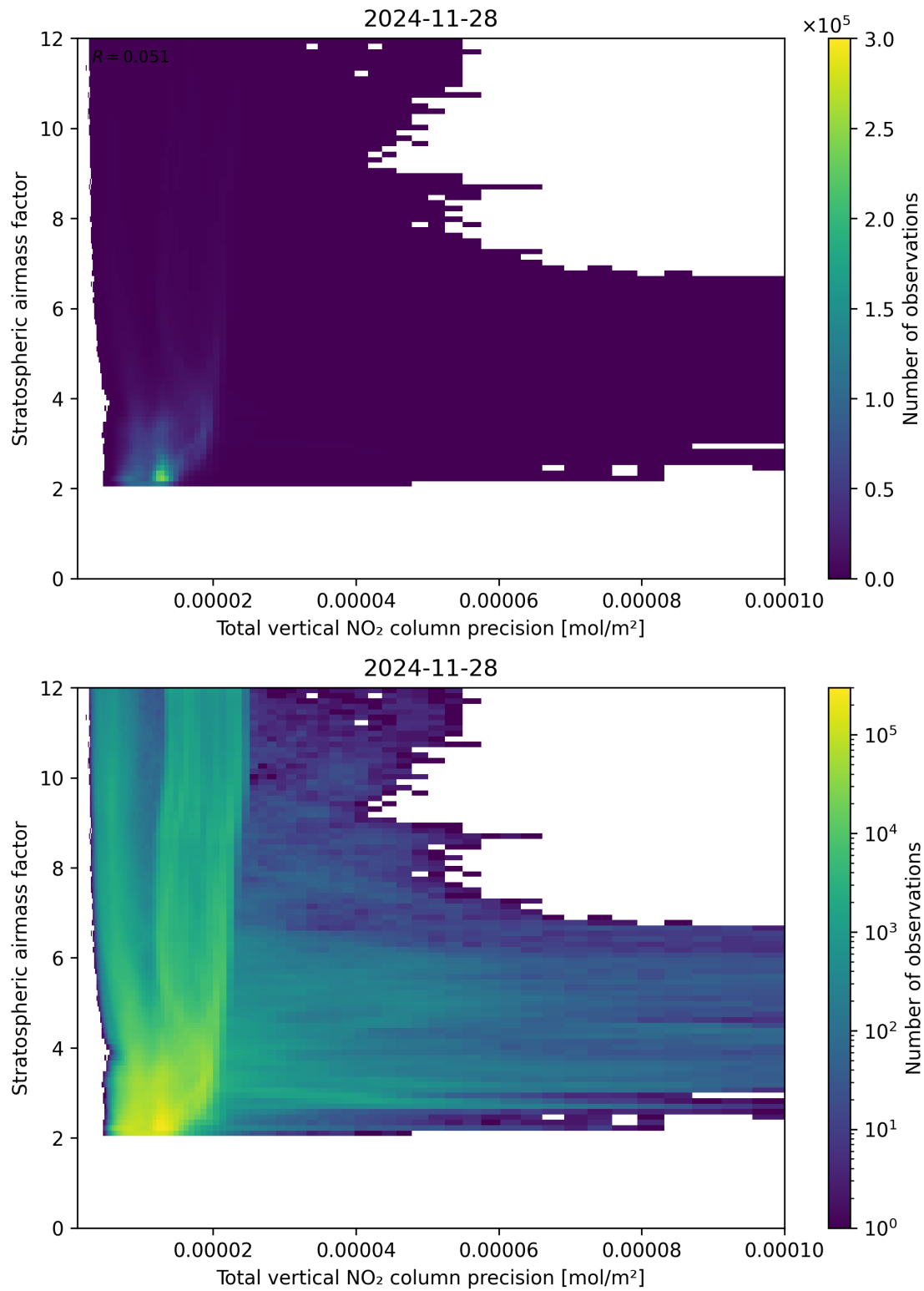
Figure 115: Scatter density plot of “Total vertical NO 2 column precision” against “Stratospheric air mass factor” for 2024-11-27 to 2024-11-29.
