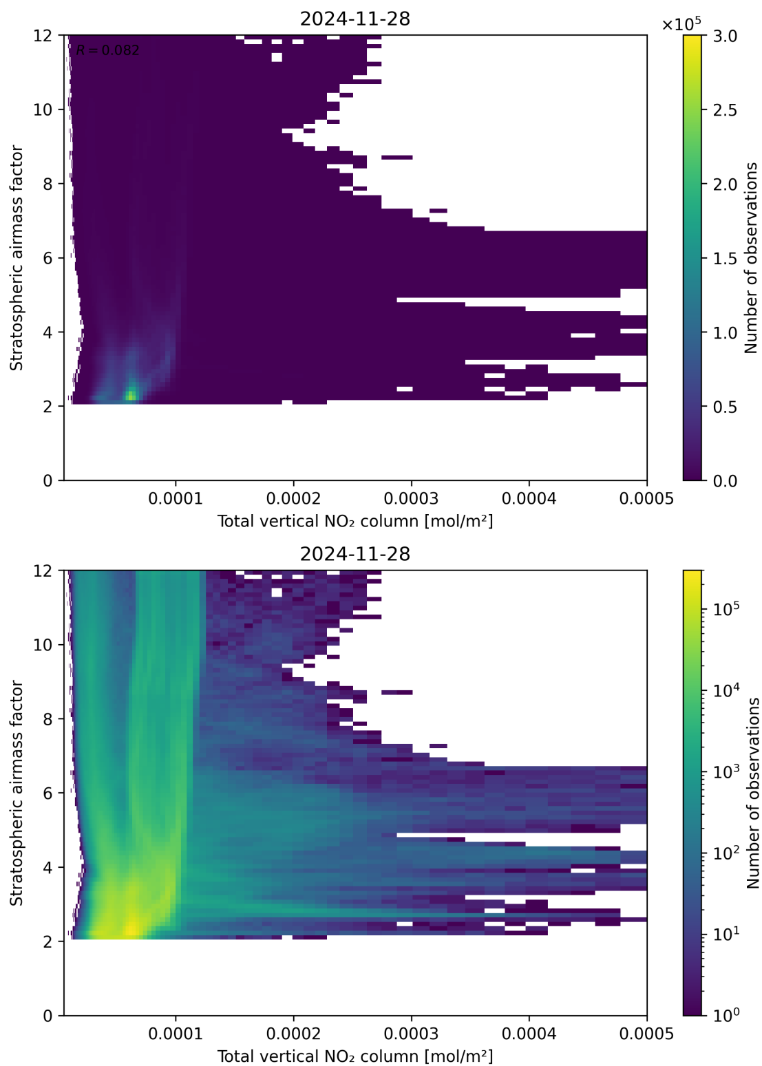
Figure 110: Scatter density plot of “Total vertical NO 2 column” against “Stratospheric airmass factor” for 2024-11-27 to 2024-11-29.
