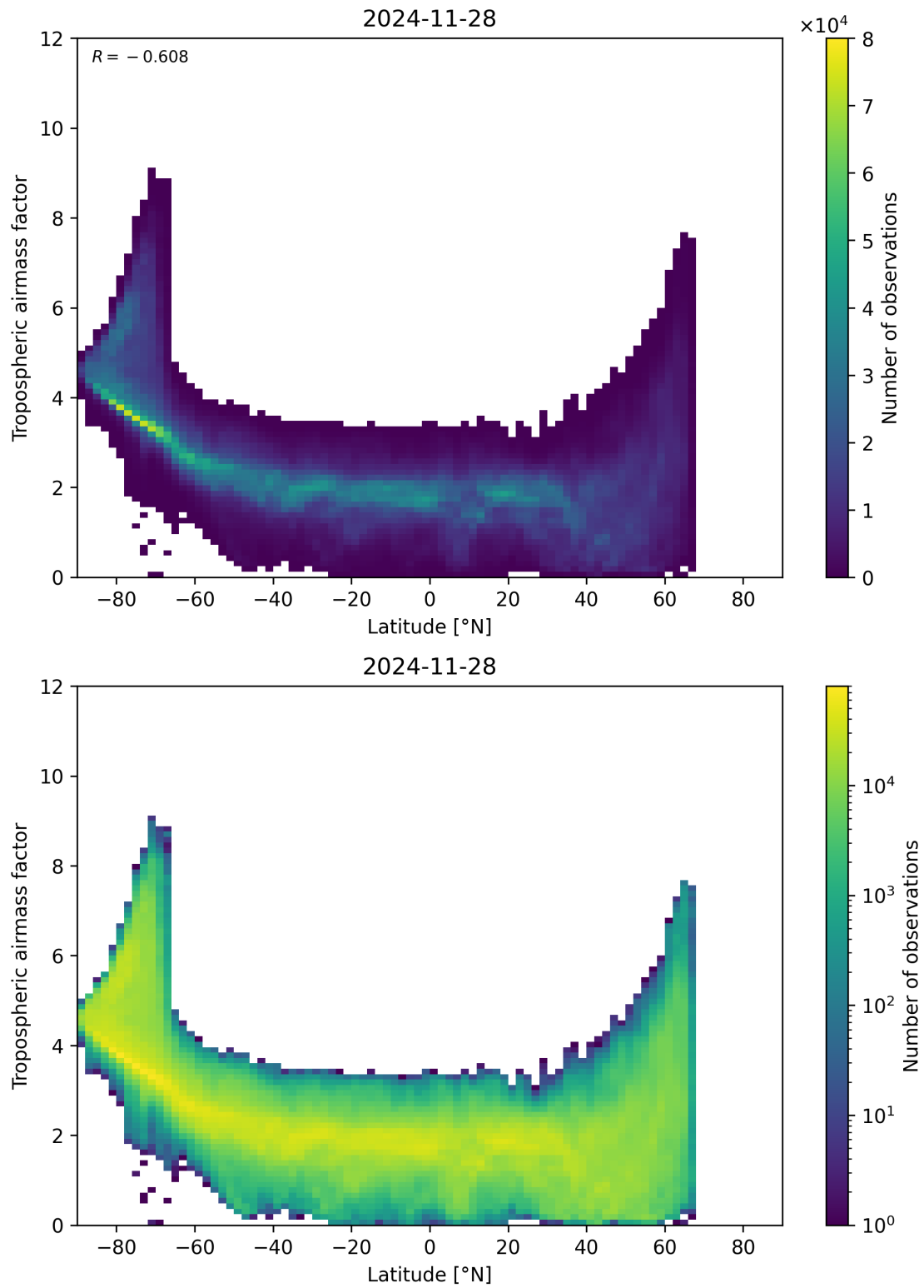
Figure 85: Scatter density plot of “Latitude” against “Tropospheric airmass factor” for 2024-11-27 to 2024-11-29.
