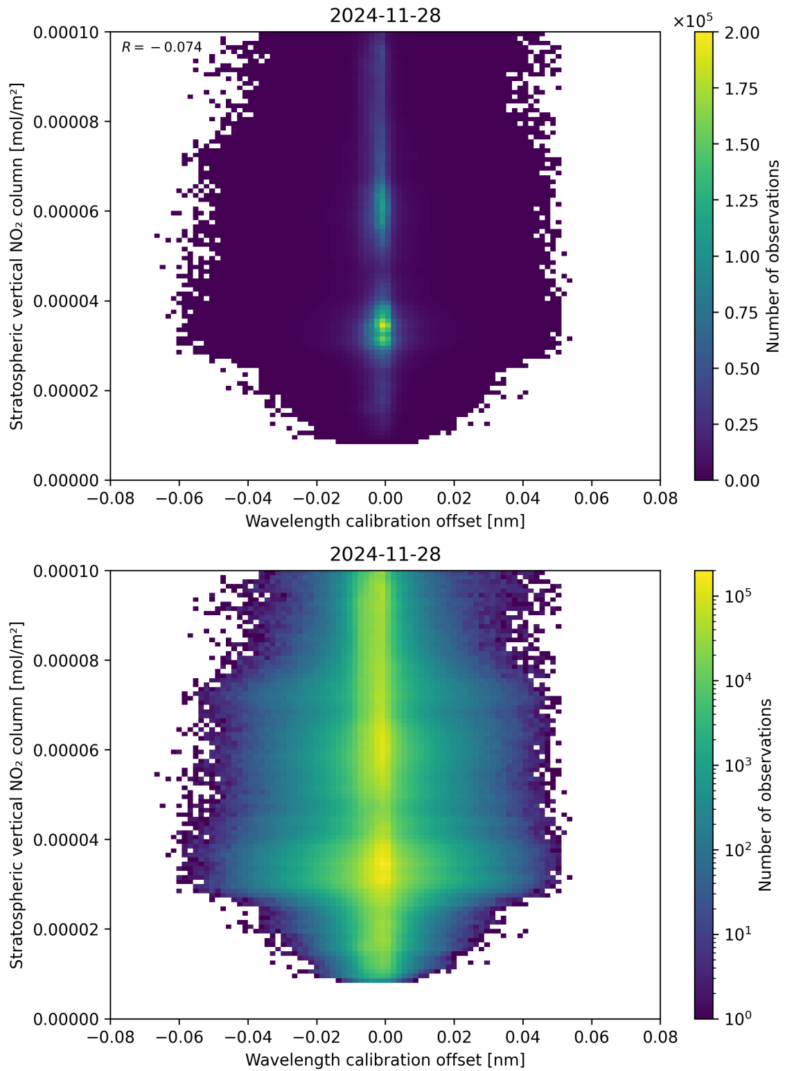
Figure 176: Scatter density plot of “Wavelength calibration offset” against “Stratospheric vertical NO 2 column” for 2024-11-27 to 2024-11-29.
