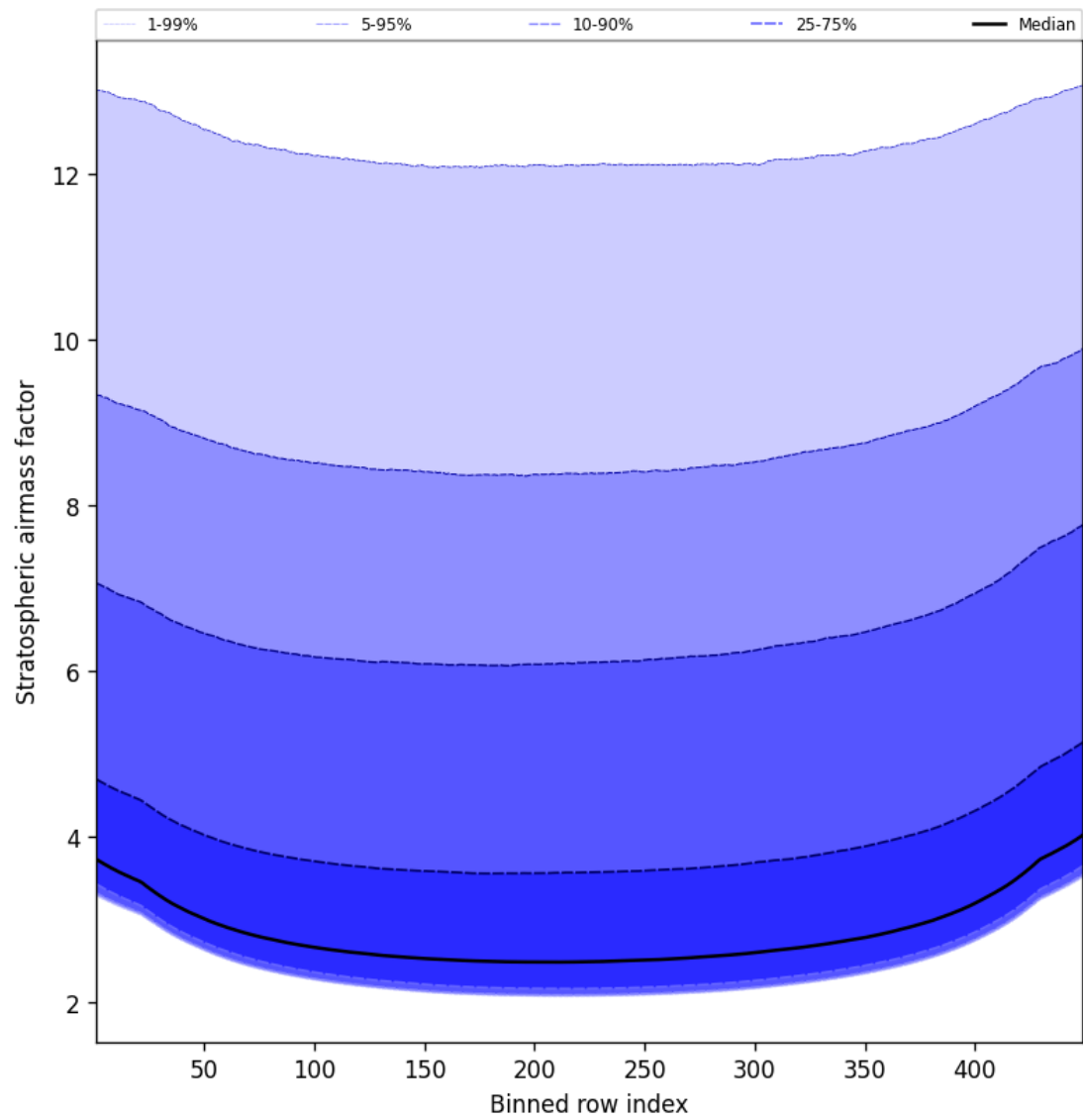
Figure 61: Along track statistics of “Stratospheric airmass factor” for 2024-11-27 to 2024-11-29
