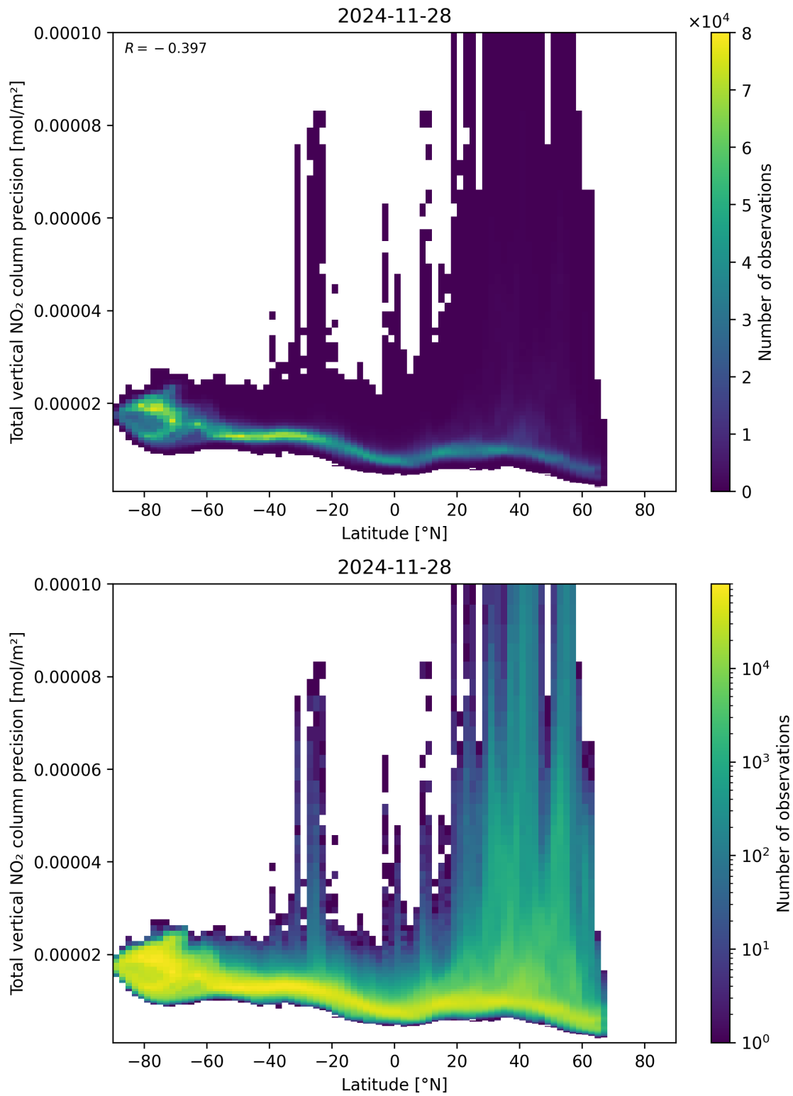
Figure 91: Scatter density plot of “Latitude” against “Total vertical NO 2 column precision” for 2024-11-27 to 2024-11-29.
