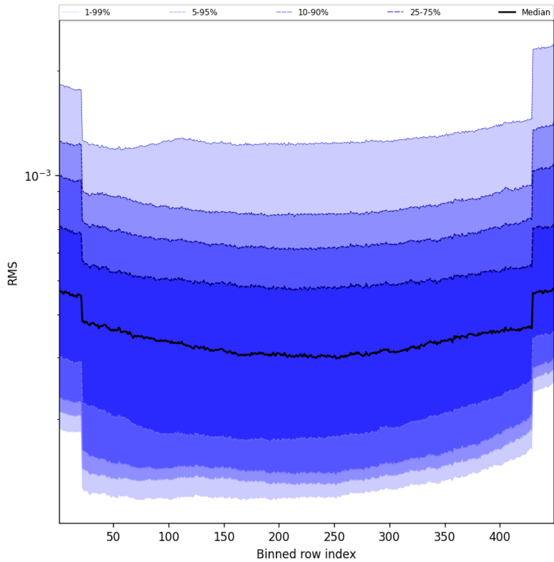
Figure 60: Along track statistics of “RMS” for 2024-11-27 to 2024-11-29
