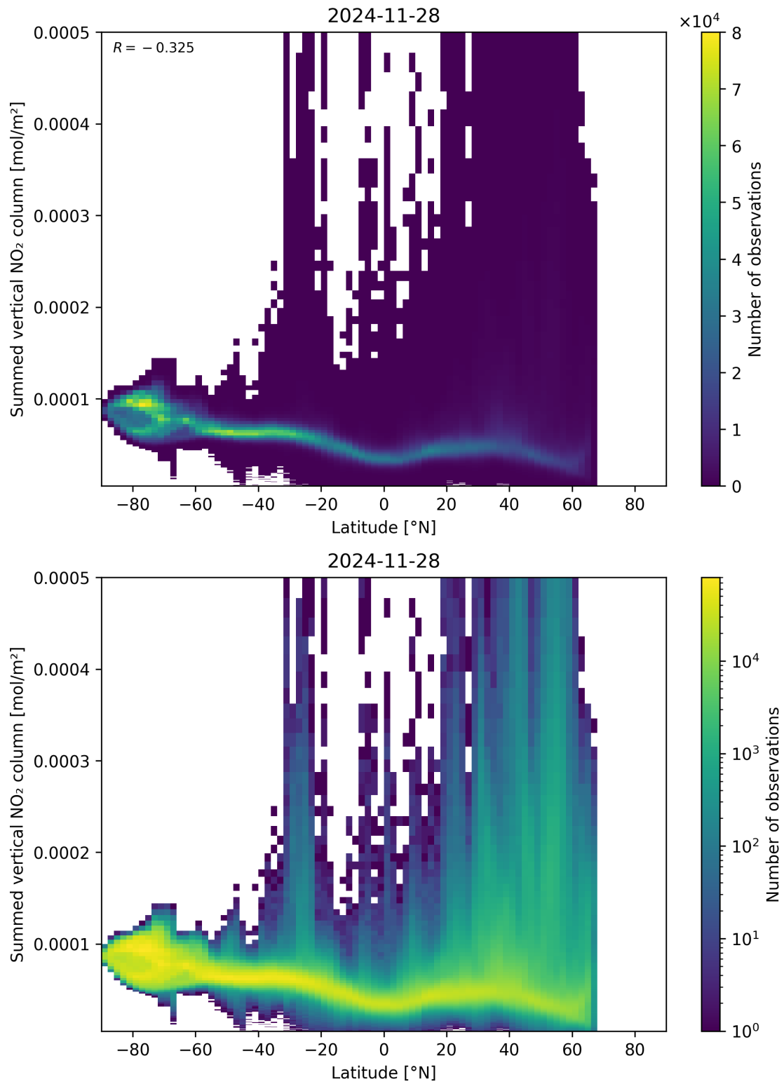
Figure 88: Scatter density plot of “Latitude” against “Summed vertical NO 2 column” for 2024-11-27 to 2024-11-29.
