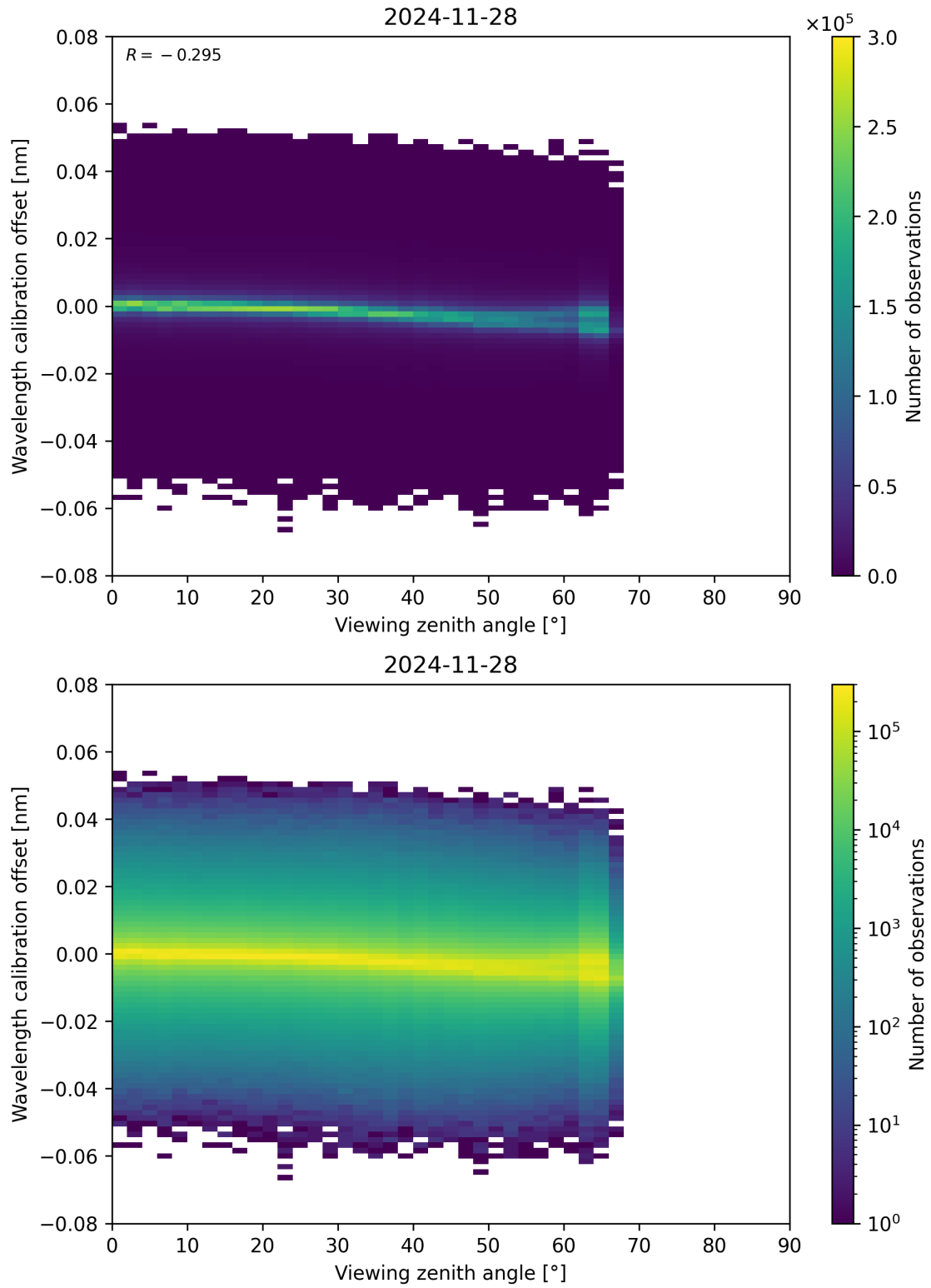
Figure 173: Scatter density plot of “Viewing zenith angle” against “Wavelength calibration offset” for 2024-11-27 to 2024-11-29.
