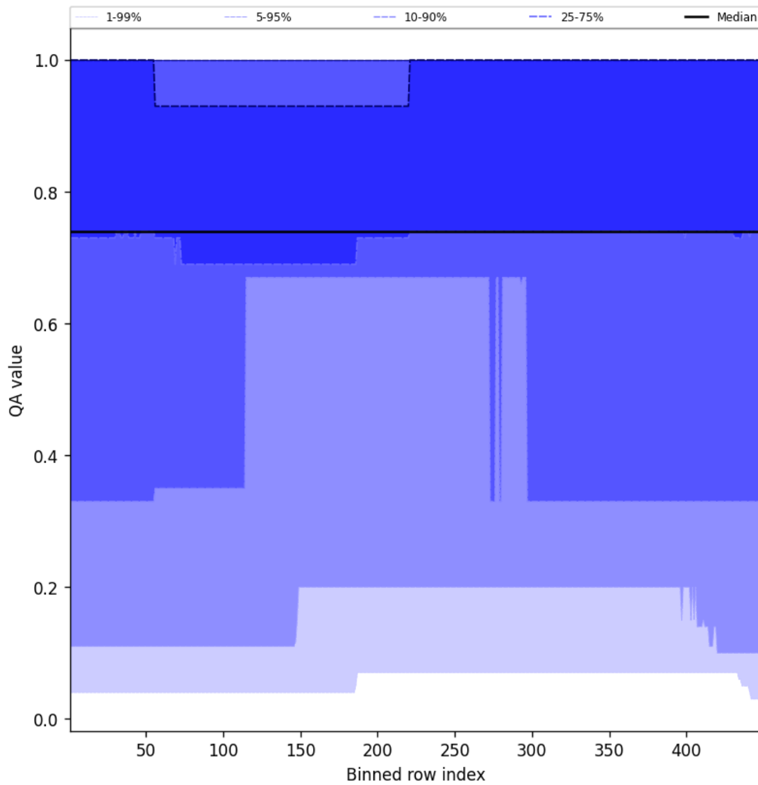
Figure 45: Along track statistics of “QA value” for 2024-11-27 to 2024-11-29
