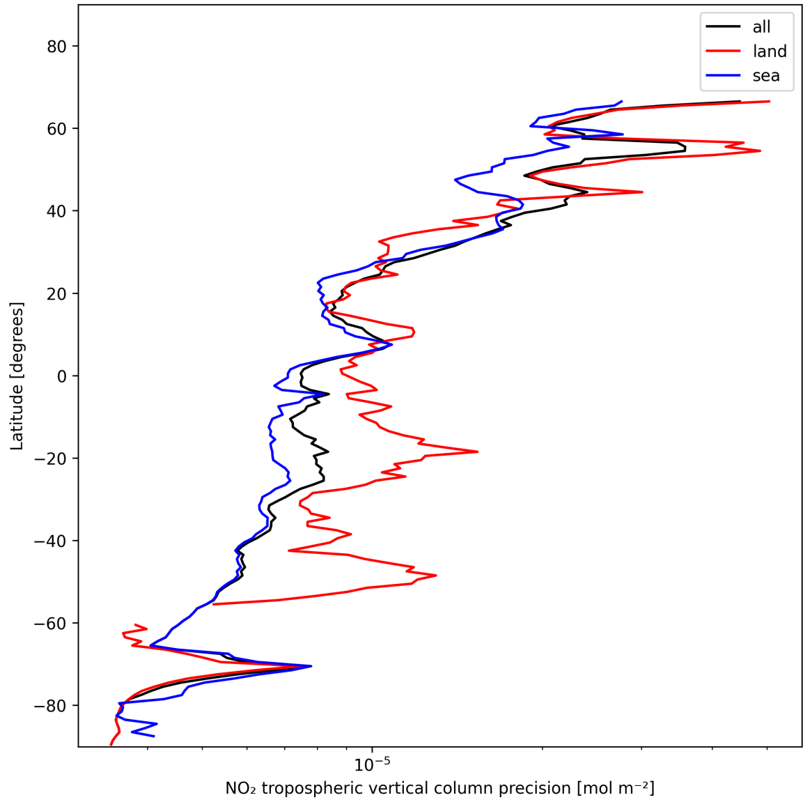
Figure 13: Zonal average of “NO 2 tropospheric vertical column precision” for 2024-11-27 to 2024-11-29.
