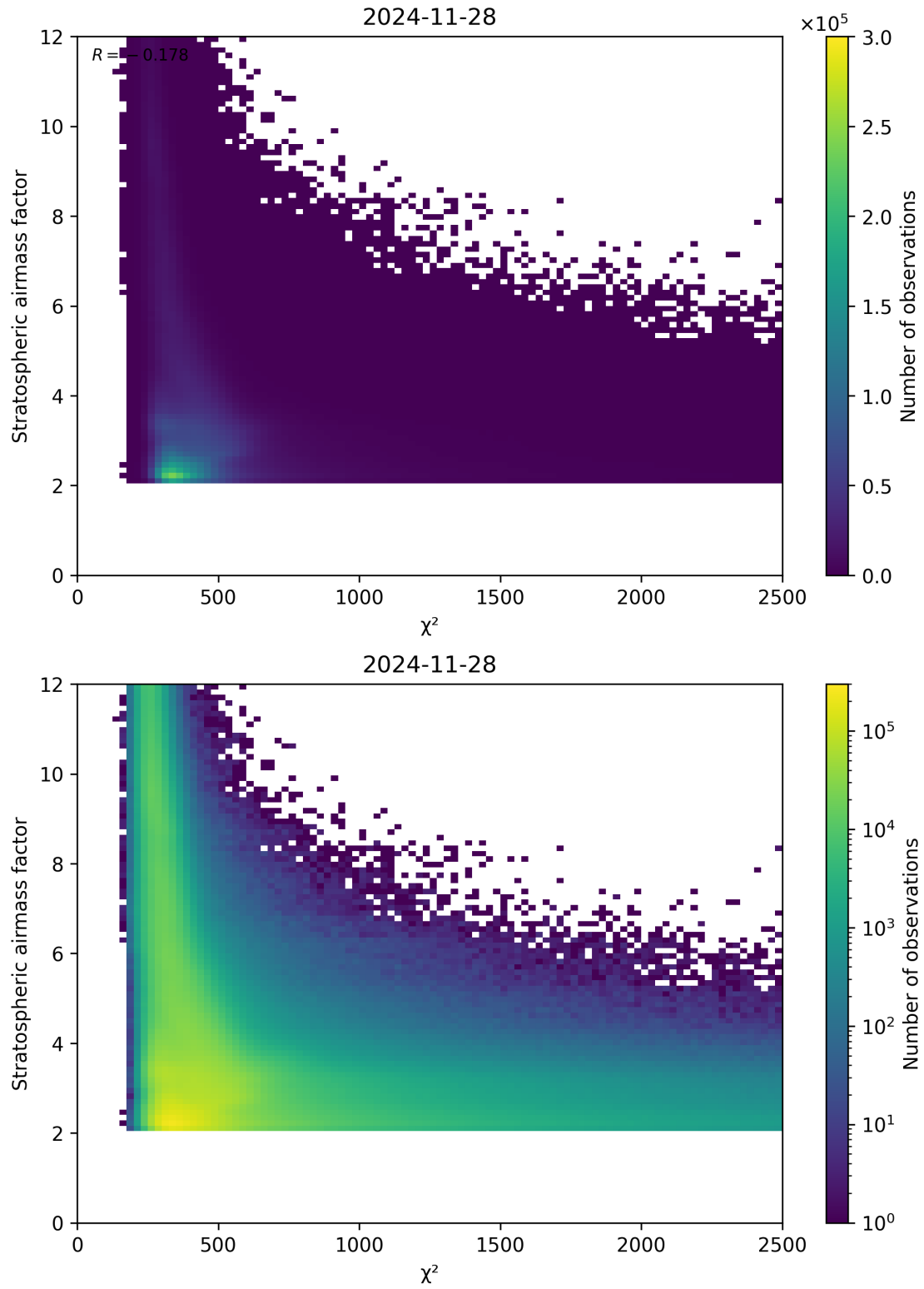
Figure 81: Scatter density plot of “ \chi^2 ” against “Stratospheric airmass factor” for 2024-11-27 to 2024-11-29.
