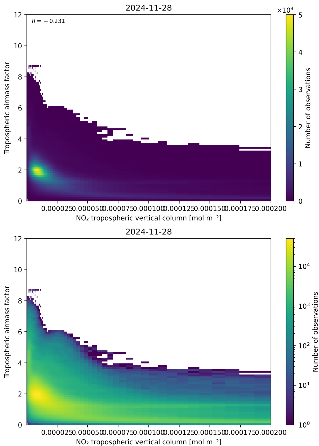
Figure 123: Scatter density plot of “NO 2 tropospheric vertical column” against “Tropospheric air mass factor” for 2024-11-27 to 2024-11-29.
