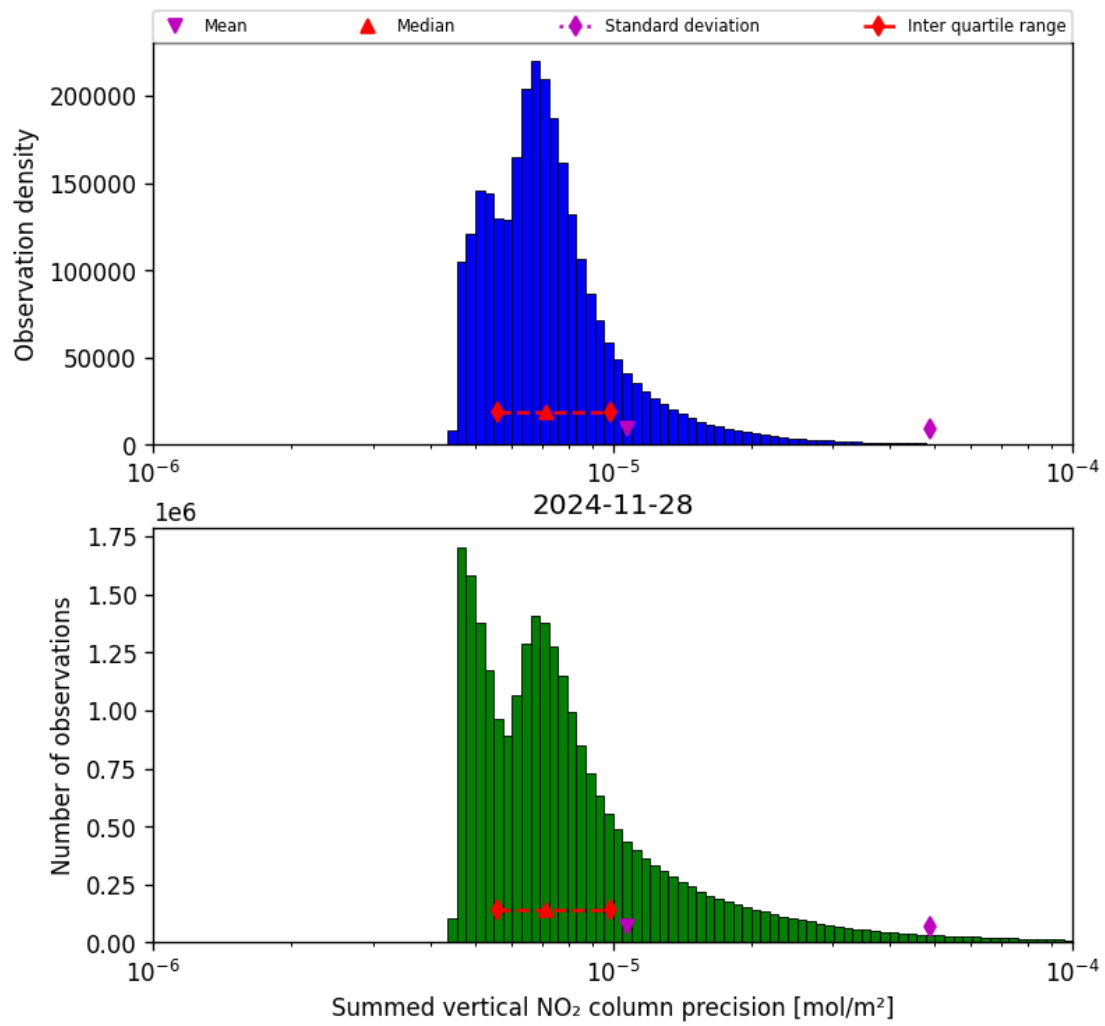
Figure 41: Histogram of “Summed vertical NO 2 column precision” for 2024-11-27 to 2024-11-29
