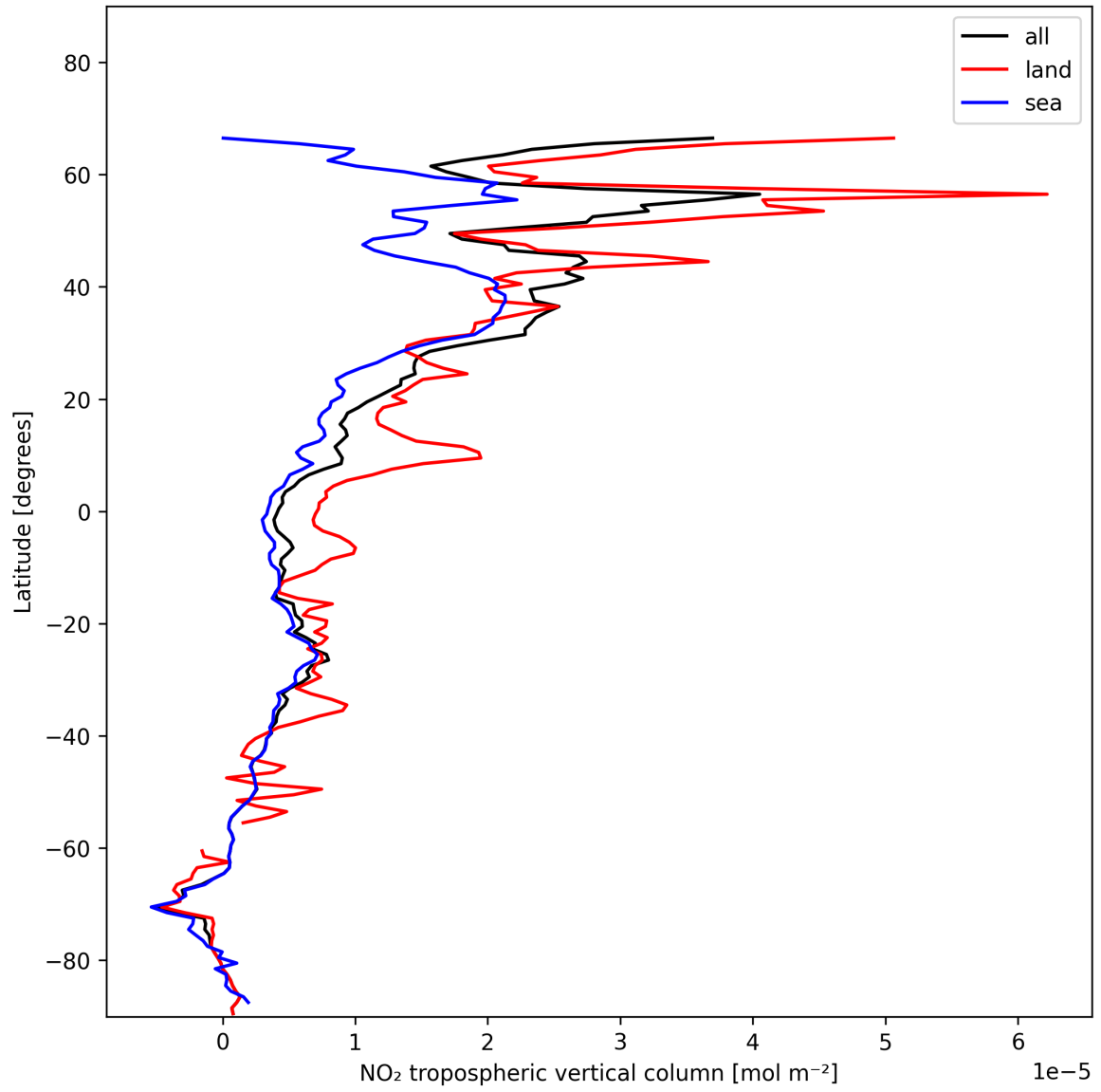
Figure 12: Zonal average of “NO 2 tropospheric vertical column” for 2024-11-27 to 2024-11-29.
