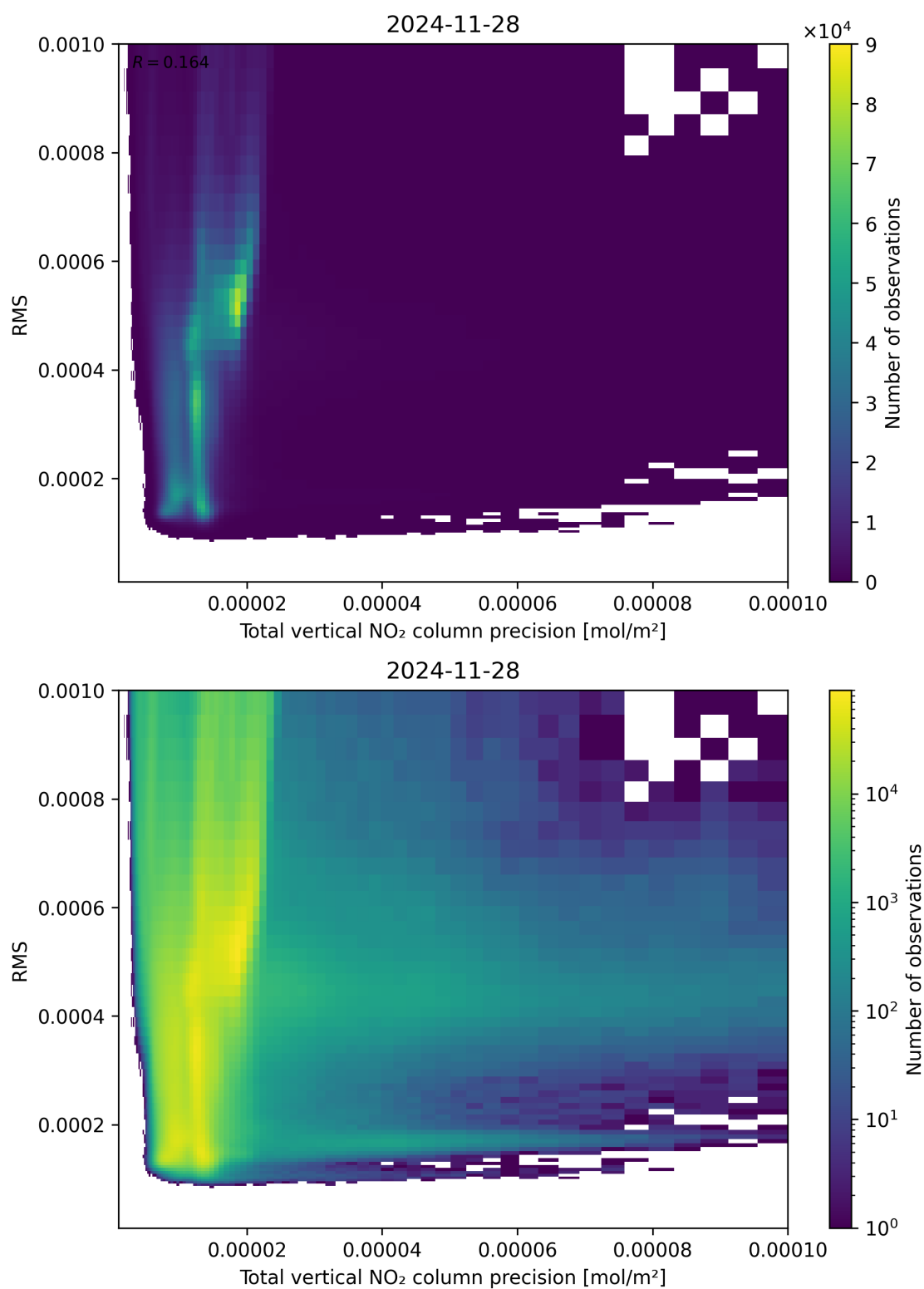
Figure 119: Scatter density plot of “Total vertical NO 2 column precision” against “RMS” for 2024-11-27 to 2024-11-29.
