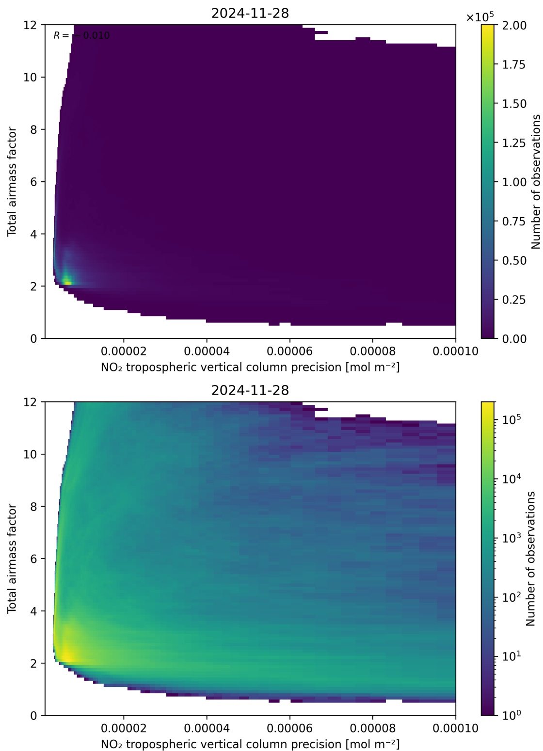
Figure 132: Scatter density plot of “NO 2 tropospheric vertical column precision” against “Total air mass factor” for 2024-11-27 to 2024-11-29.
