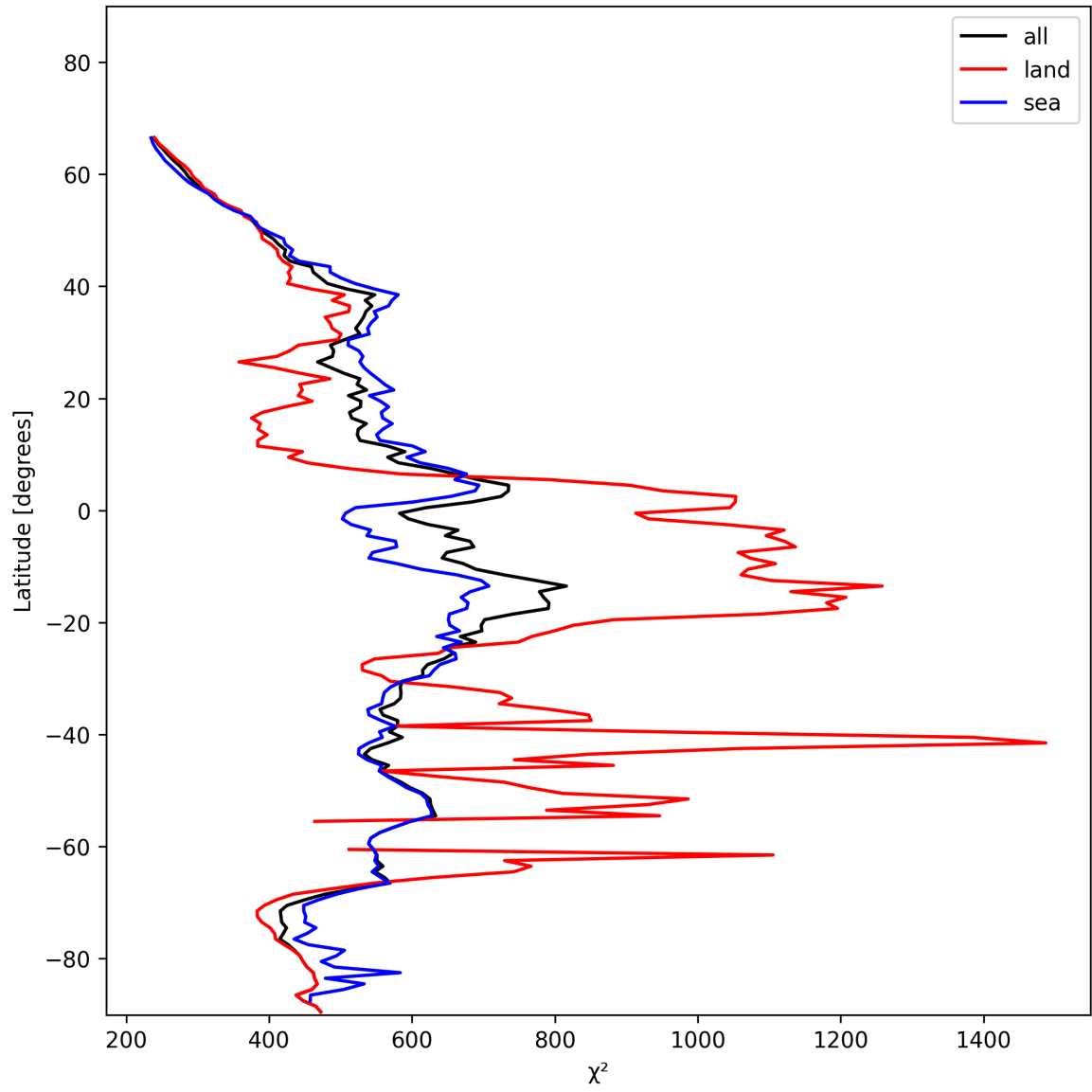
Figure 25: Zonal average of “ \chi^2 ” for 2024-11-27 to 2024-11-29.
