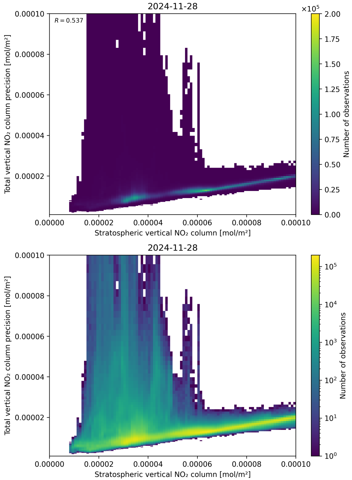
Figure 101: Scatter density plot of “Stratospheric vertical NO 2 column” against “Total vertical NO 2 column precision” for 2024-11-27 to 2024-11-29.
