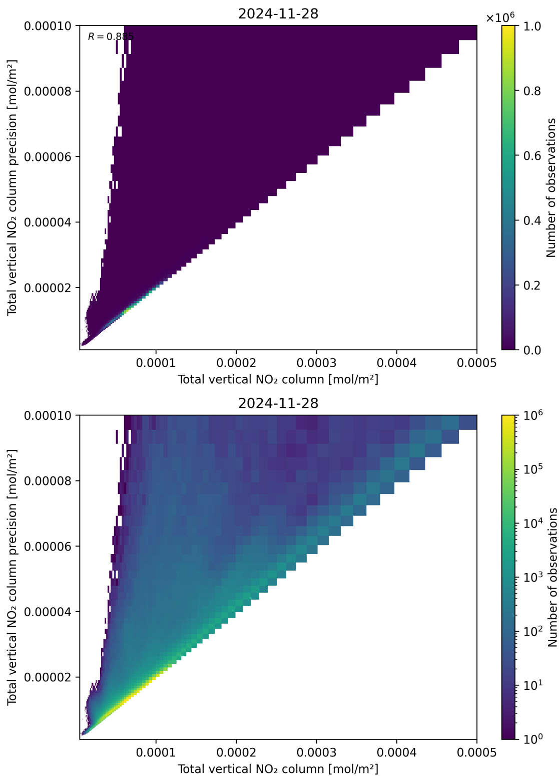
Figure 114: Scatter density plot of “Total vertical NO 2 column” against “Total vertical NO 2 column precision” for 2024-11-27 to 2024-11-29.
