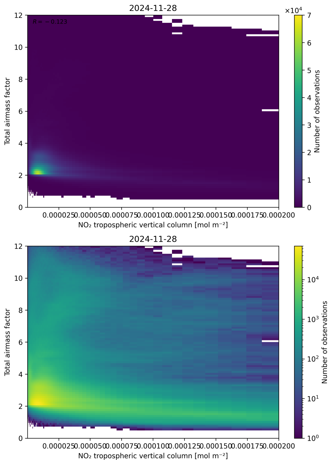
Figure 122: Scatter density plot of “NO 2 tropospheric vertical column” against “Total air mass factor” for 2024-11-27 to 2024-11-29.
