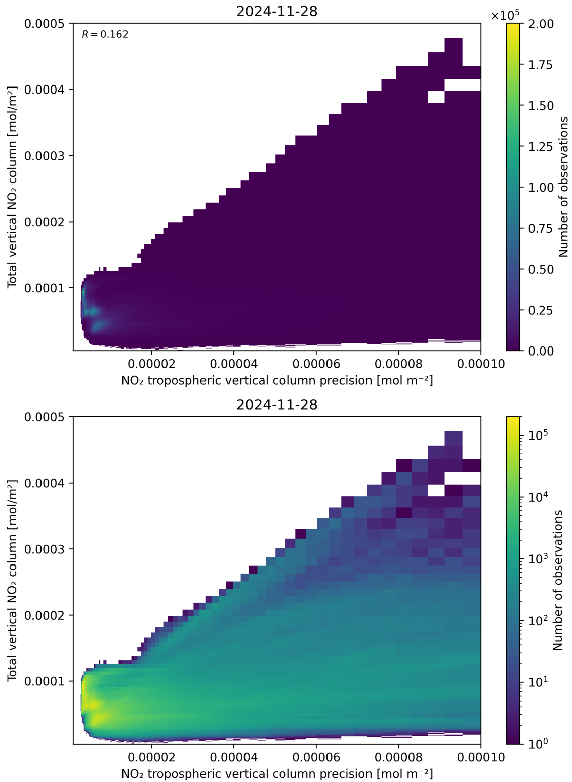
Figure 138: Scatter density plot of “NO 2 tropospheric vertical column precision” against “Total vertical NO 2 column” for 2024-11-27 to 2024-11-29.
