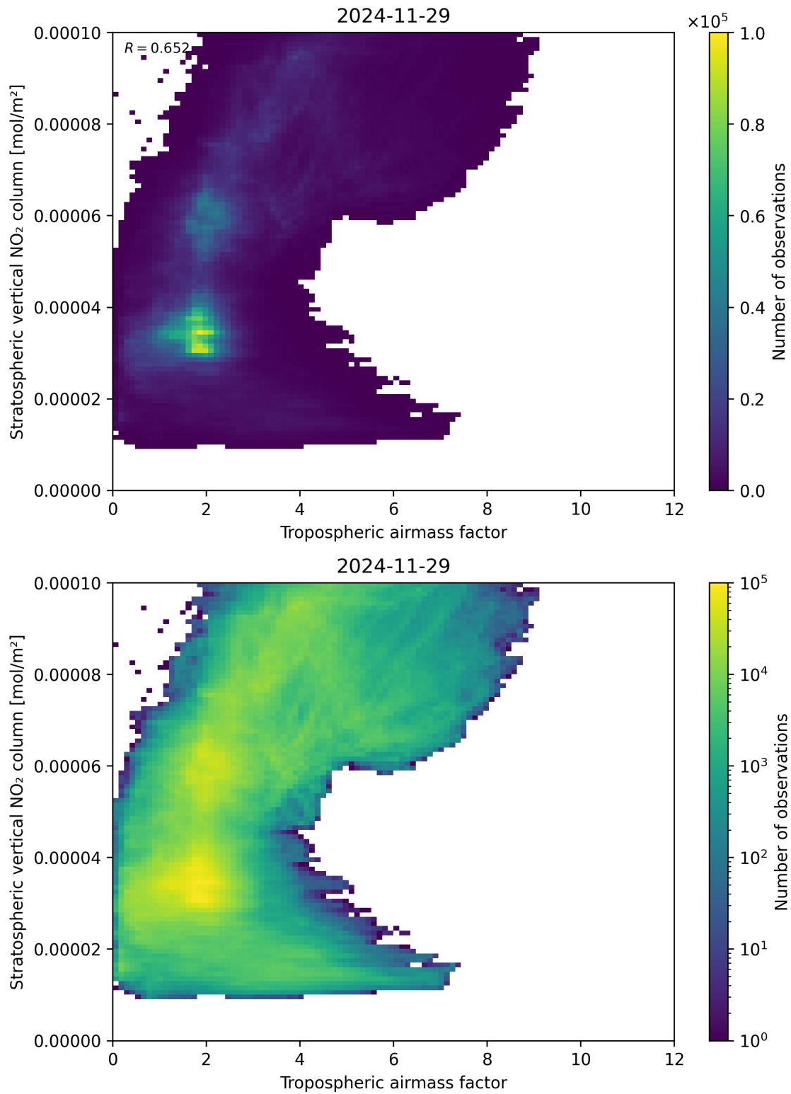
Figure 74: Scatter density plot of “Tropospheric air mass factor” against “Stratospheric vertical NO 2 column” for 2024-11-28 to 2024-11-30.
