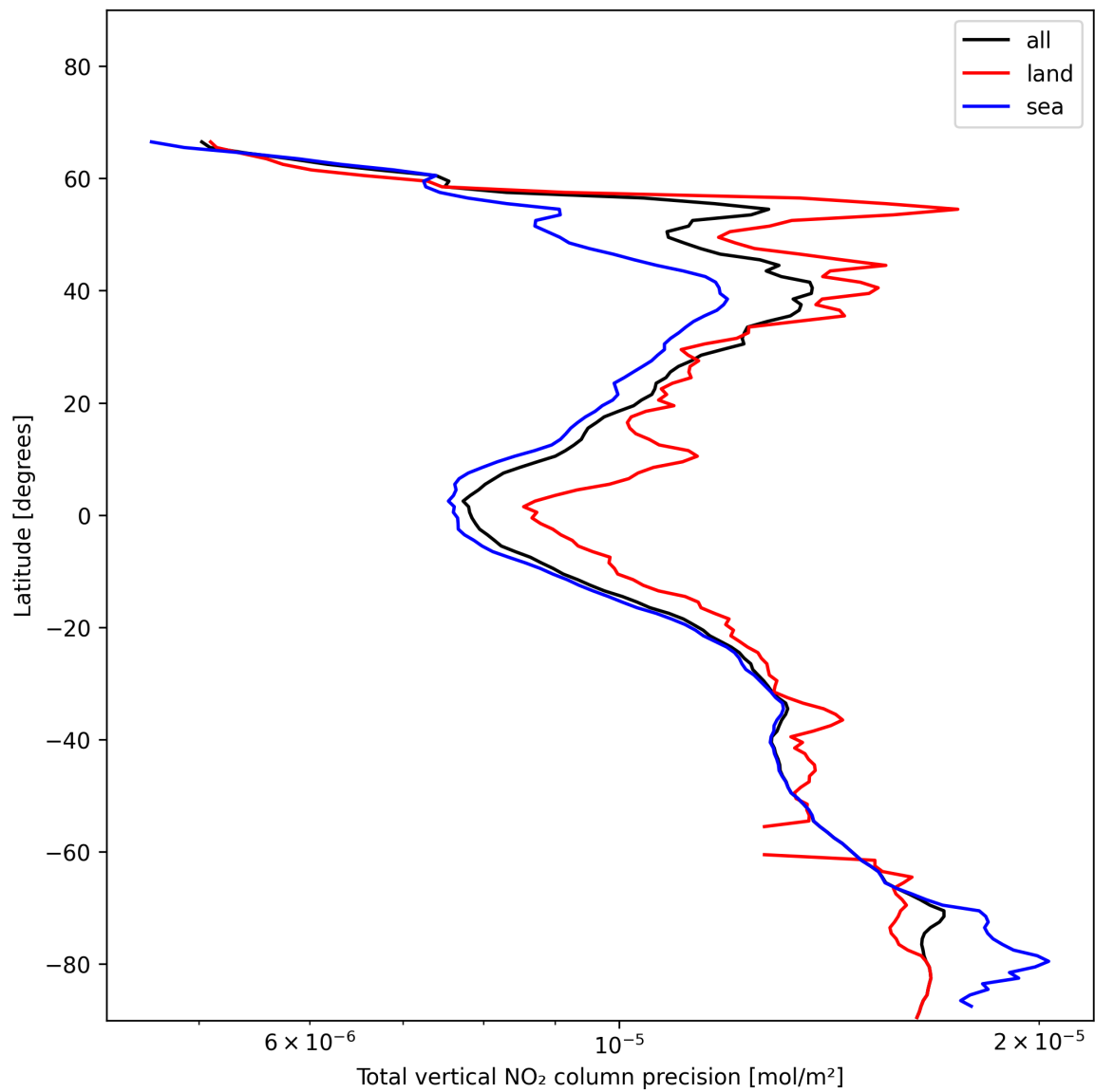
Figure 22: Zonal average of “Total vertical NO 2 column precision” for 2024-11-28 to 2024-11-30.
