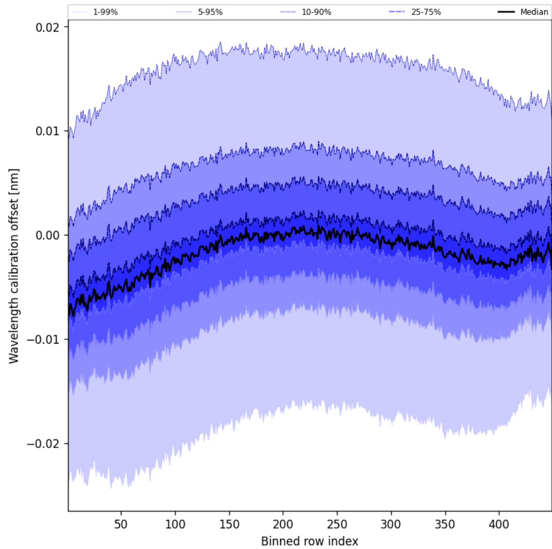
Figure 52: Along track statistics of “Wavelength calibration offset” for 2024-11-28 to 2024-11-30
