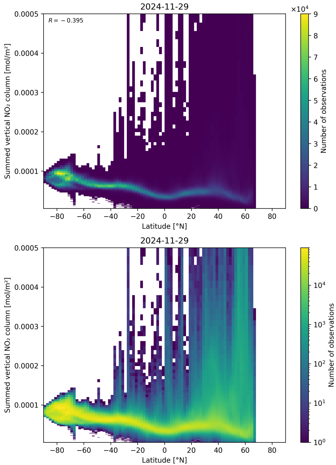
Figure 88: Scatter density plot of “Latitude” against “Summed vertical NO 2 column” for 2024-11-28 to 2024-11-30.
