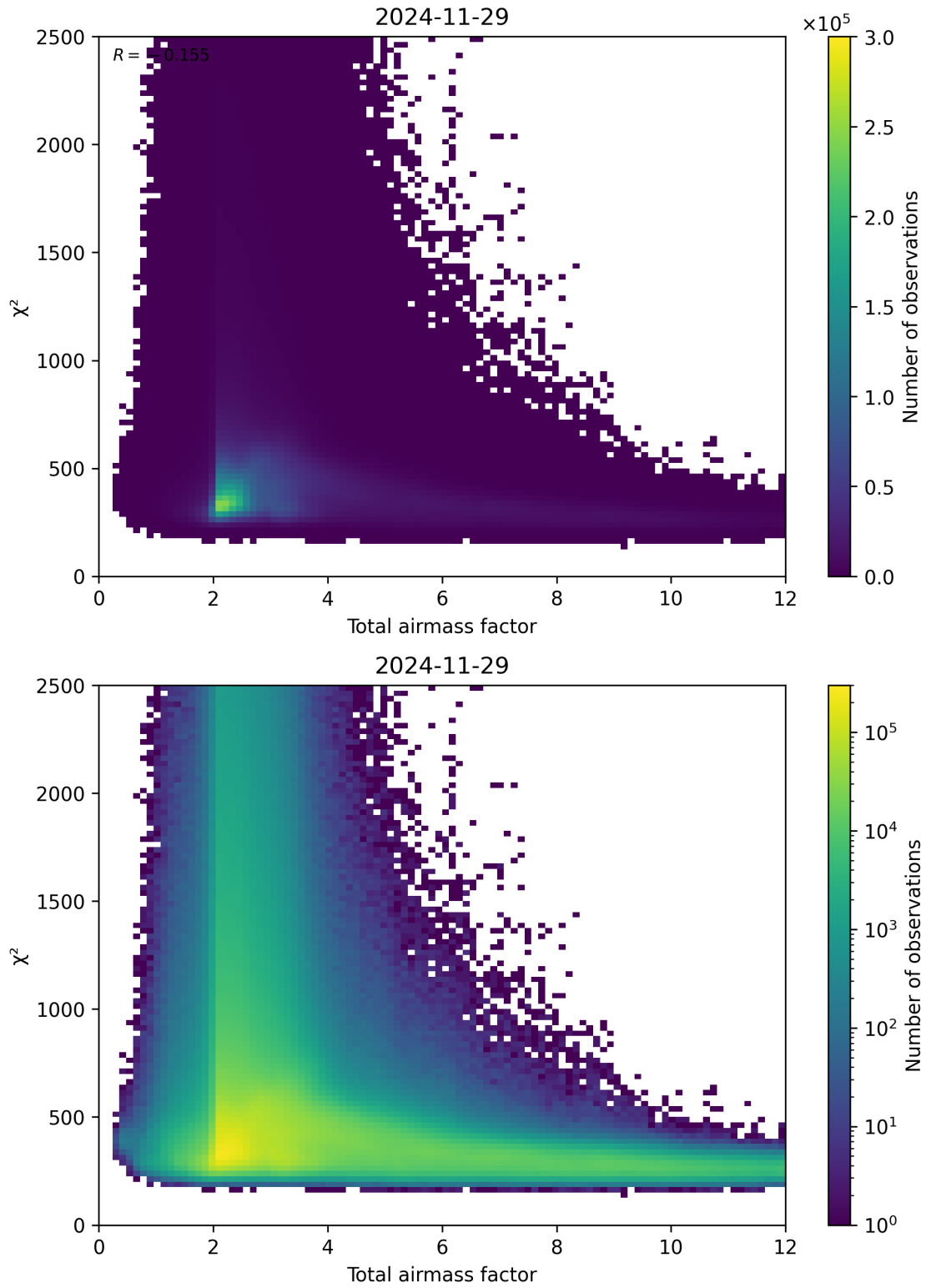
Figure 63: Scatter density plot of “Total airmass factor” against “ \chi^2 ” for 2024-11-28 to 2024-11-30.
