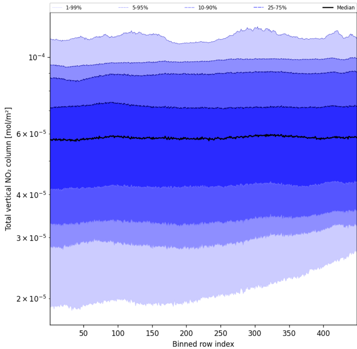
Figure 55: Along track statistics of “Total vertical NO 2 column” for 2024-11-28 to 2024-11-30
