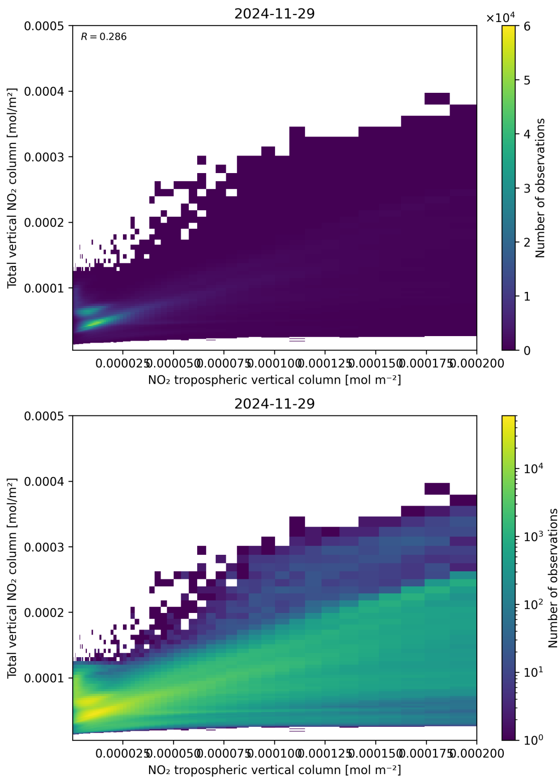
Figure 128: Scatter density plot of “NO 2 tropospheric vertical column” against “Total vertical NO 2 column” for 2024-11-28 to 2024-11-30.
