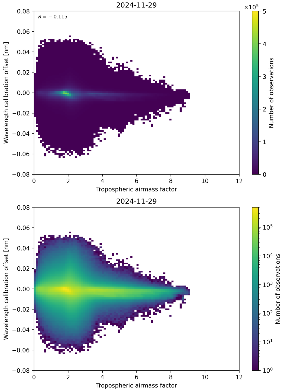
Figure 80: Scatter density plot of “Tropospheric airmass factor” against “Wavelength calibration offset” for 2024-11-28 to 2024-11-30.
