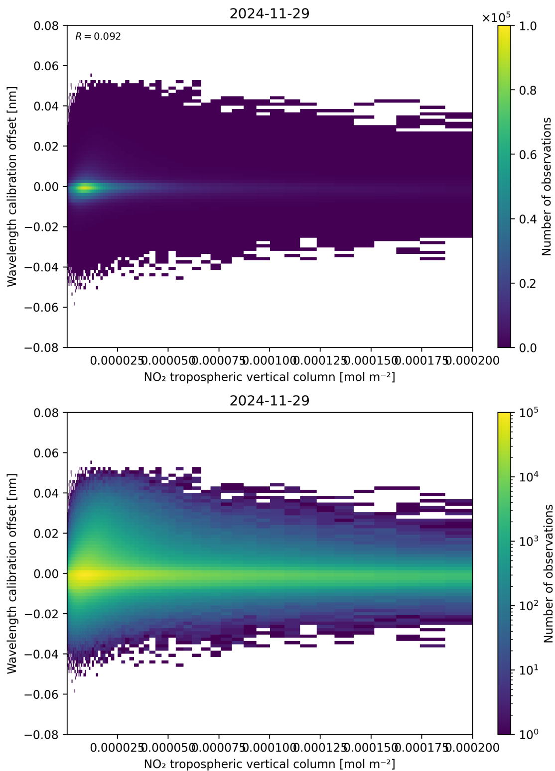
Figure 143: Scatter density plot of “NO 2 tropospheric vertical column” against “Wavelength calibration offset” for 2024-11-28 to 2024-11-30.
