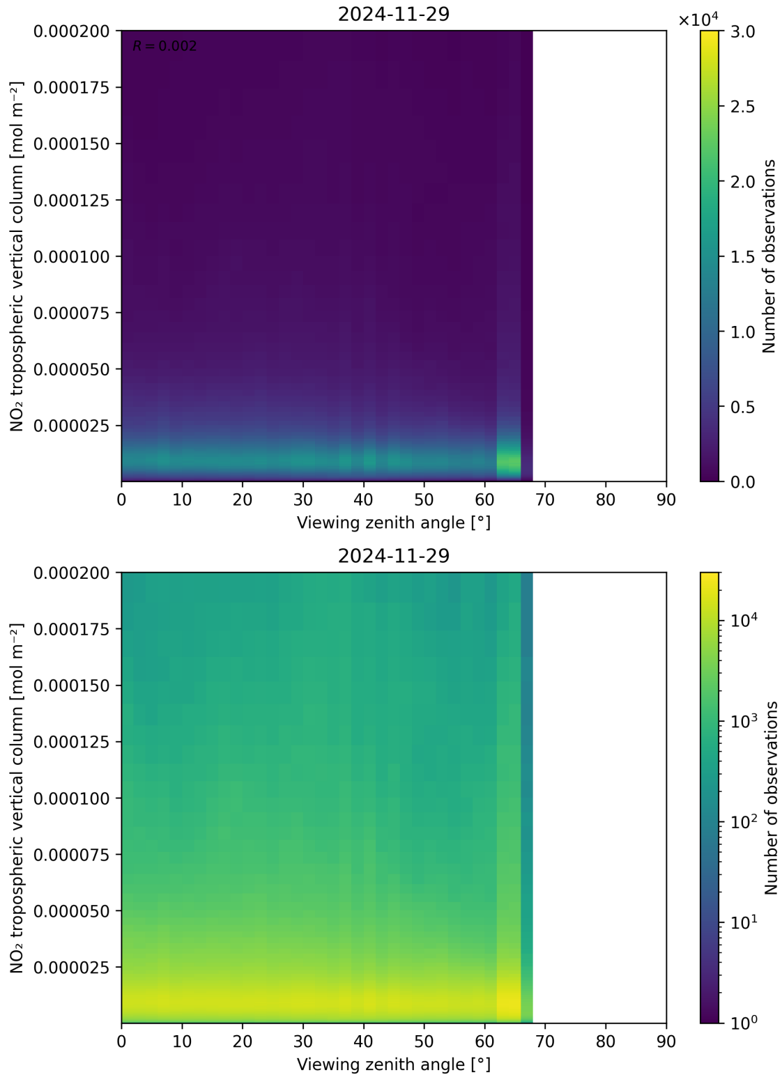
Figure 169: Scatter density plot of “Viewing zenith angle” against “NO 2 tropospheric vertical column” for 2024-11-28 to 2024-11-30.
