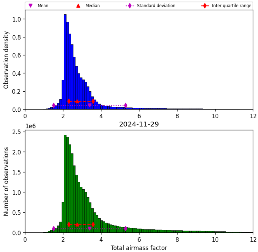
Figure 32: Histogram of “Total airmass factor” for 2024-11-28 to 2024-11-30
