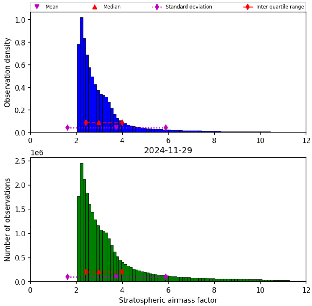
Figure 44: Histogram of “Stratospheric airmass factor” for 2024-11-28 to 2024-11-30
