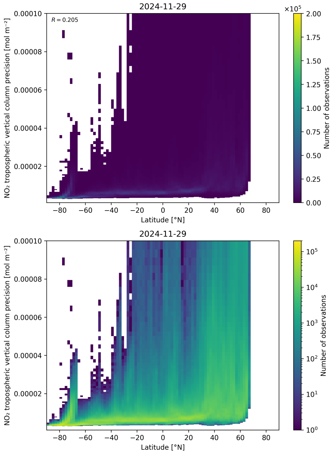
Figure 93: Scatter density plot of “Latitude” against “NO 2 tropospheric vertical column precision” for 2024-11-28 to 2024-11-30.
