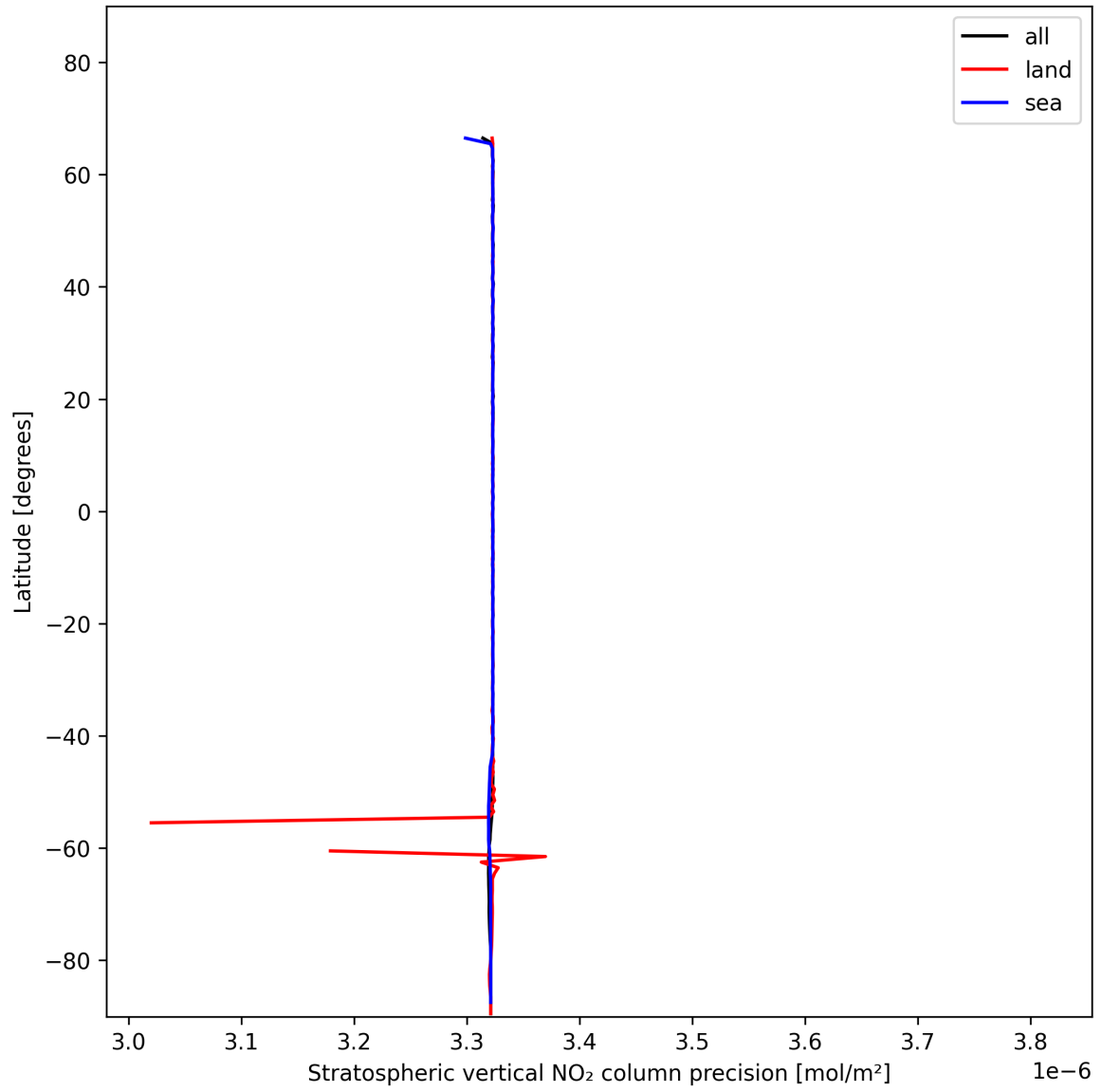
Figure 20: Zonal average of “Stratospheric vertical NO 2 column precision” for 2024-11-28 to 2024-11-30.
