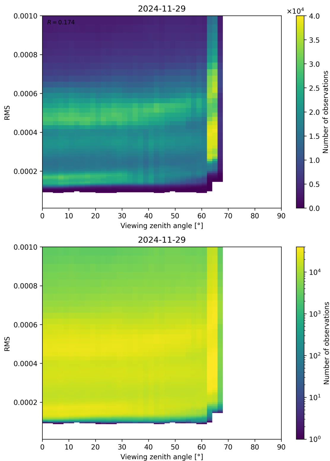
Figure 171: Scatter density plot of “Viewing zenith angle” against “RMS” for 2024-11-28 to 2024-11-30.
