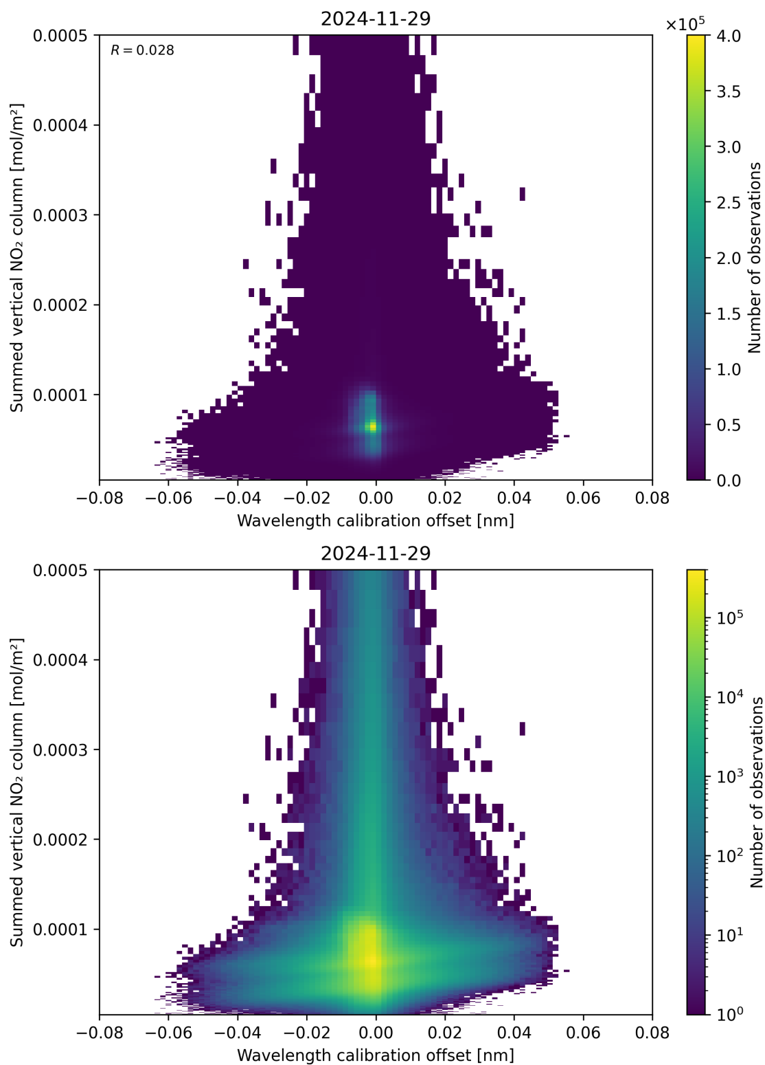
Figure 177: Scatter density plot of “Wavelength calibration offset” against “Summed vertical NO 2 column” for 2024-11-28 to 2024-11-30.
