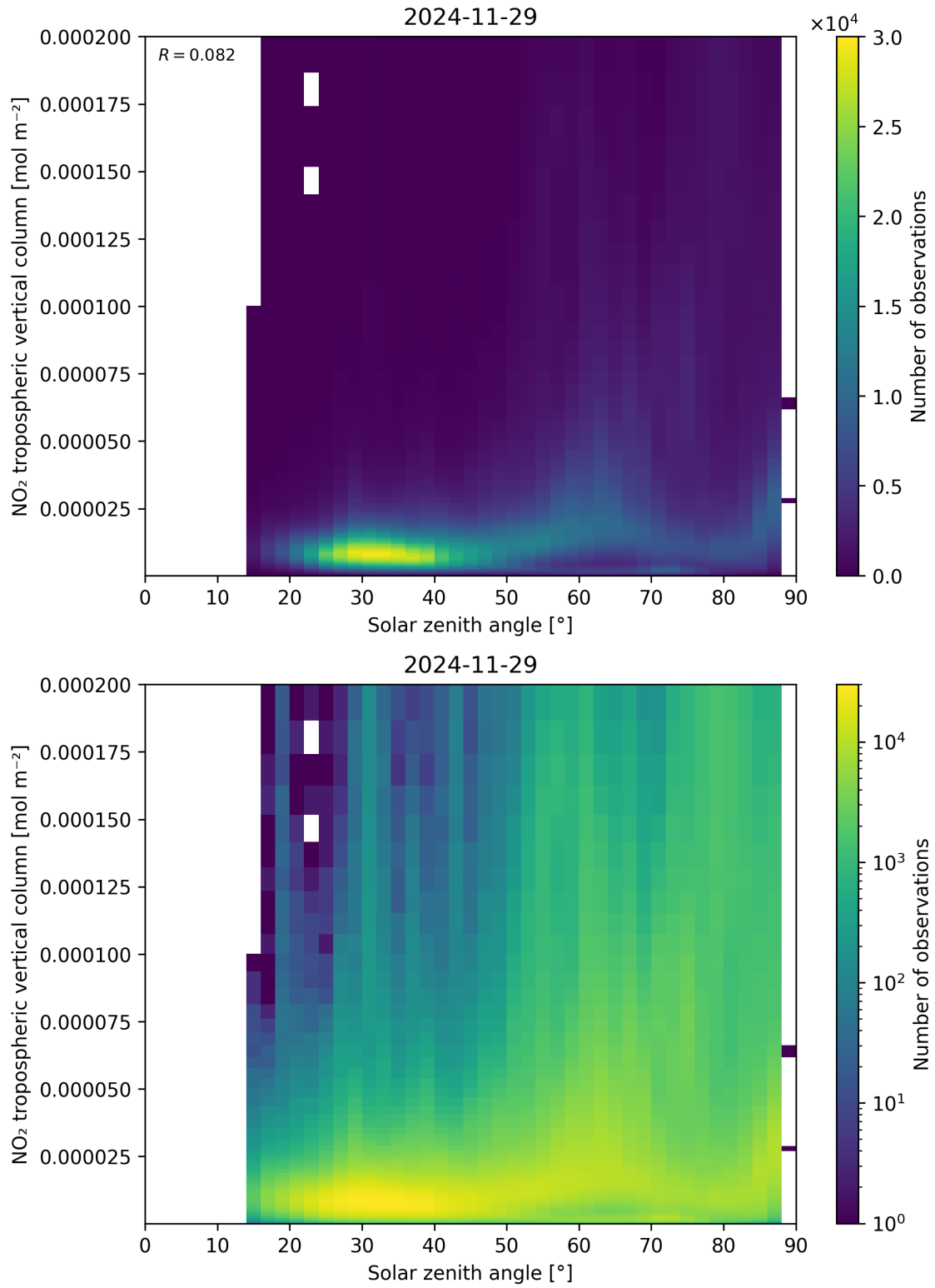
Figure 155: Scatter density plot of “Solar zenith angle” against “NO 2 tropospheric vertical column” for 2024-11-28 to 2024-11-30.
