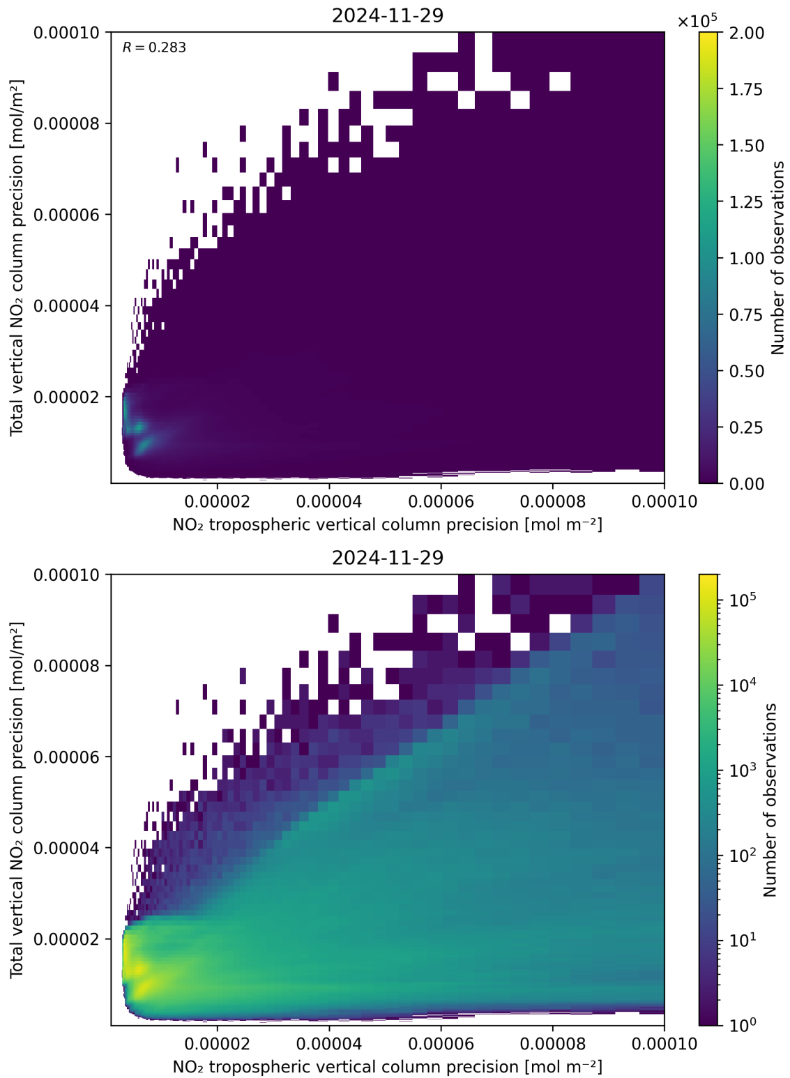
Figure 139: Scatter density plot of “NO 2 tropospheric vertical column precision” against “Total vertical NO 2 column precision” for 2024-11-28 to 2024-11-30.
