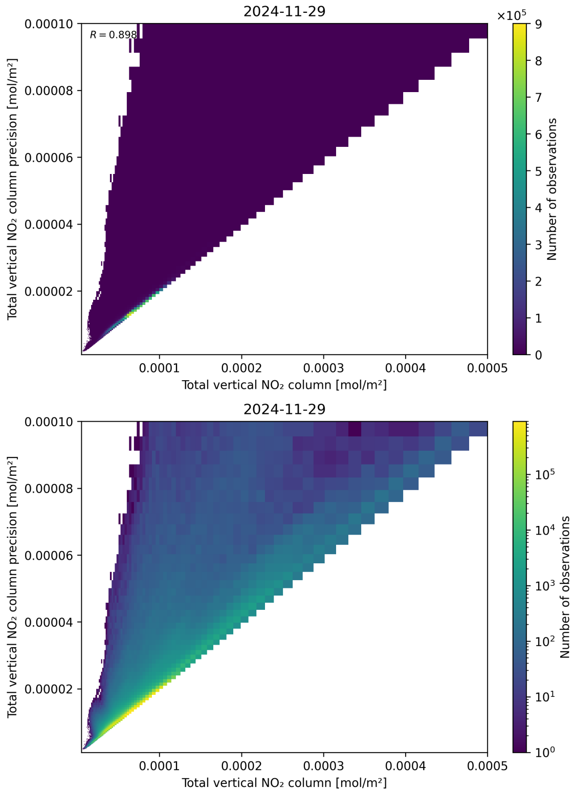
Figure 114: Scatter density plot of “Total vertical NO 2 column” against “Total vertical NO 2 column precision” for 2024-11-28 to 2024-11-30.
