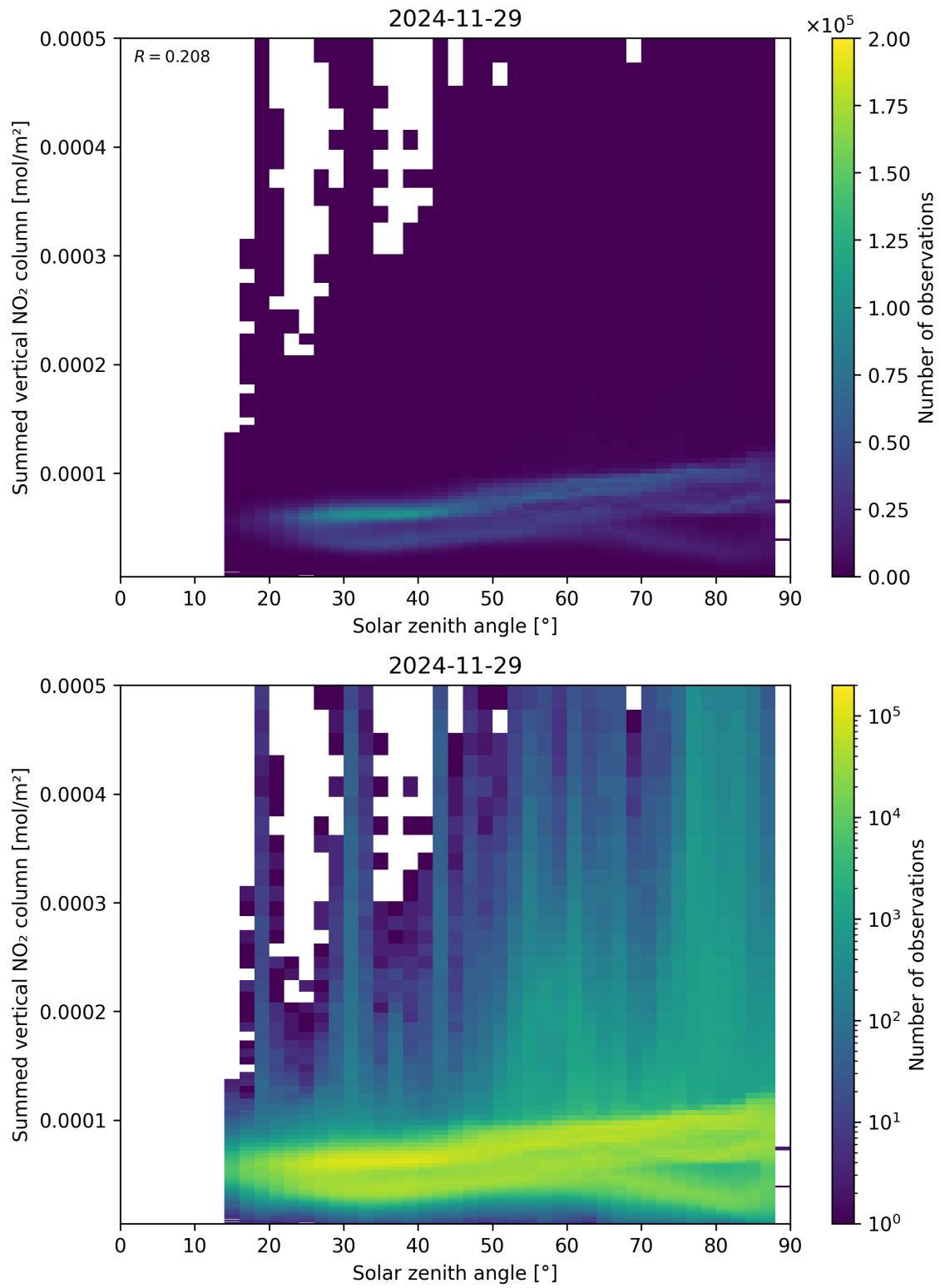
Figure 151: Scatter density plot of “Solar zenith angle” against “Summed vertical NO 2 column” for 2024-11-28 to 2024-11-30.
