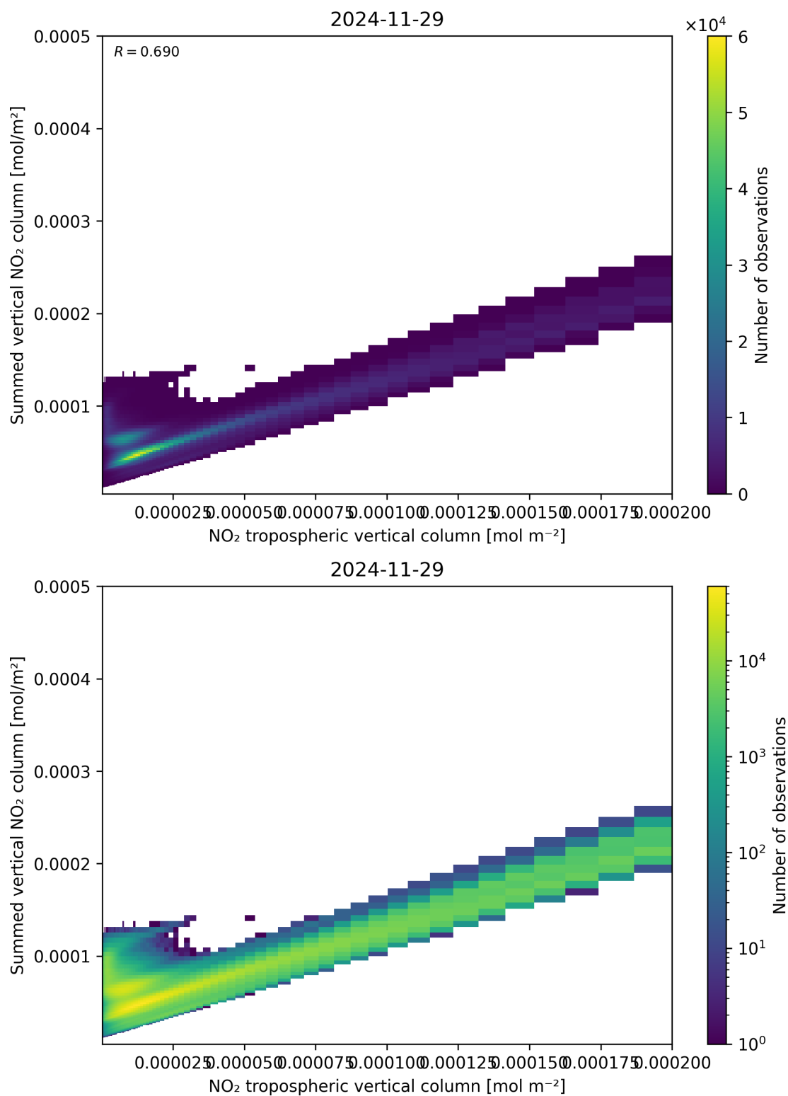
Figure 126: Scatter density plot of “NO 2 tropospheric vertical column” against “Summed vertical NO 2 column” for 2024-11-28 to 2024-11-30.
