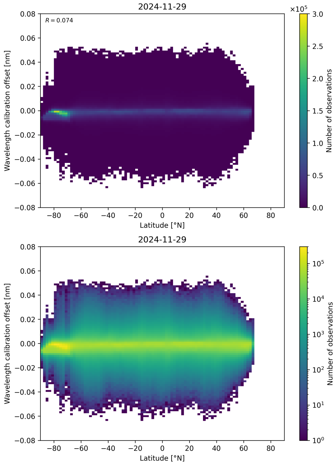
Figure 95: Scatter density plot of “Latitude” against “Wavelength calibration offset” for 2024-11-28 to 2024-11-30.
