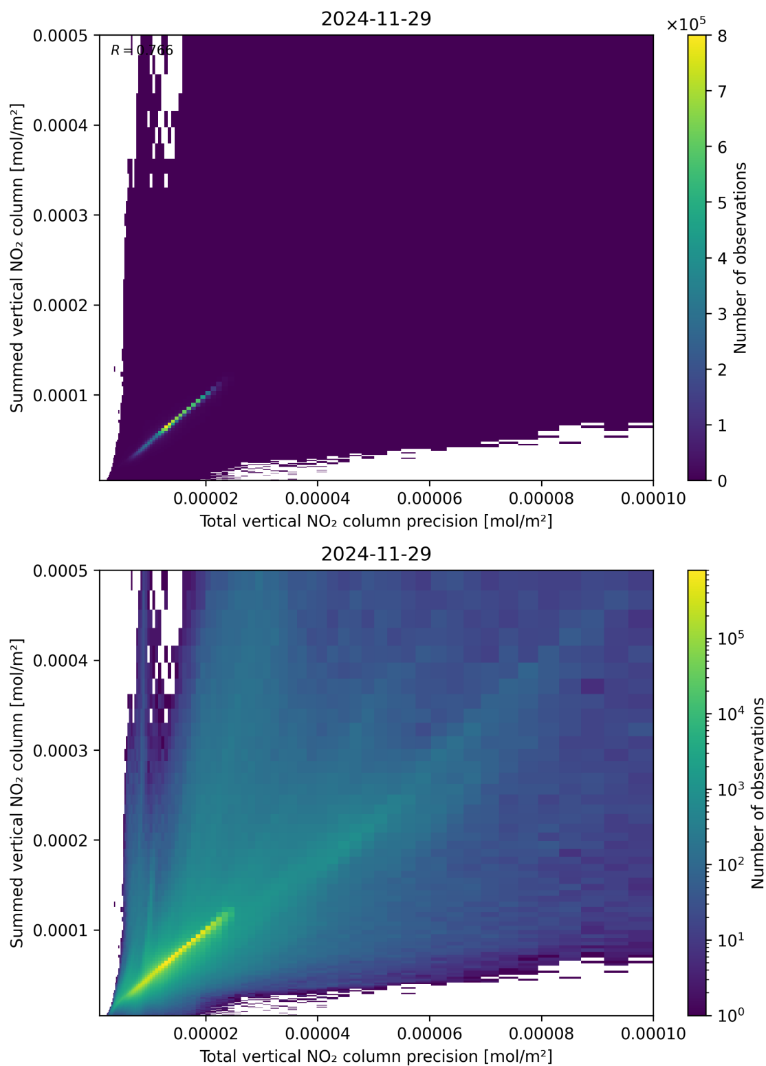
Figure 117: Scatter density plot of “Total vertical NO 2 column precision” against “Summed vertical NO 2 column” for 2024-11-28 to 2024-11-30.
