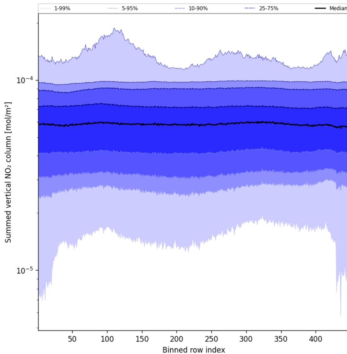
Figure 57: Along track statistics of “Summed vertical NO 2 column” for 2024-11-28 to 2024-11-30
