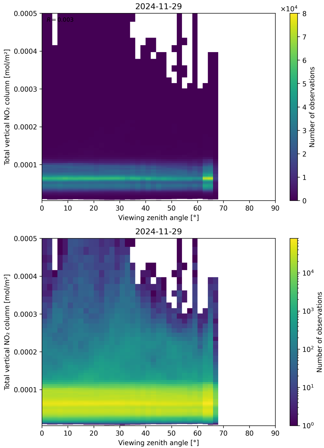
Figure 167: Scatter density plot of “Viewing zenith angle” against “Total vertical NO 2 column” for 2024-11-28 to 2024-11-30.
