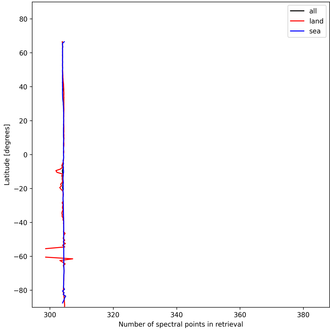
Figure 16: Zonal average of “Number of spectral points in retrieval” for 2024-11-28 to 2024-11-30.
