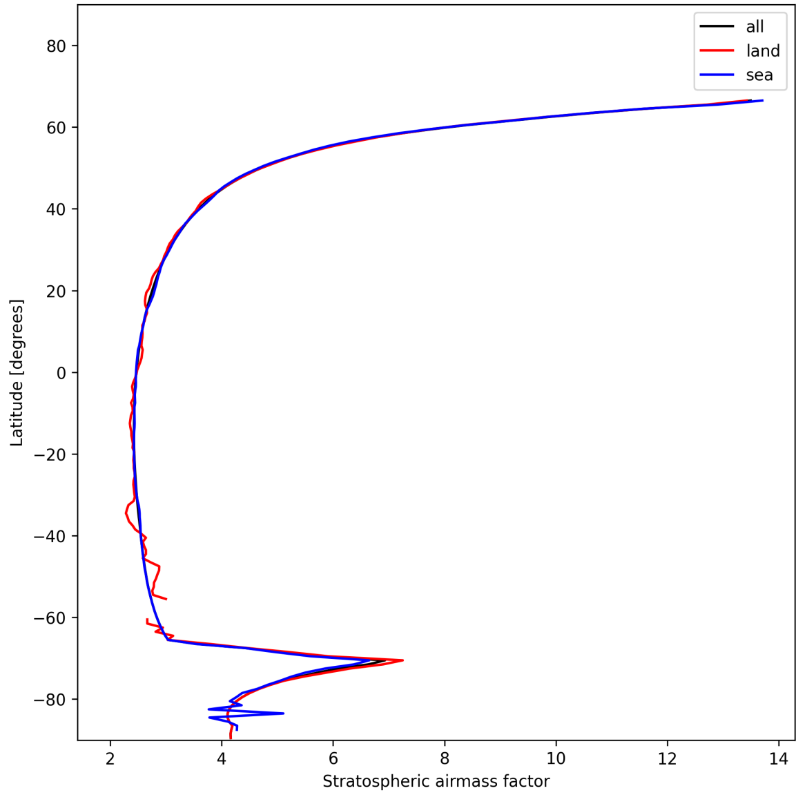
Figure 27: Zonal average of “Stratospheric airmass factor” for 2024-11-28 to 2024-11-30.
