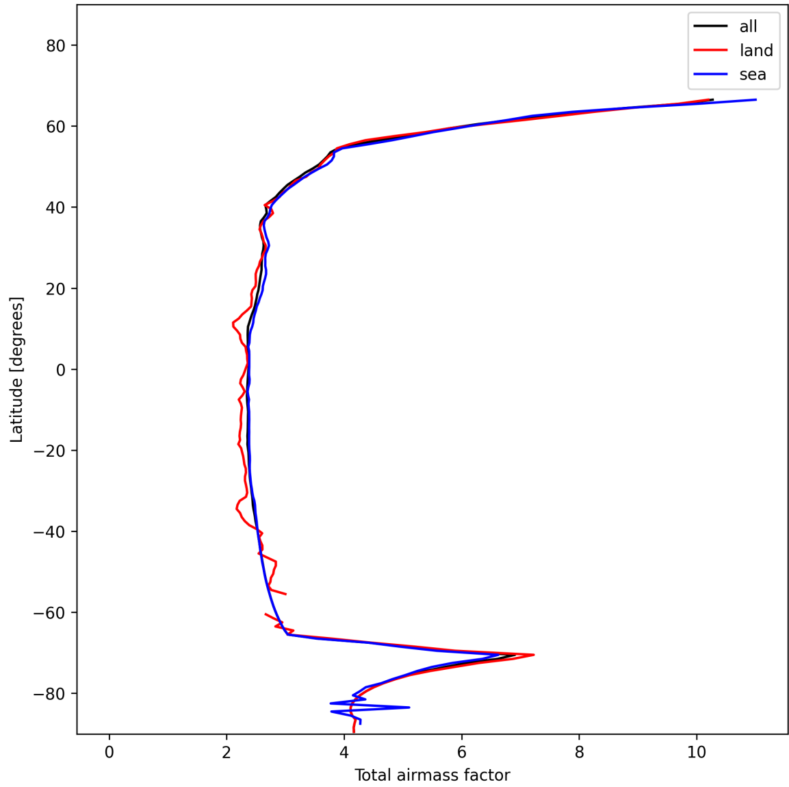
Figure 15: Zonal average of “Total airmass factor” for 2024-11-28 to 2024-11-30.
