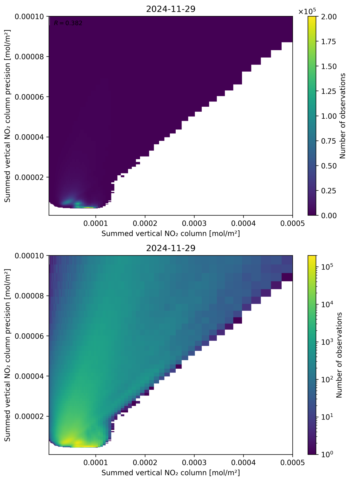
Figure 105: Scatter density plot of “Summed vertical NO 2 column” against “Summed vertical NO 2 column precision” for 2024-11-28 to 2024-11-30.
