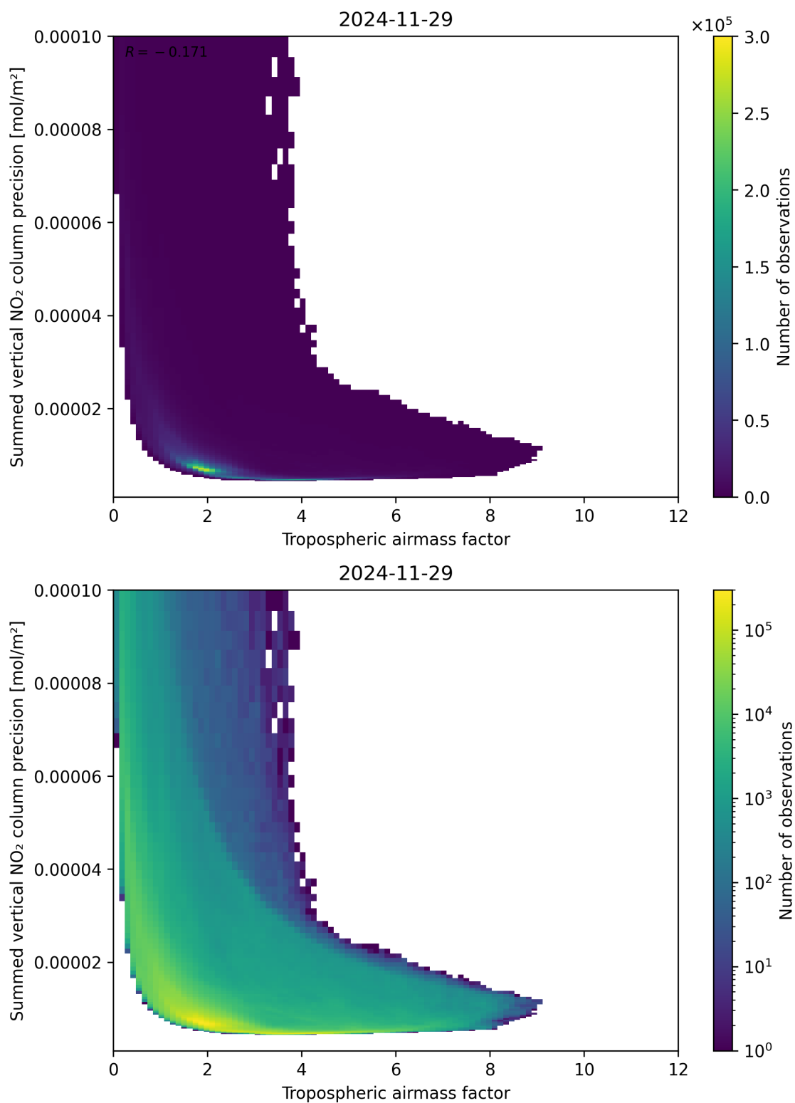
Figure 76: Scatter density plot of “Tropospheric airmass factor” against “Summed vertical NO 2 column precision” for 2024-11-28 to 2024-11-30.
