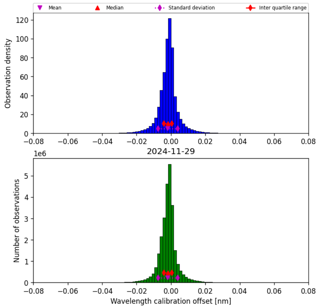
Figure 35: Histogram of “Wavelength calibration offset” for 2024-11-28 to 2024-11-30
