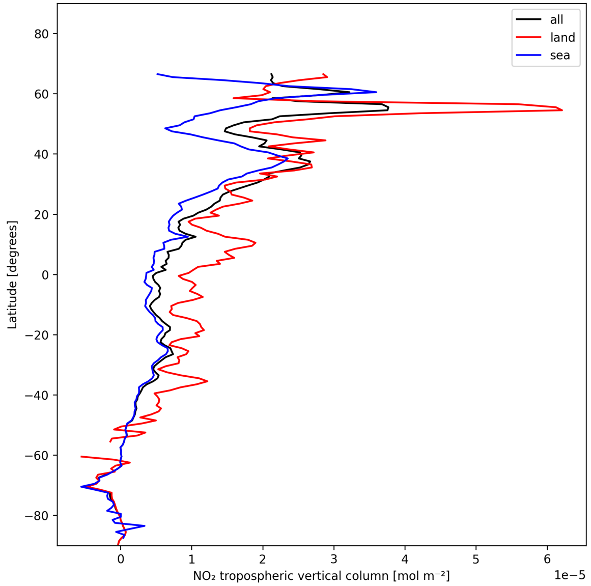
Figure 12: Zonal average of “NO 2 tropospheric vertical column” for 2024-11-28 to 2024-11-30.
