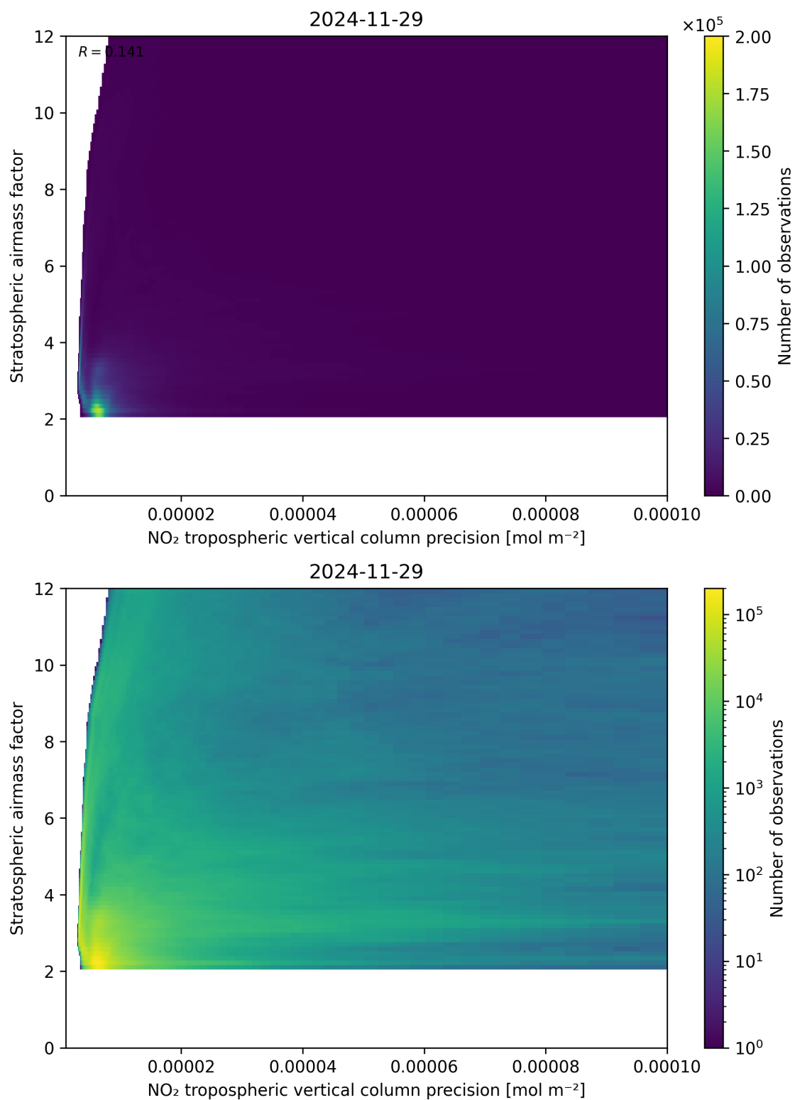
Figure 131: Scatter density plot of “NO 2 tropospheric vertical column precision” against “Stratospheric airmass factor” for 2024-11-28 to 2024-11-30.
