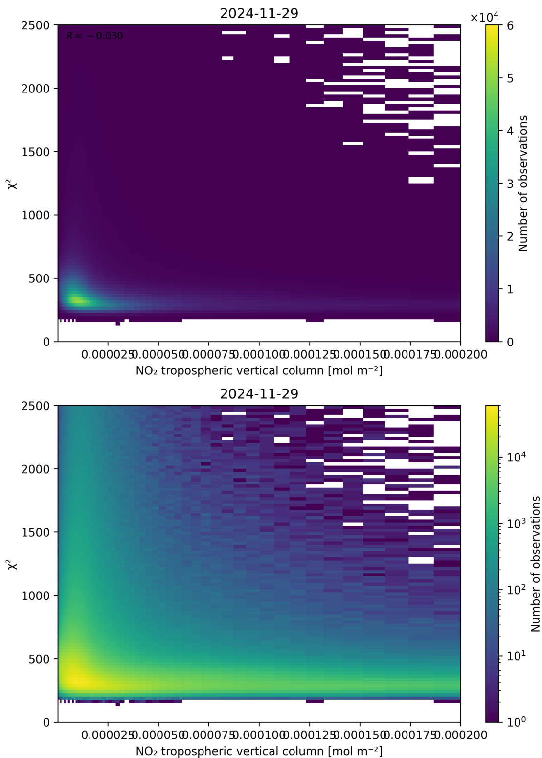
Figure 124: Scatter density plot of “NO 2 tropospheric vertical column” against “ \chi^2 ” for 2024-11-28 to 2024-11-30.
