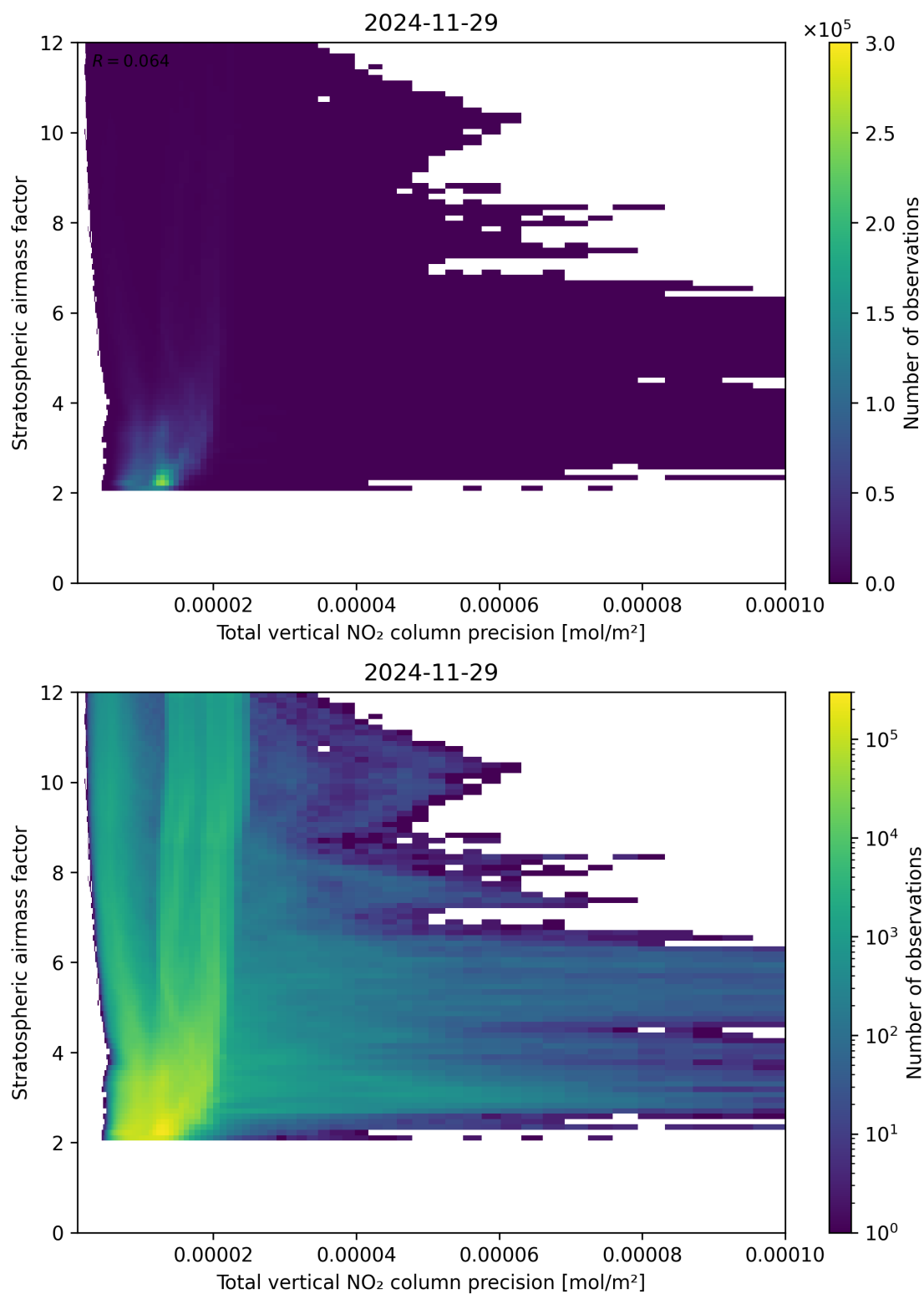
Figure 115: Scatter density plot of “Total vertical NO 2 column precision” against “Stratospheric air mass factor” for 2024-11-28 to 2024-11-30.
