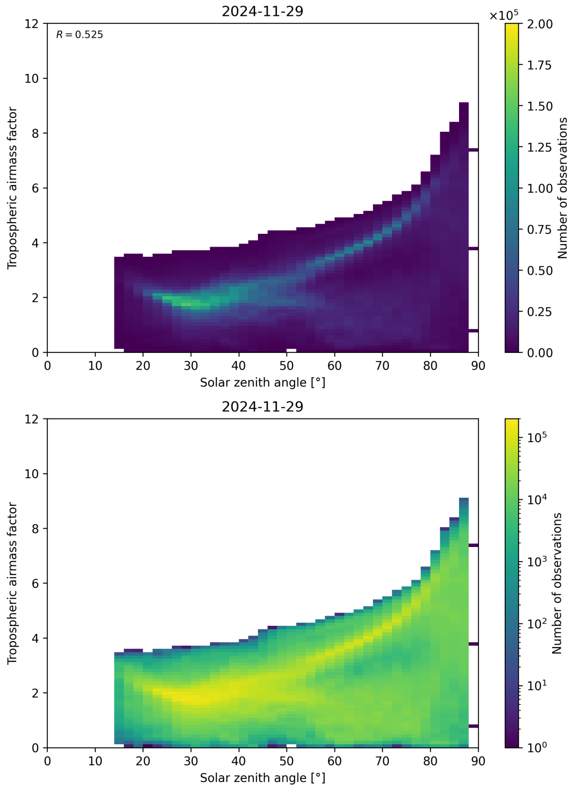
Figure 147: Scatter density plot of “Solar zenith angle” against “Tropospheric airmass factor” for 2024-11-28 to 2024-11-30.
