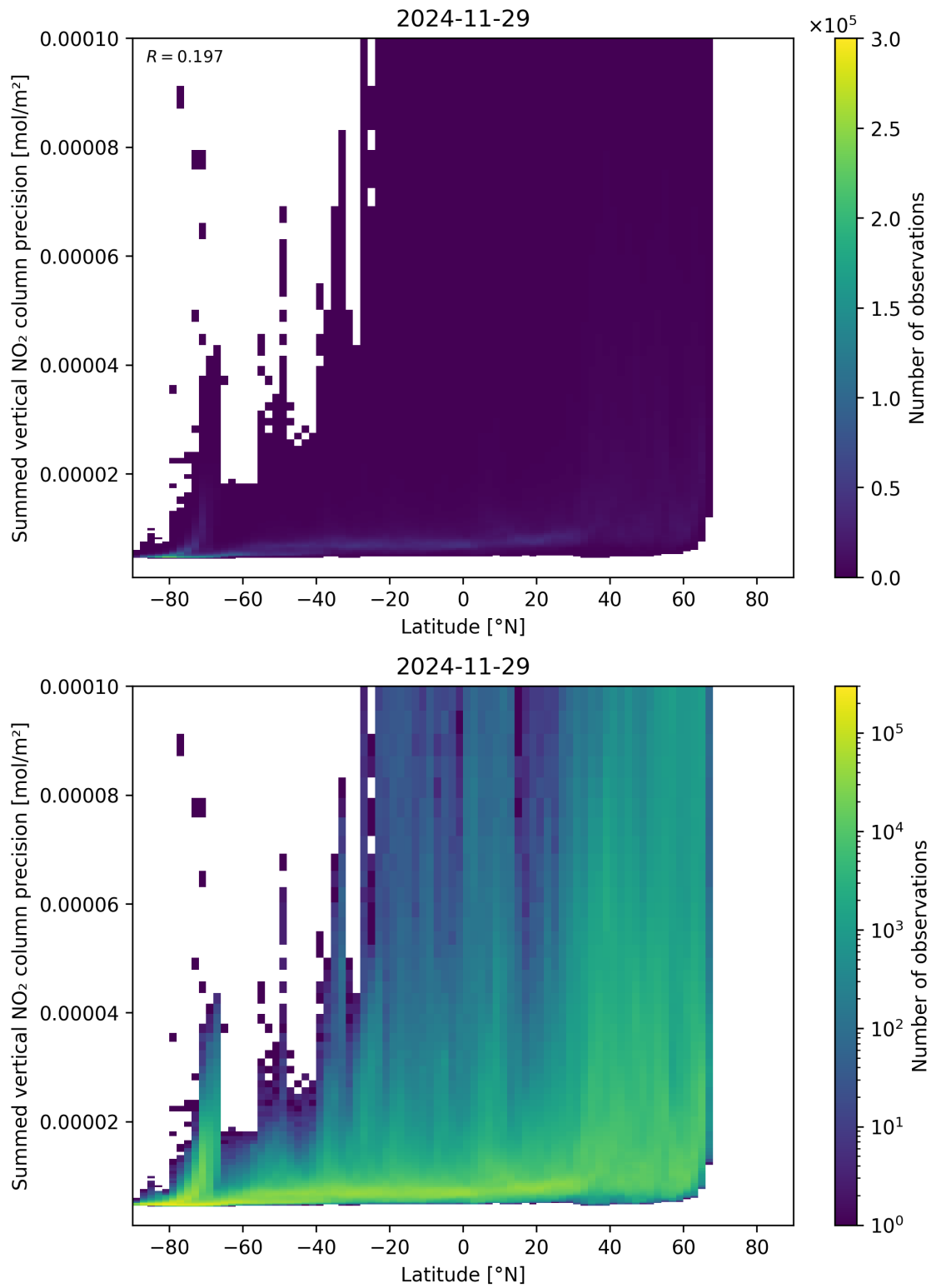
Figure 89: Scatter density plot of “Latitude” against “Summed vertical NO 2 column precision” for 2024-11-28 to 2024-11-30.
