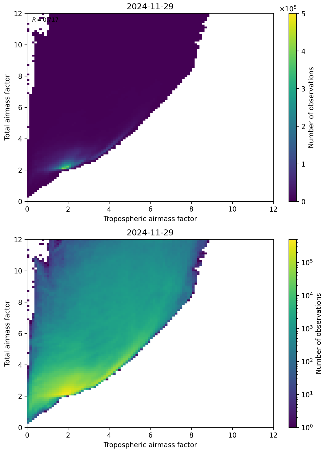
Figure 72: Scatter density plot of “Tropospheric airmass factor” against “Total airmass factor” for 2024-11-28 to 2024-11-30.
