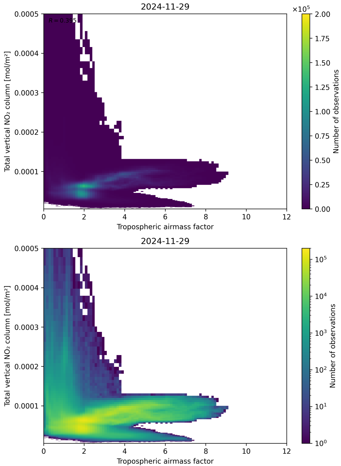
Figure 77: Scatter density plot of “Tropospheric airmass factor” against “Total vertical NO 2 column” for 2024-11-28 to 2024-11-30.
