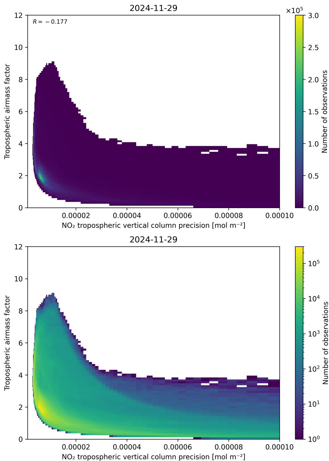
Figure 133: Scatter density plot of “NO 2 tropospheric vertical column precision” against “Tropospheric airmass factor” for 2024-11-28 to 2024-11-30.
