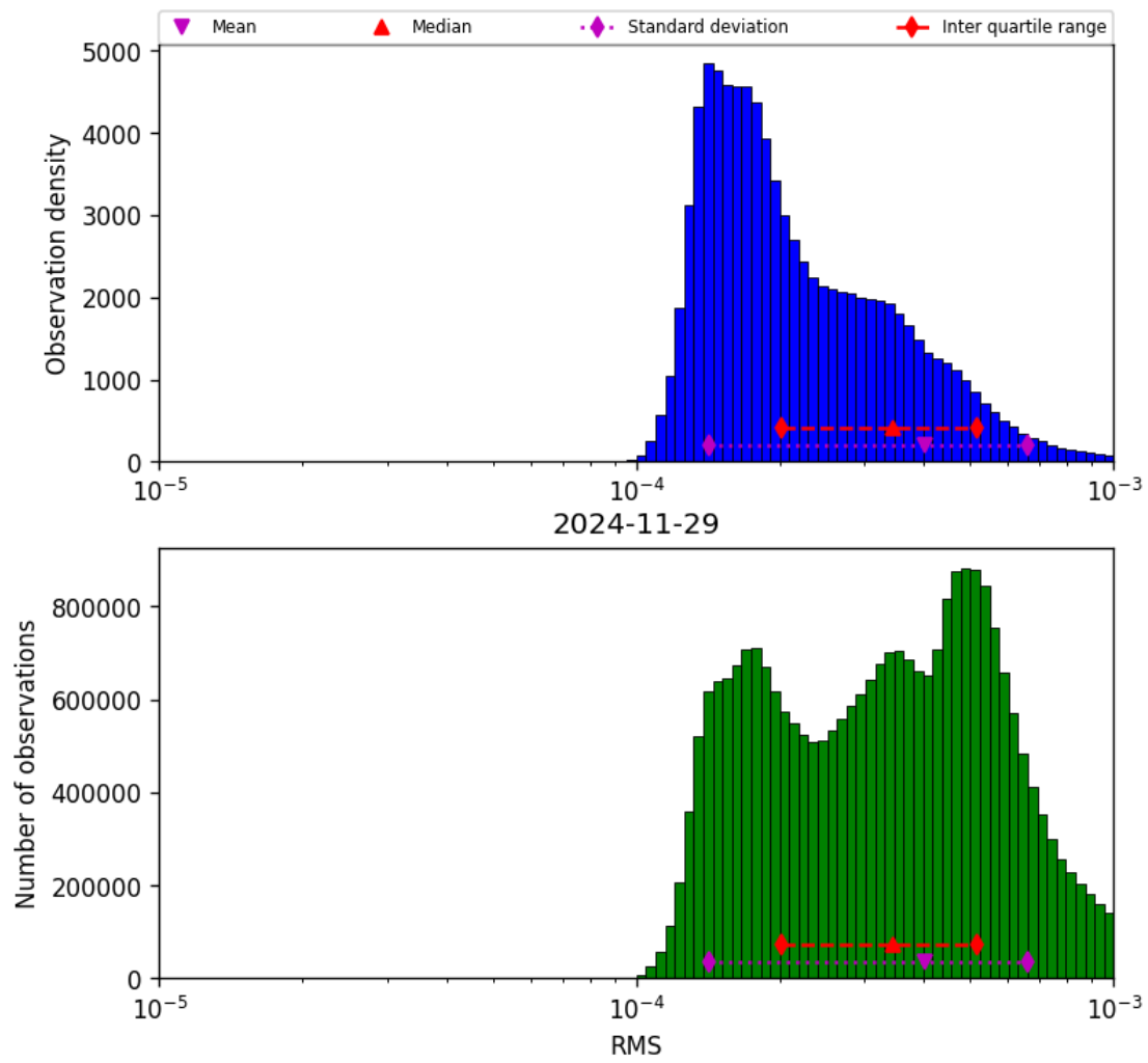
Figure 43: Histogram of “RMS” for 2024-11-28 to 2024-11-30
