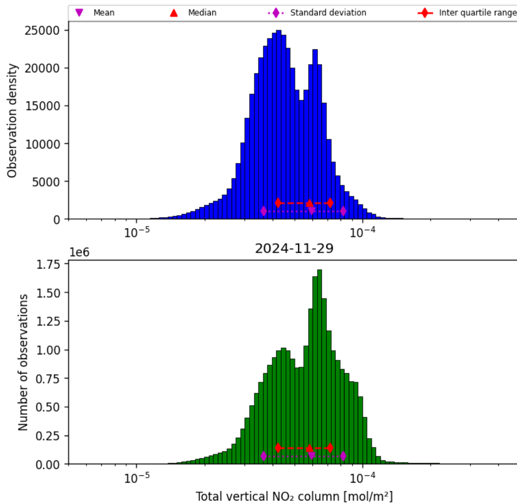
Figure 38: Histogram of “Total vertical NO 2 column” for 2024-11-28 to 2024-11-30
