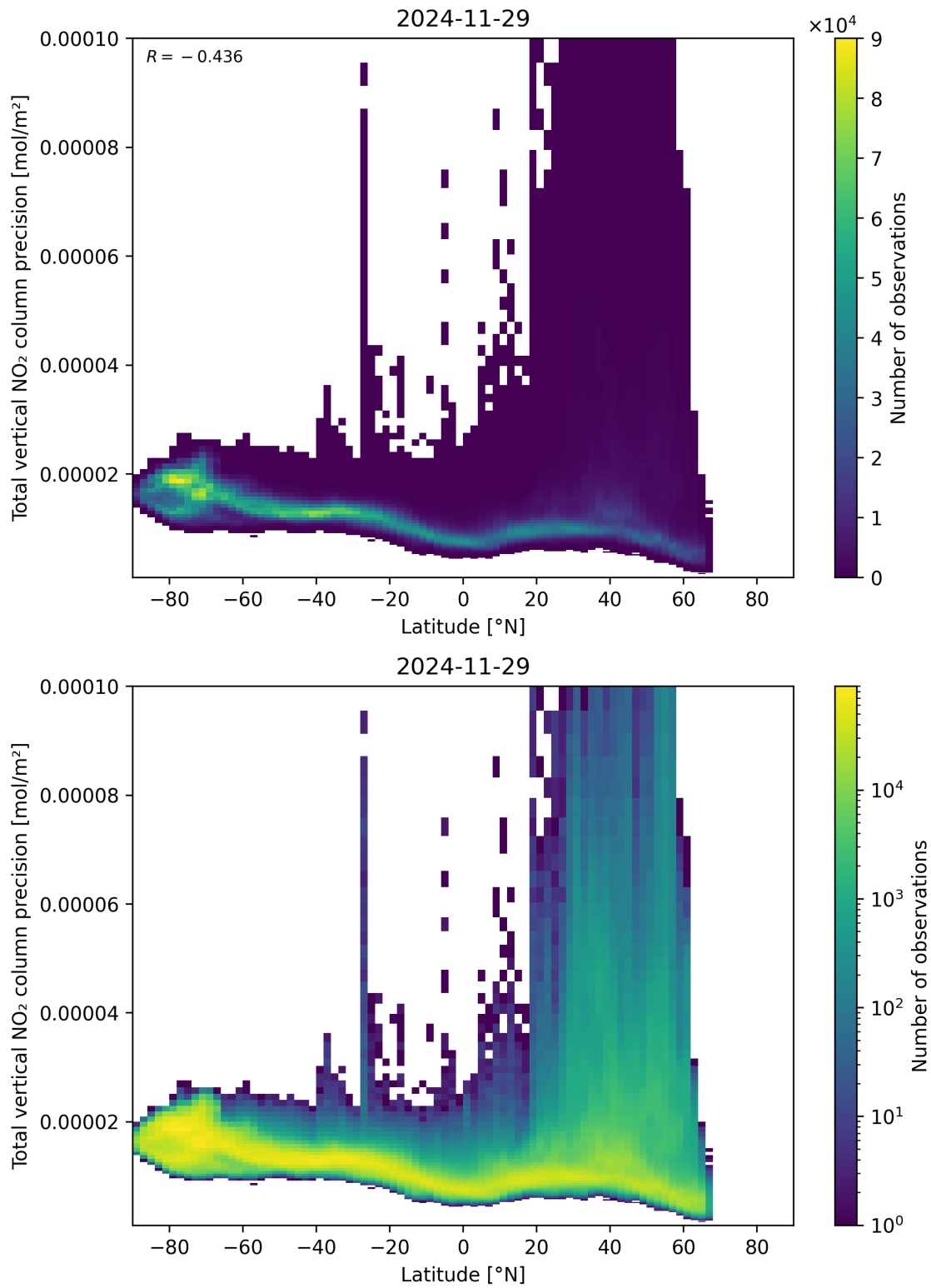
Figure 91: Scatter density plot of “Latitude” against “Total vertical NO 2 column precision” for 2024-11-28 to 2024-11-30.
