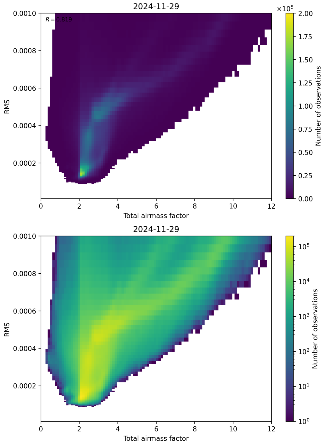
Figure 69: Scatter density plot of “Total airmass factor” against “RMS” for 2024-11-28 to 2024-11-30.
