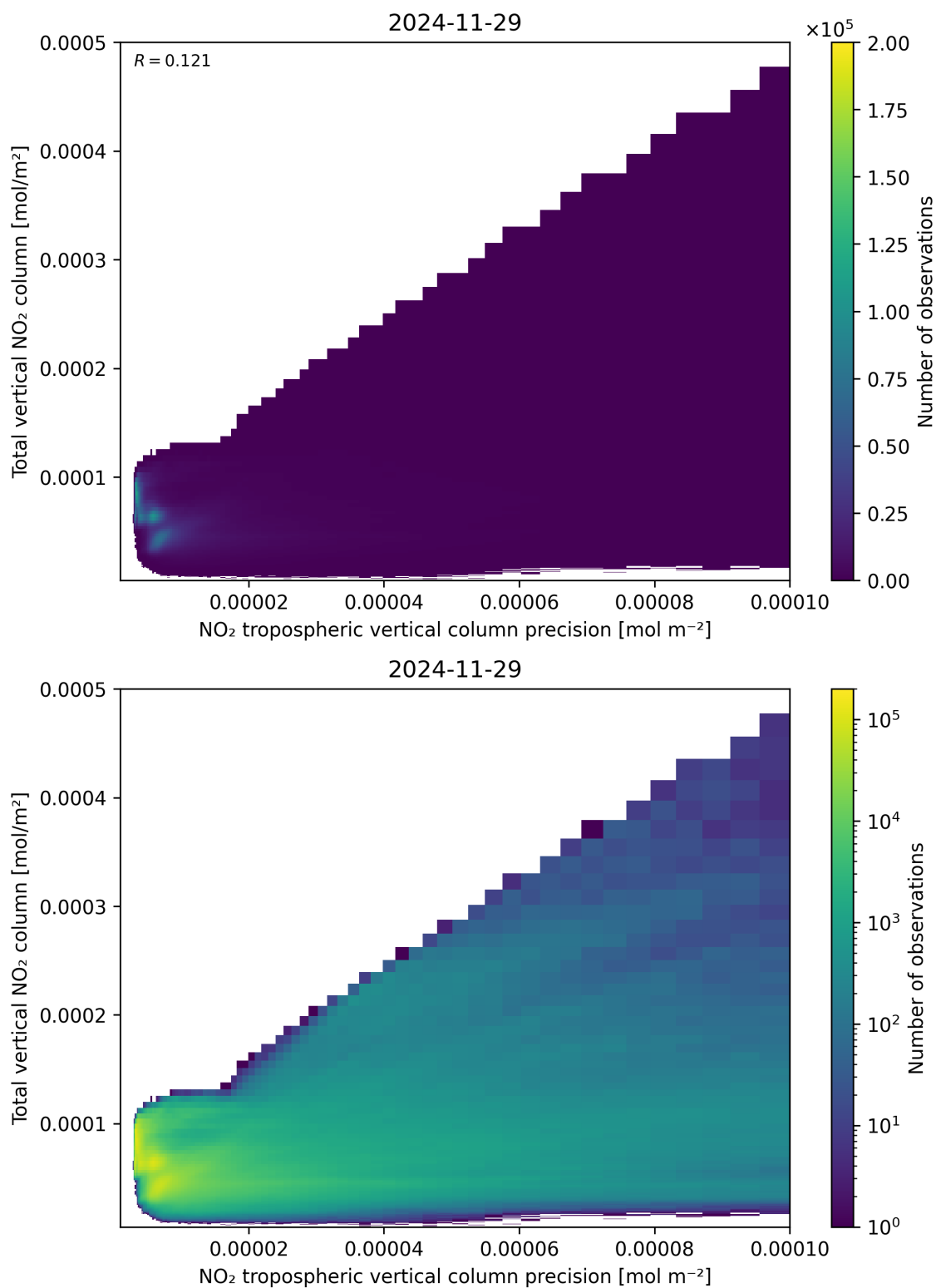
Figure 138: Scatter density plot of “NO 2 tropospheric vertical column precision” against “Total vertical NO 2 column” for 2024-11-28 to 2024-11-30.
