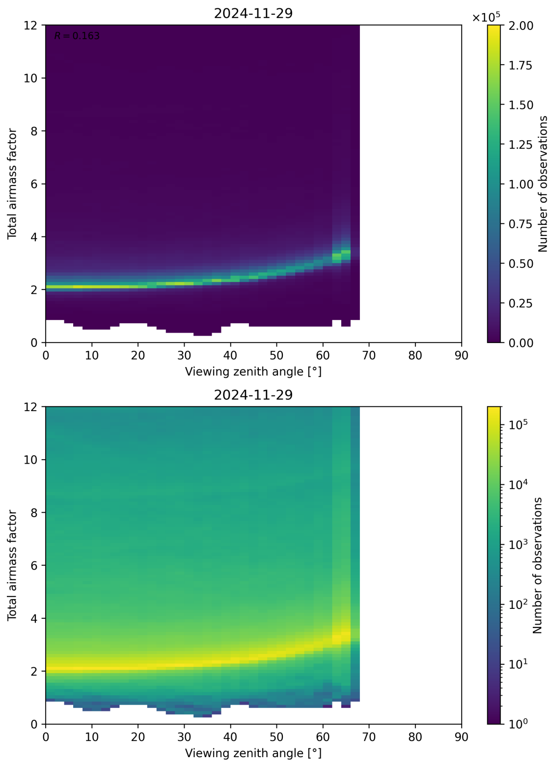
Figure 160: Scatter density plot of “Viewing zenith angle” against “Total airmass factor” for 2024-11-28 to 2024-11-30.
