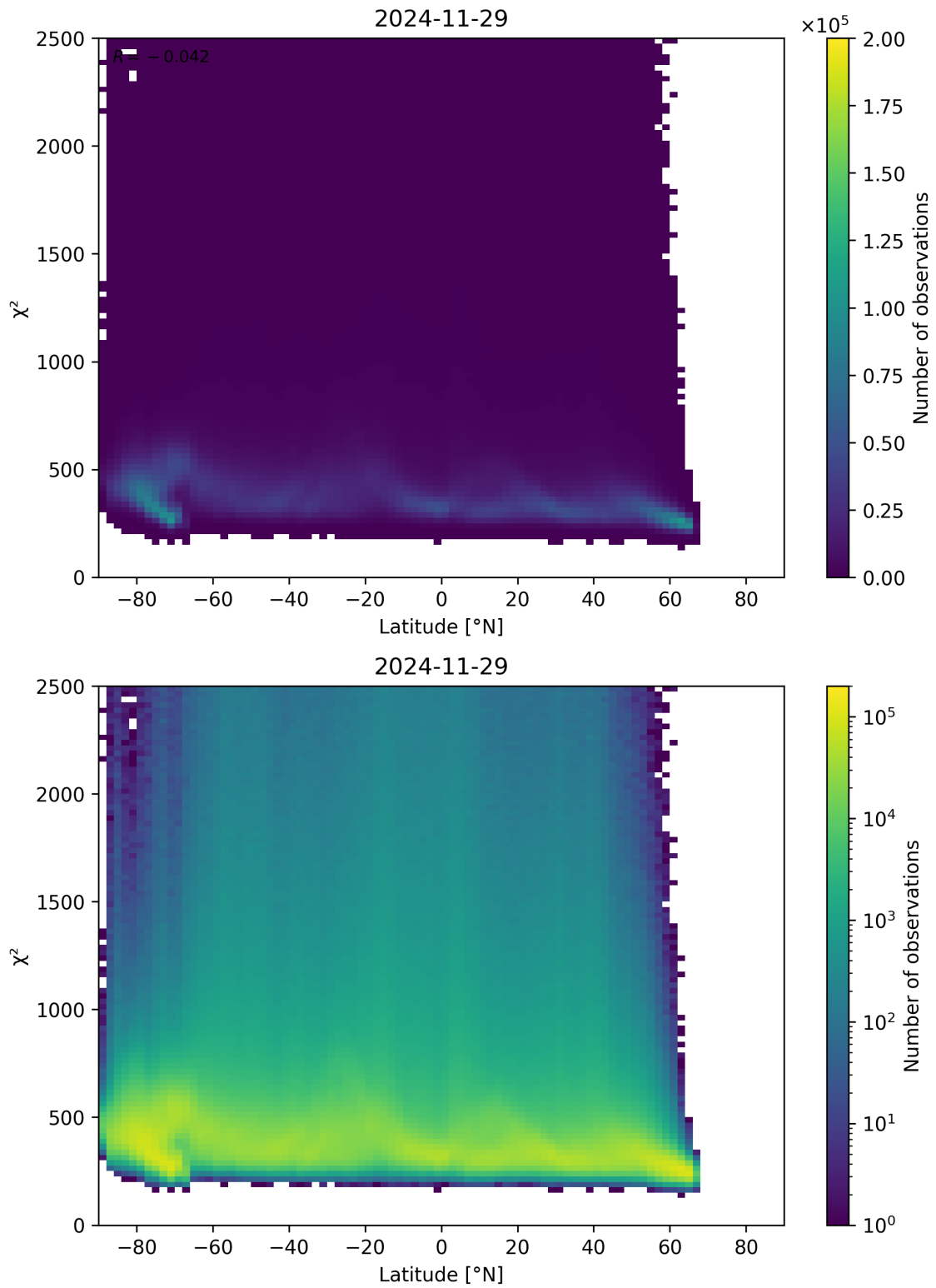
Figure 86: Scatter density plot of “Latitude” against “ \chi^2 ” for 2024-11-28 to 2024-11-30.
