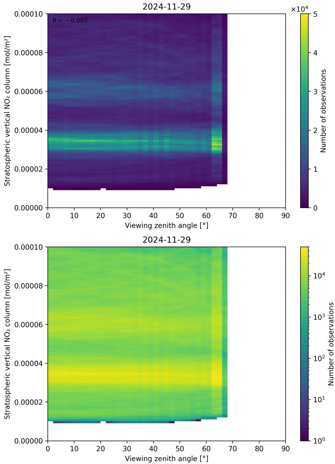
Figure 164: Scatter density plot of “Viewing zenith angle” against “Stratospheric vertical NO 2 column” for 2024-11-28 to 2024-11-30.
