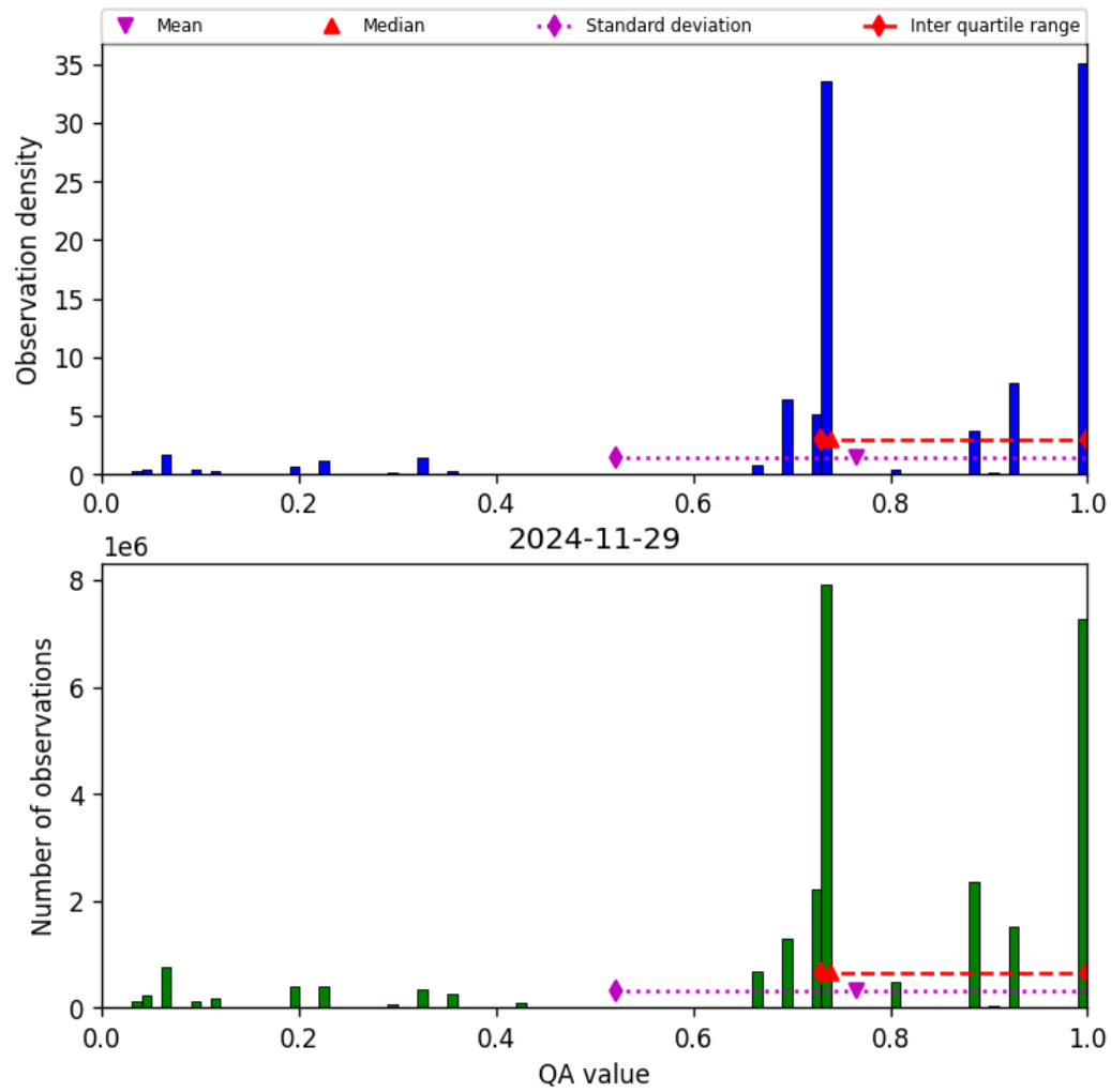
Figure 28: Histogram of “QA value” for 2024-11-28 to 2024-11-30
