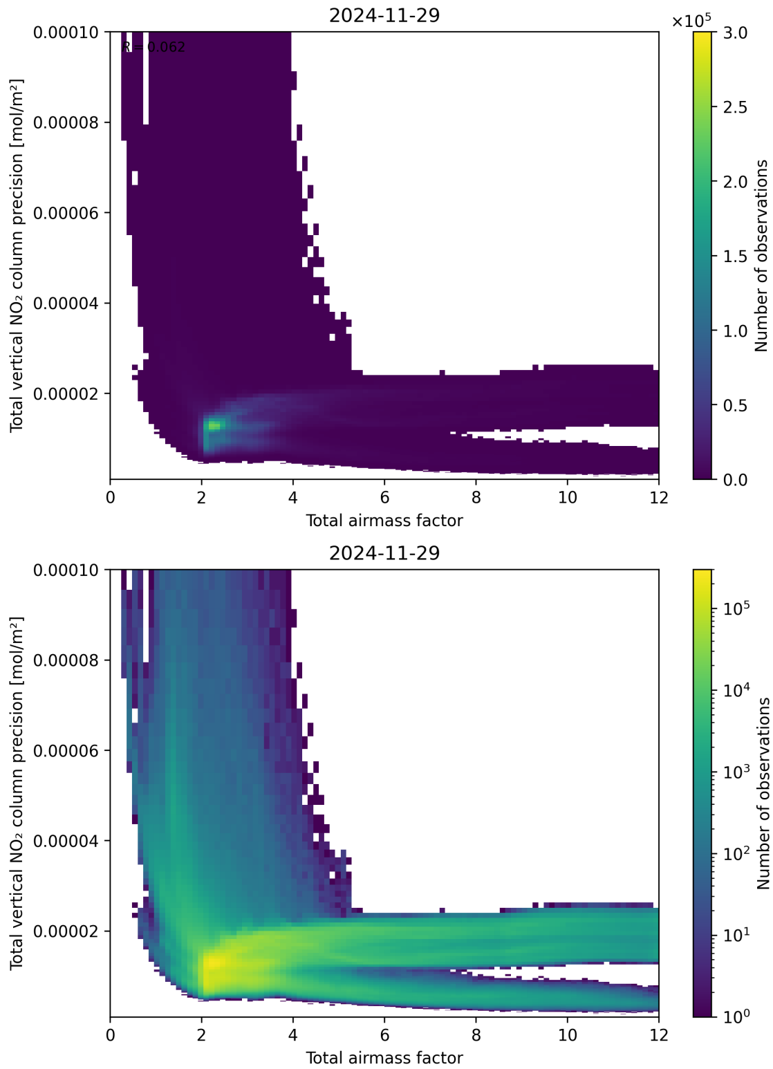
Figure 68: Scatter density plot of “Total airmass factor” against “Total vertical NO 2 column precision” for 2024-11-28 to 2024-11-30.
