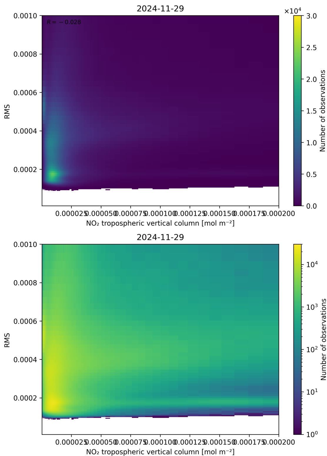
Figure 142: Scatter density plot of “NO 2 tropospheric vertical column” against “RMS” for 2024-11-28 to 2024-11-30.
