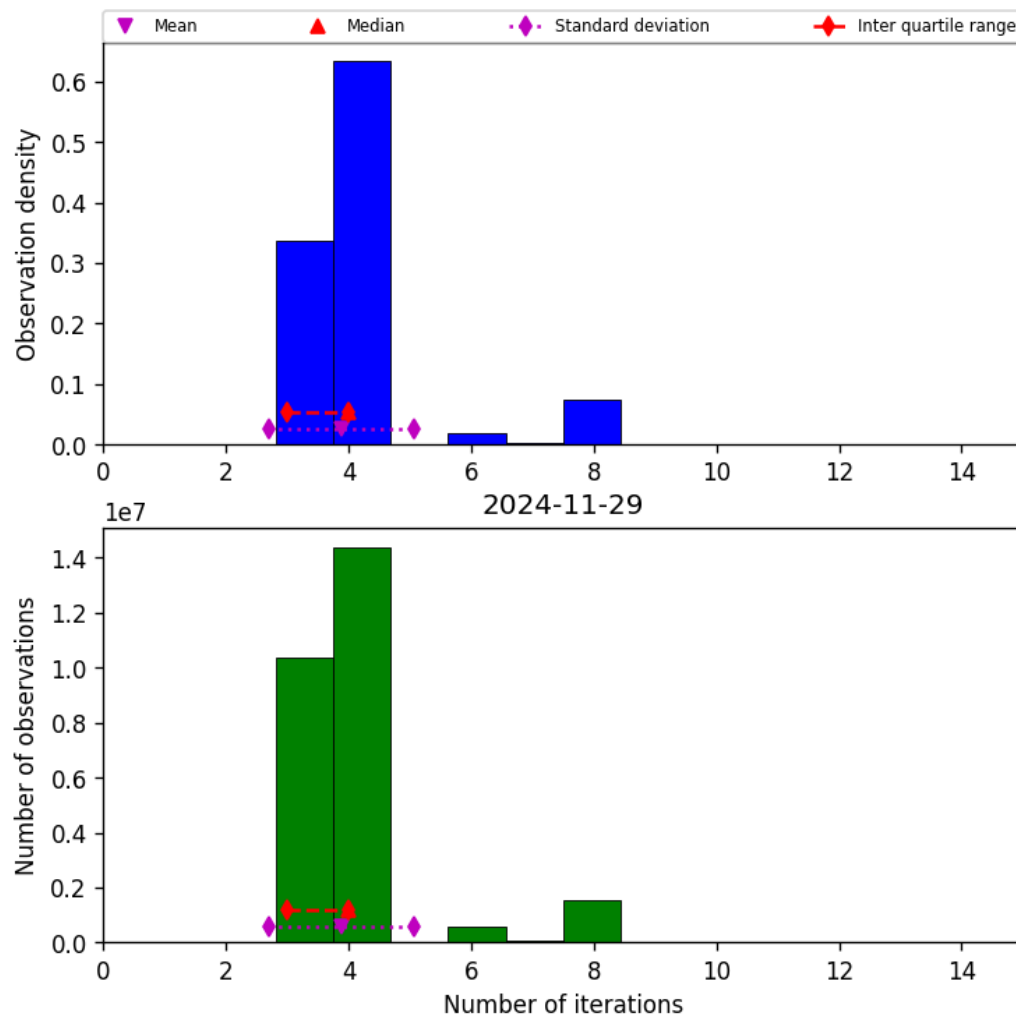
Figure 34: Histogram of “Number of iterations” for 2024-11-28 to 2024-11-30
