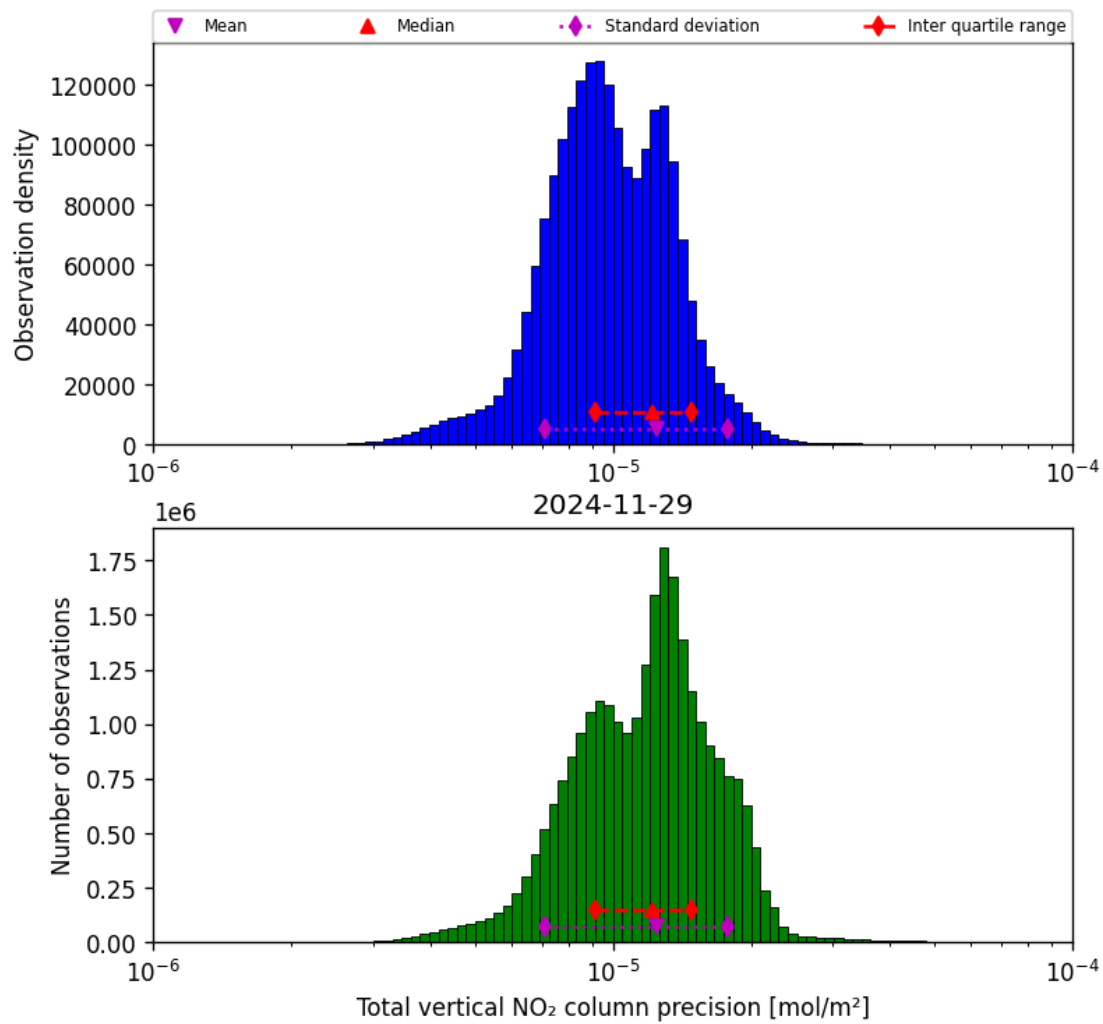
Figure 39: Histogram of “Total vertical NO 2 column precision” for 2024-11-28 to 2024-11-30
