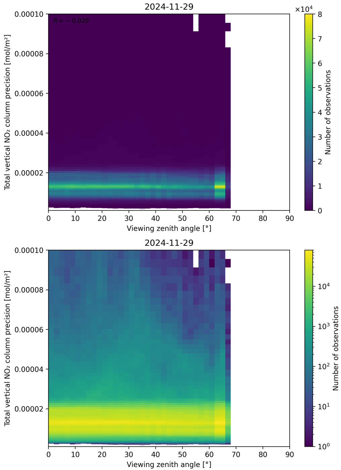
Figure 168: Scatter density plot of “Viewing zenith angle” against “Total vertical NO 2 column precision” for 2024-11-28 to 2024-11-30.
