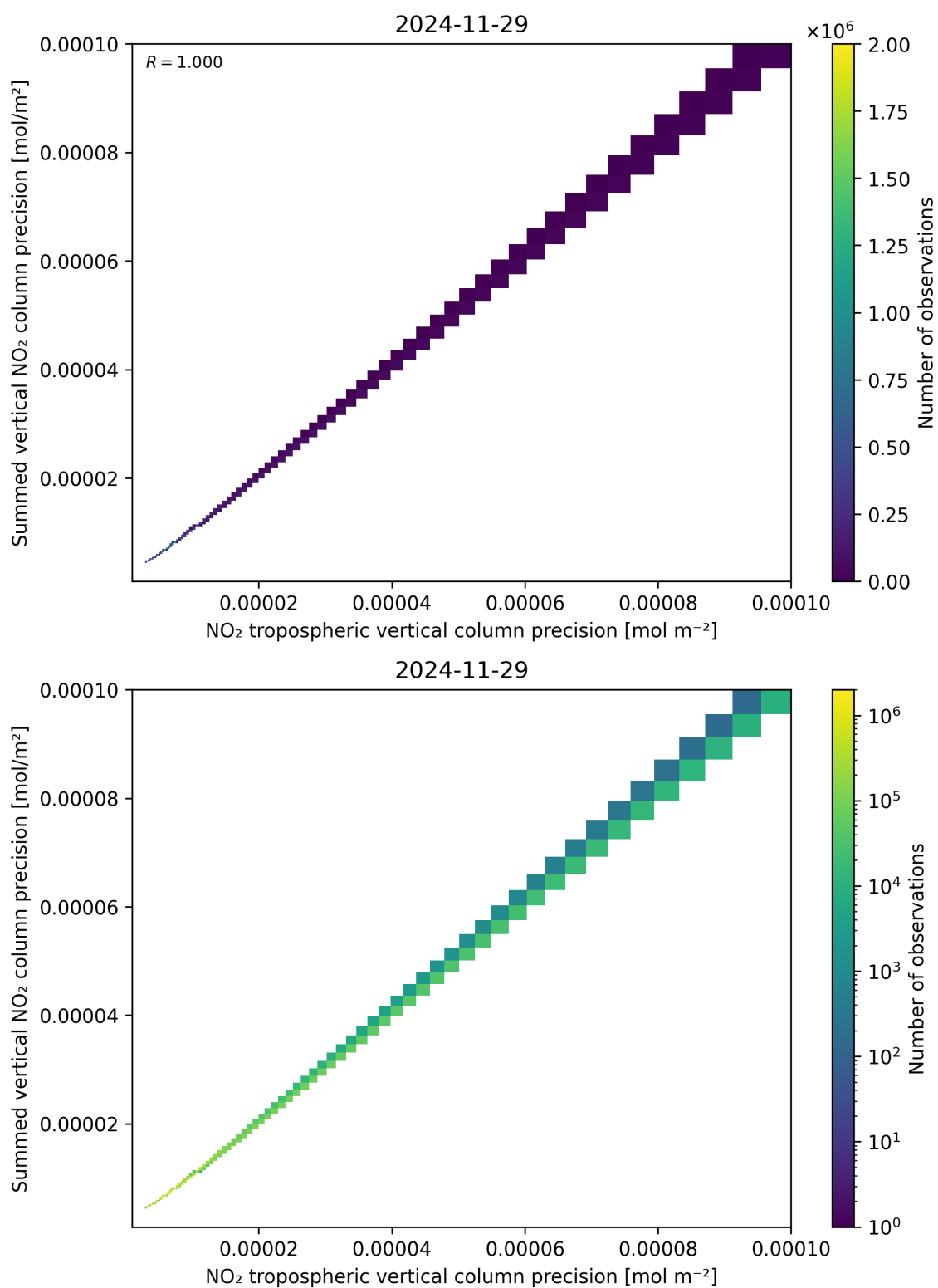
Figure 137: Scatter density plot of “NO 2 tropospheric vertical column precision” against “Summed vertical NO 2 column precision” for 2024-11-28 to 2024-11-30.
