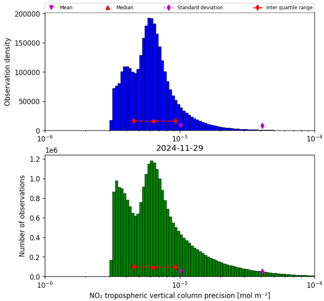
Figure 30: Histogram of “NO 2 tropospheric vertical column precision” for 2024-11-28 to 2024-11-30
