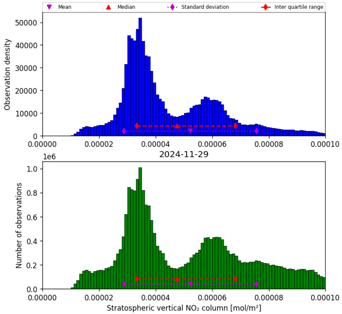
Figure 36: Histogram of “Stratospheric vertical NO 2 column” for 2024-11-28 to 2024-11-30
