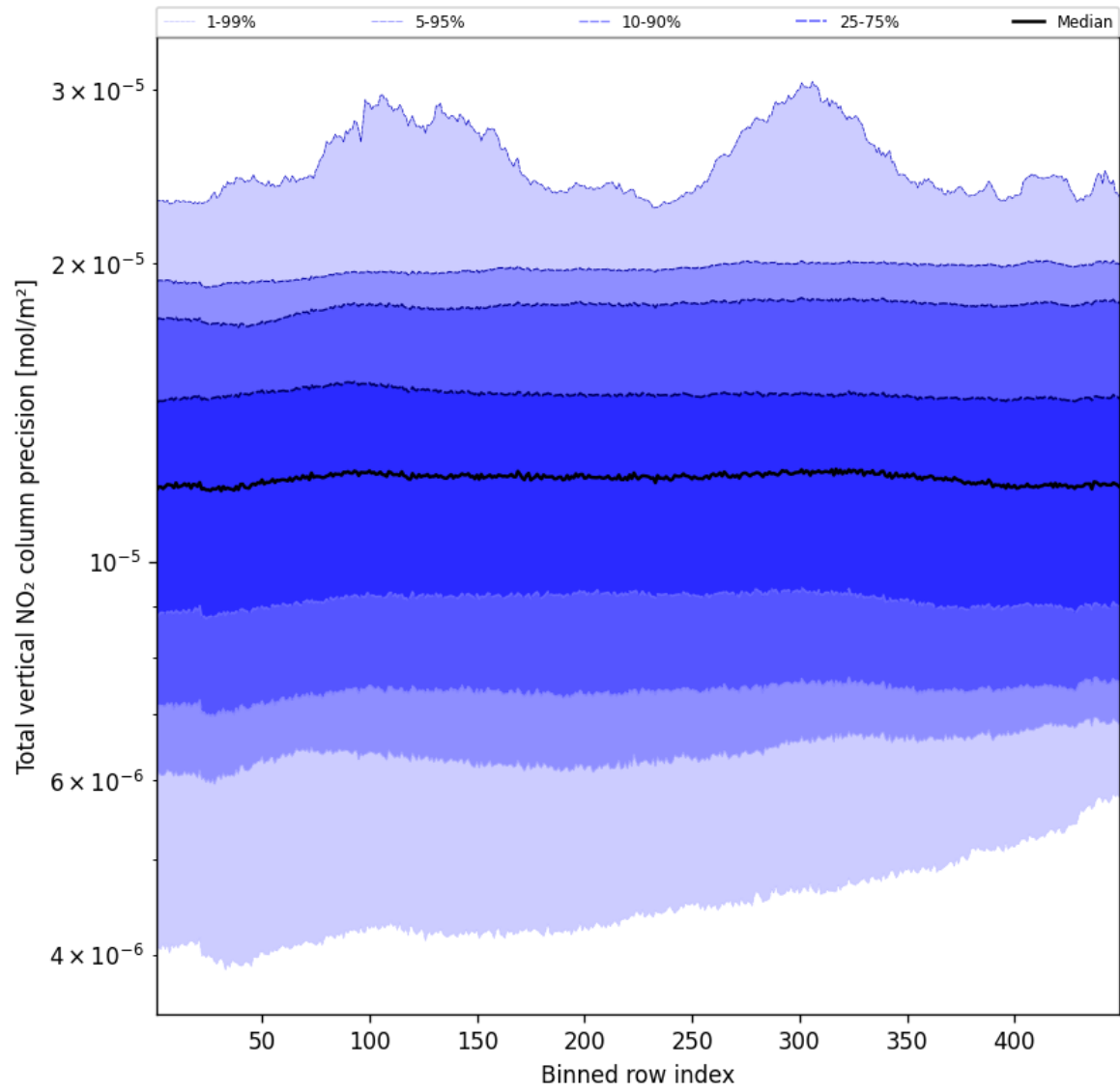
Figure 56: Along track statistics of “Total vertical NO 2 column precision” for 2024-11-28 to 2024-11-30
