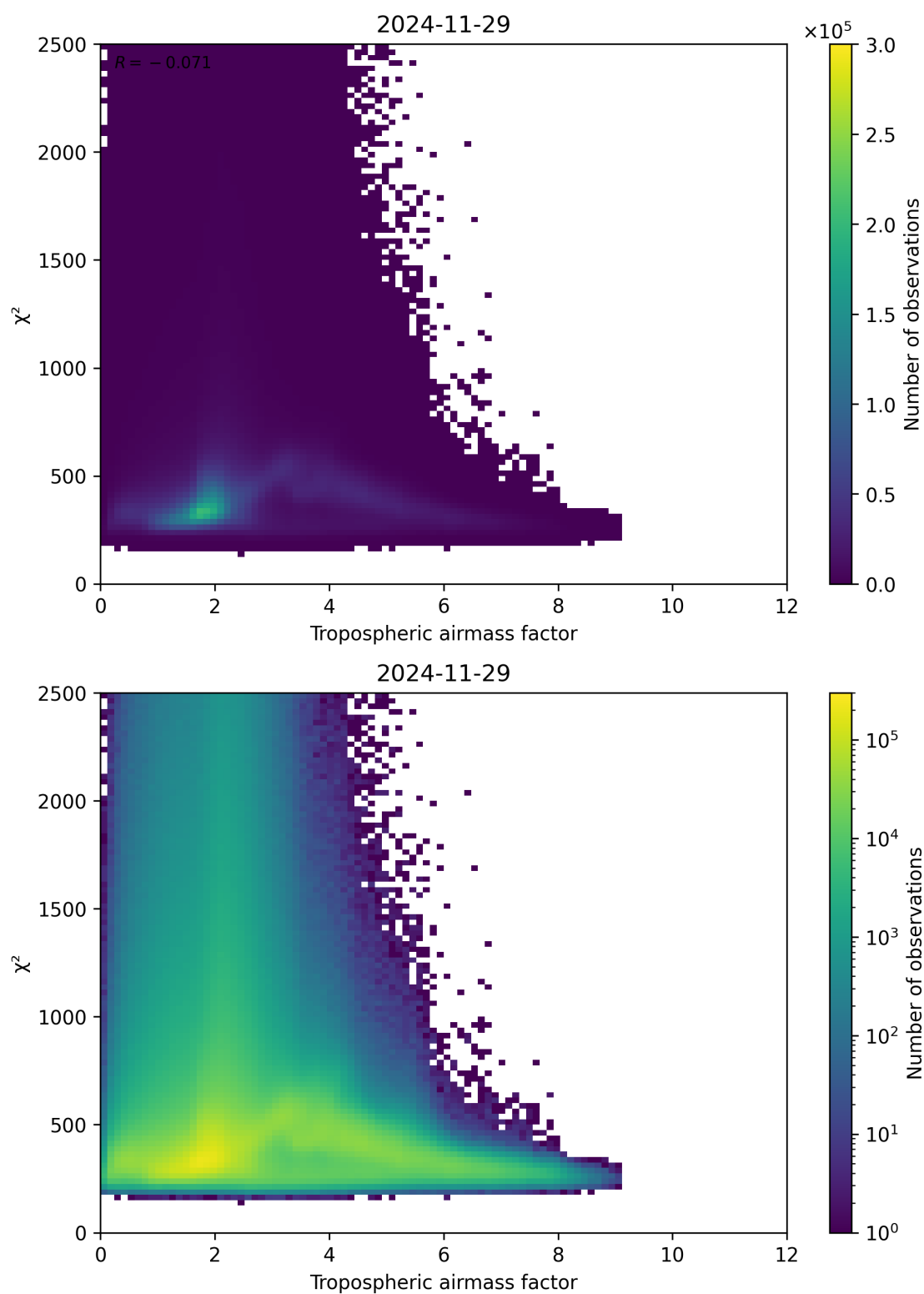
Figure 73: Scatter density plot of “Tropospheric airmass factor” against “ \chi^2 ” for 2024-11-28 to 2024-11-30.
