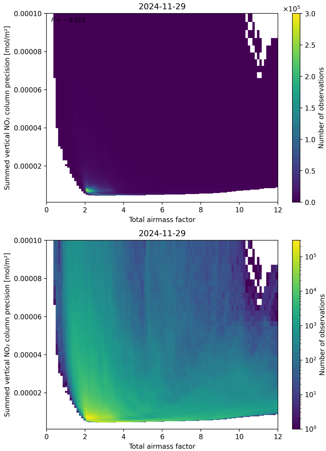
Figure 66: Scatter density plot of “Total airmass factor” against “Summed vertical NO 2 column precision” for 2024-11-28 to 2024-11-30.
