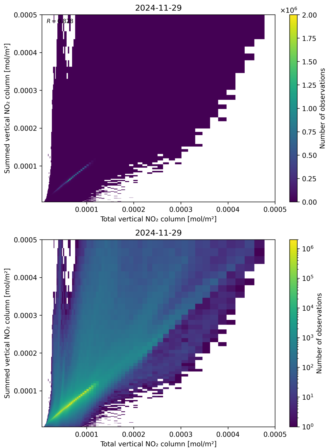
Figure 112: Scatter density plot of “Total vertical NO 2 column” against “Summed vertical NO 2 column” for 2024-11-28 to 2024-11-30.
