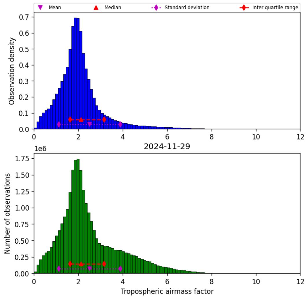
Figure 31: Histogram of “Tropospheric airmass factor” for 2024-11-28 to 2024-11-30
