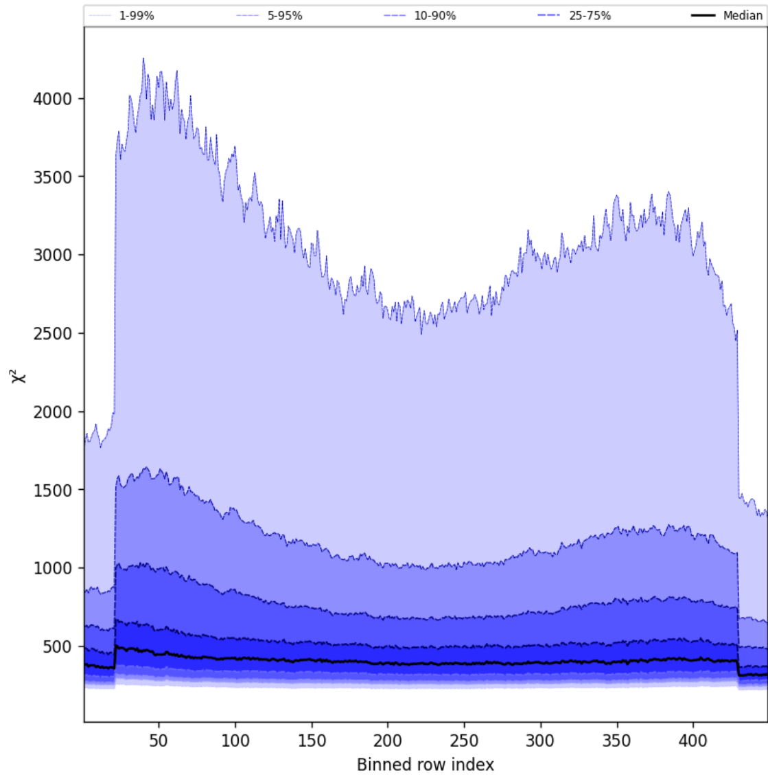
Figure 59: Along track statistics of “ \chi^2 ” for 2024-11-28 to 2024-11-30
