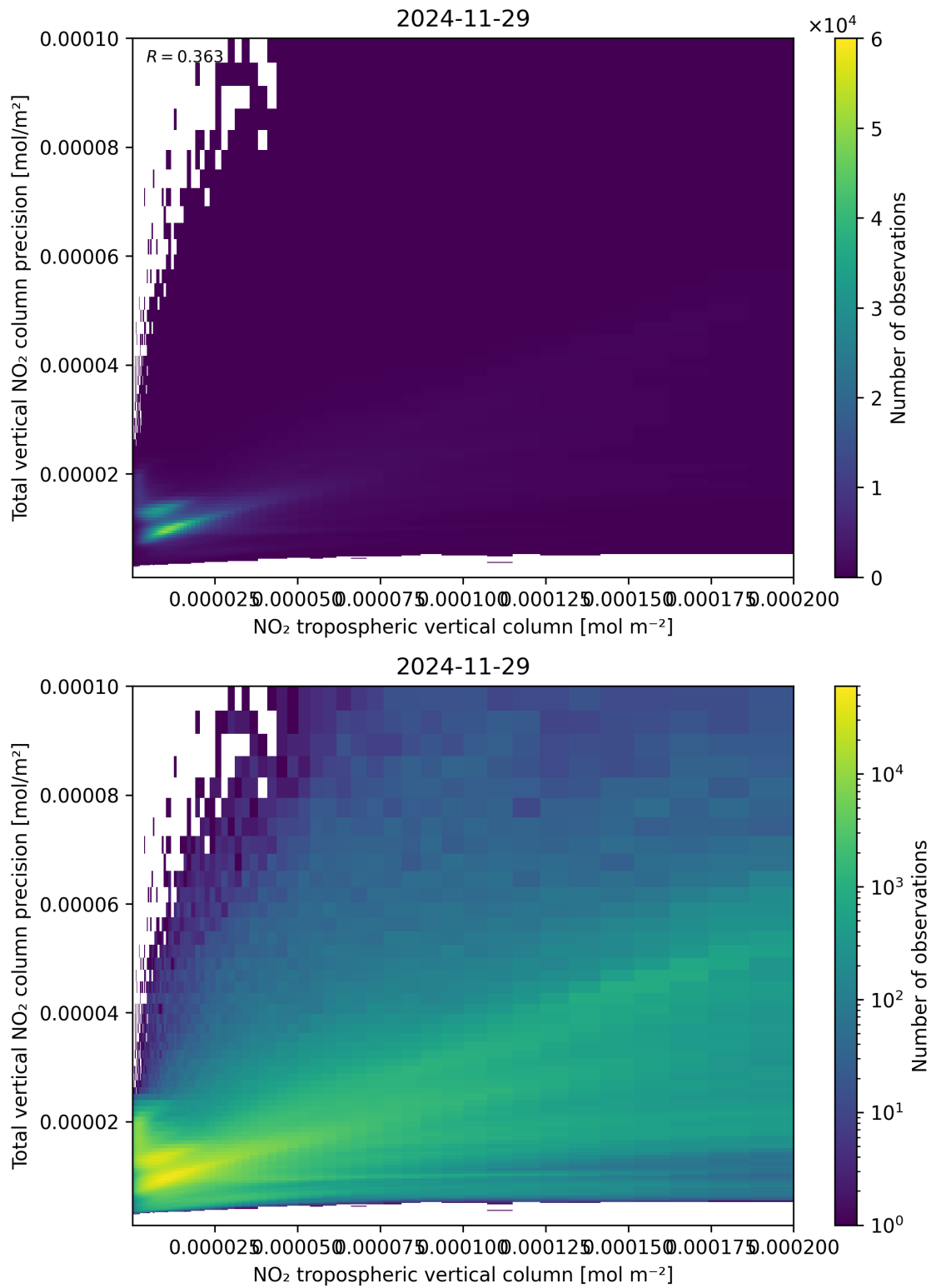
Figure 129: Scatter density plot of “NO 2 tropospheric vertical column” against “Total vertical NO 2 column precision” for 2024-11-28 to 2024-11-30.
