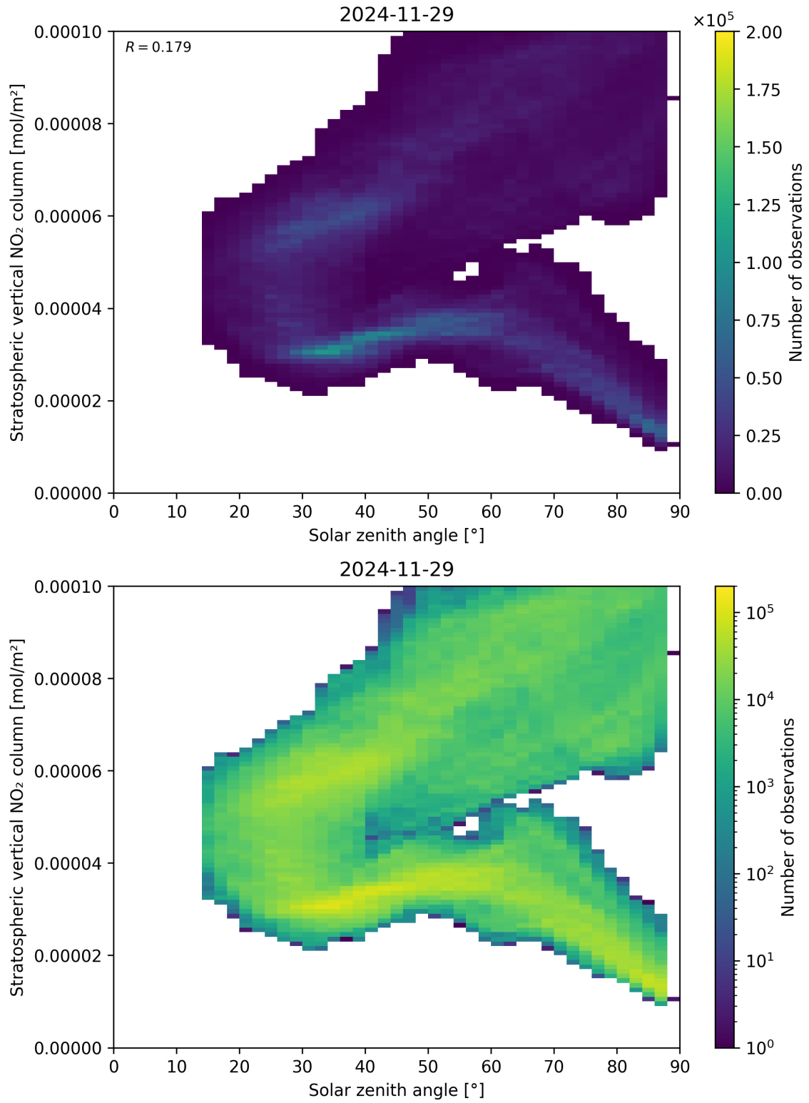
Figure 150: Scatter density plot of “Solar zenith angle” against “Stratospheric vertical NO 2 column” for 2024-11-28 to 2024-11-30.
