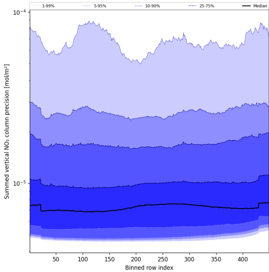
Figure 58: Along track statistics of “Summed vertical NO 2 column precision” for 2024-11-28 to 2024-11-30
