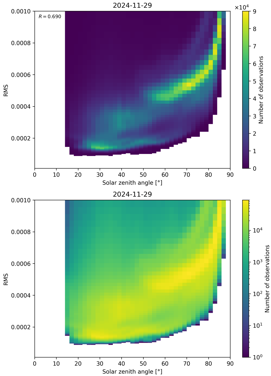
Figure 157: Scatter density plot of “Solar zenith angle” against “RMS” for 2024-11-28 to 2024-11-30.
