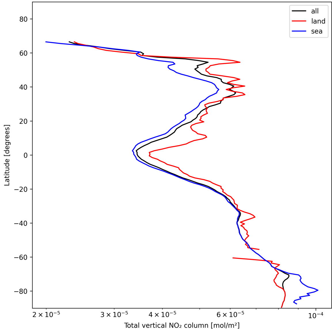
Figure 21: Zonal average of “Total vertical NO 2 column” for 2024-11-28 to 2024-11-30.
