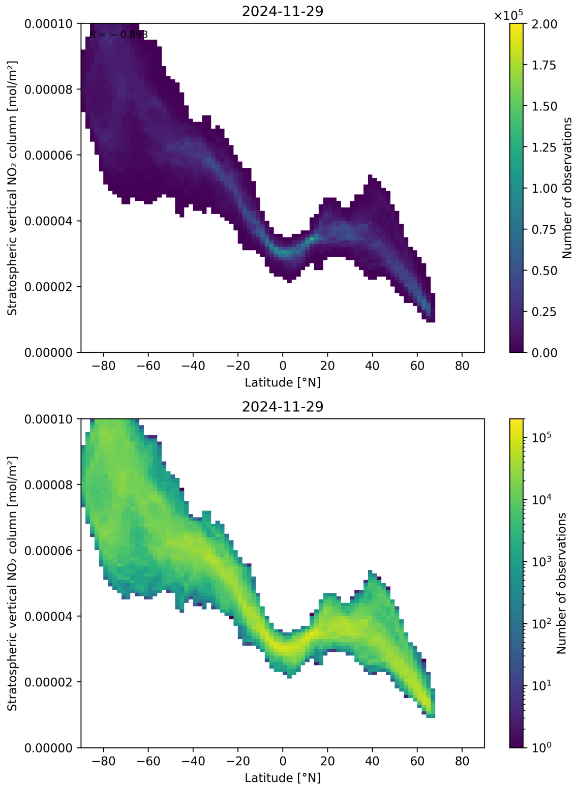
Figure 87: Scatter density plot of “Latitude” against “Stratospheric vertical NO 2 column” for 2024-11-28 to 2024-11-30.
