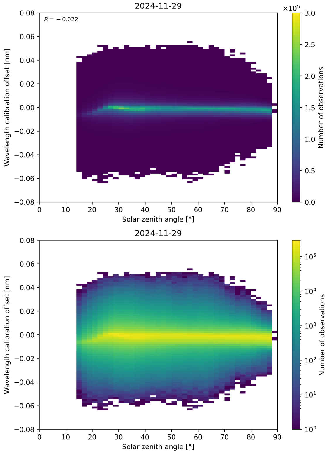
Figure 158: Scatter density plot of “Solar zenith angle” against “Wavelength calibration offset” for 2024-11-28 to 2024-11-30.
