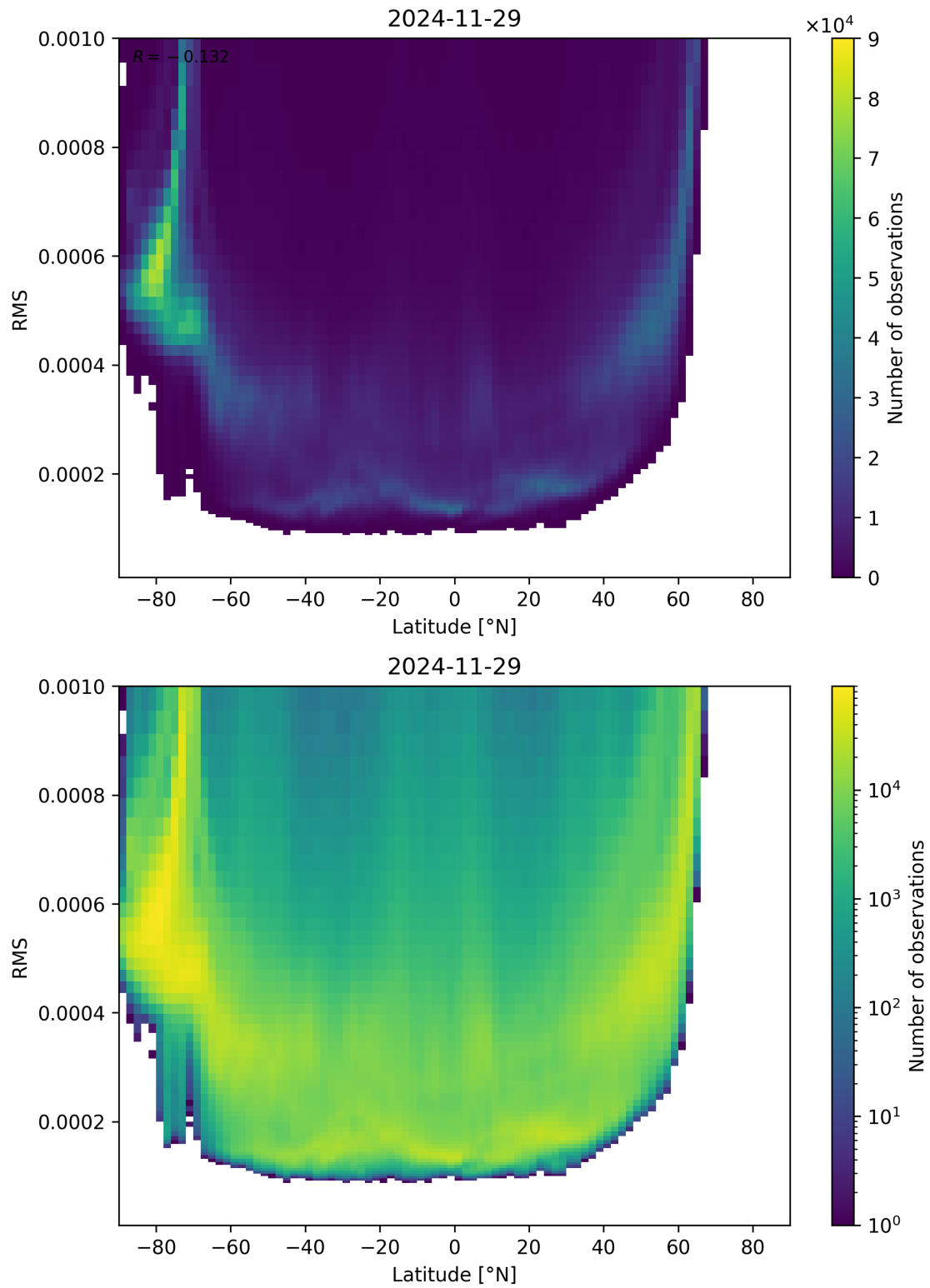
Figure 94: Scatter density plot of “Latitude” against “RMS” for 2024-11-28 to 2024-11-30.
