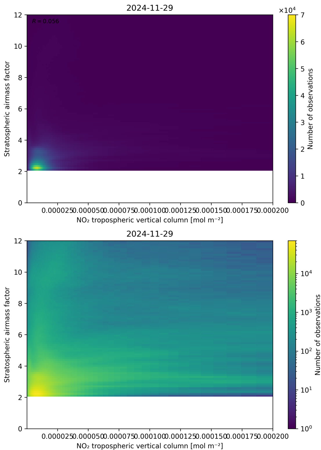
Figure 121: Scatter density plot of “NO 2 tropospheric vertical column” against “Stratospheric airmass factor” for 2024-11-28 to 2024-11-30.
