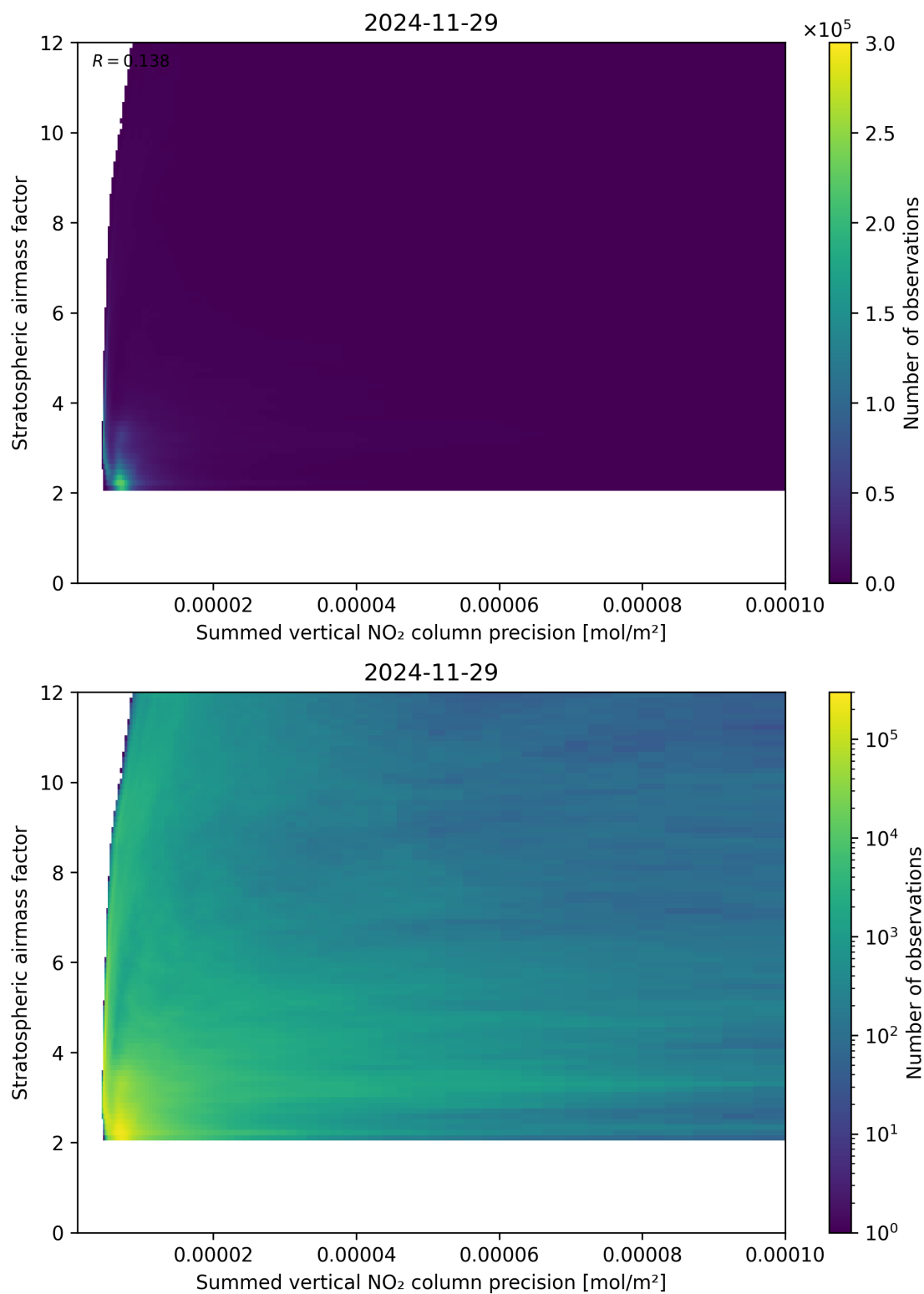
Figure 106: Scatter density plot of “Summed vertical NO 2 column precision” against “Stratospheric airmass factor” for 2024-11-28 to 2024-11-30.
