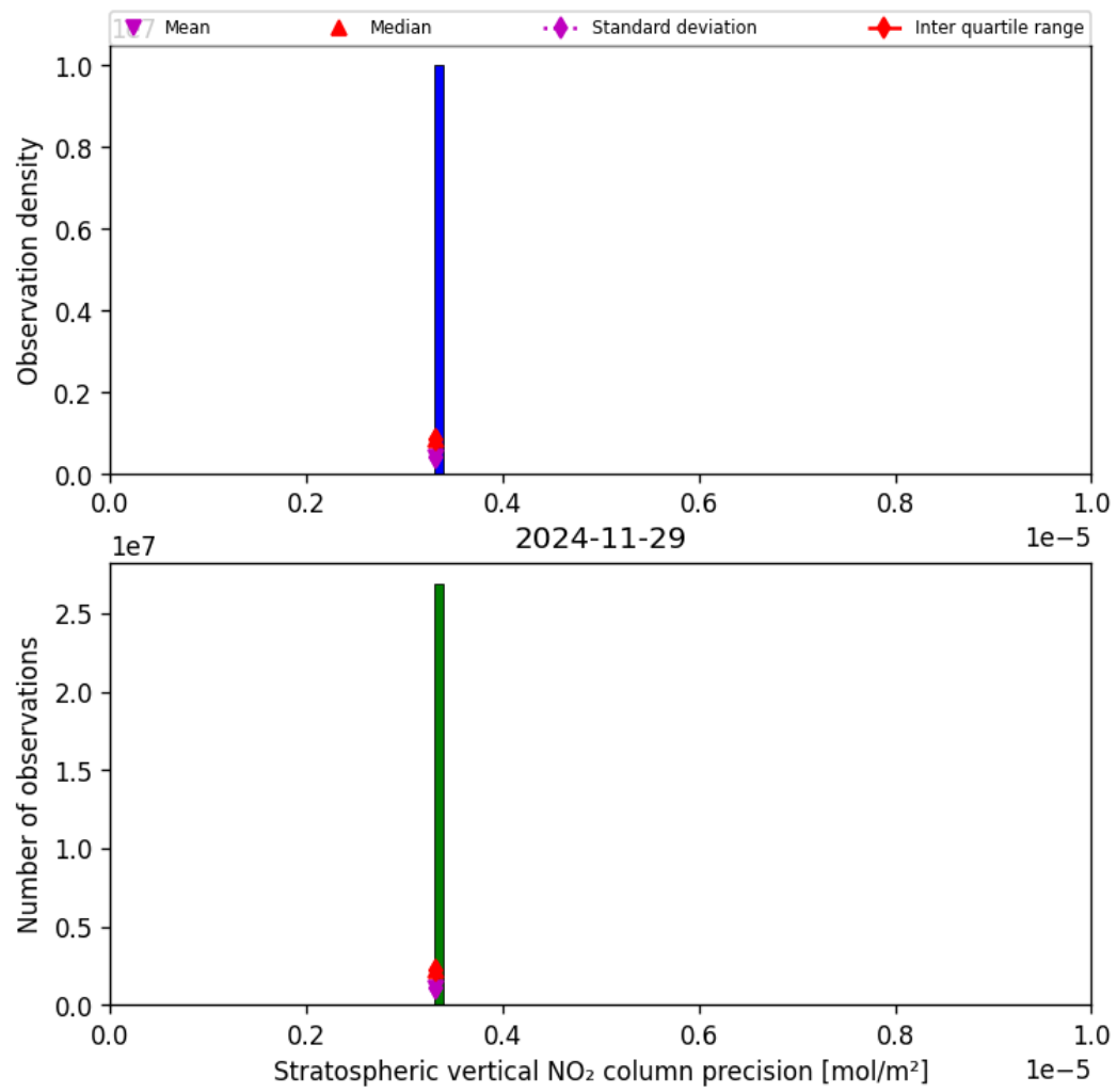
Figure 37: Histogram of “Stratospheric vertical NO 2 column precision” for 2024-11-28 to 2024-11-30
