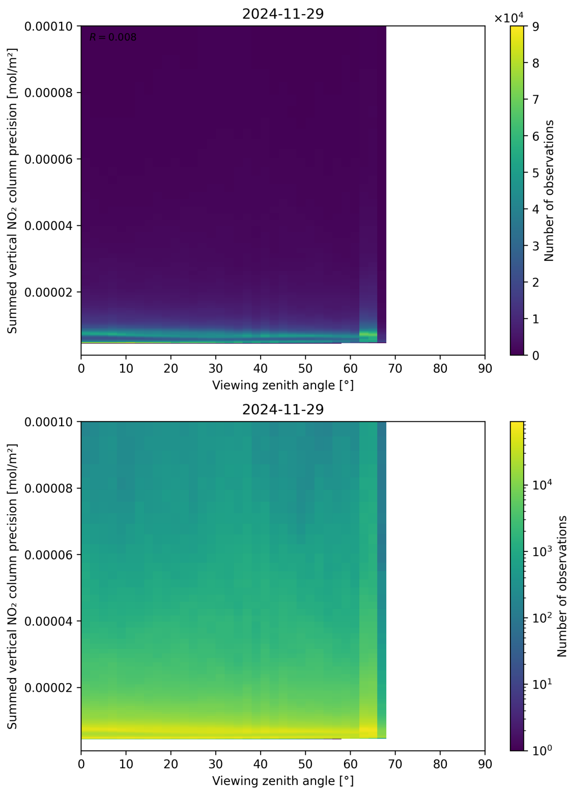
Figure 166: Scatter density plot of “Viewing zenith angle” against “Summed vertical NO 2 column precision” for 2024-11-28 to 2024-11-30.
