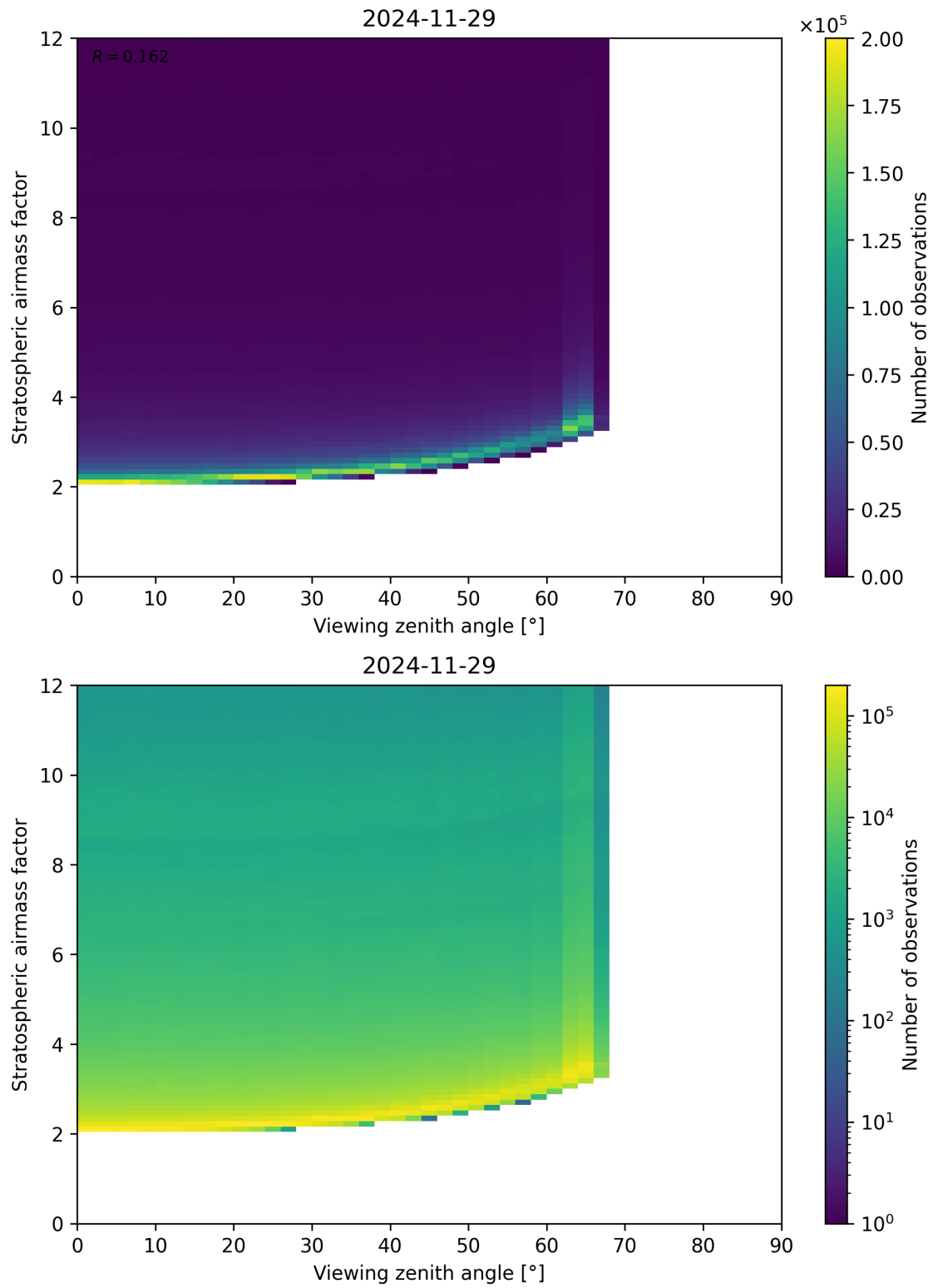
Figure 159: Scatter density plot of “Viewing zenith angle” against “Stratospheric airmass factor” for 2024-11-28 to 2024-11-30.
