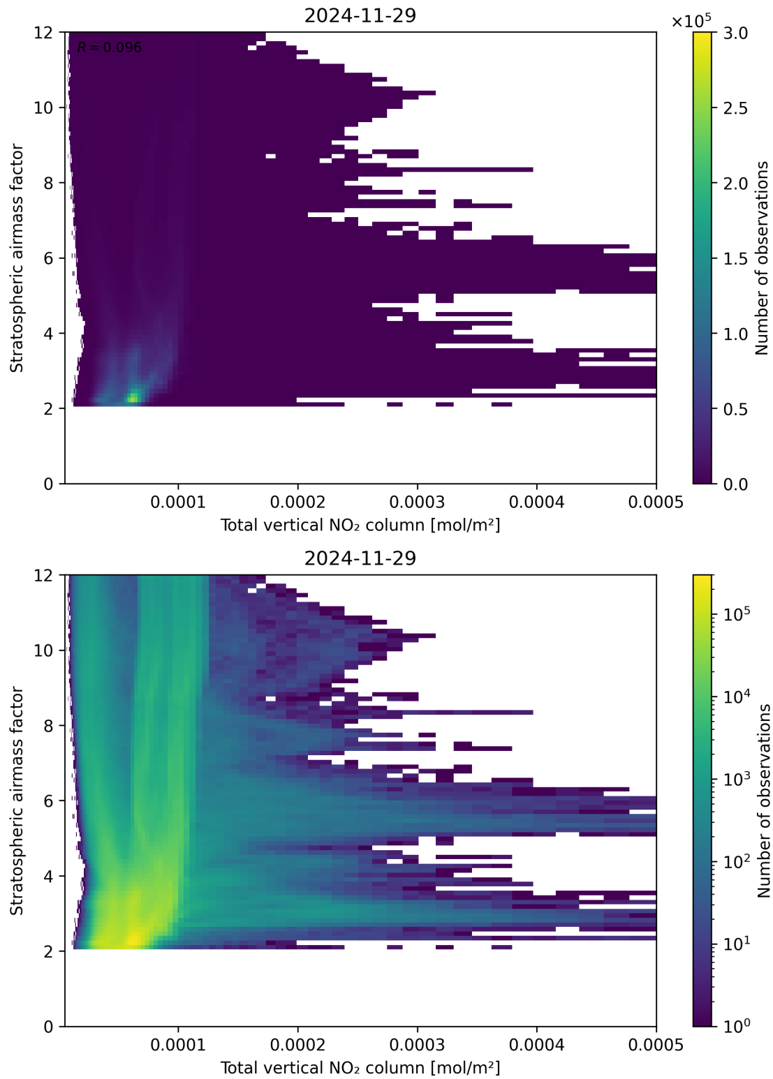
Figure 110: Scatter density plot of “Total vertical NO 2 column” against “Stratospheric airmass factor” for 2024-11-28 to 2024-11-30.
