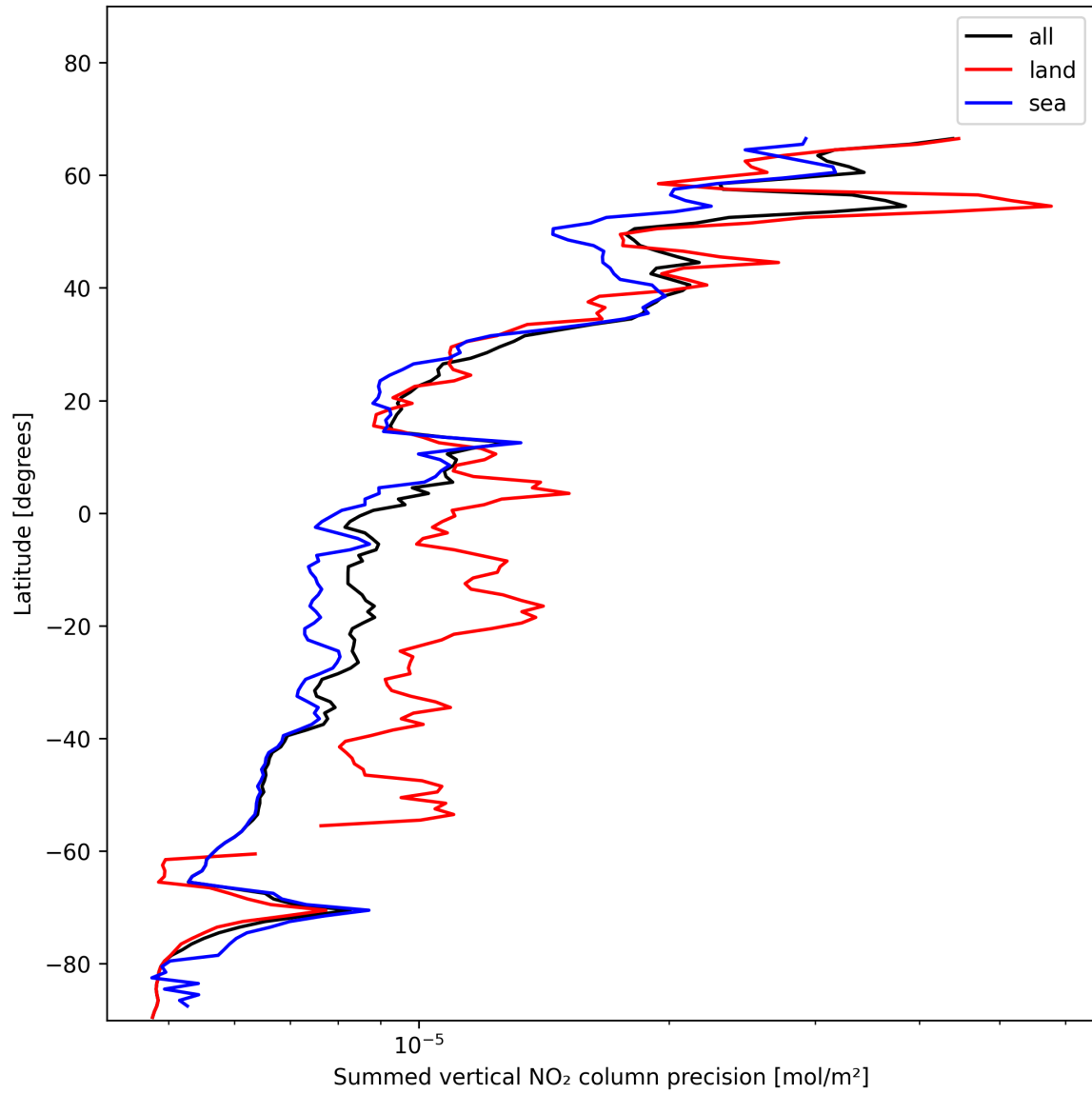
Figure 24: Zonal average of “Summed vertical NO 2 column precision” for 2024-11-28 to 2024-11-30.
