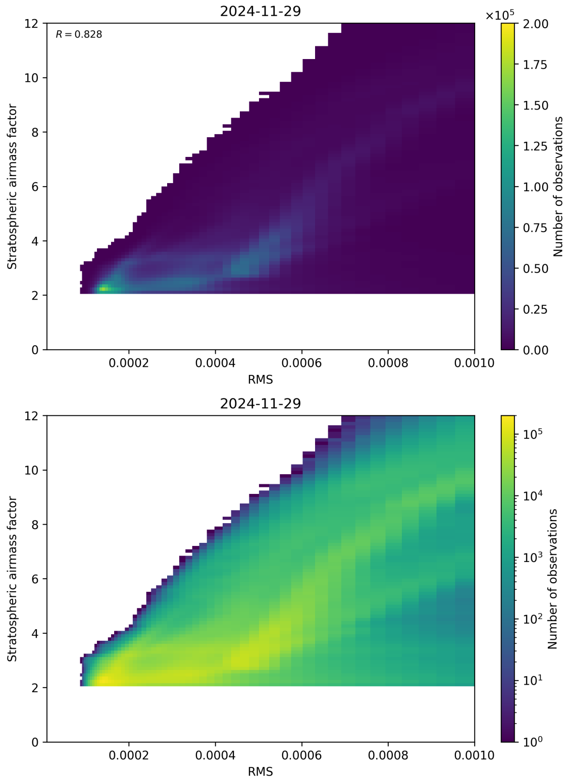
Figure 144: Scatter density plot of “RMS” against “Stratospheric airmass factor” for 2024-11-28 to 2024-11-30.
