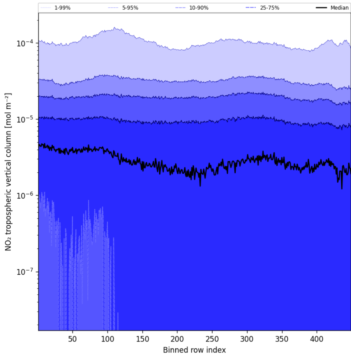
Figure 46: Along track statistics of “NO 2 tropospheric vertical column” for 2024-11-28 to 2024-11-30
