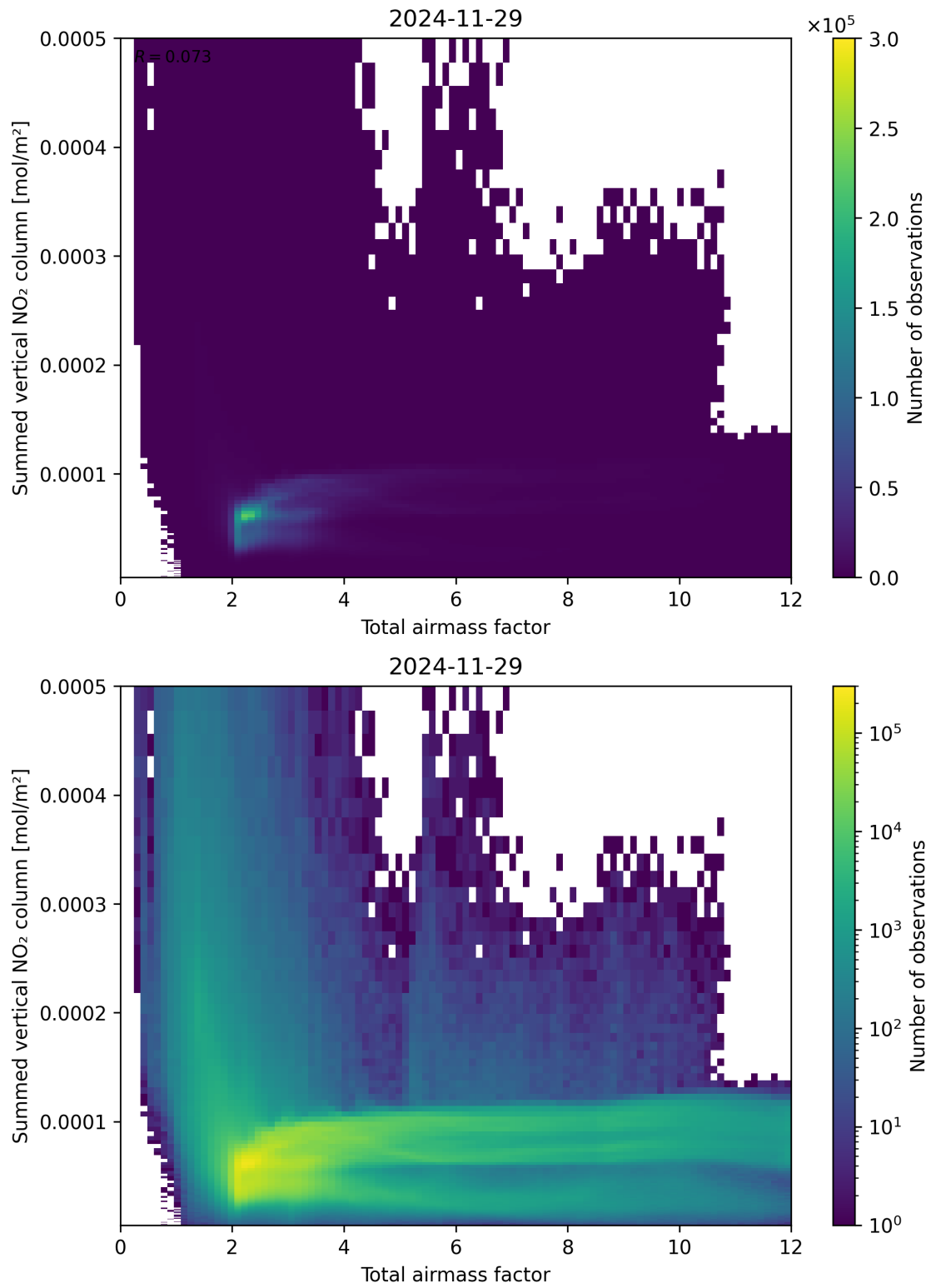
Figure 65: Scatter density plot of “Total airmass factor” against “Summed vertical NO 2 column” for 2024-11-28 to 2024-11-30.
