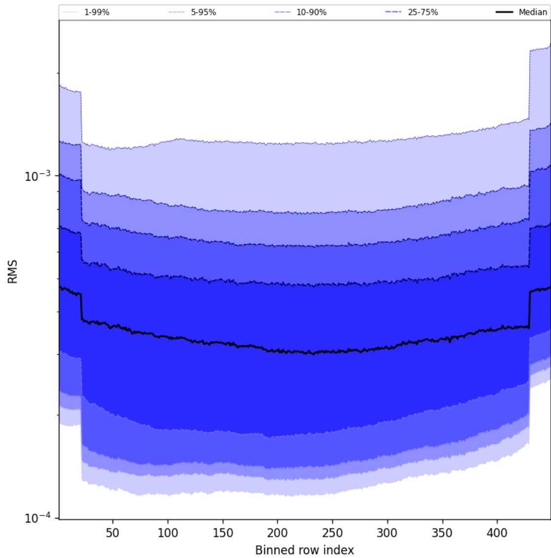
Figure 60: Along track statistics of “RMS” for 2024-11-28 to 2024-11-30
