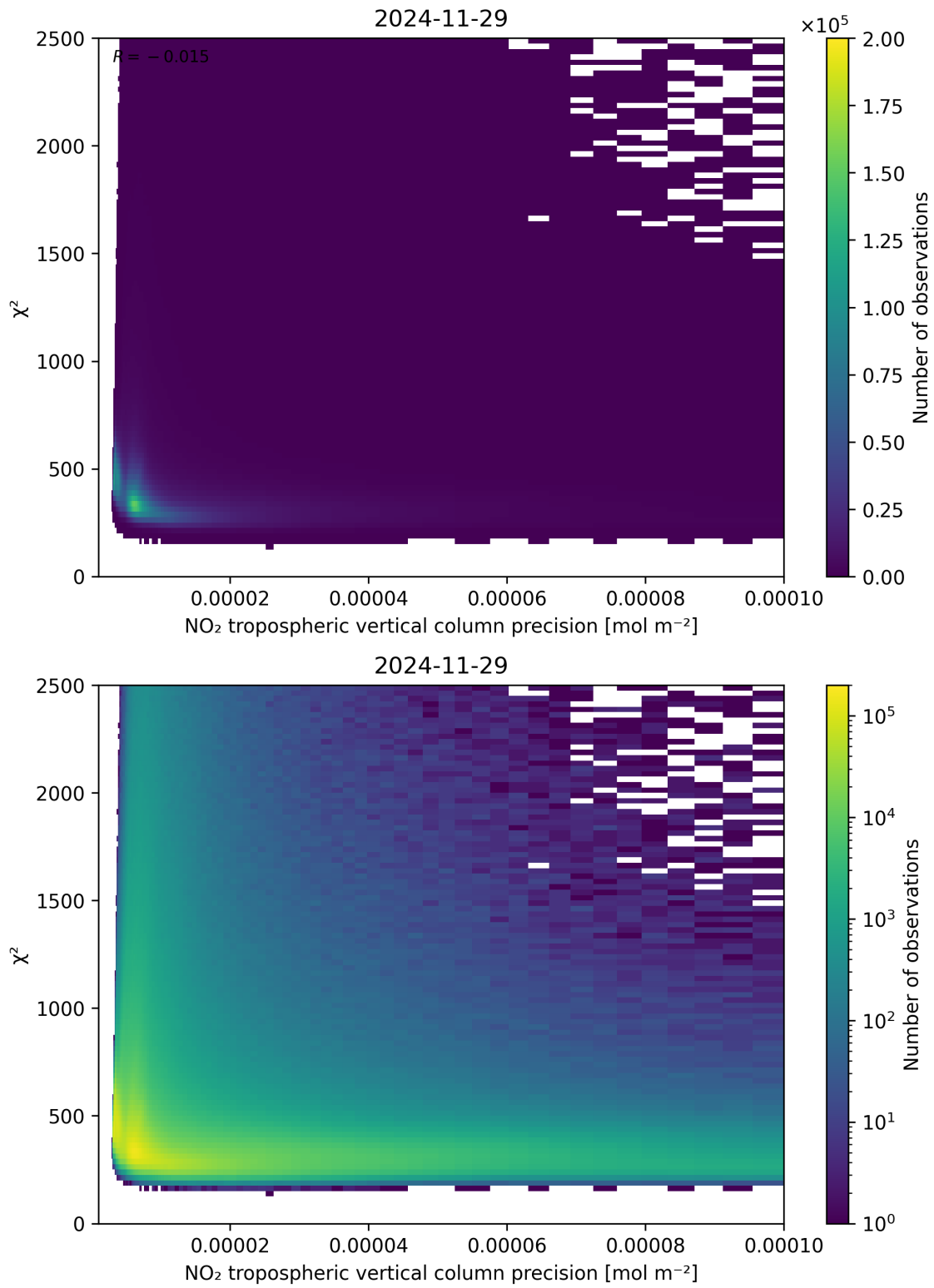
Figure 134: Scatter density plot of “NO 2 tropospheric vertical column precision” against “ \chi^2 ” for 2024-11-28 to 2024-11-30.
