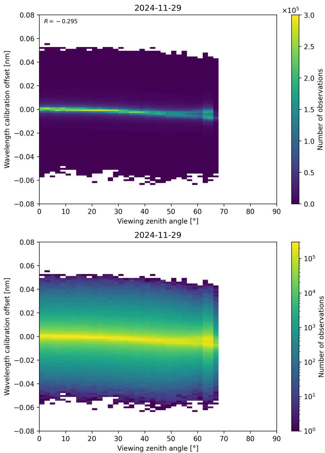
Figure 173: Scatter density plot of “Viewing zenith angle” against “Wavelength calibration offset” for 2024-11-28 to 2024-11-30.
