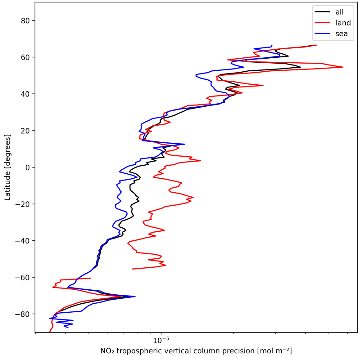
Figure 13: Zonal average of “NO 2 tropospheric vertical column precision” for 2024-11-28 to 2024-11-30.
