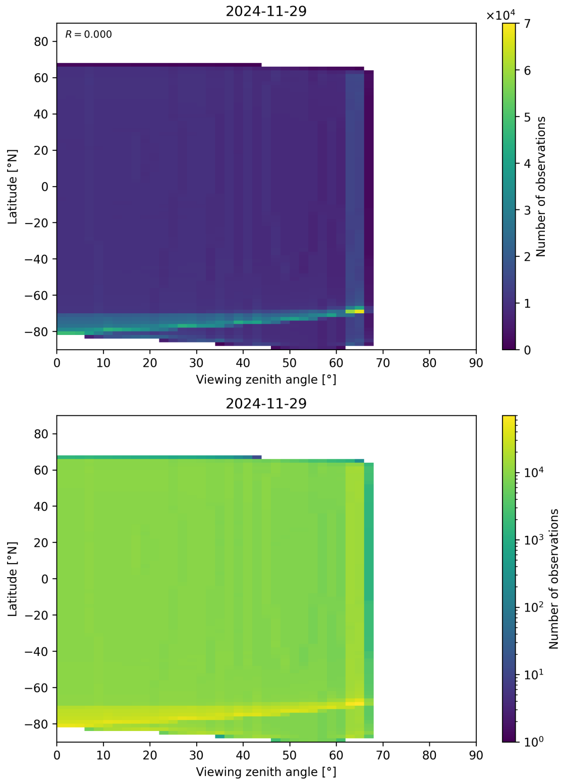
Figure 163: Scatter density plot of “Viewing zenith angle” against “Latitude” for 2024-11-28 to 2024-11-30.
