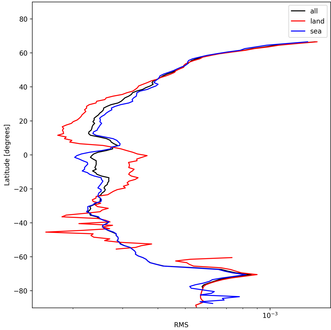
Figure 26: Zonal average of “RMS” for 2024-11-28 to 2024-11-30.
