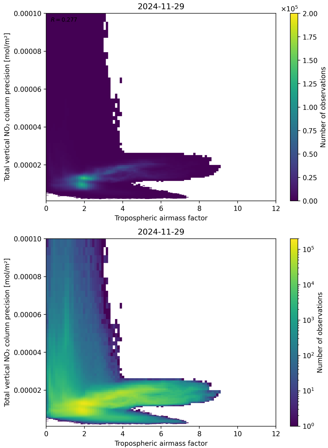
Figure 78: Scatter density plot of “Tropospheric air mass factor” against “Total vertical NO 2 column precision” for 2024-11-28 to 2024-11-30.
