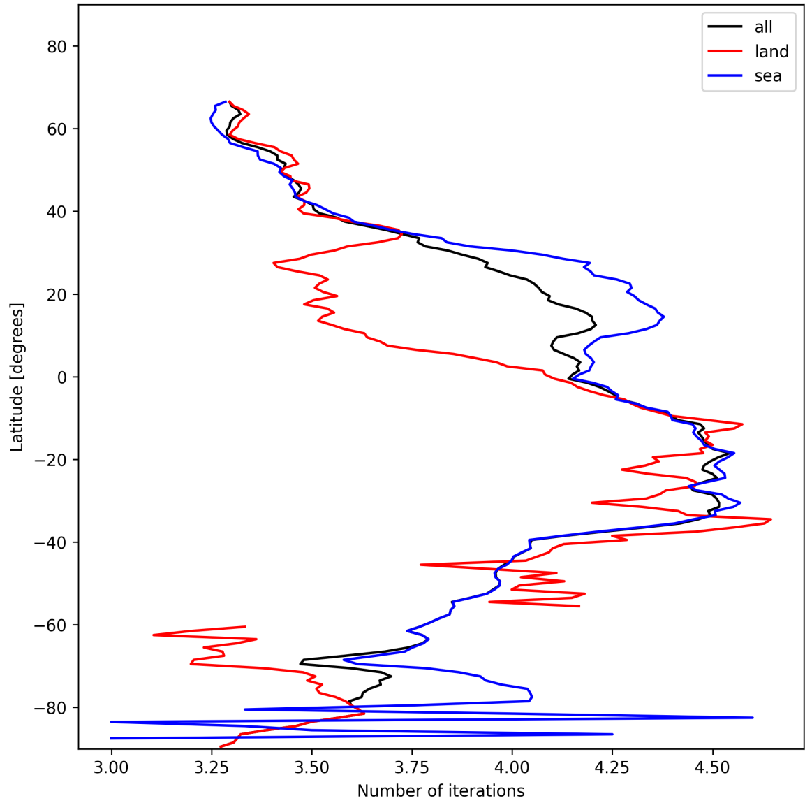
Figure 17: Zonal average of “Number of iterations” for 2024-11-28 to 2024-11-30.
