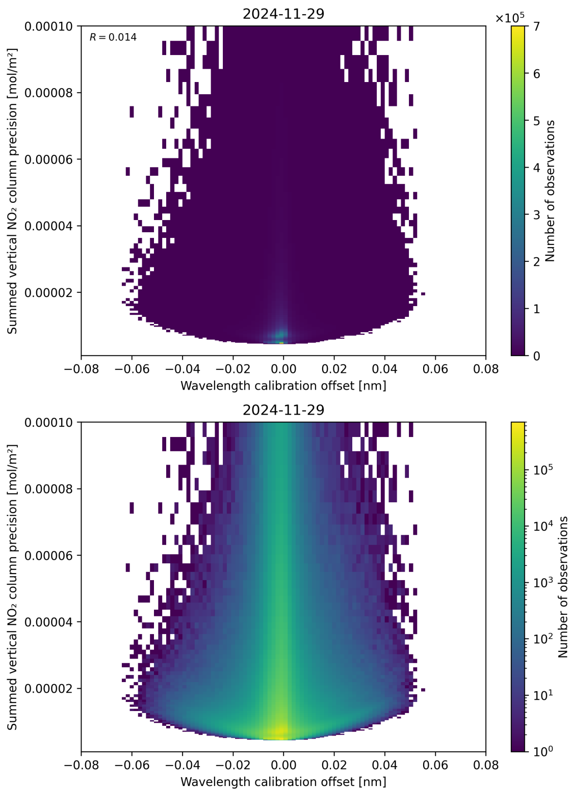
Figure 178: Scatter density plot of “Wavelength calibration offset” against “Summed vertical NO 2 column precision” for 2024-11-28 to 2024-11-30.
