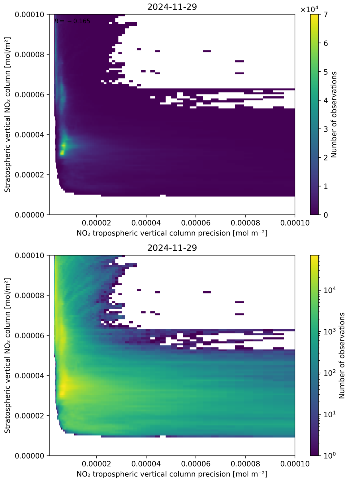
Figure 135: Scatter density plot of “NO 2 tropospheric vertical column precision” against “Stratospheric vertical NO 2 column” for 2024-11-28 to 2024-11-30.
