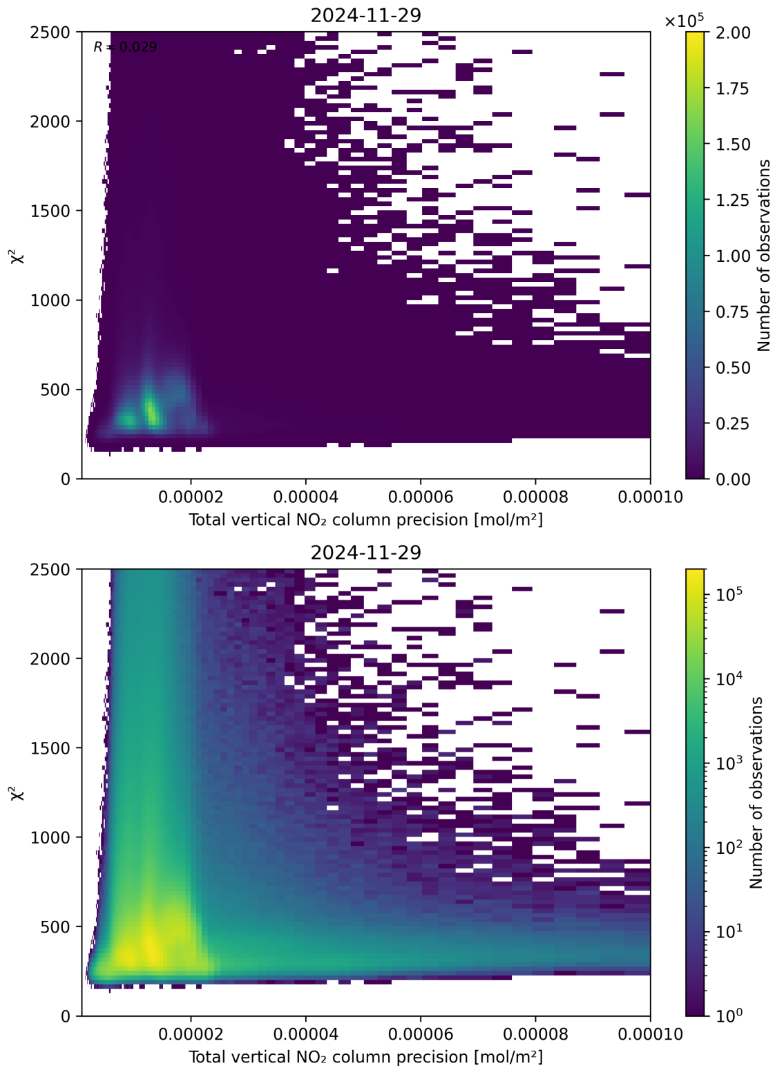
Figure 116: Scatter density plot of “Total vertical NO 2 column precision” against “ \chi^2 ” for 2024-11-28 to 2024-11-30.
