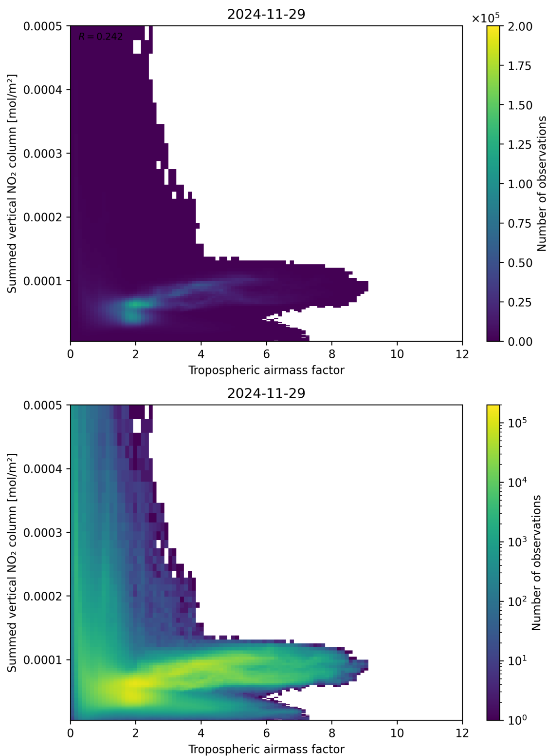
Figure 75: Scatter density plot of “Tropospheric airmass factor” against “Summed vertical NO 2 column” for 2024-11-28 to 2024-11-30.
