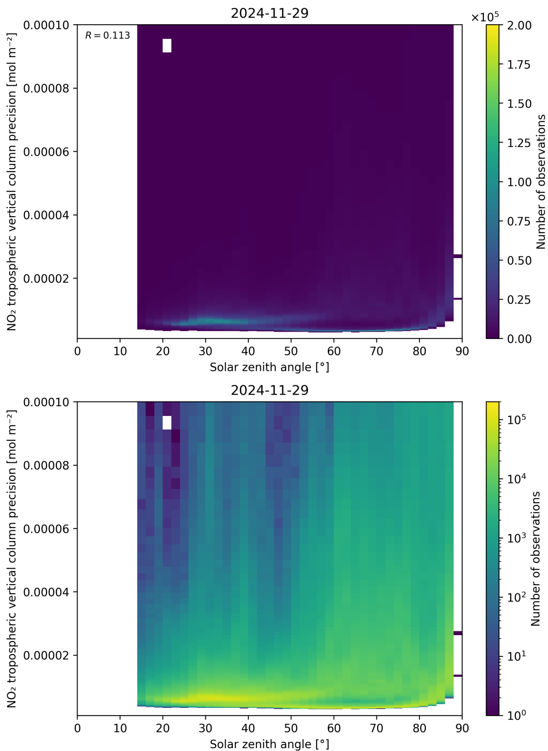
Figure 156: Scatter density plot of “Solar zenith angle” against “NO 2 tropospheric vertical column precision” for 2024-11-28 to 2024-11-30.
