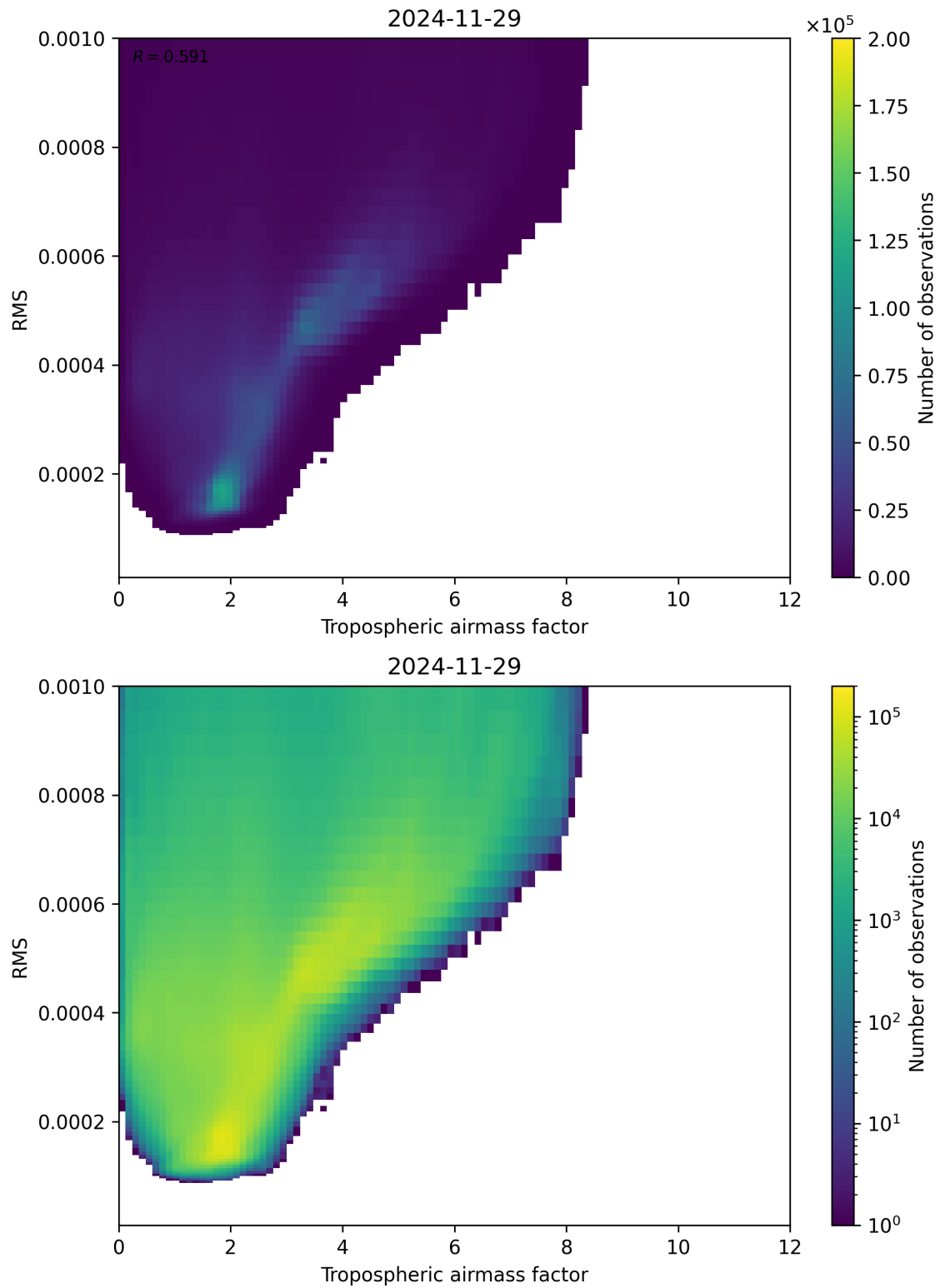
Figure 79: Scatter density plot of “Tropospheric airmass factor” against “RMS” for 2024-11-28 to 2024-11-30.
