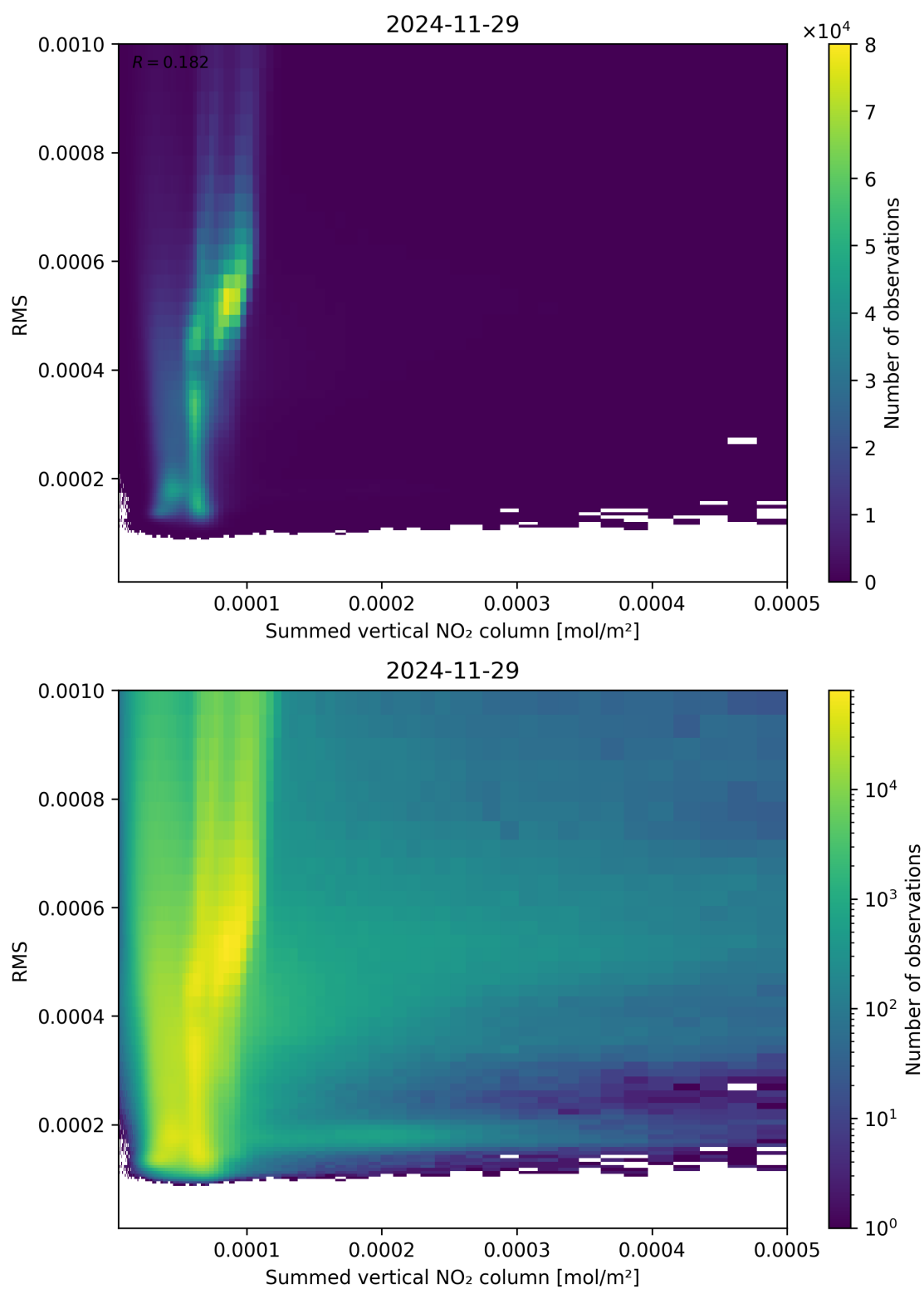
Figure 109: Scatter density plot of “Summed vertical NO 2 column” against “RMS” for 2024-11-28 to 2024-11-30.
