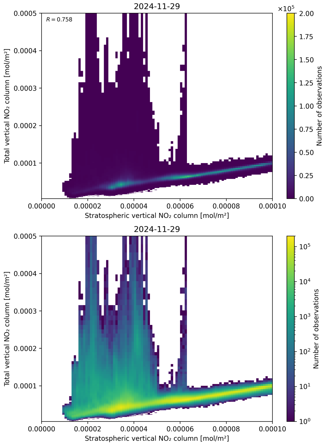
Figure 100: Scatter density plot of “Stratospheric vertical NO 2 column” against “Total vertical NO 2 column” for 2024-11-28 to 2024-11-30.
