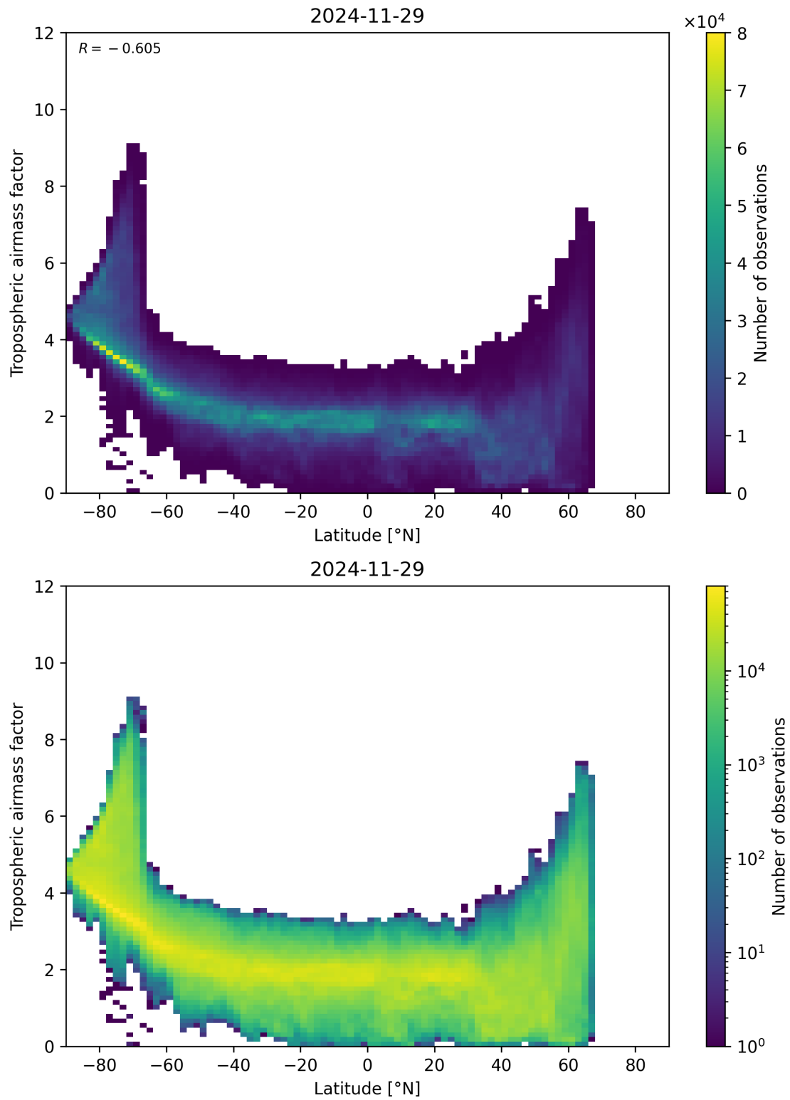
Figure 85: Scatter density plot of “Latitude” against “Tropospheric airmass factor” for 2024-11-28 to 2024-11-30.
