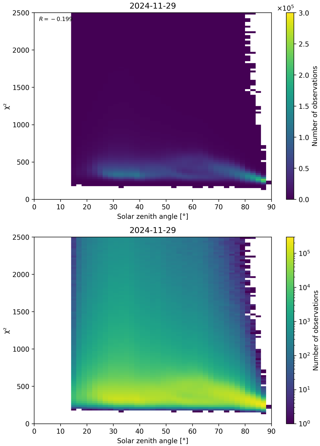
Figure 148: Scatter density plot of “Solar zenith angle” against “ \chi^2 ” for 2024-11-28 to 2024-11-30.
