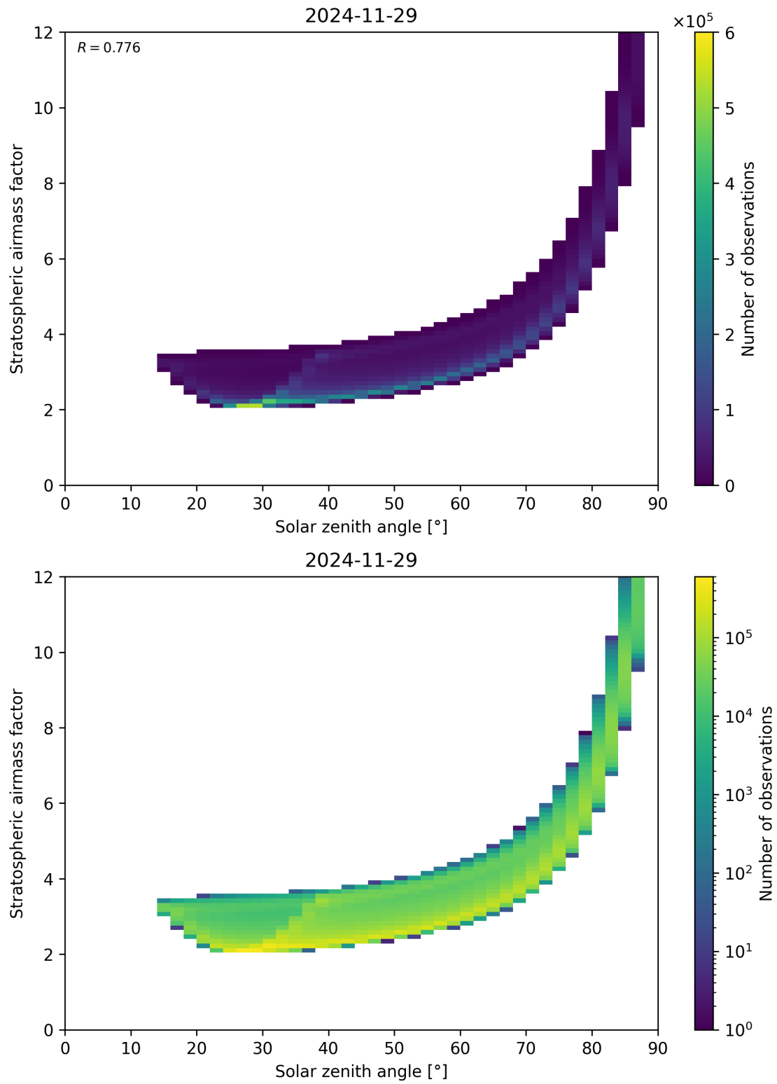
Figure 145: Scatter density plot of “Solar zenith angle” against “Stratospheric airmass factor” for 2024-11-28 to 2024-11-30.
