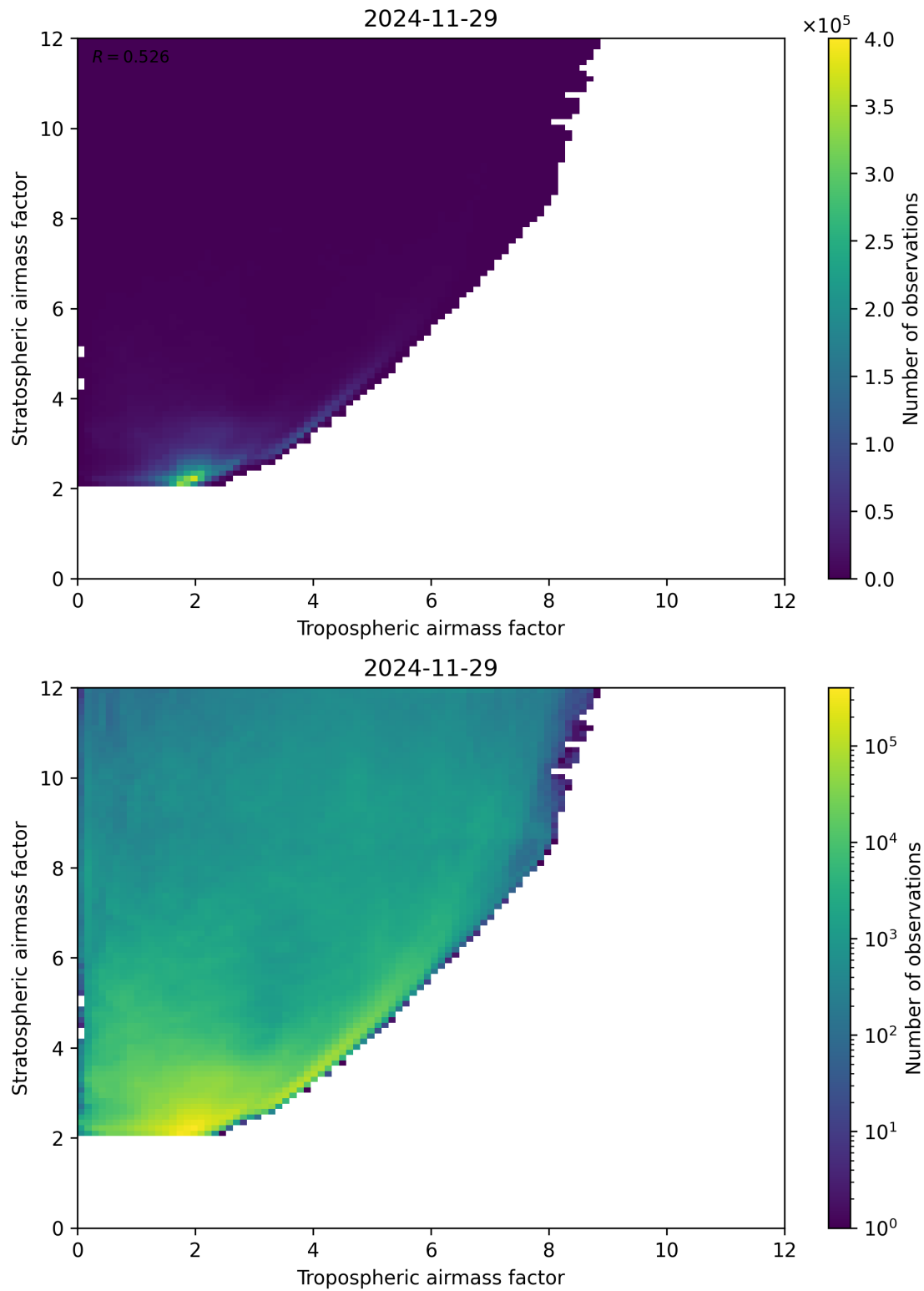
Figure 71: Scatter density plot of “Tropospheric airmass factor” against “Stratospheric airmass factor” for 2024-11-28 to 2024-11-30.
