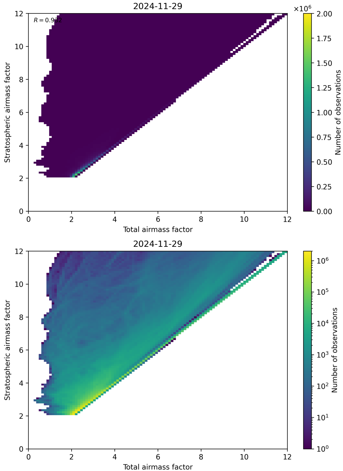
Figure 62: Scatter density plot of “Total airmass factor” against “Stratospheric airmass factor” for 2024-11-28 to 2024-11-30.
