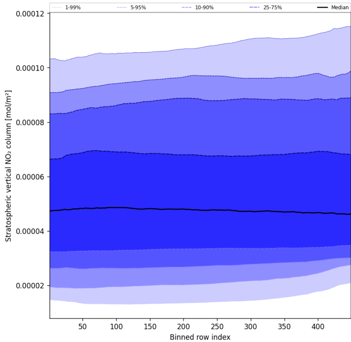
Figure 53: Along track statistics of “Stratospheric vertical NO 2 column” for 2024-11-28 to 2024-11-30
