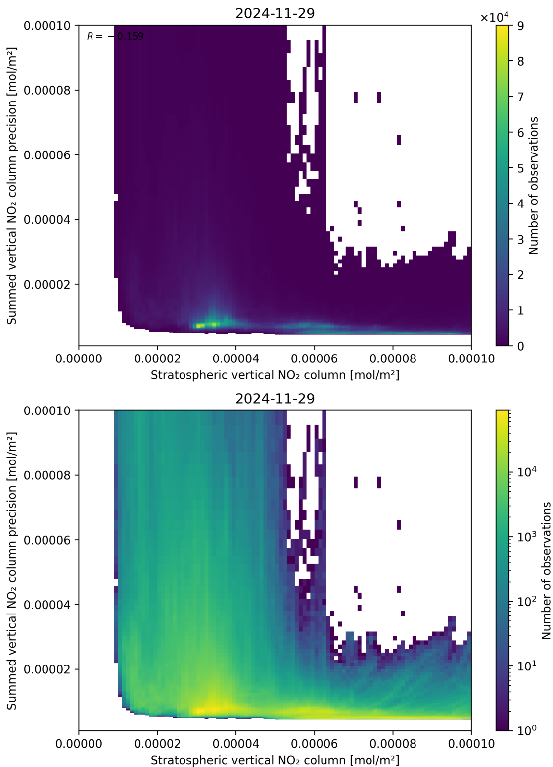
Figure 99: Scatter density plot of “Stratospheric vertical NO 2 column” against “Summed vertical NO 2 column precision” for 2024-11-28 to 2024-11-30.
