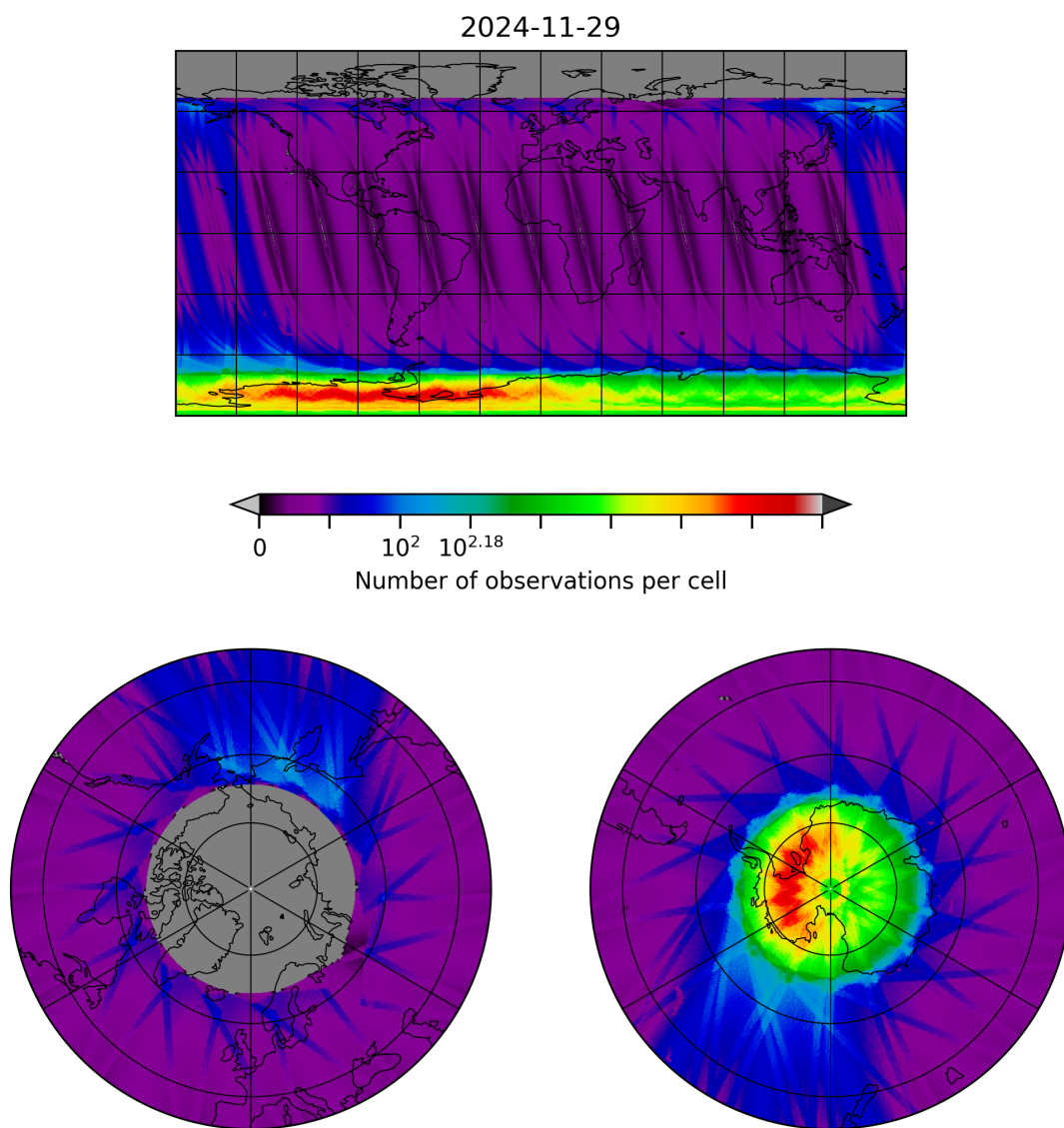
Figure 10: Map of the number of observations for 2024-11-28 to 2024-11-30
