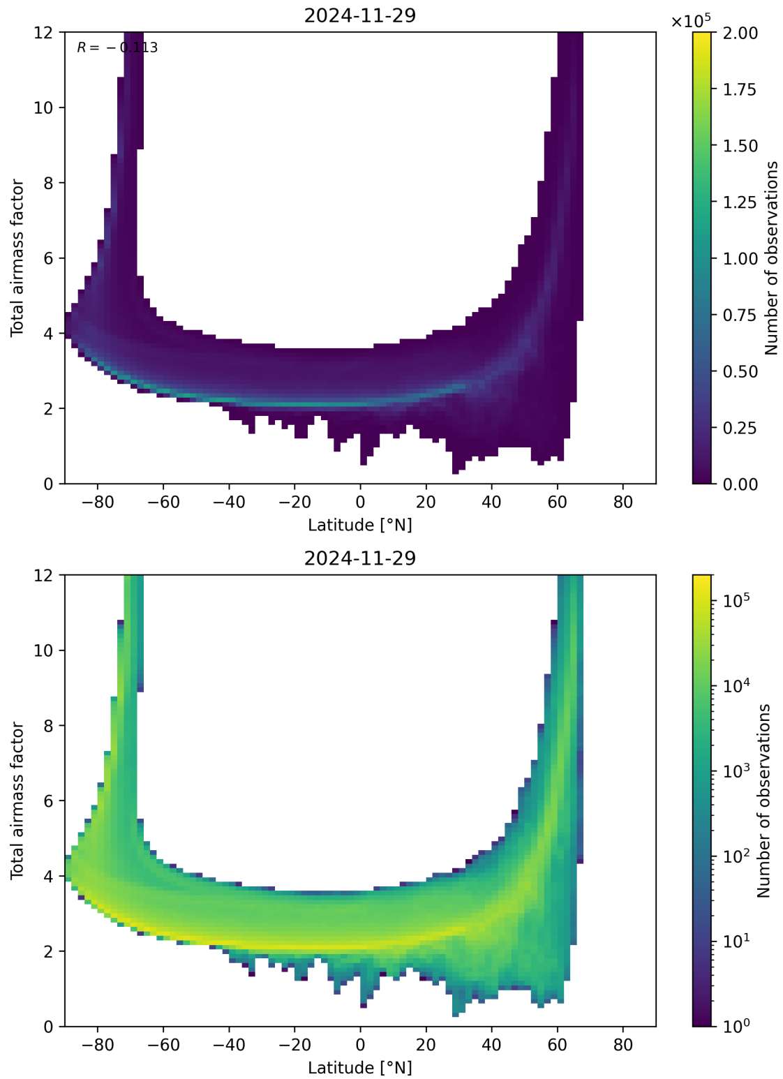
Figure 84: Scatter density plot of “Latitude” against “Total airmass factor” for 2024-11-28 to 2024-11-30.
