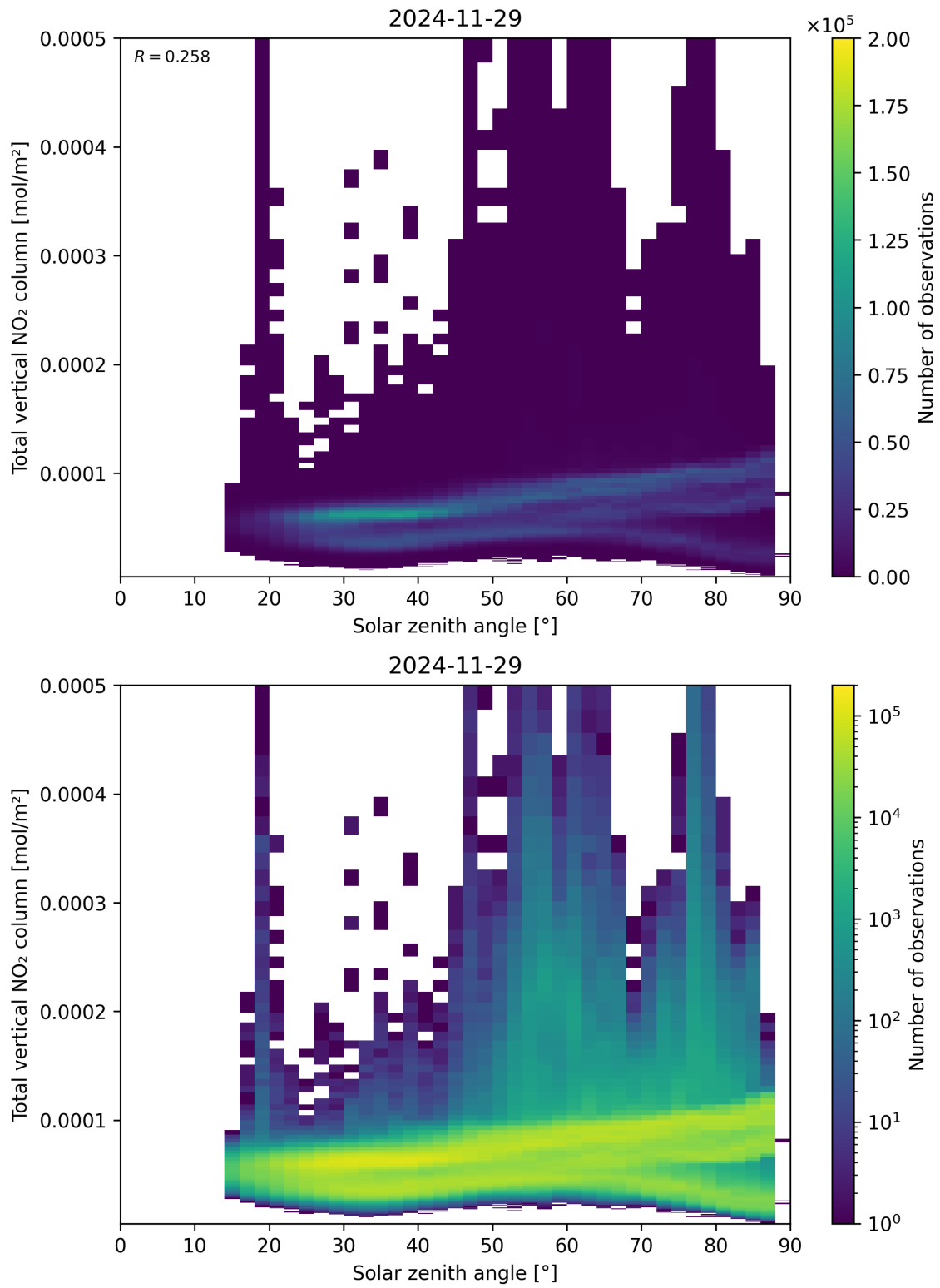
Figure 153: Scatter density plot of “Solar zenith angle” against “Total vertical NO 2 column” for 2024-11-28 to 2024-11-30.
