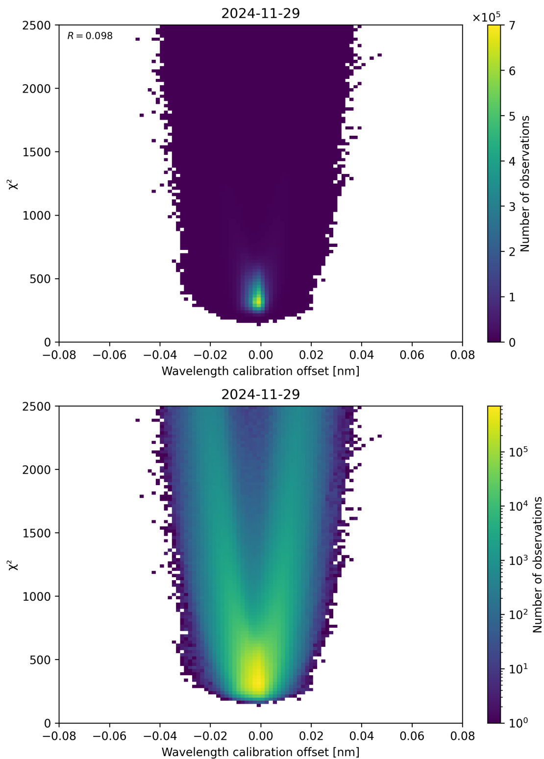
Figure 175: Scatter density plot of “Wavelength calibration offset” against “ \chi^2 ” for 2024-11-28 to 2024-11-30.
