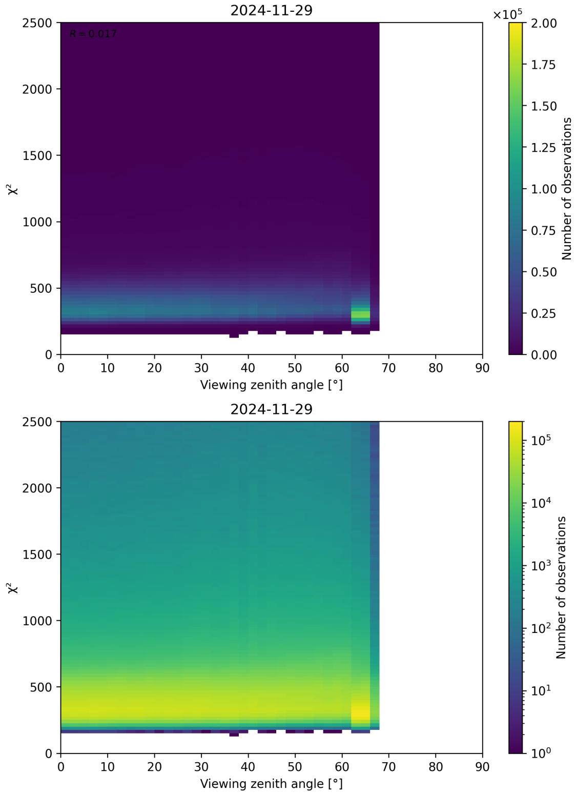
Figure 162: Scatter density plot of “Viewing zenith angle” against “ \chi^2 ” for 2024-11-28 to 2024-11-30.
