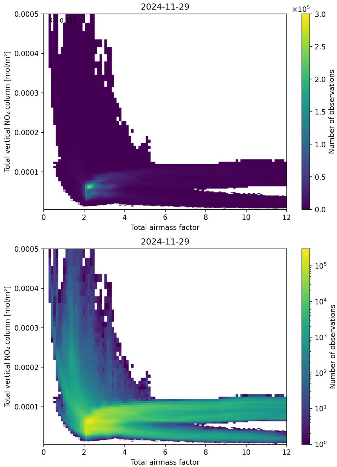
Figure 67: Scatter density plot of “Total airmass factor” against “Total vertical NO 2 column” for 2024-11-28 to 2024-11-30.
