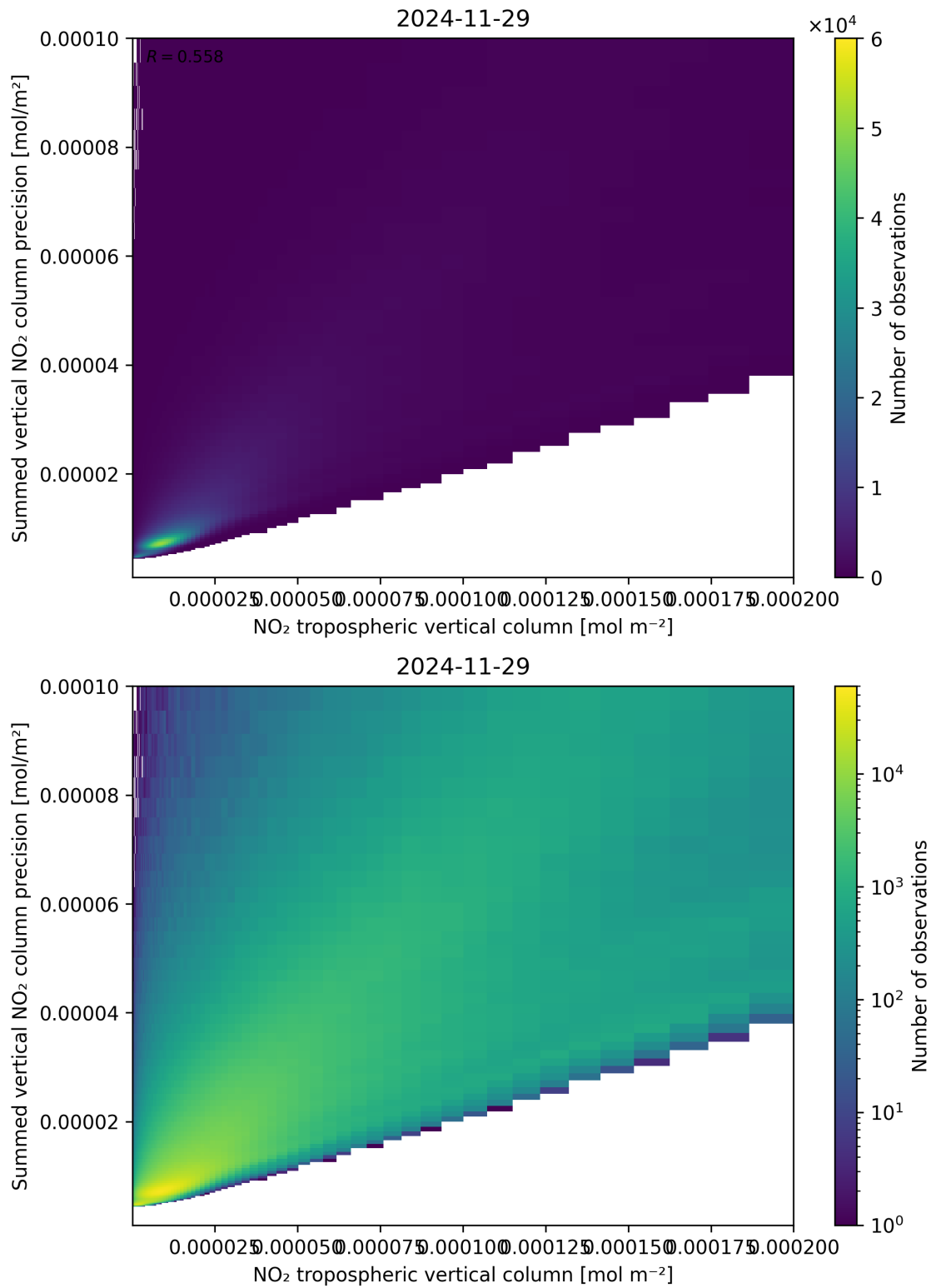
Figure 127: Scatter density plot of “NO 2 tropospheric vertical column” against “Summed vertical NO 2 column precision” for 2024-11-28 to 2024-11-30.
