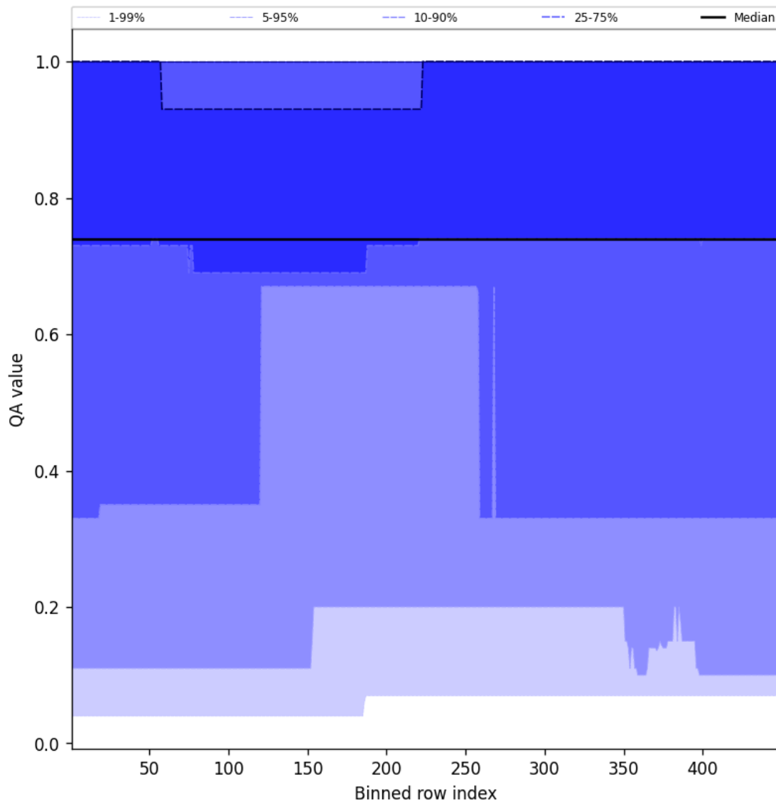
Figure 45: Along track statistics of “QA value” for 2024-11-28 to 2024-11-30
