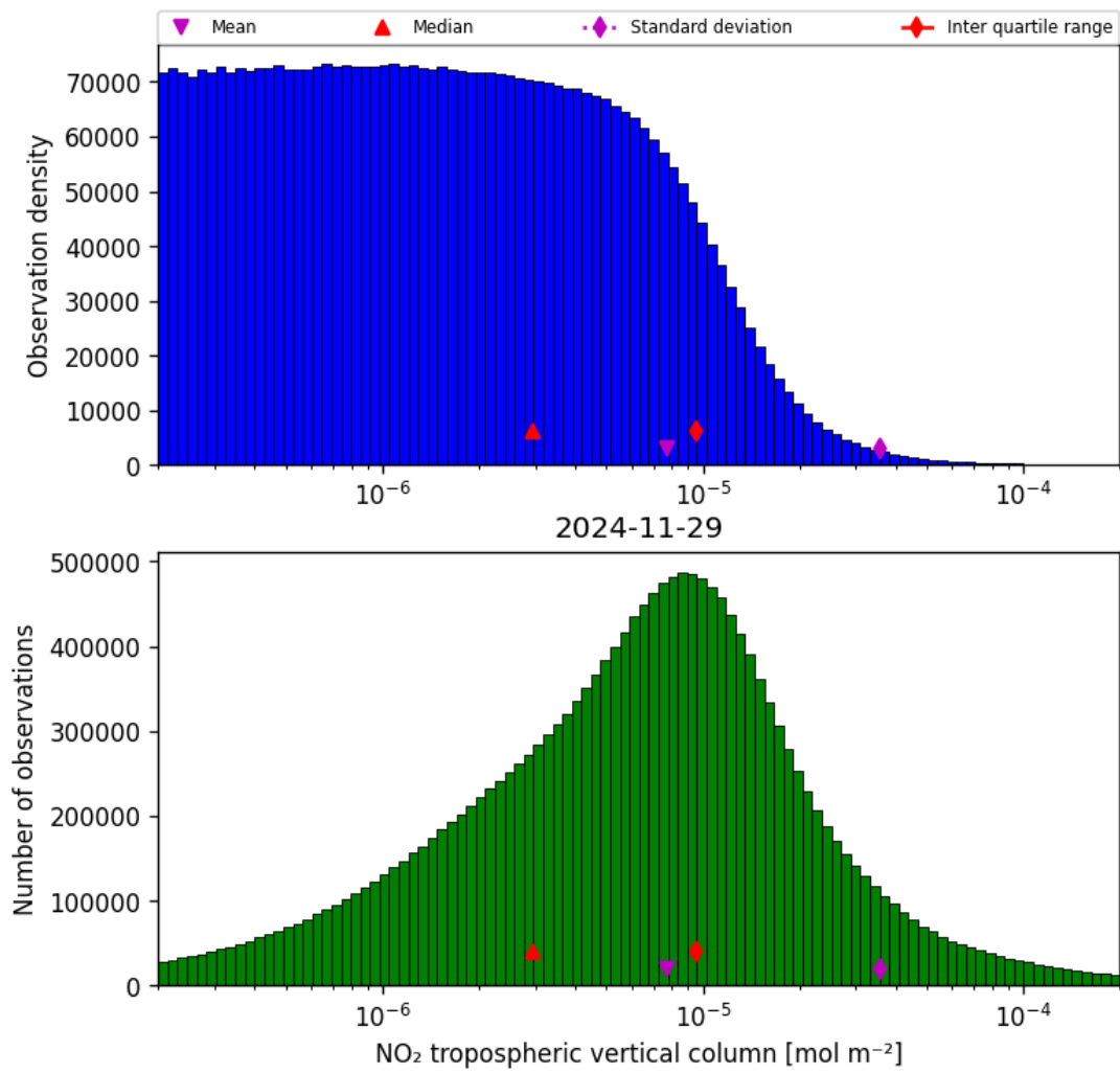
Figure 29: Histogram of “NO 2 tropospheric vertical column” for 2024-11-28 to 2024-11-30
