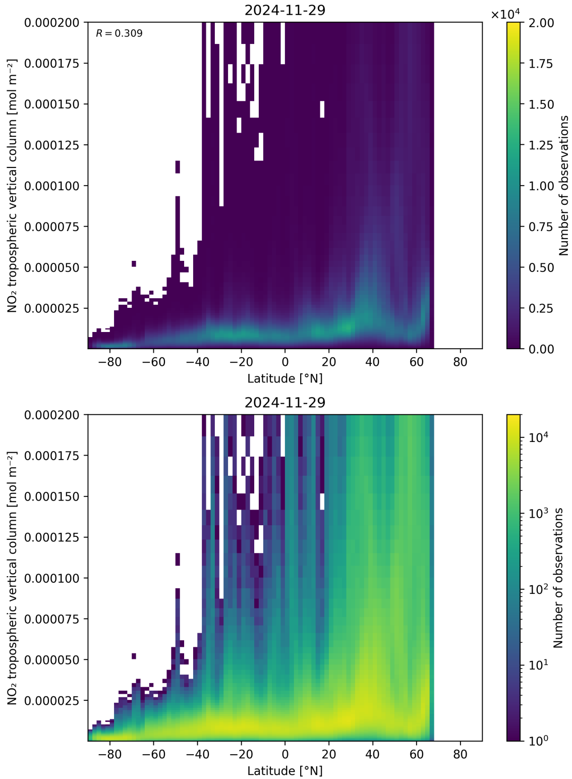
Figure 92: Scatter density plot of “Latitude” against “NO 2 tropospheric vertical column” for 2024-11-28 to 2024-11-30.
