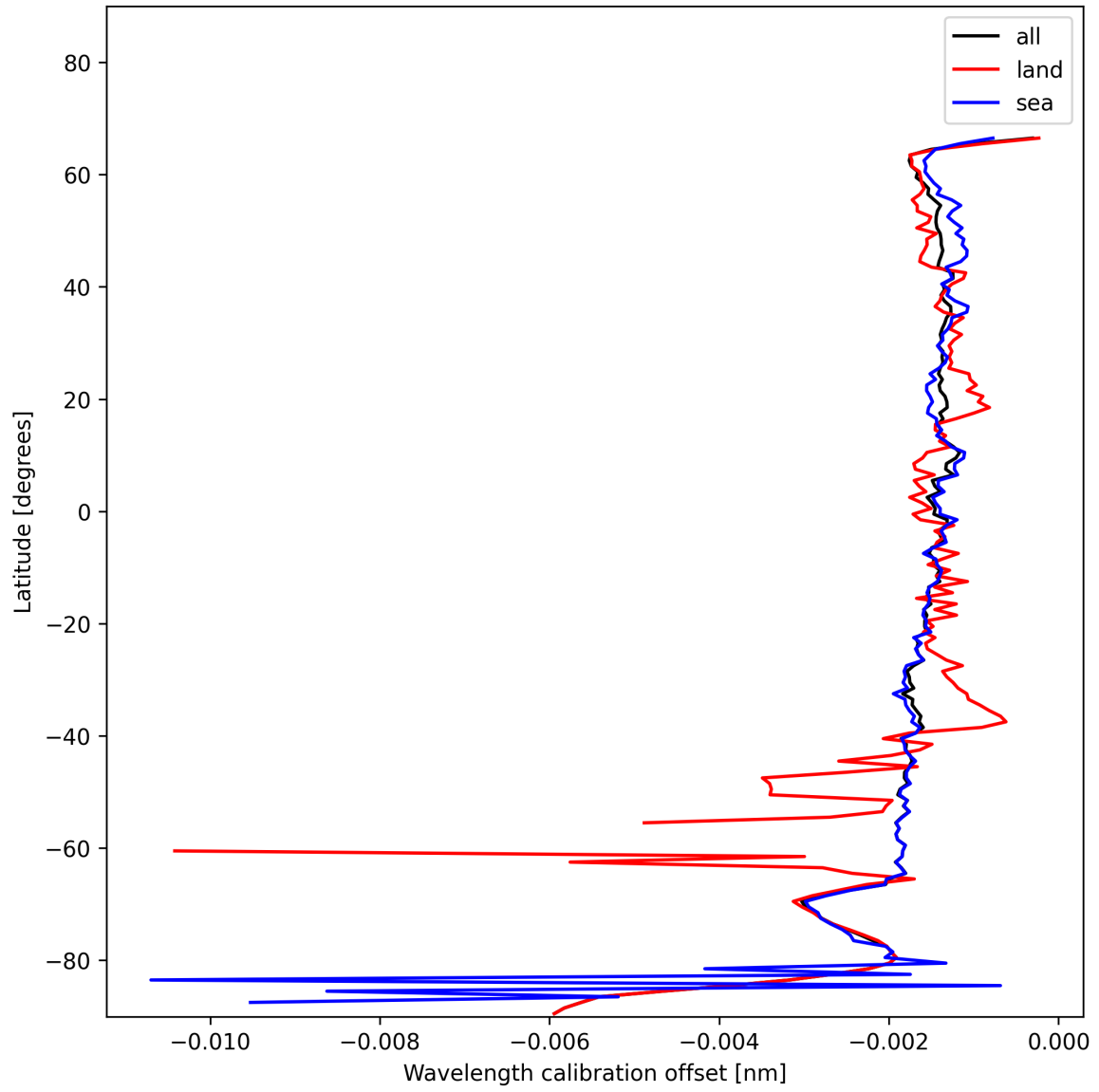
Figure 18: Zonal average of “Wavelength calibration offset” for 2024-11-28 to 2024-11-30.
