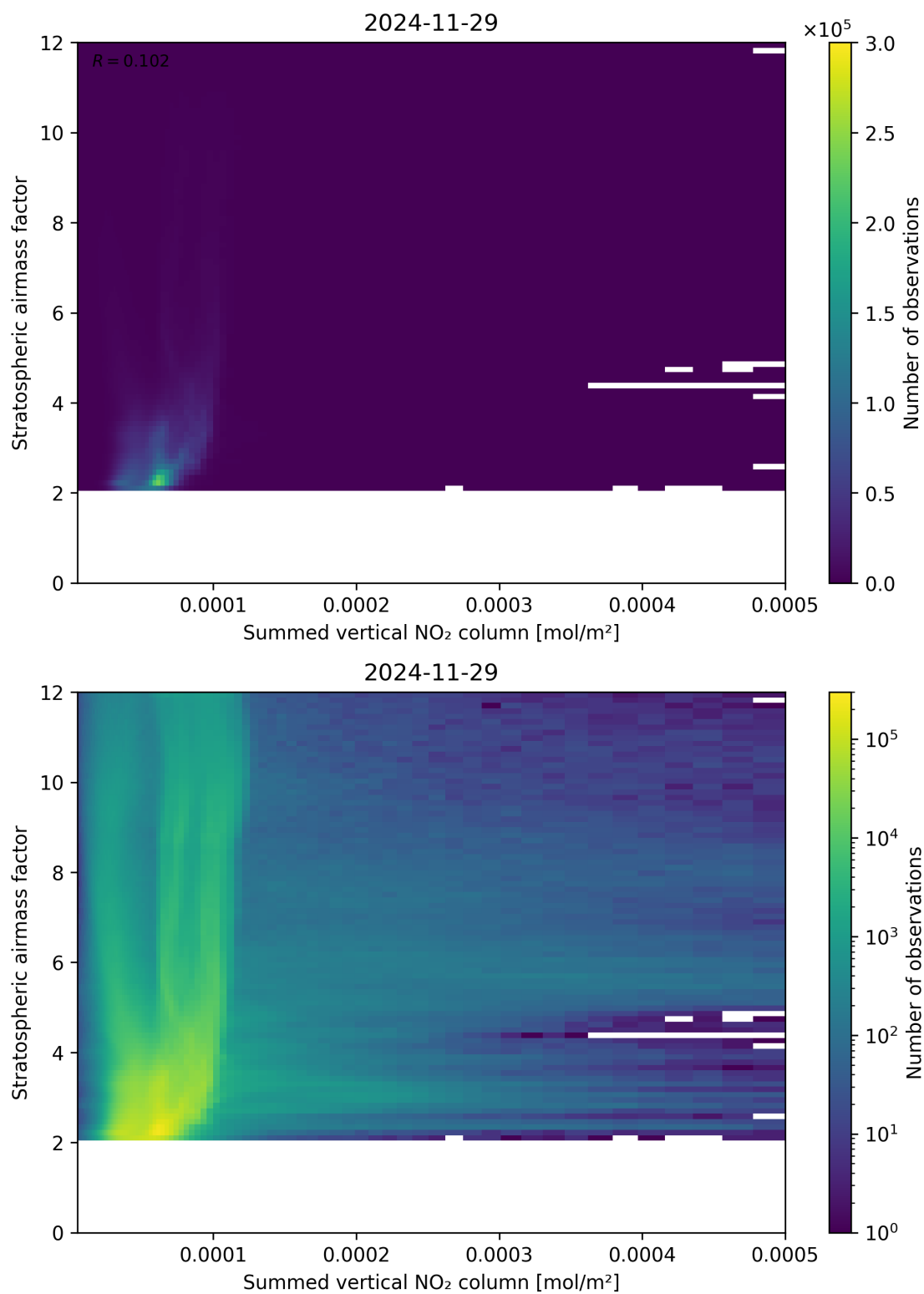
Figure 103: Scatter density plot of “Summed vertical NO 2 column” against “Stratospheric airmass factor” for 2024-11-28 to 2024-11-30.
