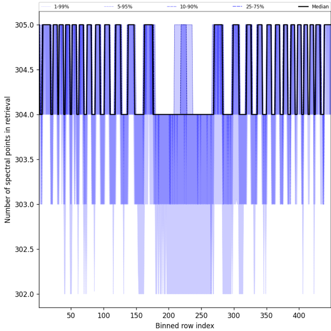
Figure 50: Along track statistics of “Number of spectral points in retrieval” for 2024-11-28 to 2024-11-30
