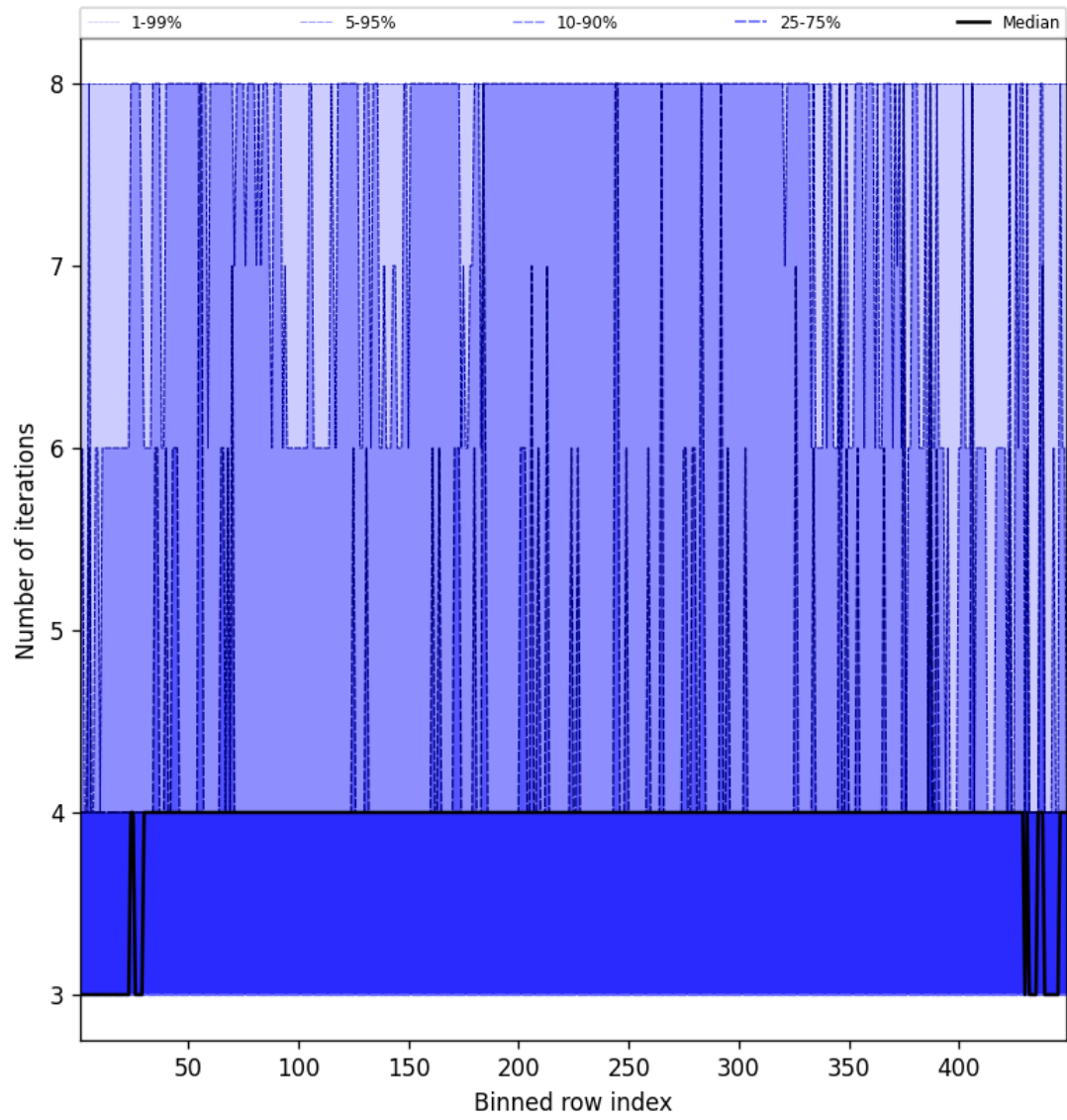
Figure 51: Along track statistics of “Number of iterations” for 2024-11-28 to 2024-11-30
