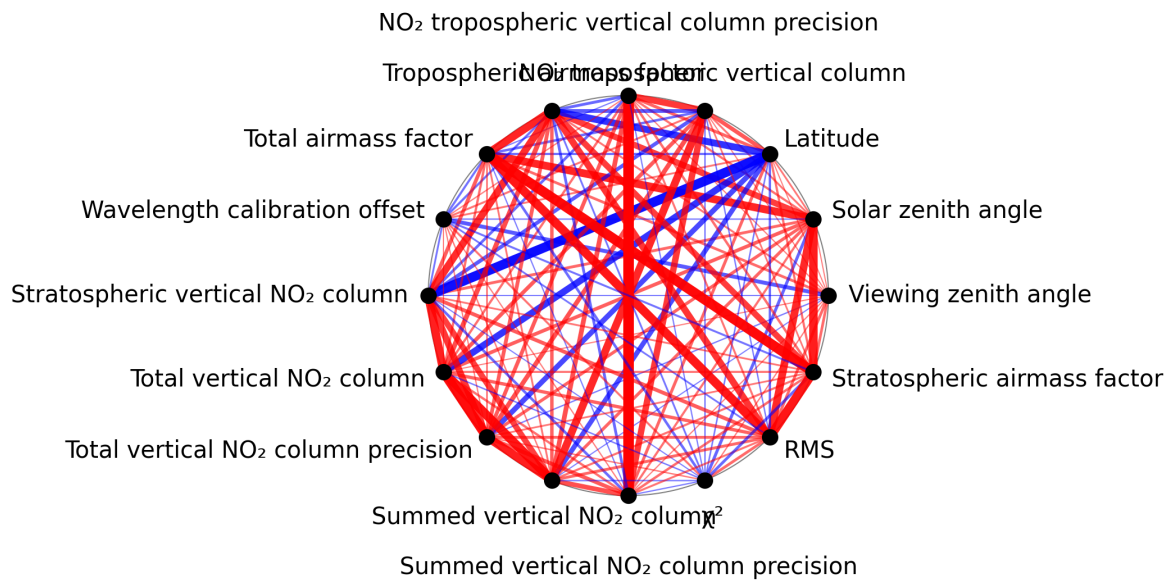
Figure 1: Map of correlation graph for 2024-11-28 to 2024-11-30.
