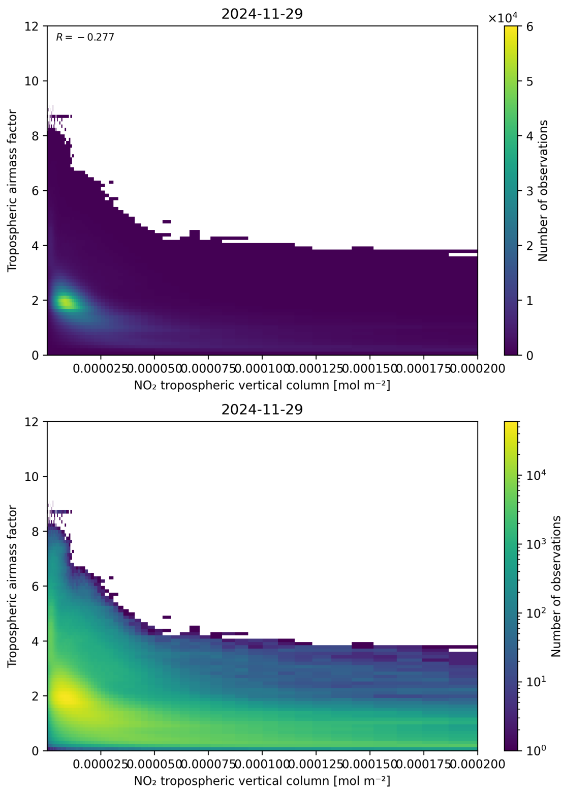
Figure 123: Scatter density plot of “NO 2 tropospheric vertical column” against “Tropospheric air mass factor” for 2024-11-28 to 2024-11-30.
