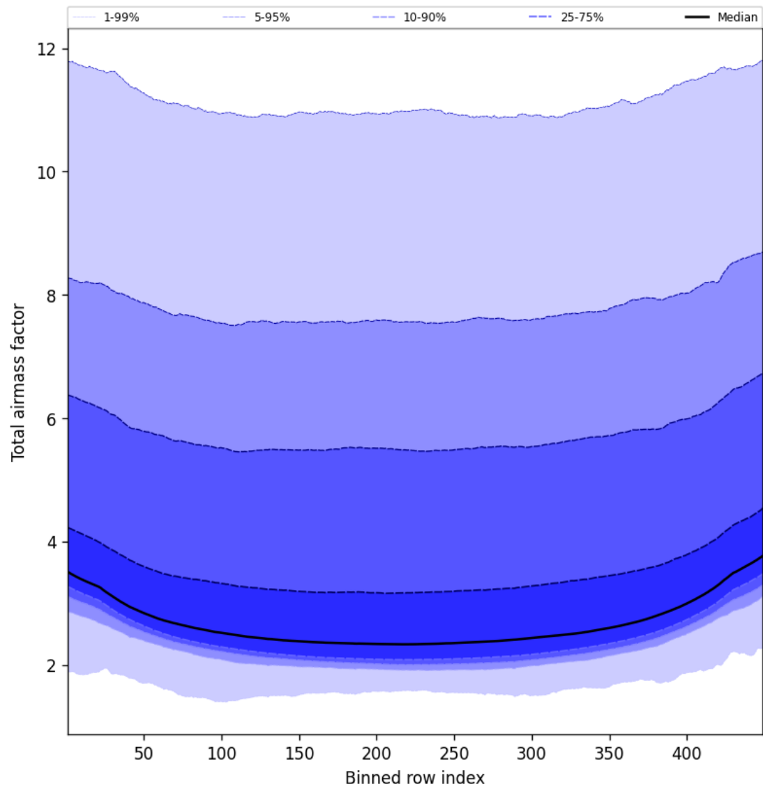
Figure 49: Along track statistics of “Total airmass factor” for 2024-11-28 to 2024-11-30
