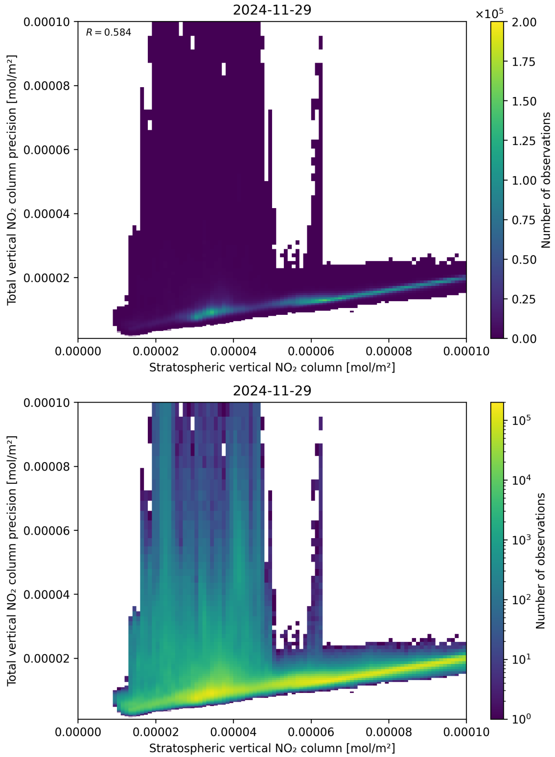
Figure 101: Scatter density plot of “Stratospheric vertical NO 2 column” against “Total vertical NO 2 column precision” for 2024-11-28 to 2024-11-30.
