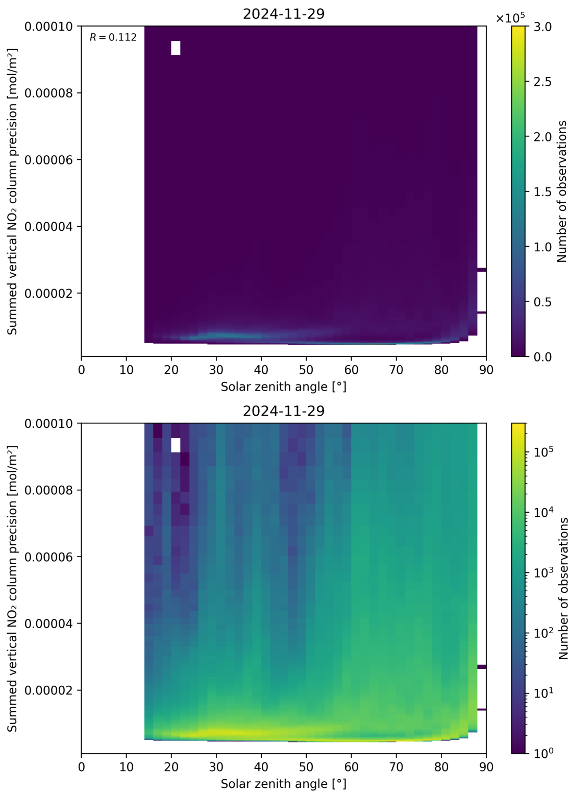
Figure 152: Scatter density plot of “Solar zenith angle” against “Summed vertical NO 2 column precision” for 2024-11-28 to 2024-11-30.
