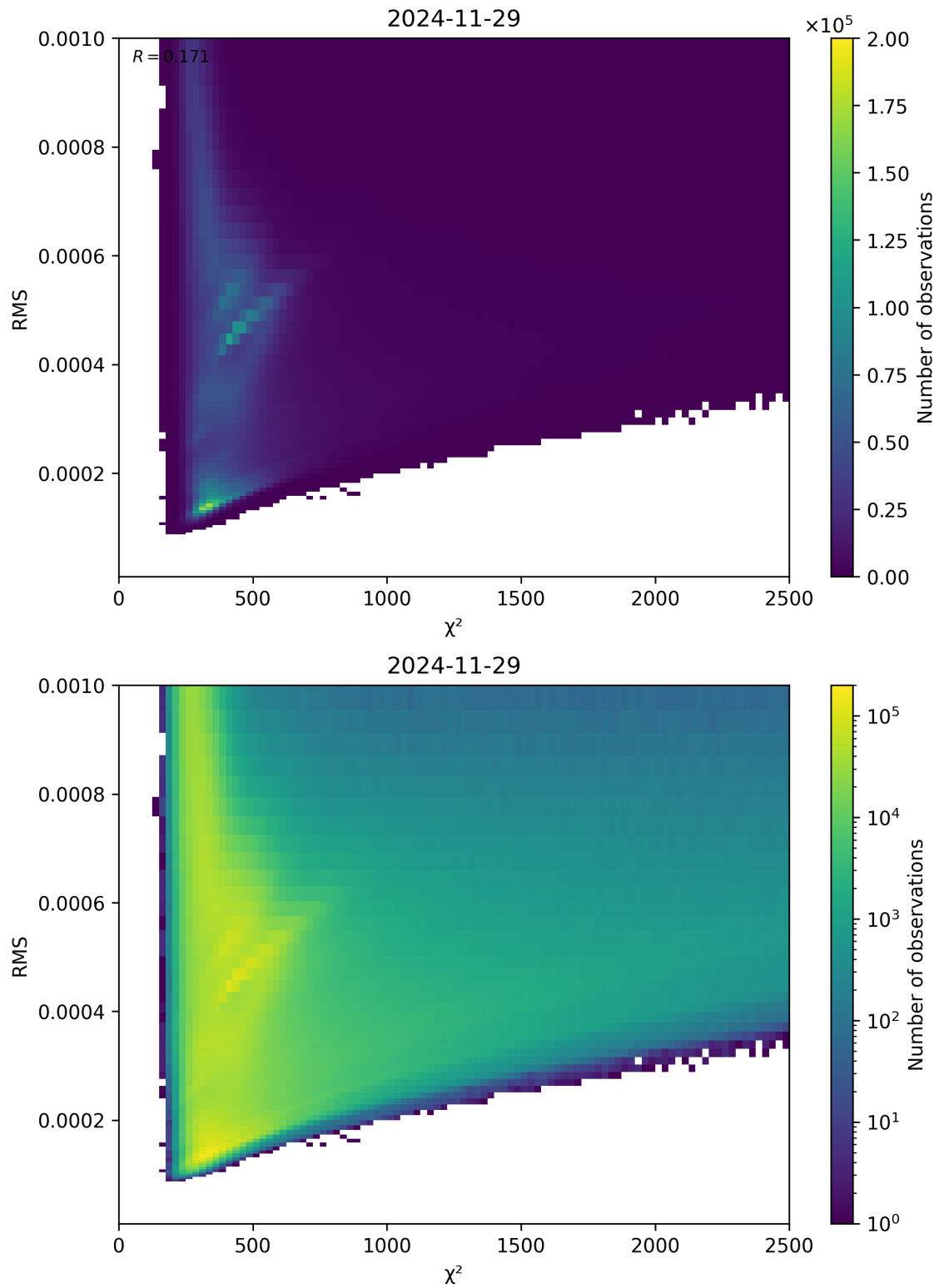
Figure 82: Scatter density plot of “ \chi^2 ” against “RMS” for 2024-11-28 to 2024-11-30.
