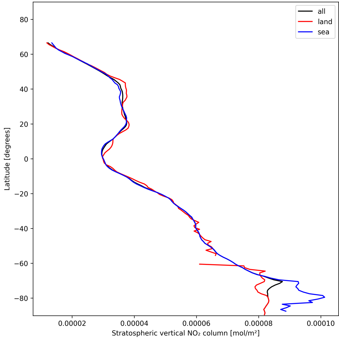
Figure 19: Zonal average of “Stratospheric vertical NO 2 column” for 2024-11-28 to 2024-11-30.
