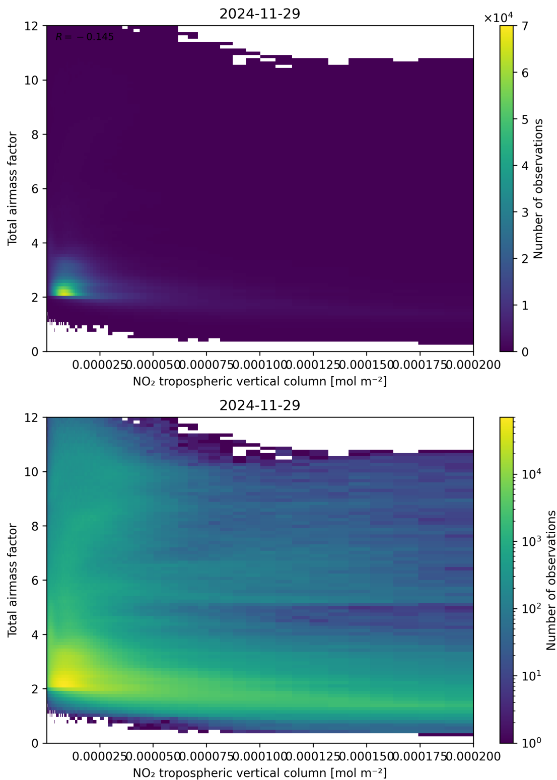
Figure 122: Scatter density plot of “NO 2 tropospheric vertical column” against “Total airmass factor” for 2024-11-28 to 2024-11-30.
