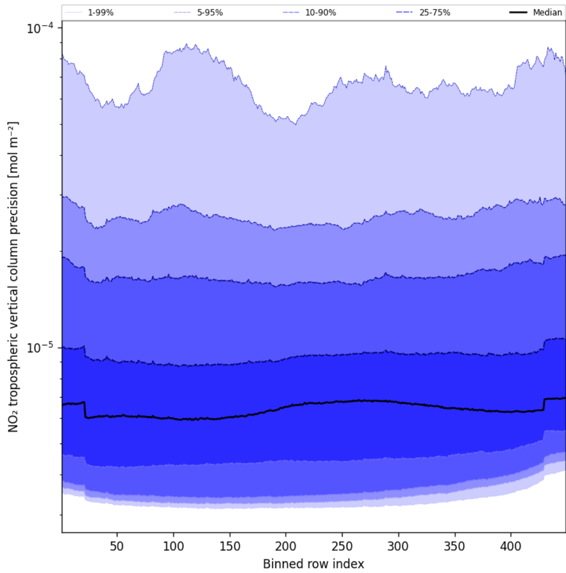
Figure 47: Along track statistics of “NO 2 tropospheric vertical column precision” for 2024-11-28 to 2024-11-30
