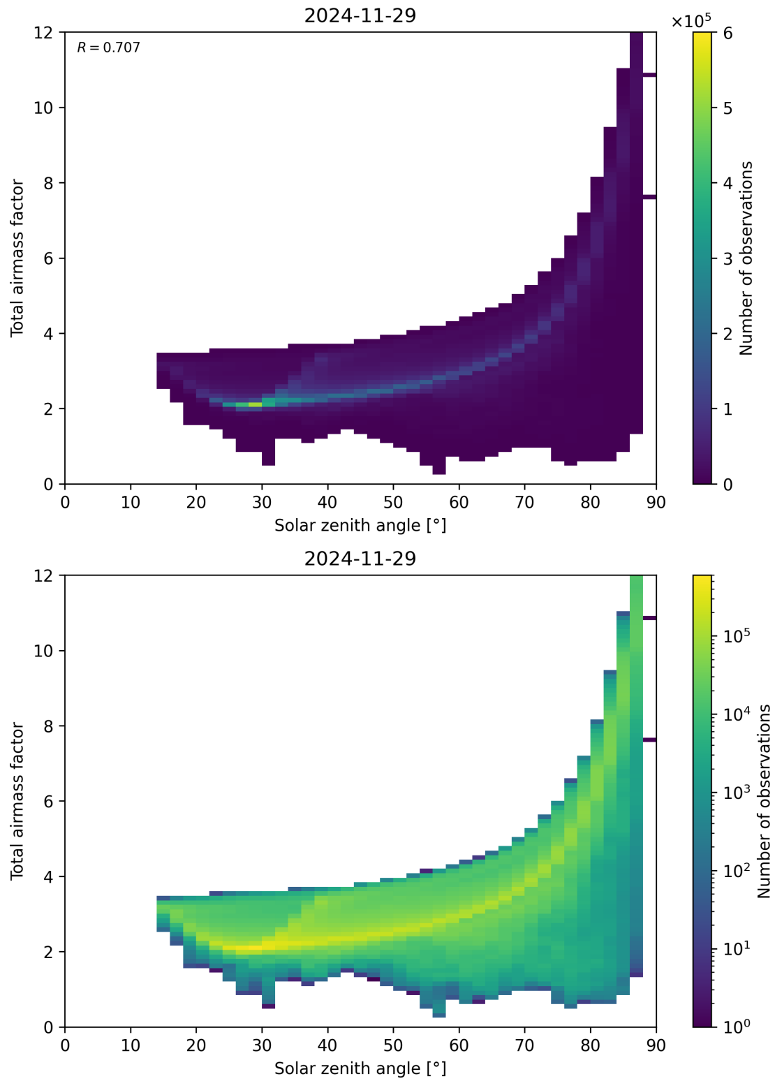
Figure 146: Scatter density plot of “Solar zenith angle” against “Total airmass factor” for 2024-11-28 to 2024-11-30.
