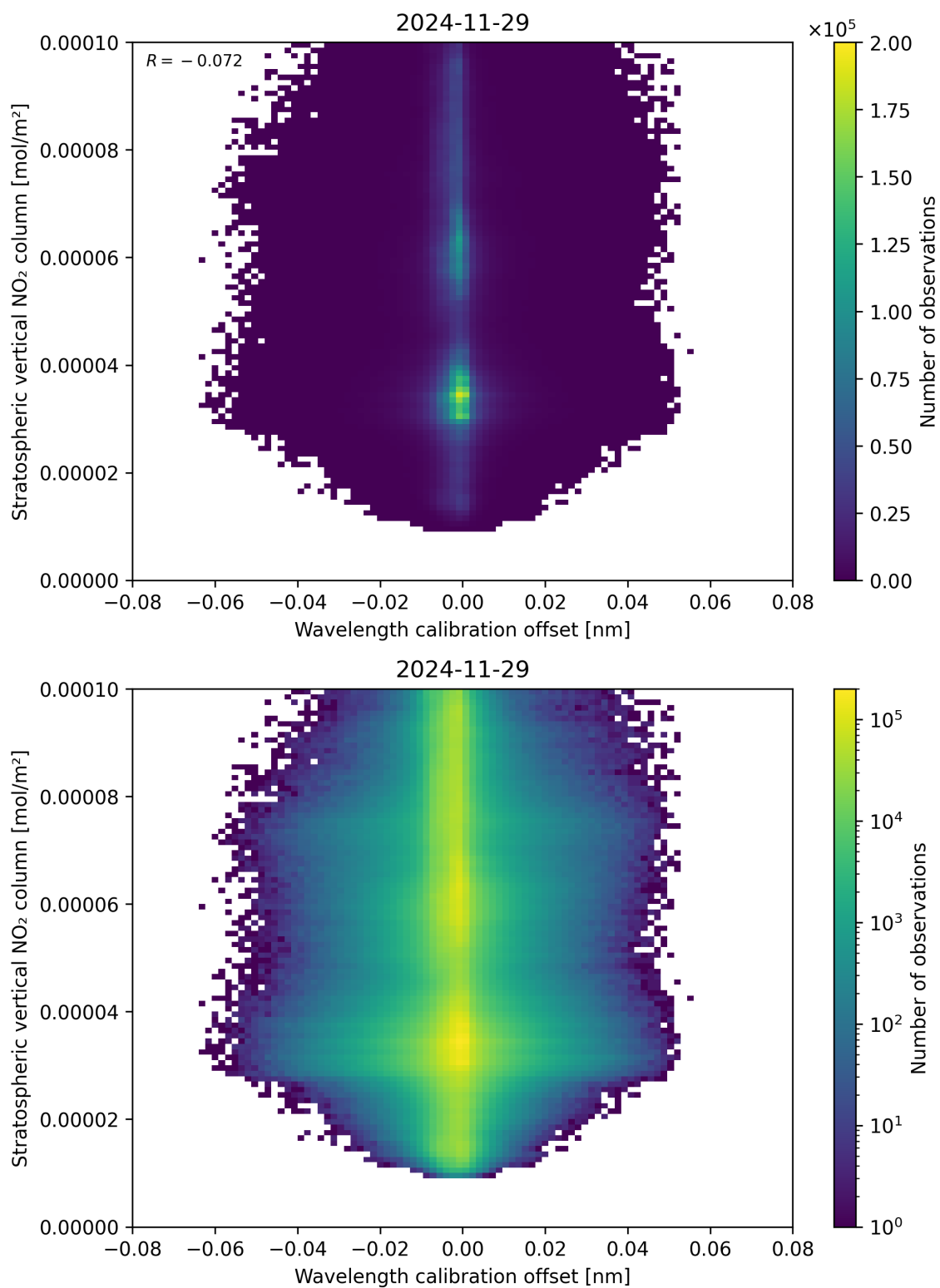
Figure 176: Scatter density plot of “Wavelength calibration offset” against “Stratospheric vertical NO 2 column” for 2024-11-28 to 2024-11-30.
