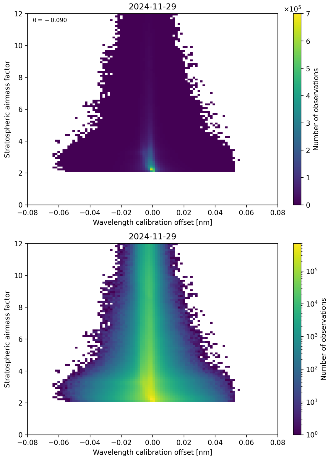
Figure 174: Scatter density plot of “Wavelength calibration offset” against “Stratospheric air mass factor” for 2024-11-28 to 2024-11-30.
