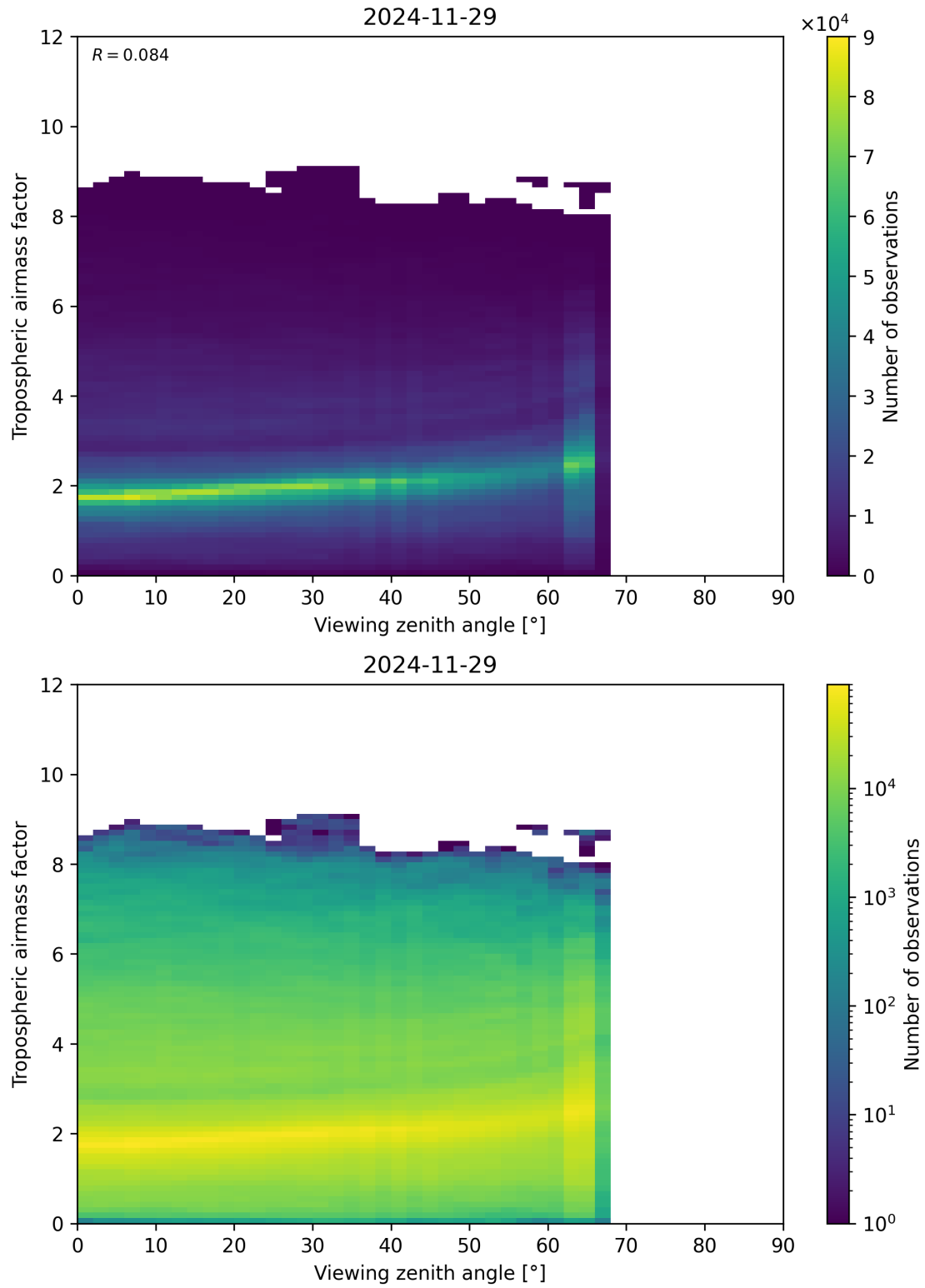
Figure 161: Scatter density plot of “Viewing zenith angle” against “Tropospheric airmass factor” for 2024-11-28 to 2024-11-30.
