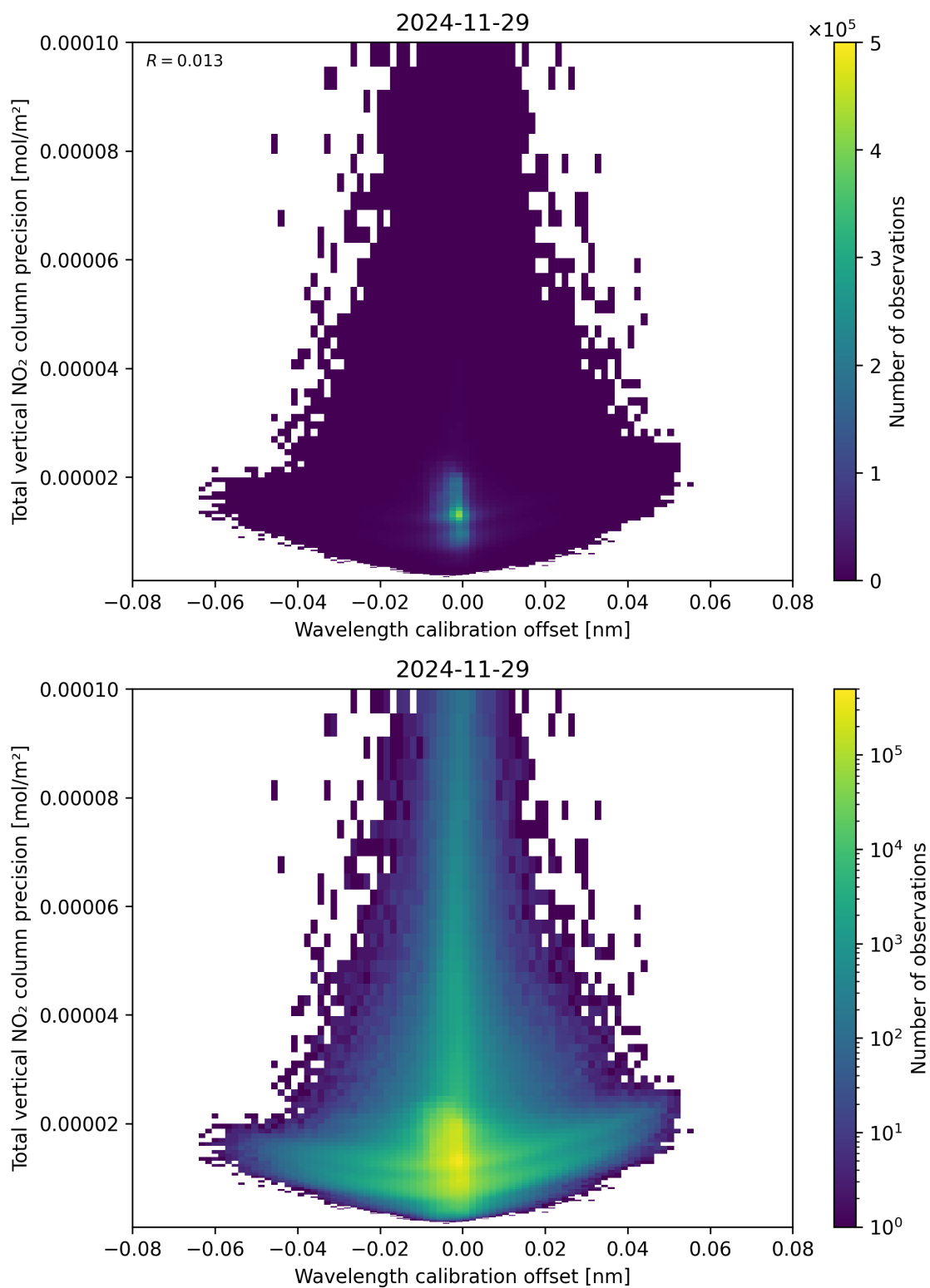
Figure 180: Scatter density plot of “Wavelength calibration offset” against “Total vertical NO 2 column precision” for 2024-11-28 to 2024-11-30.
