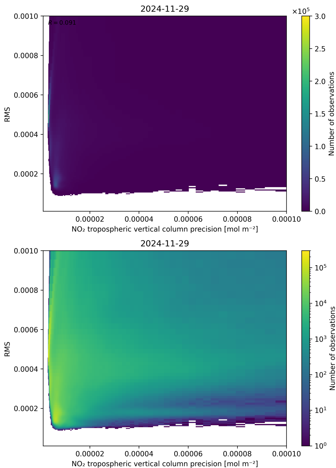
Figure 140: Scatter density plot of “NO 2 tropospheric vertical column precision” against “RMS” for 2024-11-28 to 2024-11-30.
