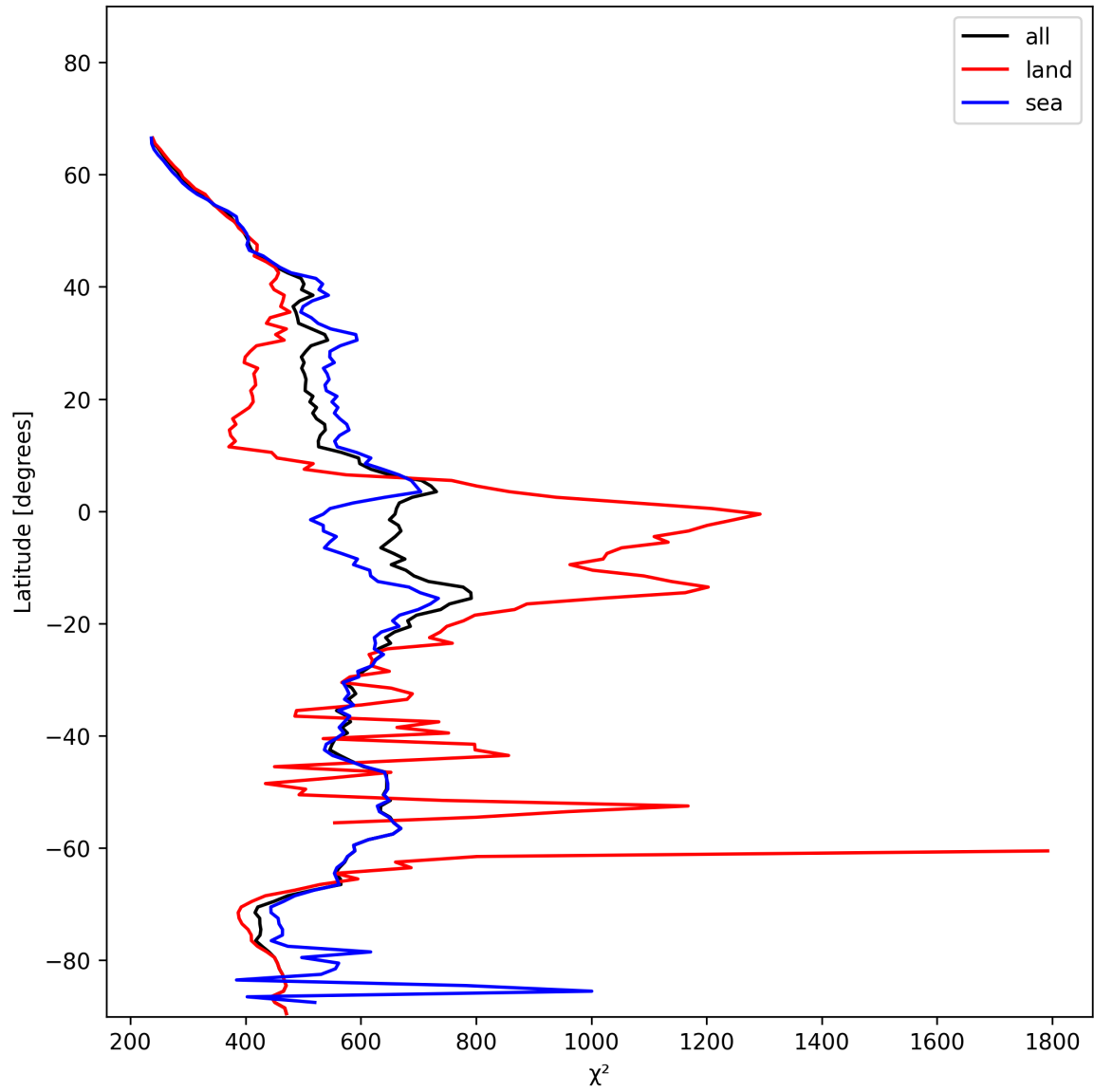
Figure 25: Zonal average of “ \chi^2 ” for 2024-11-28 to 2024-11-30.
