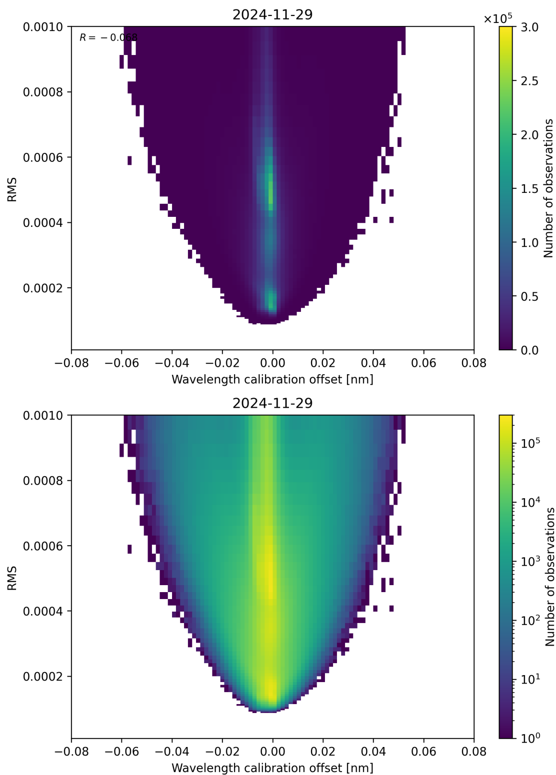
Figure 181: Scatter density plot of “Wavelength calibration offset” against “RMS” for 2024-11-28 to 2024-11-30.
