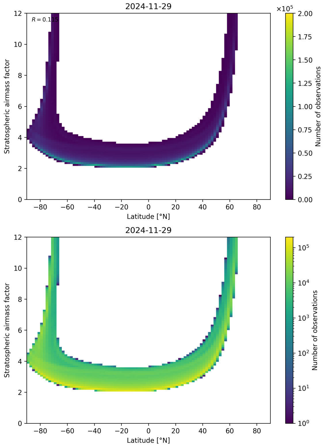
Figure 83: Scatter density plot of “Latitude” against “Stratospheric air mass factor” for 2024-11-28 to 2024-11-30.
