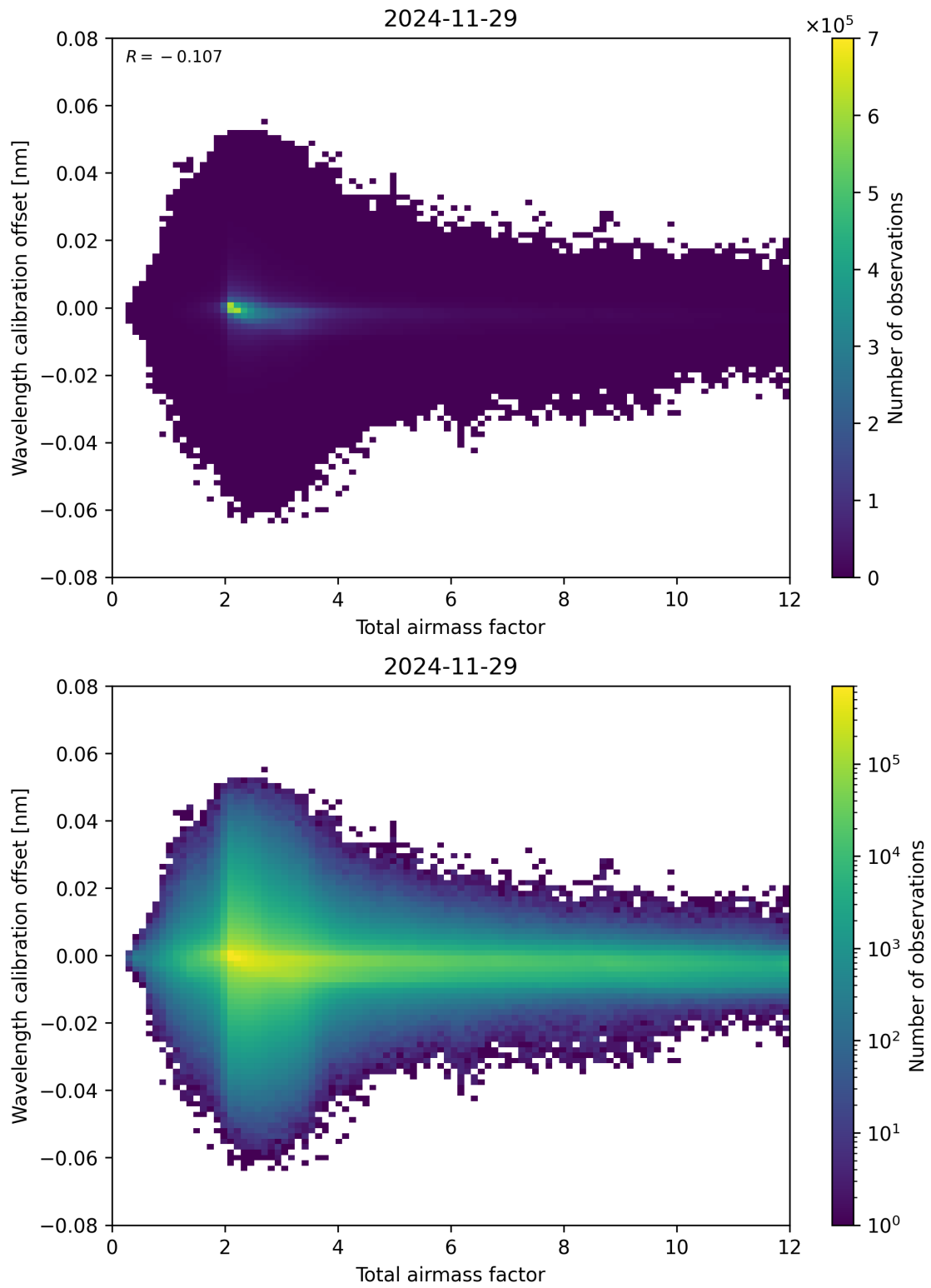
Figure 70: Scatter density plot of “Total airmass factor” against “Wavelength calibration offset” for 2024-11-28 to 2024-11-30.
