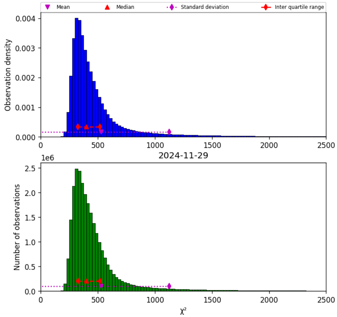
Figure 42: Histogram of “ \chi^2 ” for 2024-11-28 to 2024-11-30
