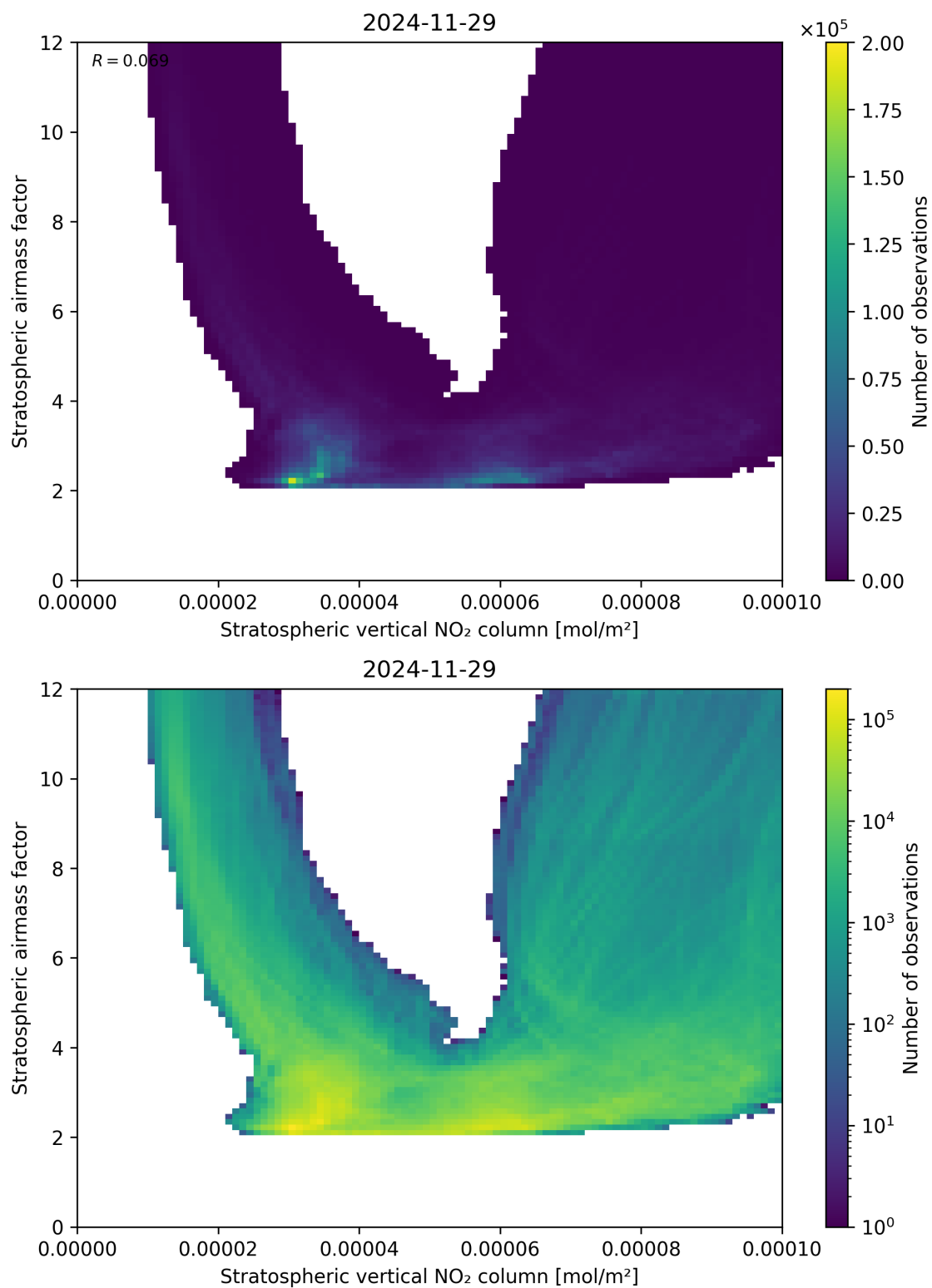
Figure 96: Scatter density plot of “Stratospheric vertical NO 2 column” against “Stratospheric airmass factor” for 2024-11-28 to 2024-11-30.
