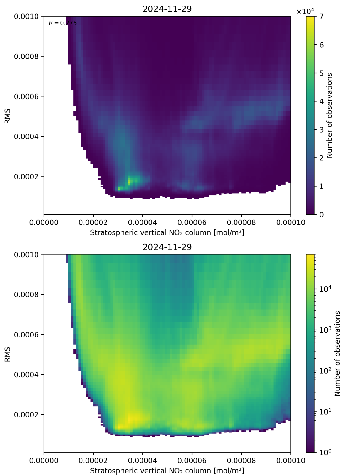
Figure 102: Scatter density plot of “Stratospheric vertical NO 2 column” against “RMS” for 2024-11-28 to 2024-11-30.
