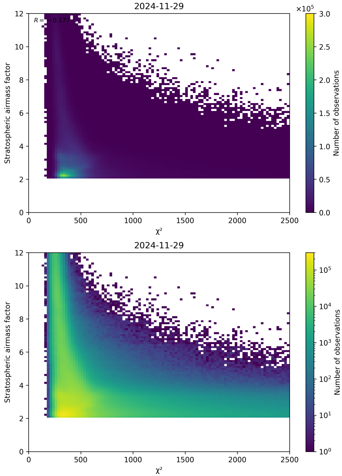
Figure 81: Scatter density plot of “ \chi^2 ” against “Stratospheric airmass factor” for 2024-11-28 to 2024-11-30.
