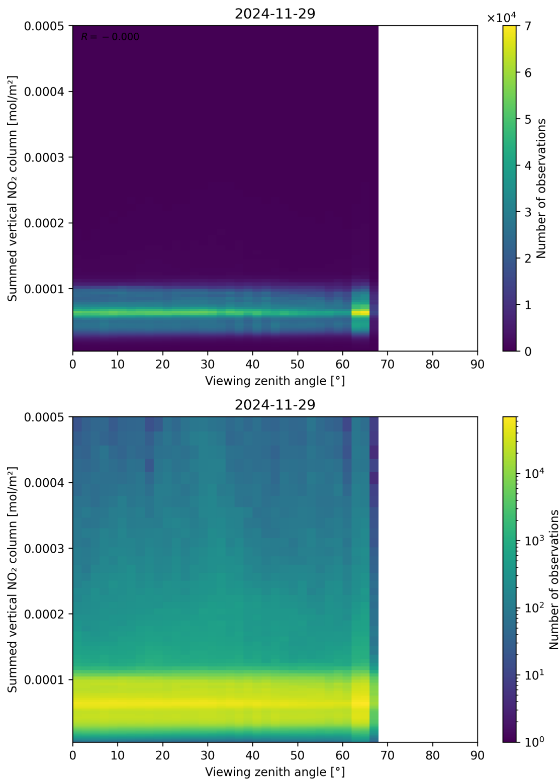
Figure 165: Scatter density plot of “Viewing zenith angle” against “Summed vertical NO 2 column” for 2024-11-28 to 2024-11-30.
