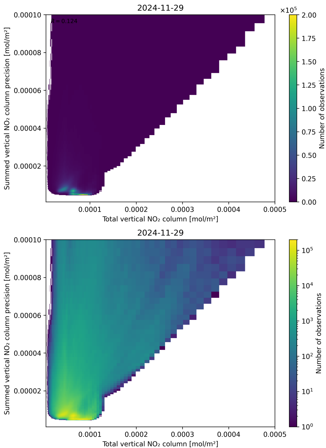
Figure 113: Scatter density plot of “Total vertical NO 2 column” against “Summed vertical NO 2 column precision” for 2024-11-28 to 2024-11-30.
