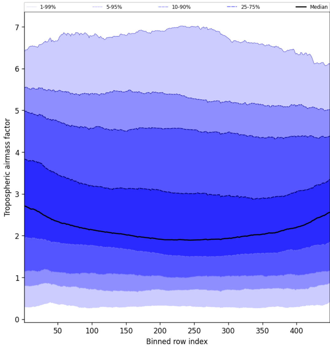
Figure 48: Along track statistics of “Tropospheric airmass factor” for 2024-11-28 to 2024-11-30
