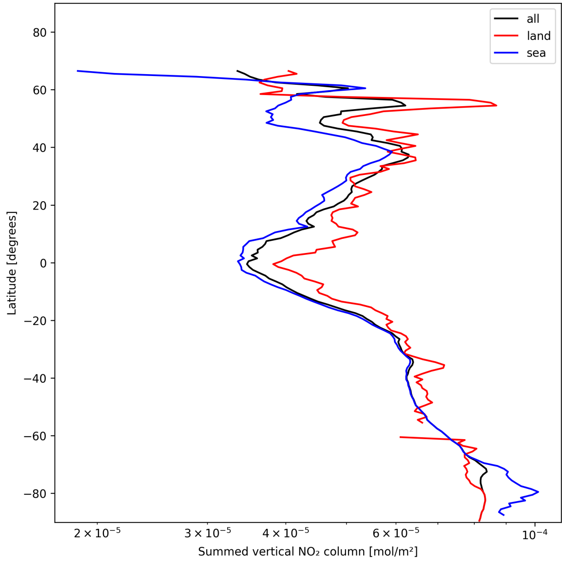
Figure 23: Zonal average of “Summed vertical NO 2 column” for 2024-11-28 to 2024-11-30.
