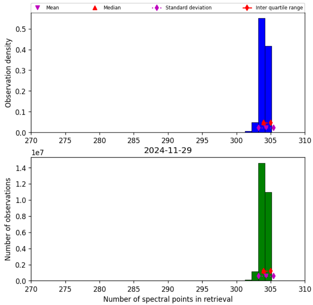
Figure 33: Histogram of “Number of spectral points in retrieval” for 2024-11-28 to 2024-11-30
