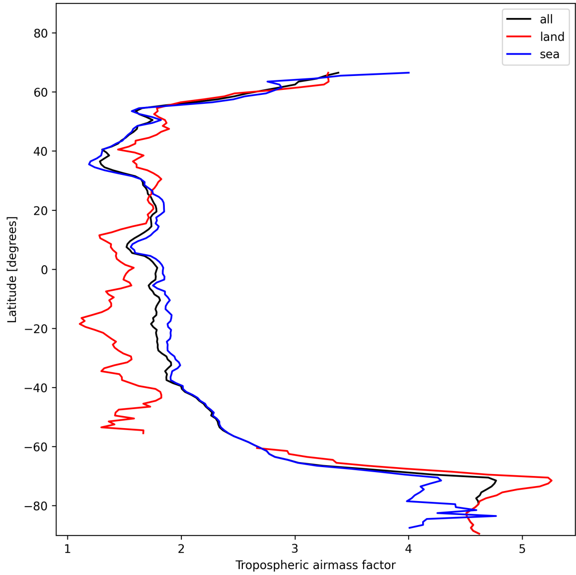
Figure 14: Zonal average of “Tropospheric airmass factor” for 2024-11-28 to 2024-11-30.
