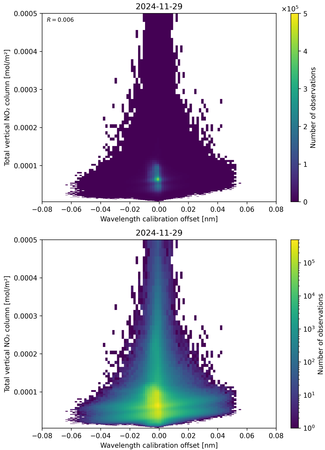
Figure 179: Scatter density plot of “Wavelength calibration offset” against “Total vertical NO 2 column” for 2024-11-28 to 2024-11-30.
