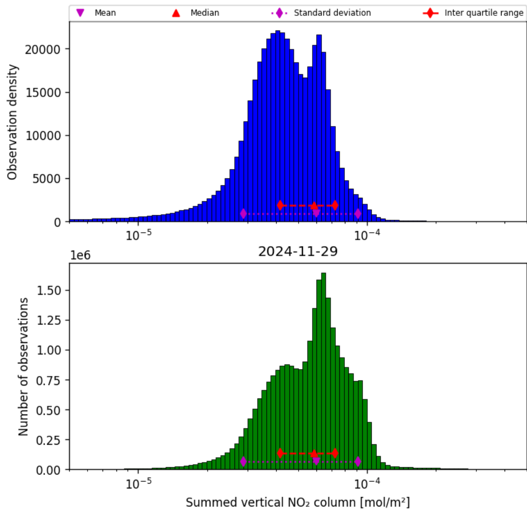
Figure 40: Histogram of “Summed vertical NO 2 column” for 2024-11-28 to 2024-11-30
