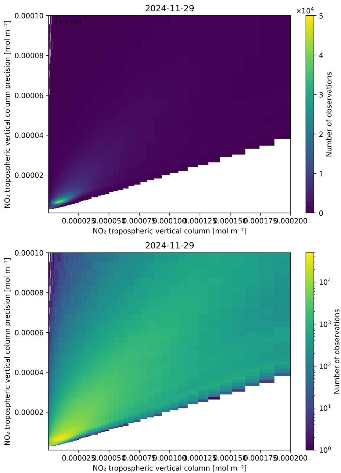
Figure 130: Scatter density plot of “NO 2 tropospheric vertical column” against “NO 2 tropospheric vertical column precision” for 2024-11-28 to 2024-11-30.
