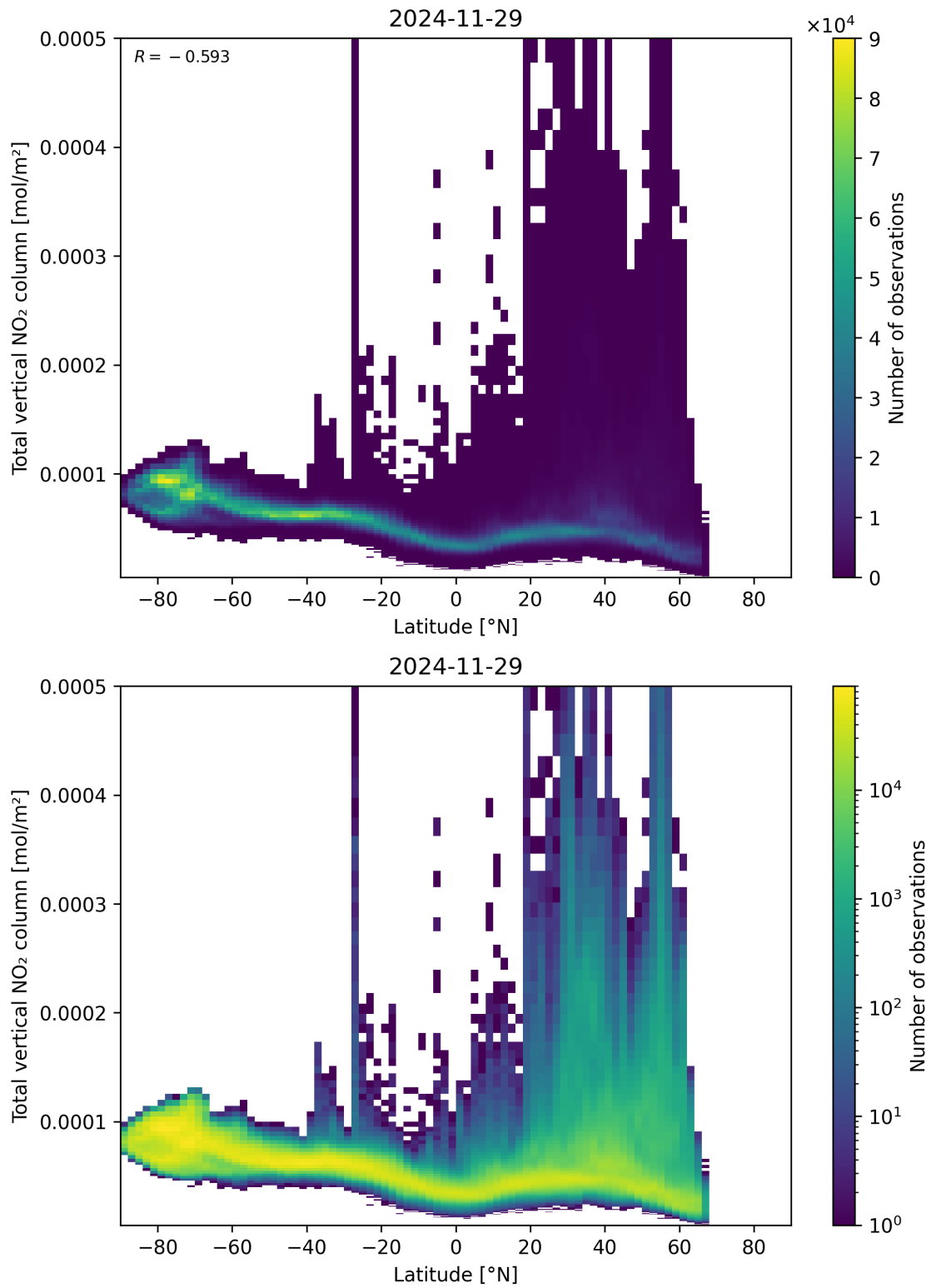
Figure 90: Scatter density plot of “Latitude” against “Total vertical NO 2 column” for 2024-11-28 to 2024-11-30.
