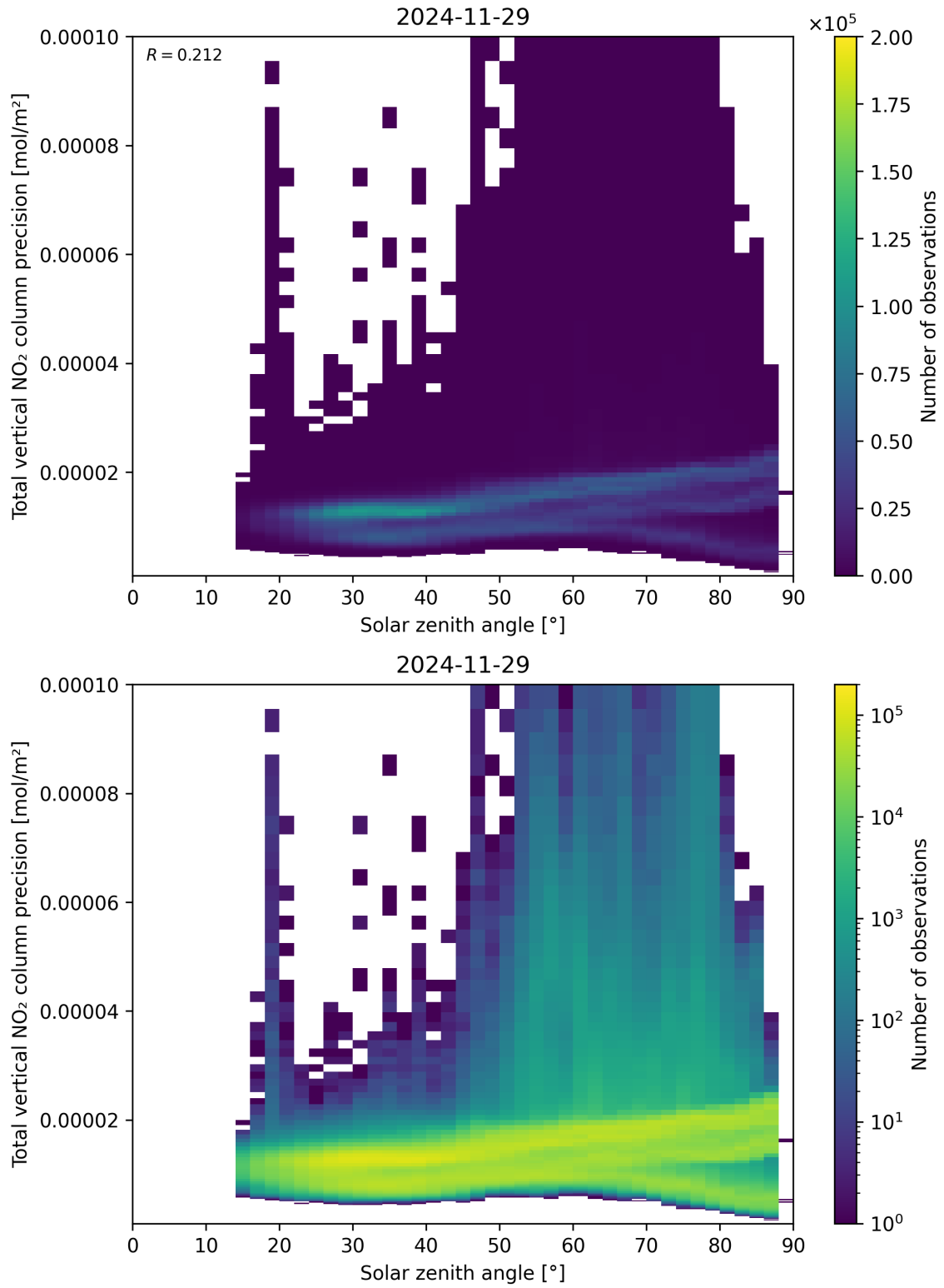
Figure 154: Scatter density plot of “Solar zenith angle” against “Total vertical NO 2 column precision” for 2024-11-28 to 2024-11-30.
