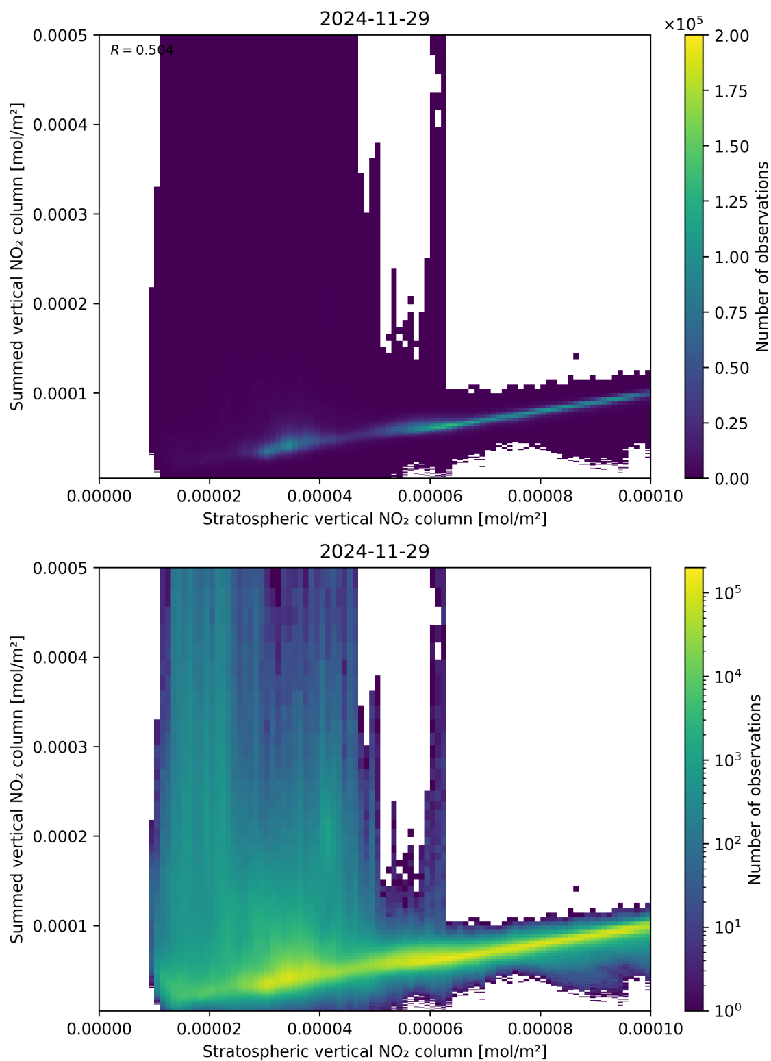
Figure 98: Scatter density plot of “Stratospheric vertical NO 2 column” against “Summed vertical NO 2 column” for 2024-11-28 to 2024-11-30.
