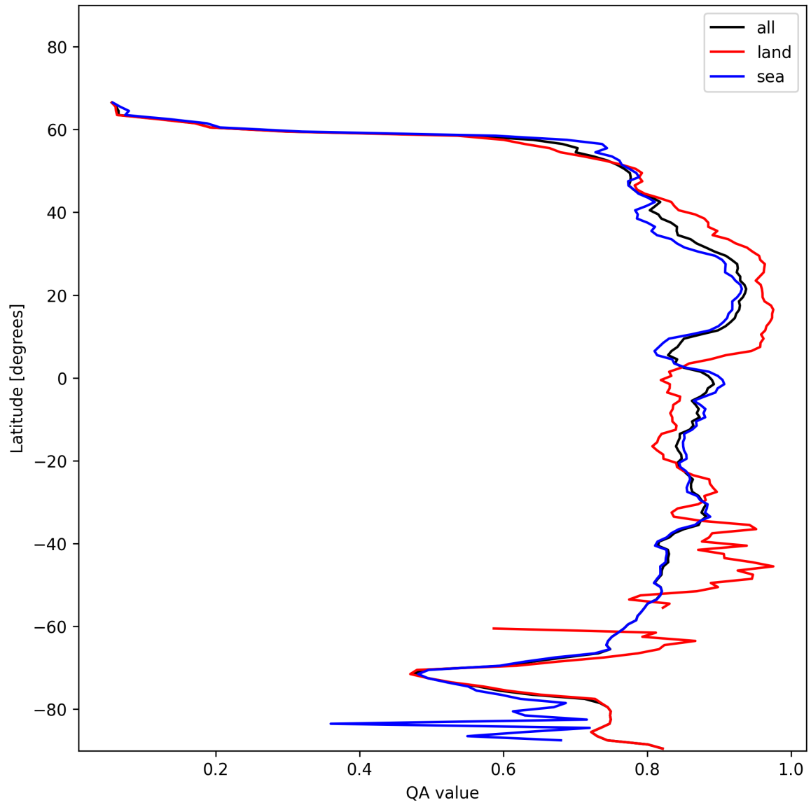
Figure 11: Zonal average of “QA value” for 2024-11-28 to 2024-11-30.
