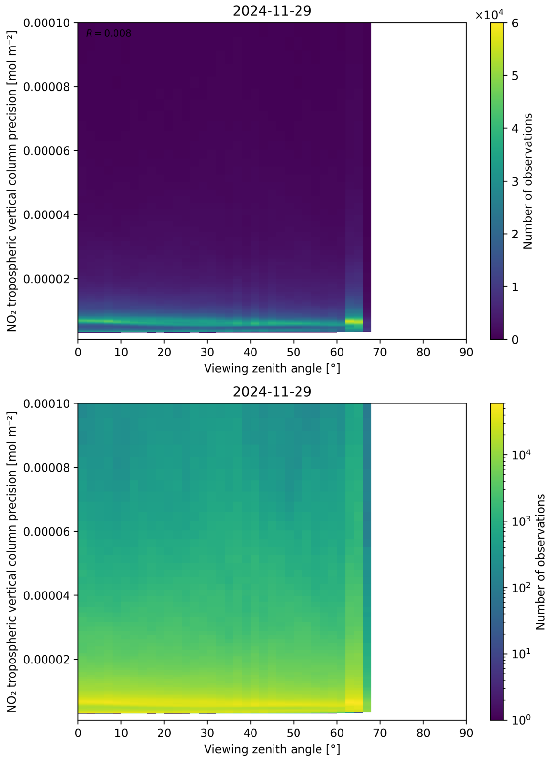
Figure 170: Scatter density plot of “Viewing zenith angle” against “NO 2 tropospheric vertical column precision” for 2024-11-28 to 2024-11-30.
