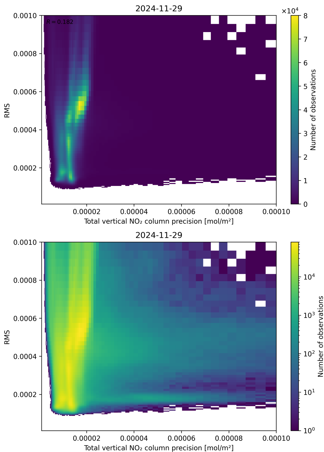
Figure 119: Scatter density plot of “Total vertical NO 2 column precision” against “RMS” for 2024-11-28 to 2024-11-30.
