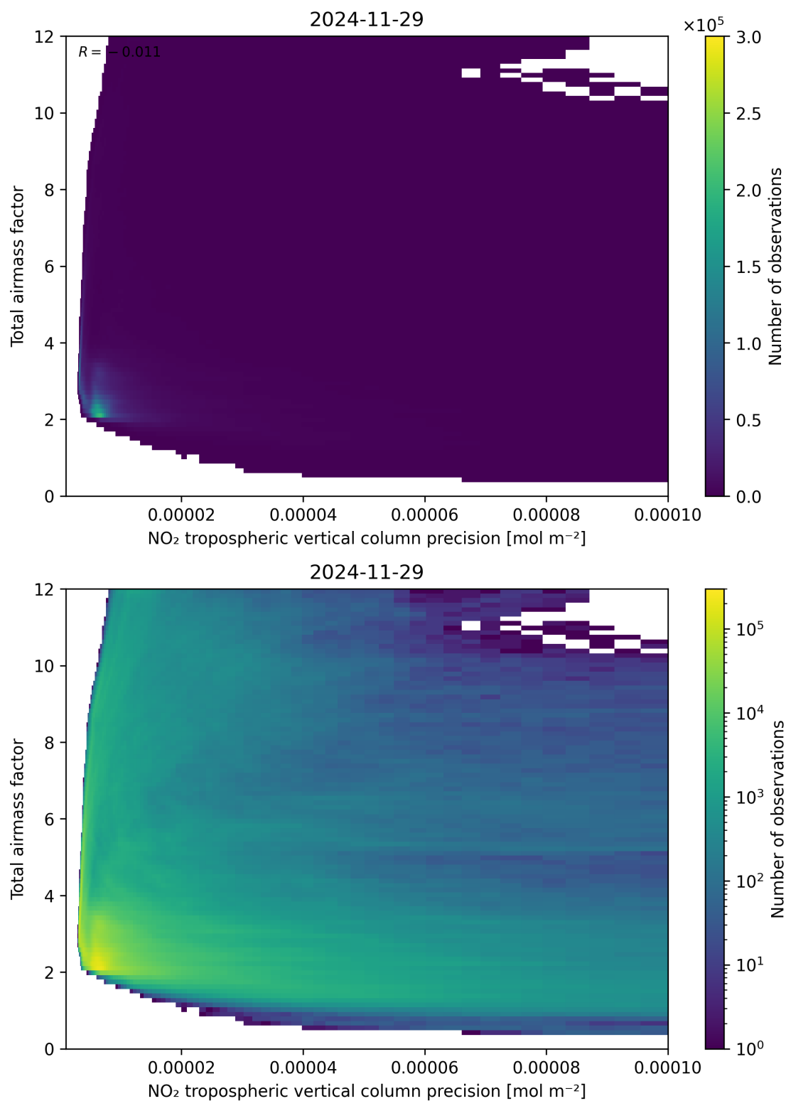
Figure 132: Scatter density plot of “NO 2 tropospheric vertical column precision” against “Total air mass factor” for 2024-11-28 to 2024-11-30.
