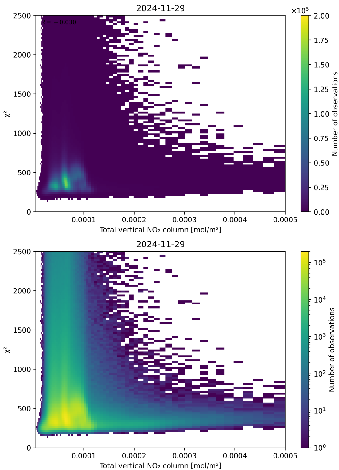
Figure 111: Scatter density plot of “Total vertical NO 2 column” against “ \chi^2 ” for 2024-11-28 to 2024-11-30.
