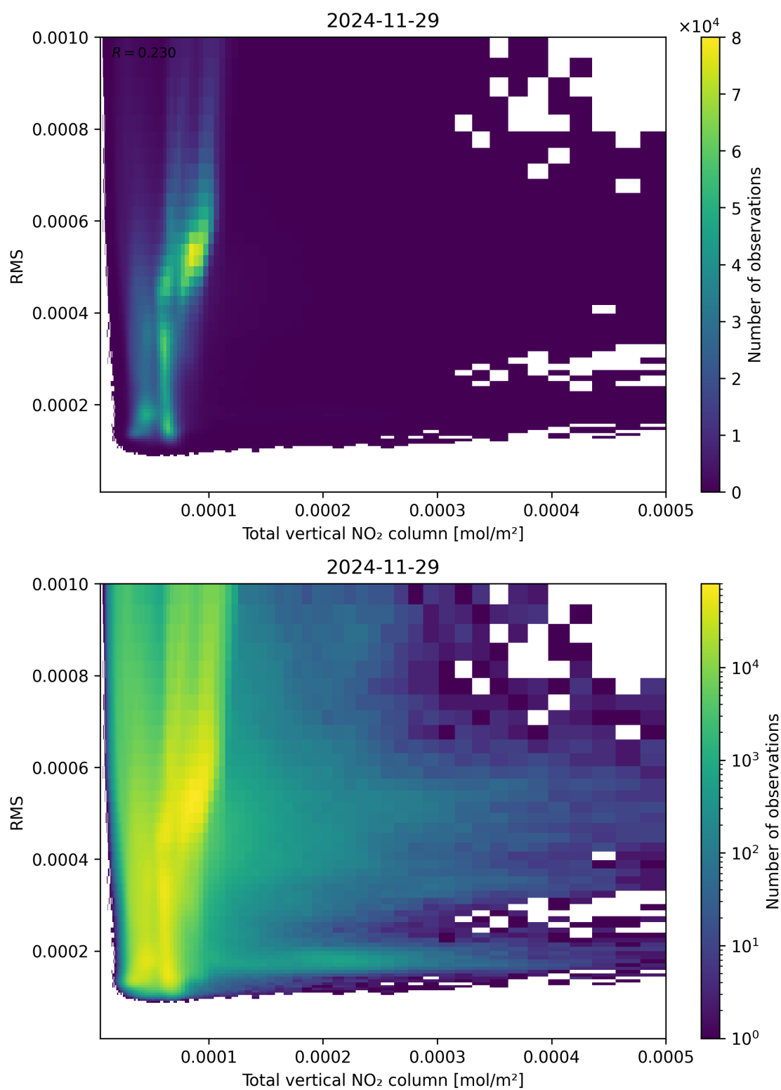
Figure 120: Scatter density plot of “Total vertical NO 2 column” against “RMS” for 2024-11-28 to 2024-11-30.
