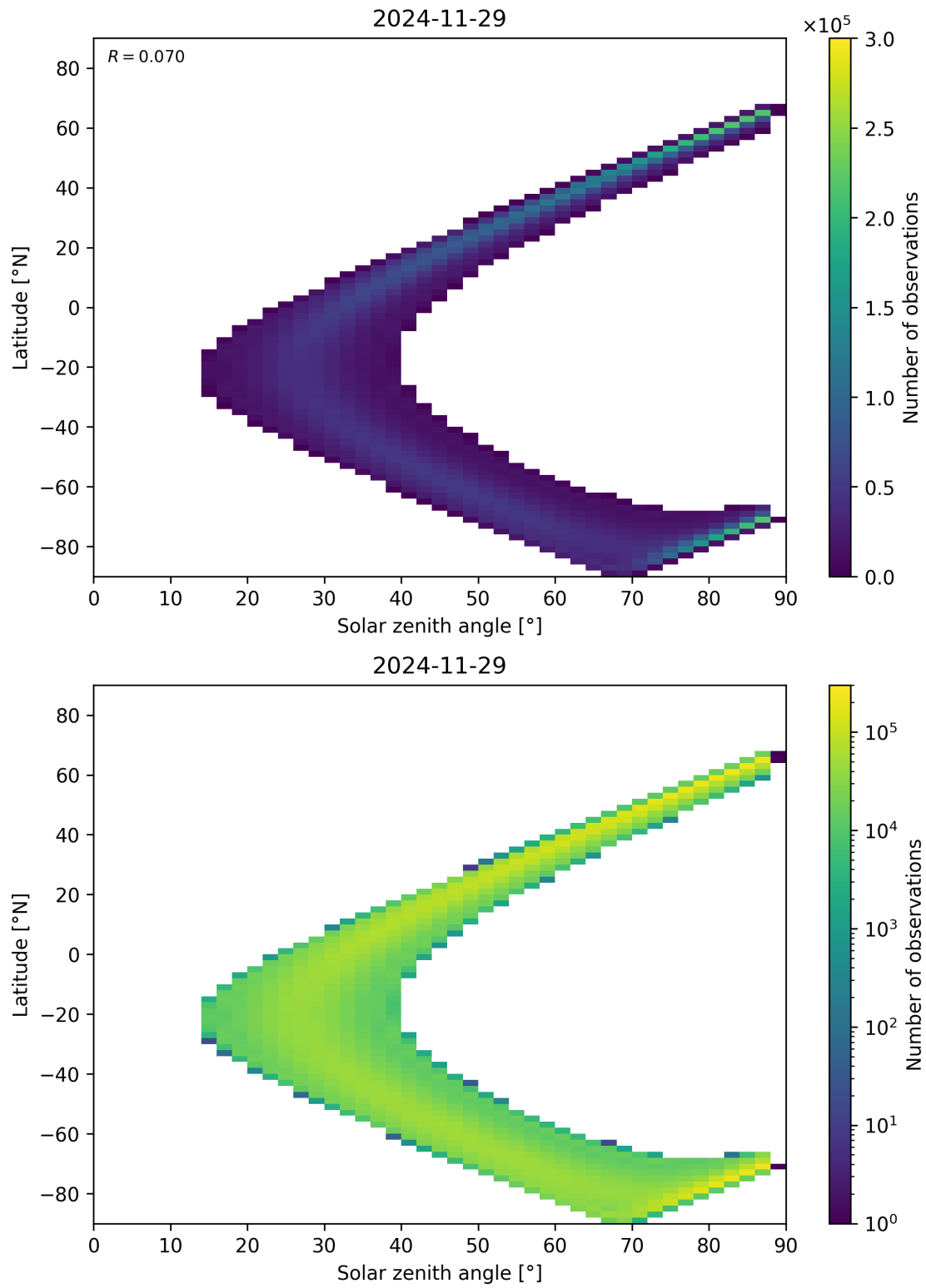
Figure 149: Scatter density plot of “Solar zenith angle” against “Latitude” for 2024-11-28 to 2024-11-30.
