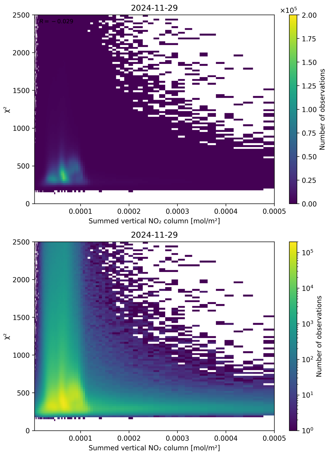
Figure 104: Scatter density plot of “Summed vertical NO 2 column” against “ \chi^2 ” for 2024-11-28 to 2024-11-30.
