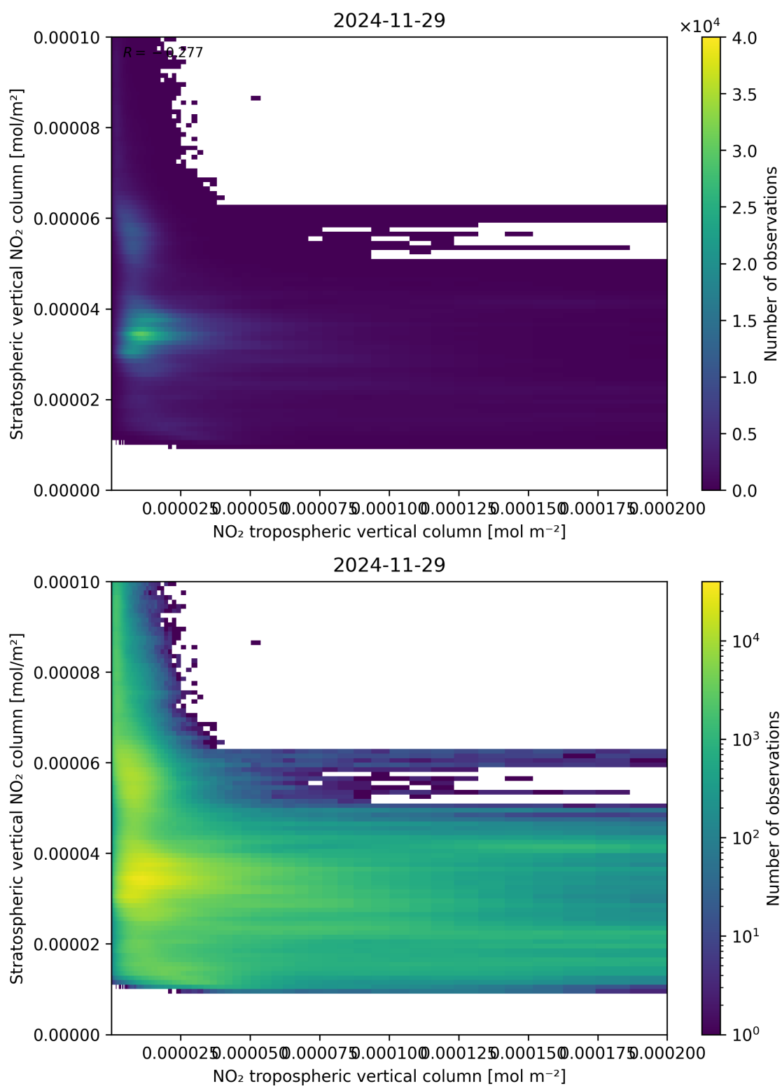
Figure 125: Scatter density plot of “NO 2 tropospheric vertical column” against “Stratospheric vertical NO 2 column” for 2024-11-28 to 2024-11-30.
