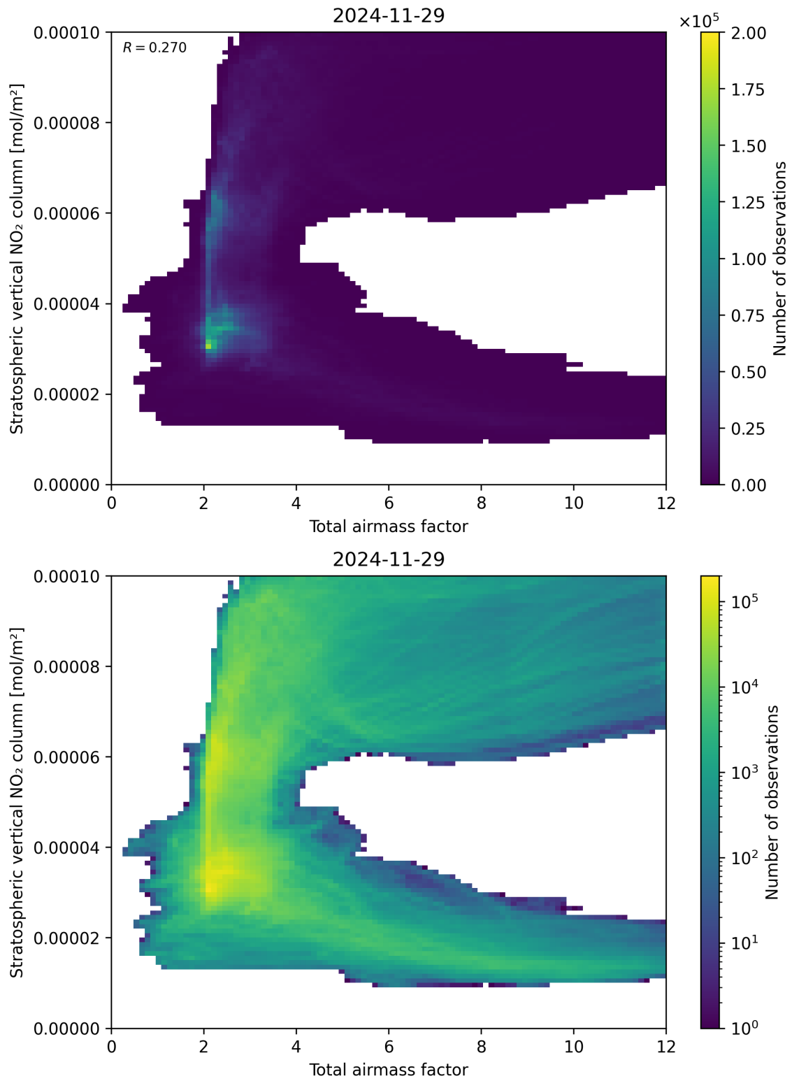
Figure 64: Scatter density plot of “Total airmass factor” against “Stratospheric vertical NO 2 column” for 2024-11-28 to 2024-11-30.
