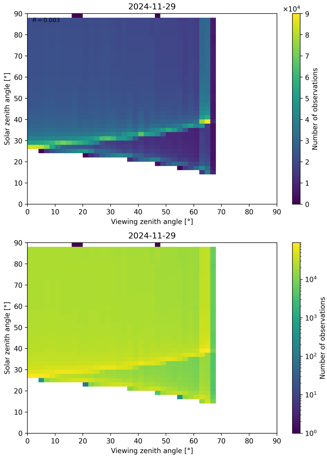
Figure 172: Scatter density plot of “Viewing zenith angle” against “Solar zenith angle” for 2024-11-28 to 2024-11-30.
