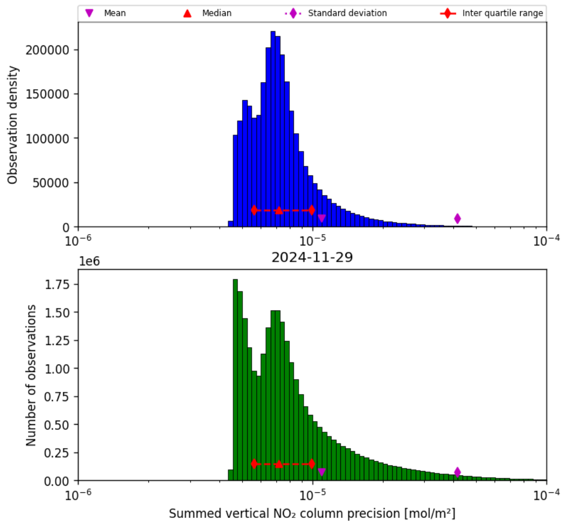
Figure 41: Histogram of "Summed vertical NO 2 column precision" for 2024-11-28 to 2024-11-30
