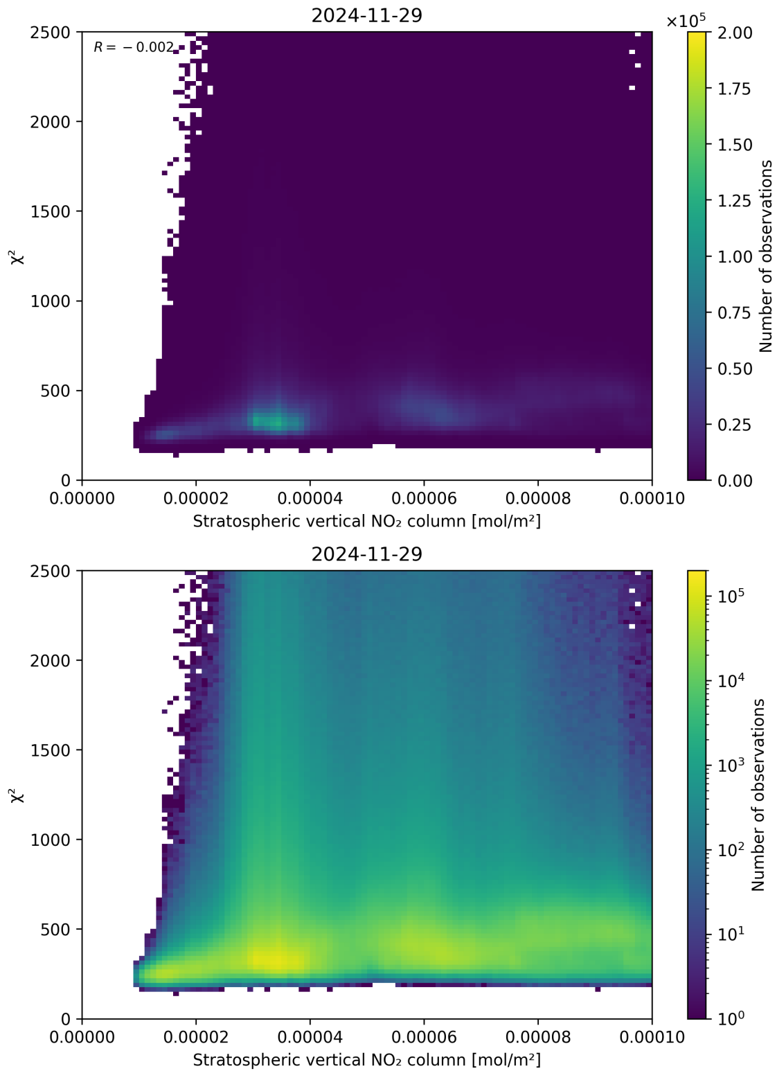
Figure 97: Scatter density plot of “Stratospheric vertical NO 2 column” against “ \chi^2 ” for 2024-11-28 to 2024-11-30.
