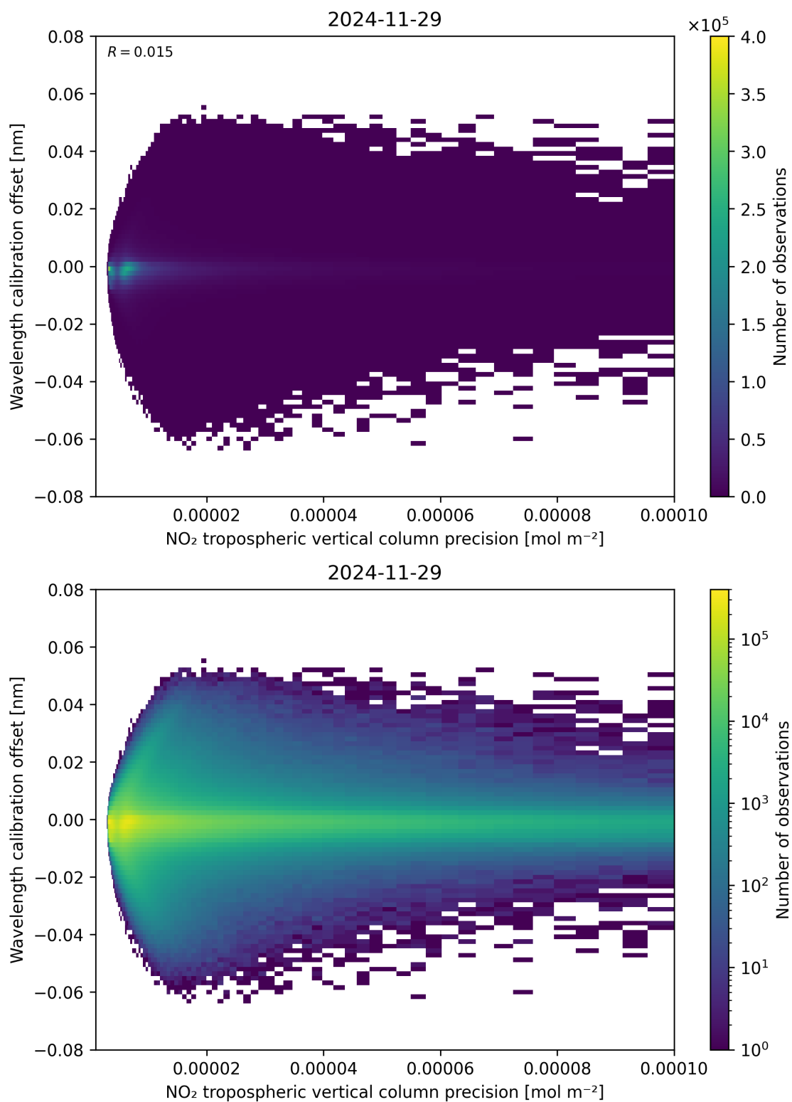
Figure 141: Scatter density plot of “NO 2 tropospheric vertical column precision” against “Wavelength calibration offset” for 2024-11-28 to 2024-11-30.
