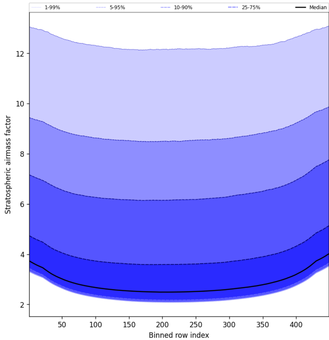
Figure 61: Along track statistics of “Stratospheric airmass factor” for 2024-11-28 to 2024-11-30
