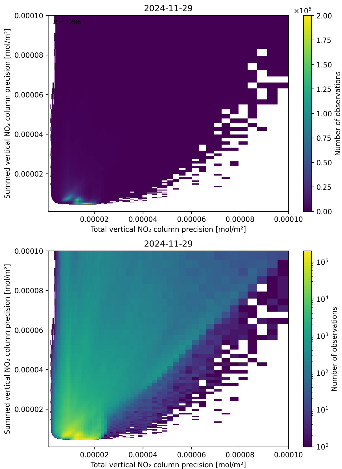
Figure 118: Scatter density plot of “Total vertical NO 2 column precision” against “Summed vertical NO 2 column precision” for 2024-11-28 to 2024-11-30.
