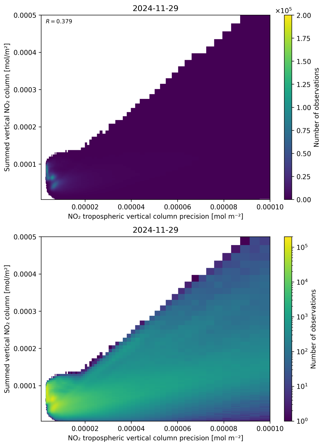
Figure 136: Scatter density plot of “NO 2 tropospheric vertical column precision” against “Summed vertical NO 2 column” for 2024-11-28 to 2024-11-30.
