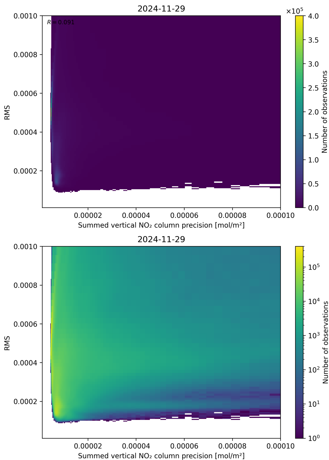
Figure 108: Scatter density plot of “Summed vertical NO 2 column precision” against “RMS” for 2024-11-28 to 2024-11-30.
