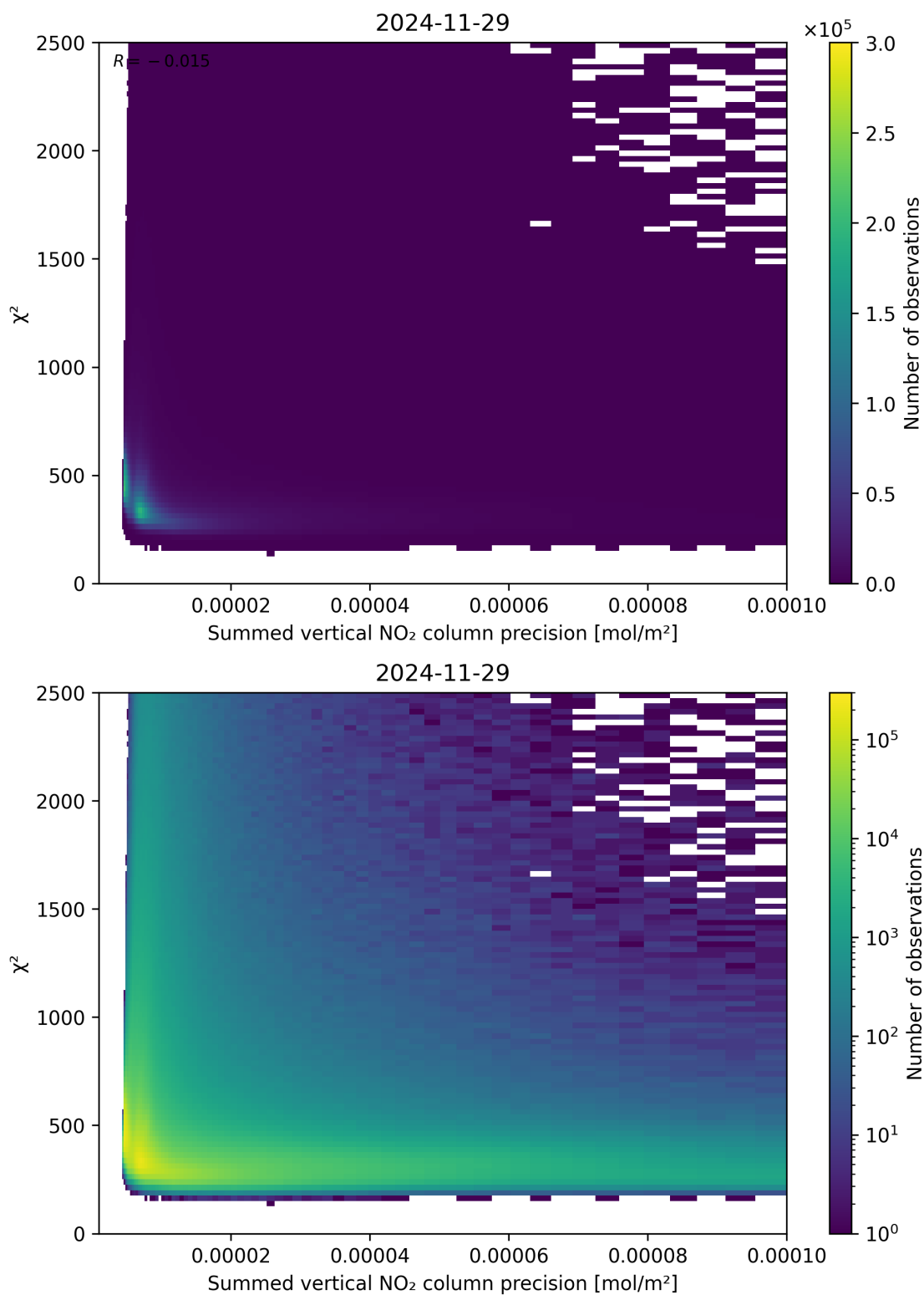
Figure 107: Scatter density plot of “Summed vertical NO 2 column precision” against “ \chi^2 ” for 2024-11-28 to 2024-11-30.
