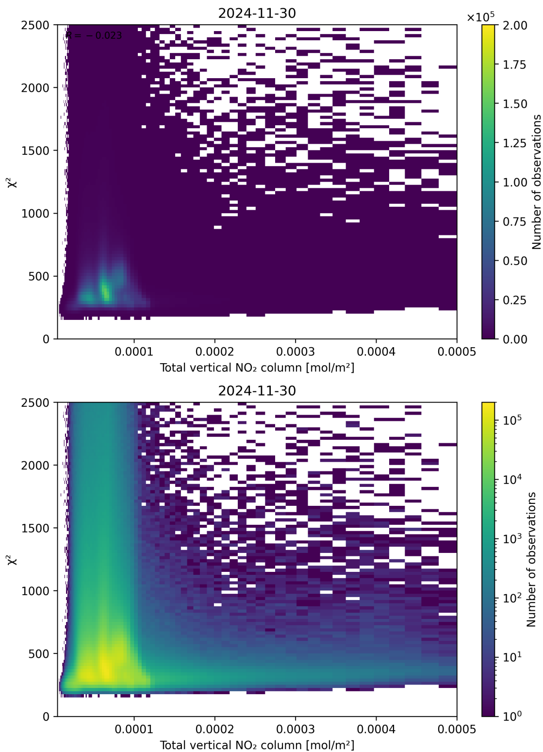
Figure 111: Scatter density plot of “Total vertical NO 2 column” against “ \chi^2 ” for 2024-11-30 to 2024-12-01.
