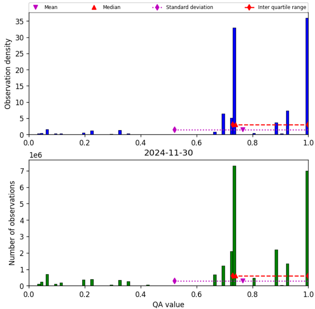
Figure 28: Histogram of “QA value” for 2024-11-30 to 2024-12-01
