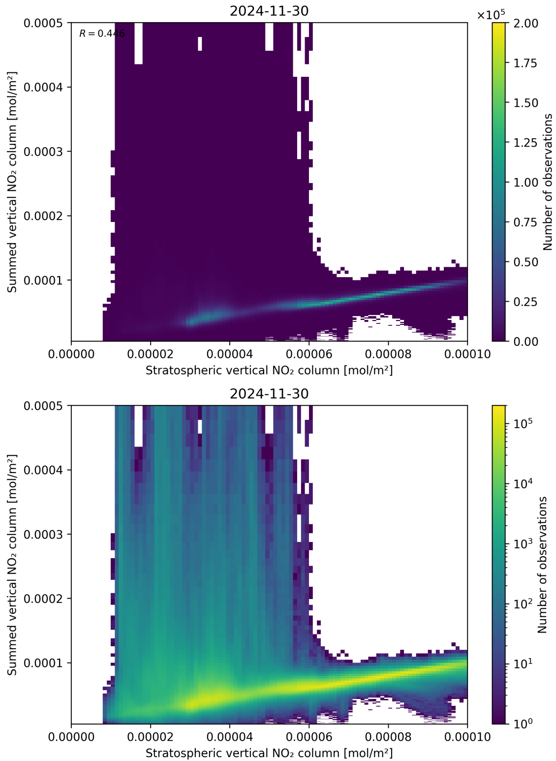
Figure 98: Scatter density plot of “Stratospheric vertical NO 2 column” against “Summed vertical NO 2 column” for 2024-11-30 to 2024-12-01.
