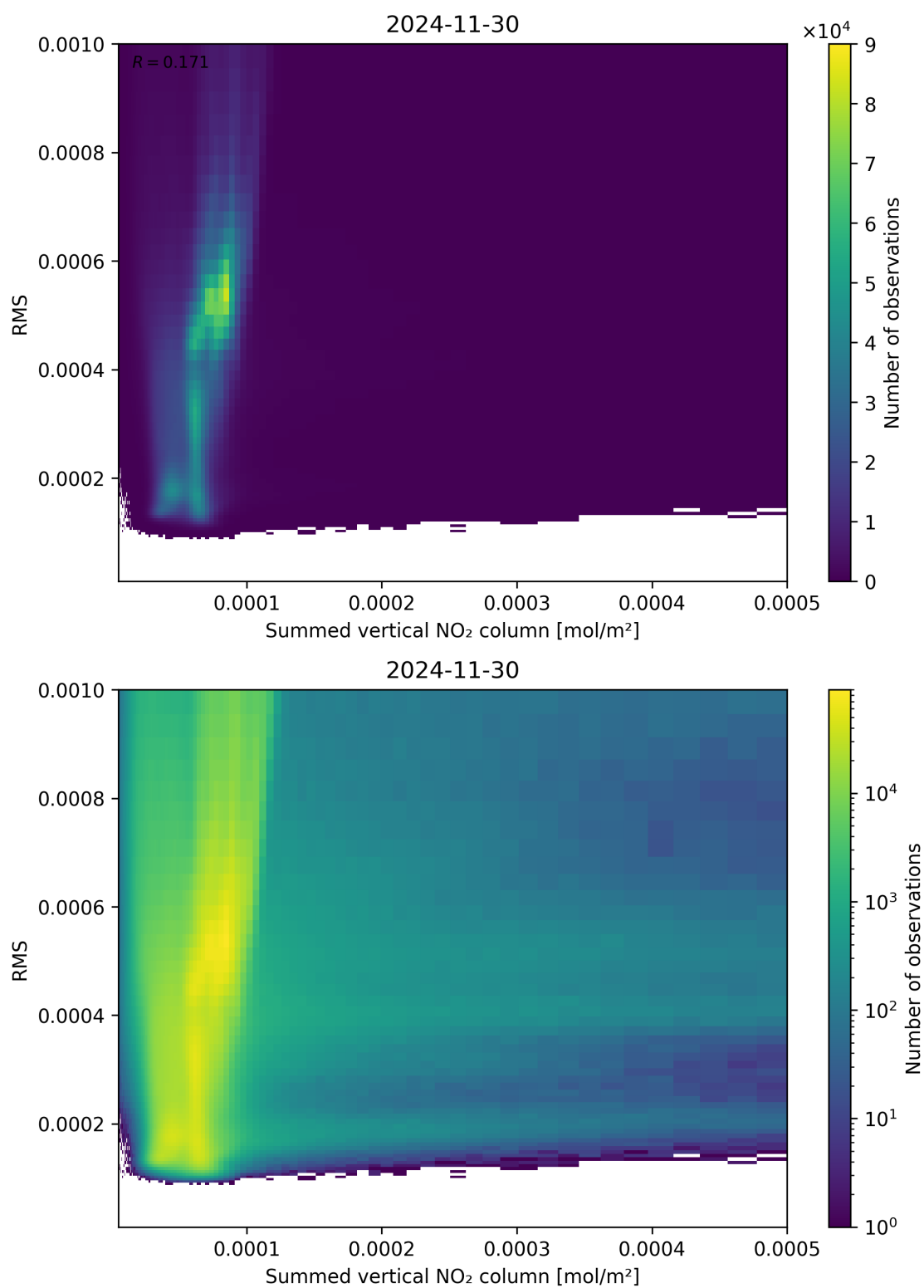
Figure 109: Scatter density plot of “Summed vertical NO 2 column” against “RMS” for 2024-11-30 to 2024-12-01.
