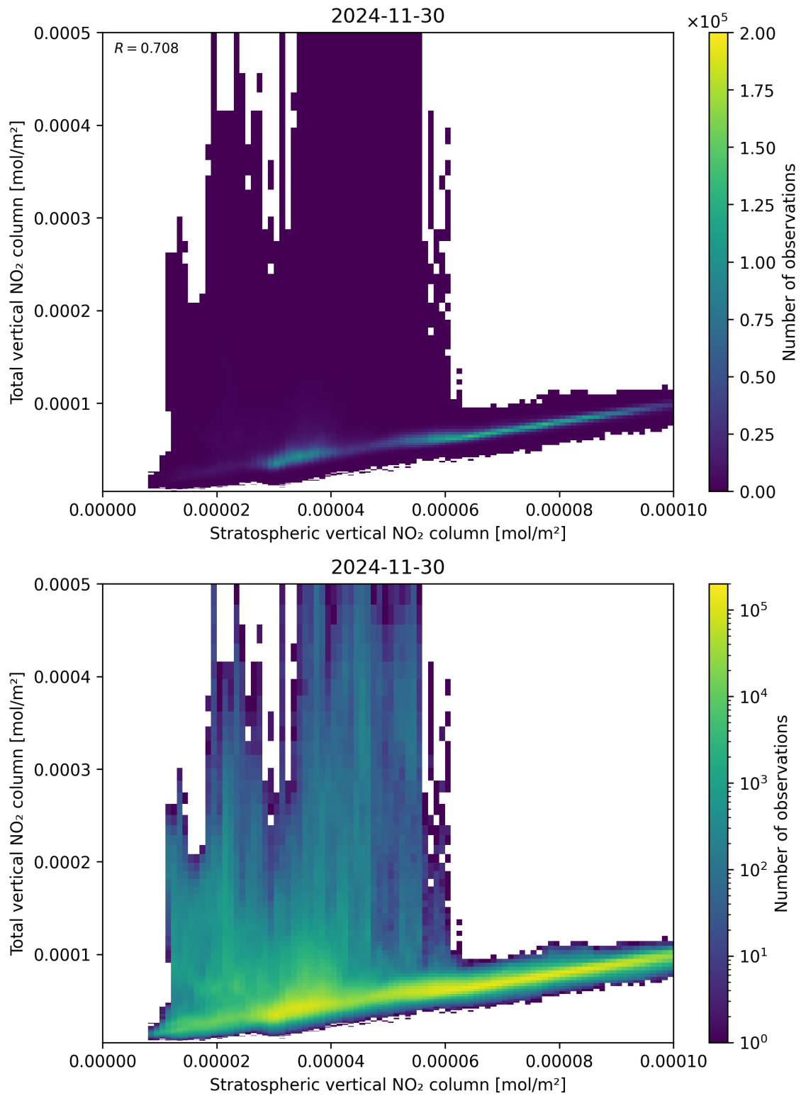
Figure 100: Scatter density plot of “Stratospheric vertical NO 2 column” against “Total vertical NO 2 column” for 2024-11-30 to 2024-12-01.
