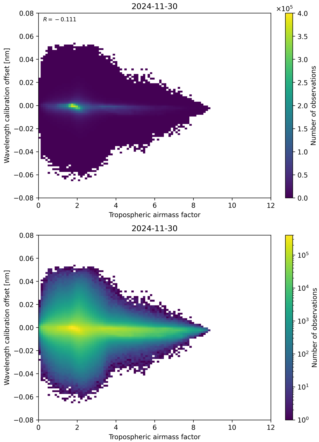
Figure 80: Scatter density plot of “Tropospheric airmass factor” against “Wavelength calibration offset” for 2024-11-30 to 2024-12-01.
