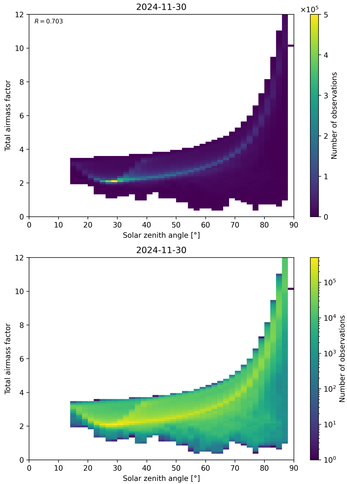
Figure 146: Scatter density plot of “Solar zenith angle” against “Total airmass factor” for 2024-11-30 to 2024-12-01.
