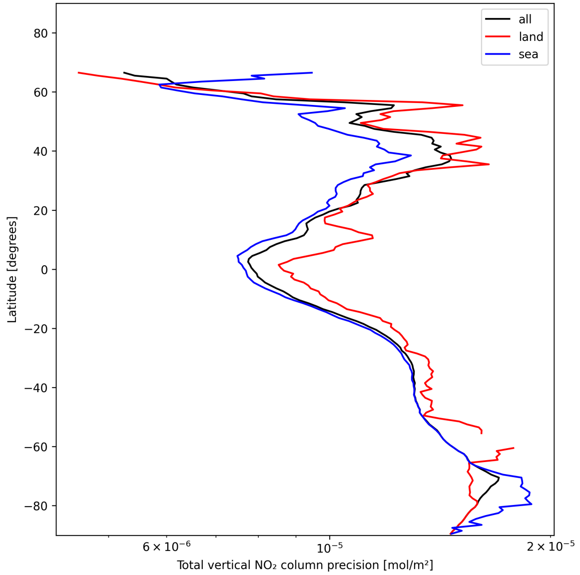
Figure 22: Zonal average of “Total vertical NO 2 column precision” for 2024-11-30 to 2024-12-01.
