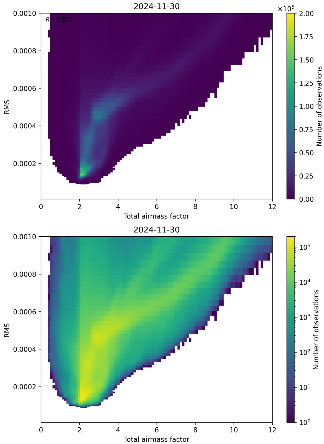
Figure 69: Scatter density plot of “Total airmass factor” against “RMS” for 2024-11-30 to 2024-12-01.
