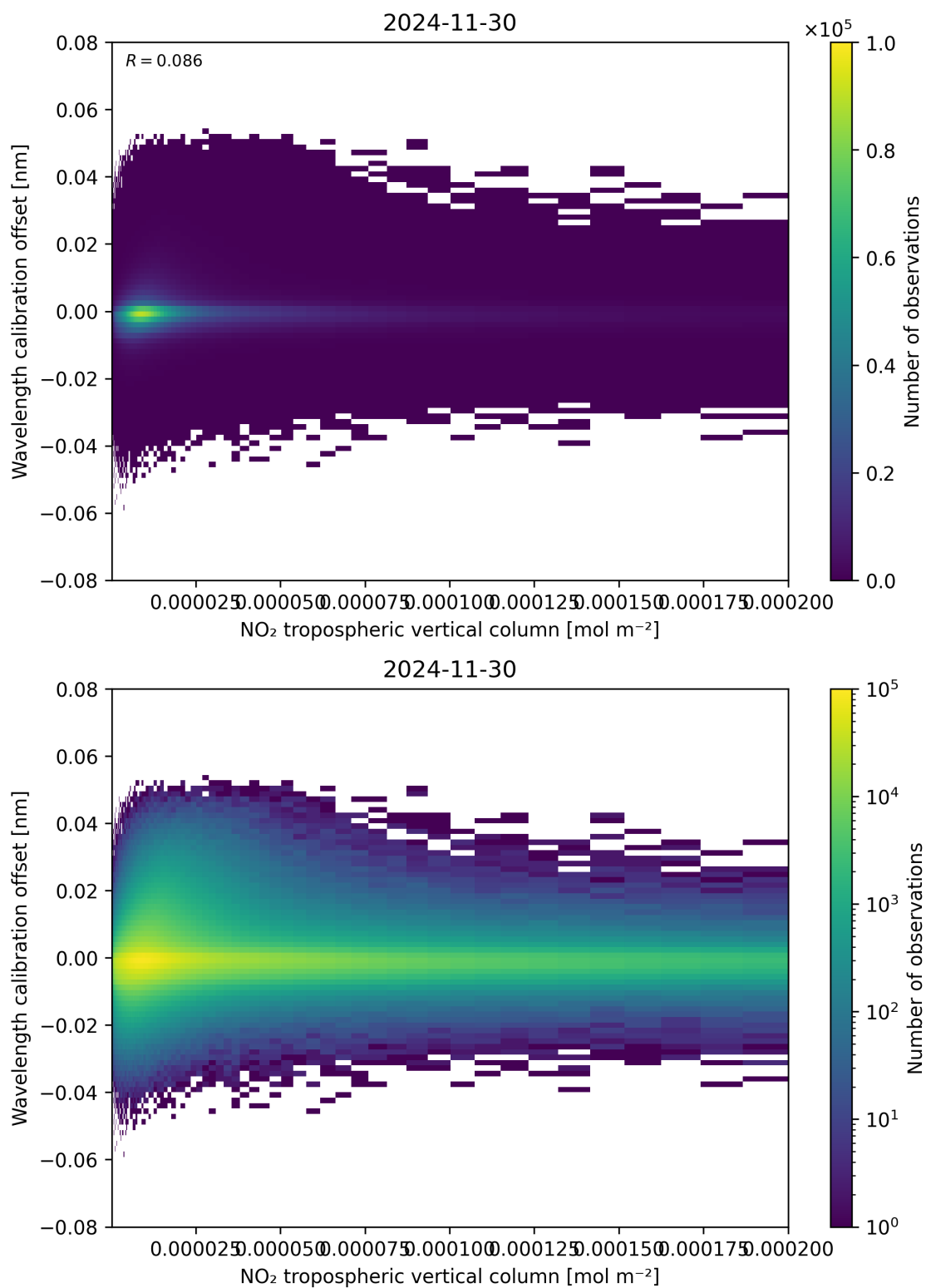
Figure 143: Scatter density plot of “NO 2 tropospheric vertical column” against “Wavelength calibration offset” for 2024-11-30 to 2024-12-01.
