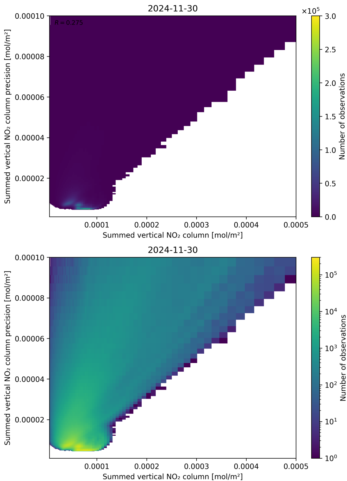
Figure 105: Scatter density plot of “Summed vertical NO 2 column” against “Summed vertical NO 2 column precision” for 2024-11-30 to 2024-12-01.
