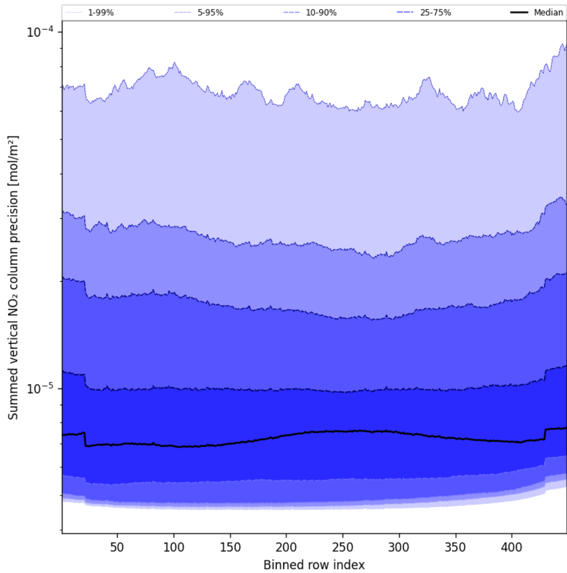
Figure 58: Along track statistics of “Summed vertical NO 2 column precision” for 2024-11-30 to 2024-12-01
