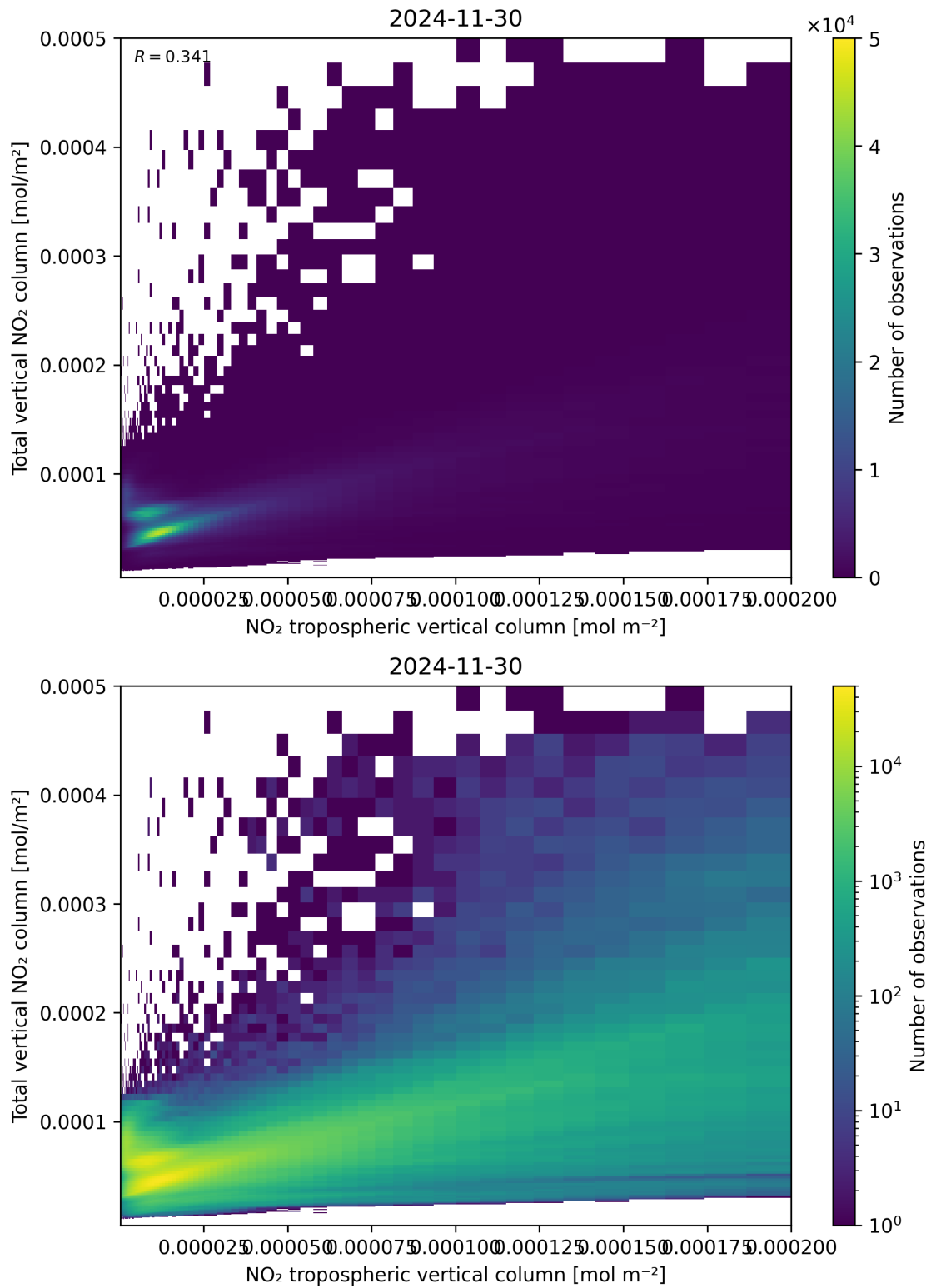
Figure 128: Scatter density plot of “NO 2 tropospheric vertical column” against “Total vertical NO 2 column” for 2024-11-30 to 2024-12-01.
