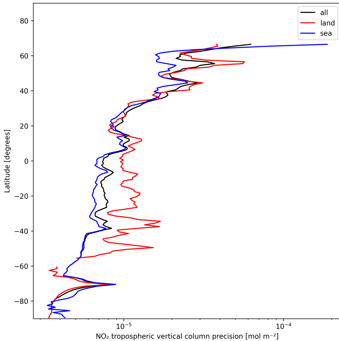
Figure 13: Zonal average of “NO 2 tropospheric vertical column precision” for 2024-11-30 to 2024-12-01.
