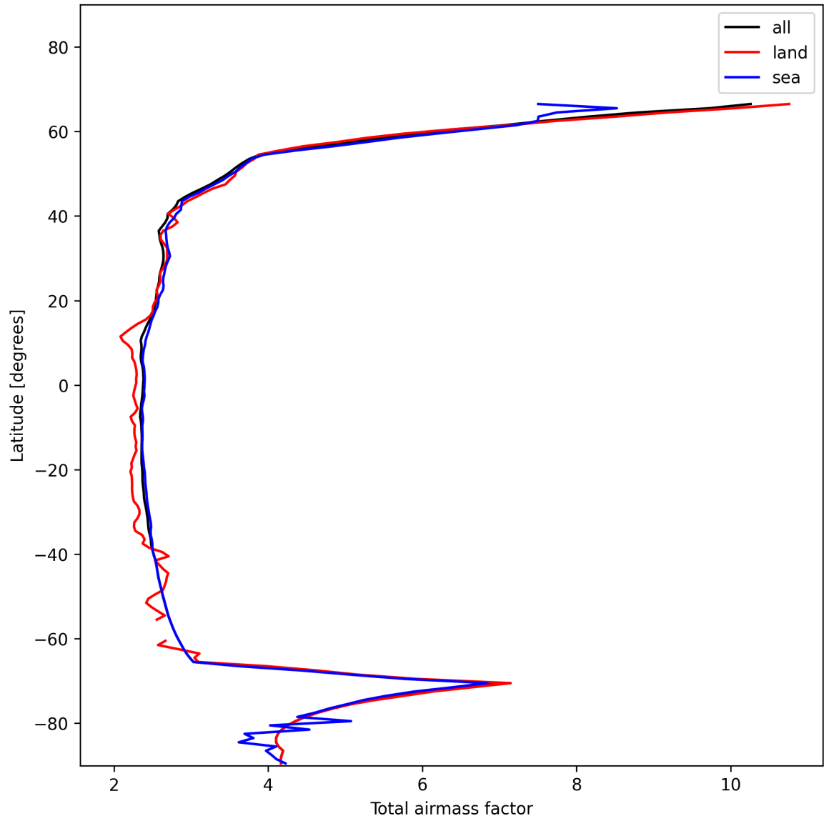
Figure 15: Zonal average of “Total airmass factor” for 2024-11-30 to 2024-12-01.
