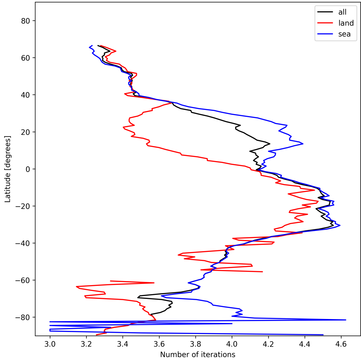
Figure 17: Zonal average of “Number of iterations” for 2024-11-30 to 2024-12-01.
