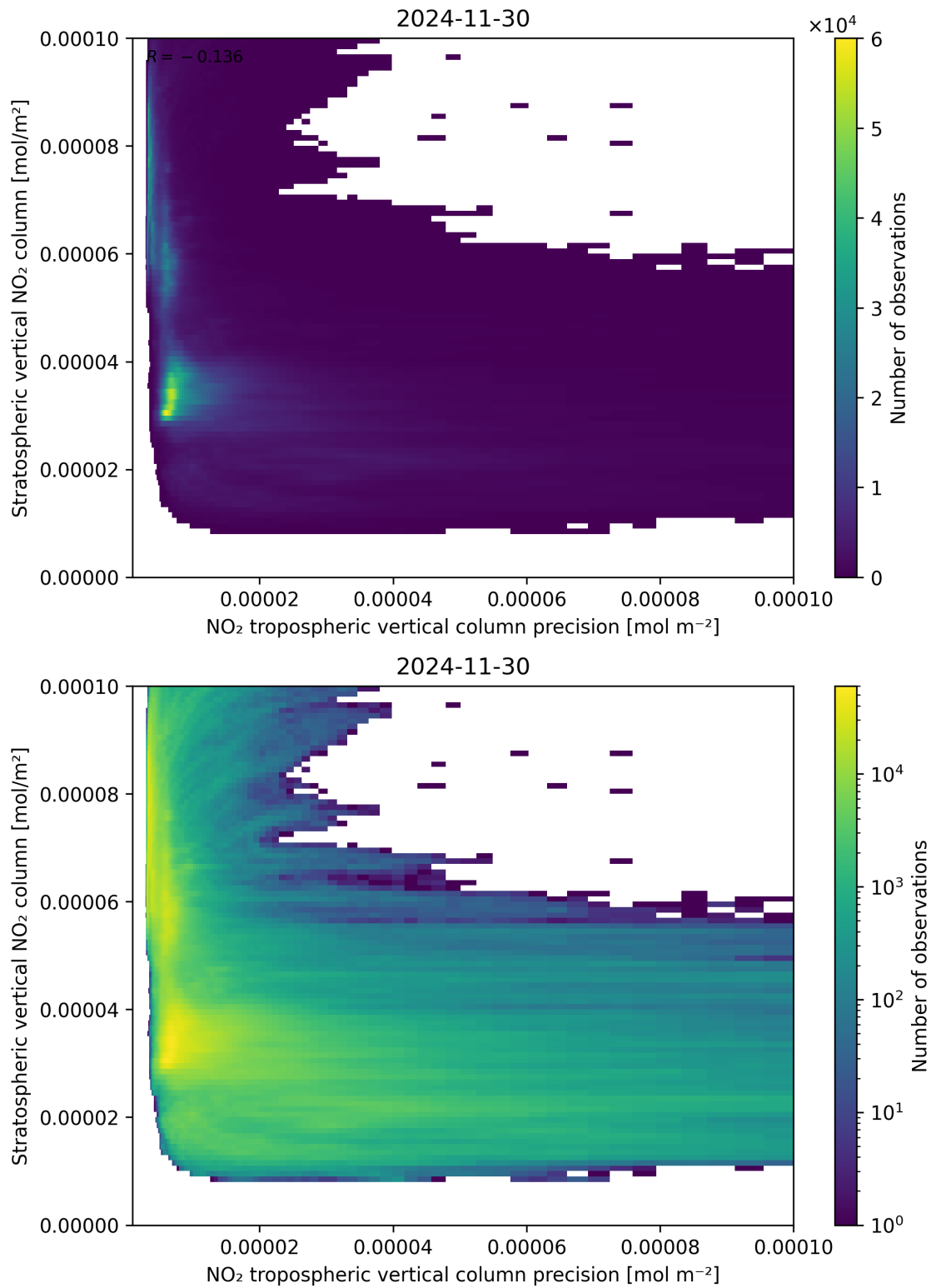
Figure 135: Scatter density plot of “NO 2 tropospheric vertical column precision” against “Stratospheric vertical NO 2 column” for 2024-11-30 to 2024-12-01.
