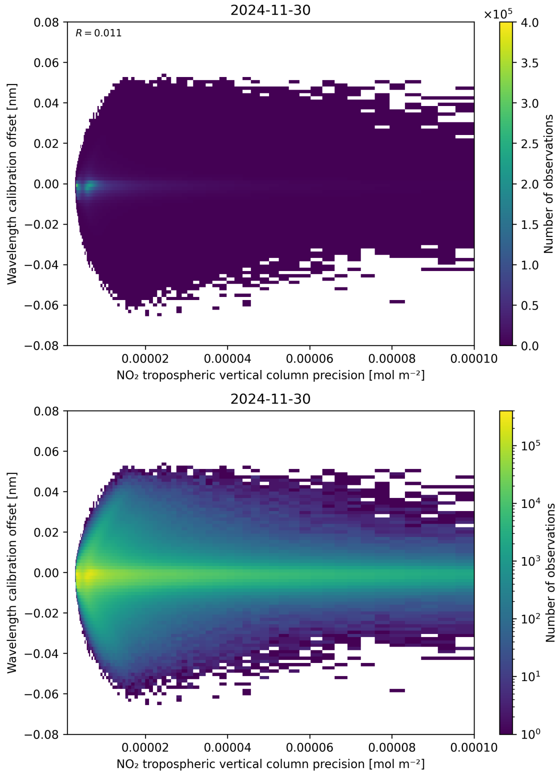
Figure 141: Scatter density plot of “NO 2 tropospheric vertical column precision” against “Wavelength calibration offset” for 2024-11-30 to 2024-12-01.
