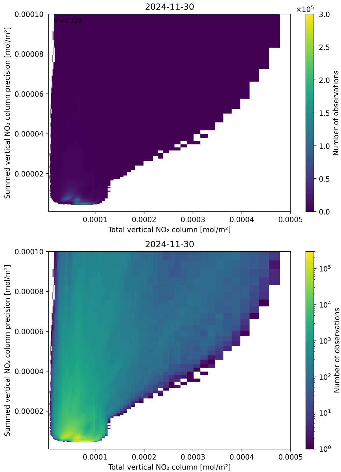
Figure 113: Scatter density plot of “Total vertical NO 2 column” against “Summed vertical NO 2 column precision” for 2024-11-30 to 2024-12-01.
