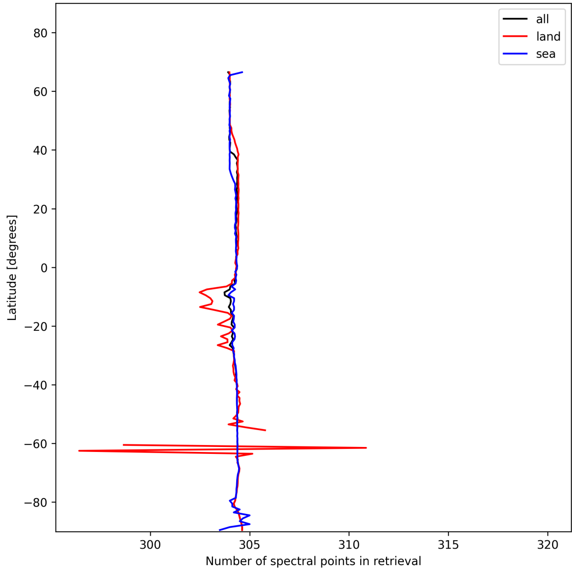
Figure 16: Zonal average of “Number of spectral points in retrieval” for 2024-11-30 to 2024-12-01.
