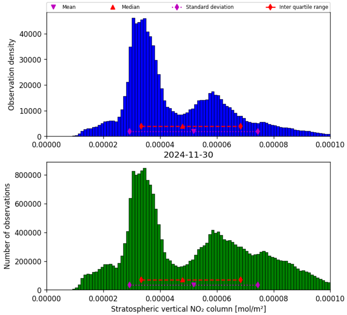
Figure 36: Histogram of “Stratospheric vertical NO 2 column” for 2024-11-30 to 2024-12-01
