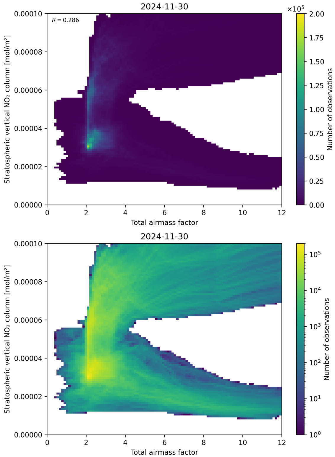
Figure 64: Scatter density plot of “Total airmass factor” against “Stratospheric vertical NO 2 column” for 2024-11-30 to 2024-12-01.
