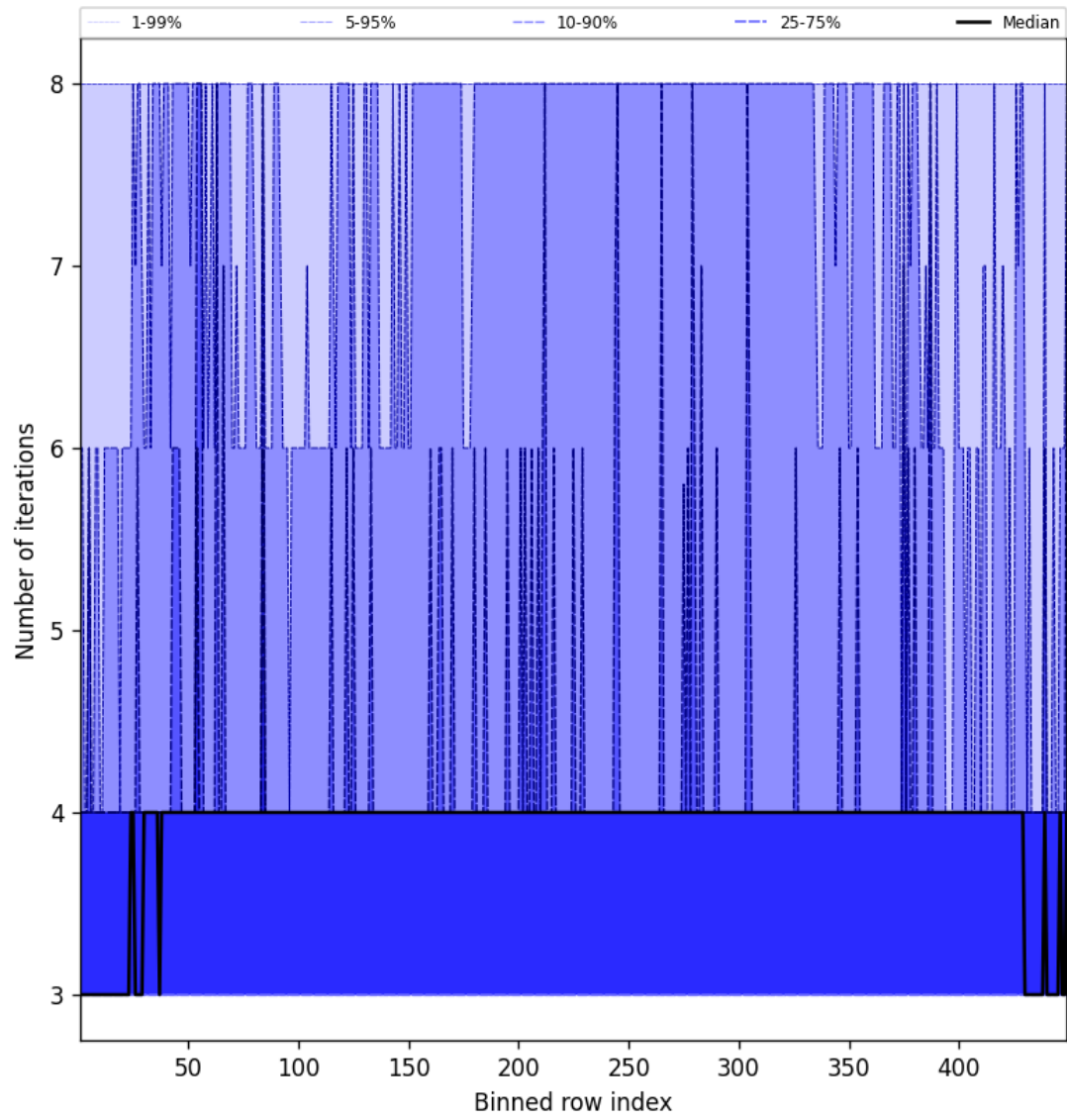
Figure 51: Along track statistics of “Number of iterations” for 2024-11-30 to 2024-12-01
