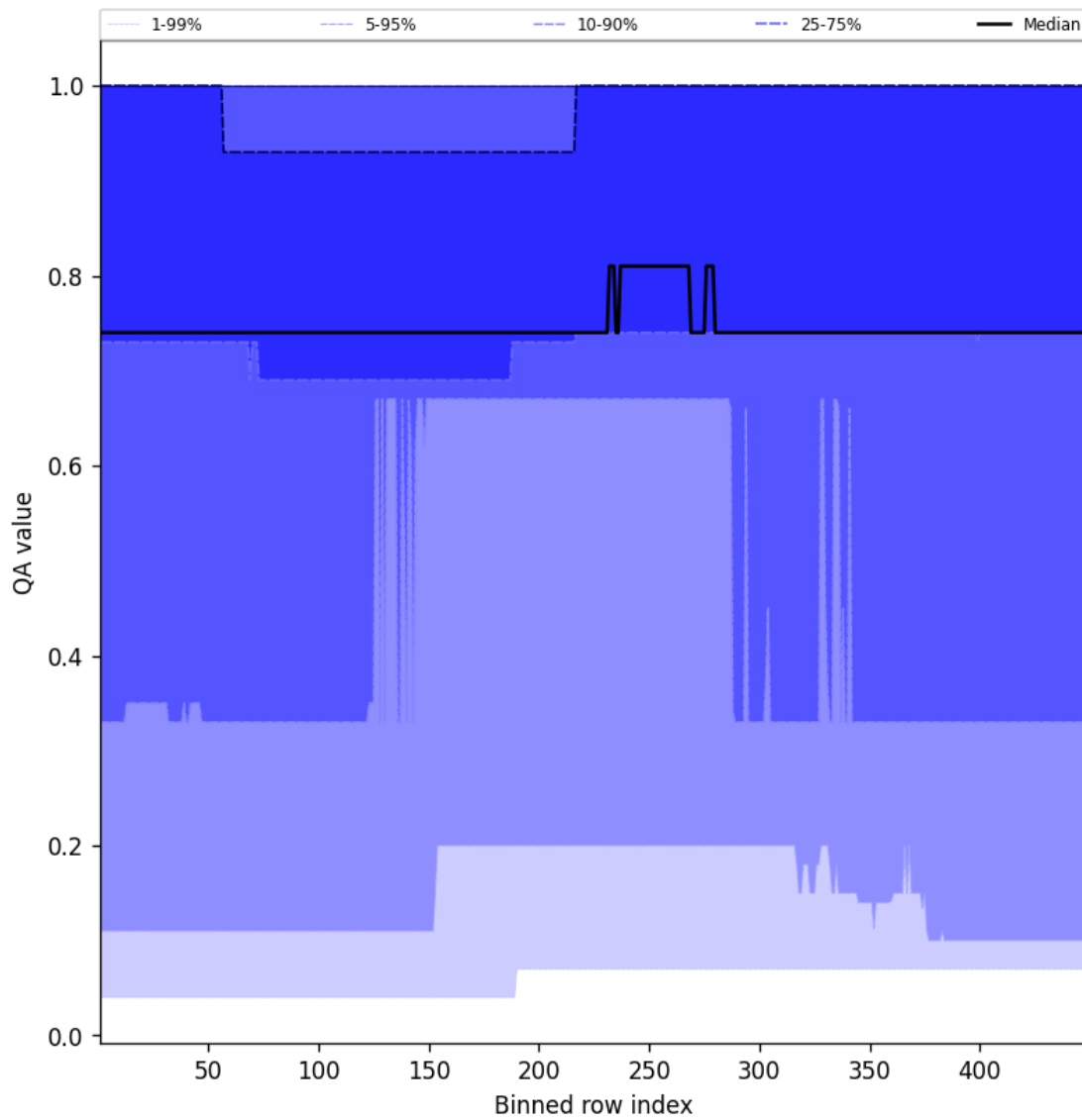
Figure 45: Along track statistics of “QA value” for 2024-11-30 to 2024-12-01
