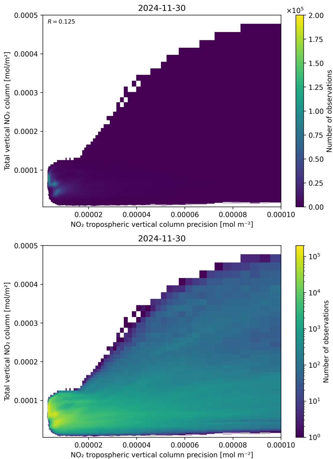
Figure 138: Scatter density plot of “NO 2 tropospheric vertical column precision” against “Total vertical NO 2 column” for 2024-11-30 to 2024-12-01.
