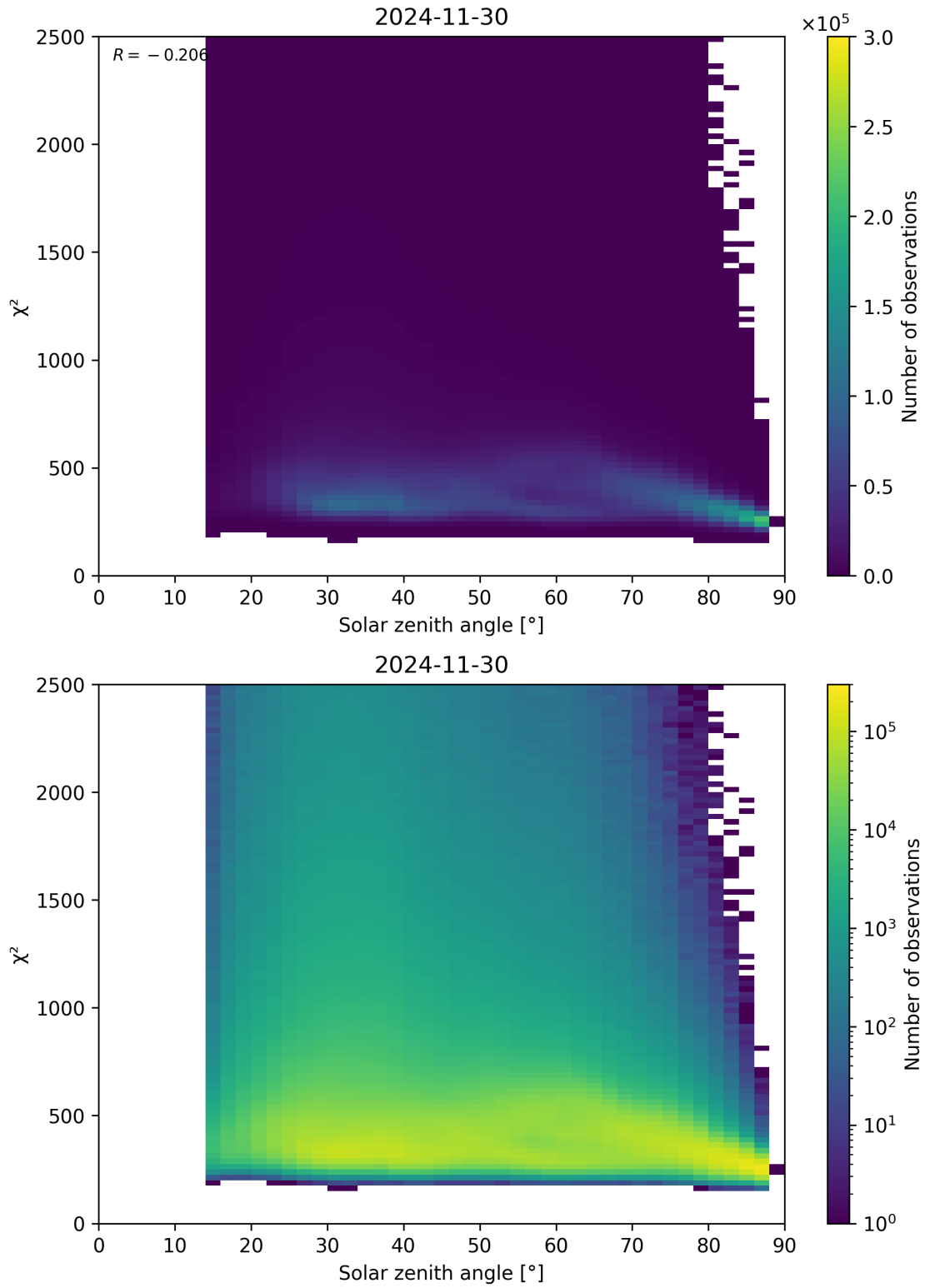
Figure 148: Scatter density plot of “Solar zenith angle” against “ \chi^2 ” for 2024-11-30 to 2024-12-01.
