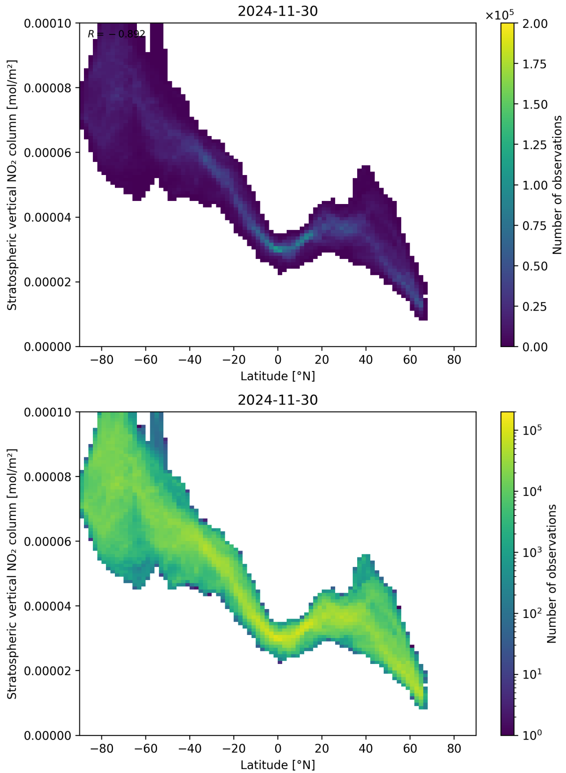
Figure 87: Scatter density plot of “Latitude” against “Stratospheric vertical NO 2 column” for 2024-11-30 to 2024-12-01.
