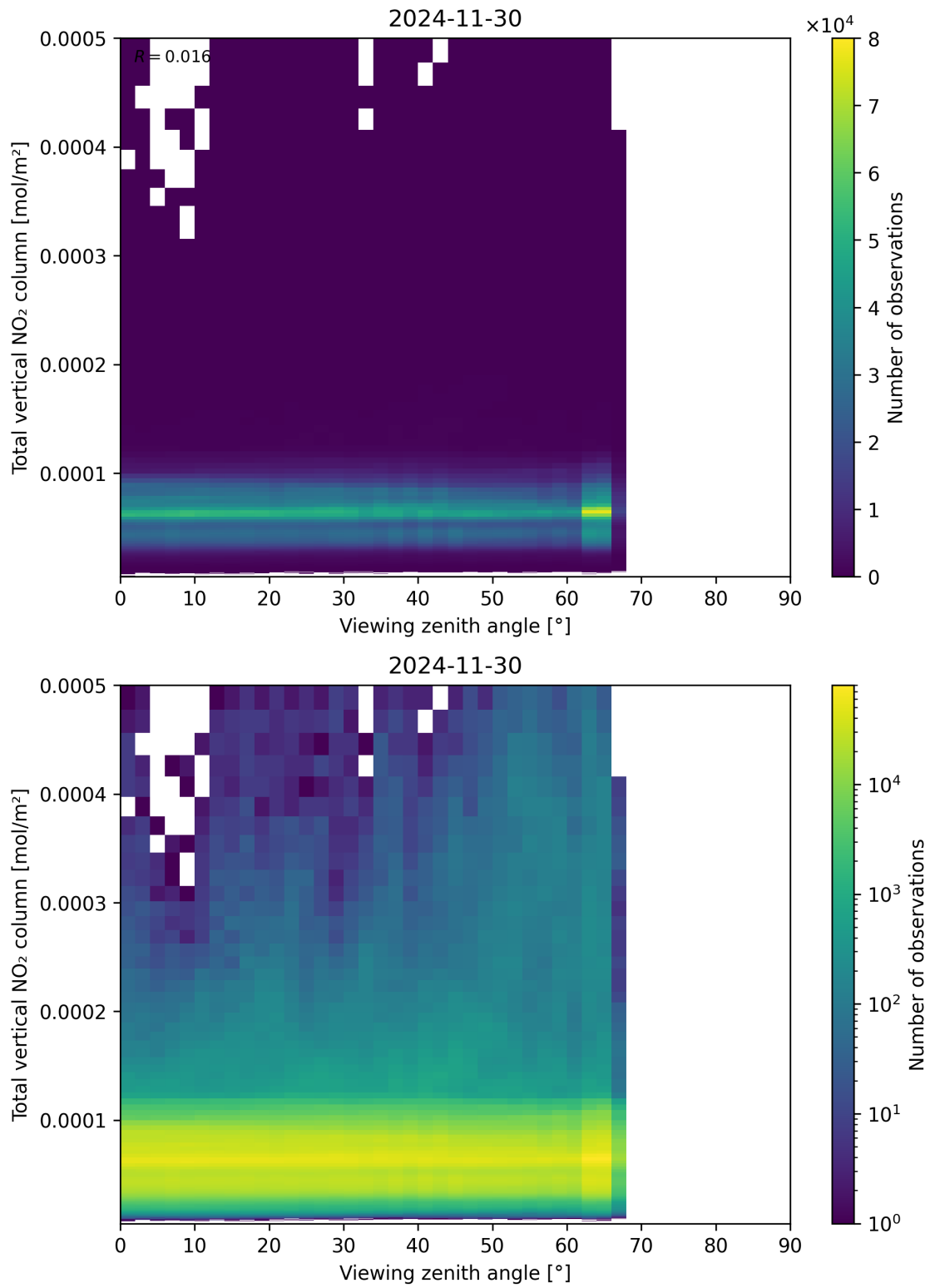
Figure 167: Scatter density plot of “Viewing zenith angle” against “Total vertical NO 2 column” for 2024-11-30 to 2024-12-01.
