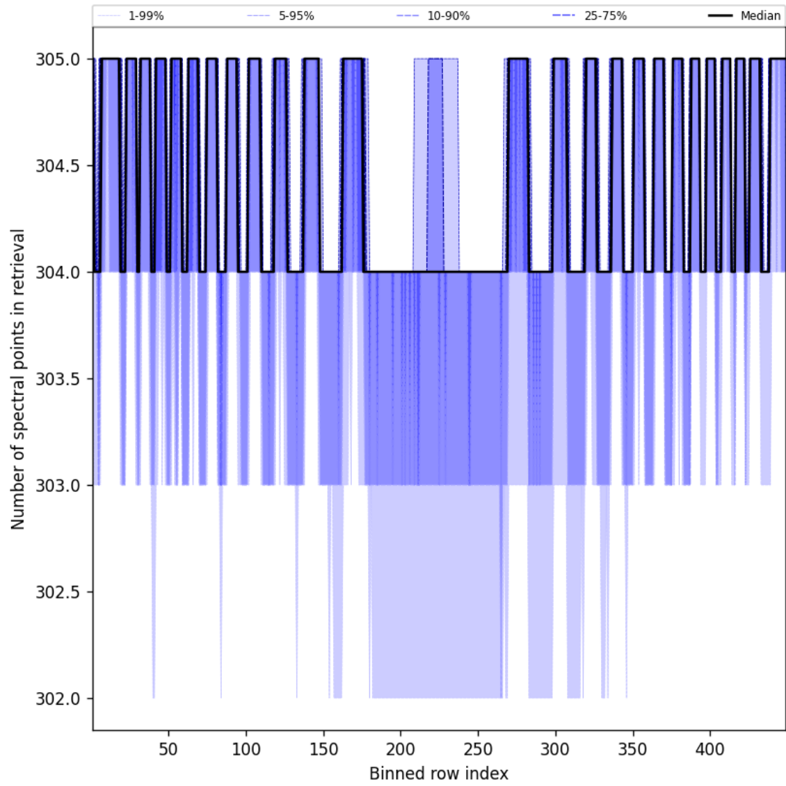
Figure 50: Along track statistics of “Number of spectral points in retrieval” for 2024-11-30 to 2024-12-01
