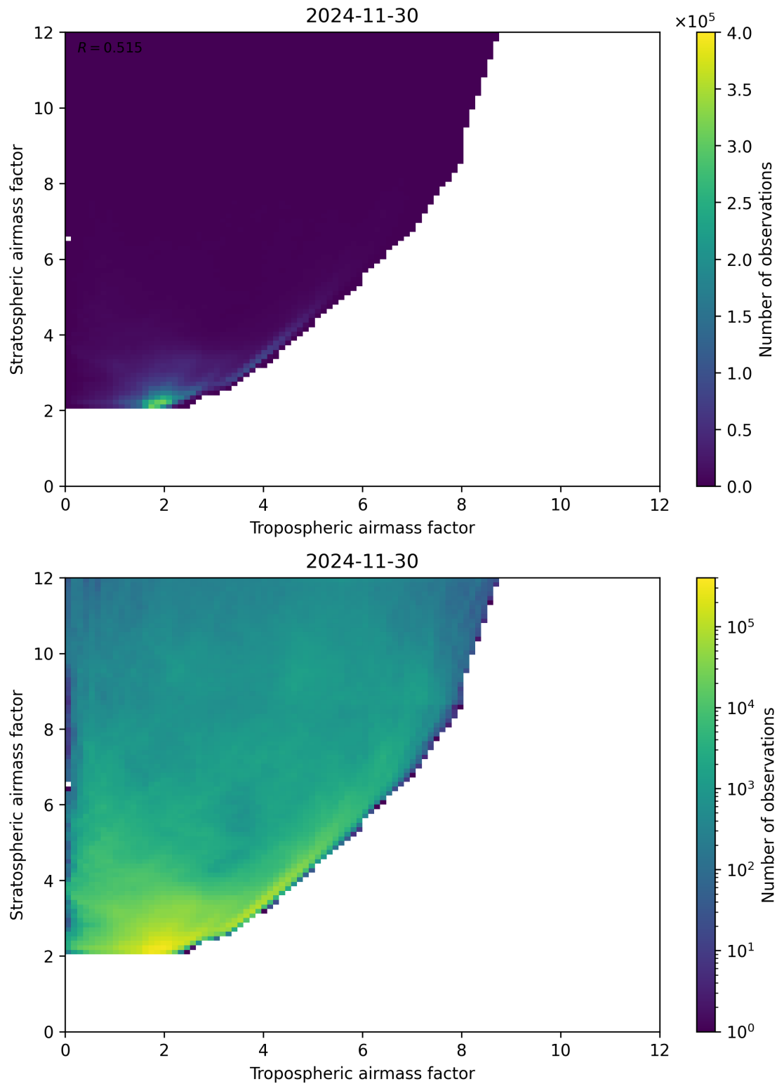
Figure 71: Scatter density plot of “Tropospheric airmass factor” against “Stratospheric airmass factor” for 2024-11-30 to 2024-12-01.
