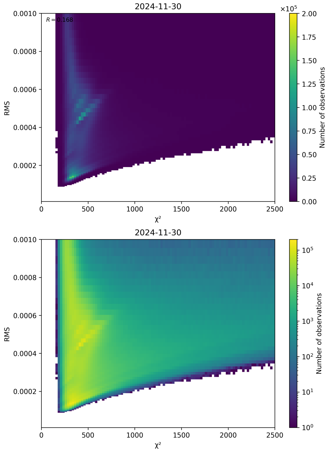
Figure 82: Scatter density plot of “ \chi^2 ” against “RMS” for 2024-11-30 to 2024-12-01.
