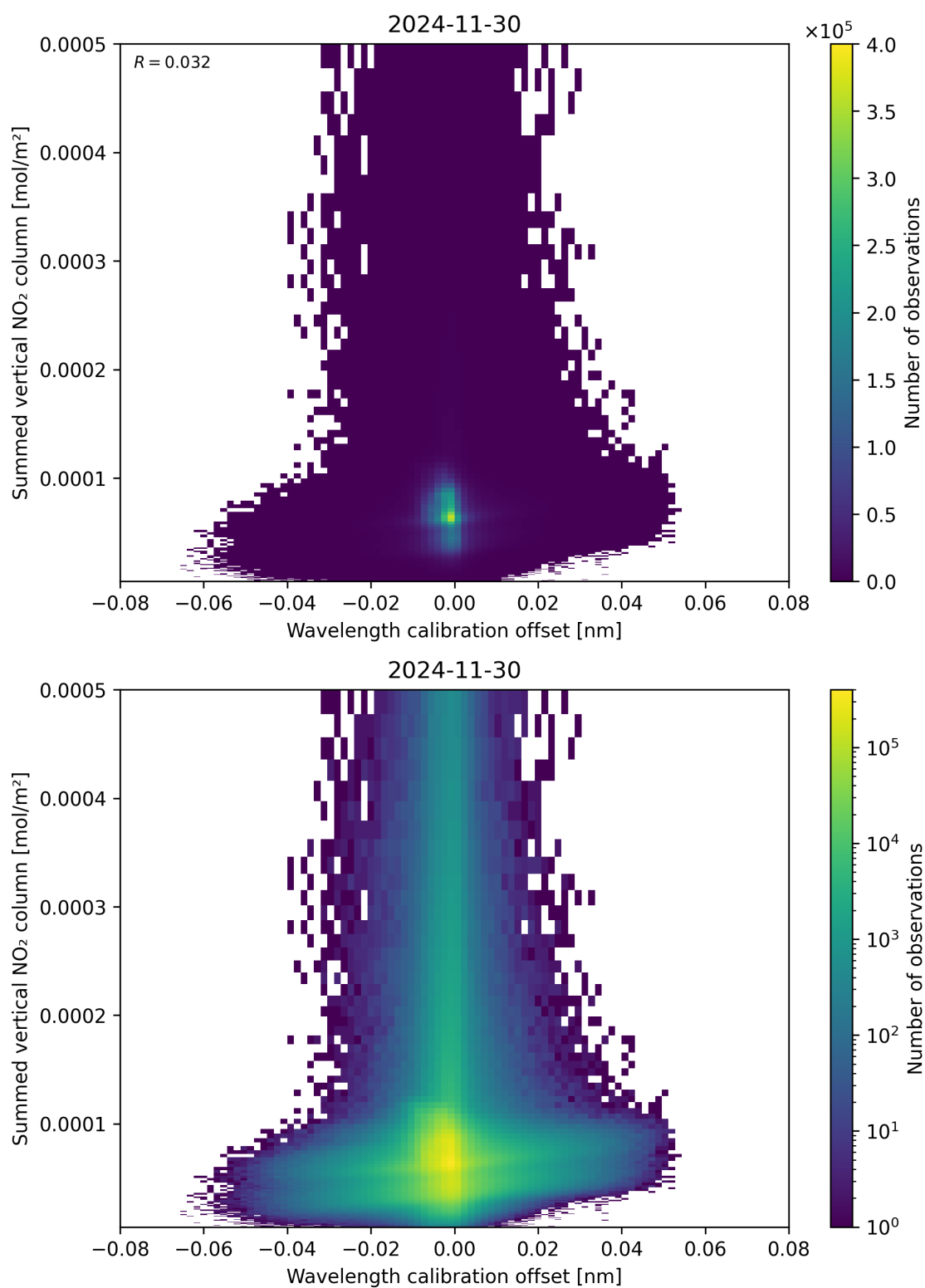
Figure 177: Scatter density plot of “Wavelength calibration offset” against “Summed vertical NO 2 column” for 2024-11-30 to 2024-12-01.
