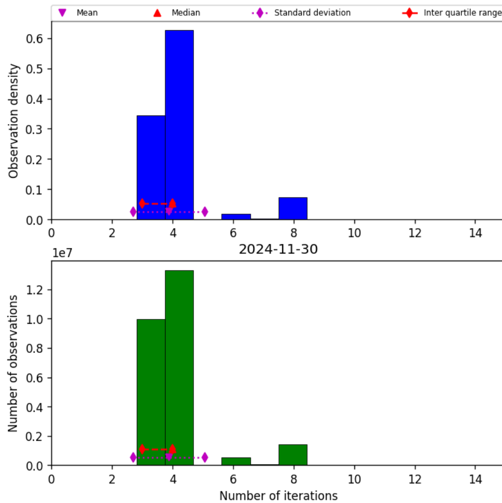
Figure 34: Histogram of “Number of iterations” for 2024-11-30 to 2024-12-01
