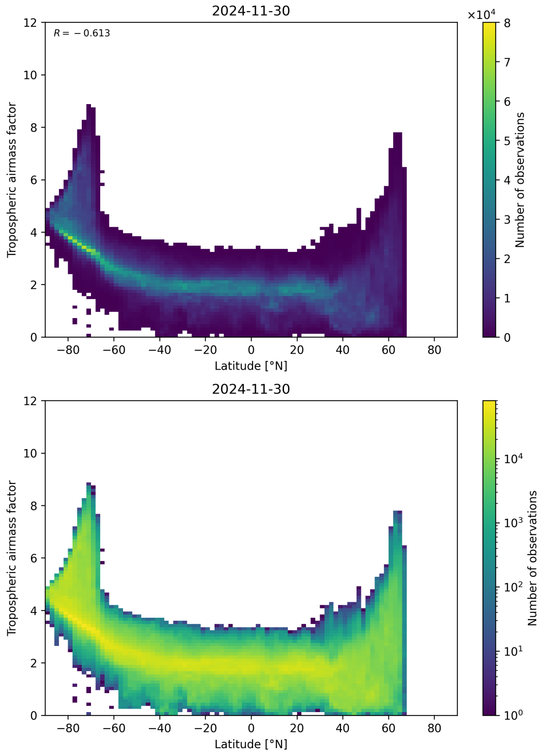
Figure 85: Scatter density plot of “Latitude” against “Tropospheric airmass factor” for 2024-11-30 to 2024-12-01.
