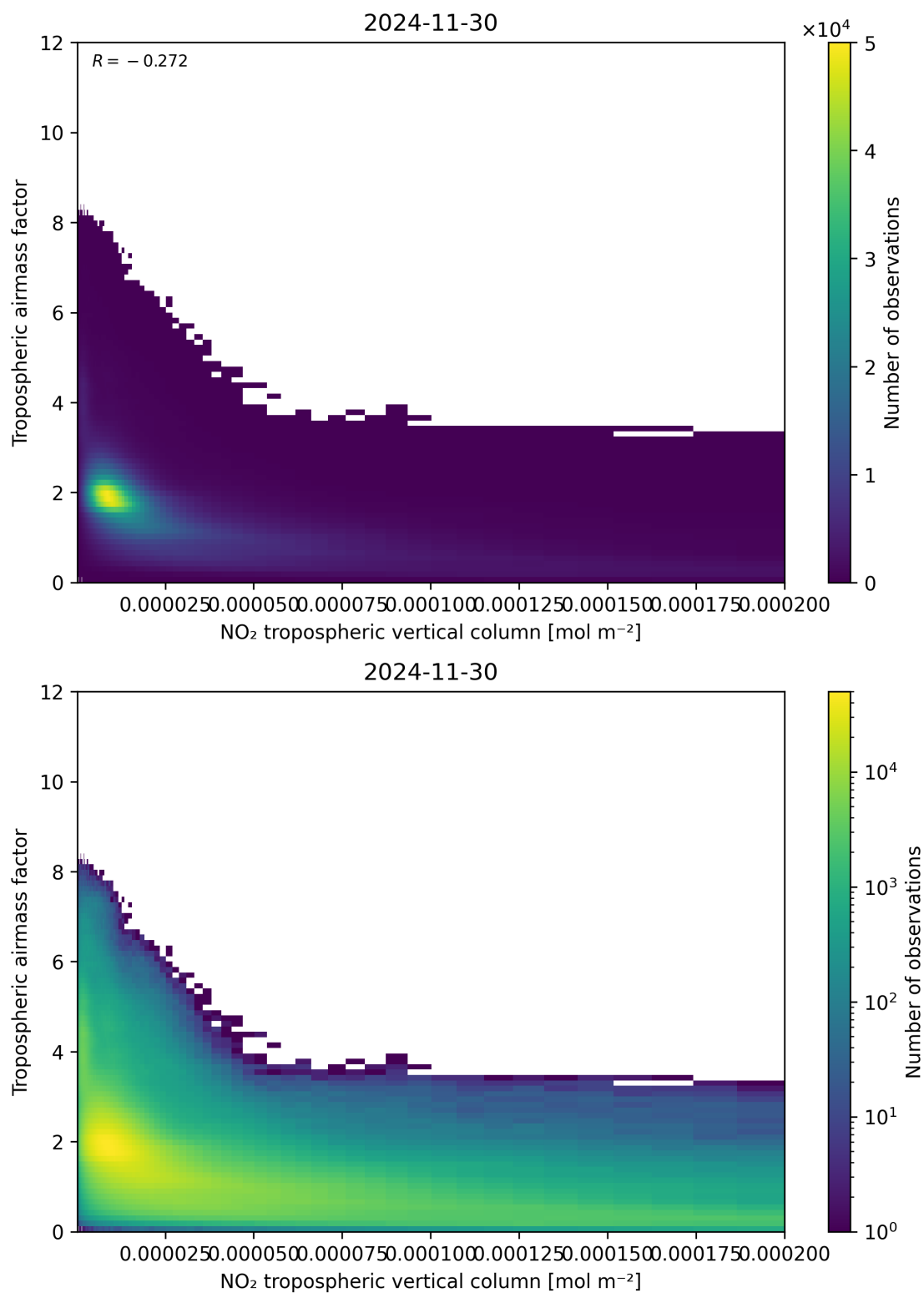
Figure 123: Scatter density plot of “NO 2 tropospheric vertical column” against “Tropospheric air mass factor” for 2024-11-30 to 2024-12-01.
