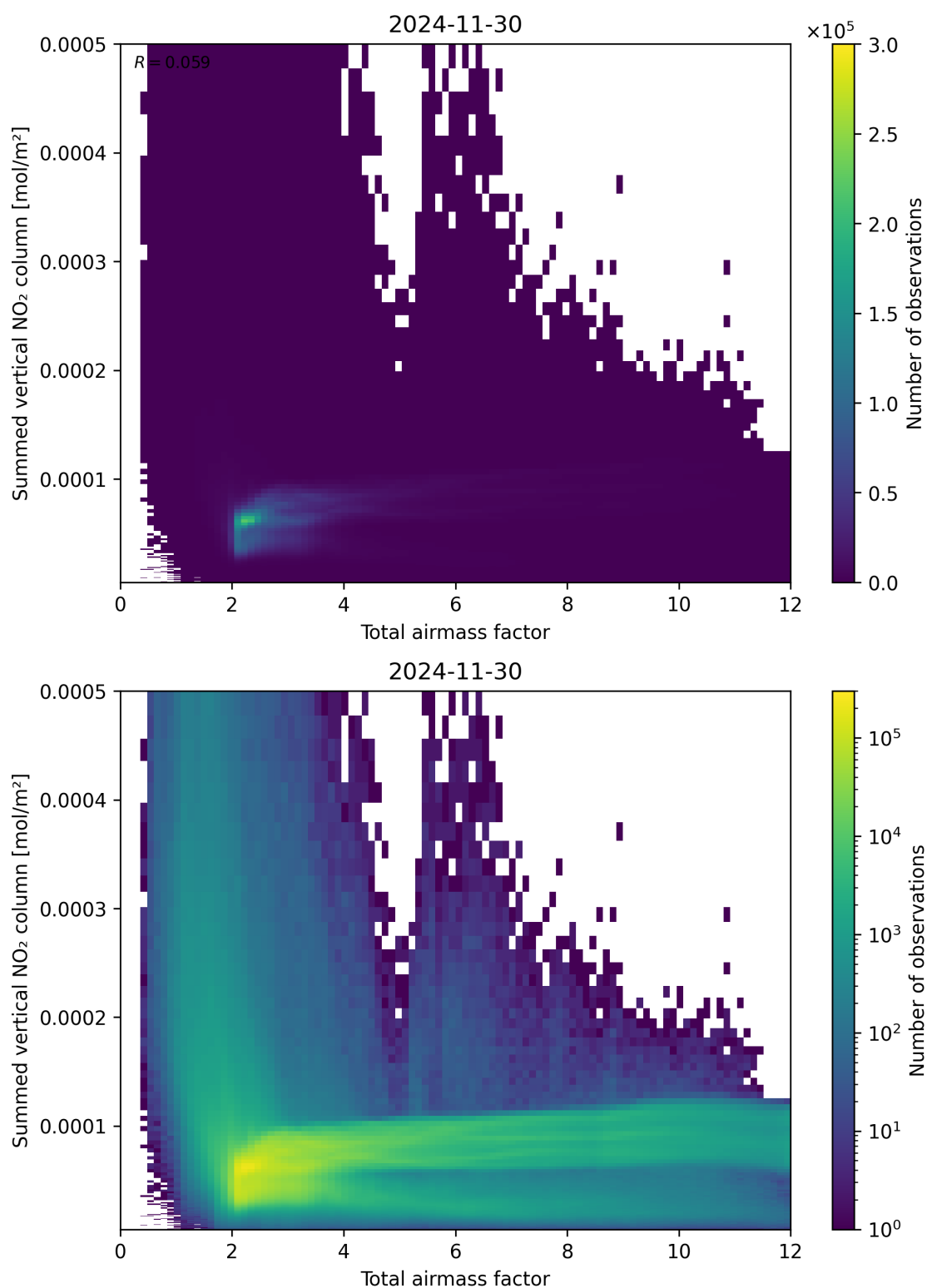
Figure 65: Scatter density plot of “Total airmass factor” against “Summed vertical NO 2 column” for 2024-11-30 to 2024-12-01.
