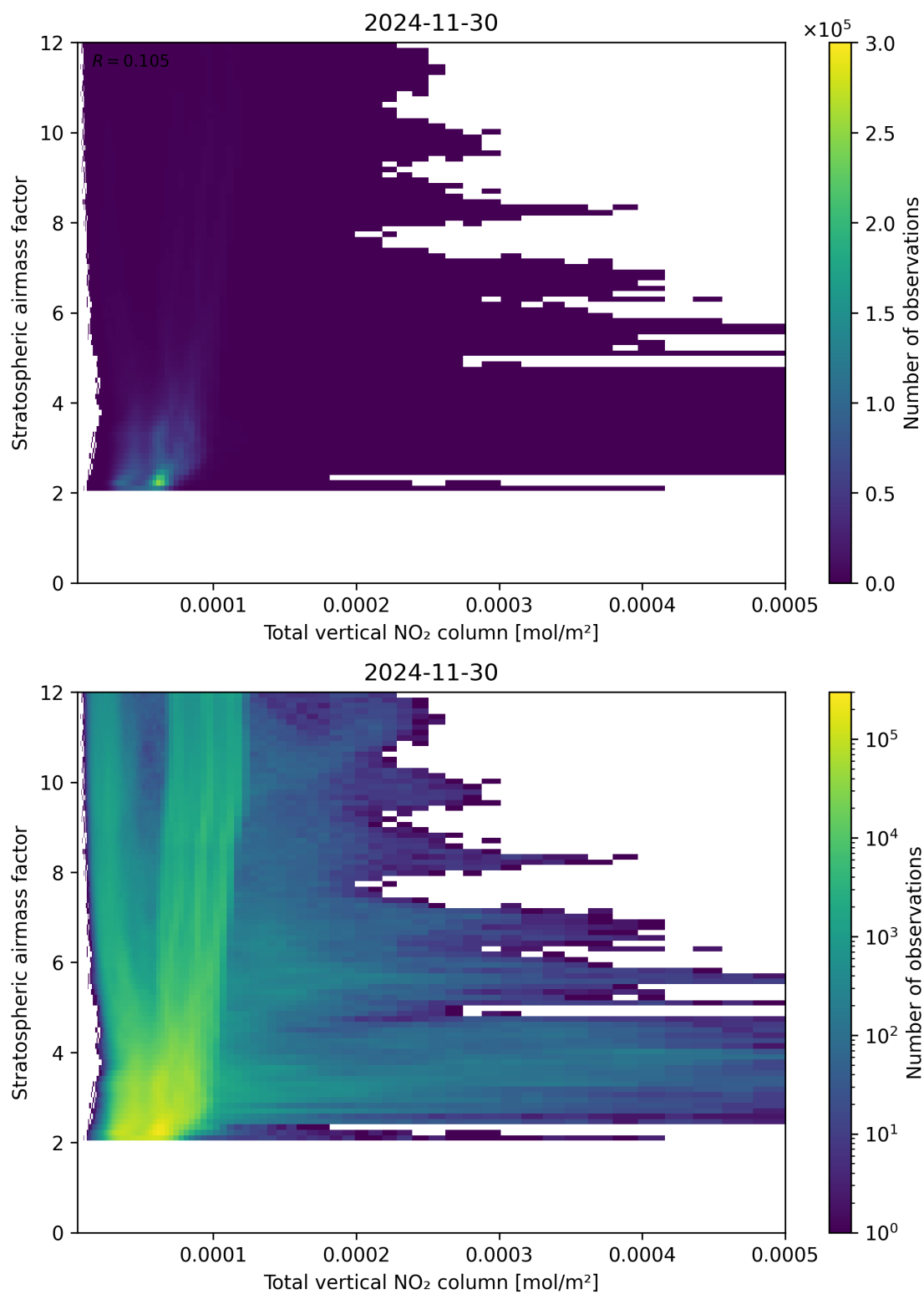
Figure 110: Scatter density plot of “Total vertical NO 2 column” against “Stratospheric airmass factor” for 2024-11-30 to 2024-12-01.
