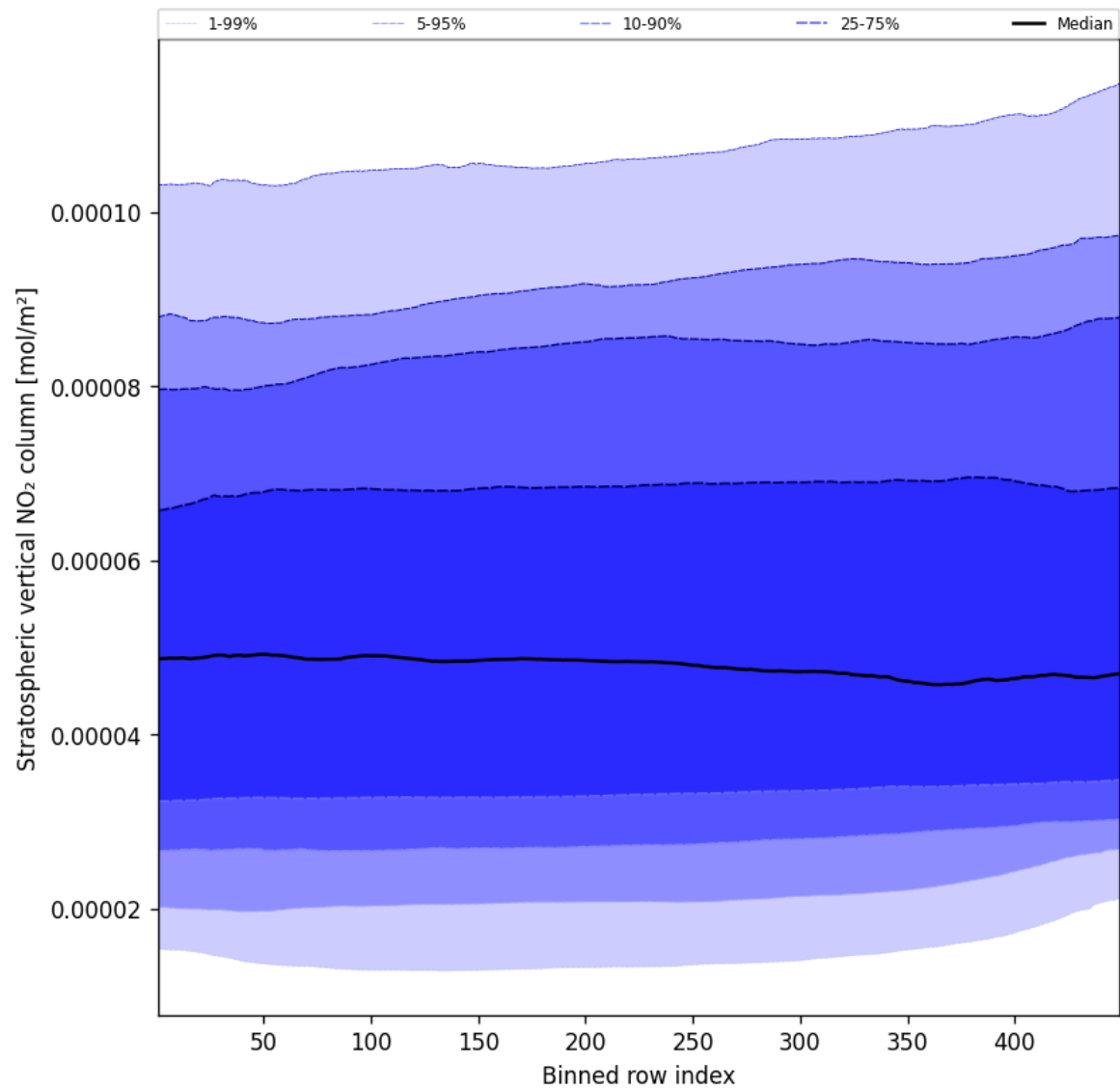
Figure 53: Along track statistics of “Stratospheric vertical NO 2 column” for 2024-11-30 to 2024-12-01
