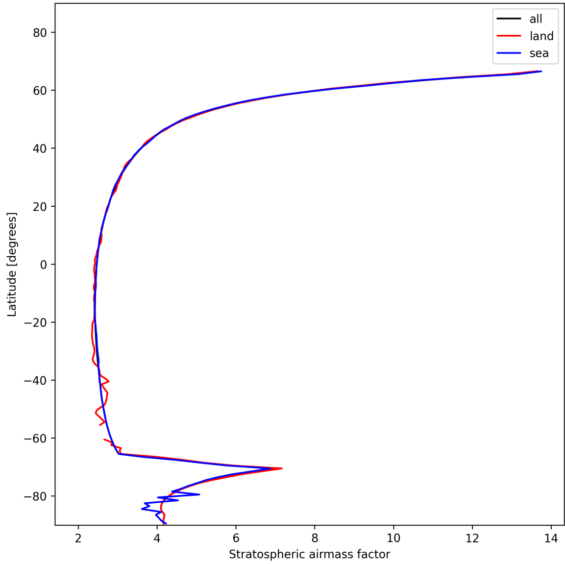
Figure 27: Zonal average of “Stratospheric air mass factor” for 2024-11-30 to 2024-12-01.
