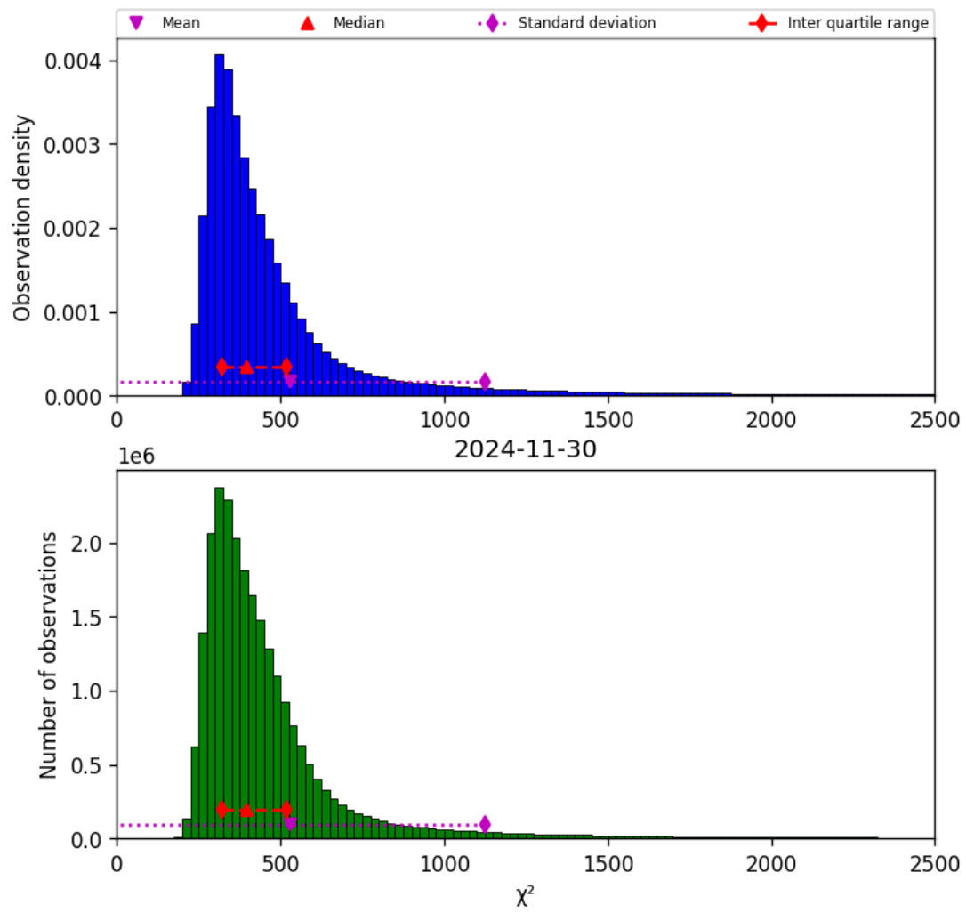
Figure 42: Histogram of “ \chi^2 ” for 2024-11-30 to 2024-12-01
