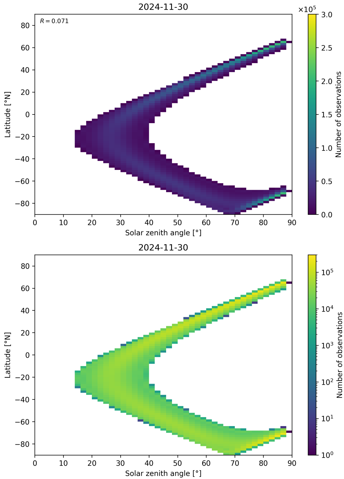
Figure 149: Scatter density plot of “Solar zenith angle” against “Latitude” for 2024-11-30 to 2024-12-01.
