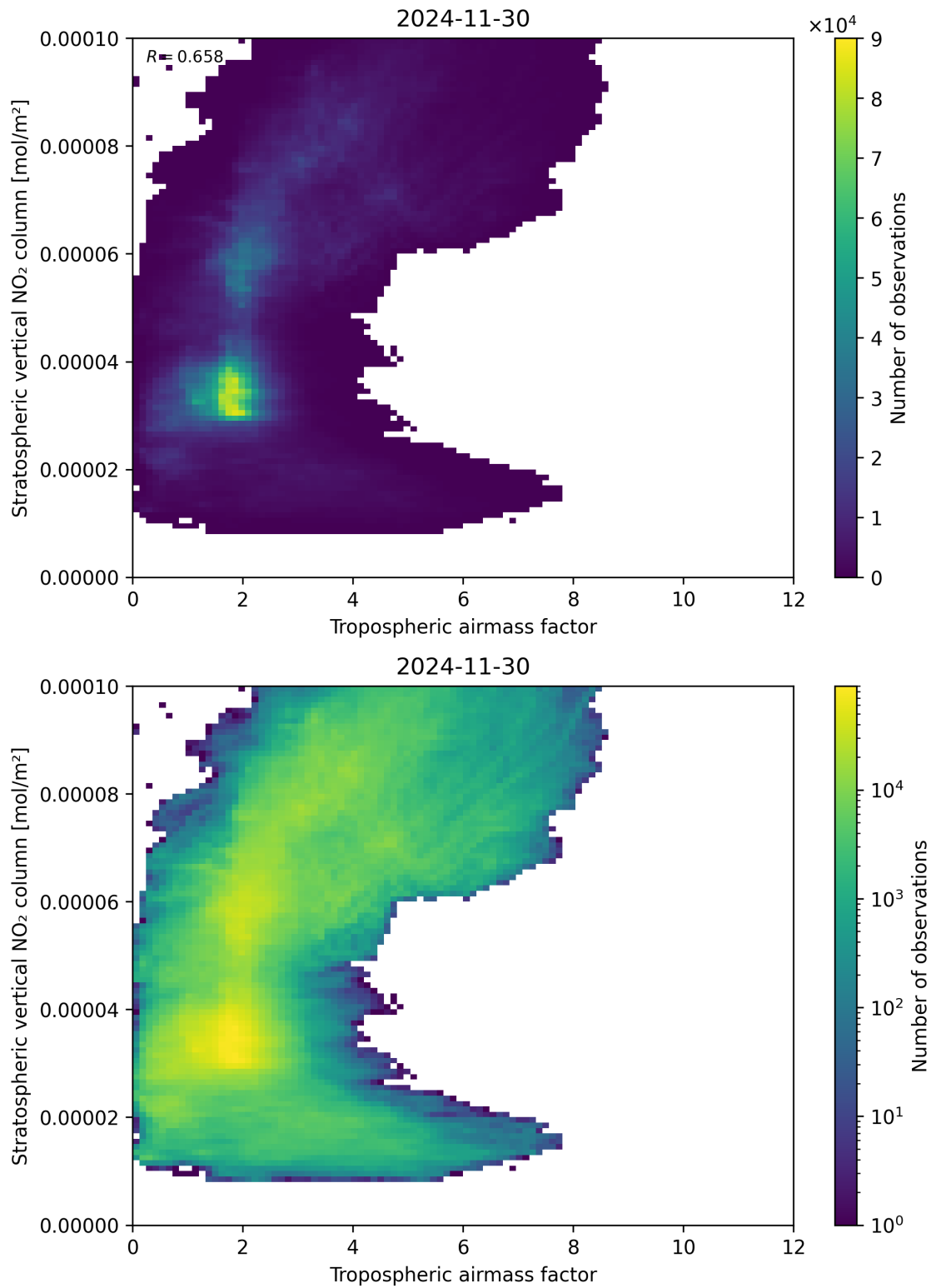
Figure 74: Scatter density plot of “Tropospheric air mass factor” against “Stratospheric vertical NO 2 column” for 2024-11-30 to 2024-12-01.
