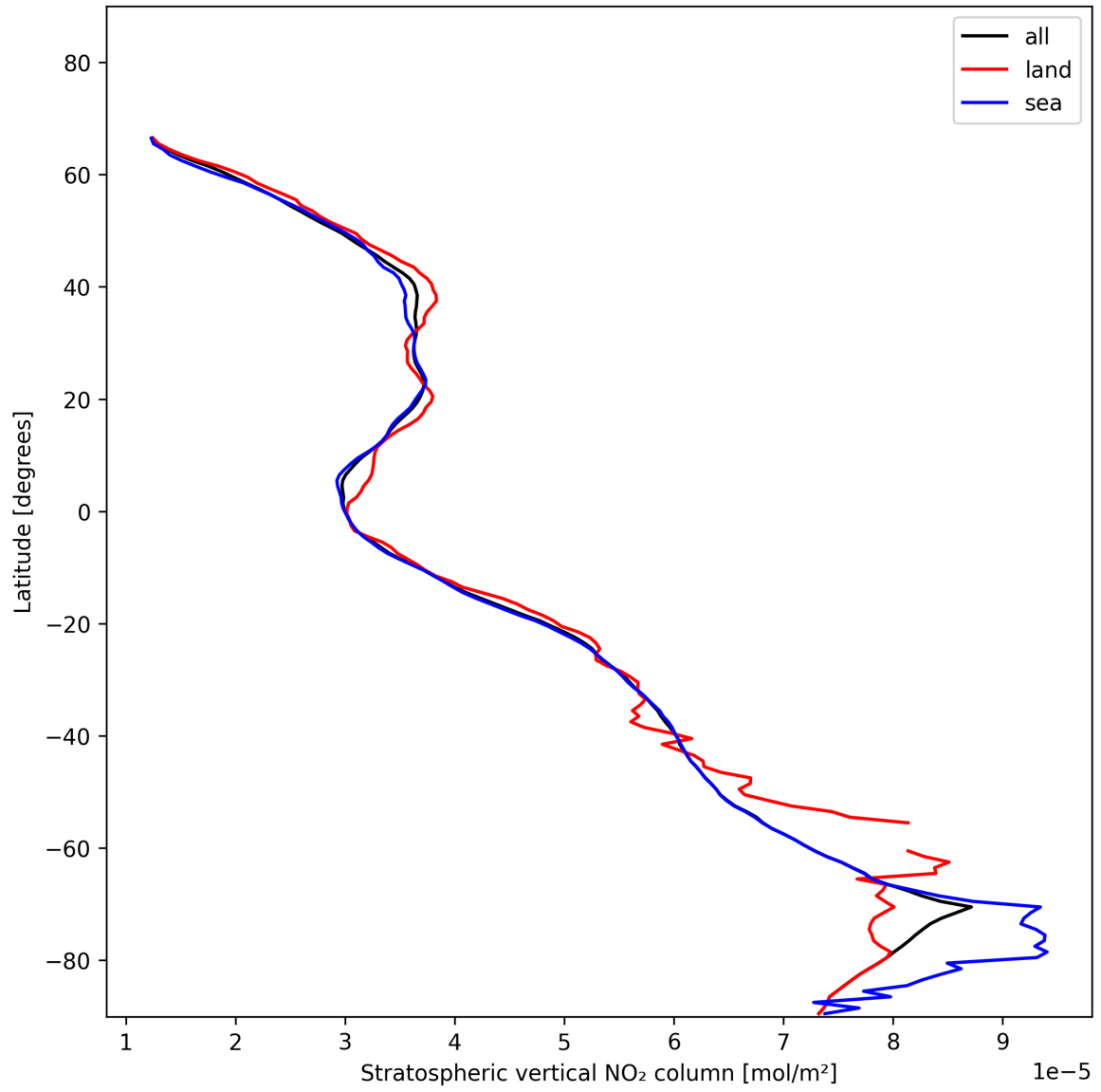
Figure 19: Zonal average of “Stratospheric vertical NO 2 column” for 2024-11-30 to 2024-12-01.
