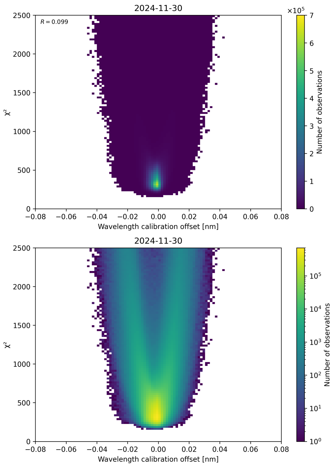
Figure 175: Scatter density plot of “Wavelength calibration offset” against “ \chi^2 ” for 2024-11-30 to 2024-12-01.
