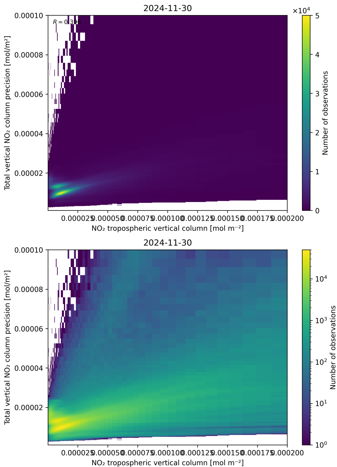
Figure 129: Scatter density plot of “NO 2 tropospheric vertical column” against “Total vertical NO 2 column precision” for 2024-11-30 to 2024-12-01.
