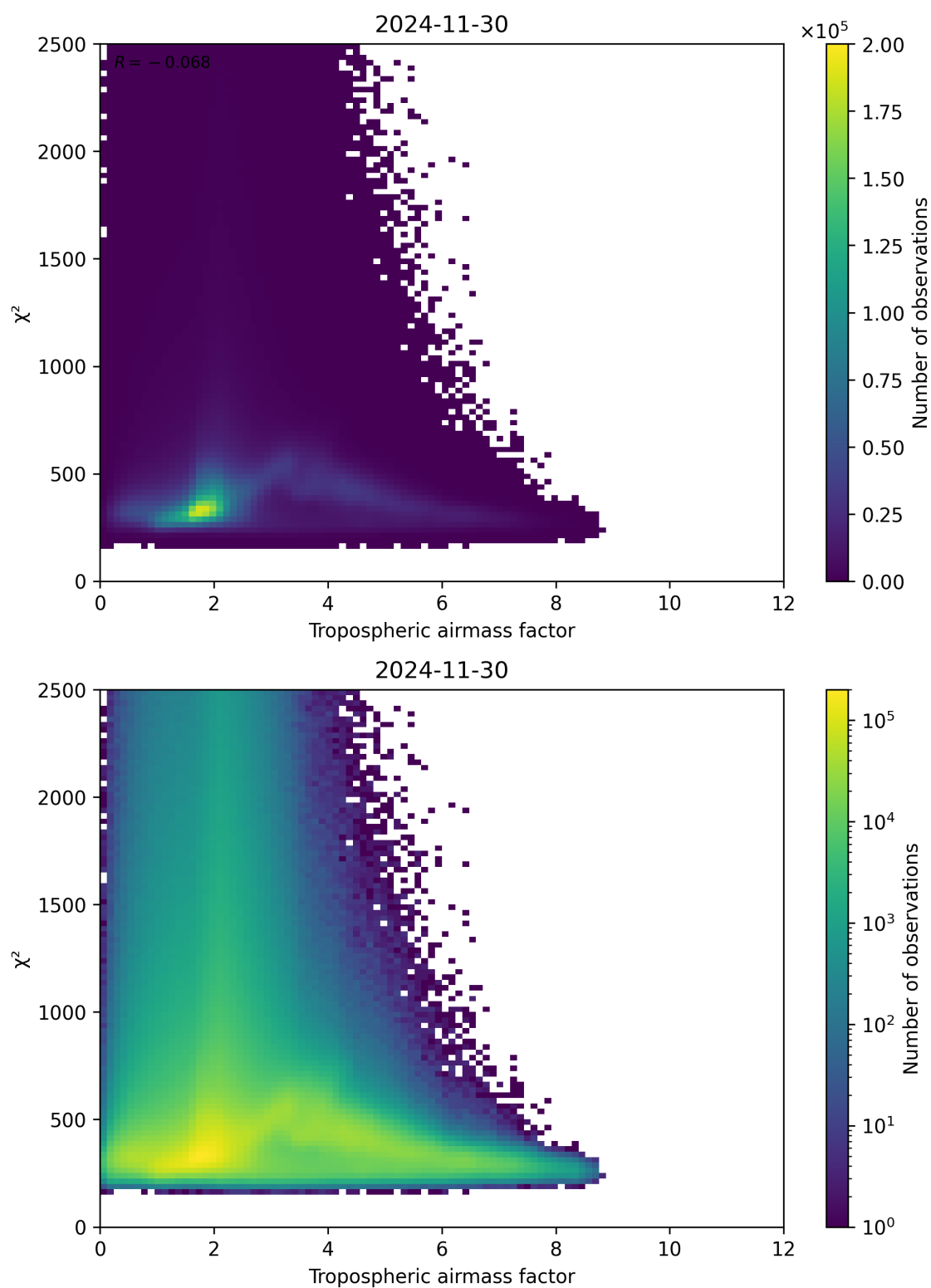
Figure 73: Scatter density plot of “Tropospheric airmass factor” against “ \chi^2 ” for 2024-11-30 to 2024-12-01.
