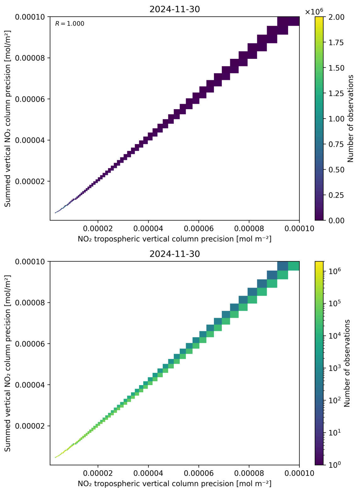
Figure 137: Scatter density plot of “NO 2 tropospheric vertical column precision” against “Summed vertical NO 2 column precision” for 2024-11-30 to 2024-12-01.
