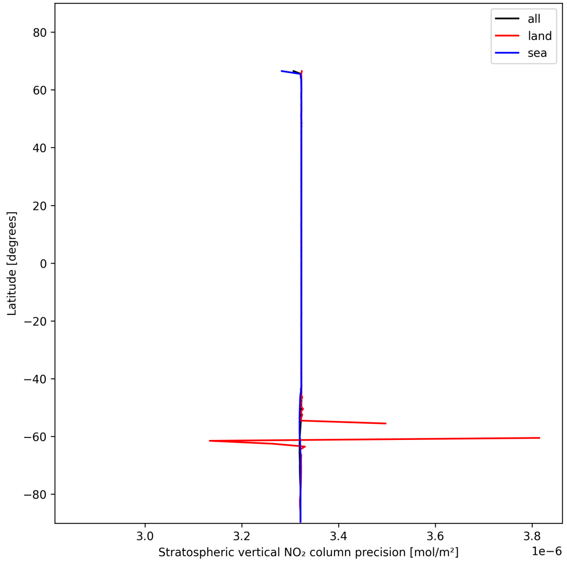
Figure 20: Zonal average of "Stratospheric vertical NO 2 column precision" for 2024-11-30 to 2024-12-01.
