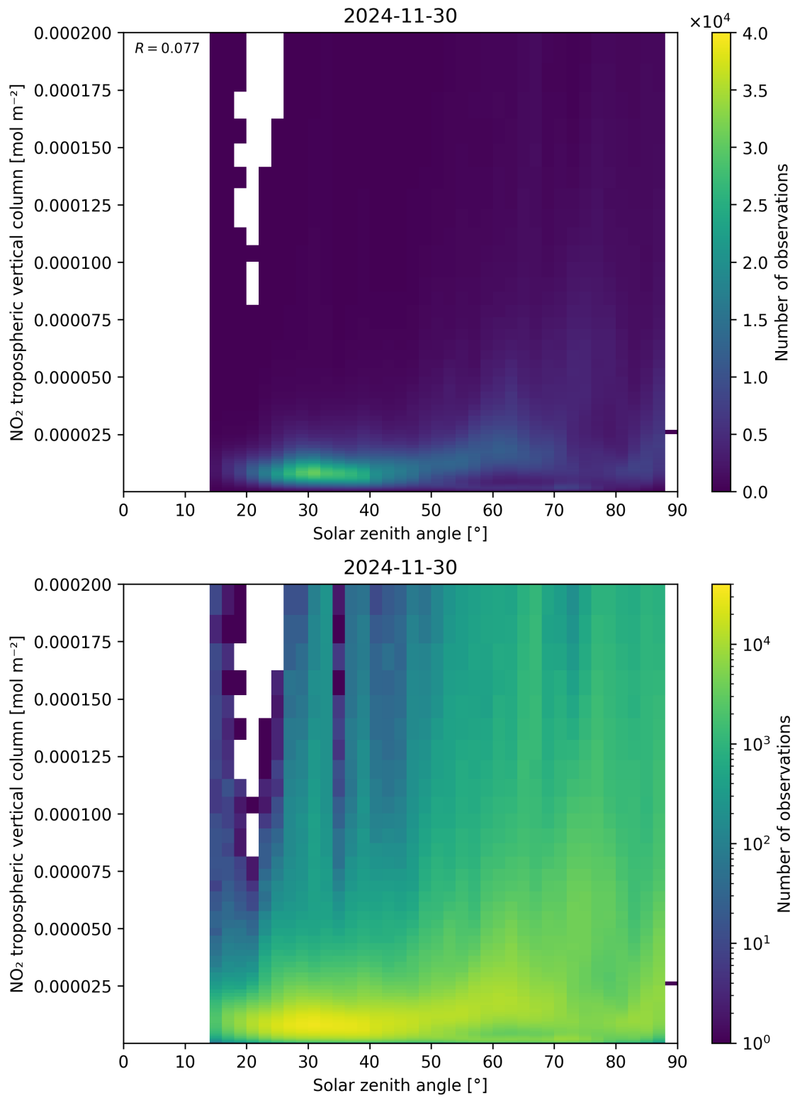
Figure 155: Scatter density plot of “Solar zenith angle” against “NO 2 tropospheric vertical column” for 2024-11-30 to 2024-12-01.
