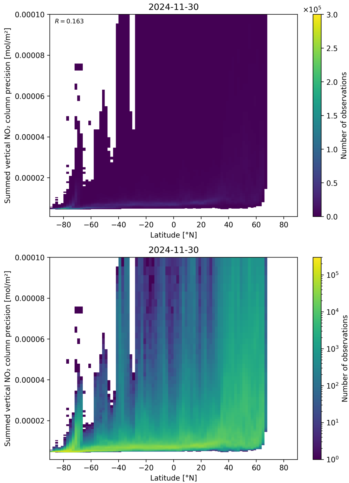
Figure 89: Scatter density plot of “Latitude” against “Summed vertical NO 2 column precision” for 2024-11-30 to 2024-12-01.
