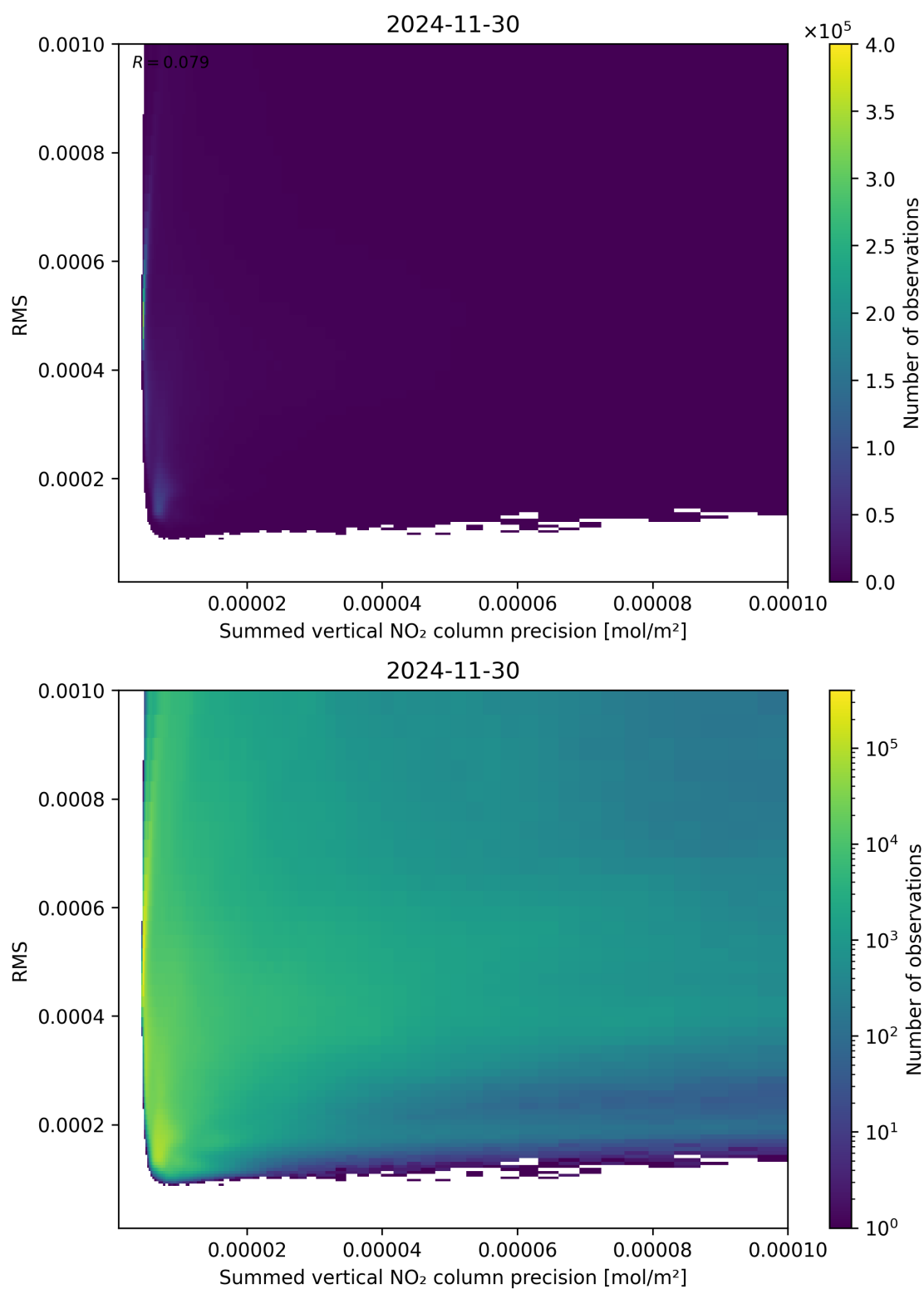
Figure 108: Scatter density plot of “Summed vertical NO 2 column precision” against “RMS” for 2024-11-30 to 2024-12-01.
