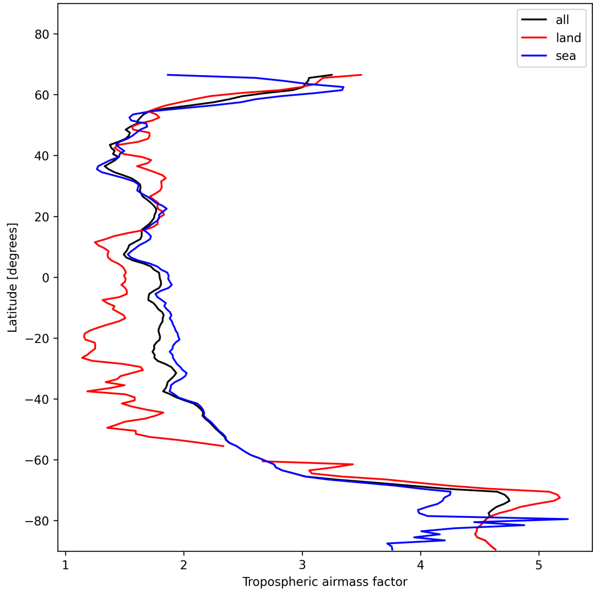
Figure 14: Zonal average of “Tropospheric airmass factor” for 2024-11-30 to 2024-12-01.
