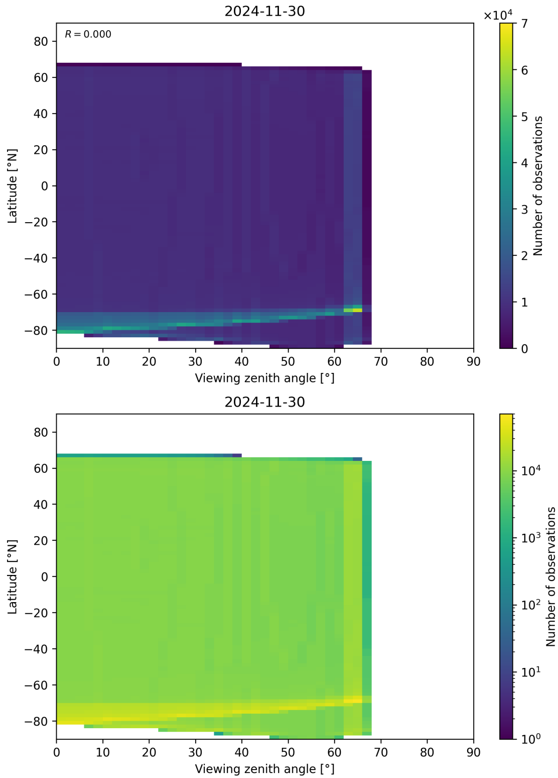
Figure 163: Scatter density plot of “Viewing zenith angle” against “Latitude” for 2024-11-30 to 2024-12-01.
