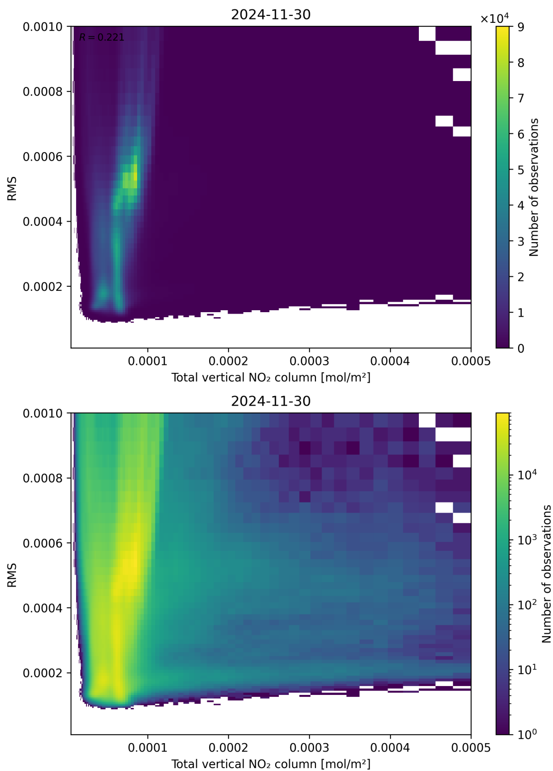
Figure 120: Scatter density plot of “Total vertical NO 2 column” against “RMS” for 2024-11-30 to 2024-12-01.
