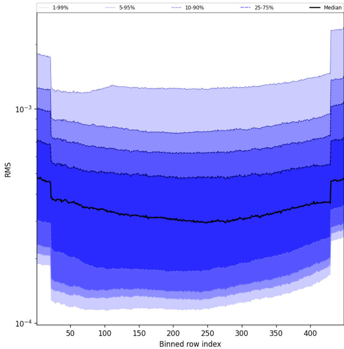
Figure 60: Along track statistics of “RMS” for 2024-11-30 to 2024-12-01
