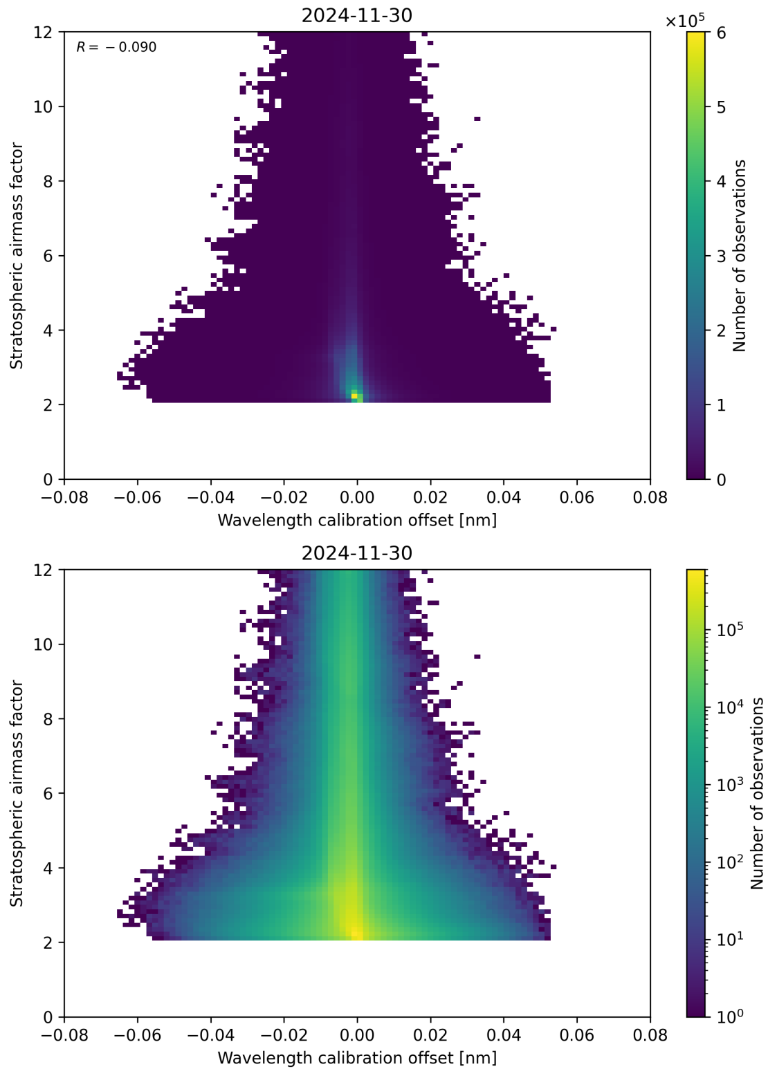
Figure 174: Scatter density plot of “Wavelength calibration offset” against “Stratospheric airmass factor” for 2024-11-30 to 2024-12-01.
