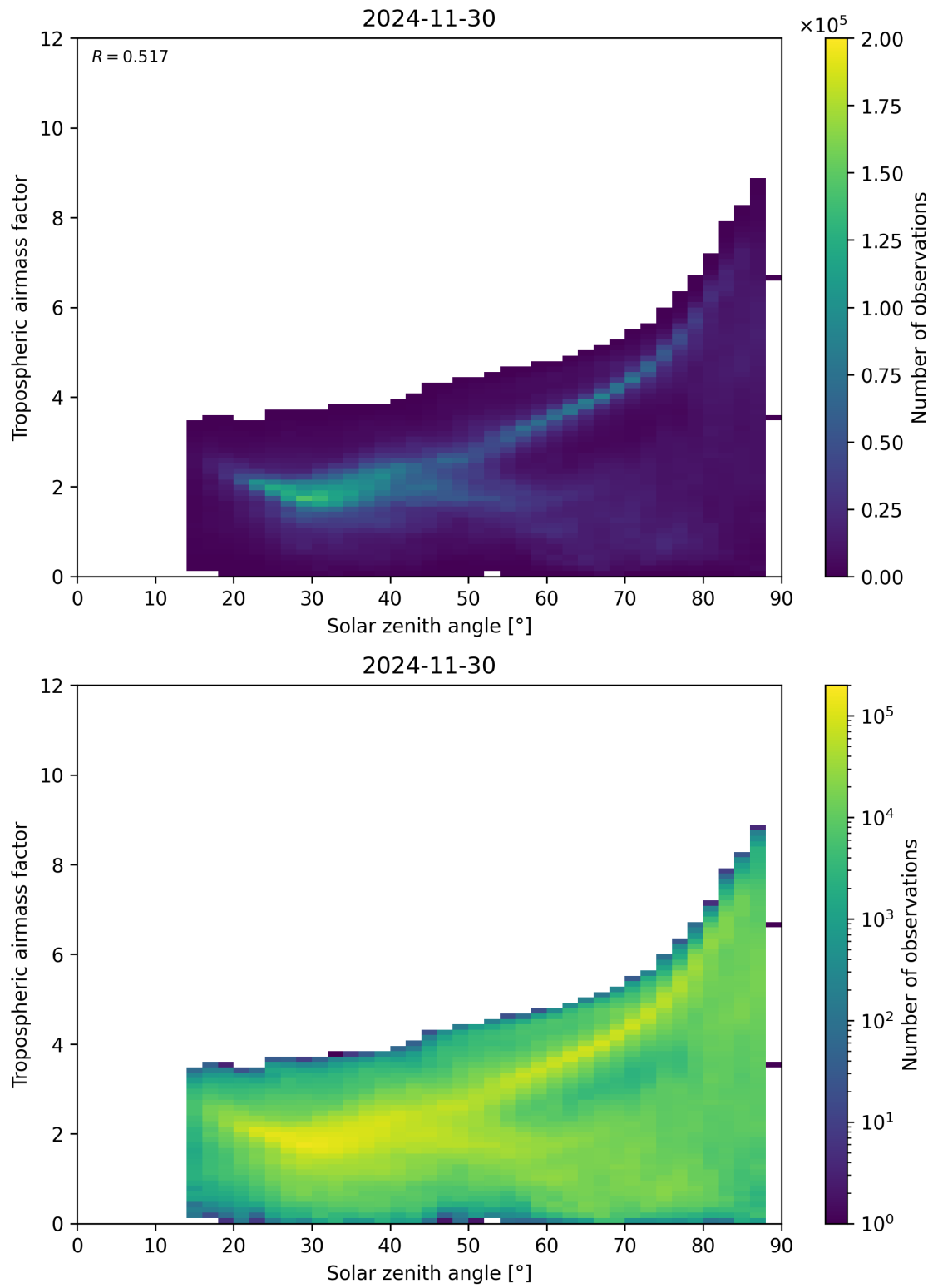
Figure 147: Scatter density plot of “Solar zenith angle” against “Tropospheric airmass factor” for 2024-11-30 to 2024-12-01.
