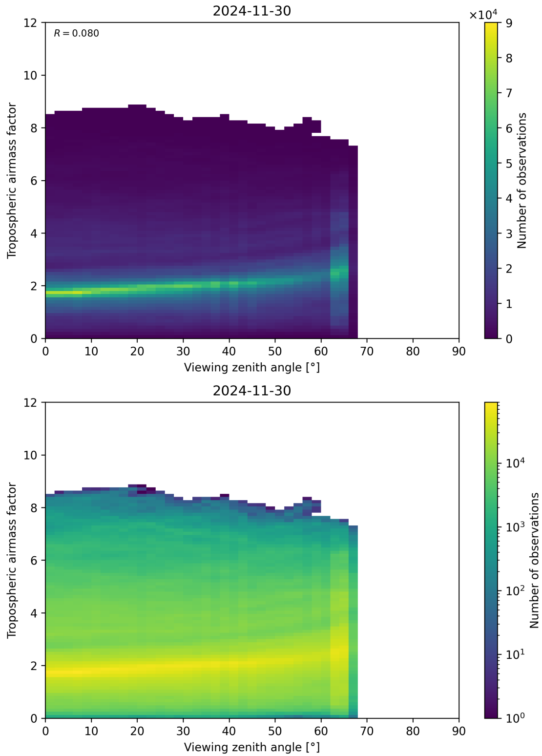
Figure 161: Scatter density plot of “Viewing zenith angle” against “Tropospheric airmass factor” for 2024-11-30 to 2024-12-01.
