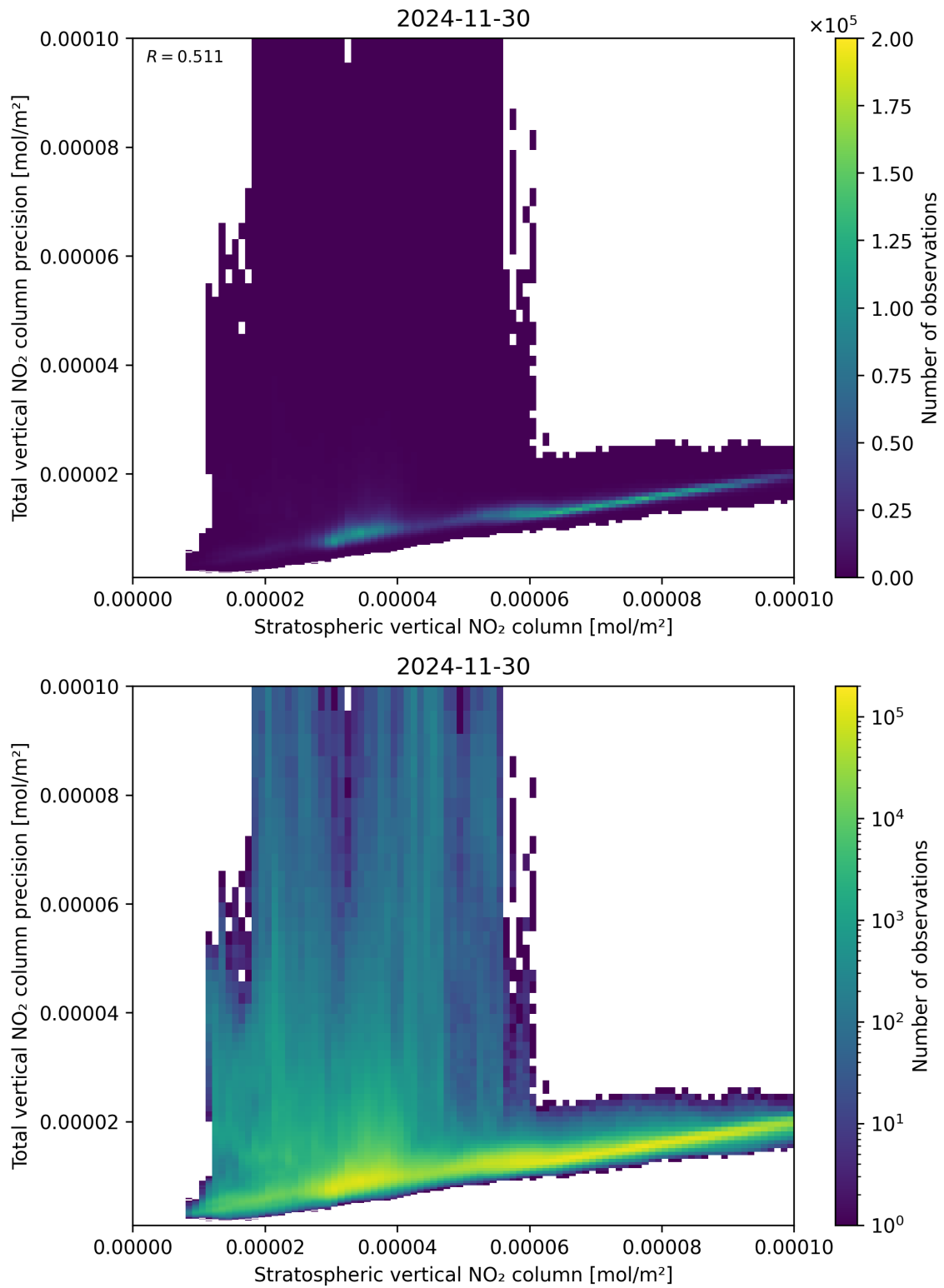
Figure 101: Scatter density plot of “Stratospheric vertical NO 2 column” against “Total vertical NO 2 column precision” for 2024-11-30 to 2024-12-01.
