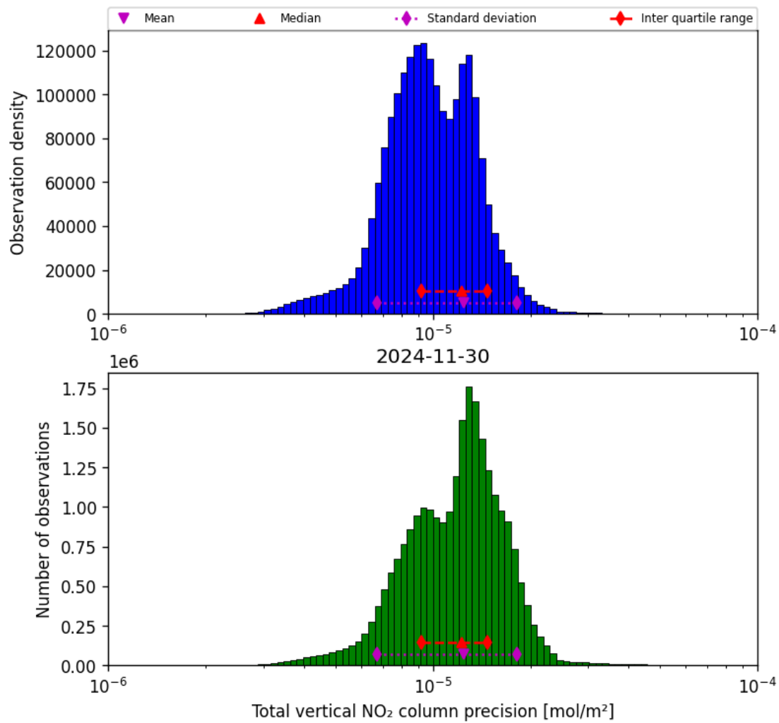
Figure 39: Histogram of “Total vertical NO 2 column precision” for 2024-11-30 to 2024-12-01
