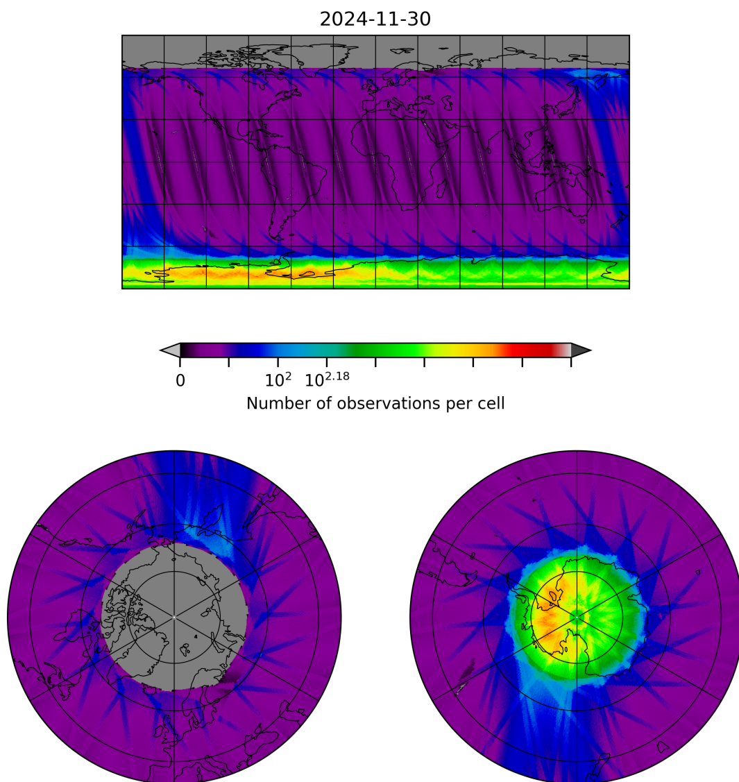
Figure 10: Map of the number of observations for 2024-11-30 to 2024-12-01
