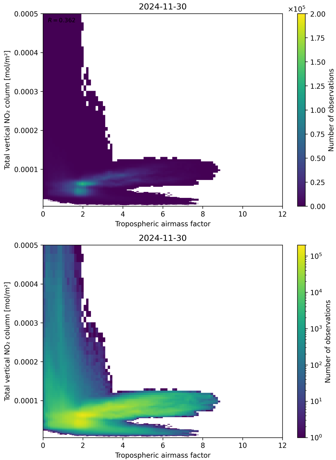
Figure 77: Scatter density plot of “Tropospheric airmass factor” against “Total vertical NO 2 column” for 2024-11-30 to 2024-12-01.
