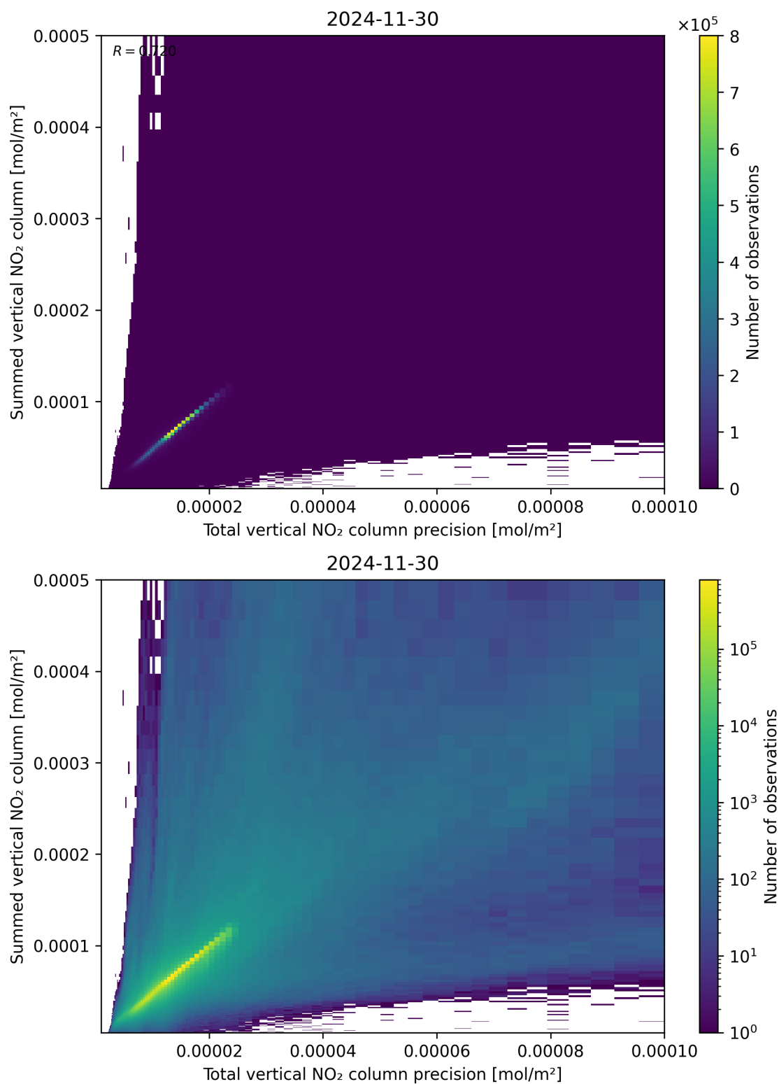
Figure 117: Scatter density plot of “Total vertical NO 2 column precision” against “Summed vertical NO 2 column” for 2024-11-30 to 2024-12-01.
