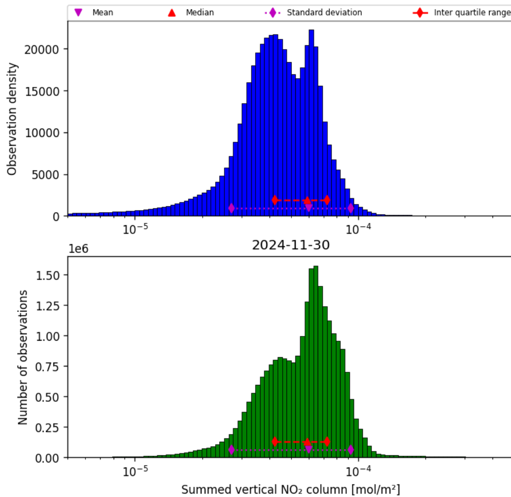
Figure 40: Histogram of “Summed vertical NO 2 column” for 2024-11-30 to 2024-12-01
