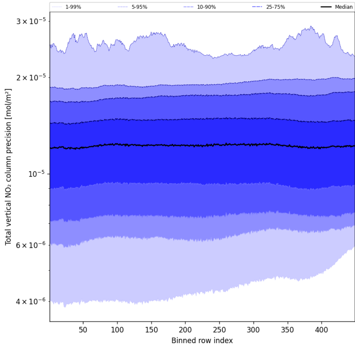
Figure 56: Along track statistics of “Total vertical NO 2 column precision” for 2024-11-30 to 2024-12-01
