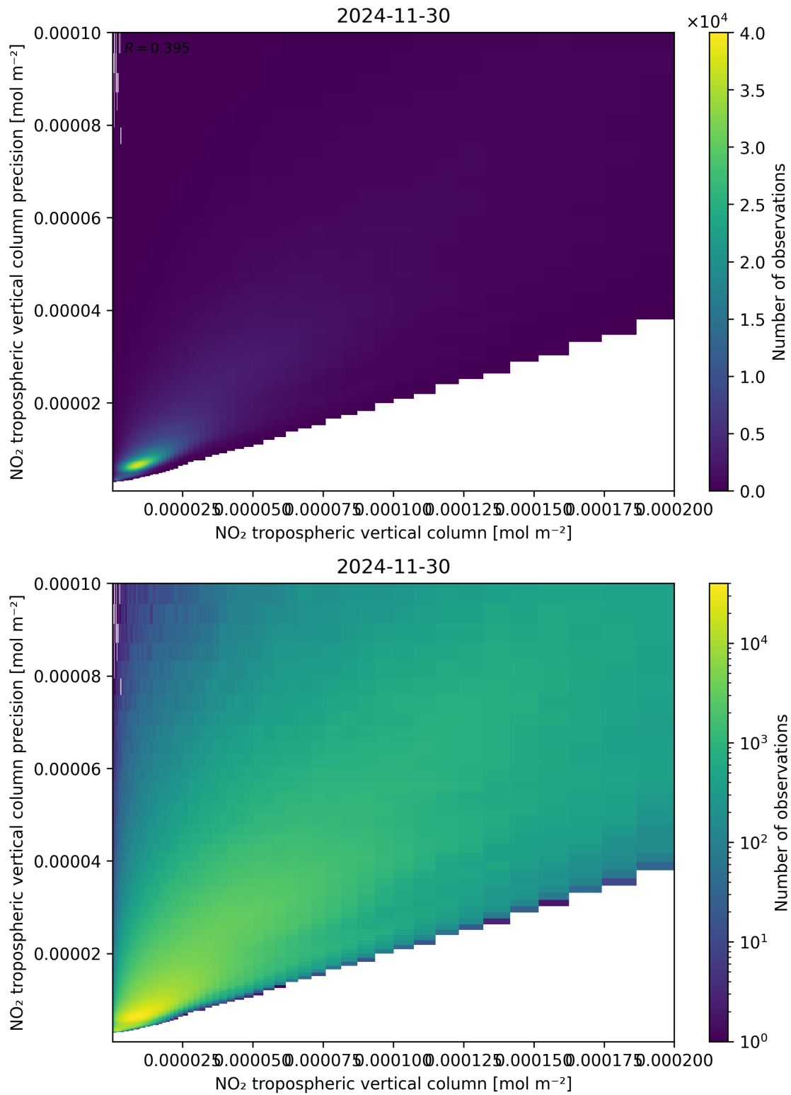
Figure 130: Scatter density plot of “NO 2 tropospheric vertical column” against “NO 2 tropospheric vertical column precision” for 2024-11-30 to 2024-12-01.
