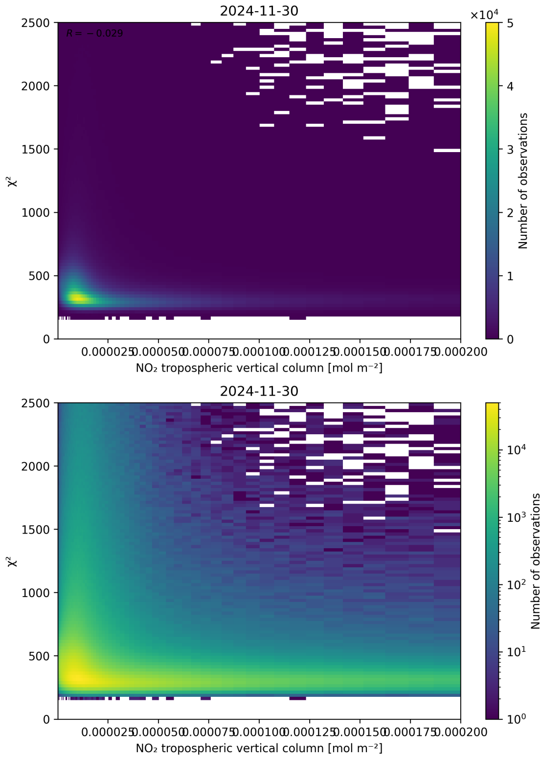
Figure 124: Scatter density plot of “NO 2 tropospheric vertical column” against “ \chi^2 ” for 2024-11-30 to 2024-12-01.
