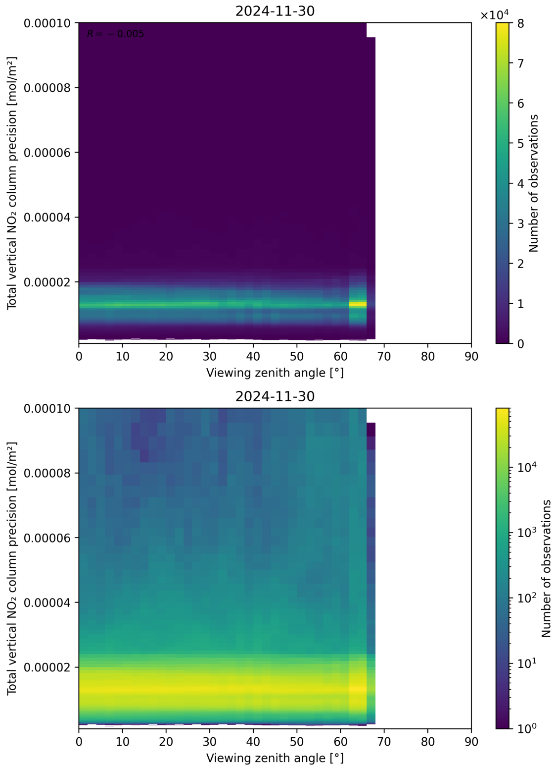
Figure 168: Scatter density plot of “Viewing zenith angle” against “Total vertical NO 2 column precision” for 2024-11-30 to 2024-12-01.
