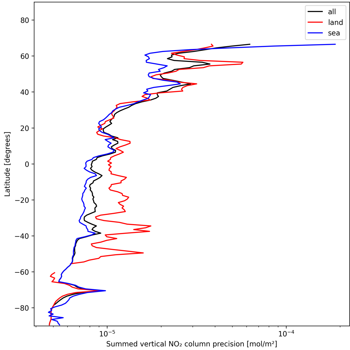
Figure 24: Zonal average of “Summed vertical NO 2 column precision” for 2024-11-30 to 2024-12-01.
