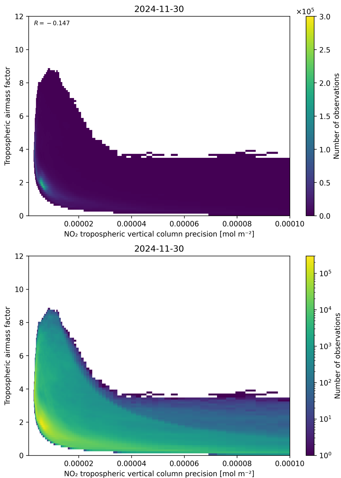
Figure 133: Scatter density plot of “NO 2 tropospheric vertical column precision” against “Tropospheric airmass factor” for 2024-11-30 to 2024-12-01.
