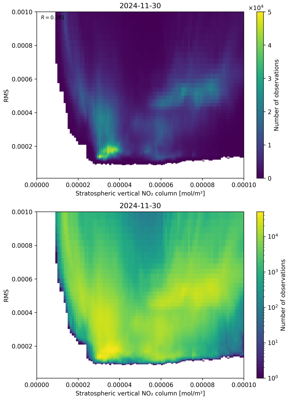
Figure 102: Scatter density plot of “Stratospheric vertical NO 2 column” against “RMS” for 2024-11-30 to 2024-12-01.
