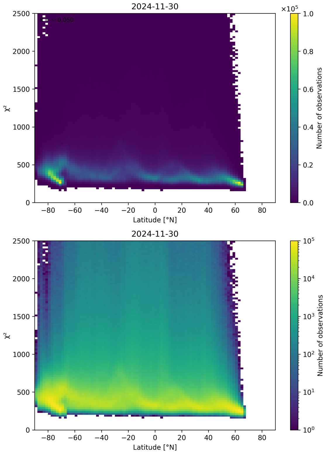
Figure 86: Scatter density plot of “Latitude” against “ \chi^2 ” for 2024-11-30 to 2024-12-01.
