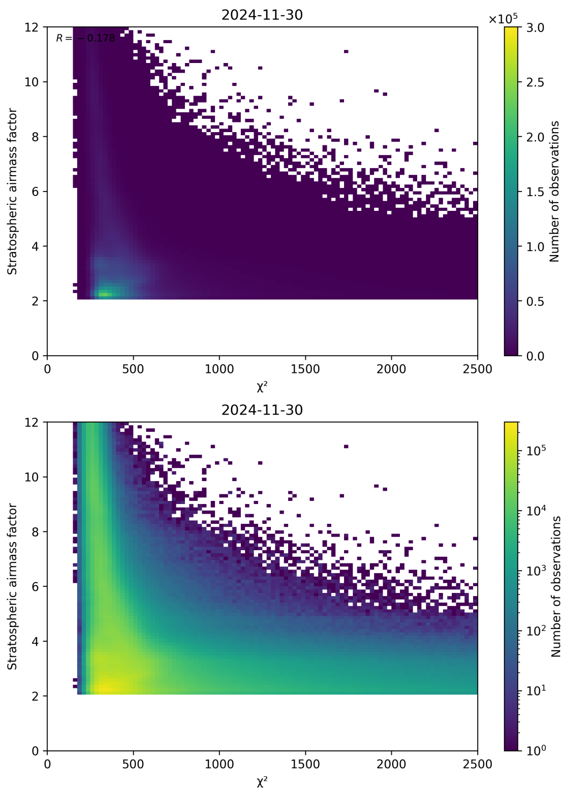
Figure 81: Scatter density plot of “ \chi^2 ” against “Stratospheric airmass factor” for 2024-11-30 to 2024-12-01.
