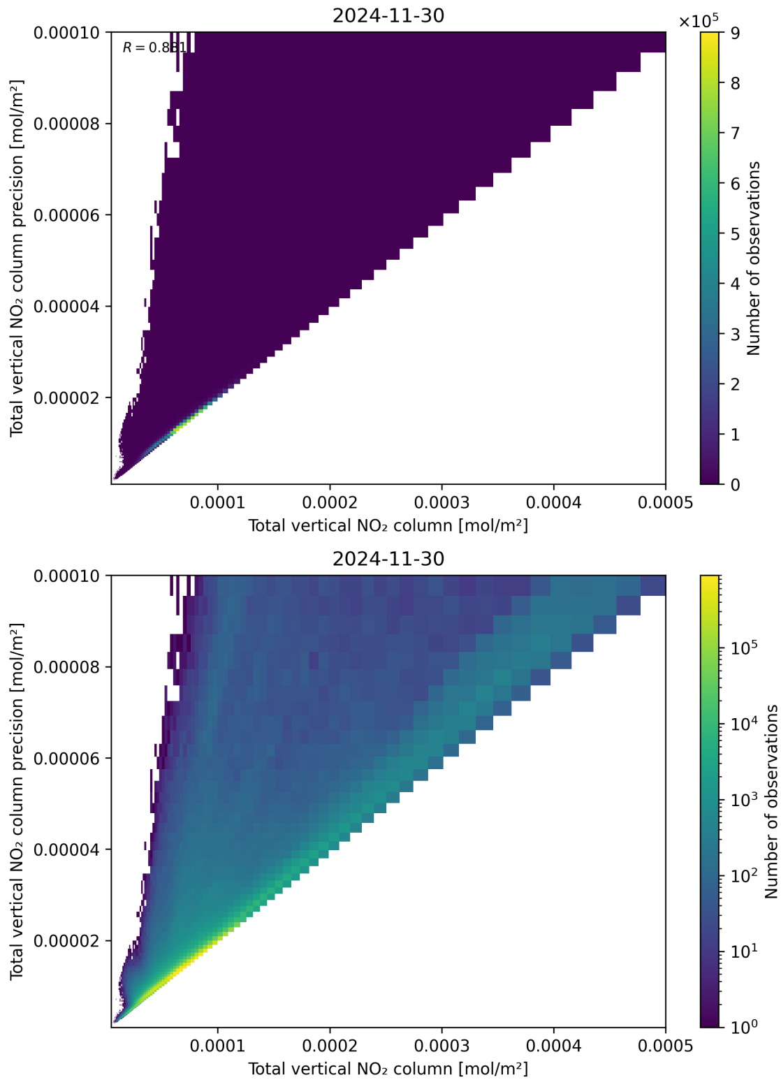
Figure 114: Scatter density plot of “Total vertical NO 2 column” against “Total vertical NO 2 column precision” for 2024-11-30 to 2024-12-01.
