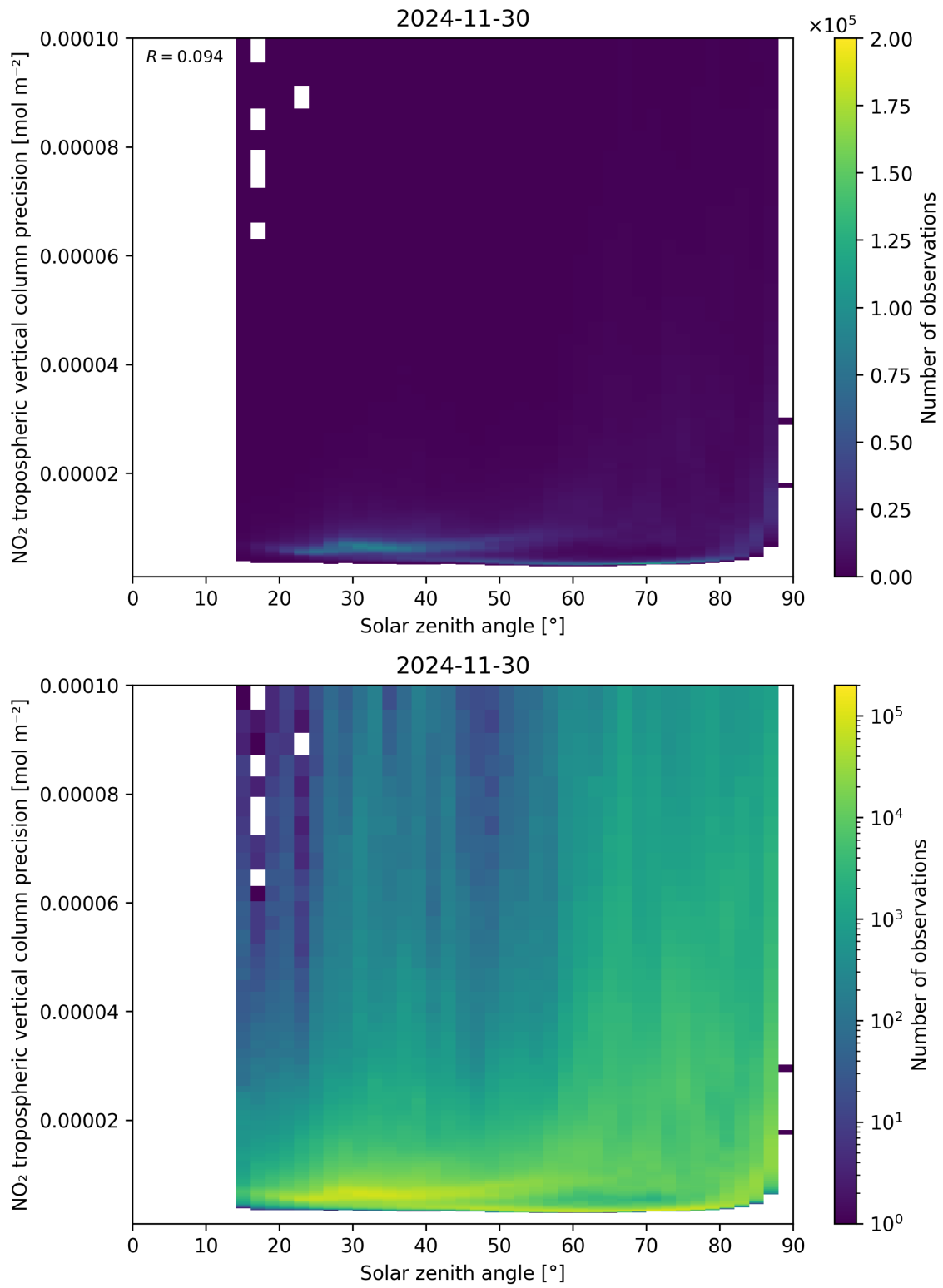
Figure 156: Scatter density plot of “Solar zenith angle” against “NO 2 tropospheric vertical column precision” for 2024-11-30 to 2024-12-01.
