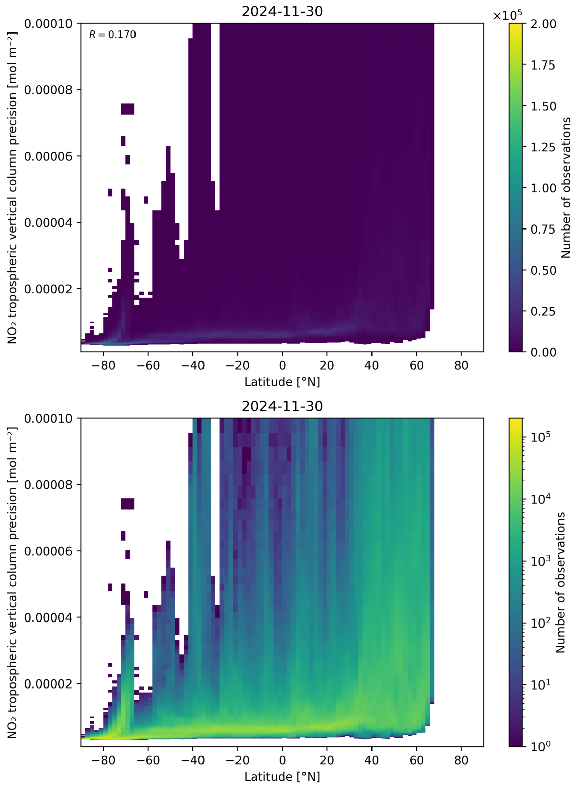
Figure 93: Scatter density plot of “Latitude” against “NO 2 tropospheric vertical column precision” for 2024-11-30 to 2024-12-01.
