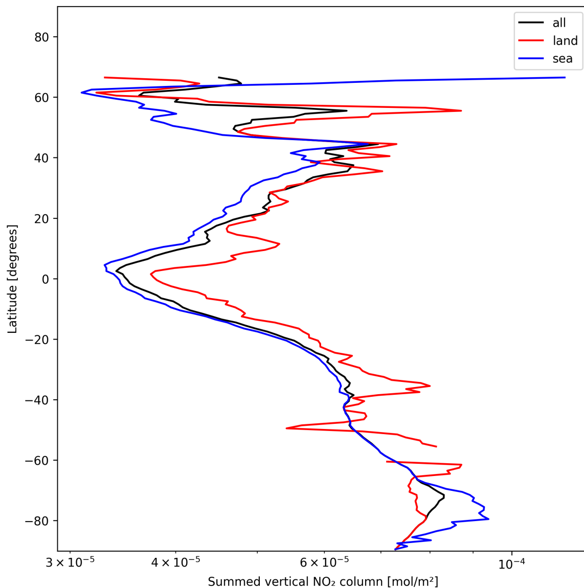
Figure 23: Zonal average of “Summed vertical NO 2 column” for 2024-11-30 to 2024-12-01.
