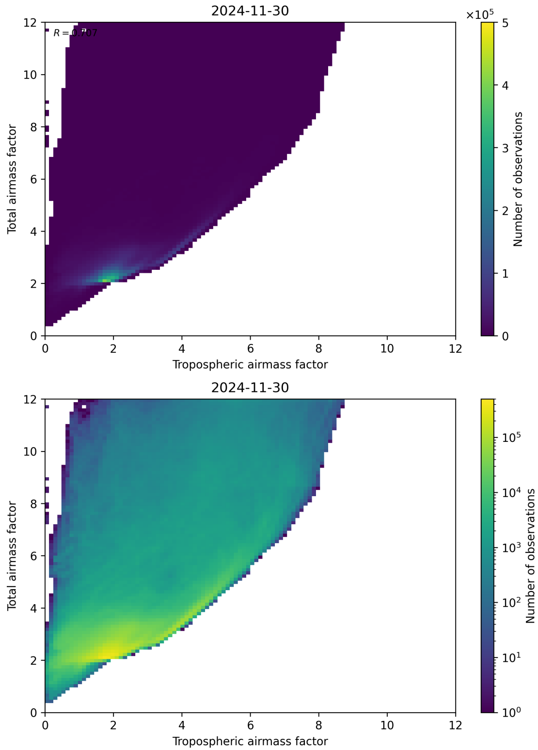
Figure 72: Scatter density plot of “Tropospheric airmass factor” against “Total airmass factor” for 2024-11-30 to 2024-12-01.
