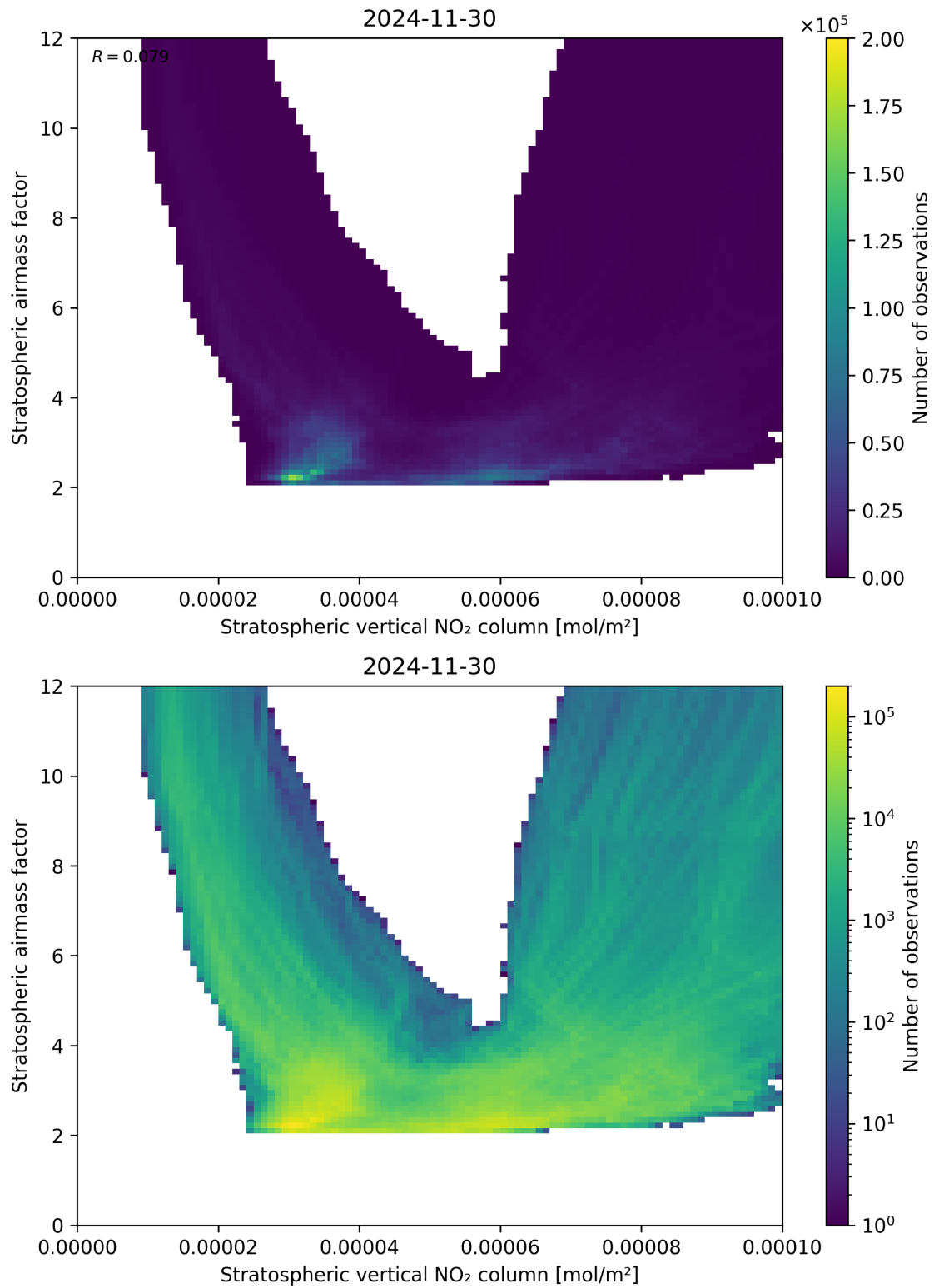
Figure 96: Scatter density plot of “Stratospheric vertical NO 2 column” against “Stratospheric airmass factor” for 2024-11-30 to 2024-12-01.
