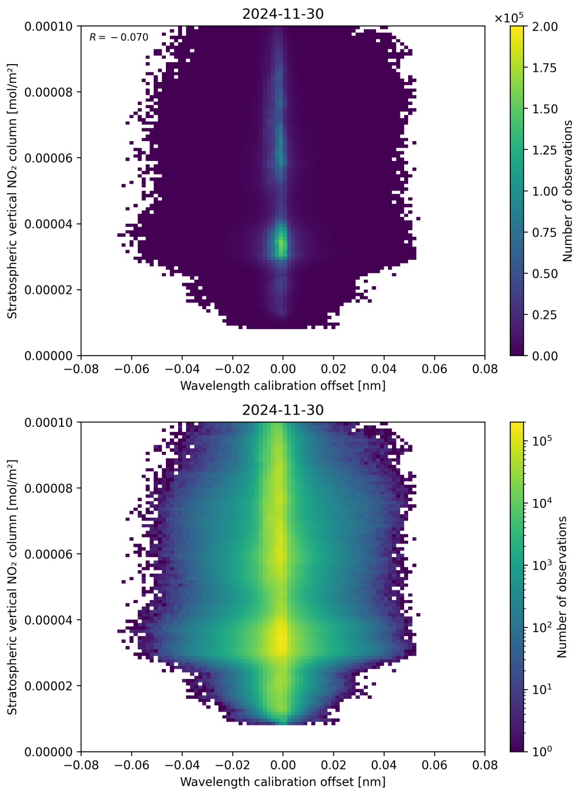
Figure 176: Scatter density plot of “Wavelength calibration offset” against “Stratospheric vertical NO 2 column” for 2024-11-30 to 2024-12-01.
