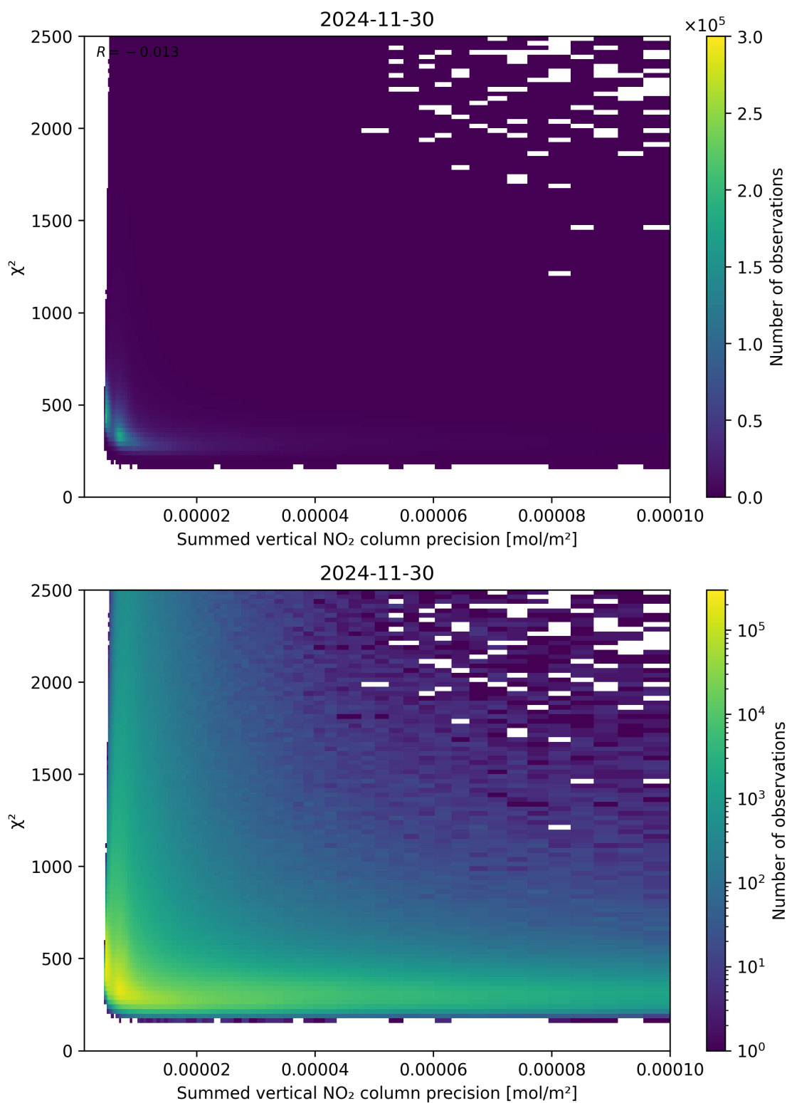
Figure 107: Scatter density plot of “Summed vertical NO 2 column precision” against “ \chi^2 ” for 2024-11-30 to 2024-12-01.
