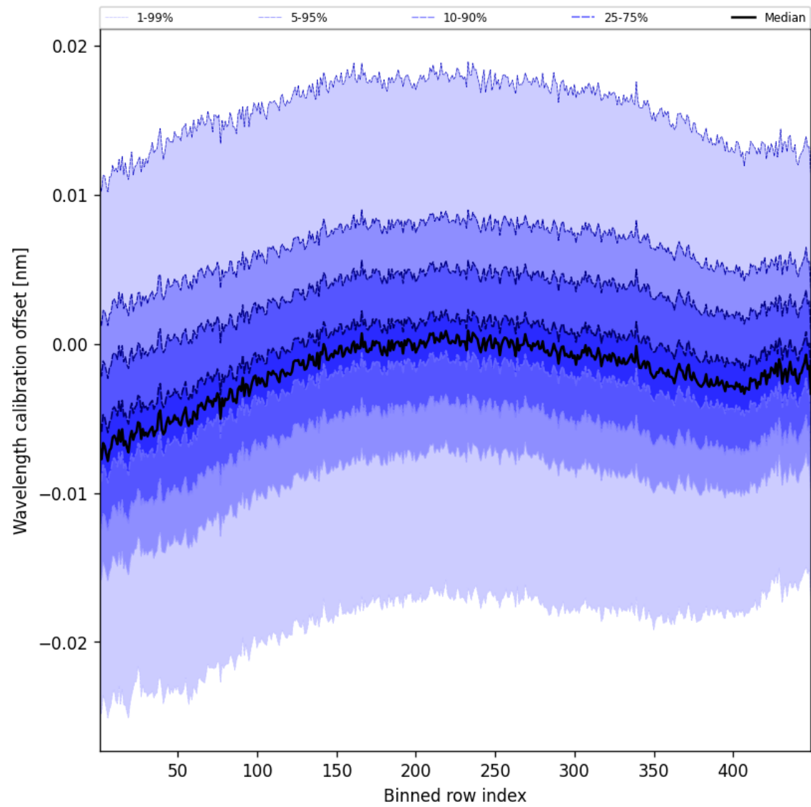
Figure 52: Along track statistics of “Wavelength calibration offset” for 2024-11-30 to 2024-12-01
