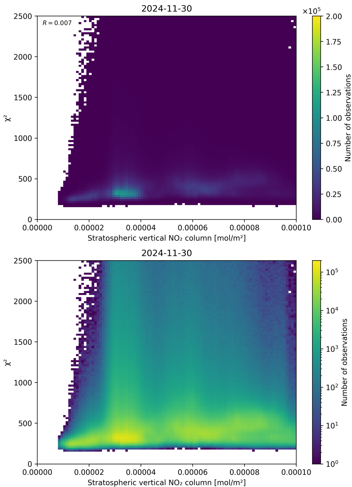
Figure 97: Scatter density plot of “Stratospheric vertical NO 2 column” against “ \chi^2 ” for 2024-11-30 to 2024-12-01.
