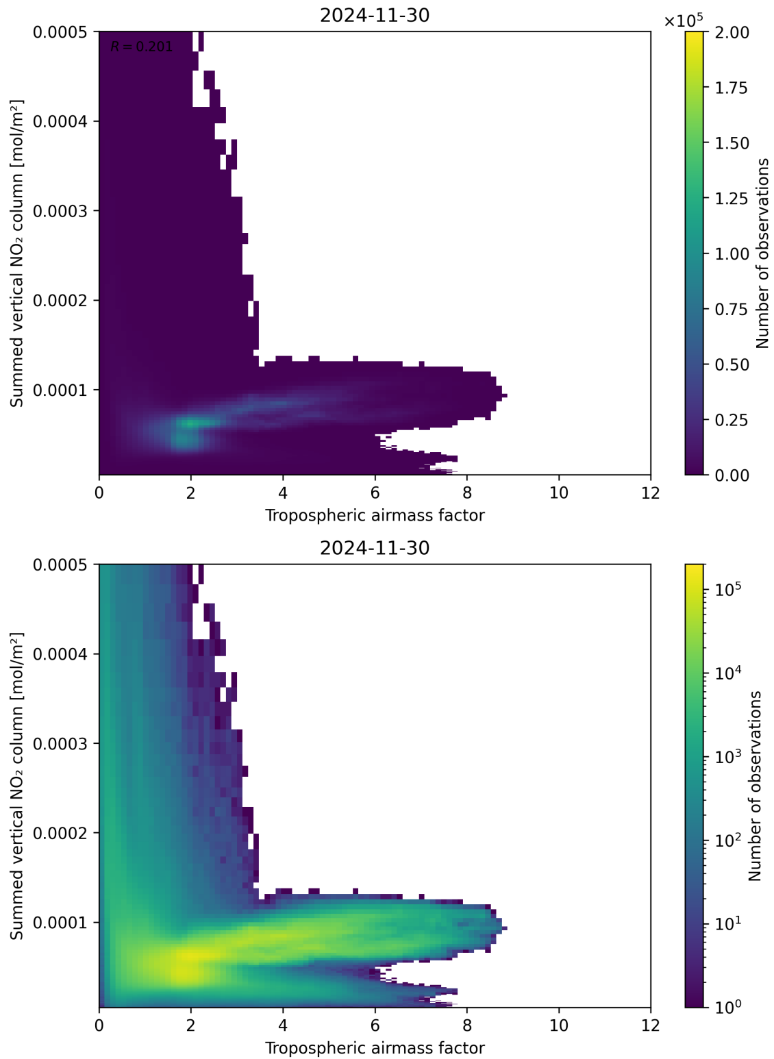
Figure 75: Scatter density plot of “Tropospheric airmass factor” against “Summed vertical NO 2 column” for 2024-11-30 to 2024-12-01.
