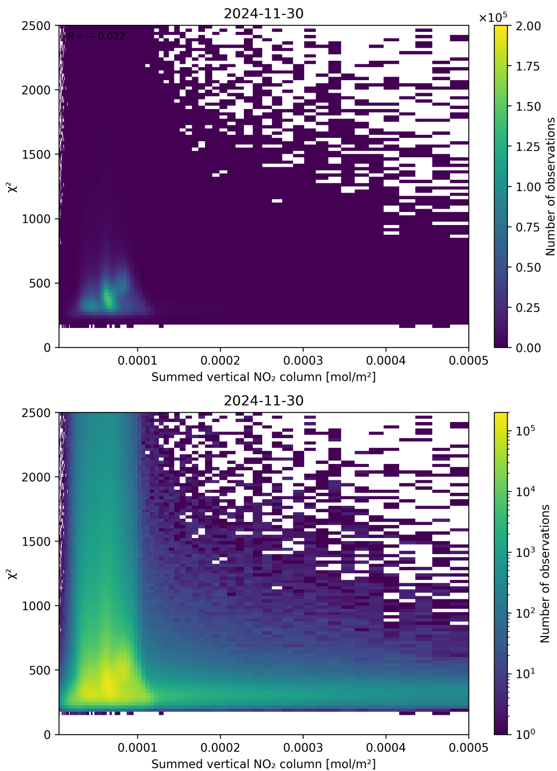
Figure 104: Scatter density plot of “Summed vertical NO 2 column” against “ \chi^2 ” for 2024-11-30 to 2024-12-01.
