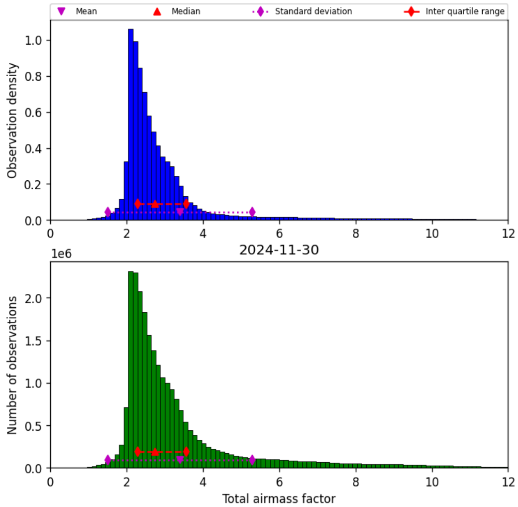
Figure 32: Histogram of “Total airmass factor” for 2024-11-30 to 2024-12-01
