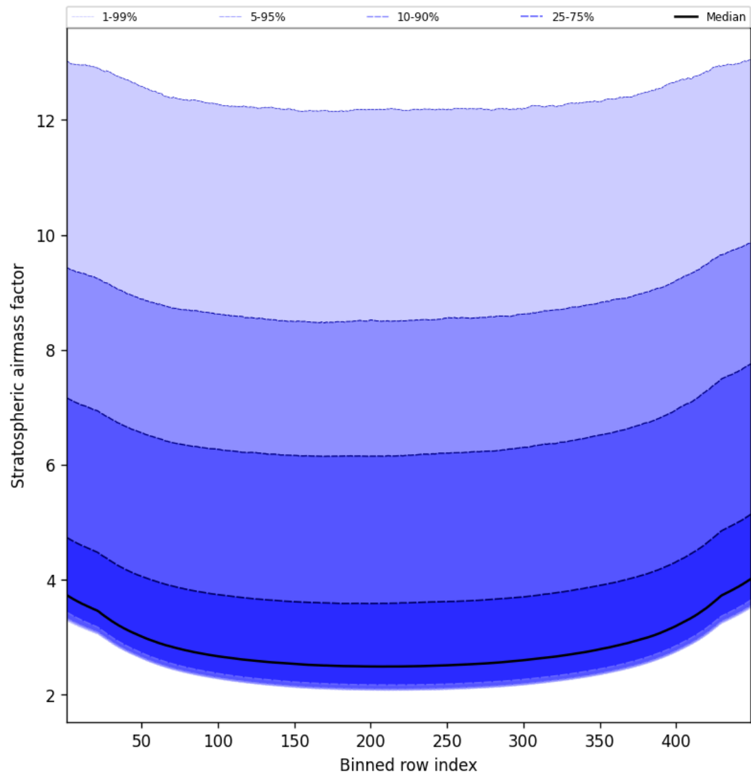
Figure 61: Along track statistics of “Stratospheric air mass factor” for 2024-11-30 to 2024-12-01
