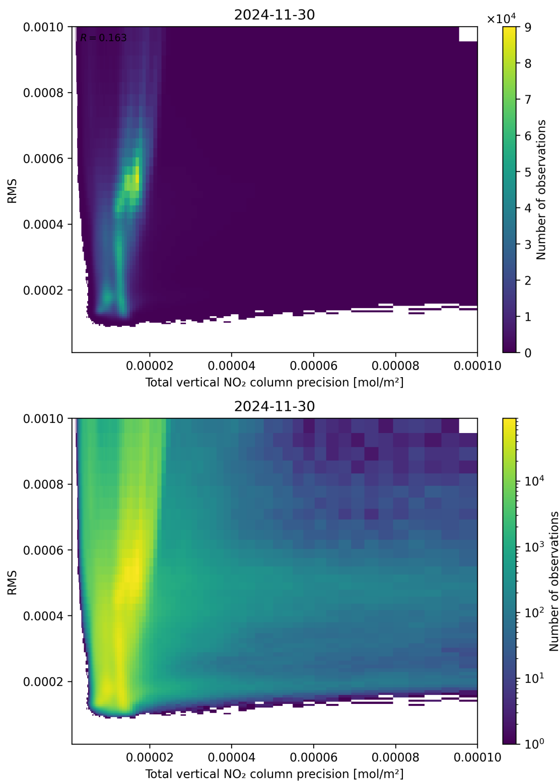
Figure 119: Scatter density plot of “Total vertical NO 2 column precision” against “RMS” for 2024-11-30 to 2024-12-01.
