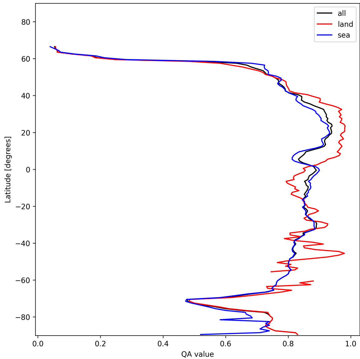
Figure 11: Zonal average of “QA value” for 2024-11-30 to 2024-12-01.
