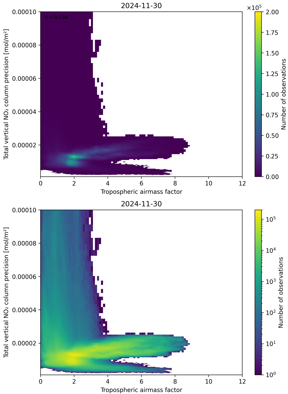
Figure 78: Scatter density plot of “Tropospheric air mass factor” against “Total vertical NO 2 column precision” for 2024-11-30 to 2024-12-01.
