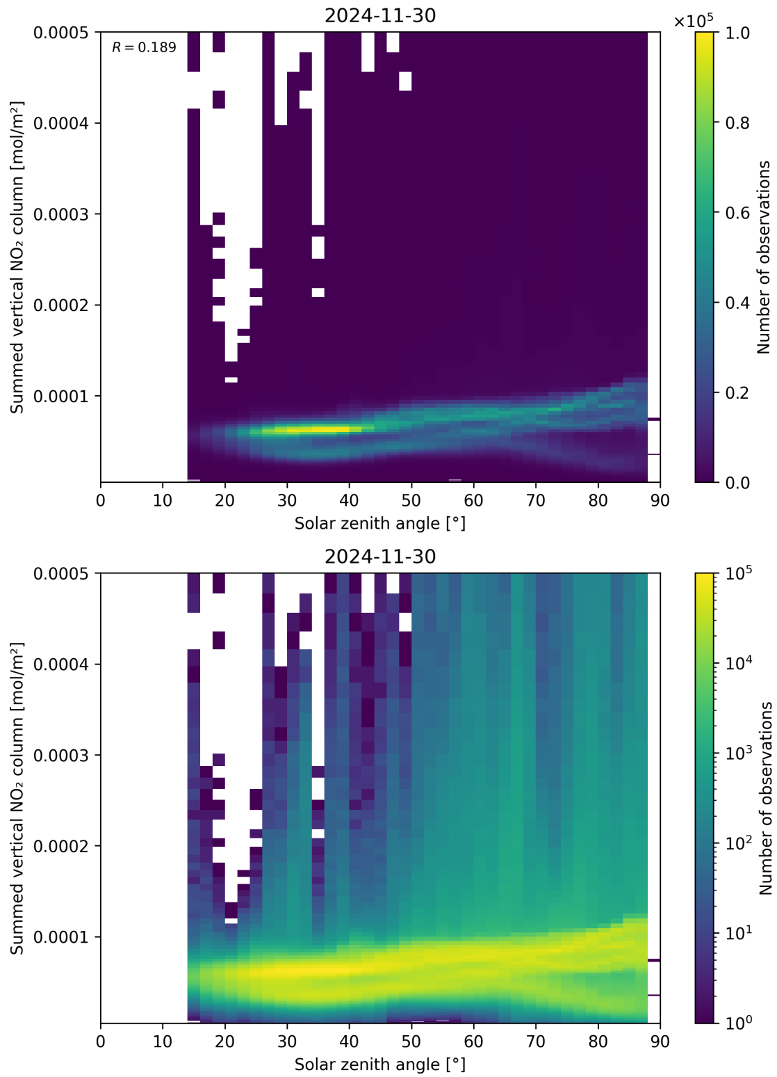
Figure 151: Scatter density plot of “Solar zenith angle” against “Summed vertical NO 2 column” for 2024-11-30 to 2024-12-01.
