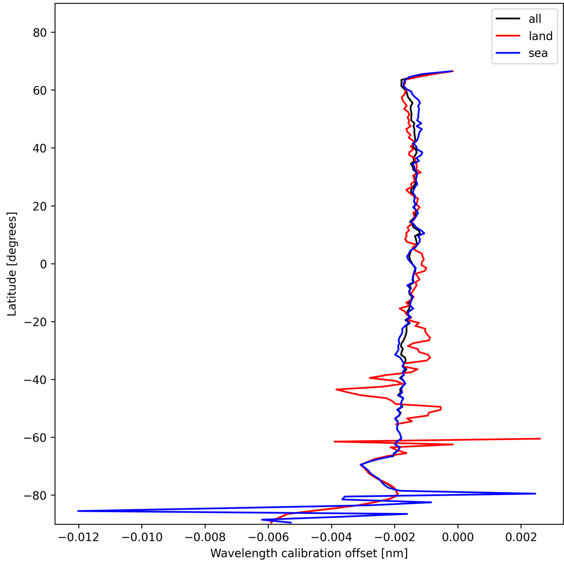
Figure 18: Zonal average of “Wavelength calibration offset” for 2024-11-30 to 2024-12-01.
