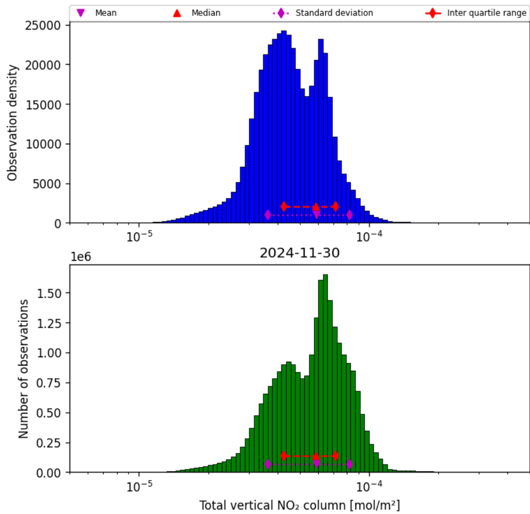
Figure 38: Histogram of “Total vertical NO 2 column” for 2024-11-30 to 2024-12-01
