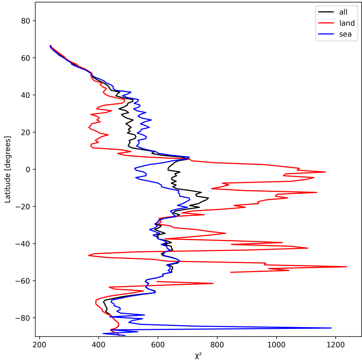
Figure 25: Zonal average of “ \chi^2 ” for 2024-11-30 to 2024-12-01.
