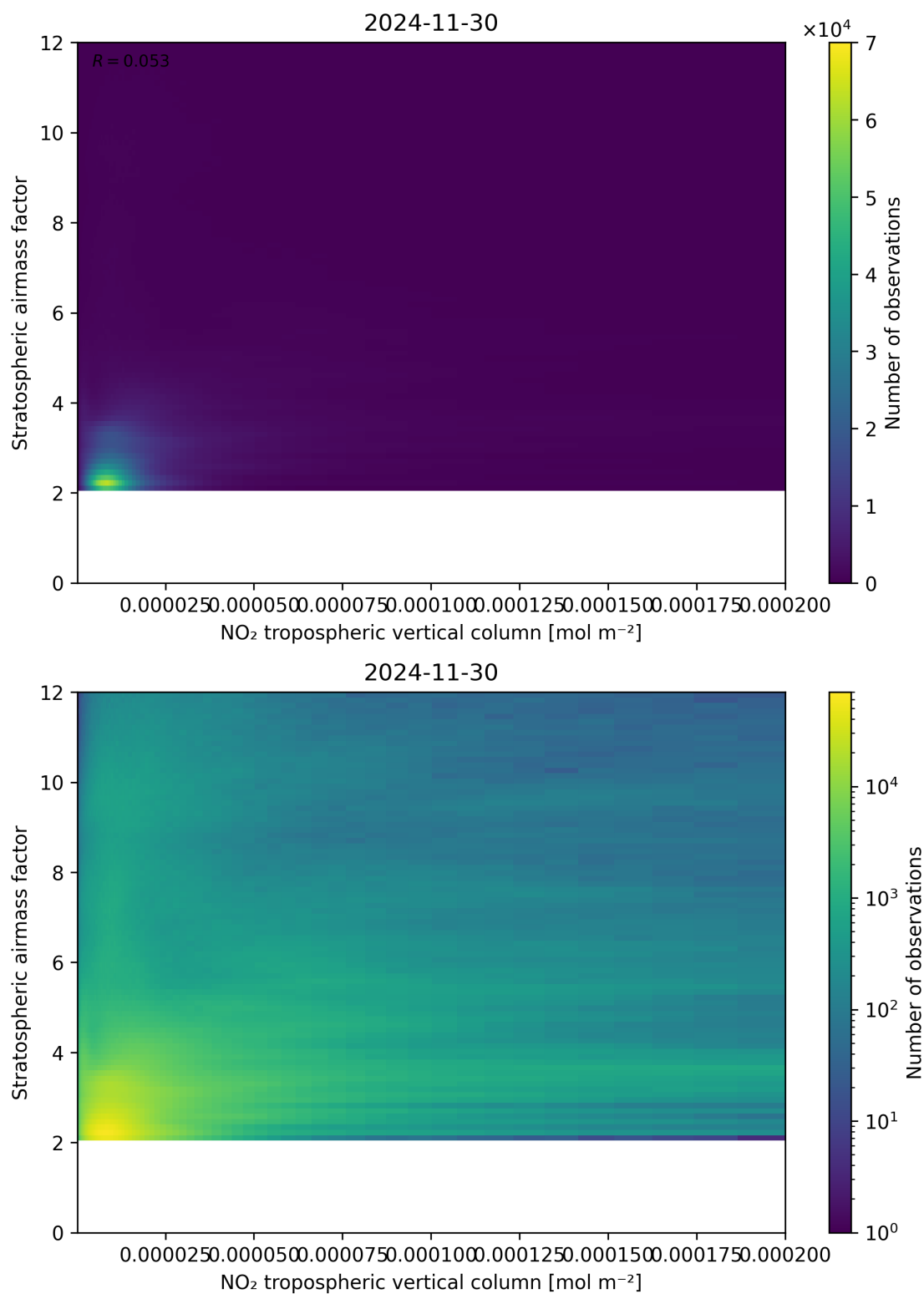
Figure 121: Scatter density plot of “NO 2 tropospheric vertical column” against “Stratospheric airmass factor” for 2024-11-30 to 2024-12-01.
