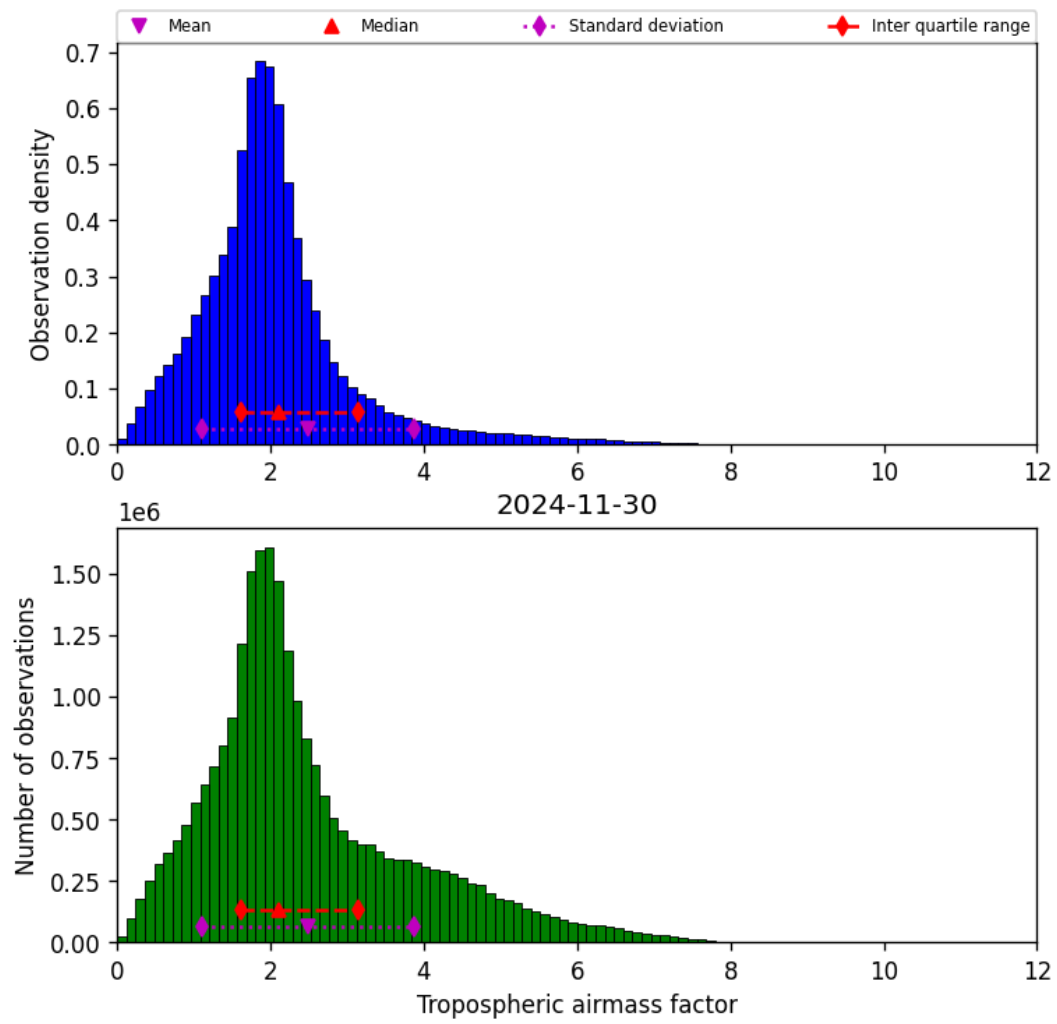
Figure 31: Histogram of “Tropospheric airmass factor” for 2024-11-30 to 2024-12-01
