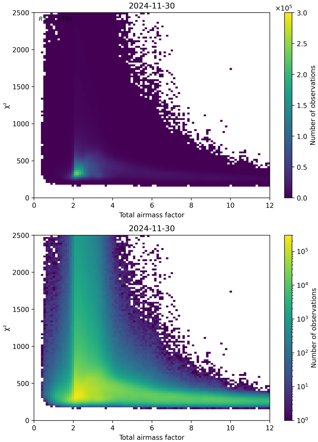
Figure 63: Scatter density plot of “Total airmass factor” against “ \chi^2 ” for 2024-11-30 to 2024-12-01.
