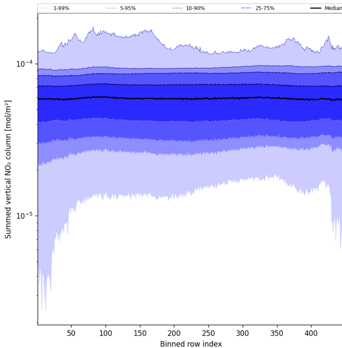
Figure 57: Along track statistics of “Summed vertical NO 2 column” for 2024-11-30 to 2024-12-01
