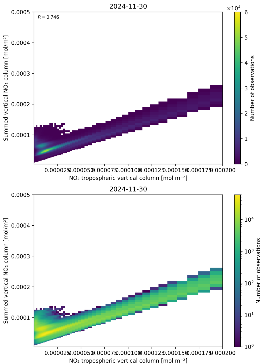
Figure 126: Scatter density plot of “NO 2 tropospheric vertical column” against “Summed vertical NO 2 column” for 2024-11-30 to 2024-12-01.
