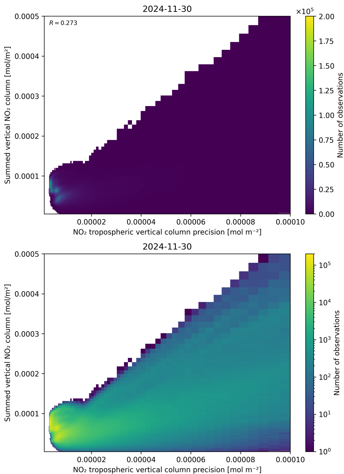
Figure 136: Scatter density plot of “NO 2 tropospheric vertical column precision” against “Summed vertical NO 2 column” for 2024-11-30 to 2024-12-01.
