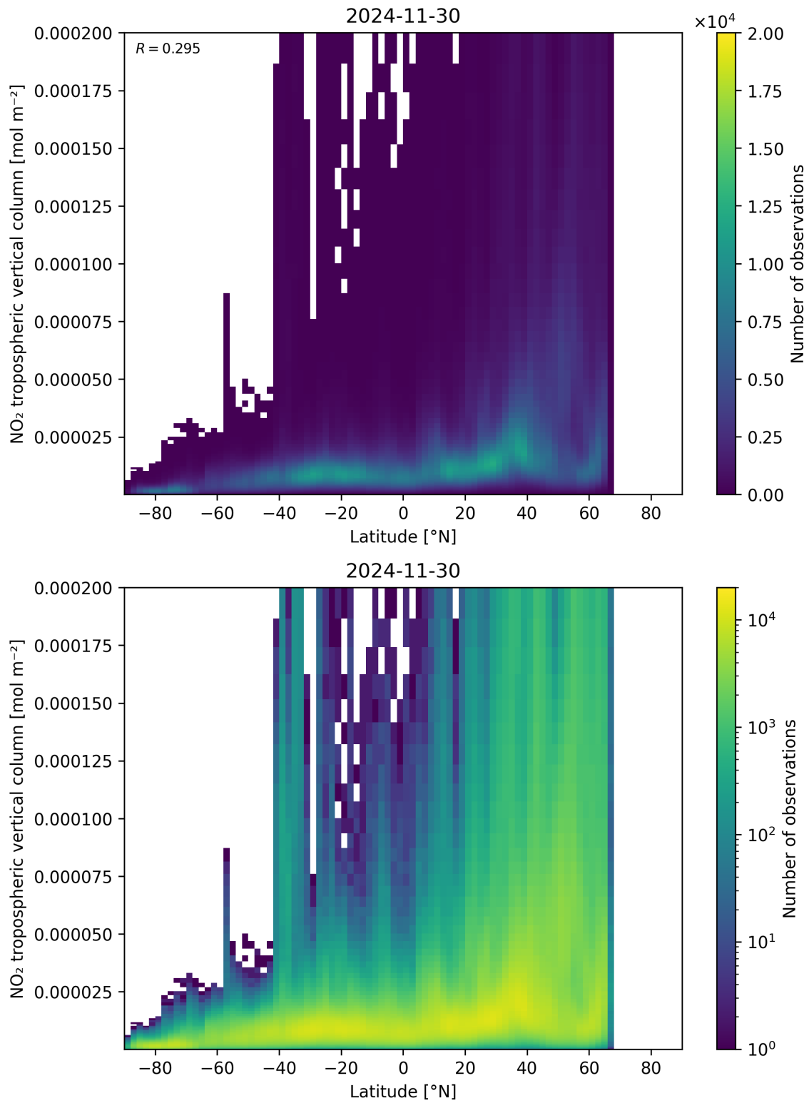
Figure 92: Scatter density plot of “Latitude” against “NO 2 tropospheric vertical column” for 2024-11-30 to 2024-12-01.
