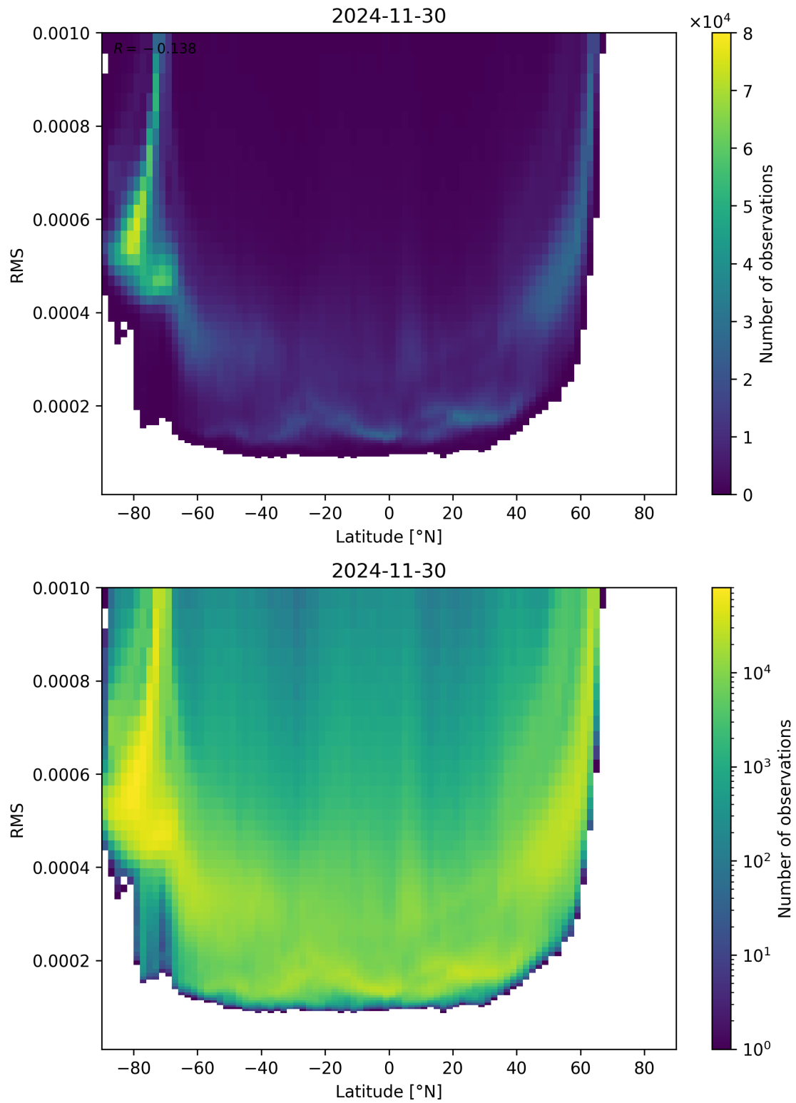
Figure 94: Scatter density plot of “Latitude” against “RMS” for 2024-11-30 to 2024-12-01.
