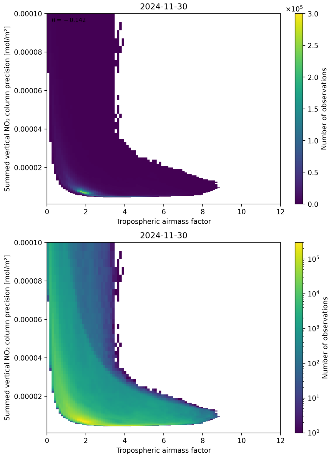
Figure 76: Scatter density plot of “Tropospheric air mass factor” against “Summed vertical NO 2 column precision” for 2024-11-30 to 2024-12-01.
