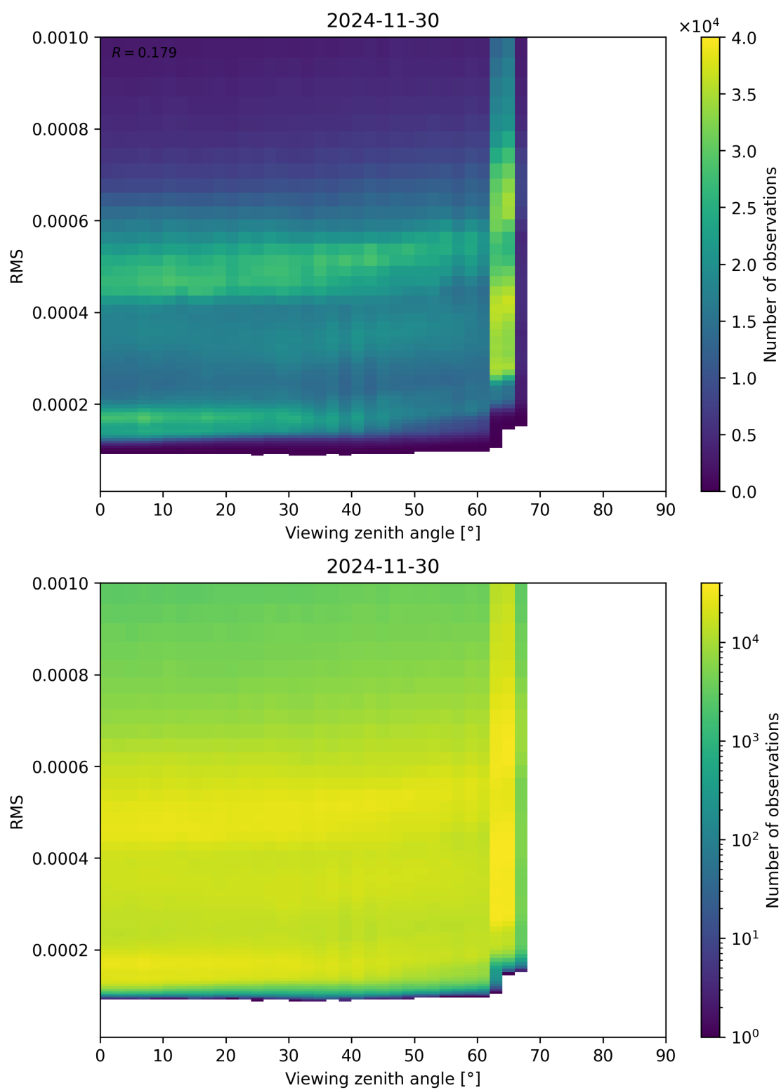
Figure 171: Scatter density plot of “Viewing zenith angle” against “RMS” for 2024-11-30 to 2024-12-01.
