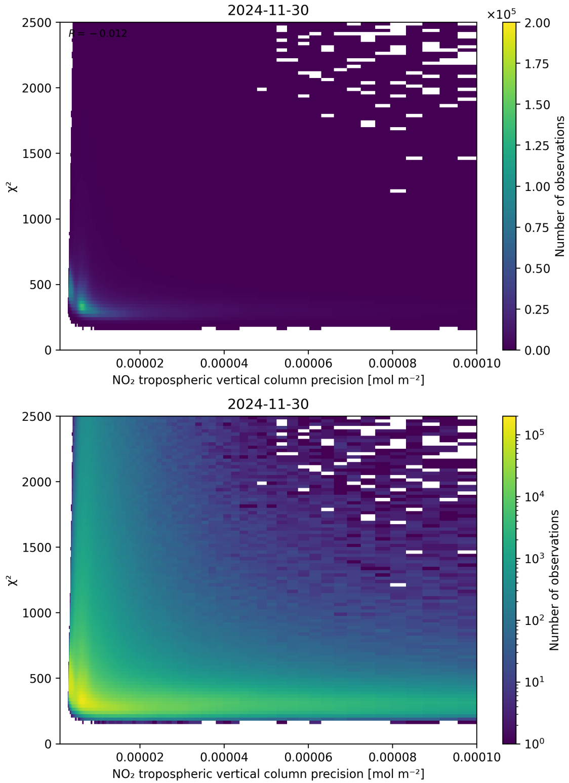
Figure 134: Scatter density plot of “NO 2 tropospheric vertical column precision” against “ \chi^2 ” for 2024-11-30 to 2024-12-01.
