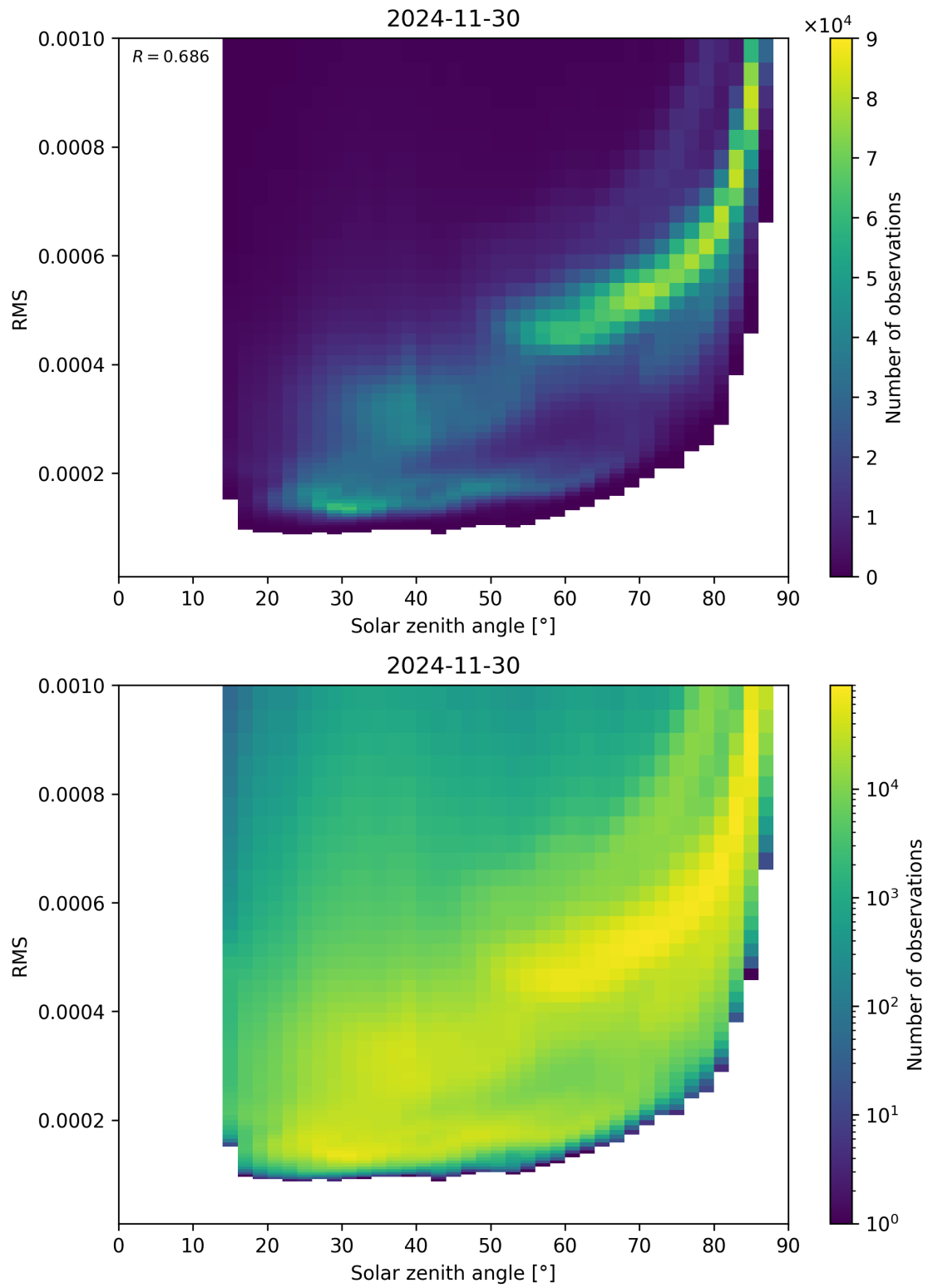
Figure 157: Scatter density plot of “Solar zenith angle” against “RMS” for 2024-11-30 to 2024-12-01.
