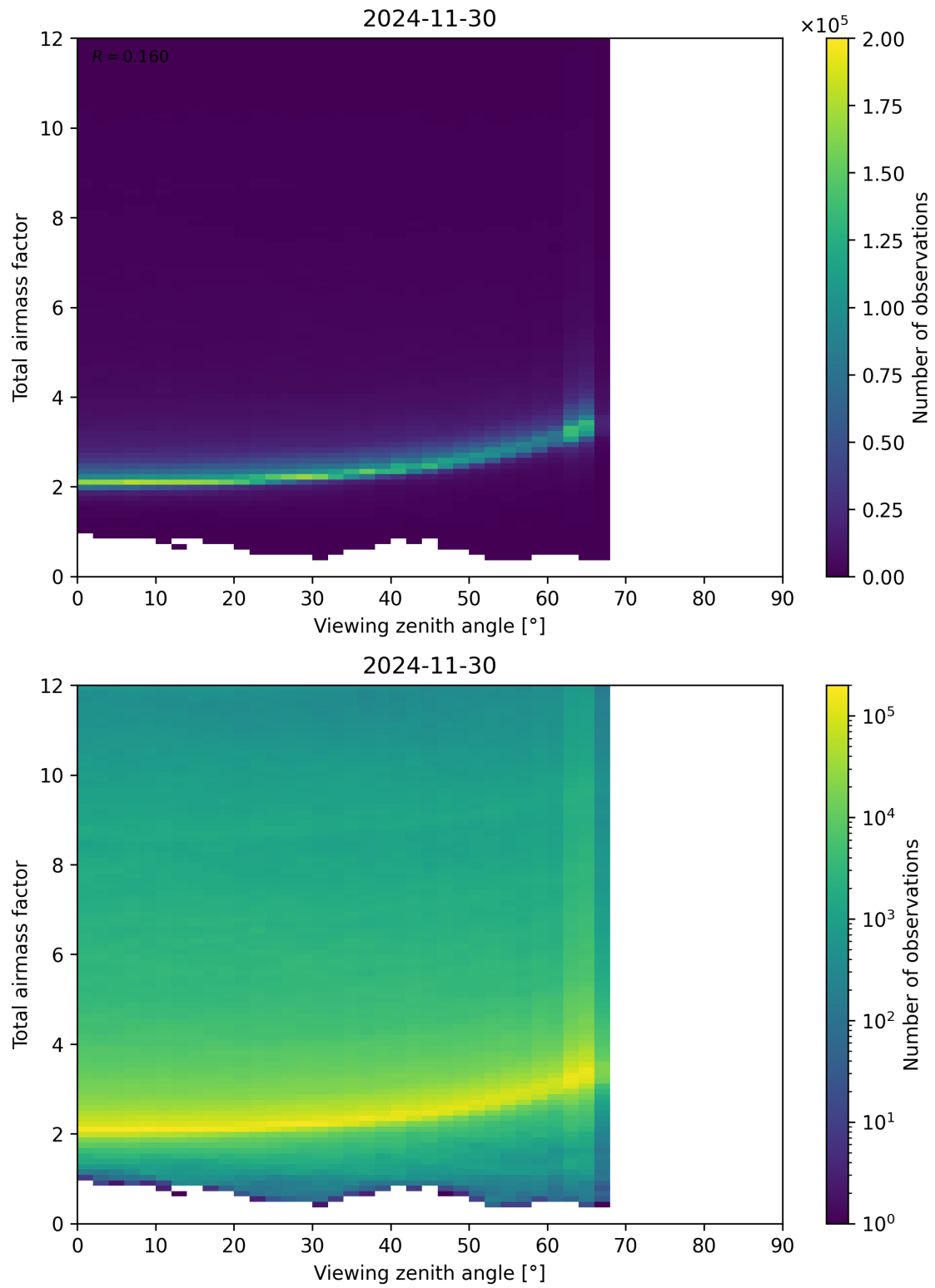
Figure 160: Scatter density plot of “Viewing zenith angle” against “Total airmass factor” for 2024-11-30 to 2024-12-01.
