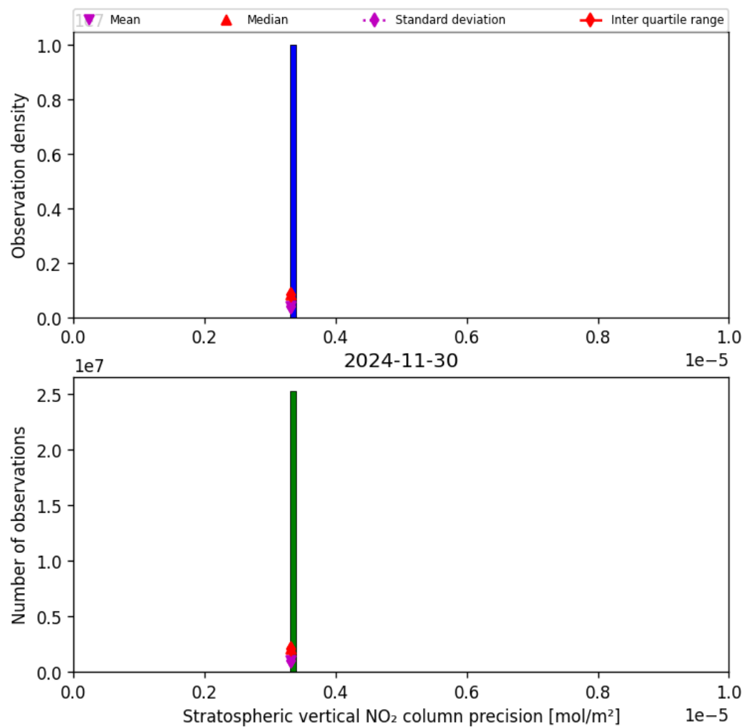
Figure 37: Histogram of “Stratospheric vertical NO 2 column precision” for 2024-11-30 to 2024-12-01
