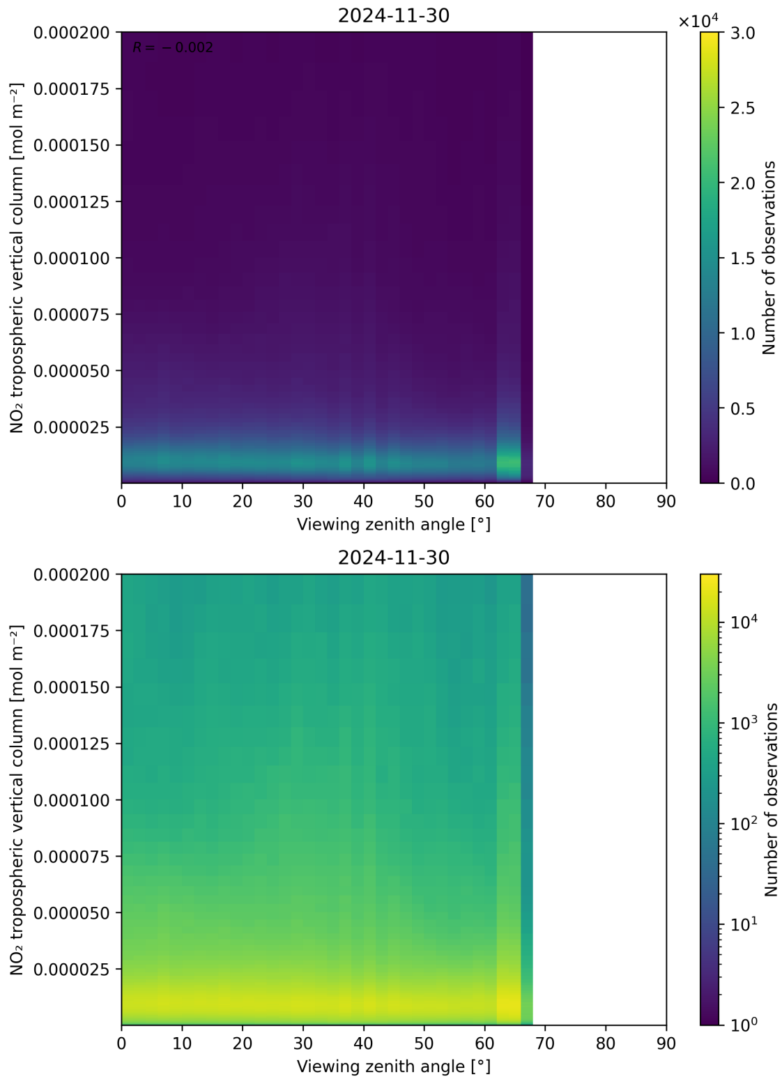
Figure 169: Scatter density plot of “Viewing zenith angle” against “NO 2 tropospheric vertical column” for 2024-11-30 to 2024-12-01.
