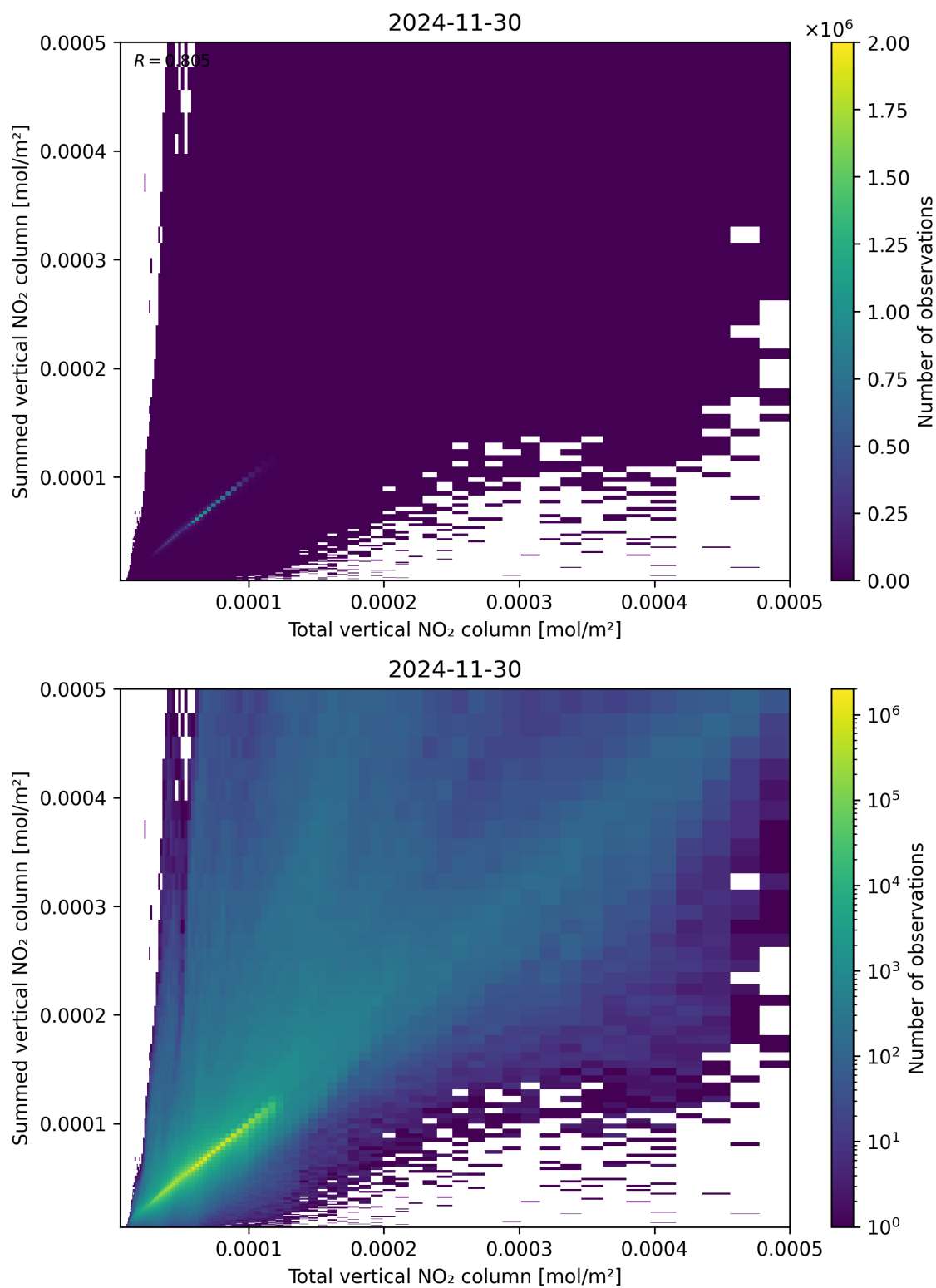
Figure 112: Scatter density plot of “Total vertical NO 2 column” against “Summed vertical NO 2 column” for 2024-11-30 to 2024-12-01.
