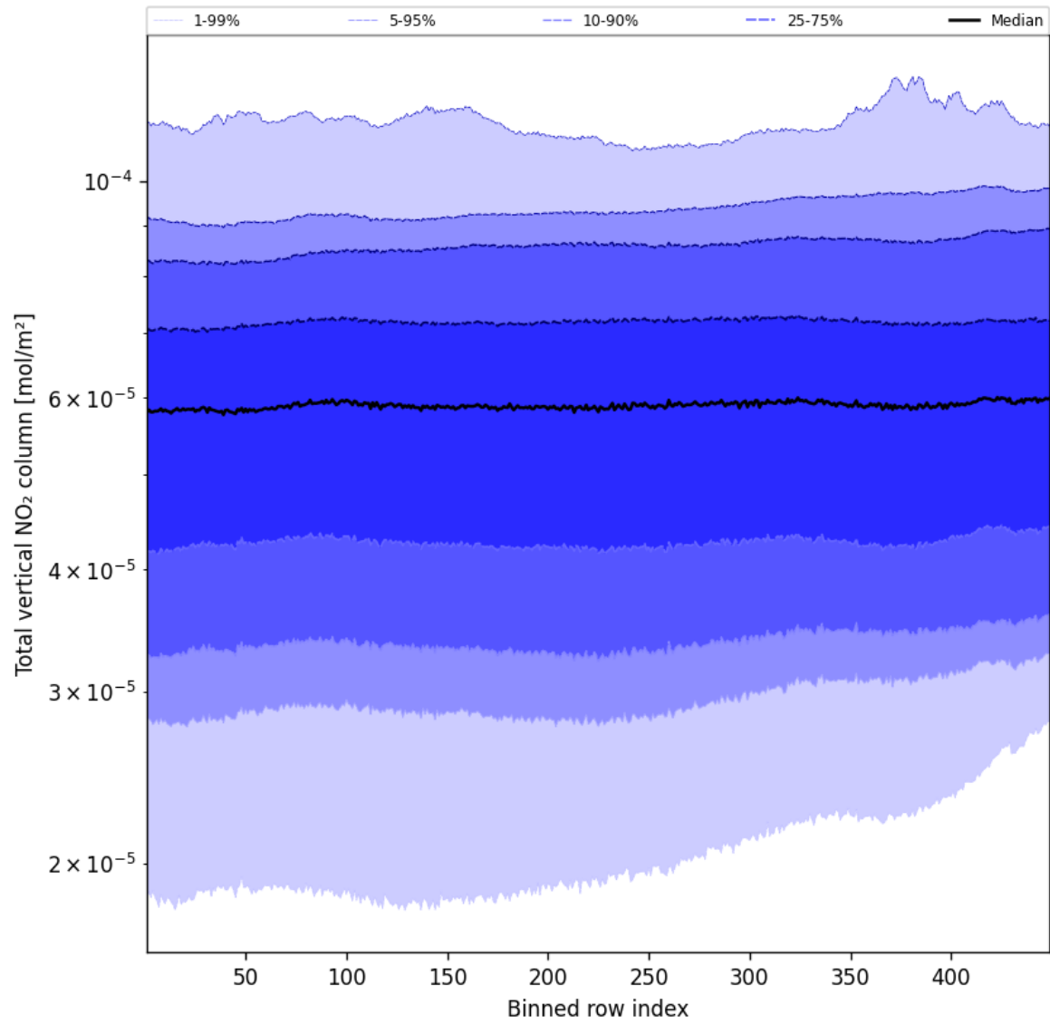
Figure 55: Along track statistics of “Total vertical NO 2 column” for 2024-11-30 to 2024-12-01
