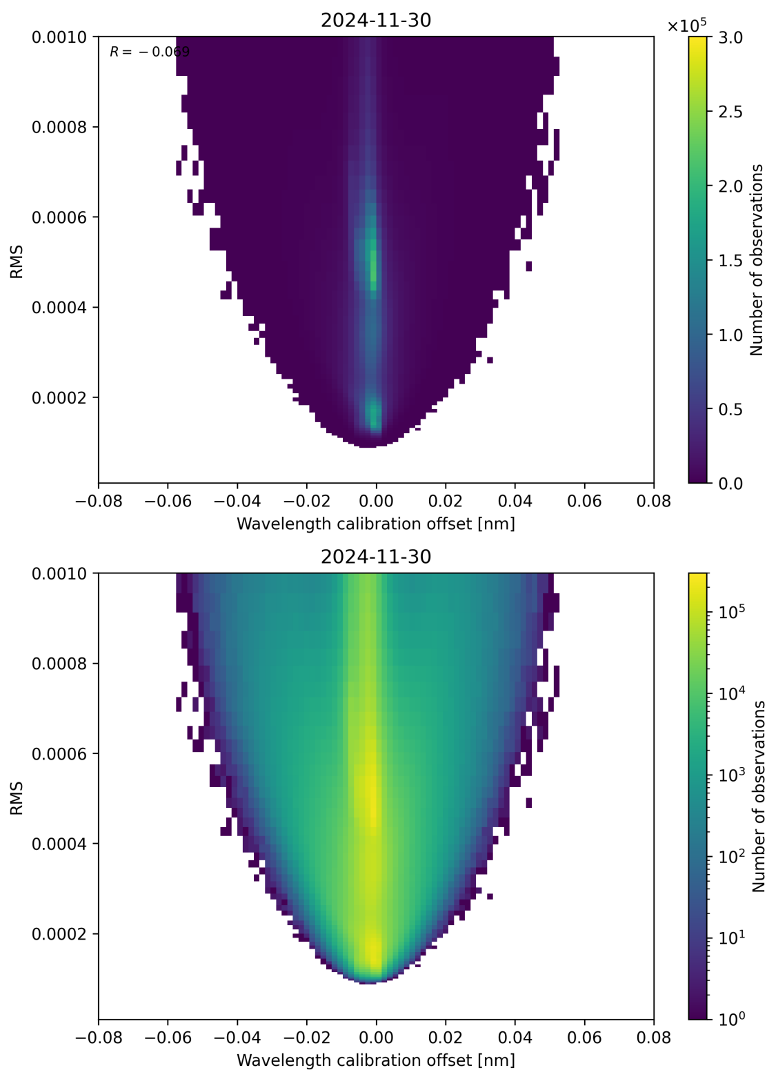
Figure 181: Scatter density plot of “Wavelength calibration offset” against “RMS” for 2024-11-30 to 2024-12-01.
