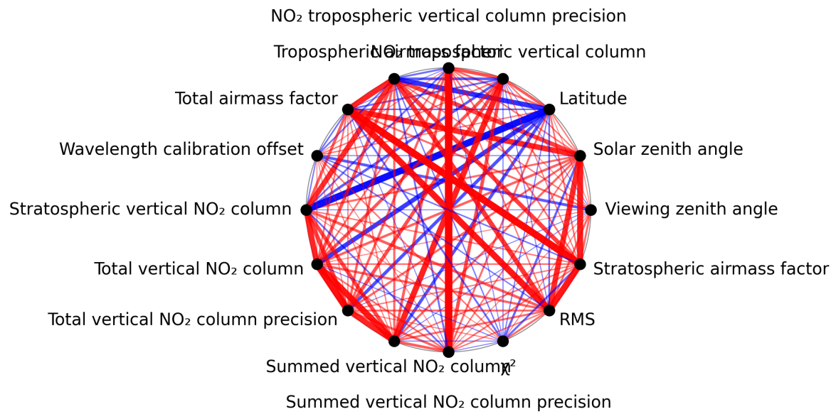
Figure 1: Map of correlation graph for 2024-11-30 to 2024-12-01.
