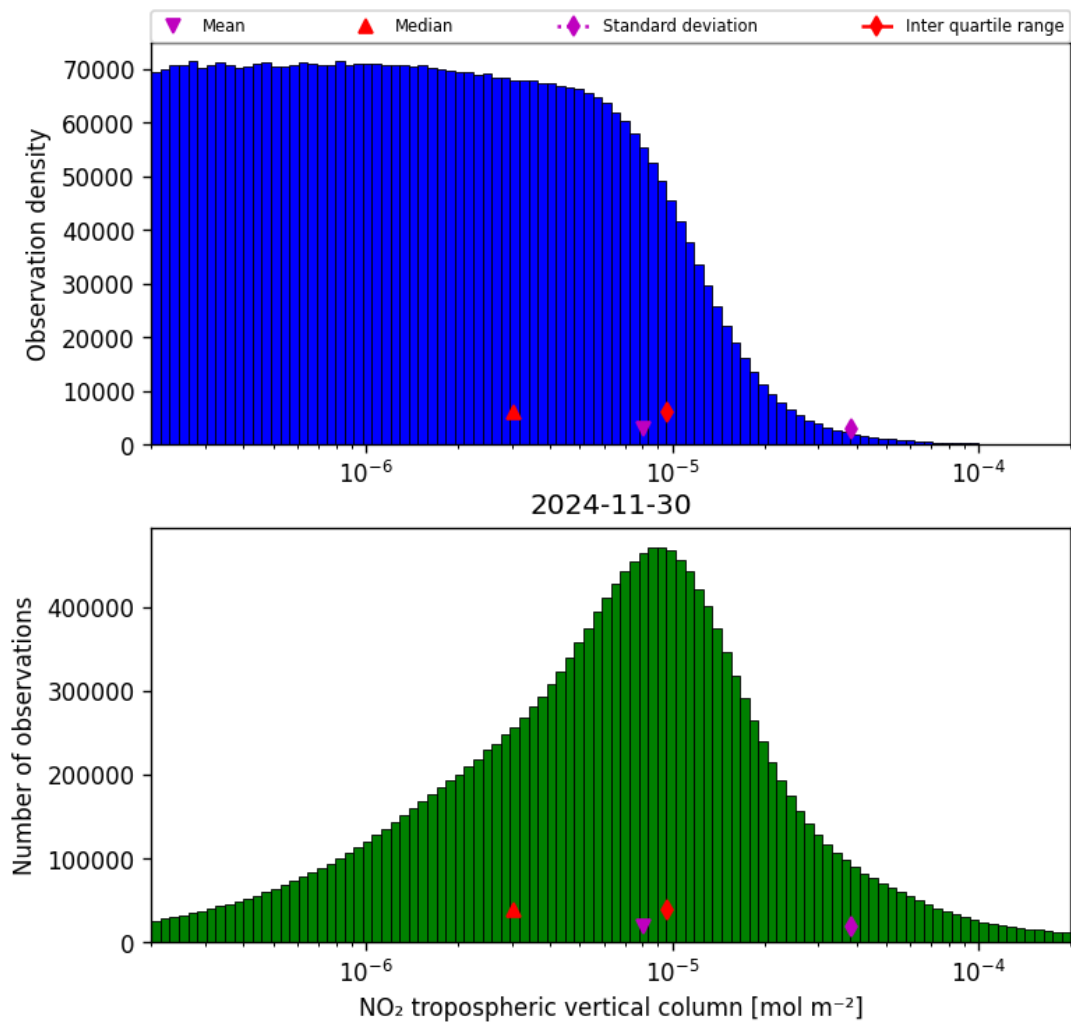
Figure 29: Histogram of “NO 2 tropospheric vertical column” for 2024-11-30 to 2024-12-01
