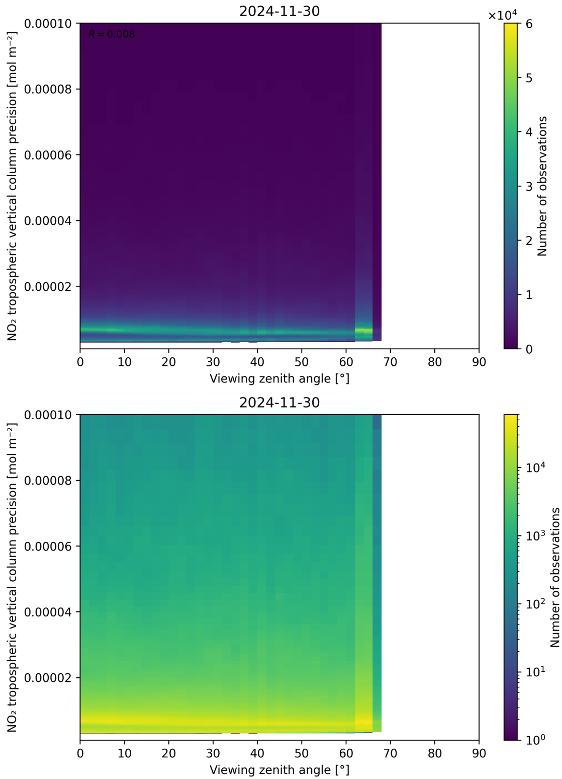
Figure 170: Scatter density plot of “Viewing zenith angle” against “NO 2 tropospheric vertical column precision” for 2024-11-30 to 2024-12-01.
