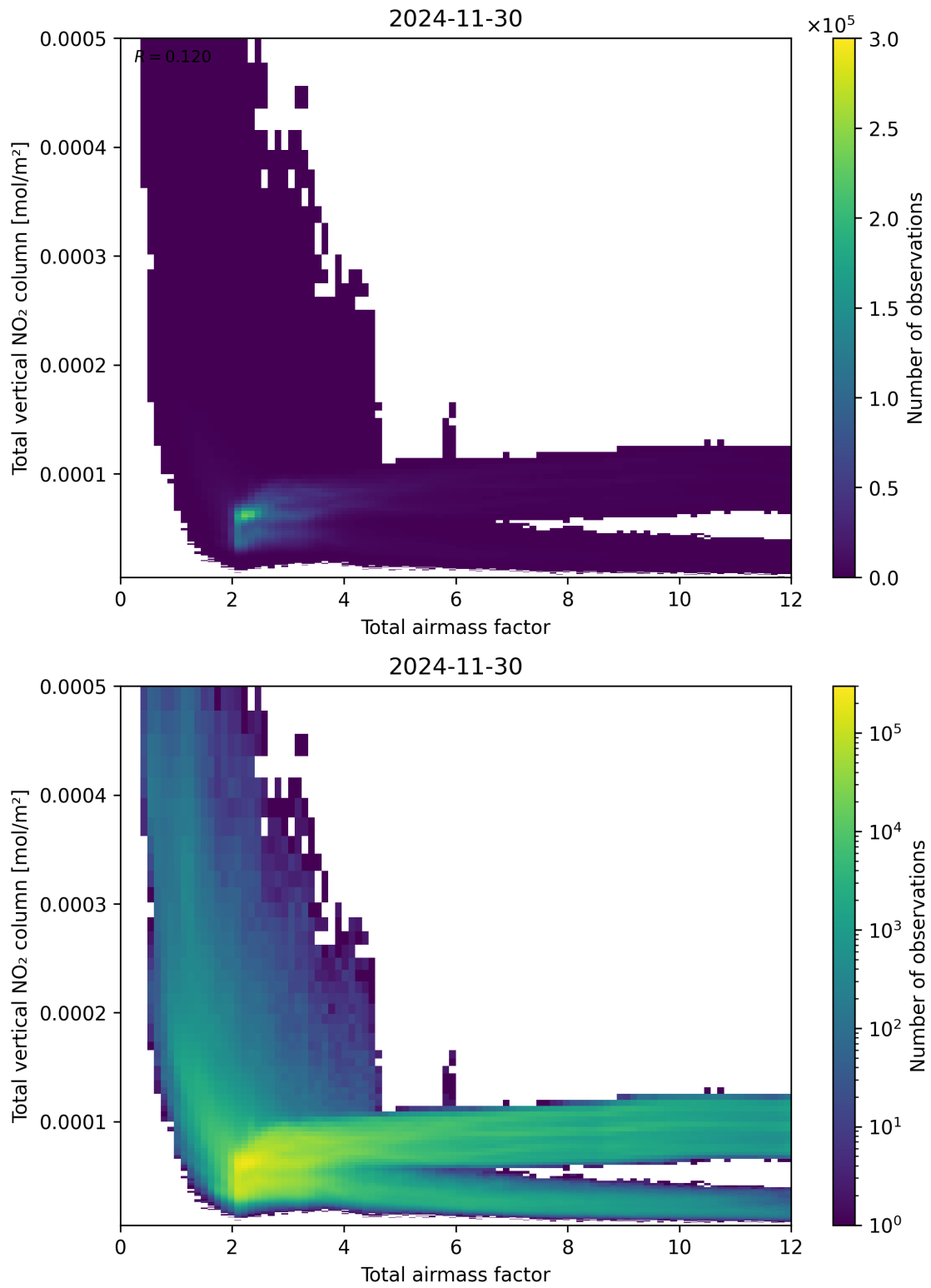
Figure 67: Scatter density plot of “Total airmass factor” against “Total vertical NO 2 column” for 2024-11-30 to 2024-12-01.
