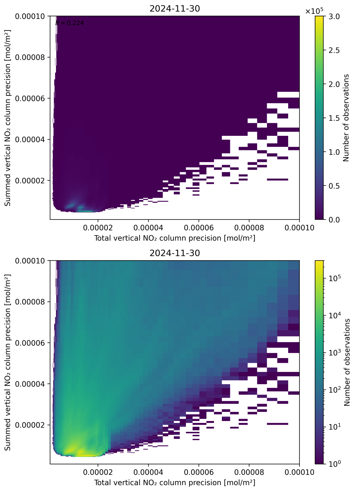
Figure 118: Scatter density plot of “Total vertical NO 2 column precision” against “Summed vertical NO 2 column precision” for 2024-11-30 to 2024-12-01.
