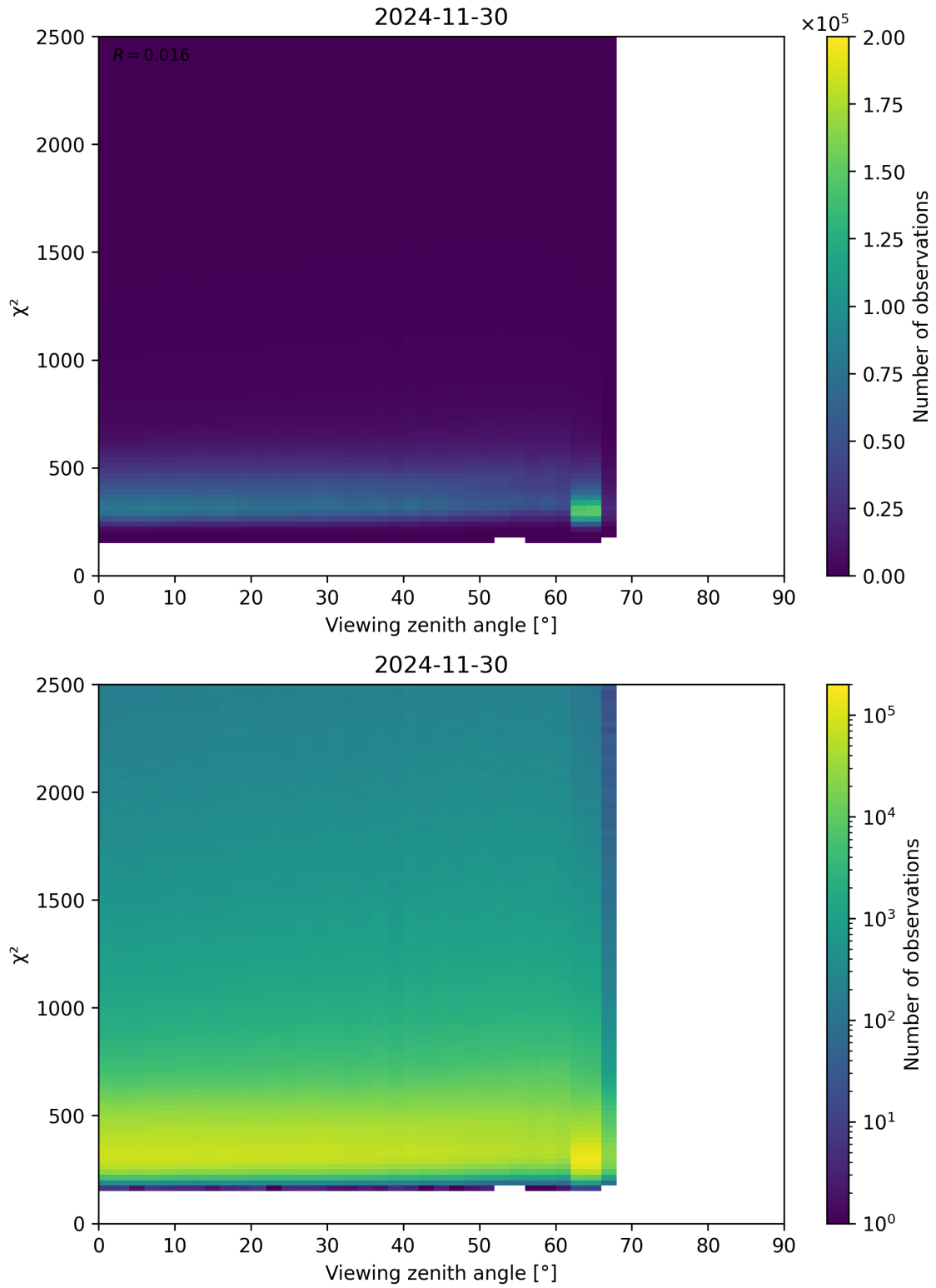
Figure 162: Scatter density plot of “Viewing zenith angle” against “ \chi^2 ” for 2024-11-30 to 2024-12-01.
