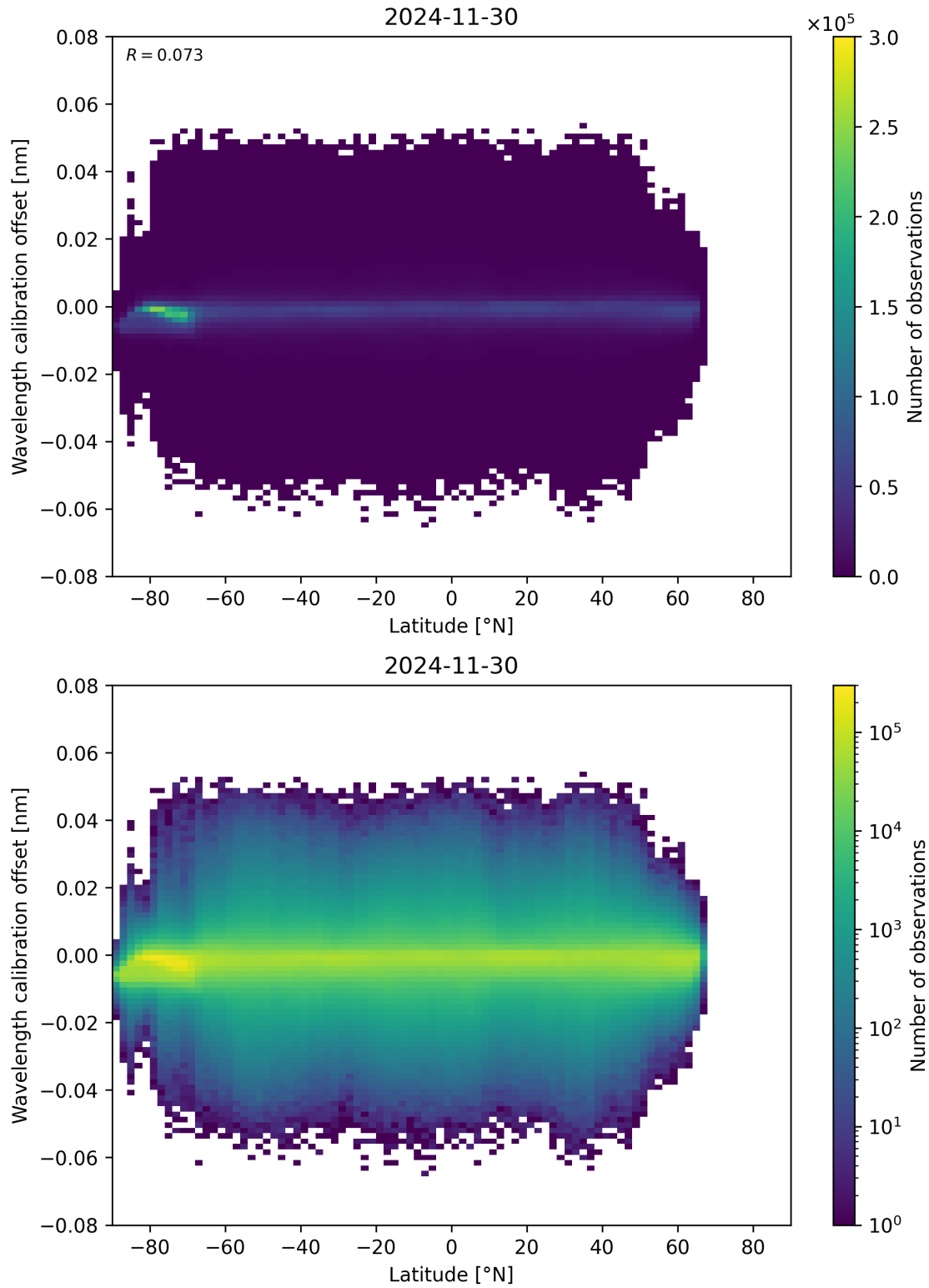
Figure 95: Scatter density plot of “Latitude” against “Wavelength calibration offset” for 2024-11-30 to 2024-12-01.
