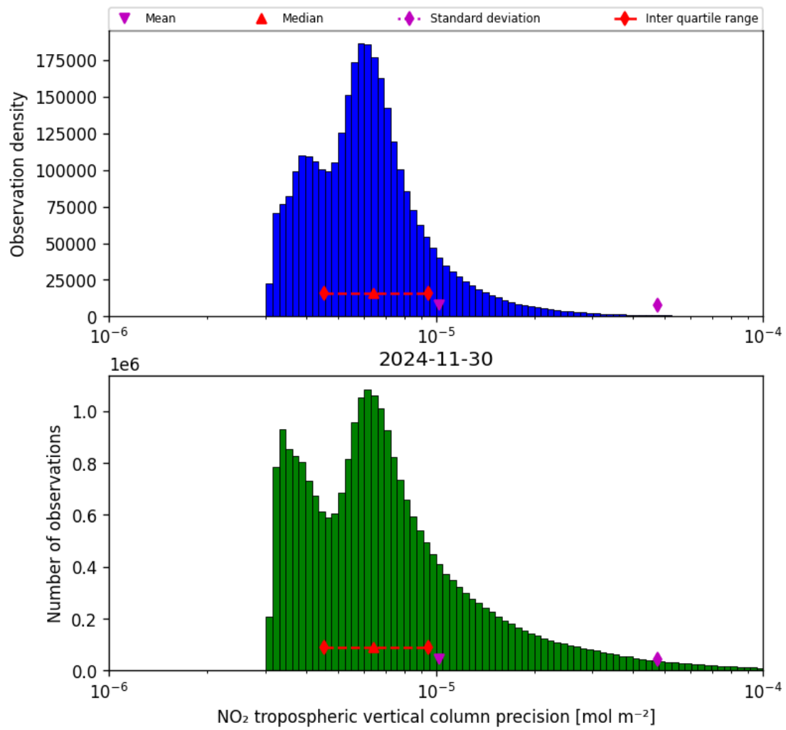
Figure 30: Histogram of “NO 2 tropospheric vertical column precision” for 2024-11-30 to 2024-12-01
