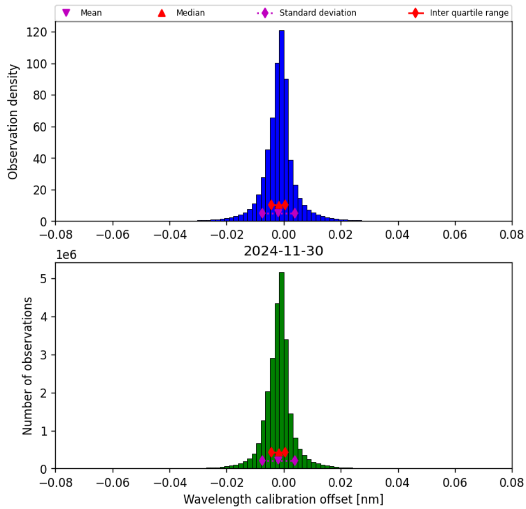
Figure 35: Histogram of “Wavelength calibration offset” for 2024-11-30 to 2024-12-01
