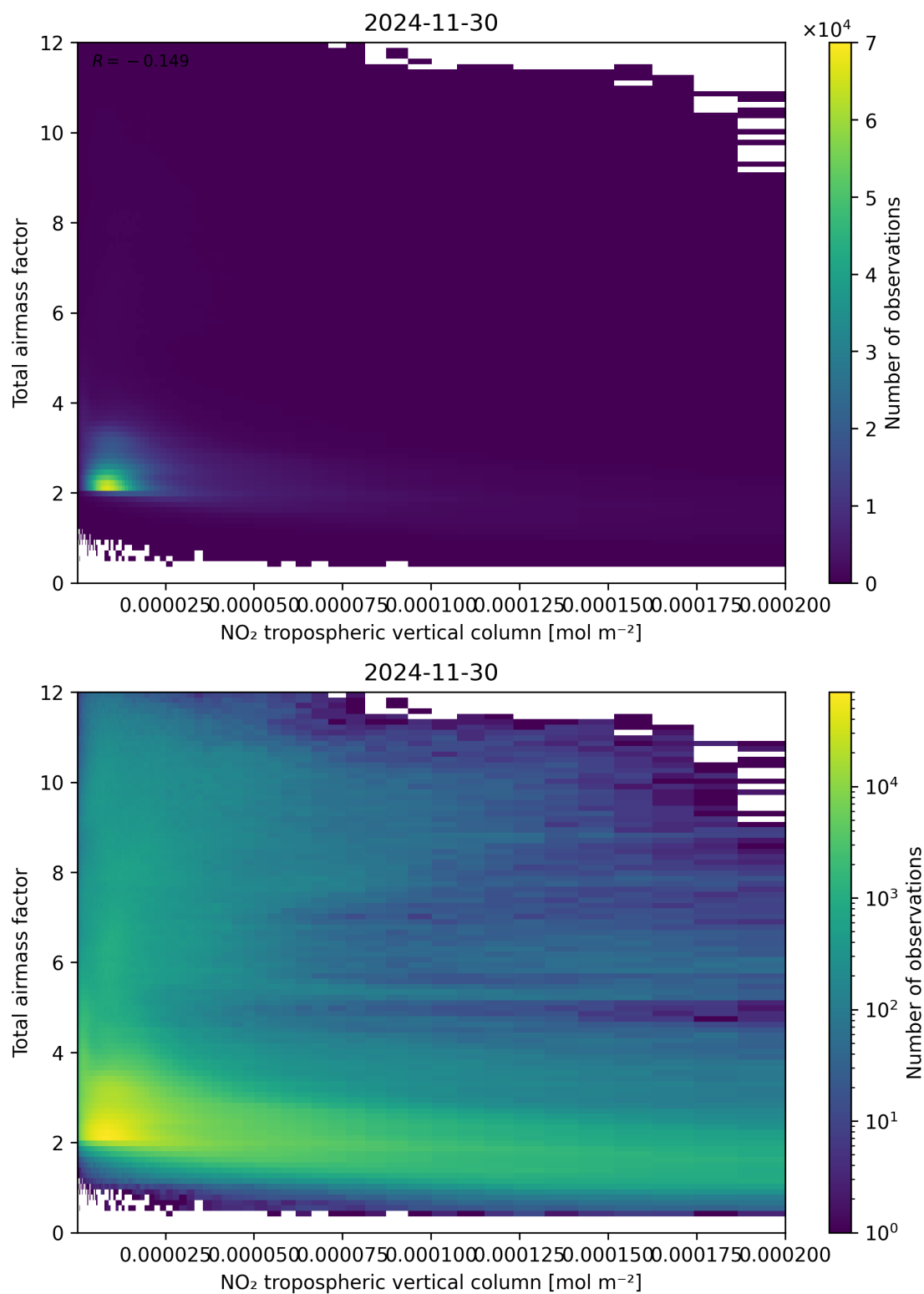
Figure 122: Scatter density plot of “NO 2 tropospheric vertical column” against “Total airmass factor” for 2024-11-30 to 2024-12-01.
