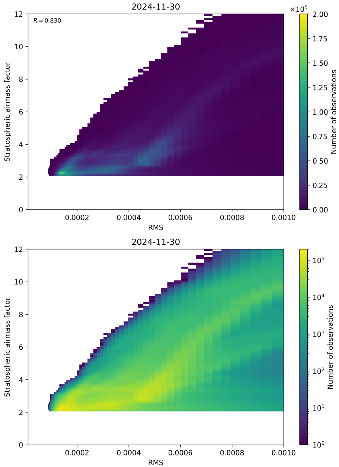
Figure 144: Scatter density plot of “RMS” against “Stratospheric airmass factor” for 2024-11-30 to 2024-12-01.
