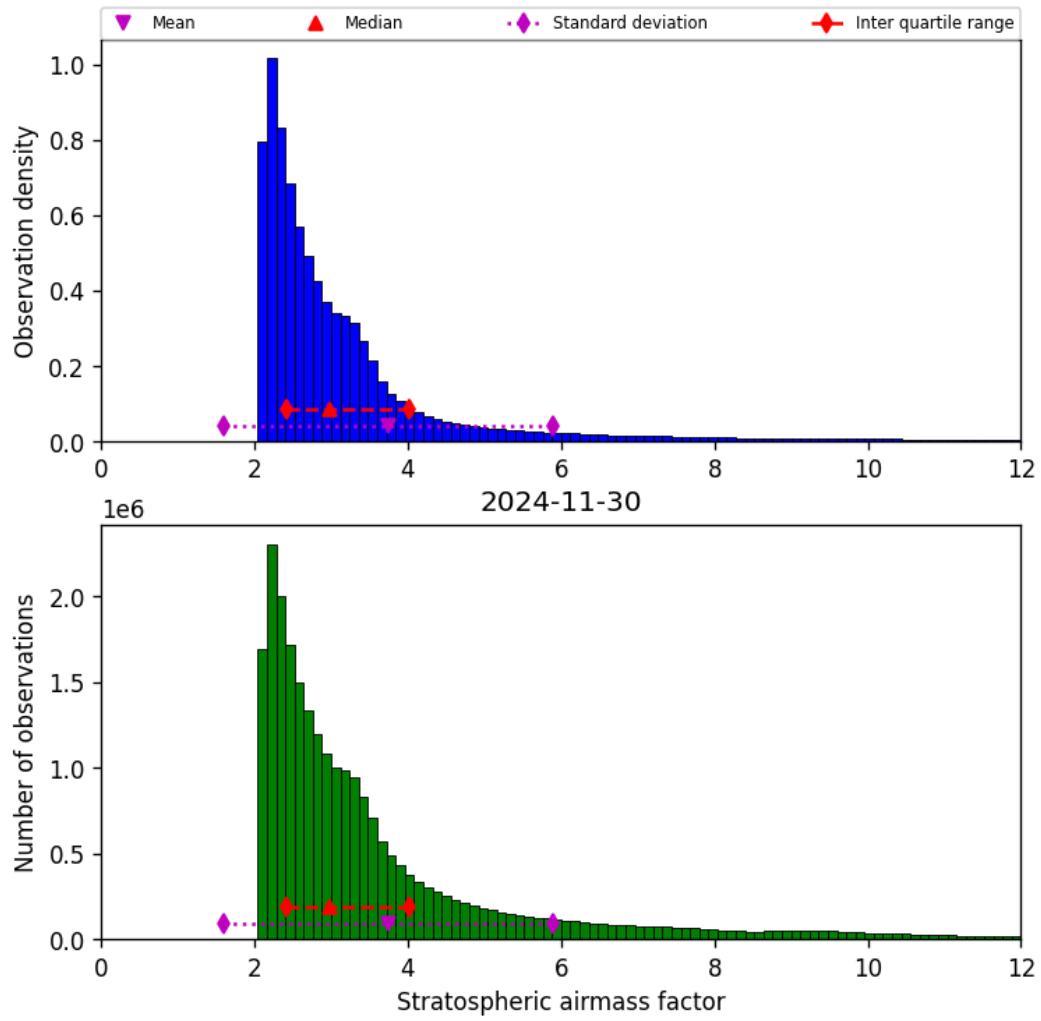
Figure 44: Histogram of “Stratospheric airmass factor” for 2024-11-30 to 2024-12-01
