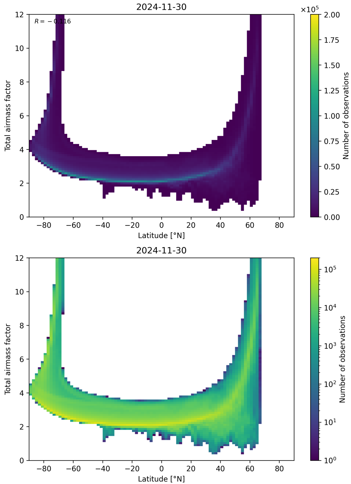
Figure 84: Scatter density plot of “Latitude” against “Total airmass factor” for 2024-11-30 to 2024-12-01.
