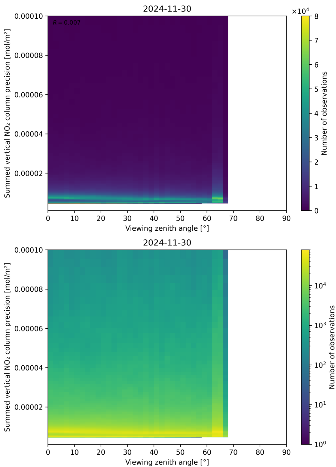
Figure 166: Scatter density plot of “Viewing zenith angle” against “Summed vertical NO 2 column precision” for 2024-11-30 to 2024-12-01.
