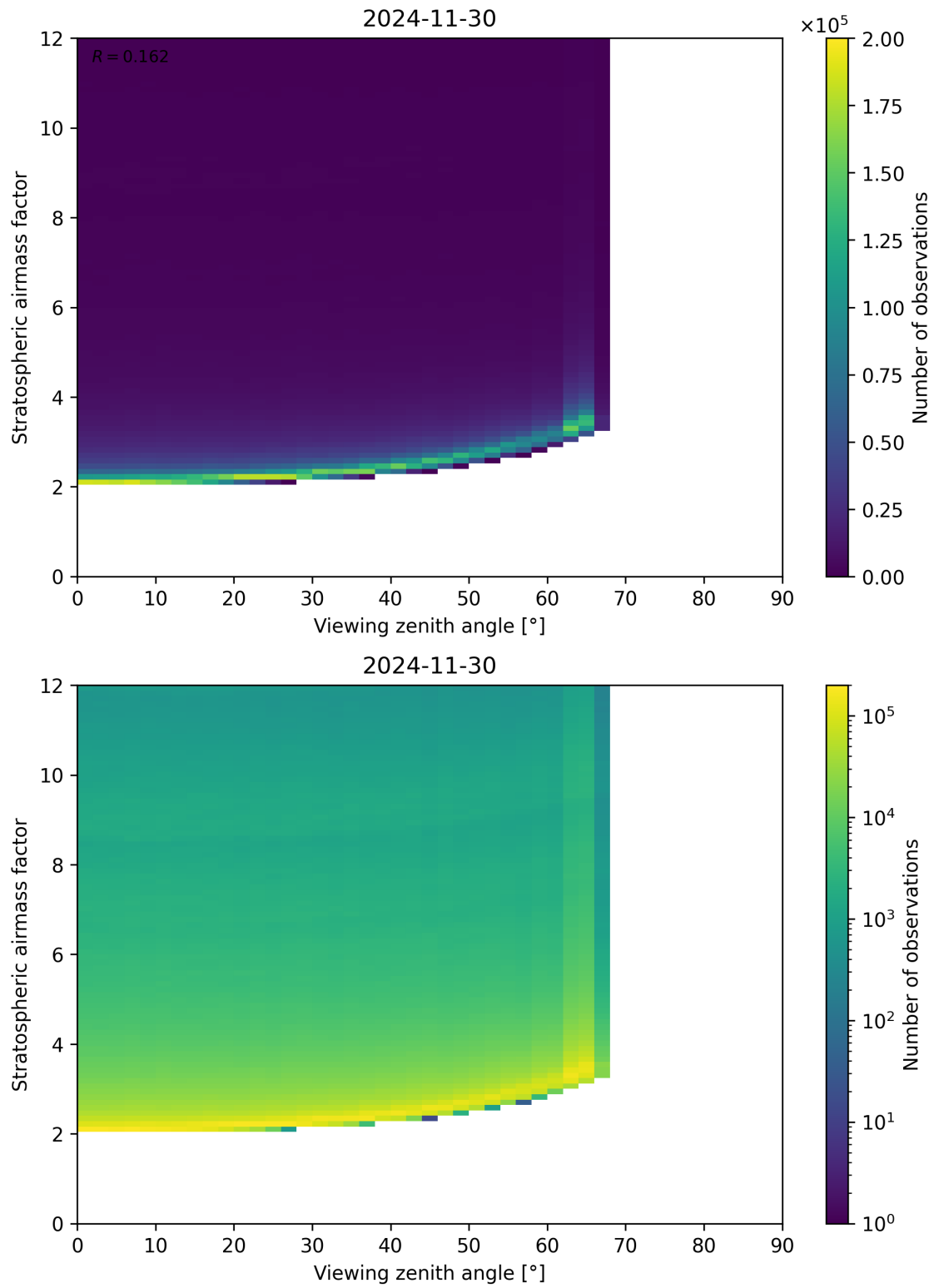
Figure 159: Scatter density plot of “Viewing zenith angle” against “Stratospheric airmass factor” for 2024-11-30 to 2024-12-01.
