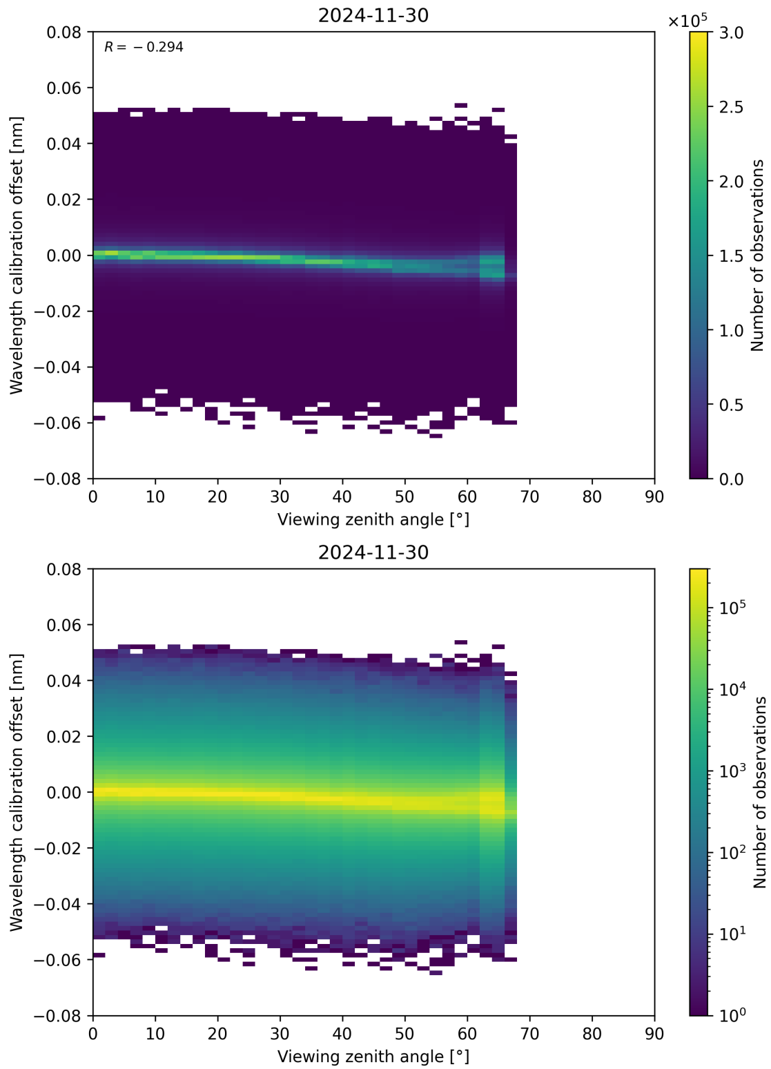
Figure 173: Scatter density plot of “Viewing zenith angle” against “Wavelength calibration offset” for 2024-11-30 to 2024-12-01.
