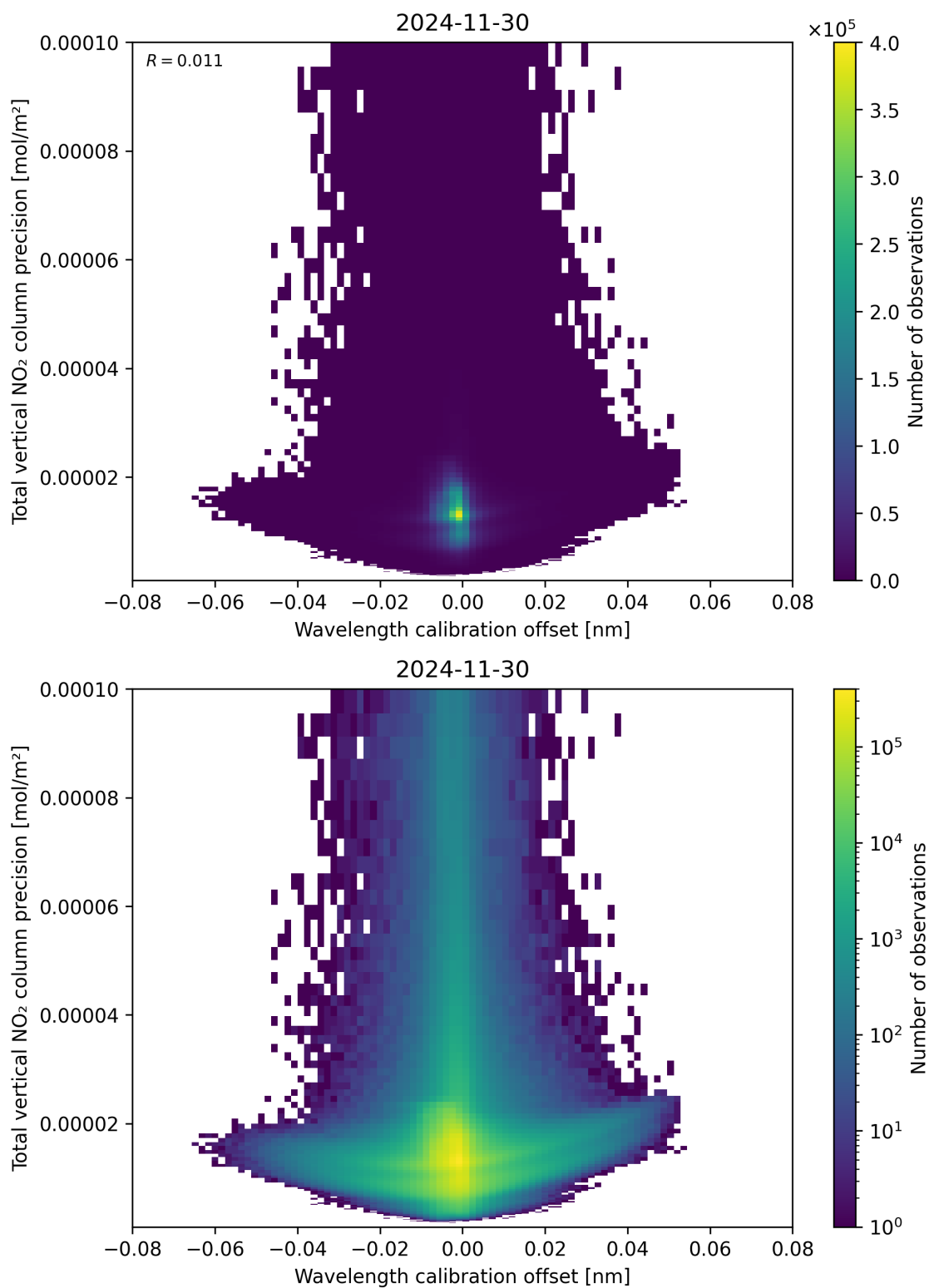
Figure 180: Scatter density plot of “Wavelength calibration offset” against “Total vertical NO 2 column precision” for 2024-11-30 to 2024-12-01.
