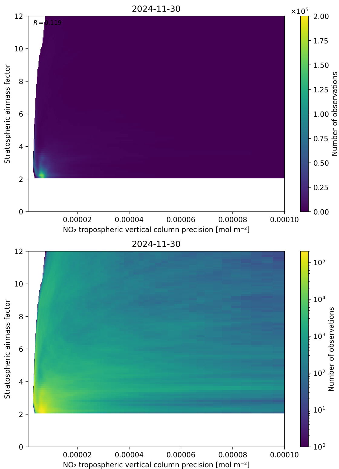
Figure 131: Scatter density plot of “NO 2 tropospheric vertical column precision” against “Stratospheric airmass factor” for 2024-11-30 to 2024-12-01.
