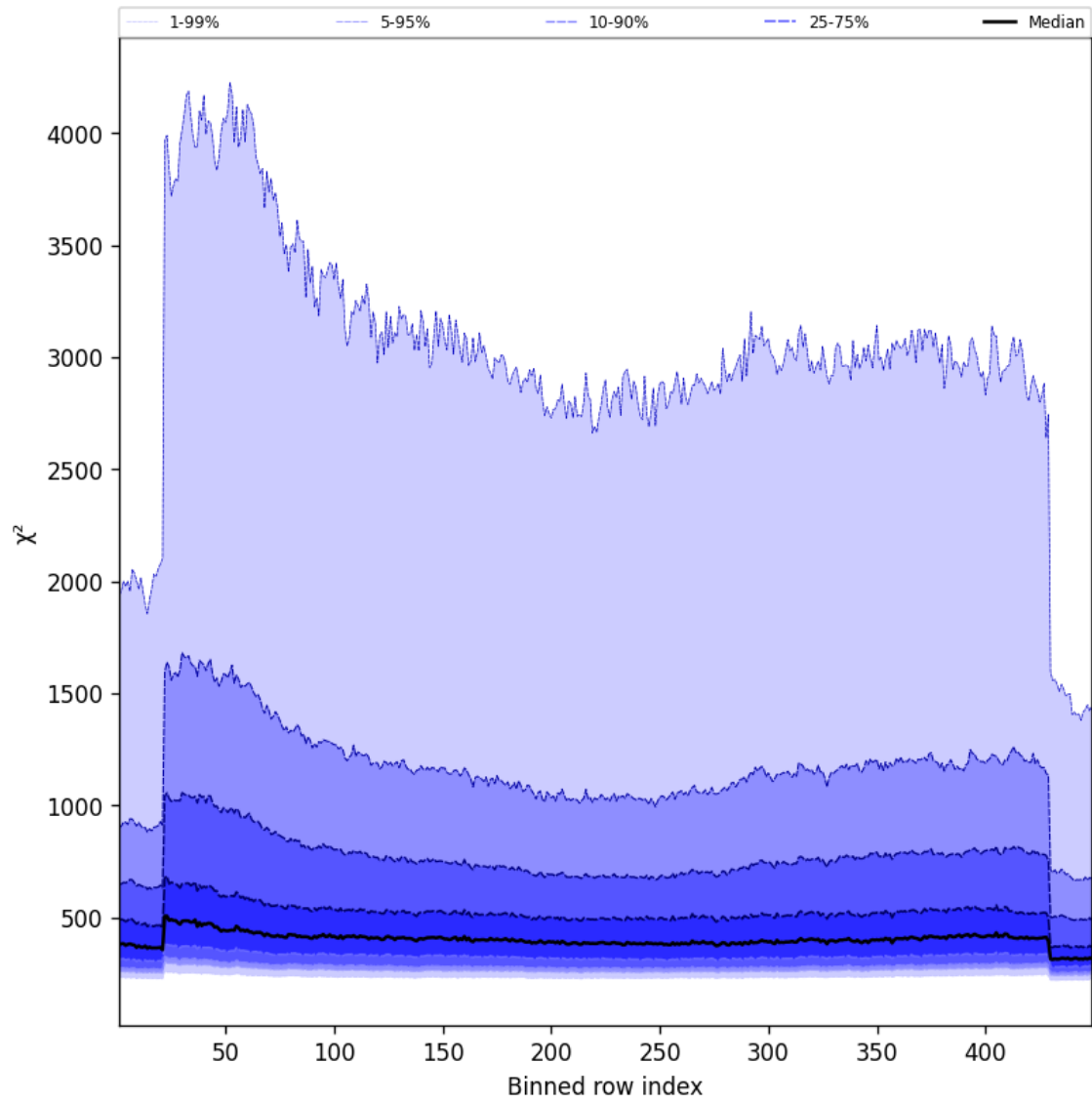
Figure 59: Along track statistics of “ \chi^2 ” for 2024-11-30 to 2024-12-01
