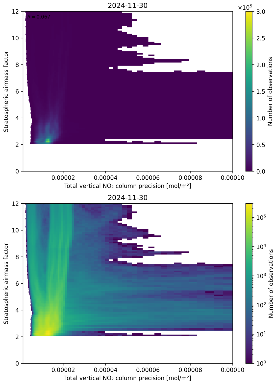
Figure 115: Scatter density plot of “Total vertical NO 2 column precision” against “Stratospheric air mass factor” for 2024-11-30 to 2024-12-01.
