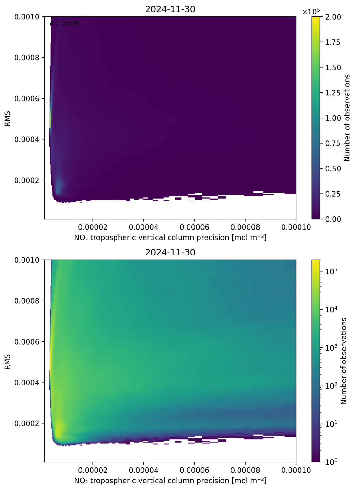
Figure 140: Scatter density plot of “NO 2 tropospheric vertical column precision” against “RMS” for 2024-11-30 to 2024-12-01.
