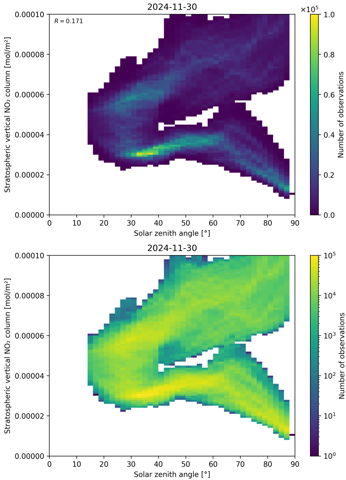
Figure 150: Scatter density plot of “Solar zenith angle” against “Stratospheric vertical NO 2 column” for 2024-11-30 to 2024-12-01.
