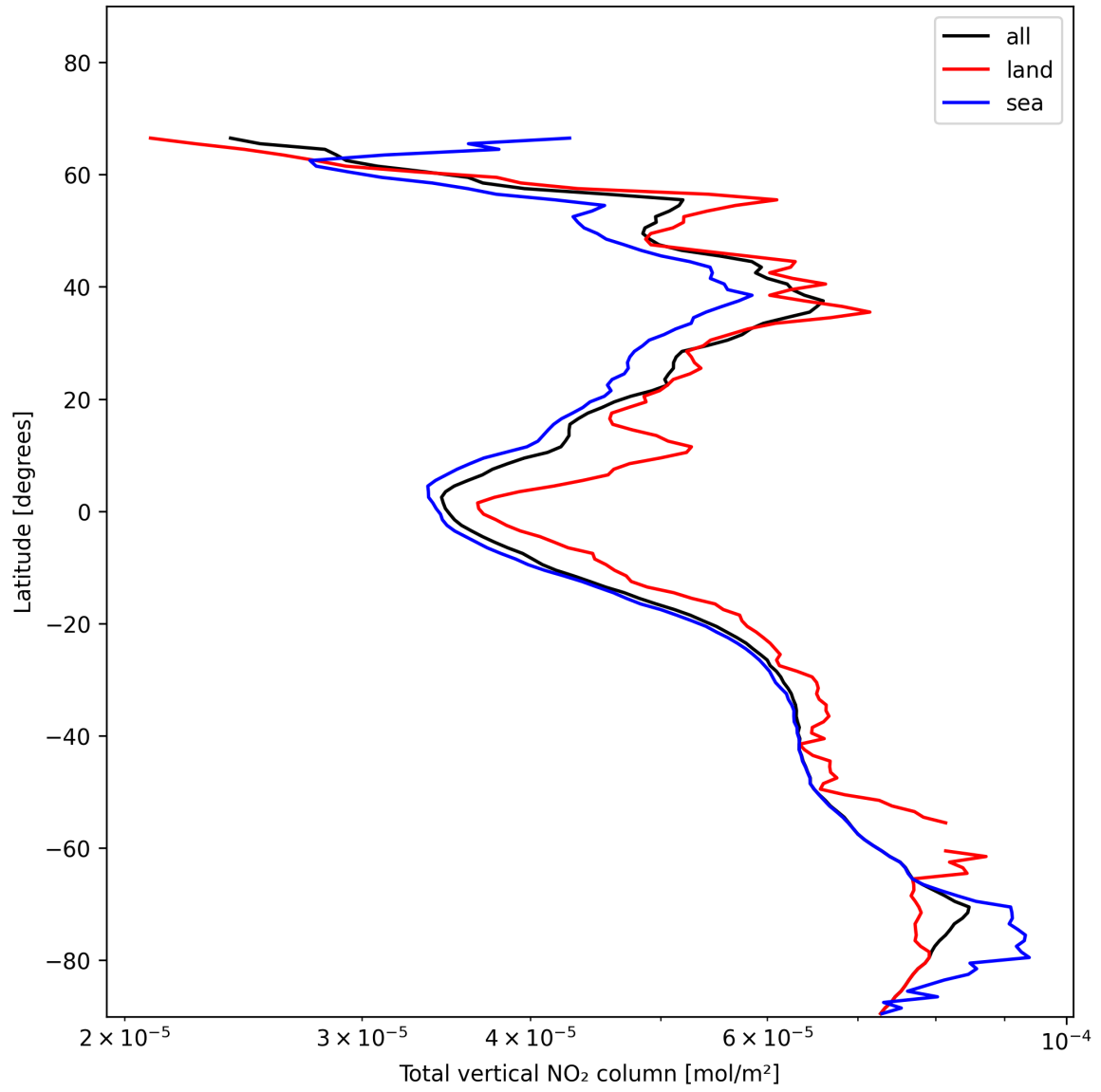
Figure 21: Zonal average of “Total vertical NO 2 column” for 2024-11-30 to 2024-12-01.
