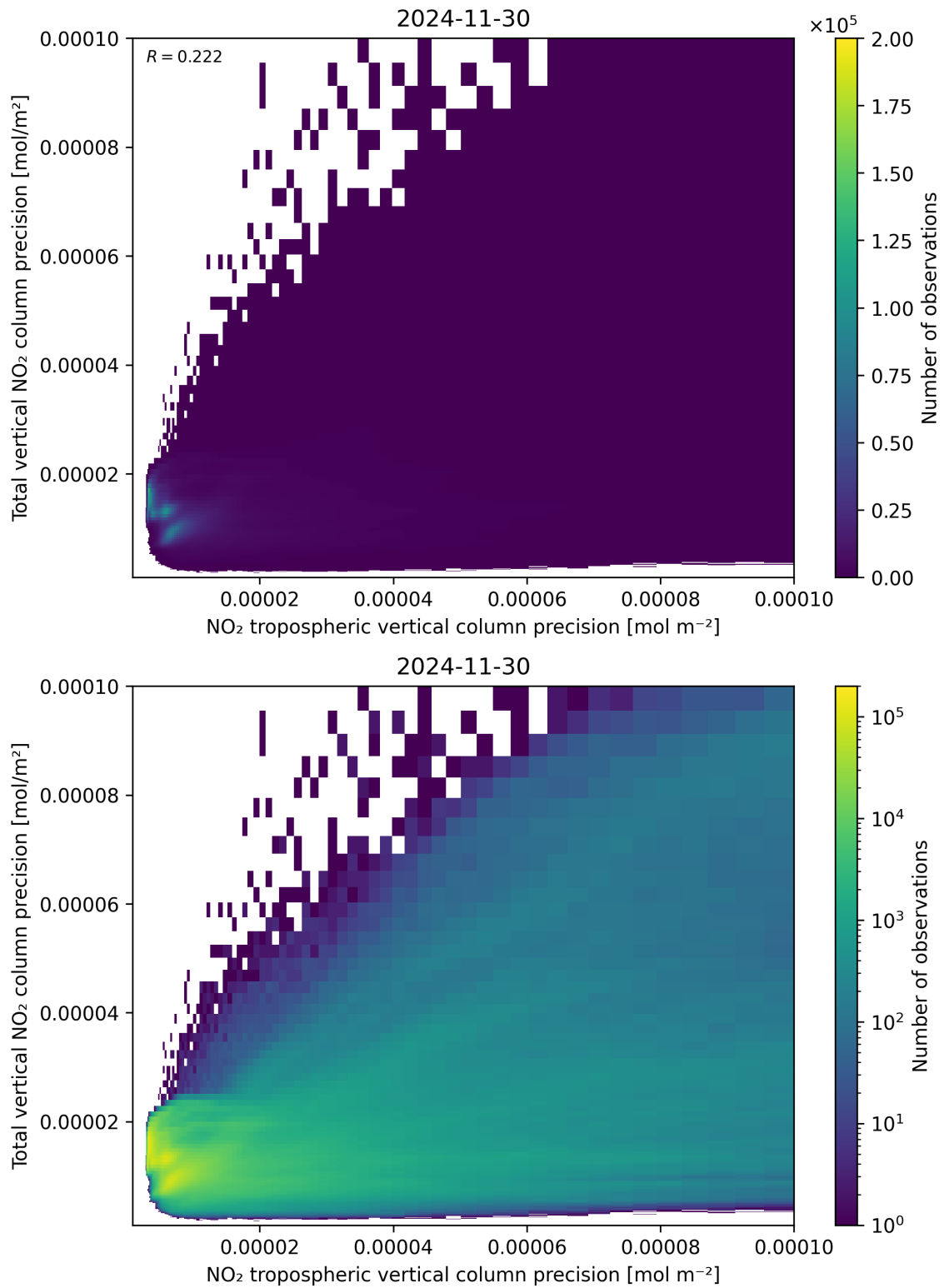
Figure 139: Scatter density plot of “NO 2 tropospheric vertical column precision” against “Total vertical NO 2 column precision” for 2024-11-30 to 2024-12-01.
