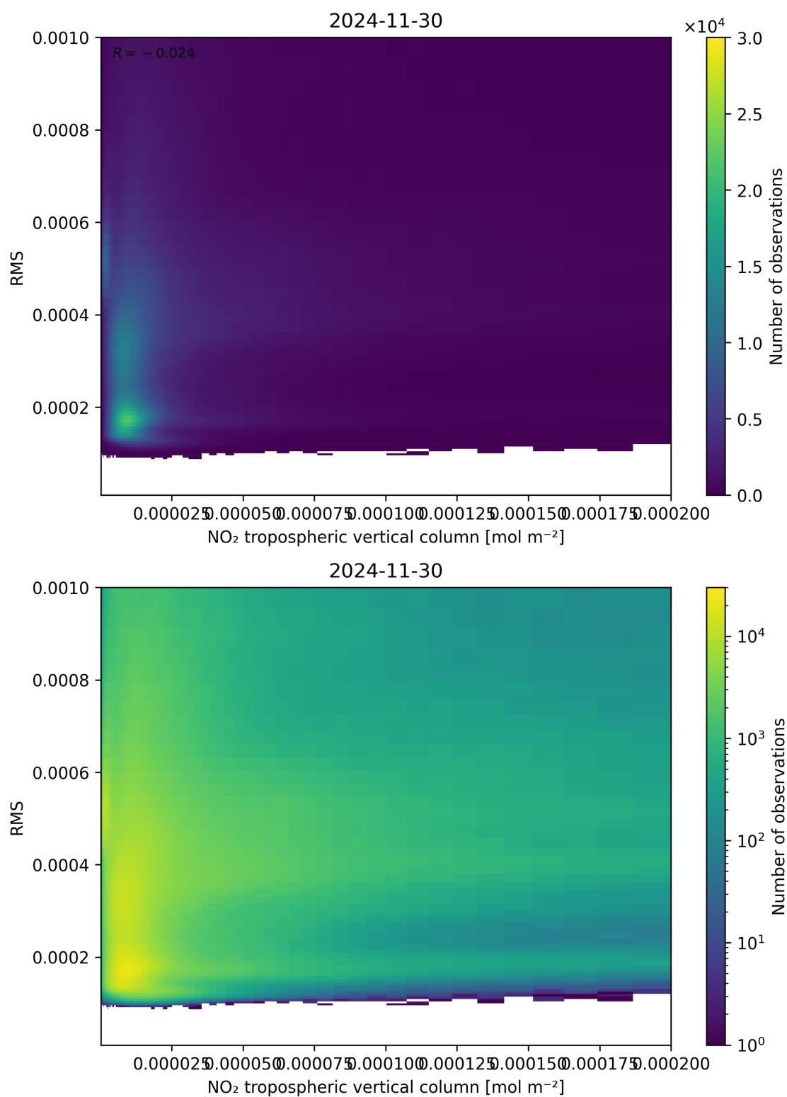
Figure 142: Scatter density plot of “NO 2 tropospheric vertical column” against “RMS” for 2024-11-30 to 2024-12-01.
