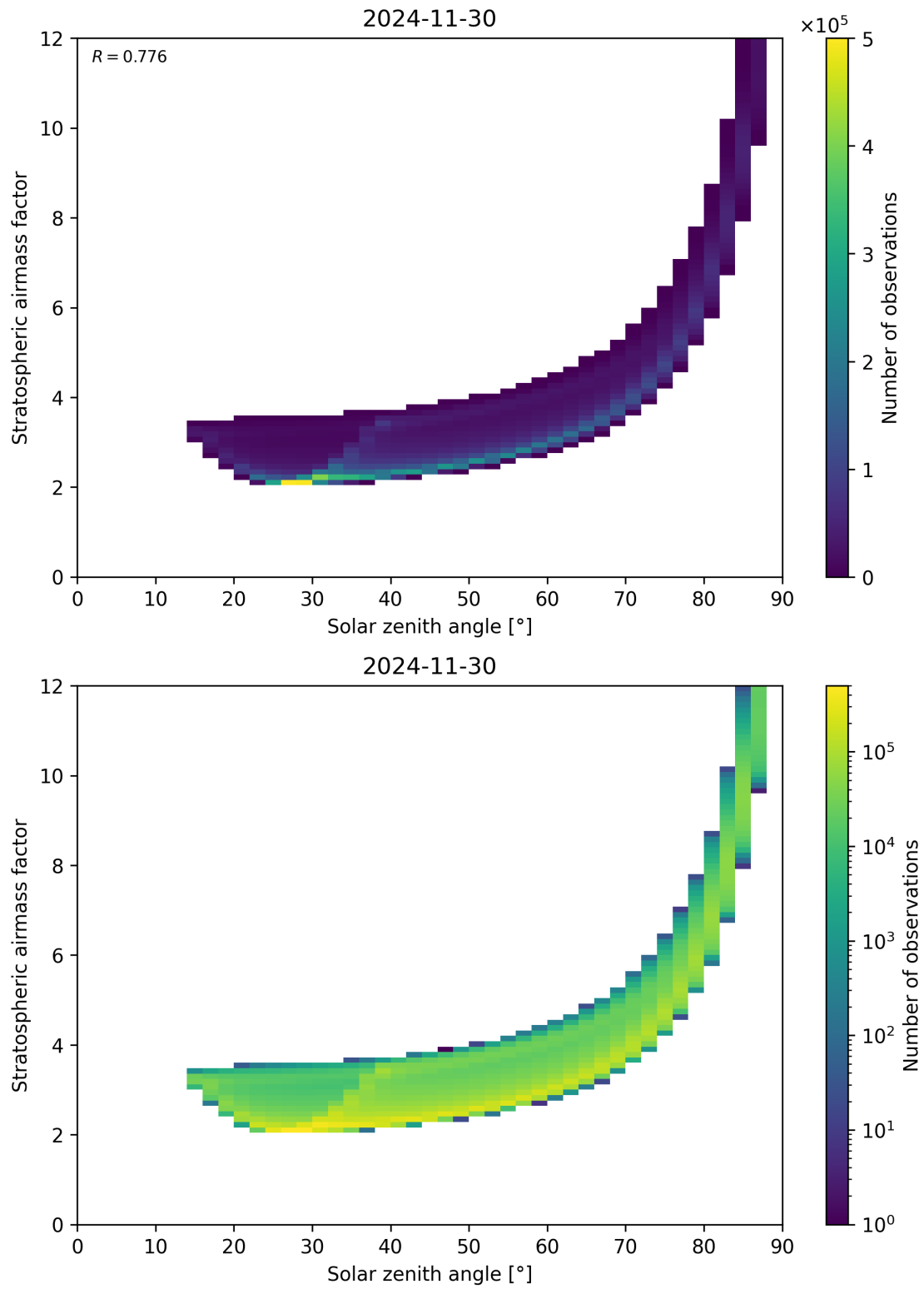
Figure 145: Scatter density plot of “Solar zenith angle” against “Stratospheric airmass factor” for 2024-11-30 to 2024-12-01.
