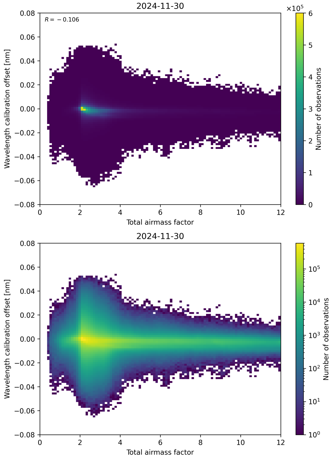
Figure 70: Scatter density plot of “Total airmass factor” against “Wavelength calibration offset” for 2024-11-30 to 2024-12-01.
