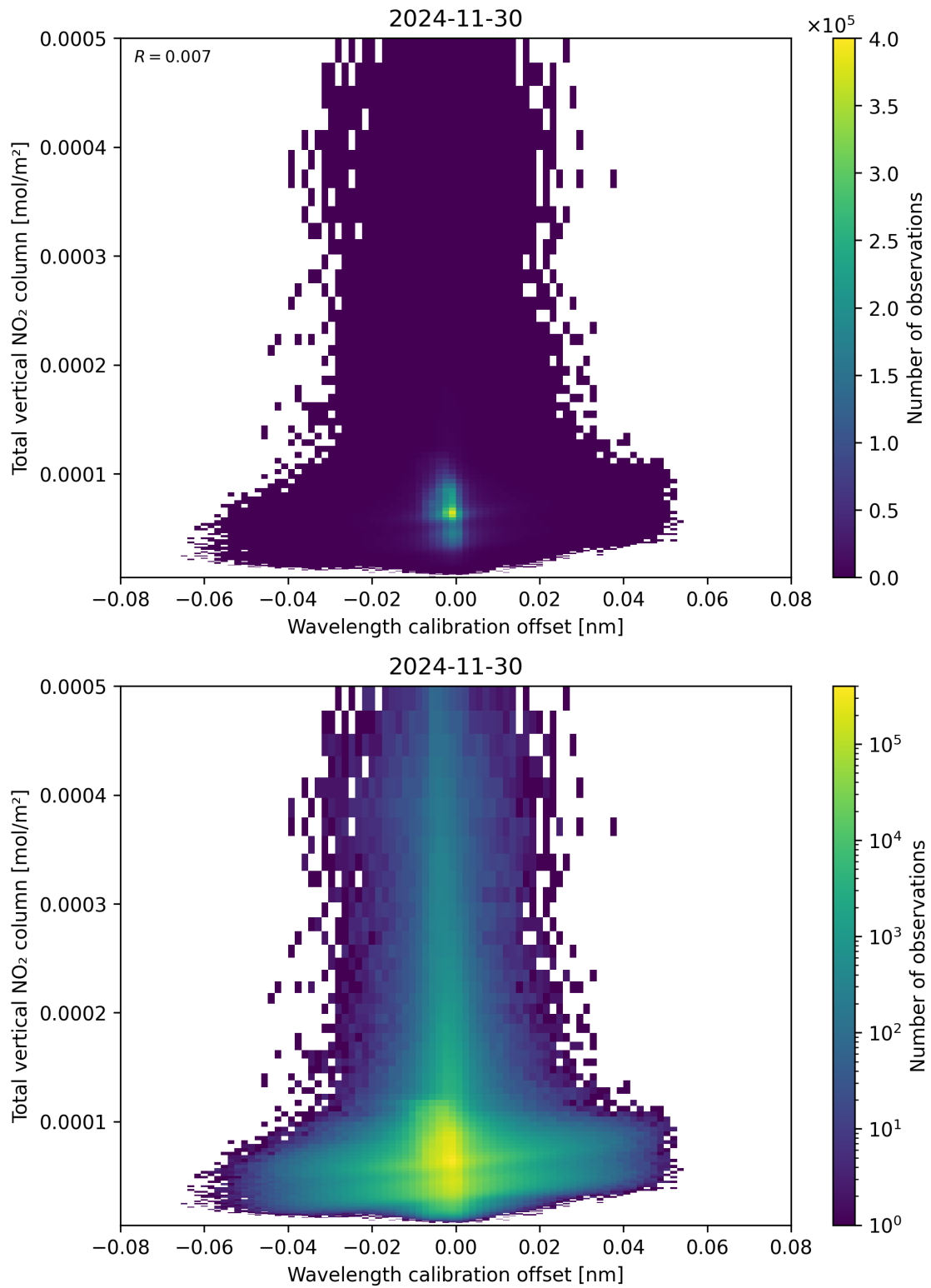
Figure 179: Scatter density plot of “Wavelength calibration offset” against “Total vertical NO 2 column” for 2024-11-30 to 2024-12-01.
