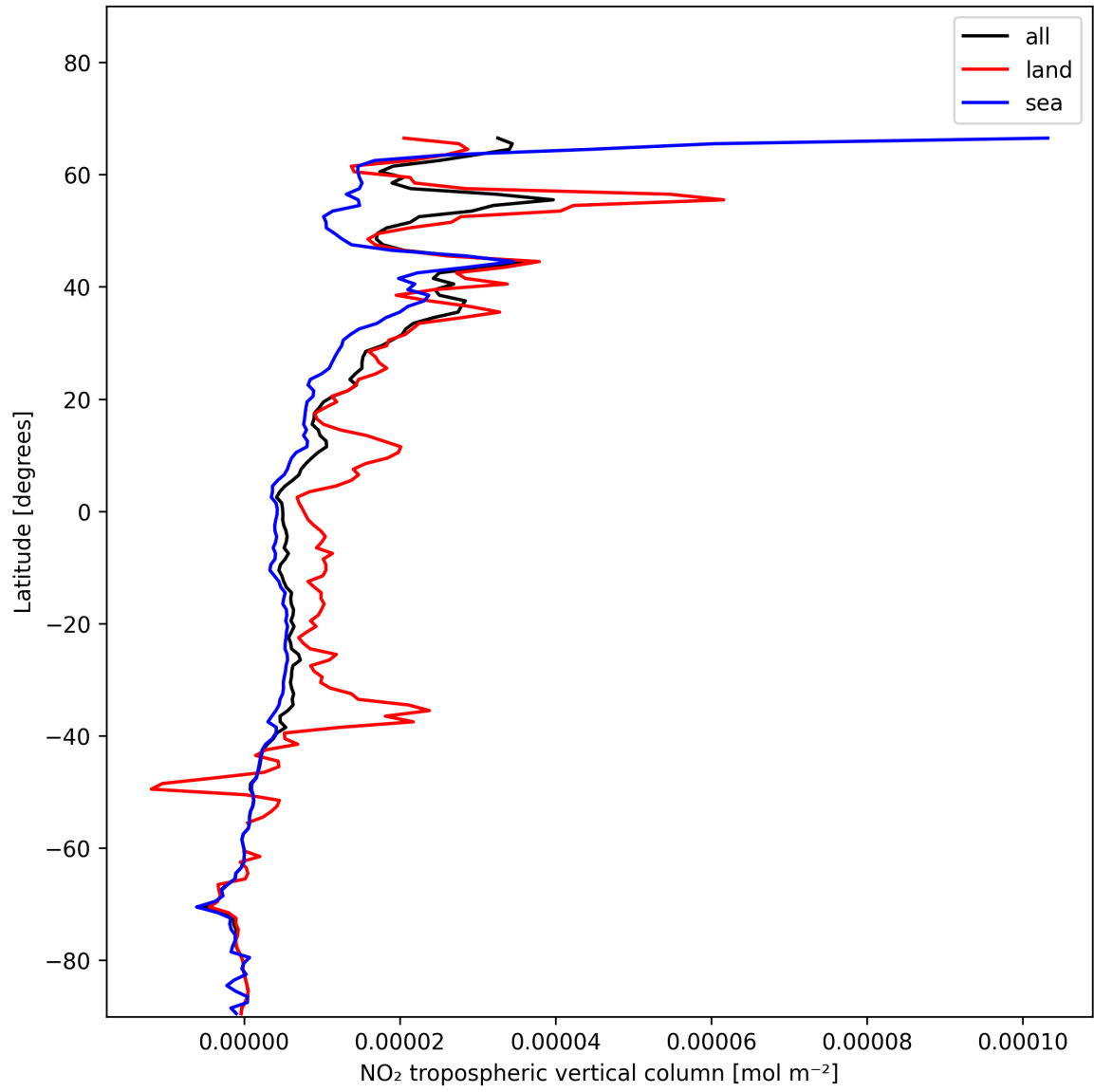
Figure 12: Zonal average of “NO 2 tropospheric vertical column” for 2024-11-30 to 2024-12-01.
