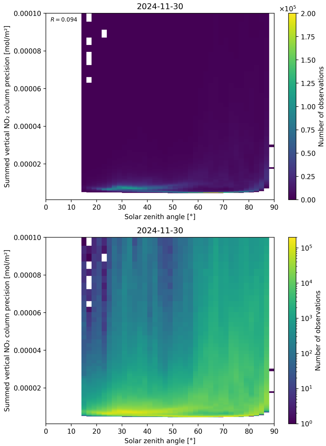
Figure 152: Scatter density plot of “Solar zenith angle” against “Summed vertical NO 2 column precision” for 2024-11-30 to 2024-12-01.
