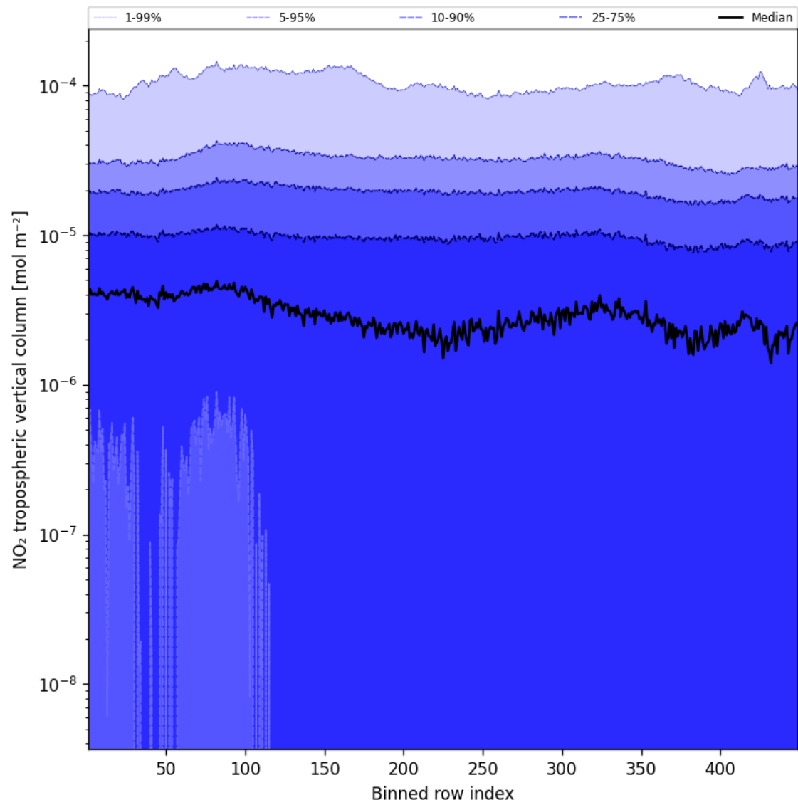
Figure 46: Along track statistics of “NO 2 tropospheric vertical column” for 2024-11-30 to 2024-12-01
