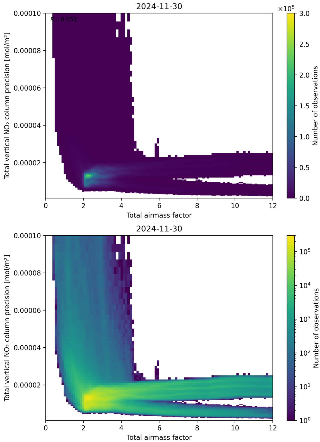
Figure 68: Scatter density plot of “Total airmass factor” against “Total vertical NO 2 column precision” for 2024-11-30 to 2024-12-01.
