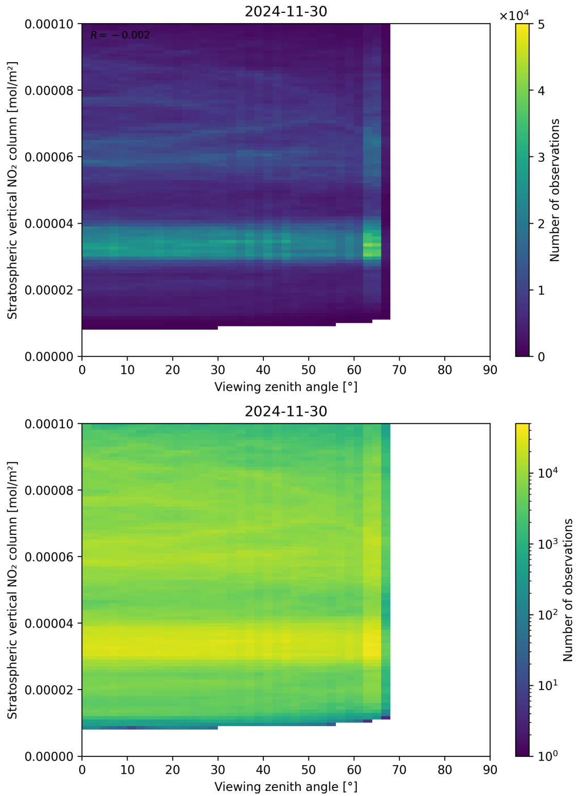
Figure 164: Scatter density plot of “Viewing zenith angle” against “Stratospheric vertical NO 2 column” for 2024-11-30 to 2024-12-01.
