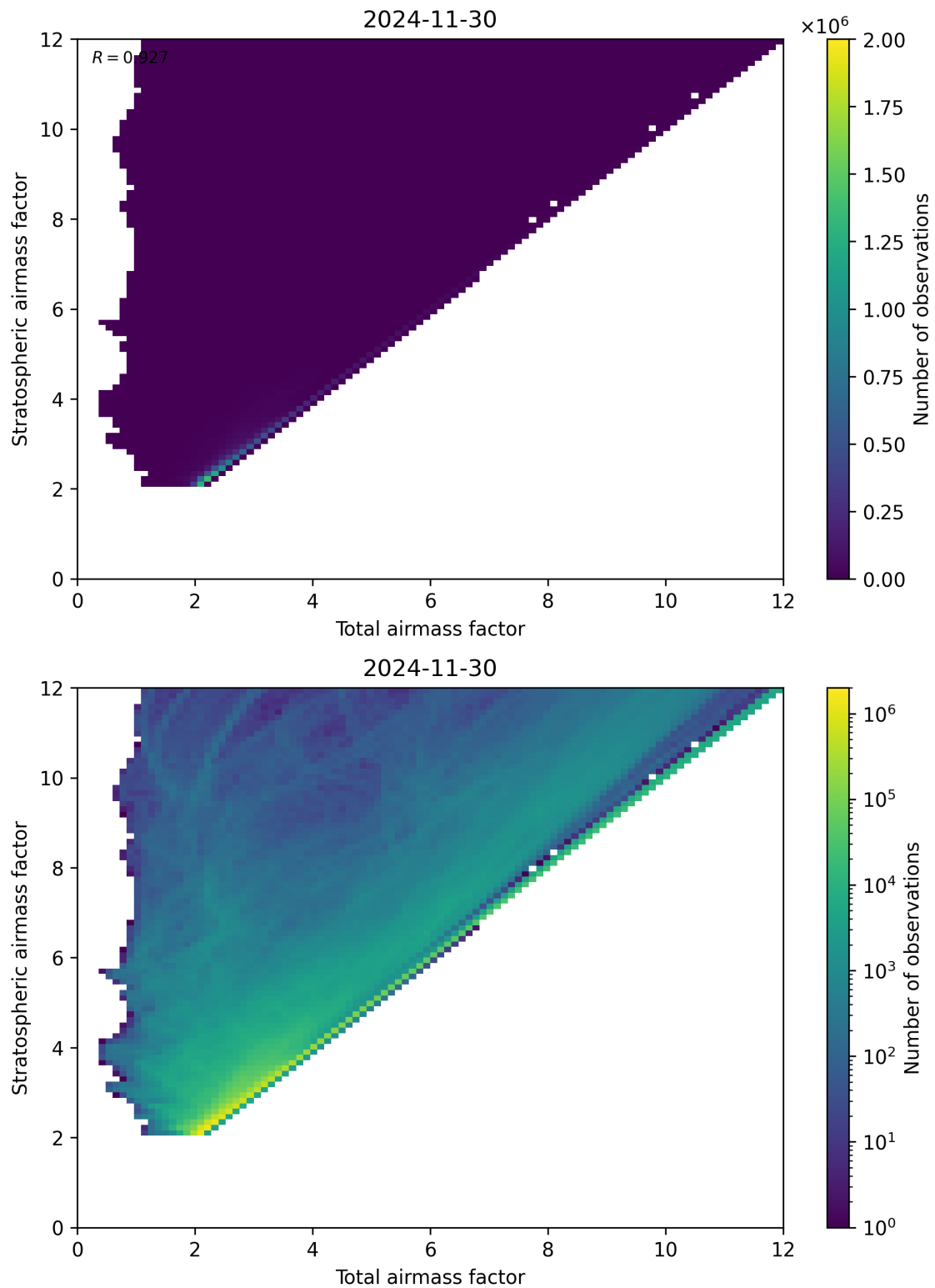
Figure 62: Scatter density plot of “Total airmass factor” against “Stratospheric airmass factor” for 2024-11-30 to 2024-12-01.
