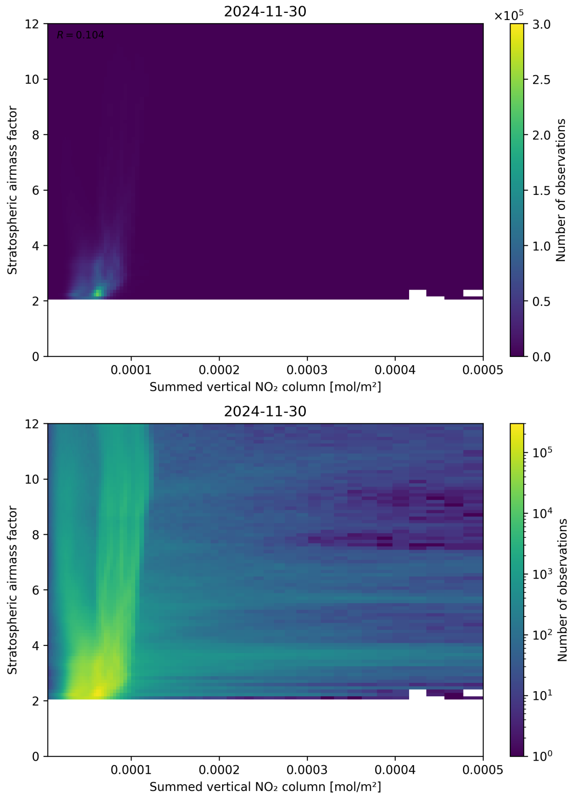
Figure 103: Scatter density plot of “Summed vertical NO 2 column” against “Stratospheric air mass factor” for 2024-11-30 to 2024-12-01.
