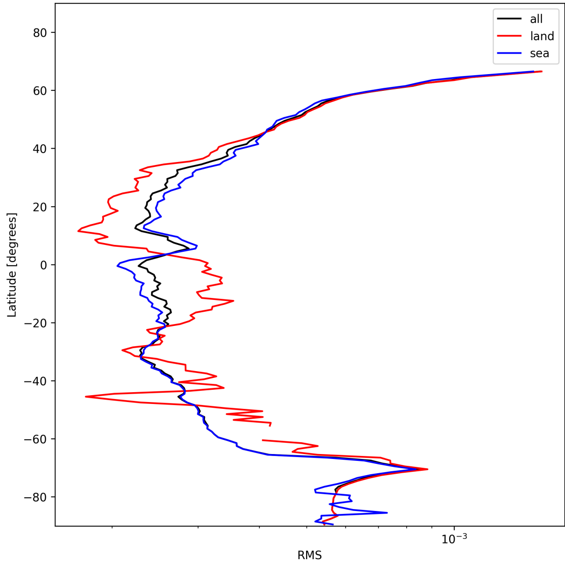
Figure 26: Zonal average of “RMS” for 2024-11-30 to 2024-12-01.
