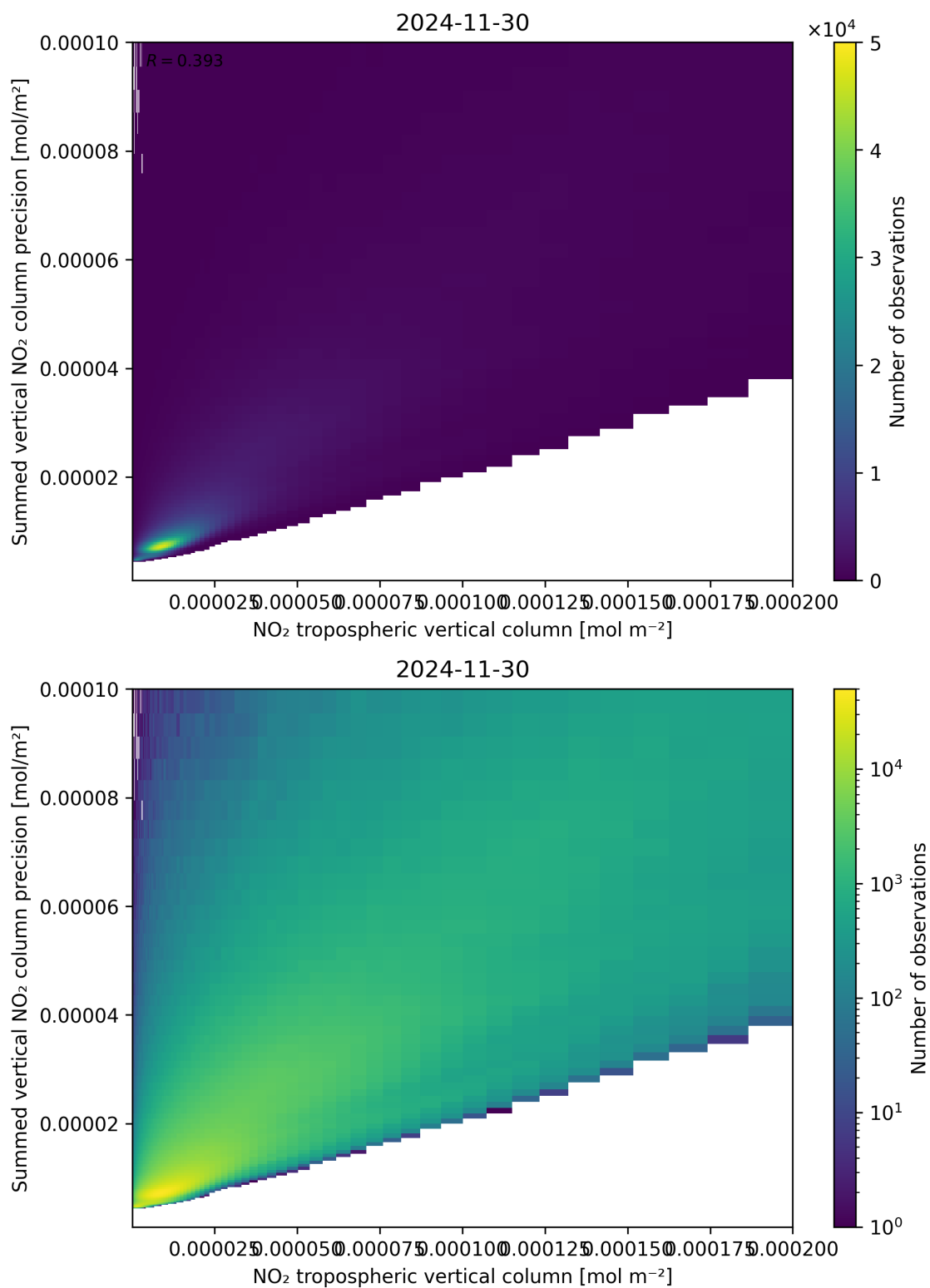
Figure 127: Scatter density plot of “NO 2 tropospheric vertical column” against “Summed vertical NO 2 column precision” for 2024-11-30 to 2024-12-01.
