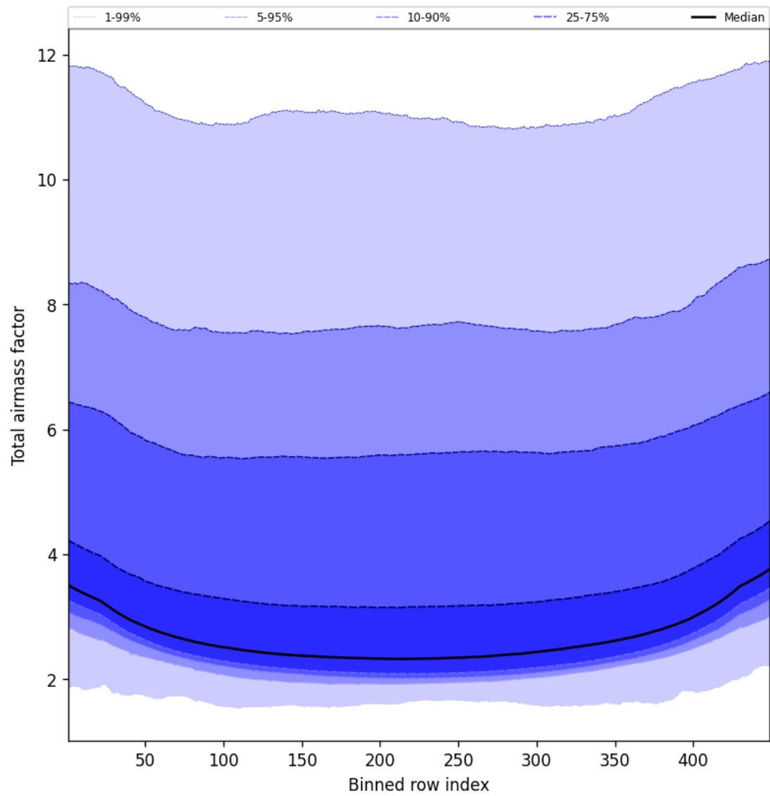
Figure 49: Along track statistics of “Total airmass factor” for 2024-11-30 to 2024-12-01
