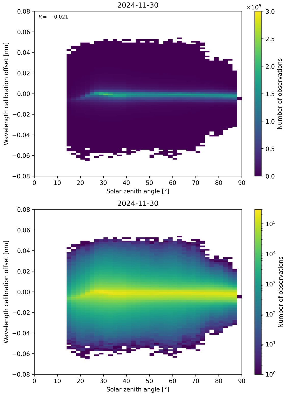
Figure 158: Scatter density plot of “Solar zenith angle” against “Wavelength calibration offset” for 2024-11-30 to 2024-12-01.
