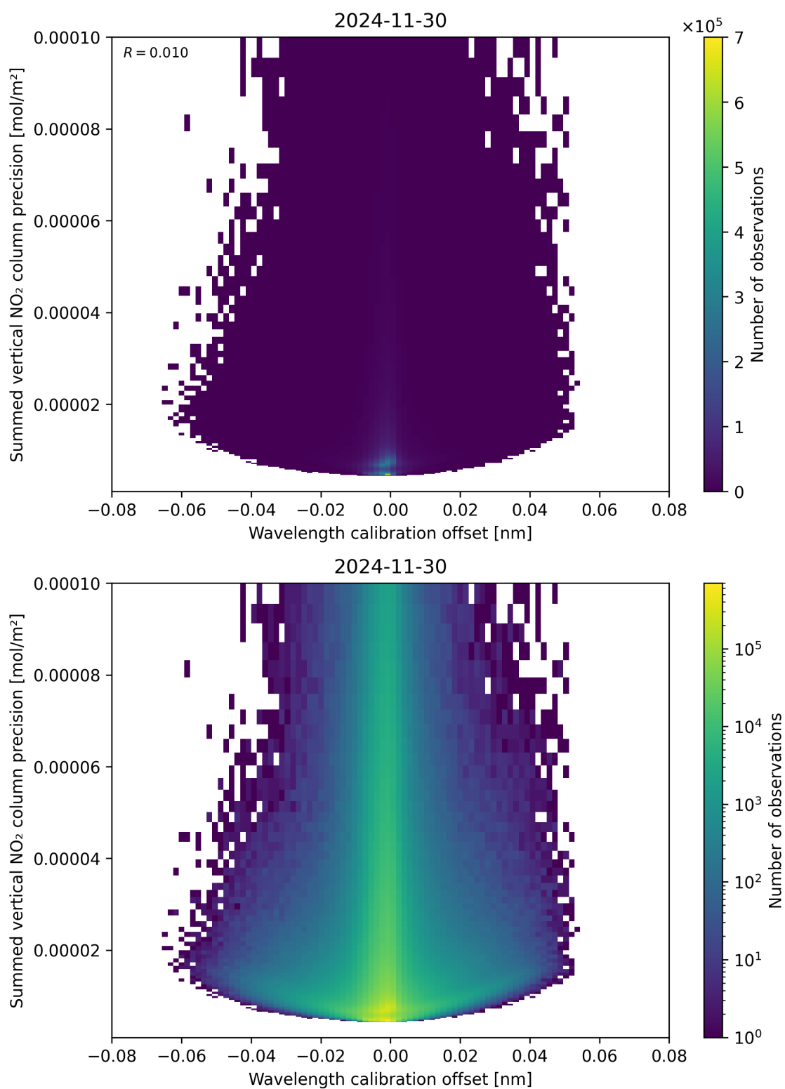
Figure 178: Scatter density plot of “Wavelength calibration offset” against “Summed vertical NO 2 column precision” for 2024-11-30 to 2024-12-01.
