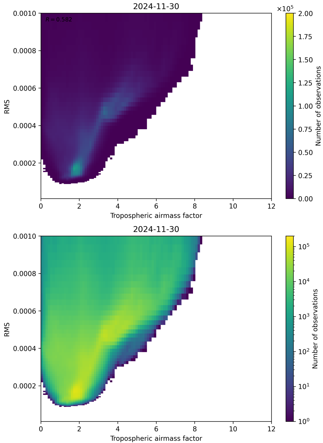
Figure 79: Scatter density plot of “Tropospheric airmass factor” against “RMS” for 2024-11-30 to 2024-12-01.
