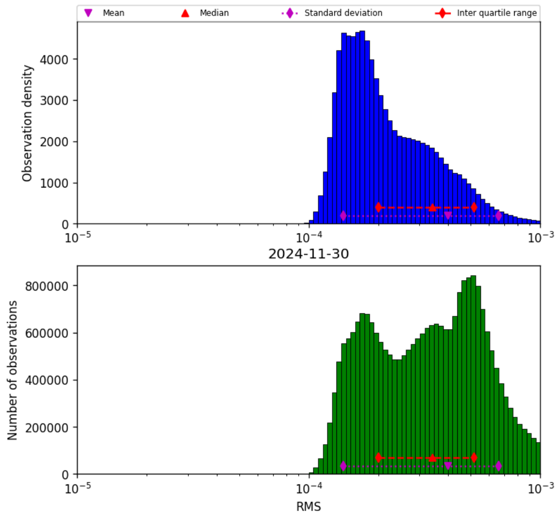
Figure 43: Histogram of “RMS” for 2024-11-30 to 2024-12-01
