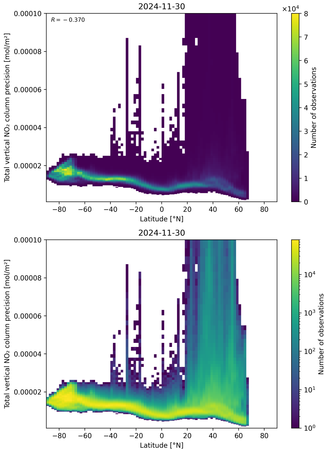
Figure 91: Scatter density plot of “Latitude” against “Total vertical NO 2 column precision” for 2024-11-30 to 2024-12-01.
