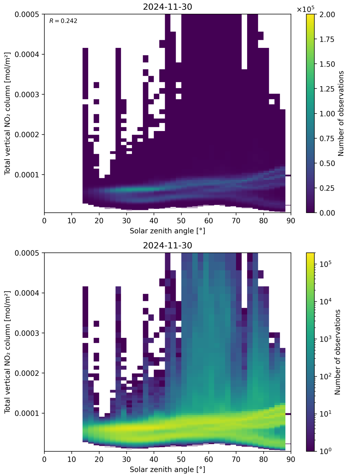
Figure 153: Scatter density plot of “Solar zenith angle” against “Total vertical NO 2 column” for 2024-11-30 to 2024-12-01.
