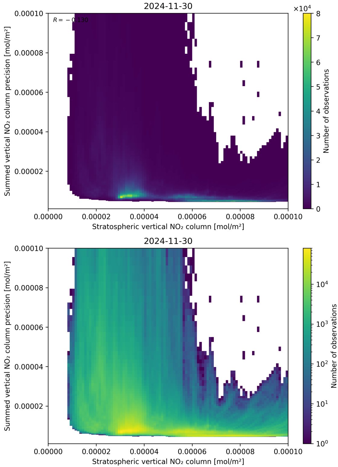
Figure 99: Scatter density plot of “Stratospheric vertical NO 2 column” against “Summed vertical NO 2 column precision” for 2024-11-30 to 2024-12-01.
