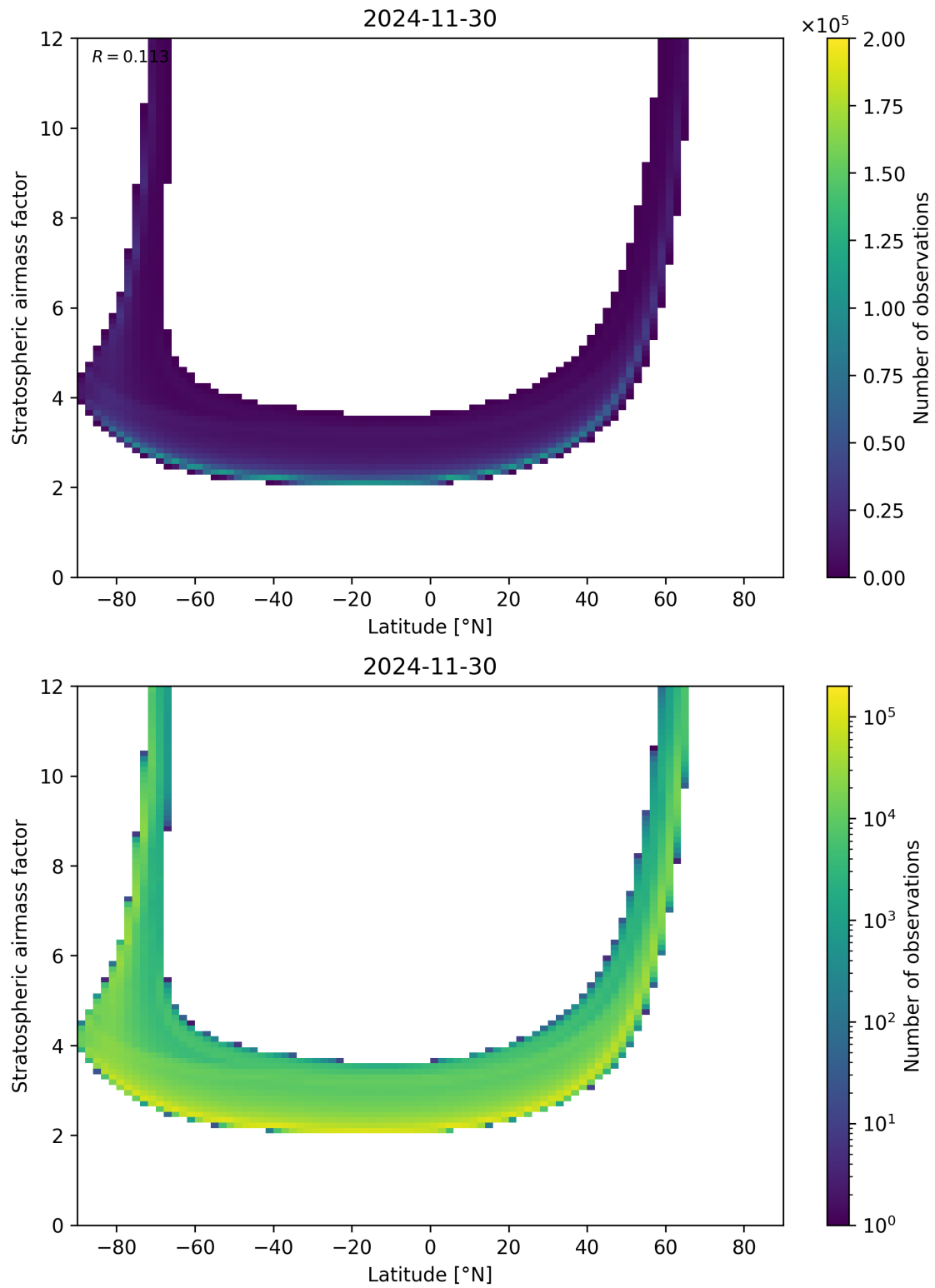
Figure 83: Scatter density plot of “Latitude” against “Stratospheric air mass factor” for 2024-11-30 to 2024-12-01.
