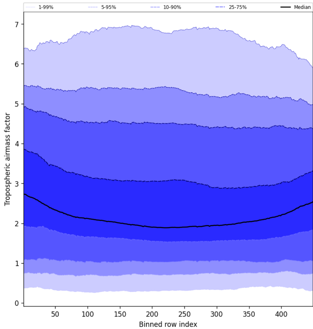
Figure 48: Along track statistics of “Tropospheric air mass factor” for 2024-11-30 to 2024-12-01
