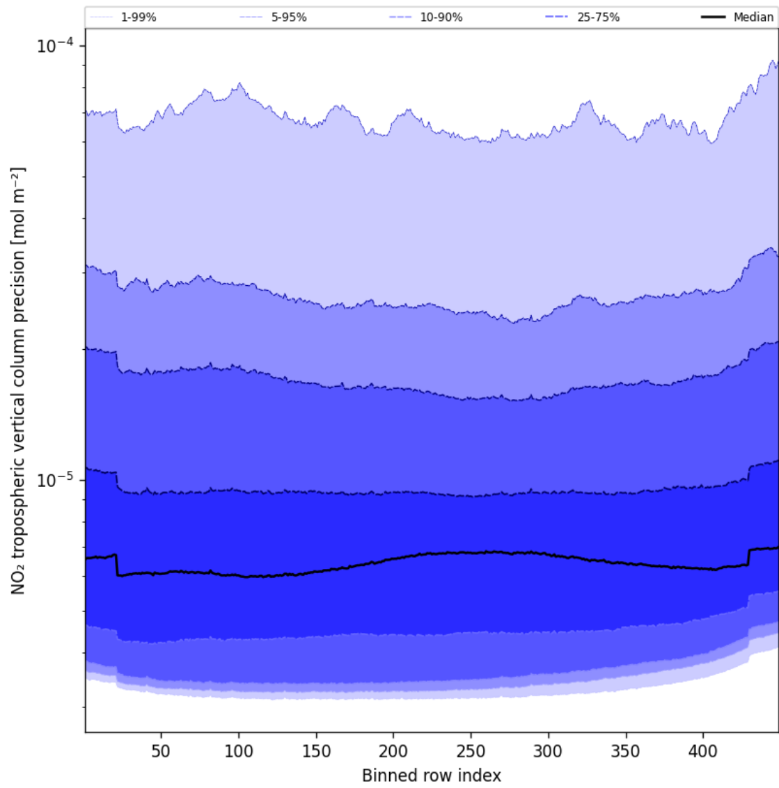
Figure 47: Along track statistics of “NO 2 tropospheric vertical column precision” for 2024-11-30 to 2024-12-01
