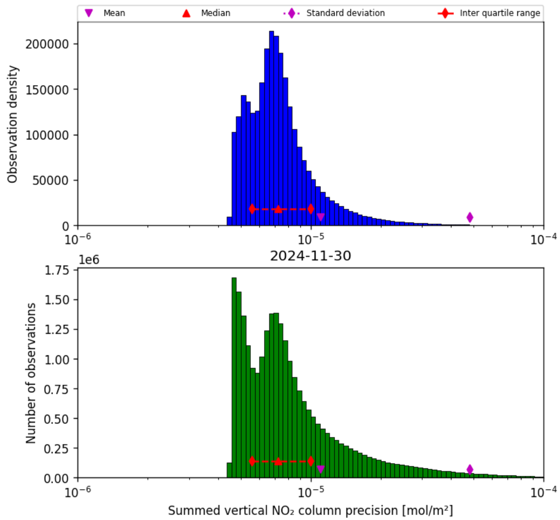
Figure 41: Histogram of "Summed vertical NO 2 column precision" for 2024-11-30 to 2024-12-01
