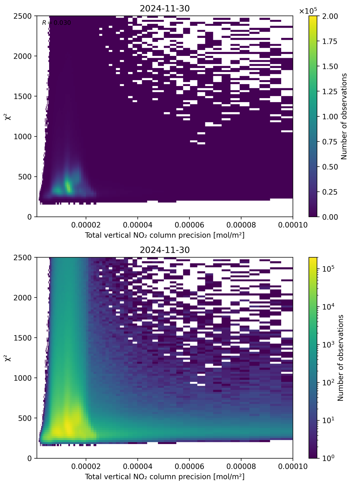
Figure 116: Scatter density plot of “Total vertical NO 2 column precision” against “ \chi^2 ” for 2024-11-30 to 2024-12-01.
