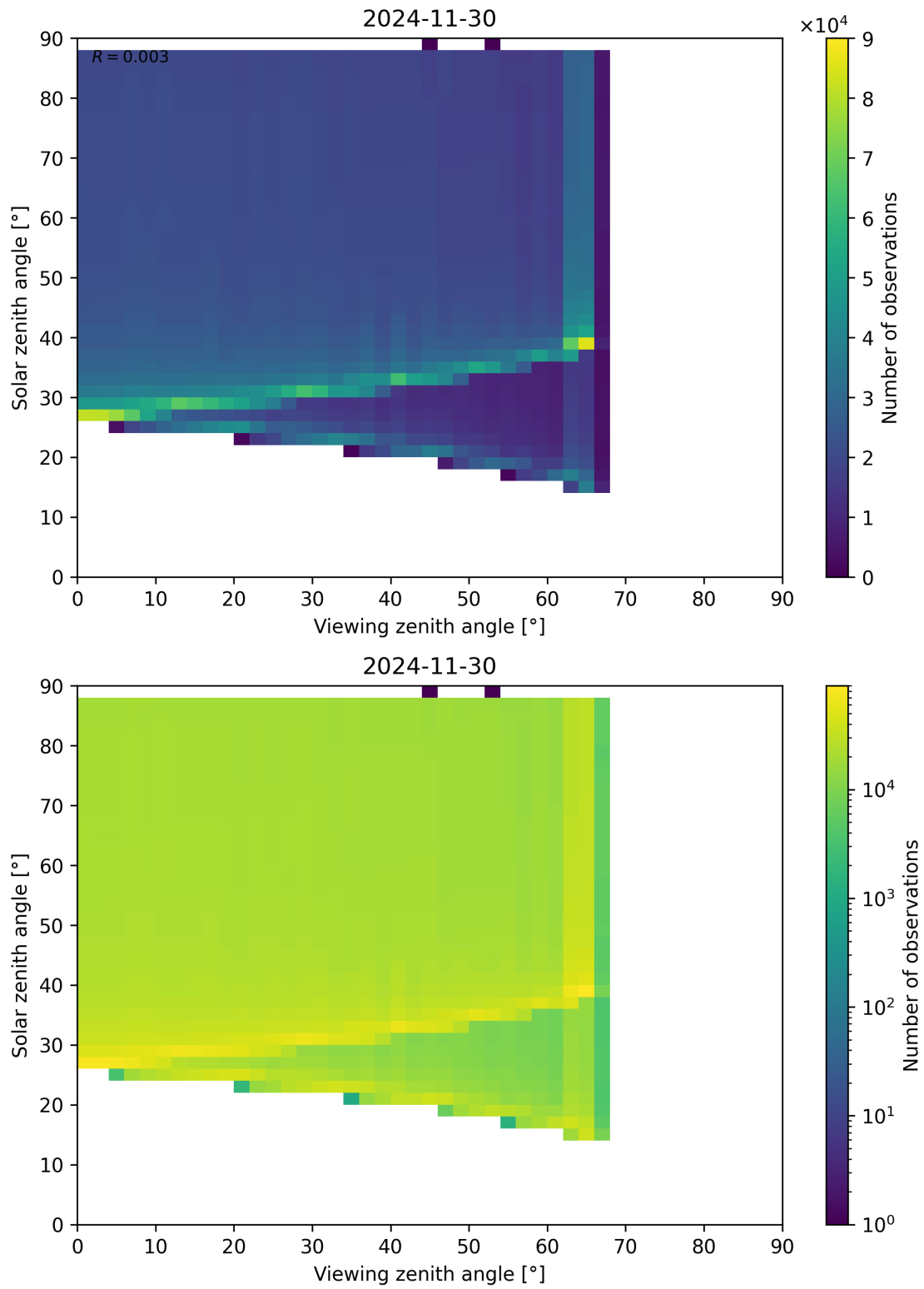
Figure 172: Scatter density plot of “Viewing zenith angle” against “Solar zenith angle” for 2024-11-30 to 2024-12-01.
