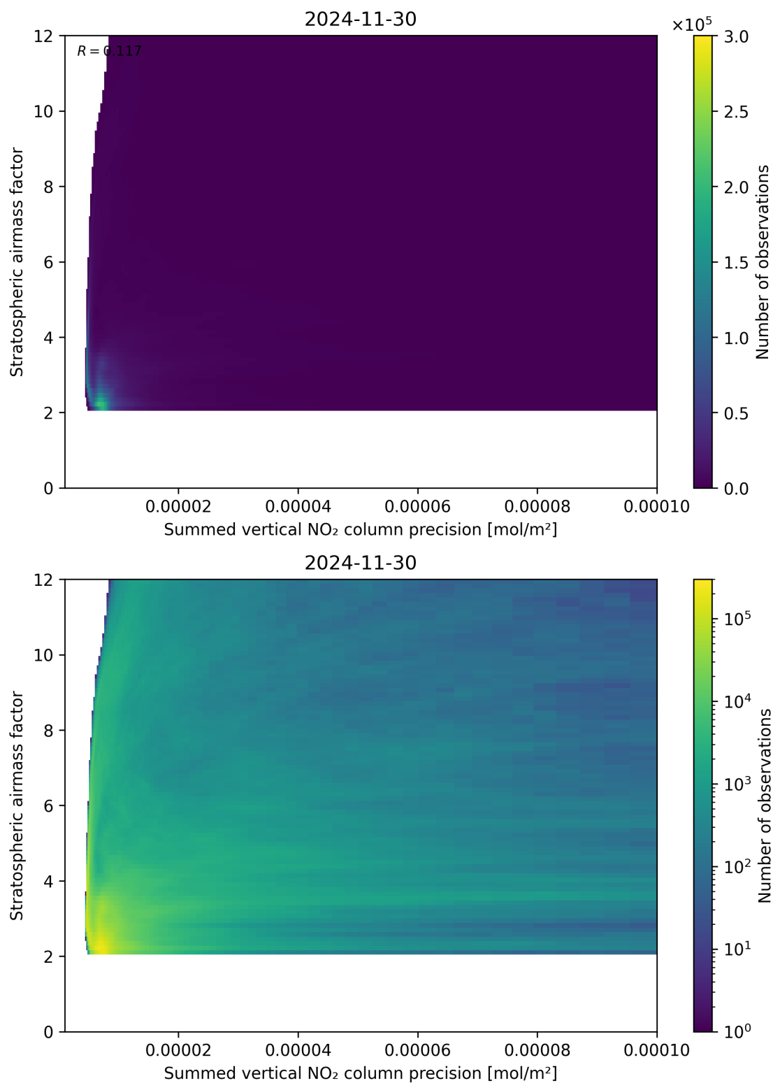
Figure 106: Scatter density plot of “Summed vertical NO 2 column precision” against “Stratospheric airmass factor” for 2024-11-30 to 2024-12-01.
