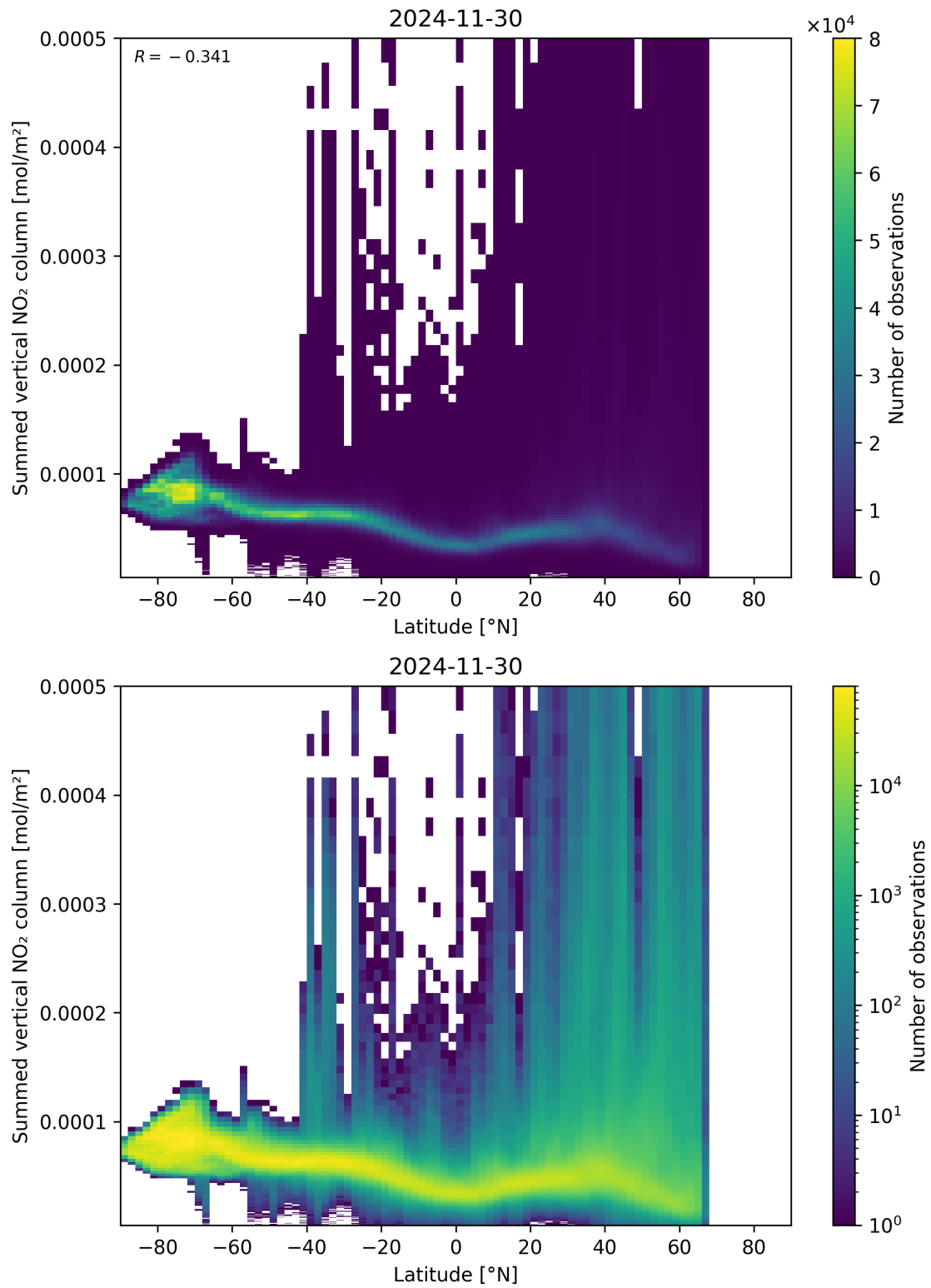
Figure 88: Scatter density plot of “Latitude” against “Summed vertical NO 2 column” for 2024-11-30 to 2024-12-01.
