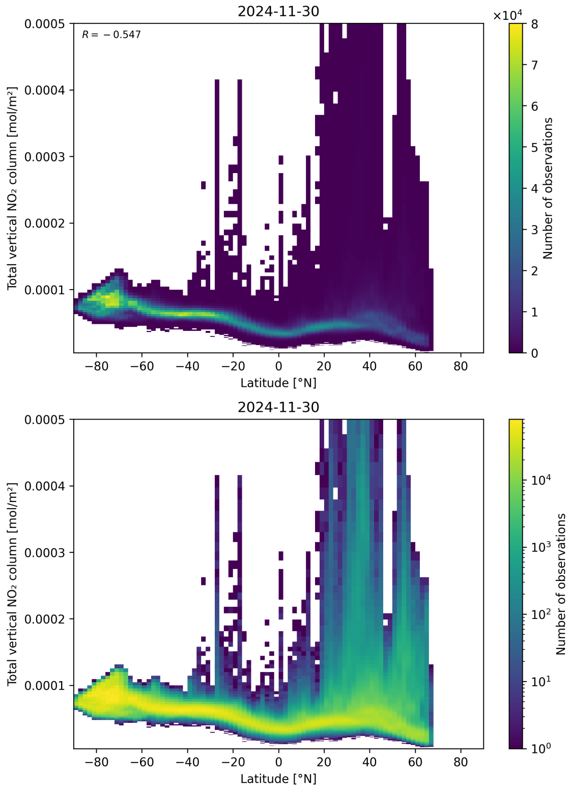
Figure 90: Scatter density plot of “Latitude” against “Total vertical NO 2 column” for 2024-11-30 to 2024-12-01.
