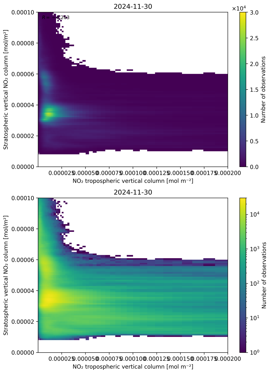
Figure 125: Scatter density plot of “NO 2 tropospheric vertical column” against “Stratospheric vertical NO 2 column” for 2024-11-30 to 2024-12-01.
