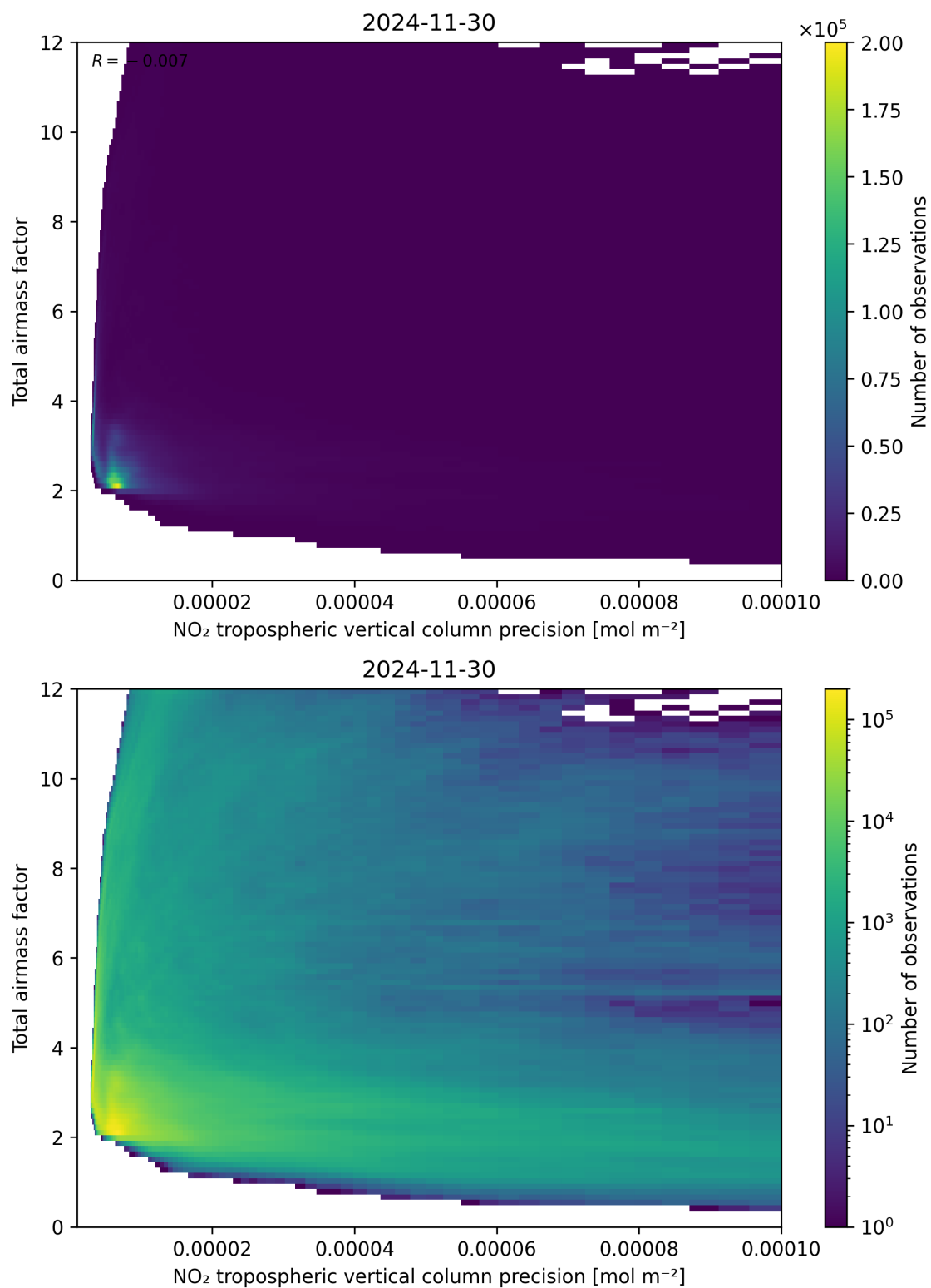
Figure 132: Scatter density plot of “NO 2 tropospheric vertical column precision” against “Total air mass factor” for 2024-11-30 to 2024-12-01.
