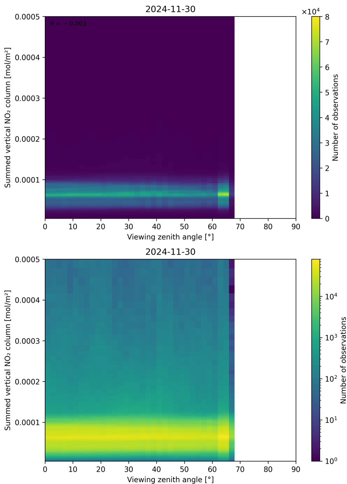
Figure 165: Scatter density plot of “Viewing zenith angle” against “Summed vertical NO 2 column” for 2024-11-30 to 2024-12-01.
