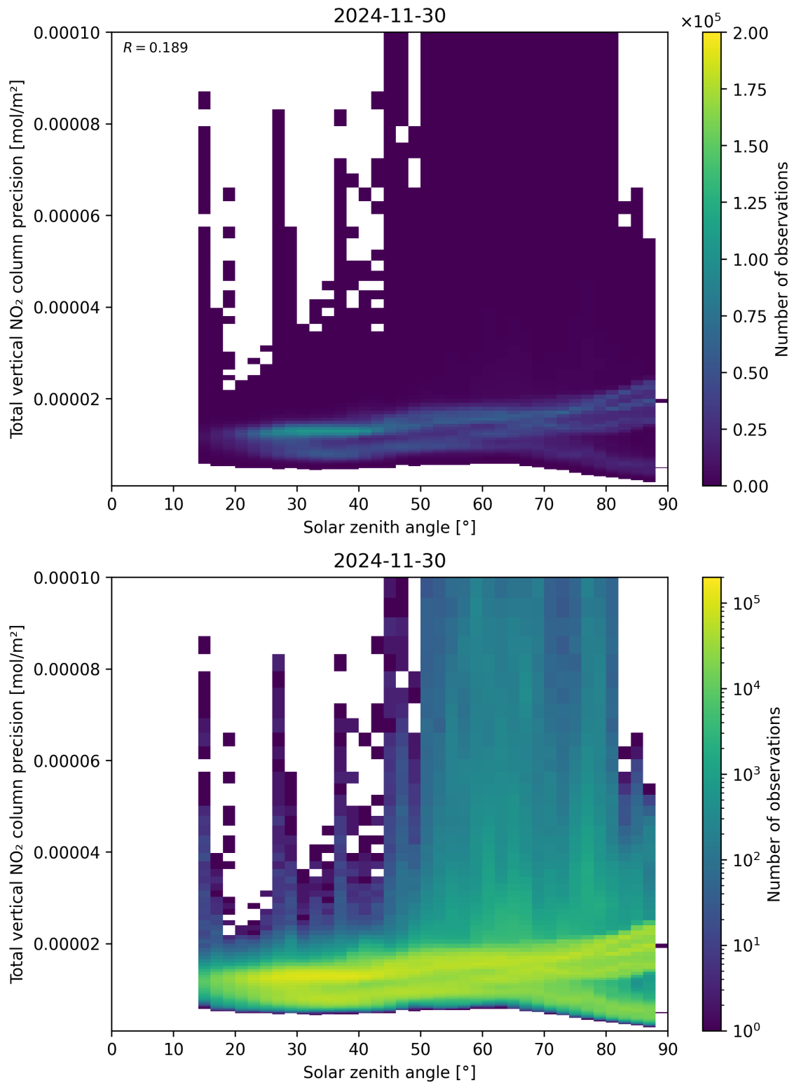
Figure 154: Scatter density plot of “Solar zenith angle” against “Total vertical NO 2 column precision” for 2024-11-30 to 2024-12-01.
