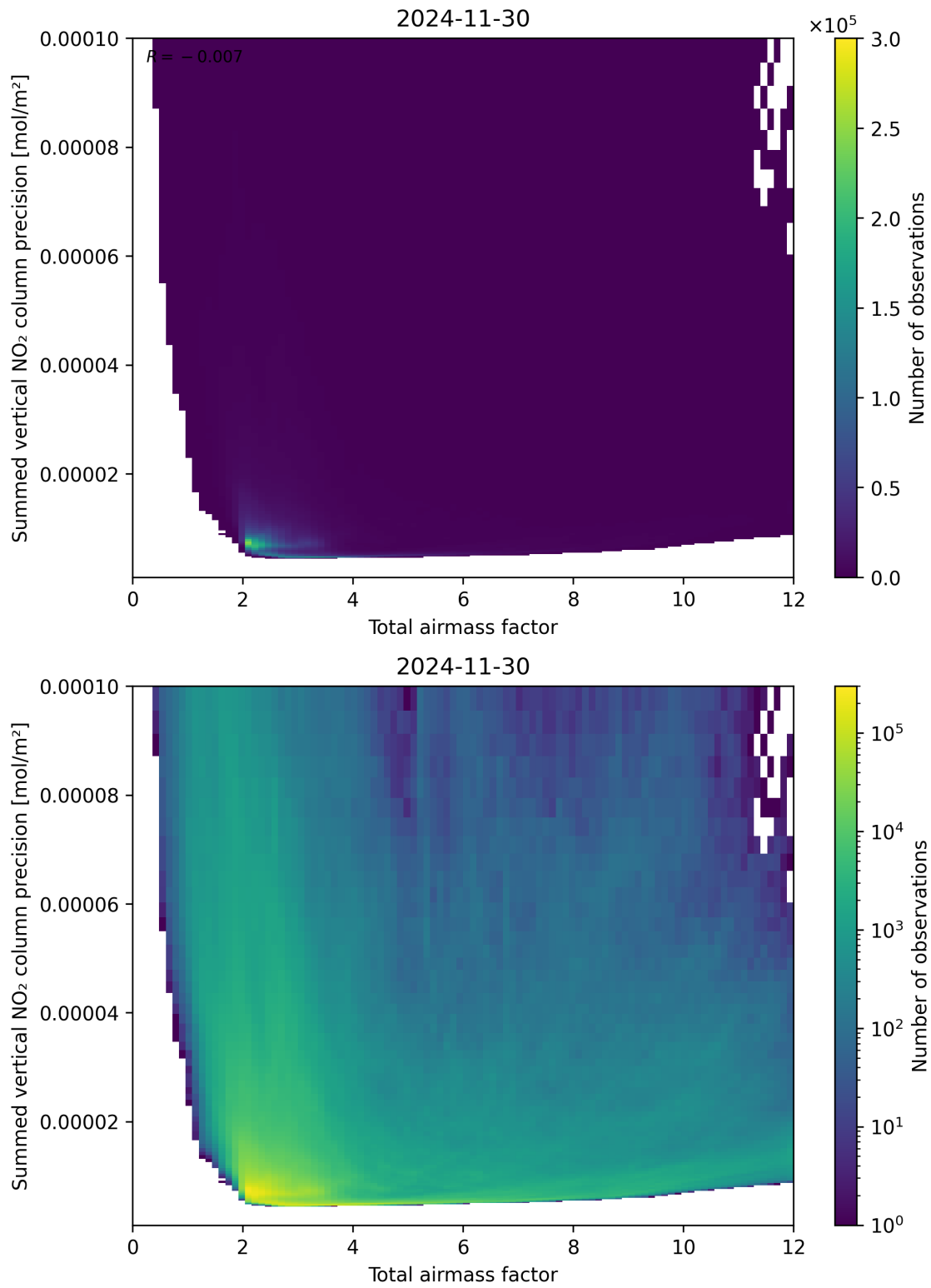
Figure 66: Scatter density plot of “Total airmass factor” against “Summed vertical NO 2 column precision” for 2024-11-30 to 2024-12-01.
