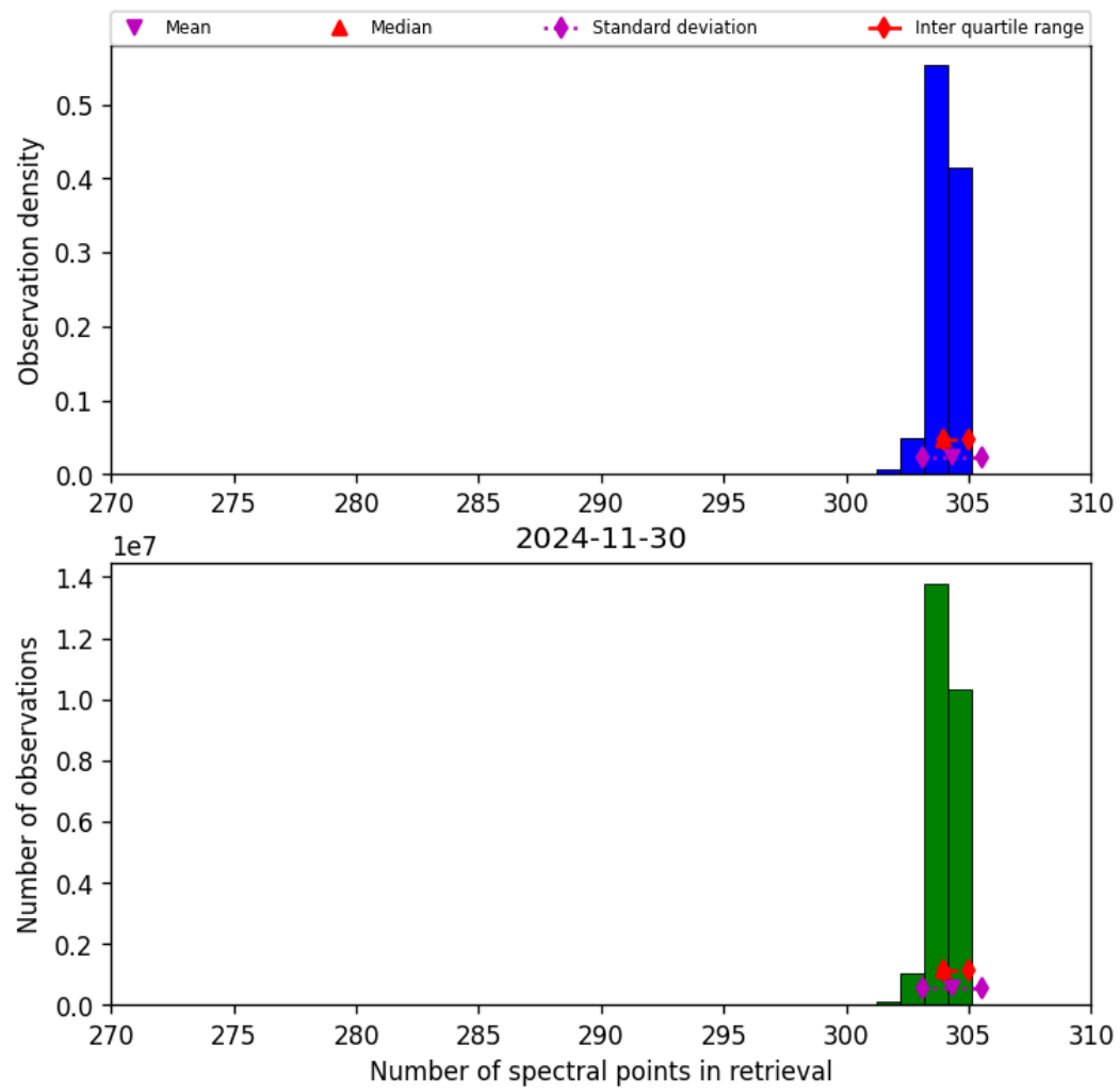
Figure 33: Histogram of “Number of spectral points in retrieval” for 2024-11-30 to 2024-12-01
