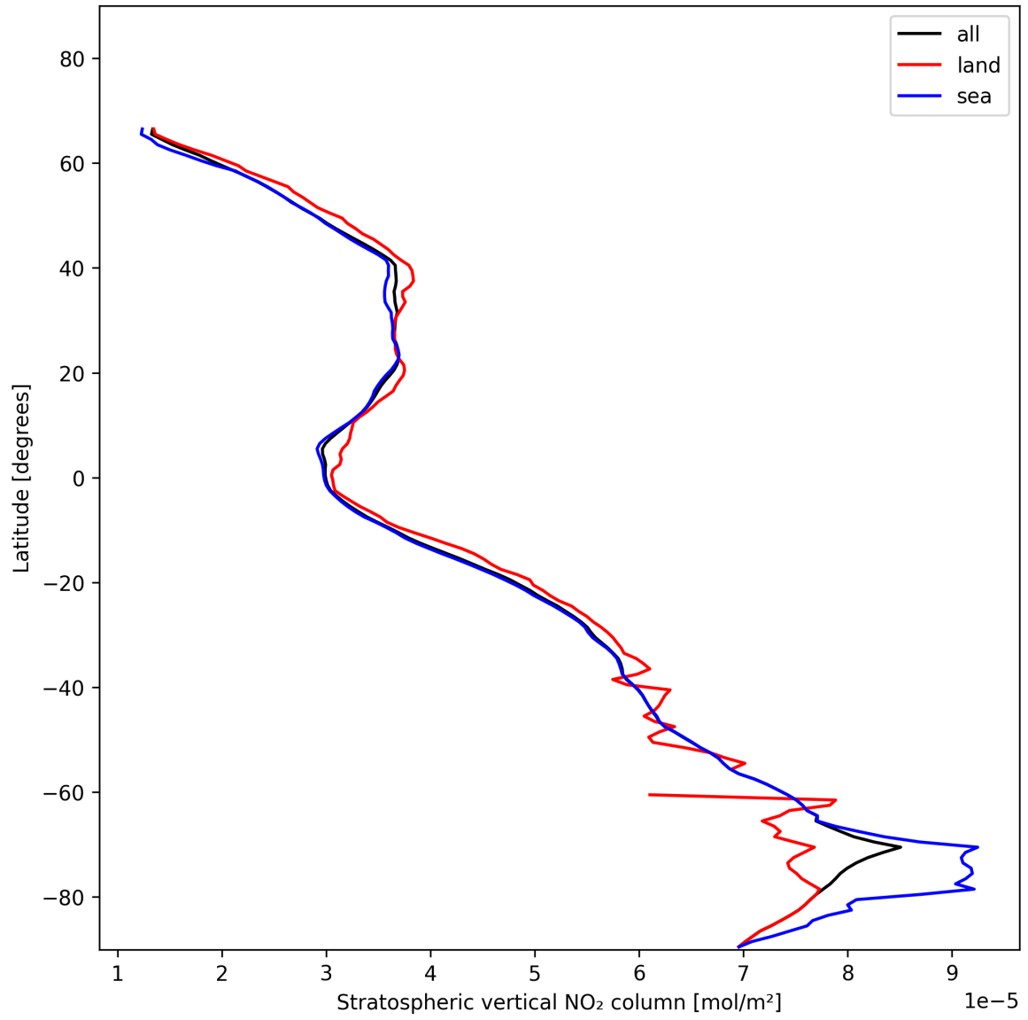
Figure 19: Zonal average of “Stratospheric vertical NO 2 column” for 2024-11-30 to 2024-12-02.
