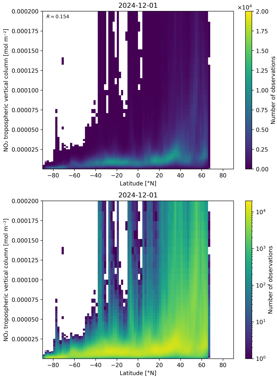
Figure 92: Scatter density plot of “Latitude” against “NO 2 tropospheric vertical column” for 2024-11-30 to 2024-12-02.
