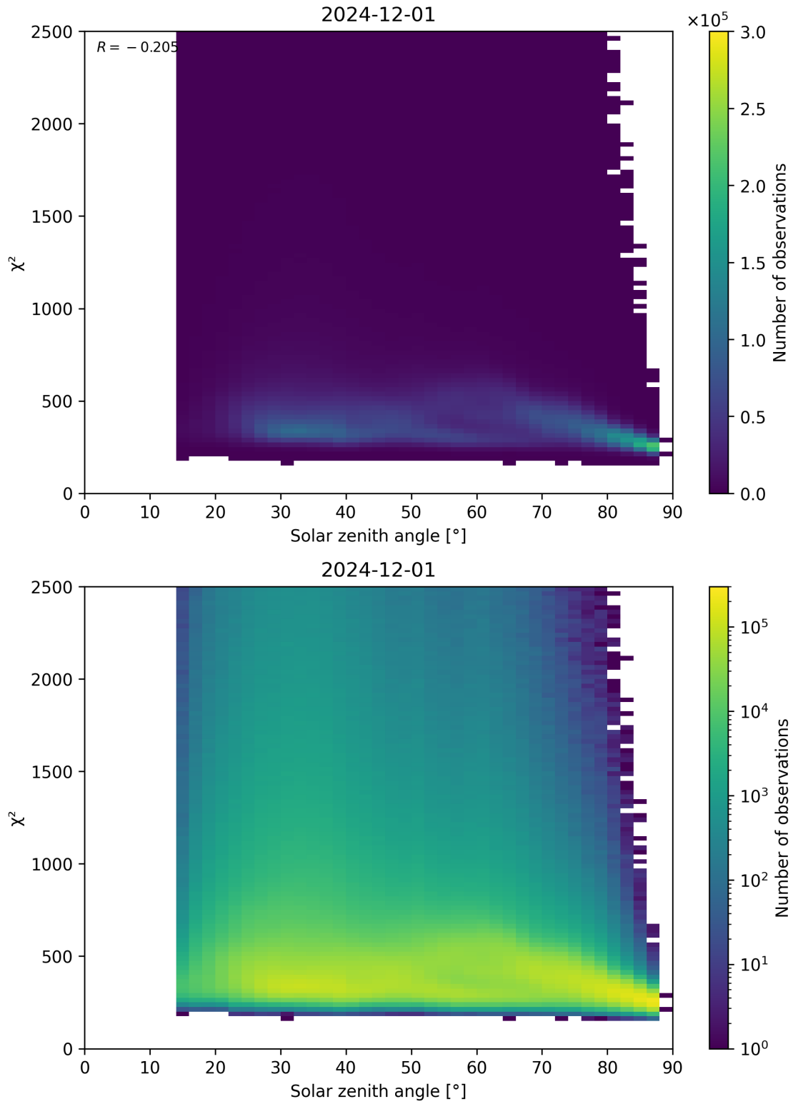
Figure 148: Scatter density plot of “Solar zenith angle” against “ \chi^2 ” for 2024-11-30 to 2024-12-02.
