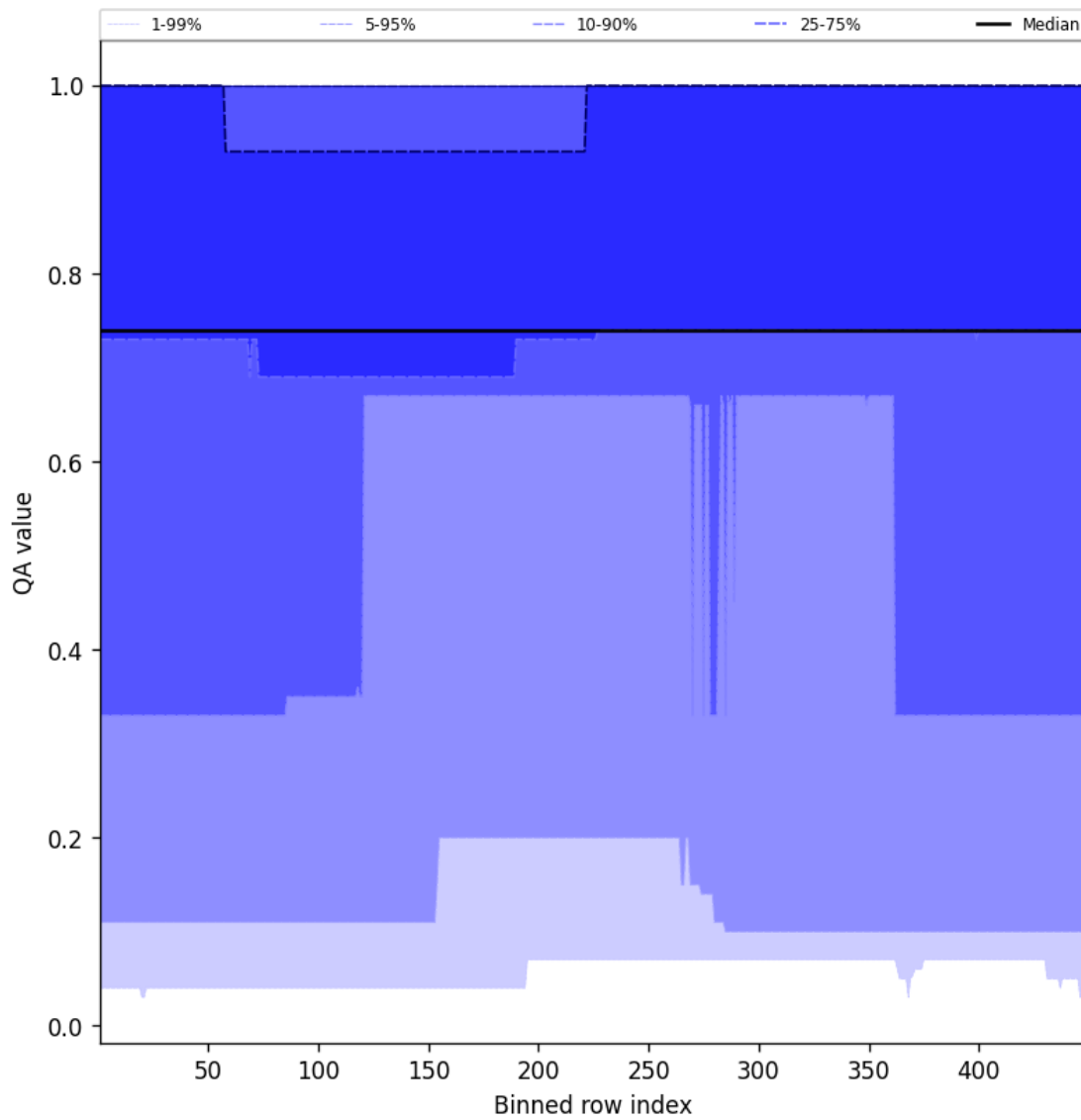
Figure 45: Along track statistics of “QA value” for 2024-11-30 to 2024-12-02
