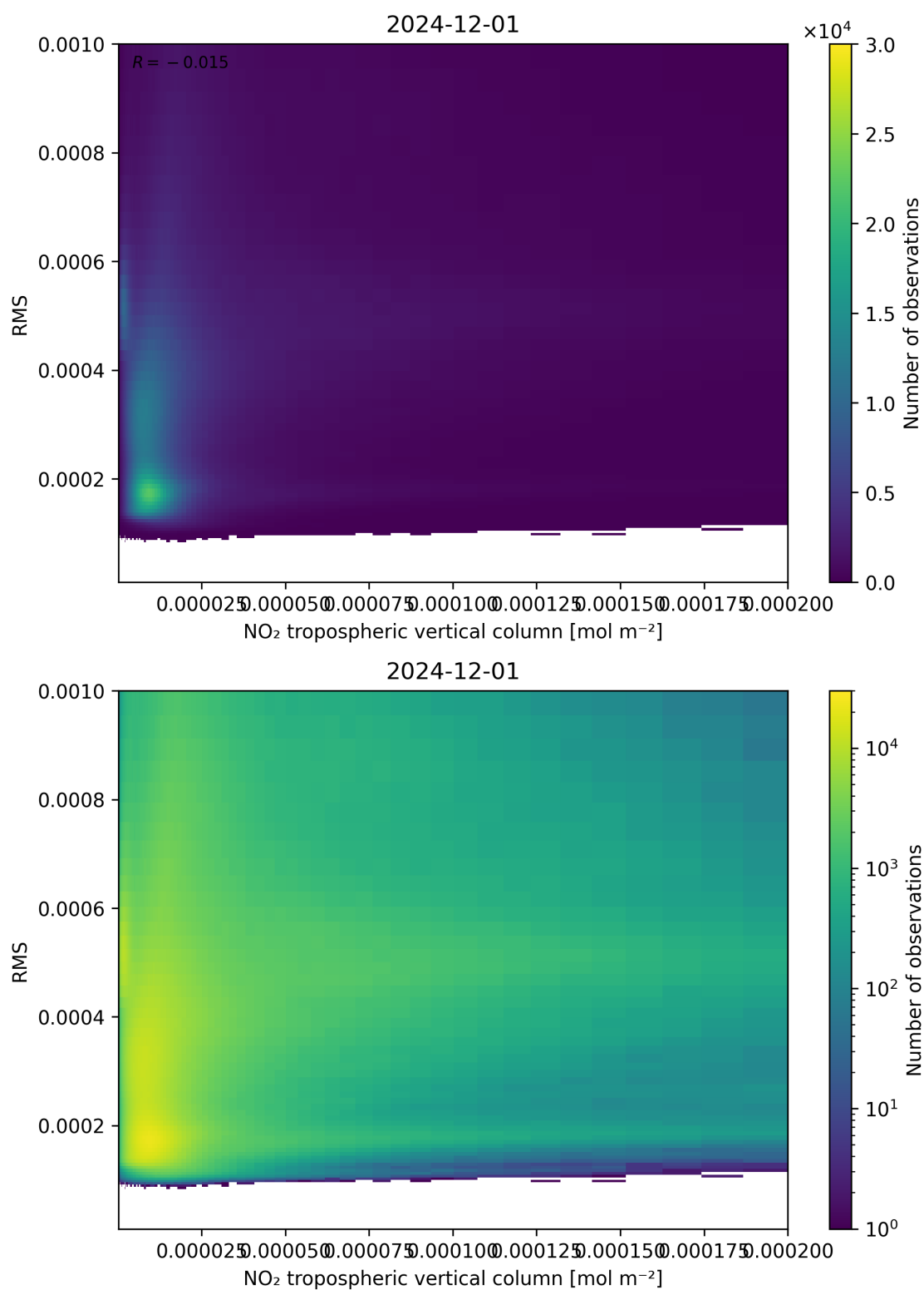
Figure 142: Scatter density plot of “NO 2 tropospheric vertical column” against “RMS” for 2024-11-30 to 2024-12-02.
