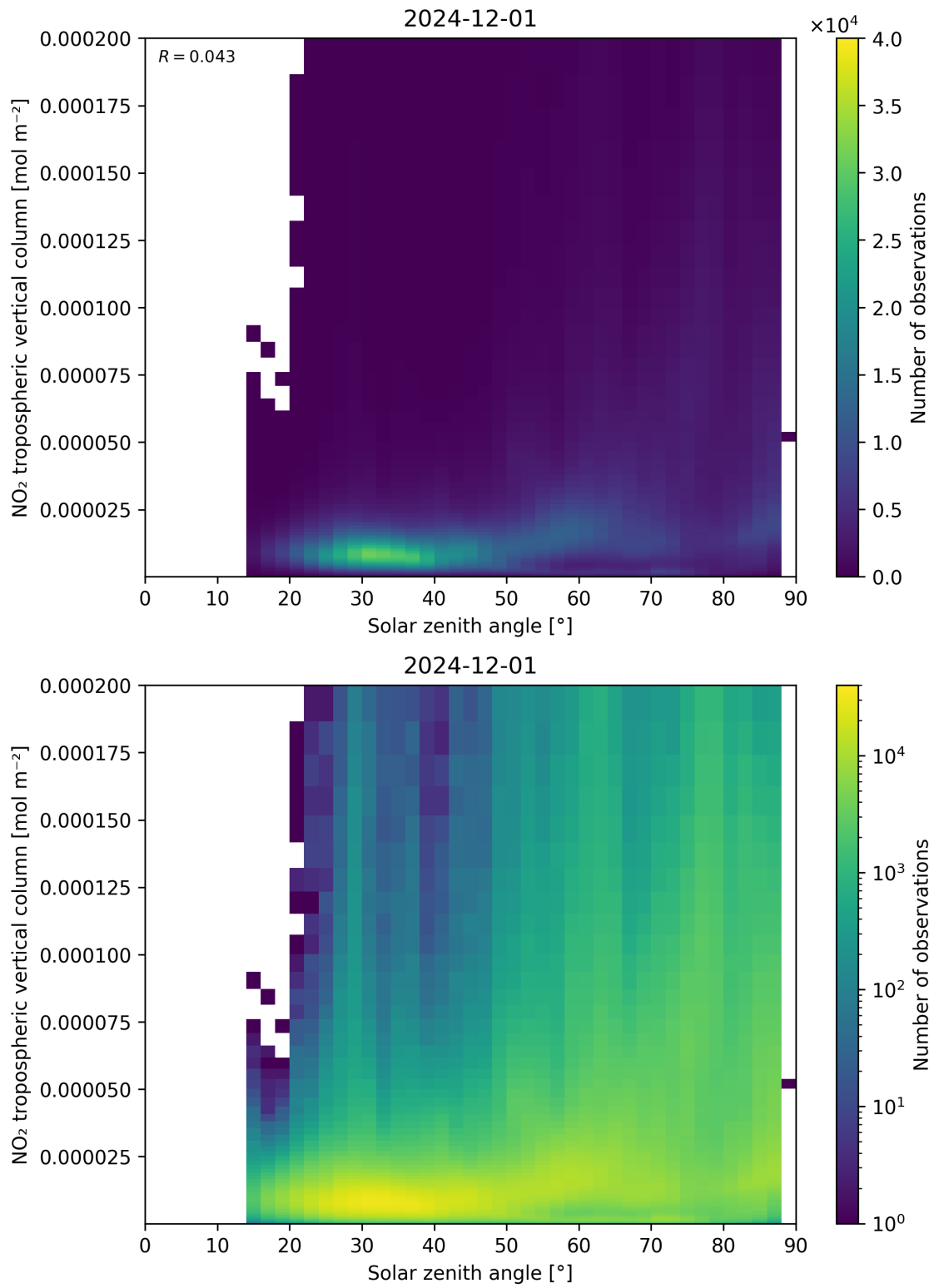
Figure 155: Scatter density plot of “Solar zenith angle” against “NO 2 tropospheric vertical column” for 2024-11-30 to 2024-12-02.
