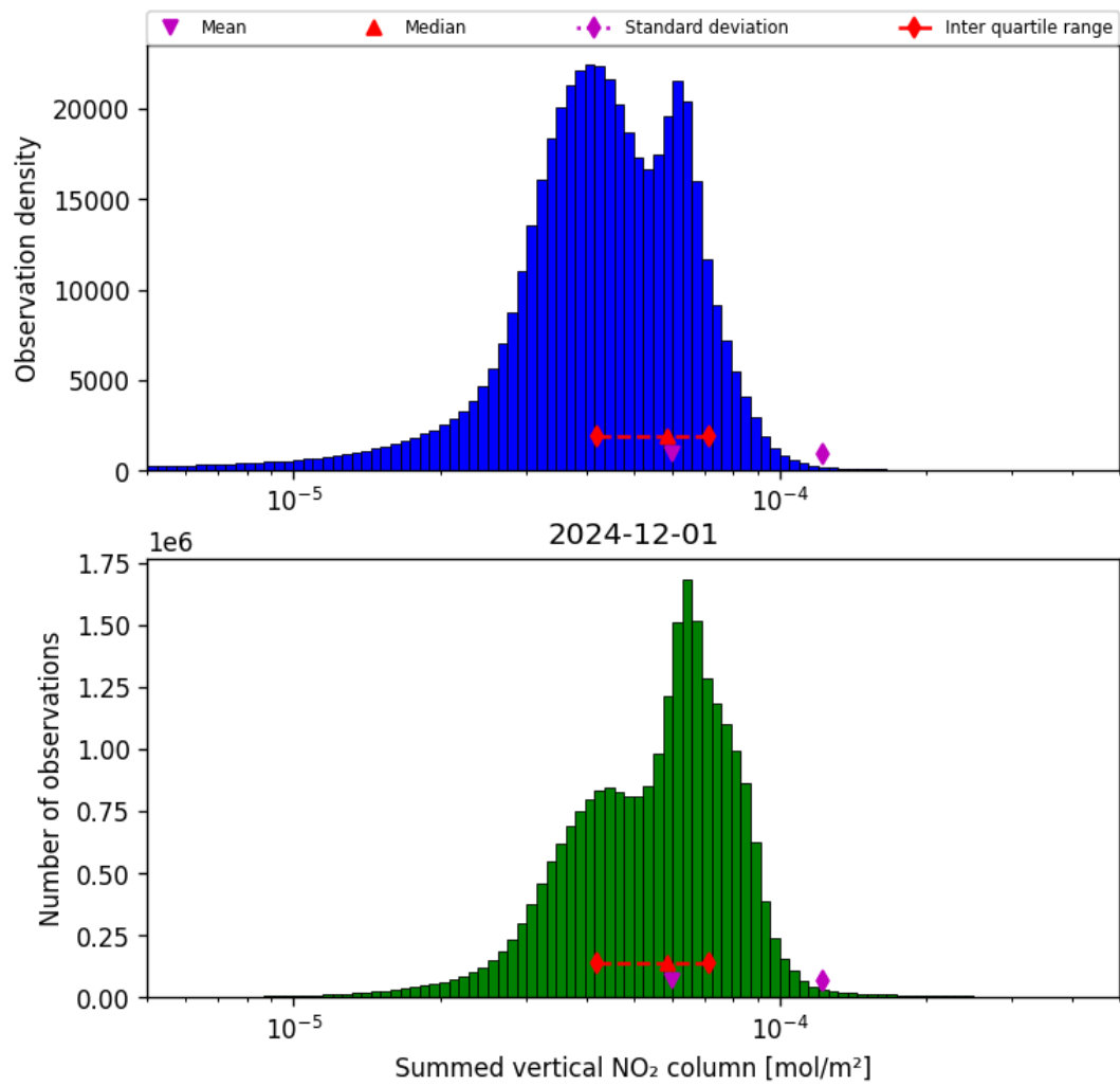
Figure 40: Histogram of “Summed vertical NO 2 column” for 2024-11-30 to 2024-12-02
