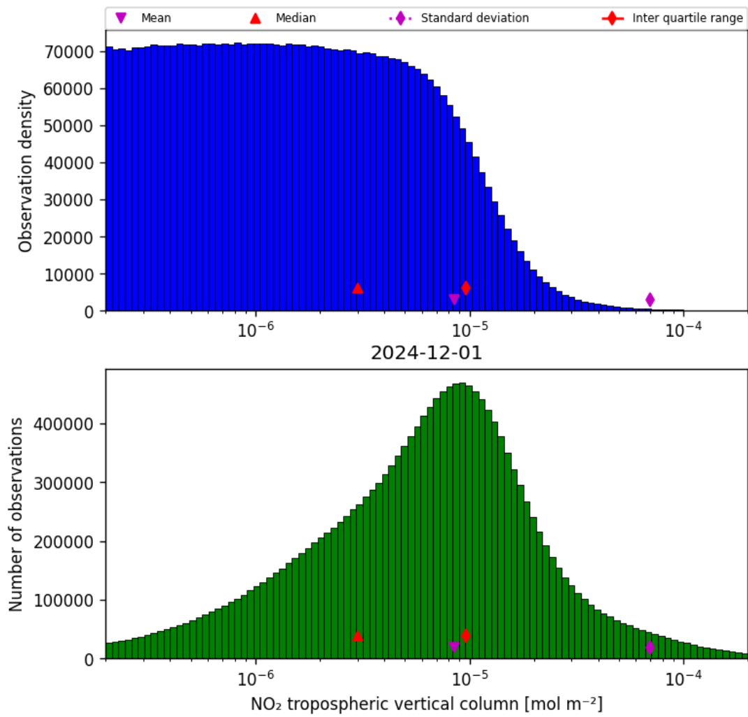
Figure 29: Histogram of “NO 2 tropospheric vertical column” for 2024-11-30 to 2024-12-02
