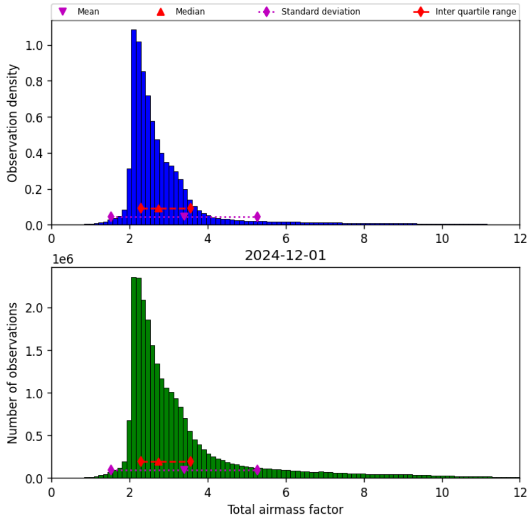
Figure 32: Histogram of “Total airmass factor” for 2024-11-30 to 2024-12-02
