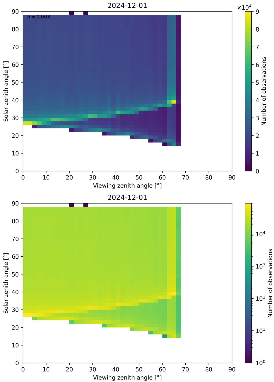
Figure 172: Scatter density plot of “Viewing zenith angle” against “Solar zenith angle” for 2024-11-30 to 2024-12-02.
