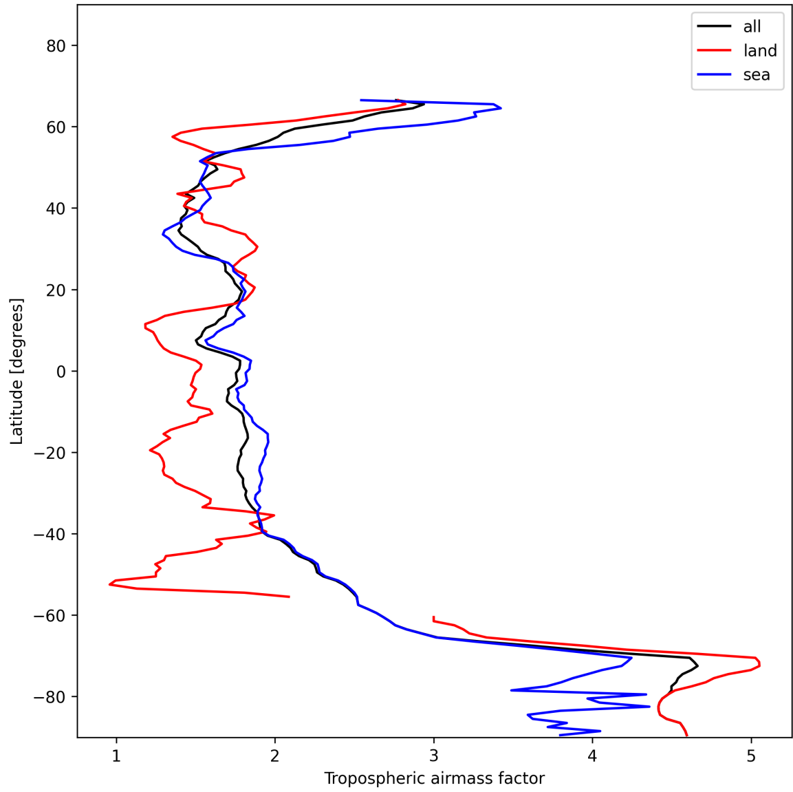
Figure 14: Zonal average of “Tropospheric airmass factor” for 2024-11-30 to 2024-12-02.
