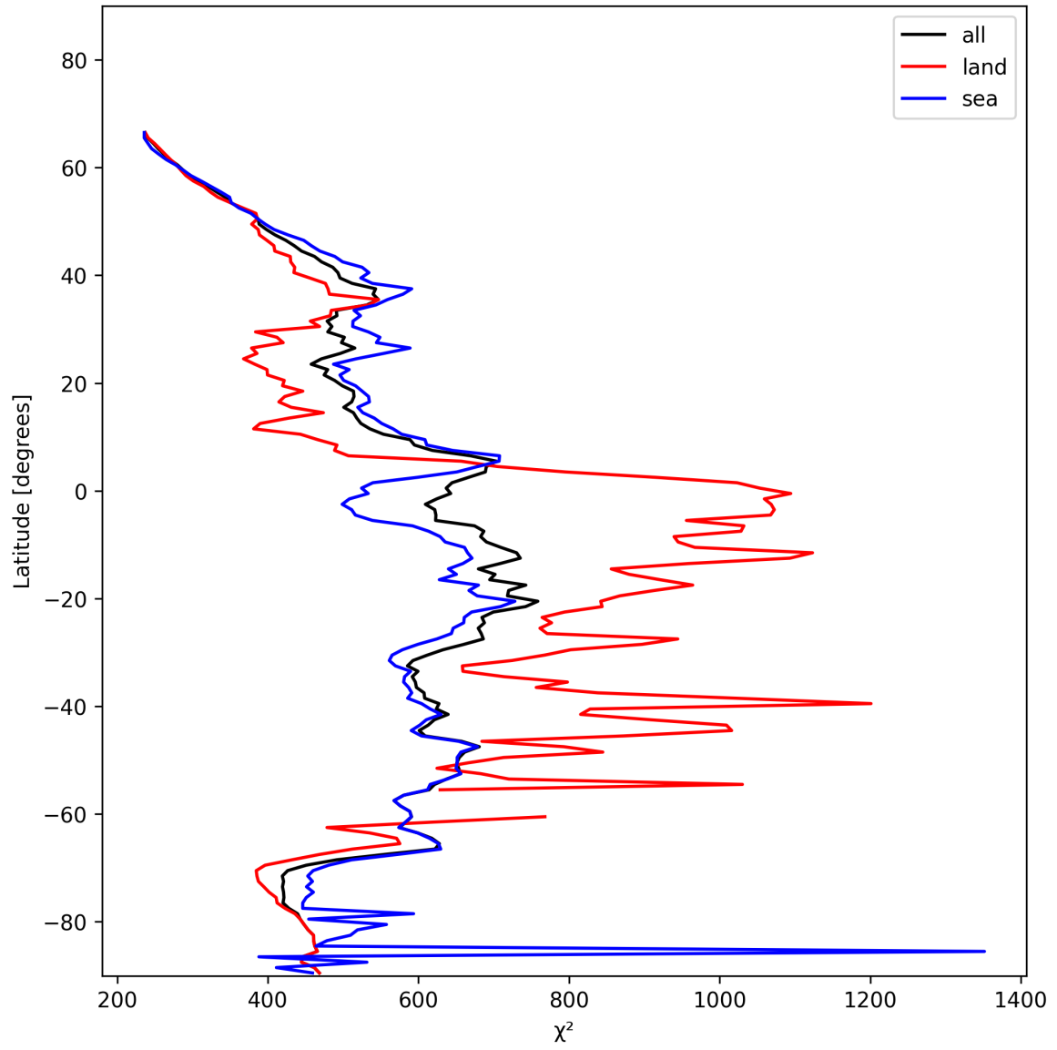
Figure 25: Zonal average of “ \chi^2 ” for 2024-11-30 to 2024-12-02.
