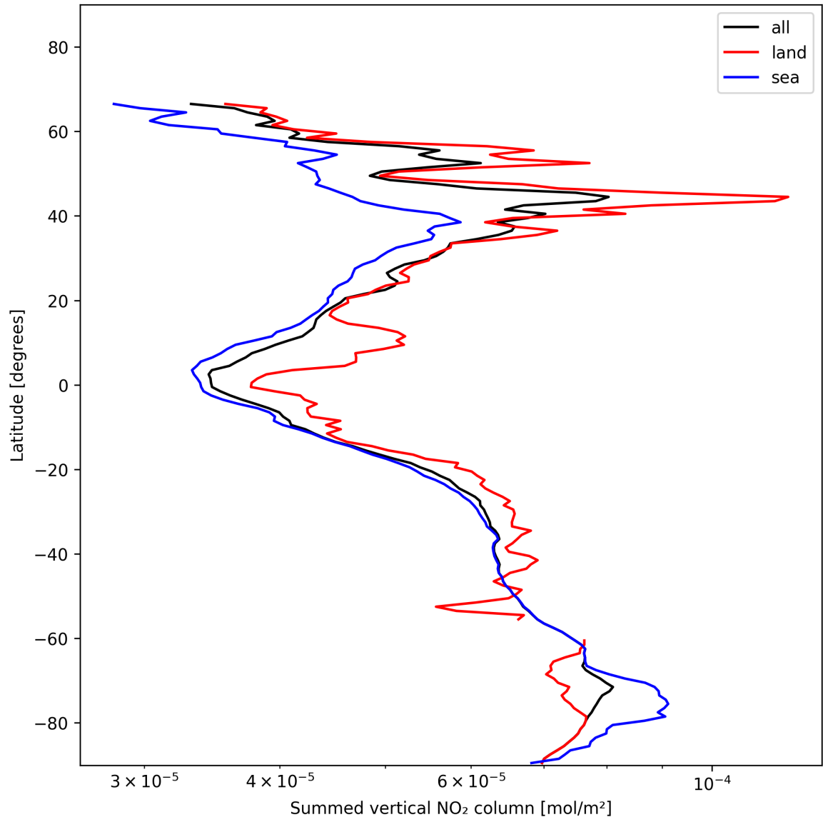
Figure 23: Zonal average of “Summed vertical NO 2 column” for 2024-11-30 to 2024-12-02.
