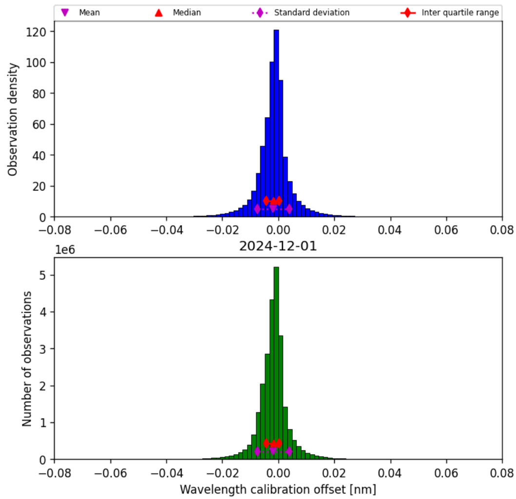
Figure 35: Histogram of “Wavelength calibration offset” for 2024-11-30 to 2024-12-02
