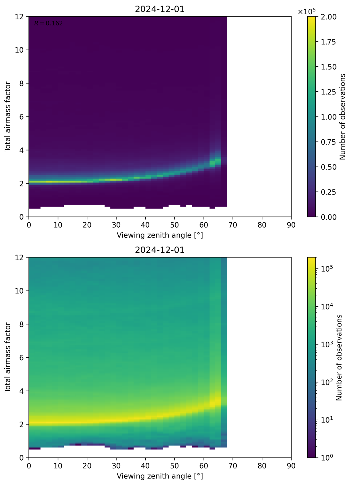
Figure 160: Scatter density plot of “Viewing zenith angle” against “Total airmass factor” for 2024-11-30 to 2024-12-02.
