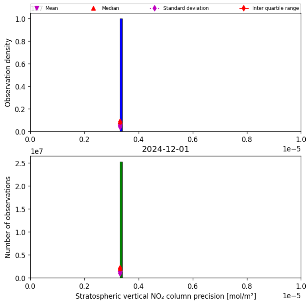
Figure 37: Histogram of “Stratospheric vertical NO 2 column precision” for 2024-11-30 to 2024-12-02
