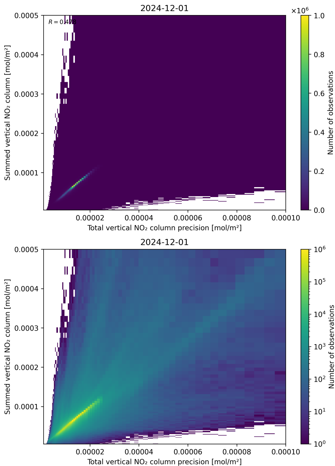
Figure 117: Scatter density plot of “Total vertical NO 2 column precision” against “Summed vertical NO 2 column” for 2024-11-30 to 2024-12-02.
