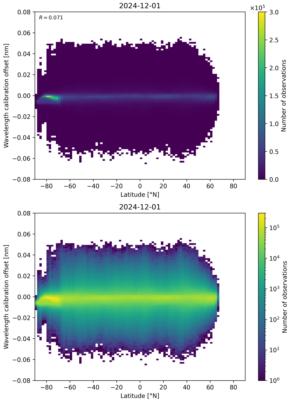
Figure 95: Scatter density plot of “Latitude” against “Wavelength calibration offset” for 2024-11-30 to 2024-12-02.
