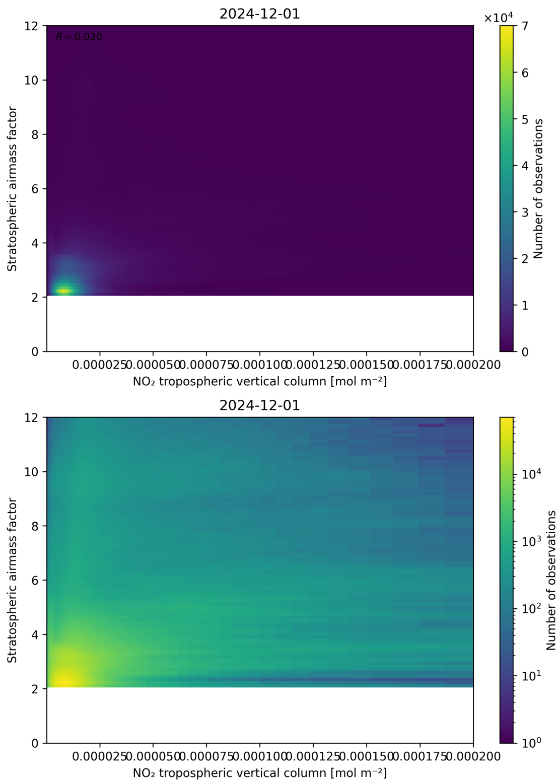
Figure 121: Scatter density plot of “NO 2 tropospheric vertical column” against “Stratospheric airmass factor” for 2024-11-30 to 2024-12-02.
