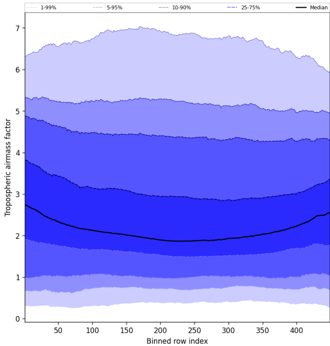
Figure 48: Along track statistics of “Tropospheric air mass factor” for 2024-11-30 to 2024-12-02
