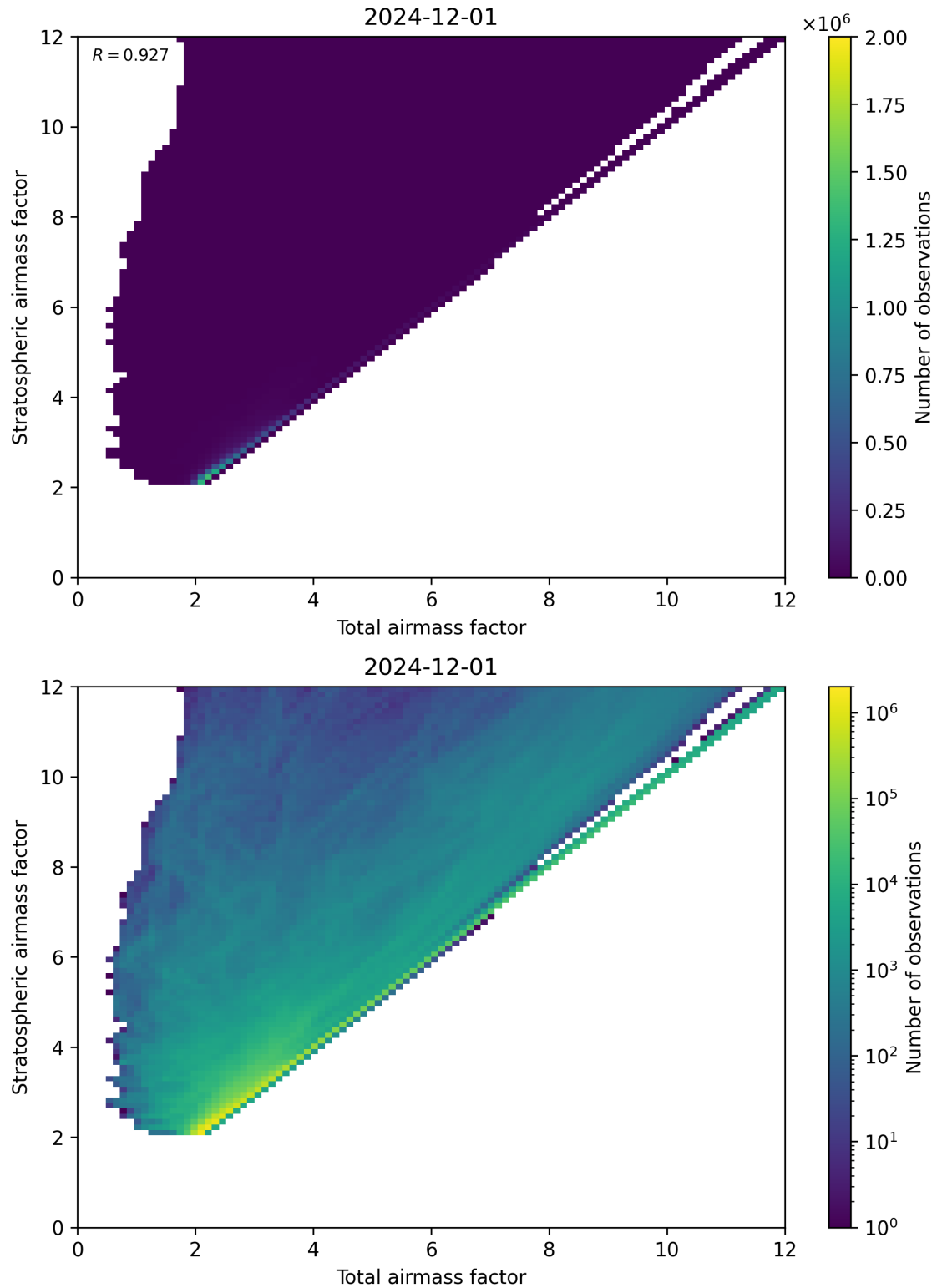
Figure 62: Scatter density plot of “Total airmass factor” against “Stratospheric airmass factor” for 2024-11-30 to 2024-12-02.
