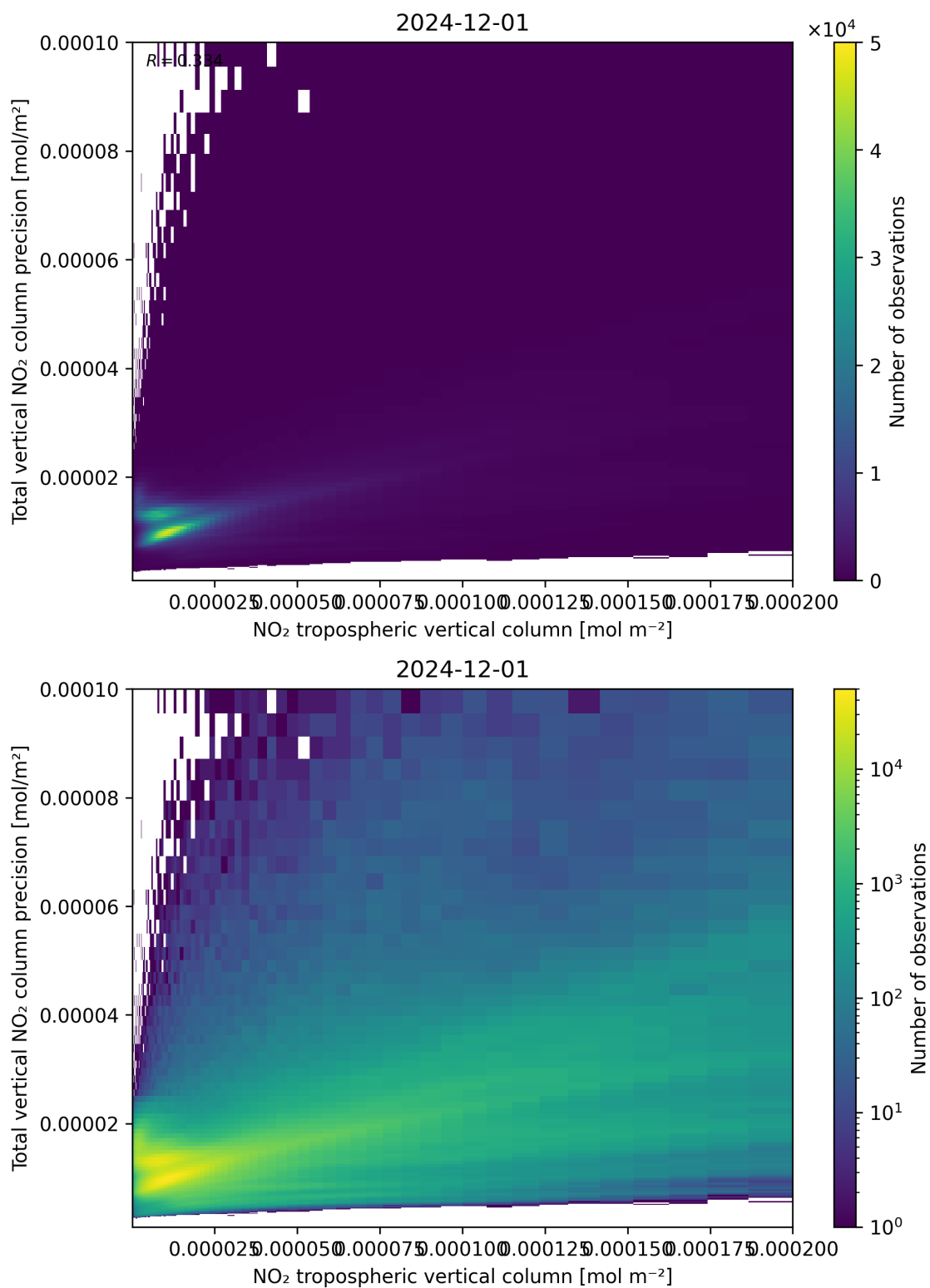
Figure 129: Scatter density plot of “NO 2 tropospheric vertical column” against “Total vertical NO 2 column precision” for 2024-11-30 to 2024-12-02.
