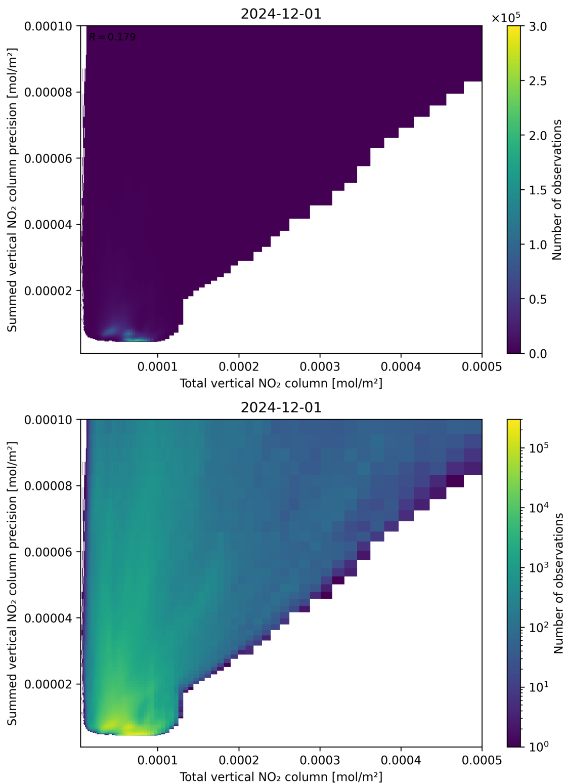
Figure 113: Scatter density plot of “Total vertical NO 2 column” against “Summed vertical NO 2 column precision” for 2024-11-30 to 2024-12-02.
