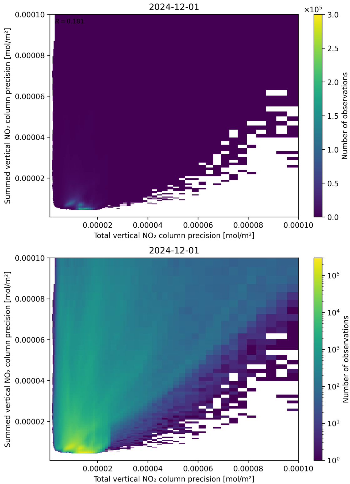
Figure 118: Scatter density plot of “Total vertical NO 2 column precision” against “Summed vertical NO 2 column precision” for 2024-11-30 to 2024-12-02.
