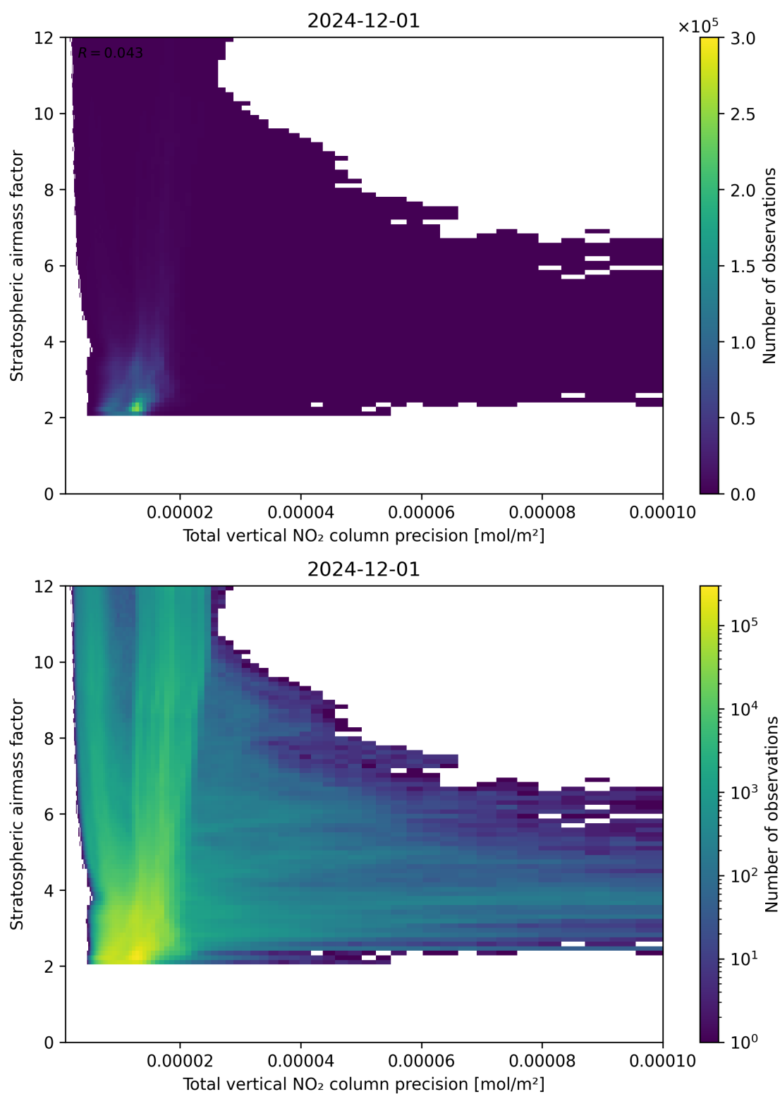
Figure 115: Scatter density plot of “Total vertical NO 2 column precision” against “Stratospheric air mass factor” for 2024-11-30 to 2024-12-02.
