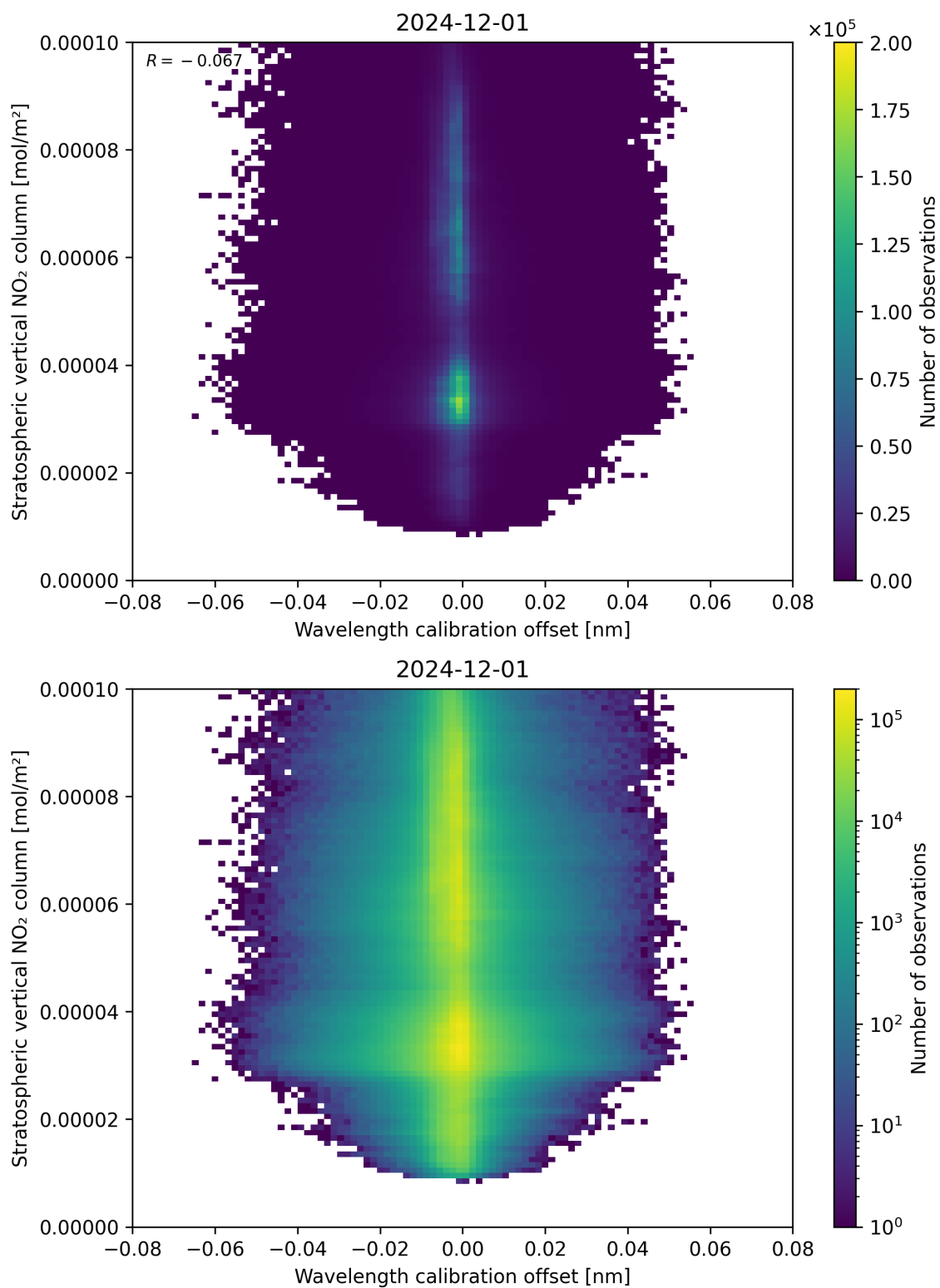
Figure 176: Scatter density plot of “Wavelength calibration offset” against “Stratospheric vertical NO 2 column” for 2024-11-30 to 2024-12-02.
