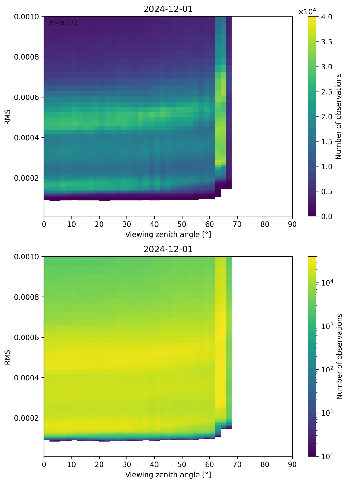
Figure 171: Scatter density plot of “Viewing zenith angle” against “RMS” for 2024-11-30 to 2024-12-02.
