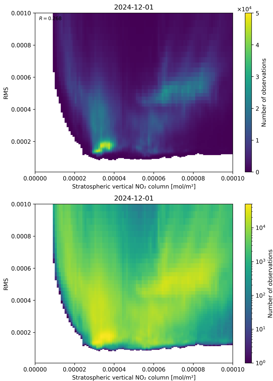
Figure 102: Scatter density plot of “Stratospheric vertical NO 2 column” against “RMS” for 2024-11-30 to 2024-12-02.
