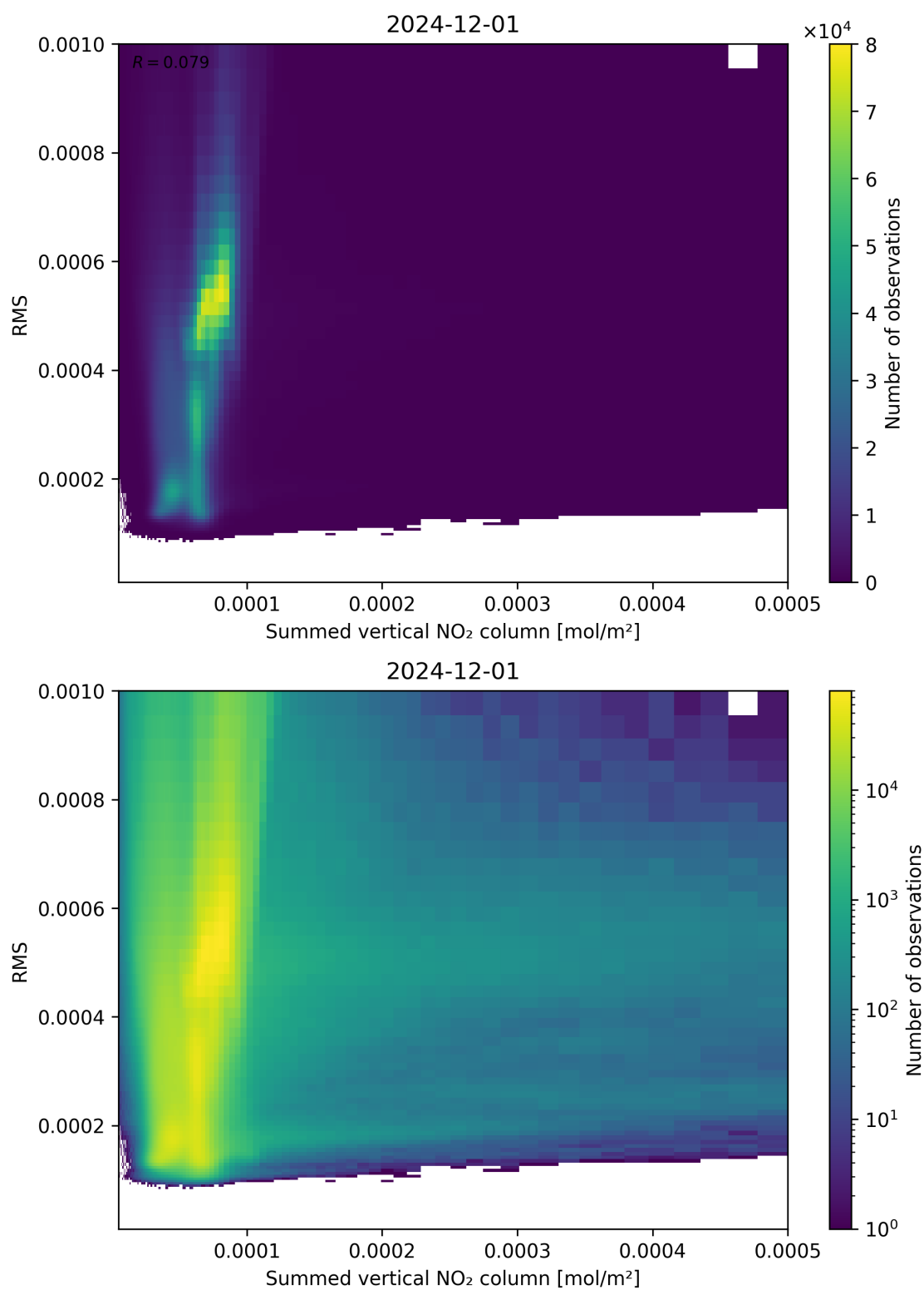
Figure 109: Scatter density plot of “Summed vertical NO 2 column” against “RMS” for 2024-11-30 to 2024-12-02.
