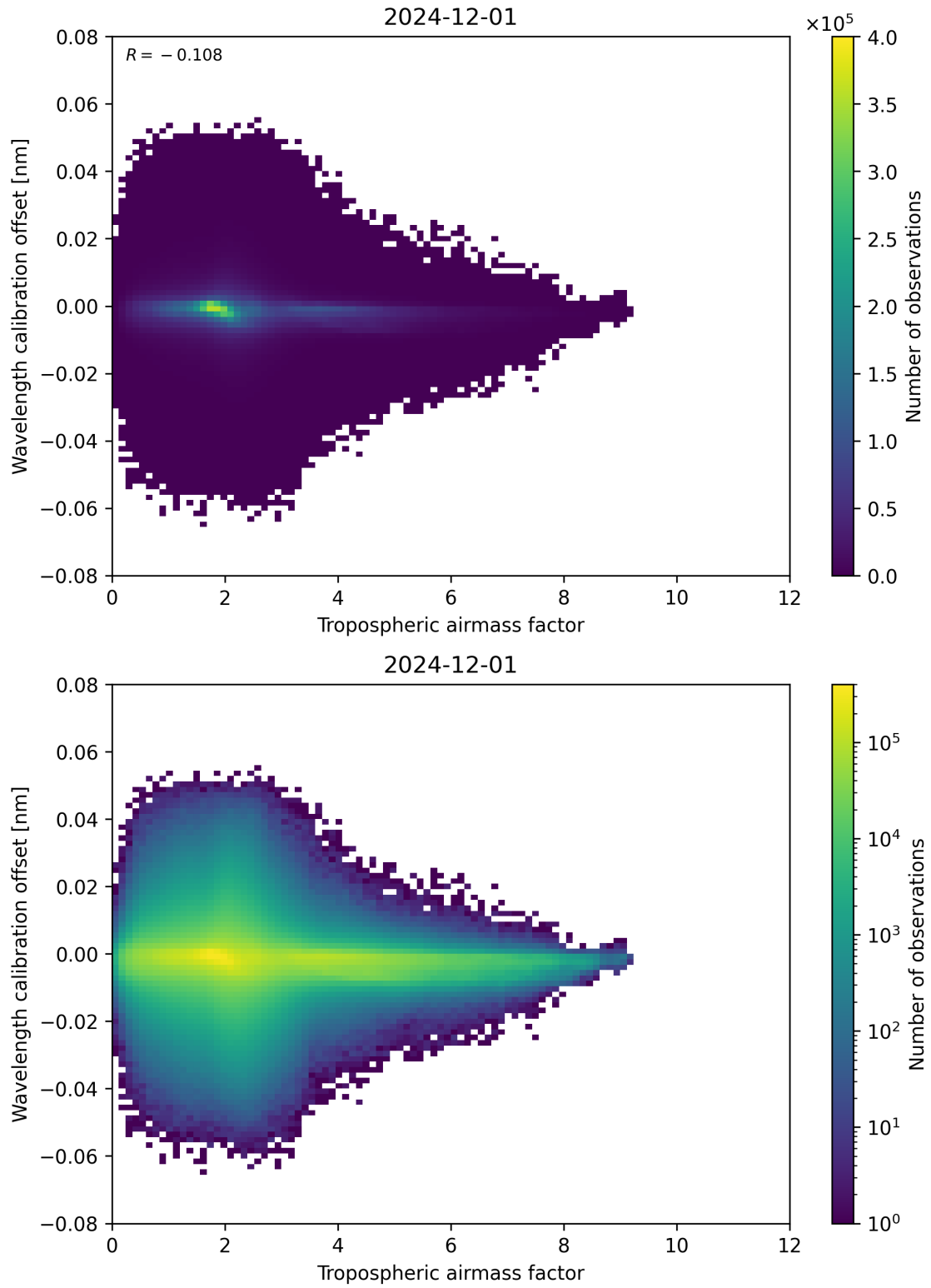
Figure 80: Scatter density plot of “Tropospheric airmass factor” against “Wavelength calibration offset” for 2024-11-30 to 2024-12-02.
