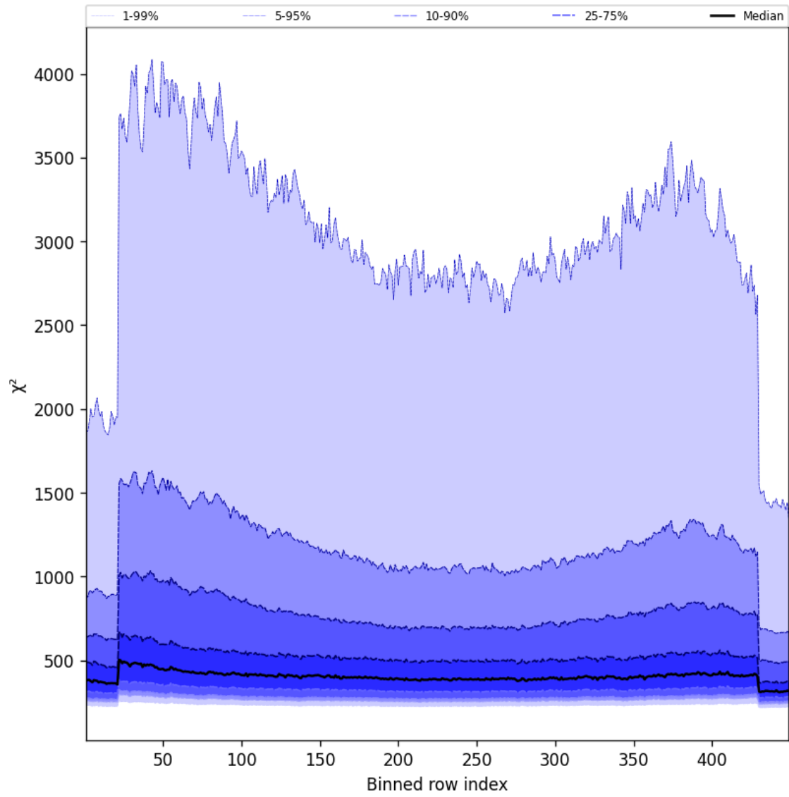
Figure 59: Along track statistics of “ \chi^2 ” for 2024-11-30 to 2024-12-02
