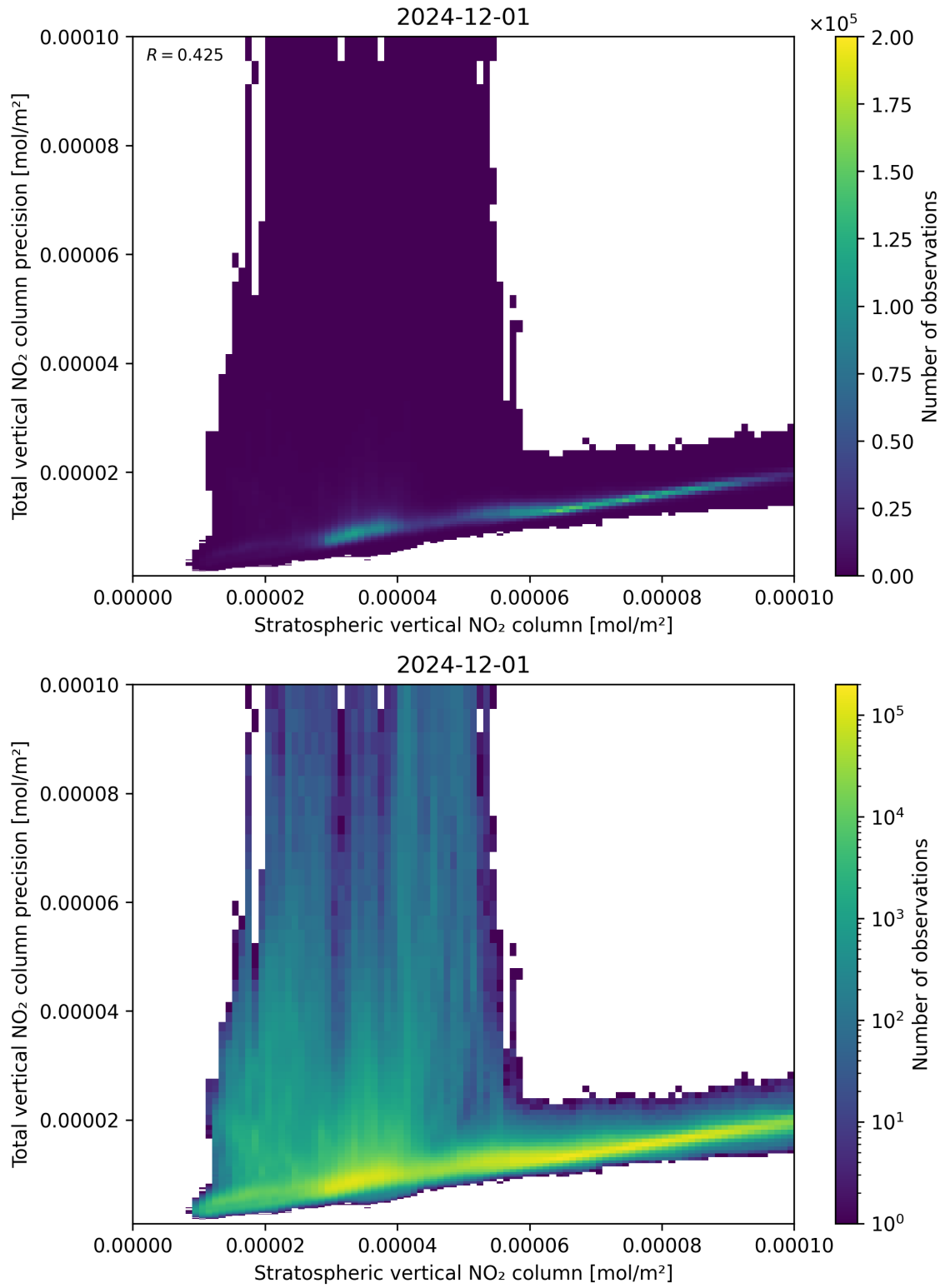
Figure 101: Scatter density plot of “Stratospheric vertical NO 2 column” against “Total vertical NO 2 column precision” for 2024-11-30 to 2024-12-02.
