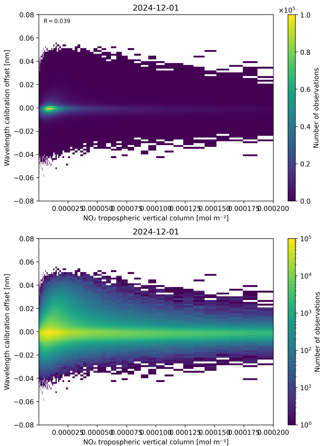
Figure 143: Scatter density plot of “NO 2 tropospheric vertical column” against “Wavelength calibration offset” for 2024-11-30 to 2024-12-02.
