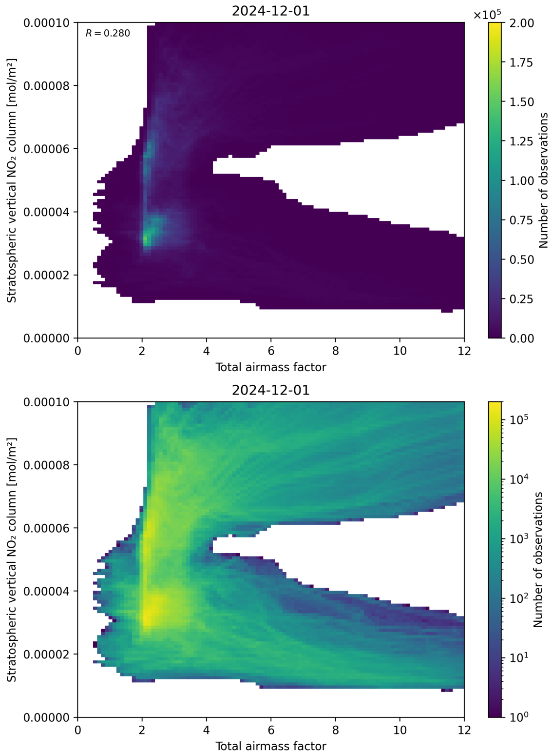
Figure 64: Scatter density plot of “Total airmass factor” against “Stratospheric vertical NO 2 column” for 2024-11-30 to 2024-12-02.
