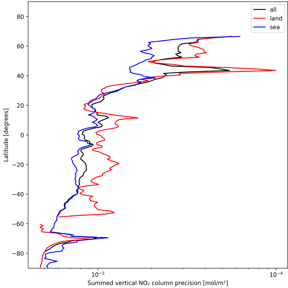
Figure 24: Zonal average of “Summed vertical NO 2 column precision” for 2024-11-30 to 2024-12-02.
