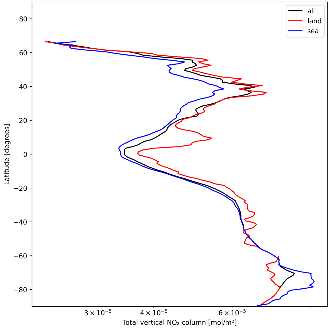
Figure 21: Zonal average of “Total vertical NO 2 column” for 2024-11-30 to 2024-12-02.
