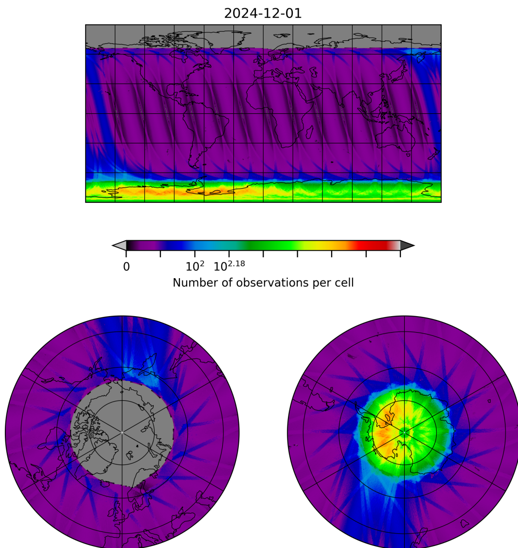
Figure 10: Map of the number of observations for 2024-11-30 to 2024-12-02
