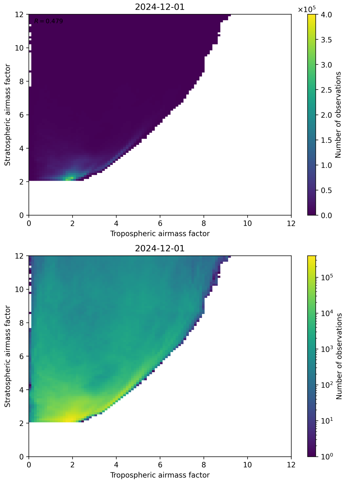
Figure 71: Scatter density plot of “Tropospheric airmass factor” against “Stratospheric airmass factor” for 2024-11-30 to 2024-12-02.
