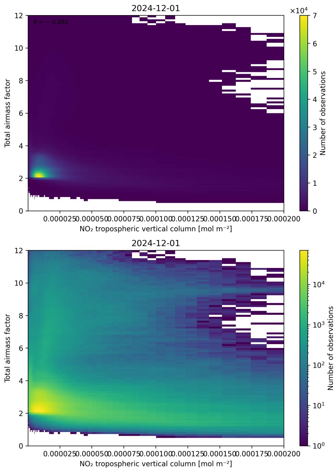
Figure 122: Scatter density plot of “NO 2 tropospheric vertical column” against “Total air mass factor” for 2024-11-30 to 2024-12-02.
