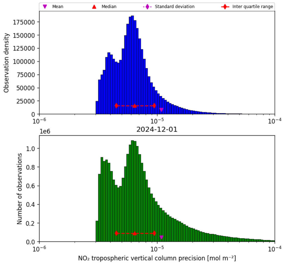
Figure 30: Histogram of “NO 2 tropospheric vertical column precision” for 2024-11-30 to 2024-12-02
