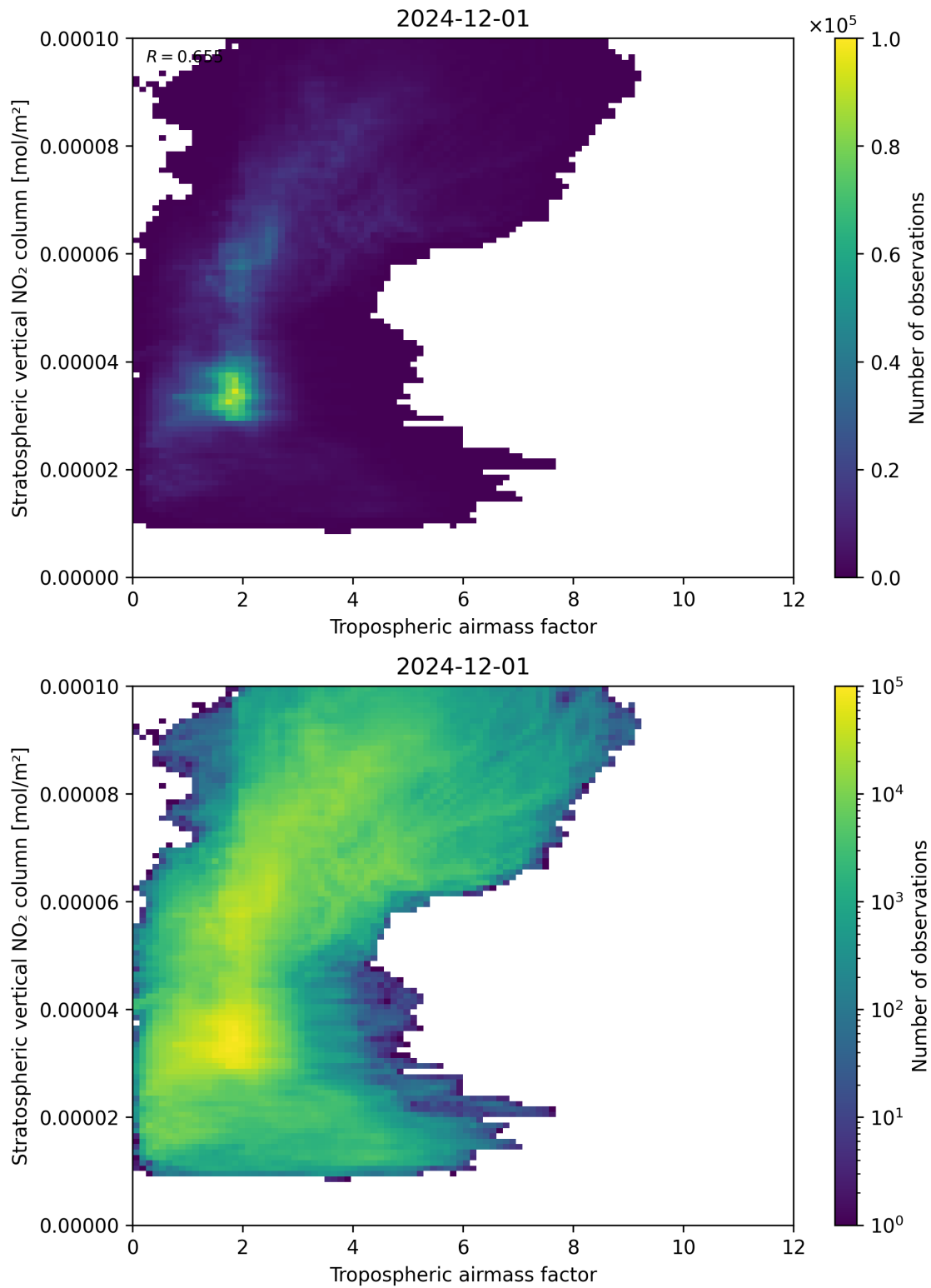
Figure 74: Scatter density plot of “Tropospheric air mass factor” against “Stratospheric vertical NO 2 column” for 2024-11-30 to 2024-12-02.
