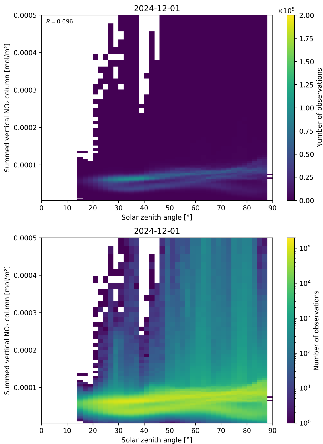
Figure 151: Scatter density plot of “Solar zenith angle” against “Summed vertical NO 2 column” for 2024-11-30 to 2024-12-02.
