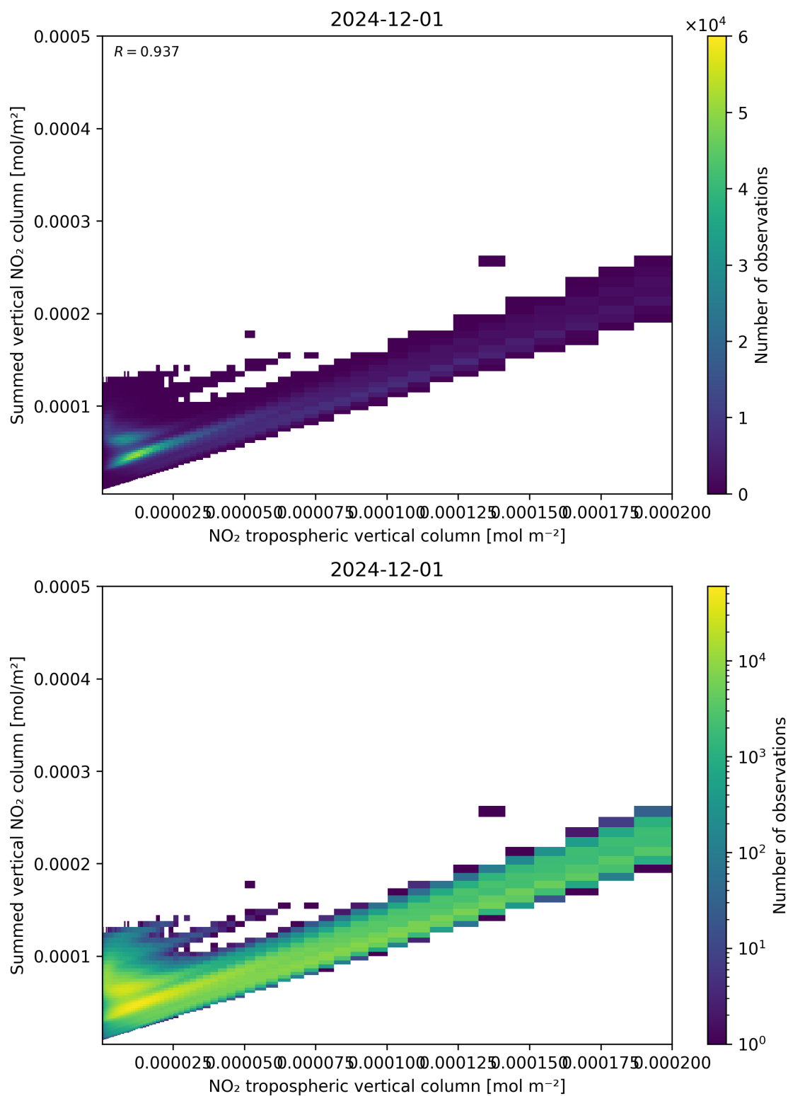
Figure 126: Scatter density plot of “NO 2 tropospheric vertical column” against “Summed vertical NO 2 column” for 2024-11-30 to 2024-12-02.
