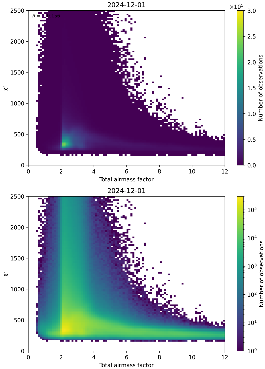
Figure 63: Scatter density plot of “Total airmass factor” against “ \chi^2 ” for 2024-11-30 to 2024-12-02.
