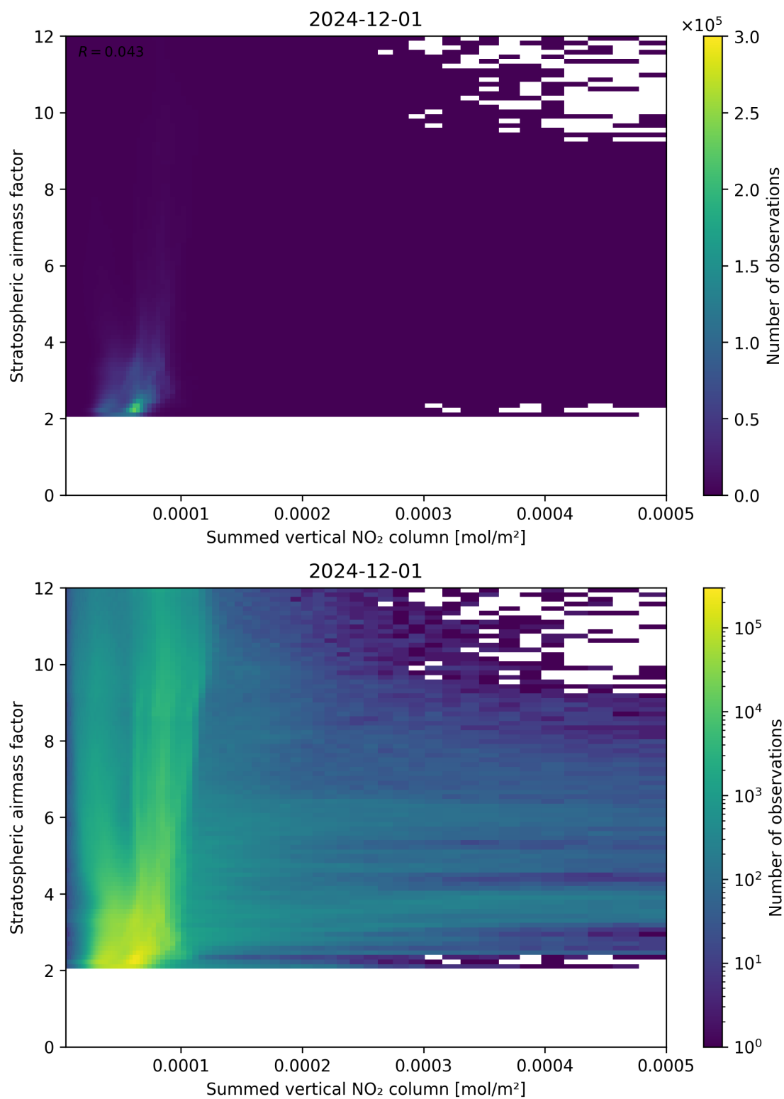
Figure 103: Scatter density plot of “Summed vertical NO 2 column” against “Stratospheric airmass factor” for 2024-11-30 to 2024-12-02.
