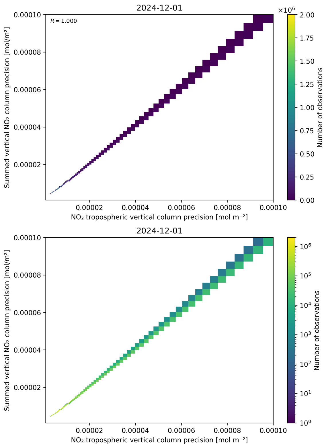
Figure 137: Scatter density plot of “NO 2 tropospheric vertical column precision” against “Summed vertical NO 2 column precision” for 2024-11-30 to 2024-12-02.
