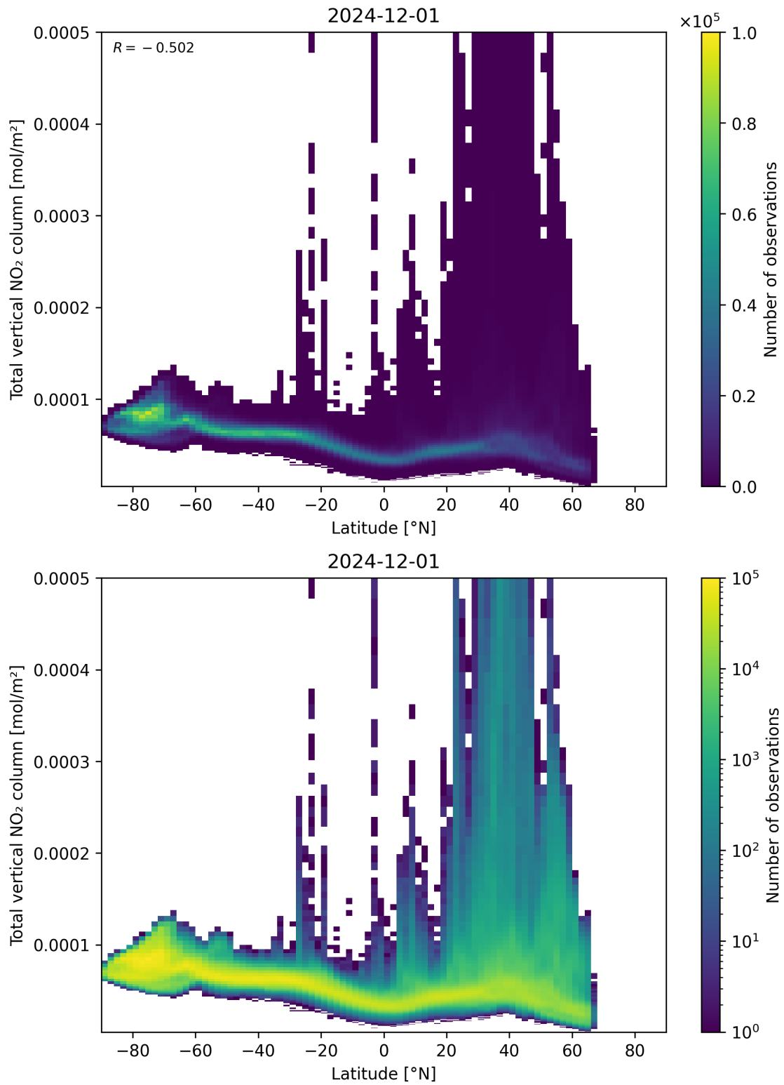
Figure 90: Scatter density plot of “Latitude” against “Total vertical NO 2 column” for 2024-11-30 to 2024-12-02.
