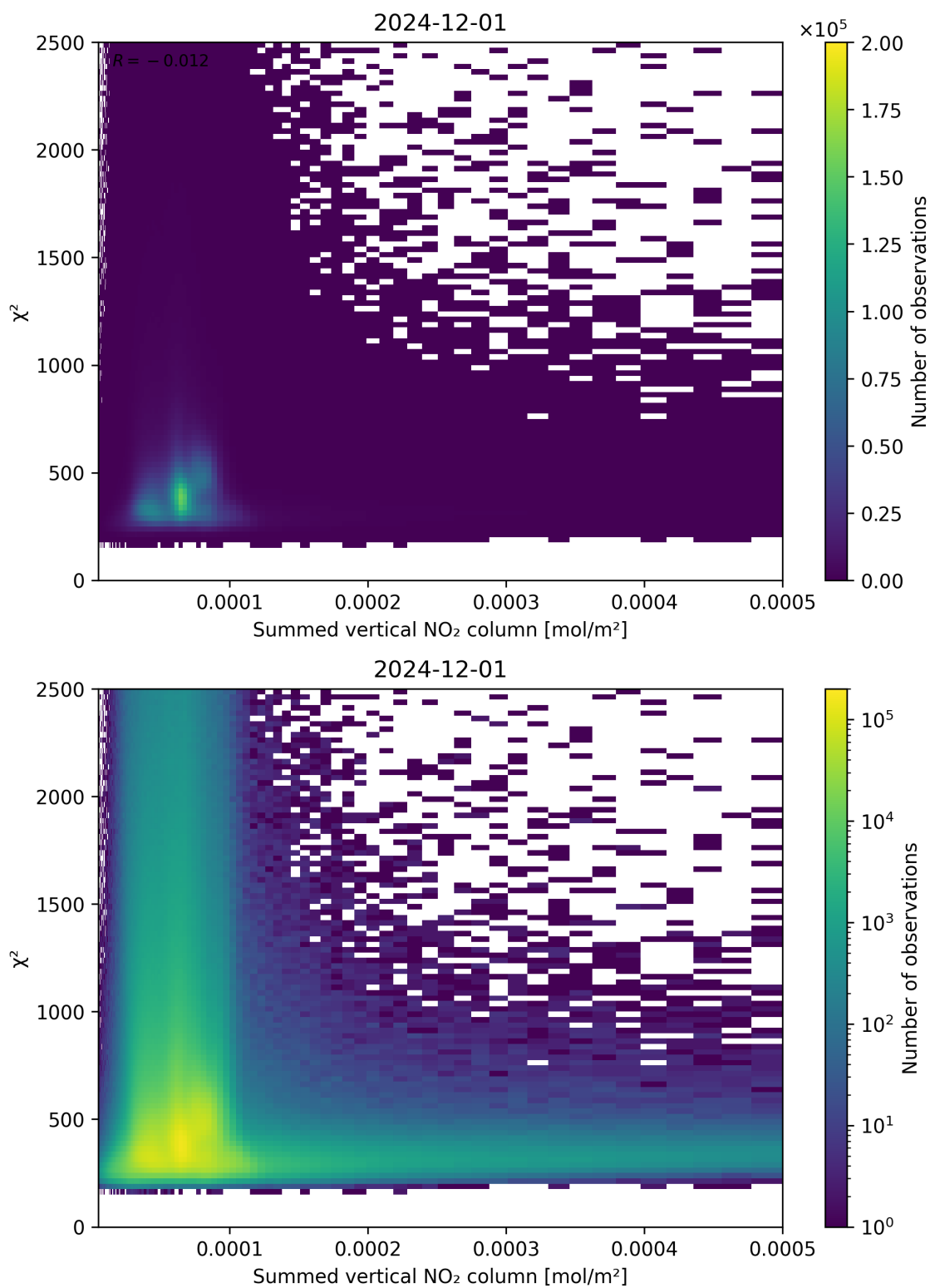
Figure 104: Scatter density plot of “Summed vertical NO 2 column” against “ \chi^2 ” for 2024-11-30 to 2024-12-02.
