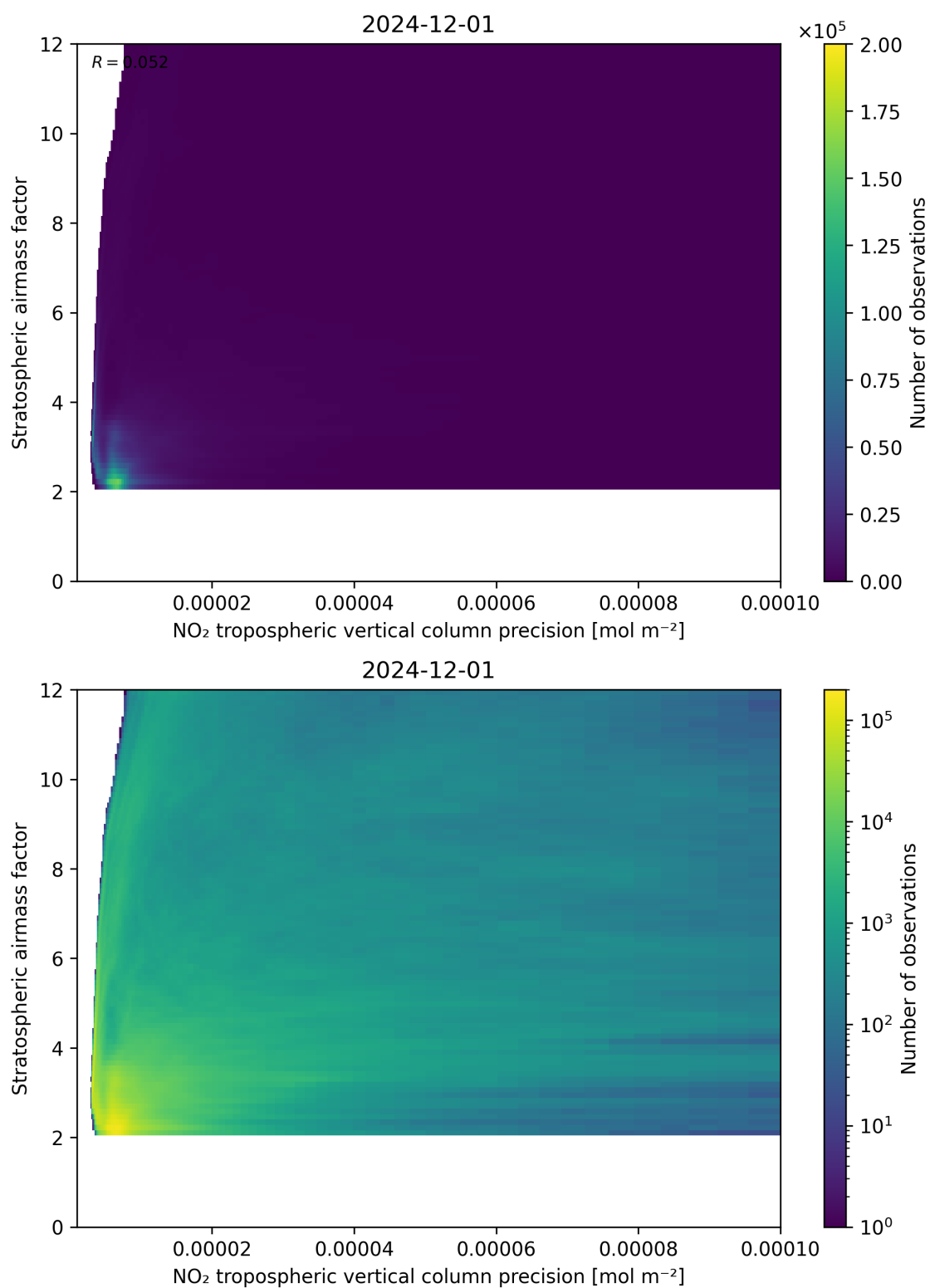
Figure 131: Scatter density plot of “NO 2 tropospheric vertical column precision” against “Stratospheric airmass factor” for 2024-11-30 to 2024-12-02.
