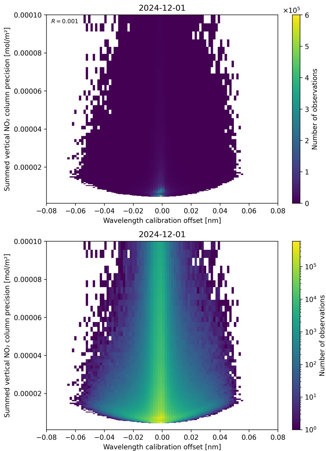
Figure 178: Scatter density plot of “Wavelength calibration offset” against “Summed vertical NO 2 column precision” for 2024-11-30 to 2024-12-02.
