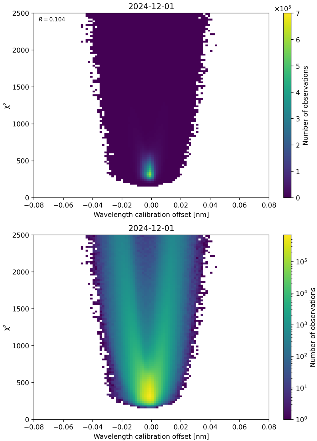
Figure 175: Scatter density plot of “Wavelength calibration offset” against “ \chi^2 ” for 2024-11-30 to 2024-12-02.
