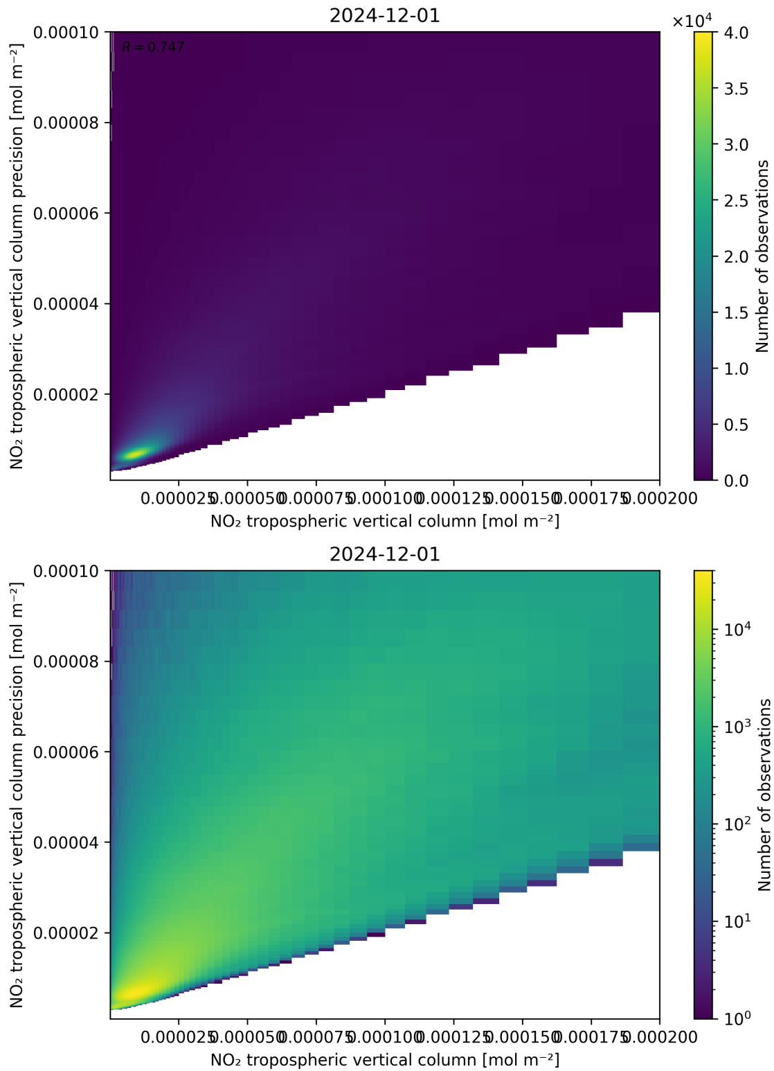
Figure 130: Scatter density plot of “NO 2 tropospheric vertical column” against “NO 2 tropospheric vertical column precision” for 2024-11-30 to 2024-12-02.
