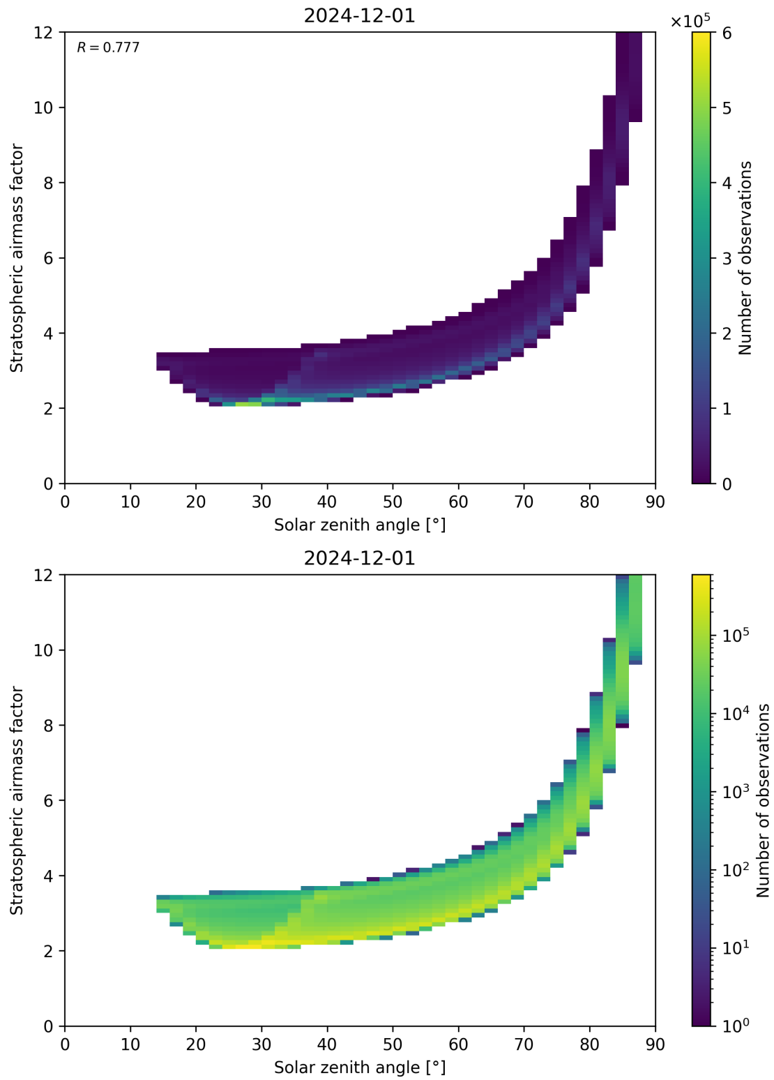
Figure 145: Scatter density plot of “Solar zenith angle” against “Stratospheric airmass factor” for 2024-11-30 to 2024-12-02.
