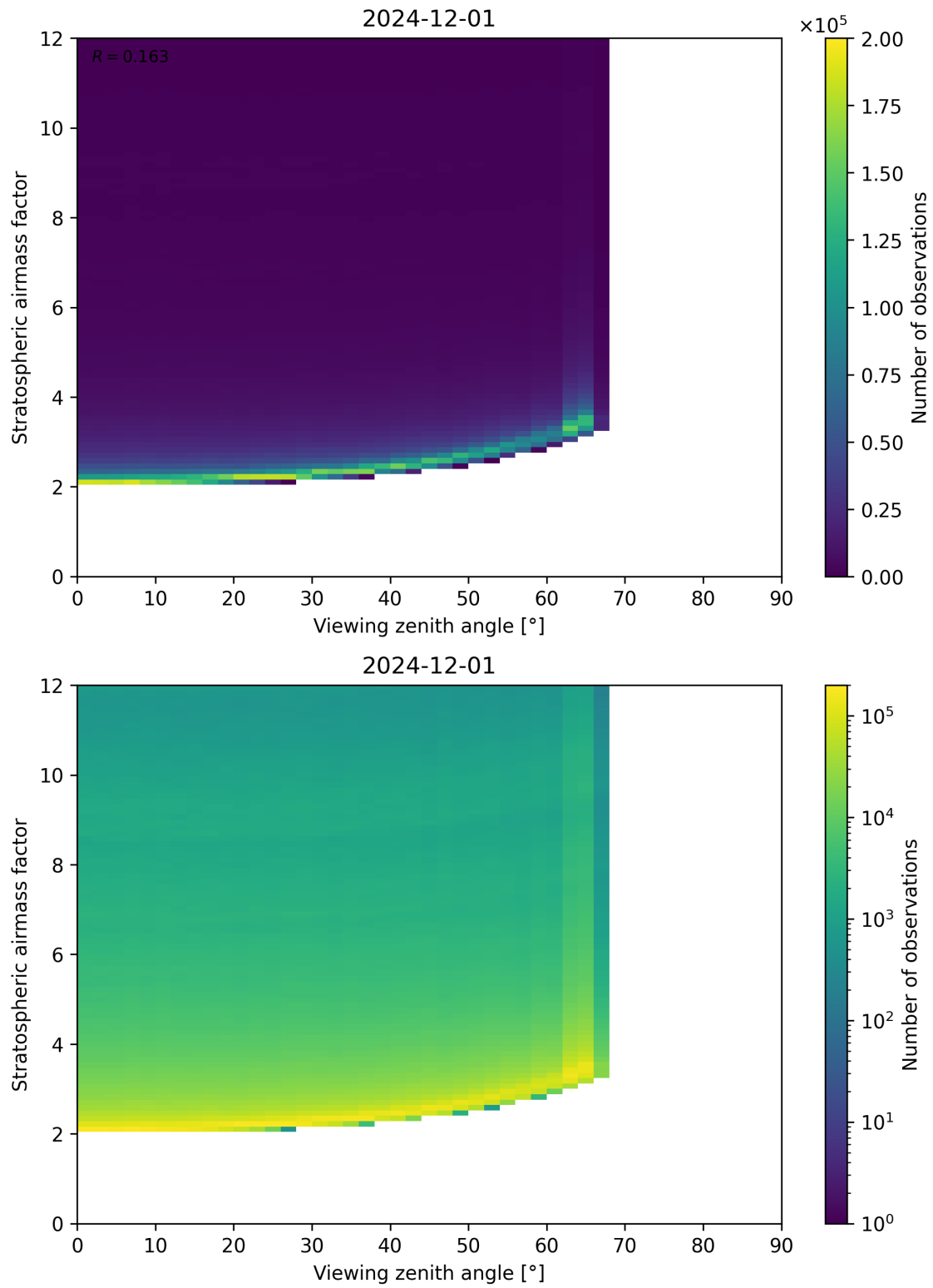
Figure 159: Scatter density plot of “Viewing zenith angle” against “Stratospheric airmass factor” for 2024-11-30 to 2024-12-02.
