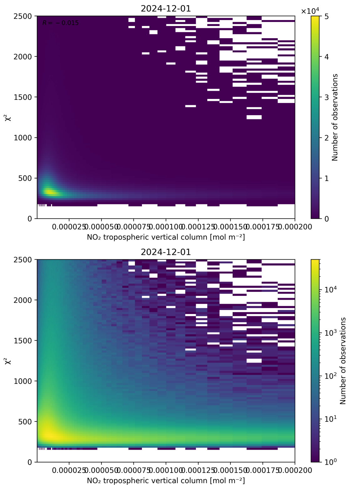
Figure 124: Scatter density plot of “NO 2 tropospheric vertical column” against “ \chi^2 ” for 2024-11-30 to 2024-12-02.
