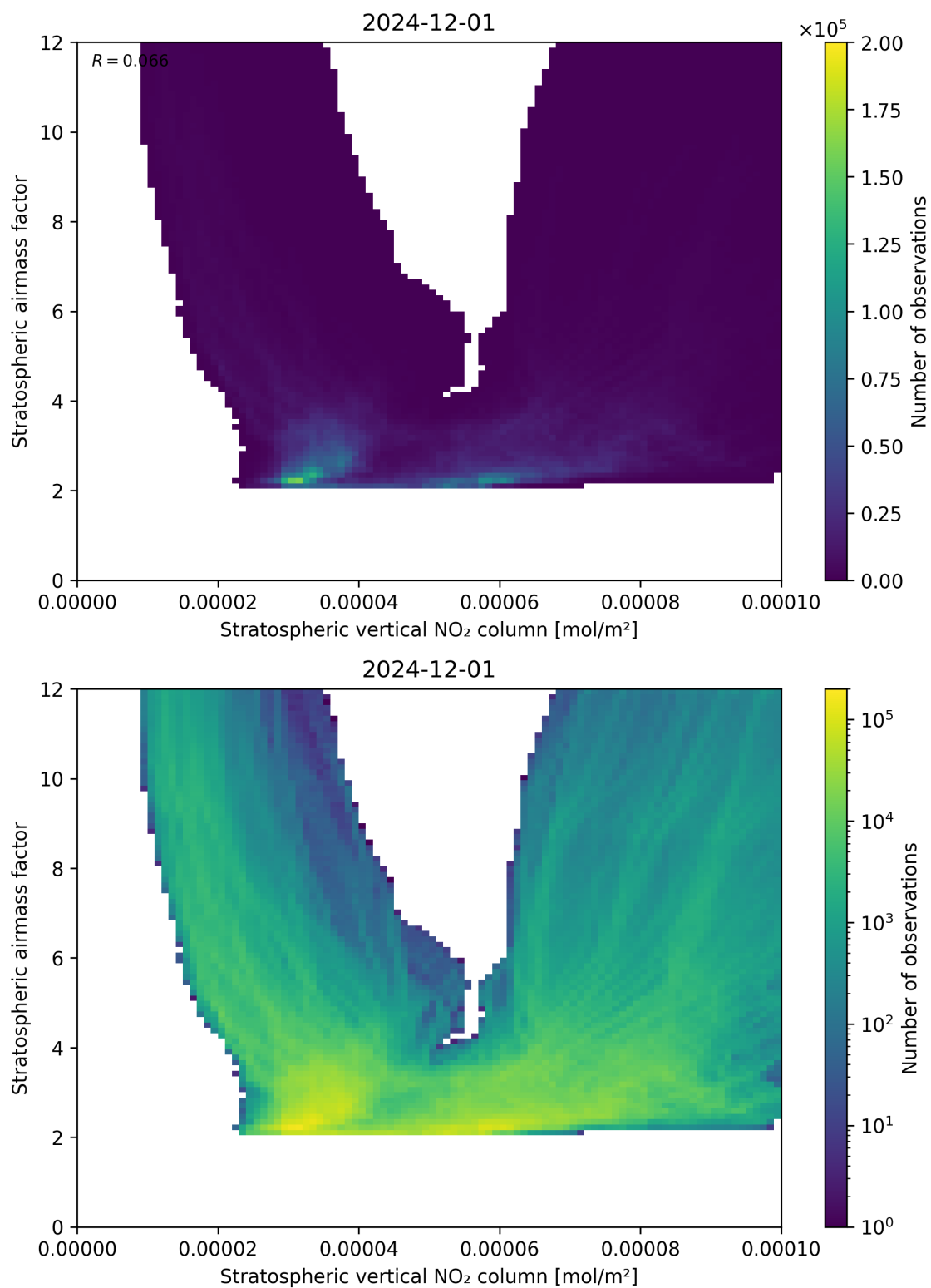
Figure 96: Scatter density plot of “Stratospheric vertical NO 2 column” against “Stratospheric airmass factor” for 2024-11-30 to 2024-12-02.
