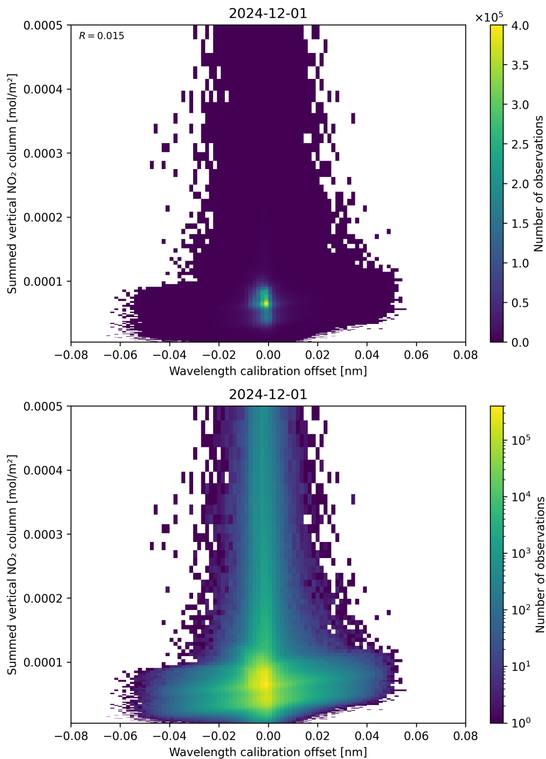
Figure 177: Scatter density plot of “Wavelength calibration offset” against “Summed vertical NO 2 column” for 2024-11-30 to 2024-12-02.
