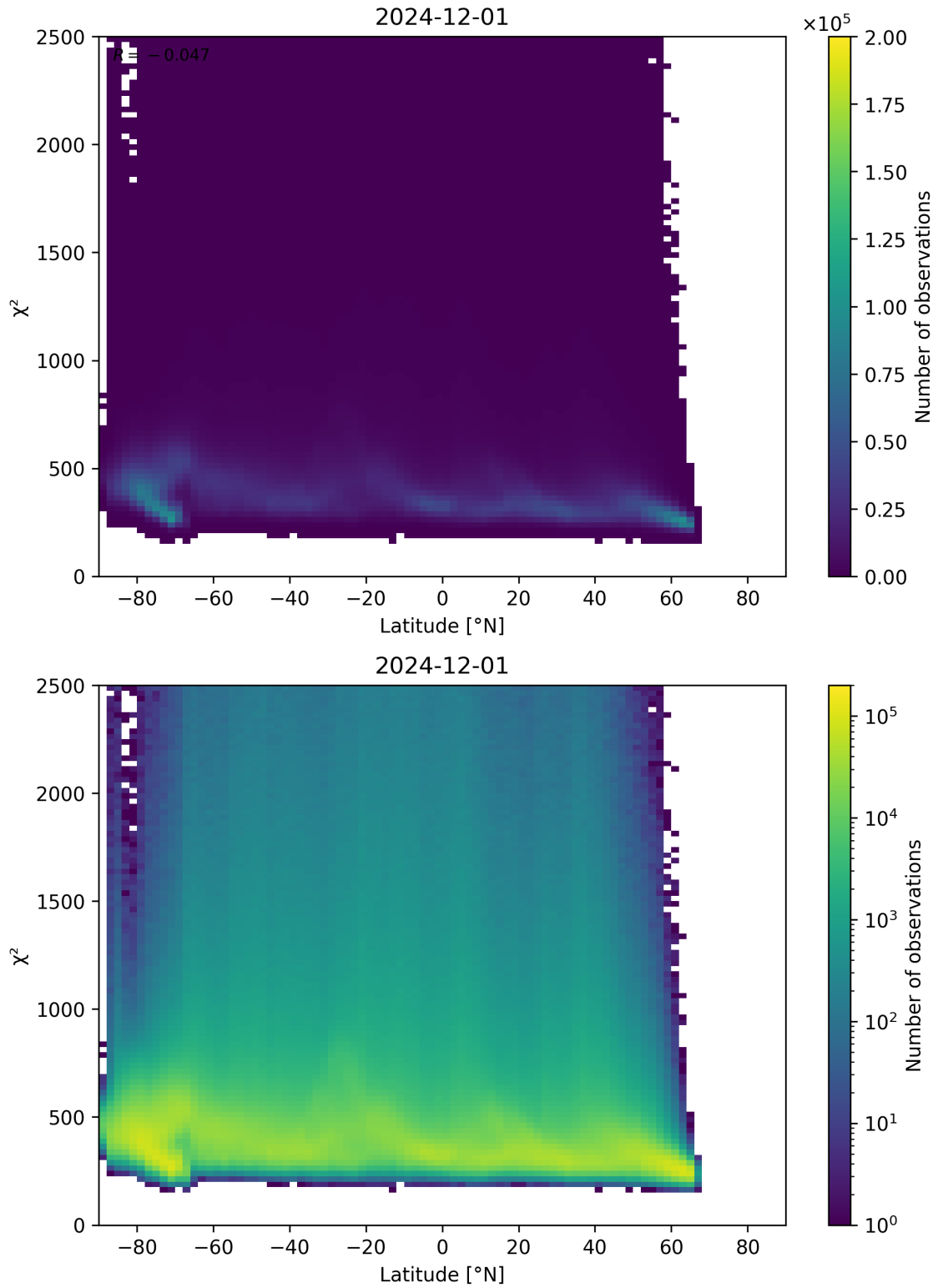
Figure 86: Scatter density plot of “Latitude” against “ \chi^2 ” for 2024-11-30 to 2024-12-02.
