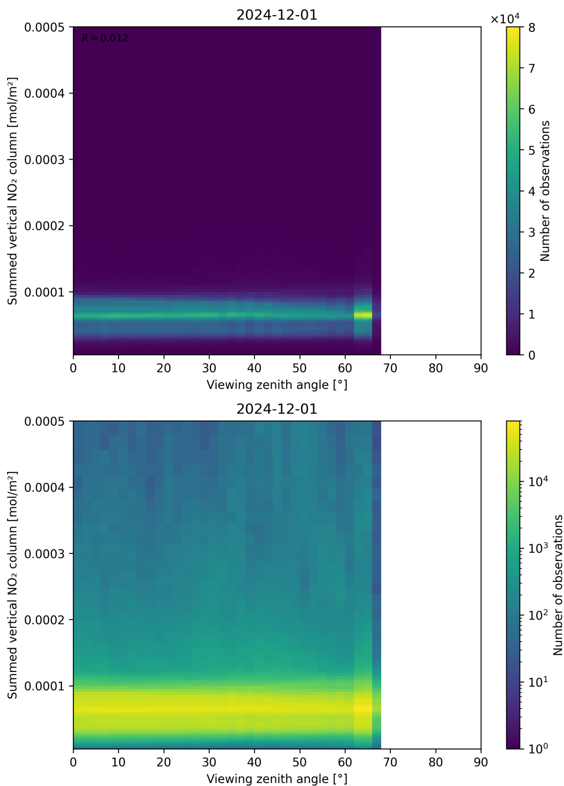
Figure 165: Scatter density plot of “Viewing zenith angle” against “Summed vertical NO 2 column” for 2024-11-30 to 2024-12-02.
