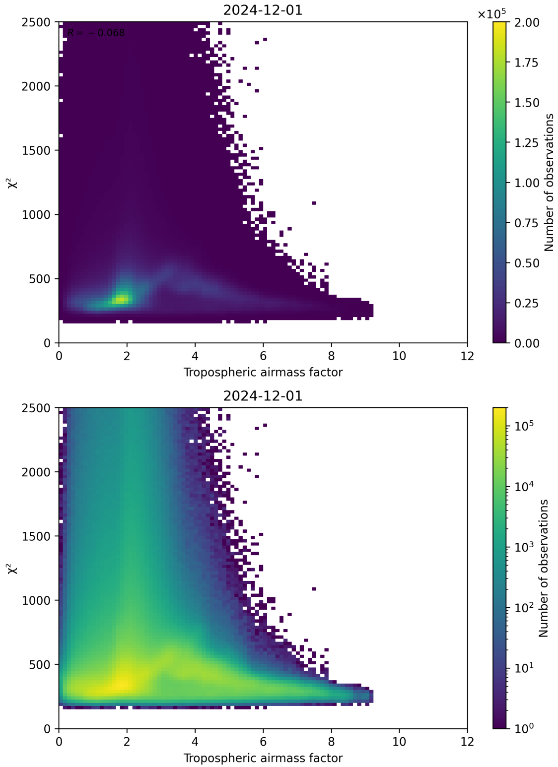
Figure 73: Scatter density plot of “Tropospheric airmass factor” against “ \chi^2 ” for 2024-11-30 to 2024-12-02.
