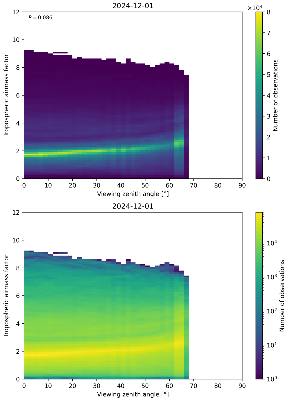
Figure 161: Scatter density plot of “Viewing zenith angle” against “Tropospheric airmass factor” for 2024-11-30 to 2024-12-02.
