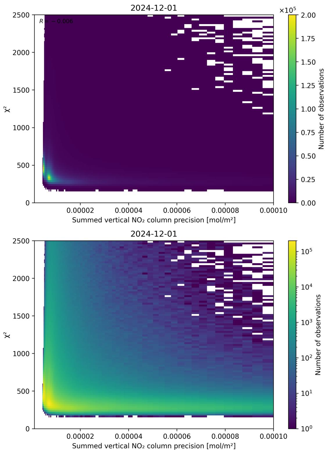
Figure 107: Scatter density plot of “Summed vertical NO 2 column precision” against “ \chi^2 ” for 2024-11-30 to 2024-12-02.
