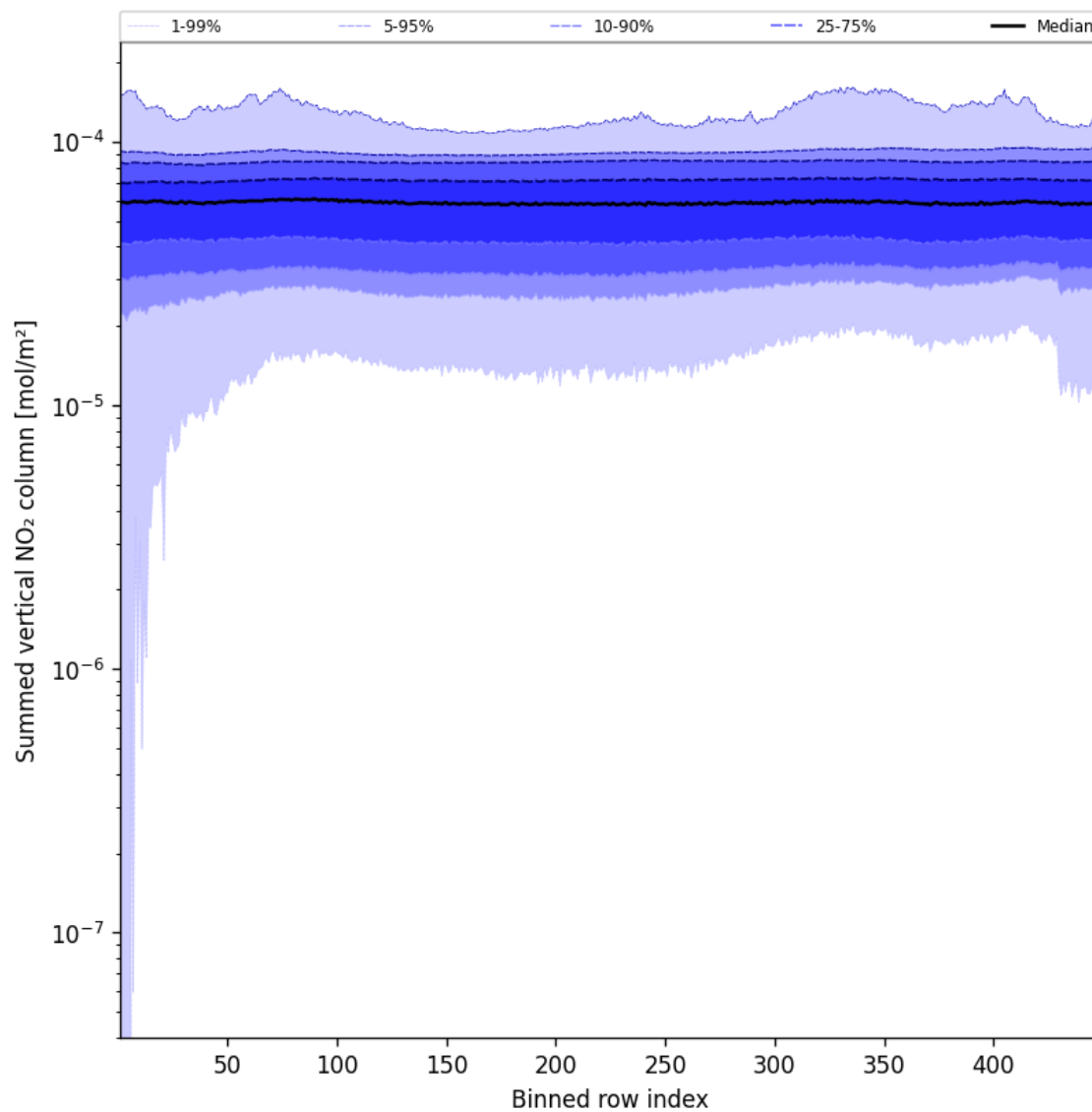
Figure 57: Along track statistics of “Summed vertical NO 2 column” for 2024-11-30 to 2024-12-02
