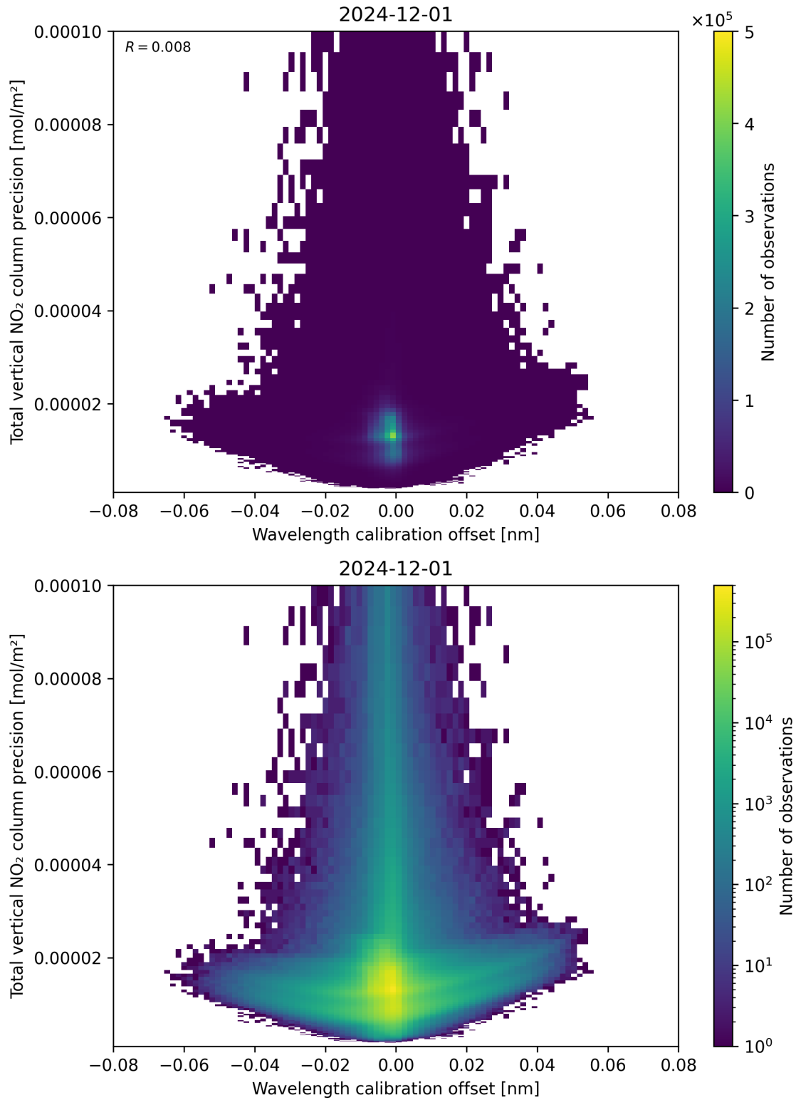
Figure 180: Scatter density plot of “Wavelength calibration offset” against “Total vertical NO 2 column precision” for 2024-11-30 to 2024-12-02.
