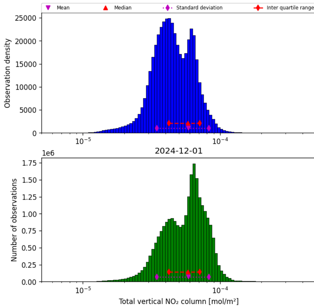
Figure 38: Histogram of “Total vertical NO 2 column” for 2024-11-30 to 2024-12-02
