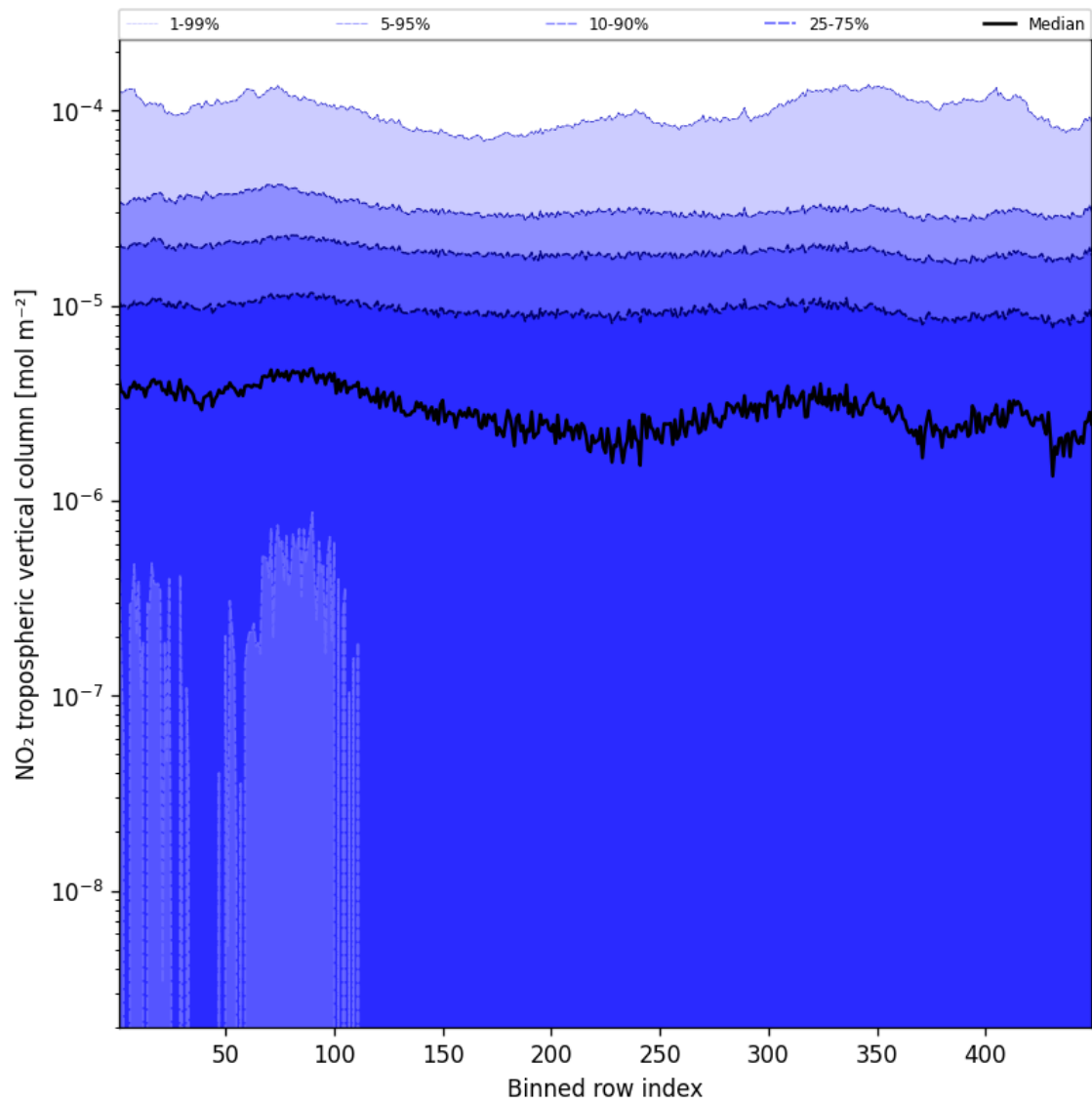
Figure 46: Along track statistics of “NO 2 tropospheric vertical column” for 2024-11-30 to 2024-12-02
