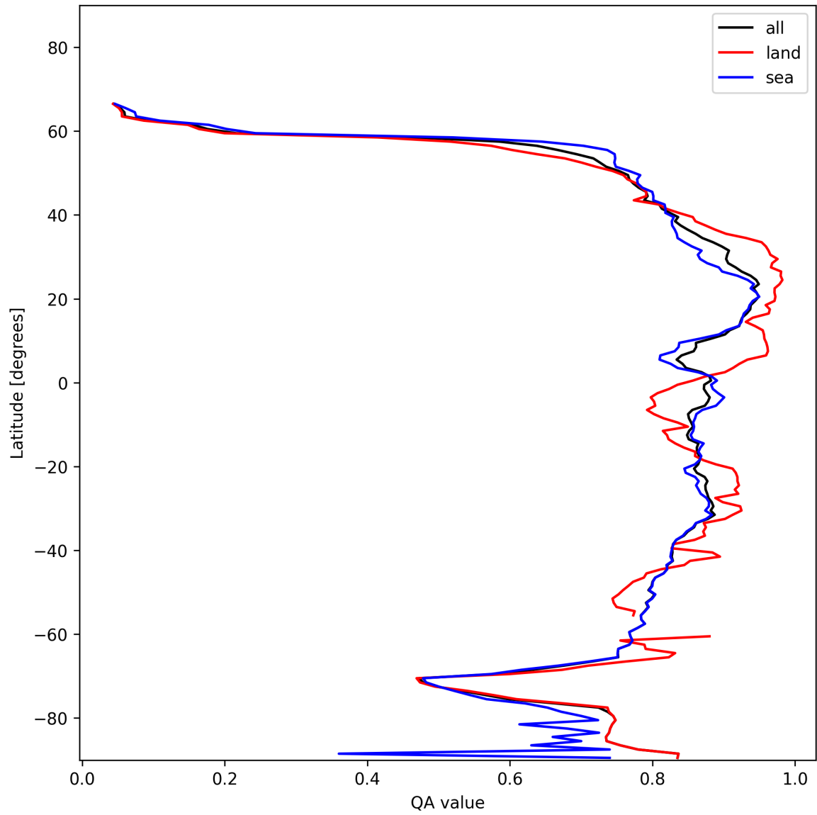
Figure 11: Zonal average of “QA value” for 2024-11-30 to 2024-12-02.
