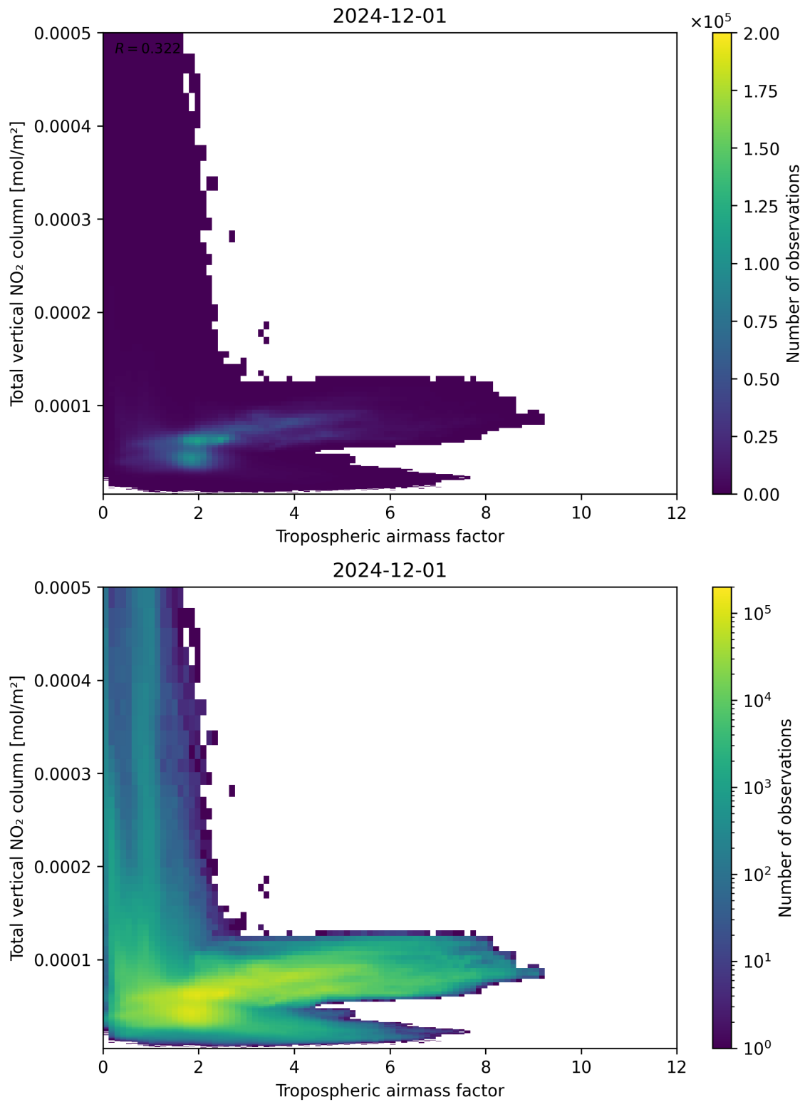
Figure 77: Scatter density plot of “Tropospheric airmass factor” against “Total vertical NO 2 column” for 2024-11-30 to 2024-12-02.
