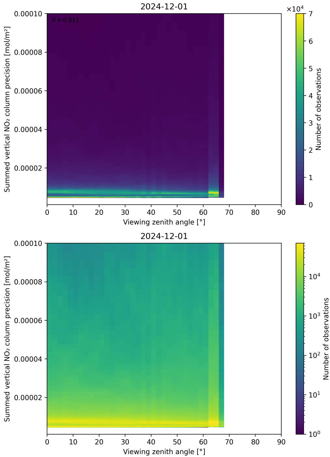
Figure 166: Scatter density plot of “Viewing zenith angle” against “Summed vertical NO 2 column precision” for 2024-11-30 to 2024-12-02.
