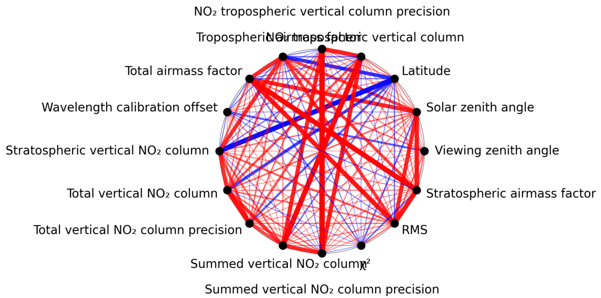
Figure 1: Map of correlation graph for 2024-11-30 to 2024-12-02.
