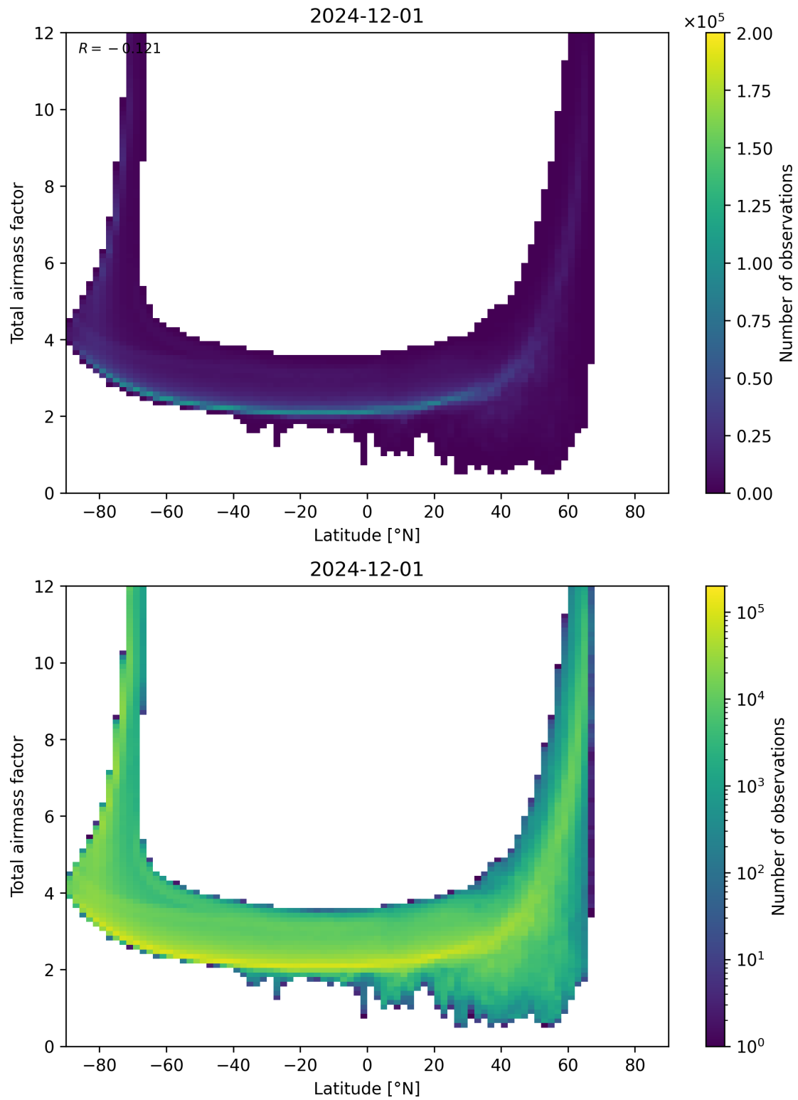
Figure 84: Scatter density plot of “Latitude” against “Total airmass factor” for 2024-11-30 to 2024-12-02.
