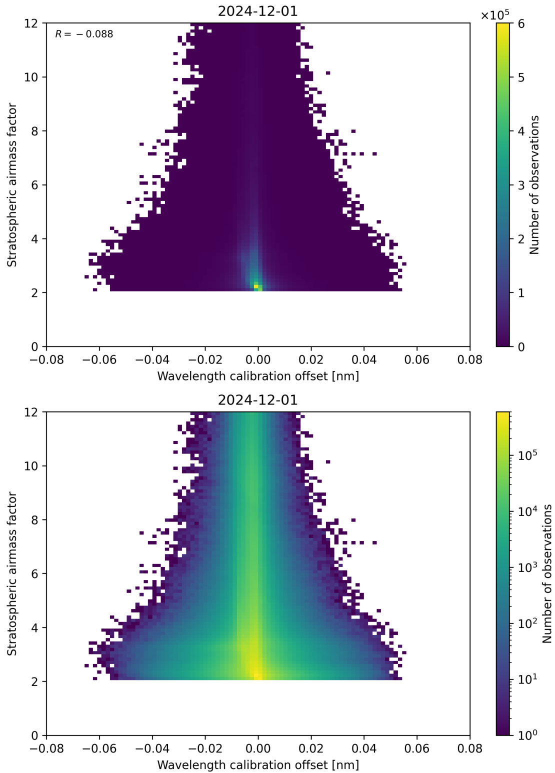
Figure 174: Scatter density plot of “Wavelength calibration offset” against “Stratospheric airmass factor” for 2024-11-30 to 2024-12-02.
