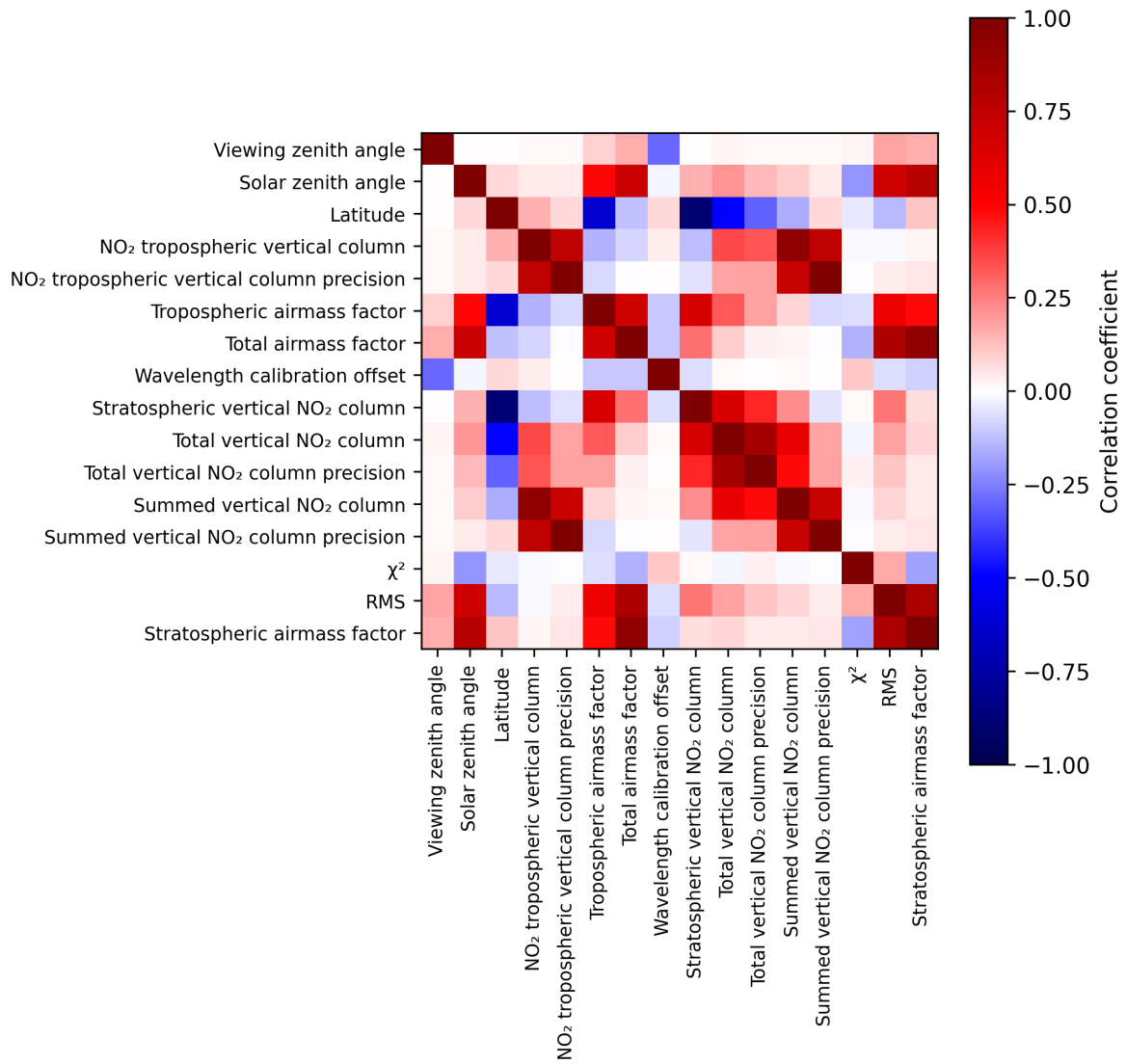
Figure 2: Map of correlation matrix for 2024-11-30 to 2024-12-02.
