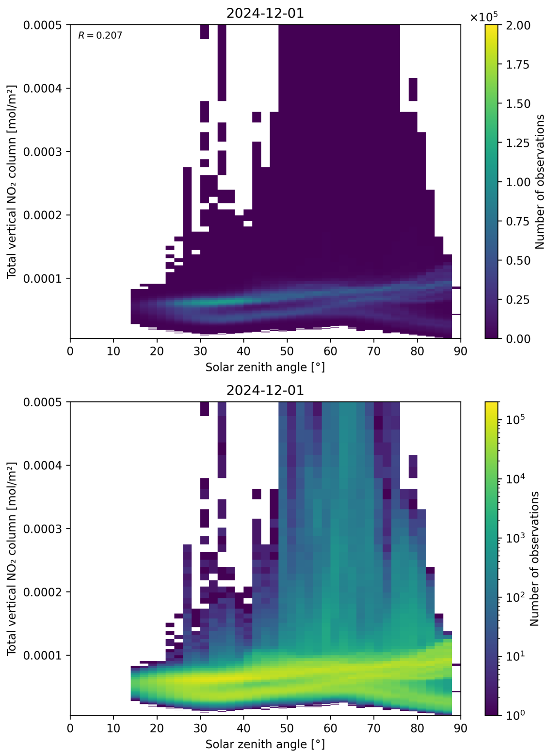
Figure 153: Scatter density plot of “Solar zenith angle” against “Total vertical NO 2 column” for 2024-11-30 to 2024-12-02.
