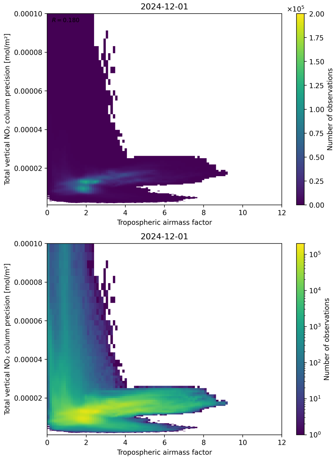
Figure 78: Scatter density plot of “Tropospheric airmass factor” against “Total vertical NO 2 column precision” for 2024-11-30 to 2024-12-02.
