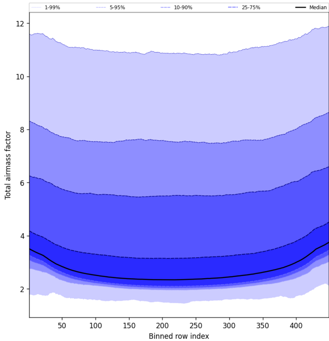
Figure 49: Along track statistics of “Total airmass factor” for 2024-11-30 to 2024-12-02
