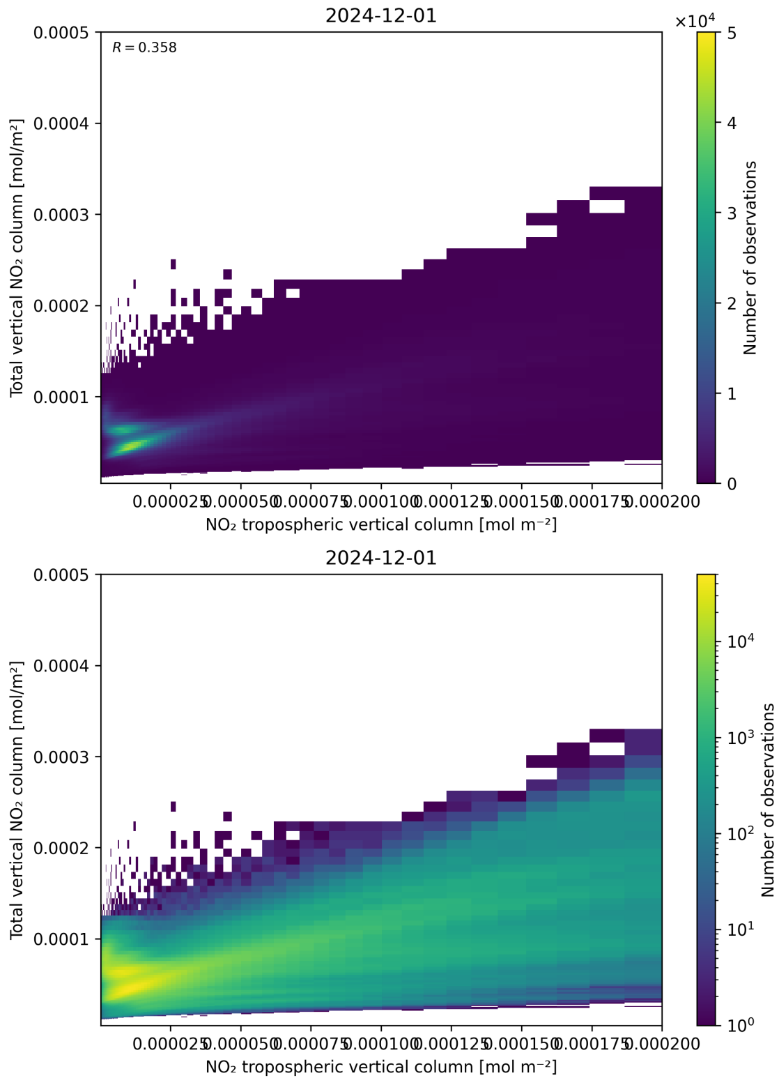
Figure 128: Scatter density plot of “NO 2 tropospheric vertical column” against “Total vertical NO 2 column” for 2024-11-30 to 2024-12-02.
