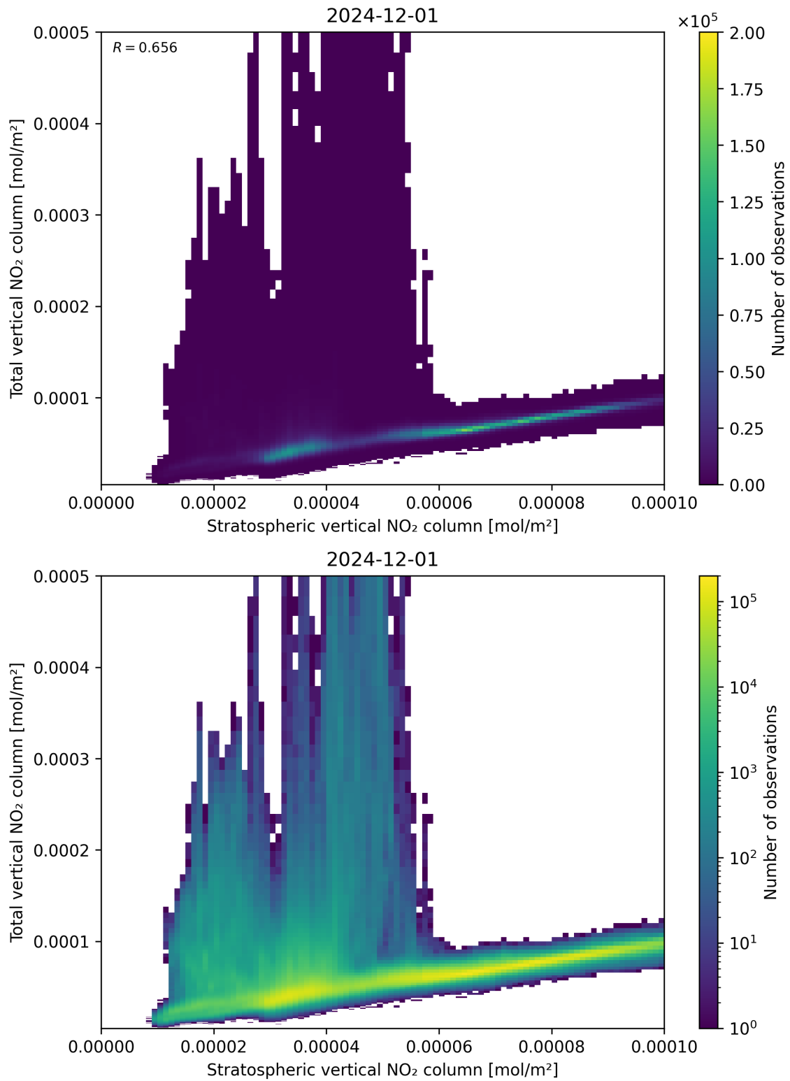
Figure 100: Scatter density plot of “Stratospheric vertical NO 2 column” against “Total vertical NO 2 column” for 2024-11-30 to 2024-12-02.
