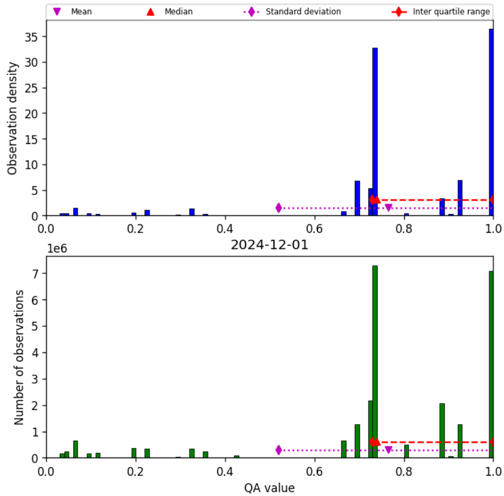
Figure 28: Histogram of “QA value” for 2024-11-30 to 2024-12-02
