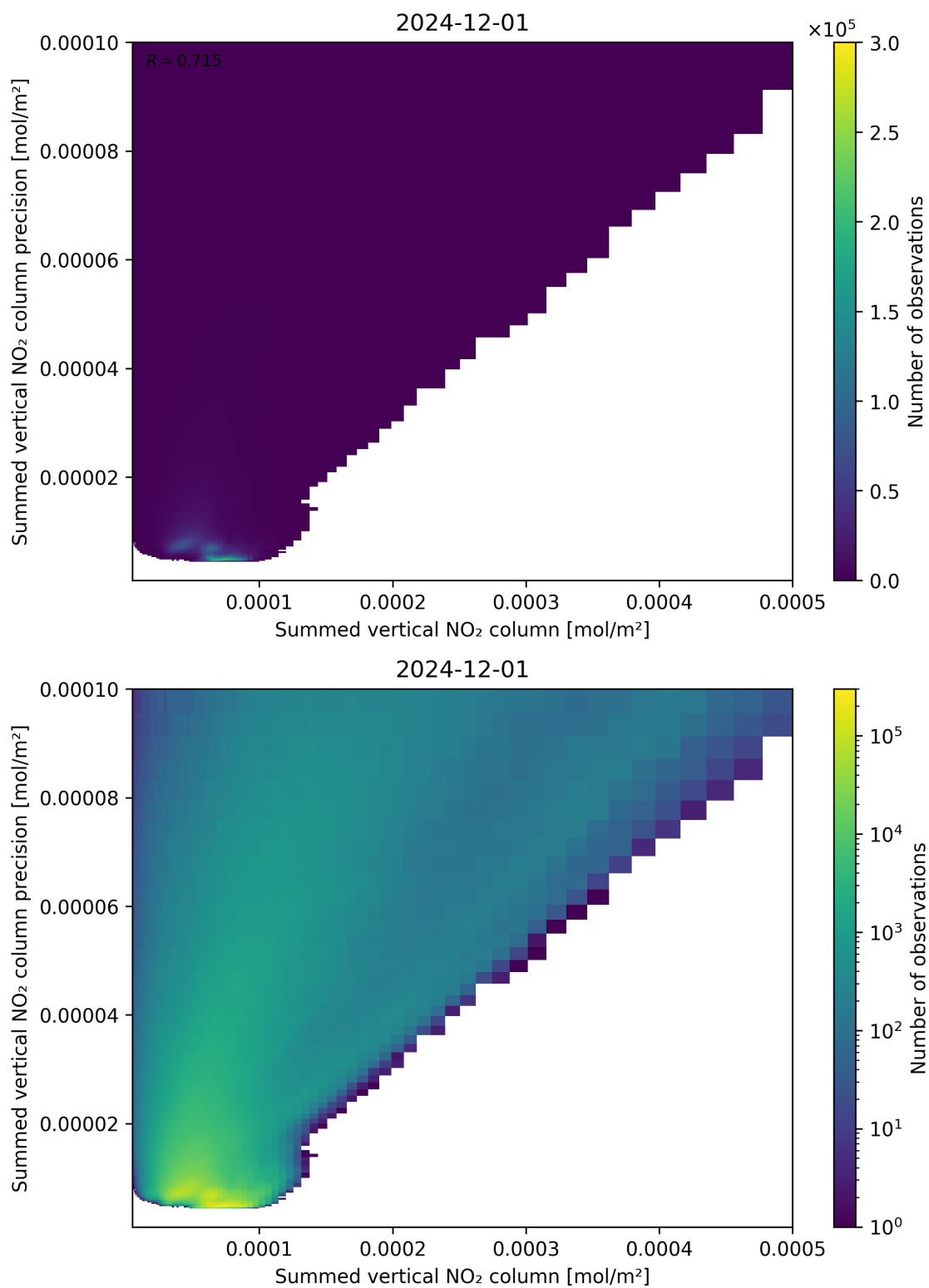
Figure 105: Scatter density plot of “Summed vertical NO 2 column” against “Summed vertical NO 2 column precision” for 2024-11-30 to 2024-12-02.
