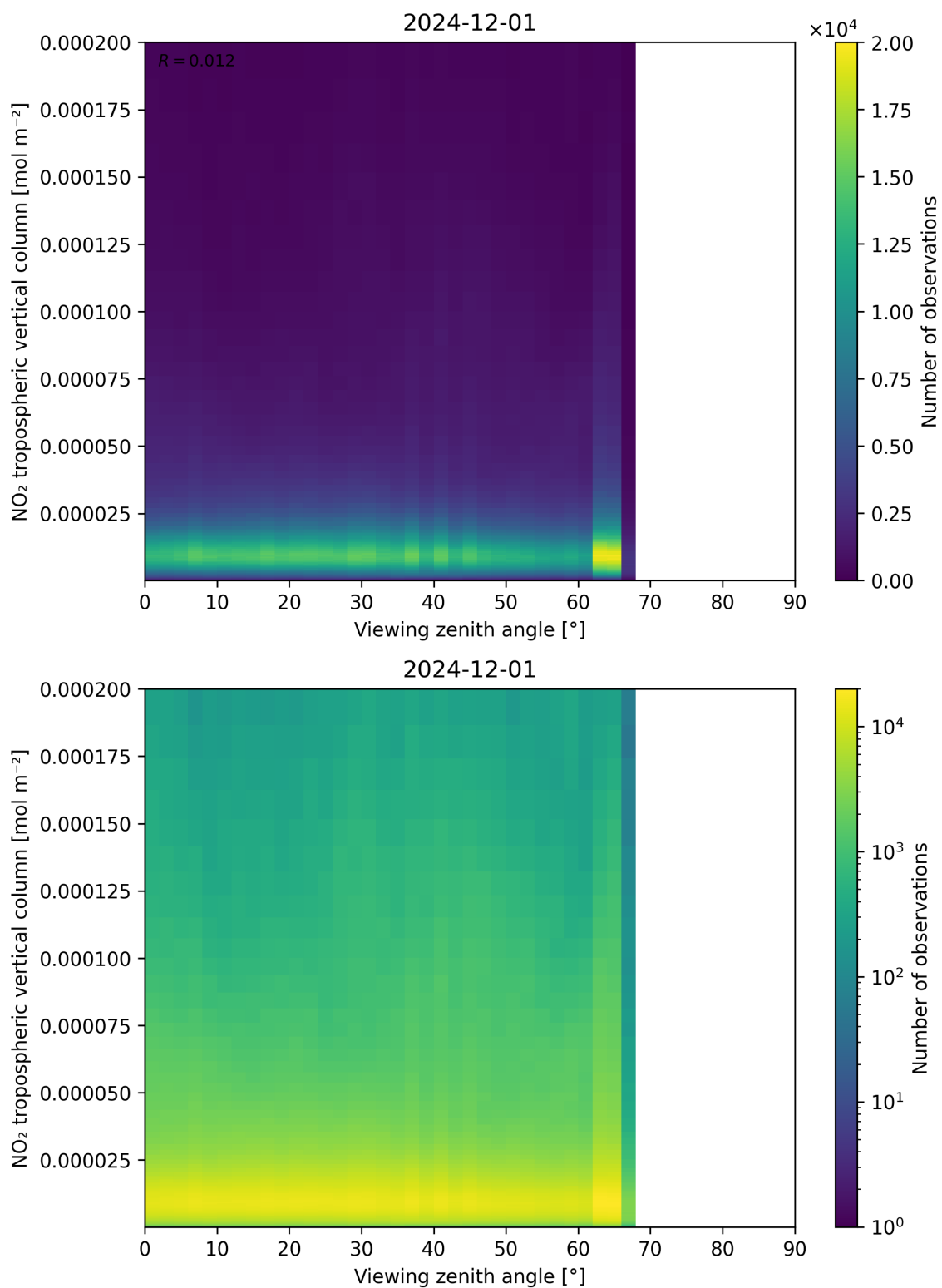
Figure 169: Scatter density plot of “Viewing zenith angle” against “NO 2 tropospheric vertical column” for 2024-11-30 to 2024-12-02.
