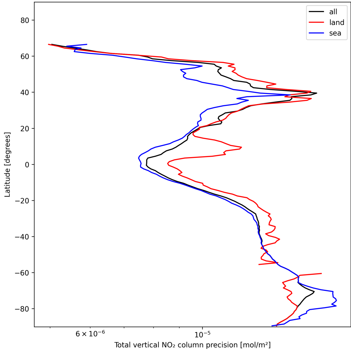
Figure 22: Zonal average of “Total vertical NO 2 column precision” for 2024-11-30 to 2024-12-02.
