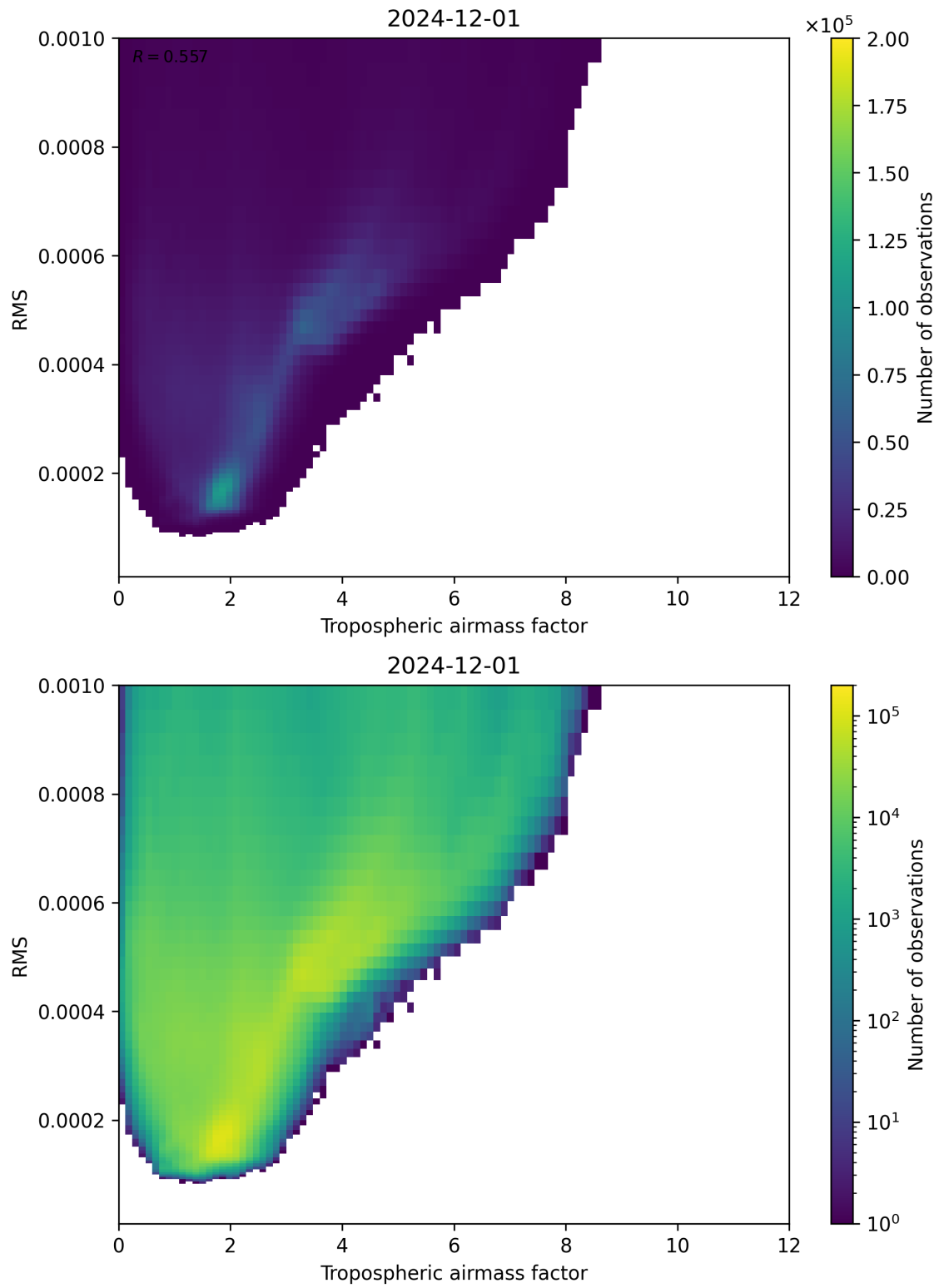
Figure 79: Scatter density plot of “Tropospheric airmass factor” against “RMS” for 2024-11-30 to 2024-12-02.
