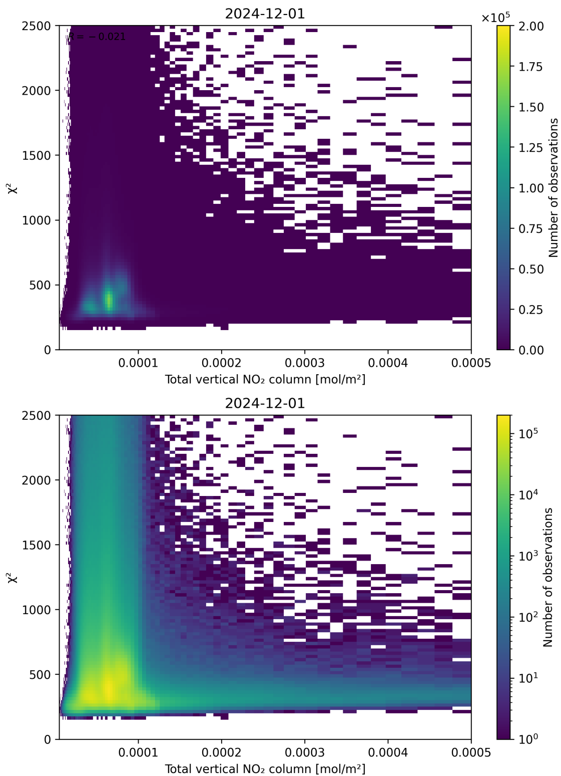
Figure 111: Scatter density plot of “Total vertical NO 2 column” against “ \chi^2 ” for 2024-11-30 to 2024-12-02.
