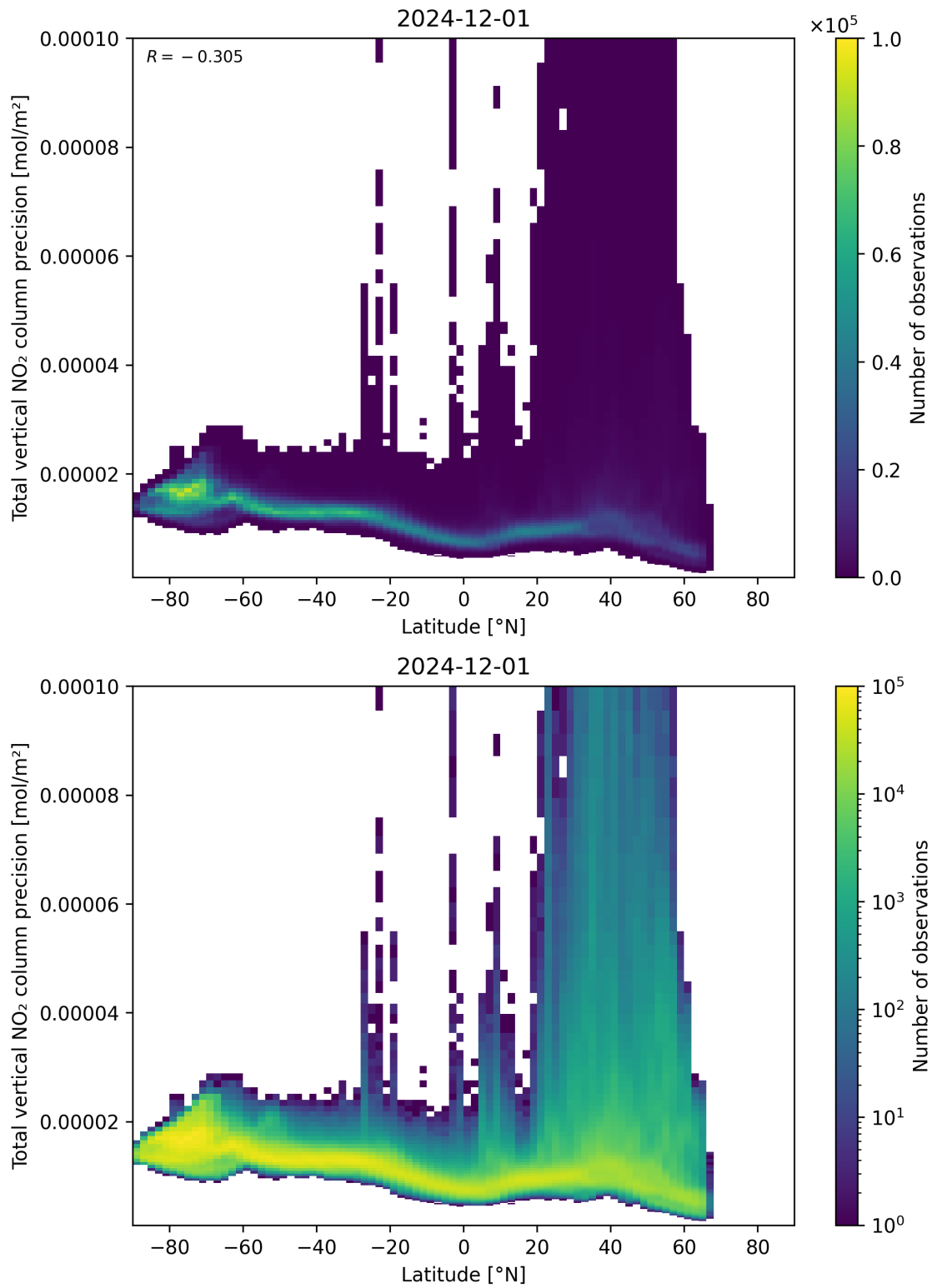
Figure 91: Scatter density plot of “Latitude” against “Total vertical NO 2 column precision” for 2024-11-30 to 2024-12-02.
