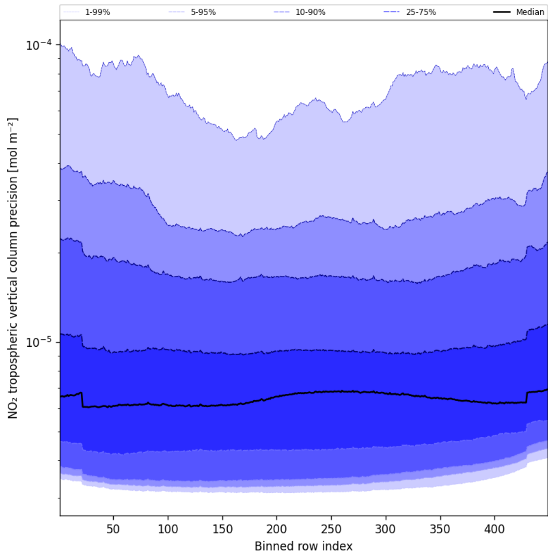
Figure 47: Along track statistics of “NO 2 tropospheric vertical column precision” for 2024-11-30 to 2024-12-02
