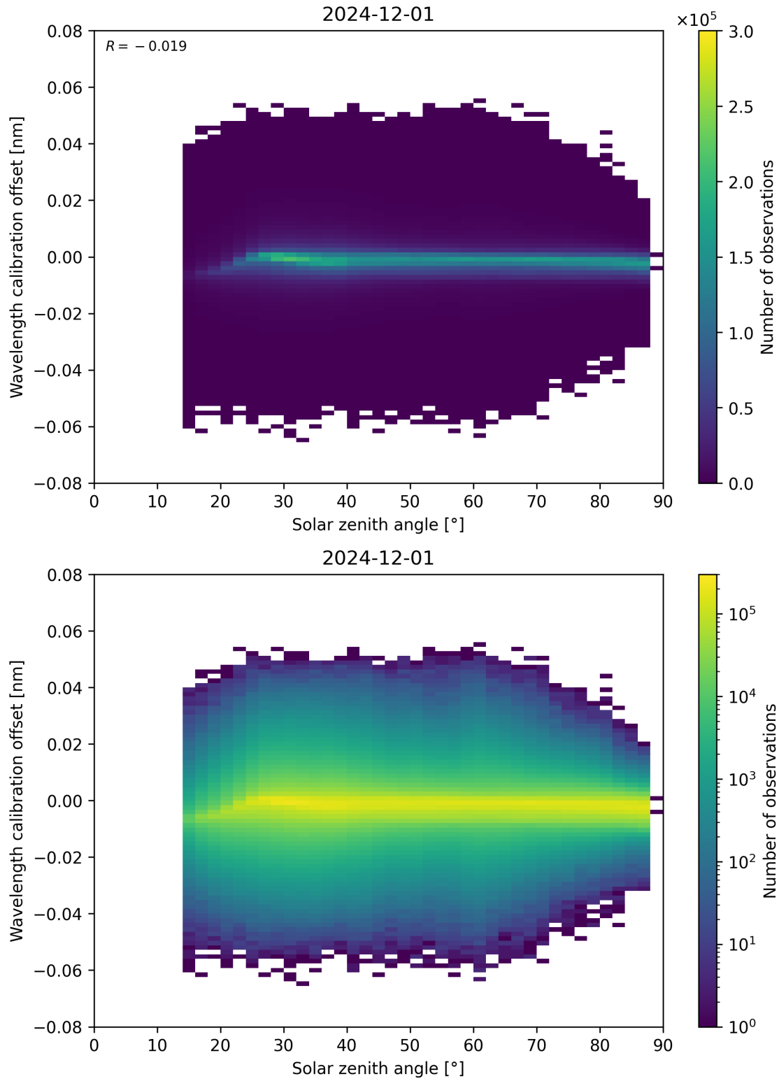
Figure 158: Scatter density plot of “Solar zenith angle” against “Wavelength calibration offset” for 2024-11-30 to 2024-12-02.
