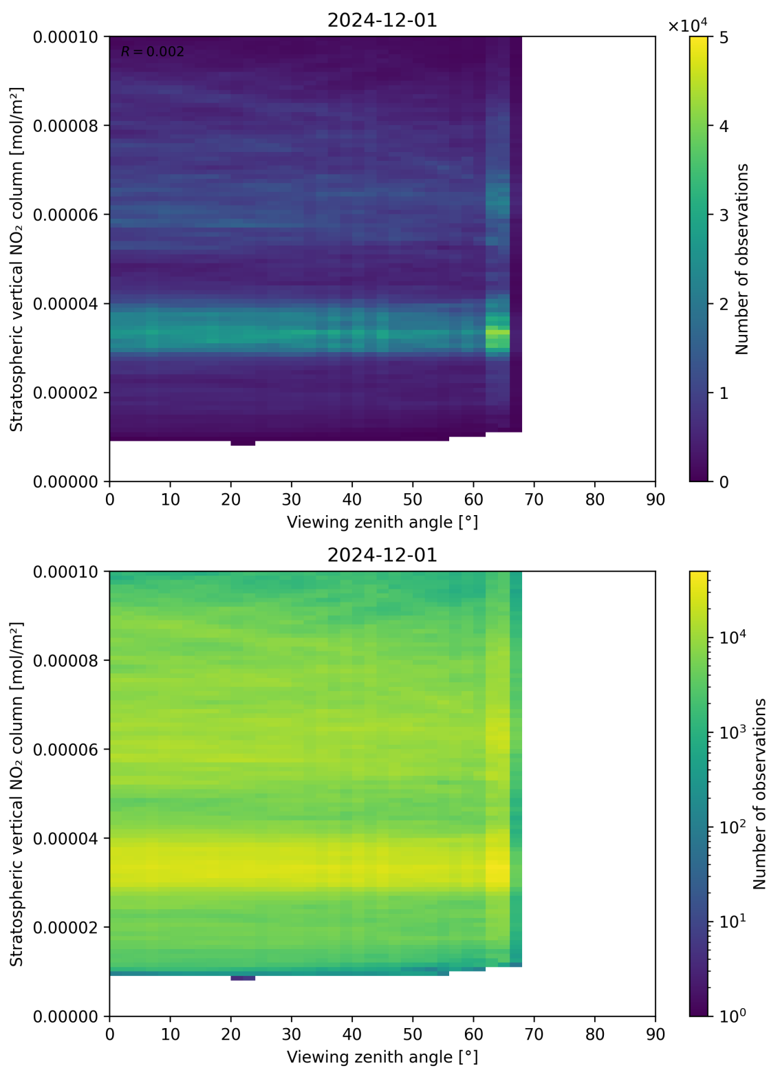
Figure 164: Scatter density plot of “Viewing zenith angle” against “Stratospheric vertical NO 2 column” for 2024-11-30 to 2024-12-02.
