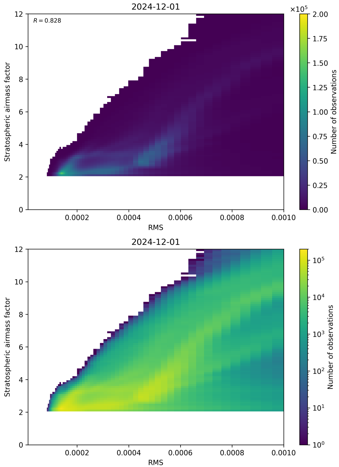
Figure 144: Scatter density plot of “RMS” against “Stratospheric airmass factor” for 2024-11-30 to 2024-12-02.
