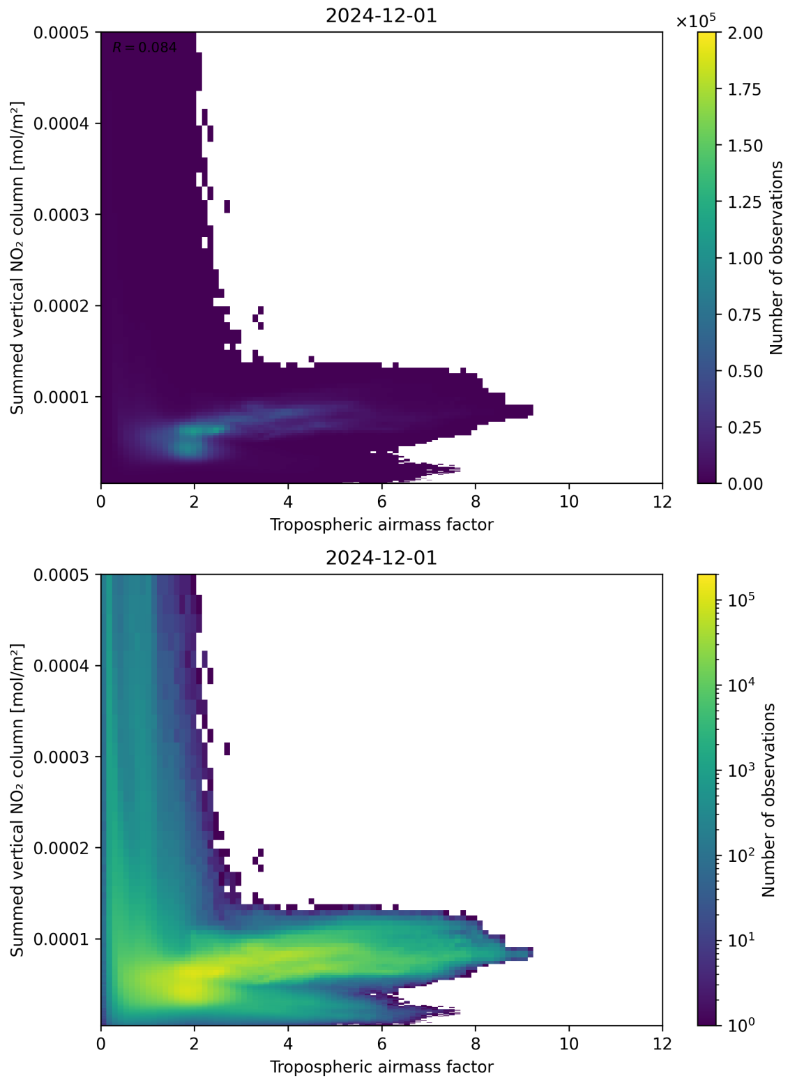
Figure 75: Scatter density plot of “Tropospheric air mass factor” against “Summed vertical NO 2 column” for 2024-11-30 to 2024-12-02.
