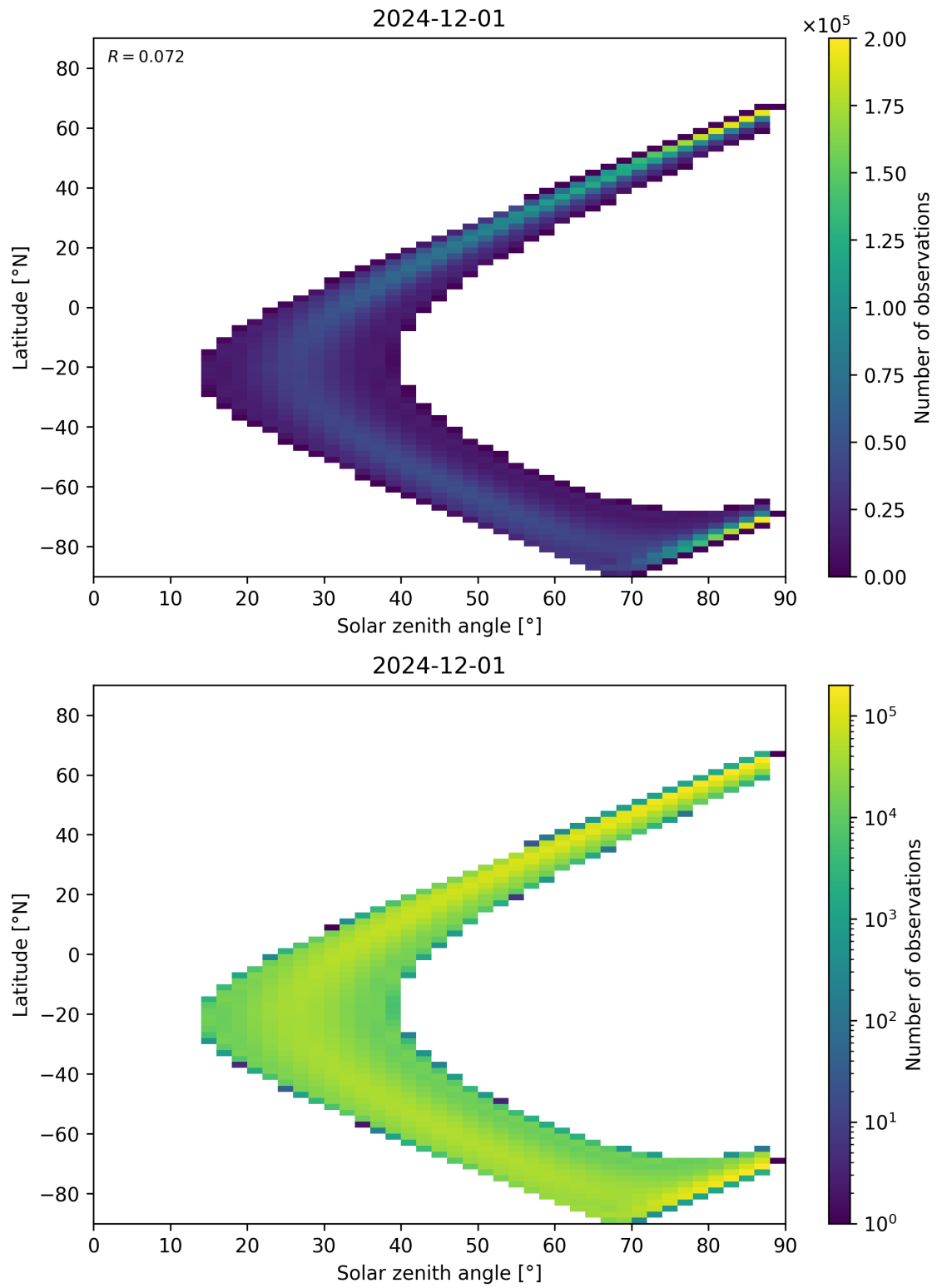
Figure 149: Scatter density plot of “Solar zenith angle” against “Latitude” for 2024-11-30 to 2024-12-02.
