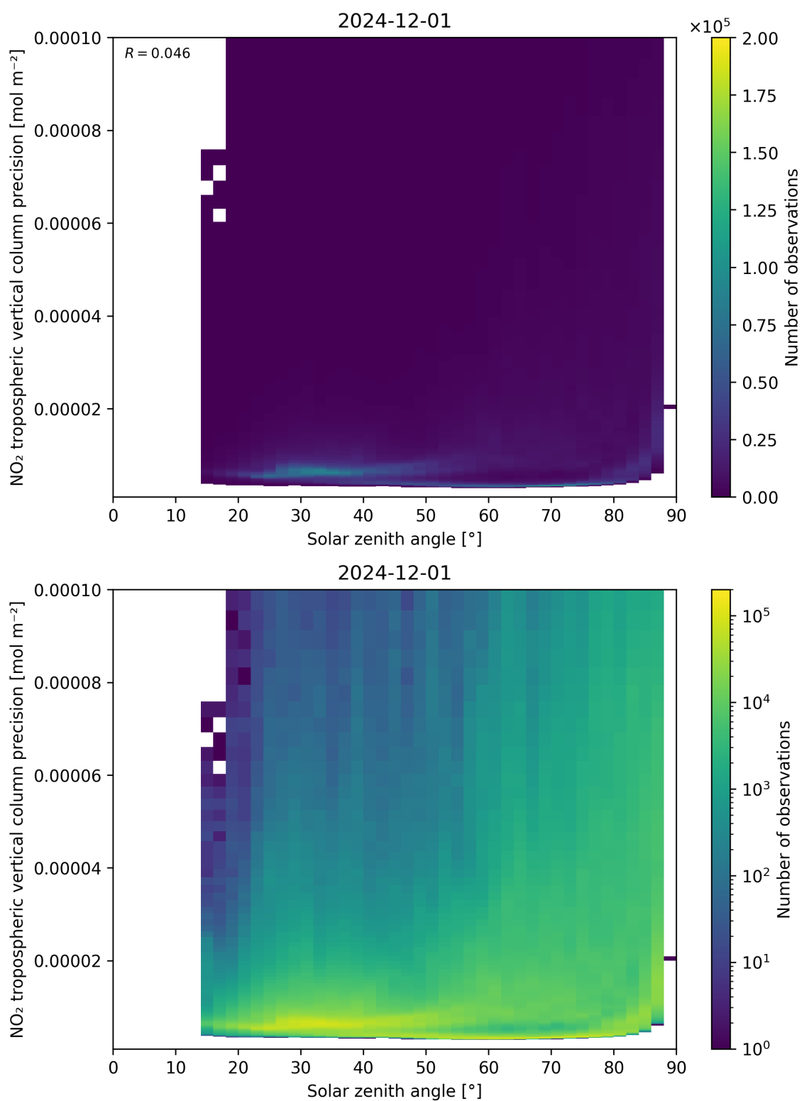
Figure 156: Scatter density plot of “Solar zenith angle” against “NO 2 tropospheric vertical column precision” for 2024-11-30 to 2024-12-02.
