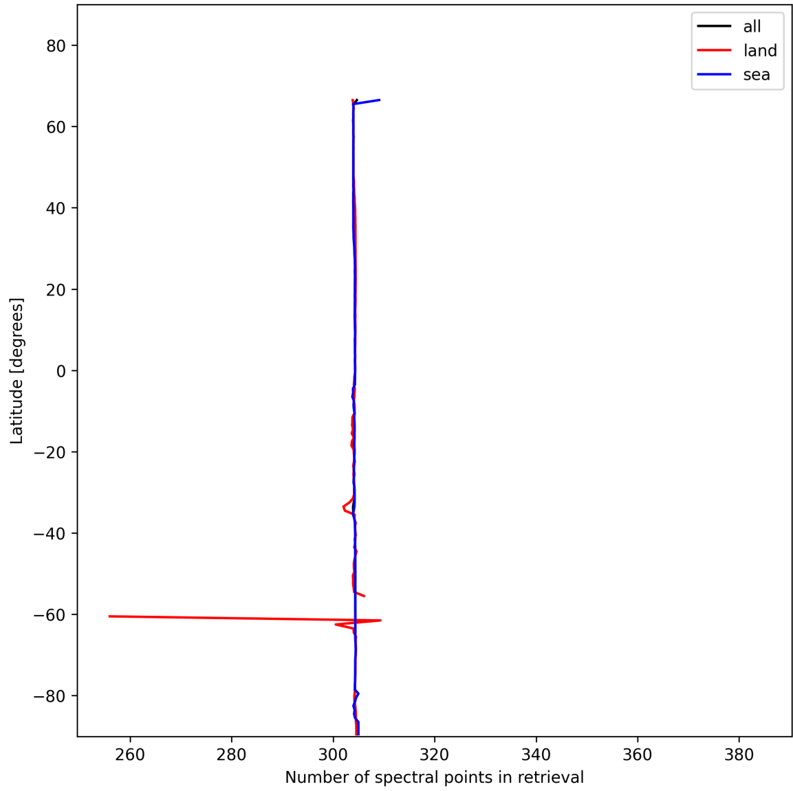
Figure 16: Zonal average of “Number of spectral points in retrieval” for 2024-11-30 to 2024-12-02.
