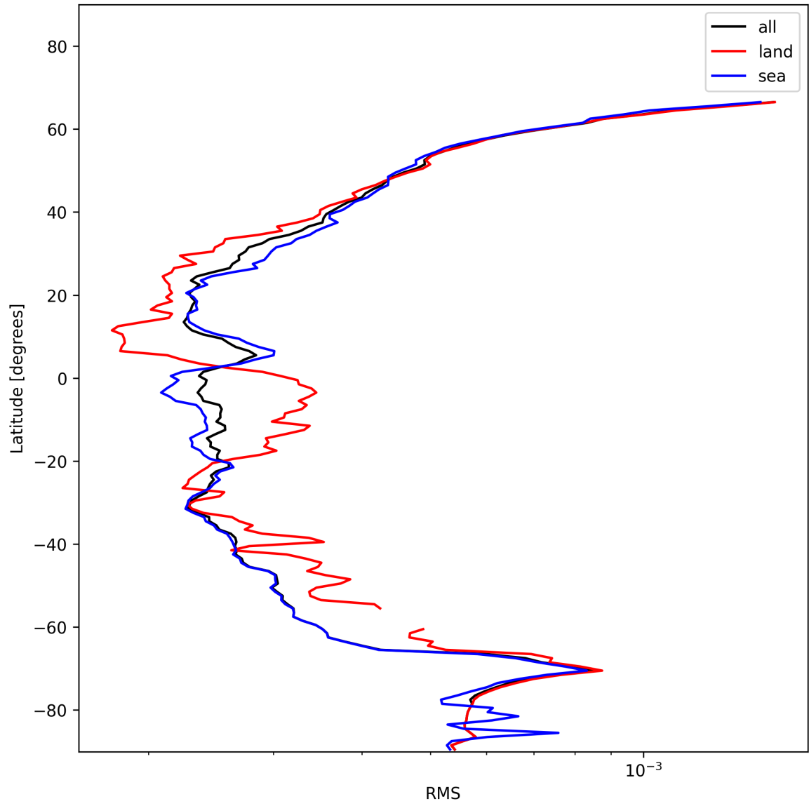
Figure 26: Zonal average of “RMS” for 2024-11-30 to 2024-12-02.
