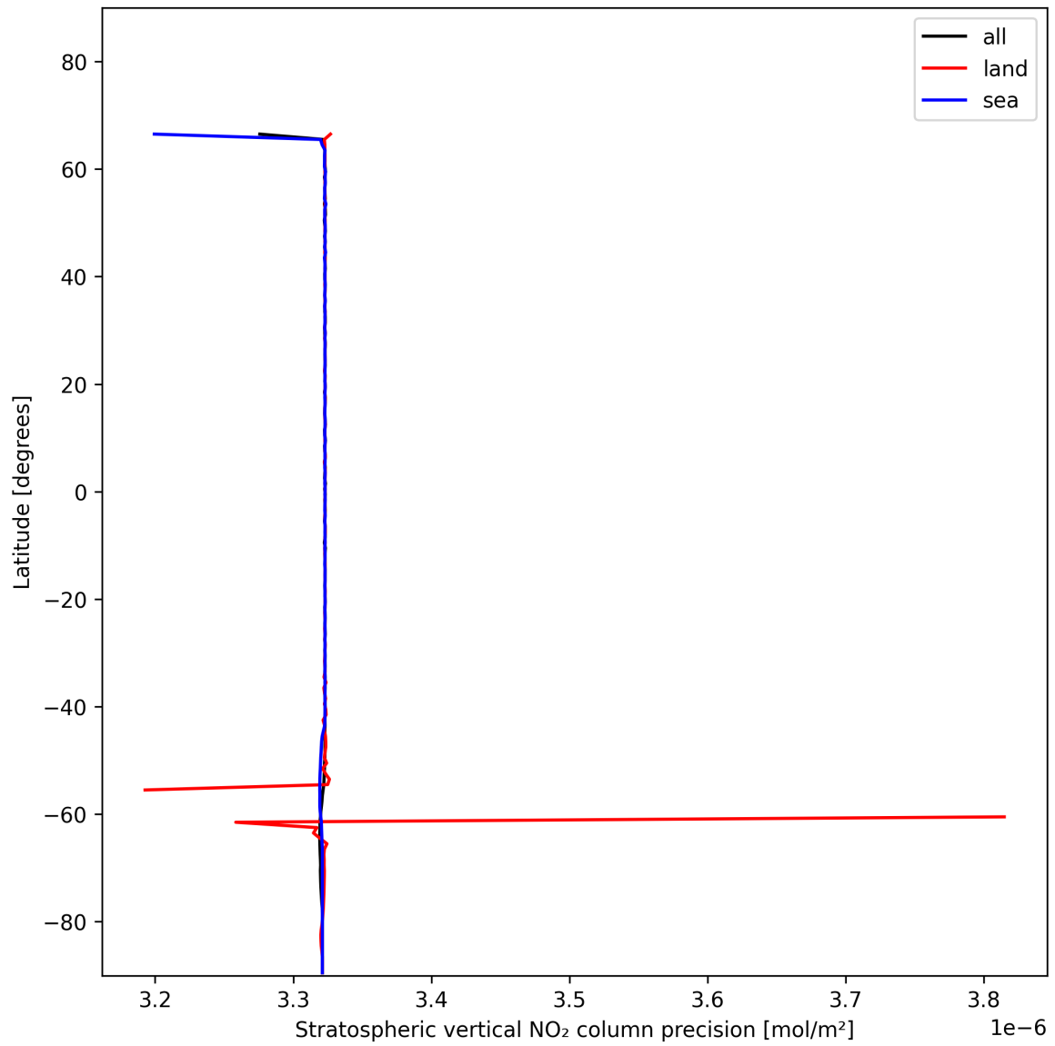
Figure 20: Zonal average of “Stratospheric vertical NO 2 column precision” for 2024-11-30 to 2024-12-02.
