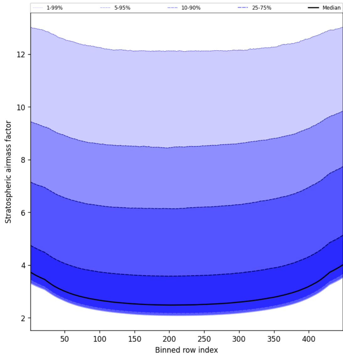
Figure 61: Along track statistics of “Stratospheric air mass factor” for 2024-11-30 to 2024-12-02
