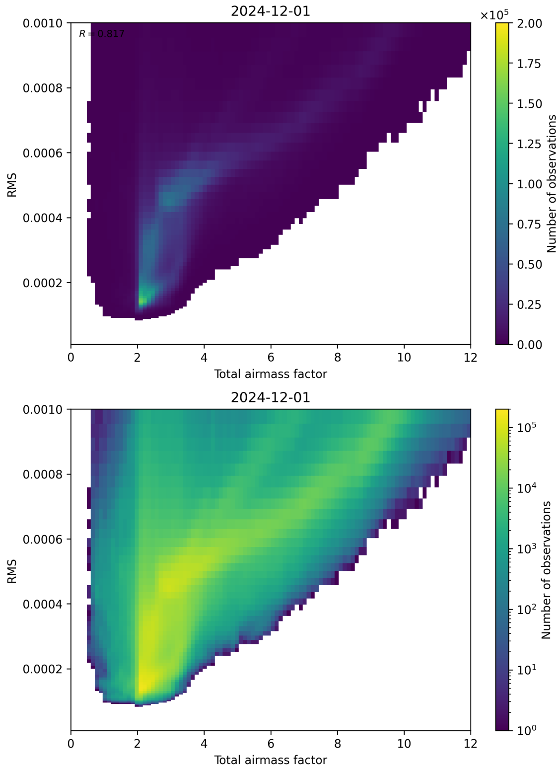
Figure 69: Scatter density plot of “Total airmass factor” against “RMS” for 2024-11-30 to 2024-12-02.
