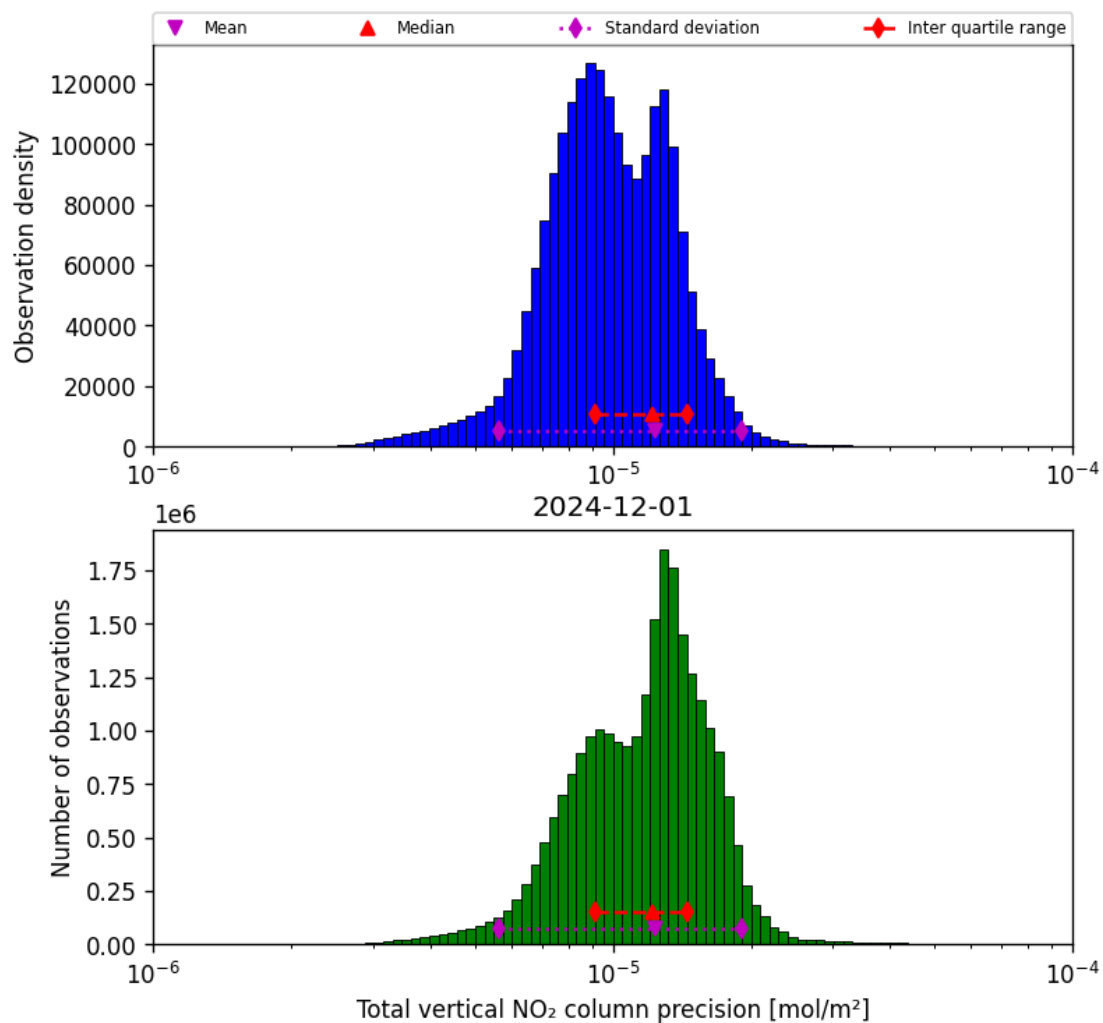
Figure 39: Histogram of “Total vertical NO 2 column precision” for 2024-11-30 to 2024-12-02
