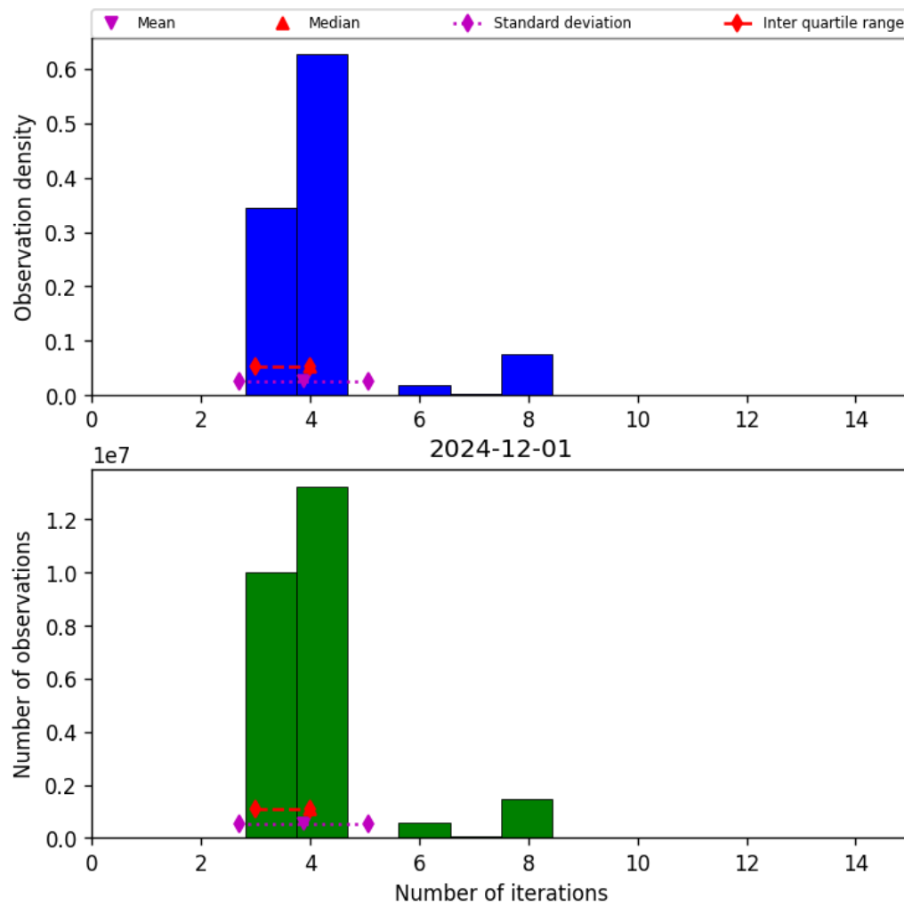
Figure 34: Histogram of “Number of iterations” for 2024-11-30 to 2024-12-02
