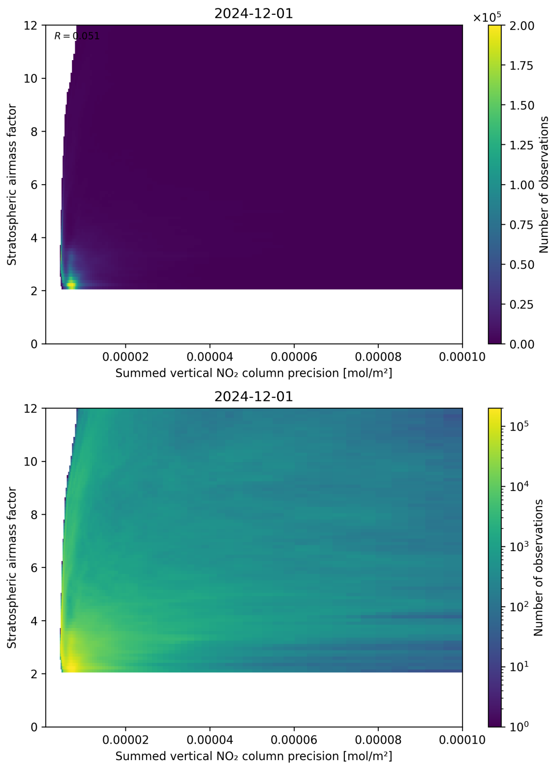
Figure 106: Scatter density plot of “Summed vertical NO 2 column precision” against “Stratospheric airmass factor” for 2024-11-30 to 2024-12-02.
