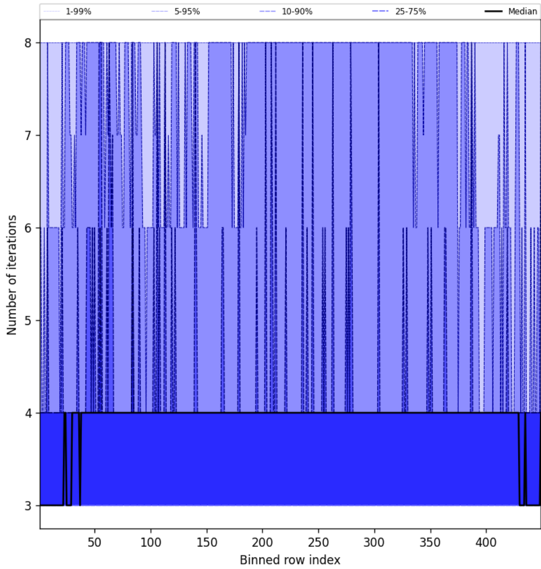
Figure 51: Along track statistics of “Number of iterations” for 2024-11-30 to 2024-12-02
