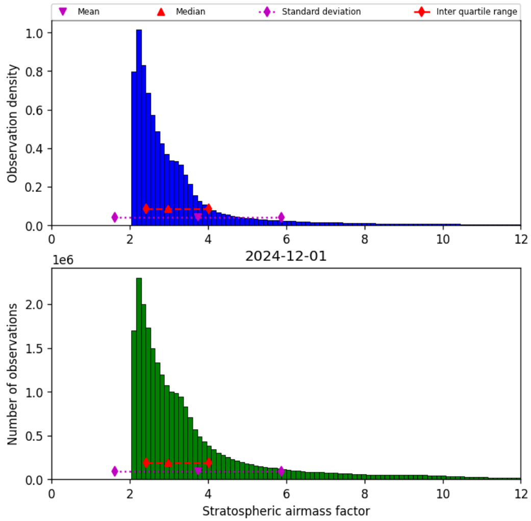
Figure 44: Histogram of “Stratospheric airmass factor” for 2024-11-30 to 2024-12-02
