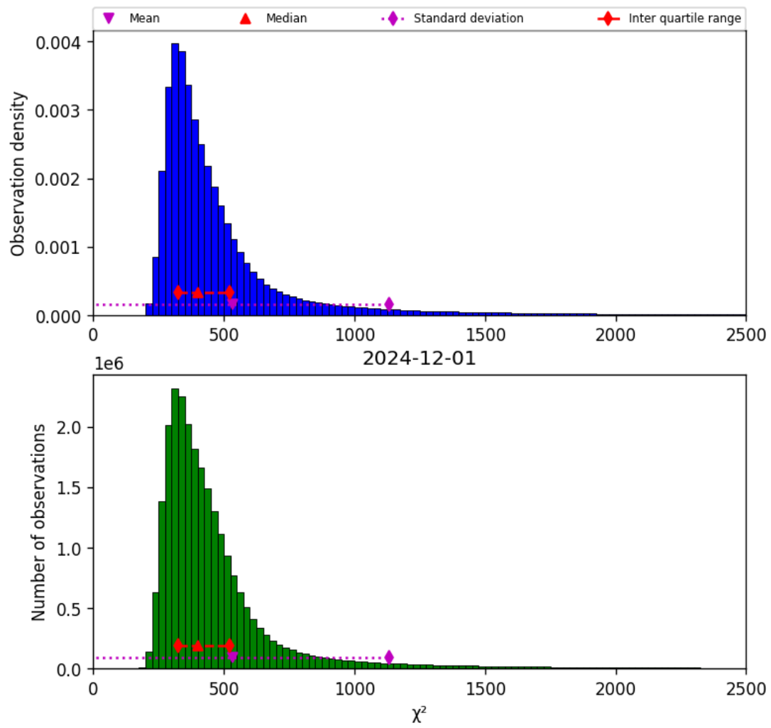
Figure 42: Histogram of " \chi^2 " for 2024-11-30 to 2024-12-02
