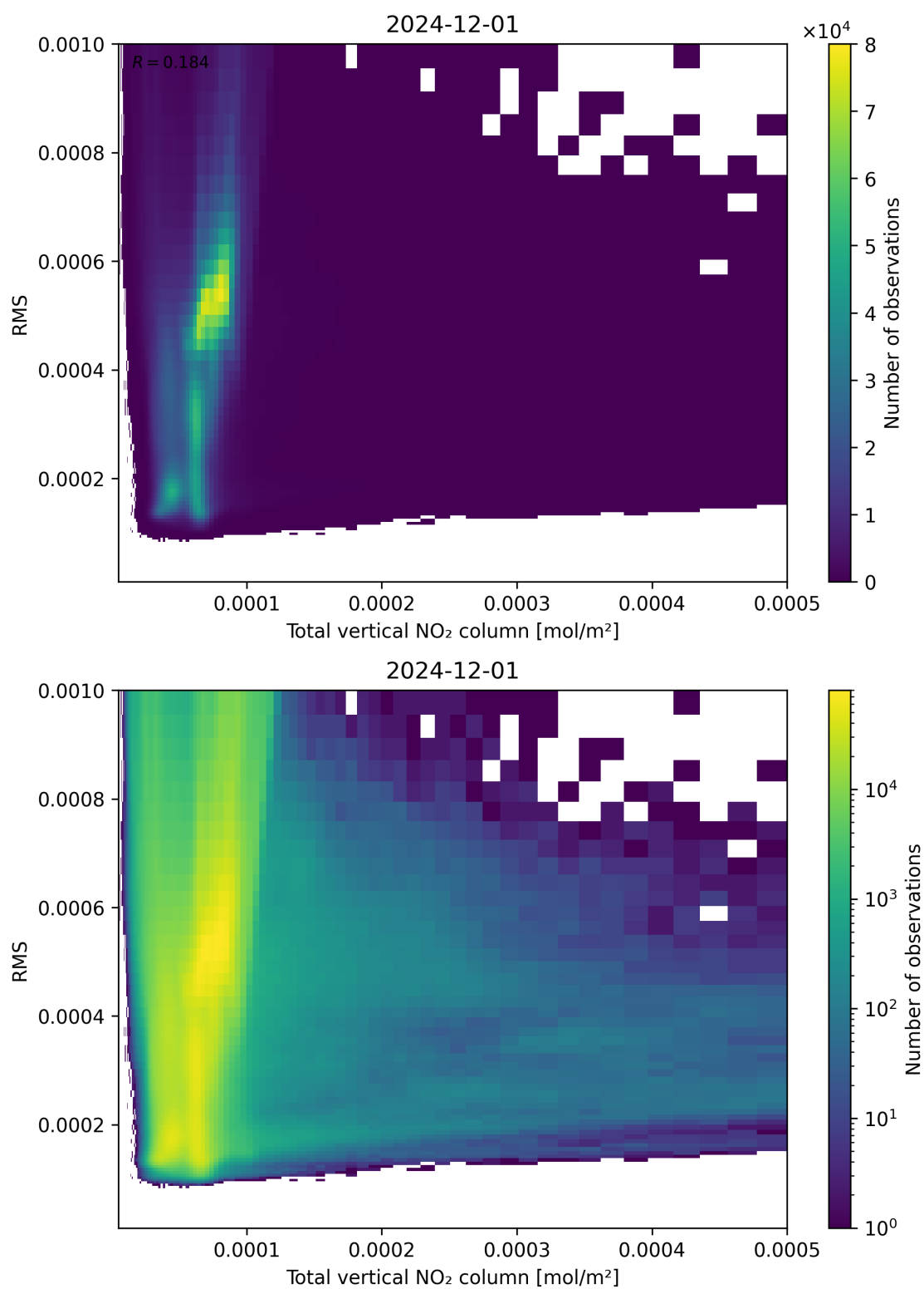
Figure 120: Scatter density plot of “Total vertical NO 2 column” against “RMS” for 2024-11-30 to 2024-12-02.
