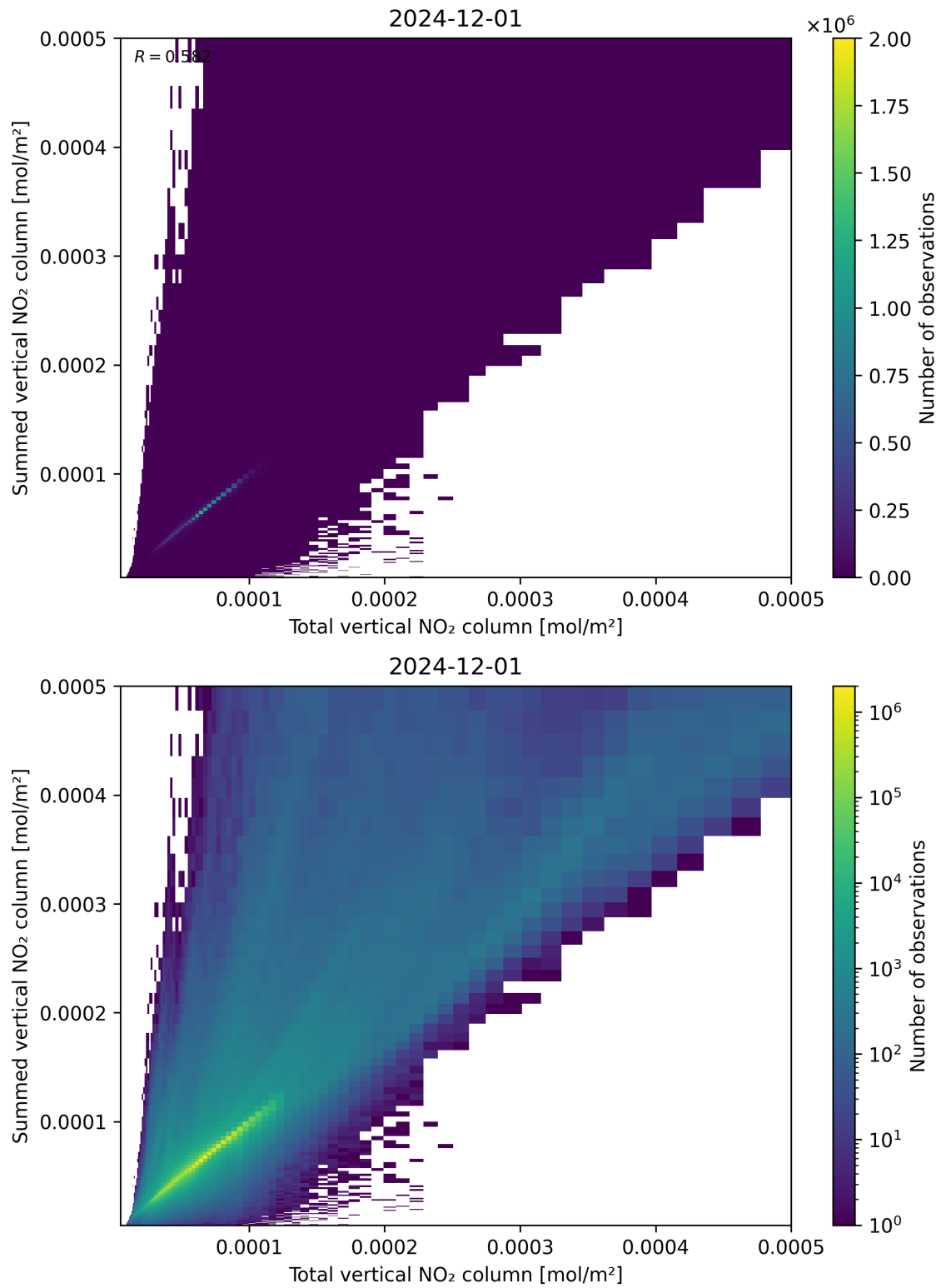
Figure 112: Scatter density plot of “Total vertical NO 2 column” against “Summed vertical NO 2 column” for 2024-11-30 to 2024-12-02.
