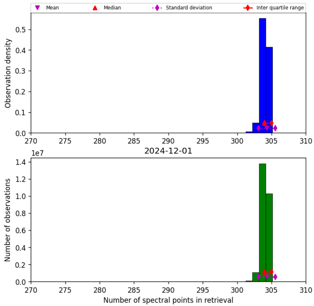
Figure 33: Histogram of “Number of spectral points in retrieval” for 2024-11-30 to 2024-12-02
