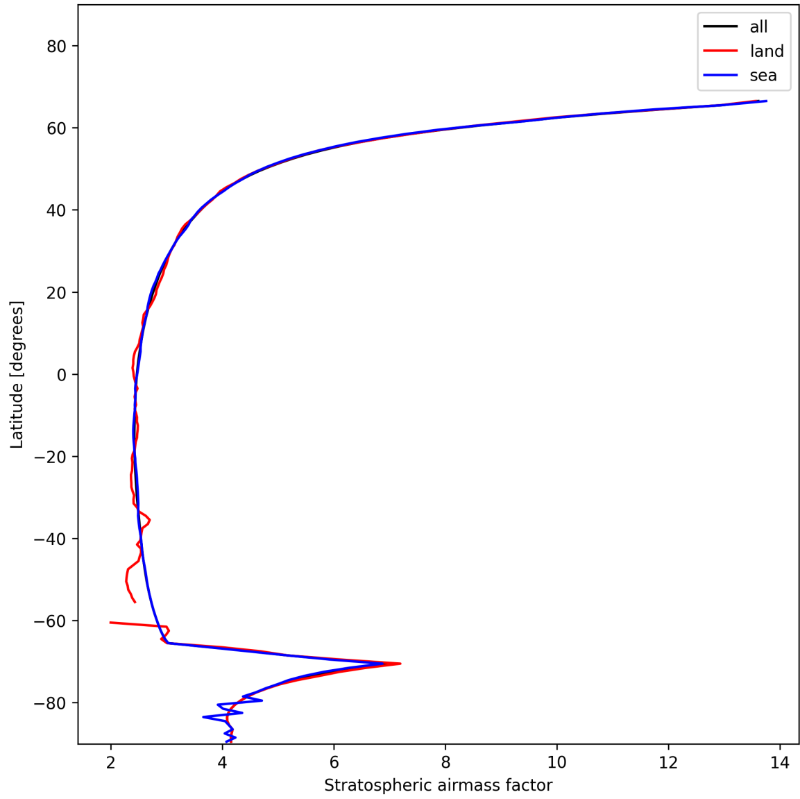
Figure 27: Zonal average of “Stratospheric air mass factor” for 2024-11-30 to 2024-12-02.
