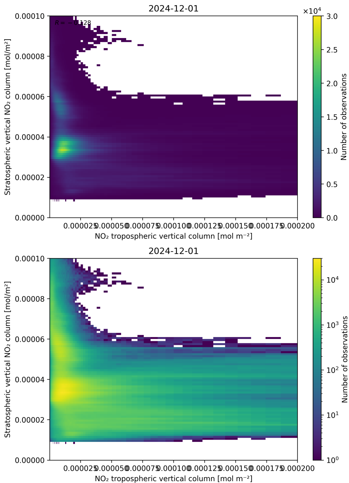
Figure 125: Scatter density plot of “NO 2 tropospheric vertical column” against “Stratospheric vertical NO 2 column” for 2024-11-30 to 2024-12-02.
