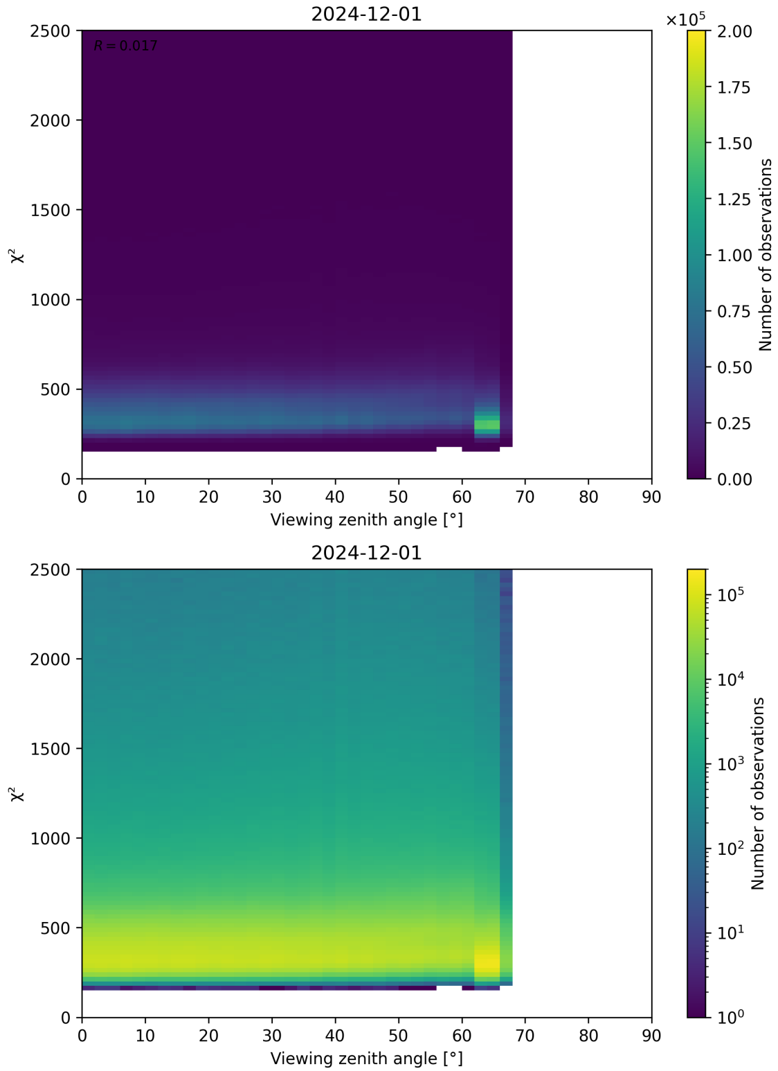
Figure 162: Scatter density plot of “Viewing zenith angle” against “ \chi^2 ” for 2024-11-30 to 2024-12-02.
