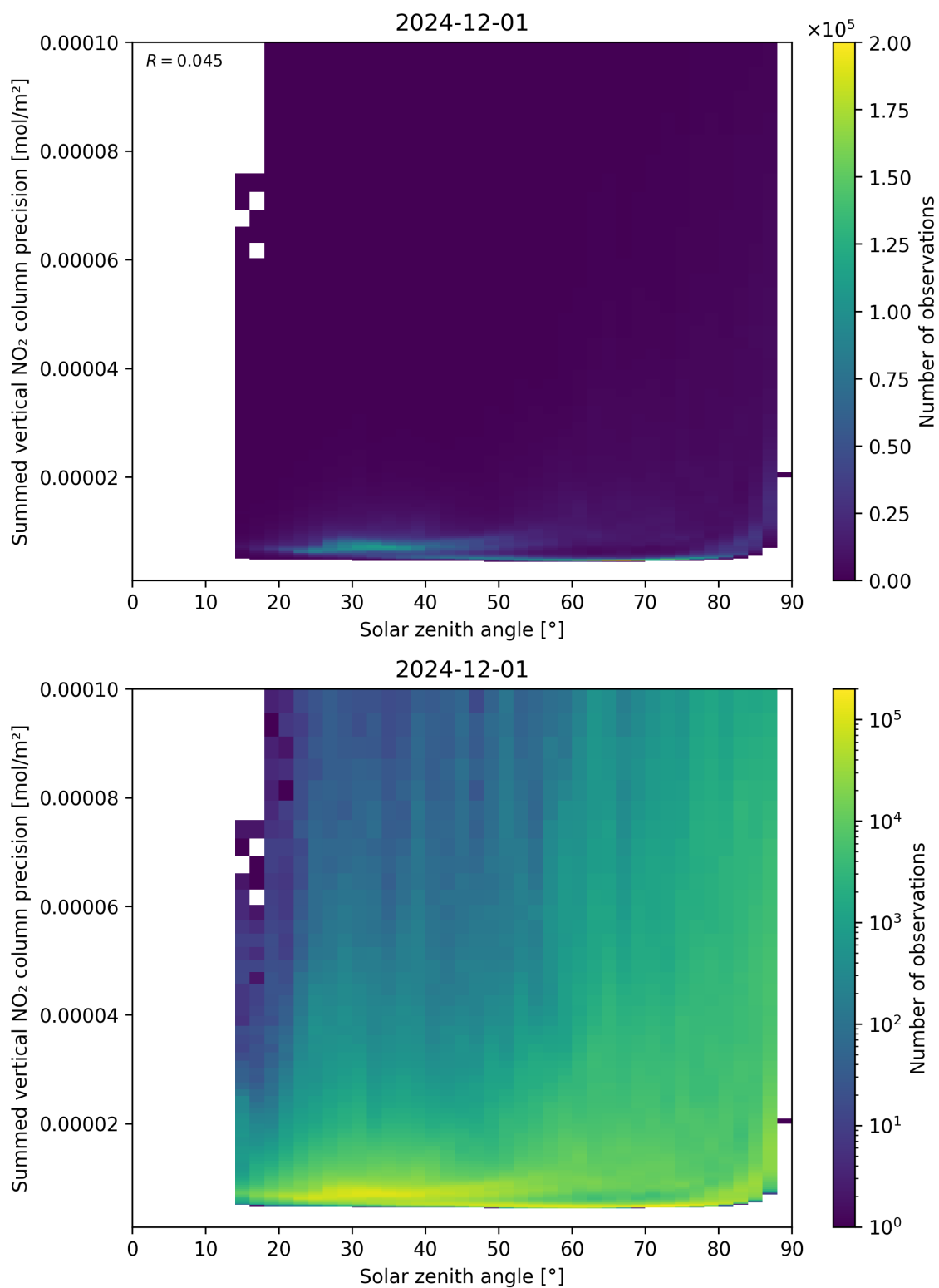
Figure 152: Scatter density plot of “Solar zenith angle” against “Summed vertical NO 2 column precision” for 2024-11-30 to 2024-12-02.
