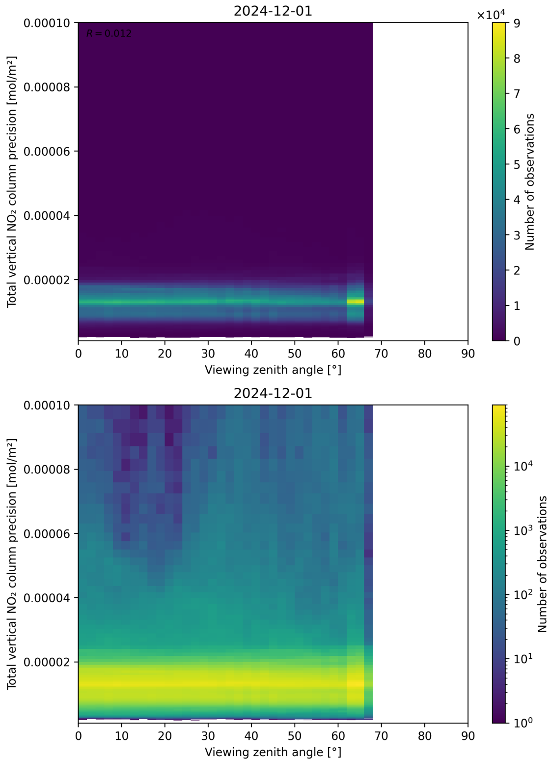
Figure 168: Scatter density plot of “Viewing zenith angle” against “Total vertical NO 2 column precision” for 2024-11-30 to 2024-12-02.
