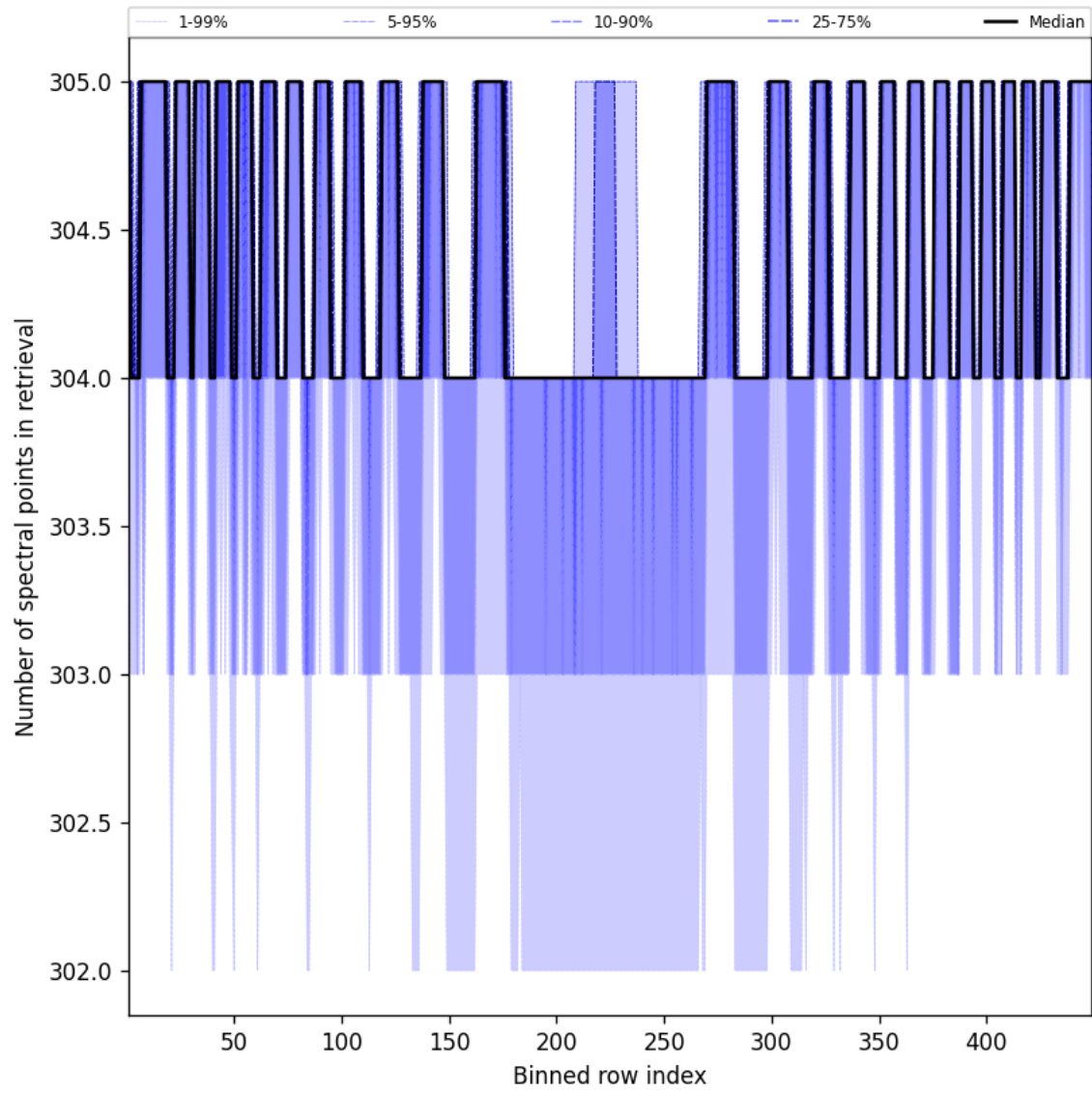
Figure 50: Along track statistics of “Number of spectral points in retrieval” for 2024-11-30 to 2024-12-02
