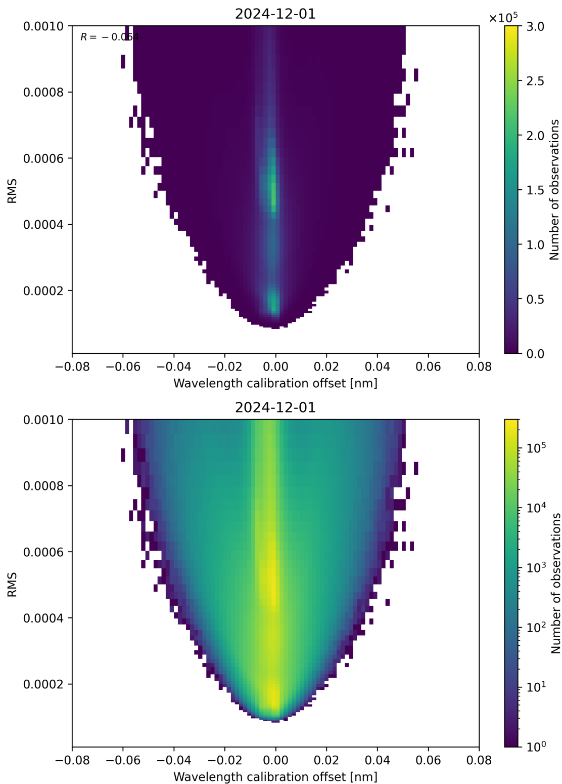
Figure 181: Scatter density plot of “Wavelength calibration offset” against “RMS” for 2024-11-30 to 2024-12-02.
