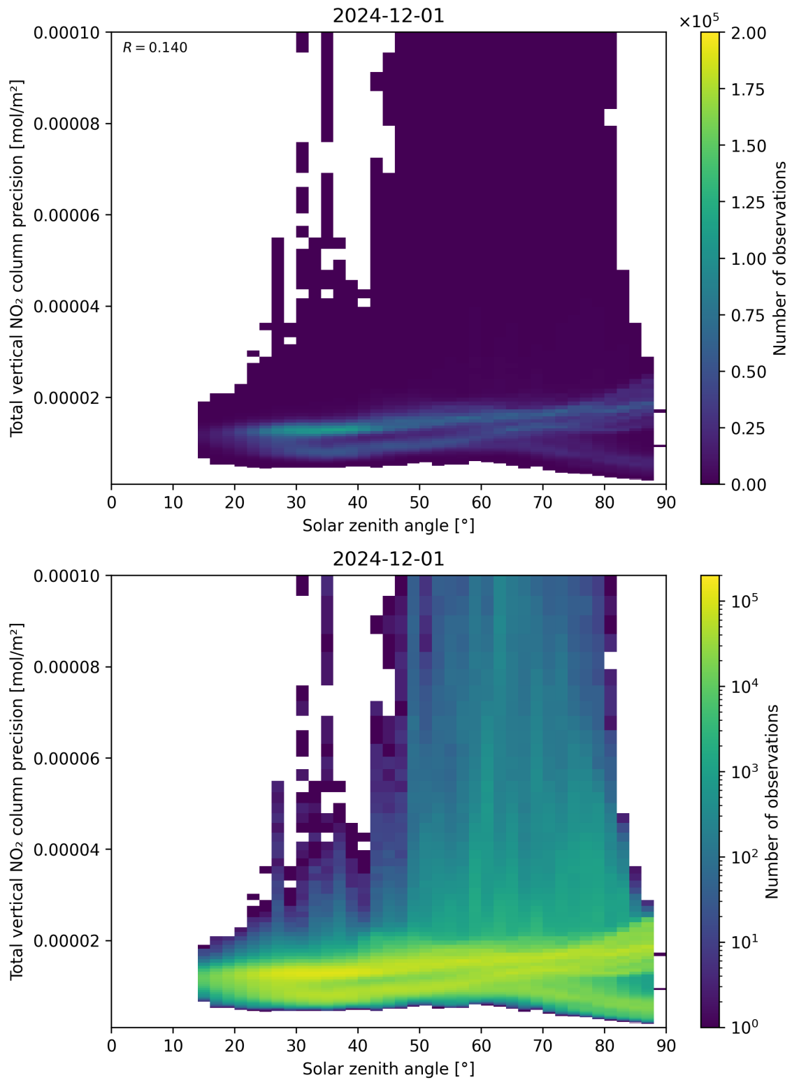
Figure 154: Scatter density plot of “Solar zenith angle” against “Total vertical NO 2 column precision” for 2024-11-30 to 2024-12-02.
