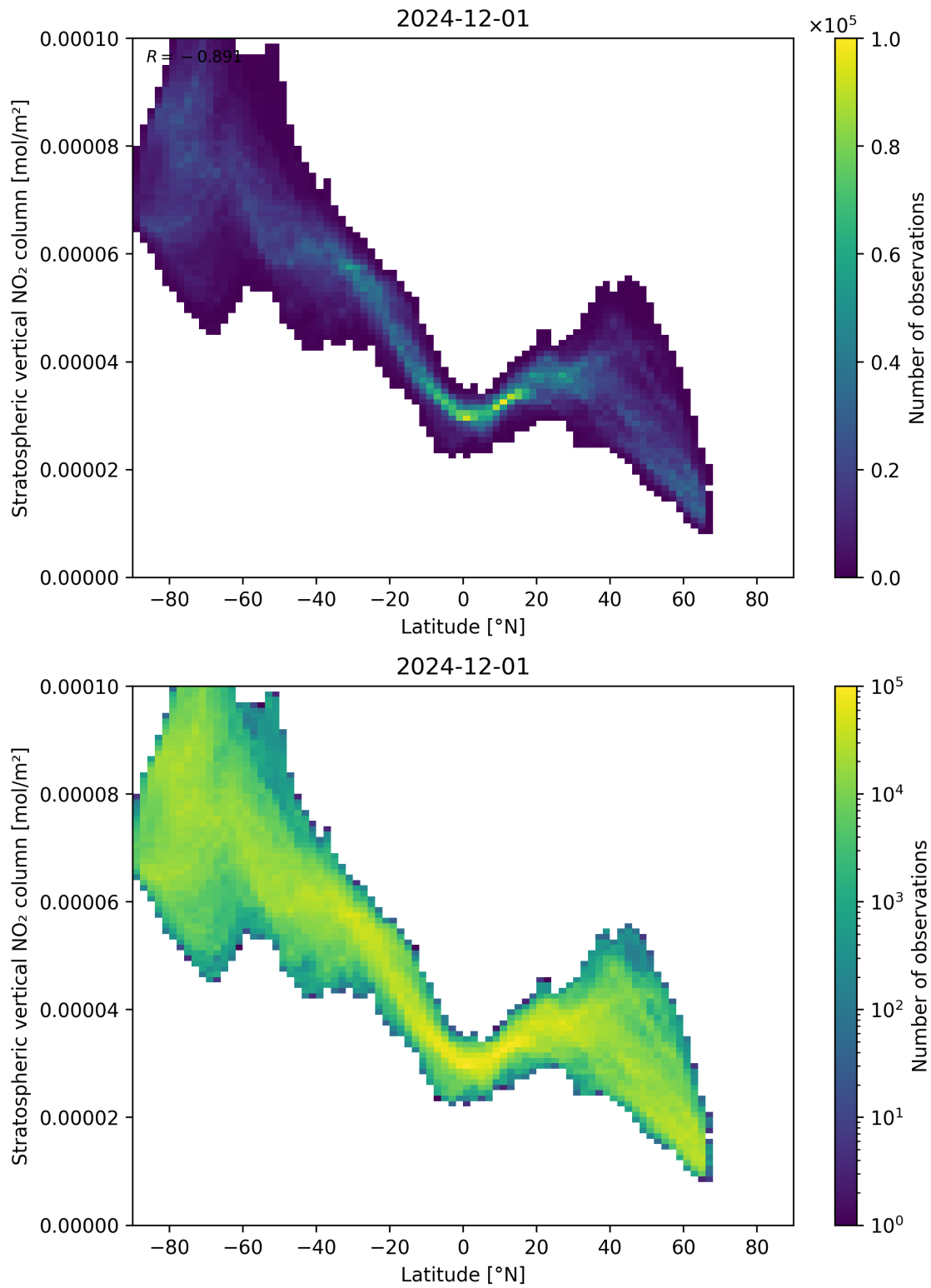
Figure 87: Scatter density plot of “Latitude” against “Stratospheric vertical NO 2 column” for 2024-11-30 to 2024-12-02.
