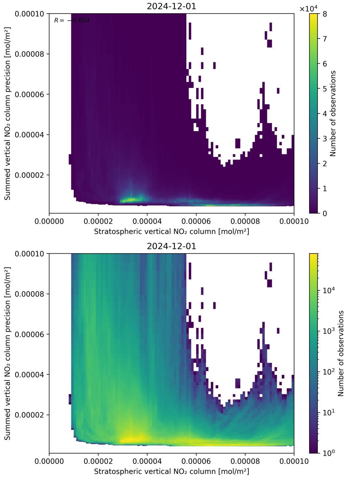
Figure 99: Scatter density plot of “Stratospheric vertical NO 2 column” against “Summed vertical NO 2 column precision” for 2024-11-30 to 2024-12-02.
