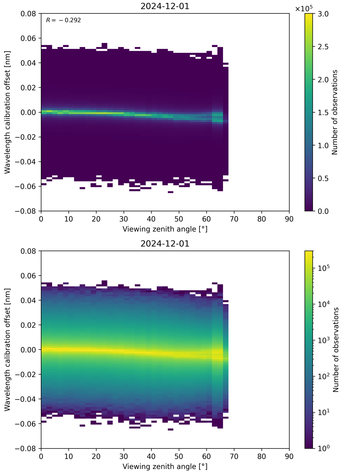
Figure 173: Scatter density plot of “Viewing zenith angle” against “Wavelength calibration offset” for 2024-11-30 to 2024-12-02.
