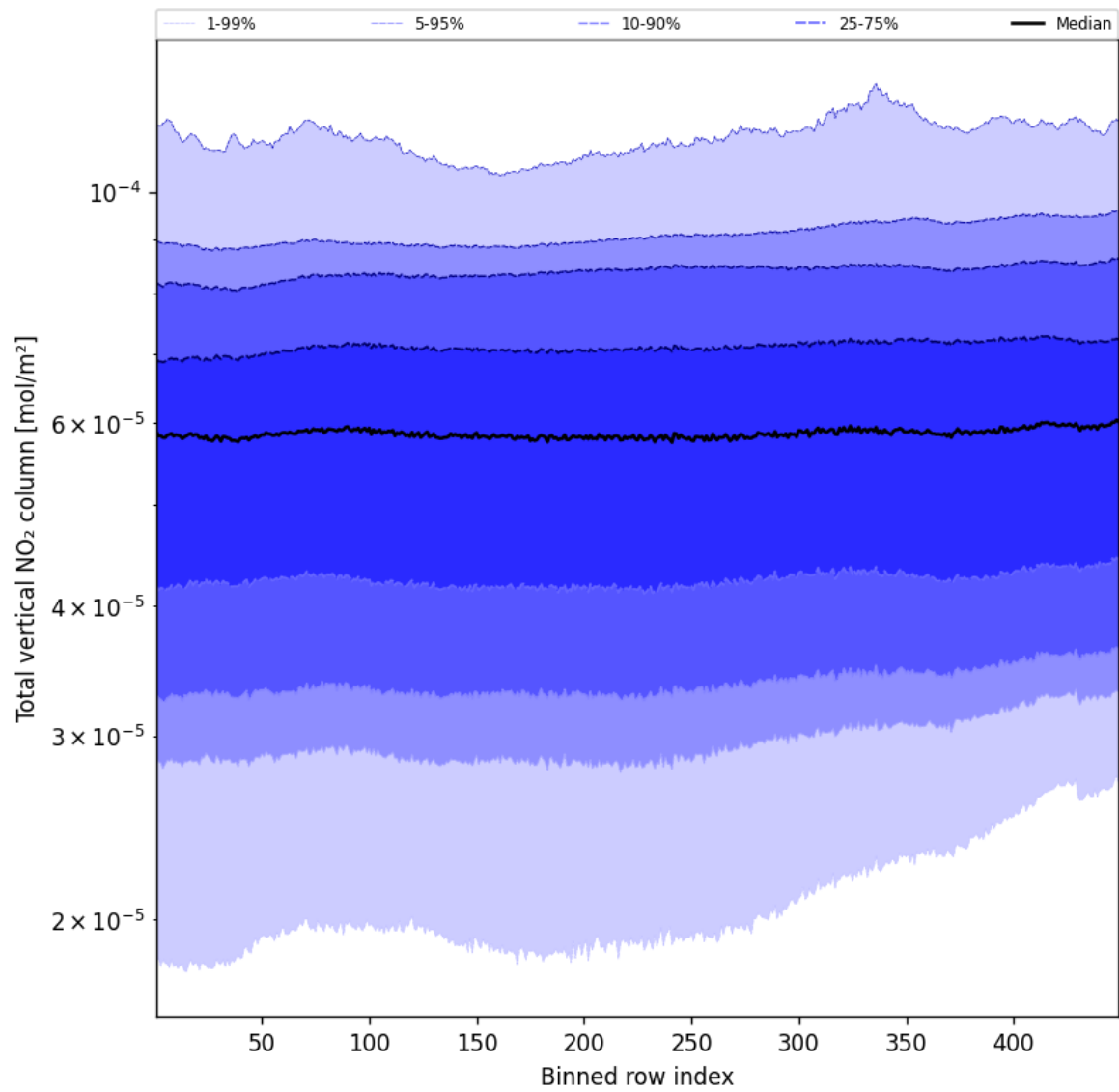
Figure 55: Along track statistics of “Total vertical NO 2 column” for 2024-11-30 to 2024-12-02
