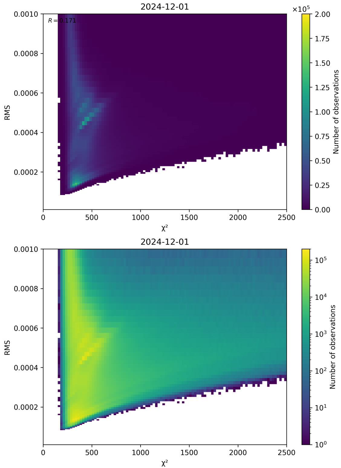
Figure 82: Scatter density plot of “ \chi^2 ” against “RMS” for 2024-11-30 to 2024-12-02.
