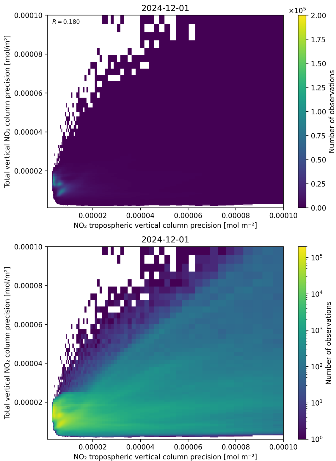
Figure 139: Scatter density plot of “NO 2 tropospheric vertical column precision” against “Total vertical NO 2 column precision” for 2024-11-30 to 2024-12-02.
