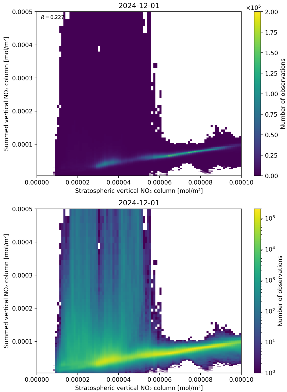
Figure 98: Scatter density plot of “Stratospheric vertical NO 2 column” against “Summed vertical NO 2 column” for 2024-11-30 to 2024-12-02.
