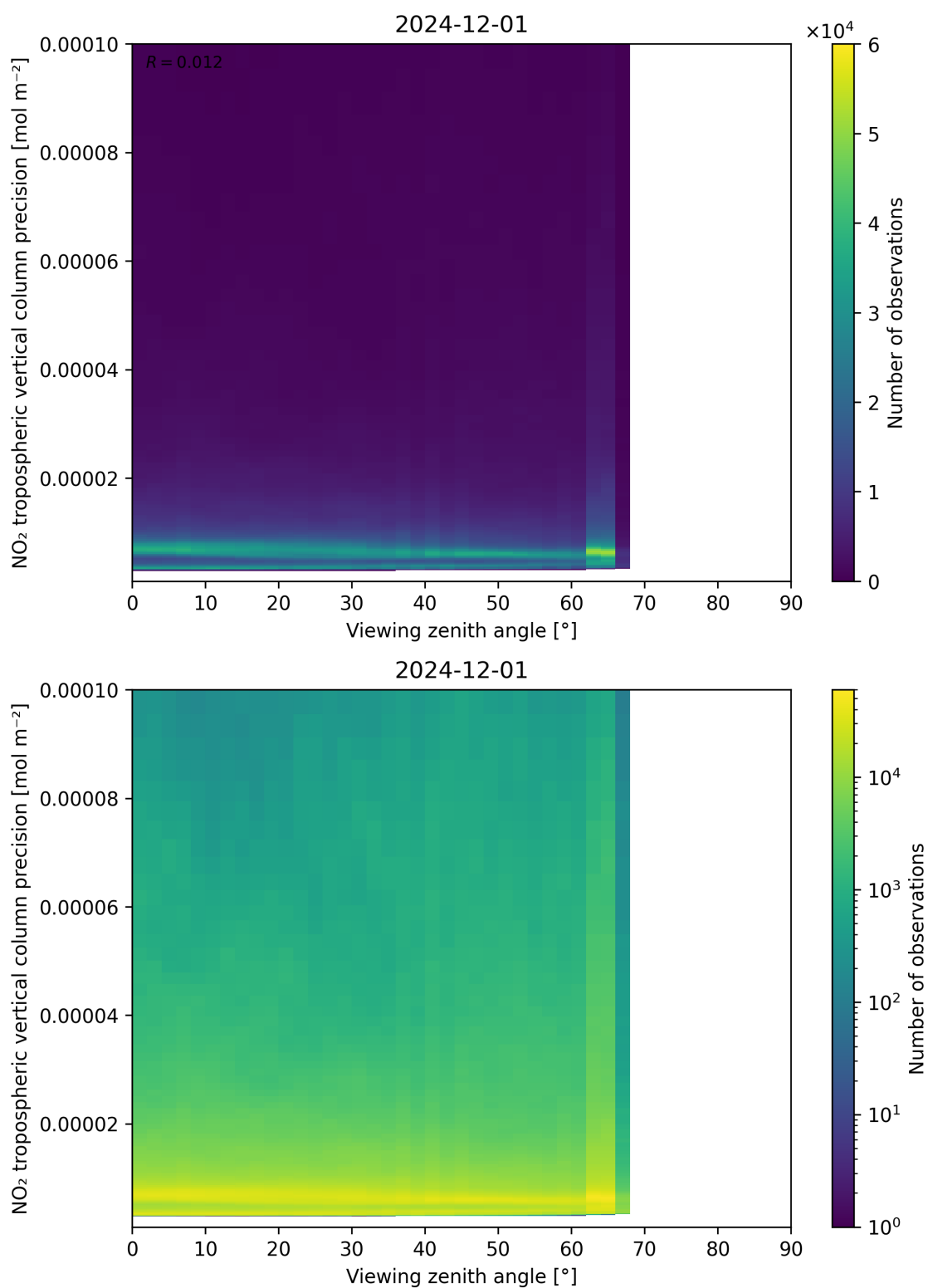
Figure 170: Scatter density plot of “Viewing zenith angle” against “NO 2 tropospheric vertical column precision” for 2024-11-30 to 2024-12-02.
