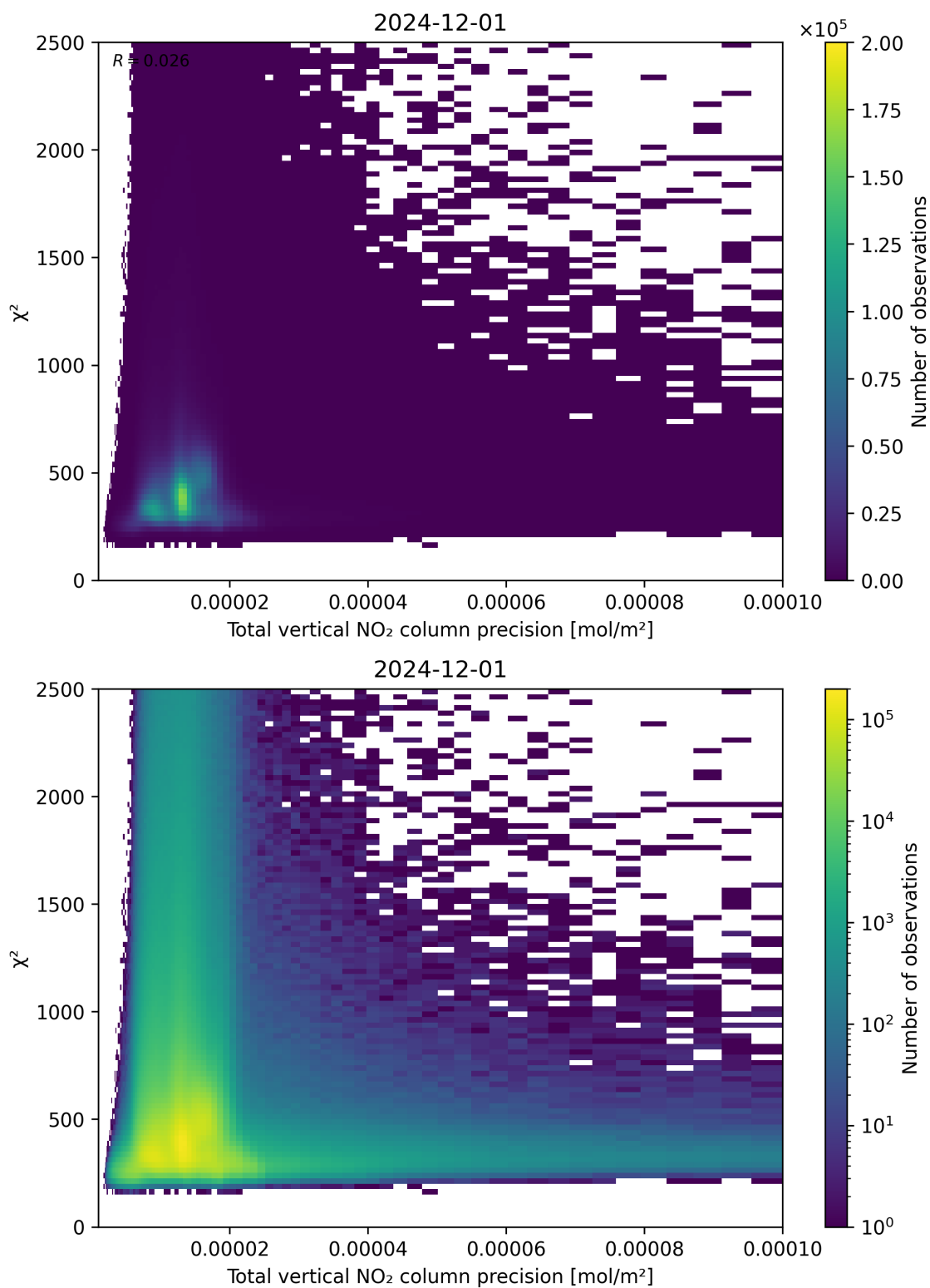
Figure 116: Scatter density plot of “Total vertical NO 2 column precision” against “ \chi^2 ” for 2024-11-30 to 2024-12-02.
