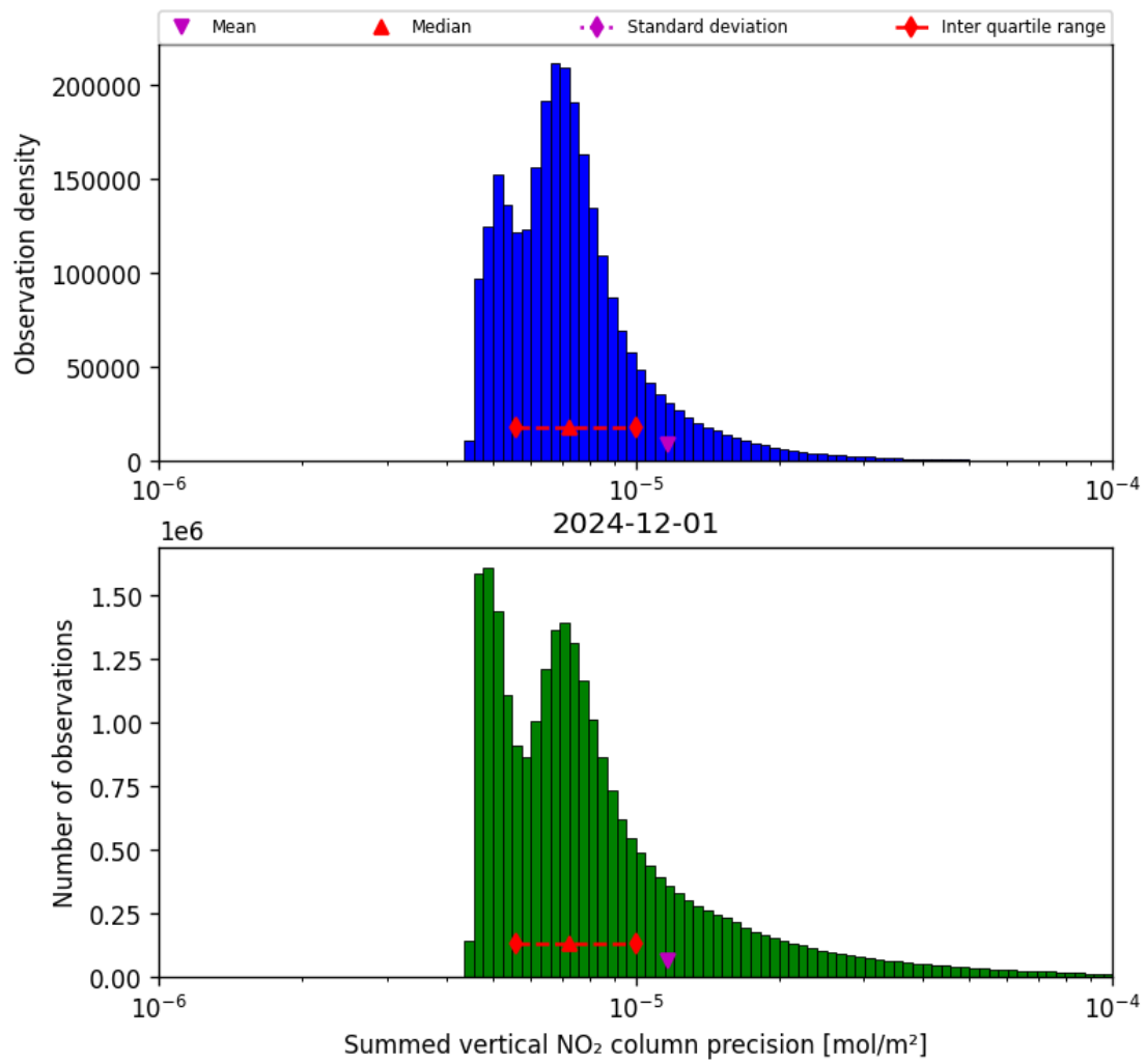
Figure 41: Histogram of “Summed vertical NO 2 column precision” for 2024-11-30 to 2024-12-02
