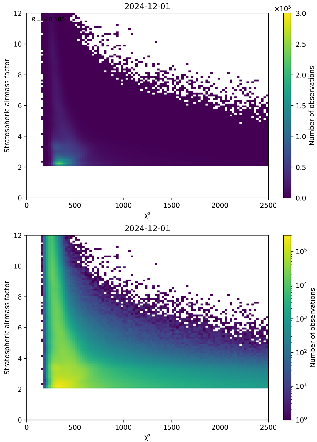
Figure 81: Scatter density plot of “ \chi^2 ” against “Stratospheric airmass factor” for 2024-11-30 to 2024-12-02.
