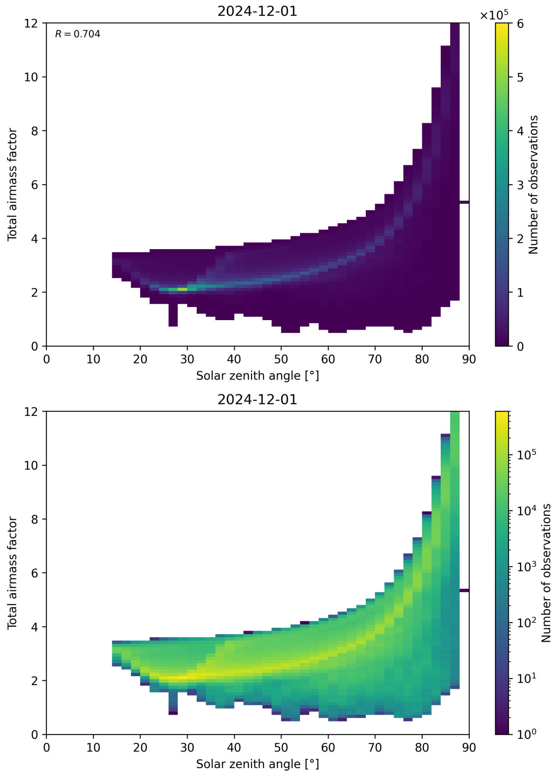
Figure 146: Scatter density plot of “Solar zenith angle” against “Total airmass factor” for 2024-11-30 to 2024-12-02.
