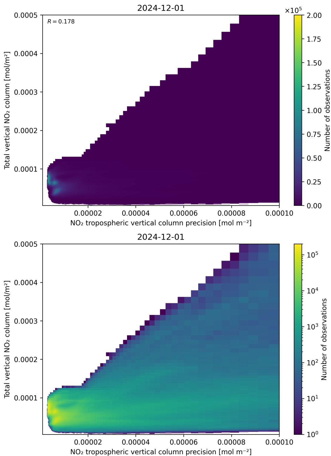
Figure 138: Scatter density plot of “NO 2 tropospheric vertical column precision” against “Total vertical NO 2 column” for 2024-11-30 to 2024-12-02.
