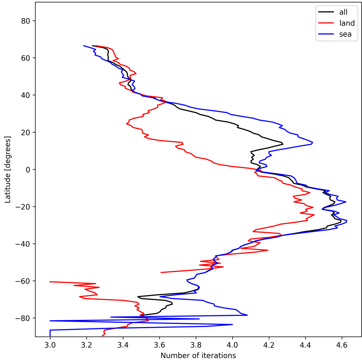
Figure 17: Zonal average of “Number of iterations” for 2024-11-30 to 2024-12-02.
