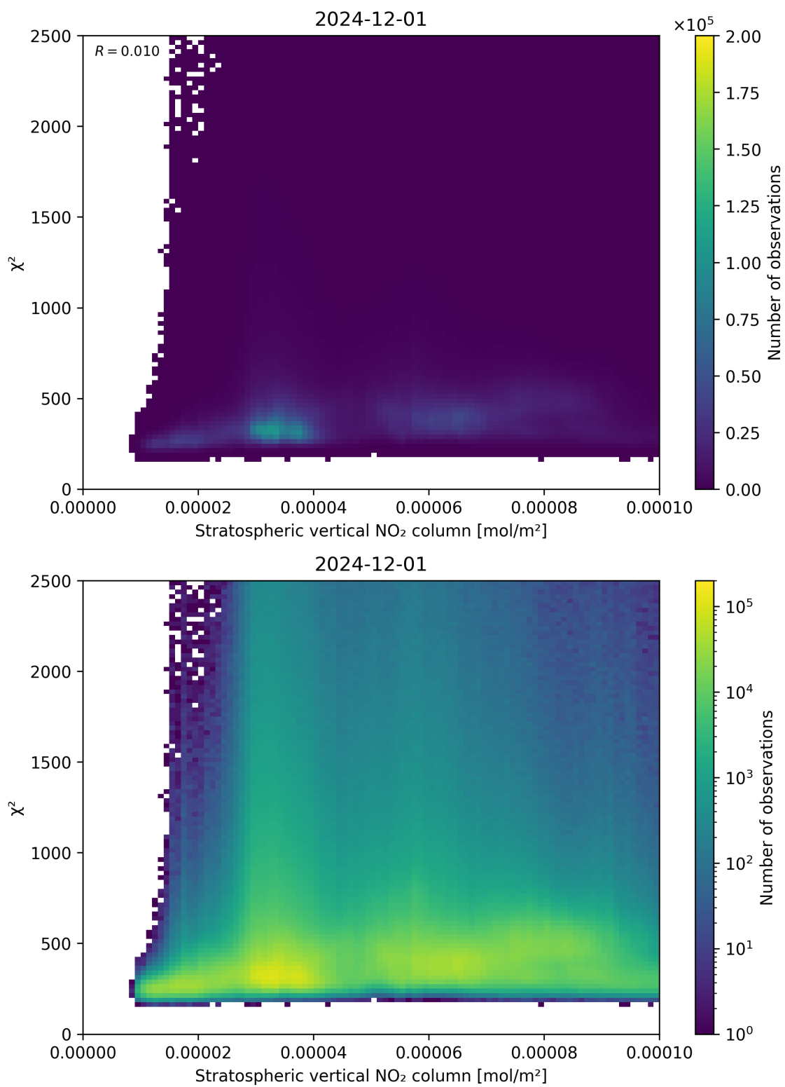
Figure 97: Scatter density plot of “Stratospheric vertical NO 2 column” against “ \chi^2 ” for 2024-11-30 to 2024-12-02.
