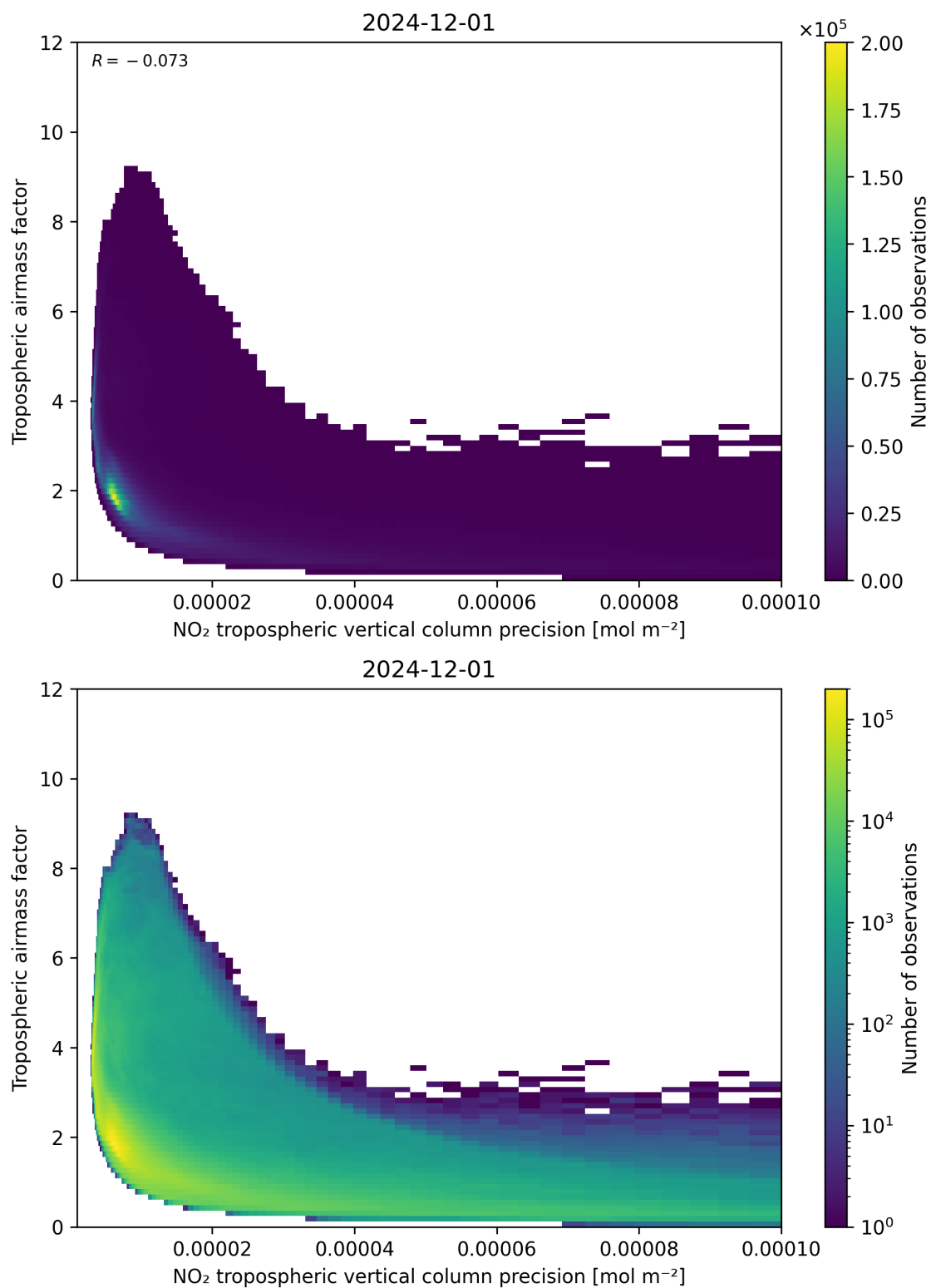
Figure 133: Scatter density plot of “NO 2 tropospheric vertical column precision” against “Tropospheric airmass factor” for 2024-11-30 to 2024-12-02.
