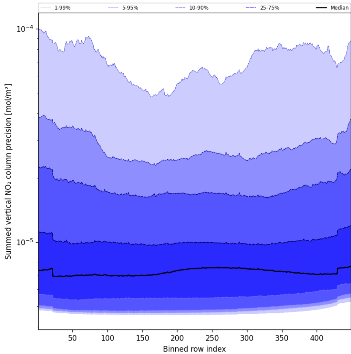
Figure 58: Along track statistics of “Summed vertical NO 2 column precision” for 2024-11-30 to 2024-12-02
