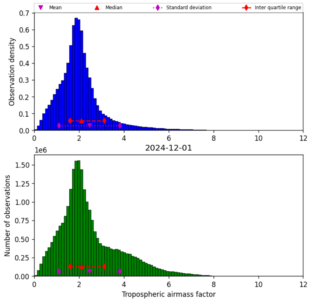
Figure 31: Histogram of “Tropospheric airmass factor” for 2024-11-30 to 2024-12-02
