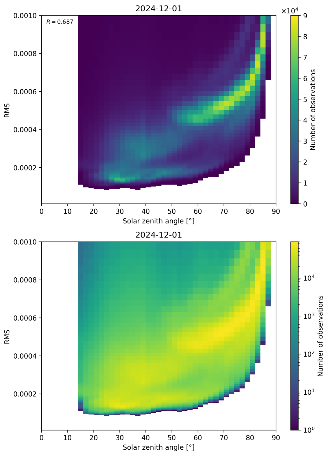
Figure 157: Scatter density plot of “Solar zenith angle” against “RMS” for 2024-11-30 to 2024-12-02.
