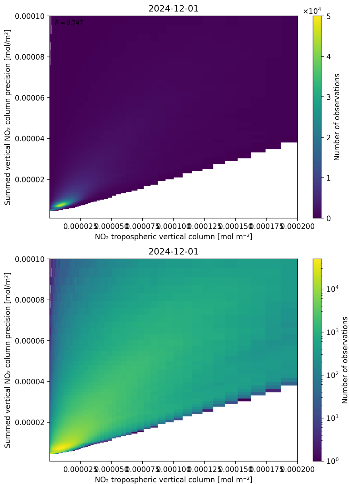
Figure 127: Scatter density plot of “NO 2 tropospheric vertical column” against “Summed vertical NO 2 column precision” for 2024-11-30 to 2024-12-02.
