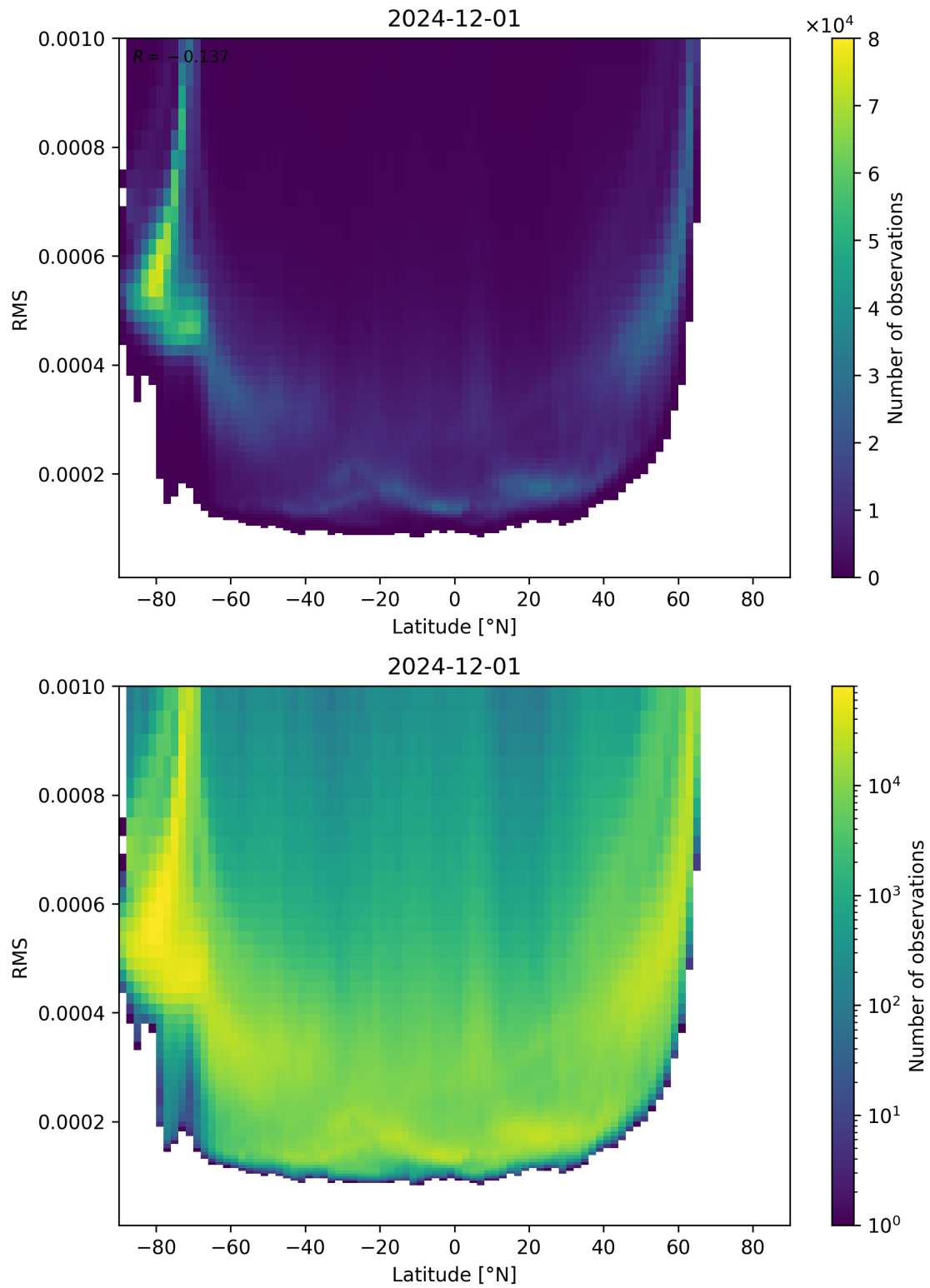
Figure 94: Scatter density plot of “Latitude” against “RMS” for 2024-11-30 to 2024-12-02.
