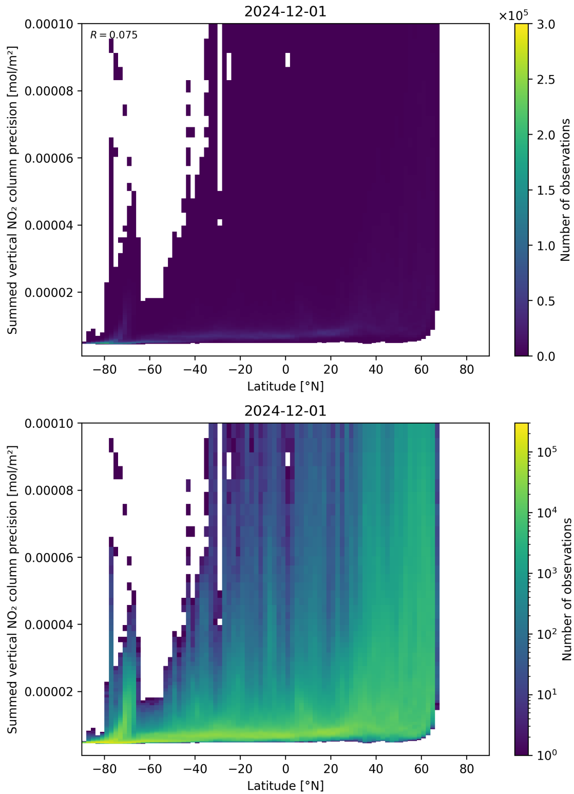
Figure 89: Scatter density plot of “Latitude” against “Summed vertical NO 2 column precision” for 2024-11-30 to 2024-12-02.
