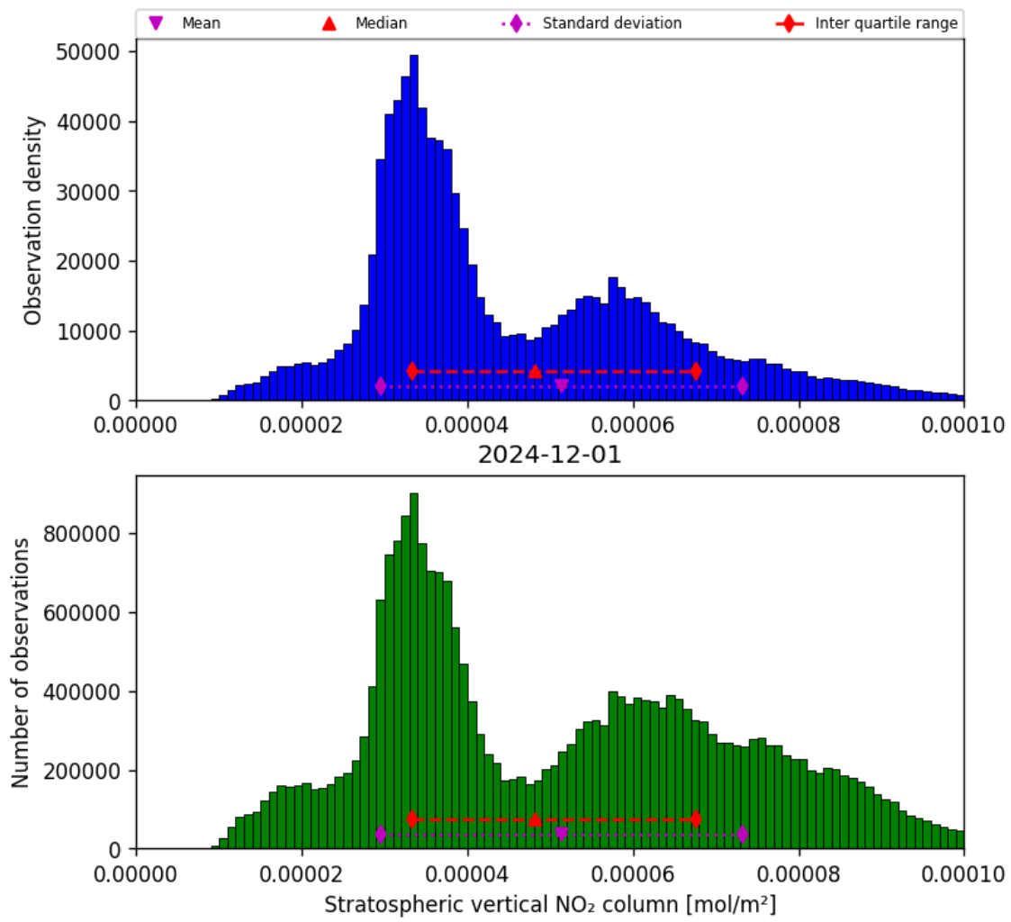
Figure 36: Histogram of “Stratospheric vertical NO 2 column” for 2024-11-30 to 2024-12-02
