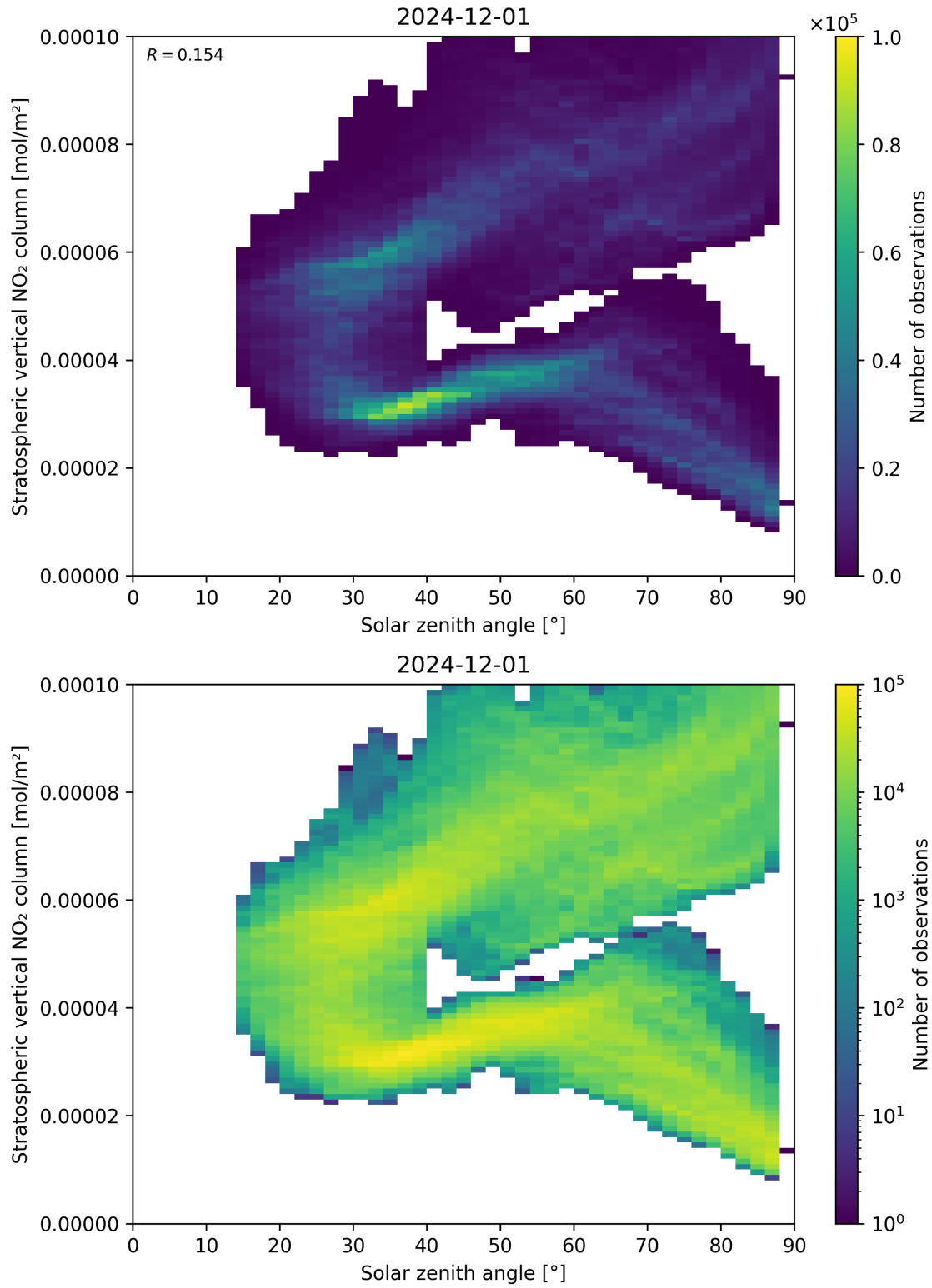
Figure 150: Scatter density plot of “Solar zenith angle” against “Stratospheric vertical NO 2 column” for 2024-11-30 to 2024-12-02.
