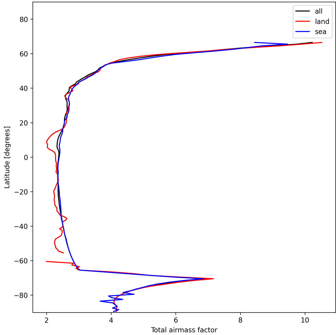
Figure 15: Zonal average of “Total airmass factor” for 2024-11-30 to 2024-12-02.
