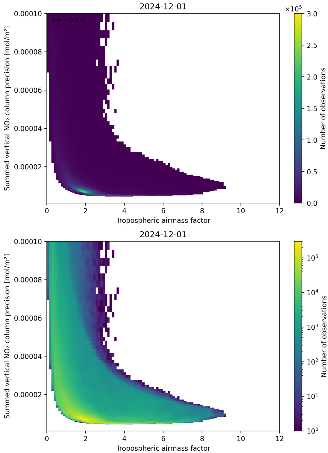
Figure 76: Scatter density plot of “Tropospheric airmass factor” against “Summed vertical NO 2 column precision” for 2024-11-30 to 2024-12-02.
