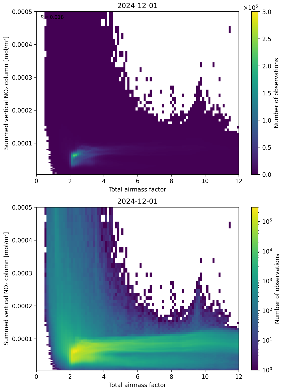
Figure 65: Scatter density plot of “Total airmass factor” against “Summed vertical NO 2 column” for 2024-11-30 to 2024-12-02.
