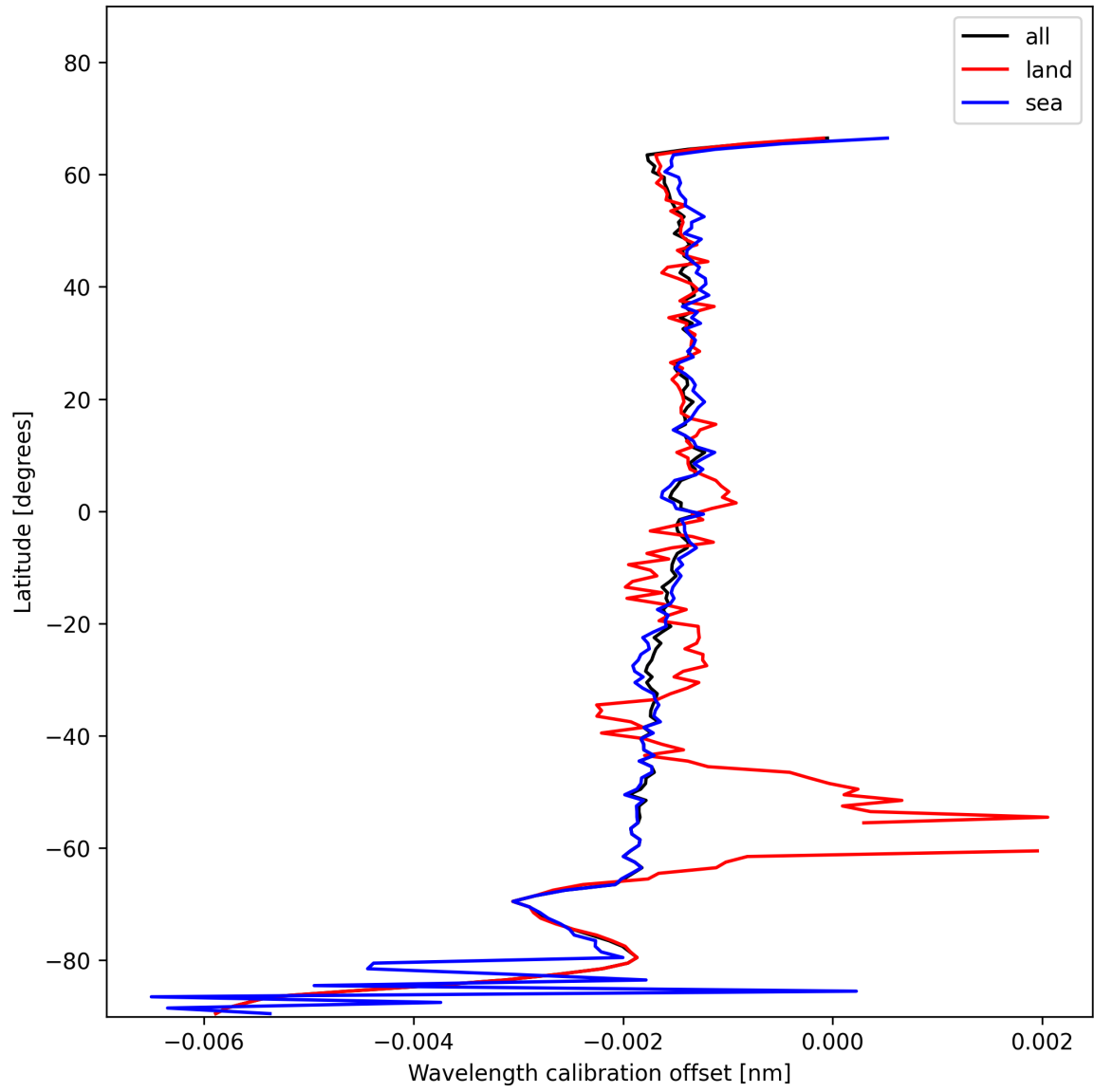
Figure 18: Zonal average of “Wavelength calibration offset” for 2024-11-30 to 2024-12-02.
