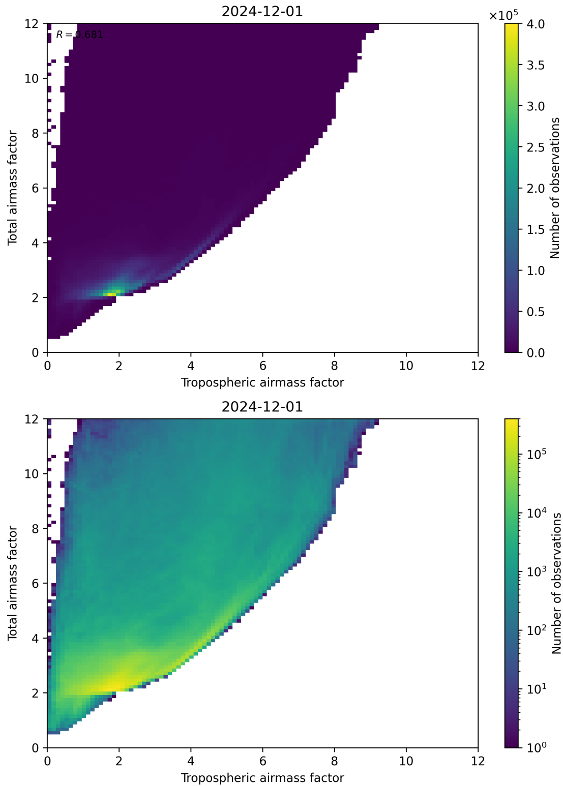
Figure 72: Scatter density plot of “Tropospheric airmass factor” against “Total airmass factor” for 2024-11-30 to 2024-12-02.
