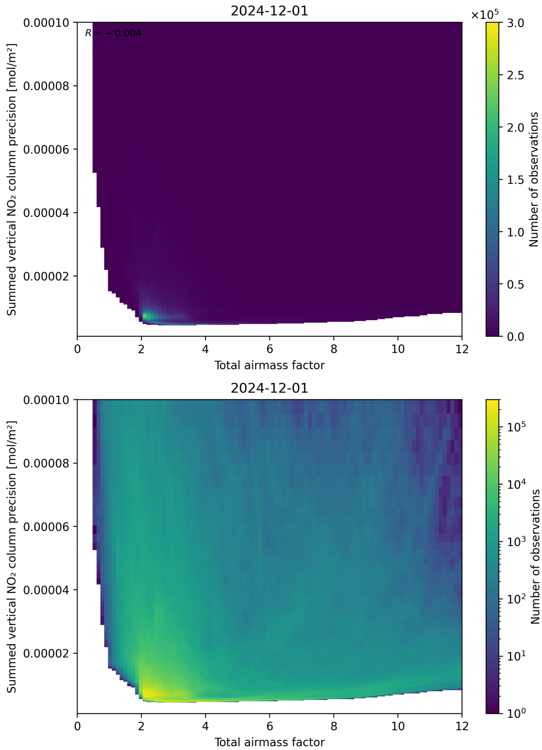
Figure 66: Scatter density plot of “Total airmass factor” against “Summed vertical NO 2 column precision” for 2024-11-30 to 2024-12-02.
