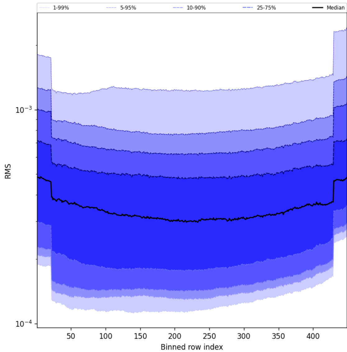
Figure 60: Along track statistics of “RMS” for 2024-11-30 to 2024-12-02
