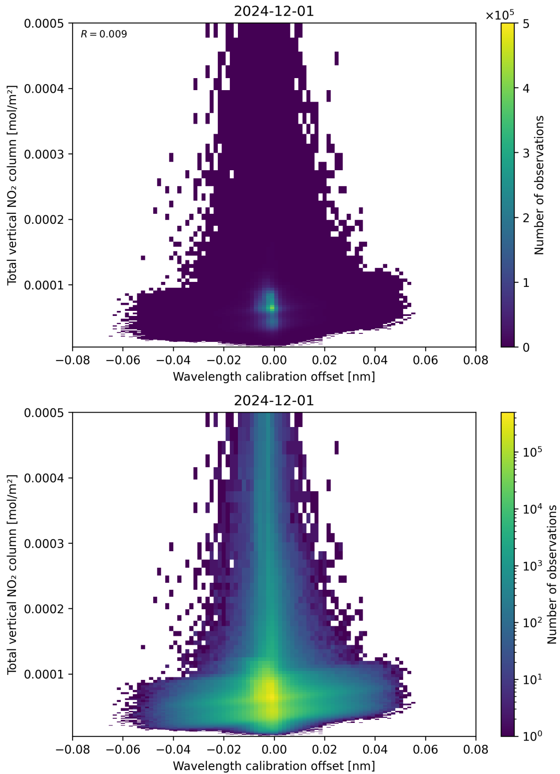
Figure 179: Scatter density plot of “Wavelength calibration offset” against “Total vertical NO 2 column” for 2024-11-30 to 2024-12-02.
