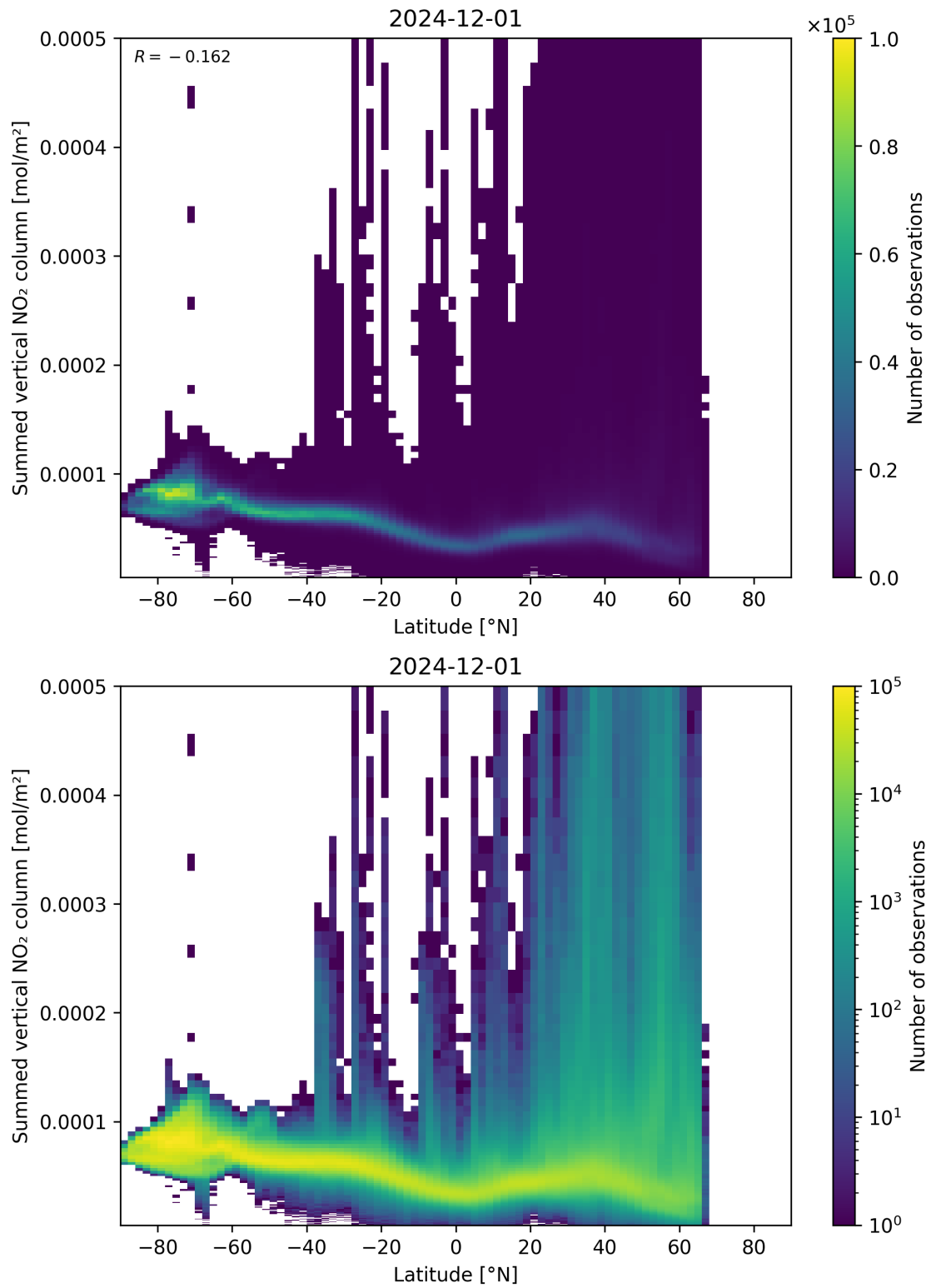
Figure 88: Scatter density plot of “Latitude” against “Summed vertical NO 2 column” for 2024-11-30 to 2024-12-02.
