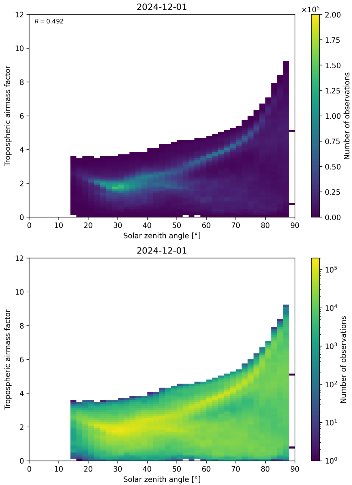
Figure 147: Scatter density plot of “Solar zenith angle” against “Tropospheric airmass factor” for 2024-11-30 to 2024-12-02.
