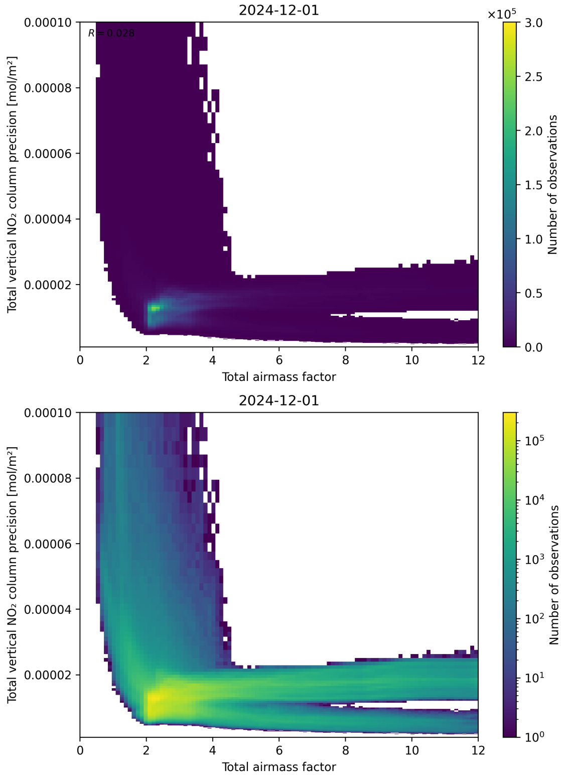
Figure 68: Scatter density plot of “Total airmass factor” against “Total vertical NO 2 column precision” for 2024-11-30 to 2024-12-02.
