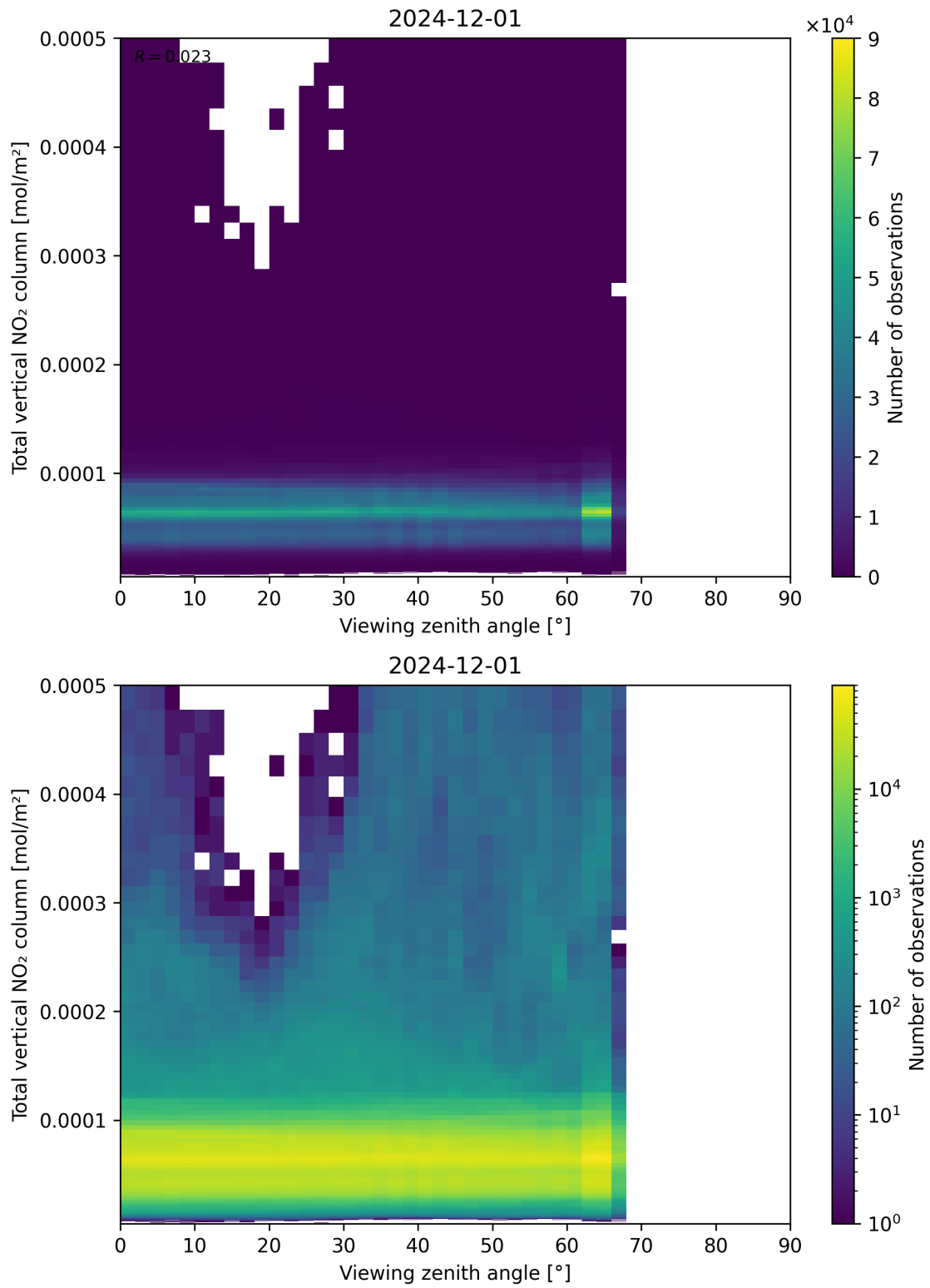
Figure 167: Scatter density plot of “Viewing zenith angle” against “Total vertical NO 2 column” for 2024-11-30 to 2024-12-02.
