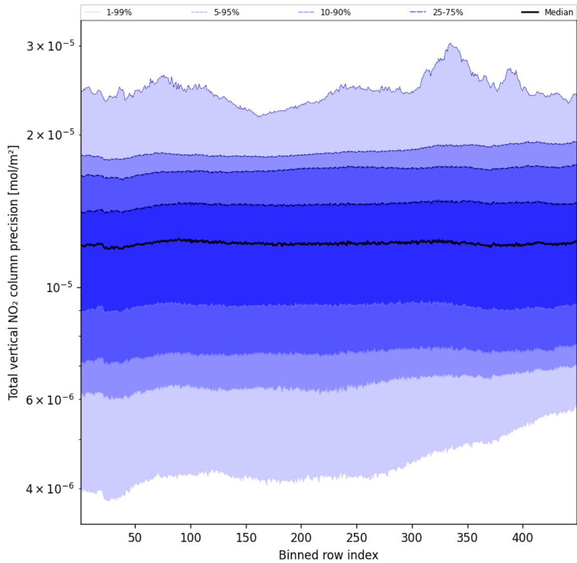
Figure 56: Along track statistics of "Total vertical NO 2 column precision" for 2024-11-30 to 2024-12-02
