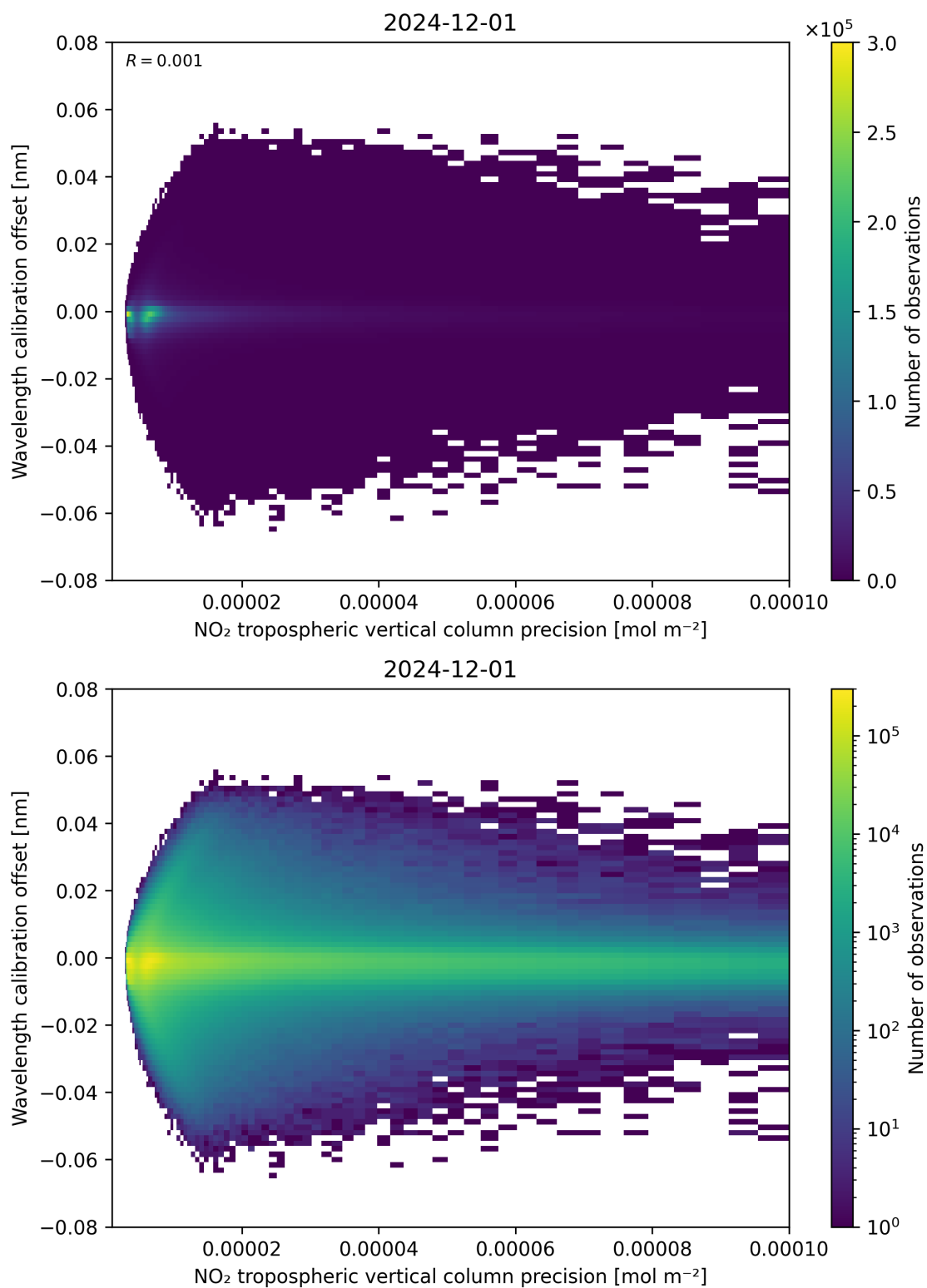
Figure 141: Scatter density plot of “NO 2 tropospheric vertical column precision” against “Wavelength calibration offset” for 2024-11-30 to 2024-12-02.
