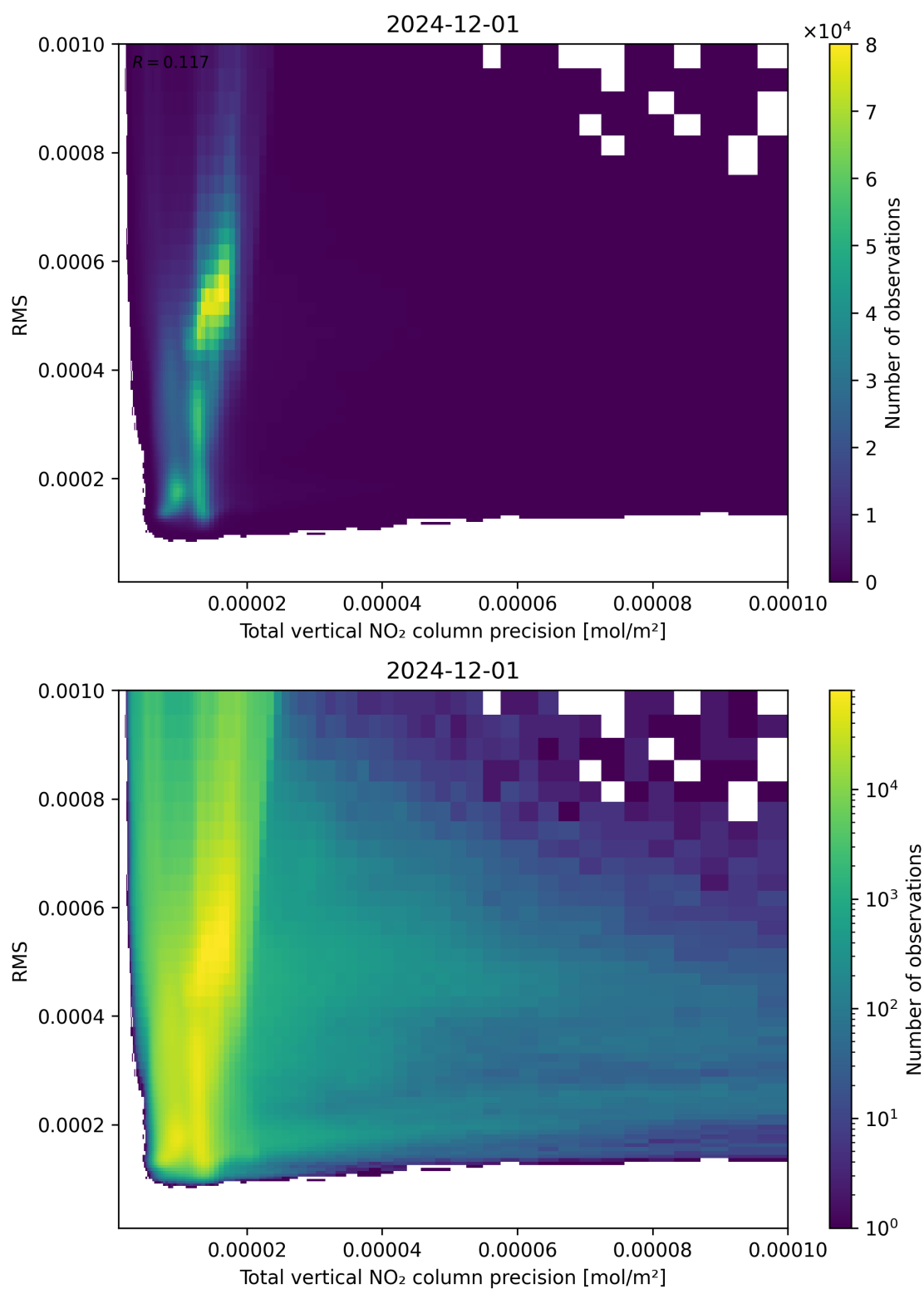
Figure 119: Scatter density plot of “Total vertical NO 2 column precision” against “RMS” for 2024-11-30 to 2024-12-02.
