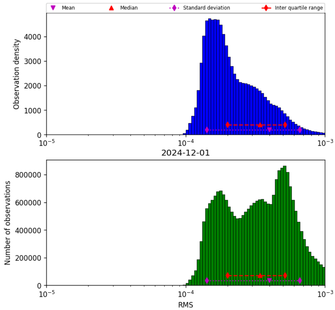
Figure 43: Histogram of “RMS” for 2024-11-30 to 2024-12-02
