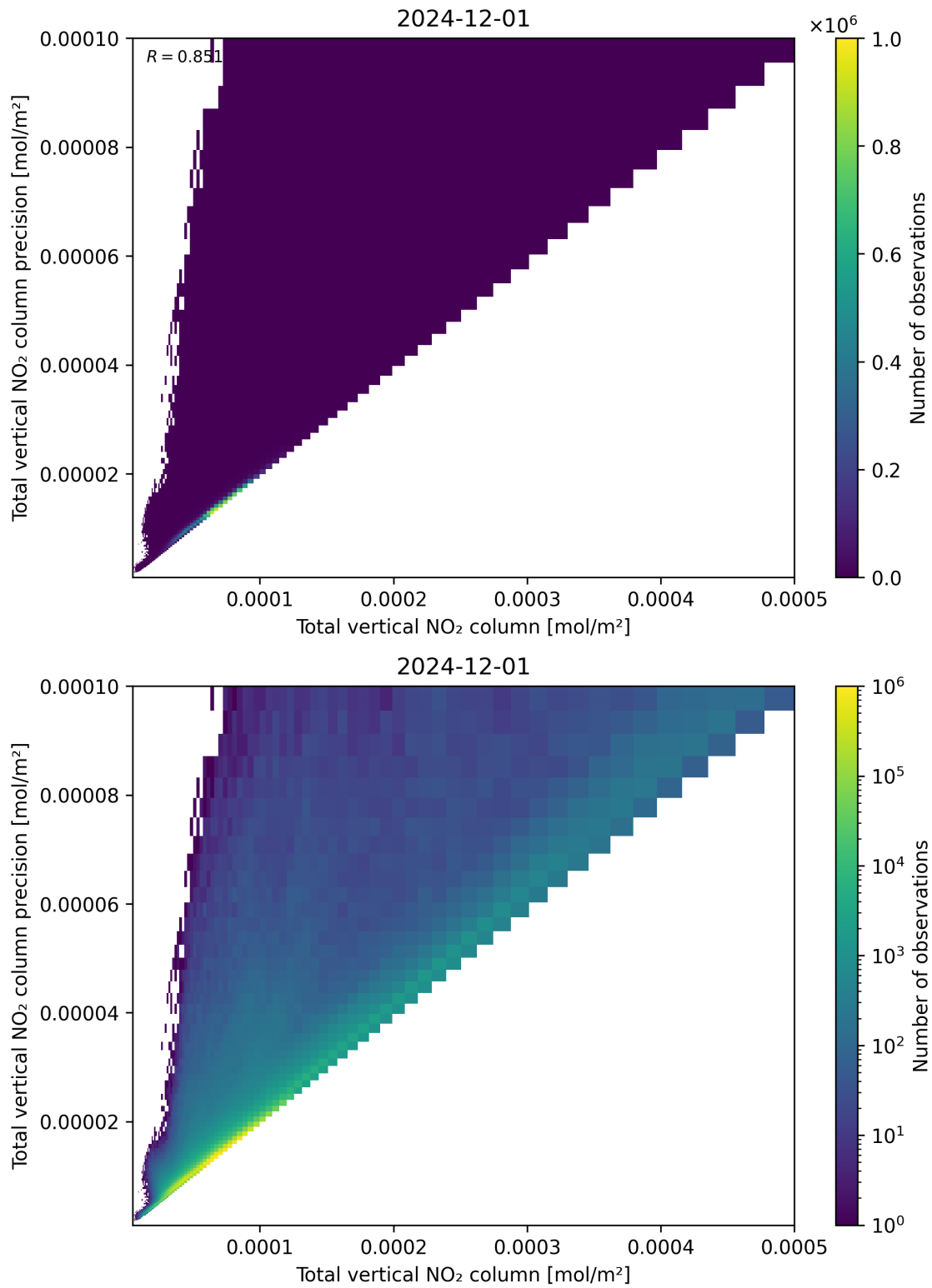
Figure 114: Scatter density plot of “Total vertical NO 2 column” against “Total vertical NO 2 column precision” for 2024-11-30 to 2024-12-02.
