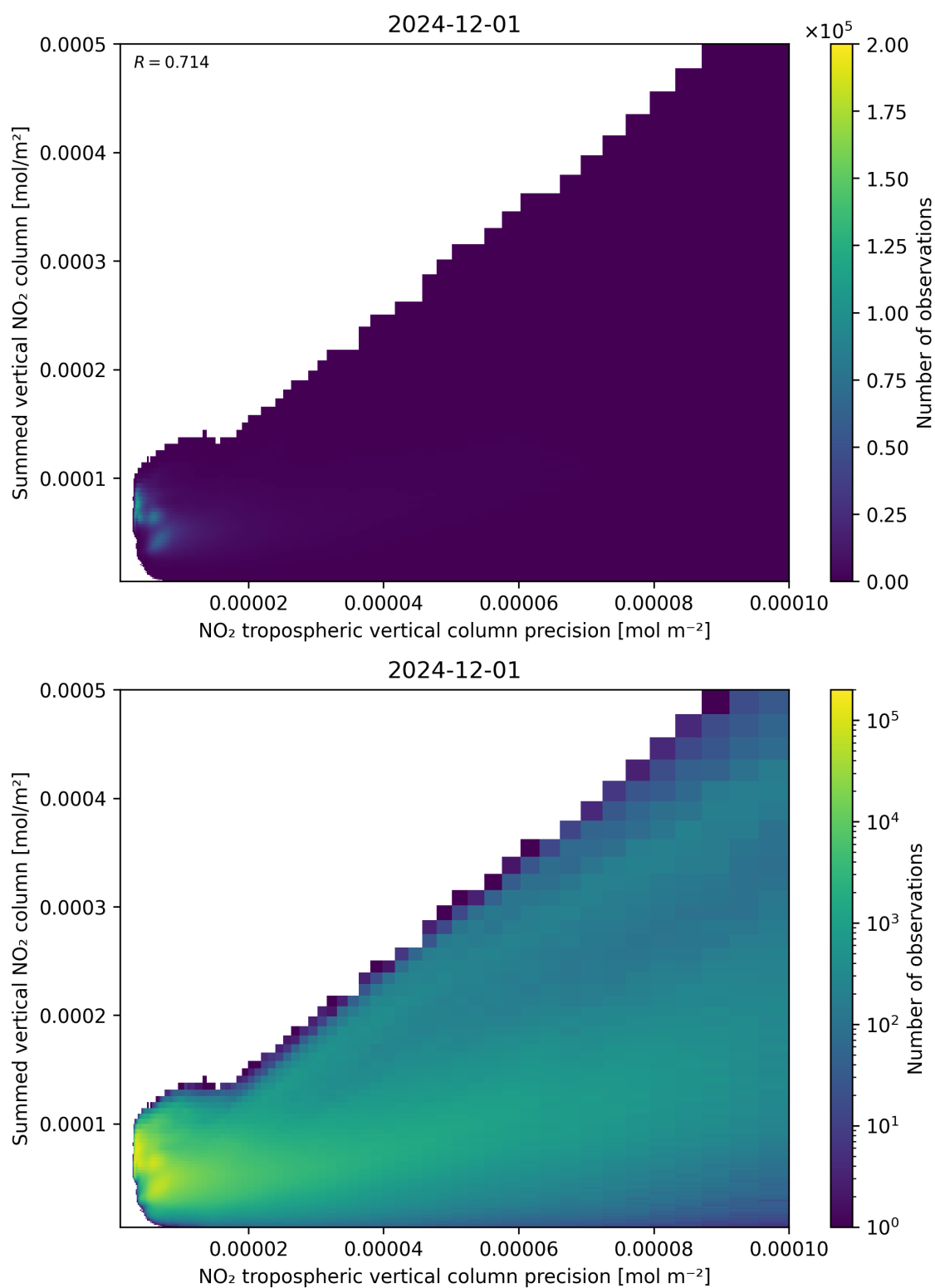
Figure 136: Scatter density plot of “NO 2 tropospheric vertical column precision” against “Summed vertical NO 2 column” for 2024-11-30 to 2024-12-02.
