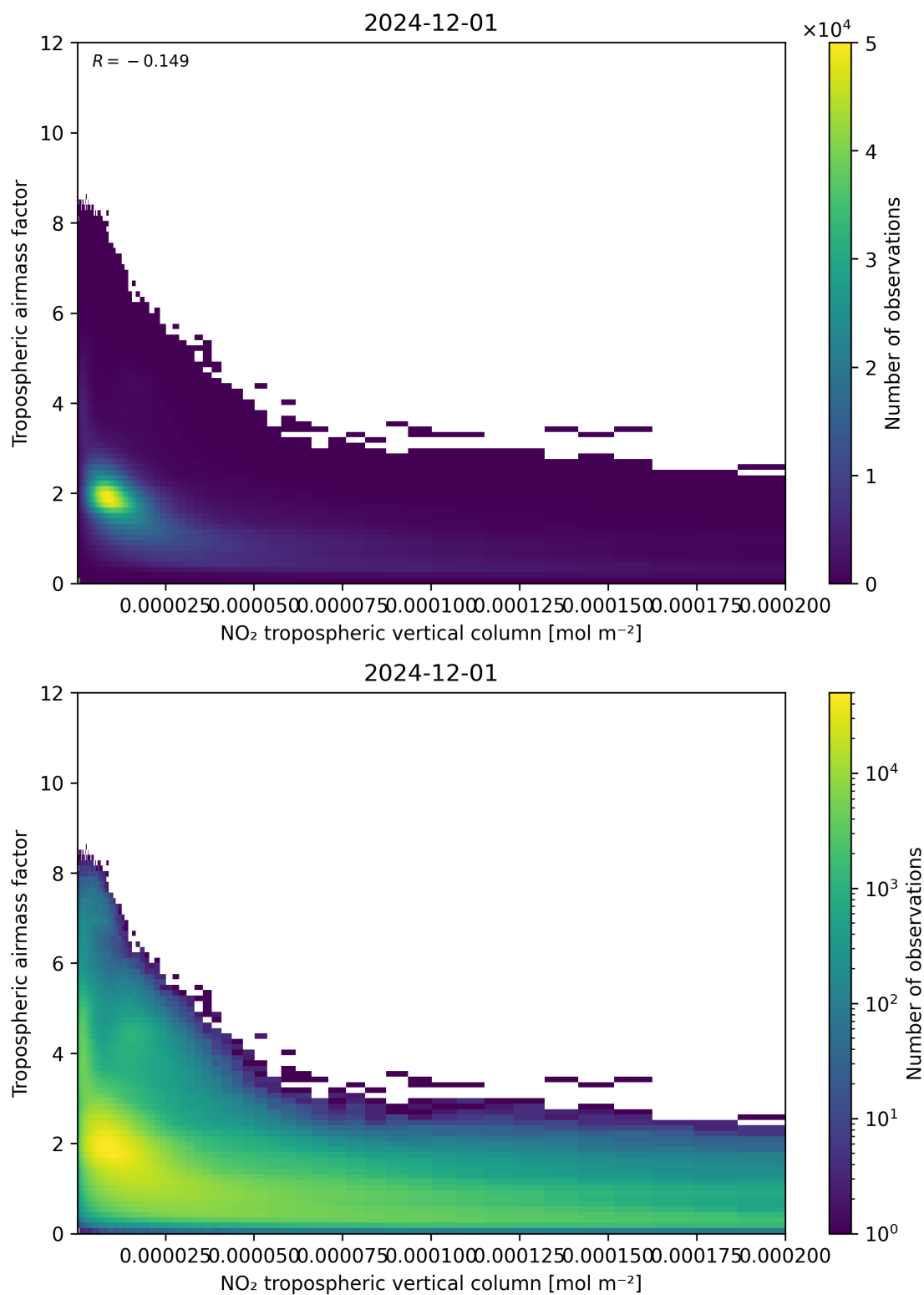
Figure 123: Scatter density plot of “NO 2 tropospheric vertical column” against “Tropospheric air mass factor” for 2024-11-30 to 2024-12-02.
