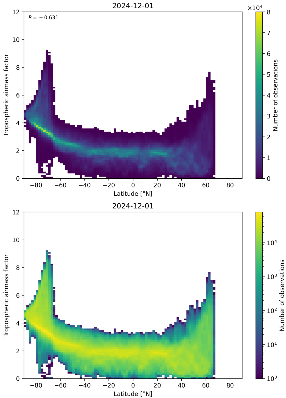
Figure 85: Scatter density plot of “Latitude” against “Tropospheric airmass factor” for 2024-11-30 to 2024-12-02.
