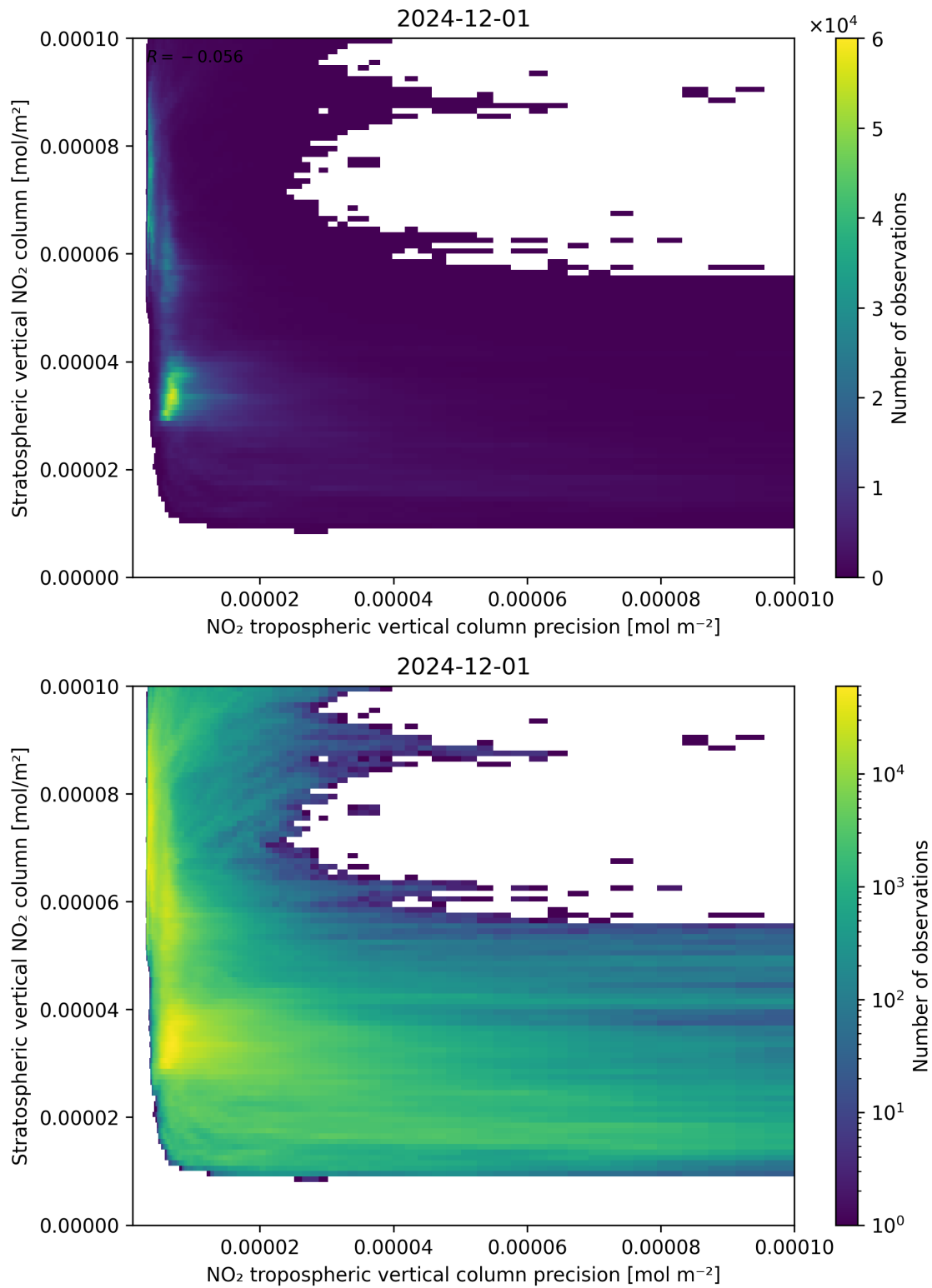
Figure 135: Scatter density plot of “NO 2 tropospheric vertical column precision” against “Stratospheric vertical NO 2 column” for 2024-11-30 to 2024-12-02.
