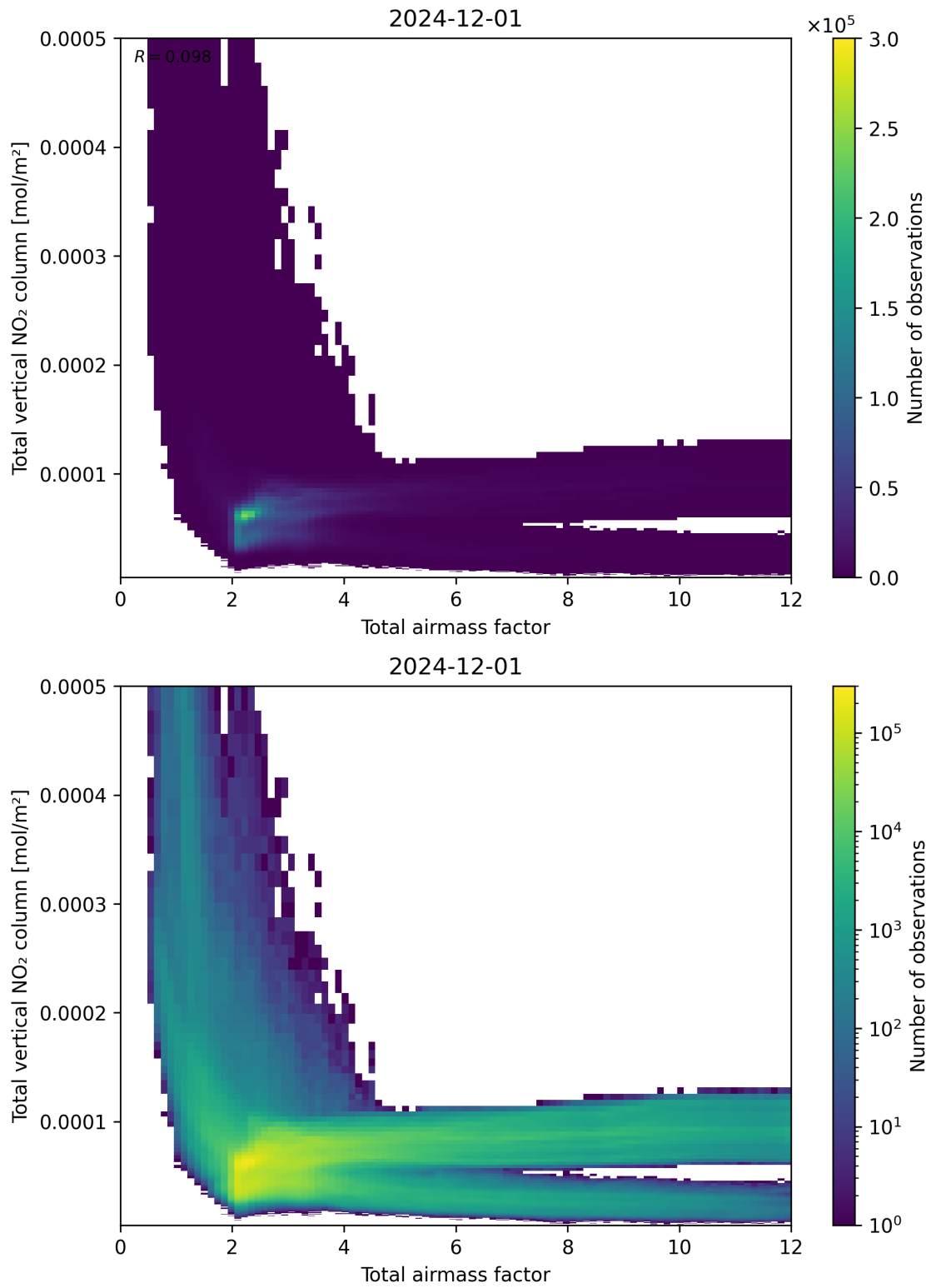
Figure 67: Scatter density plot of “Total airmass factor” against “Total vertical NO 2 column” for 2024-11-30 to 2024-12-02.
