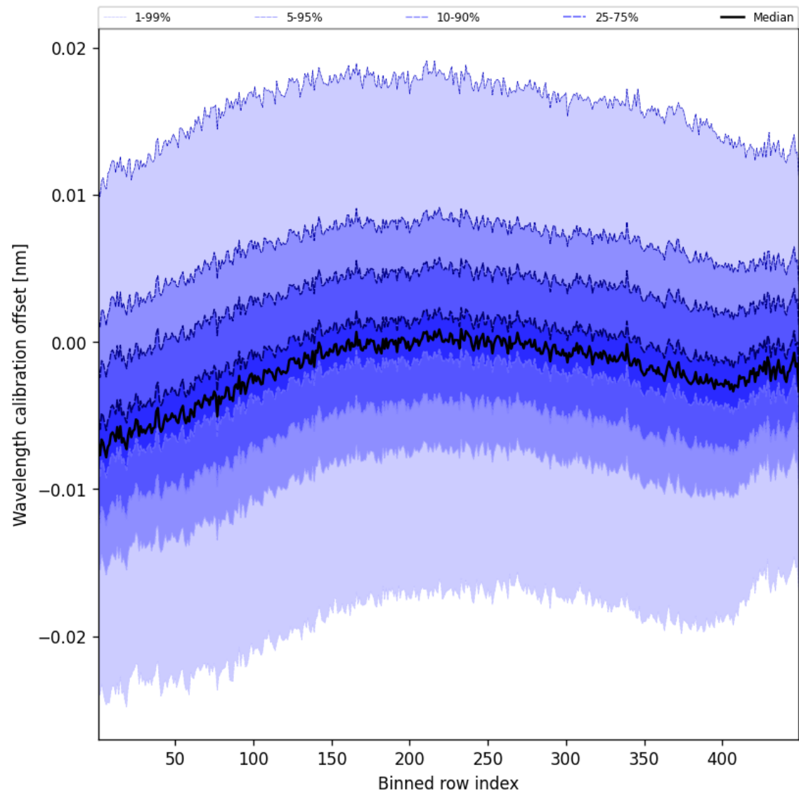
Figure 52: Along track statistics of “Wavelength calibration offset” for 2024-11-30 to 2024-12-02
