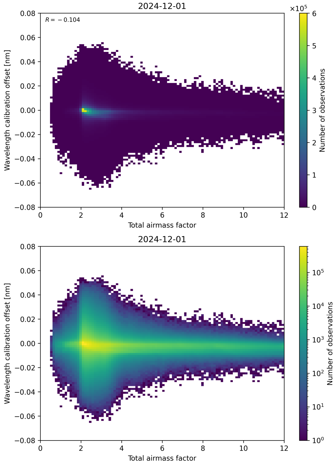
Figure 70: Scatter density plot of “Total airmass factor” against “Wavelength calibration offset” for 2024-11-30 to 2024-12-02.
