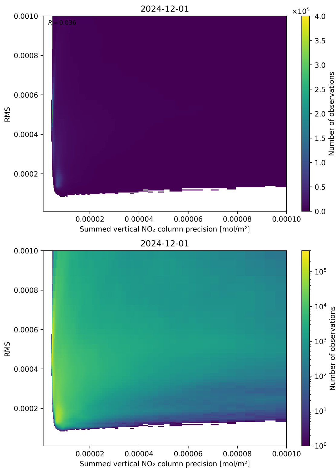
Figure 108: Scatter density plot of “Summed vertical NO 2 column precision” against “RMS” for 2024-11-30 to 2024-12-02.
