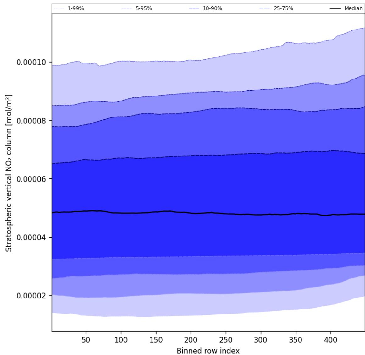
Figure 53: Along track statistics of “Stratospheric vertical NO 2 column” for 2024-11-30 to 2024-12-02
