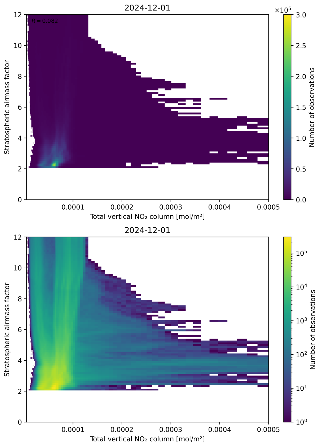
Figure 110: Scatter density plot of “Total vertical NO 2 column” against “Stratospheric airmass factor” for 2024-11-30 to 2024-12-02.
