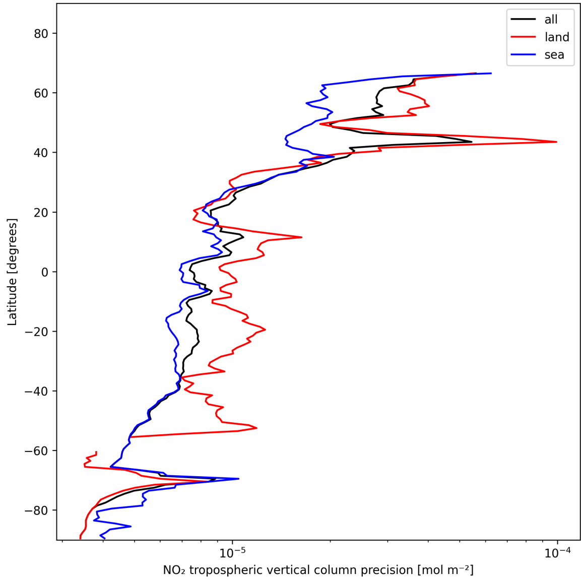
Figure 13: Zonal average of “NO 2 tropospheric vertical column precision” for 2024-11-30 to 2024-12-02.
