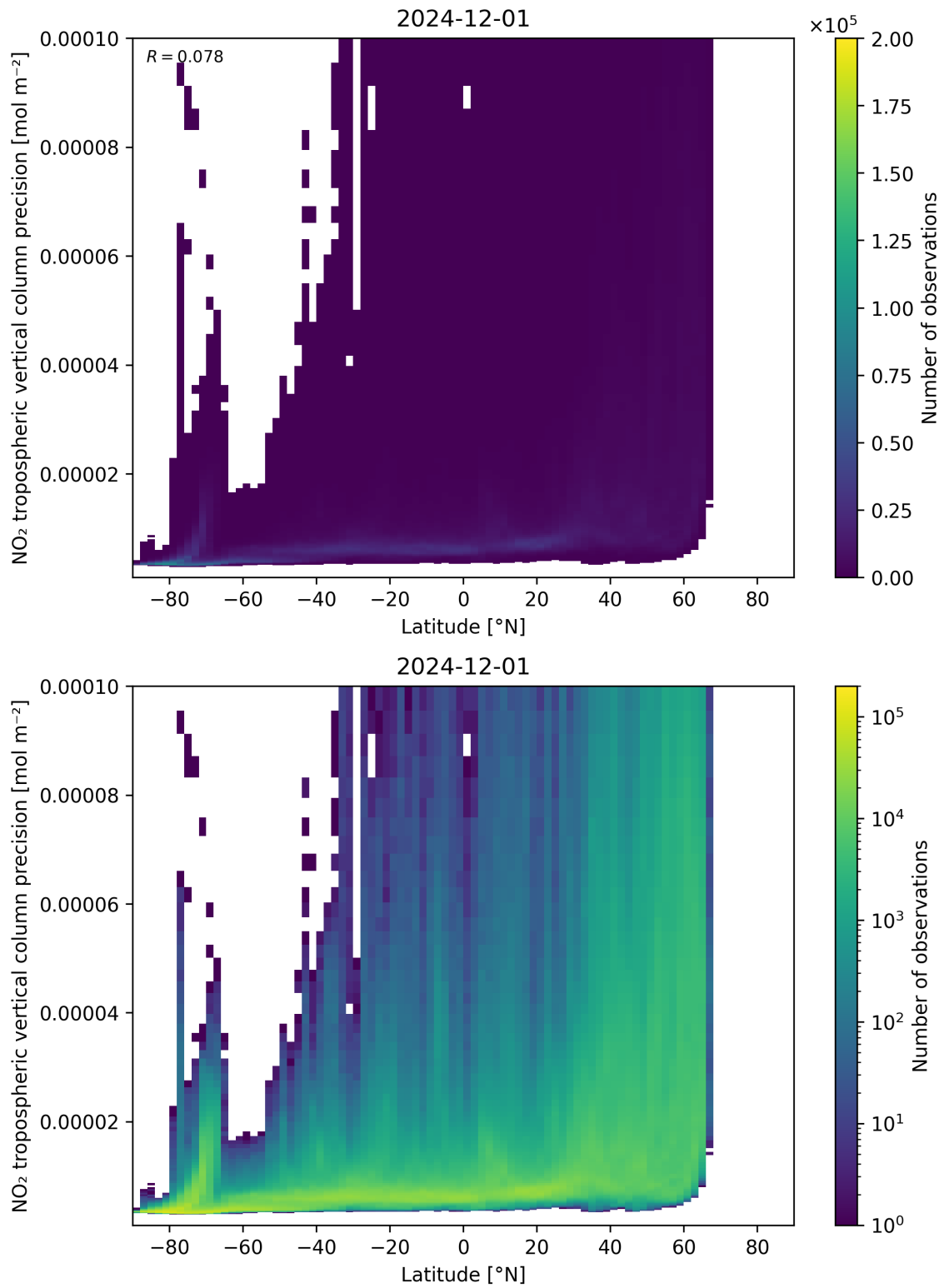
Figure 93: Scatter density plot of “Latitude” against “NO 2 tropospheric vertical column precision” for 2024-11-30 to 2024-12-02.
