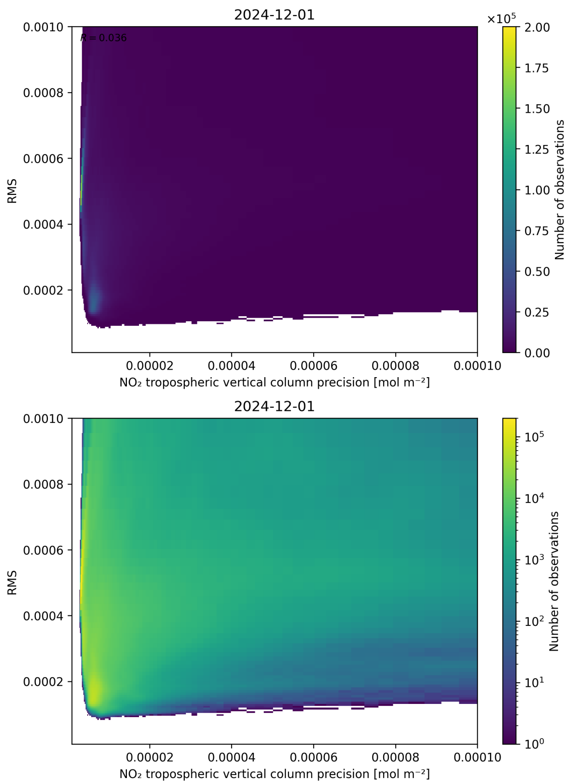
Figure 140: Scatter density plot of “NO 2 tropospheric vertical column precision” against “RMS” for 2024-11-30 to 2024-12-02.
