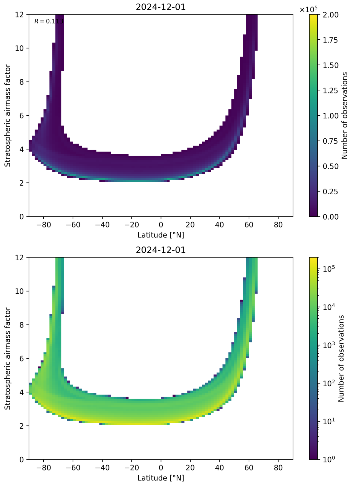
Figure 83: Scatter density plot of “Latitude” against “Stratospheric air mass factor” for 2024-11-30 to 2024-12-02.
