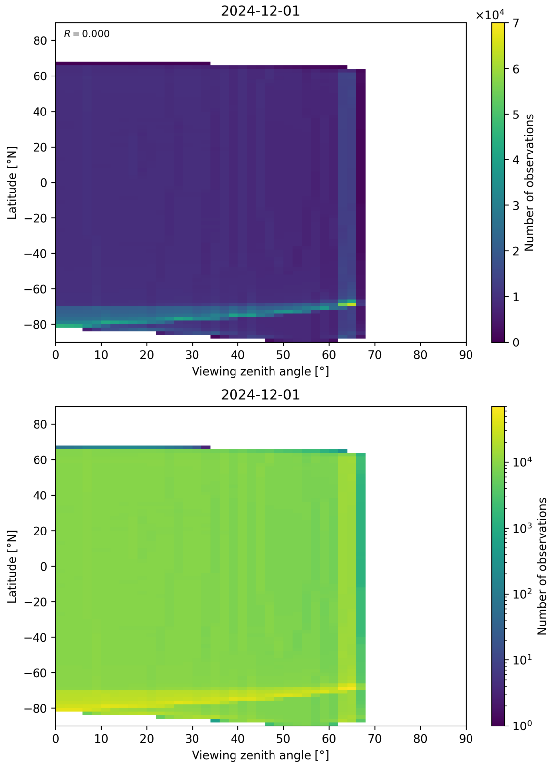
Figure 163: Scatter density plot of “Viewing zenith angle” against “Latitude” for 2024-11-30 to 2024-12-02.
