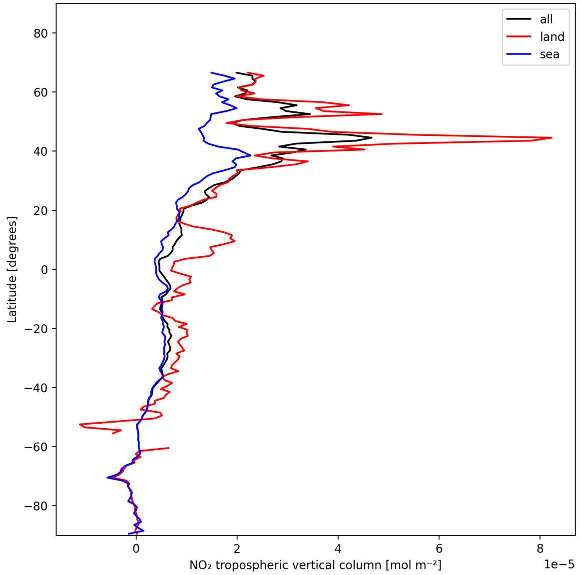
Figure 12: Zonal average of “NO 2 tropospheric vertical column” for 2024-11-30 to 2024-12-02.
