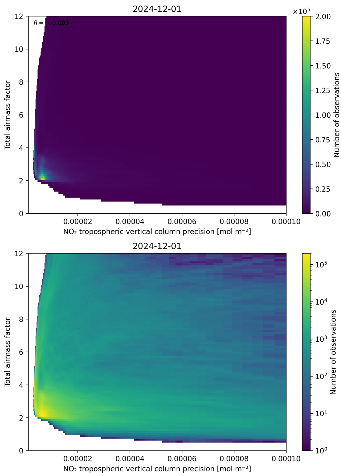
Figure 132: Scatter density plot of “NO 2 tropospheric vertical column precision” against “Total air mass factor” for 2024-11-30 to 2024-12-02.
