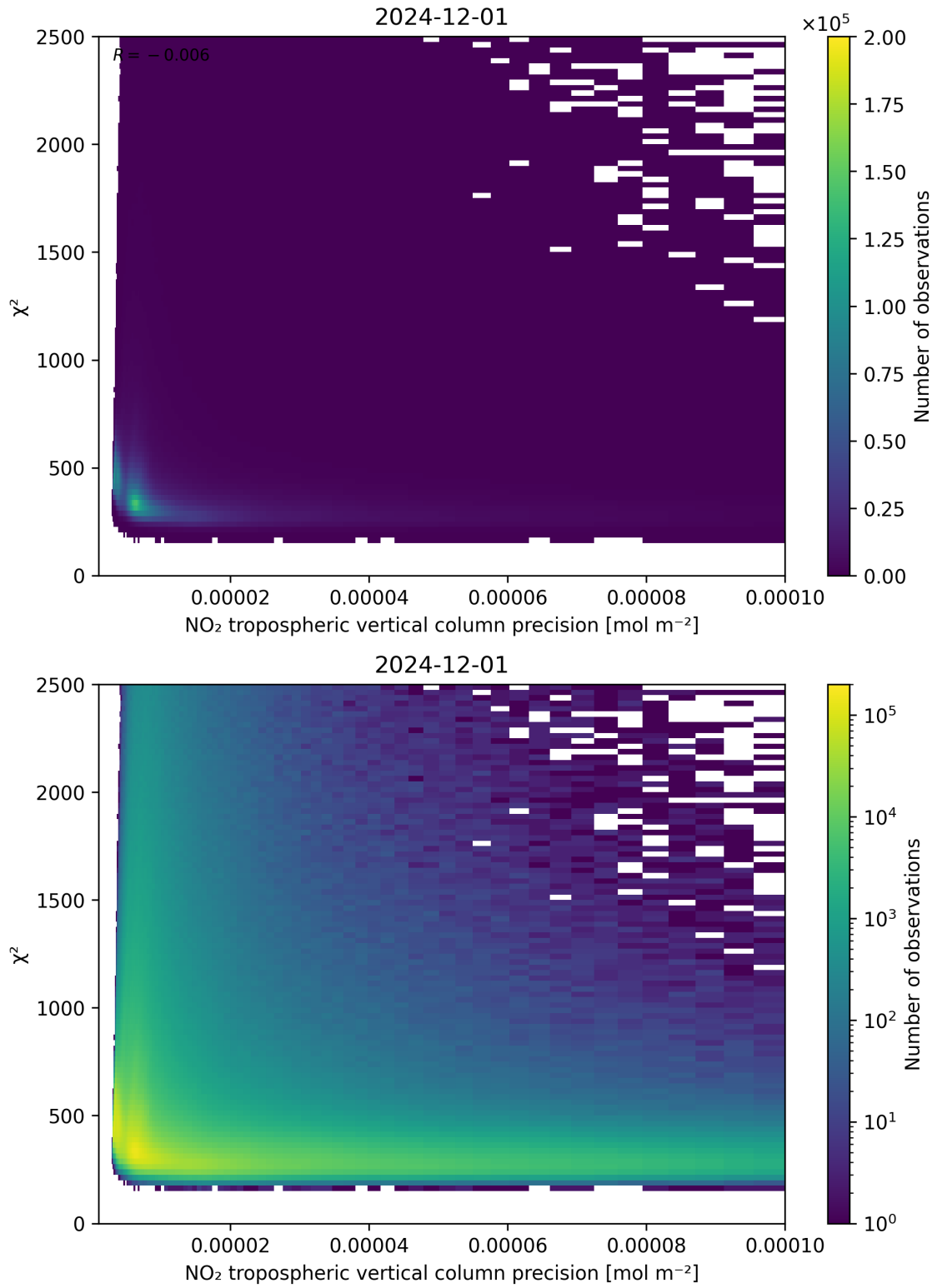
Figure 134: Scatter density plot of “NO 2 tropospheric vertical column precision” against “ \chi^2 ” for 2024-11-30 to 2024-12-02.
