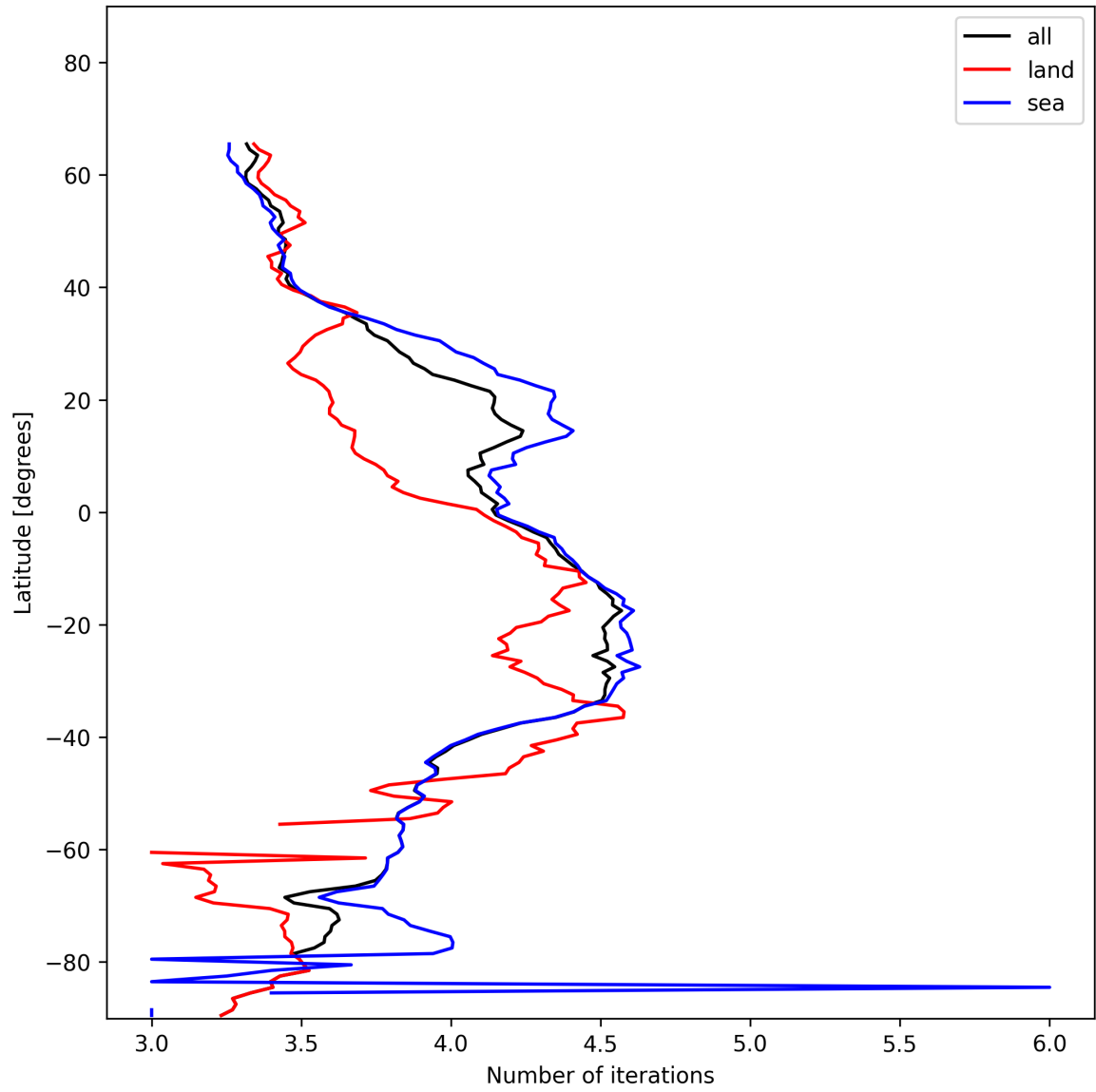
Figure 17: Zonal average of “Number of iterations” for 2024-12-01 to 2024-12-03.
