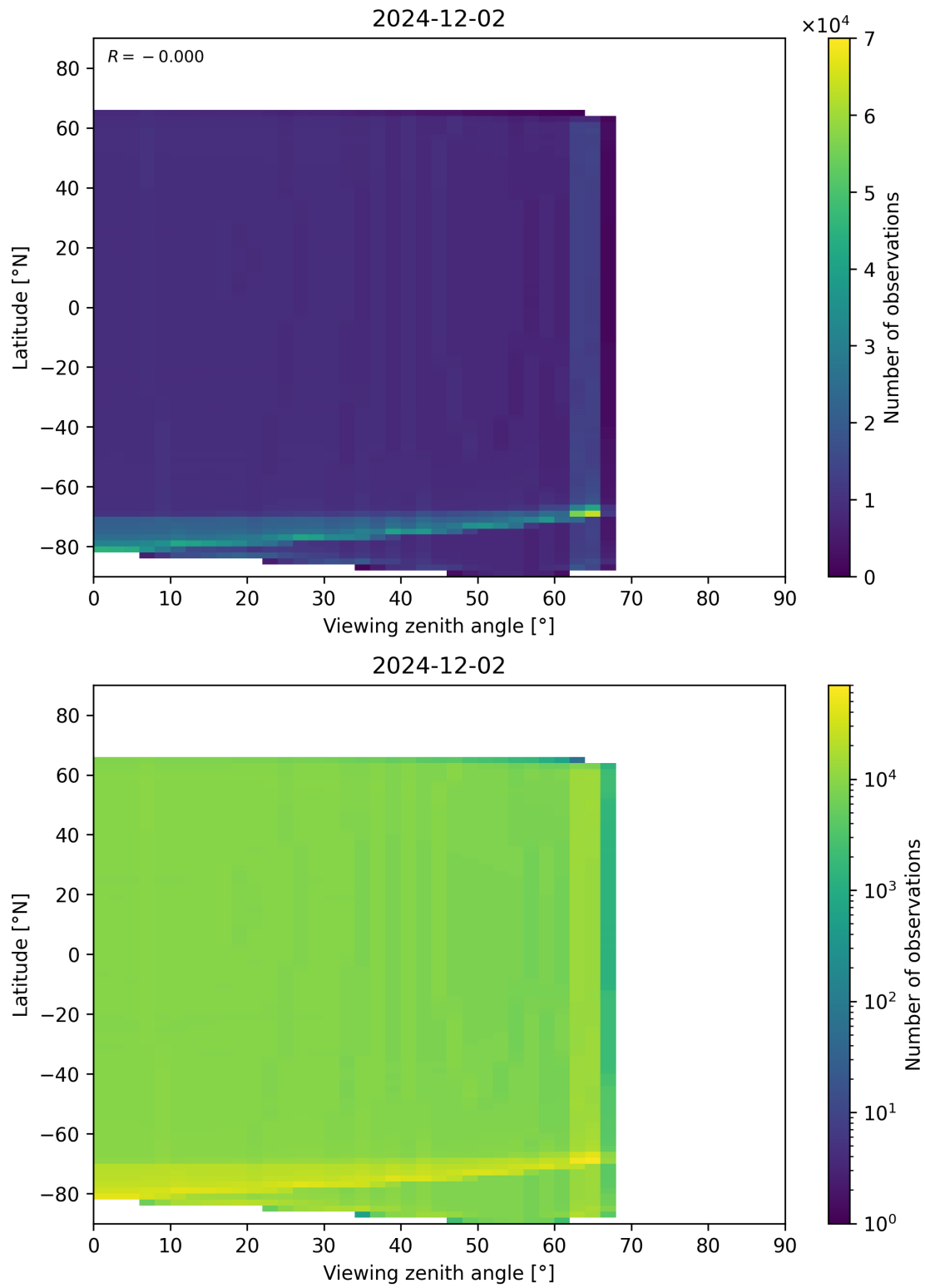
Figure 163: Scatter density plot of “Viewing zenith angle” against “Latitude” for 2024-12-01 to 2024-12-03.
