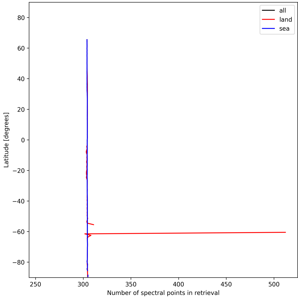
Figure 16: Zonal average of “Number of spectral points in retrieval” for 2024-12-01 to 2024-12-03.
