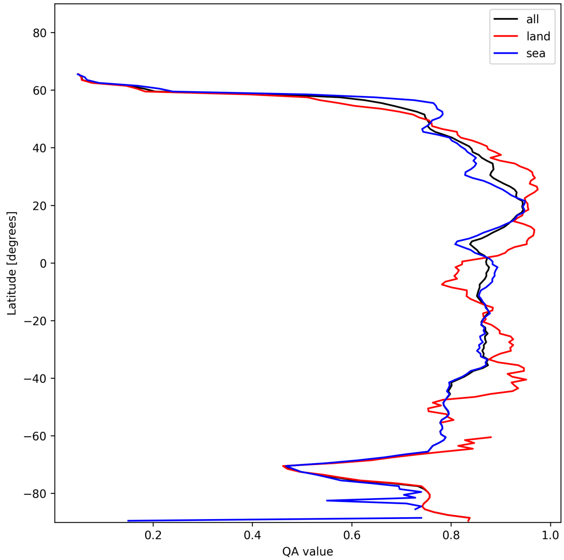
Figure 11: Zonal average of “QA value” for 2024-12-01 to 2024-12-03.
