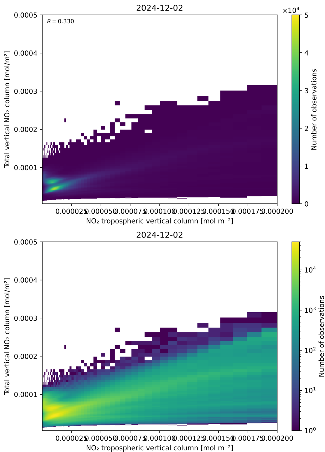
Figure 128: Scatter density plot of “NO 2 tropospheric vertical column” against “Total vertical NO 2 column” for 2024-12-01 to 2024-12-03.
