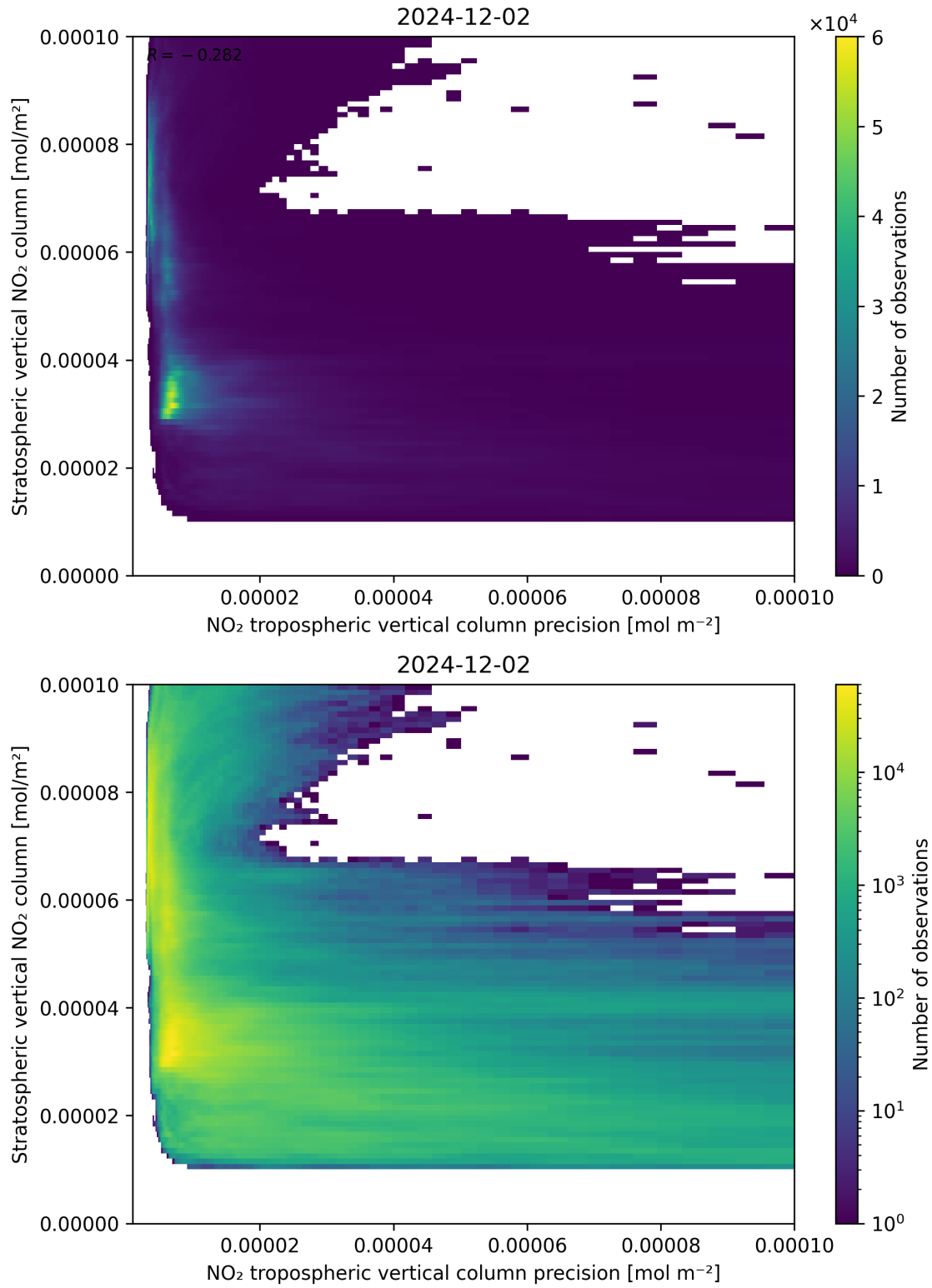
Figure 135: Scatter density plot of “NO 2 tropospheric vertical column precision” against “Stratospheric vertical NO 2 column” for 2024-12-01 to 2024-12-03.
