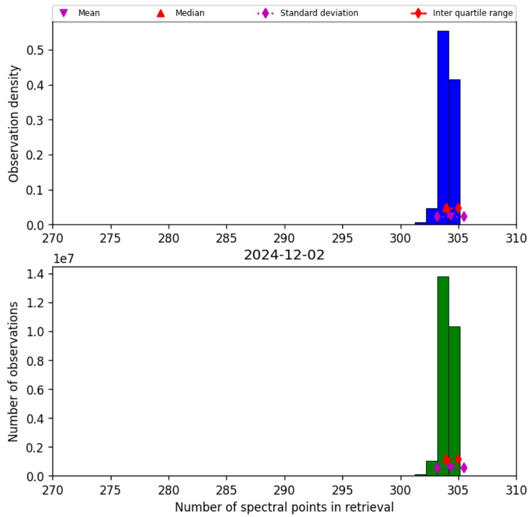
Figure 33: Histogram of “Number of spectral points in retrieval” for 2024-12-01 to 2024-12-03
