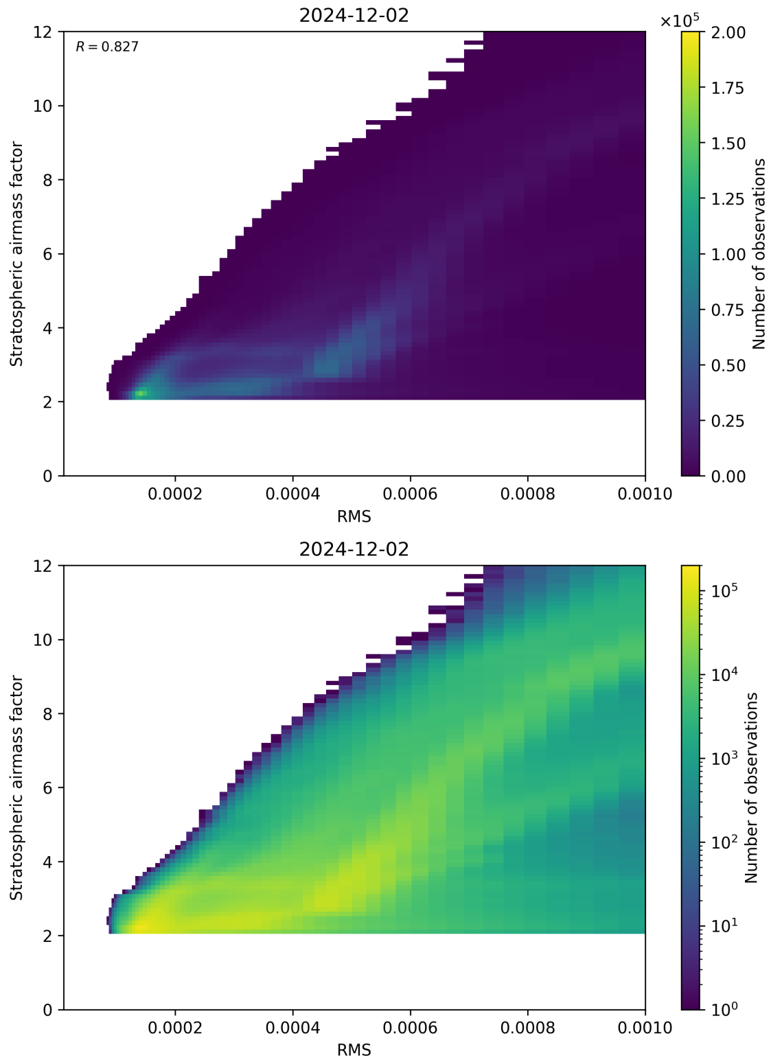
Figure 144: Scatter density plot of “RMS” against “Stratospheric airmass factor” for 2024-12-01 to 2024-12-03.
