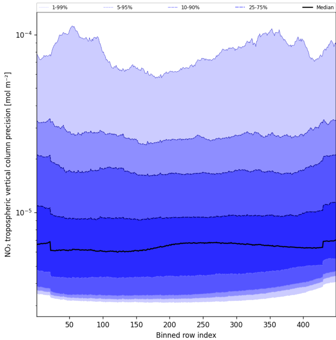
Figure 47: Along track statistics of “NO 2 tropospheric vertical column precision” for 2024-12-01 to 2024-12-03
