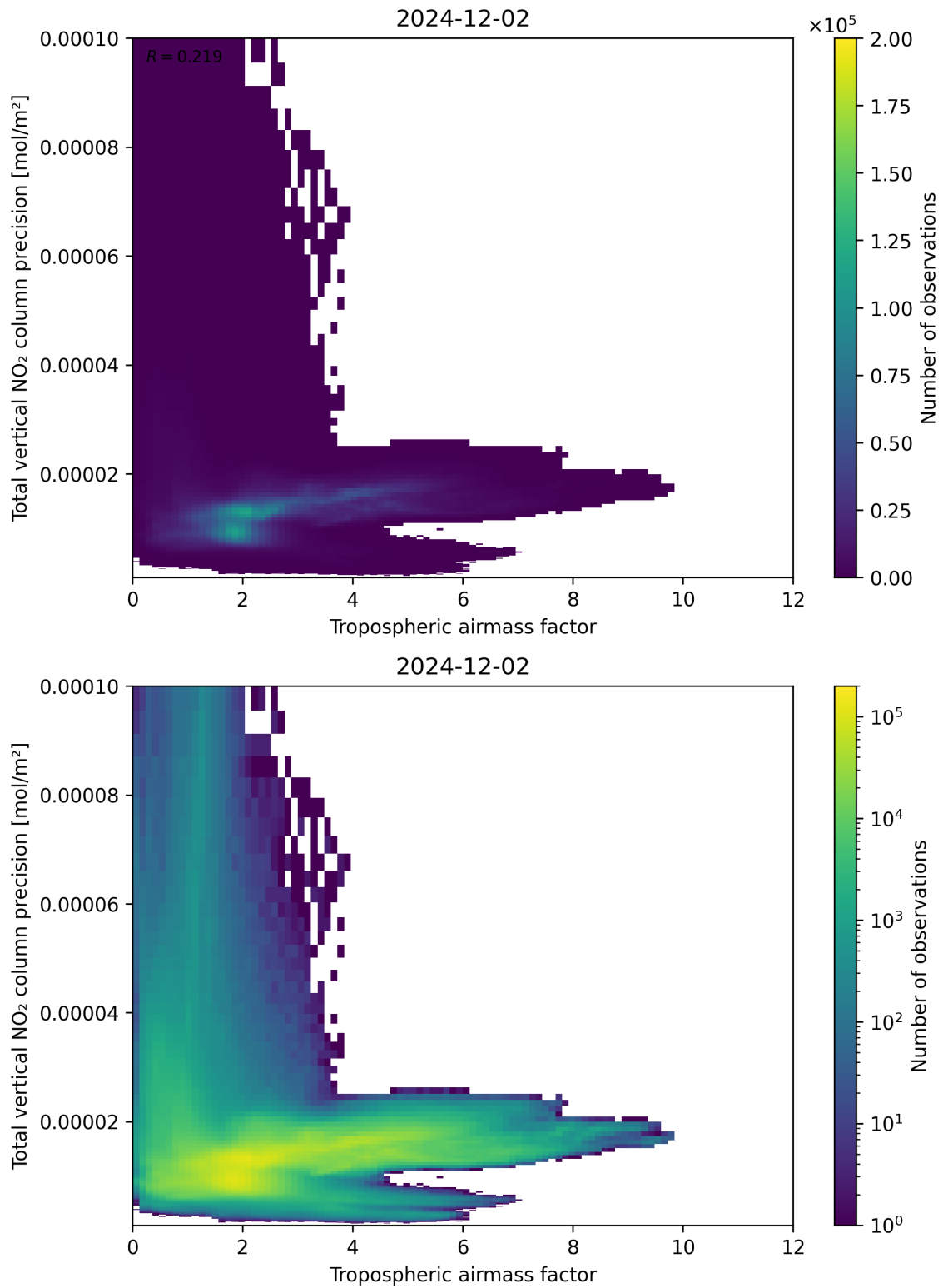
Figure 78: Scatter density plot of “Tropospheric air mass factor” against “Total vertical NO 2 column precision” for 2024-12-01 to 2024-12-03.
