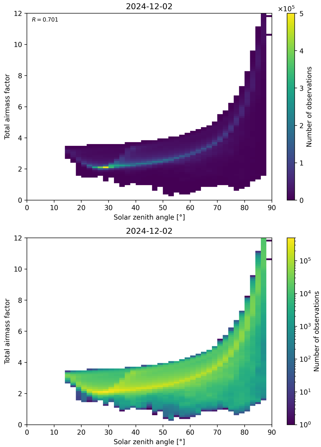
Figure 146: Scatter density plot of “Solar zenith angle” against “Total air mass factor” for 2024-12-01 to 2024-12-03.
