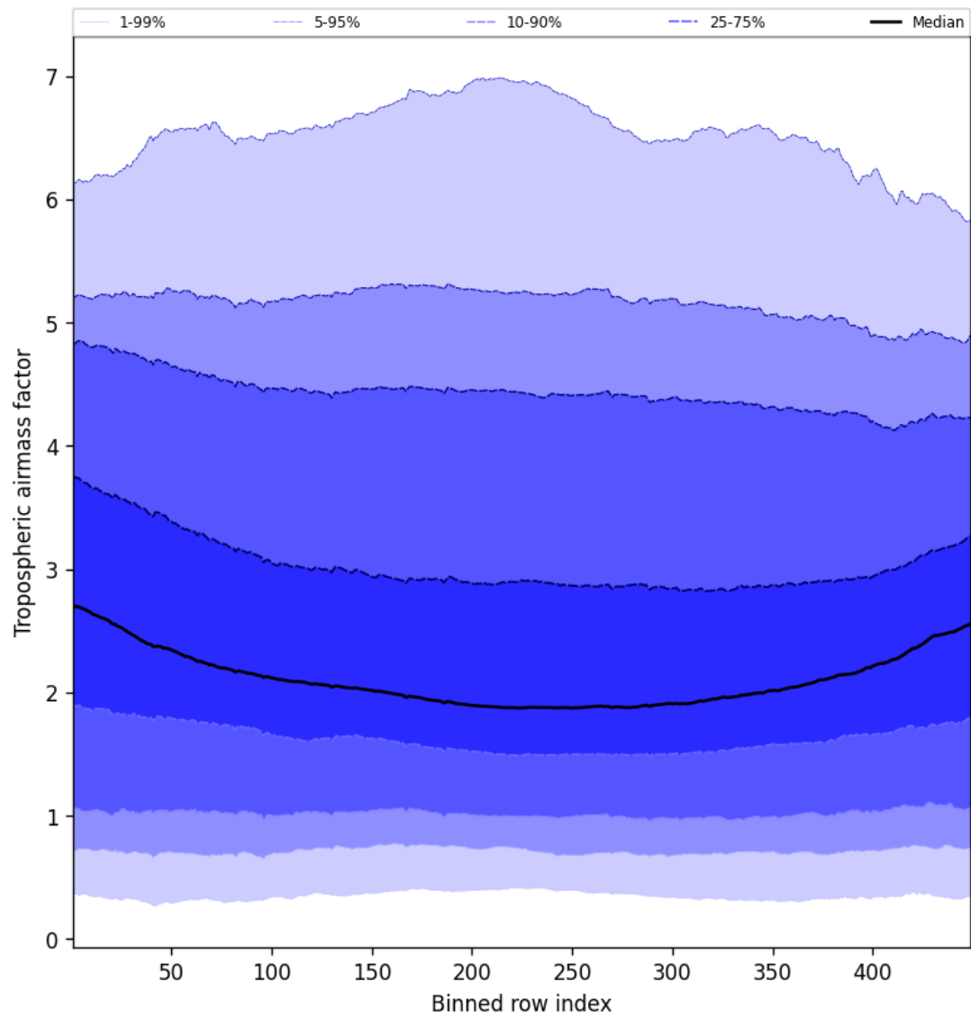
Figure 48: Along track statistics of “Tropospheric air mass factor” for 2024-12-01 to 2024-12-03
