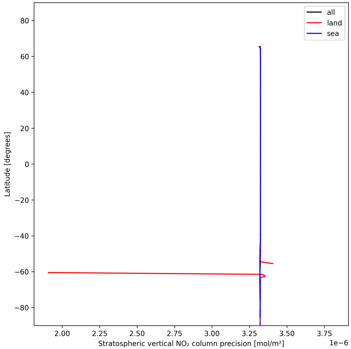
Figure 20: Zonal average of “Stratospheric vertical NO 2 column precision” for 2024-12-01 to 2024-12-03.
