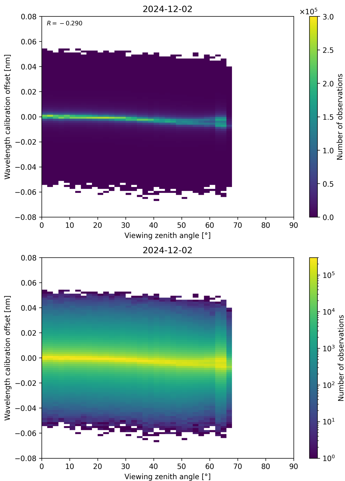
Figure 173: Scatter density plot of “Viewing zenith angle” against “Wavelength calibration offset” for 2024-12-01 to 2024-12-03.
