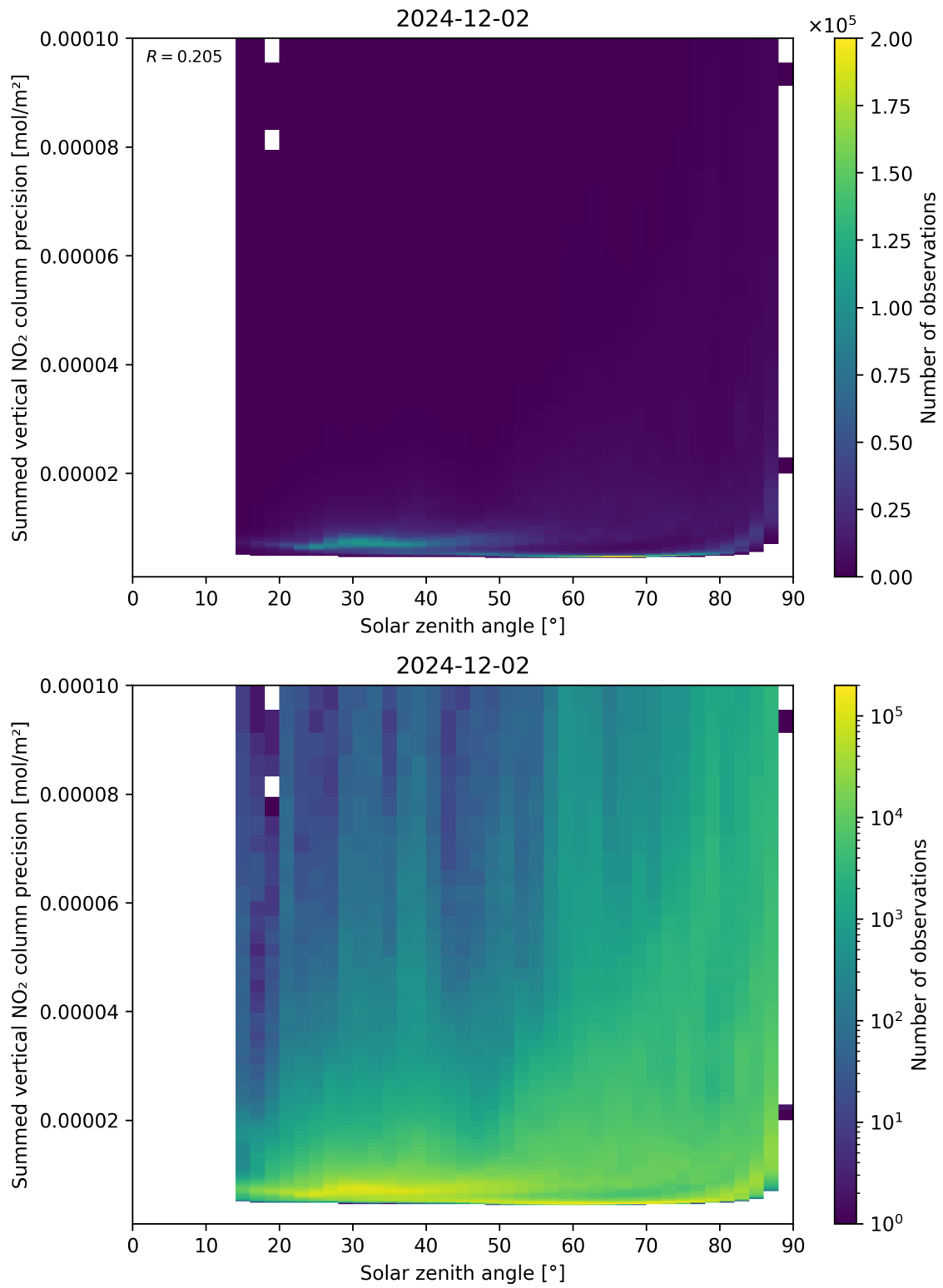
Figure 152: Scatter density plot of “Solar zenith angle” against “Summed vertical NO 2 column precision” for 2024-12-01 to 2024-12-03.
