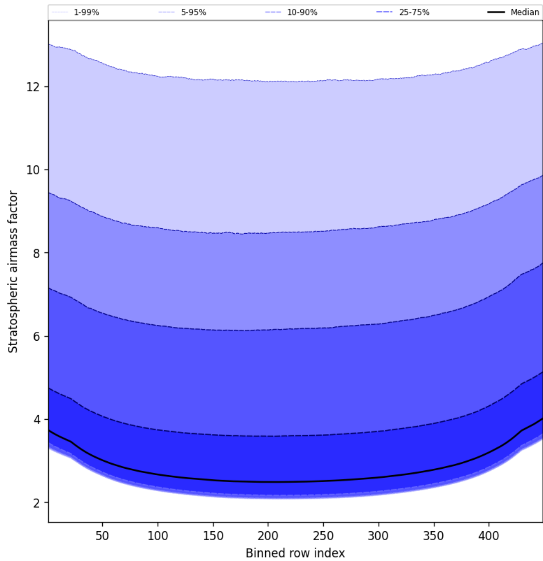
Figure 61: Along track statistics of “Stratospheric air mass factor” for 2024-12-01 to 2024-12-03
