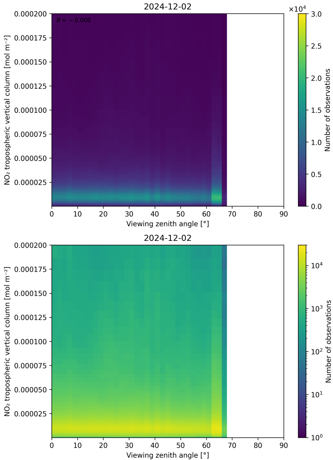
Figure 169: Scatter density plot of “Viewing zenith angle” against “NO 2 tropospheric vertical column” for 2024-12-01 to 2024-12-03.
