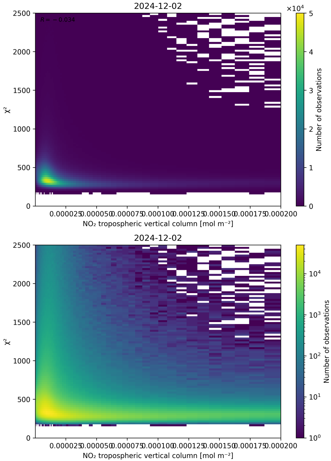
Figure 124: Scatter density plot of “NO 2 tropospheric vertical column” against “ \chi^2 ” for 2024-12-01 to 2024-12-03.
