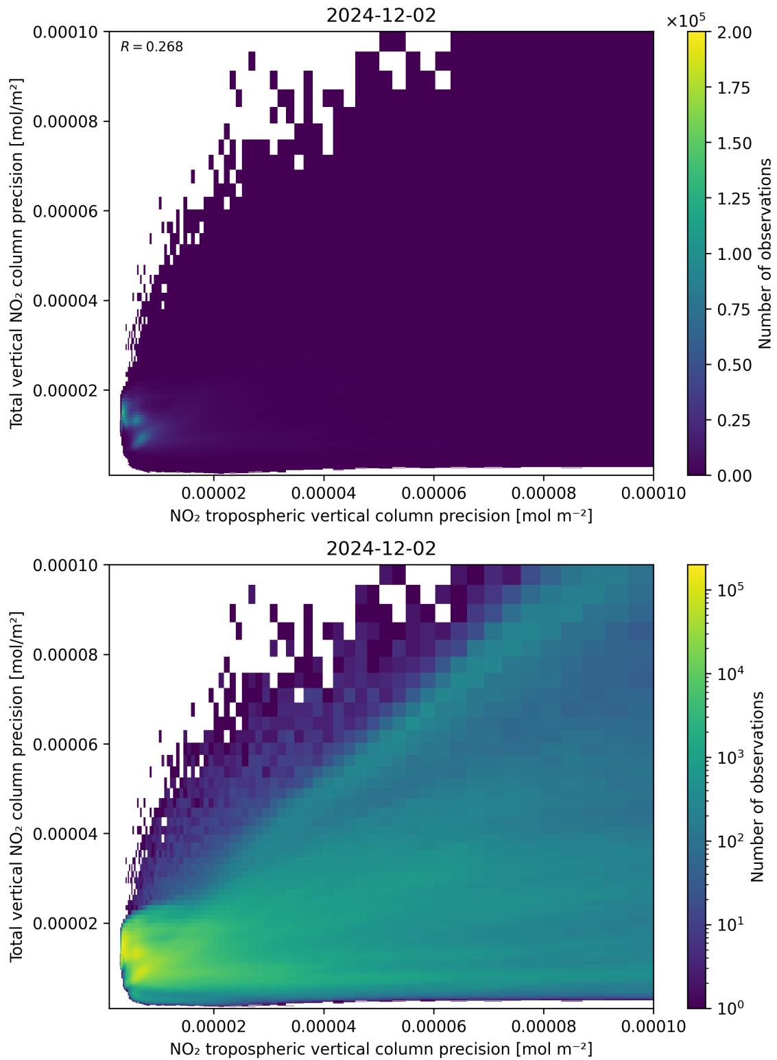
Figure 139: Scatter density plot of “NO 2 tropospheric vertical column precision” against “Total vertical NO 2 column precision” for 2024-12-01 to 2024-12-03.
