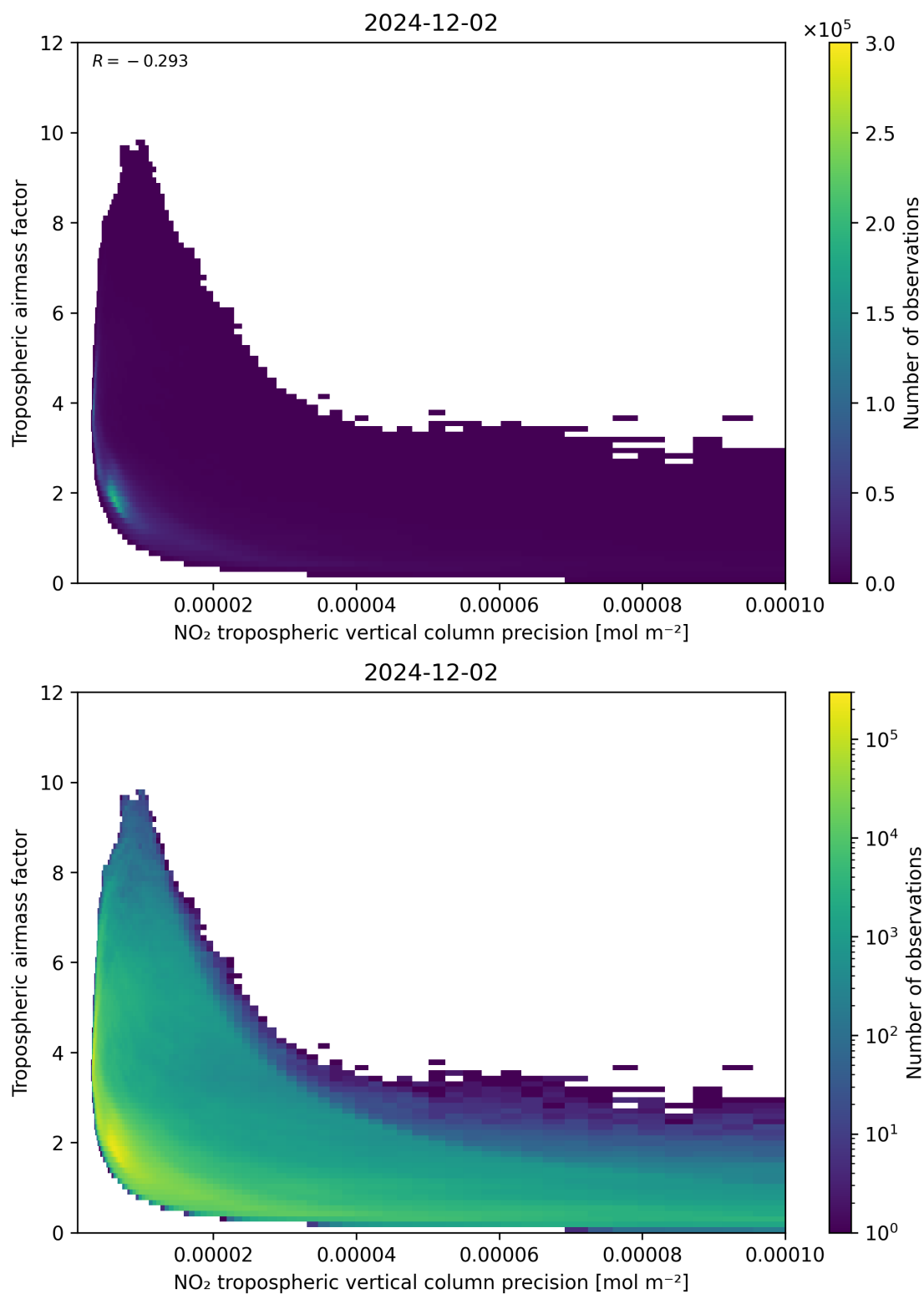
Figure 133: Scatter density plot of “NO 2 tropospheric vertical column precision” against “Tropospheric air mass factor” for 2024-12-01 to 2024-12-03.
