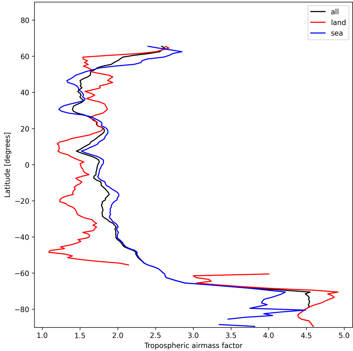
Figure 14: Zonal average of “Tropospheric airmass factor” for 2024-12-01 to 2024-12-03.
