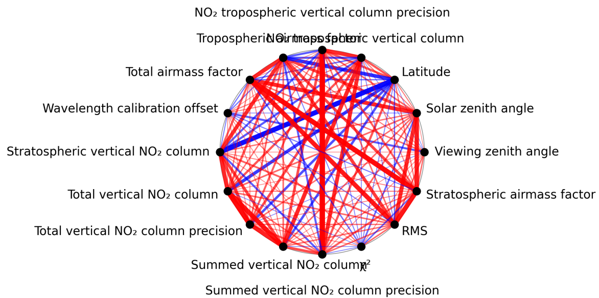
Figure 1: Map of correlation graph for 2024-12-01 to 2024-12-03.
