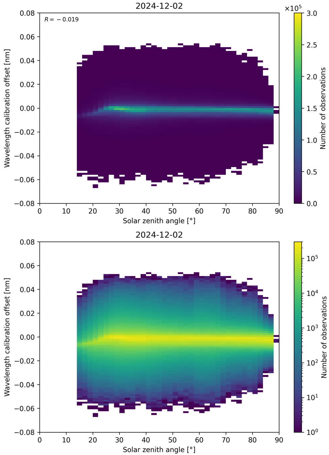
Figure 158: Scatter density plot of “Solar zenith angle” against “Wavelength calibration offset” for 2024-12-01 to 2024-12-03.
