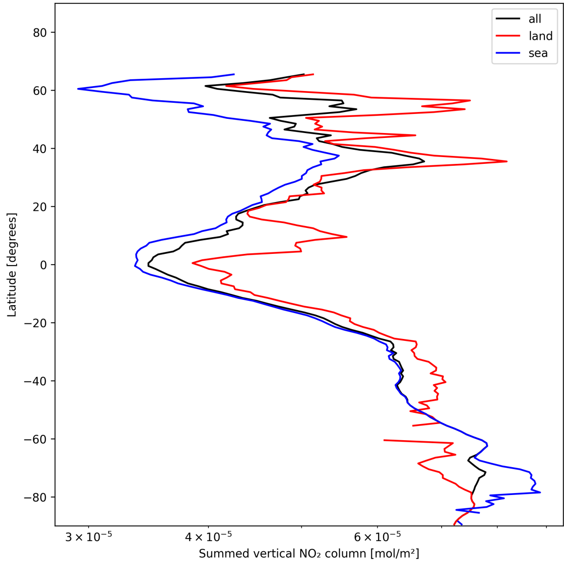
Figure 23: Zonal average of “Summed vertical NO 2 column” for 2024-12-01 to 2024-12-03.
