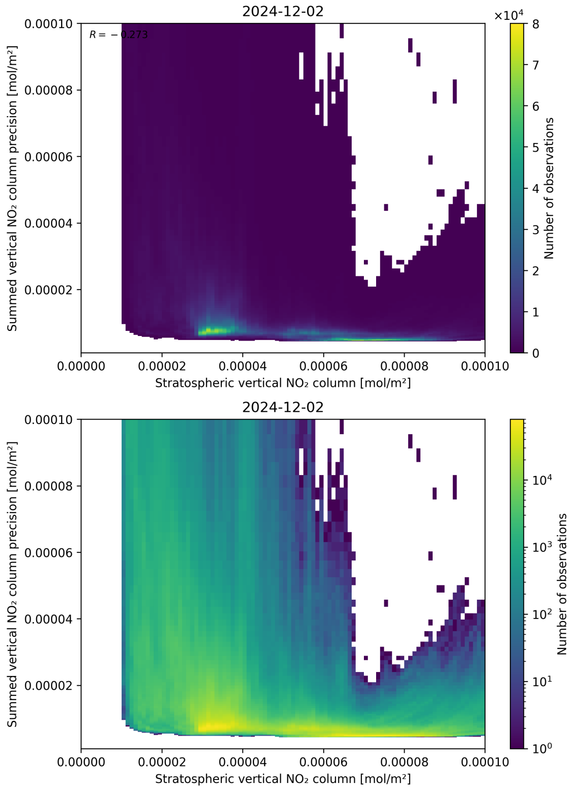
Figure 99: Scatter density plot of “Stratospheric vertical NO 2 column” against “Summed vertical NO 2 column precision” for 2024-12-01 to 2024-12-03.
