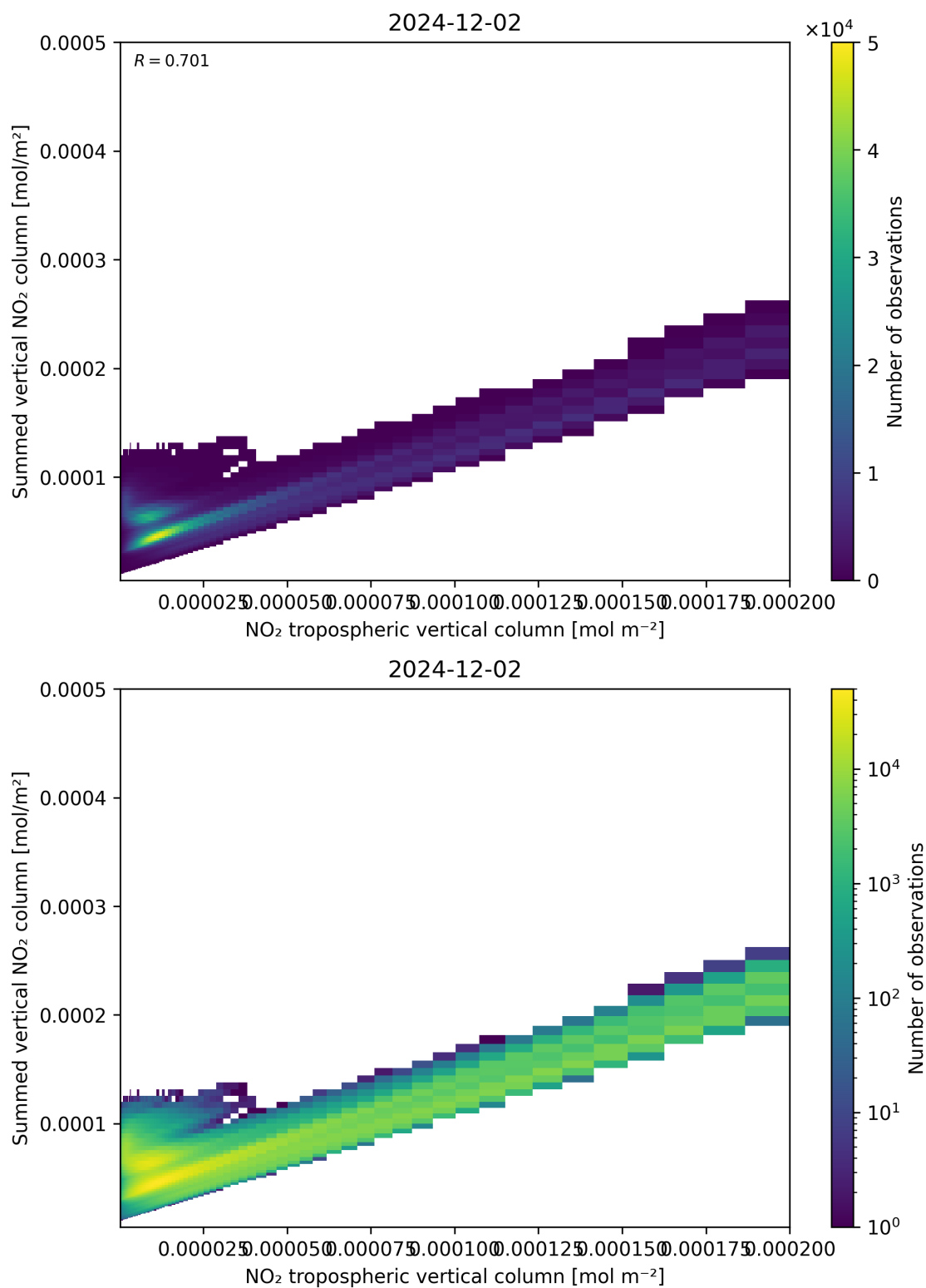
Figure 126: Scatter density plot of “NO 2 tropospheric vertical column” against “Summed vertical NO 2 column” for 2024-12-01 to 2024-12-03.
