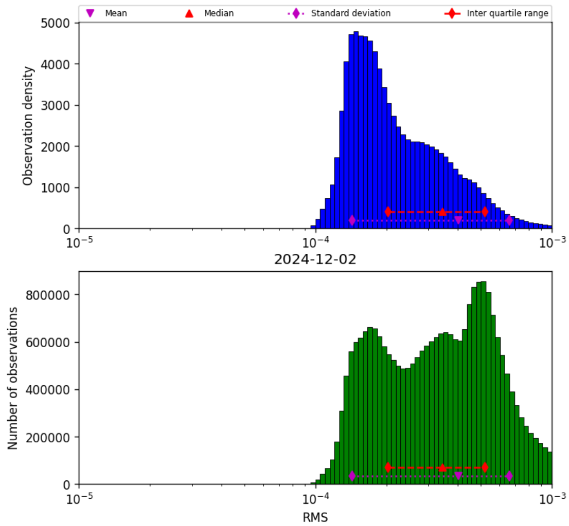
Figure 43: Histogram of “RMS” for 2024-12-01 to 2024-12-03
