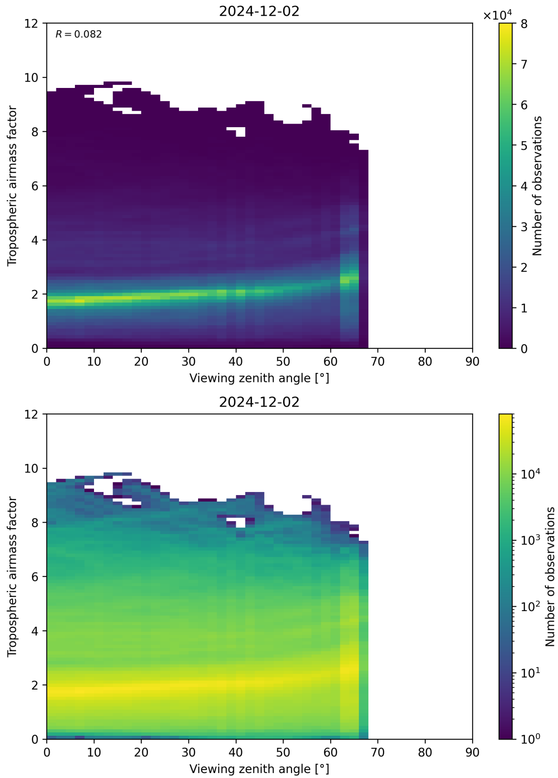
Figure 161: Scatter density plot of “Viewing zenith angle” against “Tropospheric airmass factor” for 2024-12-01 to 2024-12-03.
