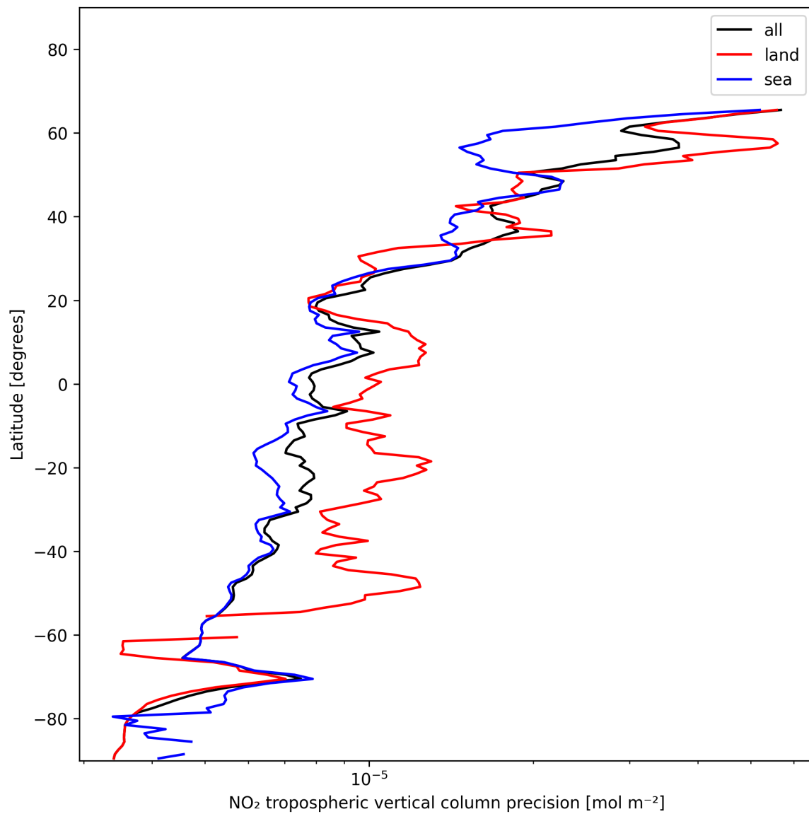
Figure 13: Zonal average of “NO 2 tropospheric vertical column precision” for 2024-12-01 to 2024-12-03.
