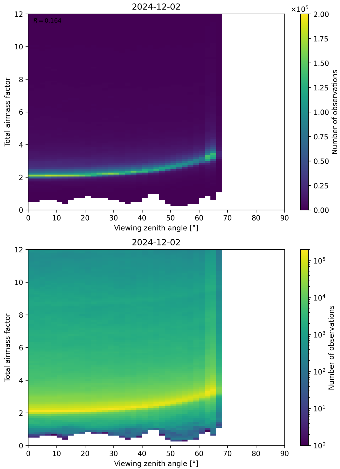
Figure 160: Scatter density plot of “Viewing zenith angle” against “Total airmass factor” for 2024-12-01 to 2024-12-03.
