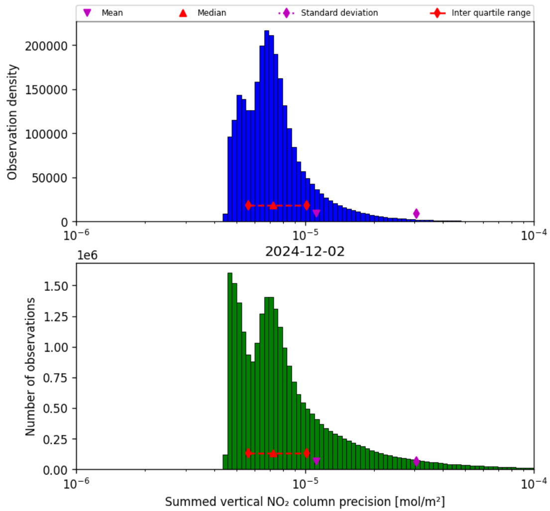
Figure 41: Histogram of “Summed vertical NO 2 column precision” for 2024-12-01 to 2024-12-03
