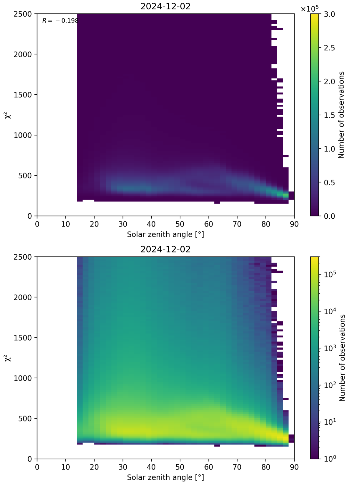
Figure 148: Scatter density plot of “Solar zenith angle” against “ \chi^2 ” for 2024-12-01 to 2024-12-03.
