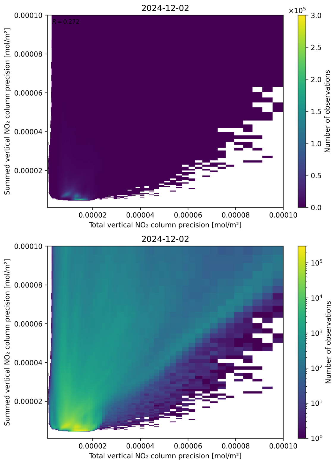
Figure 118: Scatter density plot of “Total vertical NO 2 column precision” against “Summed vertical NO 2 column precision” for 2024-12-01 to 2024-12-03.
