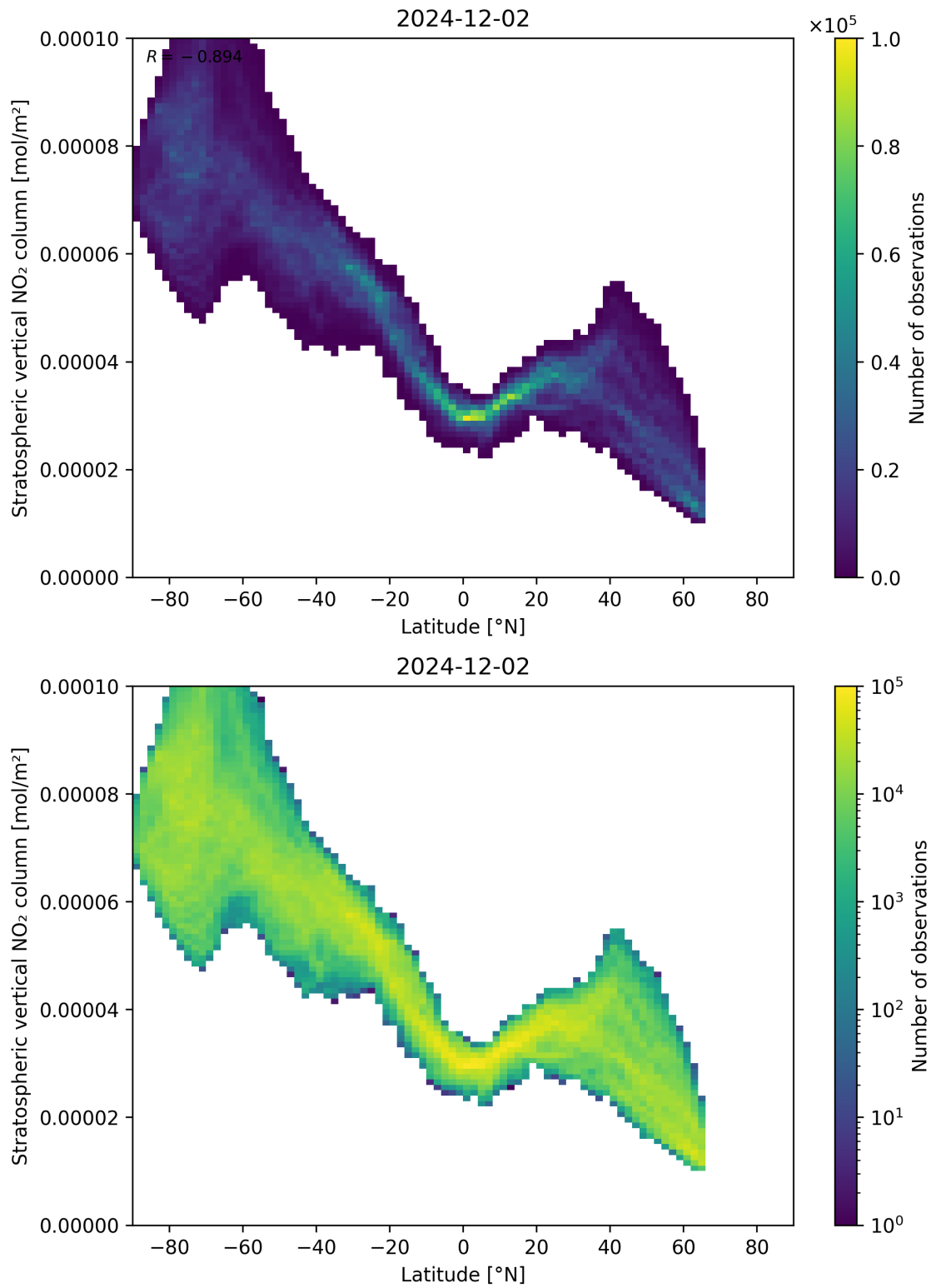
Figure 87: Scatter density plot of “Latitude” against “Stratospheric vertical NO 2 column” for 2024-12-01 to 2024-12-03.
