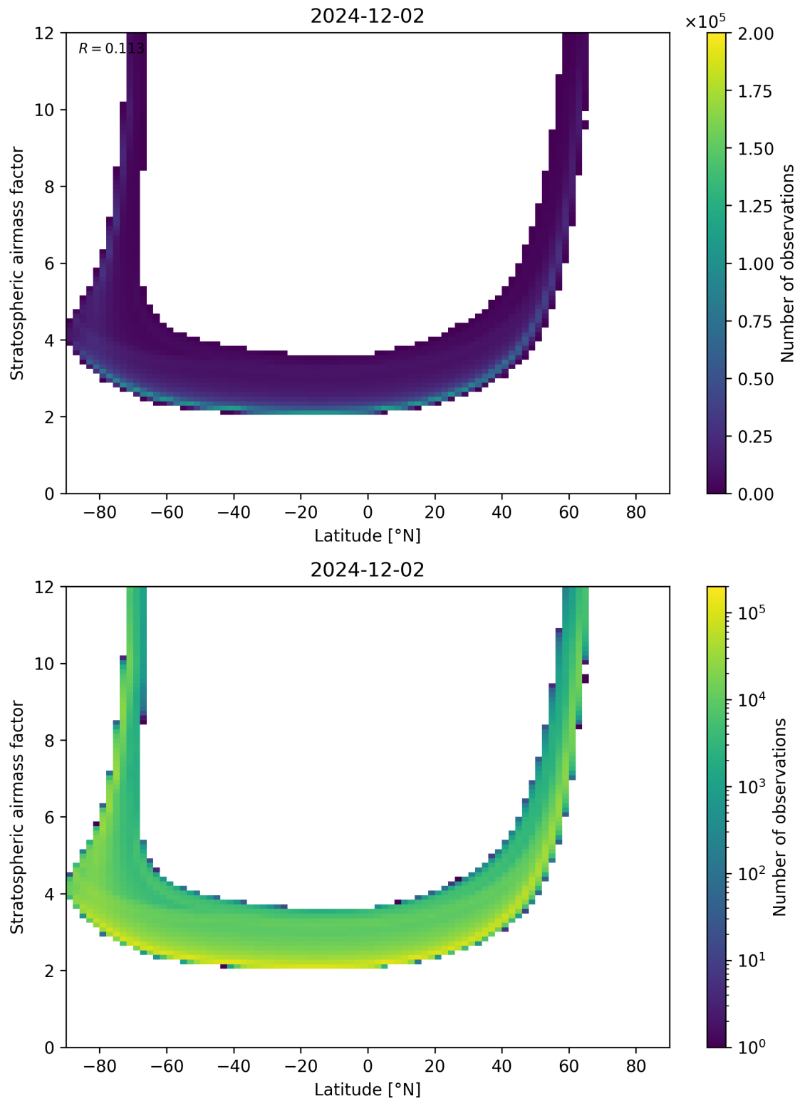
Figure 83: Scatter density plot of “Latitude” against “Stratospheric air mass factor” for 2024-12-01 to 2024-12-03.
