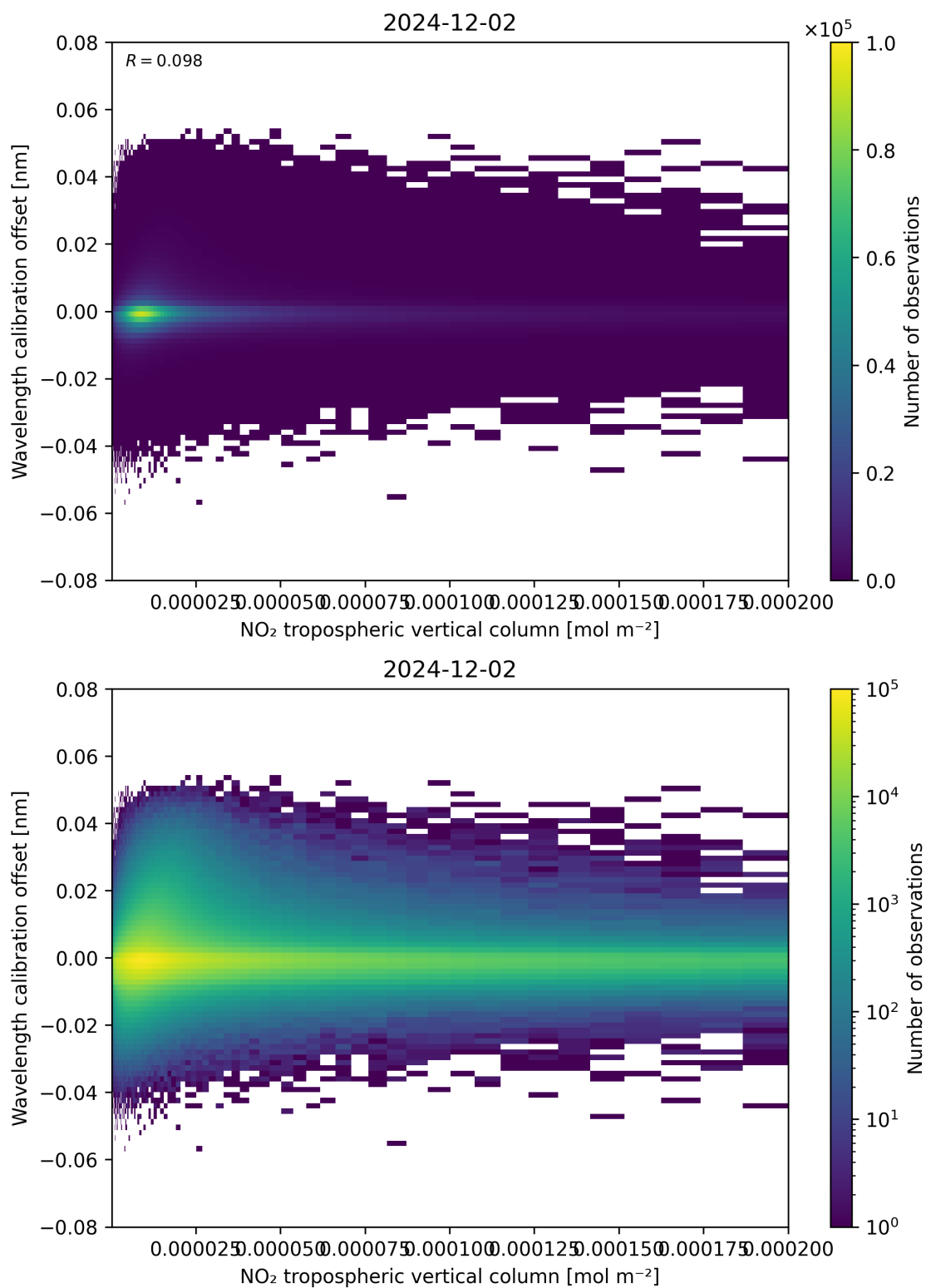
Figure 143: Scatter density plot of “NO 2 tropospheric vertical column” against “Wavelength calibration offset” for 2024-12-01 to 2024-12-03.
