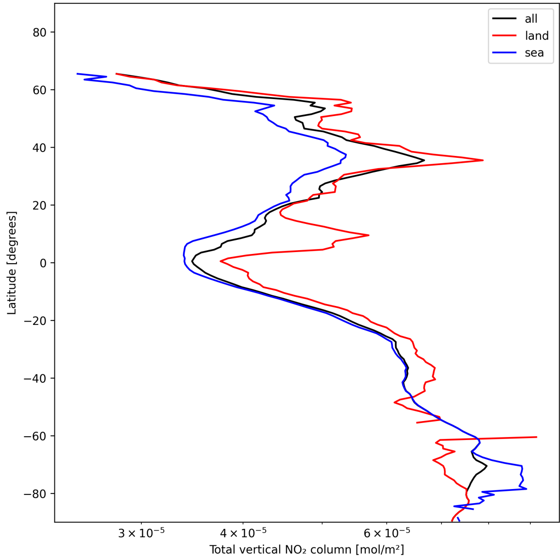
Figure 21: Zonal average of “Total vertical NO 2 column” for 2024-12-01 to 2024-12-03.
