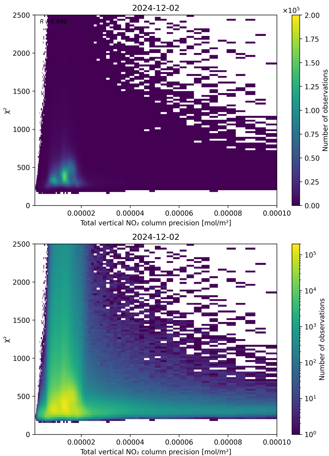
Figure 116: Scatter density plot of “Total vertical NO 2 column precision” against “ \chi^2 ” for 2024-12-01 to 2024-12-03.
