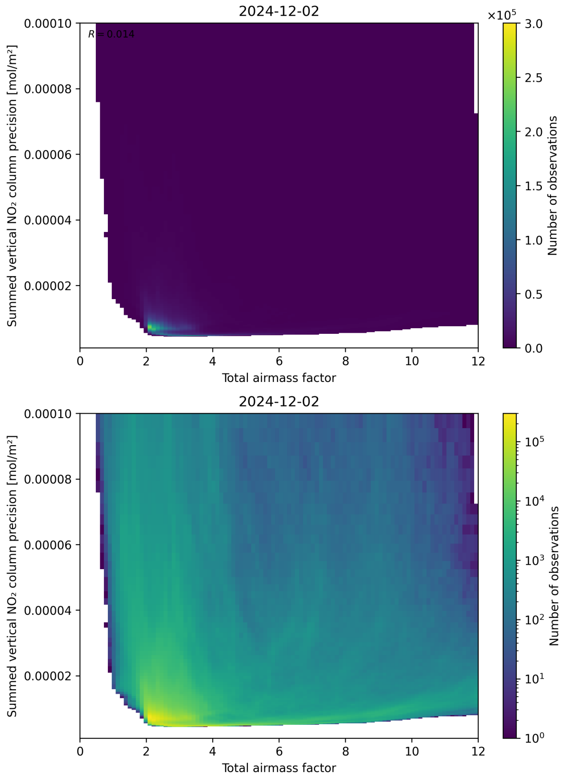
Figure 66: Scatter density plot of “Total airmass factor” against “Summed vertical NO 2 column precision” for 2024-12-01 to 2024-12-03.
