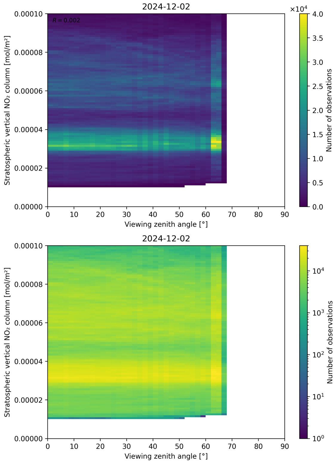
Figure 164: Scatter density plot of “Viewing zenith angle” against “Stratospheric vertical NO 2 column” for 2024-12-01 to 2024-12-03.
