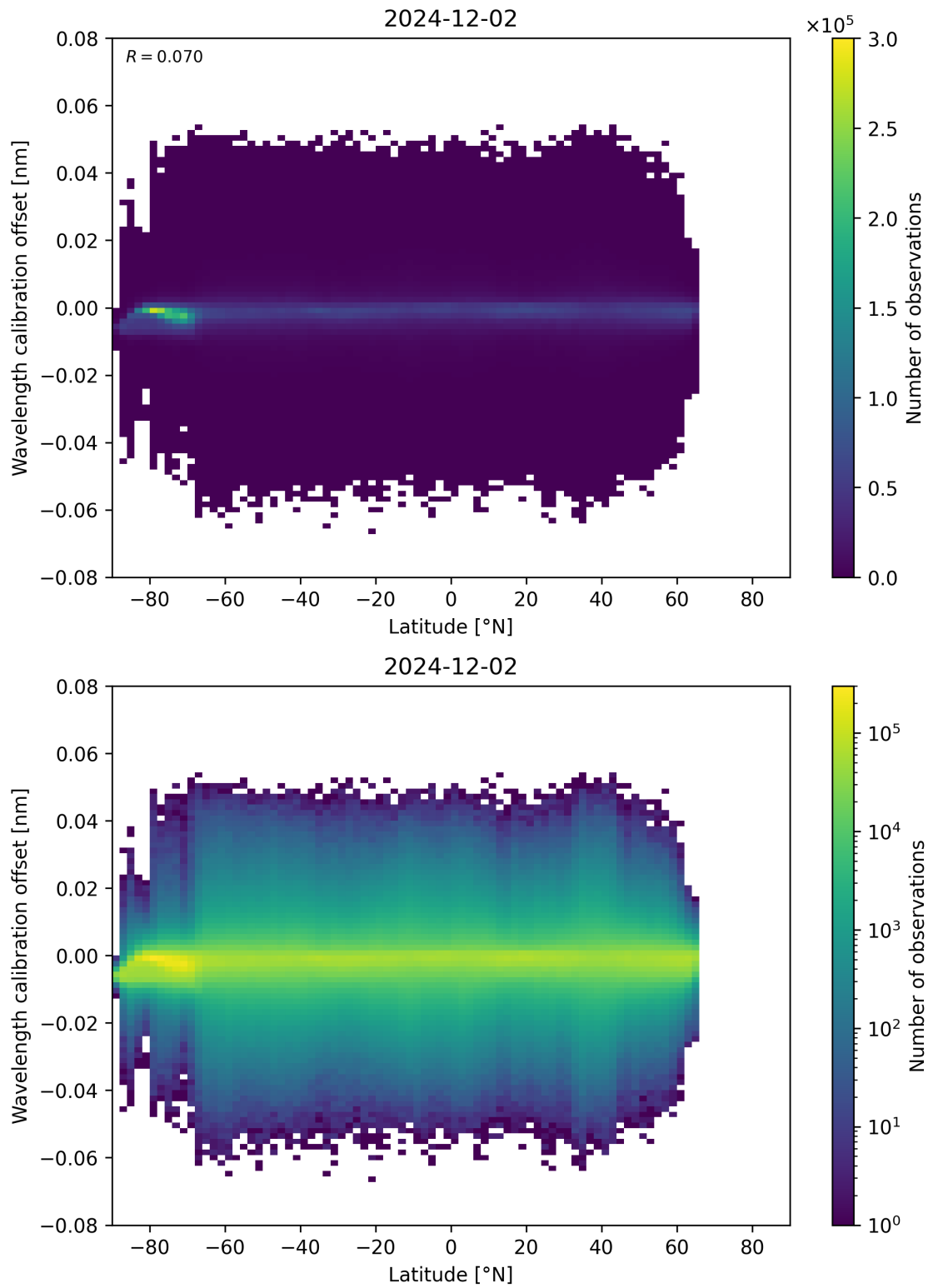
Figure 95: Scatter density plot of “Latitude” against “Wavelength calibration offset” for 2024-12-01 to 2024-12-03.
