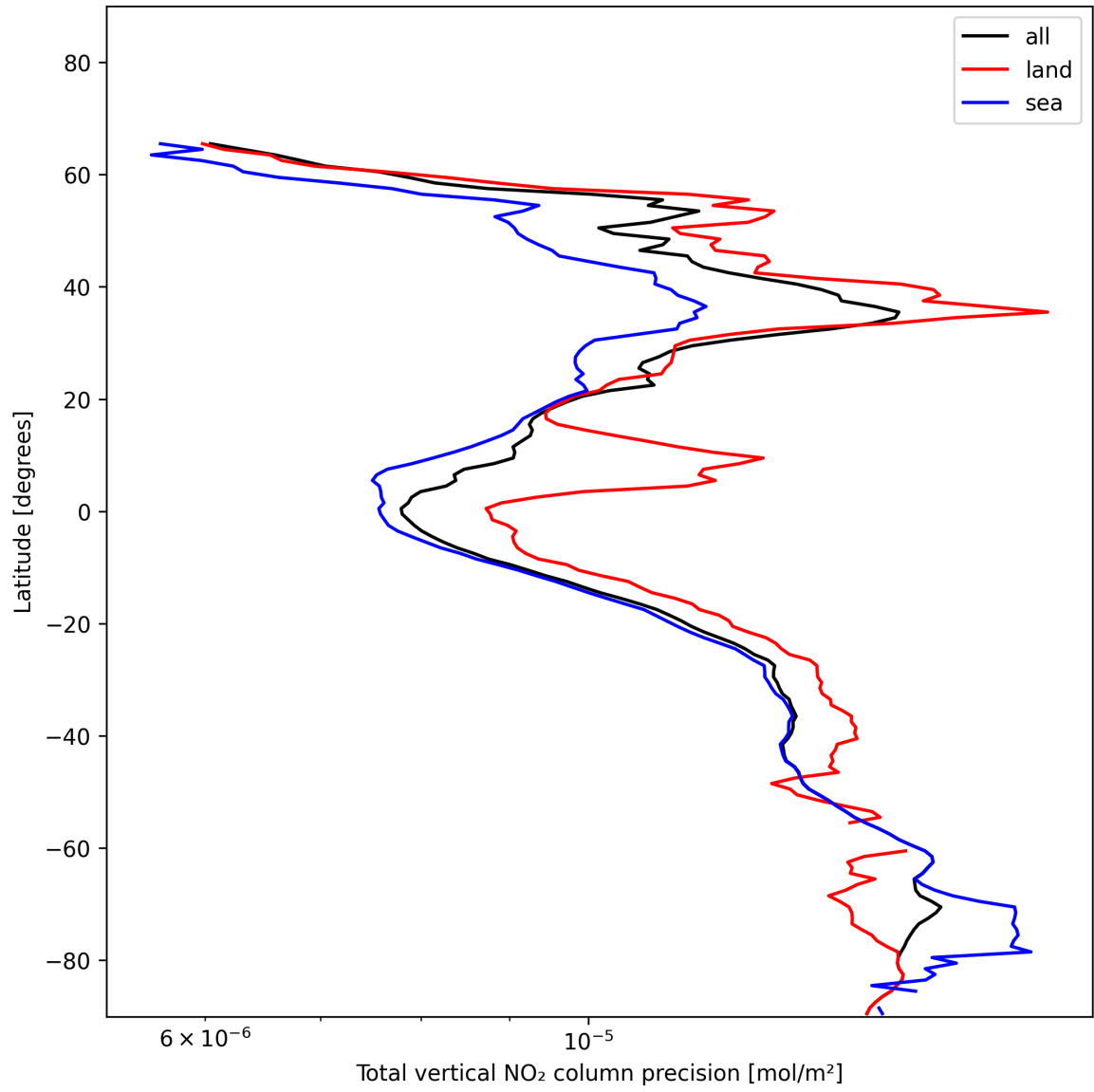
Figure 22: Zonal average of “Total vertical NO 2 column precision” for 2024-12-01 to 2024-12-03.
