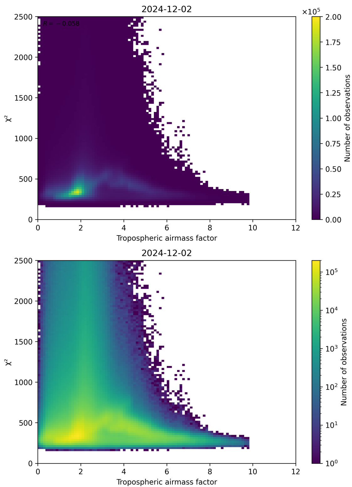
Figure 73: Scatter density plot of “Tropospheric airmass factor” against “ \chi^2 ” for 2024-12-01 to 2024-12-03.
