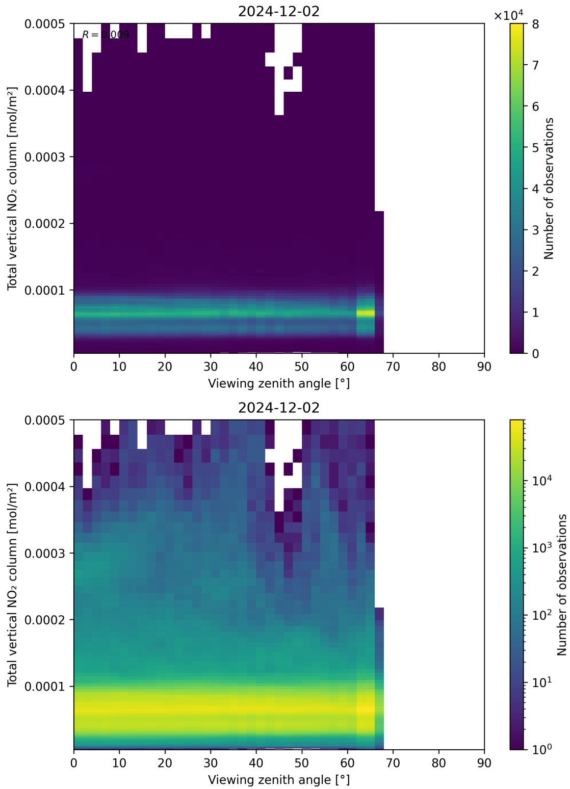
Figure 167: Scatter density plot of “Viewing zenith angle” against “Total vertical NO 2 column” for 2024-12-01 to 2024-12-03.
