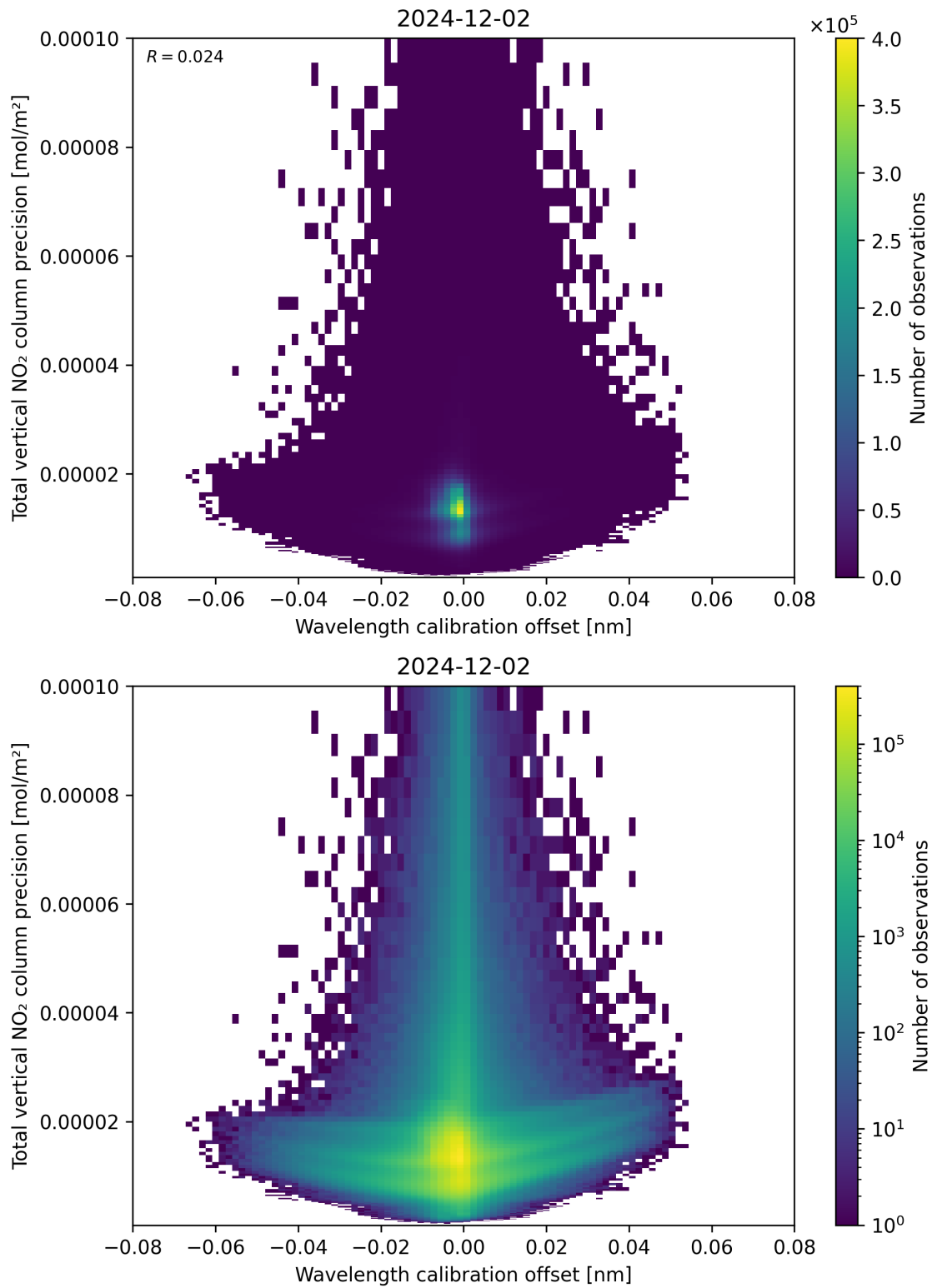
Figure 180: Scatter density plot of “Wavelength calibration offset” against “Total vertical NO 2 column precision” for 2024-12-01 to 2024-12-03.
