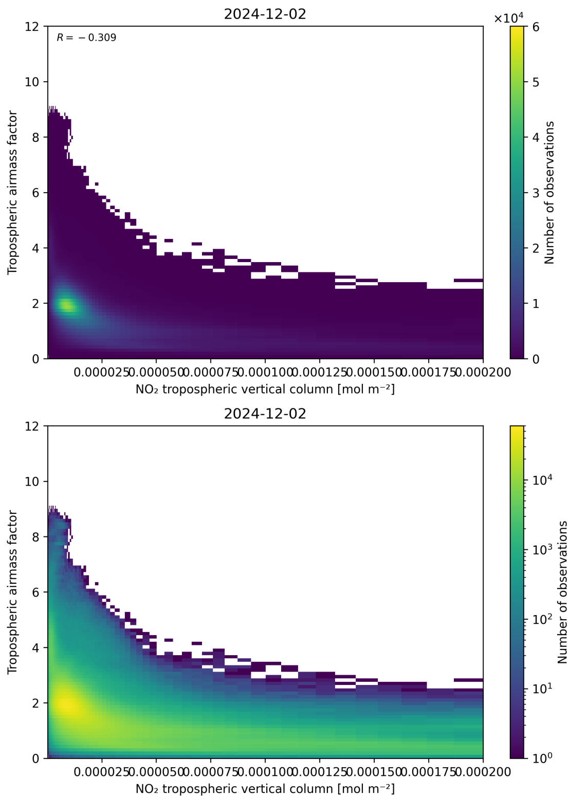
Figure 123: Scatter density plot of “NO 2 tropospheric vertical column” against “Tropospheric air mass factor” for 2024-12-01 to 2024-12-03.
