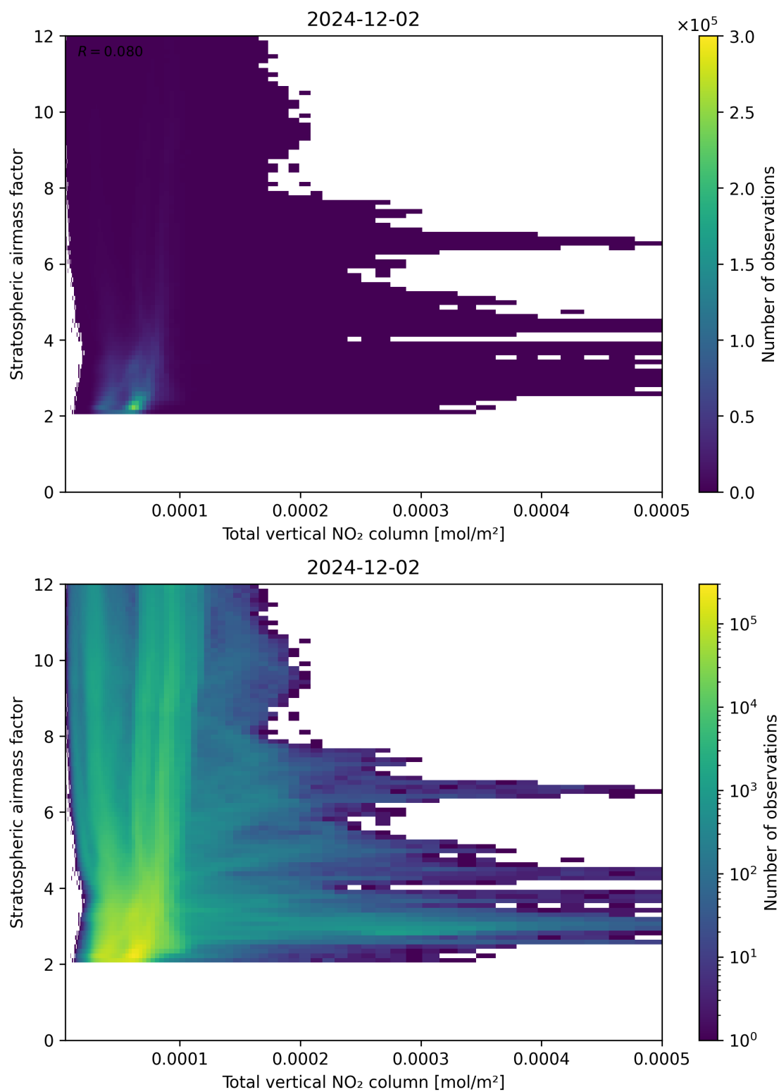
Figure 110: Scatter density plot of “Total vertical NO 2 column” against “Stratospheric airmass factor” for 2024-12-01 to 2024-12-03.
