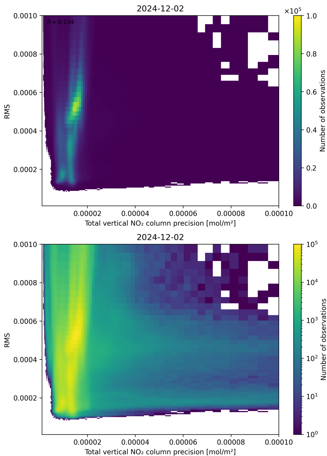
Figure 119: Scatter density plot of “Total vertical NO 2 column precision” against “RMS” for 2024-12-01 to 2024-12-03.
