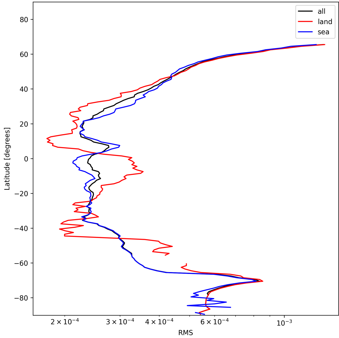
Figure 26: Zonal average of “RMS” for 2024-12-01 to 2024-12-03.
