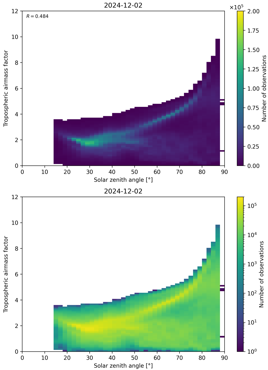
Figure 147: Scatter density plot of “Solar zenith angle” against “Tropospheric airmass factor” for 2024-12-01 to 2024-12-03.
