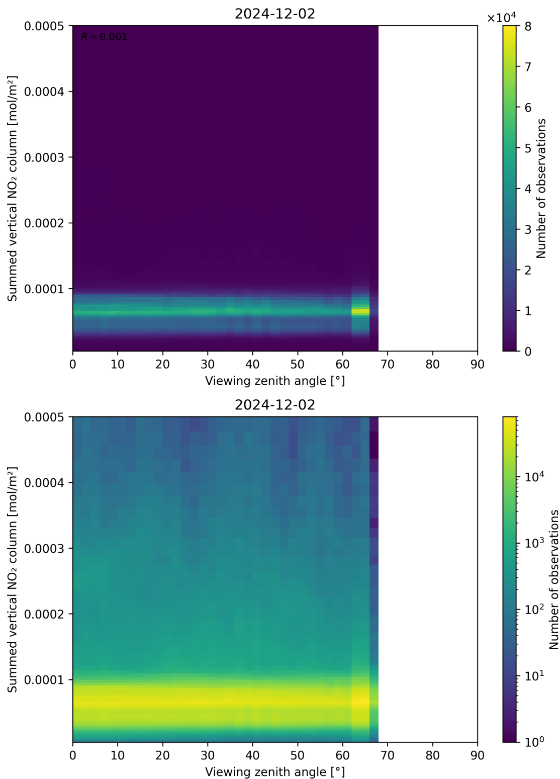
Figure 165: Scatter density plot of “Viewing zenith angle” against “Summed vertical NO 2 column” for 2024-12-01 to 2024-12-03.
