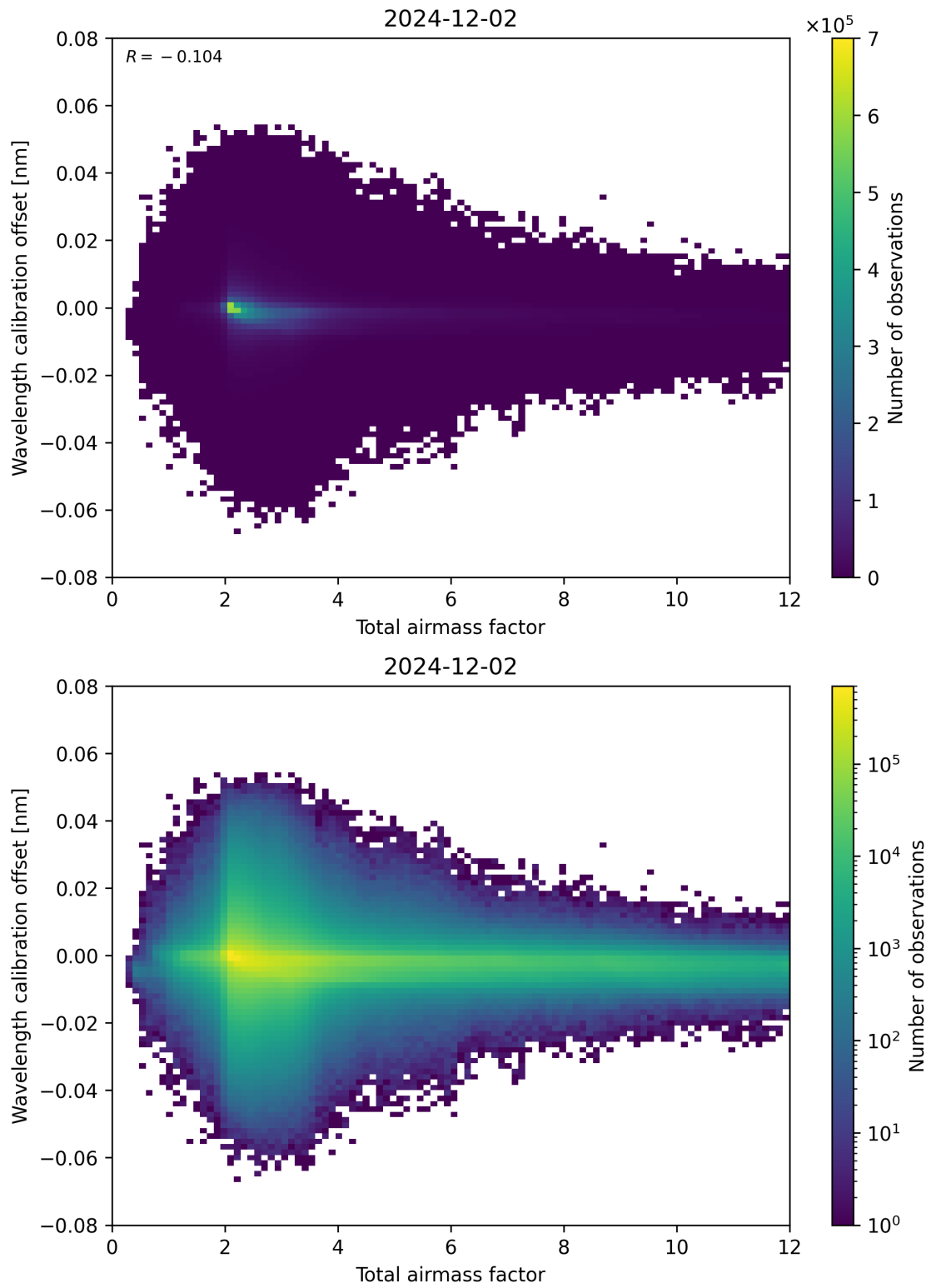
Figure 70: Scatter density plot of “Total airmass factor” against “Wavelength calibration offset” for 2024-12-01 to 2024-12-03.
