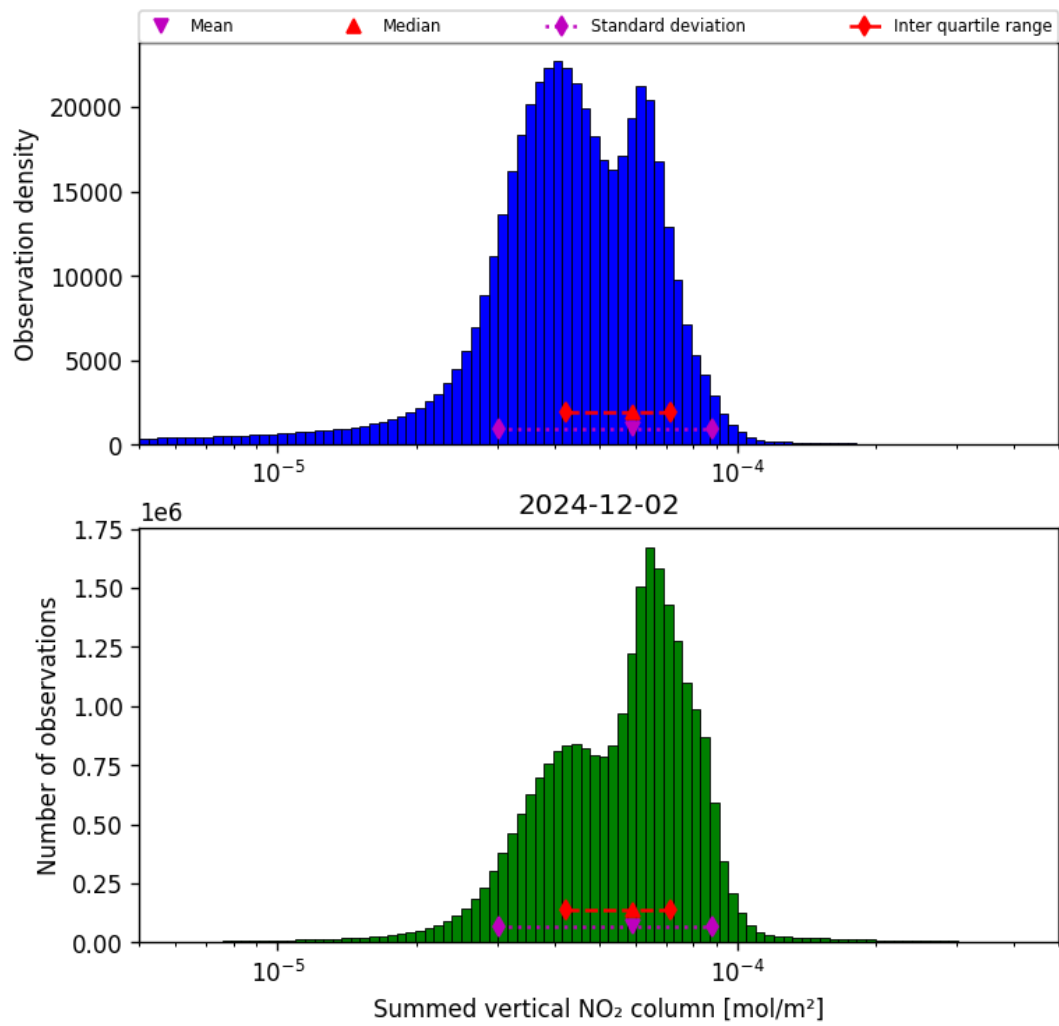
Figure 40: Histogram of “Summed vertical NO 2 column” for 2024-12-01 to 2024-12-03
