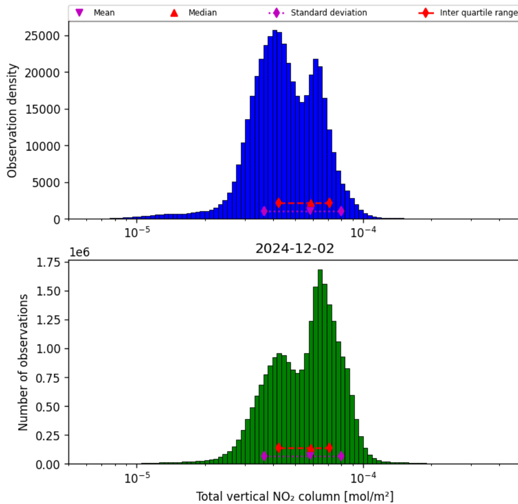
Figure 38: Histogram of “Total vertical NO 2 column” for 2024-12-01 to 2024-12-03
