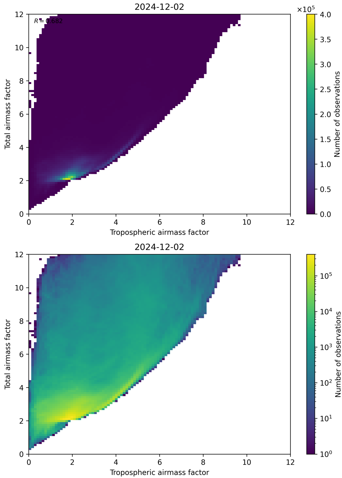
Figure 72: Scatter density plot of “Tropospheric airmass factor” against “Total airmass factor” for 2024-12-01 to 2024-12-03.
