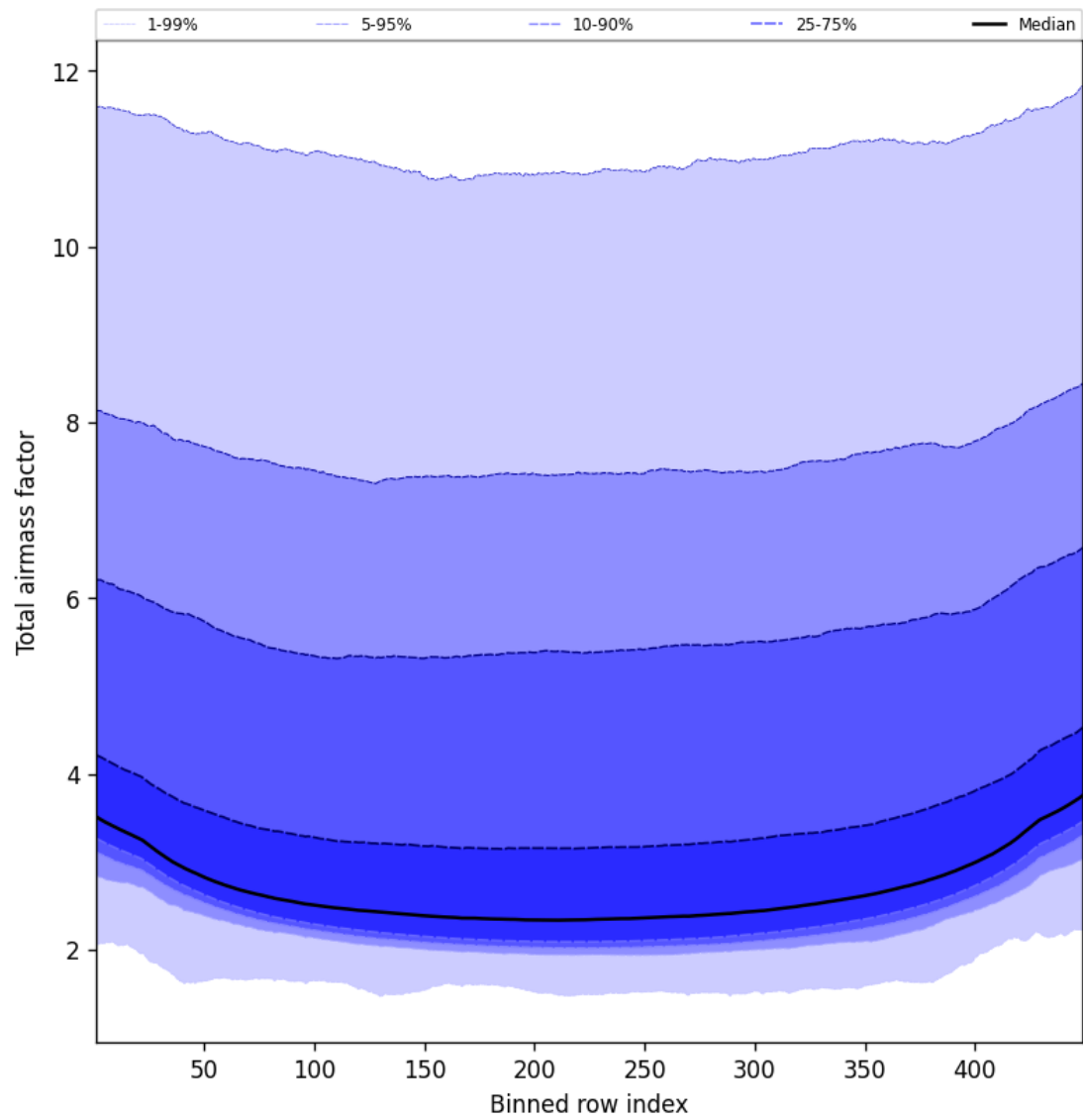
Figure 49: Along track statistics of “Total airmass factor” for 2024-12-01 to 2024-12-03
