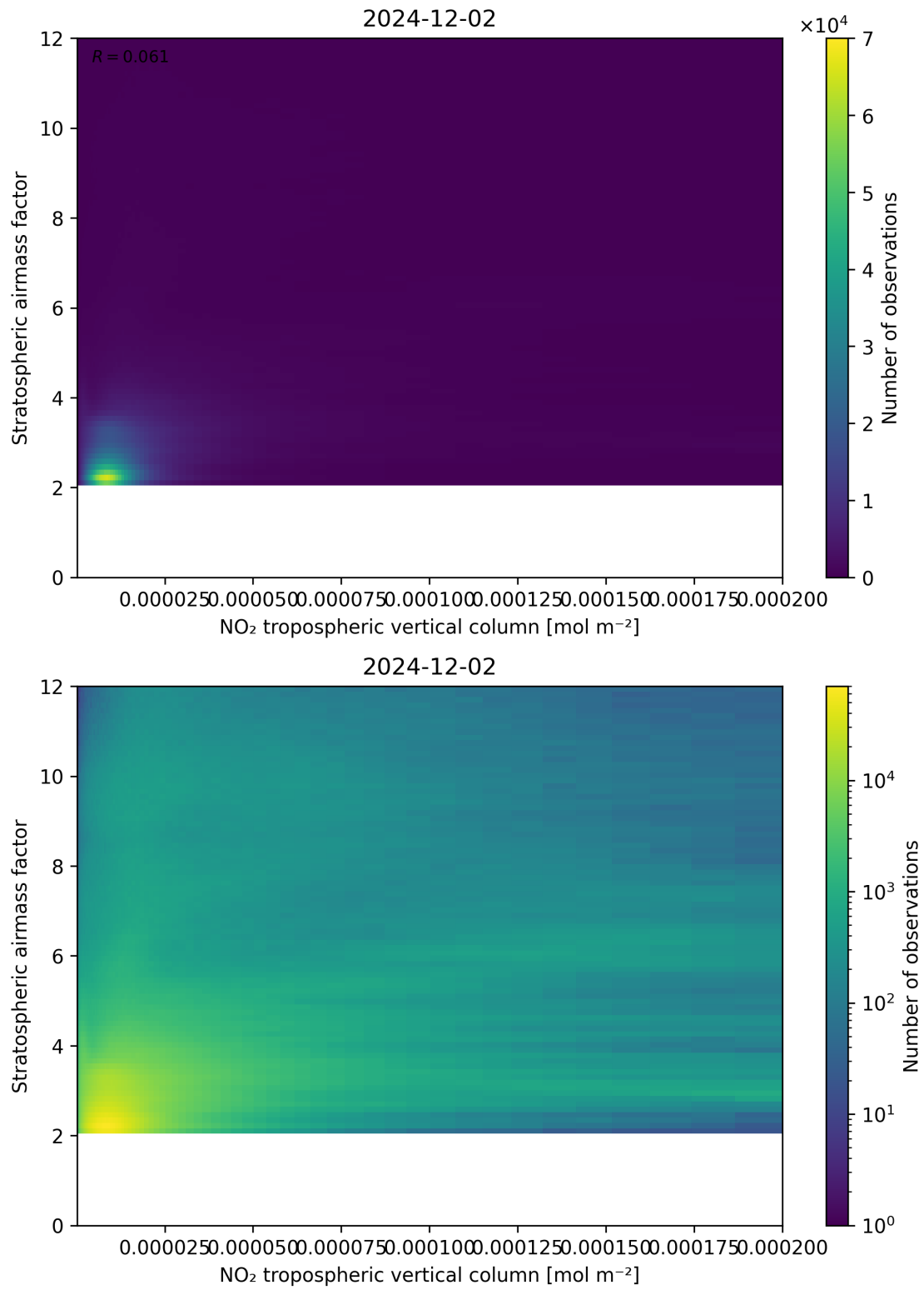
Figure 121: Scatter density plot of “NO 2 tropospheric vertical column” against “Stratospheric airmass factor” for 2024-12-01 to 2024-12-03.
