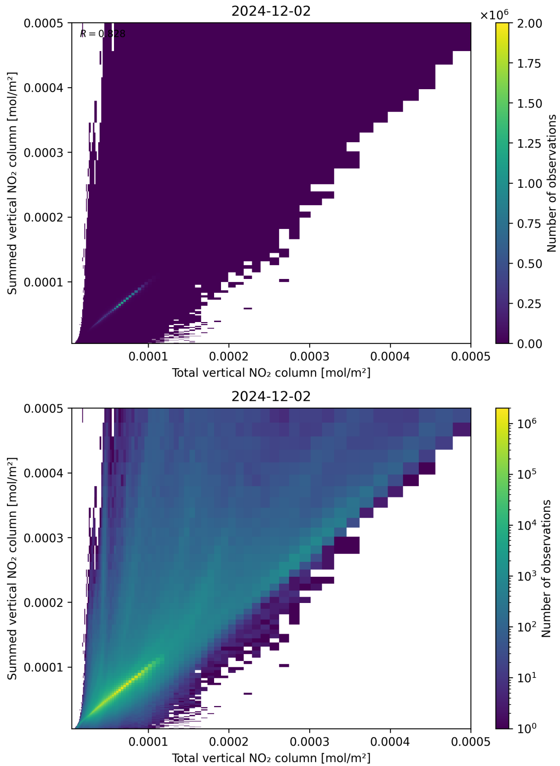
Figure 112: Scatter density plot of “Total vertical NO 2 column” against “Summed vertical NO 2 column” for 2024-12-01 to 2024-12-03.
