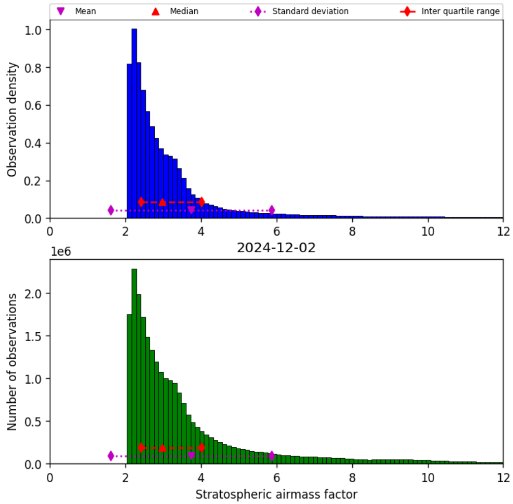
Figure 44: Histogram of “Stratospheric airmass factor” for 2024-12-01 to 2024-12-03
