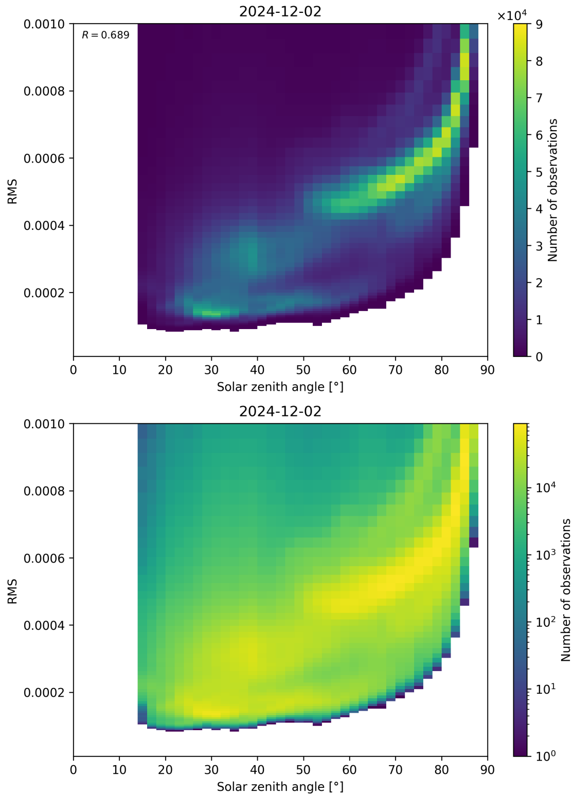
Figure 157: Scatter density plot of “Solar zenith angle” against “RMS” for 2024-12-01 to 2024-12-03.
