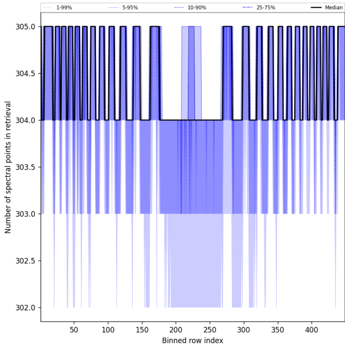
Figure 50: Along track statistics of “Number of spectral points in retrieval” for 2024-12-01 to 2024-12-03
