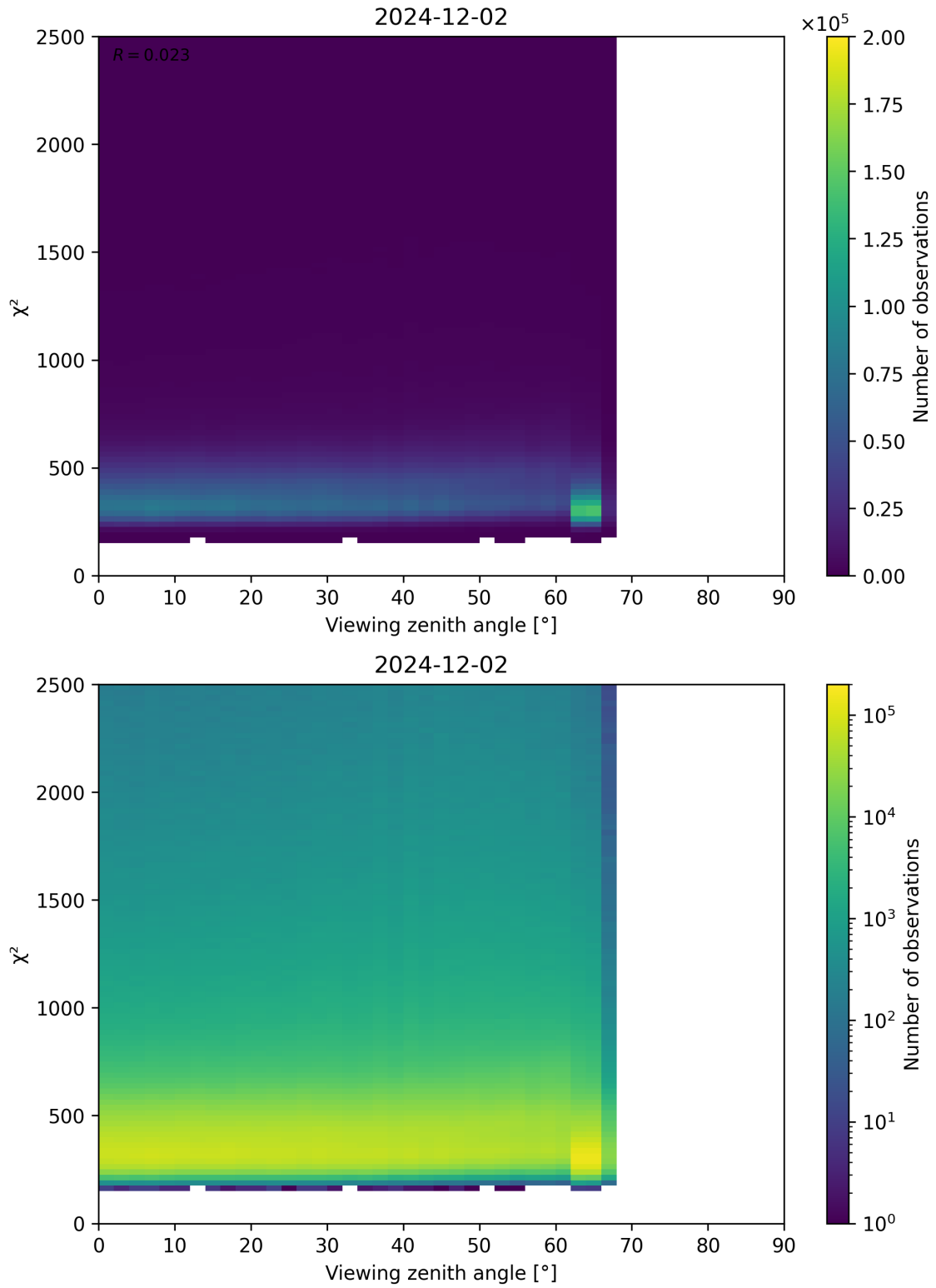
Figure 162: Scatter density plot of “Viewing zenith angle” against “ \chi^2 ” for 2024-12-01 to 2024-12-03.
