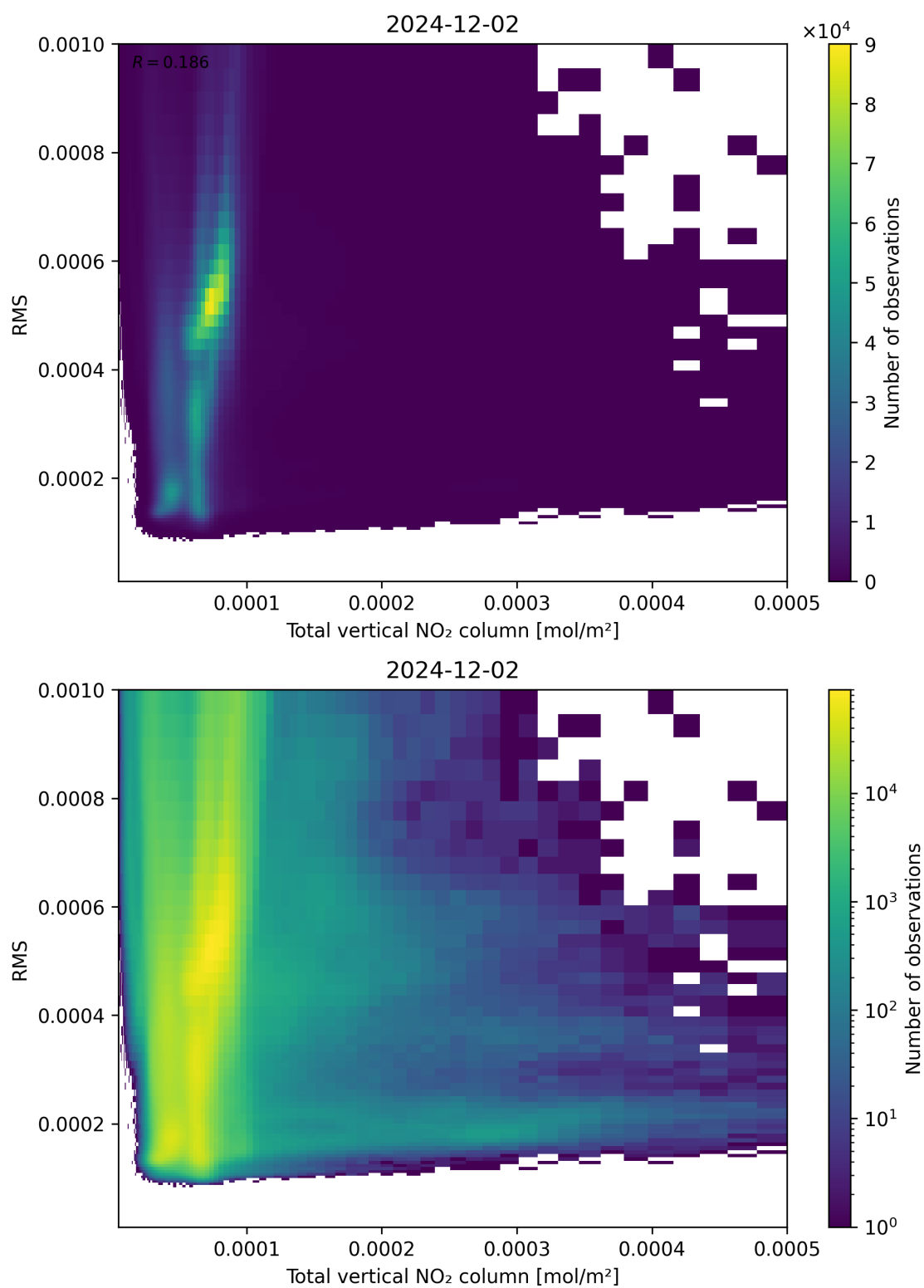
Figure 120: Scatter density plot of “Total vertical NO 2 column” against “RMS” for 2024-12-01 to 2024-12-03.
