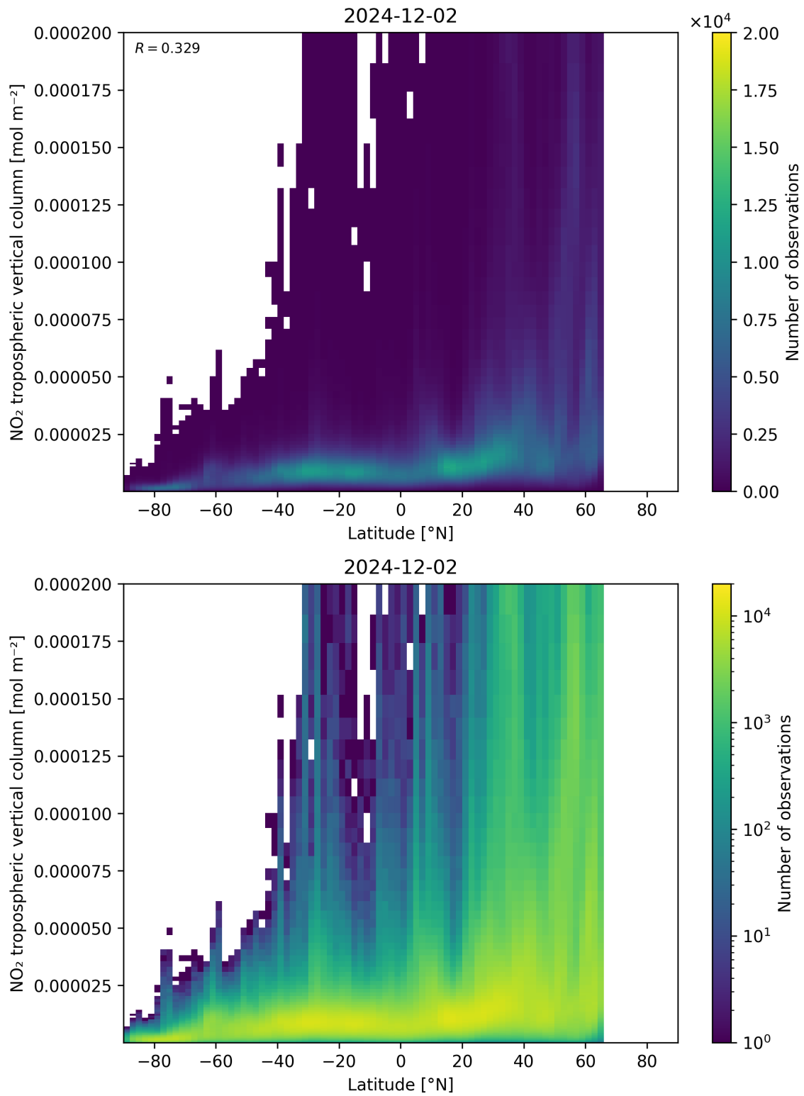
Figure 92: Scatter density plot of “Latitude” against “NO 2 tropospheric vertical column” for 2024-12-01 to 2024-12-03.
