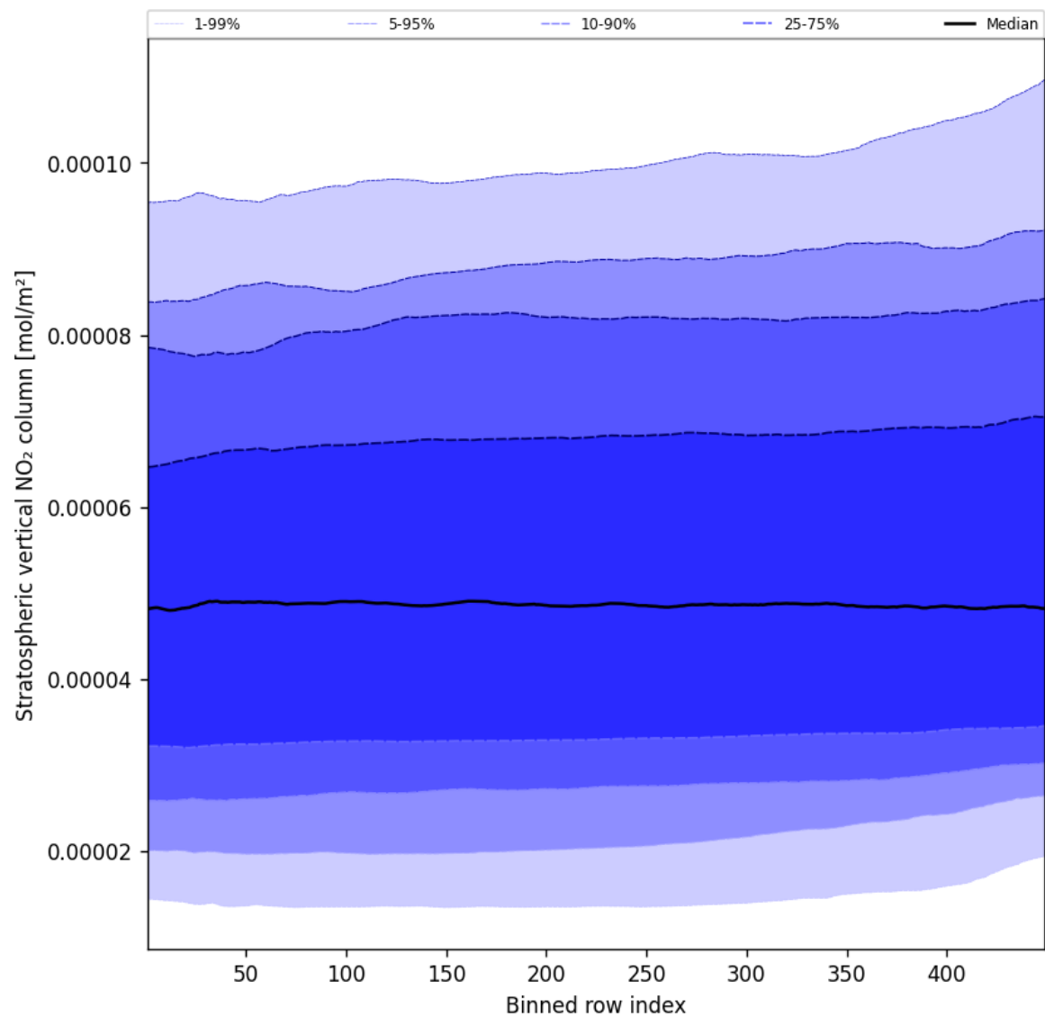
Figure 53: Along track statistics of “Stratospheric vertical NO 2 column” for 2024-12-01 to 2024-12-03
