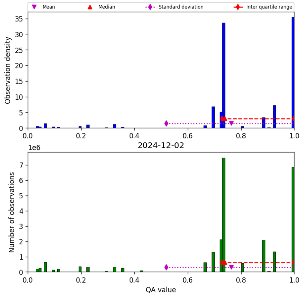
Figure 28: Histogram of “QA value” for 2024-12-01 to 2024-12-03
