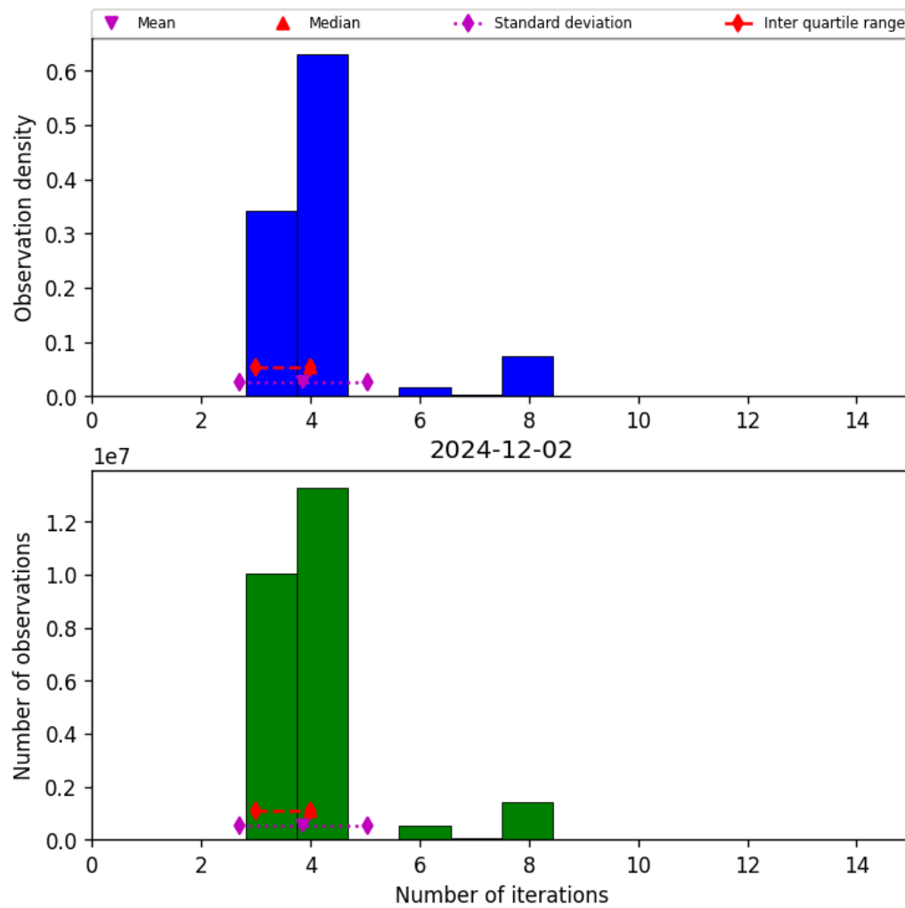
Figure 34: Histogram of “Number of iterations” for 2024-12-01 to 2024-12-03
