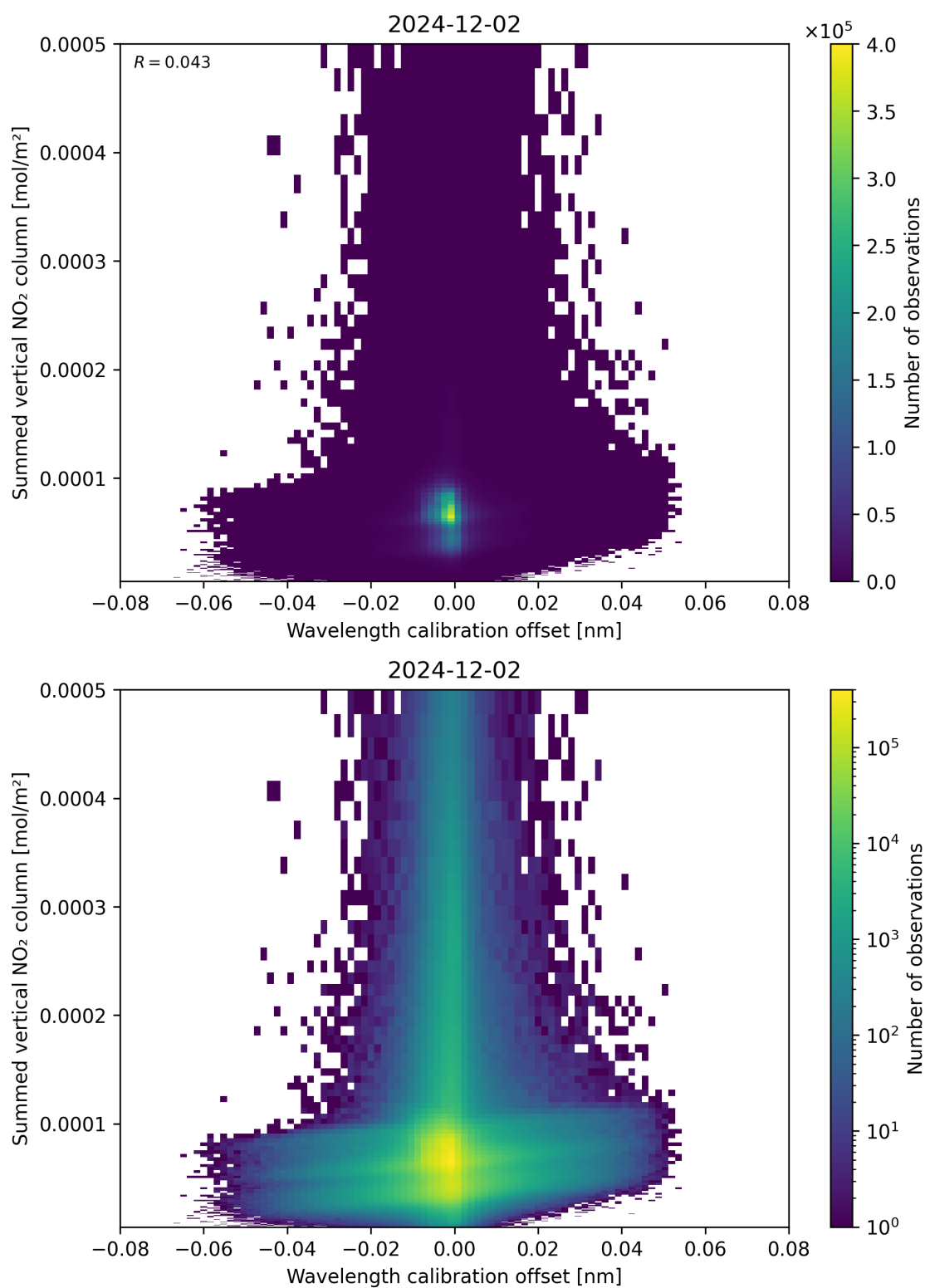
Figure 177: Scatter density plot of “Wavelength calibration offset” against “Summed vertical NO 2 column” for 2024-12-01 to 2024-12-03.
