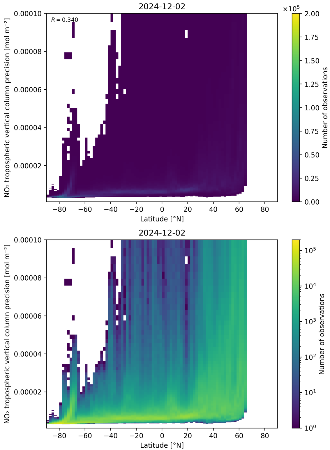
Figure 93: Scatter density plot of “Latitude” against “NO 2 tropospheric vertical column precision” for 2024-12-01 to 2024-12-03.
