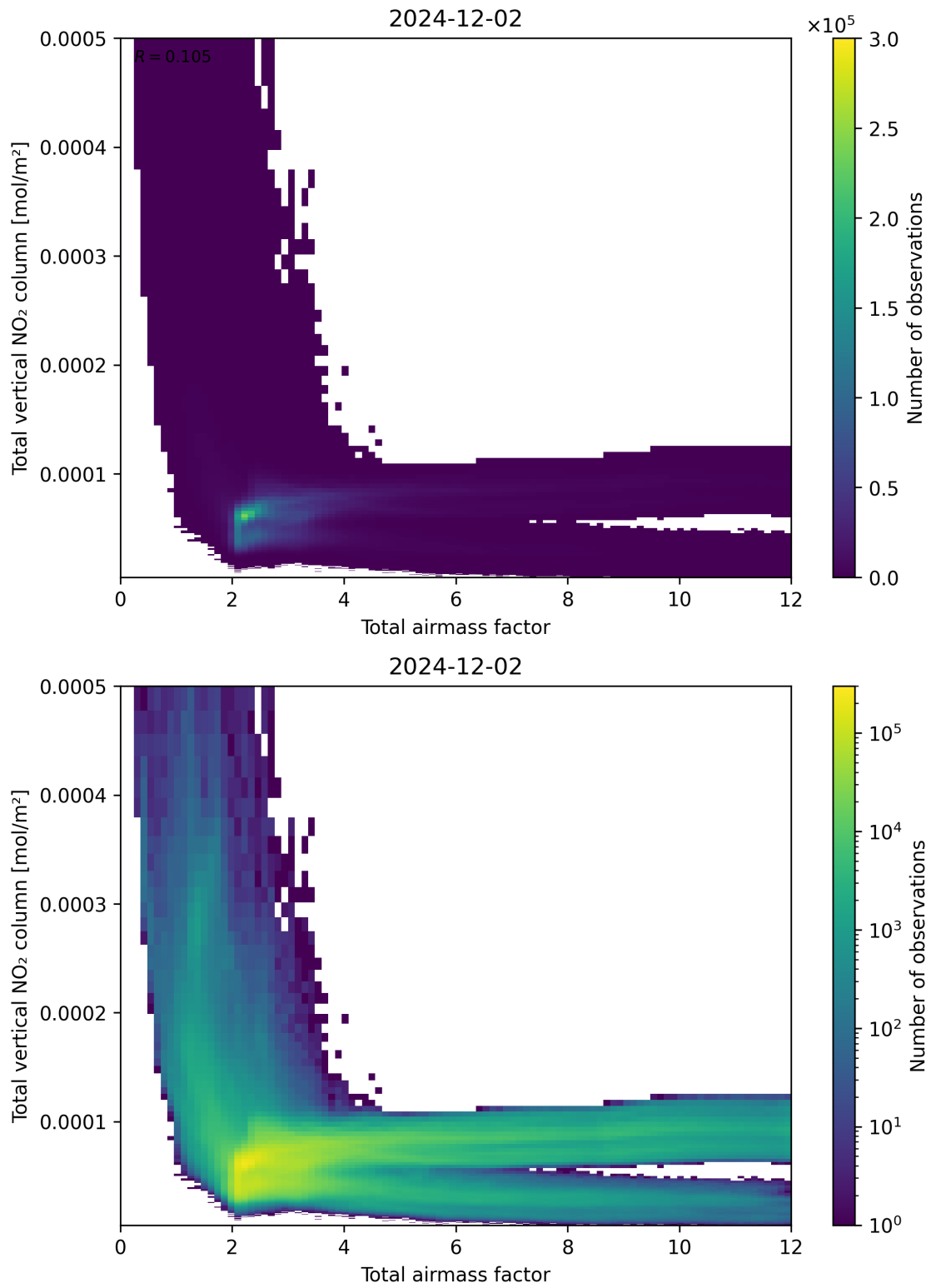
Figure 67: Scatter density plot of “Total airmass factor” against “Total vertical NO 2 column” for 2024-12-01 to 2024-12-03.
