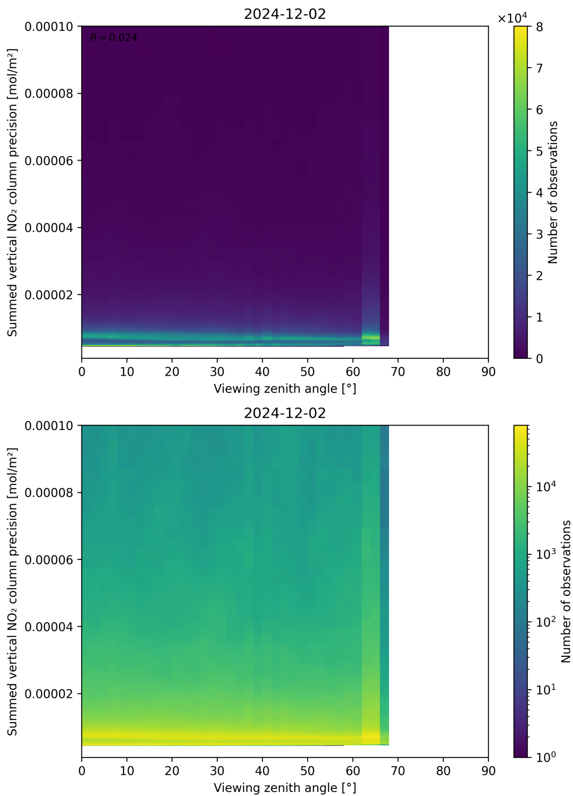
Figure 166: Scatter density plot of “Viewing zenith angle” against “Summed vertical NO 2 column precision” for 2024-12-01 to 2024-12-03.
