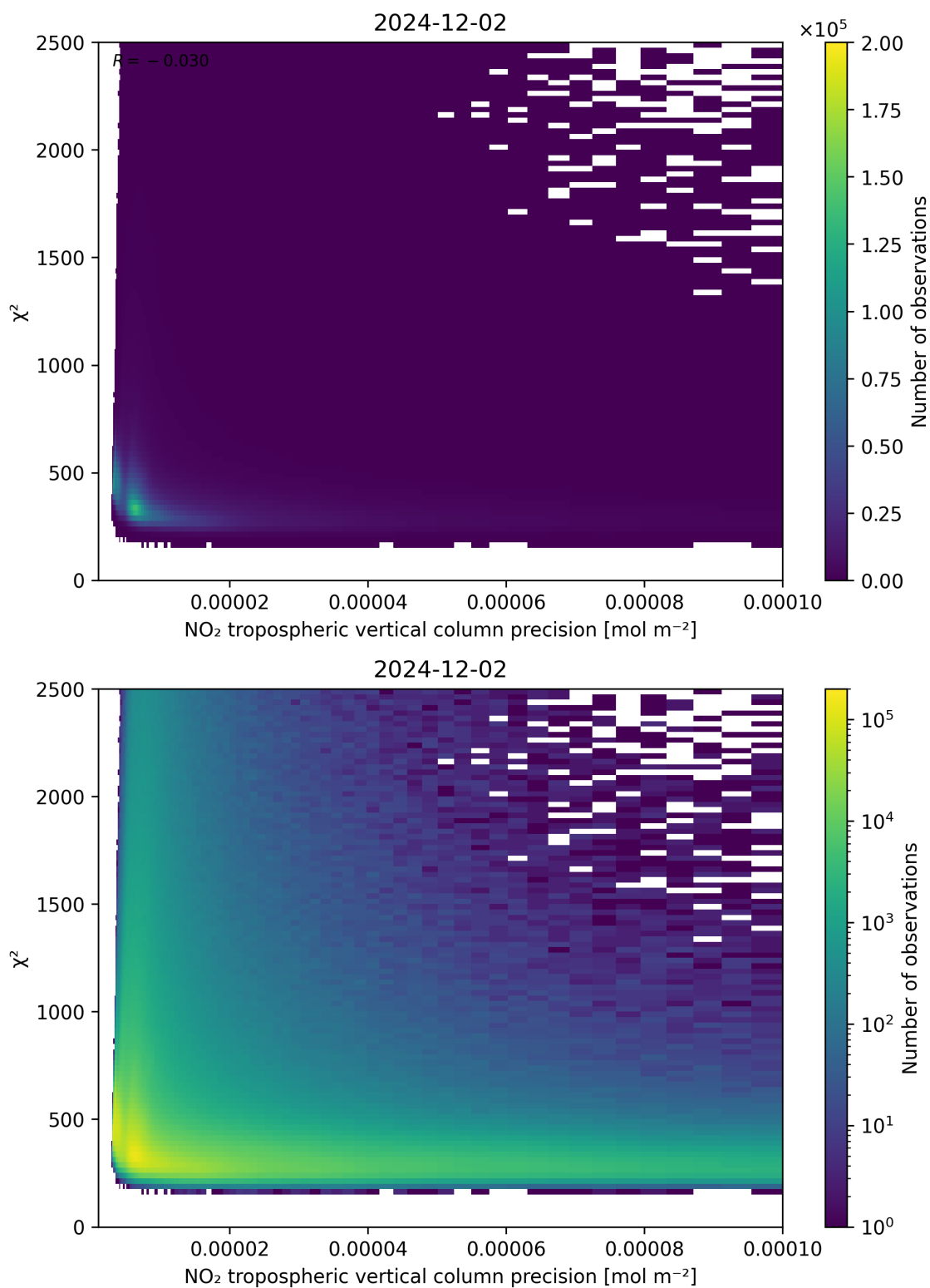
Figure 134: Scatter density plot of “NO 2 tropospheric vertical column precision” against “ \chi^2 ” for 2024-12-01 to 2024-12-03.
