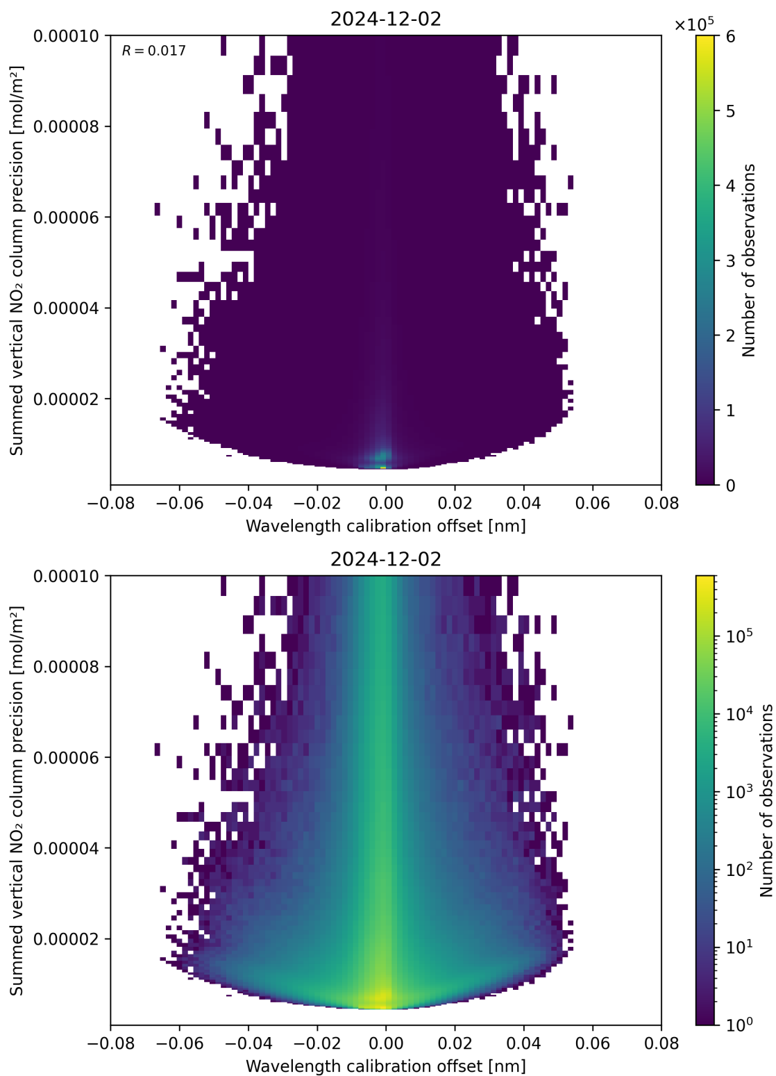
Figure 178: Scatter density plot of “Wavelength calibration offset” against “Summed vertical NO 2 column precision” for 2024-12-01 to 2024-12-03.
