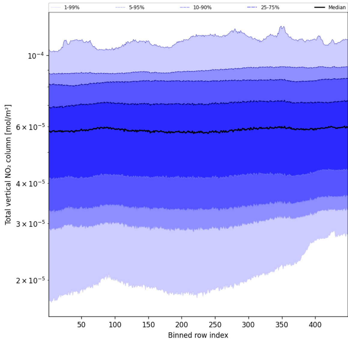
Figure 55: Along track statistics of “Total vertical NO 2 column” for 2024-12-01 to 2024-12-03
