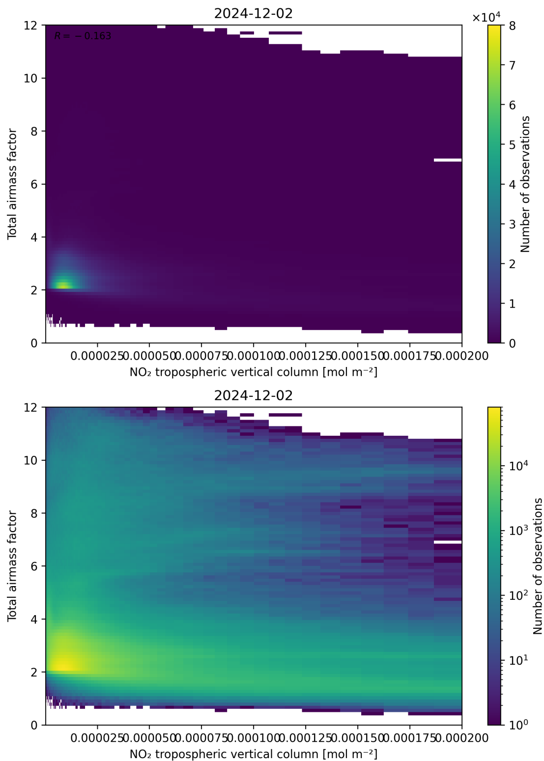
Figure 122: Scatter density plot of “NO 2 tropospheric vertical column” against “Total air mass factor” for 2024-12-01 to 2024-12-03.
