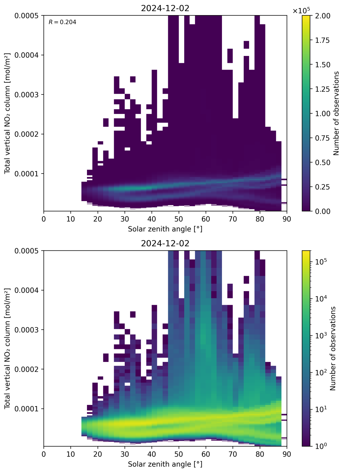
Figure 153: Scatter density plot of “Solar zenith angle” against “Total vertical NO 2 column” for 2024-12-01 to 2024-12-03.
