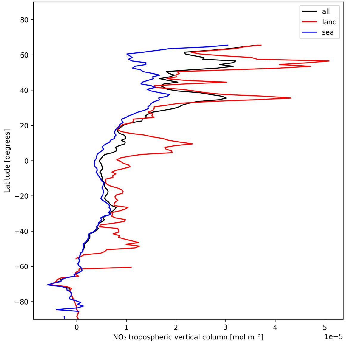
Figure 12: Zonal average of “NO 2 tropospheric vertical column” for 2024-12-01 to 2024-12-03.
