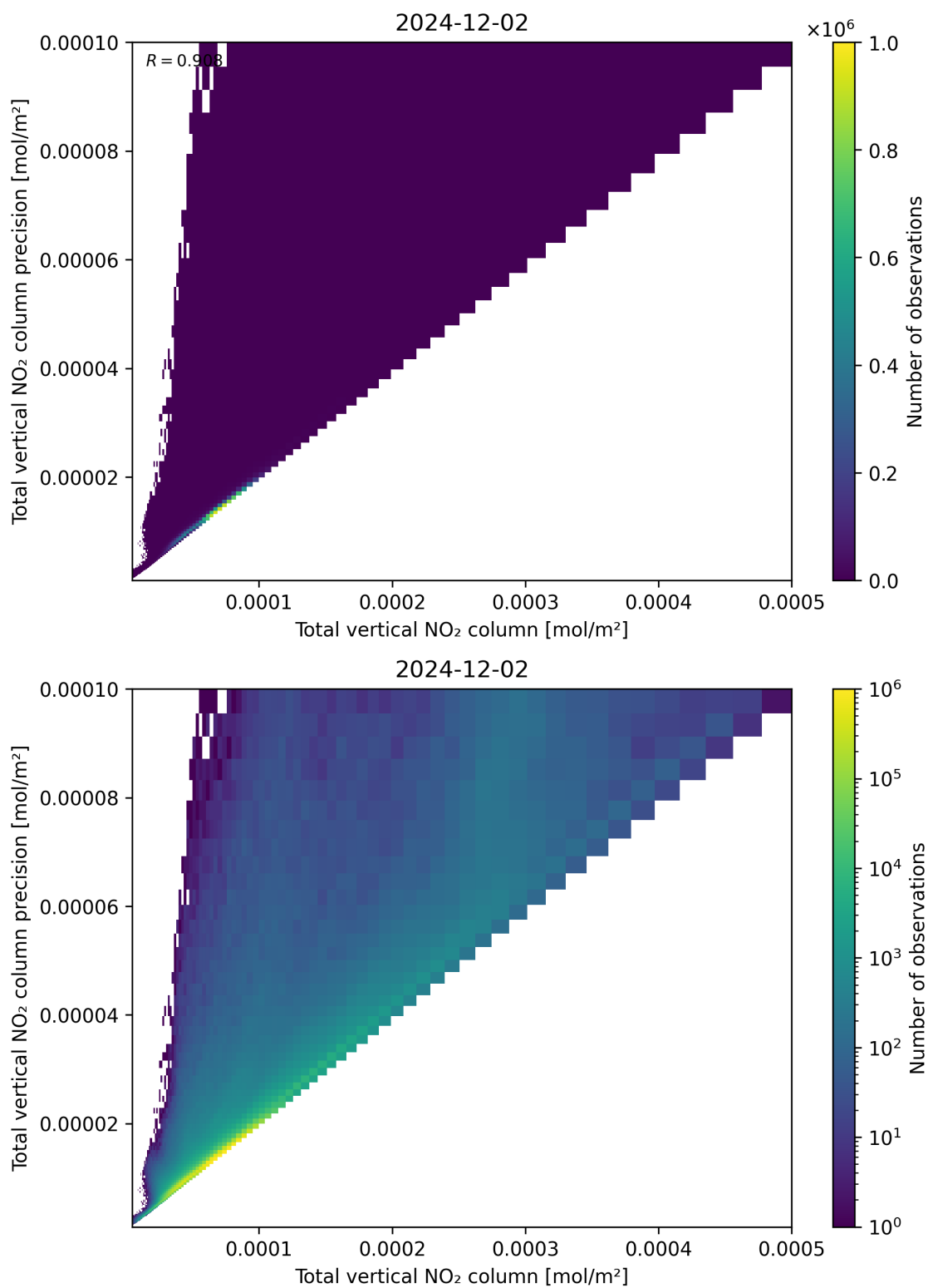
Figure 114: Scatter density plot of “Total vertical NO 2 column” against “Total vertical NO 2 column precision” for 2024-12-01 to 2024-12-03.
