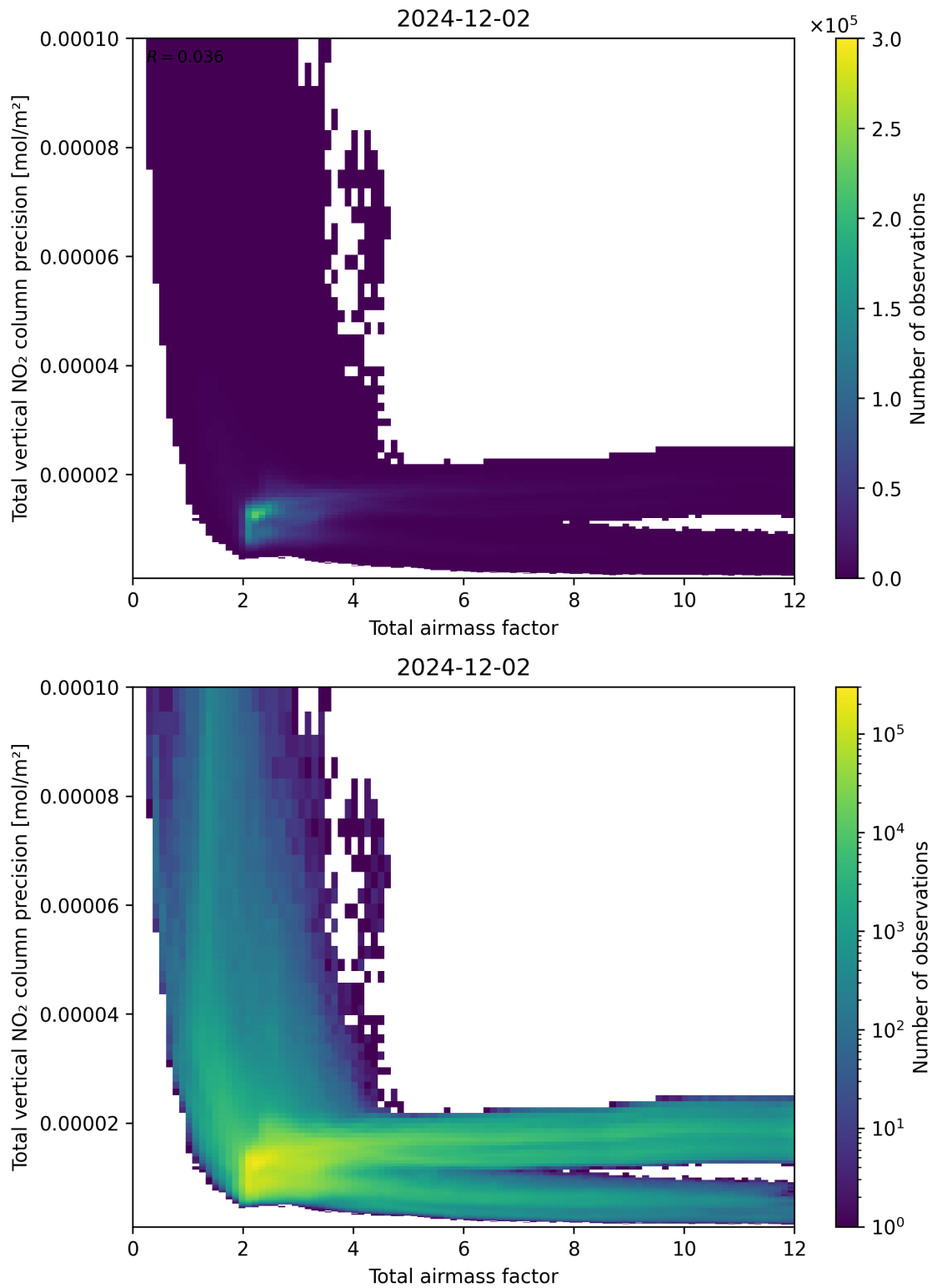
Figure 68: Scatter density plot of “Total airmass factor” against “Total vertical NO 2 column precision” for 2024-12-01 to 2024-12-03.
