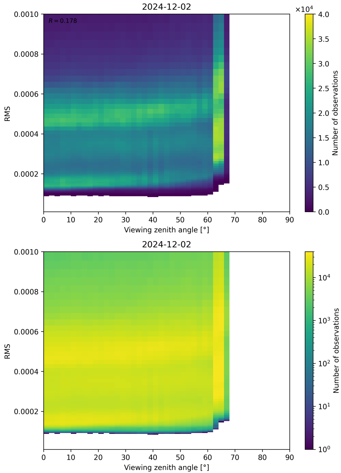
Figure 171: Scatter density plot of “Viewing zenith angle” against “RMS” for 2024-12-01 to 2024-12-03.
