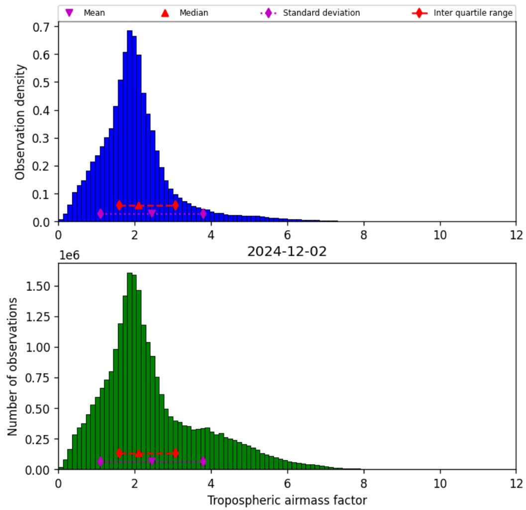
Figure 31: Histogram of “Tropospheric airmass factor” for 2024-12-01 to 2024-12-03
