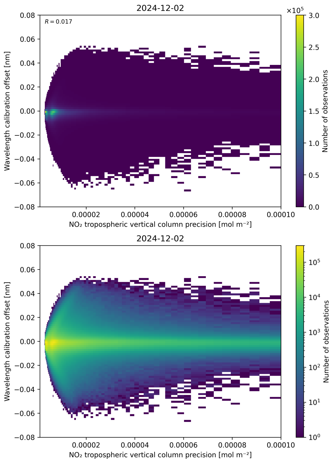
Figure 141: Scatter density plot of “NO 2 tropospheric vertical column precision” against “Wavelength calibration offset” for 2024-12-01 to 2024-12-03.
