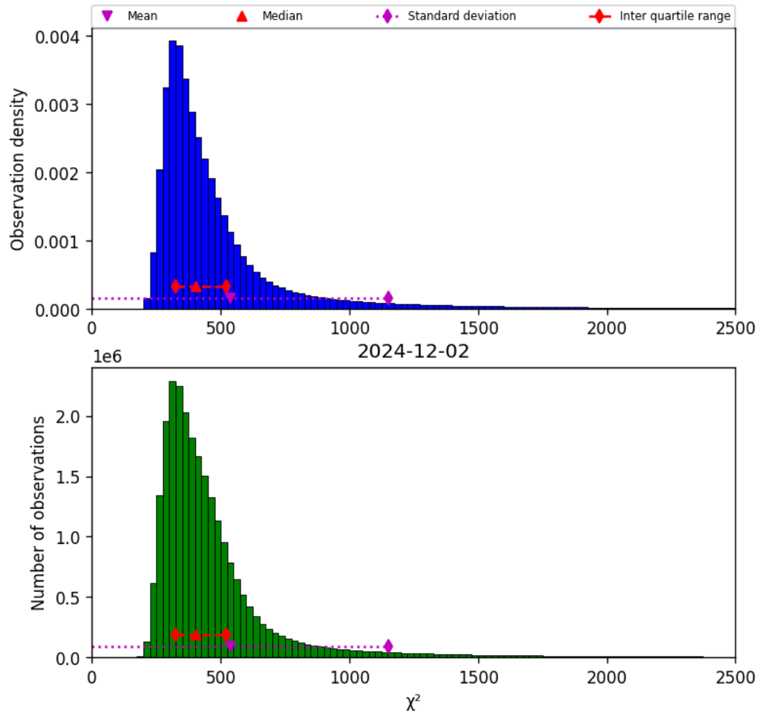
Figure 42: Histogram of “ \chi^2 ” for 2024-12-01 to 2024-12-03
