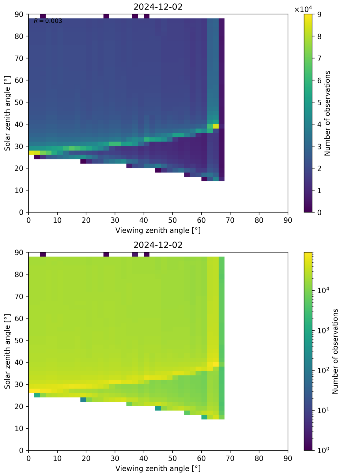
Figure 172: Scatter density plot of “Viewing zenith angle” against “Solar zenith angle” for 2024-12-01 to 2024-12-03.
