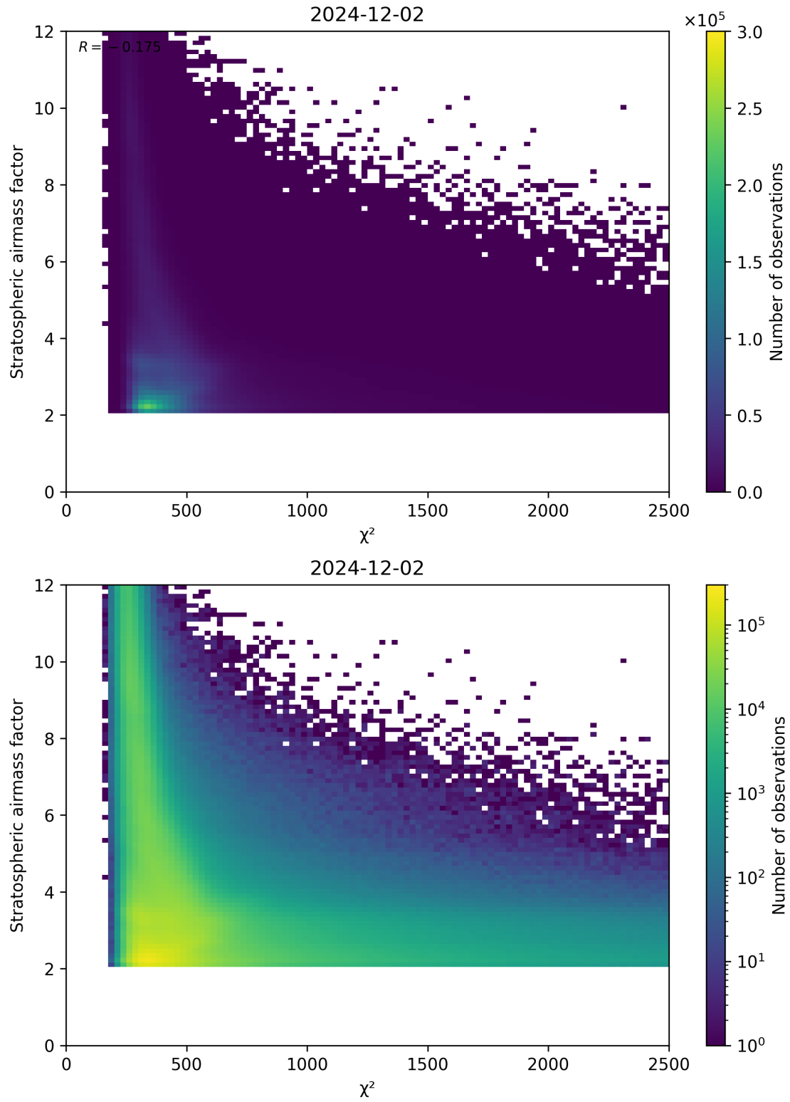
Figure 81: Scatter density plot of “ \chi^2 ” against “Stratospheric airmass factor” for 2024-12-01 to 2024-12-03.
