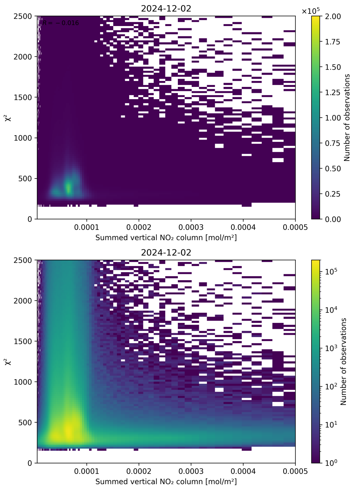
Figure 104: Scatter density plot of “Summed vertical NO 2 column” against “ \chi^2 ” for 2024-12-01 to 2024-12-03.
