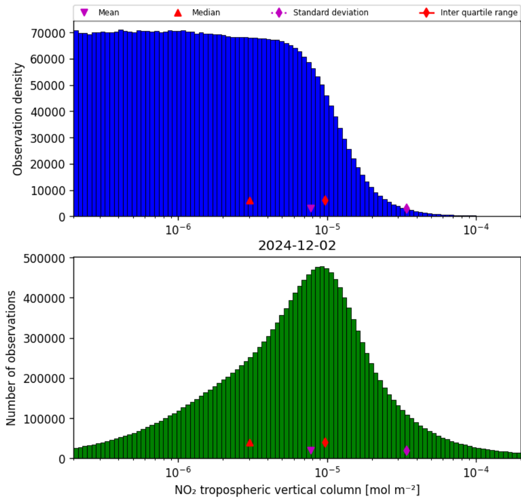
Figure 29: Histogram of “NO 2 tropospheric vertical column” for 2024-12-01 to 2024-12-03
