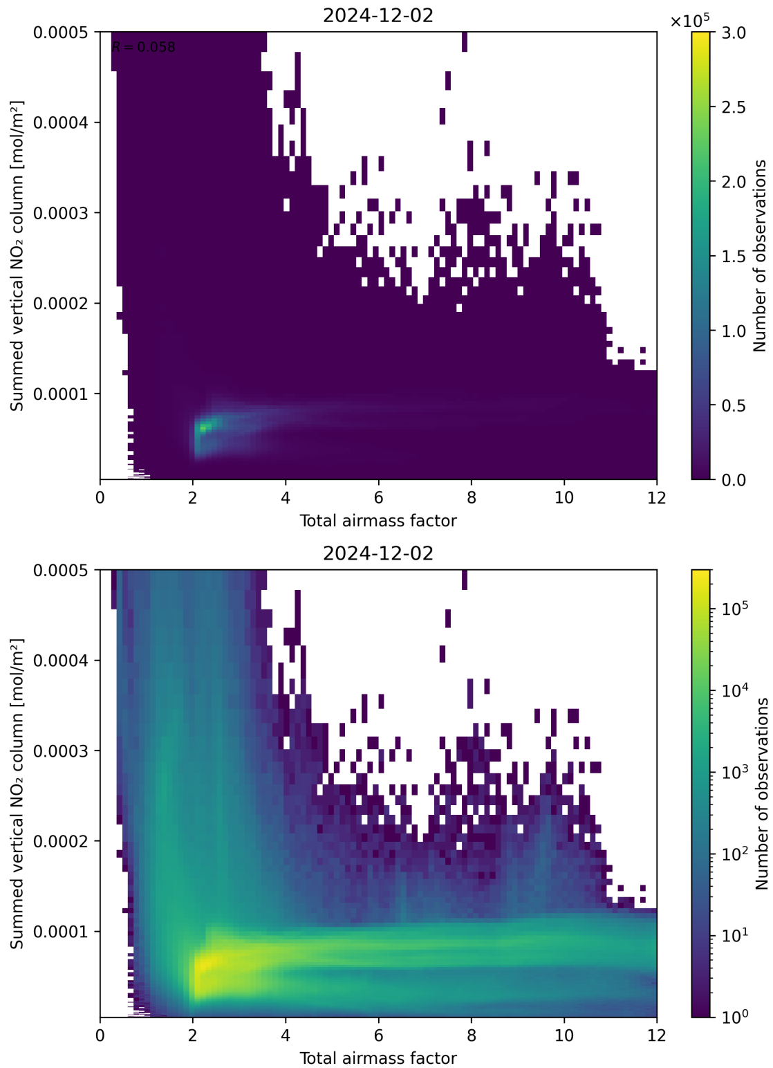
Figure 65: Scatter density plot of “Total airmass factor” against “Summed vertical NO 2 column” for 2024-12-01 to 2024-12-03.
