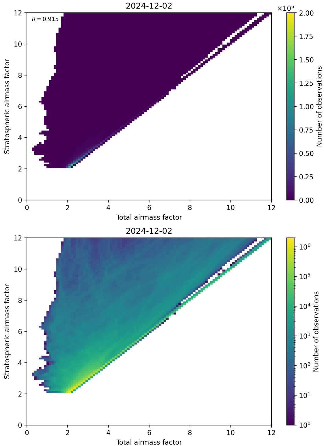
Figure 62: Scatter density plot of “Total airmass factor” against “Stratospheric airmass factor” for 2024-12-01 to 2024-12-03.
