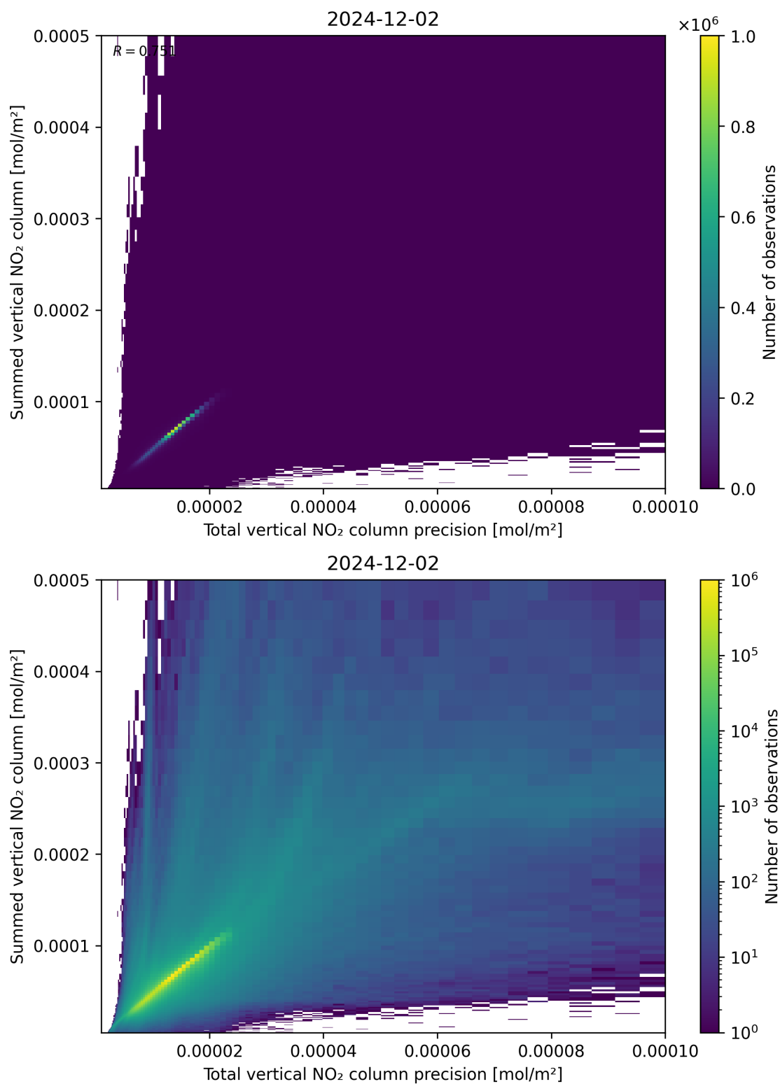
Figure 117: Scatter density plot of “Total vertical NO 2 column precision” against “Summed vertical NO 2 column” for 2024-12-01 to 2024-12-03.
