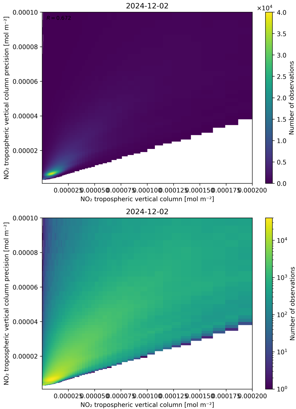
Figure 130: Scatter density plot of “NO 2 tropospheric vertical column” against “NO 2 tropospheric vertical column precision” for 2024-12-01 to 2024-12-03.
