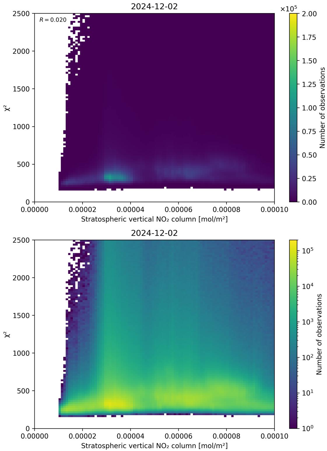
Figure 97: Scatter density plot of “Stratospheric vertical NO 2 column” against “ \chi^2 ” for 2024-12-01 to 2024-12-03.
