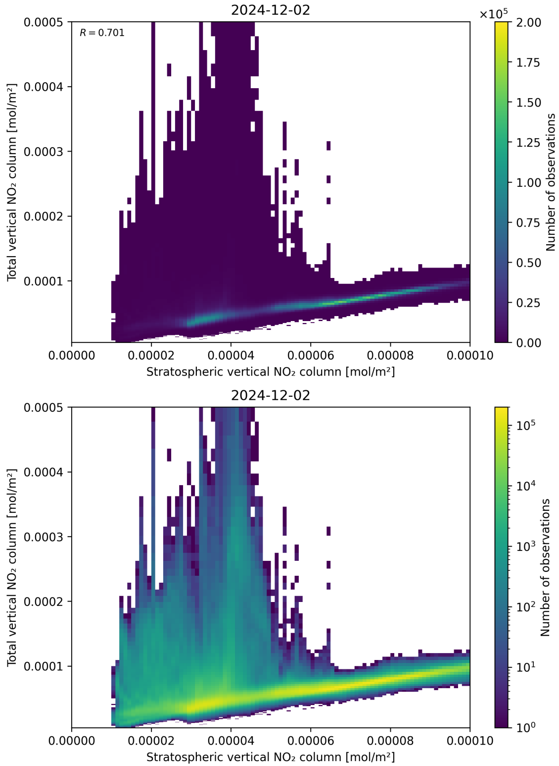
Figure 100: Scatter density plot of “Stratospheric vertical NO 2 column” against “Total vertical NO 2 column” for 2024-12-01 to 2024-12-03.
