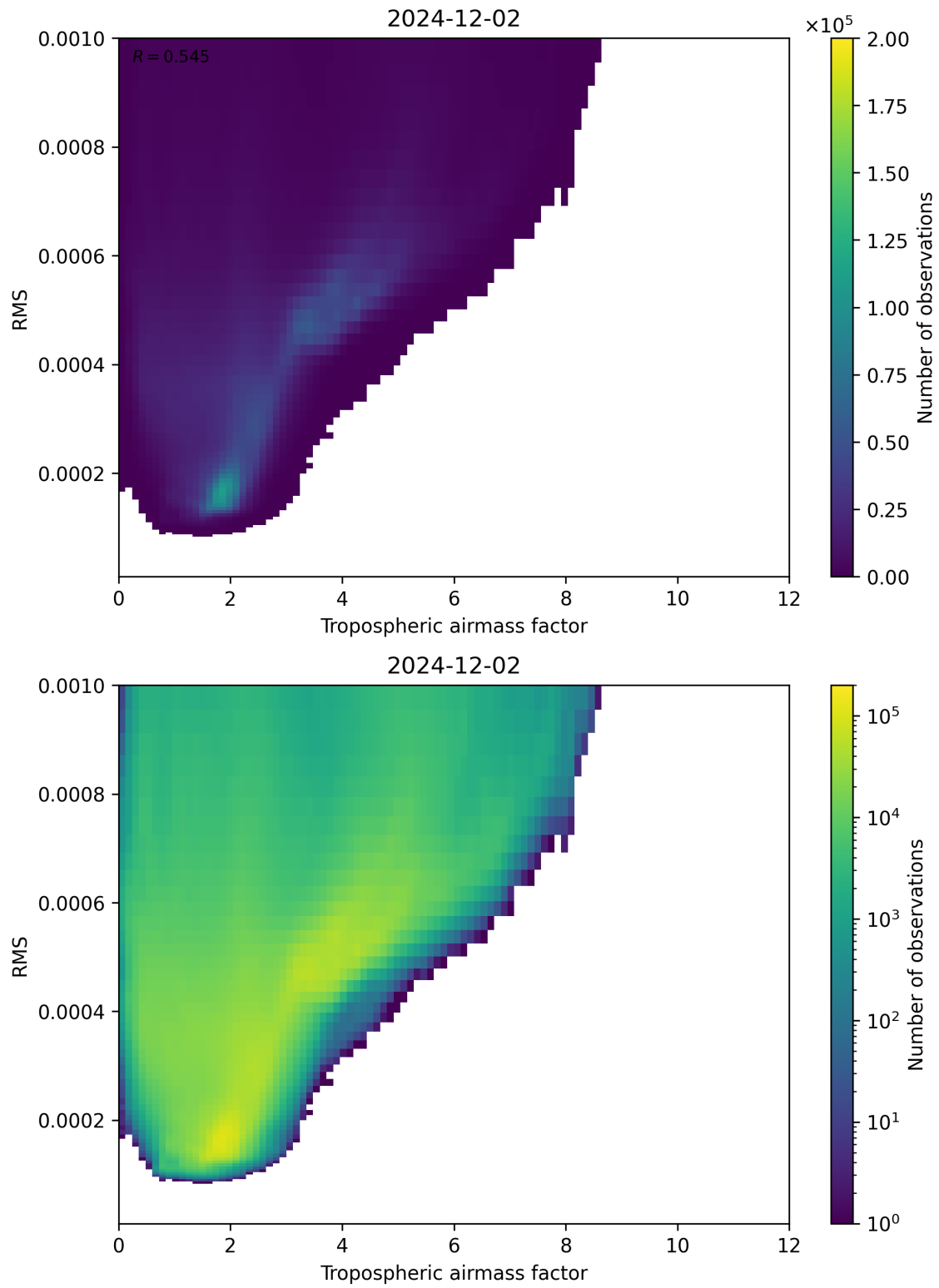
Figure 79: Scatter density plot of “Tropospheric airmass factor” against “RMS” for 2024-12-01 to 2024-12-03.
