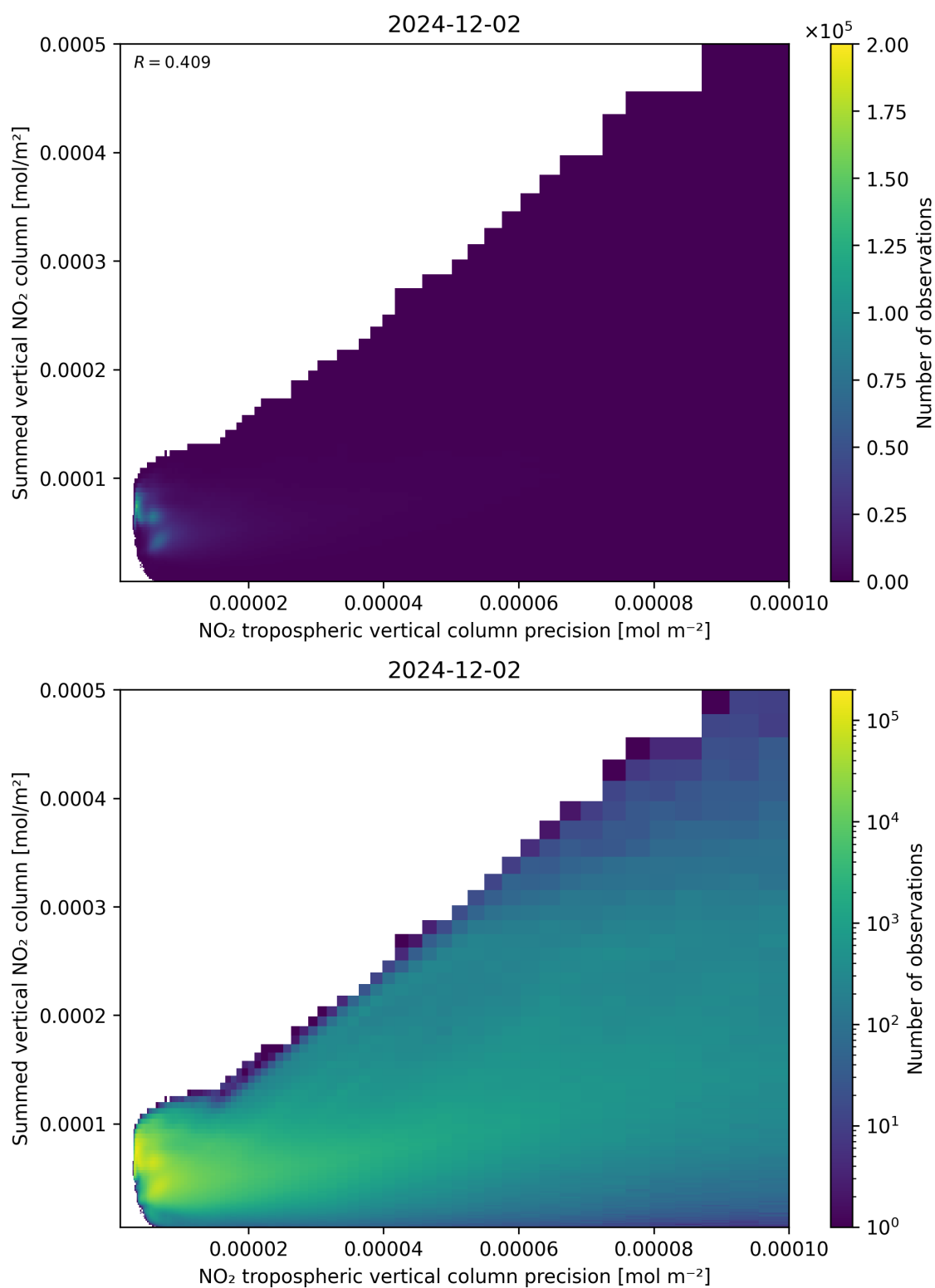
Figure 136: Scatter density plot of “NO 2 tropospheric vertical column precision” against “Summed vertical NO 2 column” for 2024-12-01 to 2024-12-03.
