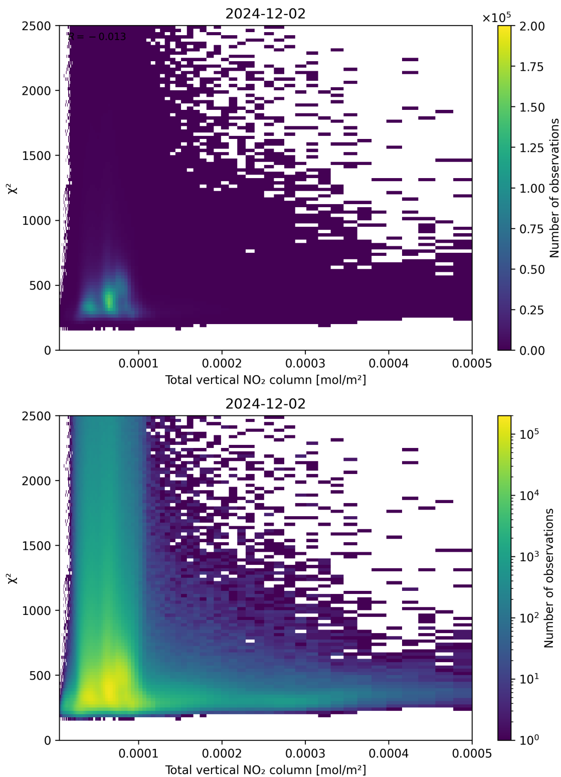
Figure 111: Scatter density plot of “Total vertical NO 2 column” against “ \chi^2 ” for 2024-12-01 to 2024-12-03.
