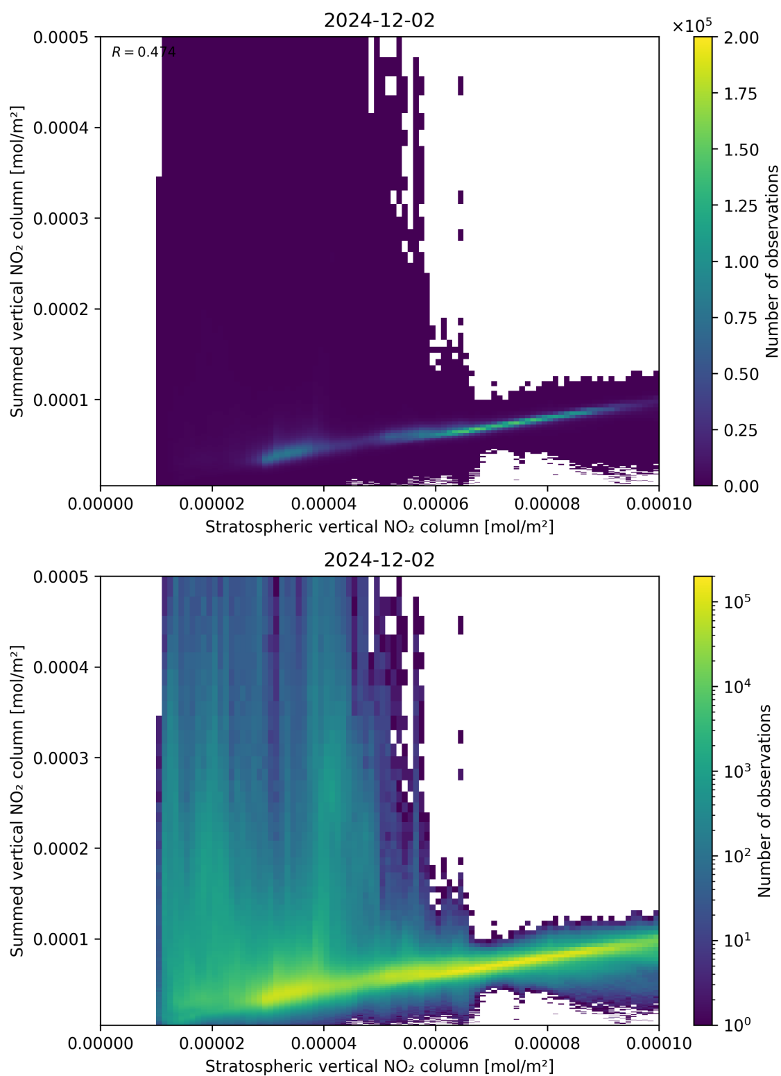
Figure 98: Scatter density plot of “Stratospheric vertical NO 2 column” against “Summed vertical NO 2 column” for 2024-12-01 to 2024-12-03.
