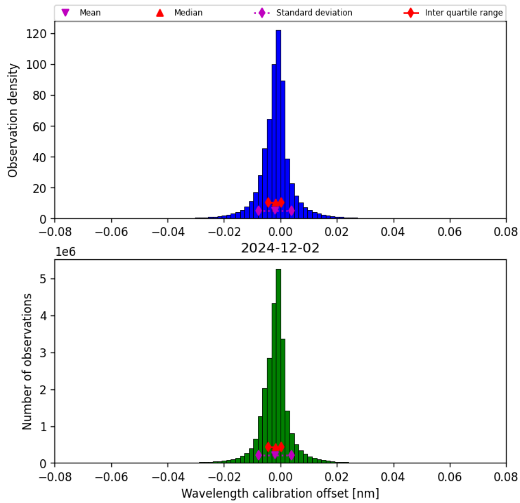
Figure 35: Histogram of “Wavelength calibration offset” for 2024-12-01 to 2024-12-03
