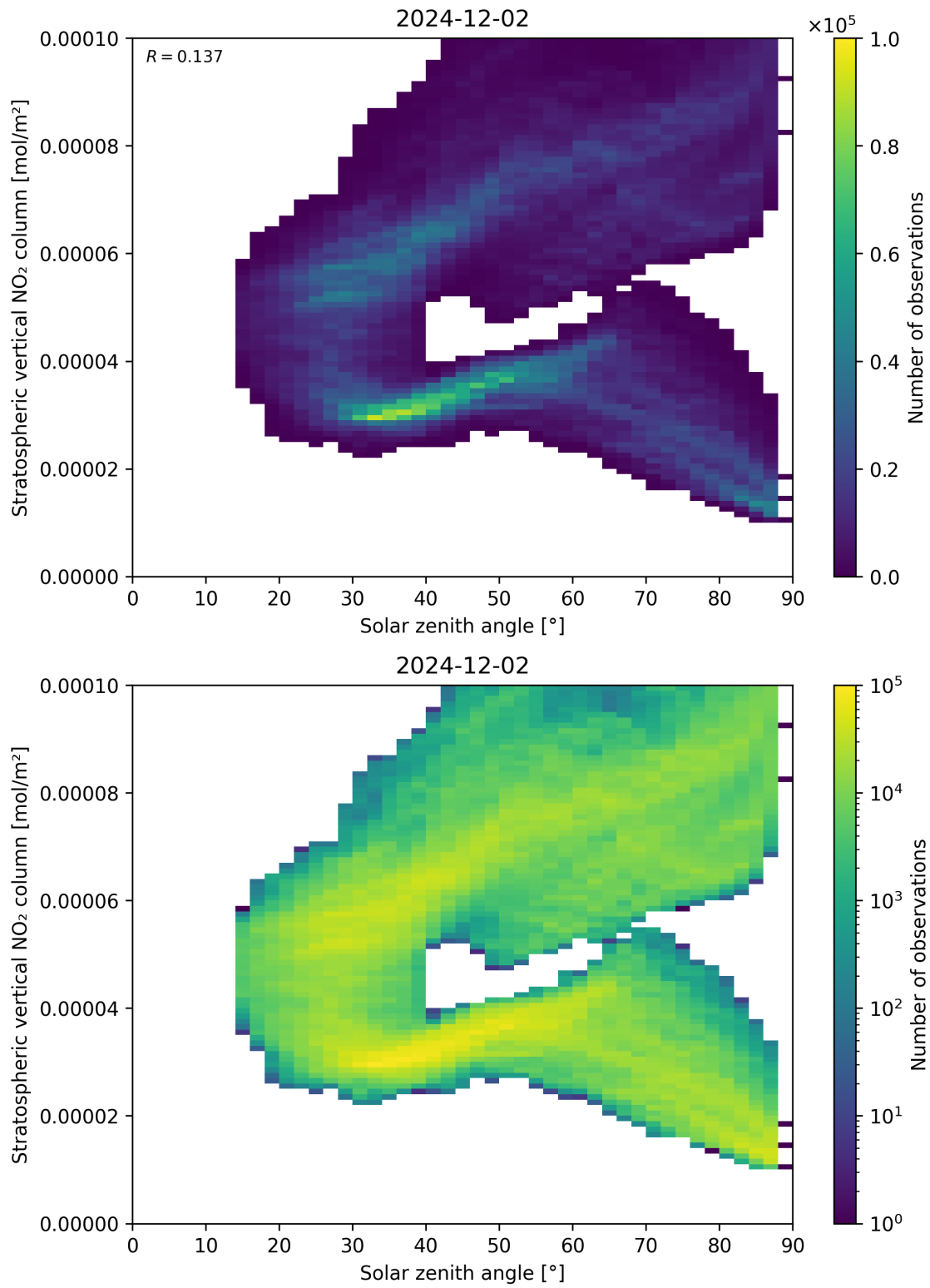
Figure 150: Scatter density plot of “Solar zenith angle” against “Stratospheric vertical NO 2 column” for 2024-12-01 to 2024-12-03.
