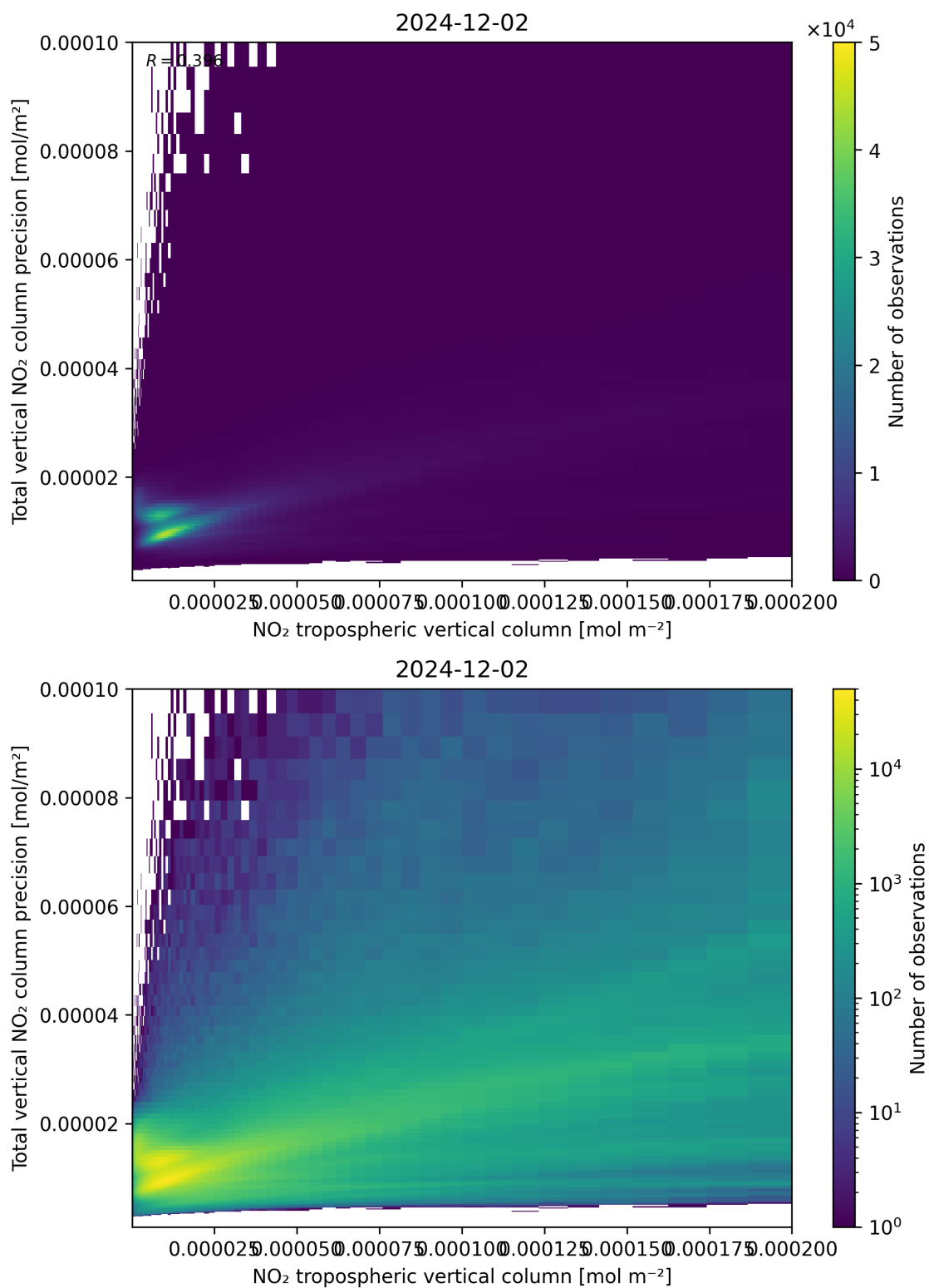
Figure 129: Scatter density plot of “NO 2 tropospheric vertical column” against “Total vertical NO 2 column precision” for 2024-12-01 to 2024-12-03.
