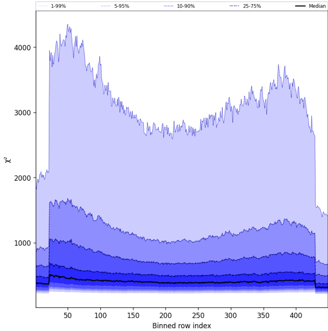
Figure 59: Along track statistics of “ \chi^2 ” for 2024-12-01 to 2024-12-03
