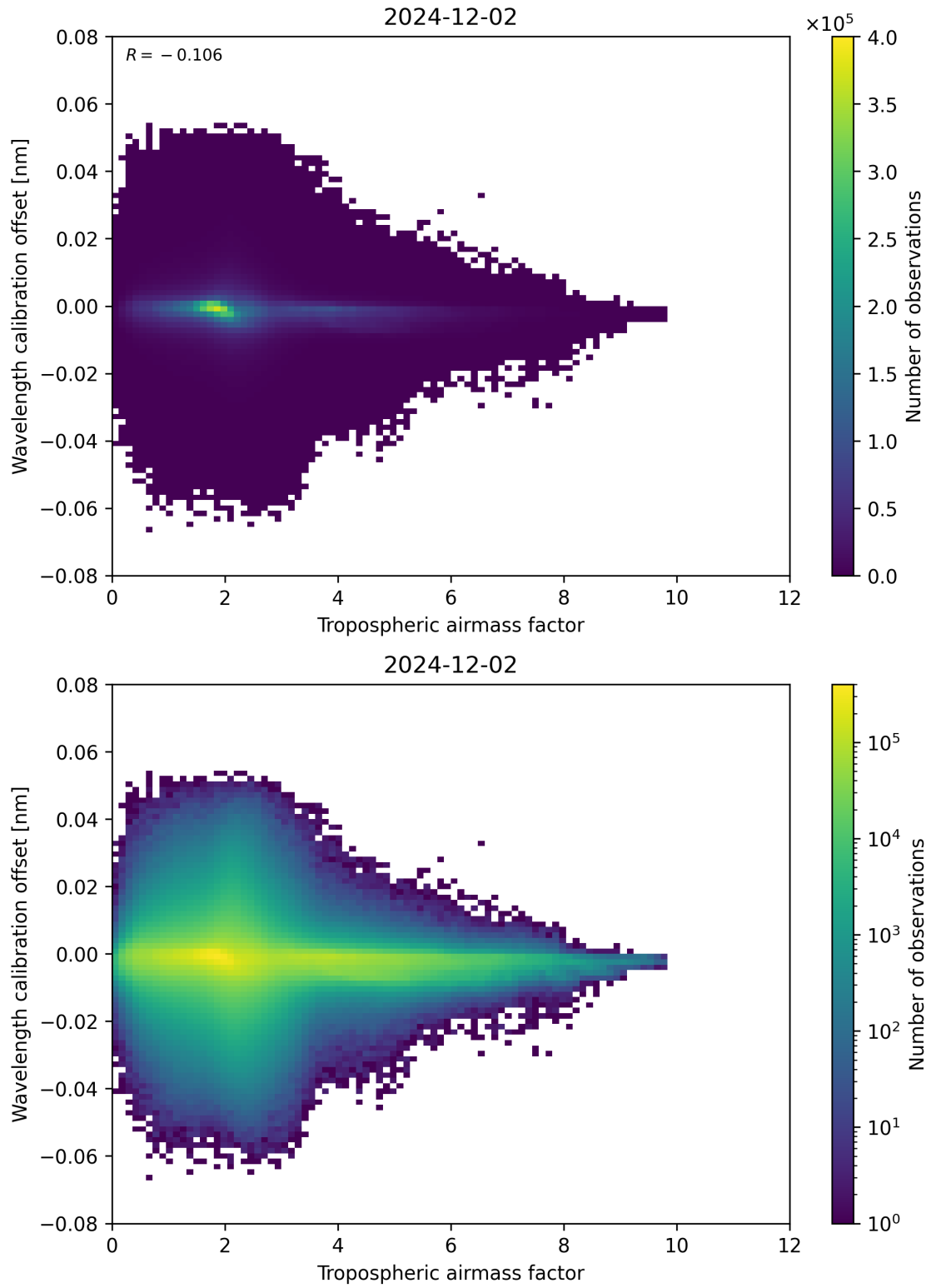
Figure 80: Scatter density plot of “Tropospheric airmass factor” against “Wavelength calibration offset” for 2024-12-01 to 2024-12-03.
