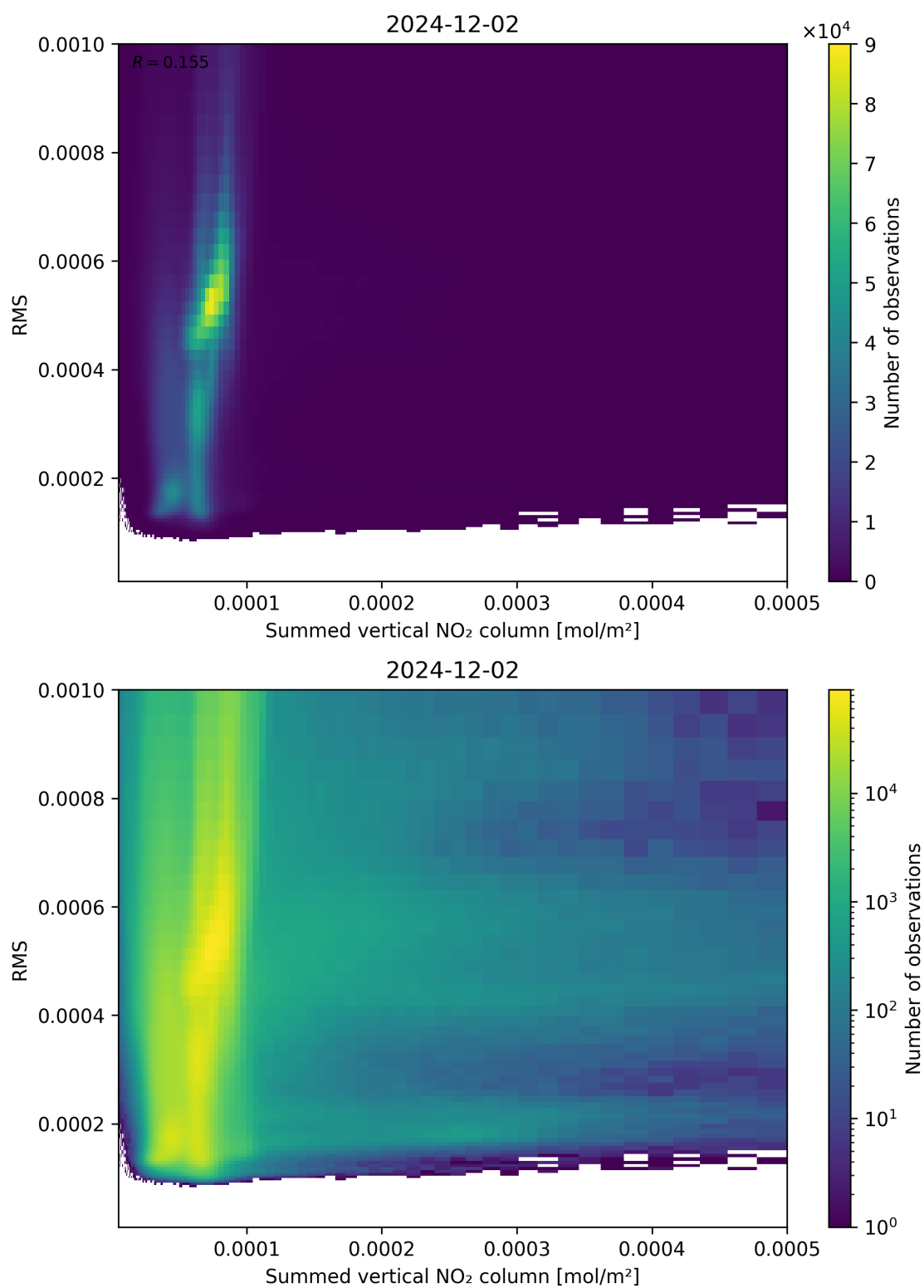
Figure 109: Scatter density plot of “Summed vertical NO 2 column” against “RMS” for 2024-12-01 to 2024-12-03.
