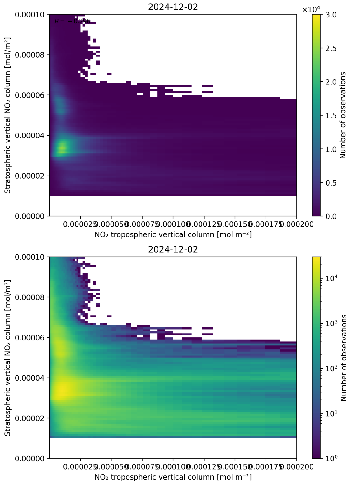
Figure 125: Scatter density plot of “NO 2 tropospheric vertical column” against “Stratospheric vertical NO 2 column” for 2024-12-01 to 2024-12-03.
