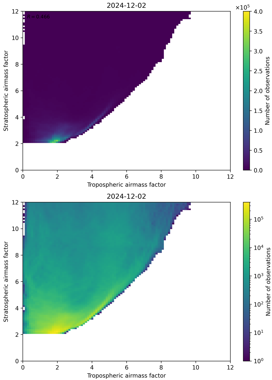
Figure 71: Scatter density plot of “Tropospheric airmass factor” against “Stratospheric airmass factor” for 2024-12-01 to 2024-12-03.
