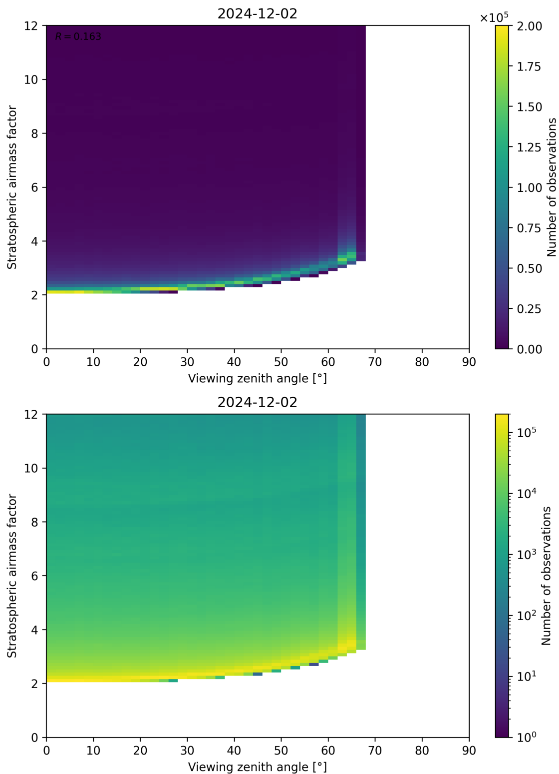
Figure 159: Scatter density plot of “Viewing zenith angle” against “Stratospheric airmass factor” for 2024-12-01 to 2024-12-03.
