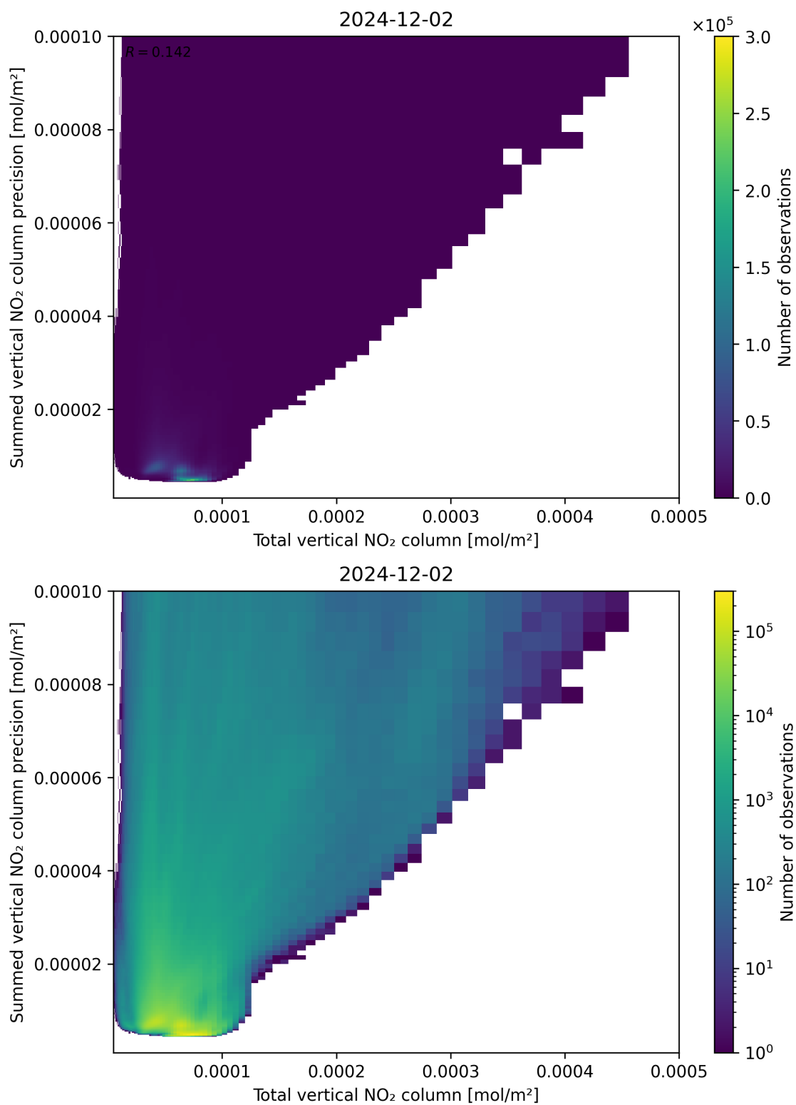
Figure 113: Scatter density plot of “Total vertical NO 2 column” against “Summed vertical NO 2 column precision” for 2024-12-01 to 2024-12-03.
