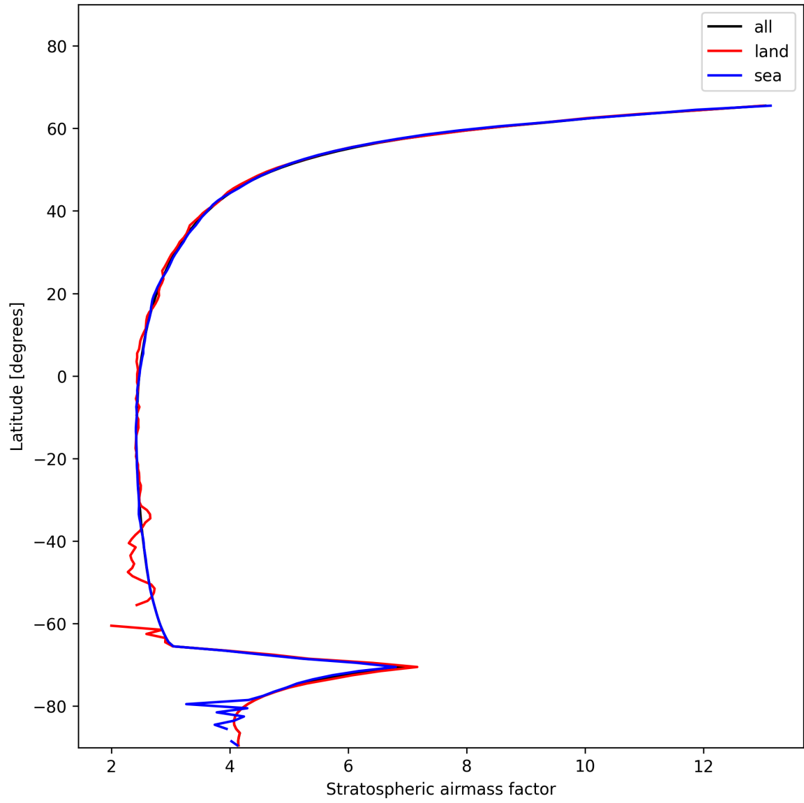
Figure 27: Zonal average of “Stratospheric airmass factor” for 2024-12-01 to 2024-12-03.
