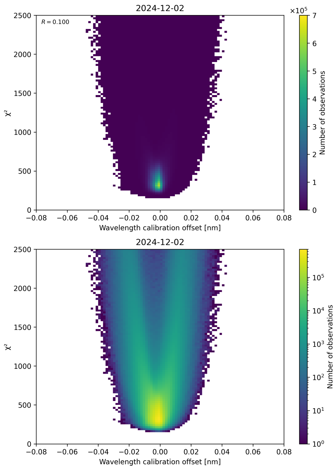
Figure 175: Scatter density plot of “Wavelength calibration offset” against “ \chi^2 ” for 2024-12-01 to 2024-12-03.
