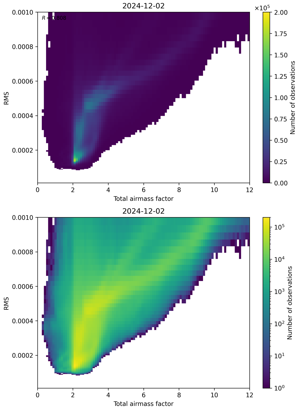
Figure 69: Scatter density plot of “Total airmass factor” against “RMS” for 2024-12-01 to 2024-12-03.
