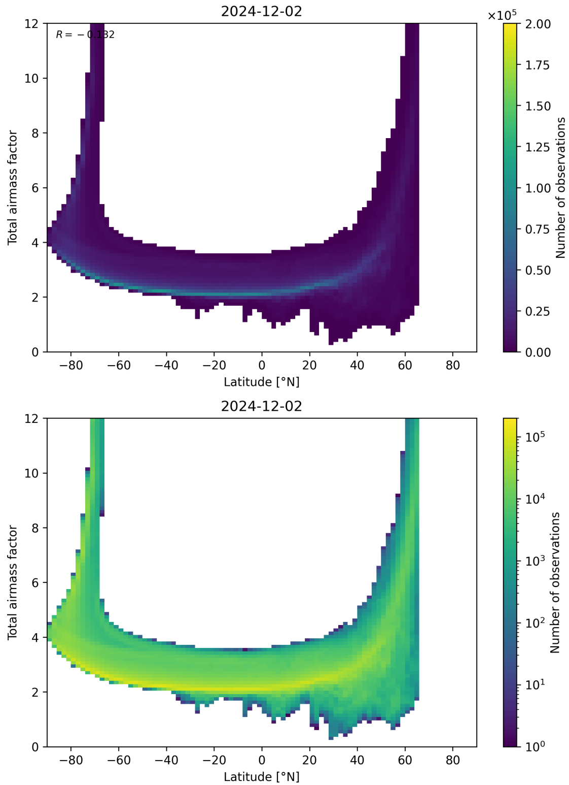
Figure 84: Scatter density plot of “Latitude” against “Total airmass factor” for 2024-12-01 to 2024-12-03.
