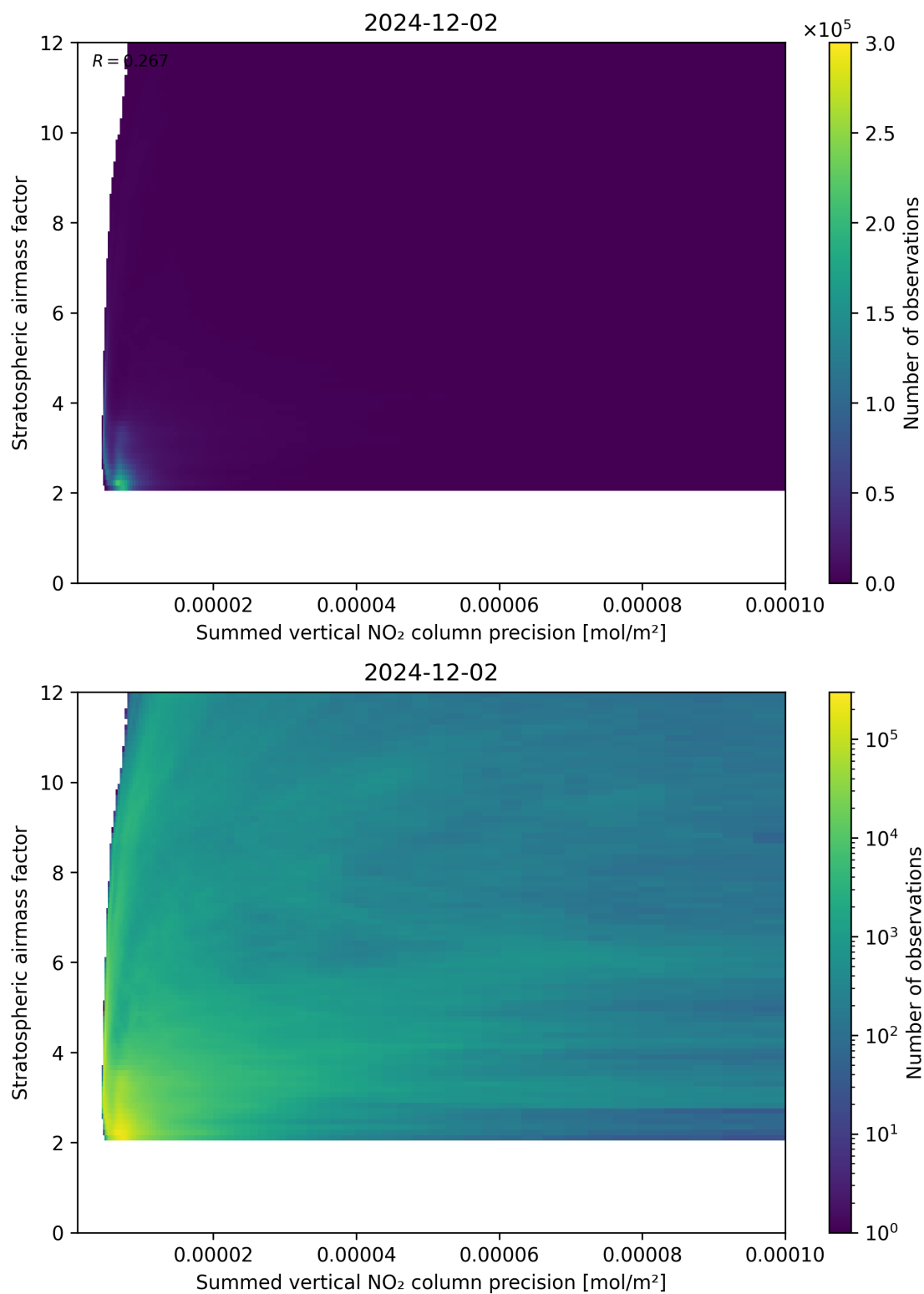
Figure 106: Scatter density plot of “Summed vertical NO 2 column precision” against “Stratospheric airmass factor” for 2024-12-01 to 2024-12-03.
