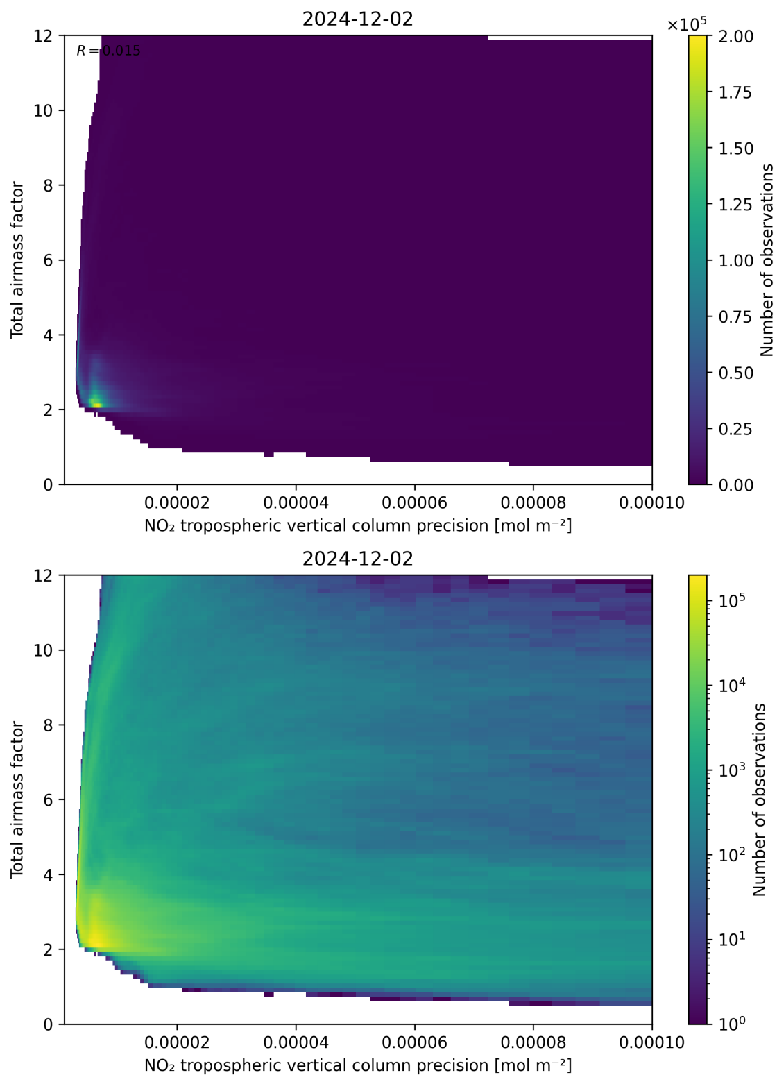
Figure 132: Scatter density plot of “NO 2 tropospheric vertical column precision” against “Total air mass factor” for 2024-12-01 to 2024-12-03.
