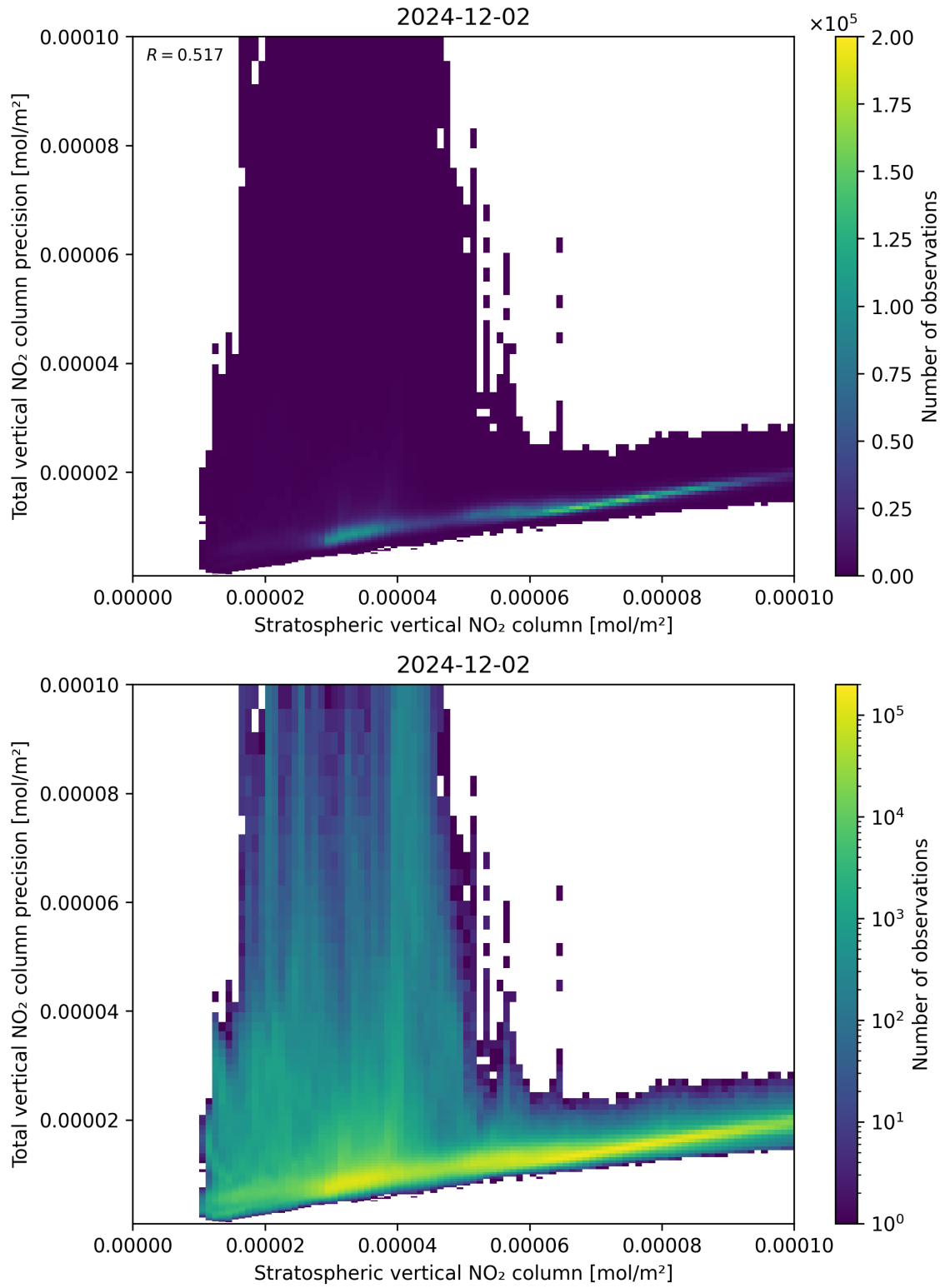
Figure 101: Scatter density plot of “Stratospheric vertical NO 2 column” against “Total vertical NO 2 column precision” for 2024-12-01 to 2024-12-03.
