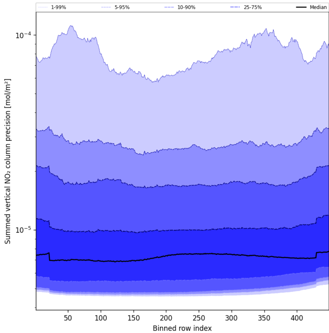
Figure 58: Along track statistics of “Summed vertical NO 2 column precision” for 2024-12-01 to 2024-12-03
