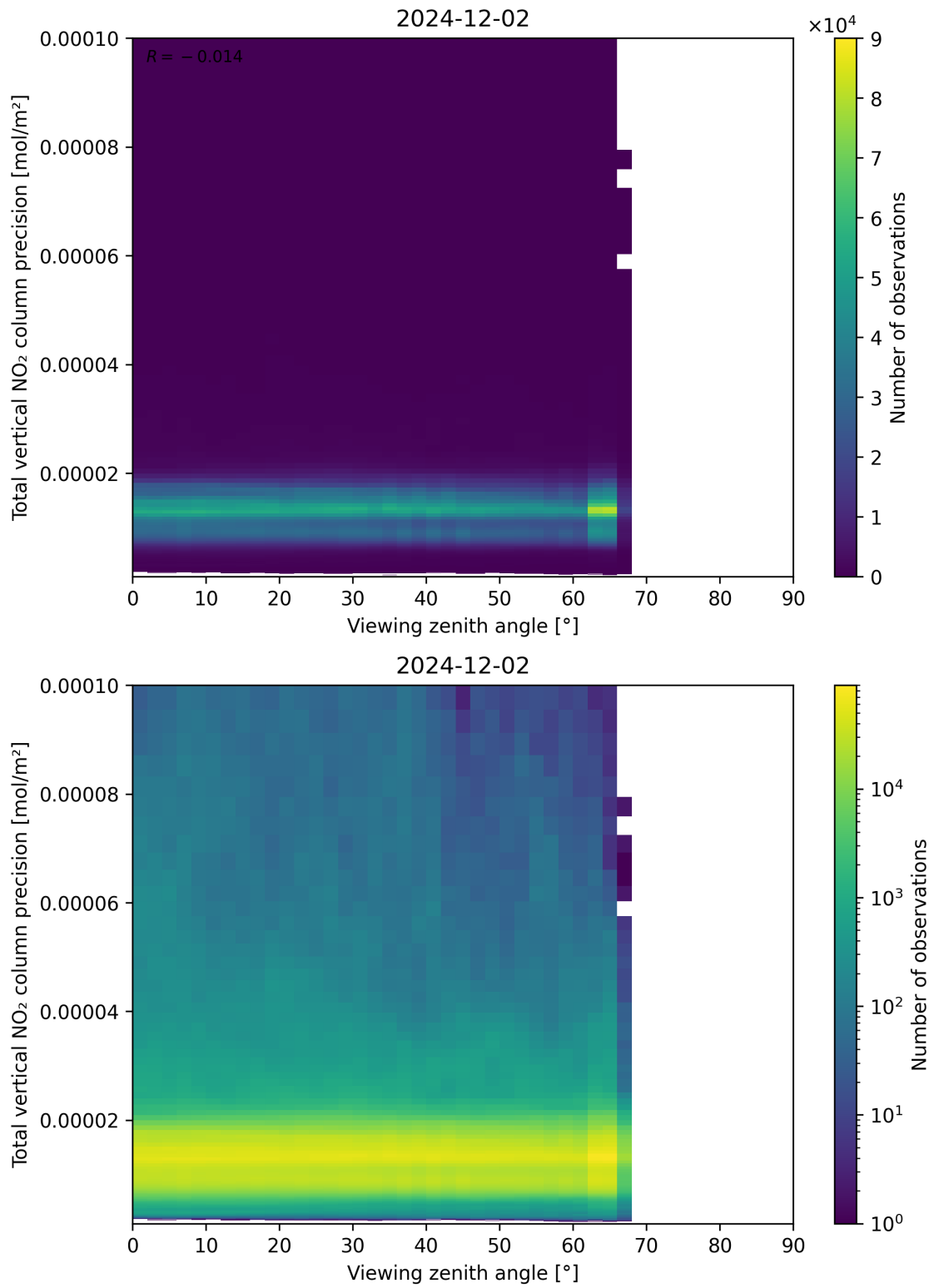
Figure 168: Scatter density plot of “Viewing zenith angle” against “Total vertical NO 2 column precision” for 2024-12-01 to 2024-12-03.
