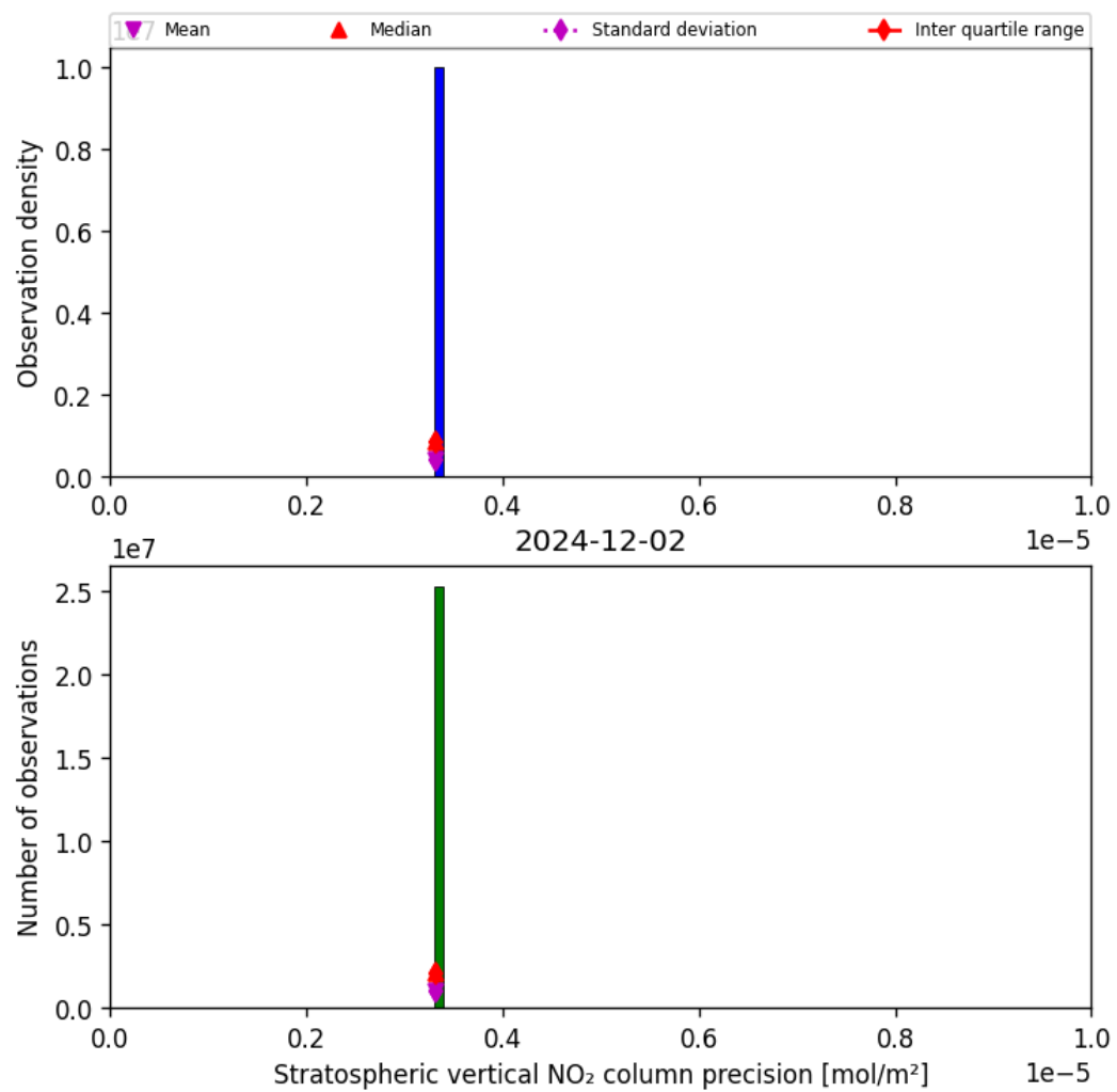
Figure 37: Histogram of “Stratospheric vertical NO 2 column precision” for 2024-12-01 to 2024-12-03
