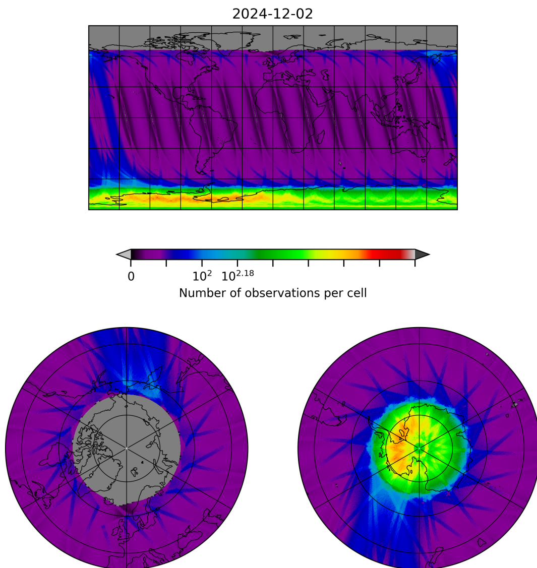
Figure 10: Map of the number of observations for 2024-12-01 to 2024-12-03
