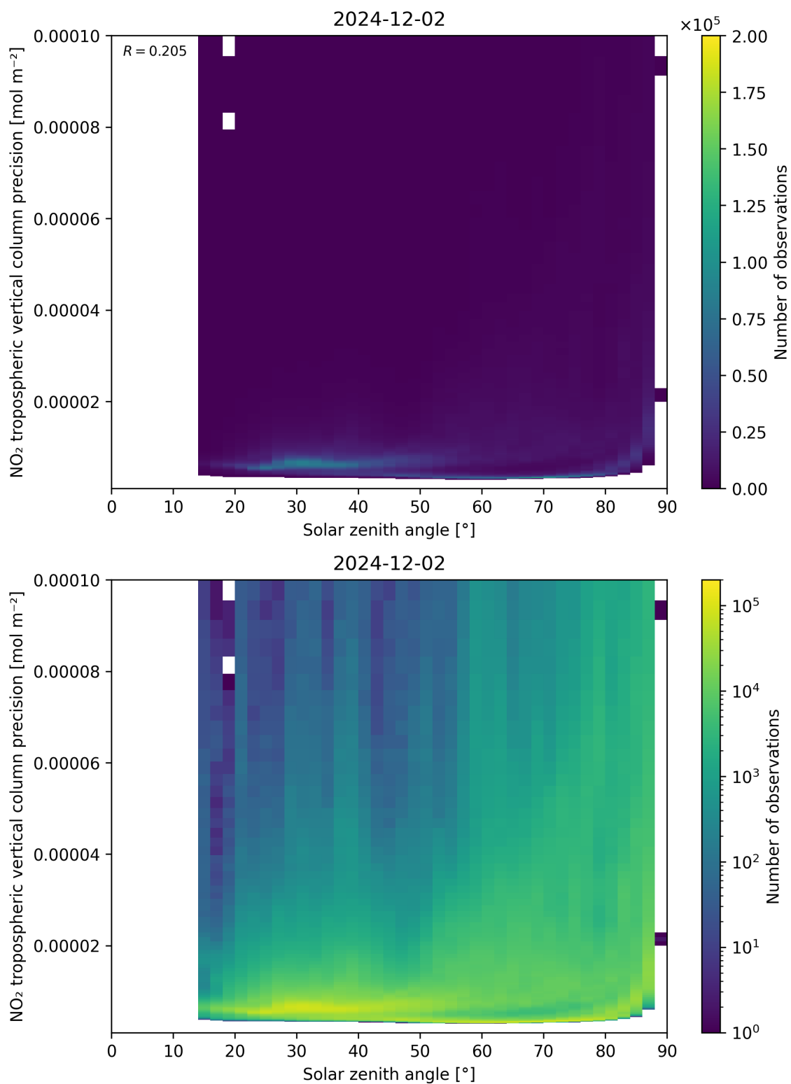
Figure 156: Scatter density plot of “Solar zenith angle” against “NO 2 tropospheric vertical column precision” for 2024-12-01 to 2024-12-03.
