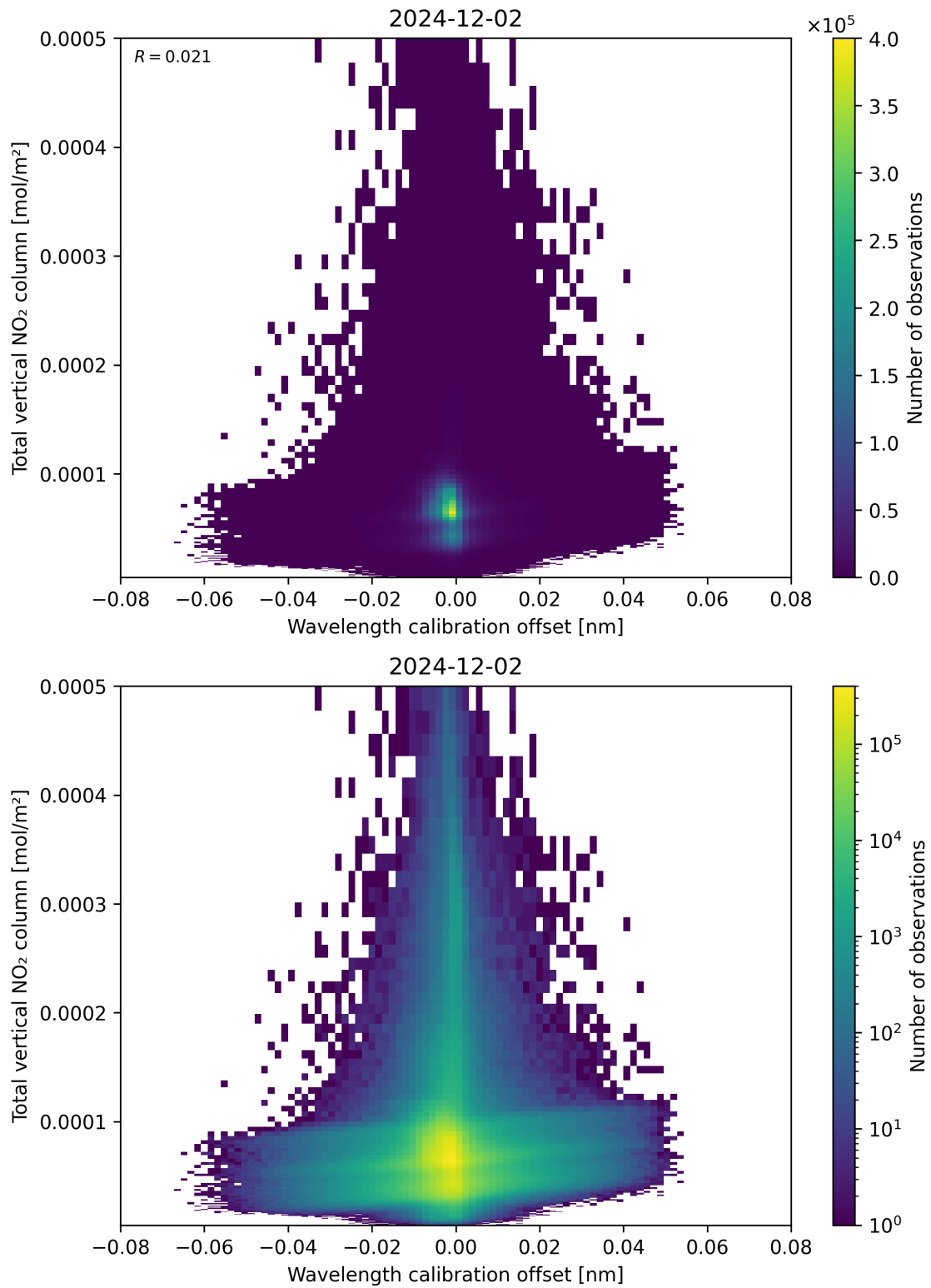
Figure 179: Scatter density plot of “Wavelength calibration offset” against “Total vertical NO 2 column” for 2024-12-01 to 2024-12-03.
