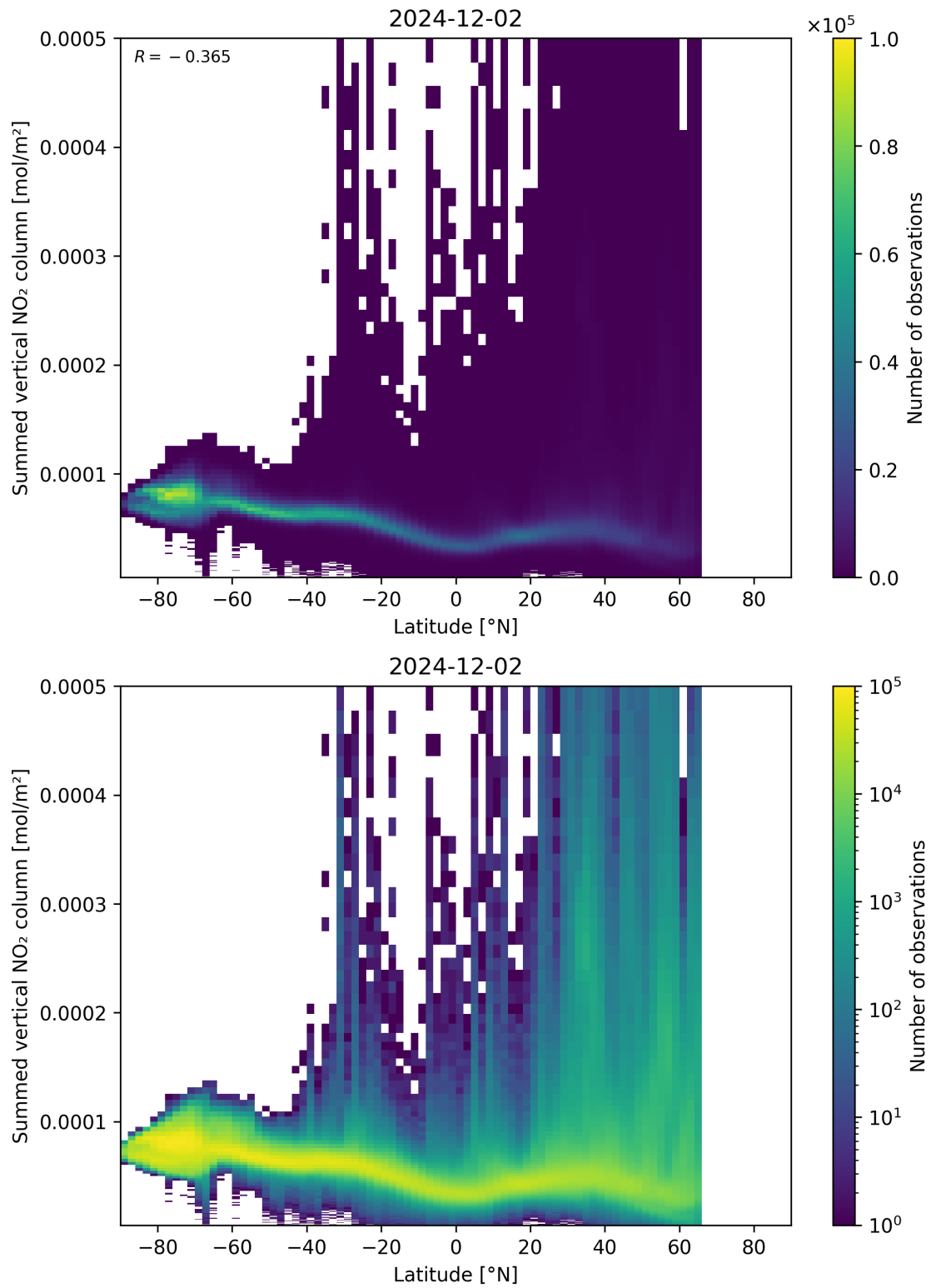
Figure 88: Scatter density plot of “Latitude” against “Summed vertical NO 2 column” for 2024-12-01 to 2024-12-03.
