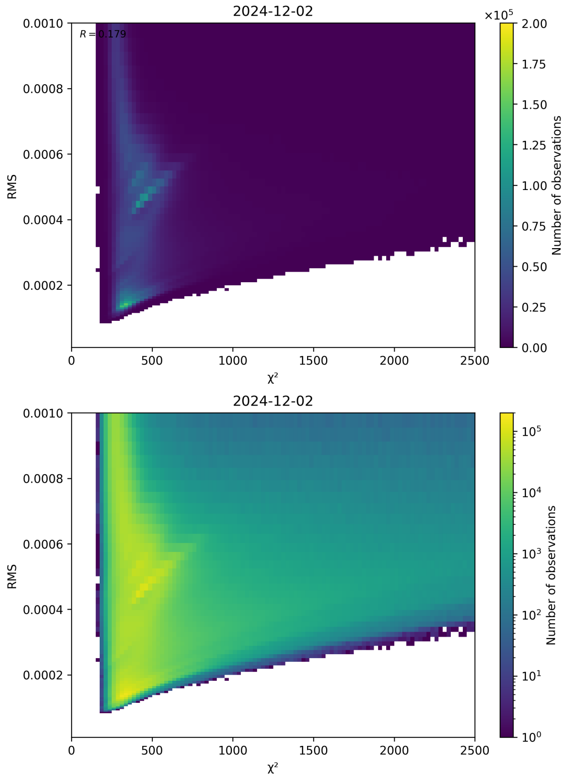
Figure 82: Scatter density plot of “ \chi^2 ” against “RMS” for 2024-12-01 to 2024-12-03.
