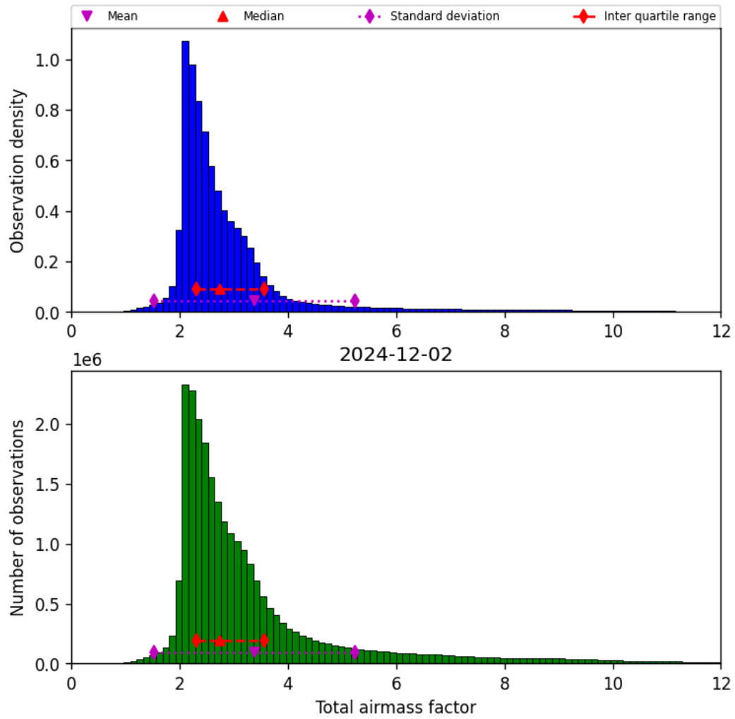
Figure 32: Histogram of “Total airmass factor” for 2024-12-01 to 2024-12-03
