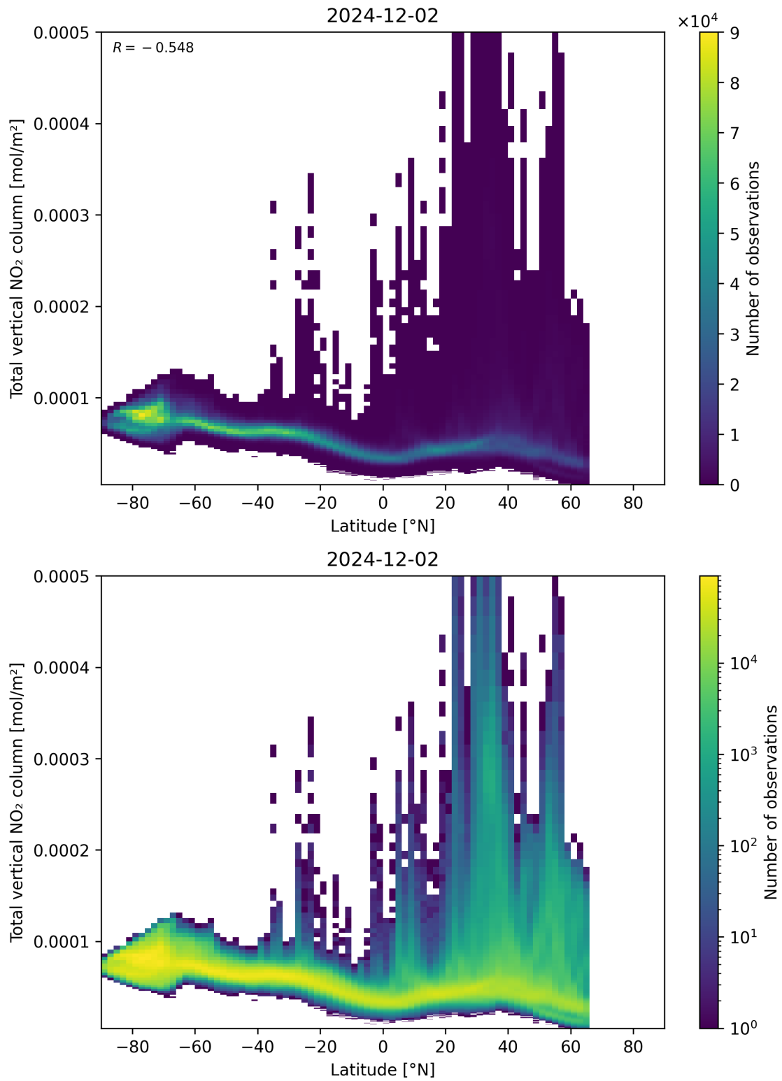
Figure 90: Scatter density plot of “Latitude” against “Total vertical NO 2 column” for 2024-12-01 to 2024-12-03.
