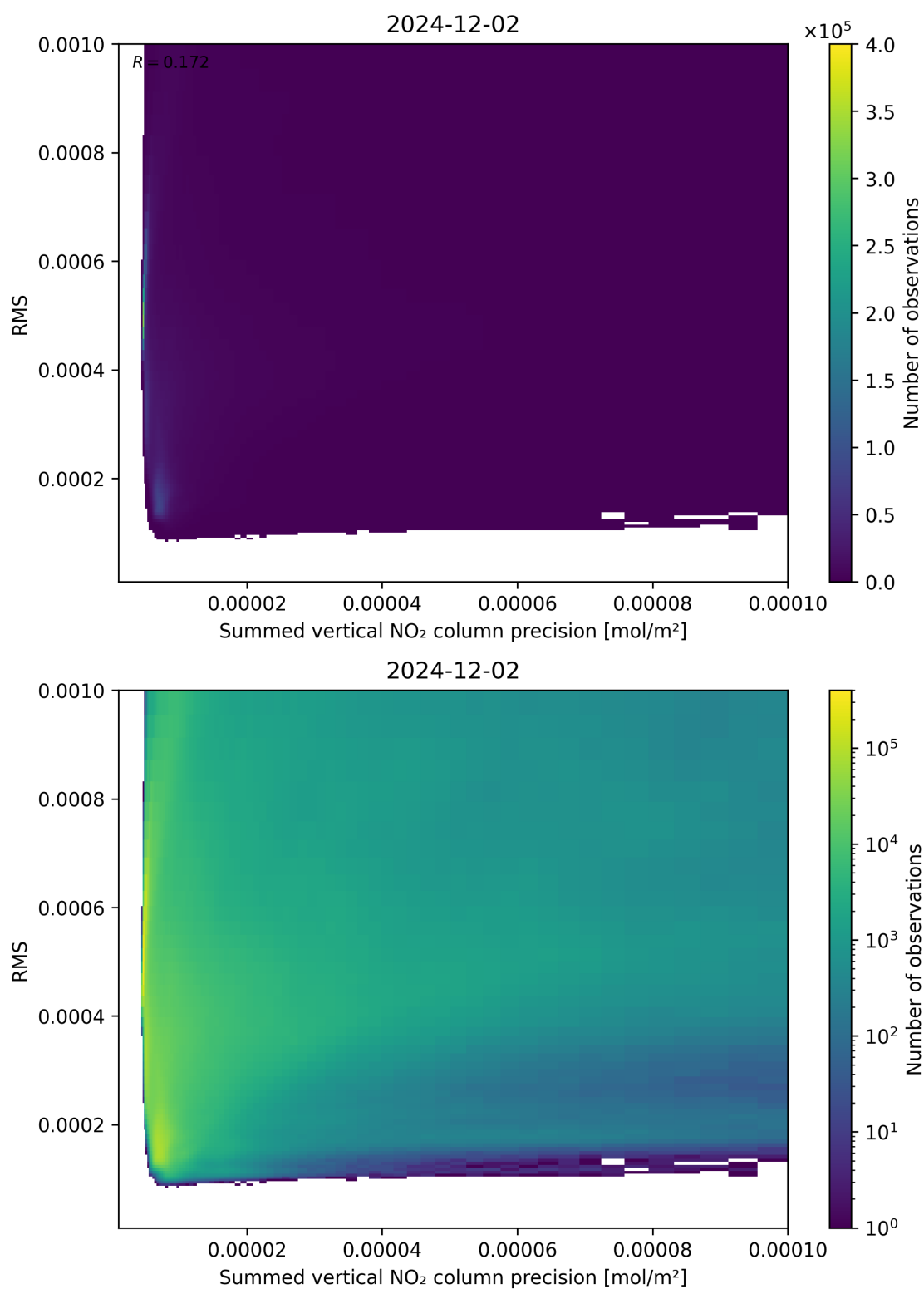
Figure 108: Scatter density plot of “Summed vertical NO 2 column precision” against “RMS” for 2024-12-01 to 2024-12-03.
