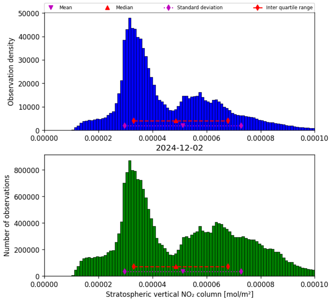
Figure 36: Histogram of “Stratospheric vertical NO 2 column” for 2024-12-01 to 2024-12-03
