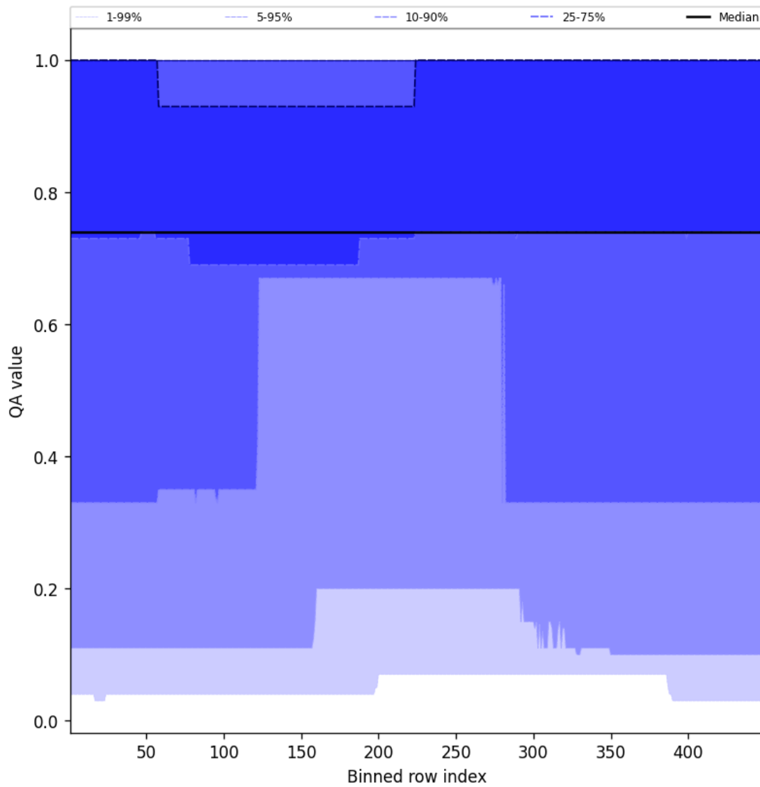
Figure 45: Along track statistics of “QA value” for 2024-12-01 to 2024-12-03
