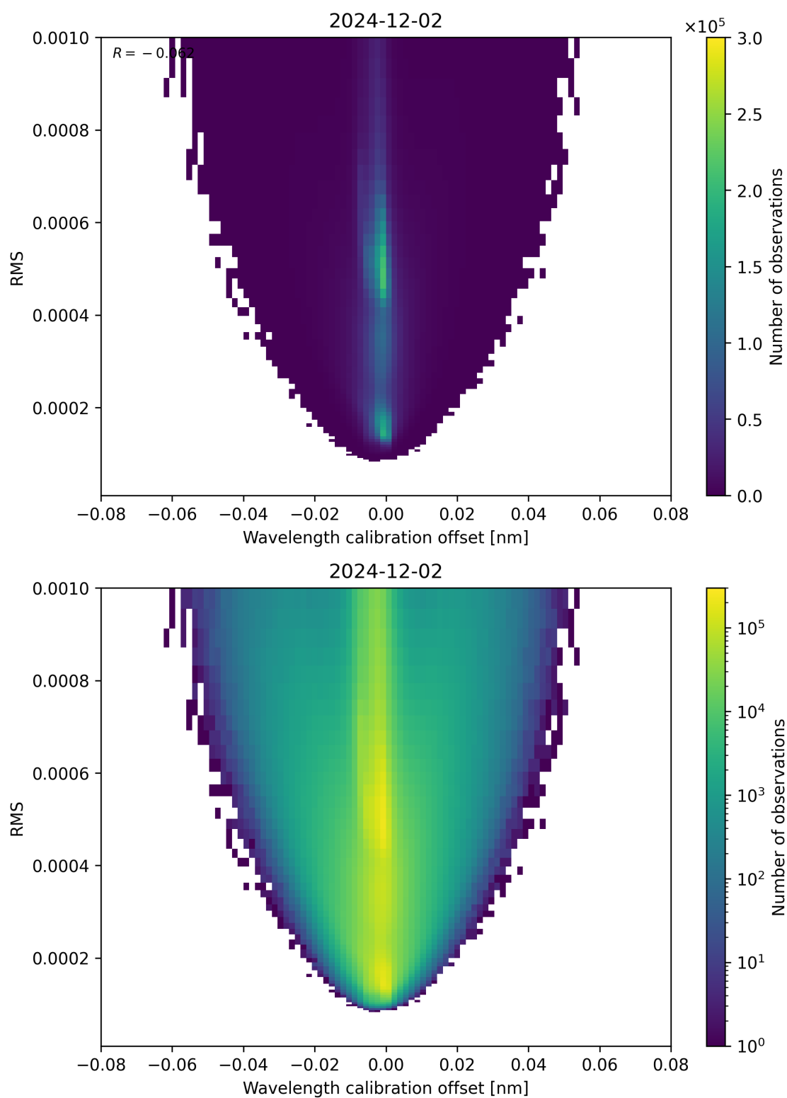
Figure 181: Scatter density plot of “Wavelength calibration offset” against “RMS” for 2024-12-01 to 2024-12-03.
