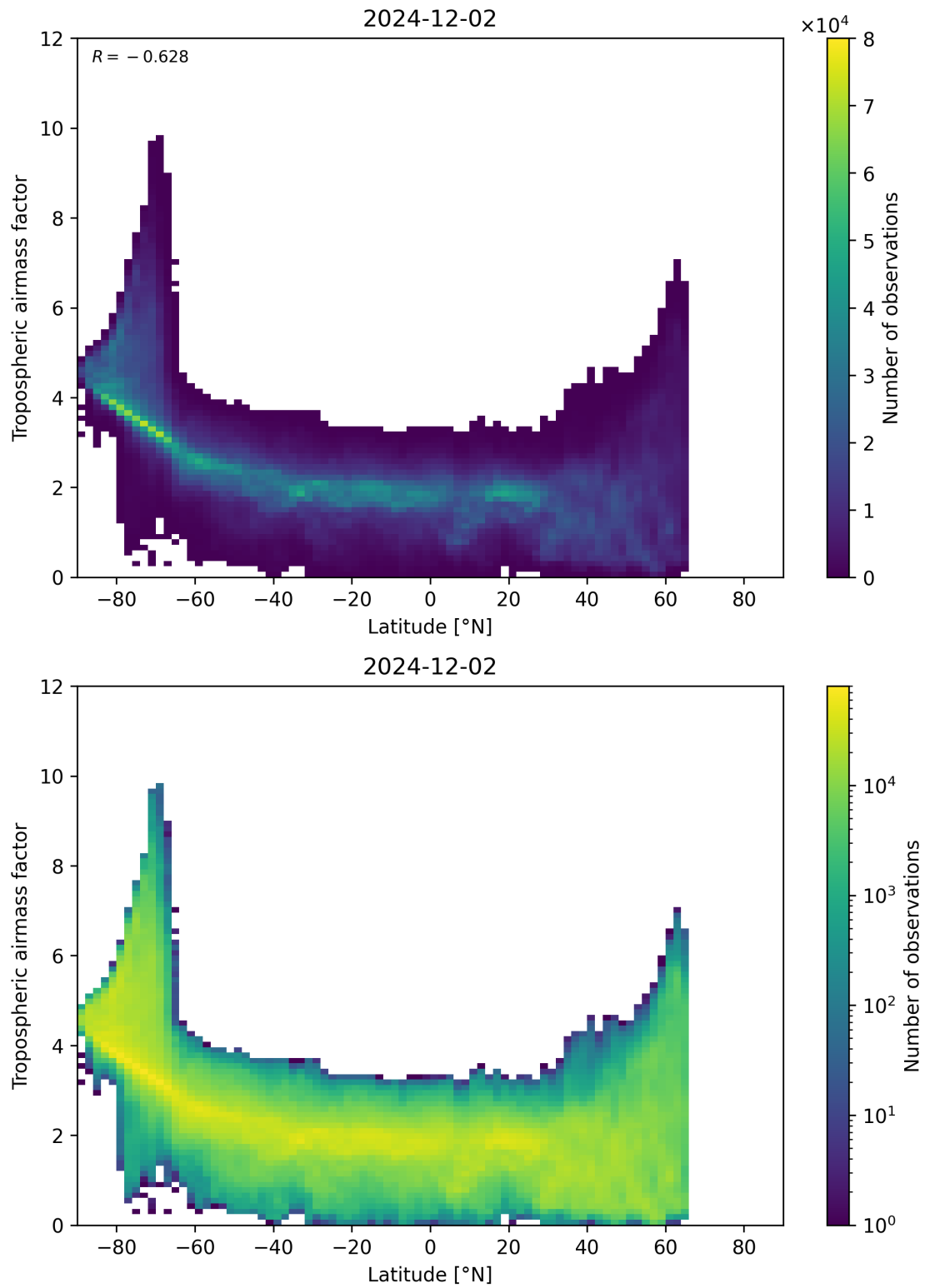
Figure 85: Scatter density plot of “Latitude” against “Tropospheric airmass factor” for 2024-12-01 to 2024-12-03.
