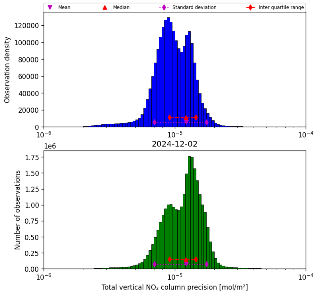
Figure 39: Histogram of “Total vertical NO 2 column precision” for 2024-12-01 to 2024-12-03
