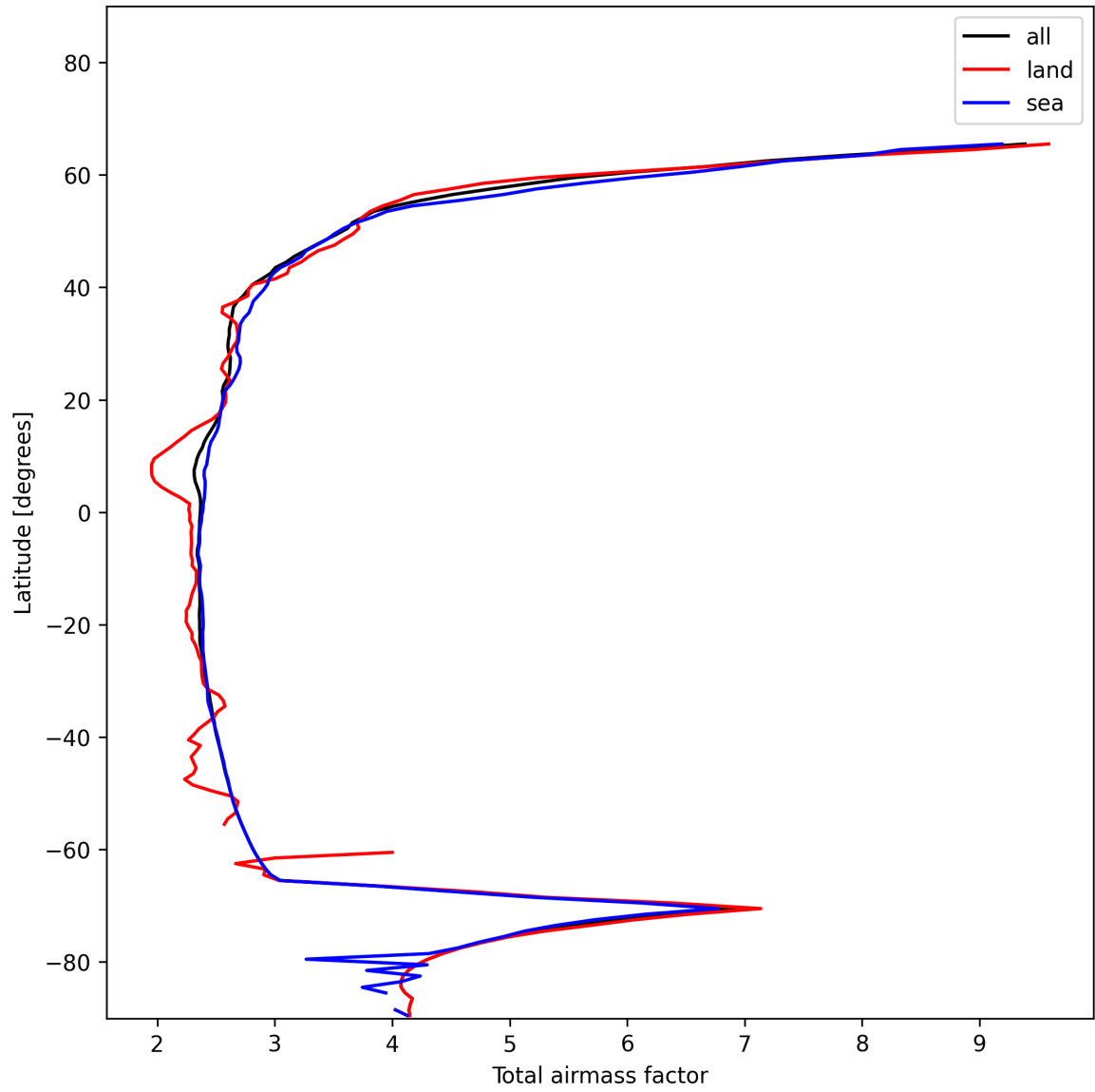
Figure 15: Zonal average of “Total airmass factor” for 2024-12-01 to 2024-12-03.
