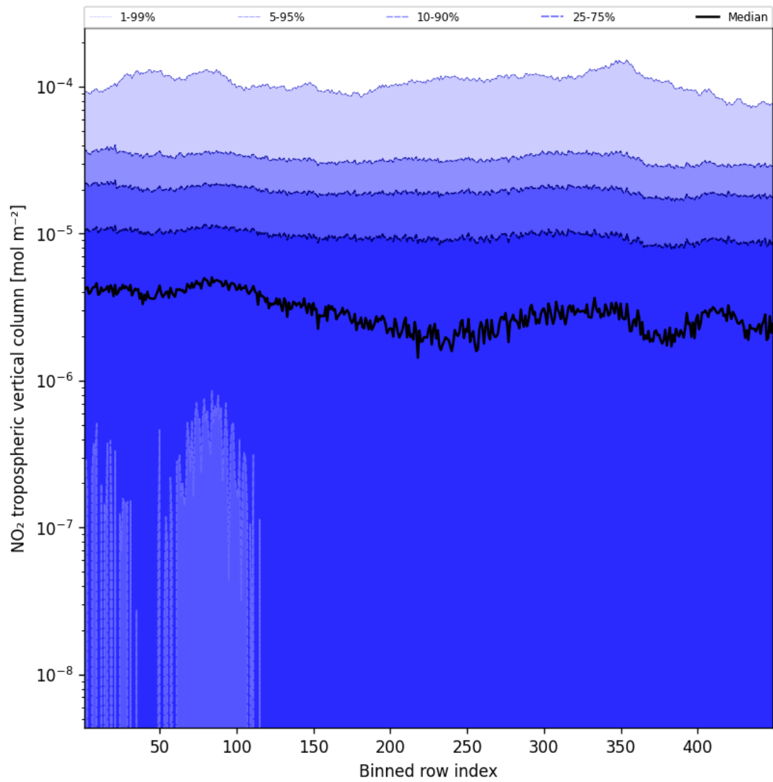
Figure 46: Along track statistics of “NO 2 tropospheric vertical column” for 2024-12-01 to 2024-12-03
