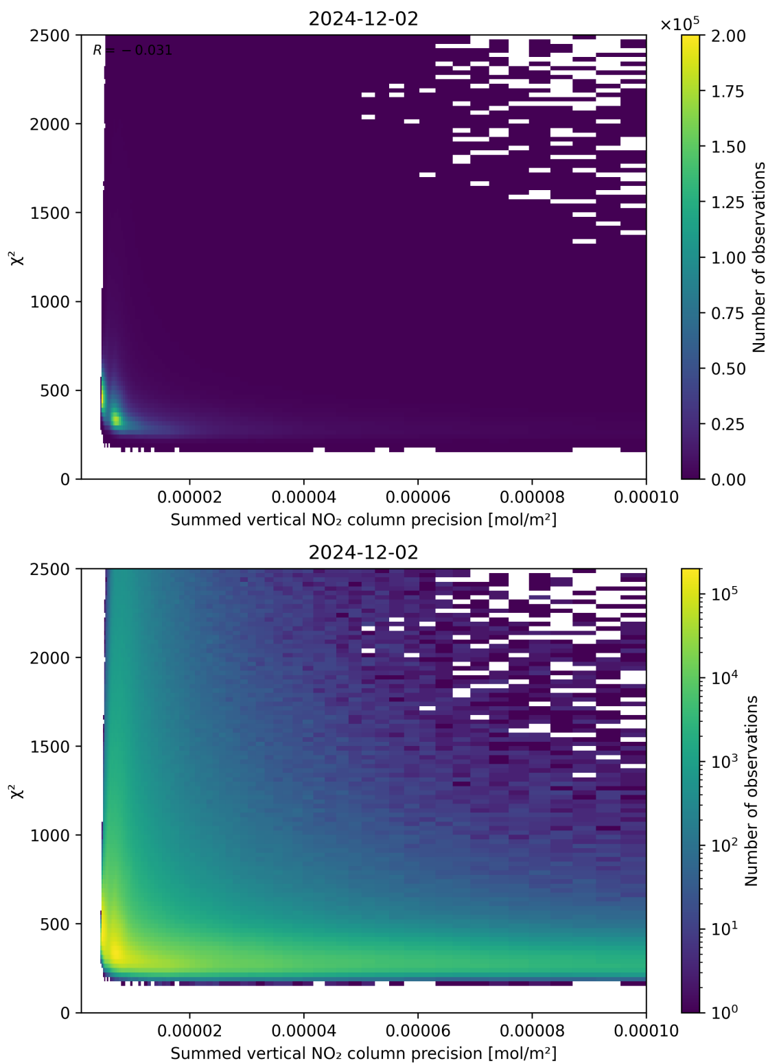
Figure 107: Scatter density plot of “Summed vertical NO 2 column precision” against “ \chi^2 ” for 2024-12-01 to 2024-12-03.
