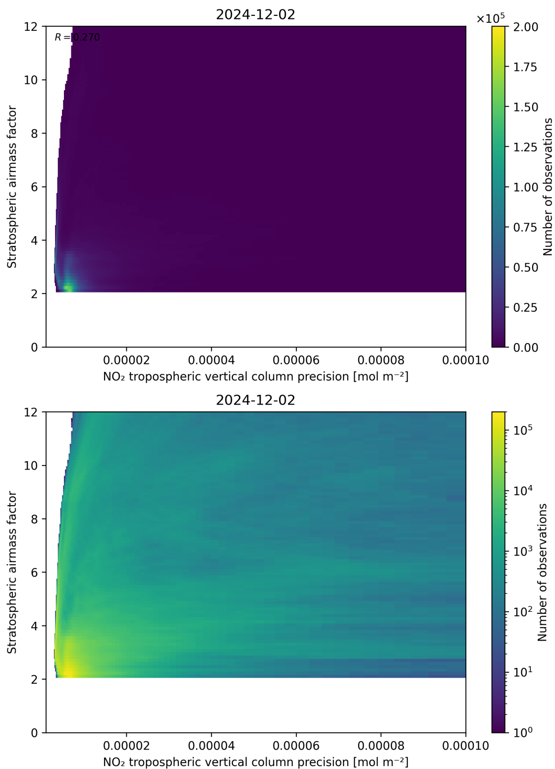
Figure 131: Scatter density plot of “NO 2 tropospheric vertical column precision” against “Stratospheric airmass factor” for 2024-12-01 to 2024-12-03.
