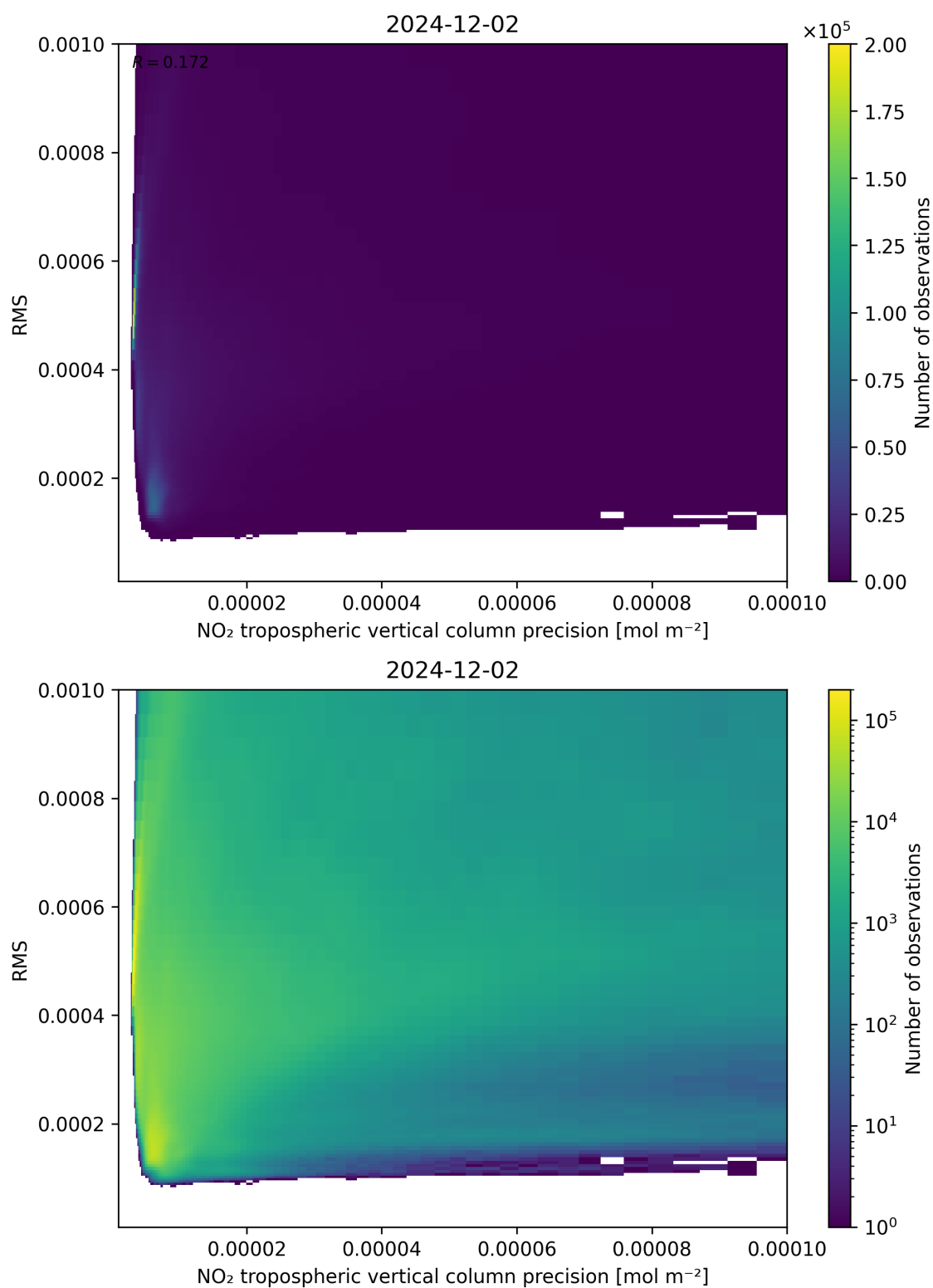
Figure 140: Scatter density plot of “NO 2 tropospheric vertical column precision” against “RMS” for 2024-12-01 to 2024-12-03.
