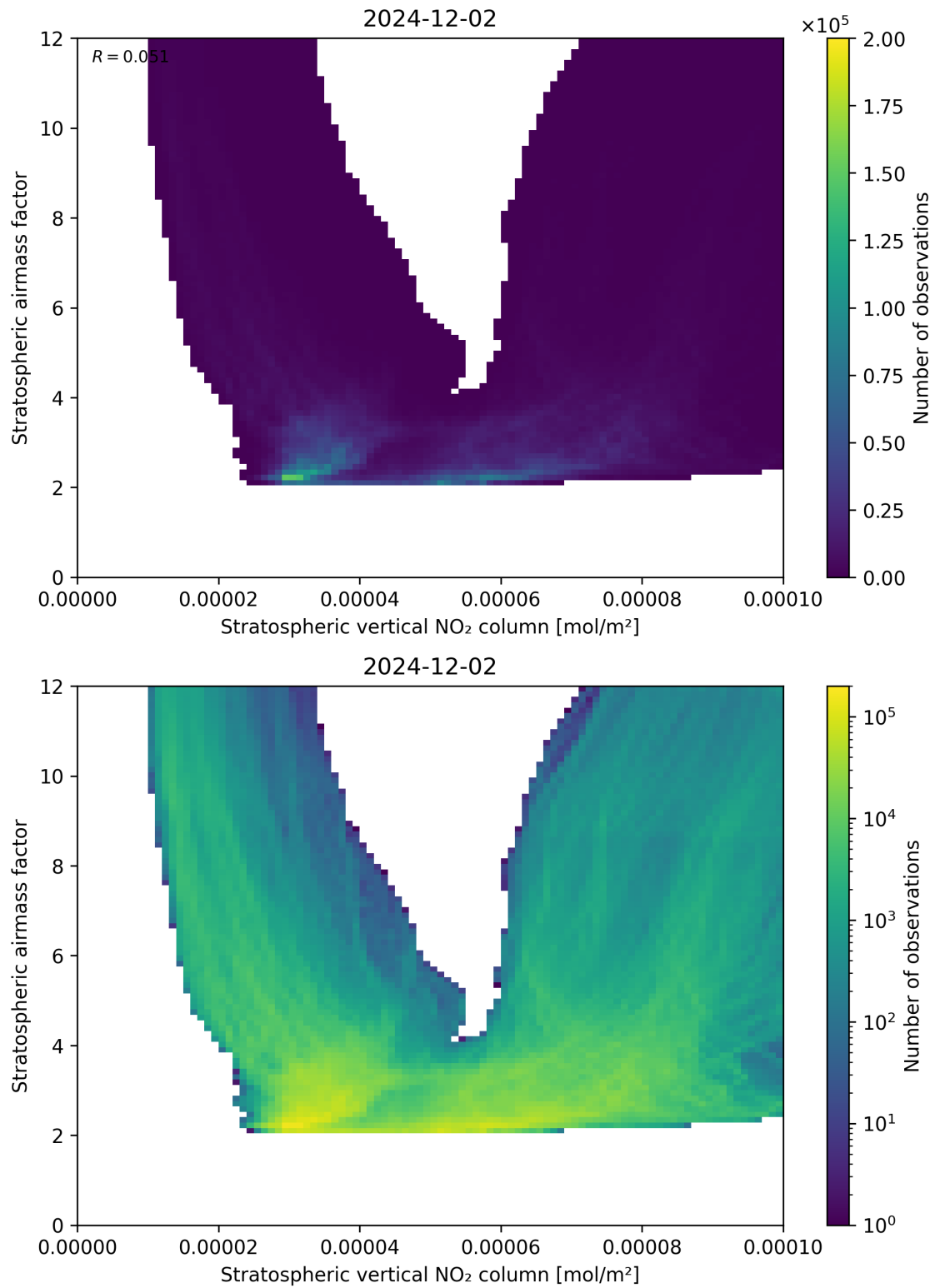
Figure 96: Scatter density plot of “Stratospheric vertical NO 2 column” against “Stratospheric airmass factor” for 2024-12-01 to 2024-12-03.
