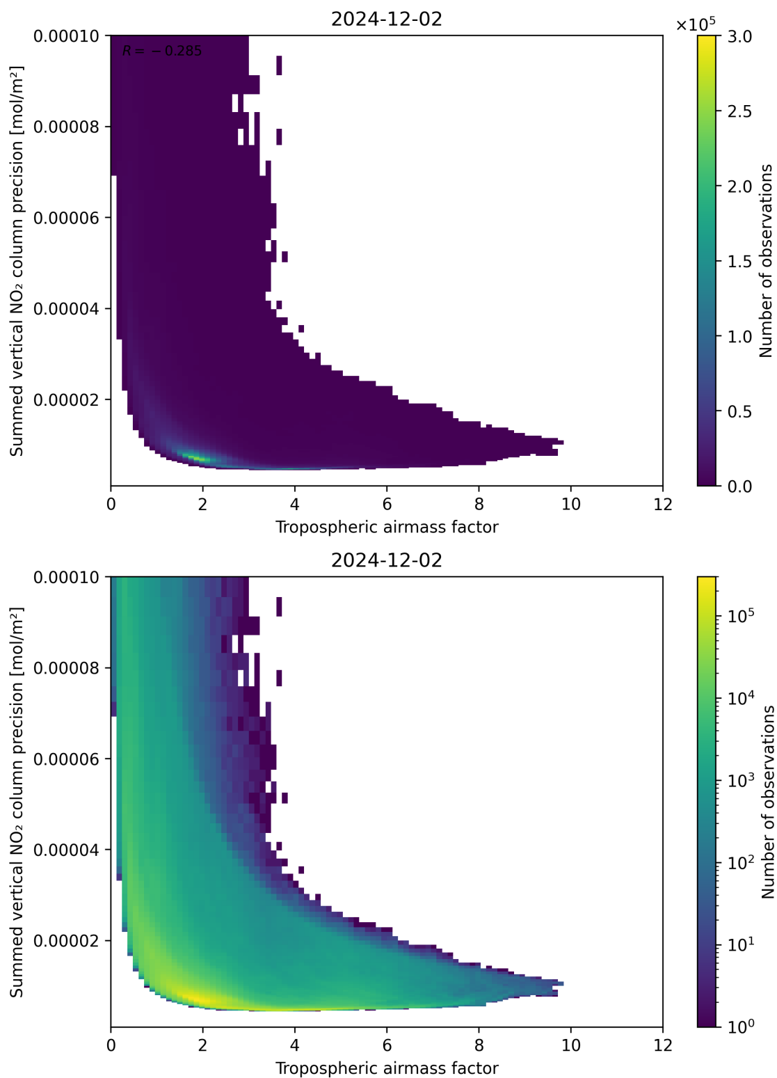
Figure 76: Scatter density plot of “Tropospheric air mass factor” against “Summed vertical NO 2 column precision” for 2024-12-01 to 2024-12-03.
