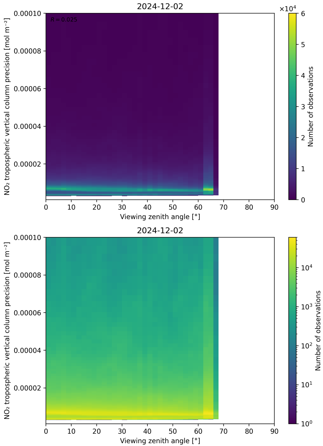
Figure 170: Scatter density plot of “Viewing zenith angle” against “NO 2 tropospheric vertical column precision” for 2024-12-01 to 2024-12-03.
