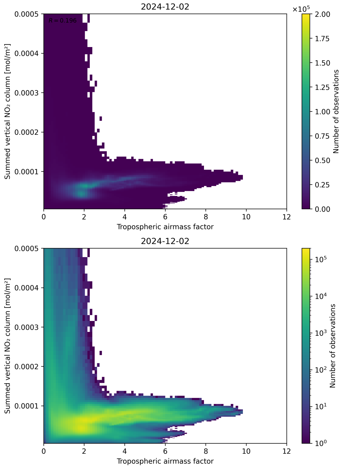
Figure 75: Scatter density plot of “Tropospheric airmass factor” against “Summed vertical NO 2 column” for 2024-12-01 to 2024-12-03.
