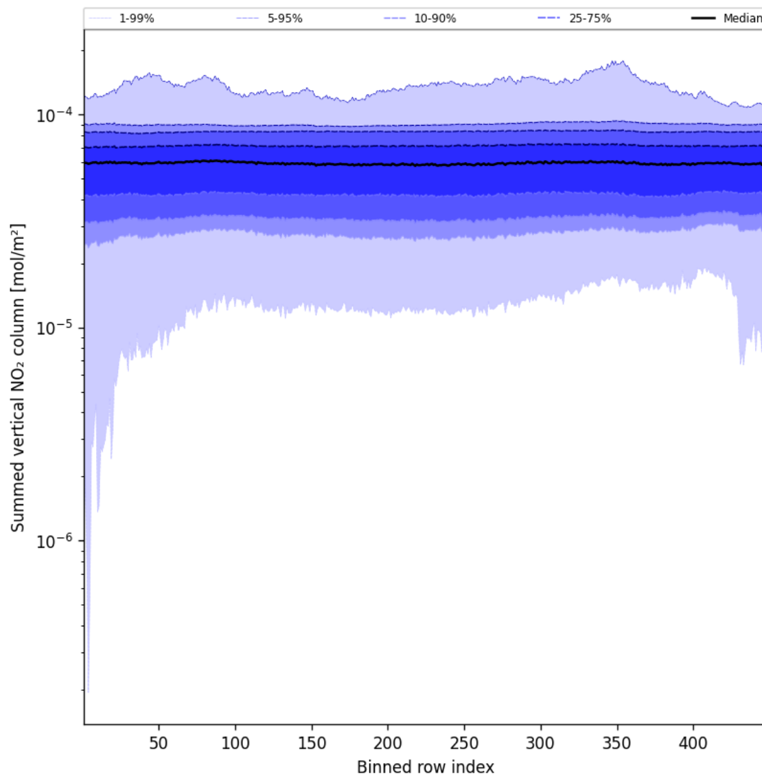
Figure 57: Along track statistics of “Summed vertical NO 2 column” for 2024-12-01 to 2024-12-03
