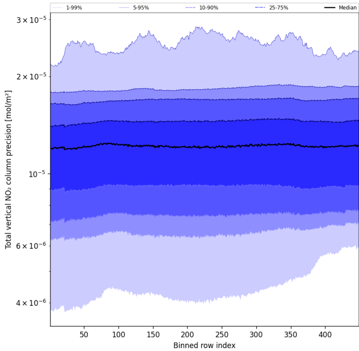
Figure 56: Along track statistics of “Total vertical NO 2 column precision” for 2024-12-01 to 2024-12-03
