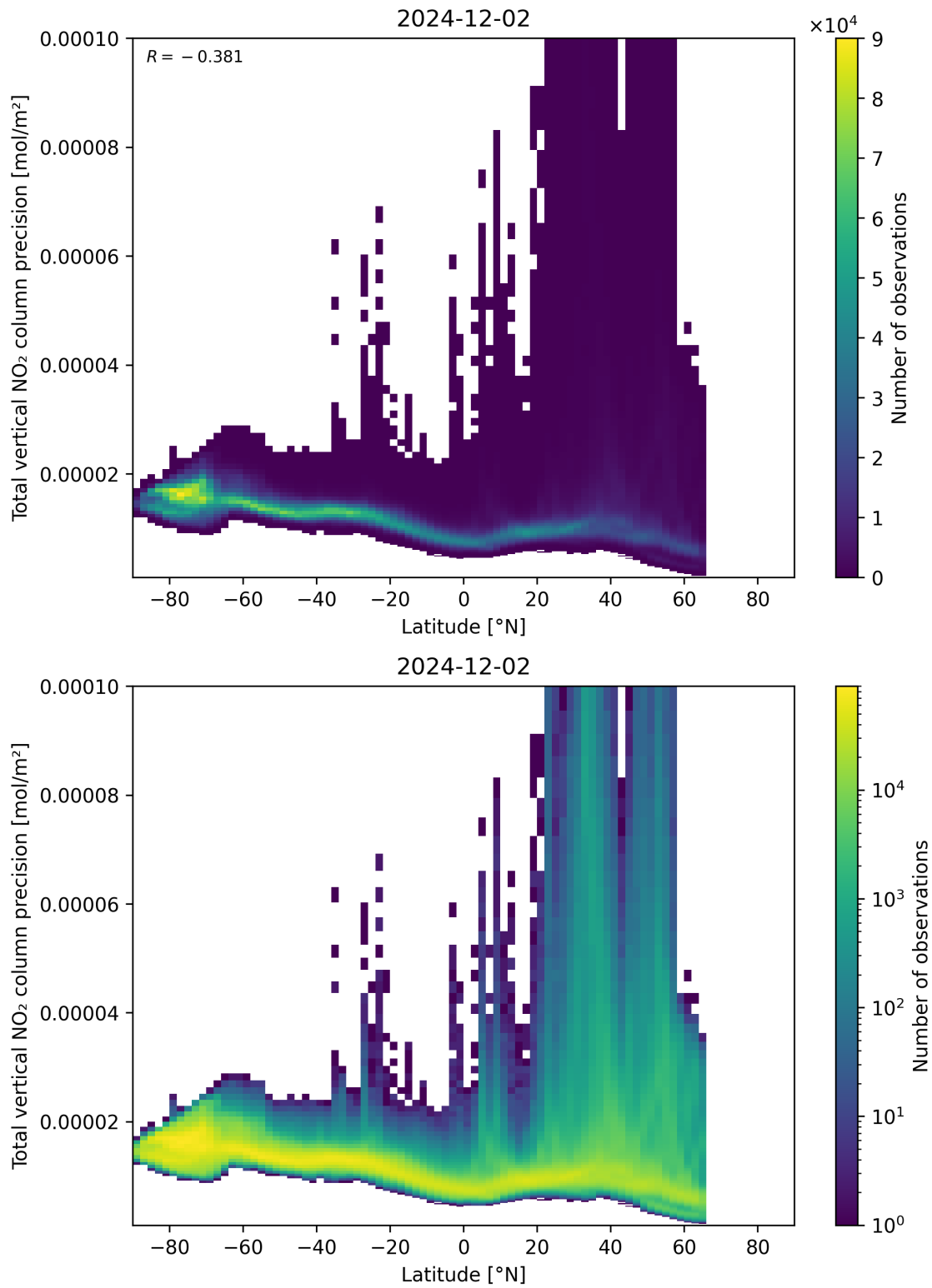
Figure 91: Scatter density plot of “Latitude” against “Total vertical NO 2 column precision” for 2024-12-01 to 2024-12-03.
