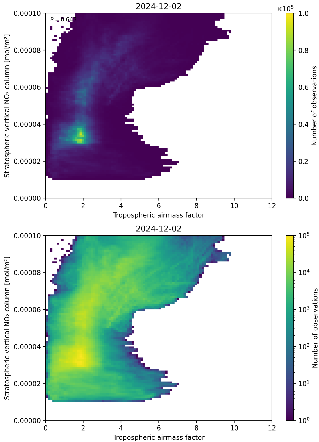
Figure 74: Scatter density plot of “Tropospheric air mass factor” against “Stratospheric vertical NO 2 column” for 2024-12-01 to 2024-12-03.
