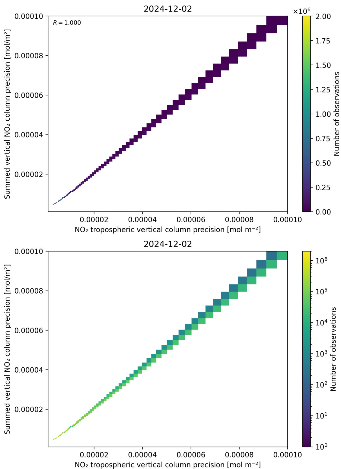
Figure 137: Scatter density plot of “NO 2 tropospheric vertical column precision” against “Summed vertical NO 2 column precision” for 2024-12-01 to 2024-12-03.
