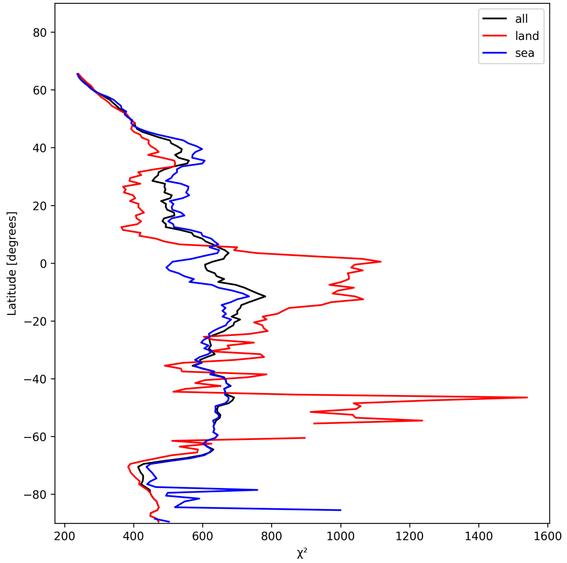
Figure 25: Zonal average of “ \chi^2 ” for 2024-12-01 to 2024-12-03.
