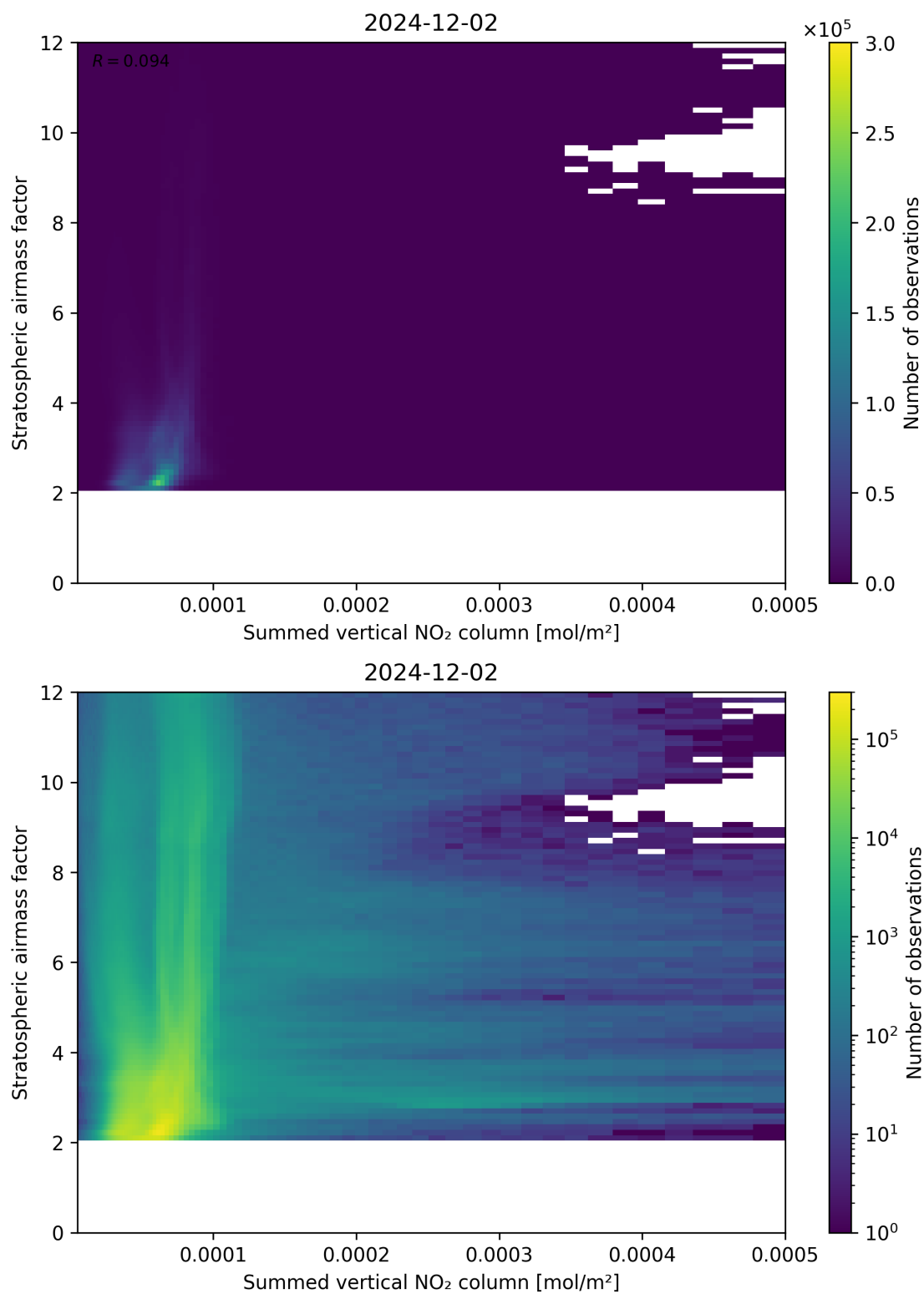
Figure 103: Scatter density plot of “Summed vertical NO 2 column” against “Stratospheric air mass factor” for 2024-12-01 to 2024-12-03.
