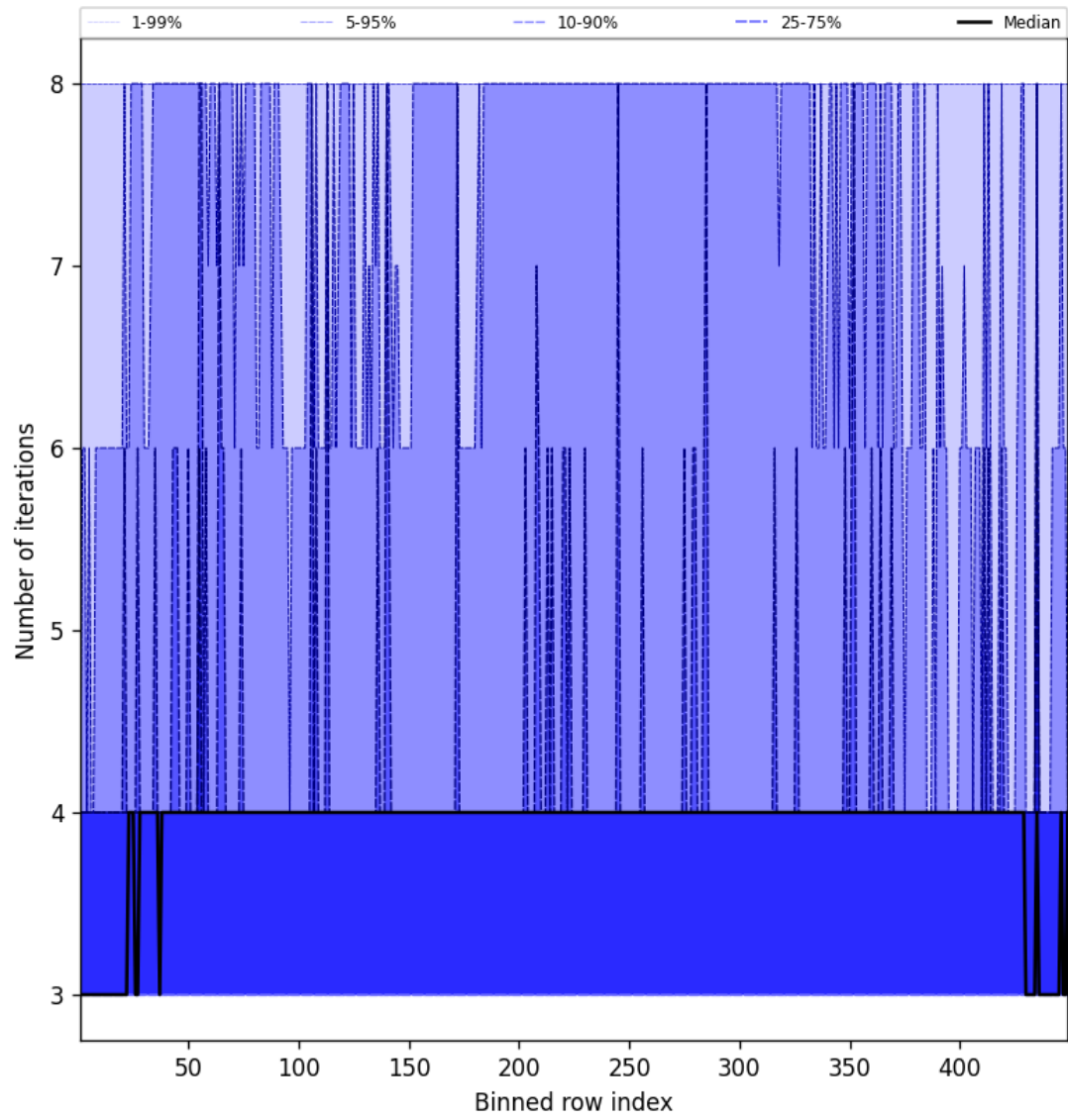
Figure 51: Along track statistics of “Number of iterations” for 2024-12-01 to 2024-12-03
