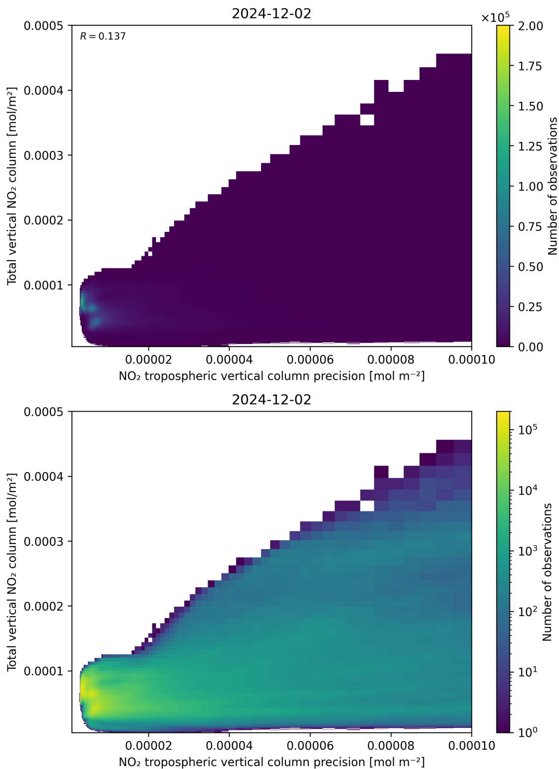
Figure 138: Scatter density plot of “NO 2 tropospheric vertical column precision” against “Total vertical NO 2 column” for 2024-12-01 to 2024-12-03.
