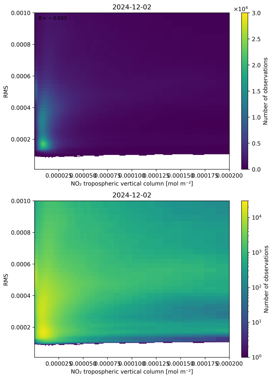
Figure 142: Scatter density plot of “NO 2 tropospheric vertical column” against “RMS” for 2024-12-01 to 2024-12-03.
