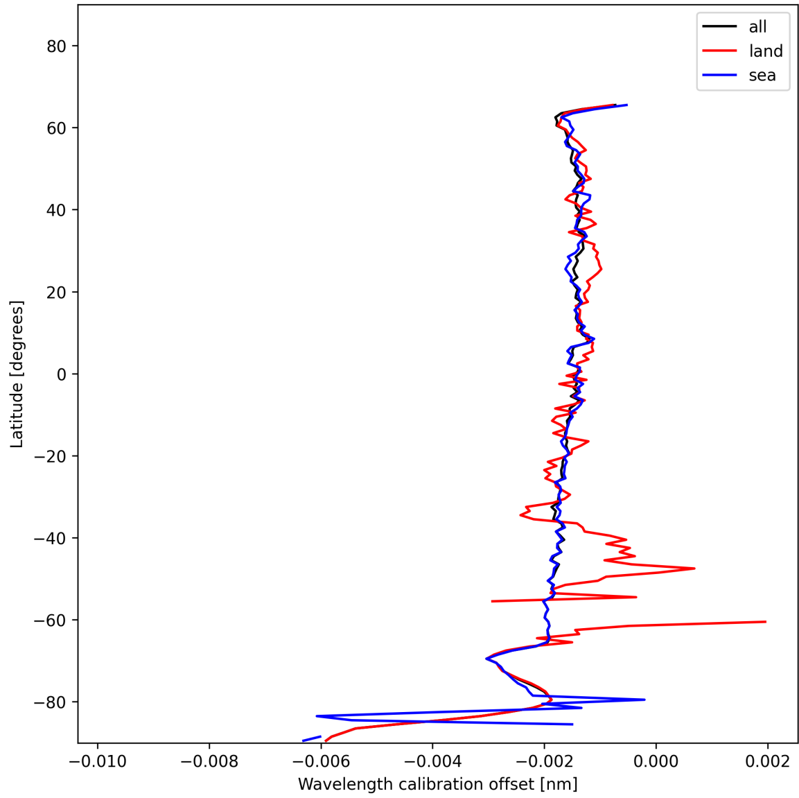
Figure 18: Zonal average of “Wavelength calibration offset” for 2024-12-01 to 2024-12-03.
