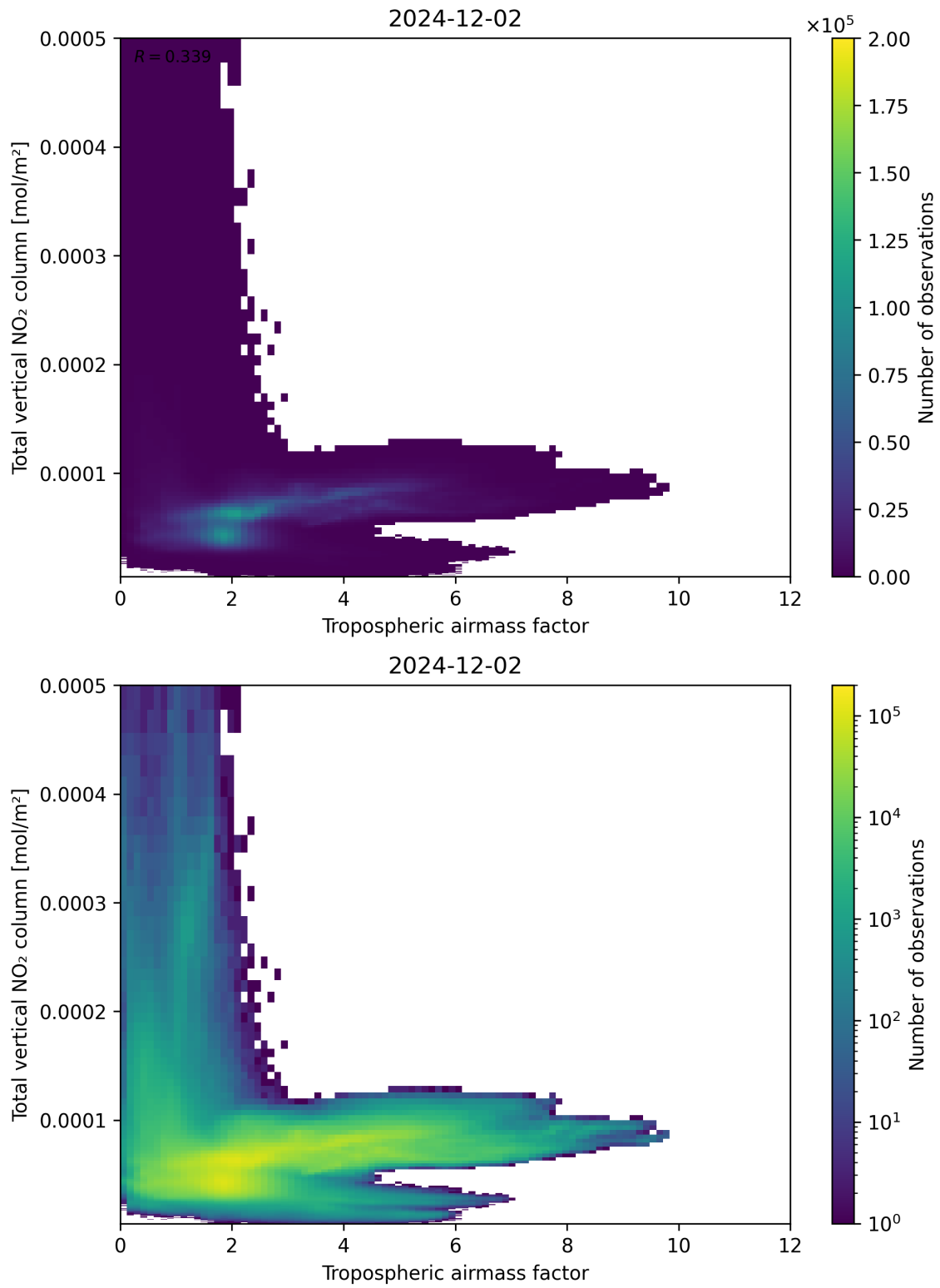
Figure 77: Scatter density plot of “Tropospheric airmass factor” against “Total vertical NO 2 column” for 2024-12-01 to 2024-12-03.
