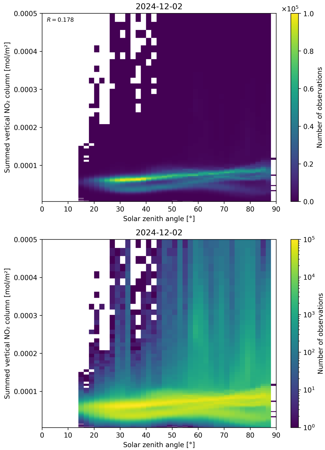
Figure 151: Scatter density plot of “Solar zenith angle” against “Summed vertical NO 2 column” for 2024-12-01 to 2024-12-03.
