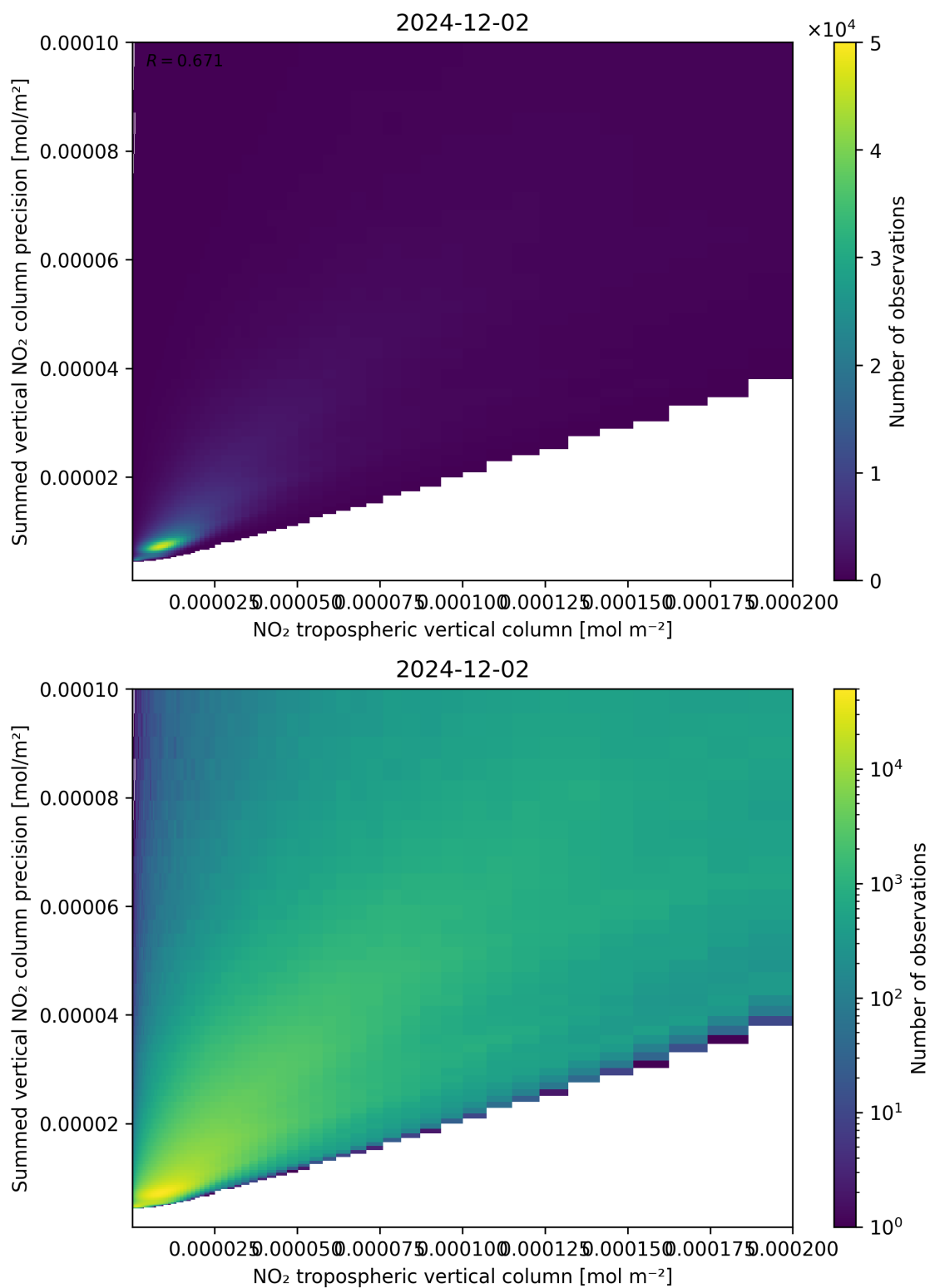
Figure 127: Scatter density plot of “NO 2 tropospheric vertical column” against “Summed vertical NO 2 column precision” for 2024-12-01 to 2024-12-03.
