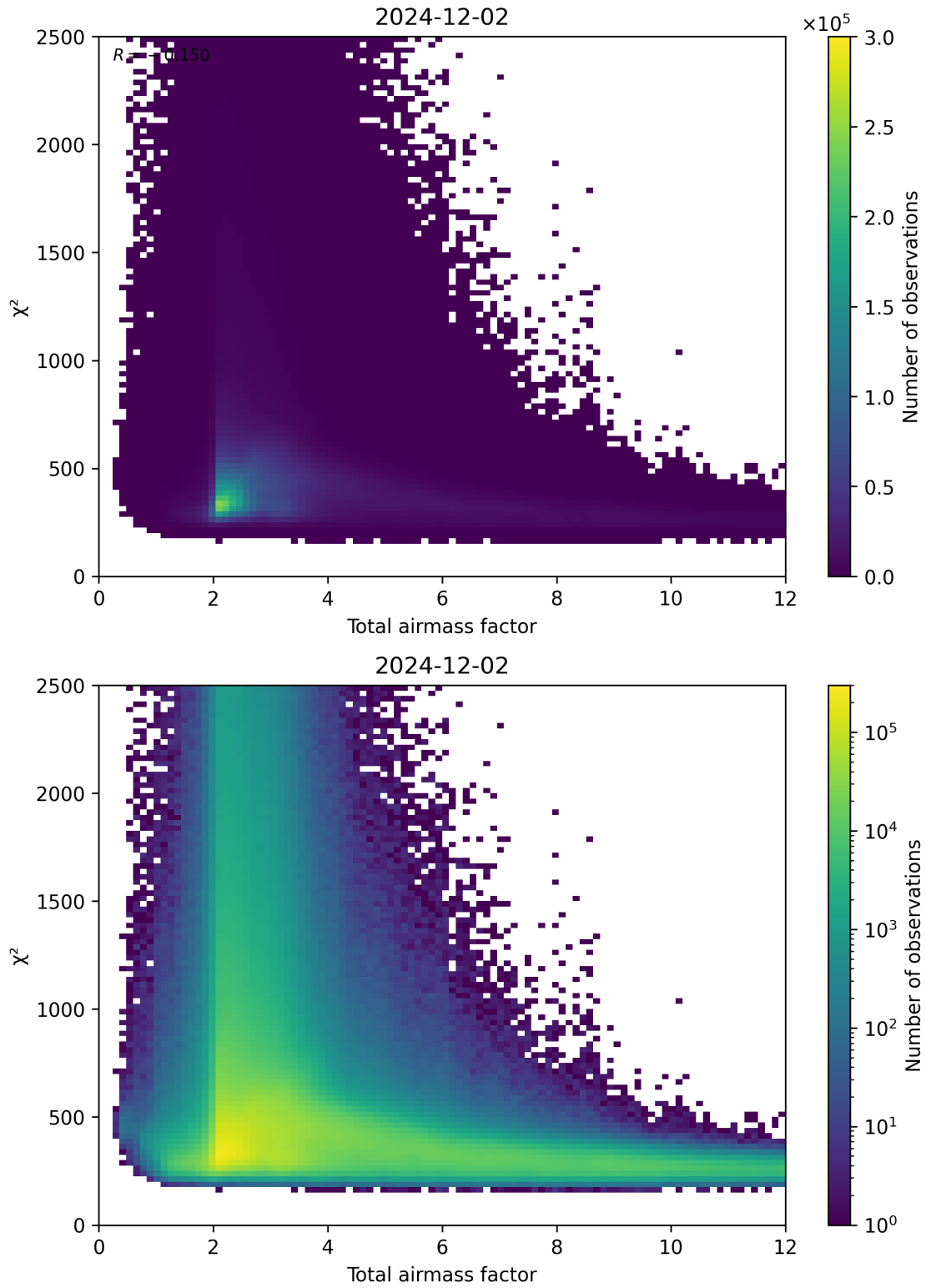
Figure 63: Scatter density plot of “Total airmass factor” against “ \chi^2 ” for 2024-12-01 to 2024-12-03.
