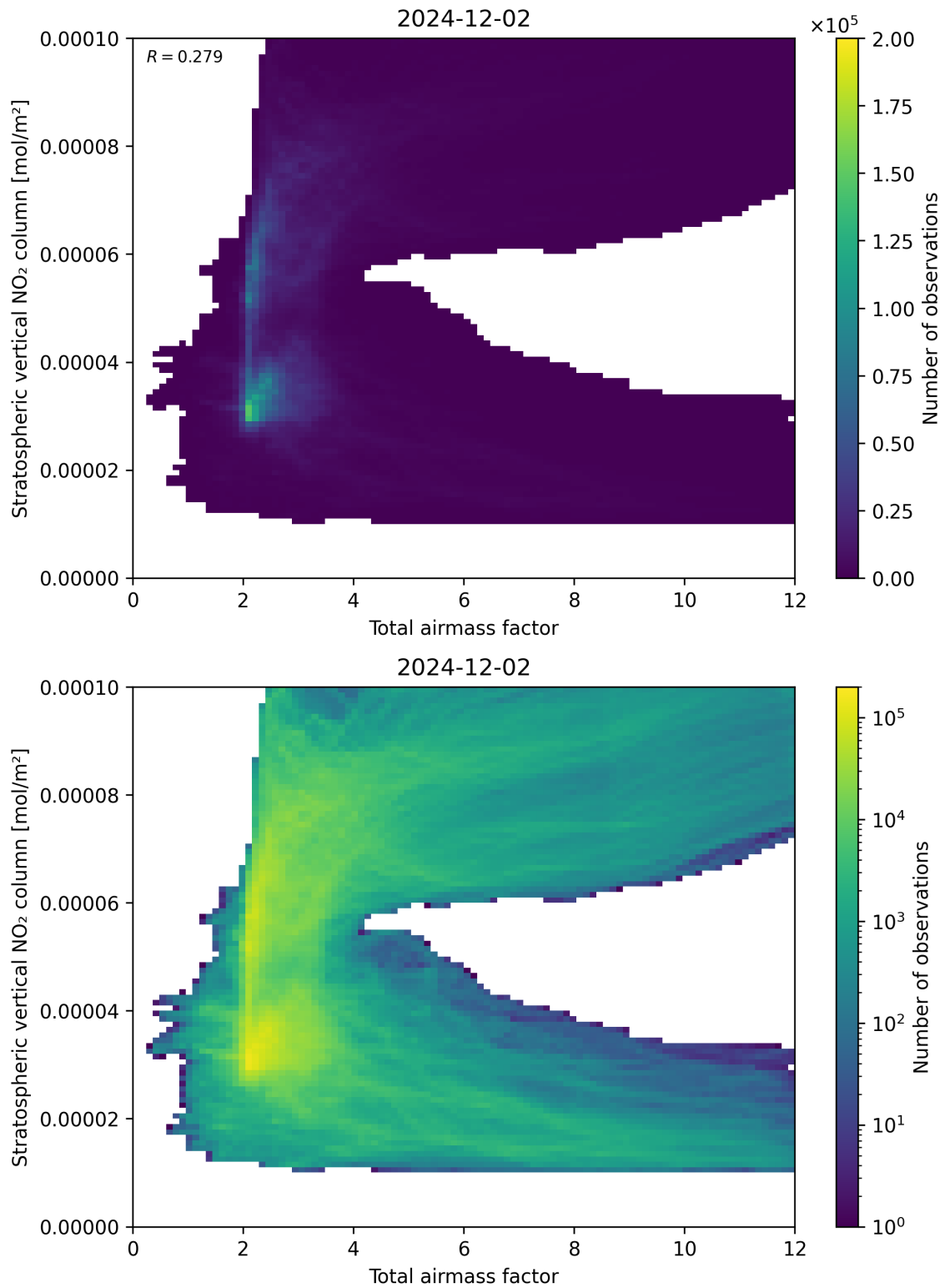
Figure 64: Scatter density plot of “Total airmass factor” against “Stratospheric vertical \text{NO}_2 column” for 2024-12-01 to 2024-12-03.
