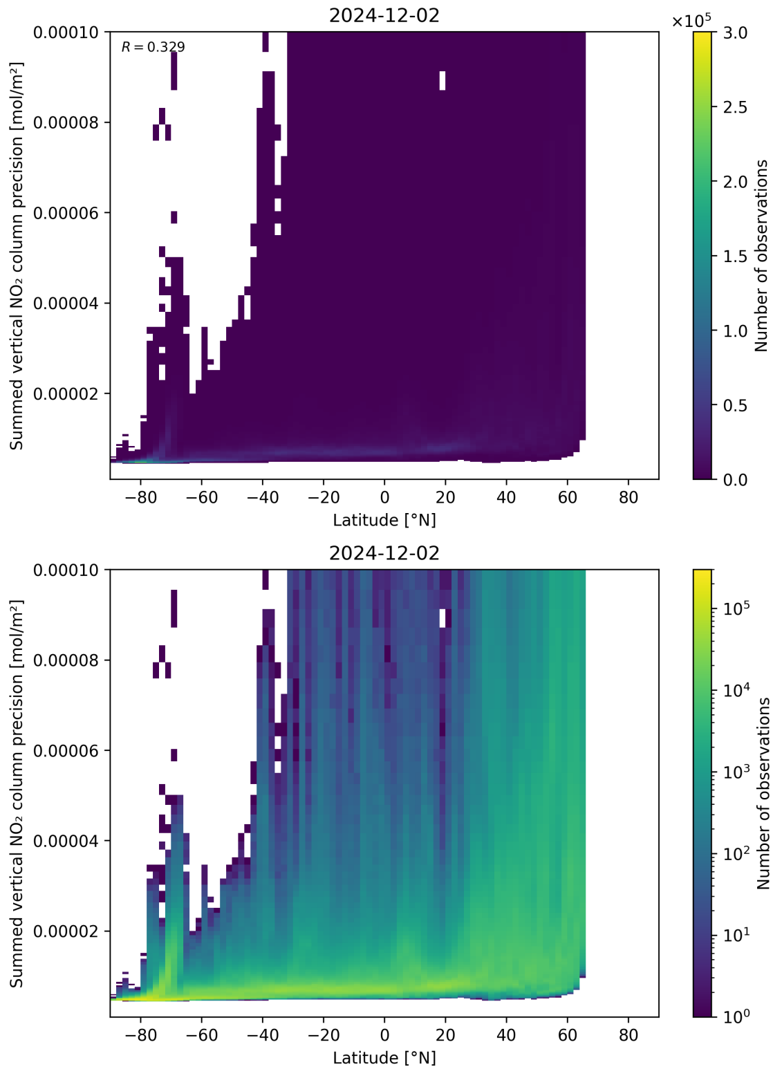
Figure 89: Scatter density plot of “Latitude” against “Summed vertical NO 2 column precision” for 2024-12-01 to 2024-12-03.
