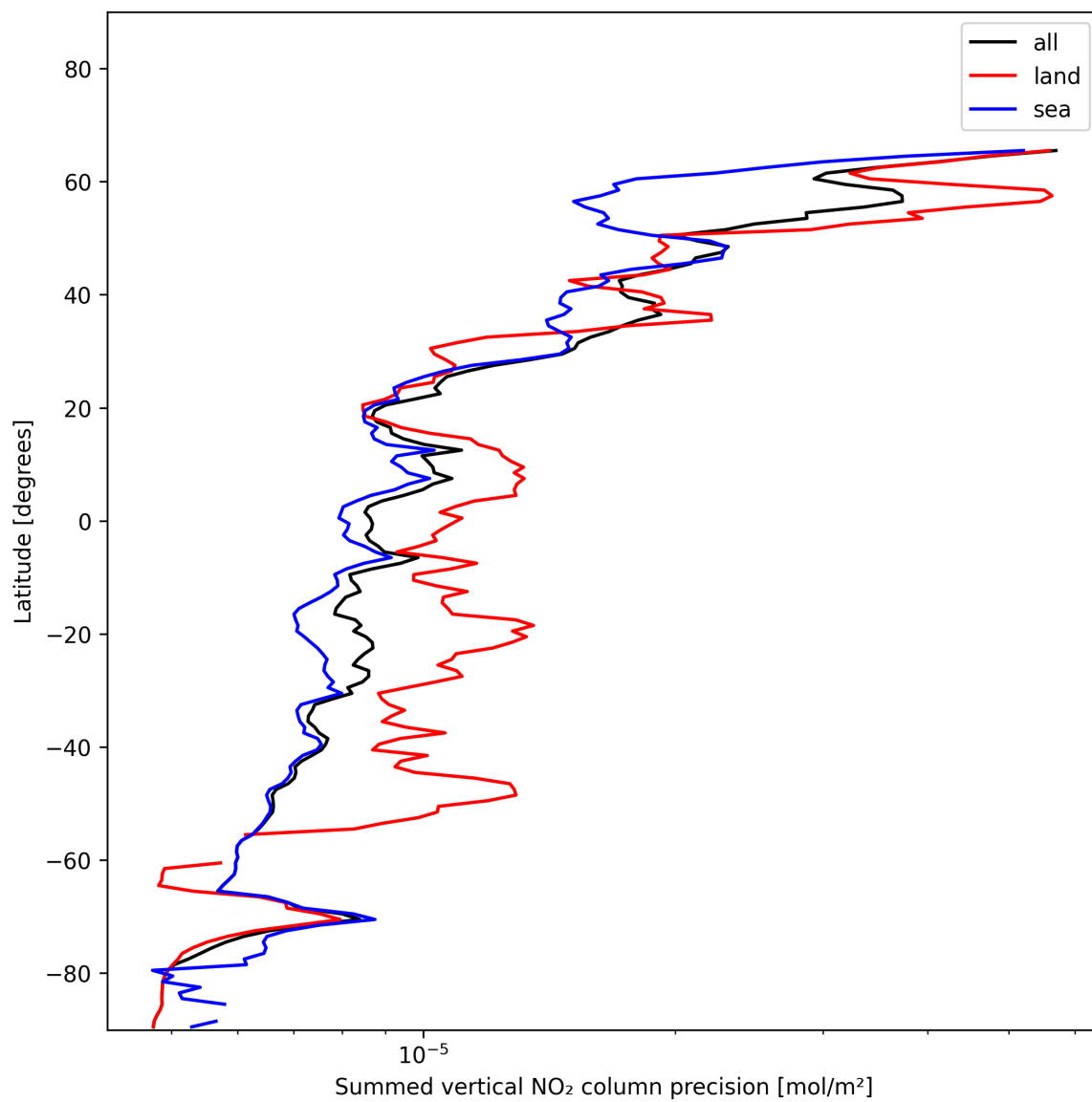
Figure 24: Zonal average of “Summed vertical NO 2 column precision” for 2024-12-01 to 2024-12-03.
