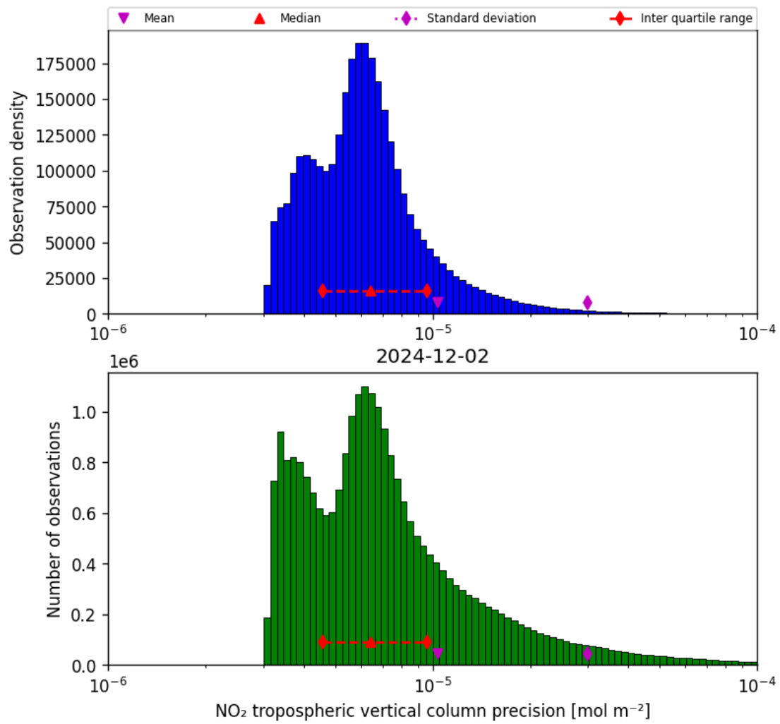
Figure 30: Histogram of “NO 2 tropospheric vertical column precision” for 2024-12-01 to 2024-12-03
