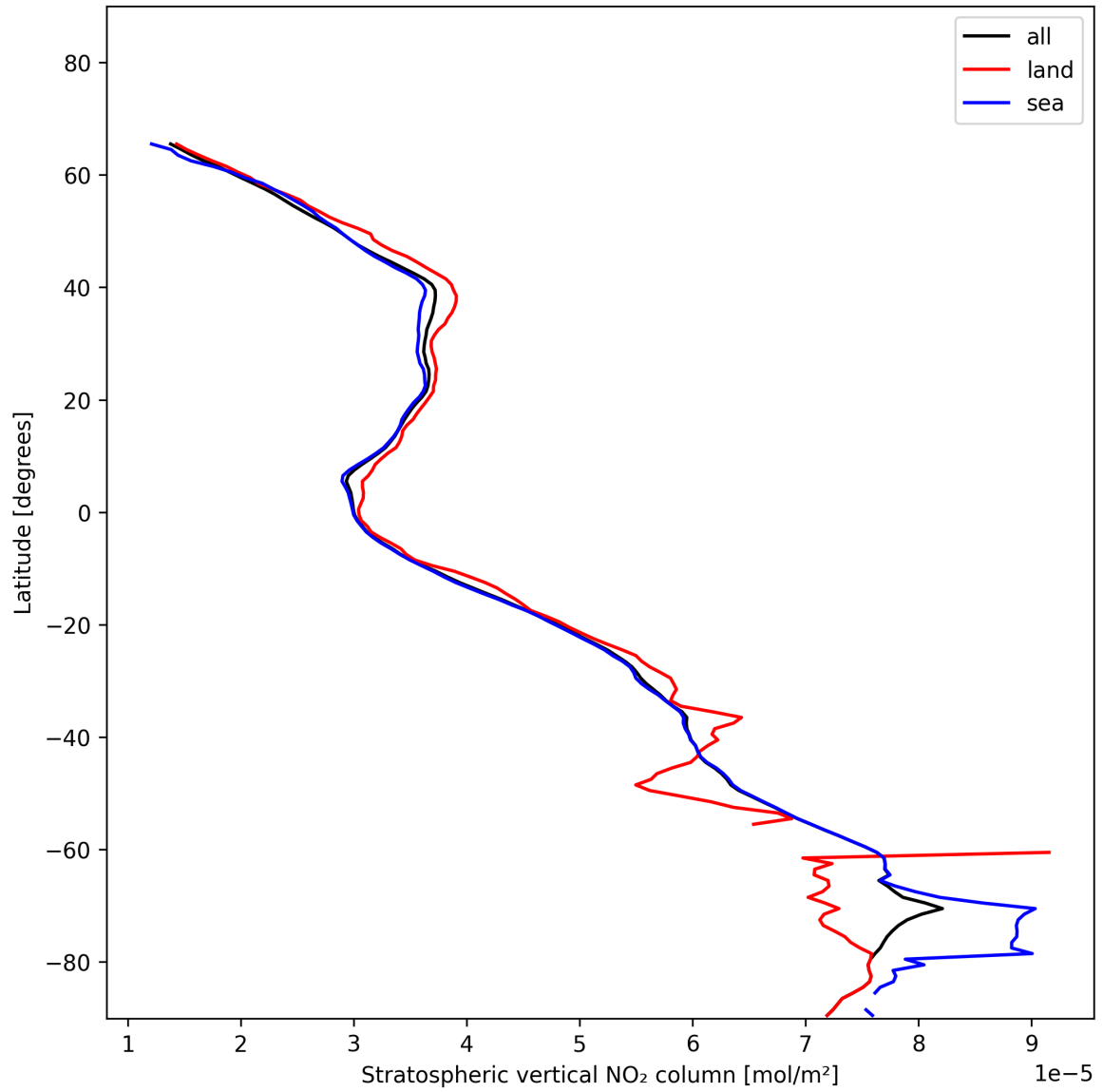
Figure 19: Zonal average of “Stratospheric vertical NO 2 column” for 2024-12-01 to 2024-12-03.
