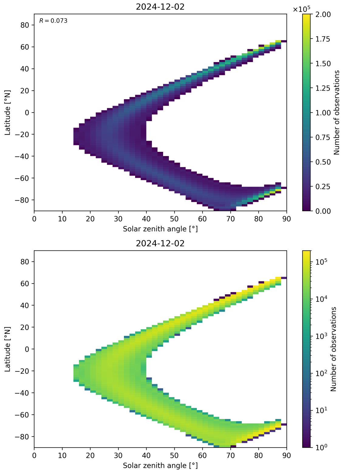
Figure 149: Scatter density plot of “Solar zenith angle” against “Latitude” for 2024-12-01 to 2024-12-03.
