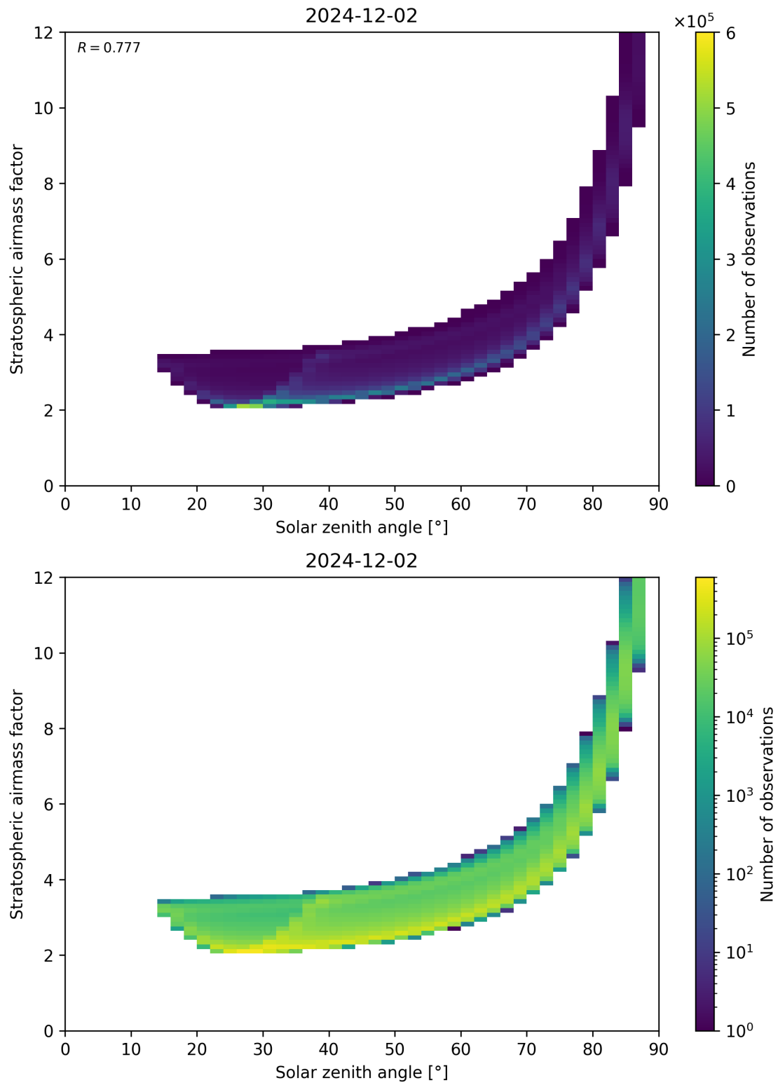
Figure 145: Scatter density plot of “Solar zenith angle” against “Stratospheric airmass factor” for 2024-12-01 to 2024-12-03.
