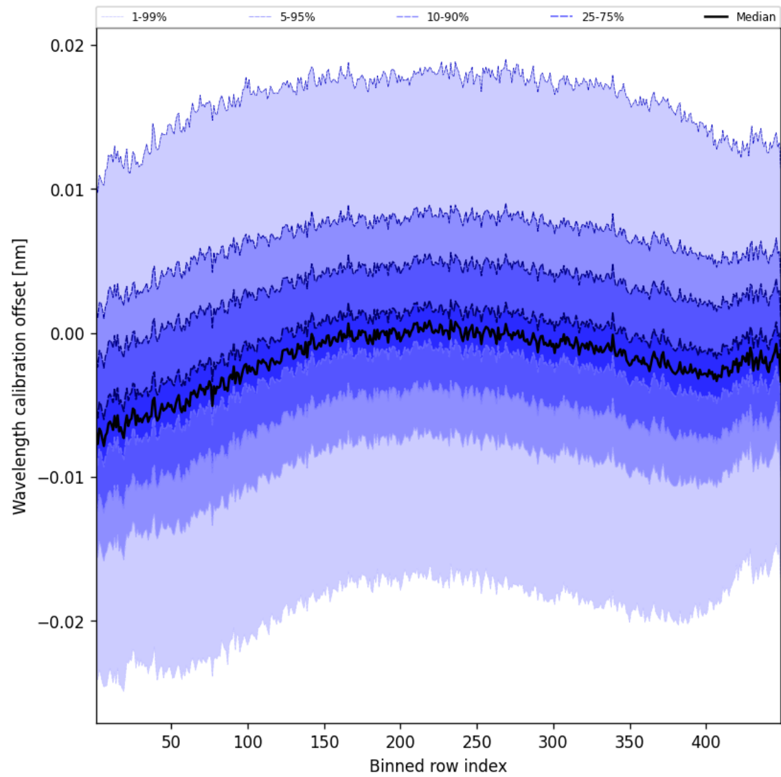
Figure 52: Along track statistics of “Wavelength calibration offset” for 2024-12-01 to 2024-12-03
