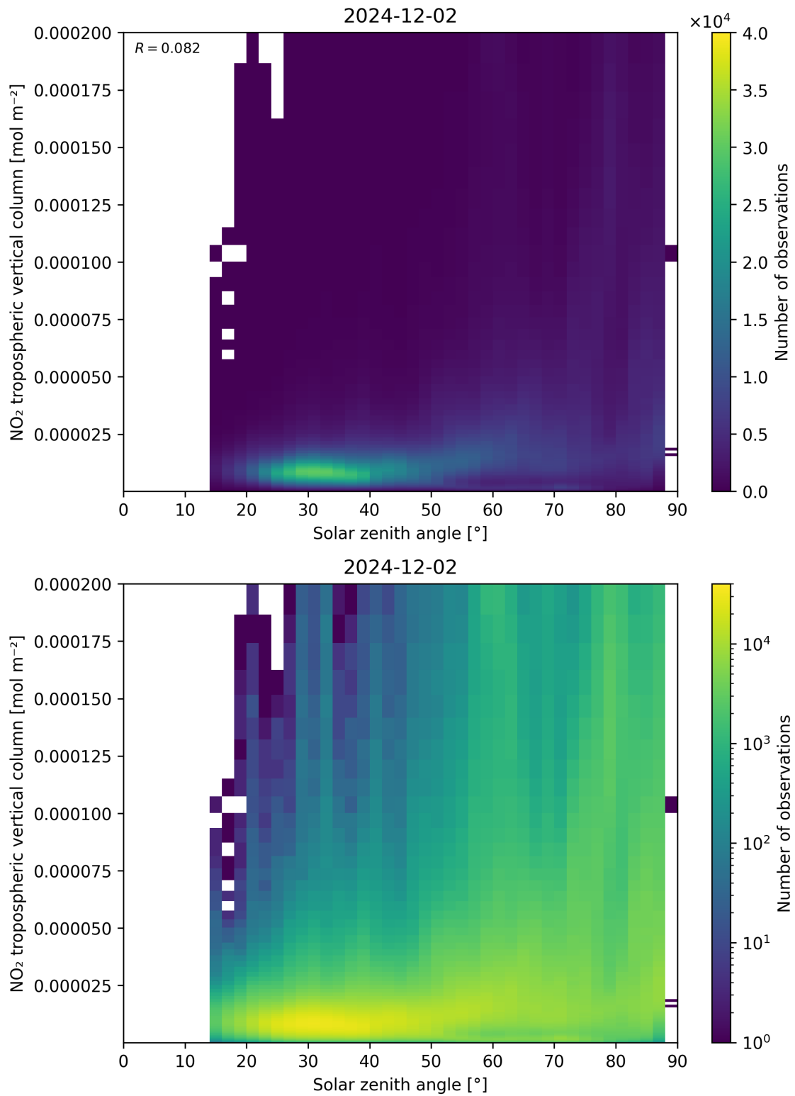
Figure 155: Scatter density plot of “Solar zenith angle” against “NO 2 tropospheric vertical column” for 2024-12-01 to 2024-12-03.
