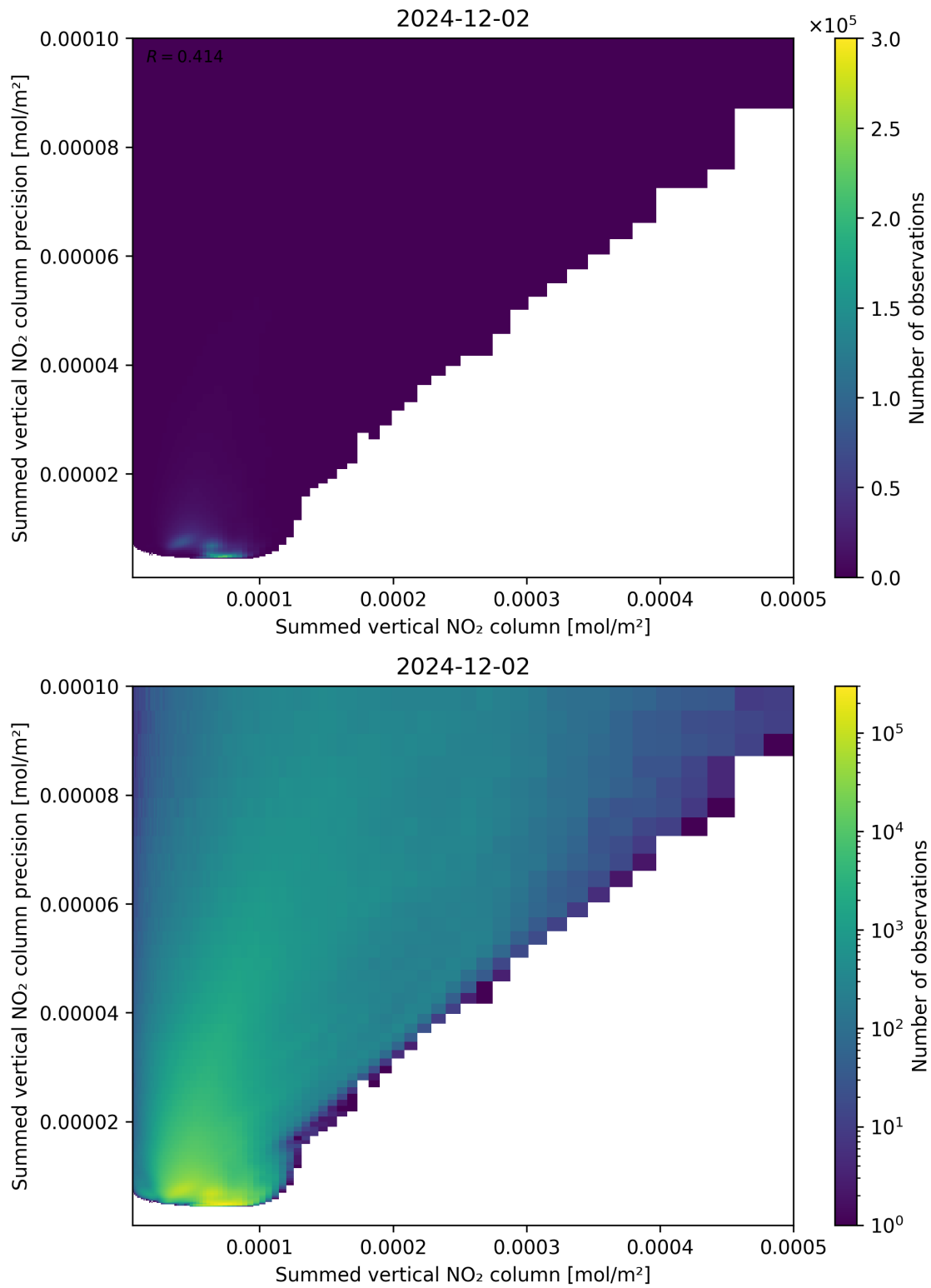
Figure 105: Scatter density plot of “Summed vertical NO 2 column” against “Summed vertical NO 2 column precision” for 2024-12-01 to 2024-12-03.
