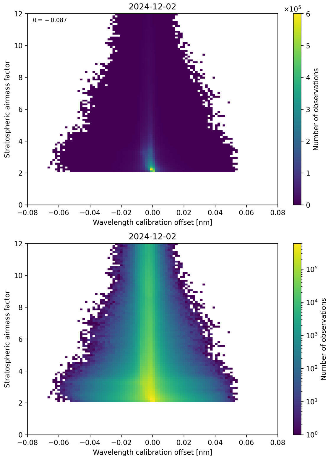
Figure 174: Scatter density plot of “Wavelength calibration offset” against “Stratospheric airmass factor” for 2024-12-01 to 2024-12-03.
