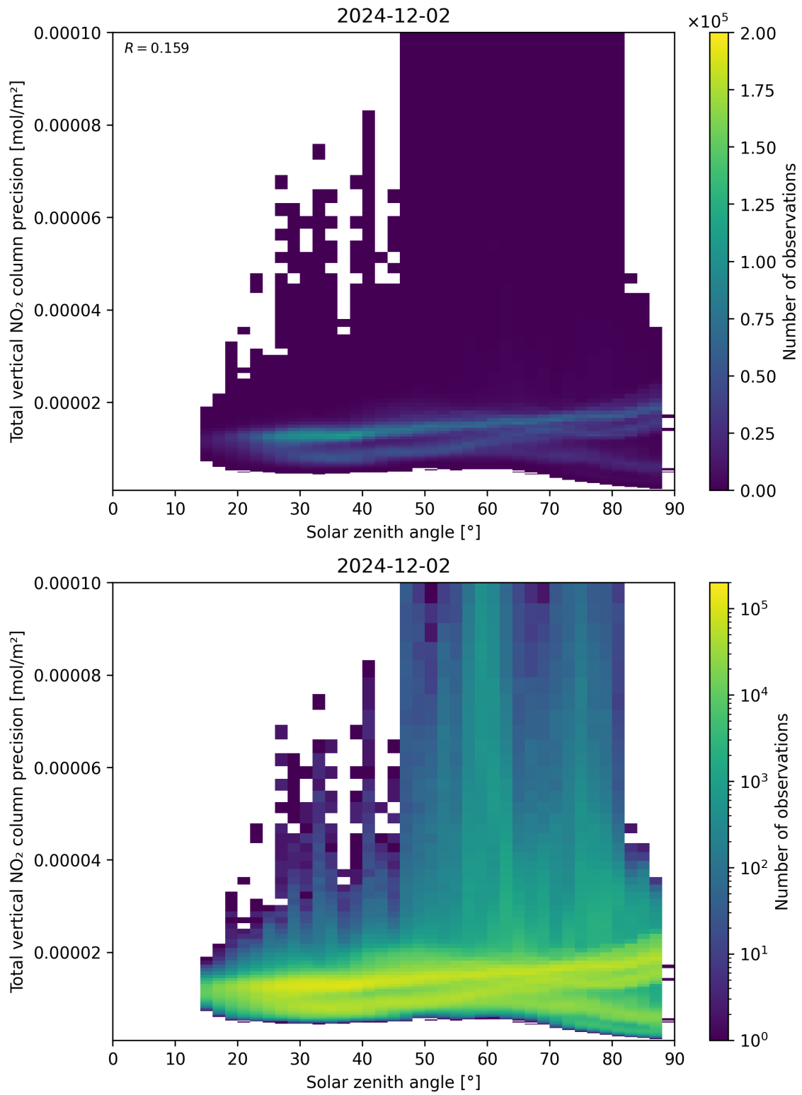
Figure 154: Scatter density plot of “Solar zenith angle” against “Total vertical NO 2 column precision” for 2024-12-01 to 2024-12-03.
