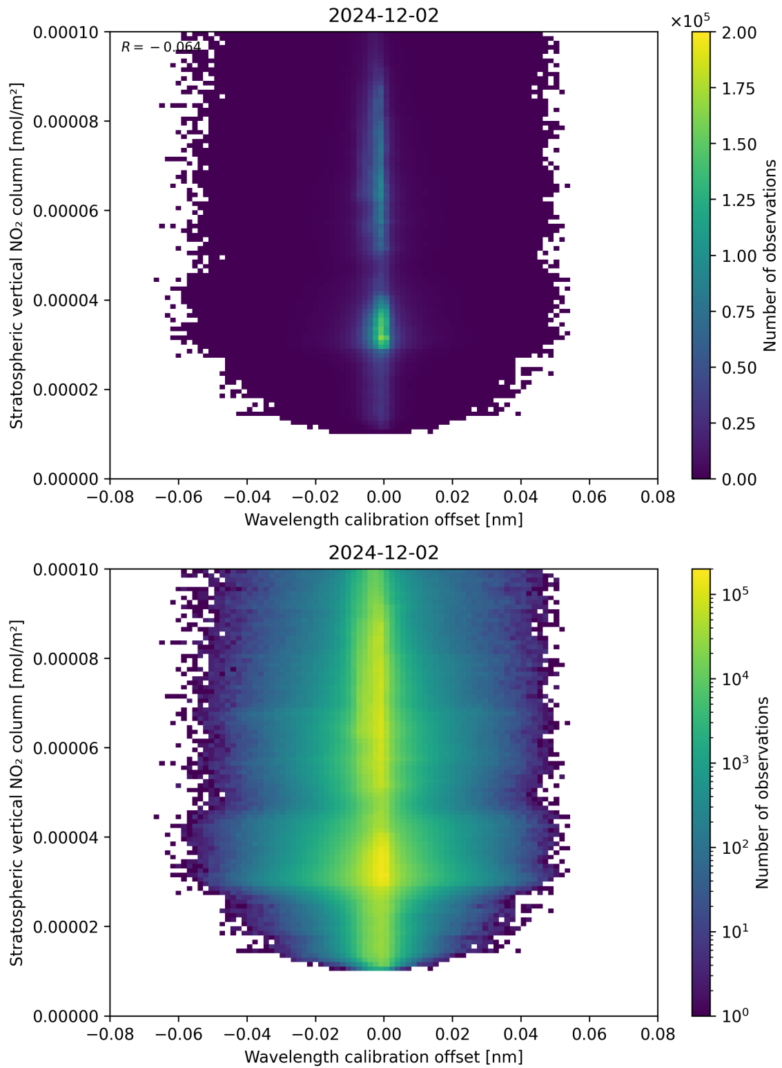
Figure 176: Scatter density plot of “Wavelength calibration offset” against “Stratospheric vertical NO 2 column” for 2024-12-01 to 2024-12-03.
