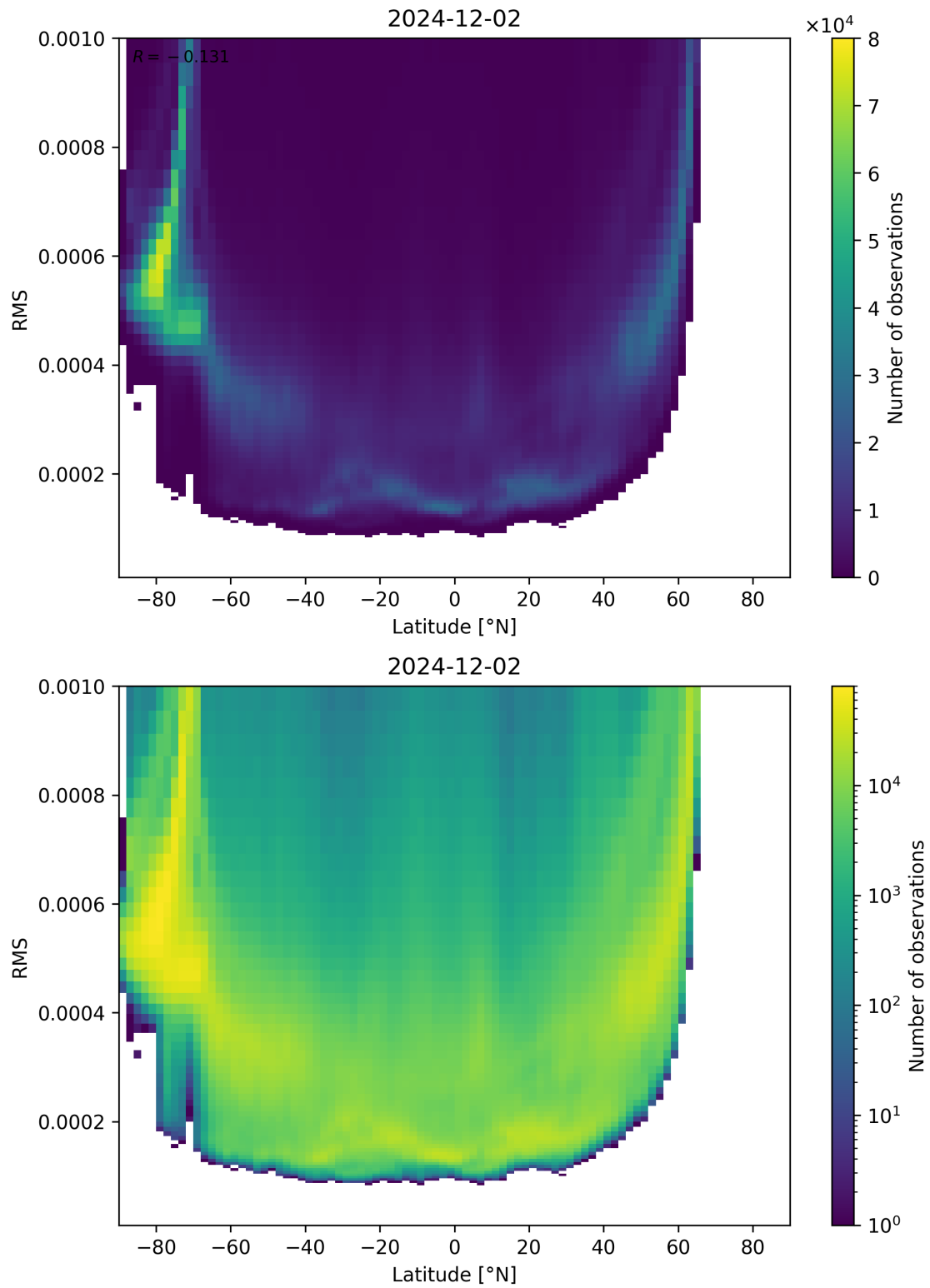
Figure 94: Scatter density plot of “Latitude” against “RMS” for 2024-12-01 to 2024-12-03.
