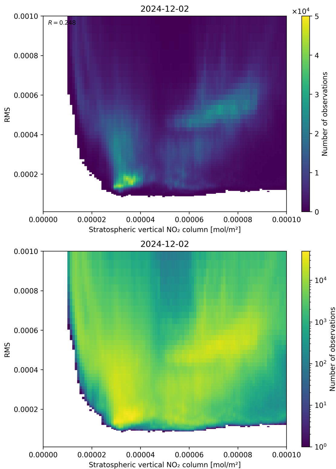
Figure 102: Scatter density plot of “Stratospheric vertical NO 2 column” against “RMS” for 2024-12-01 to 2024-12-03.
