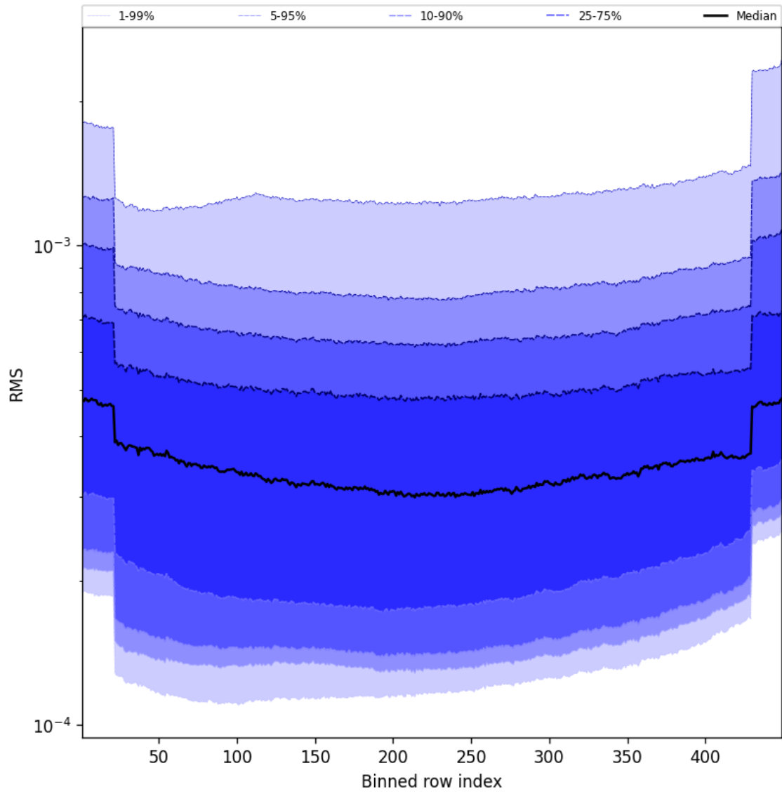
Figure 60: Along track statistics of “RMS” for 2024-12-01 to 2024-12-03
