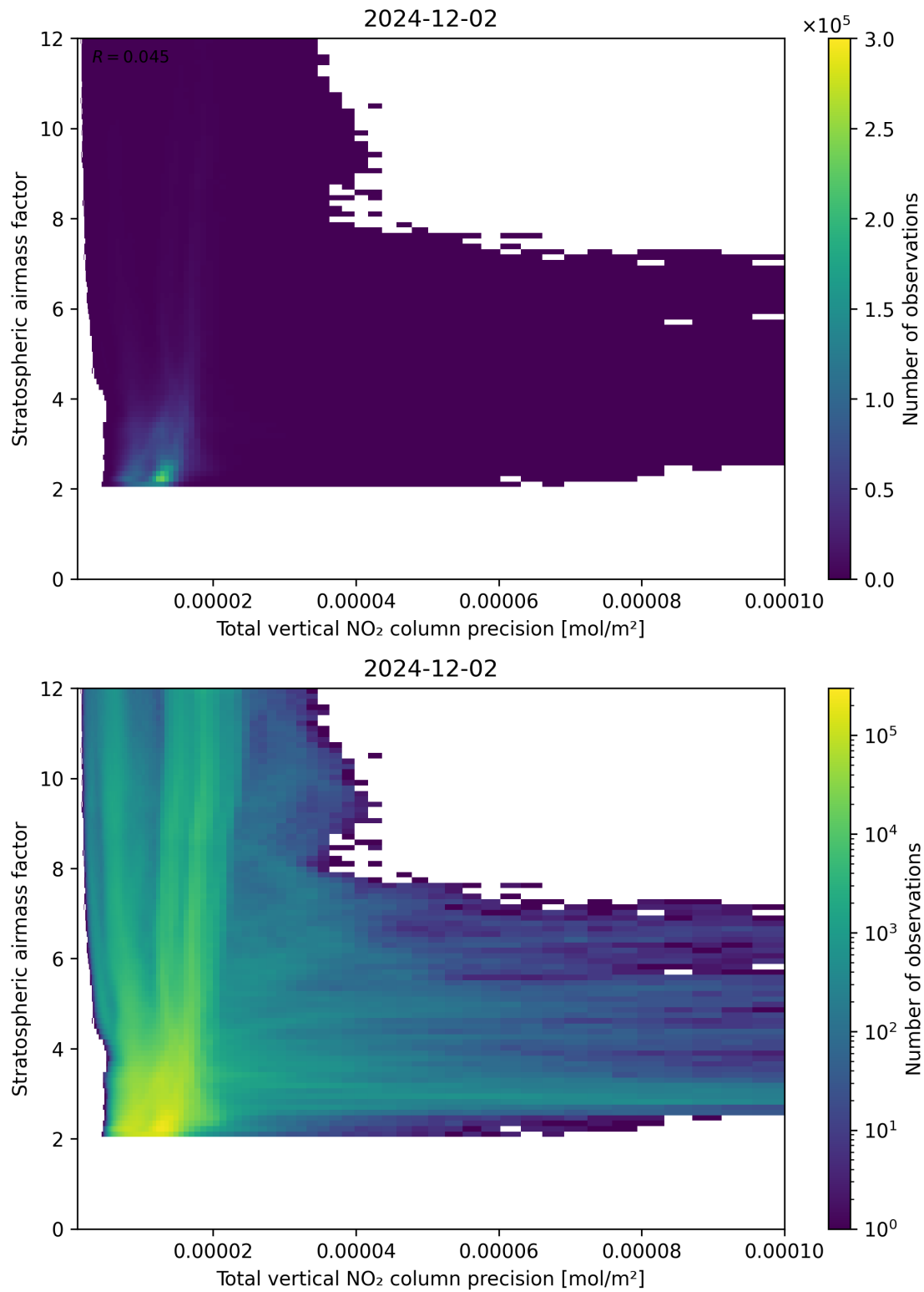
Figure 115: Scatter density plot of “Total vertical NO 2 column precision” against “Stratospheric air mass factor” for 2024-12-01 to 2024-12-03.
