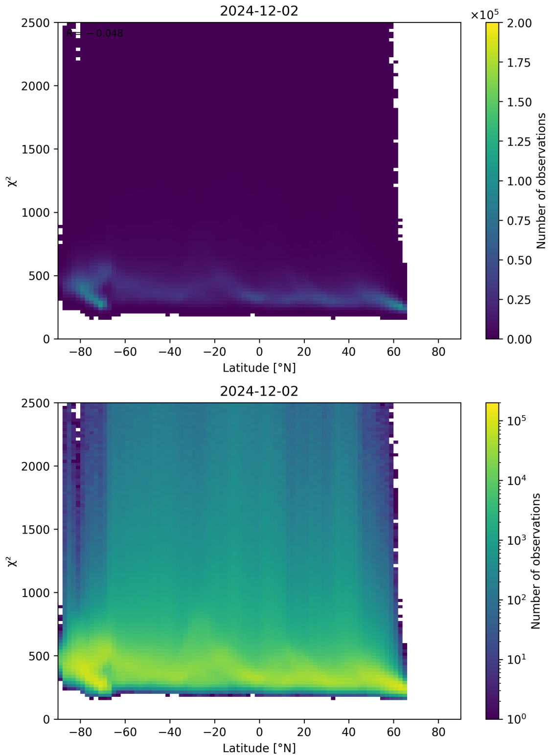
Figure 86: Scatter density plot of “Latitude” against “ \chi^2 ” for 2024-12-01 to 2024-12-03.
