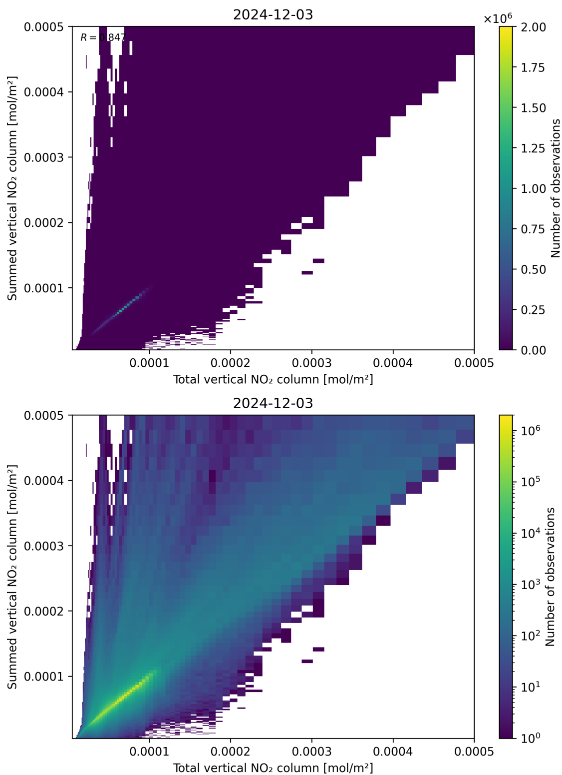
Figure 112: Scatter density plot of “Total vertical NO 2 column” against “Summed vertical NO 2 column” for 2024-12-02 to 2024-12-04.
