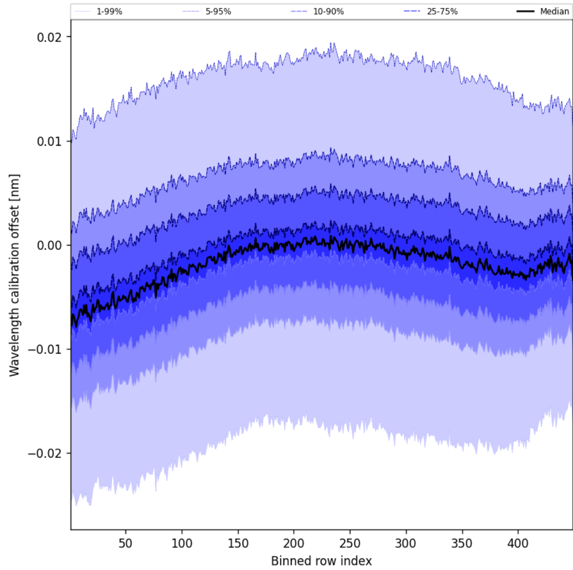
Figure 52: Along track statistics of “Wavelength calibration offset” for 2024-12-02 to 2024-12-04
