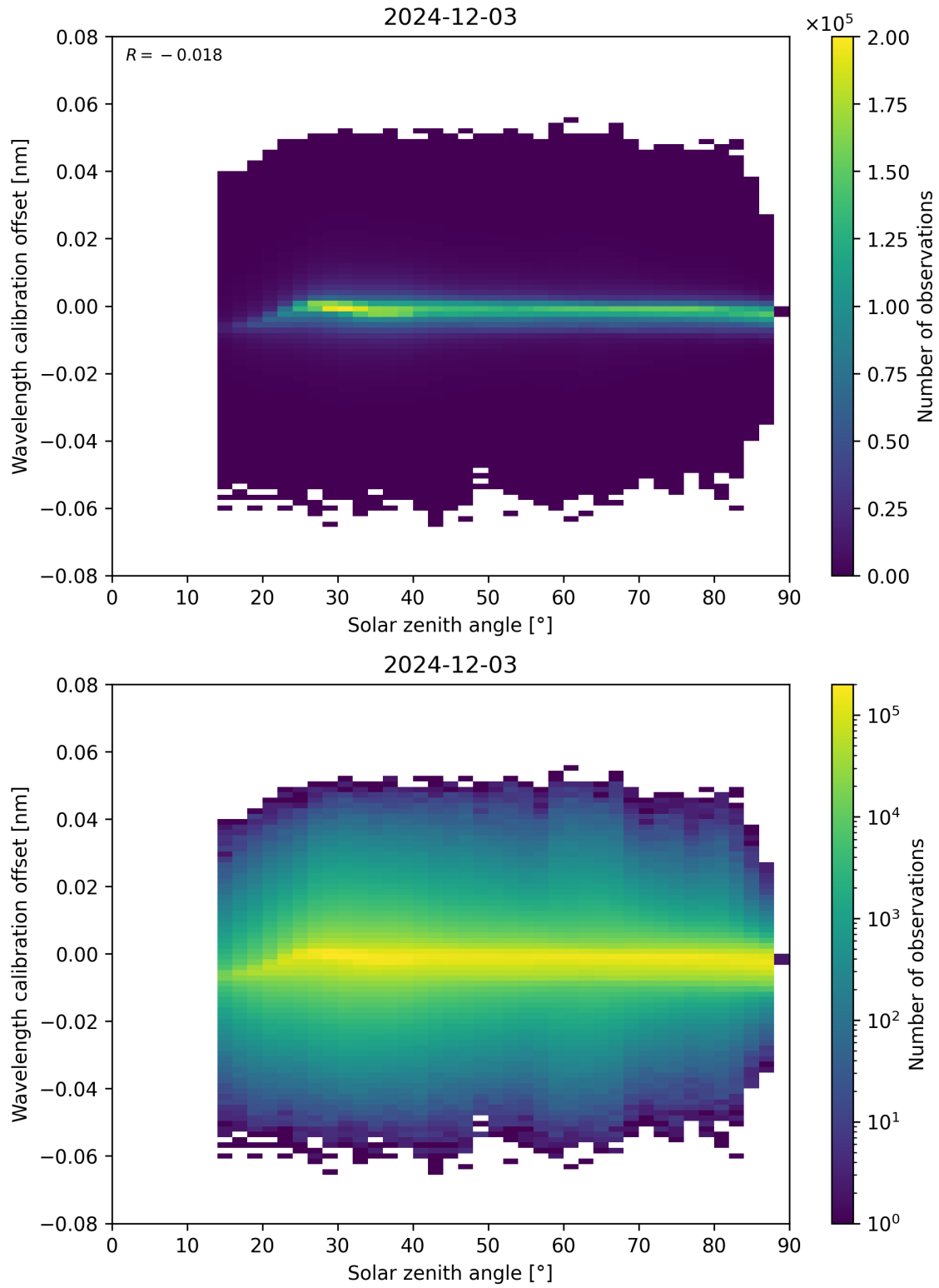
Figure 158: Scatter density plot of “Solar zenith angle” against “Wavelength calibration offset” for 2024-12-02 to 2024-12-04.
