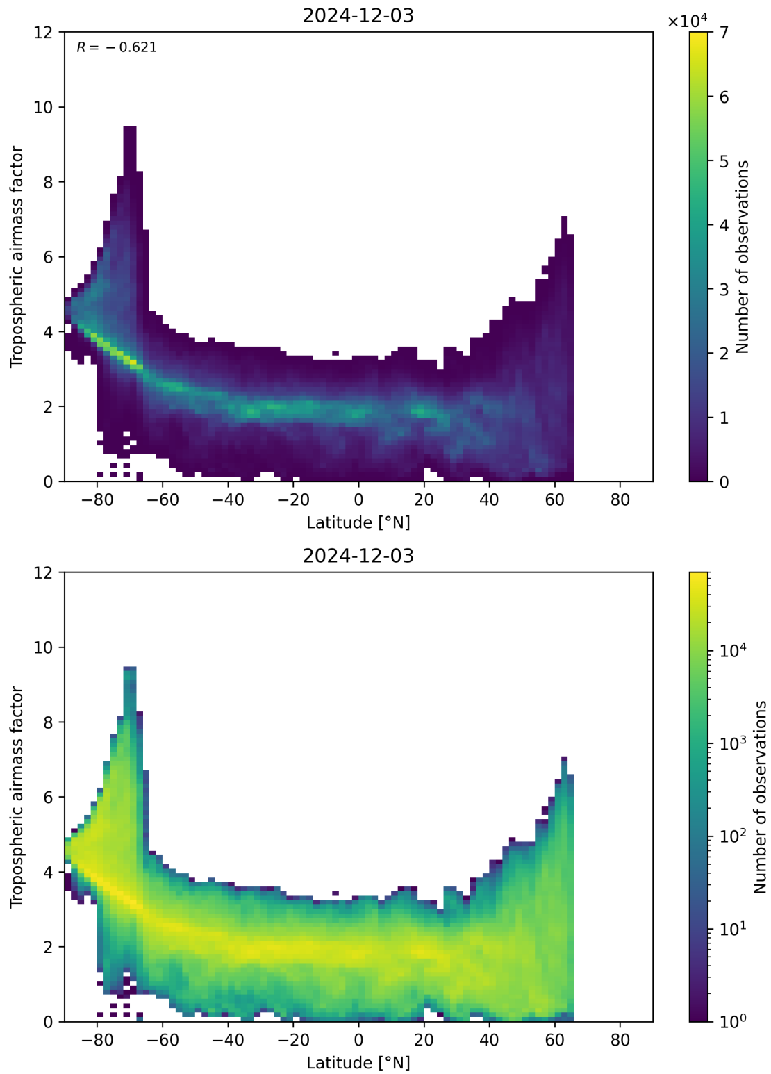
Figure 85: Scatter density plot of “Latitude” against “Tropospheric airmass factor” for 2024-12-02 to 2024-12-04.
