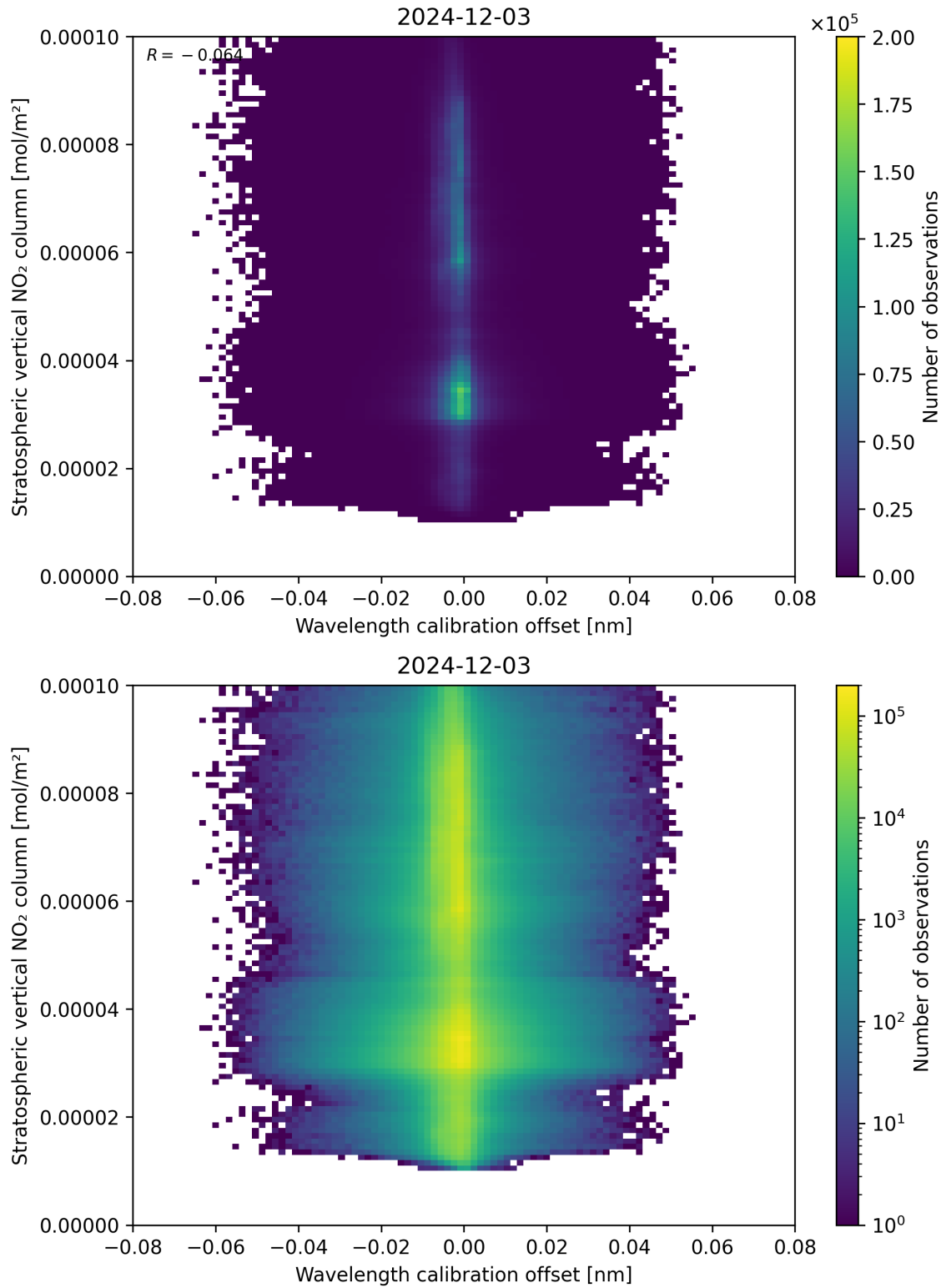
Figure 176: Scatter density plot of “Wavelength calibration offset” against “Stratospheric vertical NO 2 column” for 2024-12-02 to 2024-12-04.
