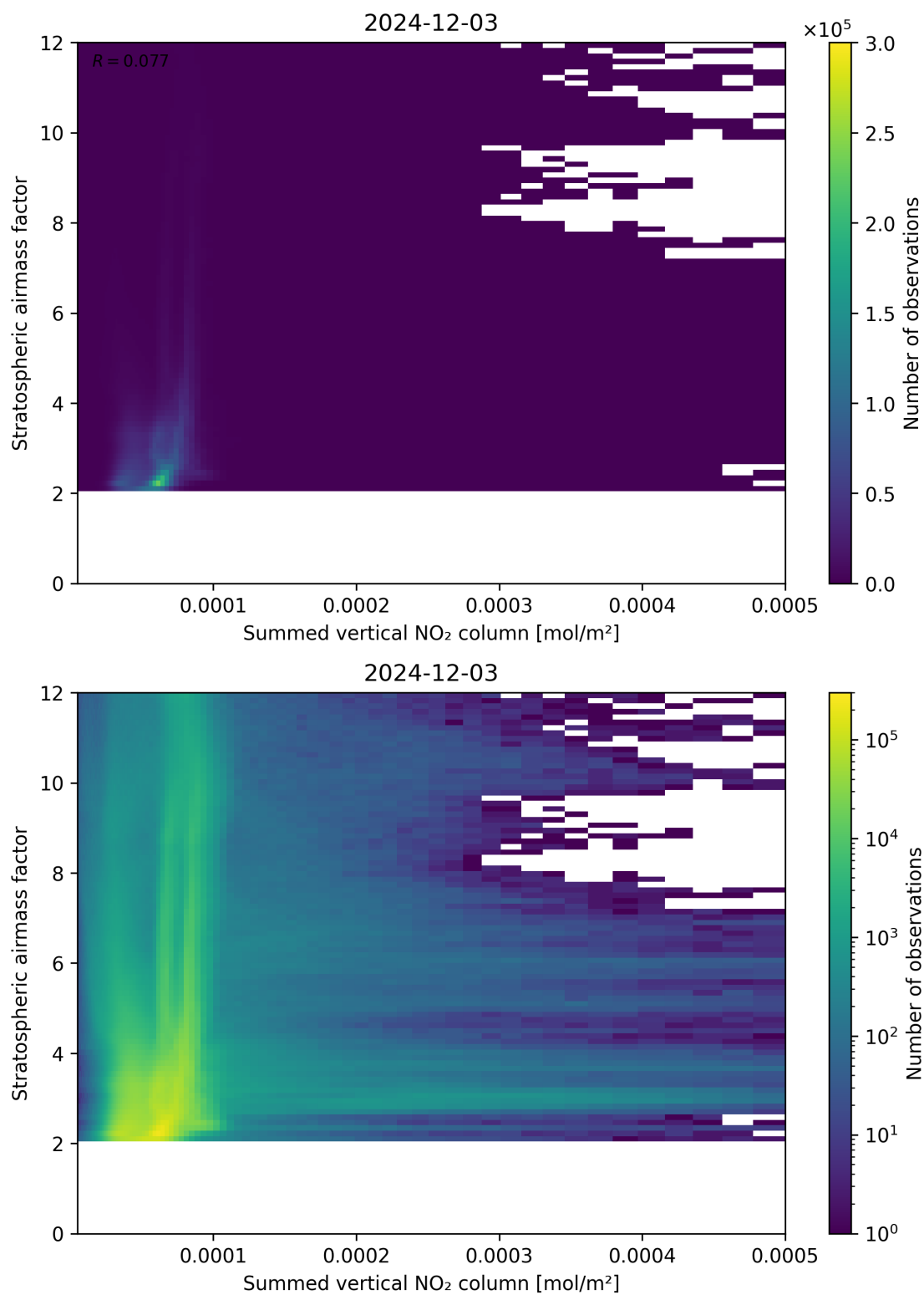
Figure 103: Scatter density plot of “Summed vertical NO 2 column” against “Stratospheric airmass factor” for 2024-12-02 to 2024-12-04.
