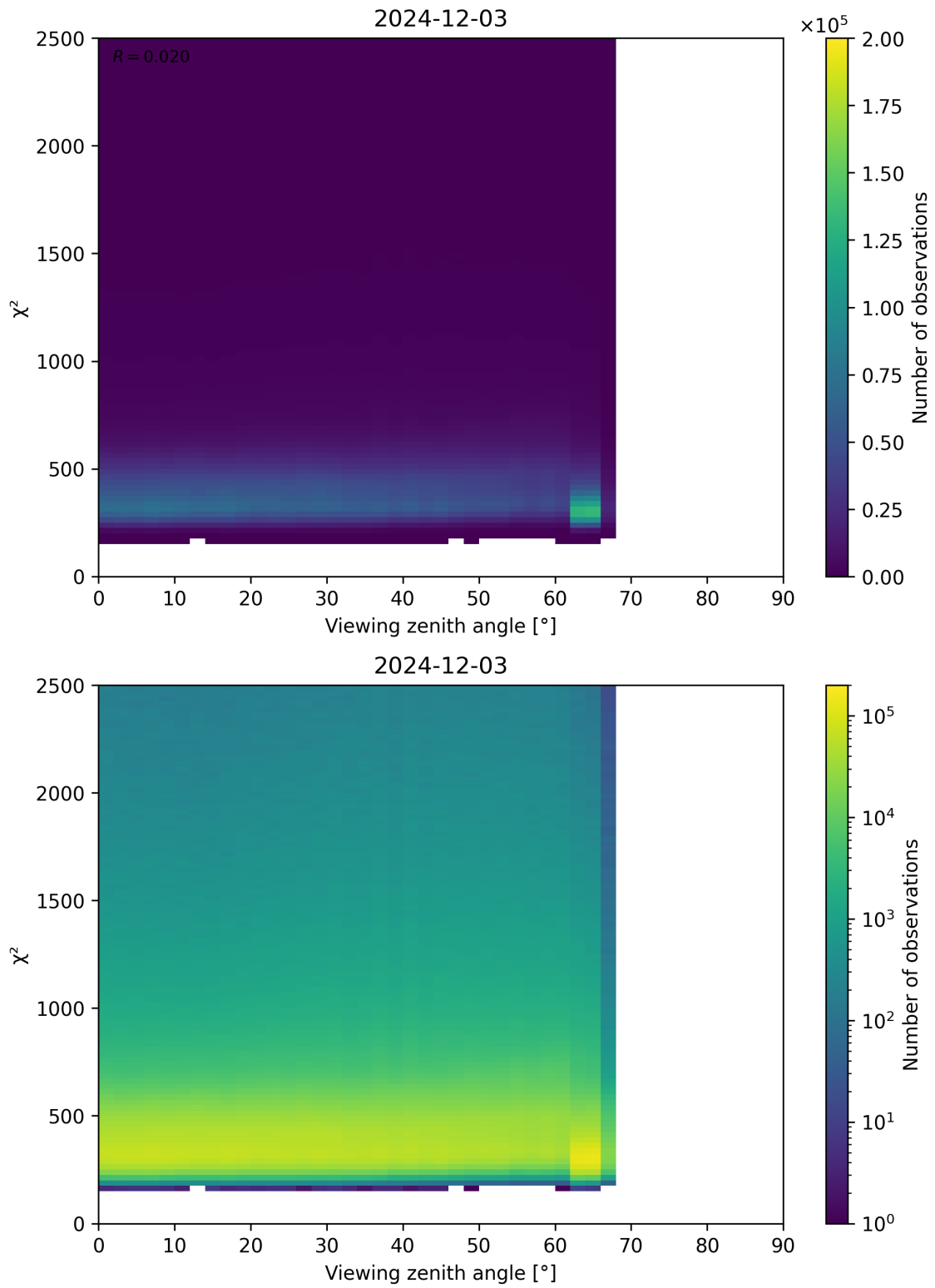
Figure 162: Scatter density plot of “Viewing zenith angle” against “ \chi^2 ” for 2024-12-02 to 2024-12-04.
