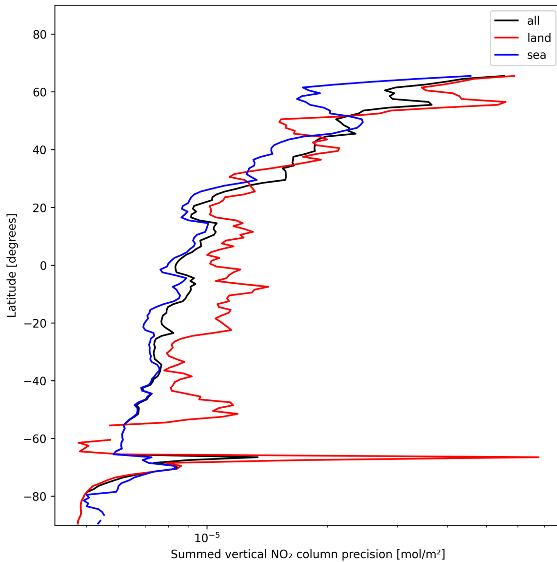
Figure 24: Zonal average of “Summed vertical NO 2 column precision” for 2024-12-02 to 2024-12-04.
