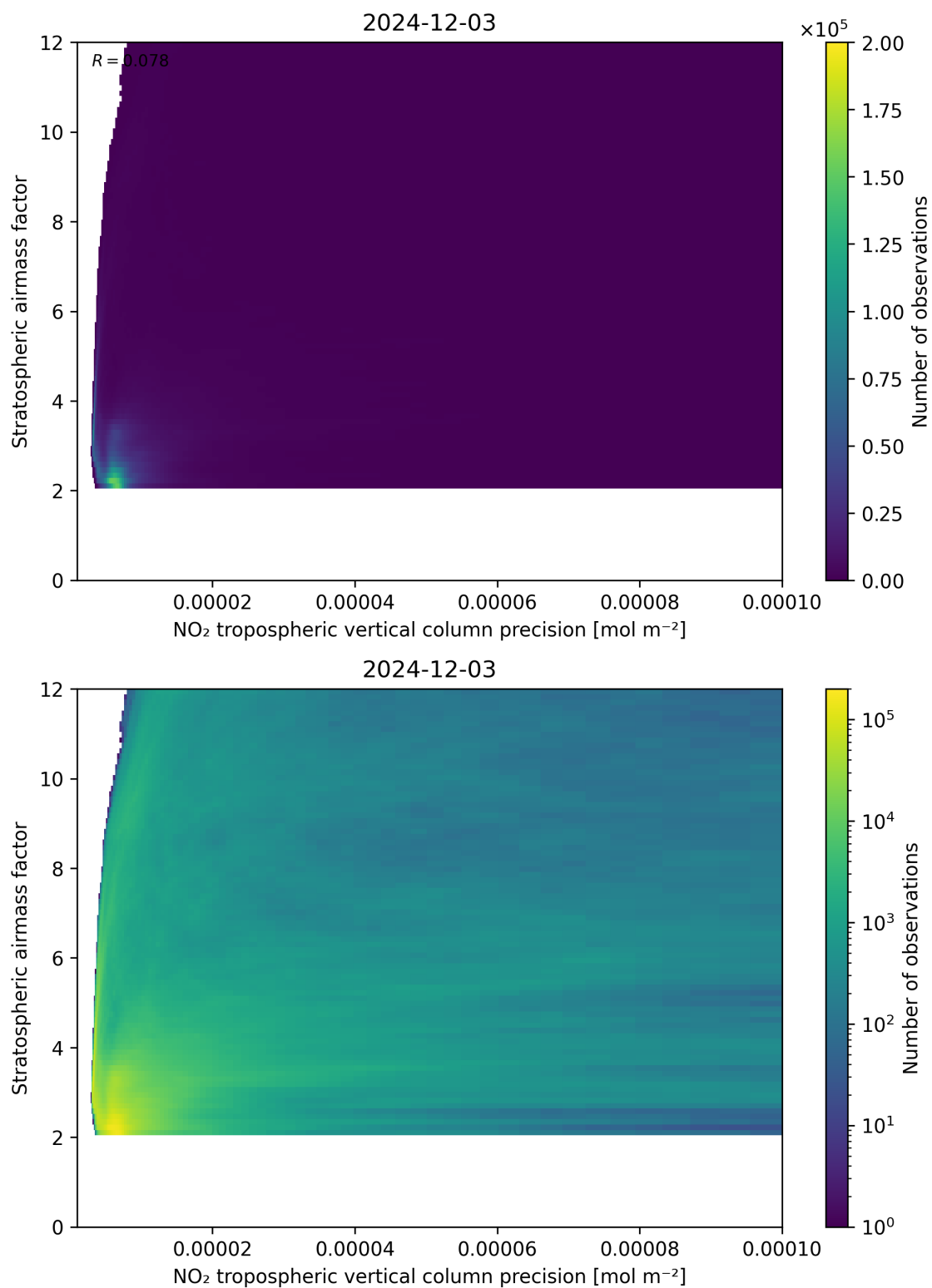
Figure 131: Scatter density plot of “NO 2 tropospheric vertical column precision” against “Stratospheric airmass factor” for 2024-12-02 to 2024-12-04.
