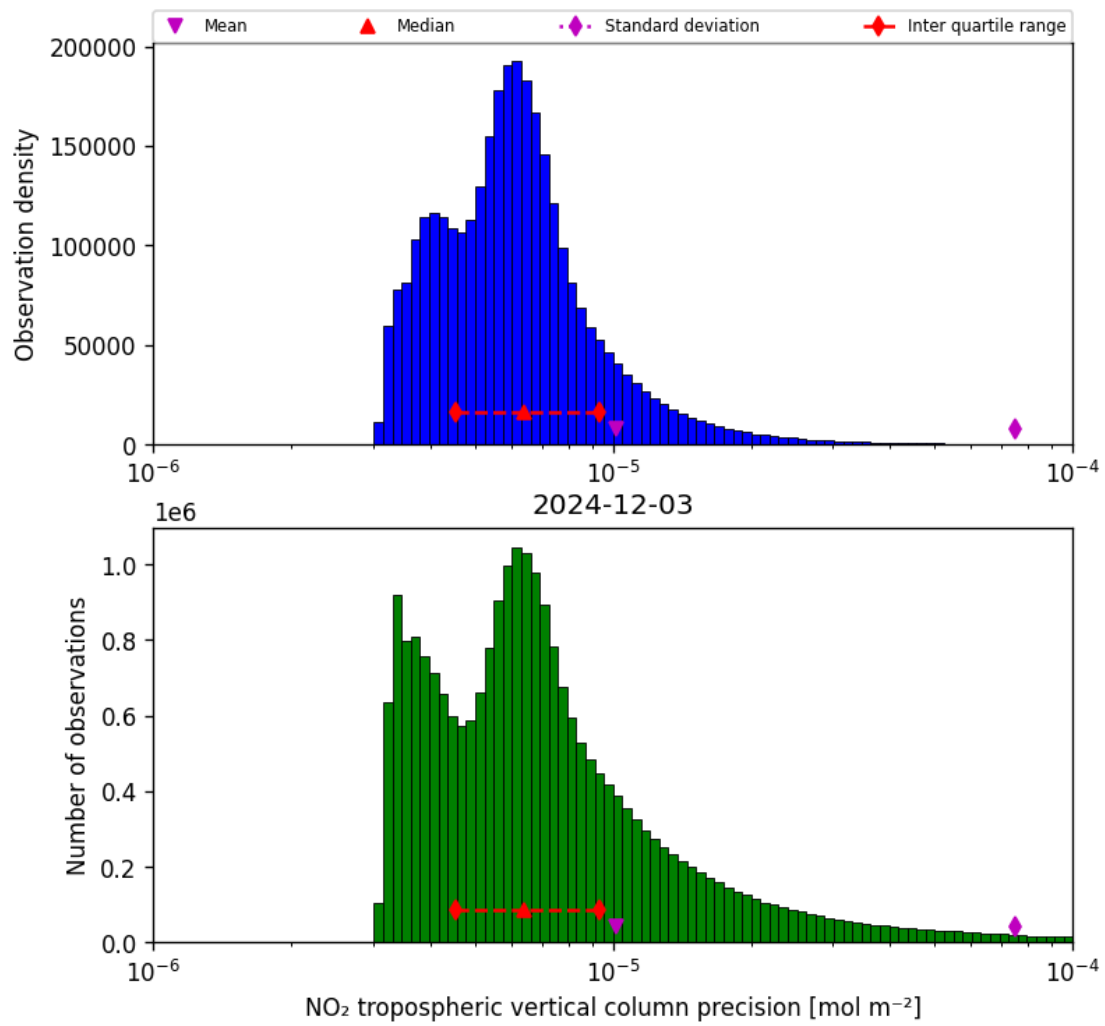
Figure 30: Histogram of “NO 2 tropospheric vertical column precision” for 2024-12-02 to 2024-12-04
