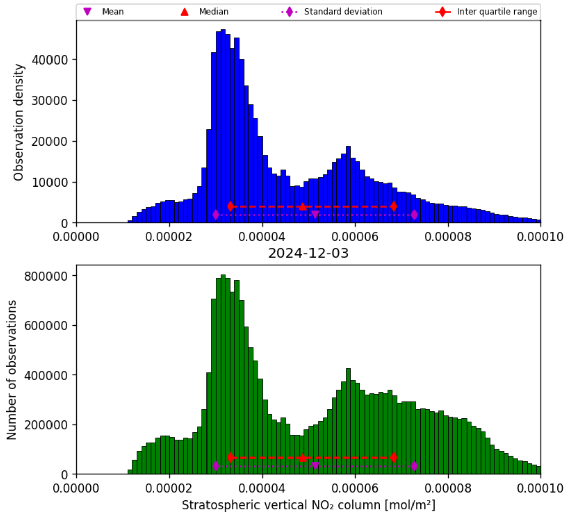
Figure 36: Histogram of “Stratospheric vertical NO 2 column” for 2024-12-02 to 2024-12-04
