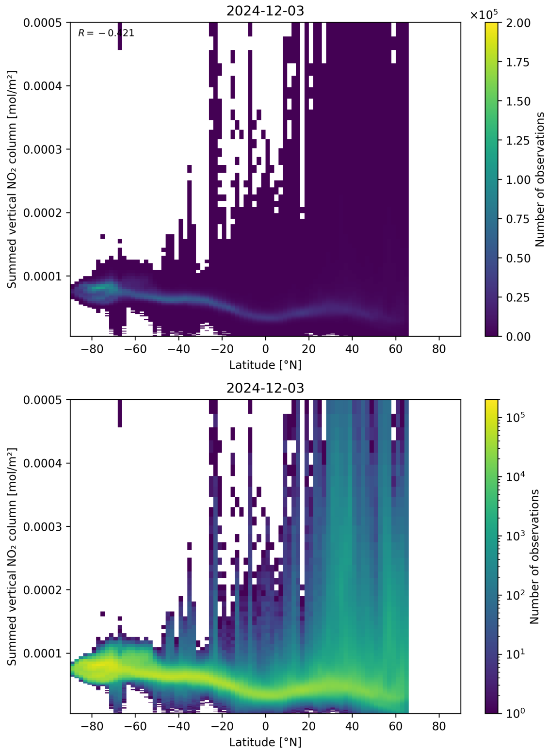
Figure 88: Scatter density plot of “Latitude” against “Summed vertical NO 2 column” for 2024-12-02 to 2024-12-04.
