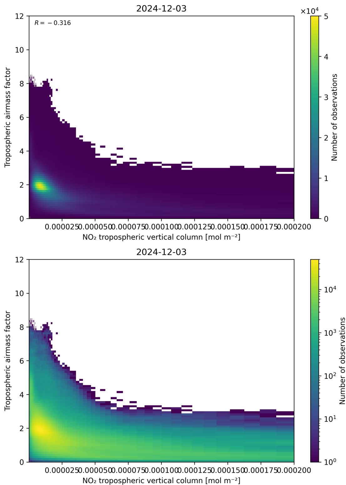
Figure 123: Scatter density plot of “NO 2 tropospheric vertical column” against “Tropospheric air mass factor” for 2024-12-02 to 2024-12-04.
