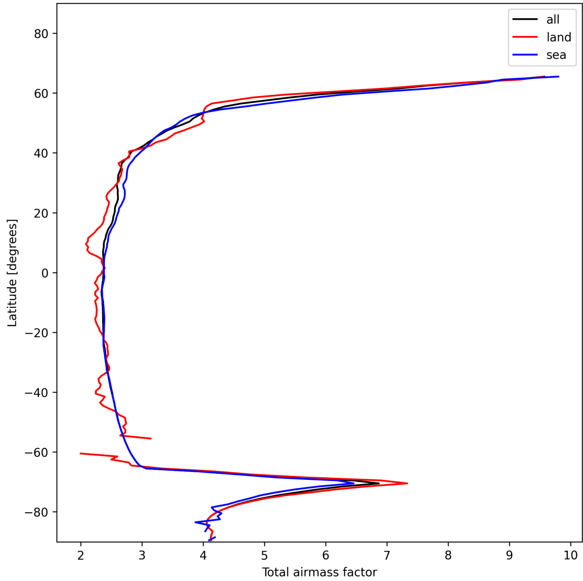
Figure 15: Zonal average of “Total airmass factor” for 2024-12-02 to 2024-12-04.
