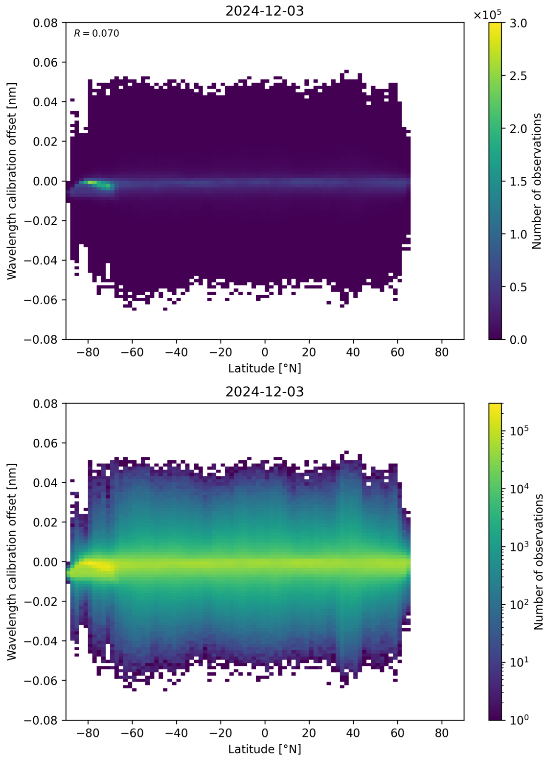
Figure 95: Scatter density plot of “Latitude” against “Wavelength calibration offset” for 2024-12-02 to 2024-12-04.
