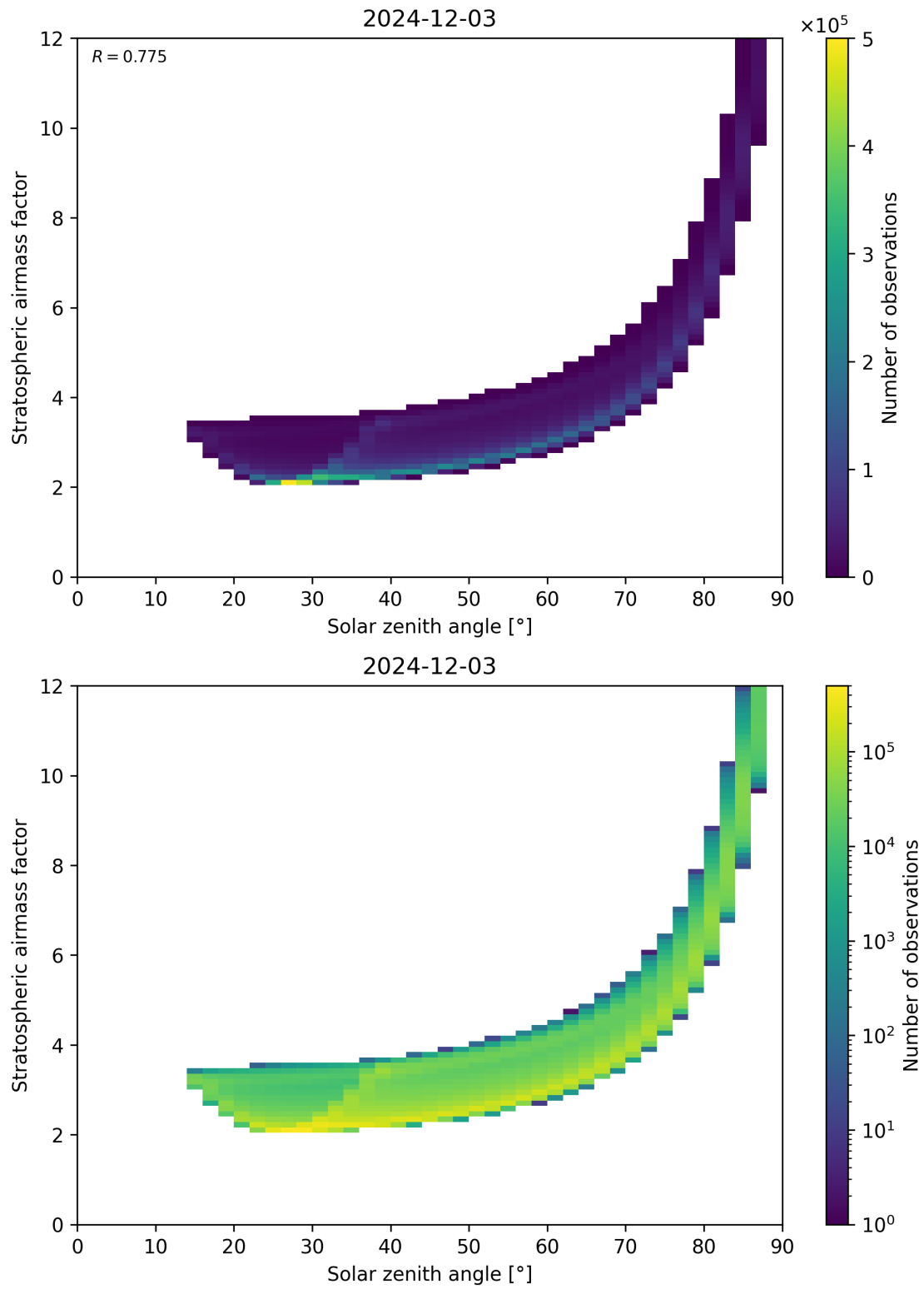
Figure 145: Scatter density plot of “Solar zenith angle” against “Stratospheric airmass factor” for 2024-12-02 to 2024-12-04.
