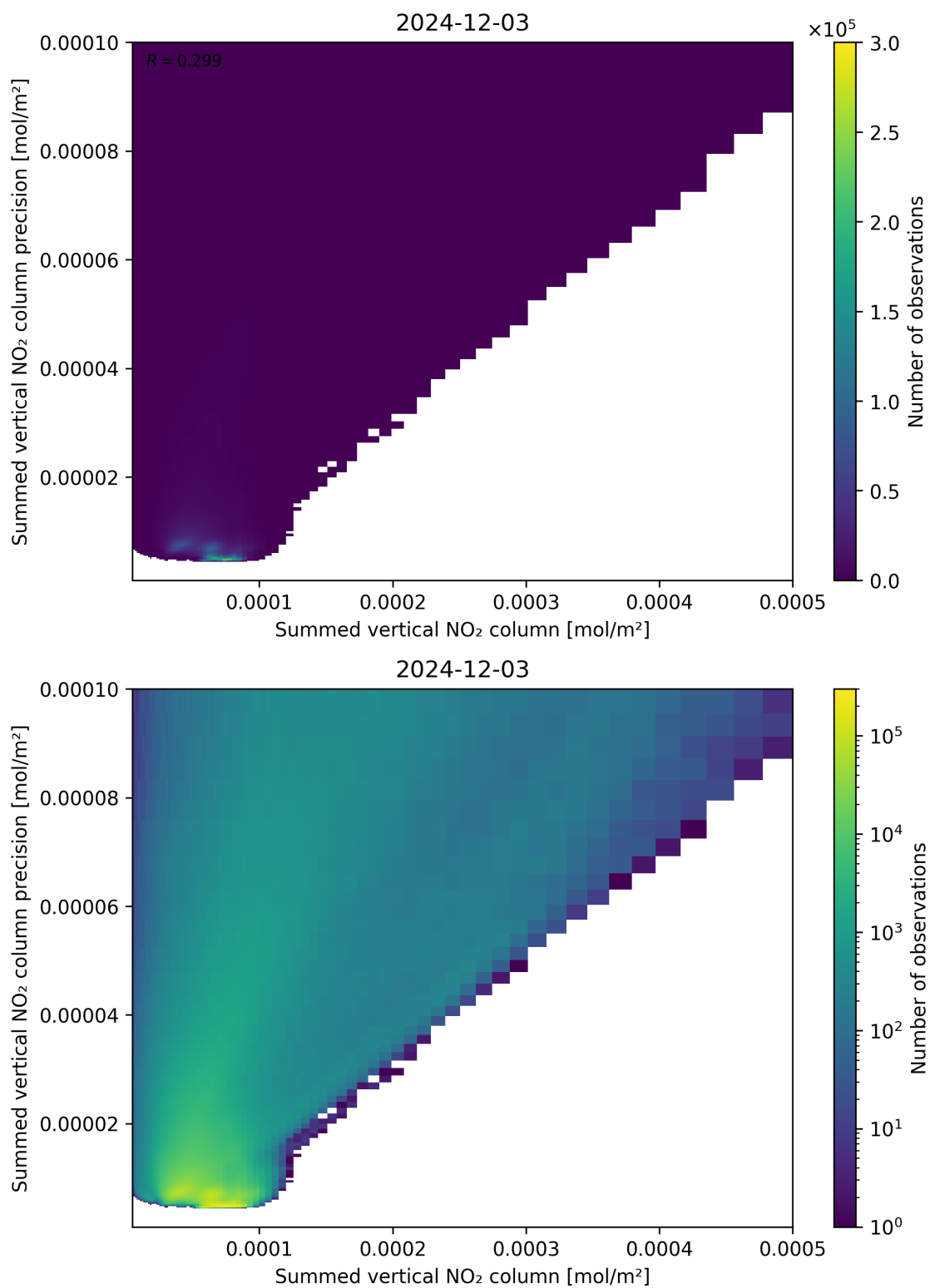
Figure 105: Scatter density plot of “Summed vertical NO 2 column” against “Summed vertical NO 2 column precision” for 2024-12-02 to 2024-12-04.
