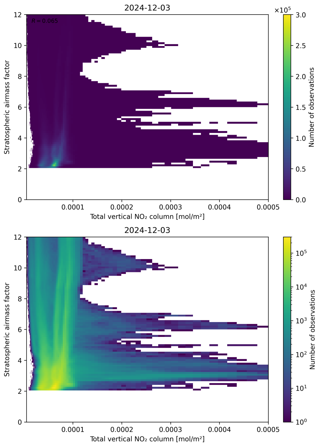
Figure 110: Scatter density plot of “Total vertical NO 2 column” against “Stratospheric airmass factor” for 2024-12-02 to 2024-12-04.
