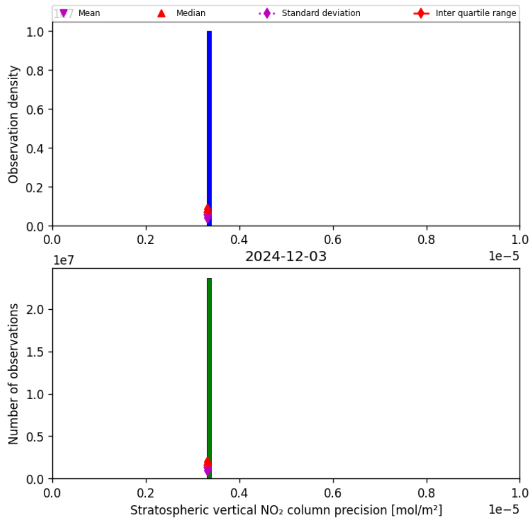
Figure 37: Histogram of “Stratospheric vertical NO 2 column precision” for 2024-12-02 to 2024-12-04
