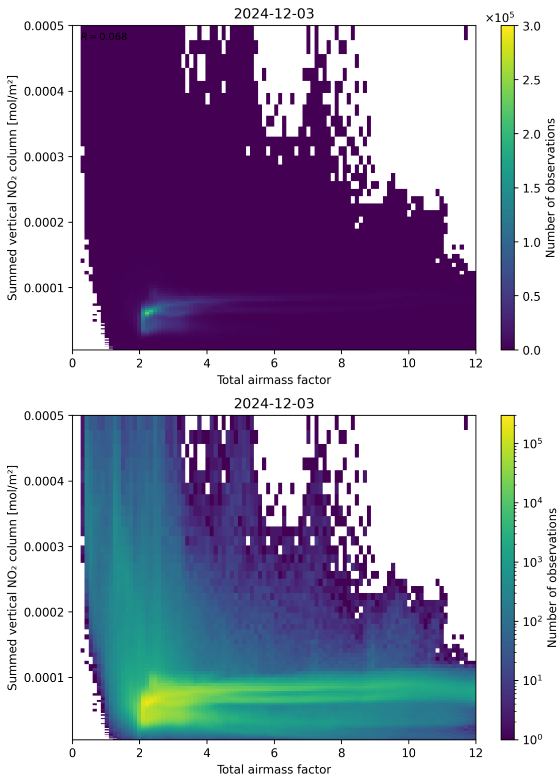
Figure 65: Scatter density plot of “Total airmass factor” against “Summed vertical NO 2 column” for 2024-12-02 to 2024-12-04.
