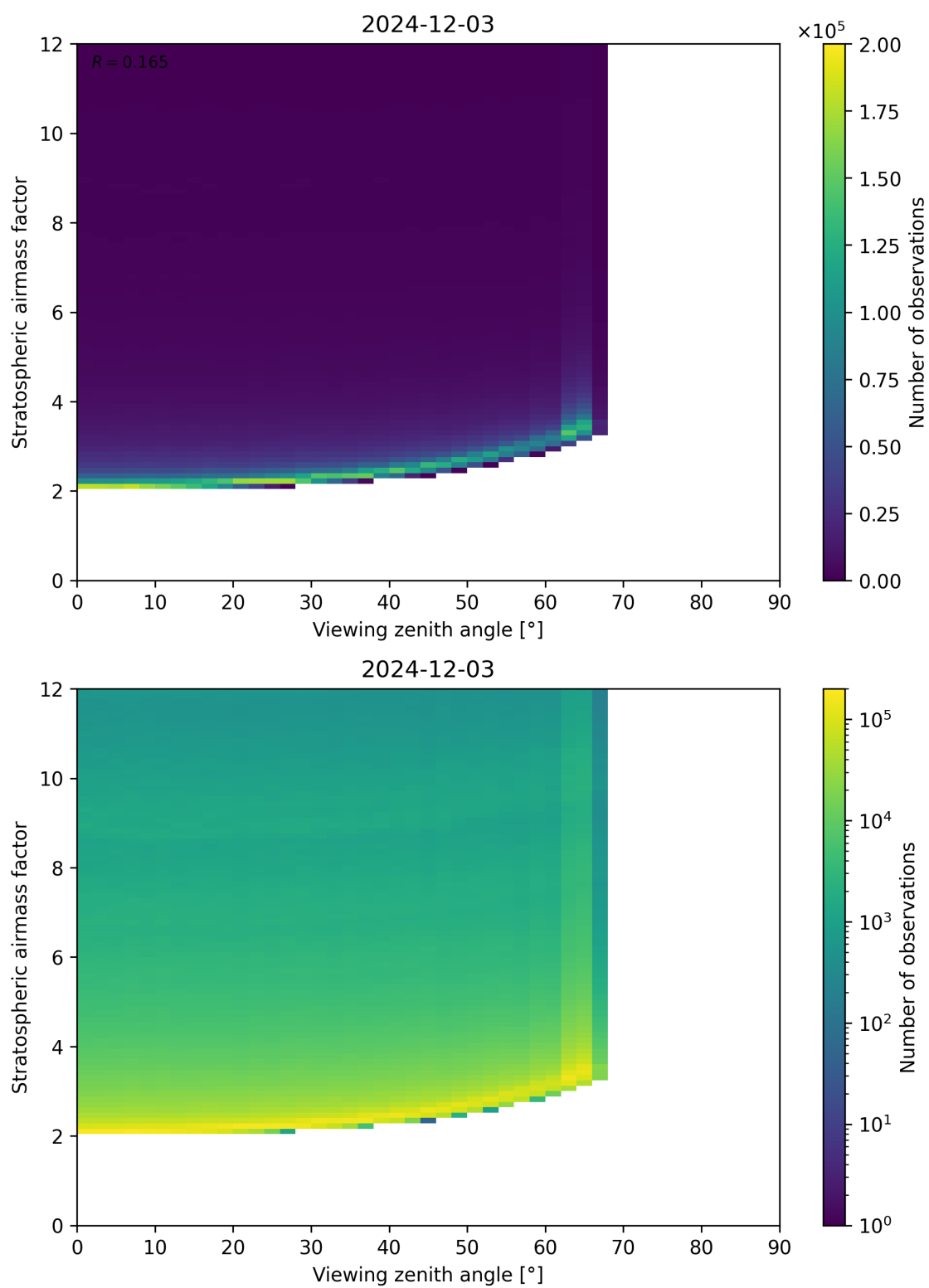
Figure 159: Scatter density plot of “Viewing zenith angle” against “Stratospheric airmass factor” for 2024-12-02 to 2024-12-04.
