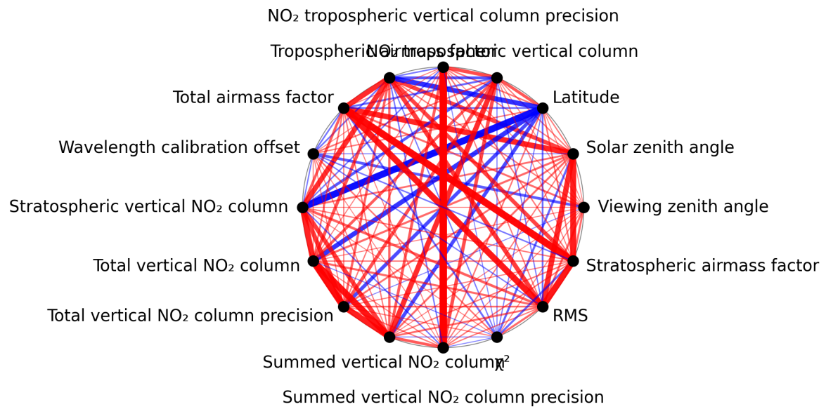
Figure 1: Map of correlation graph for 2024-12-02 to 2024-12-04.
