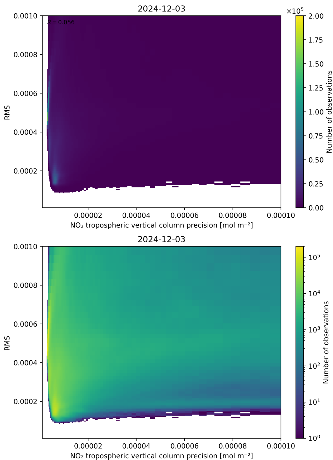
Figure 140: Scatter density plot of “NO 2 tropospheric vertical column precision” against “RMS” for 2024-12-02 to 2024-12-04.
