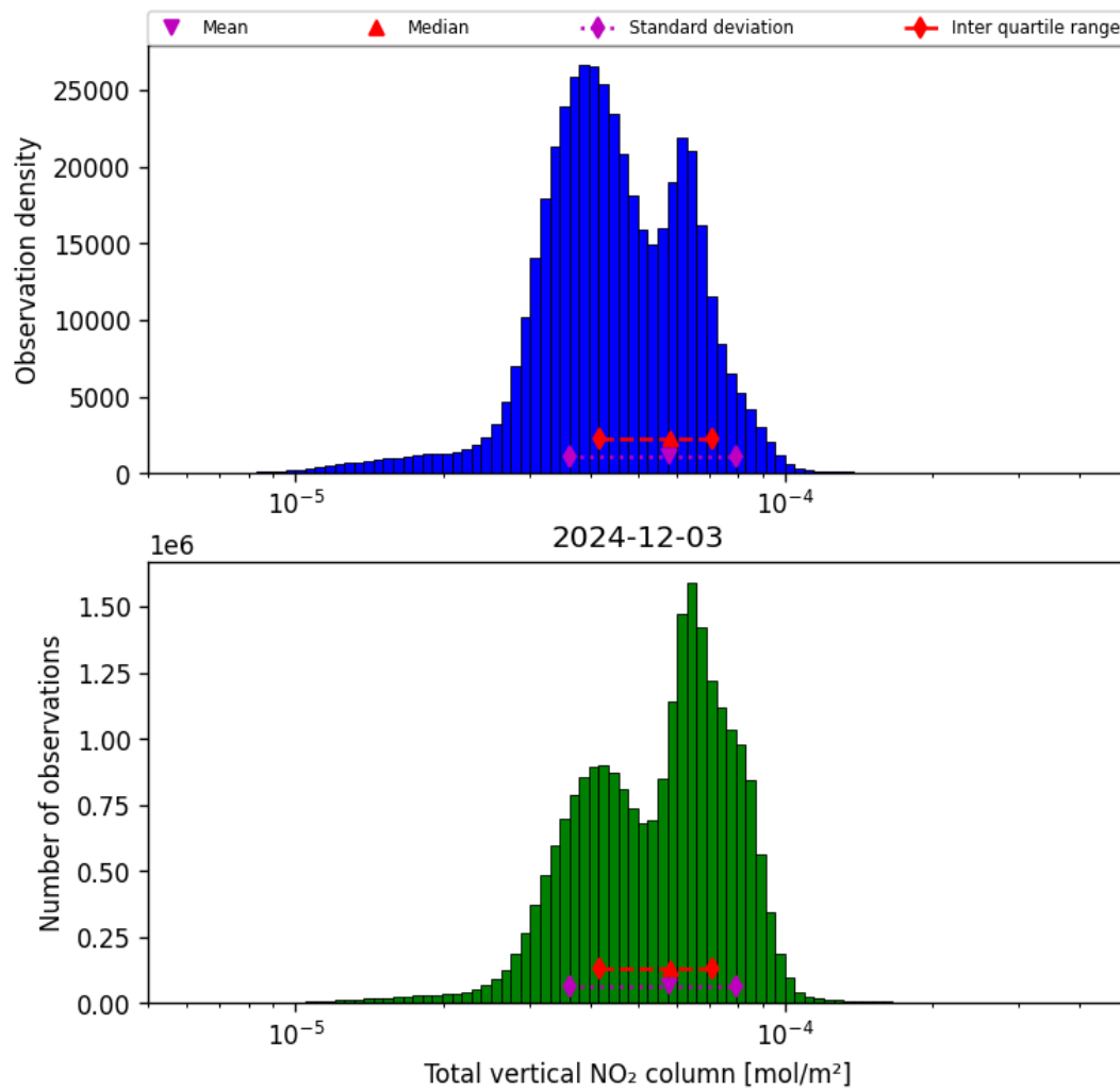
Figure 38: Histogram of “Total vertical NO 2 column” for 2024-12-02 to 2024-12-04
