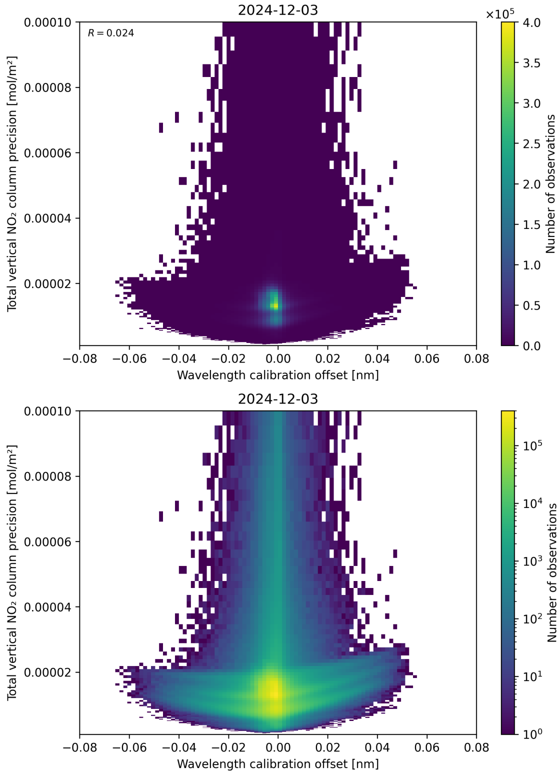
Figure 180: Scatter density plot of “Wavelength calibration offset” against “Total vertical NO 2 column precision” for 2024-12-02 to 2024-12-04.
