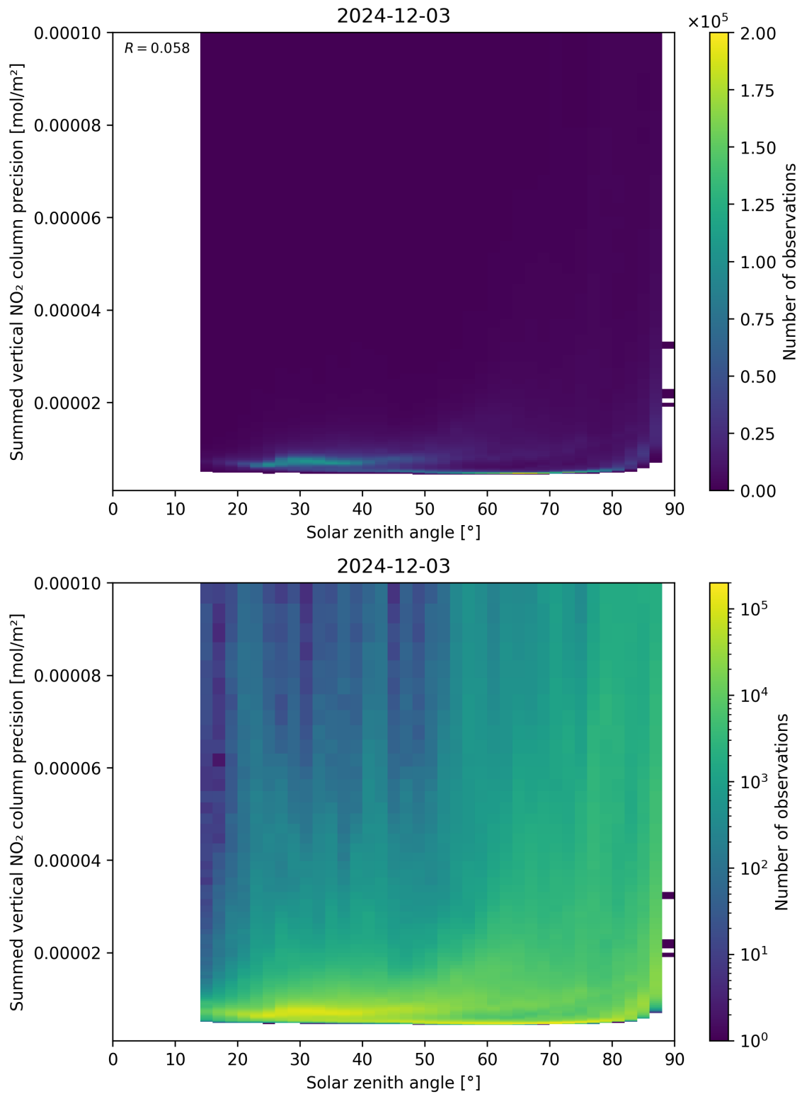
Figure 152: Scatter density plot of “Solar zenith angle” against “Summed vertical NO 2 column precision” for 2024-12-02 to 2024-12-04.
