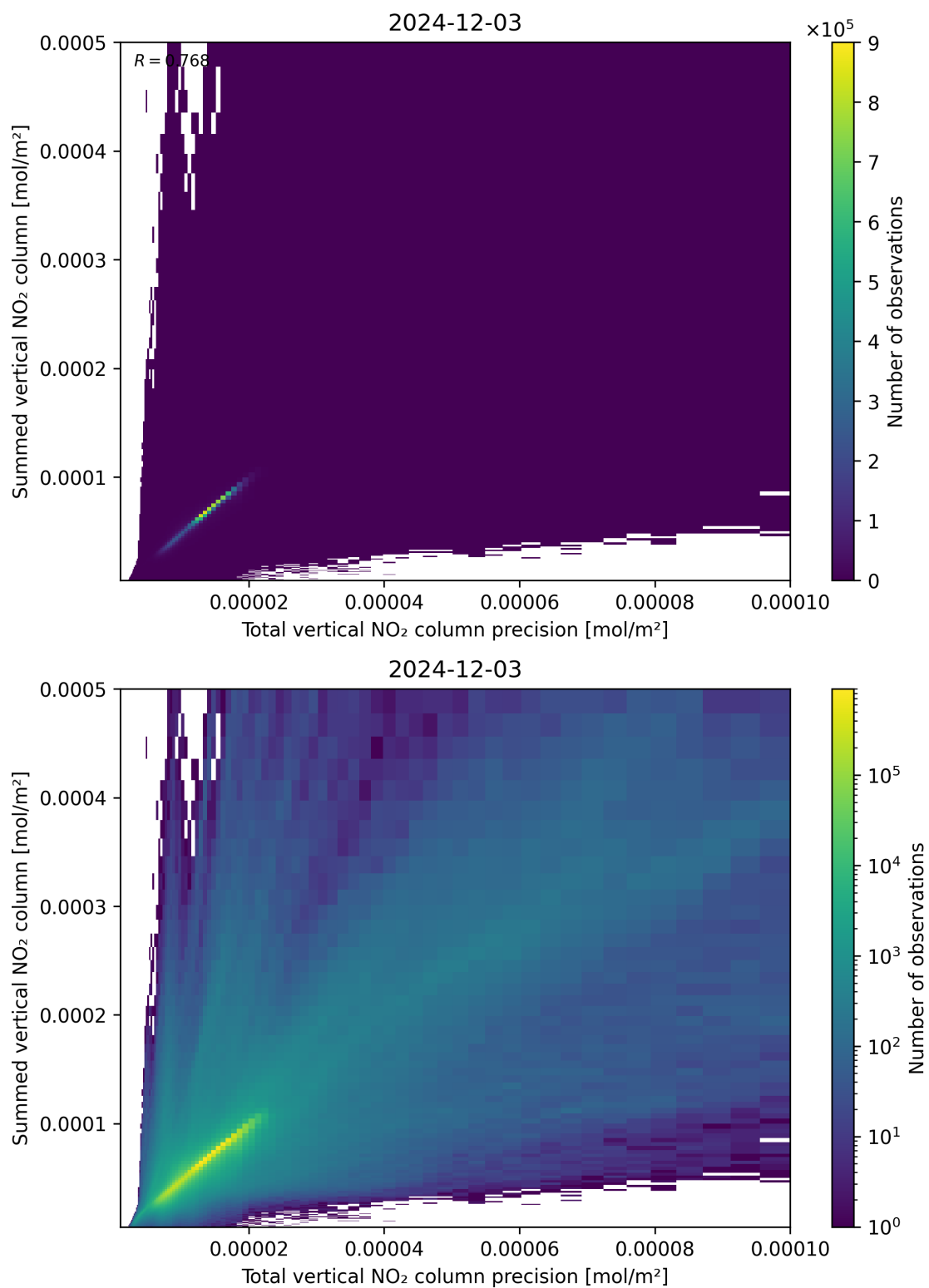
Figure 117: Scatter density plot of “Total vertical NO 2 column precision” against “Summed vertical NO 2 column” for 2024-12-02 to 2024-12-04.
