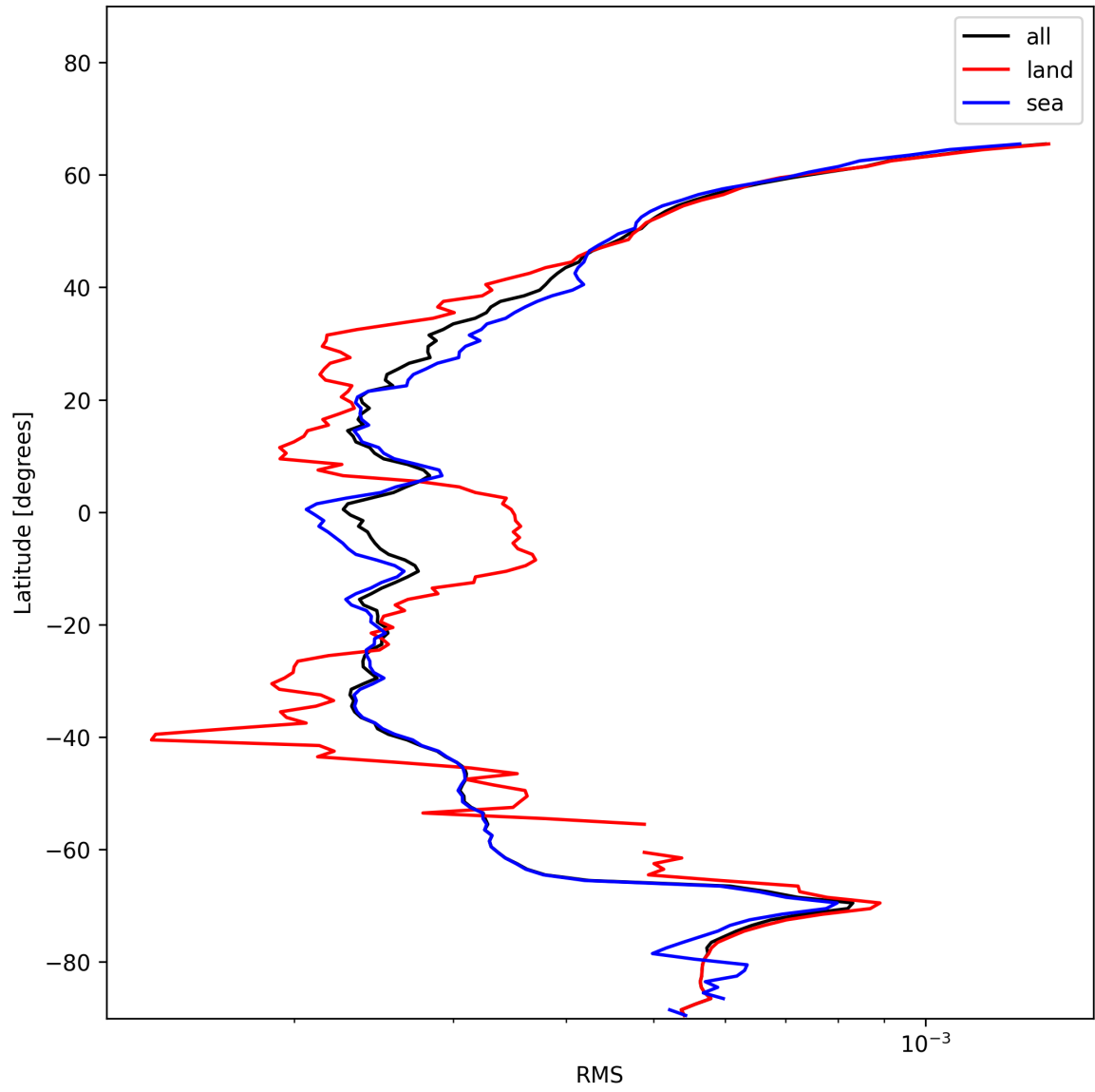
Figure 26: Zonal average of “RMS” for 2024-12-02 to 2024-12-04.
