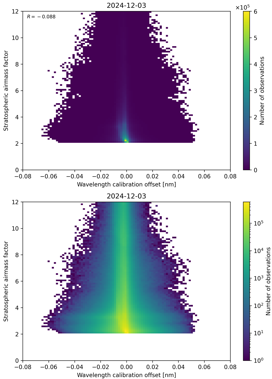
Figure 174: Scatter density plot of “Wavelength calibration offset” against “Stratospheric airmass factor” for 2024-12-02 to 2024-12-04.
