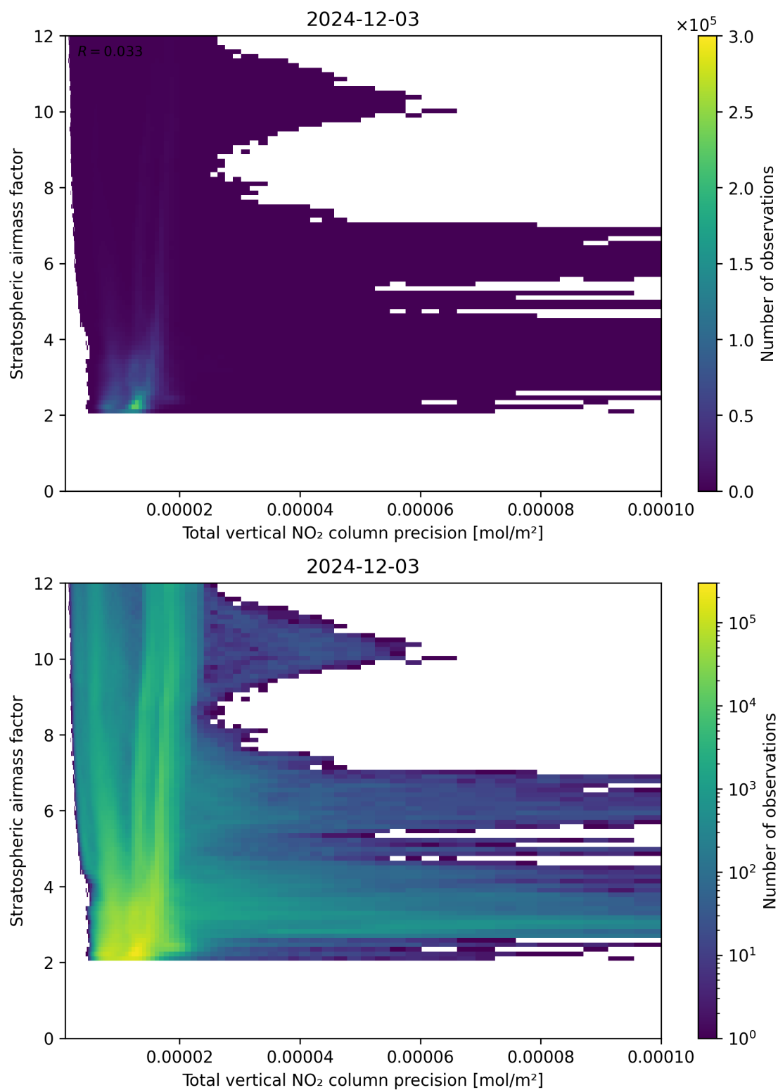
Figure 115: Scatter density plot of “Total vertical NO 2 column precision” against “Stratospheric air mass factor” for 2024-12-02 to 2024-12-04.
