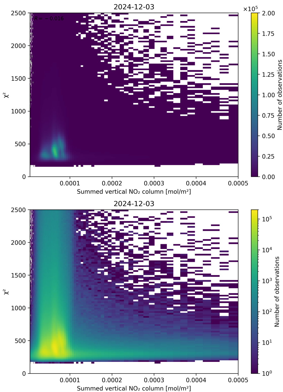
Figure 104: Scatter density plot of “Summed vertical NO 2 column” against “ \chi^2 ” for 2024-12-02 to 2024-12-04.
