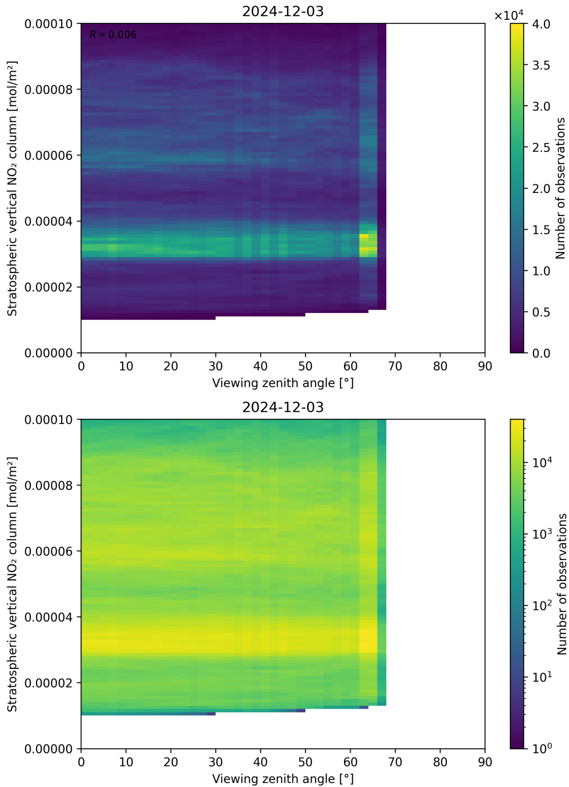
Figure 164: Scatter density plot of “Viewing zenith angle” against “Stratospheric vertical NO 2 column” for 2024-12-02 to 2024-12-04.
