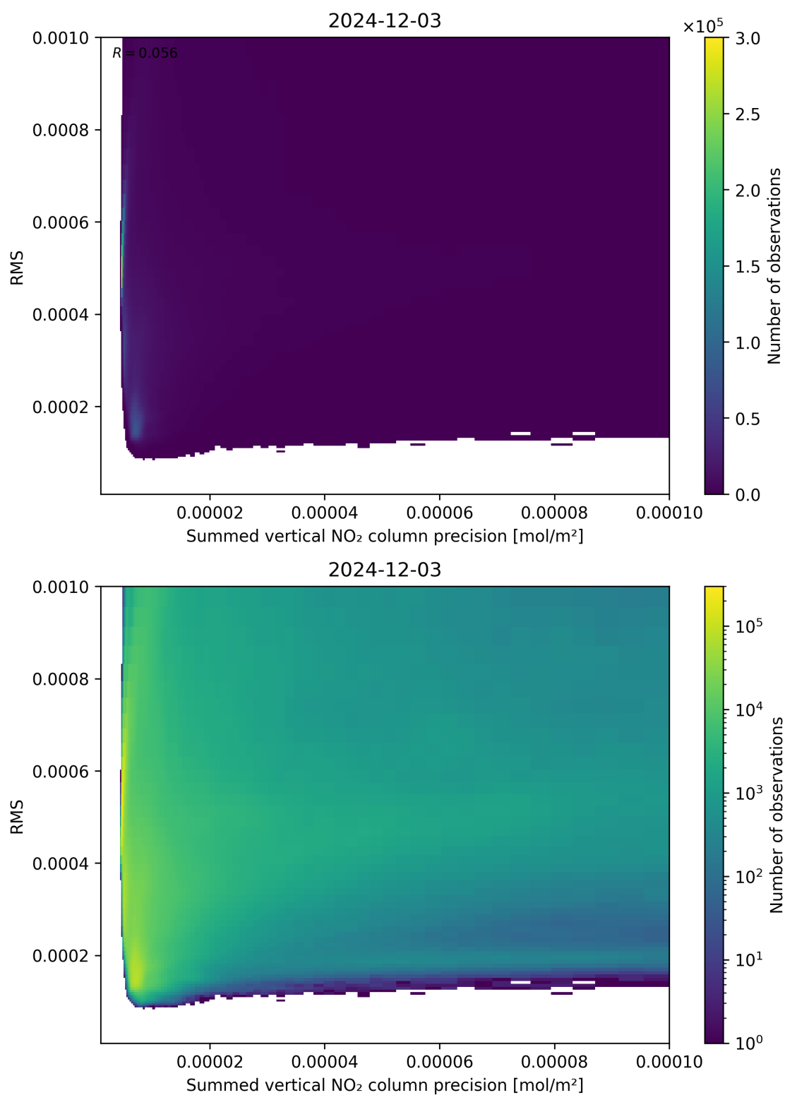
Figure 108: Scatter density plot of “Summed vertical NO 2 column precision” against “RMS” for 2024-12-02 to 2024-12-04.
