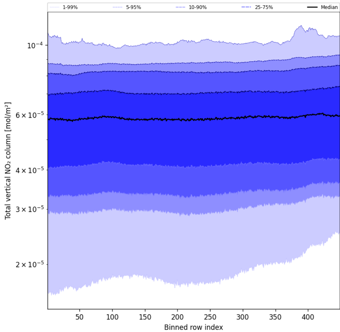
Figure 55: Along track statistics of “Total vertical NO 2 column” for 2024-12-02 to 2024-12-04
