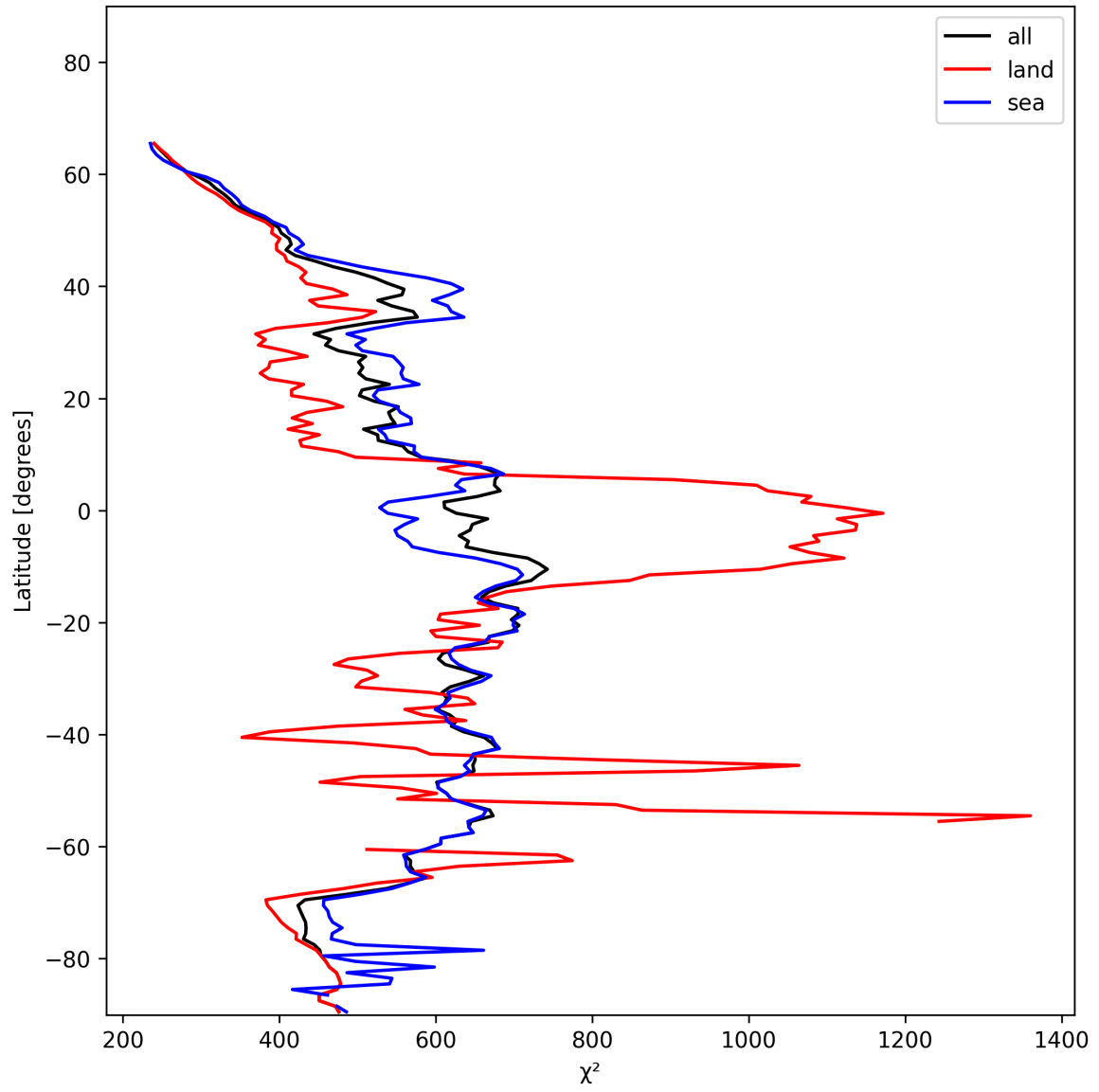
Figure 25: Zonal average of “ \chi^2 ” for 2024-12-02 to 2024-12-04.
