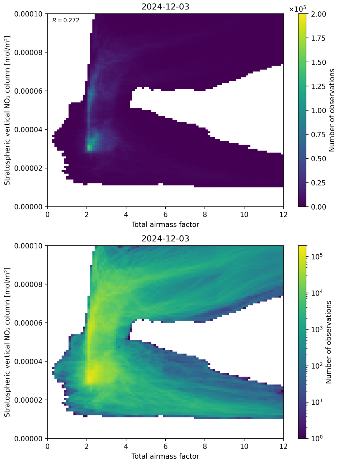
Figure 64: Scatter density plot of “Total airmass factor” against “Stratospheric vertical \text{NO}_2 column” for 2024-12-02 to 2024-12-04.
