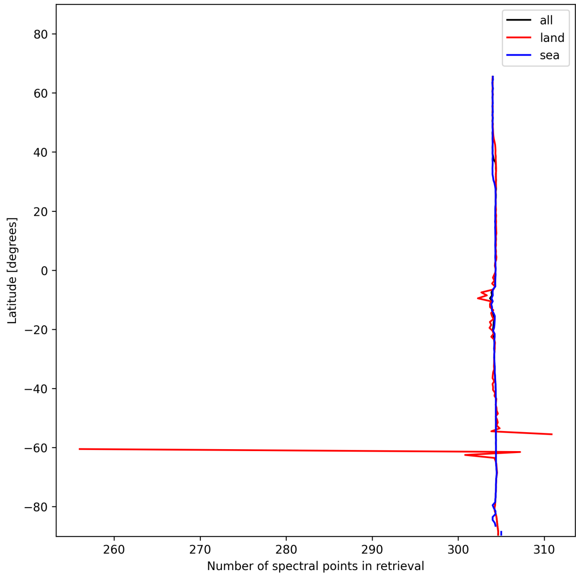
Figure 16: Zonal average of “Number of spectral points in retrieval” for 2024-12-02 to 2024-12-04.
