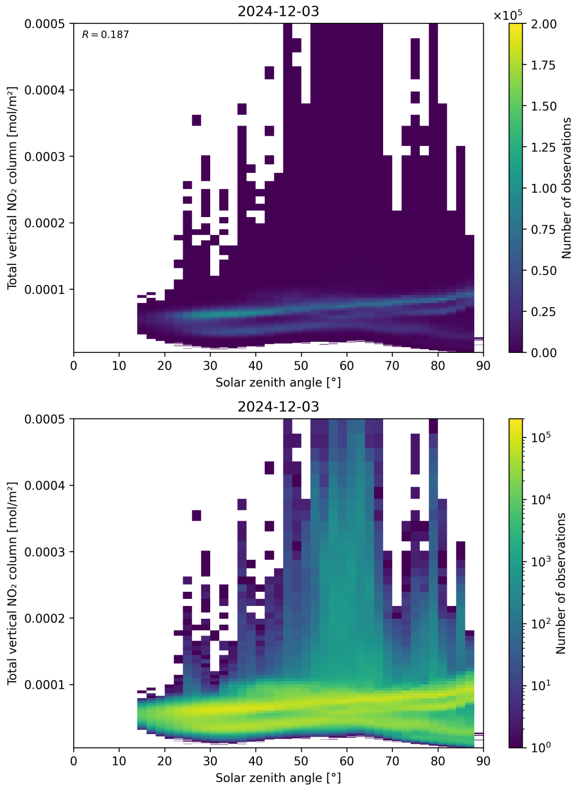
Figure 153: Scatter density plot of “Solar zenith angle” against “Total vertical NO 2 column” for 2024-12-02 to 2024-12-04.
