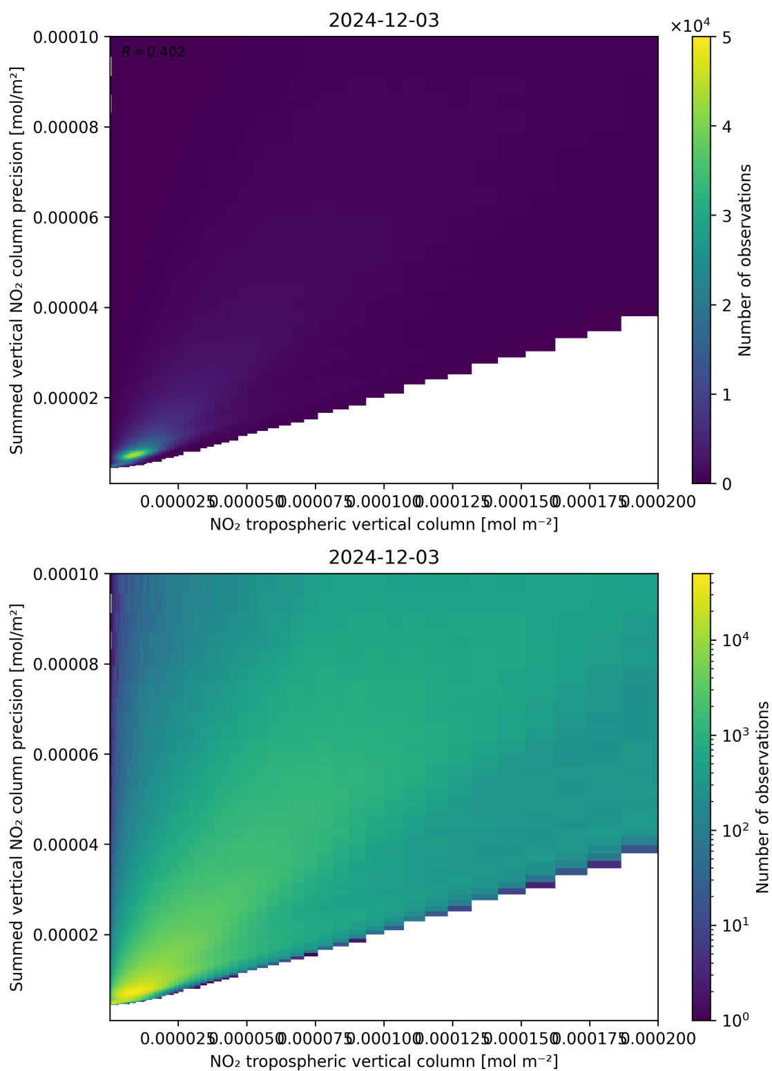
Figure 127: Scatter density plot of “NO 2 tropospheric vertical column” against “Summed vertical NO 2 column precision” for 2024-12-02 to 2024-12-04.
