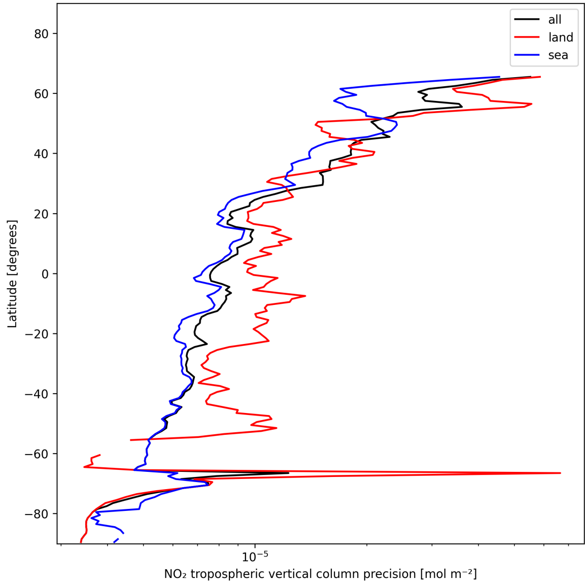
Figure 13: Zonal average of “NO 2 tropospheric vertical column precision” for 2024-12-02 to 2024-12-04.
