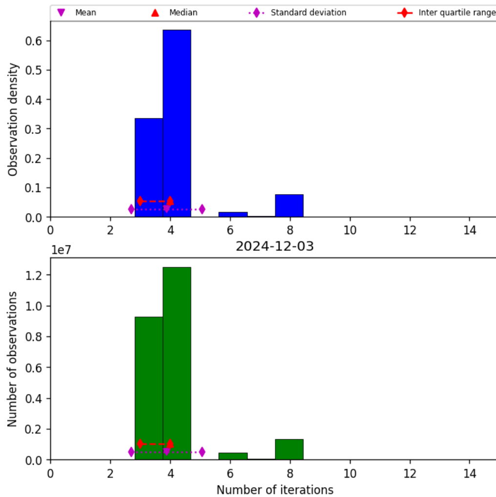
Figure 34: Histogram of “Number of iterations” for 2024-12-02 to 2024-12-04
