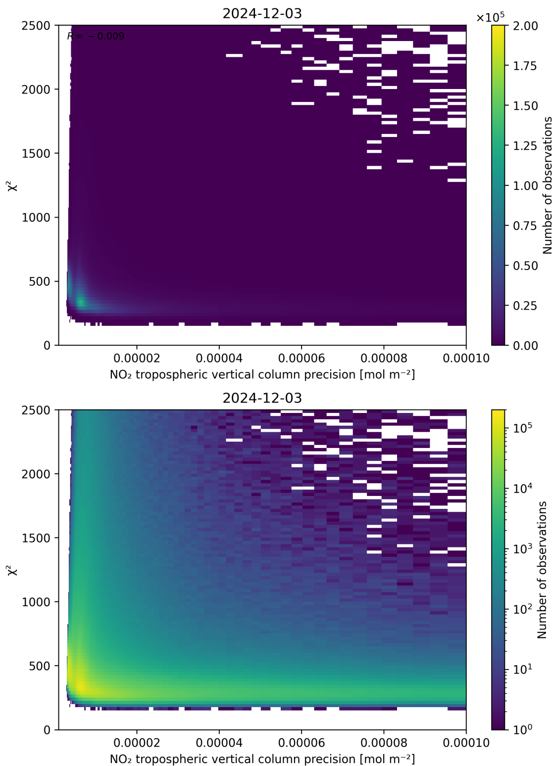
Figure 134: Scatter density plot of “NO 2 tropospheric vertical column precision” against “ \chi^2 ” for 2024-12-02 to 2024-12-04.
