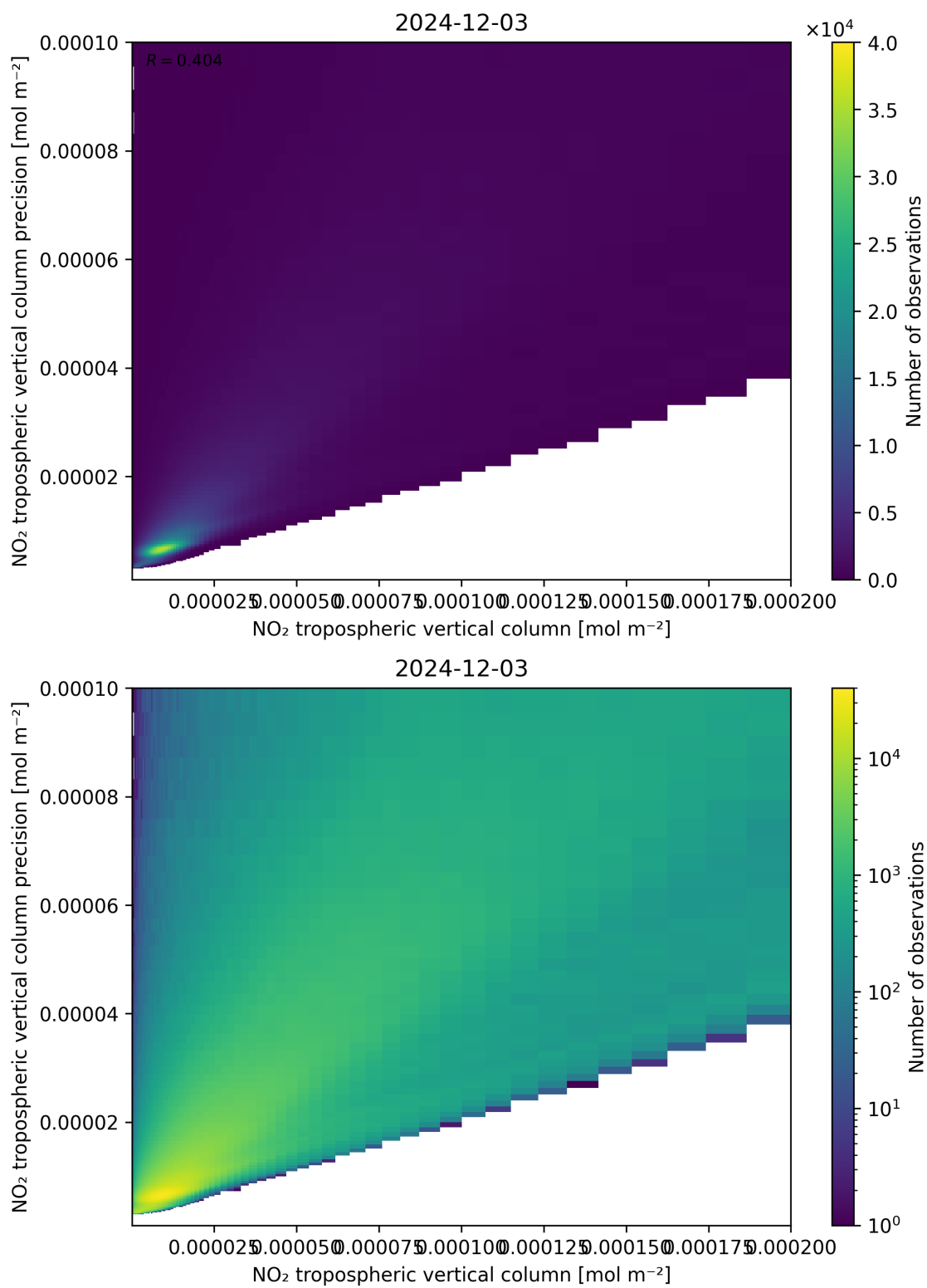
Figure 130: Scatter density plot of “NO 2 tropospheric vertical column” against “NO 2 tropospheric vertical column precision” for 2024-12-02 to 2024-12-04.
