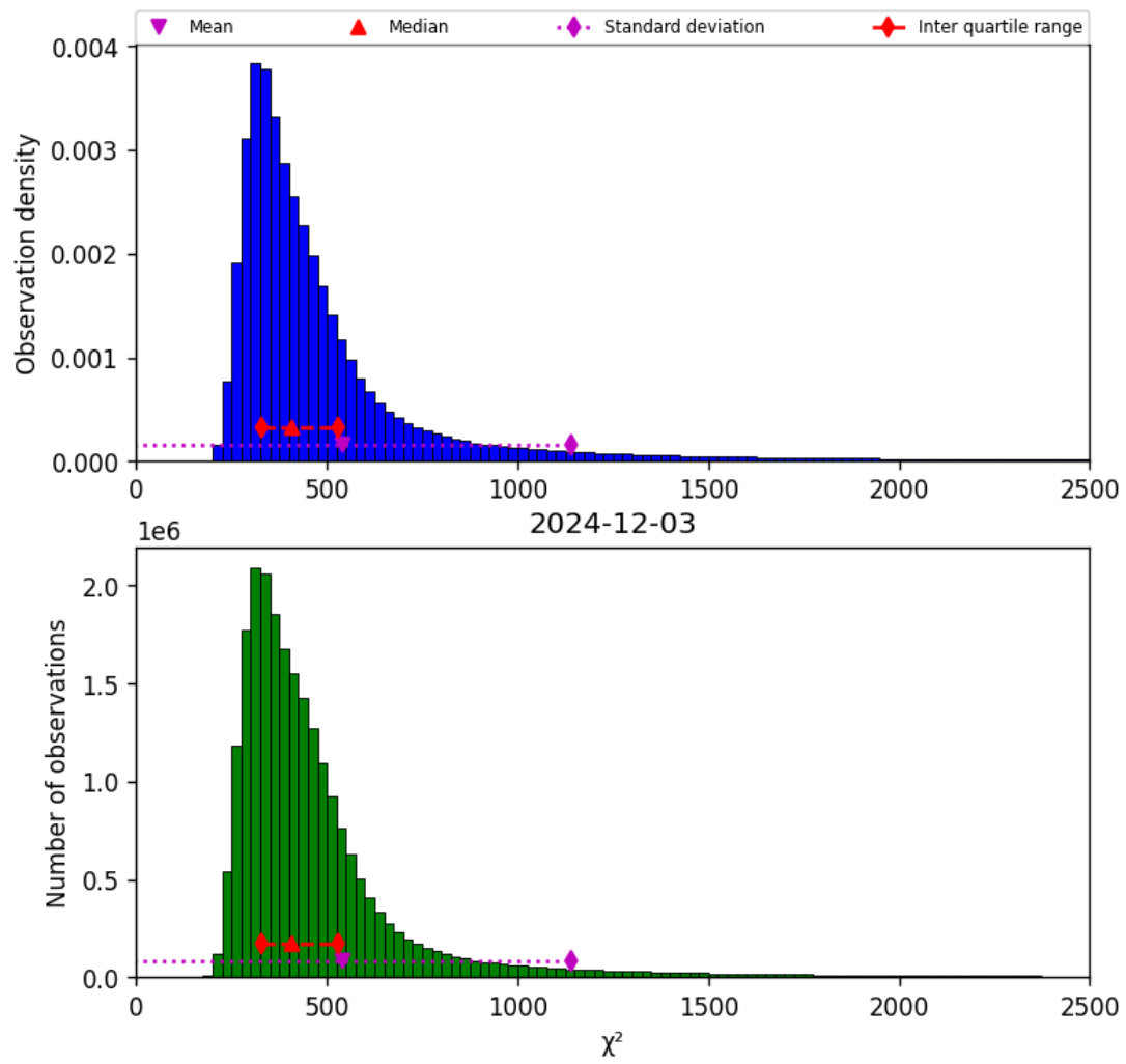
Figure 42: Histogram of " \chi^2 " for 2024-12-02 to 2024-12-04
