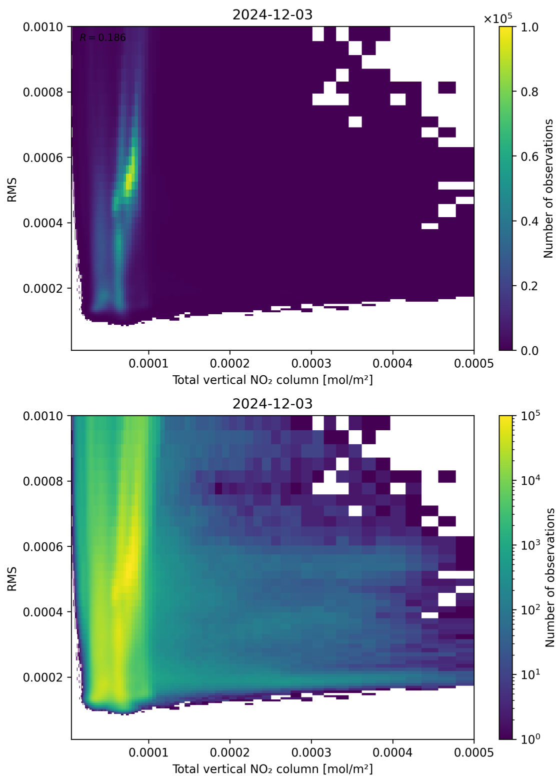
Figure 120: Scatter density plot of “Total vertical NO 2 column” against “RMS” for 2024-12-02 to 2024-12-04.
