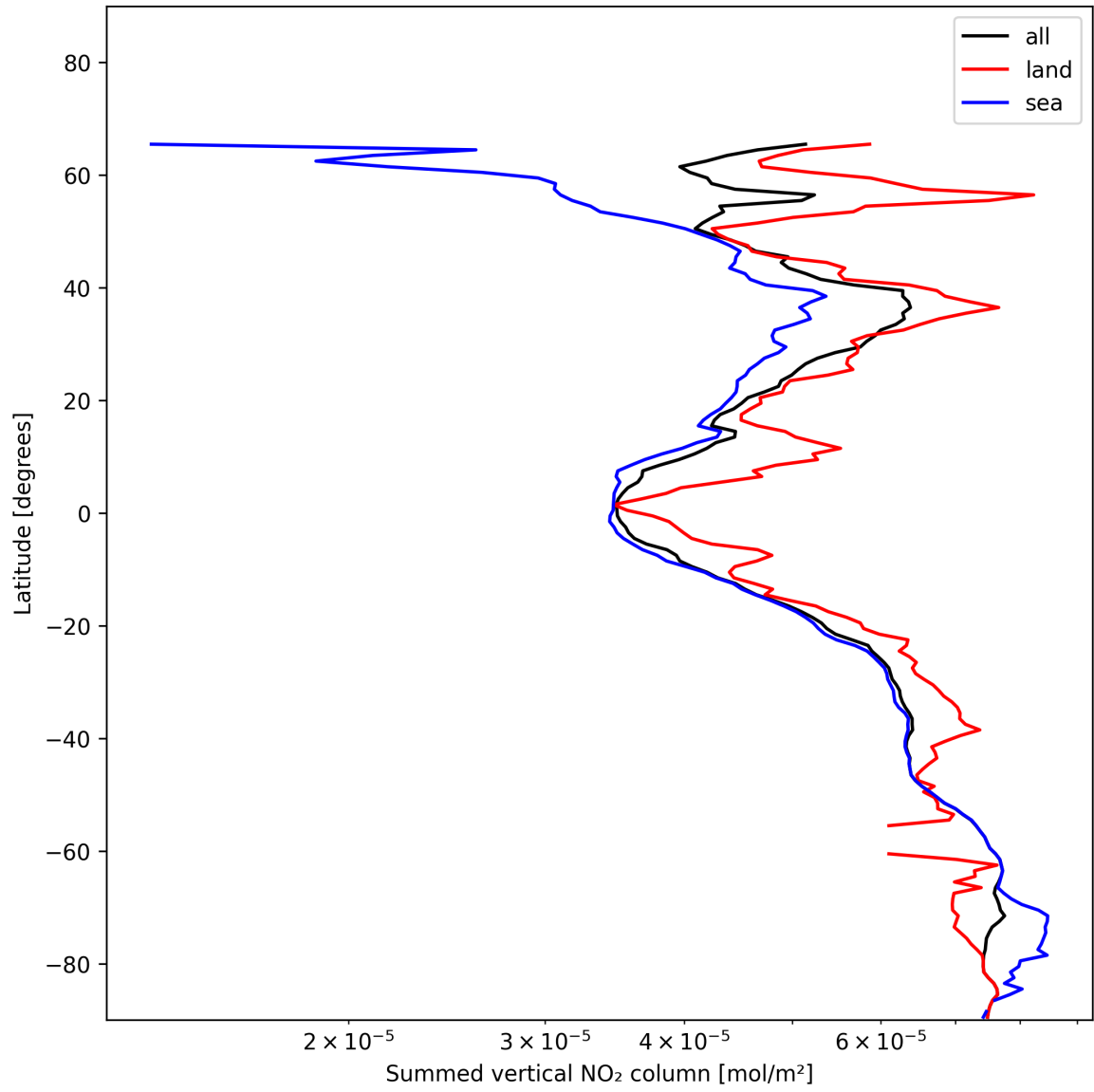
Figure 23: Zonal average of “Summed vertical NO 2 column” for 2024-12-02 to 2024-12-04.
