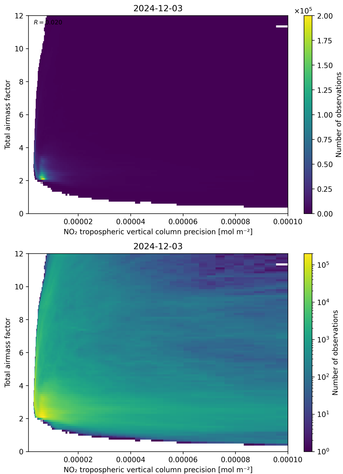
Figure 132: Scatter density plot of “NO 2 tropospheric vertical column precision” against “Total air mass factor” for 2024-12-02 to 2024-12-04.
