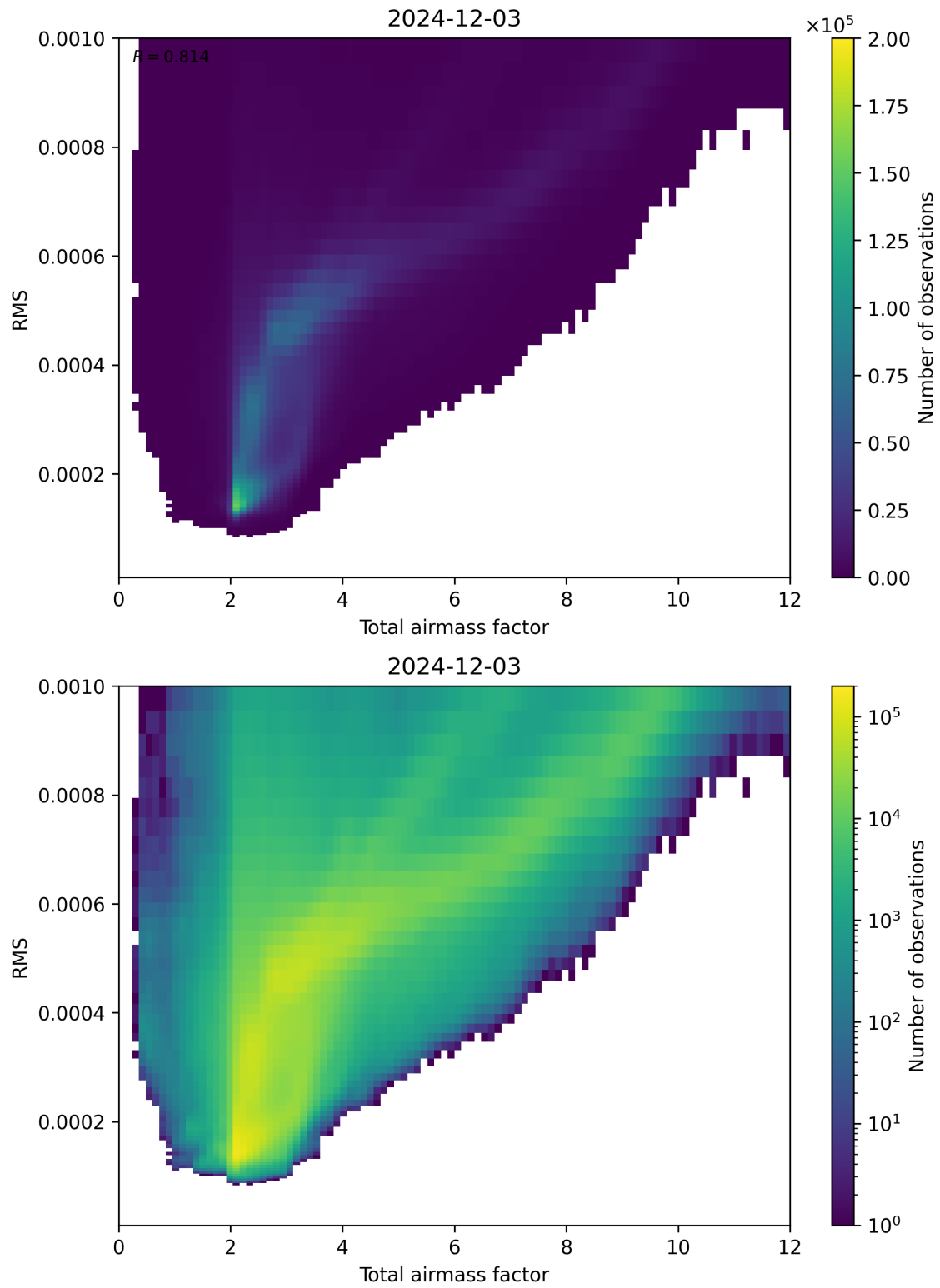
Figure 69: Scatter density plot of “Total airmass factor” against “RMS” for 2024-12-02 to 2024-12-04.
