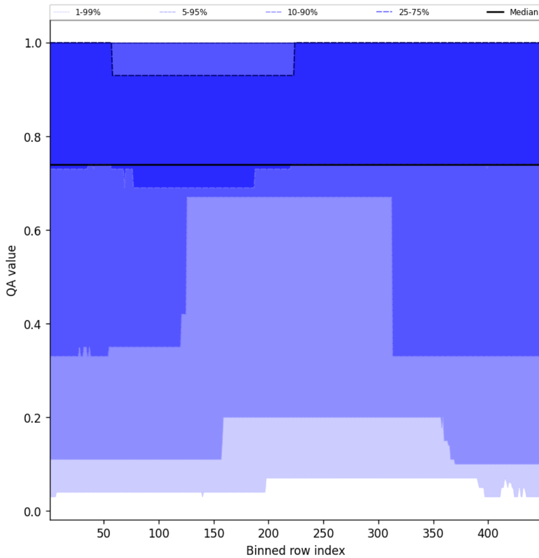
Figure 45: Along track statistics of “QA value” for 2024-12-02 to 2024-12-04
