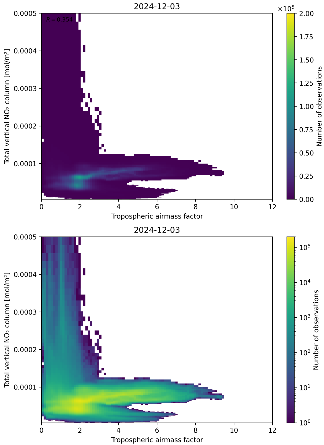
Figure 77: Scatter density plot of “Tropospheric airmass factor” against “Total vertical NO 2 column” for 2024-12-02 to 2024-12-04.
