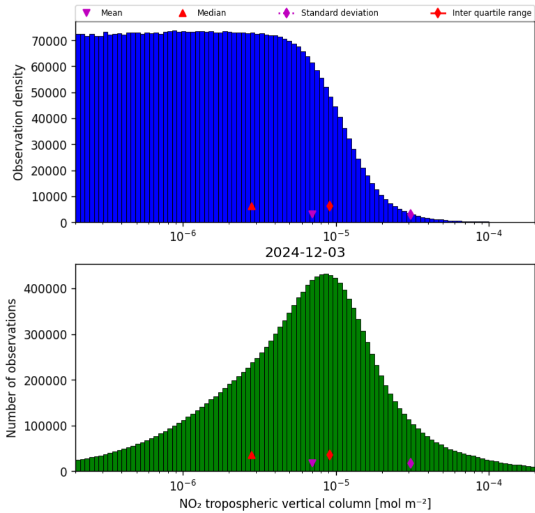
Figure 29: Histogram of “NO 2 tropospheric vertical column” for 2024-12-02 to 2024-12-04
