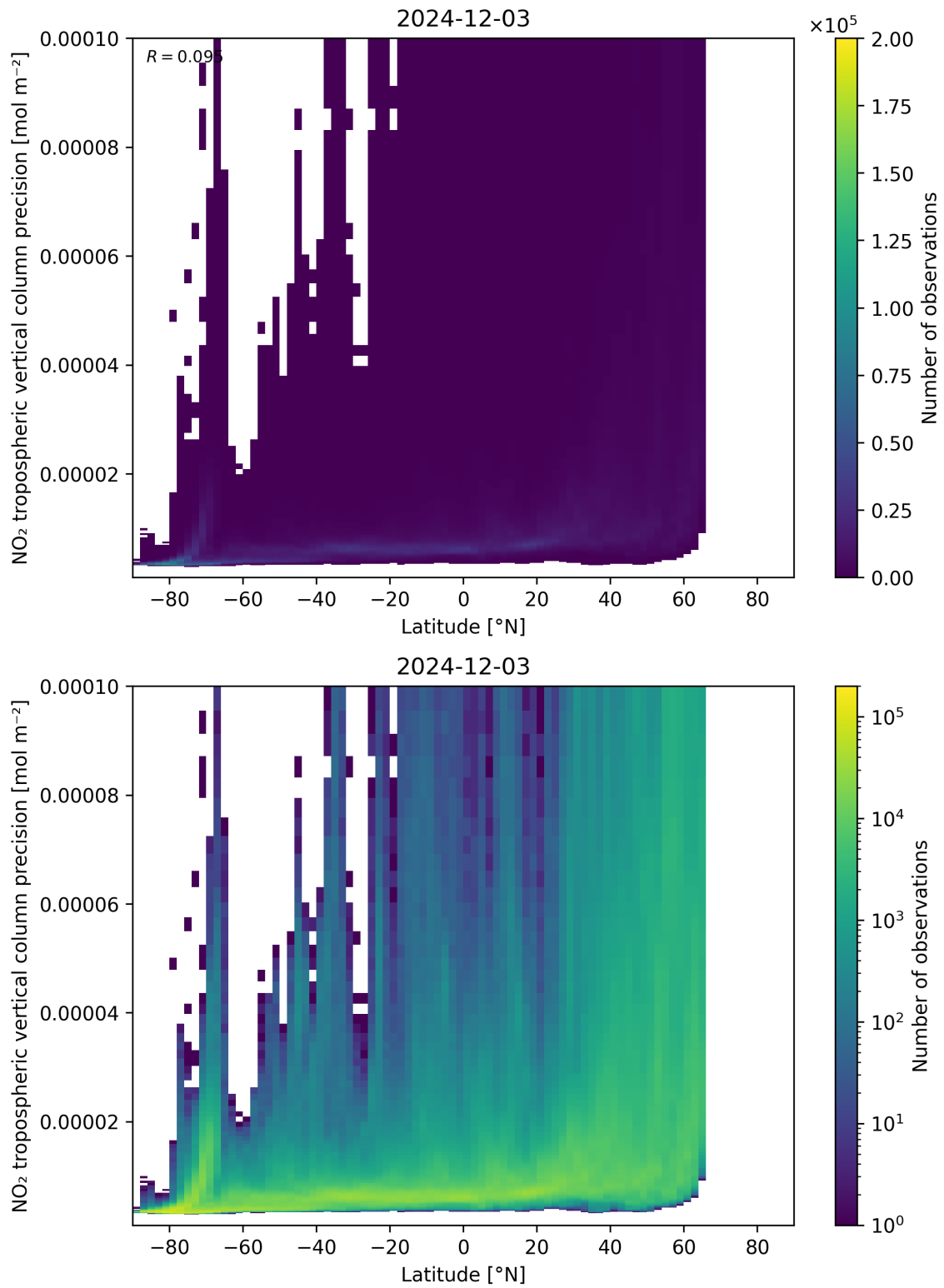
Figure 93: Scatter density plot of “Latitude” against “NO 2 tropospheric vertical column precision” for 2024-12-02 to 2024-12-04.
