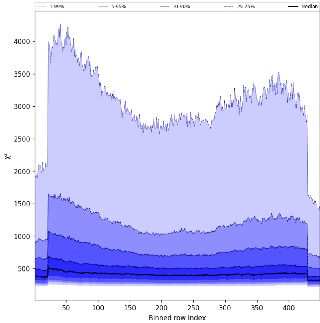
Figure 59: Along track statistics of “ \chi^2 ” for 2024-12-02 to 2024-12-04
