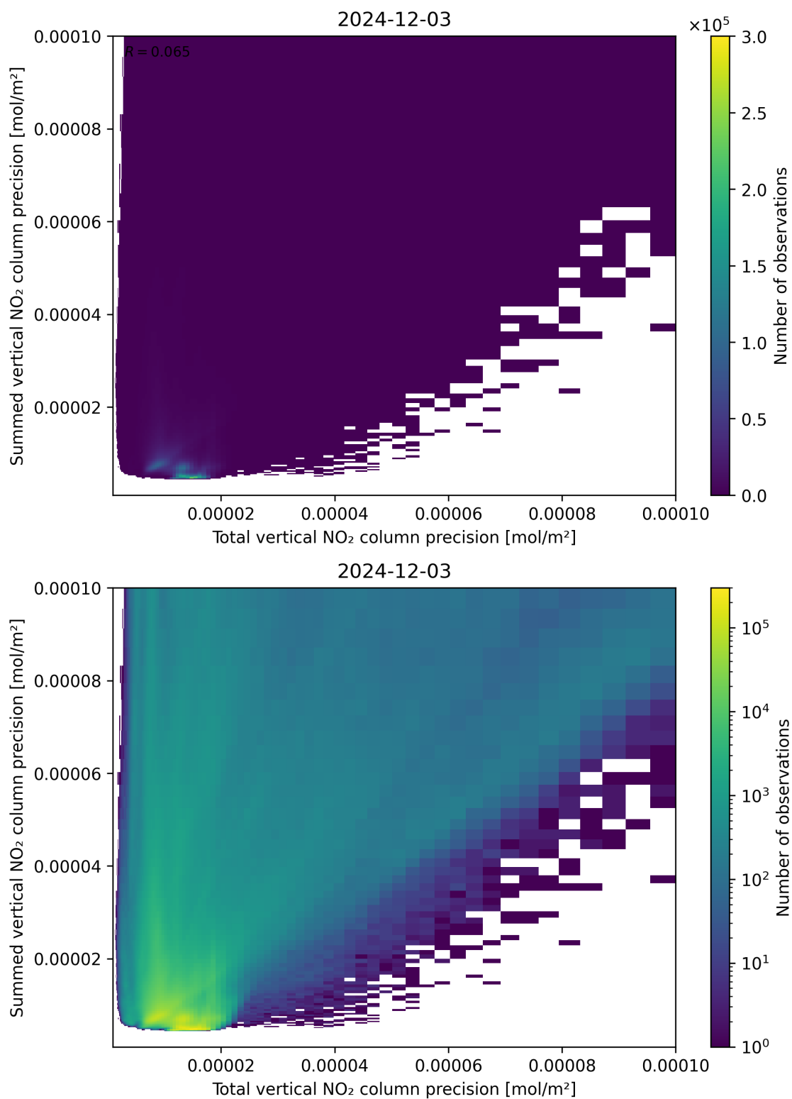
Figure 118: Scatter density plot of “Total vertical NO 2 column precision” against “Summed vertical NO 2 column precision” for 2024-12-02 to 2024-12-04.
