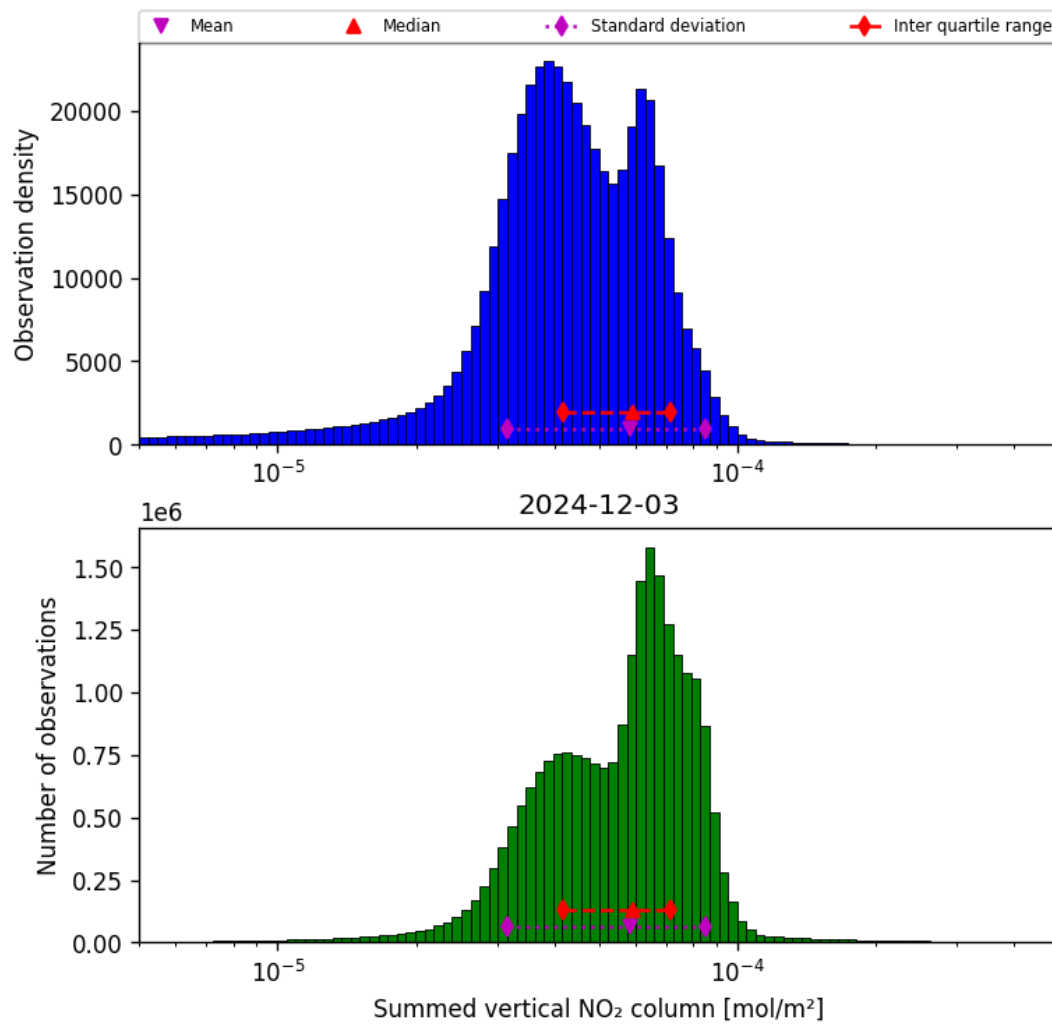
Figure 40: Histogram of “Summed vertical NO 2 column” for 2024-12-02 to 2024-12-04
