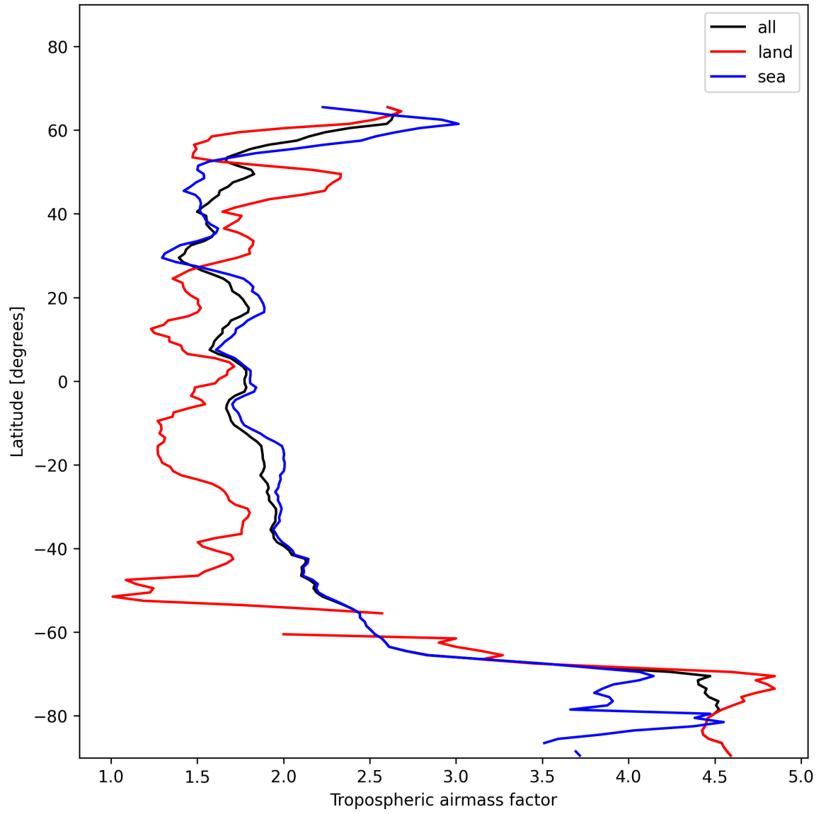
Figure 14: Zonal average of “Tropospheric airmass factor” for 2024-12-02 to 2024-12-04.
