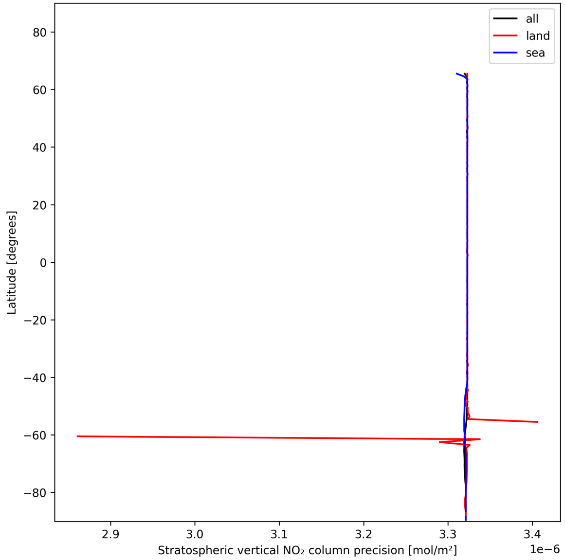
Figure 20: Zonal average of “Stratospheric vertical NO 2 column precision” for 2024-12-02 to 2024-12-04.
