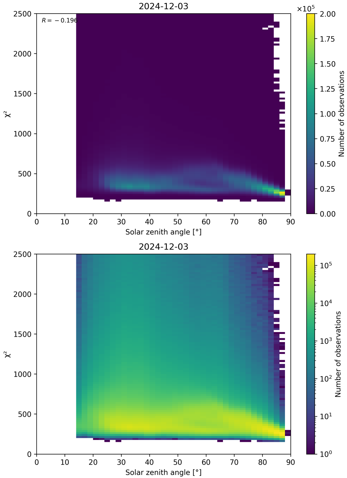
Figure 148: Scatter density plot of “Solar zenith angle” against “ \chi^2 ” for 2024-12-02 to 2024-12-04.
