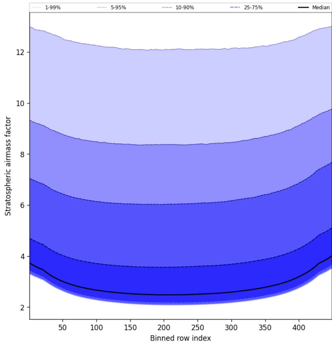
Figure 61: Along track statistics of “Stratospheric airmass factor” for 2024-12-02 to 2024-12-04
