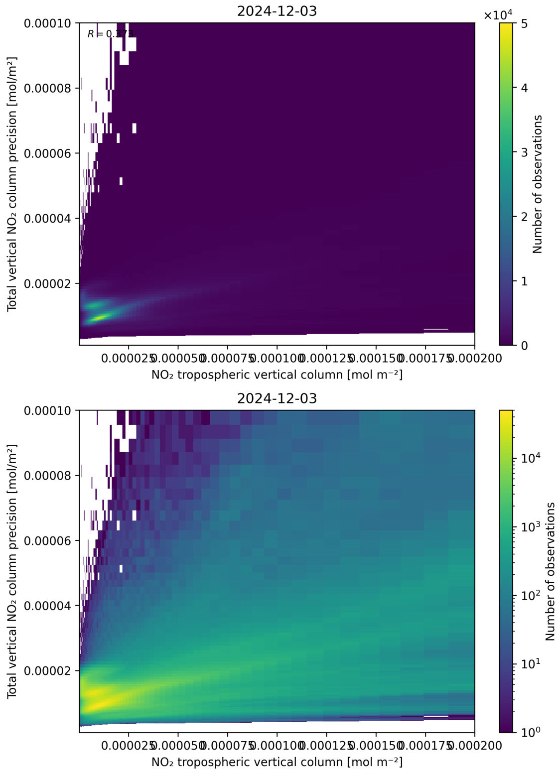
Figure 129: Scatter density plot of “NO 2 tropospheric vertical column” against “Total vertical NO 2 column precision” for 2024-12-02 to 2024-12-04.
