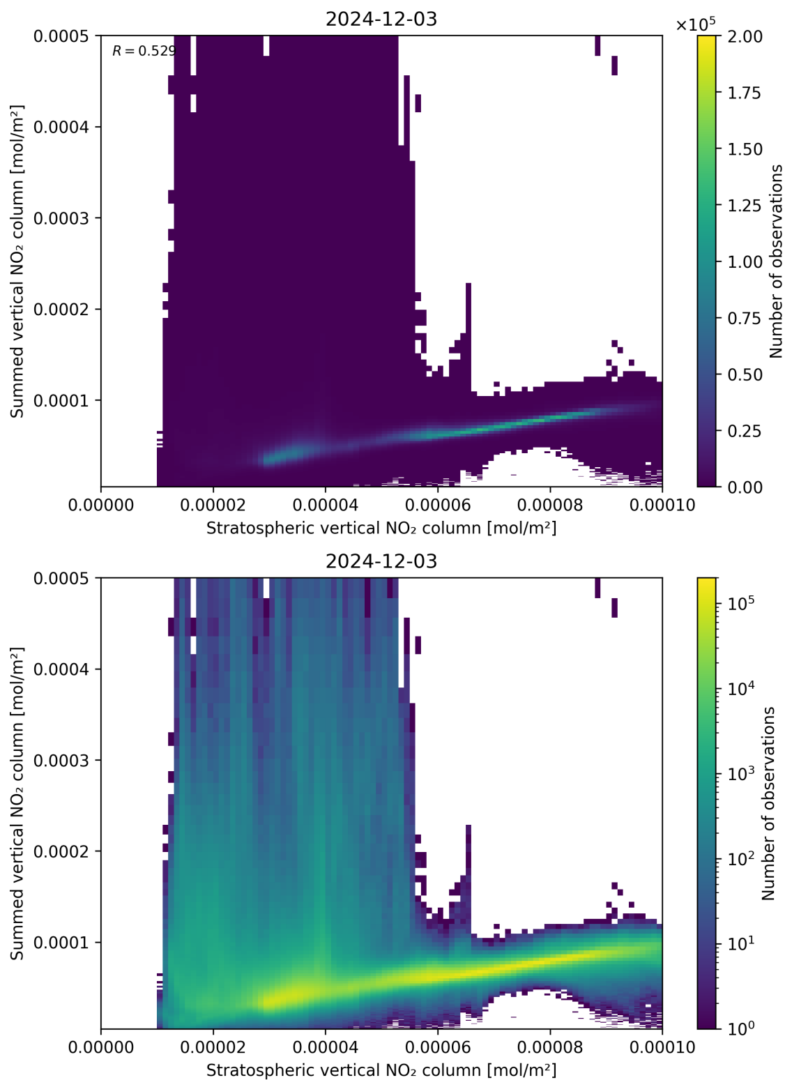
Figure 98: Scatter density plot of “Stratospheric vertical NO 2 column” against “Summed vertical NO 2 column” for 2024-12-02 to 2024-12-04.
