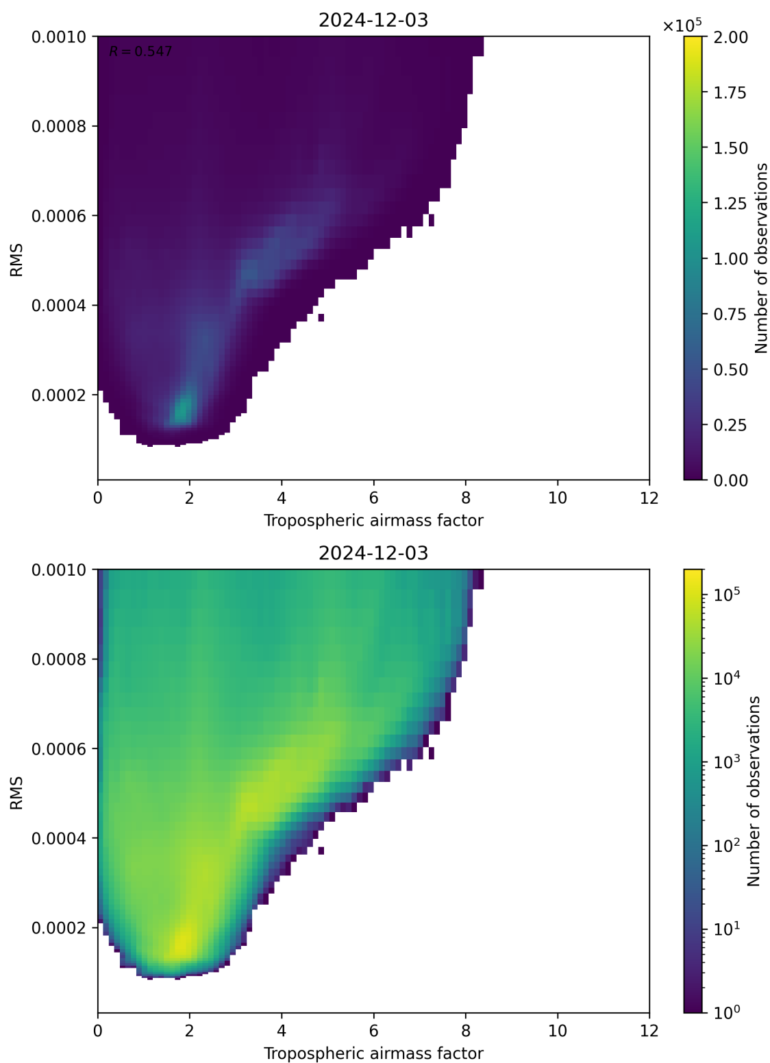
Figure 79: Scatter density plot of “Tropospheric airmass factor” against “RMS” for 2024-12-02 to 2024-12-04.
