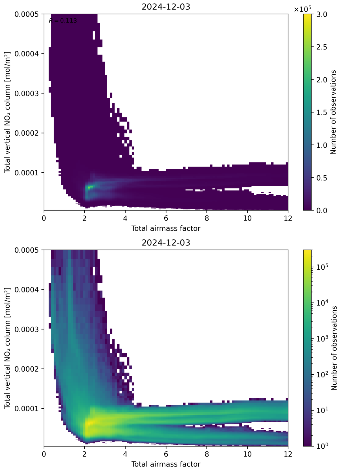
Figure 67: Scatter density plot of “Total airmass factor” against “Total vertical NO 2 column” for 2024-12-02 to 2024-12-04.
