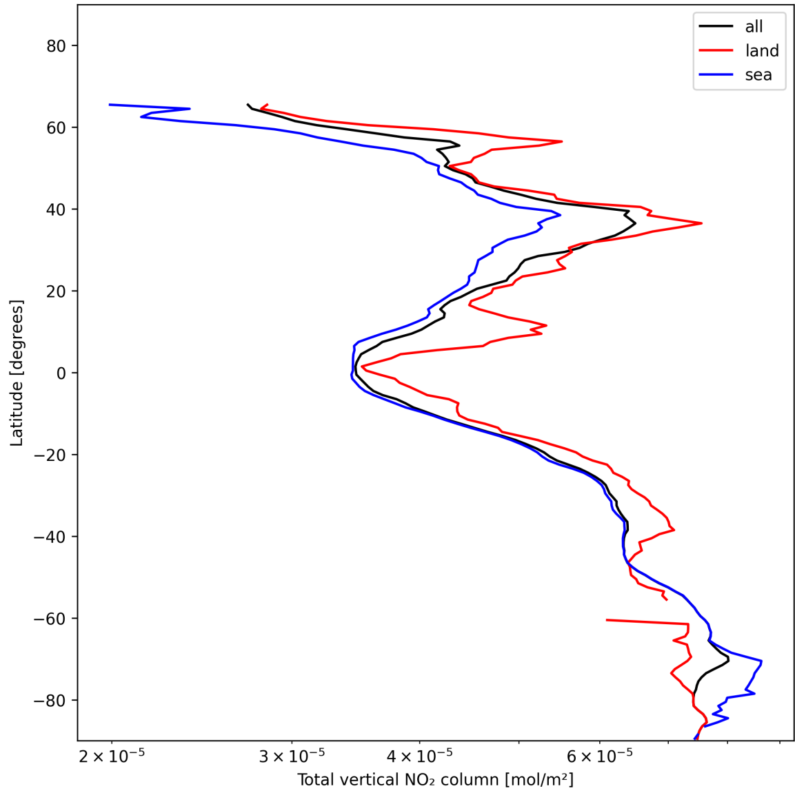
Figure 21: Zonal average of “Total vertical NO 2 column” for 2024-12-02 to 2024-12-04.
