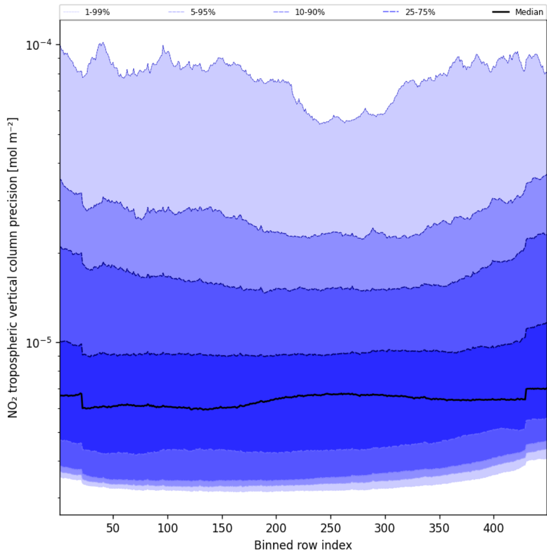
Figure 47: Along track statistics of “NO 2 tropospheric vertical column precision” for 2024-12-02 to 2024-12-04
