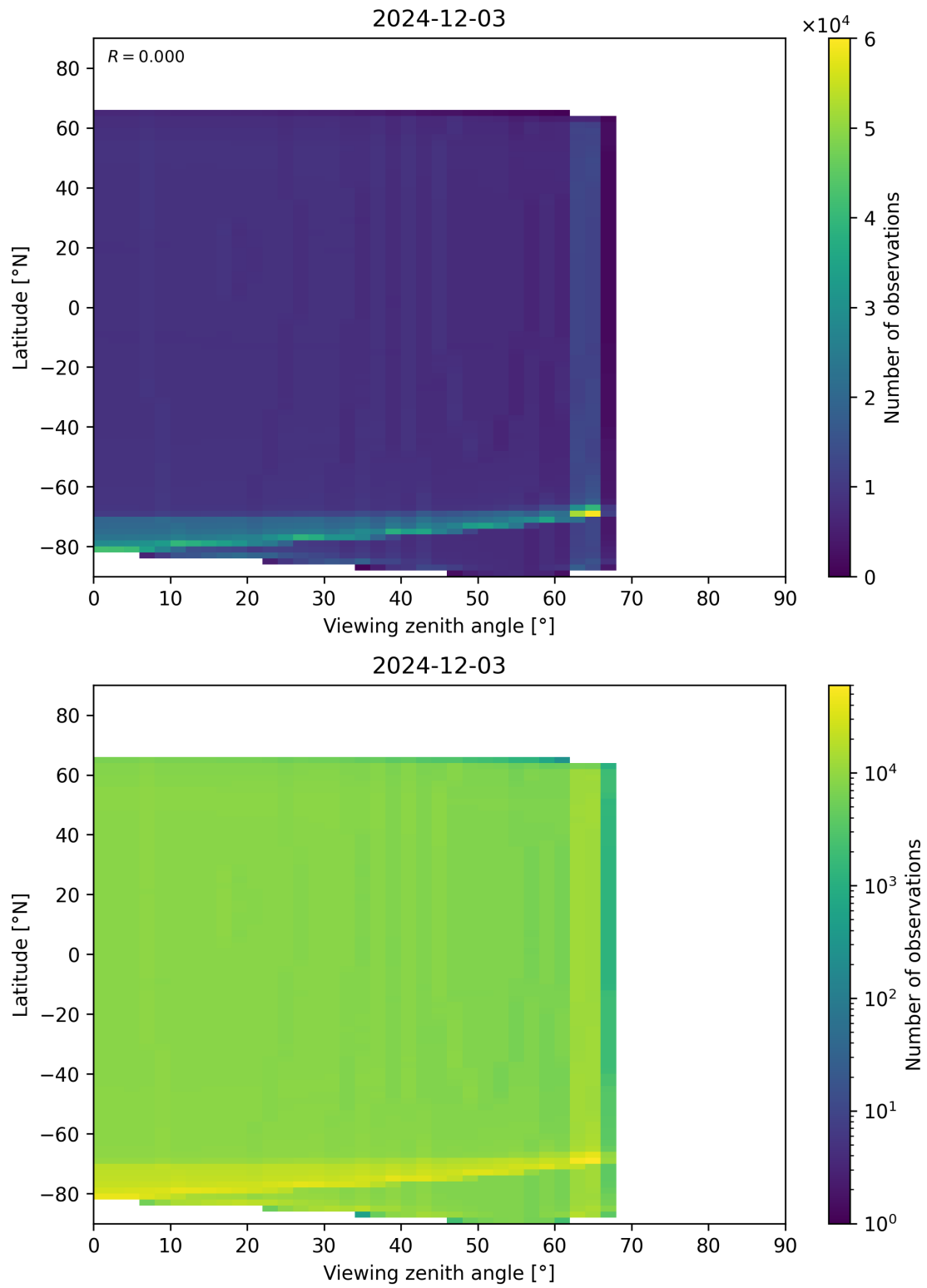
Figure 163: Scatter density plot of “Viewing zenith angle” against “Latitude” for 2024-12-02 to 2024-12-04.
