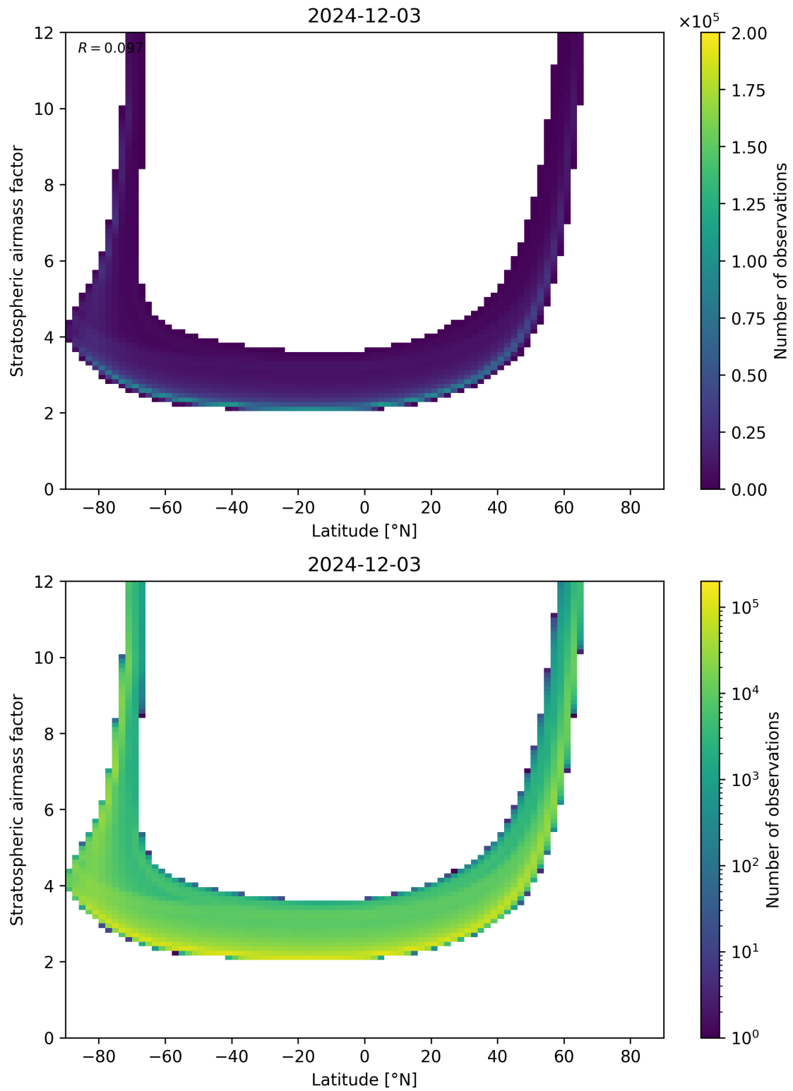
Figure 83: Scatter density plot of “Latitude” against “Stratospheric airmass factor” for 2024-12-02 to 2024-12-04.
