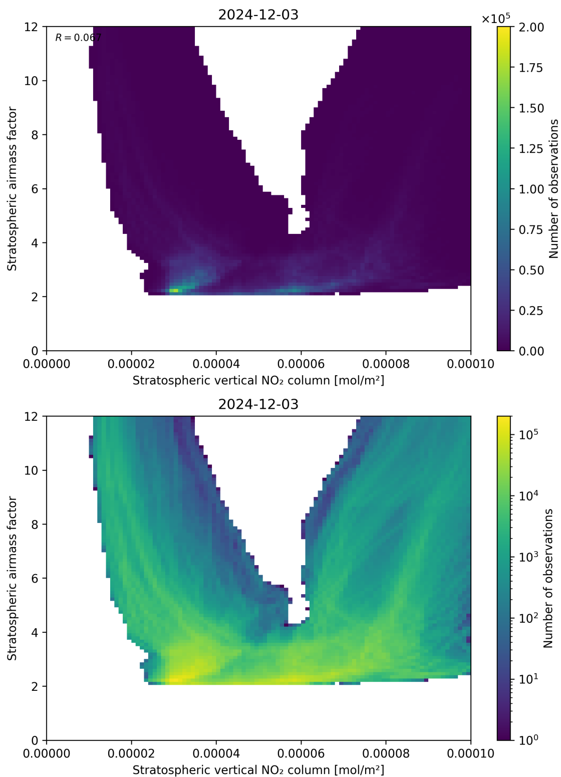
Figure 96: Scatter density plot of “Stratospheric vertical NO 2 column” against “Stratospheric airmass factor” for 2024-12-02 to 2024-12-04.
