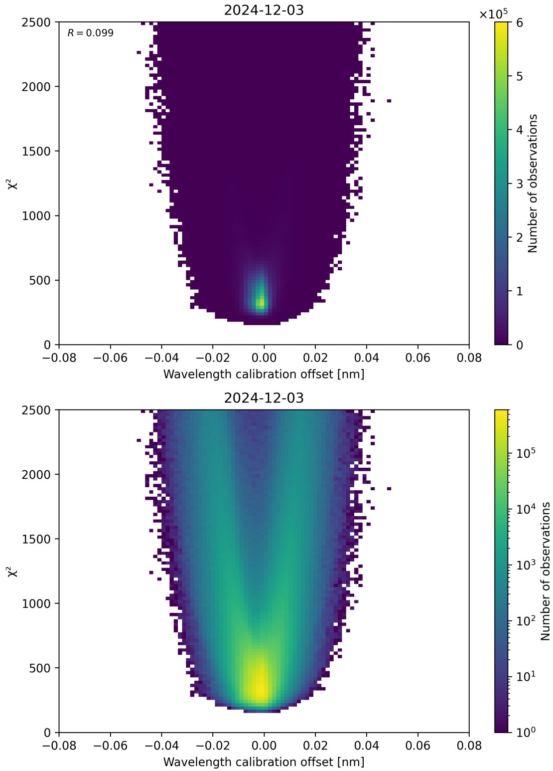
Figure 175: Scatter density plot of “Wavelength calibration offset” against “ \chi^2 ” for 2024-12-02 to 2024-12-04.
