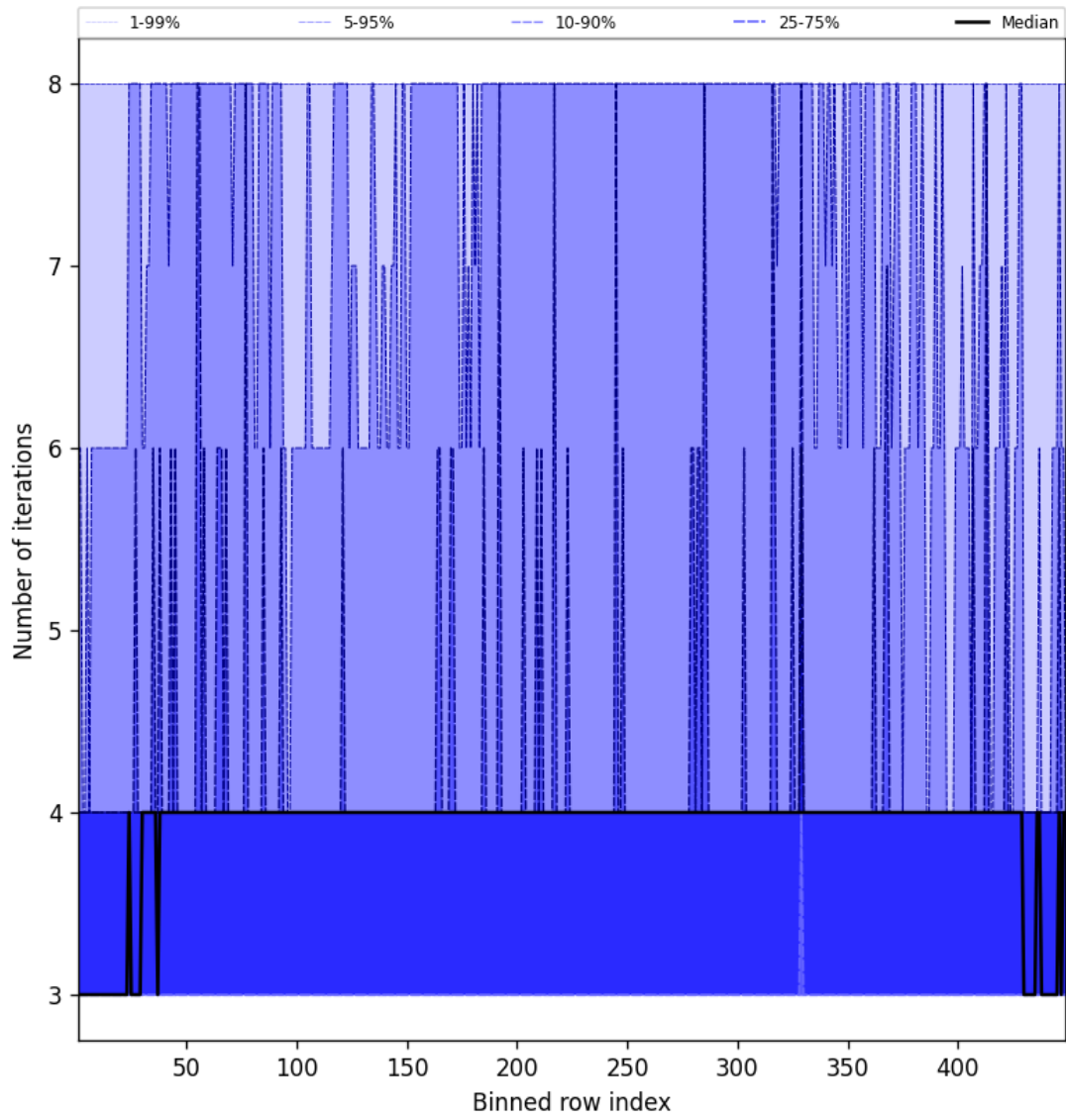
Figure 51: Along track statistics of “Number of iterations” for 2024-12-02 to 2024-12-04
