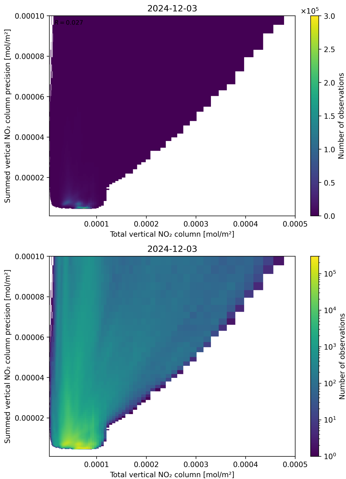
Figure 113: Scatter density plot of “Total vertical NO 2 column” against “Summed vertical NO 2 column precision” for 2024-12-02 to 2024-12-04.
