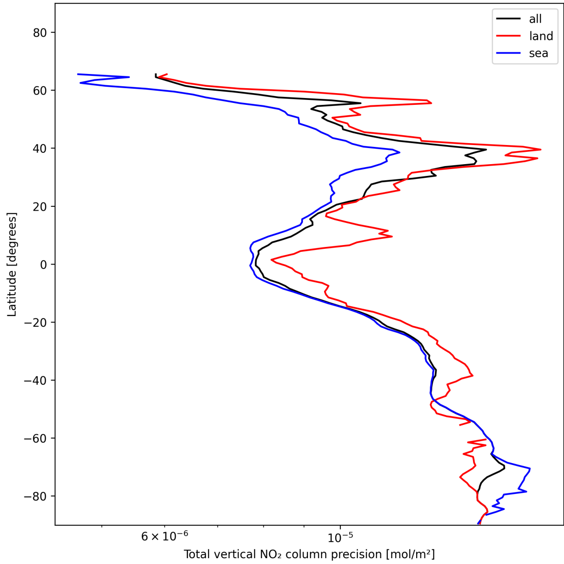
Figure 22: Zonal average of “Total vertical NO 2 column precision” for 2024-12-02 to 2024-12-04.
