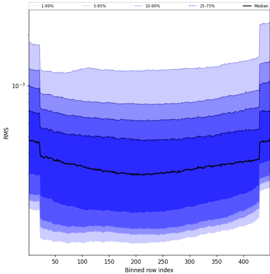
Figure 60: Along track statistics of “RMS” for 2024-12-02 to 2024-12-04
