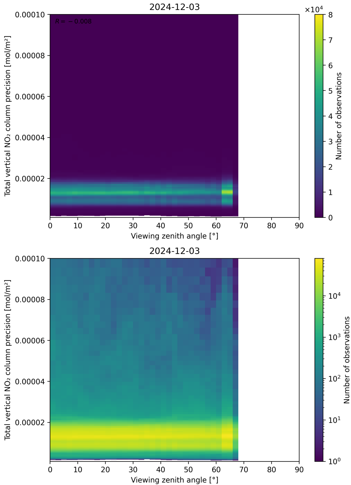
Figure 168: Scatter density plot of “Viewing zenith angle” against “Total vertical NO 2 column precision” for 2024-12-02 to 2024-12-04.
