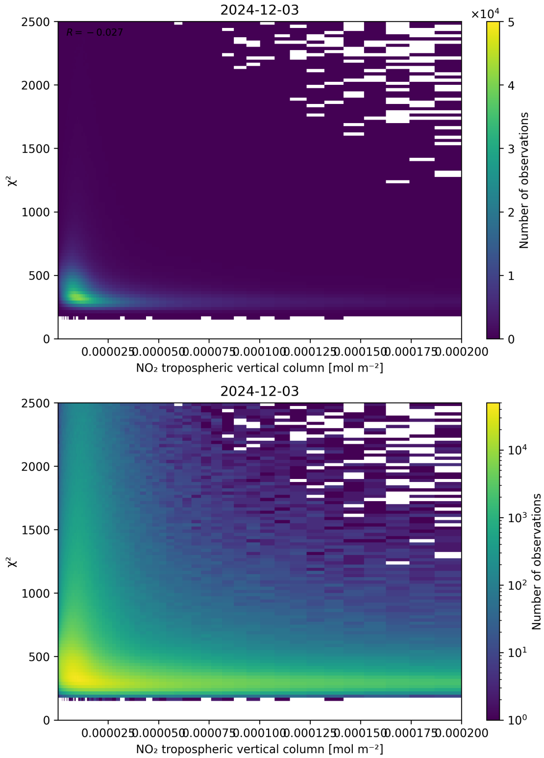
Figure 124: Scatter density plot of “NO 2 tropospheric vertical column” against “ \chi^2 ” for 2024-12-02 to 2024-12-04.
