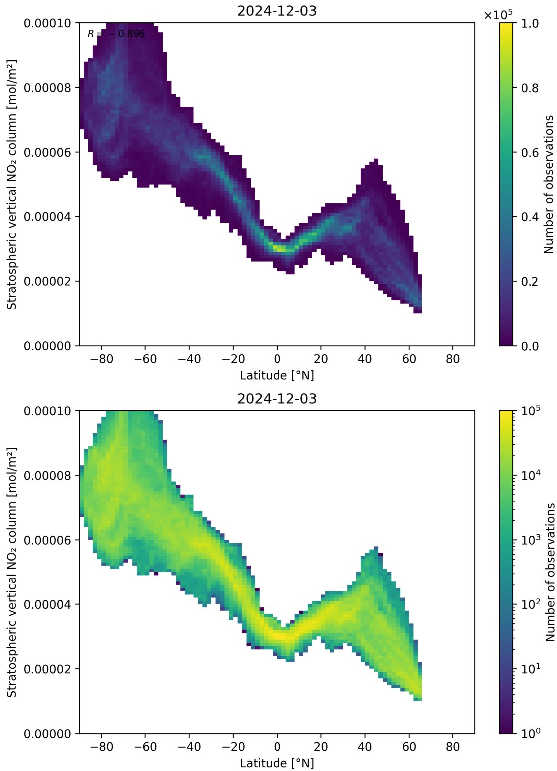
Figure 87: Scatter density plot of “Latitude” against “Stratospheric vertical NO 2 column” for 2024-12-02 to 2024-12-04.
