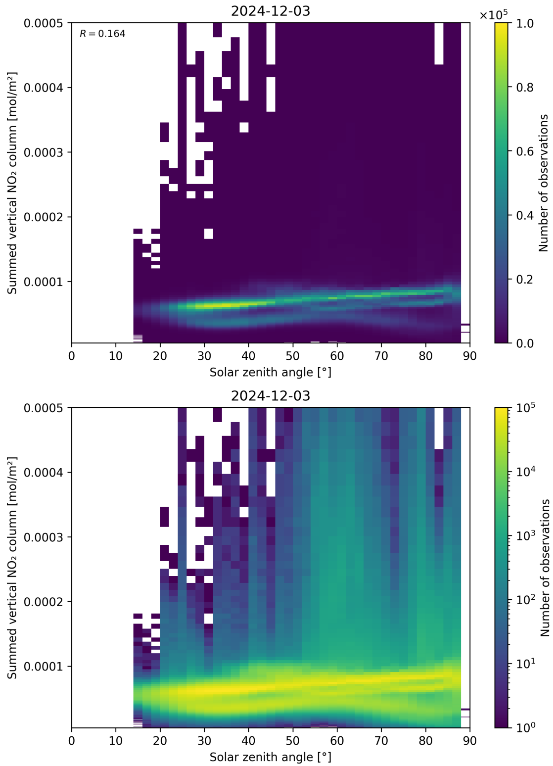
Figure 151: Scatter density plot of “Solar zenith angle” against “Summed vertical NO 2 column” for 2024-12-02 to 2024-12-04.
