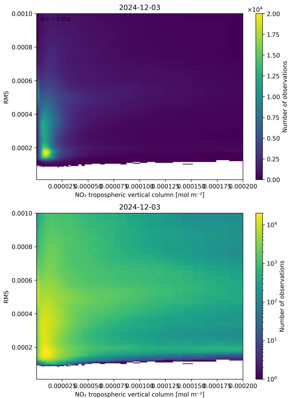
Figure 142: Scatter density plot of “NO 2 tropospheric vertical column” against “RMS” for 2024-12-02 to 2024-12-04.
