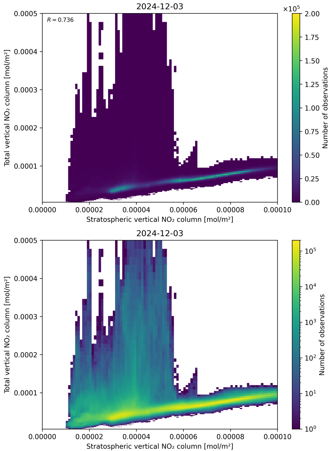
Figure 100: Scatter density plot of “Stratospheric vertical NO 2 column” against “Total vertical NO 2 column” for 2024-12-02 to 2024-12-04.
