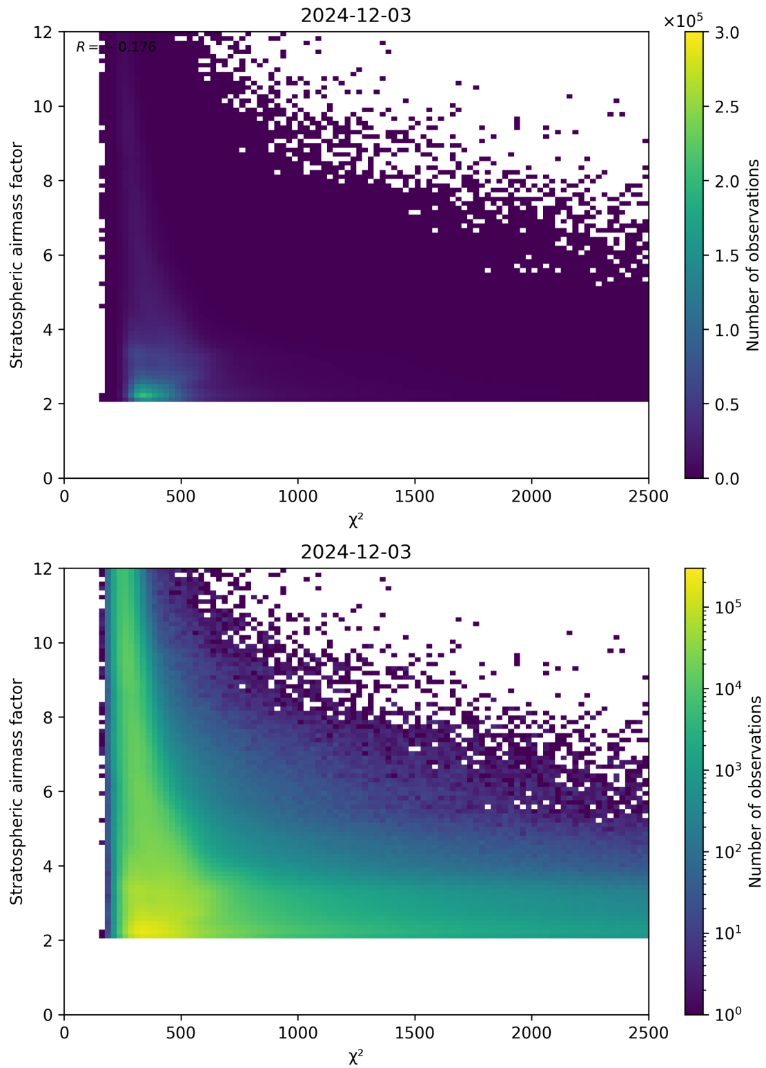
Figure 81: Scatter density plot of “ \chi^2 ” against “Stratospheric airmass factor” for 2024-12-02 to 2024-12-04.
