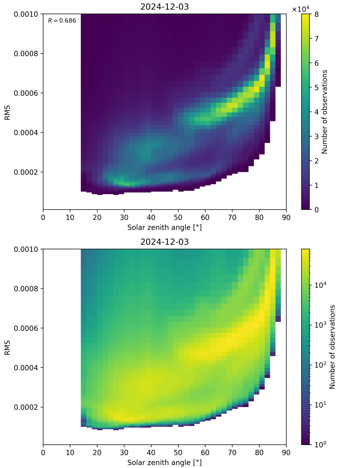
Figure 157: Scatter density plot of “Solar zenith angle” against “RMS” for 2024-12-02 to 2024-12-04.
