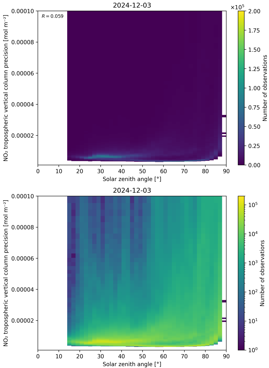
Figure 156: Scatter density plot of “Solar zenith angle” against “NO 2 tropospheric vertical column precision” for 2024-12-02 to 2024-12-04.
