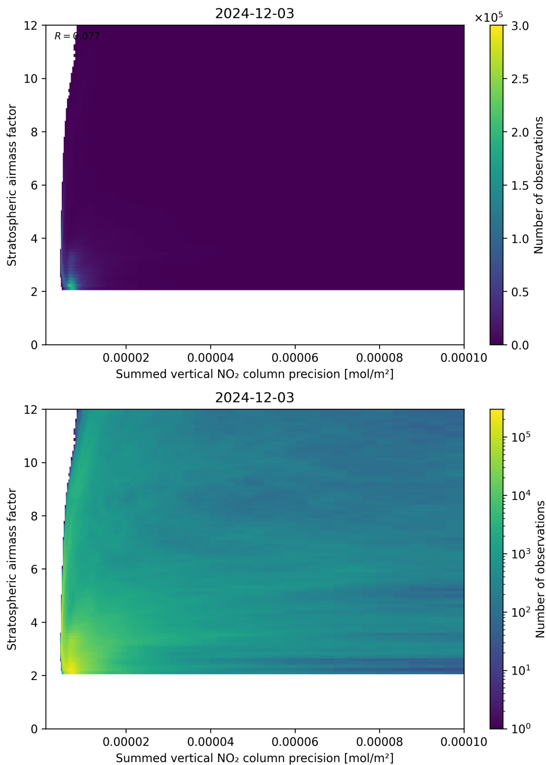
Figure 106: Scatter density plot of “Summed vertical NO 2 column precision” against “Stratospheric airmass factor” for 2024-12-02 to 2024-12-04.
