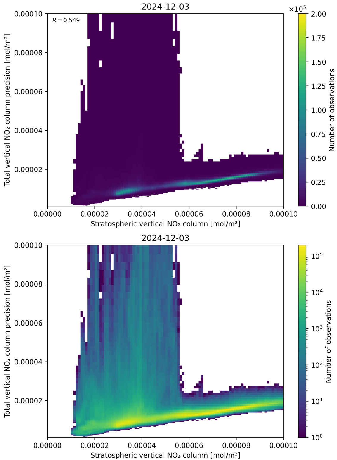
Figure 101: Scatter density plot of “Stratospheric vertical NO 2 column” against “Total vertical NO 2 column precision” for 2024-12-02 to 2024-12-04.
