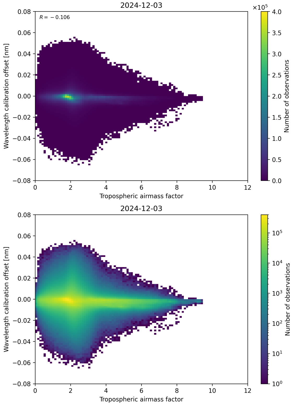
Figure 80: Scatter density plot of “Tropospheric airmass factor” against “Wavelength calibration offset” for 2024-12-02 to 2024-12-04.
