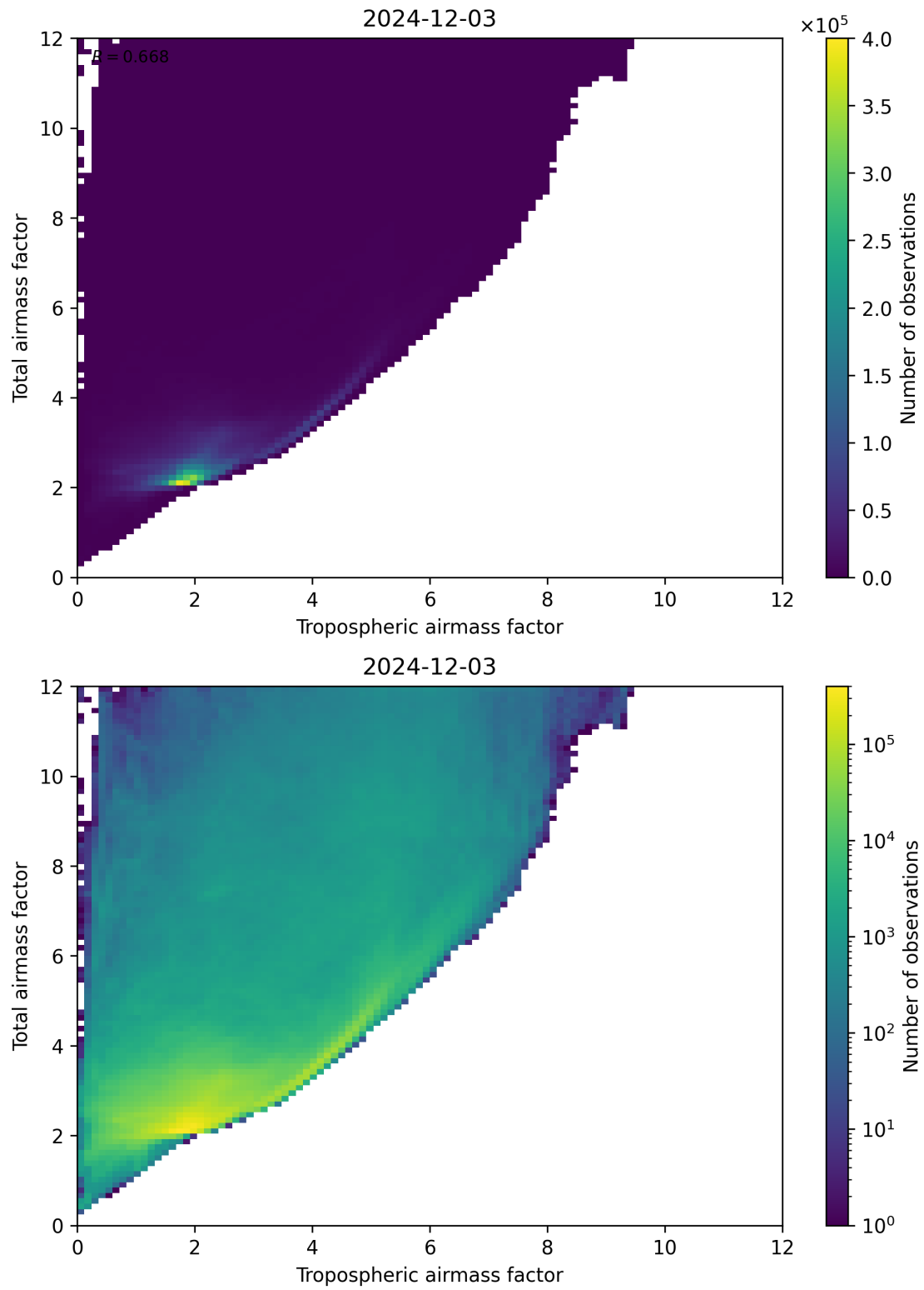
Figure 72: Scatter density plot of “Tropospheric airmass factor” against “Total airmass factor” for 2024-12-02 to 2024-12-04.
