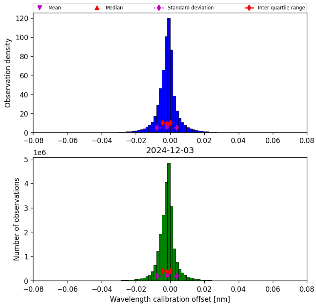
Figure 35: Histogram of “Wavelength calibration offset” for 2024-12-02 to 2024-12-04
