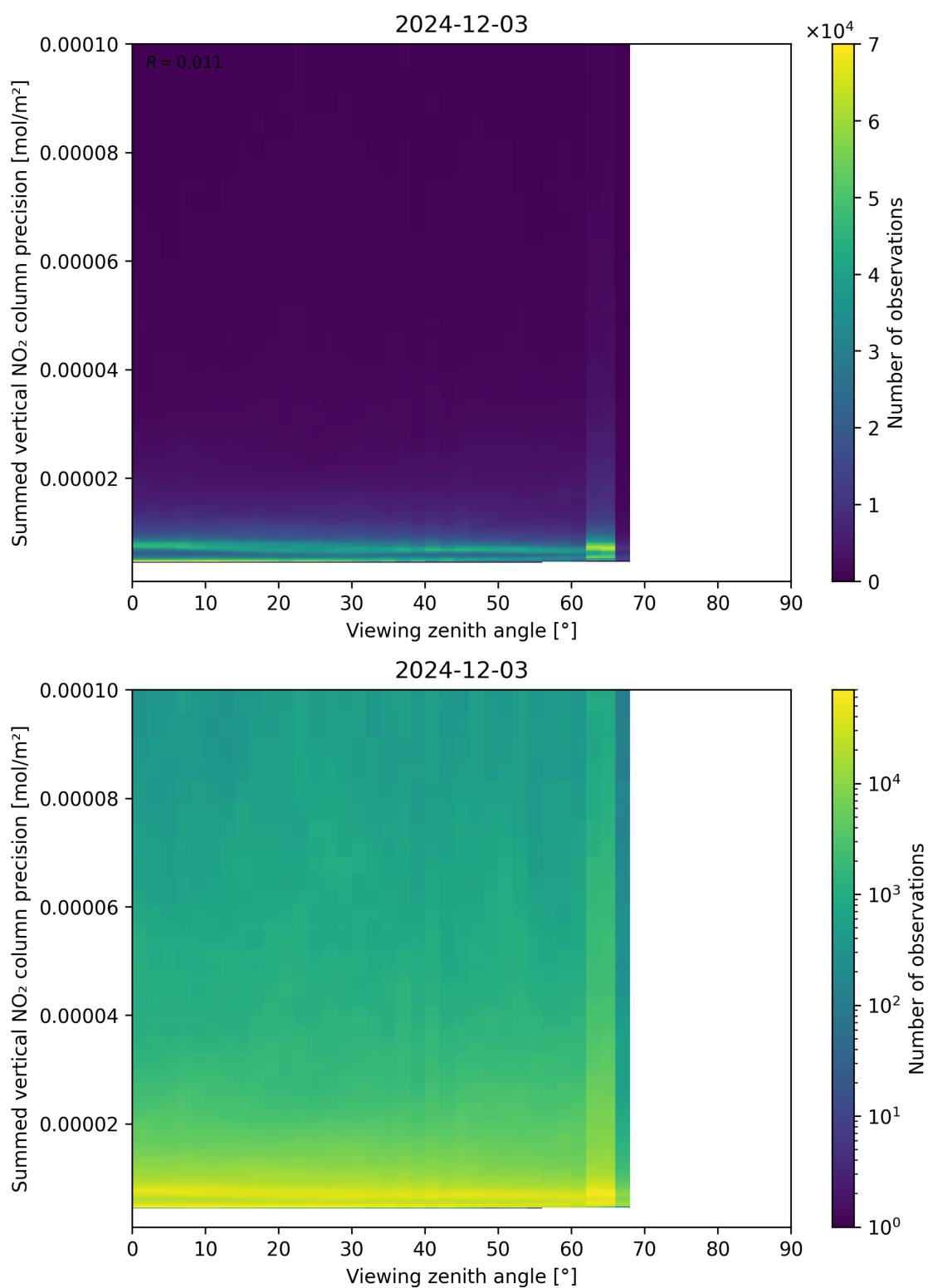
Figure 166: Scatter density plot of “Viewing zenith angle” against “Summed vertical NO 2 column precision” for 2024-12-02 to 2024-12-04.
