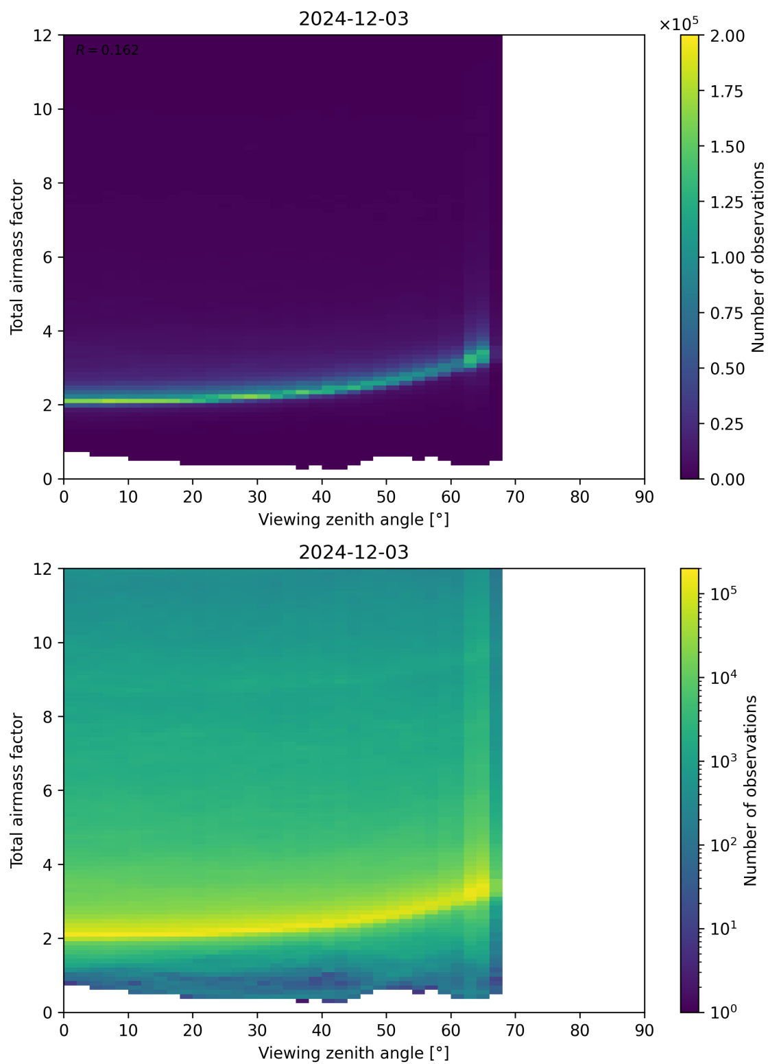
Figure 160: Scatter density plot of “Viewing zenith angle” against “Total airmass factor” for 2024-12-02 to 2024-12-04.
