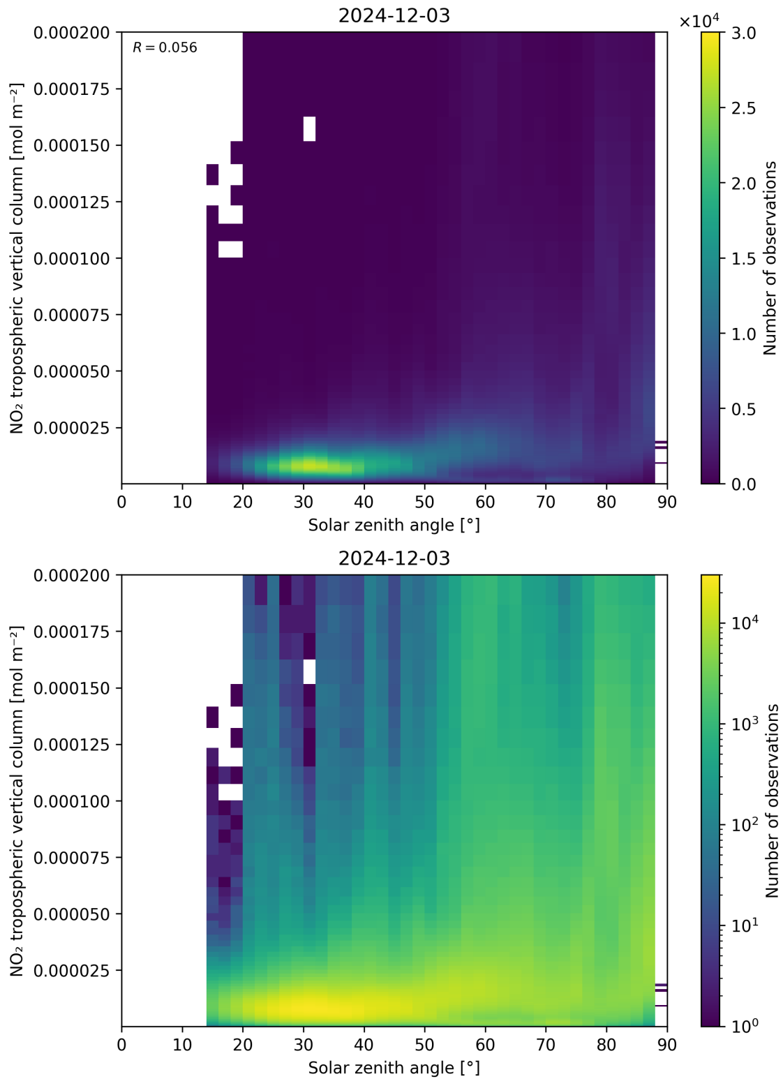
Figure 155: Scatter density plot of “Solar zenith angle” against “NO 2 tropospheric vertical column” for 2024-12-02 to 2024-12-04.
