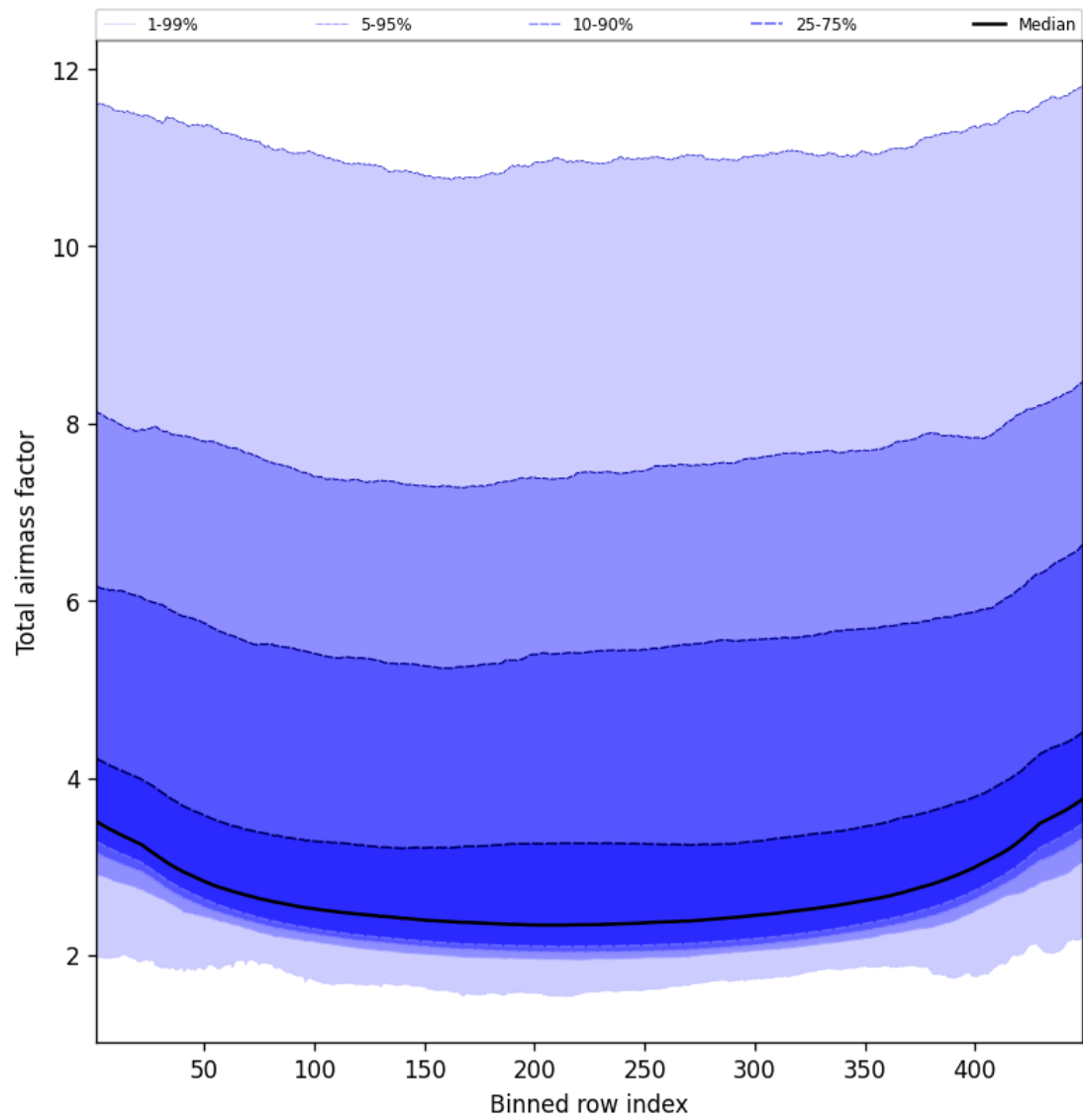
Figure 49: Along track statistics of “Total airmass factor” for 2024-12-02 to 2024-12-04
