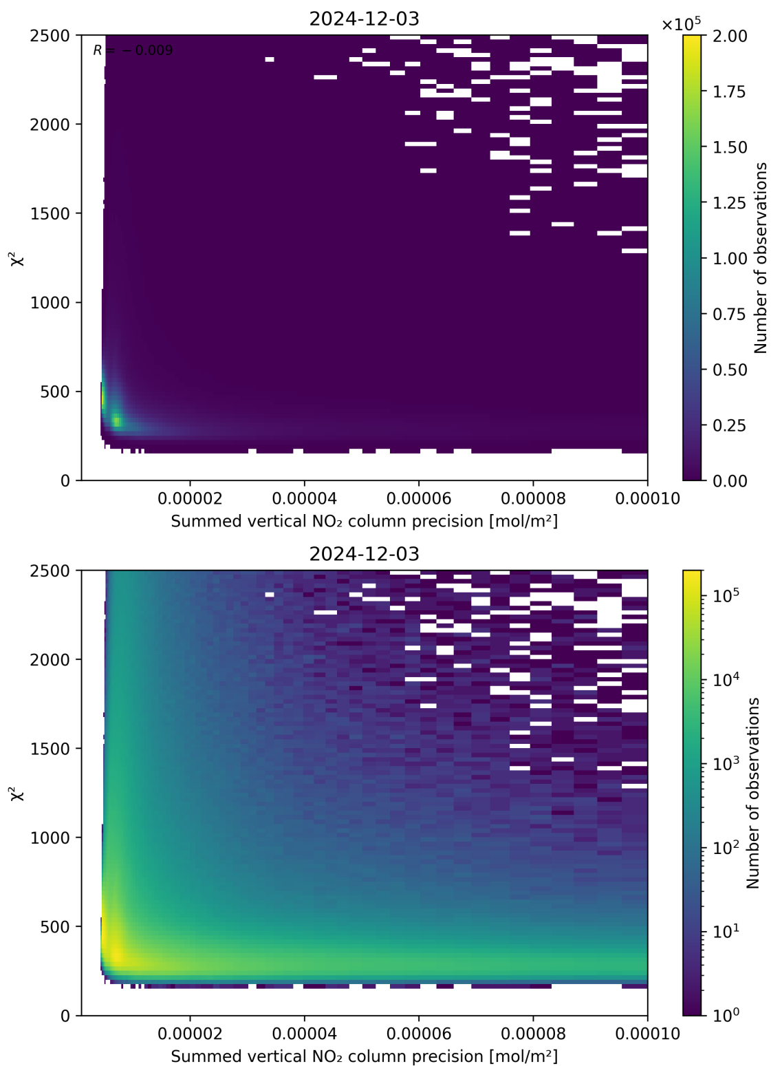
Figure 107: Scatter density plot of “Summed vertical NO 2 column precision” against “ \chi^2 ” for 2024-12-02 to 2024-12-04.
