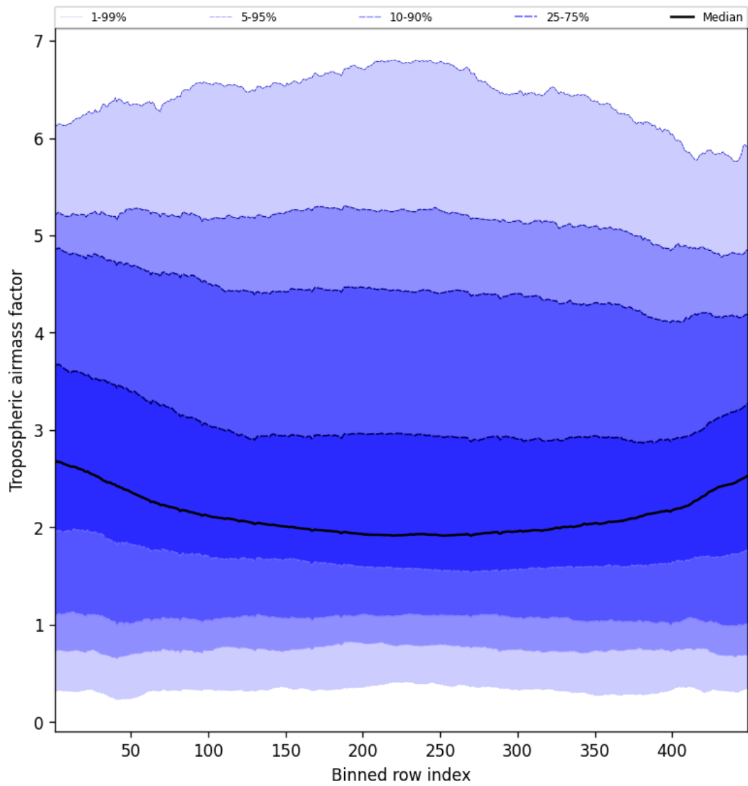
Figure 48: Along track statistics of “Tropospheric airmass factor” for 2024-12-02 to 2024-12-04
