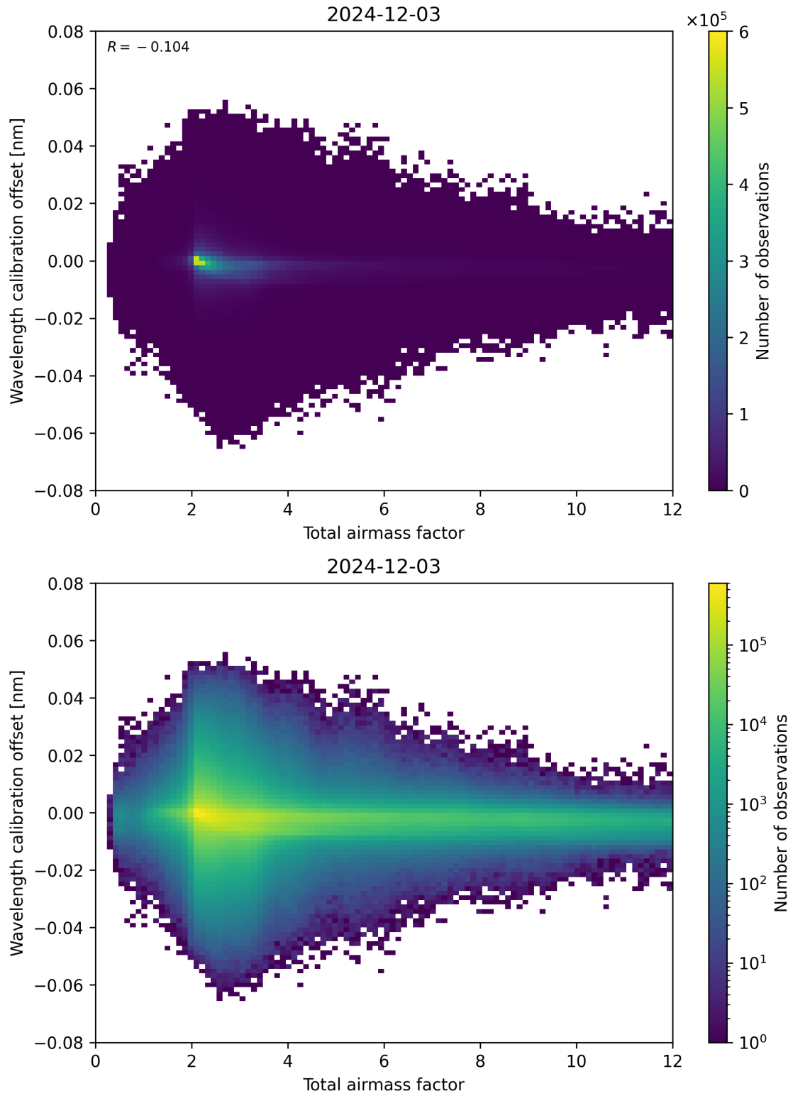
Figure 70: Scatter density plot of “Total airmass factor” against “Wavelength calibration offset” for 2024-12-02 to 2024-12-04.
