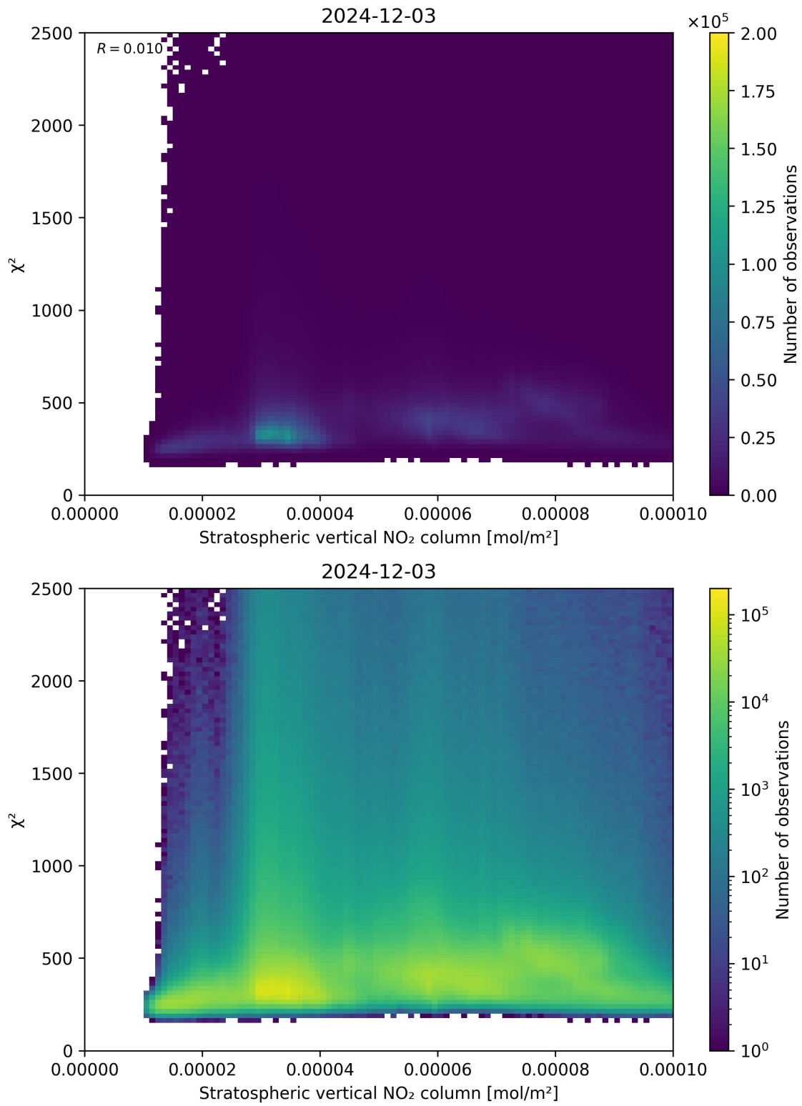
Figure 97: Scatter density plot of “Stratospheric vertical NO 2 column” against “ \chi^2 ” for 2024-12-02 to 2024-12-04.
