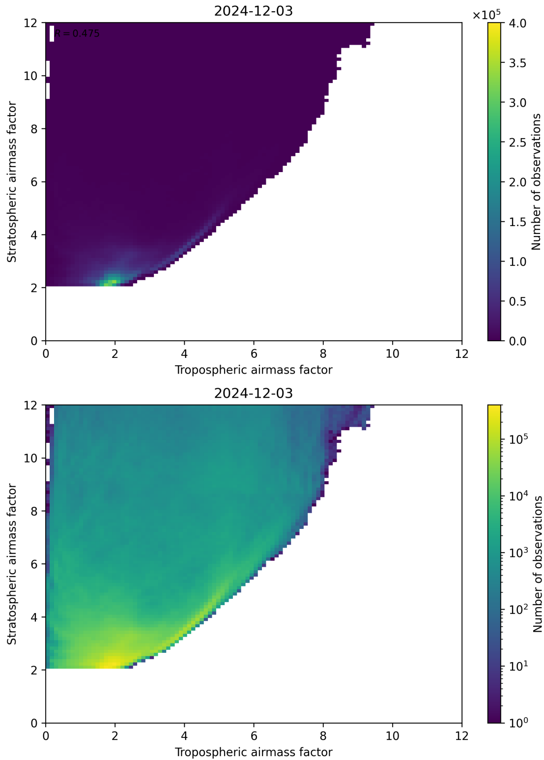
Figure 71: Scatter density plot of “Tropospheric airmass factor” against “Stratospheric airmass factor” for 2024-12-02 to 2024-12-04.
