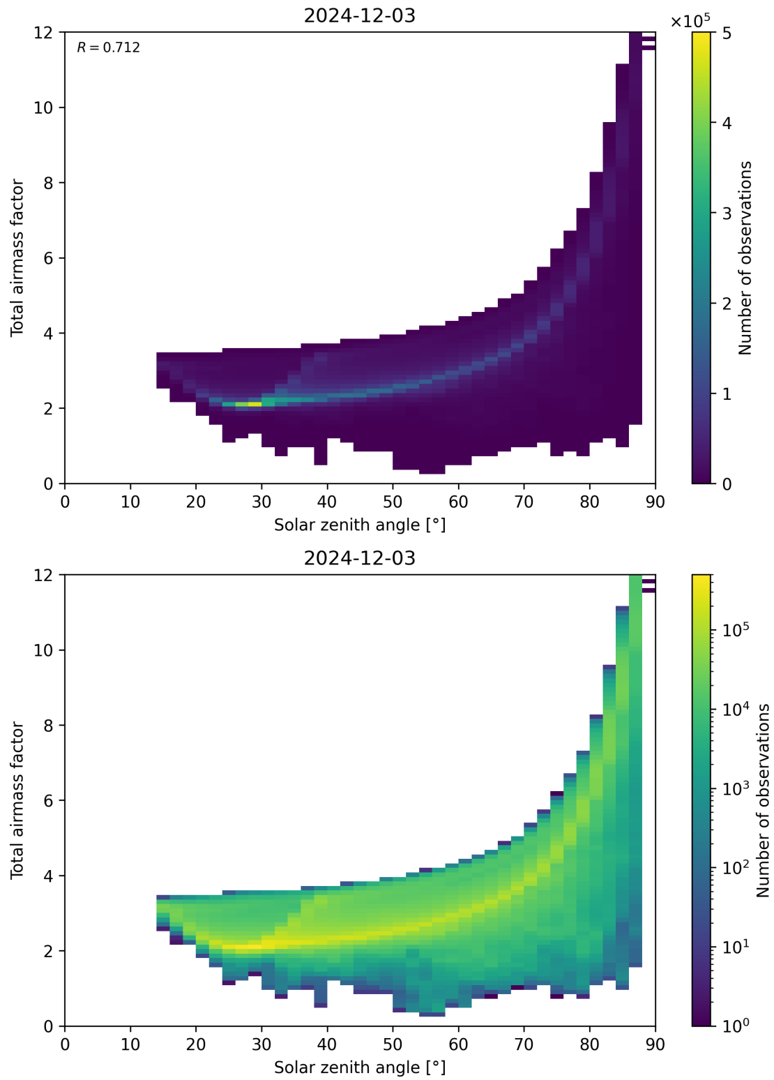
Figure 146: Scatter density plot of “Solar zenith angle” against “Total airmass factor” for 2024-12-02 to 2024-12-04.
