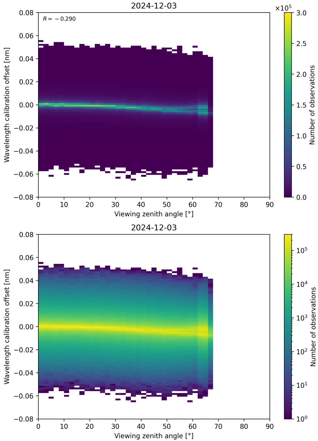
Figure 173: Scatter density plot of “Viewing zenith angle” against “Wavelength calibration offset” for 2024-12-02 to 2024-12-04.
