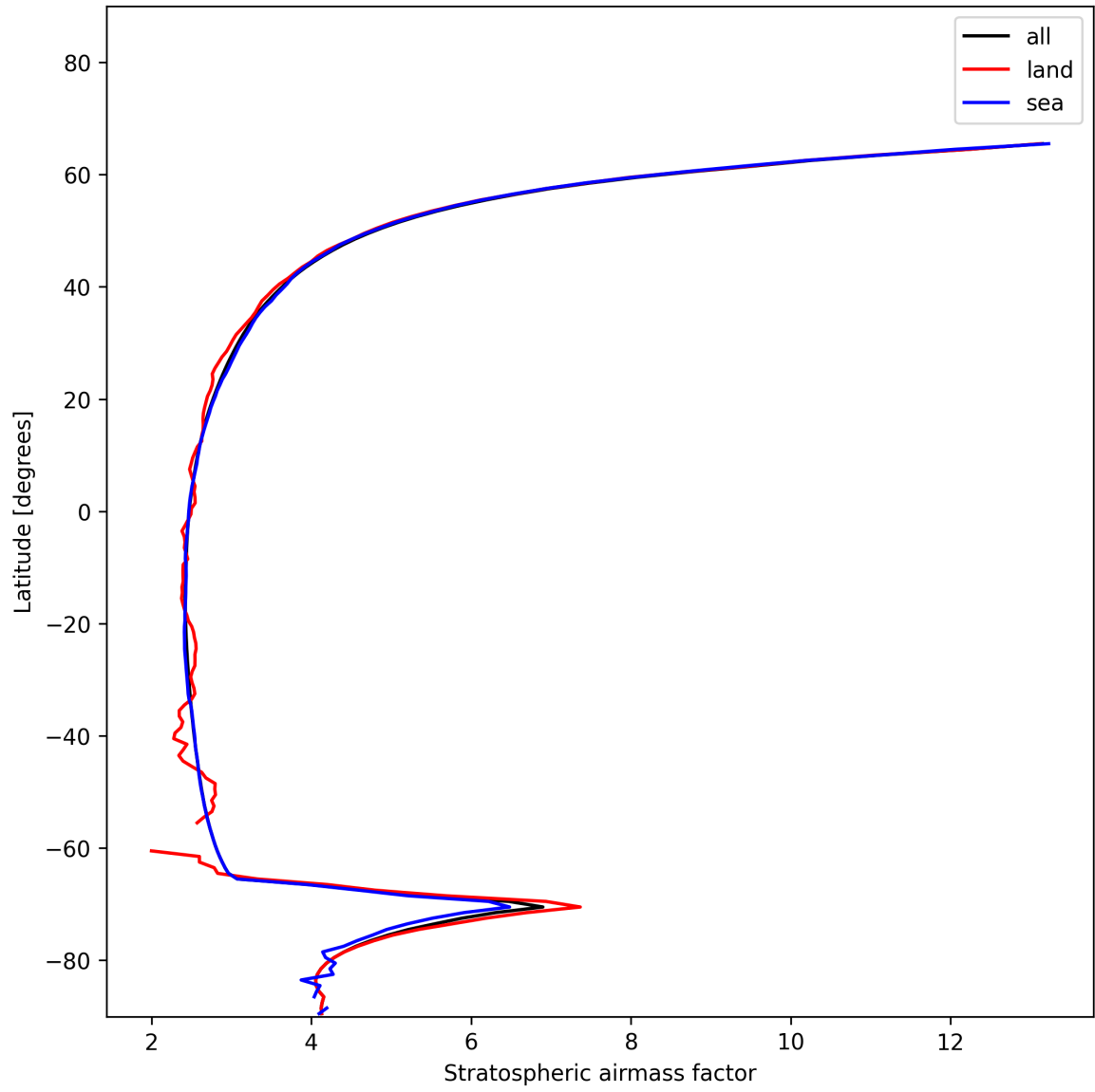
Figure 27: Zonal average of “Stratospheric air mass factor” for 2024-12-02 to 2024-12-04.
