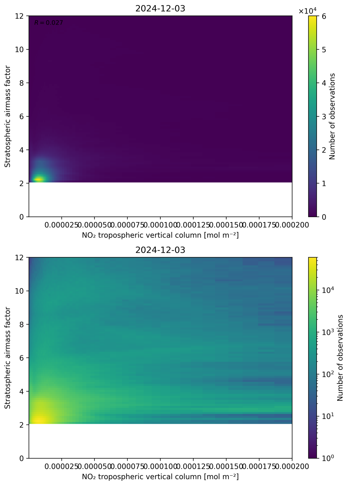
Figure 121: Scatter density plot of “NO 2 tropospheric vertical column” against “Stratospheric airmass factor” for 2024-12-02 to 2024-12-04.
