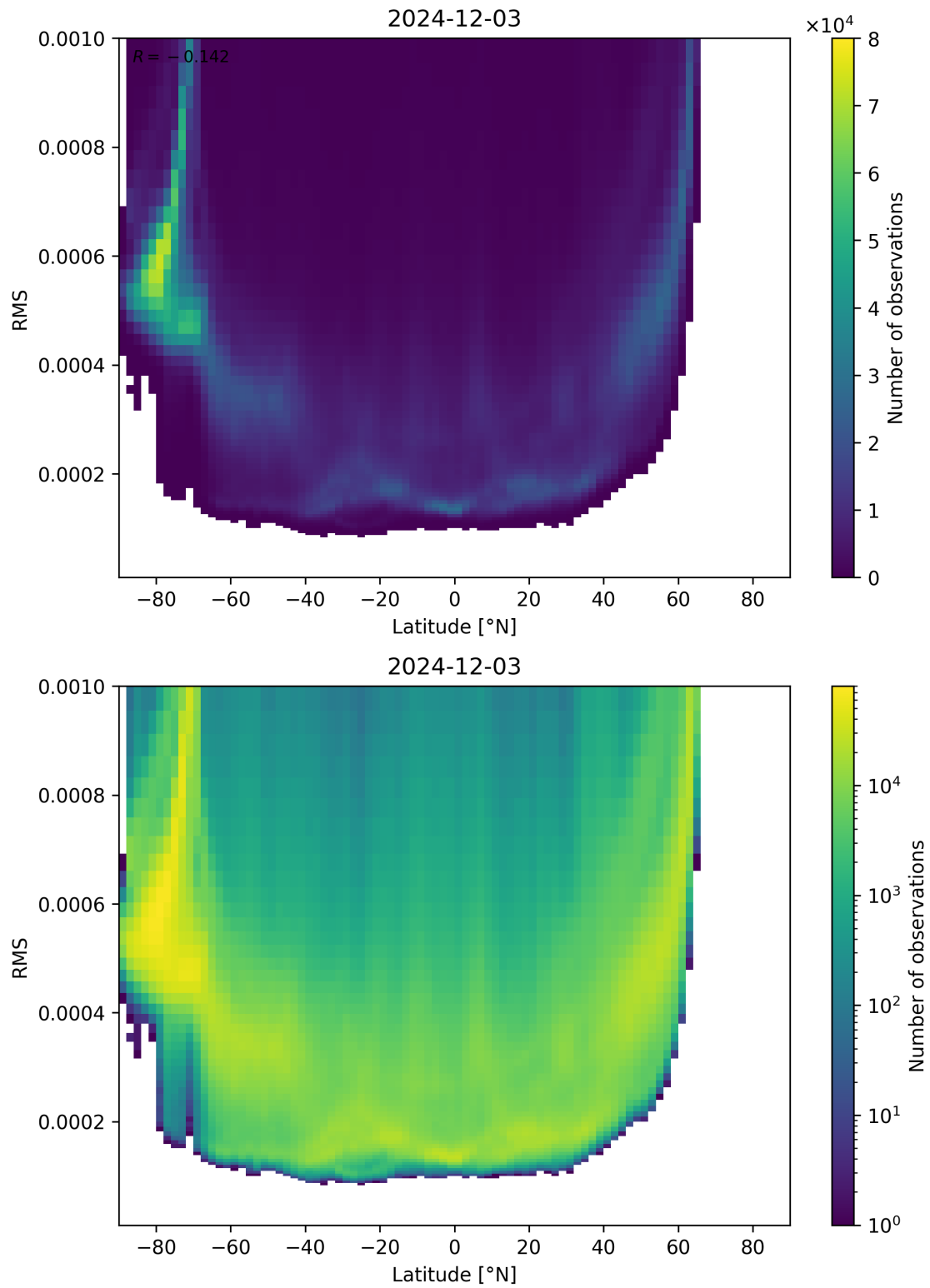
Figure 94: Scatter density plot of “Latitude” against “RMS” for 2024-12-02 to 2024-12-04.
