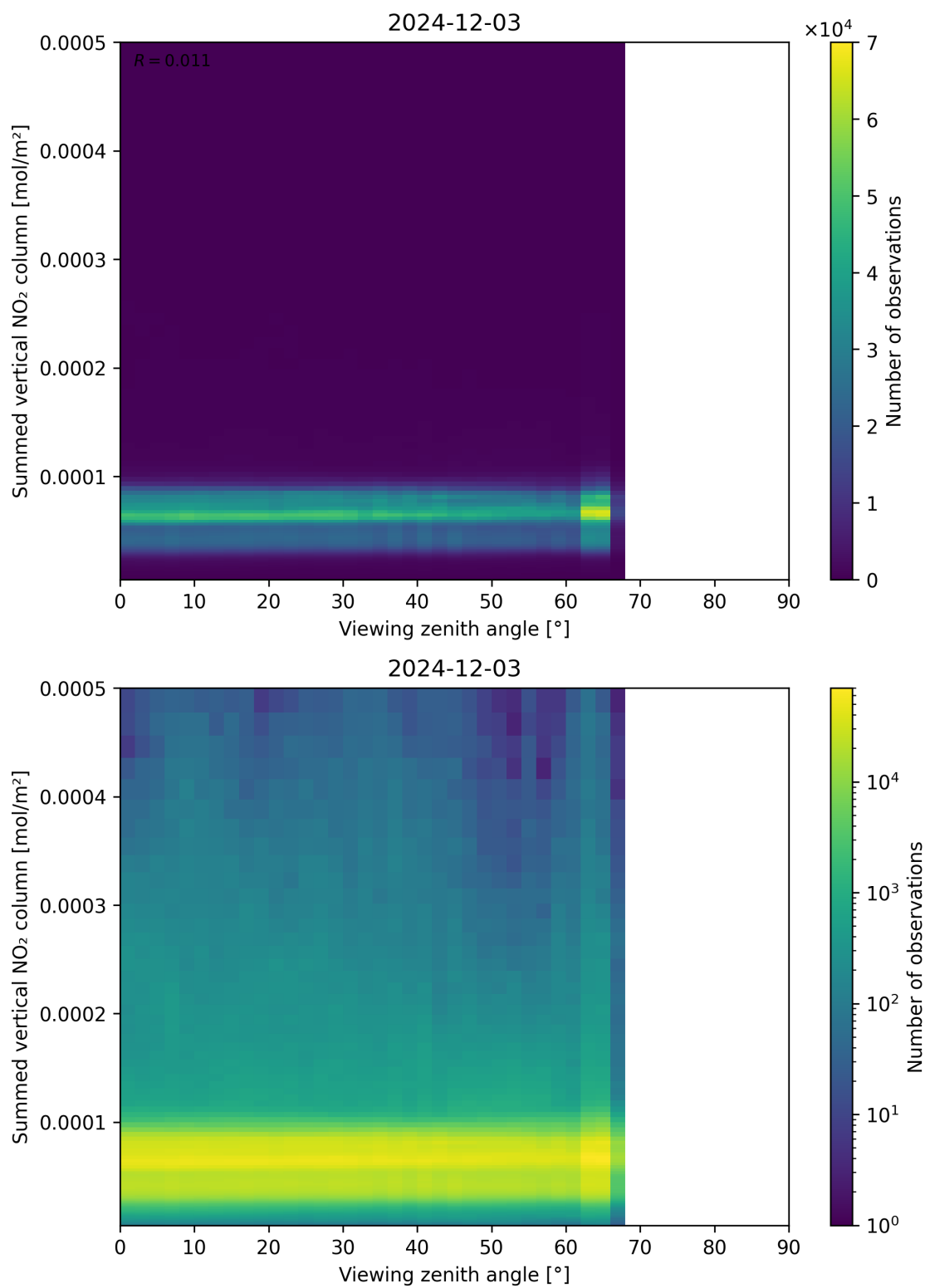
Figure 165: Scatter density plot of “Viewing zenith angle” against “Summed vertical NO 2 column” for 2024-12-02 to 2024-12-04.
