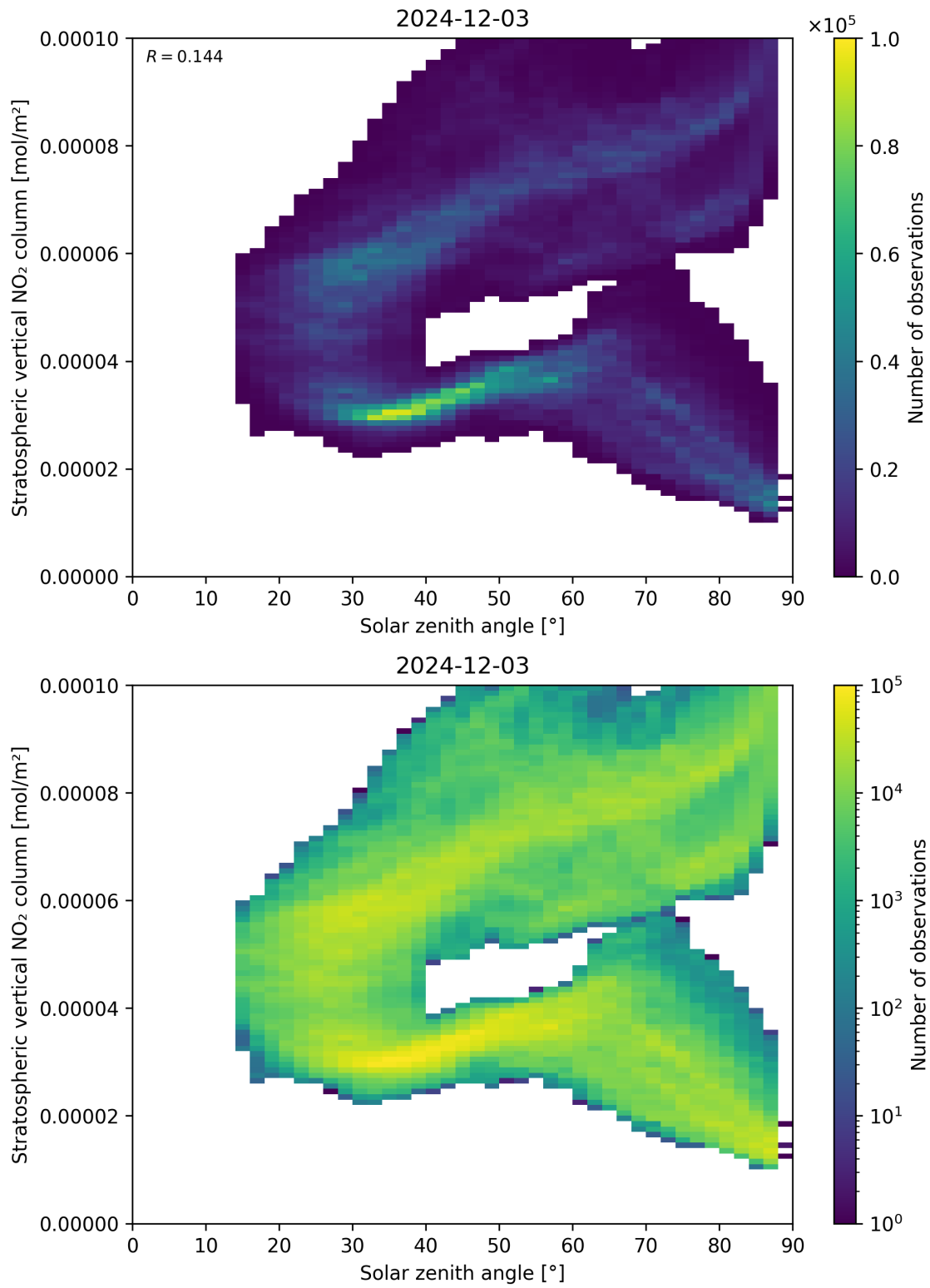
Figure 150: Scatter density plot of “Solar zenith angle” against “Stratospheric vertical NO 2 column” for 2024-12-02 to 2024-12-04.
