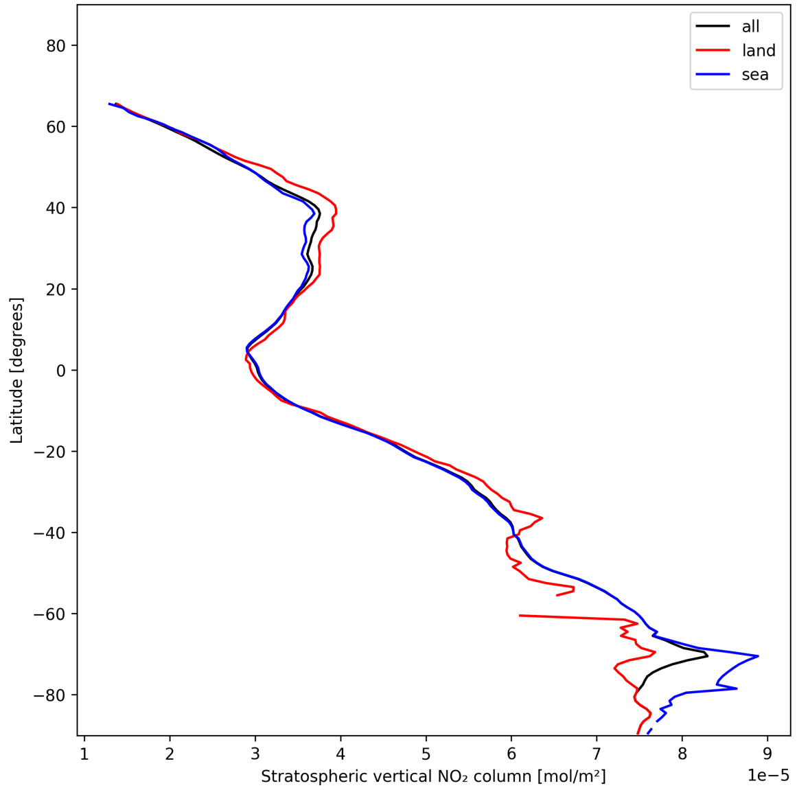
Figure 19: Zonal average of “Stratospheric vertical NO 2 column” for 2024-12-02 to 2024-12-04.
