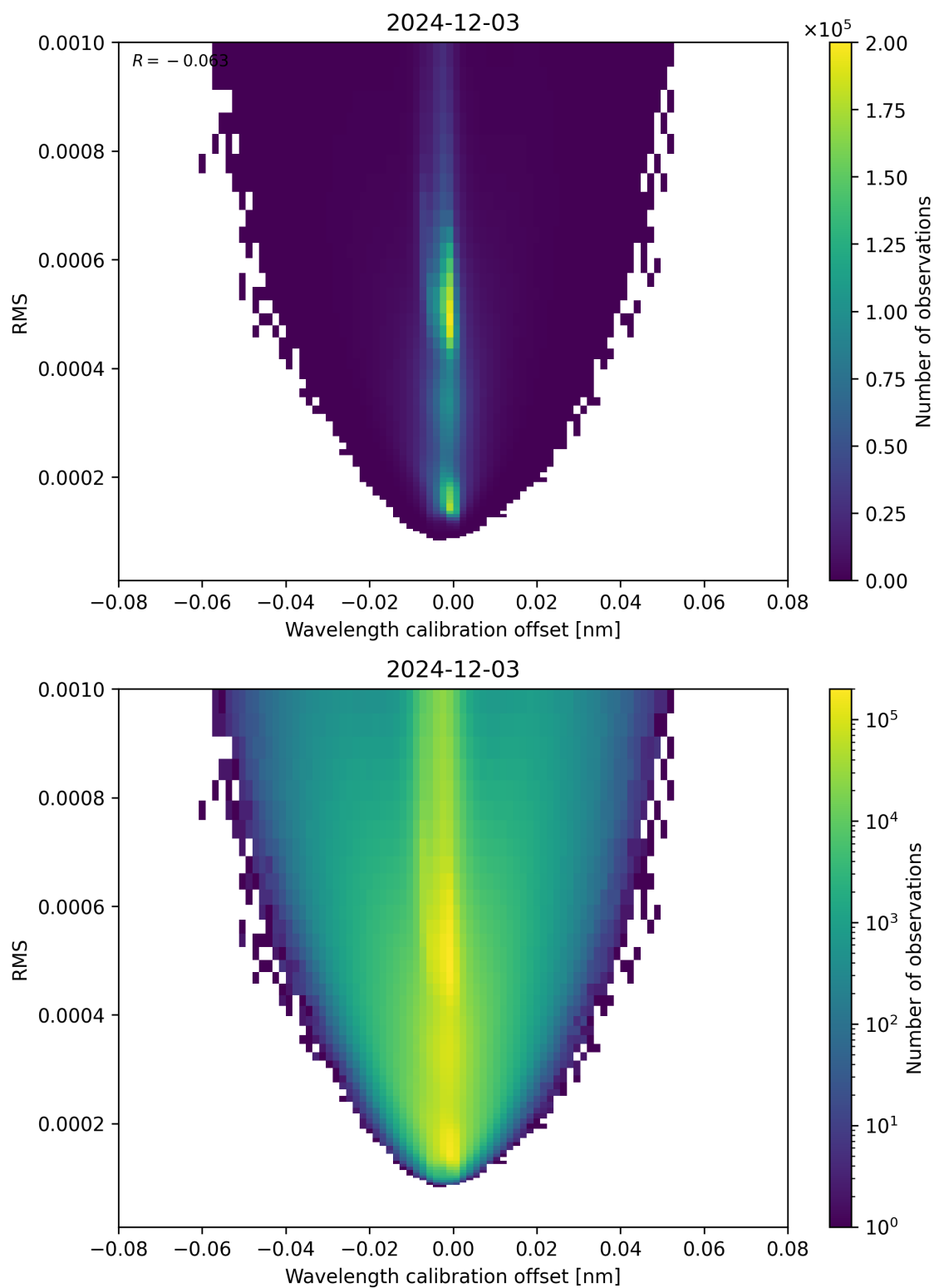
Figure 181: Scatter density plot of “Wavelength calibration offset” against “RMS” for 2024-12-02 to 2024-12-04.
