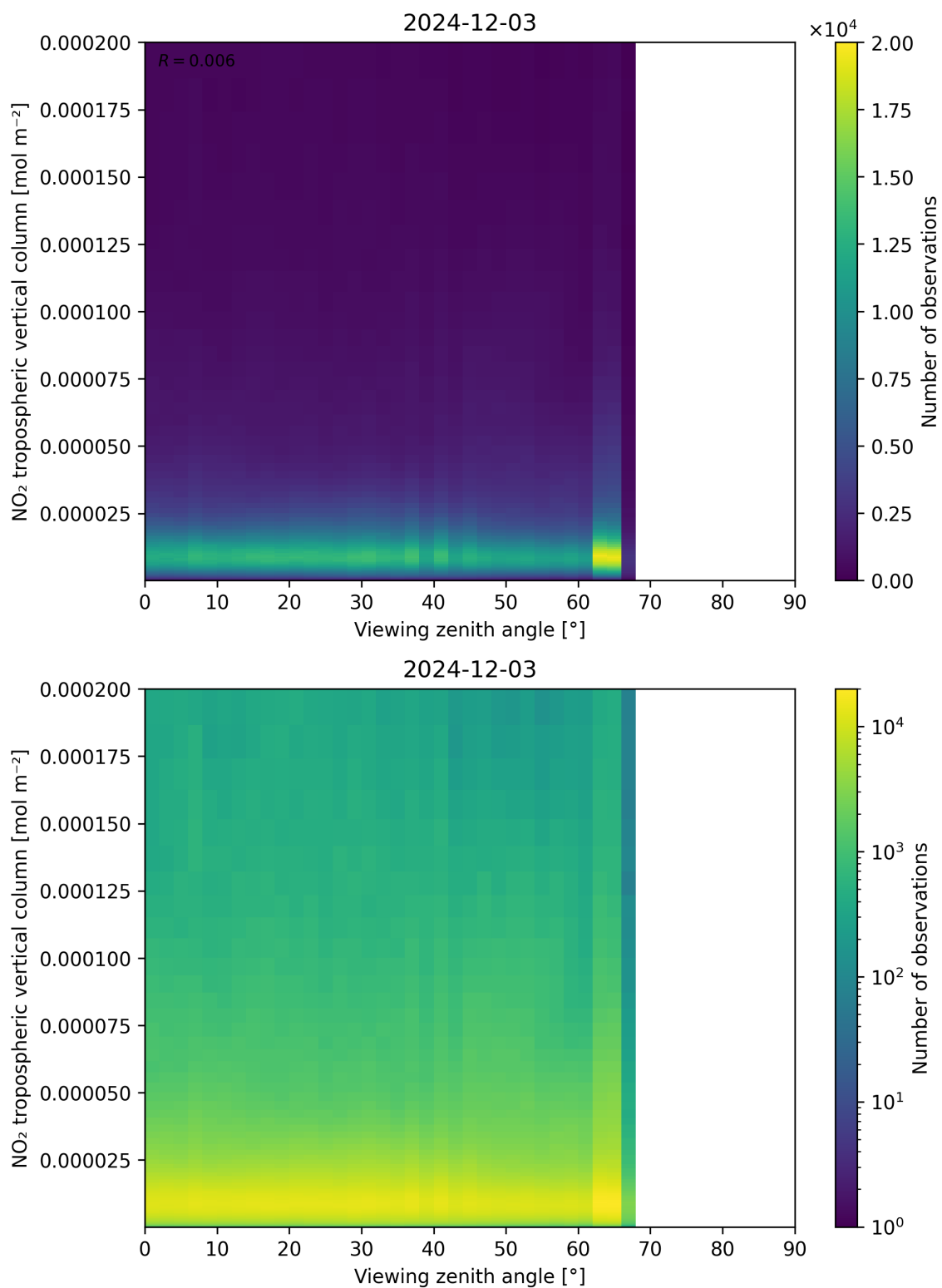
Figure 169: Scatter density plot of “Viewing zenith angle” against “NO 2 tropospheric vertical column” for 2024-12-02 to 2024-12-04.
