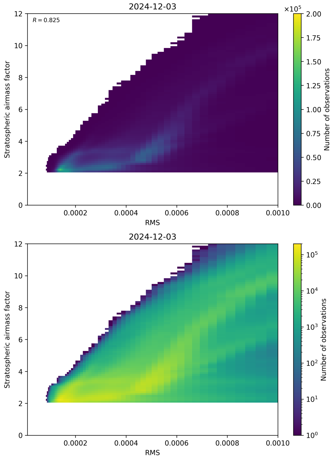
Figure 144: Scatter density plot of “RMS” against “Stratospheric airmass factor” for 2024-12-02 to 2024-12-04.
