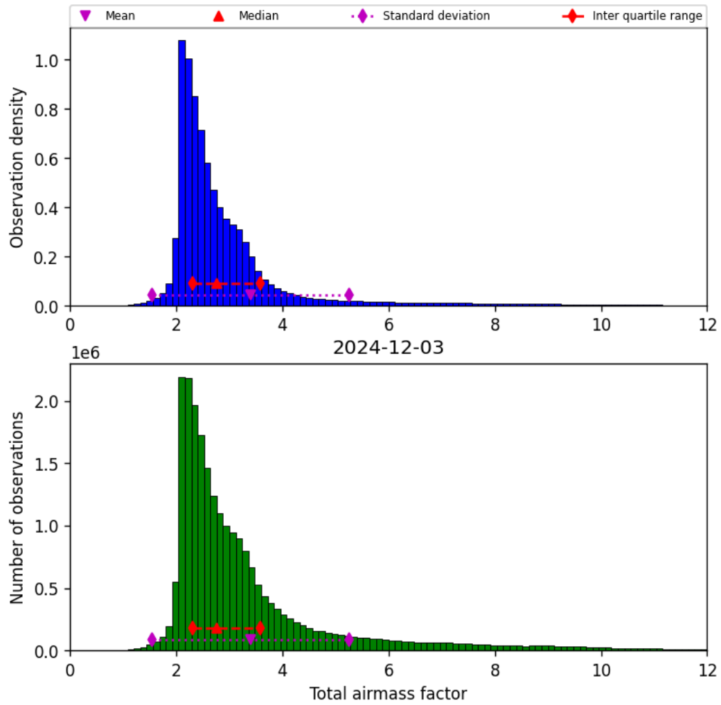
Figure 32: Histogram of “Total airmass factor” for 2024-12-02 to 2024-12-04
