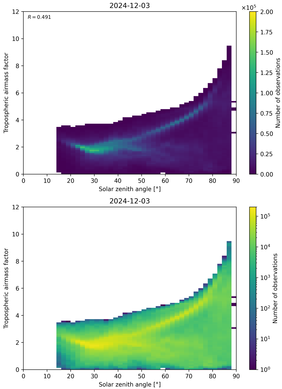
Figure 147: Scatter density plot of “Solar zenith angle” against “Tropospheric airmass factor” for 2024-12-02 to 2024-12-04.
