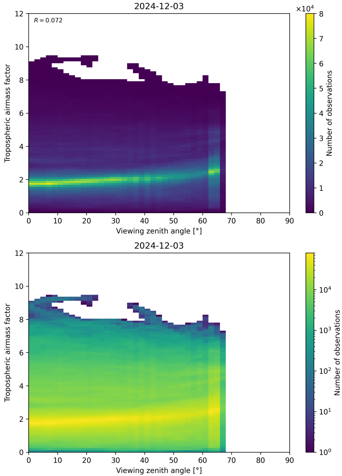
Figure 161: Scatter density plot of “Viewing zenith angle” against “Tropospheric airmass factor” for 2024-12-02 to 2024-12-04.
