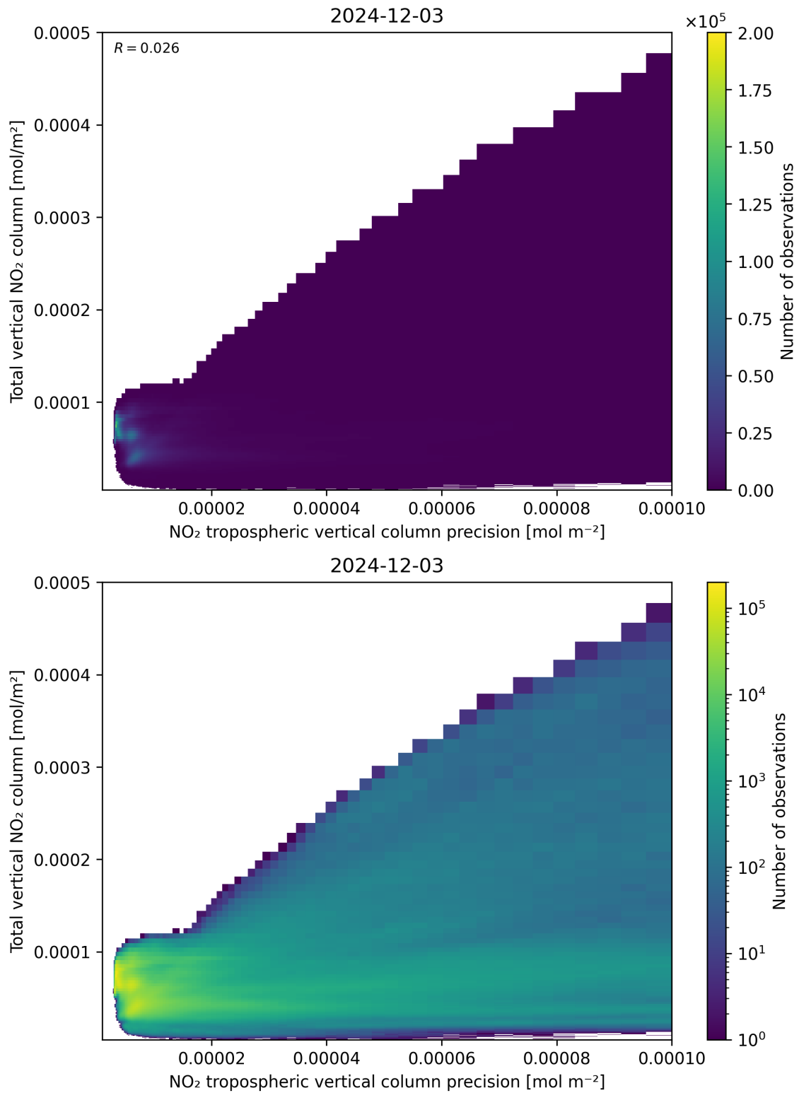
Figure 138: Scatter density plot of “NO 2 tropospheric vertical column precision” against “Total vertical NO 2 column” for 2024-12-02 to 2024-12-04.
