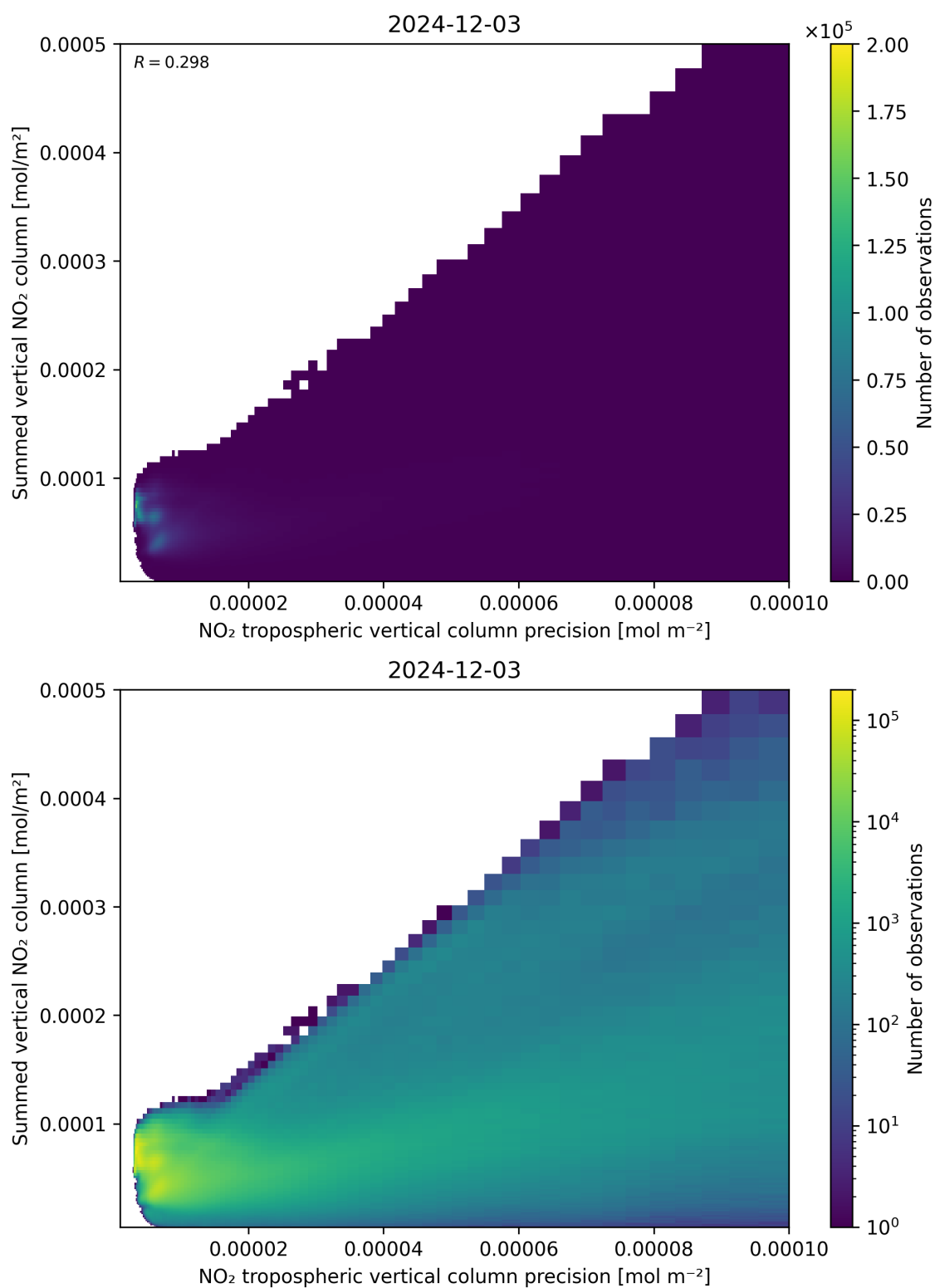
Figure 136: Scatter density plot of “NO 2 tropospheric vertical column precision” against “Summed vertical NO 2 column” for 2024-12-02 to 2024-12-04.
