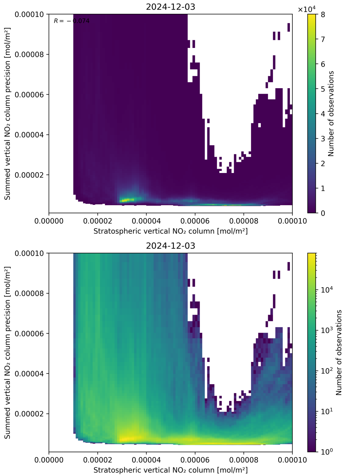
Figure 99: Scatter density plot of “Stratospheric vertical NO 2 column” against “Summed vertical NO 2 column precision” for 2024-12-02 to 2024-12-04.
