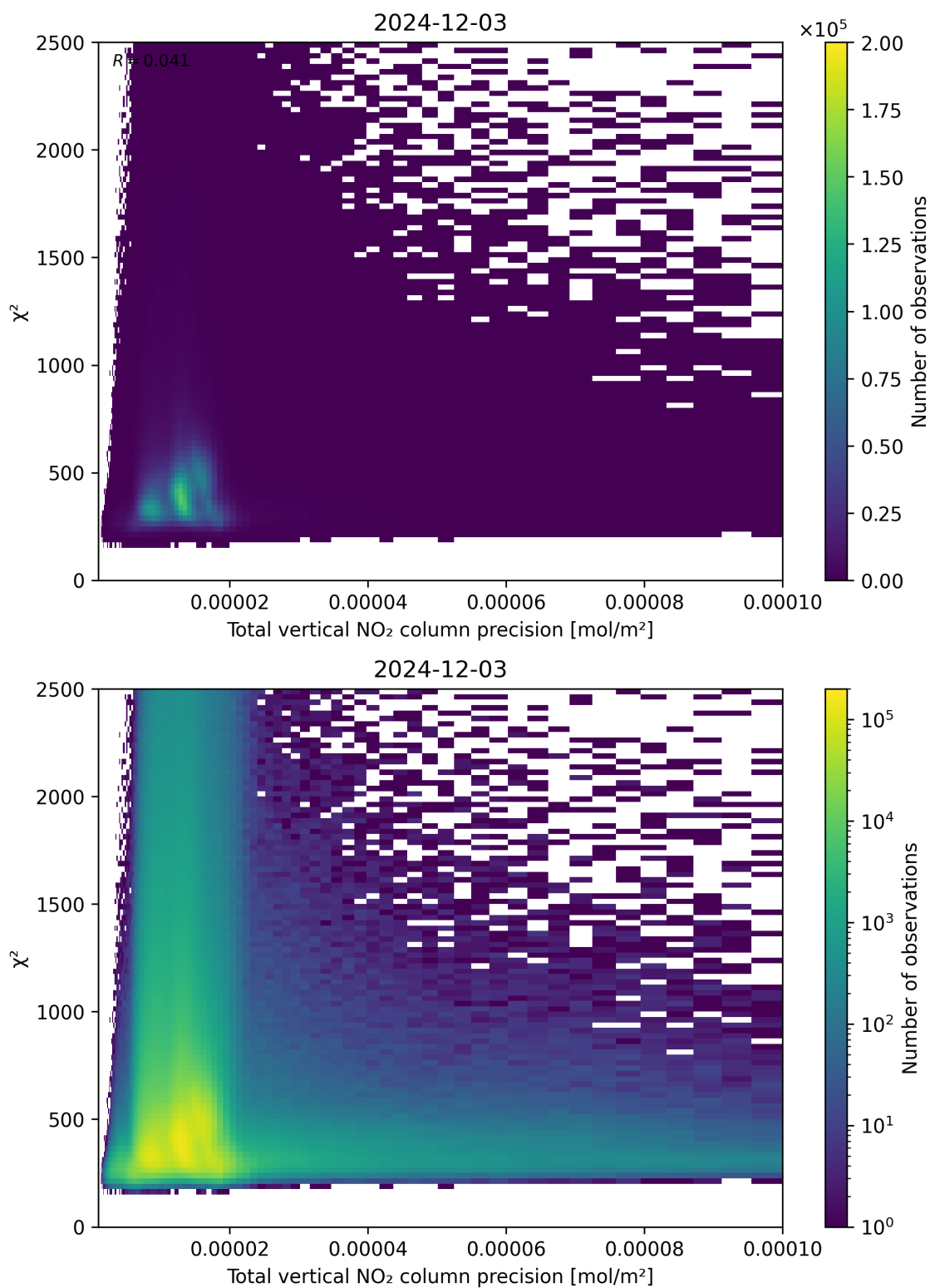
Figure 116: Scatter density plot of “Total vertical NO 2 column precision” against “ \chi^2 ” for 2024-12-02 to 2024-12-04.
