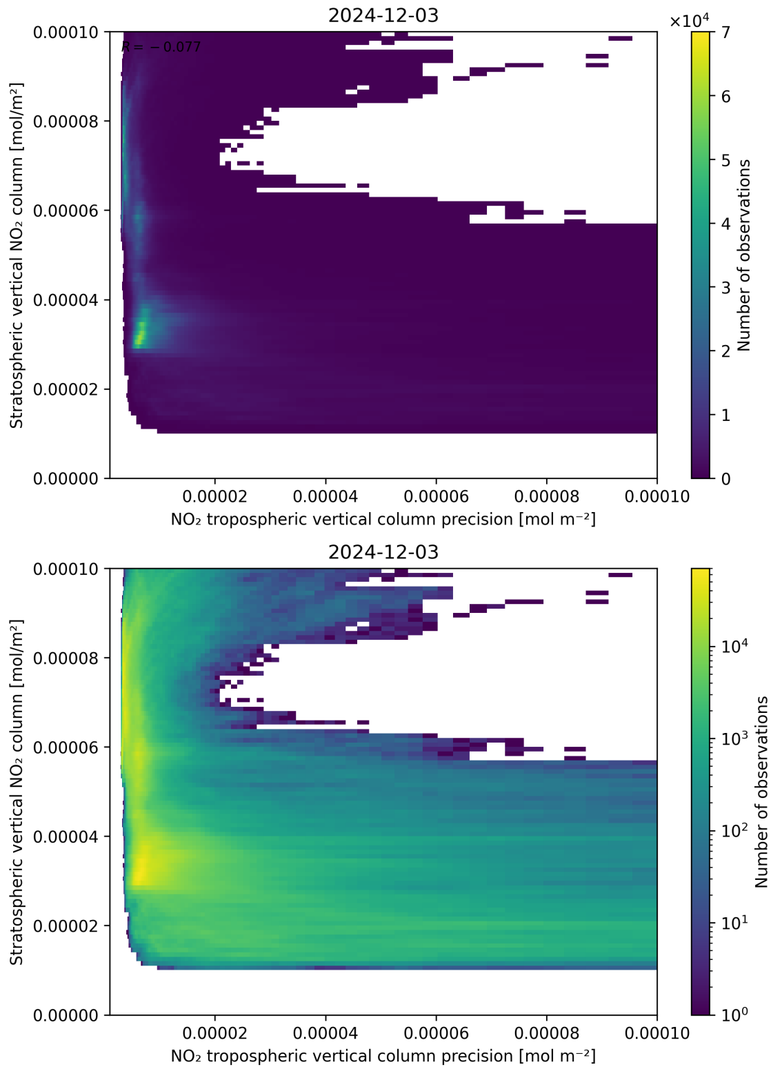
Figure 135: Scatter density plot of “NO 2 tropospheric vertical column precision” against “Stratospheric vertical NO 2 column” for 2024-12-02 to 2024-12-04.
