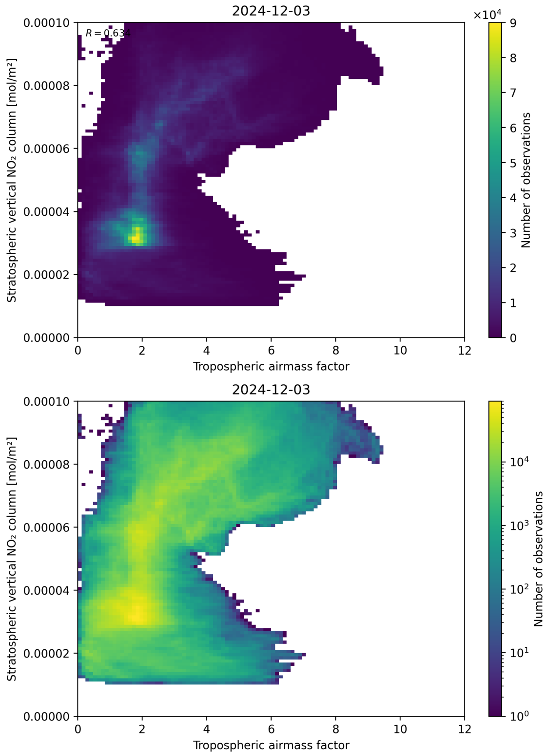
Figure 74: Scatter density plot of “Tropospheric air mass factor” against “Stratospheric vertical NO 2 column” for 2024-12-02 to 2024-12-04.
