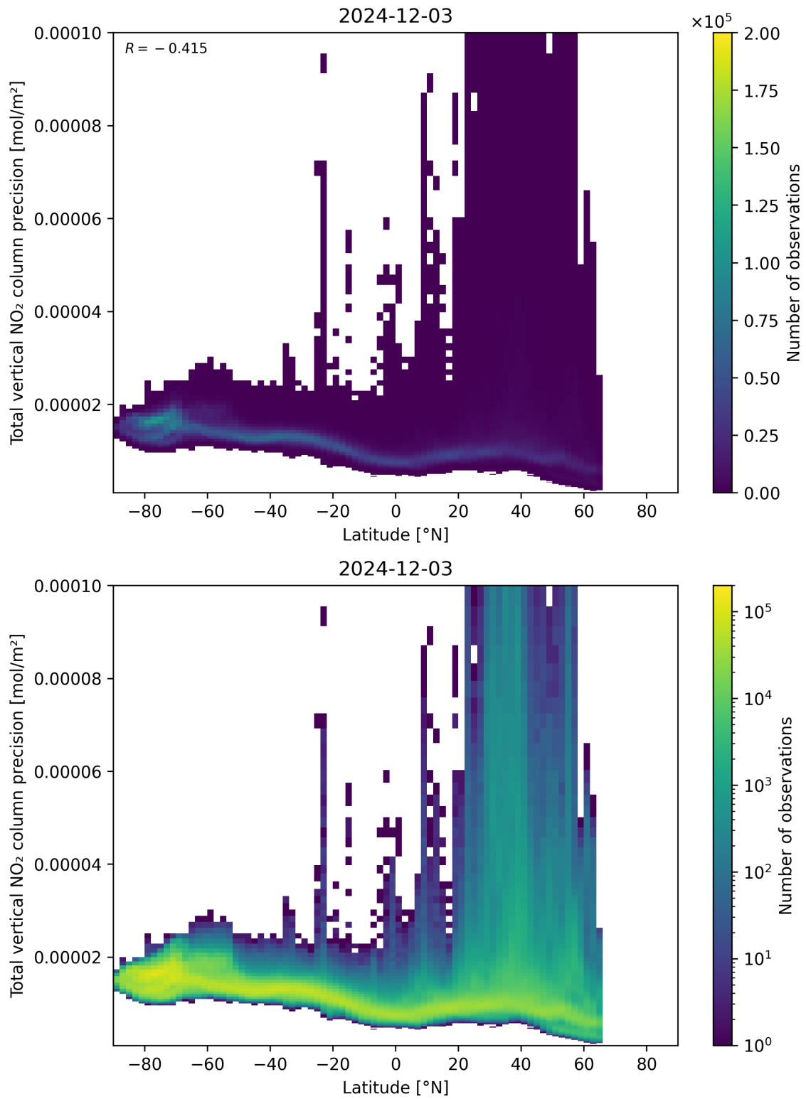
Figure 91: Scatter density plot of “Latitude” against “Total vertical NO 2 column precision” for 2024-12-02 to 2024-12-04.
