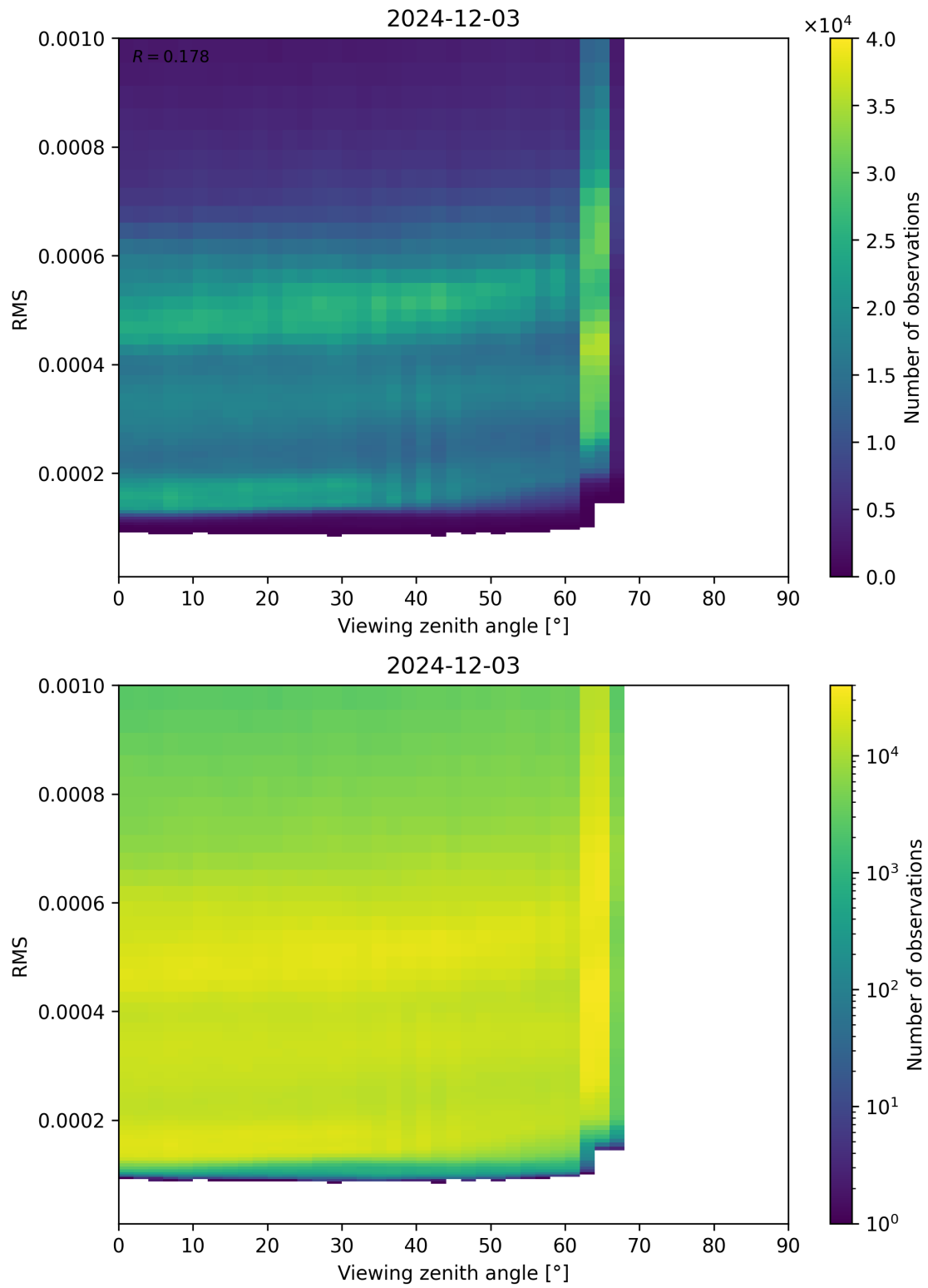
Figure 171: Scatter density plot of “Viewing zenith angle” against “RMS” for 2024-12-02 to 2024-12-04.
