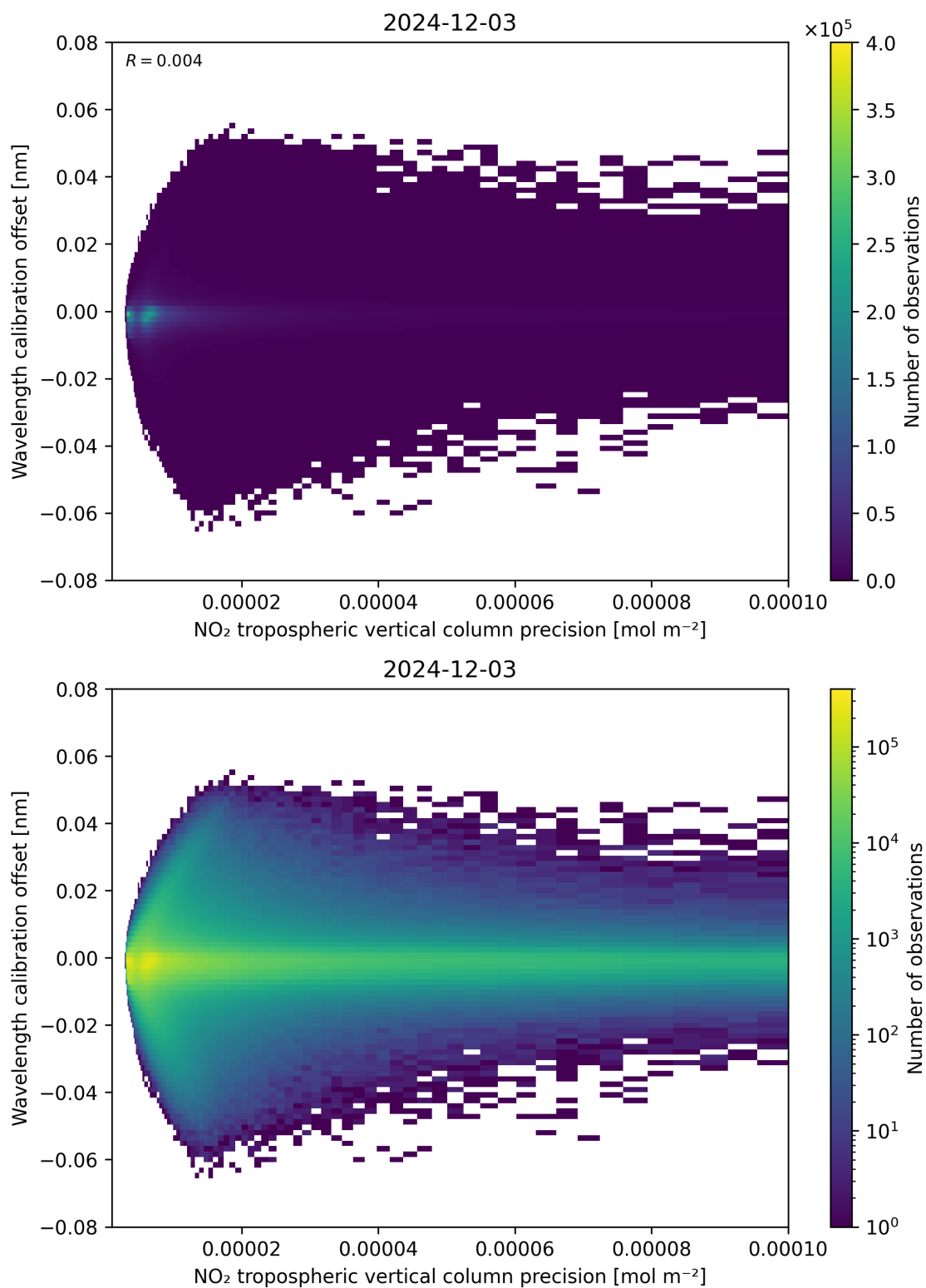
Figure 141: Scatter density plot of “NO 2 tropospheric vertical column precision” against “Wavelength calibration offset” for 2024-12-02 to 2024-12-04.
