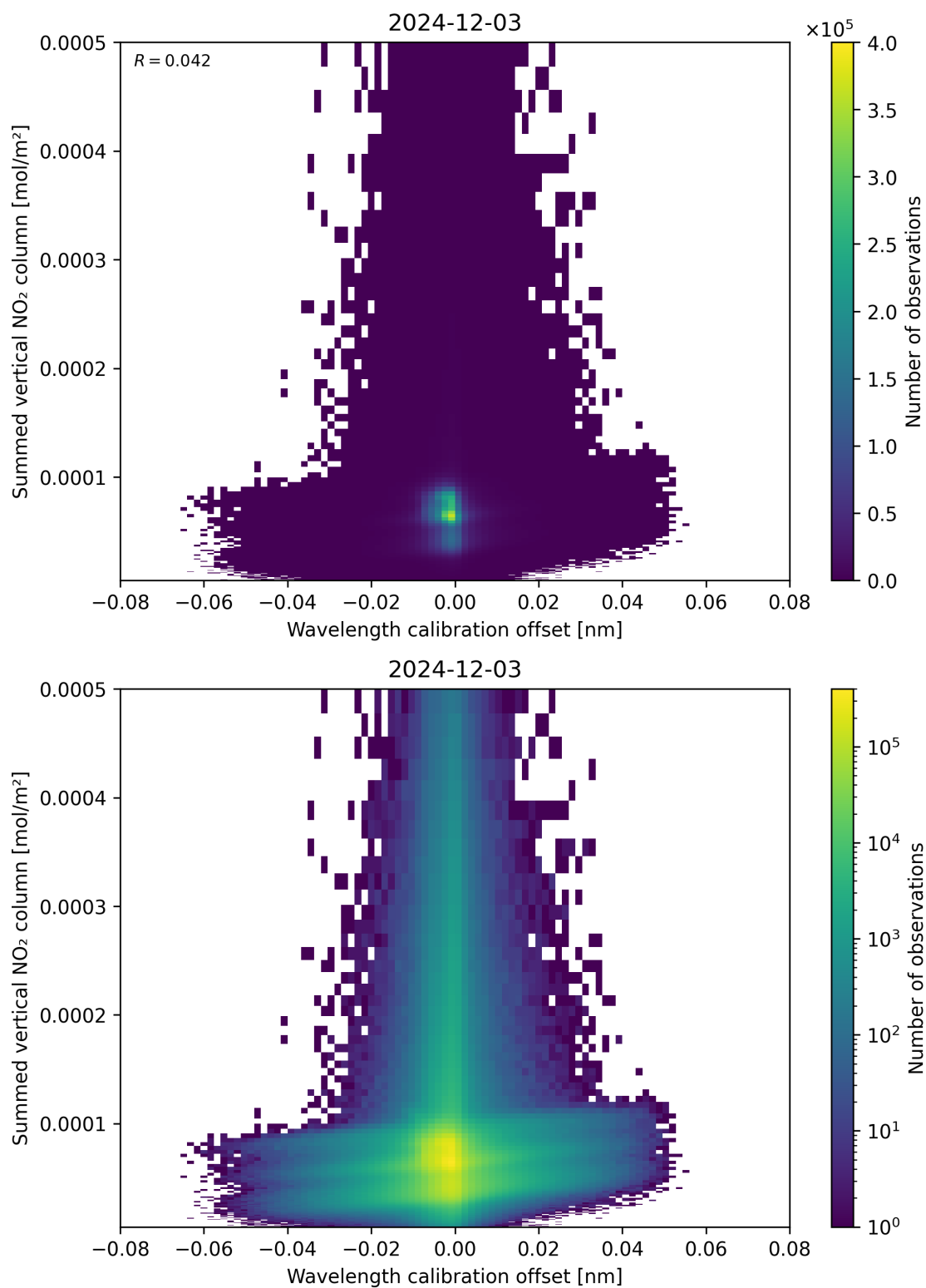
Figure 177: Scatter density plot of “Wavelength calibration offset” against “Summed vertical NO 2 column” for 2024-12-02 to 2024-12-04.
