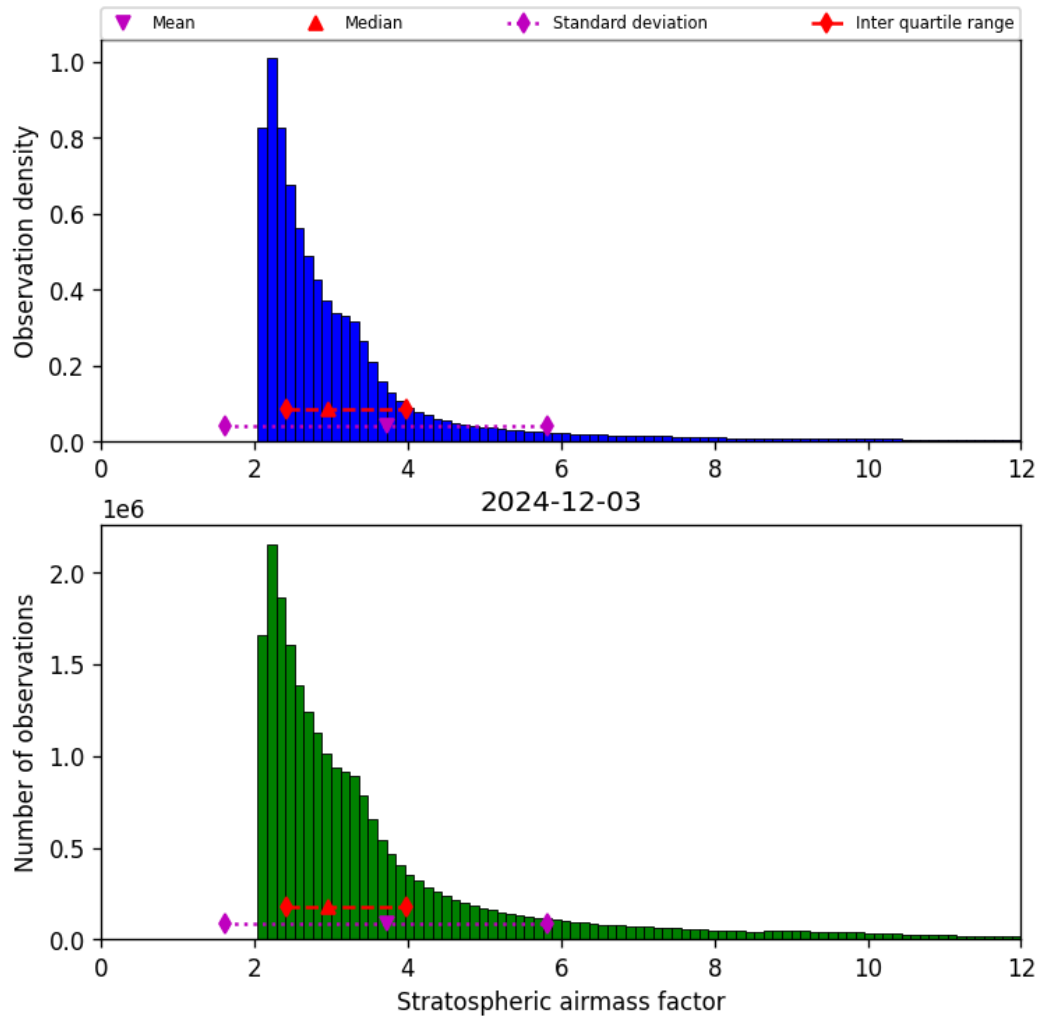
Figure 44: Histogram of “Stratospheric airmass factor” for 2024-12-02 to 2024-12-04
