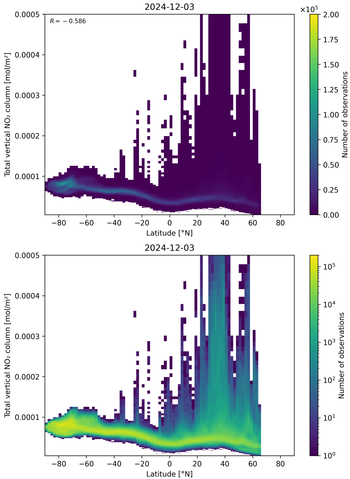
Figure 90: Scatter density plot of “Latitude” against “Total vertical NO 2 column” for 2024-12-02 to 2024-12-04.
