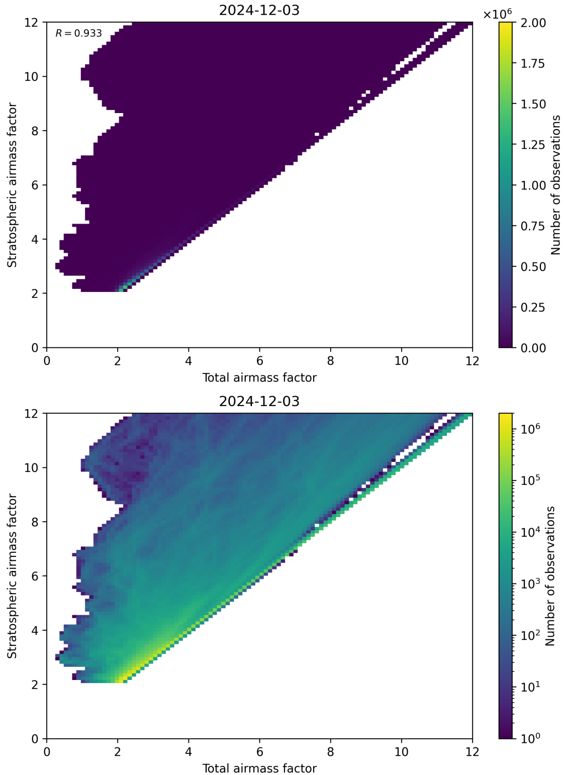
Figure 62: Scatter density plot of “Total airmass factor” against “Stratospheric airmass factor” for 2024-12-02 to 2024-12-04.
