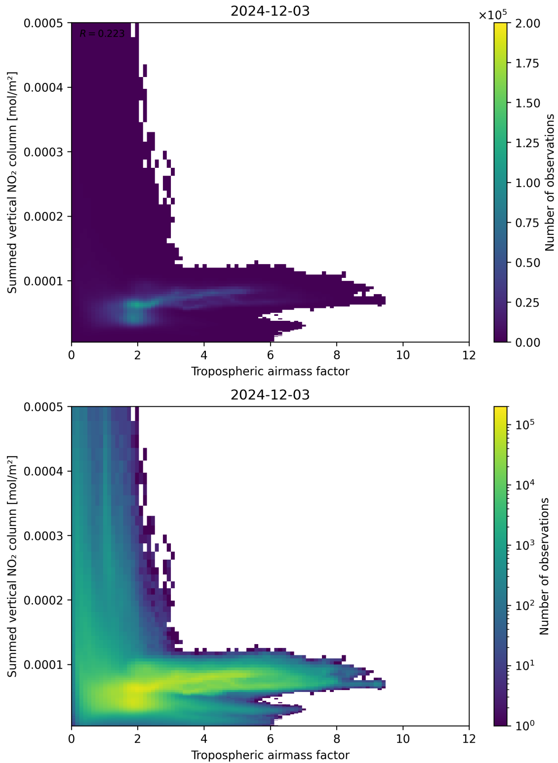
Figure 75: Scatter density plot of “Tropospheric airmass factor” against “Summed vertical NO 2 column” for 2024-12-02 to 2024-12-04.
