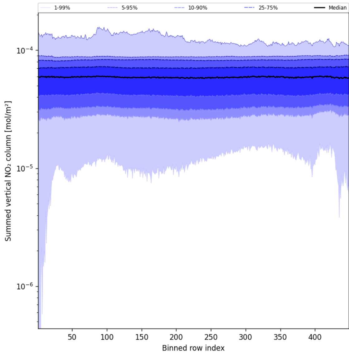
Figure 57: Along track statistics of “Summed vertical NO 2 column” for 2024-12-02 to 2024-12-04
