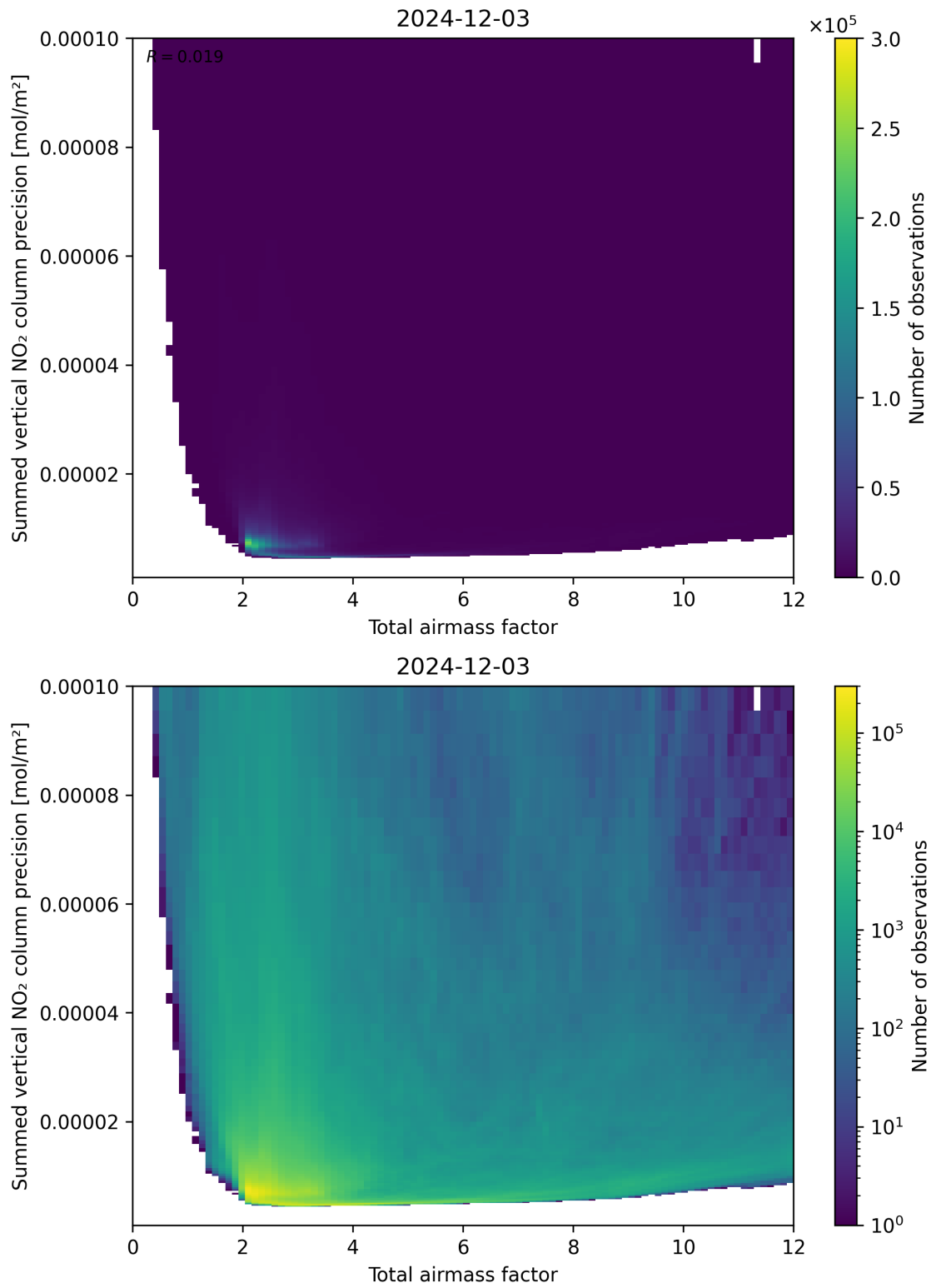
Figure 66: Scatter density plot of “Total airmass factor” against “Summed vertical NO 2 column precision” for 2024-12-02 to 2024-12-04.
