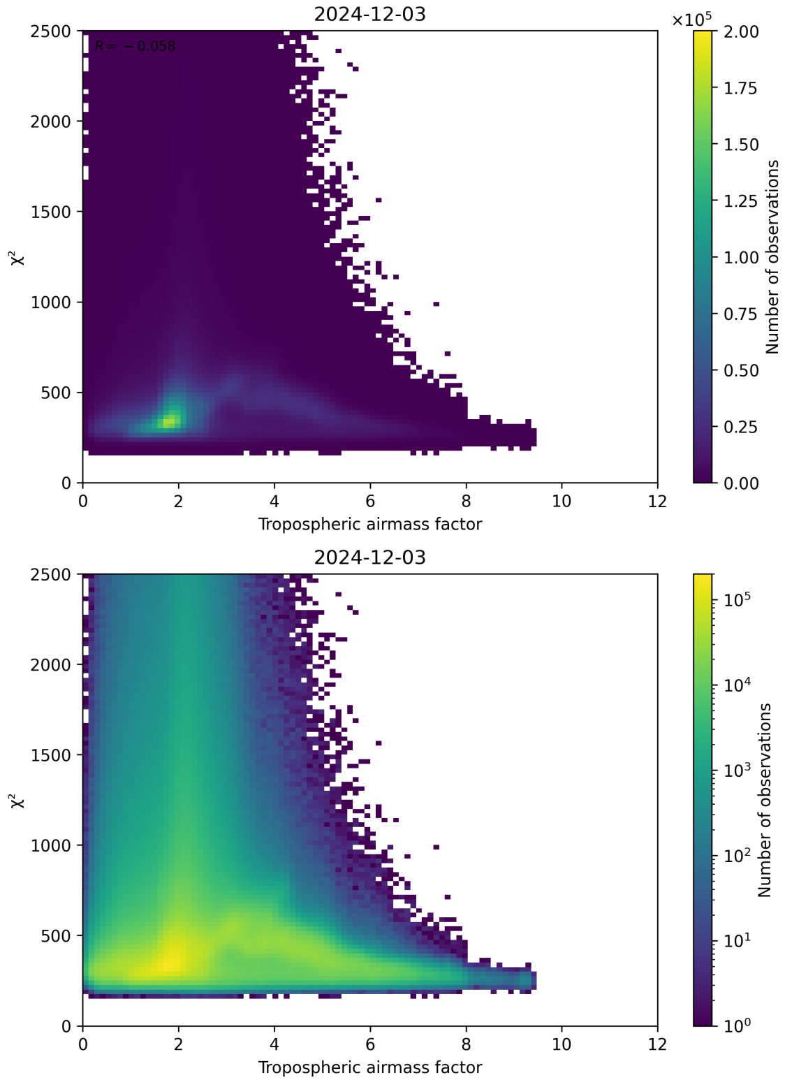
Figure 73: Scatter density plot of “Tropospheric airmass factor” against “ \chi^2 ” for 2024-12-02 to 2024-12-04.
