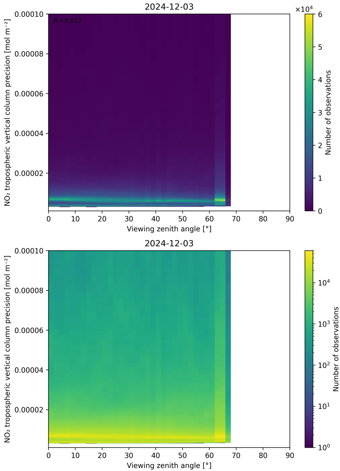
Figure 170: Scatter density plot of “Viewing zenith angle” against “NO 2 tropospheric vertical column precision” for 2024-12-02 to 2024-12-04.
