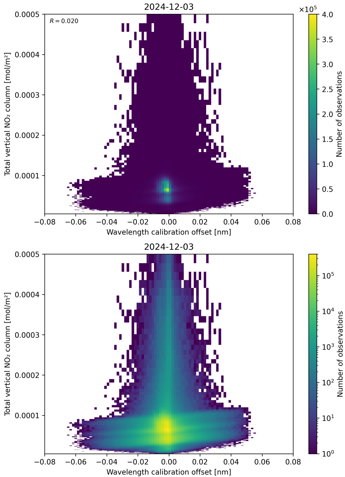
Figure 179: Scatter density plot of “Wavelength calibration offset” against “Total vertical NO 2 column” for 2024-12-02 to 2024-12-04.
