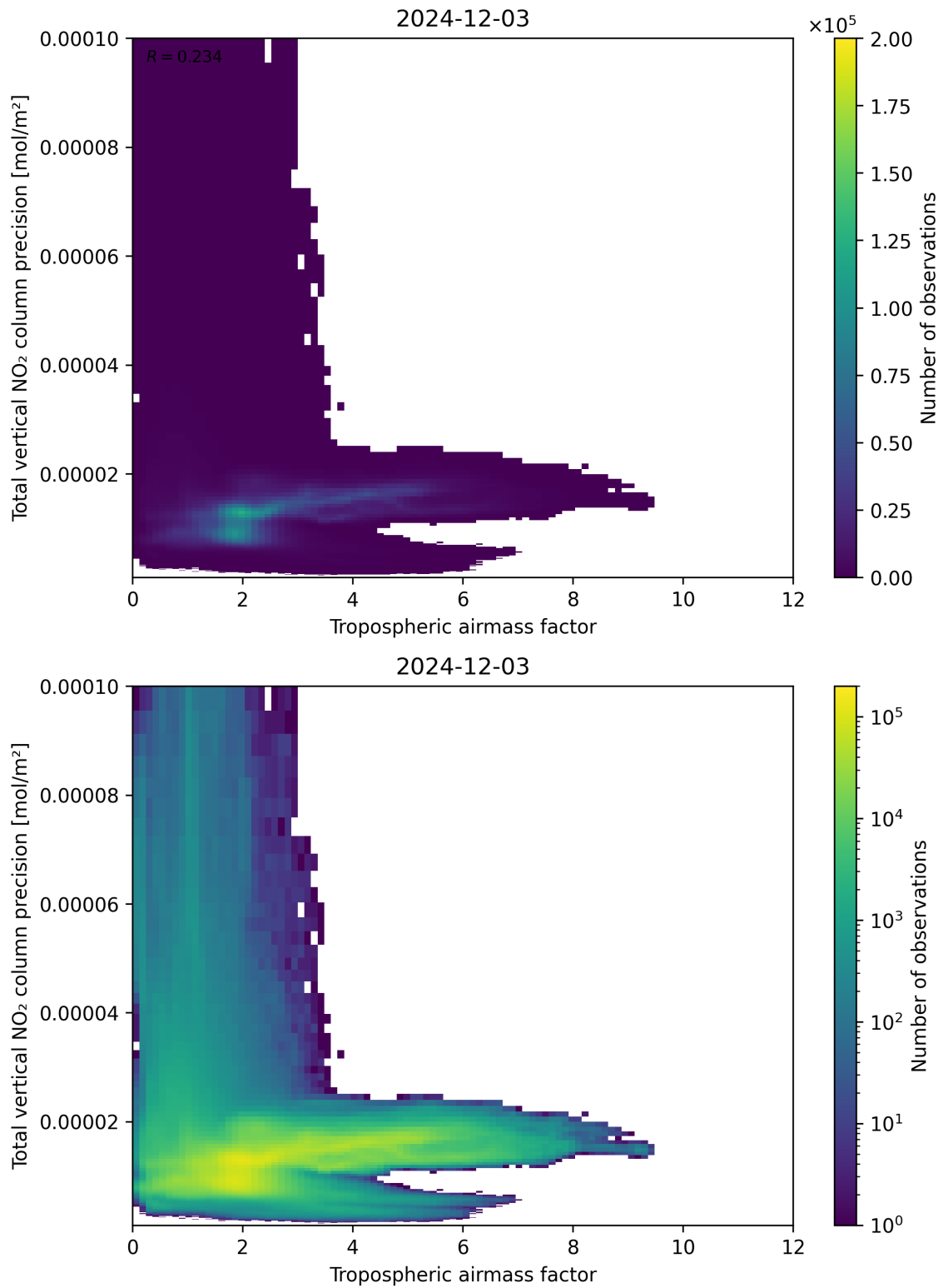
Figure 78: Scatter density plot of “Tropospheric air mass factor” against “Total vertical NO 2 column precision” for 2024-12-02 to 2024-12-04.
