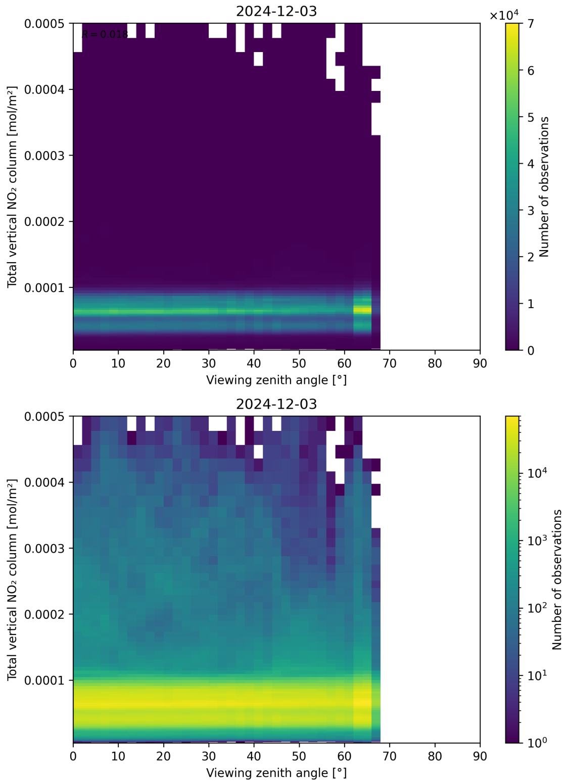
Figure 167: Scatter density plot of “Viewing zenith angle” against “Total vertical NO 2 column” for 2024-12-02 to 2024-12-04.
