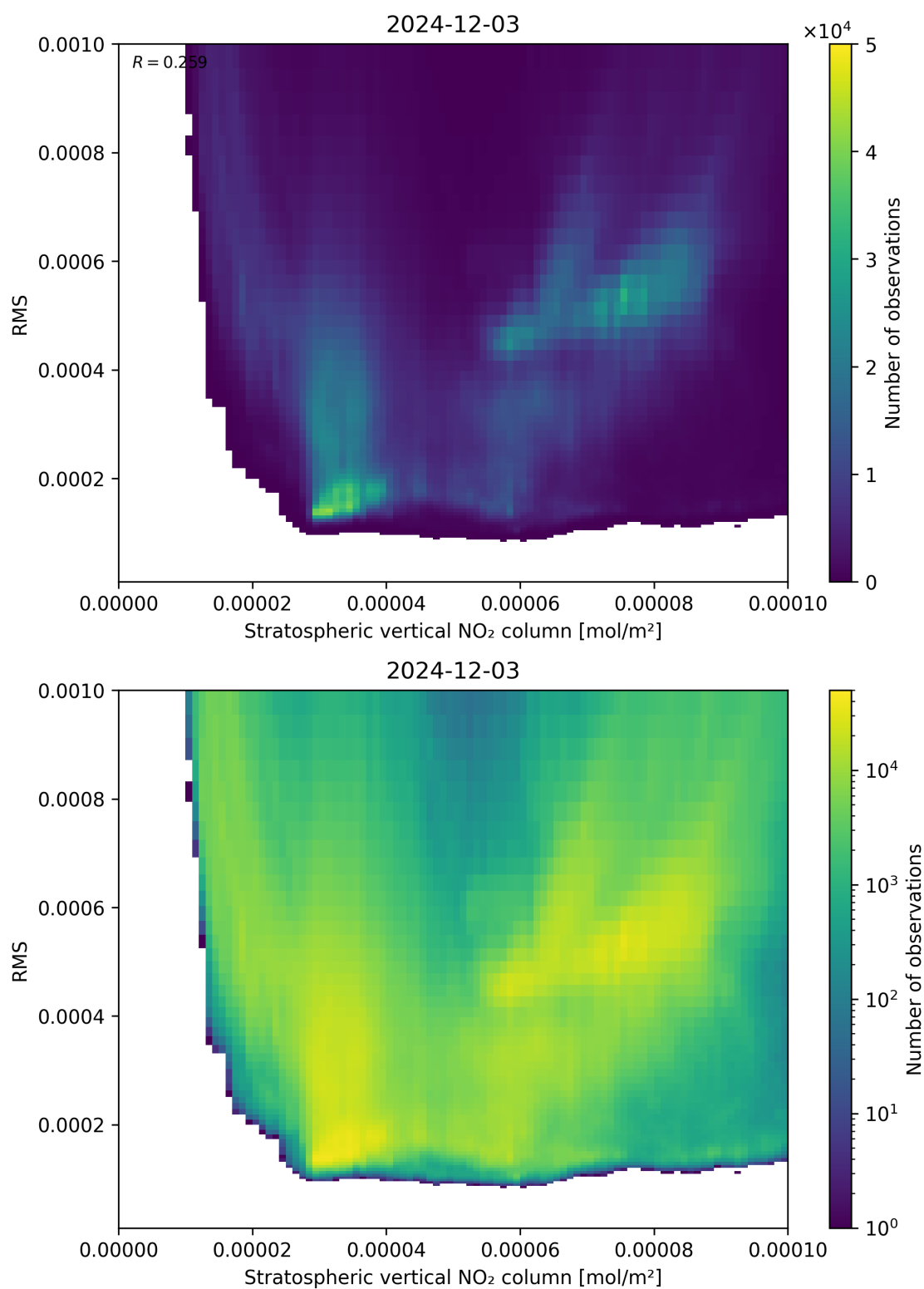
Figure 102: Scatter density plot of “Stratospheric vertical NO 2 column” against “RMS” for 2024-12-02 to 2024-12-04.
