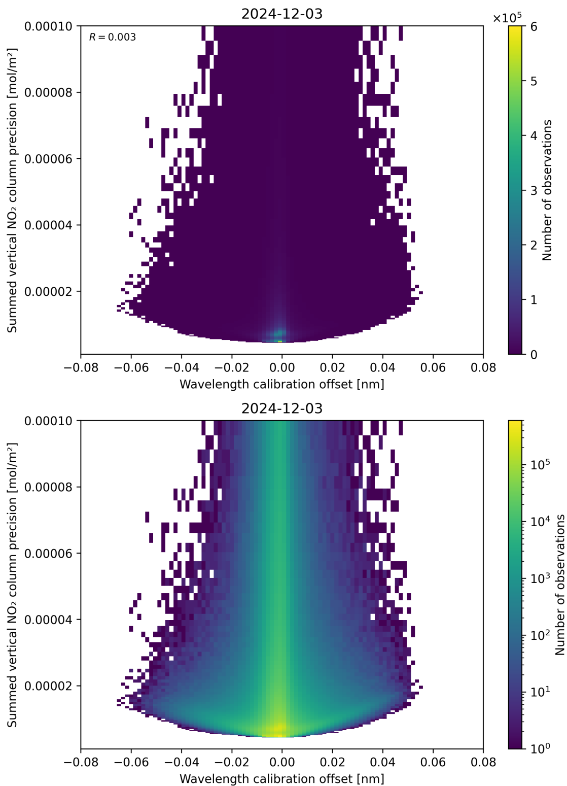
Figure 178: Scatter density plot of “Wavelength calibration offset” against “Summed vertical NO 2 column precision” for 2024-12-02 to 2024-12-04.
