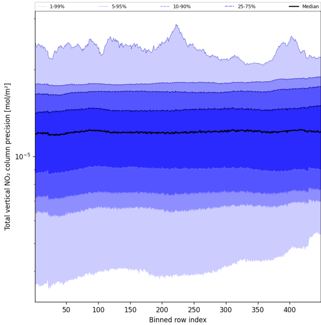
Figure 56: Along track statistics of "Total vertical NO 2 column precision" for 2024-12-02 to 2024-12-04
