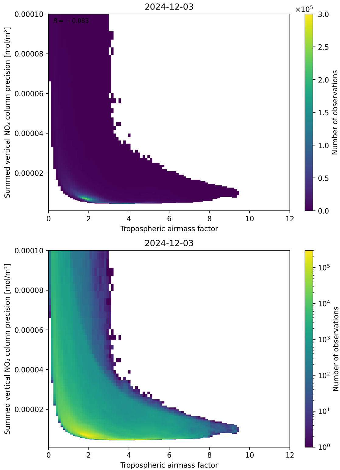
Figure 76: Scatter density plot of “Tropospheric air mass factor” against “Summed vertical NO 2 column precision” for 2024-12-02 to 2024-12-04.
