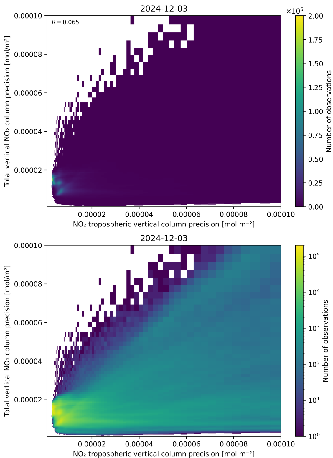
Figure 139: Scatter density plot of “NO 2 tropospheric vertical column precision” against “Total vertical NO 2 column precision” for 2024-12-02 to 2024-12-04.
