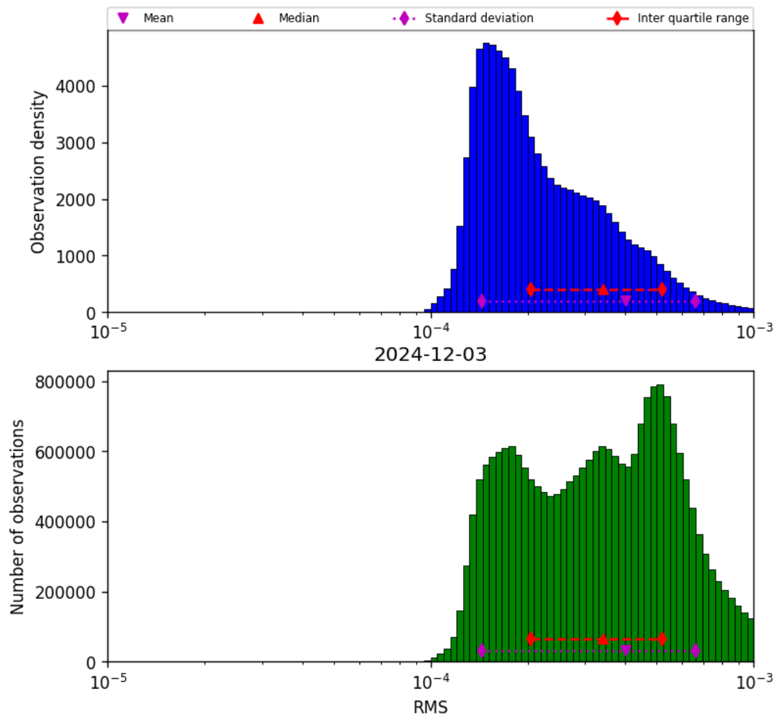
Figure 43: Histogram of “RMS” for 2024-12-02 to 2024-12-04
