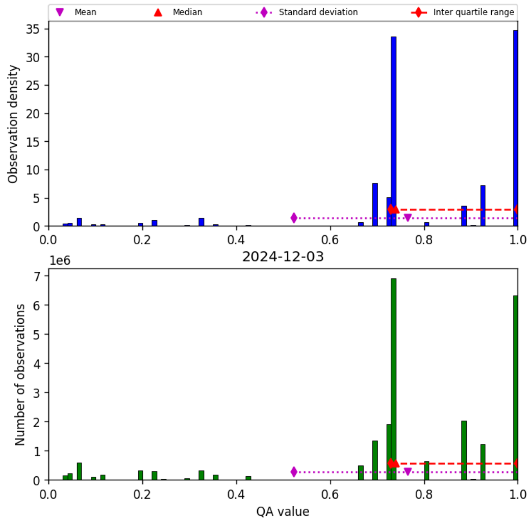
Figure 28: Histogram of “QA value” for 2024-12-02 to 2024-12-04
