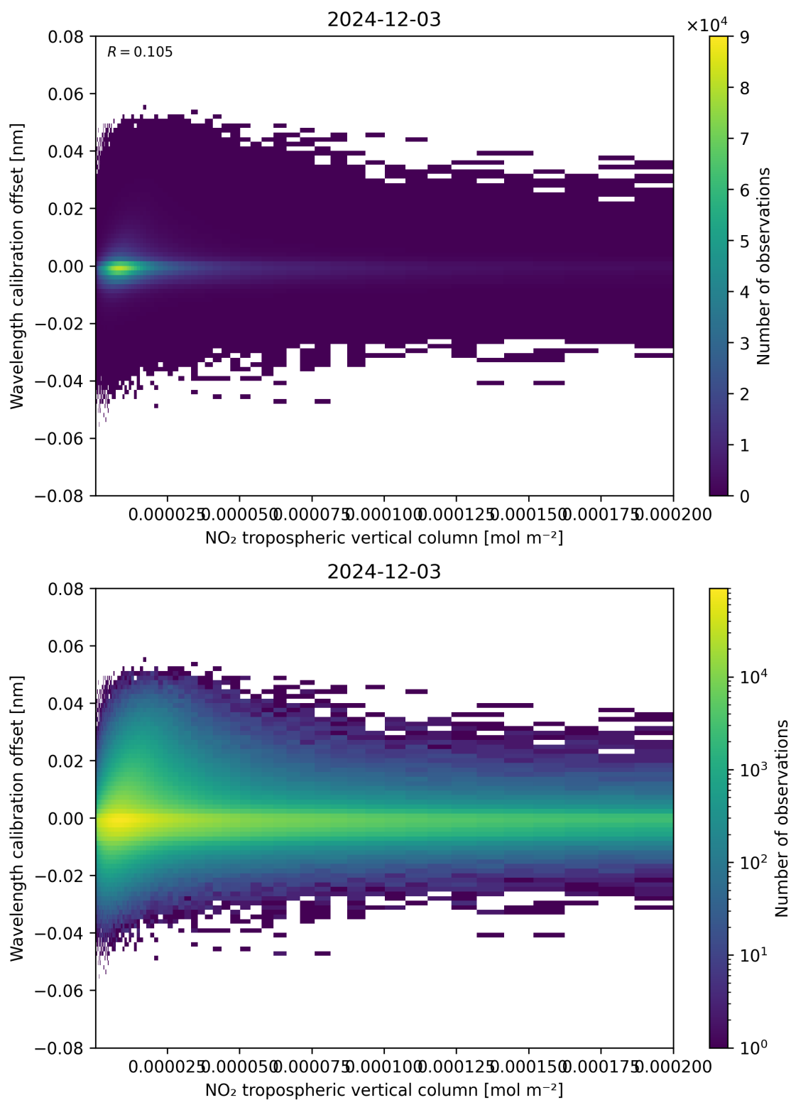
Figure 143: Scatter density plot of “NO 2 tropospheric vertical column” against “Wavelength calibration offset” for 2024-12-02 to 2024-12-04.
