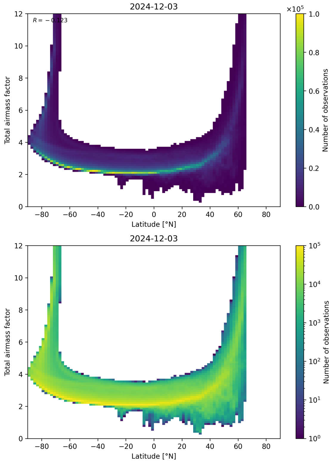
Figure 84: Scatter density plot of “Latitude” against “Total airmass factor” for 2024-12-02 to 2024-12-04.
