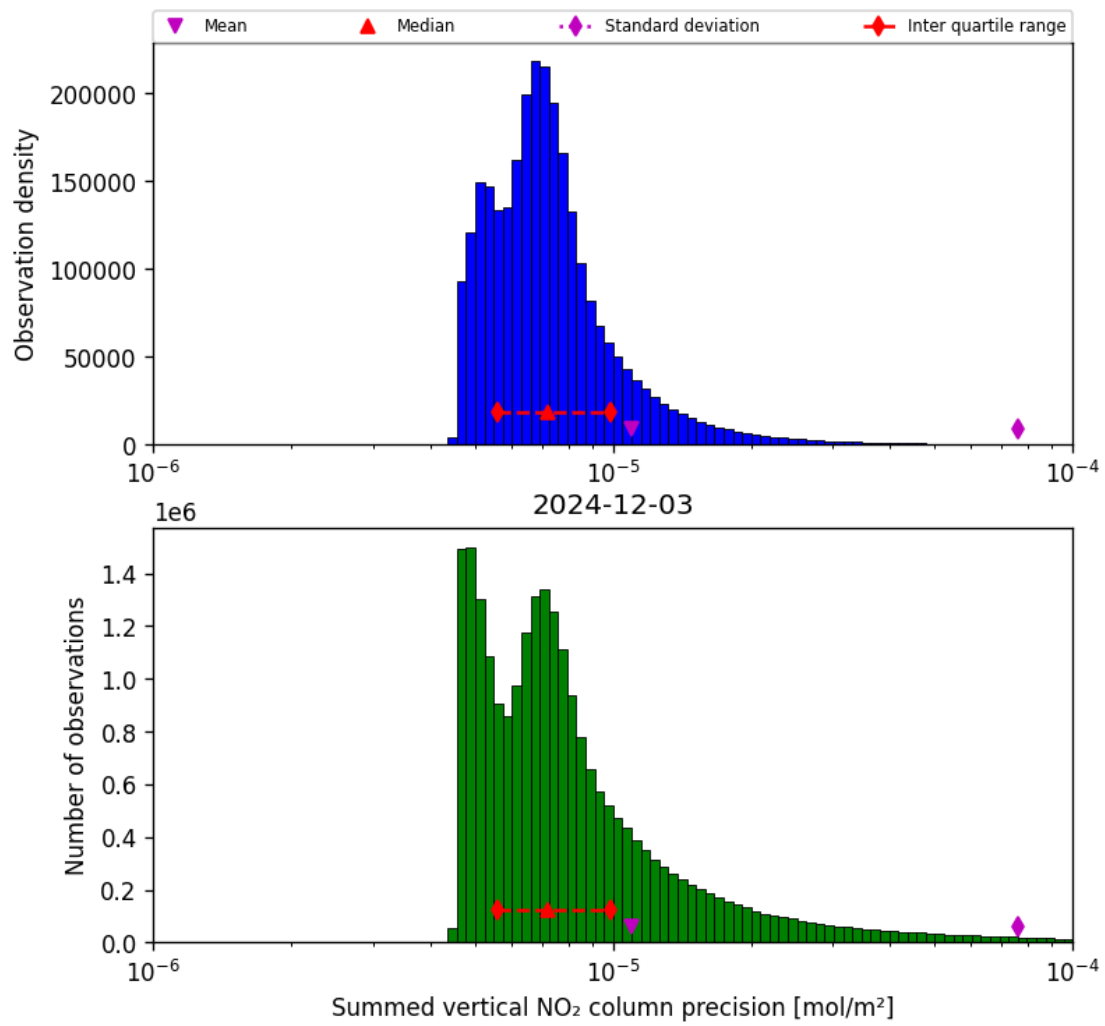
Figure 41: Histogram of “Summed vertical NO 2 column precision” for 2024-12-02 to 2024-12-04
