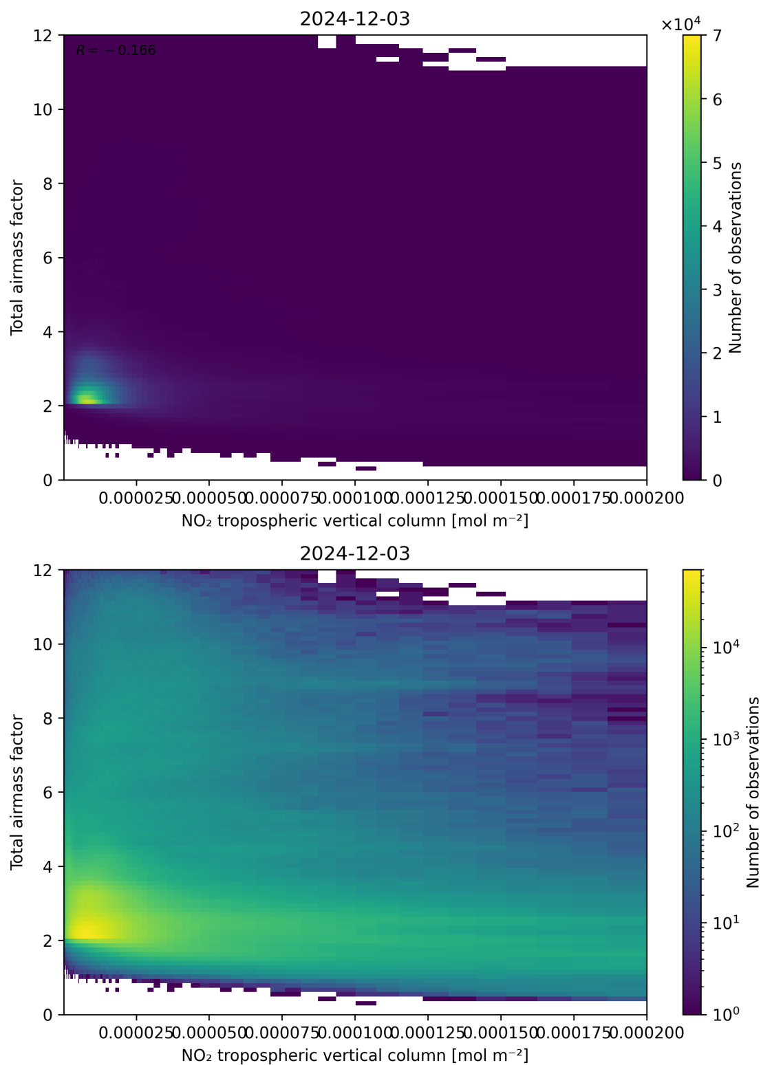
Figure 122: Scatter density plot of “NO 2 tropospheric vertical column” against “Total air mass factor” for 2024-12-02 to 2024-12-04.
