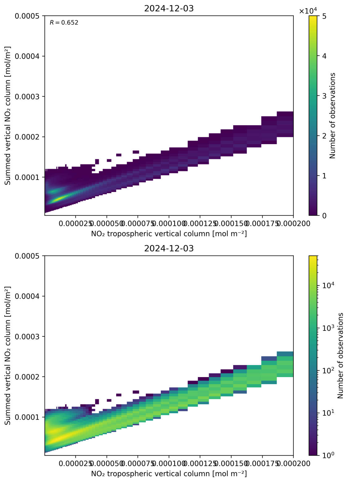
Figure 126: Scatter density plot of “NO 2 tropospheric vertical column” against “Summed vertical NO 2 column” for 2024-12-02 to 2024-12-04.
