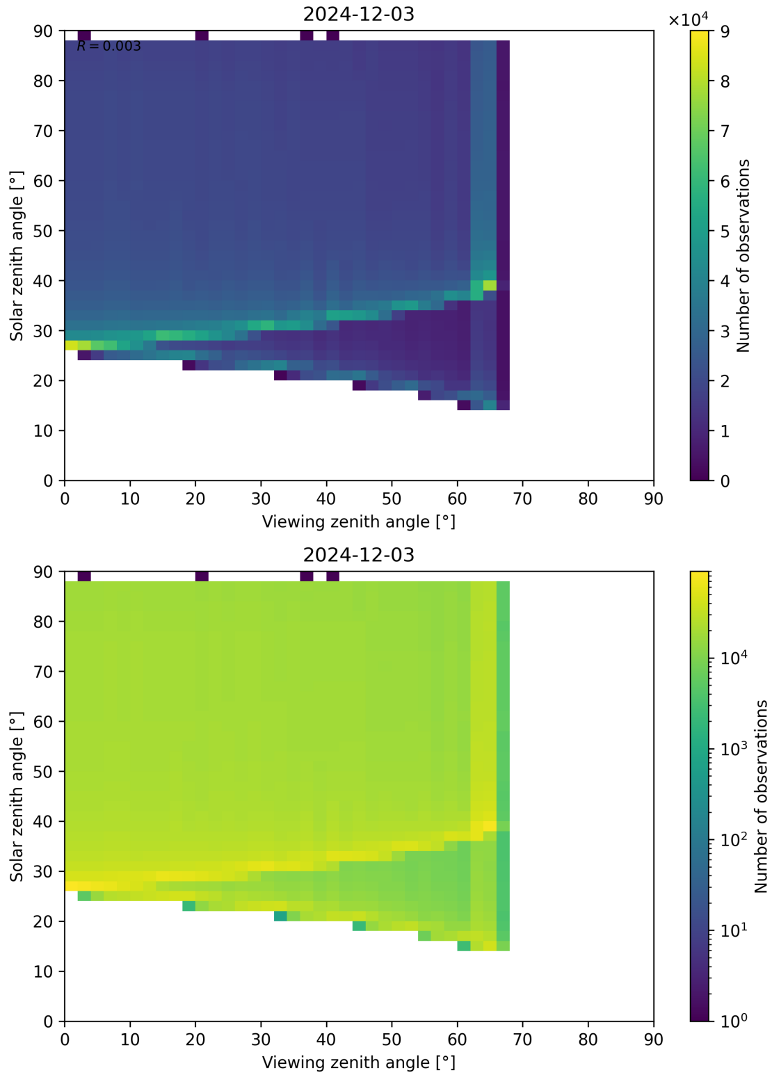
Figure 172: Scatter density plot of “Viewing zenith angle” against “Solar zenith angle” for 2024-12-02 to 2024-12-04.
