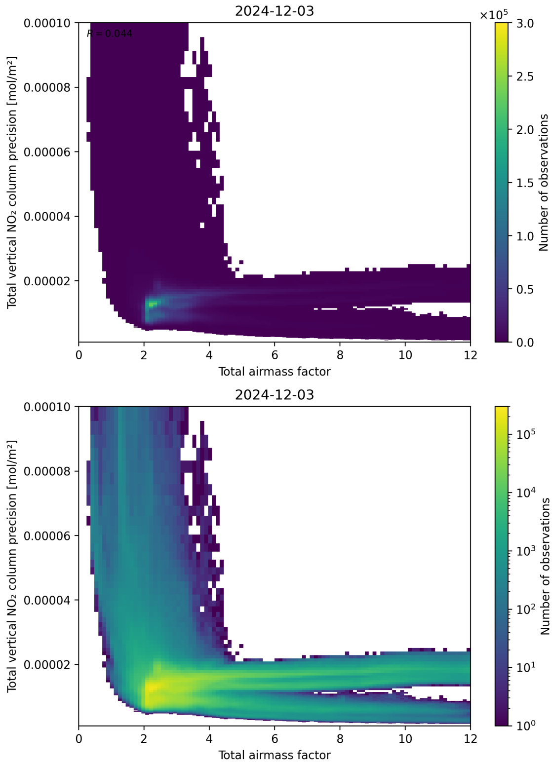
Figure 68: Scatter density plot of “Total airmass factor” against “Total vertical NO 2 column precision” for 2024-12-02 to 2024-12-04.
