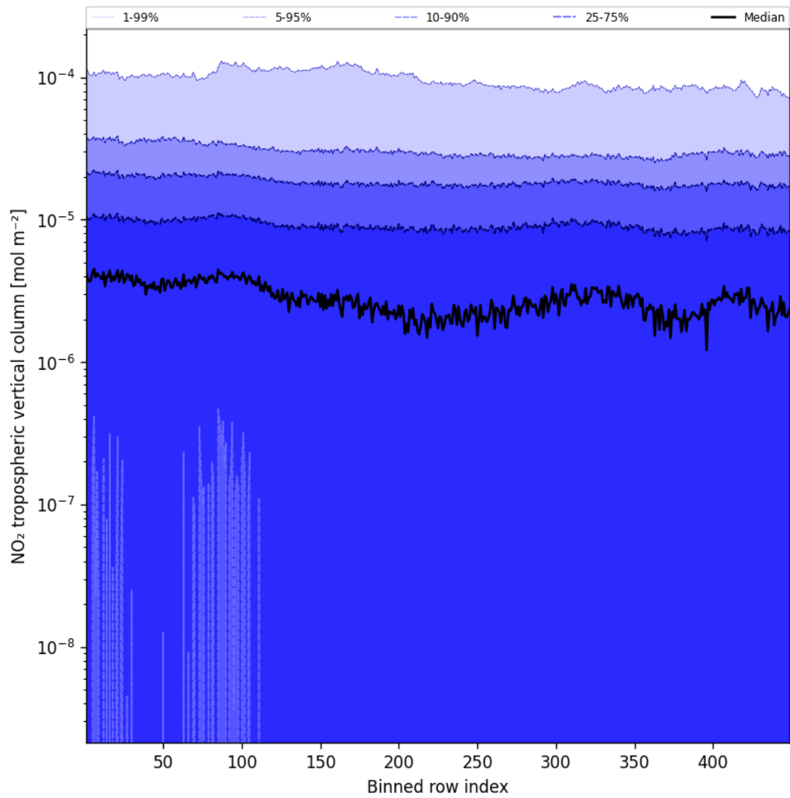
Figure 46: Along track statistics of “NO 2 tropospheric vertical column” for 2024-12-02 to 2024-12-04
