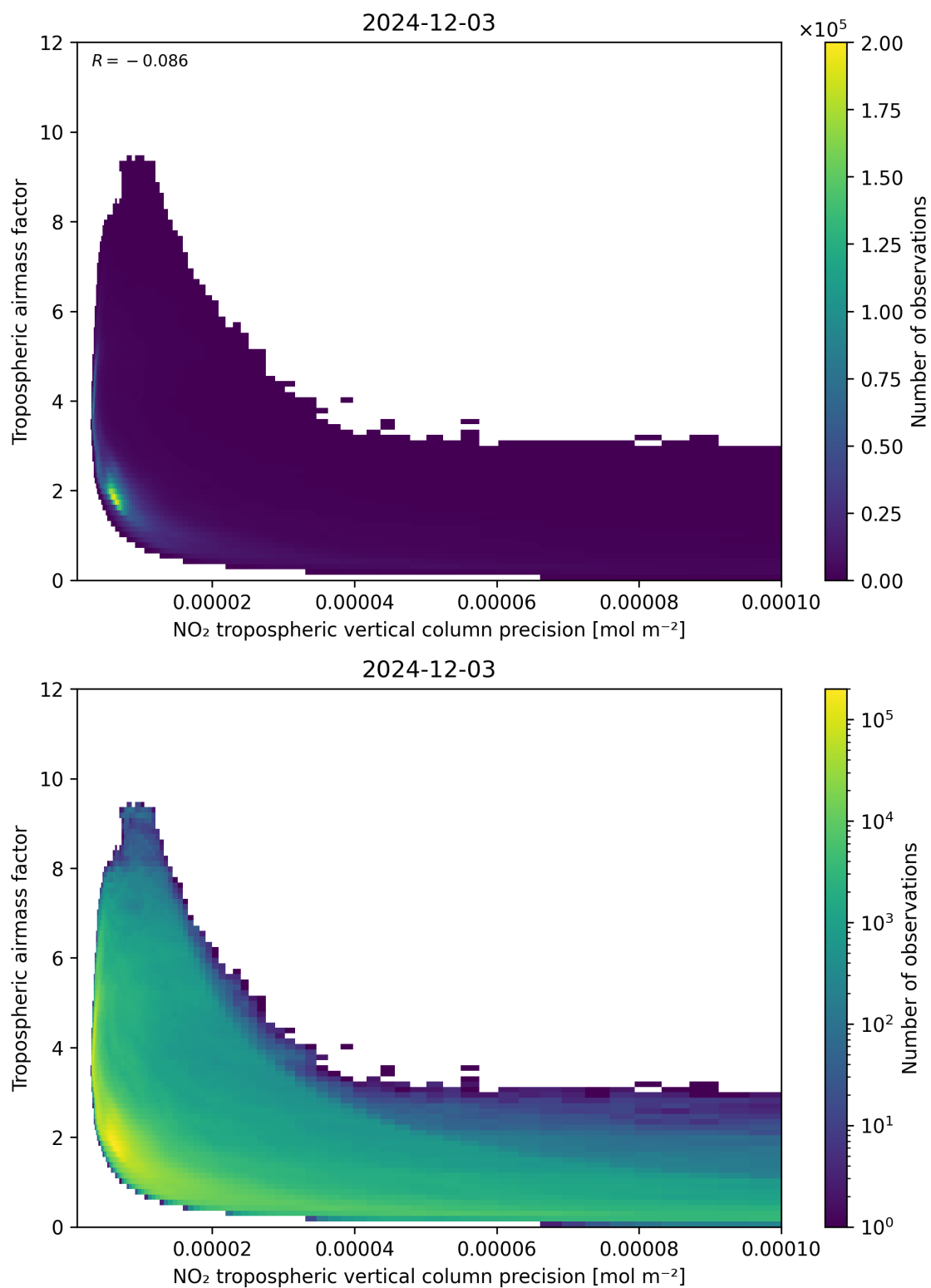
Figure 133: Scatter density plot of “NO 2 tropospheric vertical column precision” against “Tropospheric airmass factor” for 2024-12-02 to 2024-12-04.
