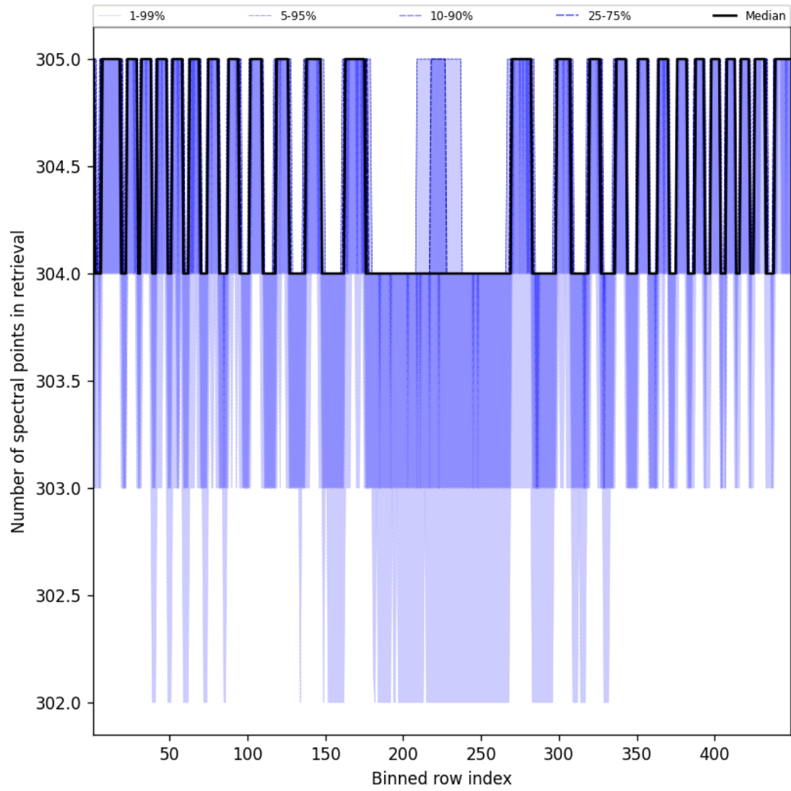
Figure 50: Along track statistics of “Number of spectral points in retrieval” for 2024-12-02 to 2024-12-04
