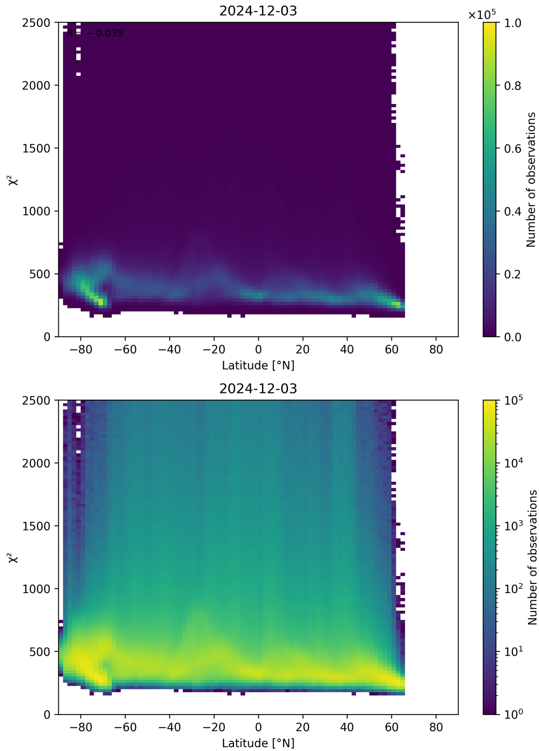
Figure 86: Scatter density plot of “Latitude” against “ \chi^2 ” for 2024-12-02 to 2024-12-04.
