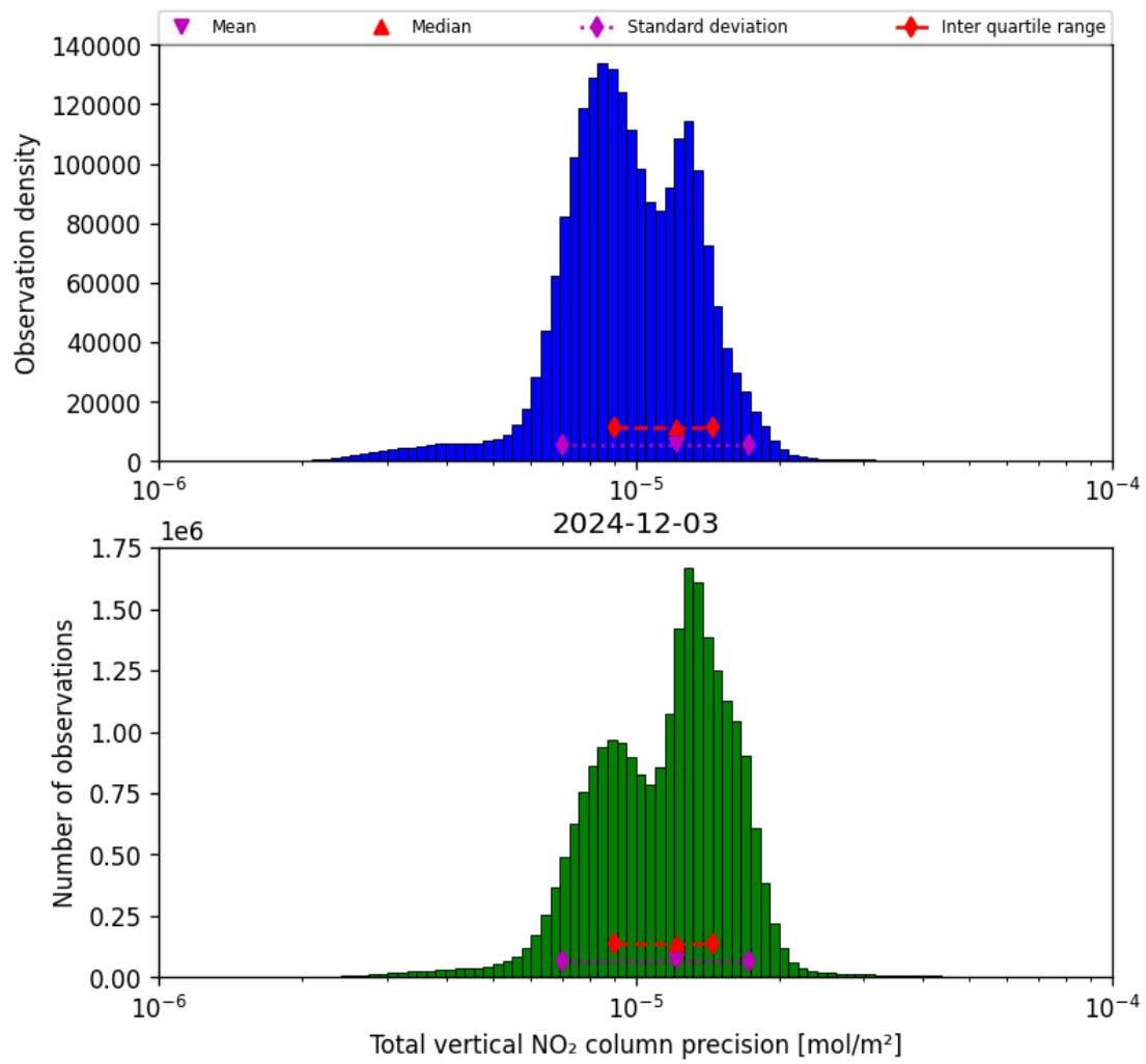
Figure 39: Histogram of “Total vertical NO 2 column precision” for 2024-12-02 to 2024-12-04
