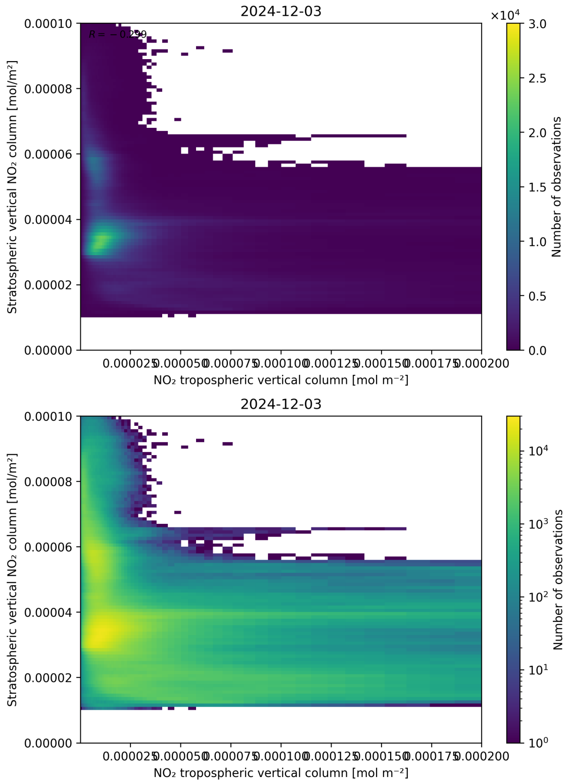
Figure 125: Scatter density plot of “NO 2 tropospheric vertical column” against “Stratospheric vertical NO 2 column” for 2024-12-02 to 2024-12-04.
