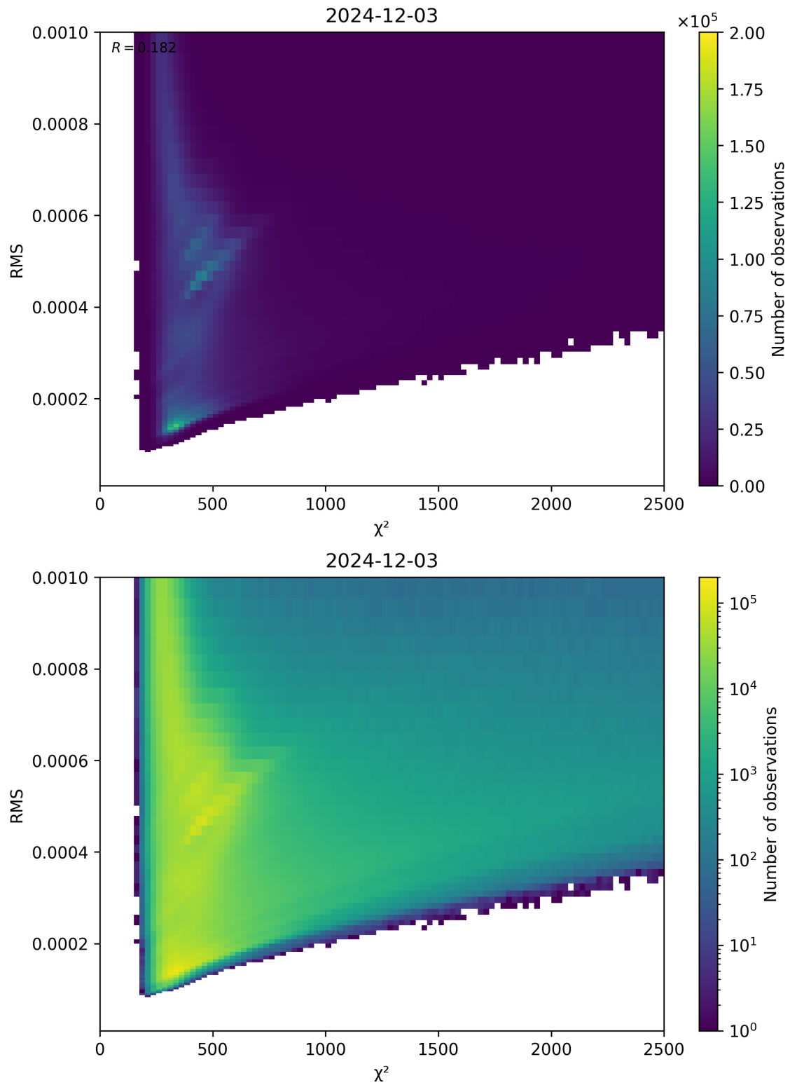
Figure 82: Scatter density plot of “ \chi^2 ” against “RMS” for 2024-12-02 to 2024-12-04.
