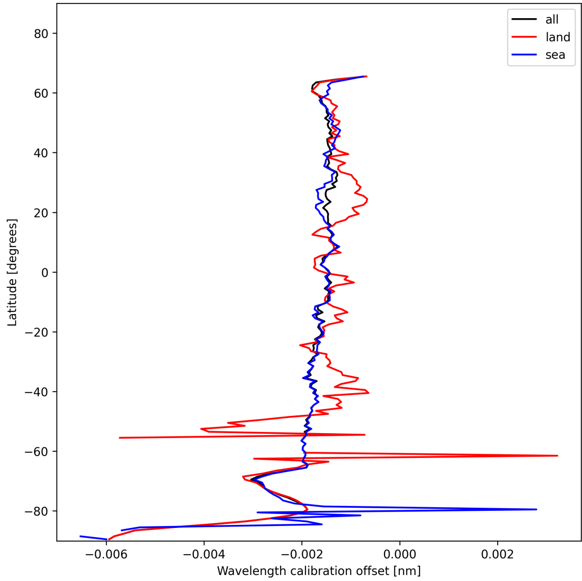
Figure 18: Zonal average of “Wavelength calibration offset” for 2024-12-02 to 2024-12-04.
