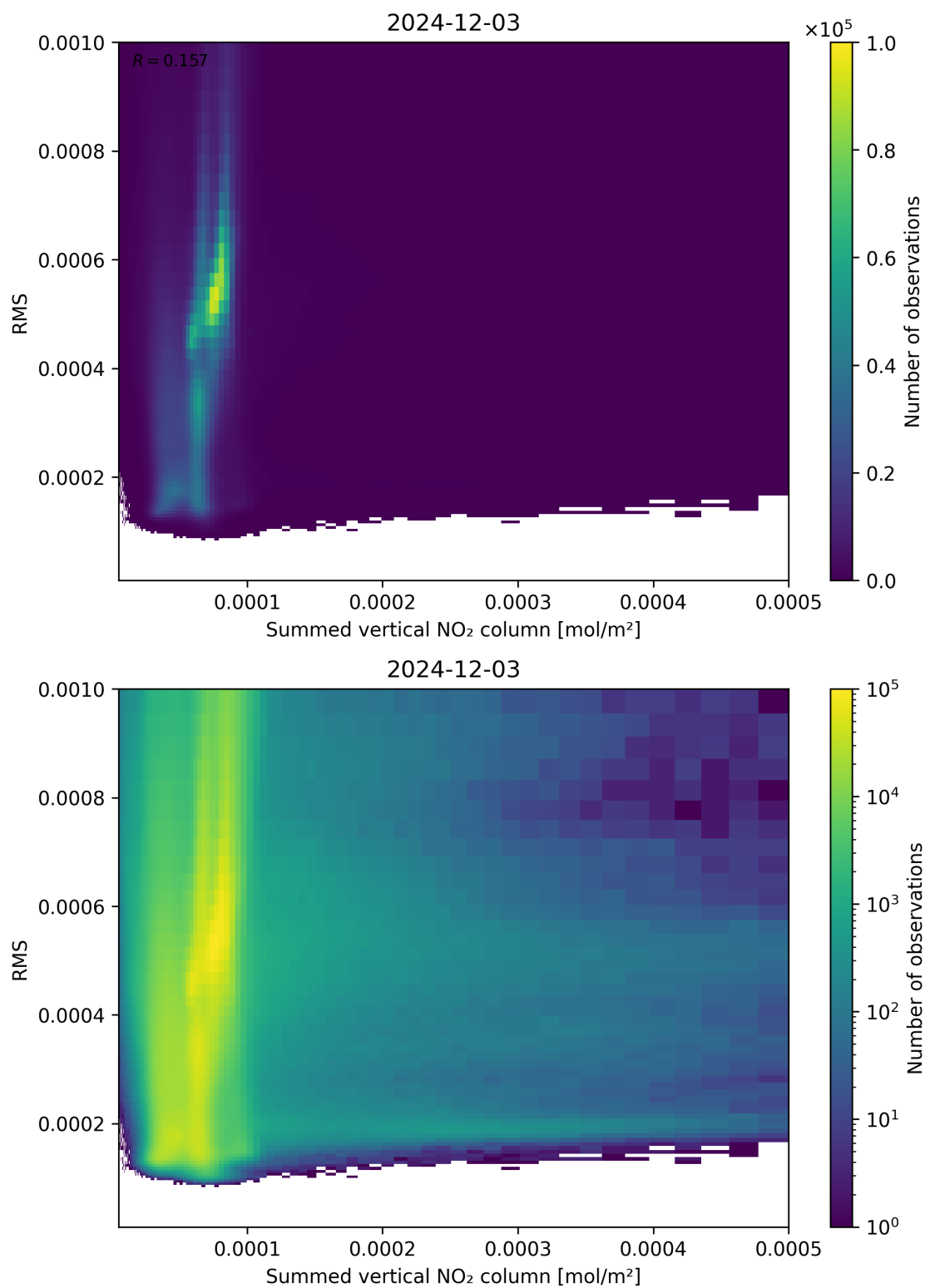
Figure 109: Scatter density plot of “Summed vertical NO 2 column” against “RMS” for 2024-12-02 to 2024-12-04.
