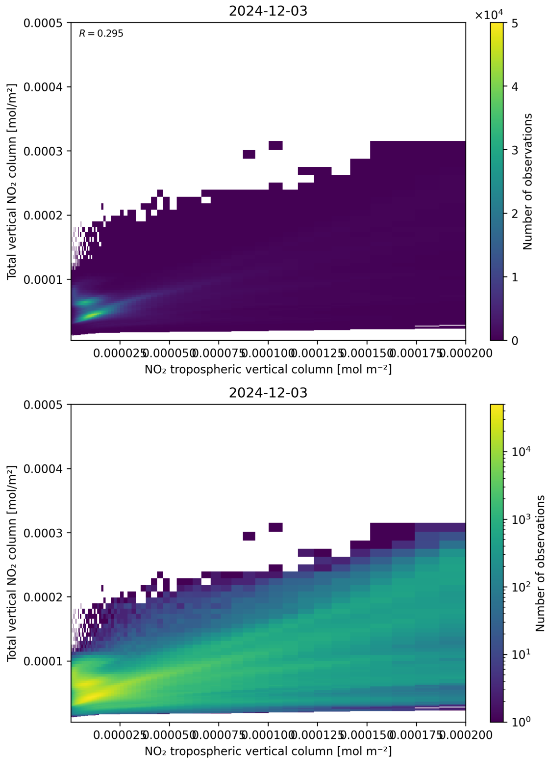
Figure 128: Scatter density plot of “NO 2 tropospheric vertical column” against “Total vertical NO 2 column” for 2024-12-02 to 2024-12-04.
