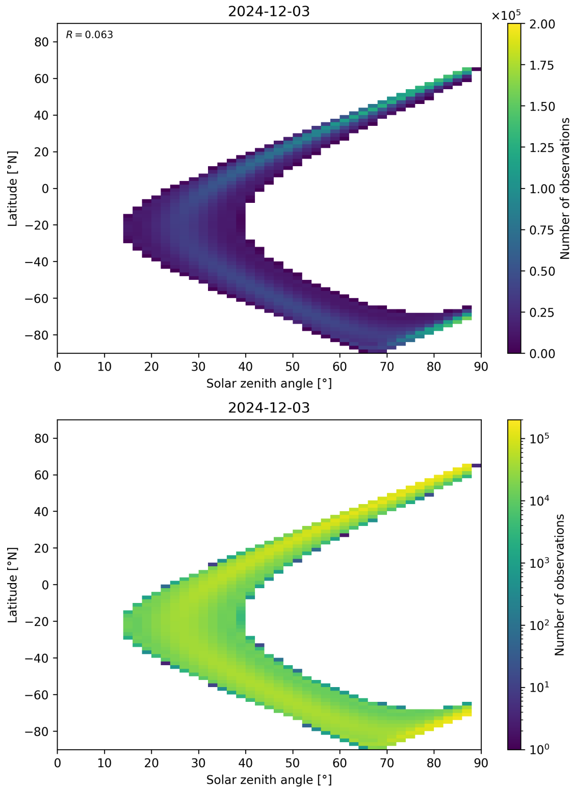
Figure 149: Scatter density plot of “Solar zenith angle” against “Latitude” for 2024-12-02 to 2024-12-04.
