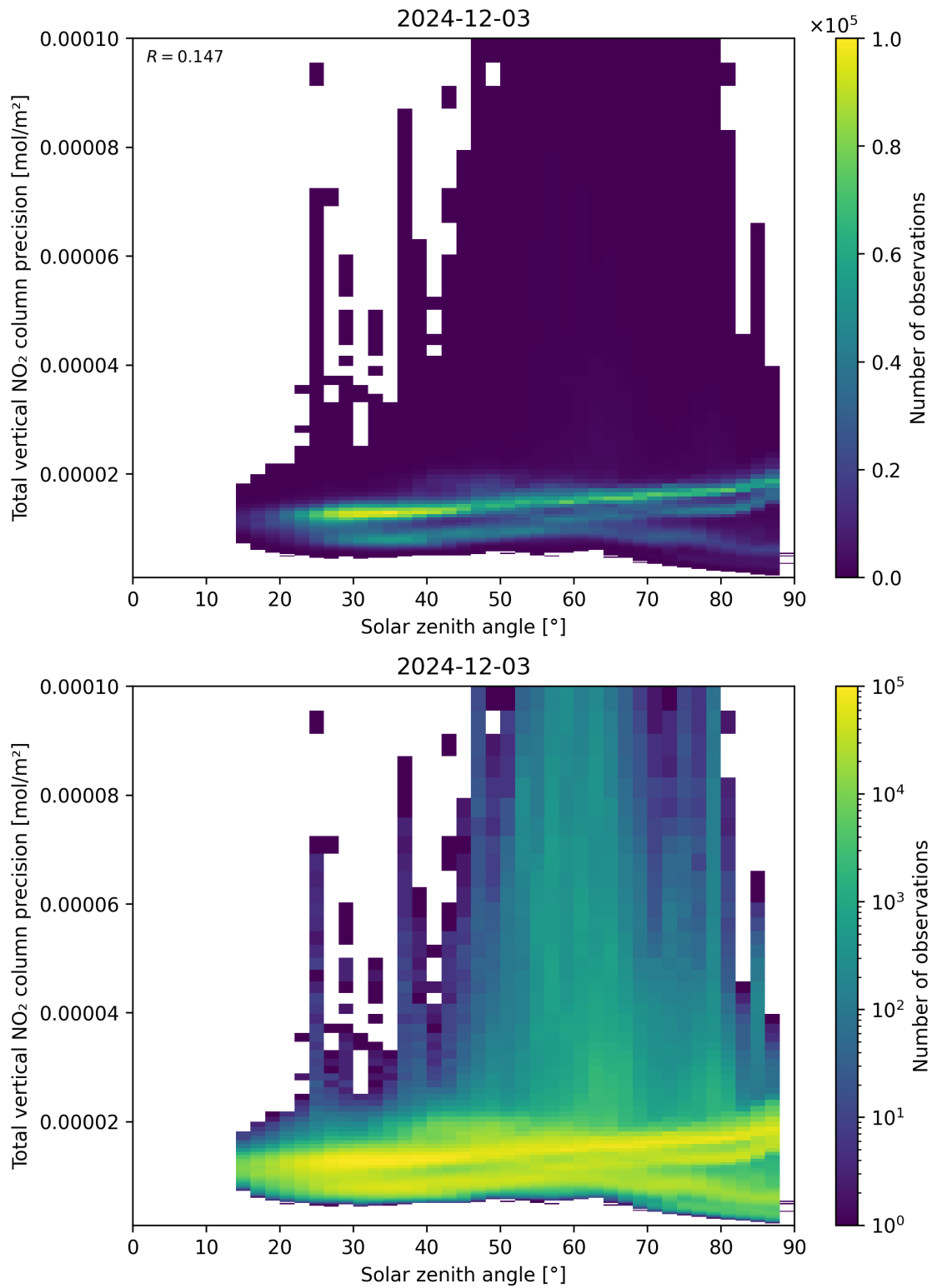
Figure 154: Scatter density plot of “Solar zenith angle” against “Total vertical NO 2 column precision” for 2024-12-02 to 2024-12-04.
