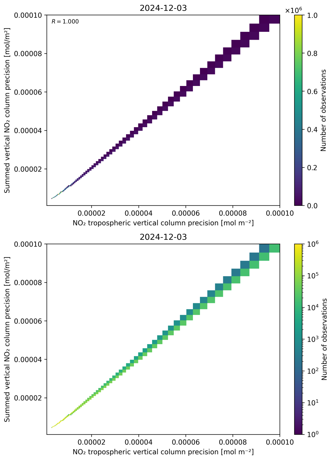
Figure 137: Scatter density plot of “NO 2 tropospheric vertical column precision” against “Summed vertical NO 2 column precision” for 2024-12-02 to 2024-12-04.
