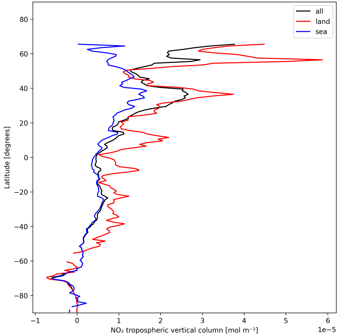
Figure 12: Zonal average of “NO 2 tropospheric vertical column” for 2024-12-02 to 2024-12-04.
