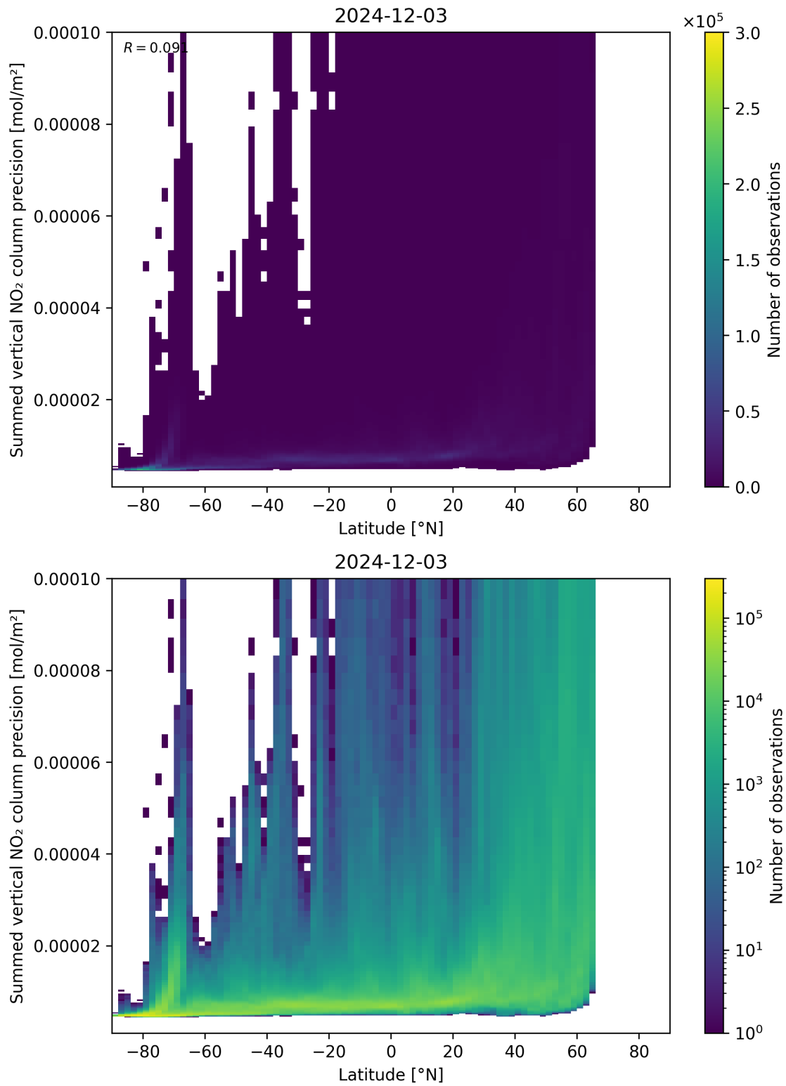
Figure 89: Scatter density plot of “Latitude” against “Summed vertical NO 2 column precision” for 2024-12-02 to 2024-12-04.
