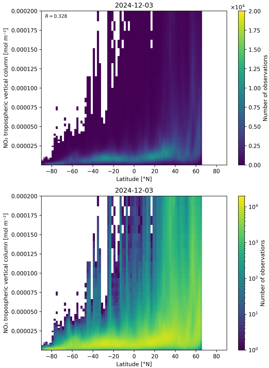
Figure 92: Scatter density plot of “Latitude” against “NO 2 tropospheric vertical column” for 2024-12-02 to 2024-12-04.
