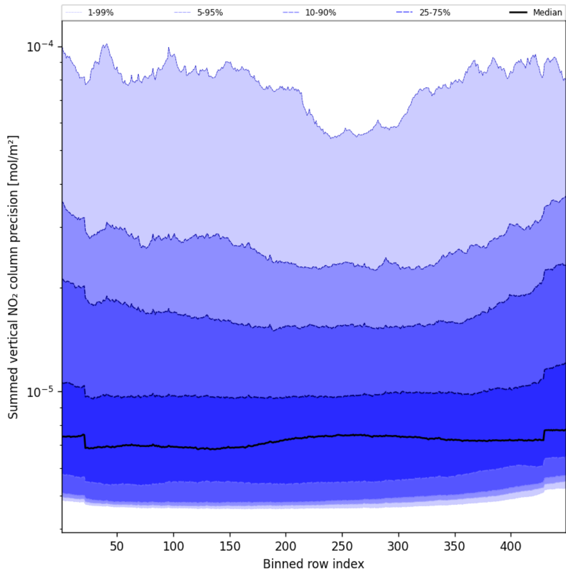
Figure 58: Along track statistics of “Summed vertical NO 2 column precision” for 2024-12-02 to 2024-12-04
