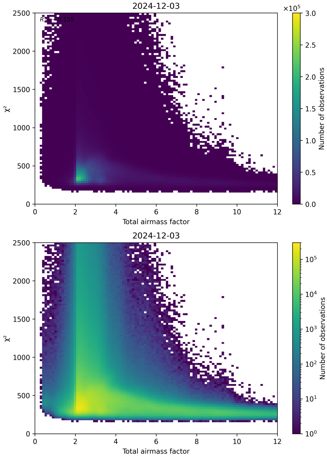
Figure 63: Scatter density plot of “Total airmass factor” against “ \chi^2 ” for 2024-12-02 to 2024-12-04.
