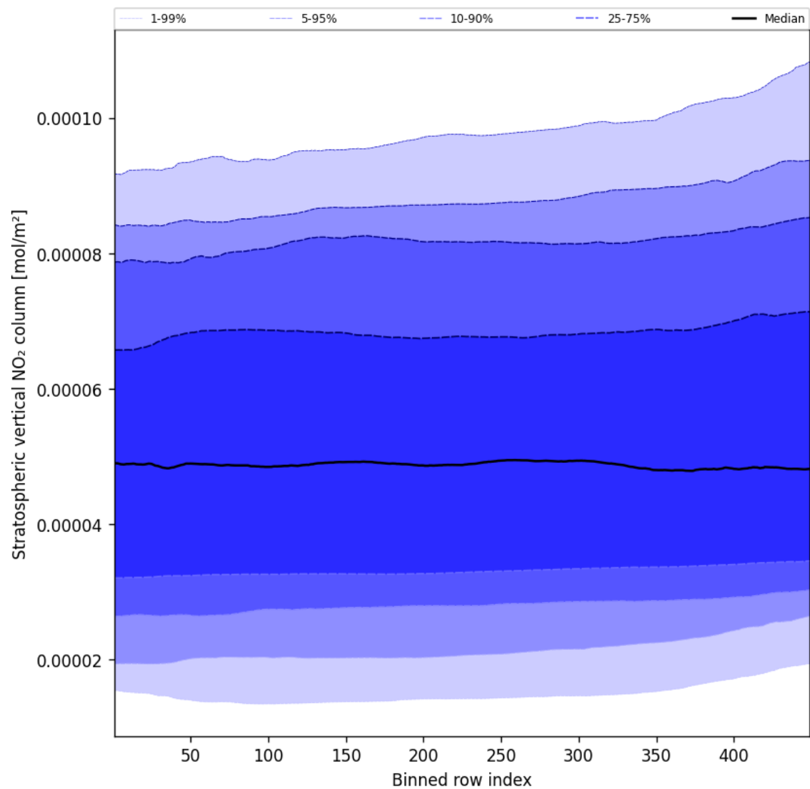
Figure 53: Along track statistics of “Stratospheric vertical NO 2 column” for 2024-12-02 to 2024-12-04
