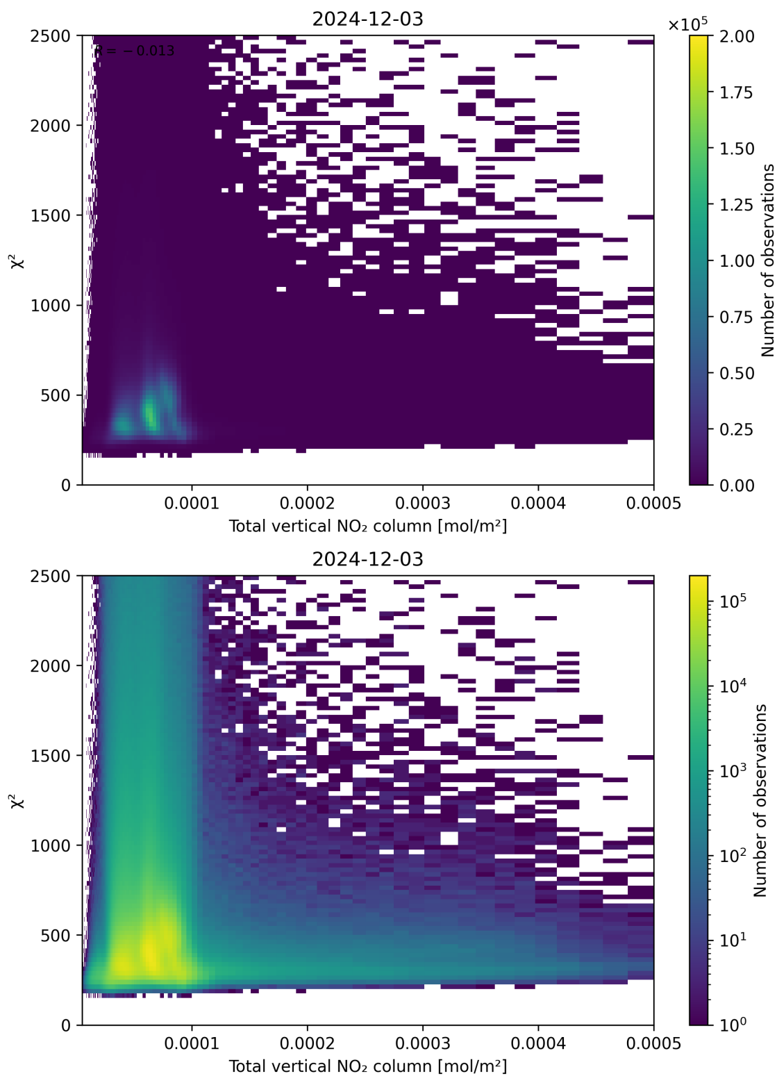
Figure 111: Scatter density plot of “Total vertical NO 2 column” against “ \chi^2 ” for 2024-12-02 to 2024-12-04.
