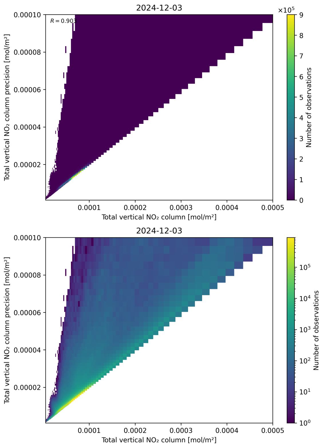
Figure 114: Scatter density plot of “Total vertical NO 2 column” against “Total vertical NO 2 column precision” for 2024-12-02 to 2024-12-04.
