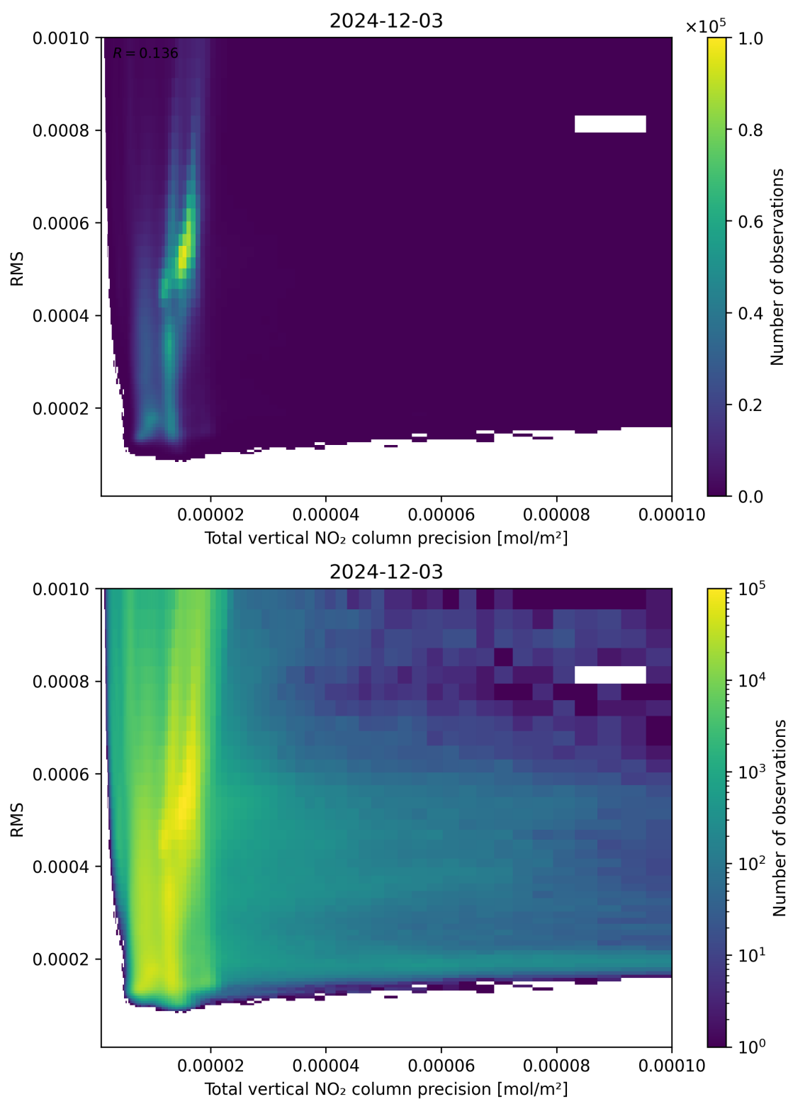
Figure 119: Scatter density plot of “Total vertical NO 2 column precision” against “RMS” for 2024-12-02 to 2024-12-04.
