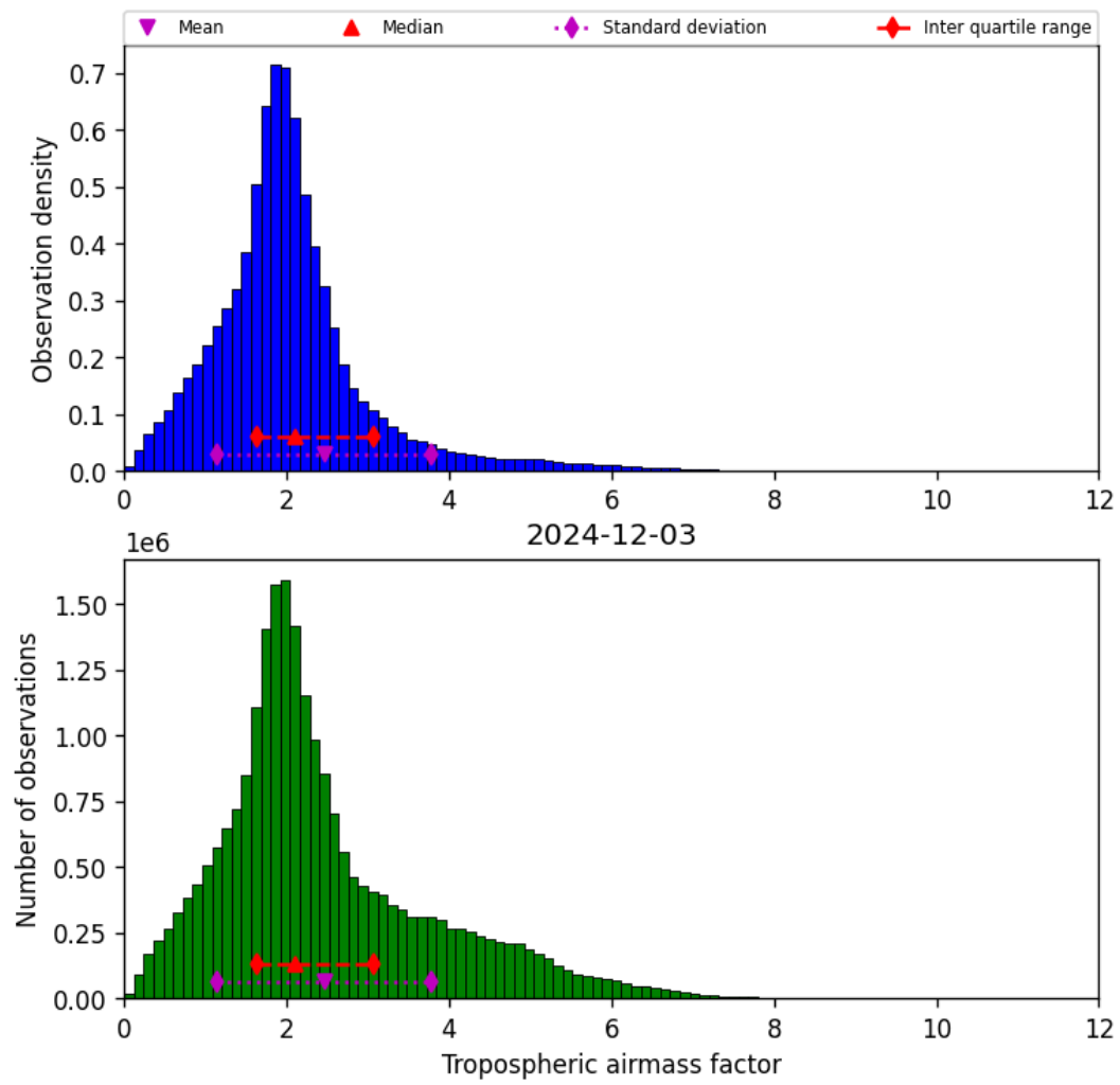
Figure 31: Histogram of “Tropospheric airmass factor” for 2024-12-02 to 2024-12-04
