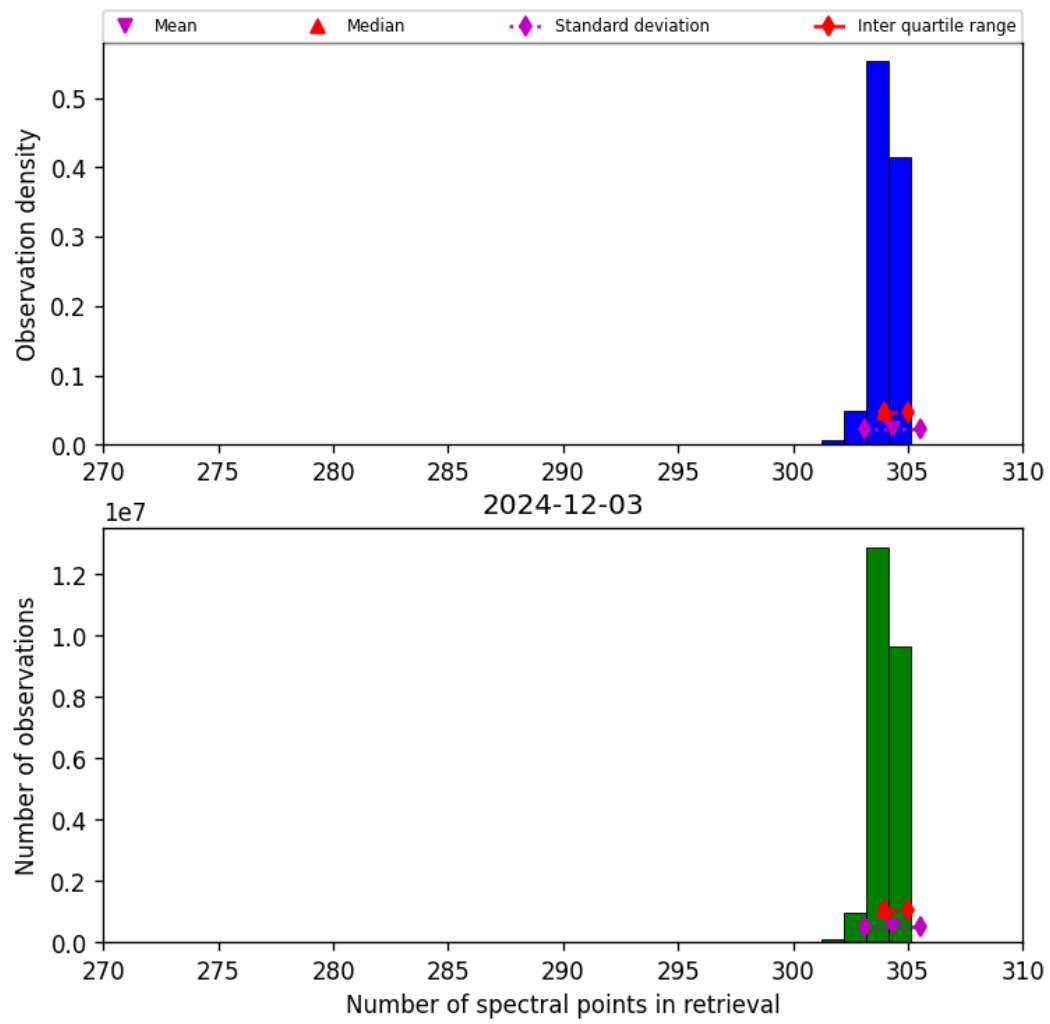
Figure 33: Histogram of “Number of spectral points in retrieval” for 2024-12-02 to 2024-12-04
