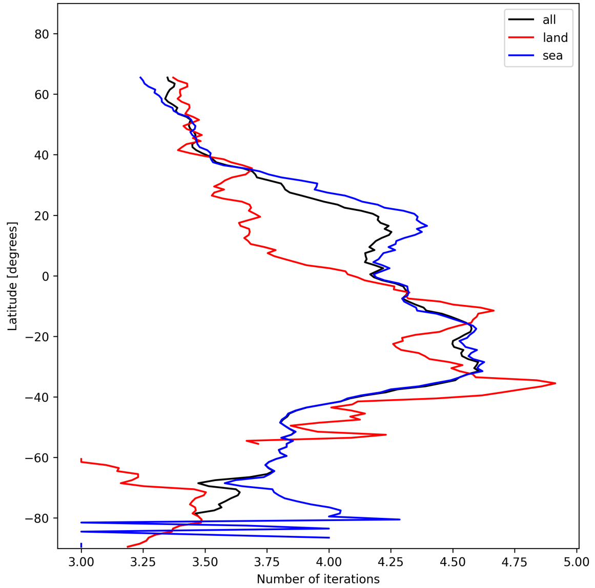
Figure 17: Zonal average of “Number of iterations” for 2024-12-02 to 2024-12-04.
