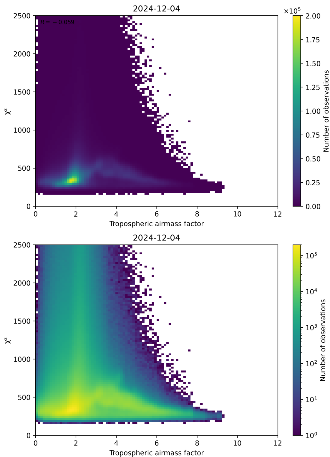
Figure 73: Scatter density plot of “Tropospheric airmass factor” against “ \chi^2 ” for 2024-12-03 to 2024-12-05.
