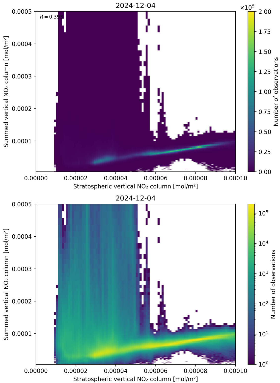
Figure 98: Scatter density plot of “Stratospheric vertical NO 2 column” against “Summed vertical NO 2 column” for 2024-12-03 to 2024-12-05.
