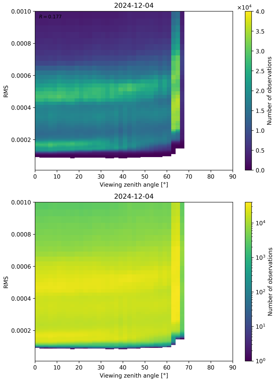
Figure 171: Scatter density plot of “Viewing zenith angle” against “RMS” for 2024-12-03 to 2024-12-05.
