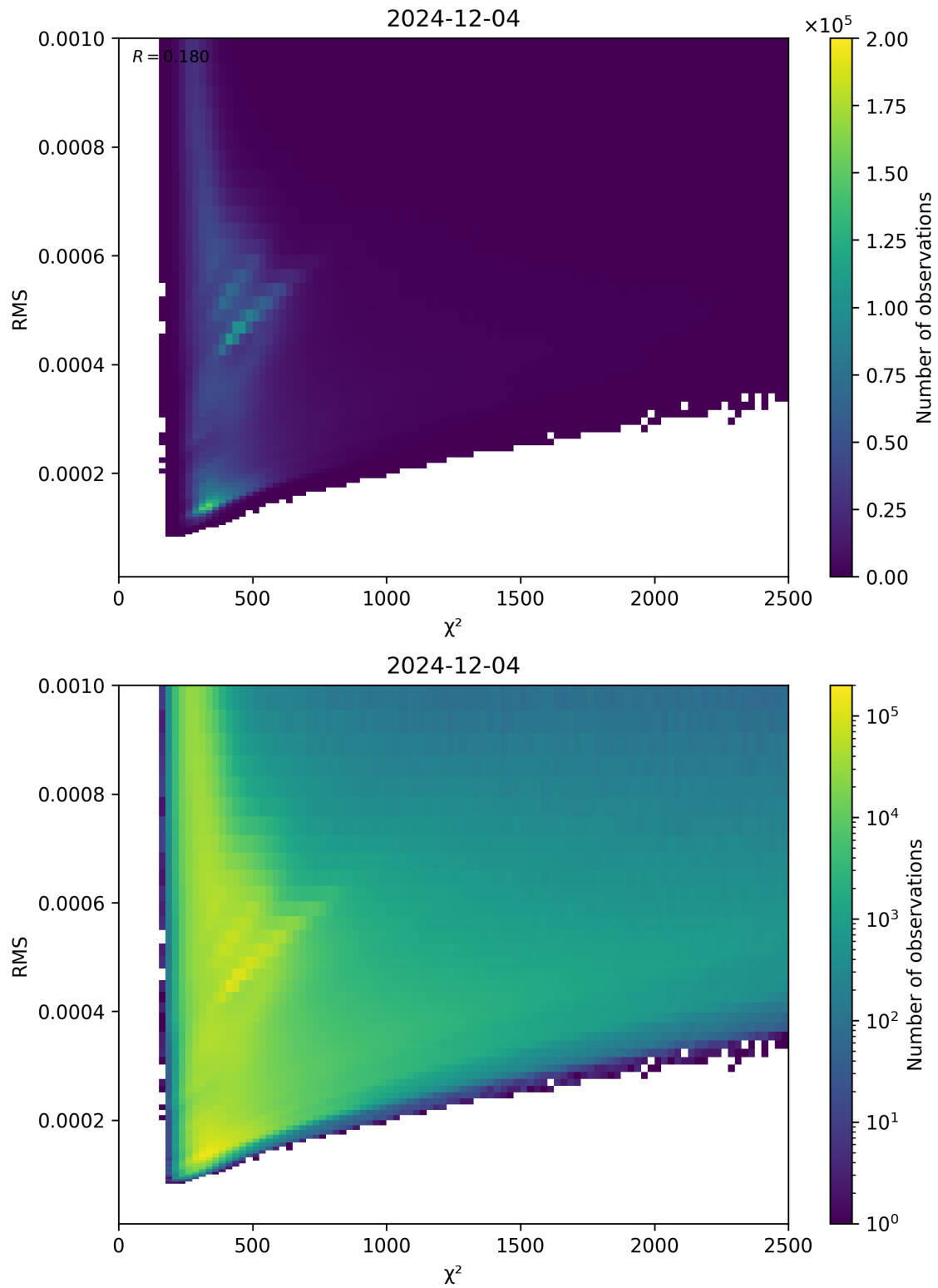
Figure 82: Scatter density plot of “ \chi^2 ” against “RMS” for 2024-12-03 to 2024-12-05.
