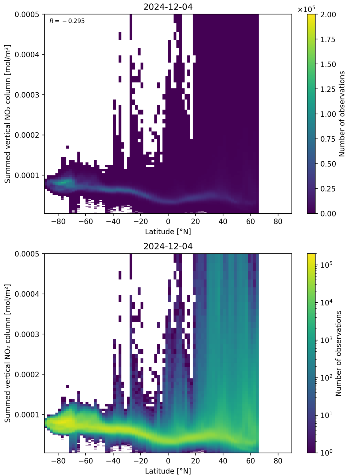
Figure 88: Scatter density plot of “Latitude” against “Summed vertical NO 2 column” for 2024-12-03 to 2024-12-05.
