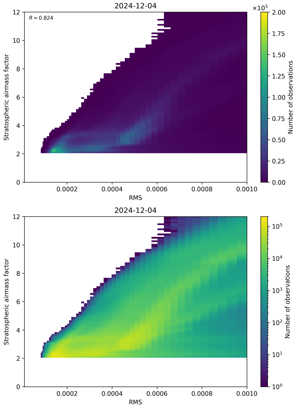
Figure 144: Scatter density plot of “RMS” against “Stratospheric airmass factor” for 2024-12-03 to 2024-12-05.
