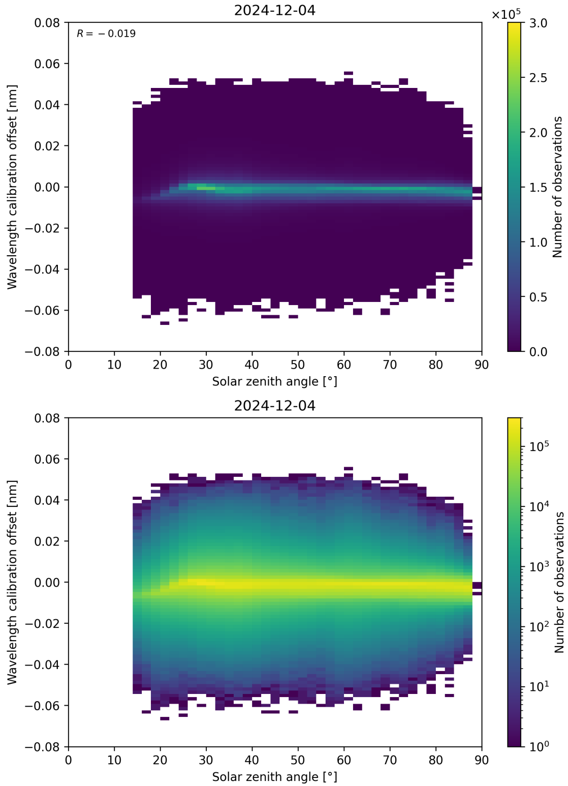
Figure 158: Scatter density plot of “Solar zenith angle” against “Wavelength calibration offset” for 2024-12-03 to 2024-12-05.
