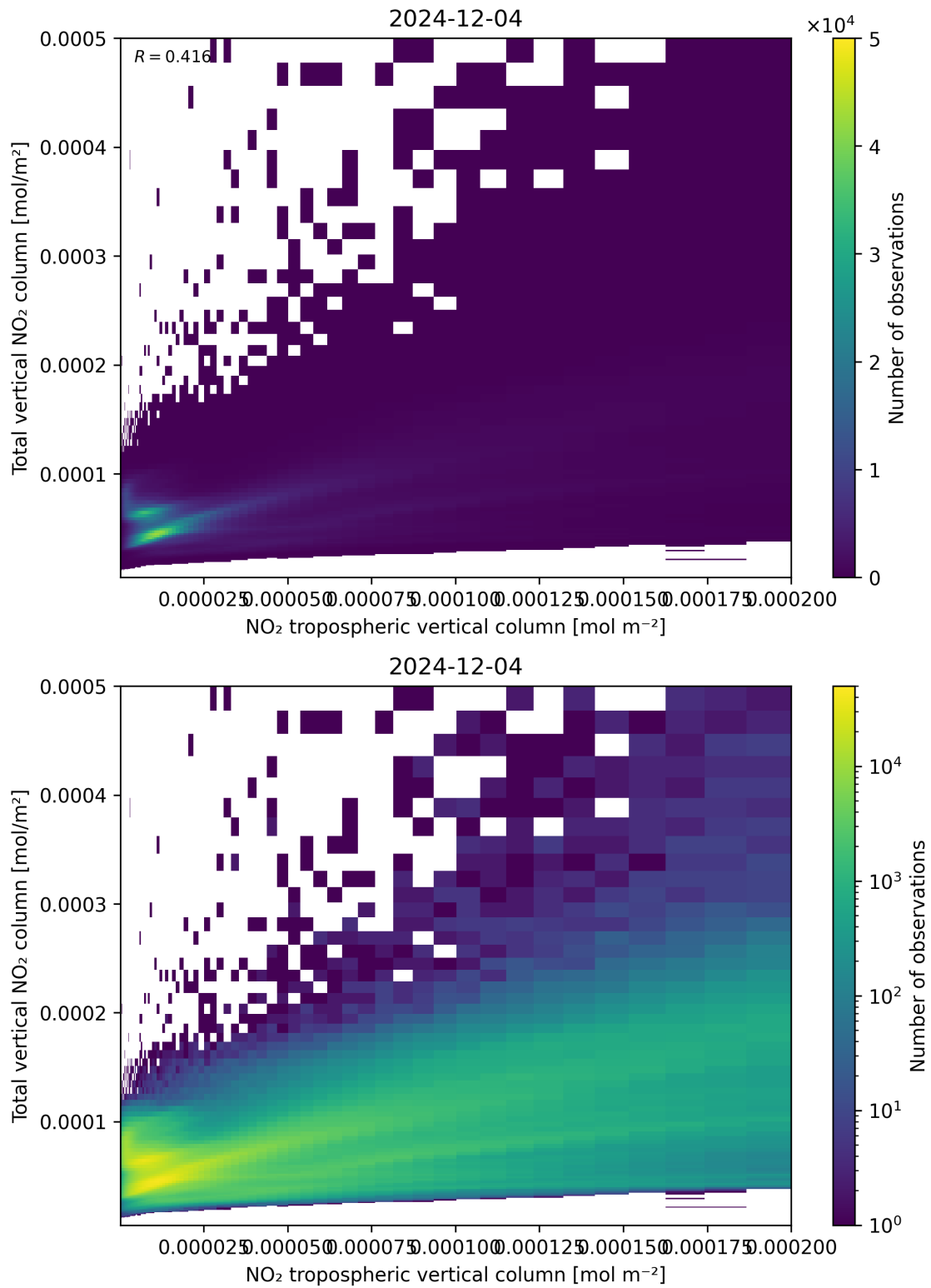
Figure 128: Scatter density plot of “NO 2 tropospheric vertical column” against “Total vertical NO 2 column” for 2024-12-03 to 2024-12-05.
