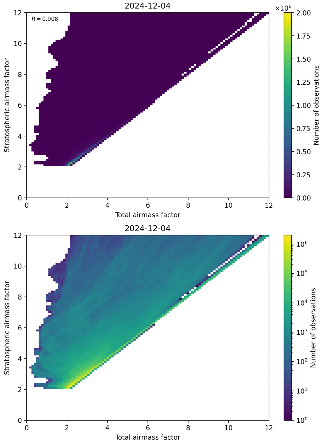
Figure 62: Scatter density plot of “Total airmass factor” against “Stratospheric airmass factor” for 2024-12-03 to 2024-12-05.
