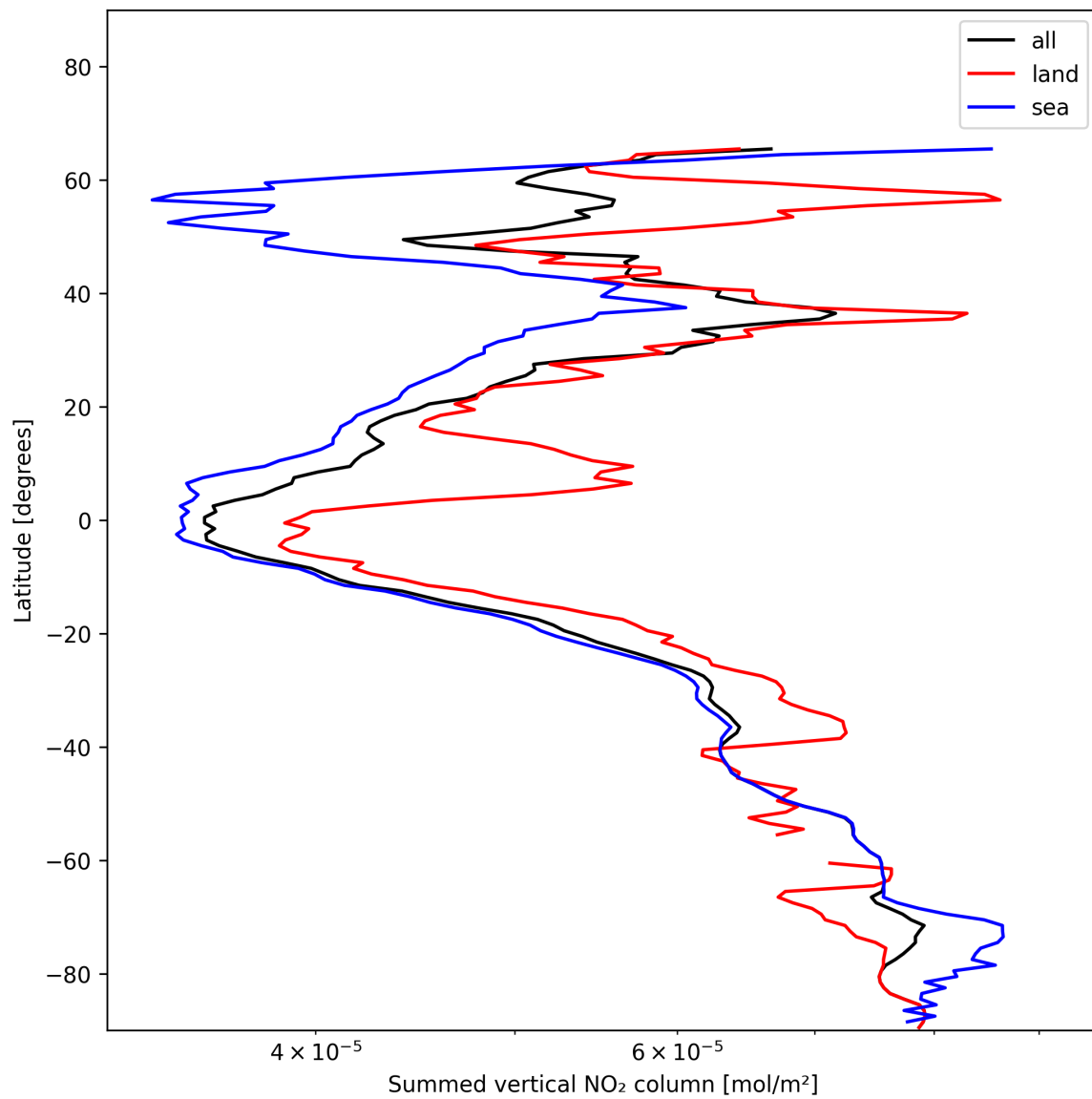
Figure 23: Zonal average of “Summed vertical NO 2 column” for 2024-12-03 to 2024-12-05.
