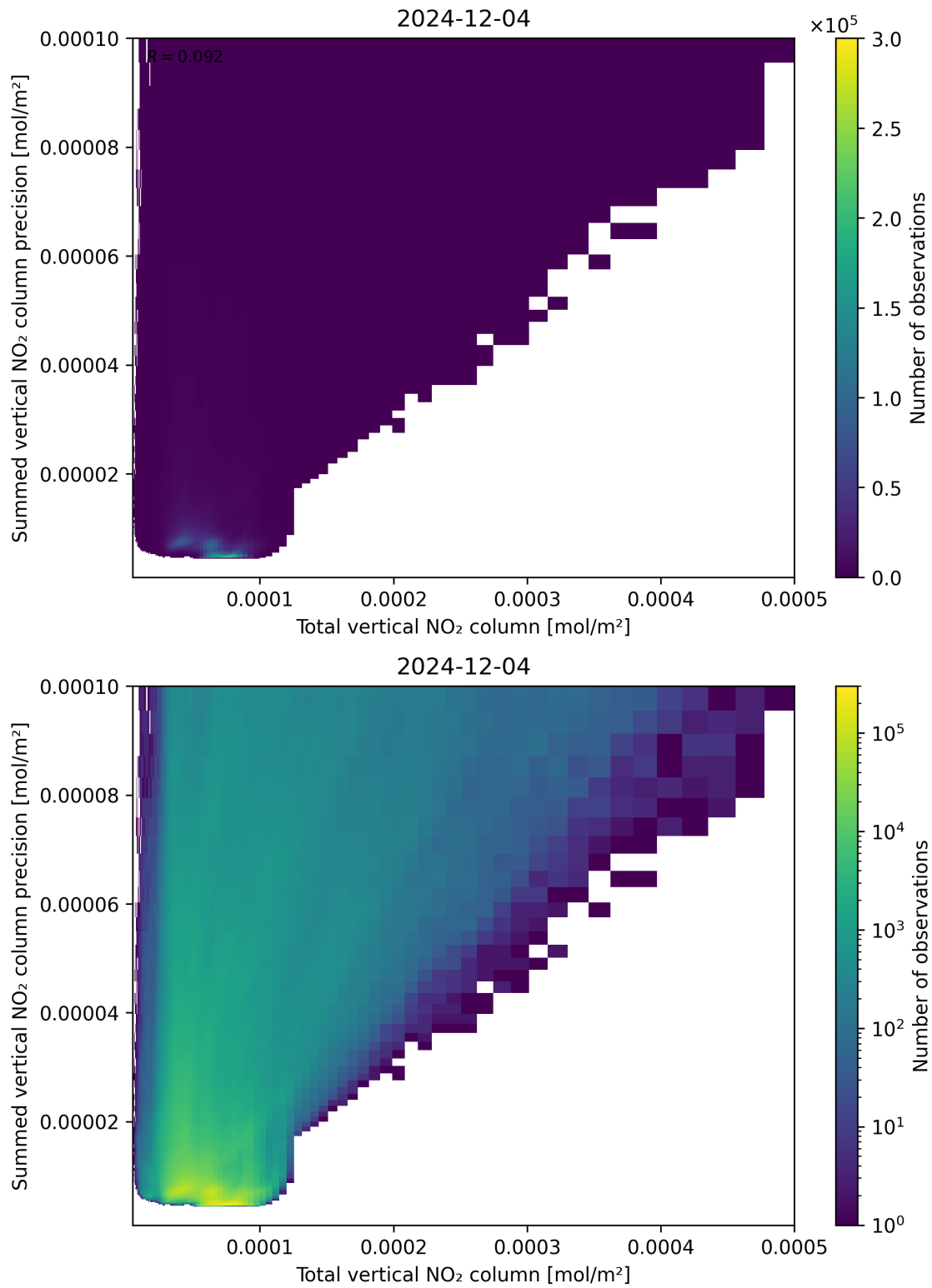
Figure 113: Scatter density plot of “Total vertical NO 2 column” against “Summed vertical NO 2 column precision” for 2024-12-03 to 2024-12-05.
