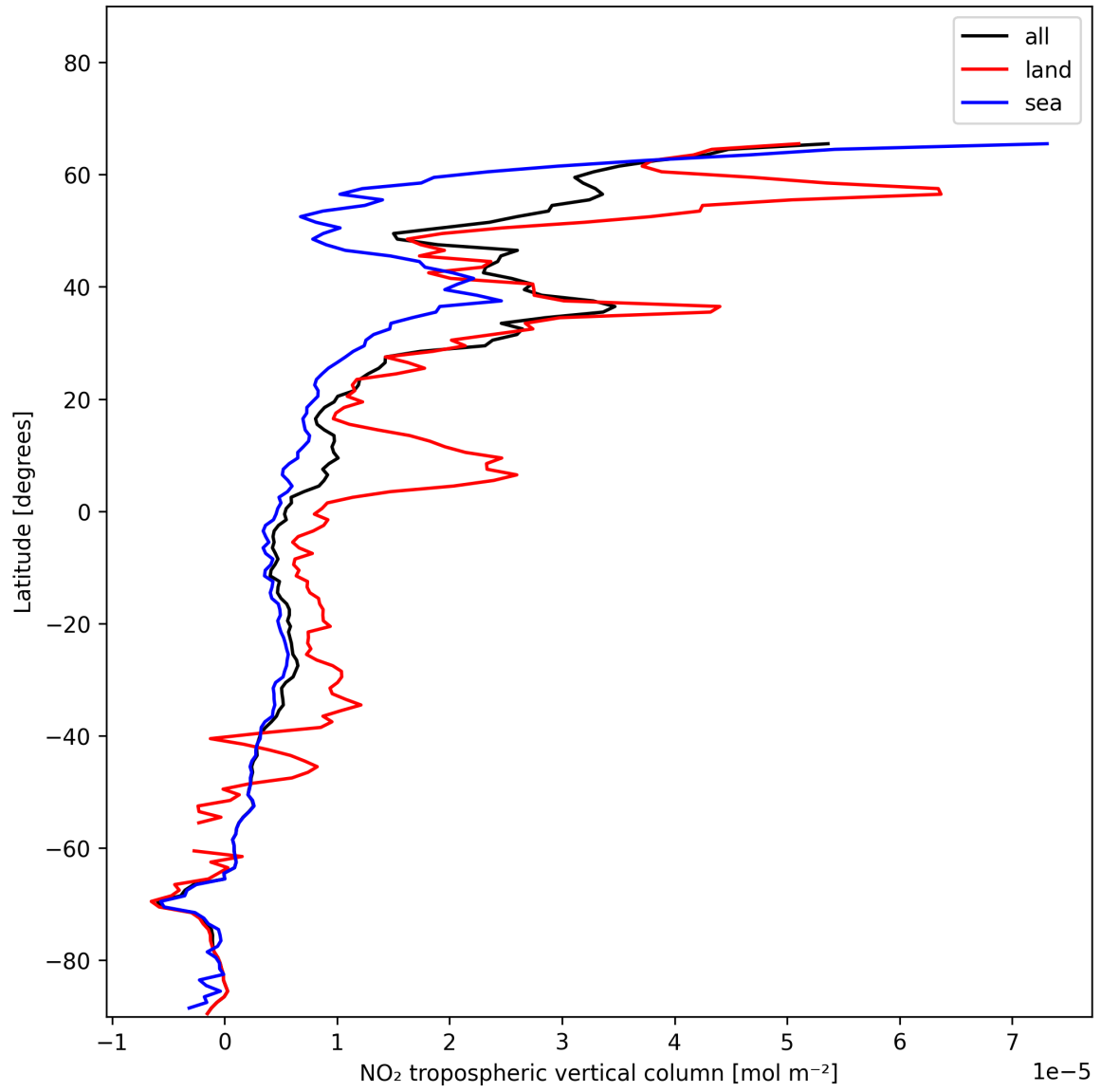
Figure 12: Zonal average of “NO 2 tropospheric vertical column” for 2024-12-03 to 2024-12-05.
