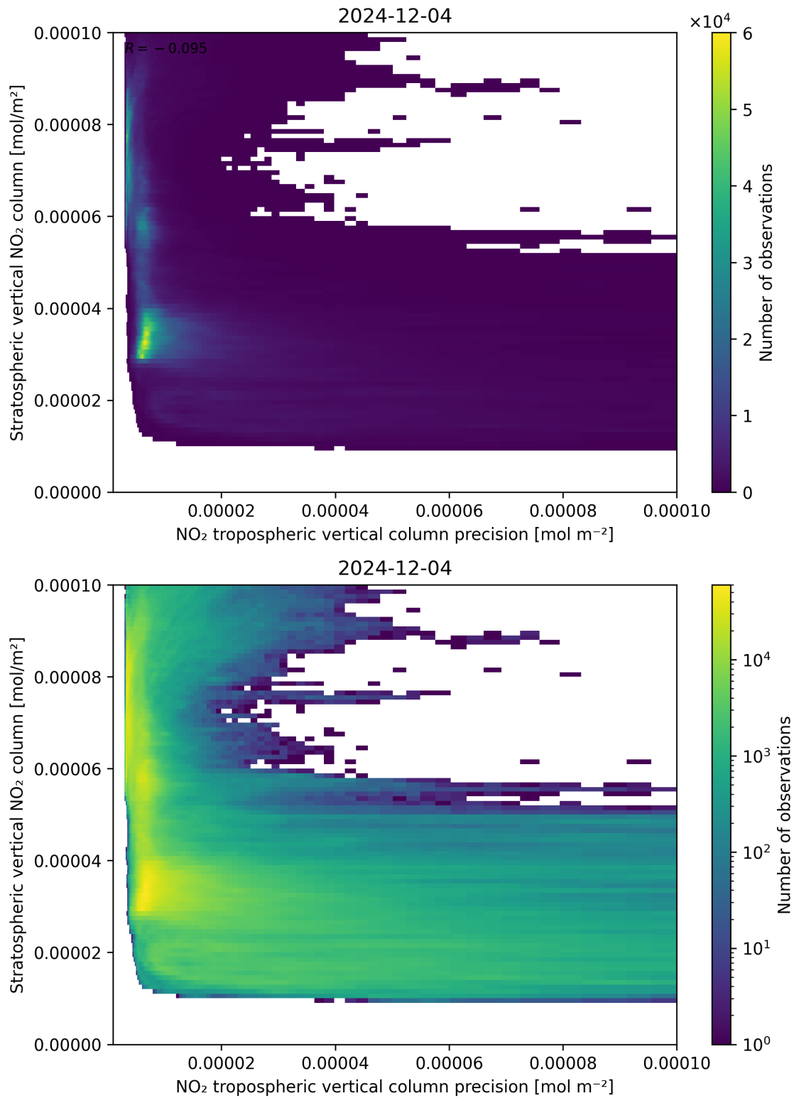
Figure 135: Scatter density plot of “NO 2 tropospheric vertical column precision” against “Stratospheric vertical NO 2 column” for 2024-12-03 to 2024-12-05.
