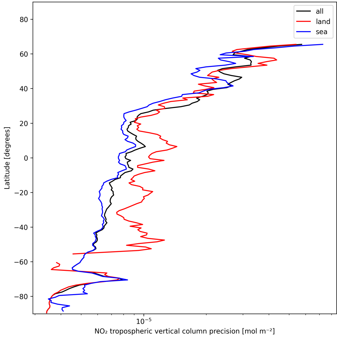
Figure 13: Zonal average of “NO 2 tropospheric vertical column precision” for 2024-12-03 to 2024-12-05.
