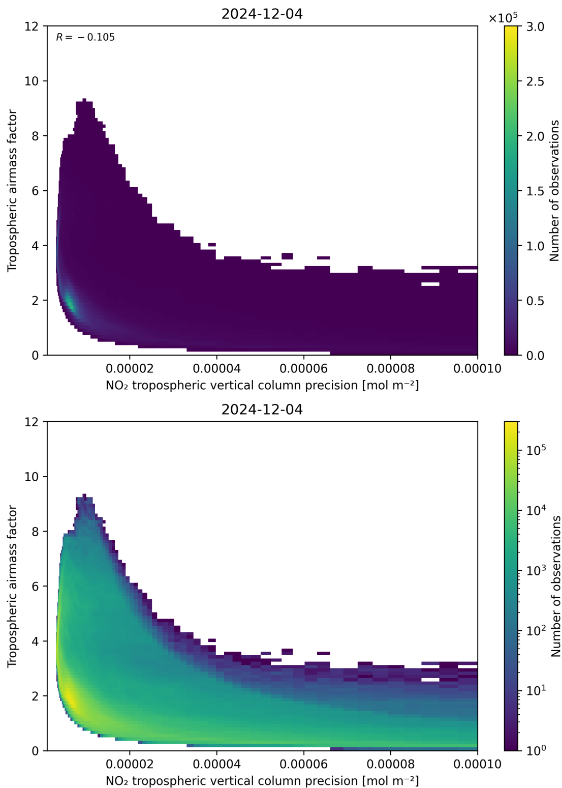
Figure 133: Scatter density plot of “NO 2 tropospheric vertical column precision” against “Tropospheric airmass factor” for 2024-12-03 to 2024-12-05.
