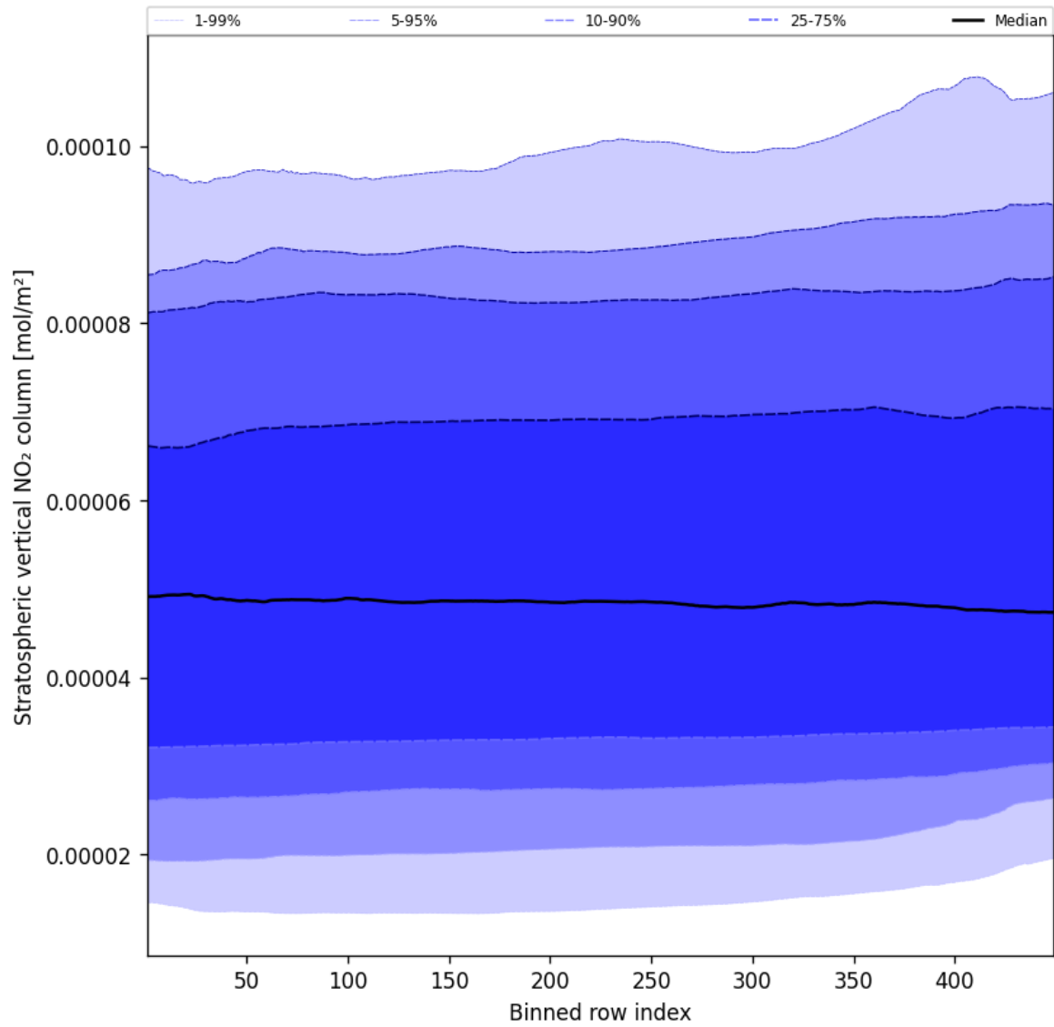
Figure 53: Along track statistics of “Stratospheric vertical NO 2 column” for 2024-12-03 to 2024-12-05
