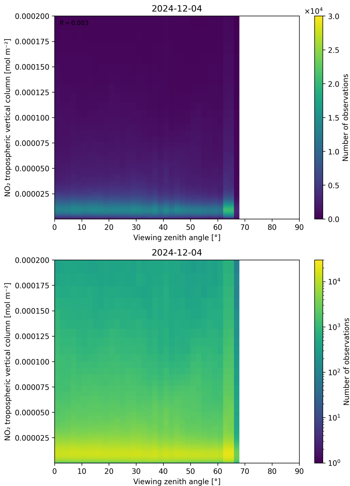
Figure 169: Scatter density plot of “Viewing zenith angle” against “NO 2 tropospheric vertical column” for 2024-12-03 to 2024-12-05.
