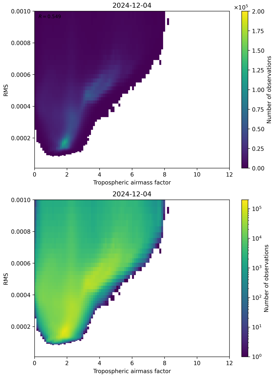
Figure 79: Scatter density plot of “Tropospheric airmass factor” against “RMS” for 2024-12-03 to 2024-12-05.
