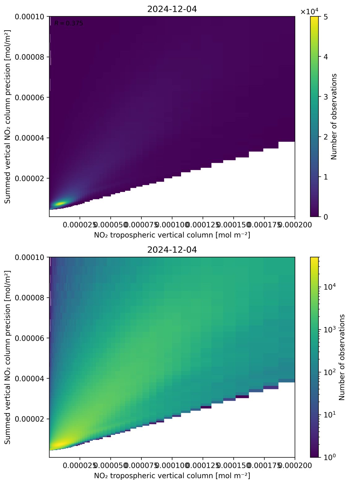
Figure 127: Scatter density plot of “NO 2 tropospheric vertical column” against “Summed vertical NO 2 column precision” for 2024-12-03 to 2024-12-05.
