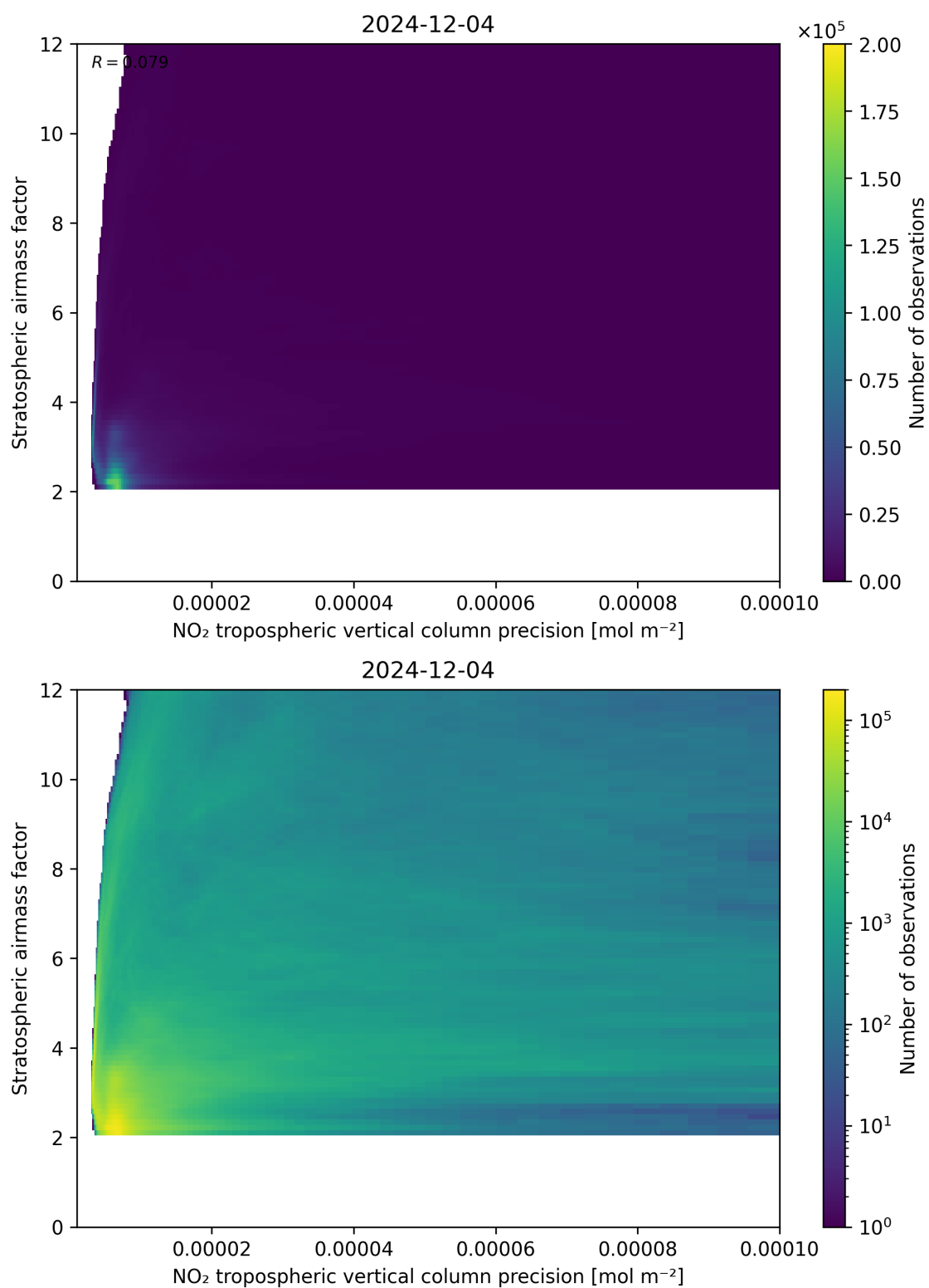
Figure 131: Scatter density plot of “NO 2 tropospheric vertical column precision” against “Stratospheric airmass factor” for 2024-12-03 to 2024-12-05.
