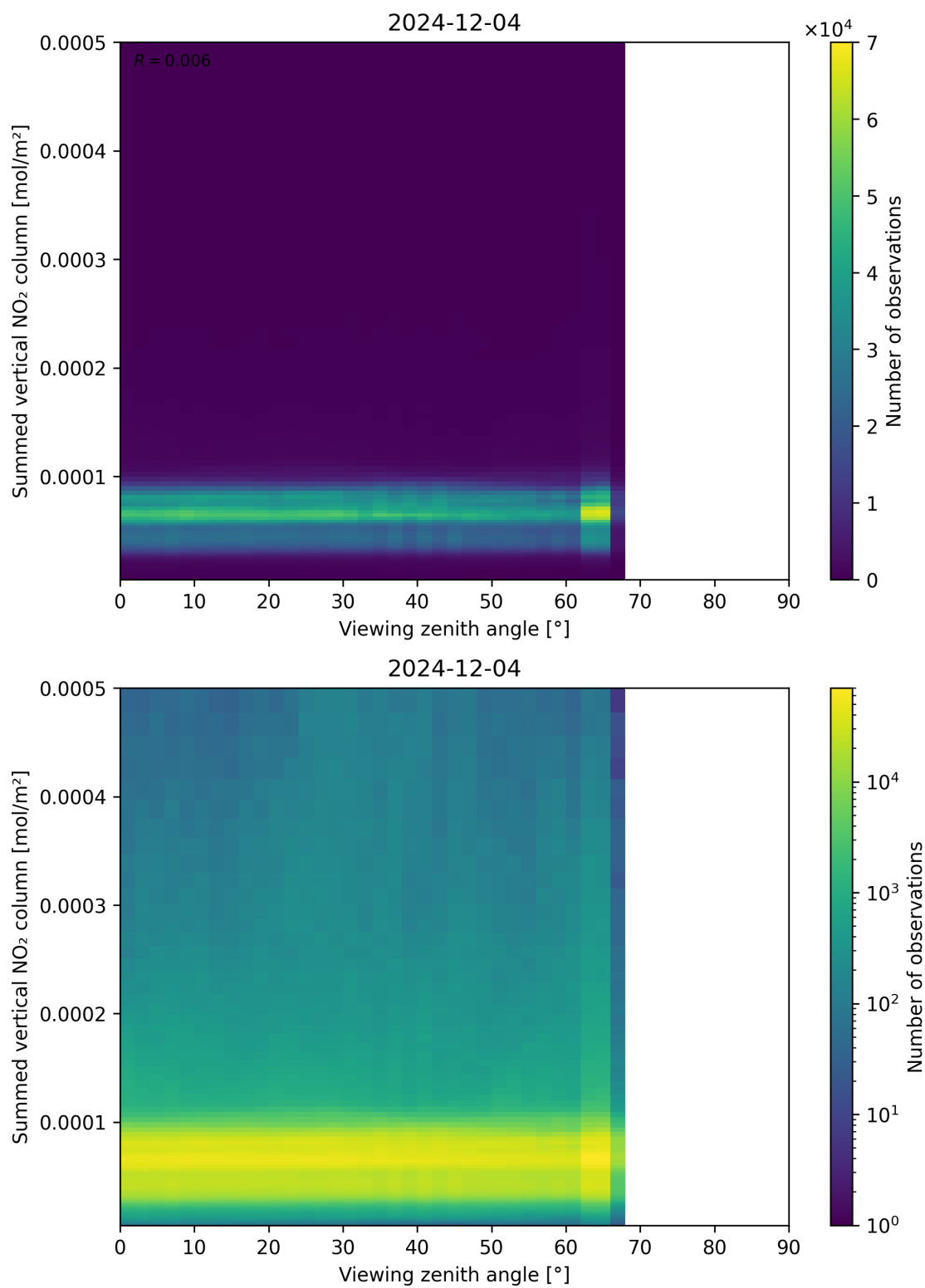
Figure 165: Scatter density plot of “Viewing zenith angle” against “Summed vertical NO 2 column” for 2024-12-03 to 2024-12-05.
