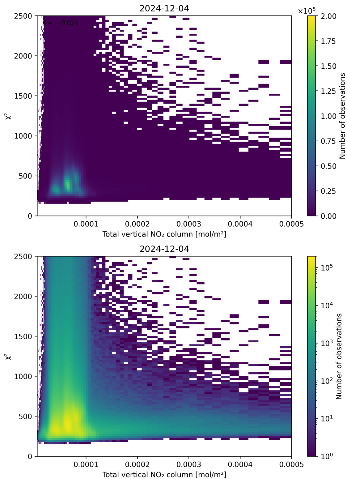
Figure 111: Scatter density plot of “Total vertical NO 2 column” against “ \chi^2 ” for 2024-12-03 to 2024-12-05.
