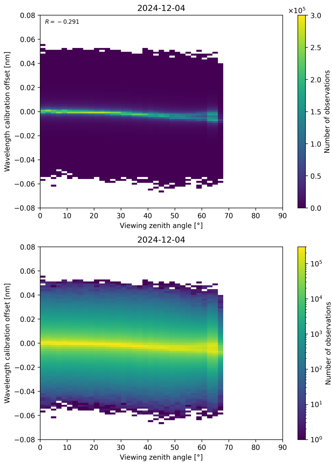
Figure 173: Scatter density plot of “Viewing zenith angle” against “Wavelength calibration offset” for 2024-12-03 to 2024-12-05.
