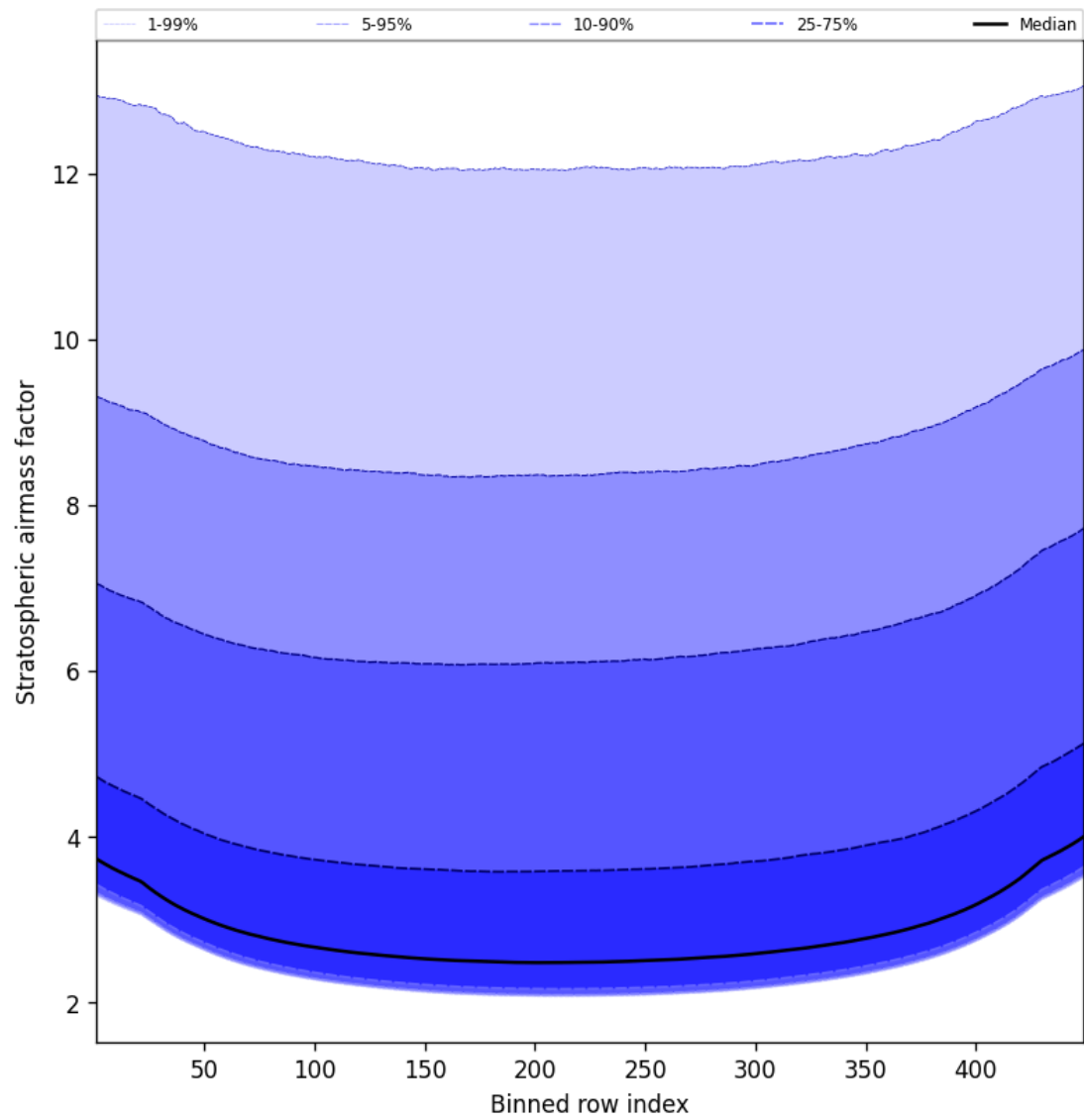
Figure 61: Along track statistics of “Stratospheric airmass factor” for 2024-12-03 to 2024-12-05
