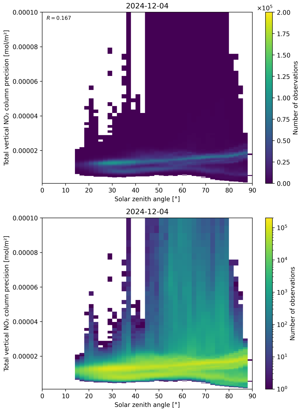
Figure 154: Scatter density plot of “Solar zenith angle” against “Total vertical NO 2 column precision” for 2024-12-03 to 2024-12-05.
