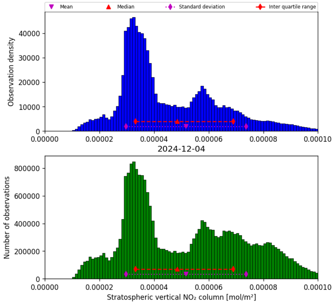
Figure 36: Histogram of “Stratospheric vertical NO 2 column” for 2024-12-03 to 2024-12-05
