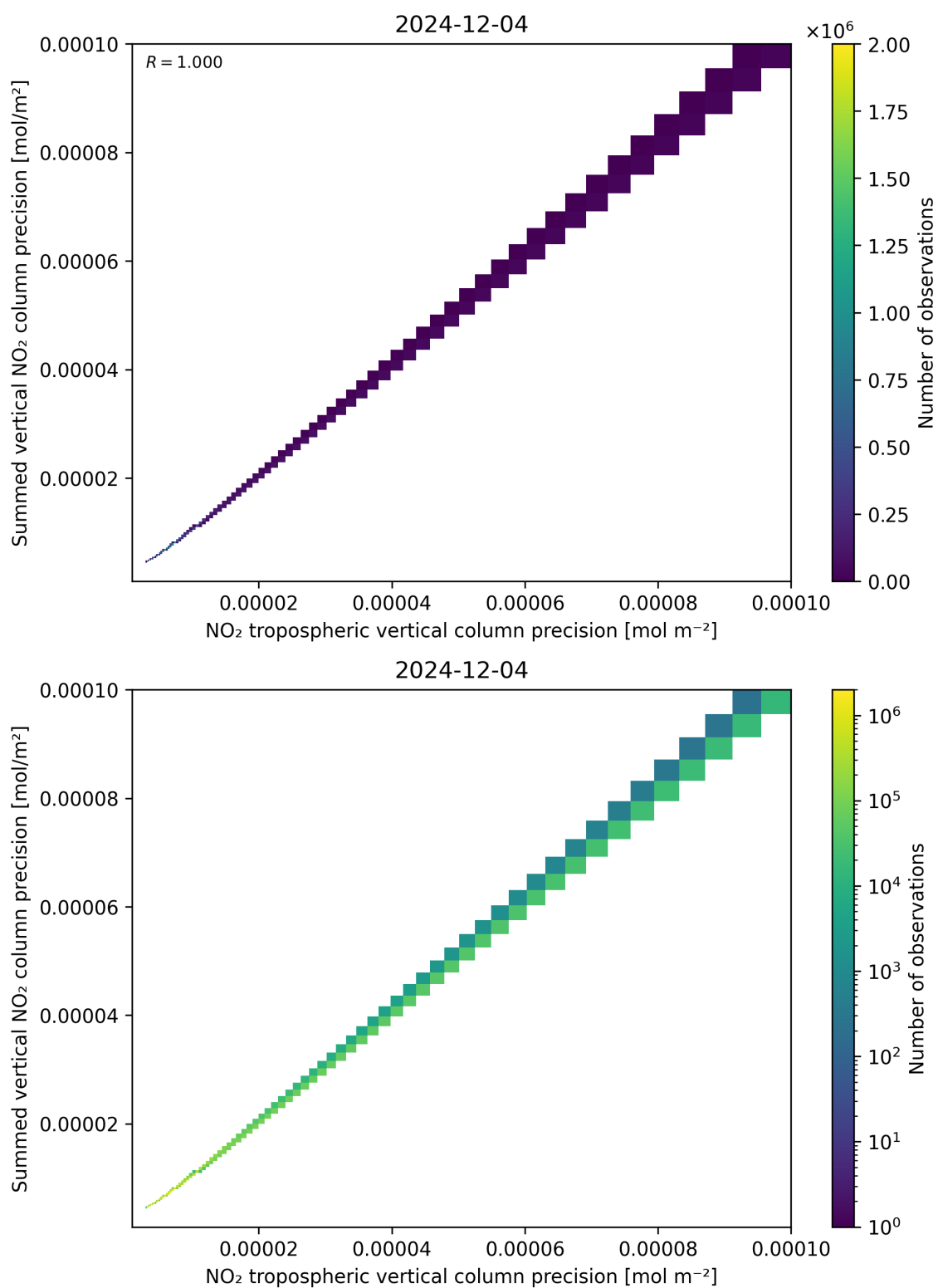
Figure 137: Scatter density plot of “NO 2 tropospheric vertical column precision” against “Summed vertical NO 2 column precision” for 2024-12-03 to 2024-12-05.
