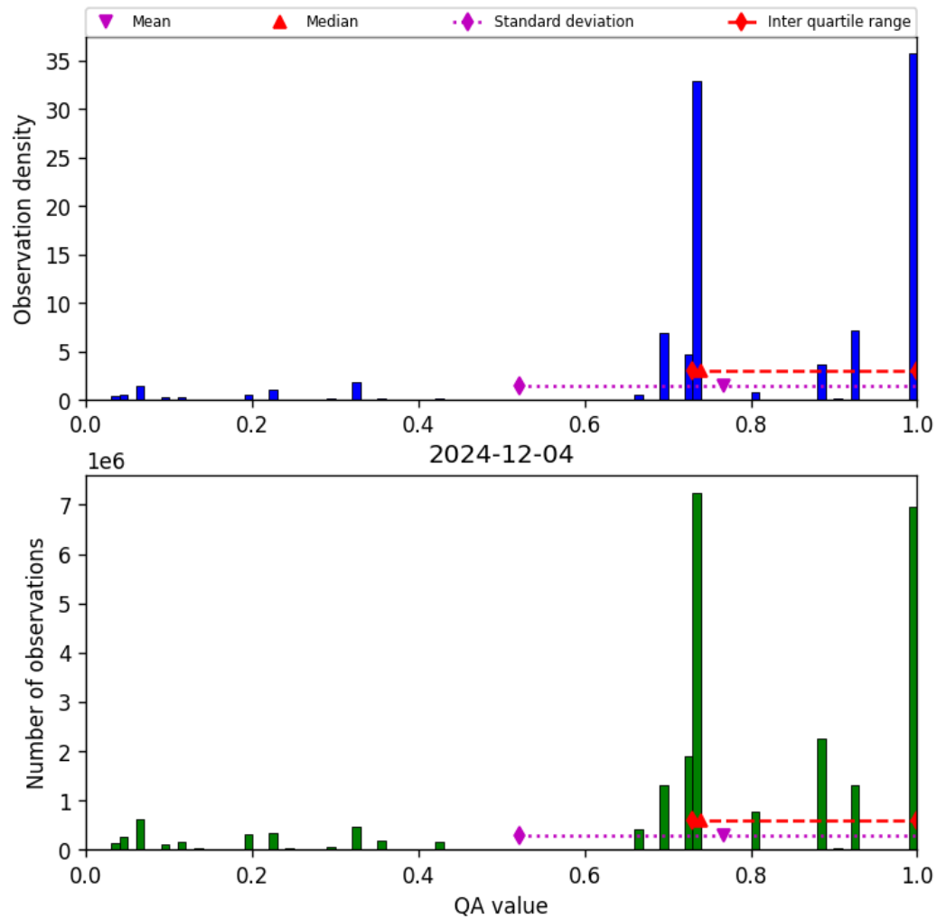
Figure 28: Histogram of “QA value” for 2024-12-03 to 2024-12-05
