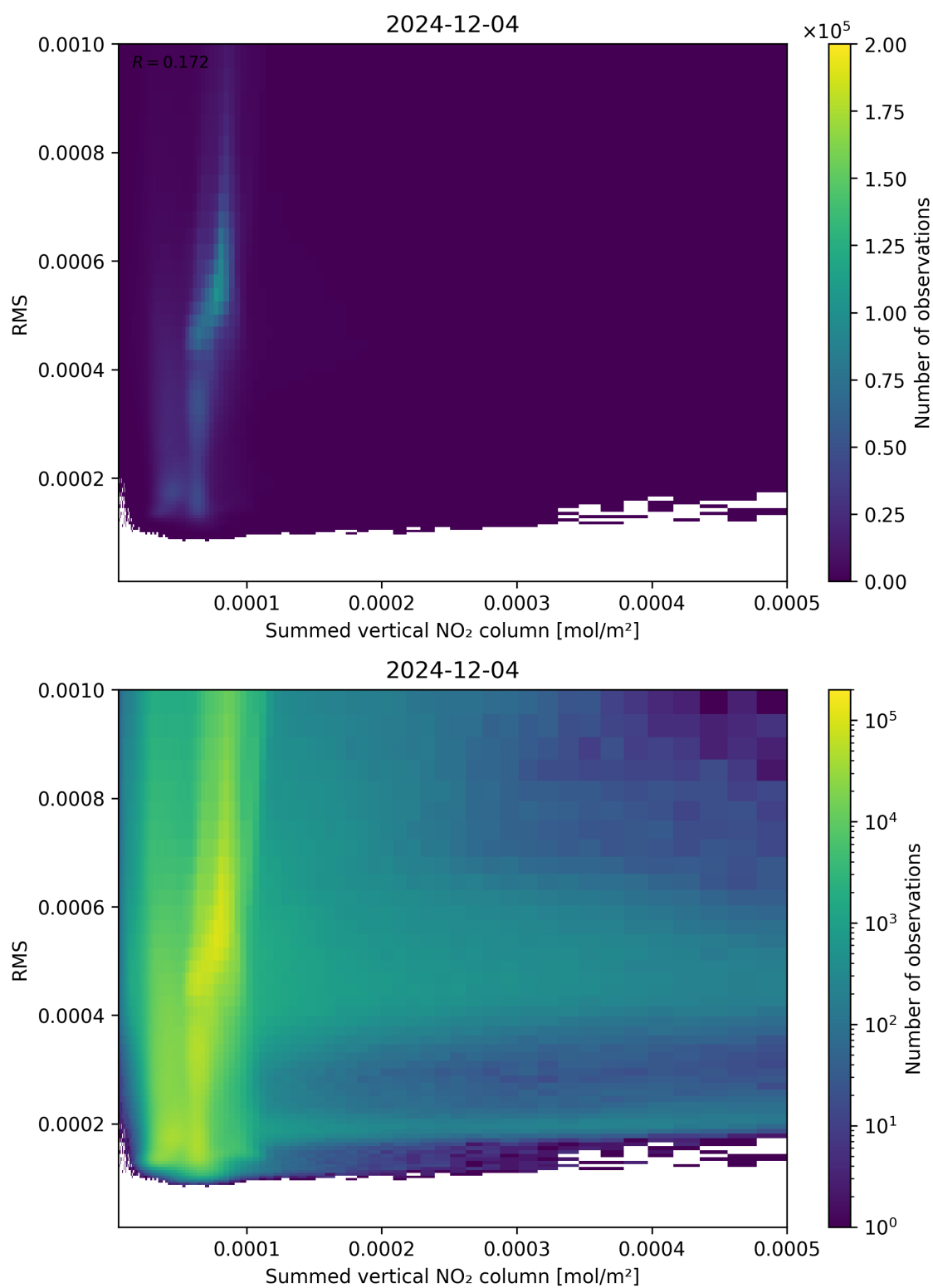
Figure 109: Scatter density plot of “Summed vertical NO 2 column” against “RMS” for 2024-12-03 to 2024-12-05.
