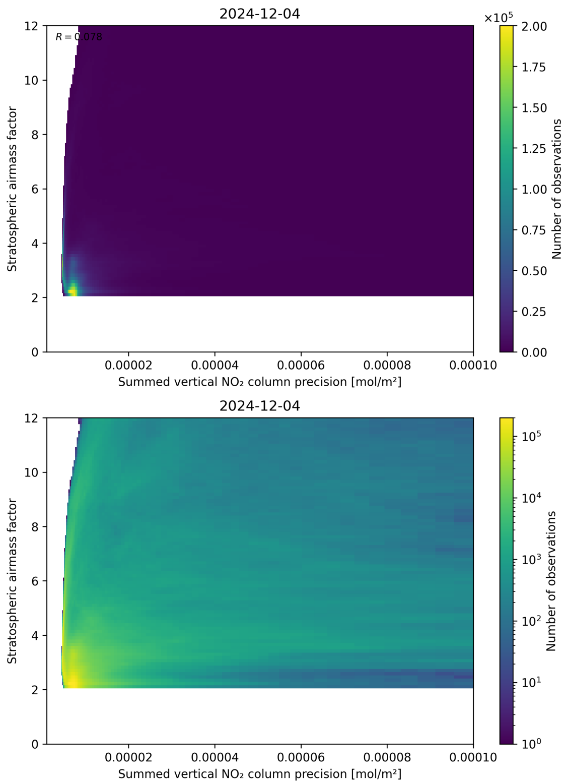
Figure 106: Scatter density plot of “Summed vertical NO 2 column precision” against “Stratospheric airmass factor” for 2024-12-03 to 2024-12-05.
