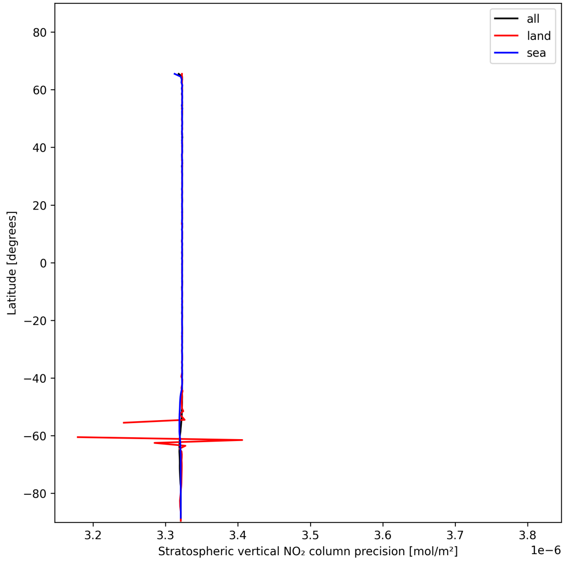
Figure 20: Zonal average of “Stratospheric vertical NO 2 column precision” for 2024-12-03 to 2024-12-05.
