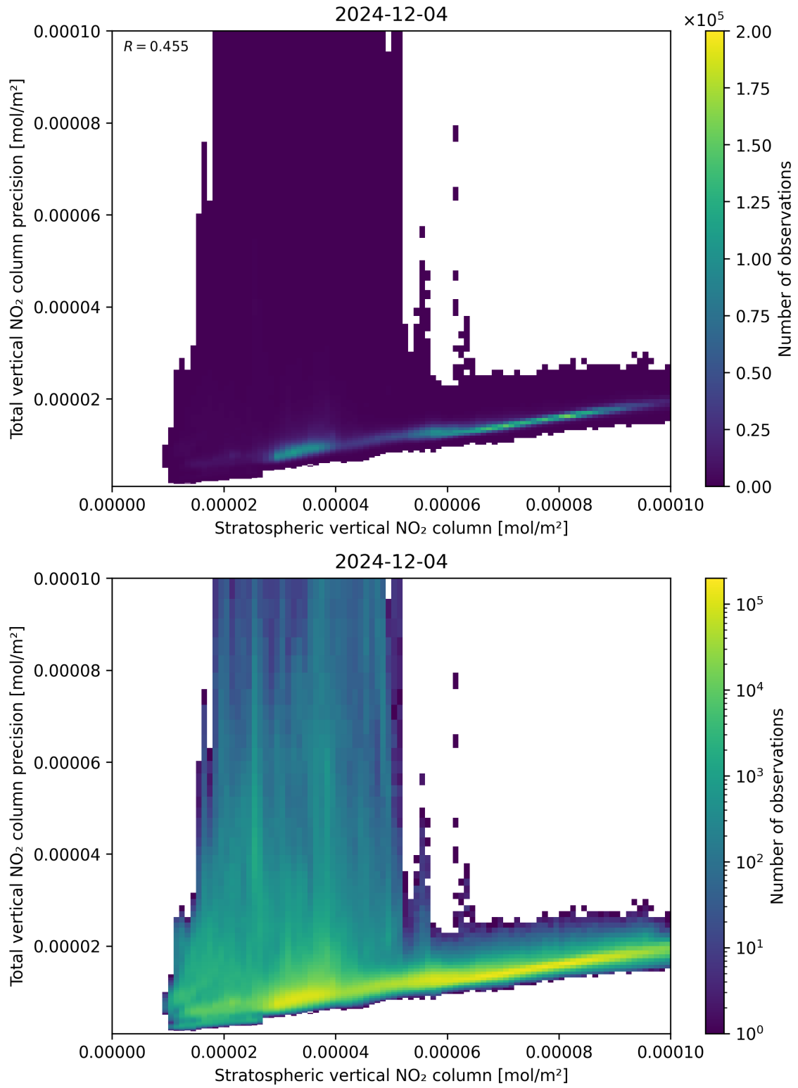
Figure 101: Scatter density plot of “Stratospheric vertical NO 2 column” against “Total vertical NO 2 column precision” for 2024-12-03 to 2024-12-05.
