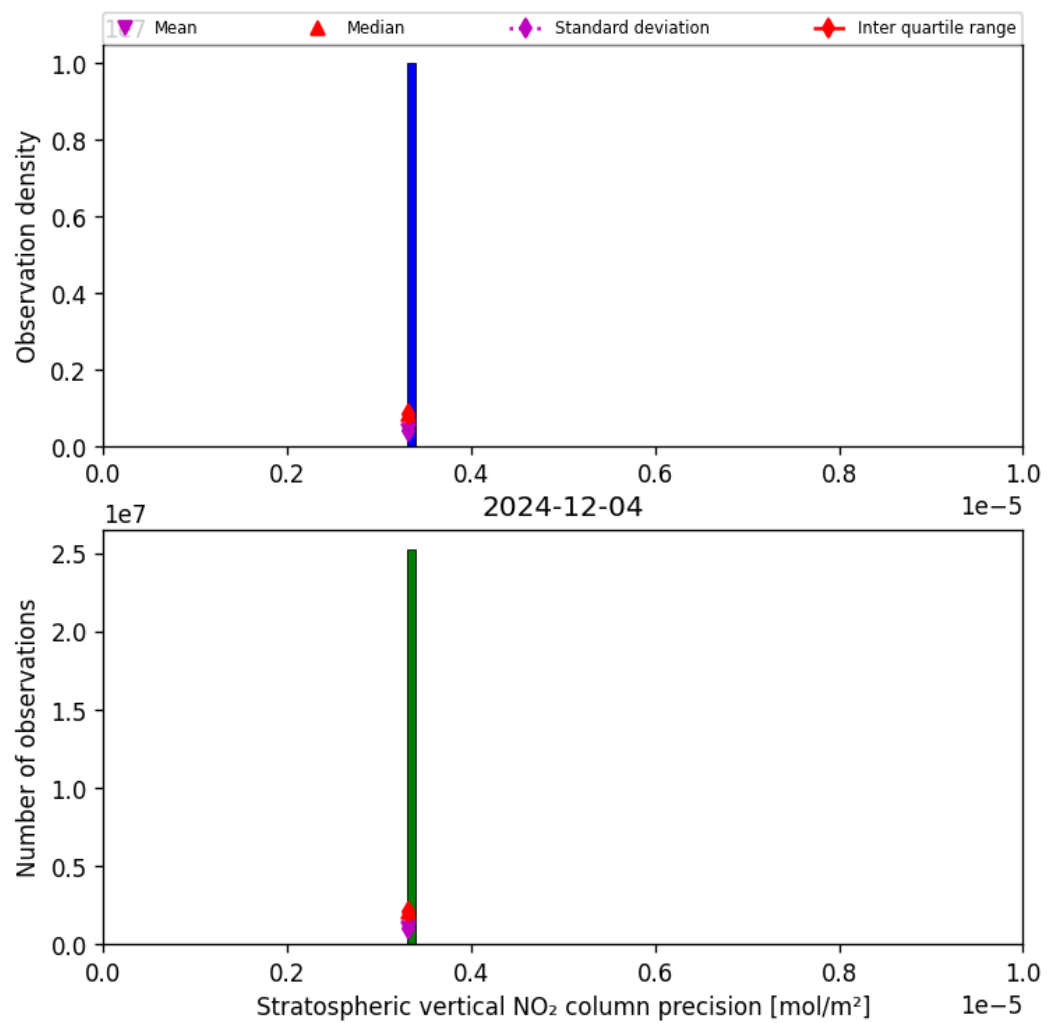
Figure 37: Histogram of “Stratospheric vertical NO 2 column precision” for 2024-12-03 to 2024-12-05
