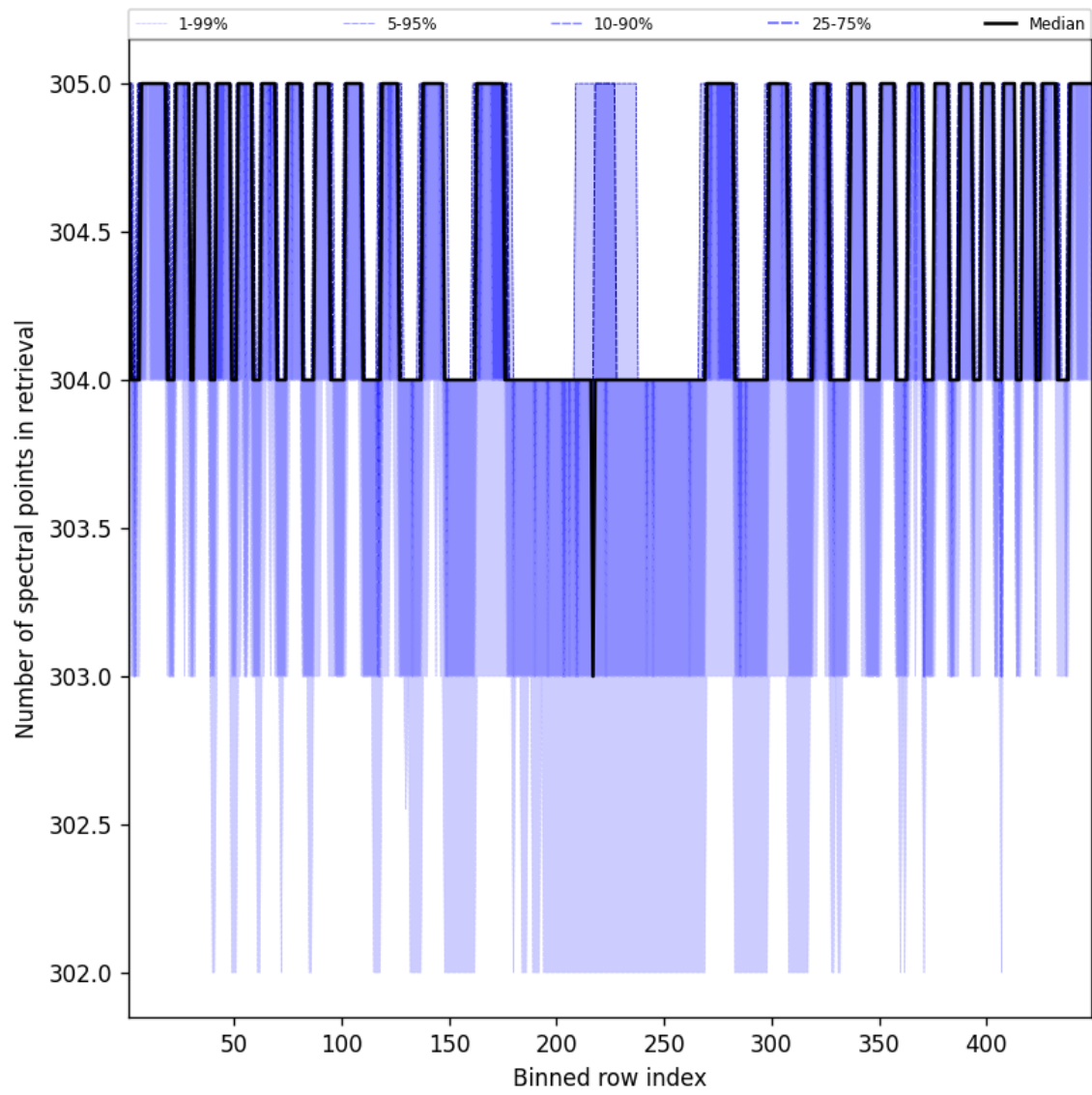
Figure 50: Along track statistics of “Number of spectral points in retrieval” for 2024-12-03 to 2024-12-05
