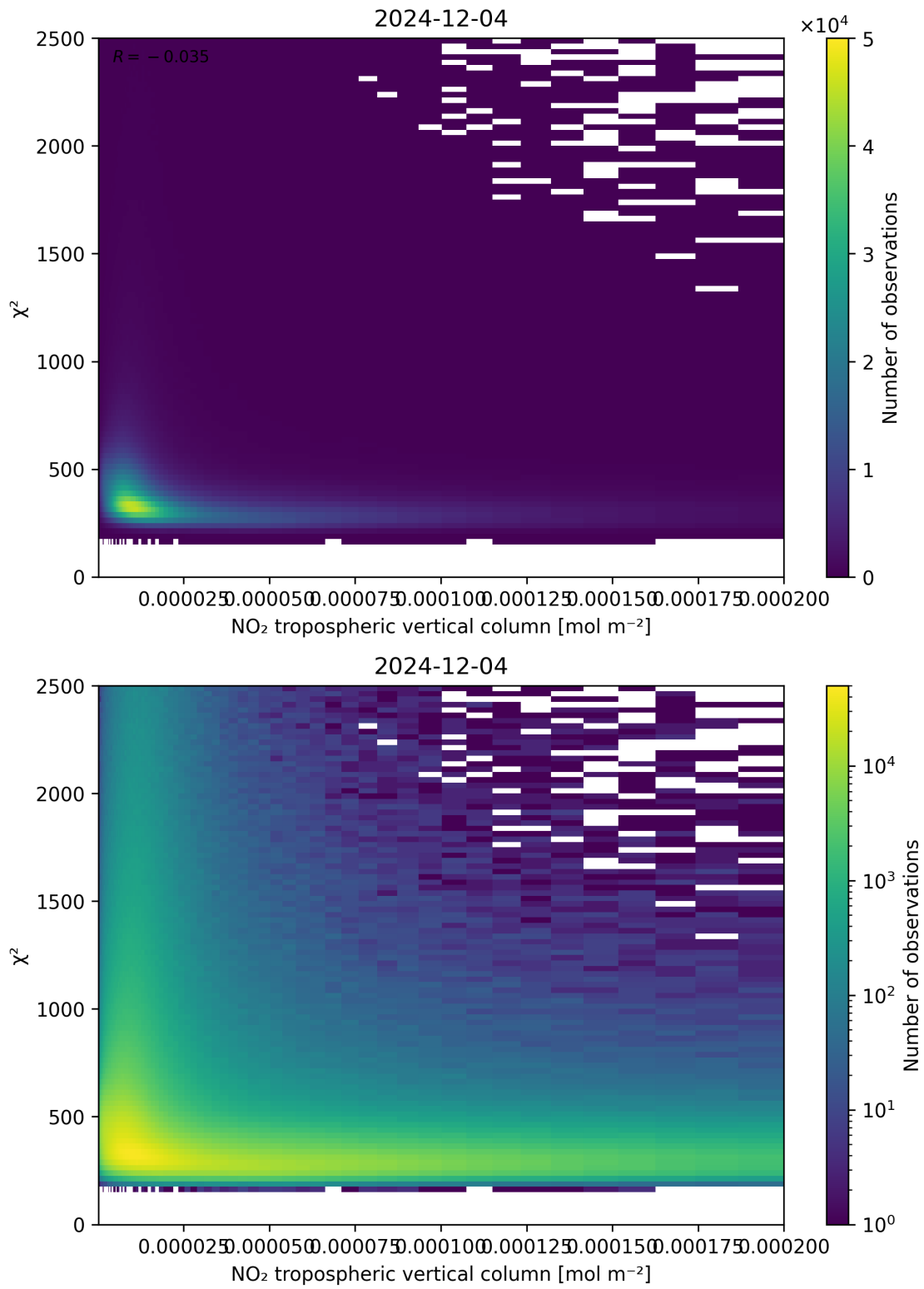
Figure 124: Scatter density plot of “NO 2 tropospheric vertical column” against “ \chi^2 ” for 2024-12-03 to 2024-12-05.
