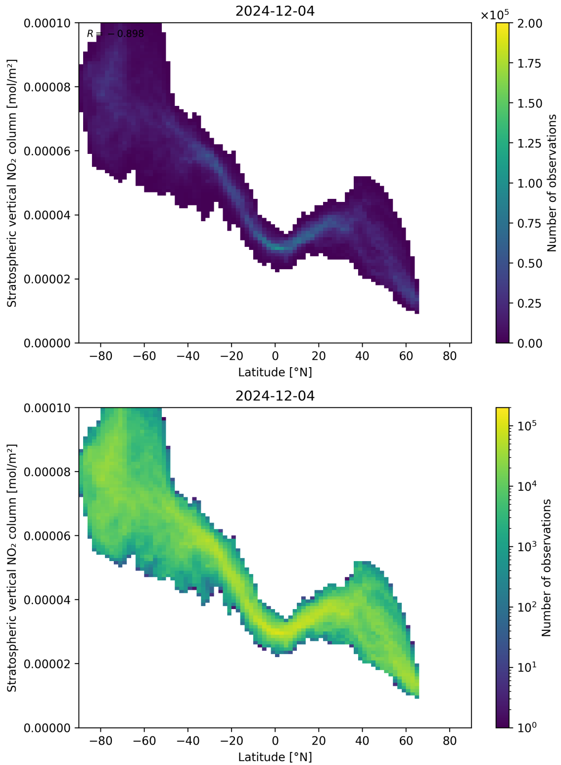
Figure 87: Scatter density plot of “Latitude” against “Stratospheric vertical NO 2 column” for 2024-12-03 to 2024-12-05.
