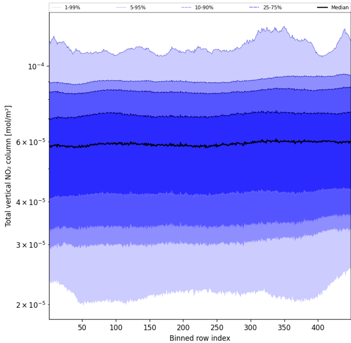
Figure 55: Along track statistics of “Total vertical NO 2 column” for 2024-12-03 to 2024-12-05
