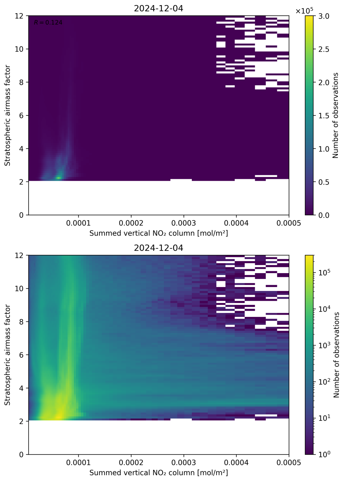
Figure 103: Scatter density plot of “Summed vertical NO 2 column” against “Stratospheric air mass factor” for 2024-12-03 to 2024-12-05.
