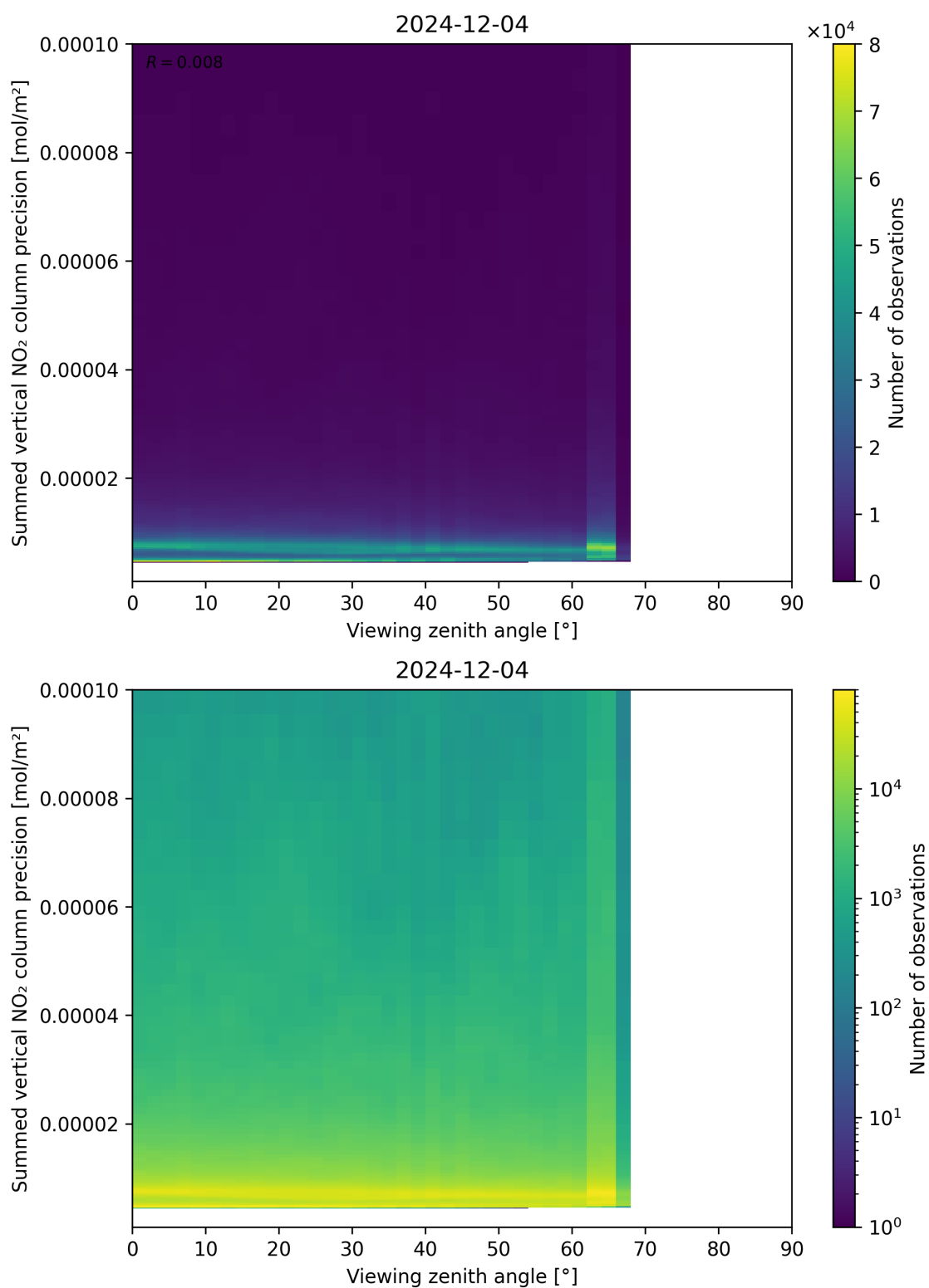
Figure 166: Scatter density plot of “Viewing zenith angle” against “Summed vertical NO 2 column precision” for 2024-12-03 to 2024-12-05.
