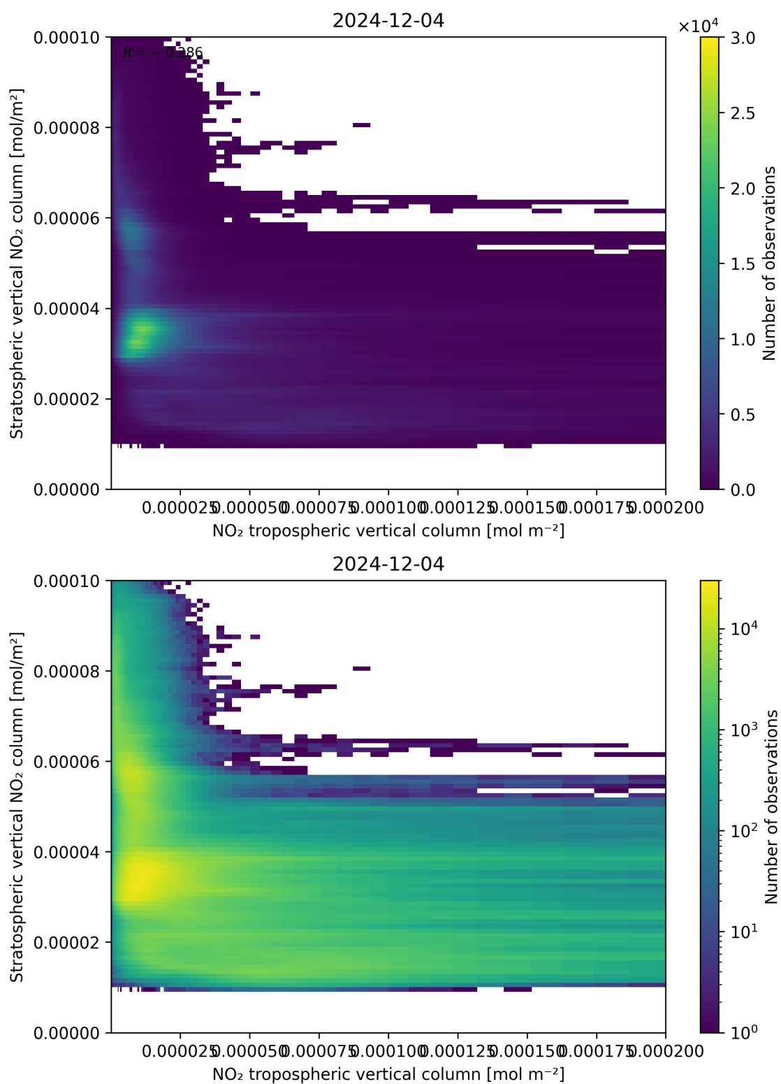
Figure 125: Scatter density plot of “NO 2 tropospheric vertical column” against “Stratospheric vertical NO 2 column” for 2024-12-03 to 2024-12-05.
