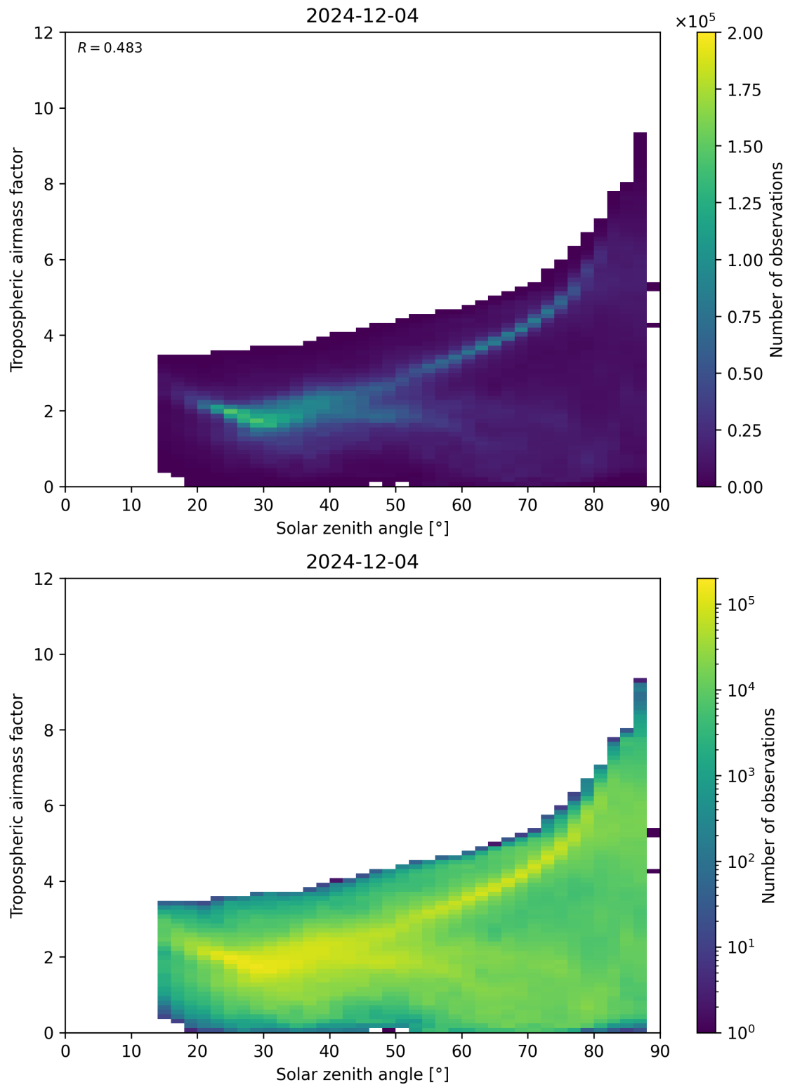
Figure 147: Scatter density plot of “Solar zenith angle” against “Tropospheric airmass factor” for 2024-12-03 to 2024-12-05.
