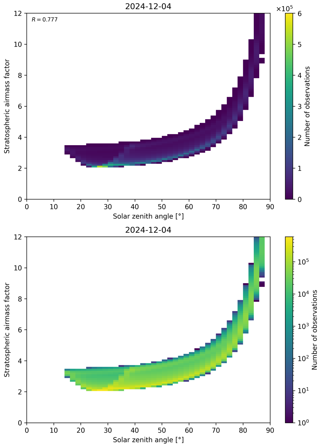
Figure 145: Scatter density plot of “Solar zenith angle” against “Stratospheric airmass factor” for 2024-12-03 to 2024-12-05.
