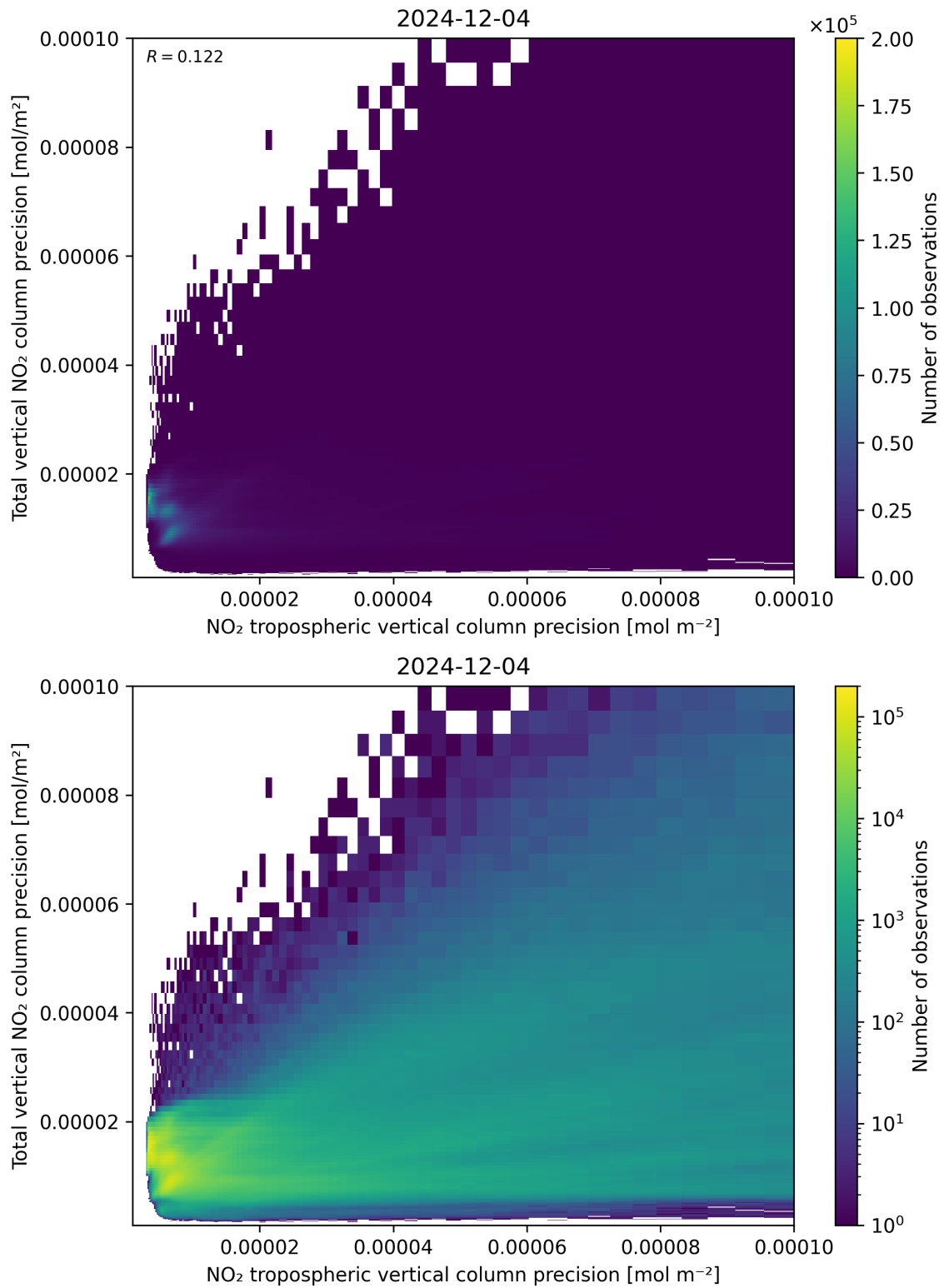
Figure 139: Scatter density plot of “NO 2 tropospheric vertical column precision” against “Total vertical NO 2 column precision” for 2024-12-03 to 2024-12-05.
