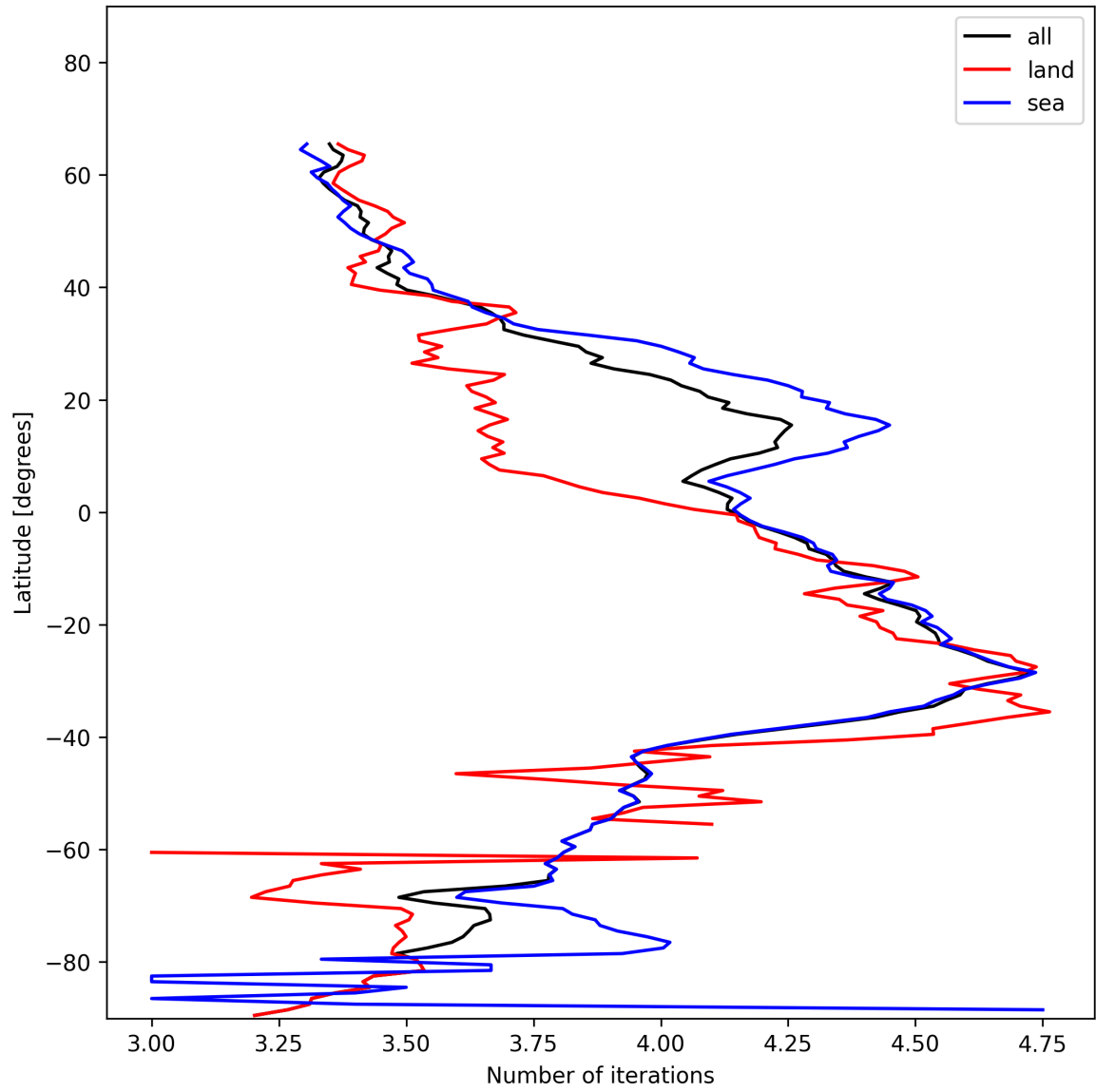
Figure 17: Zonal average of “Number of iterations” for 2024-12-03 to 2024-12-05.
