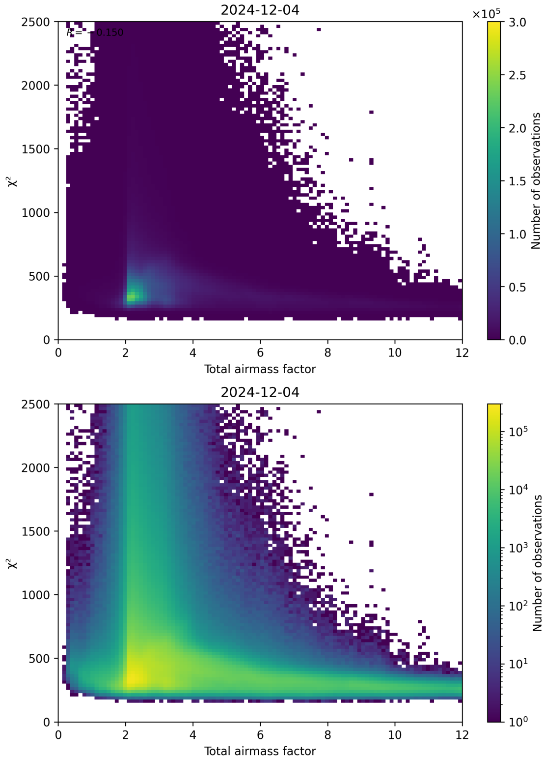
Figure 63: Scatter density plot of “Total airmass factor” against “ \chi^2 ” for 2024-12-03 to 2024-12-05.
