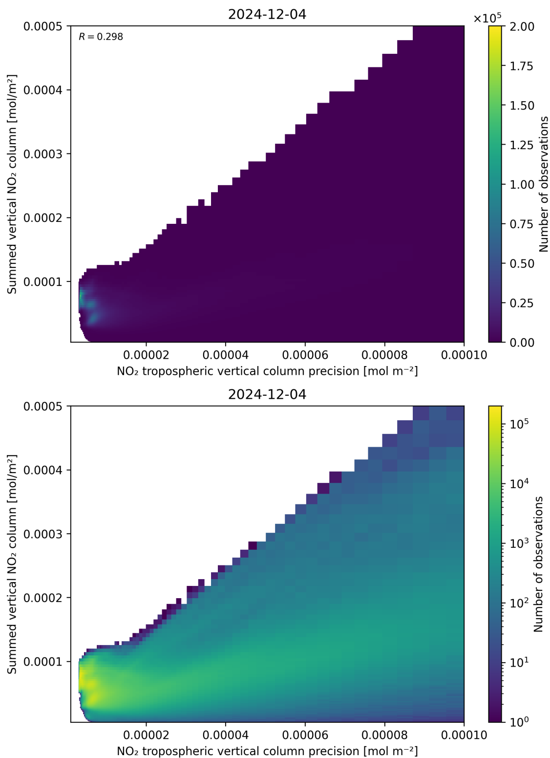
Figure 136: Scatter density plot of “NO 2 tropospheric vertical column precision” against “Summed vertical NO 2 column” for 2024-12-03 to 2024-12-05.
