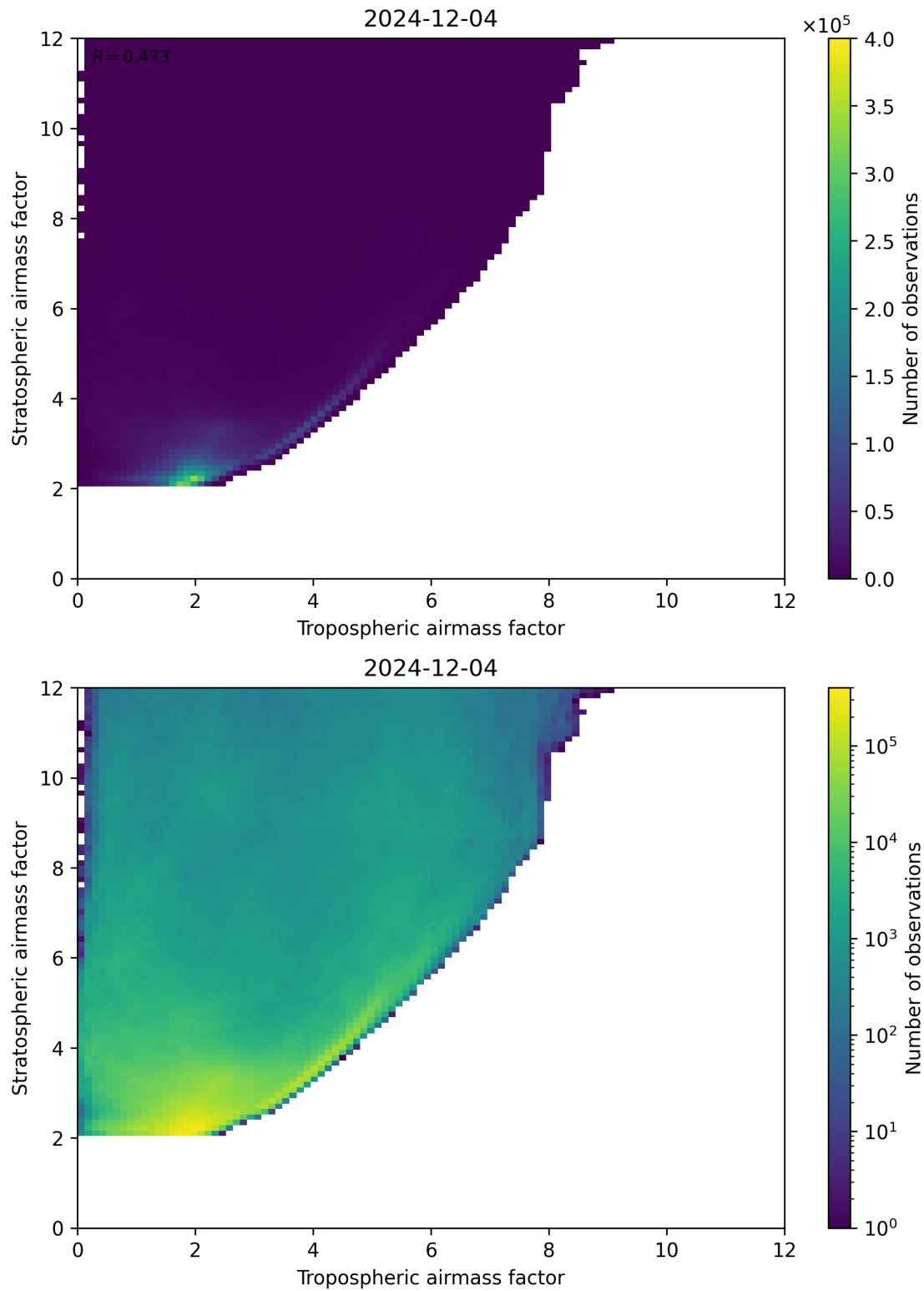
Figure 71: Scatter density plot of “Tropospheric airmass factor” against “Stratospheric airmass factor” for 2024-12-03 to 2024-12-05.
