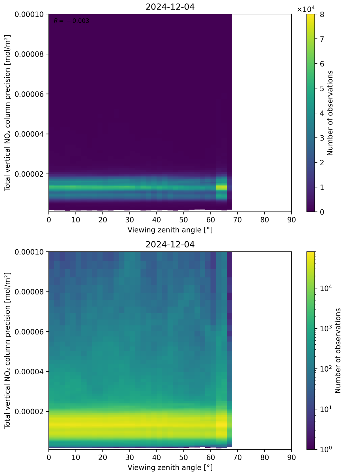
Figure 168: Scatter density plot of “Viewing zenith angle” against “Total vertical NO 2 column precision” for 2024-12-03 to 2024-12-05.
