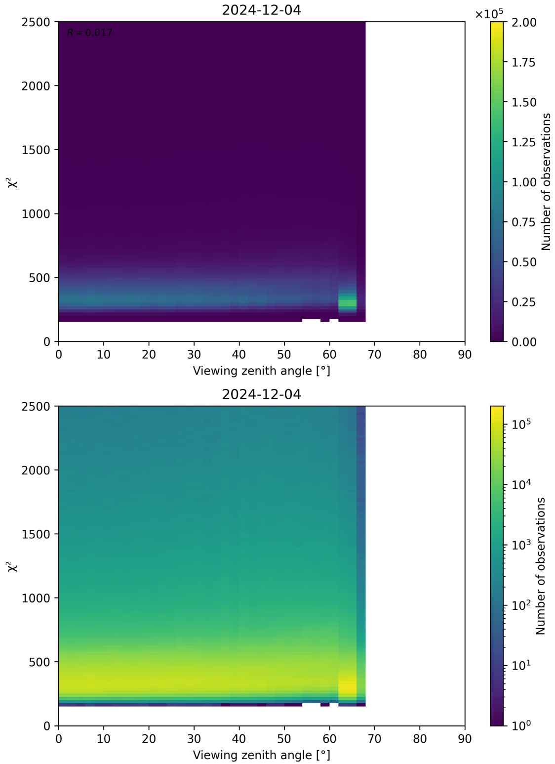
Figure 162: Scatter density plot of “Viewing zenith angle” against “ \chi^2 ” for 2024-12-03 to 2024-12-05.
