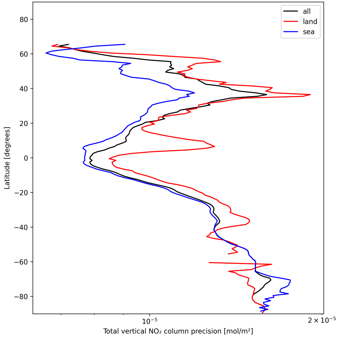
Figure 22: Zonal average of “Total vertical NO 2 column precision” for 2024-12-03 to 2024-12-05.
