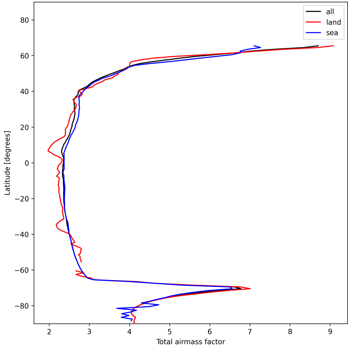
Figure 15: Zonal average of “Total airmass factor” for 2024-12-03 to 2024-12-05.
