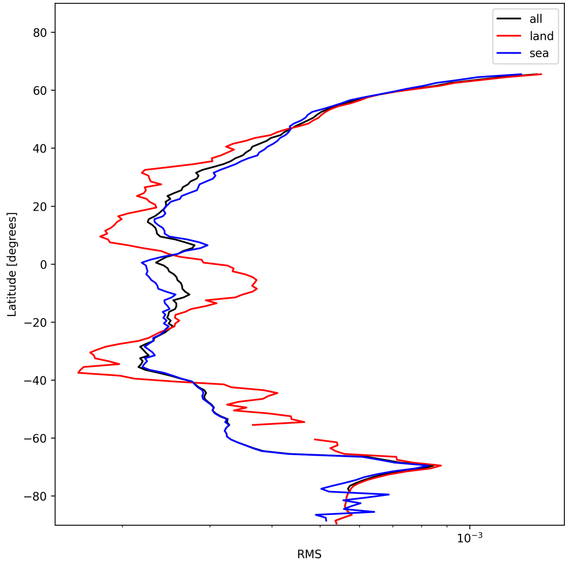
Figure 26: Zonal average of “RMS” for 2024-12-03 to 2024-12-05.
