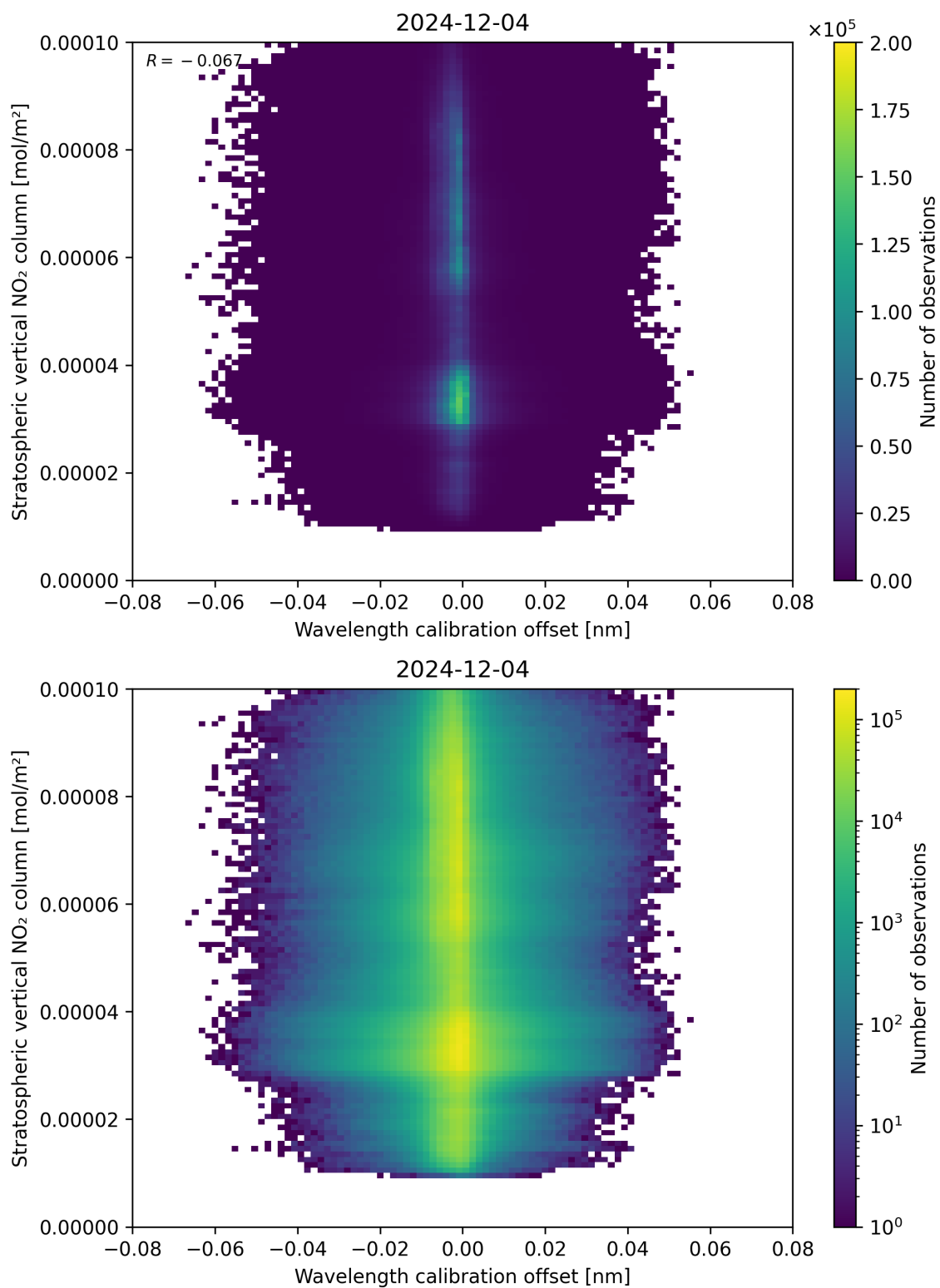
Figure 176: Scatter density plot of “Wavelength calibration offset” against “Stratospheric vertical NO 2 column” for 2024-12-03 to 2024-12-05.
