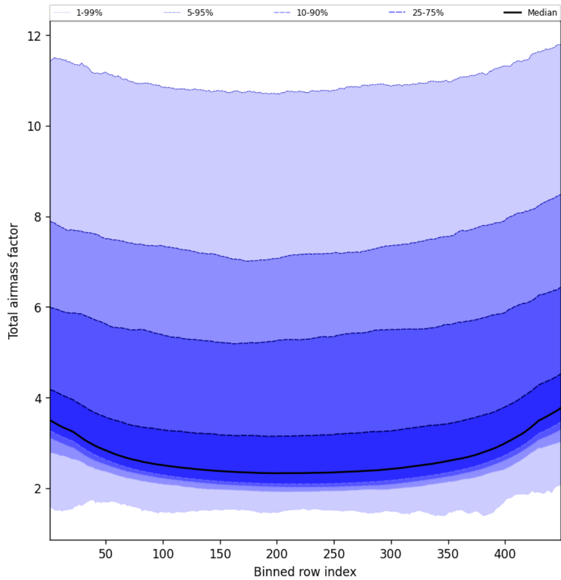
Figure 49: Along track statistics of “Total airmass factor” for 2024-12-03 to 2024-12-05
