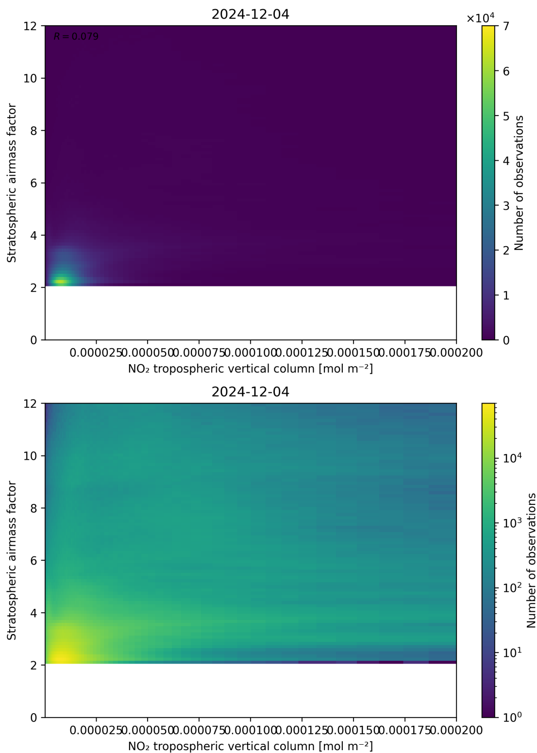
Figure 121: Scatter density plot of “NO 2 tropospheric vertical column” against “Stratospheric airmass factor” for 2024-12-03 to 2024-12-05.
