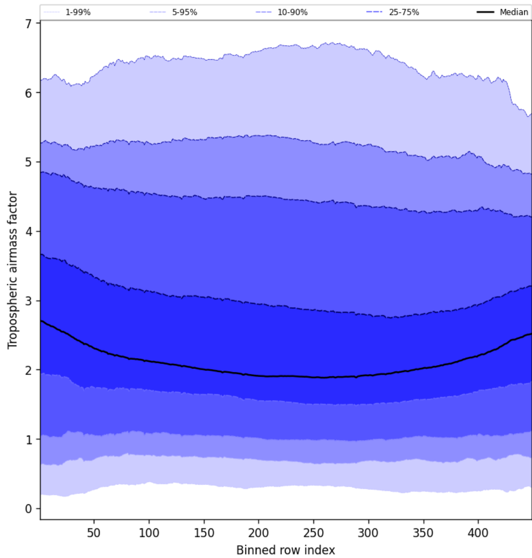
Figure 48: Along track statistics of “Tropospheric airmass factor” for 2024-12-03 to 2024-12-05
