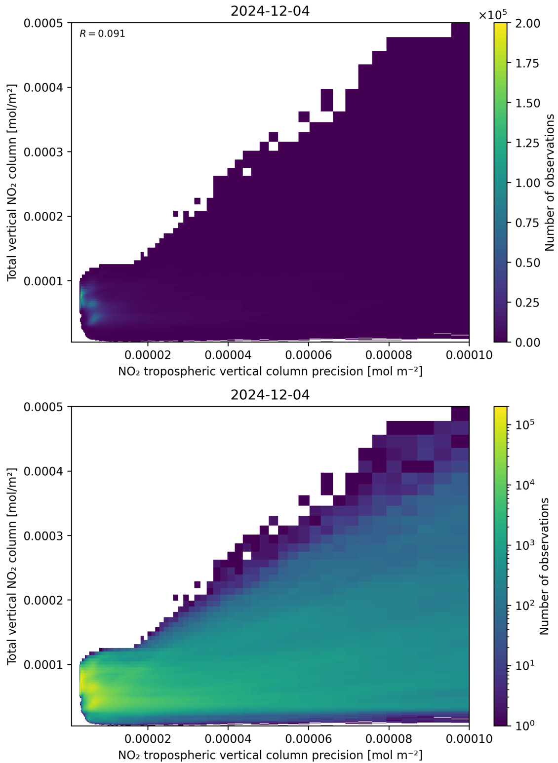
Figure 138: Scatter density plot of “NO 2 tropospheric vertical column precision” against “Total vertical NO 2 column” for 2024-12-03 to 2024-12-05.
