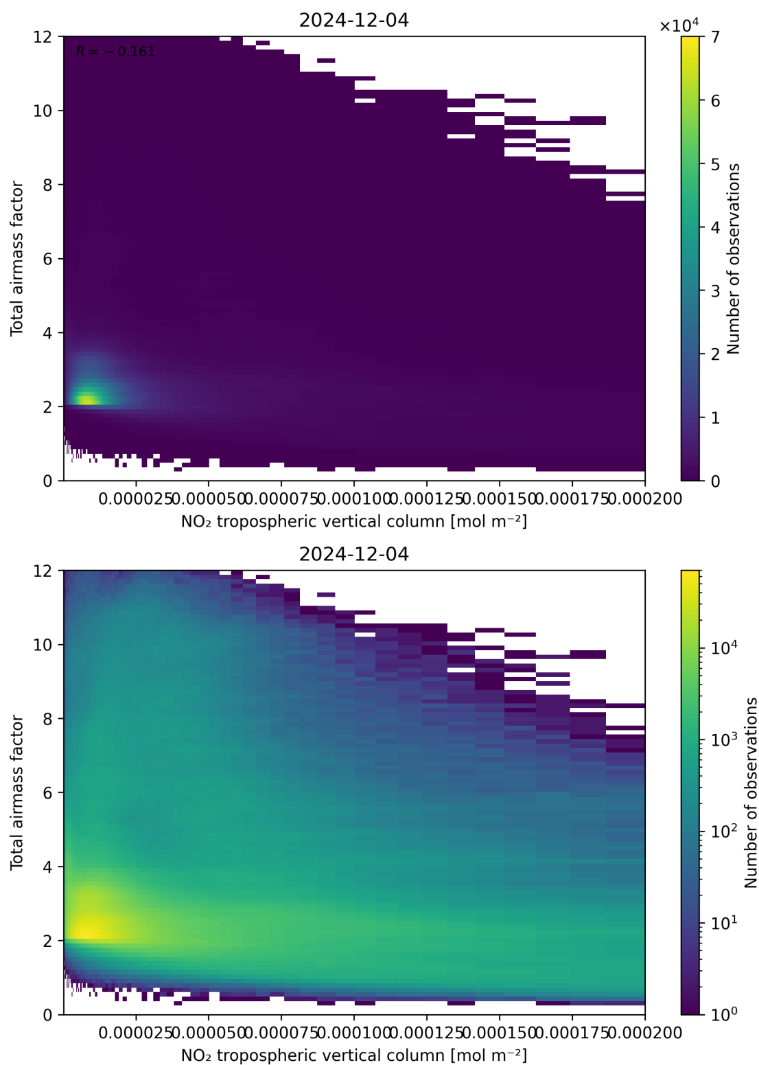
Figure 122: Scatter density plot of “NO 2 tropospheric vertical column” against “Total air mass factor” for 2024-12-03 to 2024-12-05.
