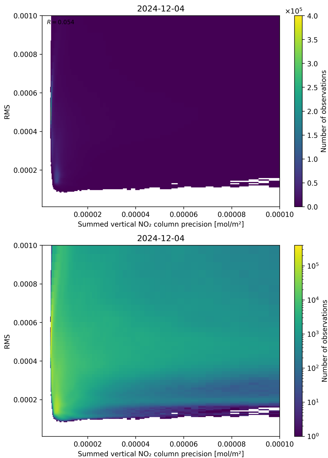
Figure 108: Scatter density plot of “Summed vertical NO 2 column precision” against “RMS” for 2024-12-03 to 2024-12-05.
