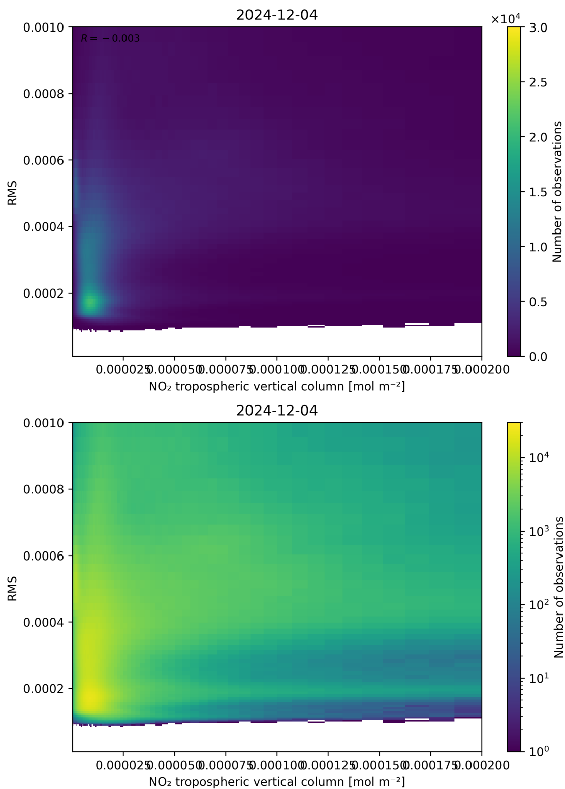
Figure 142: Scatter density plot of “NO 2 tropospheric vertical column” against “RMS” for 2024-12-03 to 2024-12-05.
