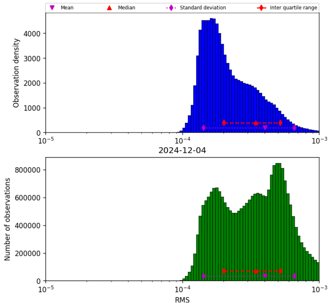
Figure 43: Histogram of “RMS” for 2024-12-03 to 2024-12-05
