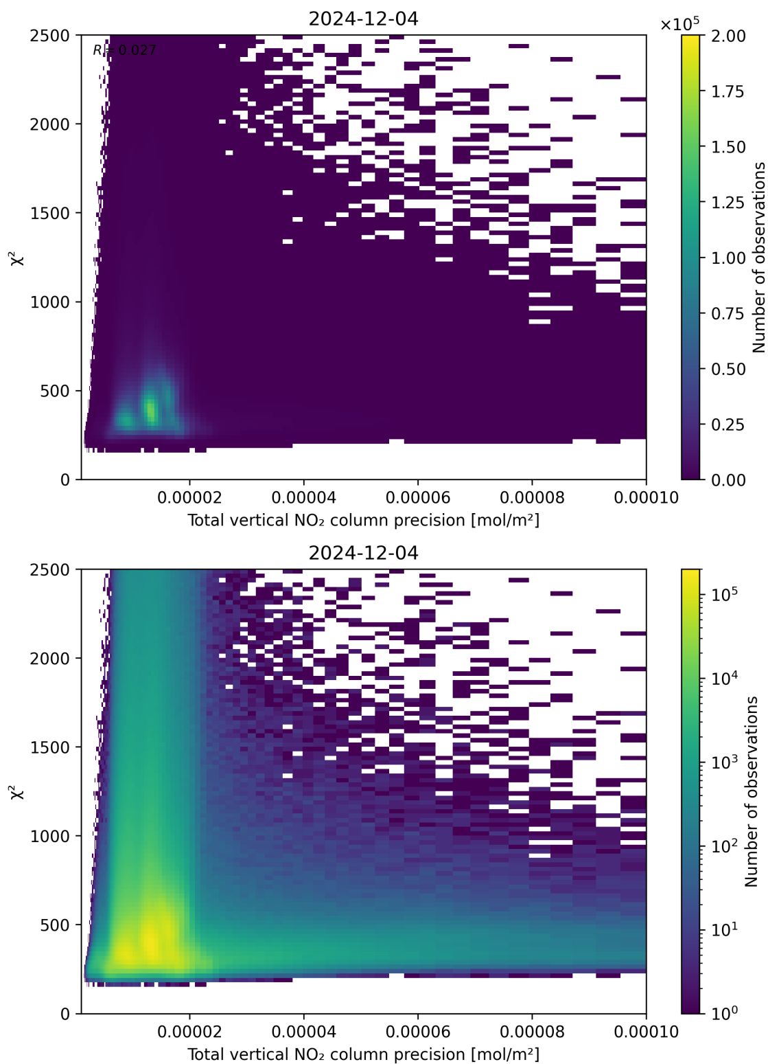
Figure 116: Scatter density plot of “Total vertical NO 2 column precision” against “ \chi^2 ” for 2024-12-03 to 2024-12-05.
