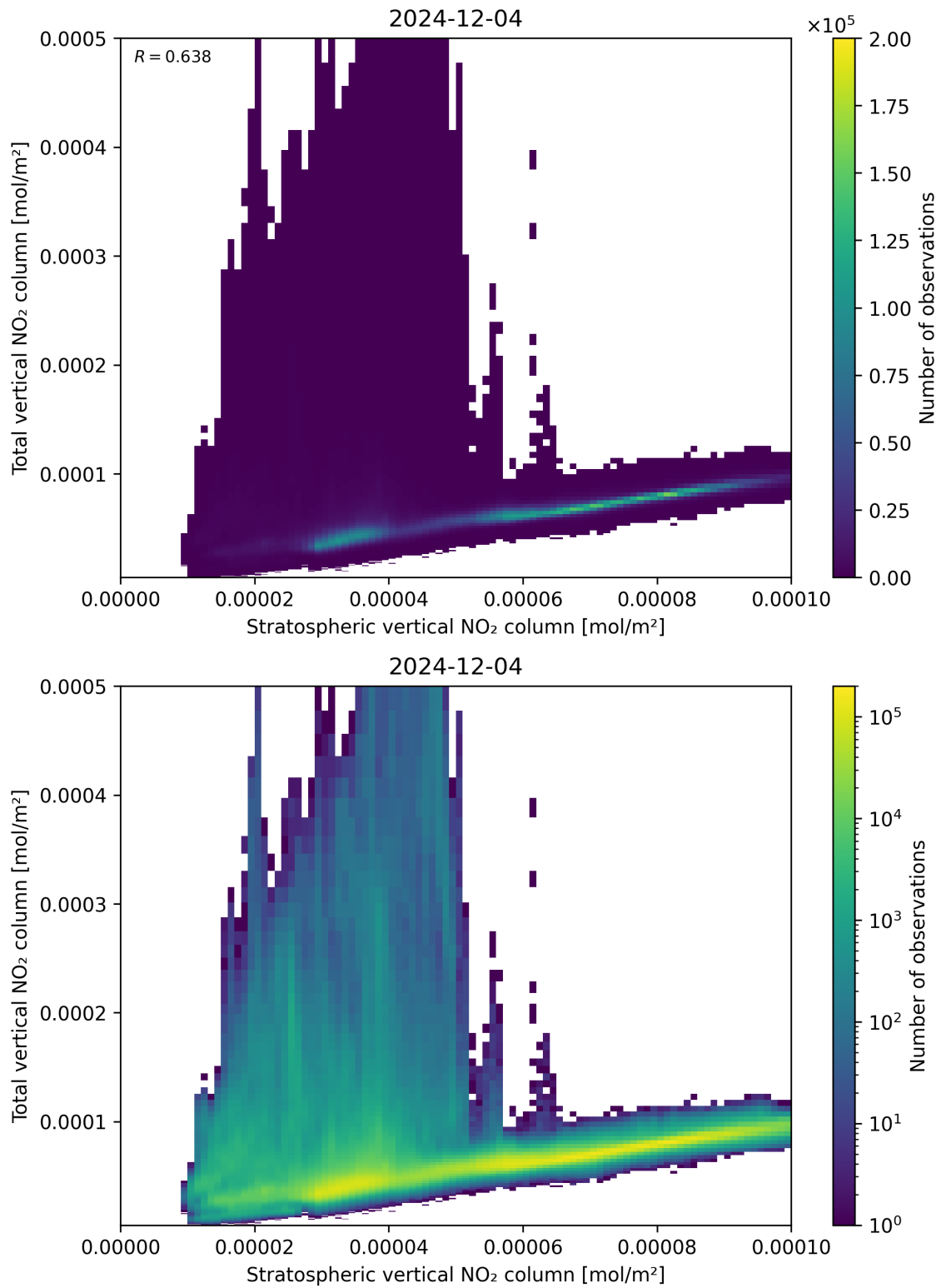
Figure 100: Scatter density plot of “Stratospheric vertical NO 2 column” against “Total vertical NO 2 column” for 2024-12-03 to 2024-12-05.
