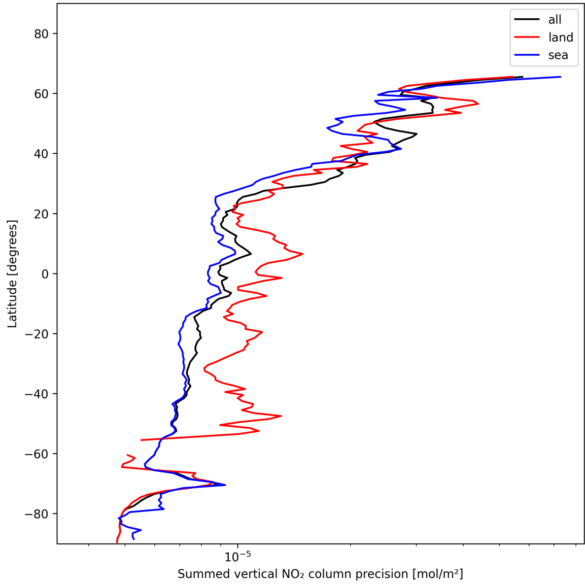
Figure 24: Zonal average of “Summed vertical NO 2 column precision” for 2024-12-03 to 2024-12-05.
