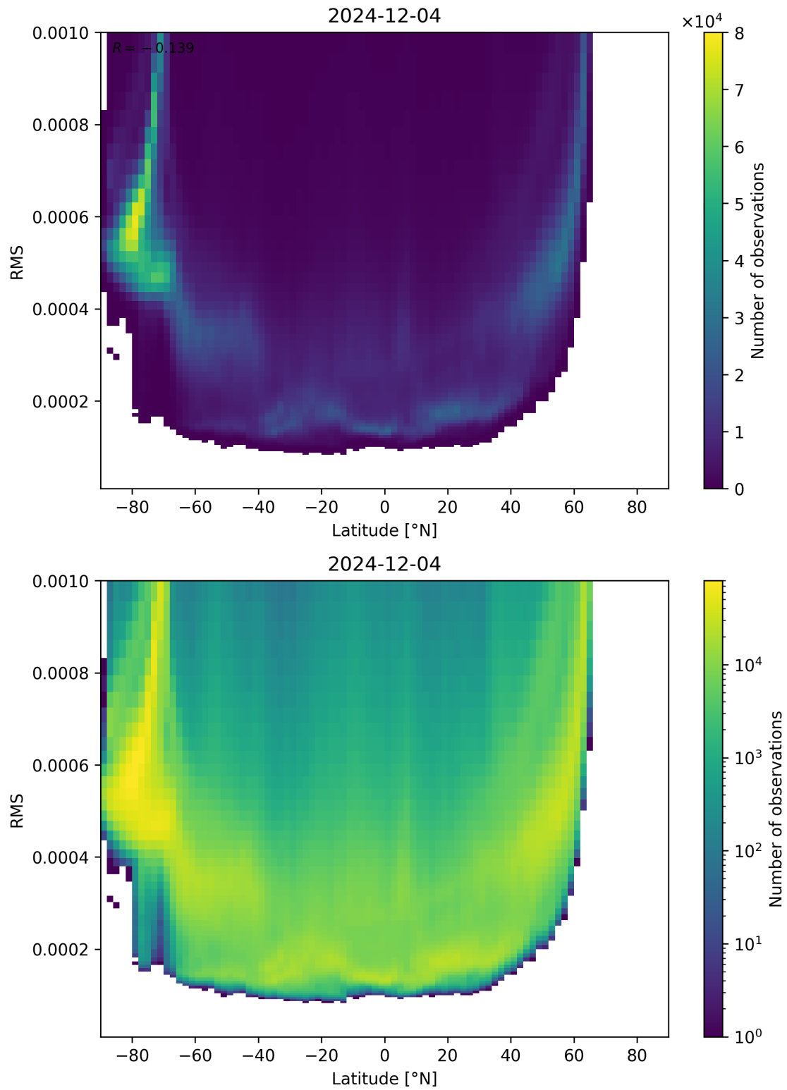
Figure 94: Scatter density plot of “Latitude” against “RMS” for 2024-12-03 to 2024-12-05.
