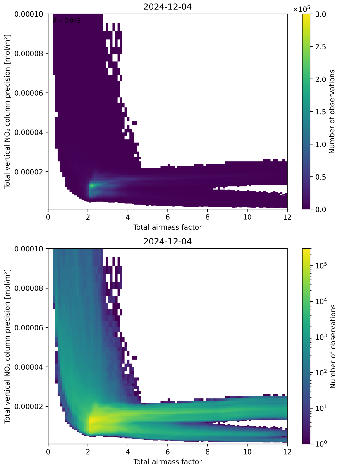
Figure 68: Scatter density plot of “Total airmass factor” against “Total vertical NO 2 column precision” for 2024-12-03 to 2024-12-05.
