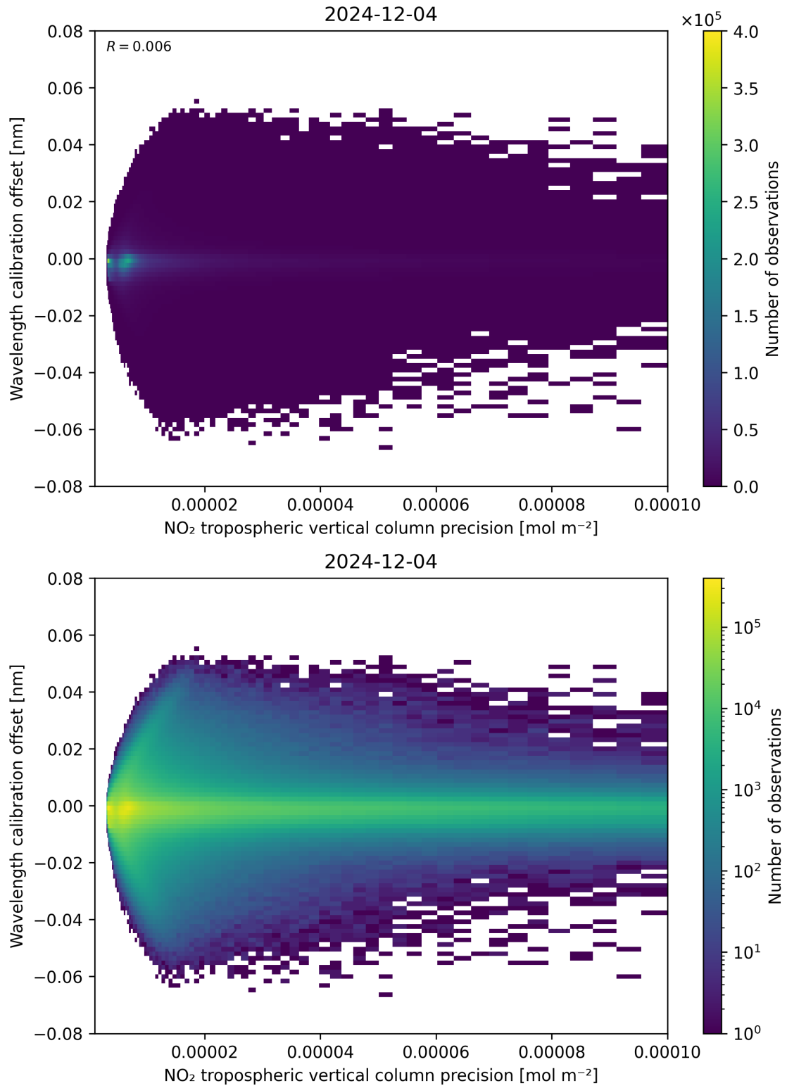
Figure 141: Scatter density plot of “NO 2 tropospheric vertical column precision” against “Wavelength calibration offset” for 2024-12-03 to 2024-12-05.
