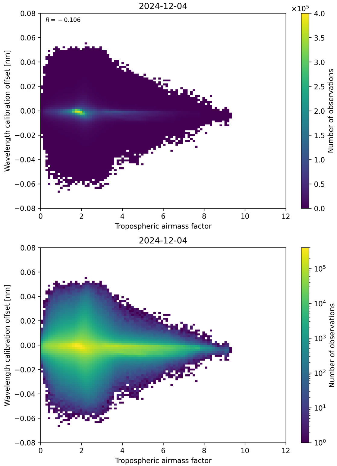
Figure 80: Scatter density plot of “Tropospheric airmass factor” against “Wavelength calibration offset” for 2024-12-03 to 2024-12-05.
