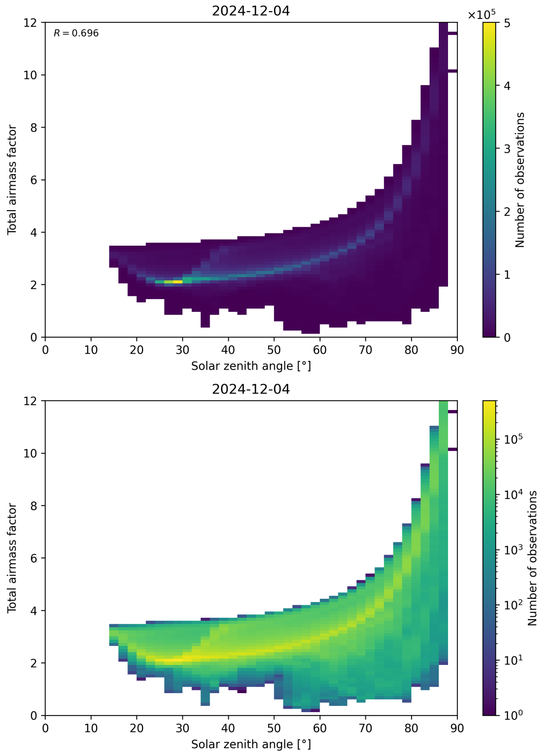
Figure 146: Scatter density plot of “Solar zenith angle” against “Total air mass factor” for 2024-12-03 to 2024-12-05.
