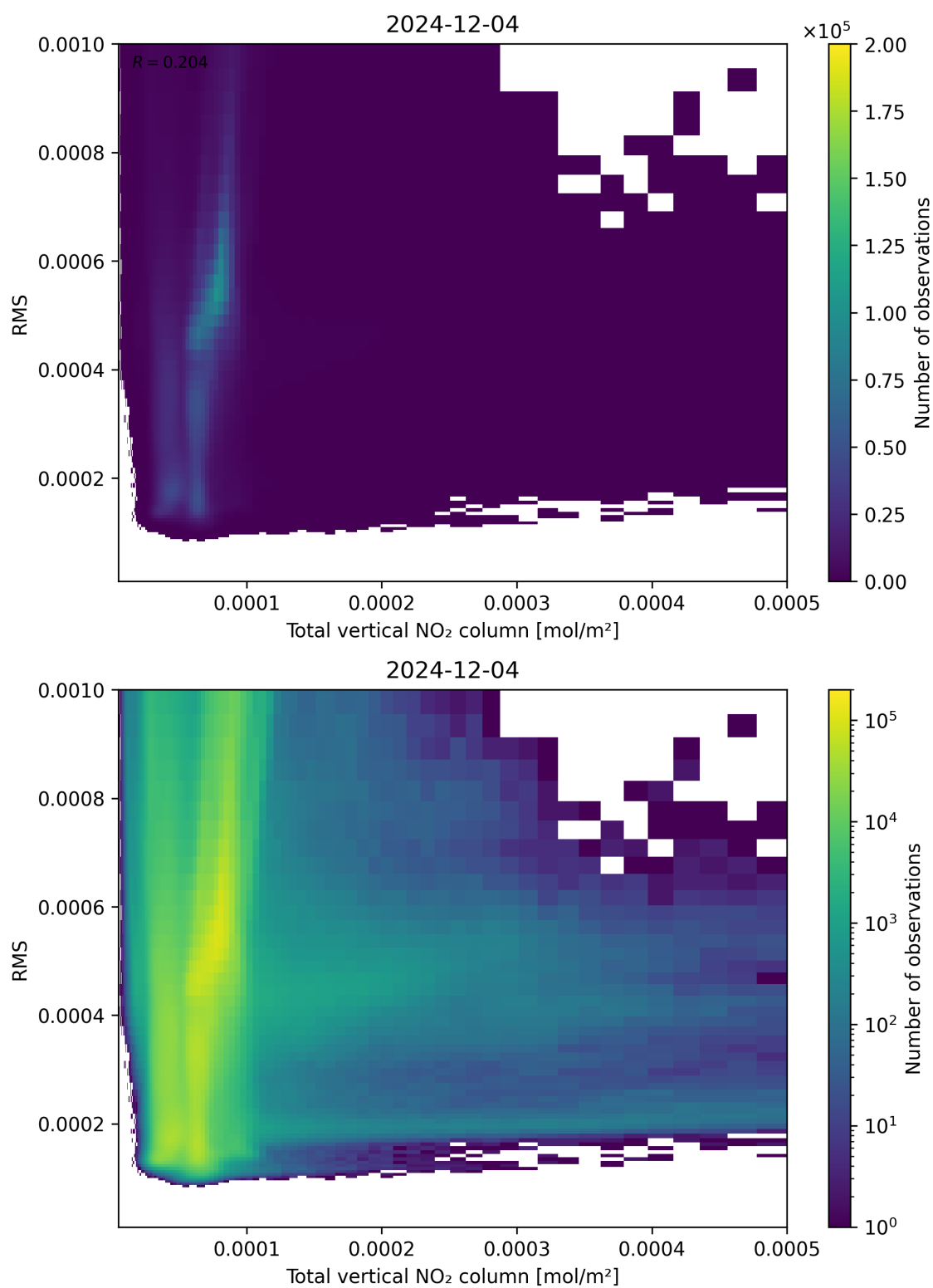
Figure 120: Scatter density plot of “Total vertical NO 2 column” against “RMS” for 2024-12-03 to 2024-12-05.
