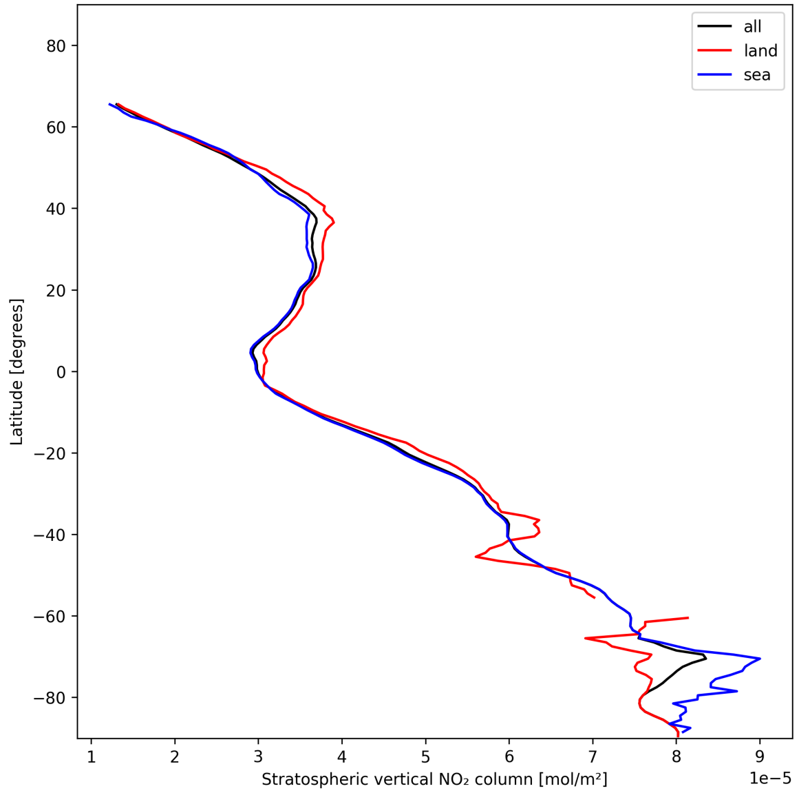
Figure 19: Zonal average of “Stratospheric vertical NO 2 column” for 2024-12-03 to 2024-12-05.
