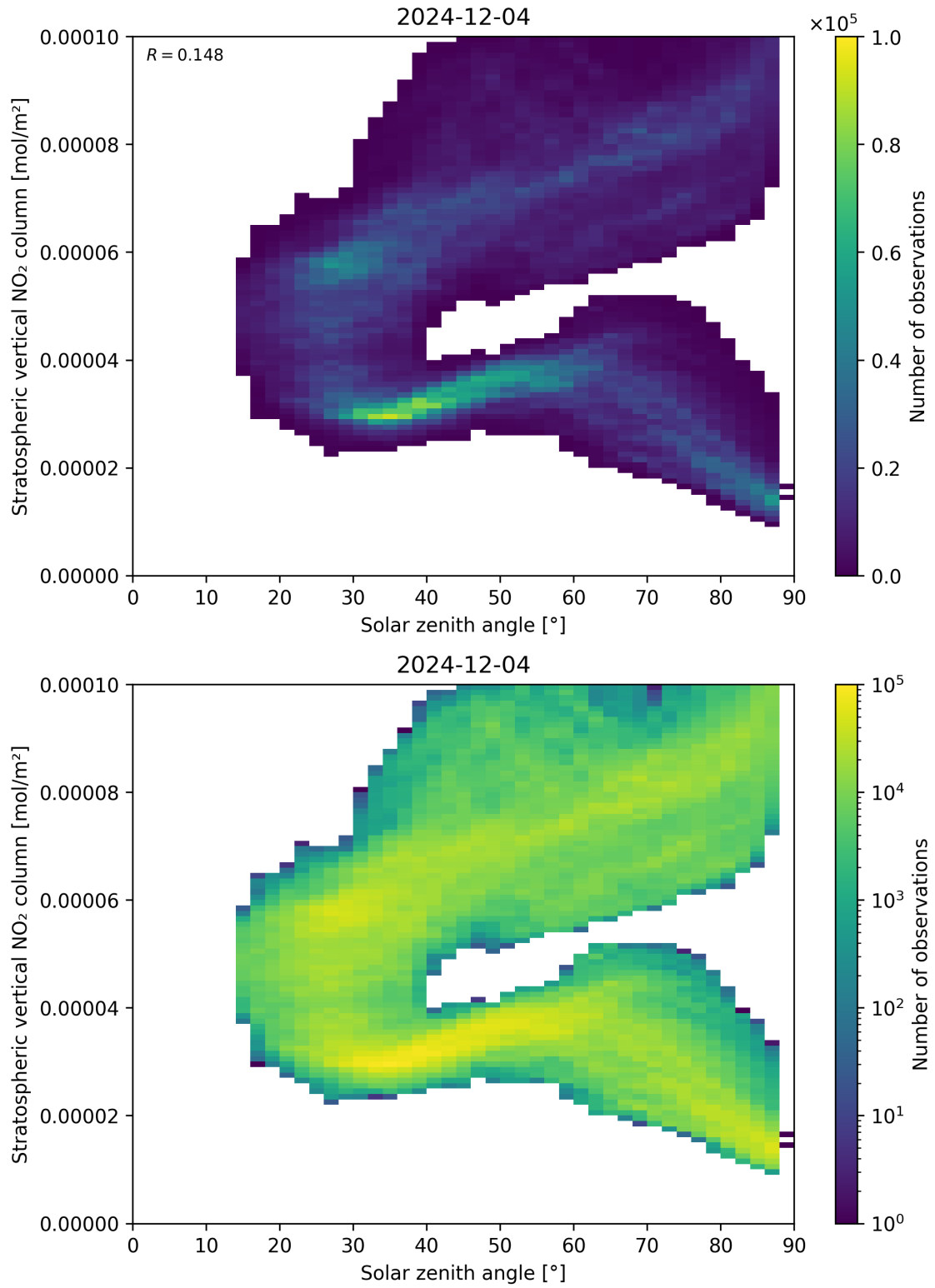
Figure 150: Scatter density plot of “Solar zenith angle” against “Stratospheric vertical NO 2 column” for 2024-12-03 to 2024-12-05.
