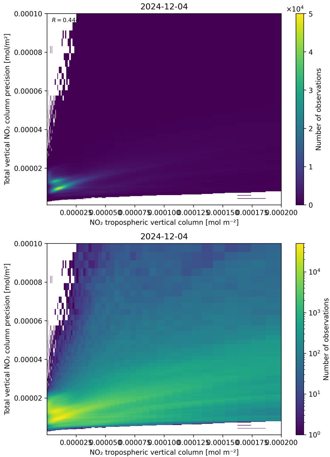
Figure 129: Scatter density plot of “NO 2 tropospheric vertical column” against “Total vertical NO 2 column precision” for 2024-12-03 to 2024-12-05.
