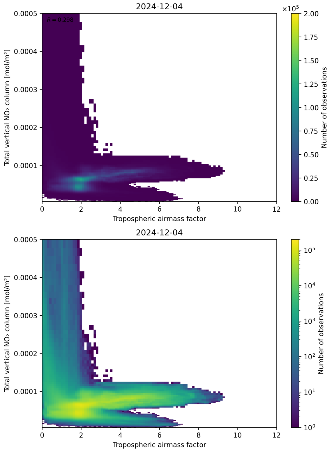
Figure 77: Scatter density plot of “Tropospheric airmass factor” against “Total vertical \text{NO}_2 column” for 2024-12-03 to 2024-12-05.
