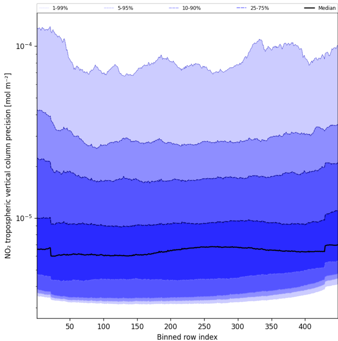
Figure 47: Along track statistics of “NO 2 tropospheric vertical column precision” for 2024-12-03 to 2024-12-05
