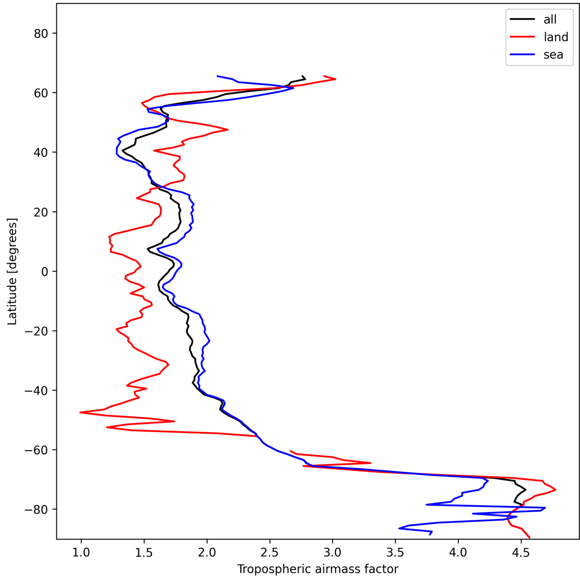
Figure 14: Zonal average of “Tropospheric airmass factor” for 2024-12-03 to 2024-12-05.
