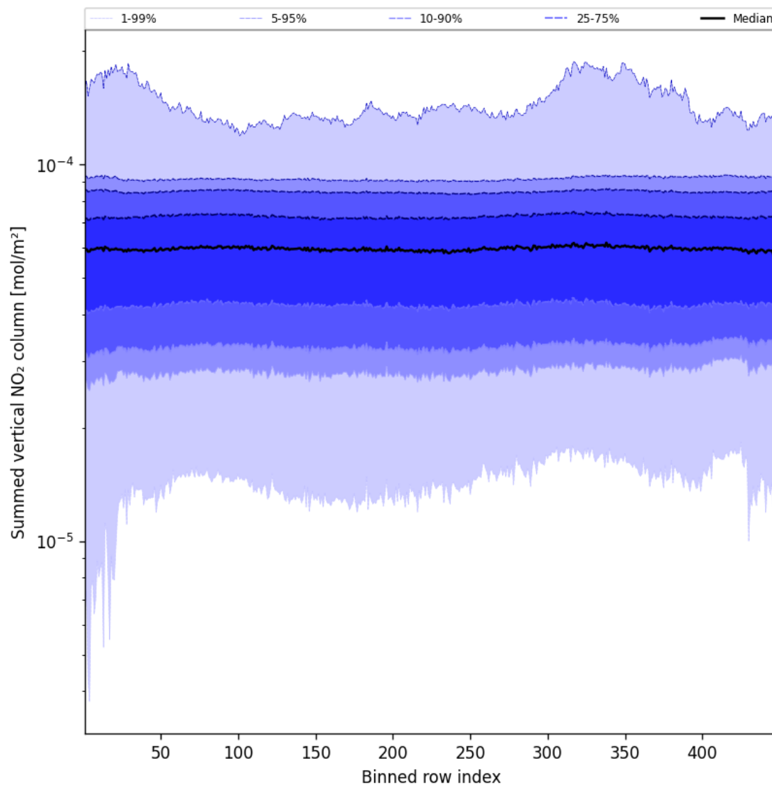
Figure 57: Along track statistics of “Summed vertical NO 2 column” for 2024-12-03 to 2024-12-05
