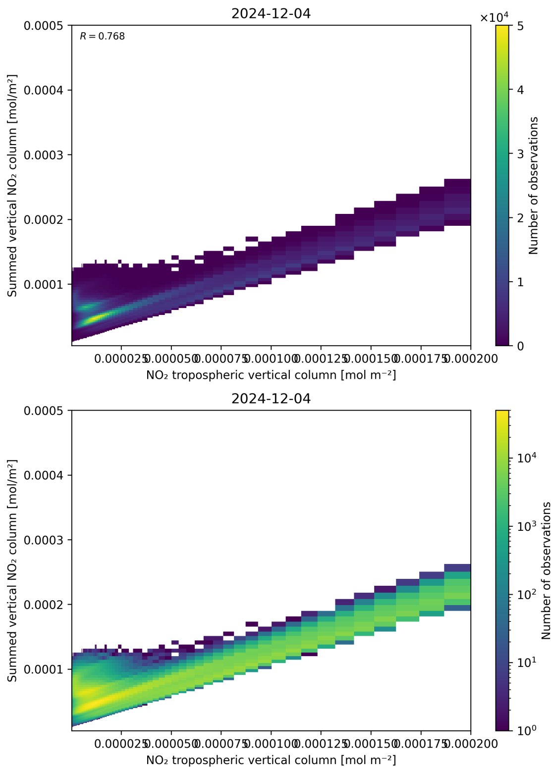
Figure 126: Scatter density plot of “NO 2 tropospheric vertical column” against “Summed vertical NO 2 column” for 2024-12-03 to 2024-12-05.
