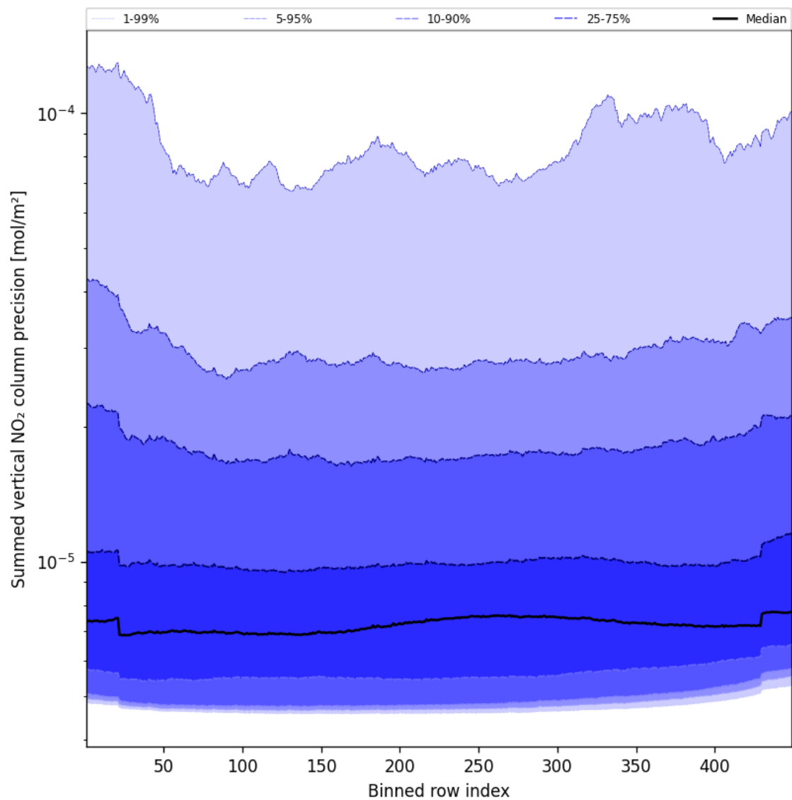
Figure 58: Along track statistics of “Summed vertical NO 2 column precision” for 2024-12-03 to 2024-12-05
