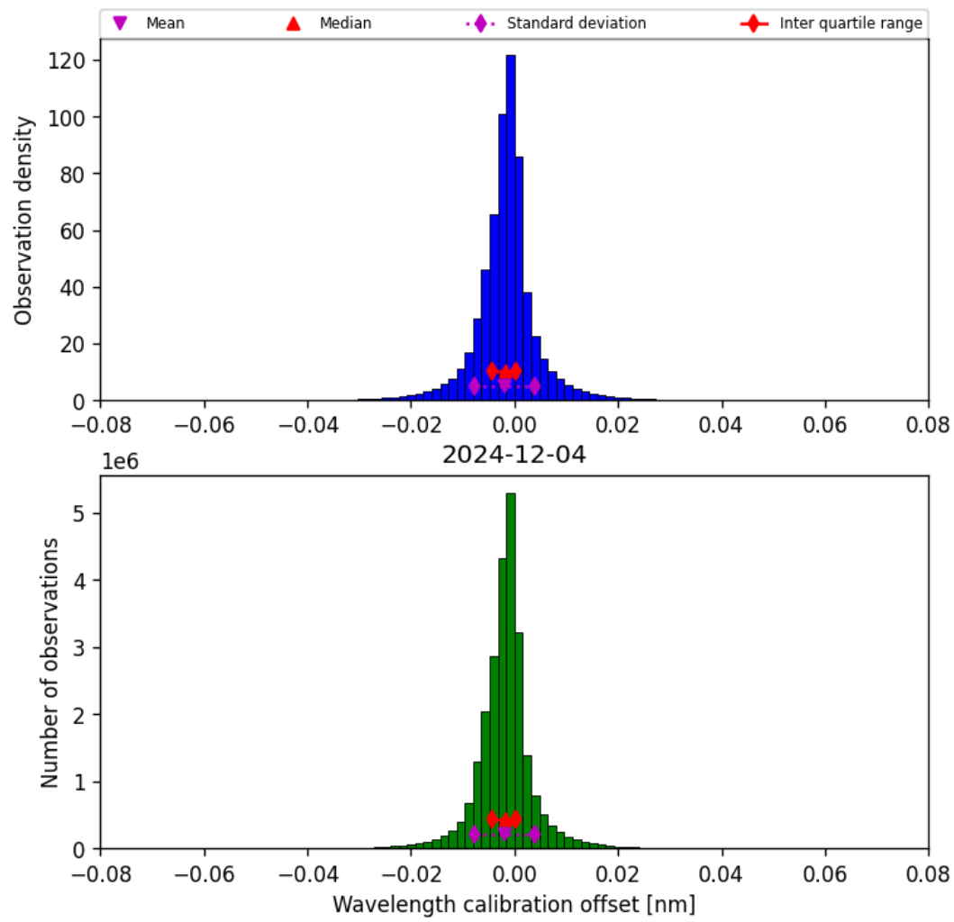
Figure 35: Histogram of “Wavelength calibration offset” for 2024-12-03 to 2024-12-05
