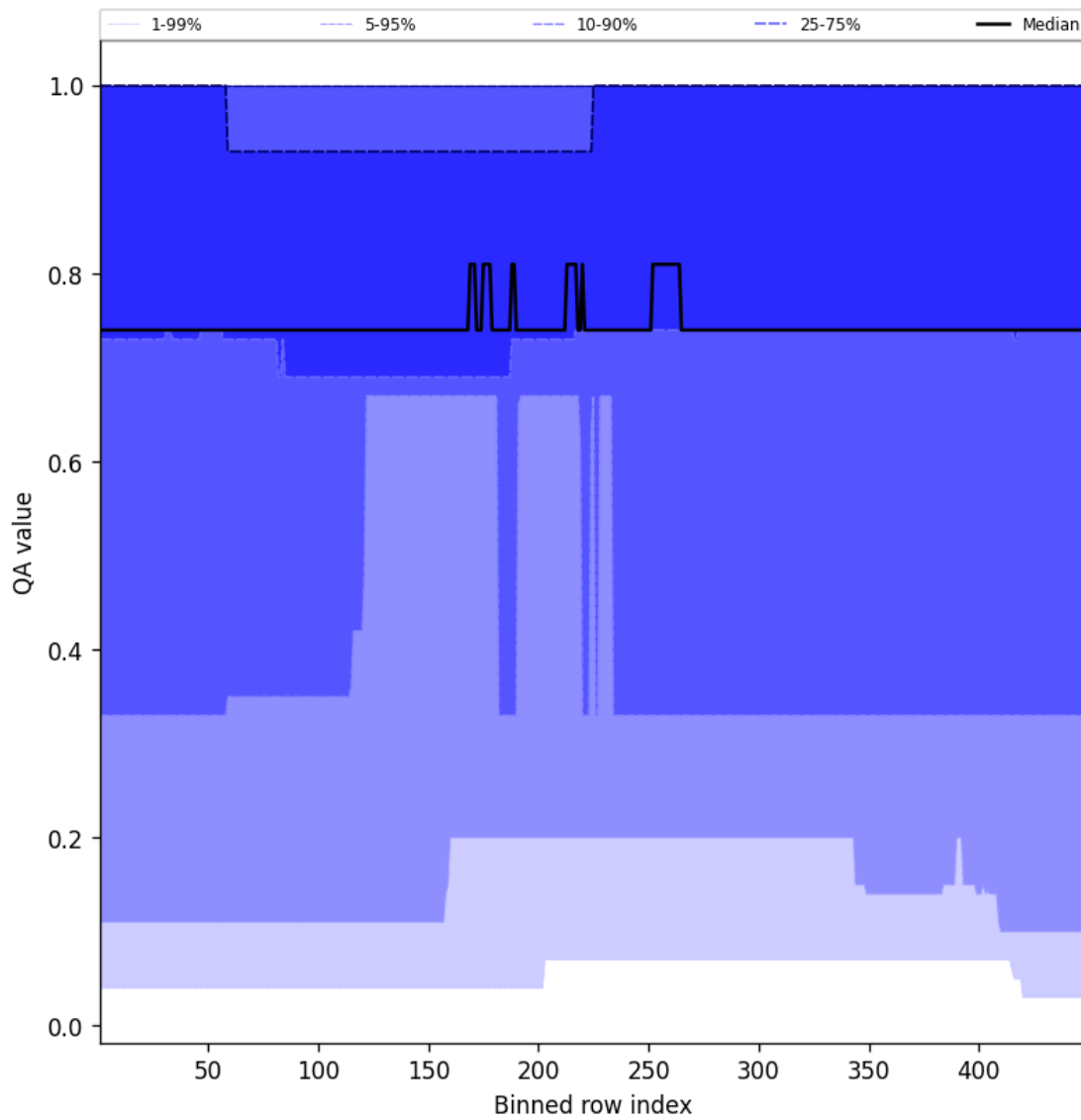
Figure 45: Along track statistics of “QA value” for 2024-12-03 to 2024-12-05
