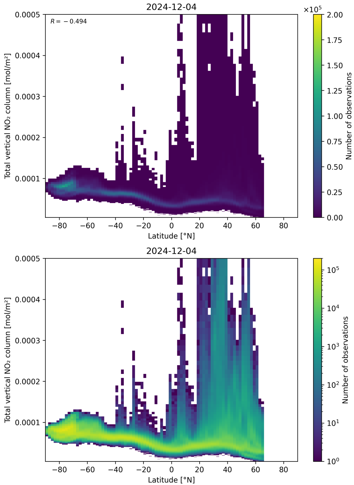
Figure 90: Scatter density plot of “Latitude” against “Total vertical NO 2 column” for 2024-12-03 to 2024-12-05.
