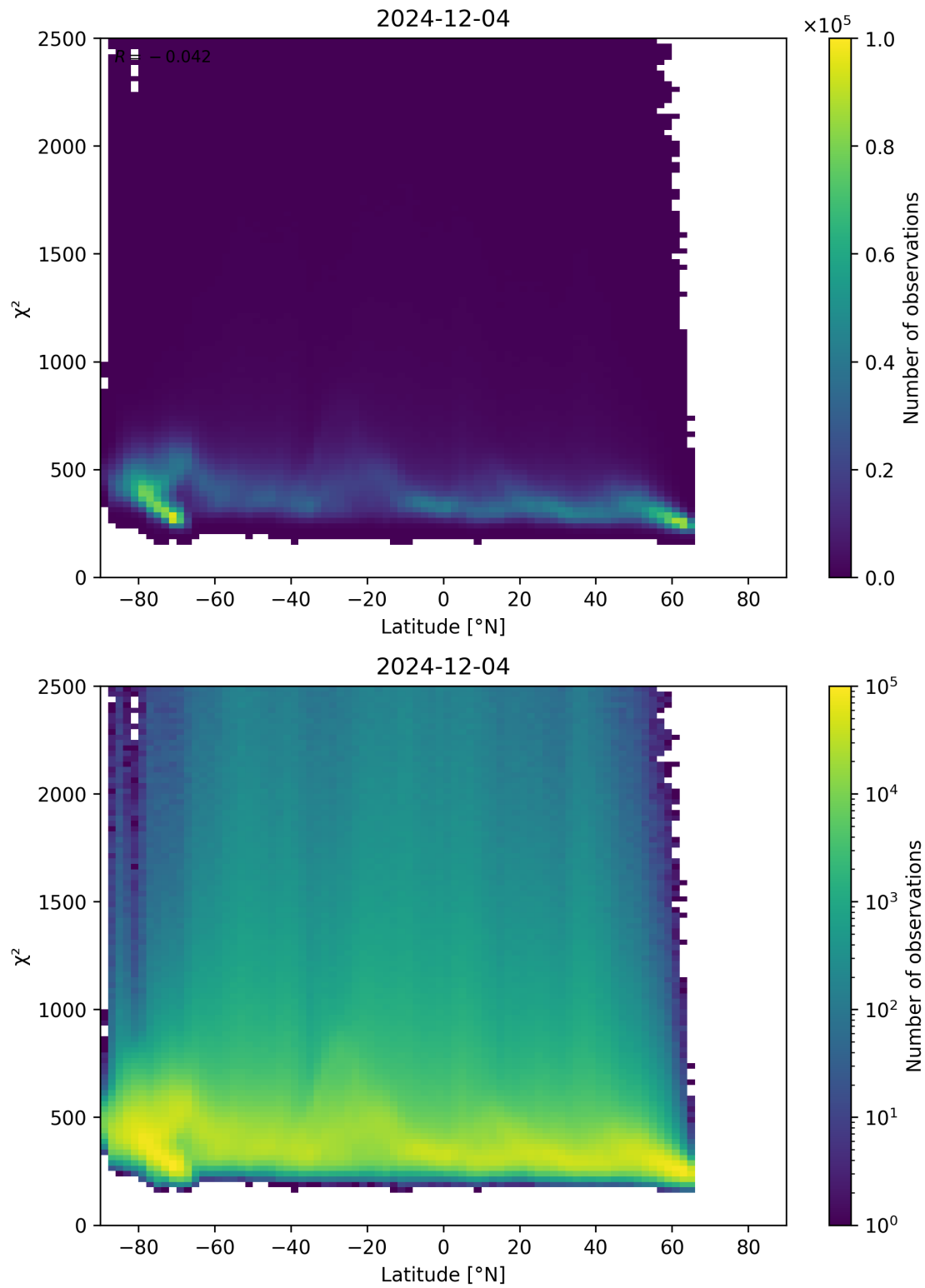
Figure 86: Scatter density plot of “Latitude” against “ \chi^2 ” for 2024-12-03 to 2024-12-05.
