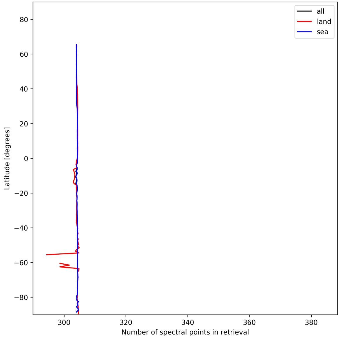
Figure 16: Zonal average of “Number of spectral points in retrieval” for 2024-12-03 to 2024-12-05.
