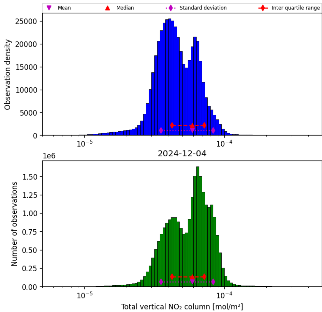
Figure 38: Histogram of “Total vertical NO 2 column” for 2024-12-03 to 2024-12-05
