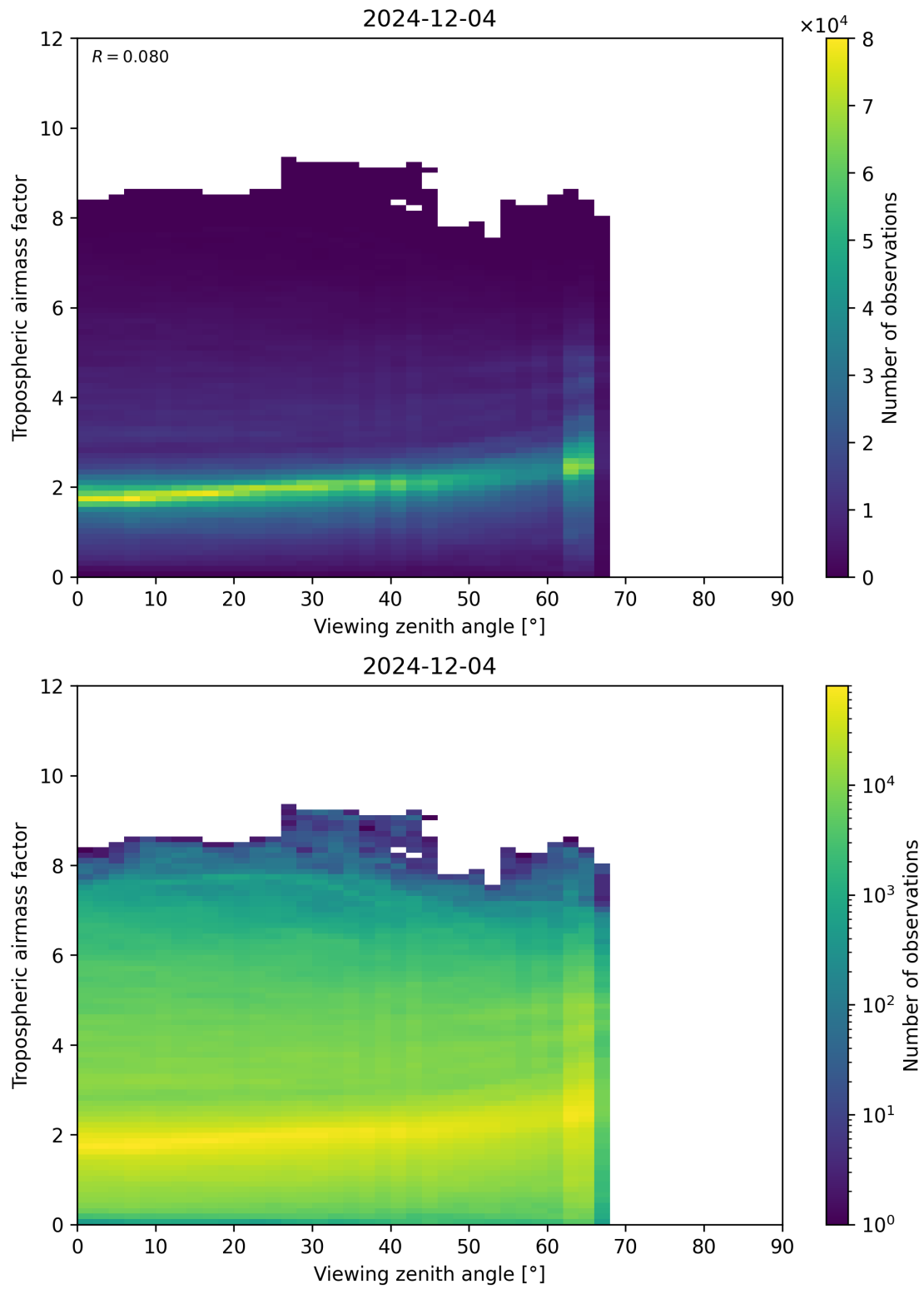
Figure 161: Scatter density plot of “Viewing zenith angle” against “Tropospheric airmass factor” for 2024-12-03 to 2024-12-05.
