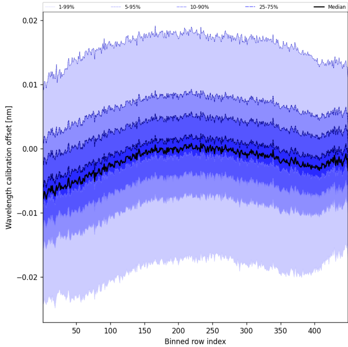
Figure 52: Along track statistics of “Wavelength calibration offset” for 2024-12-03 to 2024-12-05
