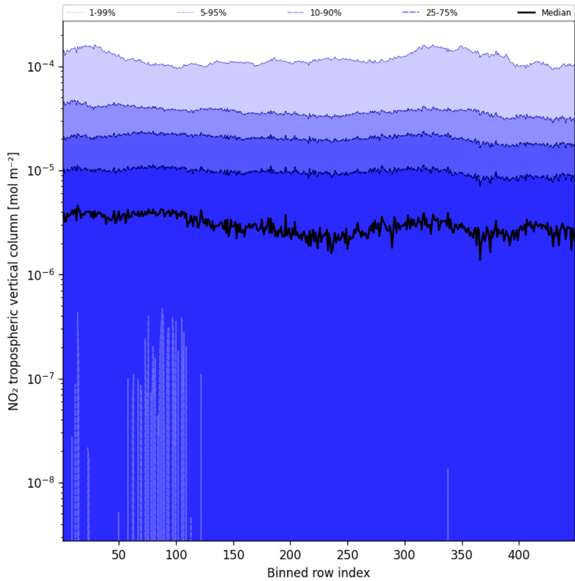
Figure 46: Along track statistics of “NO 2 tropospheric vertical column” for 2024-12-03 to 2024-12-05
