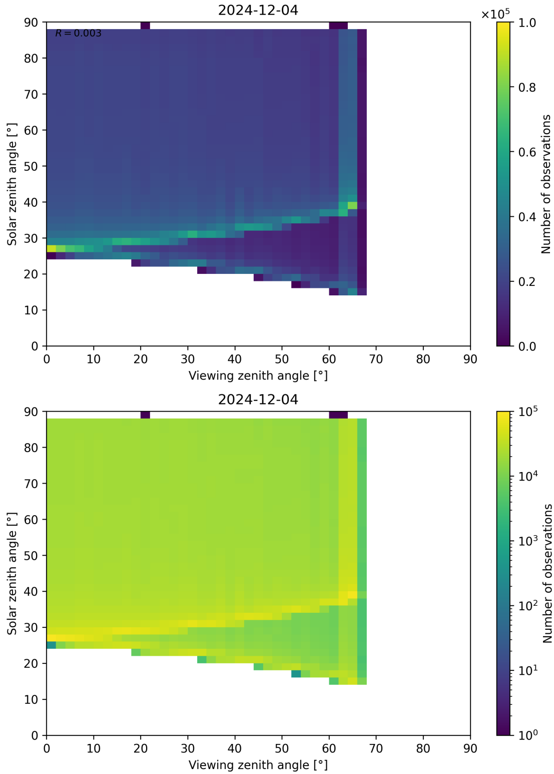
Figure 172: Scatter density plot of “Viewing zenith angle” against “Solar zenith angle” for 2024-12-03 to 2024-12-05.
