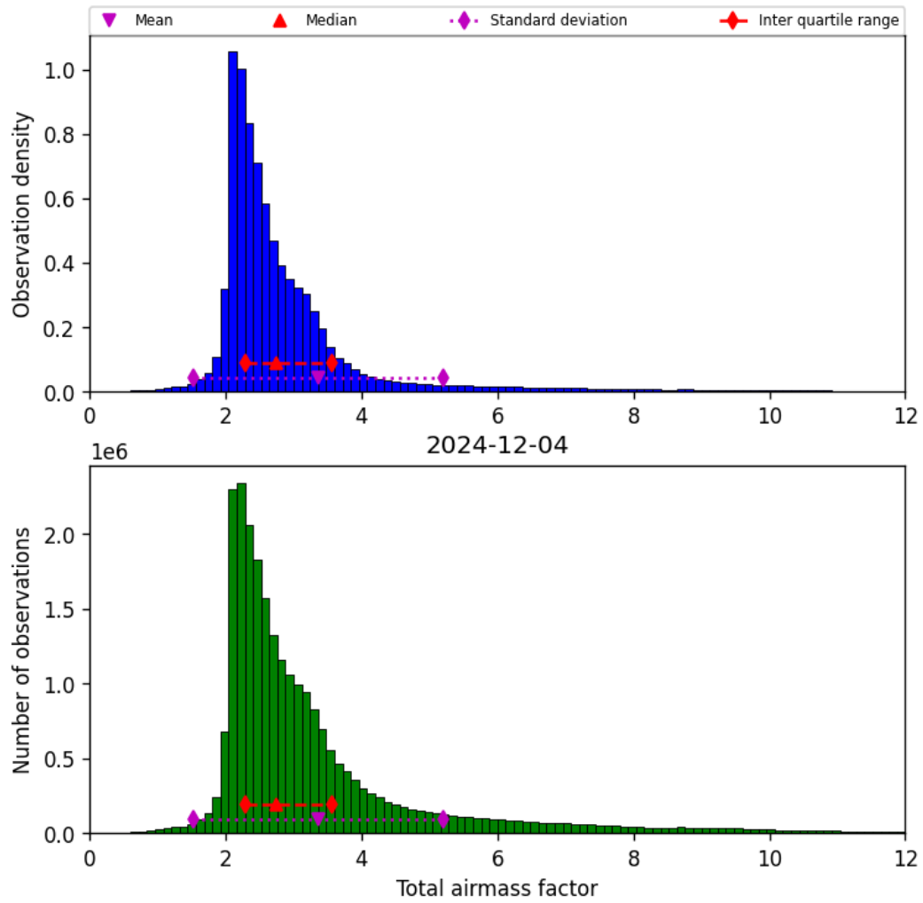
Figure 32: Histogram of “Total airmass factor” for 2024-12-03 to 2024-12-05
