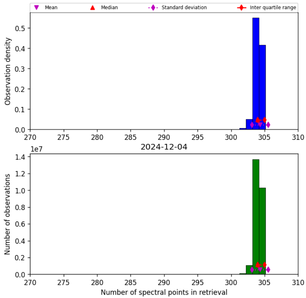
Figure 33: Histogram of “Number of spectral points in retrieval” for 2024-12-03 to 2024-12-05
