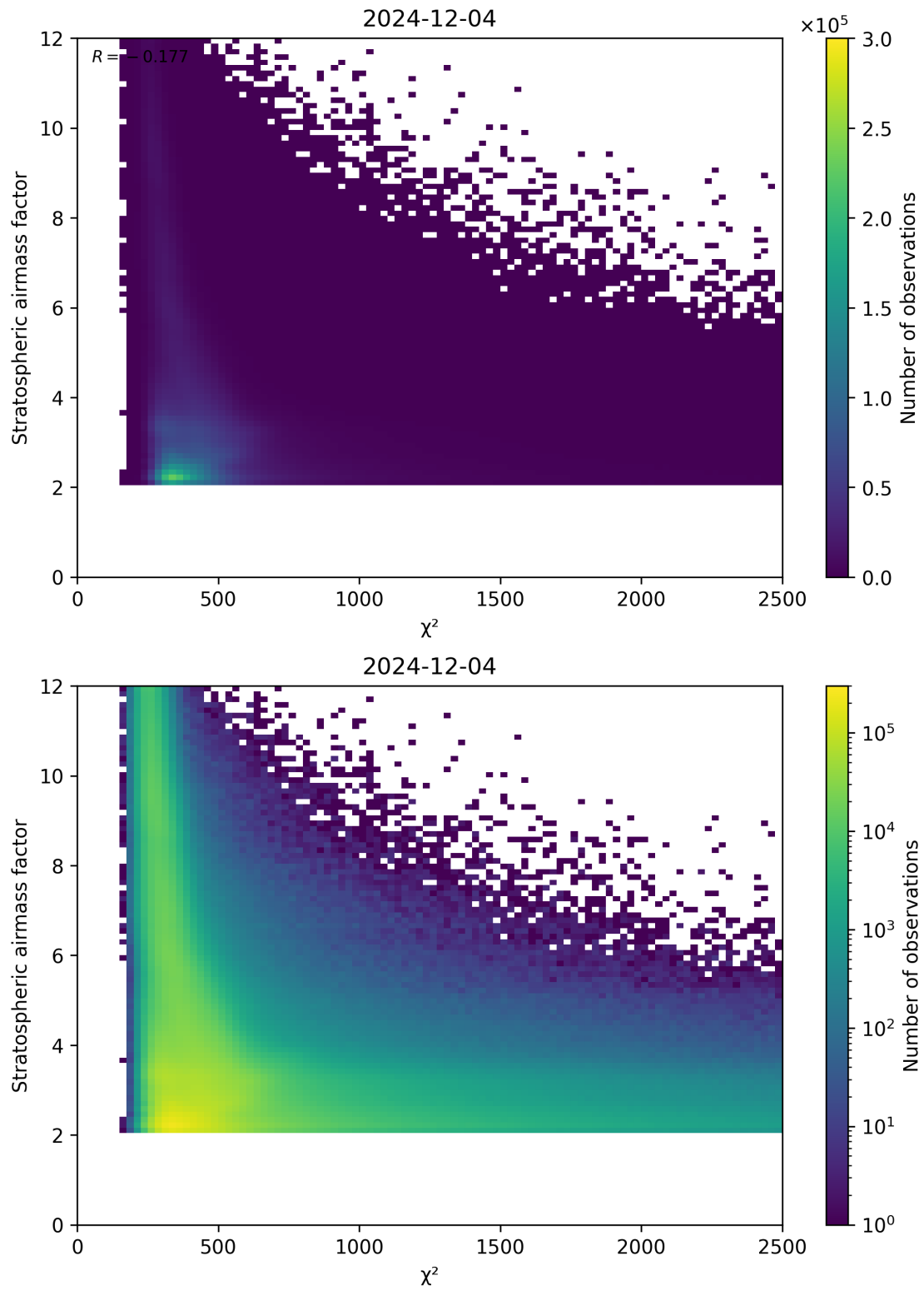
Figure 81: Scatter density plot of “ \chi^2 ” against “Stratospheric air mass factor” for 2024-12-03 to 2024-12-05.
