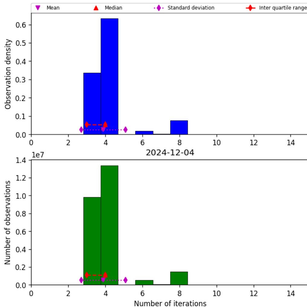
Figure 34: Histogram of “Number of iterations” for 2024-12-03 to 2024-12-05
