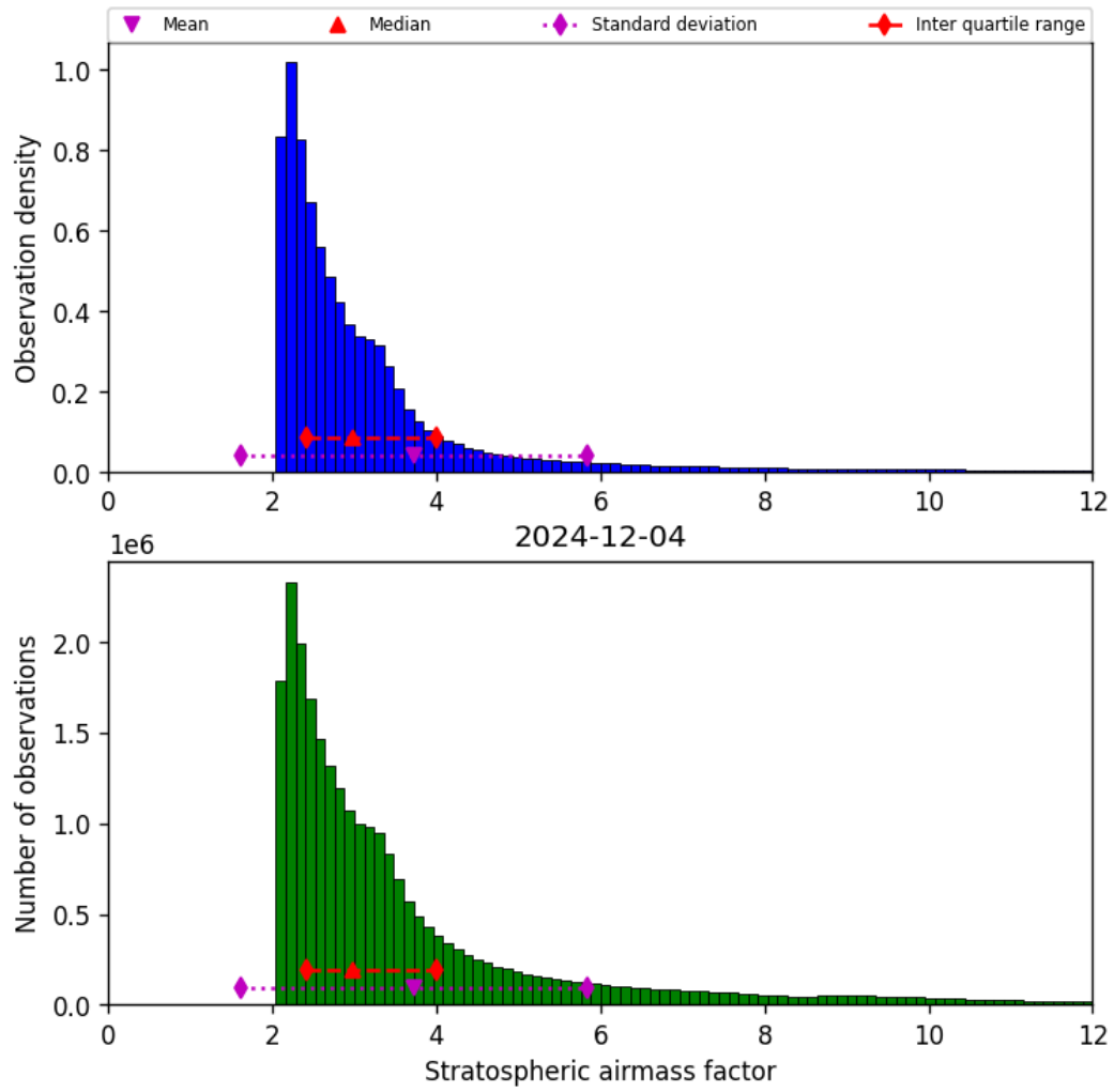
Figure 44: Histogram of “Stratospheric airmass factor” for 2024-12-03 to 2024-12-05
