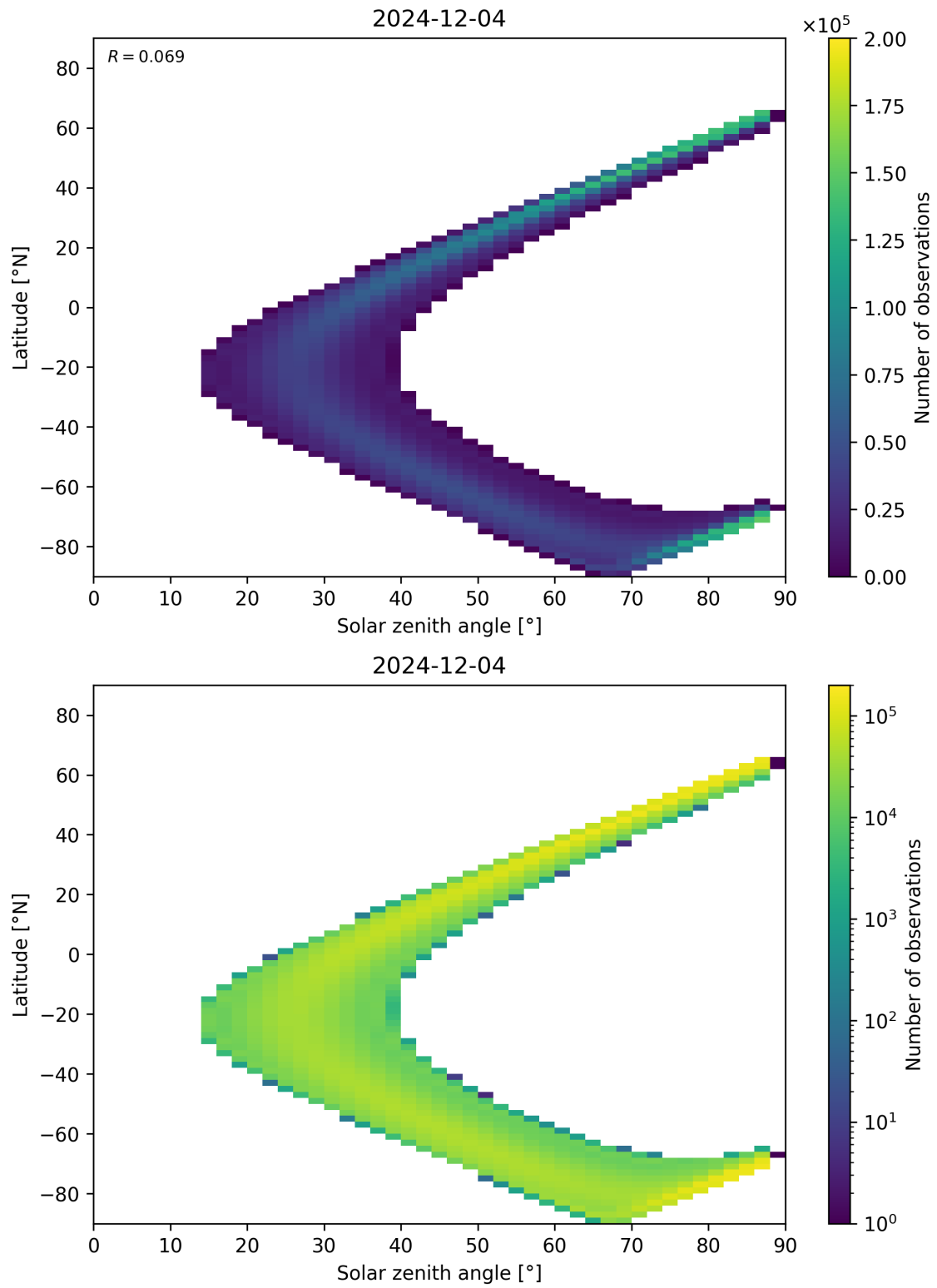
Figure 149: Scatter density plot of “Solar zenith angle” against “Latitude” for 2024-12-03 to 2024-12-05.
