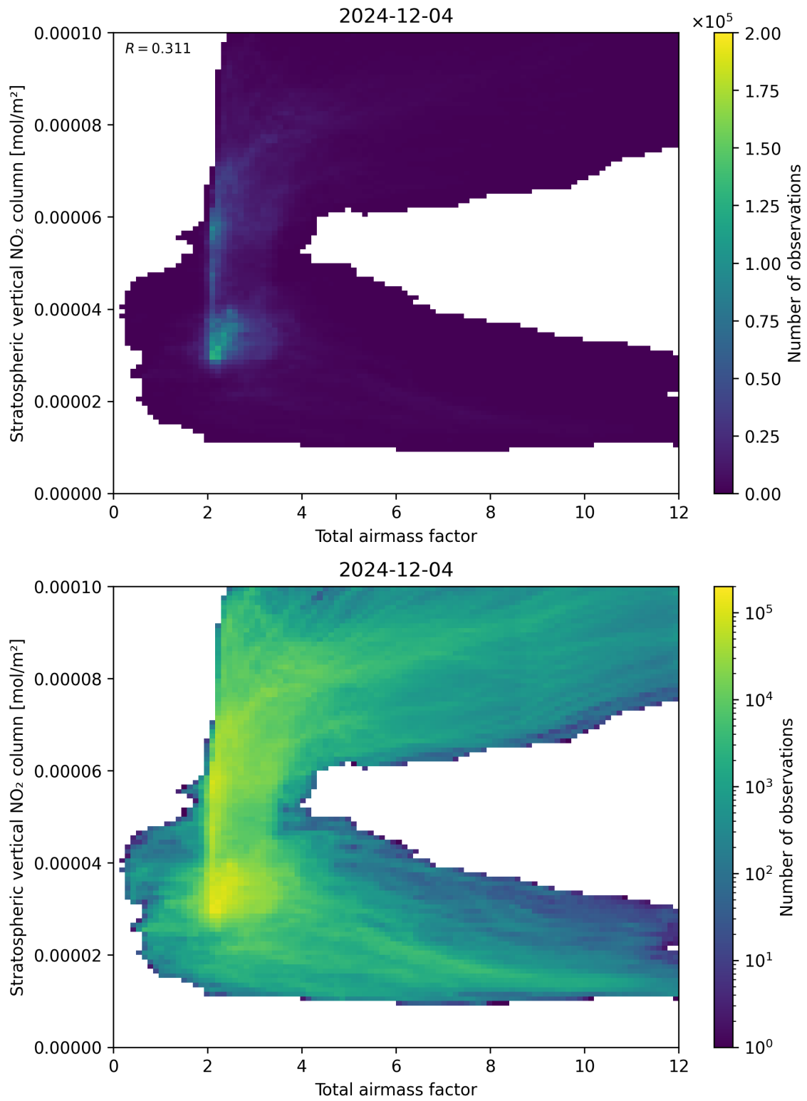
Figure 64: Scatter density plot of “Total airmass factor” against “Stratospheric vertical NO 2 column” for 2024-12-03 to 2024-12-05.
