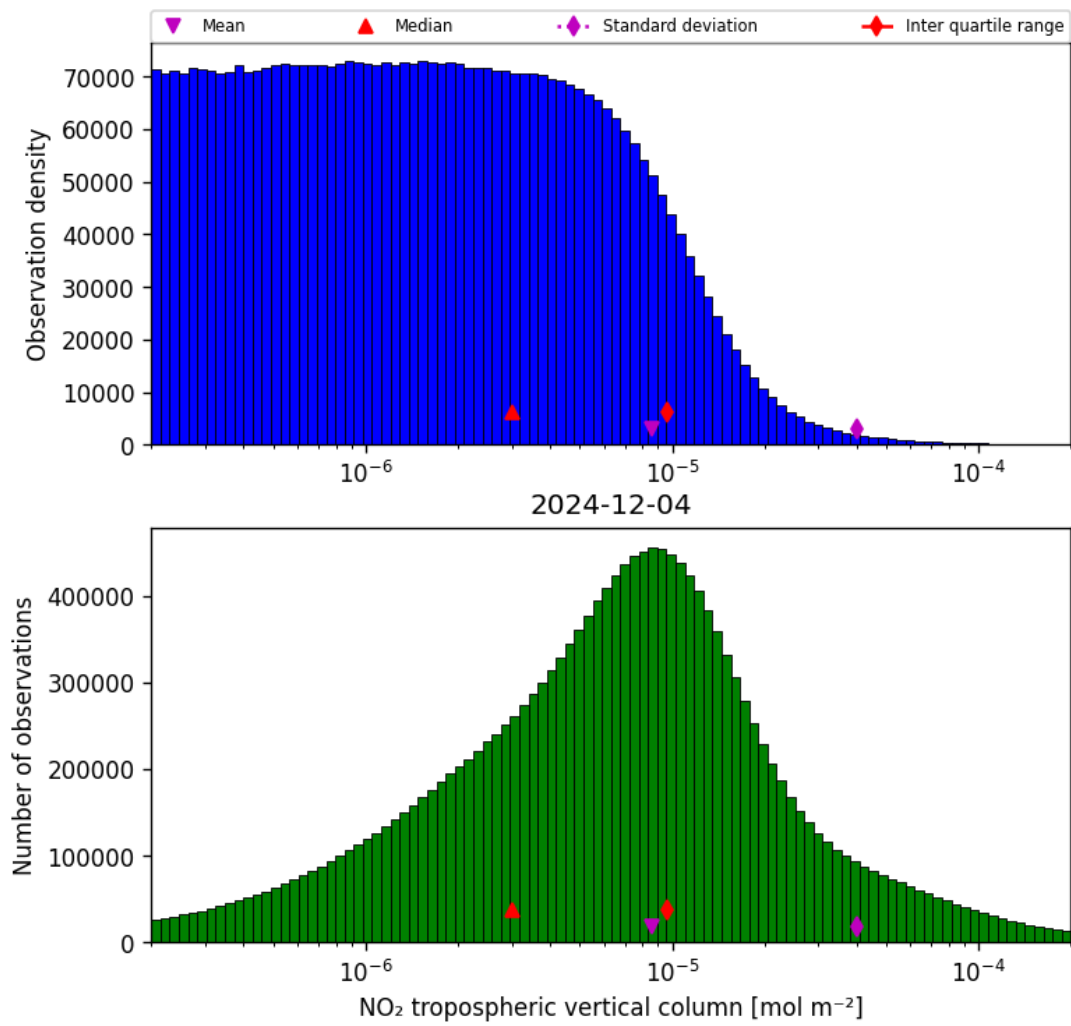
Figure 29: Histogram of “NO 2 tropospheric vertical column” for 2024-12-03 to 2024-12-05
