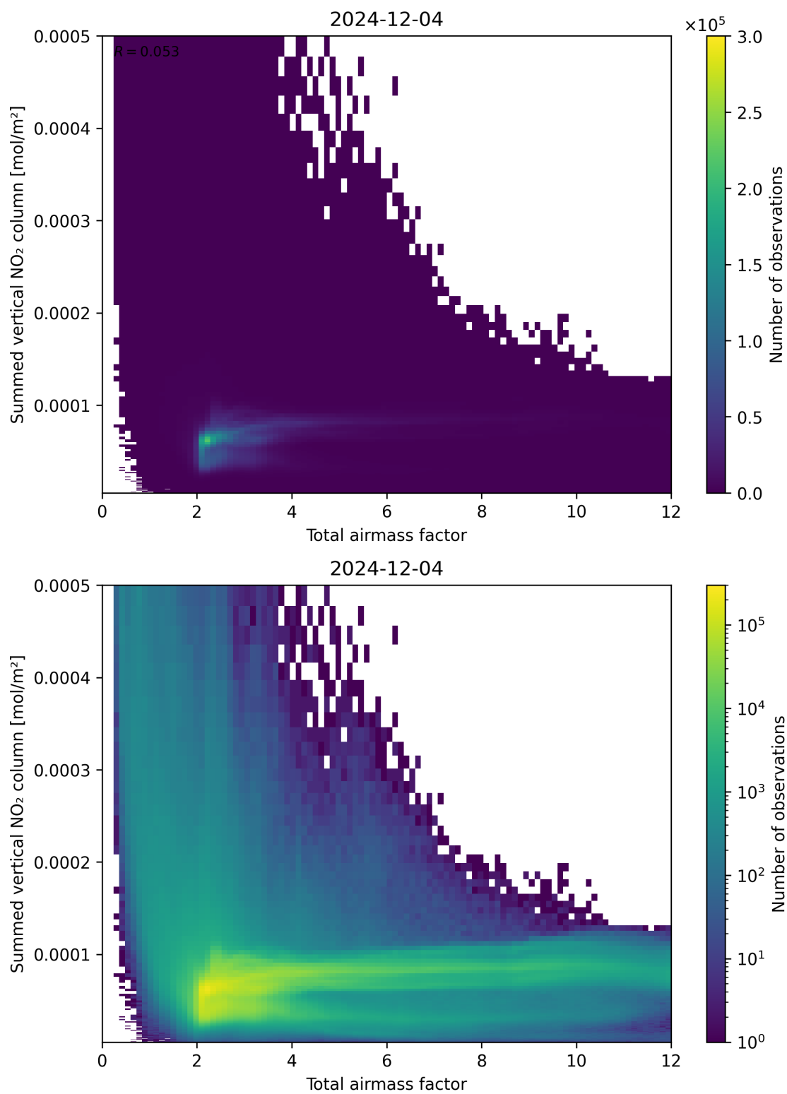
Figure 65: Scatter density plot of “Total airmass factor” against “Summed vertical NO 2 column” for 2024-12-03 to 2024-12-05.
