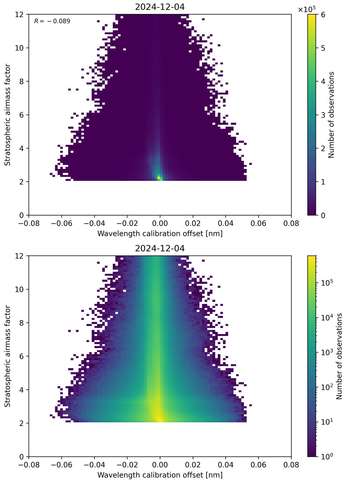
Figure 174: Scatter density plot of “Wavelength calibration offset” against “Stratospheric airmass factor” for 2024-12-03 to 2024-12-05.
