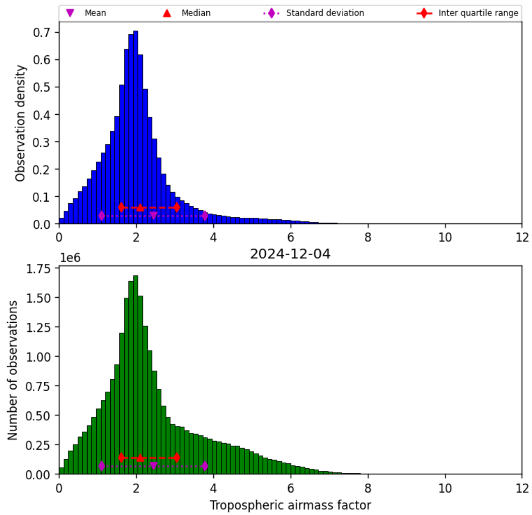
Figure 31: Histogram of “Tropospheric airmass factor” for 2024-12-03 to 2024-12-05
