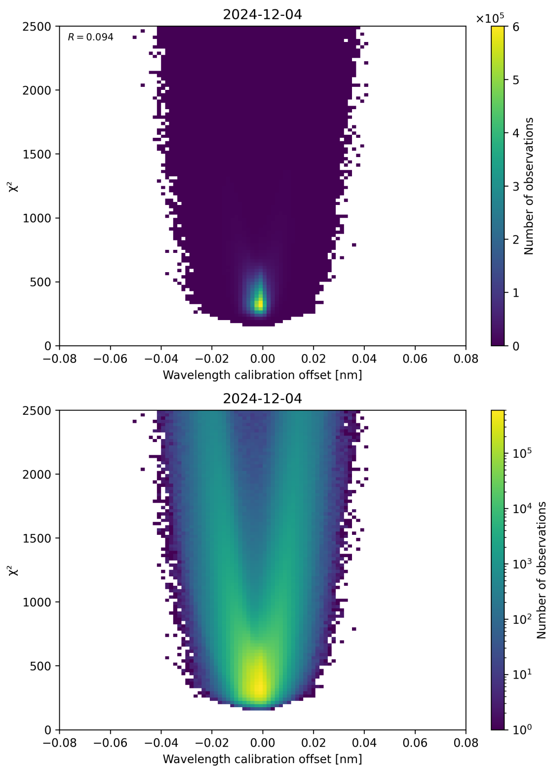
Figure 175: Scatter density plot of “Wavelength calibration offset” against “ \chi^2 ” for 2024-12-03 to 2024-12-05.
