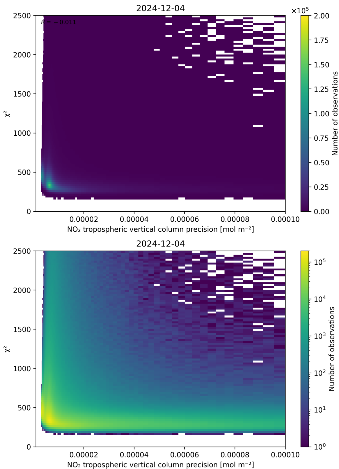
Figure 134: Scatter density plot of “NO 2 tropospheric vertical column precision” against “ \chi^2 ” for 2024-12-03 to 2024-12-05.
