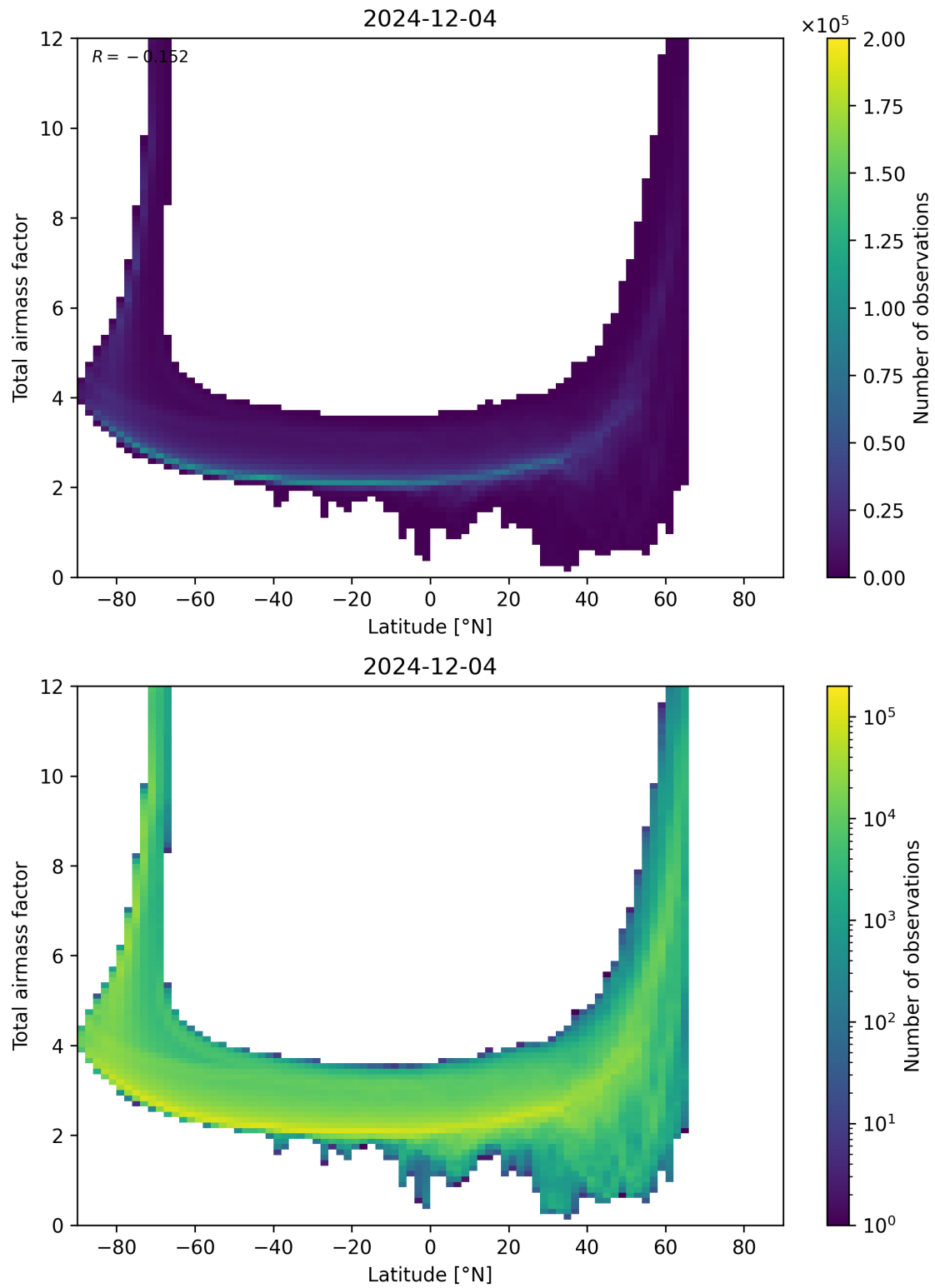
Figure 84: Scatter density plot of “Latitude” against “Total airmass factor” for 2024-12-03 to 2024-12-05.
