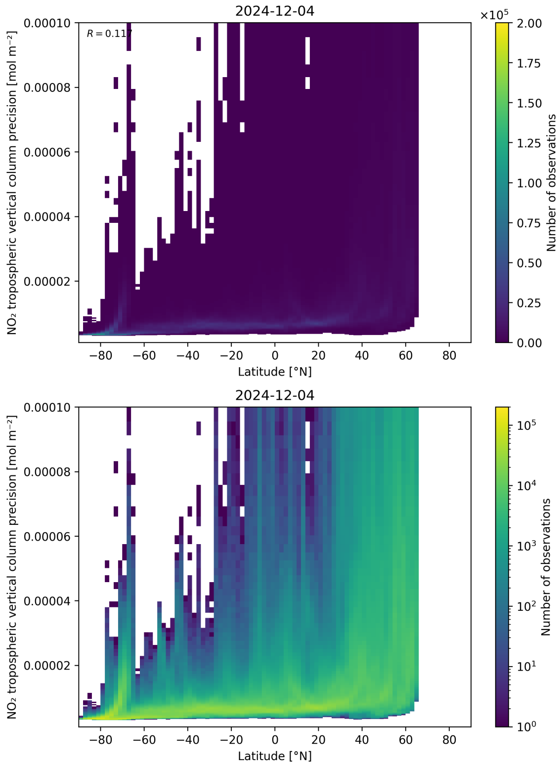
Figure 93: Scatter density plot of “Latitude” against “NO 2 tropospheric vertical column precision” for 2024-12-03 to 2024-12-05.
