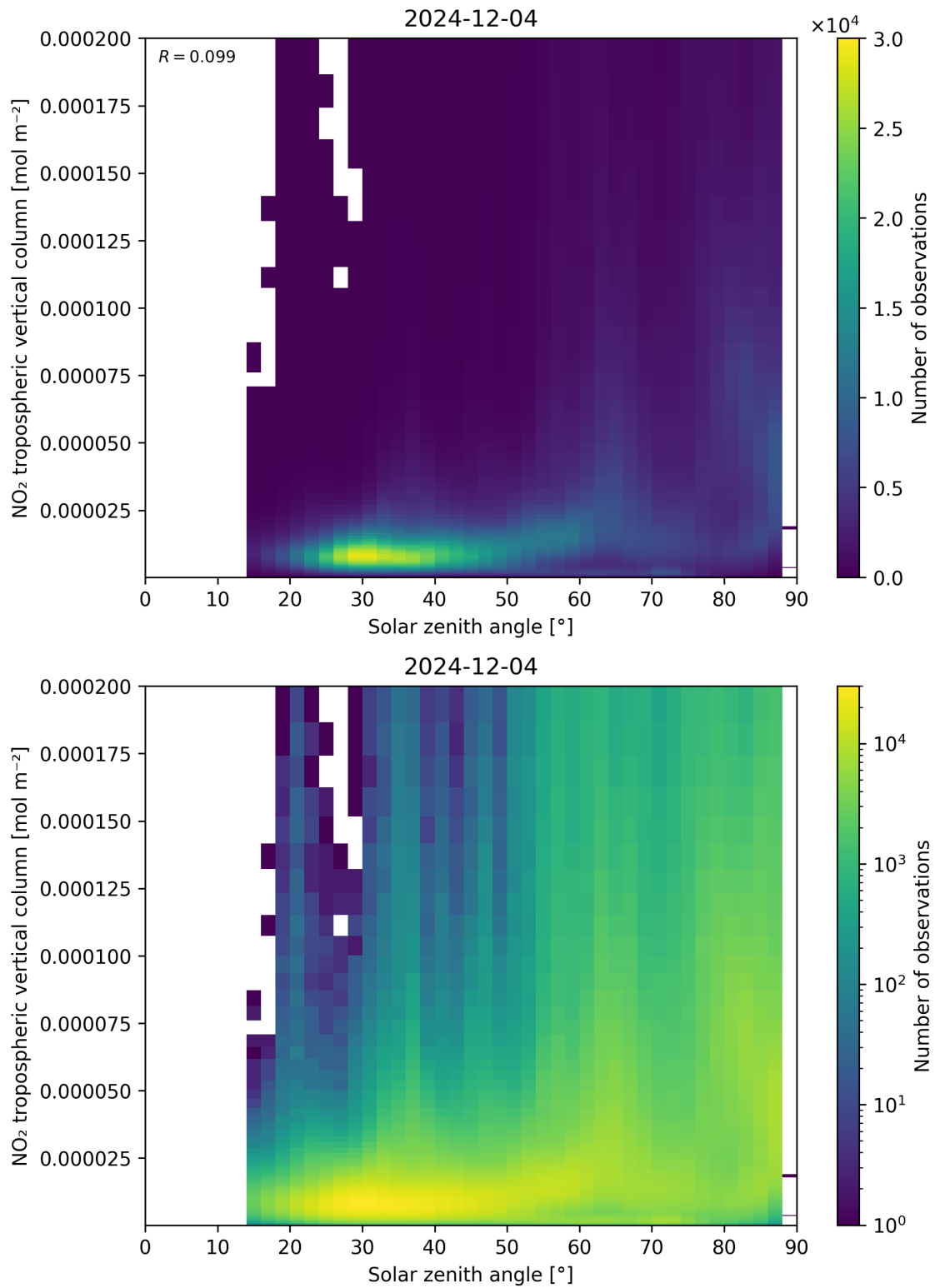
Figure 155: Scatter density plot of “Solar zenith angle” against “NO 2 tropospheric vertical column” for 2024-12-03 to 2024-12-05.
