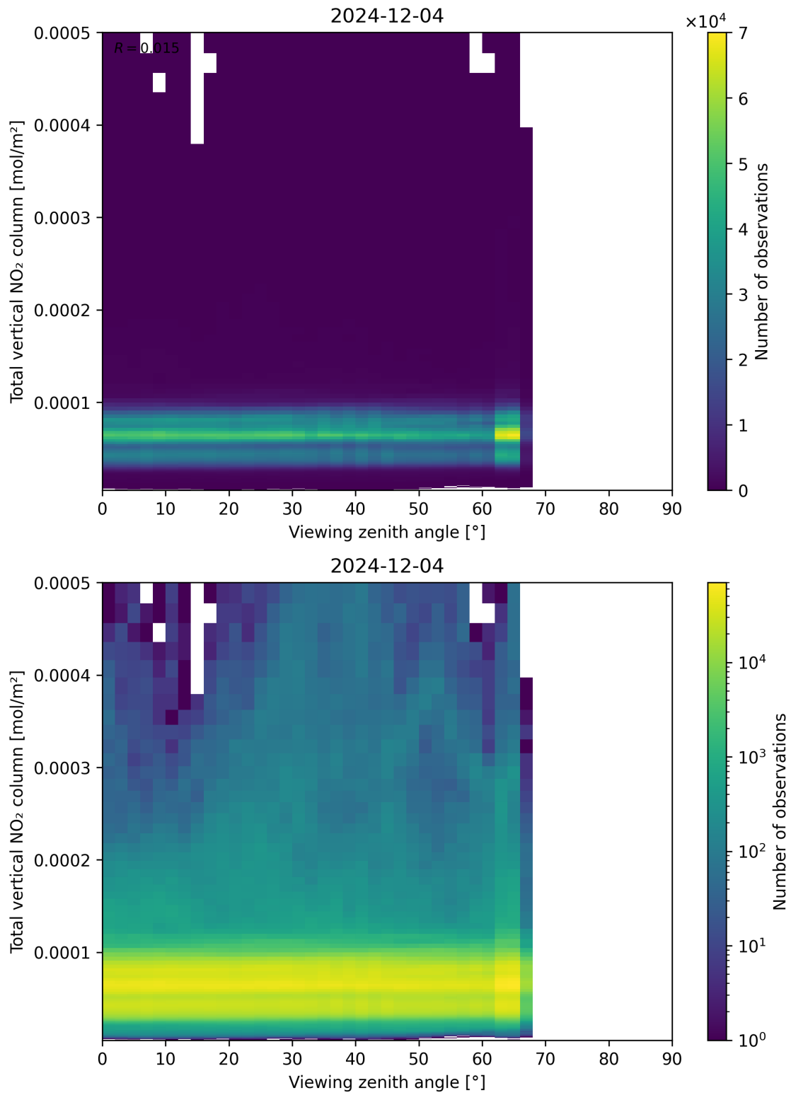
Figure 167: Scatter density plot of “Viewing zenith angle” against “Total vertical NO 2 column” for 2024-12-03 to 2024-12-05.
