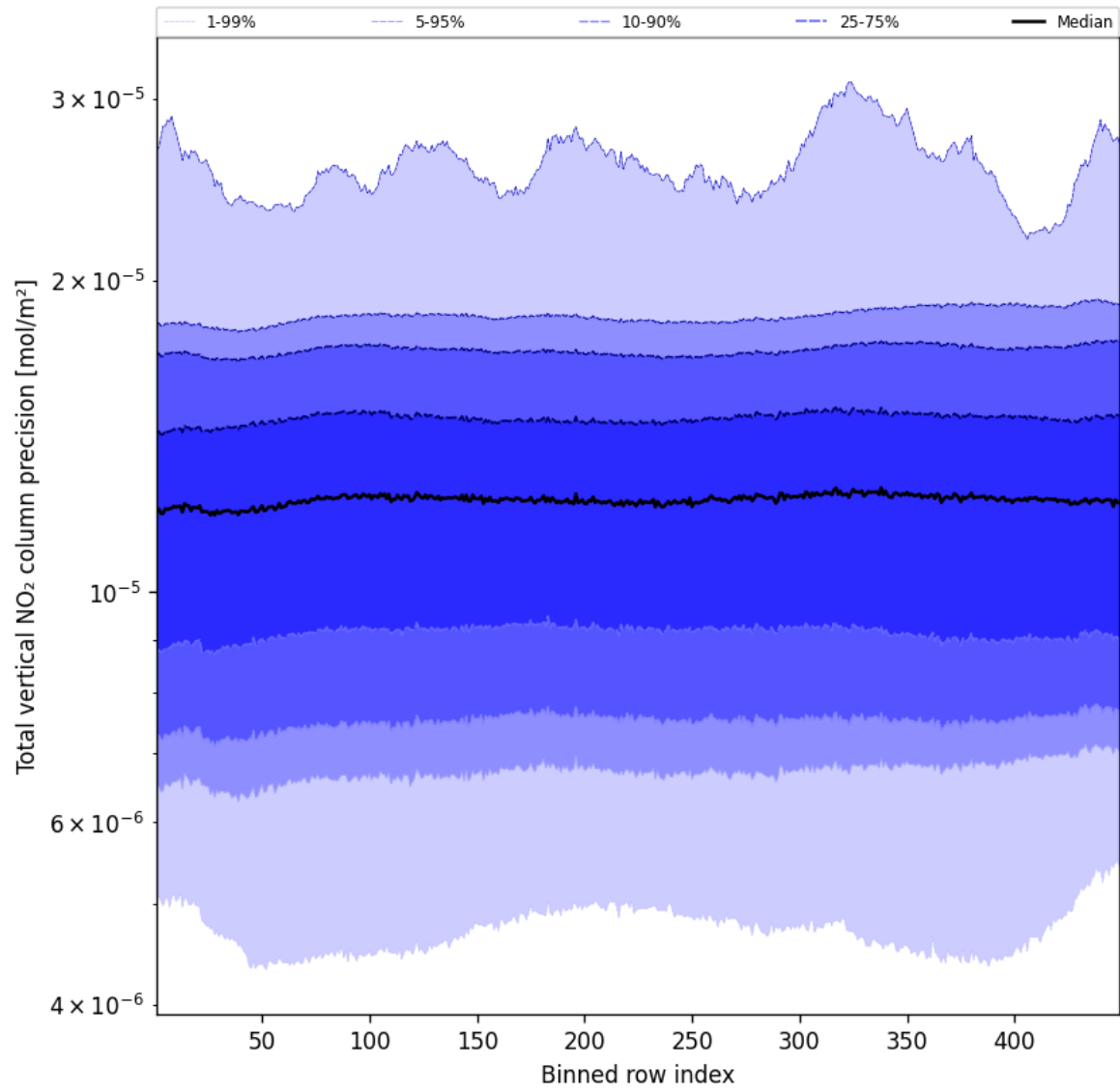
Figure 56: Along track statistics of “Total vertical NO 2 column precision” for 2024-12-03 to 2024-12-05
