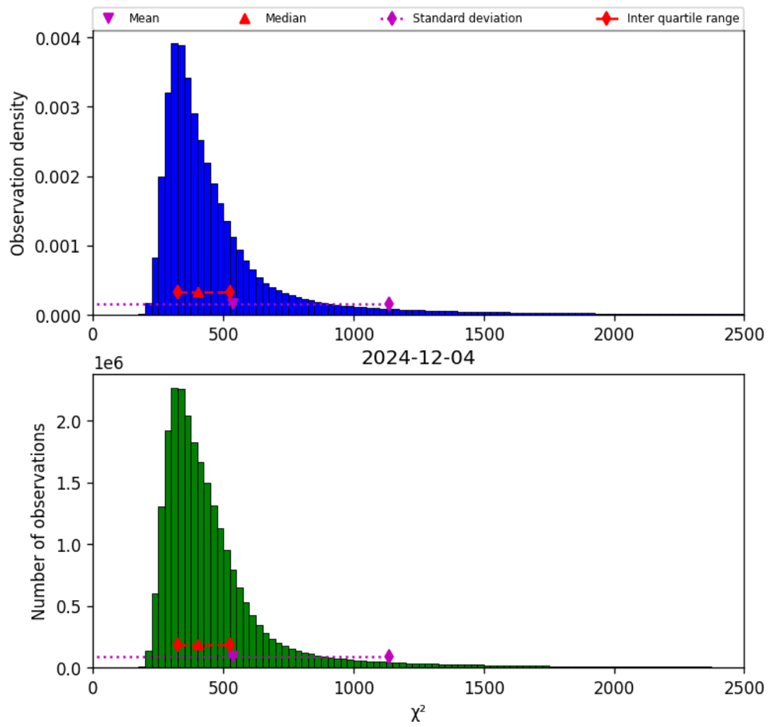
Figure 42: Histogram of “ \chi^2 ” for 2024-12-03 to 2024-12-05
