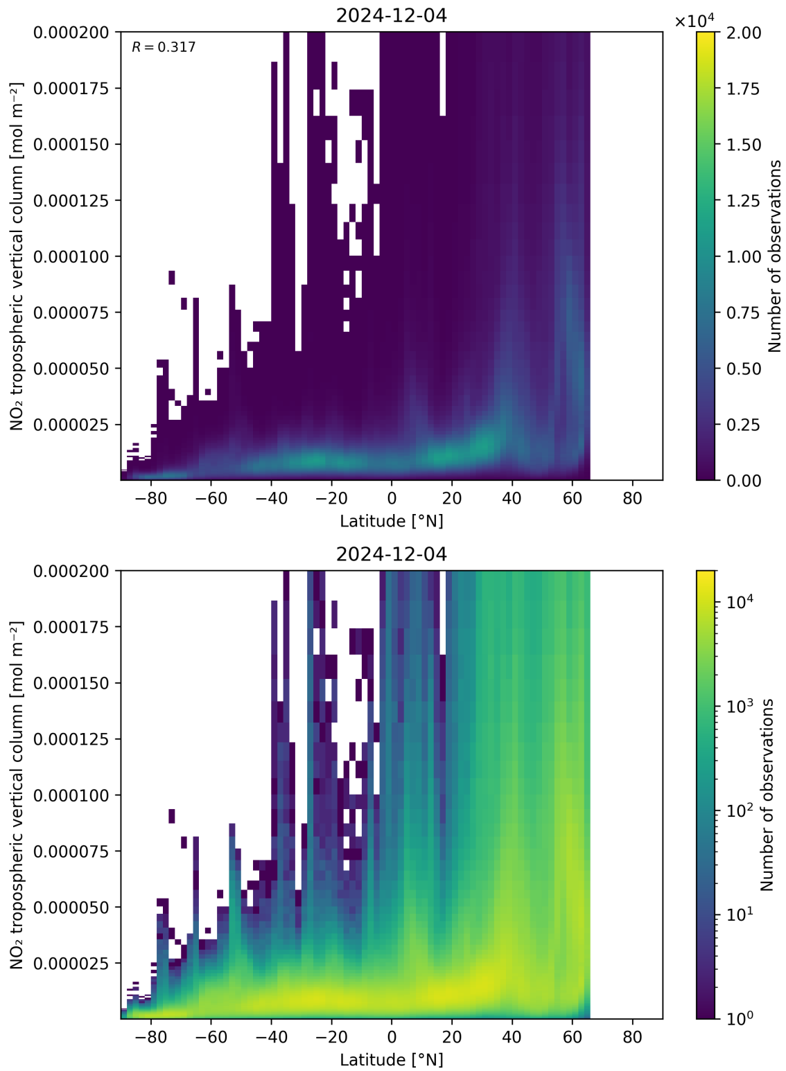
Figure 92: Scatter density plot of “Latitude” against “NO 2 tropospheric vertical column” for 2024-12-03 to 2024-12-05.
