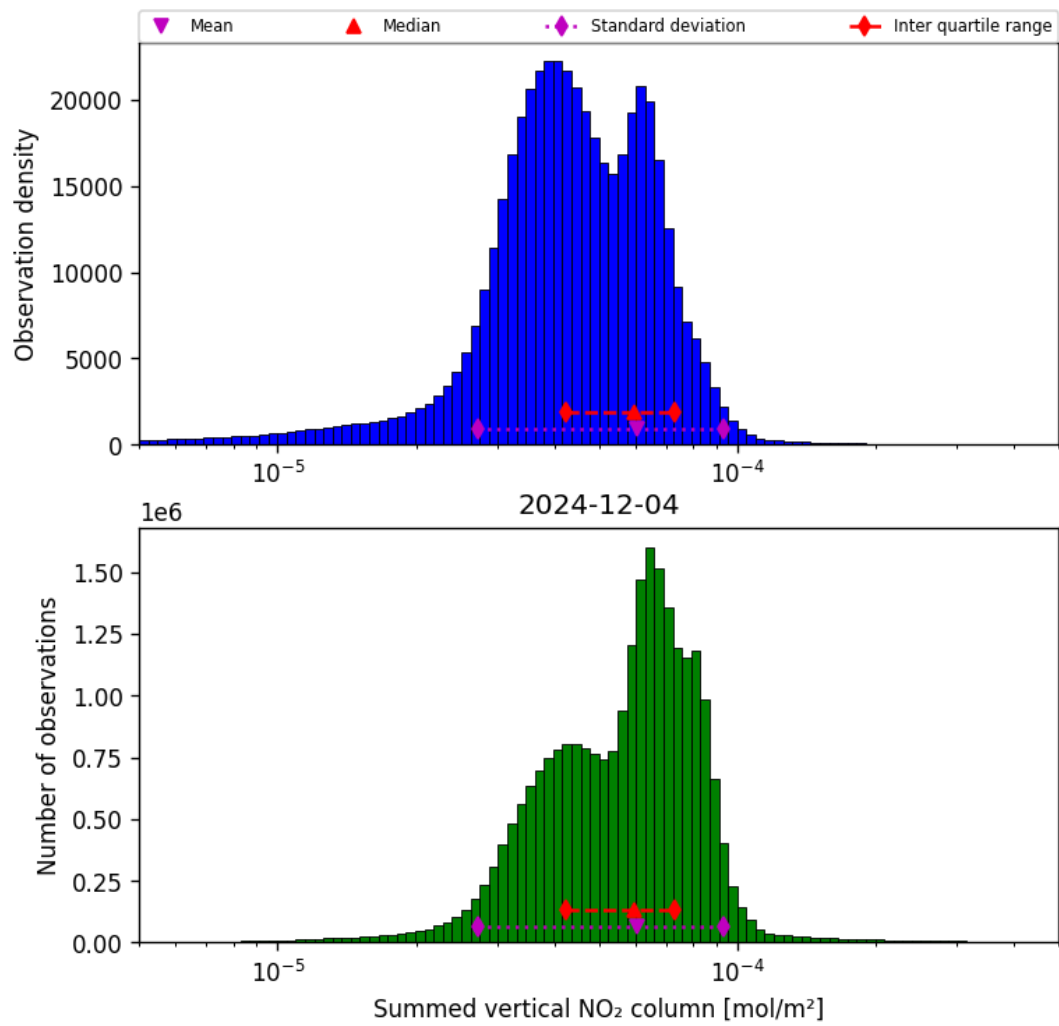
Figure 40: Histogram of “Summed vertical NO 2 column” for 2024-12-03 to 2024-12-05
