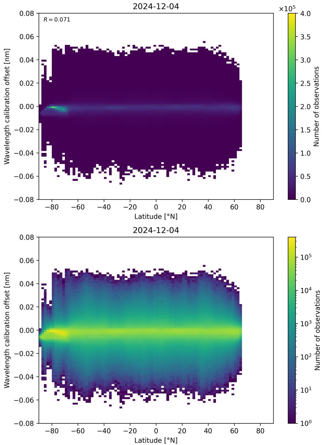
Figure 95: Scatter density plot of “Latitude” against “Wavelength calibration offset” for 2024-12-03 to 2024-12-05.
