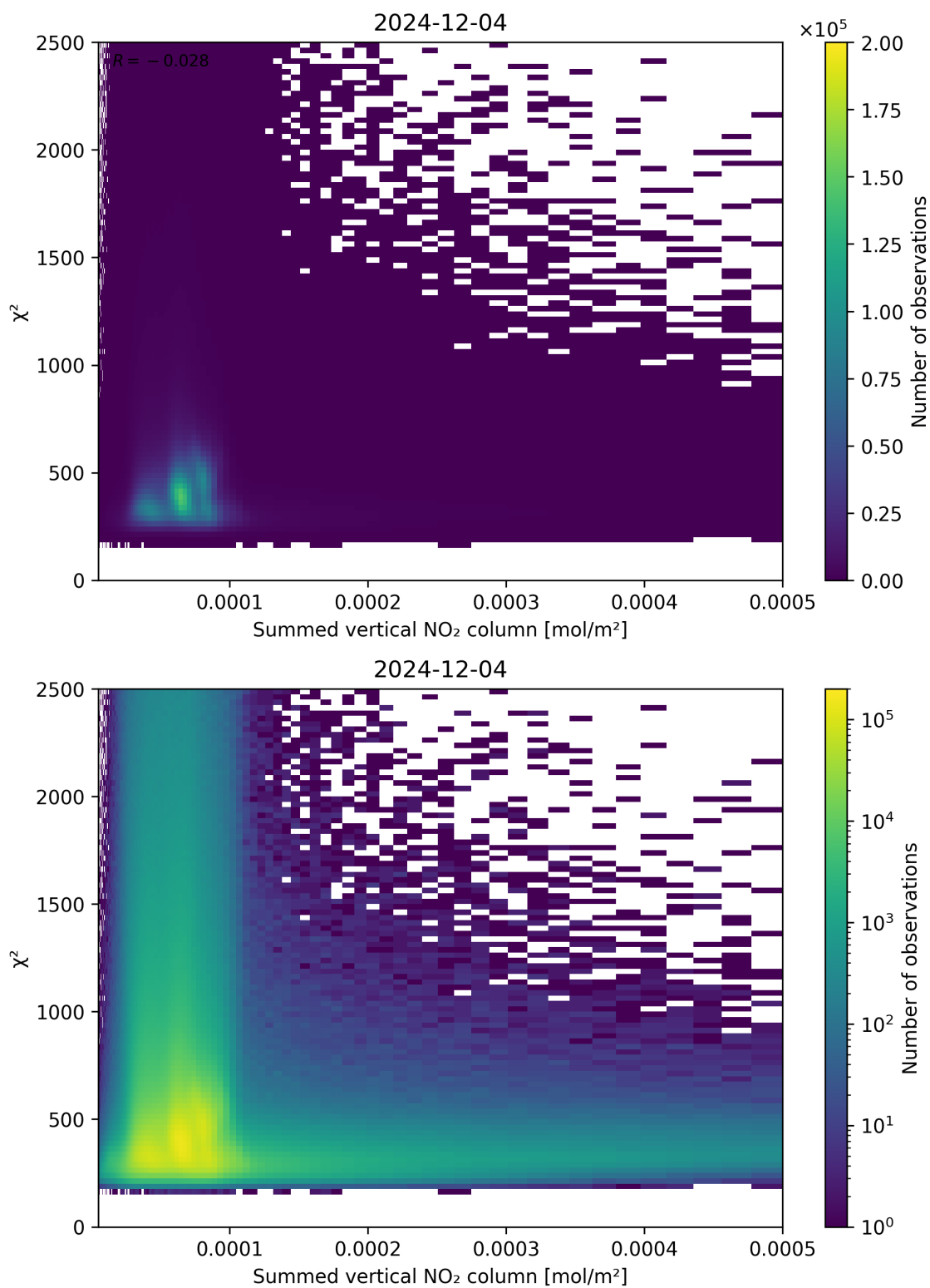
Figure 104: Scatter density plot of “Summed vertical NO 2 column” against “ \chi^2 ” for 2024-12-03 to 2024-12-05.
