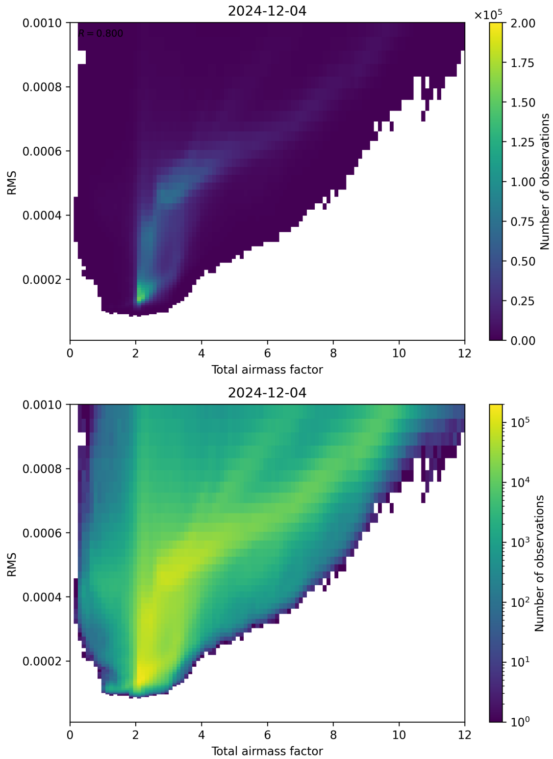
Figure 69: Scatter density plot of “Total airmass factor” against “RMS” for 2024-12-03 to 2024-12-05.
