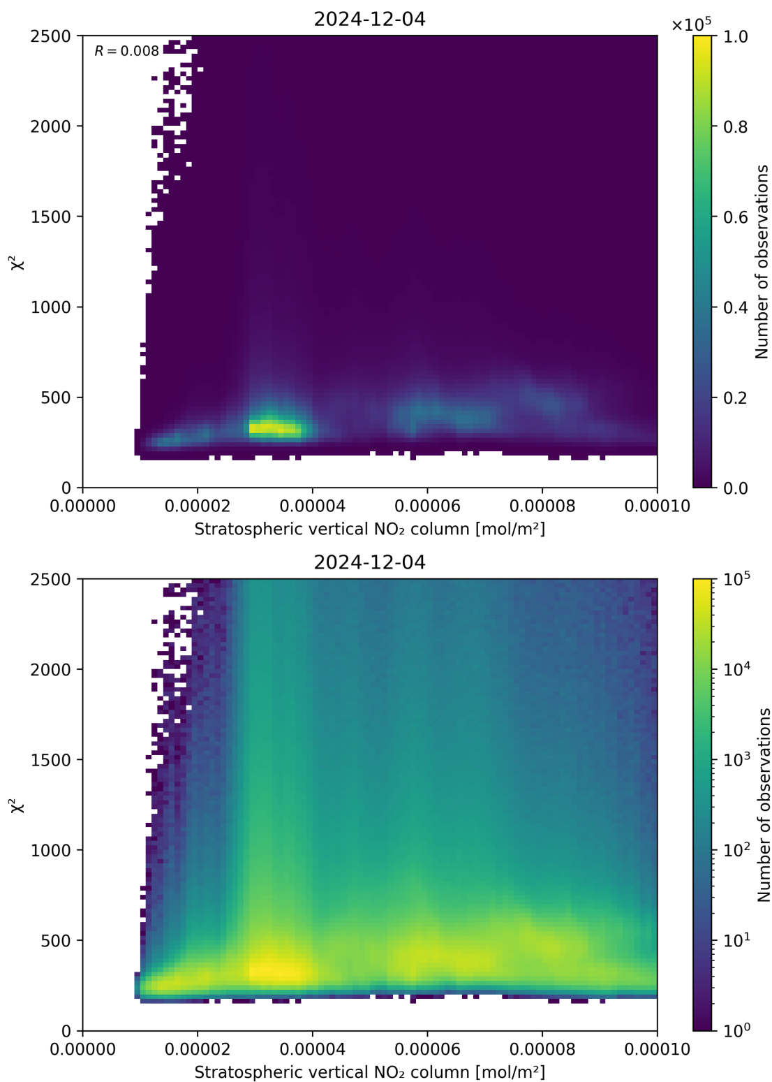
Figure 97: Scatter density plot of “Stratospheric vertical NO 2 column” against “ \chi^2 ” for 2024-12-03 to 2024-12-05.
