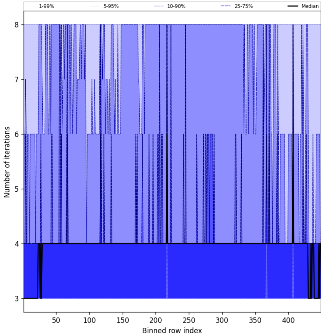
Figure 51: Along track statistics of “Number of iterations” for 2024-12-03 to 2024-12-05
