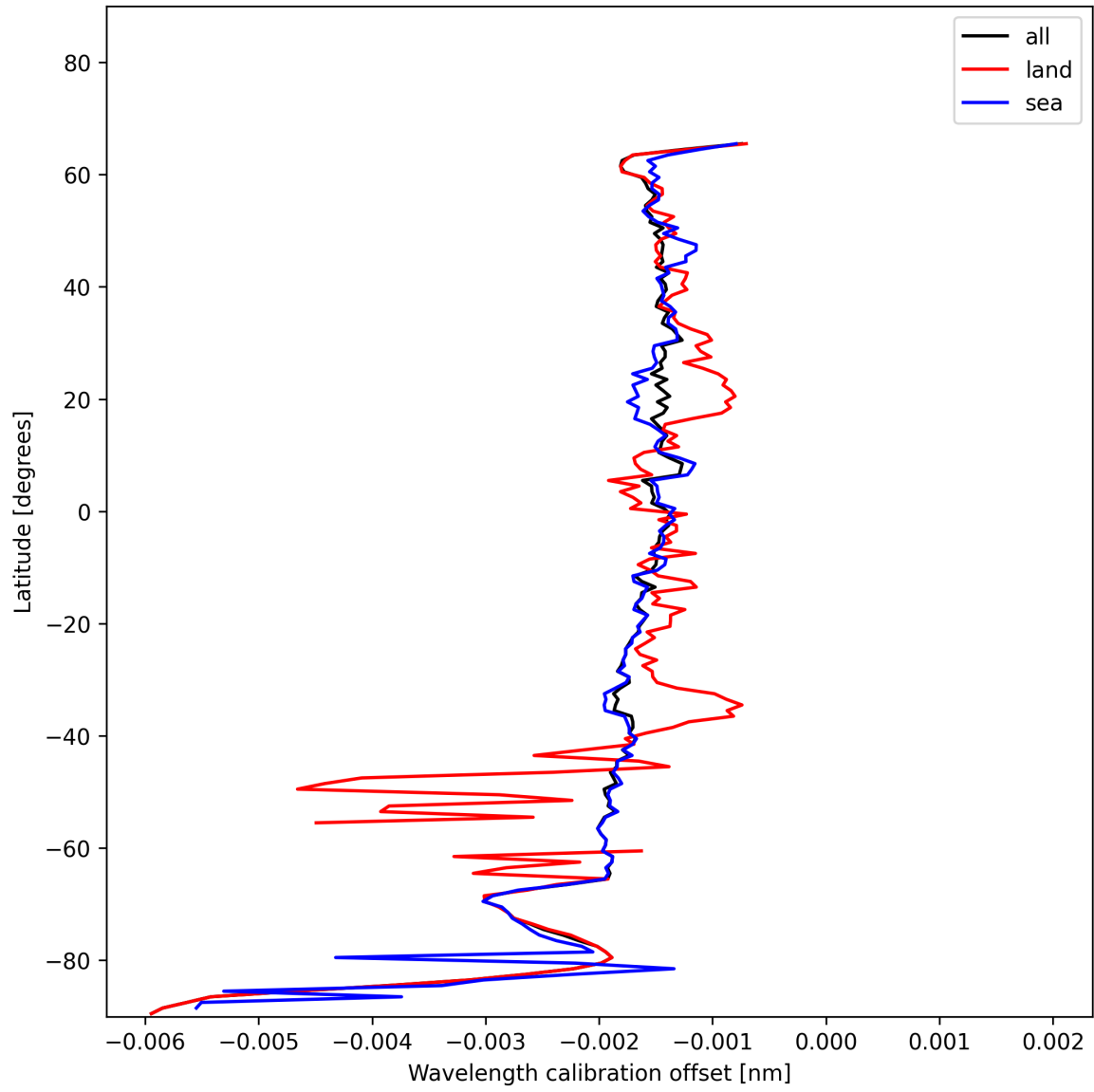
Figure 18: Zonal average of “Wavelength calibration offset” for 2024-12-03 to 2024-12-05.
