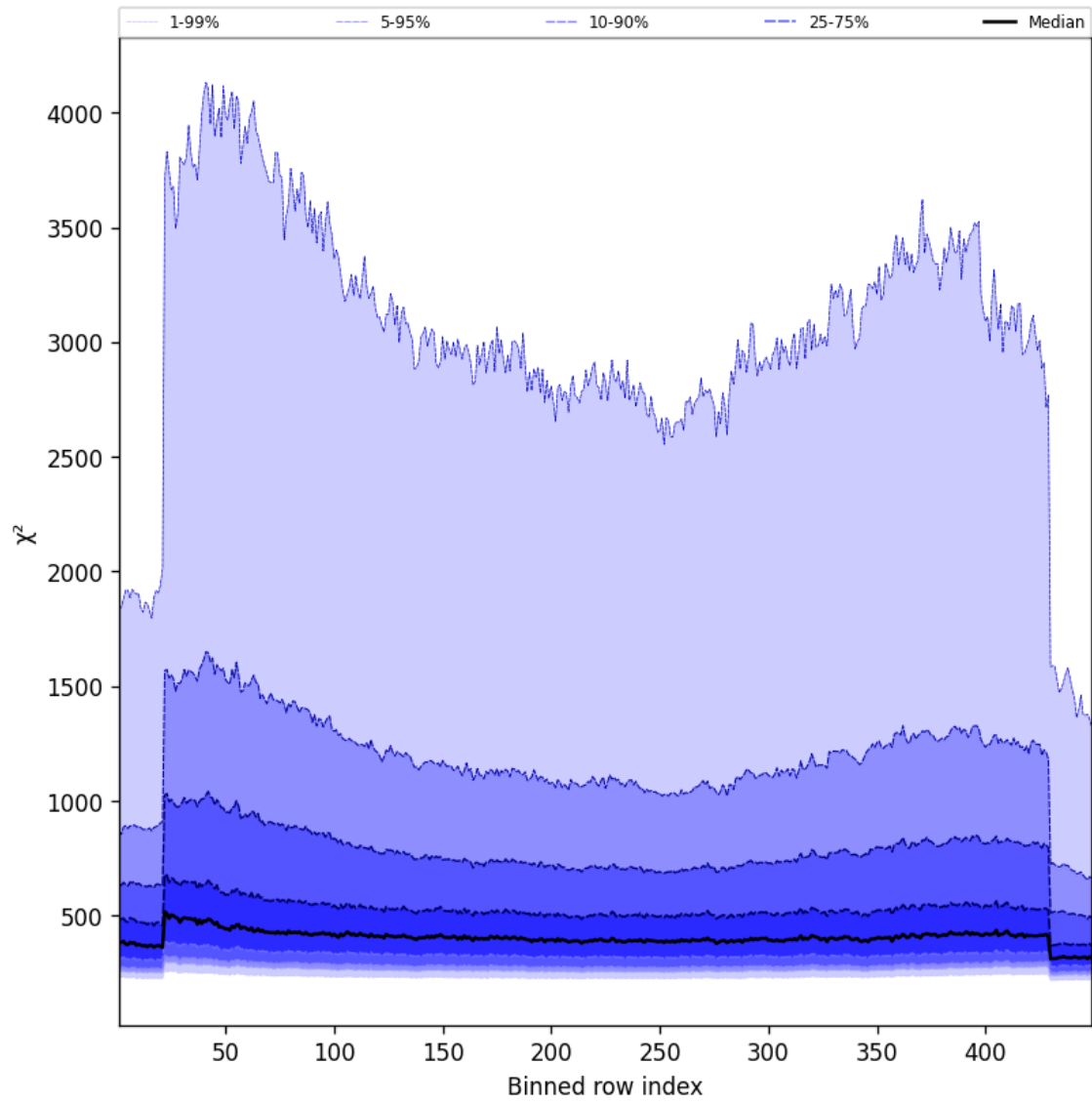
Figure 59: Along track statistics of “ \chi^2 ” for 2024-12-03 to 2024-12-05
