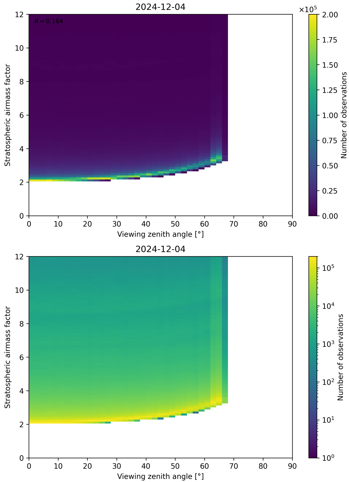
Figure 159: Scatter density plot of “Viewing zenith angle” against “Stratospheric airmass factor” for 2024-12-03 to 2024-12-05.
