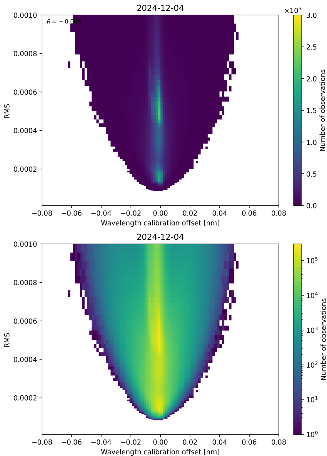
Figure 181: Scatter density plot of “Wavelength calibration offset” against “RMS” for 2024-12-03 to 2024-12-05.
