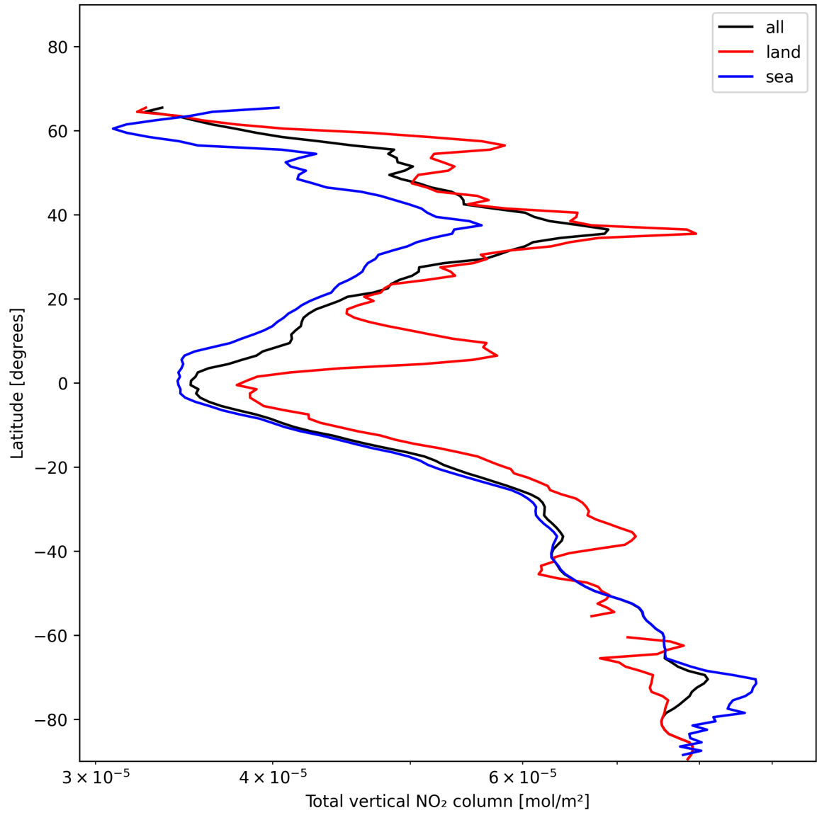
Figure 21: Zonal average of “Total vertical NO 2 column” for 2024-12-03 to 2024-12-05.
