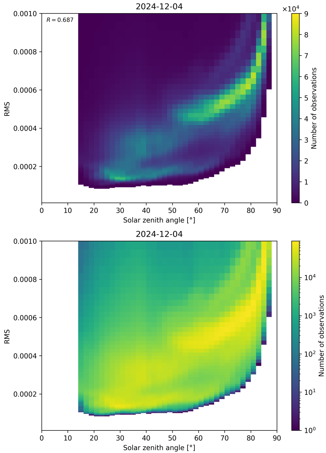
Figure 157: Scatter density plot of “Solar zenith angle” against “RMS” for 2024-12-03 to 2024-12-05.
