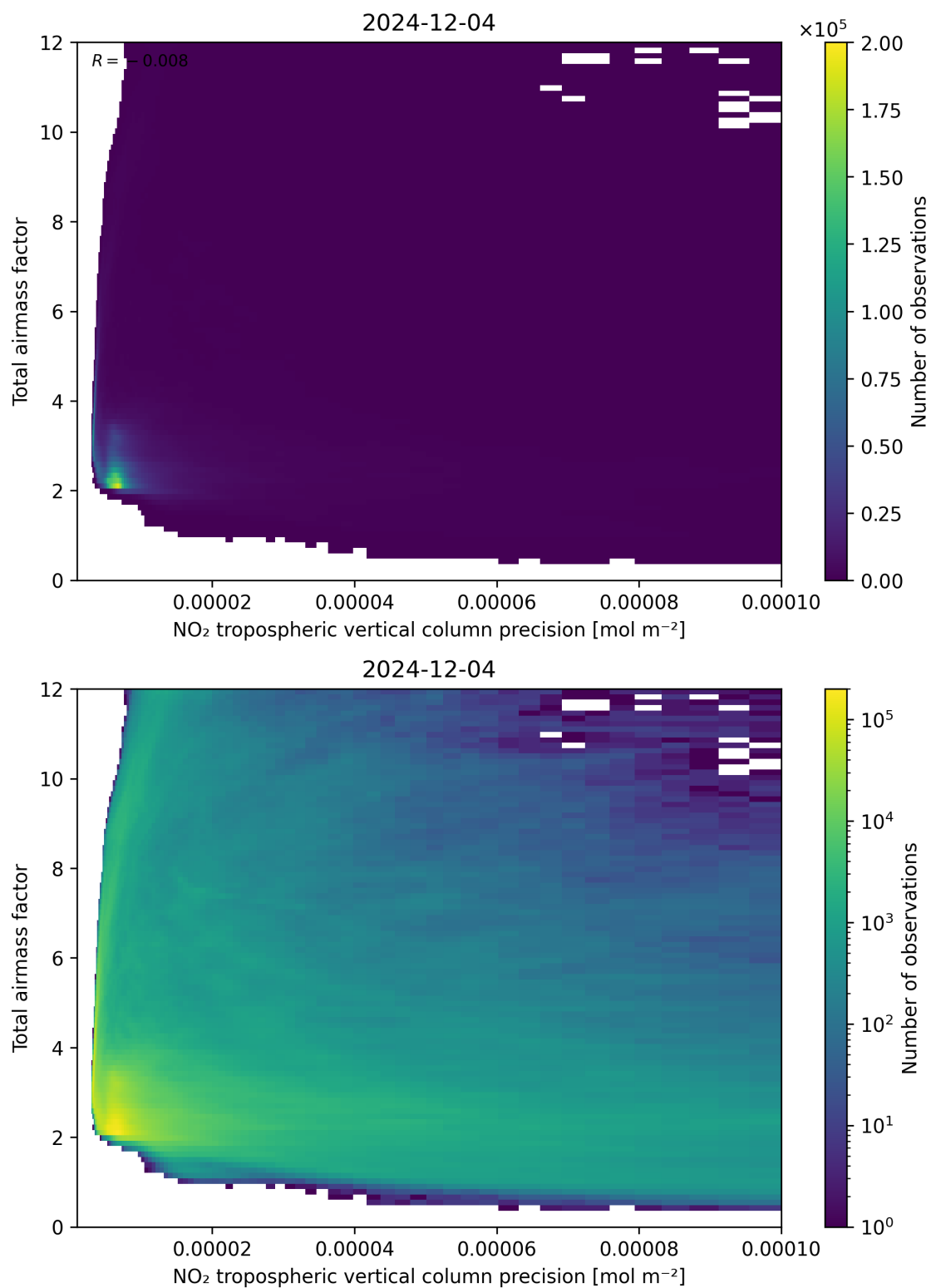
Figure 132: Scatter density plot of “NO 2 tropospheric vertical column precision” against “Total air mass factor” for 2024-12-03 to 2024-12-05.
