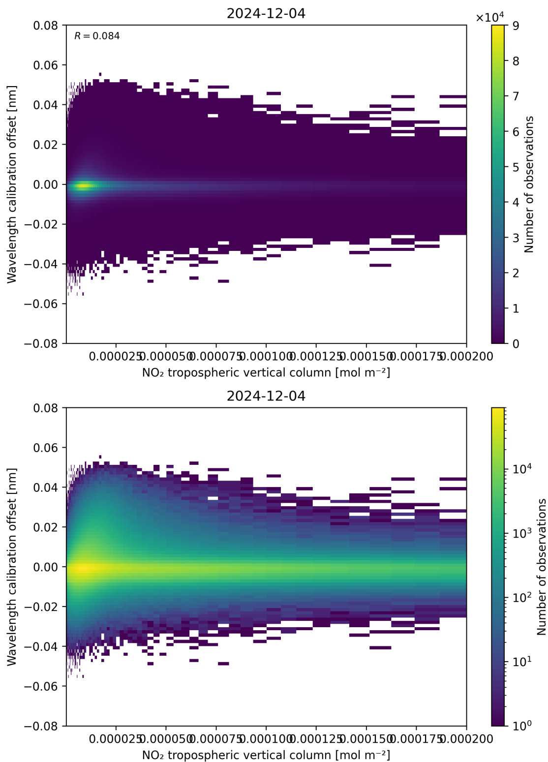
Figure 143: Scatter density plot of “NO 2 tropospheric vertical column” against “Wavelength calibration offset” for 2024-12-03 to 2024-12-05.
