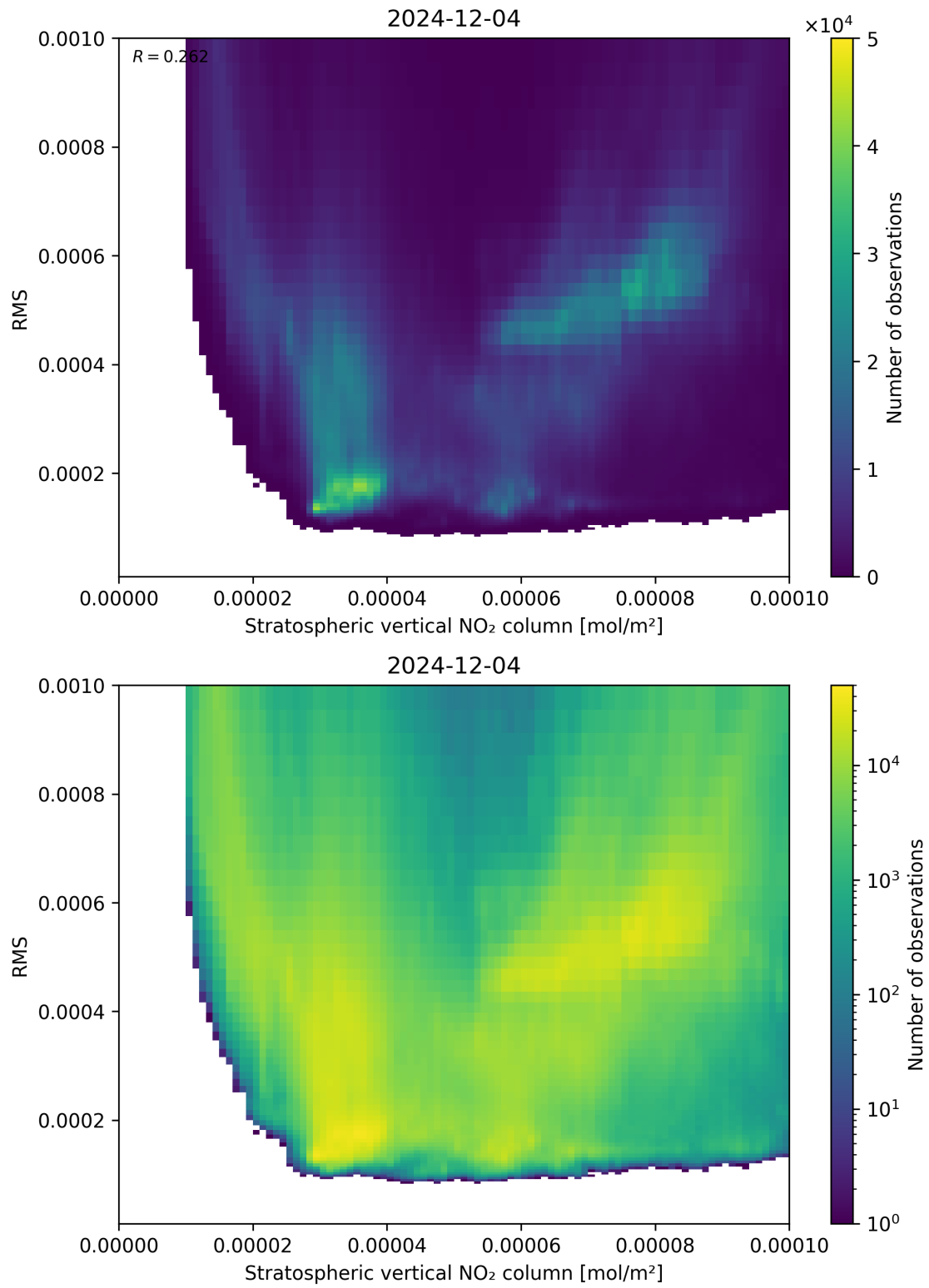
Figure 102: Scatter density plot of “Stratospheric vertical NO 2 column” against “RMS” for 2024-12-03 to 2024-12-05.
