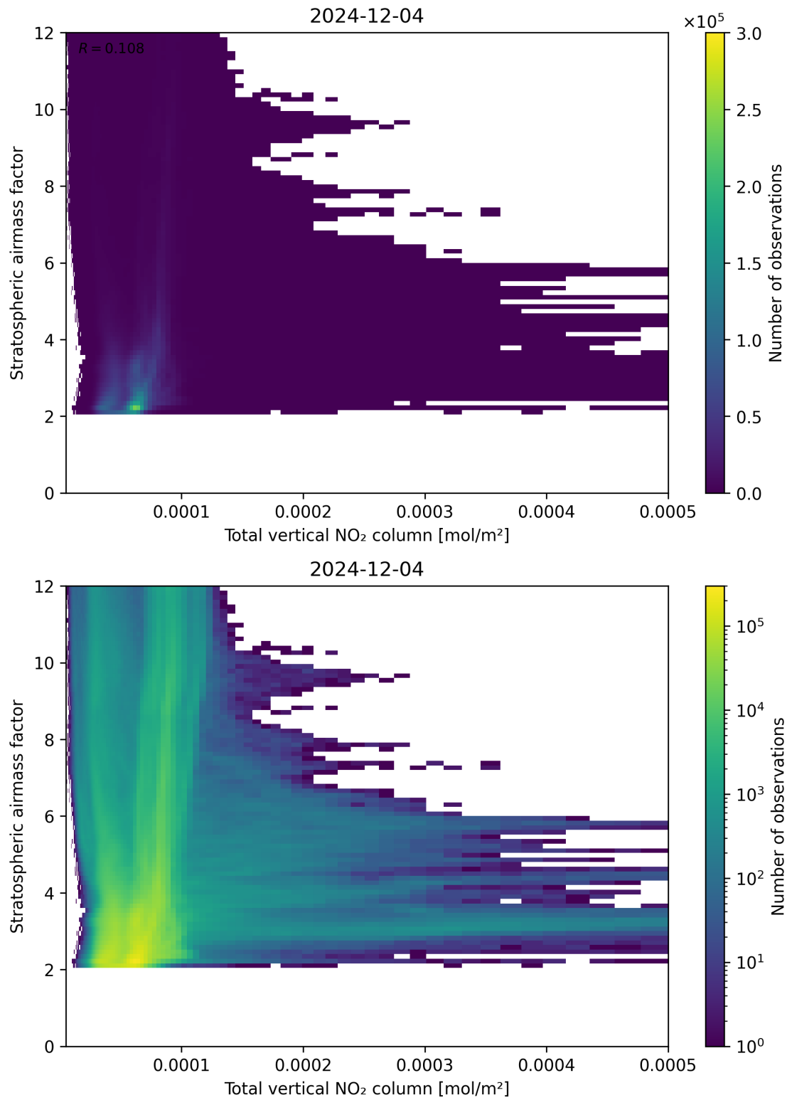
Figure 110: Scatter density plot of “Total vertical NO 2 column” against “Stratospheric airmass factor” for 2024-12-03 to 2024-12-05.
