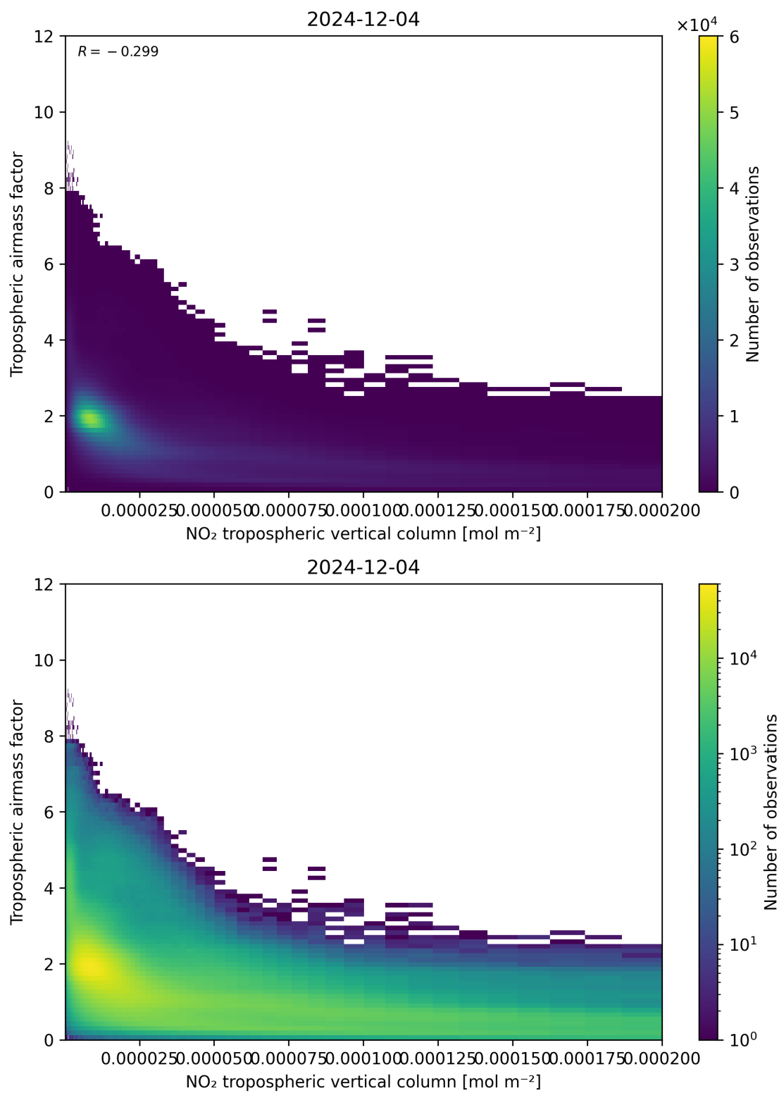
Figure 123: Scatter density plot of “NO 2 tropospheric vertical column” against “Tropospheric air mass factor” for 2024-12-03 to 2024-12-05.
