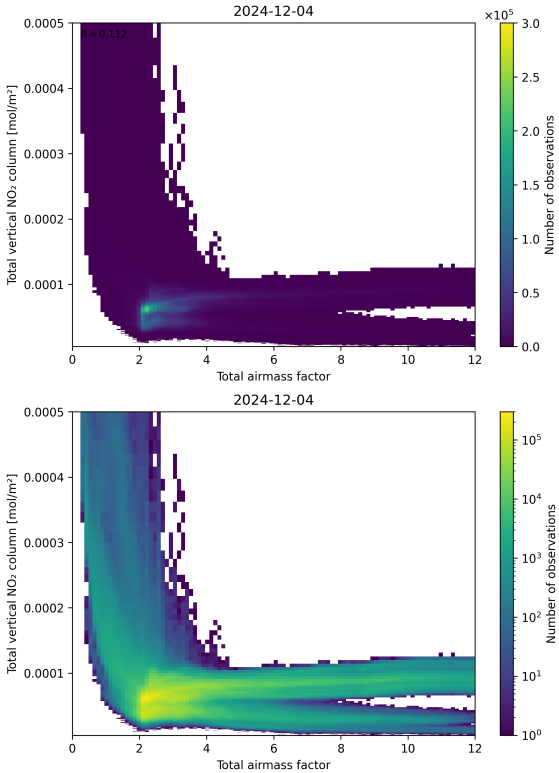
Figure 67: Scatter density plot of “Total airmass factor” against “Total vertical NO 2 column” for 2024-12-03 to 2024-12-05.
