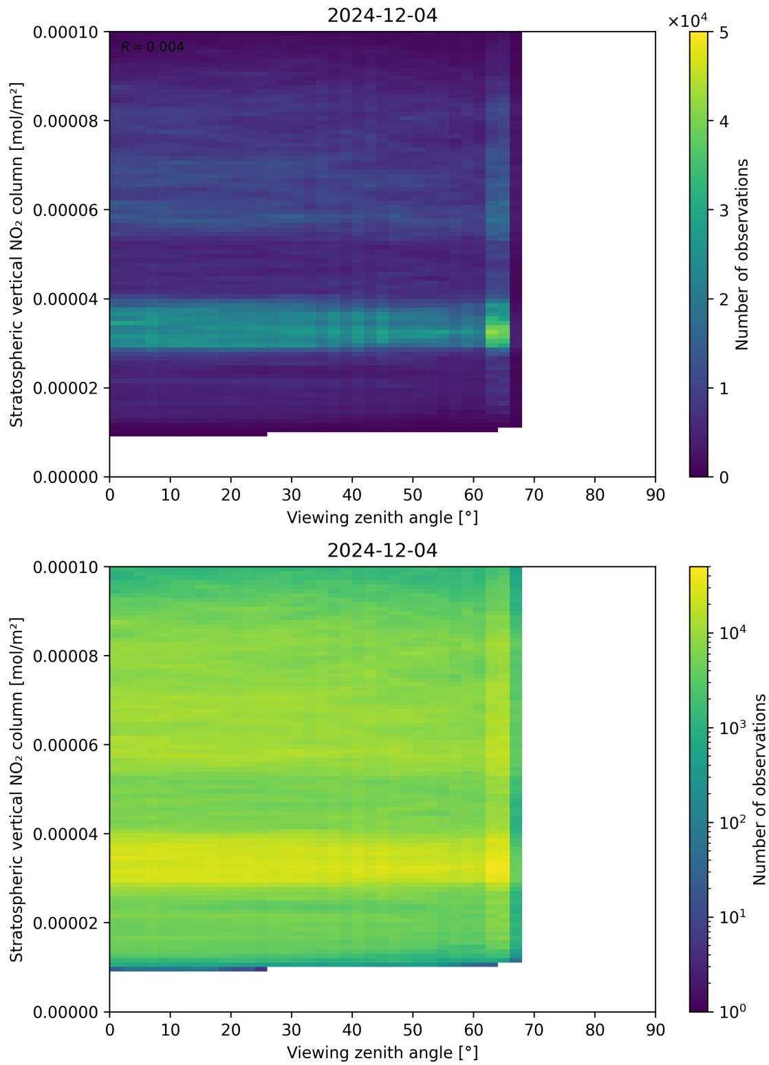
Figure 164: Scatter density plot of “Viewing zenith angle” against “Stratospheric vertical NO 2 column” for 2024-12-03 to 2024-12-05.
