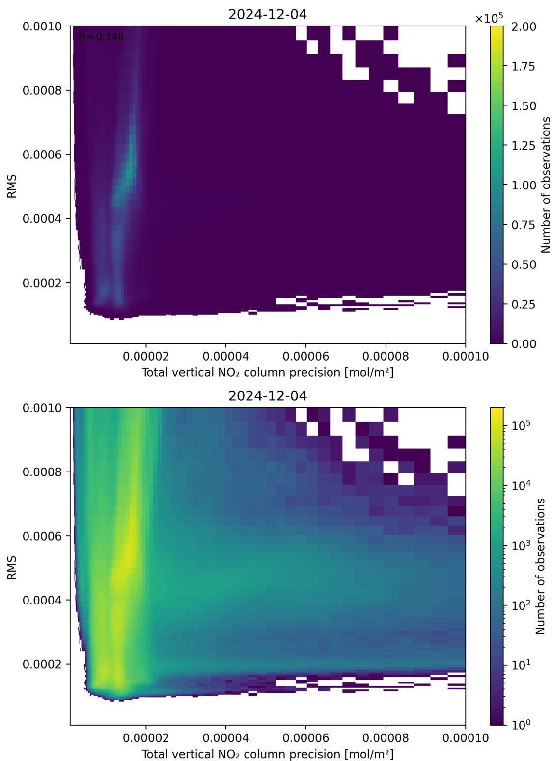
Figure 119: Scatter density plot of “Total vertical NO 2 column precision” against “RMS” for 2024-12-03 to 2024-12-05.
