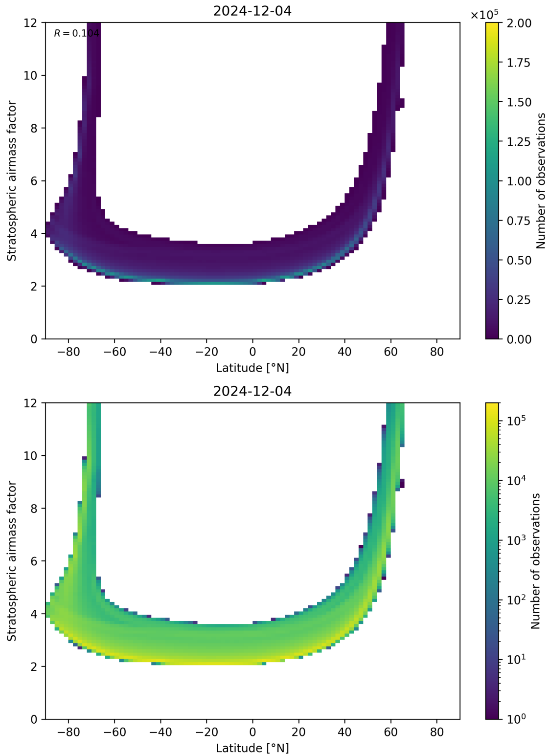
Figure 83: Scatter density plot of “Latitude” against “Stratospheric airmass factor” for 2024-12-03 to 2024-12-05.
