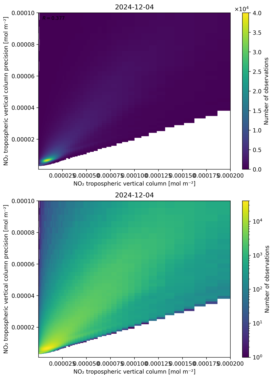
Figure 130: Scatter density plot of “NO 2 tropospheric vertical column” against “NO 2 tropospheric vertical column precision” for 2024-12-03 to 2024-12-05.
