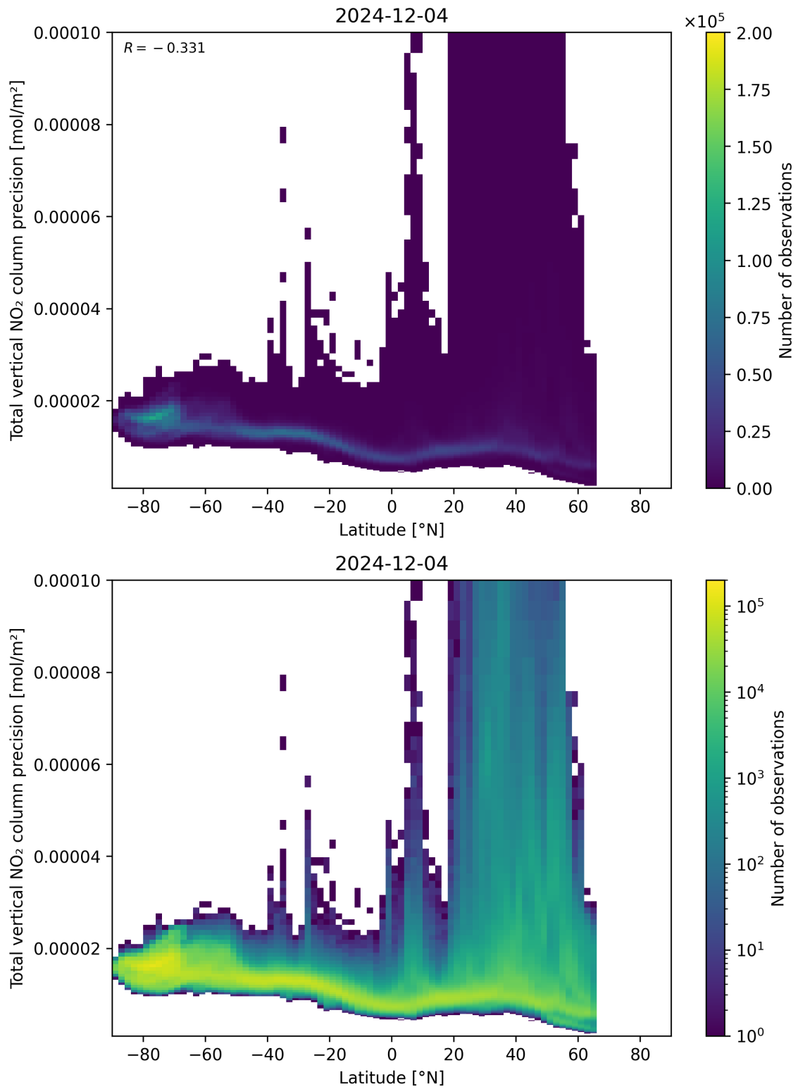
Figure 91: Scatter density plot of “Latitude” against “Total vertical NO 2 column precision” for 2024-12-03 to 2024-12-05.
