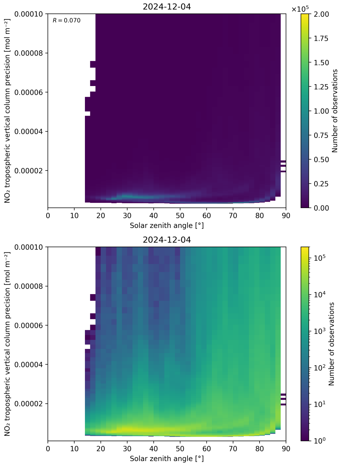
Figure 156: Scatter density plot of “Solar zenith angle” against “NO 2 tropospheric vertical column precision” for 2024-12-03 to 2024-12-05.
