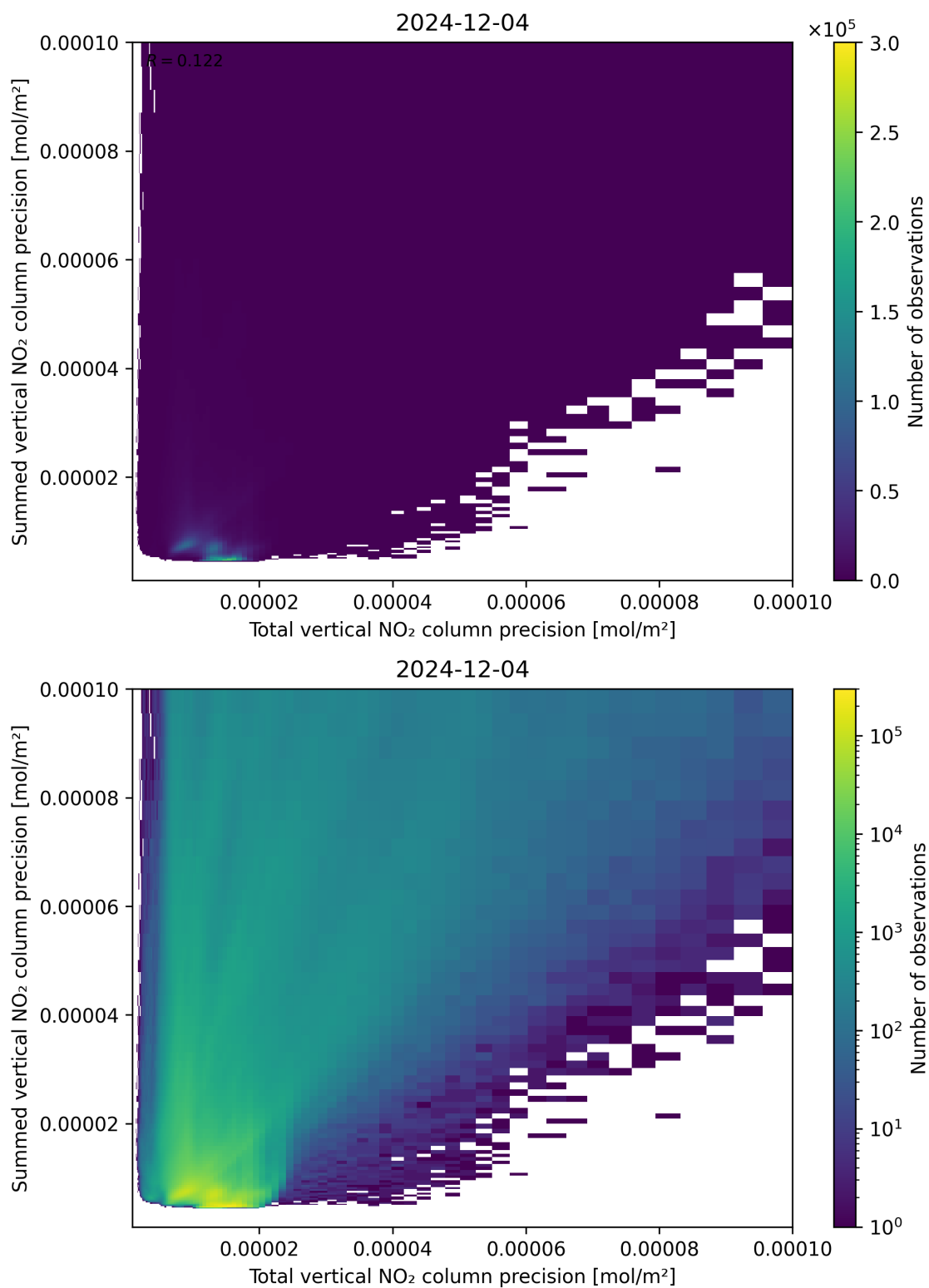
Figure 118: Scatter density plot of “Total vertical NO 2 column precision” against “Summed vertical NO 2 column precision” for 2024-12-03 to 2024-12-05.
