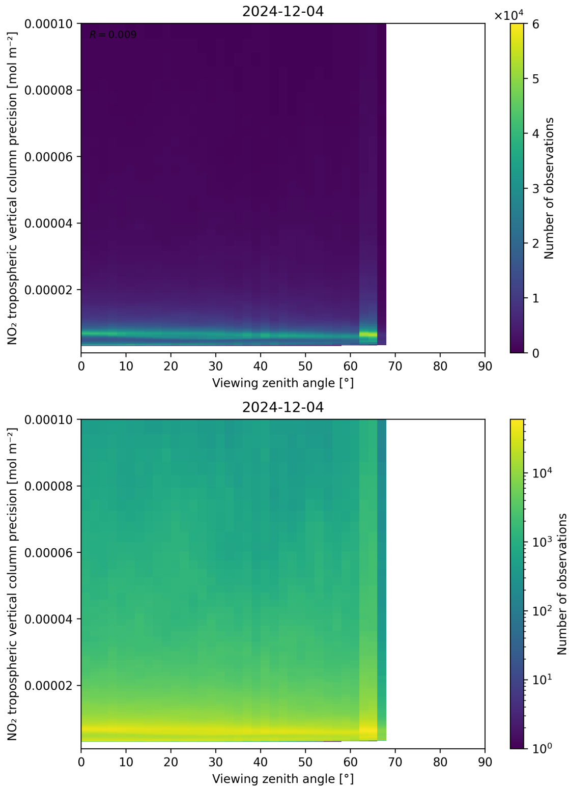
Figure 170: Scatter density plot of “Viewing zenith angle” against “NO 2 tropospheric vertical column precision” for 2024-12-03 to 2024-12-05.
