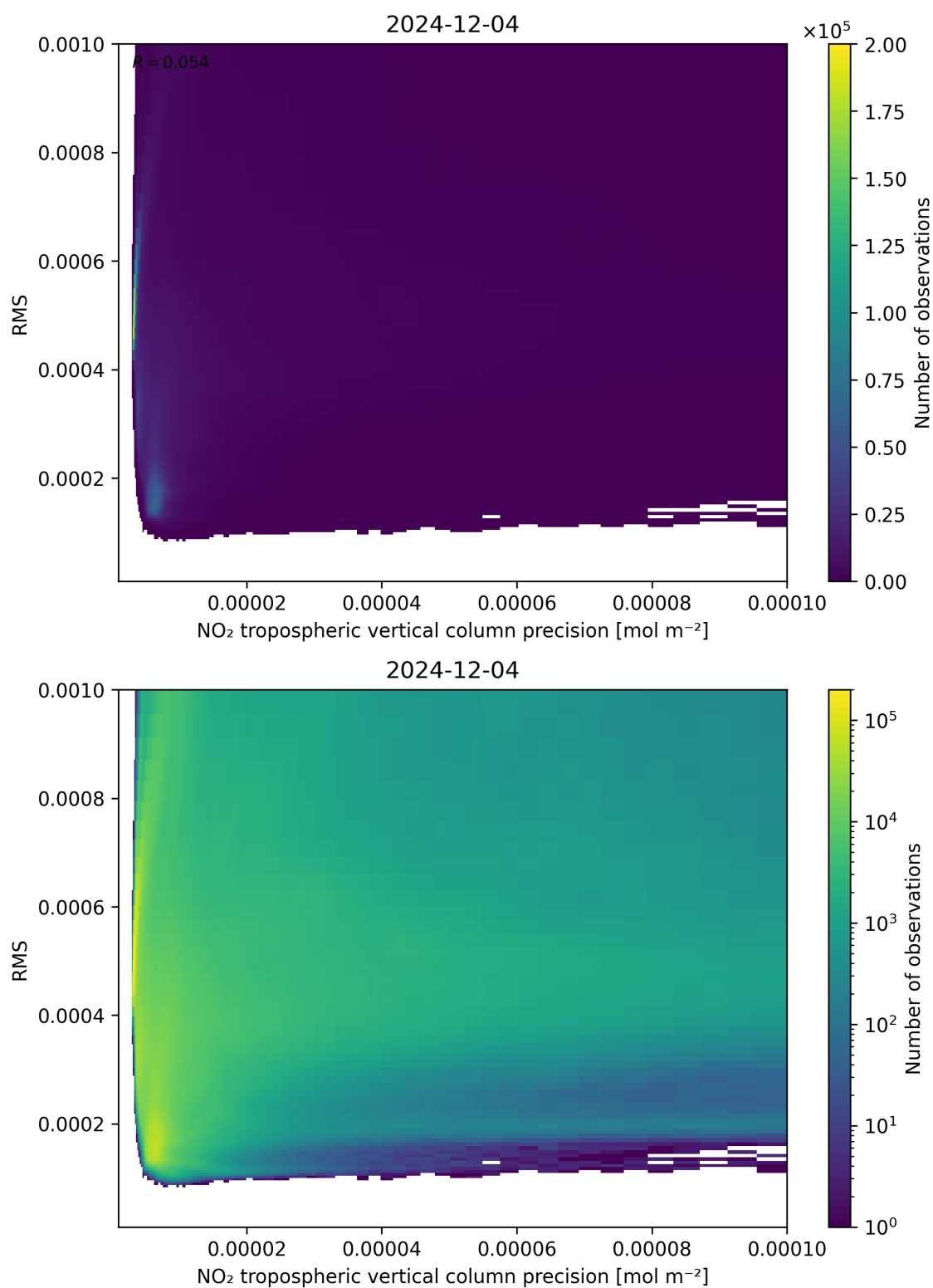
Figure 140: Scatter density plot of “NO 2 tropospheric vertical column precision” against “RMS” for 2024-12-03 to 2024-12-05.
