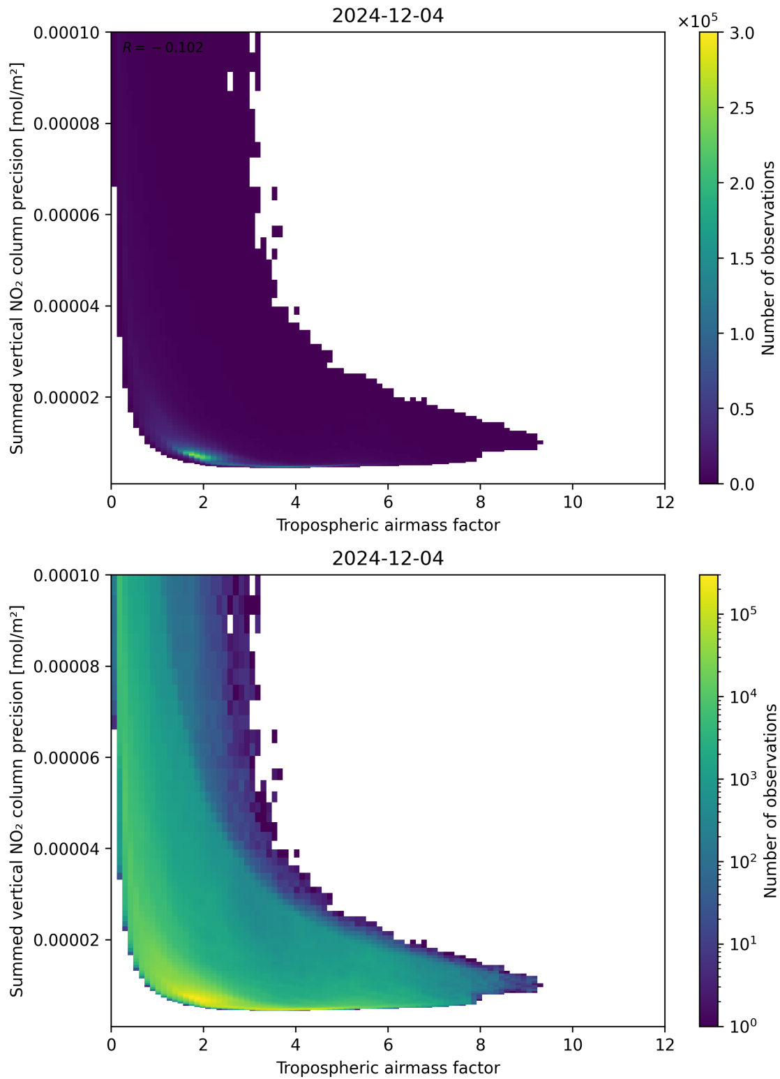
Figure 76: Scatter density plot of “Tropospheric air mass factor” against “Summed vertical NO 2 column precision” for 2024-12-03 to 2024-12-05.
