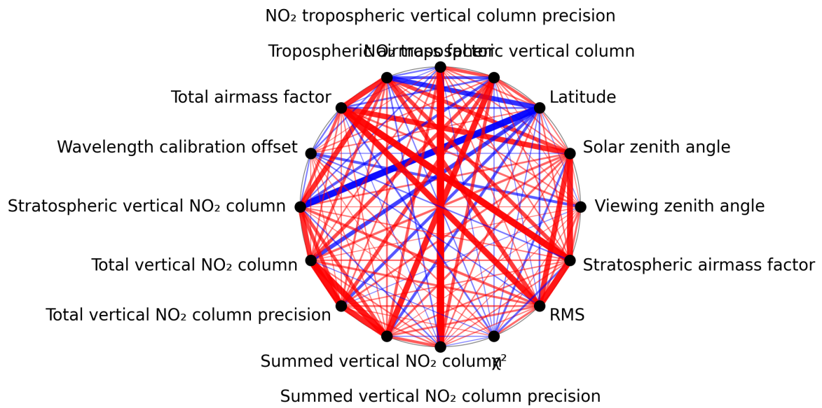
Figure 1: Map of correlation graph for 2024-12-03 to 2024-12-05.
