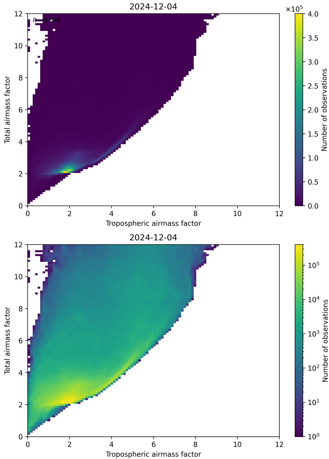
Figure 72: Scatter density plot of “Tropospheric airmass factor” against “Total airmass factor” for 2024-12-03 to 2024-12-05.
