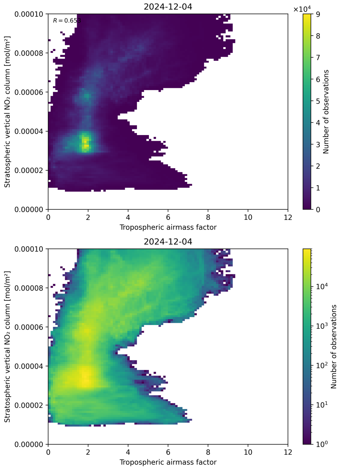
Figure 74: Scatter density plot of “Tropospheric air mass factor” against “Stratospheric vertical NO 2 column” for 2024-12-03 to 2024-12-05.
