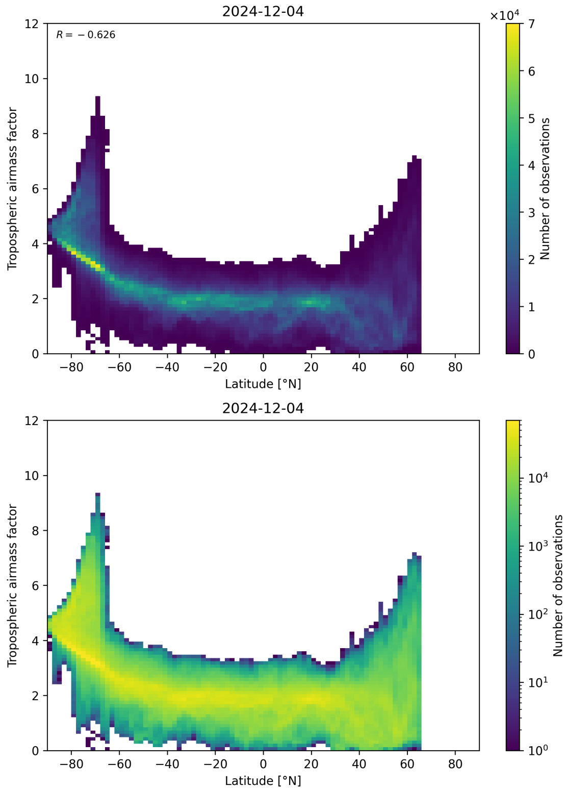
Figure 85: Scatter density plot of “Latitude” against “Tropospheric airmass factor” for 2024-12-03 to 2024-12-05.
