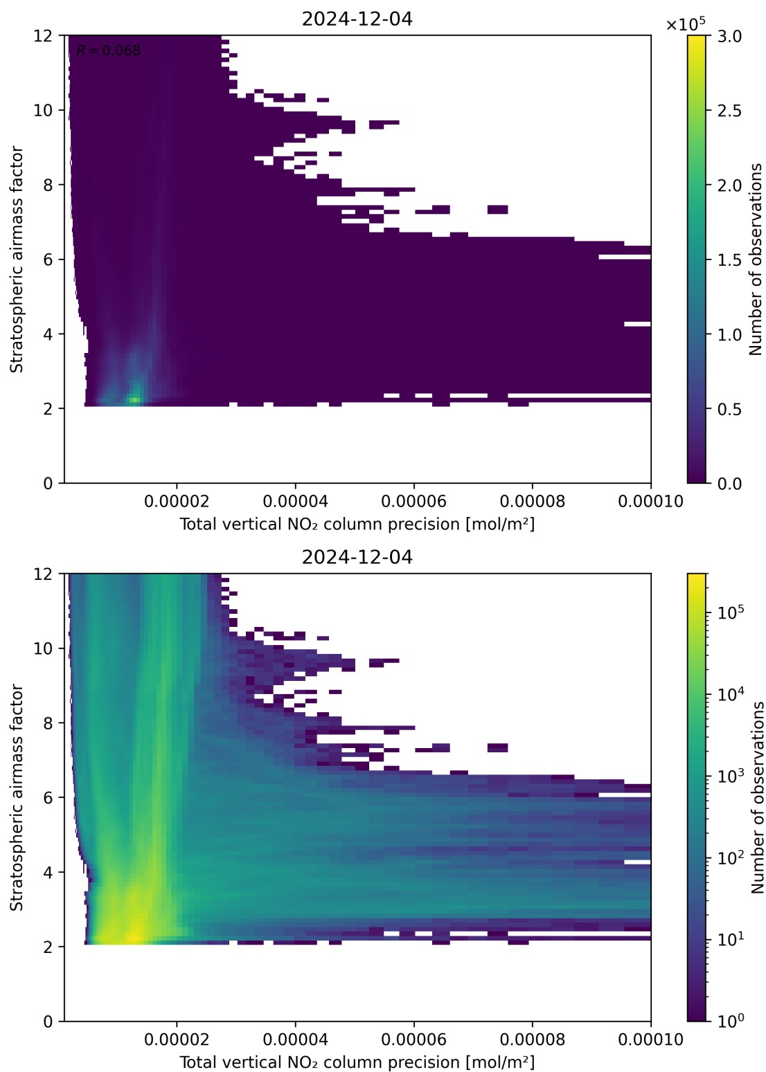
Figure 115: Scatter density plot of “Total vertical NO 2 column precision” against “Stratospheric air mass factor” for 2024-12-03 to 2024-12-05.
