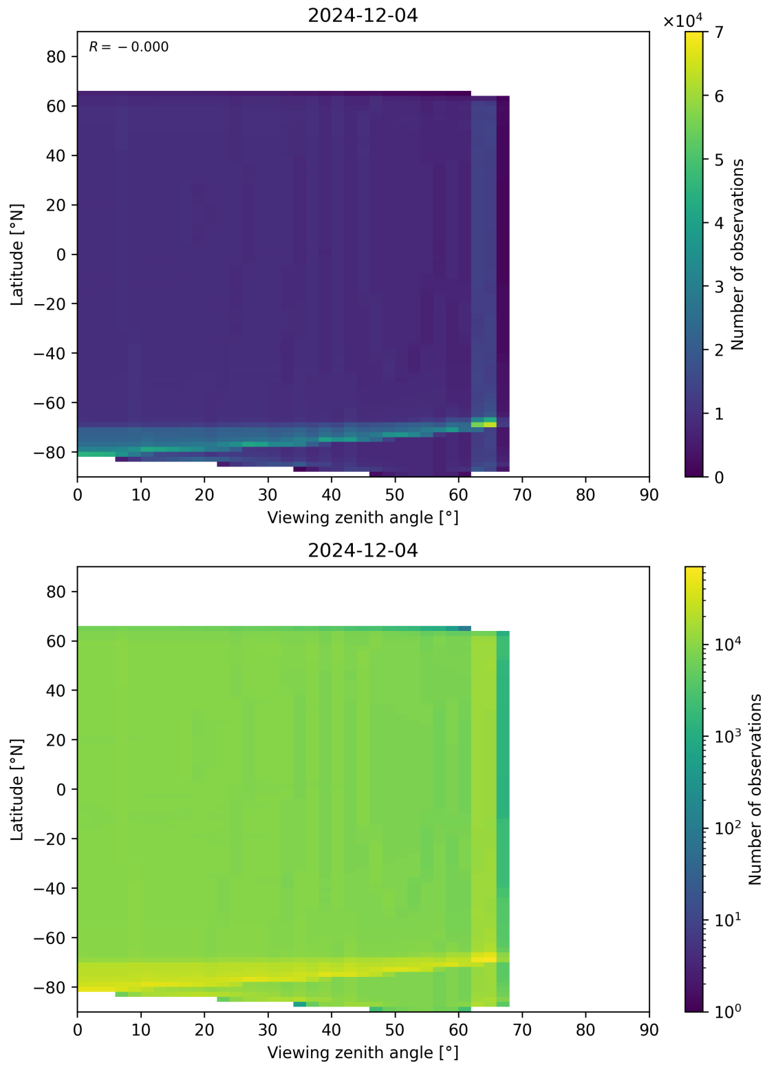
Figure 163: Scatter density plot of “Viewing zenith angle” against “Latitude” for 2024-12-03 to 2024-12-05.
