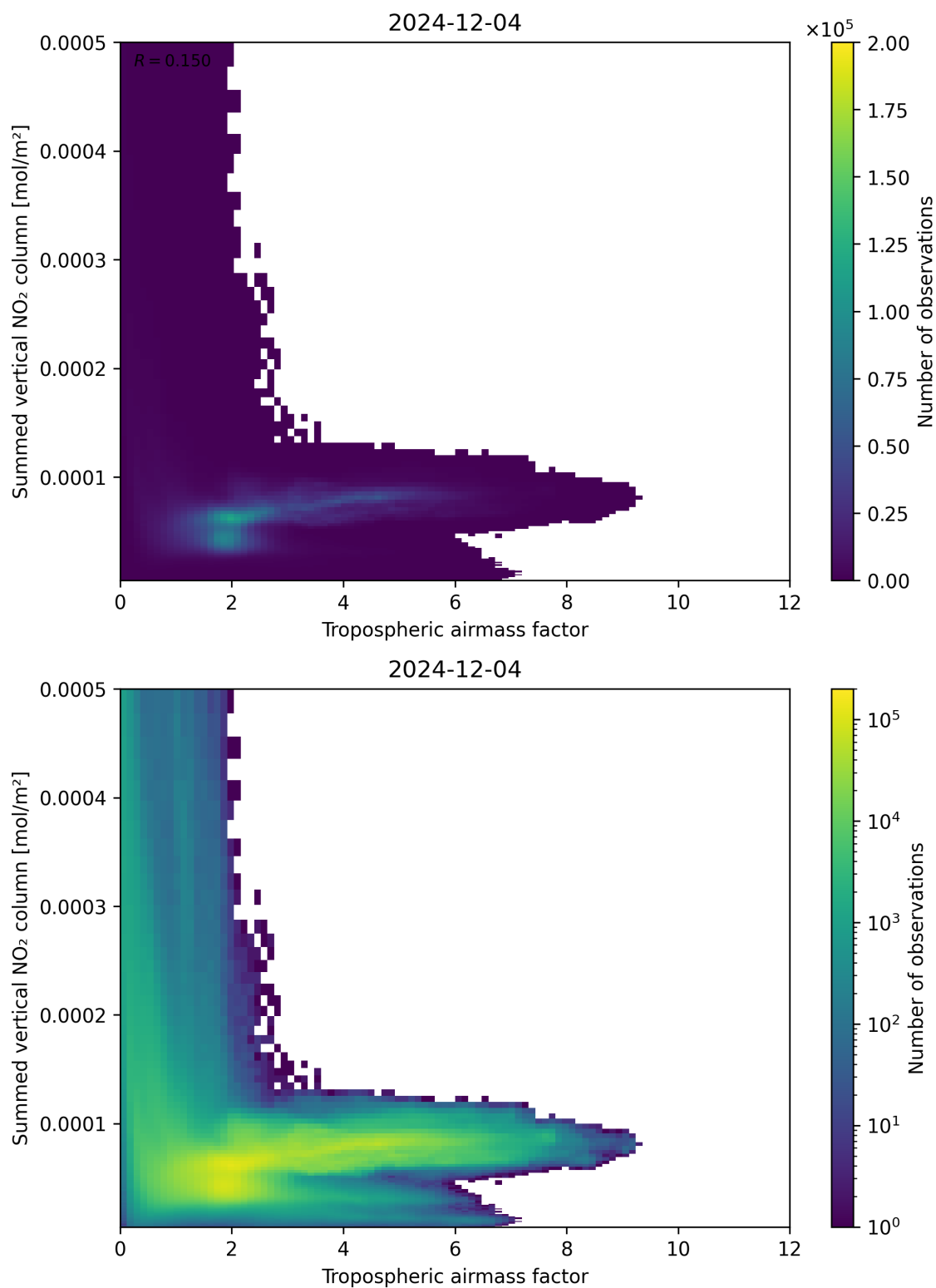
Figure 75: Scatter density plot of “Tropospheric air mass factor” against “Summed vertical NO 2 column” for 2024-12-03 to 2024-12-05.
