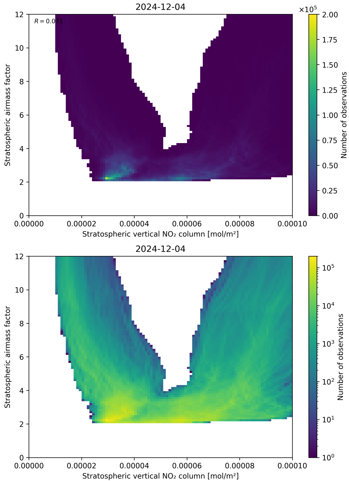
Figure 96: Scatter density plot of “Stratospheric vertical NO 2 column” against “Stratospheric airmass factor” for 2024-12-03 to 2024-12-05.
