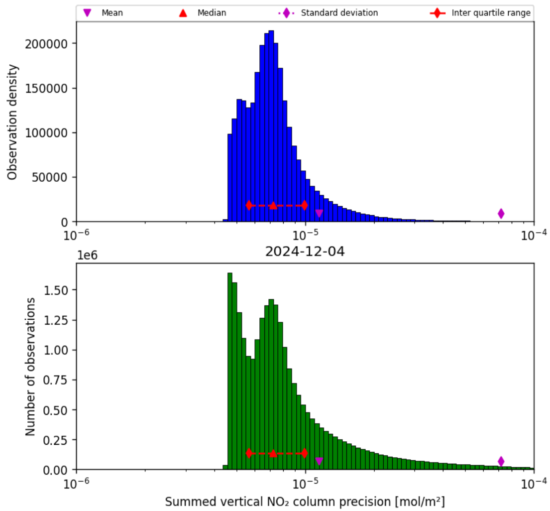
Figure 41: Histogram of “Summed vertical NO 2 column precision” for 2024-12-03 to 2024-12-05
