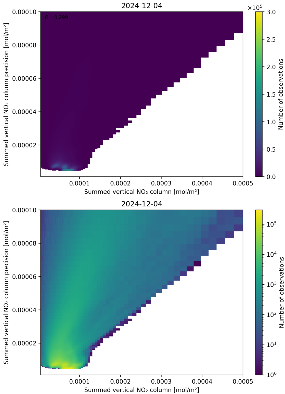
Figure 105: Scatter density plot of “Summed vertical NO 2 column” against “Summed vertical NO 2 column precision” for 2024-12-03 to 2024-12-05.
