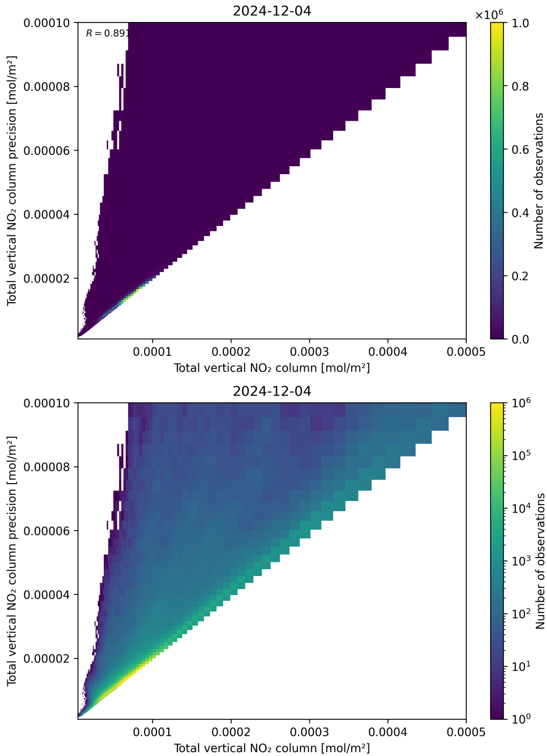
Figure 114: Scatter density plot of “Total vertical NO 2 column” against “Total vertical NO 2 column precision” for 2024-12-03 to 2024-12-05.
