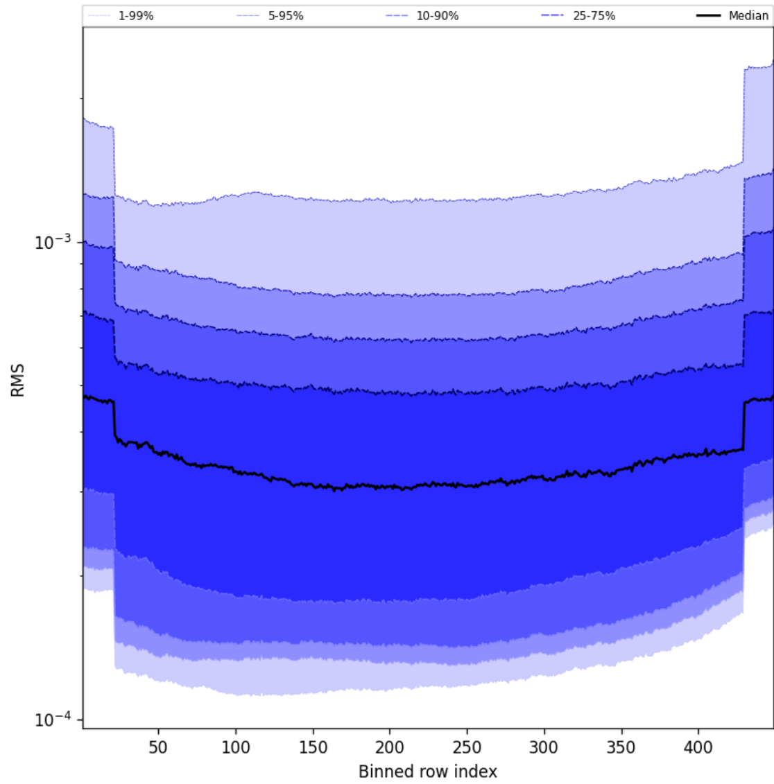
Figure 60: Along track statistics of “RMS” for 2024-12-03 to 2024-12-05
