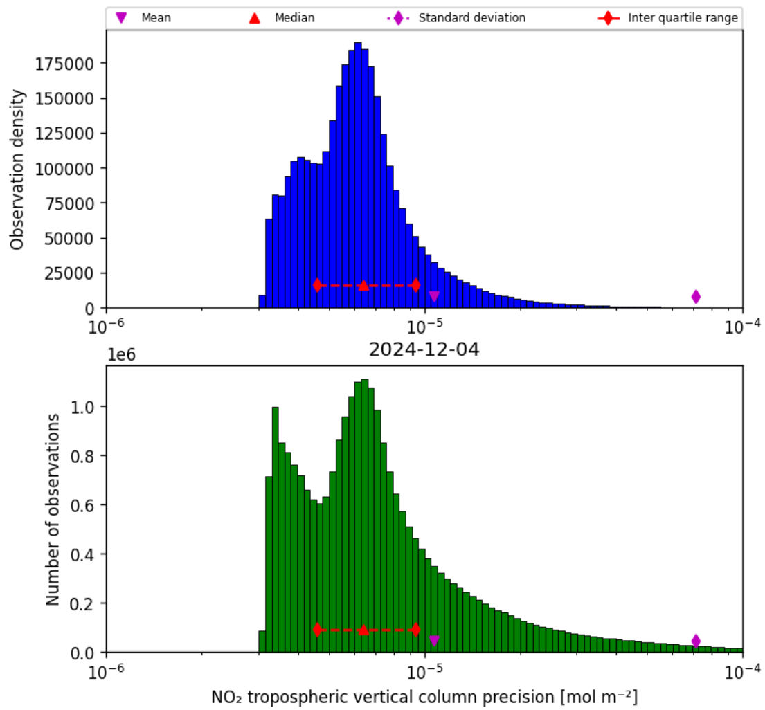
Figure 30: Histogram of “NO 2 tropospheric vertical column precision” for 2024-12-03 to 2024-12-05
