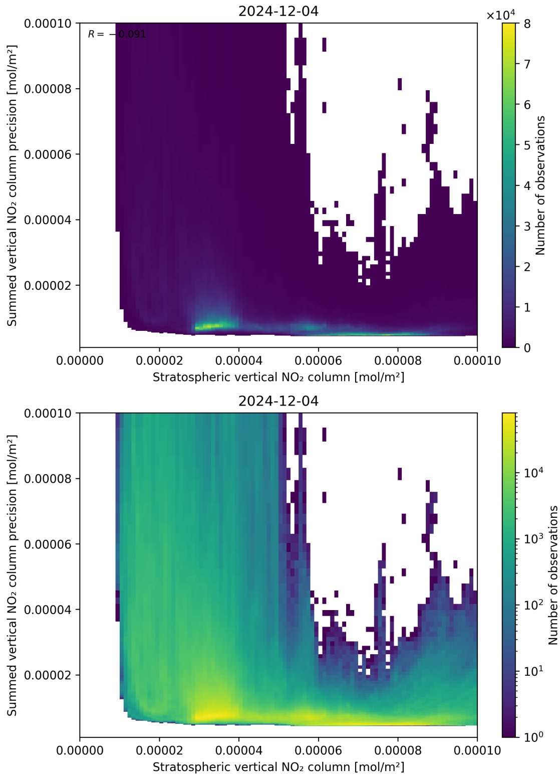
Figure 99: Scatter density plot of “Stratospheric vertical NO 2 column” against “Summed vertical NO 2 column precision” for 2024-12-03 to 2024-12-05.
