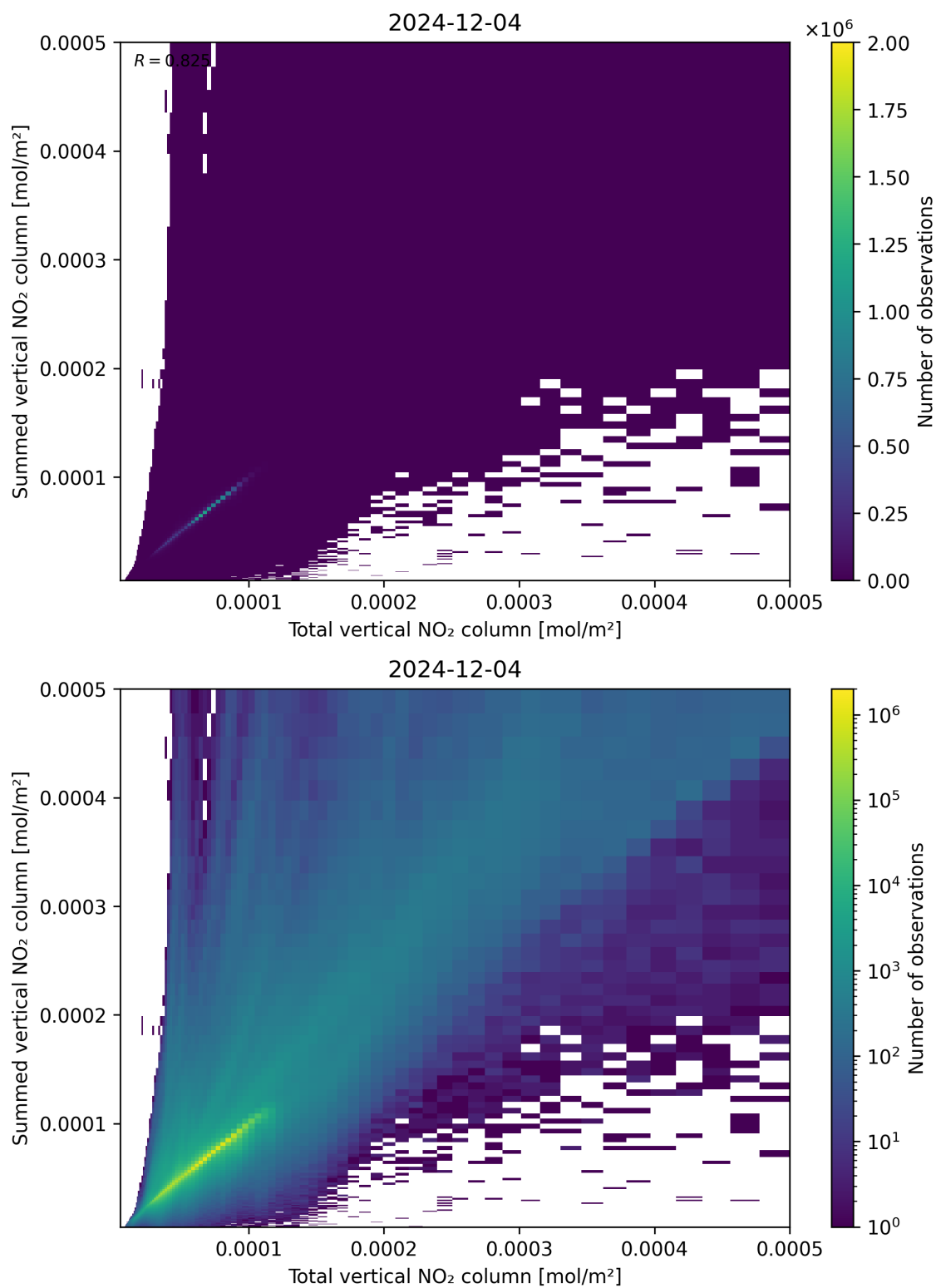
Figure 112: Scatter density plot of “Total vertical NO 2 column” against “Summed vertical NO 2 column” for 2024-12-03 to 2024-12-05.
