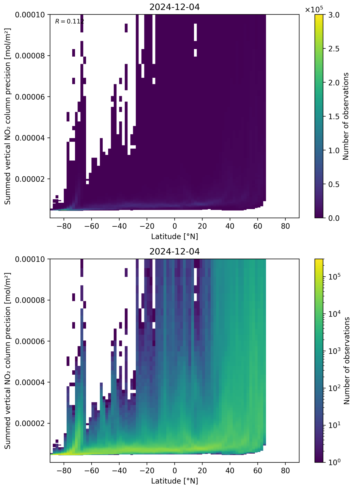
Figure 89: Scatter density plot of “Latitude” against “Summed vertical NO 2 column precision” for 2024-12-03 to 2024-12-05.
