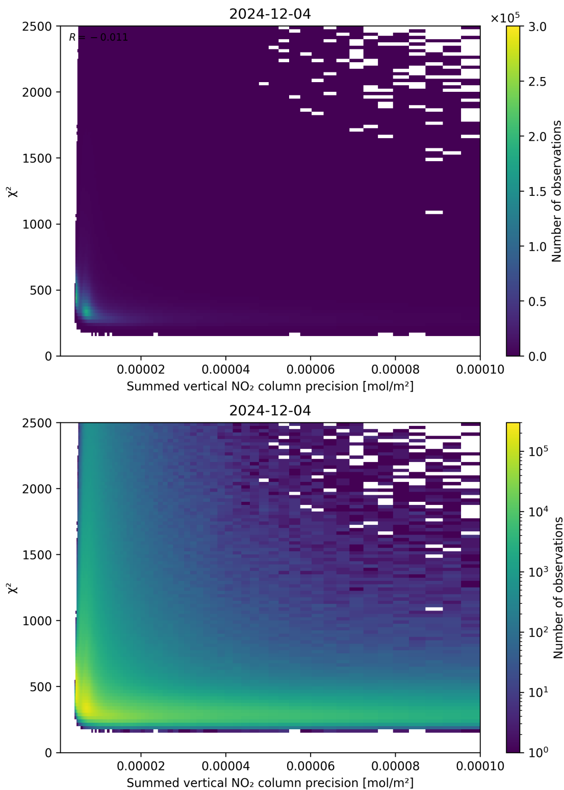
Figure 107: Scatter density plot of “Summed vertical NO 2 column precision” against “ \chi^2 ” for 2024-12-03 to 2024-12-05.
