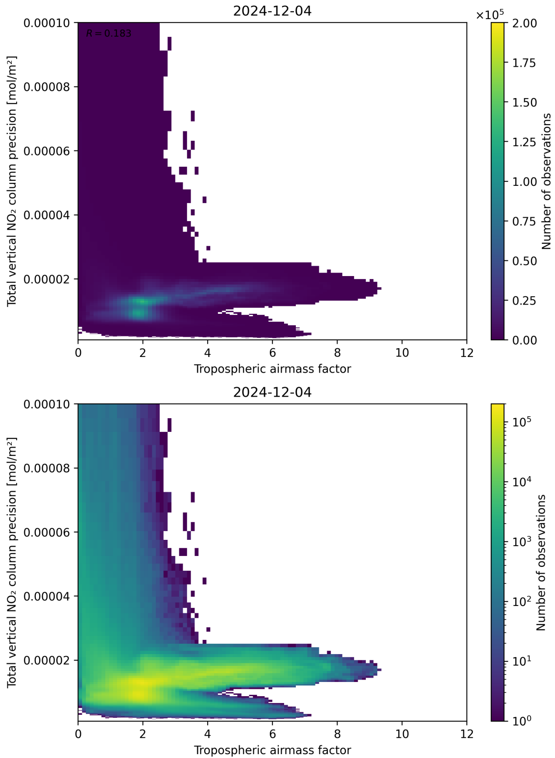
Figure 78: Scatter density plot of “Tropospheric air mass factor” against “Total vertical NO 2 column precision” for 2024-12-03 to 2024-12-05.
