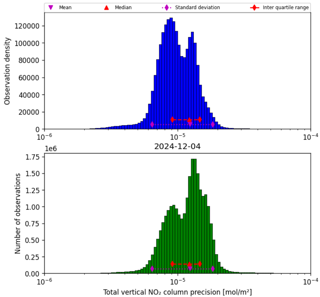
Figure 39: Histogram of "Total vertical NO 2 column precision" for 2024-12-03 to 2024-12-05
