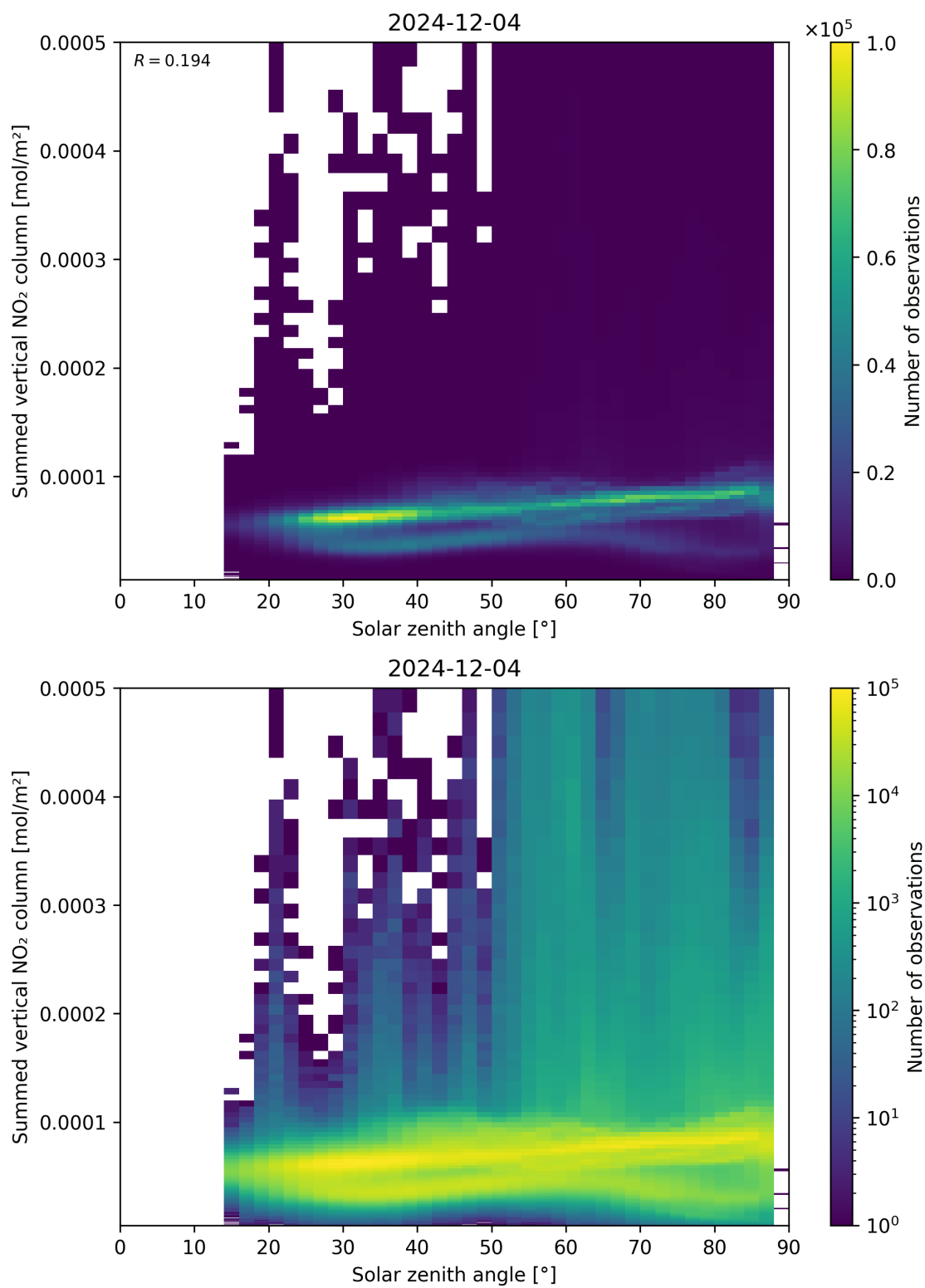
Figure 151: Scatter density plot of “Solar zenith angle” against “Summed vertical NO 2 column” for 2024-12-03 to 2024-12-05.
