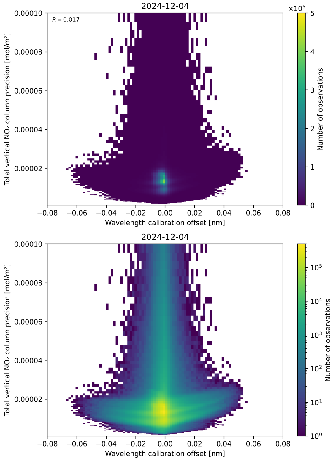
Figure 180: Scatter density plot of “Wavelength calibration offset” against “Total vertical NO 2 column precision” for 2024-12-03 to 2024-12-05.
