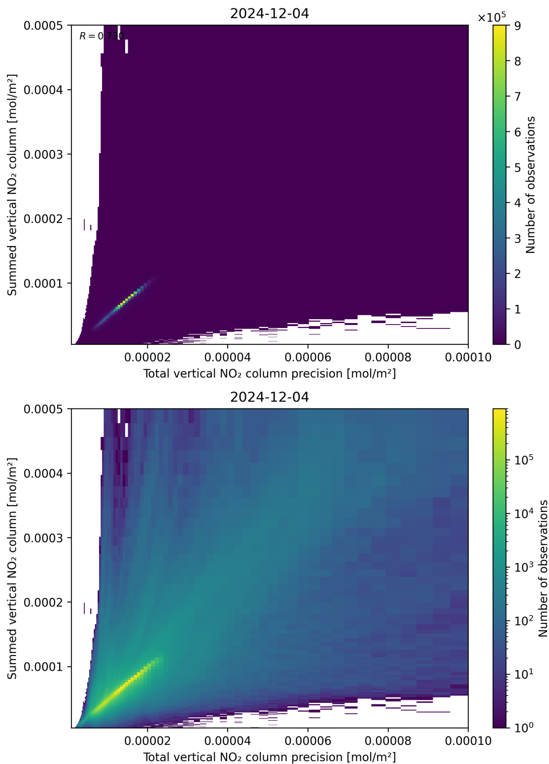
Figure 117: Scatter density plot of “Total vertical NO 2 column precision” against “Summed vertical NO 2 column” for 2024-12-03 to 2024-12-05.
