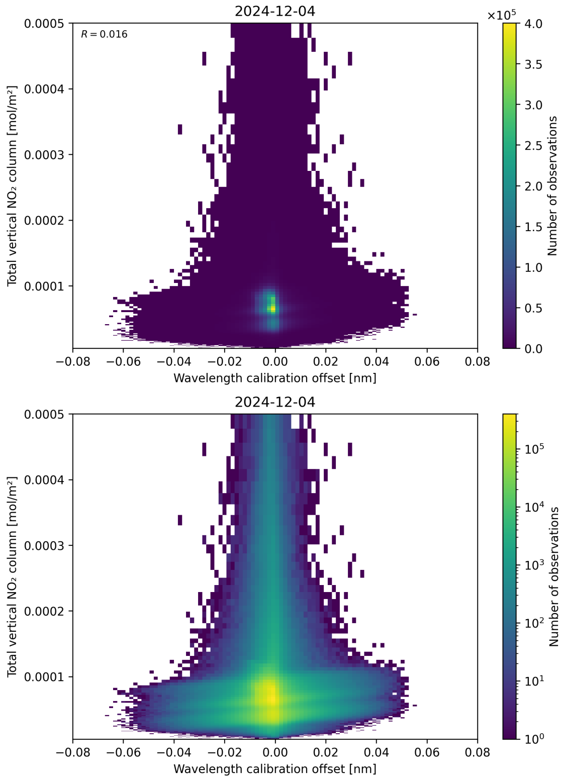
Figure 179: Scatter density plot of “Wavelength calibration offset” against “Total vertical NO 2 column” for 2024-12-03 to 2024-12-05.
