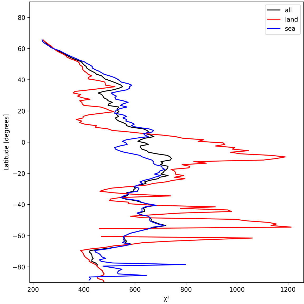
Figure 25: Zonal average of “ \chi^2 ” for 2024-12-03 to 2024-12-05.
