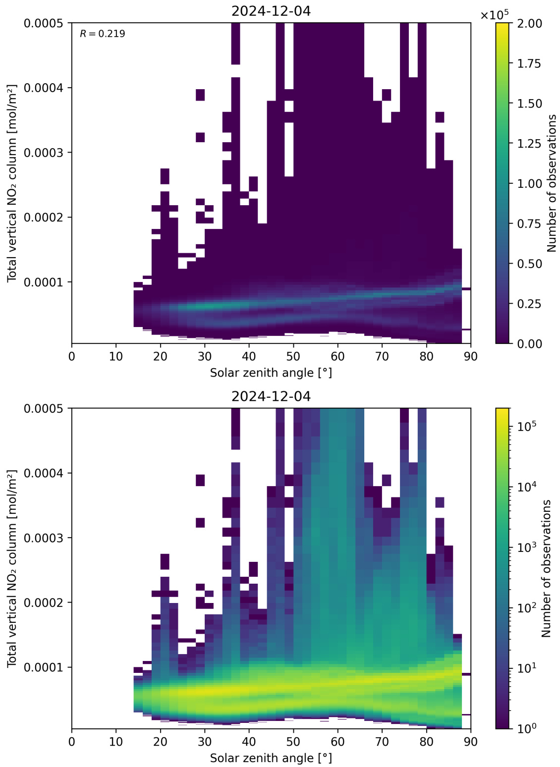
Figure 153: Scatter density plot of “Solar zenith angle” against “Total vertical NO 2 column” for 2024-12-03 to 2024-12-05.
