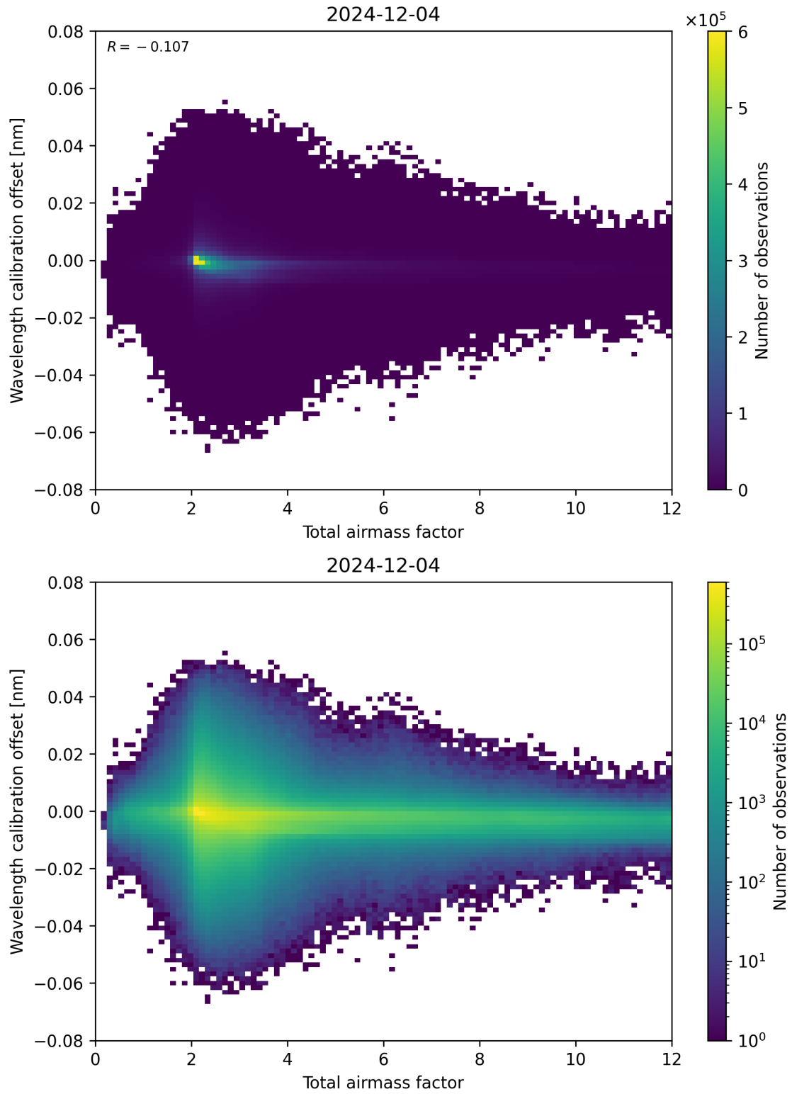
Figure 70: Scatter density plot of “Total airmass factor” against “Wavelength calibration offset” for 2024-12-03 to 2024-12-05.
