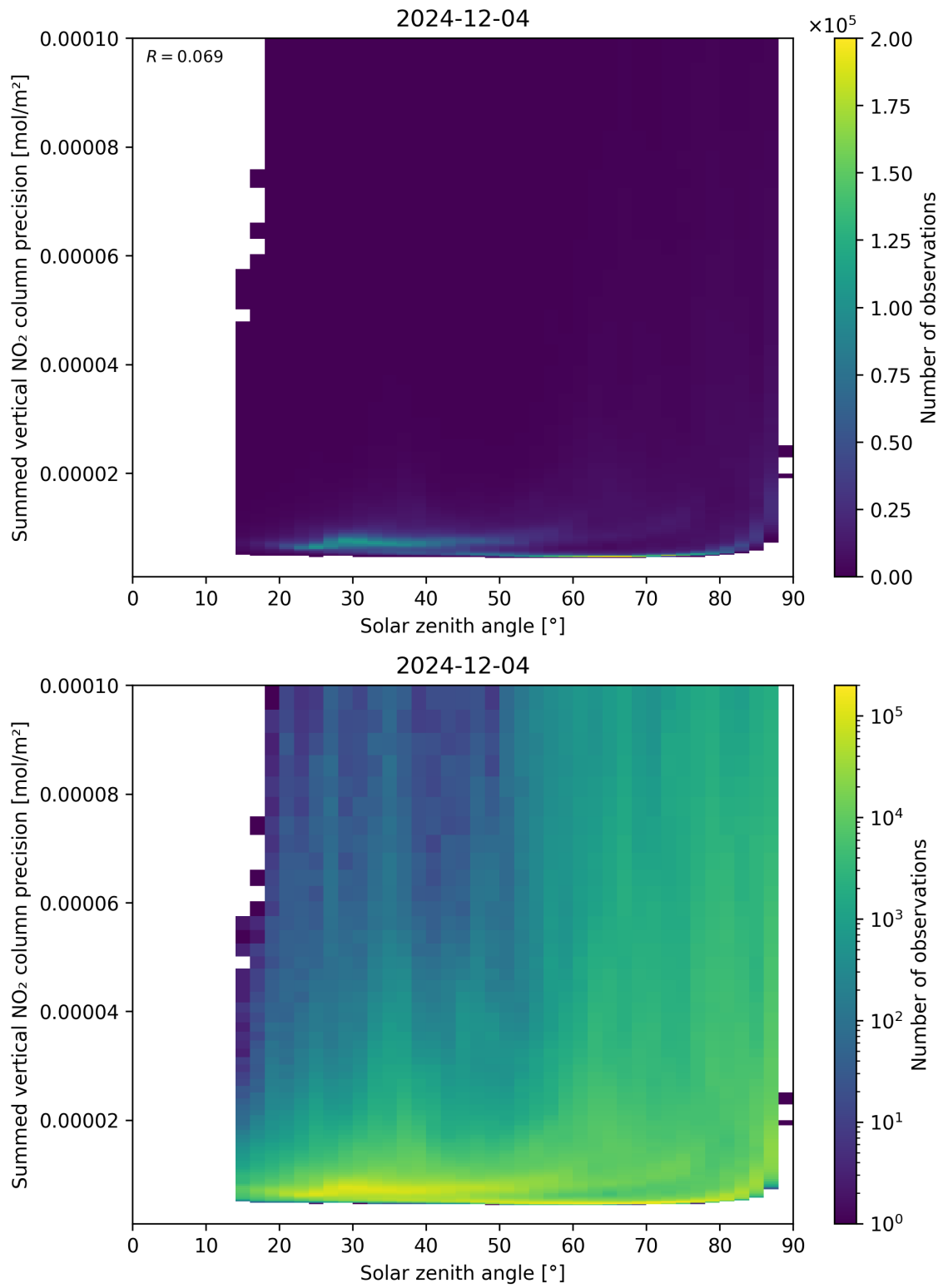
Figure 152: Scatter density plot of “Solar zenith angle” against “Summed vertical NO 2 column precision” for 2024-12-03 to 2024-12-05.
