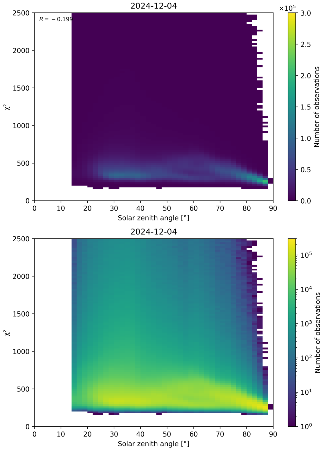
Figure 148: Scatter density plot of “Solar zenith angle” against “ \chi^2 ” for 2024-12-03 to 2024-12-05.
