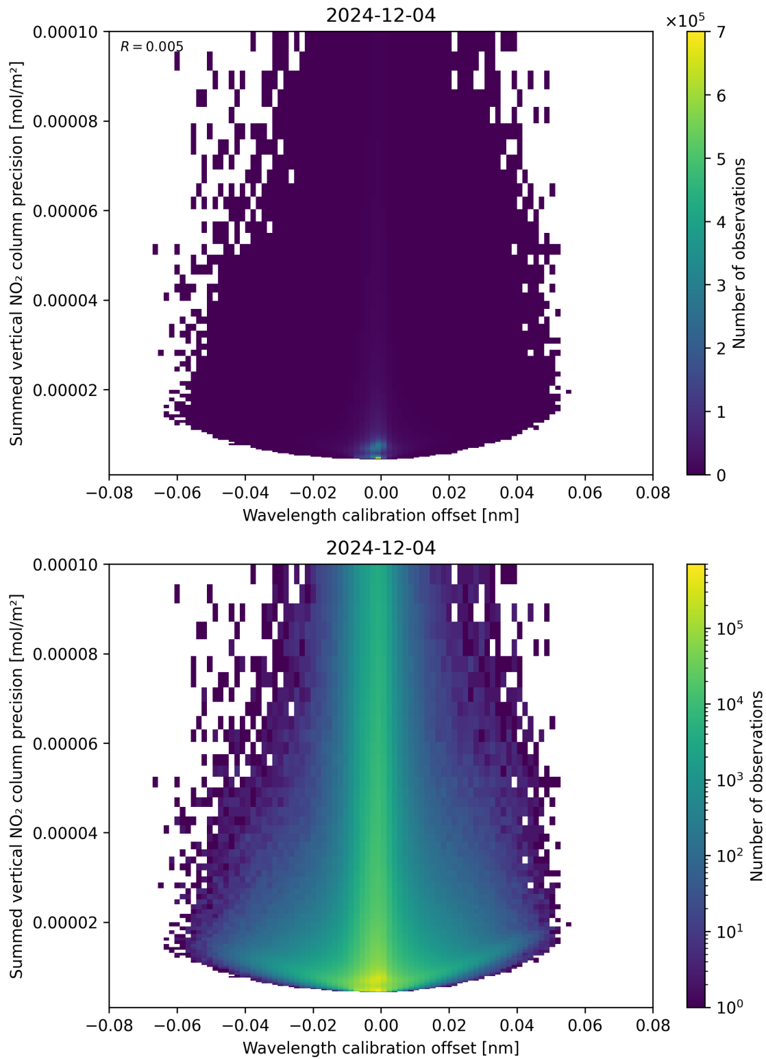
Figure 178: Scatter density plot of “Wavelength calibration offset” against “Summed vertical NO 2 column precision” for 2024-12-03 to 2024-12-05.
