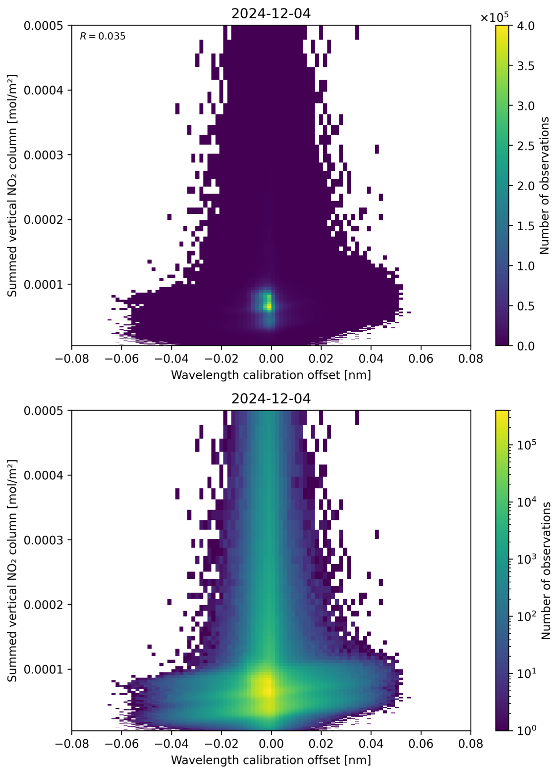
Figure 177: Scatter density plot of “Wavelength calibration offset” against “Summed vertical NO 2 column” for 2024-12-03 to 2024-12-05.
