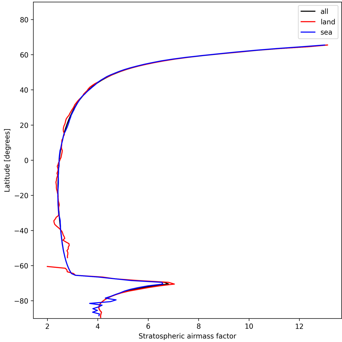
Figure 27: Zonal average of “Stratospheric airmass factor” for 2024-12-03 to 2024-12-05.
