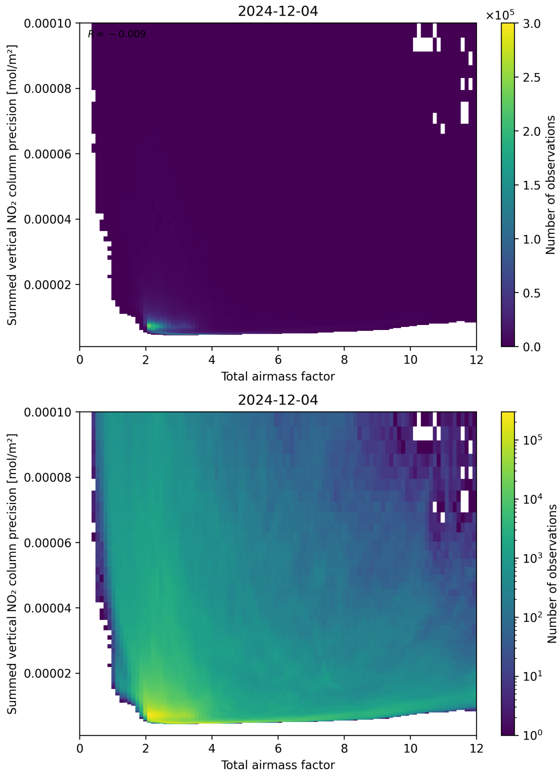
Figure 66: Scatter density plot of “Total airmass factor” against “Summed vertical NO 2 column precision” for 2024-12-03 to 2024-12-05.
