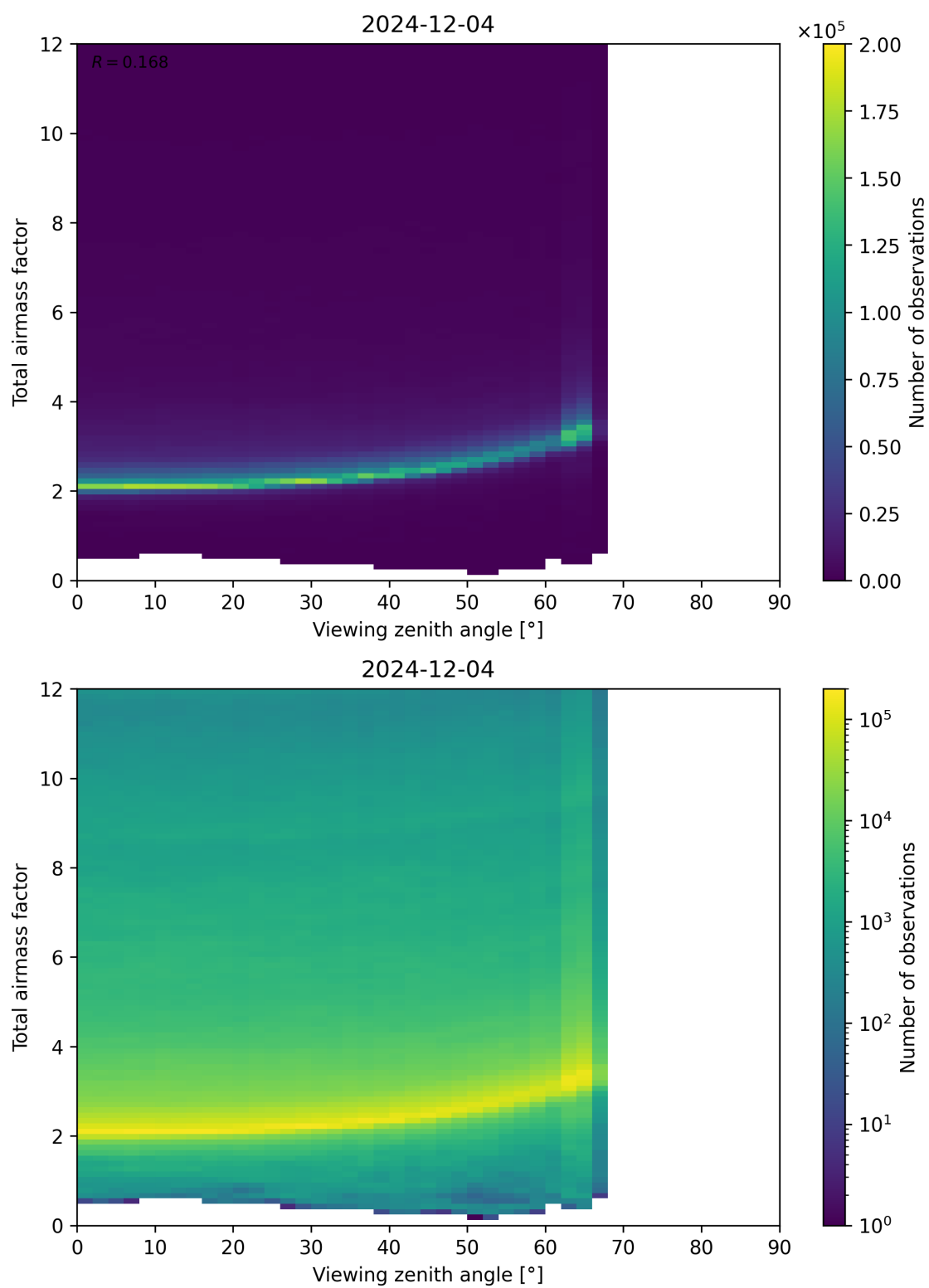
Figure 160: Scatter density plot of “Viewing zenith angle” against “Total airmass factor” for 2024-12-03 to 2024-12-05.
