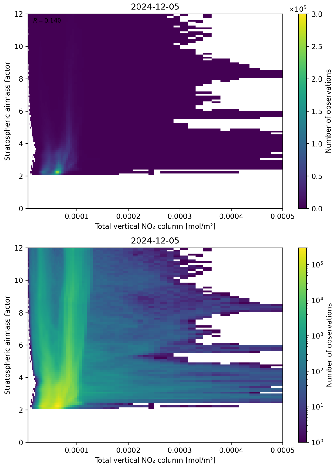
Figure 110: Scatter density plot of “Total vertical NO 2 column” against “Stratospheric airmass factor” for 2024-12-04 to 2024-12-06.
