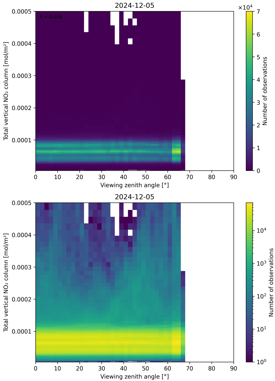
Figure 167: Scatter density plot of “Viewing zenith angle” against “Total vertical NO 2 column” for 2024-12-04 to 2024-12-06.
