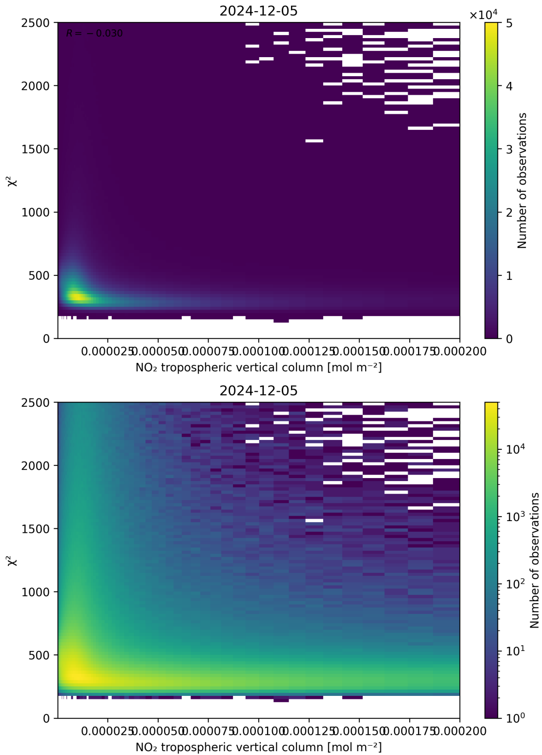
Figure 124: Scatter density plot of “NO 2 tropospheric vertical column” against “ \chi^2 ” for 2024-12-04 to 2024-12-06.
