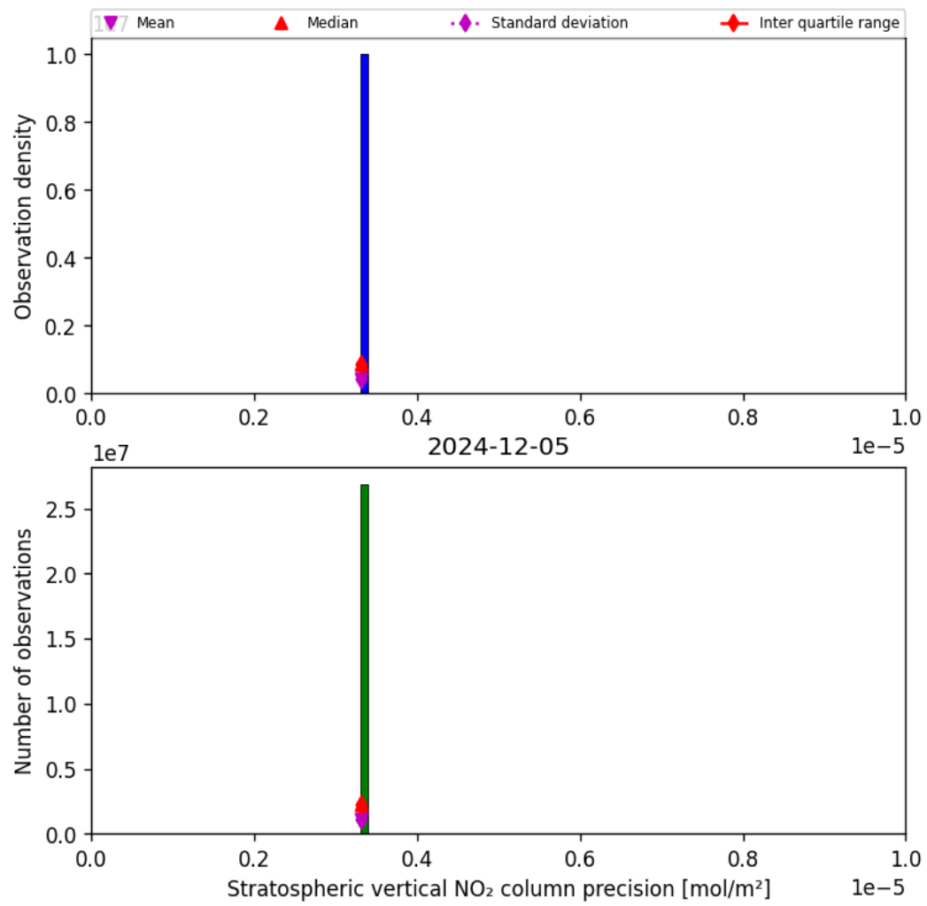
Figure 37: Histogram of “Stratospheric vertical NO 2 column precision” for 2024-12-04 to 2024-12-06
