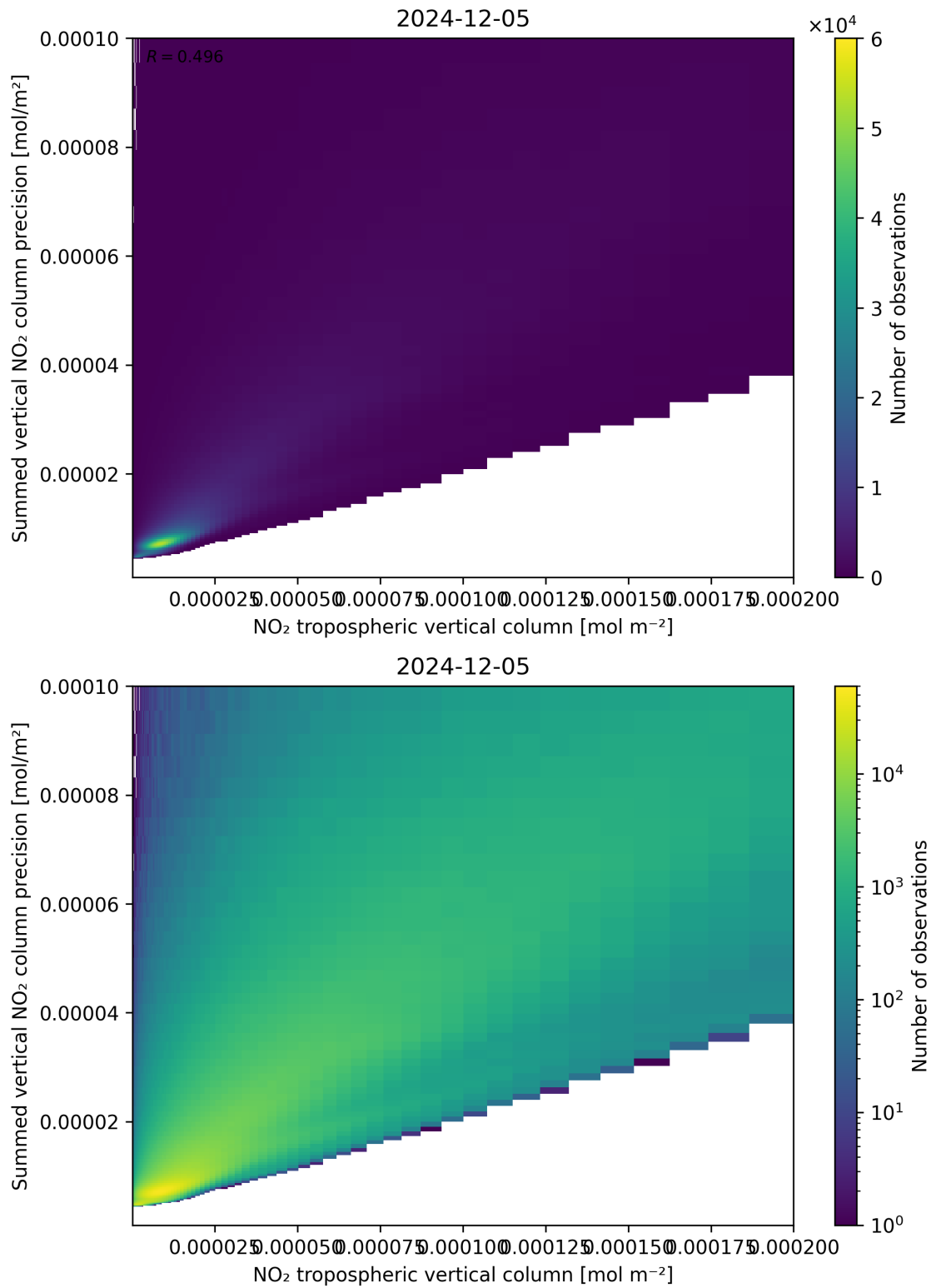
Figure 127: Scatter density plot of “NO 2 tropospheric vertical column” against “Summed vertical NO 2 column precision” for 2024-12-04 to 2024-12-06.
