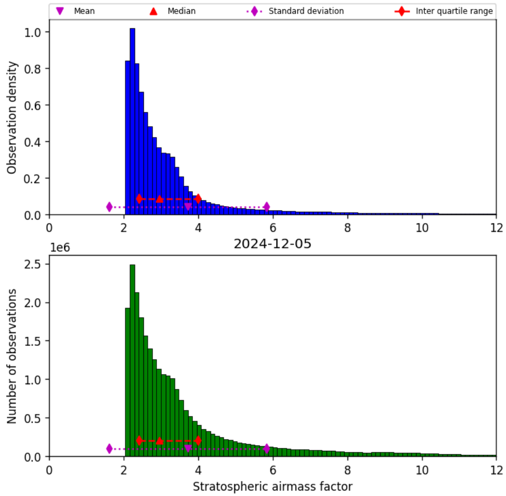
Figure 44: Histogram of “Stratospheric airmass factor” for 2024-12-04 to 2024-12-06
