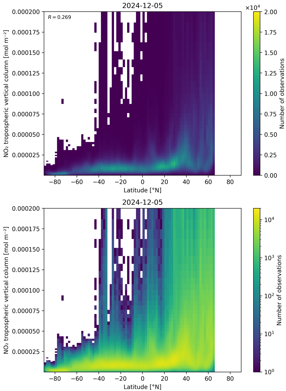
Figure 92: Scatter density plot of “Latitude” against “NO 2 tropospheric vertical column” for 2024-12-04 to 2024-12-06.
