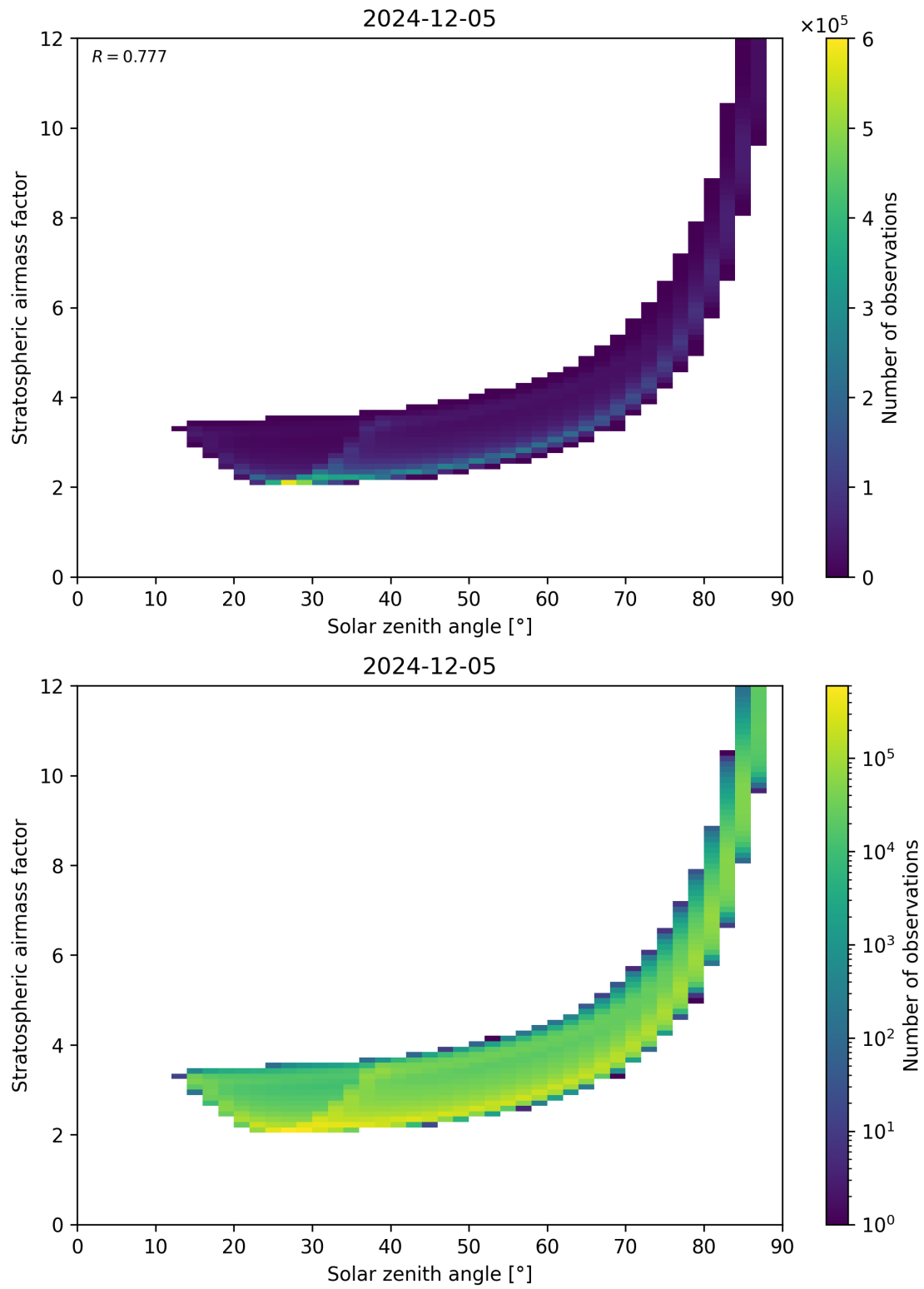
Figure 145: Scatter density plot of “Solar zenith angle” against “Stratospheric airmass factor” for 2024-12-04 to 2024-12-06.
