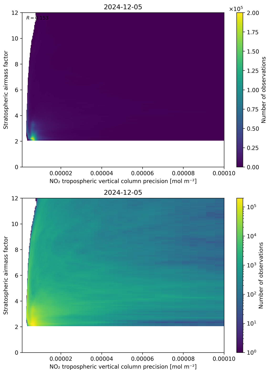
Figure 131: Scatter density plot of “NO 2 tropospheric vertical column precision” against “Stratospheric airmass factor” for 2024-12-04 to 2024-12-06.
