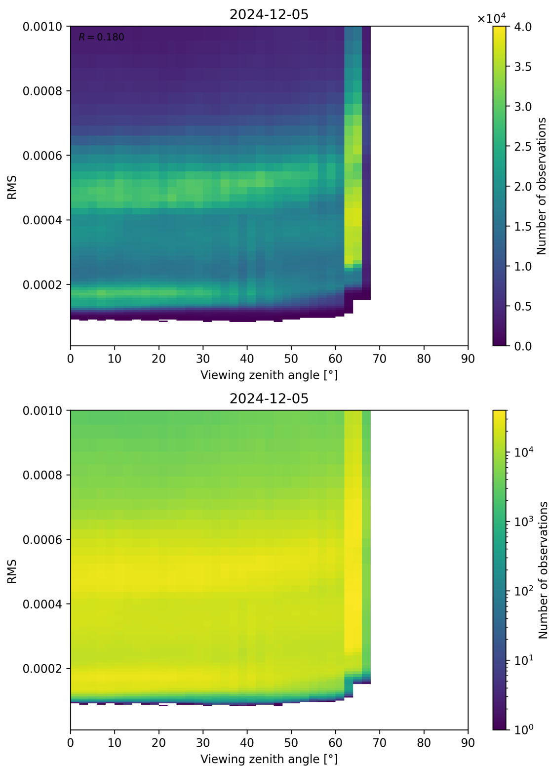
Figure 171: Scatter density plot of “Viewing zenith angle” against “RMS” for 2024-12-04 to 2024-12-06.
