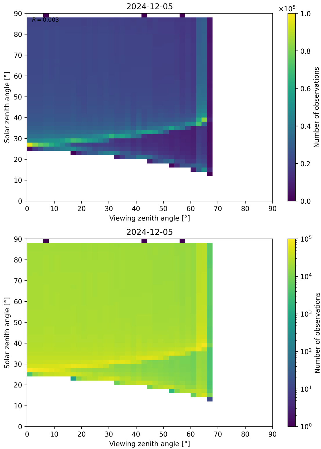
Figure 172: Scatter density plot of “Viewing zenith angle” against “Solar zenith angle” for 2024-12-04 to 2024-12-06.
