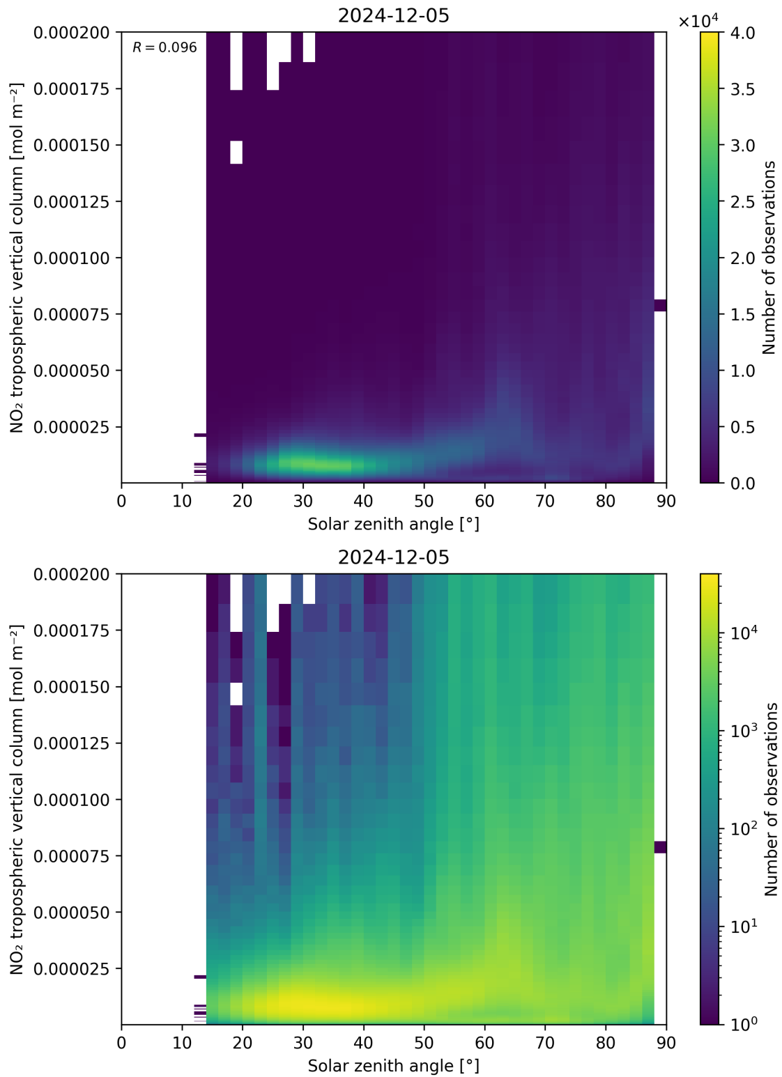
Figure 155: Scatter density plot of “Solar zenith angle” against “NO 2 tropospheric vertical column” for 2024-12-04 to 2024-12-06.
