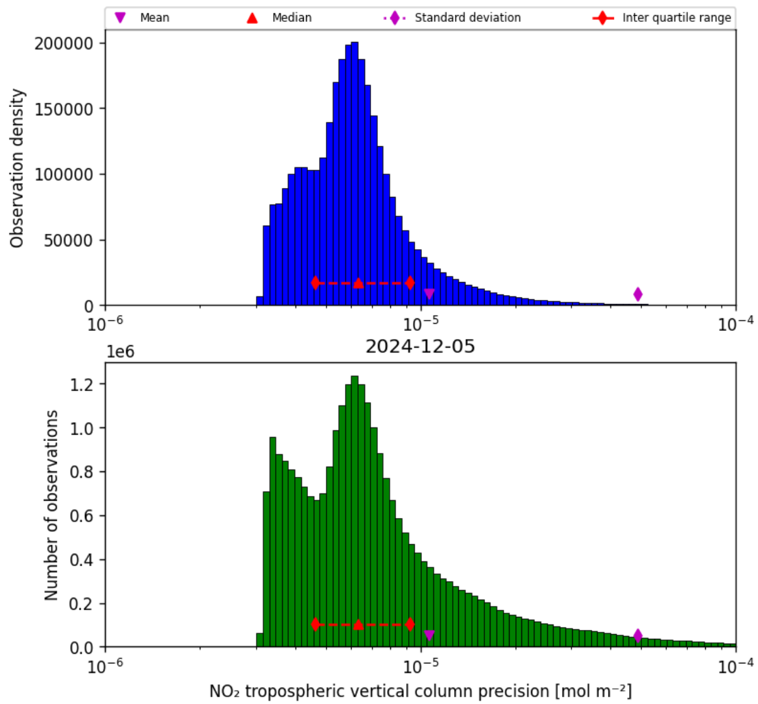
Figure 30: Histogram of “NO 2 tropospheric vertical column precision” for 2024-12-04 to 2024-12-06
