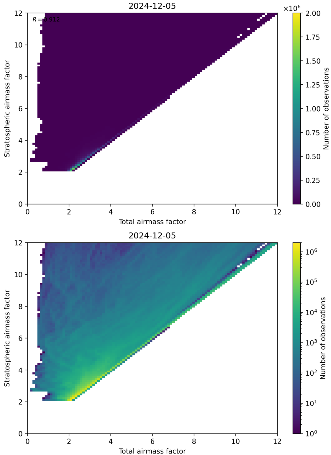
Figure 62: Scatter density plot of “Total airmass factor” against “Stratospheric airmass factor” for 2024-12-04 to 2024-12-06.
