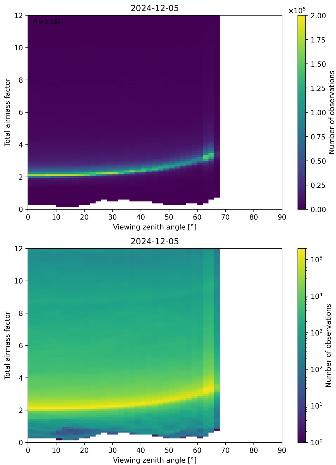
Figure 160: Scatter density plot of “Viewing zenith angle” against “Total airmass factor” for 2024-12-04 to 2024-12-06.
