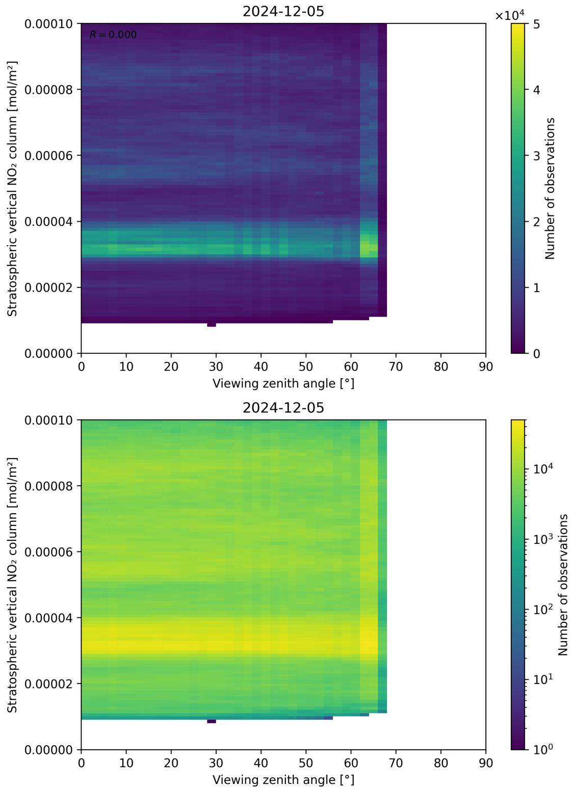
Figure 164: Scatter density plot of “Viewing zenith angle” against “Stratospheric vertical NO 2 column” for 2024-12-04 to 2024-12-06.
