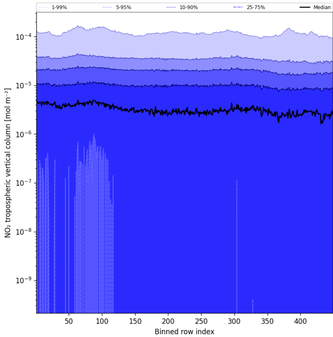
Figure 46: Along track statistics of “ \text{NO}_2 tropospheric vertical column” for 2024-12-04 to 2024-12-06
