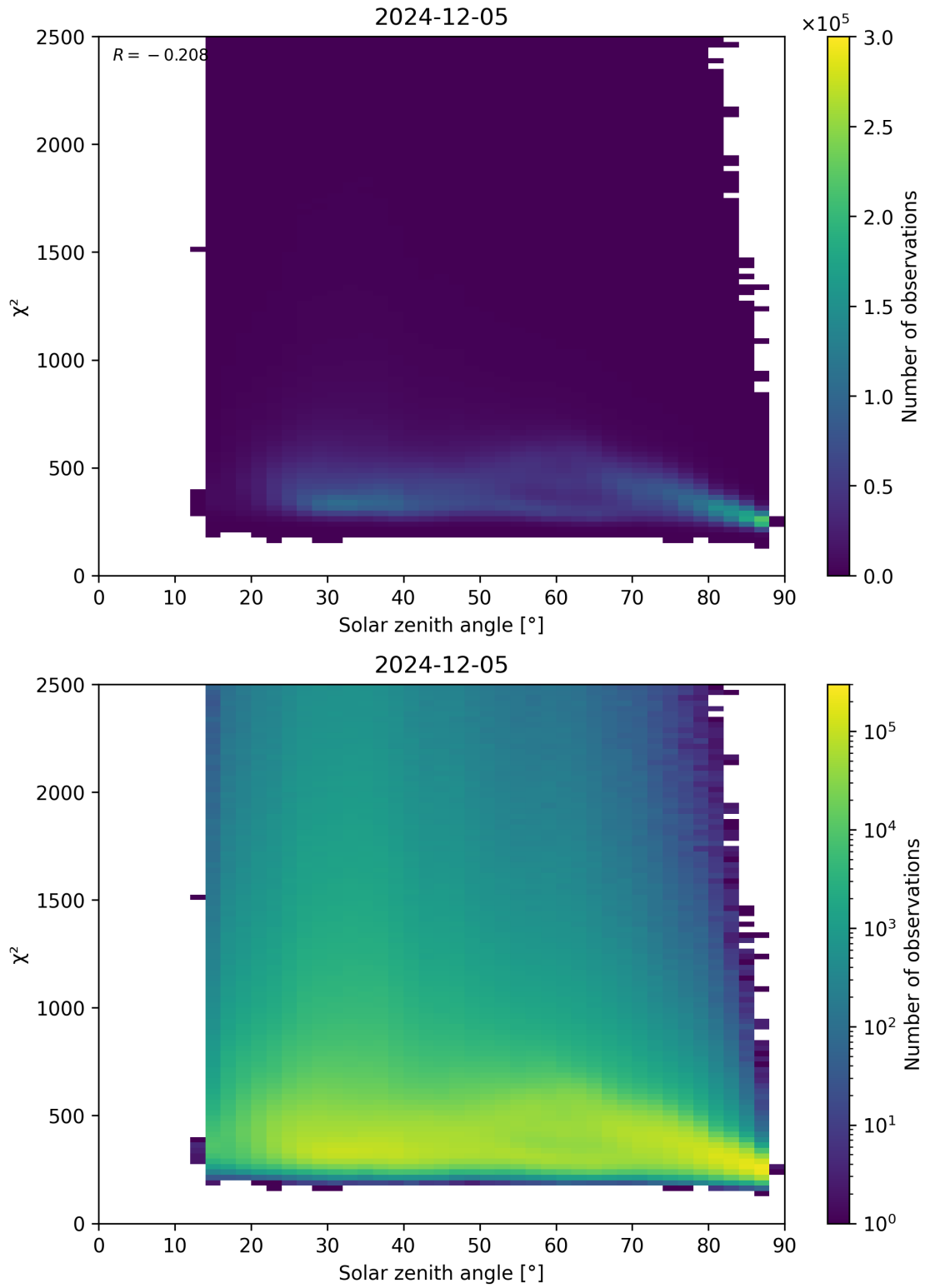
Figure 148: Scatter density plot of “Solar zenith angle” against “ \chi^2 ” for 2024-12-04 to 2024-12-06.
