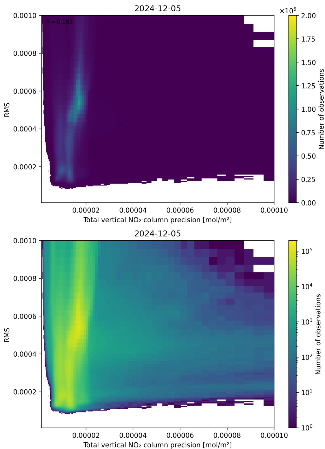
Figure 119: Scatter density plot of “Total vertical NO 2 column precision” against “RMS” for 2024-12-04 to 2024-12-06.
