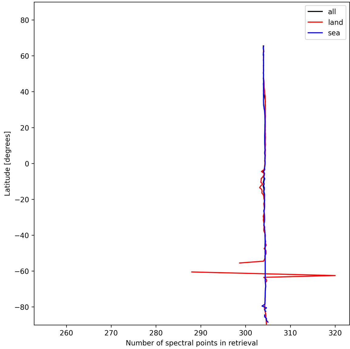
Figure 16: Zonal average of “Number of spectral points in retrieval” for 2024-12-04 to 2024-12-06.
