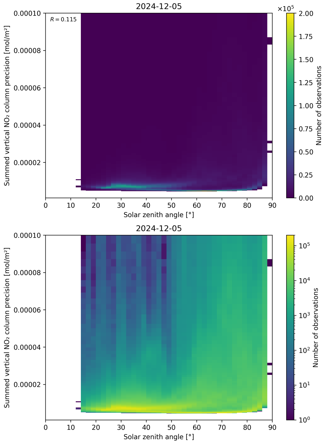
Figure 152: Scatter density plot of “Solar zenith angle” against “Summed vertical NO 2 column precision” for 2024-12-04 to 2024-12-06.
