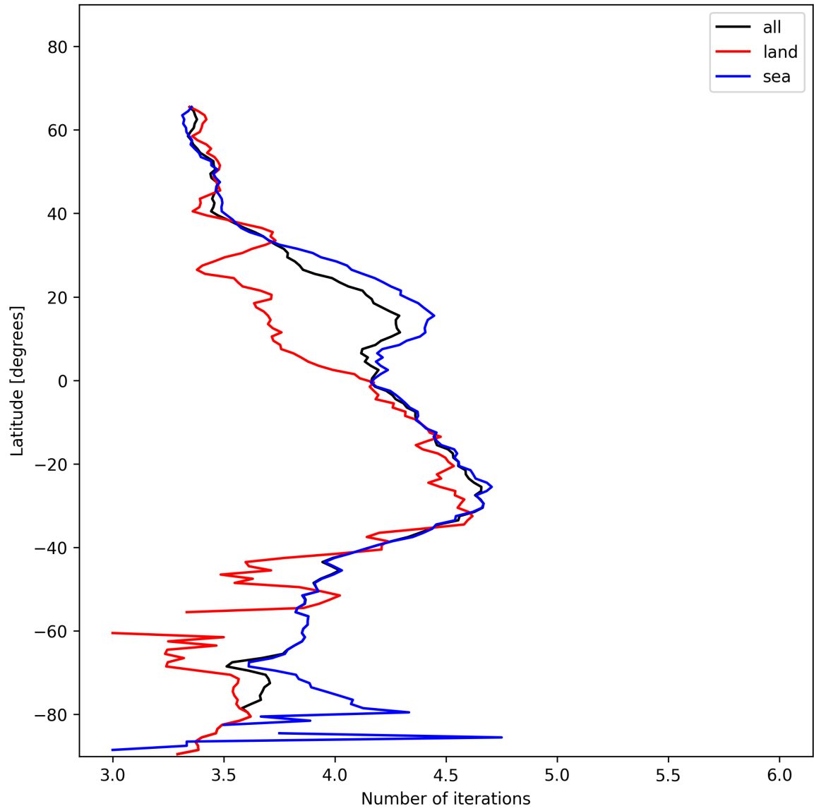
Figure 17: Zonal average of “Number of iterations” for 2024-12-04 to 2024-12-06.
