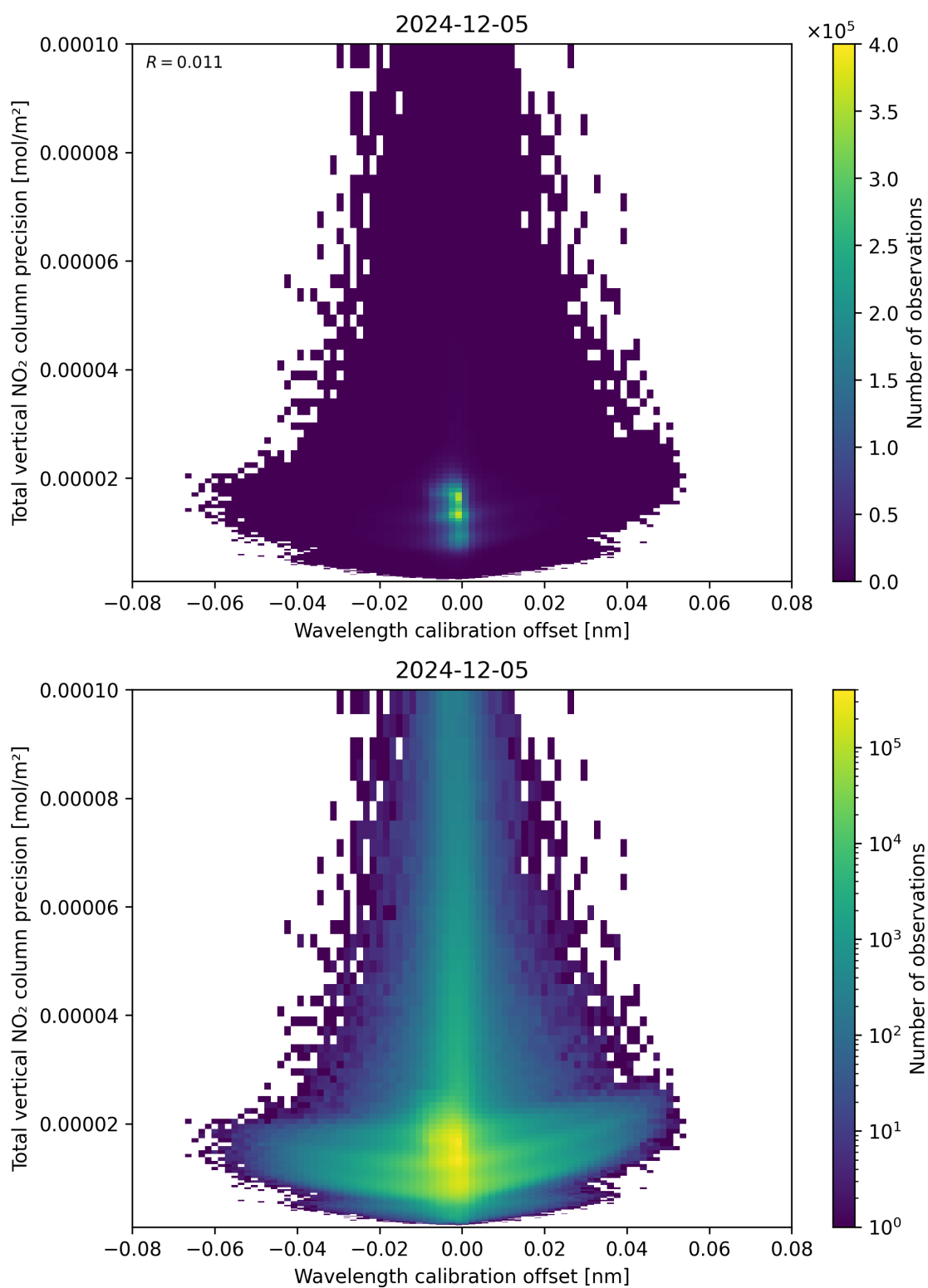
Figure 180: Scatter density plot of “Wavelength calibration offset” against “Total vertical NO 2 column precision” for 2024-12-04 to 2024-12-06.
