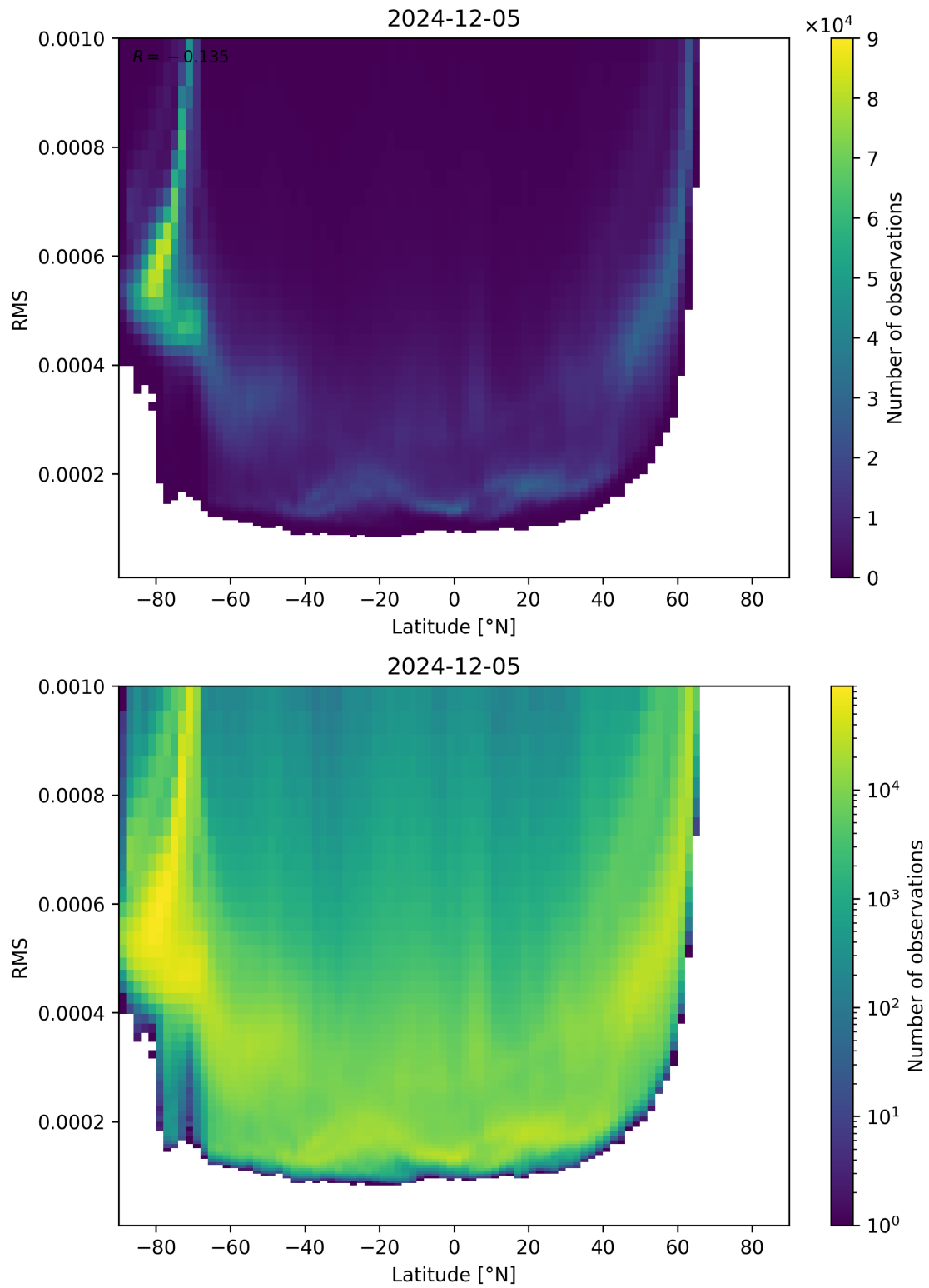
Figure 94: Scatter density plot of “Latitude” against “RMS” for 2024-12-04 to 2024-12-06.
