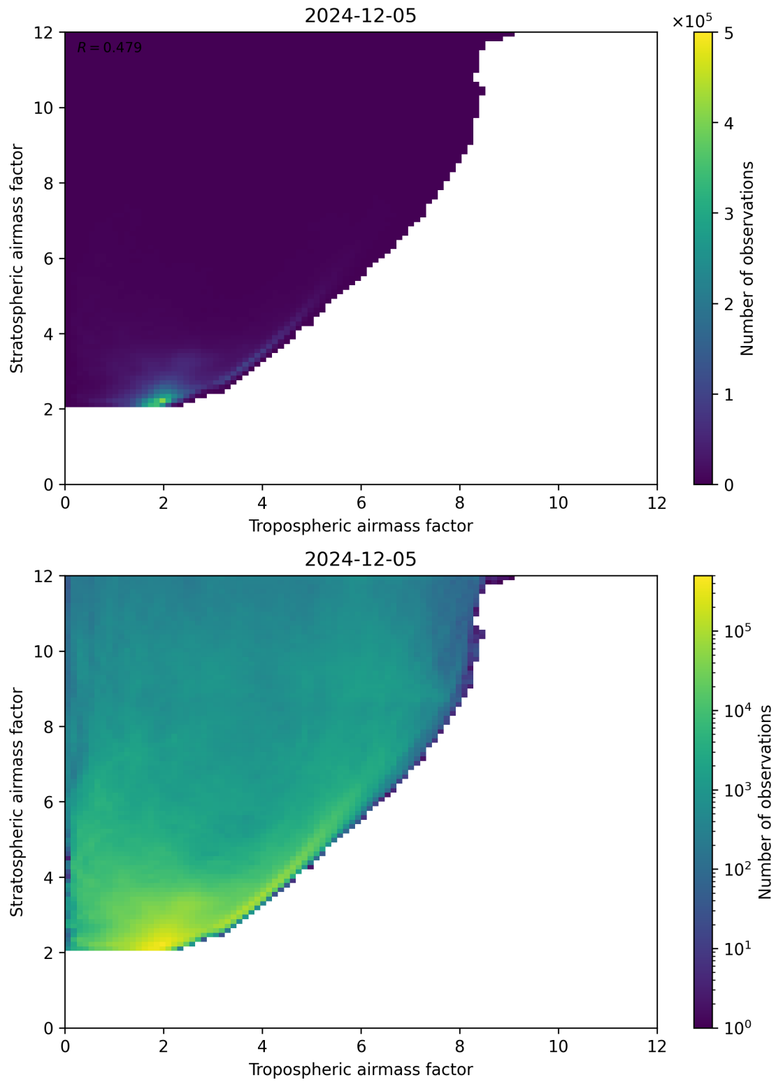
Figure 71: Scatter density plot of “Tropospheric airmass factor” against “Stratospheric airmass factor” for 2024-12-04 to 2024-12-06.
