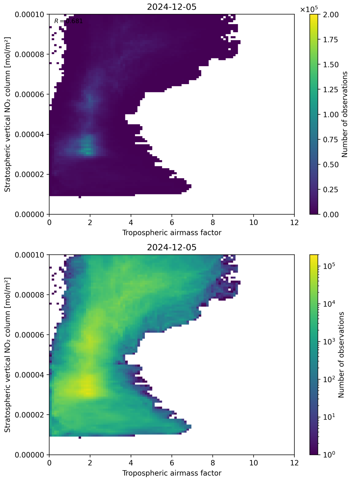
Figure 74: Scatter density plot of “Tropospheric air mass factor” against “Stratospheric vertical NO 2 column” for 2024-12-04 to 2024-12-06.
