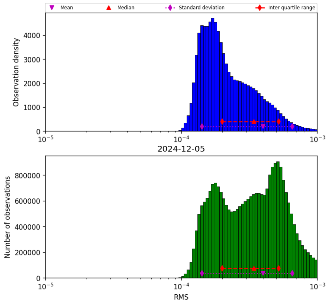
Figure 43: Histogram of “RMS” for 2024-12-04 to 2024-12-06
