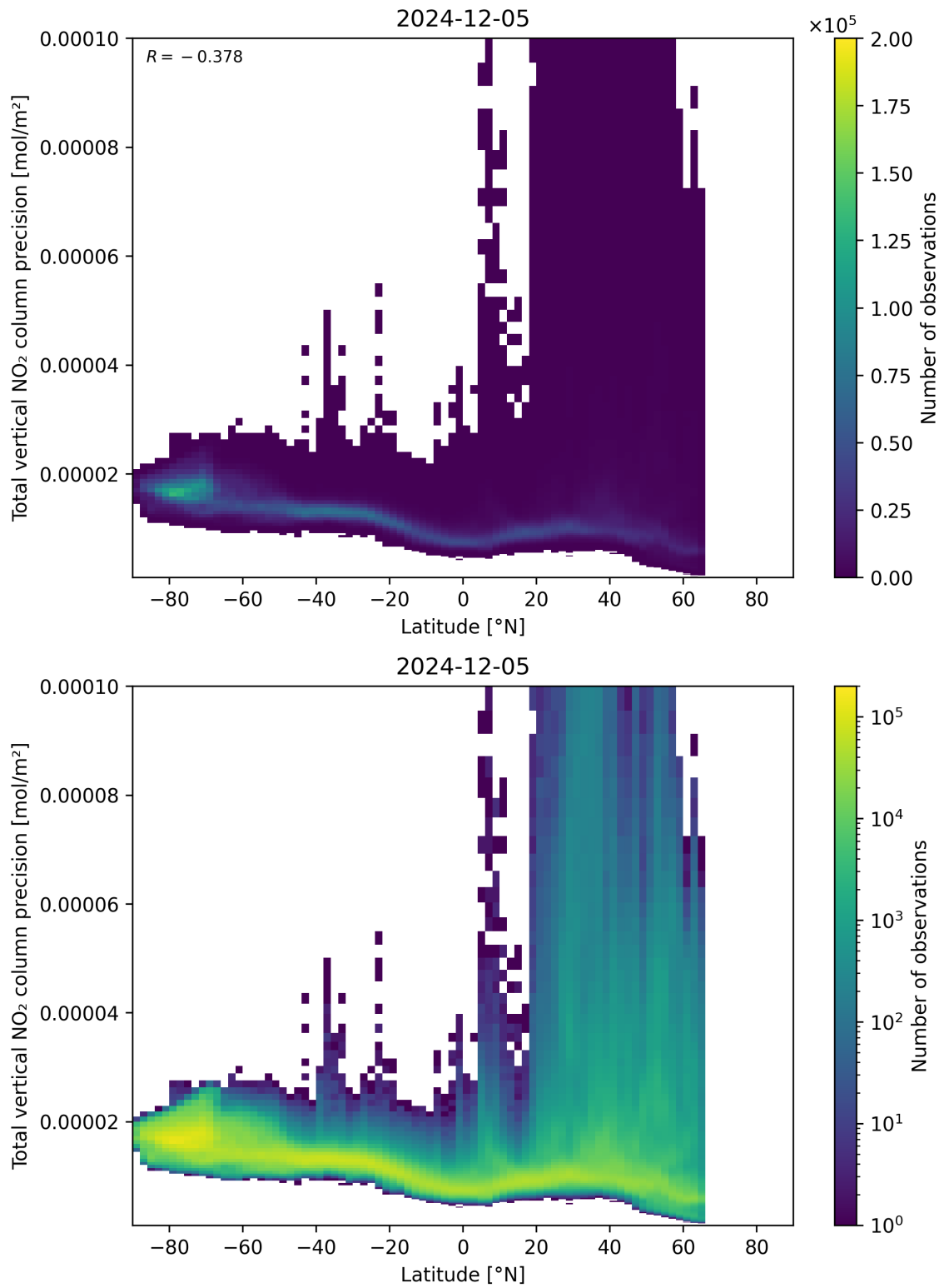
Figure 91: Scatter density plot of “Latitude” against “Total vertical NO 2 column precision” for 2024-12-04 to 2024-12-06.
