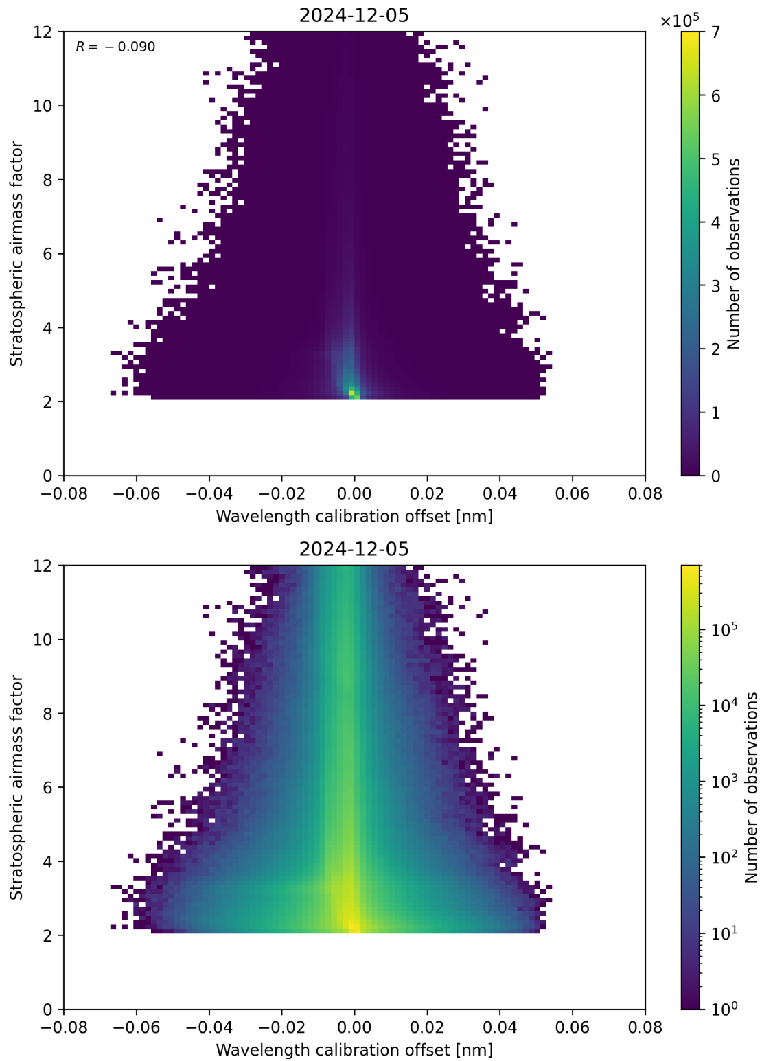
Figure 174: Scatter density plot of “Wavelength calibration offset” against “Stratospheric airmass factor” for 2024-12-04 to 2024-12-06.
