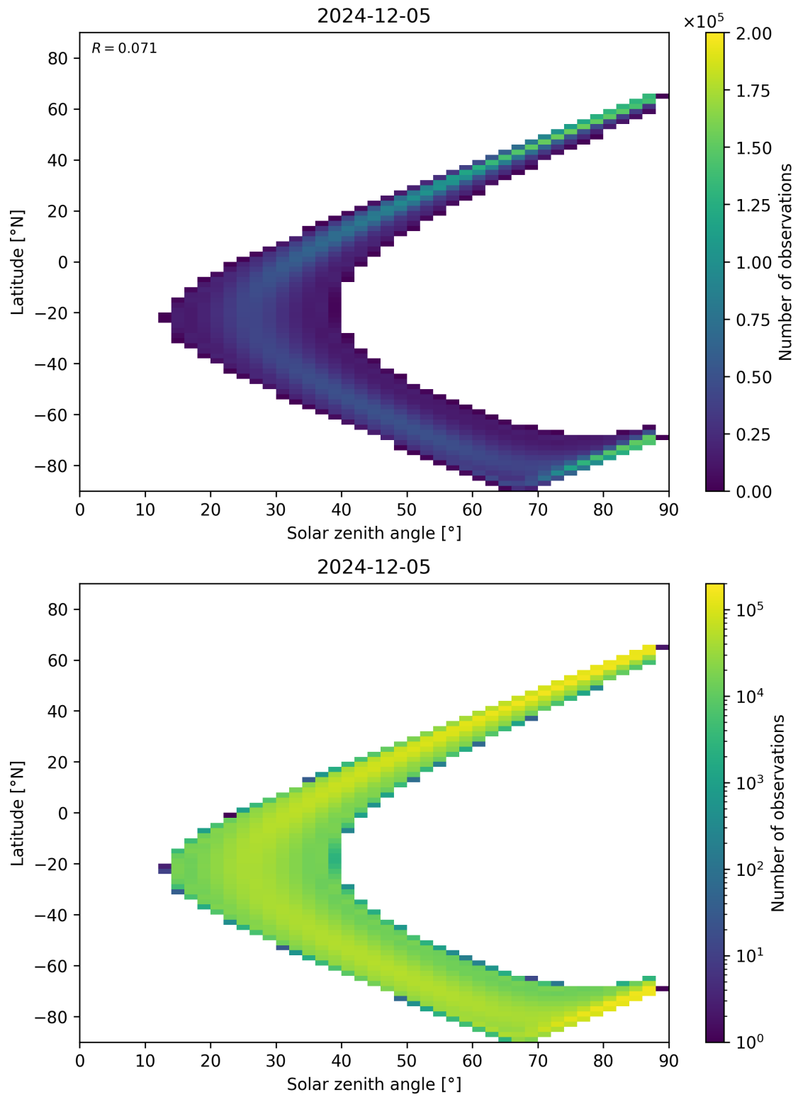
Figure 149: Scatter density plot of “Solar zenith angle” against “Latitude” for 2024-12-04 to 2024-12-06.
