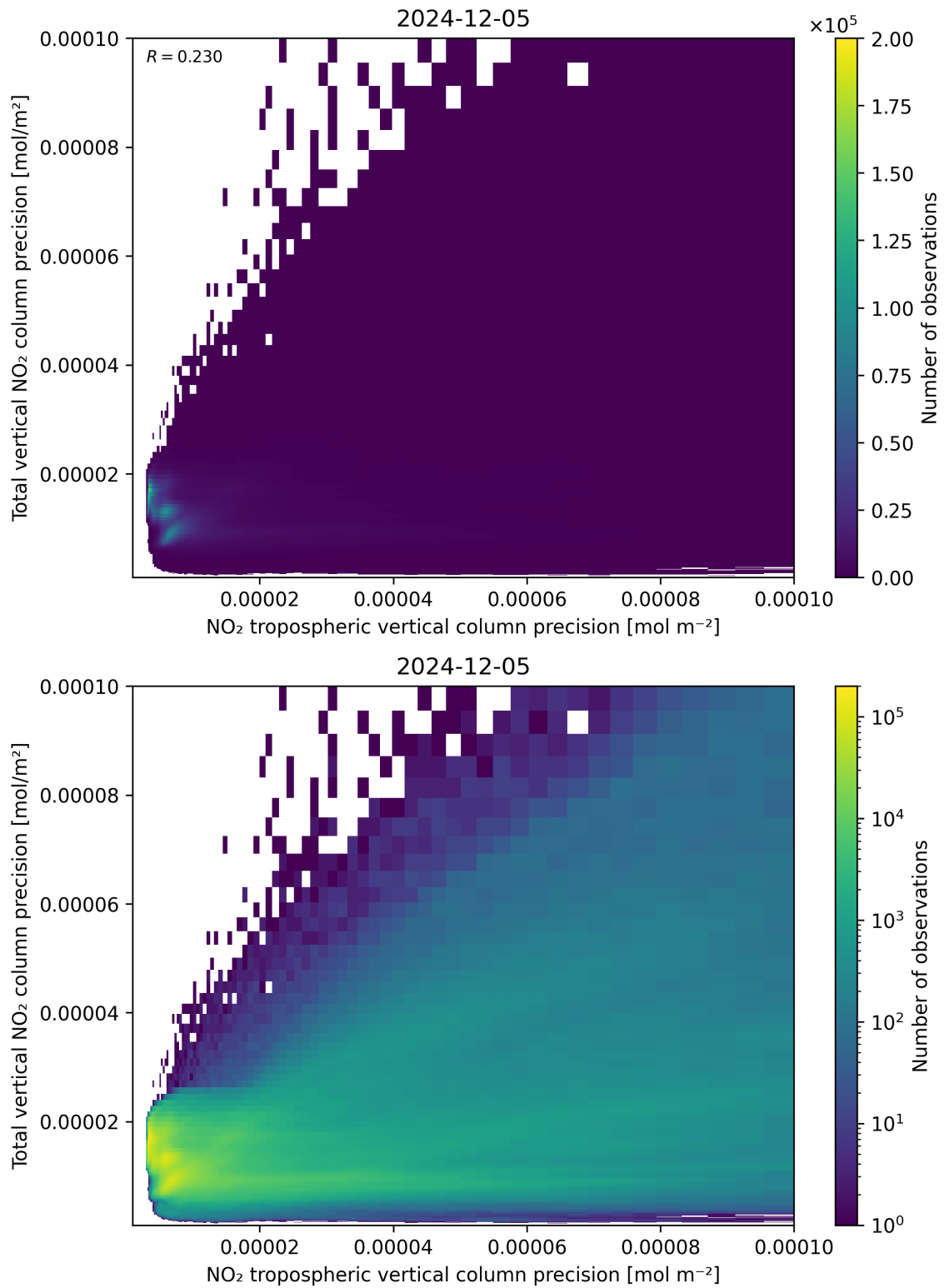
Figure 139: Scatter density plot of “NO 2 tropospheric vertical column precision” against “Total vertical NO 2 column precision” for 2024-12-04 to 2024-12-06.
