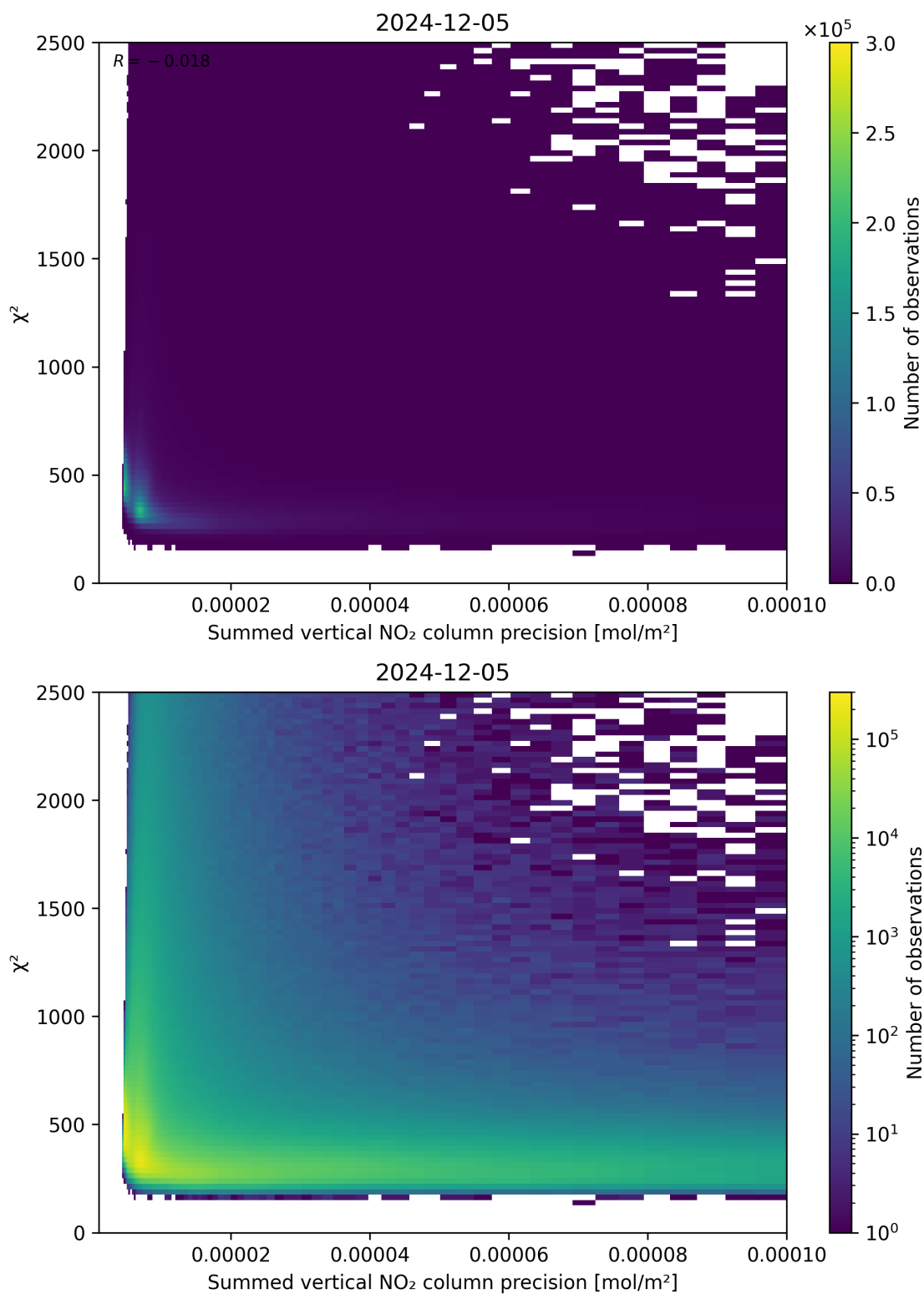
Figure 107: Scatter density plot of “Summed vertical NO 2 column precision” against “ \chi^2 ” for 2024-12-04 to 2024-12-06.
