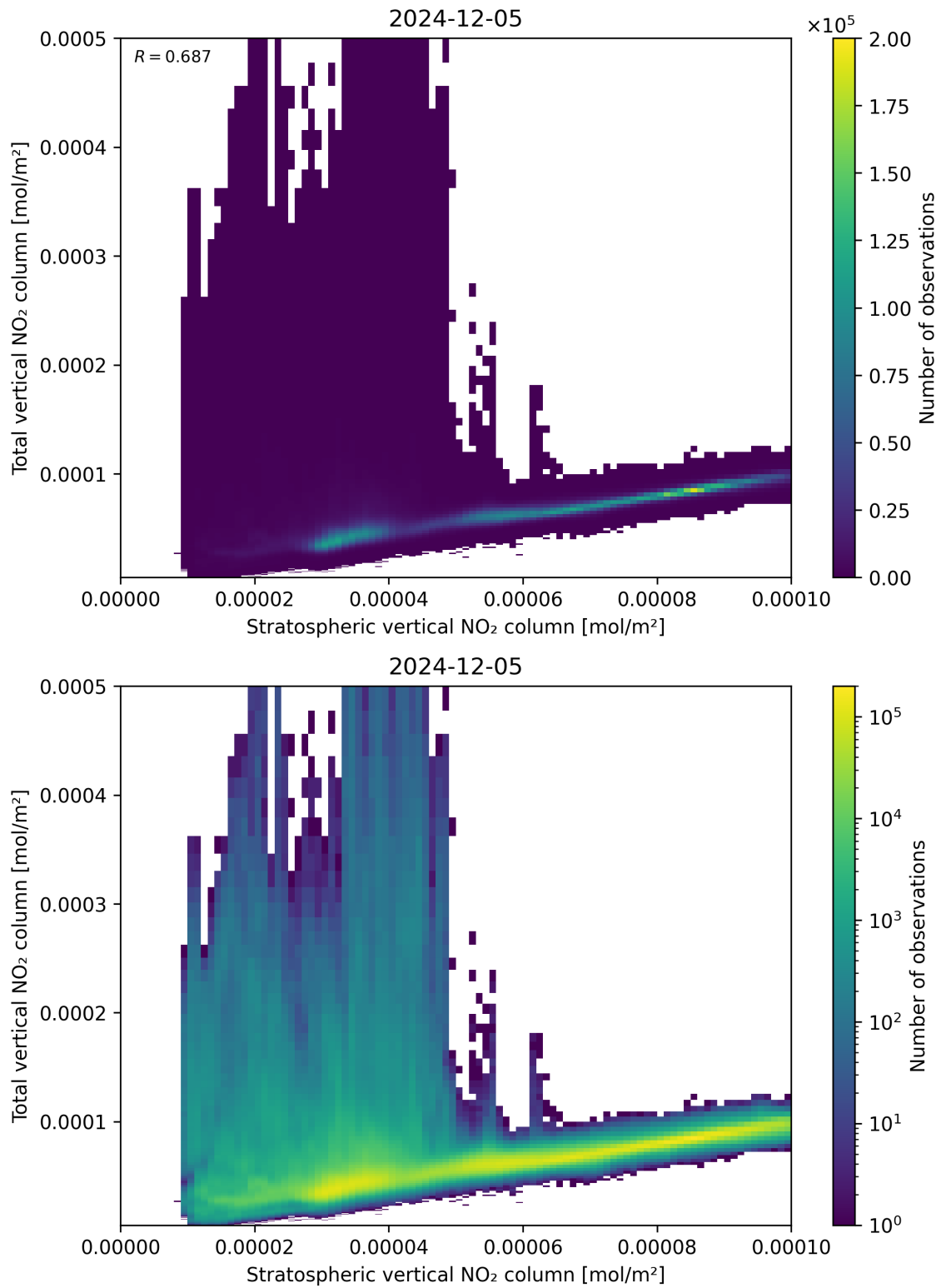
Figure 100: Scatter density plot of “Stratospheric vertical NO 2 column” against “Total vertical NO 2 column” for 2024-12-04 to 2024-12-06.
