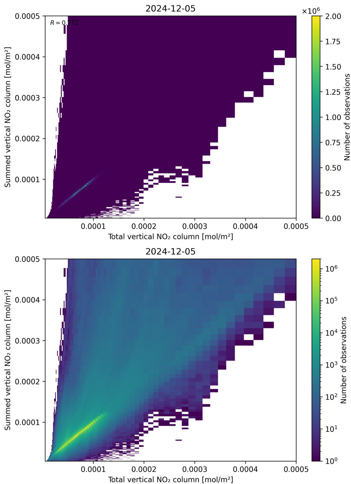
Figure 112: Scatter density plot of “Total vertical NO 2 column” against “Summed vertical NO 2 column” for 2024-12-04 to 2024-12-06.
