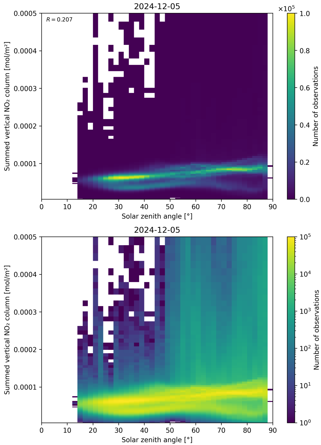
Figure 151: Scatter density plot of “Solar zenith angle” against “Summed vertical NO 2 column” for 2024-12-04 to 2024-12-06.
