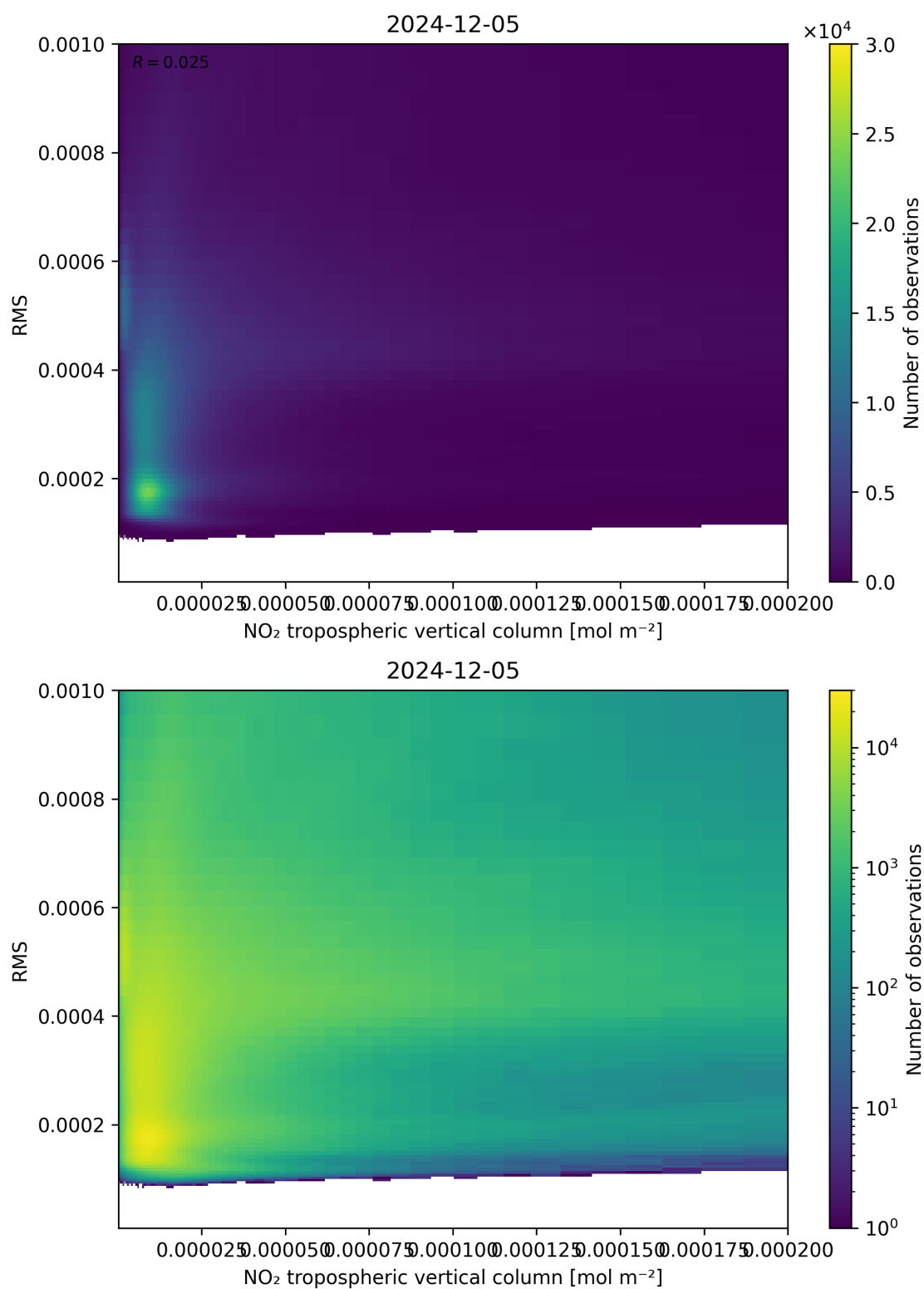
Figure 142: Scatter density plot of “NO 2 tropospheric vertical column” against “RMS” for 2024-12-04 to 2024-12-06.
