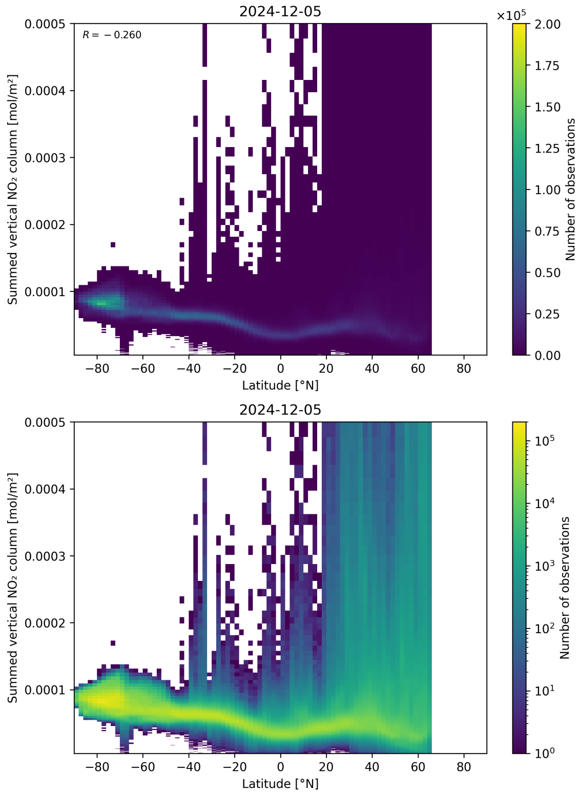
Figure 88: Scatter density plot of “Latitude” against “Summed vertical NO 2 column” for 2024-12-04 to 2024-12-06.
