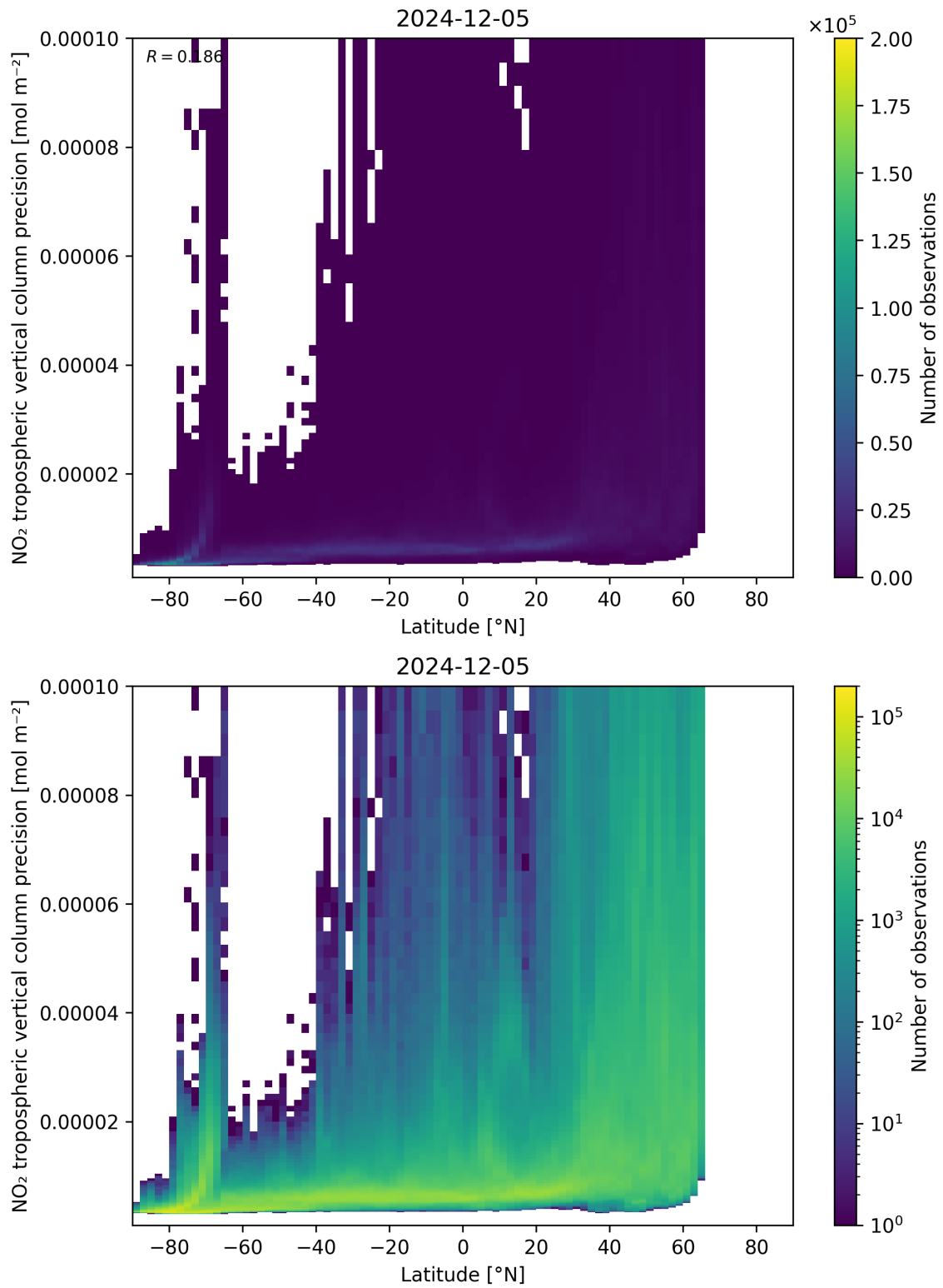
Figure 93: Scatter density plot of “Latitude” against “NO 2 tropospheric vertical column precision” for 2024-12-04 to 2024-12-06.
