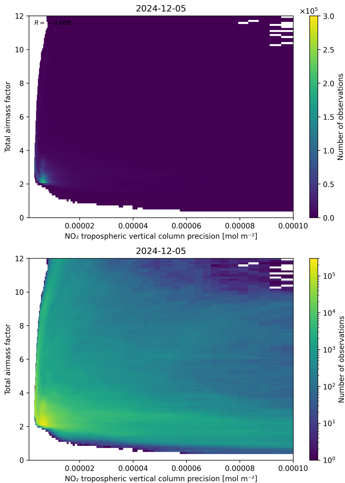
Figure 132: Scatter density plot of “NO 2 tropospheric vertical column precision” against “Total airmass factor” for 2024-12-04 to 2024-12-06.
