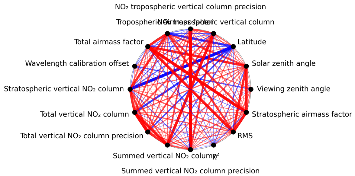
Figure 1: Map of correlation graph for 2024-12-04 to 2024-12-06.
