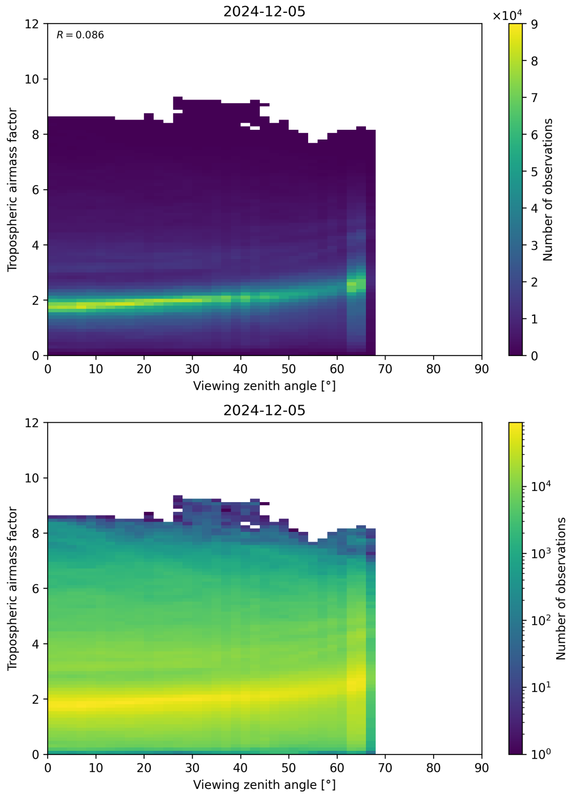
Figure 161: Scatter density plot of “Viewing zenith angle” against “Tropospheric airmass factor” for 2024-12-04 to 2024-12-06.
