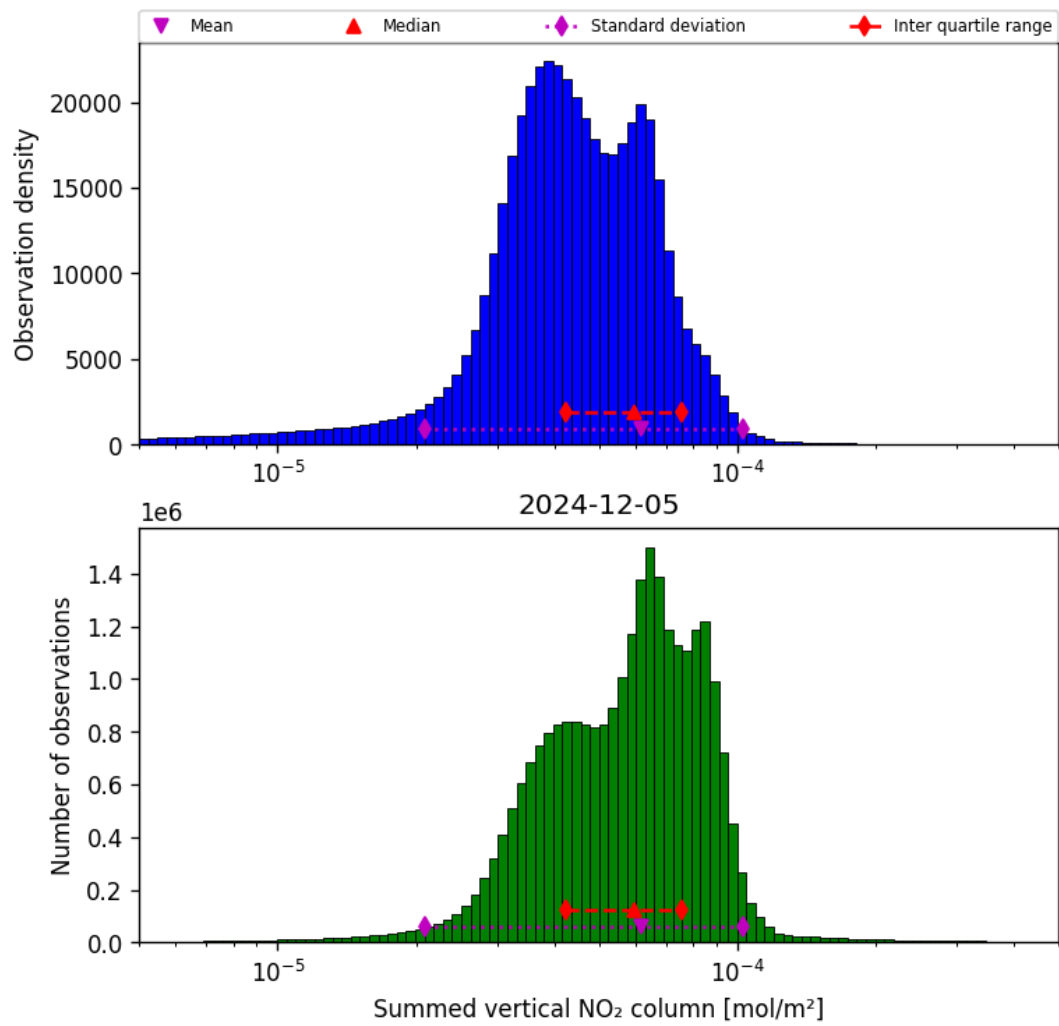
Figure 40: Histogram of “Summed vertical NO 2 column” for 2024-12-04 to 2024-12-06
