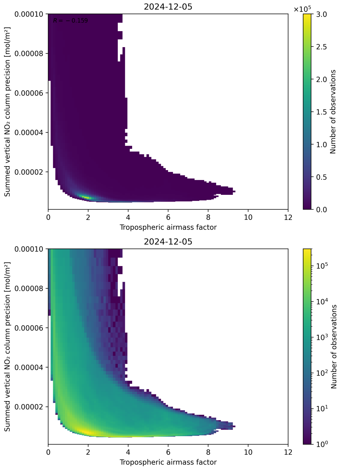
Figure 76: Scatter density plot of “Tropospheric air mass factor” against “Summed vertical NO 2 column precision” for 2024-12-04 to 2024-12-06.
