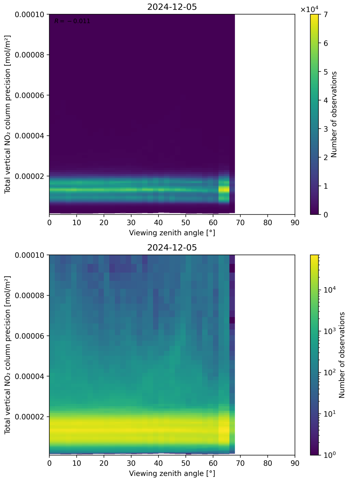
Figure 168: Scatter density plot of “Viewing zenith angle” against “Total vertical NO 2 column precision” for 2024-12-04 to 2024-12-06.
