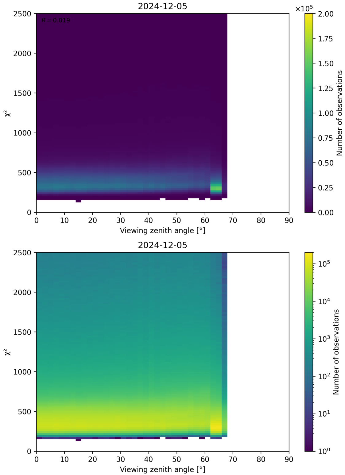
Figure 162: Scatter density plot of “Viewing zenith angle” against “ \chi^2 ” for 2024-12-04 to 2024-12-06.
