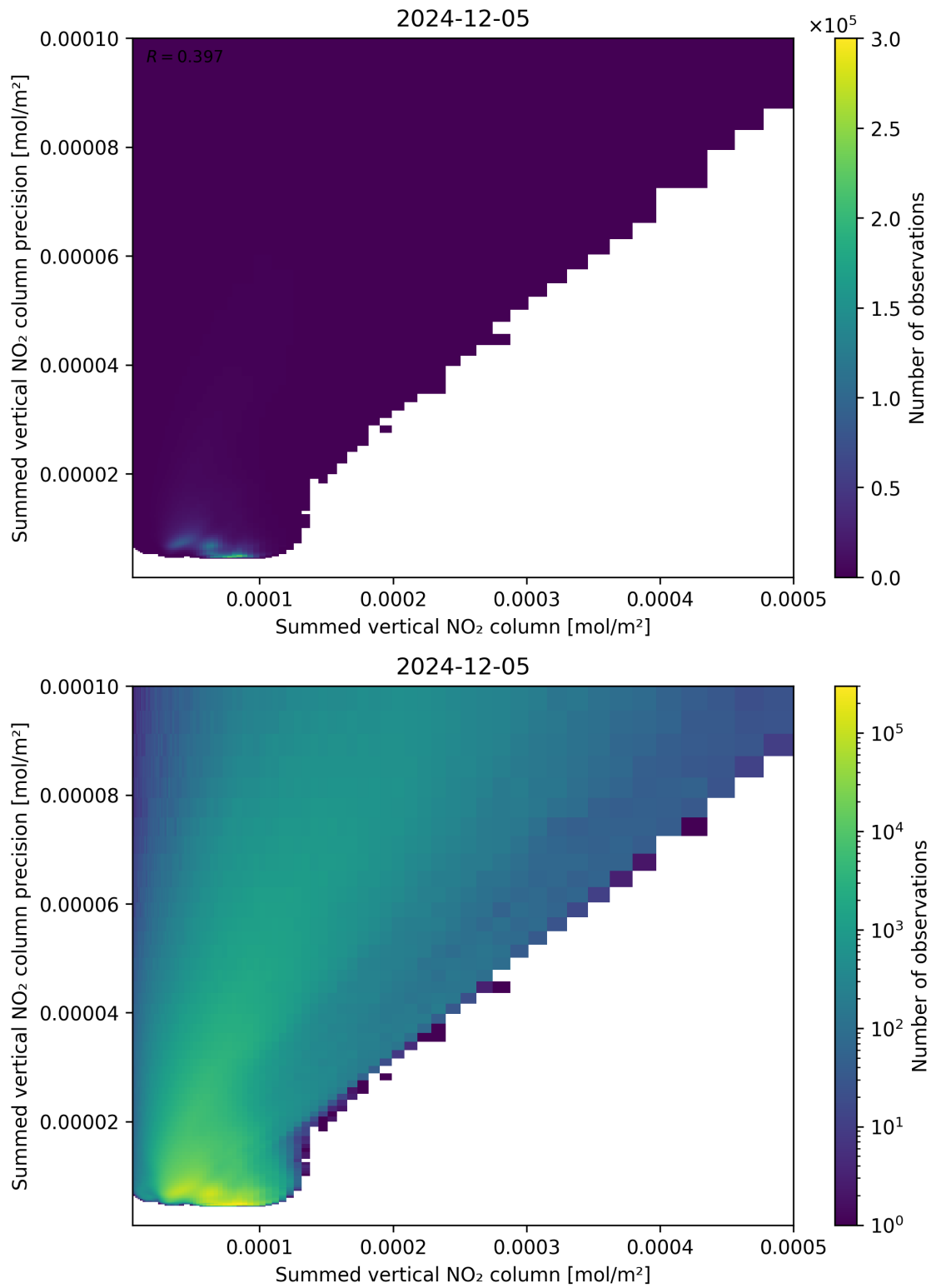
Figure 105: Scatter density plot of “Summed vertical NO 2 column” against “Summed vertical NO 2 column precision” for 2024-12-04 to 2024-12-06.
