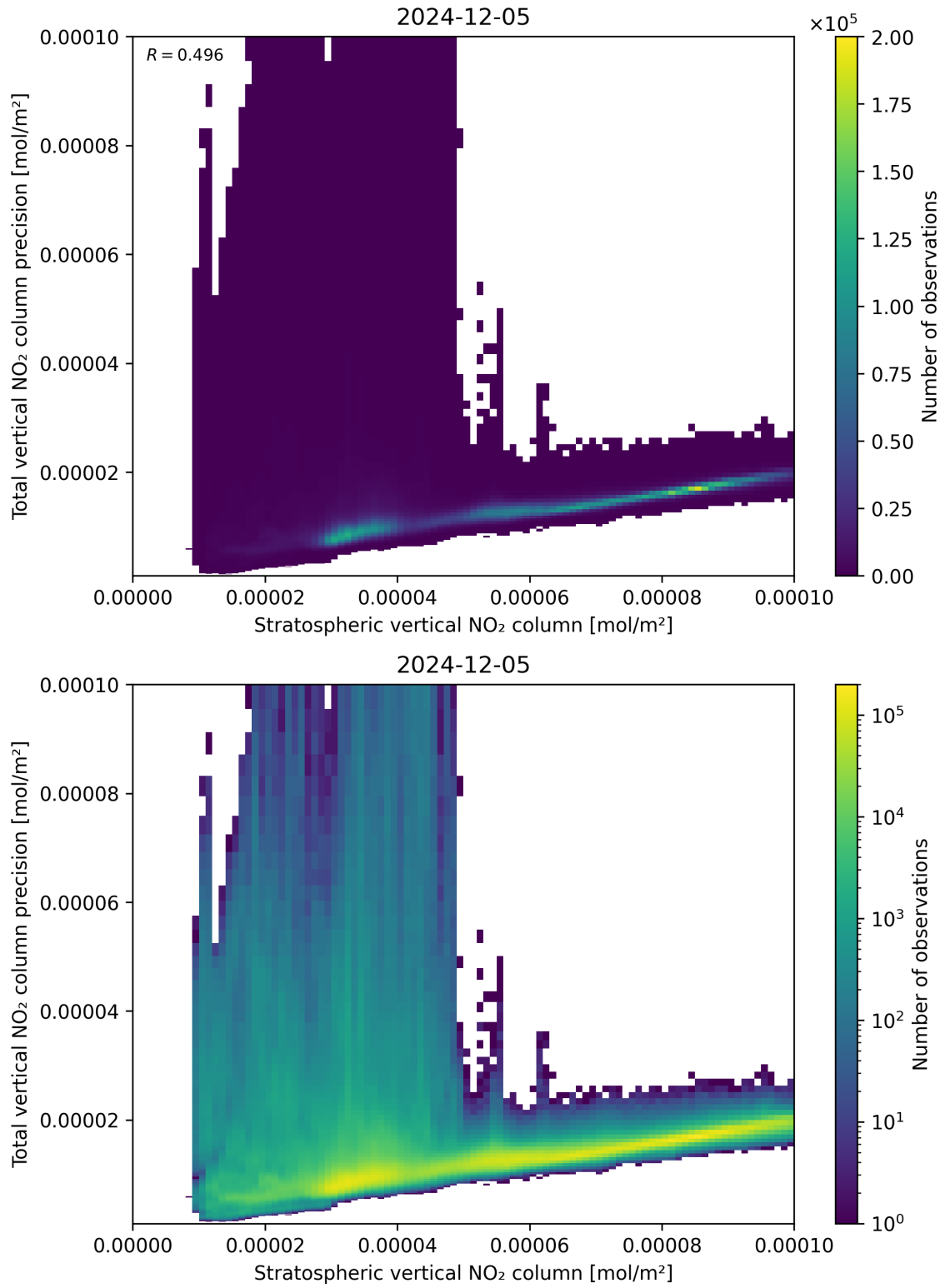
Figure 101: Scatter density plot of “Stratospheric vertical NO 2 column” against “Total vertical NO 2 column precision” for 2024-12-04 to 2024-12-06.
