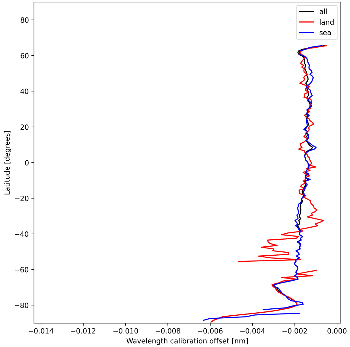
Figure 18: Zonal average of “Wavelength calibration offset” for 2024-12-04 to 2024-12-06.
