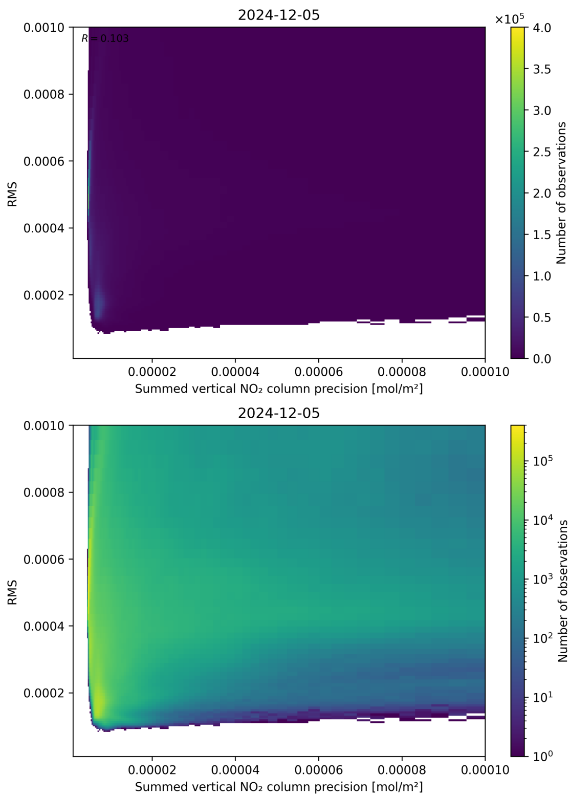
Figure 108: Scatter density plot of “Summed vertical NO 2 column precision” against “RMS” for 2024-12-04 to 2024-12-06.
