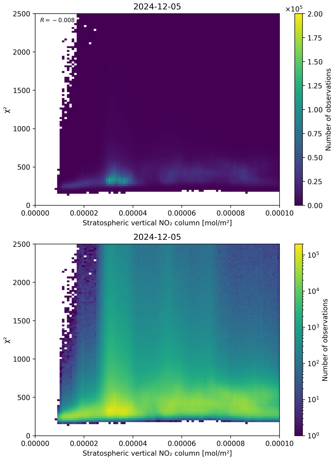
Figure 97: Scatter density plot of “Stratospheric vertical NO 2 column” against “ \chi^2 ” for 2024-12-04 to 2024-12-06.
