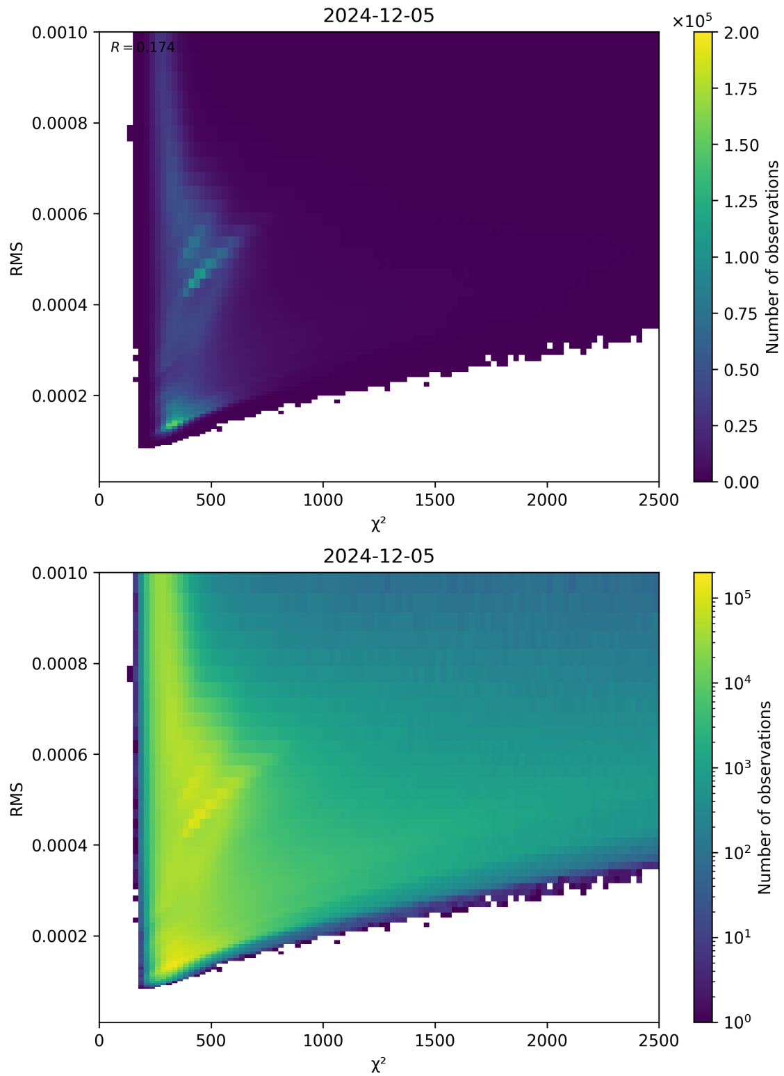
Figure 82: Scatter density plot of “ \chi^2 ” against “RMS” for 2024-12-04 to 2024-12-06.
