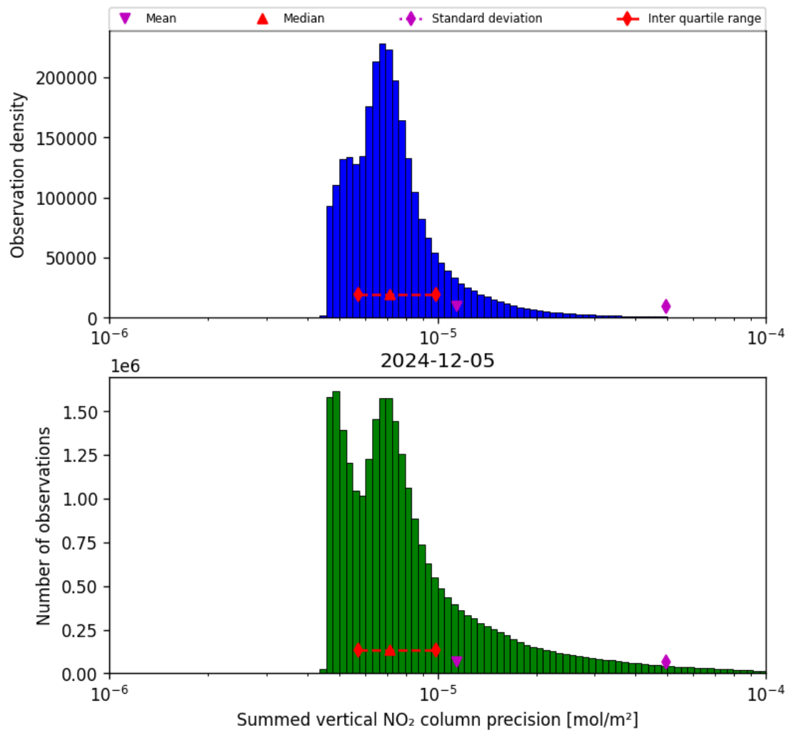
Figure 41: Histogram of “Summed vertical NO 2 column precision” for 2024-12-04 to 2024-12-06
