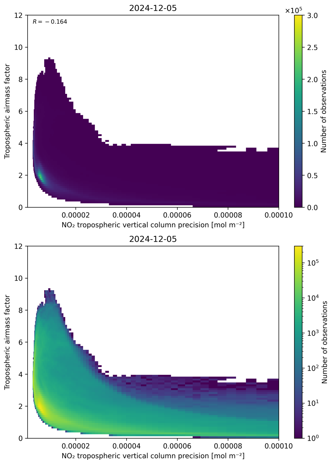
Figure 133: Scatter density plot of “NO 2 tropospheric vertical column precision” against “Tropospheric air mass factor” for 2024-12-04 to 2024-12-06.
