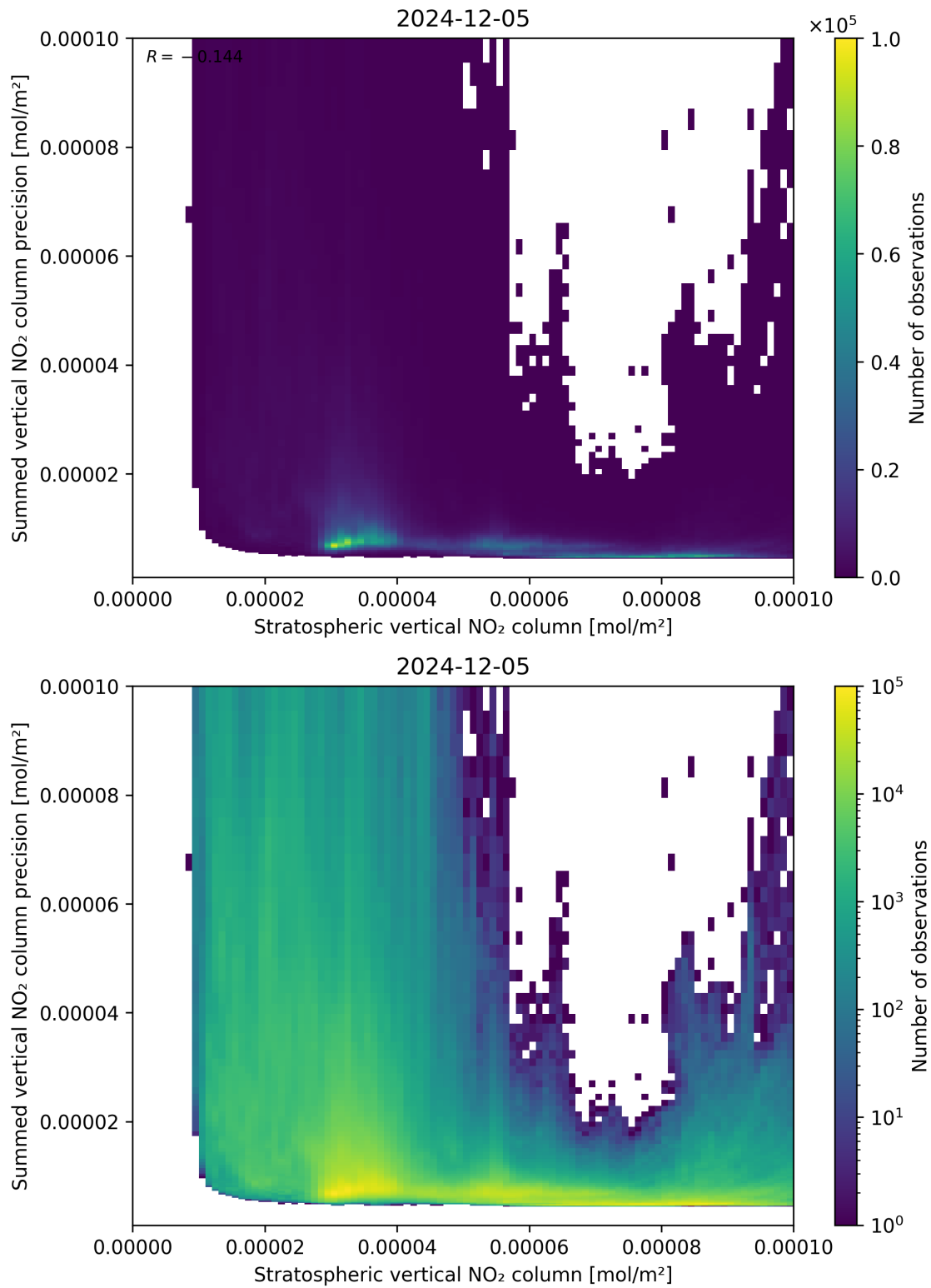
Figure 99: Scatter density plot of “Stratospheric vertical NO 2 column” against “Summed vertical NO 2 column precision” for 2024-12-04 to 2024-12-06.
