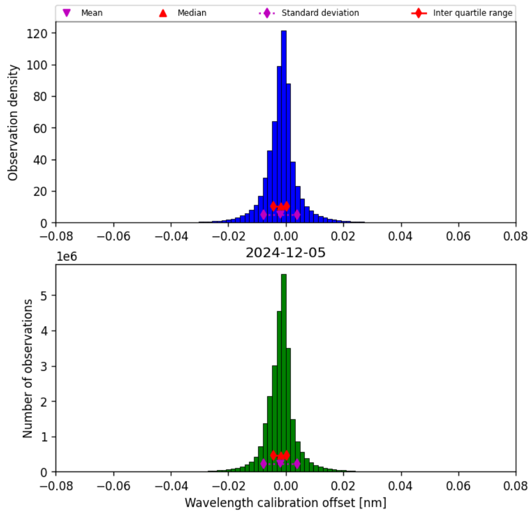
Figure 35: Histogram of “Wavelength calibration offset” for 2024-12-04 to 2024-12-06
