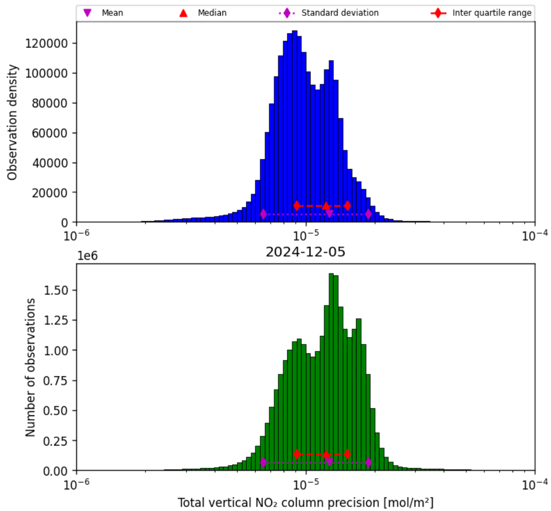
Figure 39: Histogram of “Total vertical NO 2 column precision” for 2024-12-04 to 2024-12-06
