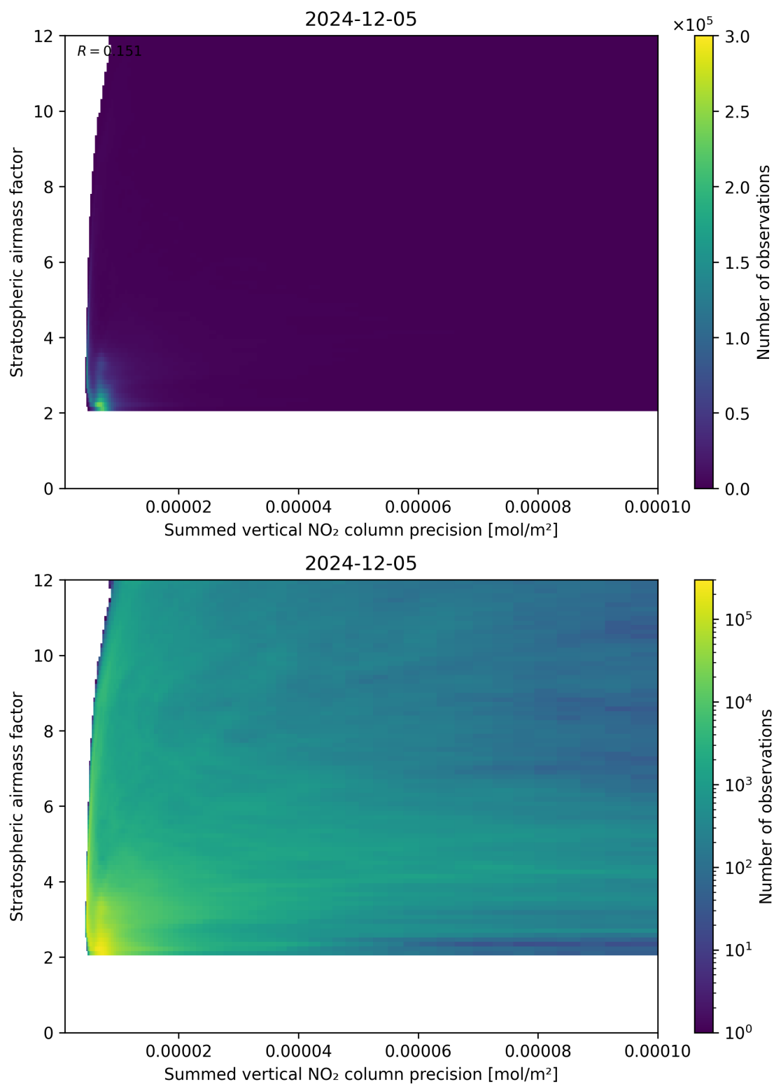
Figure 106: Scatter density plot of “Summed vertical NO 2 column precision” against “Stratospheric airmass factor” for 2024-12-04 to 2024-12-06.
