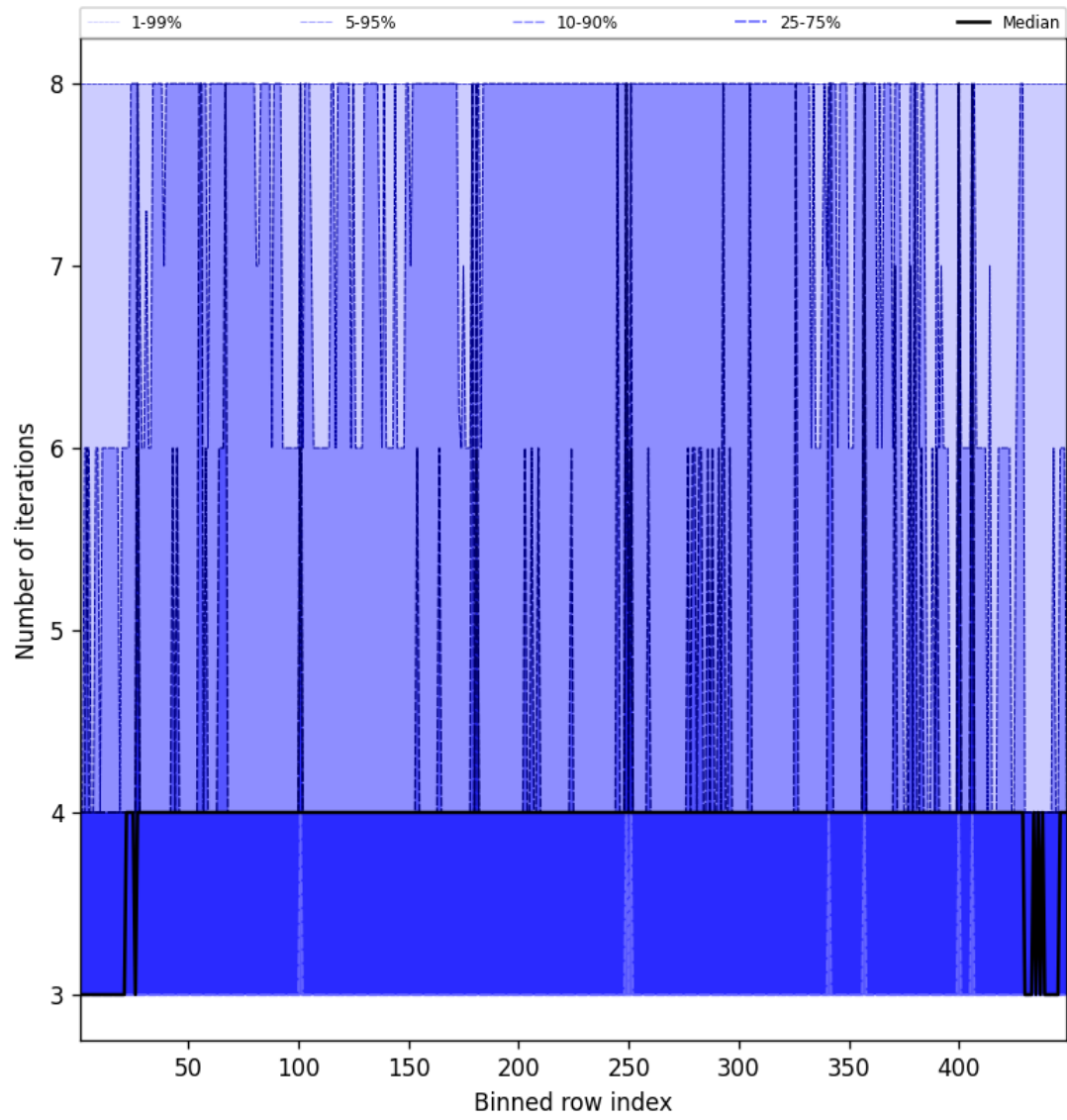
Figure 51: Along track statistics of “Number of iterations” for 2024-12-04 to 2024-12-06
