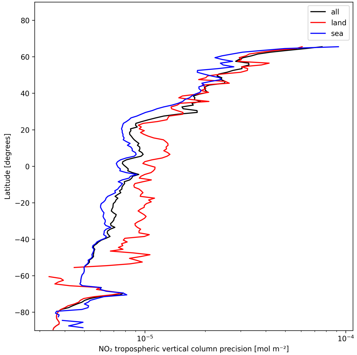
Figure 13: Zonal average of “NO 2 tropospheric vertical column precision” for 2024-12-04 to 2024-12-06.
