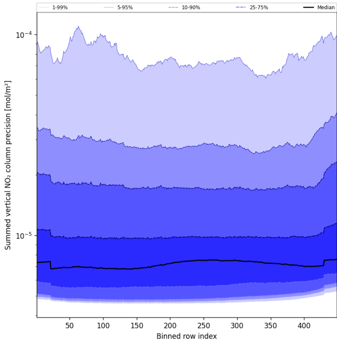
Figure 58: Along track statistics of “Summed vertical NO 2 column precision” for 2024-12-04 to 2024-12-06
