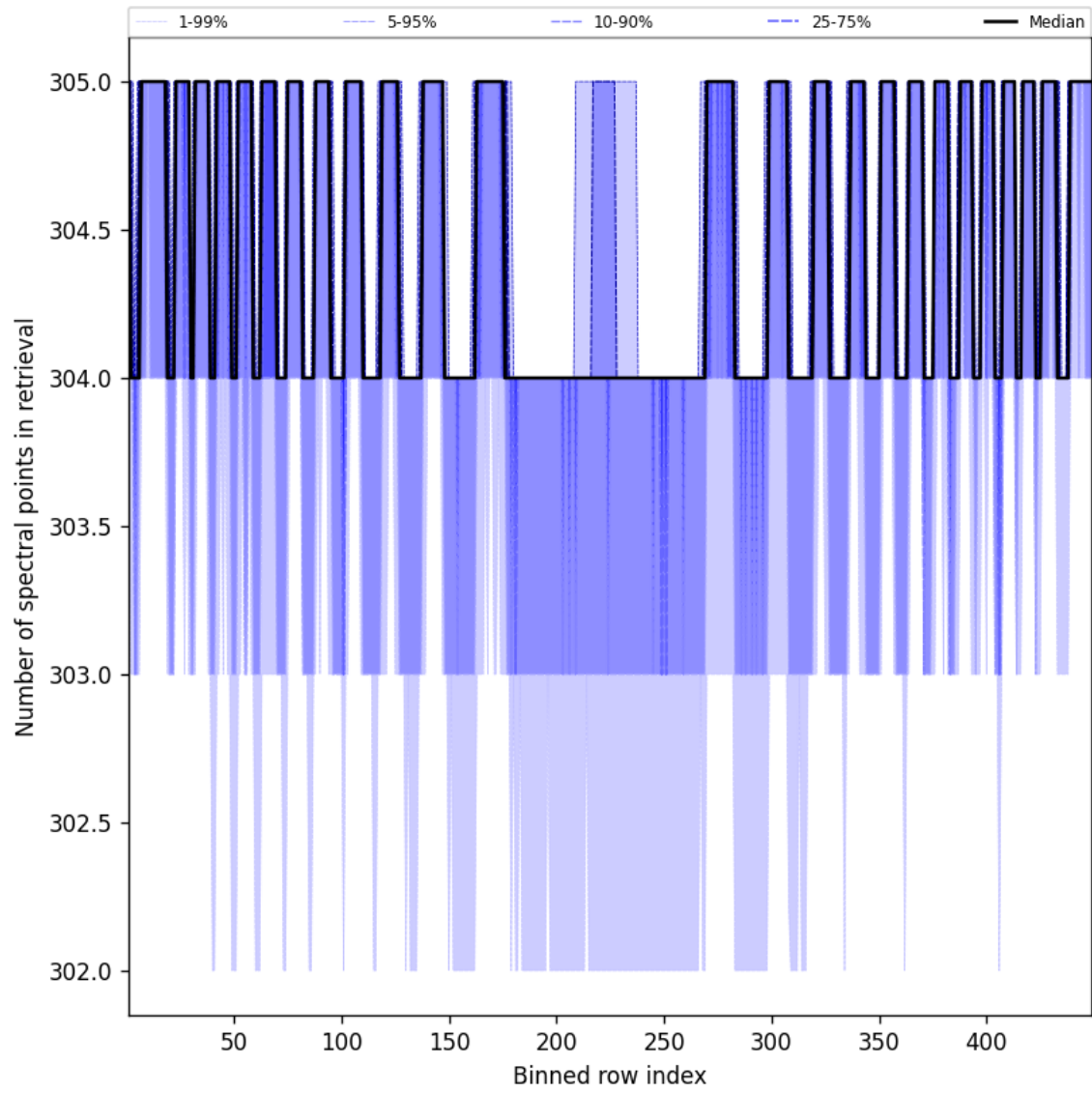
Figure 50: Along track statistics of “Number of spectral points in retrieval” for 2024-12-04 to 2024-12-06
