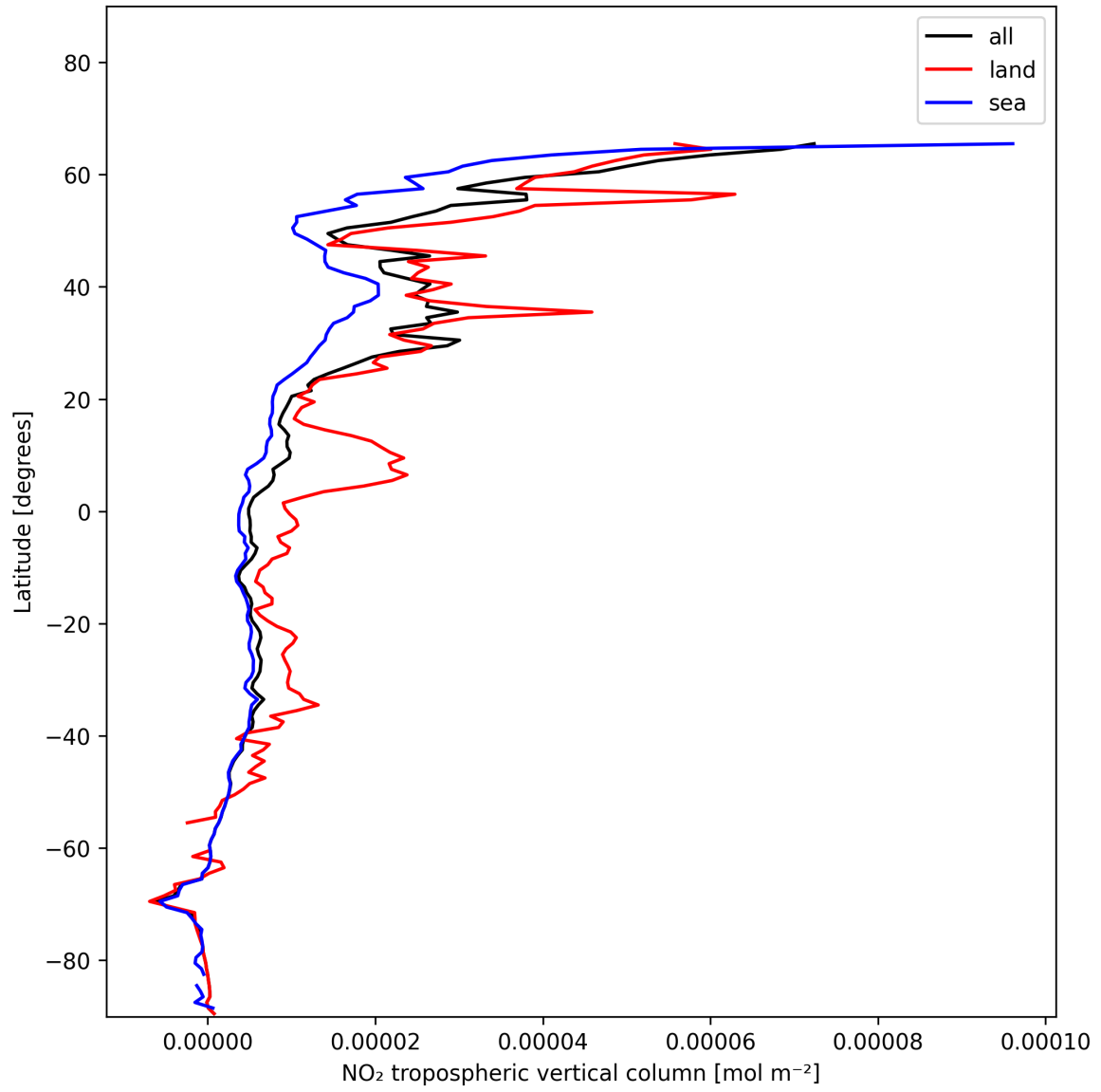
Figure 12: Zonal average of “NO 2 tropospheric vertical column” for 2024-12-04 to 2024-12-06.
