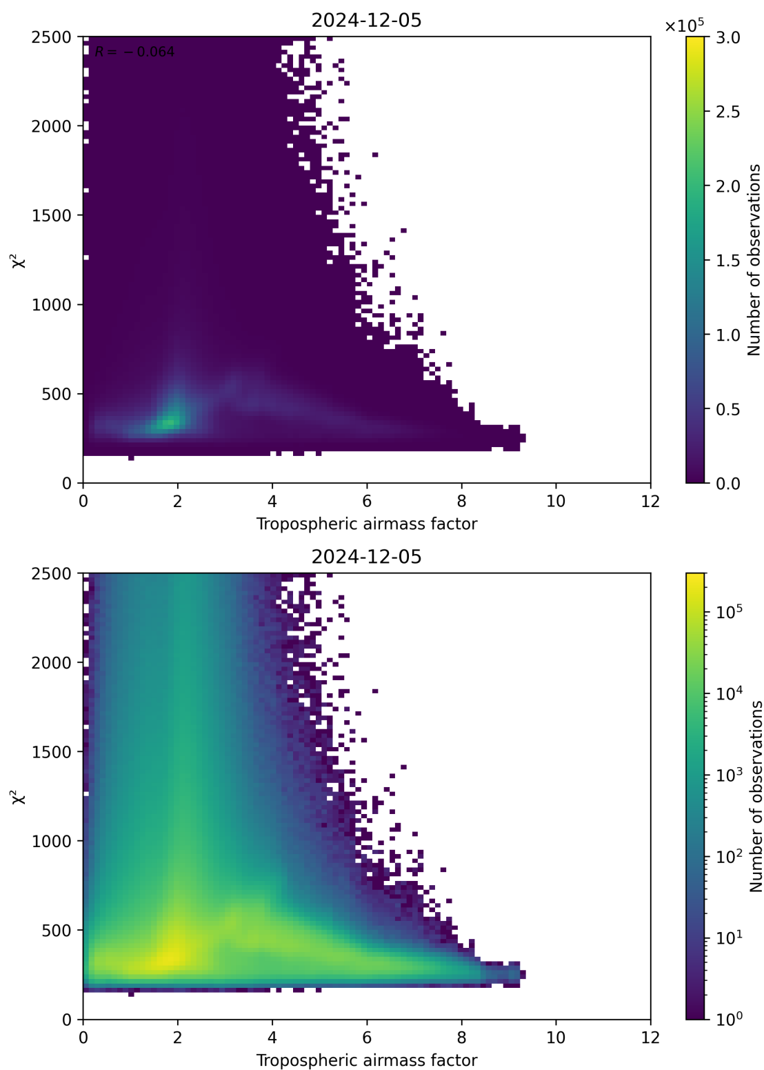
Figure 73: Scatter density plot of “Tropospheric airmass factor” against “ \chi^2 ” for 2024-12-04 to 2024-12-06.
