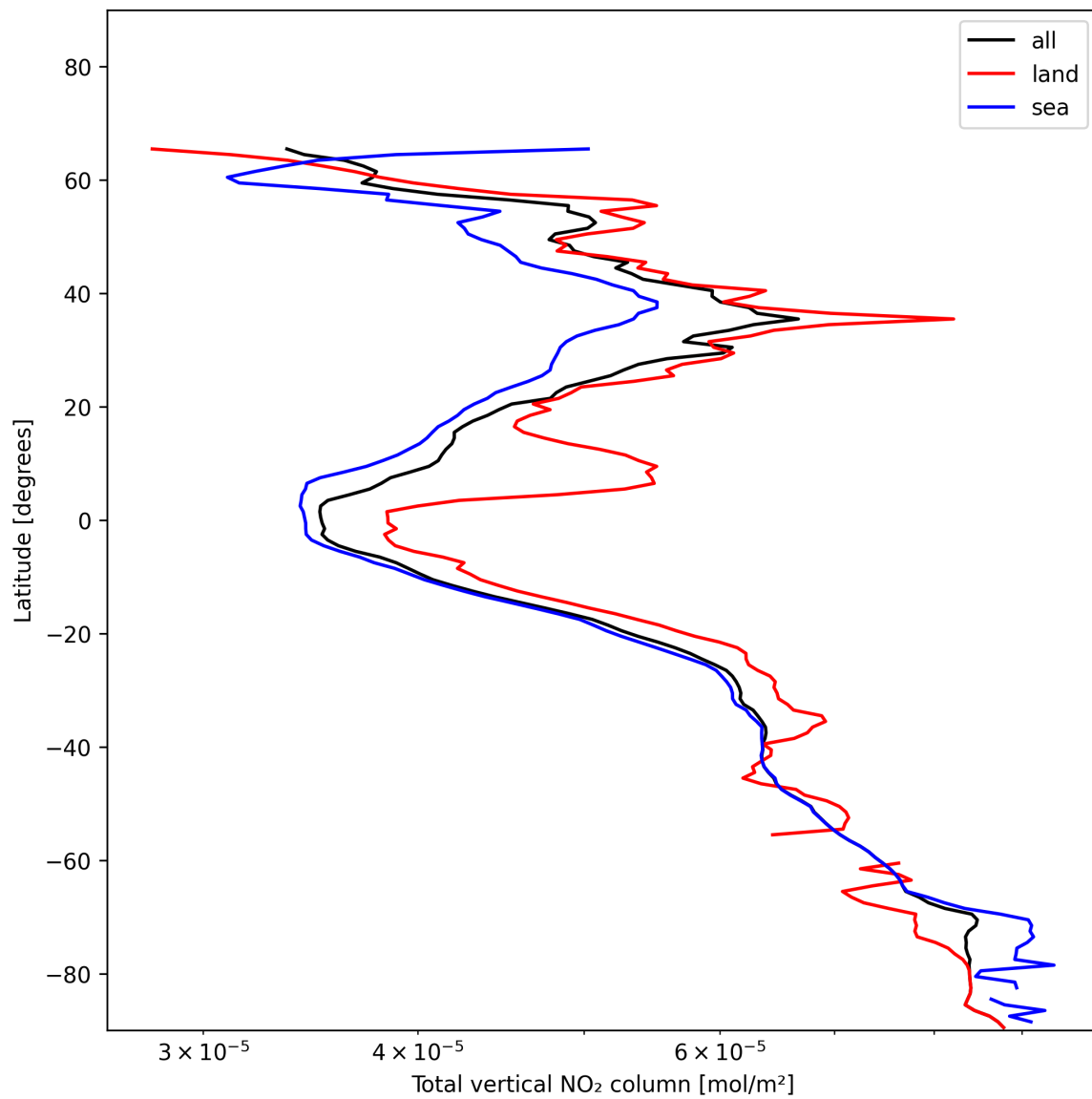
Figure 21: Zonal average of “Total vertical NO 2 column” for 2024-12-04 to 2024-12-06.
