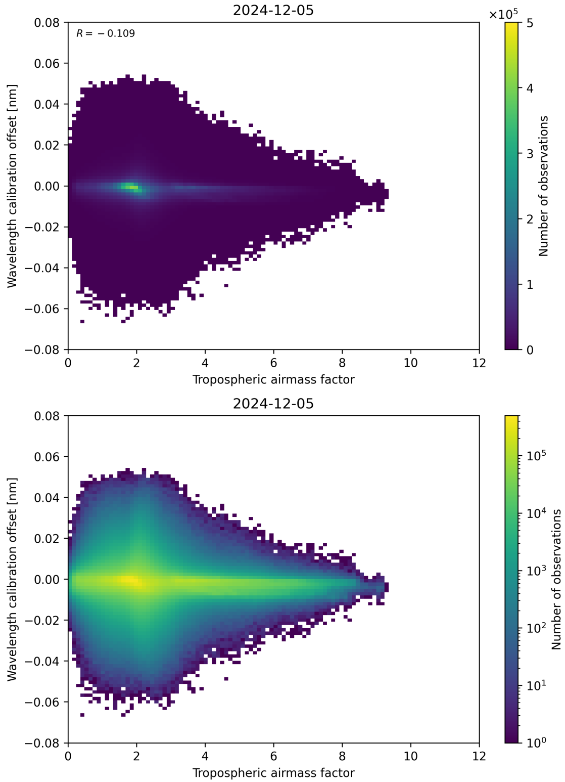
Figure 80: Scatter density plot of “Tropospheric airmass factor” against “Wavelength calibration offset” for 2024-12-04 to 2024-12-06.
