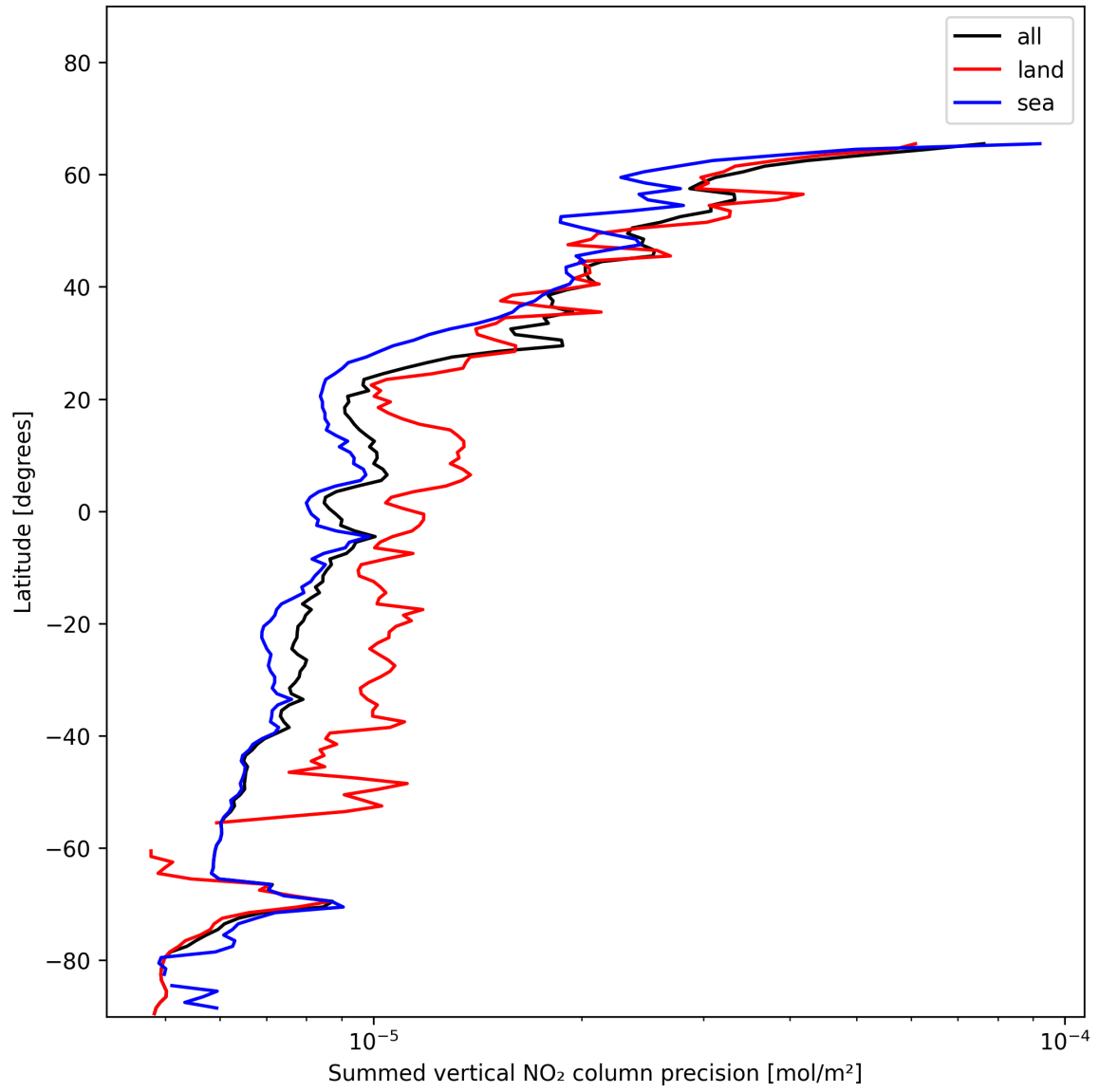
Figure 24: Zonal average of “Summed vertical NO 2 column precision” for 2024-12-04 to 2024-12-06.
