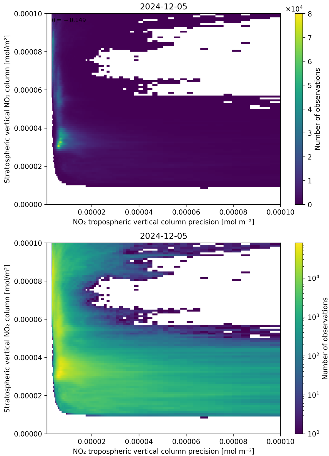
Figure 135: Scatter density plot of “NO 2 tropospheric vertical column precision” against “Stratospheric vertical NO 2 column” for 2024-12-04 to 2024-12-06.
