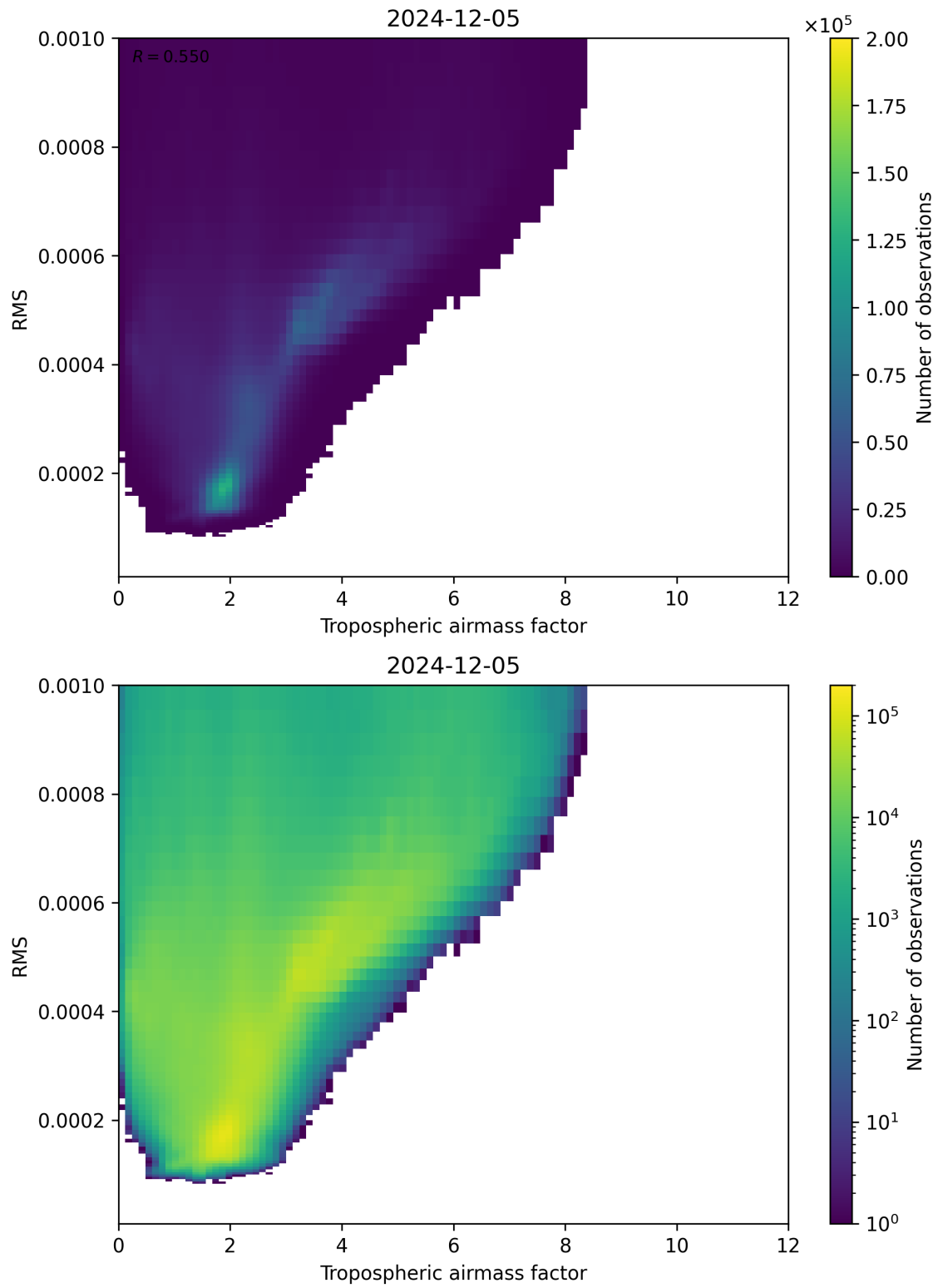
Figure 79: Scatter density plot of “Tropospheric airmass factor” against “RMS” for 2024-12-04 to 2024-12-06.
