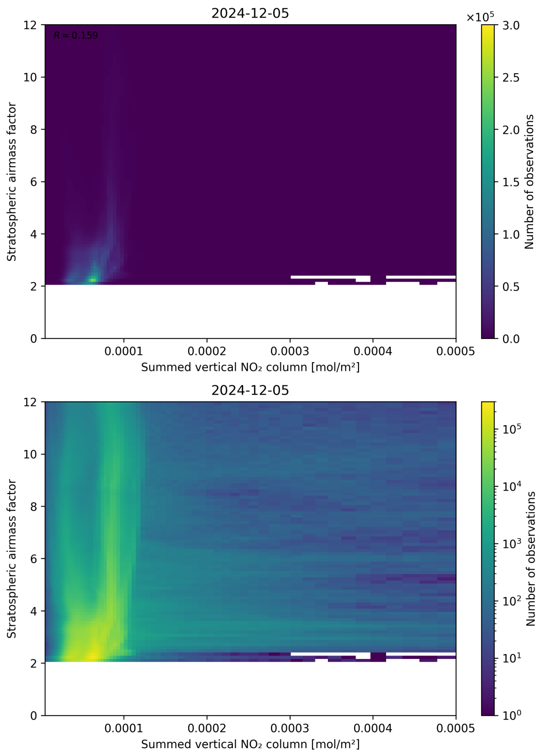
Figure 103: Scatter density plot of “Summed vertical NO 2 column” against “Stratospheric air mass factor” for 2024-12-04 to 2024-12-06.
