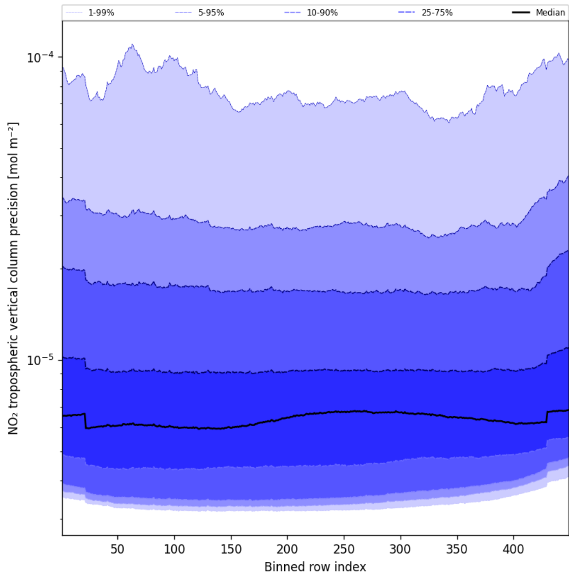
Figure 47: Along track statistics of “NO 2 tropospheric vertical column precision” for 2024-12-04 to 2024-12-06
