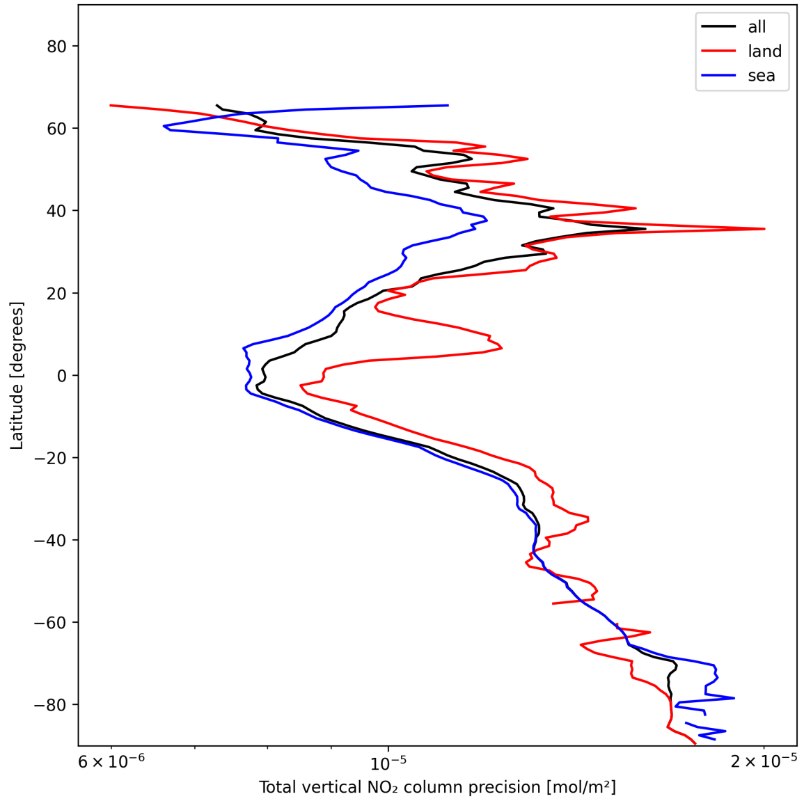
Figure 22: Zonal average of “Total vertical NO 2 column precision” for 2024-12-04 to 2024-12-06.
