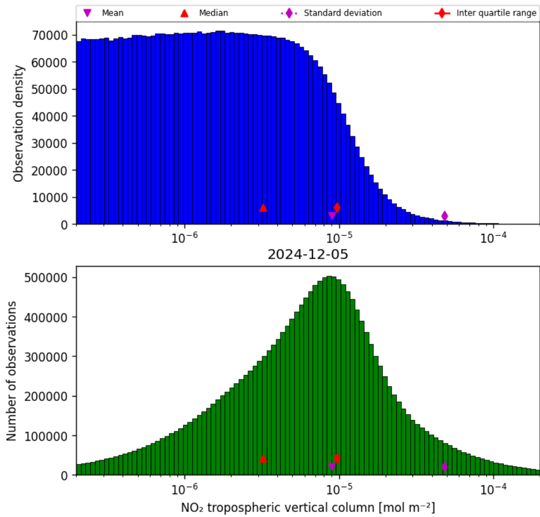
Figure 29: Histogram of “NO 2 tropospheric vertical column” for 2024-12-04 to 2024-12-06
