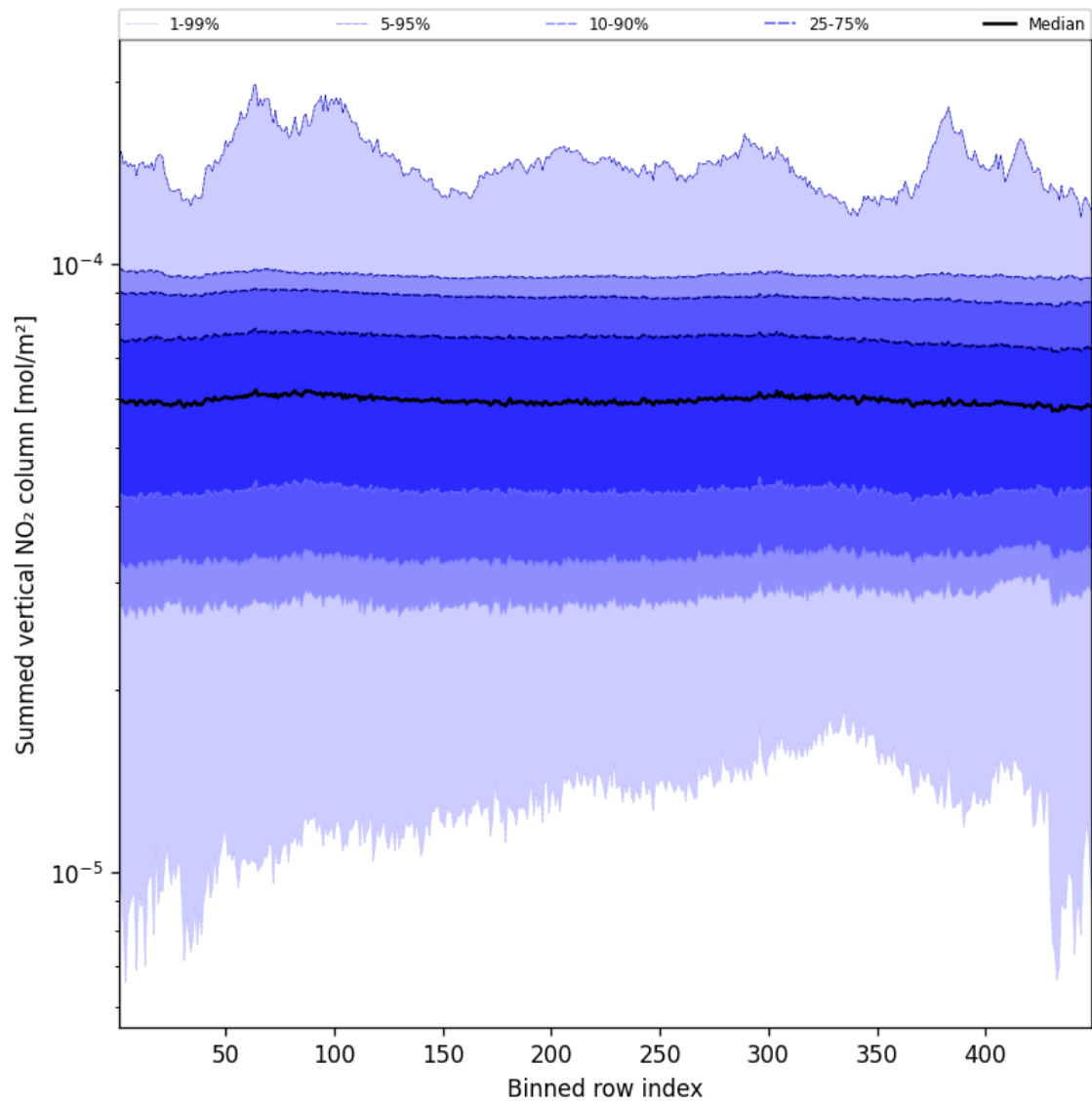
Figure 57: Along track statistics of “Summed vertical NO 2 column” for 2024-12-04 to 2024-12-06
