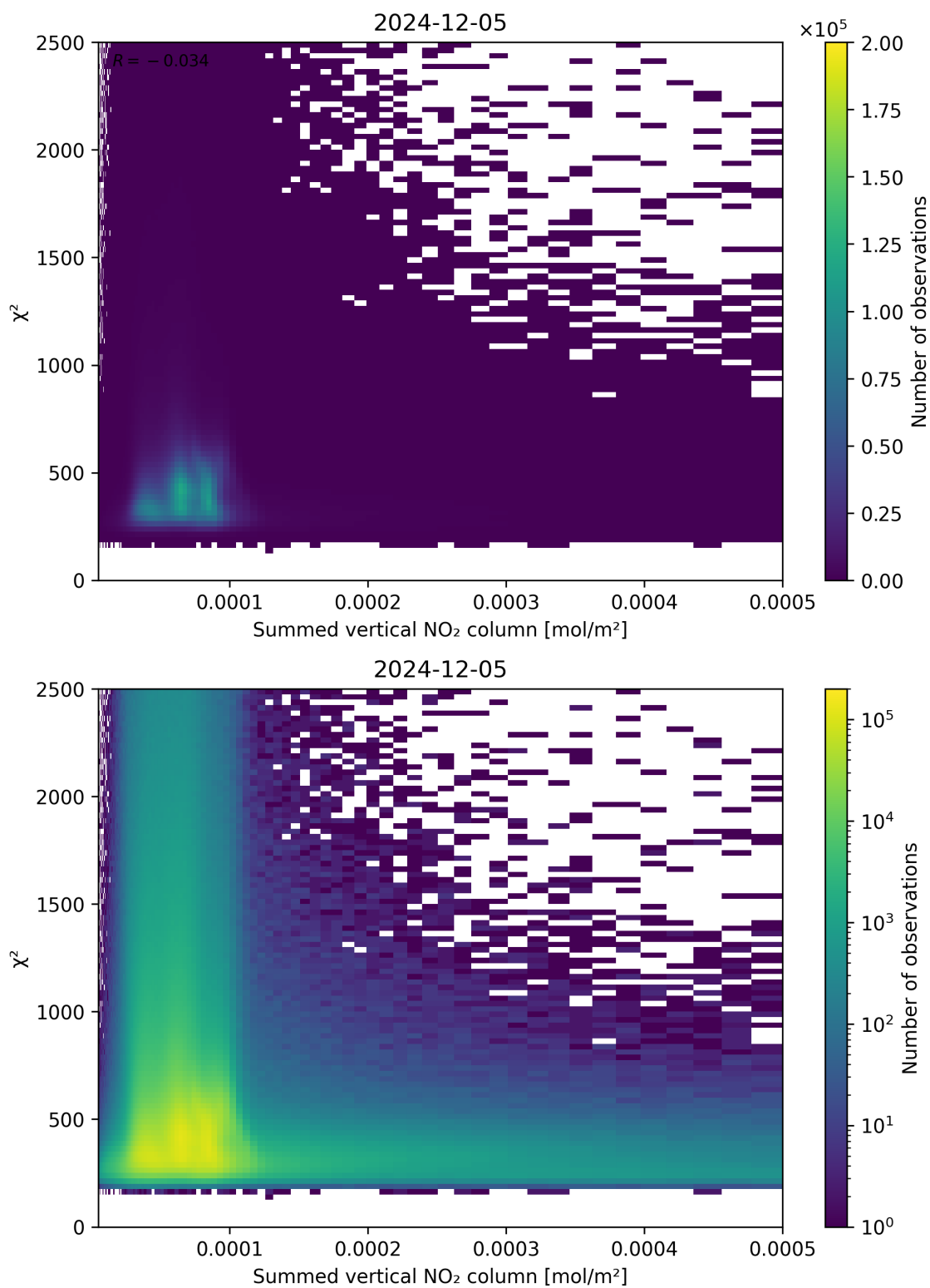
Figure 104: Scatter density plot of “Summed vertical NO 2 column” against “ \chi^2 ” for 2024-12-04 to 2024-12-06.
