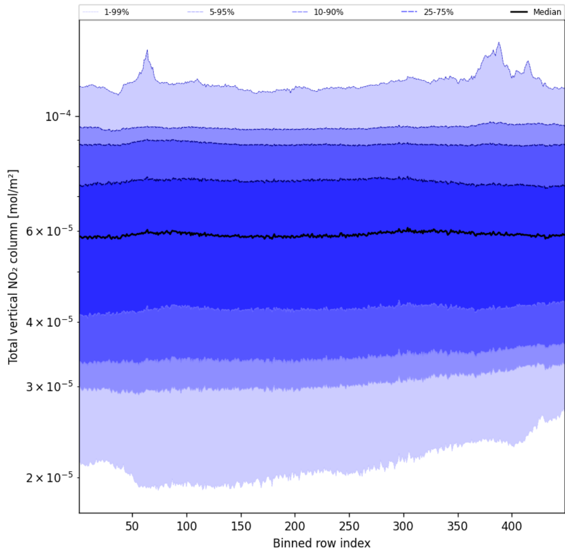
Figure 55: Along track statistics of “Total vertical NO 2 column” for 2024-12-04 to 2024-12-06
