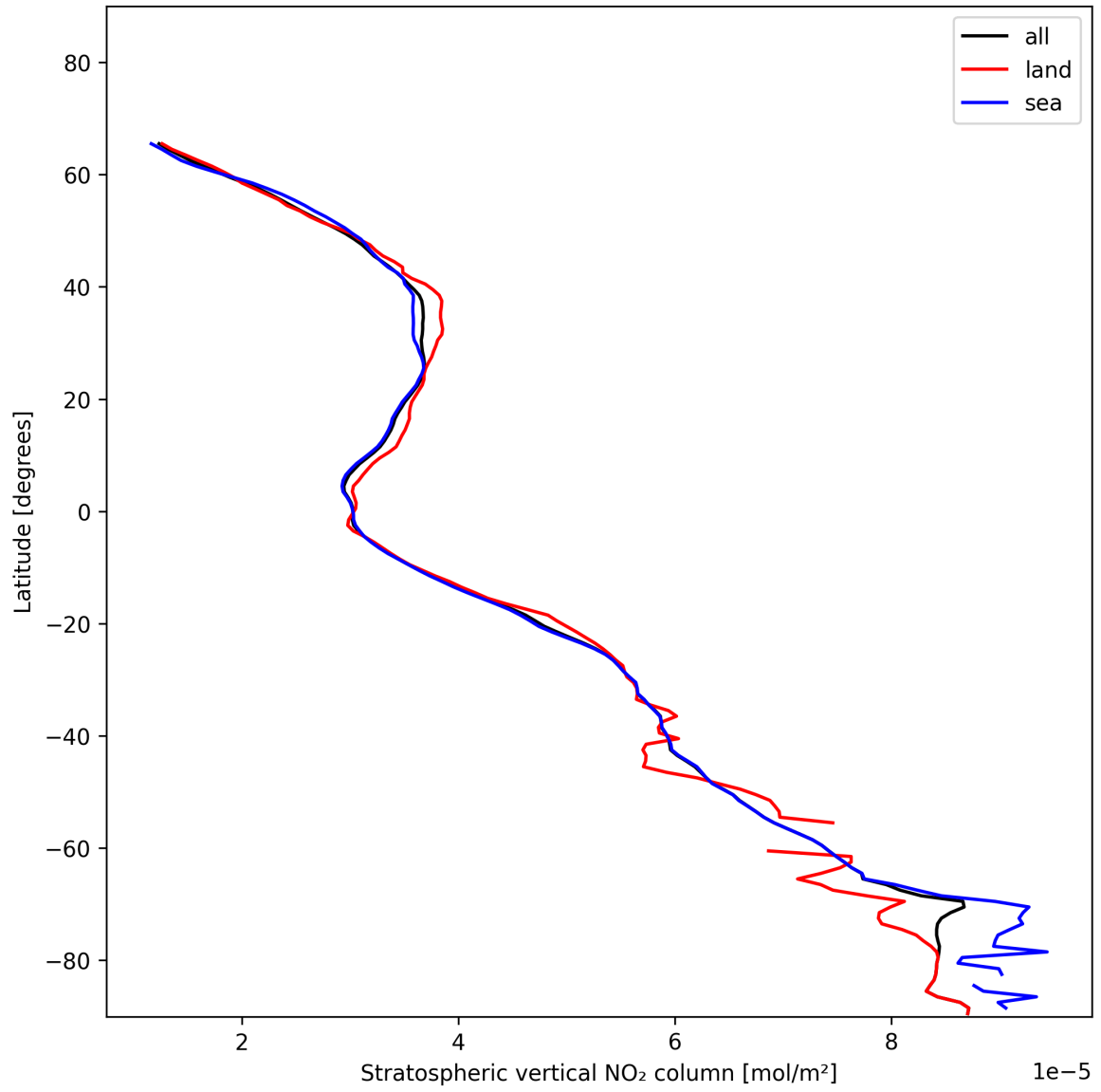
Figure 19: Zonal average of “Stratospheric vertical NO 2 column” for 2024-12-04 to 2024-12-06.
