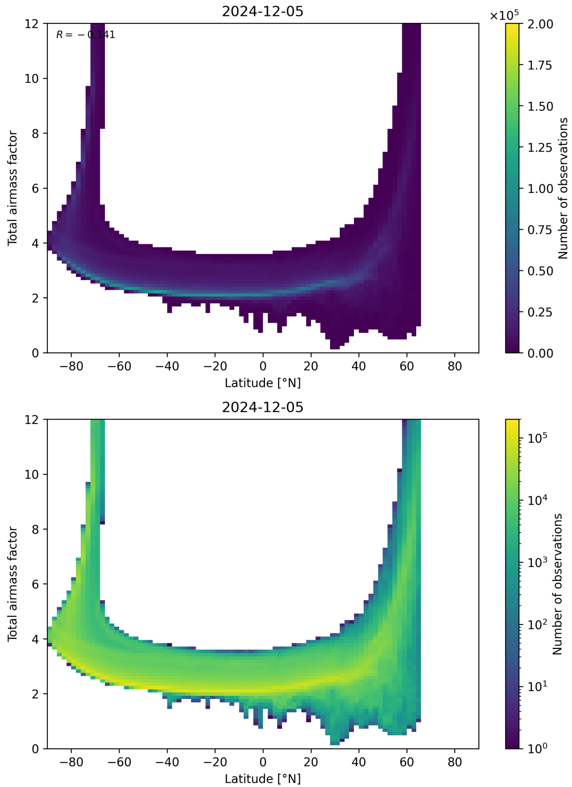
Figure 84: Scatter density plot of “Latitude” against “Total airmass factor” for 2024-12-04 to 2024-12-06.
