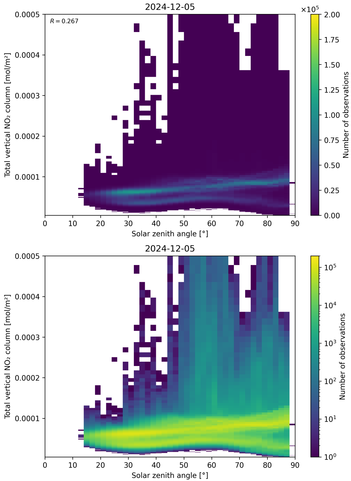
Figure 153: Scatter density plot of “Solar zenith angle” against “Total vertical NO 2 column” for 2024-12-04 to 2024-12-06.
