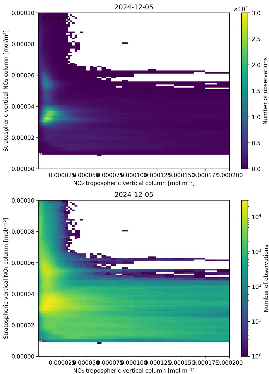
Figure 125: Scatter density plot of “NO 2 tropospheric vertical column” against “Stratospheric vertical NO 2 column” for 2024-12-04 to 2024-12-06.
