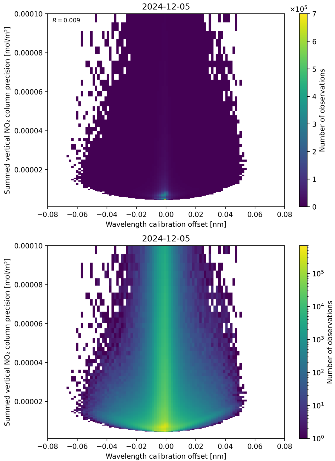
Figure 178: Scatter density plot of “Wavelength calibration offset” against “Summed vertical NO 2 column precision” for 2024-12-04 to 2024-12-06.
