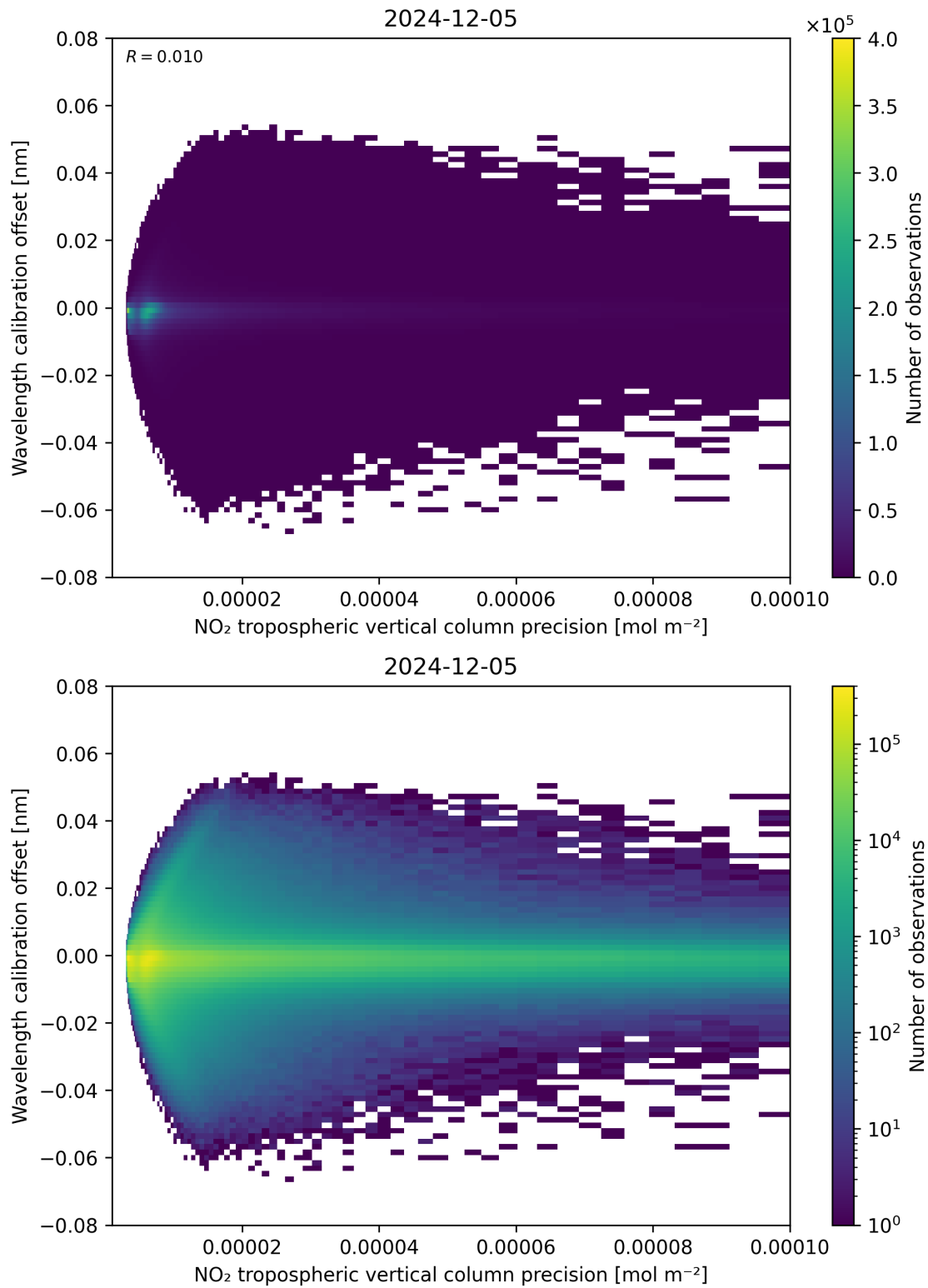
Figure 141: Scatter density plot of “NO 2 tropospheric vertical column precision” against “Wavelength calibration offset” for 2024-12-04 to 2024-12-06.
