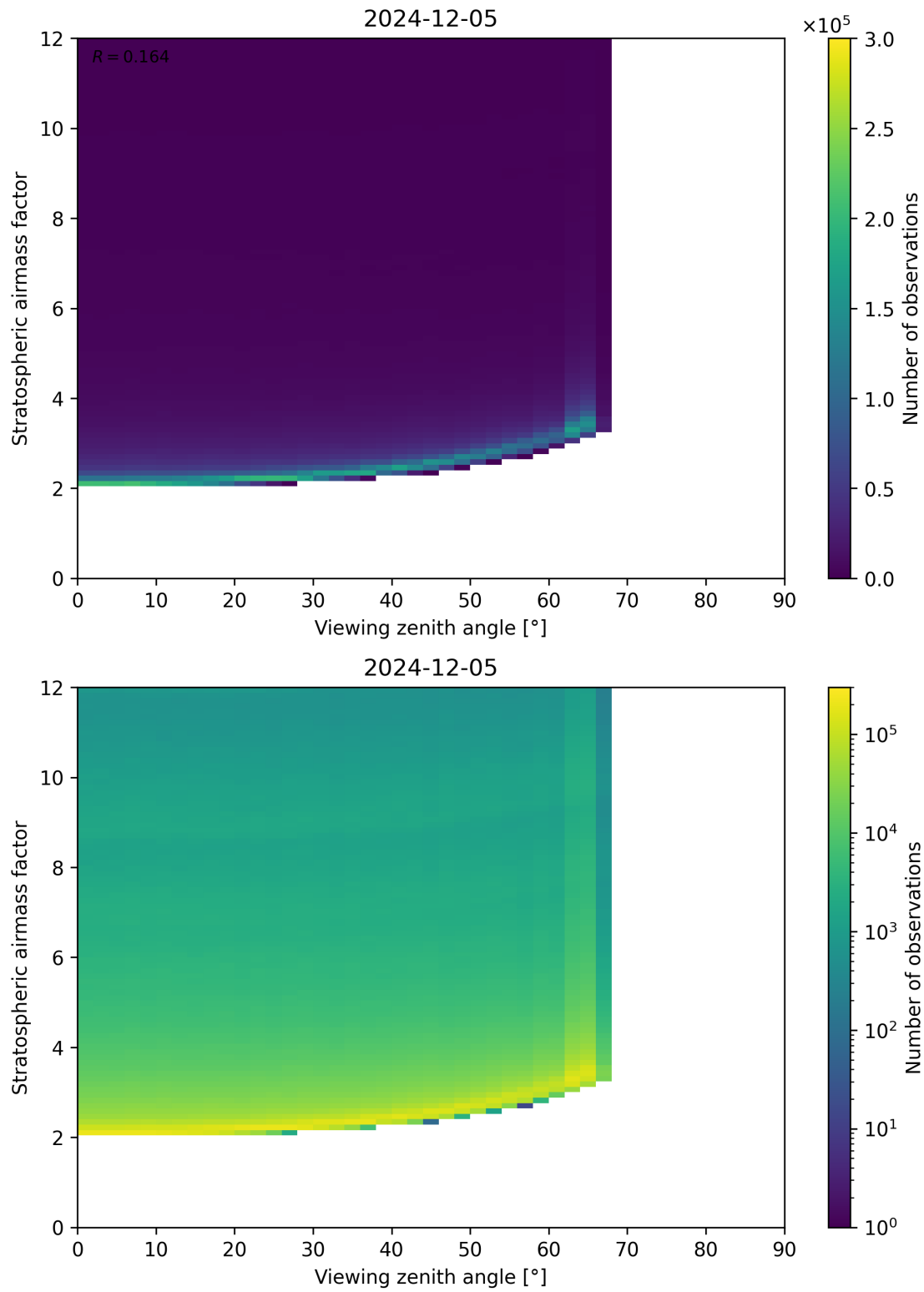
Figure 159: Scatter density plot of “Viewing zenith angle” against “Stratospheric airmass factor” for 2024-12-04 to 2024-12-06.
