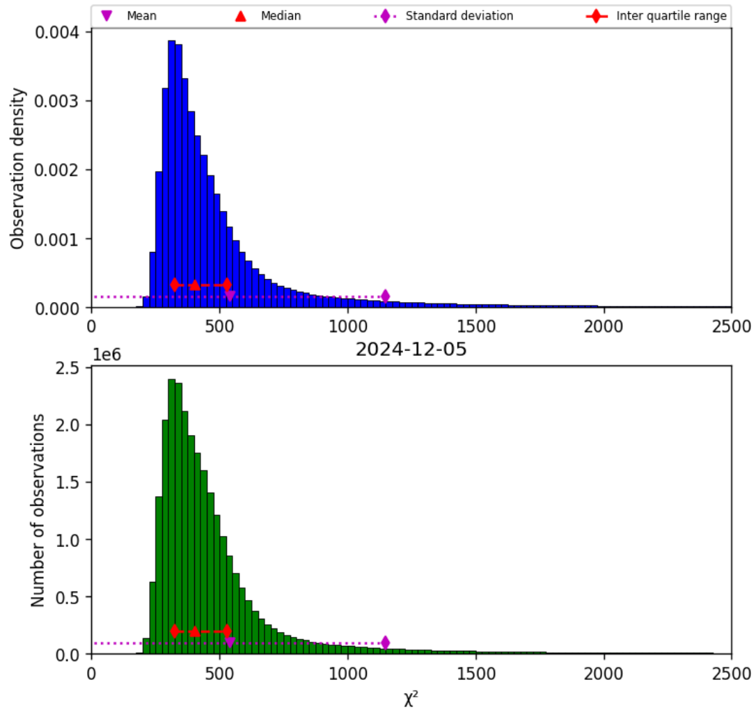
Figure 42: Histogram of “ \chi^2 ” for 2024-12-04 to 2024-12-06
