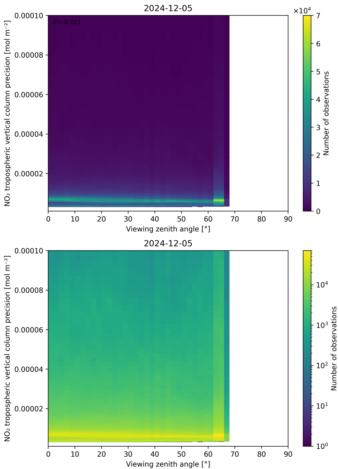
Figure 170: Scatter density plot of “Viewing zenith angle” against “NO 2 tropospheric vertical column precision” for 2024-12-04 to 2024-12-06.
