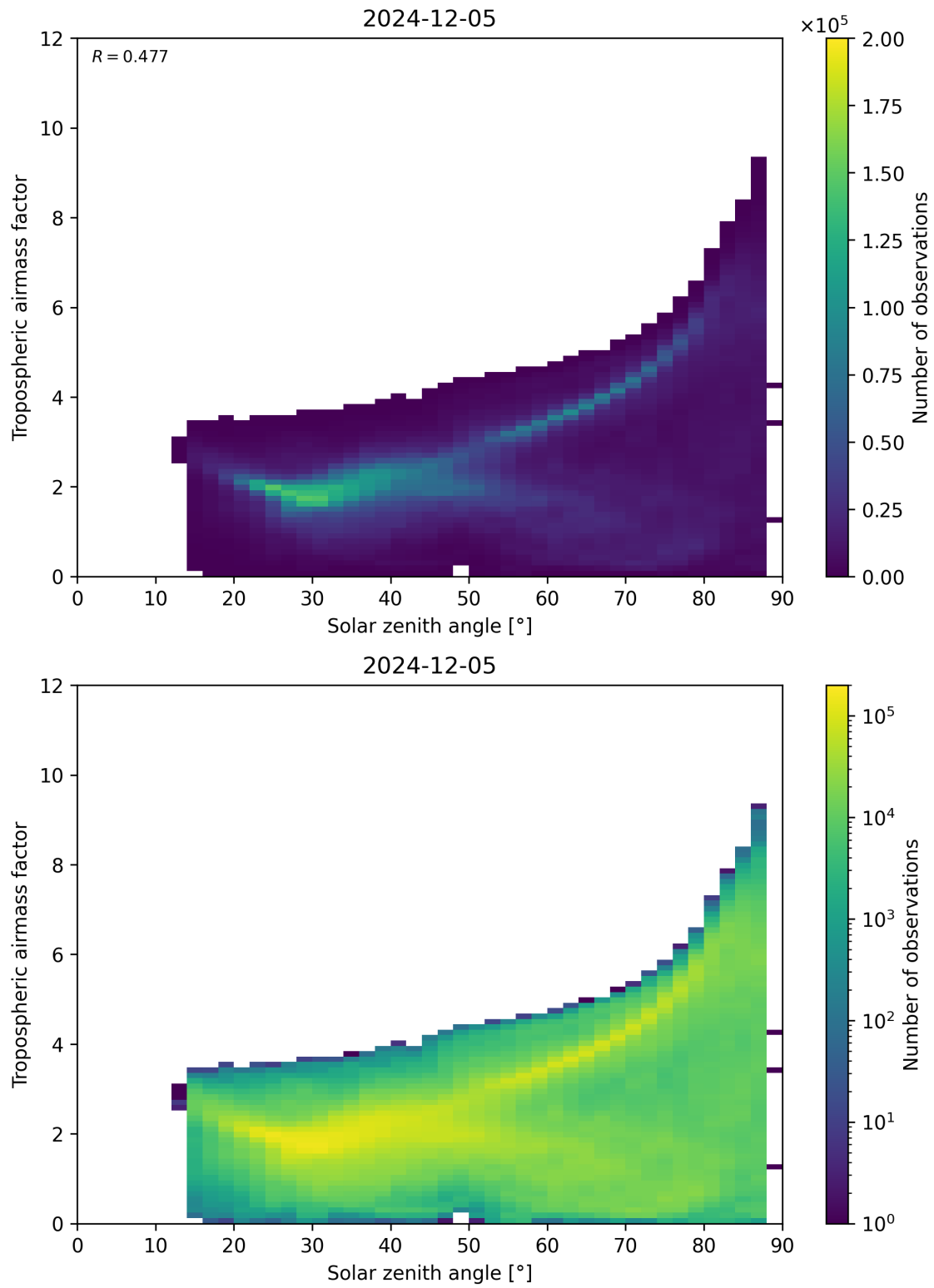
Figure 147: Scatter density plot of “Solar zenith angle” against “Tropospheric airmass factor” for 2024-12-04 to 2024-12-06.
