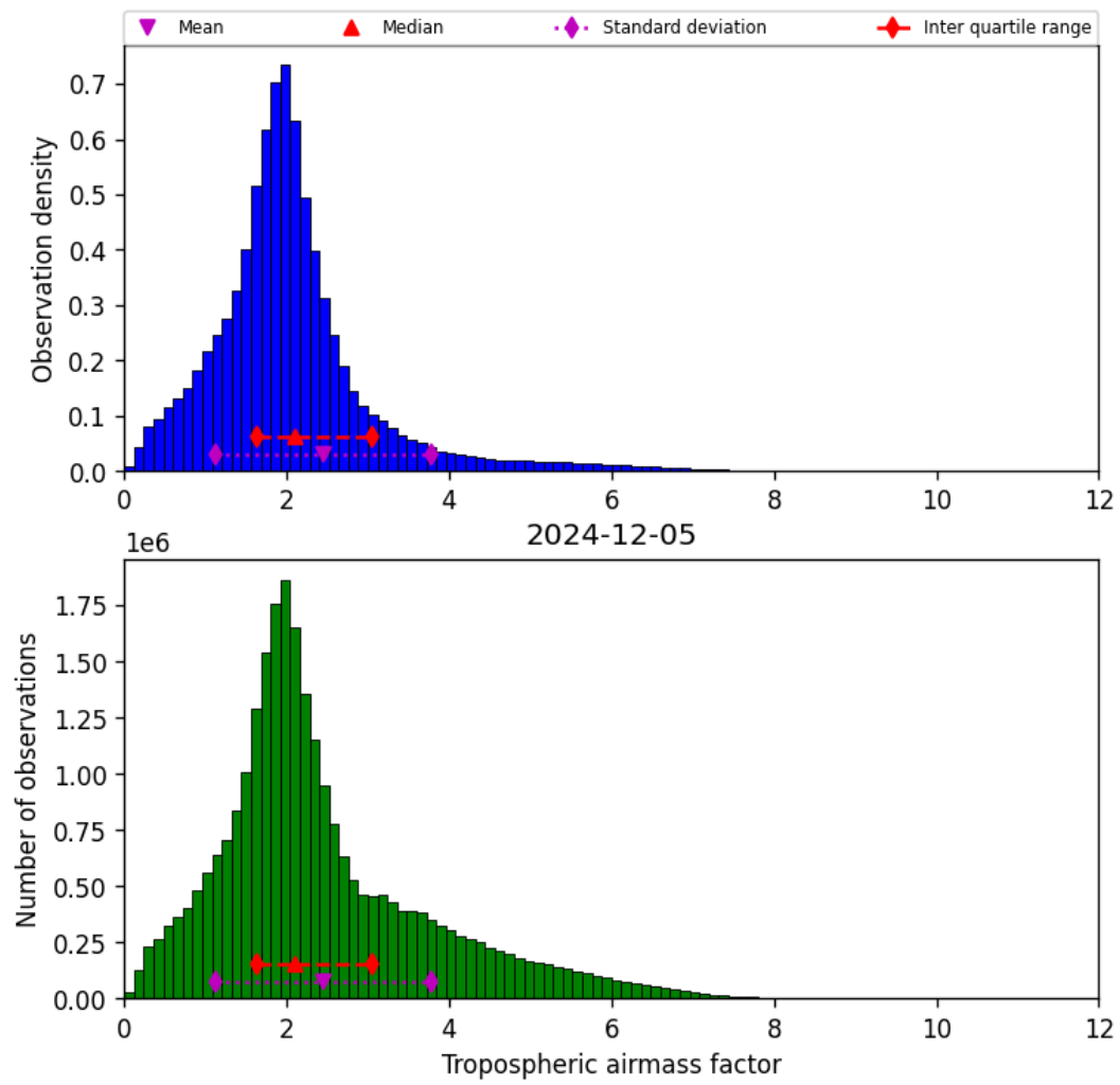
Figure 31: Histogram of “Tropospheric airmass factor” for 2024-12-04 to 2024-12-06
