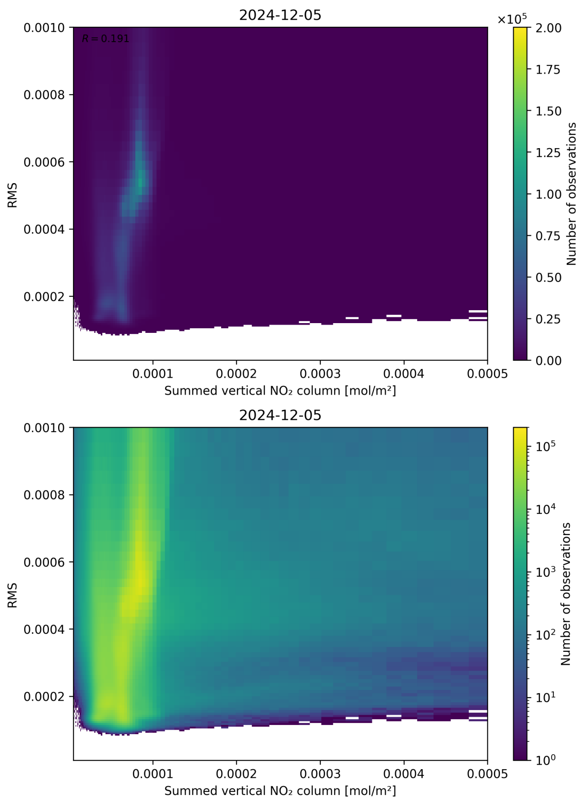
Figure 109: Scatter density plot of “Summed vertical NO 2 column” against “RMS” for 2024-12-04 to 2024-12-06.
