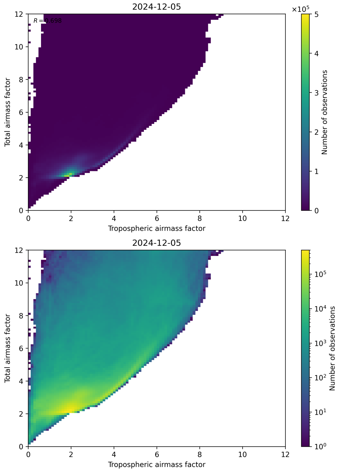
Figure 72: Scatter density plot of “Tropospheric airmass factor” against “Total airmass factor” for 2024-12-04 to 2024-12-06.
