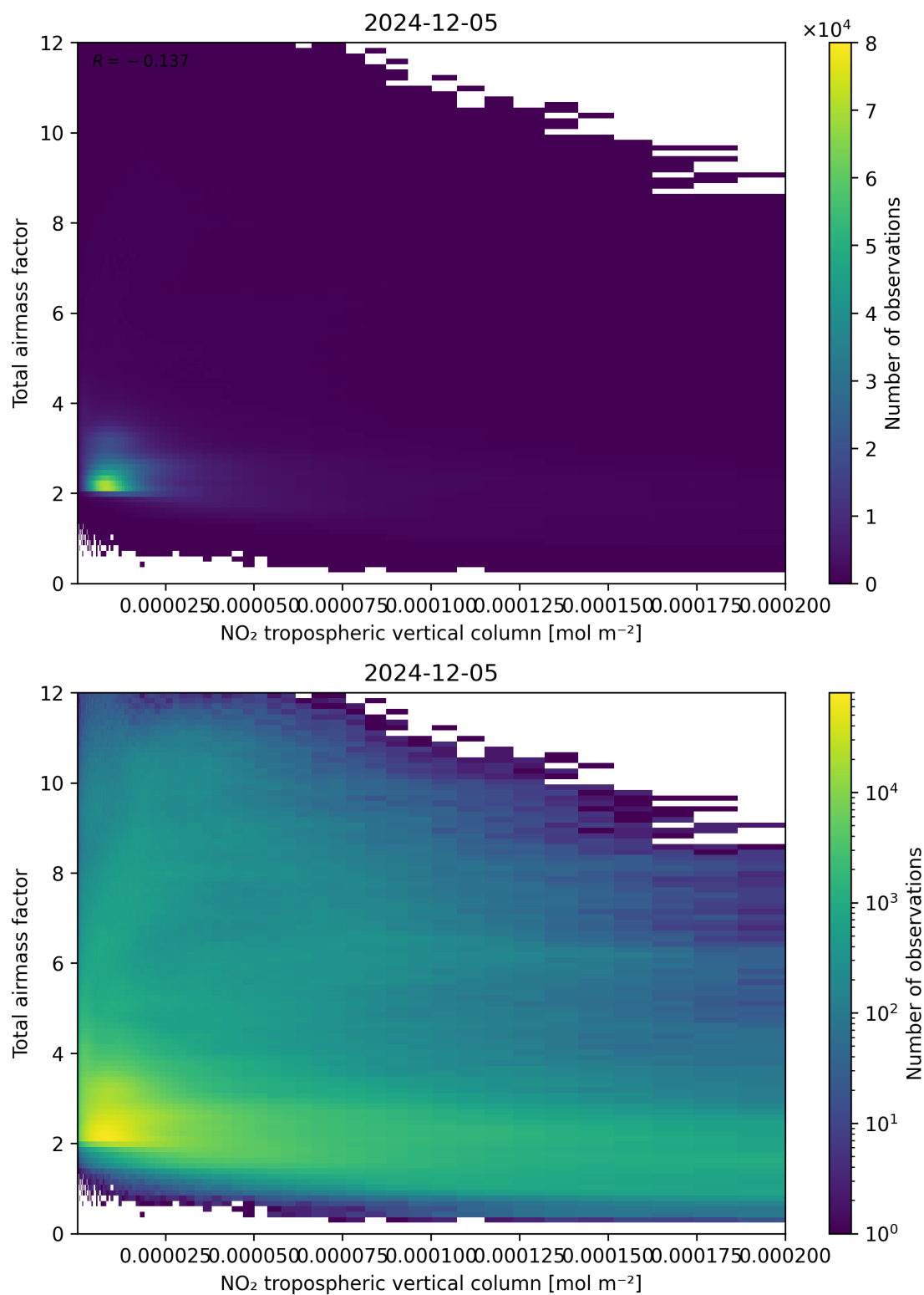
Figure 122: Scatter density plot of “NO 2 tropospheric vertical column” against “Total air mass factor” for 2024-12-04 to 2024-12-06.
