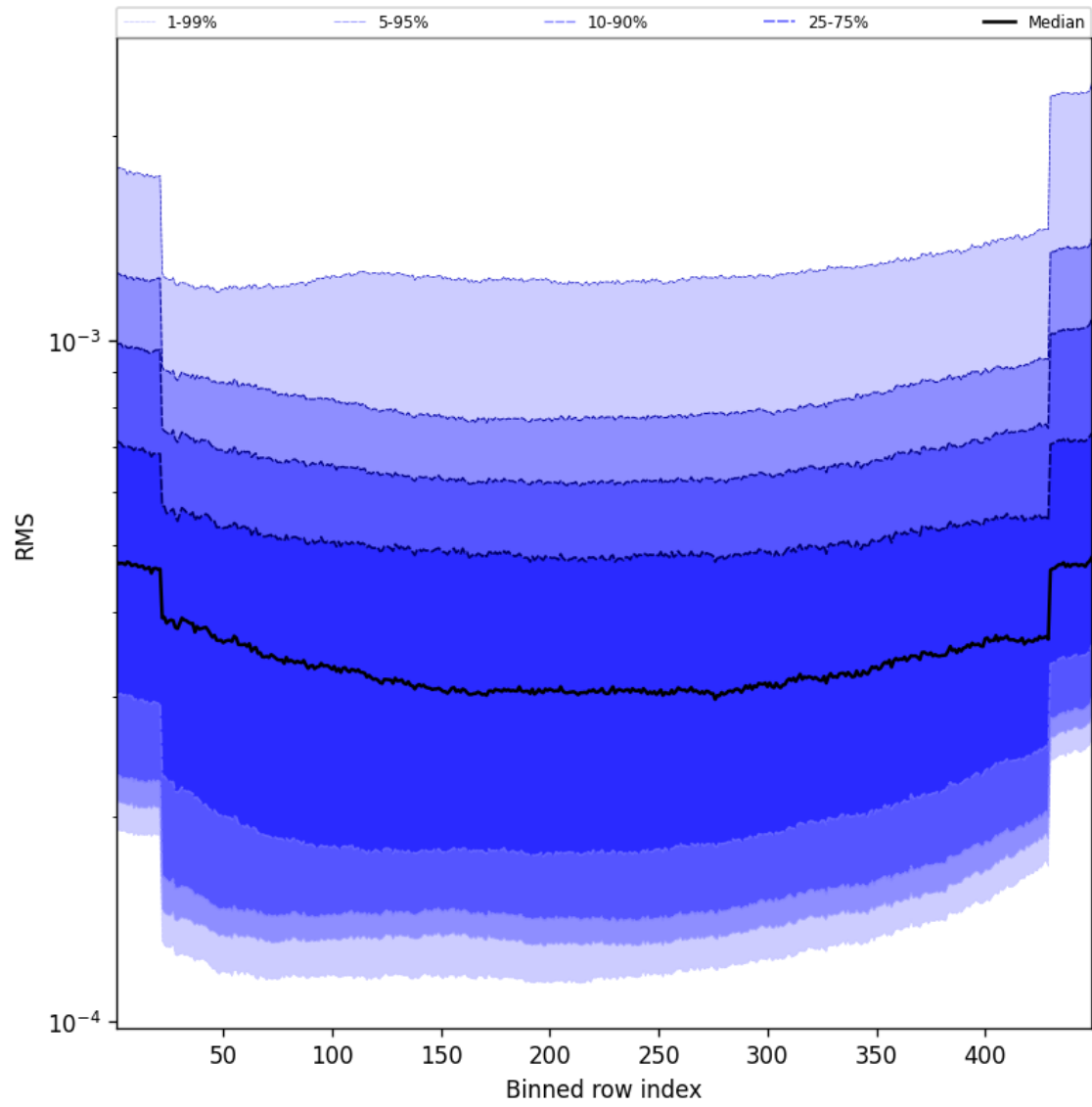
Figure 60: Along track statistics of “RMS” for 2024-12-04 to 2024-12-06
