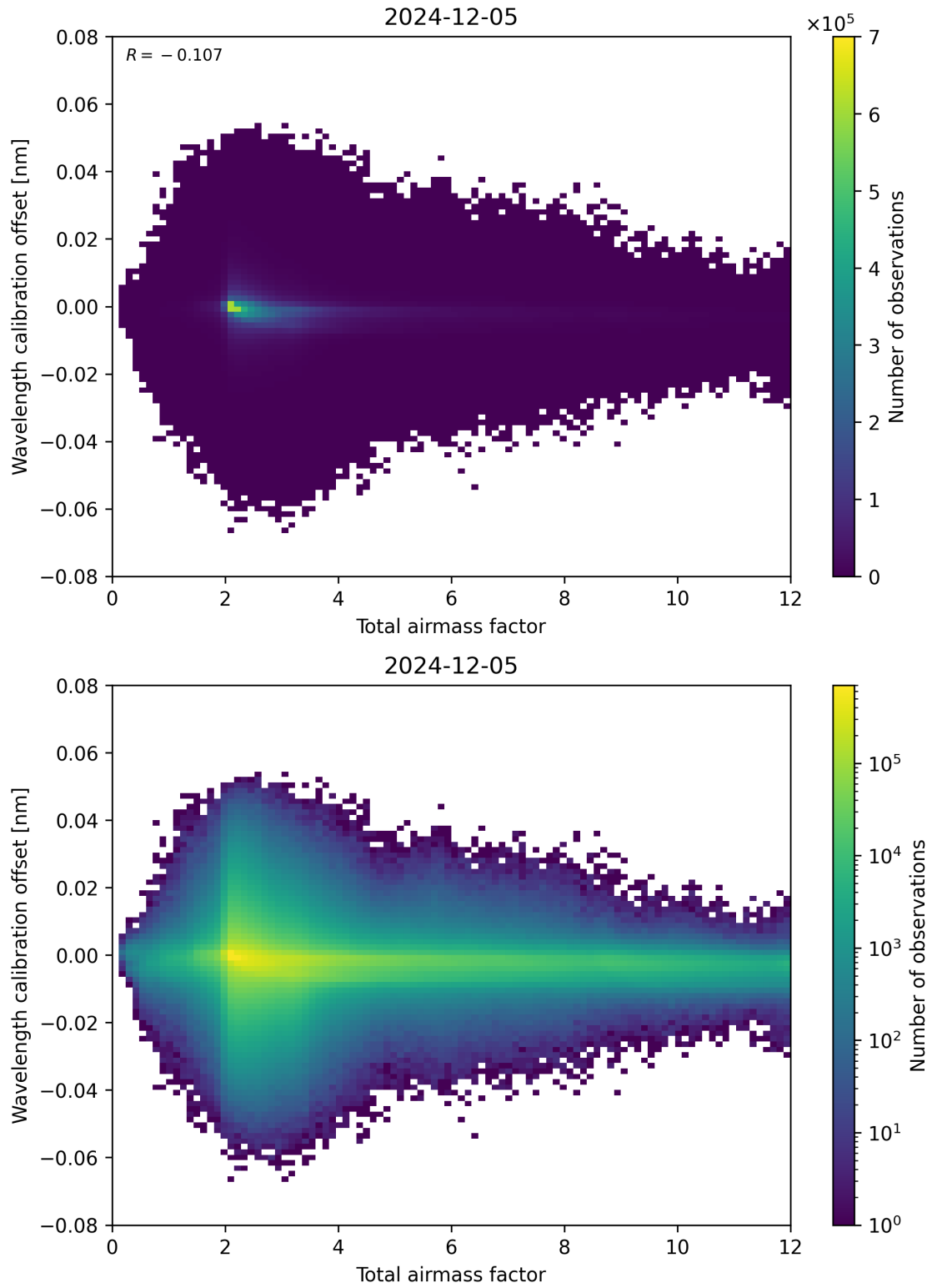
Figure 70: Scatter density plot of “Total airmass factor” against “Wavelength calibration offset” for 2024-12-04 to 2024-12-06.
