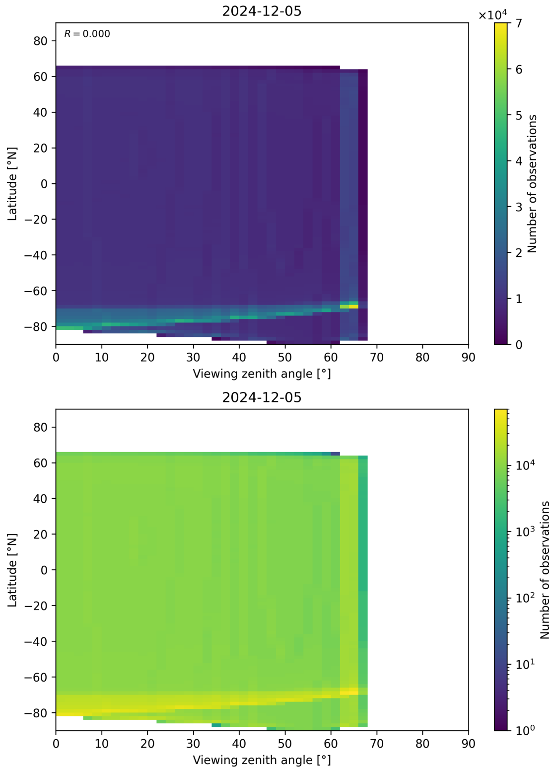
Figure 163: Scatter density plot of “Viewing zenith angle” against “Latitude” for 2024-12-04 to 2024-12-06.
