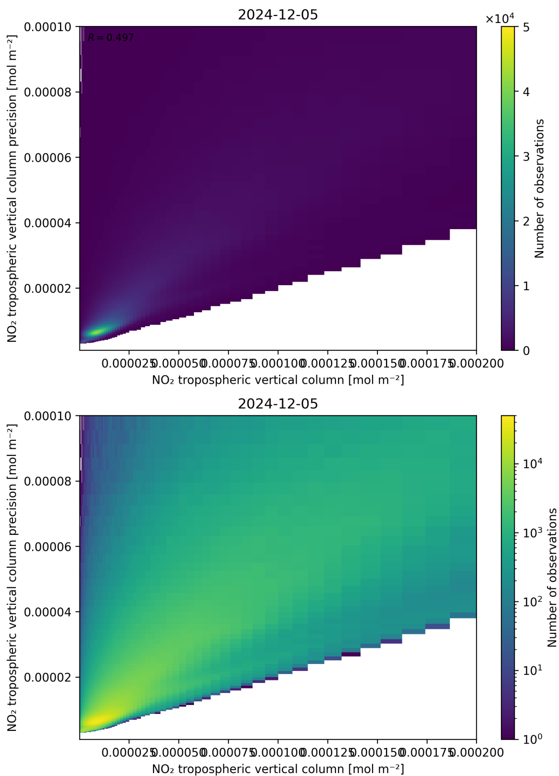
Figure 130: Scatter density plot of “NO 2 tropospheric vertical column” against “NO 2 tropospheric vertical column precision” for 2024-12-04 to 2024-12-06.
