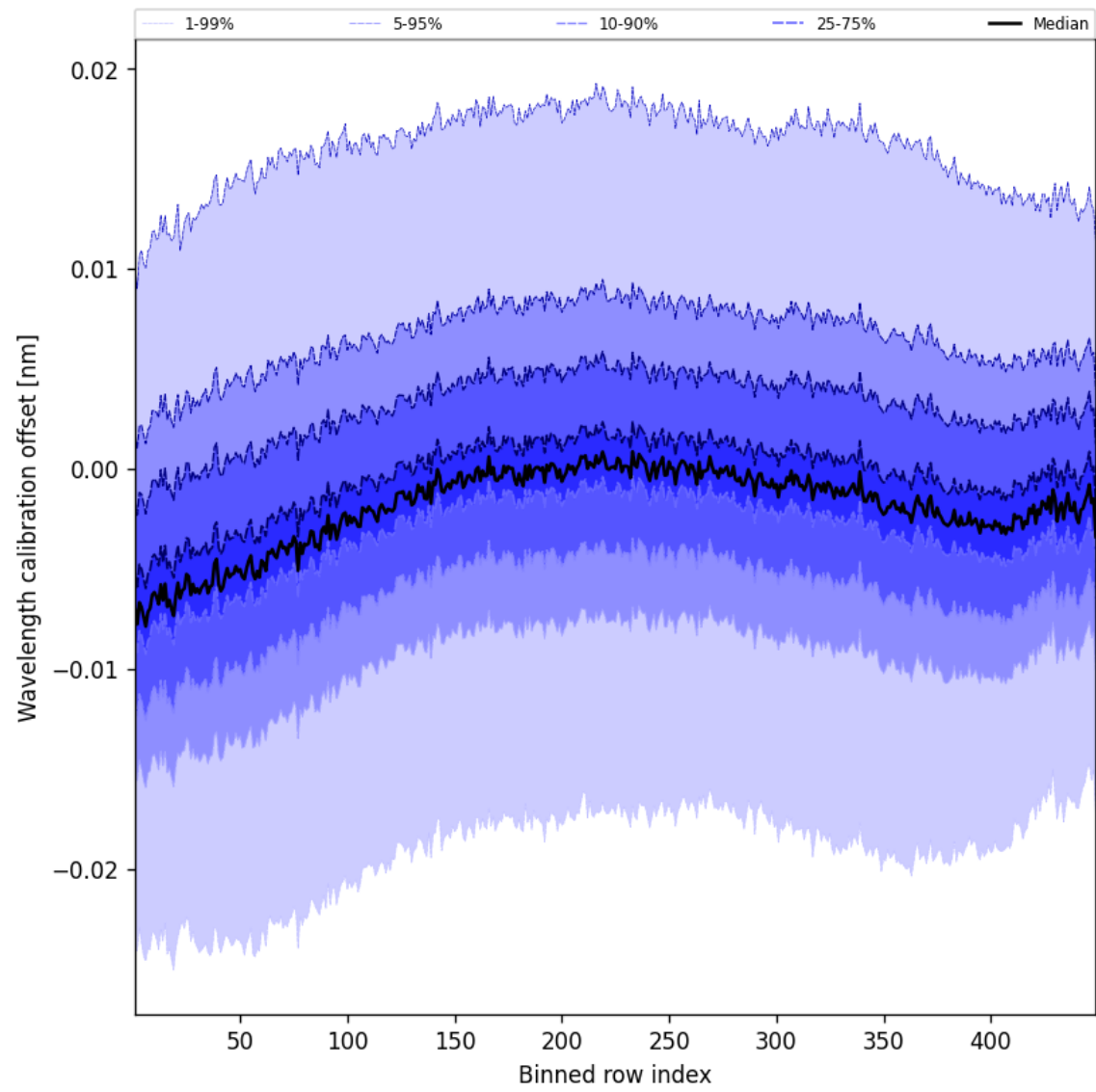
Figure 52: Along track statistics of “Wavelength calibration offset” for 2024-12-04 to 2024-12-06
