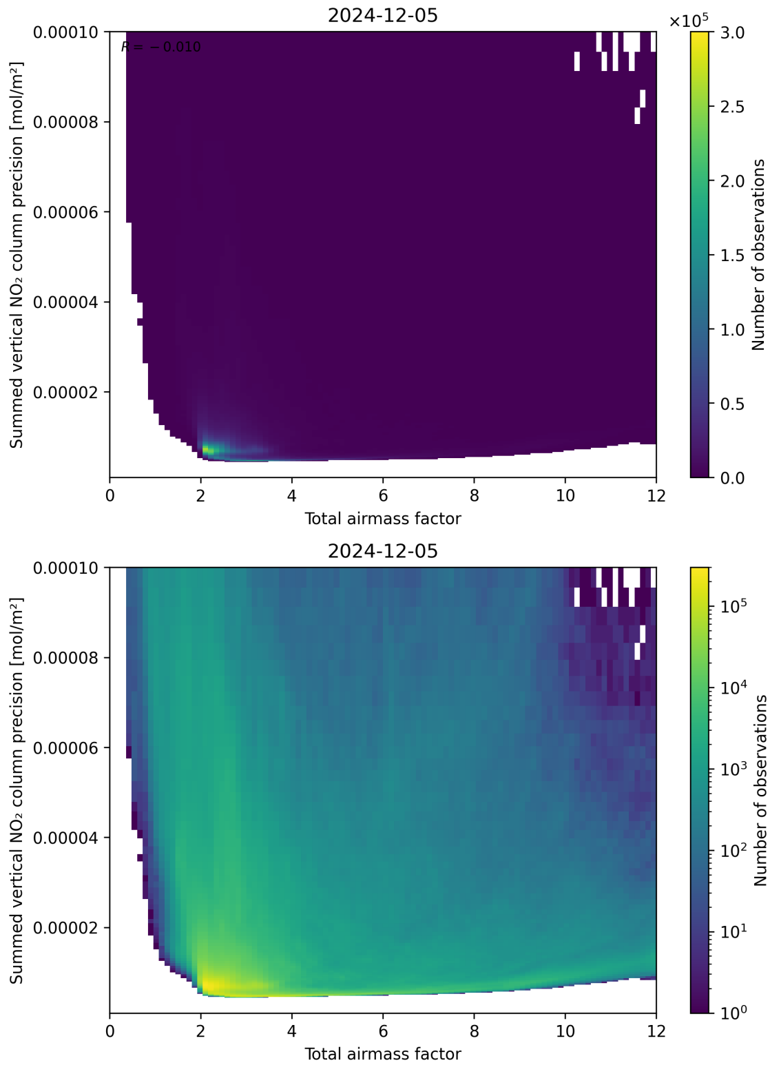
Figure 66: Scatter density plot of “Total airmass factor” against “Summed vertical NO 2 column precision” for 2024-12-04 to 2024-12-06.
