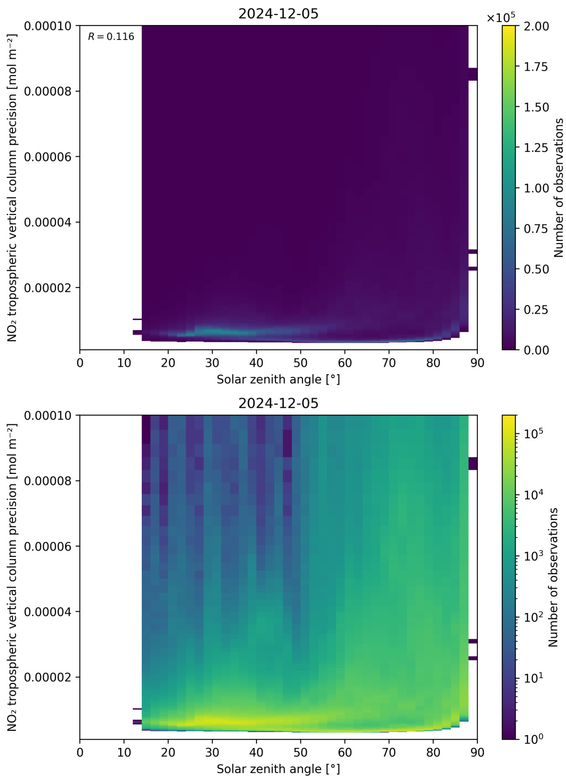
Figure 156: Scatter density plot of “Solar zenith angle” against “NO 2 tropospheric vertical column precision” for 2024-12-04 to 2024-12-06.
