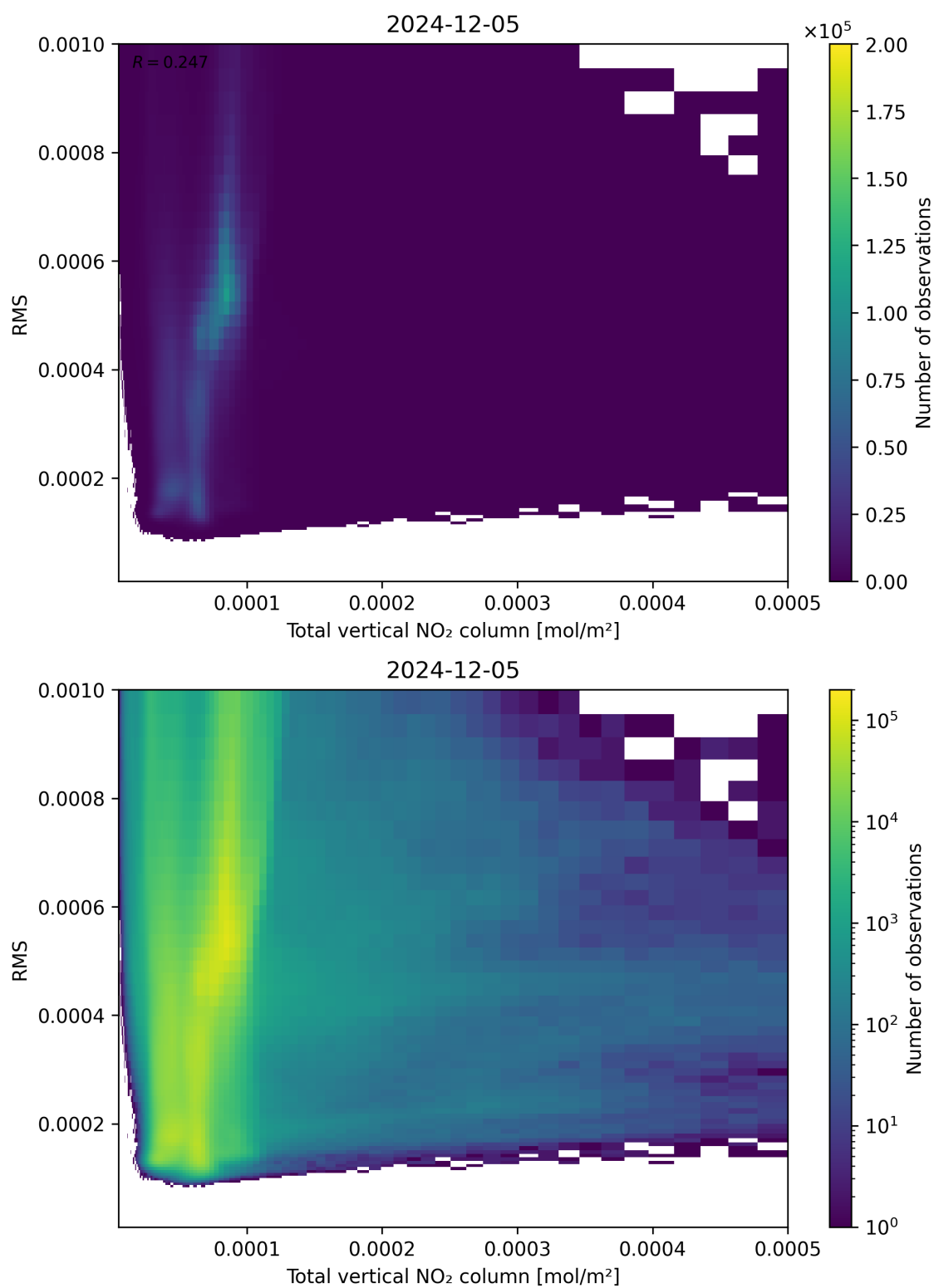
Figure 120: Scatter density plot of “Total vertical NO 2 column” against “RMS” for 2024-12-04 to 2024-12-06.
