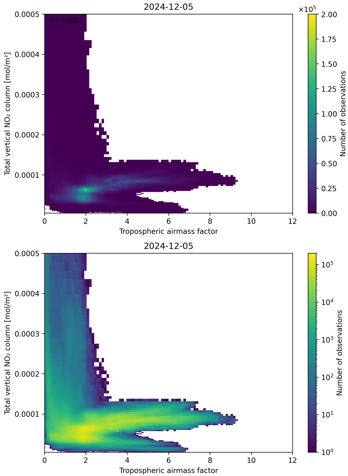
Figure 77: Scatter density plot of “Tropospheric airmass factor” against “Total vertical NO 2 column” for 2024-12-04 to 2024-12-06.
