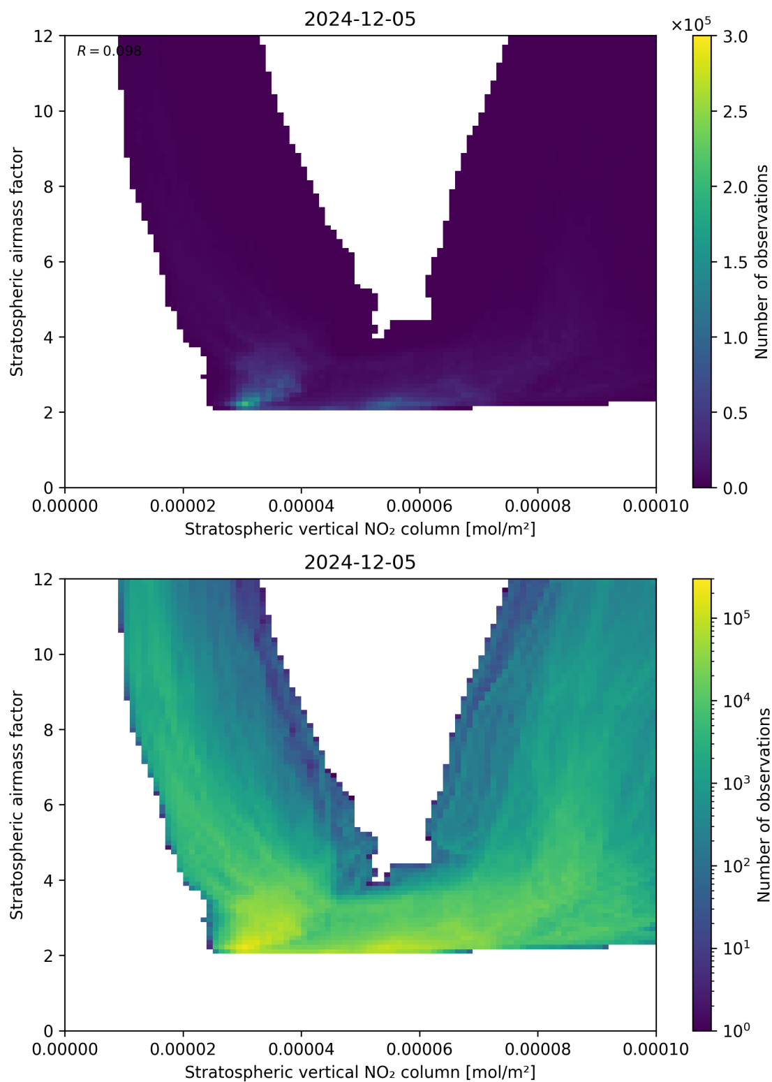
Figure 96: Scatter density plot of “Stratospheric vertical NO 2 column” against “Stratospheric airmass factor” for 2024-12-04 to 2024-12-06.
