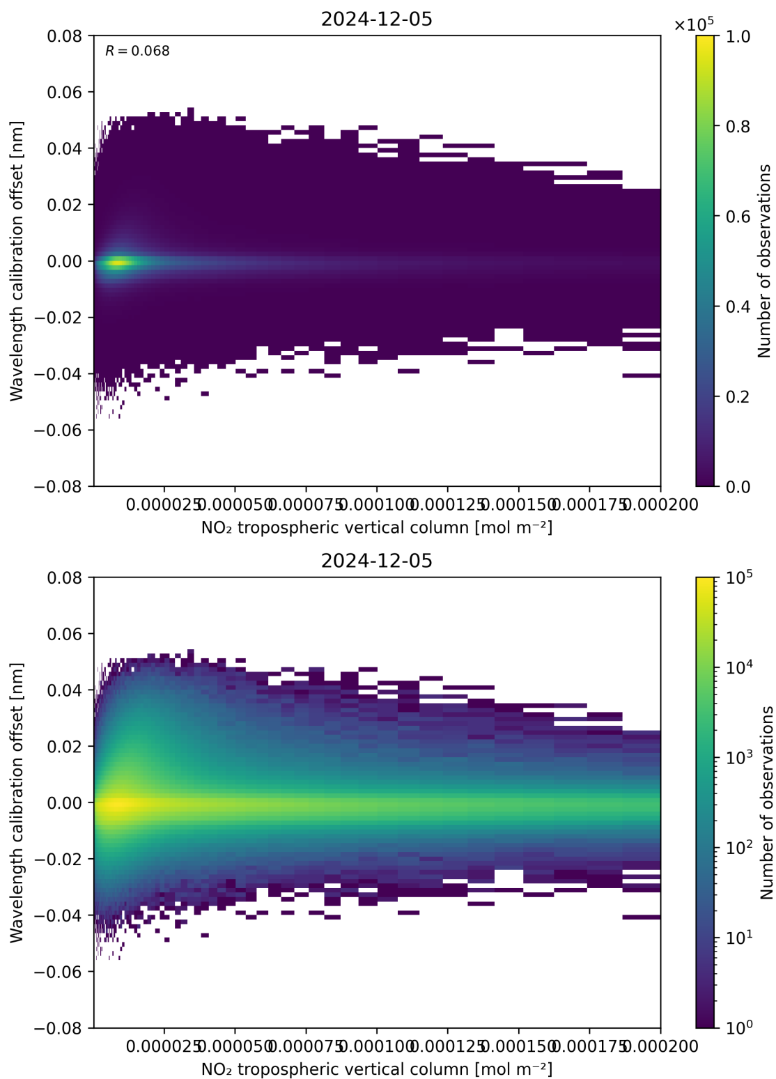
Figure 143: Scatter density plot of “NO 2 tropospheric vertical column” against “Wavelength calibration offset” for 2024-12-04 to 2024-12-06.
