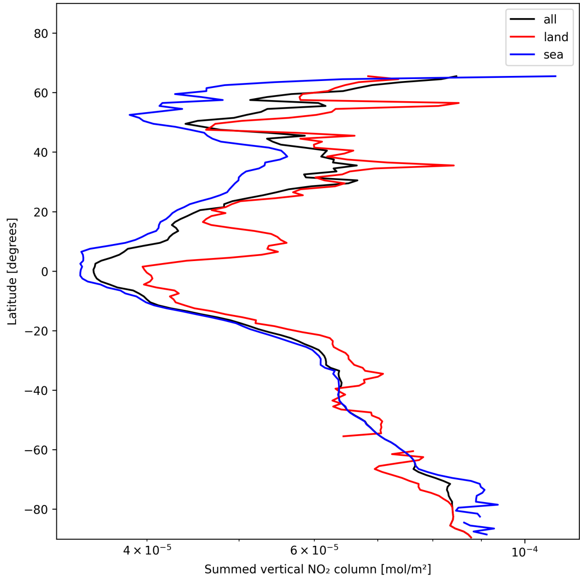
Figure 23: Zonal average of “Summed vertical NO 2 column” for 2024-12-04 to 2024-12-06.
