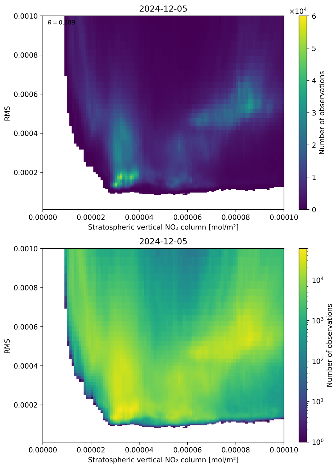
Figure 102: Scatter density plot of “Stratospheric vertical NO 2 column” against “RMS” for 2024-12-04 to 2024-12-06.
