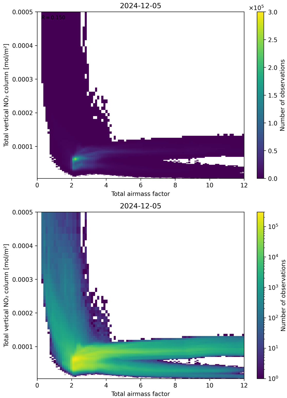
Figure 67: Scatter density plot of “Total airmass factor” against “Total vertical NO 2 column” for 2024-12-04 to 2024-12-06.
