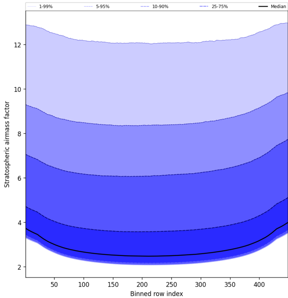
Figure 61: Along track statistics of “Stratospheric air mass factor” for 2024-12-04 to 2024-12-06
