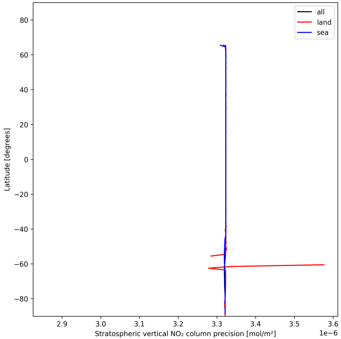
Figure 20: Zonal average of “Stratospheric vertical NO 2 column precision” for 2024-12-04 to 2024-12-06.
