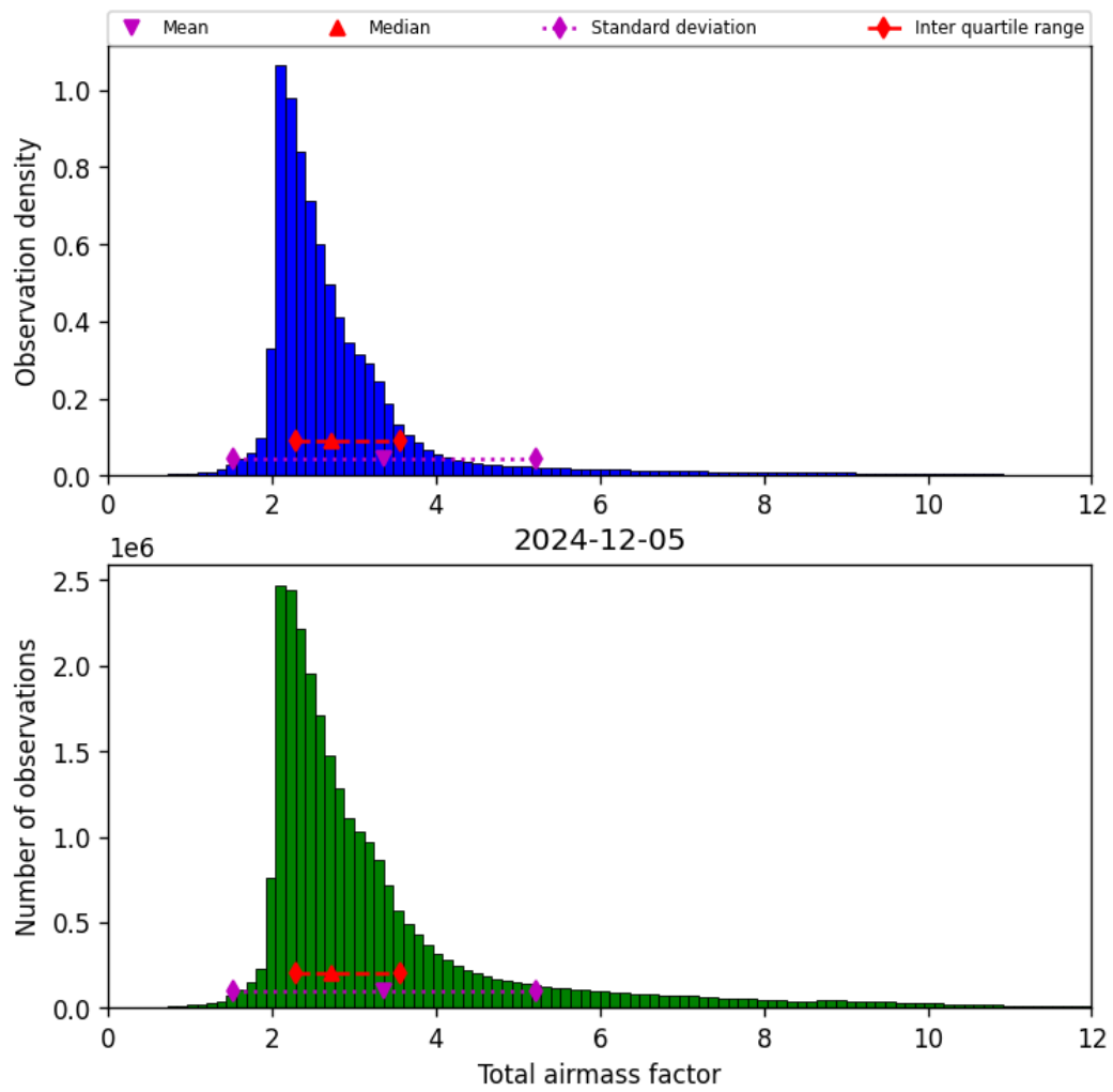
Figure 32: Histogram of “Total airmass factor” for 2024-12-04 to 2024-12-06
