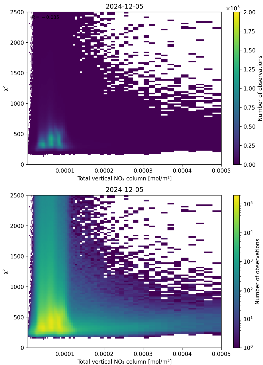
Figure 111: Scatter density plot of “Total vertical NO 2 column” against “ \chi^2 ” for 2024-12-04 to 2024-12-06.
