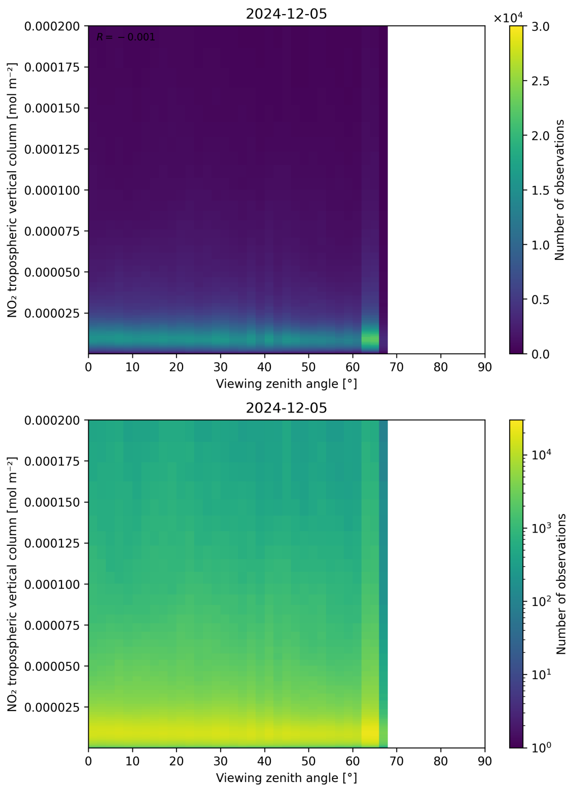
Figure 169: Scatter density plot of “Viewing zenith angle” against “NO 2 tropospheric vertical column” for 2024-12-04 to 2024-12-06.
