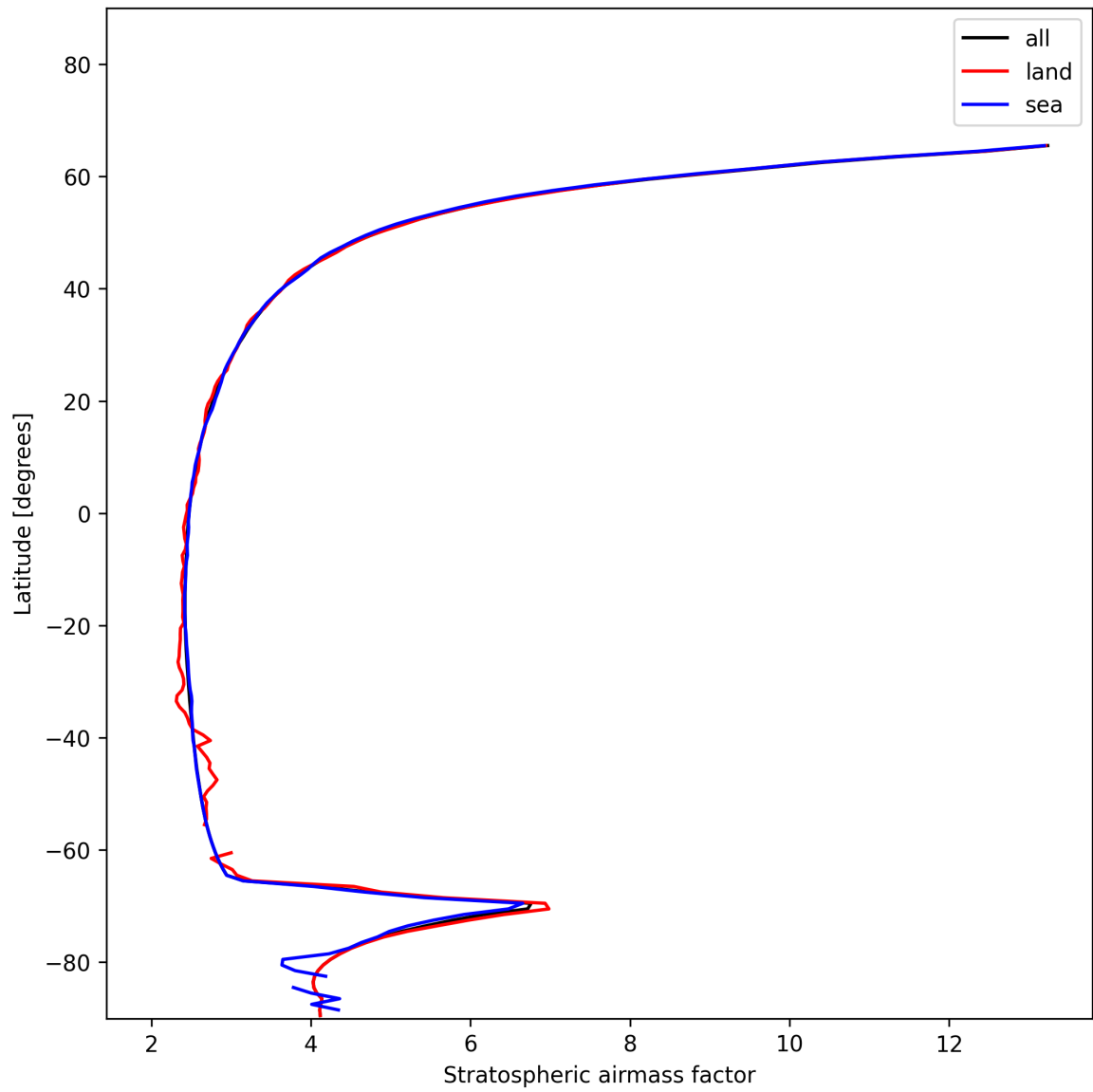
Figure 27: Zonal average of “Stratospheric air mass factor” for 2024-12-04 to 2024-12-06.
