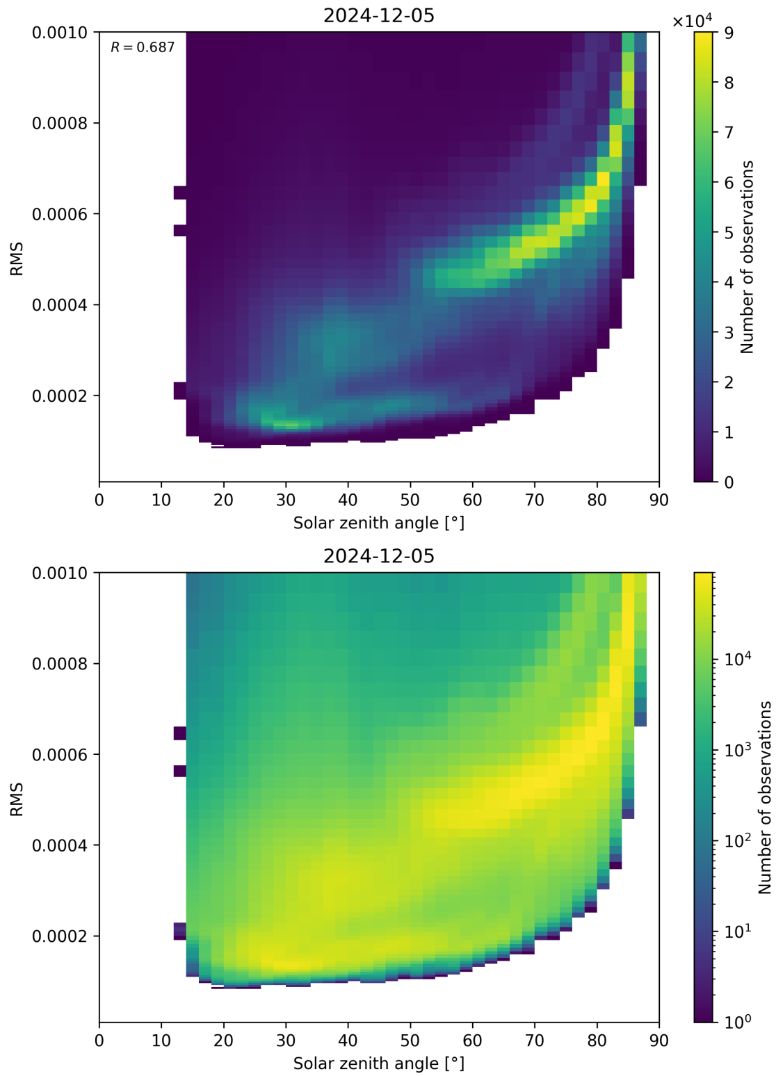
Figure 157: Scatter density plot of “Solar zenith angle” against “RMS” for 2024-12-04 to 2024-12-06.
