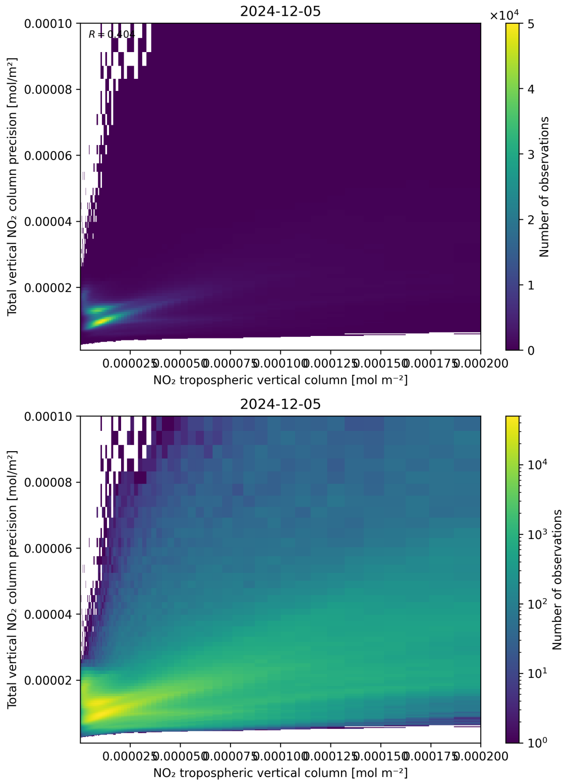
Figure 129: Scatter density plot of “NO 2 tropospheric vertical column” against “Total vertical NO 2 column precision” for 2024-12-04 to 2024-12-06.
