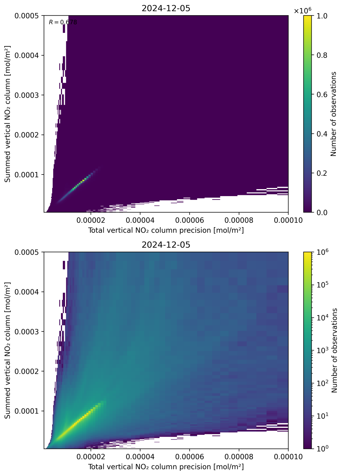
Figure 117: Scatter density plot of “Total vertical NO 2 column precision” against “Summed vertical NO 2 column” for 2024-12-04 to 2024-12-06.
