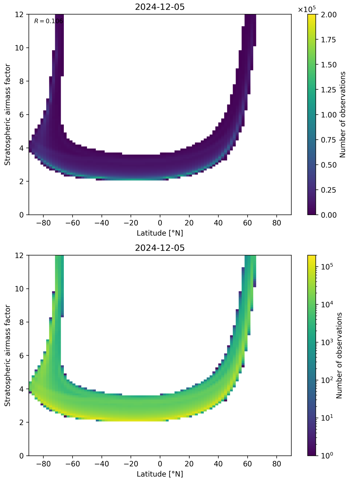
Figure 83: Scatter density plot of “Latitude” against “Stratospheric air mass factor” for 2024-12-04 to 2024-12-06.
