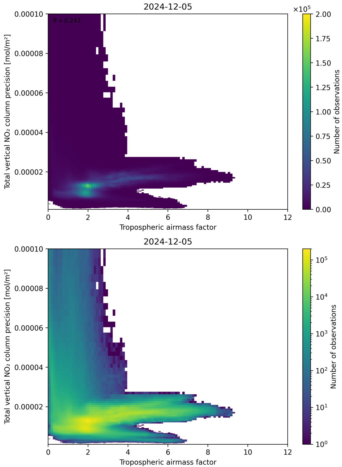
Figure 78: Scatter density plot of “Tropospheric air mass factor” against “Total vertical NO 2 column precision” for 2024-12-04 to 2024-12-06.
