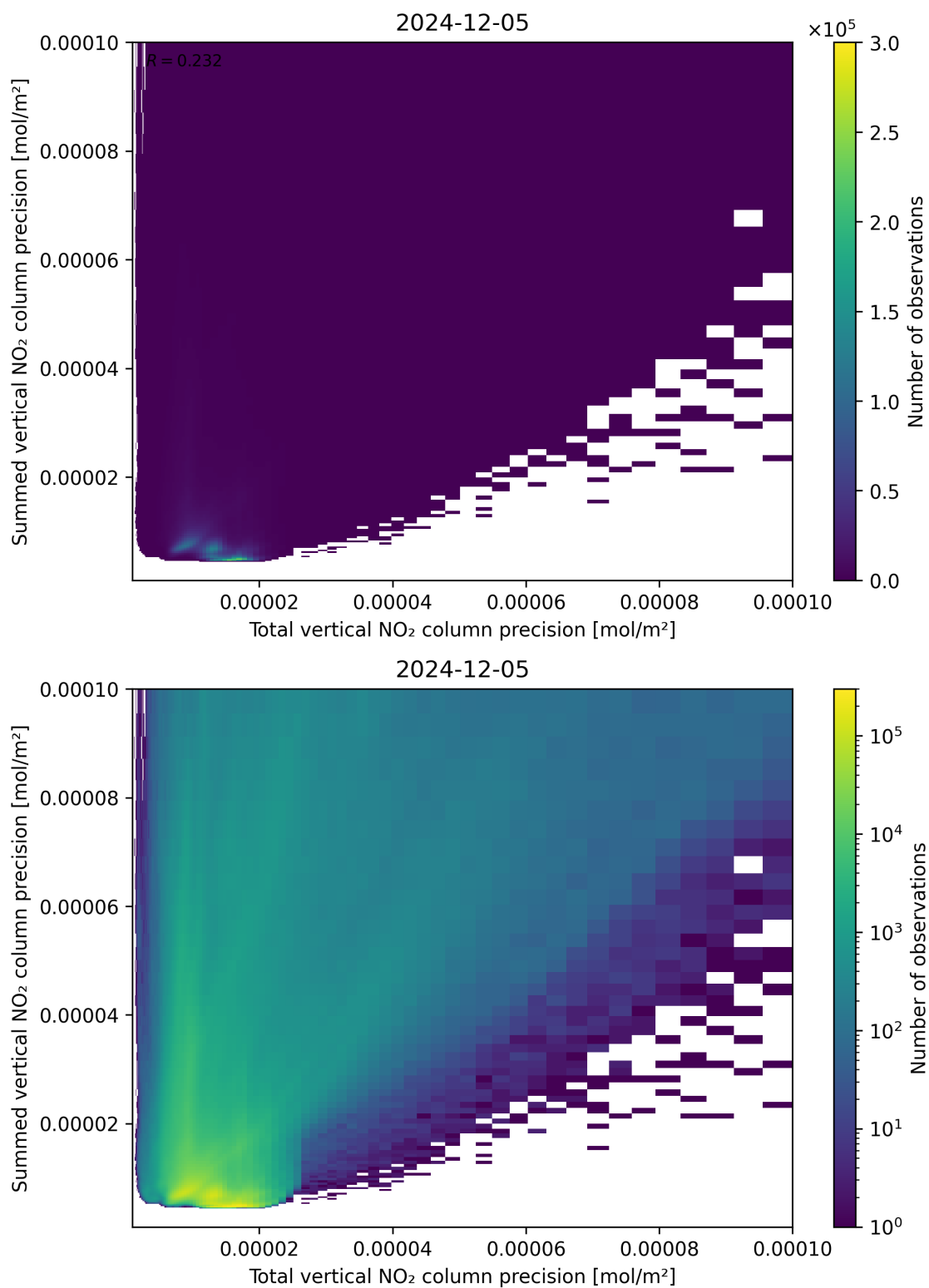
Figure 118: Scatter density plot of “Total vertical NO 2 column precision” against “Summed vertical NO 2 column precision” for 2024-12-04 to 2024-12-06.
