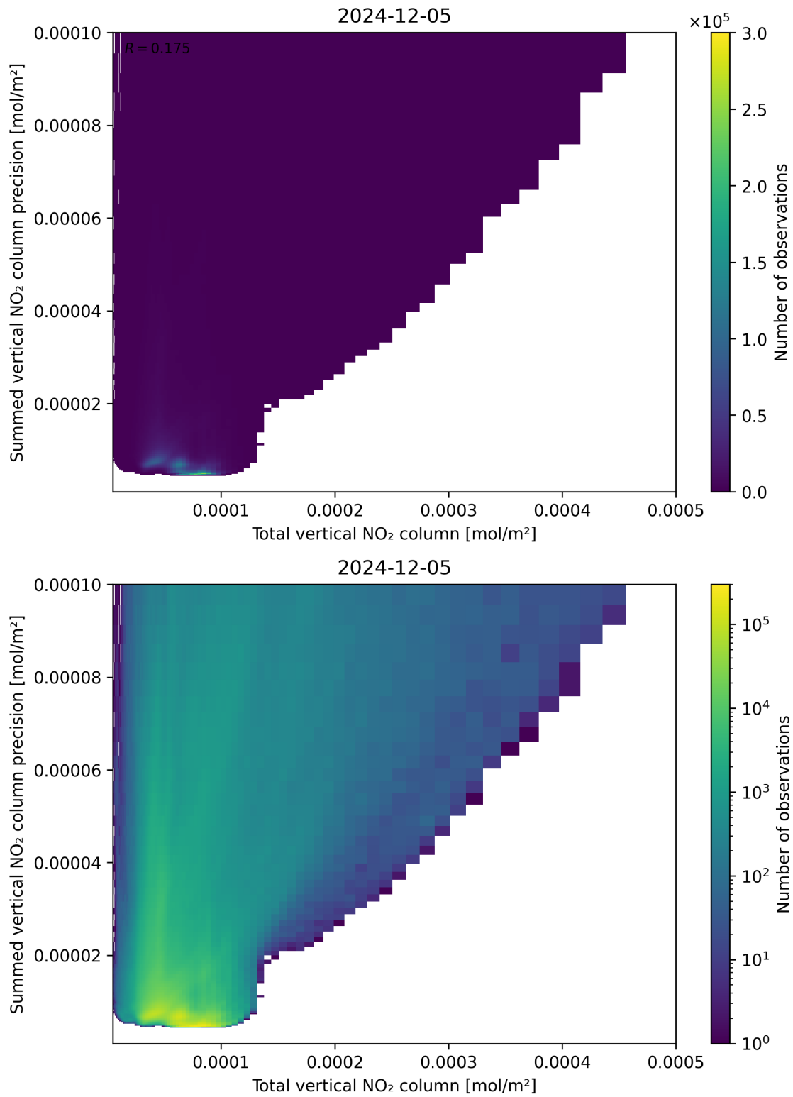
Figure 113: Scatter density plot of “Total vertical NO 2 column” against “Summed vertical NO 2 column precision” for 2024-12-04 to 2024-12-06.
