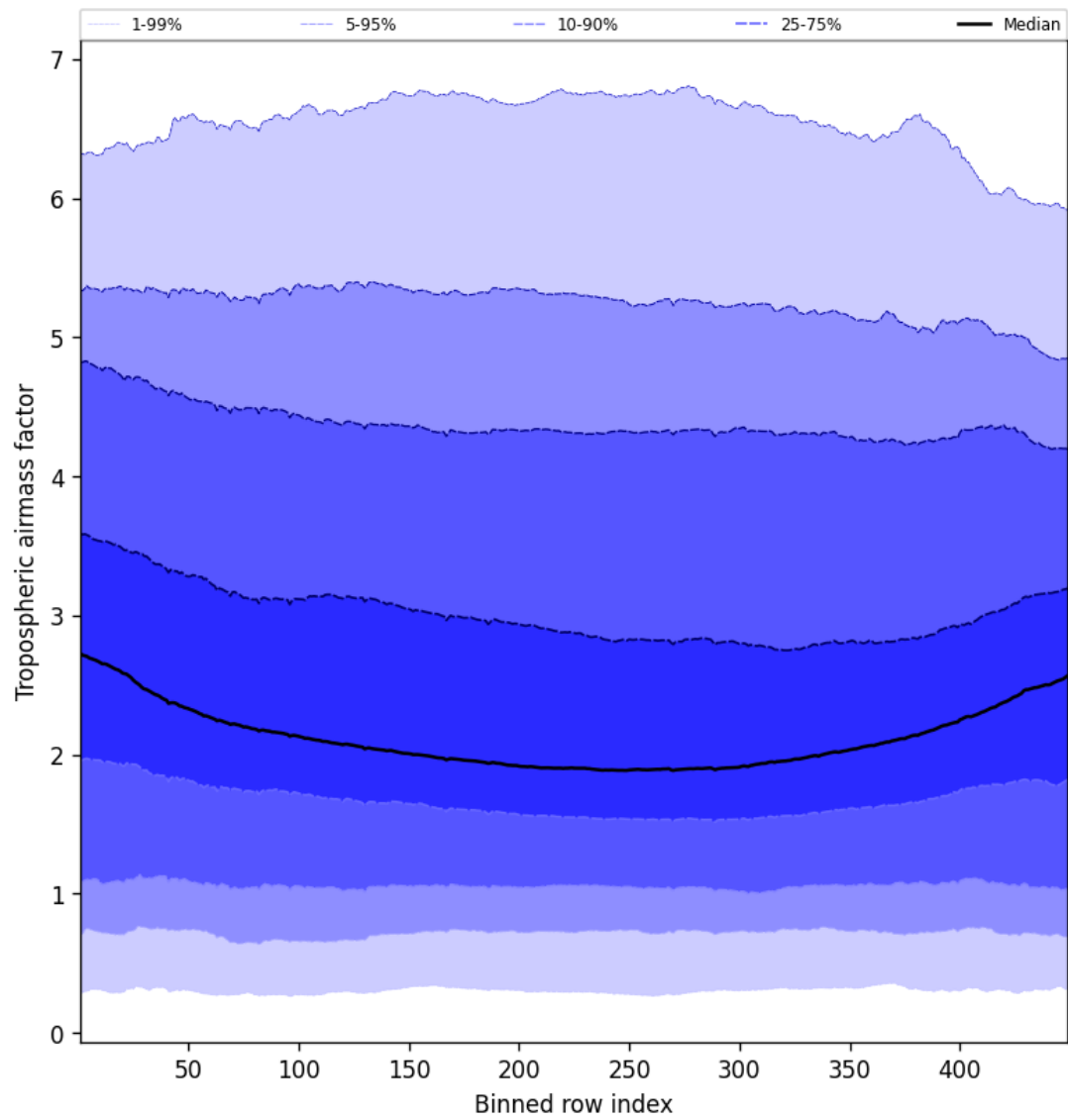
Figure 48: Along track statistics of “Tropospheric airmass factor” for 2024-12-04 to 2024-12-06
