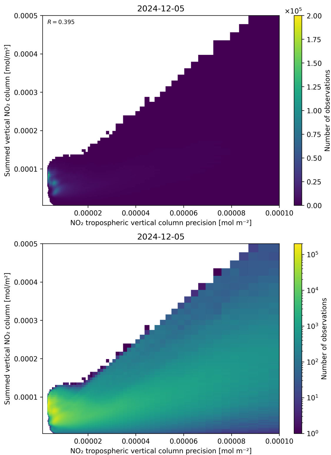
Figure 136: Scatter density plot of “NO 2 tropospheric vertical column precision” against “Summed vertical NO 2 column” for 2024-12-04 to 2024-12-06.
