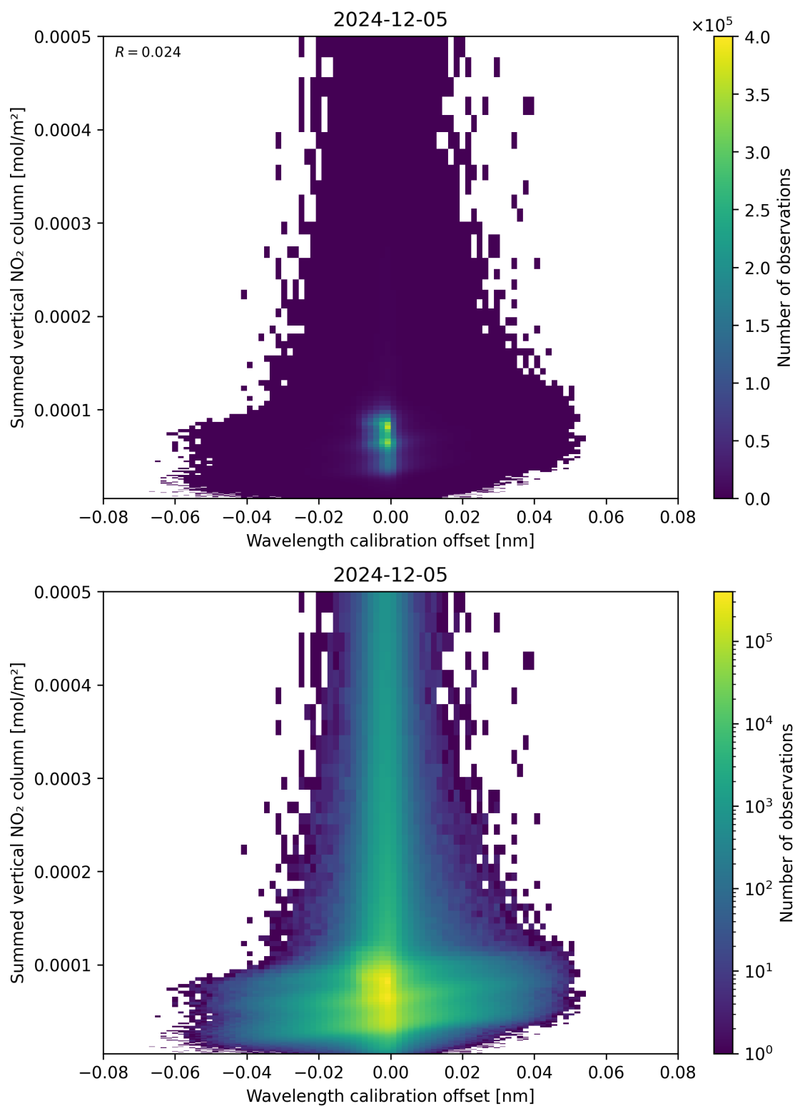
Figure 177: Scatter density plot of “Wavelength calibration offset” against “Summed vertical NO 2 column” for 2024-12-04 to 2024-12-06.
