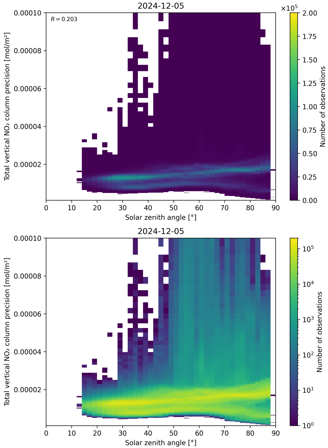
Figure 154: Scatter density plot of “Solar zenith angle” against “Total vertical NO 2 column precision” for 2024-12-04 to 2024-12-06.
