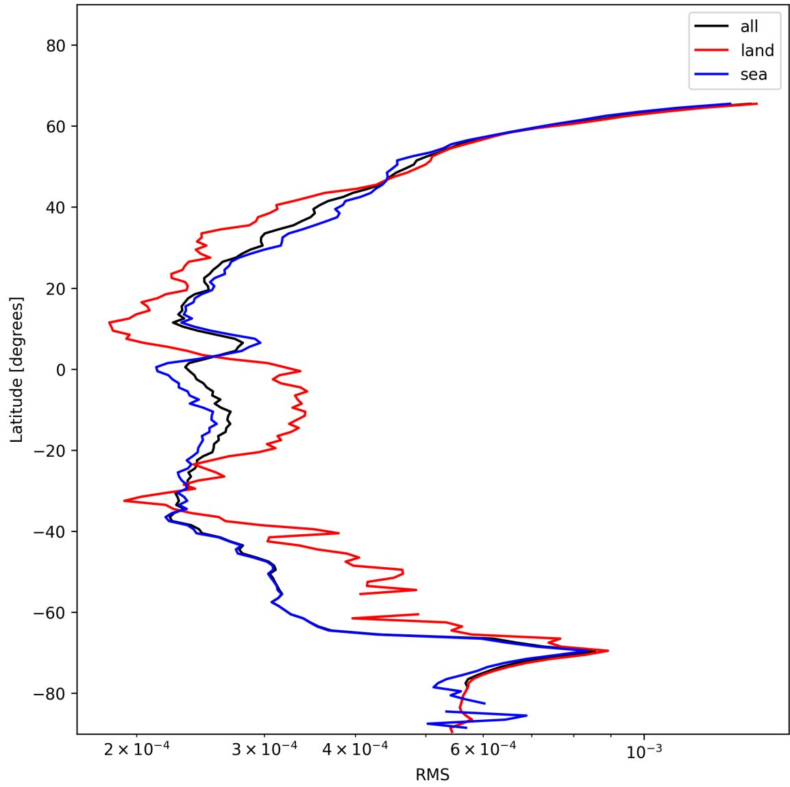
Figure 26: Zonal average of “RMS” for 2024-12-04 to 2024-12-06.
