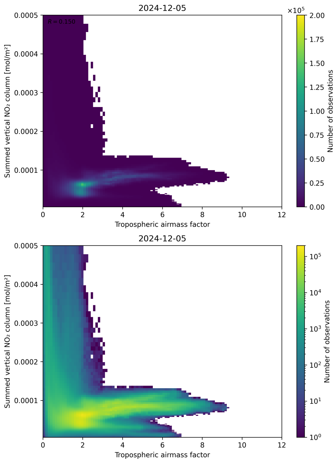
Figure 75: Scatter density plot of “Tropospheric air mass factor” against “Summed vertical NO 2 column” for 2024-12-04 to 2024-12-06.
