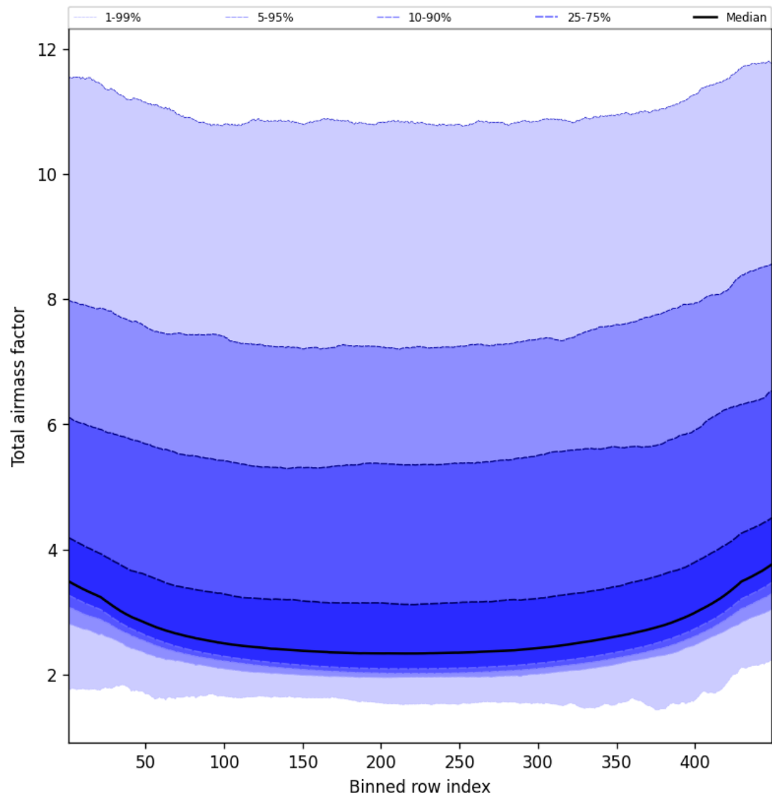
Figure 49: Along track statistics of “Total airmass factor” for 2024-12-04 to 2024-12-06
