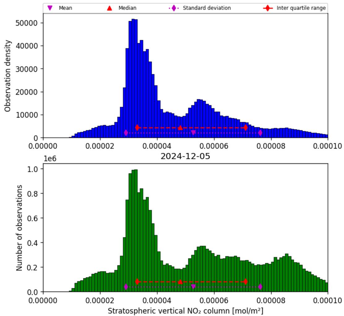
Figure 36: Histogram of “Stratospheric vertical NO 2 column” for 2024-12-04 to 2024-12-06
