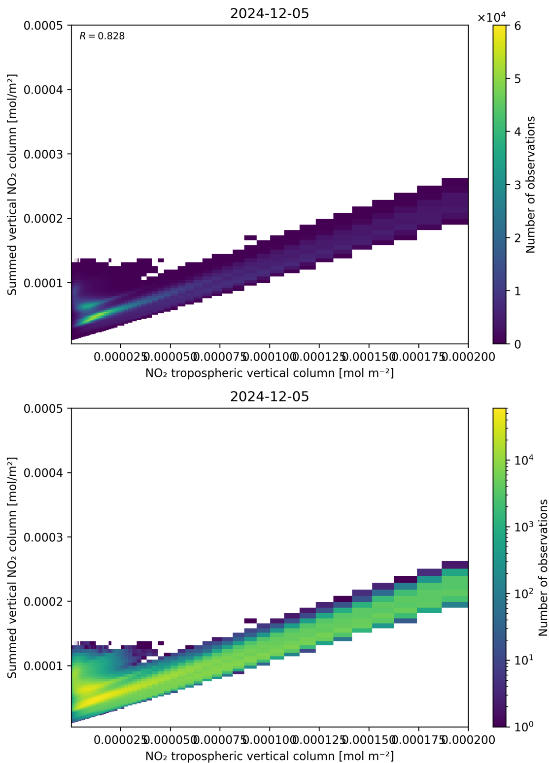
Figure 126: Scatter density plot of “NO 2 tropospheric vertical column” against “Summed vertical NO 2 column” for 2024-12-04 to 2024-12-06.
