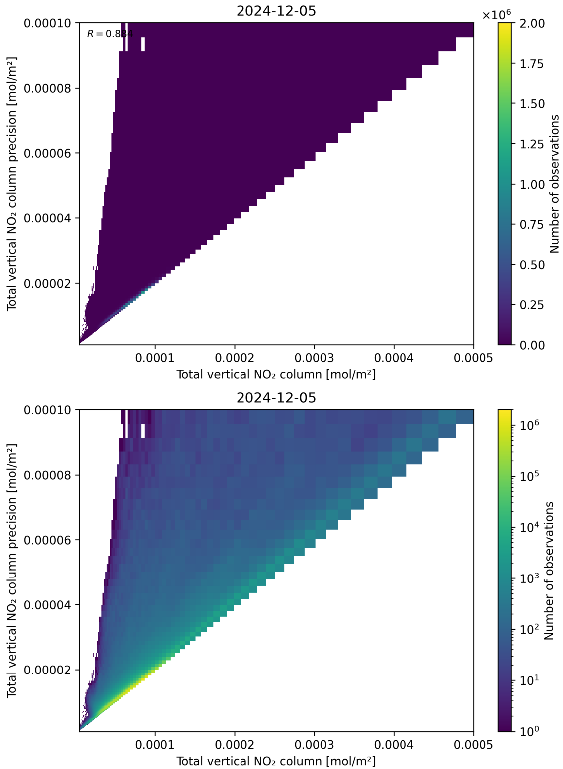
Figure 114: Scatter density plot of “Total vertical NO 2 column” against “Total vertical NO 2 column precision” for 2024-12-04 to 2024-12-06.
