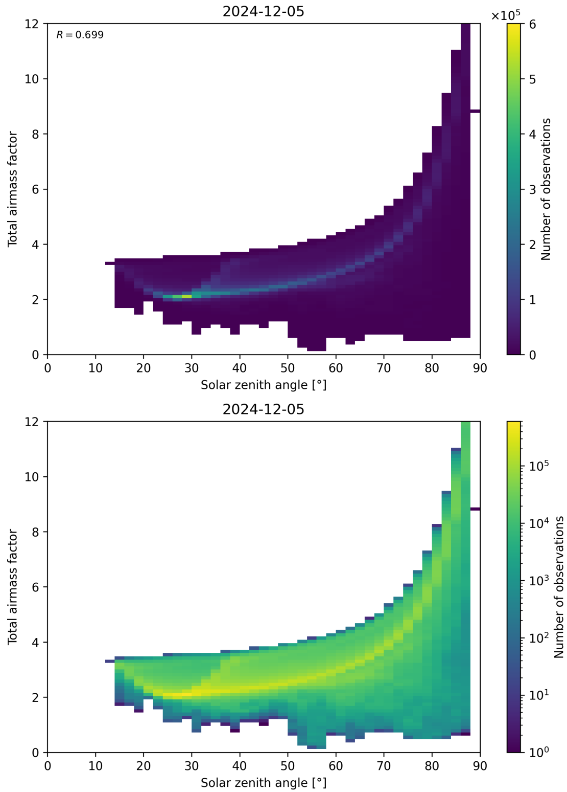
Figure 146: Scatter density plot of “Solar zenith angle” against “Total air mass factor” for 2024-12-04 to 2024-12-06.
