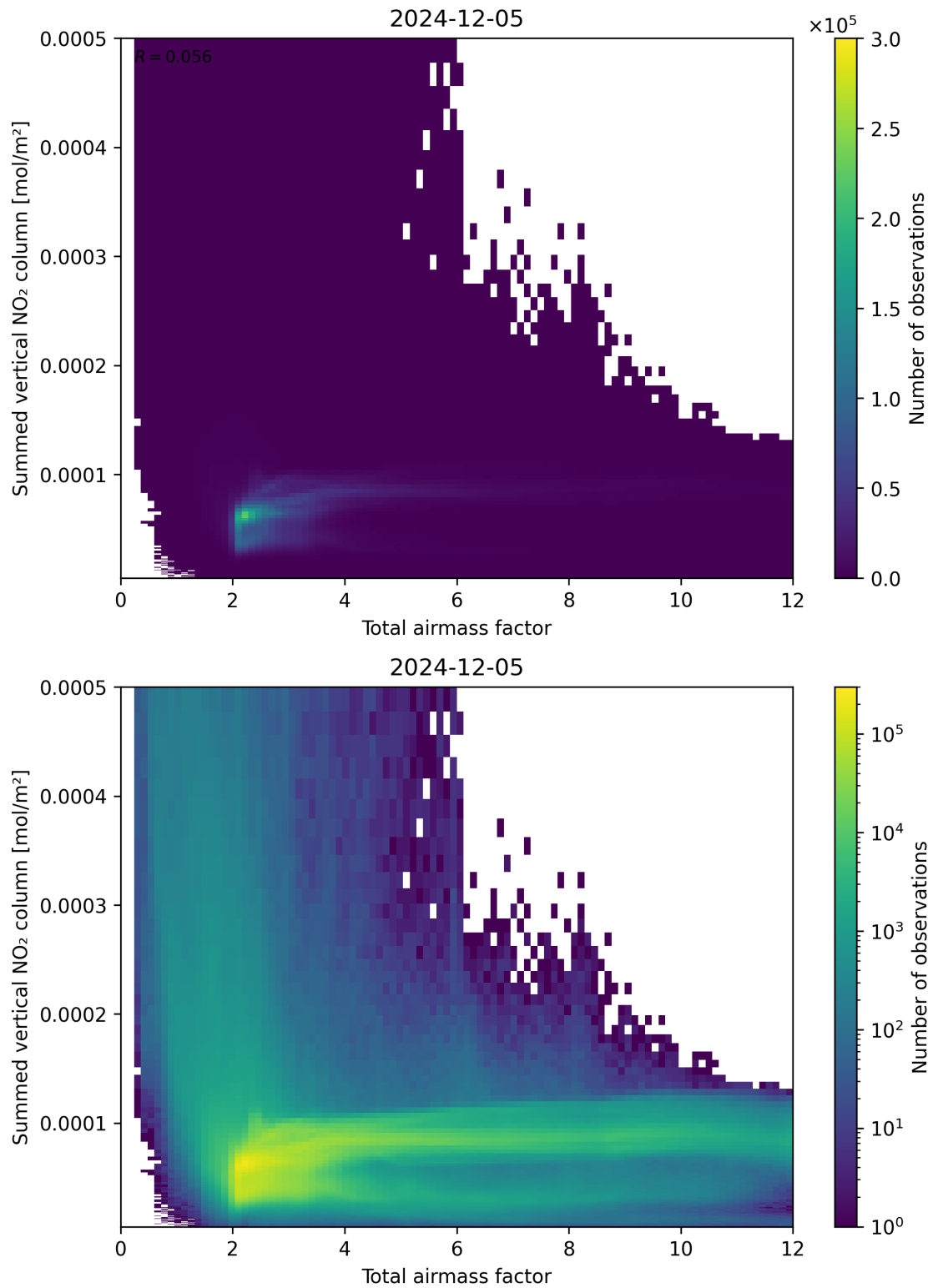
Figure 65: Scatter density plot of “Total airmass factor” against “Summed vertical NO 2 column” for 2024-12-04 to 2024-12-06.
