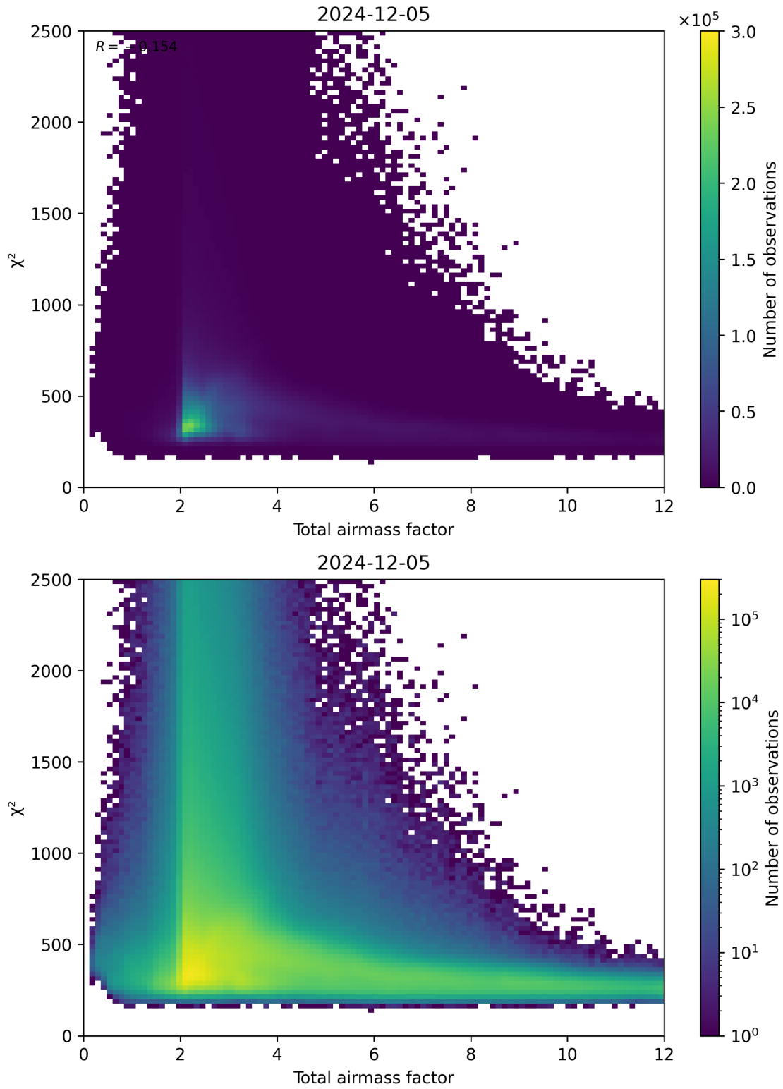
Figure 63: Scatter density plot of “Total airmass factor” against “ \chi^2 ” for 2024-12-04 to 2024-12-06.
