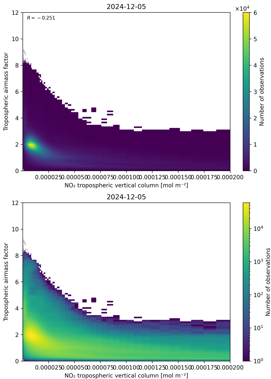
Figure 123: Scatter density plot of “NO 2 tropospheric vertical column” against “Tropospheric air mass factor” for 2024-12-04 to 2024-12-06.
