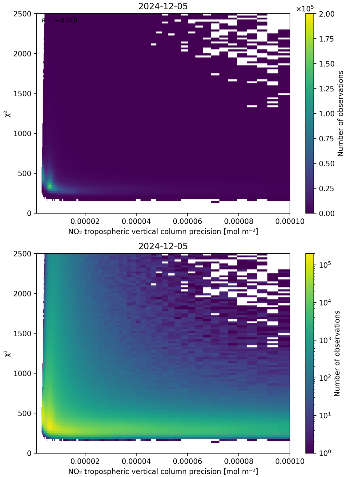
Figure 134: Scatter density plot of “NO 2 tropospheric vertical column precision” against “ \chi^2 ” for 2024-12-04 to 2024-12-06.
