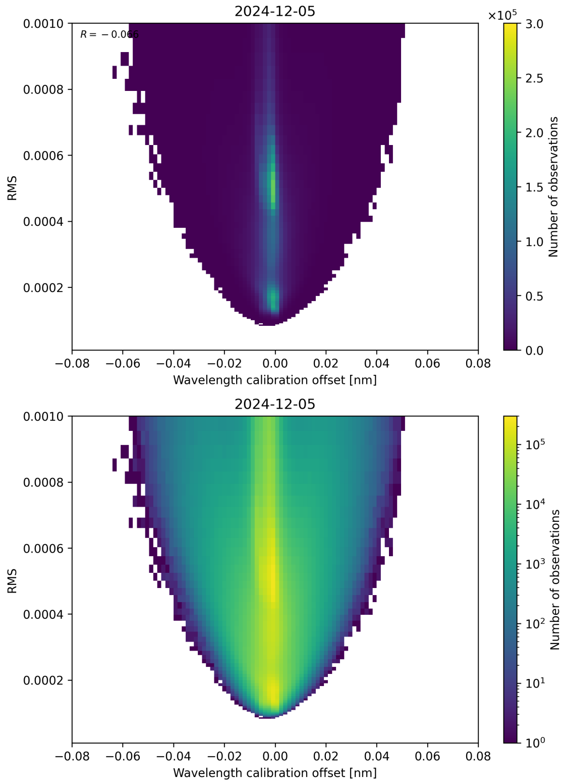
Figure 181: Scatter density plot of “Wavelength calibration offset” against “RMS” for 2024-12-04 to 2024-12-06.
