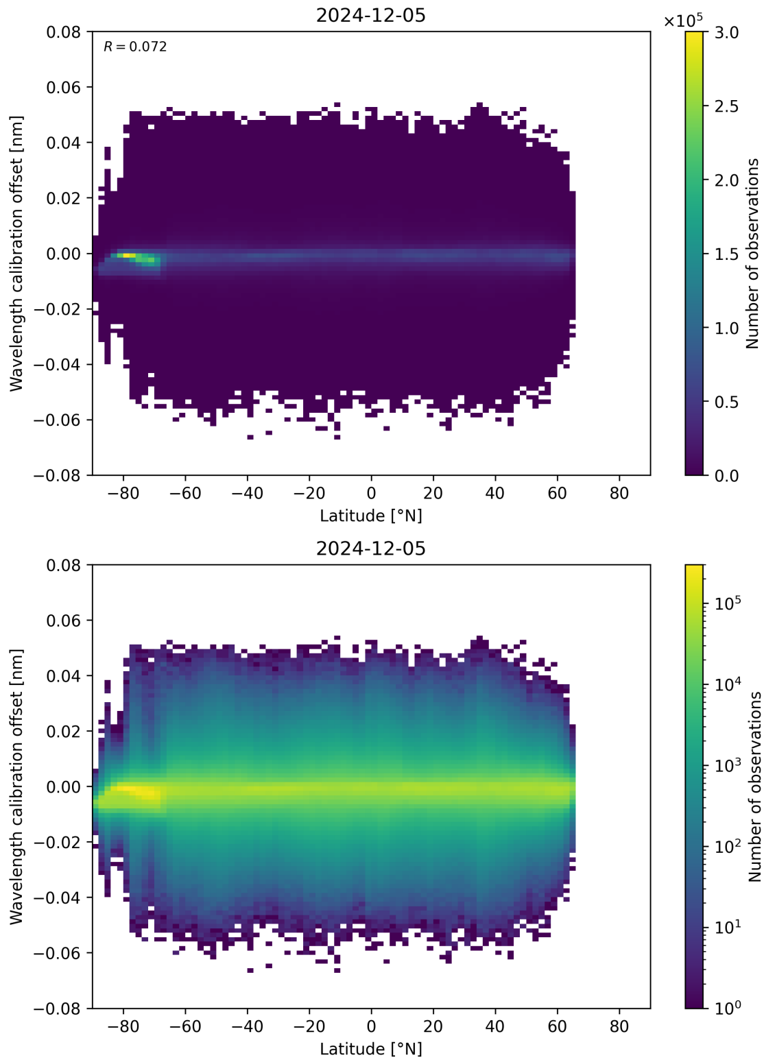
Figure 95: Scatter density plot of “Latitude” against “Wavelength calibration offset” for 2024-12-04 to 2024-12-06.
