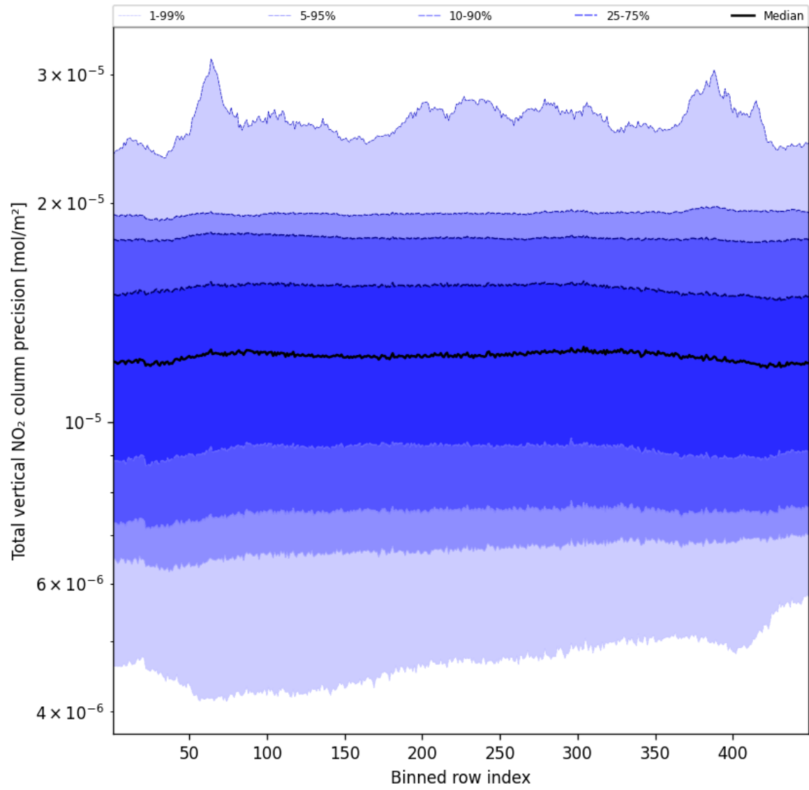
Figure 56: Along track statistics of “Total vertical NO 2 column precision” for 2024-12-04 to 2024-12-06
