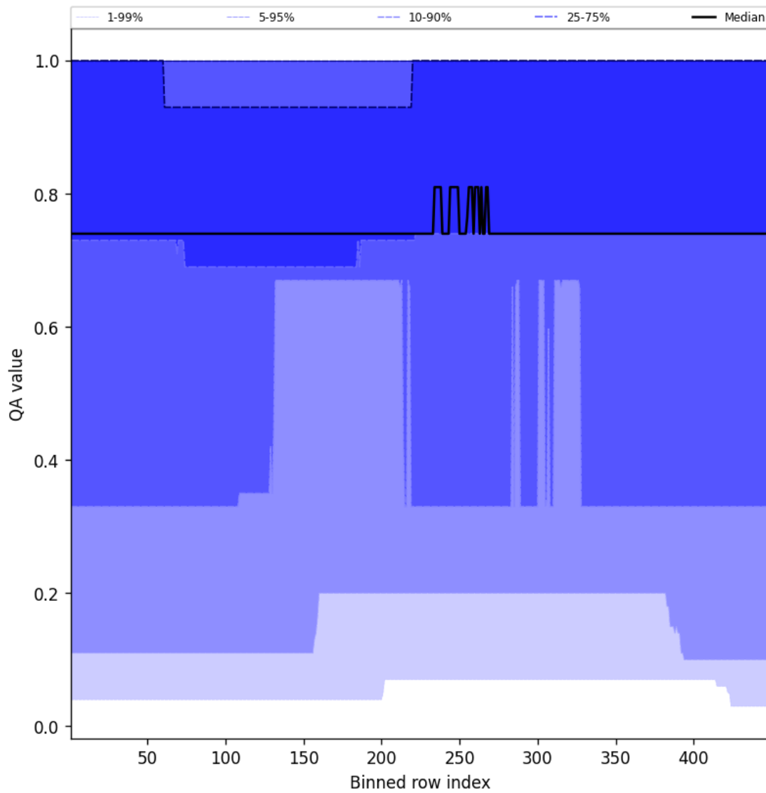
Figure 45: Along track statistics of “QA value” for 2024-12-04 to 2024-12-06
