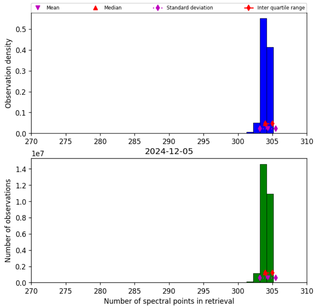
Figure 33: Histogram of “Number of spectral points in retrieval” for 2024-12-04 to 2024-12-06
