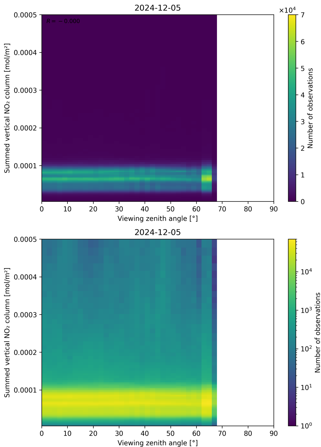
Figure 165: Scatter density plot of “Viewing zenith angle” against “Summed vertical NO 2 column” for 2024-12-04 to 2024-12-06.
