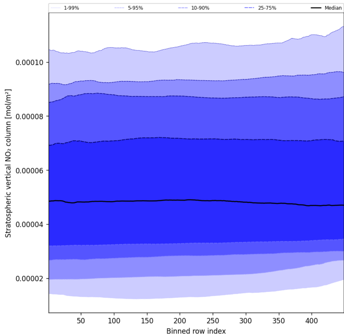
Figure 53: Along track statistics of “Stratospheric vertical NO 2 column” for 2024-12-04 to 2024-12-06
