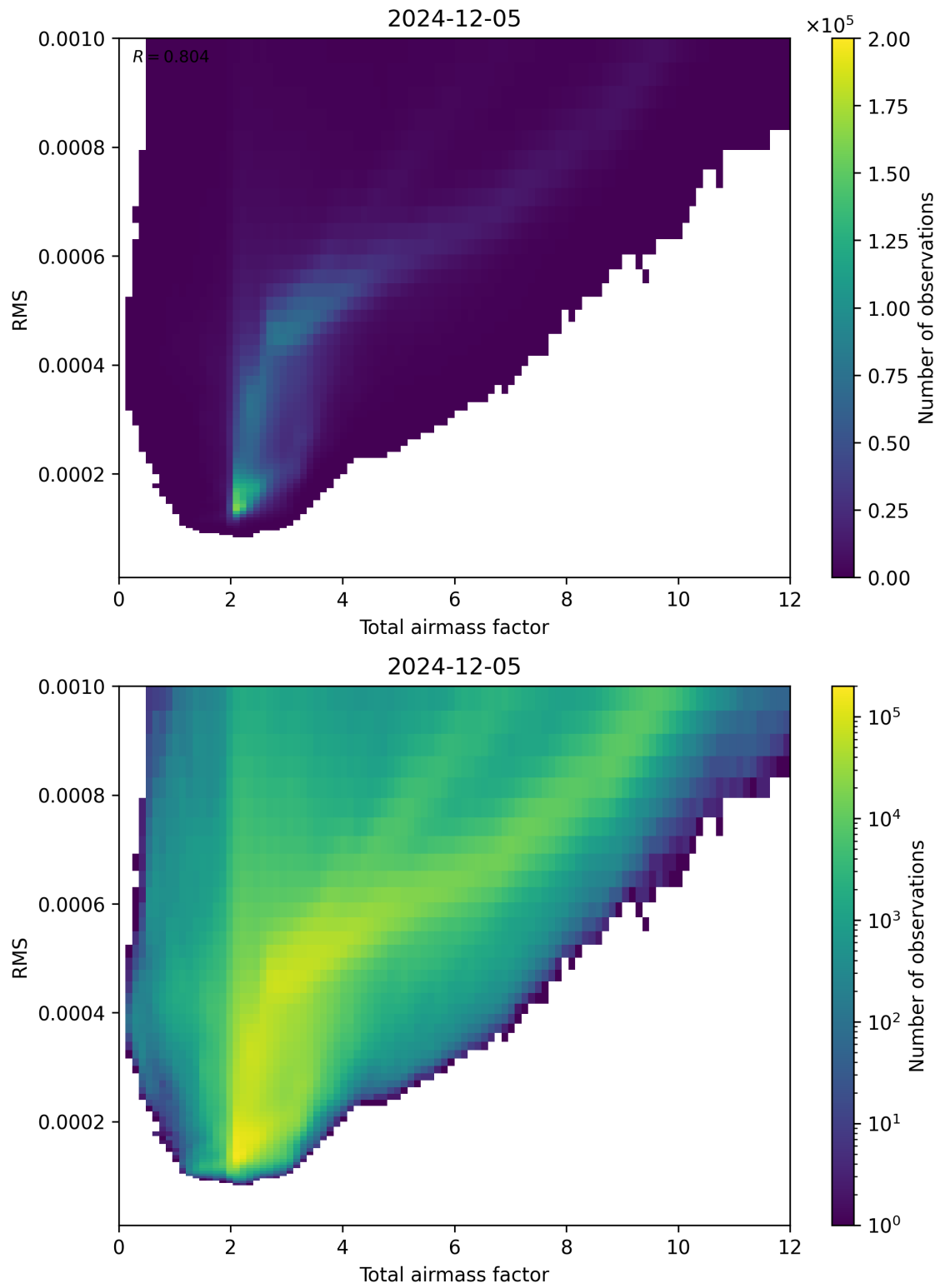
Figure 69: Scatter density plot of “Total airmass factor” against “RMS” for 2024-12-04 to 2024-12-06.
