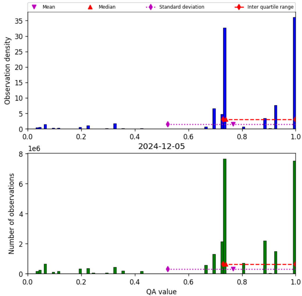
Figure 28: Histogram of “QA value” for 2024-12-04 to 2024-12-06
