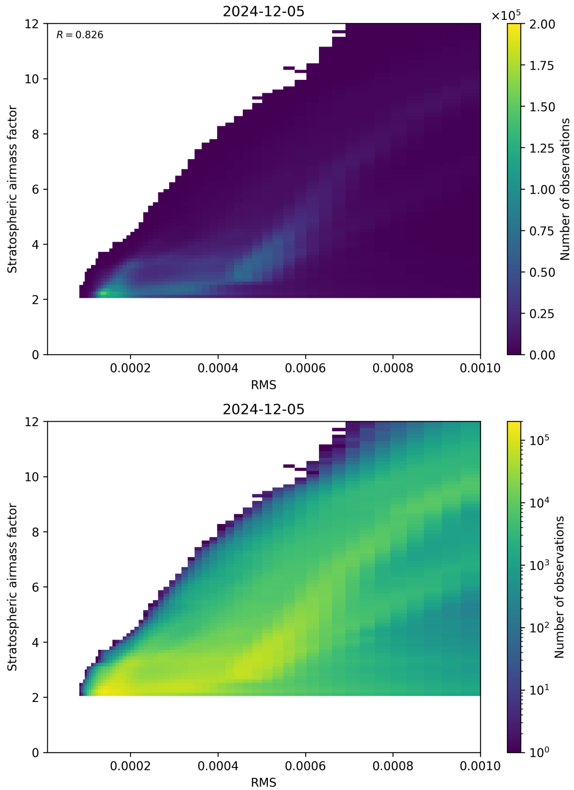
Figure 144: Scatter density plot of “RMS” against “Stratospheric airmass factor” for 2024-12-04 to 2024-12-06.
