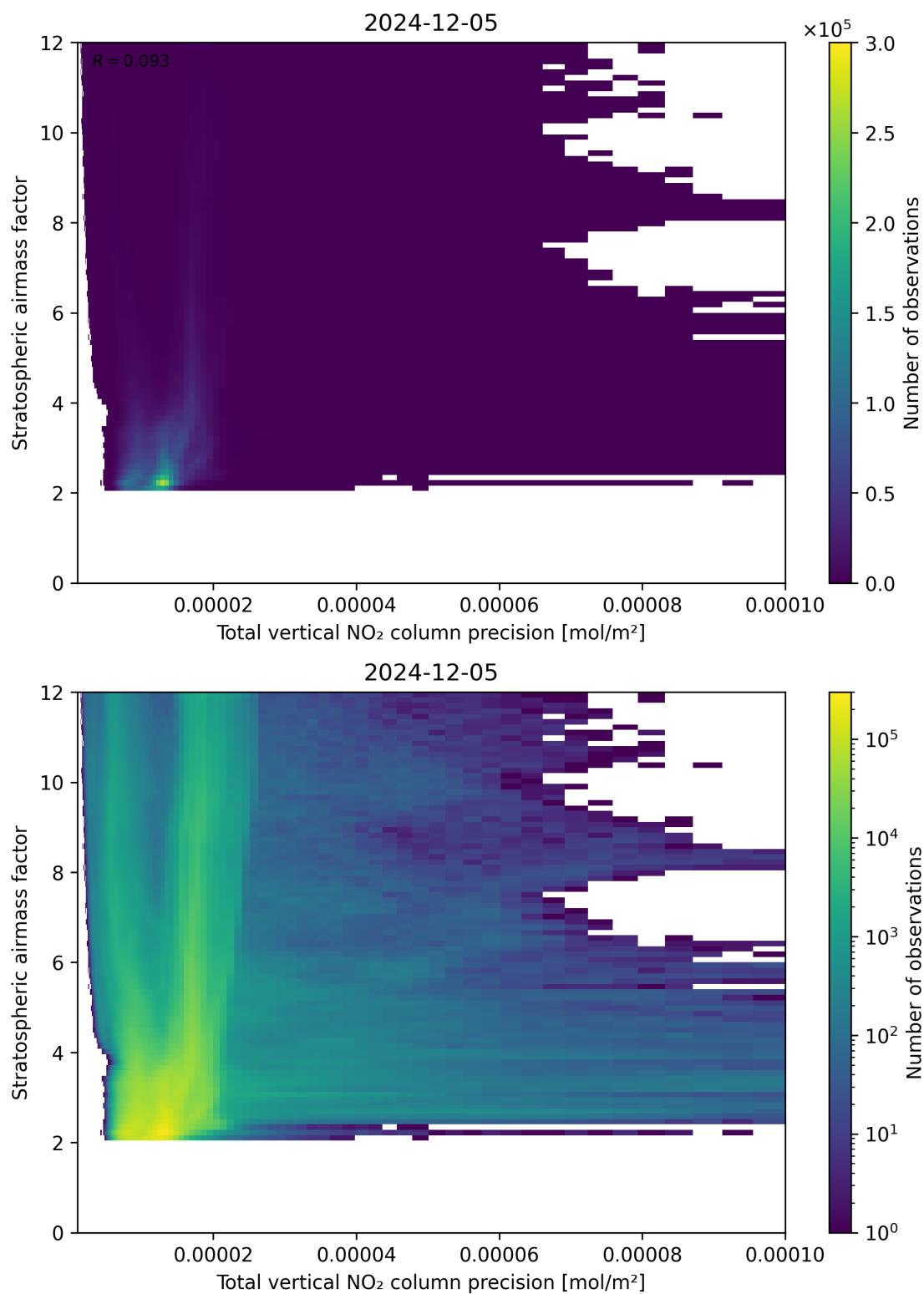
Figure 115: Scatter density plot of “Total vertical NO 2 column precision” against “Stratospheric air mass factor” for 2024-12-04 to 2024-12-06.
