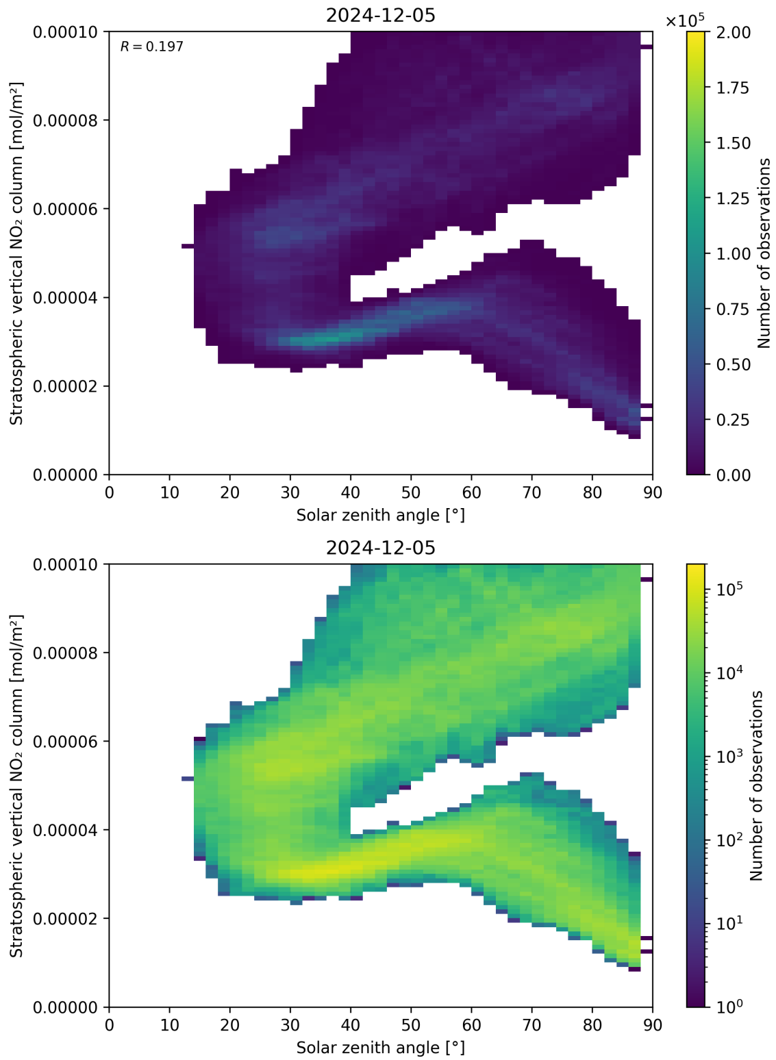
Figure 150: Scatter density plot of “Solar zenith angle” against “Stratospheric vertical NO 2 column” for 2024-12-04 to 2024-12-06.
