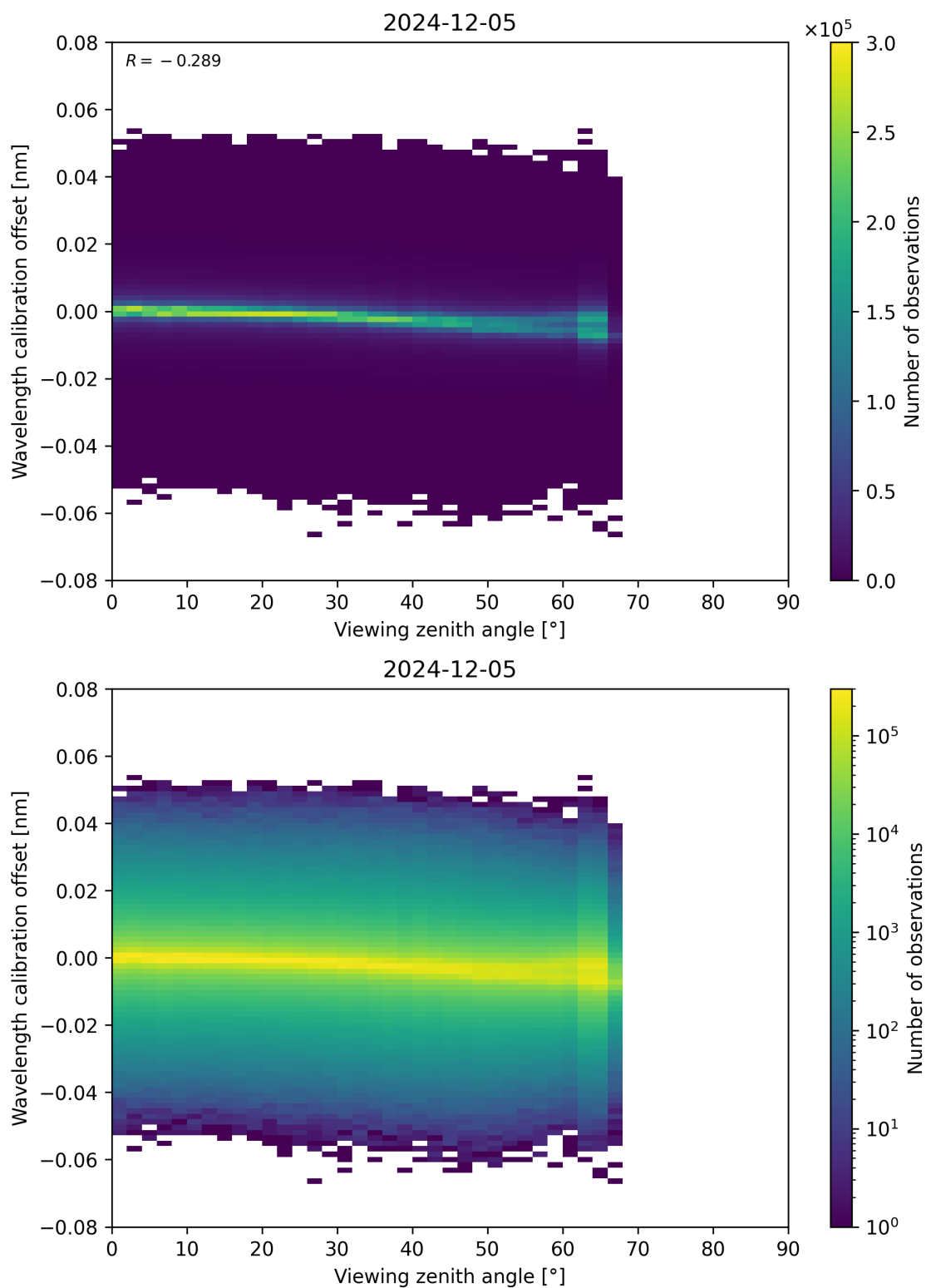
Figure 173: Scatter density plot of “Viewing zenith angle” against “Wavelength calibration offset” for 2024-12-04 to 2024-12-06.
