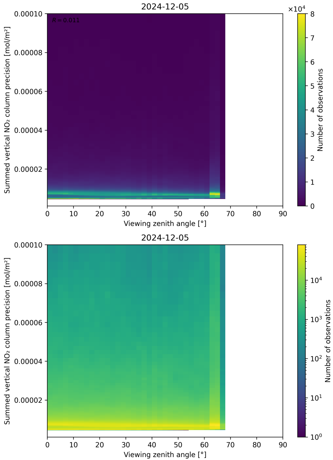
Figure 166: Scatter density plot of “Viewing zenith angle” against “Summed vertical NO 2 column precision” for 2024-12-04 to 2024-12-06.
