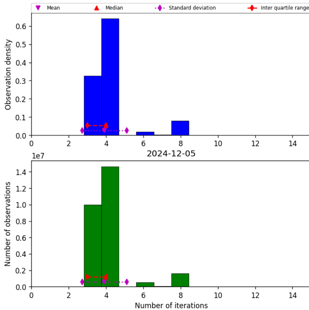
Figure 34: Histogram of “Number of iterations” for 2024-12-04 to 2024-12-06
