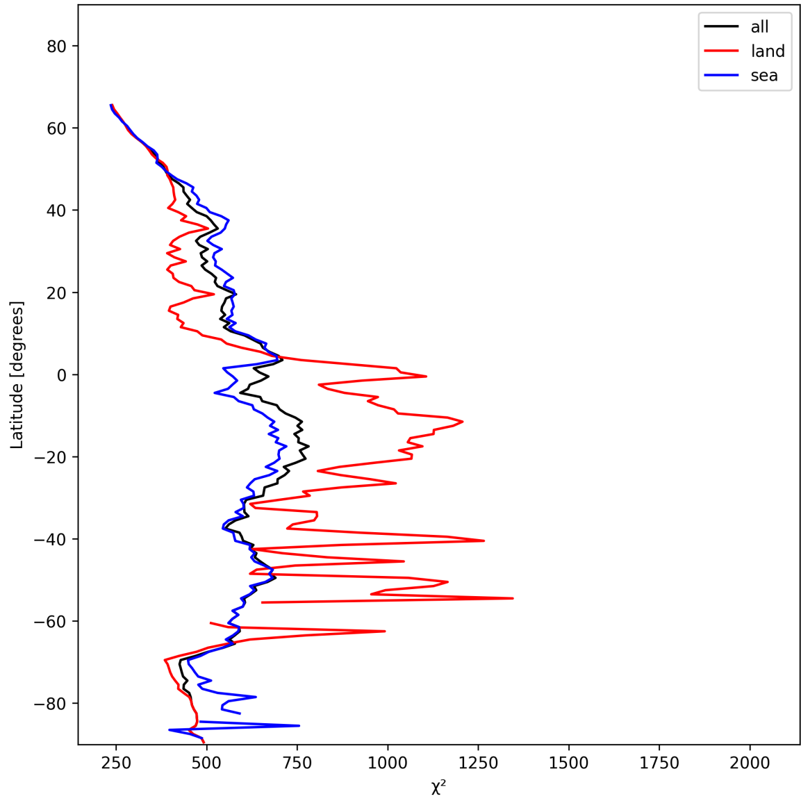
Figure 25: Zonal average of “ \chi^2 ” for 2024-12-04 to 2024-12-06.
