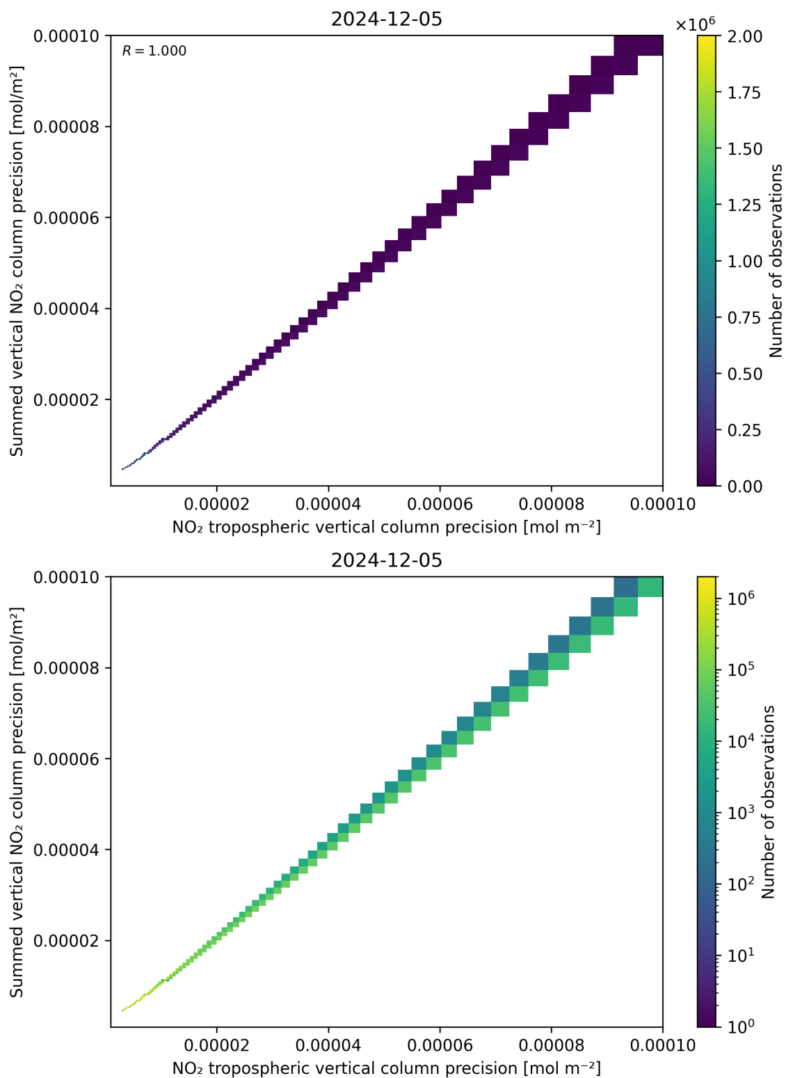
Figure 137: Scatter density plot of “NO 2 tropospheric vertical column precision” against “Summed vertical NO 2 column precision” for 2024-12-04 to 2024-12-06.
