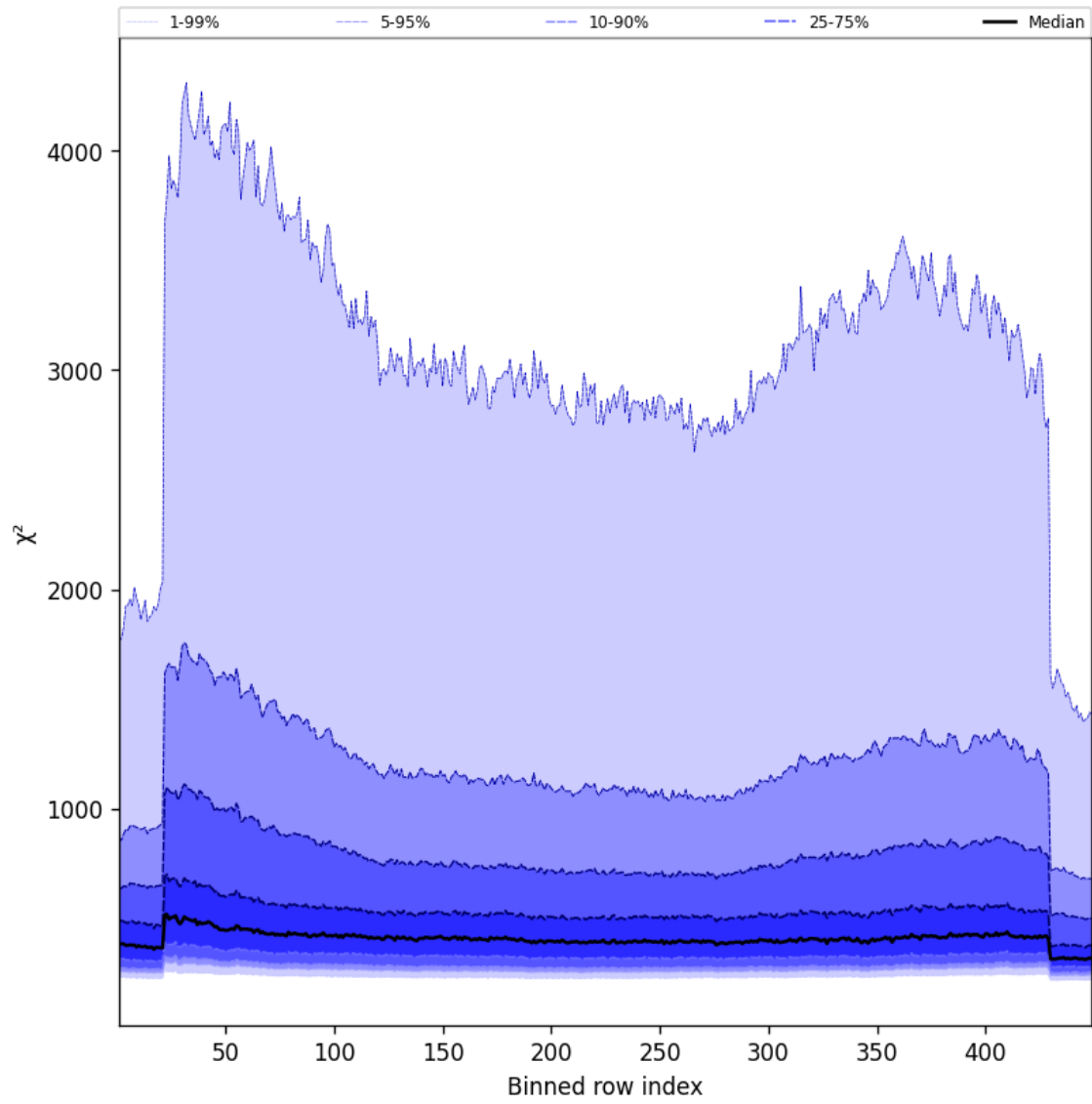
Figure 59: Along track statistics of “ \chi^2 ” for 2024-12-04 to 2024-12-06
