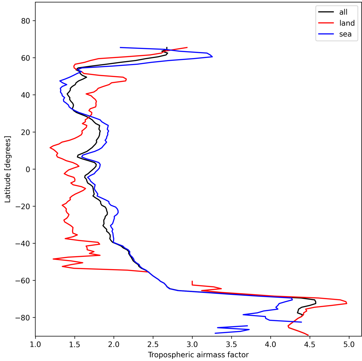
Figure 14: Zonal average of “Tropospheric airmass factor” for 2024-12-04 to 2024-12-06.
