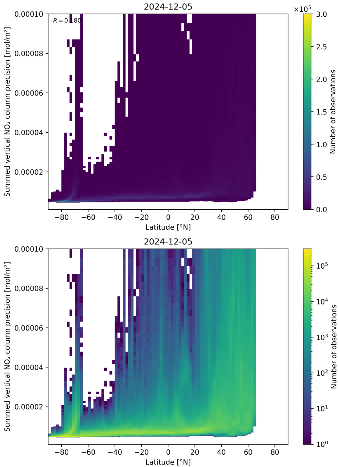
Figure 89: Scatter density plot of “Latitude” against “Summed vertical NO 2 column precision” for 2024-12-04 to 2024-12-06.
