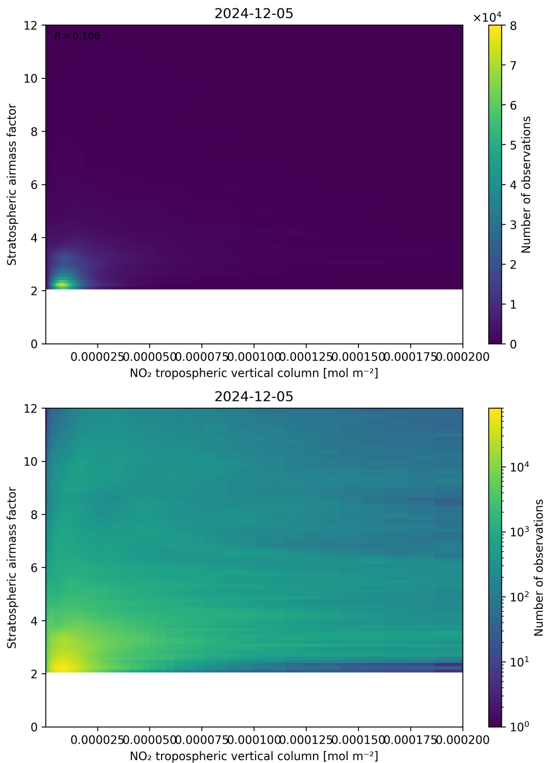
Figure 121: Scatter density plot of “NO 2 tropospheric vertical column” against “Stratospheric airmass factor” for 2024-12-04 to 2024-12-06.
