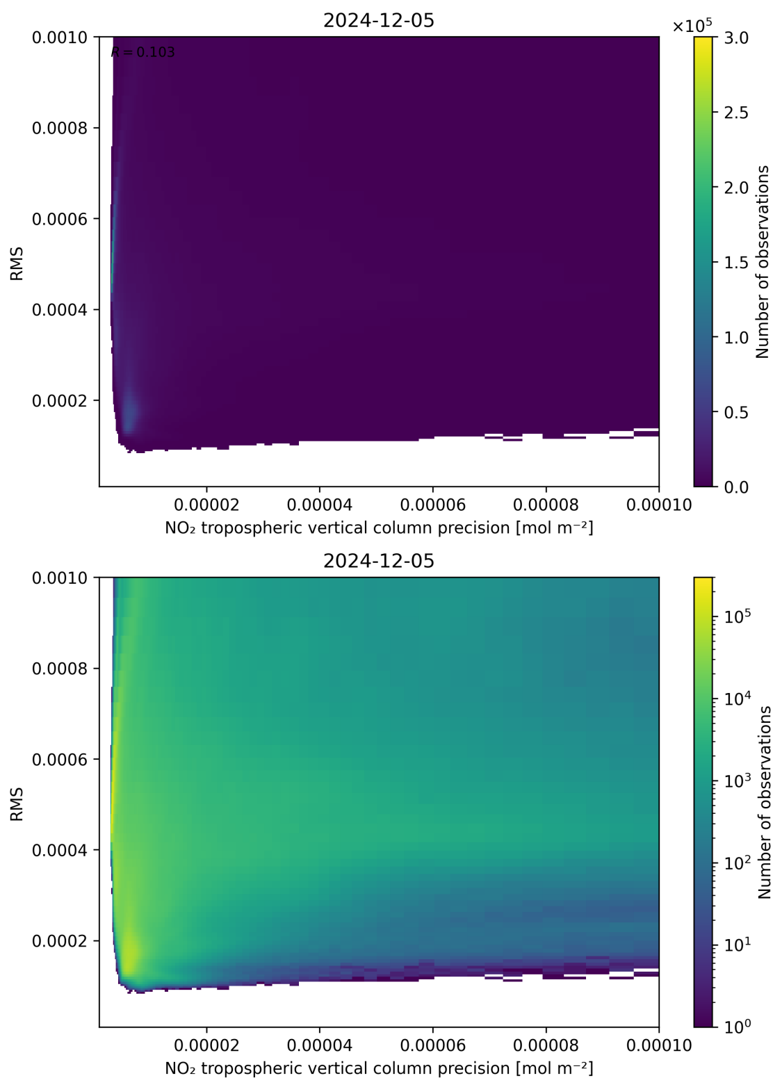
Figure 140: Scatter density plot of “NO 2 tropospheric vertical column precision” against “RMS” for 2024-12-04 to 2024-12-06.
