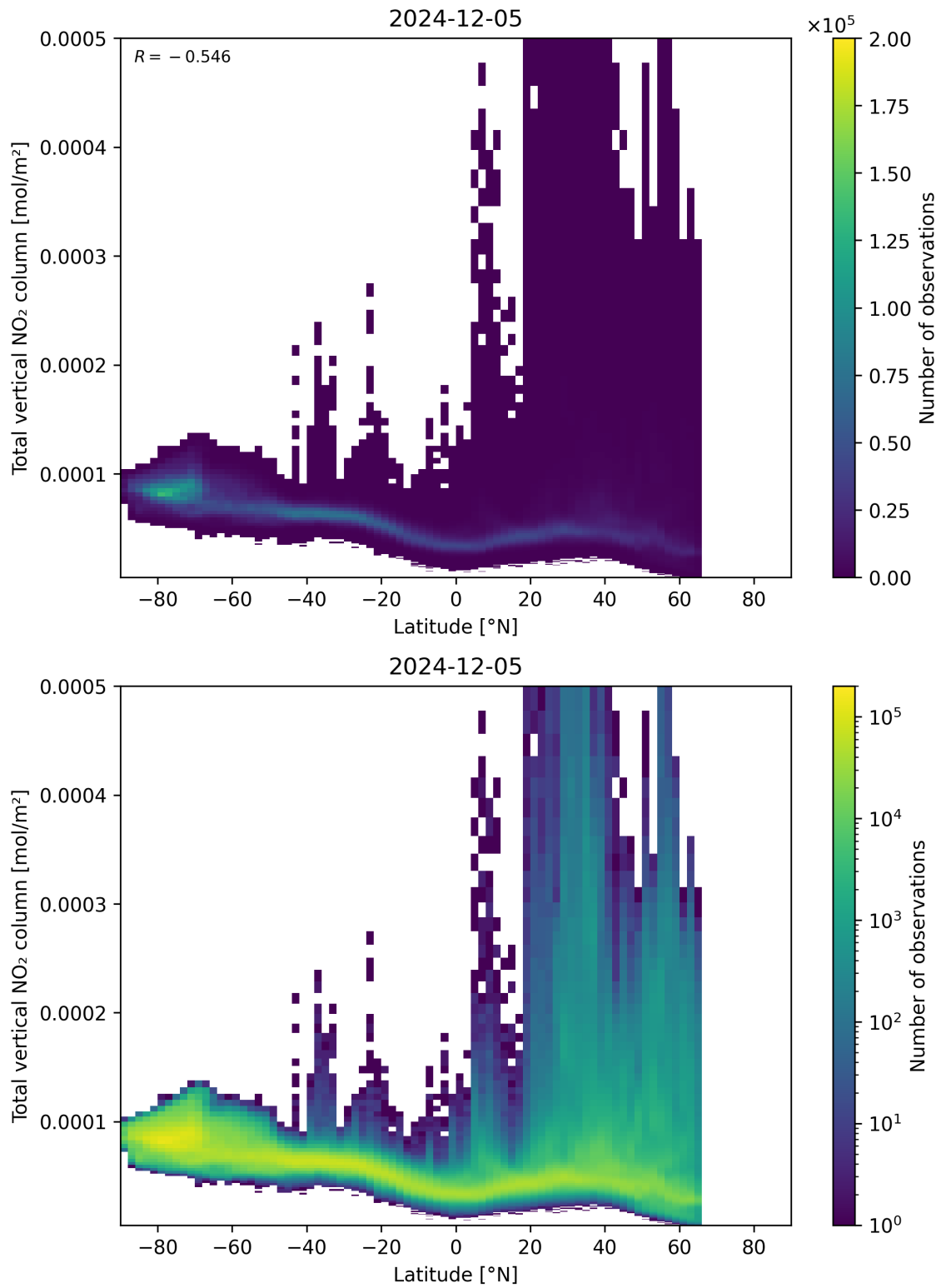
Figure 90: Scatter density plot of “Latitude” against “Total vertical NO 2 column” for 2024-12-04 to 2024-12-06.
