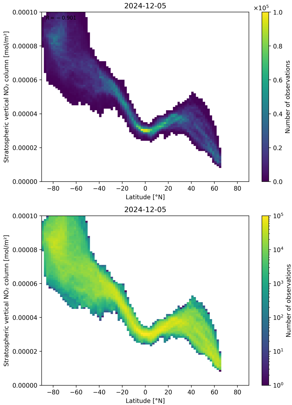
Figure 87: Scatter density plot of “Latitude” against “Stratospheric vertical NO 2 column” for 2024-12-04 to 2024-12-06.
