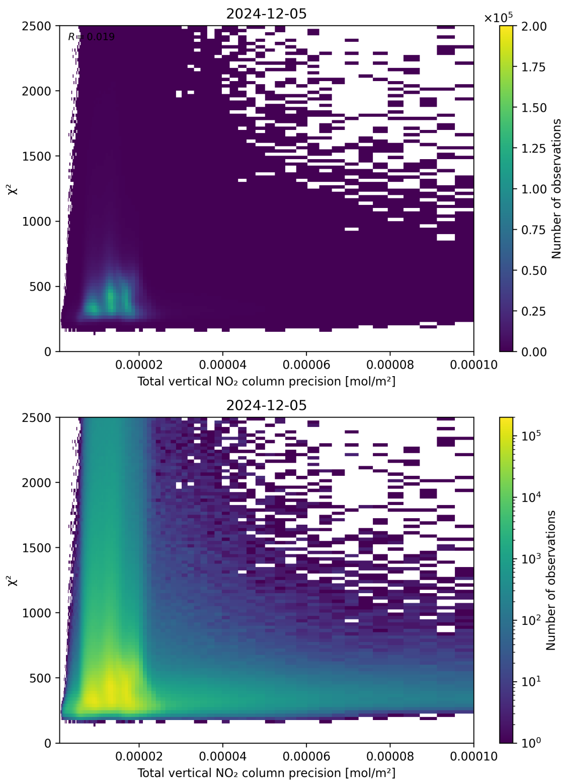
Figure 116: Scatter density plot of “Total vertical NO 2 column precision” against “ \chi^2 ” for 2024-12-04 to 2024-12-06.
