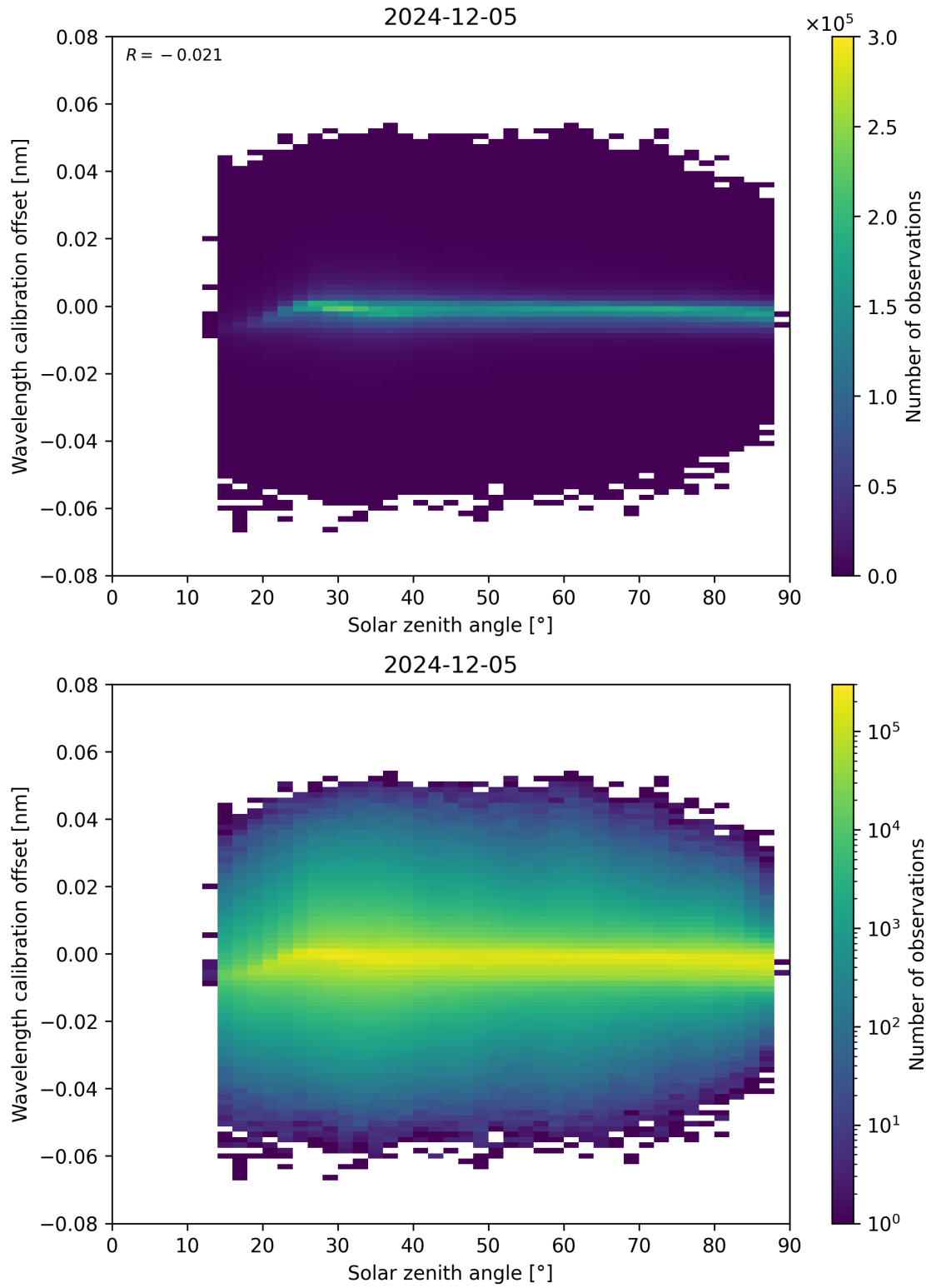
Figure 158: Scatter density plot of “Solar zenith angle” against “Wavelength calibration offset” for 2024-12-04 to 2024-12-06.
