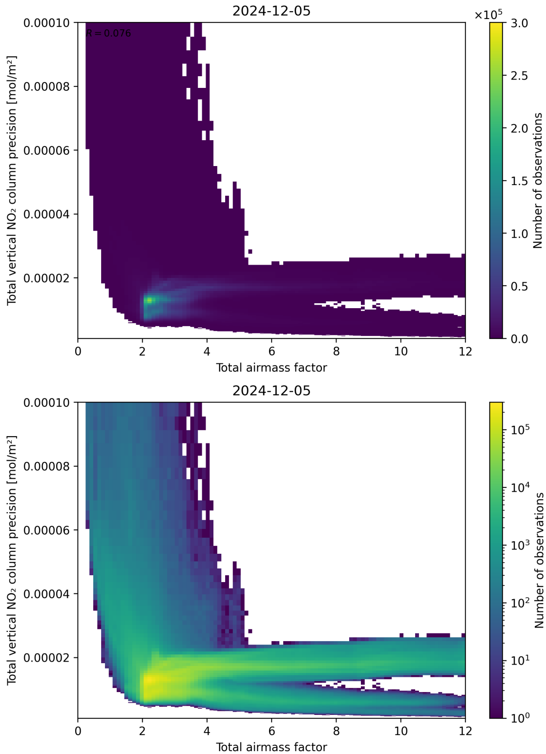
Figure 68: Scatter density plot of “Total airmass factor” against “Total vertical NO 2 column precision” for 2024-12-04 to 2024-12-06.
