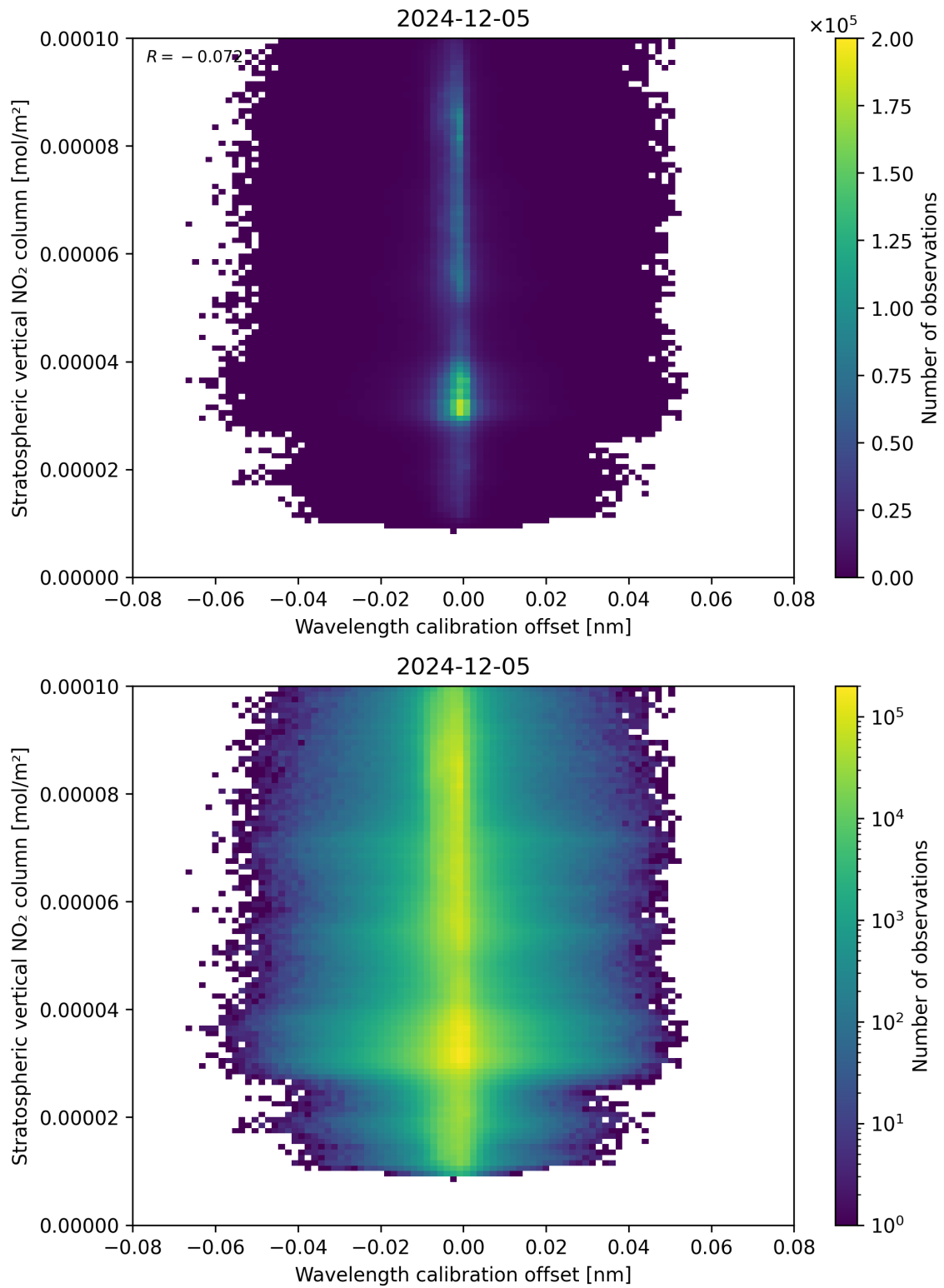
Figure 176: Scatter density plot of “Wavelength calibration offset” against “Stratospheric vertical NO 2 column” for 2024-12-04 to 2024-12-06.
