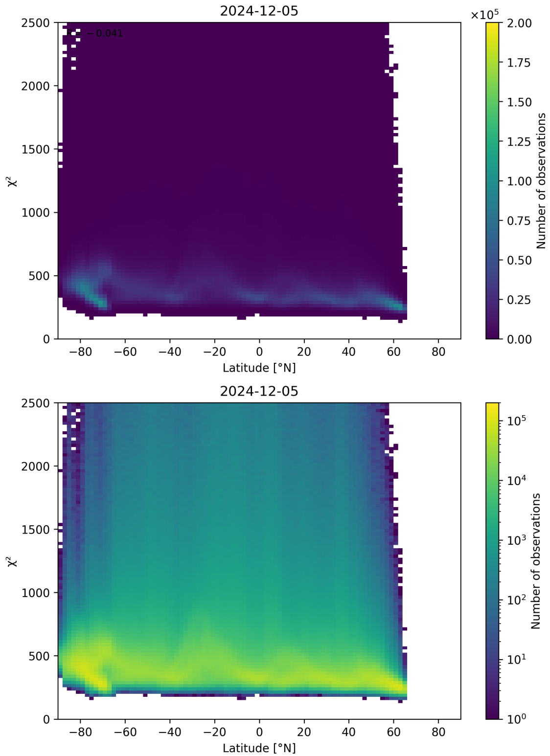
Figure 86: Scatter density plot of “Latitude” against “ \chi^2 ” for 2024-12-04 to 2024-12-06.
