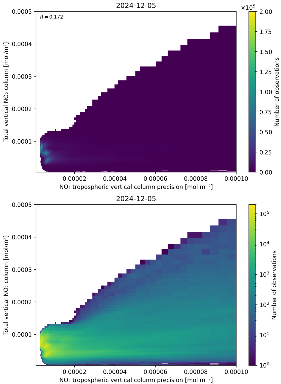
Figure 138: Scatter density plot of “NO 2 tropospheric vertical column precision” against “Total vertical NO 2 column” for 2024-12-04 to 2024-12-06.
