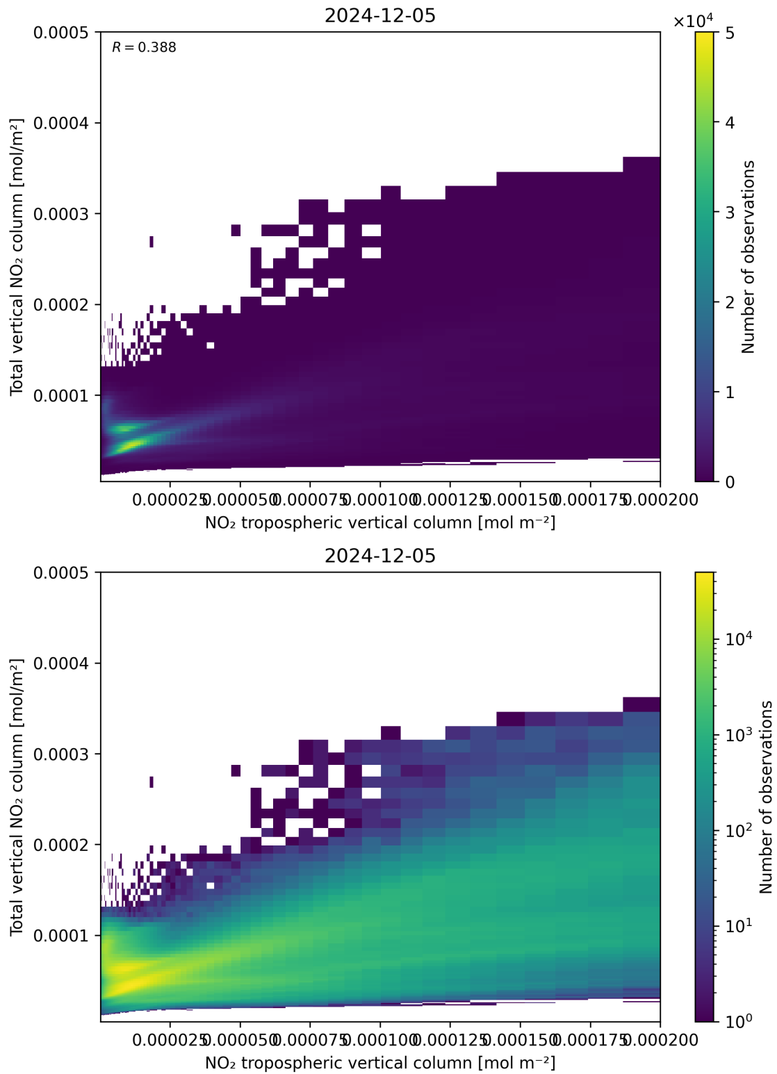
Figure 128: Scatter density plot of “NO 2 tropospheric vertical column” against “Total vertical NO 2 column” for 2024-12-04 to 2024-12-06.
