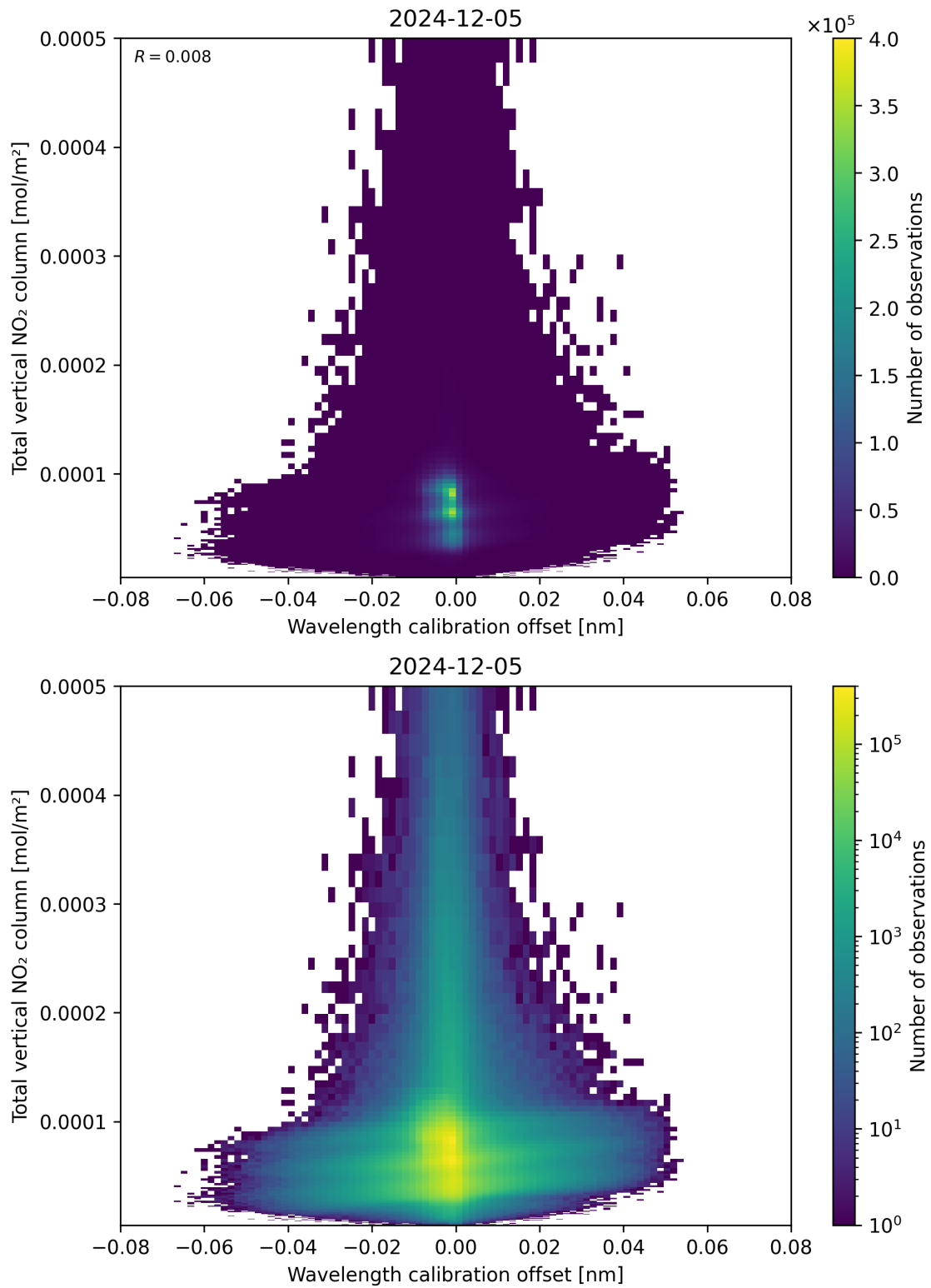
Figure 179: Scatter density plot of “Wavelength calibration offset” against “Total vertical NO 2 column” for 2024-12-04 to 2024-12-06.
