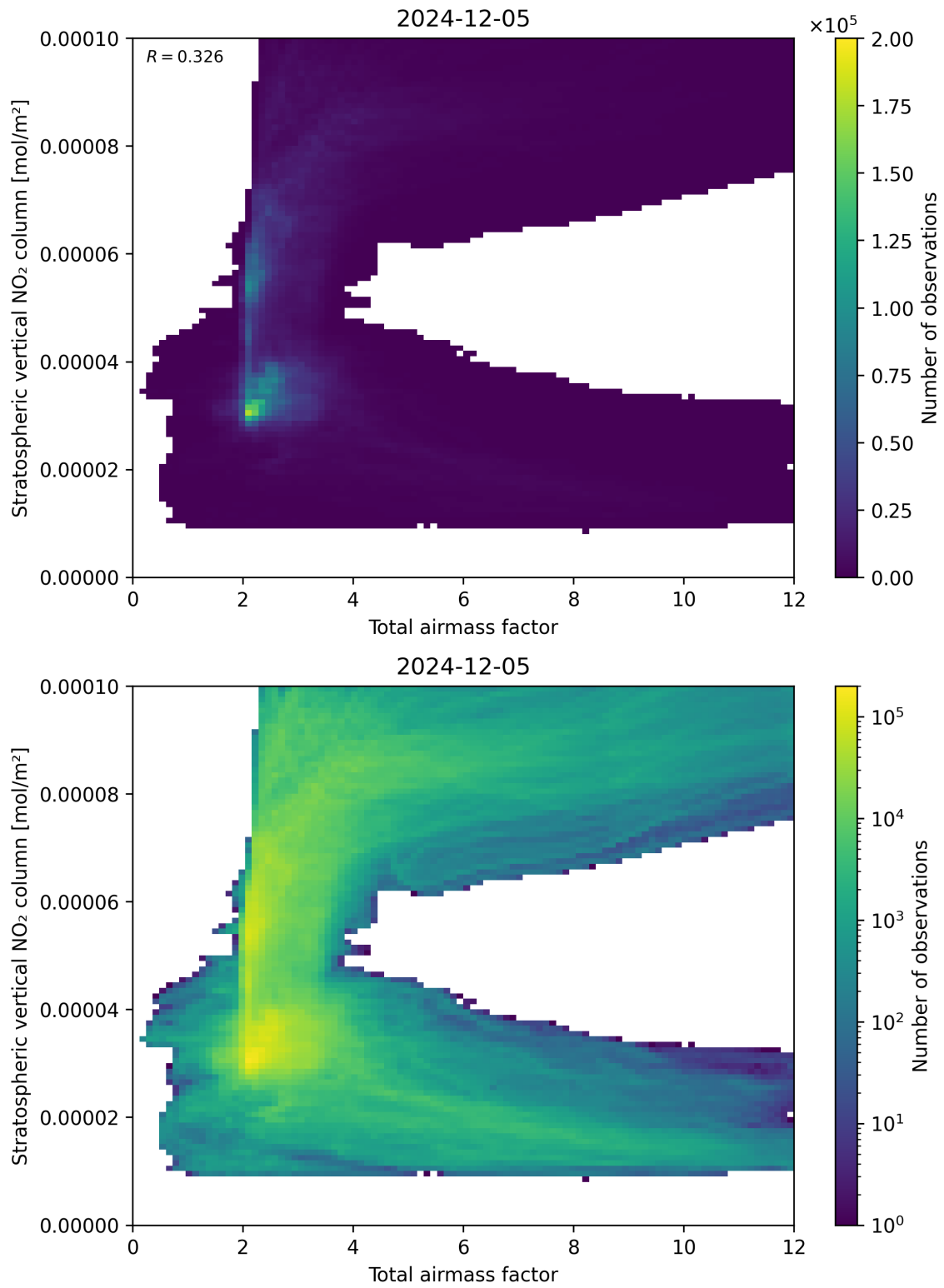
Figure 64: Scatter density plot of “Total airmass factor” against “Stratospheric vertical NO 2 column” for 2024-12-04 to 2024-12-06.
