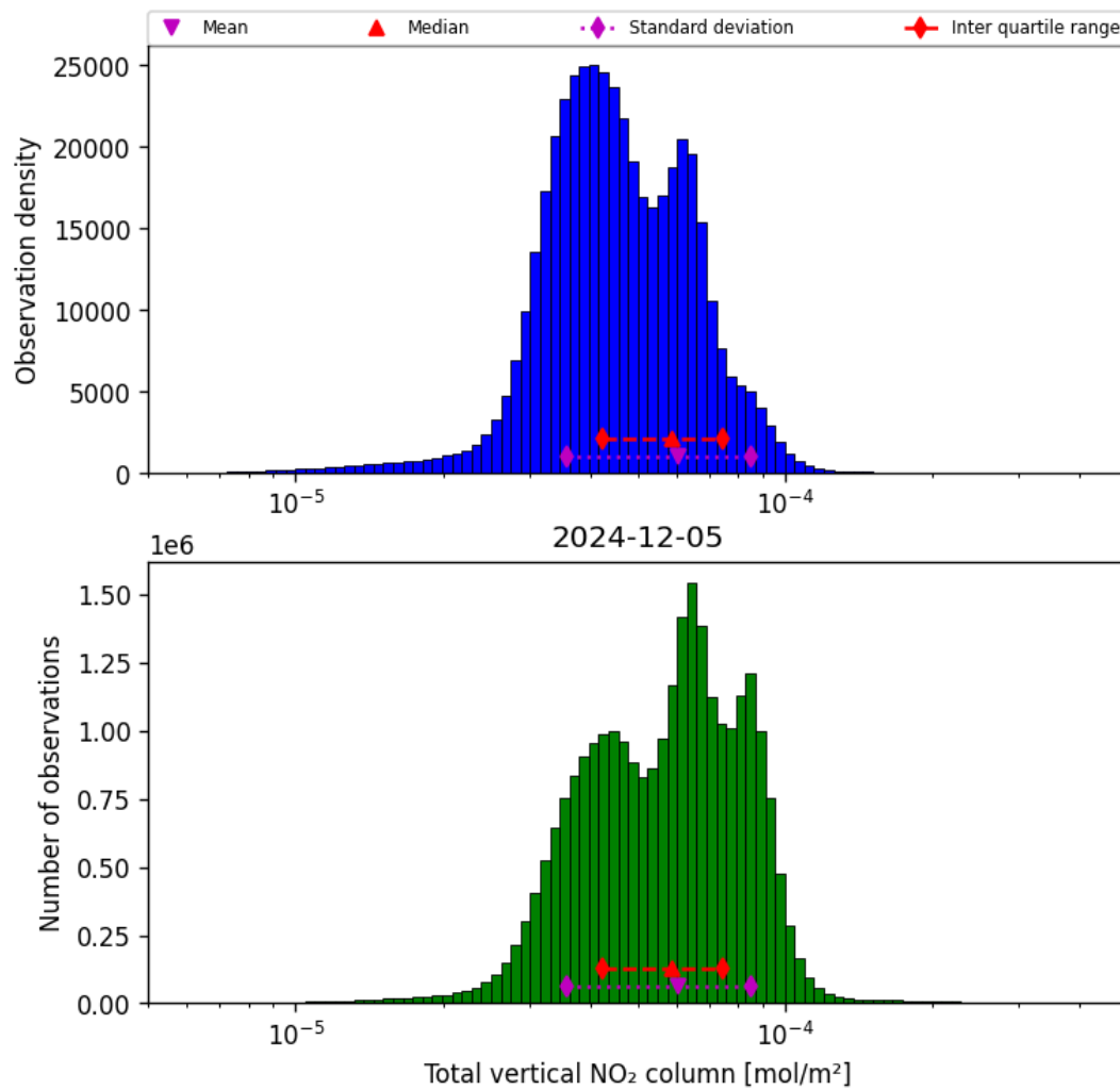
Figure 38: Histogram of “Total vertical NO 2 column” for 2024-12-04 to 2024-12-06
