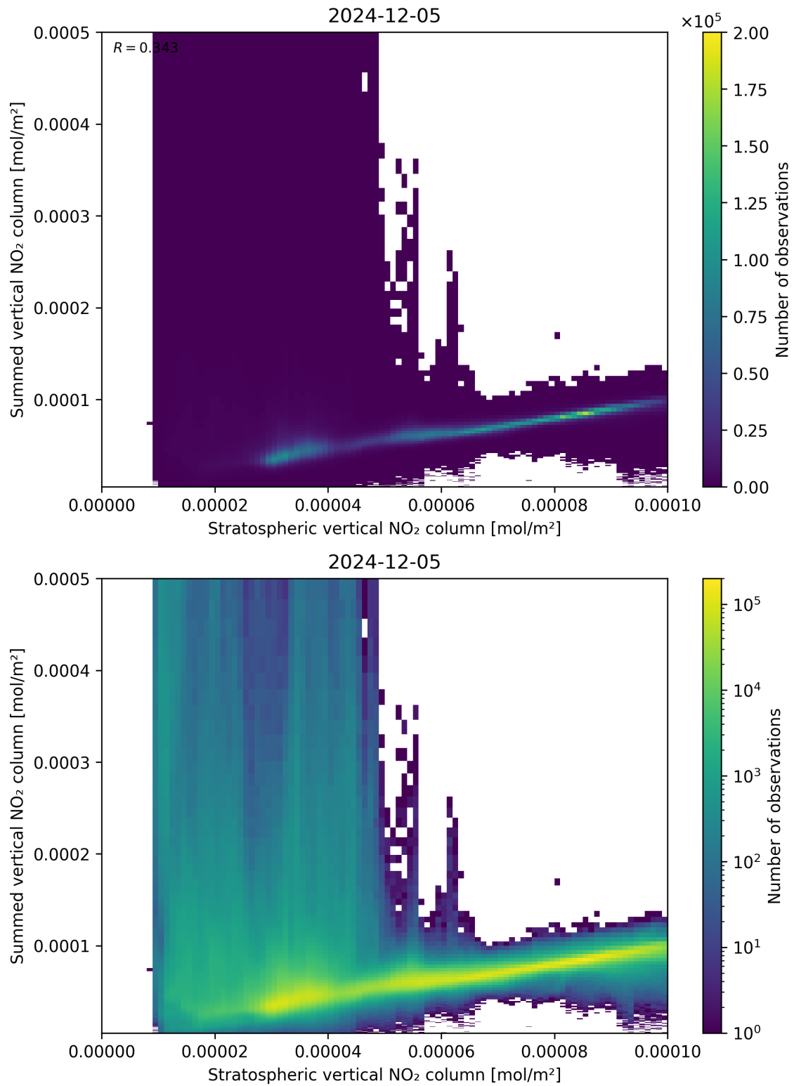
Figure 98: Scatter density plot of “Stratospheric vertical NO 2 column” against “Summed vertical NO 2 column” for 2024-12-04 to 2024-12-06.
