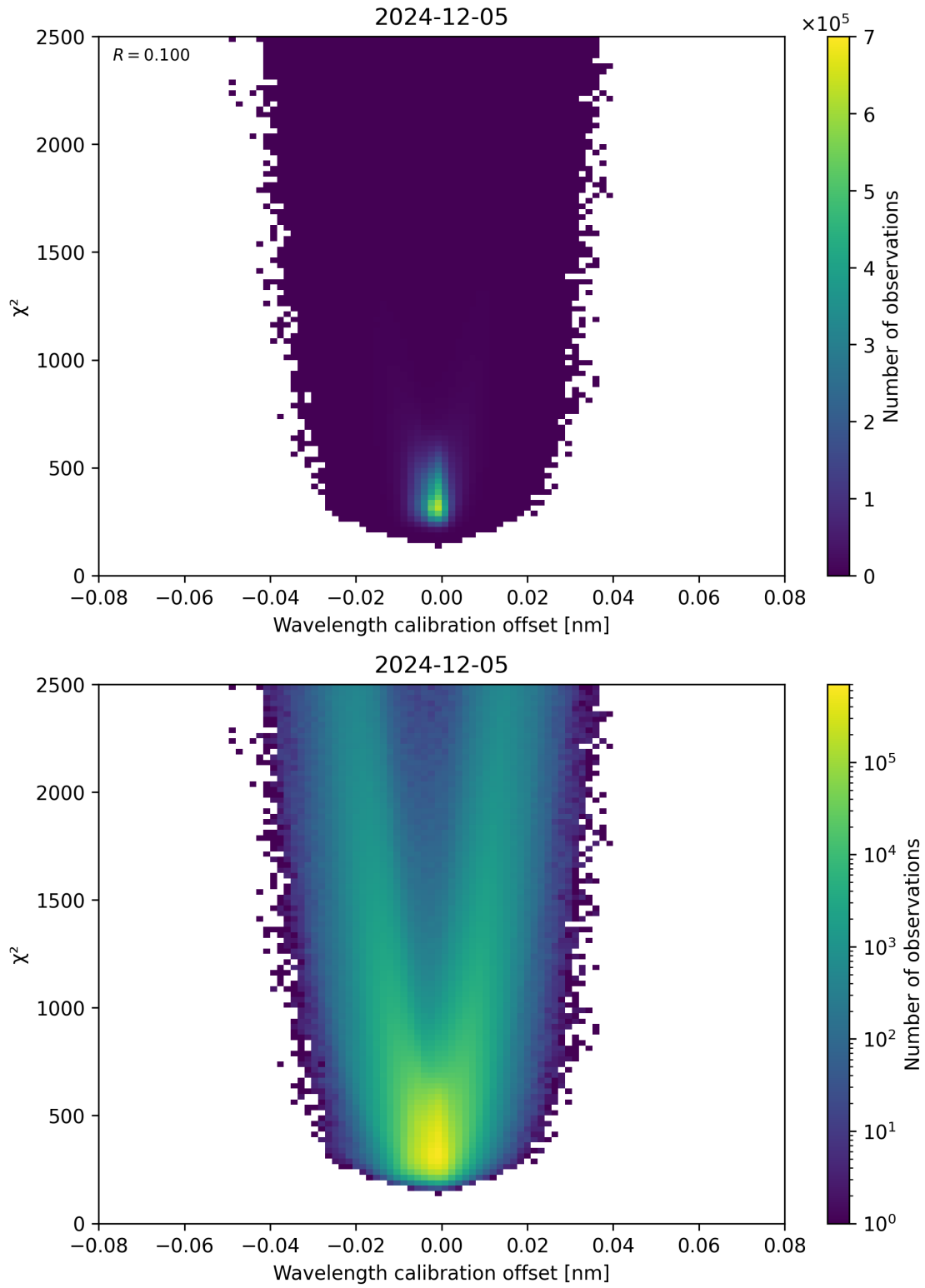
Figure 175: Scatter density plot of “Wavelength calibration offset” against “ \chi^2 ” for 2024-12-04 to 2024-12-06.
