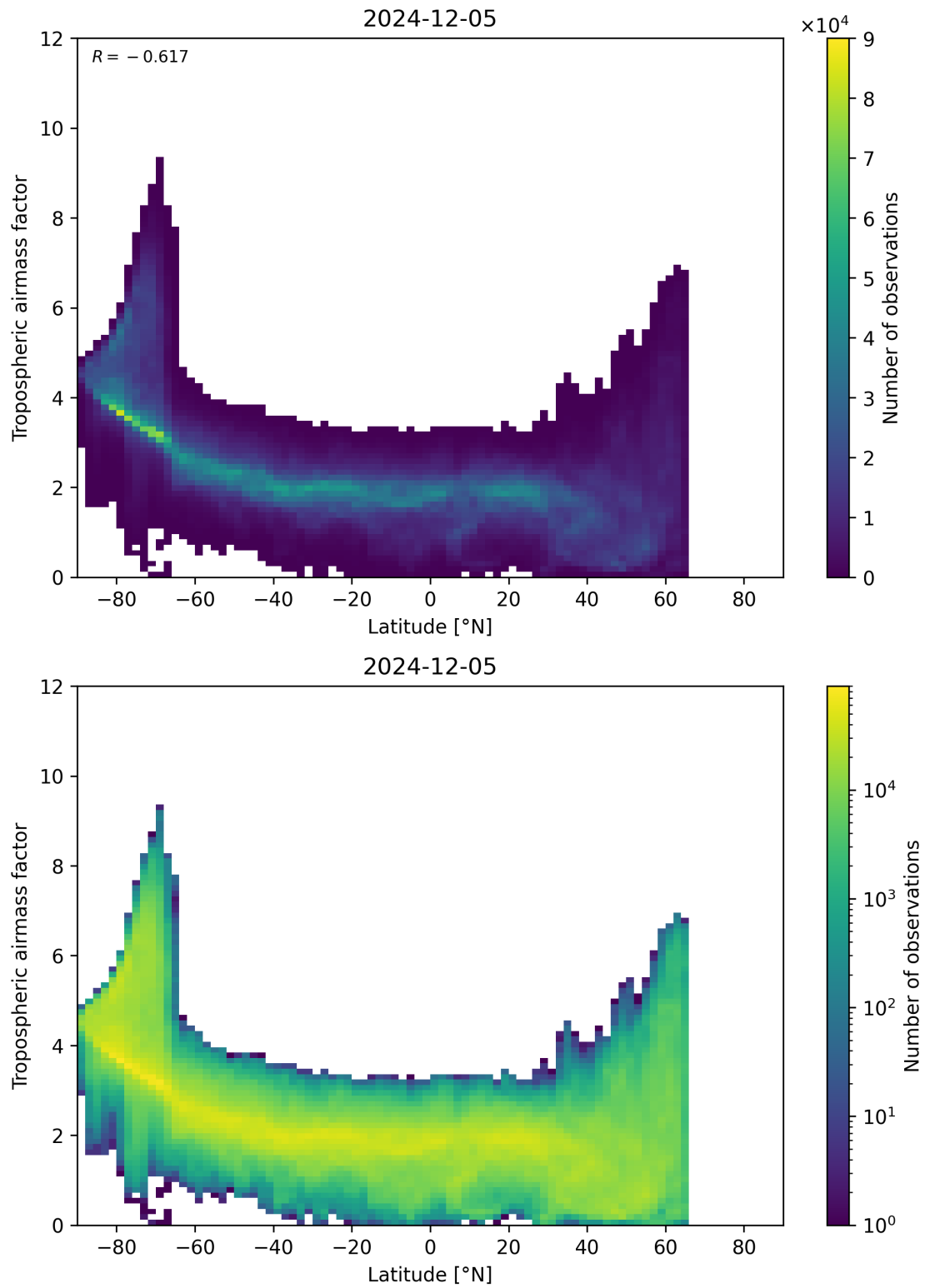
Figure 85: Scatter density plot of “Latitude” against “Tropospheric air mass factor” for 2024-12-04 to 2024-12-06.
