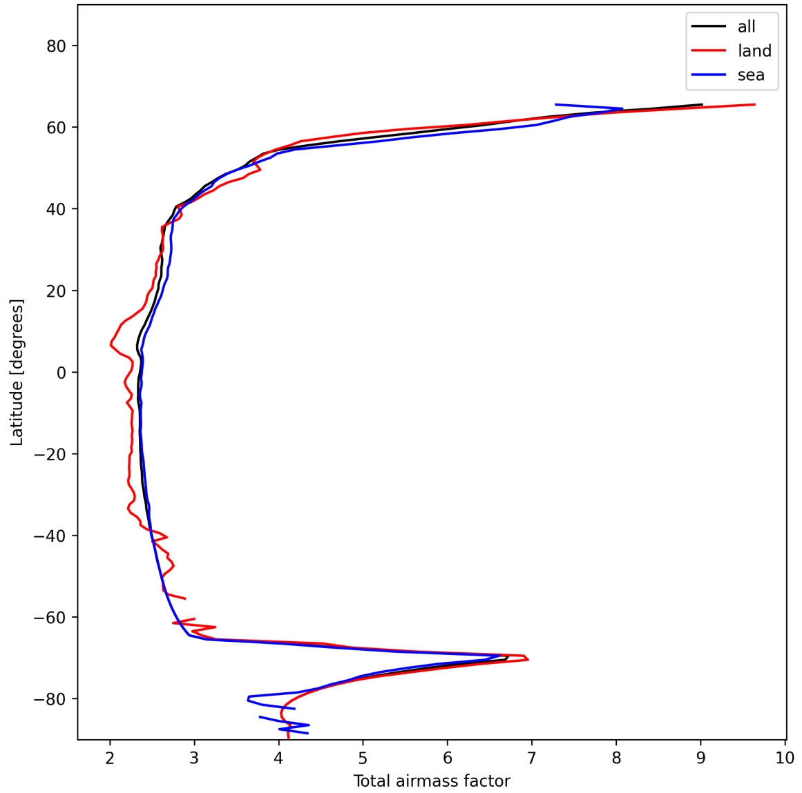
Figure 15: Zonal average of “Total airmass factor” for 2024-12-04 to 2024-12-06.
