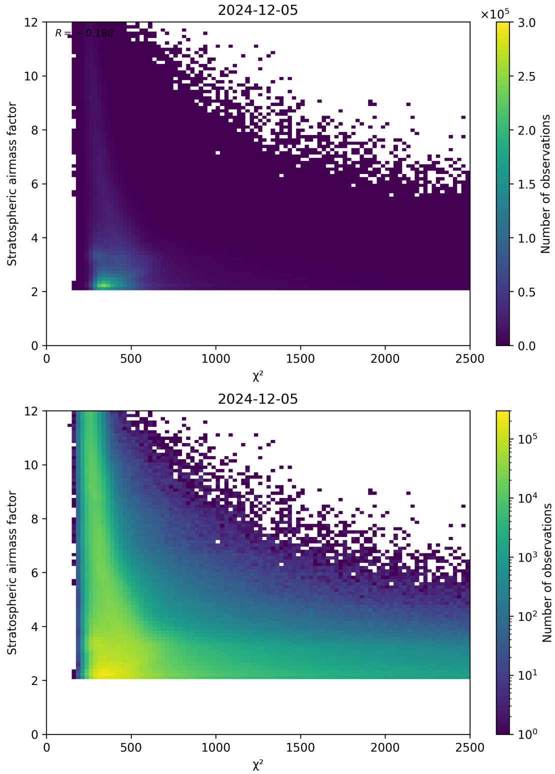
Figure 81: Scatter density plot of “ \chi^2 ” against “Stratospheric airmass factor” for 2024-12-04 to 2024-12-06.
