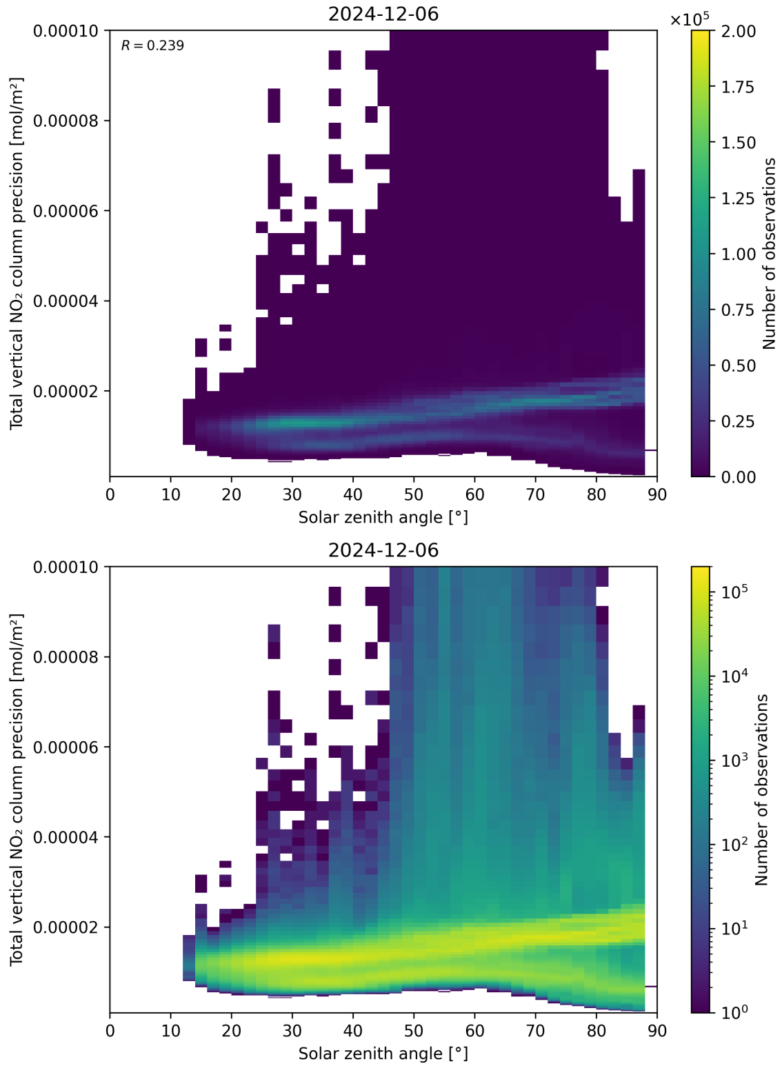
Figure 154: Scatter density plot of “Solar zenith angle” against “Total vertical NO 2 column precision” for 2024-12-06 to 2024-12-07.
