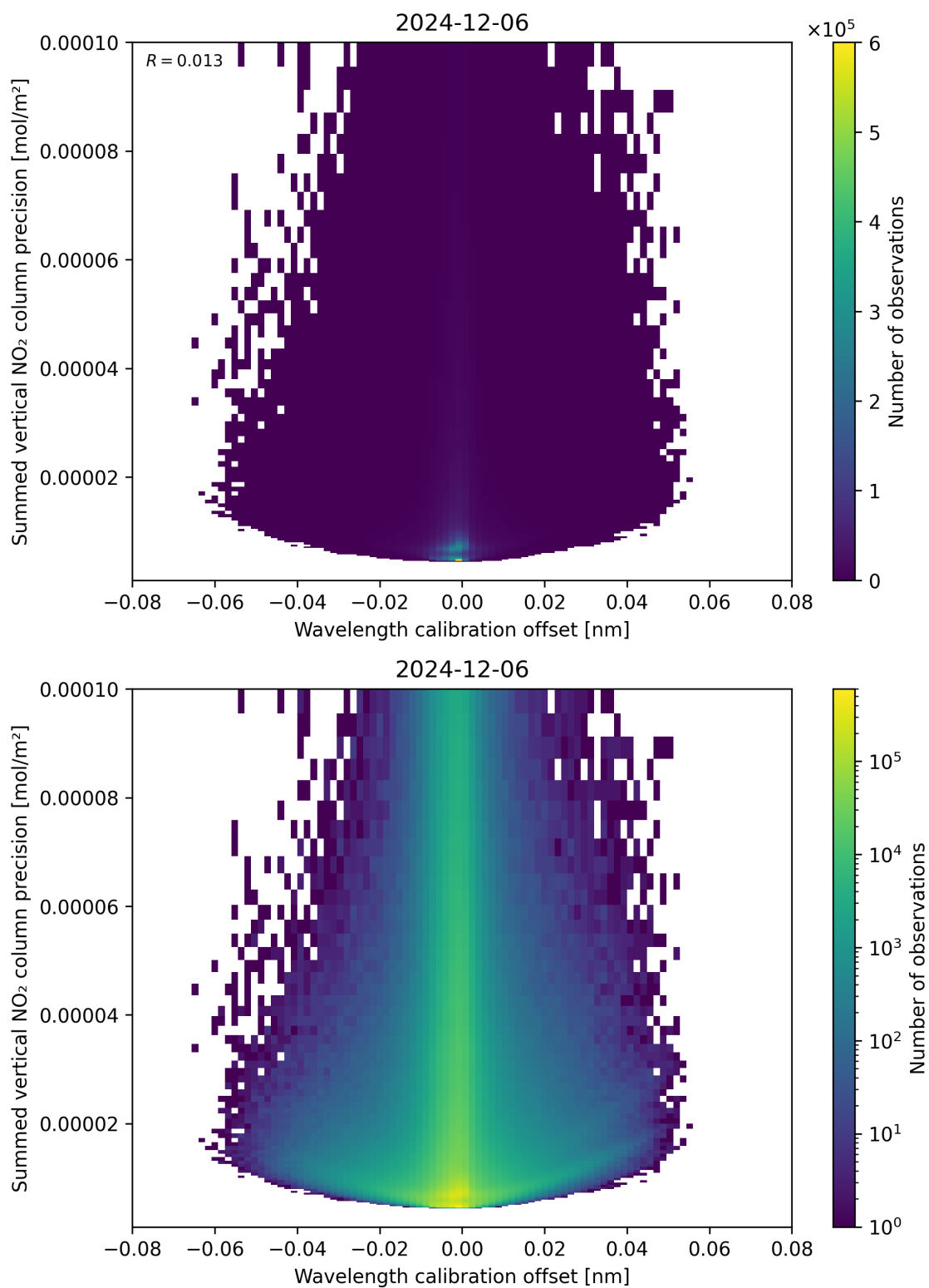
Figure 178: Scatter density plot of “Wavelength calibration offset” against “Summed vertical NO 2 column precision” for 2024-12-06 to 2024-12-07.
