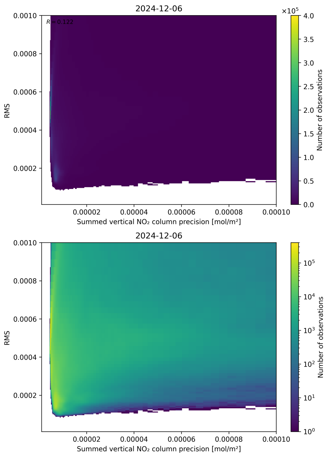
Figure 108: Scatter density plot of “Summed vertical NO 2 column precision” against “RMS” for 2024-12-06 to 2024-12-07.
