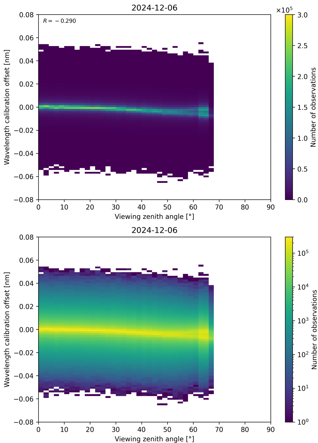
Figure 173: Scatter density plot of “Viewing zenith angle” against “Wavelength calibration offset” for 2024-12-06 to 2024-12-07.
