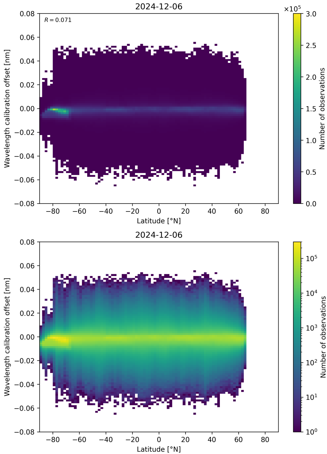
Figure 95: Scatter density plot of “Latitude” against “Wavelength calibration offset” for 2024-12-06 to 2024-12-07.
