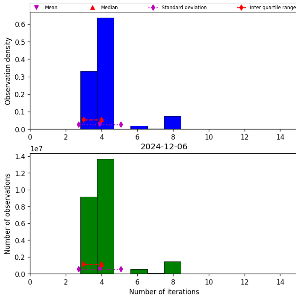
Figure 34: Histogram of “Number of iterations” for 2024-12-06 to 2024-12-07
