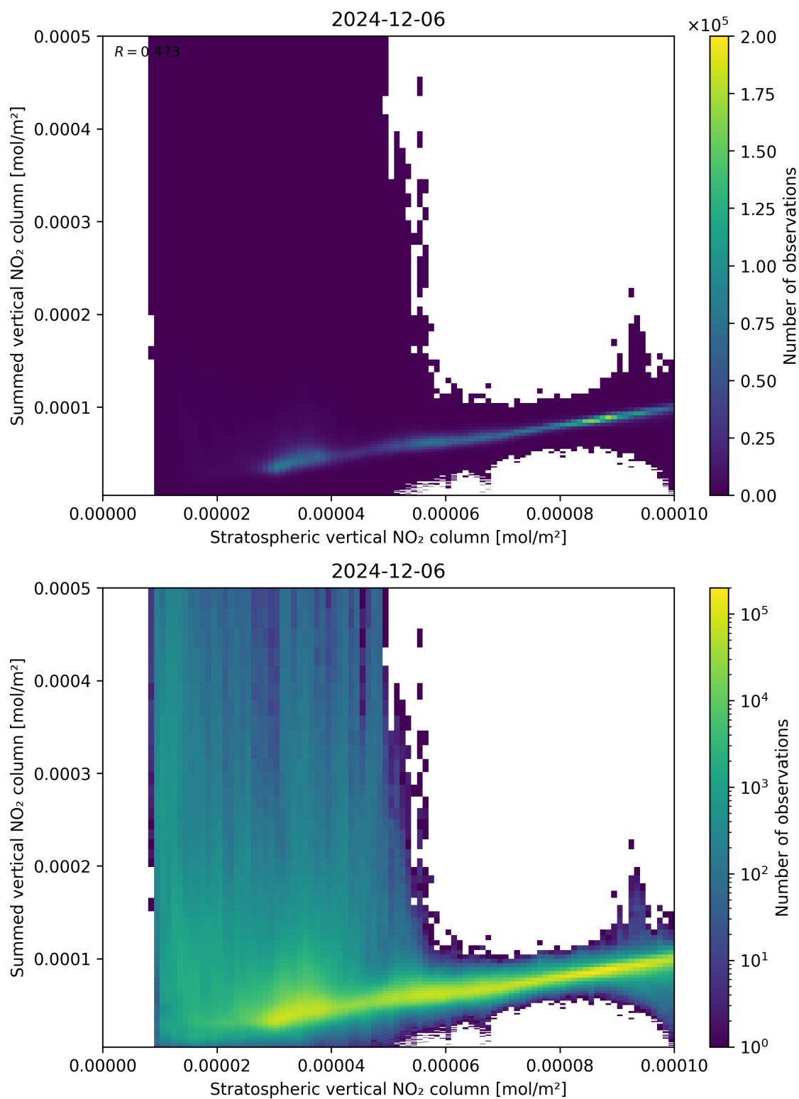
Figure 98: Scatter density plot of “Stratospheric vertical NO 2 column” against “Summed vertical NO 2 column” for 2024-12-06 to 2024-12-07.
