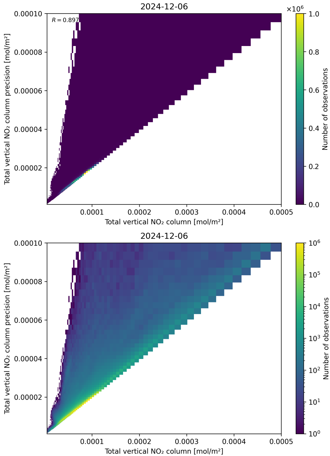
Figure 114: Scatter density plot of “Total vertical NO 2 column” against “Total vertical NO 2 column precision” for 2024-12-06 to 2024-12-07.
