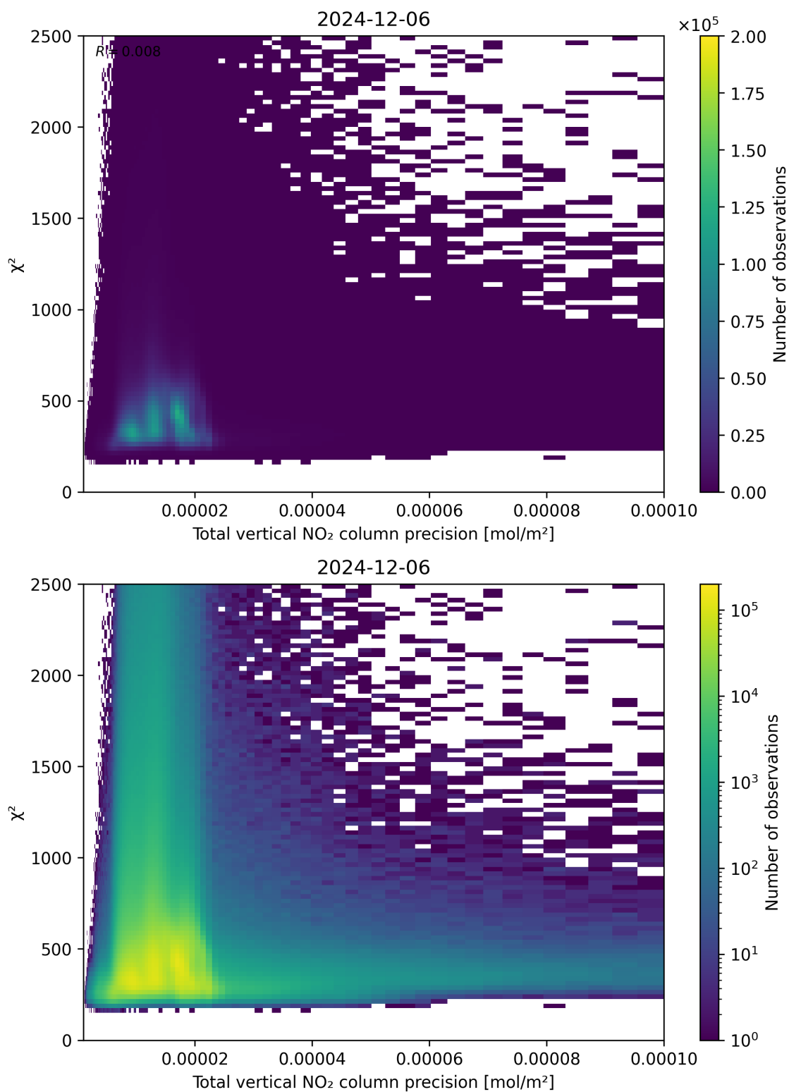
Figure 116: Scatter density plot of “Total vertical NO 2 column precision” against “ \chi^2 ” for 2024-12-06 to 2024-12-07.
