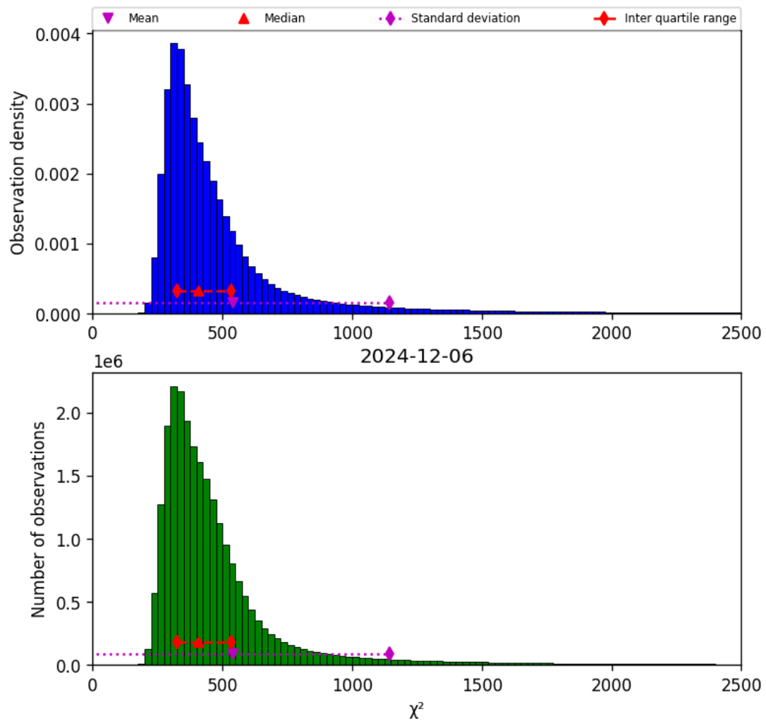
Figure 42: Histogram of “ \chi^2 ” for 2024-12-06 to 2024-12-07
