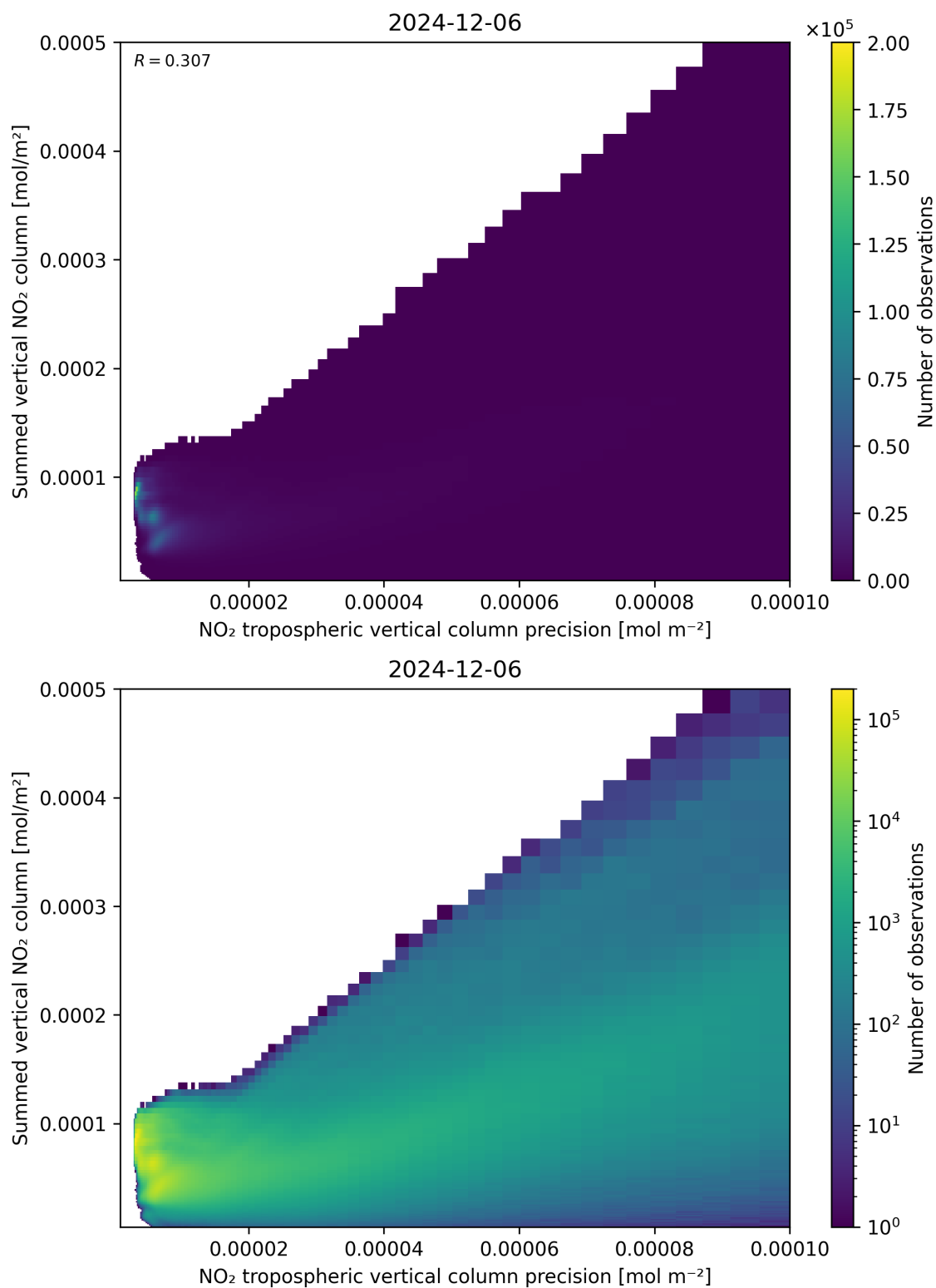
Figure 136: Scatter density plot of “NO 2 tropospheric vertical column precision” against “Summed vertical NO 2 column” for 2024-12-06 to 2024-12-07.
