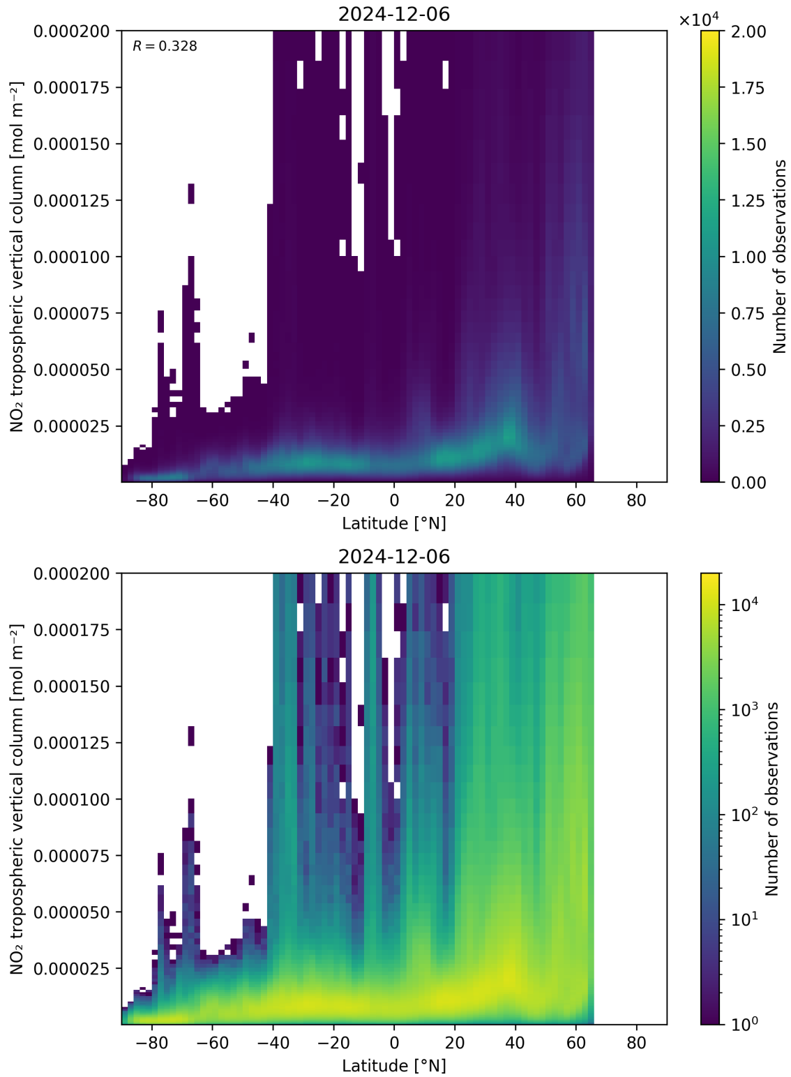
Figure 92: Scatter density plot of “Latitude” against “NO 2 tropospheric vertical column” for 2024-12-06 to 2024-12-07.
