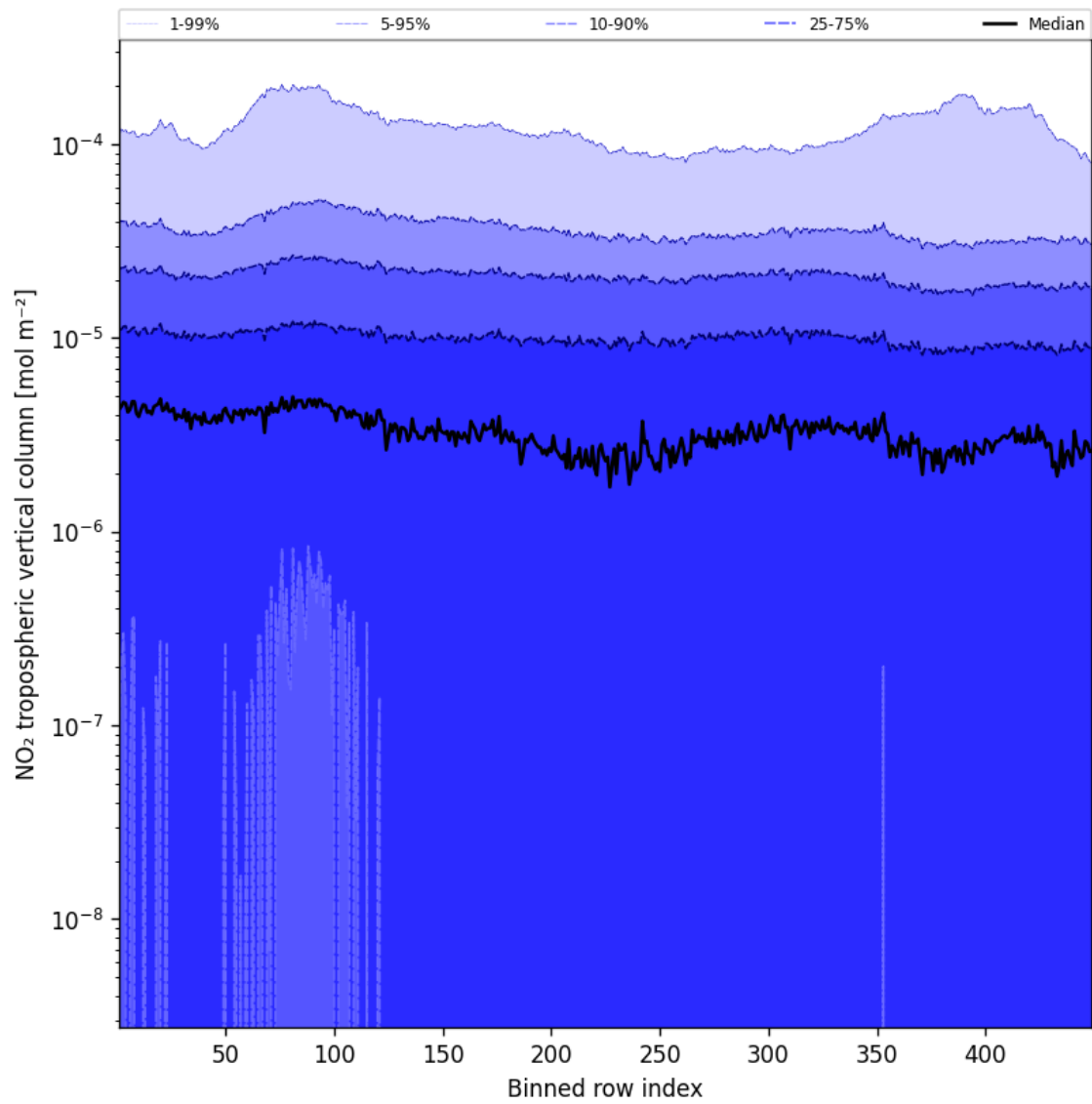
Figure 46: Along track statistics of “NO 2 tropospheric vertical column” for 2024-12-06 to 2024-12-07
