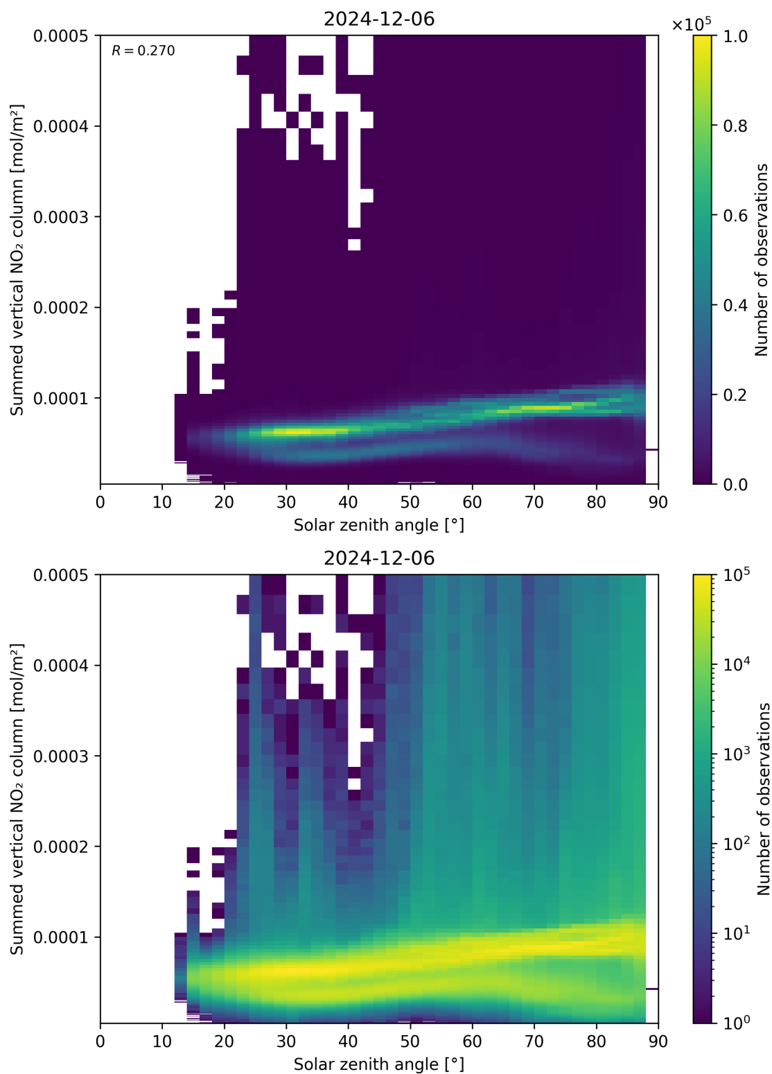
Figure 151: Scatter density plot of “Solar zenith angle” against “Summed vertical NO 2 column” for 2024-12-06 to 2024-12-07.
