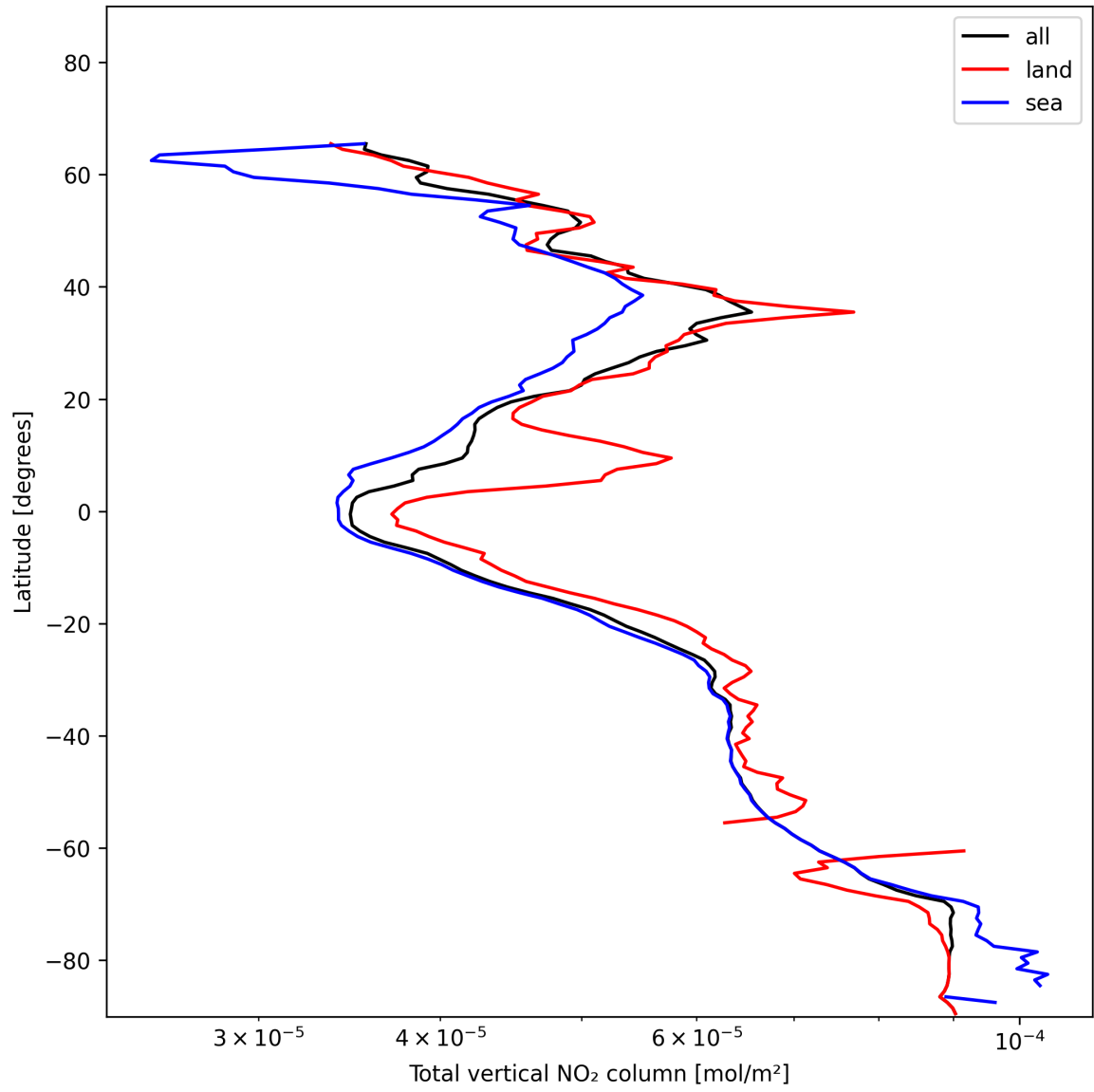
Figure 21: Zonal average of “Total vertical NO 2 column” for 2024-12-06 to 2024-12-07.
