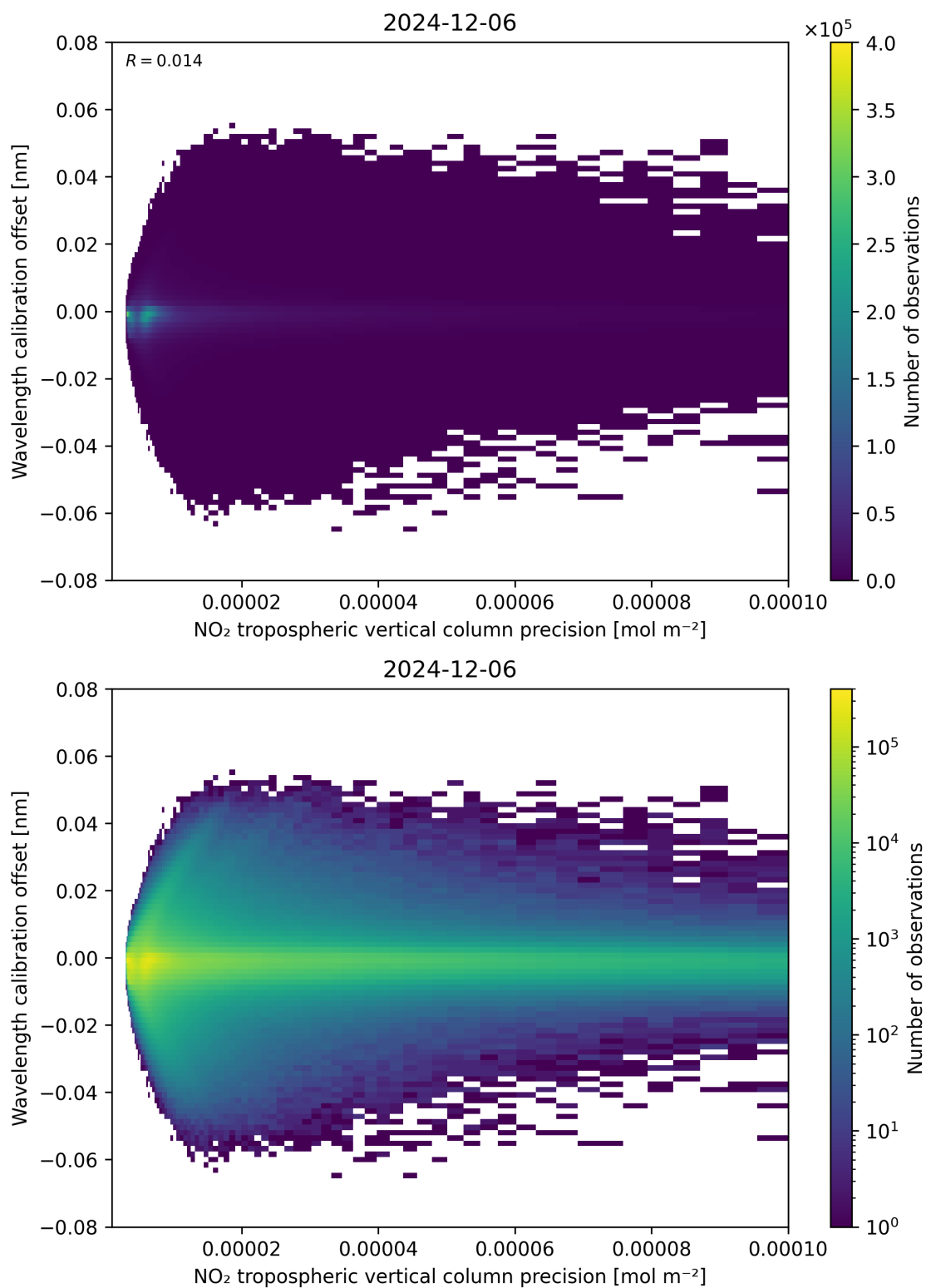
Figure 141: Scatter density plot of “NO 2 tropospheric vertical column precision” against “Wavelength calibration offset” for 2024-12-06 to 2024-12-07.
