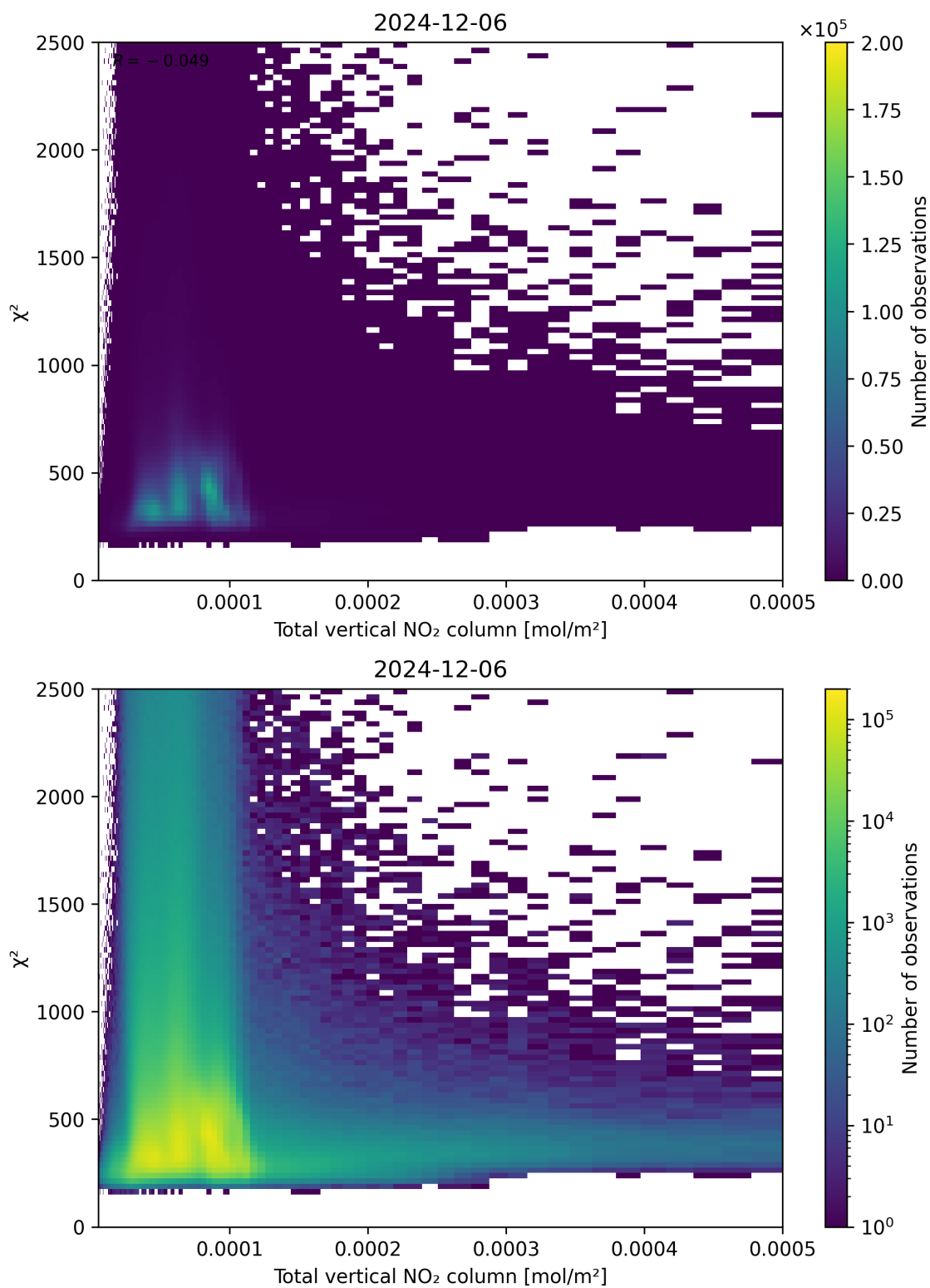
Figure 111: Scatter density plot of “Total vertical NO 2 column” against “ \chi^2 ” for 2024-12-06 to 2024-12-07.
