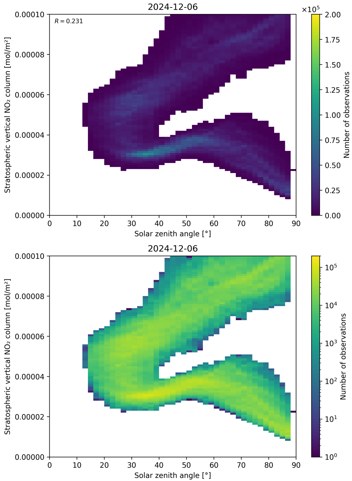
Figure 150: Scatter density plot of “Solar zenith angle” against “Stratospheric vertical NO 2 column” for 2024-12-06 to 2024-12-07.
