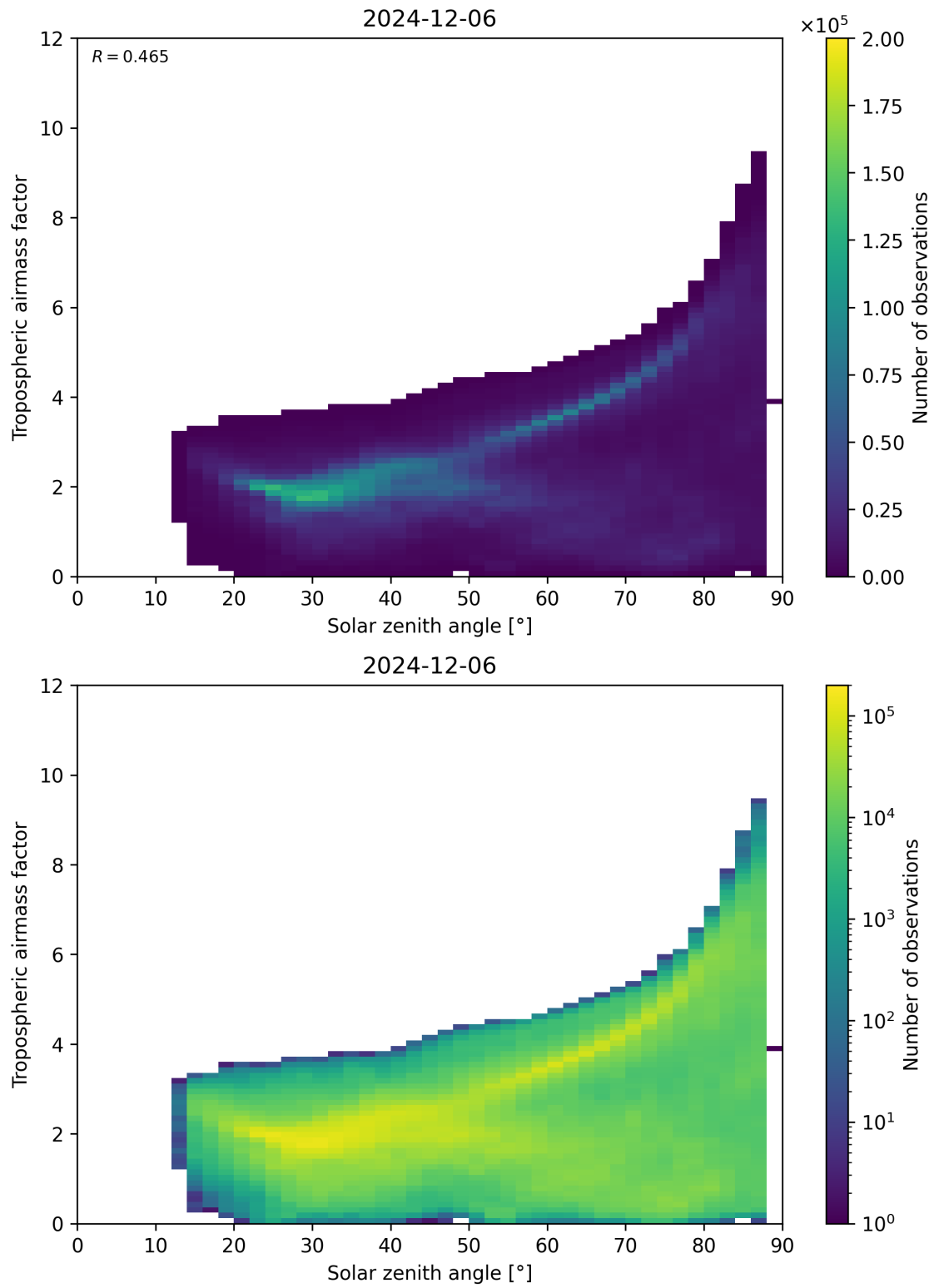
Figure 147: Scatter density plot of “Solar zenith angle” against “Tropospheric airmass factor” for 2024-12-06 to 2024-12-07.
