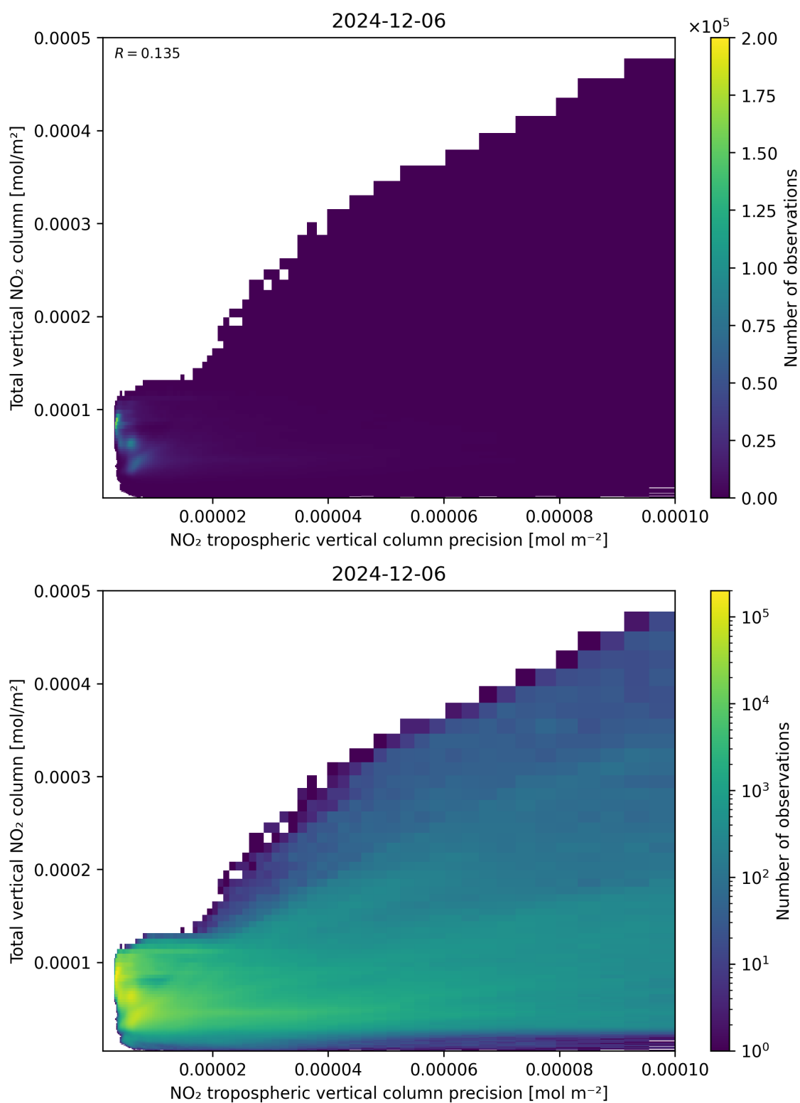
Figure 138: Scatter density plot of “NO 2 tropospheric vertical column precision” against “Total vertical NO 2 column” for 2024-12-06 to 2024-12-07.
