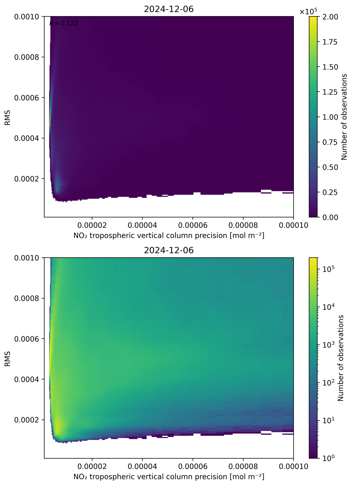
Figure 140: Scatter density plot of “NO 2 tropospheric vertical column precision” against “RMS” for 2024-12-06 to 2024-12-07.
