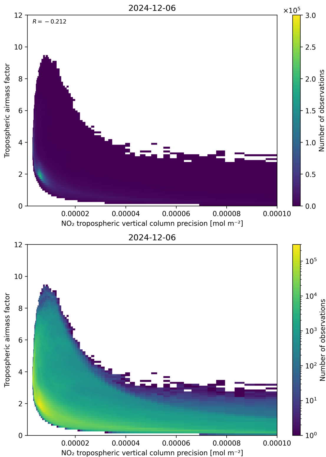
Figure 133: Scatter density plot of “NO 2 tropospheric vertical column precision” against “Tropospheric air mass factor” for 2024-12-06 to 2024-12-07.
