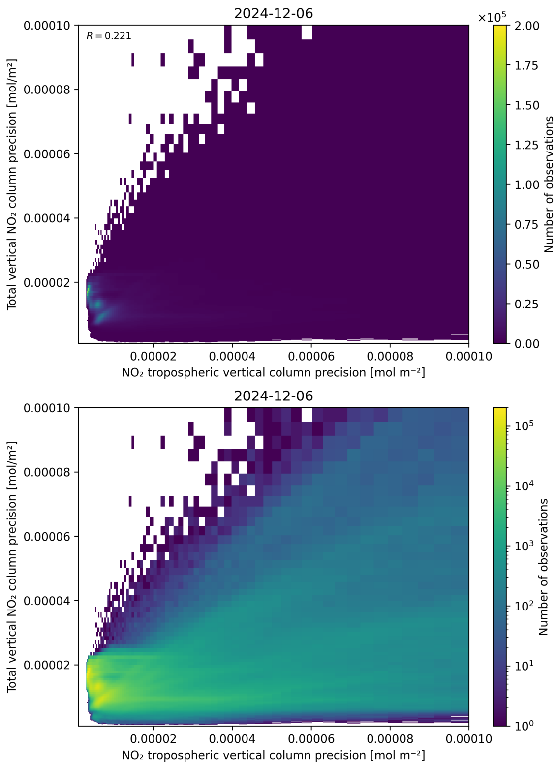
Figure 139: Scatter density plot of “NO 2 tropospheric vertical column precision” against “Total vertical NO 2 column precision” for 2024-12-06 to 2024-12-07.
