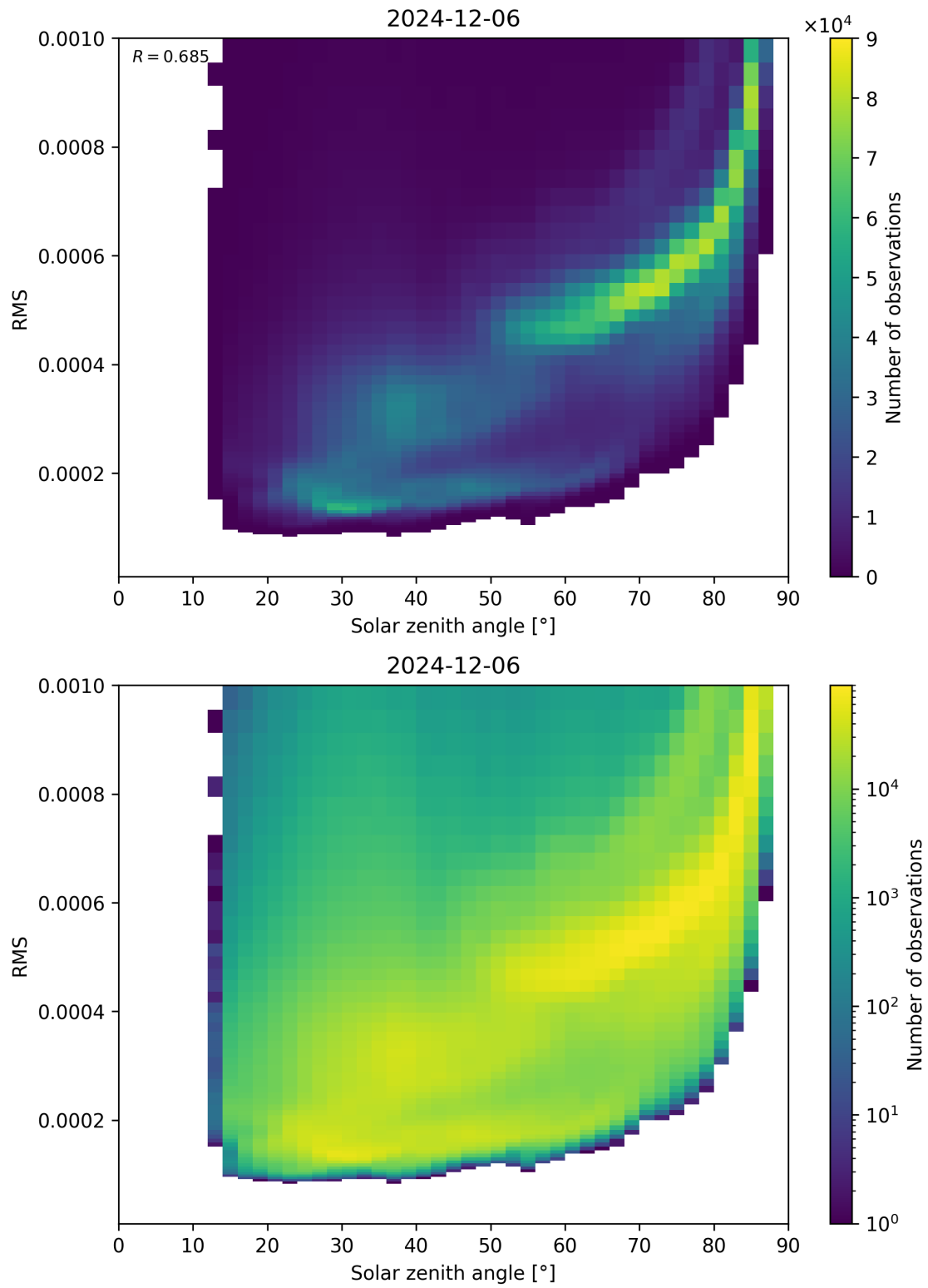
Figure 157: Scatter density plot of “Solar zenith angle” against “RMS” for 2024-12-06 to 2024-12-07.
