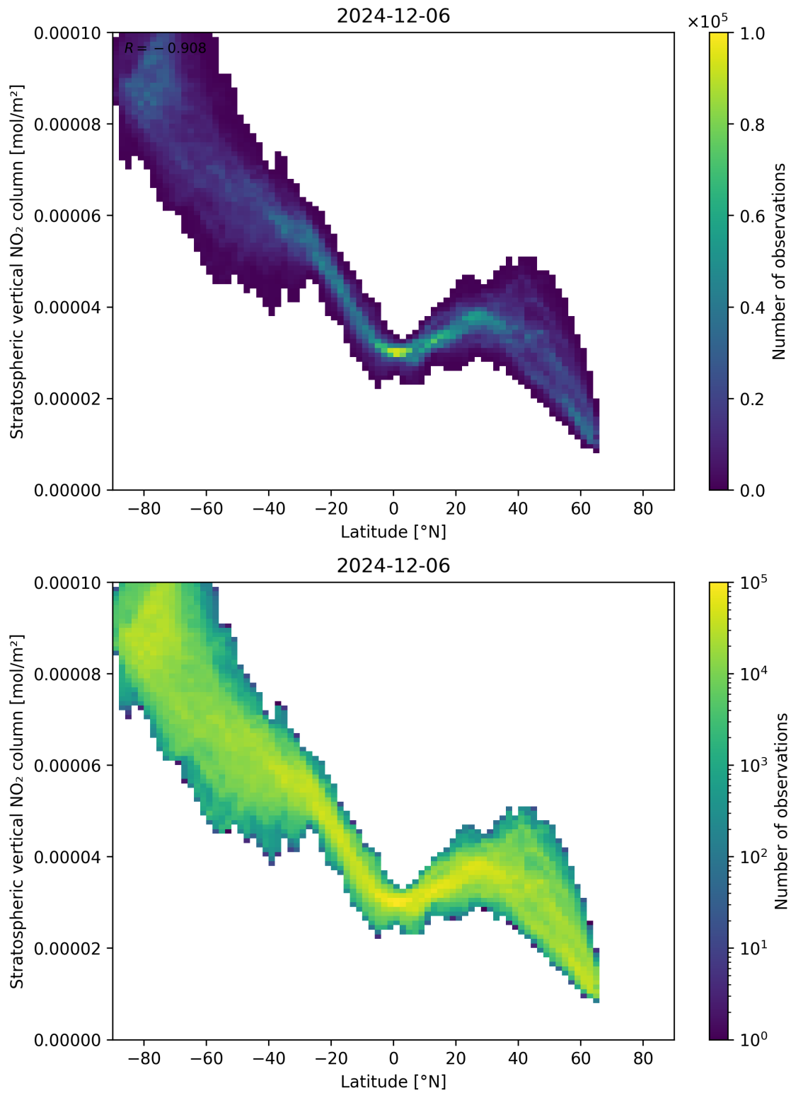
Figure 87: Scatter density plot of “Latitude” against “Stratospheric vertical NO 2 column” for 2024-12-06 to 2024-12-07.
