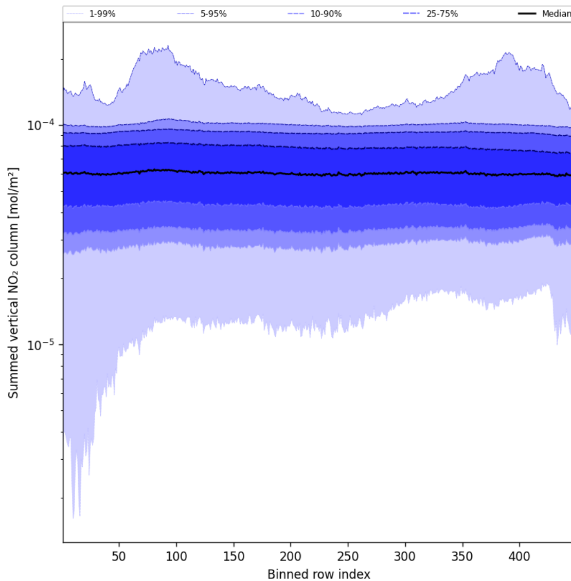
Figure 57: Along track statistics of “Summed vertical NO 2 column” for 2024-12-06 to 2024-12-07
