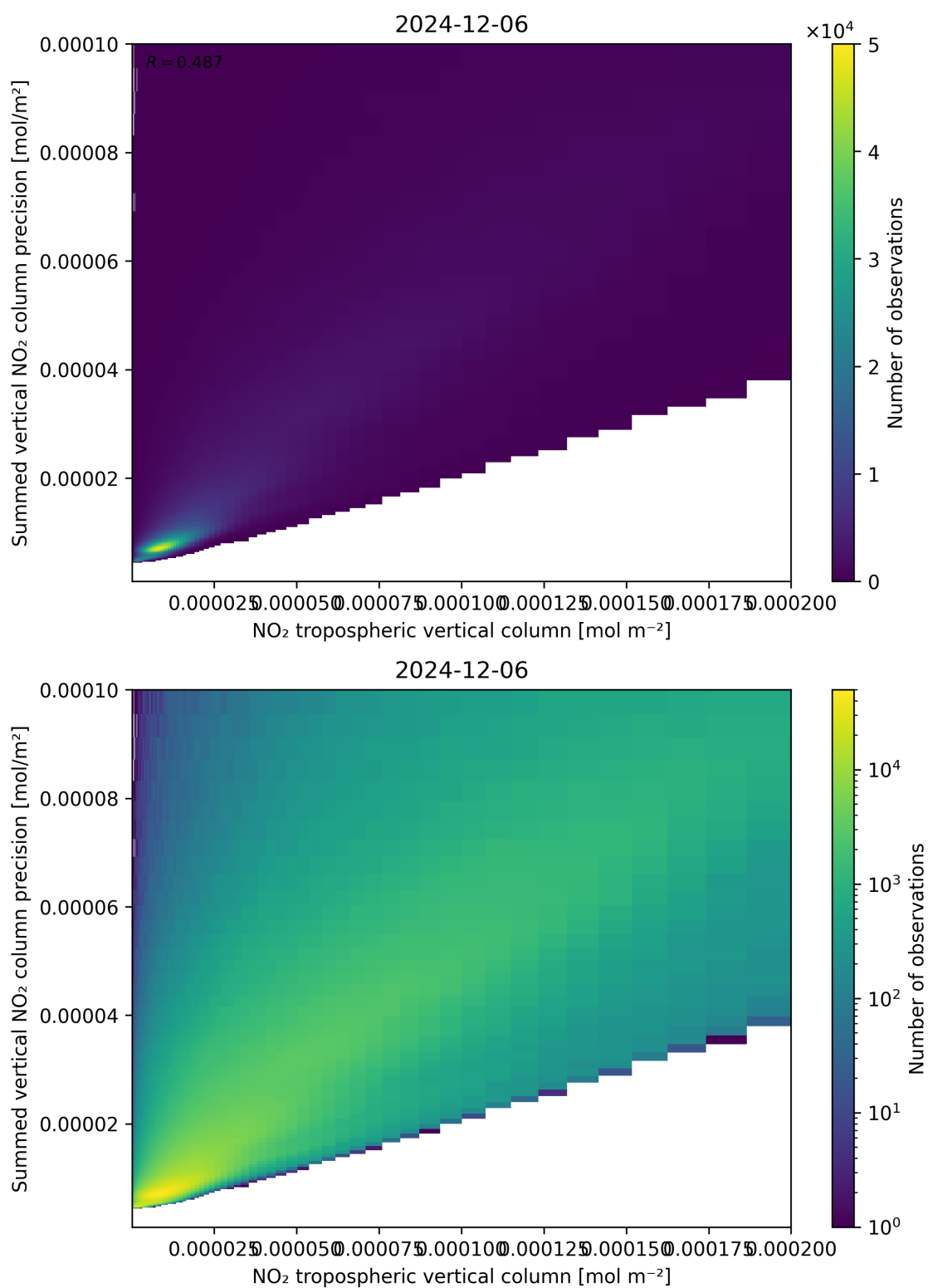
Figure 127: Scatter density plot of “NO 2 tropospheric vertical column” against “Summed vertical NO 2 column precision” for 2024-12-06 to 2024-12-07.
