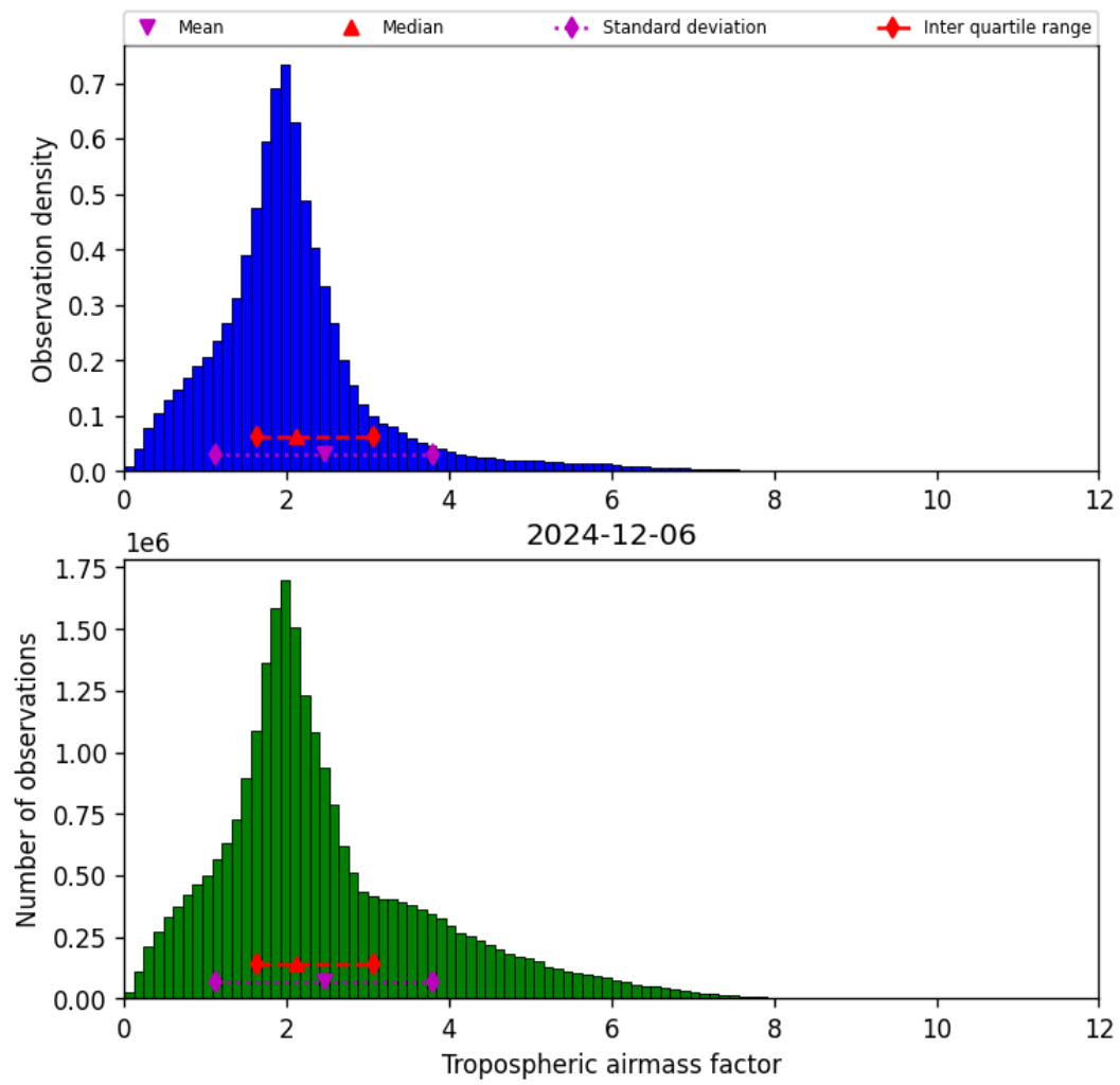
Figure 31: Histogram of “Tropospheric airmass factor” for 2024-12-06 to 2024-12-07
