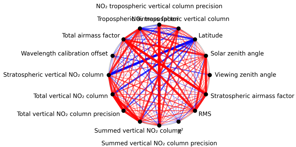
Figure 1: Map of correlation graph for 2024-12-06 to 2024-12-07.
