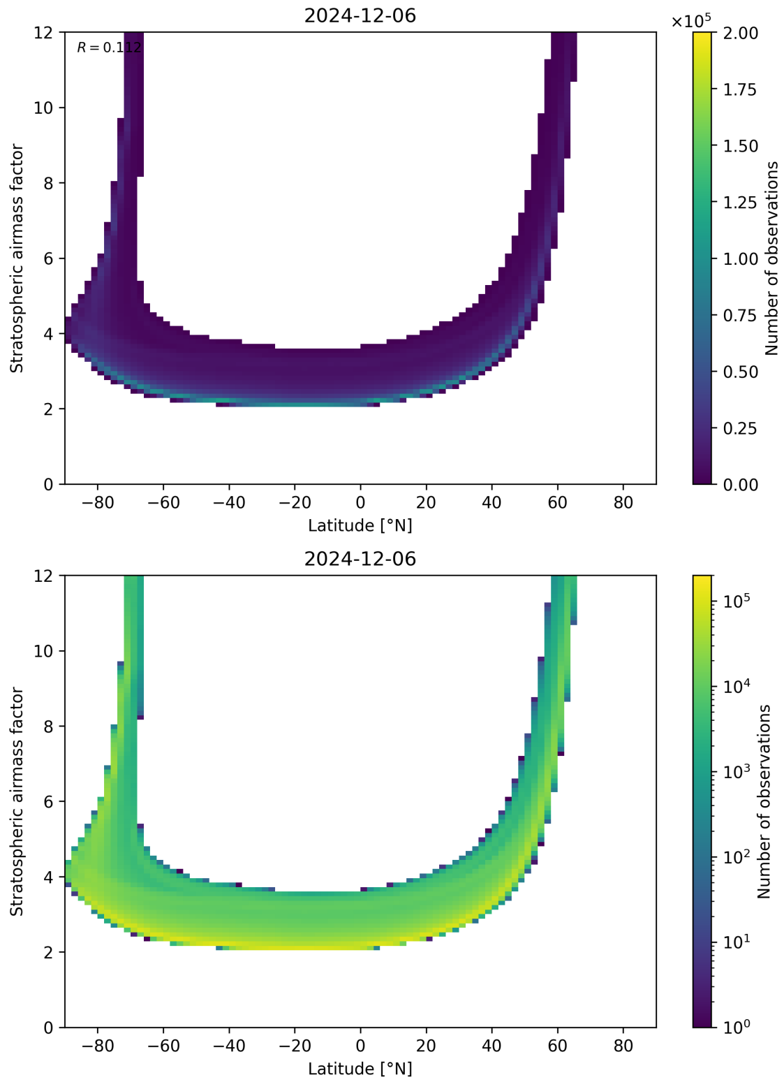
Figure 83: Scatter density plot of “Latitude” against “Stratospheric air mass factor” for 2024-12-06 to 2024-12-07.
