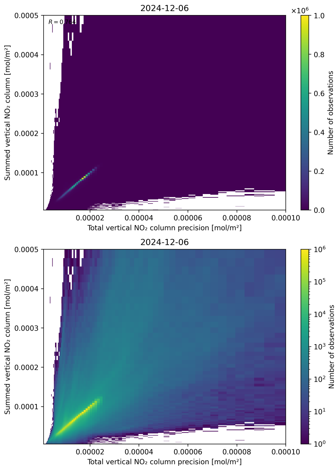
Figure 117: Scatter density plot of “Total vertical NO 2 column precision” against “Summed vertical NO 2 column” for 2024-12-06 to 2024-12-07.
