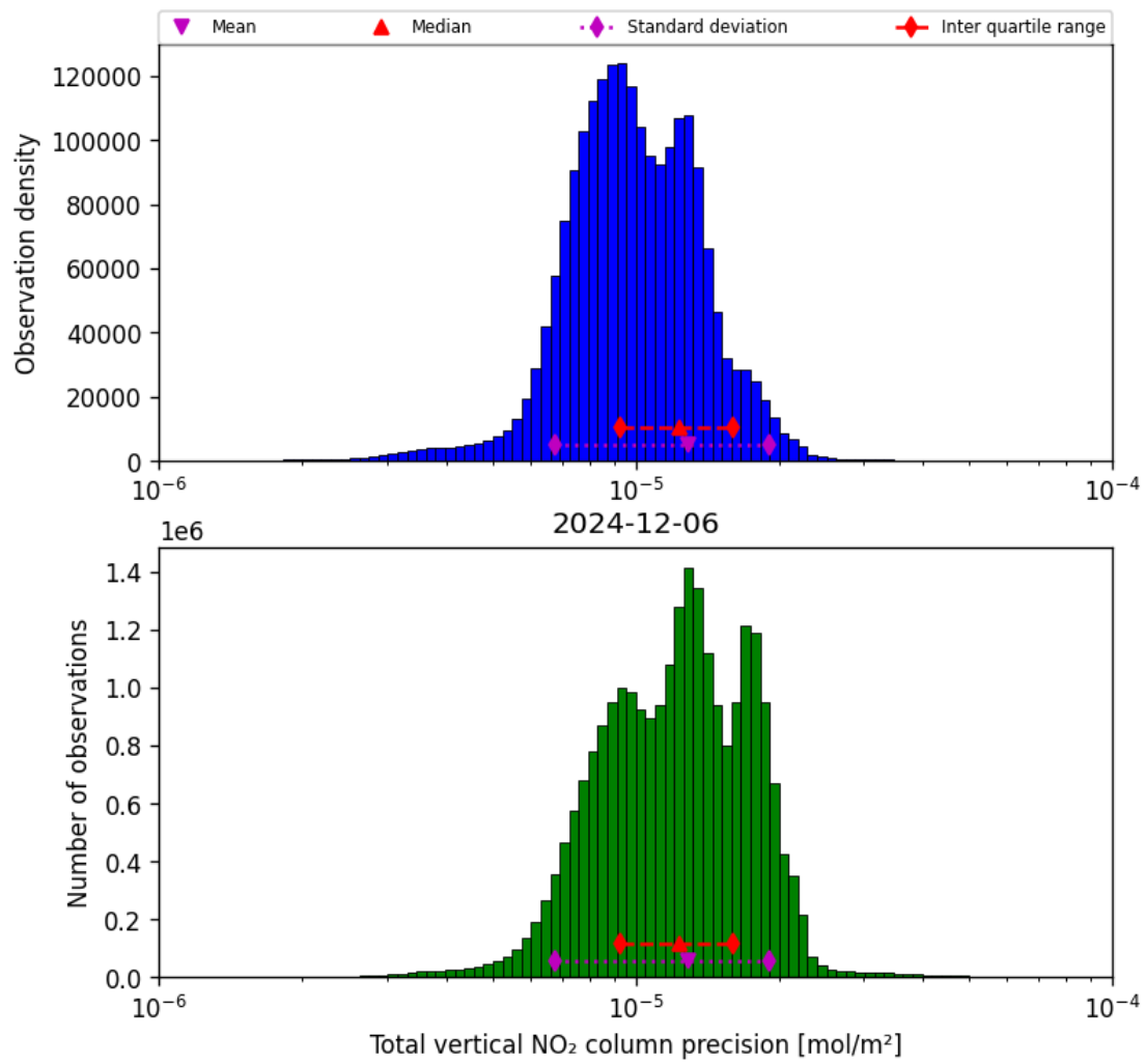
Figure 39: Histogram of “Total vertical NO 2 column precision” for 2024-12-06 to 2024-12-07
