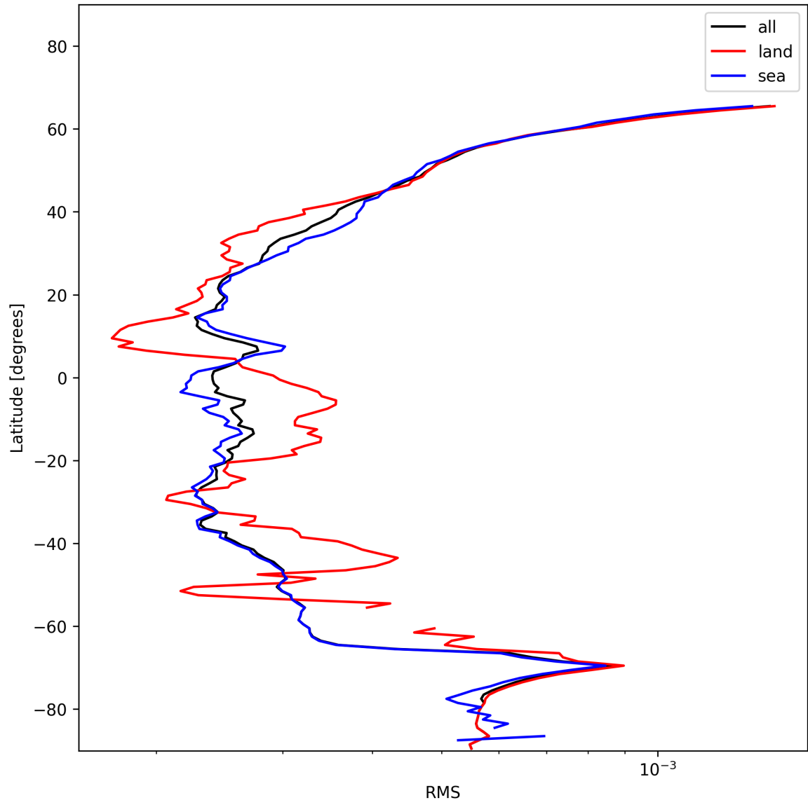
Figure 26: Zonal average of “RMS” for 2024-12-06 to 2024-12-07.
