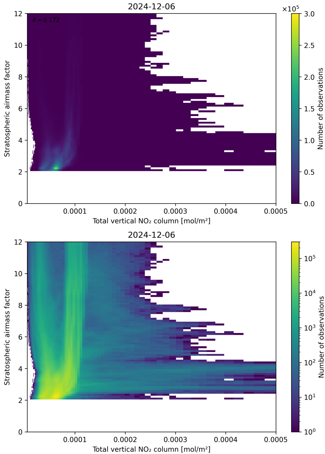
Figure 110: Scatter density plot of “Total vertical NO 2 column” against “Stratospheric airmass factor” for 2024-12-06 to 2024-12-07.
