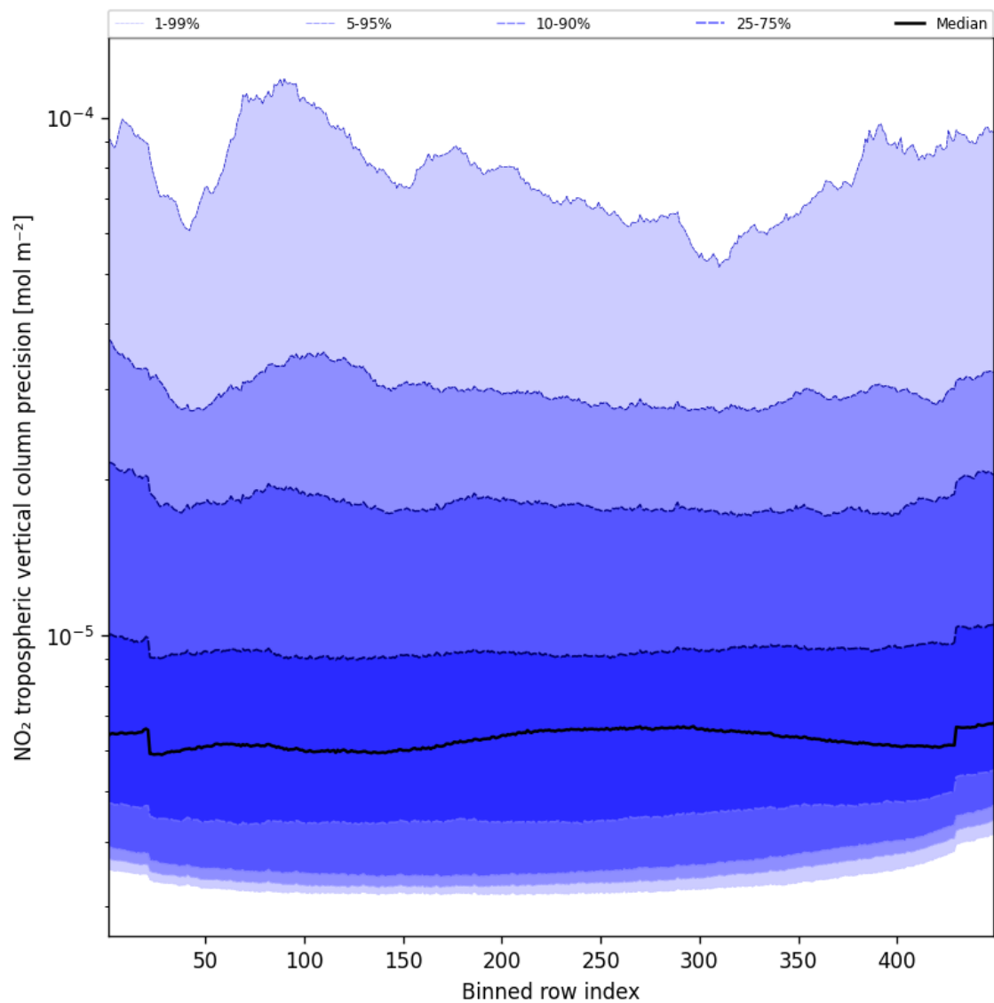
Figure 47: Along track statistics of “NO 2 tropospheric vertical column precision” for 2024-12-06 to 2024-12-07
