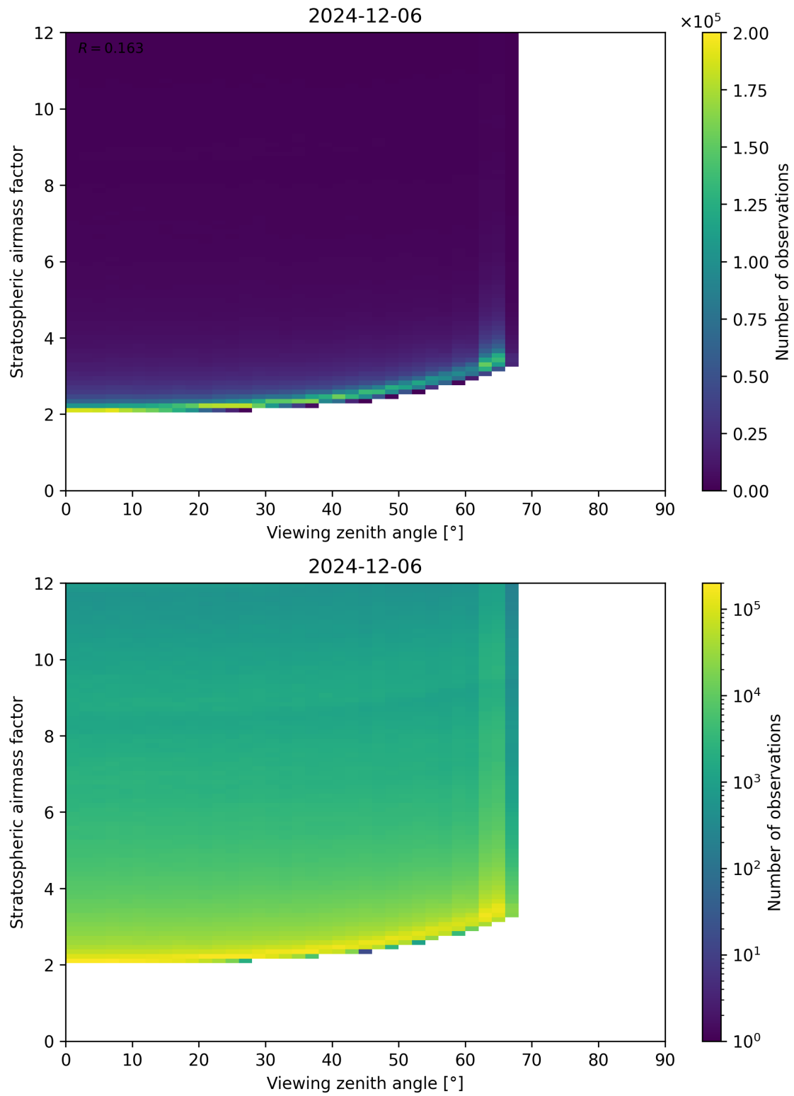
Figure 159: Scatter density plot of “Viewing zenith angle” against “Stratospheric airmass factor” for 2024-12-06 to 2024-12-07.
