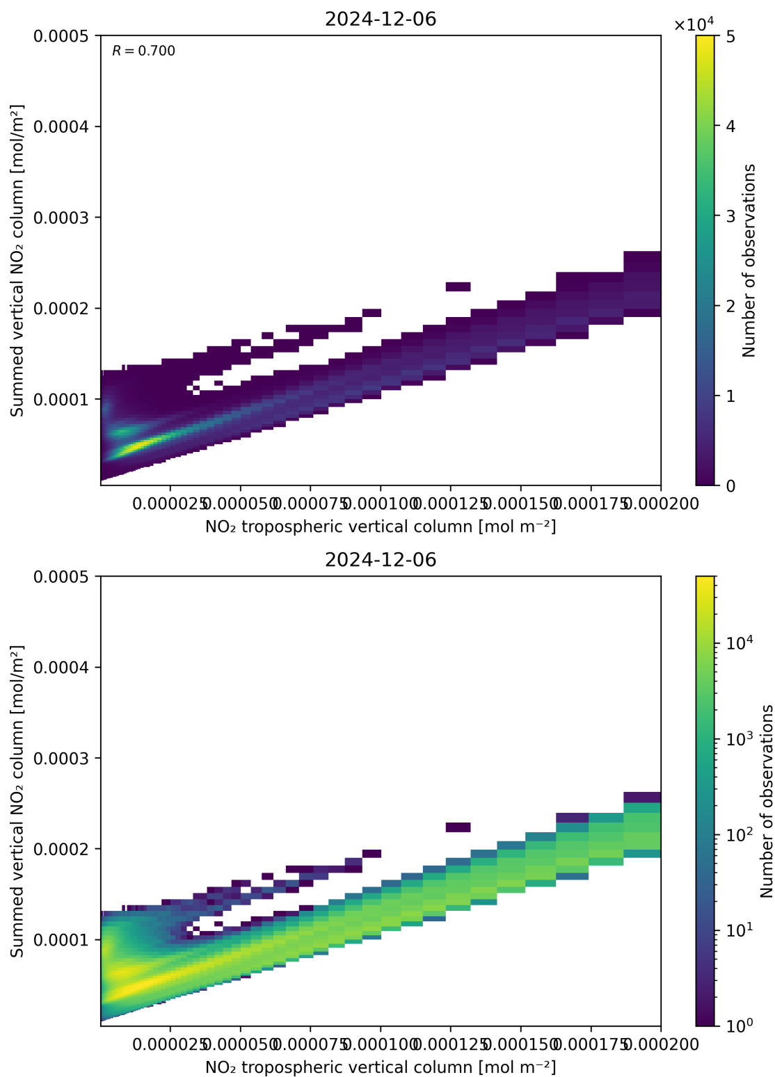
Figure 126: Scatter density plot of “NO 2 tropospheric vertical column” against “Summed vertical NO 2 column” for 2024-12-06 to 2024-12-07.
