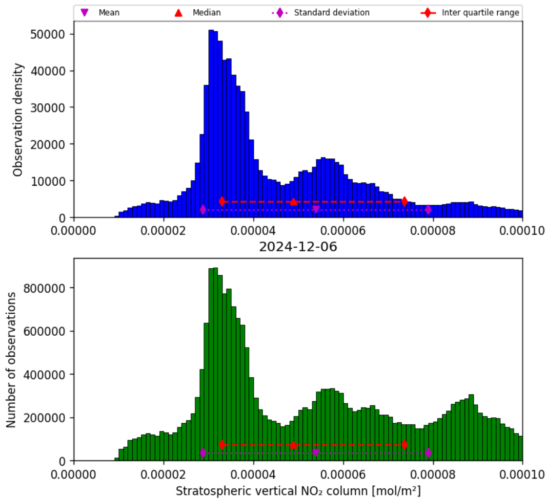
Figure 36: Histogram of “Stratospheric vertical NO 2 column” for 2024-12-06 to 2024-12-07
