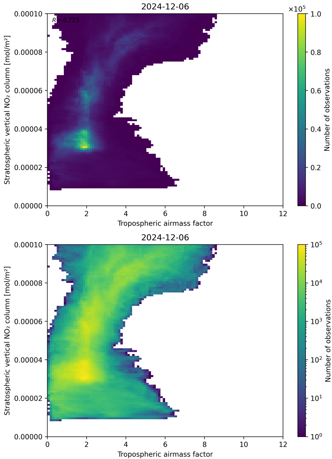
Figure 74: Scatter density plot of “Tropospheric airmass factor” against “Stratospheric vertical NO 2 column” for 2024-12-06 to 2024-12-07.
