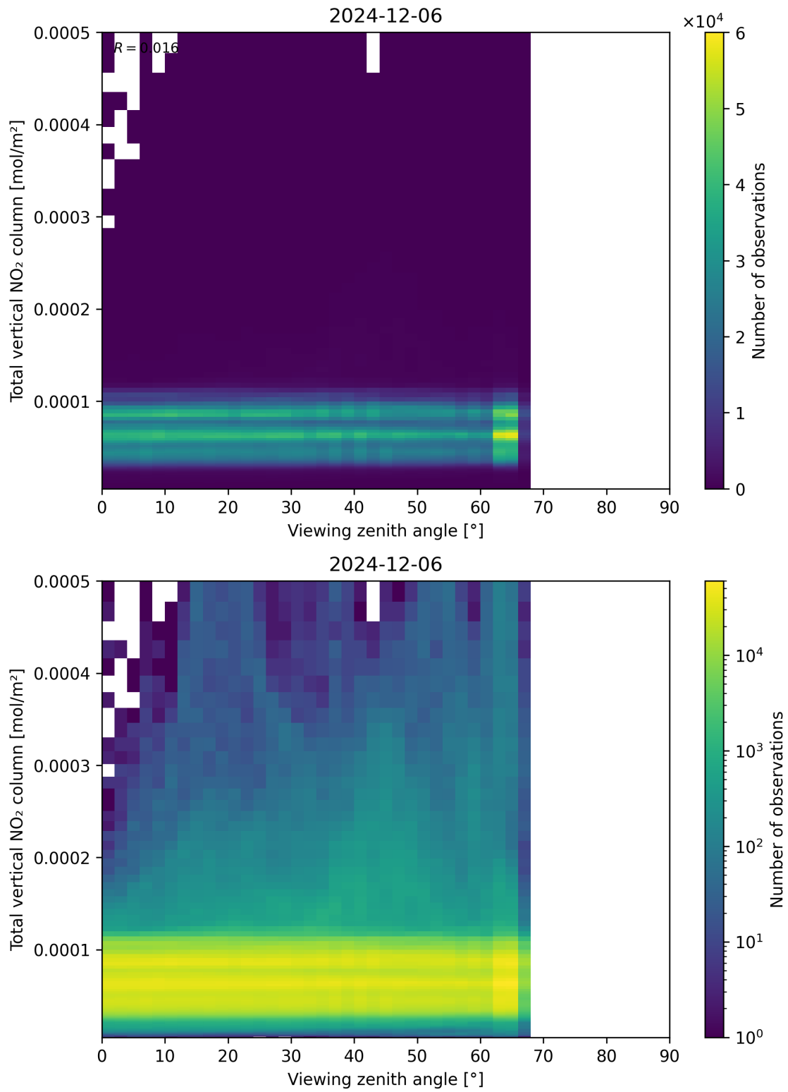
Figure 167: Scatter density plot of “Viewing zenith angle” against “Total vertical NO 2 column” for 2024-12-06 to 2024-12-07.
