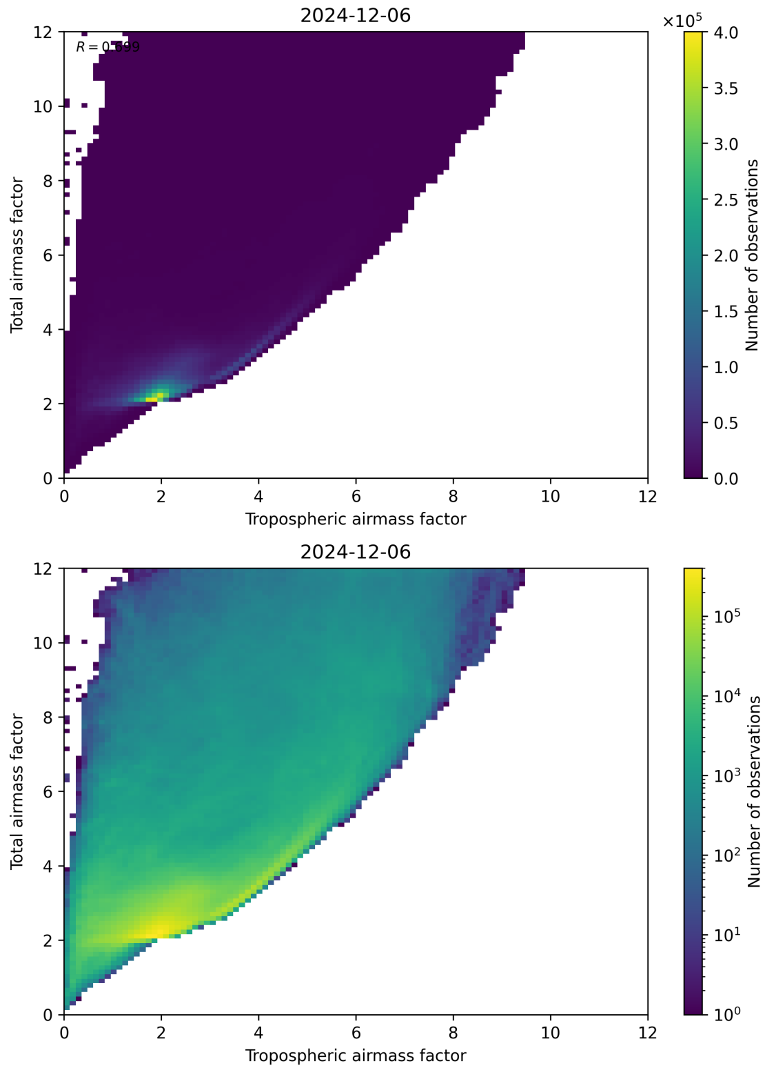
Figure 72: Scatter density plot of “Tropospheric airmass factor” against “Total airmass factor” for 2024-12-06 to 2024-12-07.
