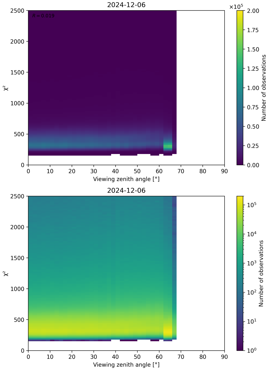
Figure 162: Scatter density plot of “Viewing zenith angle” against “ \chi^2 ” for 2024-12-06 to 2024-12-07.
