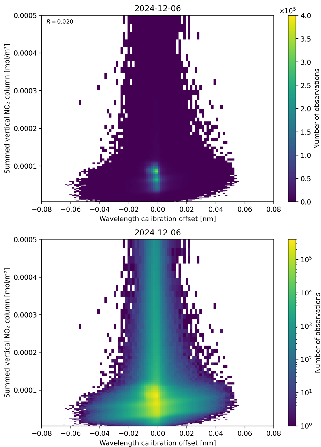
Figure 177: Scatter density plot of “Wavelength calibration offset” against “Summed vertical NO 2 column” for 2024-12-06 to 2024-12-07.
