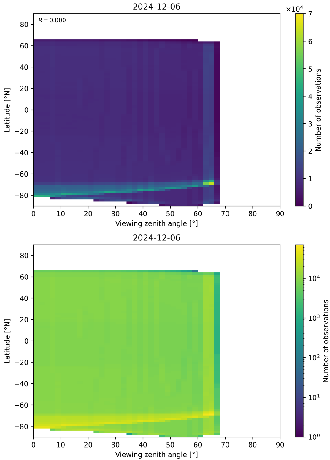
Figure 163: Scatter density plot of “Viewing zenith angle” against “Latitude” for 2024-12-06 to 2024-12-07.
