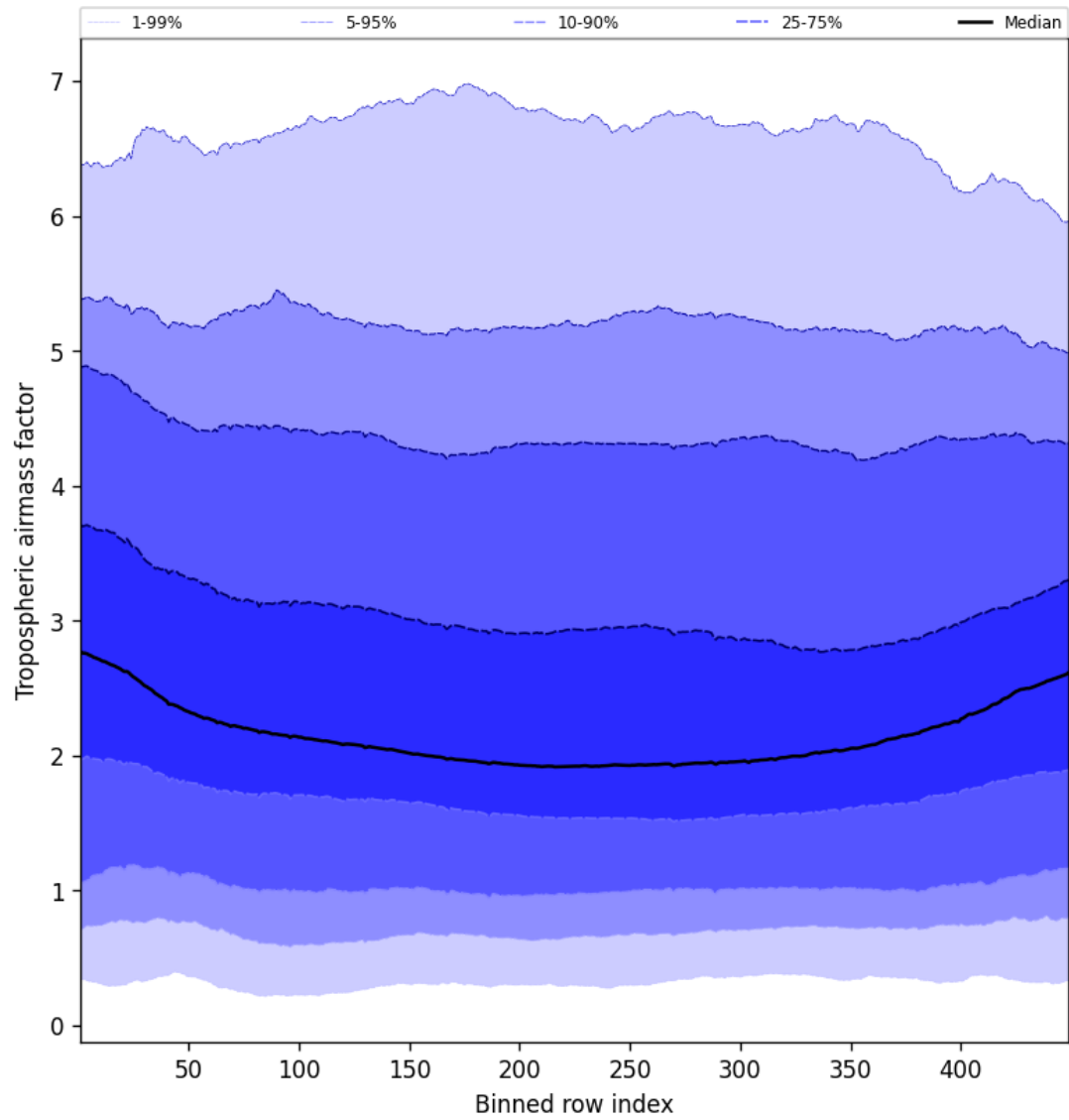
Figure 48: Along track statistics of “Tropospheric airmass factor” for 2024-12-06 to 2024-12-07
