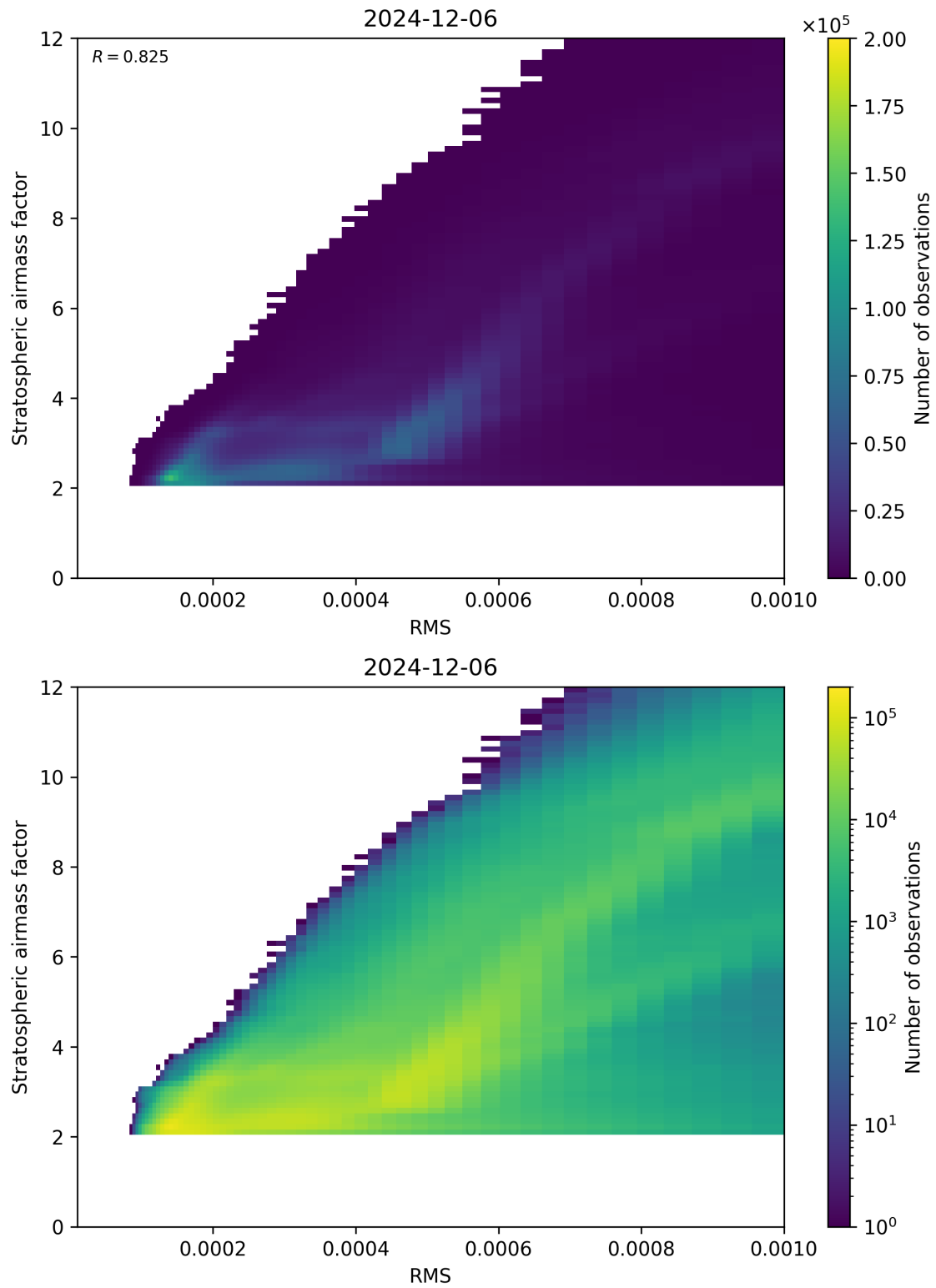
Figure 144: Scatter density plot of “RMS” against “Stratospheric airmass factor” for 2024-12-06 to 2024-12-07.
