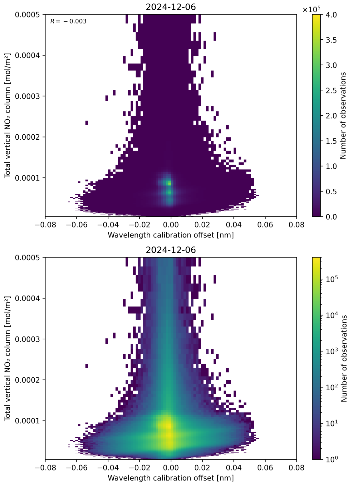
Figure 179: Scatter density plot of “Wavelength calibration offset” against “Total vertical NO 2 column” for 2024-12-06 to 2024-12-07.
