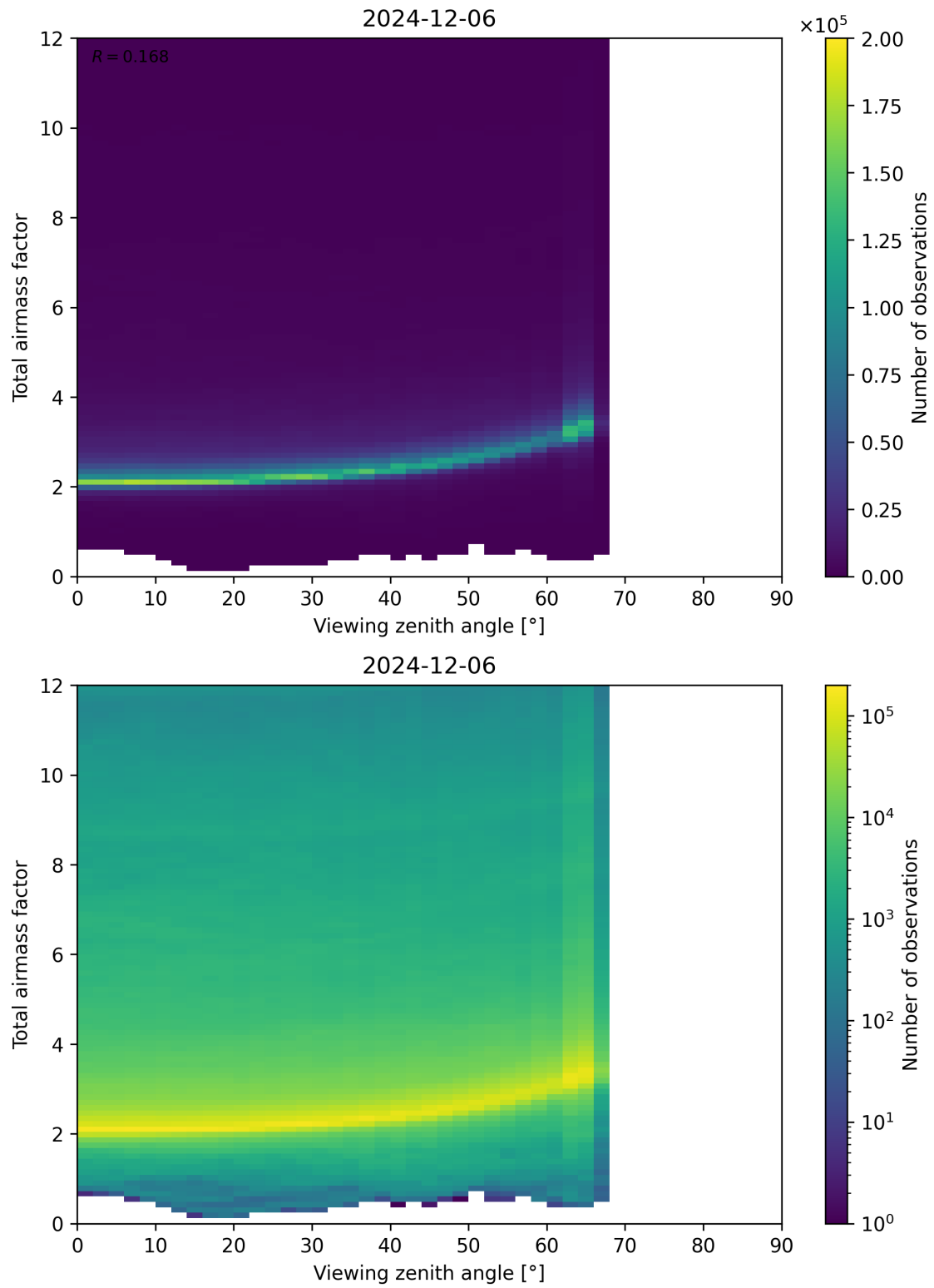
Figure 160: Scatter density plot of “Viewing zenith angle” against “Total airmass factor” for 2024-12-06 to 2024-12-07.
