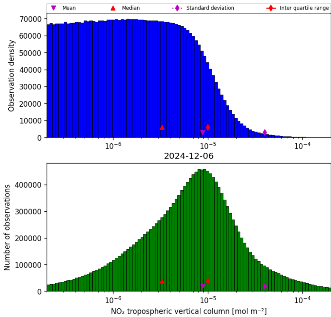
Figure 29: Histogram of “NO 2 tropospheric vertical column” for 2024-12-06 to 2024-12-07
