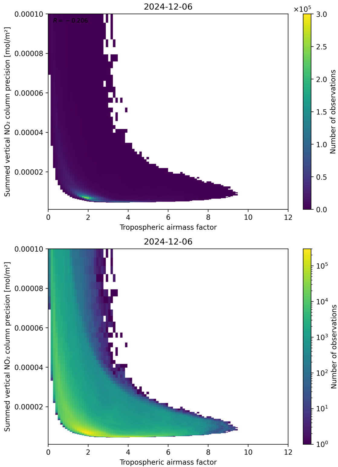
Figure 76: Scatter density plot of “Tropospheric air mass factor” against “Summed vertical NO 2 column precision” for 2024-12-06 to 2024-12-07.
