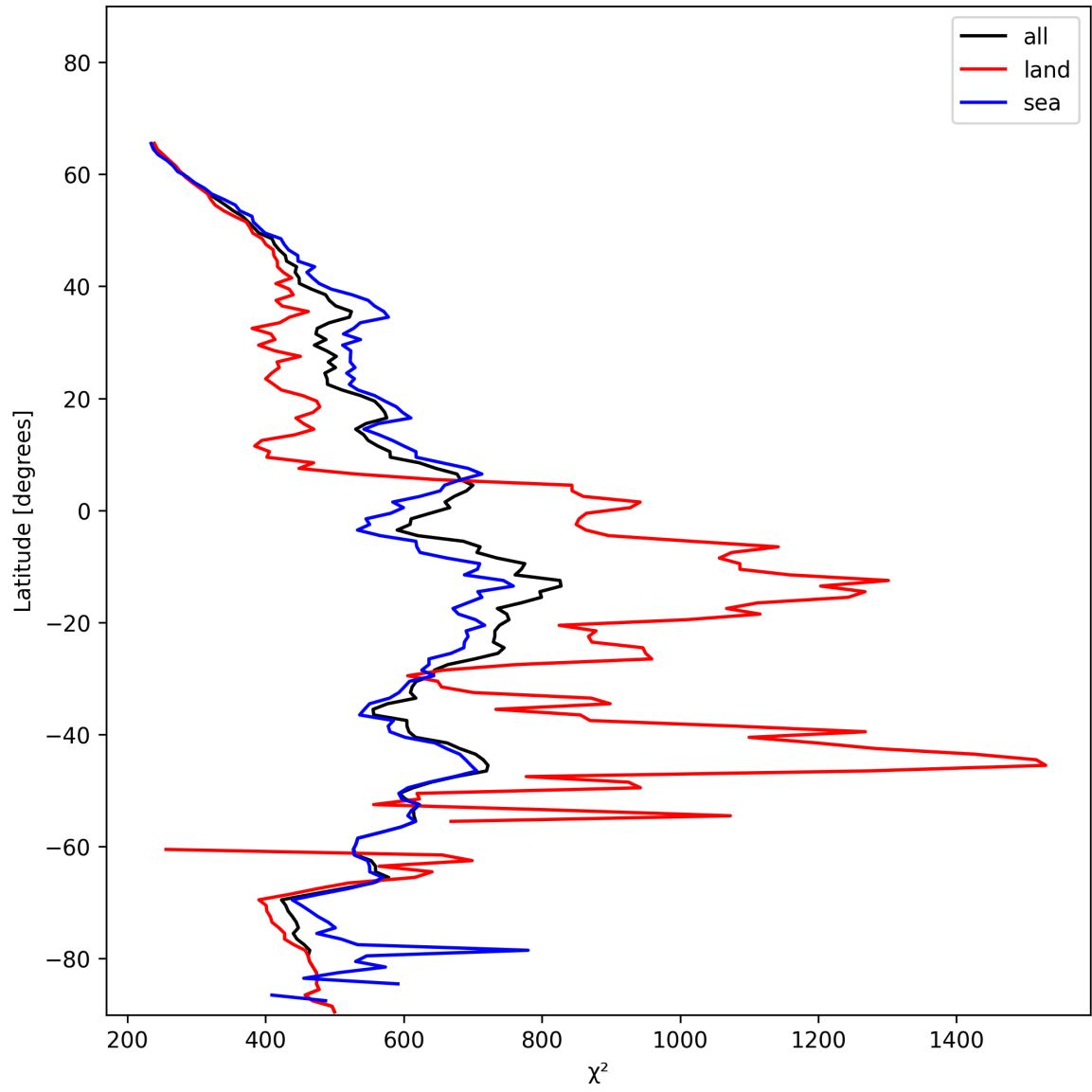
Figure 25: Zonal average of “ \chi^2 ” for 2024-12-06 to 2024-12-07.
