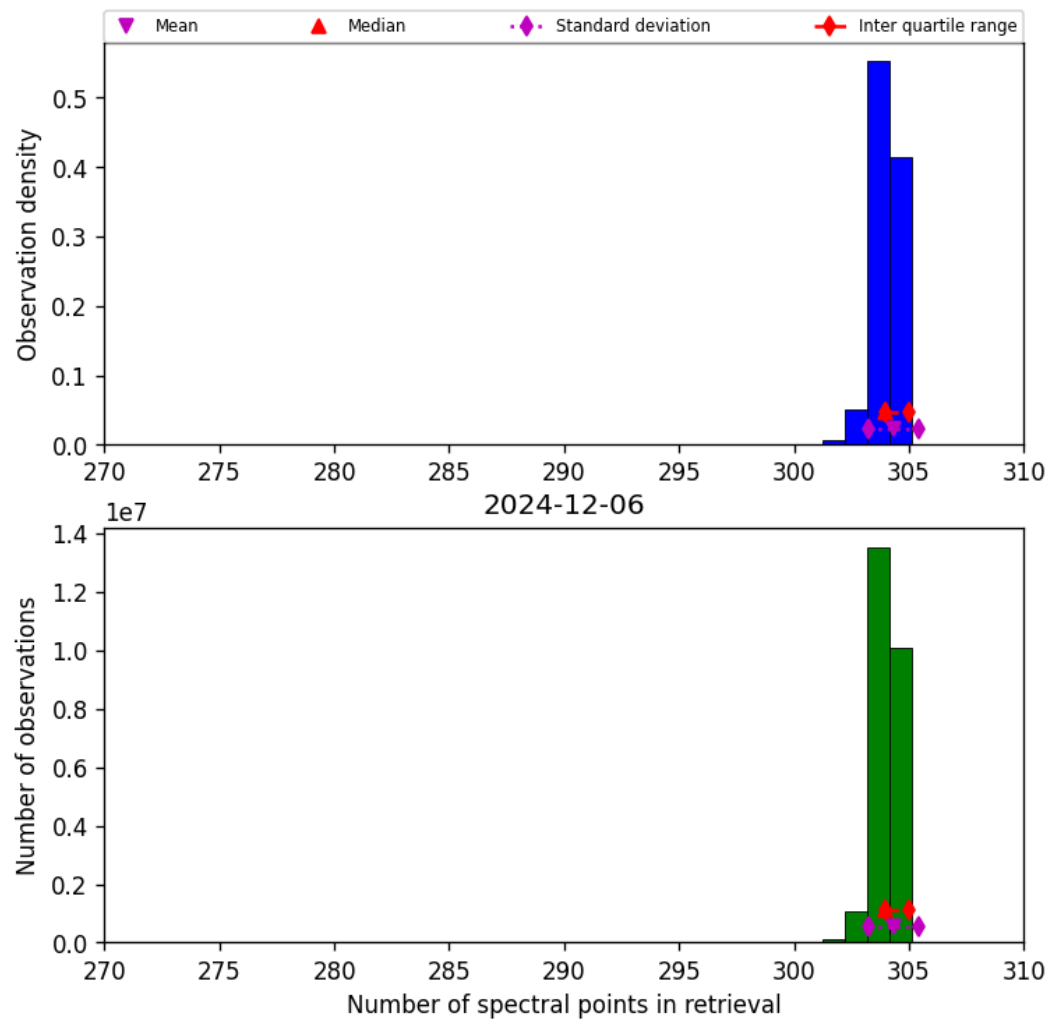
Figure 33: Histogram of “Number of spectral points in retrieval” for 2024-12-06 to 2024-12-07
