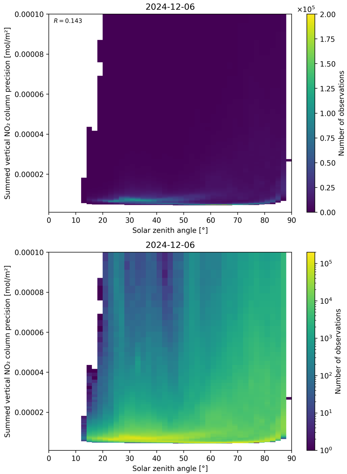
Figure 152: Scatter density plot of “Solar zenith angle” against “Summed vertical NO 2 column precision” for 2024-12-06 to 2024-12-07.
