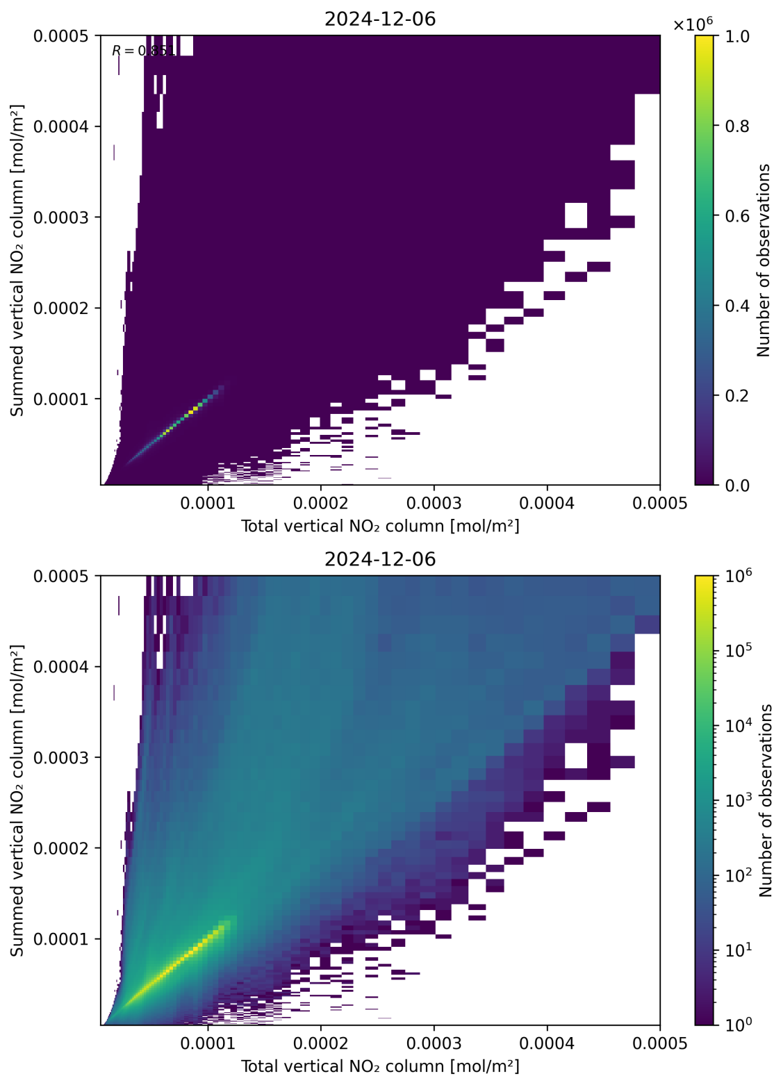
Figure 112: Scatter density plot of “Total vertical NO 2 column” against “Summed vertical NO 2 column” for 2024-12-06 to 2024-12-07.
