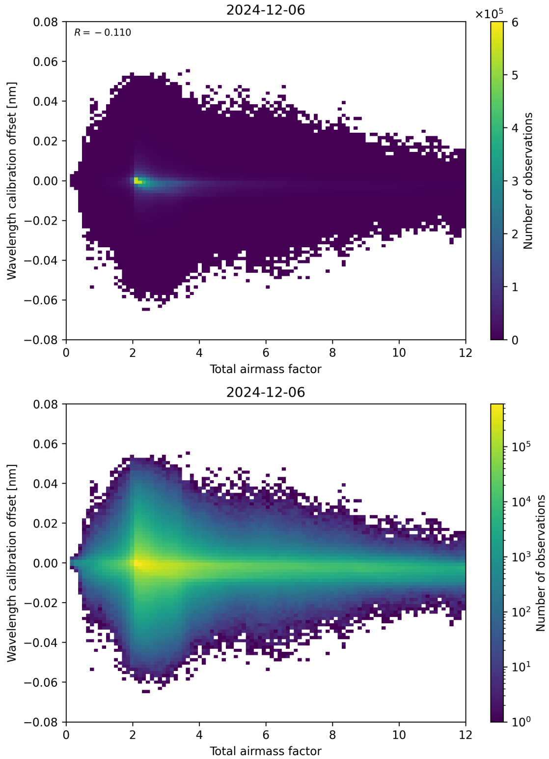
Figure 70: Scatter density plot of “Total airmass factor” against “Wavelength calibration offset” for 2024-12-06 to 2024-12-07.
