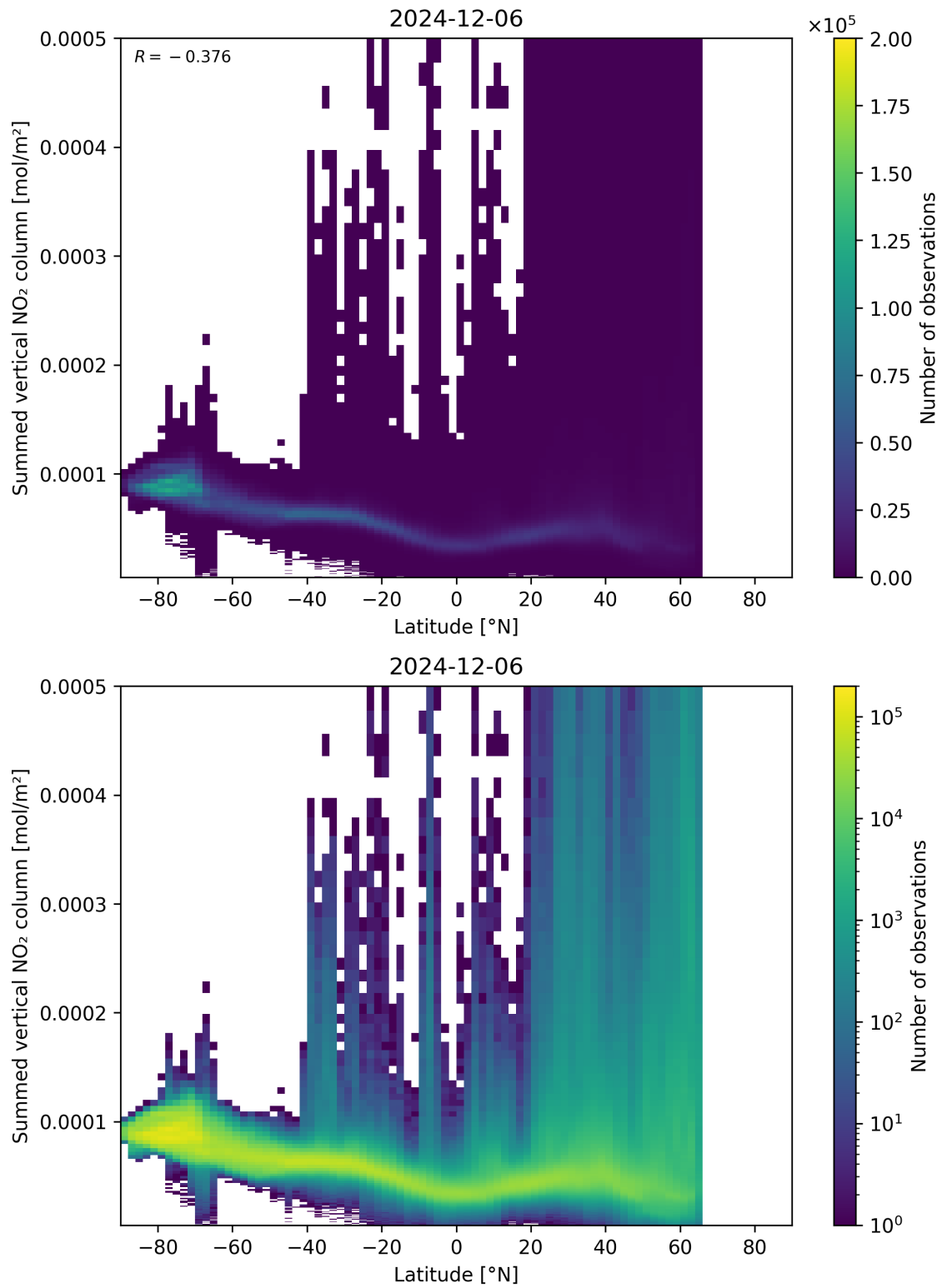
Figure 88: Scatter density plot of “Latitude” against “Summed vertical NO 2 column” for 2024-12-06 to 2024-12-07.
