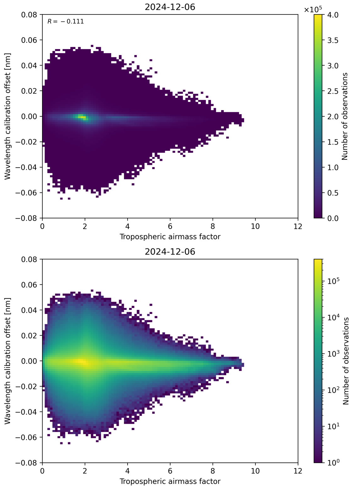
Figure 80: Scatter density plot of “Tropospheric air mass factor” against “Wavelength calibration offset” for 2024-12-06 to 2024-12-07.
