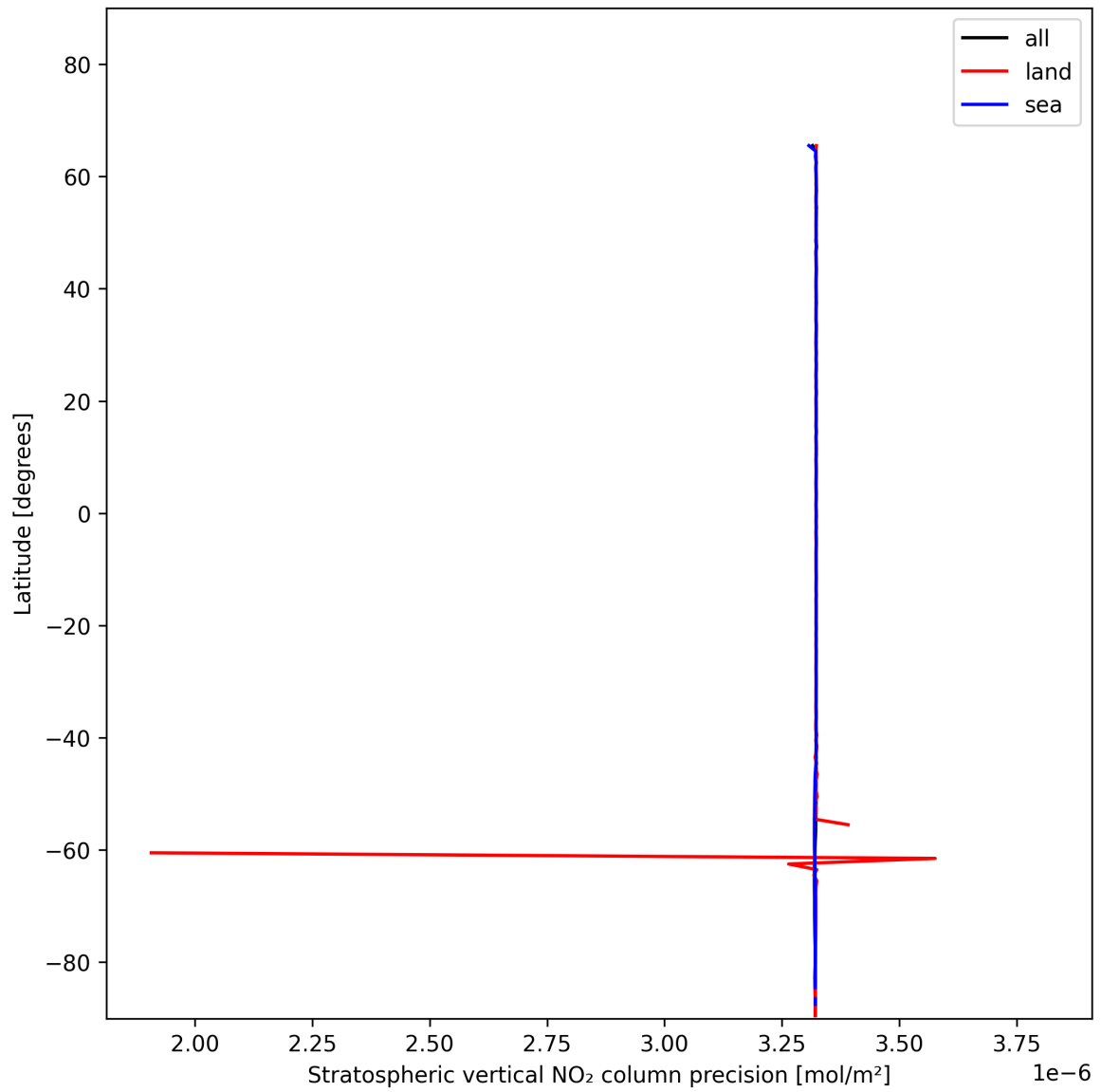
Figure 20: Zonal average of “Stratospheric vertical NO 2 column precision” for 2024-12-06 to 2024-12-07.
