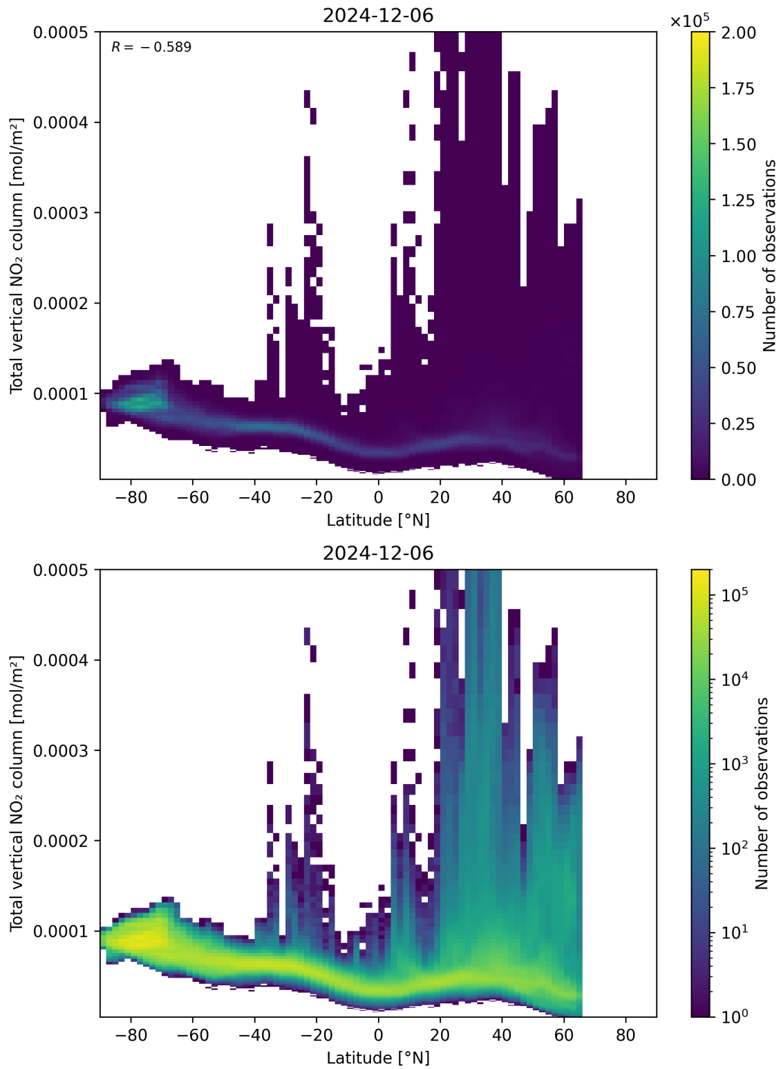
Figure 90: Scatter density plot of “Latitude” against “Total vertical NO 2 column” for 2024-12-06 to 2024-12-07.
