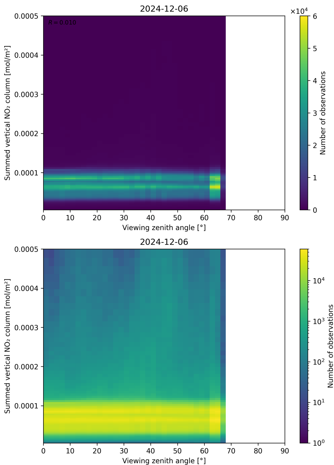
Figure 165: Scatter density plot of “Viewing zenith angle” against “Summed vertical NO 2 column” for 2024-12-06 to 2024-12-07.
