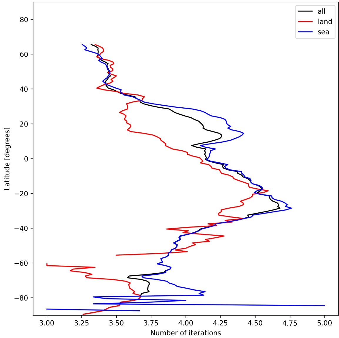
Figure 17: Zonal average of “Number of iterations” for 2024-12-06 to 2024-12-07.
