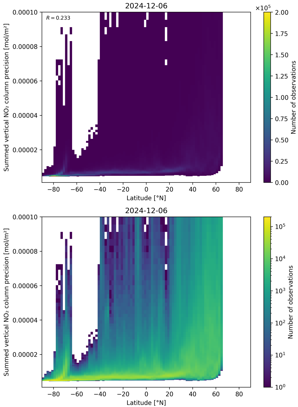
Figure 89: Scatter density plot of “Latitude” against “Summed vertical NO 2 column precision” for 2024-12-06 to 2024-12-07.
