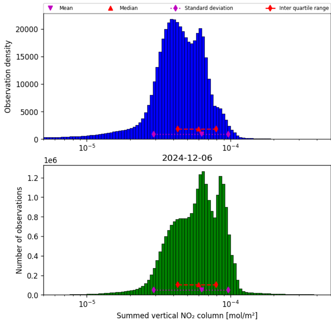
Figure 40: Histogram of “Summed vertical NO 2 column” for 2024-12-06 to 2024-12-07
