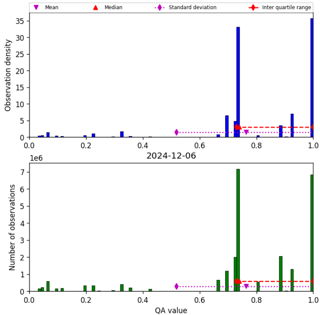
Figure 28: Histogram of “QA value” for 2024-12-06 to 2024-12-07
