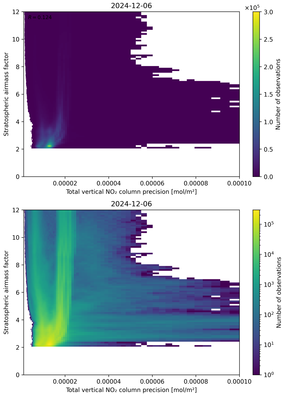
Figure 115: Scatter density plot of “Total vertical NO 2 column precision” against “Stratospheric air mass factor” for 2024-12-06 to 2024-12-07.
