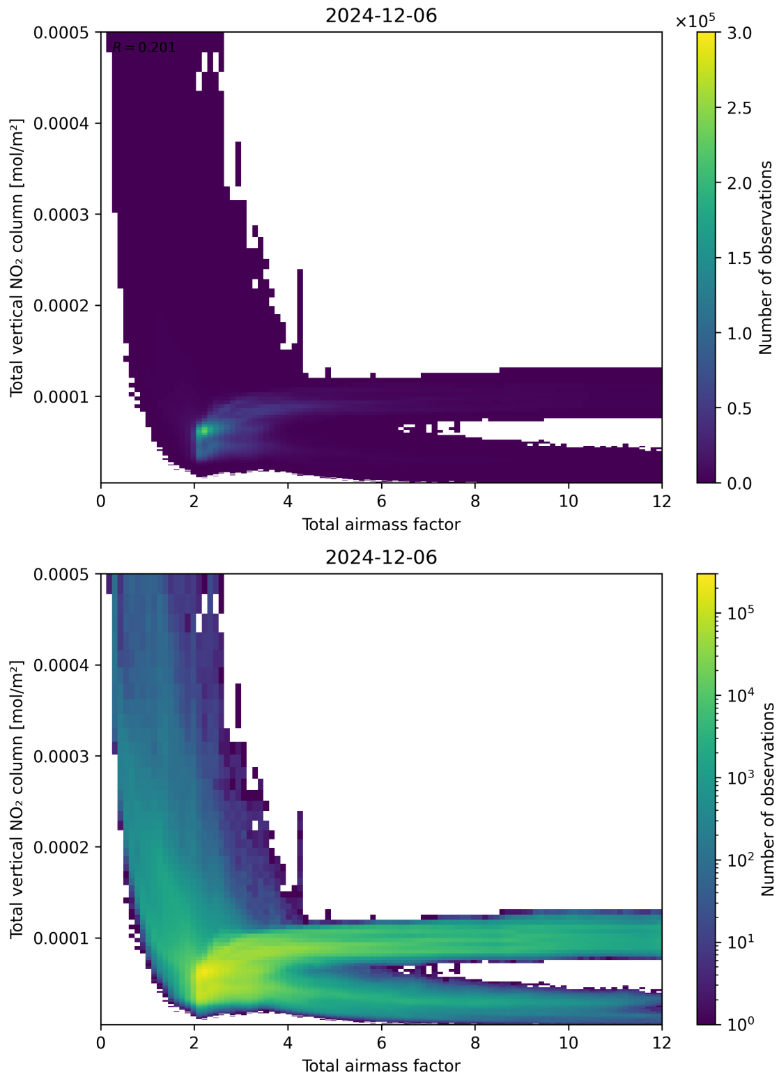
Figure 67: Scatter density plot of “Total airmass factor” against “Total vertical NO 2 column” for 2024-12-06 to 2024-12-07.
