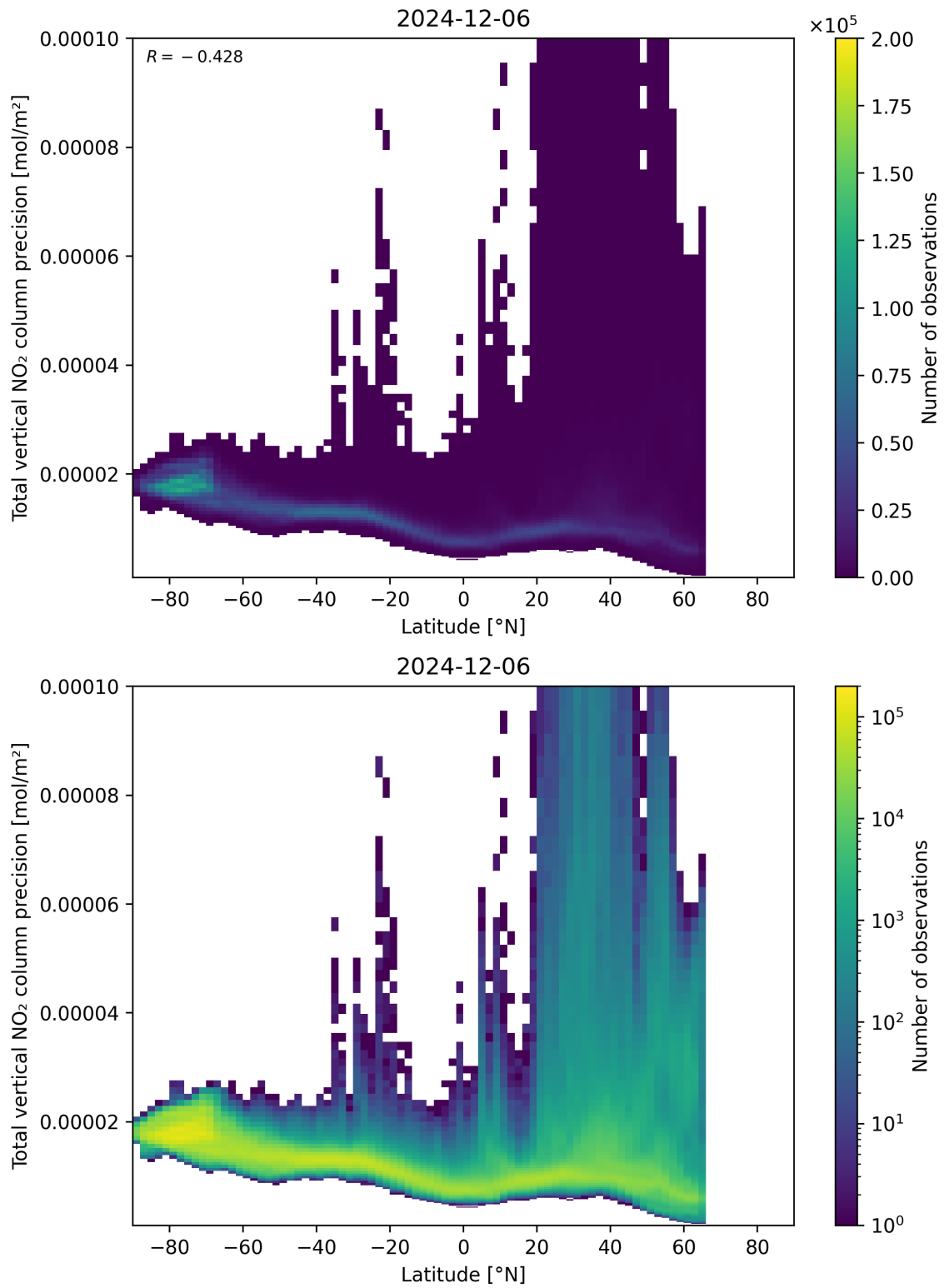
Figure 91: Scatter density plot of “Latitude” against “Total vertical NO 2 column precision” for 2024-12-06 to 2024-12-07.
