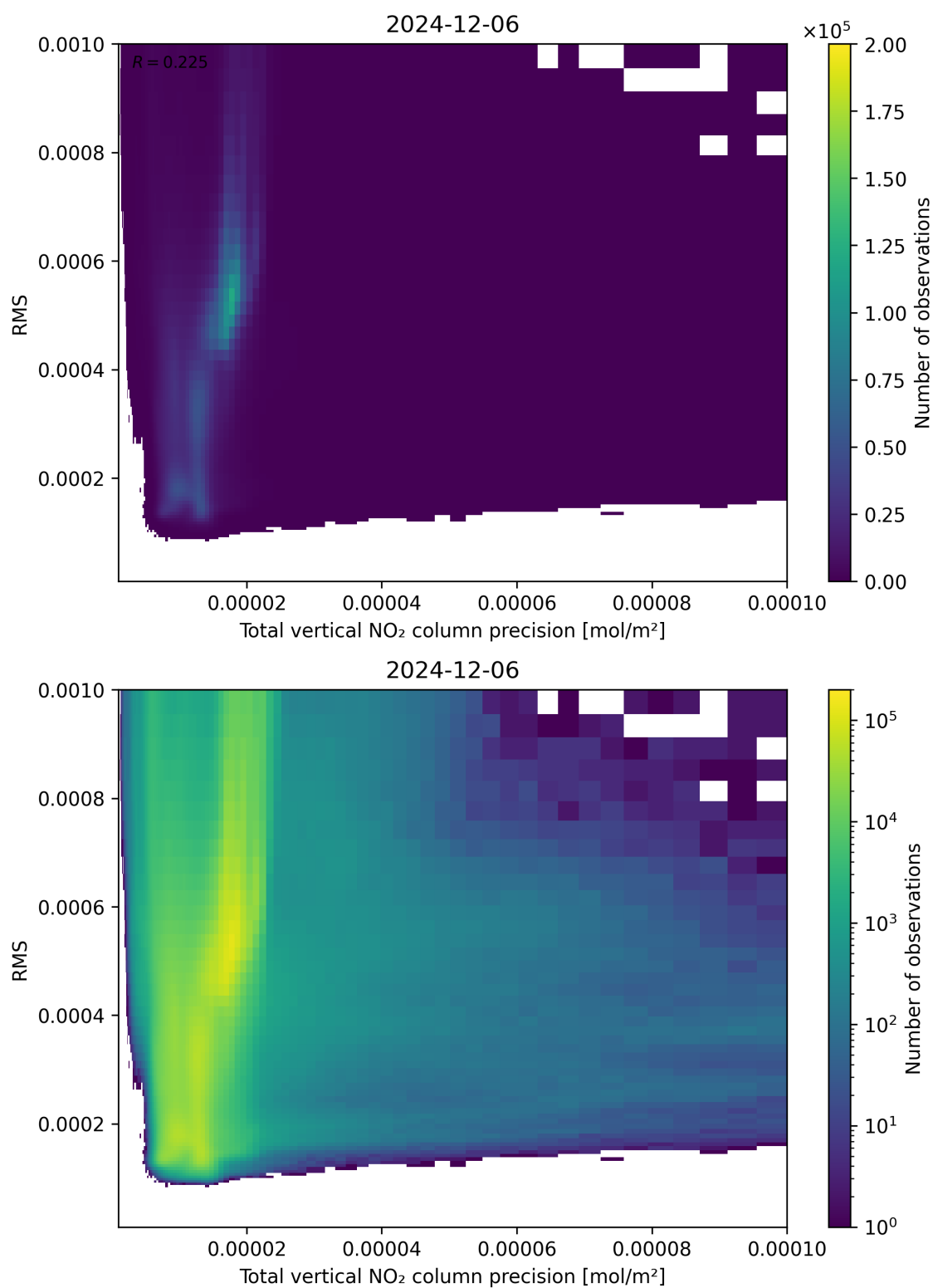
Figure 119: Scatter density plot of “Total vertical NO 2 column precision” against “RMS” for 2024-12-06 to 2024-12-07.
