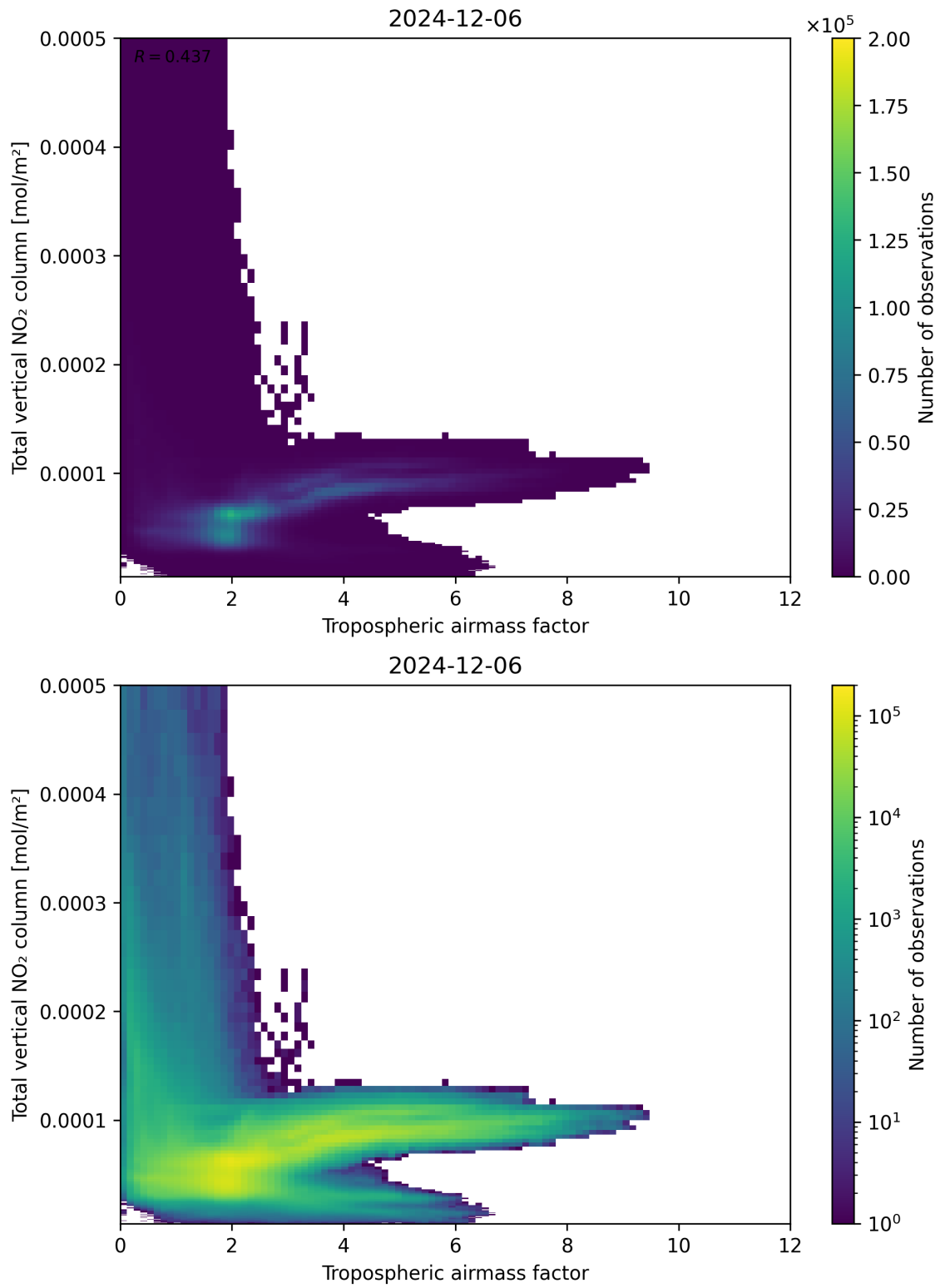
Figure 77: Scatter density plot of “Tropospheric airmass factor” against “Total vertical NO 2 column” for 2024-12-06 to 2024-12-07.
