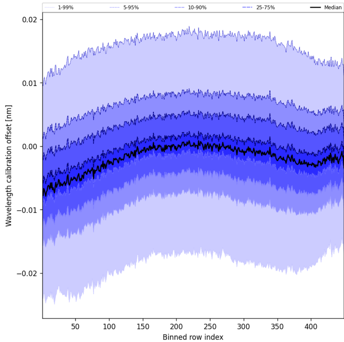
Figure 52: Along track statistics of “Wavelength calibration offset” for 2024-12-06 to 2024-12-07
