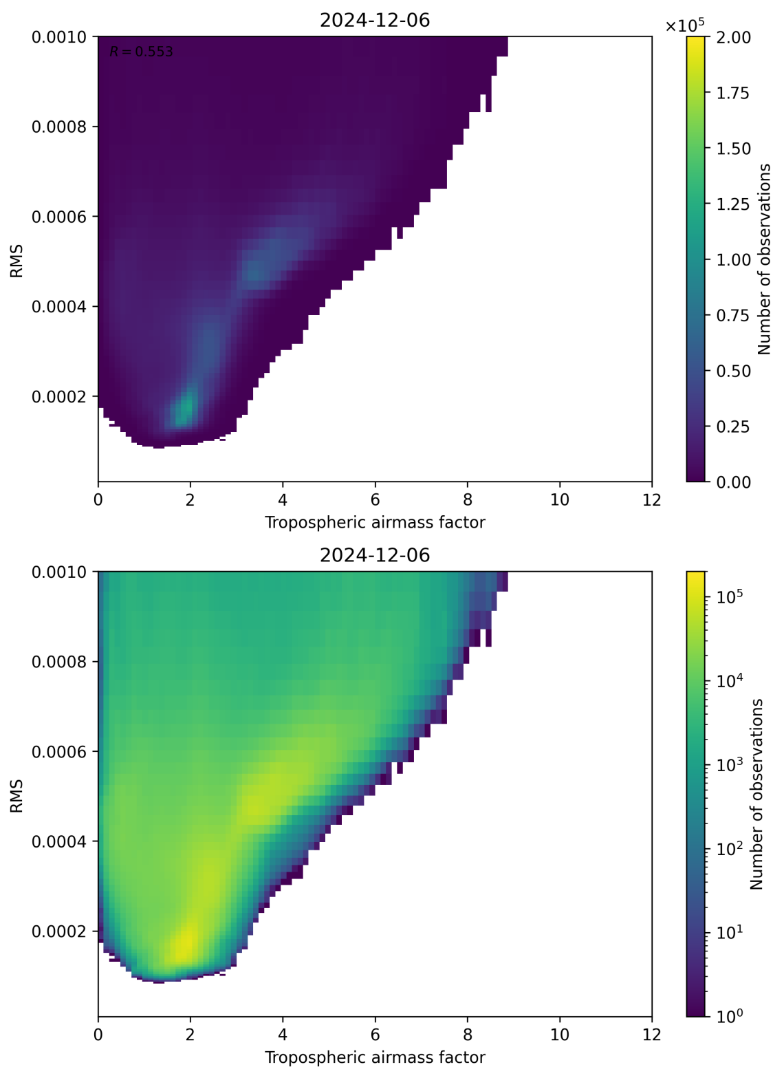
Figure 79: Scatter density plot of “Tropospheric airmass factor” against “RMS” for 2024-12-06 to 2024-12-07.
