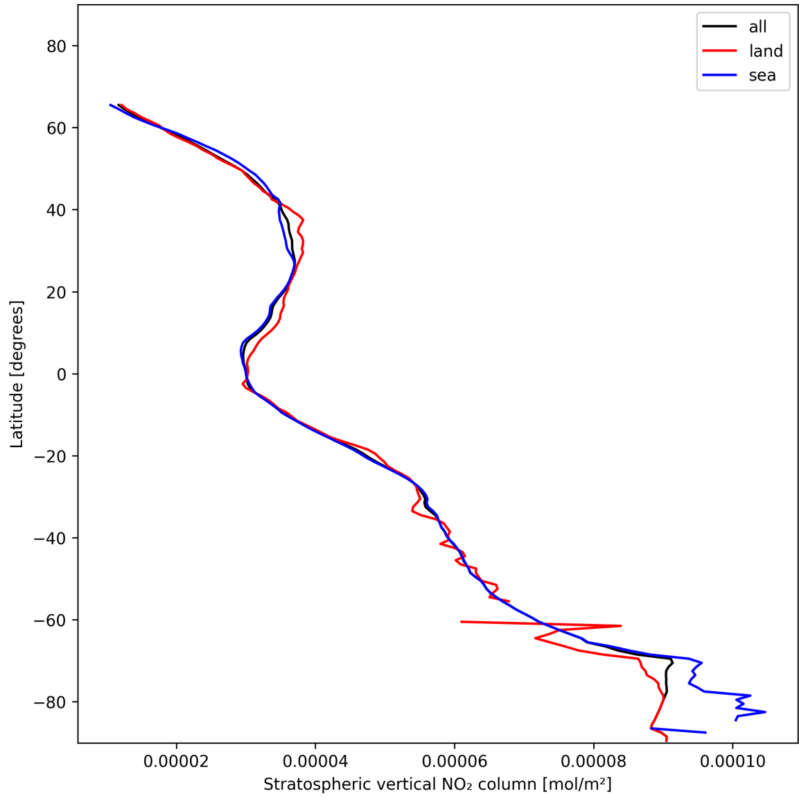
Figure 19: Zonal average of “Stratospheric vertical NO 2 column” for 2024-12-06 to 2024-12-07.
