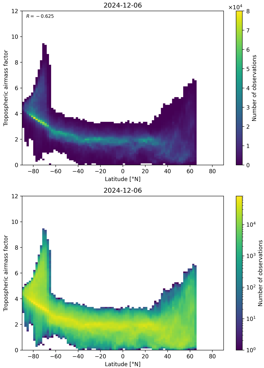
Figure 85: Scatter density plot of “Latitude” against “Tropospheric airmass factor” for 2024-12-06 to 2024-12-07.
