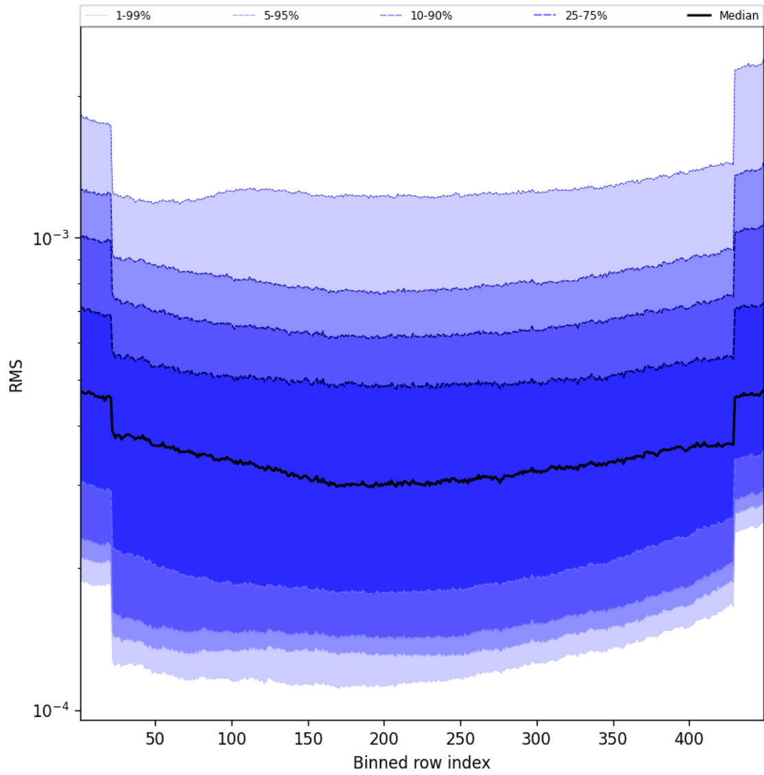
Figure 60: Along track statistics of “RMS” for 2024-12-06 to 2024-12-07
