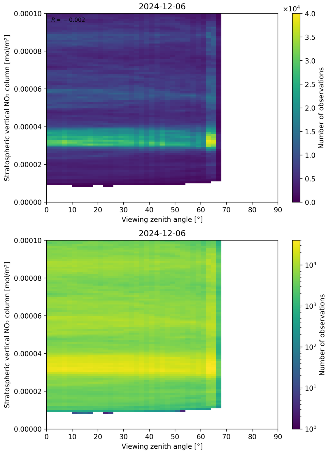
Figure 164: Scatter density plot of “Viewing zenith angle” against “Stratospheric vertical NO 2 column” for 2024-12-06 to 2024-12-07.
