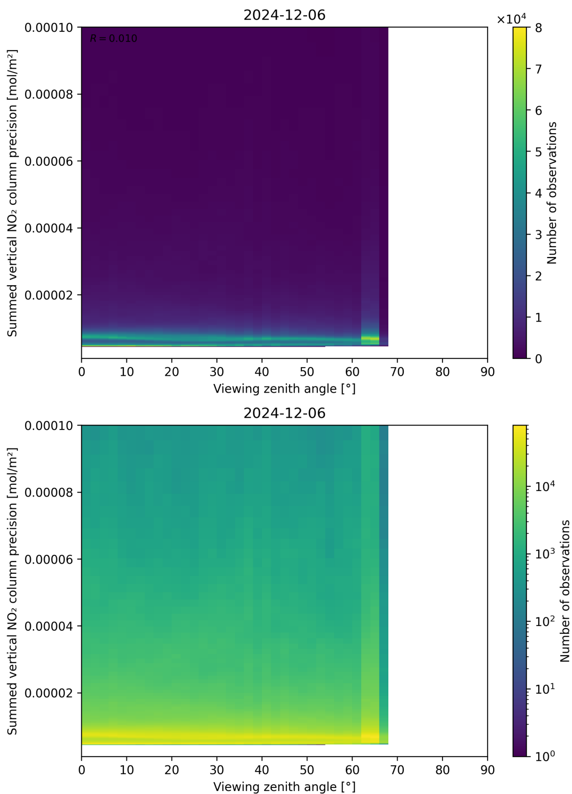
Figure 166: Scatter density plot of “Viewing zenith angle” against “Summed vertical NO 2 column precision” for 2024-12-06 to 2024-12-07.
