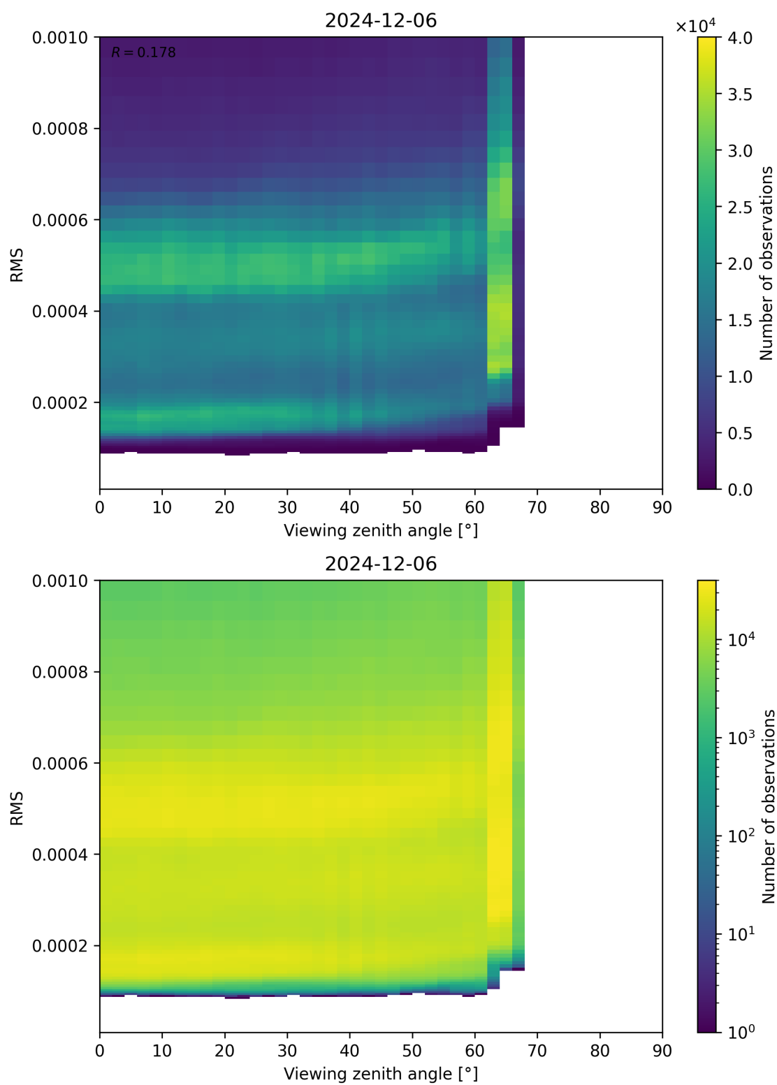
Figure 171: Scatter density plot of “Viewing zenith angle” against “RMS” for 2024-12-06 to 2024-12-07.
