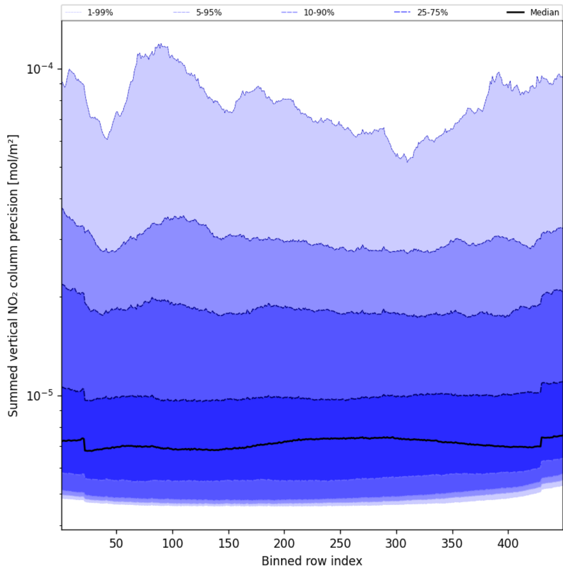
Figure 58: Along track statistics of “Summed vertical NO 2 column precision” for 2024-12-06 to 2024-12-07
