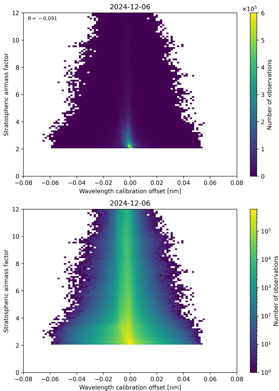
Figure 174: Scatter density plot of “Wavelength calibration offset” against “Stratospheric airmass factor” for 2024-12-06 to 2024-12-07.
