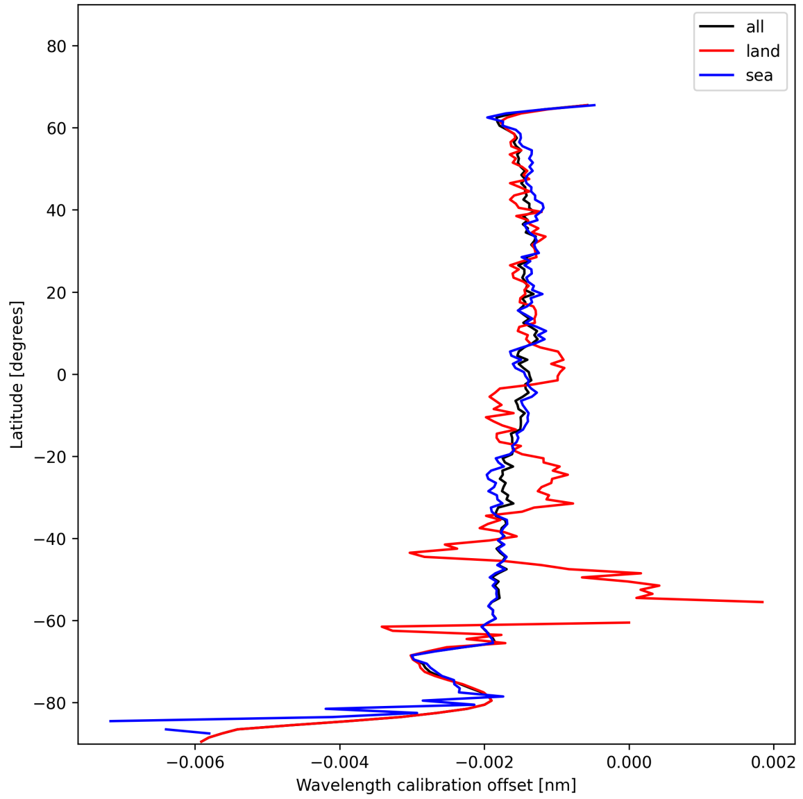
Figure 18: Zonal average of “Wavelength calibration offset” for 2024-12-06 to 2024-12-07.
