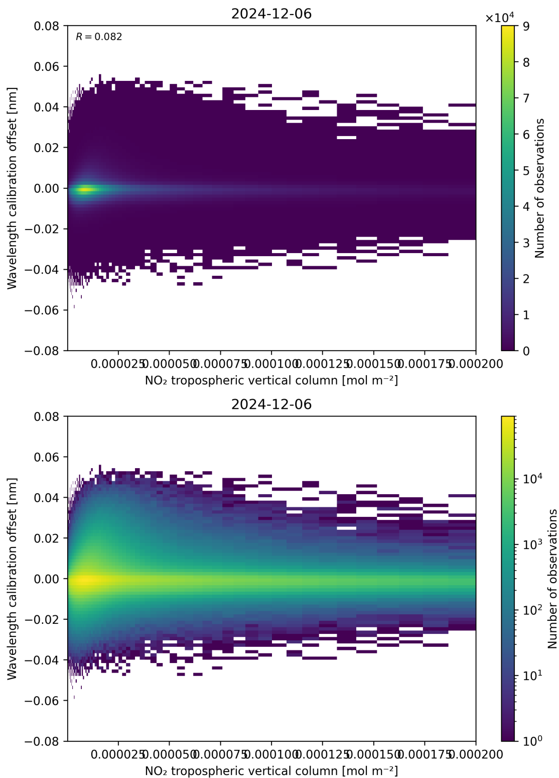
Figure 143: Scatter density plot of “NO 2 tropospheric vertical column” against “Wavelength calibration offset” for 2024-12-06 to 2024-12-07.
