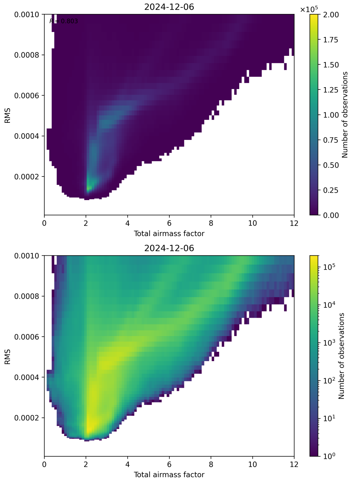
Figure 69: Scatter density plot of “Total airmass factor” against “RMS” for 2024-12-06 to 2024-12-07.
