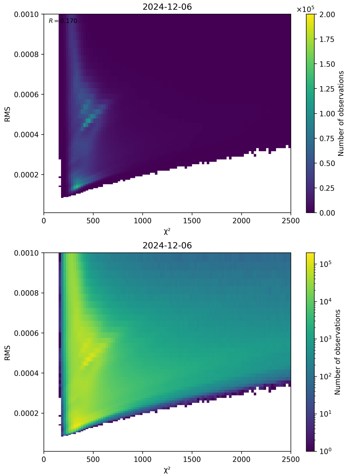
Figure 82: Scatter density plot of “ \chi^2 ” against “RMS” for 2024-12-06 to 2024-12-07.
