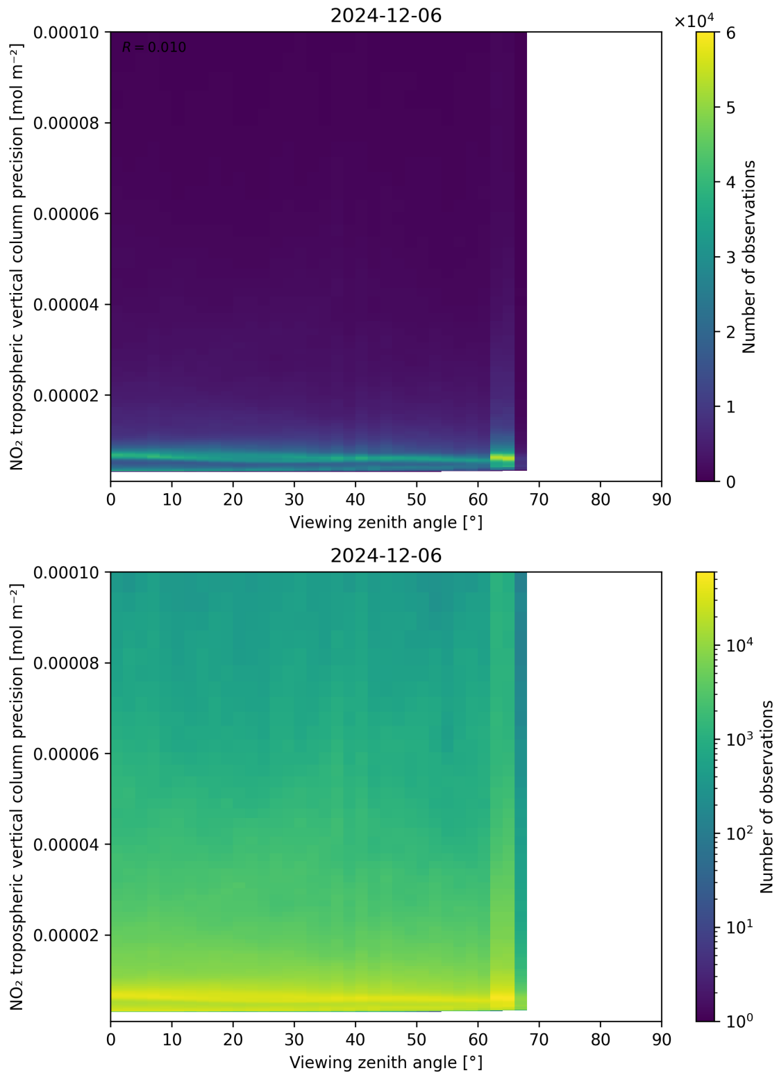
Figure 170: Scatter density plot of “Viewing zenith angle” against “NO 2 tropospheric vertical column precision” for 2024-12-06 to 2024-12-07.
