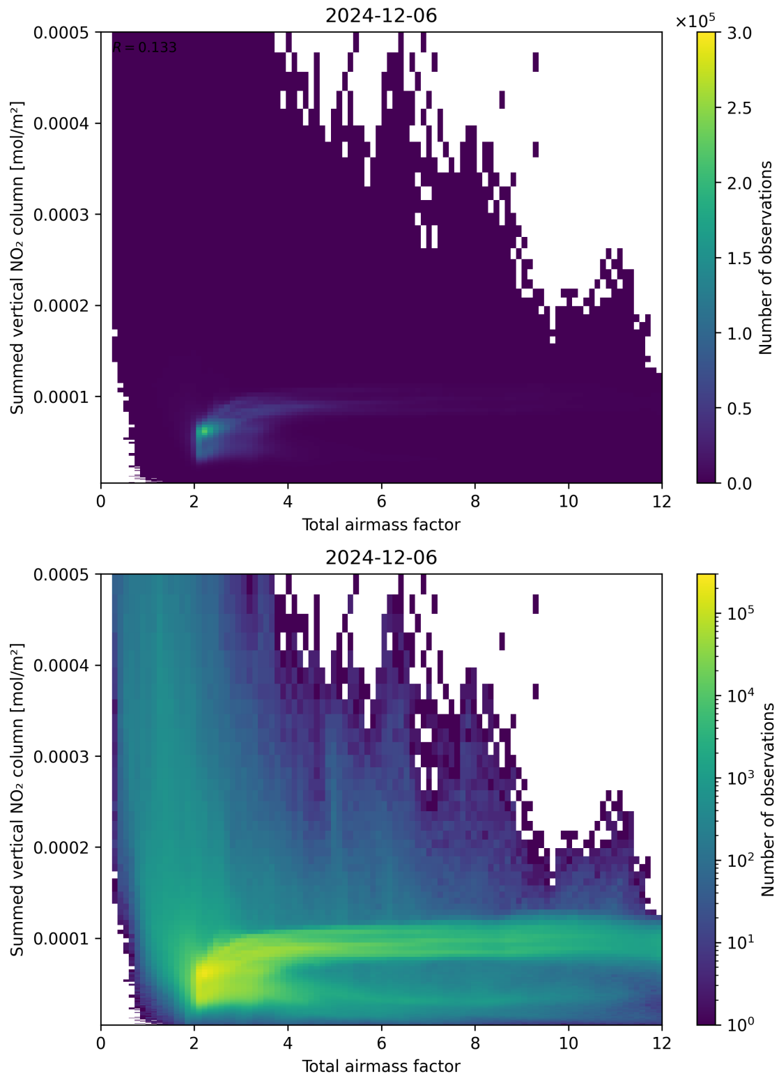
Figure 65: Scatter density plot of “Total airmass factor” against “Summed vertical NO 2 column” for 2024-12-06 to 2024-12-07.
