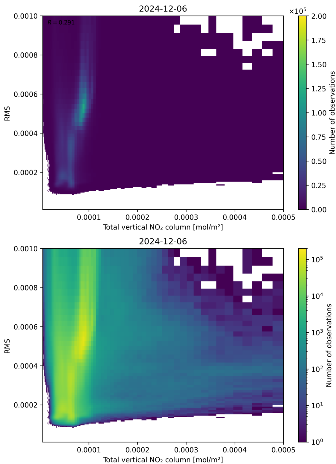
Figure 120: Scatter density plot of “Total vertical NO 2 column” against “RMS” for 2024-12-06 to 2024-12-07.
