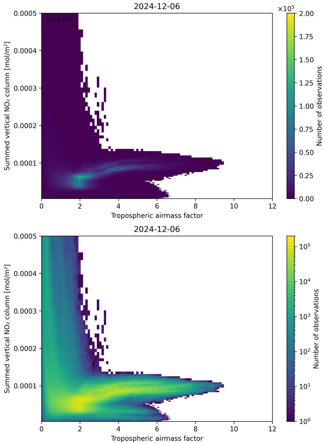
Figure 75: Scatter density plot of “Tropospheric air mass factor” against “Summed vertical NO 2 column” for 2024-12-06 to 2024-12-07.
