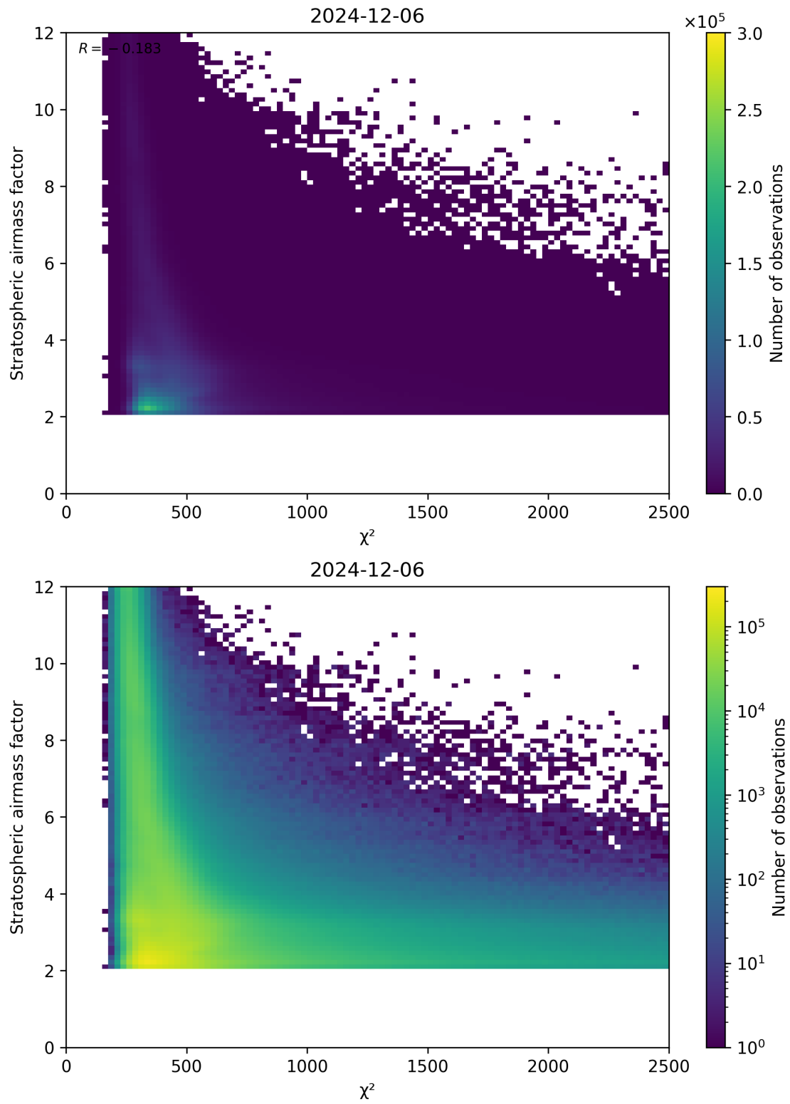
Figure 81: Scatter density plot of “ \chi^2 ” against “Stratospheric airmass factor” for 2024-12-06 to 2024-12-07.
