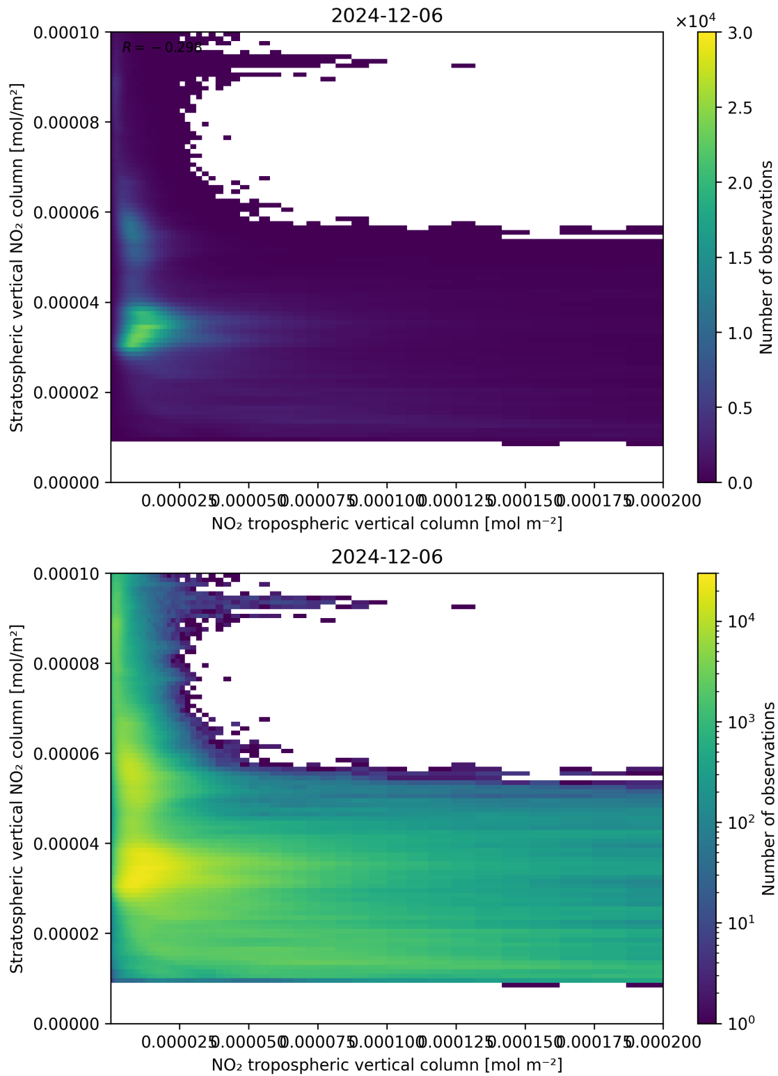
Figure 125: Scatter density plot of “NO 2 tropospheric vertical column” against “Stratospheric vertical NO 2 column” for 2024-12-06 to 2024-12-07.
