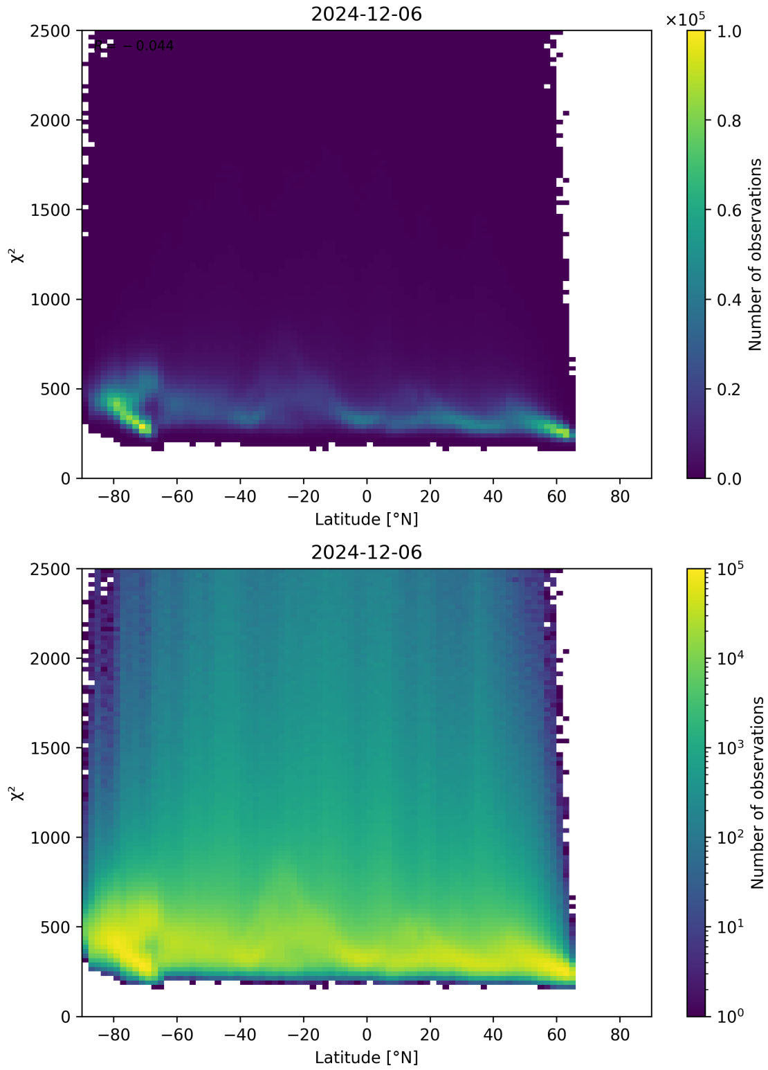
Figure 86: Scatter density plot of “Latitude” against “ \chi^2 ” for 2024-12-06 to 2024-12-07.
