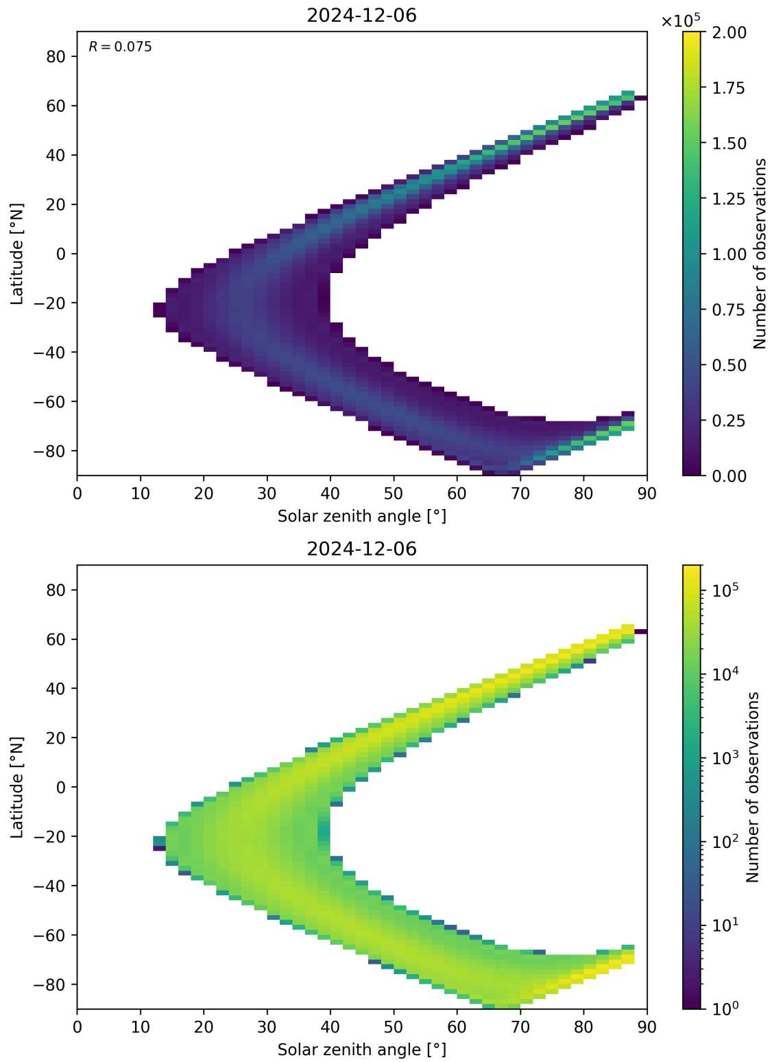
Figure 149: Scatter density plot of “Solar zenith angle” against “Latitude” for 2024-12-06 to 2024-12-07.
