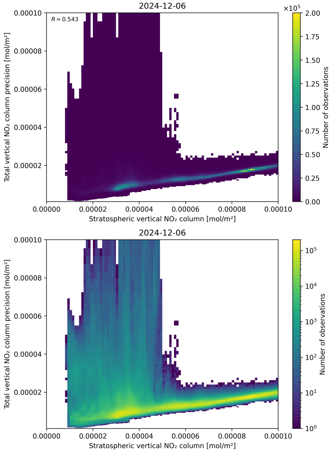
Figure 101: Scatter density plot of “Stratospheric vertical NO 2 column” against “Total vertical NO 2 column precision” for 2024-12-06 to 2024-12-07.
