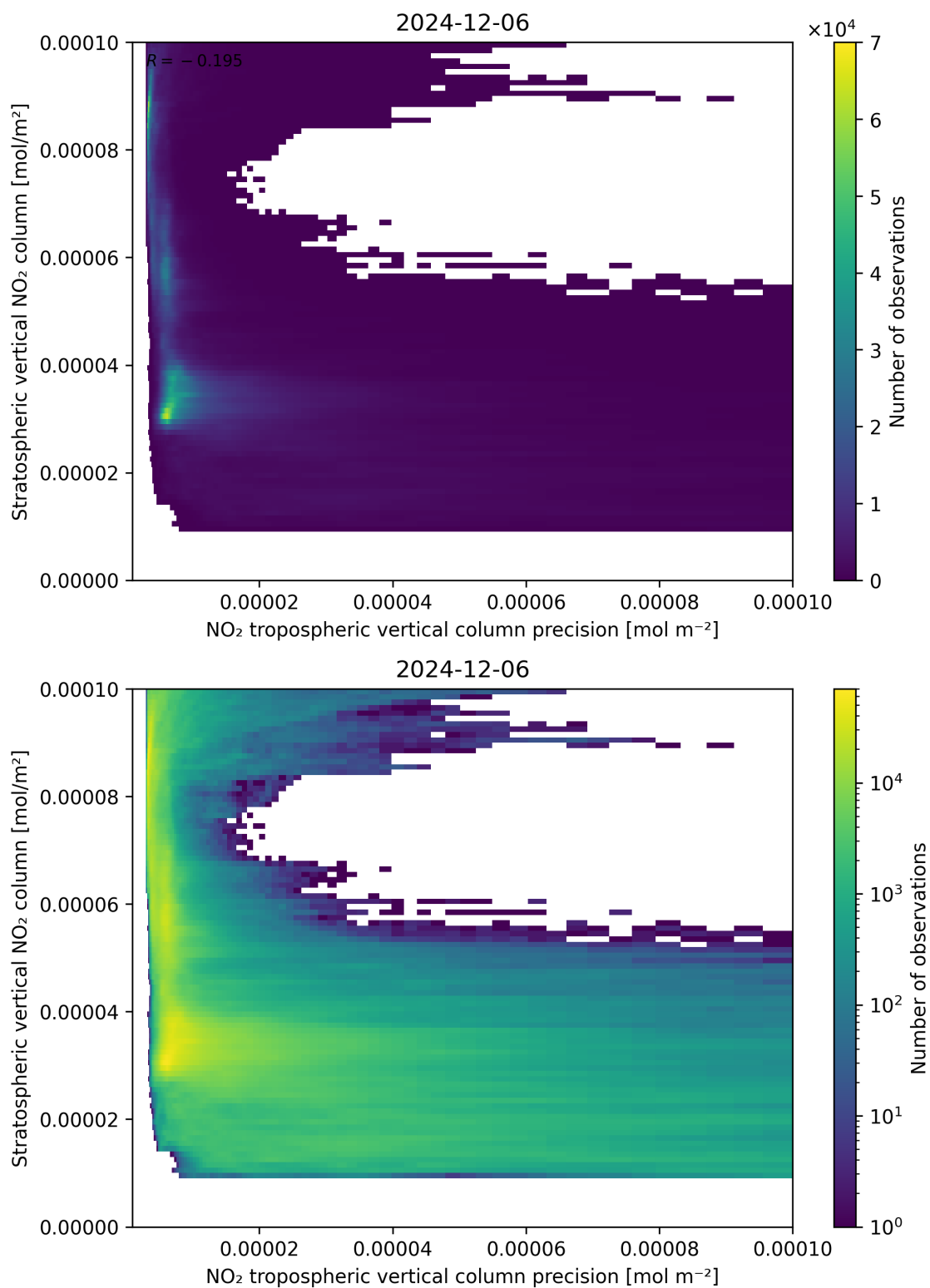
Figure 135: Scatter density plot of “NO 2 tropospheric vertical column precision” against “Stratospheric vertical NO 2 column” for 2024-12-06 to 2024-12-07.
