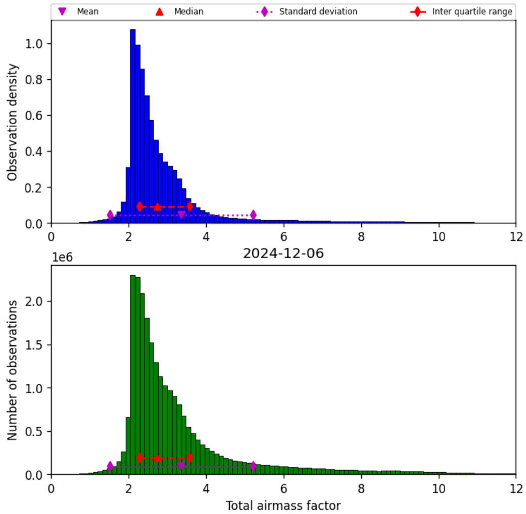
Figure 32: Histogram of “Total airmass factor” for 2024-12-06 to 2024-12-07
