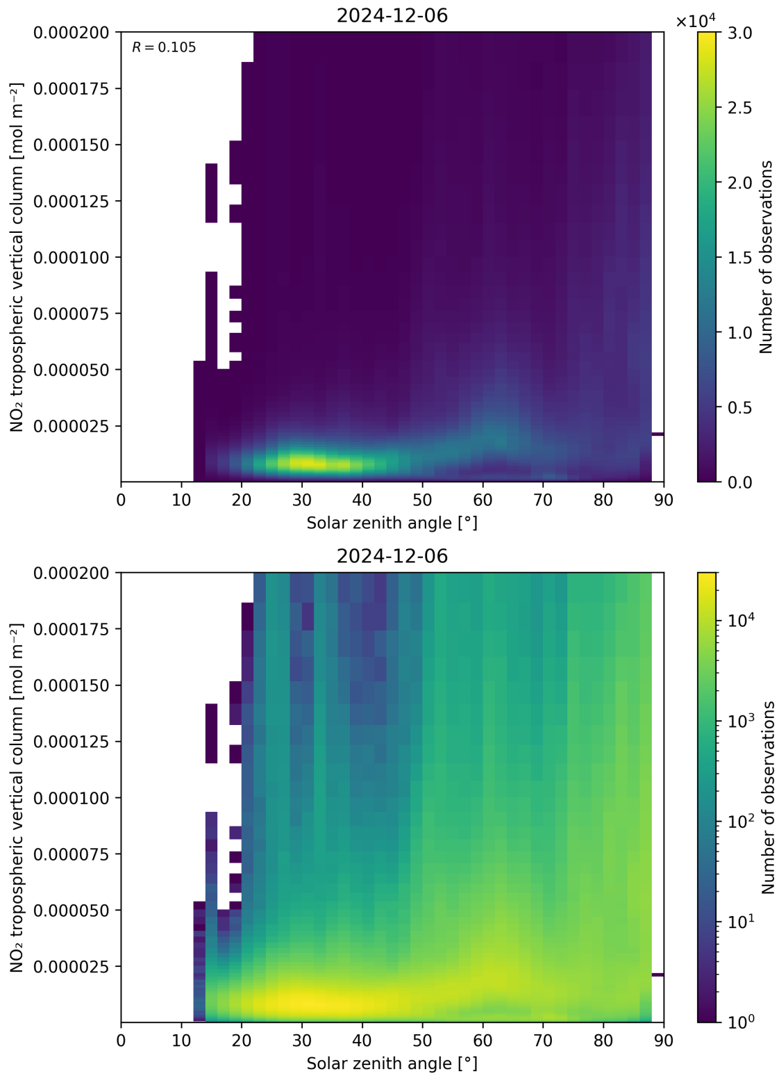
Figure 155: Scatter density plot of “Solar zenith angle” against “NO 2 tropospheric vertical column” for 2024-12-06 to 2024-12-07.
