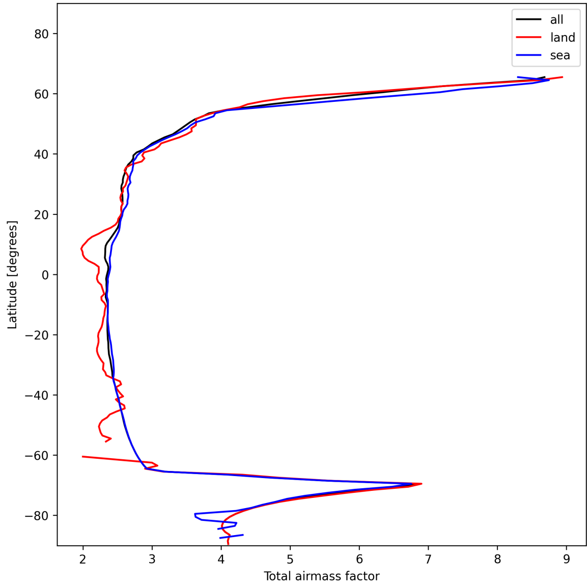
Figure 15: Zonal average of “Total airmass factor” for 2024-12-06 to 2024-12-07.
