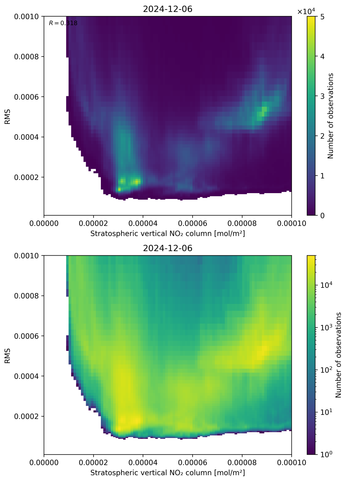
Figure 102: Scatter density plot of “Stratospheric vertical NO 2 column” against “RMS” for 2024-12-06 to 2024-12-07.
