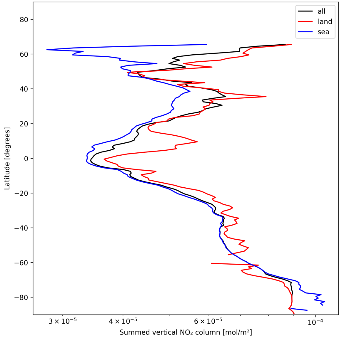
Figure 23: Zonal average of “Summed vertical NO 2 column” for 2024-12-06 to 2024-12-07.
