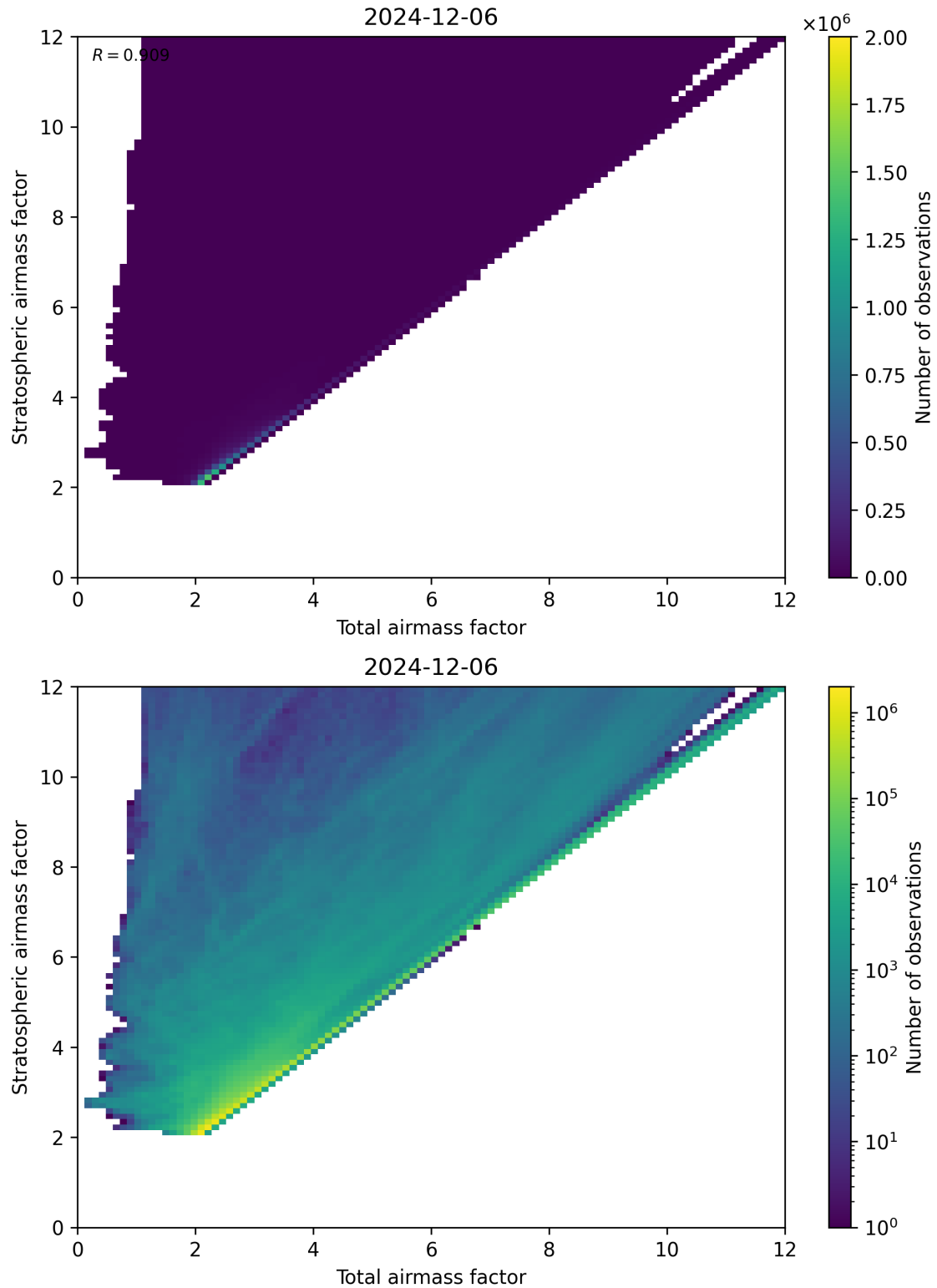
Figure 62: Scatter density plot of “Total airmass factor” against “Stratospheric airmass factor” for 2024-12-06 to 2024-12-07.
