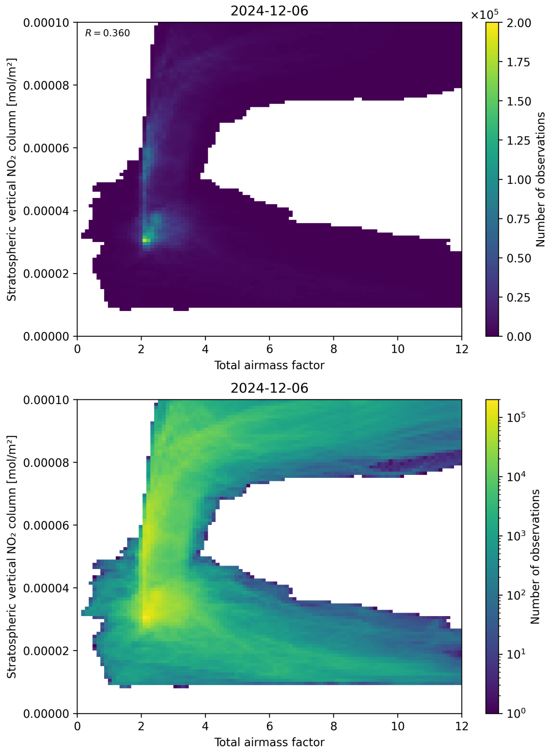
Figure 64: Scatter density plot of “Total airmass factor” against “Stratospheric vertical NO 2 column” for 2024-12-06 to 2024-12-07.
