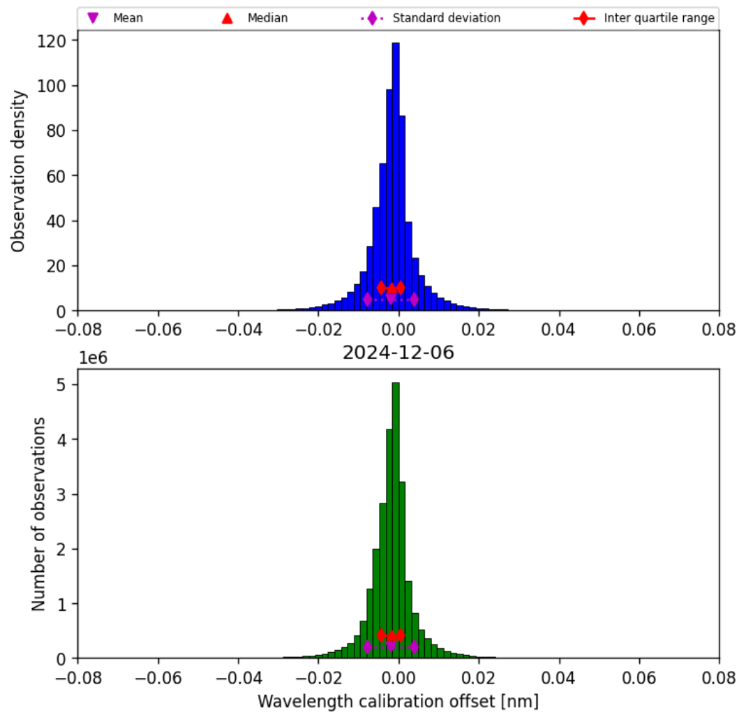
Figure 35: Histogram of “Wavelength calibration offset” for 2024-12-06 to 2024-12-07
