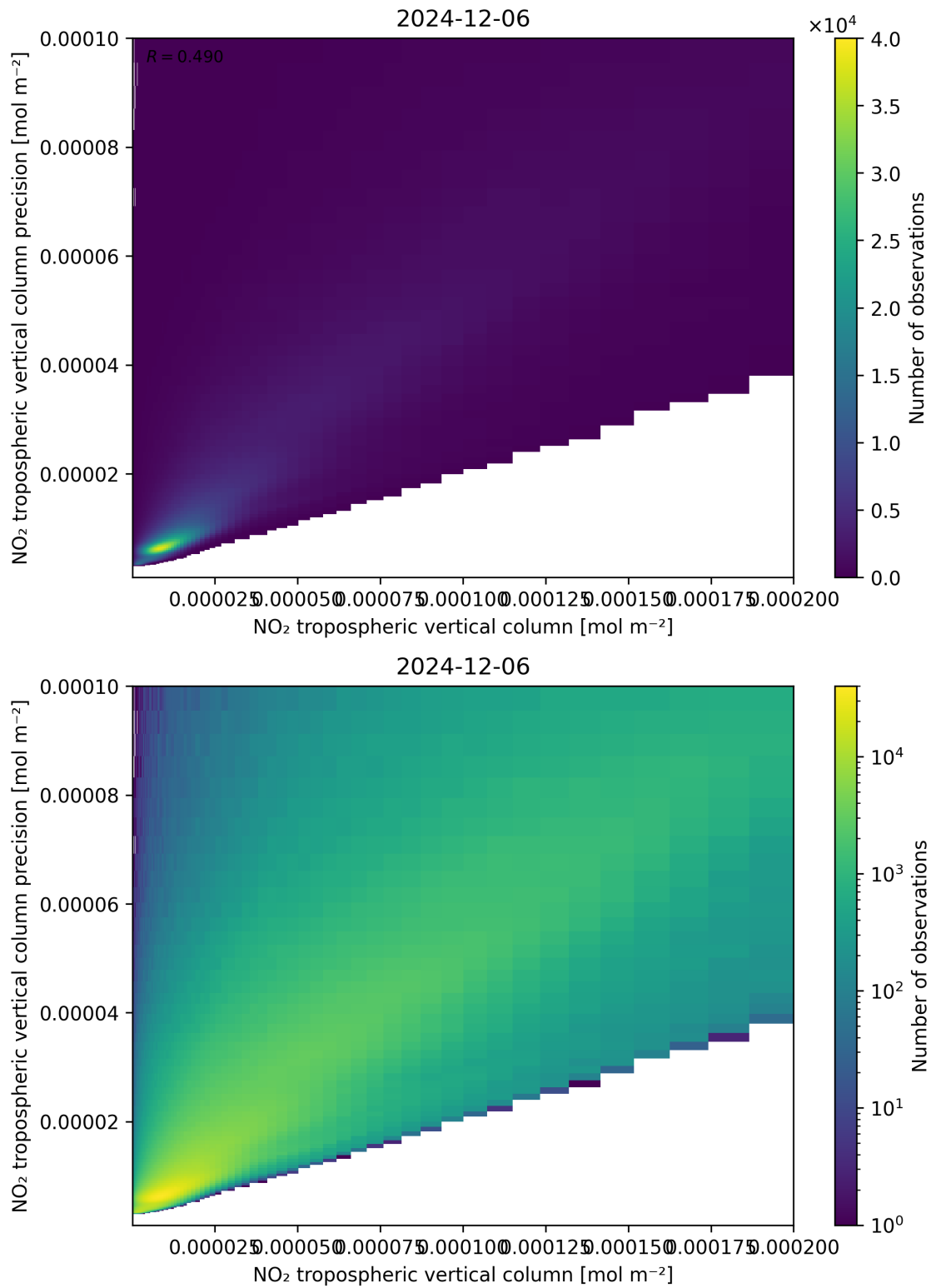
Figure 130: Scatter density plot of “NO 2 tropospheric vertical column” against “NO 2 tropospheric vertical column precision” for 2024-12-06 to 2024-12-07.
