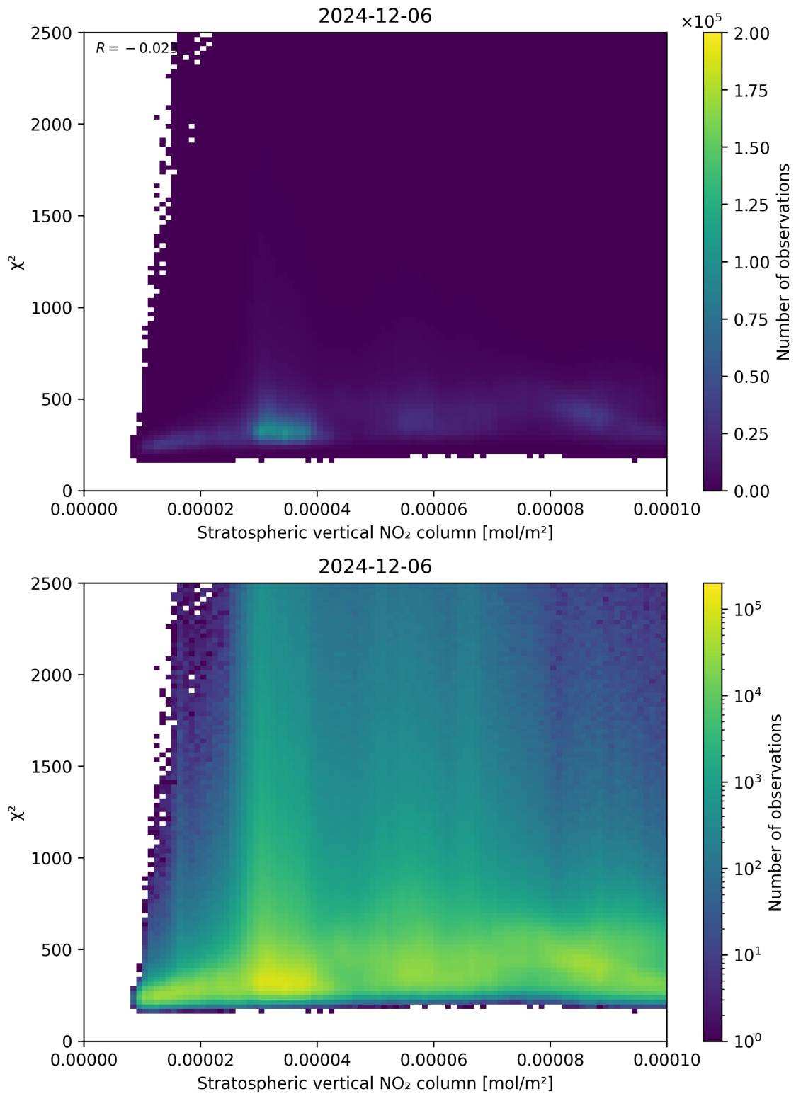
Figure 97: Scatter density plot of “Stratospheric vertical NO 2 column” against “ \chi^2 ” for 2024-12-06 to 2024-12-07.
