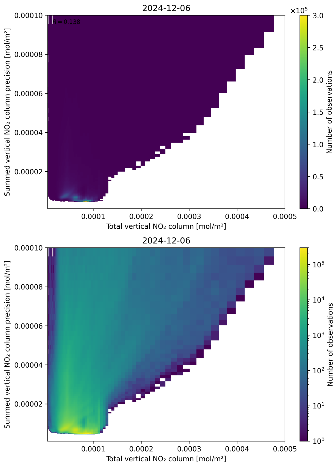
Figure 113: Scatter density plot of “Total vertical NO 2 column” against “Summed vertical NO 2 column precision” for 2024-12-06 to 2024-12-07.
