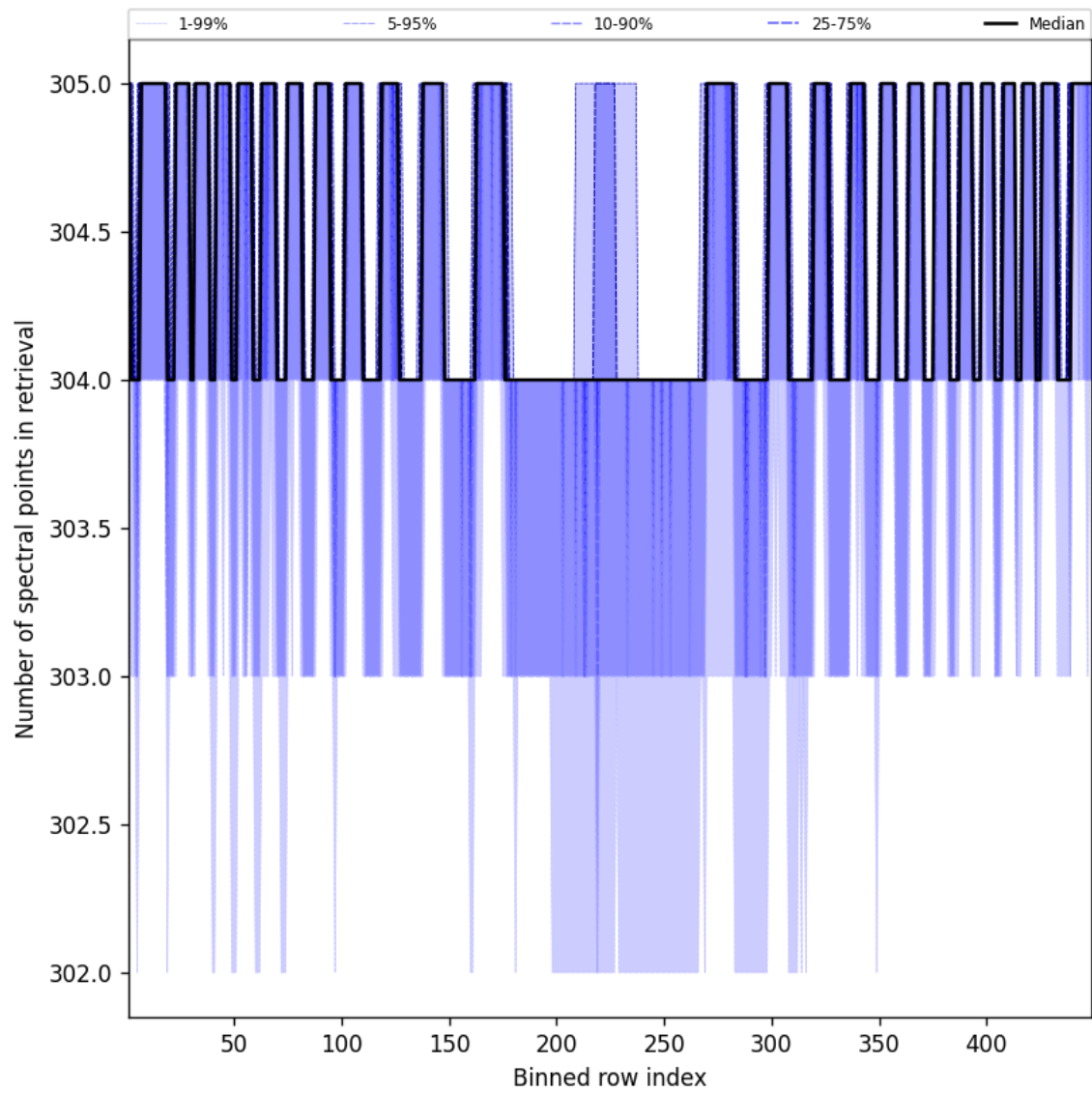
Figure 50: Along track statistics of “Number of spectral points in retrieval” for 2024-12-06 to 2024-12-07
