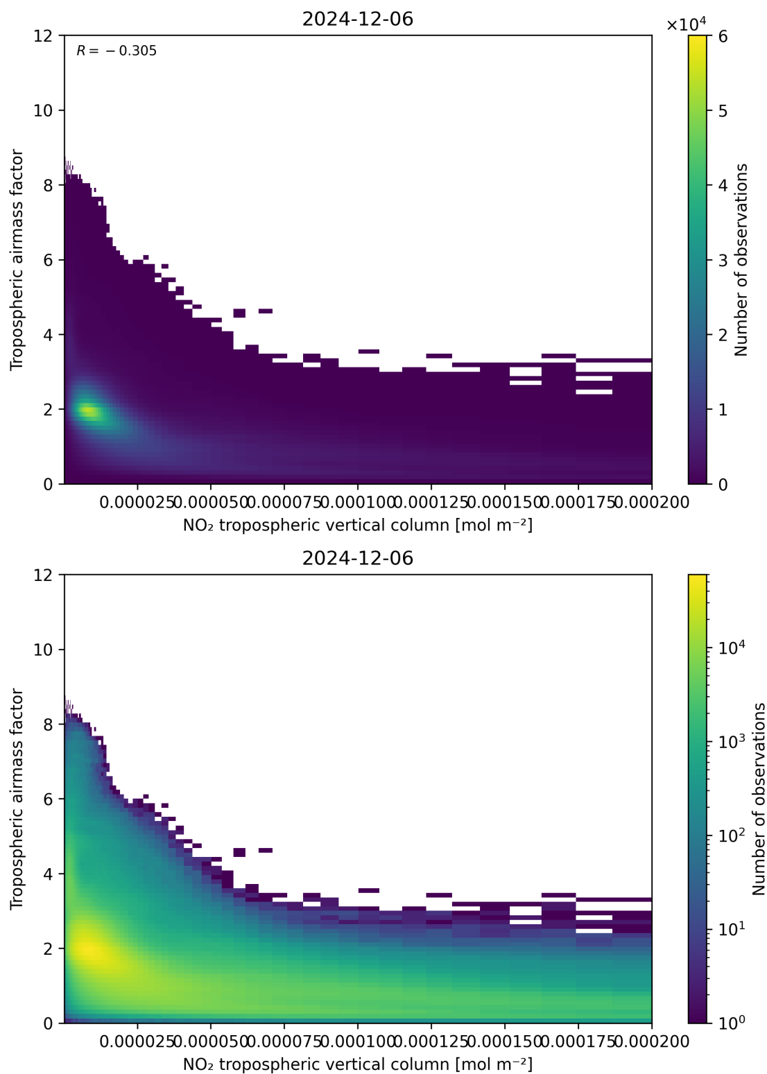
Figure 123: Scatter density plot of “NO 2 tropospheric vertical column” against “Tropospheric air mass factor” for 2024-12-06 to 2024-12-07.
