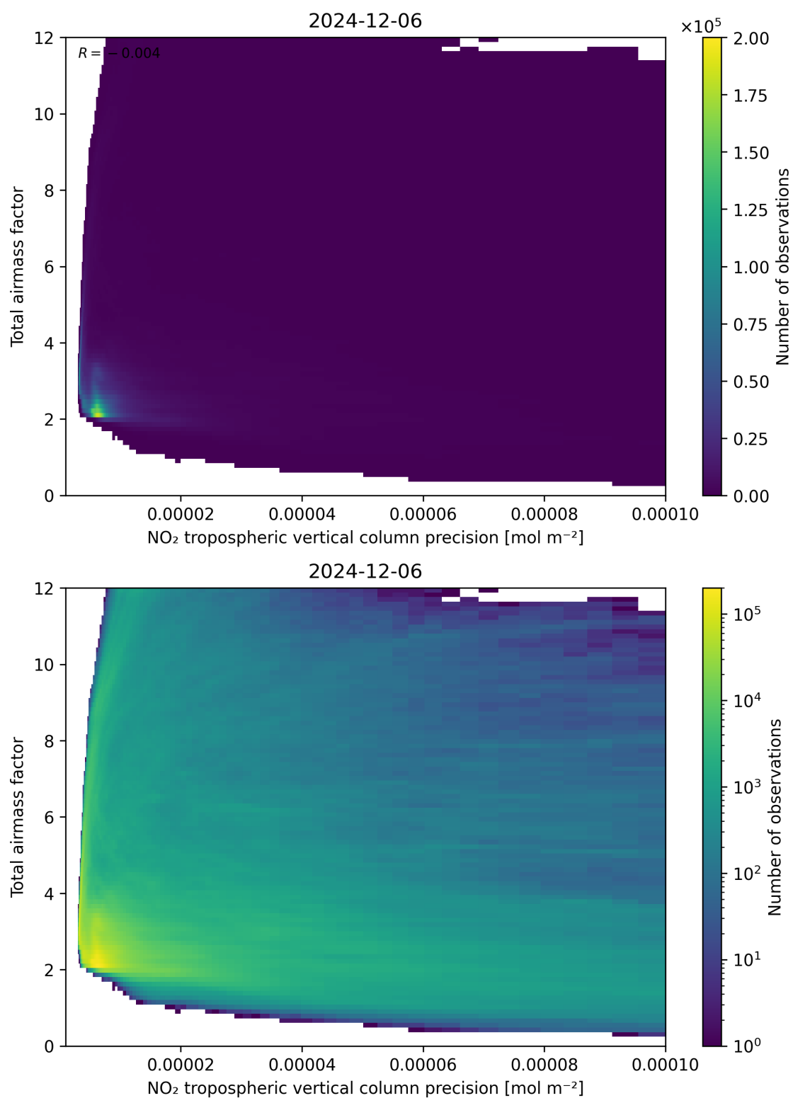
Figure 132: Scatter density plot of “NO 2 tropospheric vertical column precision” against “Total air mass factor” for 2024-12-06 to 2024-12-07.
