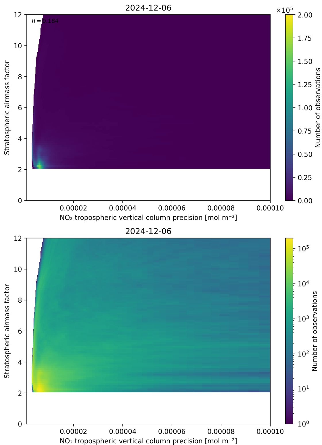
Figure 131: Scatter density plot of “NO 2 tropospheric vertical column precision” against “Stratospheric airmass factor” for 2024-12-06 to 2024-12-07.
