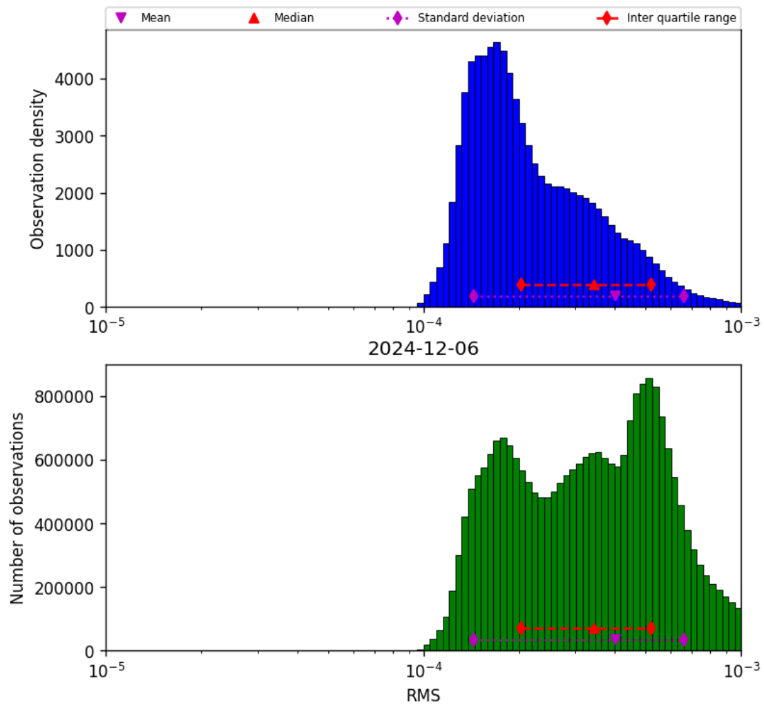
Figure 43: Histogram of “RMS” for 2024-12-06 to 2024-12-07
