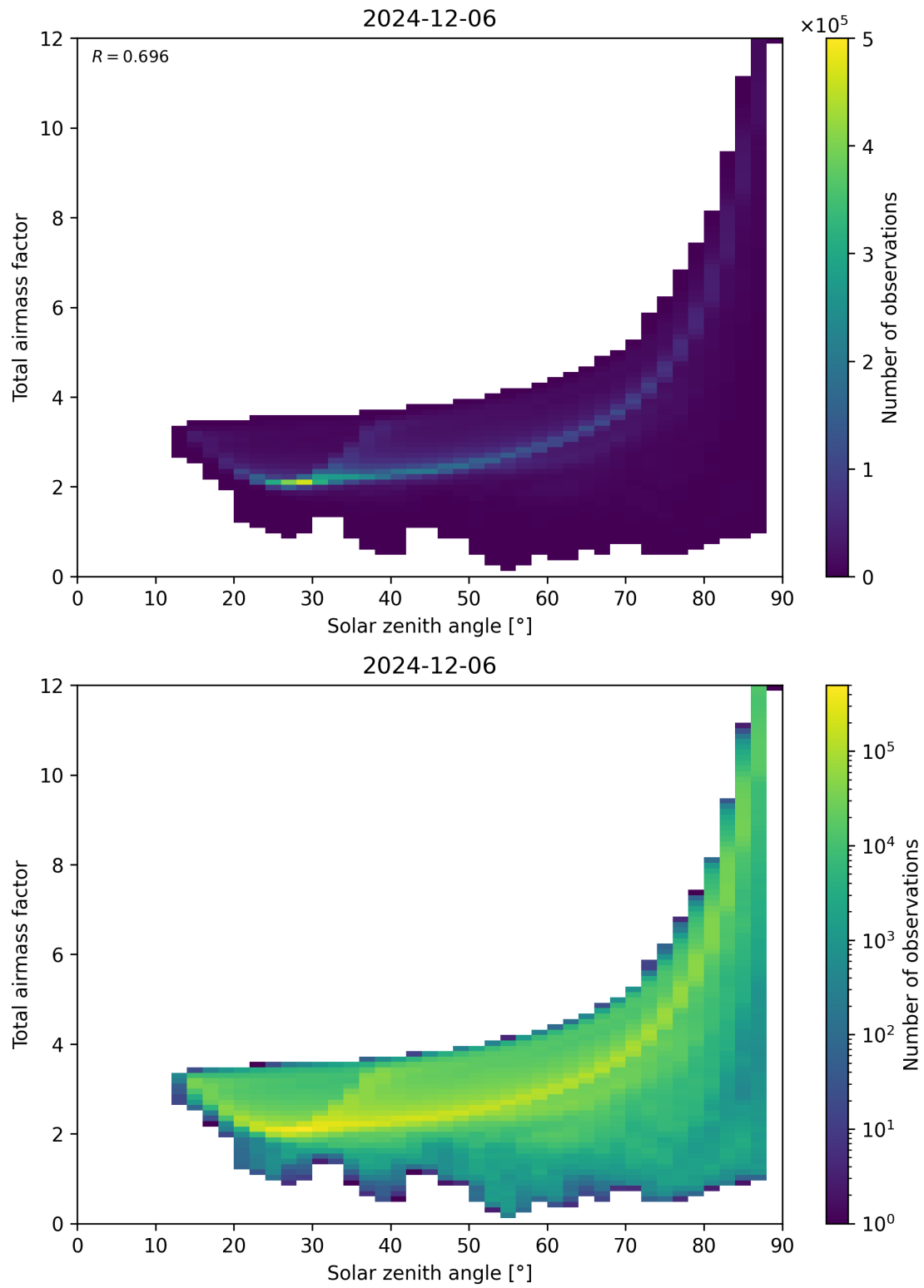
Figure 146: Scatter density plot of “Solar zenith angle” against “Total airmass factor” for 2024-12-06 to 2024-12-07.
