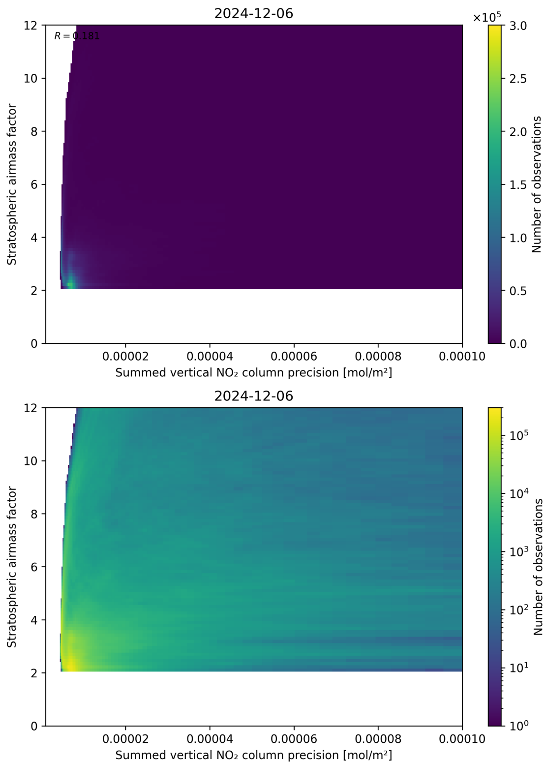
Figure 106: Scatter density plot of “Summed vertical NO 2 column precision” against “Stratospheric airmass factor” for 2024-12-06 to 2024-12-07.
