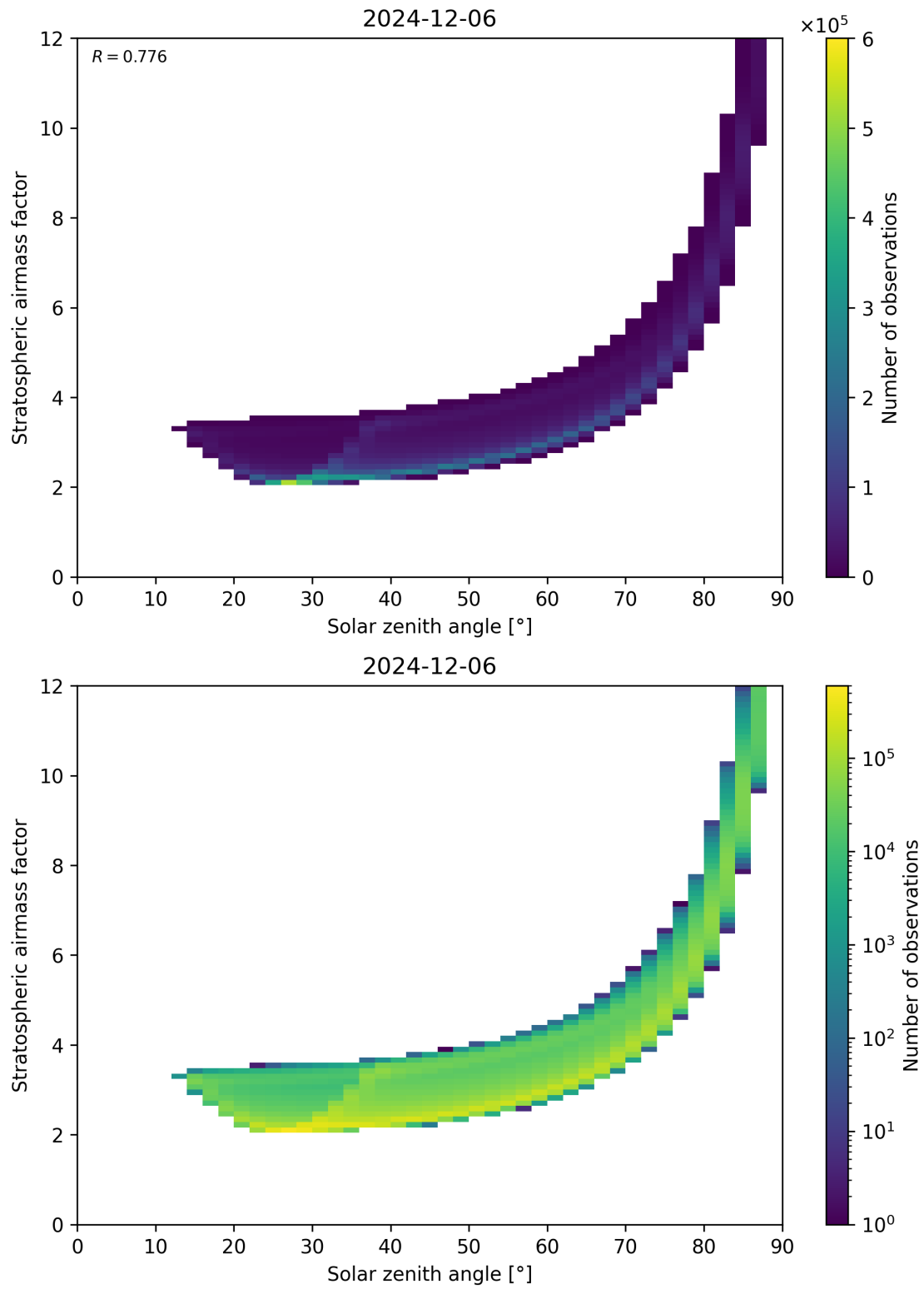
Figure 145: Scatter density plot of “Solar zenith angle” against “Stratospheric airmass factor” for 2024-12-06 to 2024-12-07.
