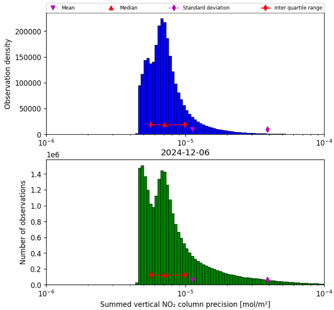
Figure 41: Histogram of “Summed vertical NO 2 column precision” for 2024-12-06 to 2024-12-07
