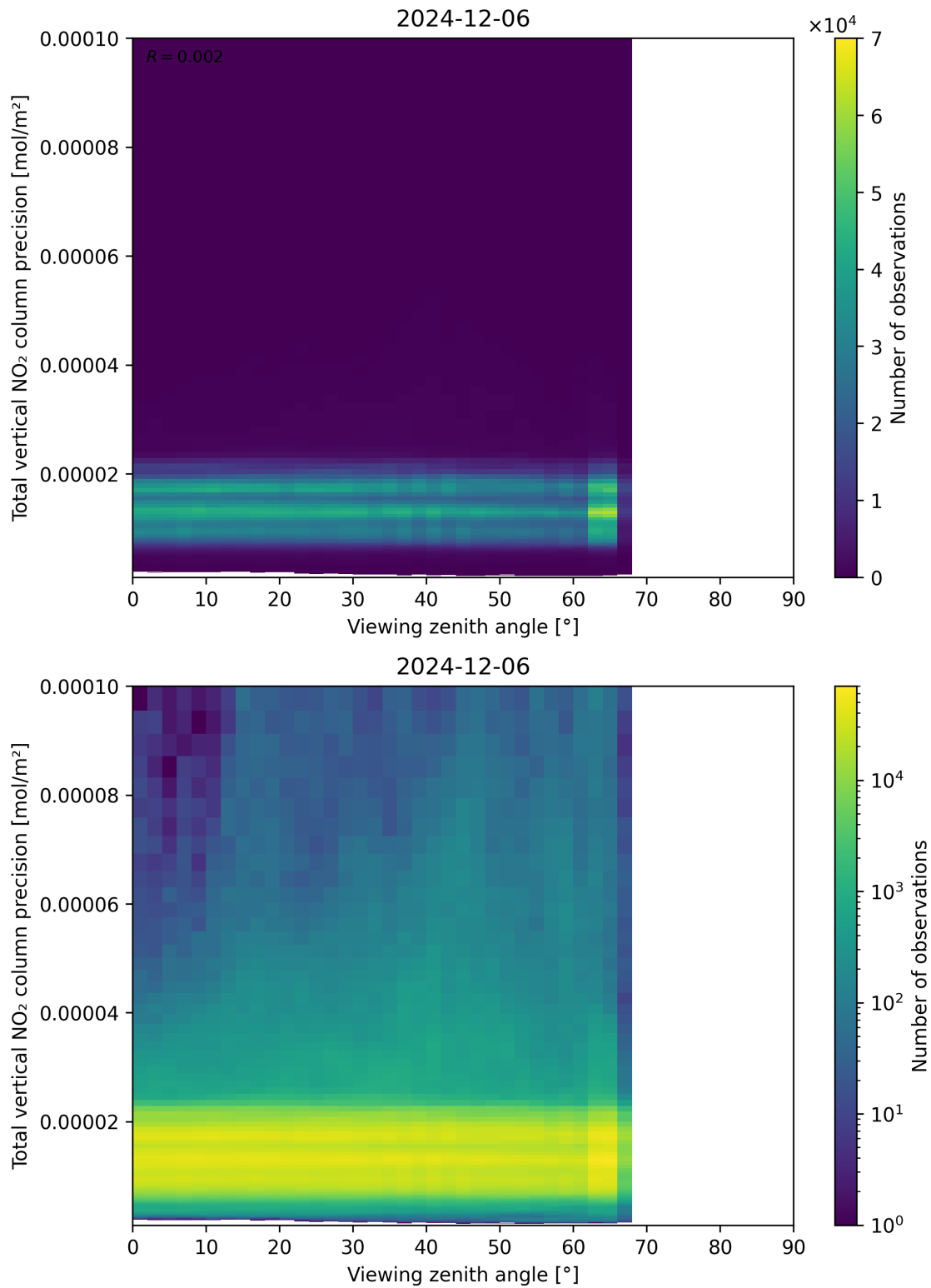
Figure 168: Scatter density plot of “Viewing zenith angle” against “Total vertical NO 2 column precision” for 2024-12-06 to 2024-12-07.
