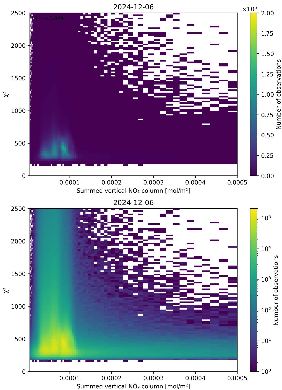
Figure 104: Scatter density plot of “Summed vertical NO 2 column” against “ \chi^2 ” for 2024-12-06 to 2024-12-07.
