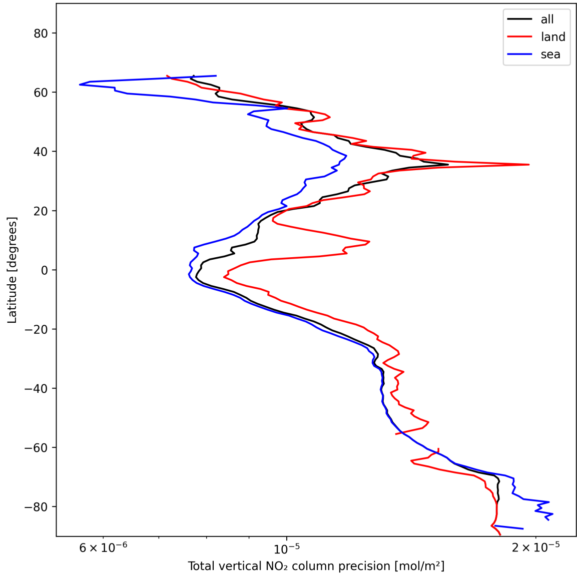
Figure 22: Zonal average of “Total vertical NO 2 column precision” for 2024-12-06 to 2024-12-07.
