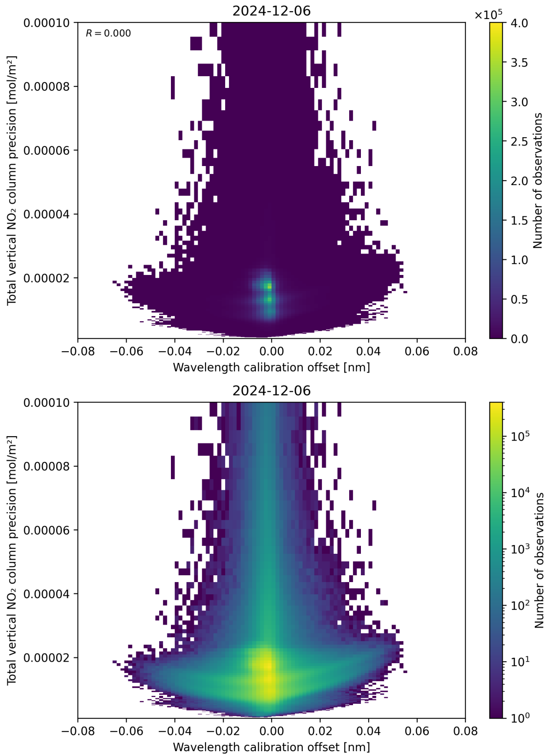
Figure 180: Scatter density plot of “Wavelength calibration offset” against “Total vertical NO 2 column precision” for 2024-12-06 to 2024-12-07.
