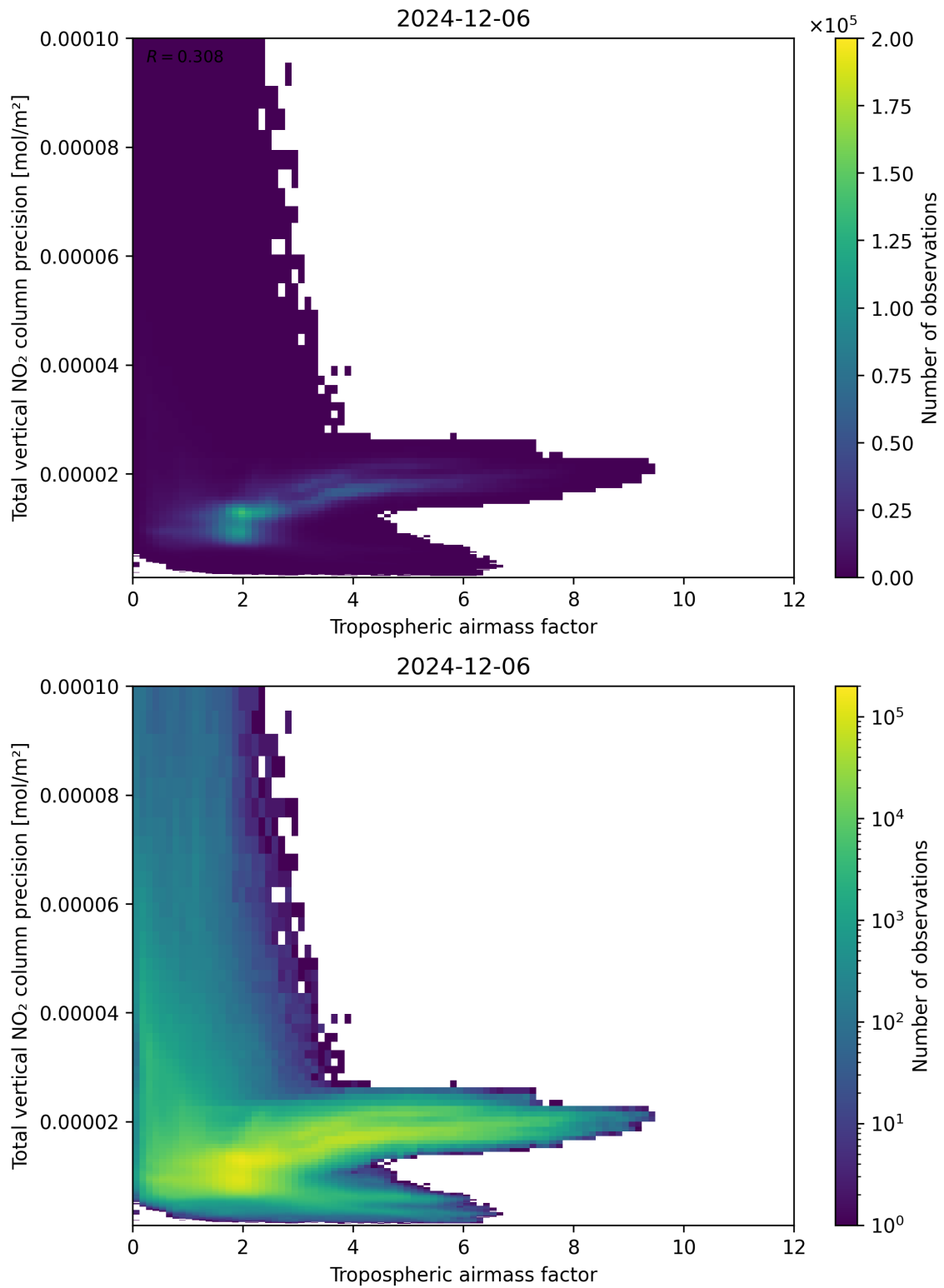
Figure 78: Scatter density plot of “Tropospheric air mass factor” against “Total vertical NO 2 column precision” for 2024-12-06 to 2024-12-07.
