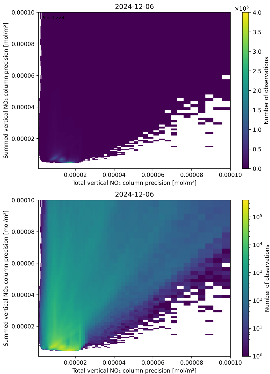
Figure 118: Scatter density plot of “Total vertical NO 2 column precision” against “Summed vertical NO 2 column precision” for 2024-12-06 to 2024-12-07.
