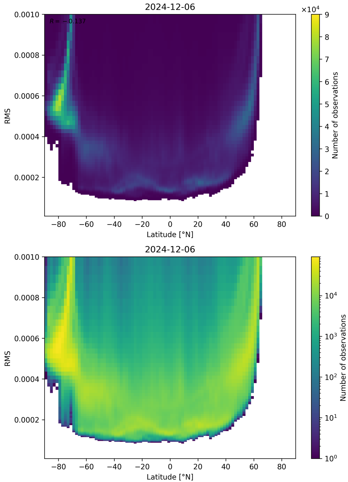
Figure 94: Scatter density plot of “Latitude” against “RMS” for 2024-12-06 to 2024-12-07.
