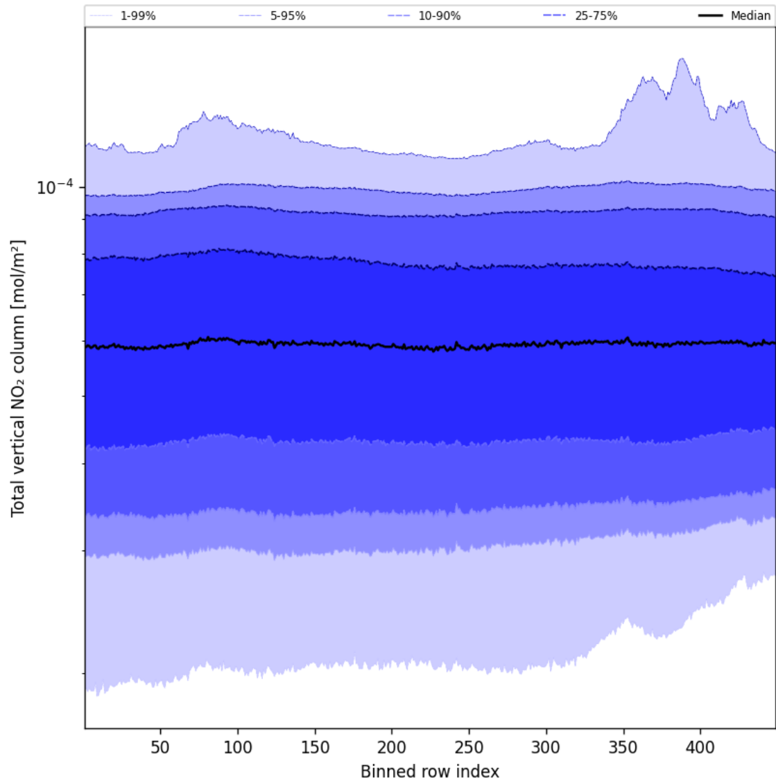
Figure 55: Along track statistics of “Total vertical NO 2 column” for 2024-12-06 to 2024-12-07
