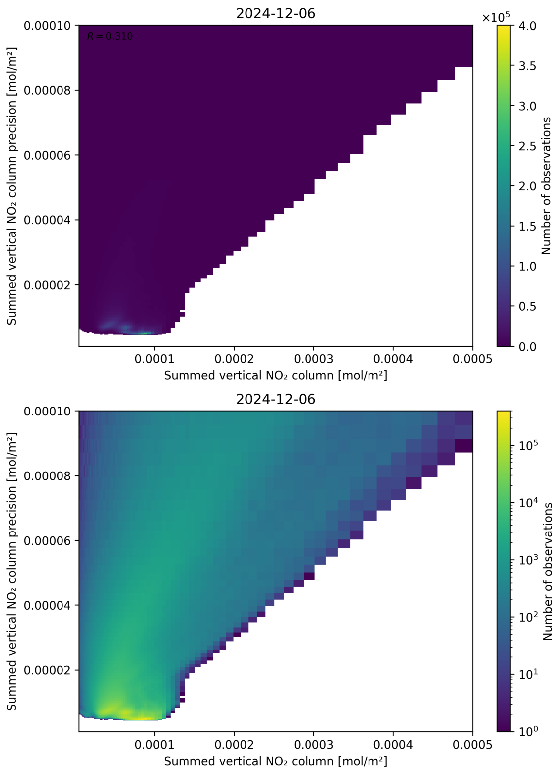
Figure 105: Scatter density plot of “Summed vertical NO 2 column” against “Summed vertical NO 2 column precision” for 2024-12-06 to 2024-12-07.
