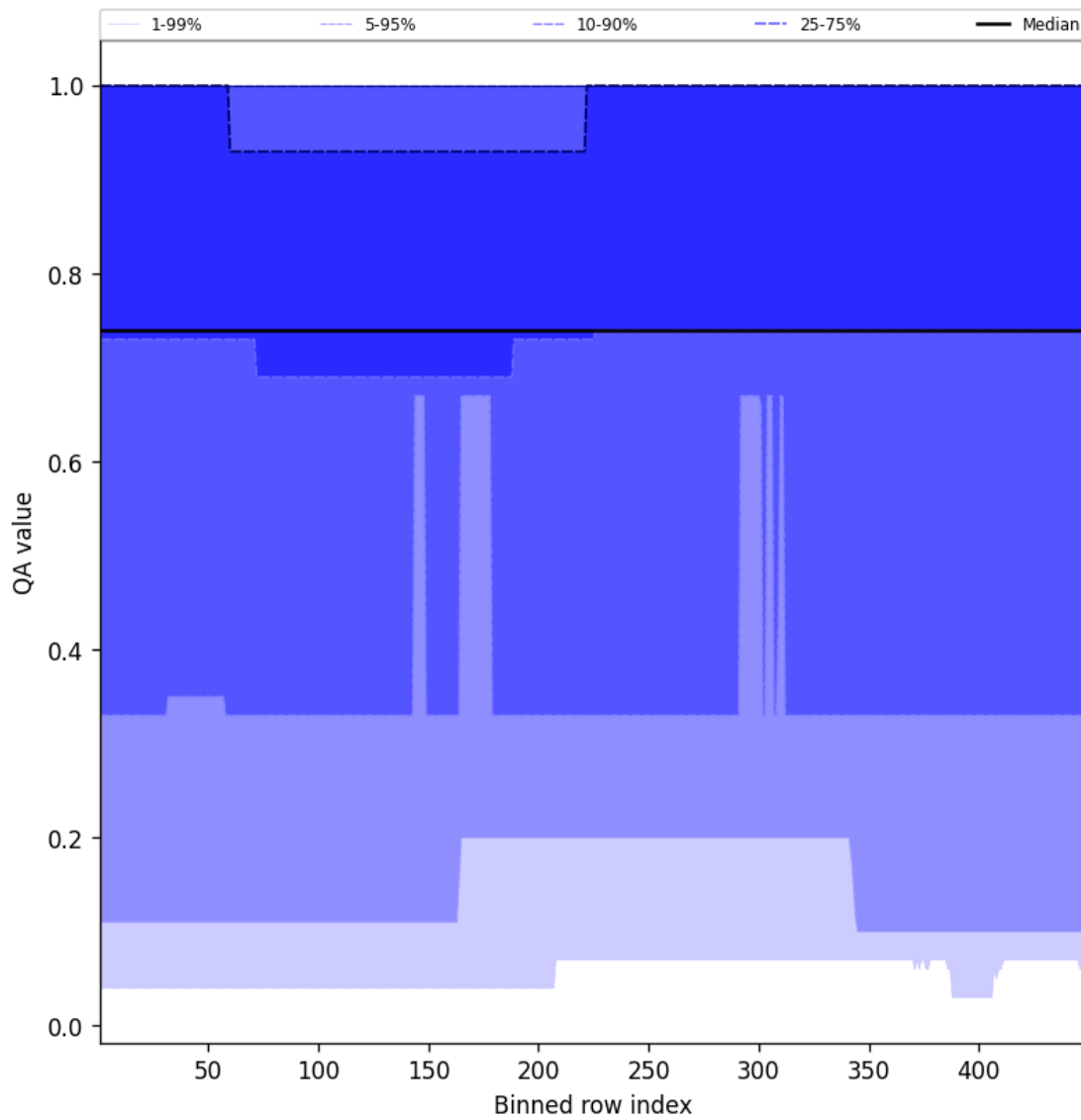
Figure 45: Along track statistics of “QA value” for 2024-12-06 to 2024-12-07
