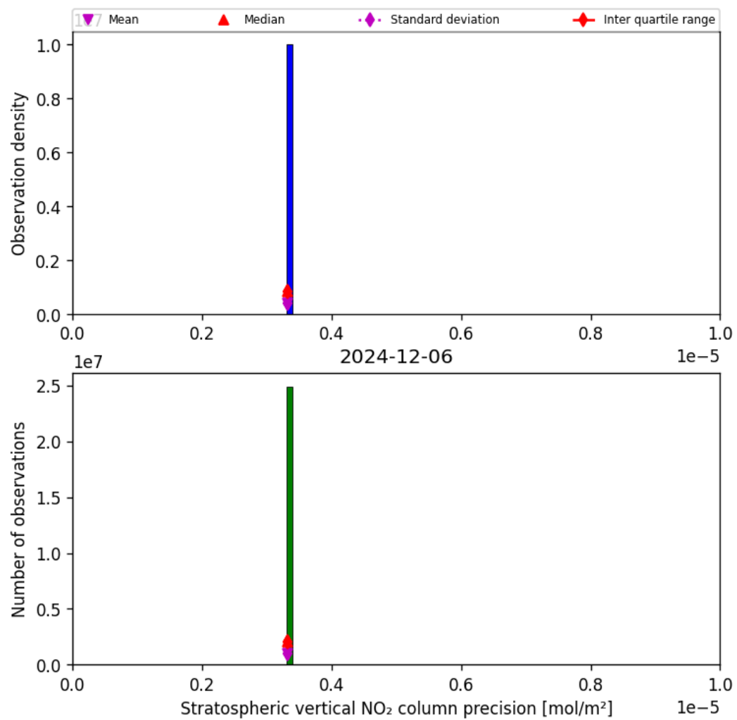
Figure 37: Histogram of “Stratospheric vertical NO 2 column precision” for 2024-12-06 to 2024-12-07
