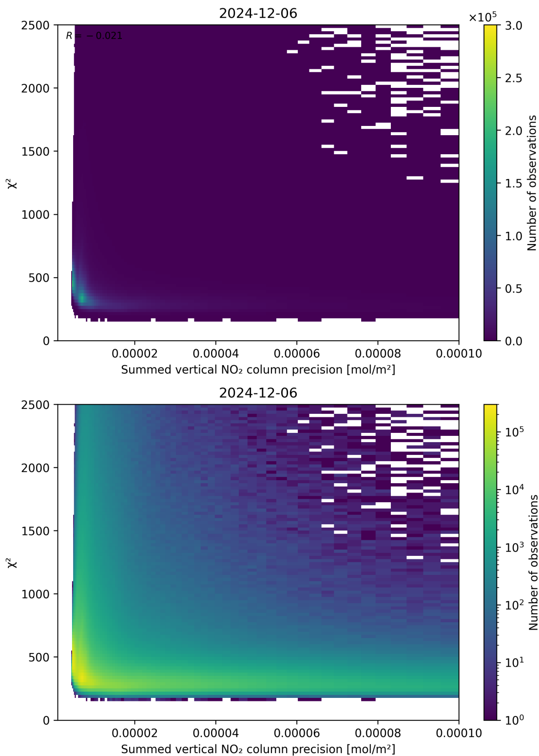
Figure 107: Scatter density plot of “Summed vertical NO 2 column precision” against “ \chi^2 ” for 2024-12-06 to 2024-12-07.
