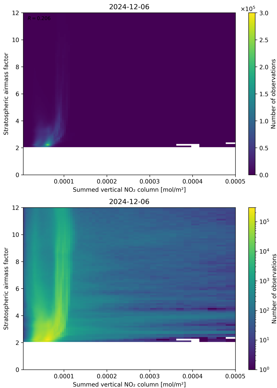
Figure 103: Scatter density plot of “Summed vertical NO 2 column” against “Stratospheric air mass factor” for 2024-12-06 to 2024-12-07.
