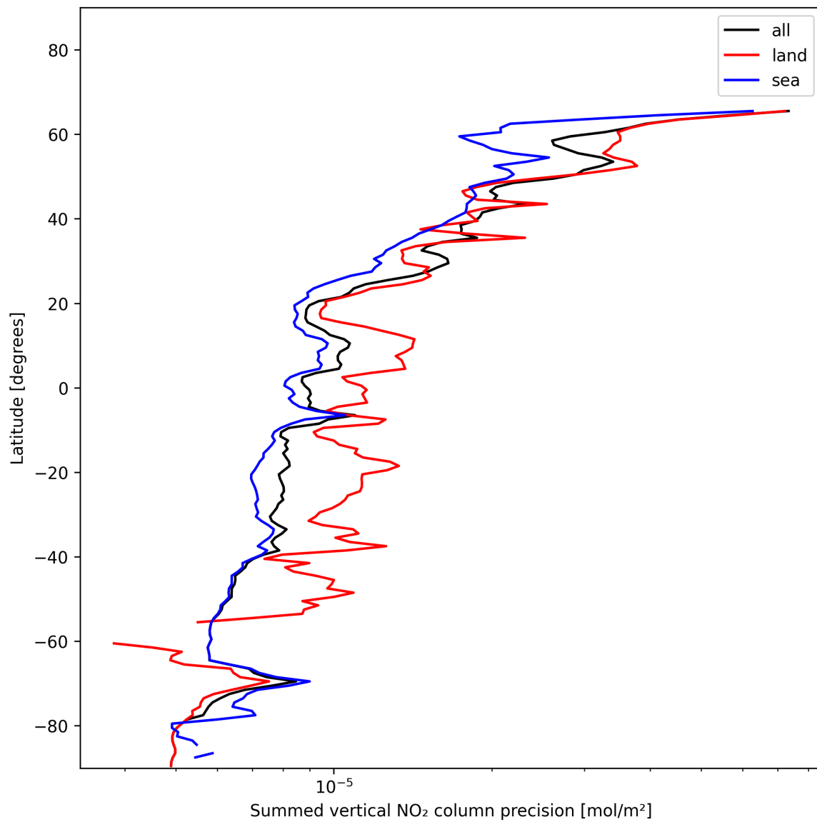
Figure 24: Zonal average of “Summed vertical NO 2 column precision” for 2024-12-06 to 2024-12-07.
