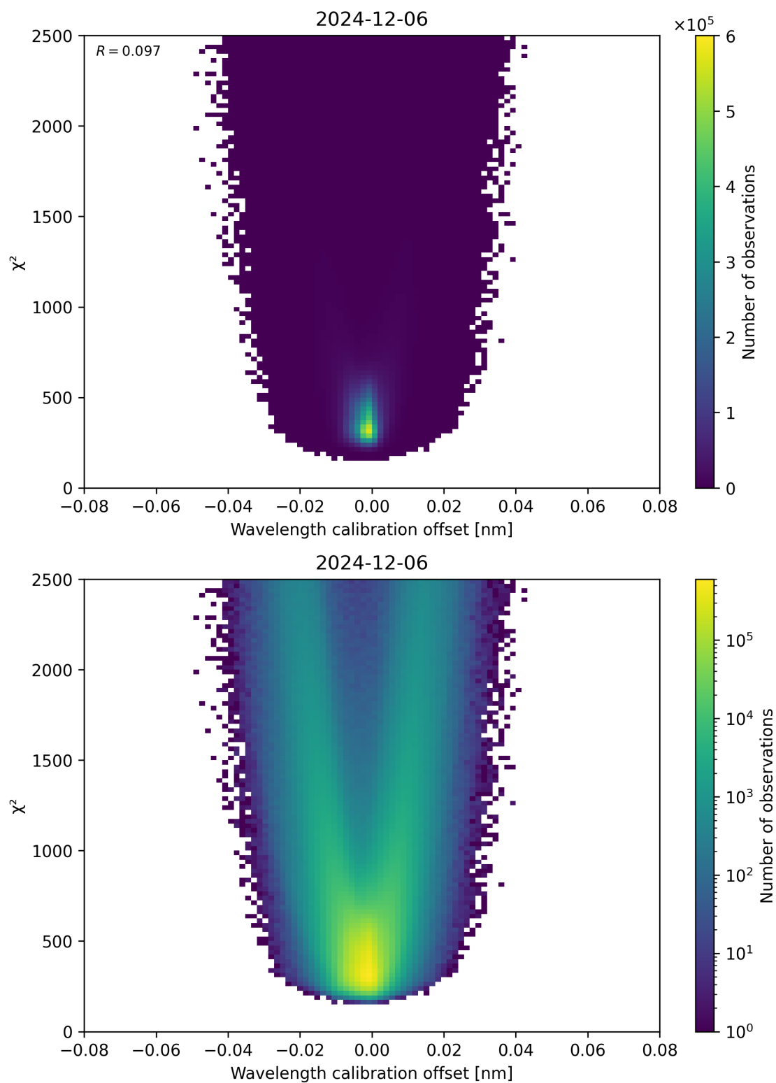
Figure 175: Scatter density plot of “Wavelength calibration offset” against “ \chi^2 ” for 2024-12-06 to 2024-12-07.
