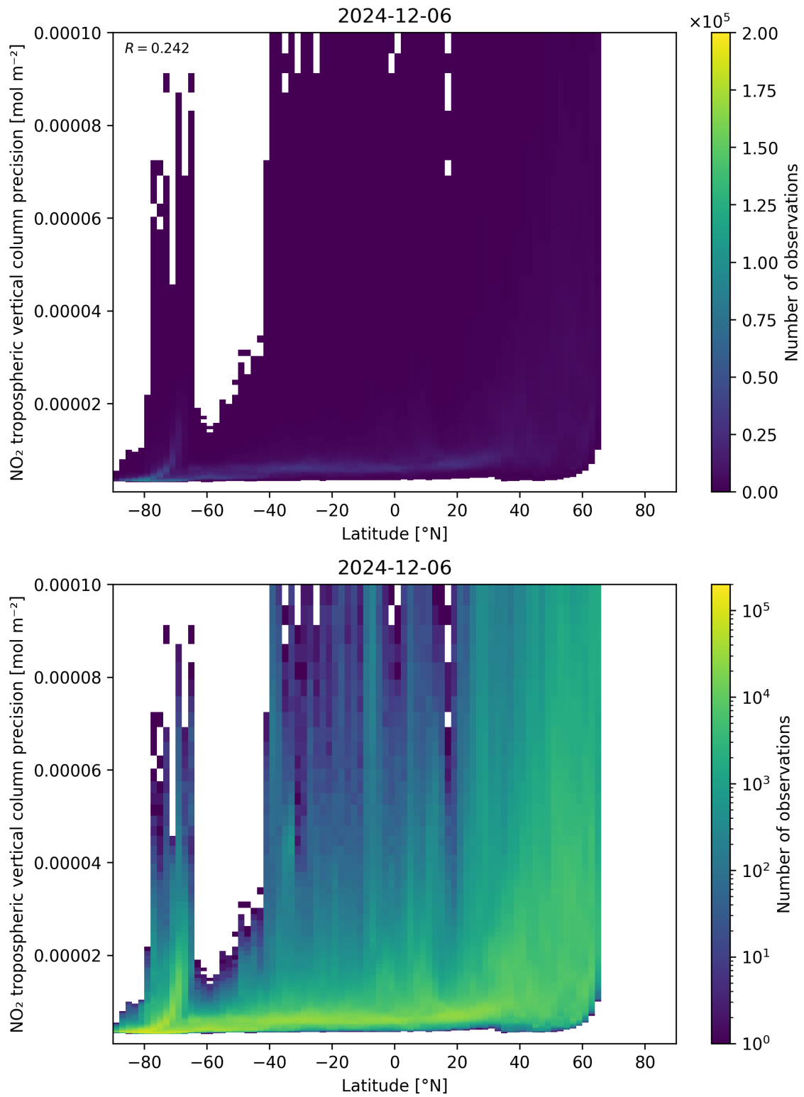
Figure 93: Scatter density plot of “Latitude” against “NO 2 tropospheric vertical column precision” for 2024-12-06 to 2024-12-07.
