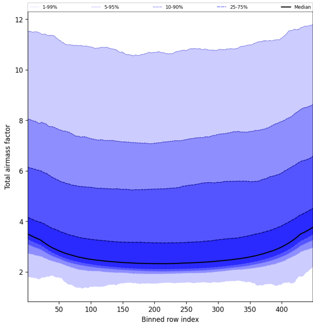
Figure 49: Along track statistics of “Total airmass factor” for 2024-12-06 to 2024-12-07
