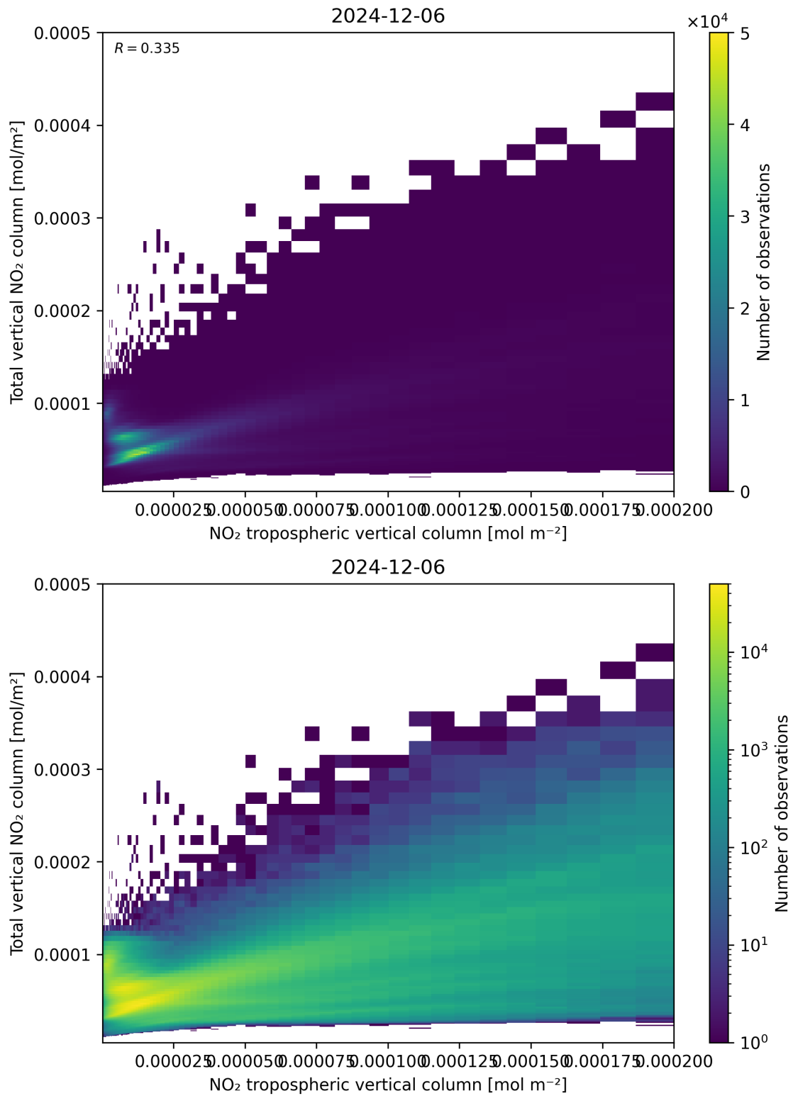
Figure 128: Scatter density plot of “NO 2 tropospheric vertical column” against “Total vertical NO 2 column” for 2024-12-06 to 2024-12-07.
