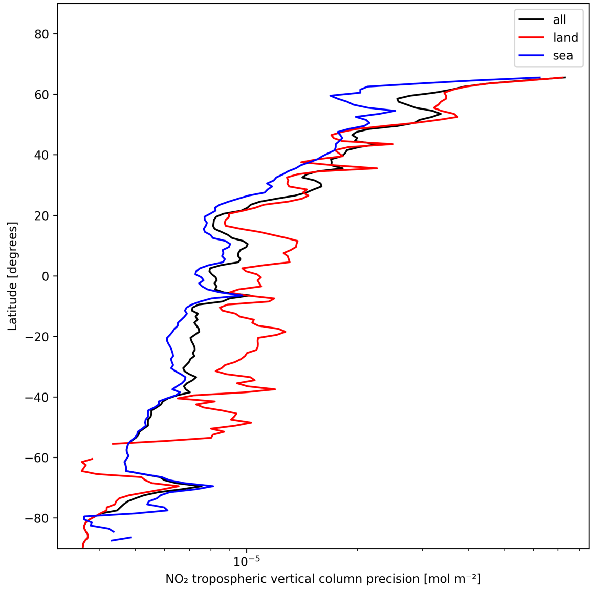
Figure 13: Zonal average of “NO 2 tropospheric vertical column precision” for 2024-12-06 to 2024-12-07.
