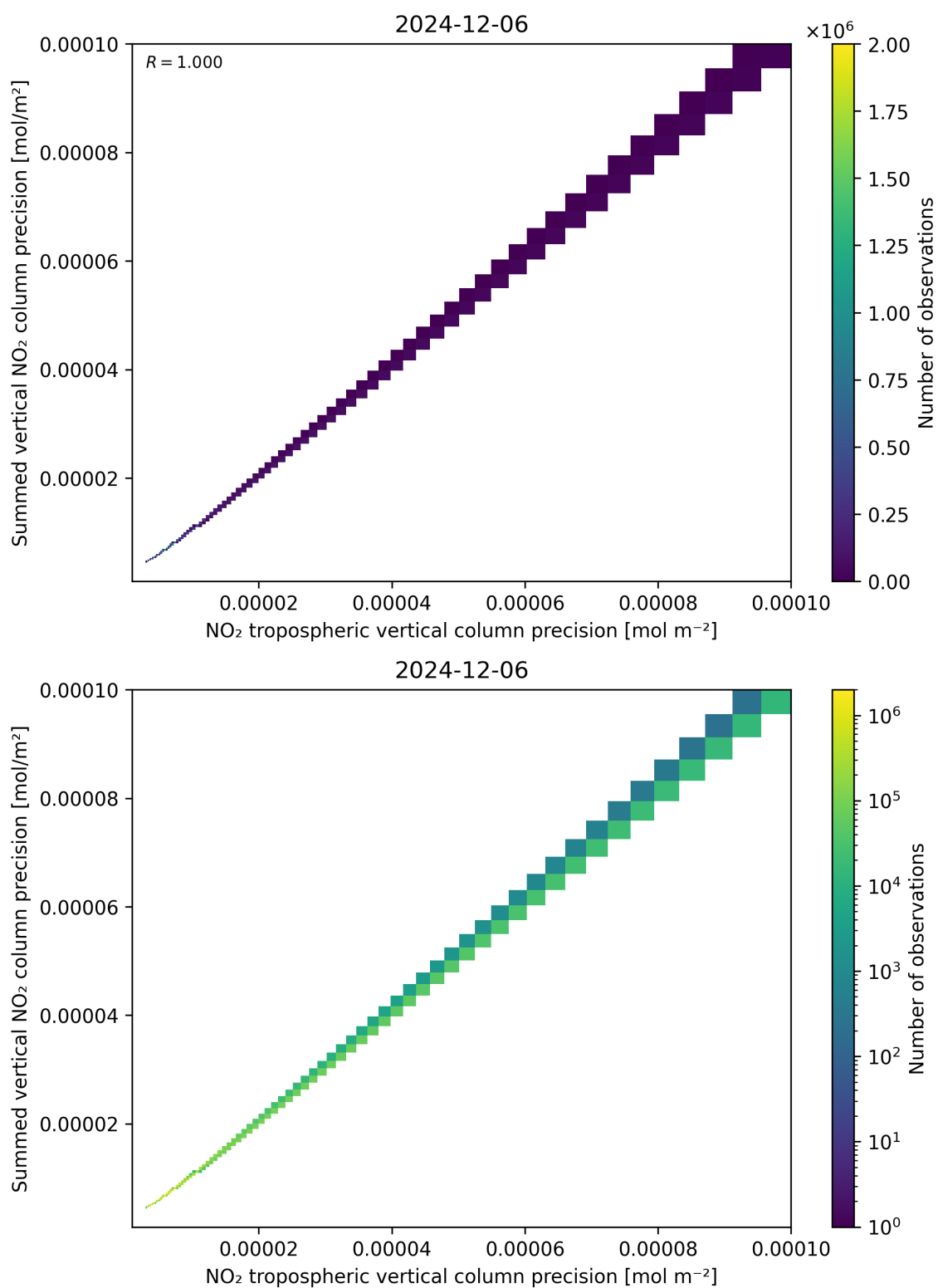
Figure 137: Scatter density plot of “NO 2 tropospheric vertical column precision” against “Summed vertical NO 2 column precision” for 2024-12-06 to 2024-12-07.
