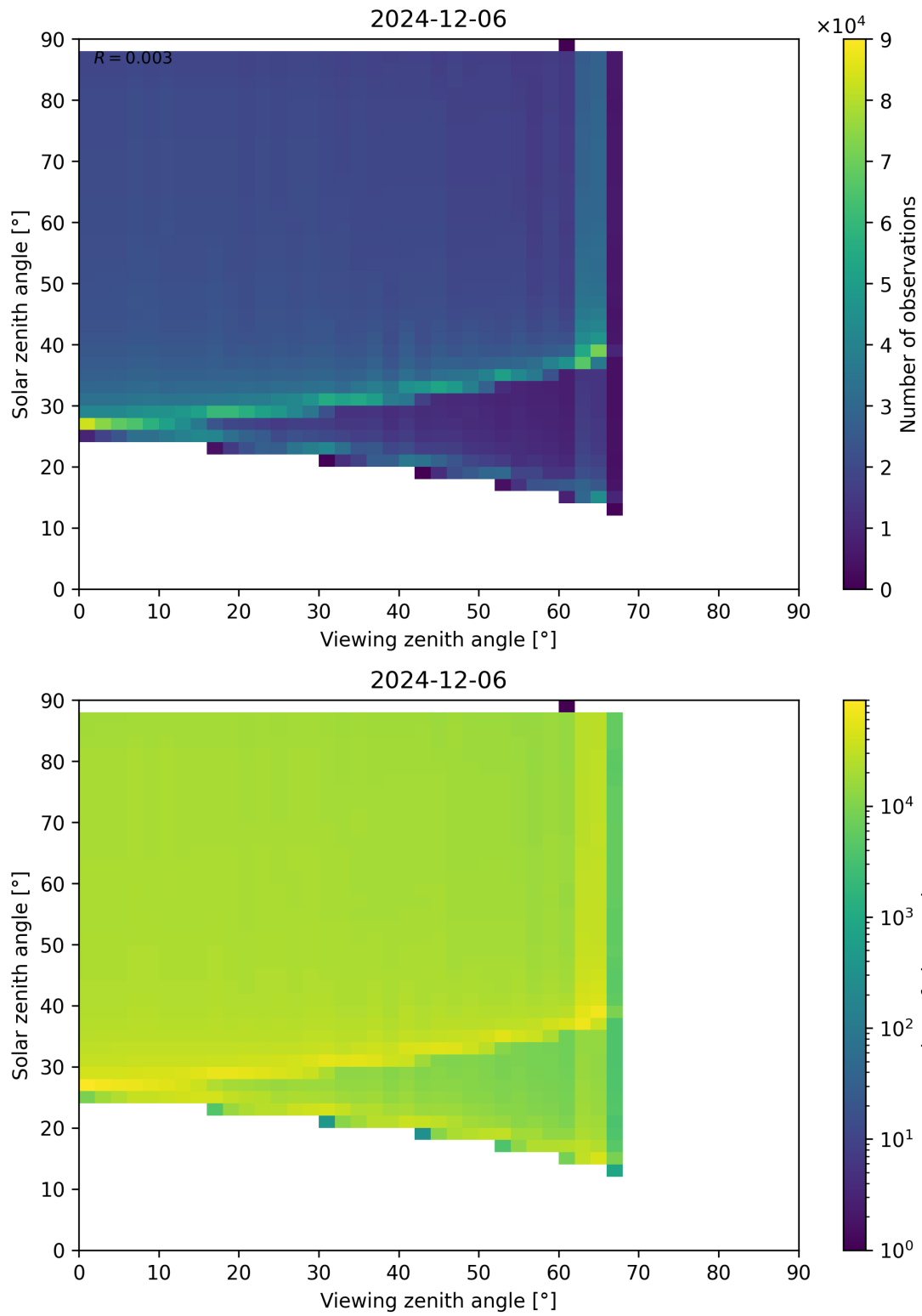
Figure 172: Scatter density plot of “Viewing zenith angle” against “Solar zenith angle” for 2024-12-06 to 2024-12-07.
