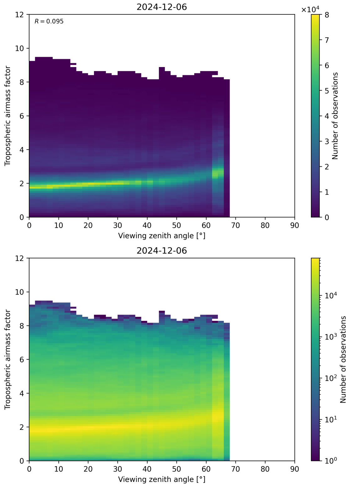
Figure 161: Scatter density plot of “Viewing zenith angle” against “Tropospheric airmass factor” for 2024-12-06 to 2024-12-07.
