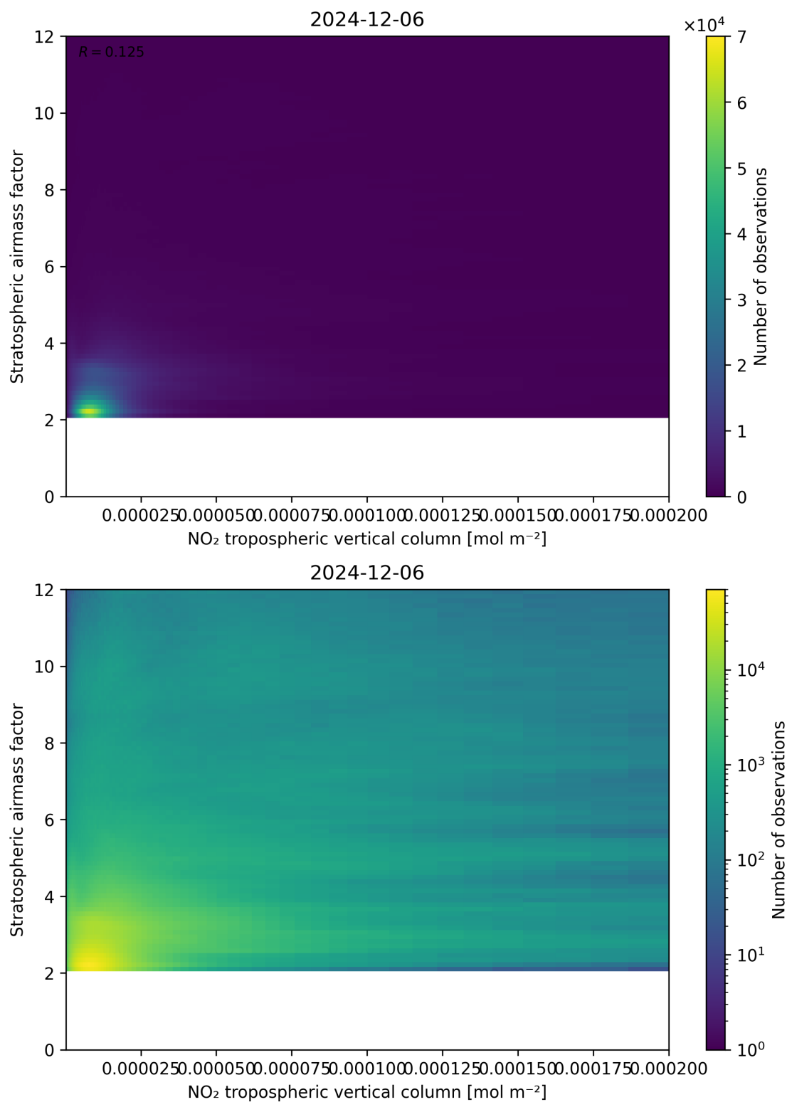
Figure 121: Scatter density plot of “NO 2 tropospheric vertical column” against “Stratospheric airmass factor” for 2024-12-06 to 2024-12-07.
