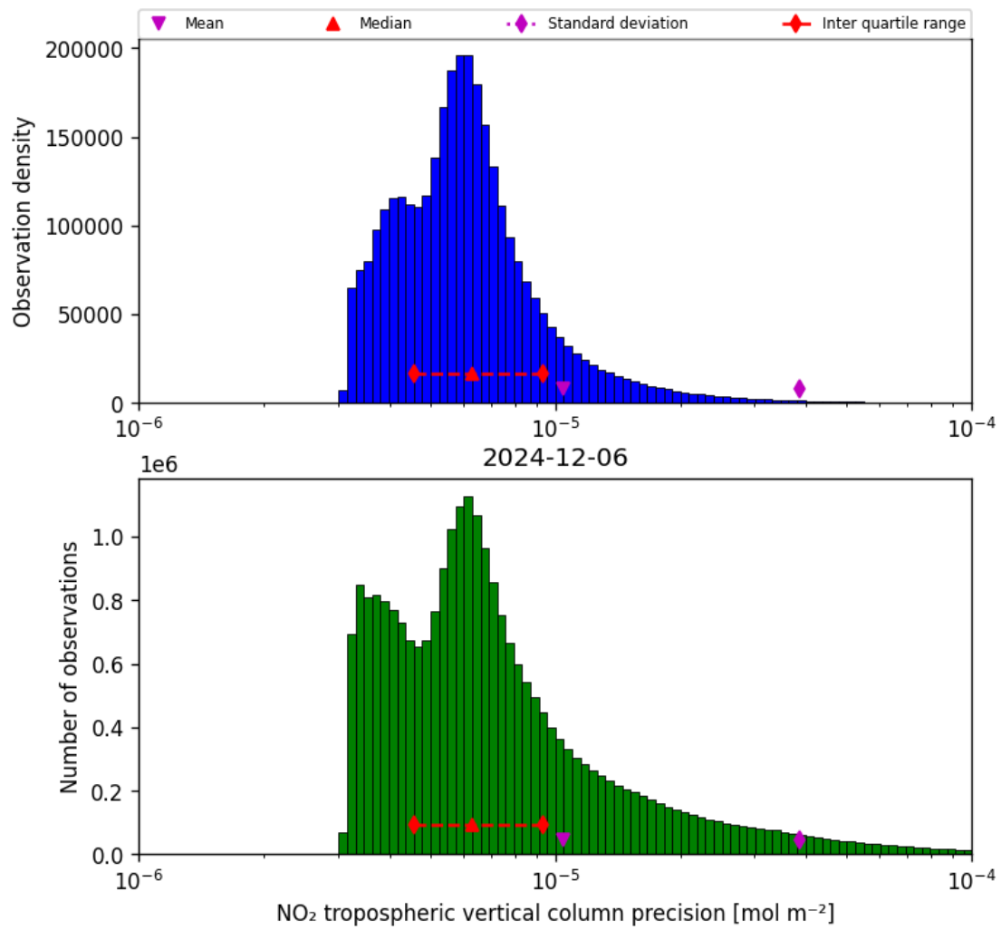
Figure 30: Histogram of “NO 2 tropospheric vertical column precision” for 2024-12-06 to 2024-12-07
