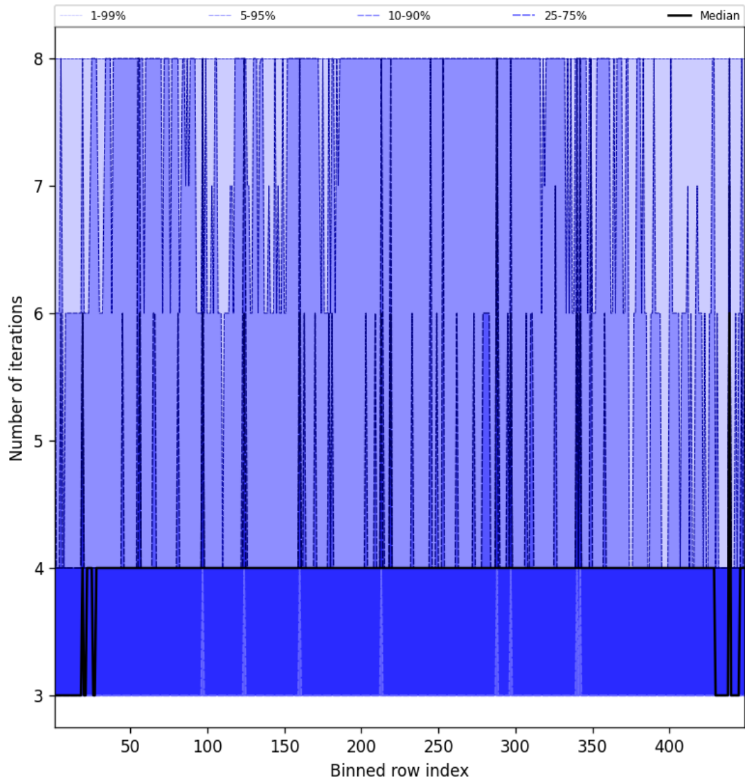
Figure 51: Along track statistics of “Number of iterations” for 2024-12-06 to 2024-12-07
