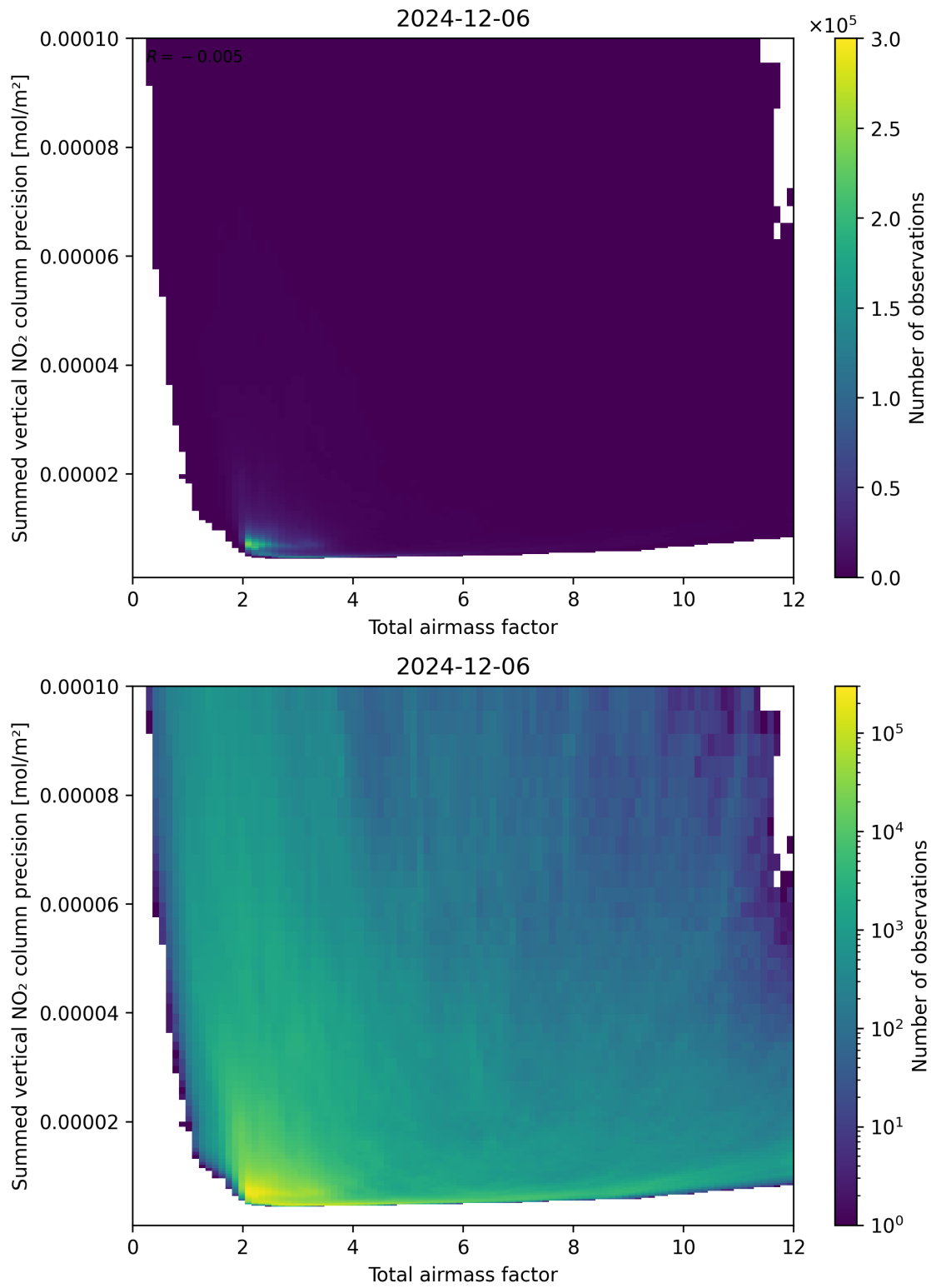
Figure 66: Scatter density plot of “Total airmass factor” against “Summed vertical NO 2 column precision” for 2024-12-06 to 2024-12-07.
