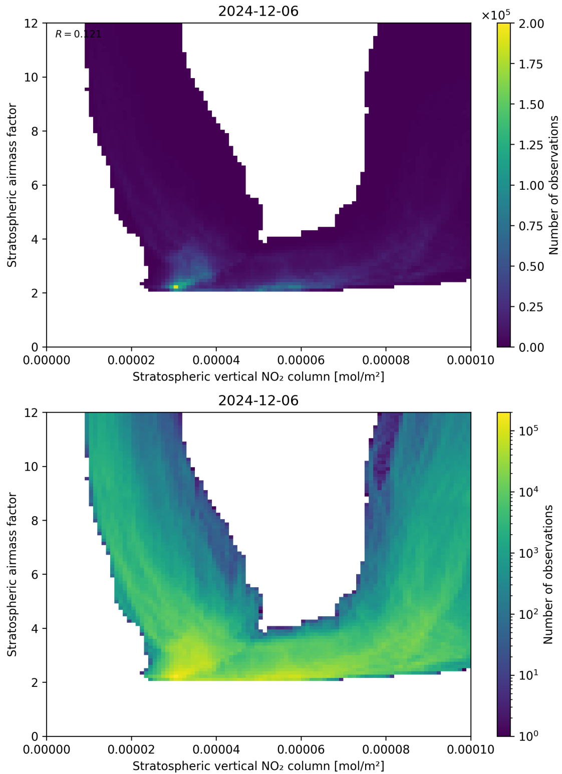
Figure 96: Scatter density plot of “Stratospheric vertical NO 2 column” against “Stratospheric airmass factor” for 2024-12-06 to 2024-12-07.
