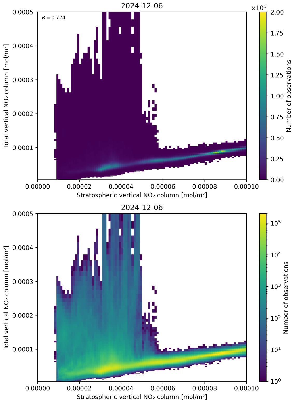
Figure 100: Scatter density plot of “Stratospheric vertical NO 2 column” against “Total vertical NO 2 column” for 2024-12-06 to 2024-12-07.
