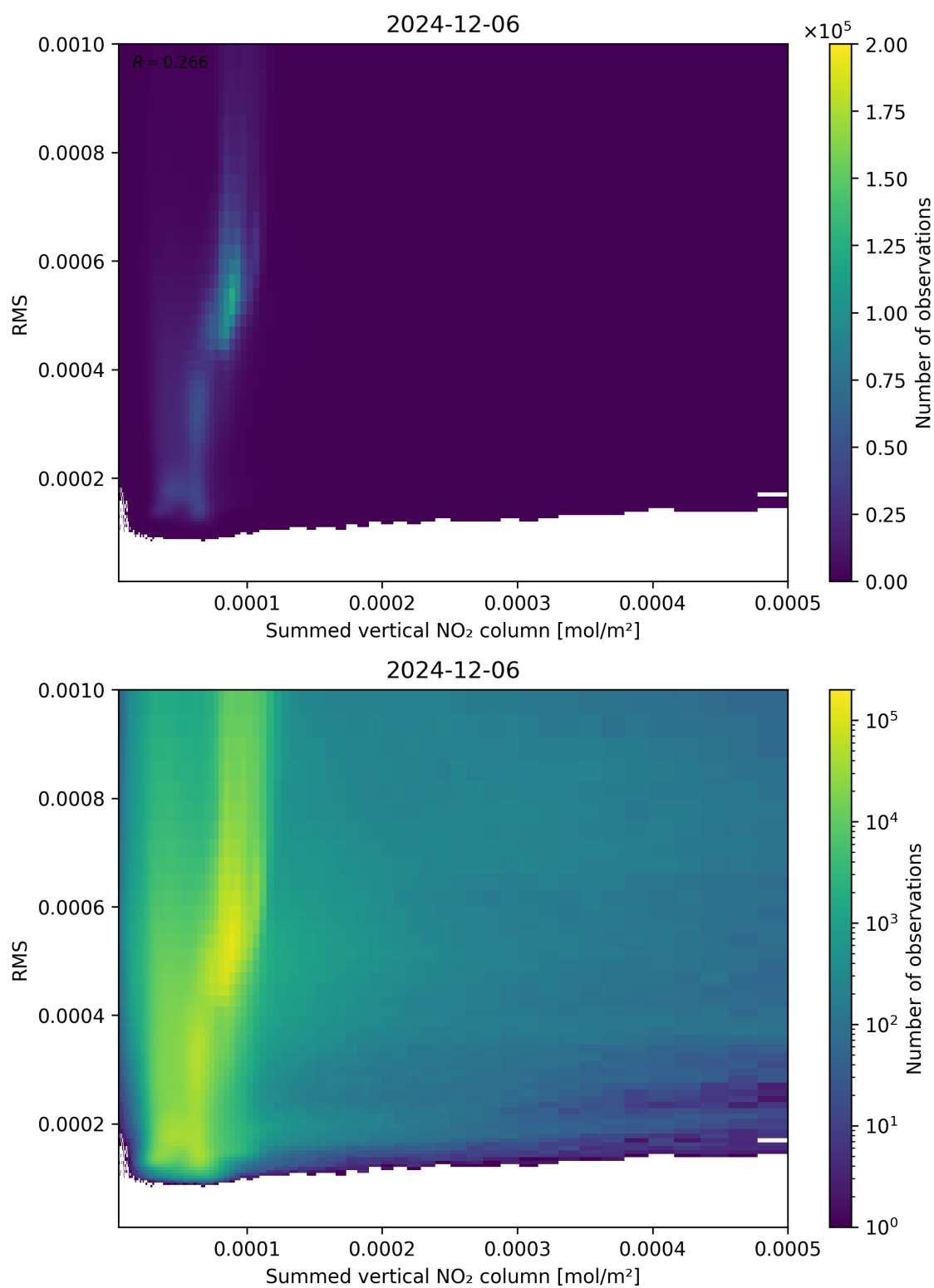
Figure 109: Scatter density plot of “Summed vertical NO 2 column” against “RMS” for 2024-12-06 to 2024-12-07.
