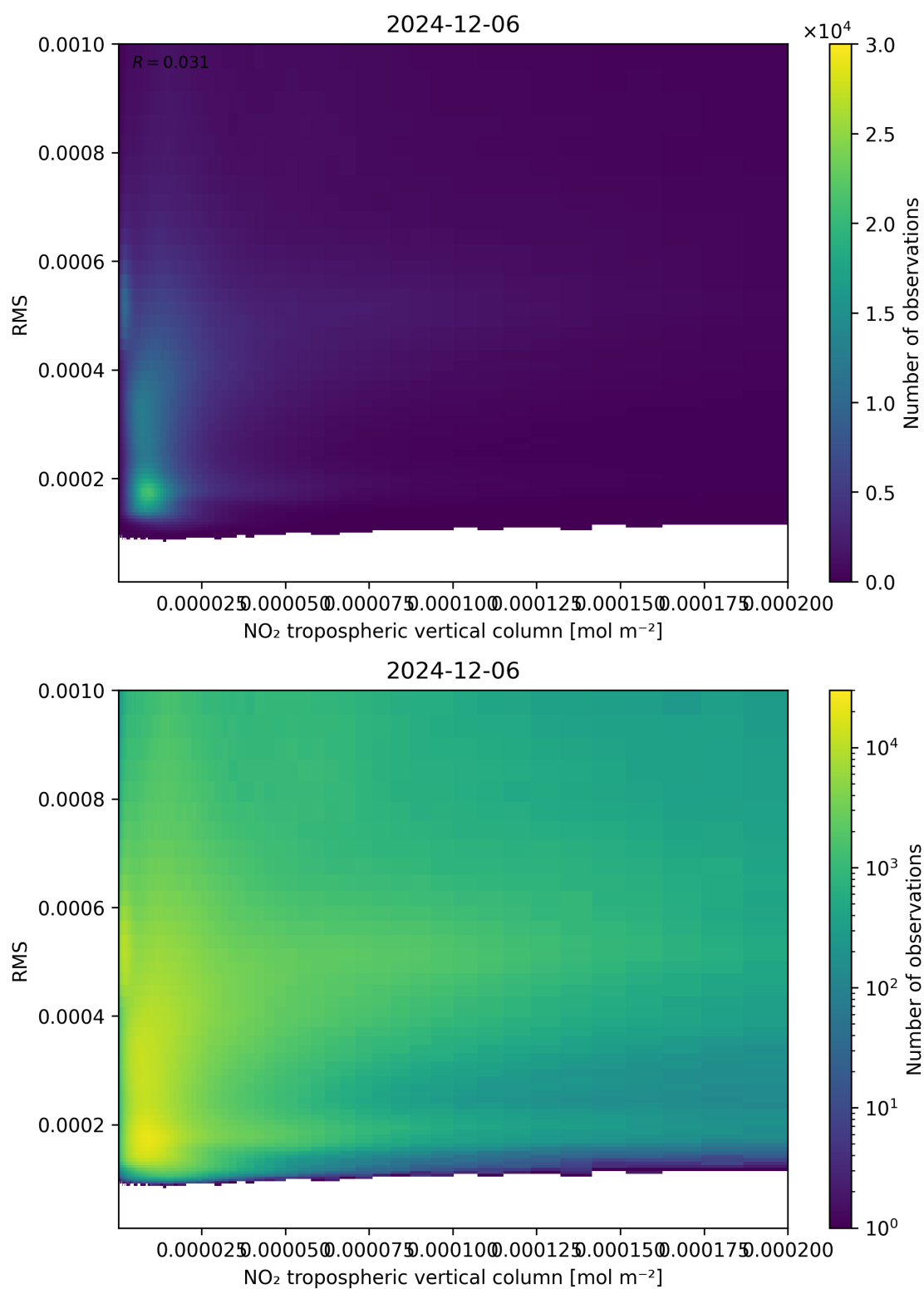
Figure 142: Scatter density plot of “NO 2 tropospheric vertical column” against “RMS” for 2024-12-06 to 2024-12-07.
