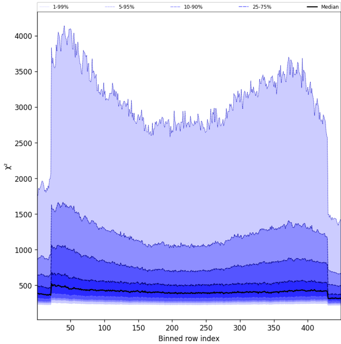
Figure 59: Along track statistics of “ \chi^2 ” for 2024-12-06 to 2024-12-07
