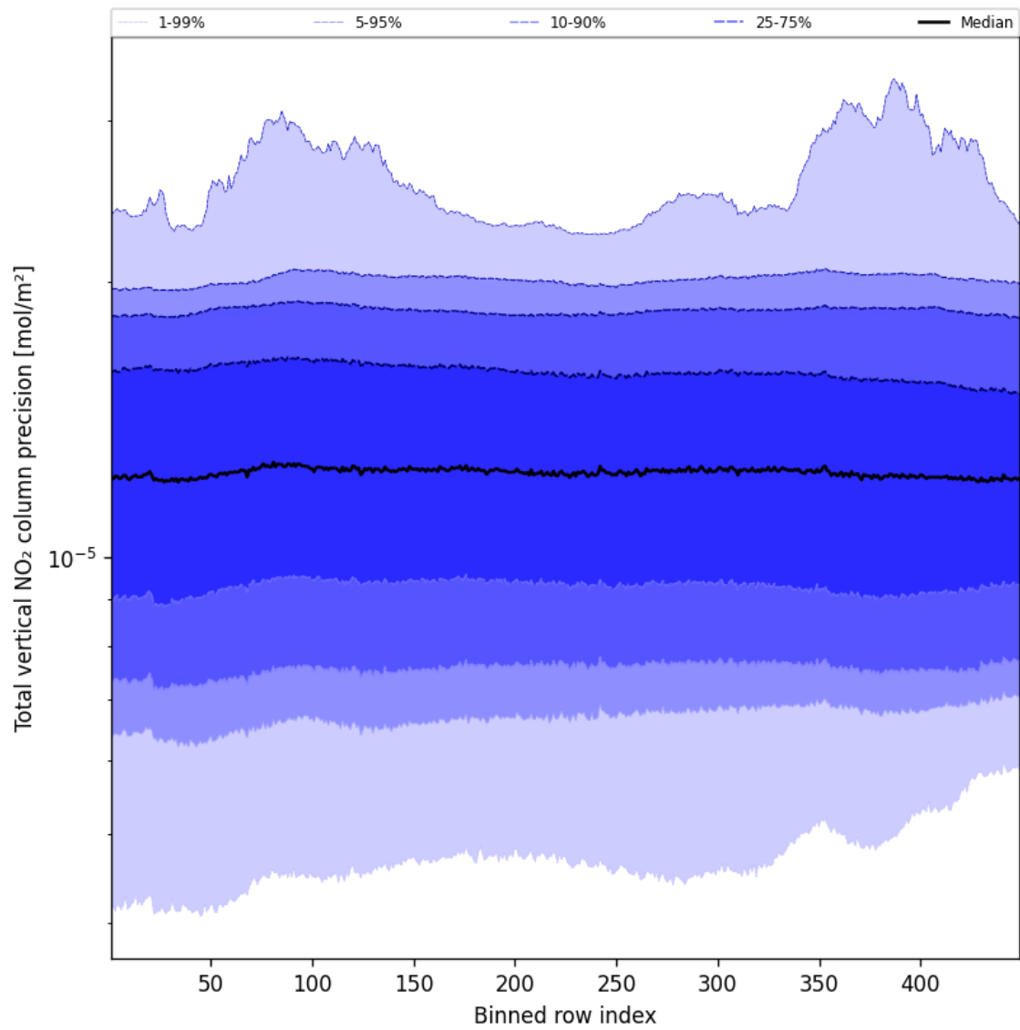
Figure 56: Along track statistics of “Total vertical NO 2 column precision” for 2024-12-06 to 2024-12-07
