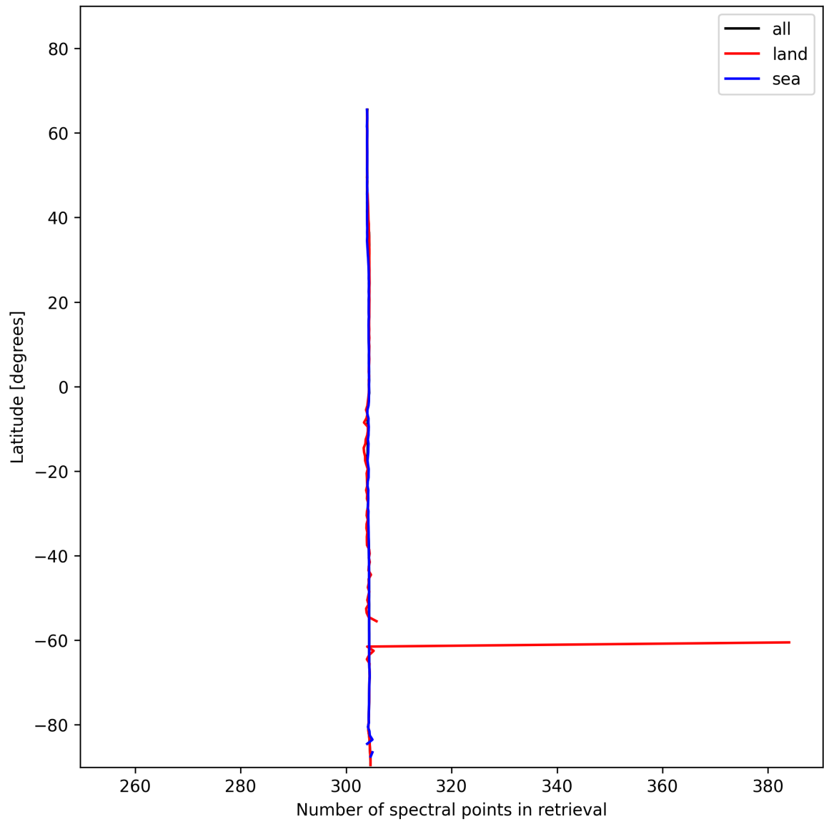
Figure 16: Zonal average of “Number of spectral points in retrieval” for 2024-12-06 to 2024-12-07.
