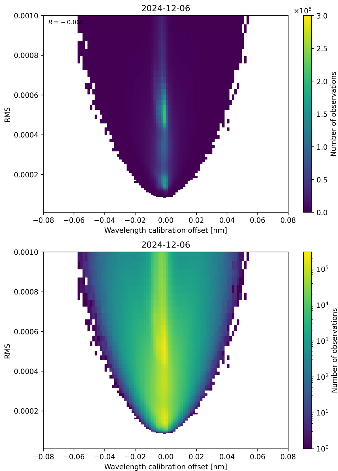
Figure 181: Scatter density plot of “Wavelength calibration offset” against “RMS” for 2024-12-06 to 2024-12-07.
