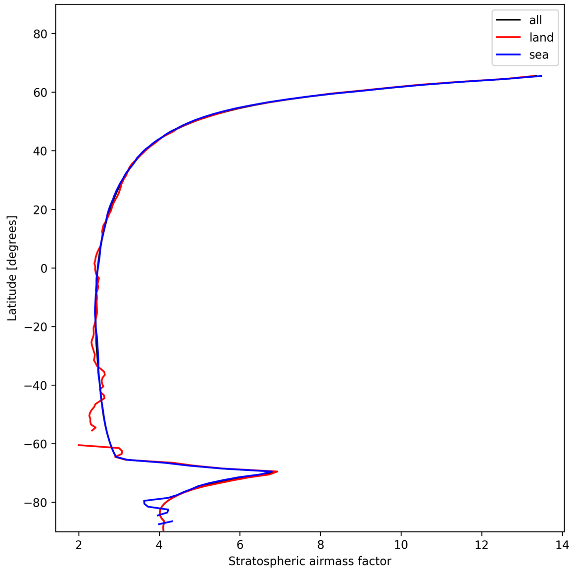
Figure 27: Zonal average of “Stratospheric airmass factor” for 2024-12-06 to 2024-12-07.
