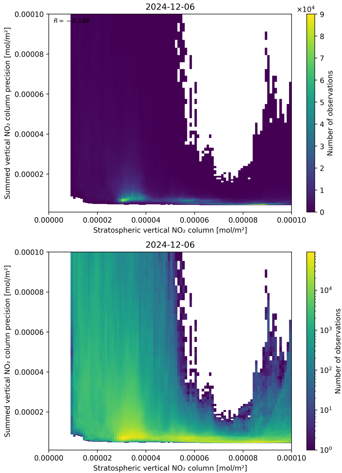
Figure 99: Scatter density plot of “Stratospheric vertical NO 2 column” against “Summed vertical NO 2 column precision” for 2024-12-06 to 2024-12-07.
