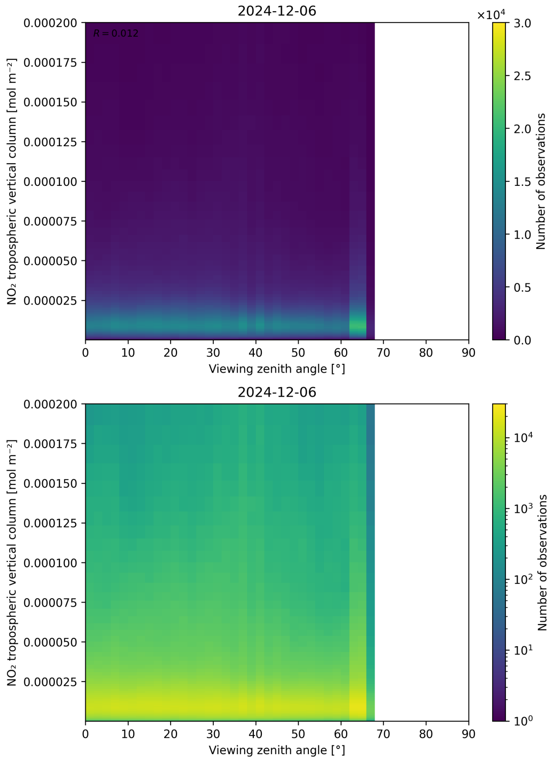
Figure 169: Scatter density plot of “Viewing zenith angle” against “NO 2 tropospheric vertical column” for 2024-12-06 to 2024-12-07.
