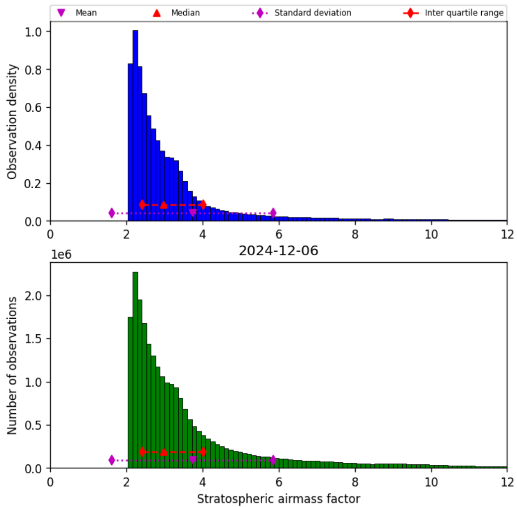
Figure 44: Histogram of “Stratospheric airmass factor” for 2024-12-06 to 2024-12-07
