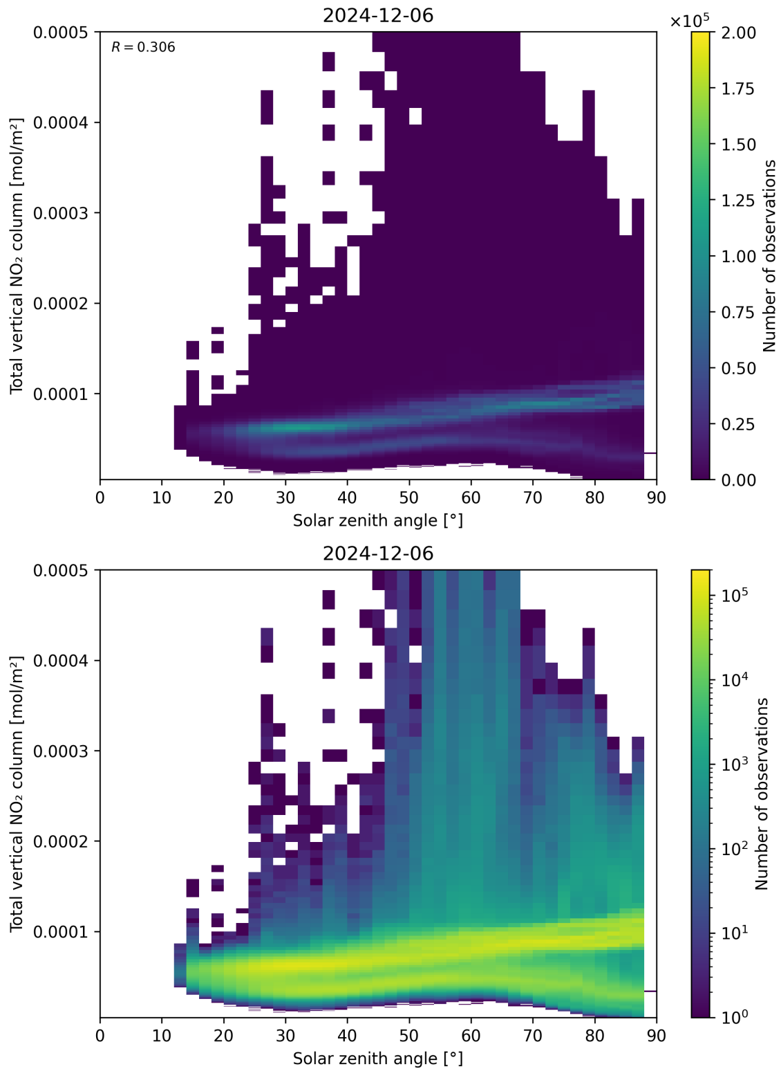
Figure 153: Scatter density plot of “Solar zenith angle” against “Total vertical NO 2 column” for 2024-12-06 to 2024-12-07.
