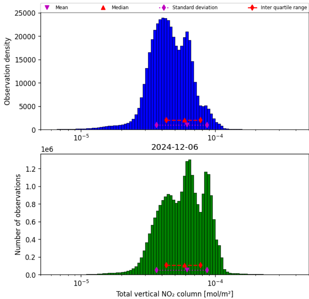
Figure 38: Histogram of "Total vertical NO 2 column" for 2024-12-06 to 2024-12-07
