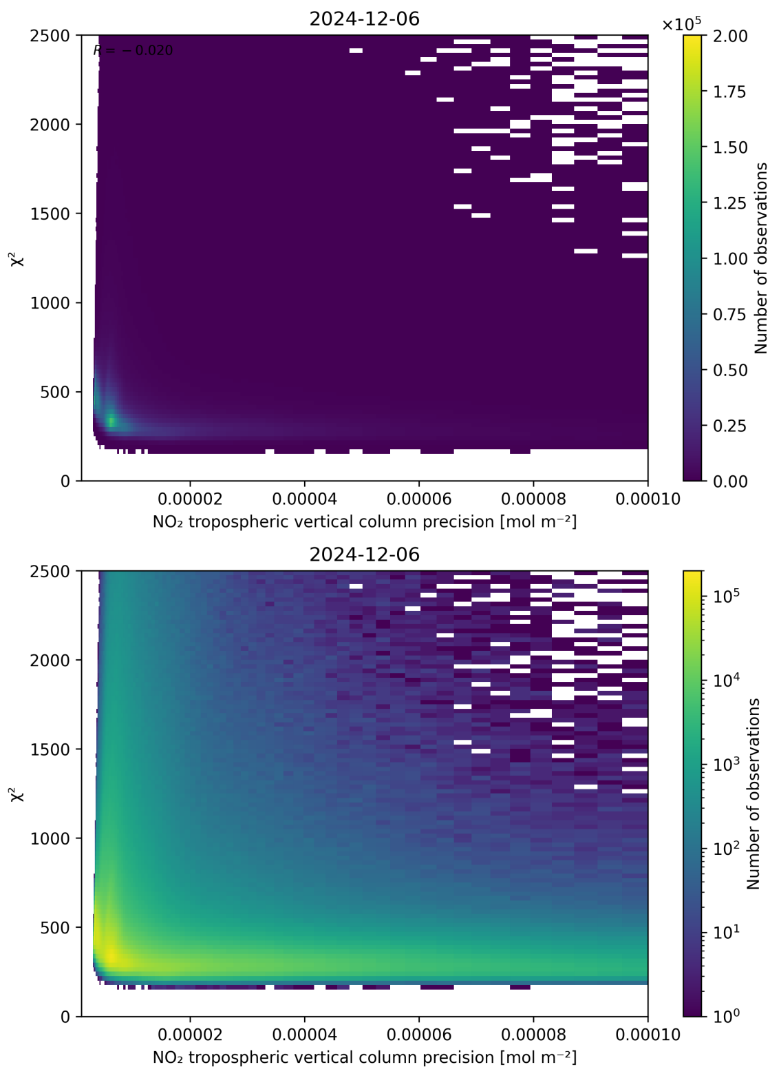
Figure 134: Scatter density plot of “NO 2 tropospheric vertical column precision” against “ \chi^2 ” for 2024-12-06 to 2024-12-07.
