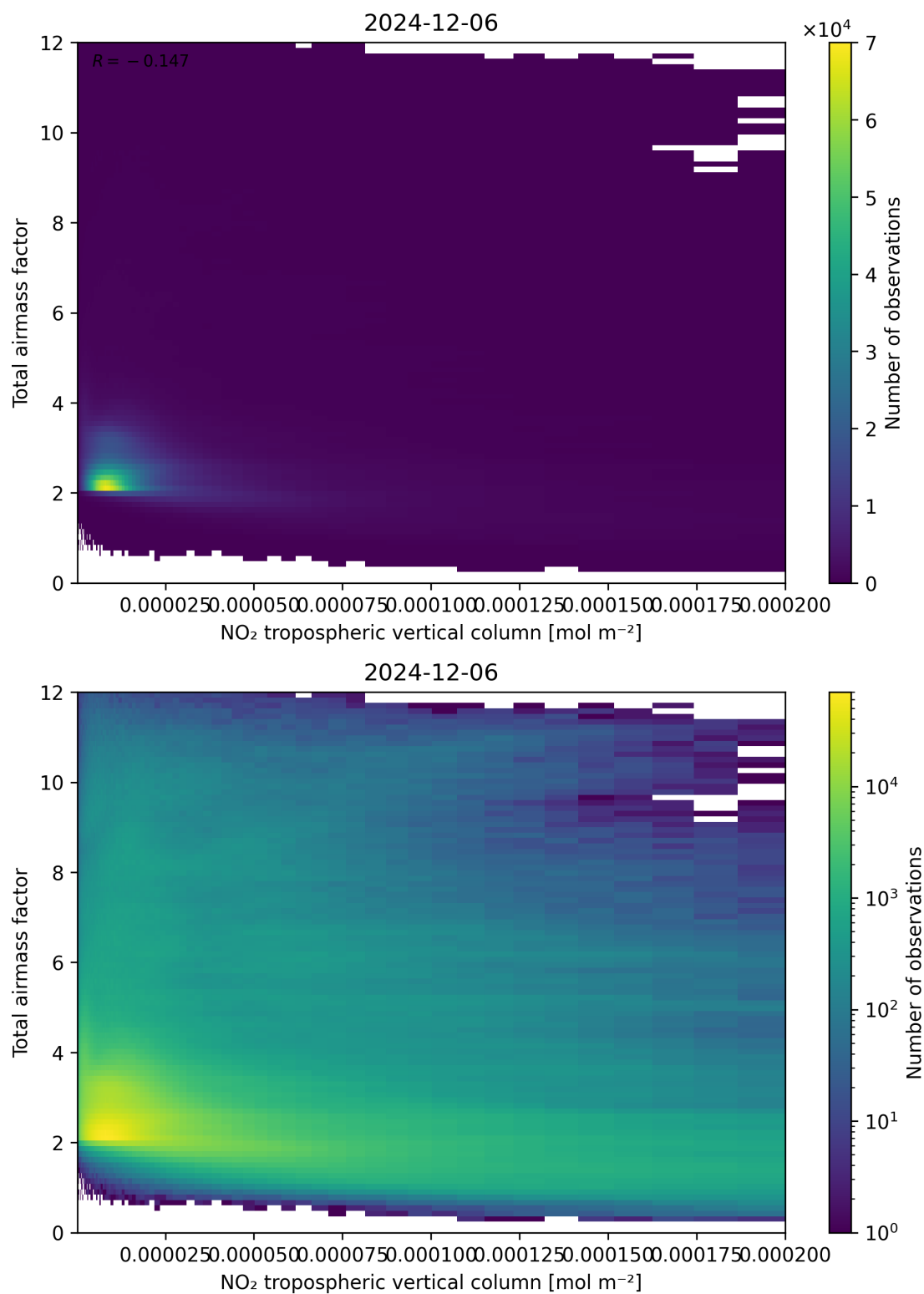
Figure 122: Scatter density plot of “NO 2 tropospheric vertical column” against “Total airmass factor” for 2024-12-06 to 2024-12-07.
