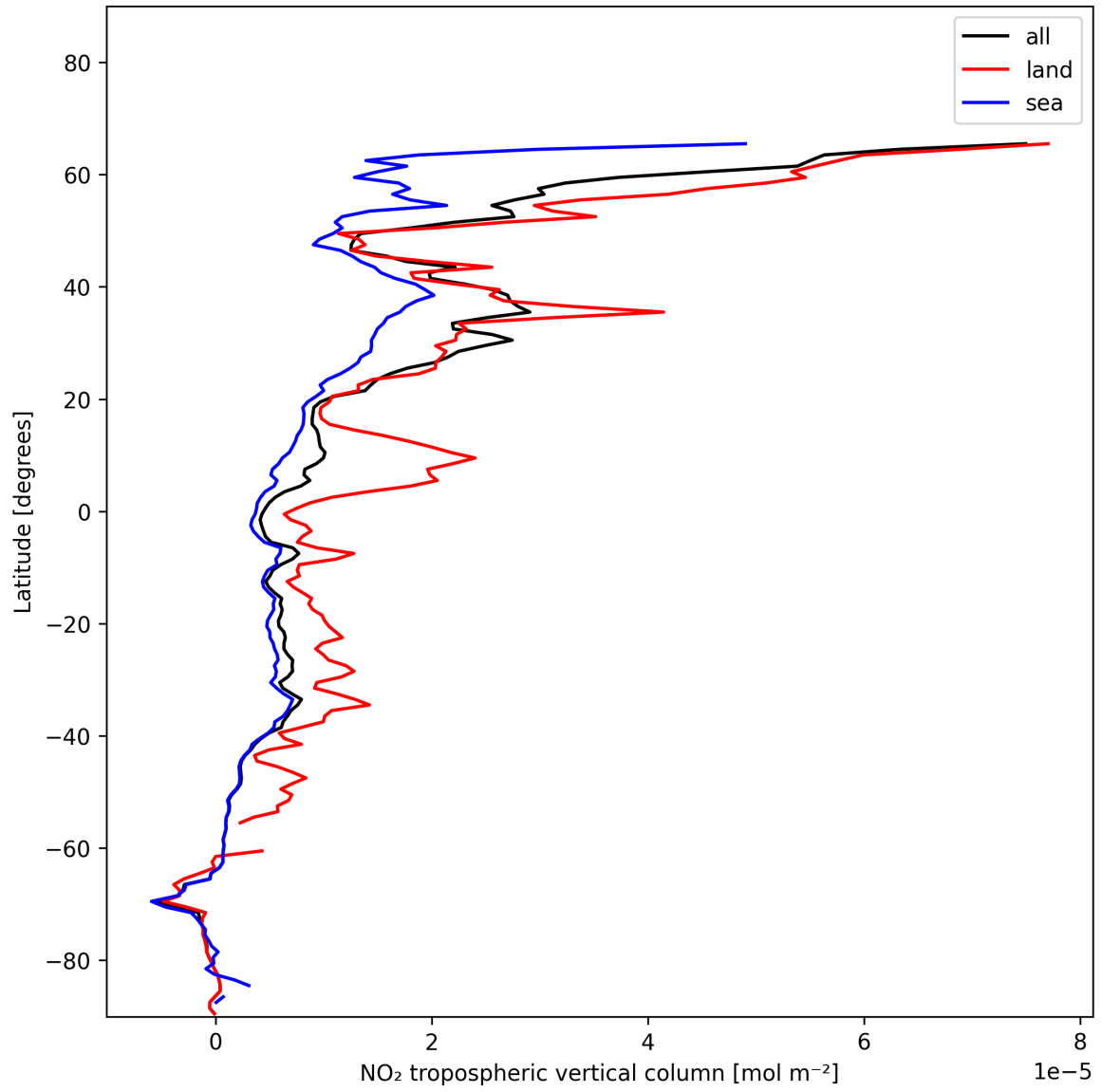
Figure 12: Zonal average of “NO 2 tropospheric vertical column” for 2024-12-06 to 2024-12-07.
