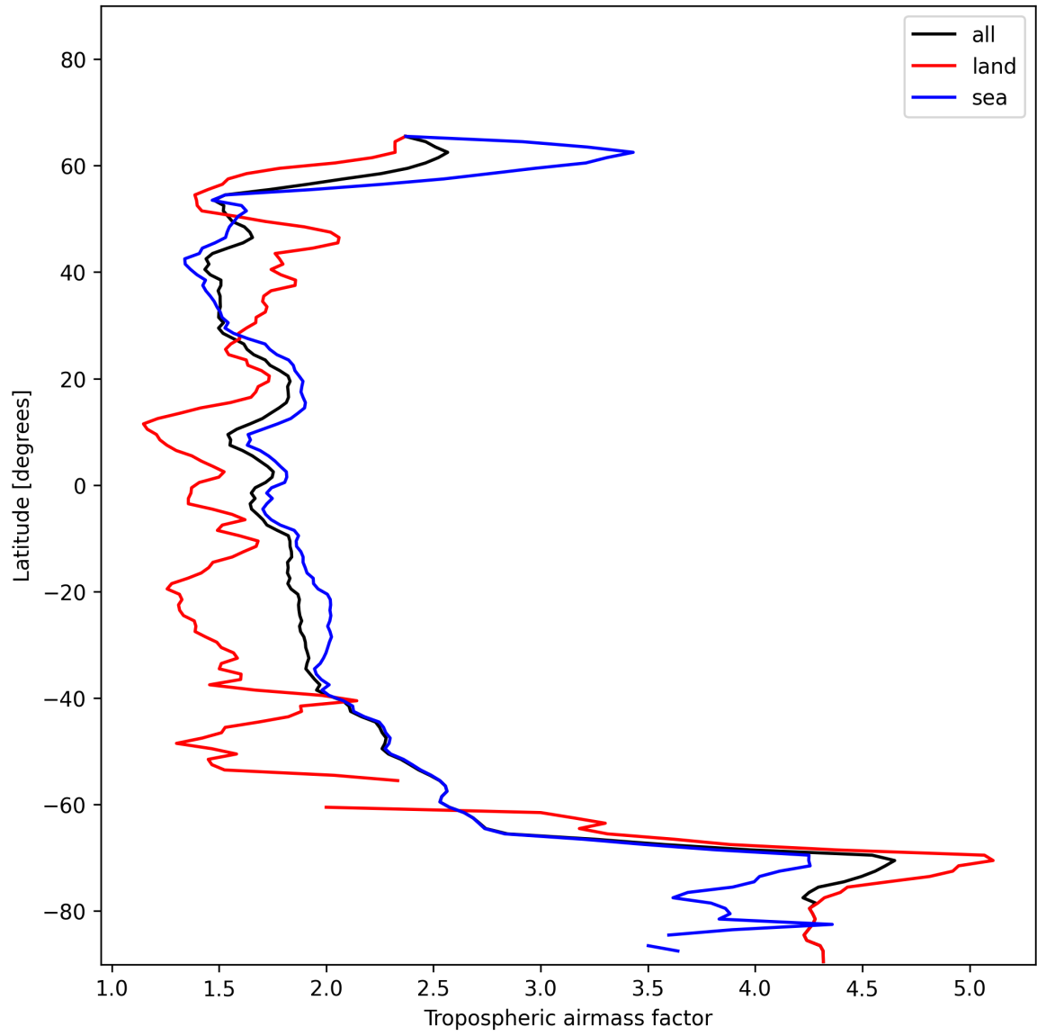
Figure 14: Zonal average of “Tropospheric airmass factor” for 2024-12-06 to 2024-12-07.
