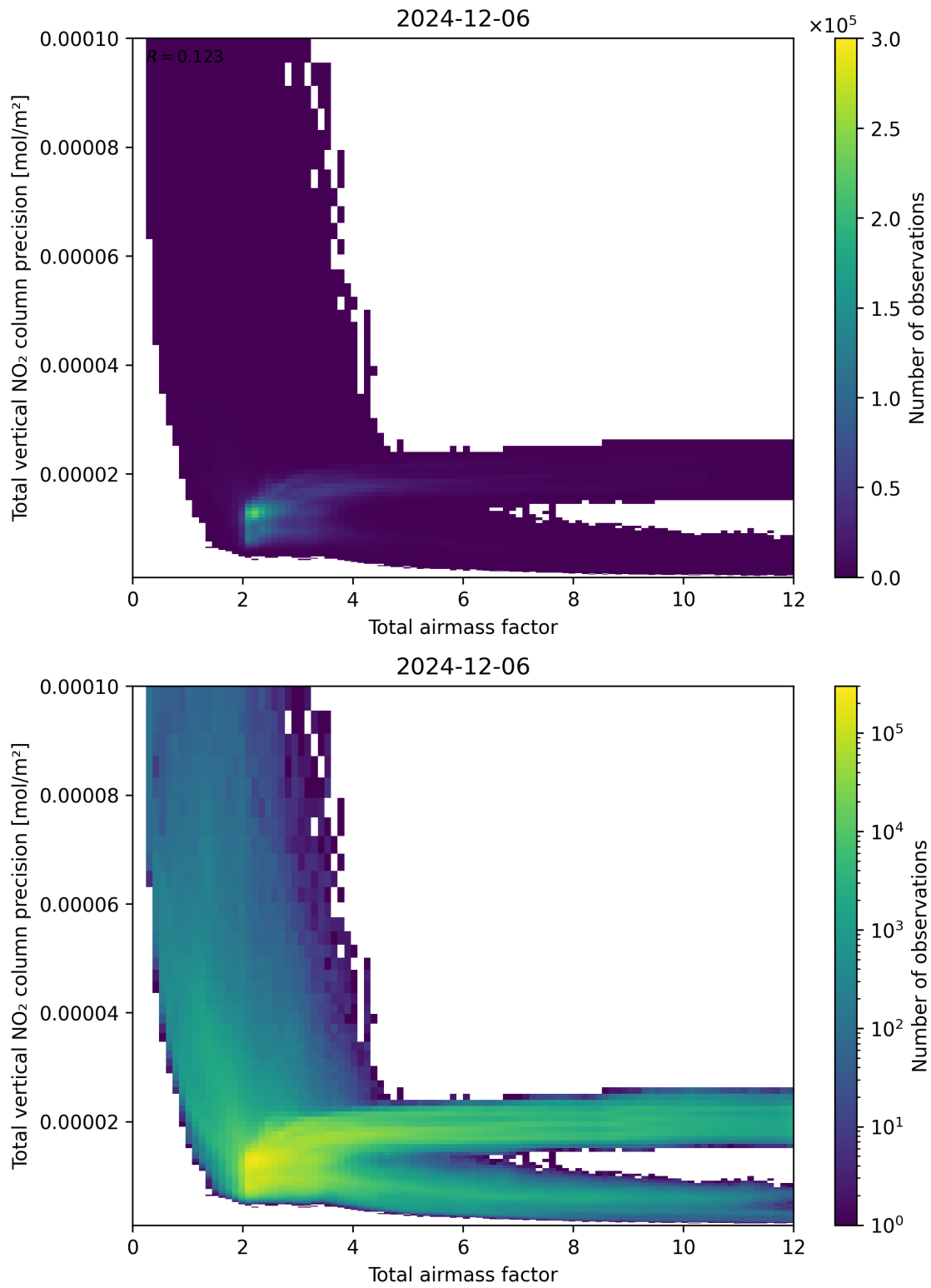
Figure 68: Scatter density plot of “Total airmass factor” against “Total vertical NO 2 column precision” for 2024-12-06 to 2024-12-07.
