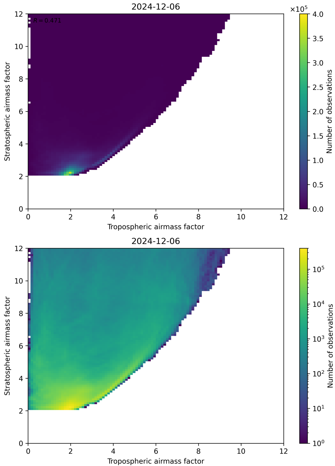
Figure 71: Scatter density plot of “Tropospheric airmass factor” against “Stratospheric airmass factor” for 2024-12-06 to 2024-12-07.
