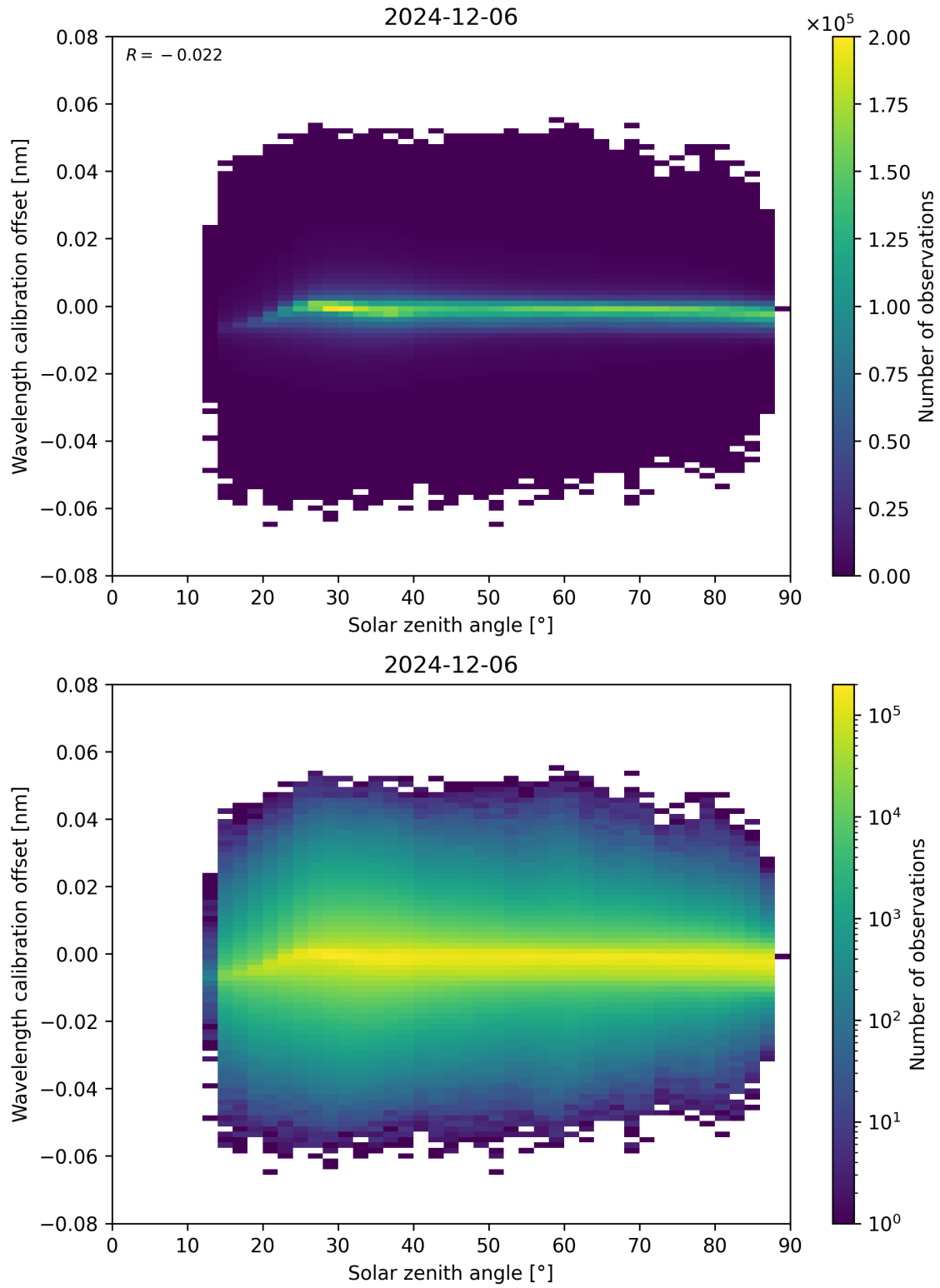
Figure 158: Scatter density plot of “Solar zenith angle” against “Wavelength calibration offset” for 2024-12-06 to 2024-12-07.
