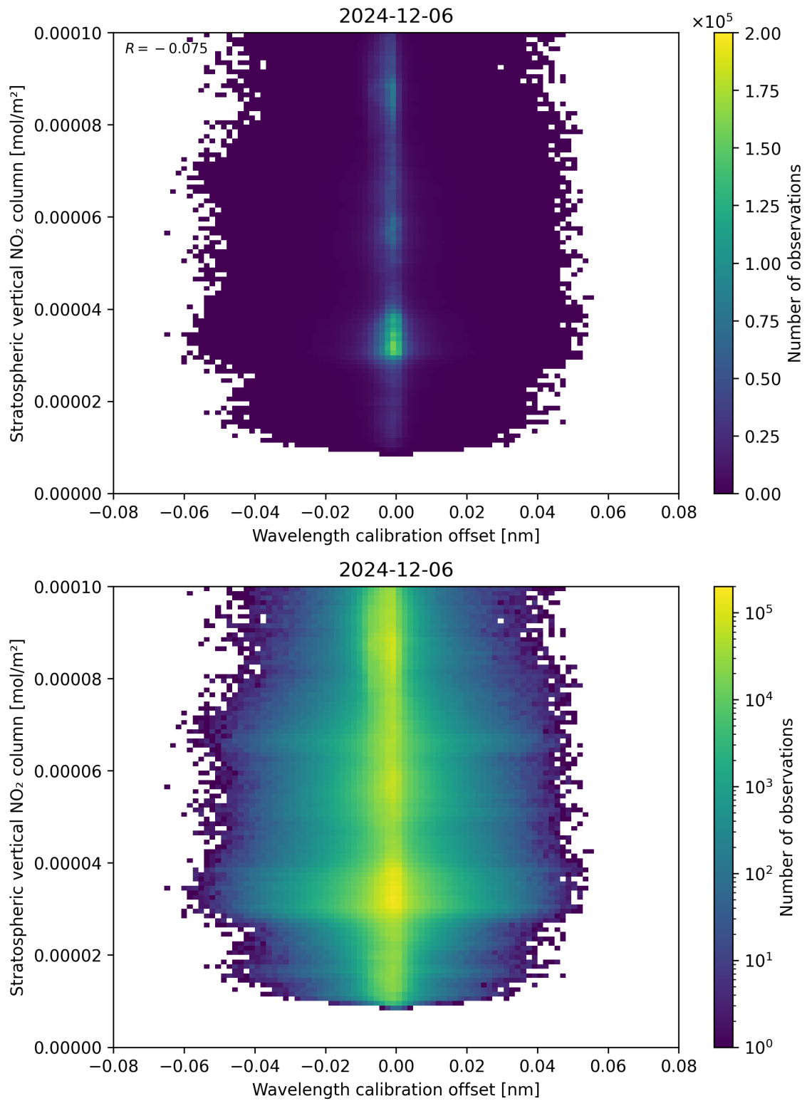
Figure 176: Scatter density plot of “Wavelength calibration offset” against “Stratospheric vertical NO 2 column” for 2024-12-06 to 2024-12-07.
