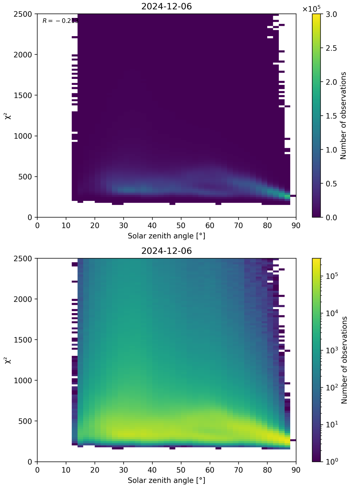
Figure 148: Scatter density plot of “Solar zenith angle” against “ \chi^2 ” for 2024-12-06 to 2024-12-07.
