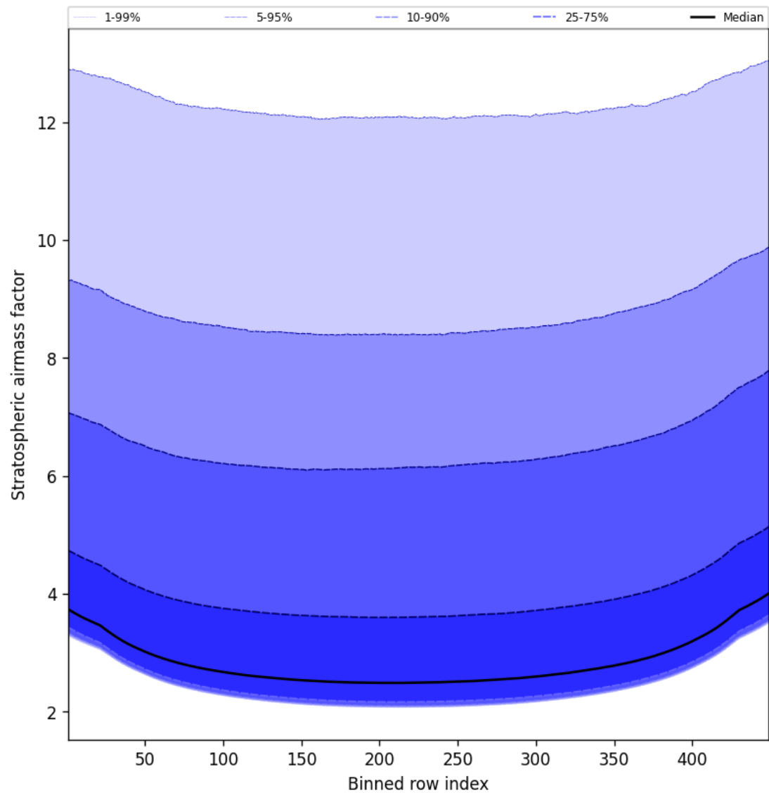
Figure 61: Along track statistics of “Stratospheric air mass factor” for 2024-12-06 to 2024-12-07
