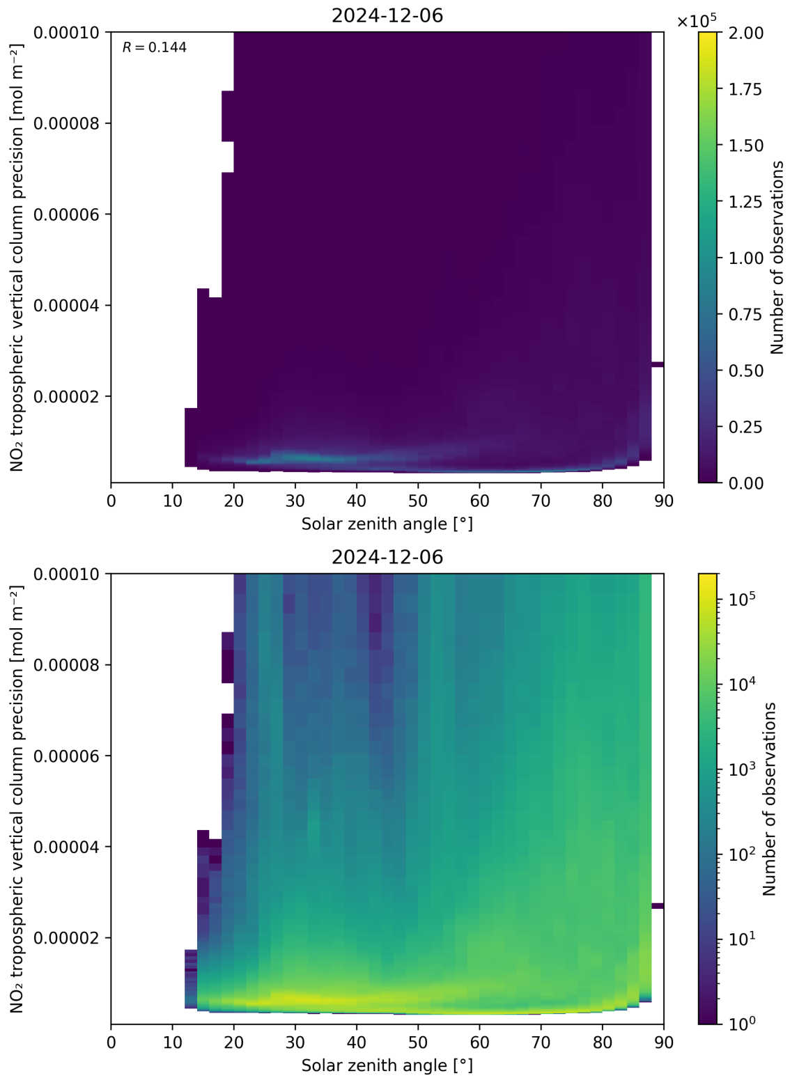
Figure 156: Scatter density plot of “Solar zenith angle” against “NO 2 tropospheric vertical column precision” for 2024-12-06 to 2024-12-07.
