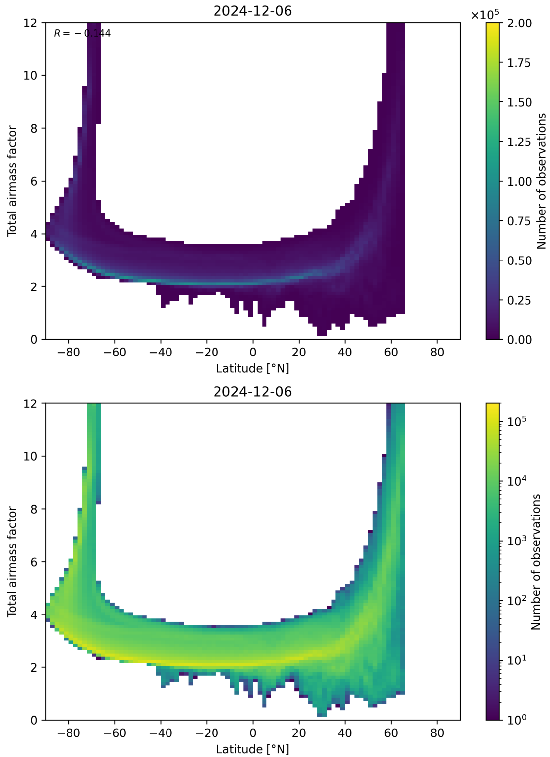
Figure 84: Scatter density plot of “Latitude” against “Total airmass factor” for 2024-12-06 to 2024-12-07.
