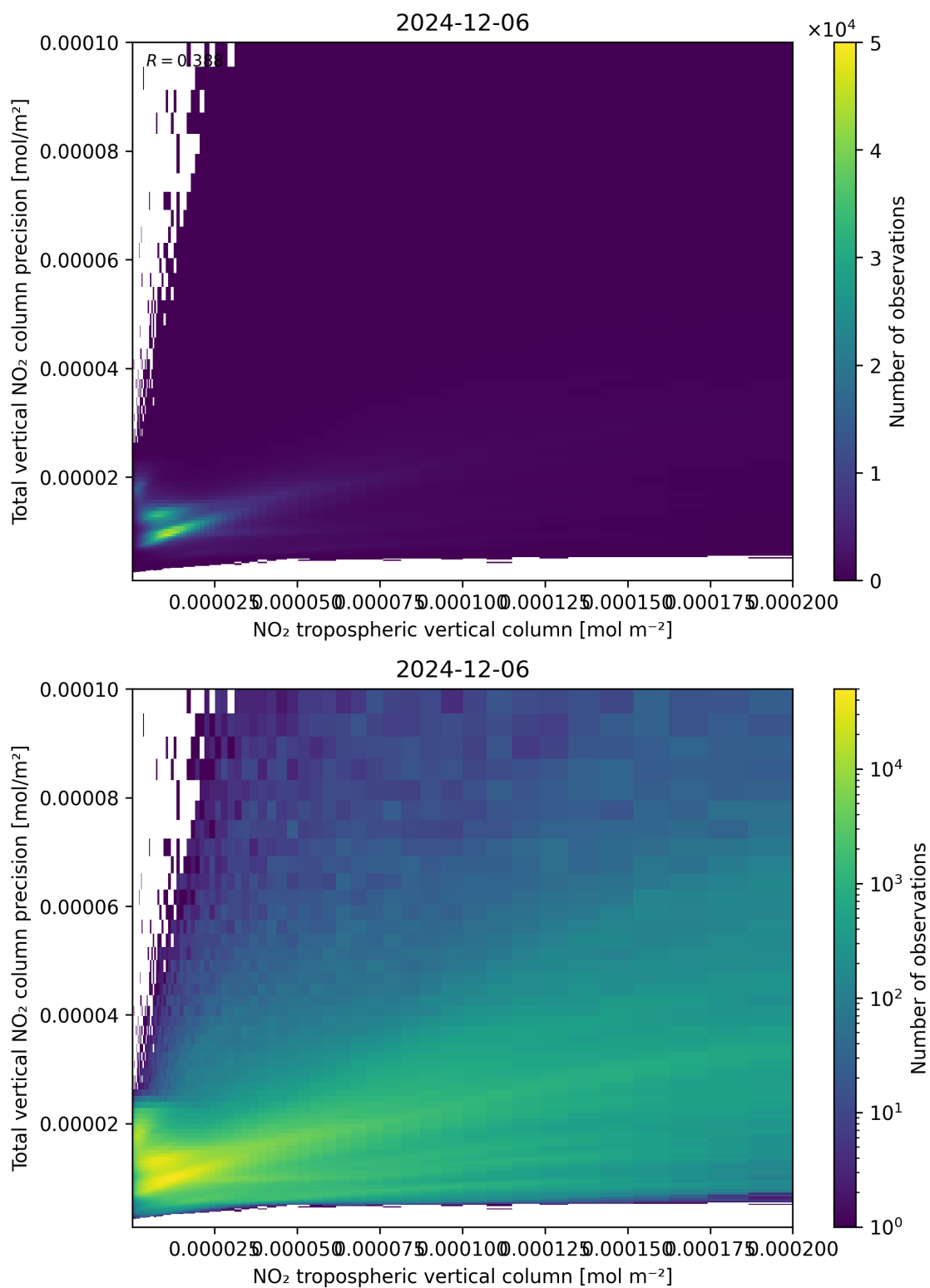
Figure 129: Scatter density plot of “NO 2 tropospheric vertical column” against “Total vertical NO 2 column precision” for 2024-12-06 to 2024-12-07.
