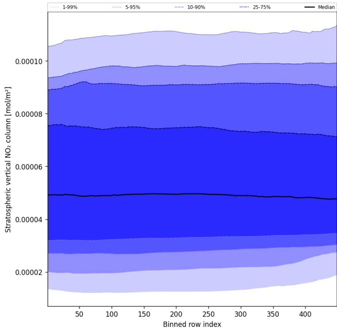
Figure 53: Along track statistics of “Stratospheric vertical NO 2 column” for 2024-12-06 to 2024-12-07
