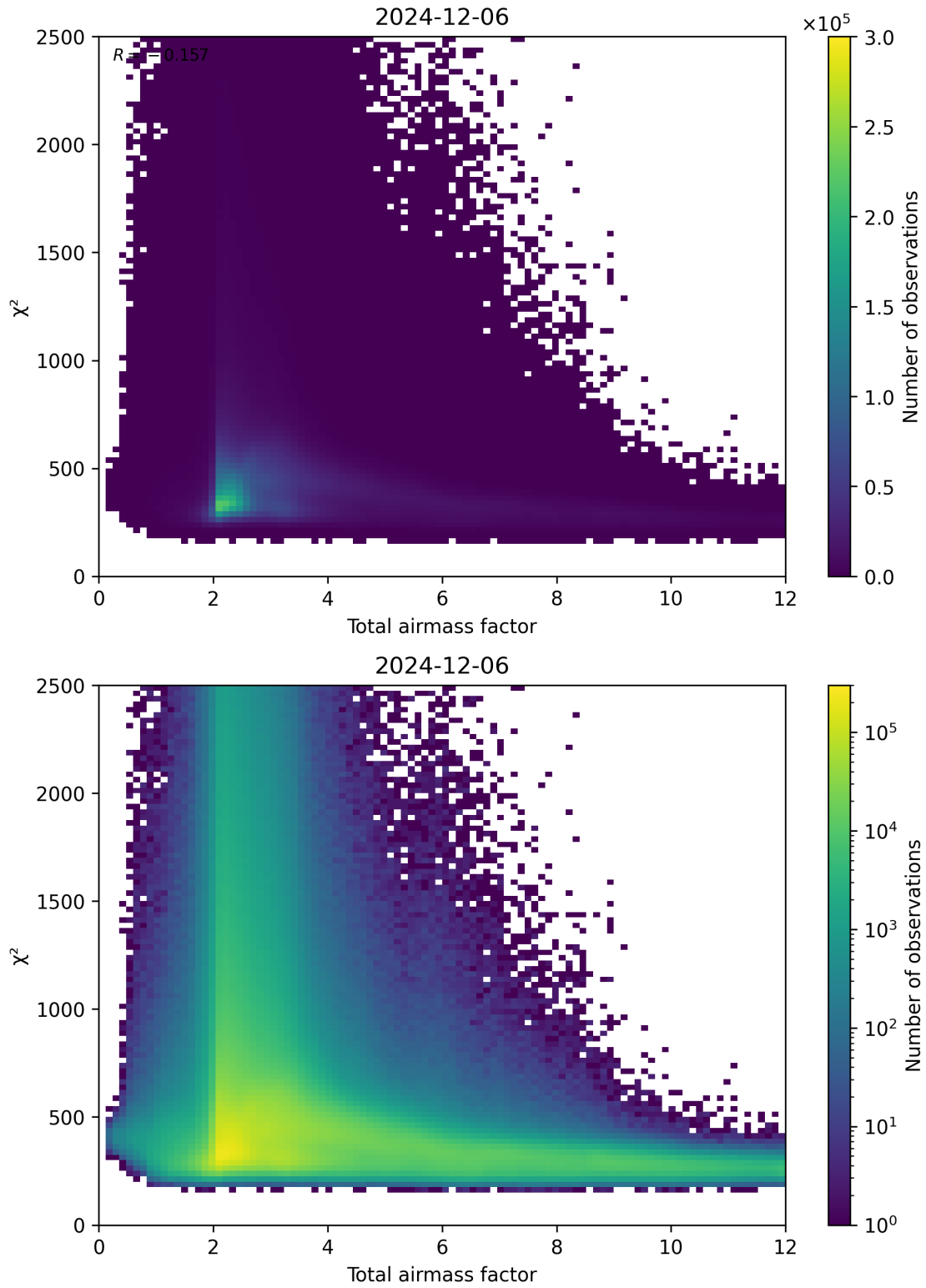
Figure 63: Scatter density plot of “Total airmass factor” against “ \chi^2 ” for 2024-12-06 to 2024-12-07.
