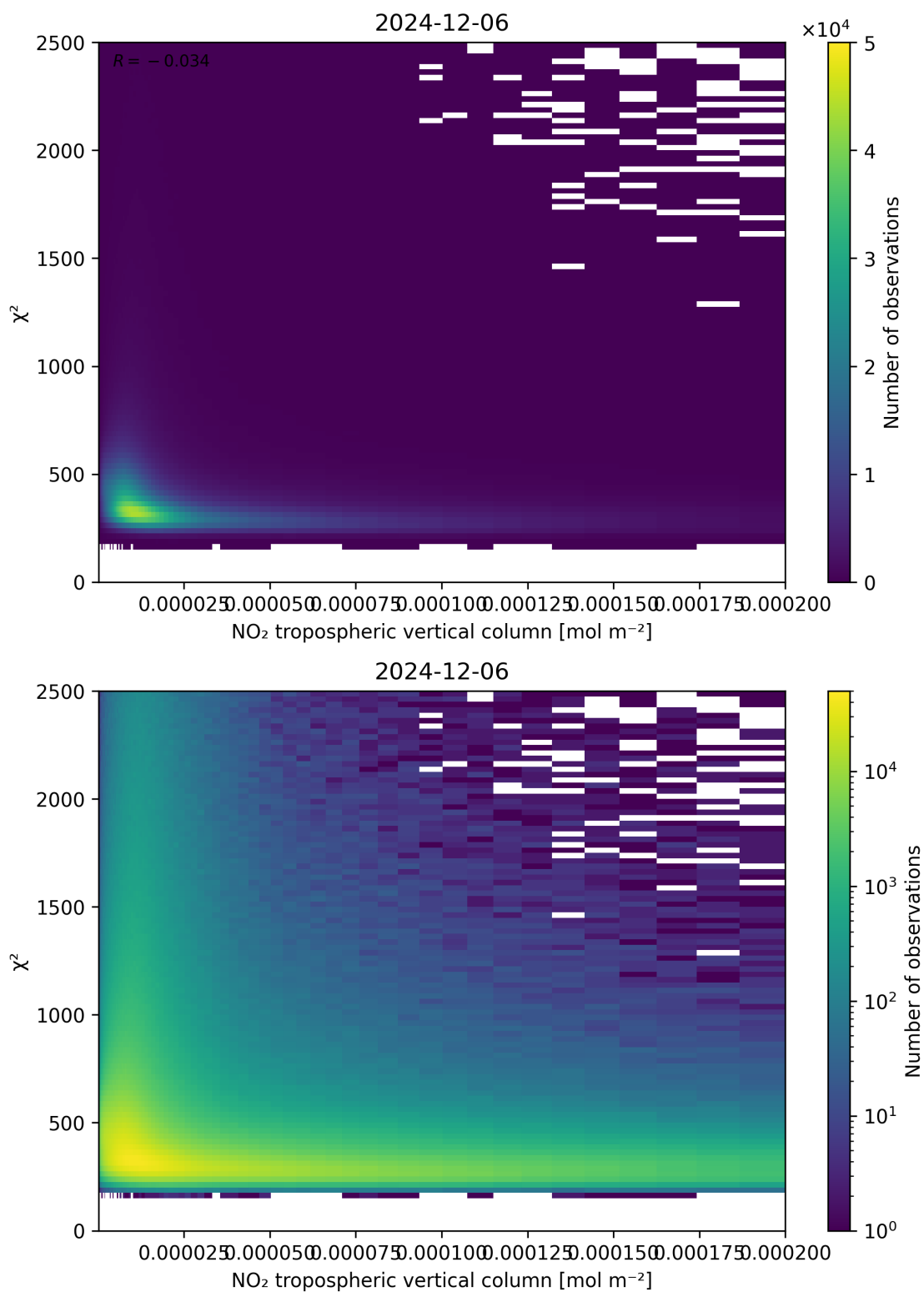
Figure 124: Scatter density plot of “NO 2 tropospheric vertical column” against “ \chi^2 ” for 2024-12-06 to 2024-12-07.
