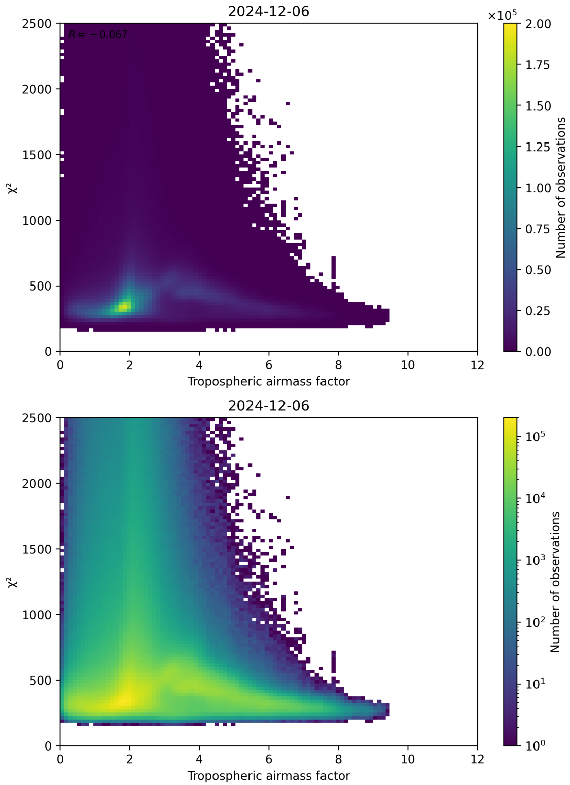
Figure 73: Scatter density plot of “Tropospheric airmass factor” against “ \chi^2 ” for 2024-12-06 to 2024-12-07.
