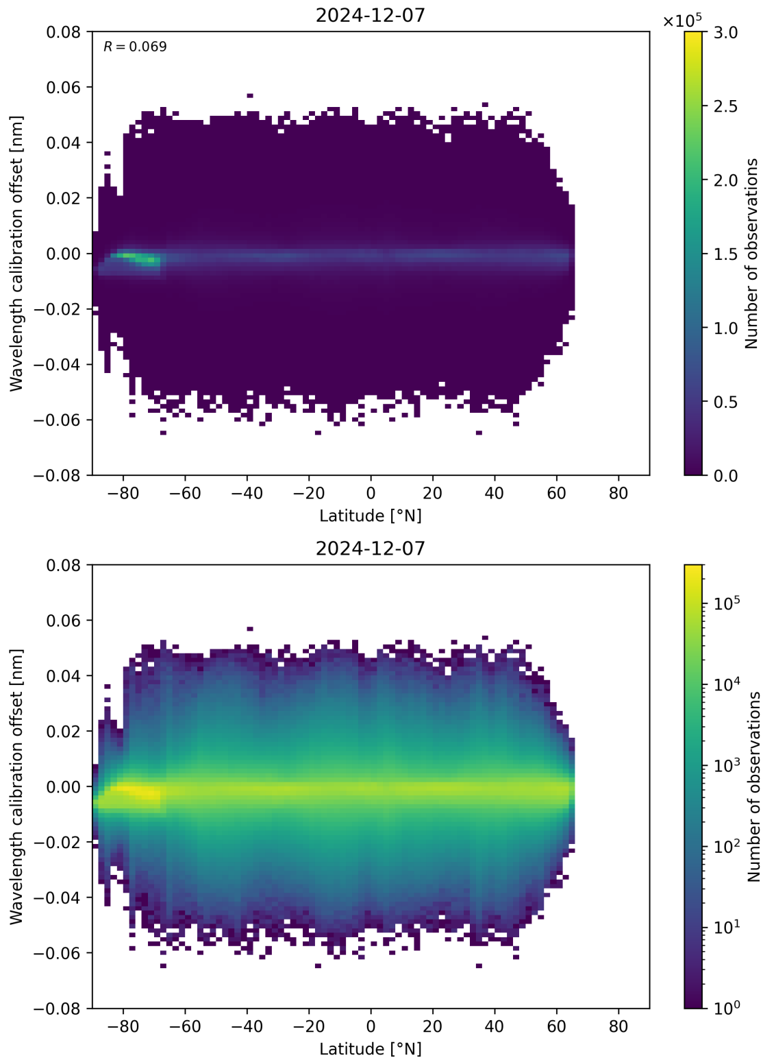
Figure 95: Scatter density plot of “Latitude” against “Wavelength calibration offset” for 2024-12-06 to 2024-12-08.
