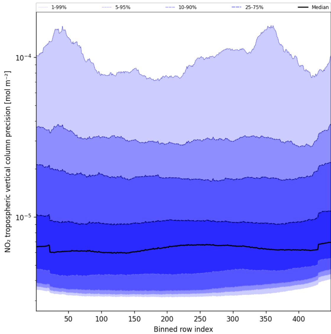
Figure 47: Along track statistics of “NO 2 tropospheric vertical column precision” for 2024-12-06 to 2024-12-08
