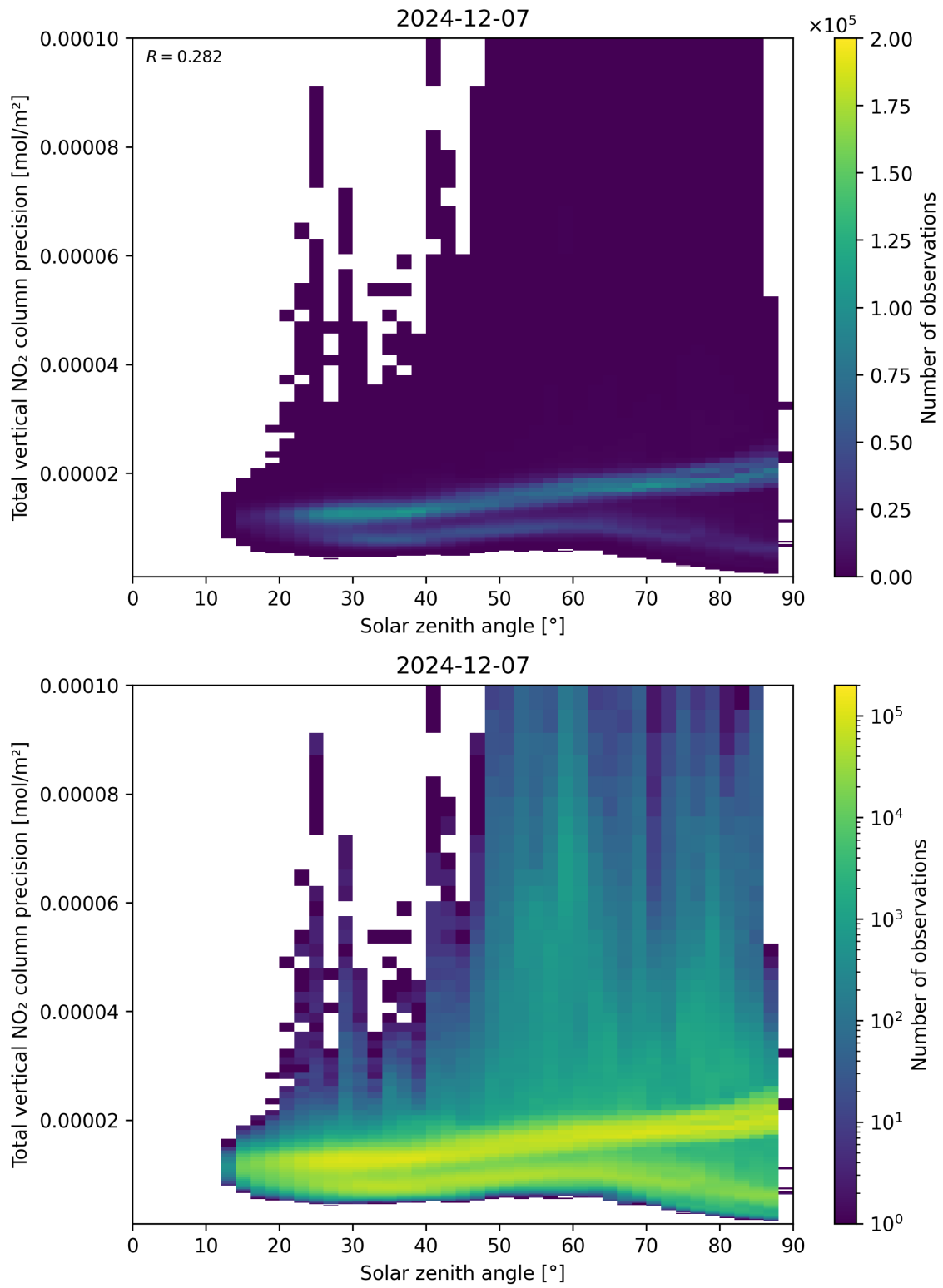
Figure 154: Scatter density plot of “Solar zenith angle” against “Total vertical NO 2 column precision” for 2024-12-06 to 2024-12-08.
