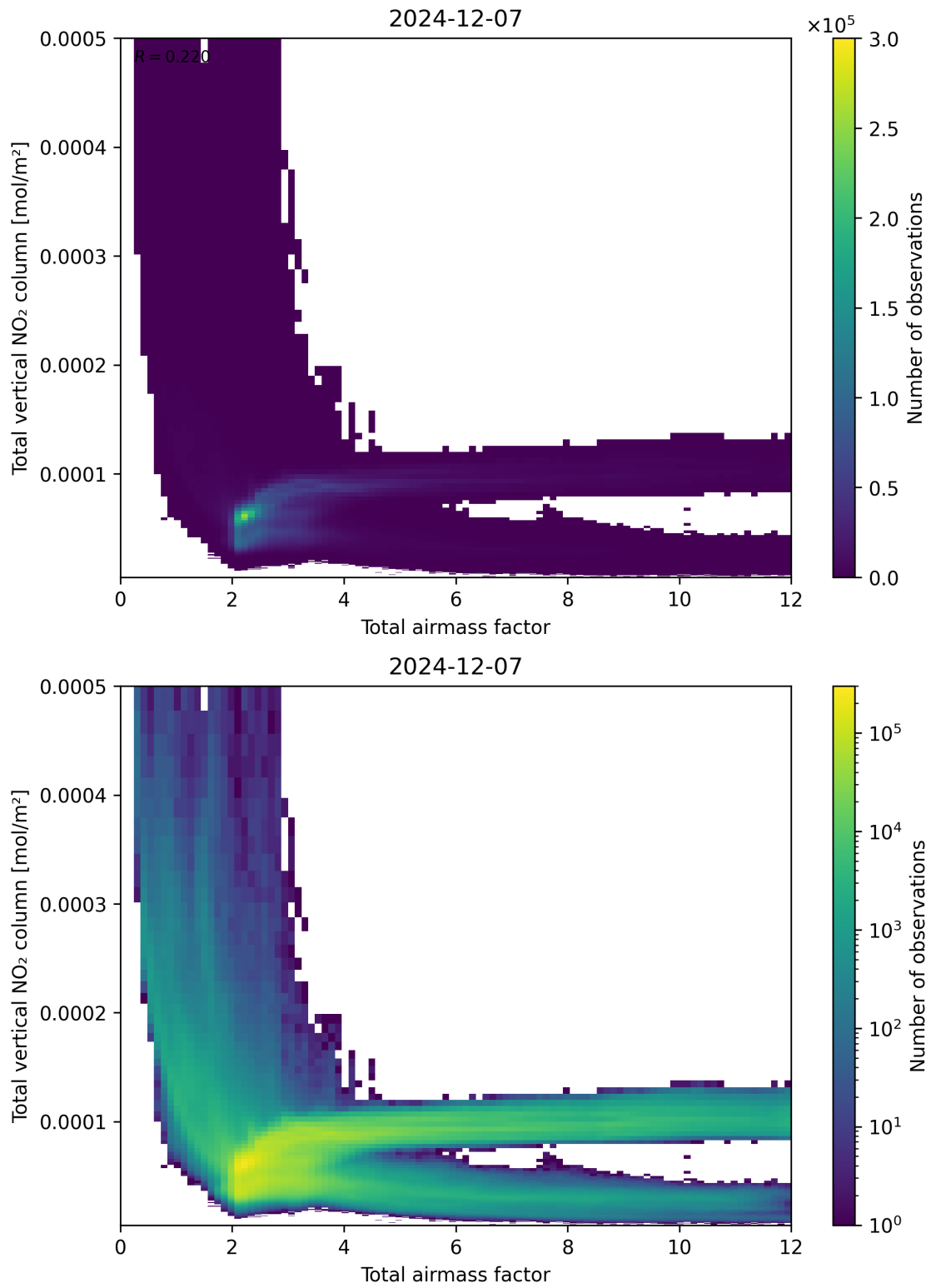
Figure 67: Scatter density plot of “Total air mass factor” against “Total vertical NO 2 column” for 2024-12-06 to 2024-12-08.
