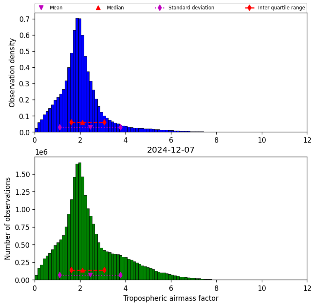
Figure 31: Histogram of “Tropospheric airmass factor” for 2024-12-06 to 2024-12-08
