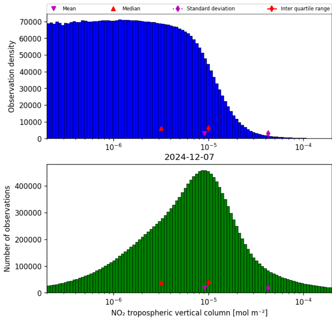
Figure 29: Histogram of “NO 2 tropospheric vertical column” for 2024-12-06 to 2024-12-08
