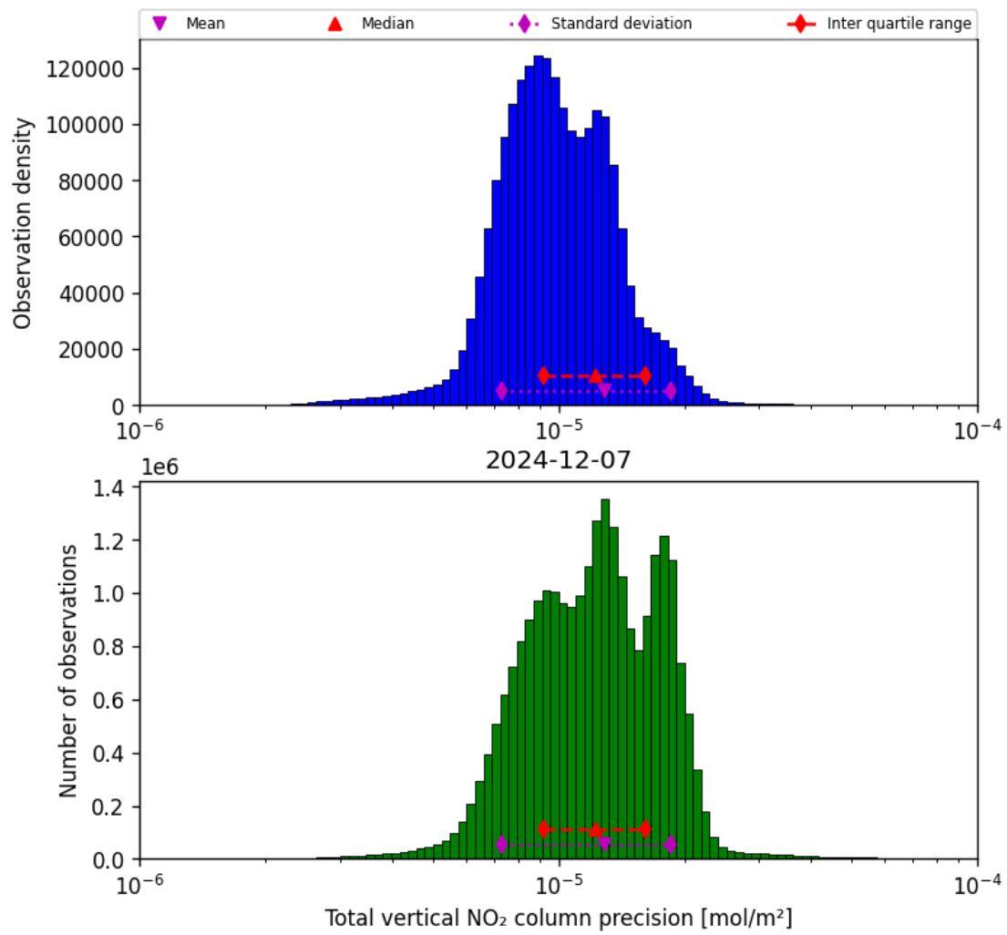
Figure 39: Histogram of “Total vertical NO 2 column precision” for 2024-12-06 to 2024-12-08
