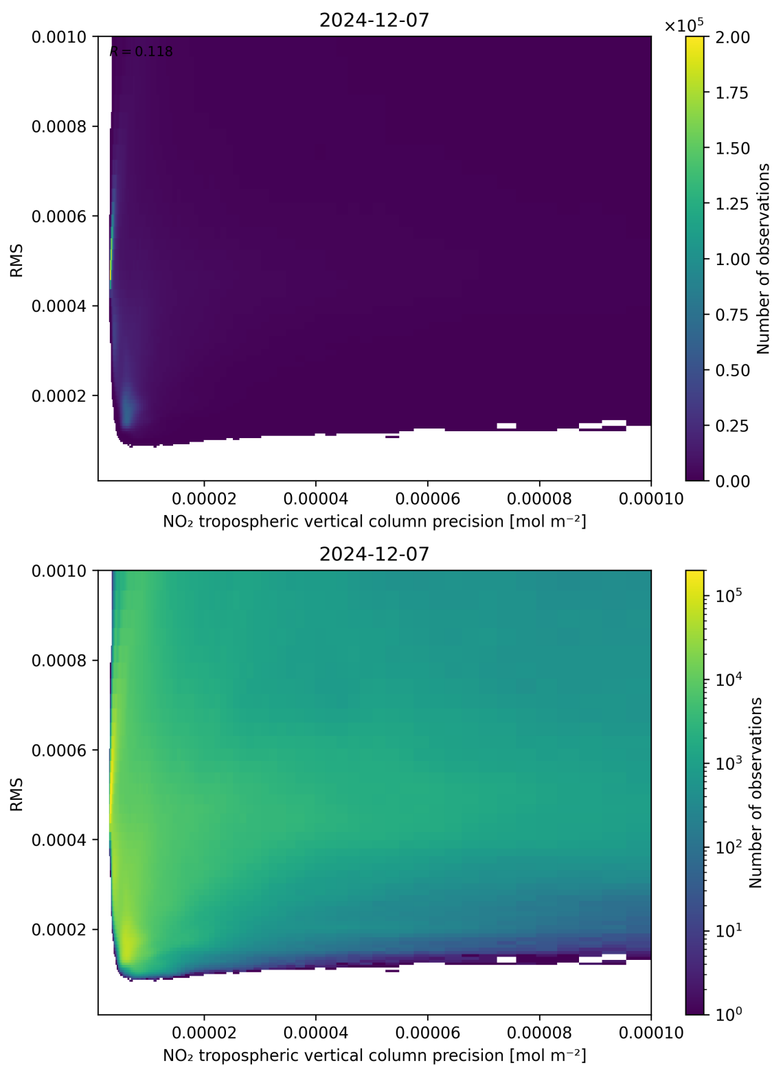
Figure 140: Scatter density plot of “NO 2 tropospheric vertical column precision” against “RMS” for 2024-12-06 to 2024-12-08.
