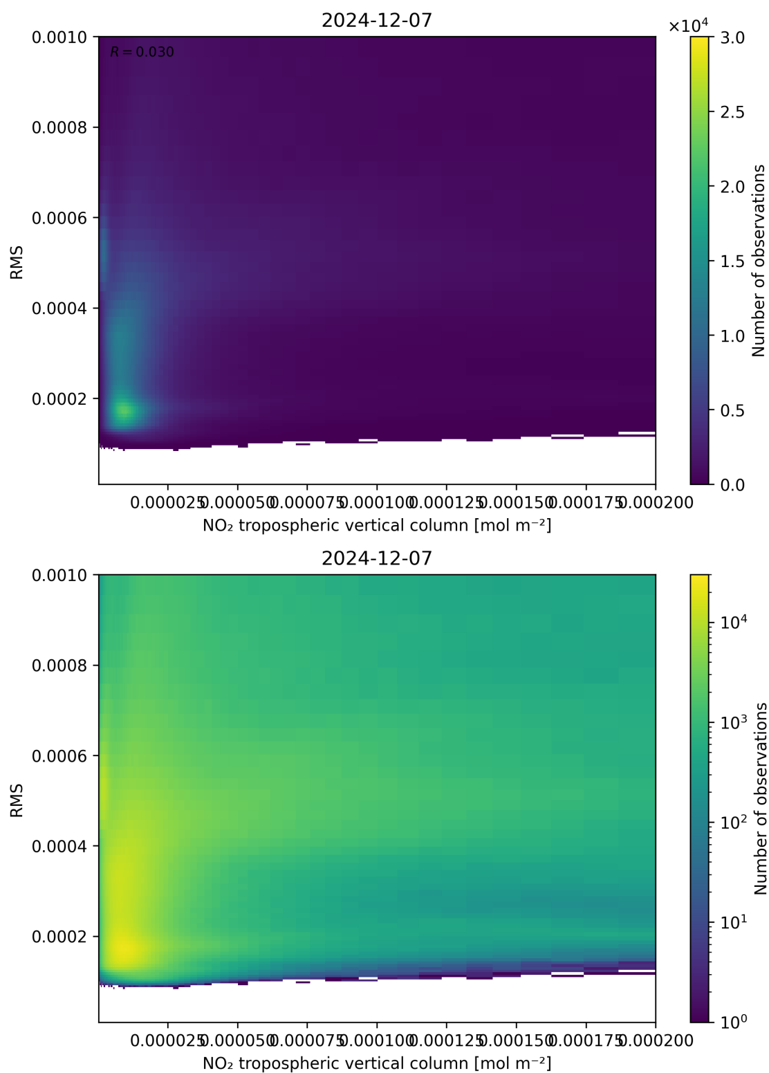
Figure 142: Scatter density plot of “NO 2 tropospheric vertical column” against “RMS” for 2024-12-06 to 2024-12-08.
