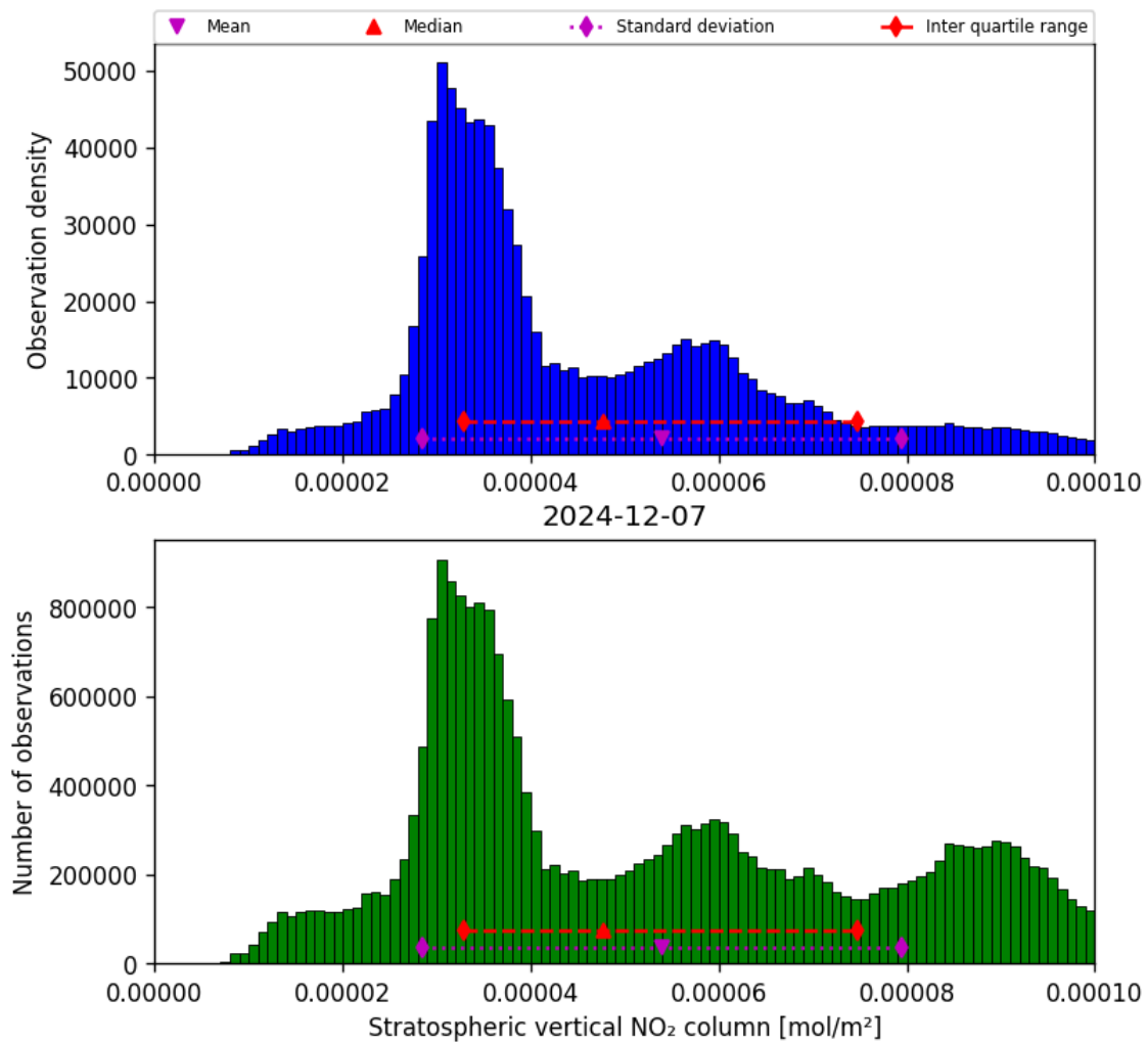
Figure 36: Histogram of “Stratospheric vertical NO 2 column” for 2024-12-06 to 2024-12-08
