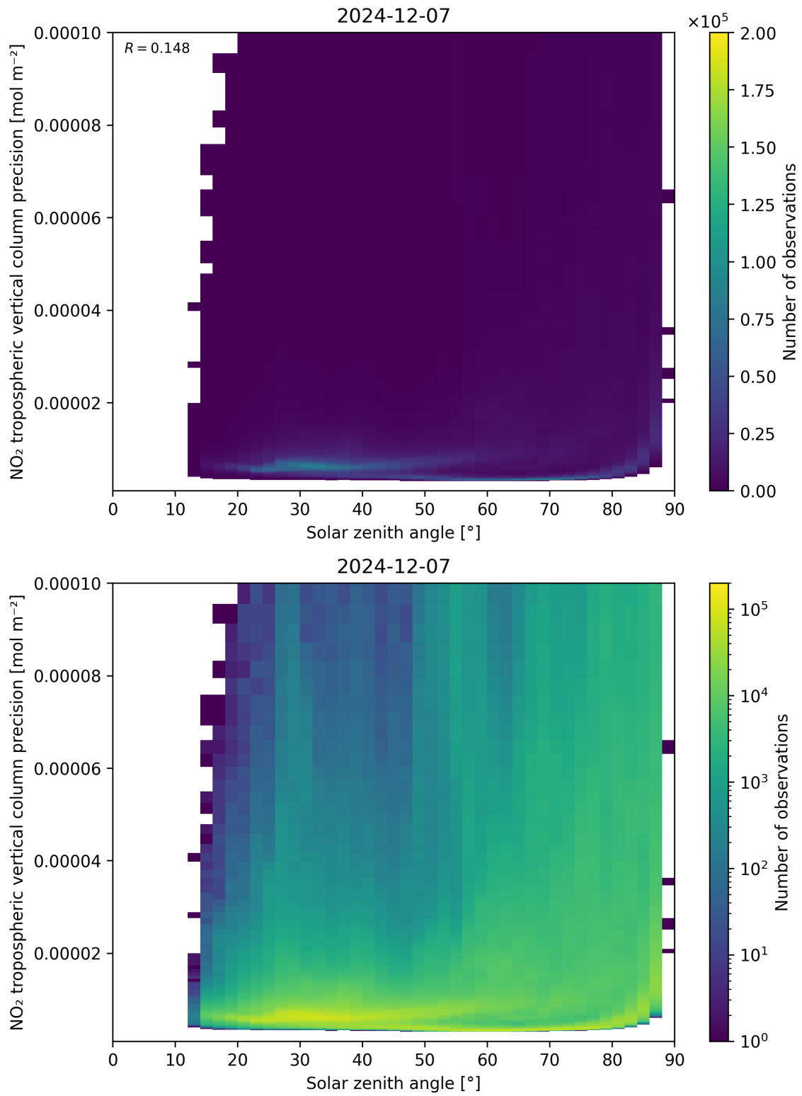
Figure 156: Scatter density plot of “Solar zenith angle” against “NO 2 tropospheric vertical column precision” for 2024-12-06 to 2024-12-08.
