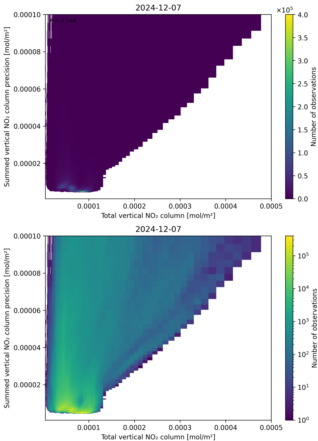
Figure 113: Scatter density plot of “Total vertical NO 2 column” against “Summed vertical NO 2 column precision” for 2024-12-06 to 2024-12-08.
