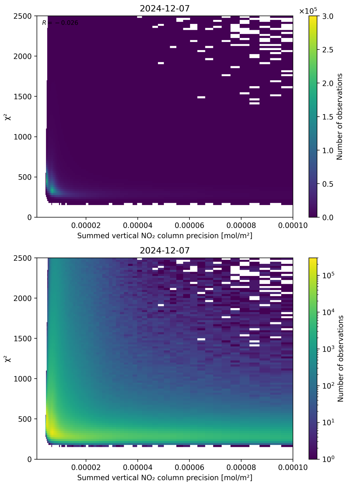
Figure 107: Scatter density plot of “Summed vertical NO 2 column precision” against “ \chi^2 ” for 2024-12-06 to 2024-12-08.
