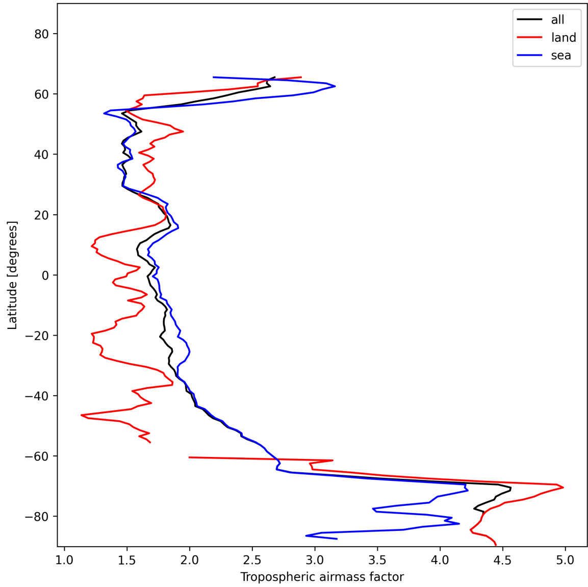
Figure 14: Zonal average of “Tropospheric air mass factor” for 2024-12-06 to 2024-12-08.
