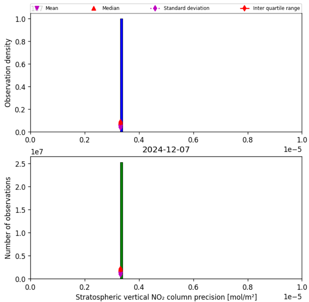
Figure 37: Histogram of “Stratospheric vertical NO 2 column precision” for 2024-12-06 to 2024-12-08
