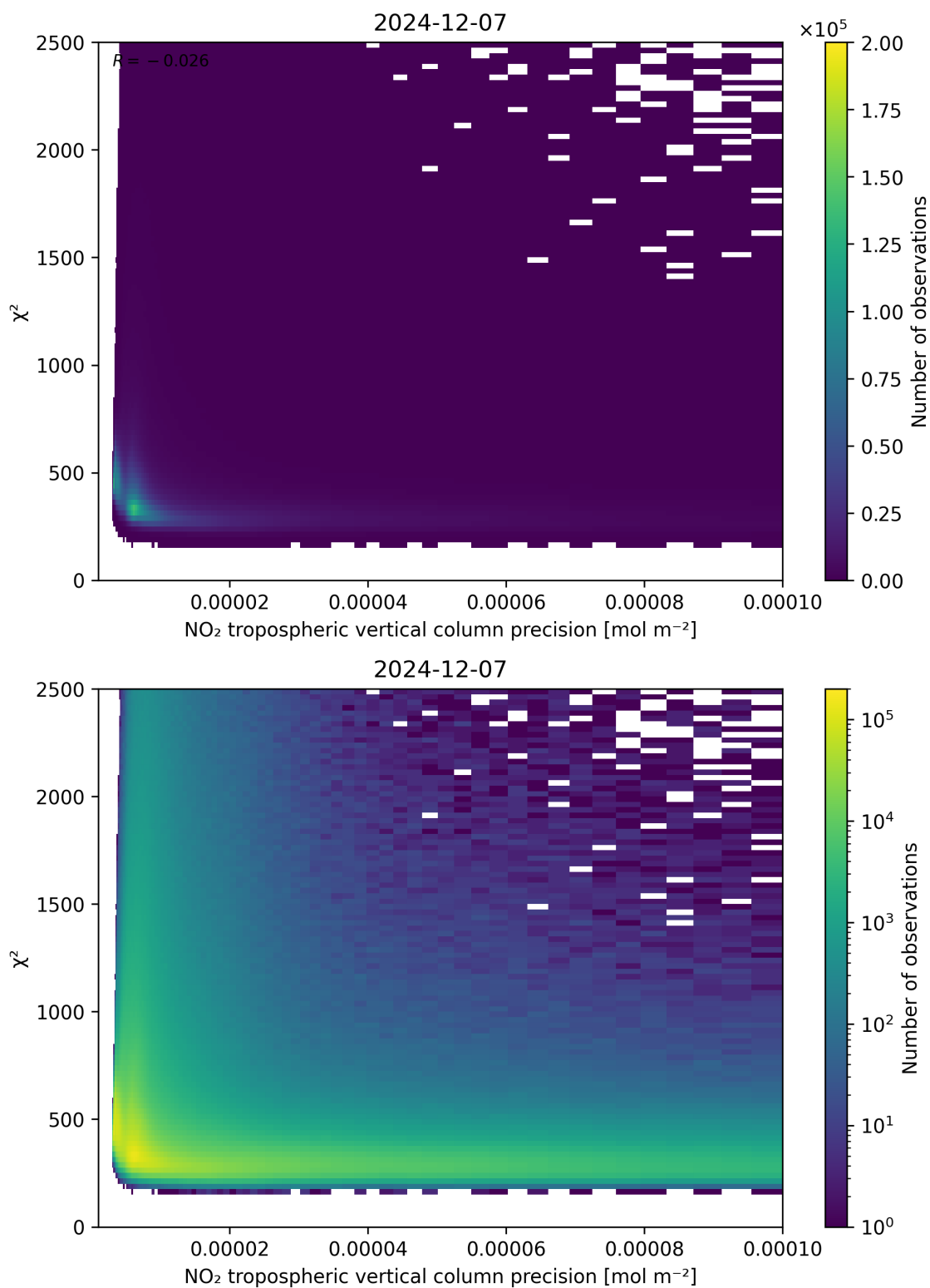
Figure 134: Scatter density plot of “NO 2 tropospheric vertical column precision” against “ \chi^2 ” for 2024-12-06 to 2024-12-08.
