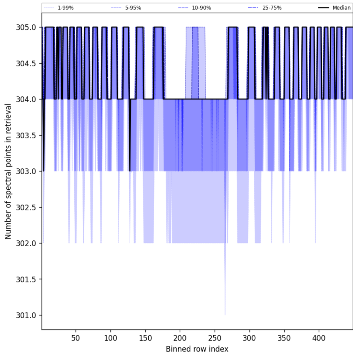
Figure 50: Along track statistics of “Number of spectral points in retrieval” for 2024-12-06 to 2024-12-08
