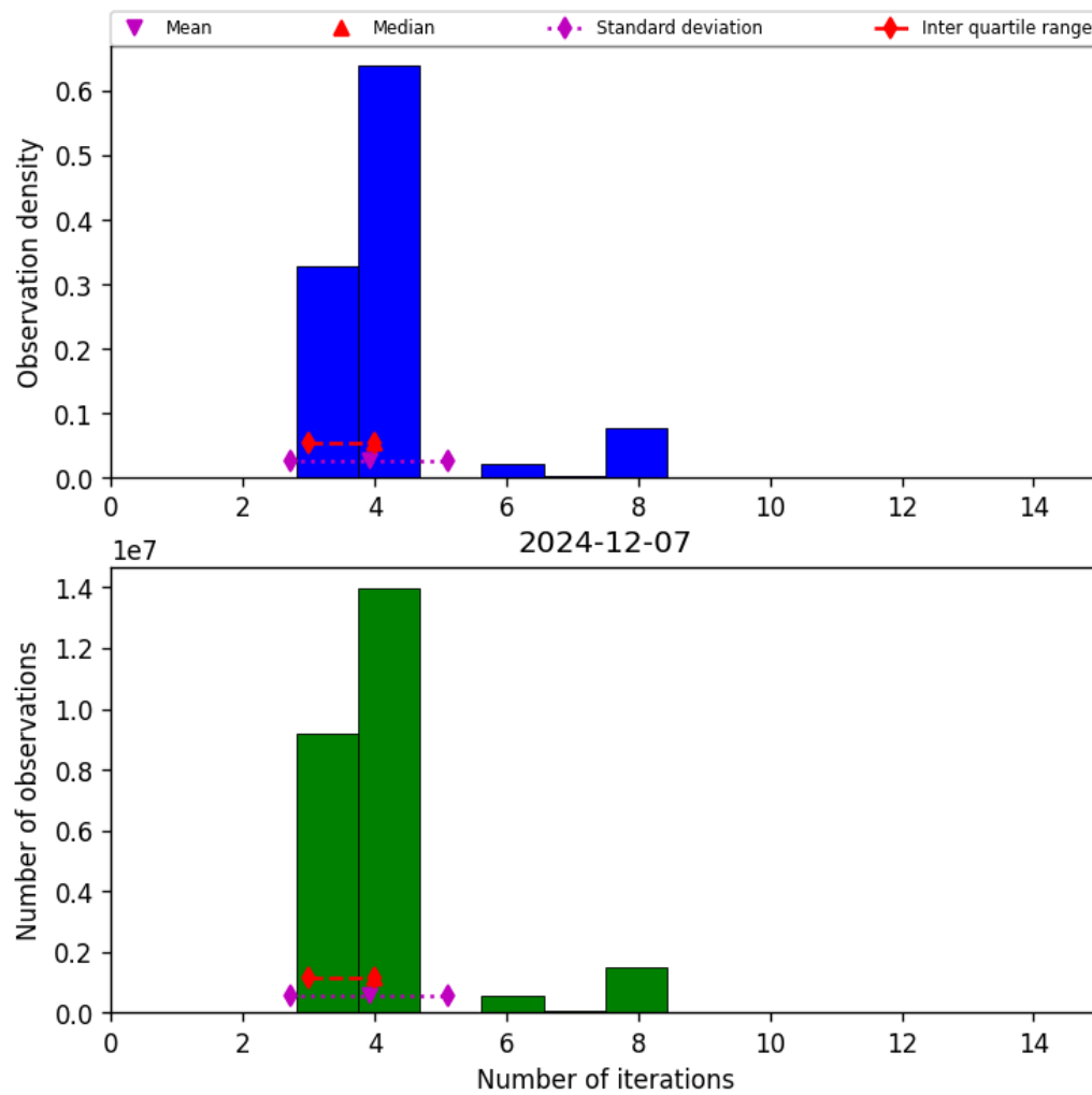
Figure 34: Histogram of “Number of iterations” for 2024-12-06 to 2024-12-08
