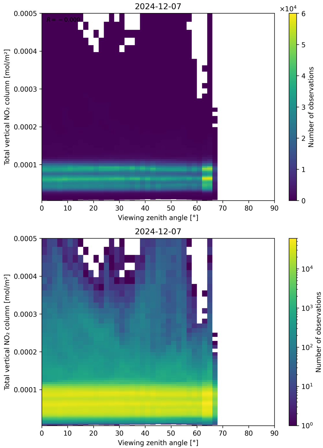
Figure 167: Scatter density plot of “Viewing zenith angle” against “Total vertical NO 2 column” for 2024-12-06 to 2024-12-08.
