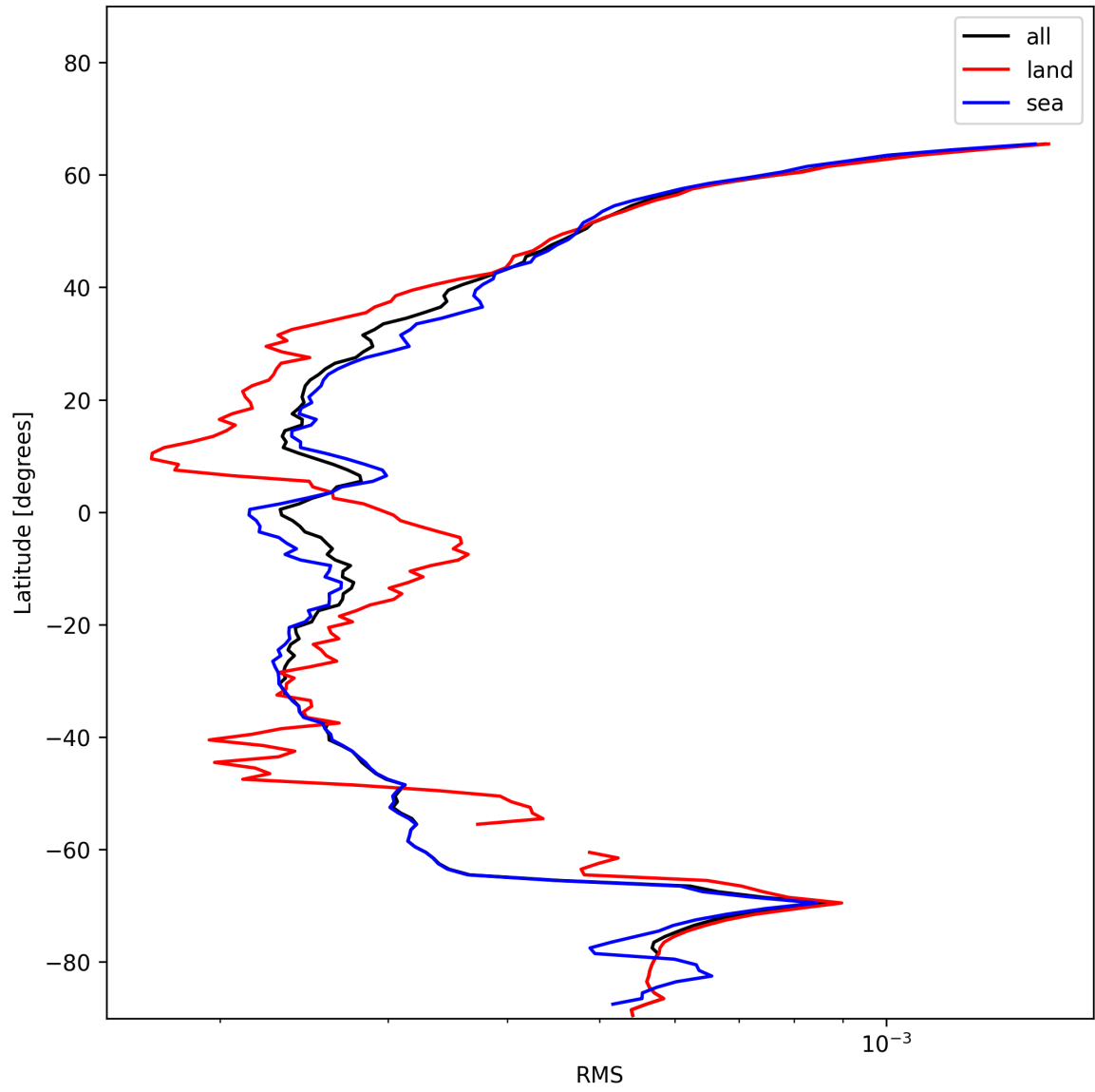
Figure 26: Zonal average of “RMS” for 2024-12-06 to 2024-12-08.
