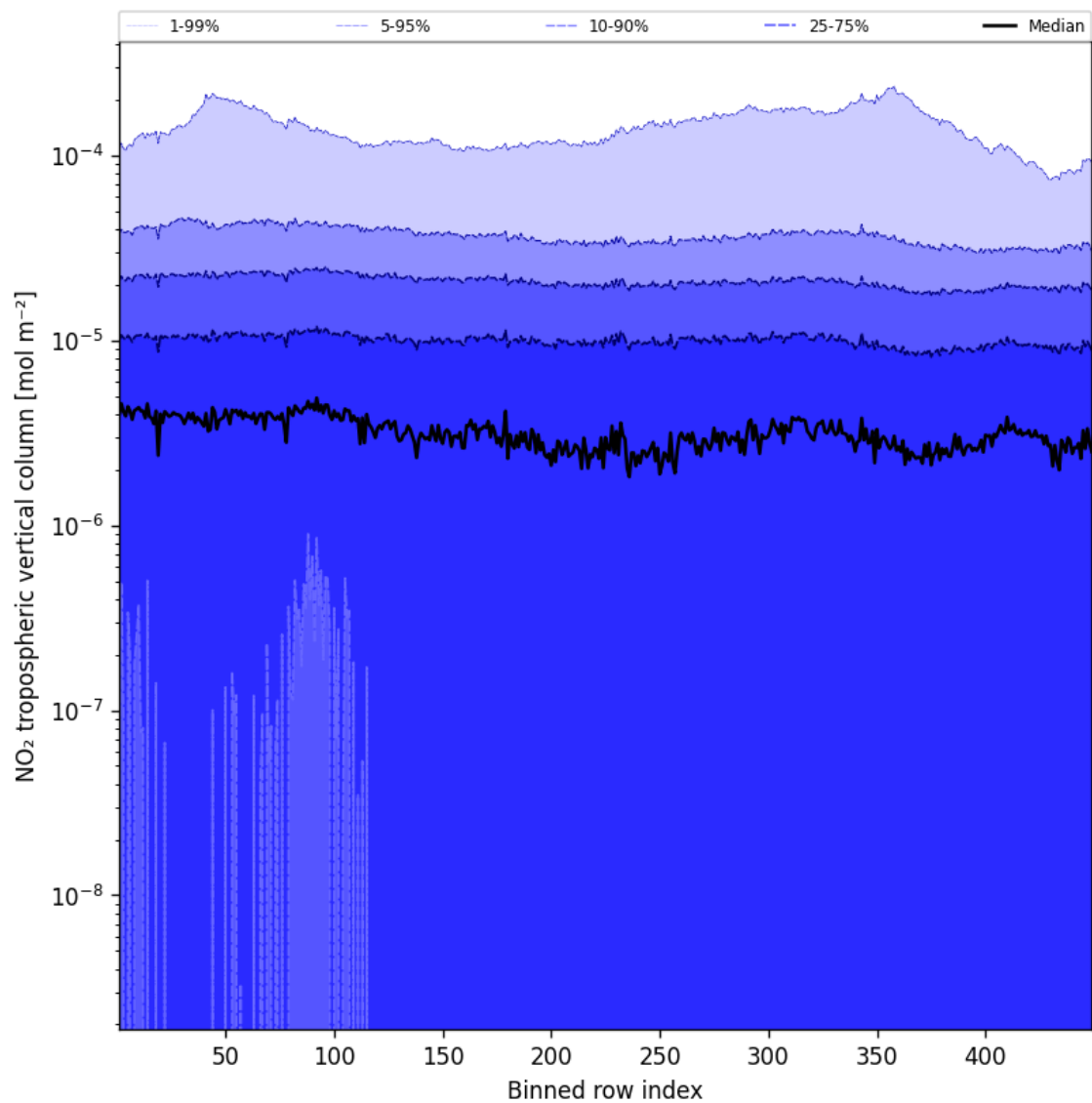
Figure 46: Along track statistics of “ \text{NO}_2 tropospheric vertical column” for 2024-12-06 to 2024-12-08
