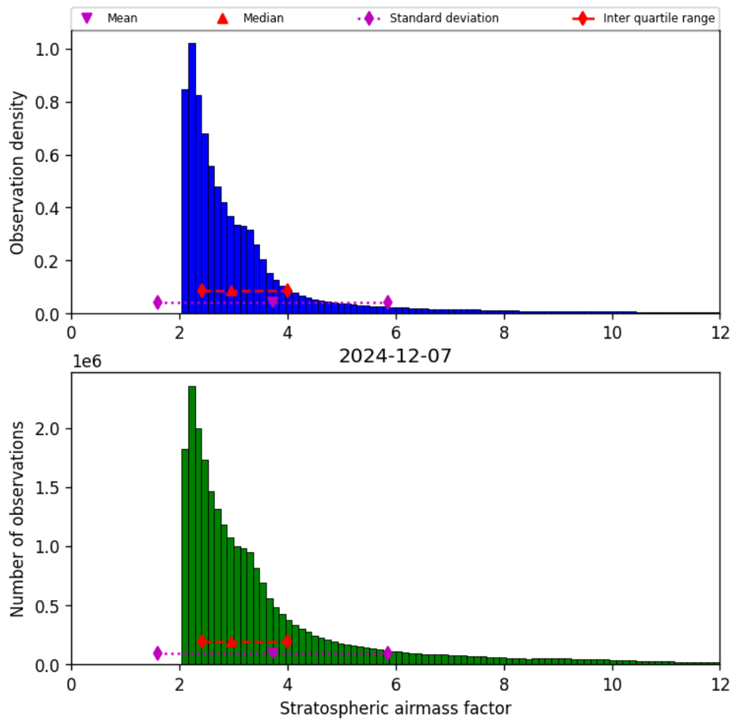
Figure 44: Histogram of “Stratospheric airmass factor” for 2024-12-06 to 2024-12-08
