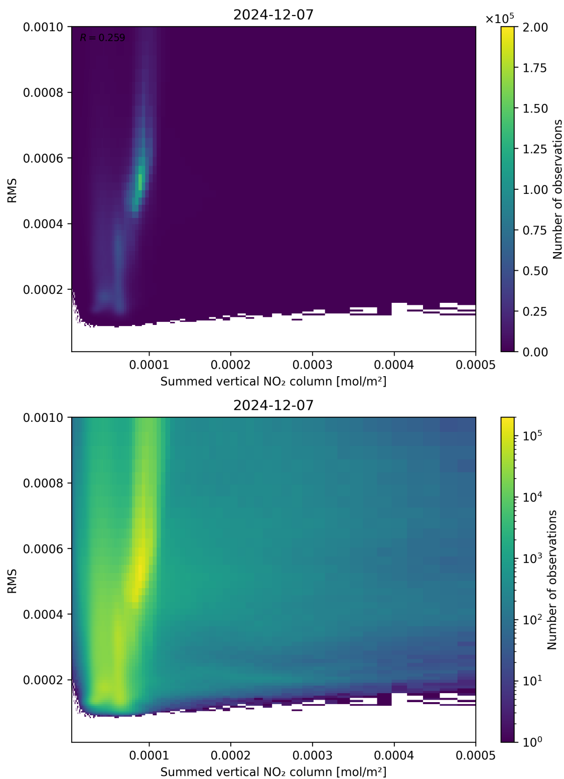
Figure 109: Scatter density plot of “Summed vertical NO 2 column” against “RMS” for 2024-12-06 to 2024-12-08.
