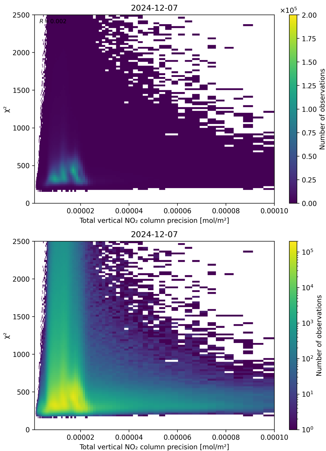
Figure 116: Scatter density plot of “Total vertical NO 2 column precision” against “ \chi^2 ” for 2024-12-06 to 2024-12-08.
