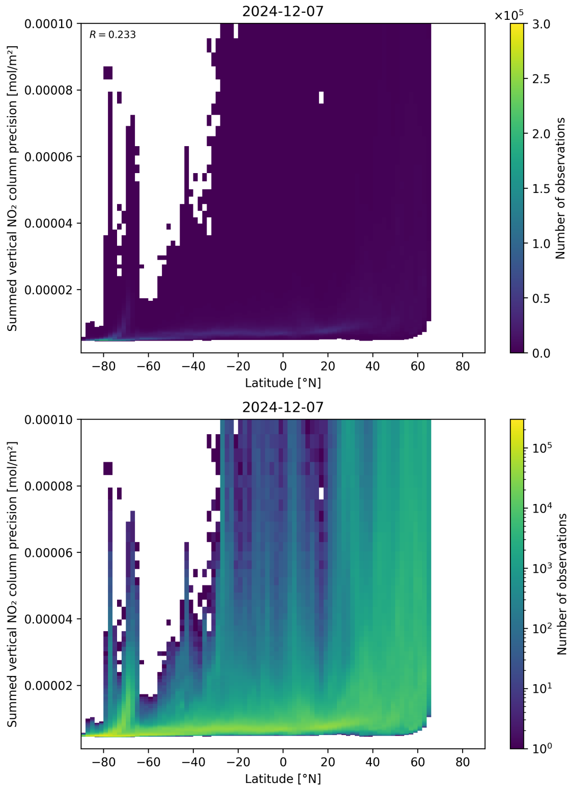
Figure 89: Scatter density plot of “Latitude” against “Summed vertical NO 2 column precision” for 2024-12-06 to 2024-12-08.
