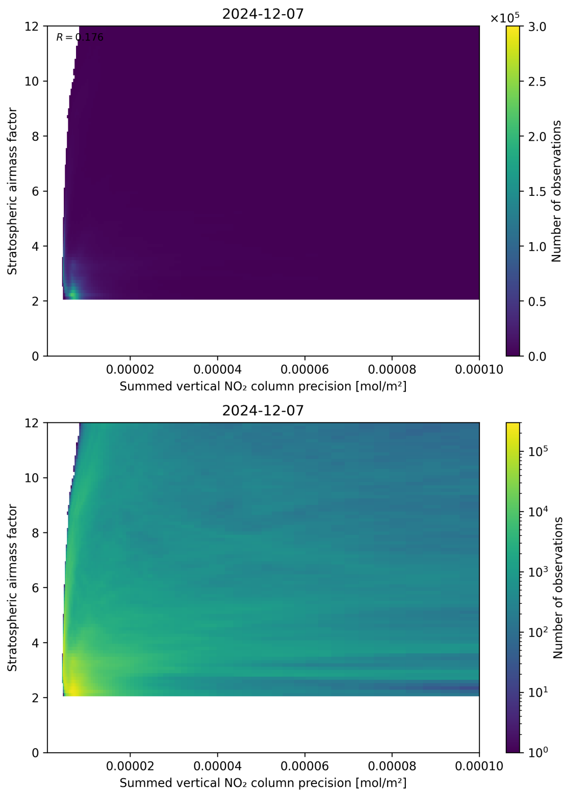
Figure 106: Scatter density plot of “Summed vertical NO 2 column precision” against “Stratospheric airmass factor” for 2024-12-06 to 2024-12-08.
