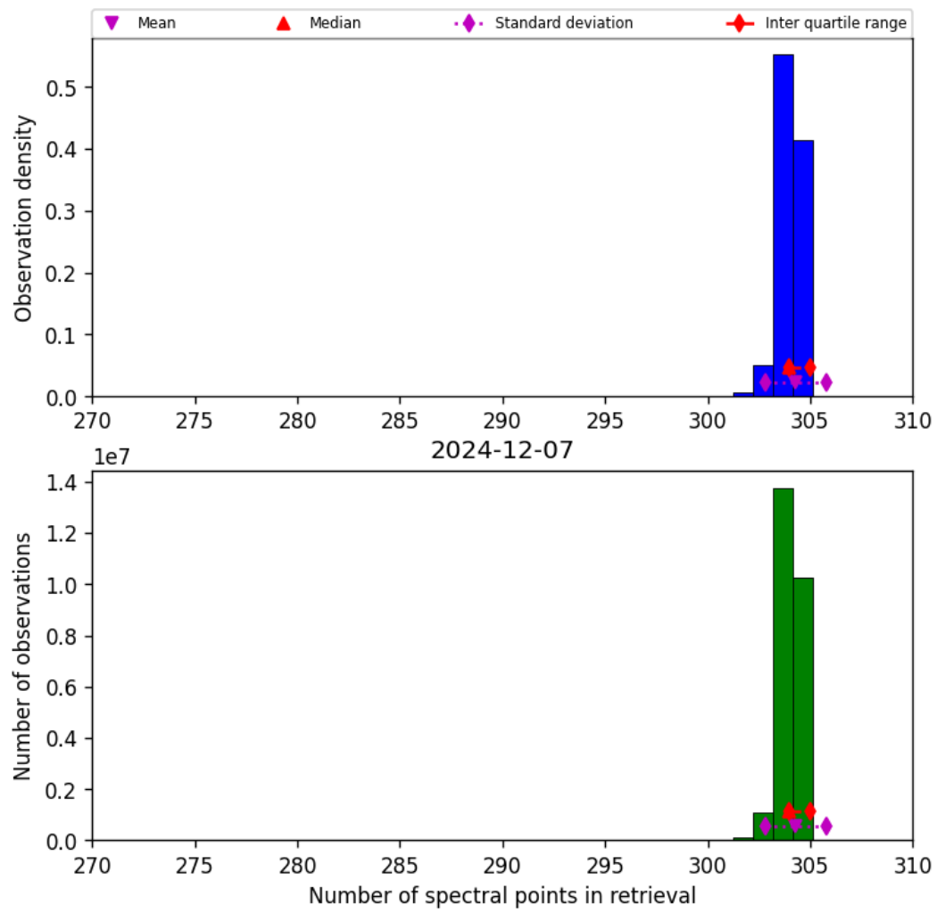
Figure 33: Histogram of “Number of spectral points in retrieval” for 2024-12-06 to 2024-12-08
