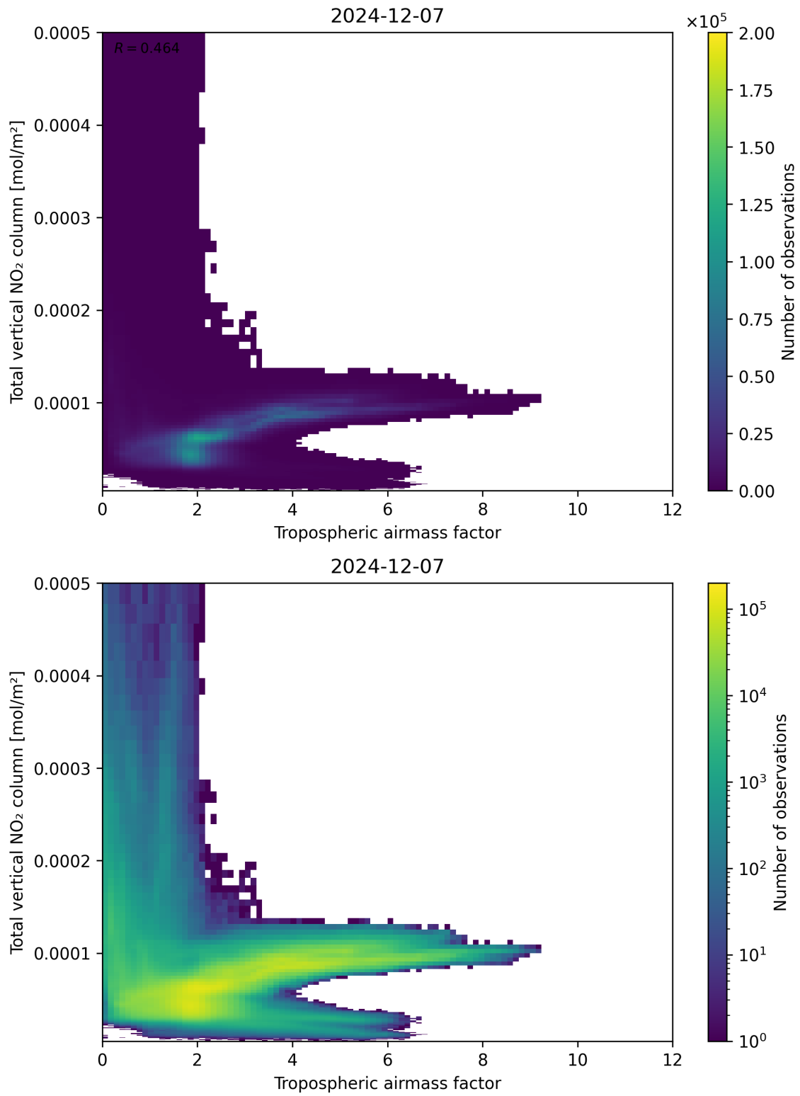
Figure 77: Scatter density plot of “Tropospheric airmass factor” against “Total vertical NO 2 column” for 2024-12-06 to 2024-12-08.
