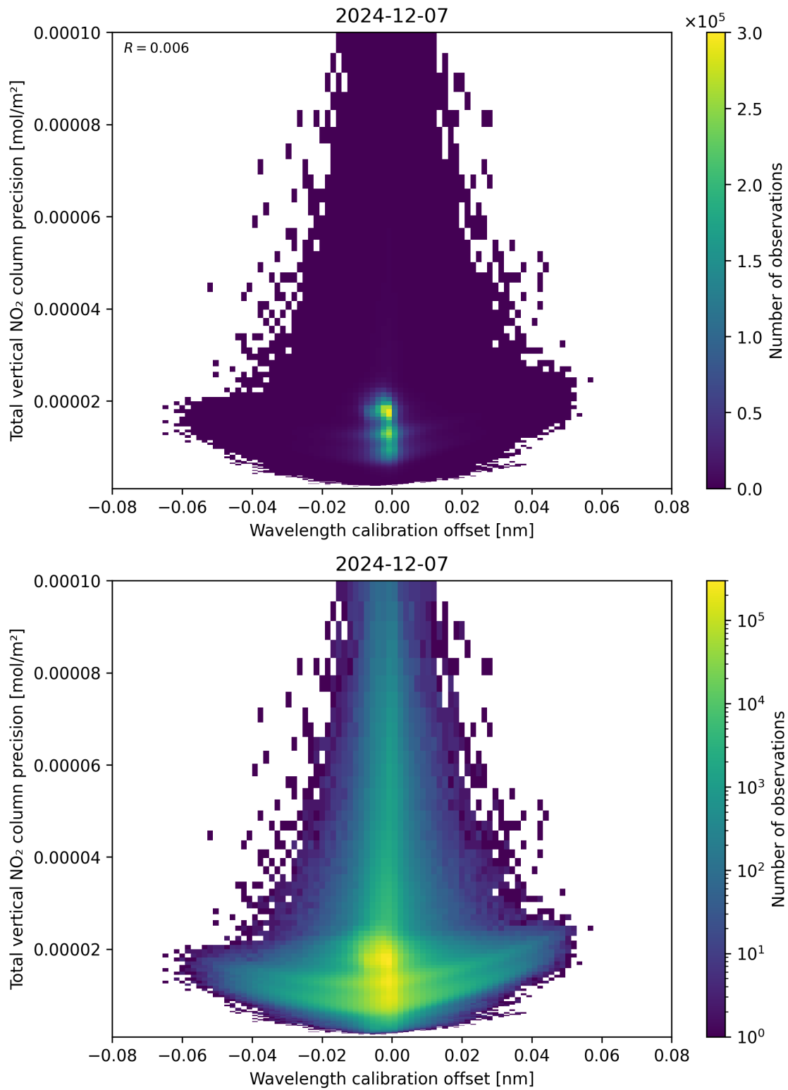
Figure 180: Scatter density plot of “Wavelength calibration offset” against “Total vertical NO 2 column precision” for 2024-12-06 to 2024-12-08.
