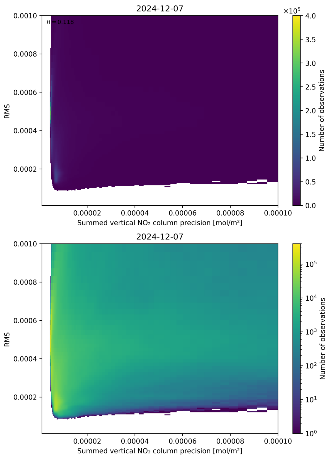
Figure 108: Scatter density plot of “Summed vertical NO 2 column precision” against “RMS” for 2024-12-06 to 2024-12-08.
