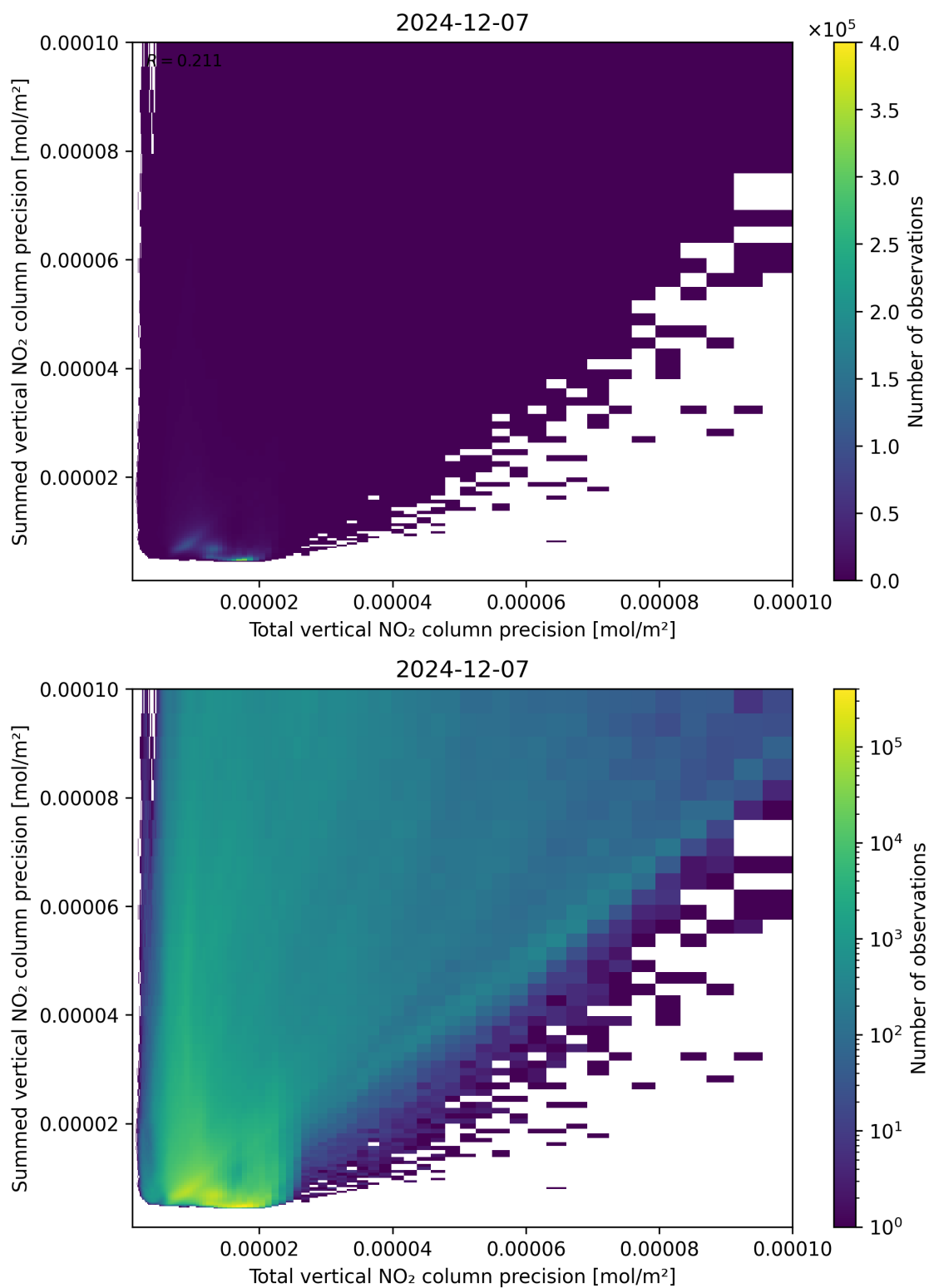
Figure 118: Scatter density plot of “Total vertical NO 2 column precision” against “Summed vertical NO 2 column precision” for 2024-12-06 to 2024-12-08.
