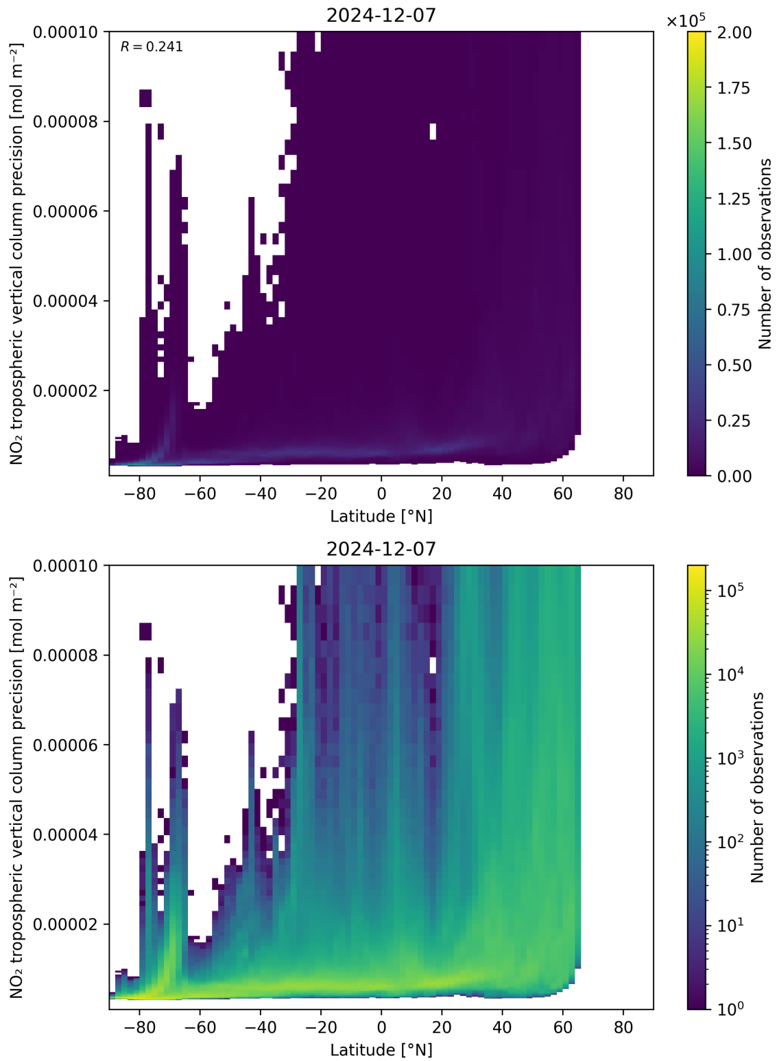
Figure 93: Scatter density plot of “Latitude” against “NO 2 tropospheric vertical column precision” for 2024-12-06 to 2024-12-08.
