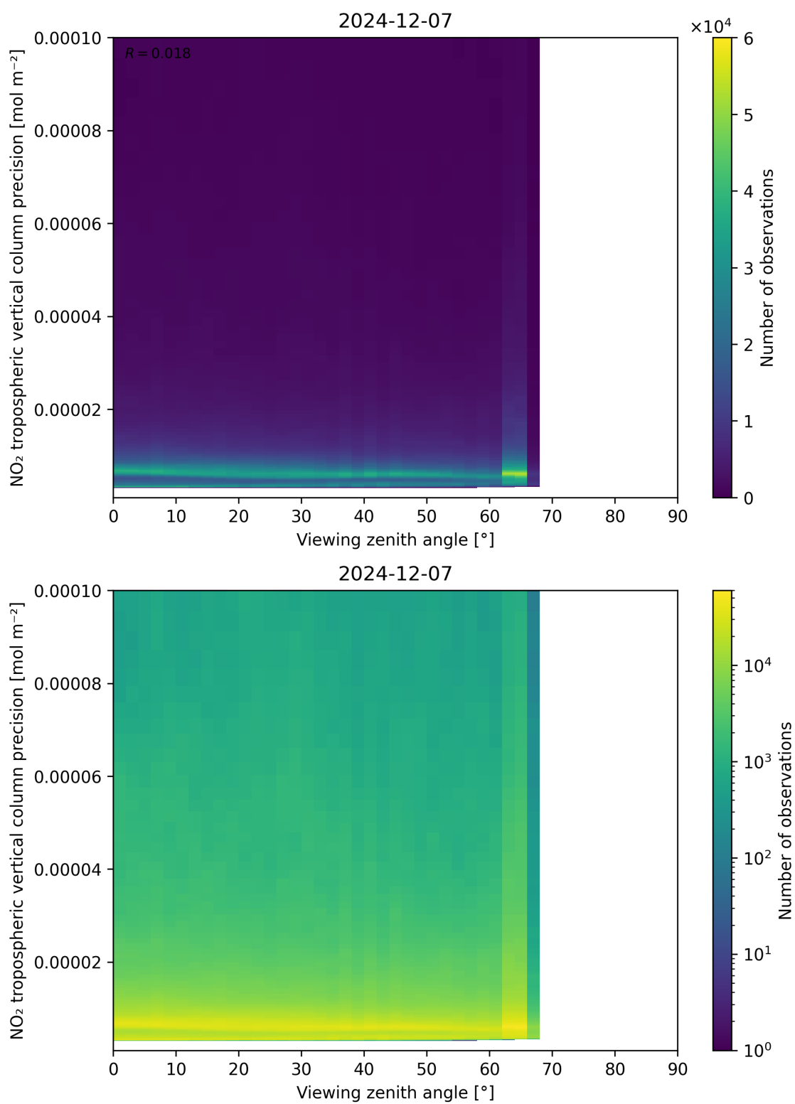
Figure 170: Scatter density plot of “Viewing zenith angle” against “NO 2 tropospheric vertical column precision” for 2024-12-06 to 2024-12-08.
