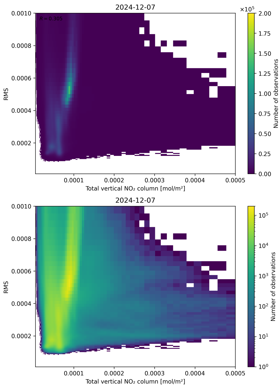
Figure 120: Scatter density plot of “Total vertical NO 2 column” against “RMS” for 2024-12-06 to 2024-12-08.
