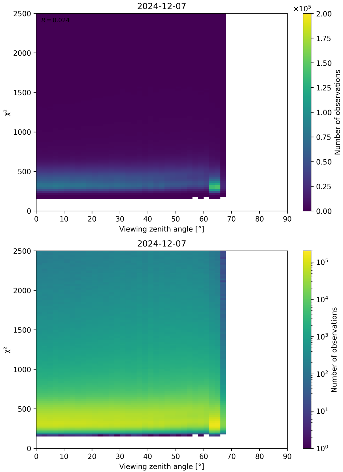
Figure 162: Scatter density plot of “Viewing zenith angle” against “ \chi^2 ” for 2024-12-06 to 2024-12-08.
