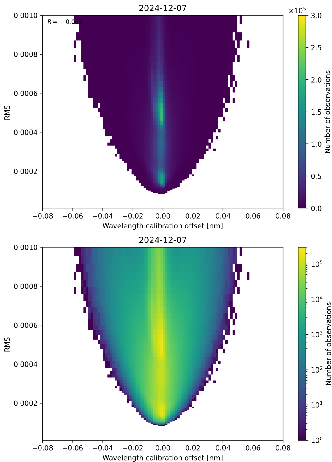
Figure 181: Scatter density plot of “Wavelength calibration offset” against “RMS” for 2024-12-06 to 2024-12-08.
