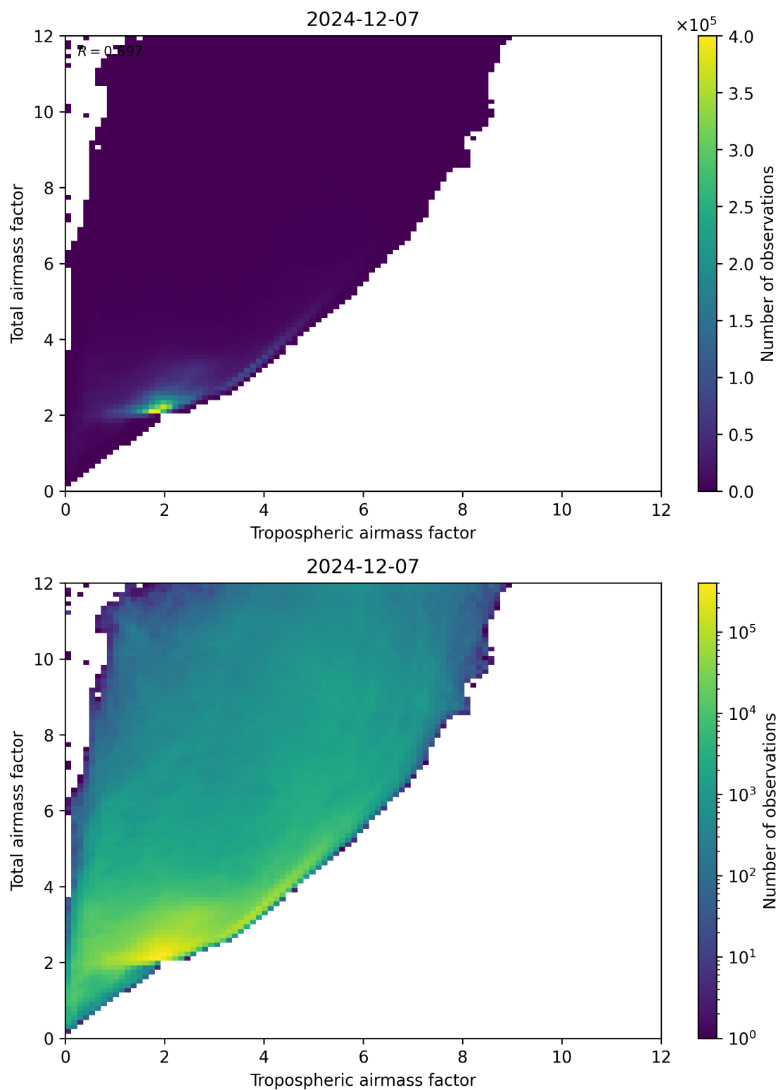
Figure 72: Scatter density plot of “Tropospheric airmass factor” against “Total airmass factor” for 2024-12-06 to 2024-12-08.
