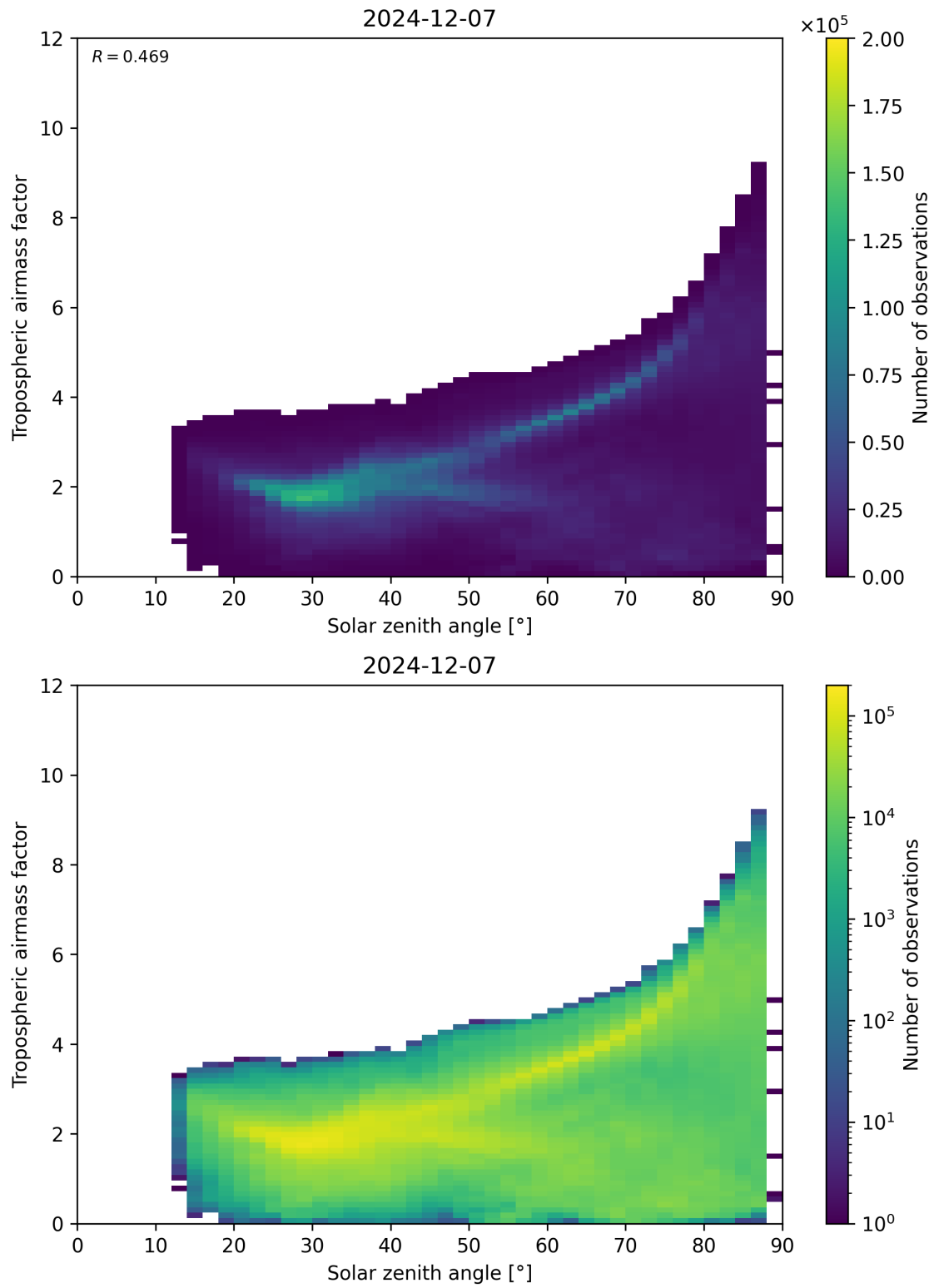
Figure 147: Scatter density plot of “Solar zenith angle” against “Tropospheric airmass factor” for 2024-12-06 to 2024-12-08.
