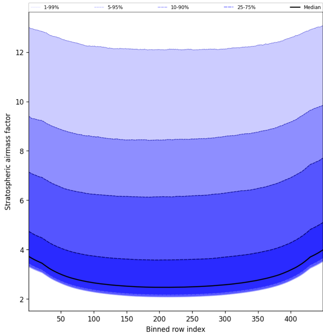
Figure 61: Along track statistics of “Stratospheric air mass factor” for 2024-12-06 to 2024-12-08
