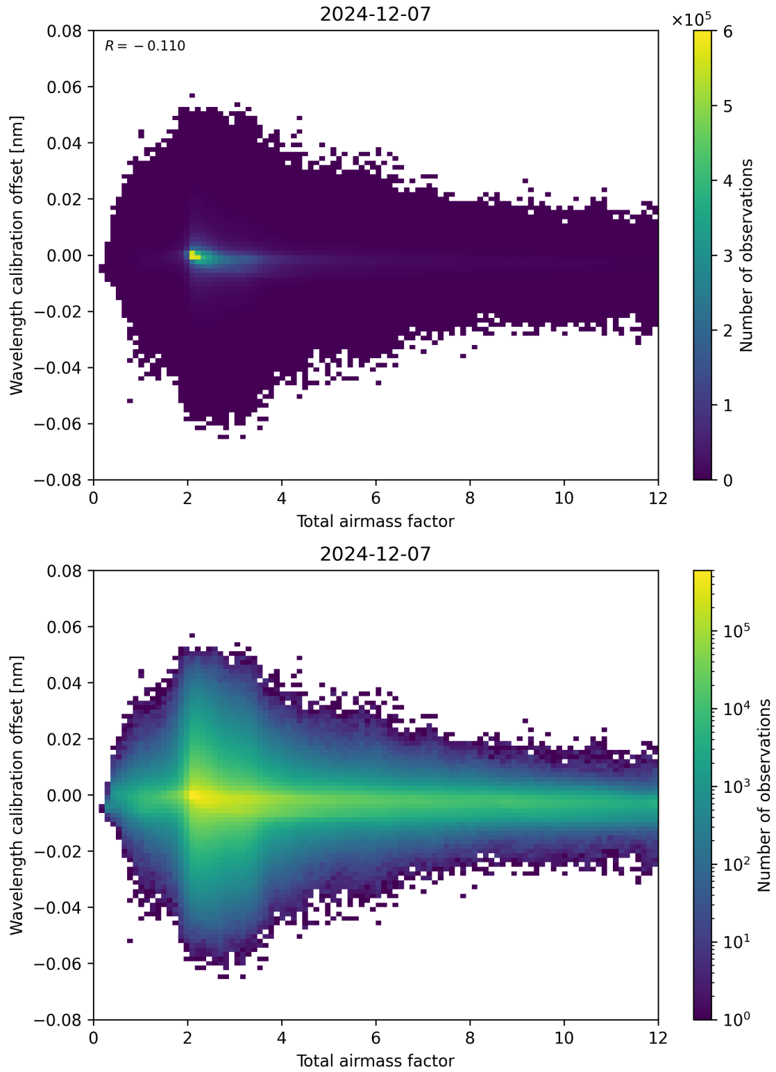
Figure 70: Scatter density plot of “Total airmass factor” against “Wavelength calibration offset” for 2024-12-06 to 2024-12-08.
