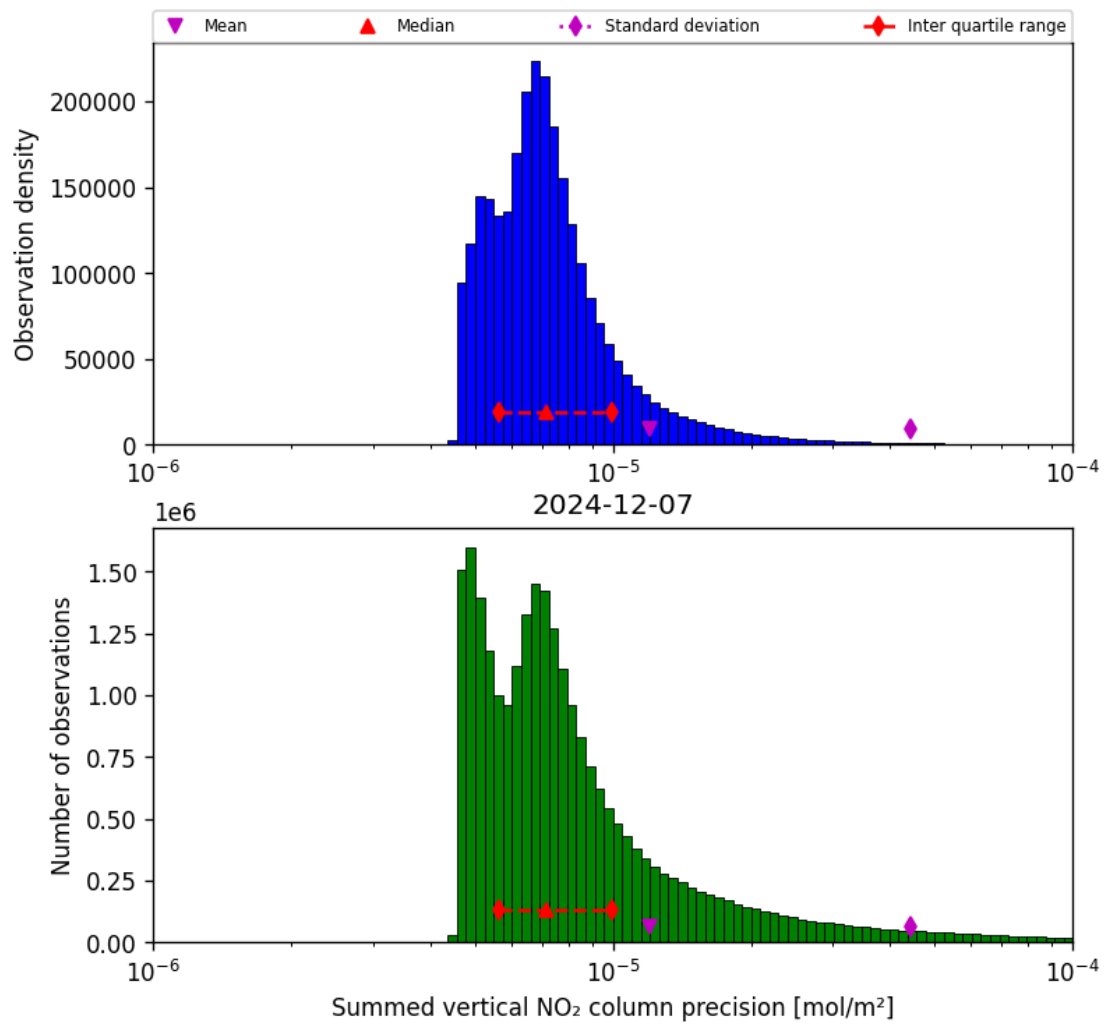
Figure 41: Histogram of “Summed vertical NO 2 column precision” for 2024-12-06 to 2024-12-08
