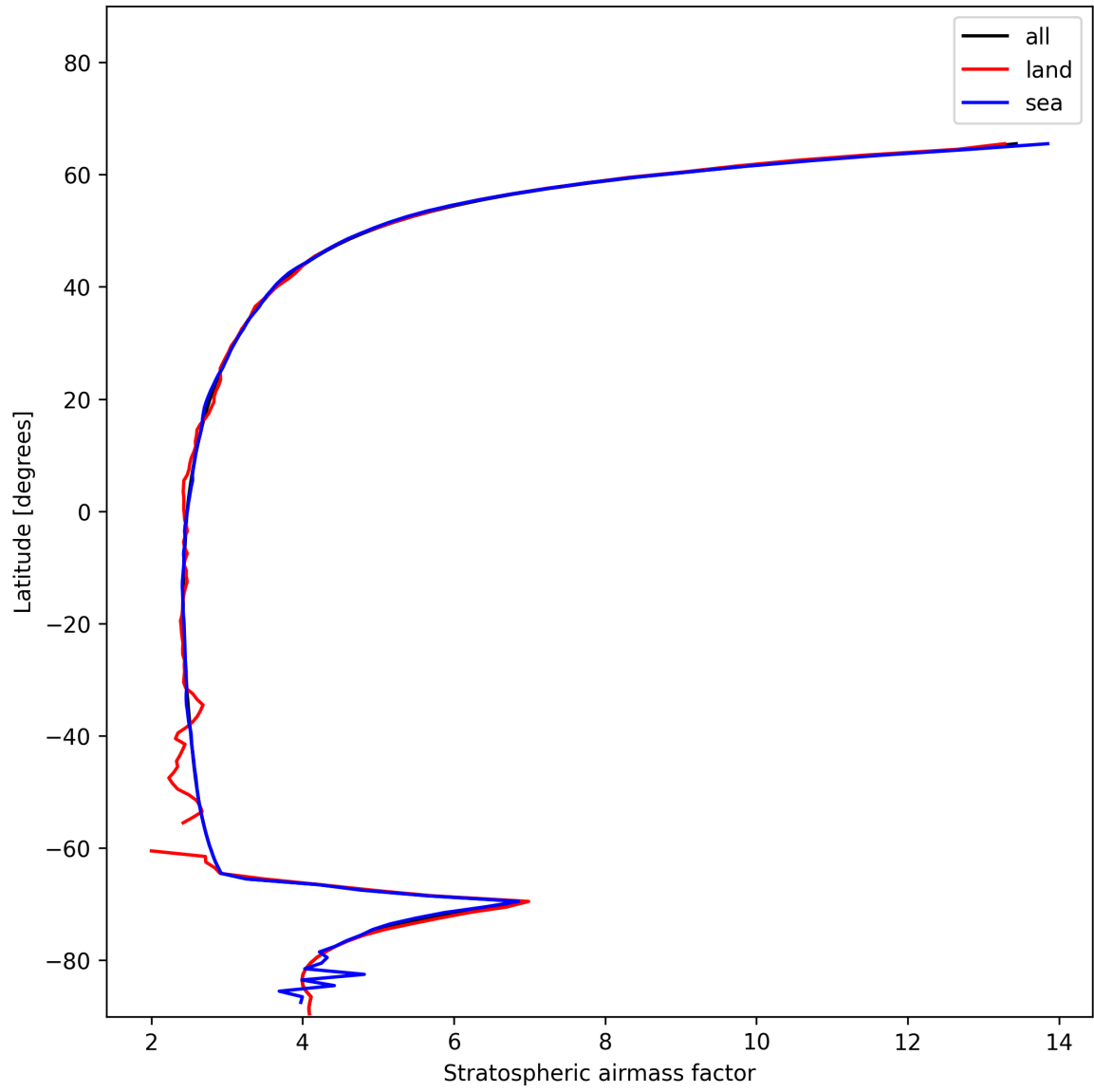
Figure 27: Zonal average of “Stratospheric air mass factor” for 2024-12-06 to 2024-12-08.
