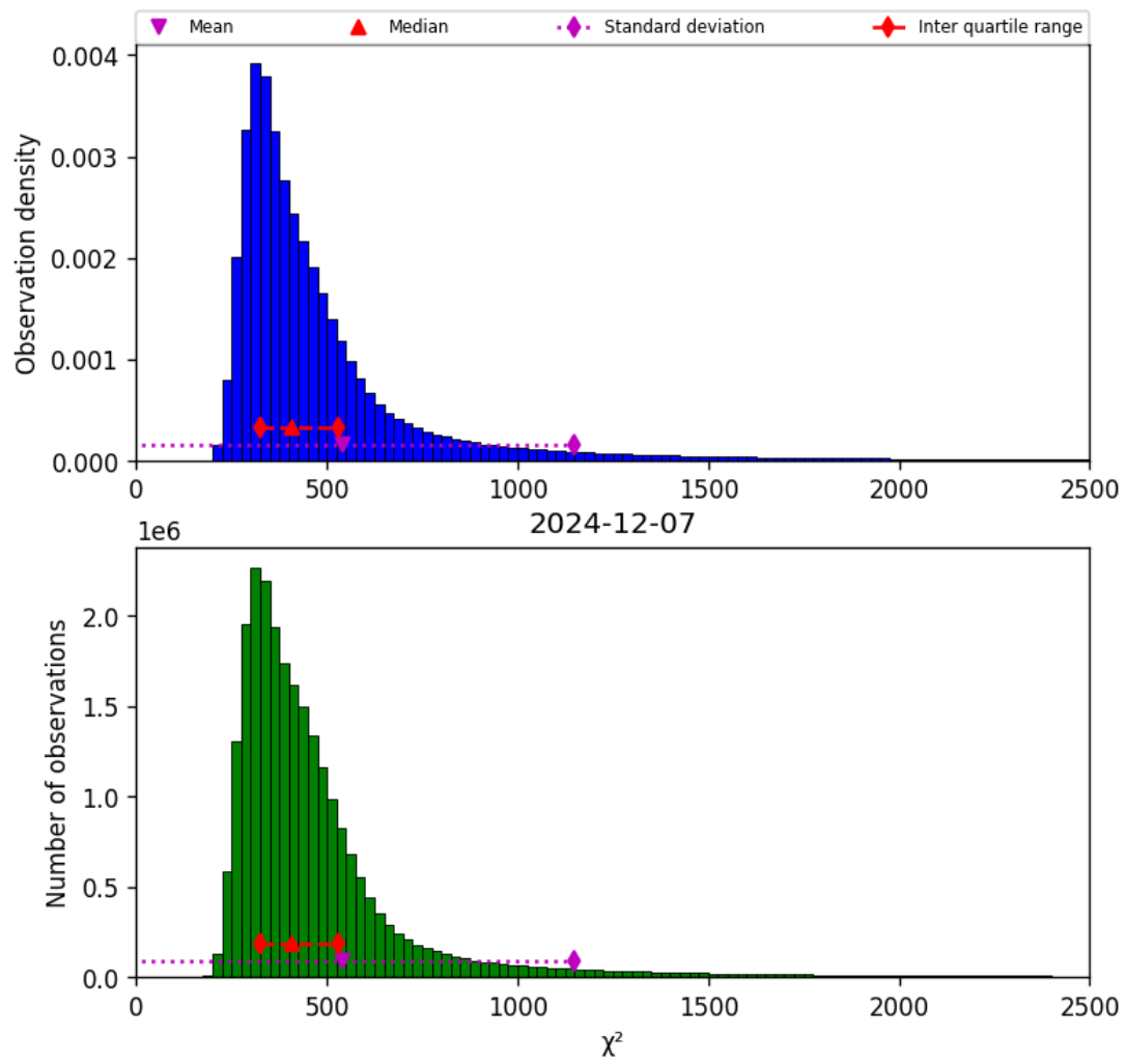
Figure 42: Histogram of “ \chi^2 ” for 2024-12-06 to 2024-12-08
