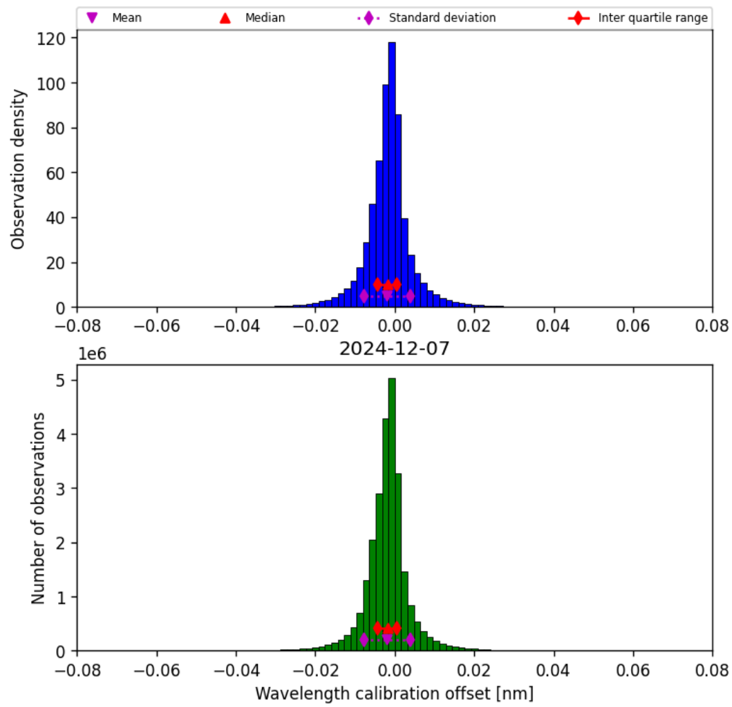
Figure 35: Histogram of “Wavelength calibration offset” for 2024-12-06 to 2024-12-08
