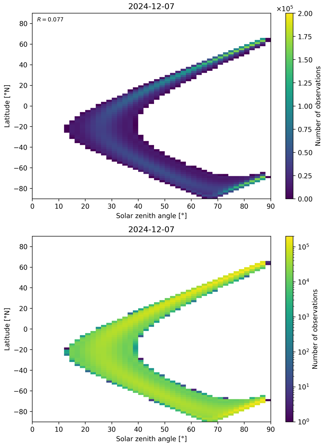
Figure 149: Scatter density plot of “Solar zenith angle” against “Latitude” for 2024-12-06 to 2024-12-08.
