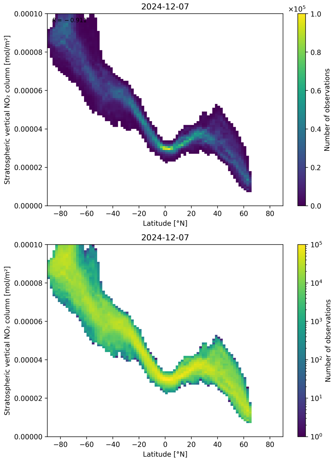
Figure 87: Scatter density plot of “Latitude” against “Stratospheric vertical NO 2 column” for 2024-12-06 to 2024-12-08.
