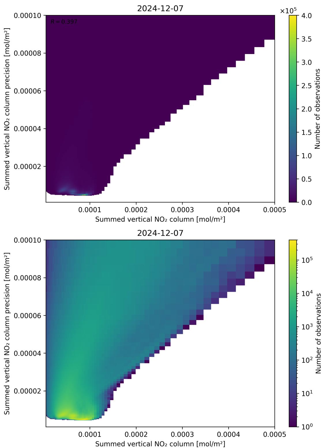
Figure 105: Scatter density plot of “Summed vertical NO 2 column” against “Summed vertical NO 2 column precision” for 2024-12-06 to 2024-12-08.
