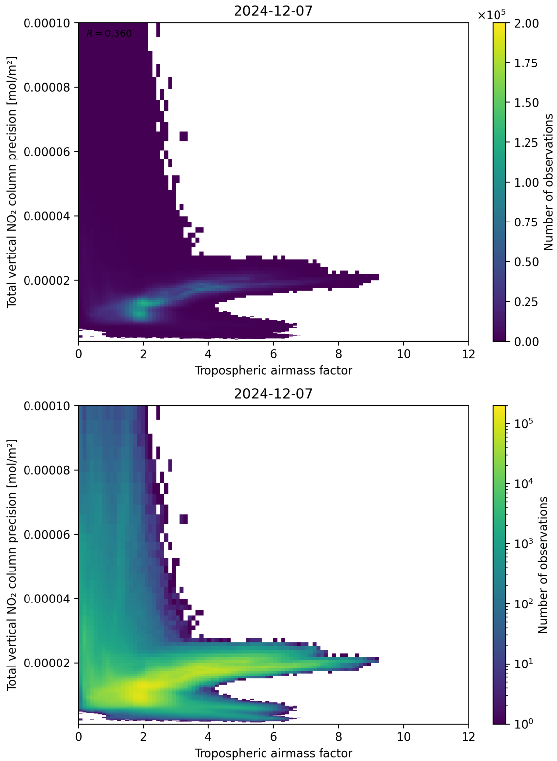
Figure 78: Scatter density plot of “Tropospheric air mass factor” against “Total vertical NO 2 column precision” for 2024-12-06 to 2024-12-08.
