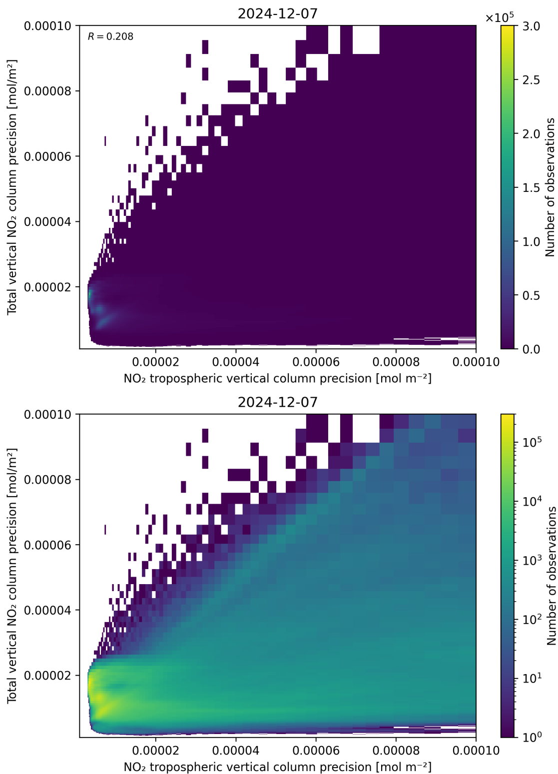
Figure 139: Scatter density plot of “NO 2 tropospheric vertical column precision” against “Total vertical NO 2 column precision” for 2024-12-06 to 2024-12-08.
