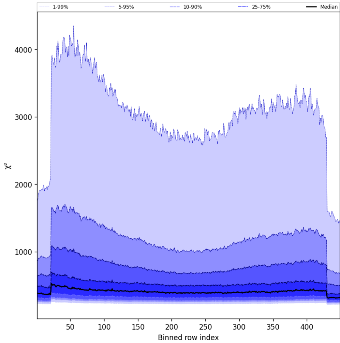
Figure 59: Along track statistics of “ \chi^2 ” for 2024-12-06 to 2024-12-08
