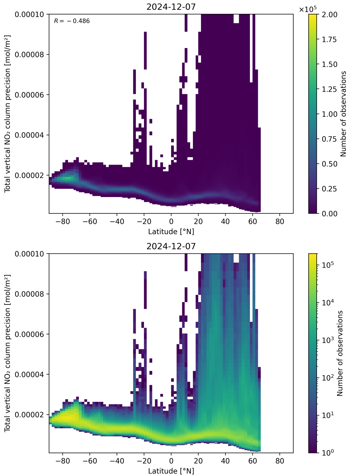
Figure 91: Scatter density plot of “Latitude” against “Total vertical NO 2 column precision” for 2024-12-06 to 2024-12-08.
