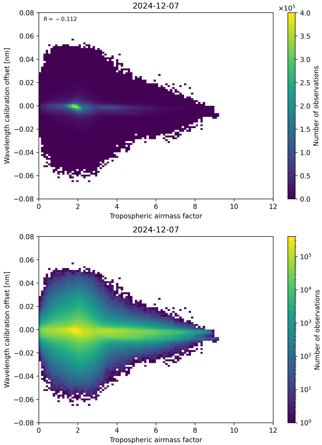
Figure 80: Scatter density plot of “Tropospheric airmass factor” against “Wavelength calibration offset” for 2024-12-06 to 2024-12-08.
