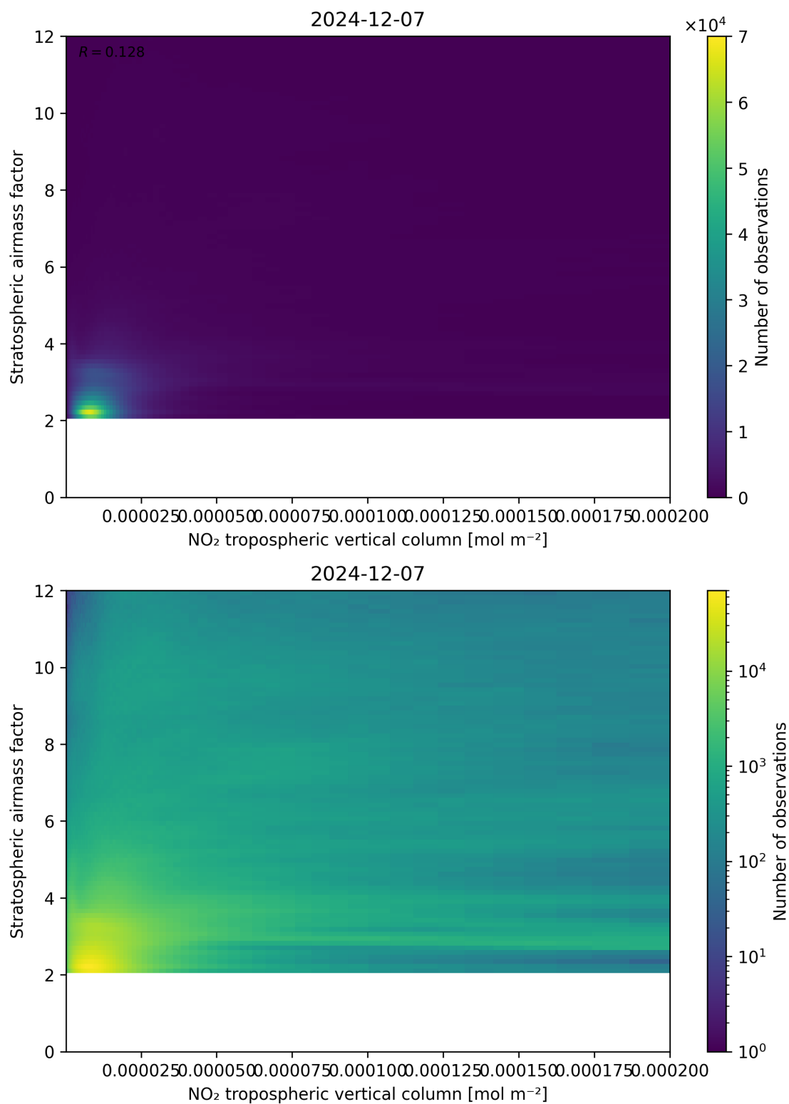
Figure 121: Scatter density plot of “NO 2 tropospheric vertical column” against “Stratospheric airmass factor” for 2024-12-06 to 2024-12-08.
