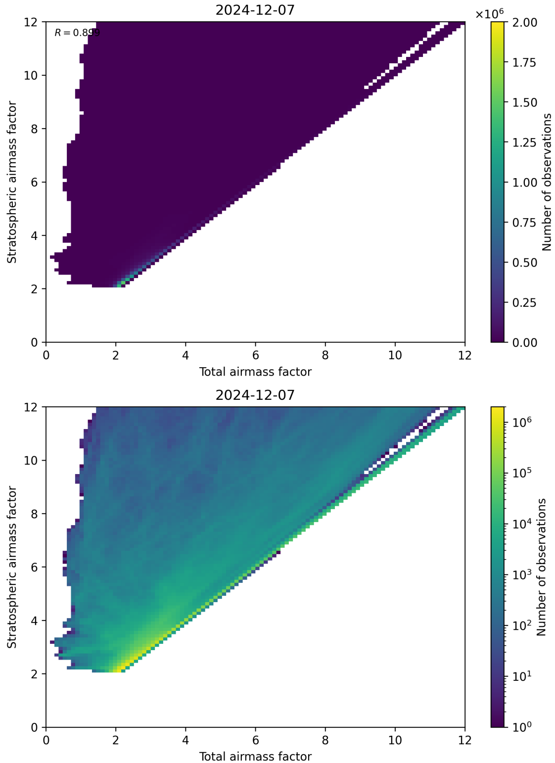
Figure 62: Scatter density plot of “Total airmass factor” against “Stratospheric airmass factor” for 2024-12-06 to 2024-12-08.
