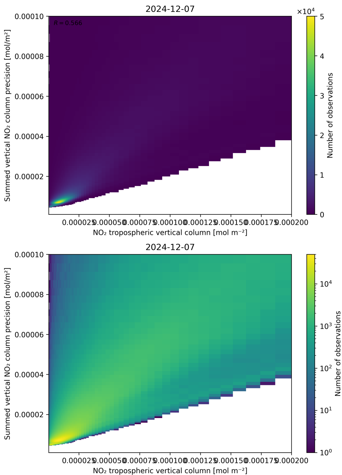
Figure 127: Scatter density plot of “NO 2 tropospheric vertical column” against “Summed vertical NO 2 column precision” for 2024-12-06 to 2024-12-08.
