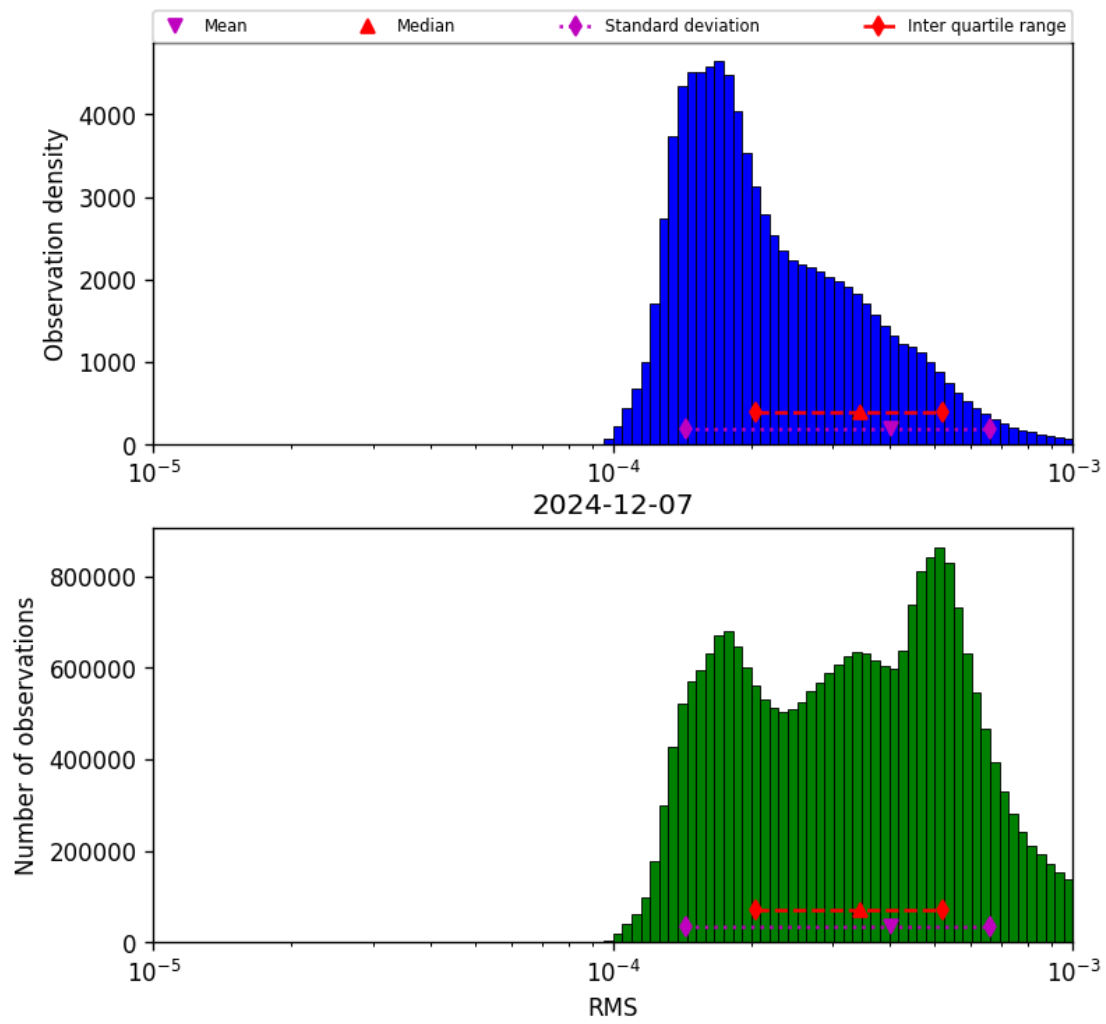
Figure 43: Histogram of “RMS” for 2024-12-06 to 2024-12-08
