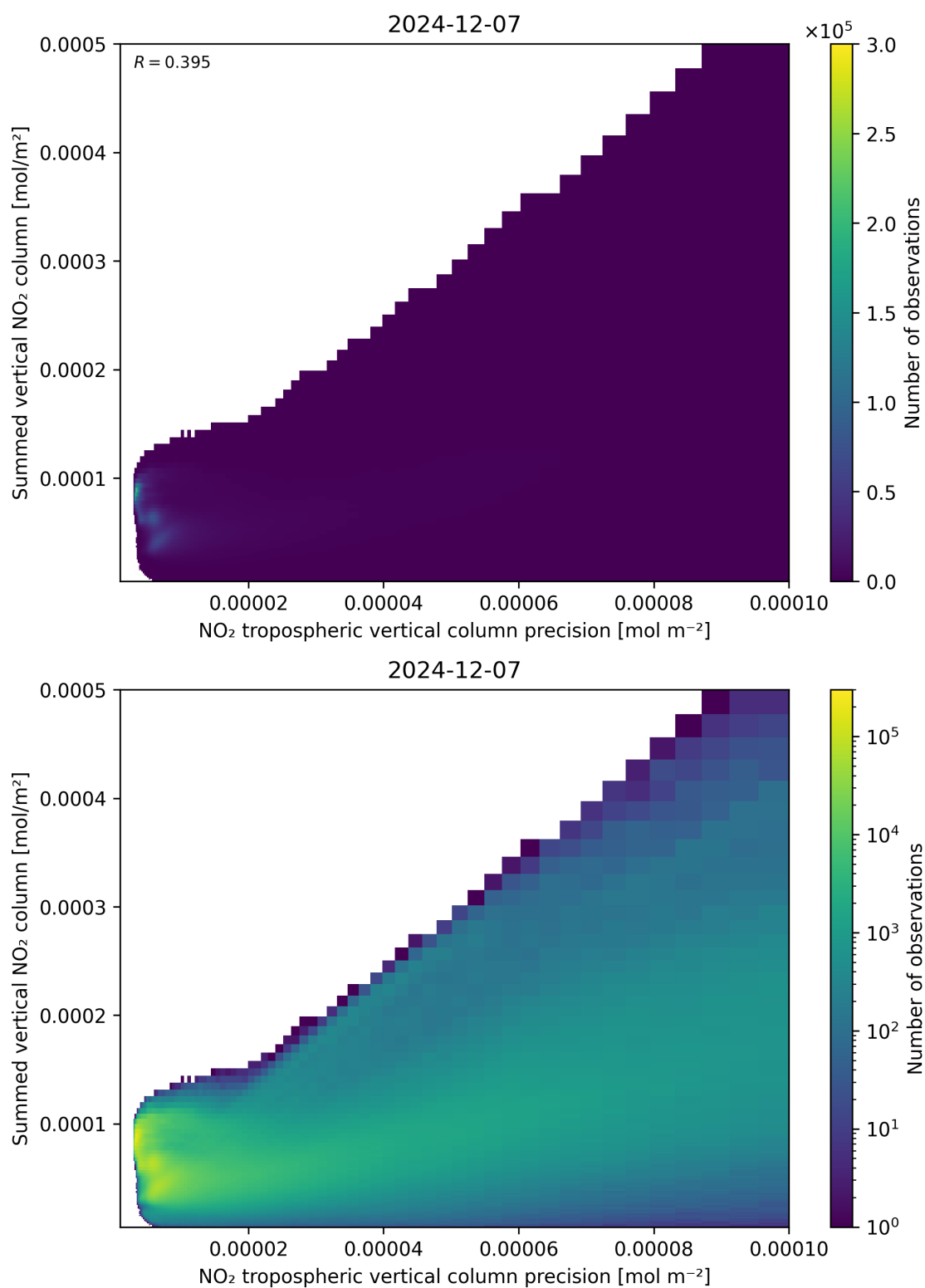
Figure 136: Scatter density plot of “NO 2 tropospheric vertical column precision” against “Summed vertical NO 2 column” for 2024-12-06 to 2024-12-08.
