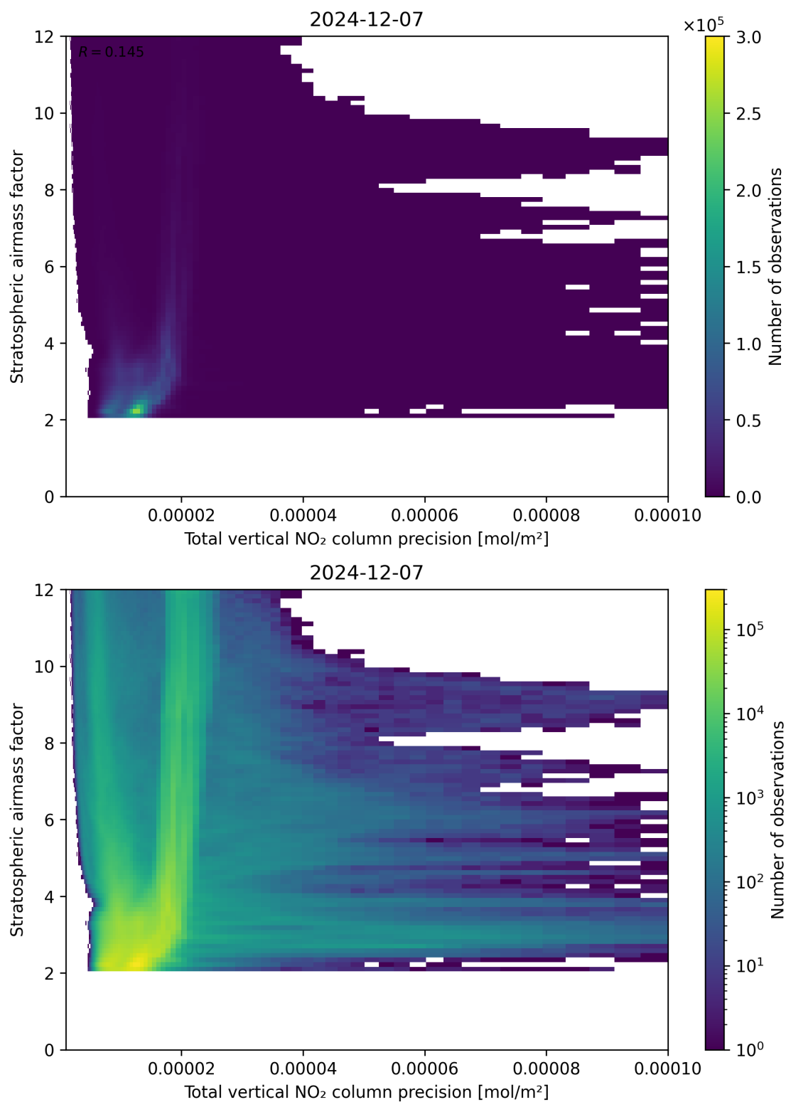
Figure 115: Scatter density plot of “Total vertical NO 2 column precision” against “Stratospheric air mass factor” for 2024-12-06 to 2024-12-08.
