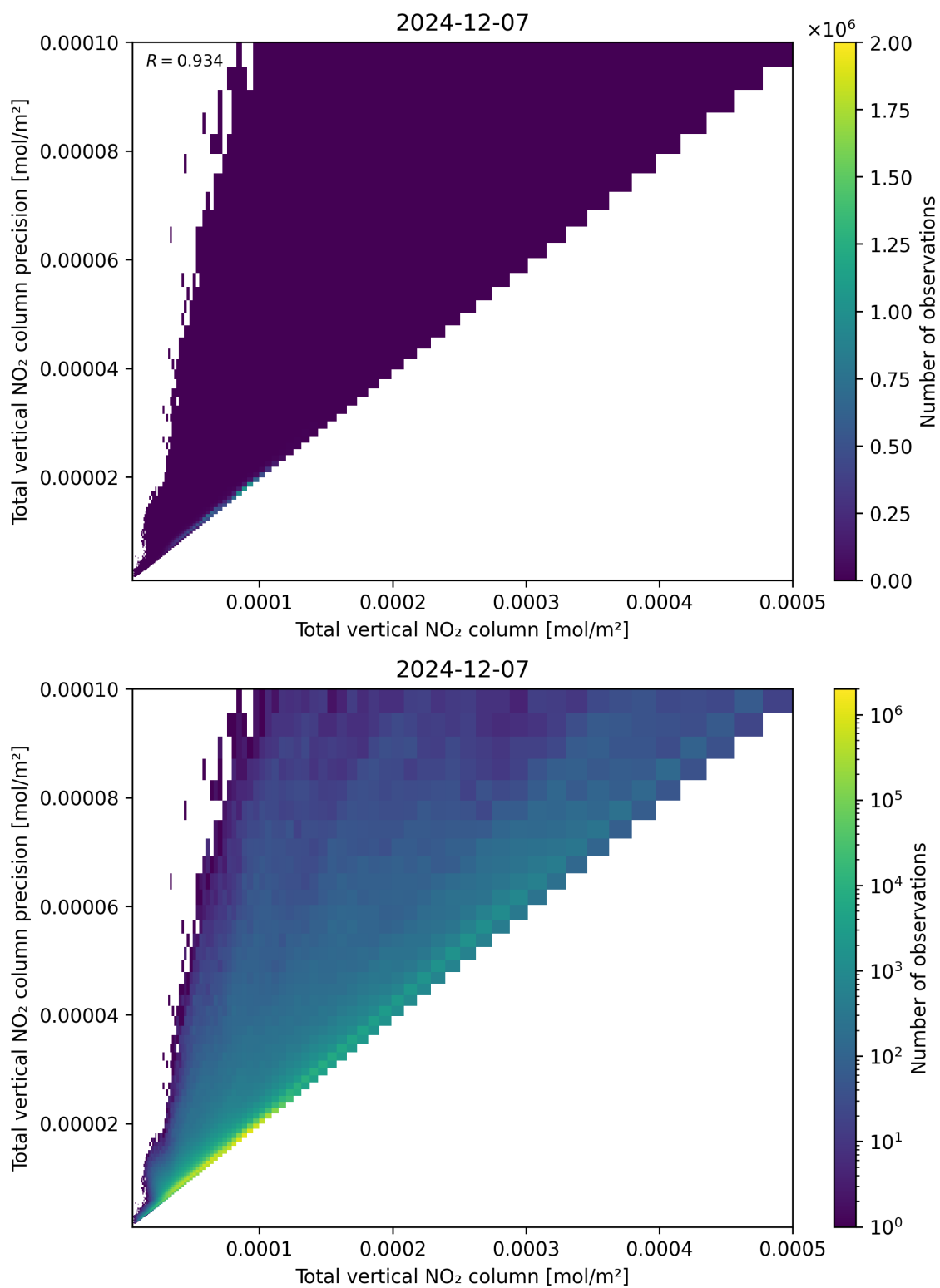
Figure 114: Scatter density plot of “Total vertical NO 2 column” against “Total vertical NO 2 column precision” for 2024-12-06 to 2024-12-08.
