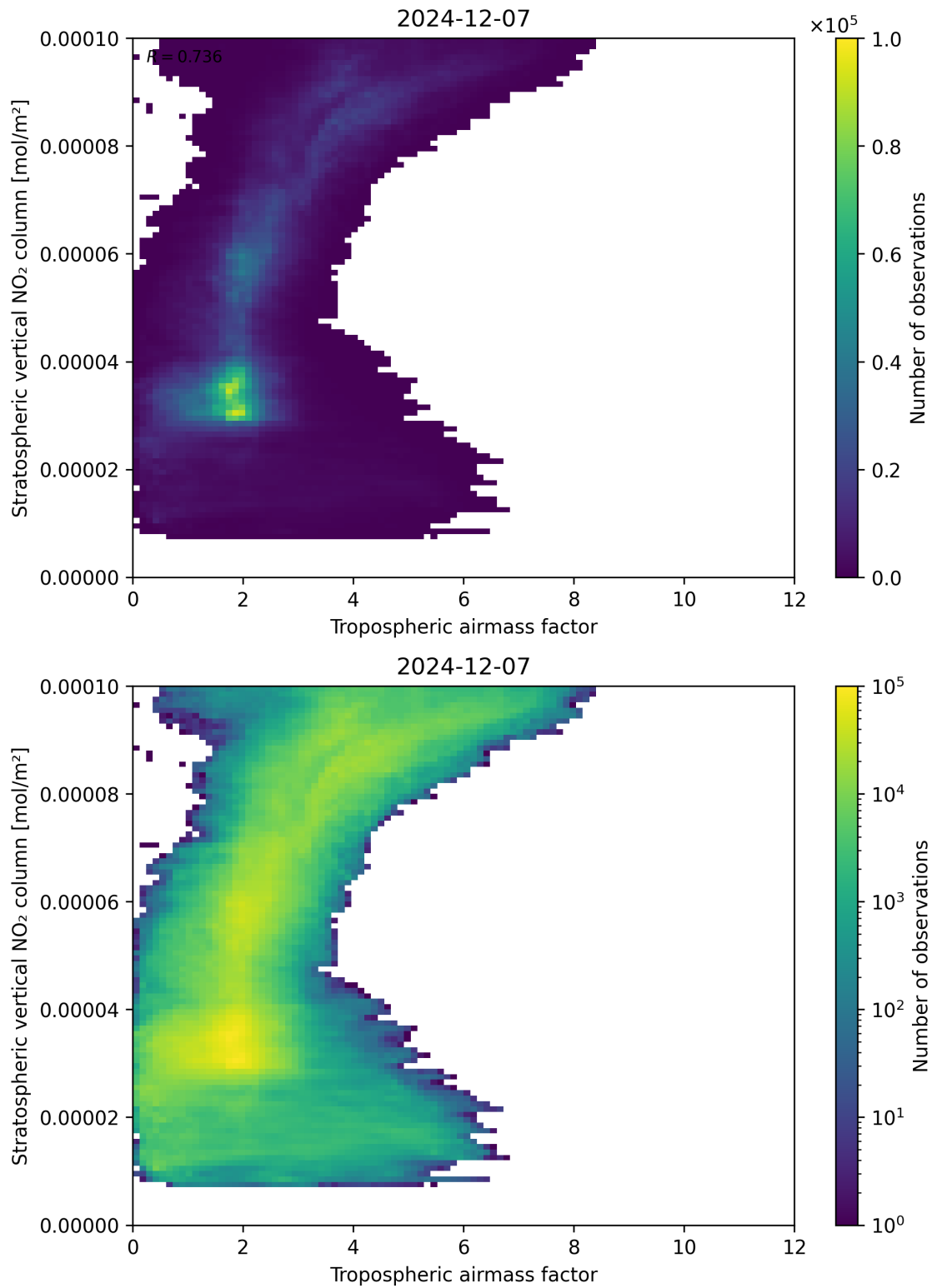
Figure 74: Scatter density plot of “Tropospheric airmass factor” against “Stratospheric vertical NO 2 column” for 2024-12-06 to 2024-12-08.
