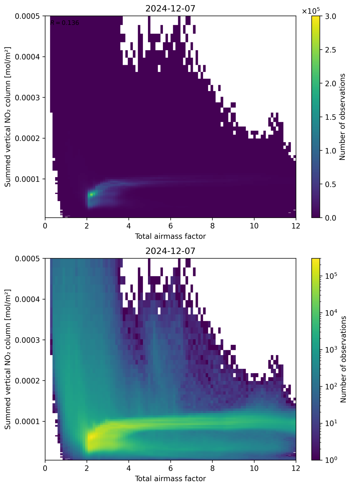
Figure 65: Scatter density plot of “Total airmass factor” against “Summed vertical NO 2 column” for 2024-12-06 to 2024-12-08.
