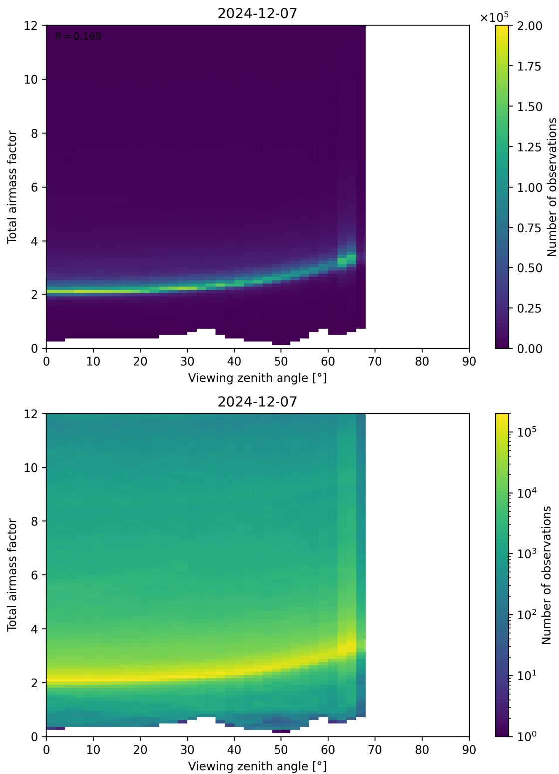
Figure 160: Scatter density plot of “Viewing zenith angle” against “Total airmass factor” for 2024-12-06 to 2024-12-08.
