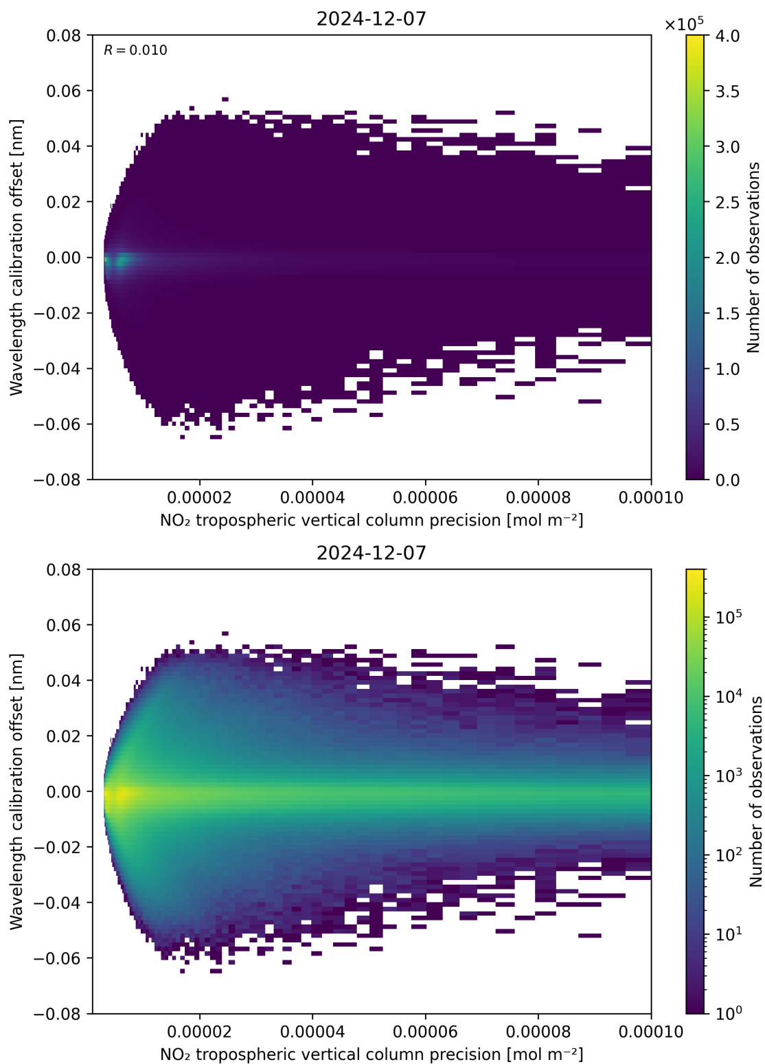
Figure 141: Scatter density plot of “NO 2 tropospheric vertical column precision” against “Wavelength calibration offset” for 2024-12-06 to 2024-12-08.
