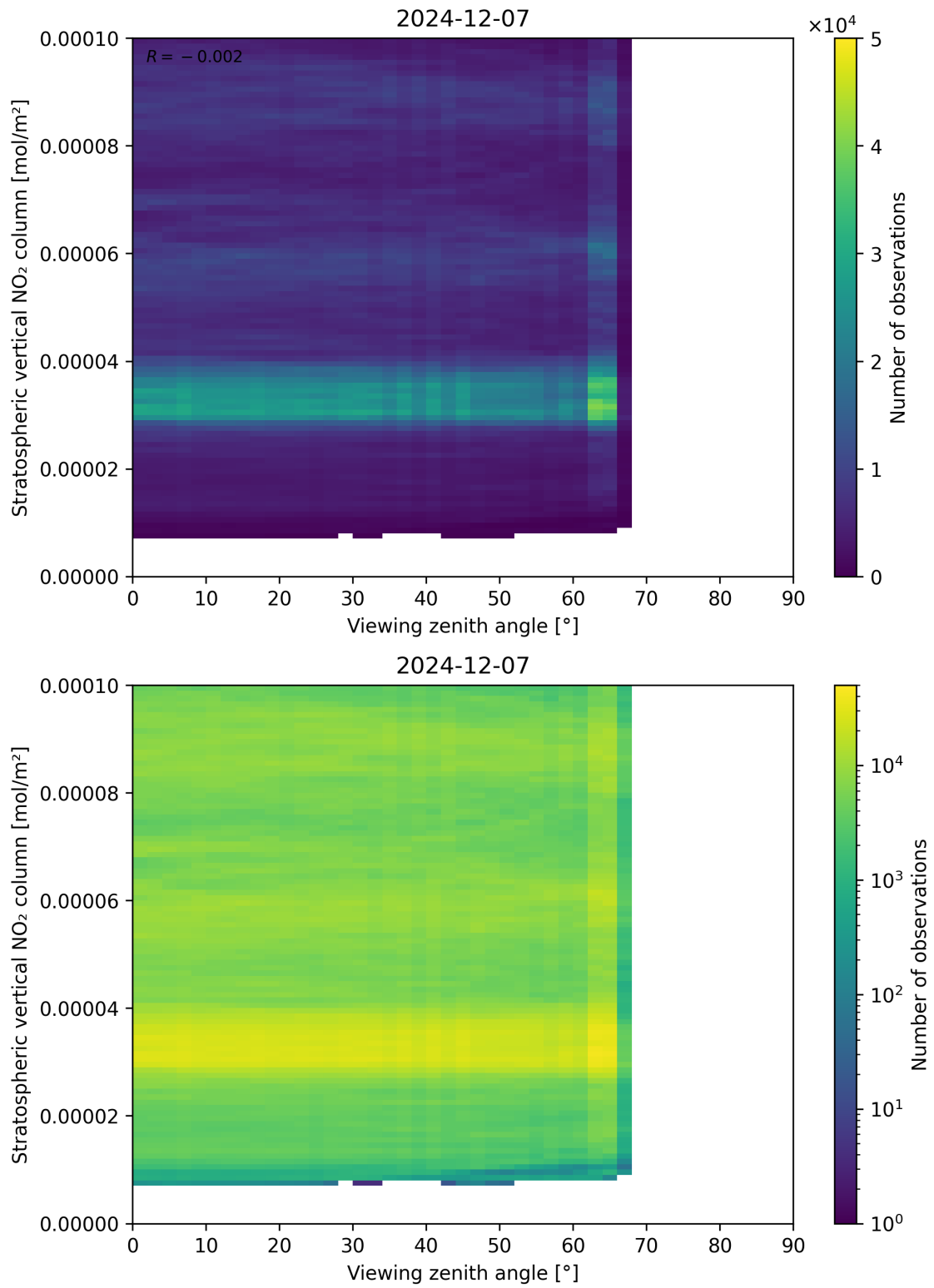
Figure 164: Scatter density plot of “Viewing zenith angle” against “Stratospheric vertical NO 2 column” for 2024-12-06 to 2024-12-08.
