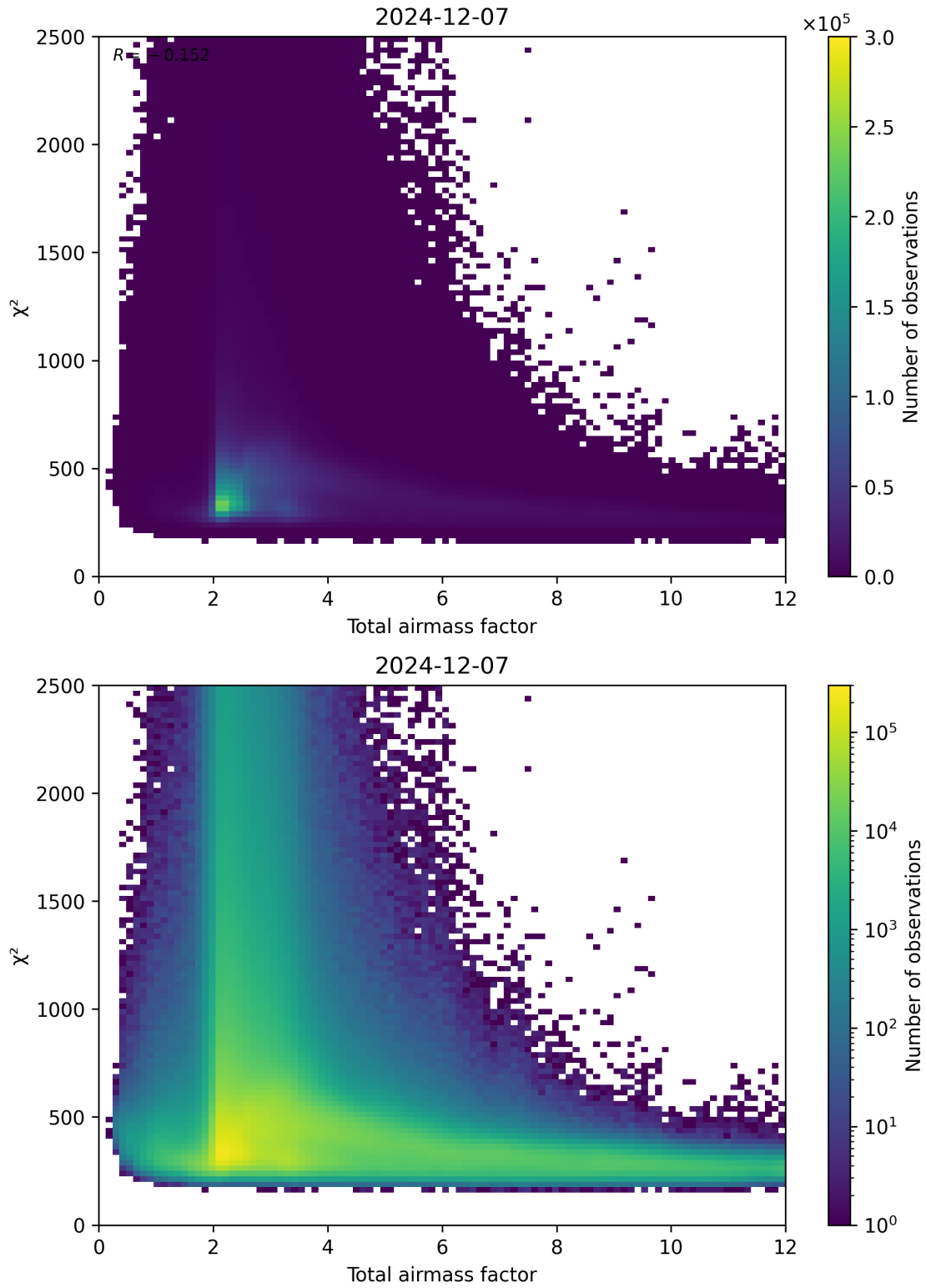
Figure 63: Scatter density plot of “Total airmass factor” against “ \chi^2 ” for 2024-12-06 to 2024-12-08.
