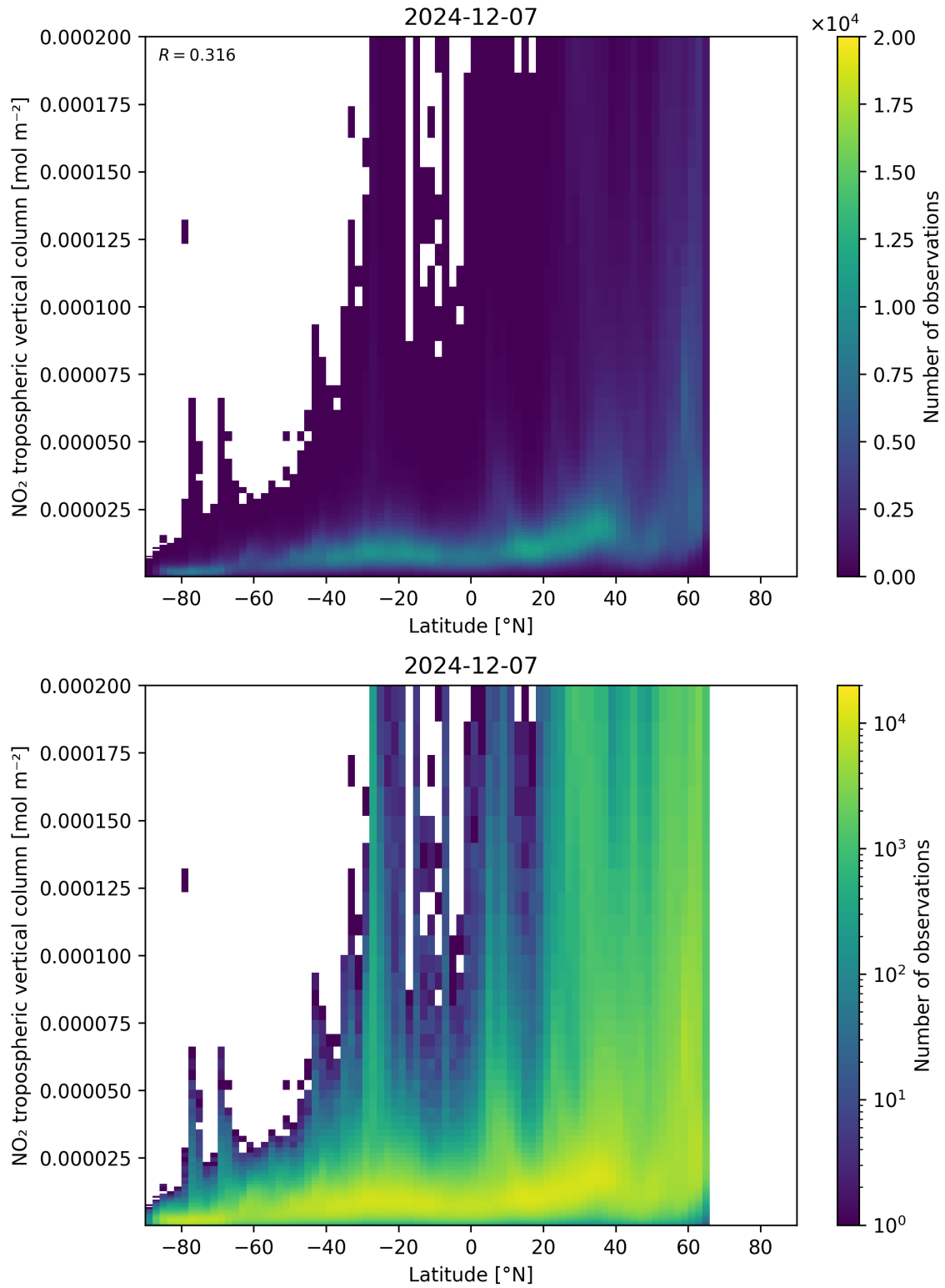
Figure 92: Scatter density plot of “Latitude” against “NO 2 tropospheric vertical column” for 2024-12-06 to 2024-12-08.
