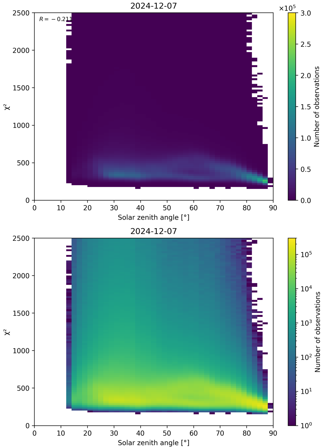
Figure 148: Scatter density plot of “Solar zenith angle” against “ \chi^2 ” for 2024-12-06 to 2024-12-08.
