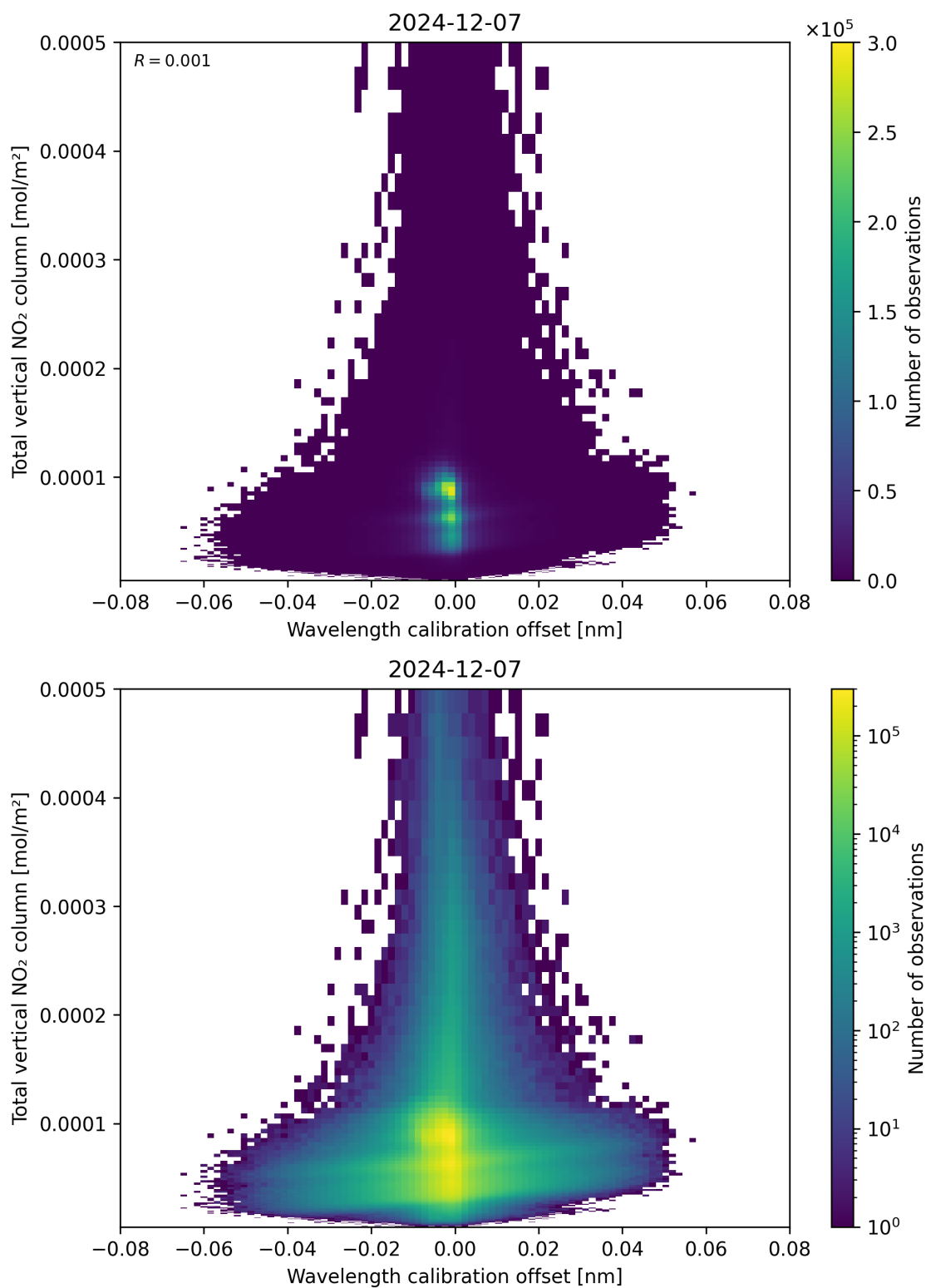
Figure 179: Scatter density plot of “Wavelength calibration offset” against “Total vertical NO 2 column” for 2024-12-06 to 2024-12-08.
