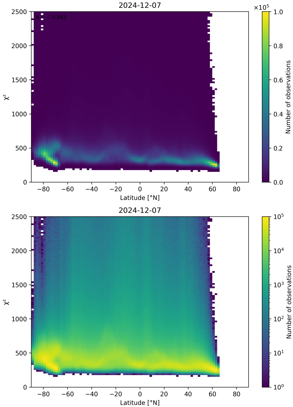
Figure 86: Scatter density plot of “Latitude” against “ \chi^2 ” for 2024-12-06 to 2024-12-08.
