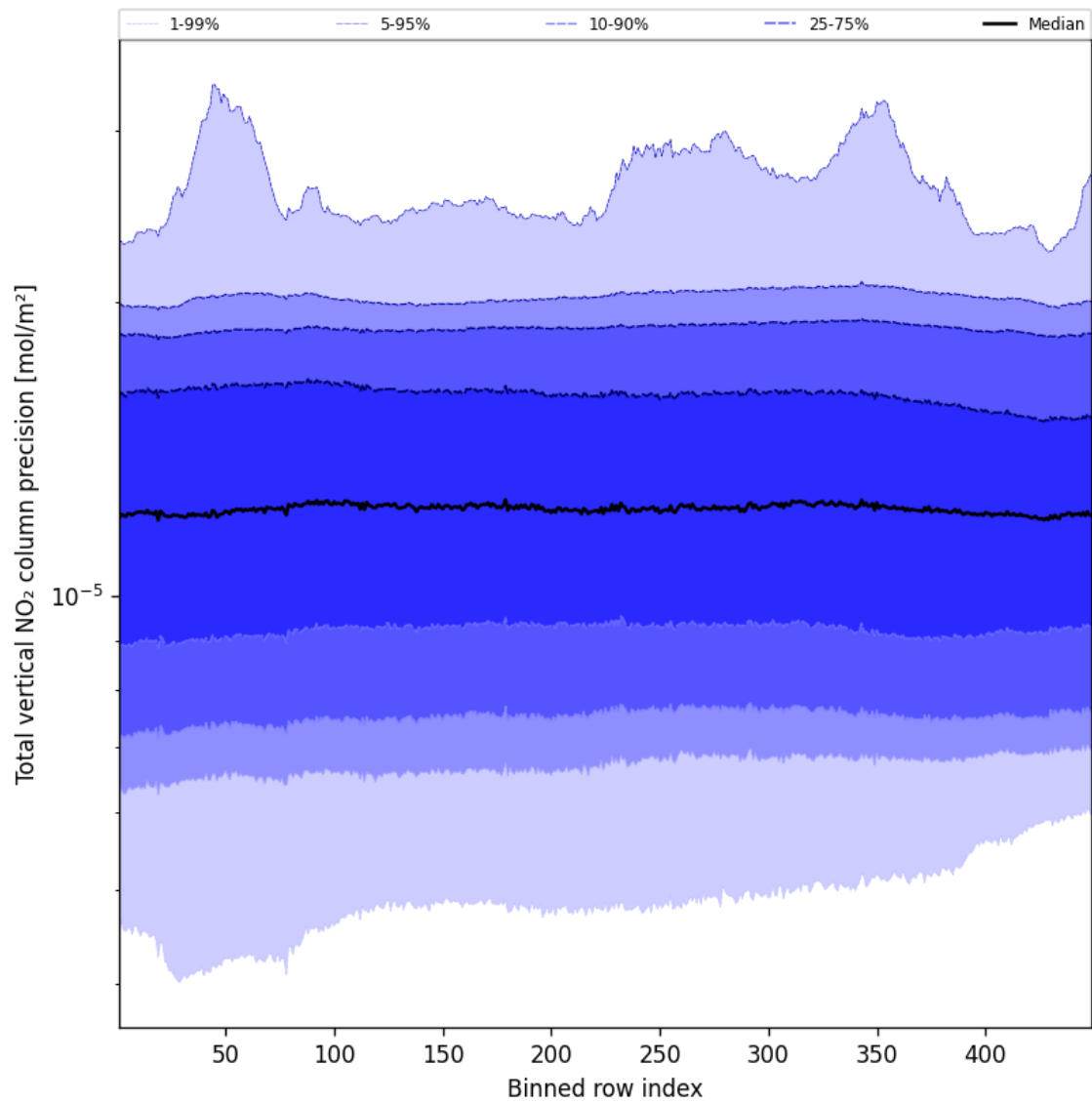
Figure 56: Along track statistics of “Total vertical NO 2 column precision” for 2024-12-06 to 2024-12-08
