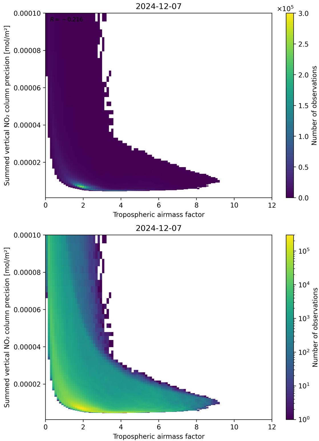
Figure 76: Scatter density plot of “Tropospheric air mass factor” against “Summed vertical NO 2 column precision” for 2024-12-06 to 2024-12-08.
