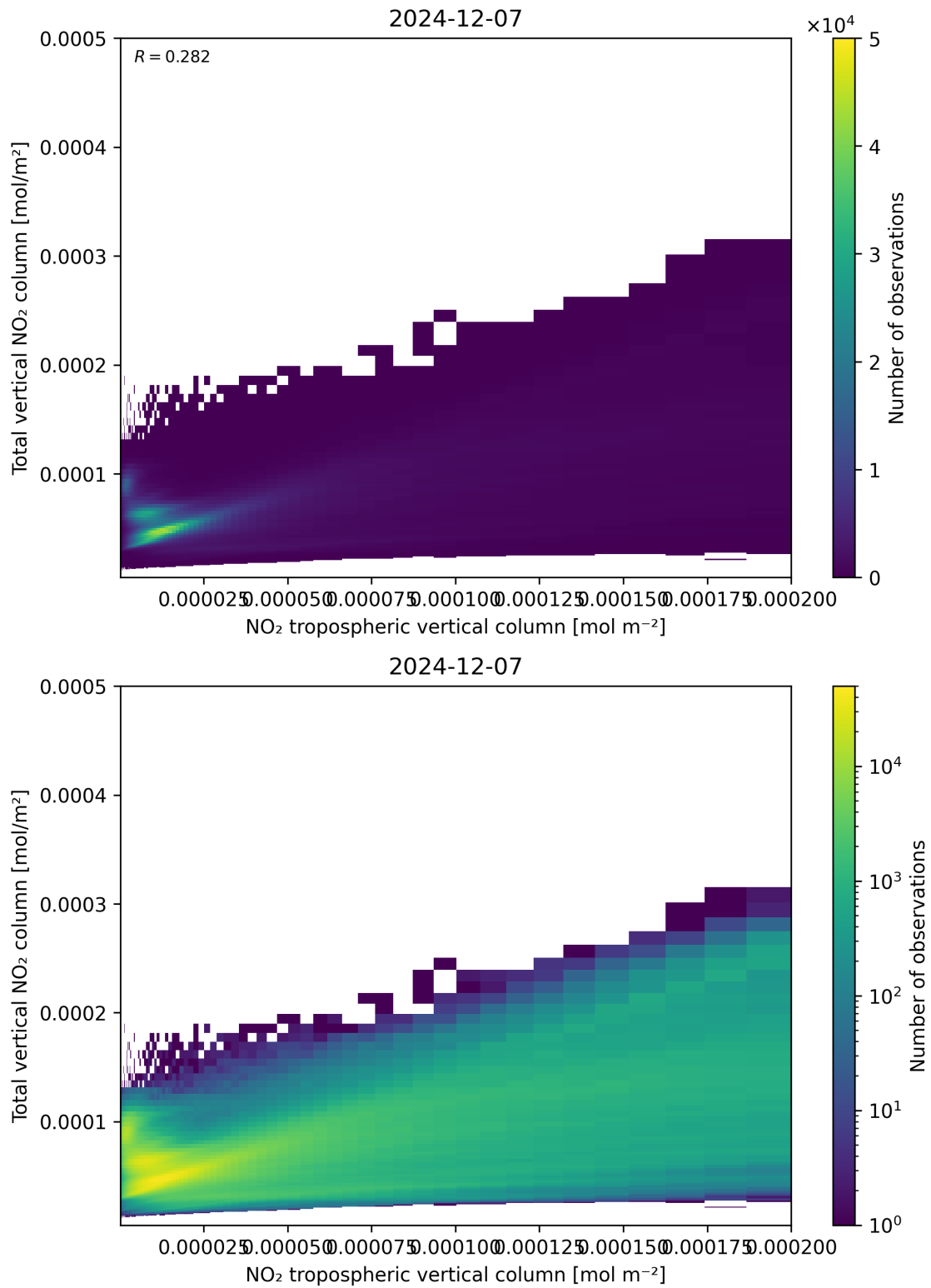
Figure 128: Scatter density plot of “NO 2 tropospheric vertical column” against “Total vertical NO 2 column” for 2024-12-06 to 2024-12-08.
