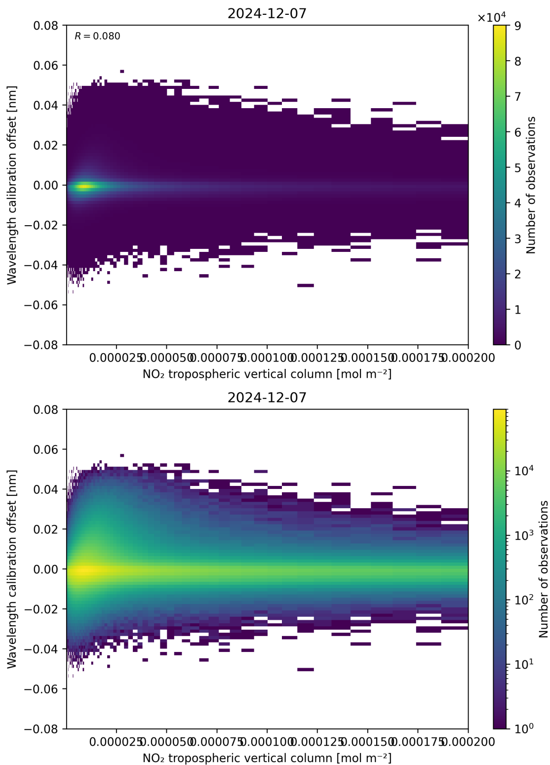
Figure 143: Scatter density plot of “NO 2 tropospheric vertical column” against “Wavelength calibration offset” for 2024-12-06 to 2024-12-08.
