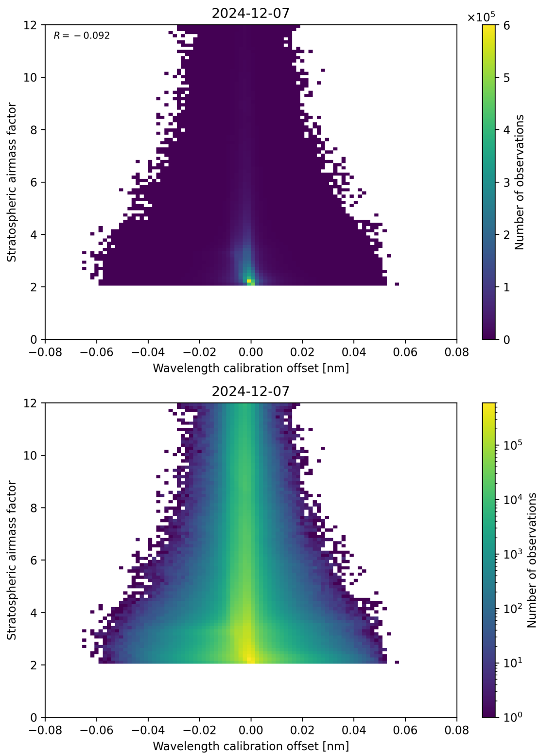
Figure 174: Scatter density plot of “Wavelength calibration offset” against “Stratospheric airmass factor” for 2024-12-06 to 2024-12-08.
