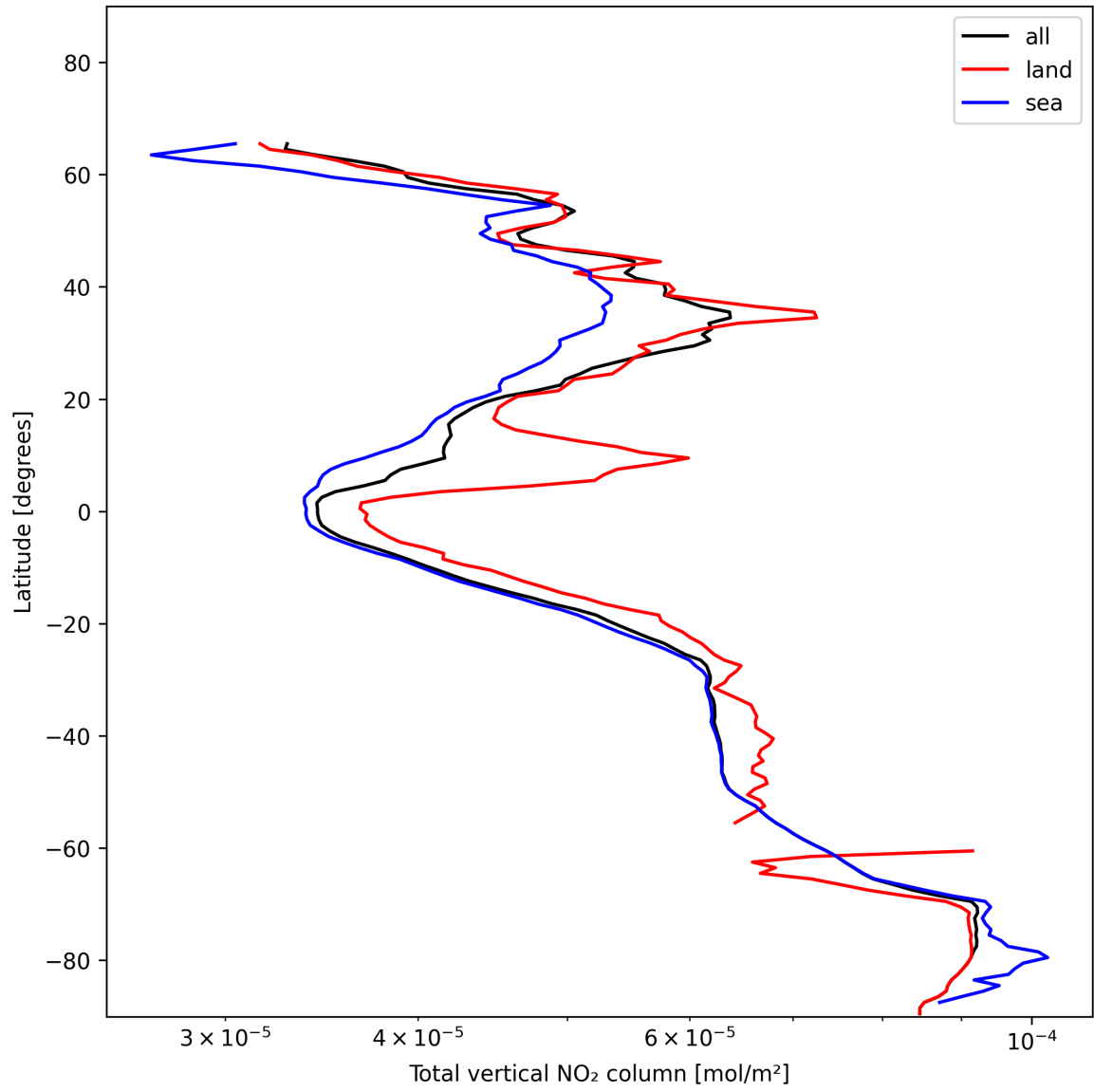
Figure 21: Zonal average of “Total vertical NO 2 column” for 2024-12-06 to 2024-12-08.
