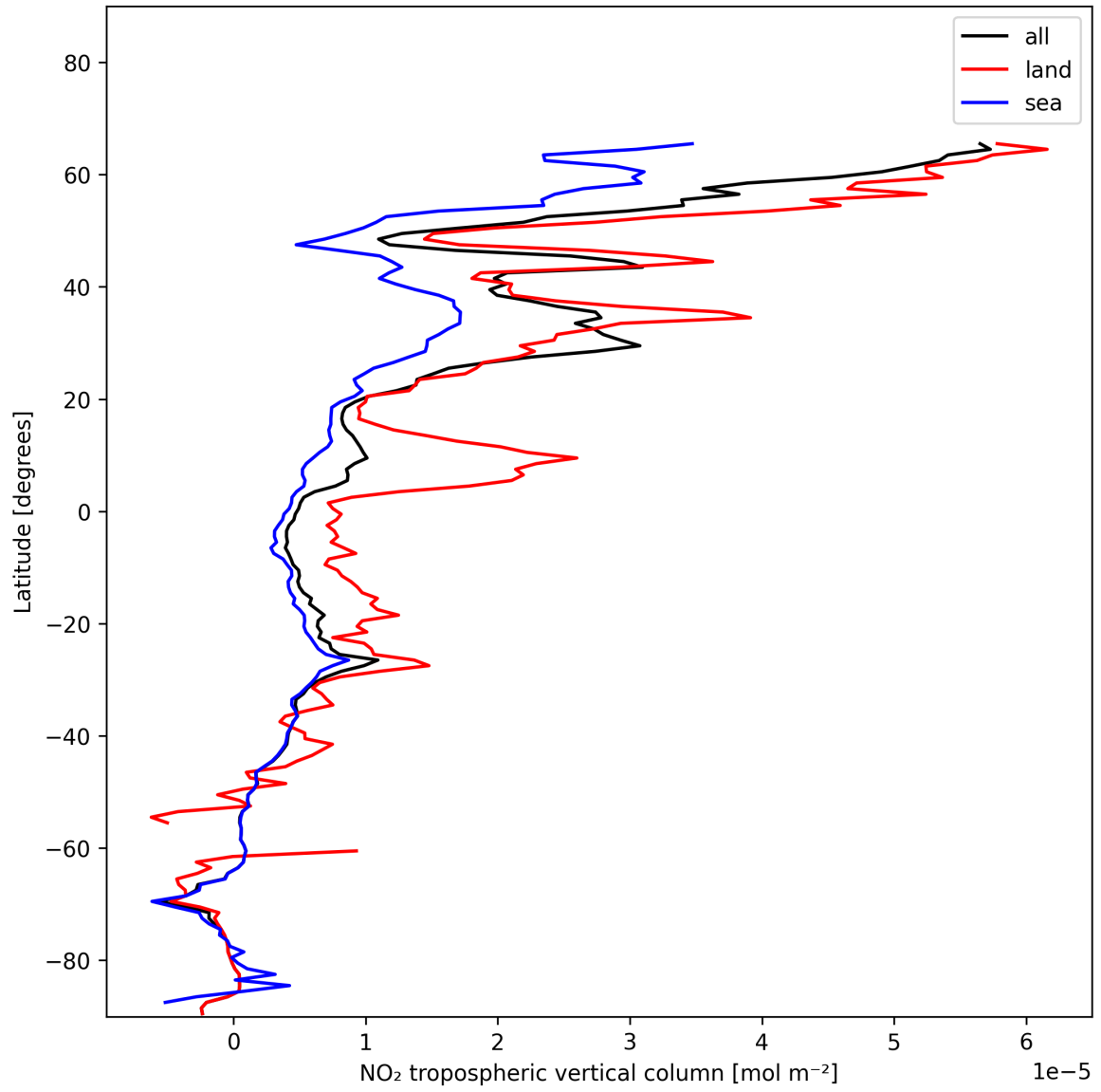
Figure 12: Zonal average of “NO 2 tropospheric vertical column” for 2024-12-06 to 2024-12-08.
