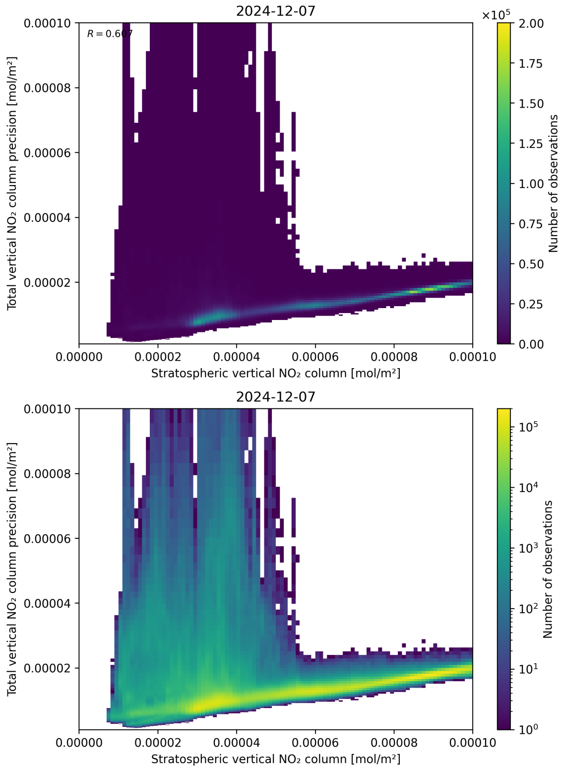
Figure 101: Scatter density plot of “Stratospheric vertical NO 2 column” against “Total vertical NO 2 column precision” for 2024-12-06 to 2024-12-08.
