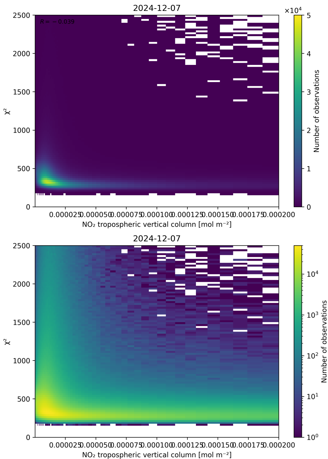
Figure 124: Scatter density plot of “NO 2 tropospheric vertical column” against “ \chi^2 ” for 2024-12-06 to 2024-12-08.
