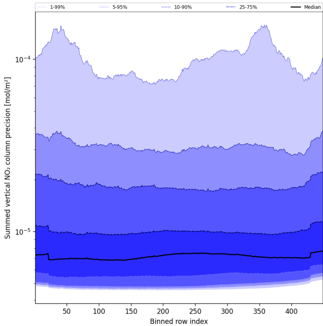
Figure 58: Along track statistics of “Summed vertical NO 2 column precision” for 2024-12-06 to 2024-12-08
