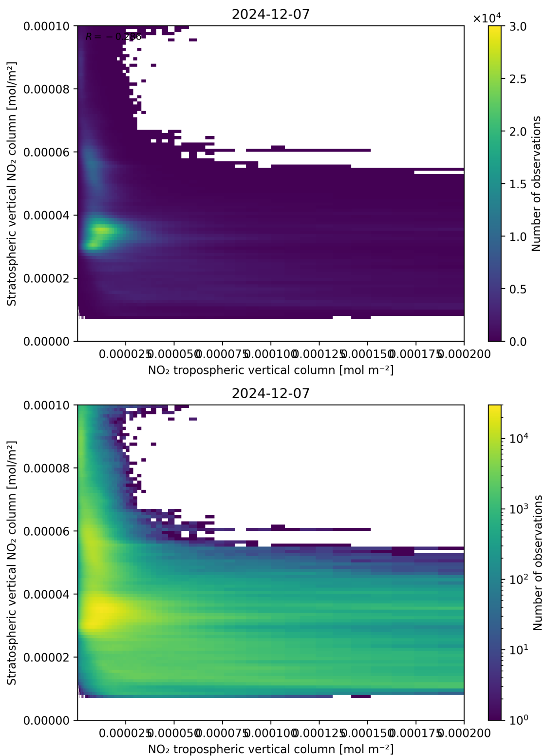
Figure 125: Scatter density plot of “NO 2 tropospheric vertical column” against “Stratospheric vertical NO 2 column” for 2024-12-06 to 2024-12-08.
