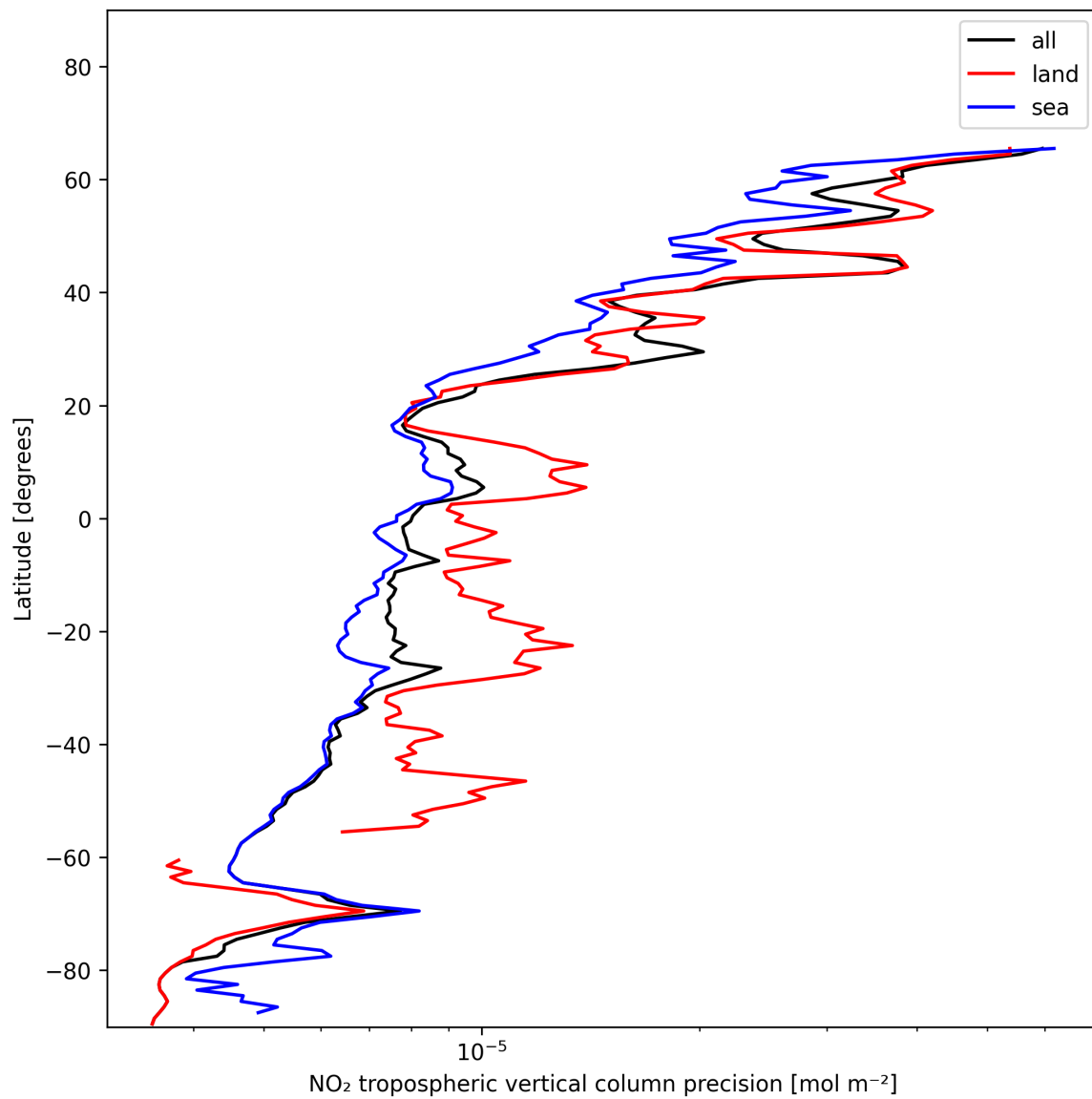
Figure 13: Zonal average of “NO 2 tropospheric vertical column precision” for 2024-12-06 to 2024-12-08.
