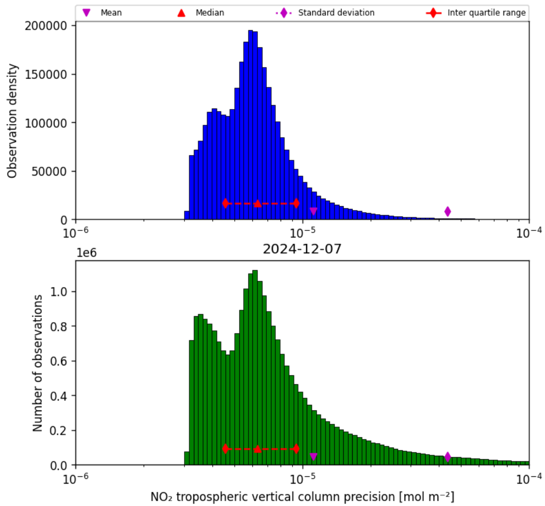
Figure 30: Histogram of “NO 2 tropospheric vertical column precision” for 2024-12-06 to 2024-12-08
