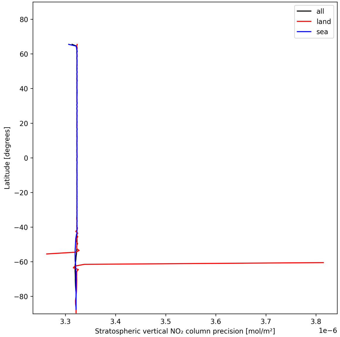
Figure 20: Zonal average of “Stratospheric vertical NO 2 column precision” for 2024-12-06 to 2024-12-08.
