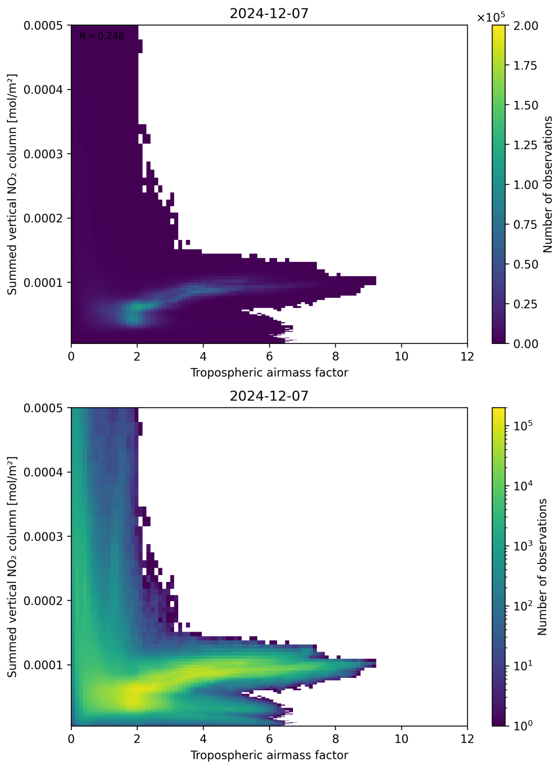
Figure 75: Scatter density plot of “Tropospheric airmass factor” against “Summed vertical NO 2 column” for 2024-12-06 to 2024-12-08.
