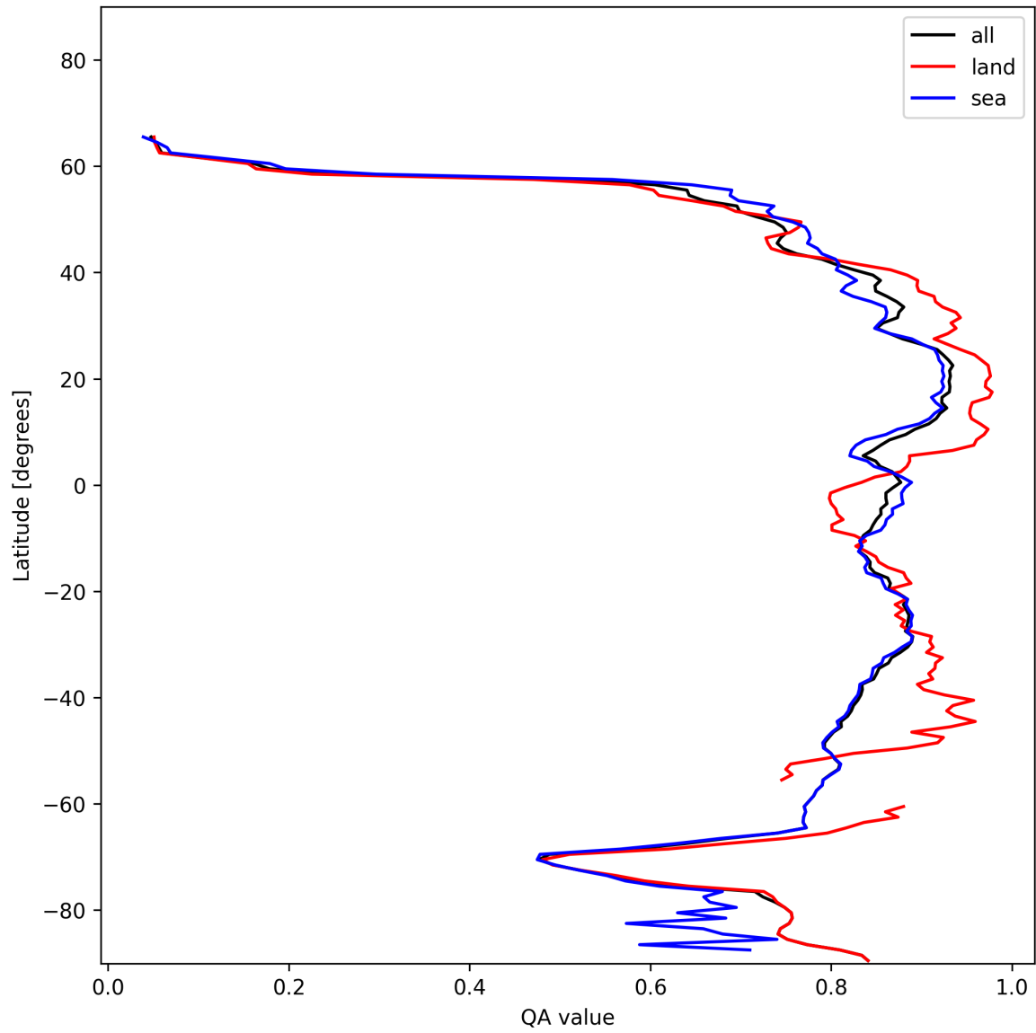
Figure 11: Zonal average of “QA value” for 2024-12-06 to 2024-12-08.
