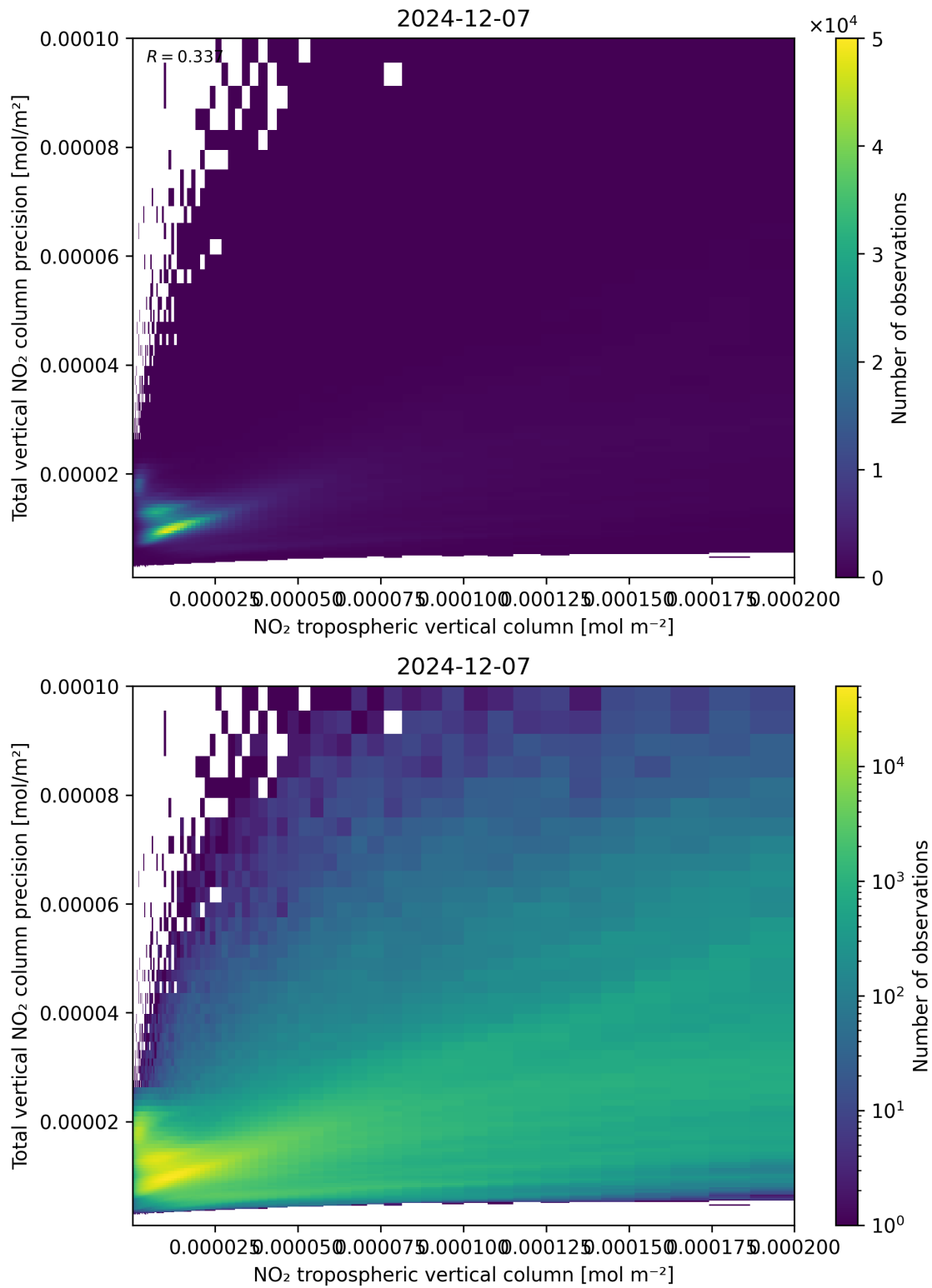
Figure 129: Scatter density plot of “NO 2 tropospheric vertical column” against “Total vertical NO 2 column precision” for 2024-12-06 to 2024-12-08.
