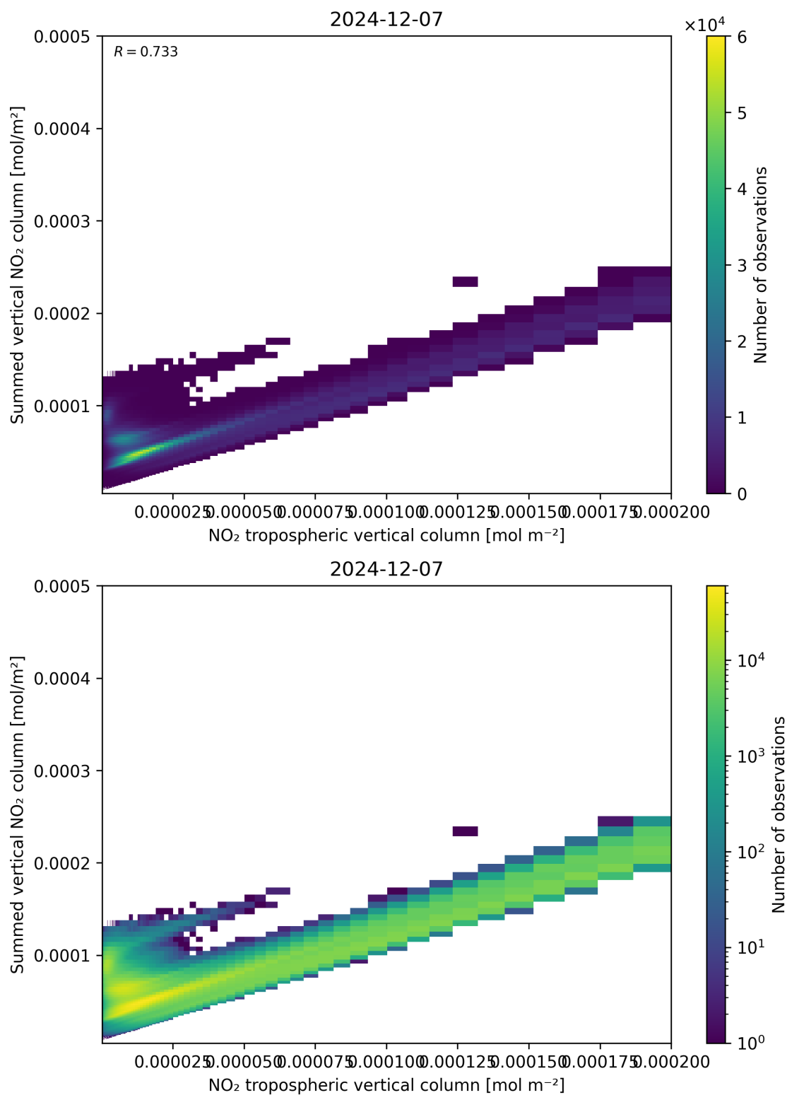
Figure 126: Scatter density plot of “NO 2 tropospheric vertical column” against “Summed vertical NO 2 column” for 2024-12-06 to 2024-12-08.
