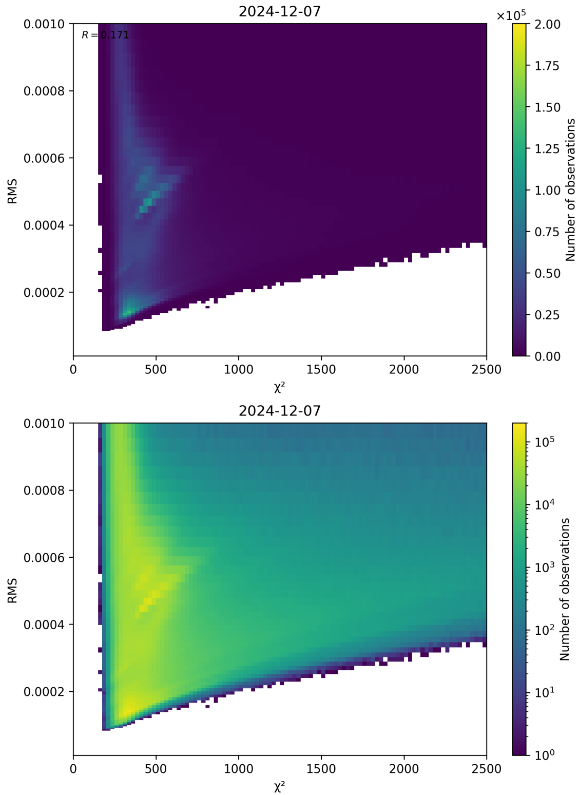
Figure 82: Scatter density plot of “ \chi^2 ” against “RMS” for 2024-12-06 to 2024-12-08.
