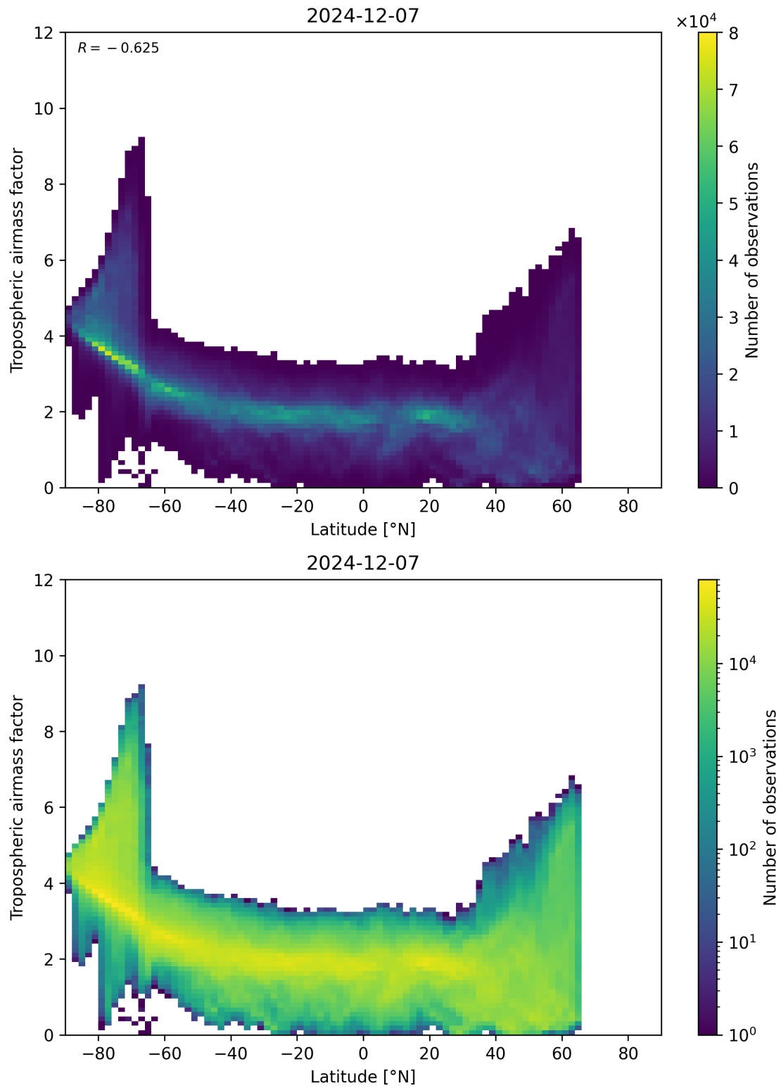
Figure 85: Scatter density plot of “Latitude” against “Tropospheric airmass factor” for 2024-12-06 to 2024-12-08.
