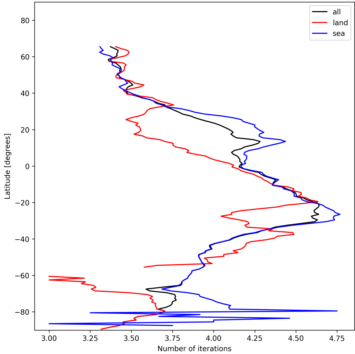
Figure 17: Zonal average of “Number of iterations” for 2024-12-06 to 2024-12-08.
