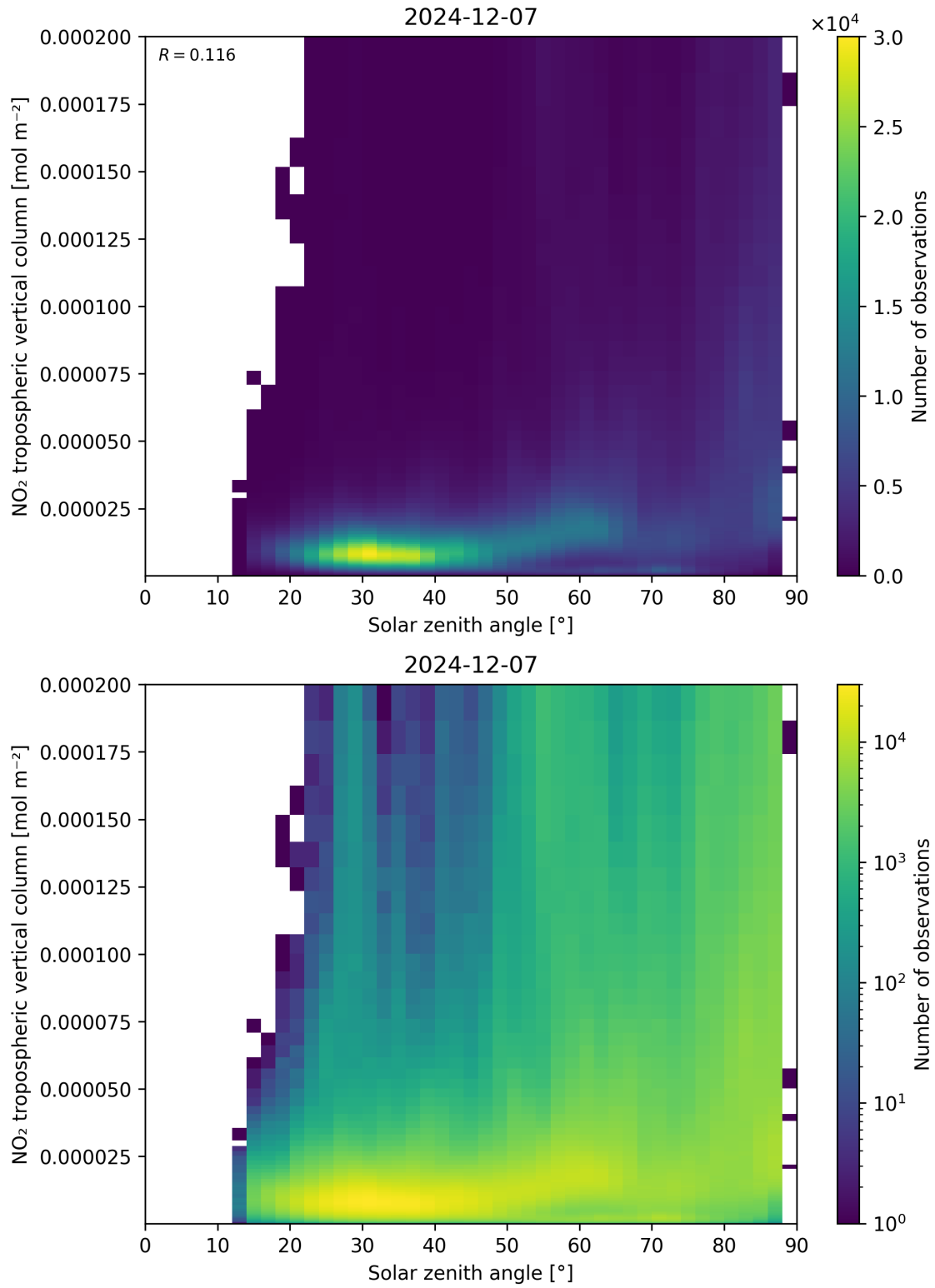
Figure 155: Scatter density plot of “Solar zenith angle” against “NO 2 tropospheric vertical column” for 2024-12-06 to 2024-12-08.
