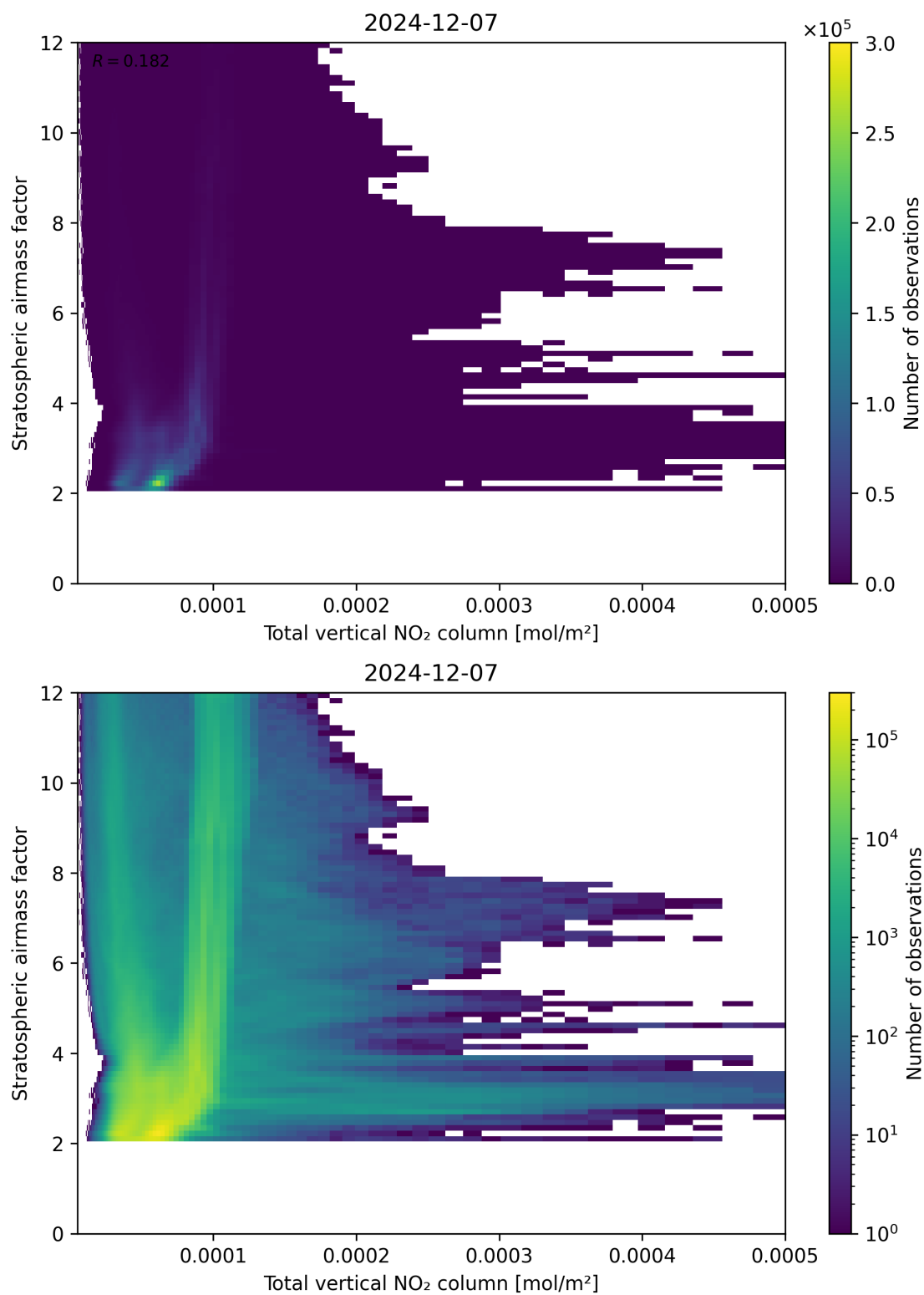
Figure 110: Scatter density plot of “Total vertical NO 2 column” against “Stratospheric air mass factor” for 2024-12-06 to 2024-12-08.
