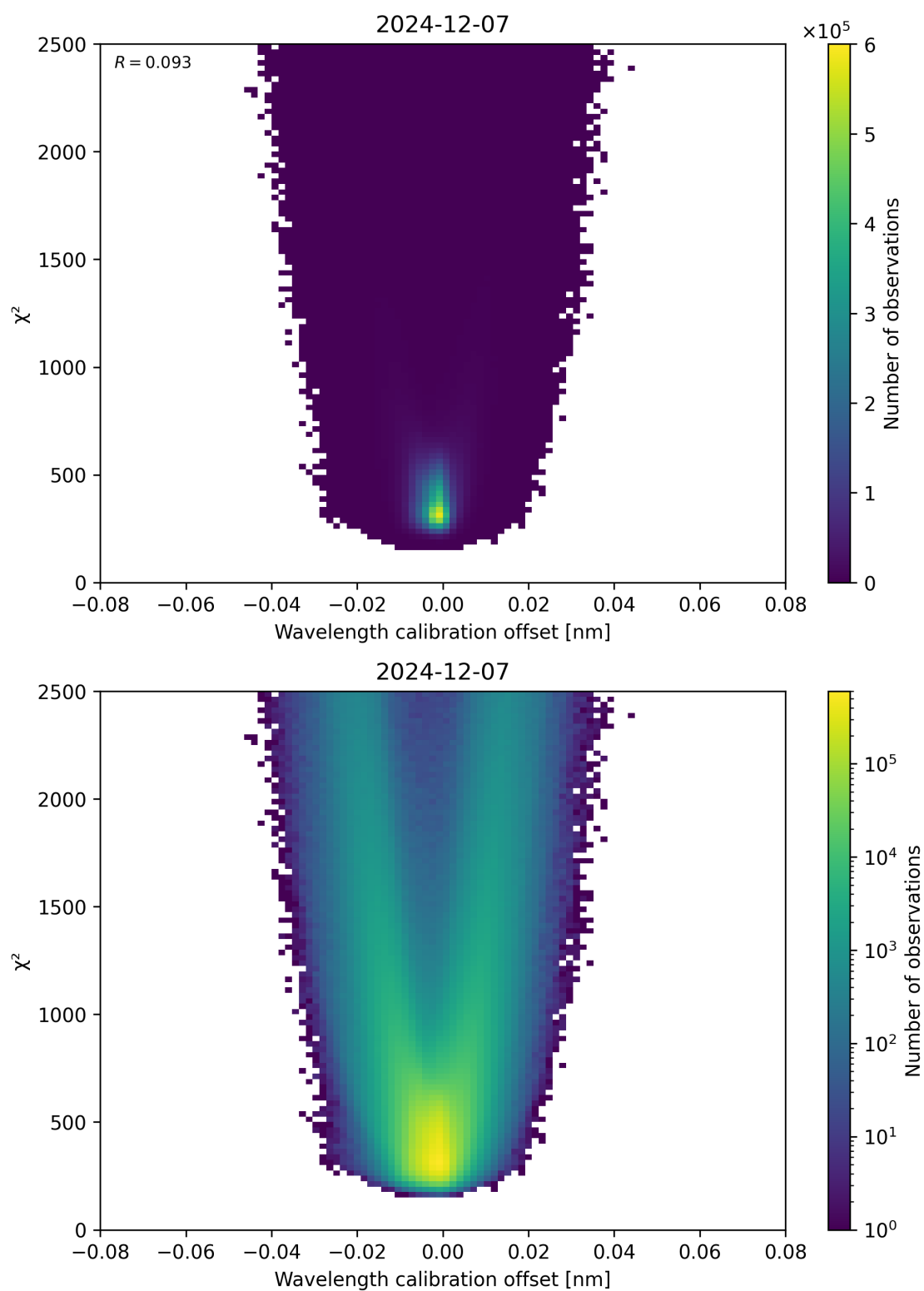
Figure 175: Scatter density plot of “Wavelength calibration offset” against “ \chi^2 ” for 2024-12-06 to 2024-12-08.
