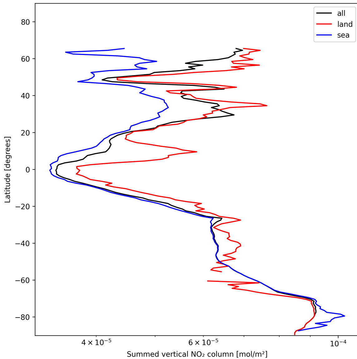
Figure 23: Zonal average of “Summed vertical NO 2 column” for 2024-12-06 to 2024-12-08.
