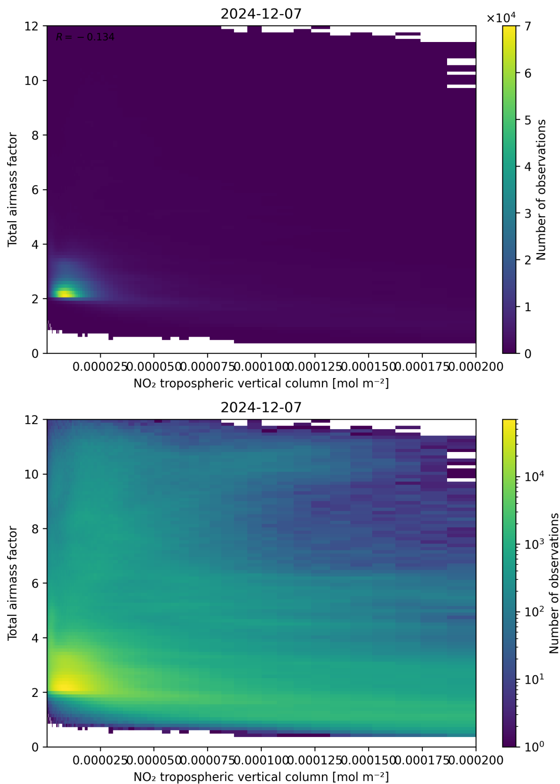
Figure 122: Scatter density plot of “NO 2 tropospheric vertical column” against “Total airmass factor” for 2024-12-06 to 2024-12-08.
