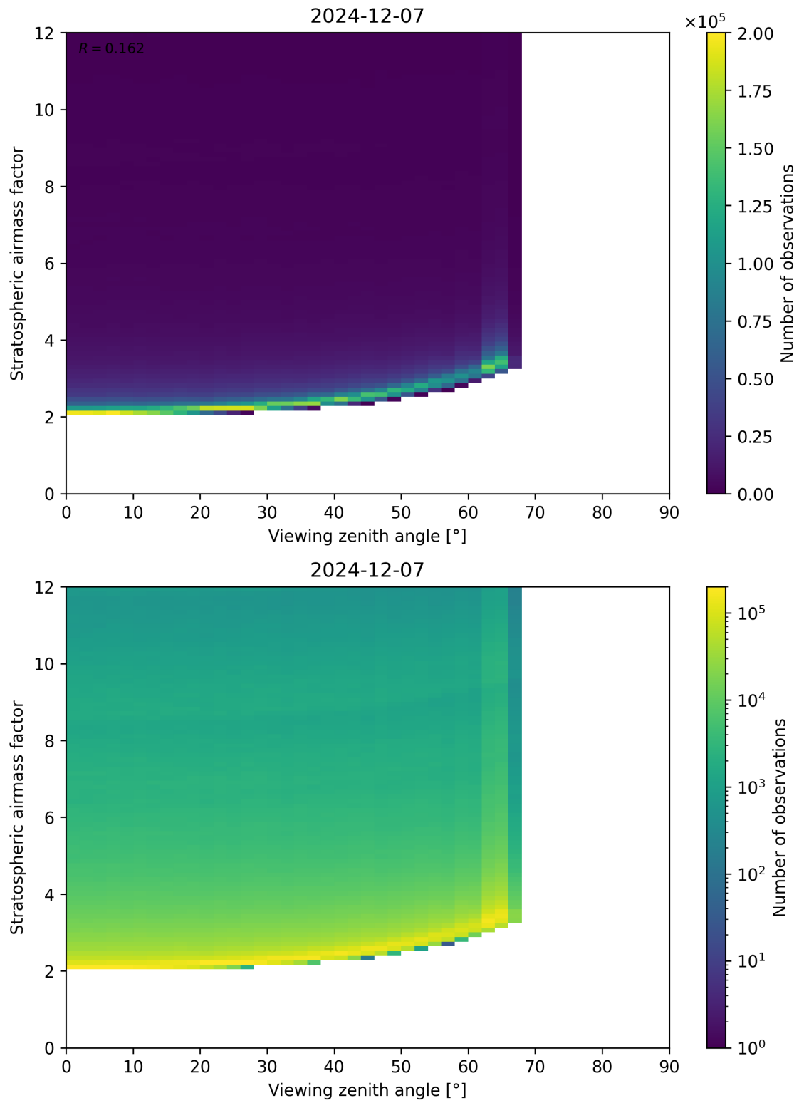
Figure 159: Scatter density plot of “Viewing zenith angle” against “Stratospheric airmass factor” for 2024-12-06 to 2024-12-08.
