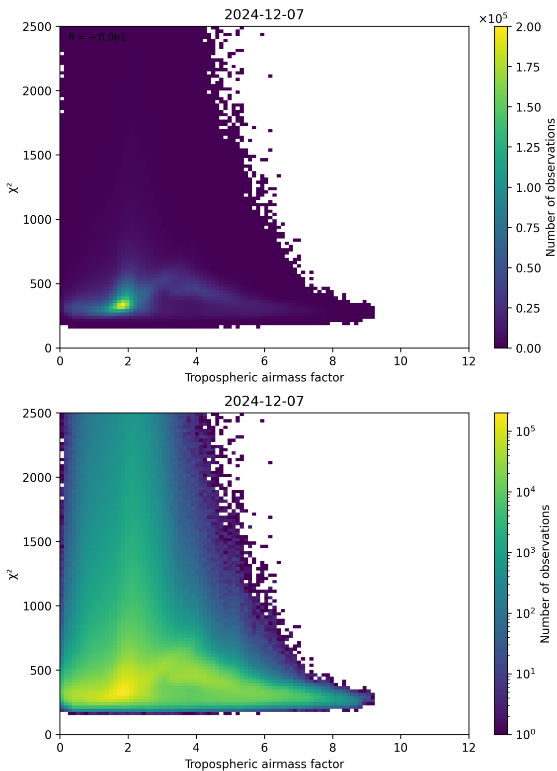
Figure 73: Scatter density plot of “Tropospheric airmass factor” against “ \chi^2 ” for 2024-12-06 to 2024-12-08.
