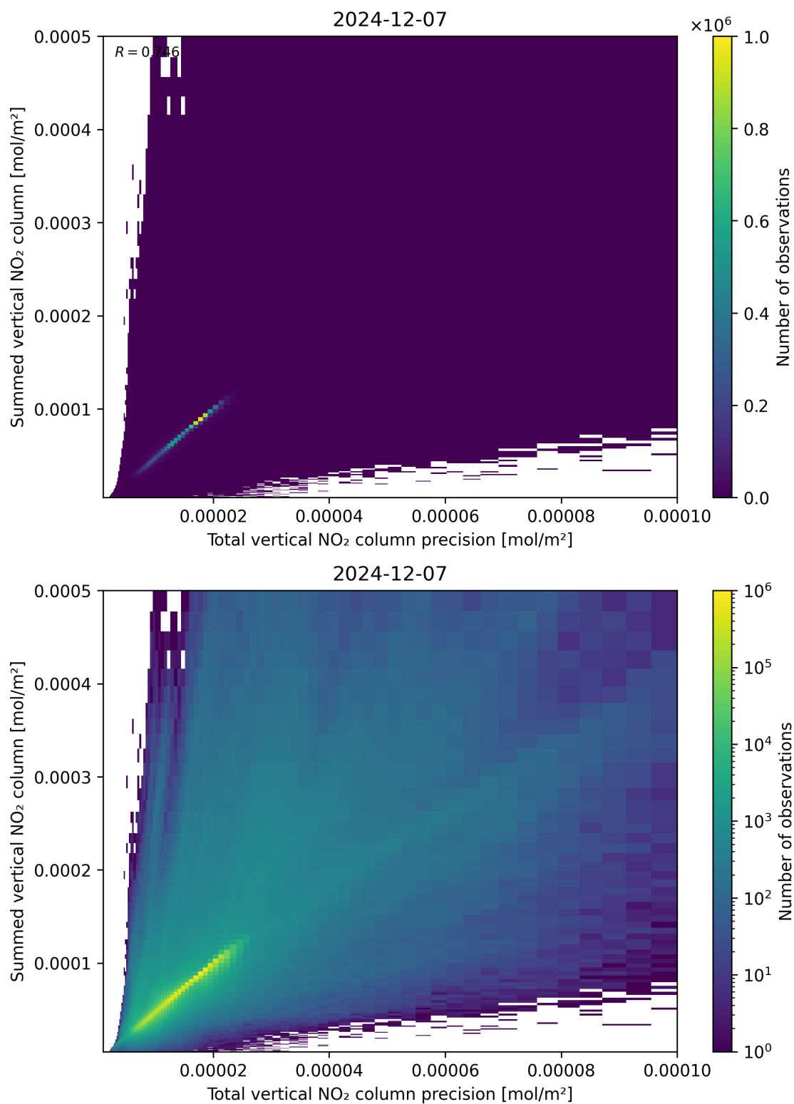
Figure 117: Scatter density plot of “Total vertical NO 2 column precision” against “Summed vertical NO 2 column” for 2024-12-06 to 2024-12-08.
