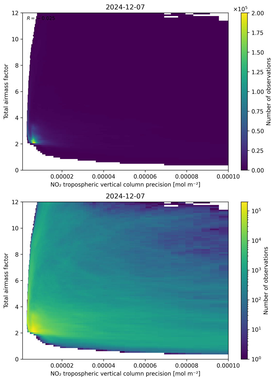
Figure 132: Scatter density plot of “NO 2 tropospheric vertical column precision” against “Total air mass factor” for 2024-12-06 to 2024-12-08.
