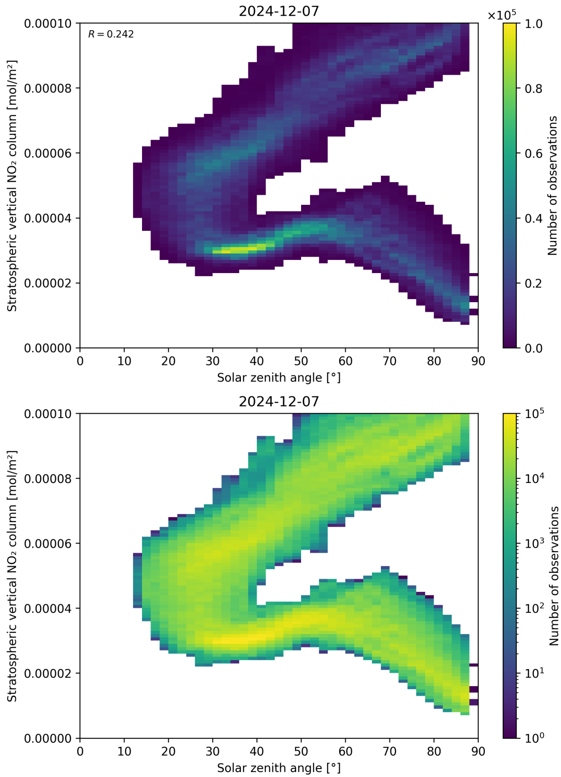
Figure 150: Scatter density plot of “Solar zenith angle” against “Stratospheric vertical NO 2 column” for 2024-12-06 to 2024-12-08.
