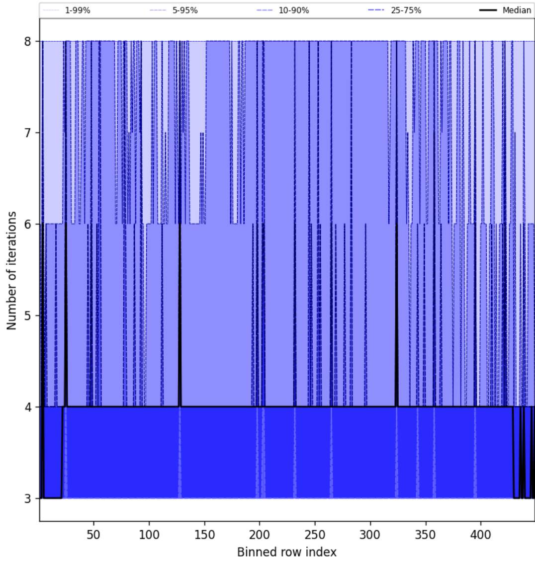
Figure 51: Along track statistics of “Number of iterations” for 2024-12-06 to 2024-12-08
