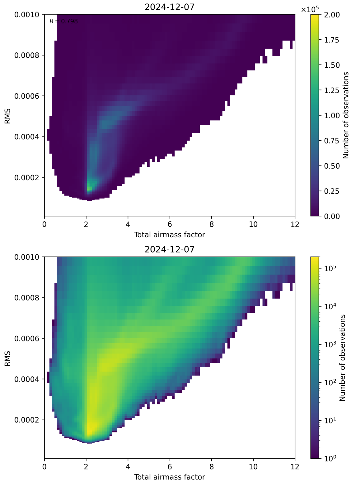
Figure 69: Scatter density plot of “Total airmass factor” against “RMS” for 2024-12-06 to 2024-12-08.
