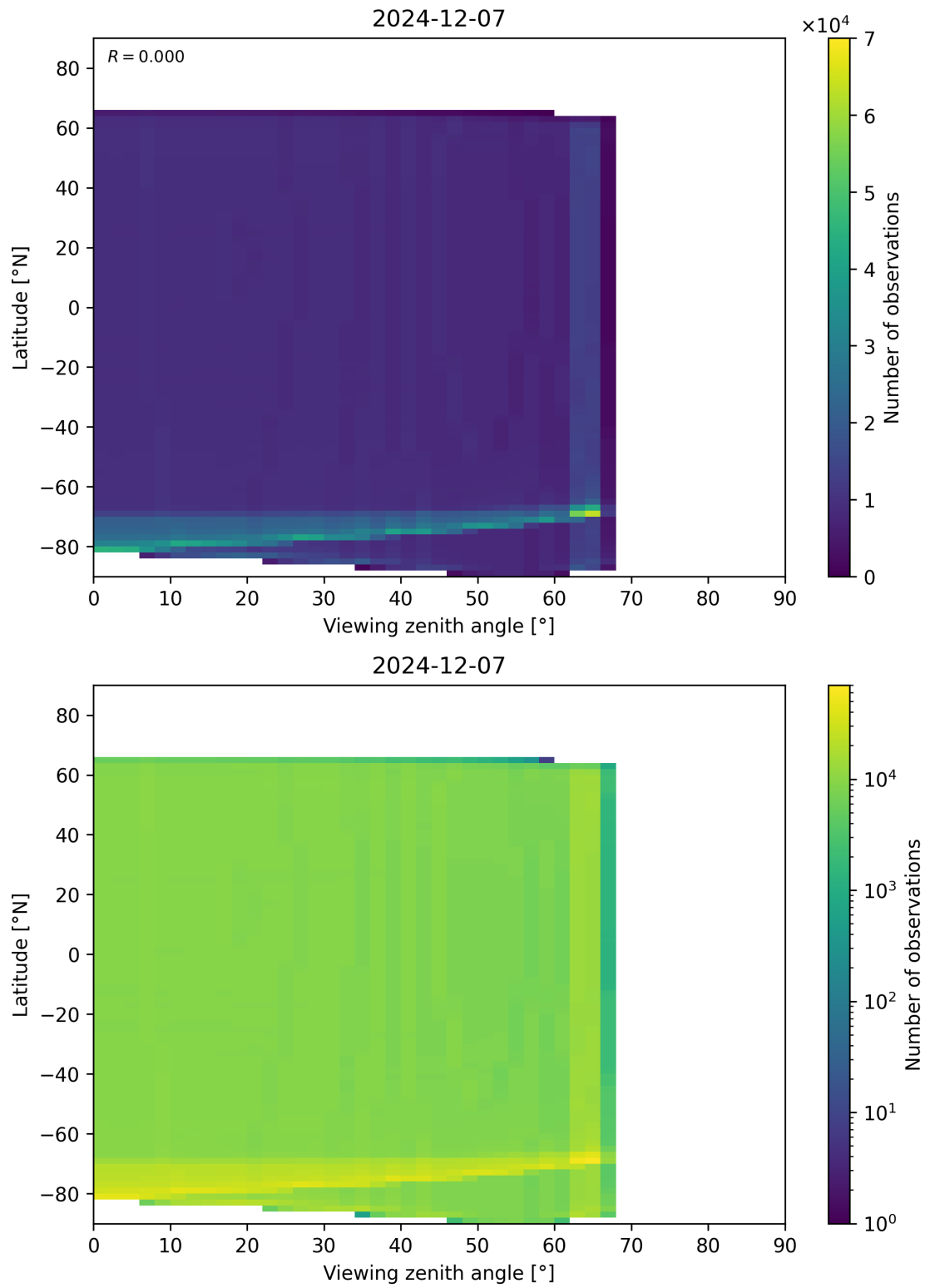
Figure 163: Scatter density plot of “Viewing zenith angle” against “Latitude” for 2024-12-06 to 2024-12-08.
