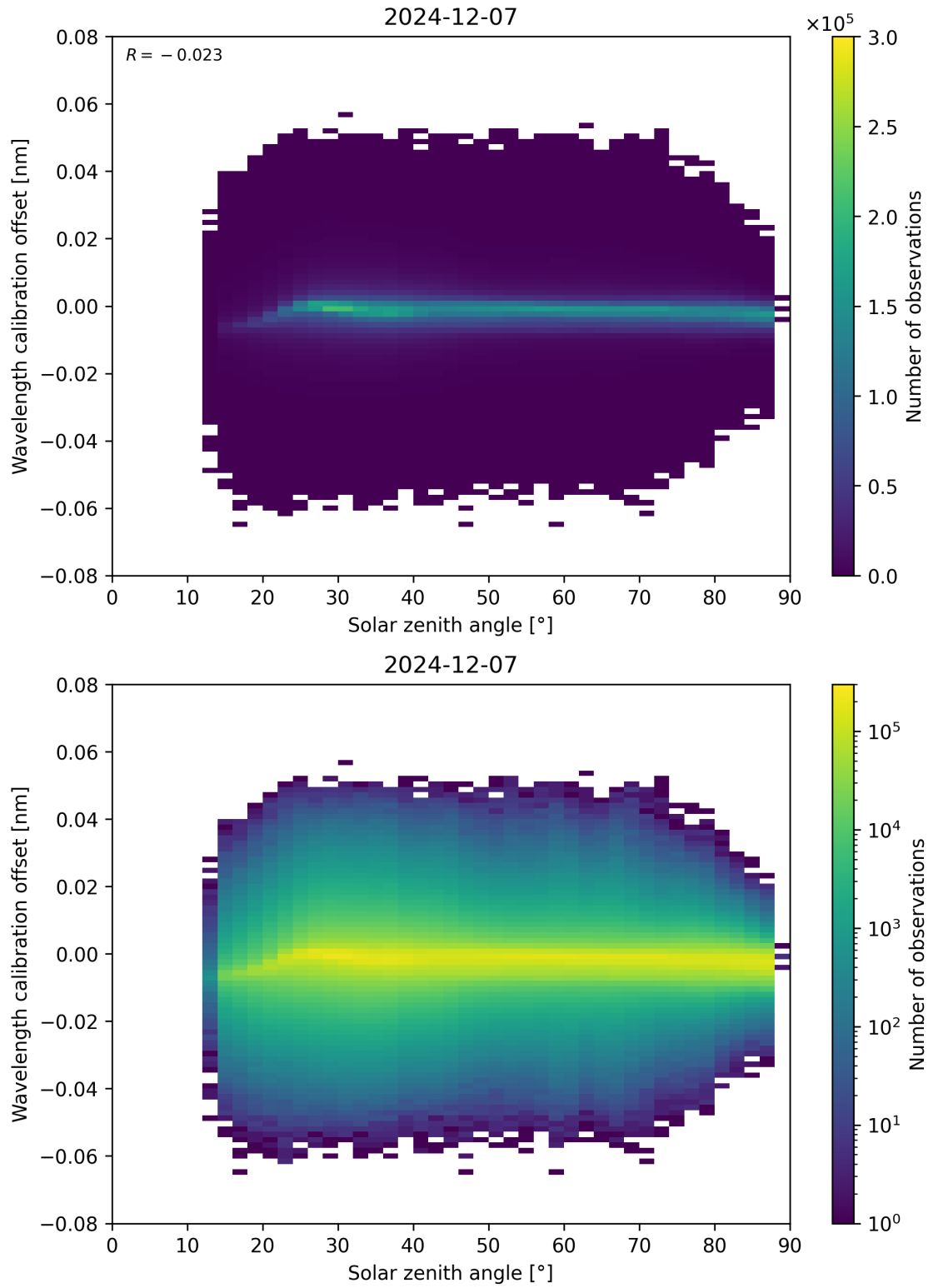
Figure 158: Scatter density plot of “Solar zenith angle” against “Wavelength calibration offset” for 2024-12-06 to 2024-12-08.
