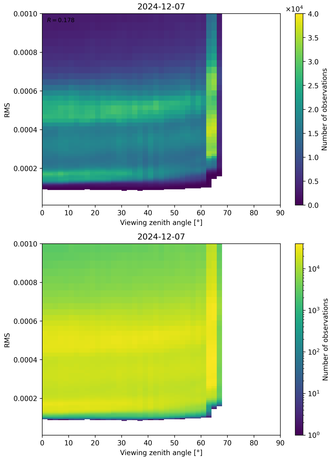
Figure 171: Scatter density plot of “Viewing zenith angle” against “RMS” for 2024-12-06 to 2024-12-08.
