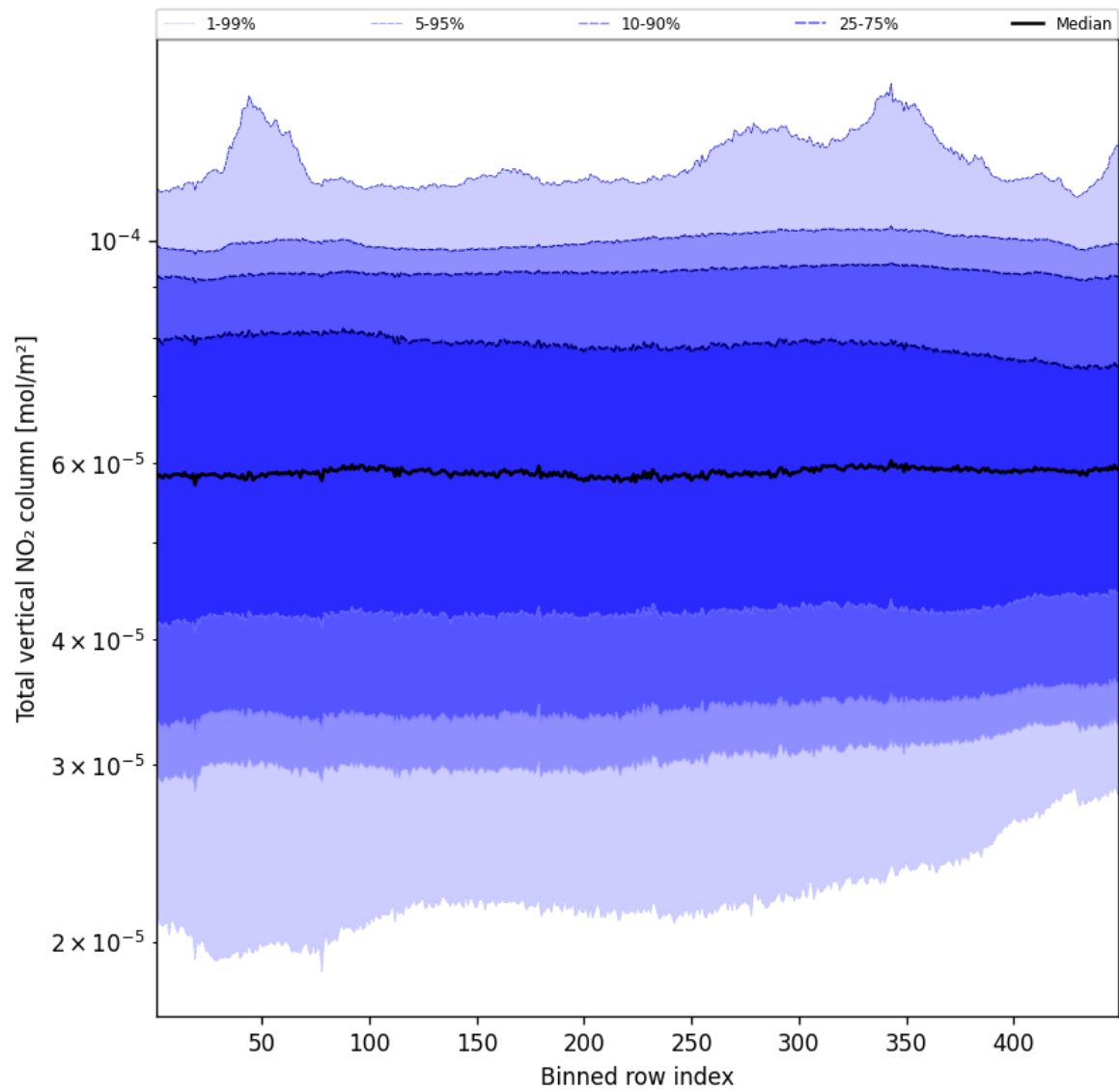
Figure 55: Along track statistics of “Total vertical NO 2 column” for 2024-12-06 to 2024-12-08
