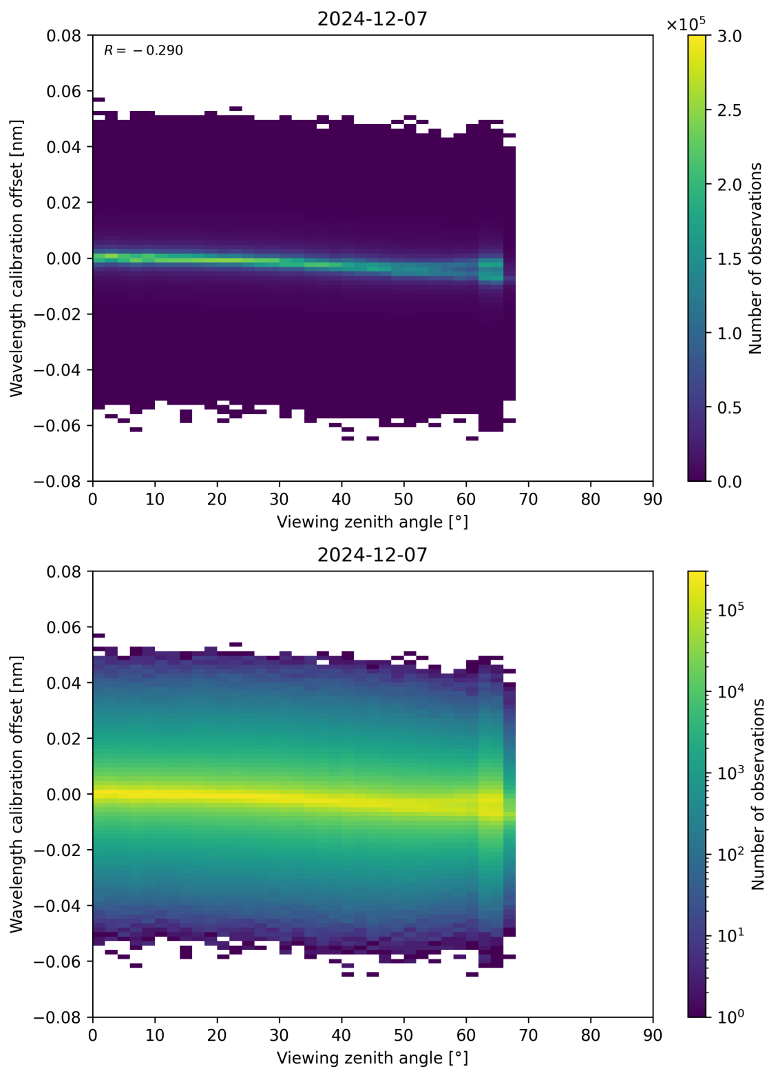
Figure 173: Scatter density plot of “Viewing zenith angle” against “Wavelength calibration offset” for 2024-12-06 to 2024-12-08.
