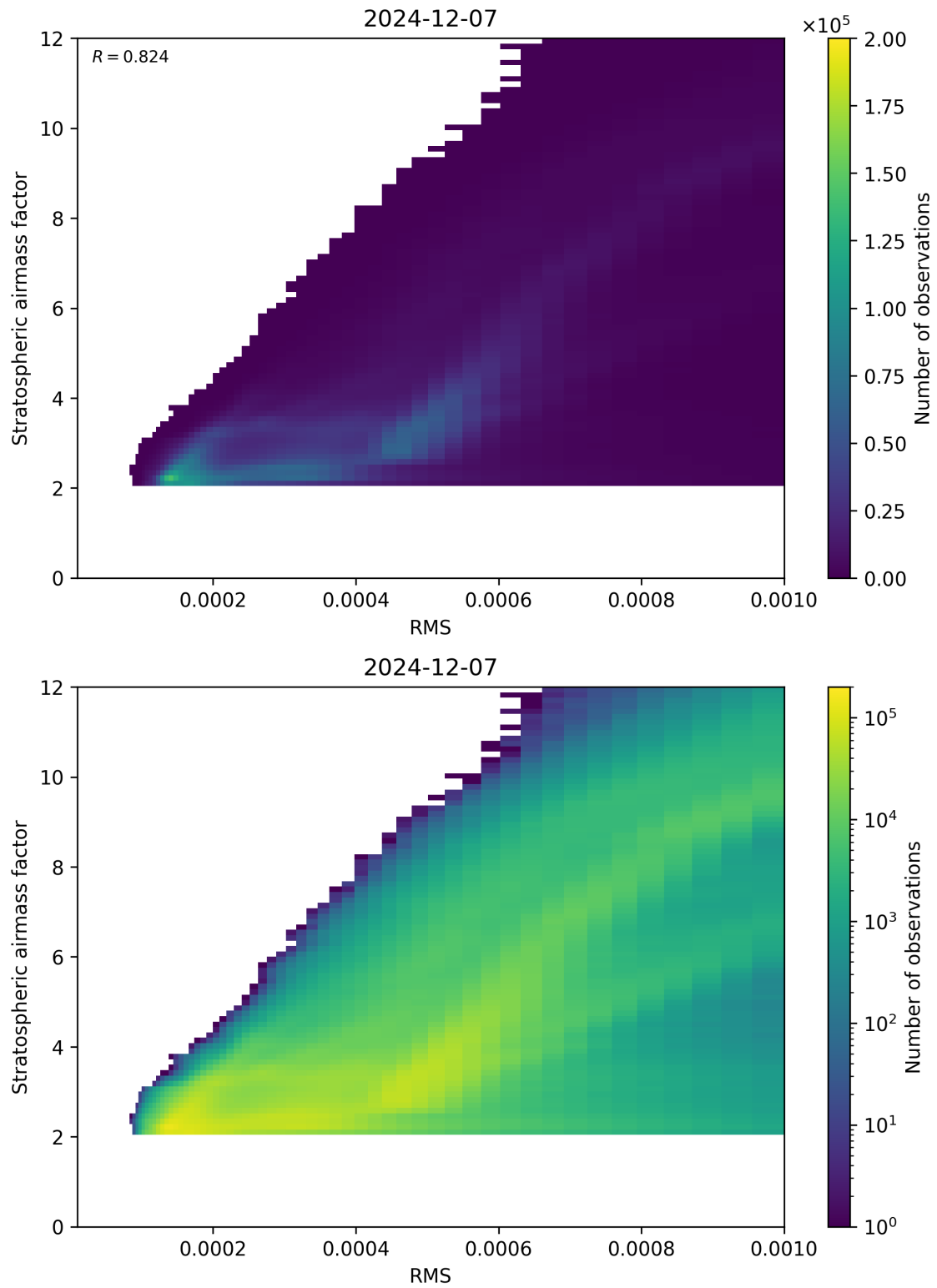
Figure 144: Scatter density plot of “RMS” against “Stratospheric airmass factor” for 2024-12-06 to 2024-12-08.
