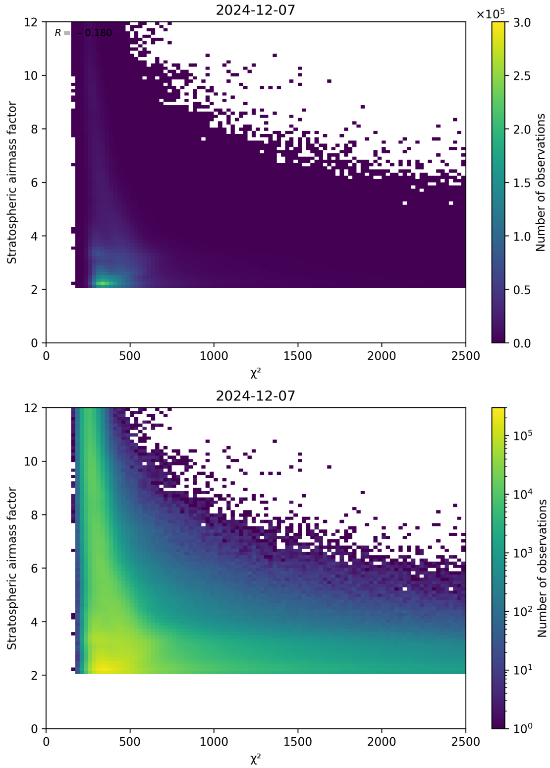
Figure 81: Scatter density plot of “ \chi^2 ” against “Stratospheric airmass factor” for 2024-12-06 to 2024-12-08.
