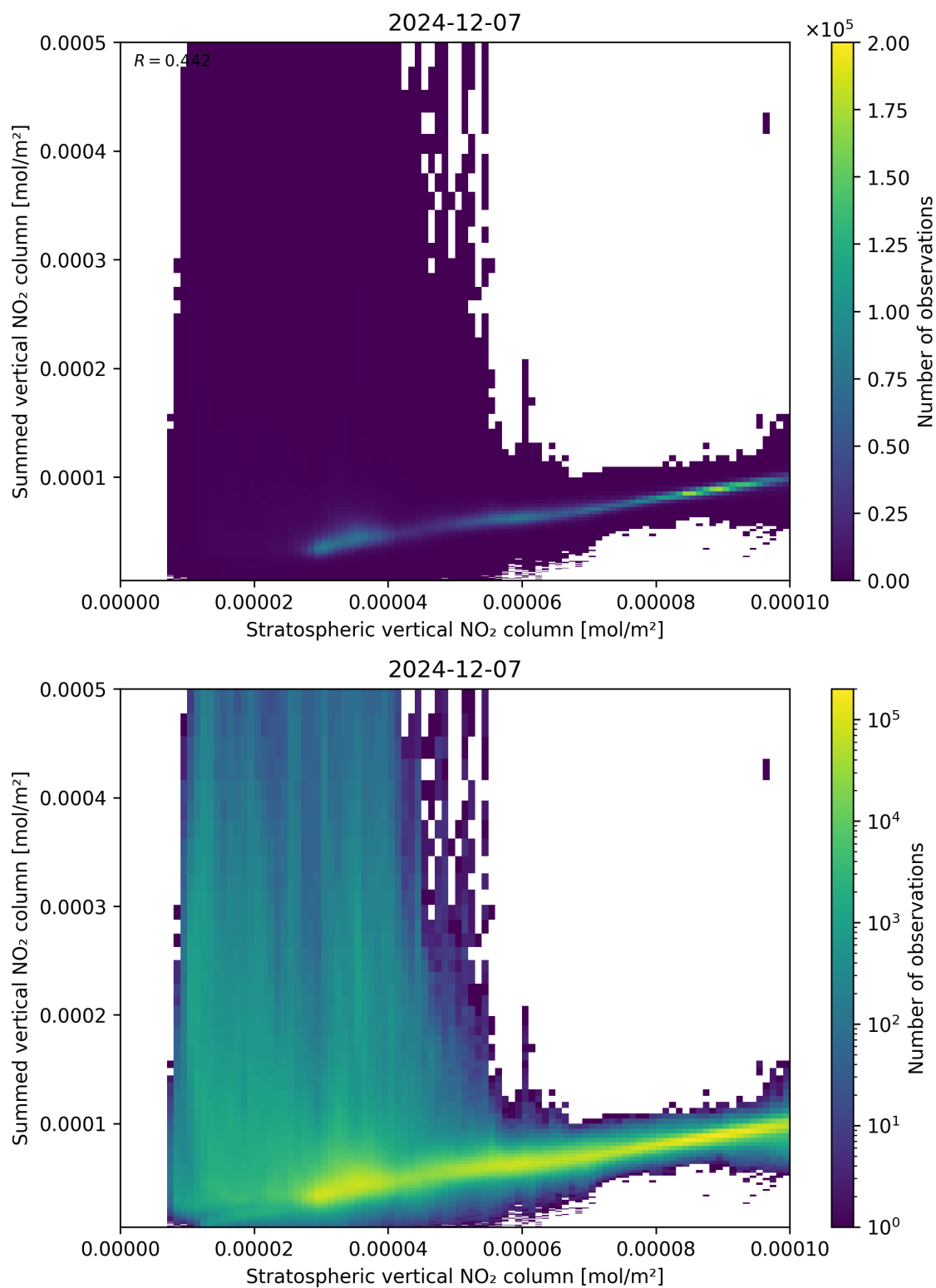
Figure 98: Scatter density plot of “Stratospheric vertical NO 2 column” against “Summed vertical NO 2 column” for 2024-12-06 to 2024-12-08.
