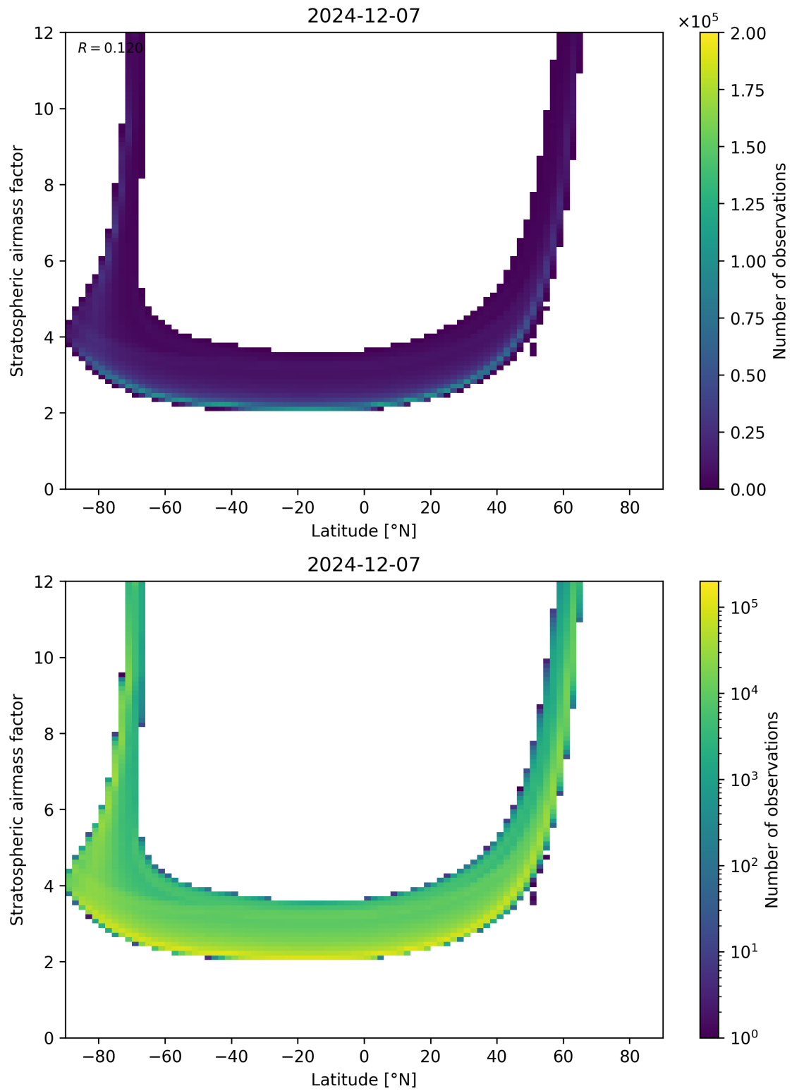
Figure 83: Scatter density plot of “Latitude” against “Stratospheric air mass factor” for 2024-12-06 to 2024-12-08.
