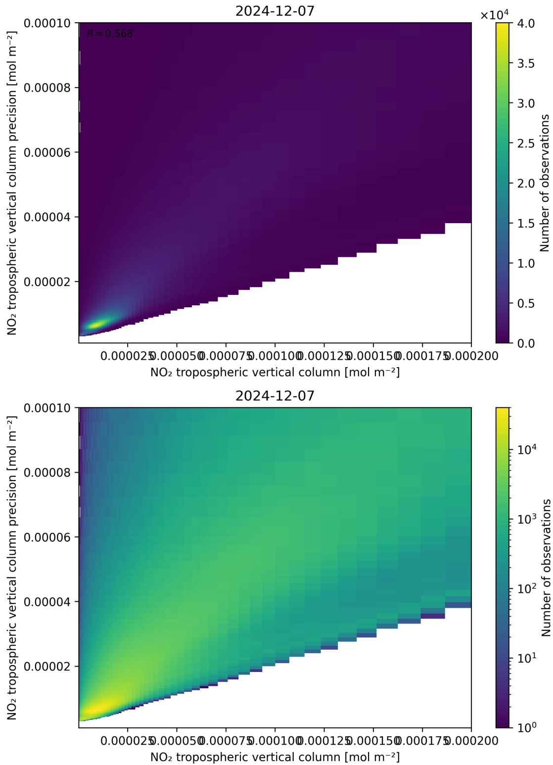
Figure 130: Scatter density plot of “NO 2 tropospheric vertical column” against “NO 2 tropospheric vertical column precision” for 2024-12-06 to 2024-12-08.
