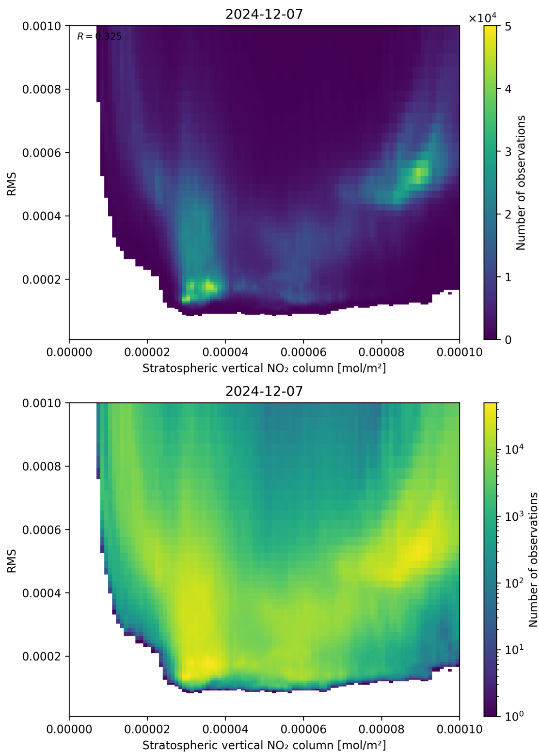
Figure 102: Scatter density plot of “Stratospheric vertical NO 2 column” against “RMS” for 2024-12-06 to 2024-12-08.
