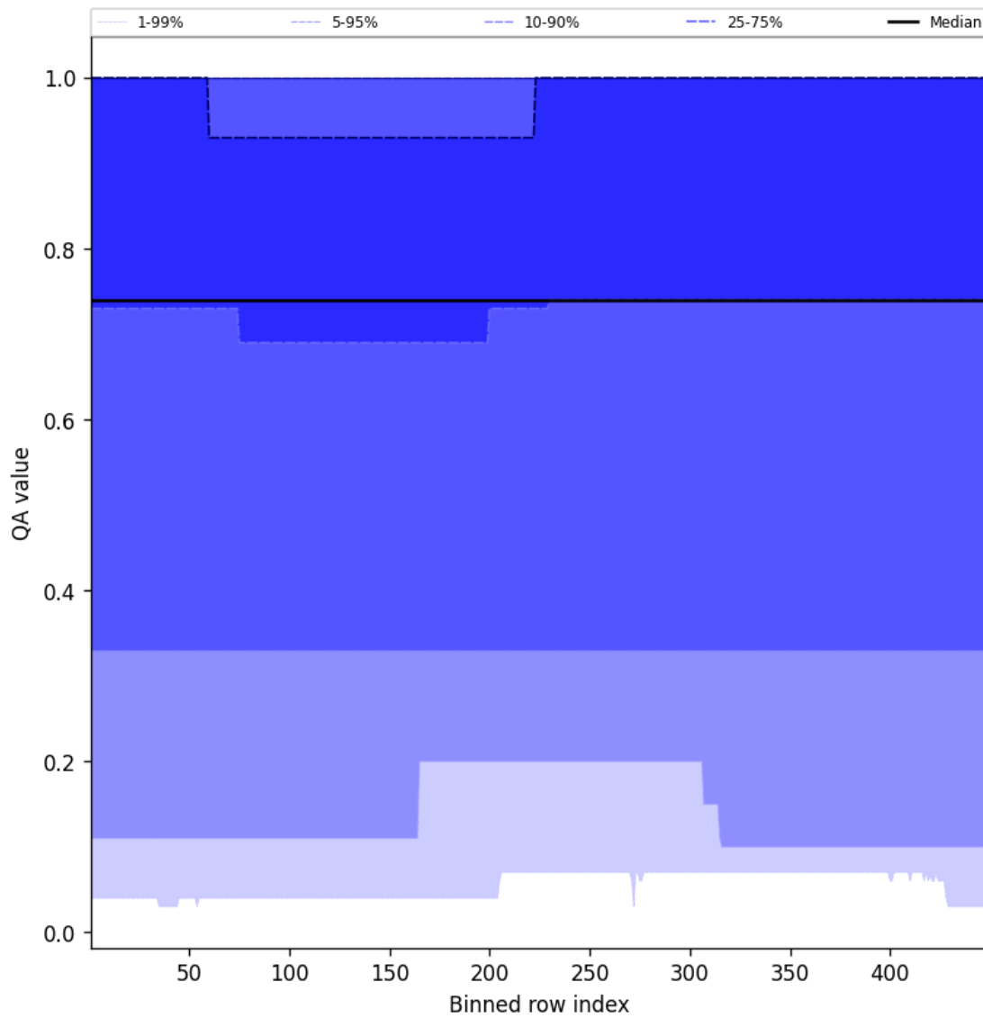
Figure 45: Along track statistics of “QA value” for 2024-12-06 to 2024-12-08
