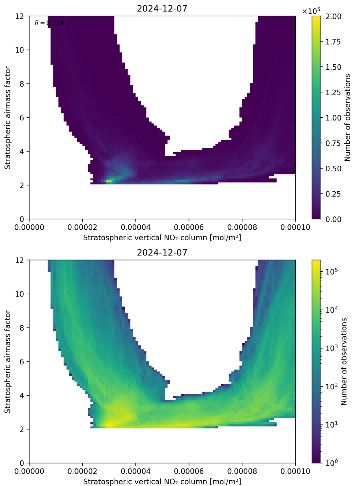
Figure 96: Scatter density plot of “Stratospheric vertical NO 2 column” against “Stratospheric airmass factor” for 2024-12-06 to 2024-12-08.
