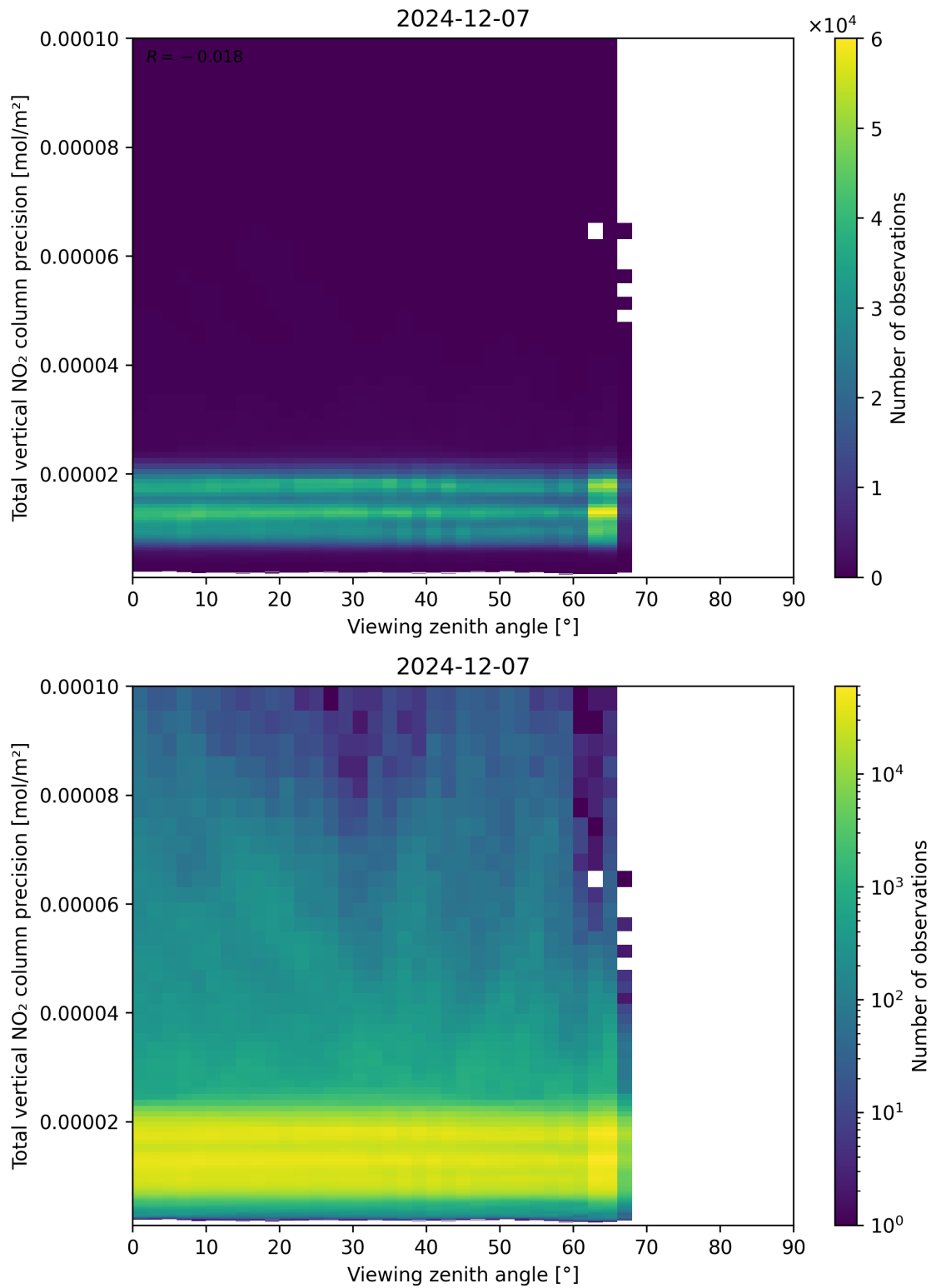
Figure 168: Scatter density plot of “Viewing zenith angle” against “Total vertical NO 2 column precision” for 2024-12-06 to 2024-12-08.
