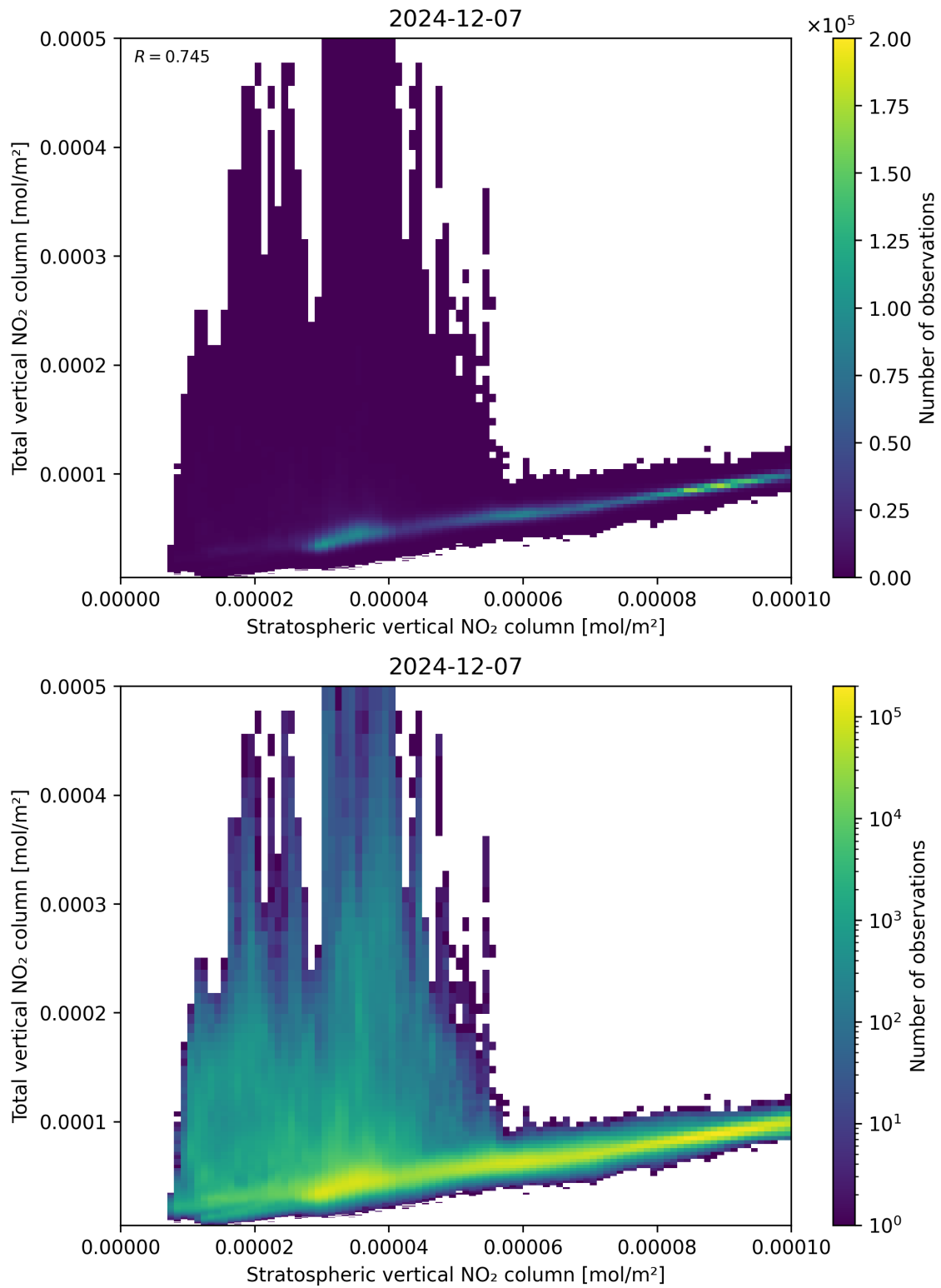
Figure 100: Scatter density plot of “Stratospheric vertical NO 2 column” against “Total vertical NO 2 column” for 2024-12-06 to 2024-12-08.
