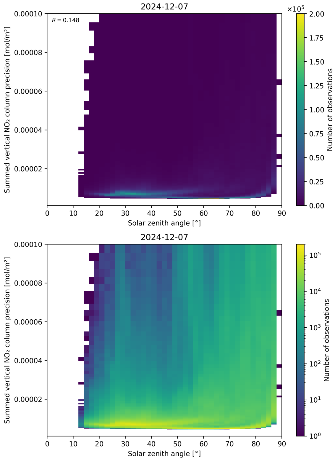
Figure 152: Scatter density plot of “Solar zenith angle” against “Summed vertical NO 2 column precision” for 2024-12-06 to 2024-12-08.
