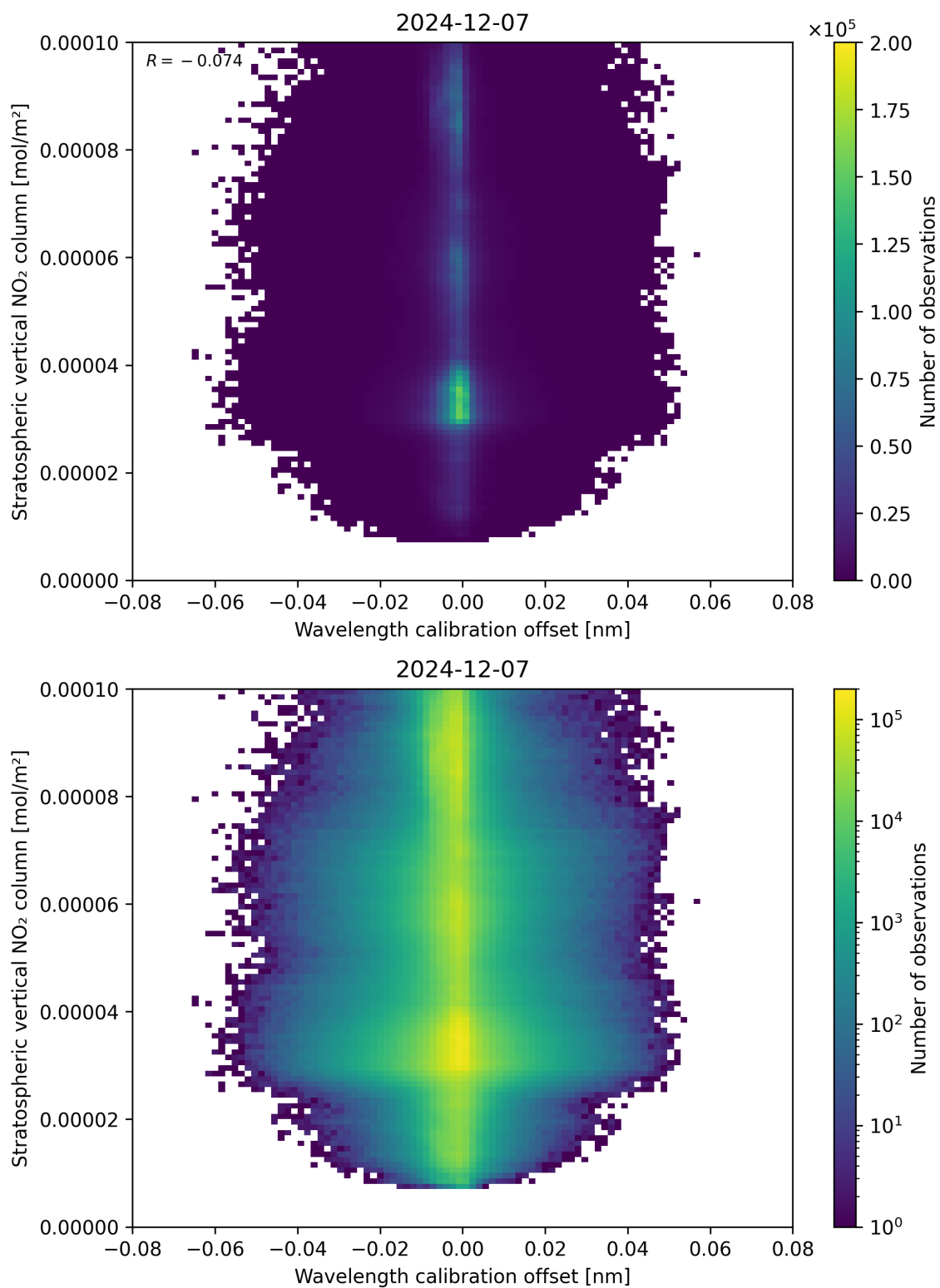
Figure 176: Scatter density plot of “Wavelength calibration offset” against “Stratospheric vertical NO 2 column” for 2024-12-06 to 2024-12-08.
