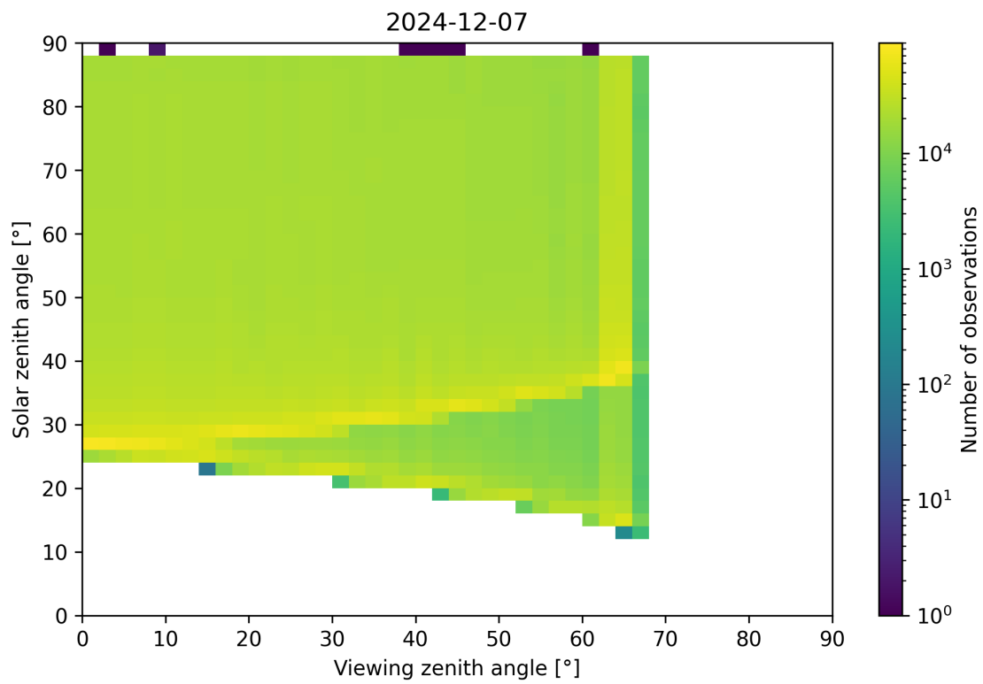
Figure 172: Scatter density plot of “Viewing zenith angle” against “Solar zenith angle” for 2024-12-06 to 2024-12-08.
