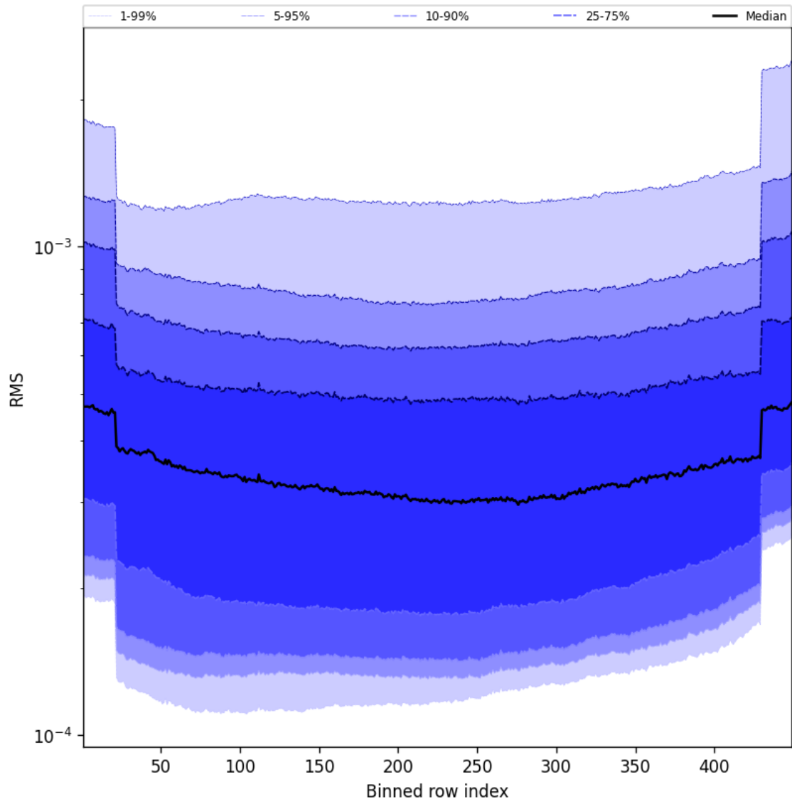
Figure 60: Along track statistics of “RMS” for 2024-12-06 to 2024-12-08
