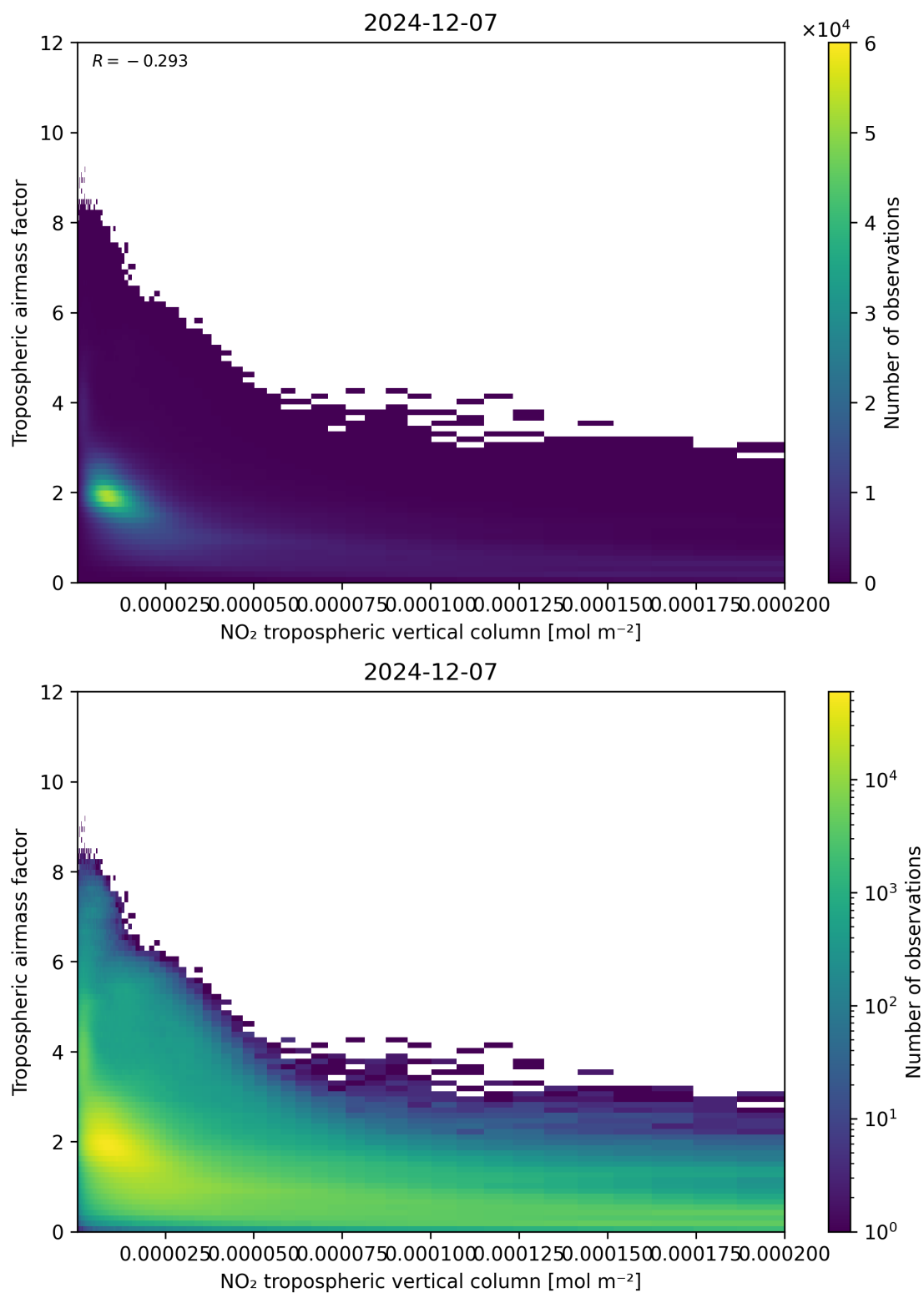
Figure 123: Scatter density plot of “NO 2 tropospheric vertical column” against “Tropospheric air mass factor” for 2024-12-06 to 2024-12-08.
