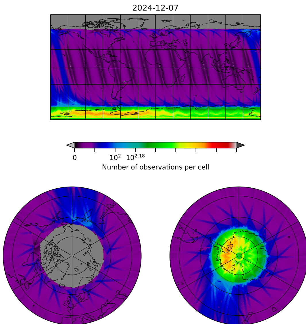
Figure 10: Map of the number of observations for 2024-12-06 to 2024-12-08
