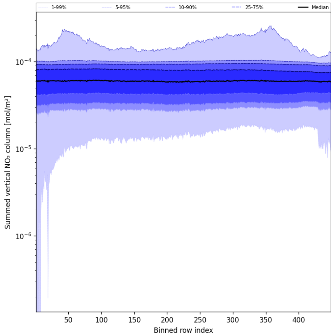
Figure 57: Along track statistics of “Summed vertical NO 2 column” for 2024-12-06 to 2024-12-08
