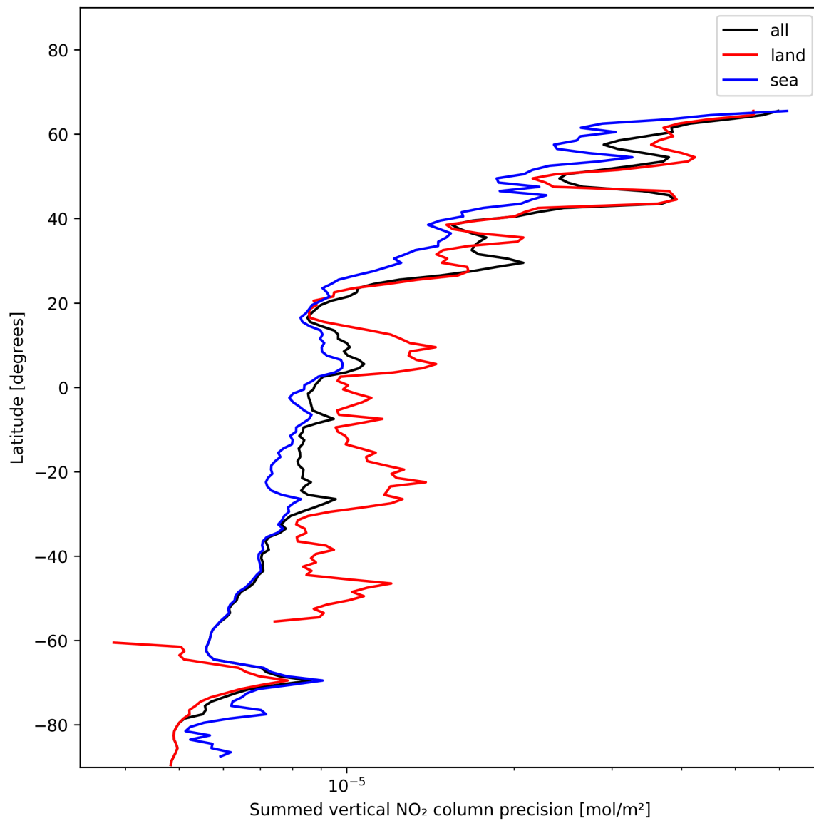
Figure 24: Zonal average of “Summed vertical NO 2 column precision” for 2024-12-06 to 2024-12-08.
