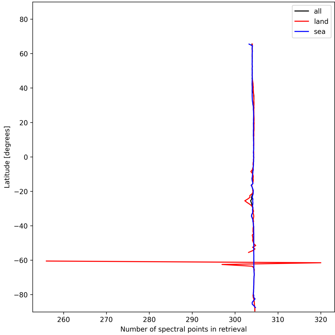
Figure 16: Zonal average of “Number of spectral points in retrieval” for 2024-12-06 to 2024-12-08.
