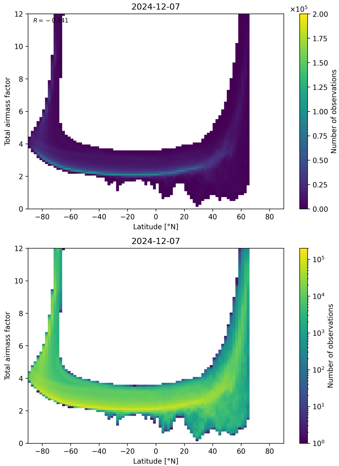
Figure 84: Scatter density plot of “Latitude” against “Total airmass factor” for 2024-12-06 to 2024-12-08.
