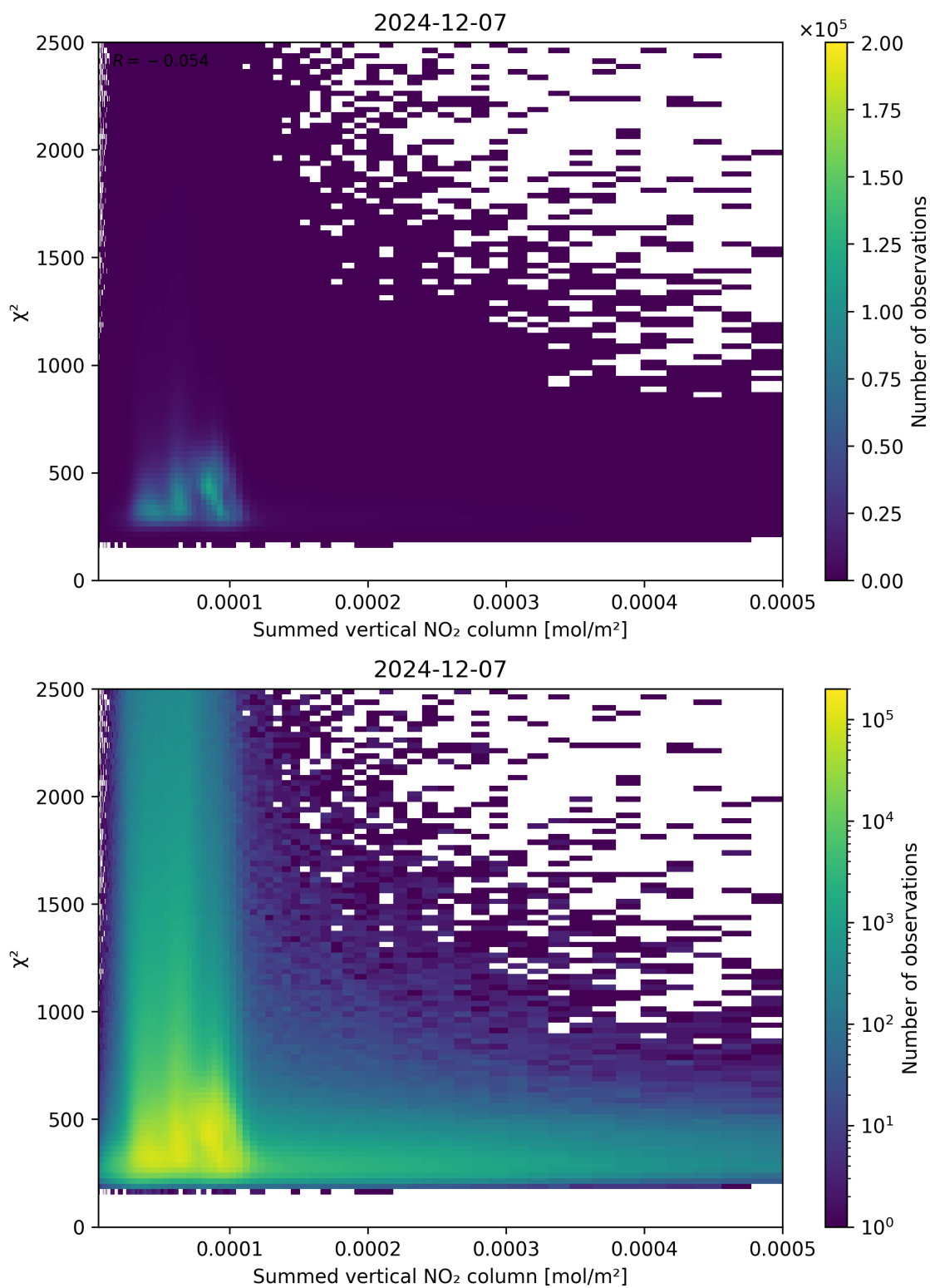
Figure 104: Scatter density plot of “Summed vertical NO 2 column” against “ \chi^2 ” for 2024-12-06 to 2024-12-08.
