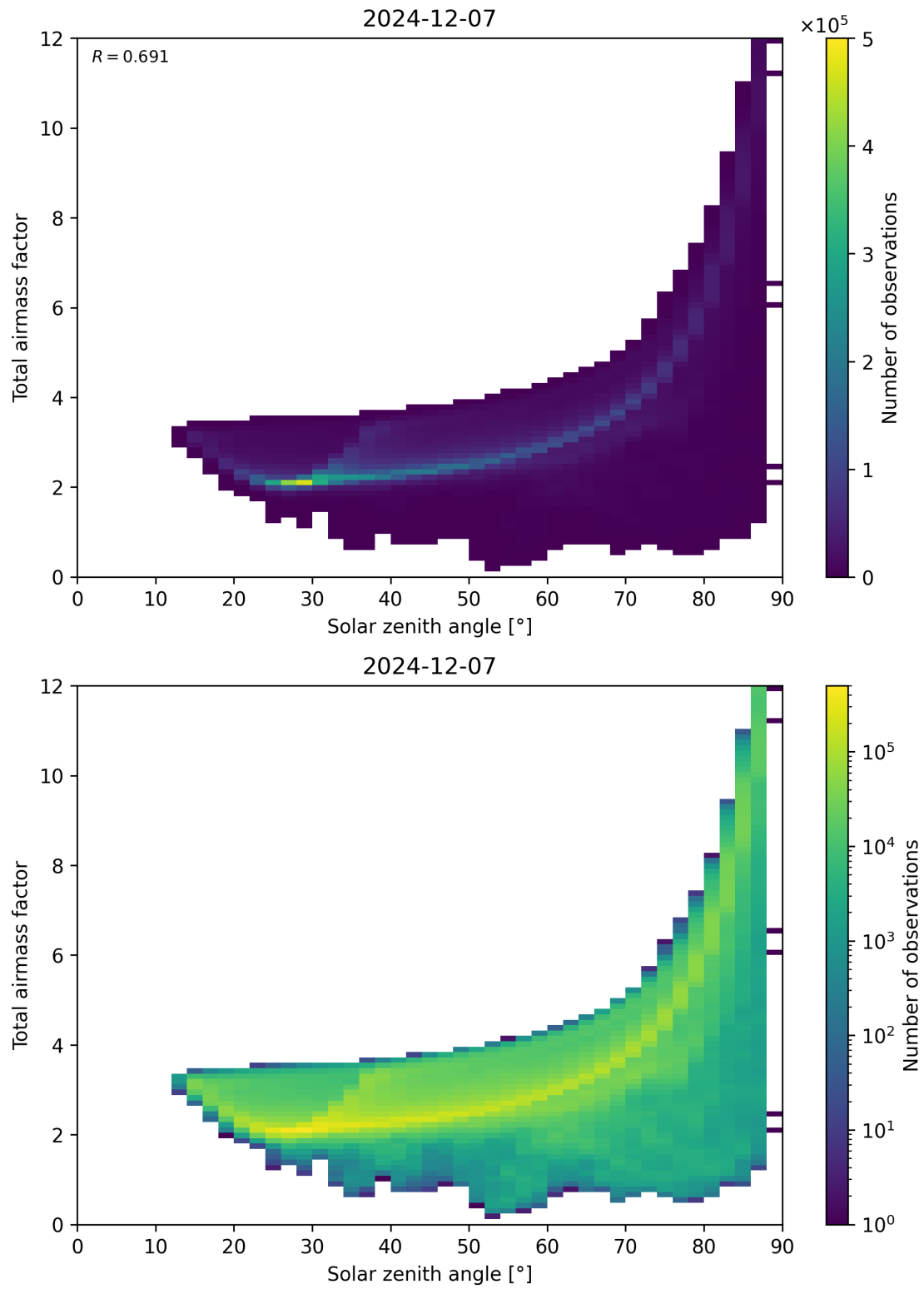
Figure 146: Scatter density plot of “Solar zenith angle” against “Total air mass factor” for 2024-12-06 to 2024-12-08.
