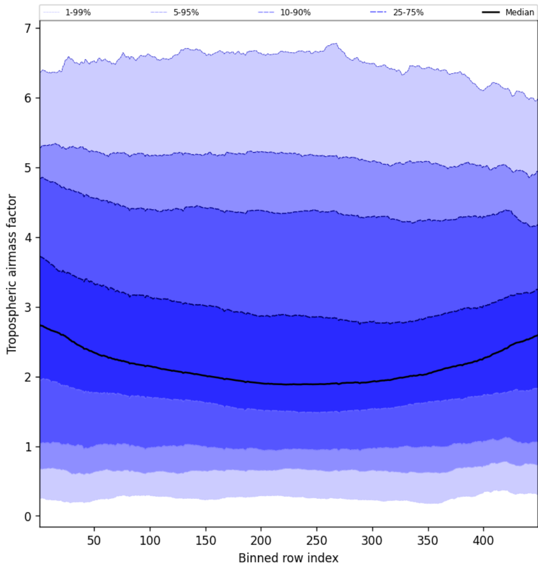
Figure 48: Along track statistics of “Tropospheric airmass factor” for 2024-12-06 to 2024-12-08
