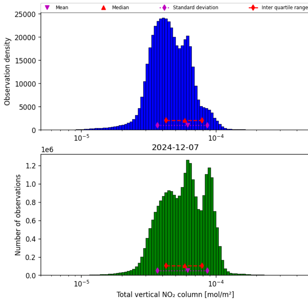
Figure 38: Histogram of “Total vertical NO 2 column” for 2024-12-06 to 2024-12-08
