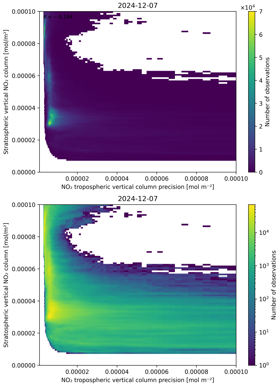
Figure 135: Scatter density plot of “NO 2 tropospheric vertical column precision” against “Stratospheric vertical NO 2 column” for 2024-12-06 to 2024-12-08.
