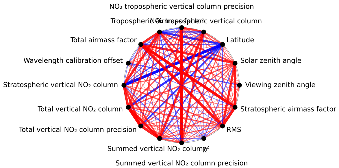
Figure 1: Map of correlation graph for 2024-12-06 to 2024-12-08.
