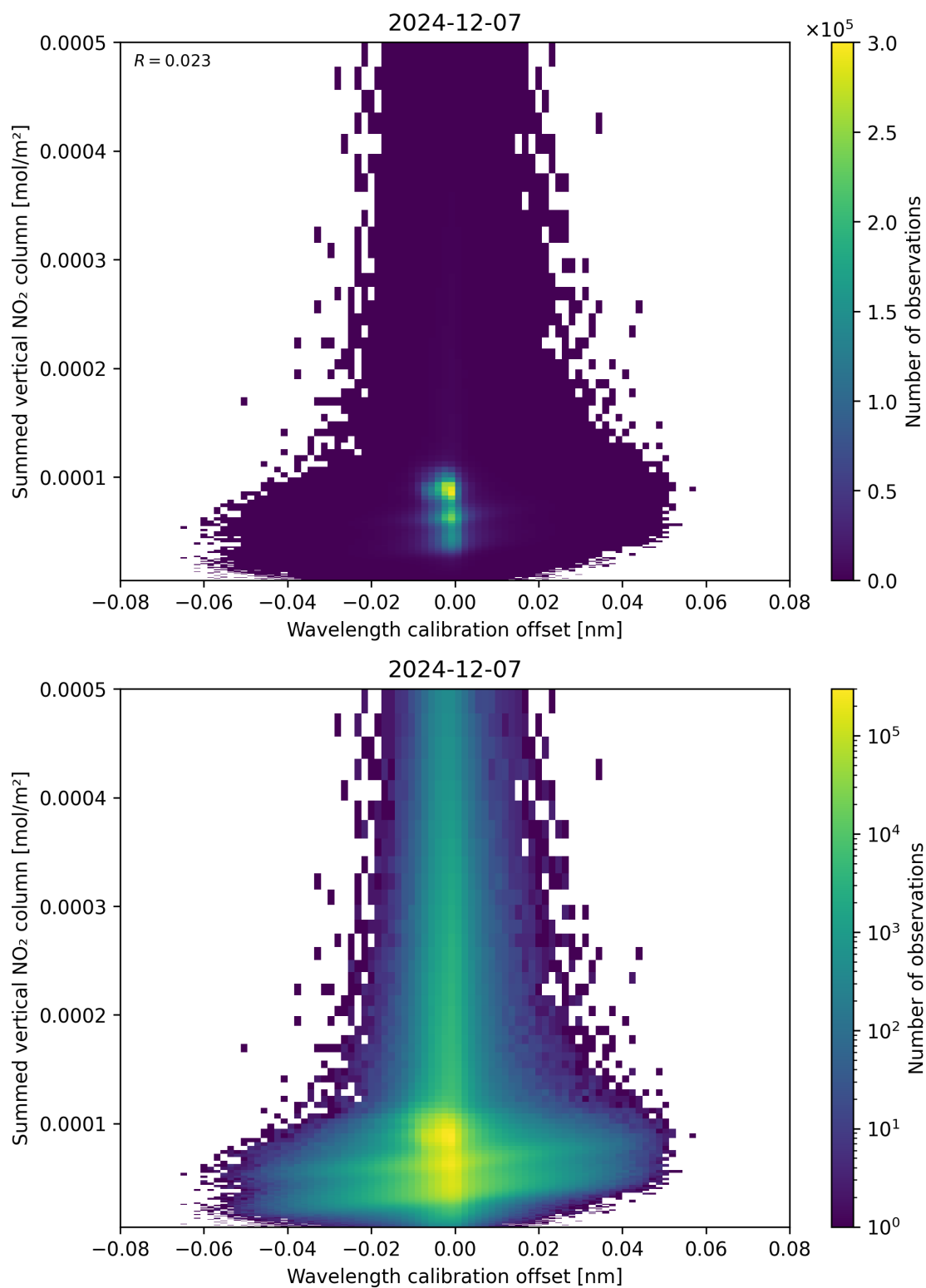
Figure 177: Scatter density plot of “Wavelength calibration offset” against “Summed vertical NO 2 column” for 2024-12-06 to 2024-12-08.
