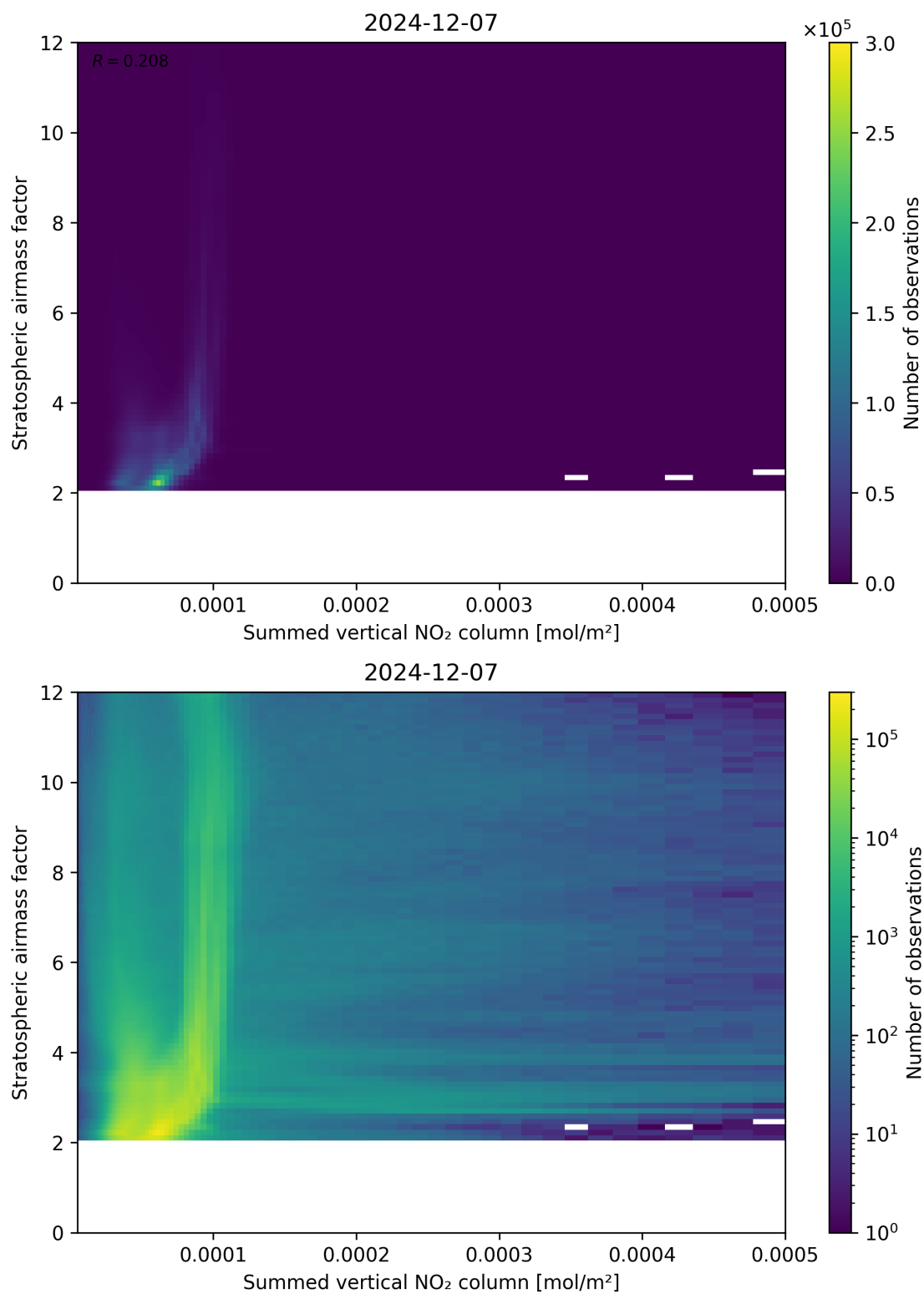
Figure 103: Scatter density plot of “Summed vertical NO 2 column” against “Stratospheric airmass factor” for 2024-12-06 to 2024-12-08.
