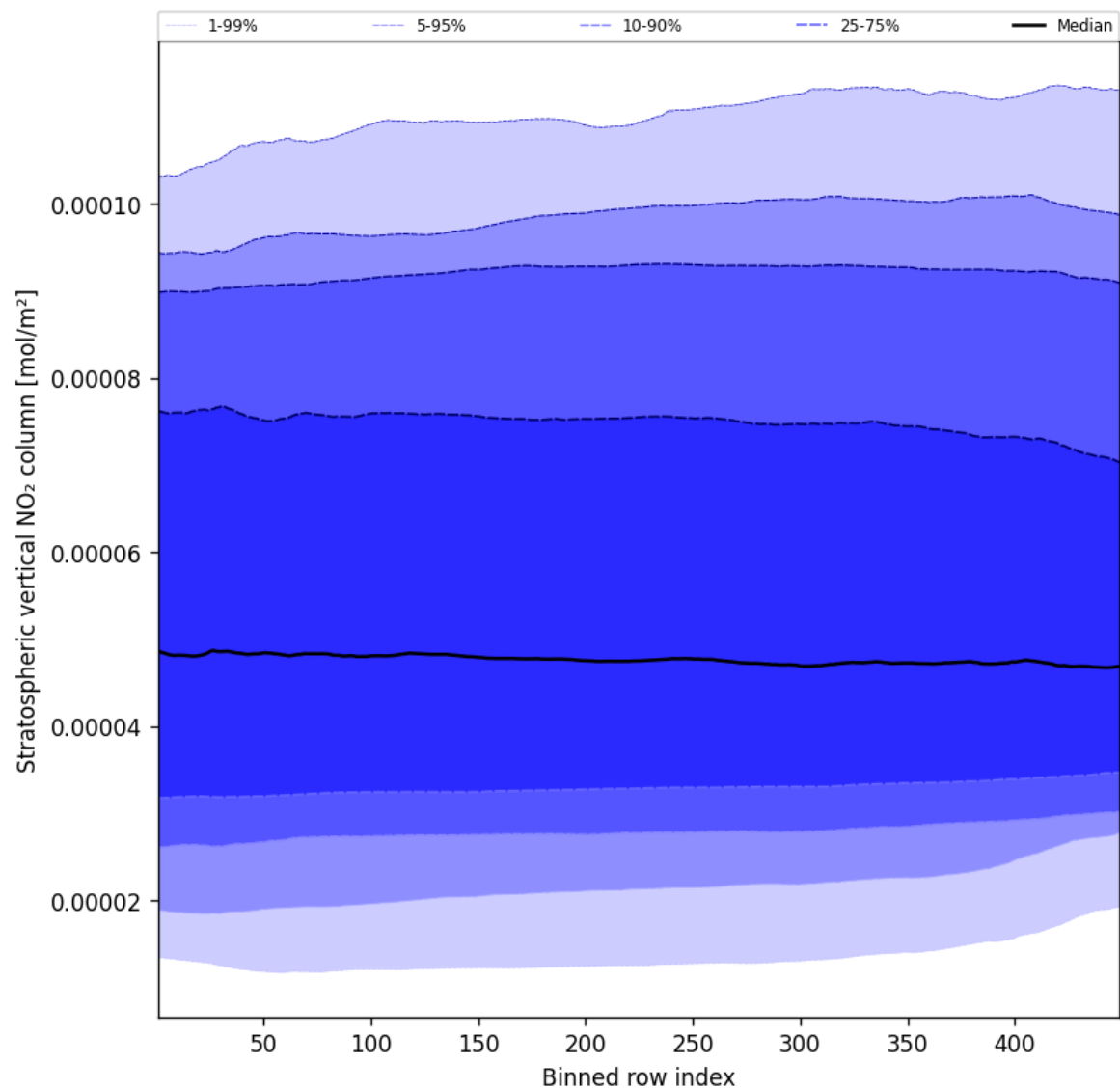
Figure 53: Along track statistics of “Stratospheric vertical NO 2 column” for 2024-12-06 to 2024-12-08
