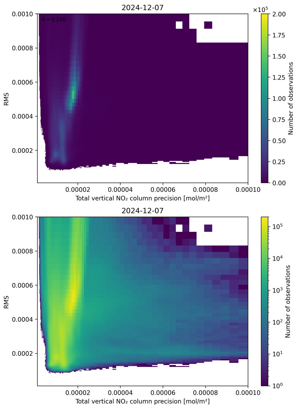
Figure 119: Scatter density plot of “Total vertical NO 2 column precision” against “RMS” for 2024-12-06 to 2024-12-08.
