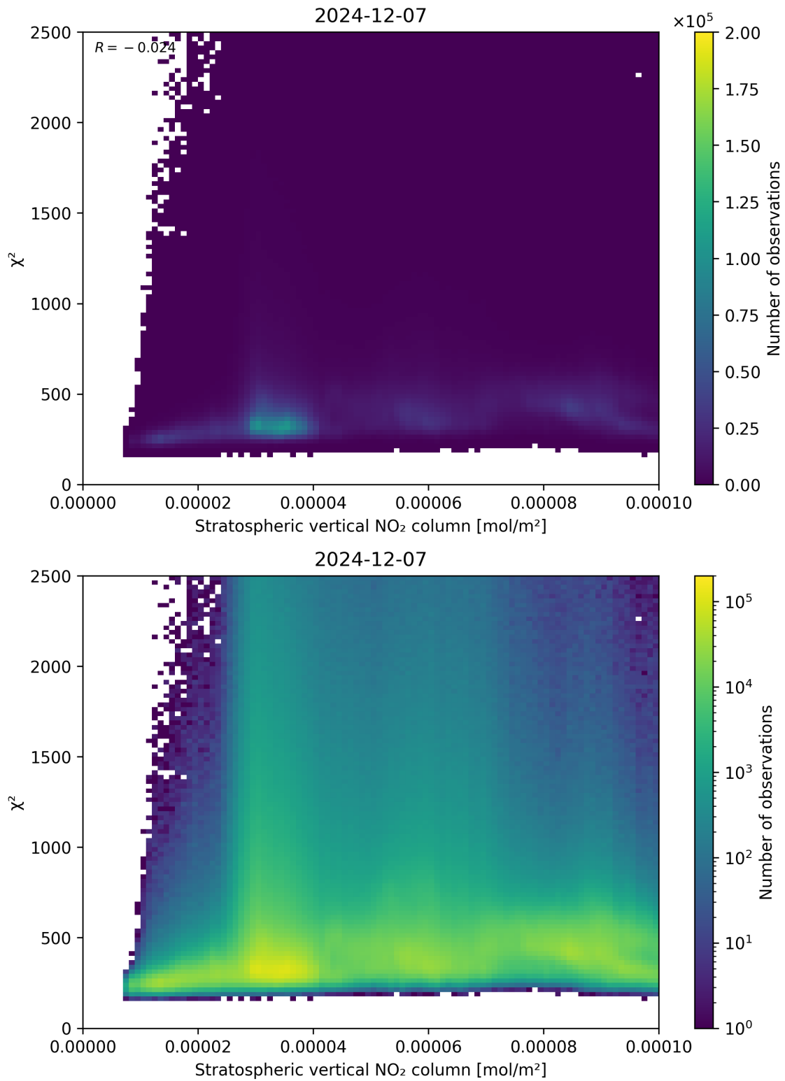
Figure 97: Scatter density plot of “Stratospheric vertical NO 2 column” against “ \chi^2 ” for 2024-12-06 to 2024-12-08.
