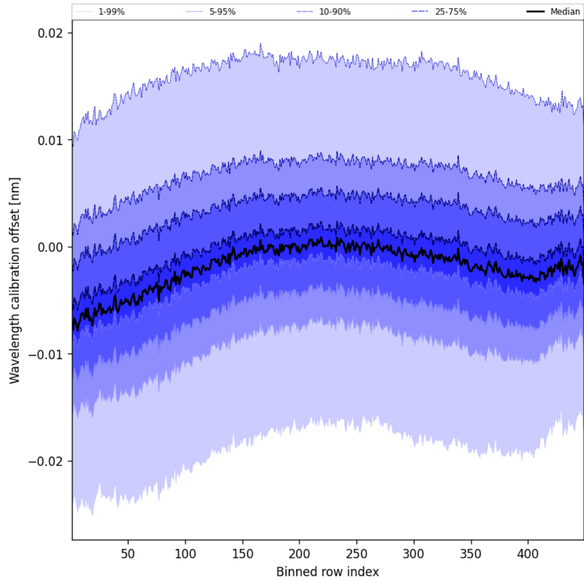
Figure 52: Along track statistics of “Wavelength calibration offset” for 2024-12-06 to 2024-12-08
