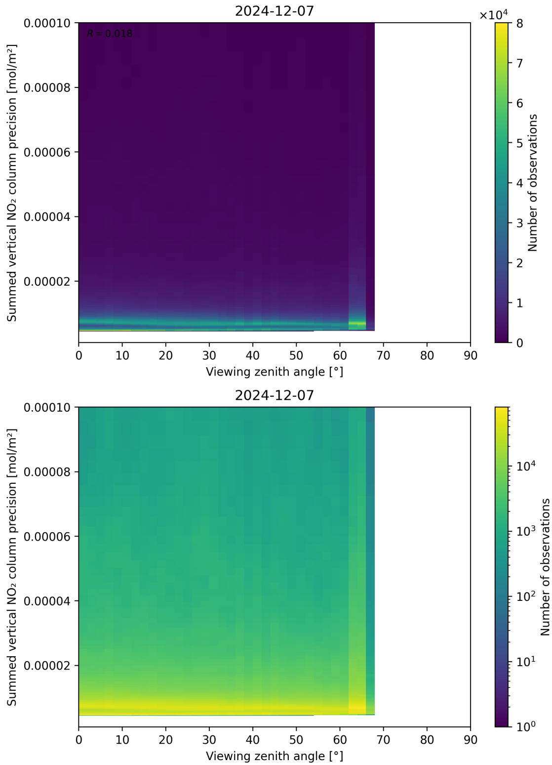
Figure 166: Scatter density plot of “Viewing zenith angle” against “Summed vertical NO 2 column precision” for 2024-12-06 to 2024-12-08.
