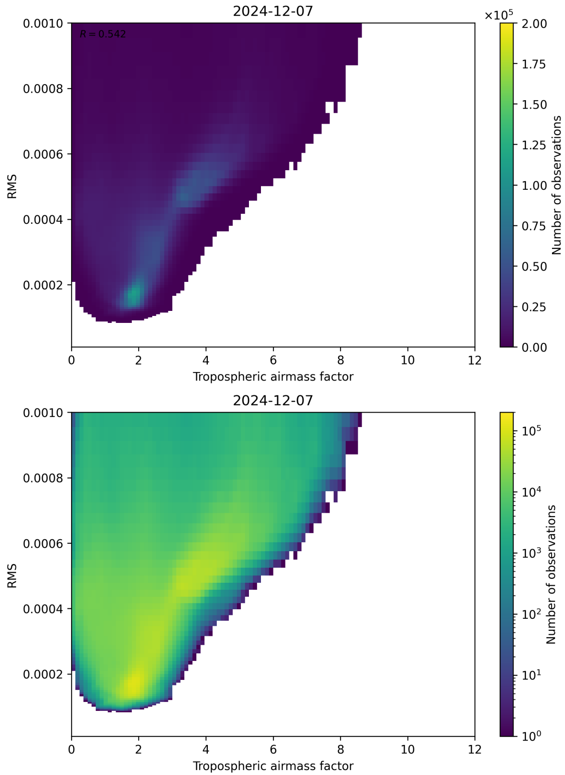
Figure 79: Scatter density plot of “Tropospheric airmass factor” against “RMS” for 2024-12-06 to 2024-12-08.
