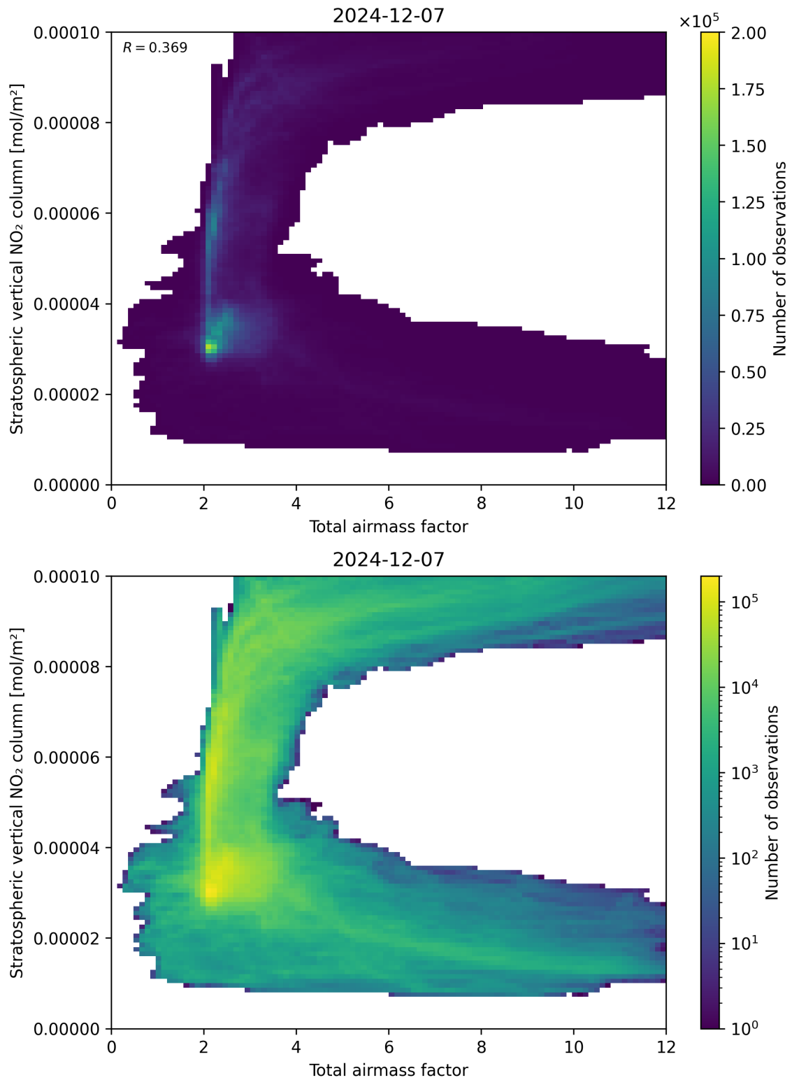
Figure 64: Scatter density plot of “Total airmass factor” against “Stratospheric vertical NO 2 column” for 2024-12-06 to 2024-12-08.
