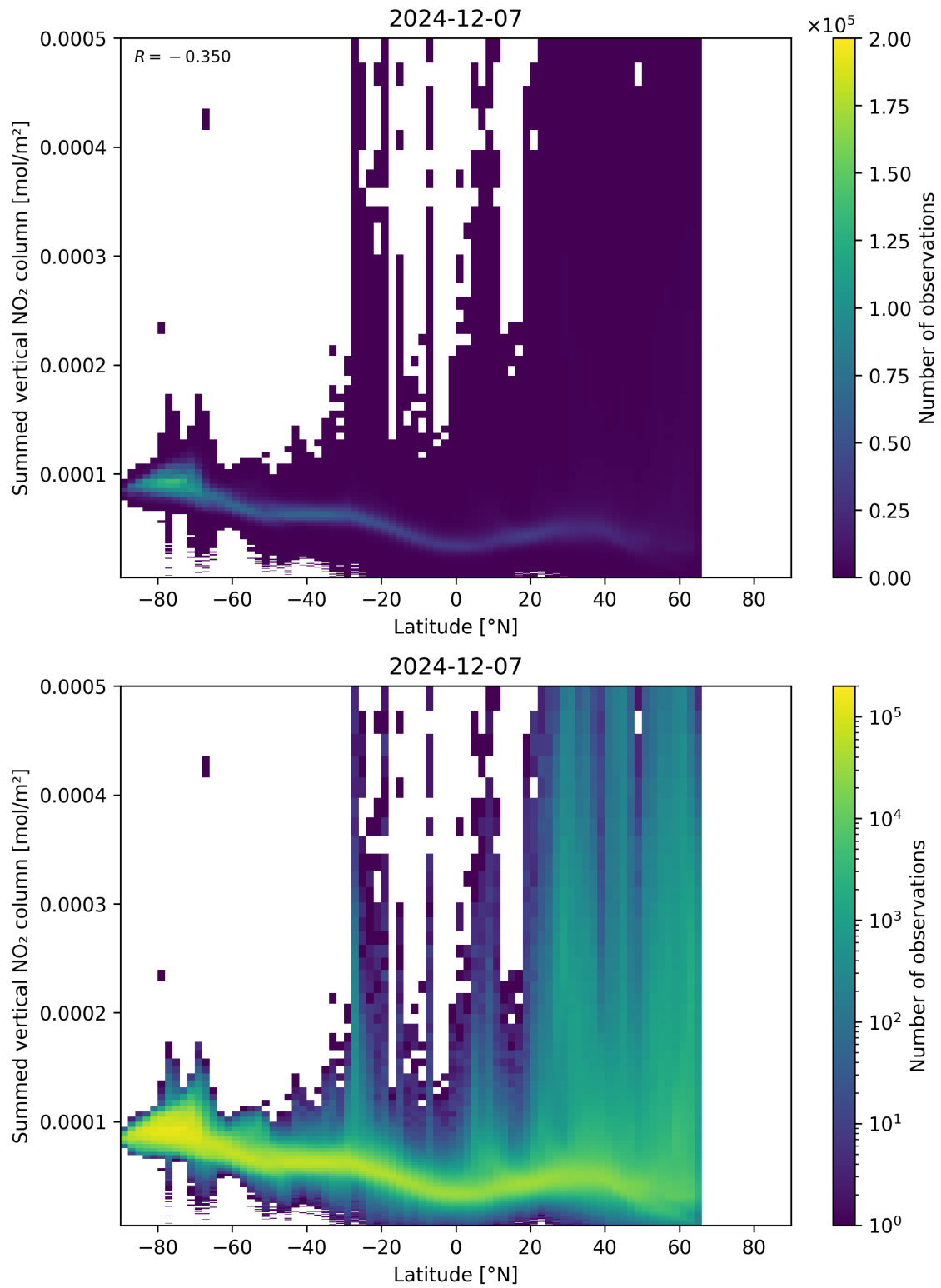
Figure 88: Scatter density plot of “Latitude” against “Summed vertical NO 2 column” for 2024-12-06 to 2024-12-08.
