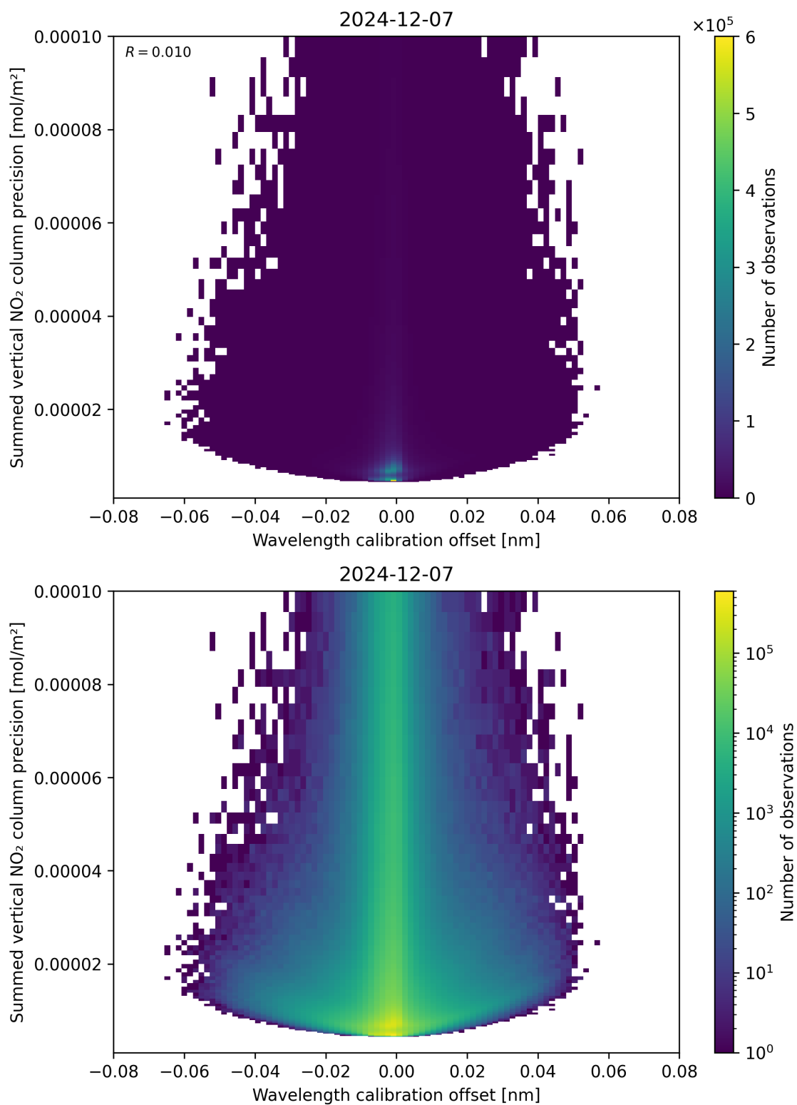
Figure 178: Scatter density plot of “Wavelength calibration offset” against “Summed vertical NO 2 column precision” for 2024-12-06 to 2024-12-08.
