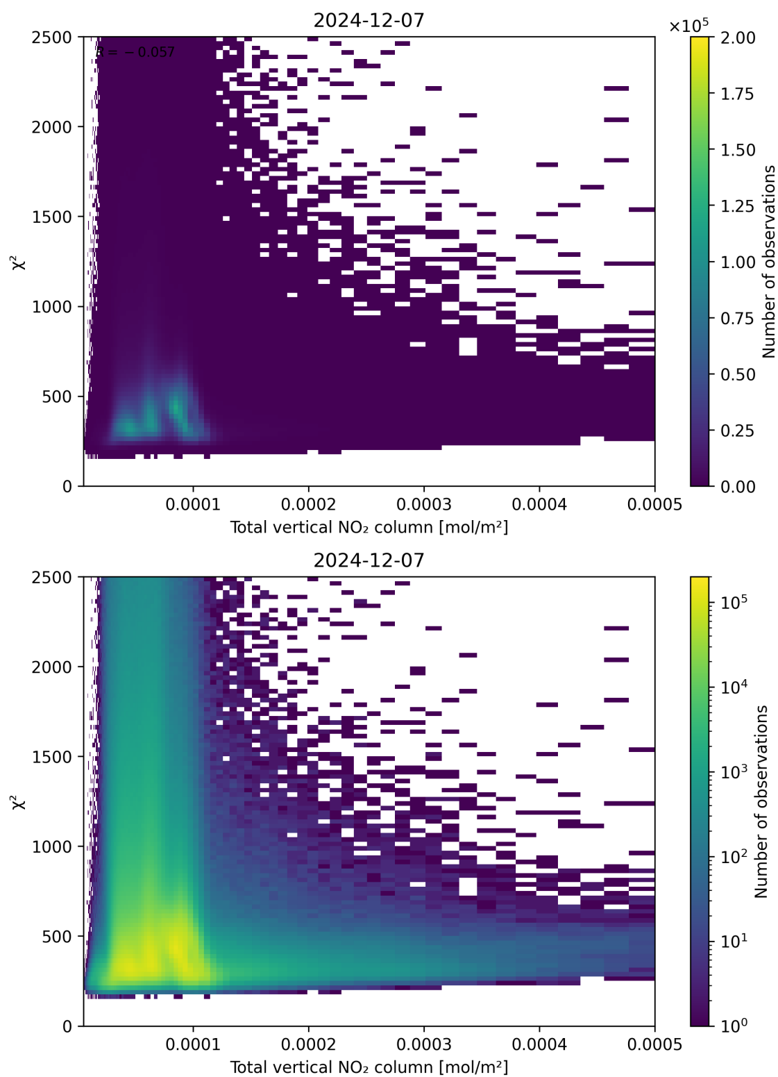
Figure 111: Scatter density plot of “Total vertical NO 2 column” against “ \chi^2 ” for 2024-12-06 to 2024-12-08.
