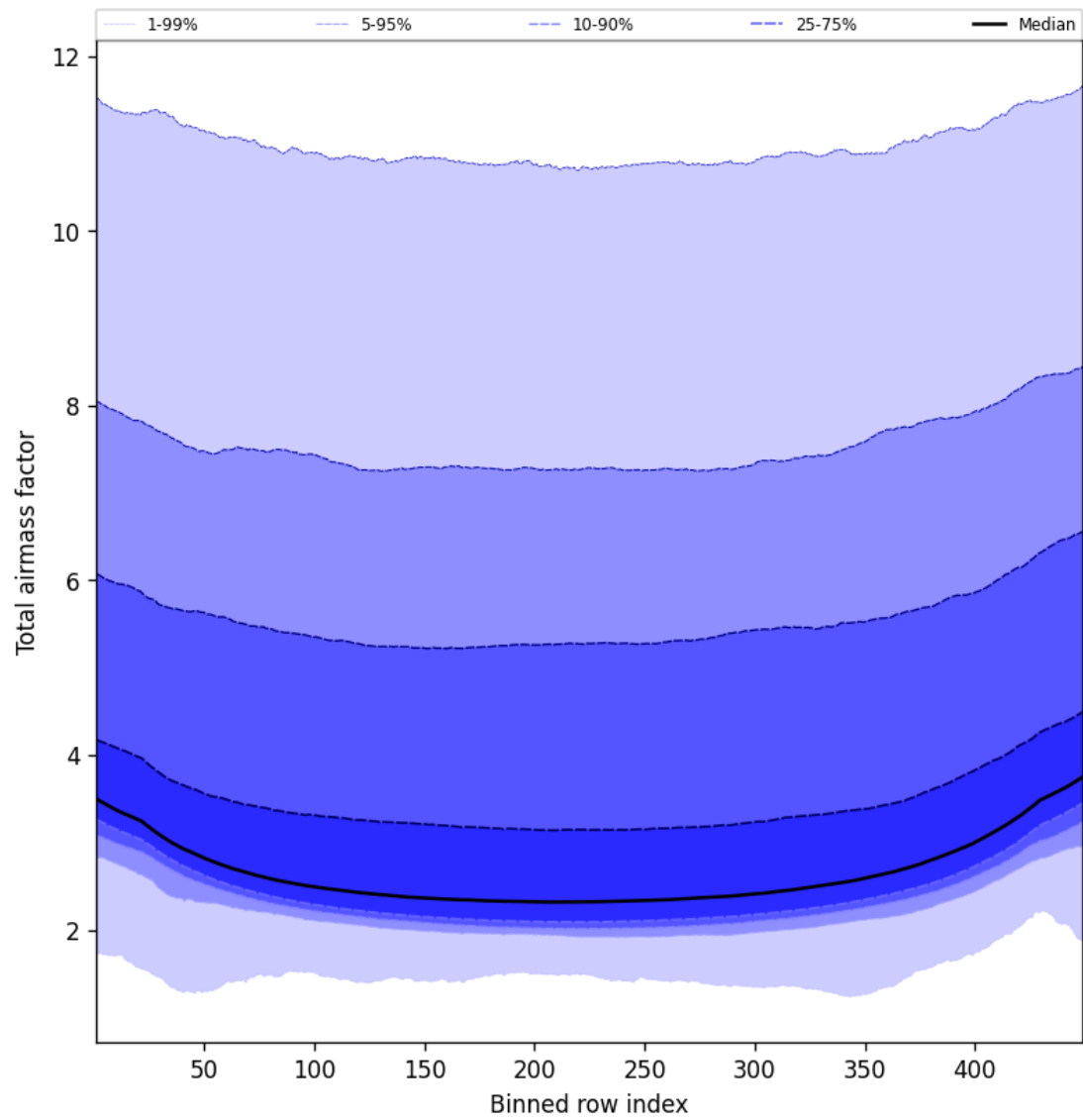
Figure 49: Along track statistics of “Total airmass factor” for 2024-12-06 to 2024-12-08
