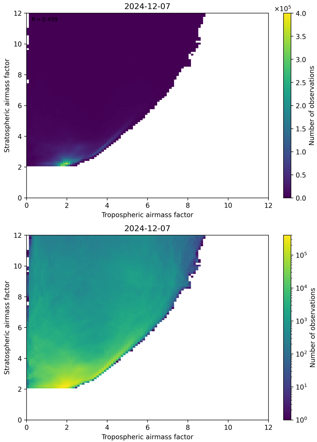
Figure 71: Scatter density plot of “Tropospheric airmass factor” against “Stratospheric airmass factor” for 2024-12-06 to 2024-12-08.
