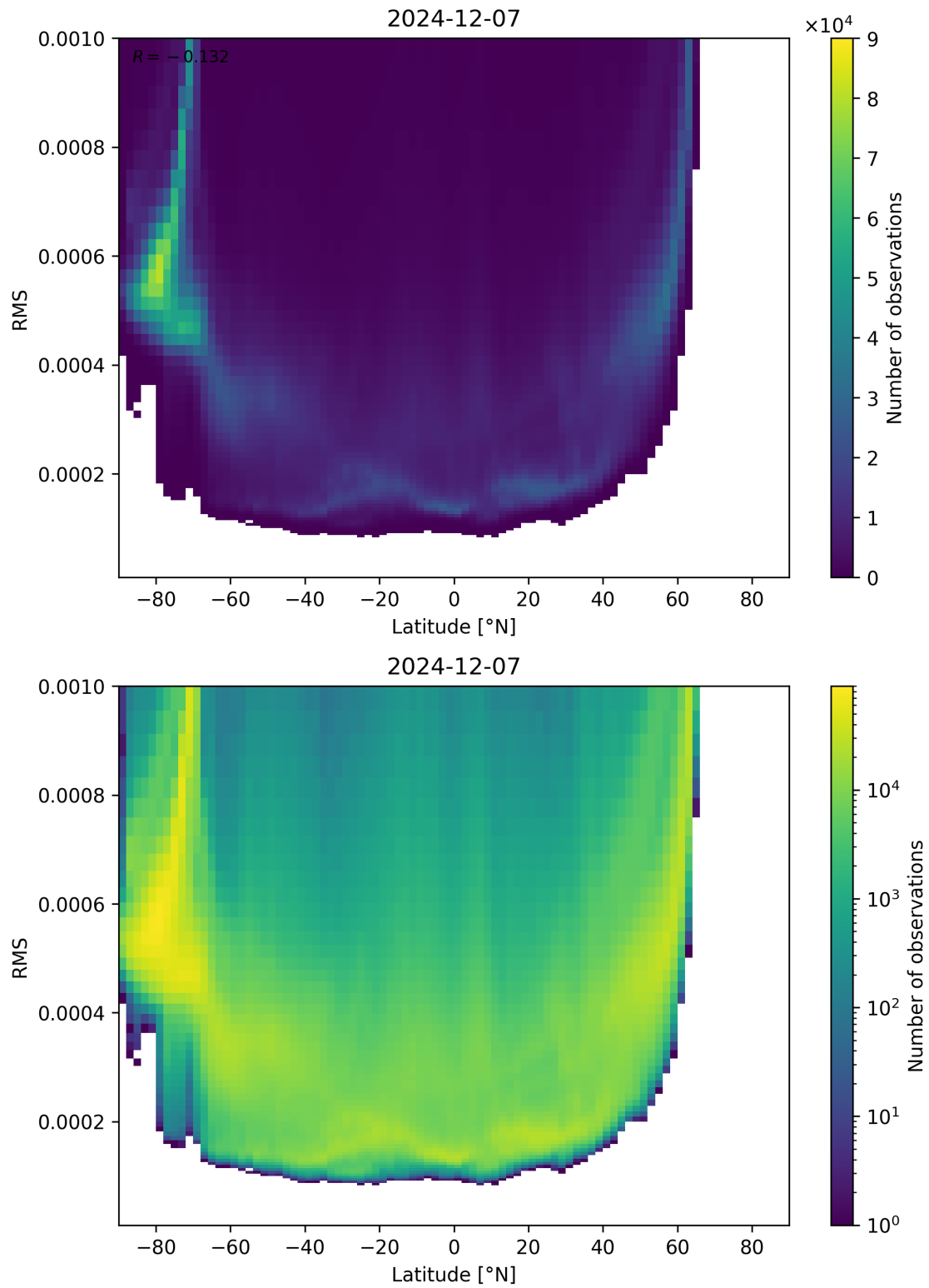
Figure 94: Scatter density plot of “Latitude” against “RMS” for 2024-12-06 to 2024-12-08.
