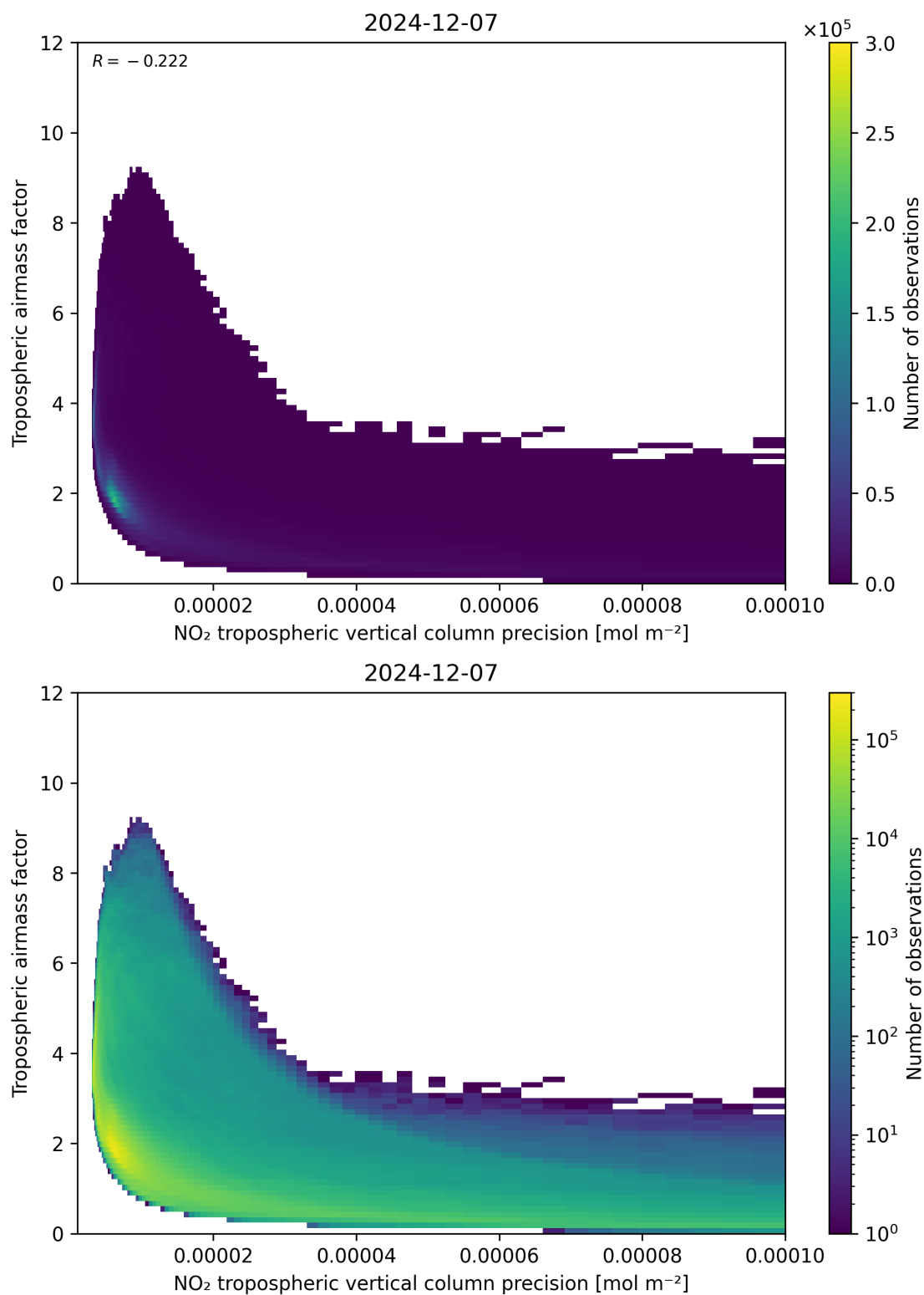
Figure 133: Scatter density plot of “NO 2 tropospheric vertical column precision” against “Tropospheric airmass factor” for 2024-12-06 to 2024-12-08.
