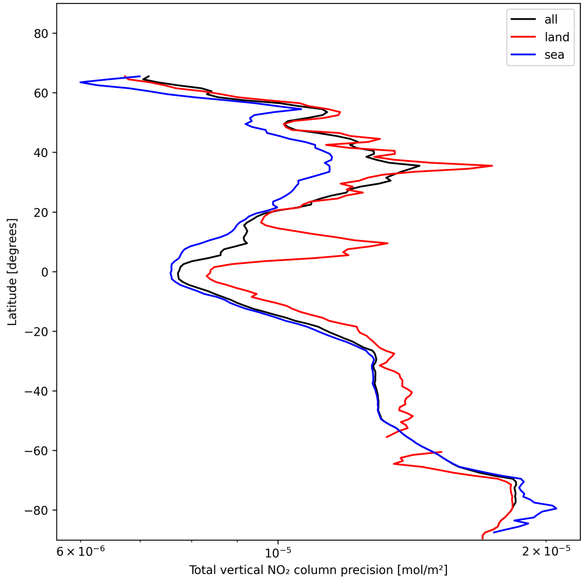
Figure 22: Zonal average of “Total vertical NO 2 column precision” for 2024-12-06 to 2024-12-08.
