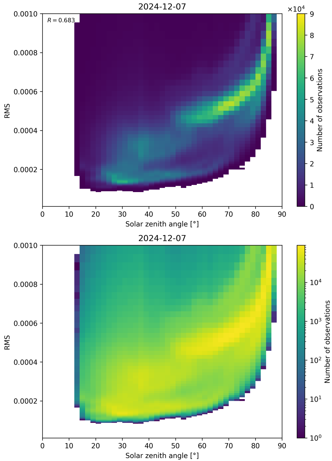
Figure 157: Scatter density plot of “Solar zenith angle” against “RMS” for 2024-12-06 to 2024-12-08.
