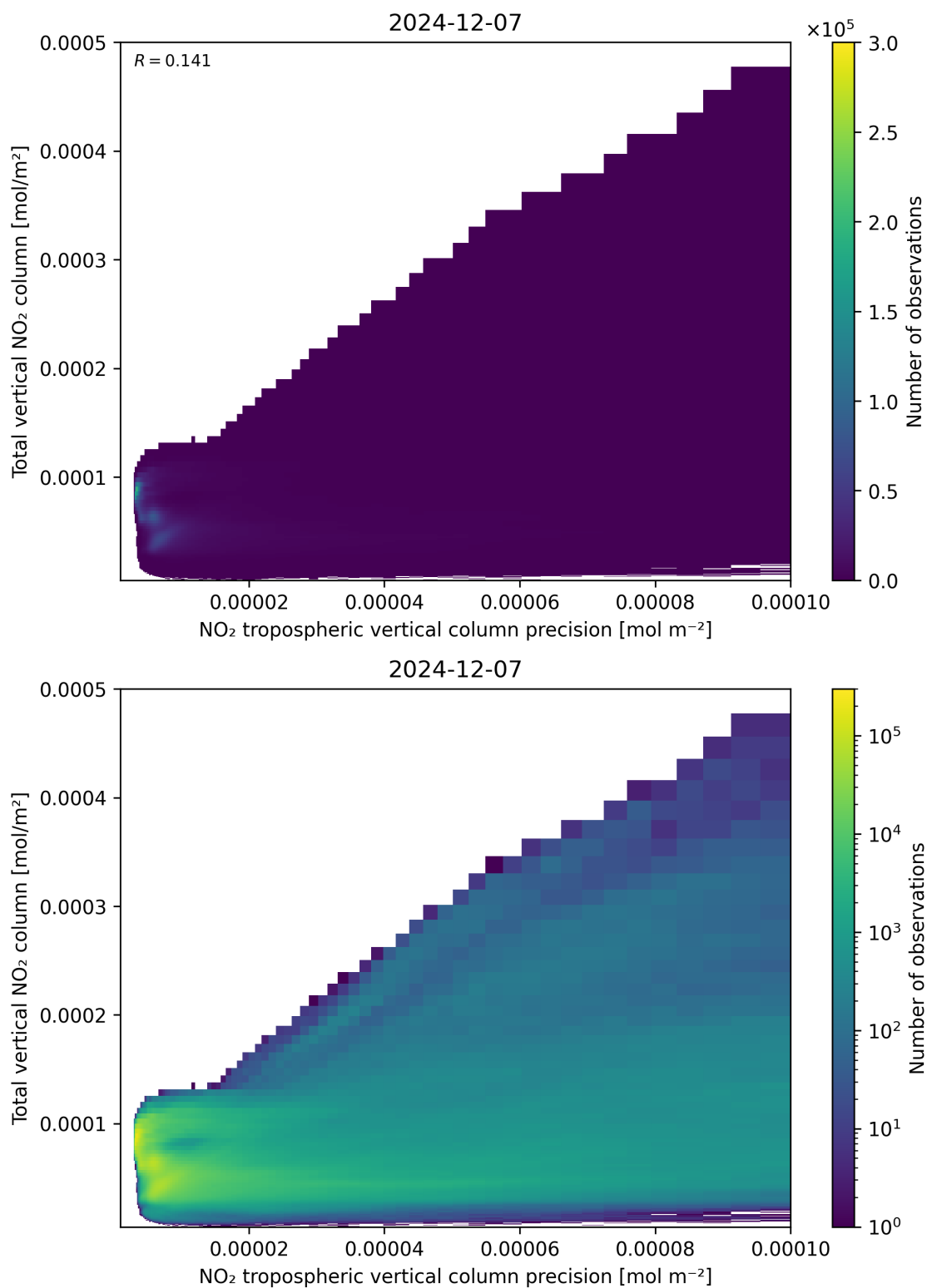
Figure 138: Scatter density plot of “NO 2 tropospheric vertical column precision” against “Total vertical NO 2 column” for 2024-12-06 to 2024-12-08.
