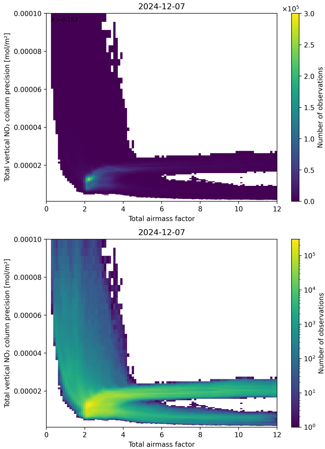
Figure 68: Scatter density plot of “Total airmass factor” against “Total vertical NO 2 column precision” for 2024-12-06 to 2024-12-08.
