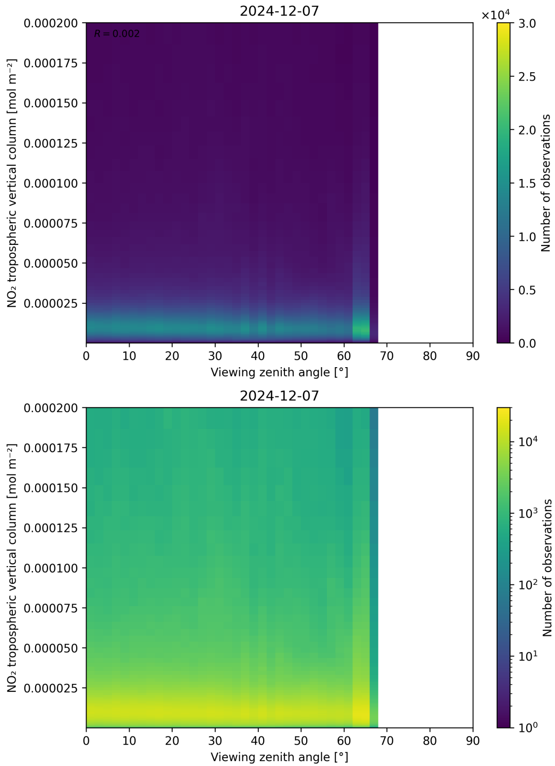
Figure 169: Scatter density plot of “Viewing zenith angle” against “NO 2 tropospheric vertical column” for 2024-12-06 to 2024-12-08.
