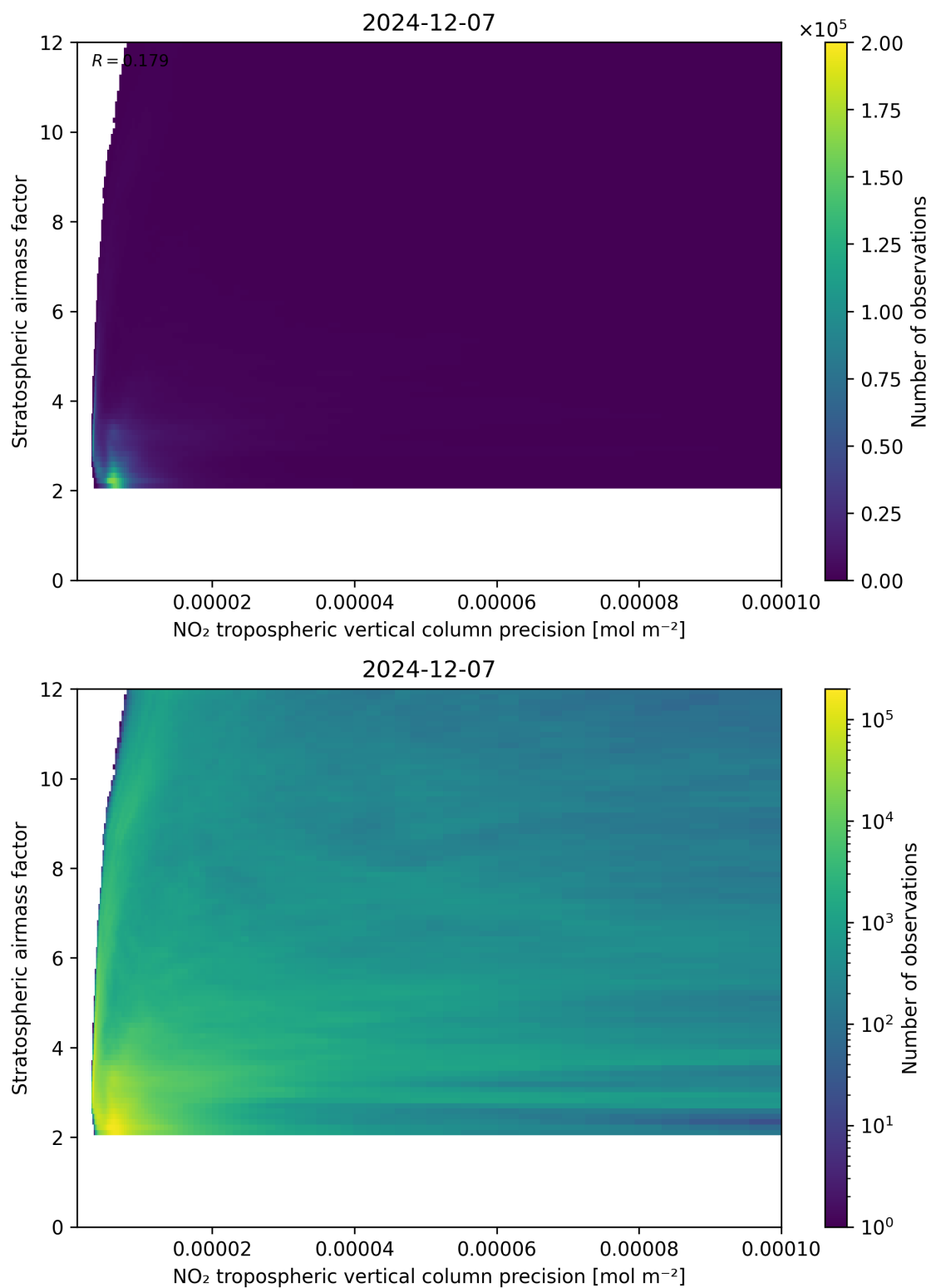
Figure 131: Scatter density plot of “NO 2 tropospheric vertical column precision” against “Stratospheric airmass factor” for 2024-12-06 to 2024-12-08.
