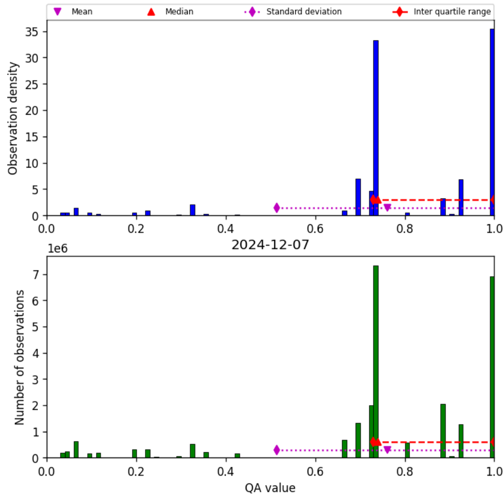
Figure 28: Histogram of “QA value” for 2024-12-06 to 2024-12-08
