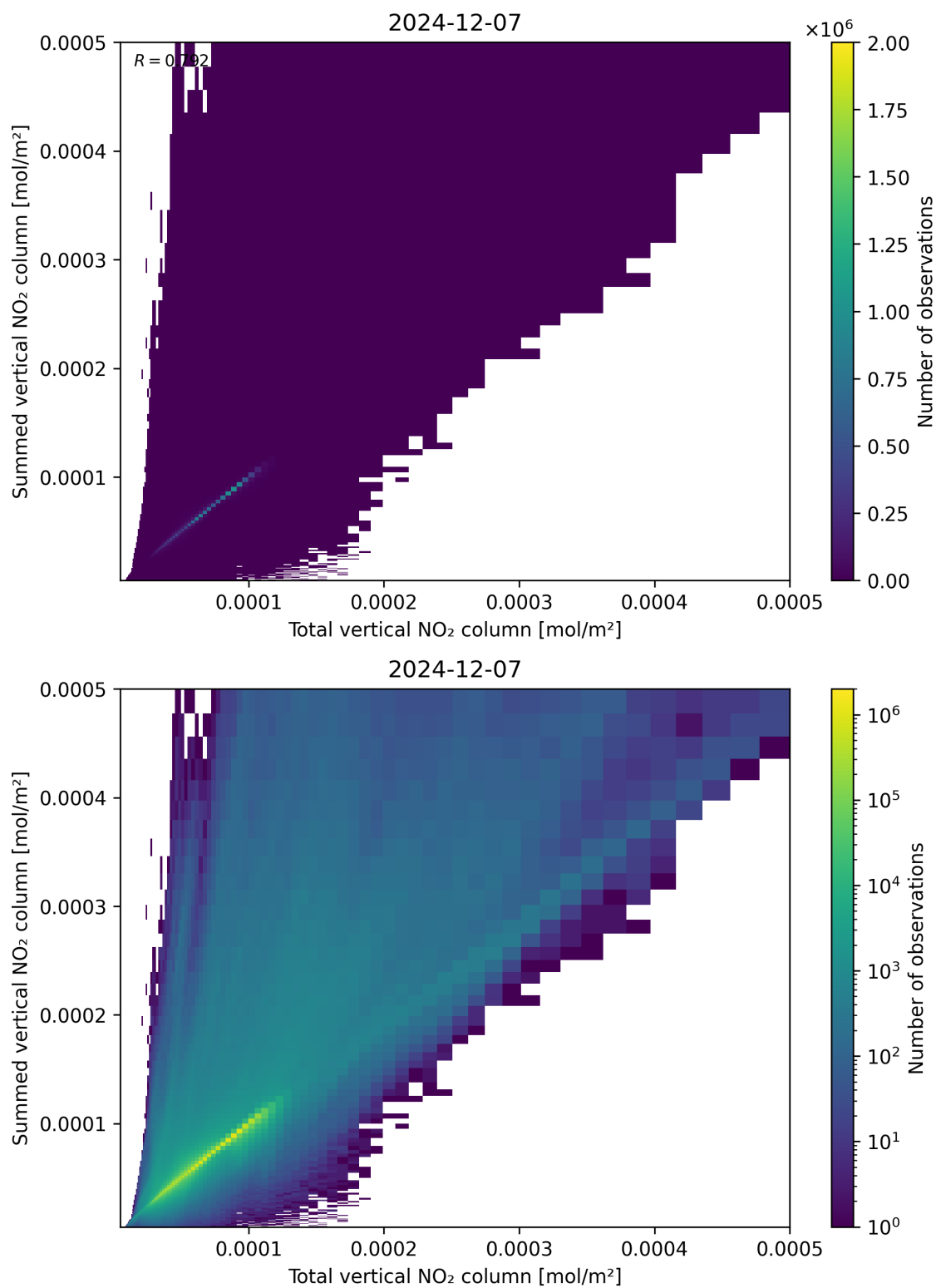
Figure 112: Scatter density plot of “Total vertical NO 2 column” against “Summed vertical NO 2 column” for 2024-12-06 to 2024-12-08.
