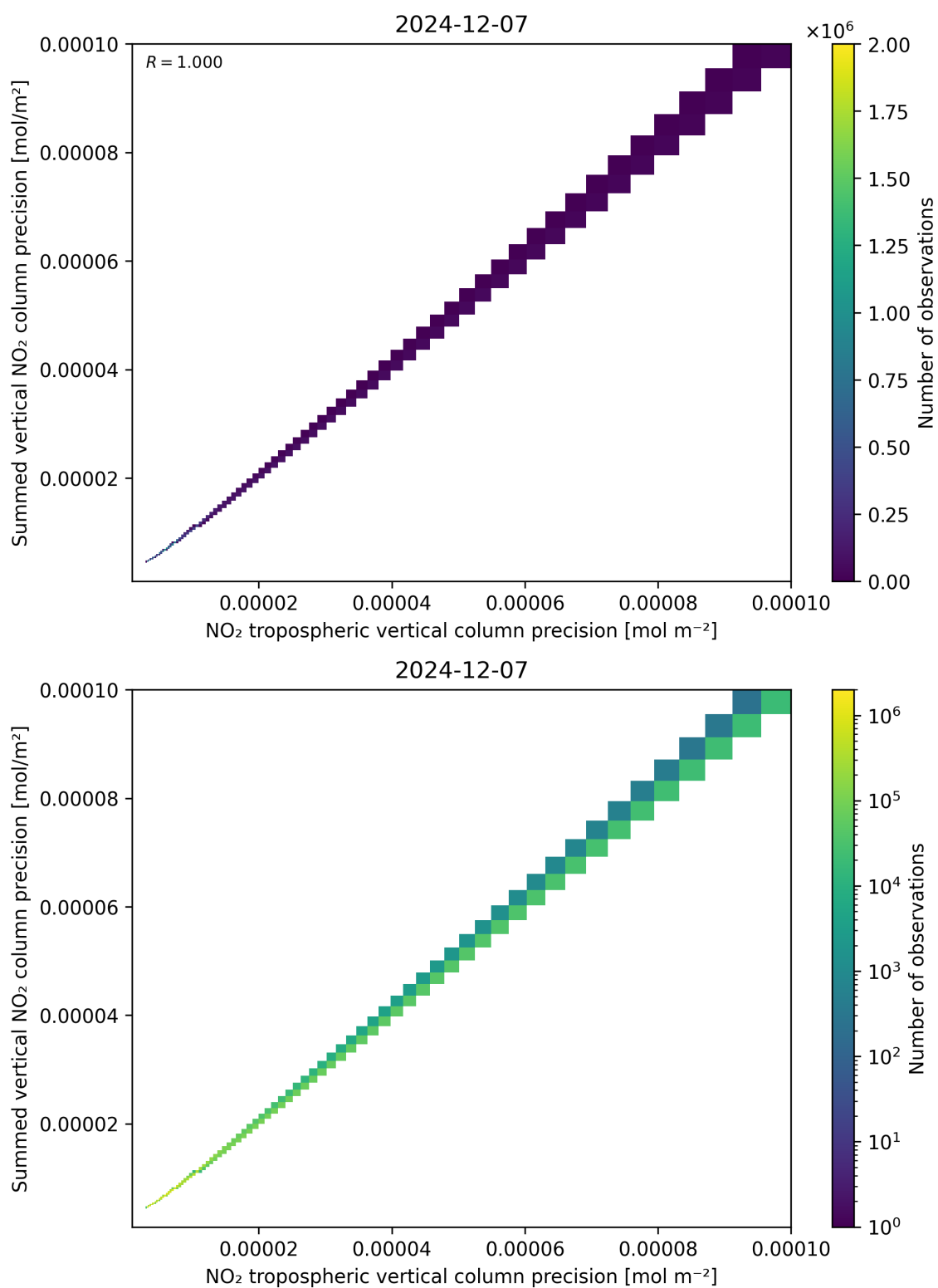
Figure 137: Scatter density plot of “NO 2 tropospheric vertical column precision” against “Summed vertical NO 2 column precision” for 2024-12-06 to 2024-12-08.
