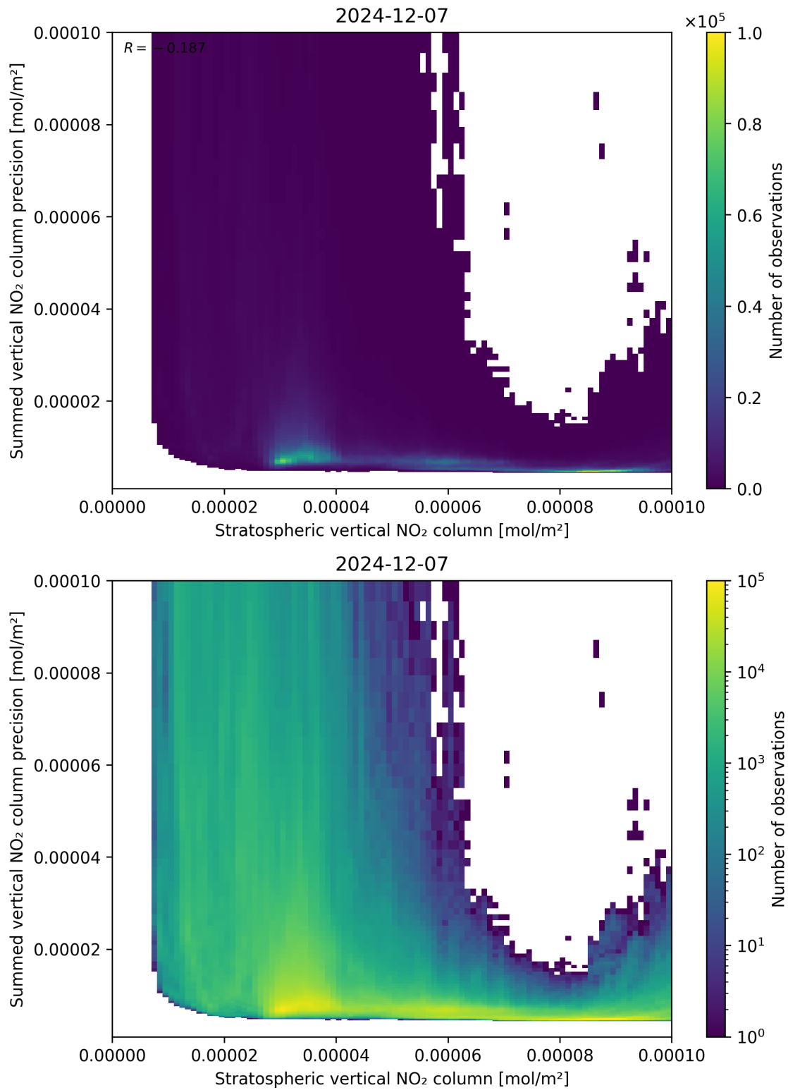
Figure 99: Scatter density plot of “Stratospheric vertical NO 2 column” against “Summed vertical NO 2 column precision” for 2024-12-06 to 2024-12-08.
