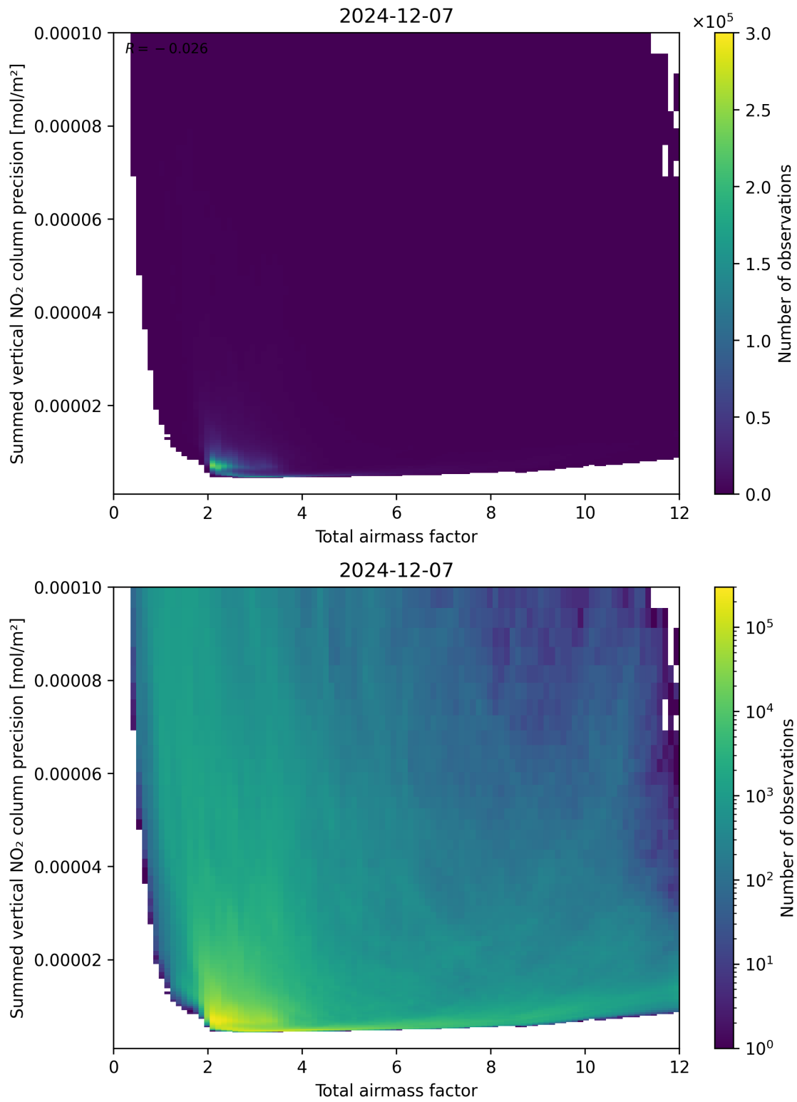
Figure 66: Scatter density plot of “Total airmass factor” against “Summed vertical NO 2 column precision” for 2024-12-06 to 2024-12-08.
