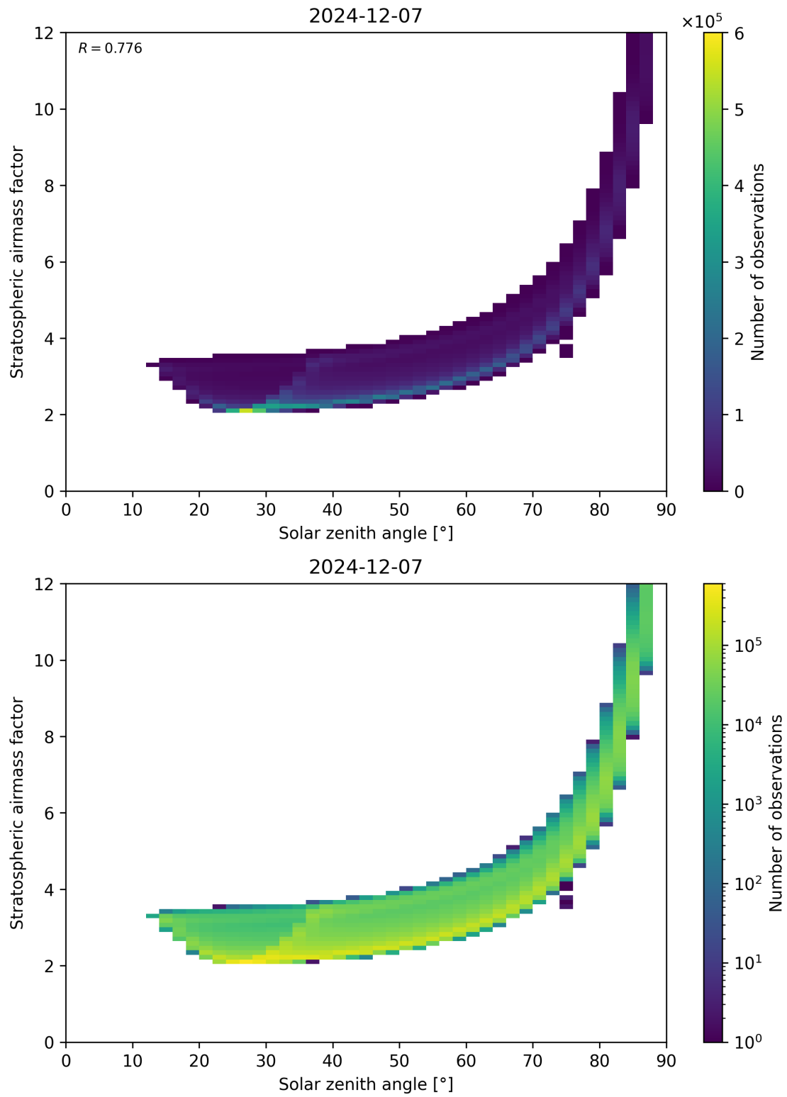
Figure 145: Scatter density plot of “Solar zenith angle” against “Stratospheric airmass factor” for 2024-12-06 to 2024-12-08.
