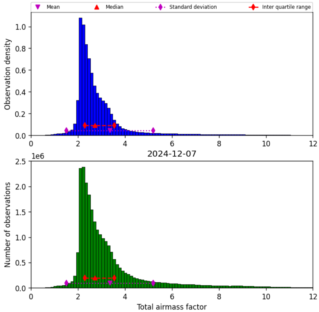
Figure 32: Histogram of “Total airmass factor” for 2024-12-06 to 2024-12-08
