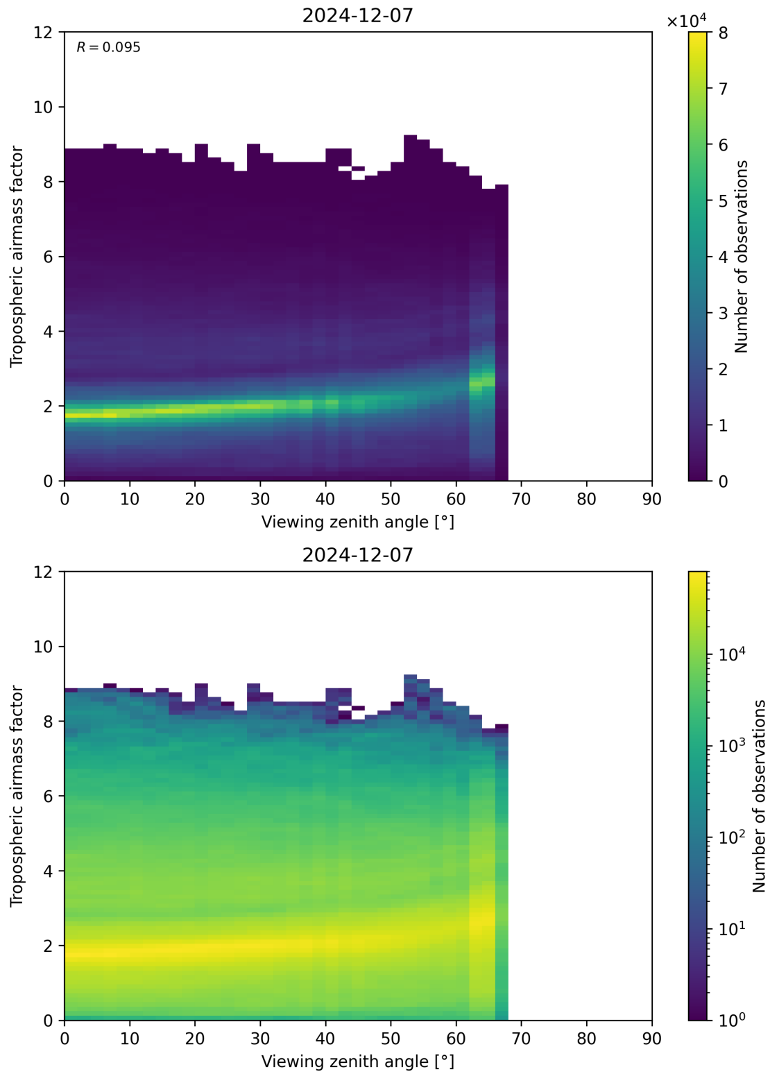
Figure 161: Scatter density plot of “Viewing zenith angle” against “Tropospheric airmass factor” for 2024-12-06 to 2024-12-08.
