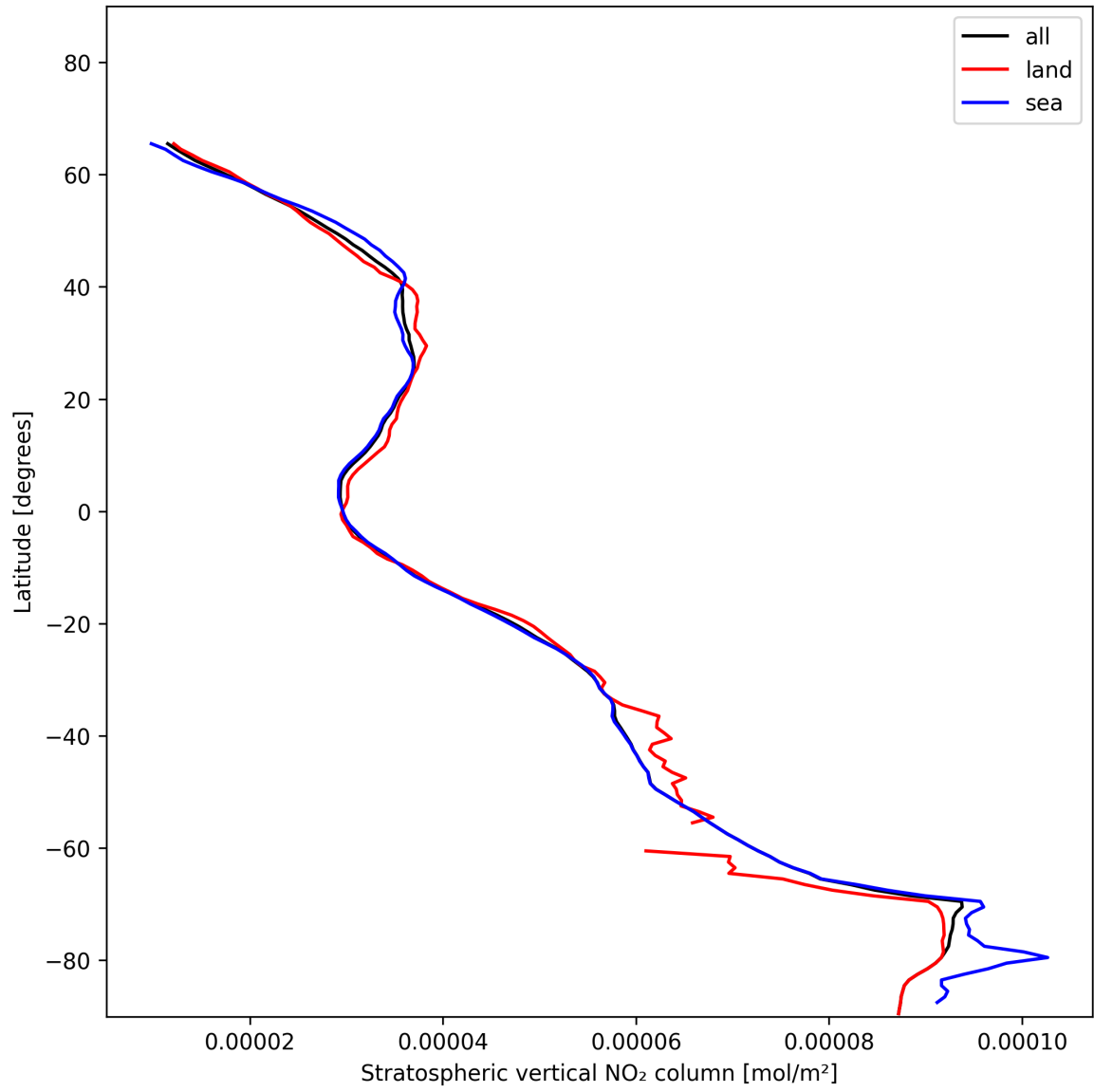
Figure 19: Zonal average of “Stratospheric vertical NO 2 column” for 2024-12-06 to 2024-12-08.
