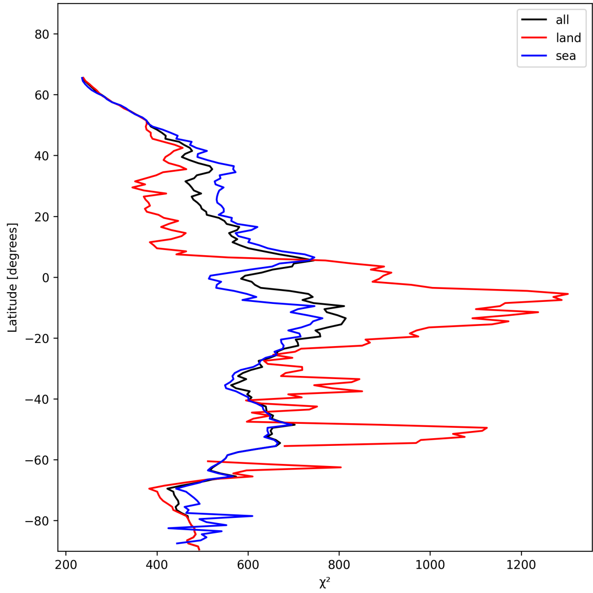
Figure 25: Zonal average of “ \chi^2 ” for 2024-12-06 to 2024-12-08.
