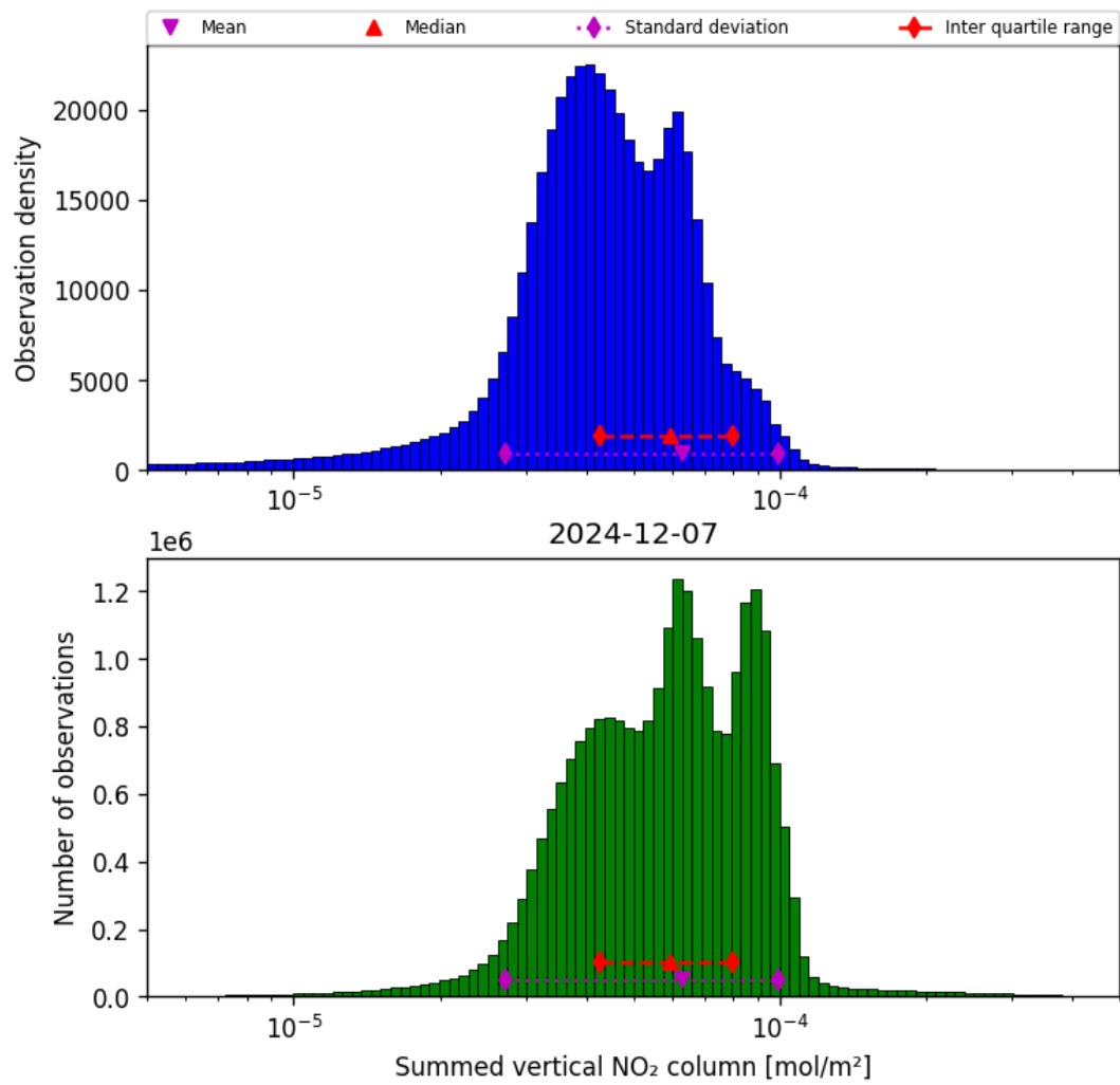
Figure 40: Histogram of “Summed vertical NO 2 column” for 2024-12-06 to 2024-12-08
