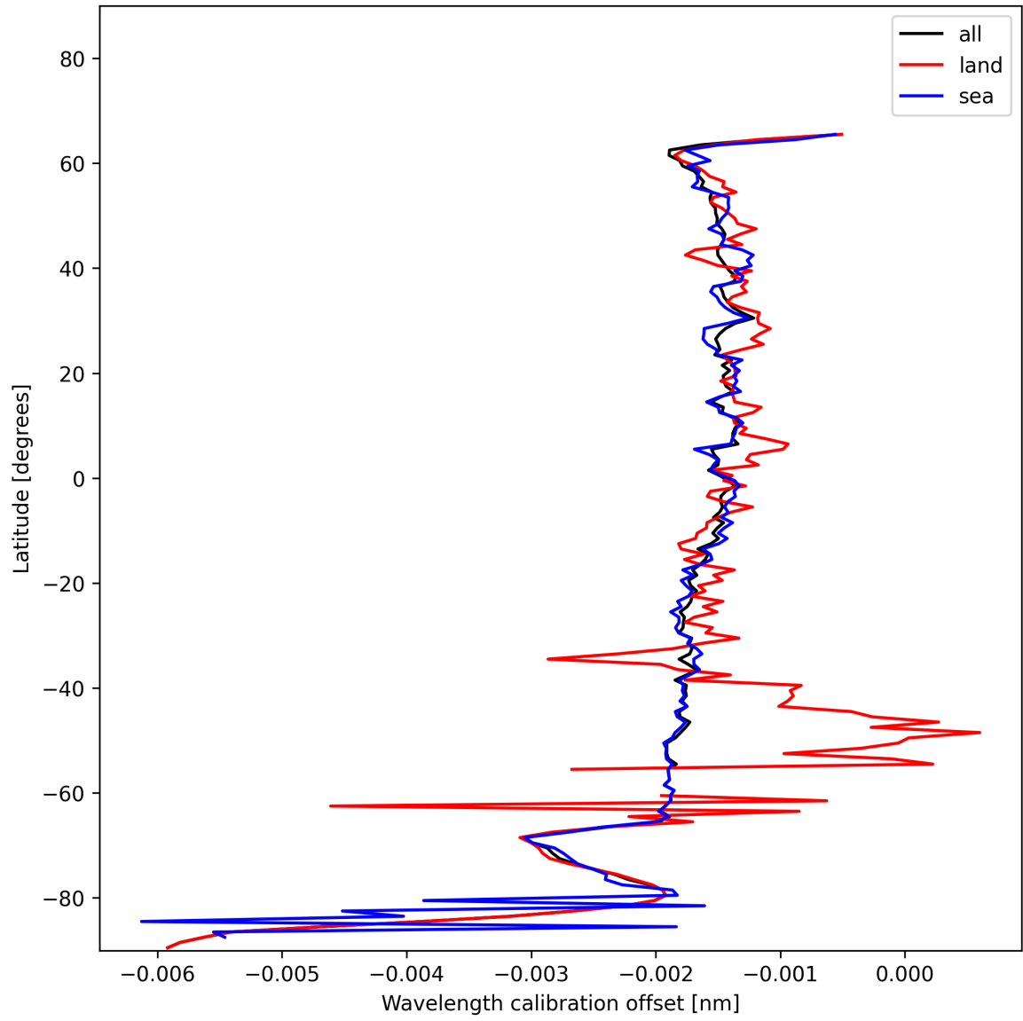
Figure 18: Zonal average of “Wavelength calibration offset” for 2024-12-06 to 2024-12-08.
