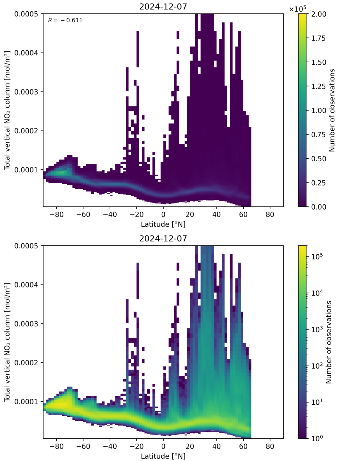
Figure 90: Scatter density plot of “Latitude” against “Total vertical NO 2 column” for 2024-12-06 to 2024-12-08.
