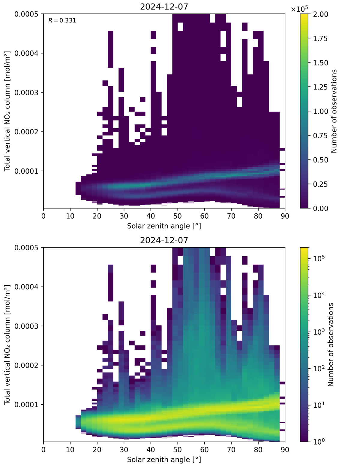
Figure 153: Scatter density plot of “Solar zenith angle” against “Total vertical NO 2 column” for 2024-12-06 to 2024-12-08.
