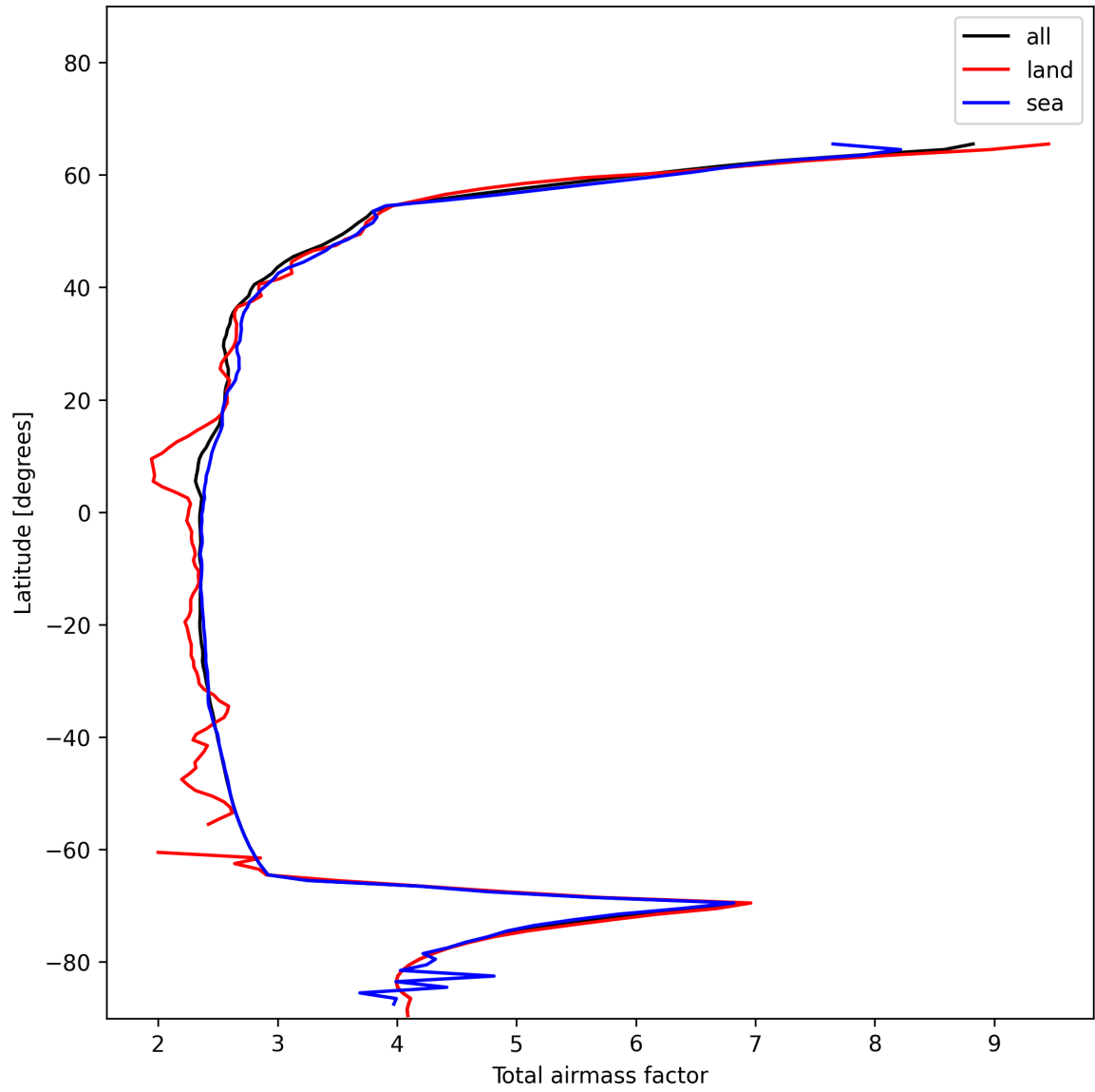
Figure 15: Zonal average of “Total airmass factor” for 2024-12-06 to 2024-12-08.
