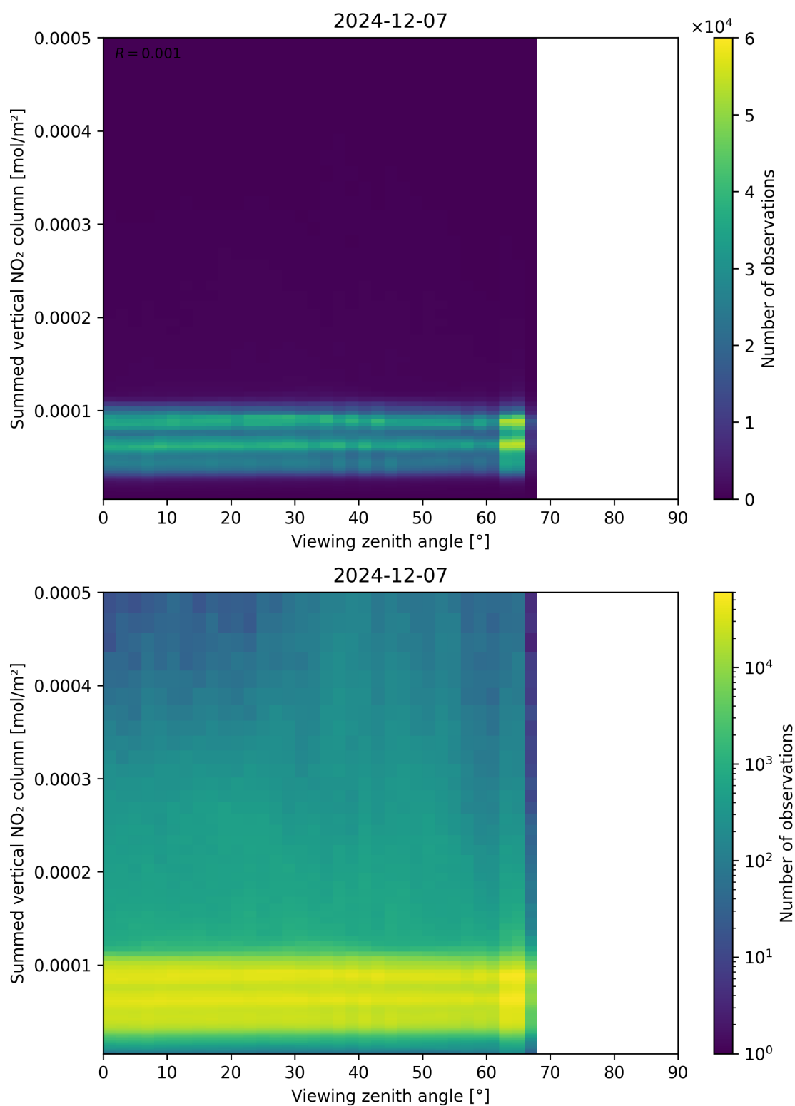
Figure 165: Scatter density plot of “Viewing zenith angle” against “Summed vertical NO 2 column” for 2024-12-06 to 2024-12-08.
