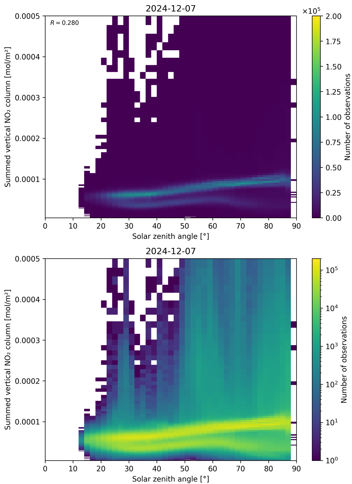
Figure 151: Scatter density plot of “Solar zenith angle” against “Summed vertical NO 2 column” for 2024-12-06 to 2024-12-08.
