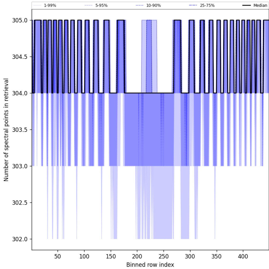
Figure 50: Along track statistics of “Number of spectral points in retrieval” for 2024-12-07 to 2024-12-09
