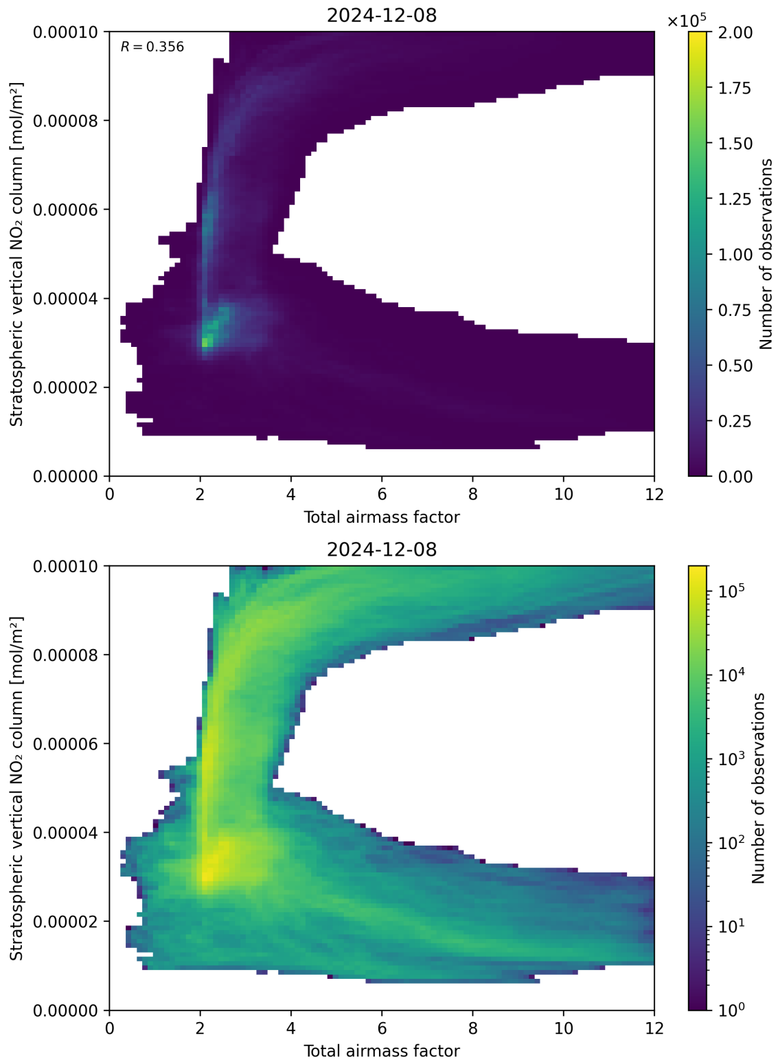
Figure 64: Scatter density plot of “Total airmass factor” against “Stratospheric vertical NO 2 column” for 2024-12-07 to 2024-12-09.
