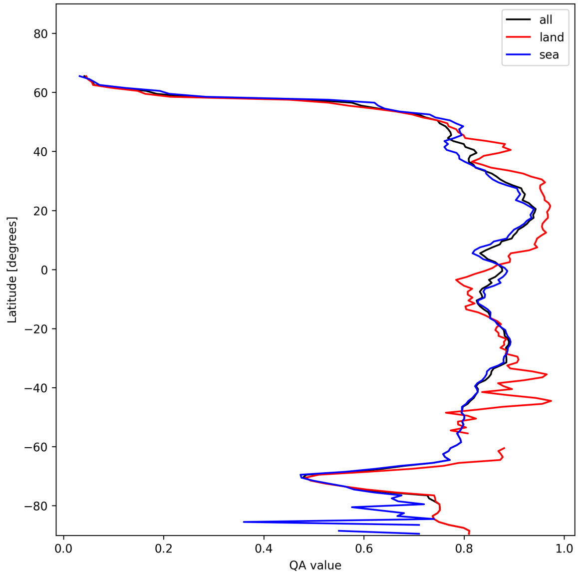
Figure 11: Zonal average of “QA value” for 2024-12-07 to 2024-12-09.
