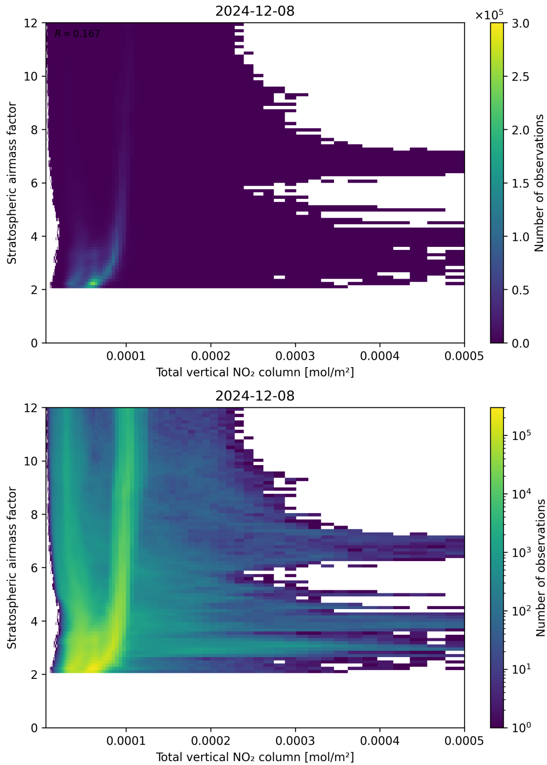
Figure 110: Scatter density plot of “Total vertical NO 2 column” against “Stratospheric airmass factor” for 2024-12-07 to 2024-12-09.
