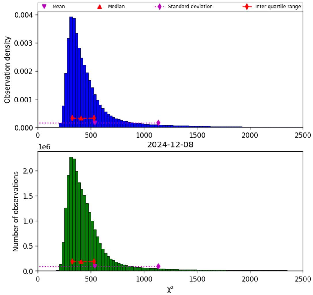
Figure 42: Histogram of “ \chi^2 ” for 2024-12-07 to 2024-12-09
