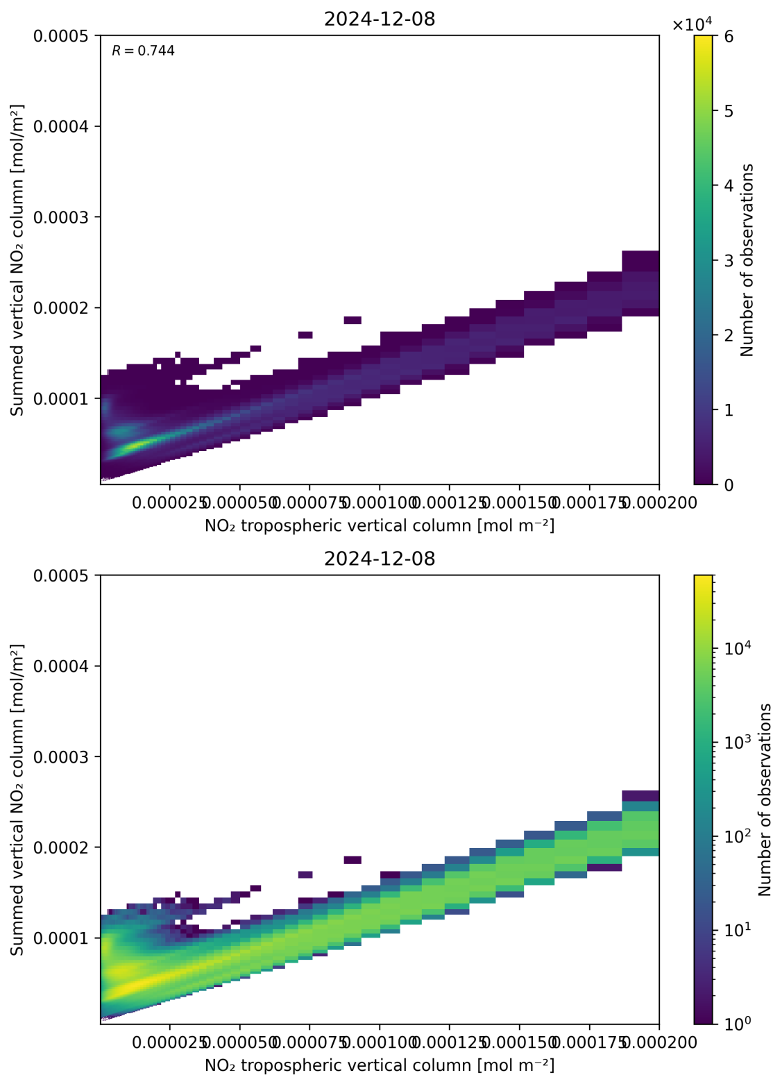
Figure 126: Scatter density plot of “NO 2 tropospheric vertical column” against “Summed vertical NO 2 column” for 2024-12-07 to 2024-12-09.
