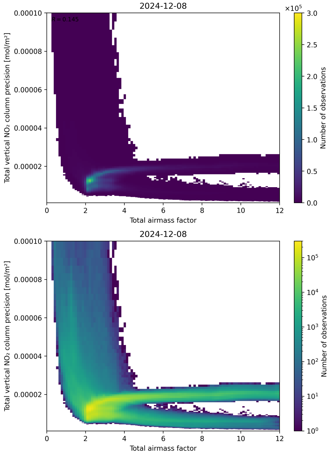
Figure 68: Scatter density plot of “Total airmass factor” against “Total vertical NO 2 column precision” for 2024-12-07 to 2024-12-09.
