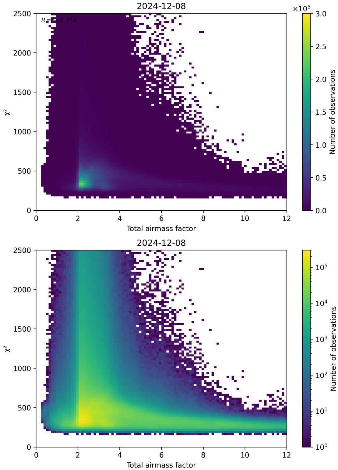
Figure 63: Scatter density plot of “Total airmass factor” against “ \chi^2 ” for 2024-12-07 to 2024-12-09.
