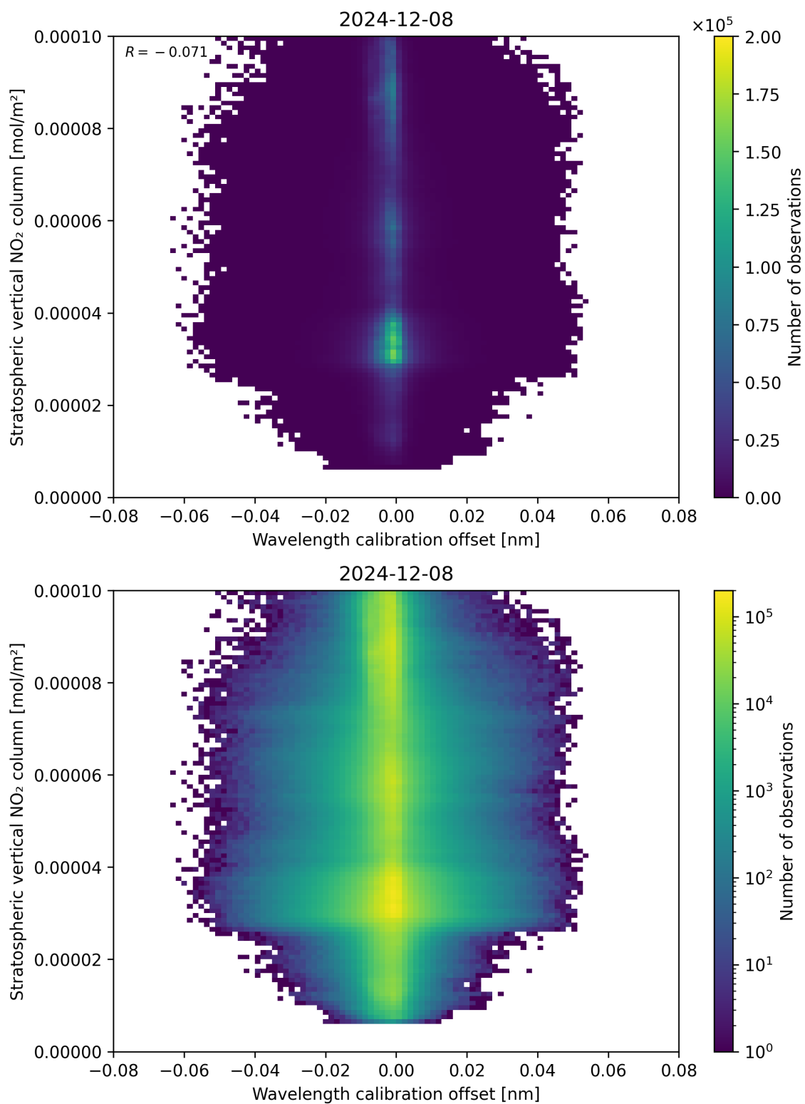
Figure 176: Scatter density plot of “Wavelength calibration offset” against “Stratospheric vertical NO 2 column” for 2024-12-07 to 2024-12-09.
