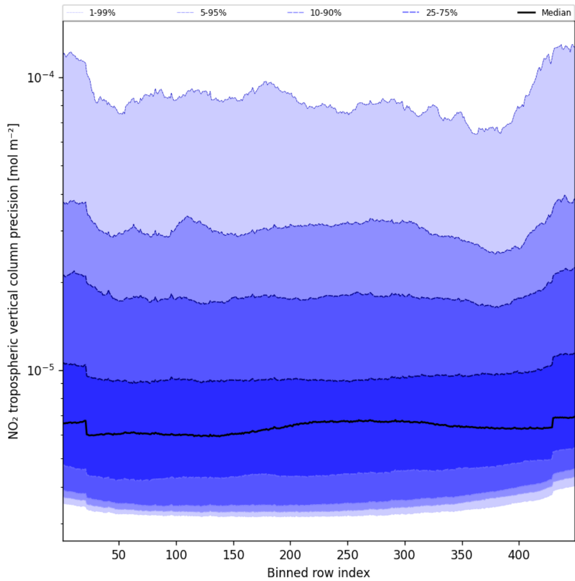
Figure 47: Along track statistics of “NO 2 tropospheric vertical column precision” for 2024-12-07 to 2024-12-09
