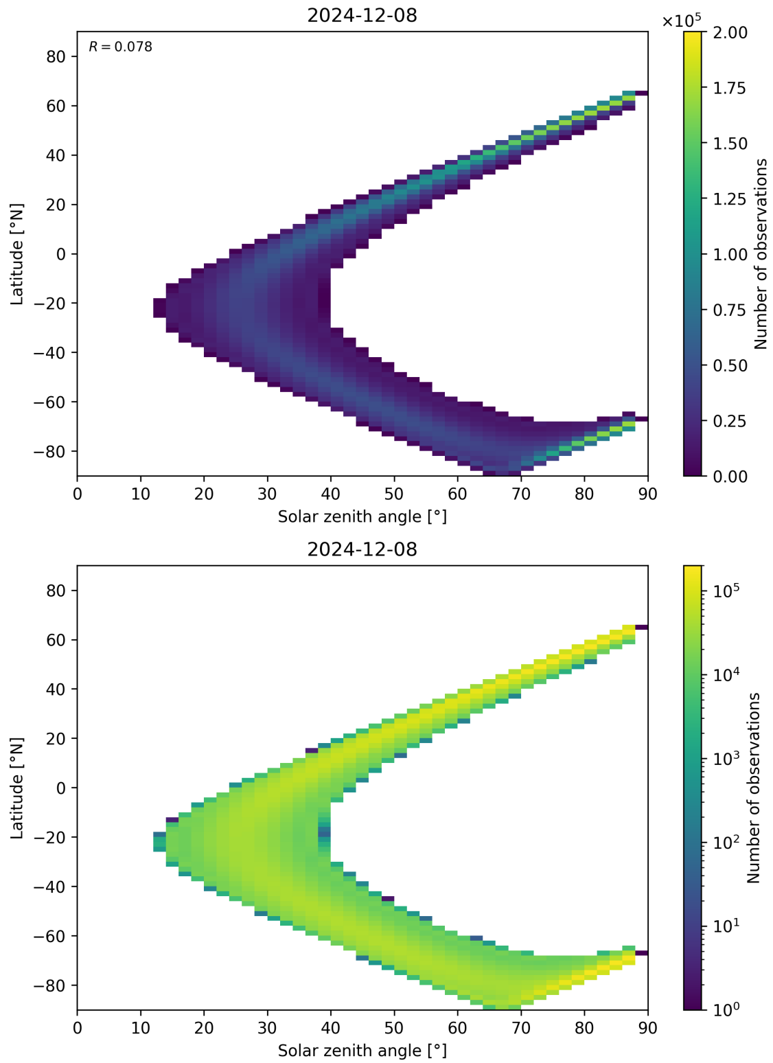
Figure 149: Scatter density plot of “Solar zenith angle” against “Latitude” for 2024-12-07 to 2024-12-09.
