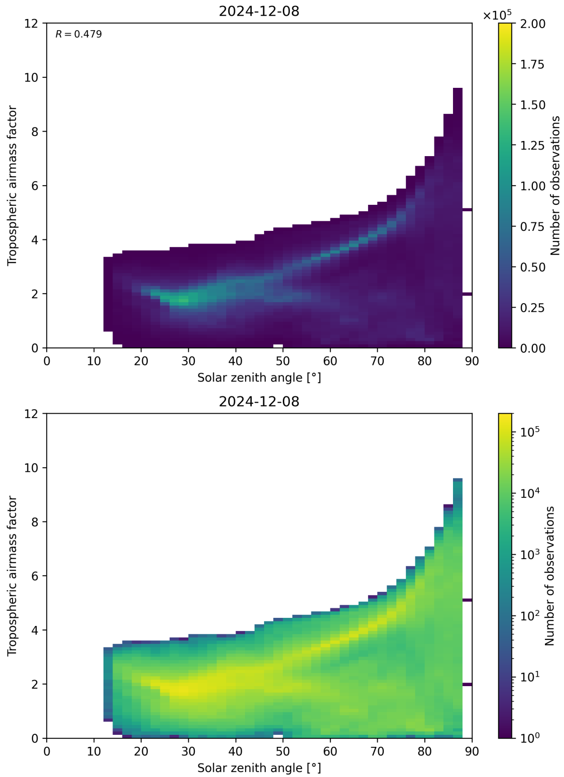
Figure 147: Scatter density plot of “Solar zenith angle” against “Tropospheric airmass factor” for 2024-12-07 to 2024-12-09.
