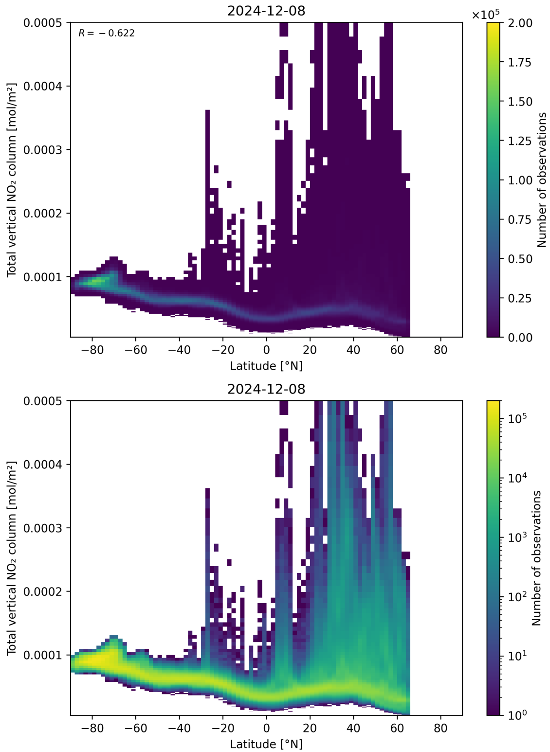
Figure 90: Scatter density plot of “Latitude” against “Total vertical NO 2 column” for 2024-12-07 to 2024-12-09.
