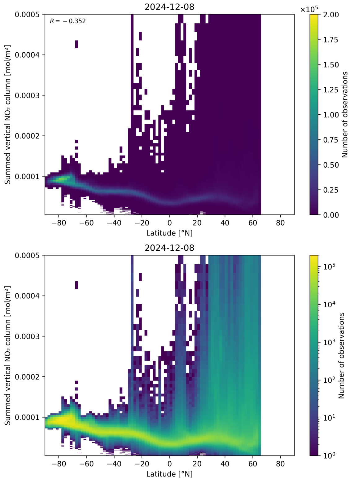
Figure 88: Scatter density plot of “Latitude” against “Summed vertical NO 2 column” for 2024-12-07 to 2024-12-09.
