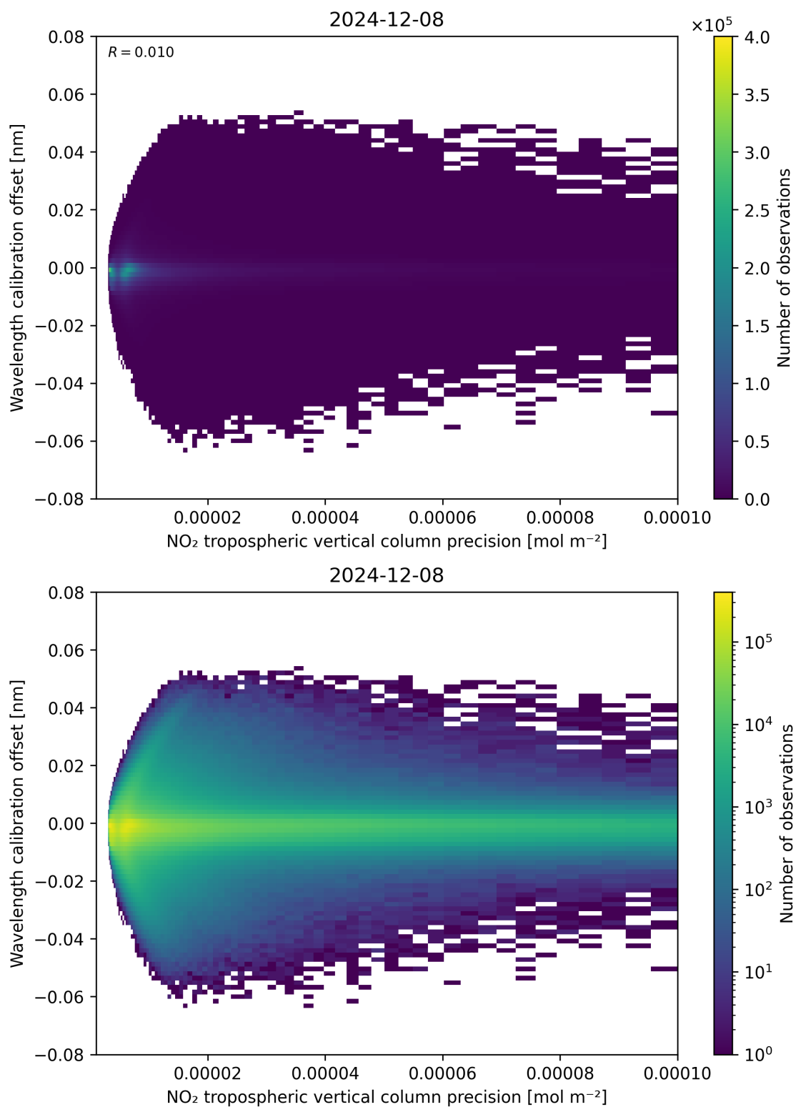
Figure 141: Scatter density plot of “NO 2 tropospheric vertical column precision” against “Wavelength calibration offset” for 2024-12-07 to 2024-12-09.
