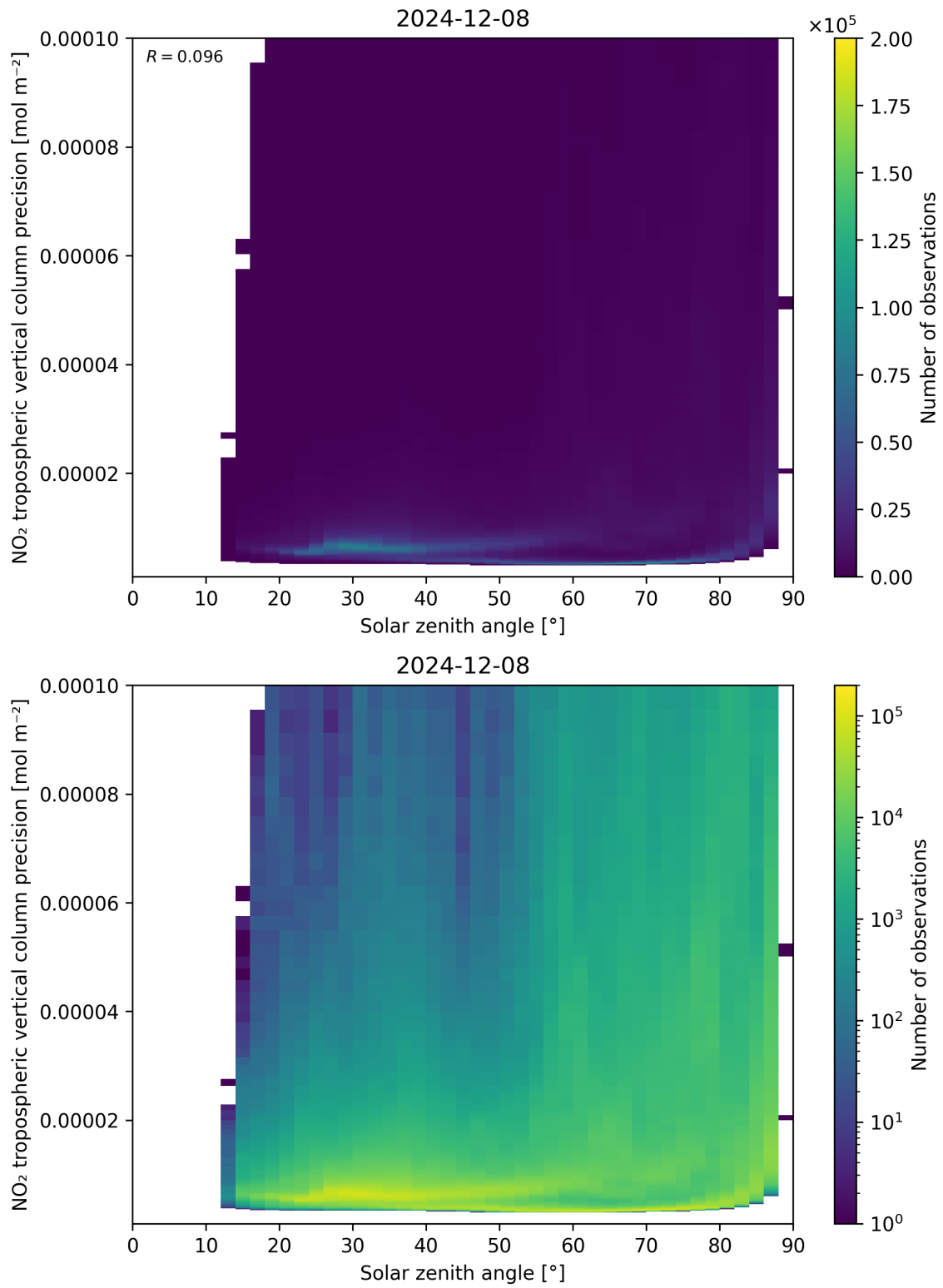
Figure 156: Scatter density plot of “Solar zenith angle” against “NO 2 tropospheric vertical column precision” for 2024-12-07 to 2024-12-09.
