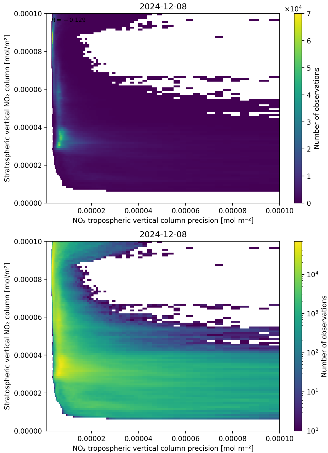
Figure 135: Scatter density plot of “NO 2 tropospheric vertical column precision” against “Stratospheric vertical NO 2 column” for 2024-12-07 to 2024-12-09.
