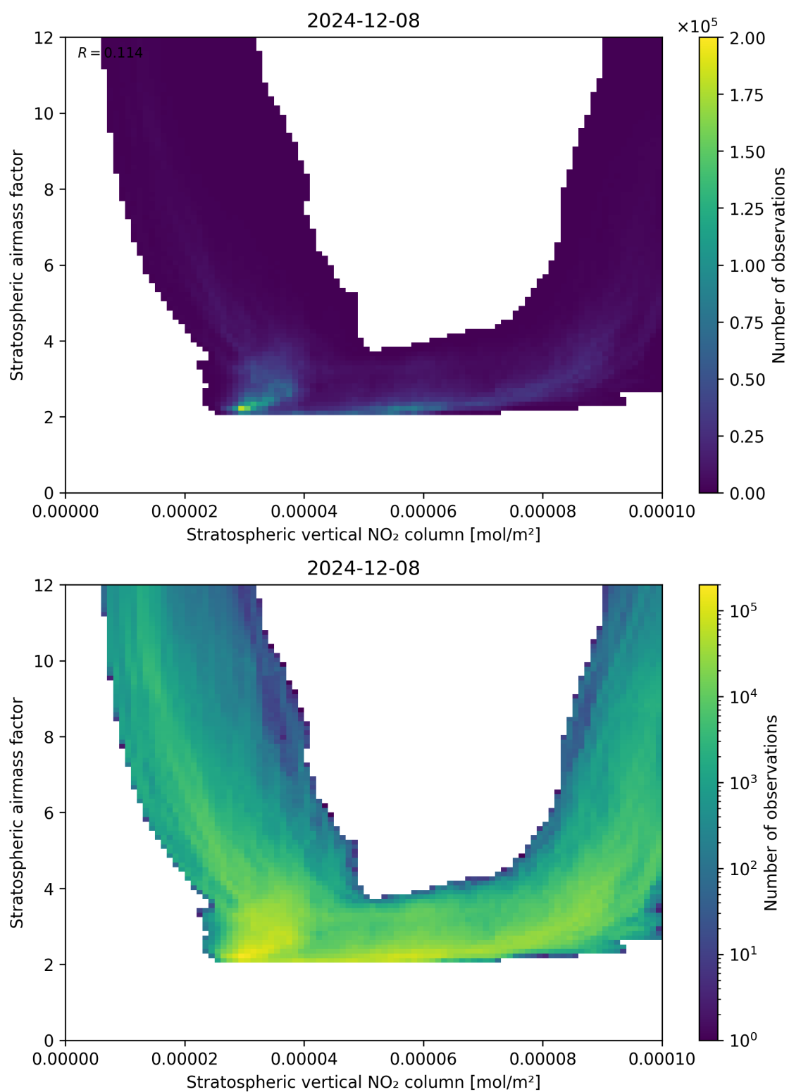
Figure 96: Scatter density plot of “Stratospheric vertical NO 2 column” against “Stratospheric airmass factor” for 2024-12-07 to 2024-12-09.
