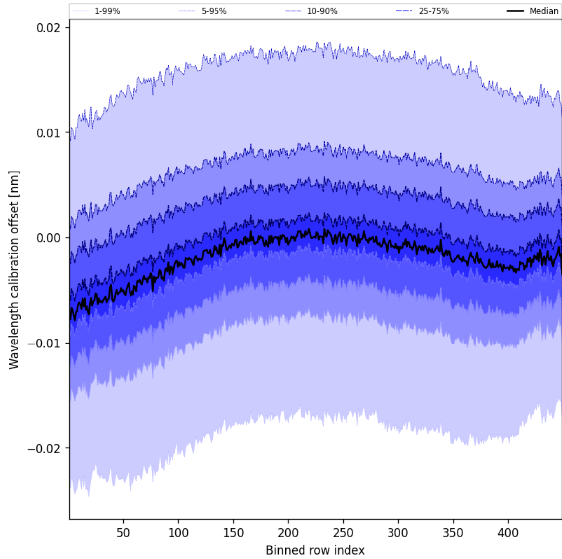
Figure 52: Along track statistics of “Wavelength calibration offset” for 2024-12-07 to 2024-12-09
