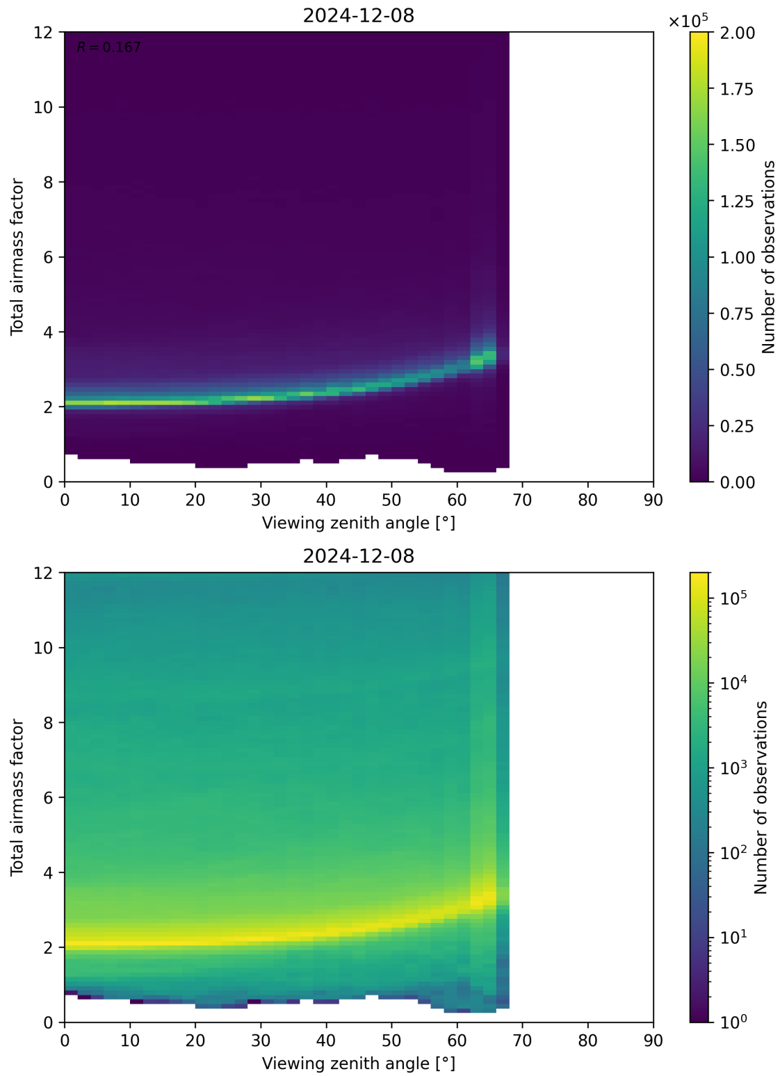
Figure 160: Scatter density plot of “Viewing zenith angle” against “Total airmass factor” for 2024-12-07 to 2024-12-09.
