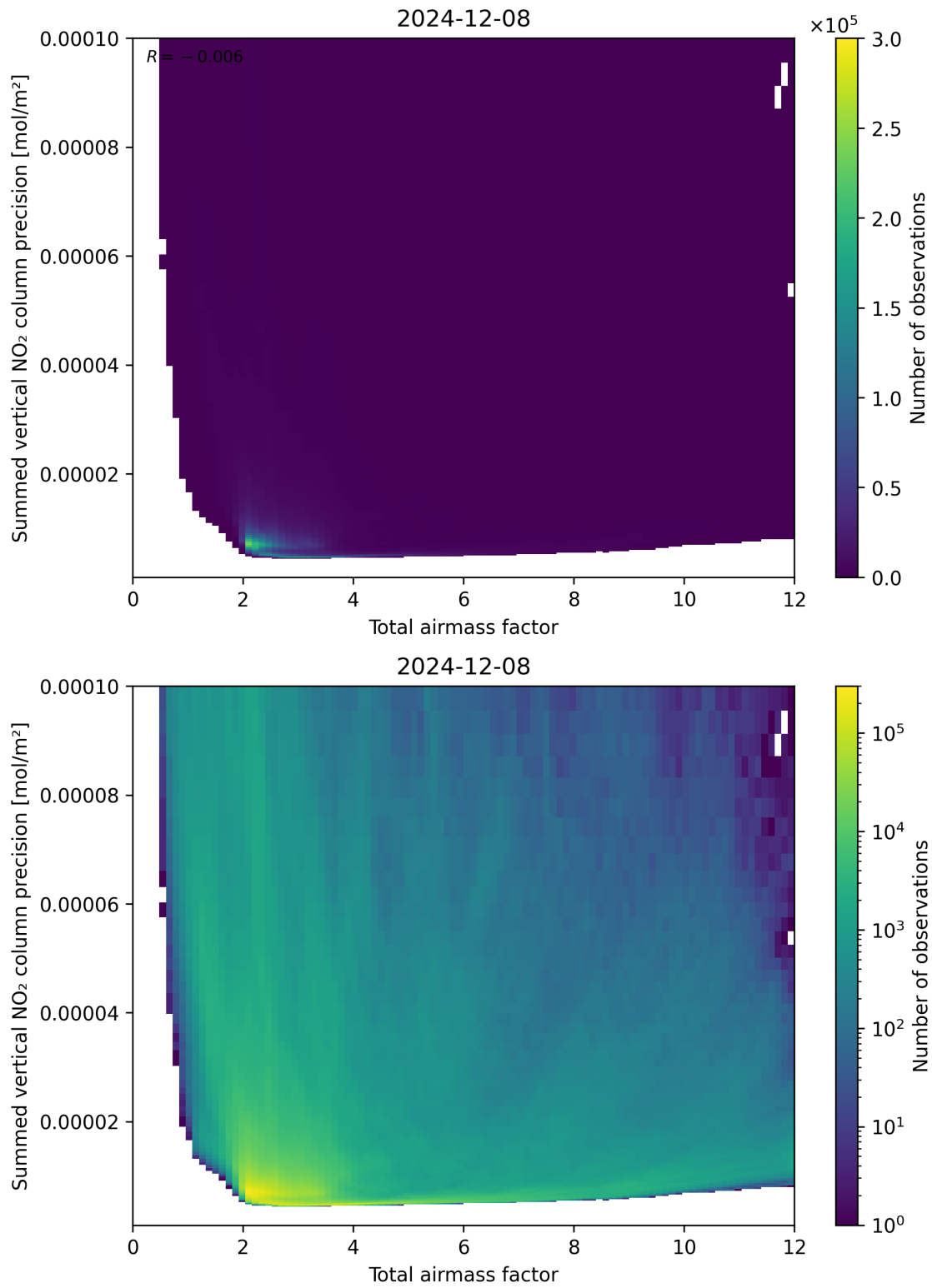
Figure 66: Scatter density plot of “Total airmass factor” against “Summed vertical NO 2 column precision” for 2024-12-07 to 2024-12-09.
