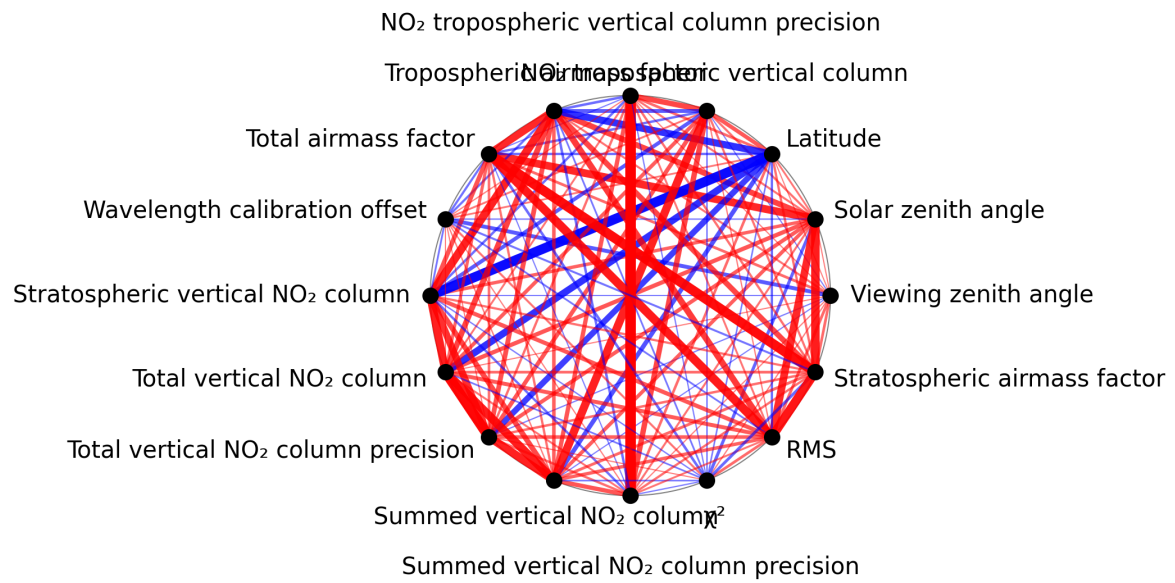
Figure 1: Map of correlation graph for 2024-12-07 to 2024-12-09.
