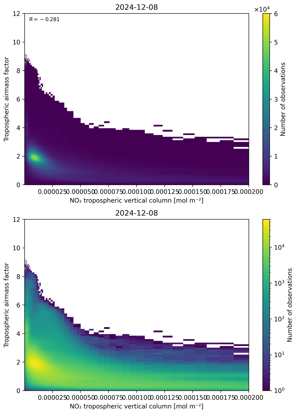
Figure 123: Scatter density plot of “NO 2 tropospheric vertical column” against “Tropospheric air mass factor” for 2024-12-07 to 2024-12-09.
