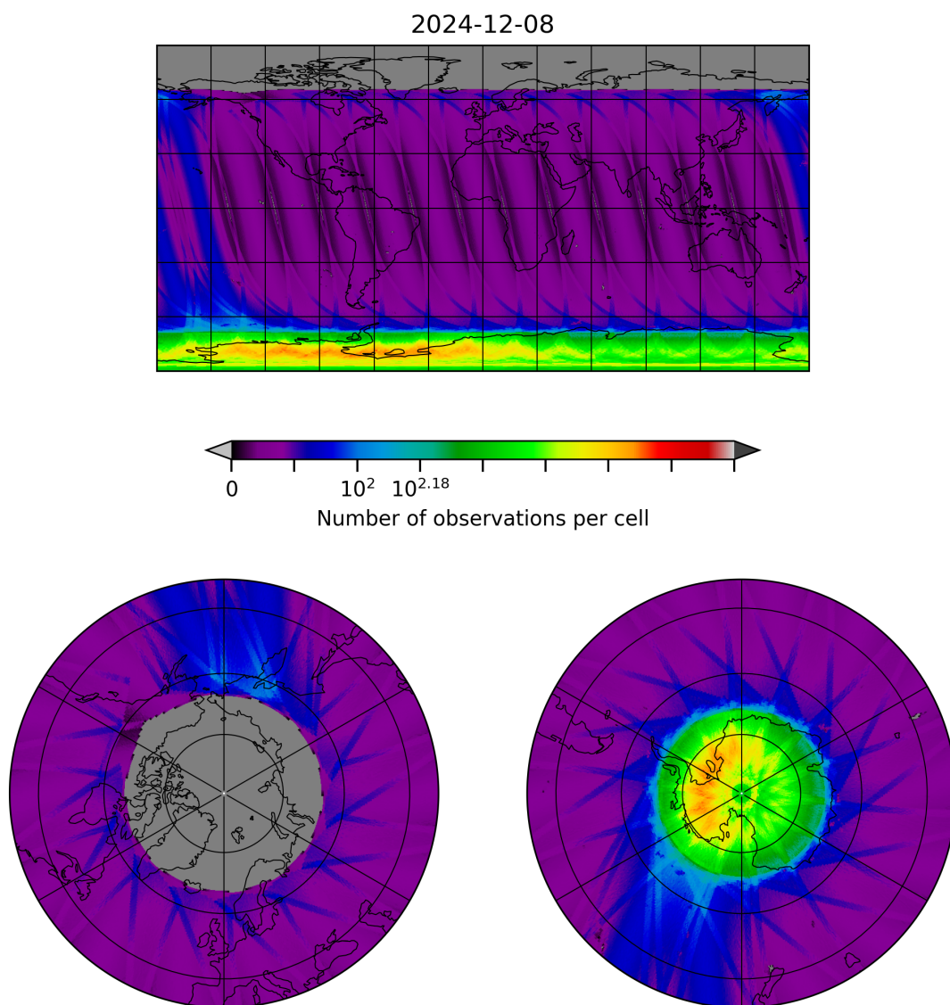
Figure 10: Map of the number of observations for 2024-12-07 to 2024-12-09
