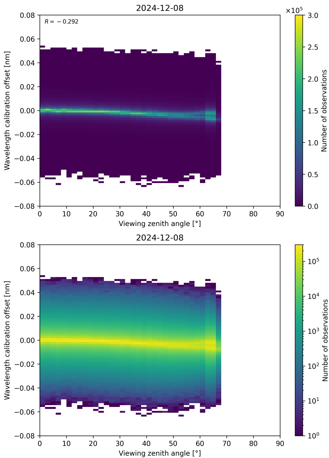
Figure 173: Scatter density plot of “Viewing zenith angle” against “Wavelength calibration offset” for 2024-12-07 to 2024-12-09.
