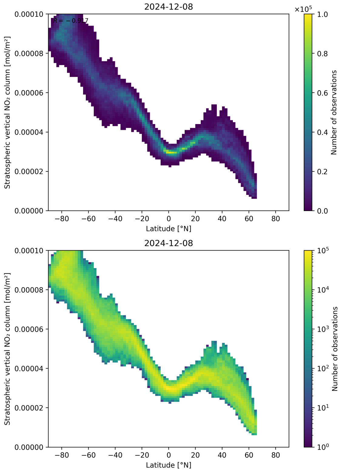
Figure 87: Scatter density plot of “Latitude” against “Stratospheric vertical NO 2 column” for 2024-12-07 to 2024-12-09.
