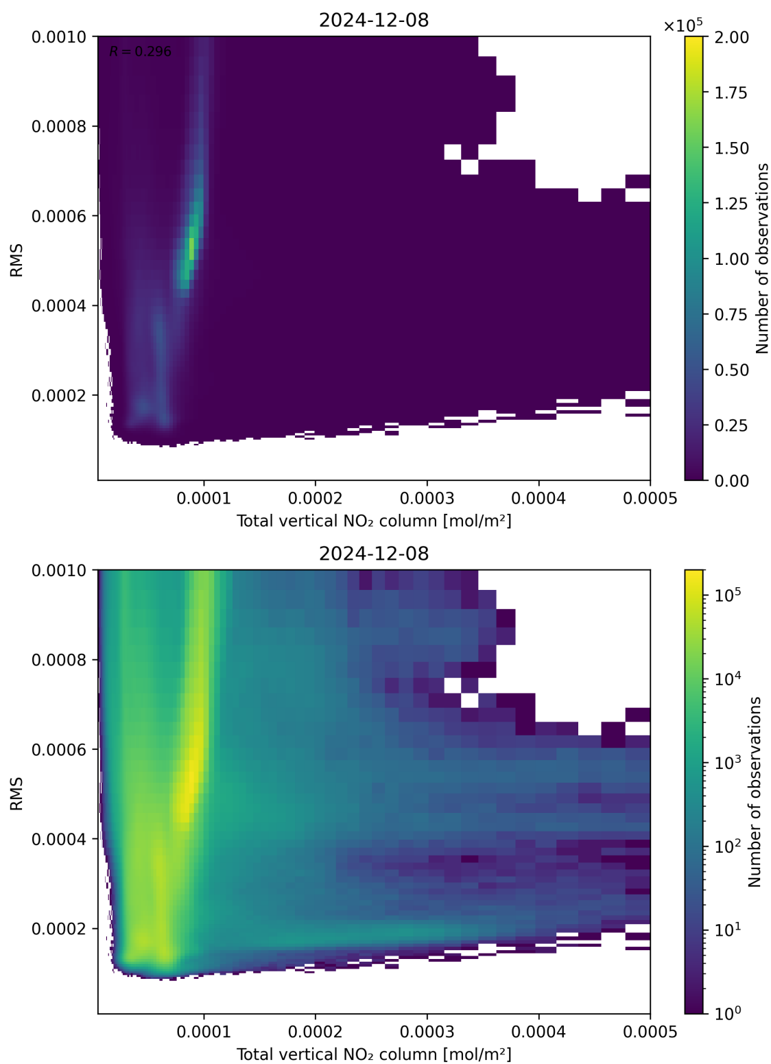
Figure 120: Scatter density plot of “Total vertical NO 2 column” against “RMS” for 2024-12-07 to 2024-12-09.
