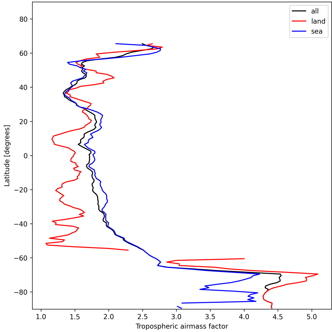
Figure 14: Zonal average of “Tropospheric airmass factor” for 2024-12-07 to 2024-12-09.
