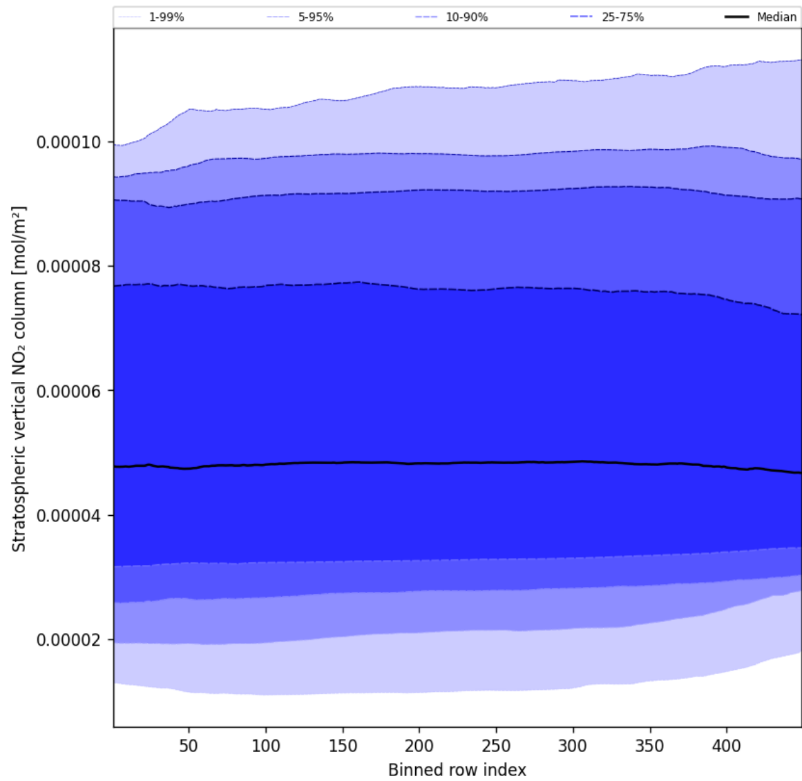
Figure 53: Along track statistics of “Stratospheric vertical NO 2 column” for 2024-12-07 to 2024-12-09
