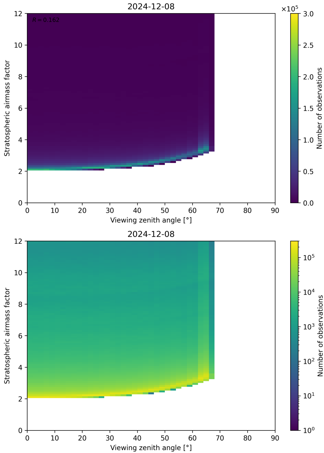
Figure 159: Scatter density plot of “Viewing zenith angle” against “Stratospheric airmass factor” for 2024-12-07 to 2024-12-09.
