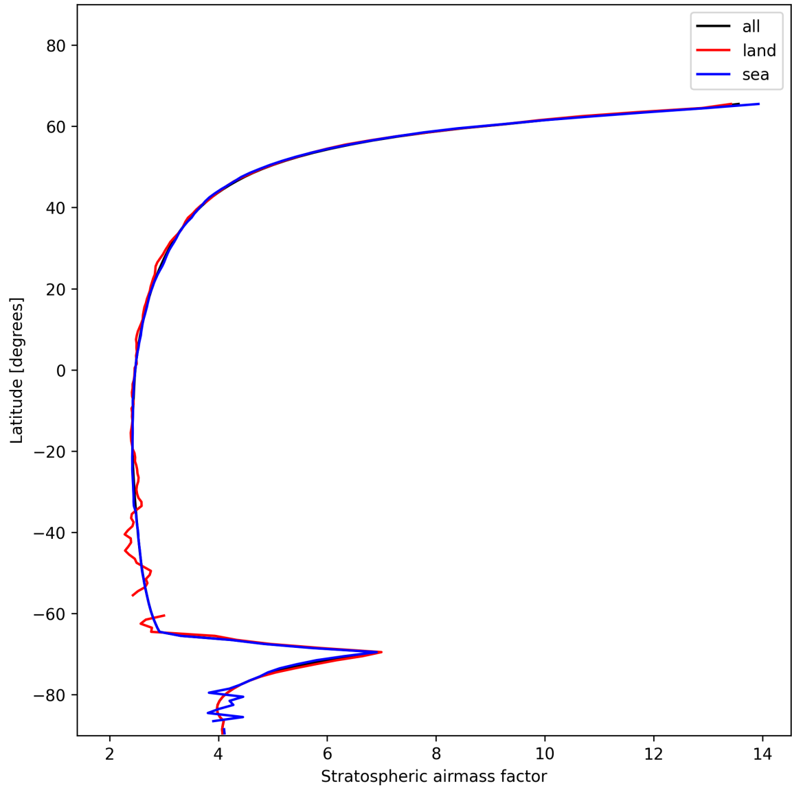
Figure 27: Zonal average of “Stratospheric air mass factor” for 2024-12-07 to 2024-12-09.
