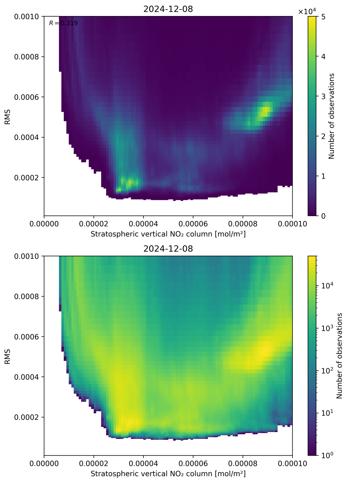
Figure 102: Scatter density plot of “Stratospheric vertical NO 2 column” against “RMS” for 2024-12-07 to 2024-12-09.
