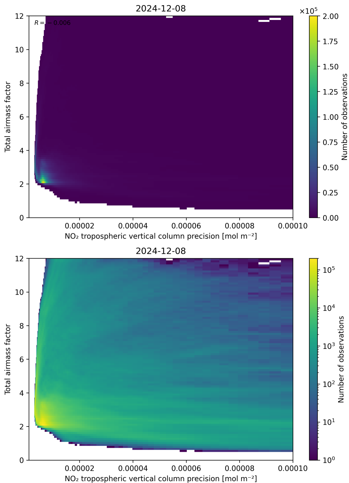
Figure 132: Scatter density plot of “NO 2 tropospheric vertical column precision” against “Total air mass factor” for 2024-12-07 to 2024-12-09.
