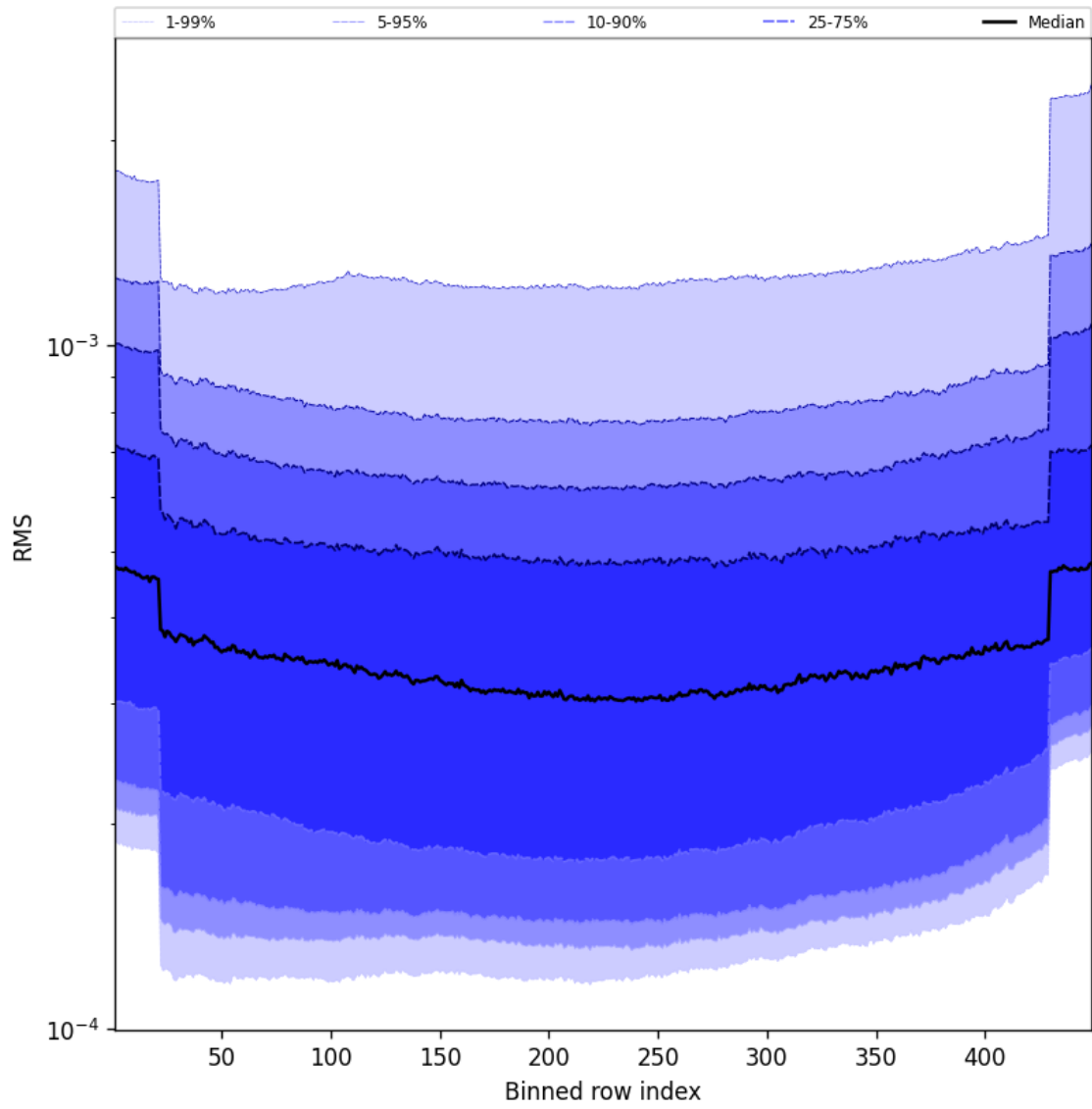
Figure 60: Along track statistics of “RMS” for 2024-12-07 to 2024-12-09
