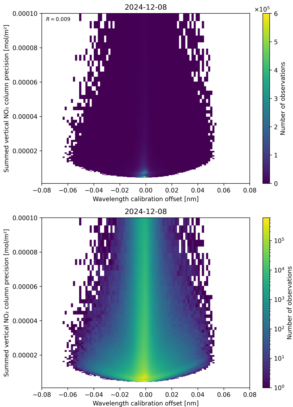
Figure 178: Scatter density plot of “Wavelength calibration offset” against “Summed vertical NO 2 column precision” for 2024-12-07 to 2024-12-09.
