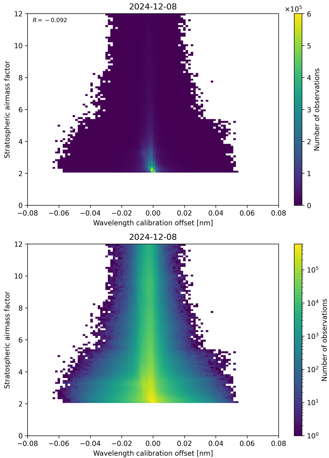
Figure 174: Scatter density plot of “Wavelength calibration offset” against “Stratospheric airmass factor” for 2024-12-07 to 2024-12-09.
