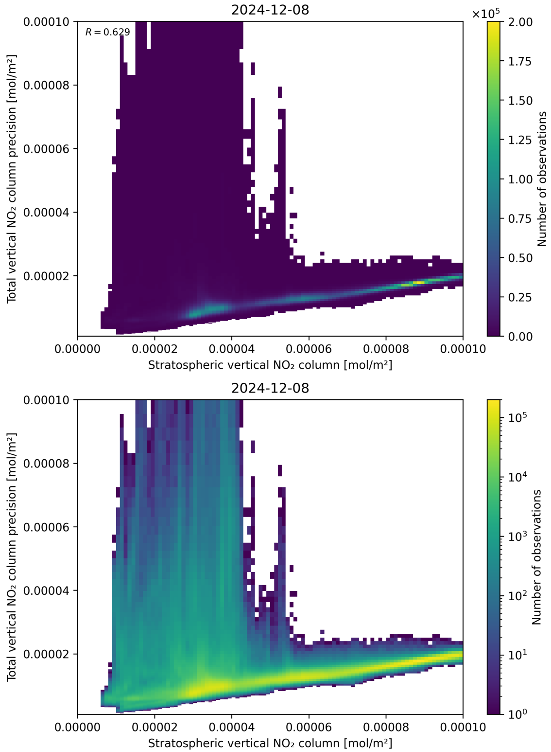
Figure 101: Scatter density plot of “Stratospheric vertical NO 2 column” against “Total vertical NO 2 column precision” for 2024-12-07 to 2024-12-09.
