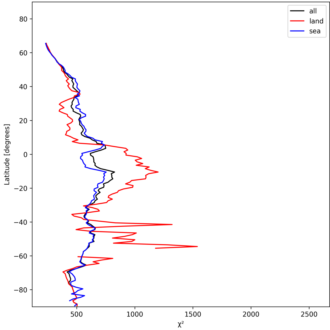
Figure 25: Zonal average of “ \chi^2 ” for 2024-12-07 to 2024-12-09.
