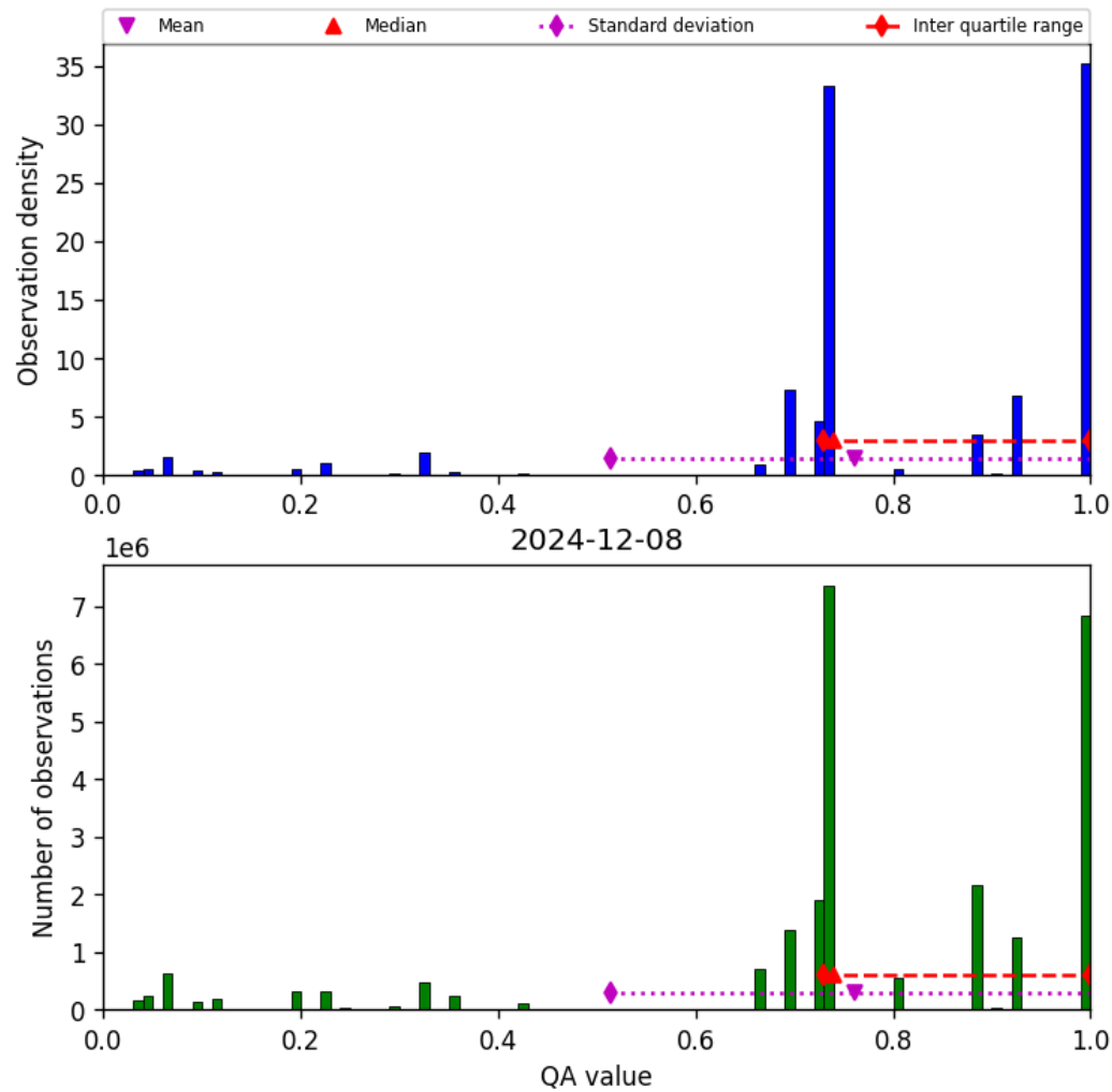
Figure 28: Histogram of “QA value” for 2024-12-07 to 2024-12-09
