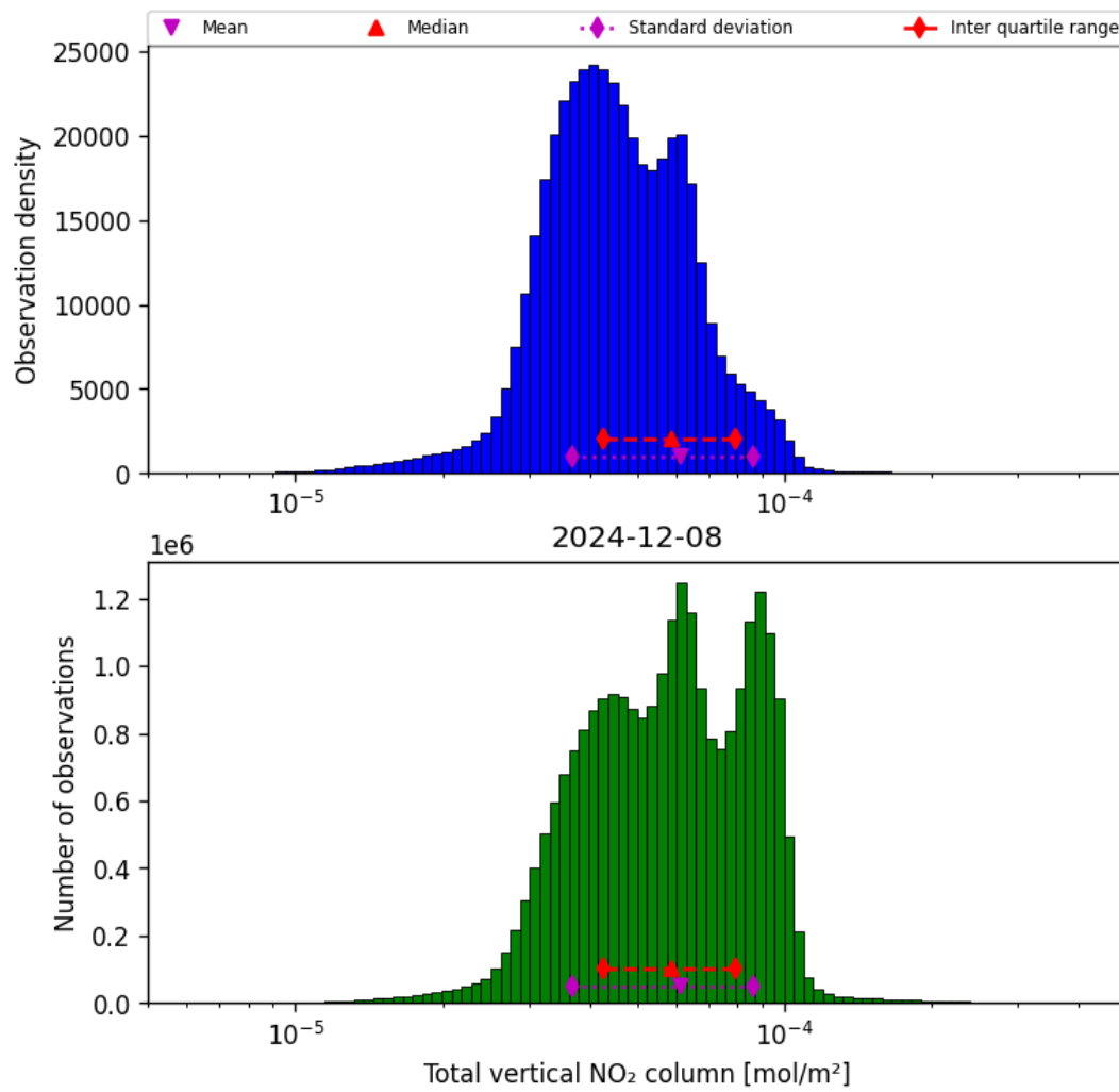
Figure 38: Histogram of “Total vertical NO 2 column” for 2024-12-07 to 2024-12-09
