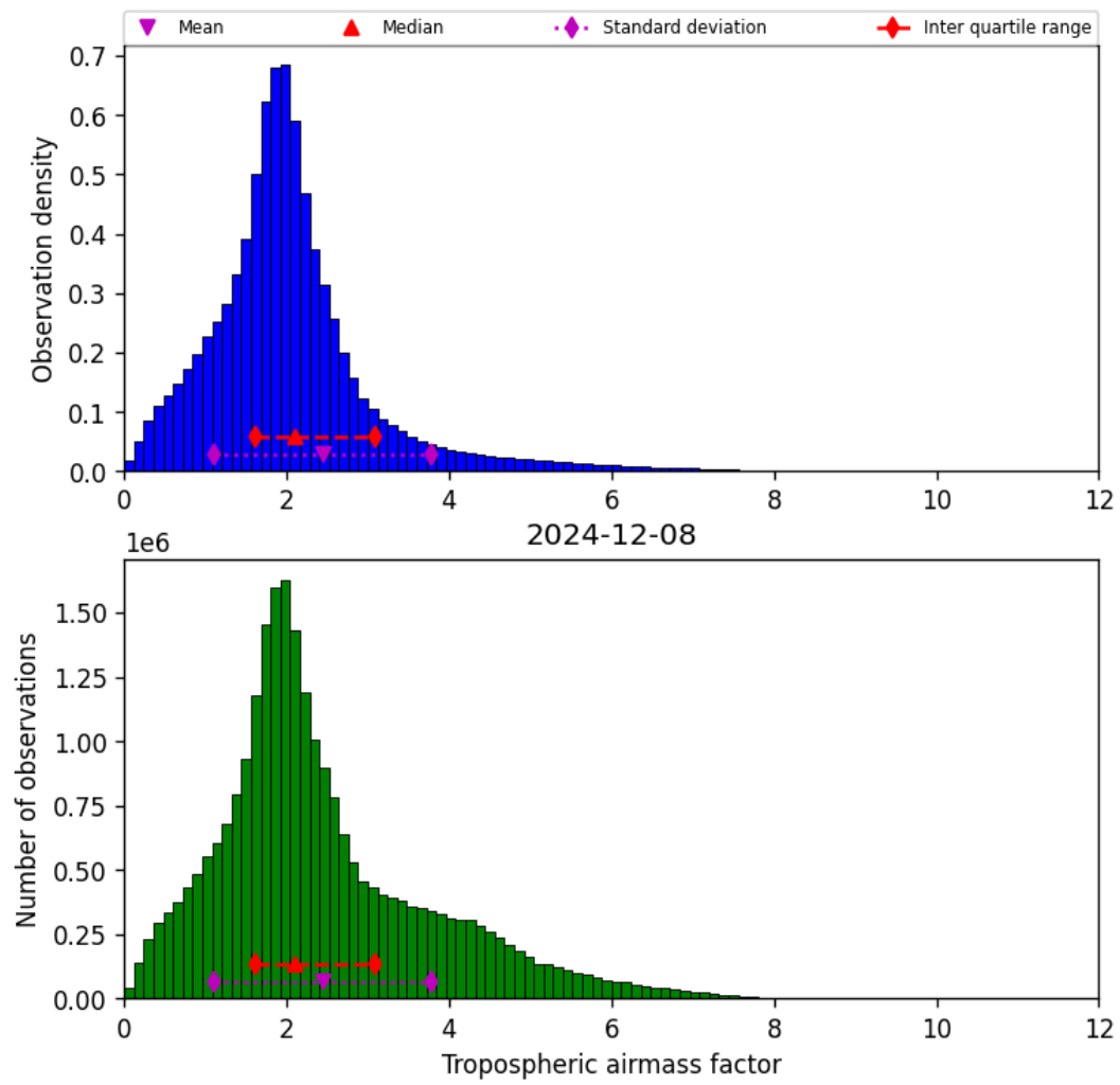
Figure 31: Histogram of “Tropospheric airmass factor” for 2024-12-07 to 2024-12-09
