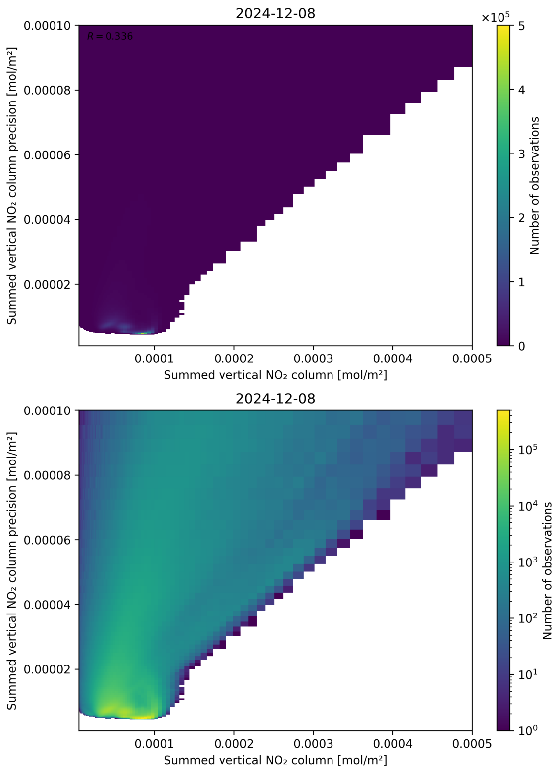
Figure 105: Scatter density plot of “Summed vertical NO 2 column” against “Summed vertical NO 2 column precision” for 2024-12-07 to 2024-12-09.
