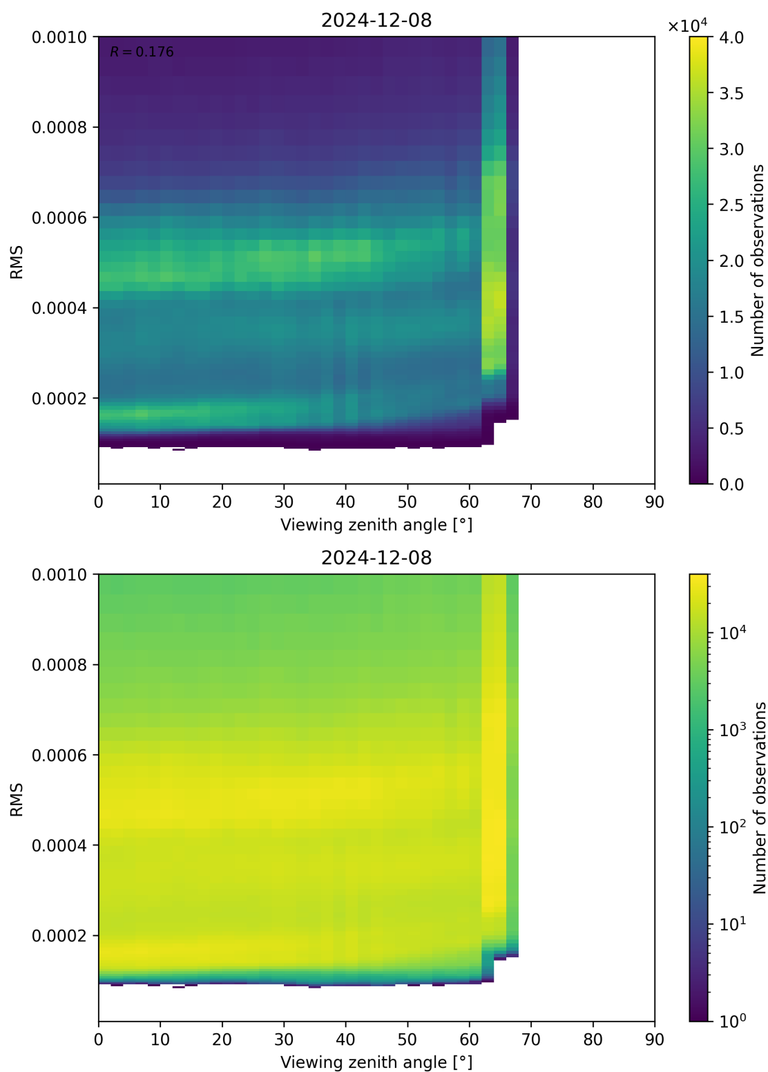
Figure 171: Scatter density plot of “Viewing zenith angle” against “RMS” for 2024-12-07 to 2024-12-09.
