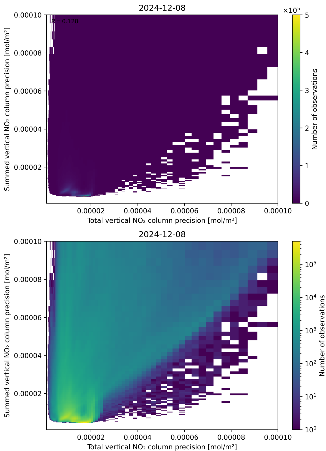
Figure 118: Scatter density plot of “Total vertical NO 2 column precision” against “Summed vertical NO 2 column precision” for 2024-12-07 to 2024-12-09.
