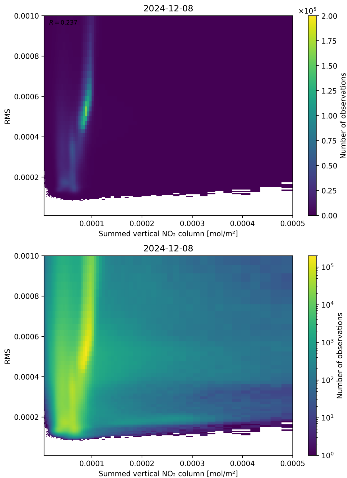
Figure 109: Scatter density plot of “Summed vertical NO 2 column” against “RMS” for 2024-12-07 to 2024-12-09.
