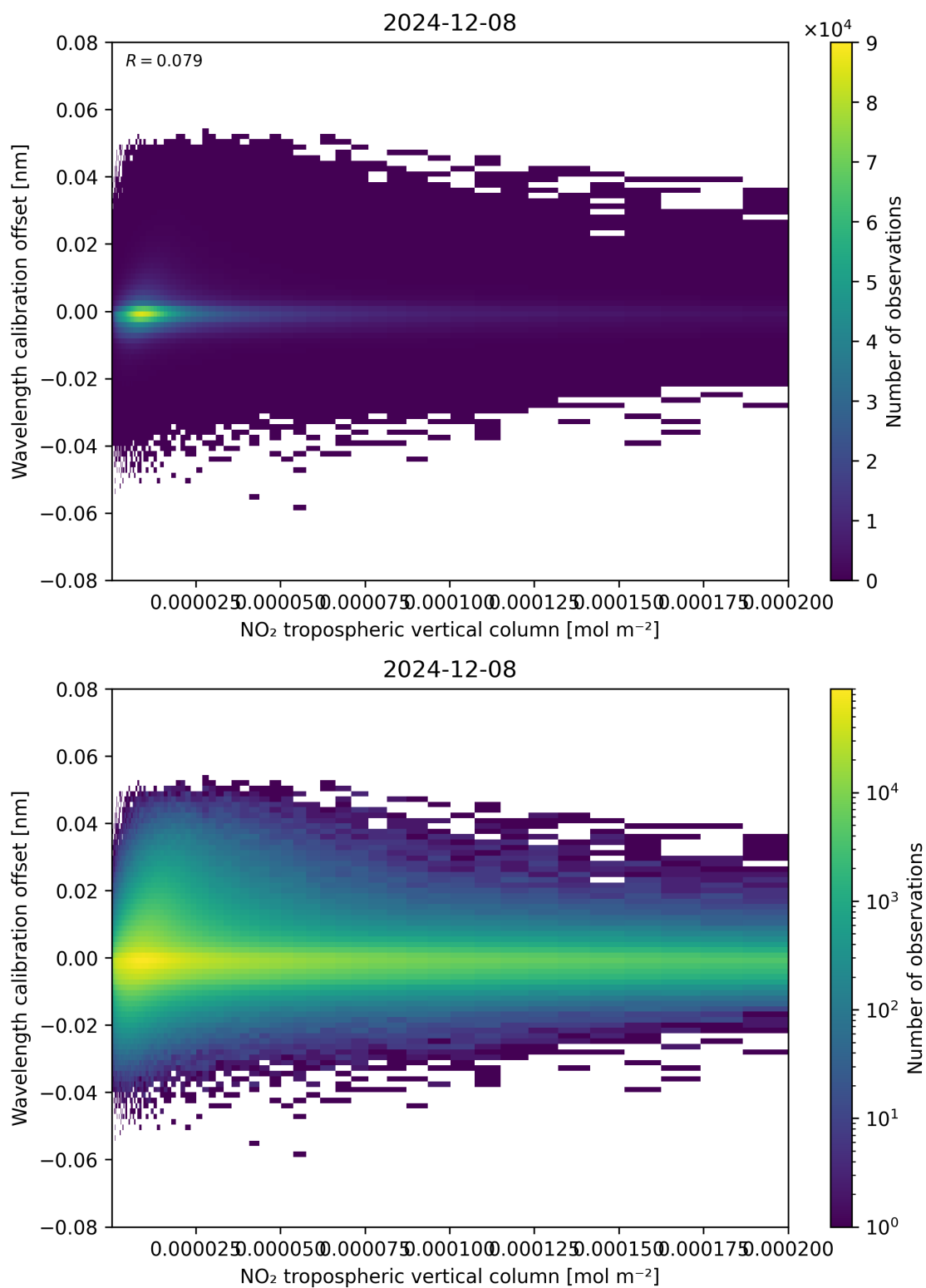
Figure 143: Scatter density plot of “NO 2 tropospheric vertical column” against “Wavelength calibration offset” for 2024-12-07 to 2024-12-09.
