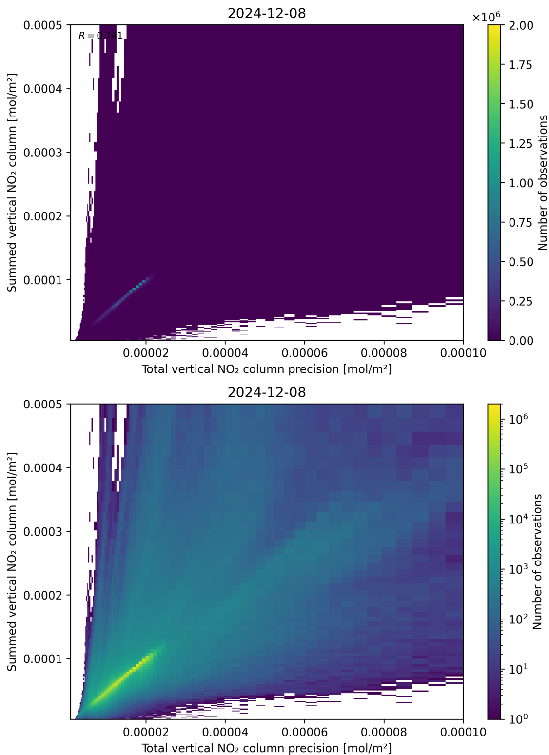
Figure 117: Scatter density plot of “Total vertical NO 2 column precision” against “Summed vertical NO 2 column” for 2024-12-07 to 2024-12-09.
