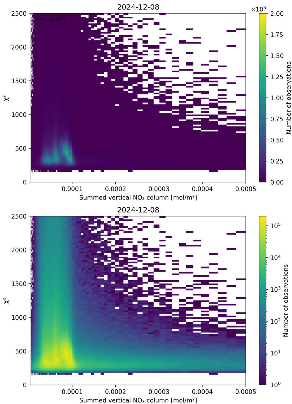
Figure 104: Scatter density plot of “Summed vertical NO 2 column” against “ \chi^2 ” for 2024-12-07 to 2024-12-09.
