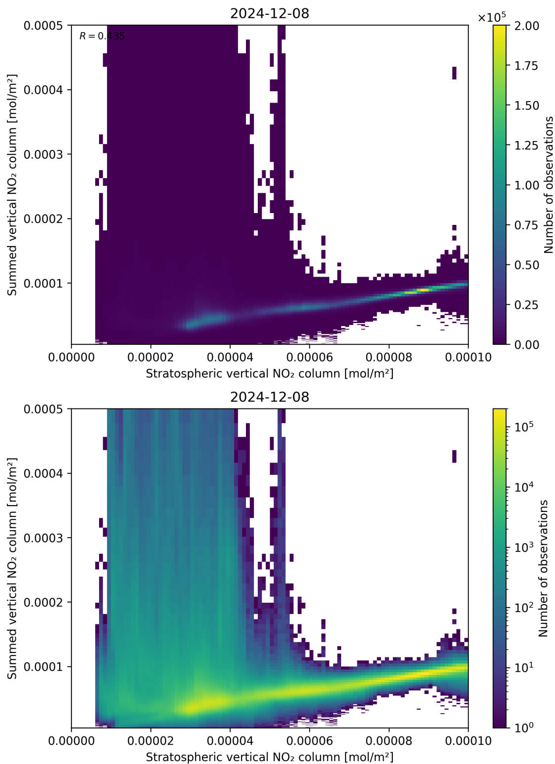
Figure 98: Scatter density plot of “Stratospheric vertical NO 2 column” against “Summed vertical NO 2 column” for 2024-12-07 to 2024-12-09.
