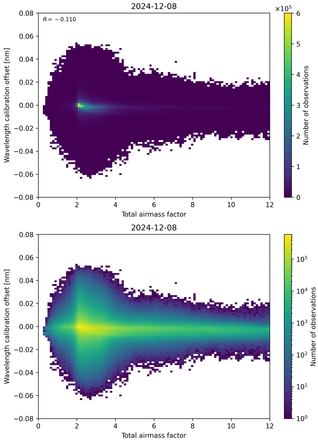
Figure 70: Scatter density plot of “Total airmass factor” against “Wavelength calibration offset” for 2024-12-07 to 2024-12-09.
