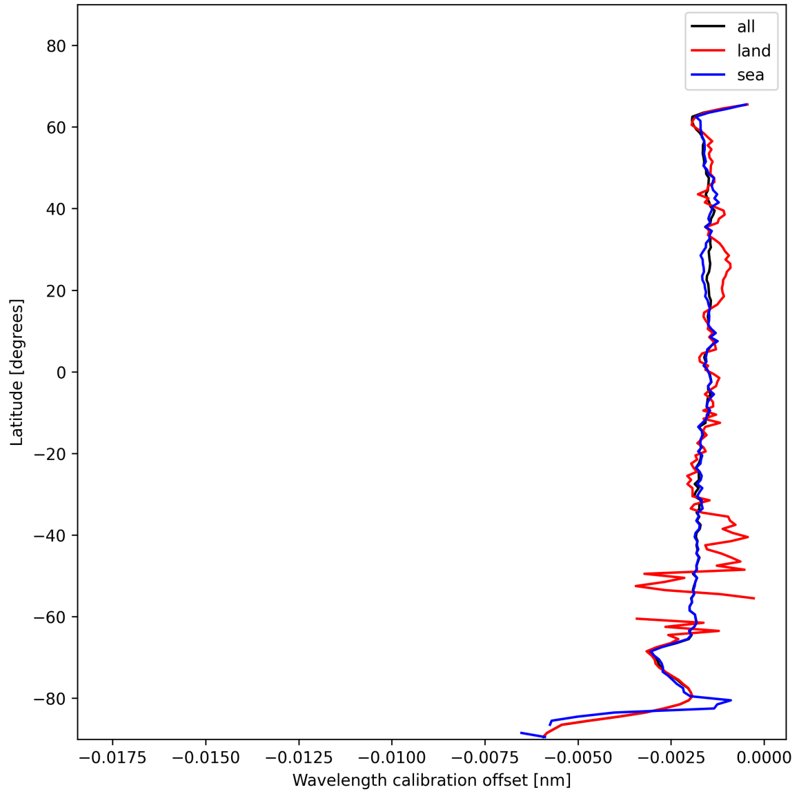
Figure 18: Zonal average of “Wavelength calibration offset” for 2024-12-07 to 2024-12-09.
