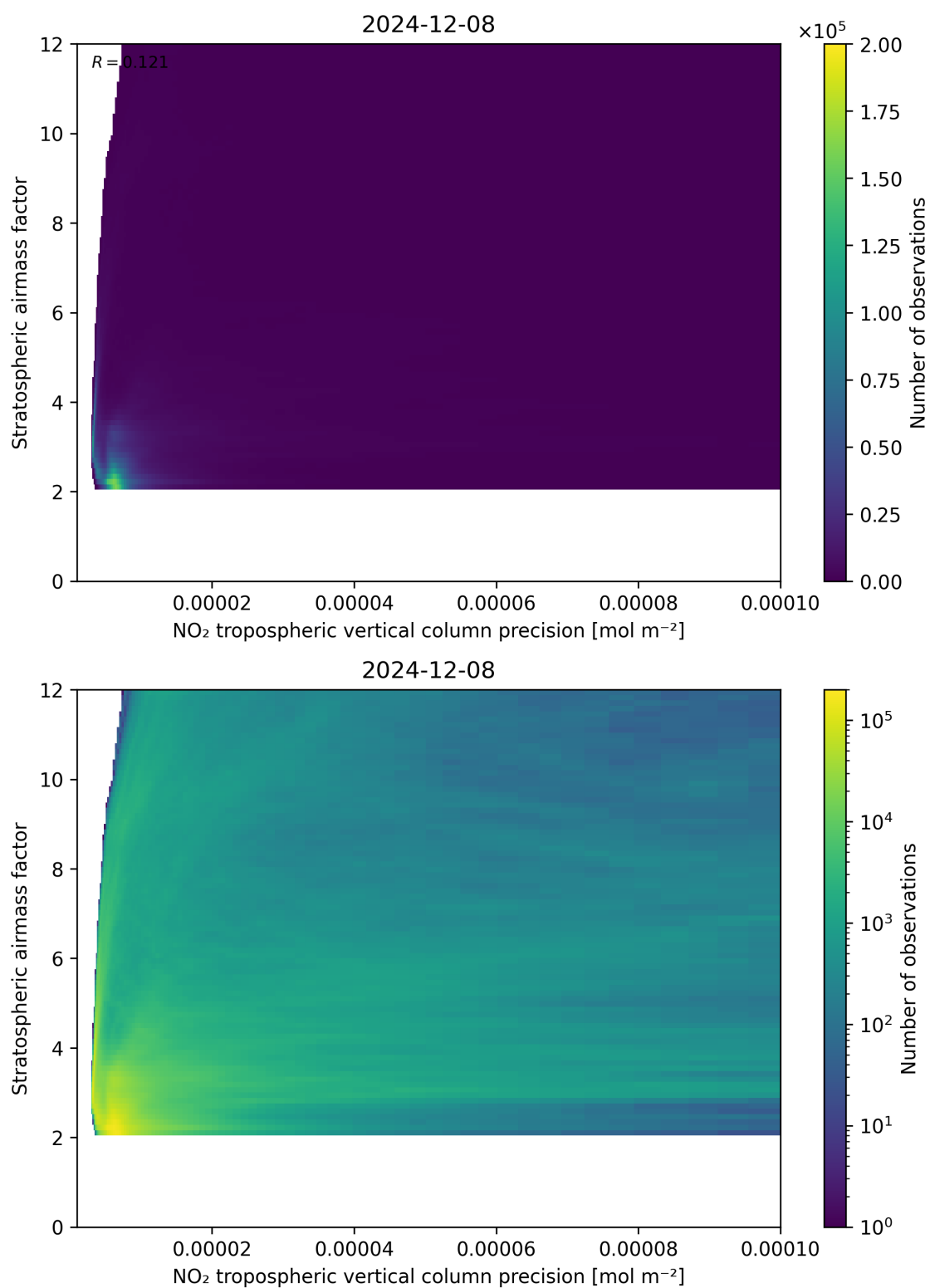
Figure 131: Scatter density plot of “NO 2 tropospheric vertical column precision” against “Stratospheric airmass factor” for 2024-12-07 to 2024-12-09.
