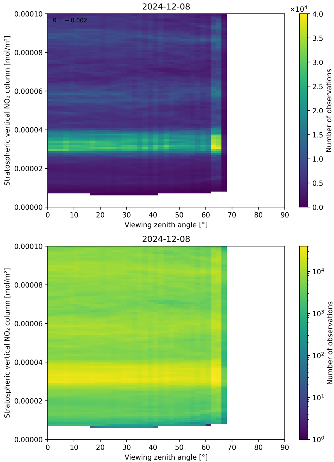
Figure 164: Scatter density plot of “Viewing zenith angle” against “Stratospheric vertical NO 2 column” for 2024-12-07 to 2024-12-09.
