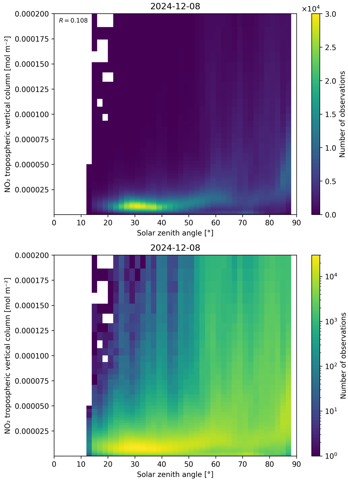
Figure 155: Scatter density plot of “Solar zenith angle” against “NO 2 tropospheric vertical column” for 2024-12-07 to 2024-12-09.
