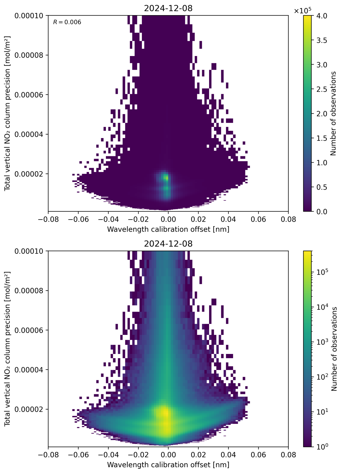
Figure 180: Scatter density plot of “Wavelength calibration offset” against “Total vertical NO 2 column precision” for 2024-12-07 to 2024-12-09.
