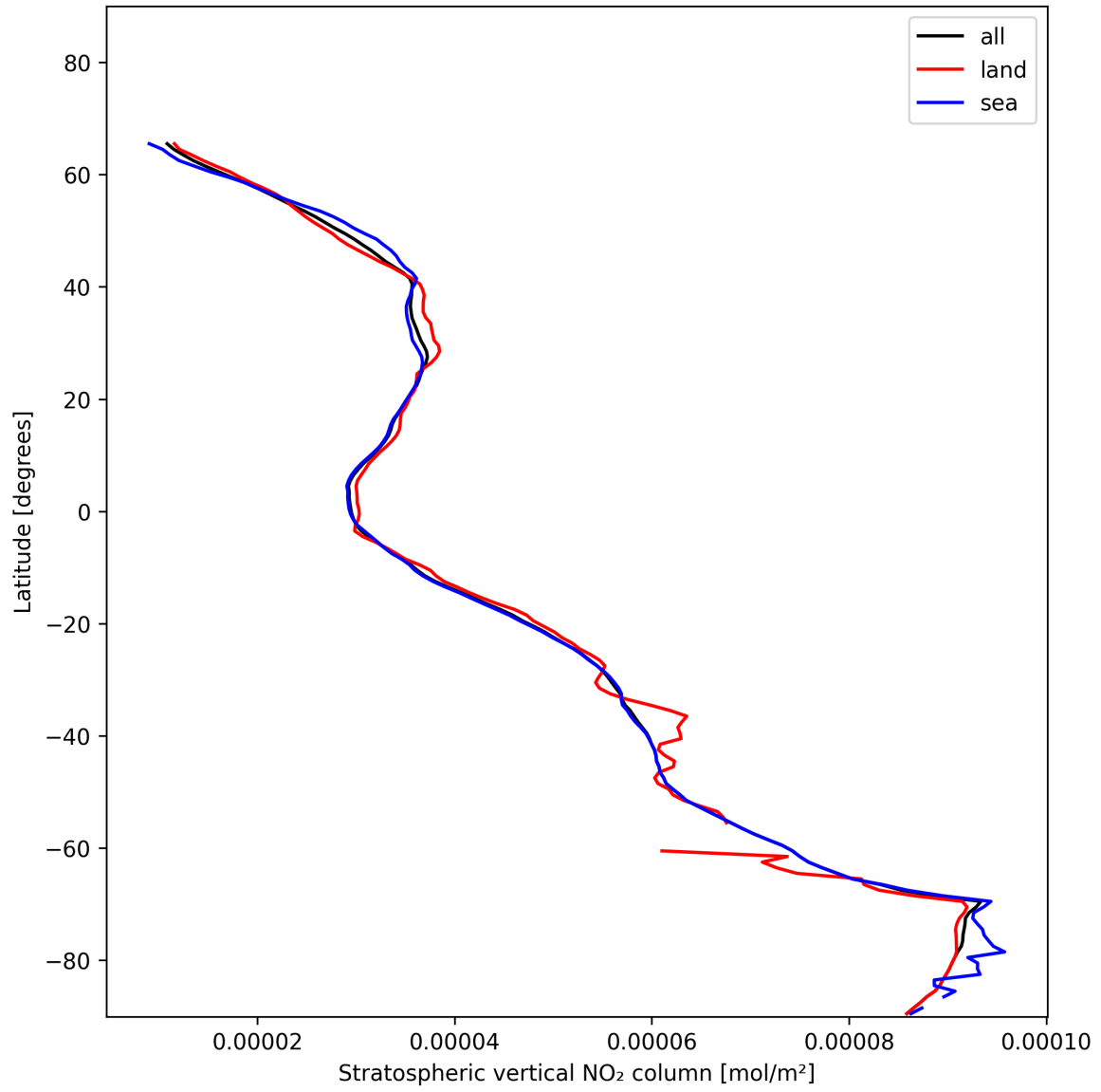
Figure 19: Zonal average of “Stratospheric vertical NO 2 column” for 2024-12-07 to 2024-12-09.
