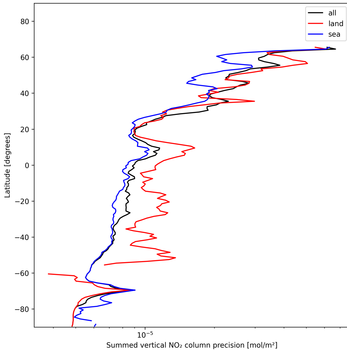
Figure 24: Zonal average of “Summed vertical NO 2 column precision” for 2024-12-07 to 2024-12-09.
