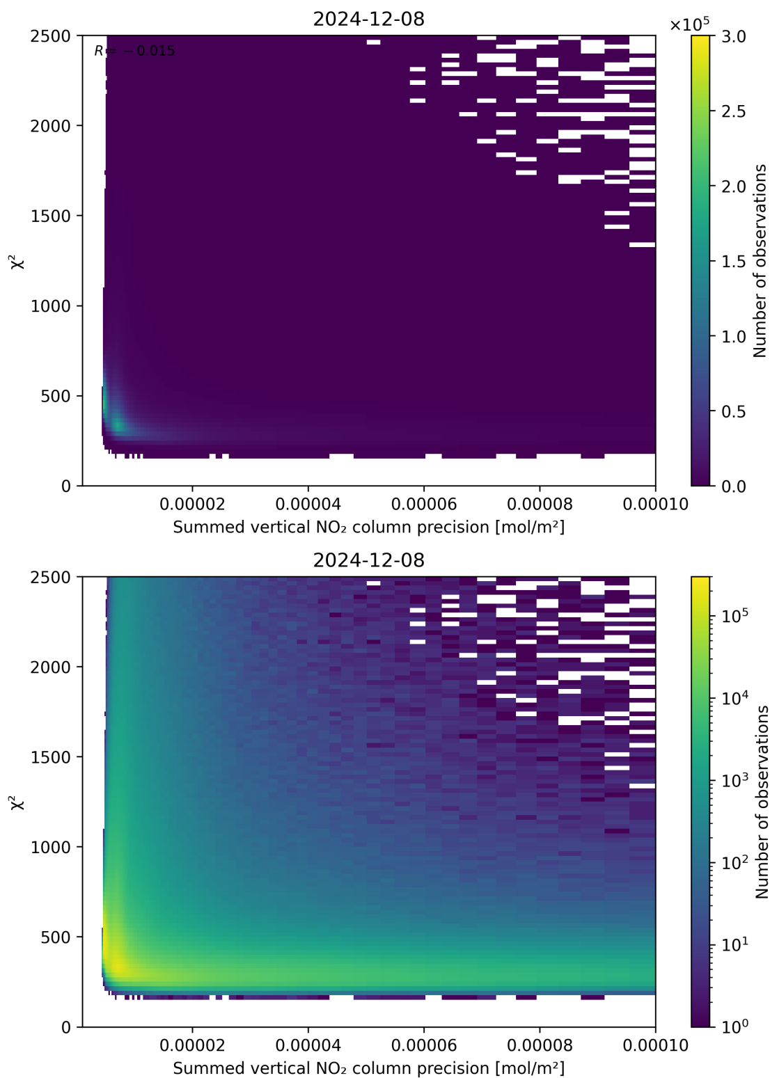
Figure 107: Scatter density plot of “Summed vertical NO 2 column precision” against “ \chi^2 ” for 2024-12-07 to 2024-12-09.
