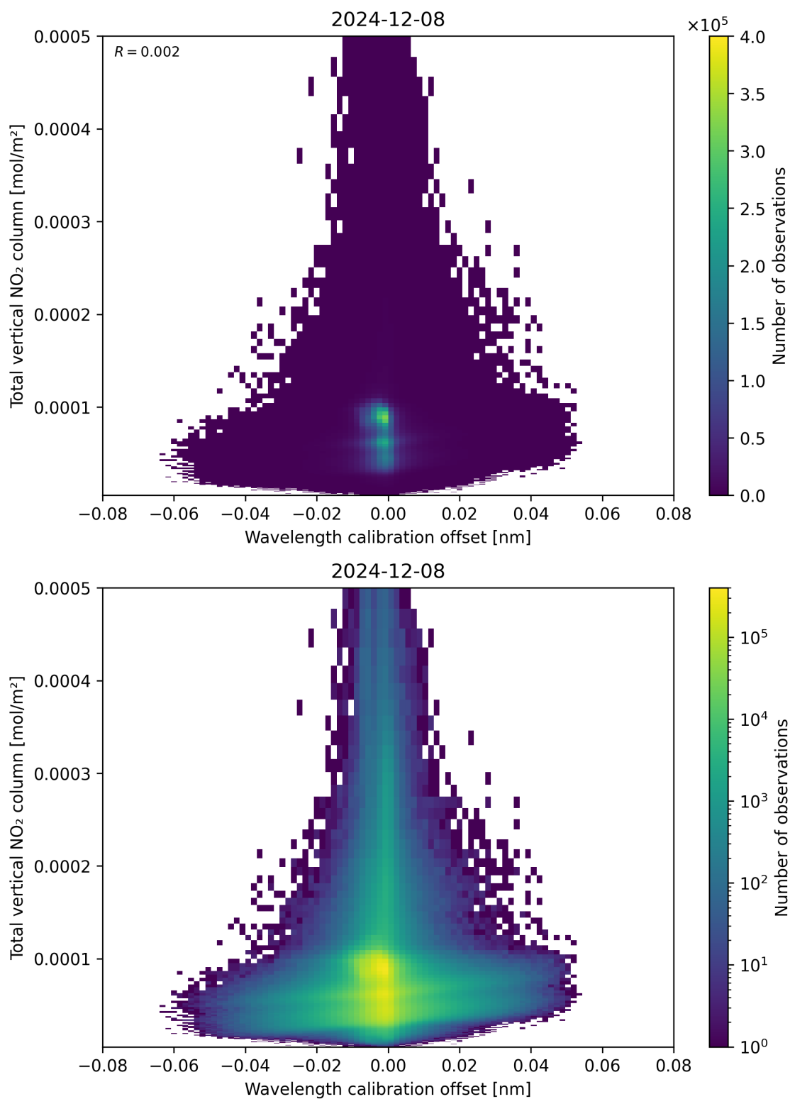
Figure 179: Scatter density plot of “Wavelength calibration offset” against “Total vertical NO 2 column” for 2024-12-07 to 2024-12-09.
