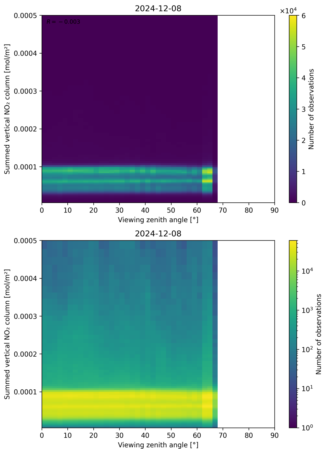
Figure 165: Scatter density plot of “Viewing zenith angle” against “Summed vertical NO 2 column” for 2024-12-07 to 2024-12-09.
