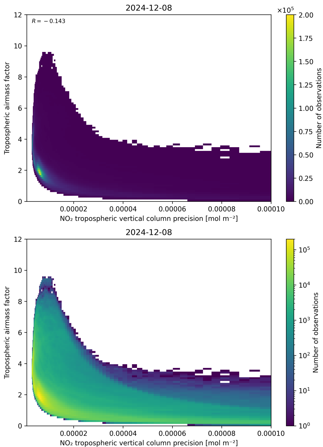
Figure 133: Scatter density plot of “NO 2 tropospheric vertical column precision” against “Tropospheric air mass factor” for 2024-12-07 to 2024-12-09.
