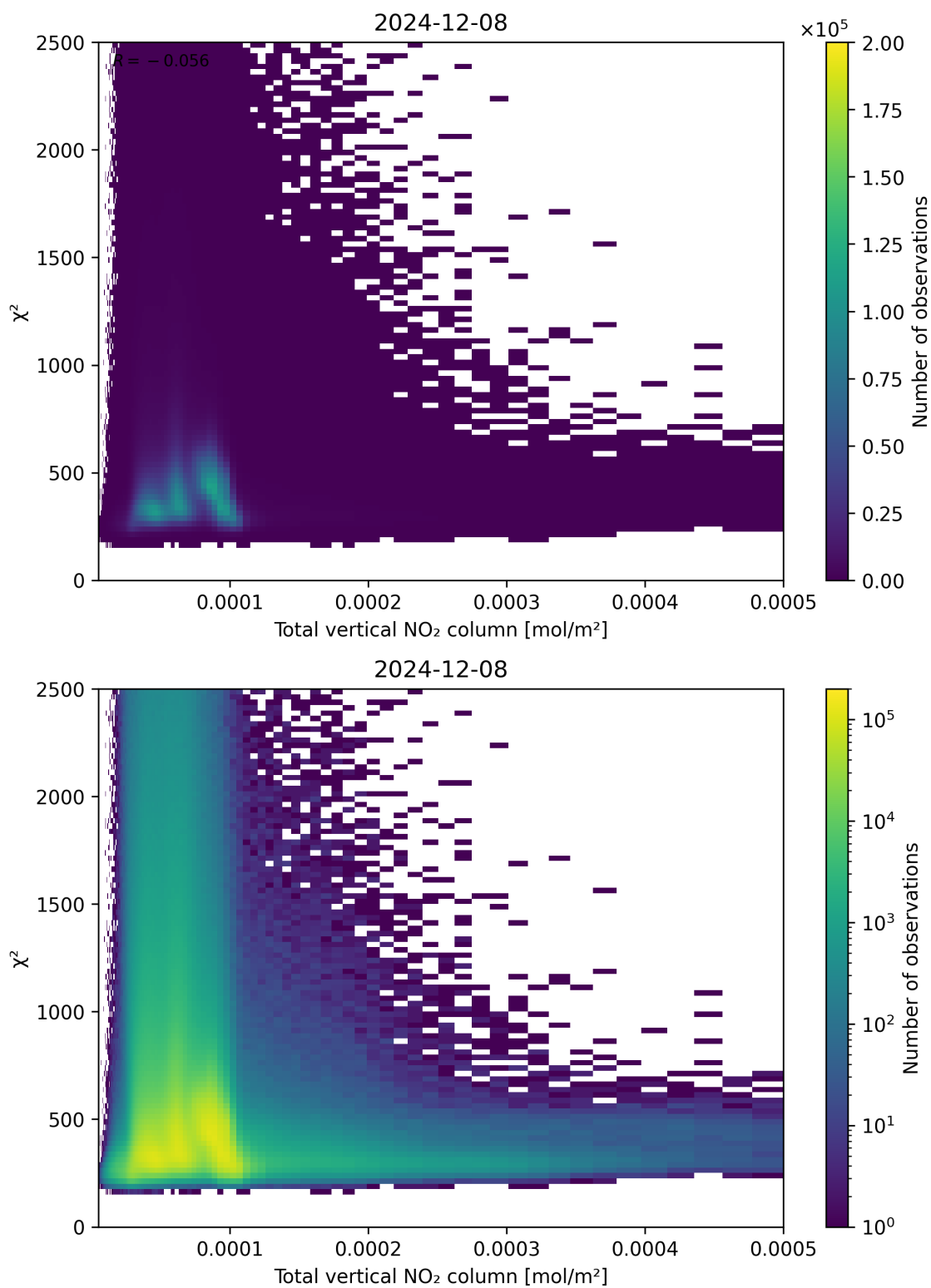
Figure 111: Scatter density plot of “Total vertical NO 2 column” against “ \chi^2 ” for 2024-12-07 to 2024-12-09.
