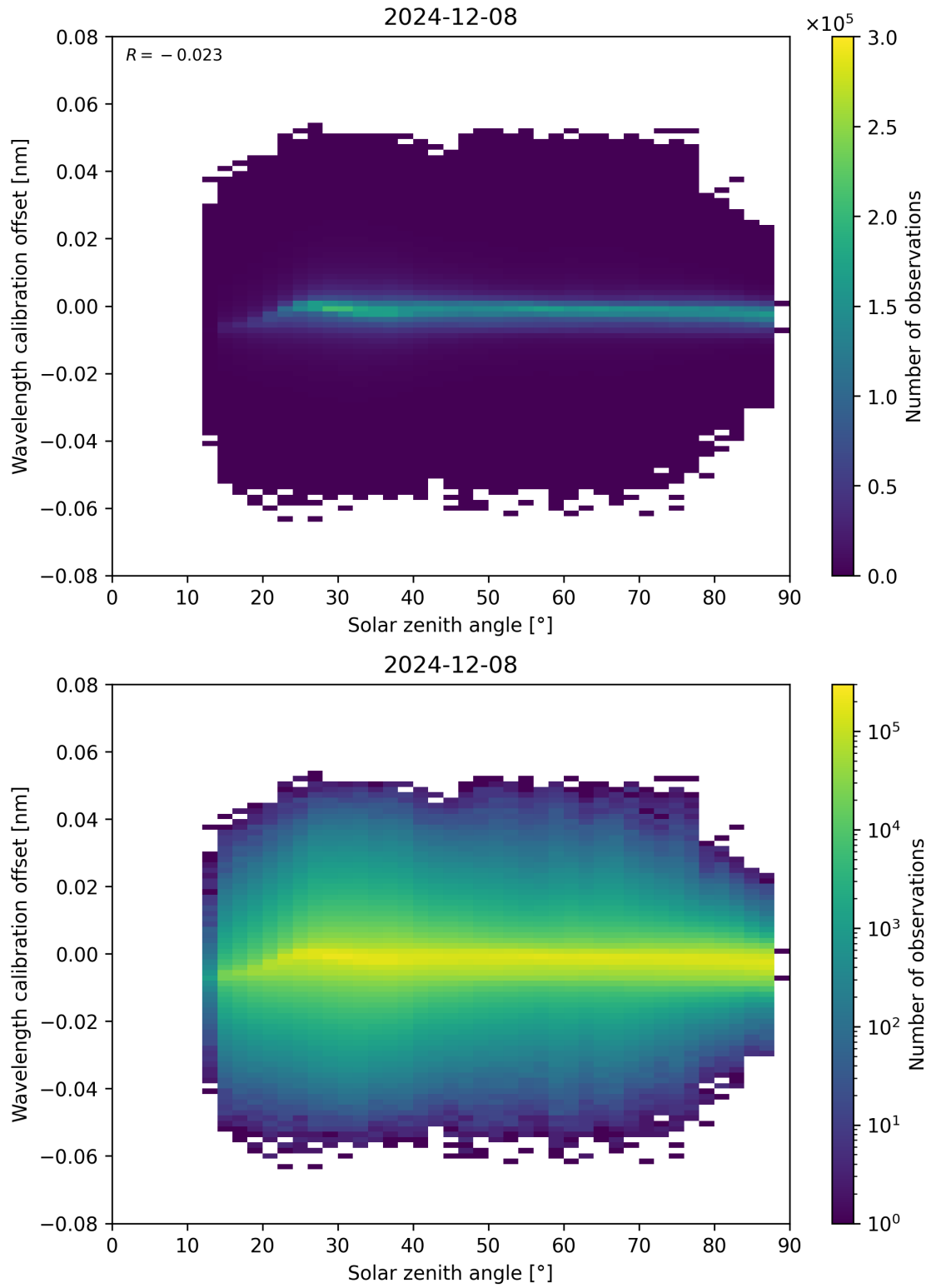
Figure 158: Scatter density plot of “Solar zenith angle” against “Wavelength calibration offset” for 2024-12-07 to 2024-12-09.
