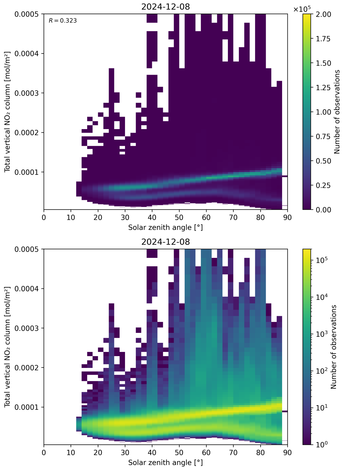
Figure 153: Scatter density plot of “Solar zenith angle” against “Total vertical NO 2 column” for 2024-12-07 to 2024-12-09.
