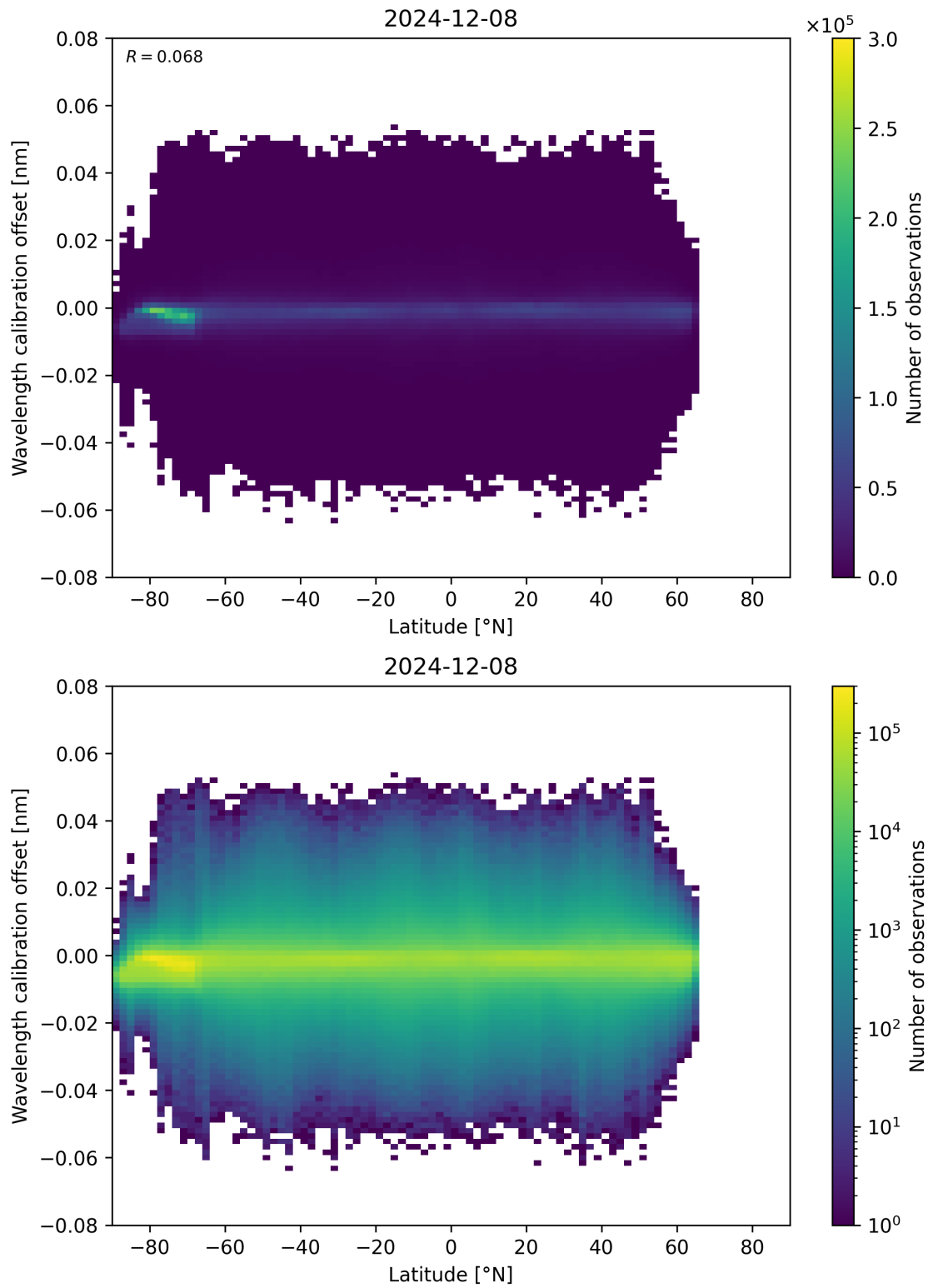
Figure 95: Scatter density plot of “Latitude” against “Wavelength calibration offset” for 2024-12-07 to 2024-12-09.
