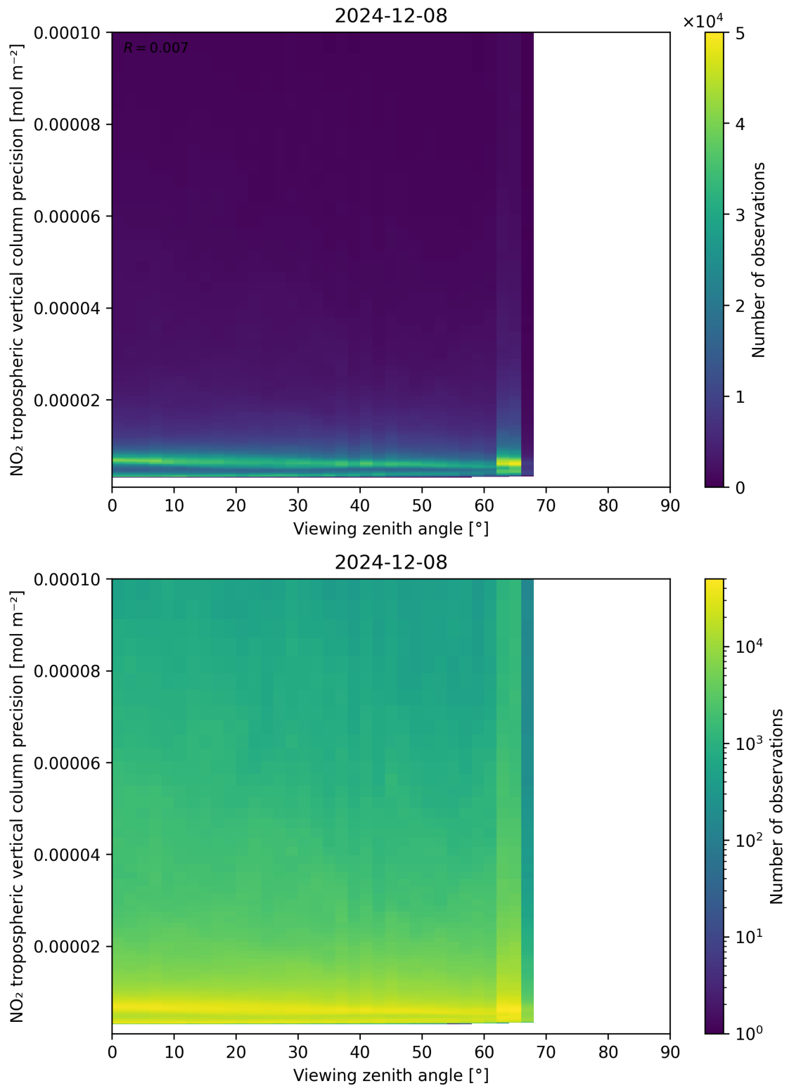
Figure 170: Scatter density plot of “Viewing zenith angle” against “NO 2 tropospheric vertical column precision” for 2024-12-07 to 2024-12-09.
