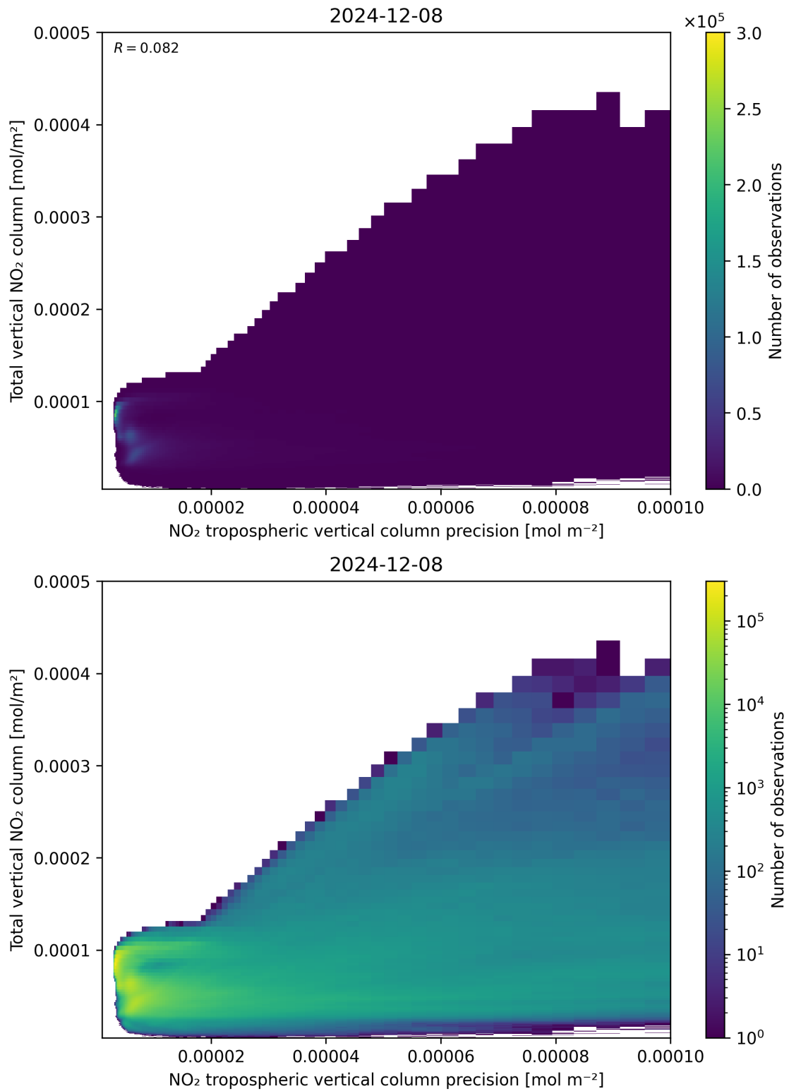
Figure 138: Scatter density plot of “NO 2 tropospheric vertical column precision” against “Total vertical NO 2 column” for 2024-12-07 to 2024-12-09.
