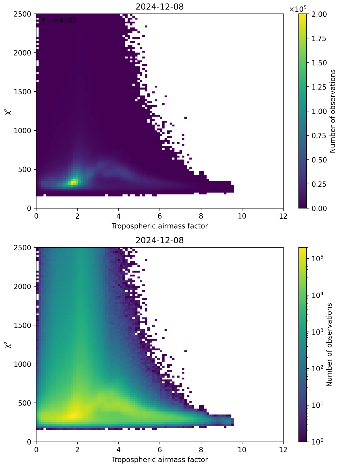
Figure 73: Scatter density plot of “Tropospheric airmass factor” against “ \chi^2 ” for 2024-12-07 to 2024-12-09.
