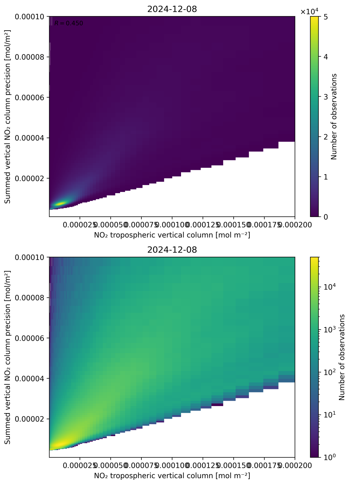
Figure 127: Scatter density plot of “NO 2 tropospheric vertical column” against “Summed vertical NO 2 column precision” for 2024-12-07 to 2024-12-09.
