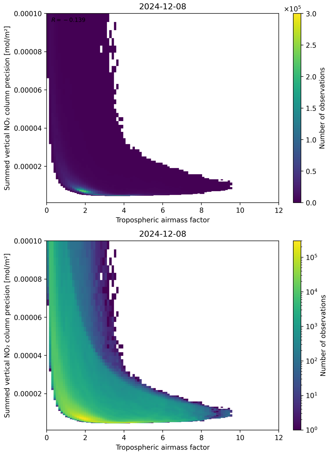
Figure 76: Scatter density plot of “Tropospheric air mass factor” against “Summed vertical NO 2 column precision” for 2024-12-07 to 2024-12-09.
