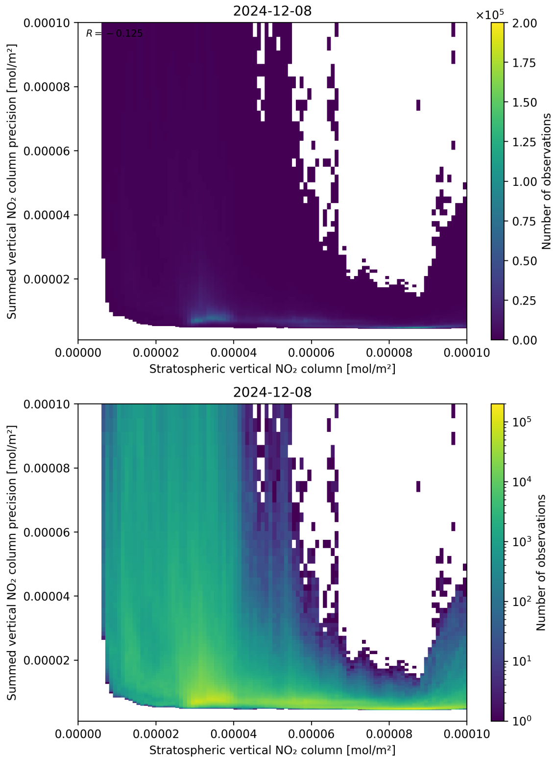
Figure 99: Scatter density plot of “Stratospheric vertical NO 2 column” against “Summed vertical NO 2 column precision” for 2024-12-07 to 2024-12-09.
