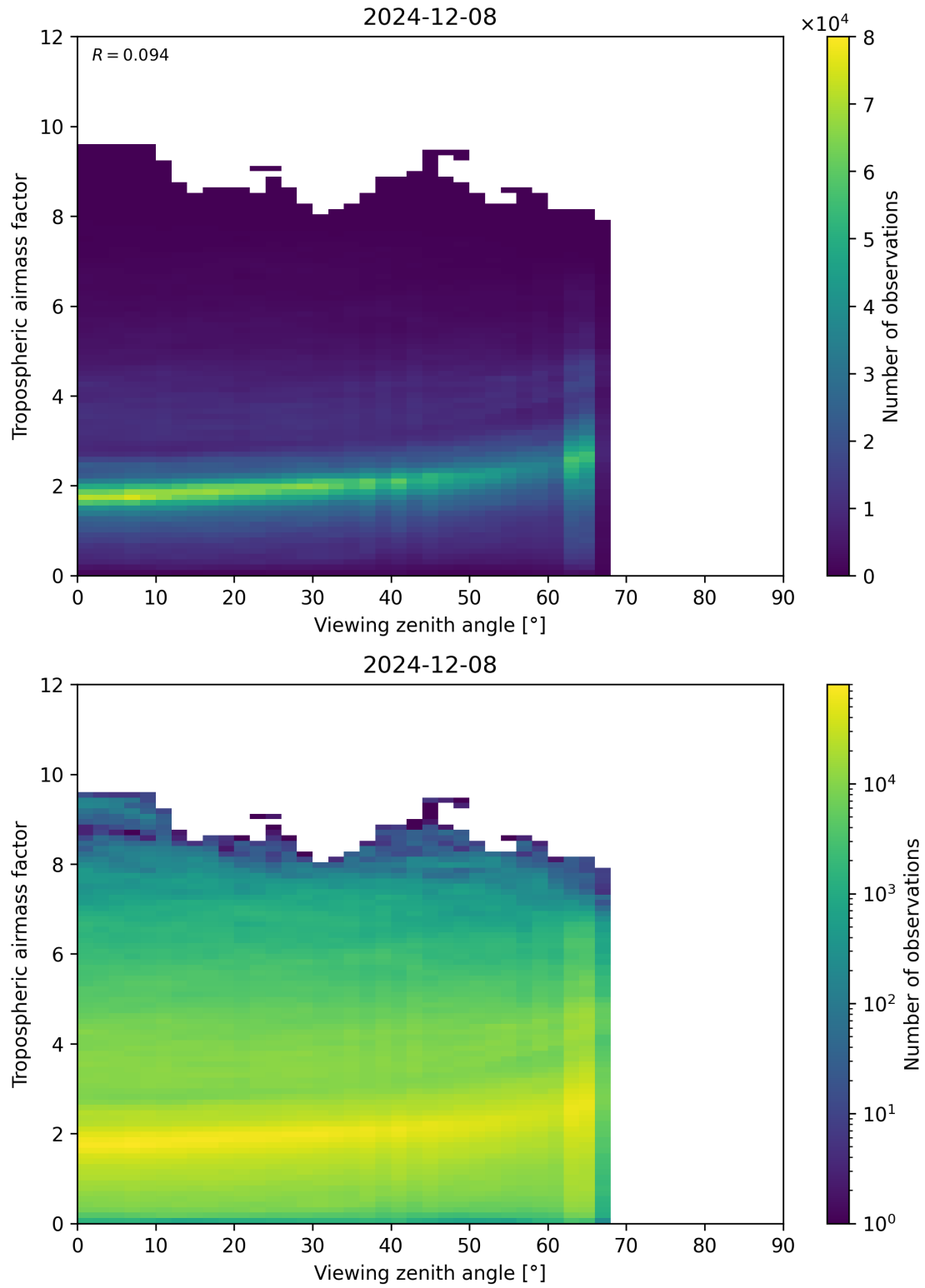
Figure 161: Scatter density plot of “Viewing zenith angle” against “Tropospheric airmass factor” for 2024-12-07 to 2024-12-09.
