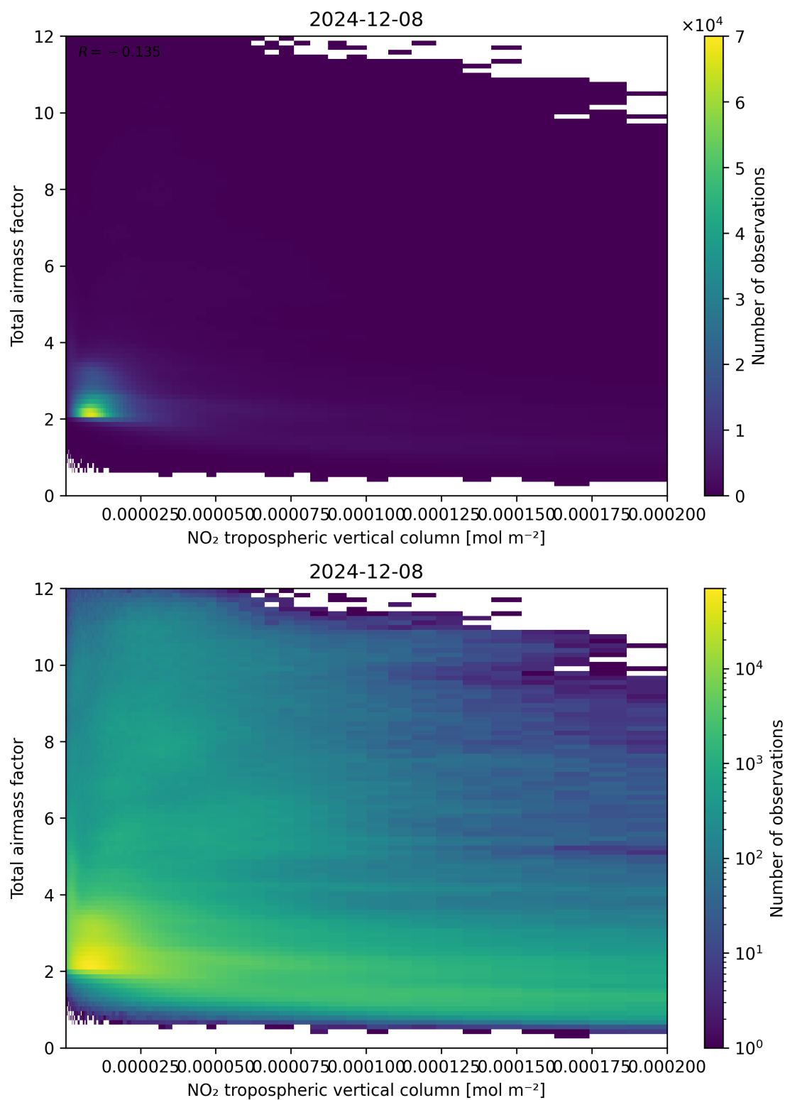
Figure 122: Scatter density plot of “NO 2 tropospheric vertical column” against “Total air mass factor” for 2024-12-07 to 2024-12-09.
