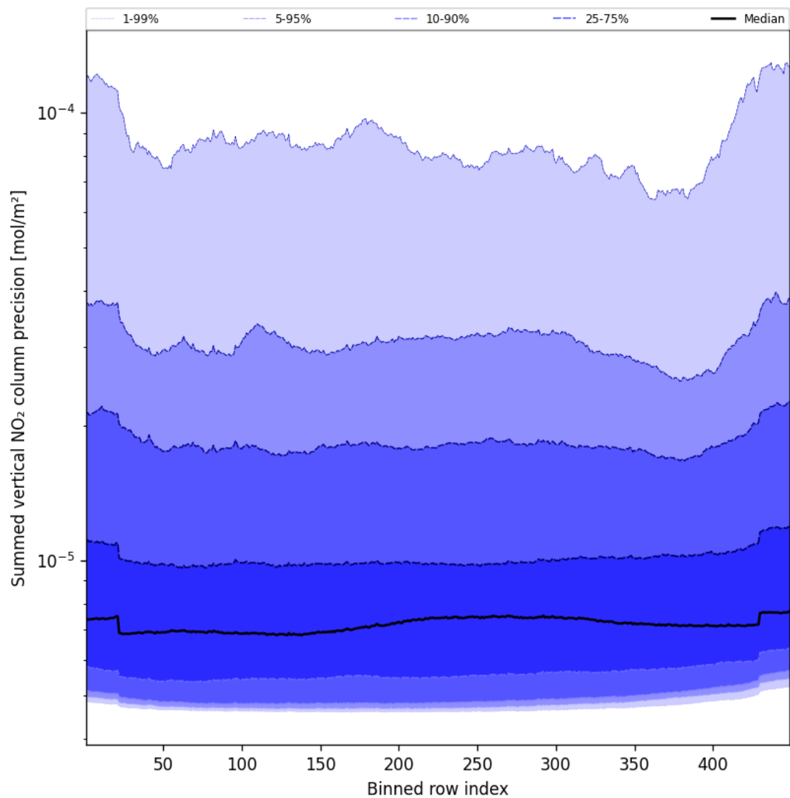
Figure 58: Along track statistics of “Summed vertical NO 2 column precision” for 2024-12-07 to 2024-12-09
