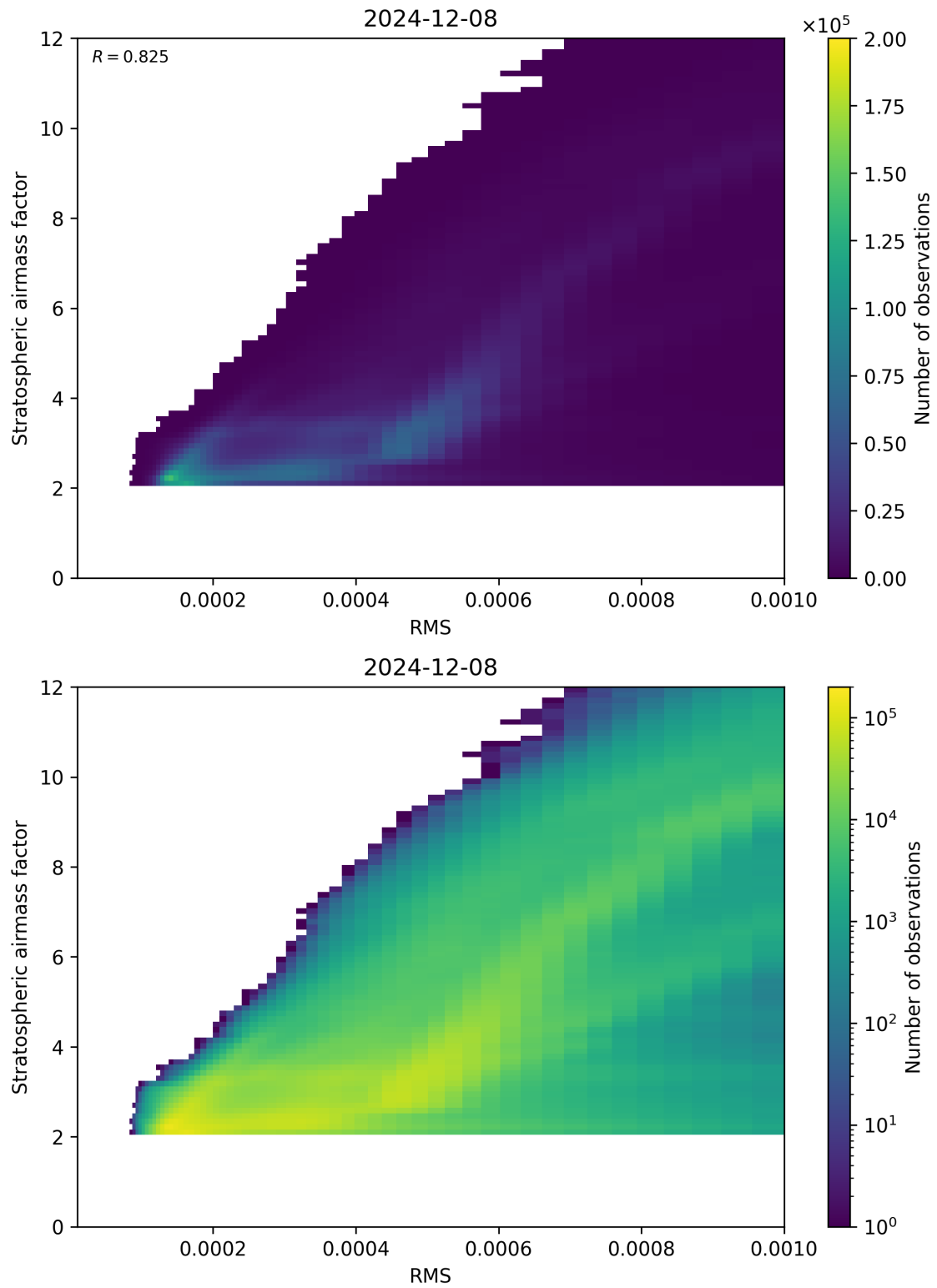
Figure 144: Scatter density plot of “RMS” against “Stratospheric airmass factor” for 2024-12-07 to 2024-12-09.
