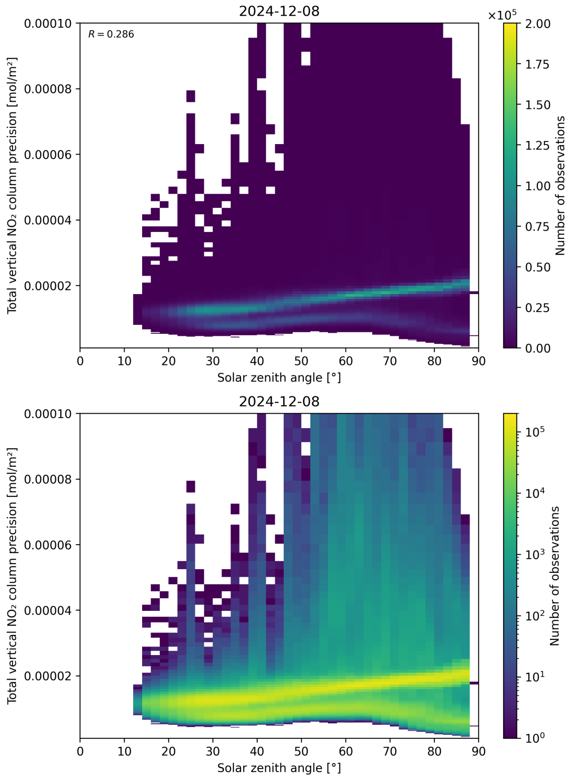
Figure 154: Scatter density plot of “Solar zenith angle” against “Total vertical NO 2 column precision” for 2024-12-07 to 2024-12-09.
