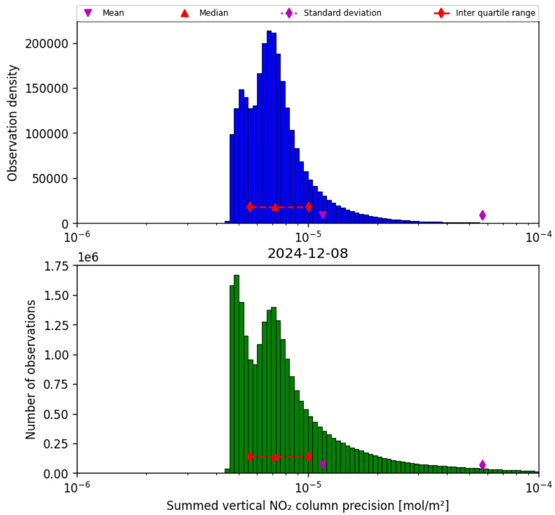
Figure 41: Histogram of “Summed vertical NO 2 column precision” for 2024-12-07 to 2024-12-09
