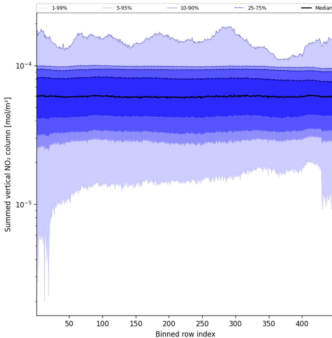
Figure 57: Along track statistics of “Summed vertical NO 2 column” for 2024-12-07 to 2024-12-09
