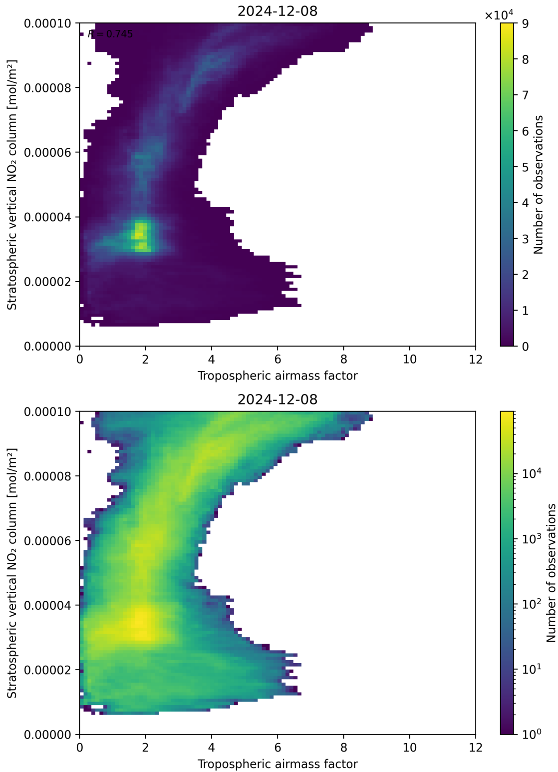
Figure 74: Scatter density plot of “Tropospheric air mass factor” against “Stratospheric vertical NO 2 column” for 2024-12-07 to 2024-12-09.
