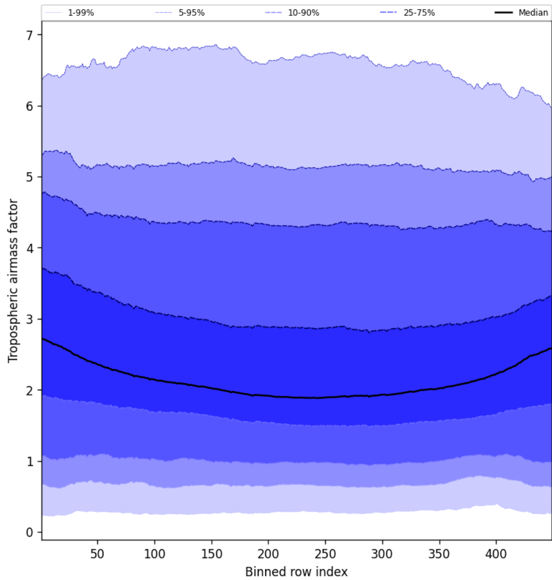
Figure 48: Along track statistics of “Tropospheric air mass factor” for 2024-12-07 to 2024-12-09
