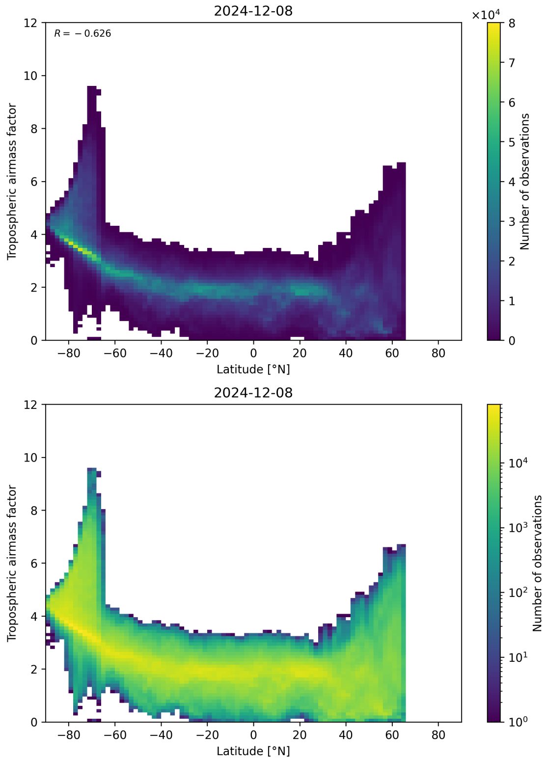
Figure 85: Scatter density plot of “Latitude” against “Tropospheric airmass factor” for 2024-12-07 to 2024-12-09.
