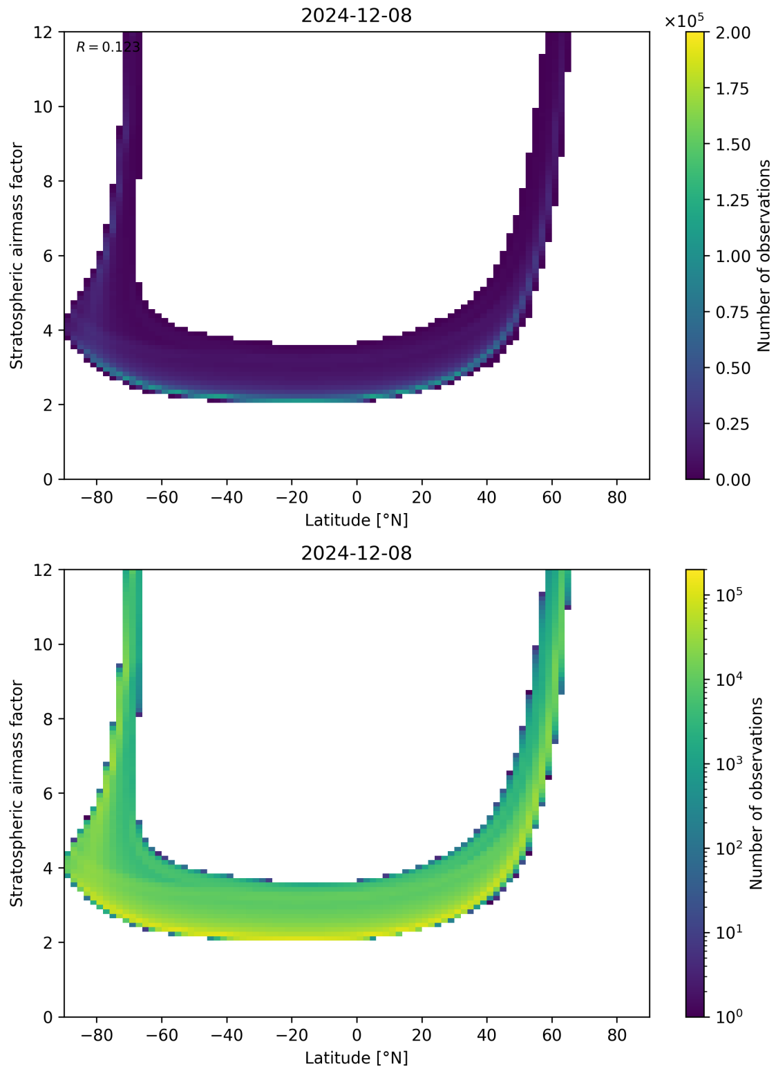
Figure 83: Scatter density plot of “Latitude” against “Stratospheric air mass factor” for 2024-12-07 to 2024-12-09.
