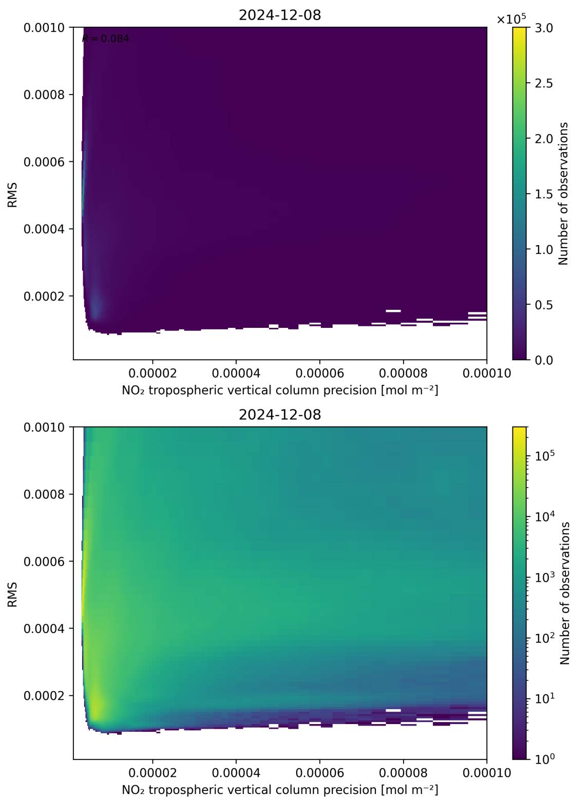
Figure 140: Scatter density plot of “NO 2 tropospheric vertical column precision” against “RMS” for 2024-12-07 to 2024-12-09.
