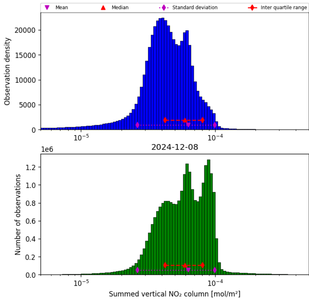
Figure 40: Histogram of “Summed vertical NO 2 column” for 2024-12-07 to 2024-12-09
