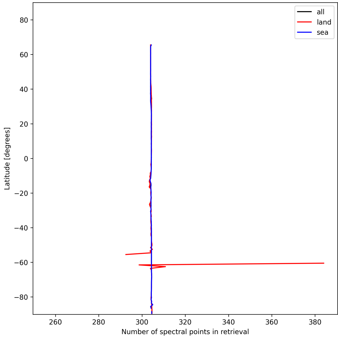
Figure 16: Zonal average of “Number of spectral points in retrieval” for 2024-12-07 to 2024-12-09.
