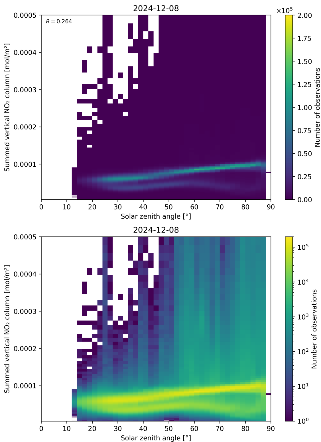
Figure 151: Scatter density plot of “Solar zenith angle” against “Summed vertical NO 2 column” for 2024-12-07 to 2024-12-09.
