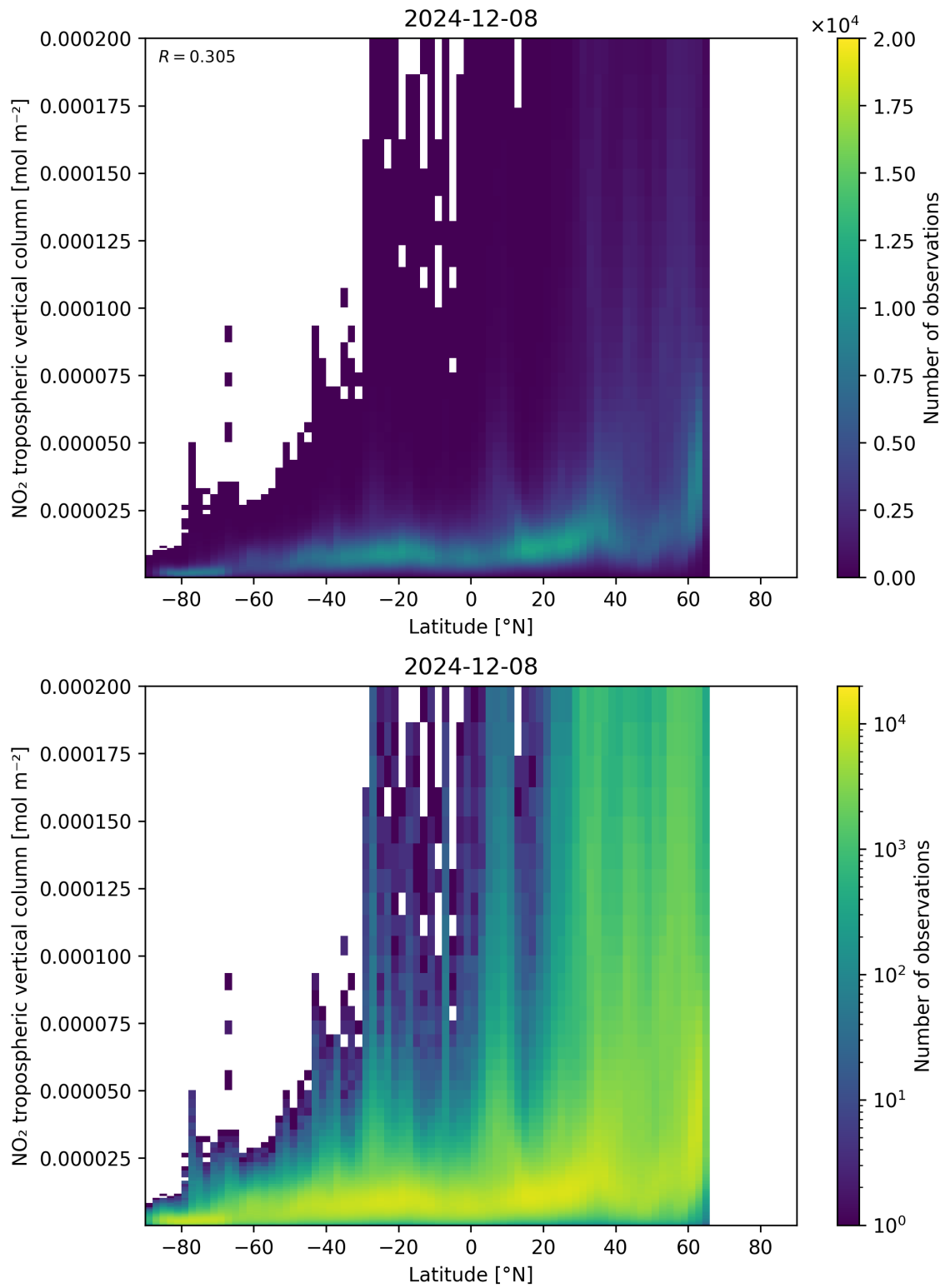
Figure 92: Scatter density plot of “Latitude” against “NO 2 tropospheric vertical column” for 2024-12-07 to 2024-12-09.
