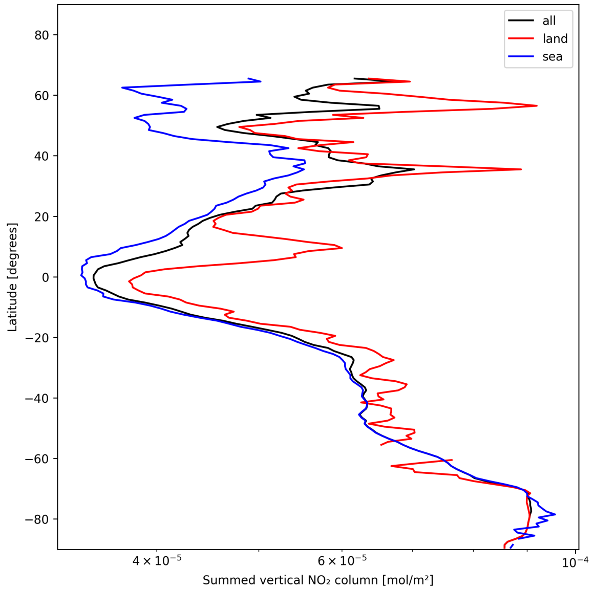
Figure 23: Zonal average of “Summed vertical NO 2 column” for 2024-12-07 to 2024-12-09.
