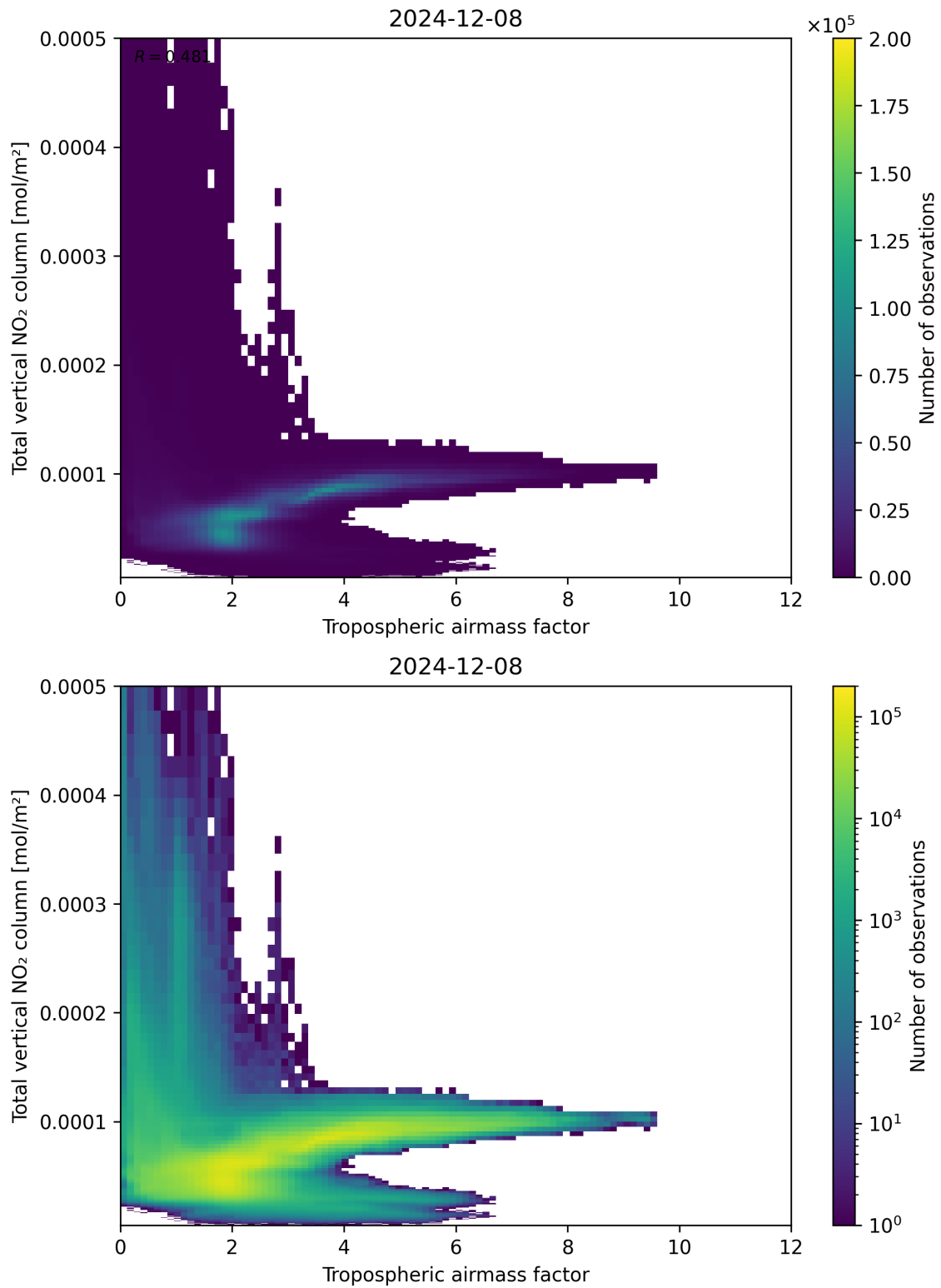
Figure 77: Scatter density plot of “Tropospheric airmass factor” against “Total vertical NO 2 column” for 2024-12-07 to 2024-12-09.
