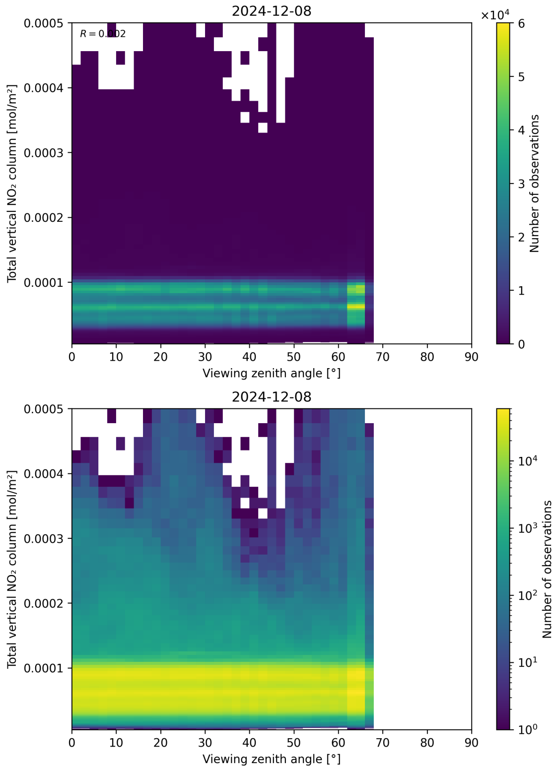
Figure 167: Scatter density plot of “Viewing zenith angle” against “Total vertical NO 2 column” for 2024-12-07 to 2024-12-09.
