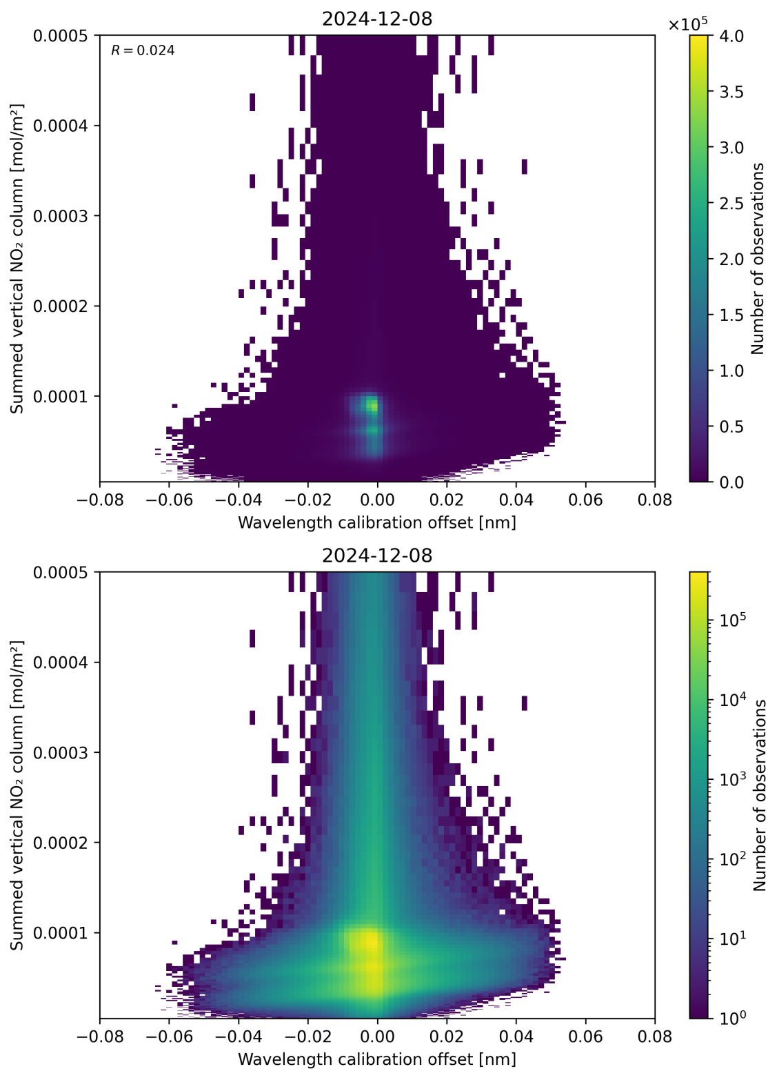
Figure 177: Scatter density plot of “Wavelength calibration offset” against “Summed vertical NO 2 column” for 2024-12-07 to 2024-12-09.
