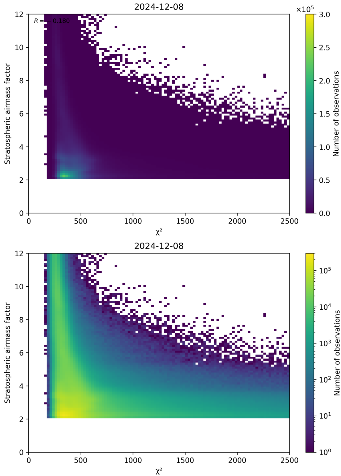
Figure 81: Scatter density plot of “ \chi^2 ” against “Stratospheric airmass factor” for 2024-12-07 to 2024-12-09.
