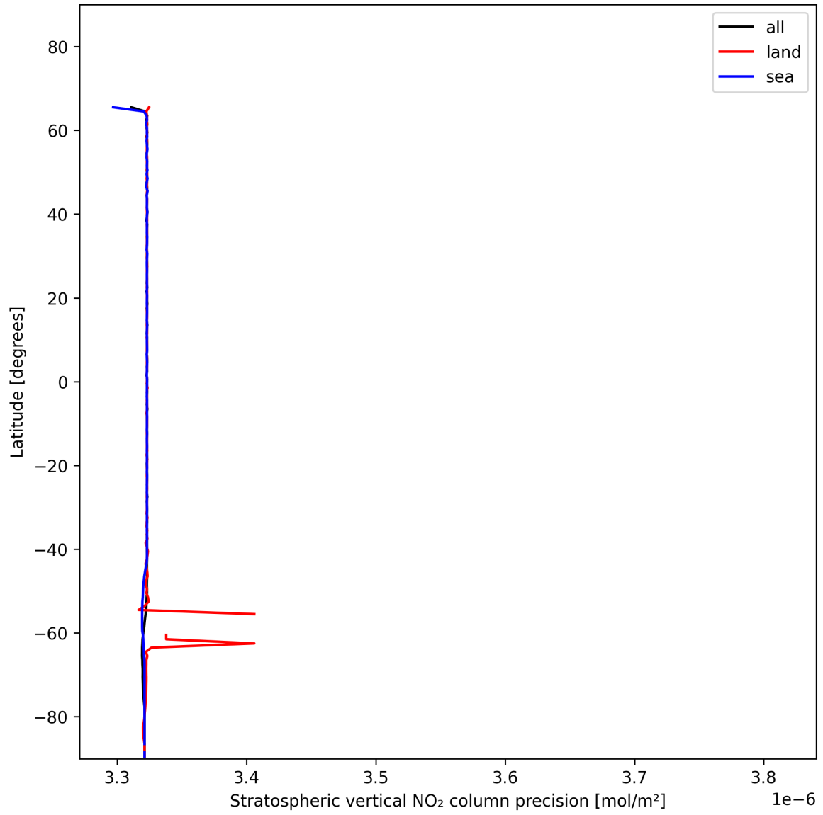
Figure 20: Zonal average of "Stratospheric vertical NO 2 column precision" for 2024-12-07 to 2024-12-09.
