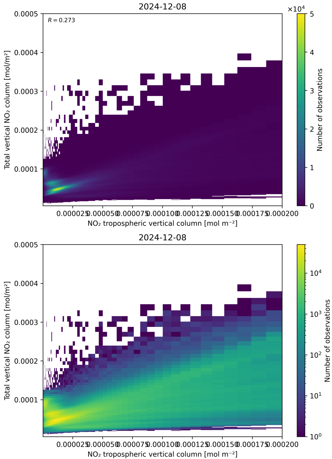
Figure 128: Scatter density plot of “NO 2 tropospheric vertical column” against “Total vertical NO 2 column” for 2024-12-07 to 2024-12-09.
