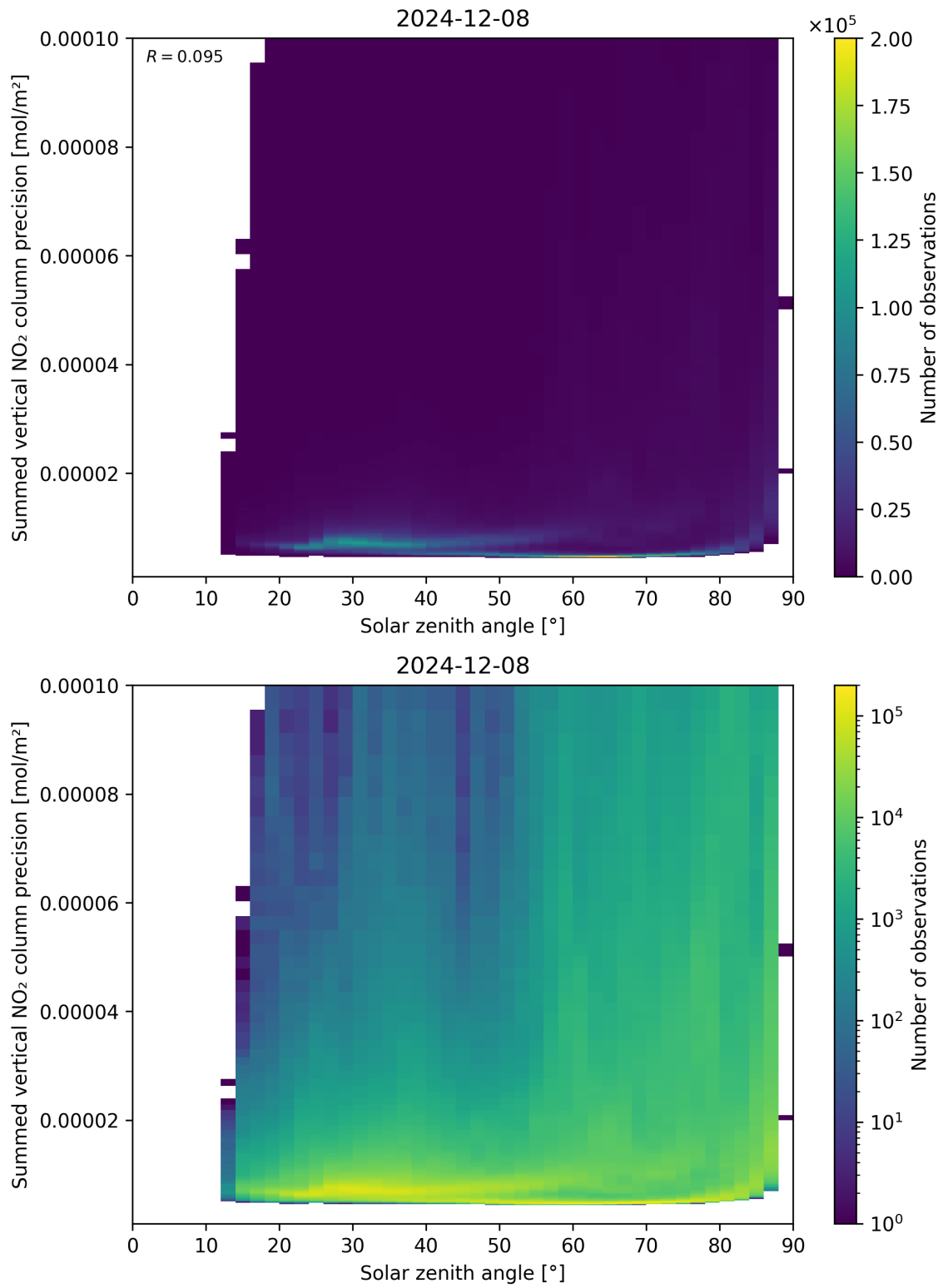
Figure 152: Scatter density plot of “Solar zenith angle” against “Summed vertical NO 2 column precision” for 2024-12-07 to 2024-12-09.
