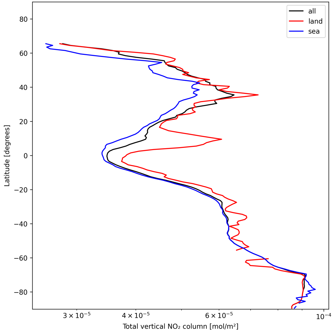
Figure 21: Zonal average of “Total vertical NO 2 column” for 2024-12-07 to 2024-12-09.
