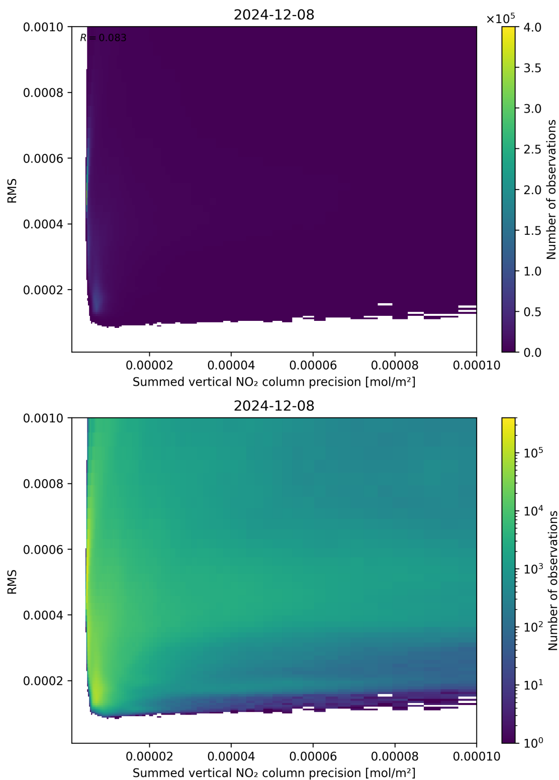
Figure 108: Scatter density plot of “Summed vertical NO 2 column precision” against “RMS” for 2024-12-07 to 2024-12-09.
