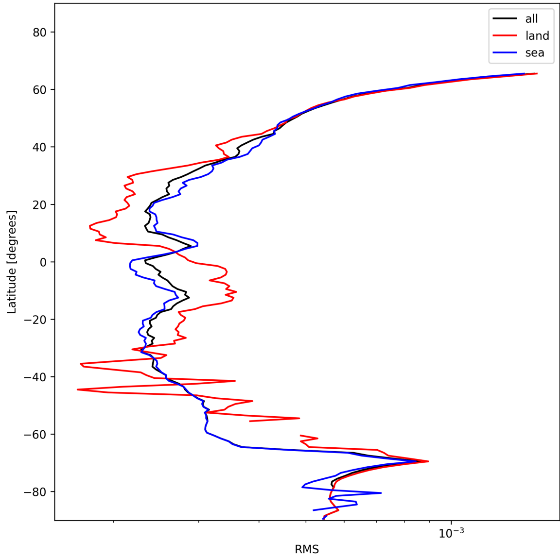
Figure 26: Zonal average of “RMS” for 2024-12-07 to 2024-12-09.
