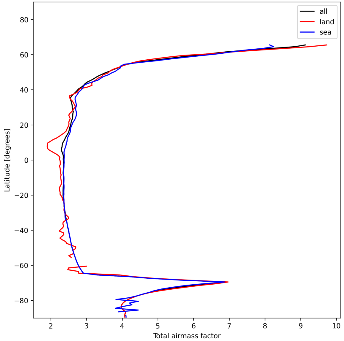
Figure 15: Zonal average of “Total airmass factor” for 2024-12-07 to 2024-12-09.
