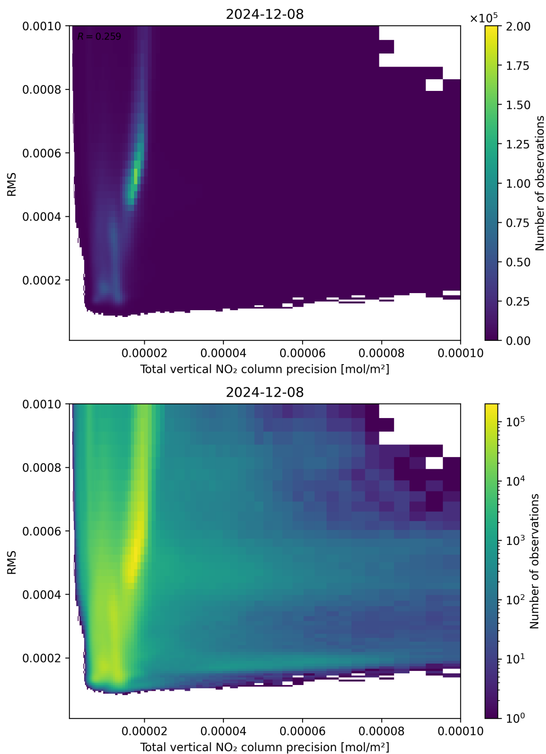
Figure 119: Scatter density plot of “Total vertical NO 2 column precision” against “RMS” for 2024-12-07 to 2024-12-09.
