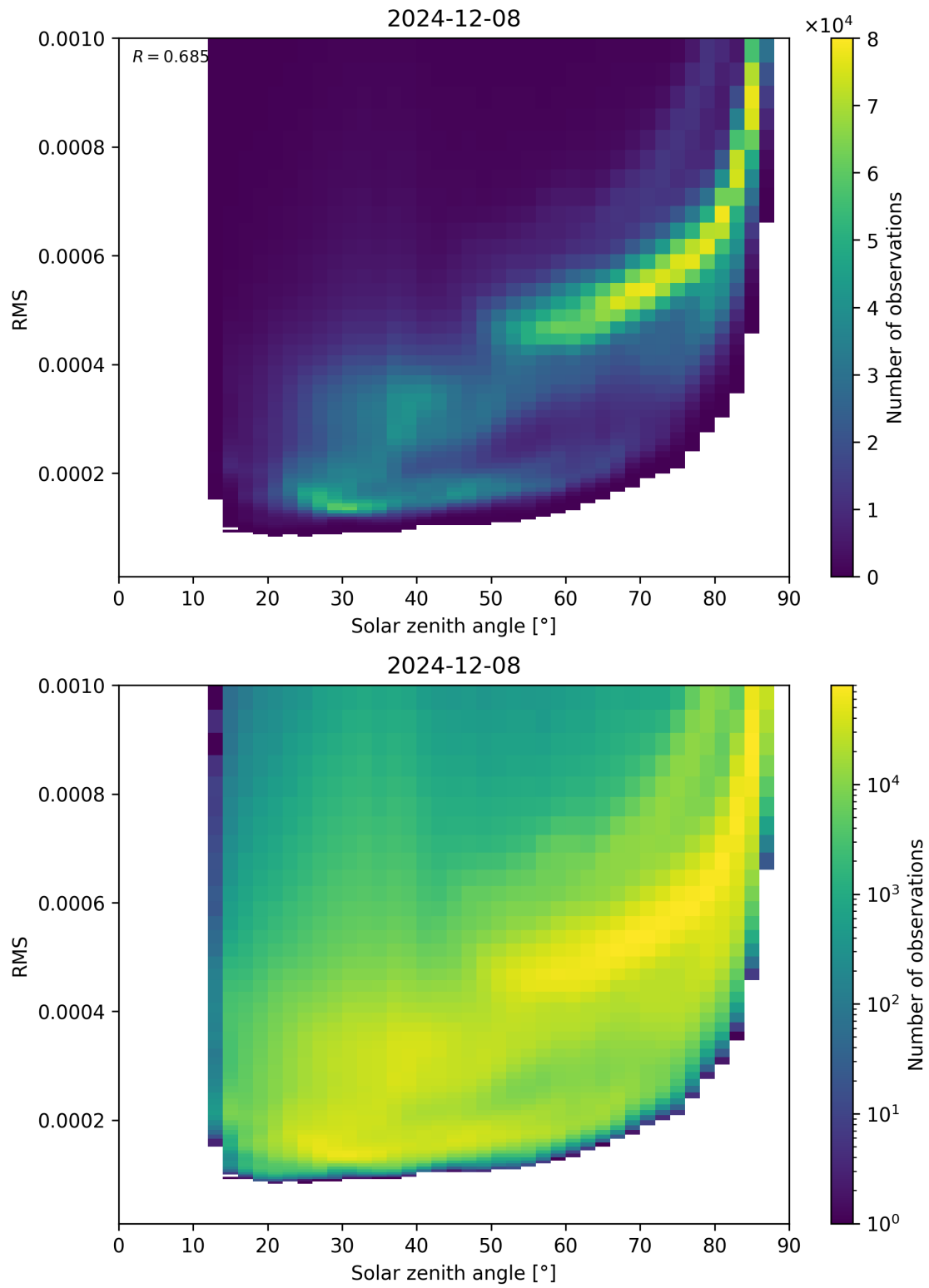
Figure 157: Scatter density plot of “Solar zenith angle” against “RMS” for 2024-12-07 to 2024-12-09.
