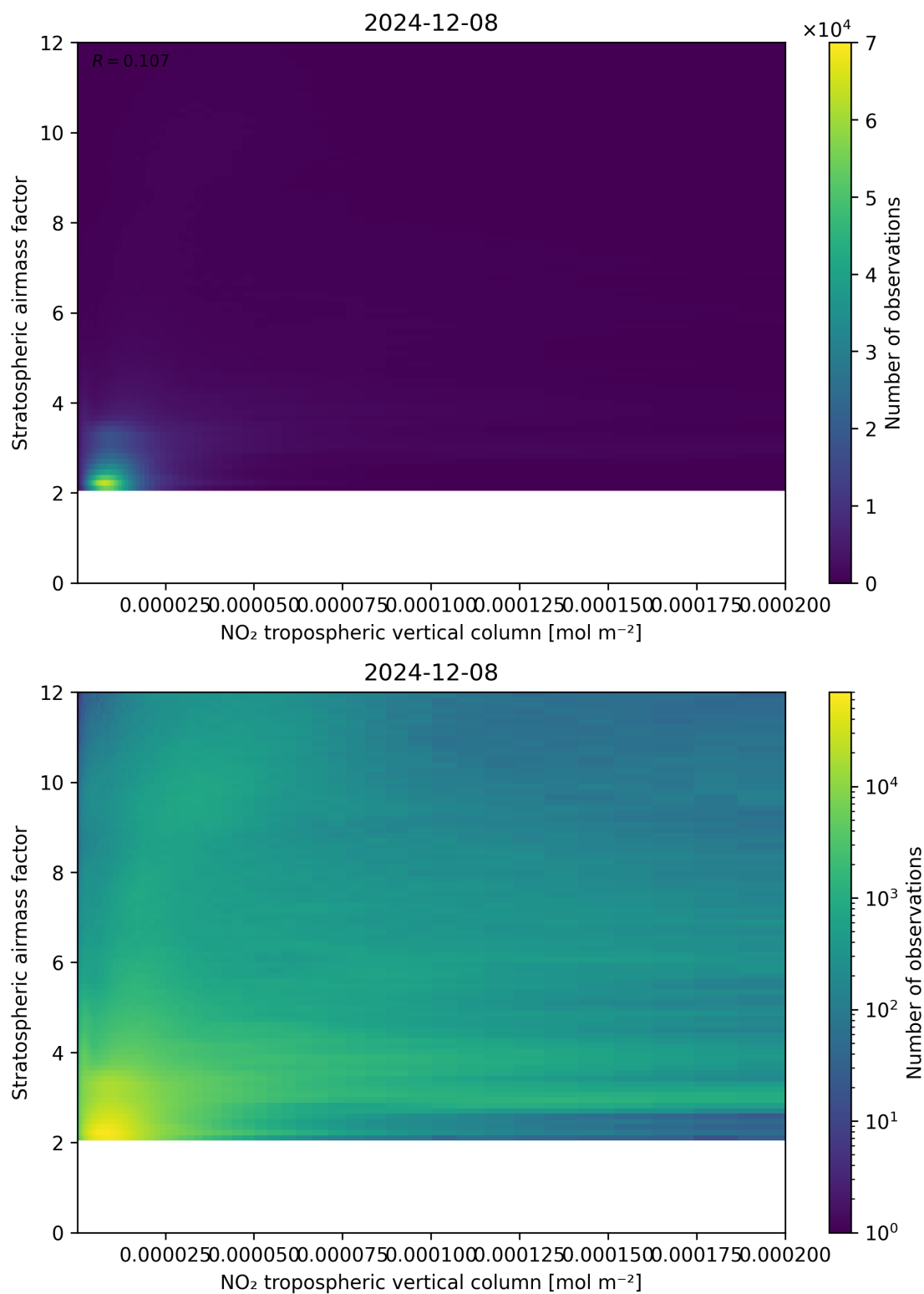
Figure 121: Scatter density plot of “NO 2 tropospheric vertical column” against “Stratospheric airmass factor” for 2024-12-07 to 2024-12-09.
