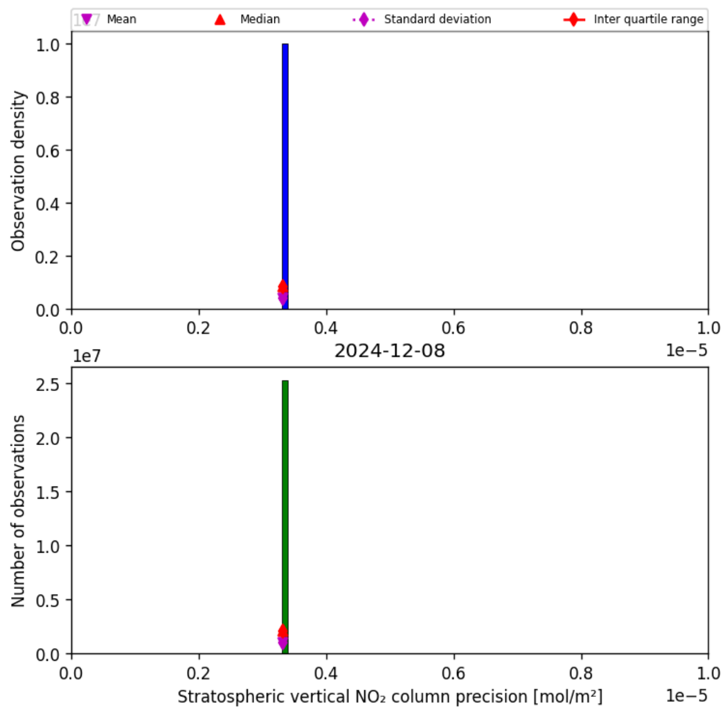
Figure 37: Histogram of “Stratospheric vertical NO 2 column precision” for 2024-12-07 to 2024-12-09
