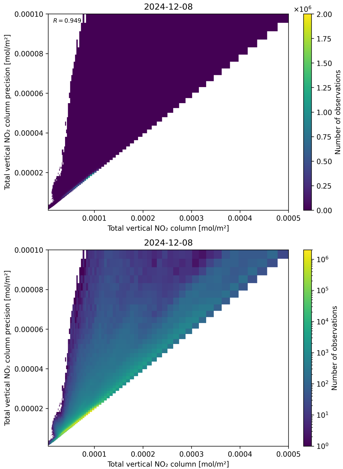
Figure 114: Scatter density plot of “Total vertical NO 2 column” against “Total vertical NO 2 column precision” for 2024-12-07 to 2024-12-09.
