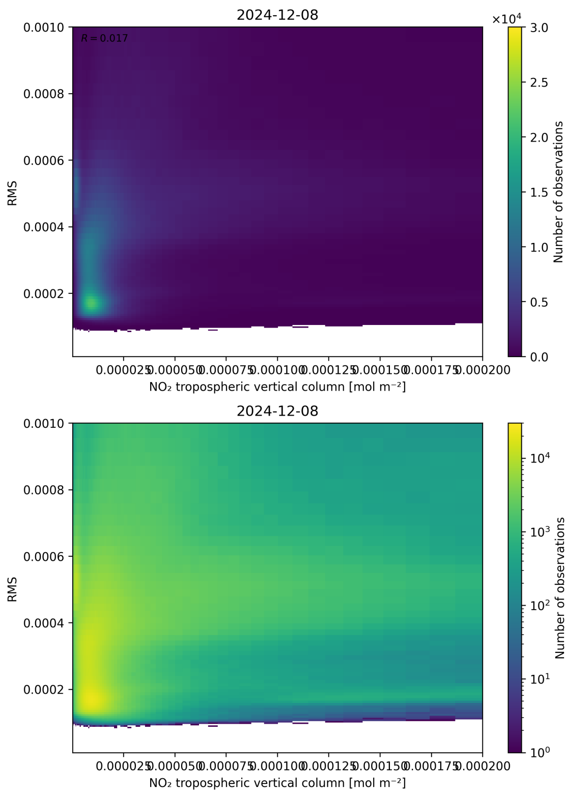
Figure 142: Scatter density plot of “NO 2 tropospheric vertical column” against “RMS” for 2024-12-07 to 2024-12-09.
