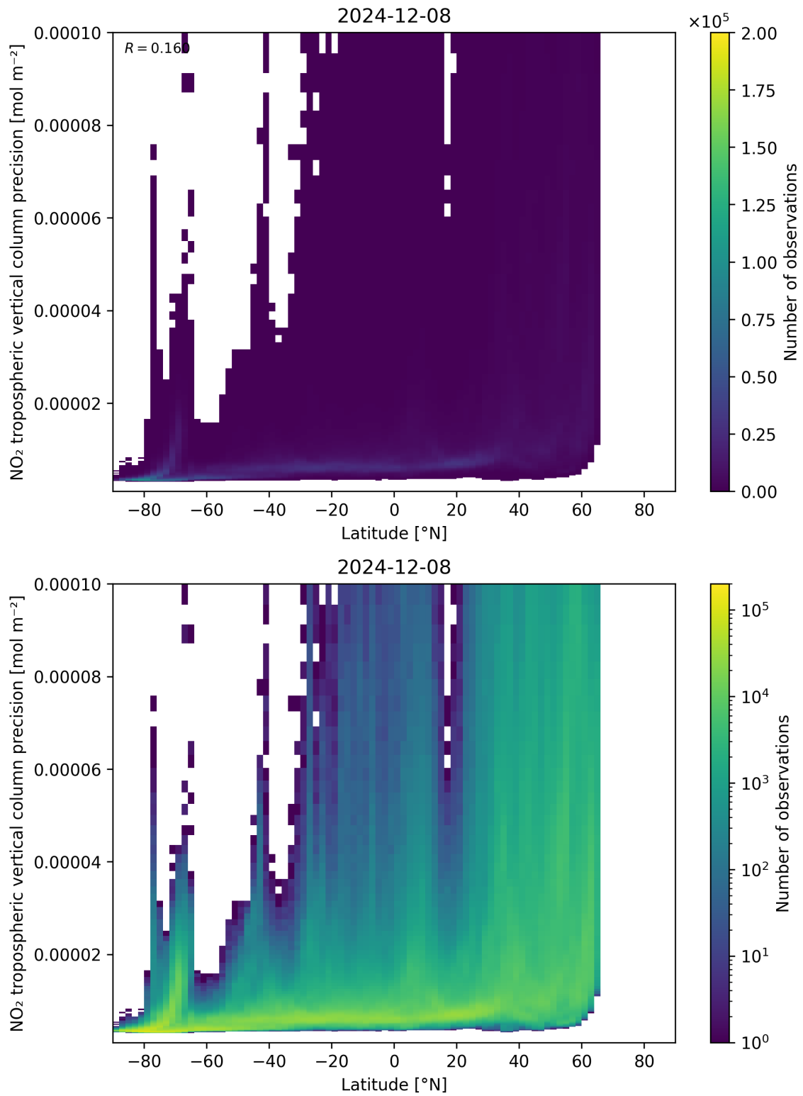
Figure 93: Scatter density plot of “Latitude” against “NO 2 tropospheric vertical column precision” for 2024-12-07 to 2024-12-09.
