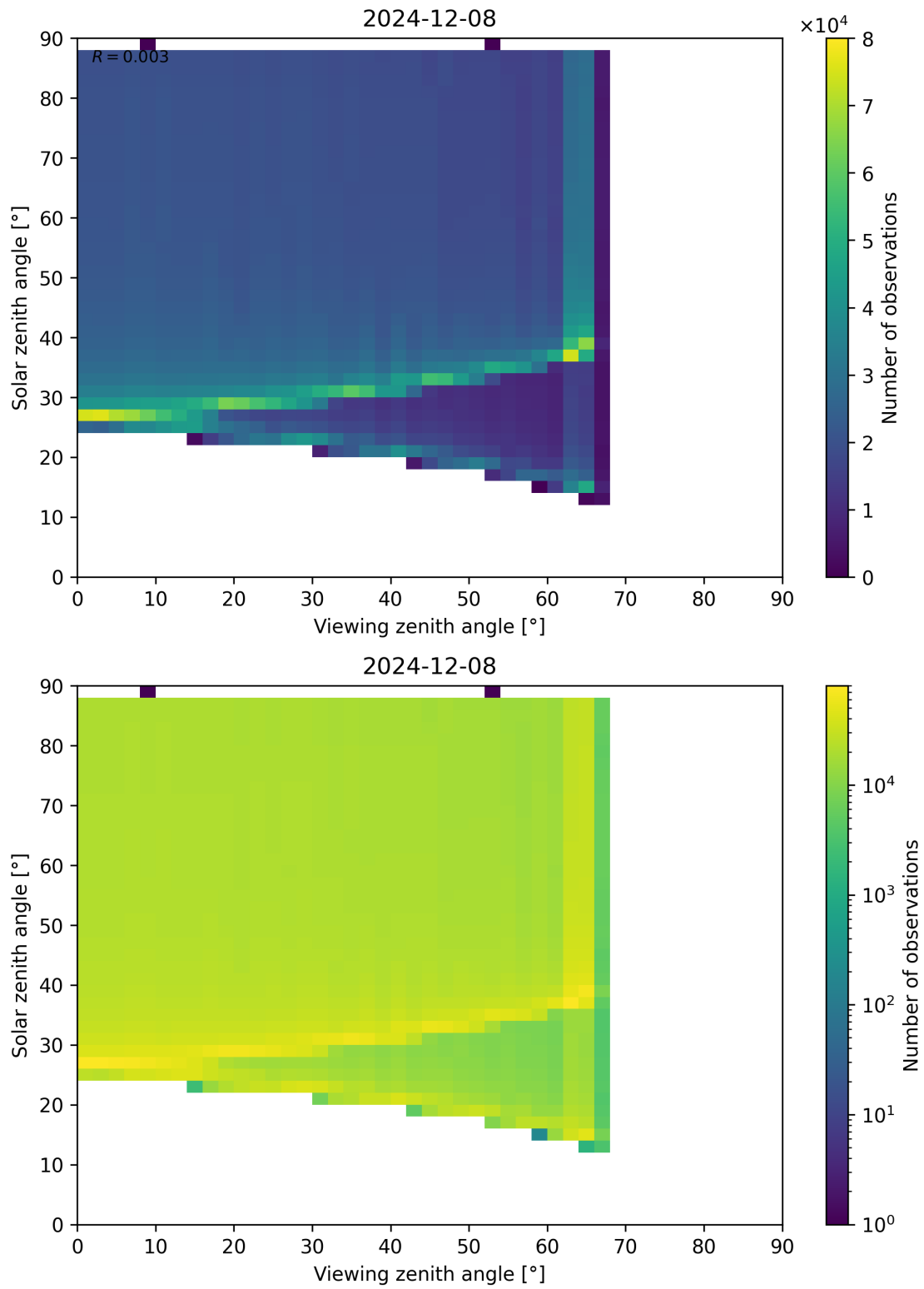
Figure 172: Scatter density plot of “Viewing zenith angle” against “Solar zenith angle” for 2024-12-07 to 2024-12-09.
