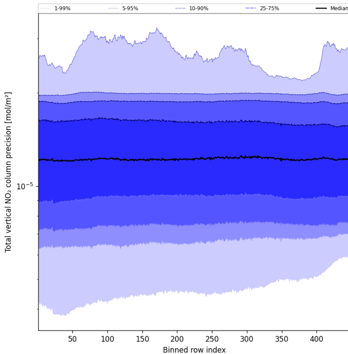
Figure 56: Along track statistics of “Total vertical NO 2 column precision” for 2024-12-07 to 2024-12-09
