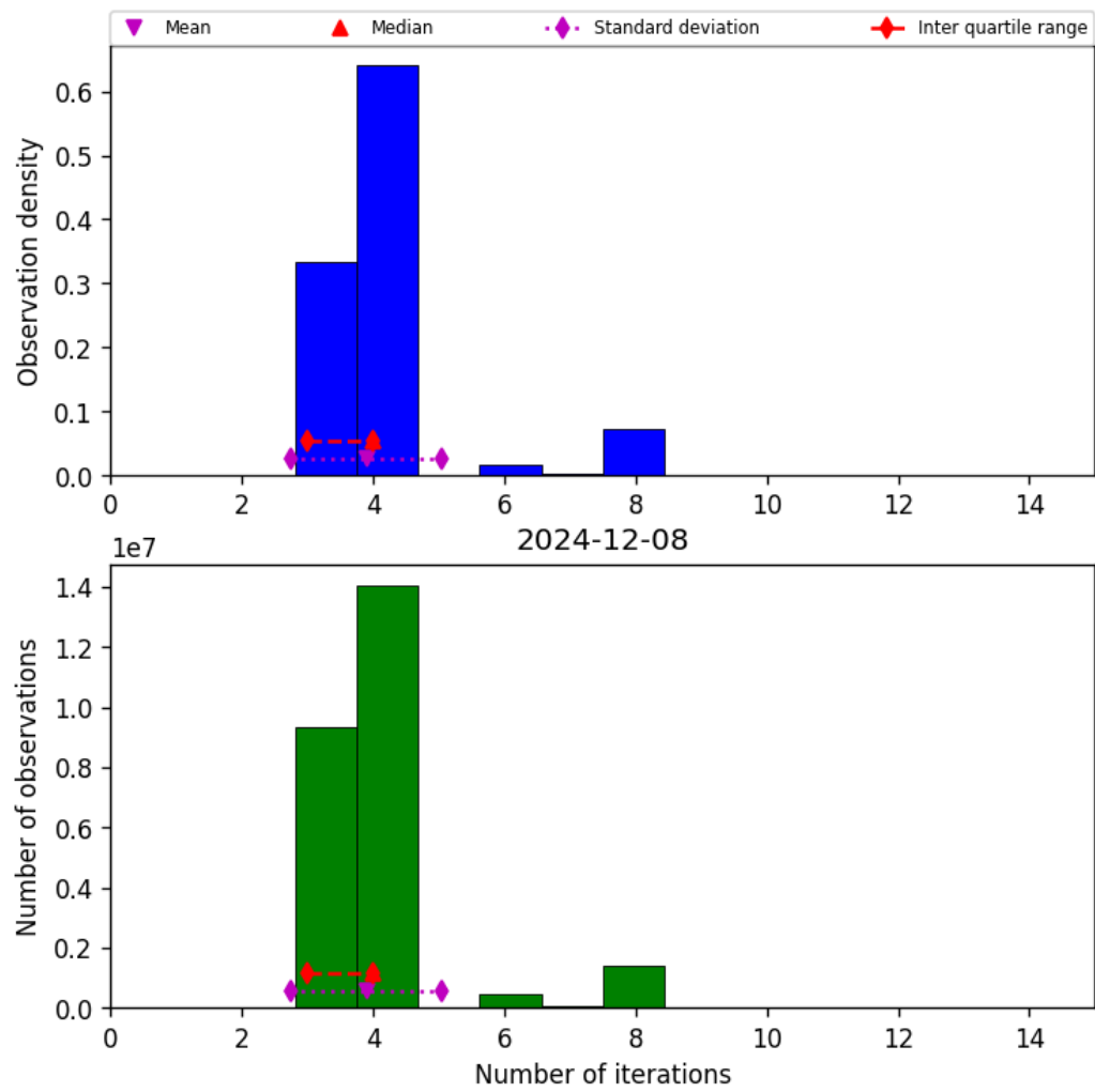
Figure 34: Histogram of “Number of iterations” for 2024-12-07 to 2024-12-09
