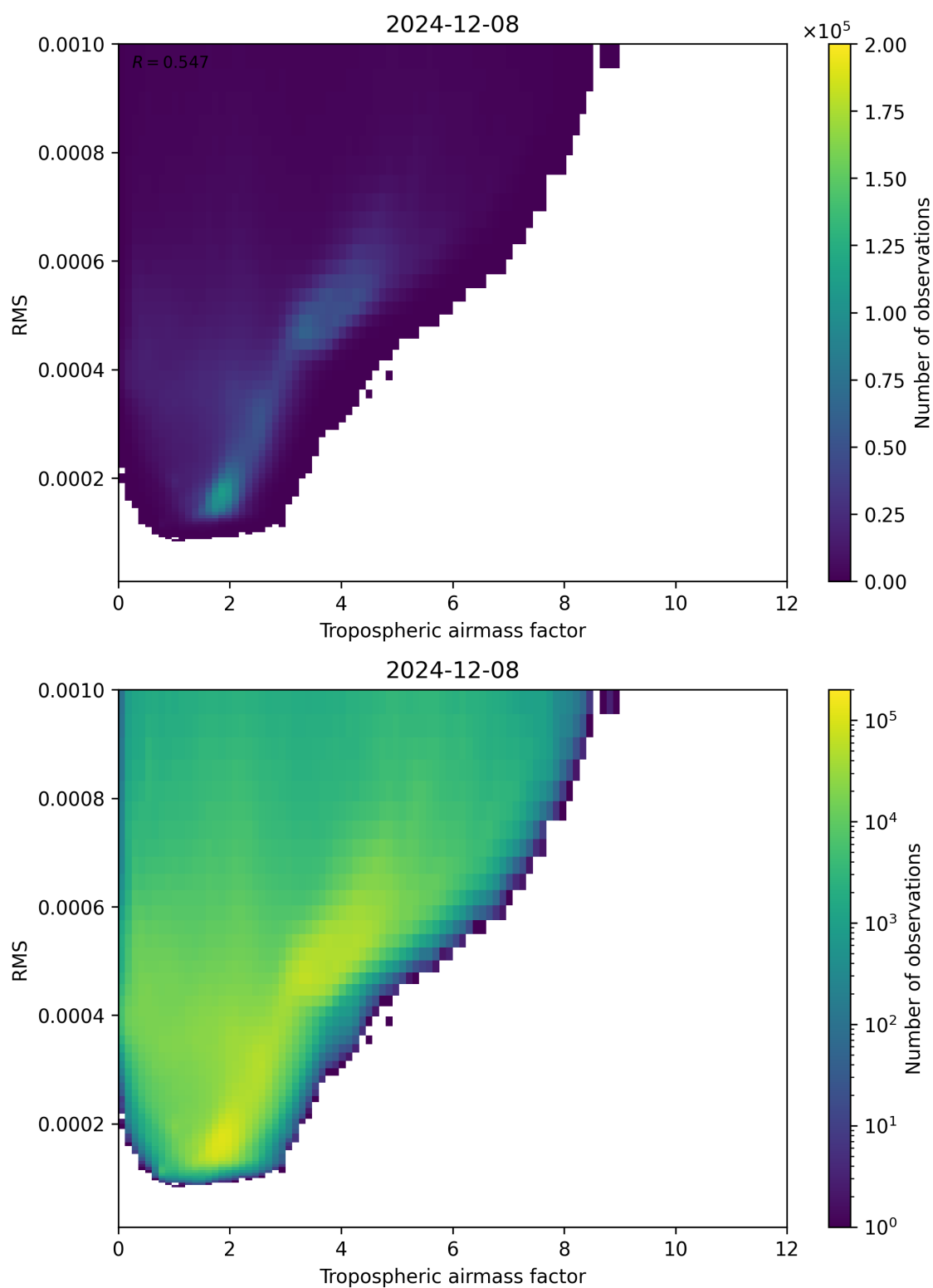
Figure 79: Scatter density plot of “Tropospheric airmass factor” against “RMS” for 2024-12-07 to 2024-12-09.
