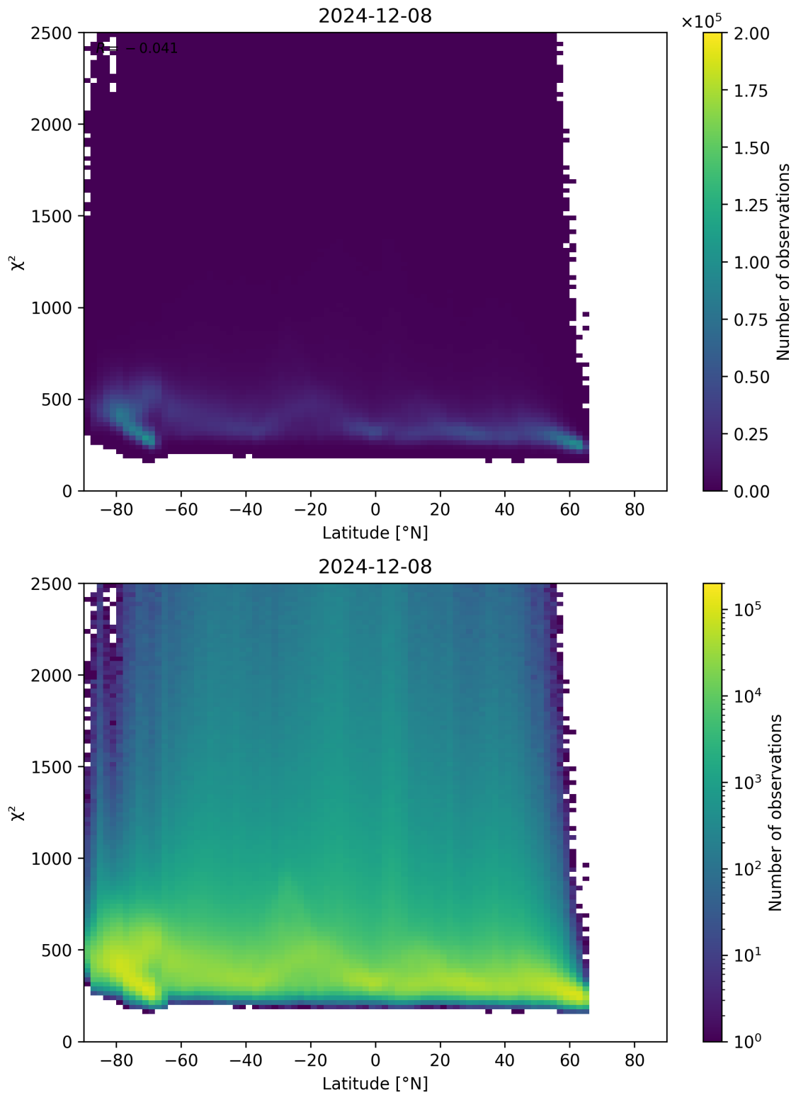
Figure 86: Scatter density plot of “Latitude” against “ \chi^2 ” for 2024-12-07 to 2024-12-09.
