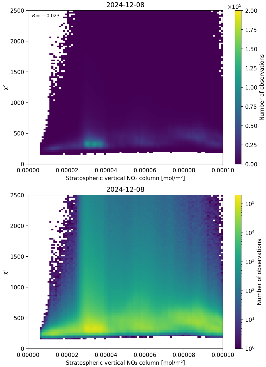
Figure 97: Scatter density plot of “Stratospheric vertical NO 2 column” against “ \chi^2 ” for 2024-12-07 to 2024-12-09.
