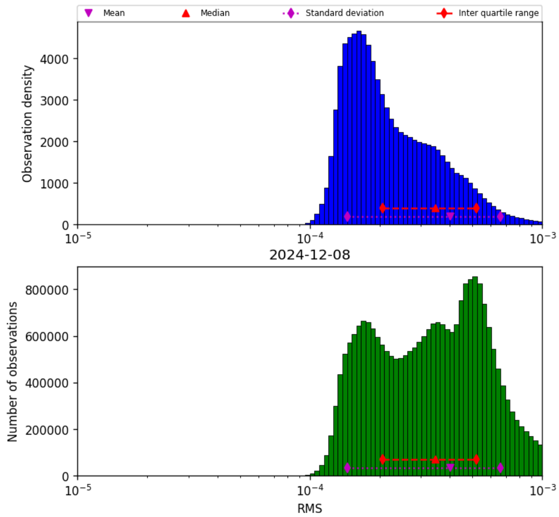
Figure 43: Histogram of “RMS” for 2024-12-07 to 2024-12-09
