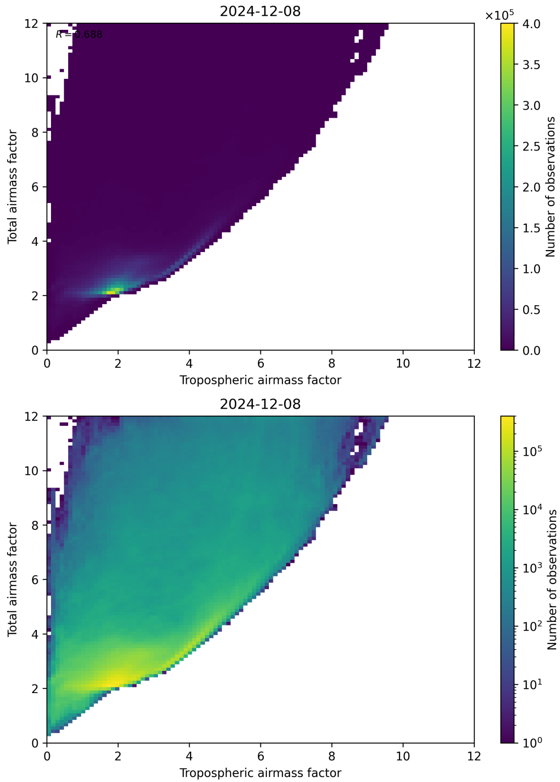
Figure 72: Scatter density plot of “Tropospheric airmass factor” against “Total airmass factor” for 2024-12-07 to 2024-12-09.
