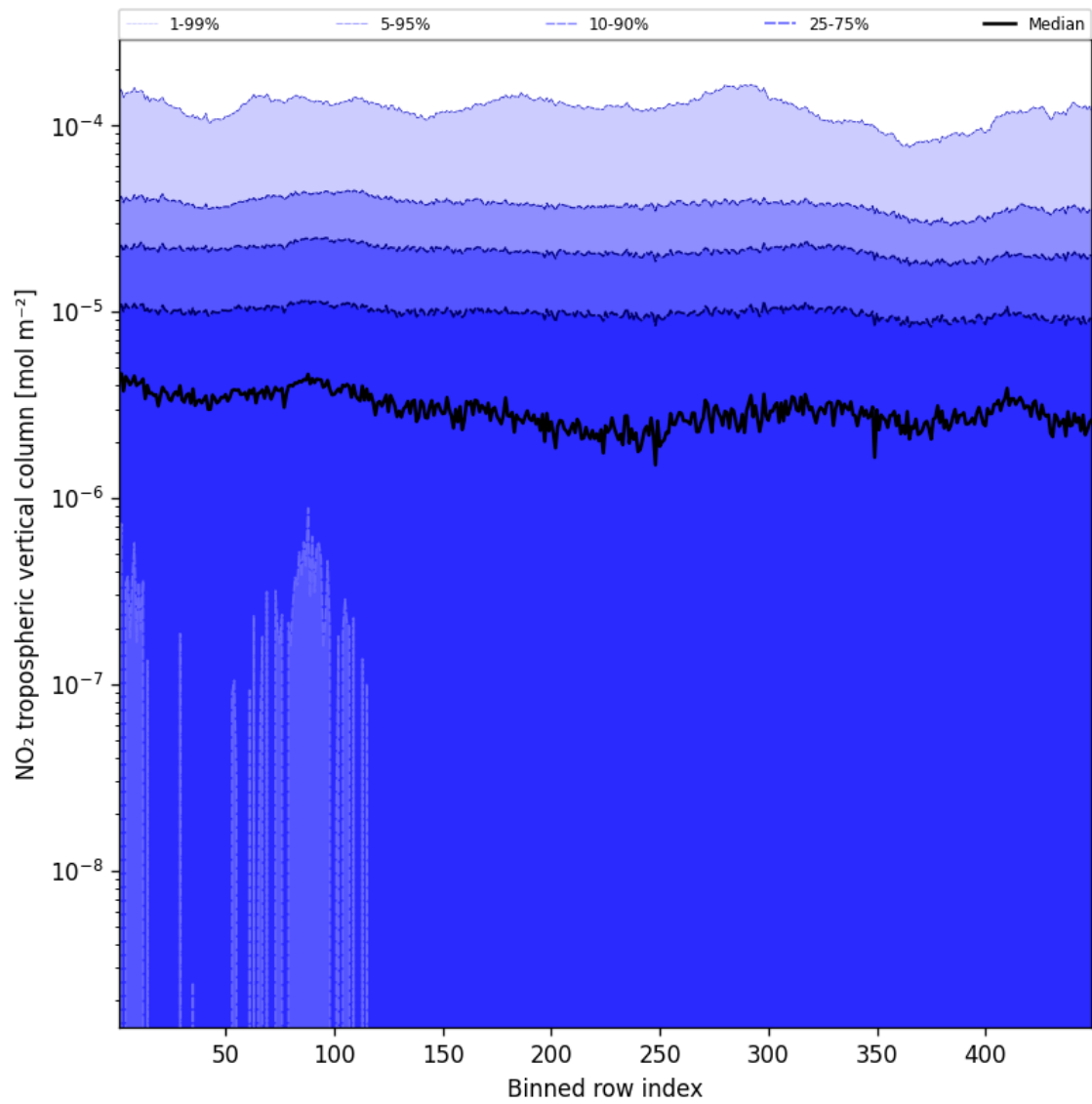
Figure 46: Along track statistics of “NO 2 tropospheric vertical column” for 2024-12-07 to 2024-12-09
