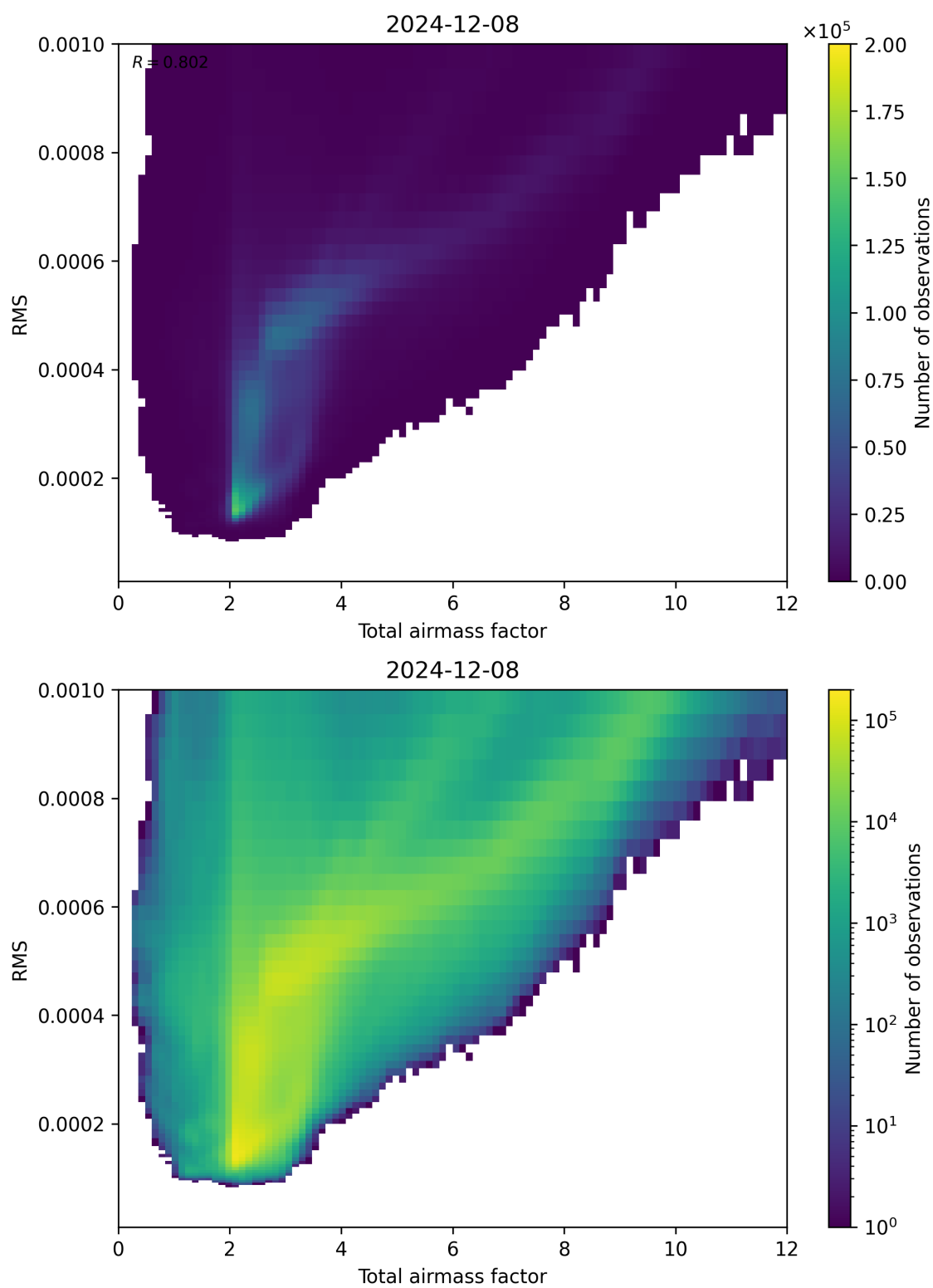
Figure 69: Scatter density plot of “Total airmass factor” against “RMS” for 2024-12-07 to 2024-12-09.
