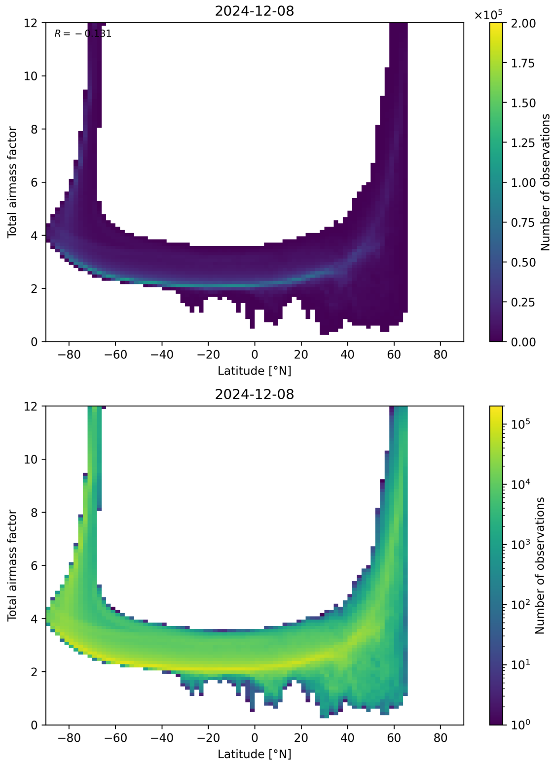
Figure 84: Scatter density plot of “Latitude” against “Total airmass factor” for 2024-12-07 to 2024-12-09.
