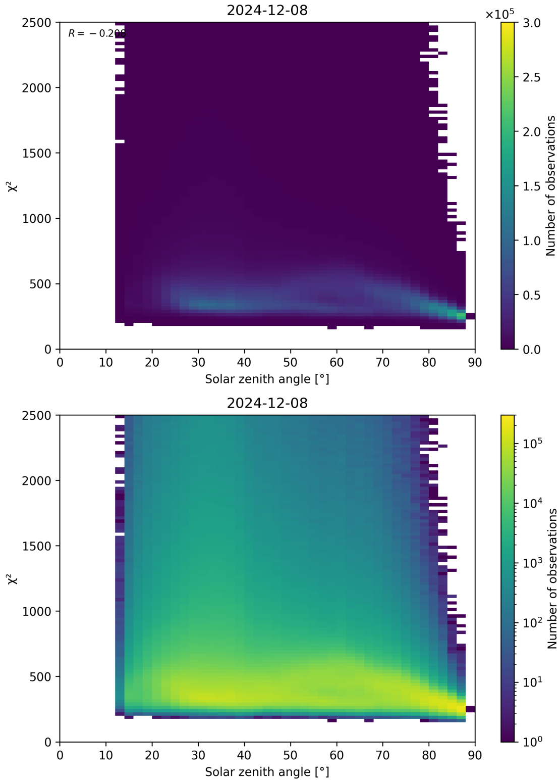
Figure 148: Scatter density plot of “Solar zenith angle” against “ \chi^2 ” for 2024-12-07 to 2024-12-09.
