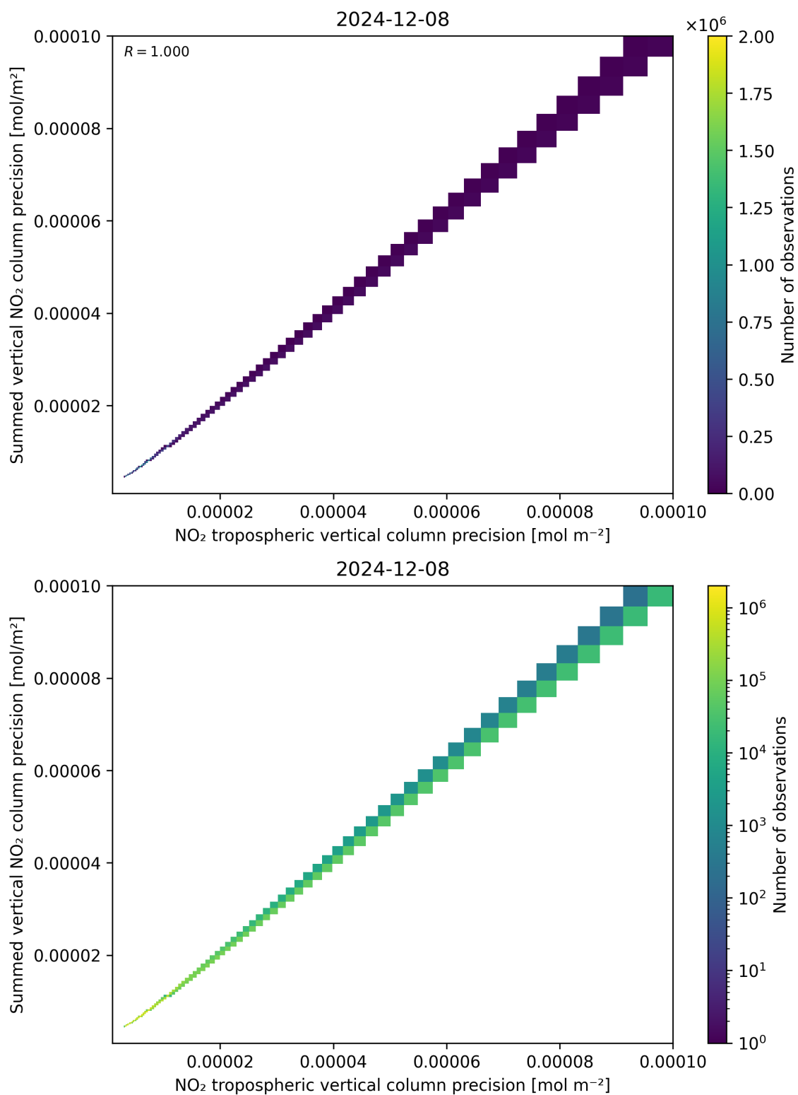
Figure 137: Scatter density plot of “NO 2 tropospheric vertical column precision” against “Summed vertical NO 2 column precision” for 2024-12-07 to 2024-12-09.
