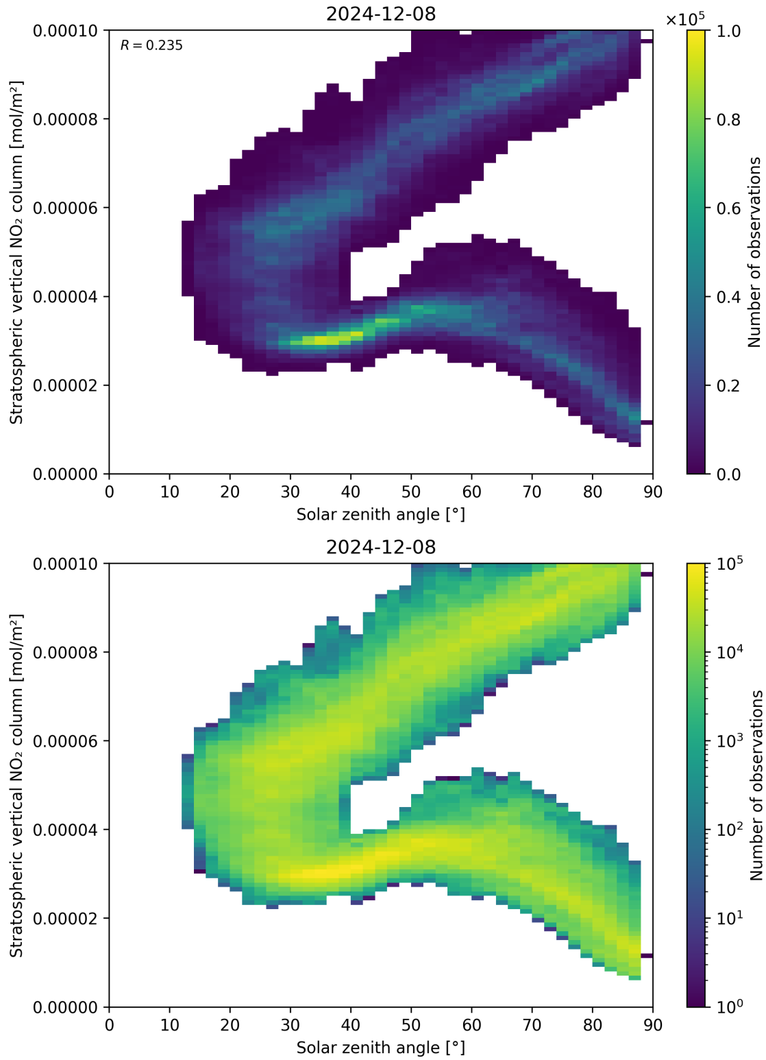
Figure 150: Scatter density plot of “Solar zenith angle” against “Stratospheric vertical NO 2 column” for 2024-12-07 to 2024-12-09.
