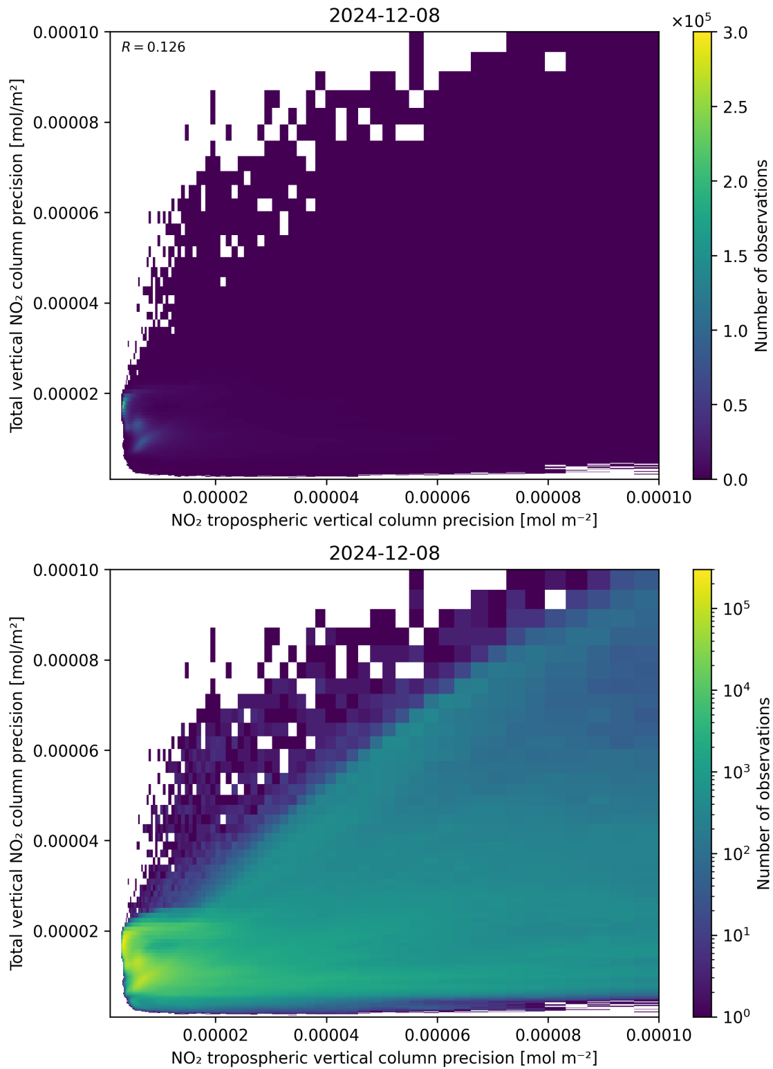
Figure 139: Scatter density plot of “NO 2 tropospheric vertical column precision” against “Total vertical NO 2 column precision” for 2024-12-07 to 2024-12-09.
