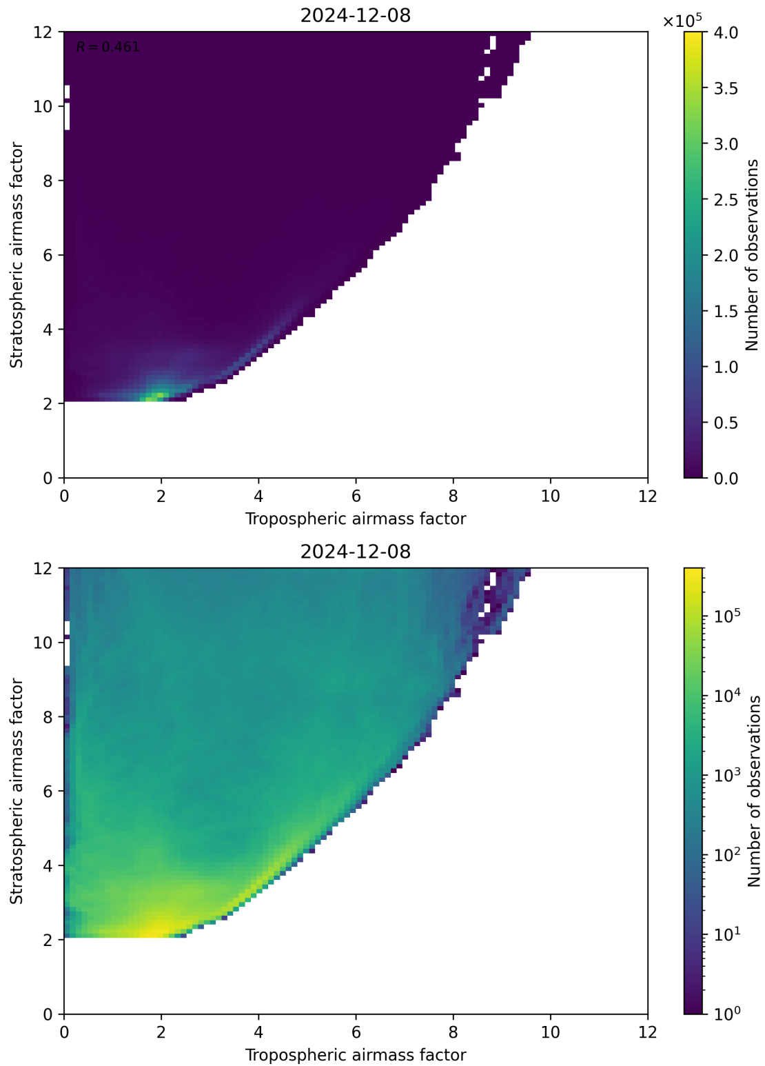
Figure 71: Scatter density plot of “Tropospheric airmass factor” against “Stratospheric airmass factor” for 2024-12-07 to 2024-12-09.
