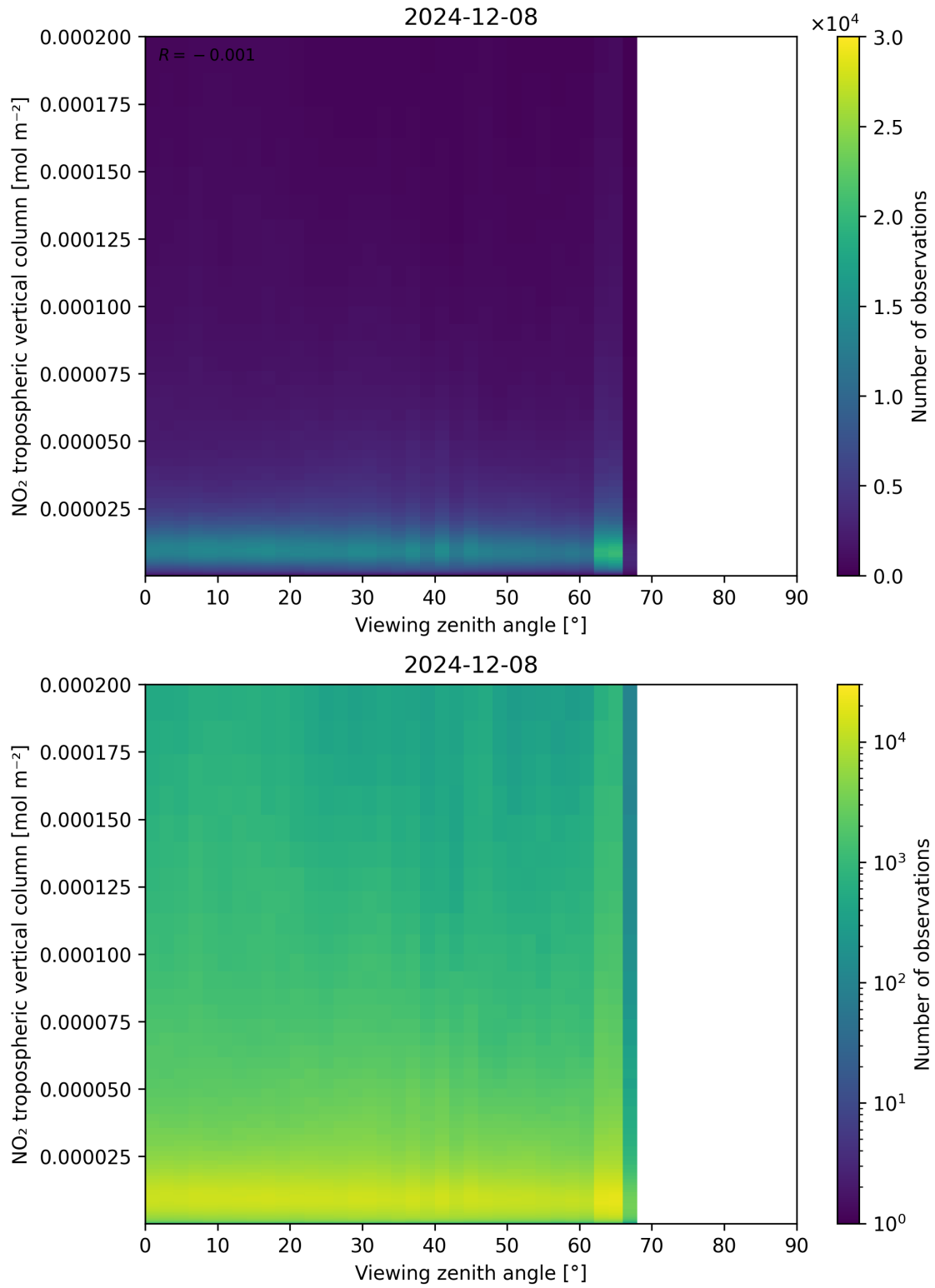
Figure 169: Scatter density plot of “Viewing zenith angle” against “NO 2 tropospheric vertical column” for 2024-12-07 to 2024-12-09.
