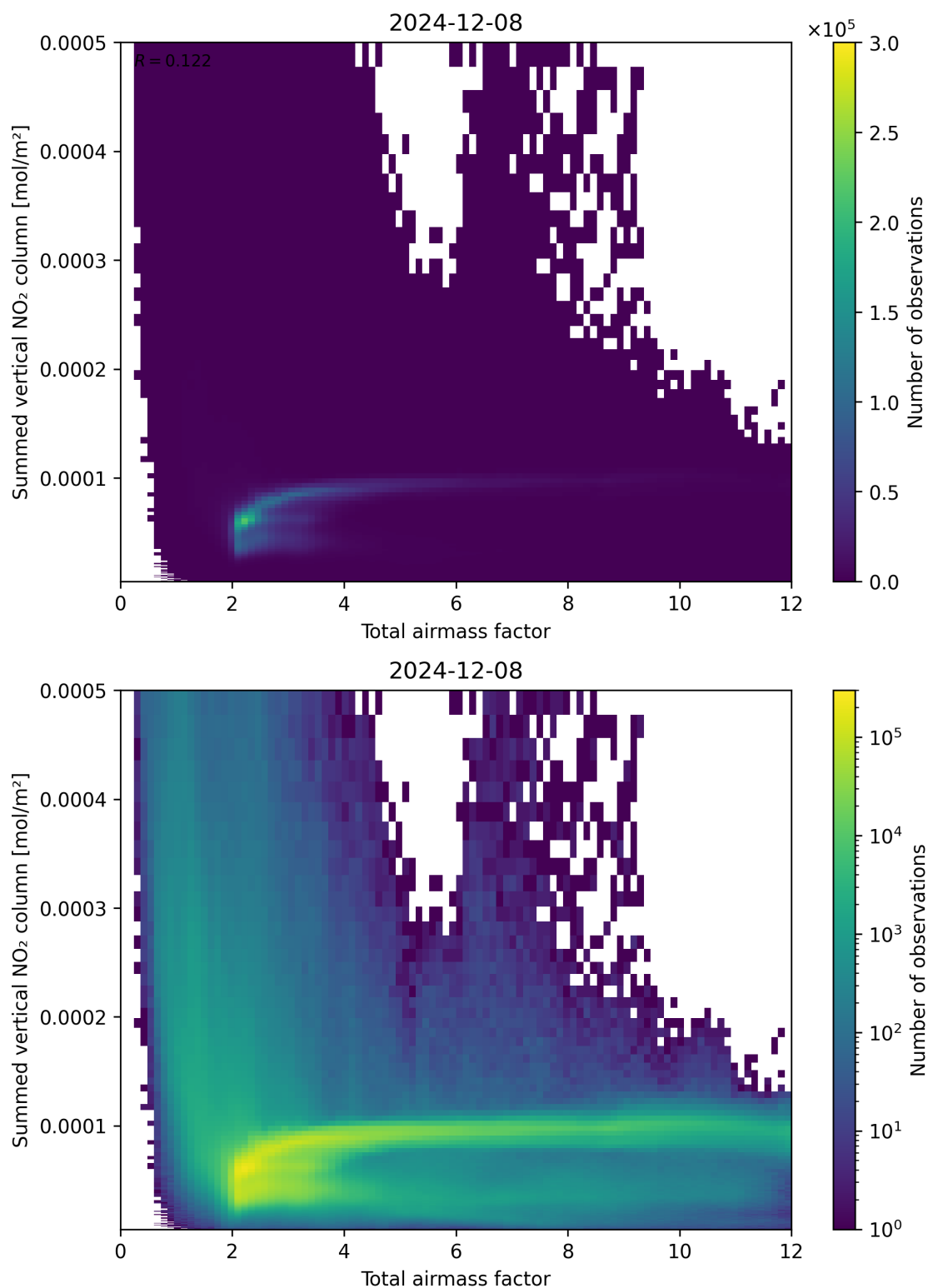
Figure 65: Scatter density plot of “Total airmass factor” against “Summed vertical NO 2 column” for 2024-12-07 to 2024-12-09.
