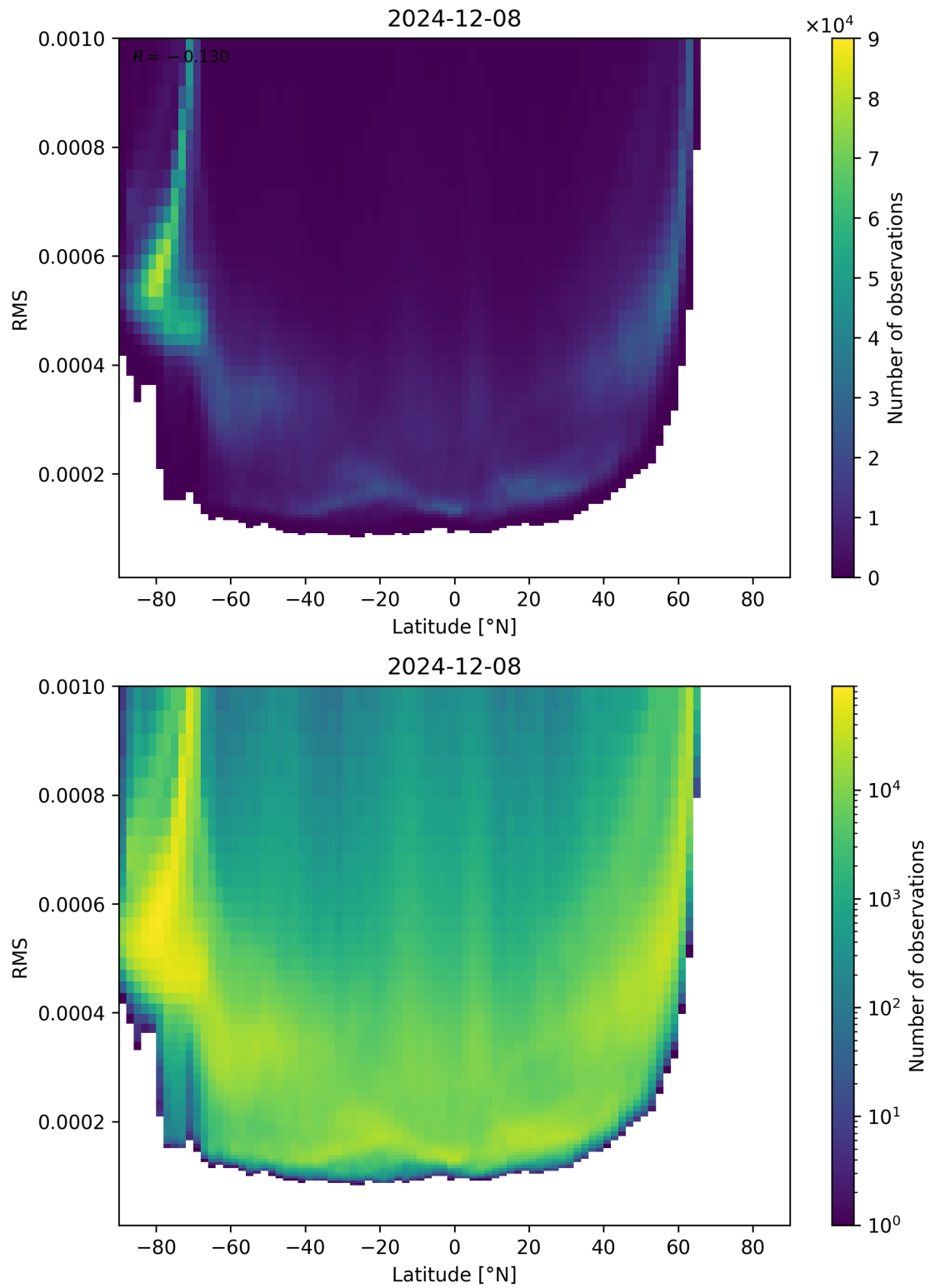
Figure 94: Scatter density plot of “Latitude” against “RMS” for 2024-12-07 to 2024-12-09.
