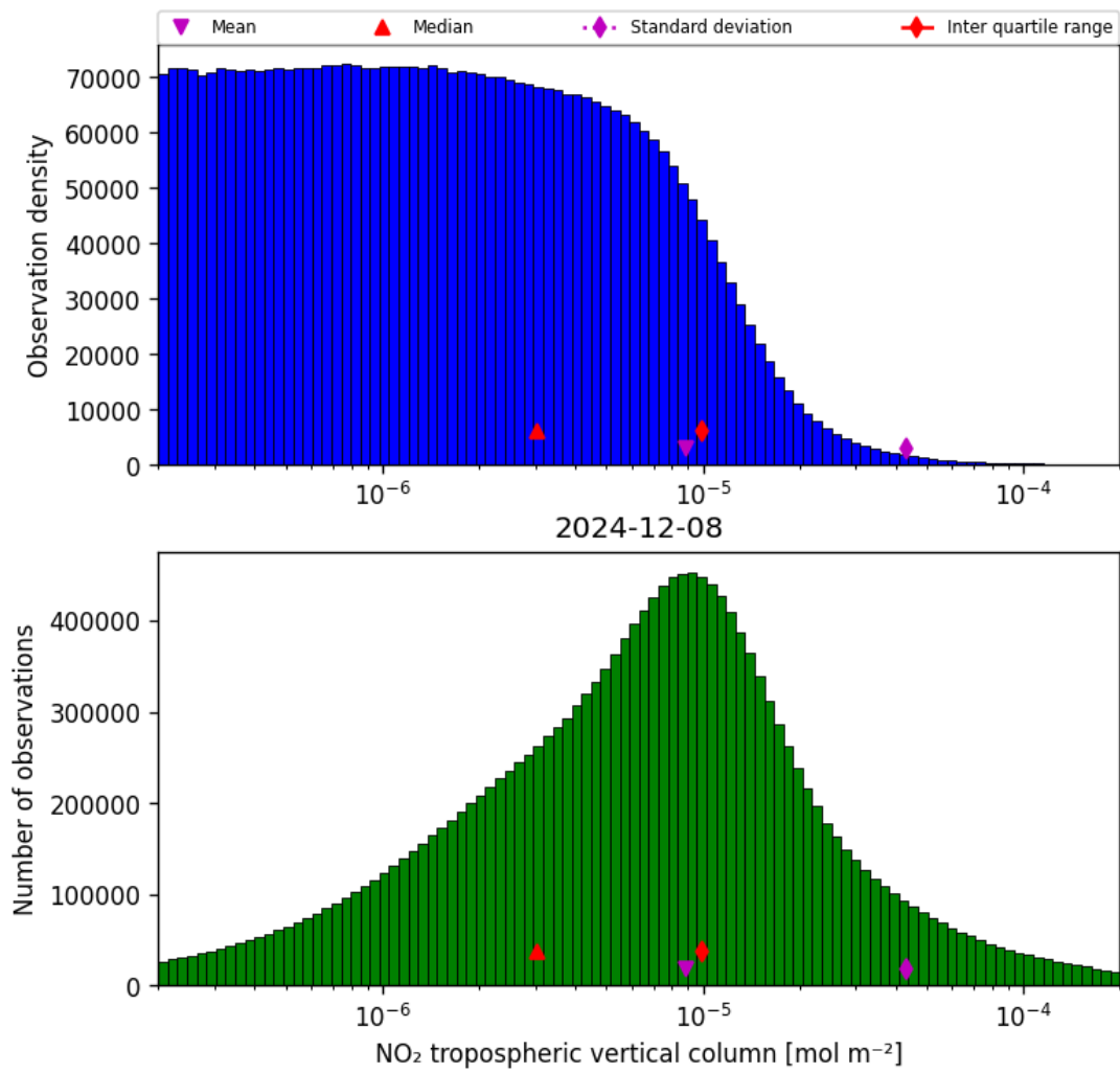
Figure 29: Histogram of “NO 2 tropospheric vertical column” for 2024-12-07 to 2024-12-09
