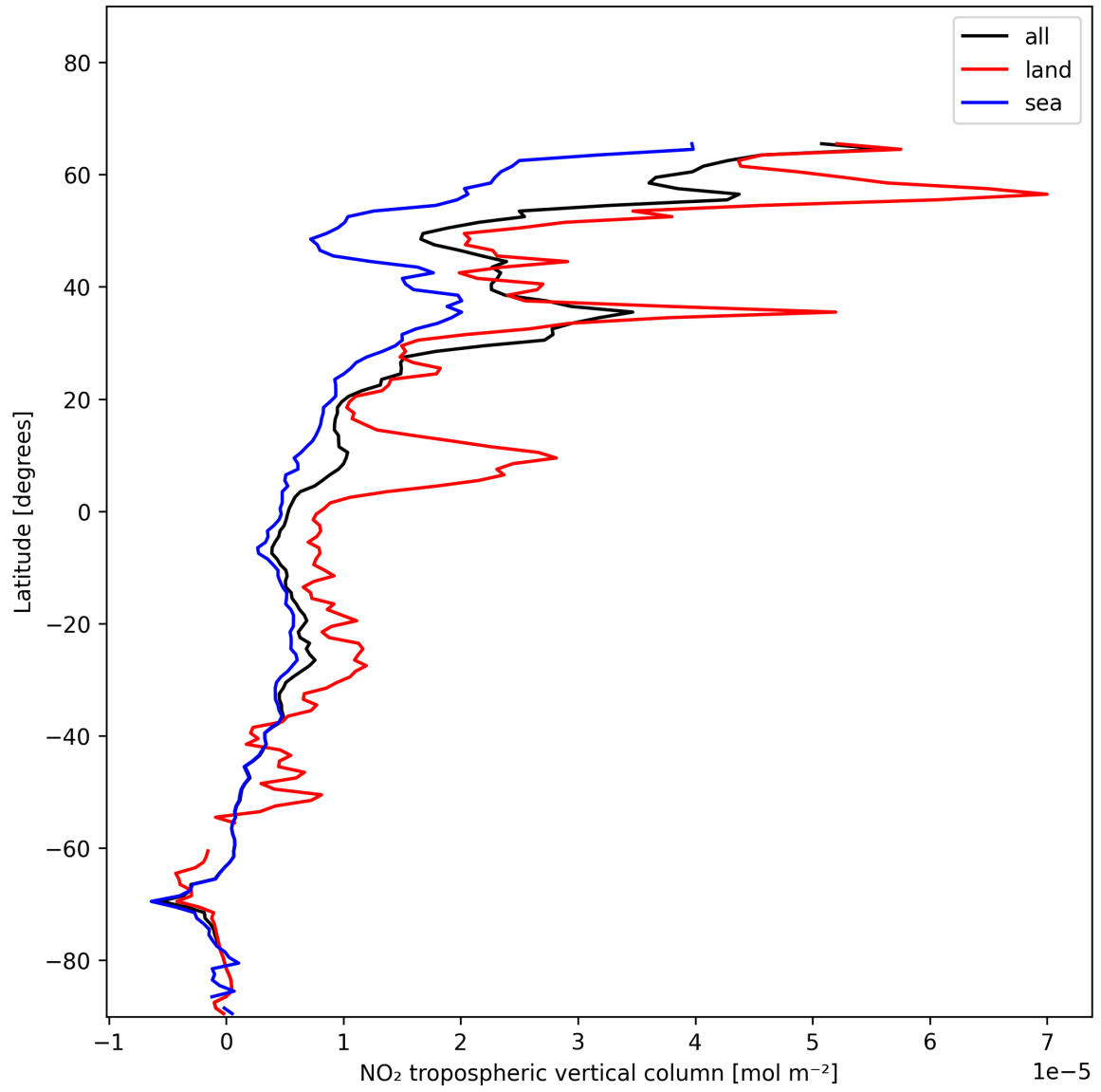
Figure 12: Zonal average of “NO 2 tropospheric vertical column” for 2024-12-07 to 2024-12-09.
