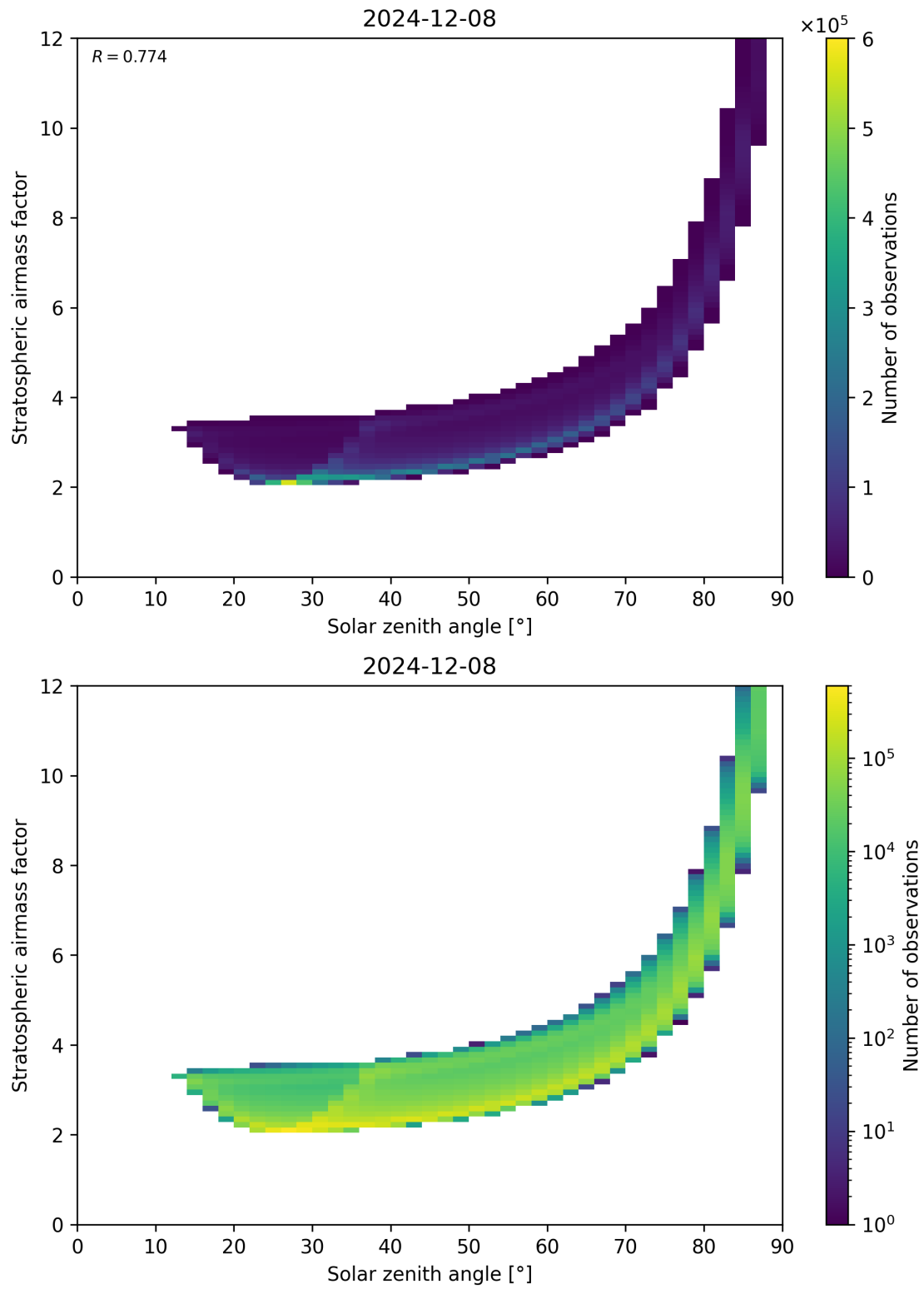
Figure 145: Scatter density plot of “Solar zenith angle” against “Stratospheric airmass factor” for 2024-12-07 to 2024-12-09.
