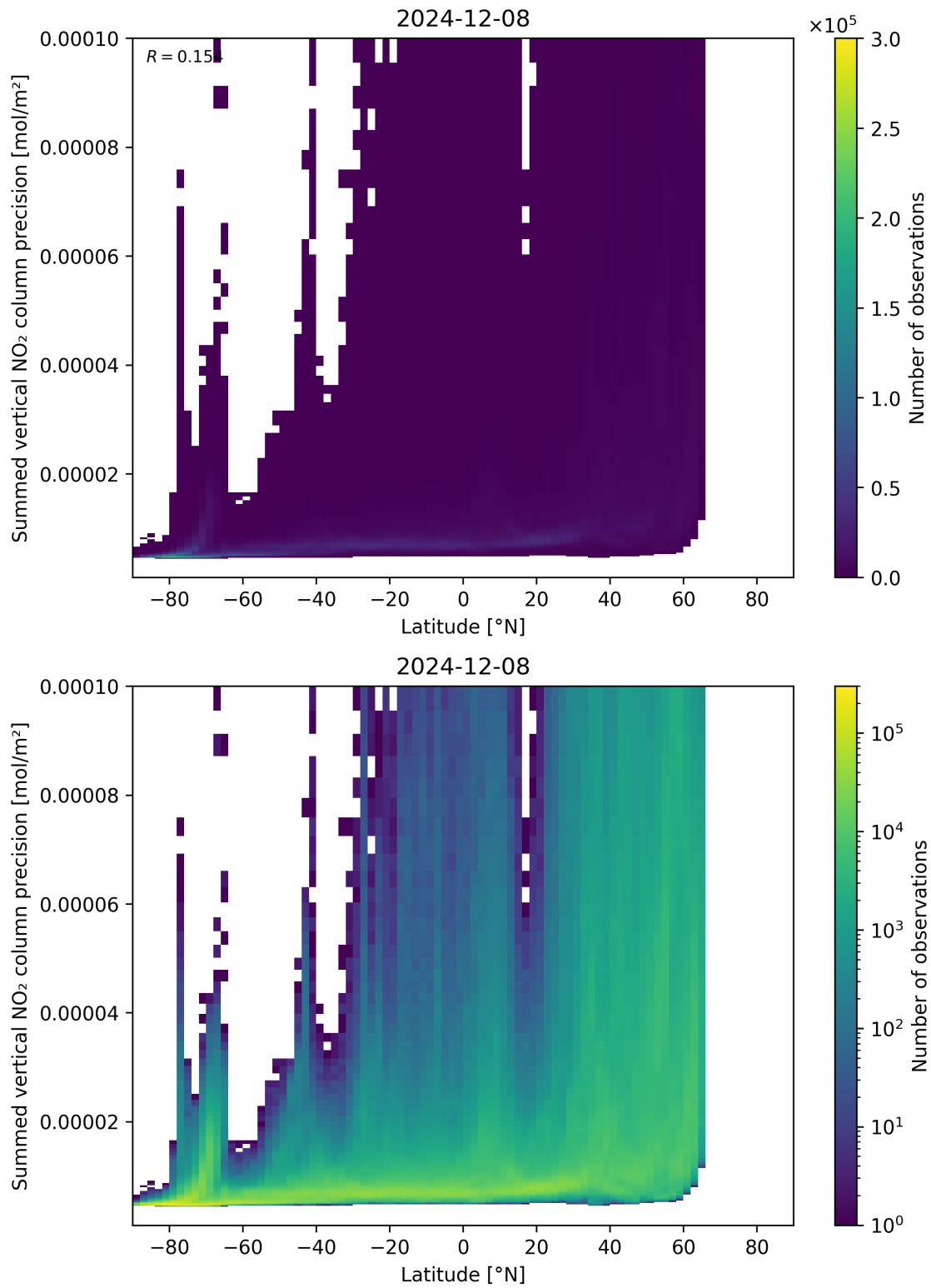
Figure 89: Scatter density plot of “Latitude” against “Summed vertical NO 2 column precision” for 2024-12-07 to 2024-12-09.
