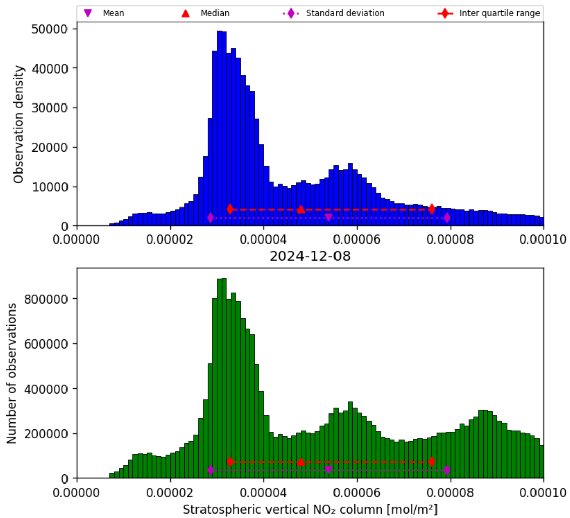
Figure 36: Histogram of “Stratospheric vertical NO 2 column” for 2024-12-07 to 2024-12-09
