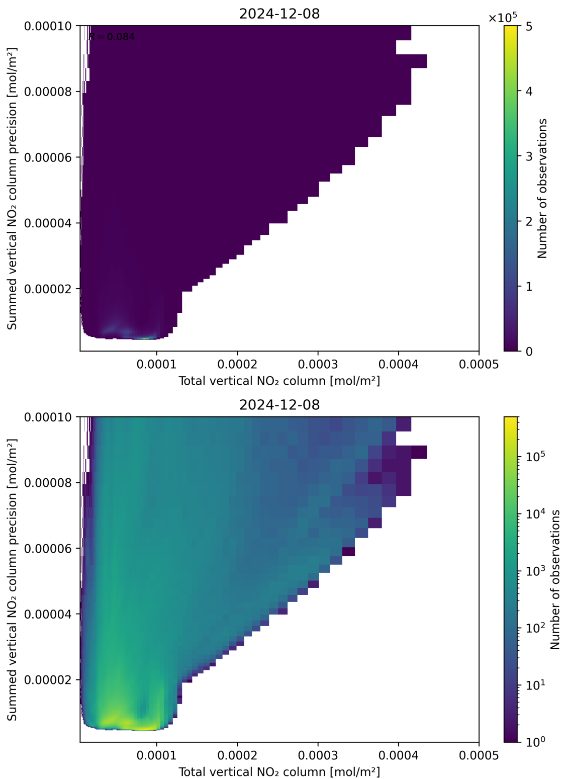
Figure 113: Scatter density plot of “Total vertical NO 2 column” against “Summed vertical NO 2 column precision” for 2024-12-07 to 2024-12-09.
