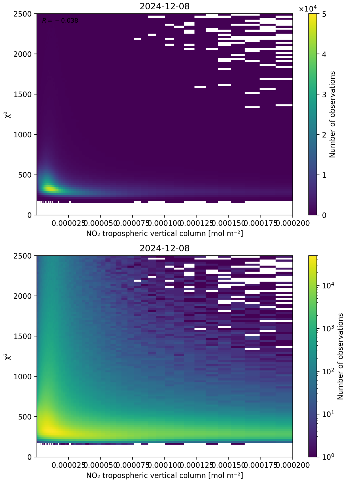
Figure 124: Scatter density plot of “NO 2 tropospheric vertical column” against “ \chi^2 ” for 2024-12-07 to 2024-12-09.
