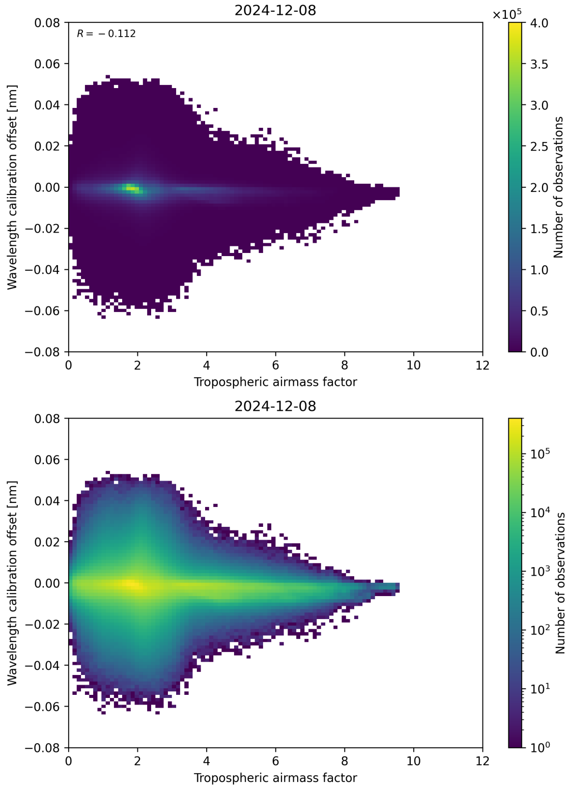
Figure 80: Scatter density plot of “Tropospheric airmass factor” against “Wavelength calibration offset” for 2024-12-07 to 2024-12-09.
