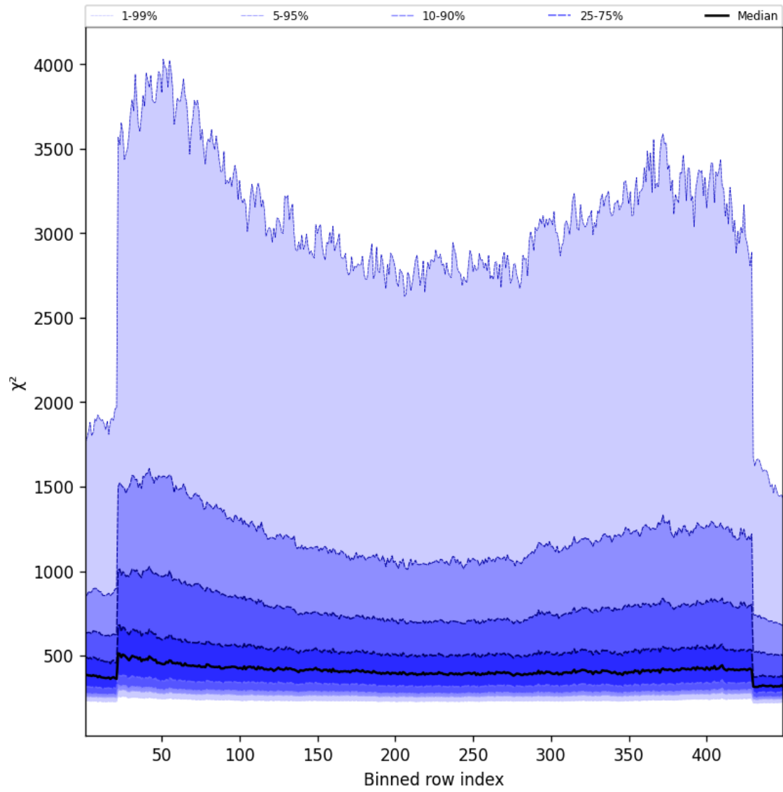
Figure 59: Along track statistics of “ \chi^2 ” for 2024-12-07 to 2024-12-09
