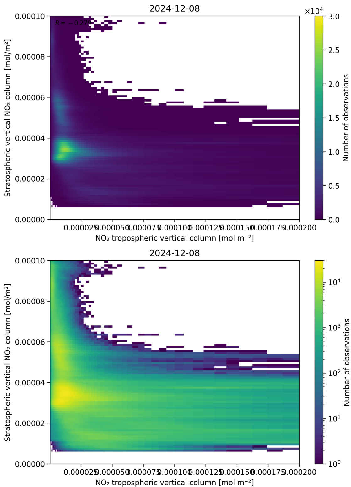
Figure 125: Scatter density plot of “NO 2 tropospheric vertical column” against “Stratospheric vertical NO 2 column” for 2024-12-07 to 2024-12-09.
