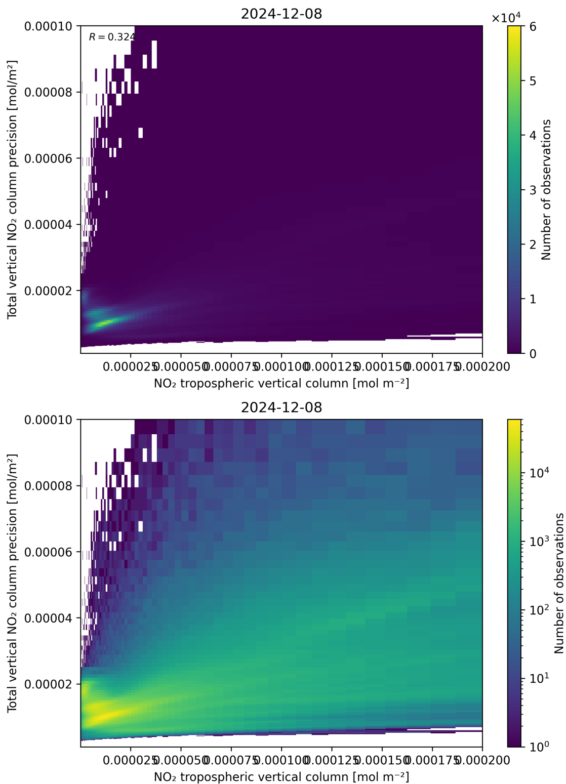
Figure 129: Scatter density plot of “NO 2 tropospheric vertical column” against “Total vertical NO 2 column precision” for 2024-12-07 to 2024-12-09.
