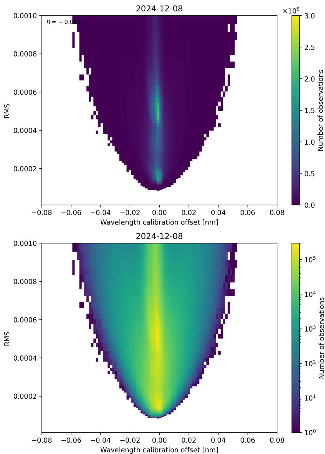
Figure 181: Scatter density plot of “Wavelength calibration offset” against “RMS” for 2024-12-07 to 2024-12-09.
