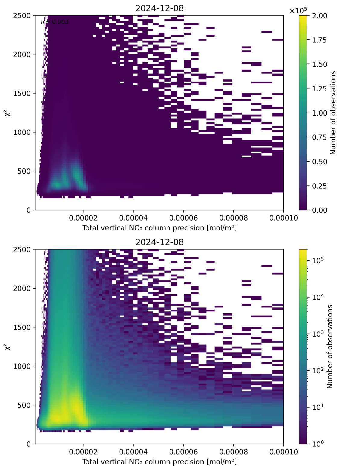
Figure 116: Scatter density plot of “Total vertical NO 2 column precision” against “ \chi^2 ” for 2024-12-07 to 2024-12-09.
