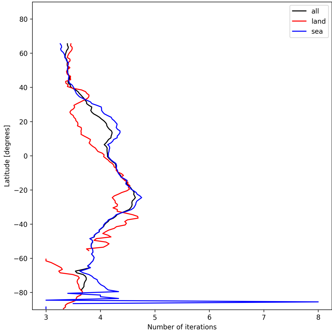
Figure 17: Zonal average of “Number of iterations” for 2024-12-07 to 2024-12-09.
