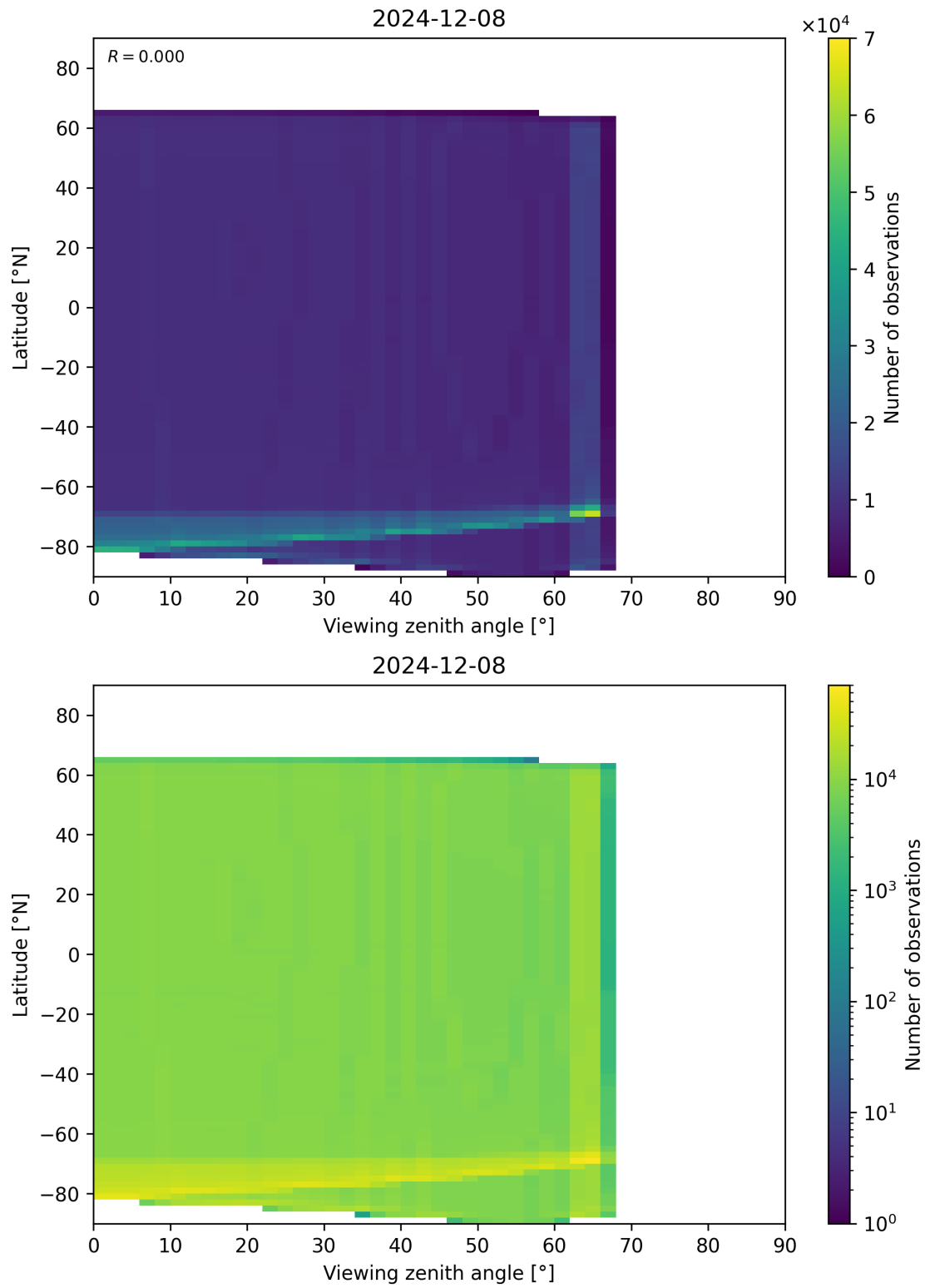
Figure 163: Scatter density plot of “Viewing zenith angle” against “Latitude” for 2024-12-07 to 2024-12-09.
