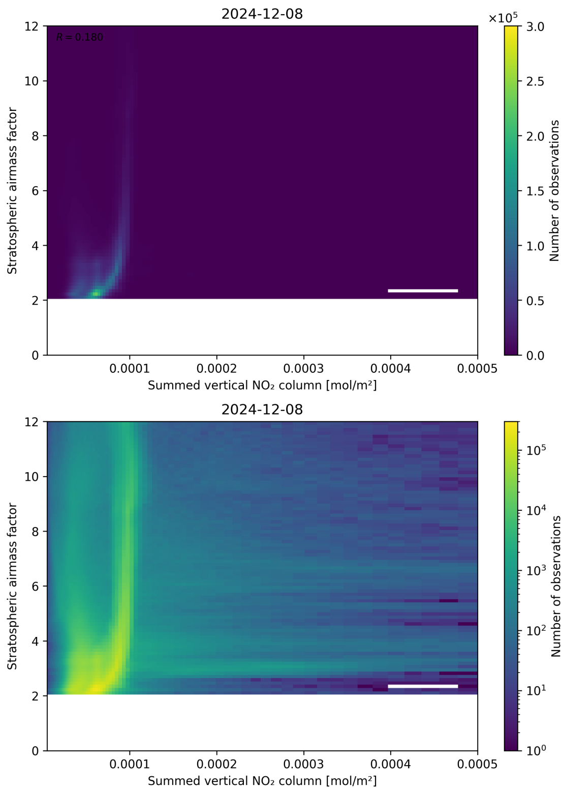
Figure 103: Scatter density plot of “Summed vertical NO 2 column” against “Stratospheric airmass factor” for 2024-12-07 to 2024-12-09.
