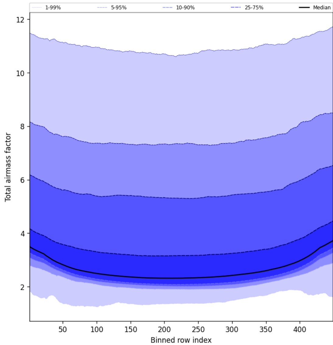
Figure 49: Along track statistics of “Total airmass factor” for 2024-12-07 to 2024-12-09
