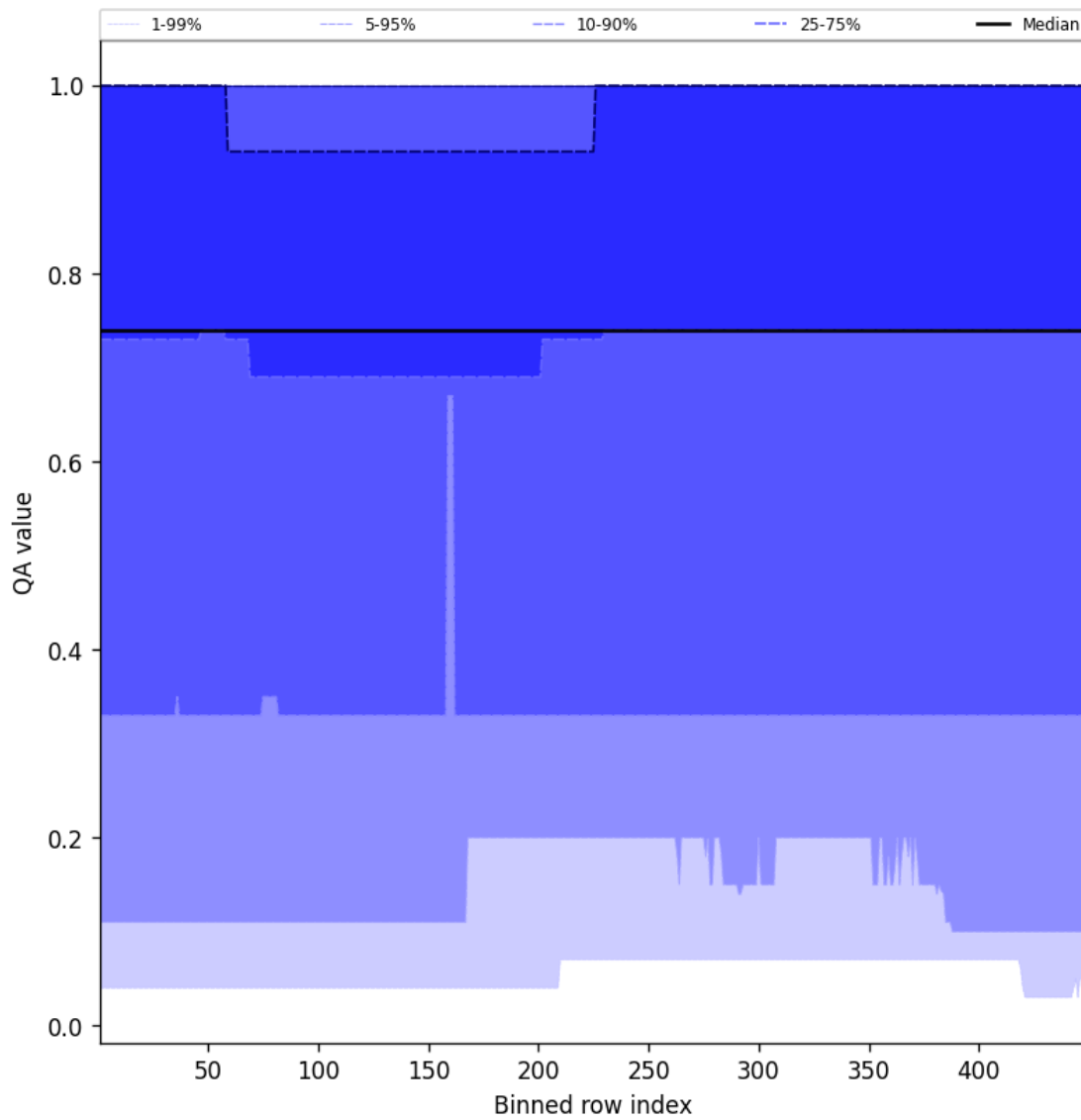
Figure 45: Along track statistics of “QA value” for 2024-12-07 to 2024-12-09
