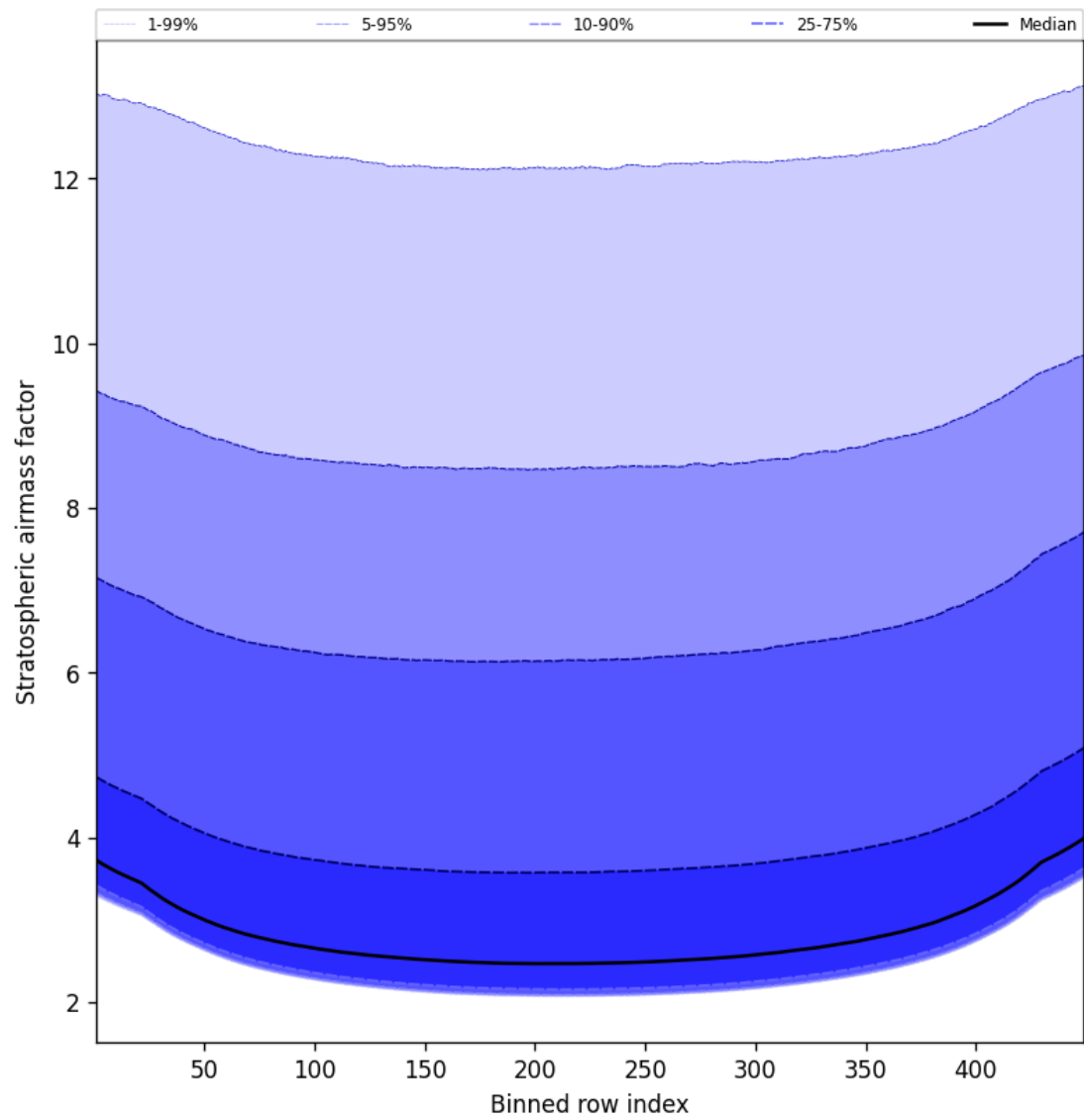
Figure 61: Along track statistics of “Stratospheric airmass factor” for 2024-12-07 to 2024-12-09
