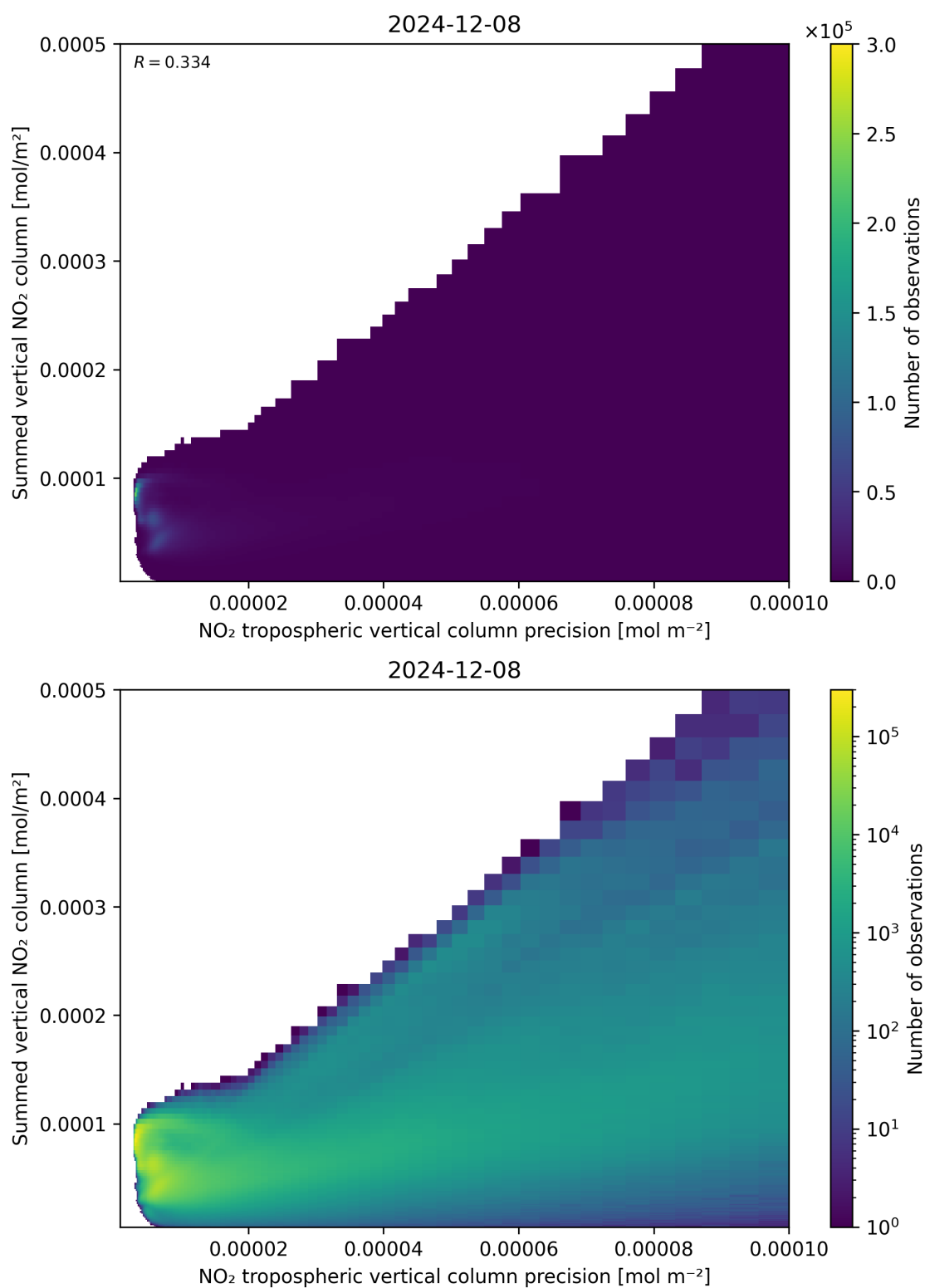
Figure 136: Scatter density plot of “NO 2 tropospheric vertical column precision” against “Summed vertical NO 2 column” for 2024-12-07 to 2024-12-09.
