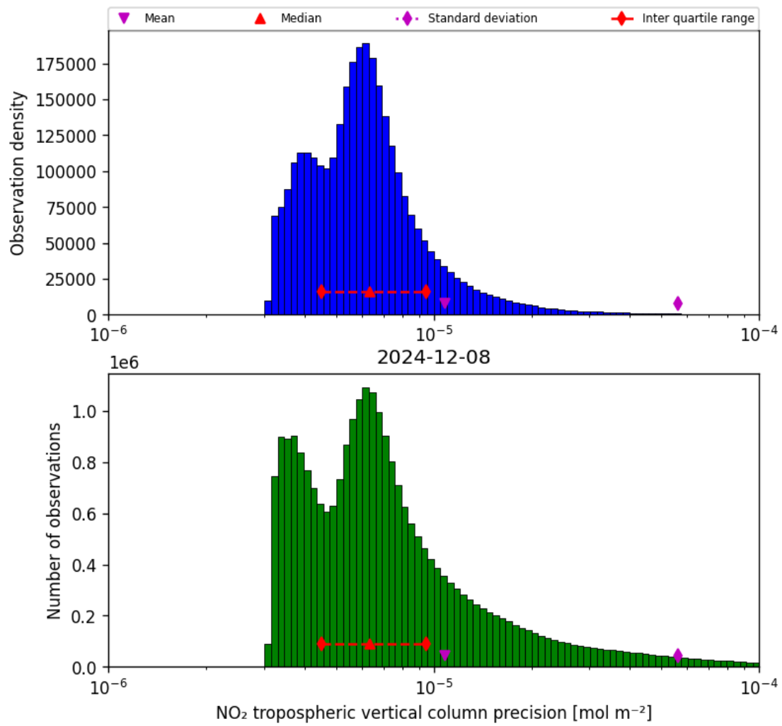
Figure 30: Histogram of “NO 2 tropospheric vertical column precision” for 2024-12-07 to 2024-12-09
