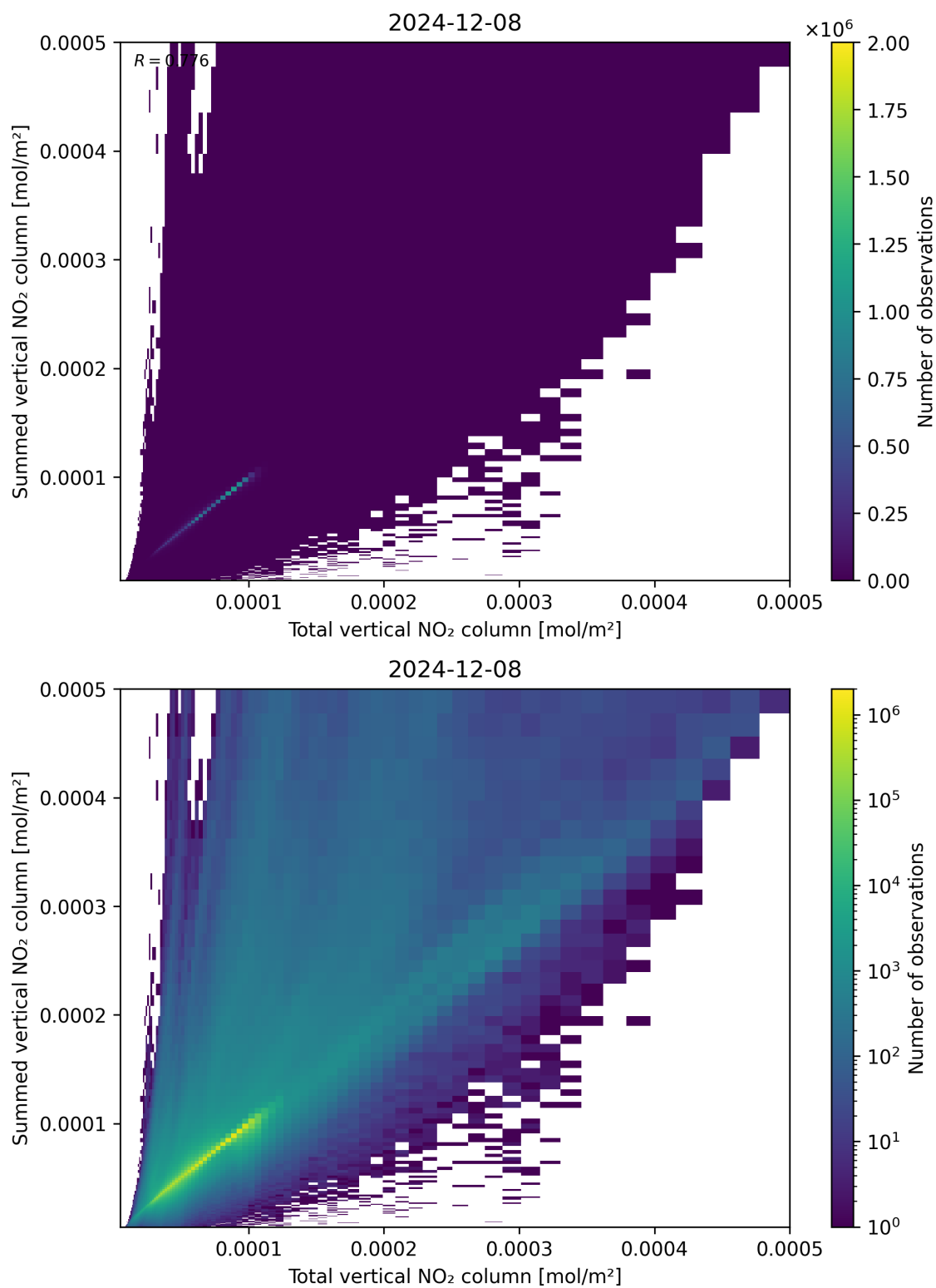
Figure 112: Scatter density plot of “Total vertical NO 2 column” against “Summed vertical NO 2 column” for 2024-12-07 to 2024-12-09.
