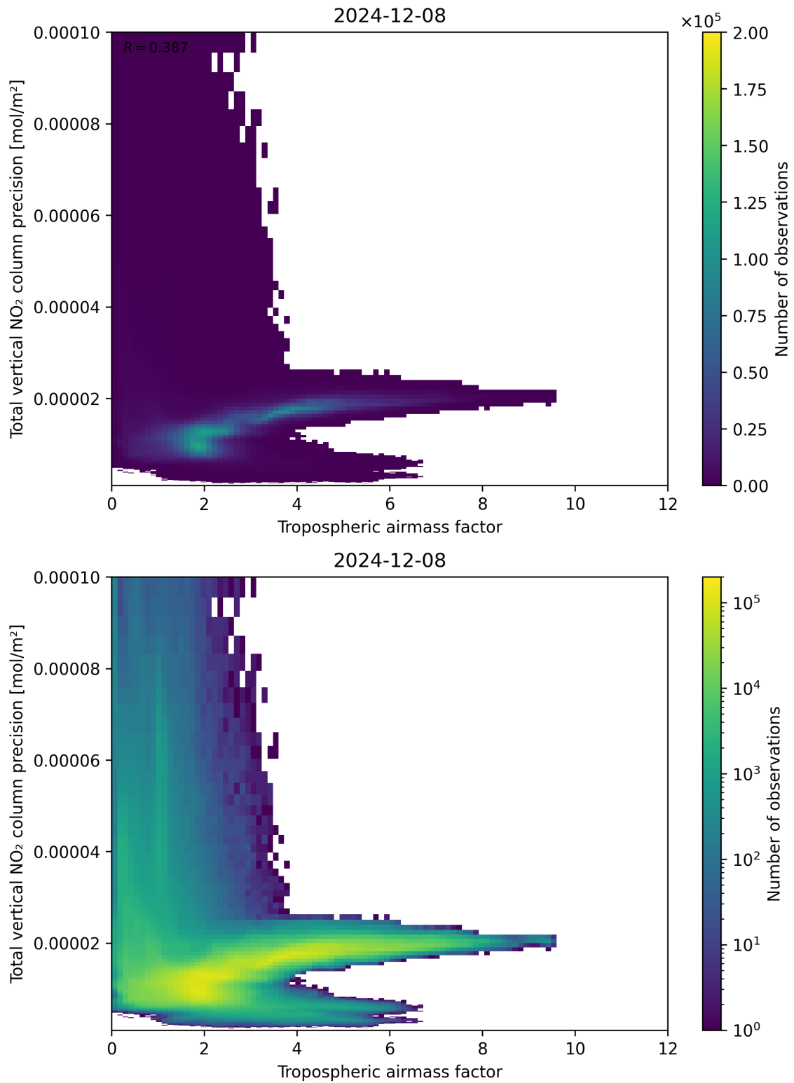
Figure 78: Scatter density plot of “Tropospheric air mass factor” against “Total vertical NO 2 column precision” for 2024-12-07 to 2024-12-09.
