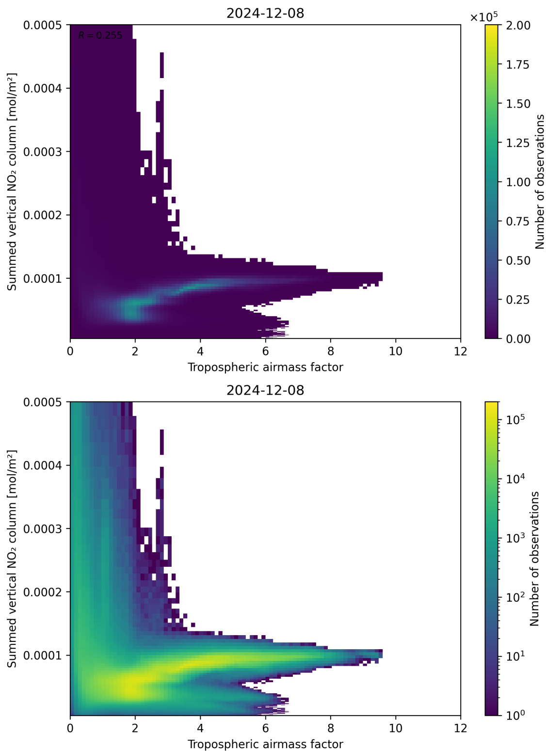
Figure 75: Scatter density plot of “Tropospheric airmass factor” against “Summed vertical NO 2 column” for 2024-12-07 to 2024-12-09.
