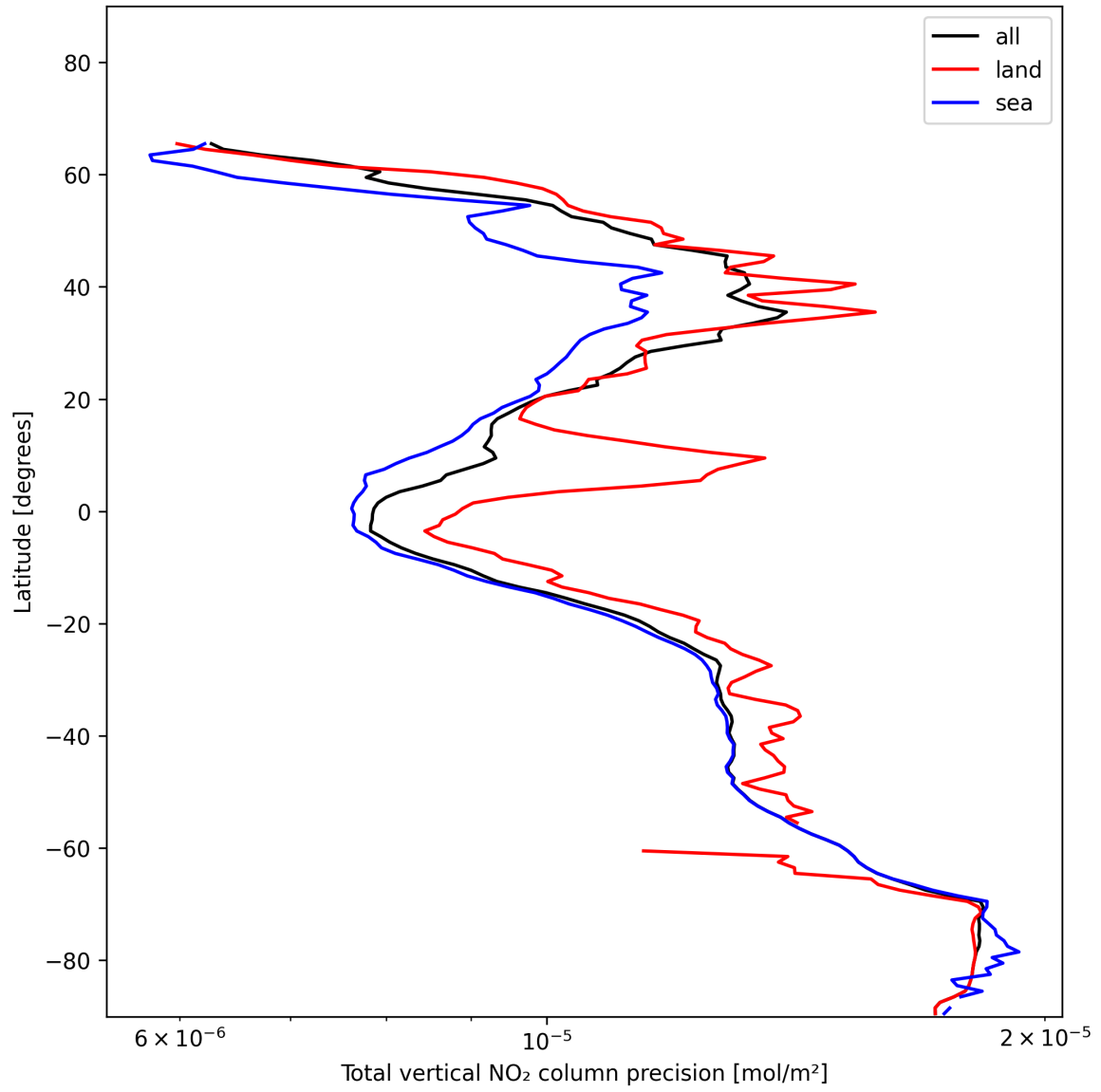
Figure 22: Zonal average of “Total vertical NO 2 column precision” for 2024-12-07 to 2024-12-09.
