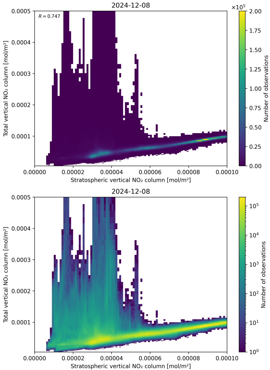
Figure 100: Scatter density plot of “Stratospheric vertical NO 2 column” against “Total vertical NO 2 column” for 2024-12-07 to 2024-12-09.
