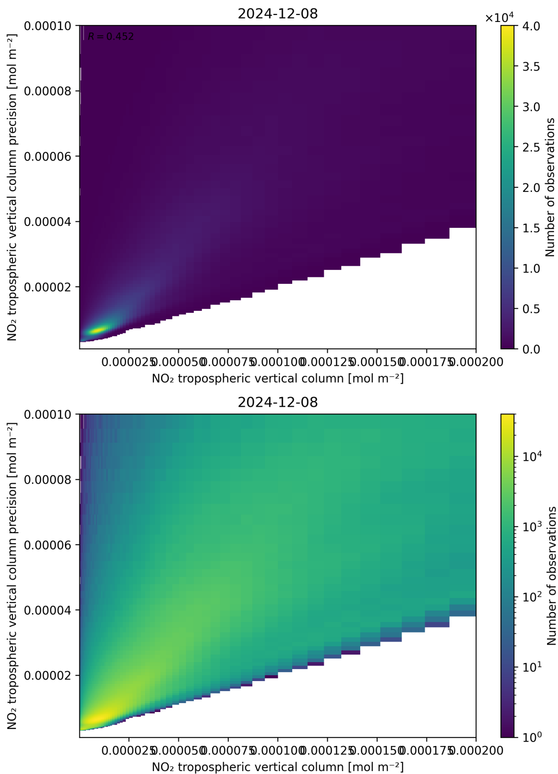
Figure 130: Scatter density plot of “NO 2 tropospheric vertical column” against “NO 2 tropospheric vertical column precision” for 2024-12-07 to 2024-12-09.
