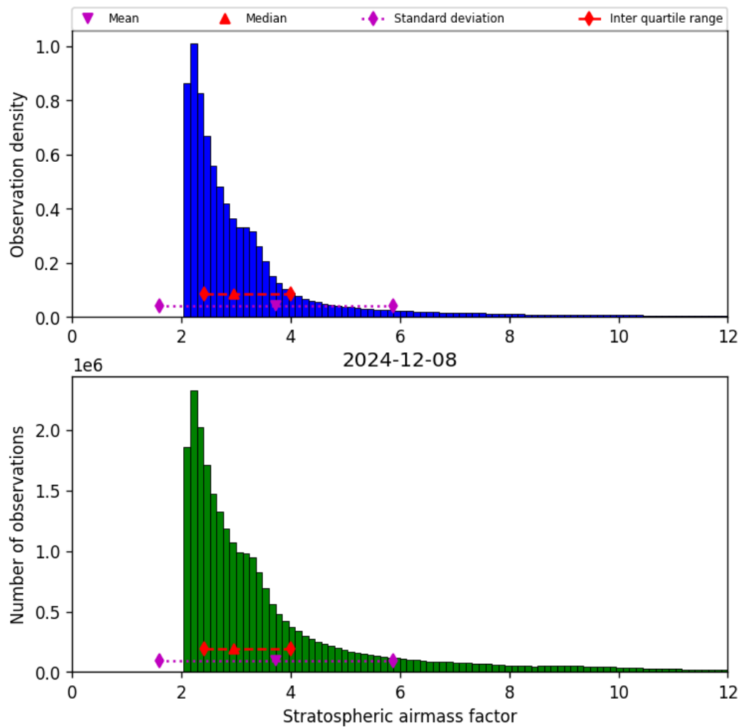
Figure 44: Histogram of “Stratospheric airmass factor” for 2024-12-07 to 2024-12-09
