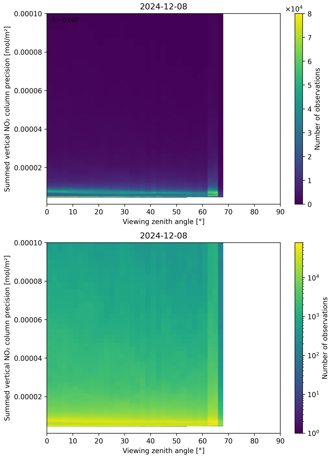
Figure 166: Scatter density plot of “Viewing zenith angle” against “Summed vertical NO 2 column precision” for 2024-12-07 to 2024-12-09.
