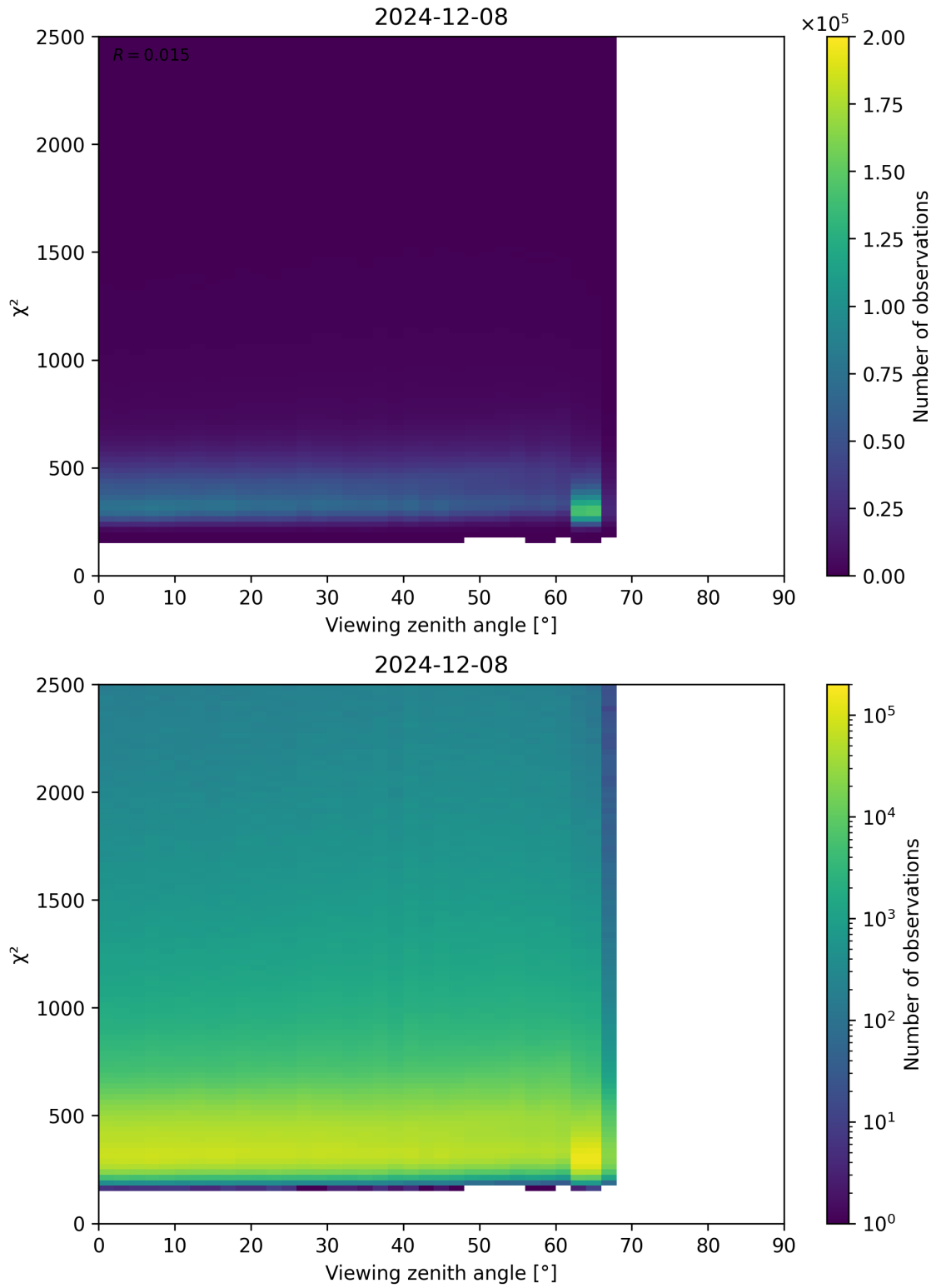
Figure 162: Scatter density plot of “Viewing zenith angle” against “ \chi^2 ” for 2024-12-07 to 2024-12-09.
