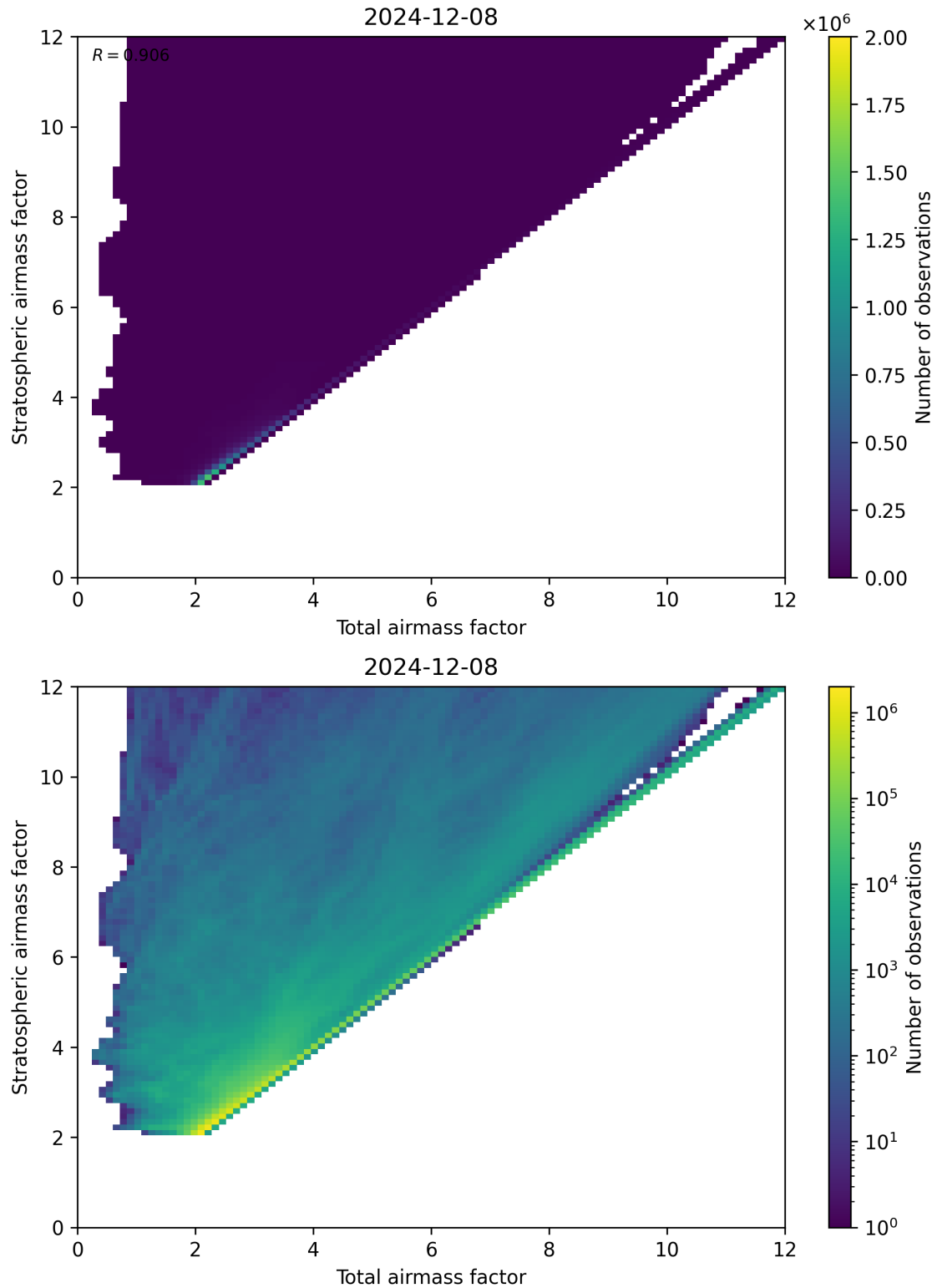
Figure 62: Scatter density plot of “Total airmass factor” against “Stratospheric airmass factor” for 2024-12-07 to 2024-12-09.
