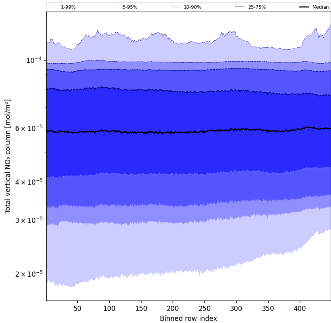
Figure 55: Along track statistics of “Total vertical NO 2 column” for 2024-12-07 to 2024-12-09
