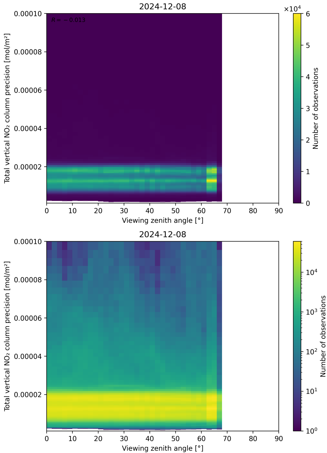
Figure 168: Scatter density plot of “Viewing zenith angle” against “Total vertical NO 2 column precision” for 2024-12-07 to 2024-12-09.
