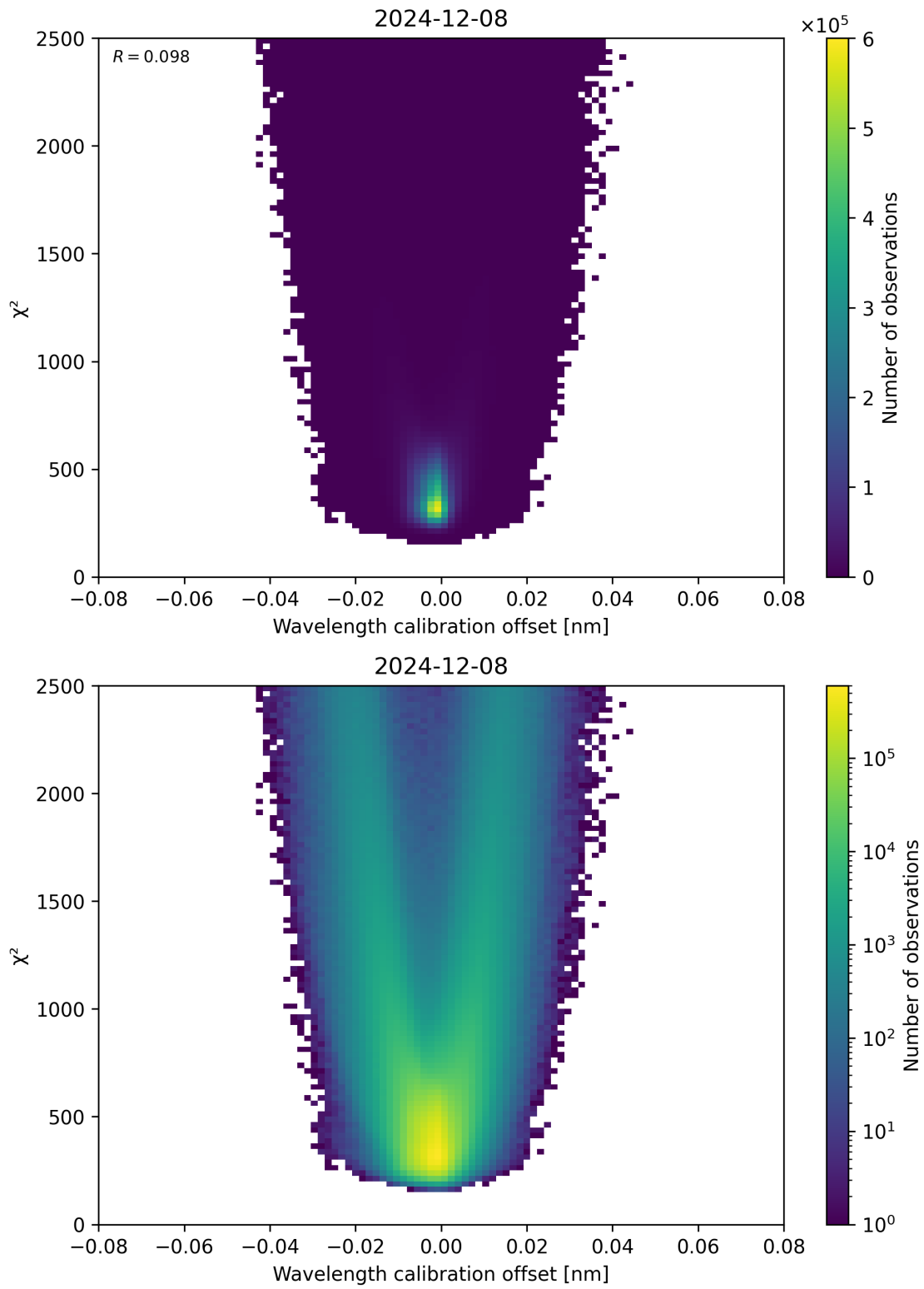
Figure 175: Scatter density plot of “Wavelength calibration offset” against “ \chi^2 ” for 2024-12-07 to 2024-12-09.
