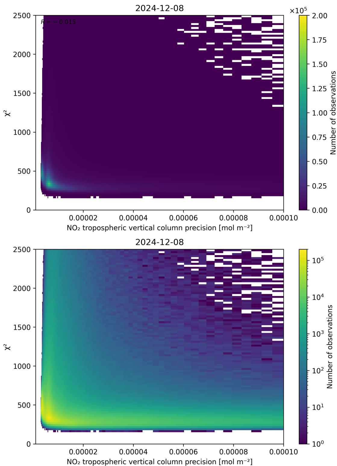
Figure 134: Scatter density plot of “NO 2 tropospheric vertical column precision” against “ \chi^2 ” for 2024-12-07 to 2024-12-09.
