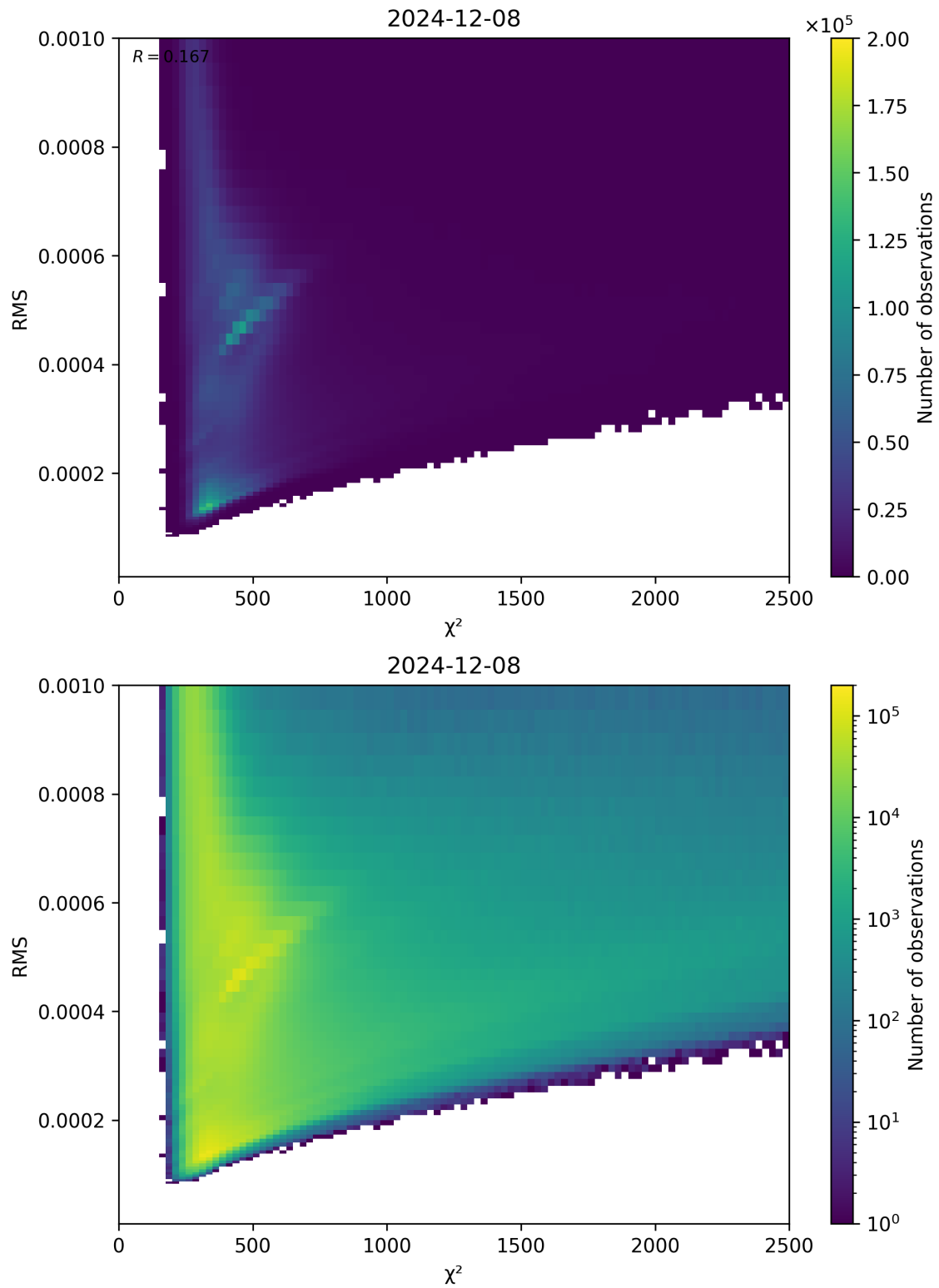
Figure 82: Scatter density plot of “ \chi^2 ” against “RMS” for 2024-12-07 to 2024-12-09.
