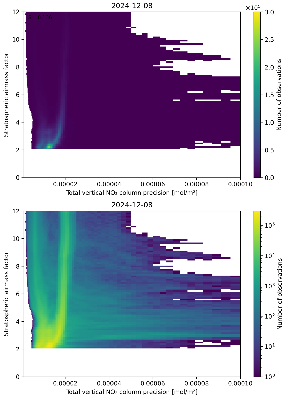
Figure 115: Scatter density plot of “Total vertical NO 2 column precision” against “Stratospheric air mass factor” for 2024-12-07 to 2024-12-09.
