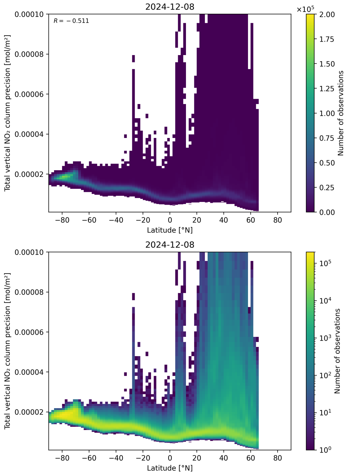
Figure 91: Scatter density plot of “Latitude” against “Total vertical NO 2 column precision” for 2024-12-07 to 2024-12-09.
