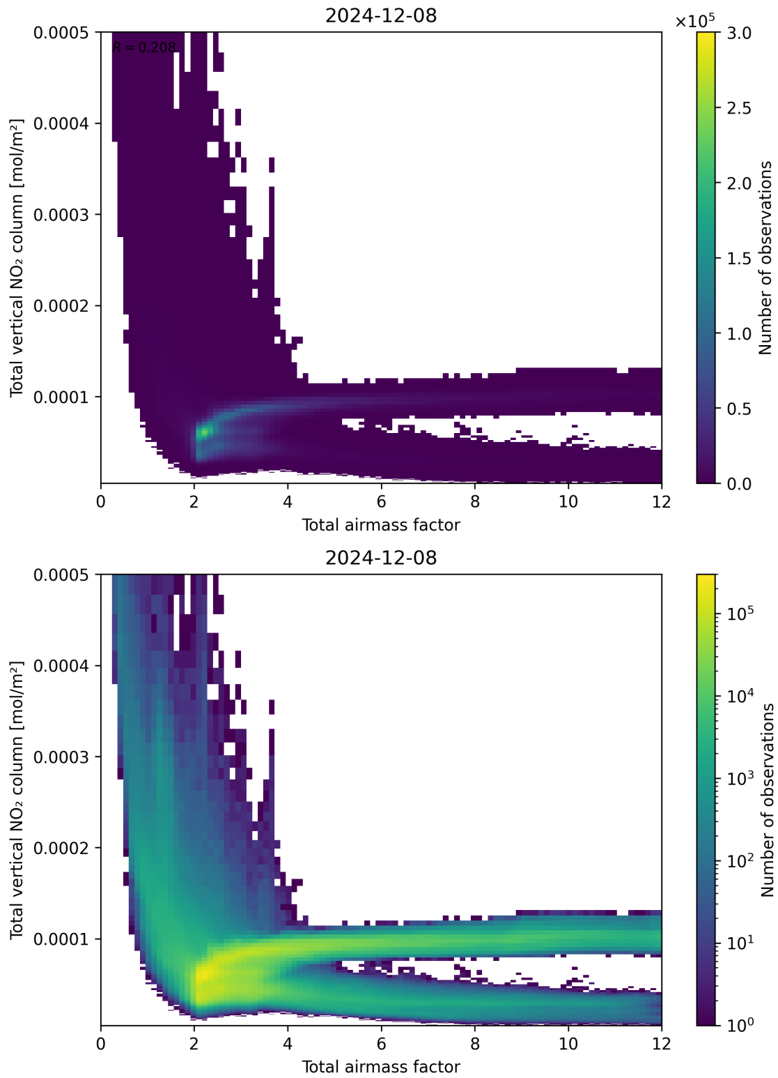
Figure 67: Scatter density plot of “Total airmass factor” against “Total vertical NO 2 column” for 2024-12-07 to 2024-12-09.
