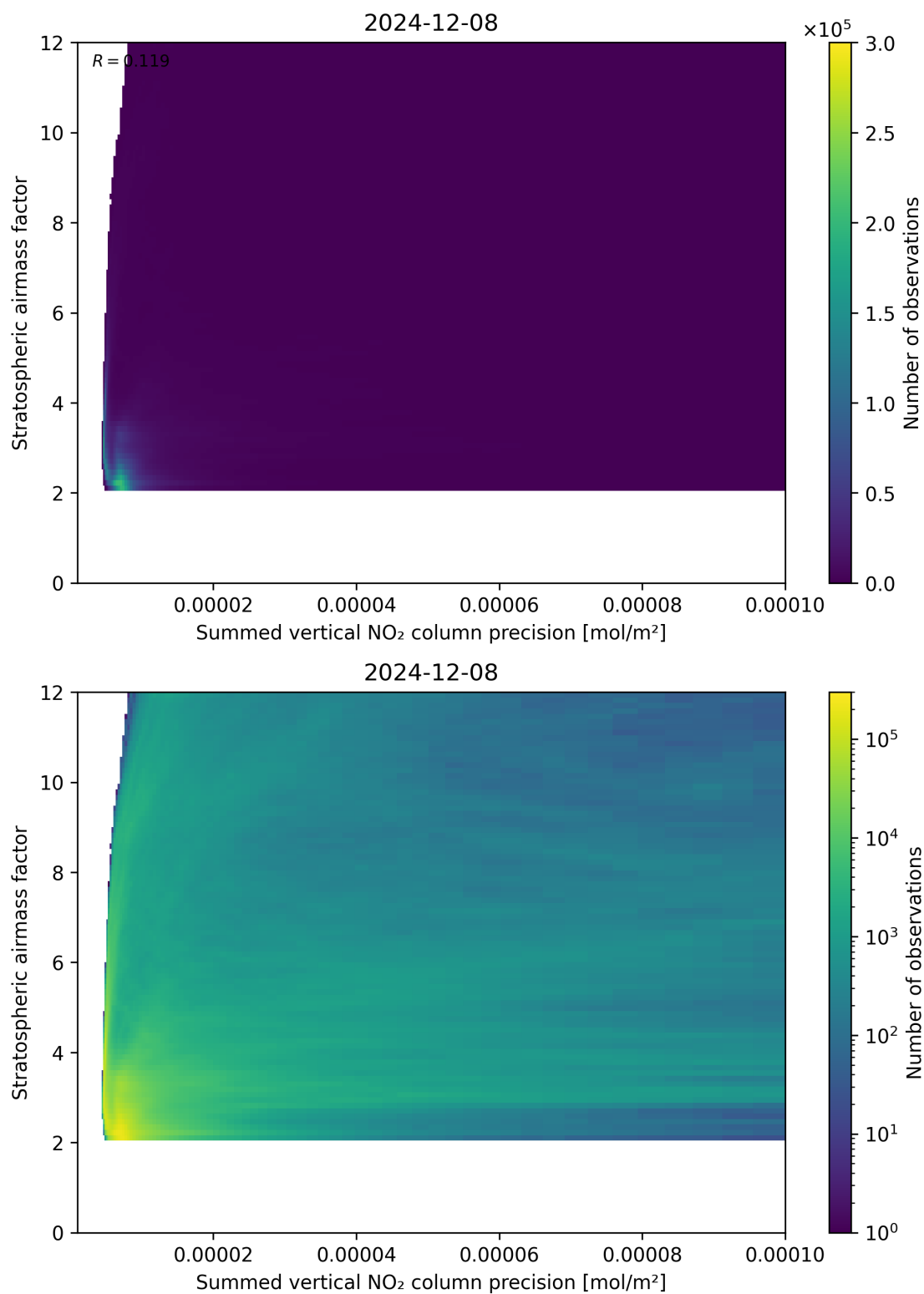
Figure 106: Scatter density plot of “Summed vertical NO 2 column precision” against “Stratospheric airmass factor” for 2024-12-07 to 2024-12-09.
