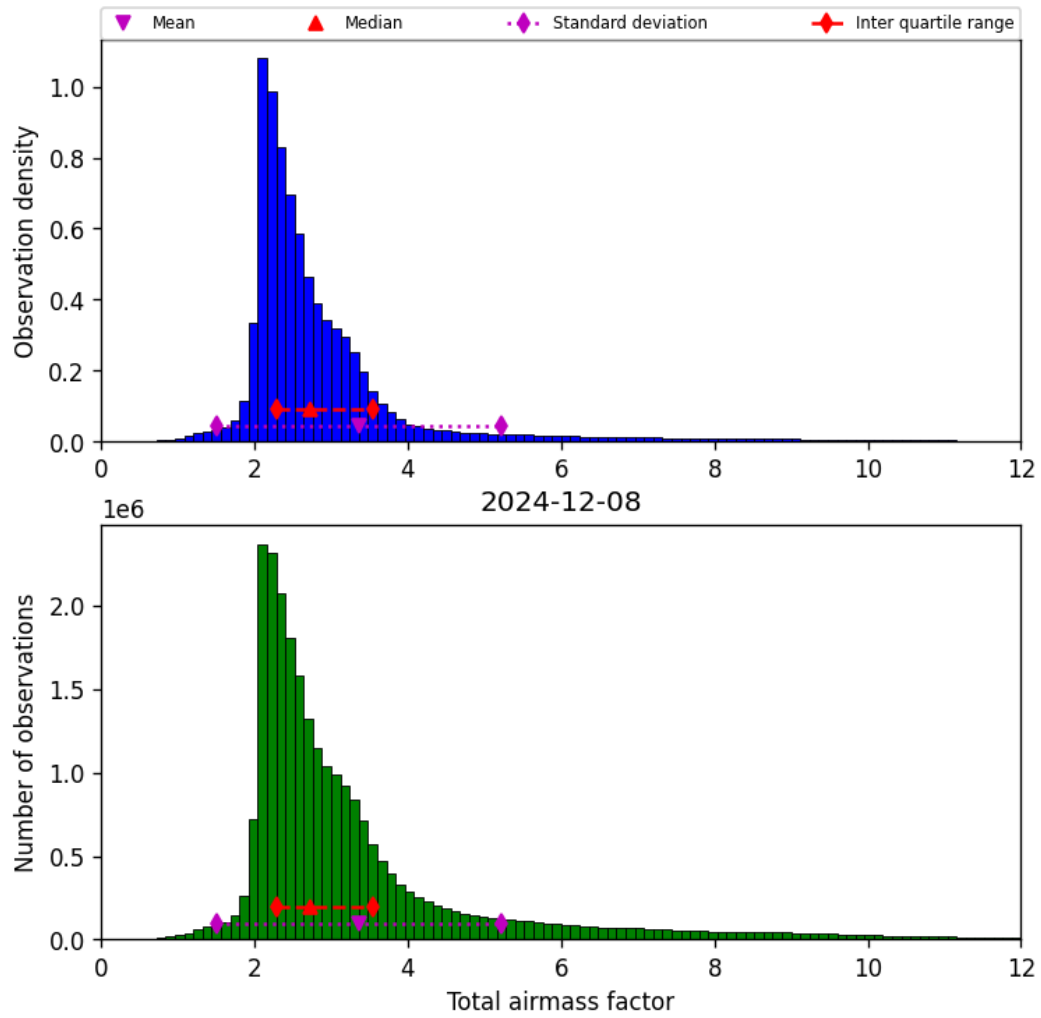
Figure 32: Histogram of “Total airmass factor” for 2024-12-07 to 2024-12-09
