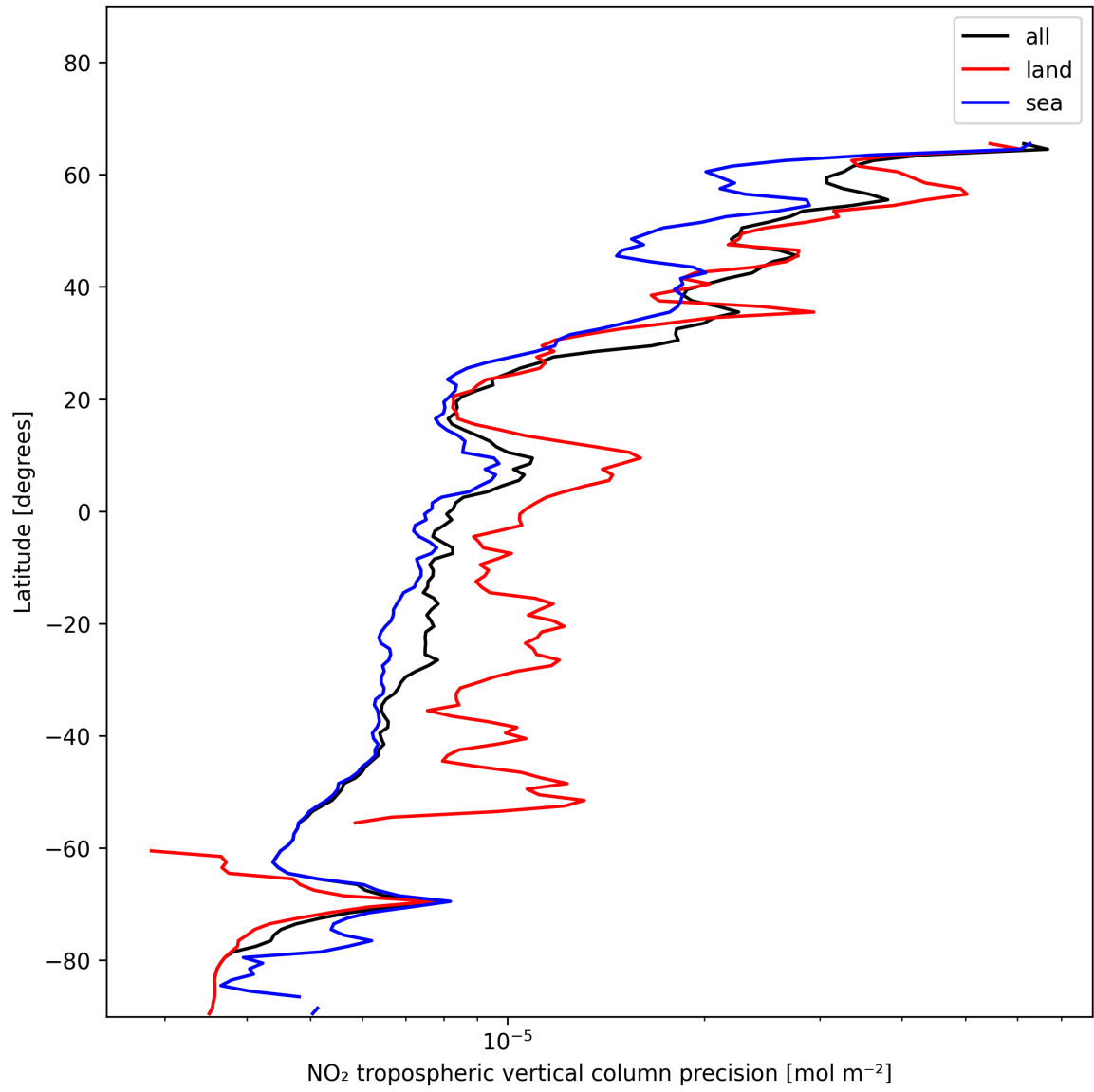
Figure 13: Zonal average of “NO 2 tropospheric vertical column precision” for 2024-12-07 to 2024-12-09.
