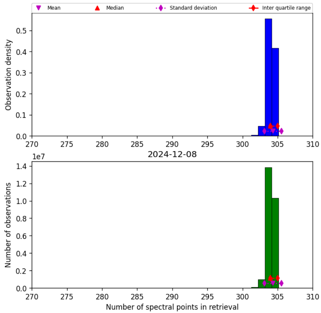
Figure 33: Histogram of “Number of spectral points in retrieval” for 2024-12-07 to 2024-12-09
