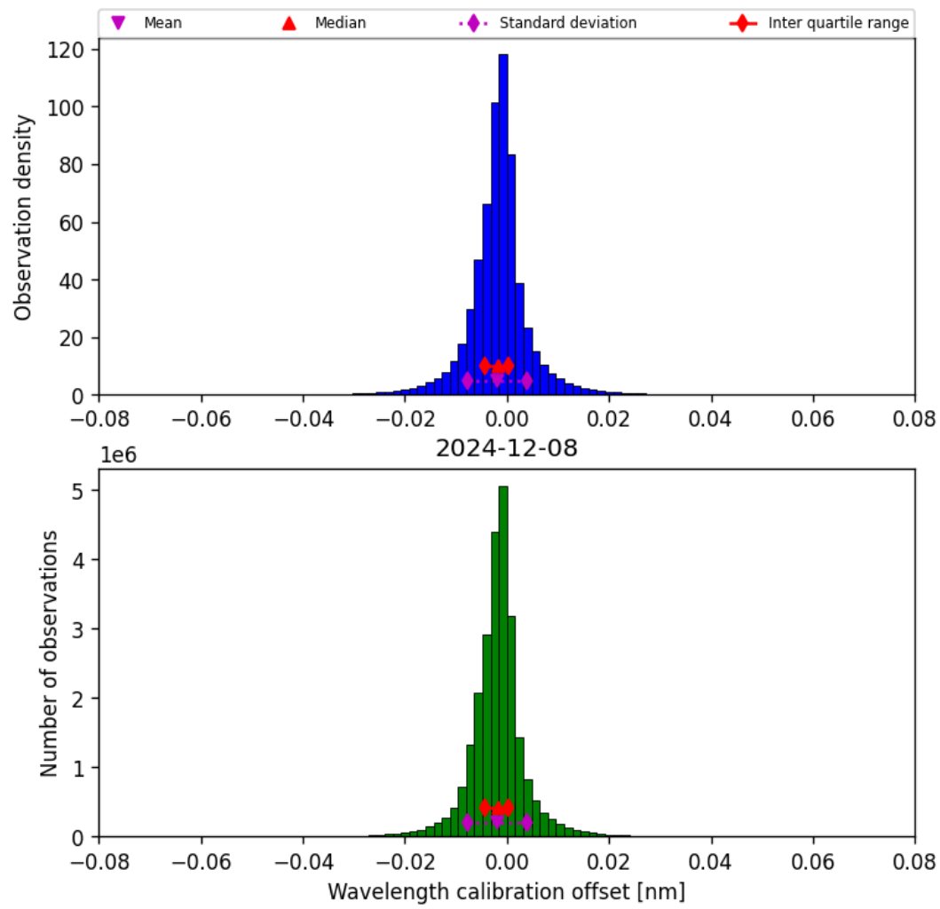
Figure 35: Histogram of “Wavelength calibration offset” for 2024-12-07 to 2024-12-09
