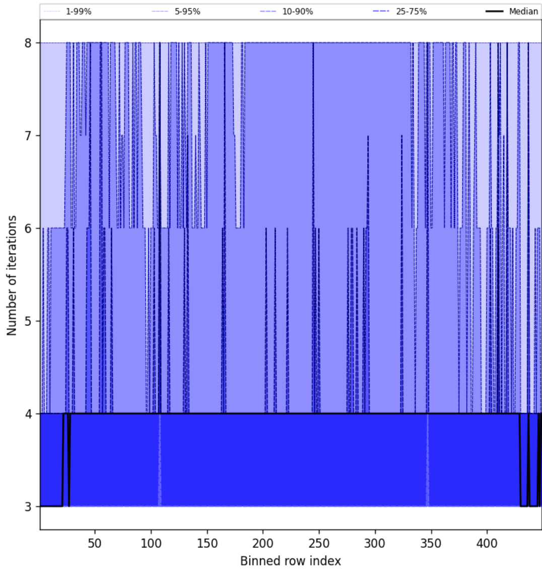
Figure 51: Along track statistics of “Number of iterations” for 2024-12-07 to 2024-12-09
