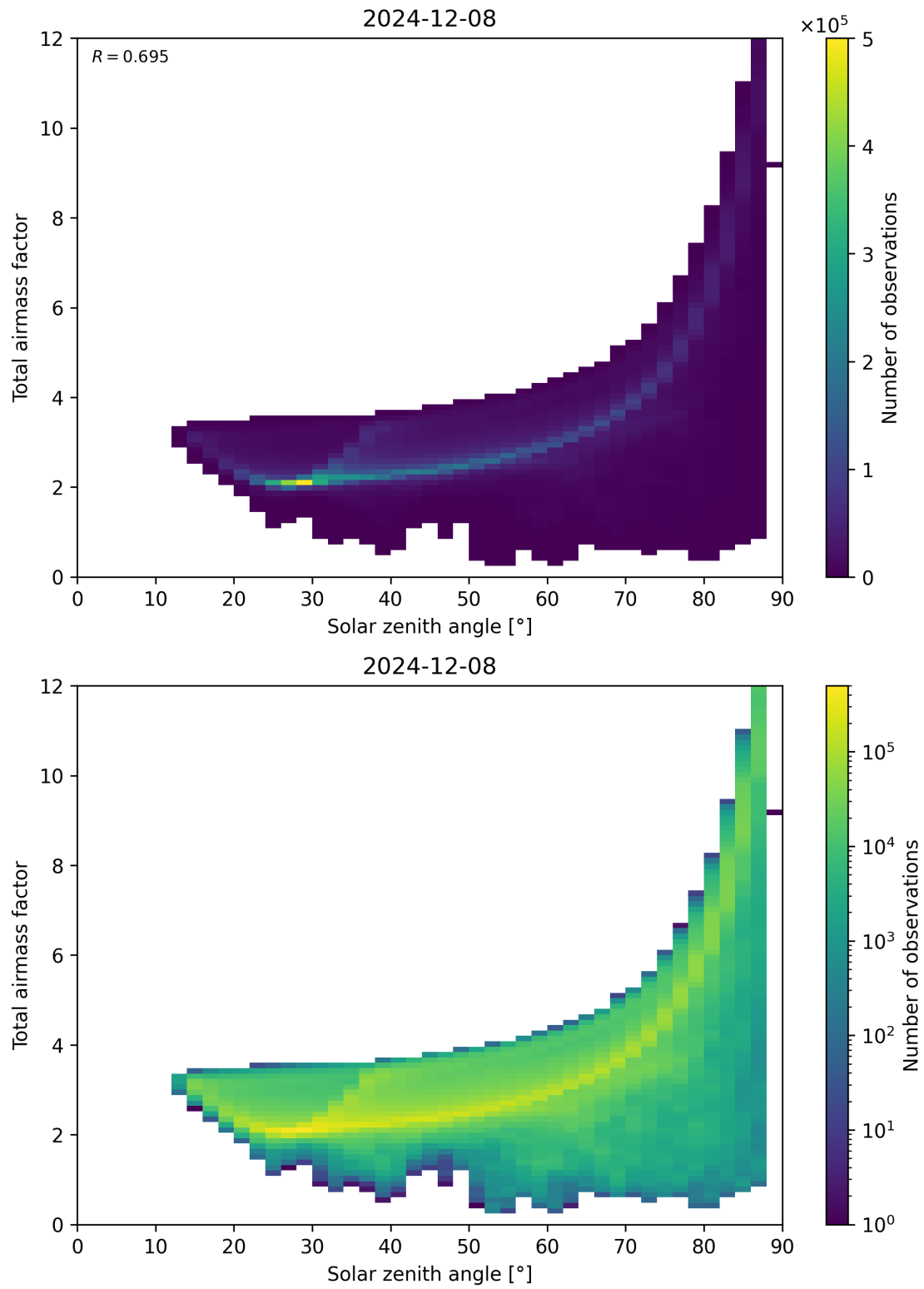
Figure 146: Scatter density plot of “Solar zenith angle” against “Total air mass factor” for 2024-12-07 to 2024-12-09.
