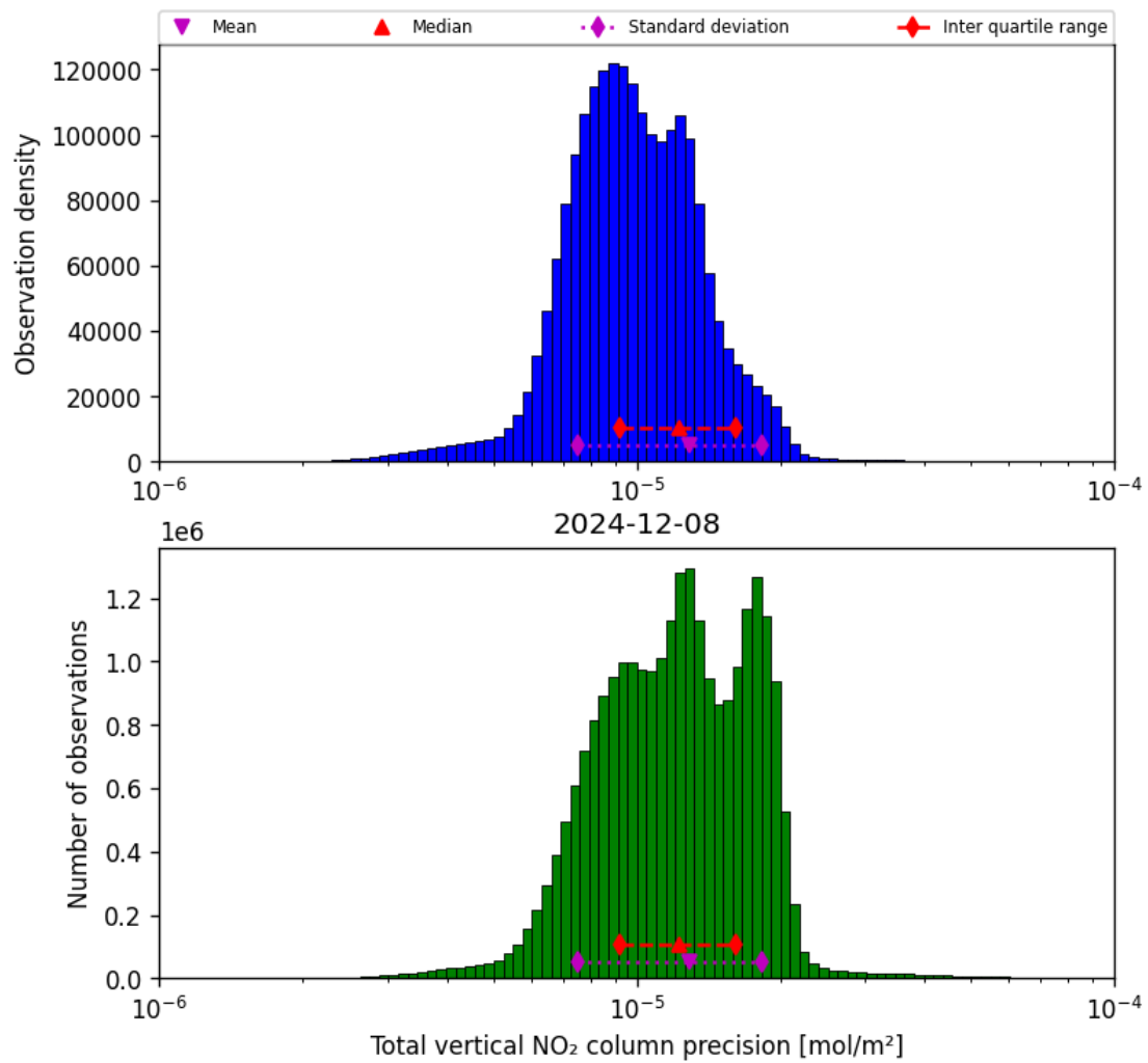
Figure 39: Histogram of “Total vertical NO 2 column precision” for 2024-12-07 to 2024-12-09
