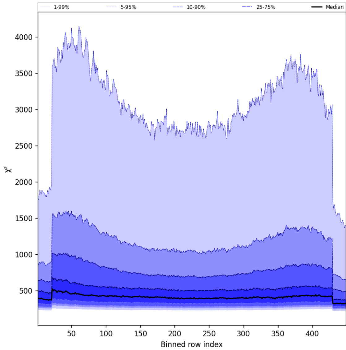
Figure 59: Along track statistics of “ \chi^2 ” for 2024-12-08 to 2024-12-10
