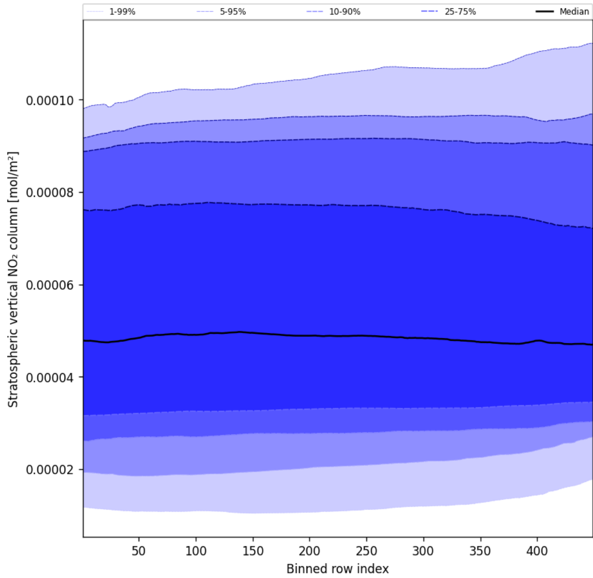
Figure 53: Along track statistics of “Stratospheric vertical NO 2 column” for 2024-12-08 to 2024-12-10
