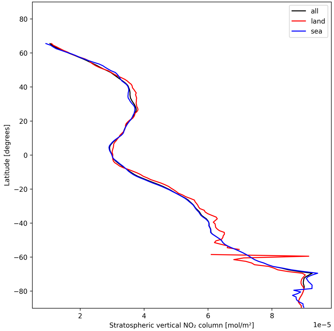
Figure 19: Zonal average of “Stratospheric vertical NO 2 column” for 2024-12-08 to 2024-12-10.
