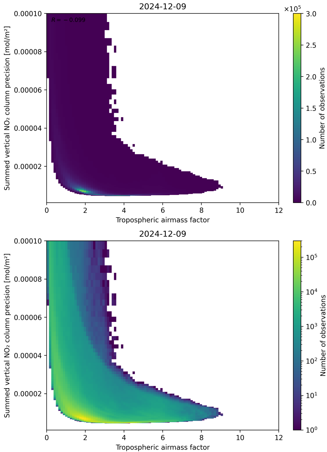
Figure 76: Scatter density plot of “Tropospheric air mass factor” against “Summed vertical NO 2 column precision” for 2024-12-08 to 2024-12-10.
