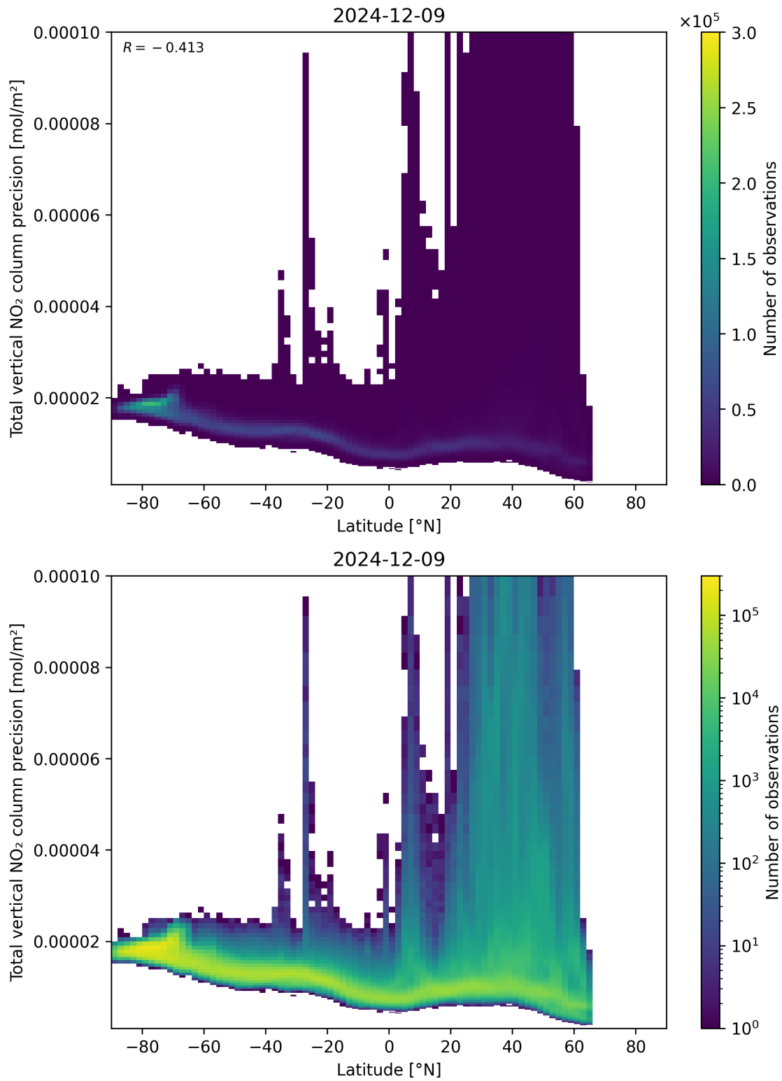
Figure 91: Scatter density plot of “Latitude” against “Total vertical NO 2 column precision” for 2024-12-08 to 2024-12-10.
