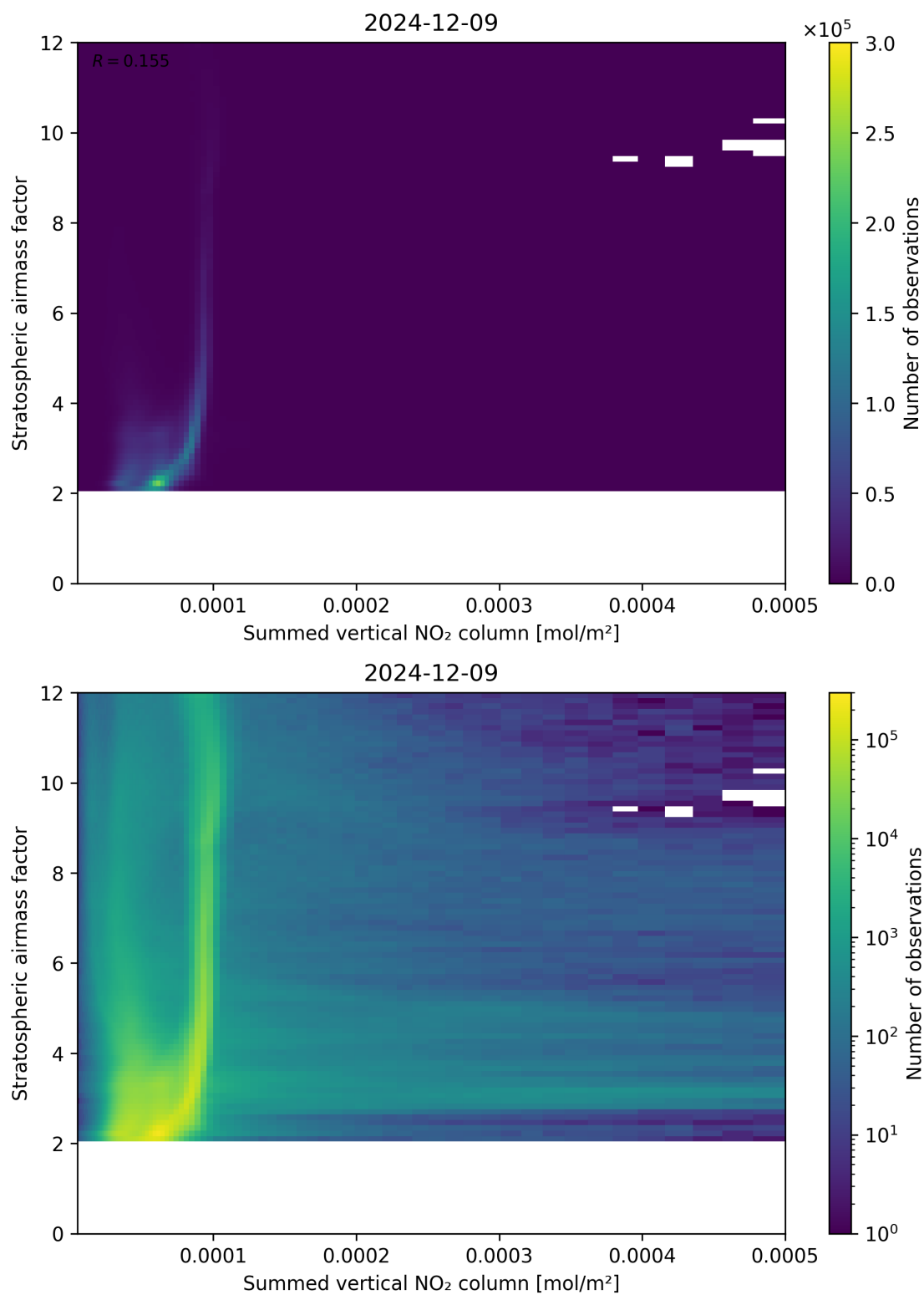
Figure 103: Scatter density plot of “Summed vertical NO 2 column” against “Stratospheric airmass factor” for 2024-12-08 to 2024-12-10.
