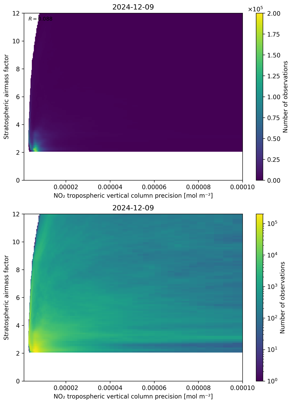
Figure 131: Scatter density plot of “NO 2 tropospheric vertical column precision” against “Stratospheric airmass factor” for 2024-12-08 to 2024-12-10.
