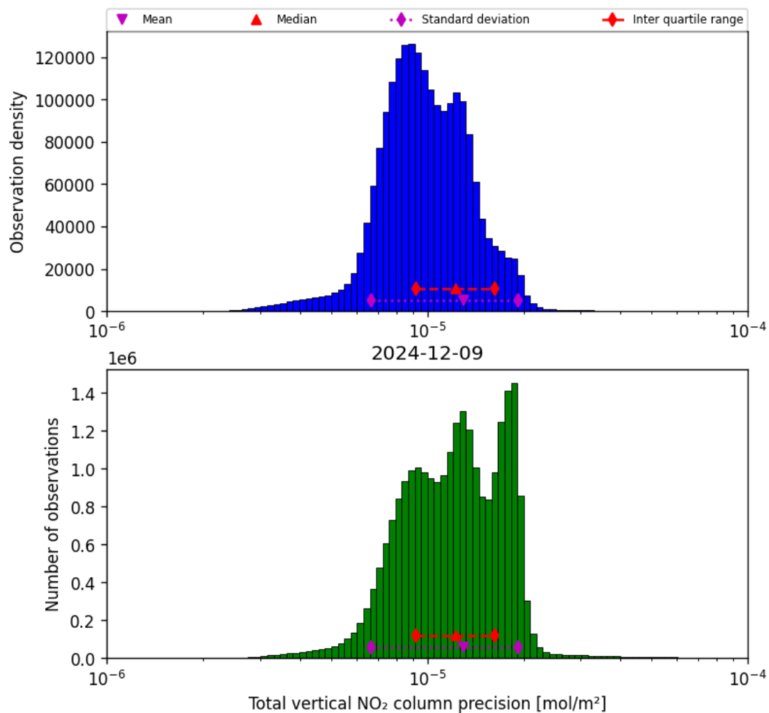
Figure 39: Histogram of “Total vertical NO 2 column precision” for 2024-12-08 to 2024-12-10
