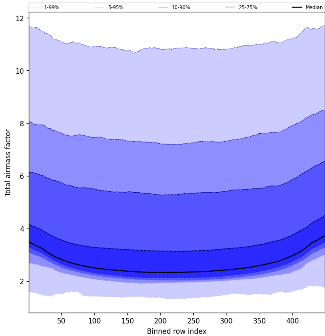
Figure 49: Along track statistics of “Total airmass factor” for 2024-12-08 to 2024-12-10
