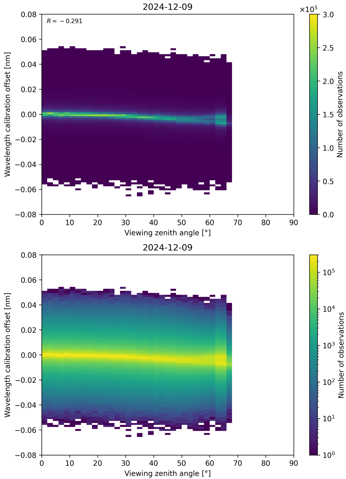
Figure 173: Scatter density plot of “Viewing zenith angle” against “Wavelength calibration offset” for 2024-12-08 to 2024-12-10.
