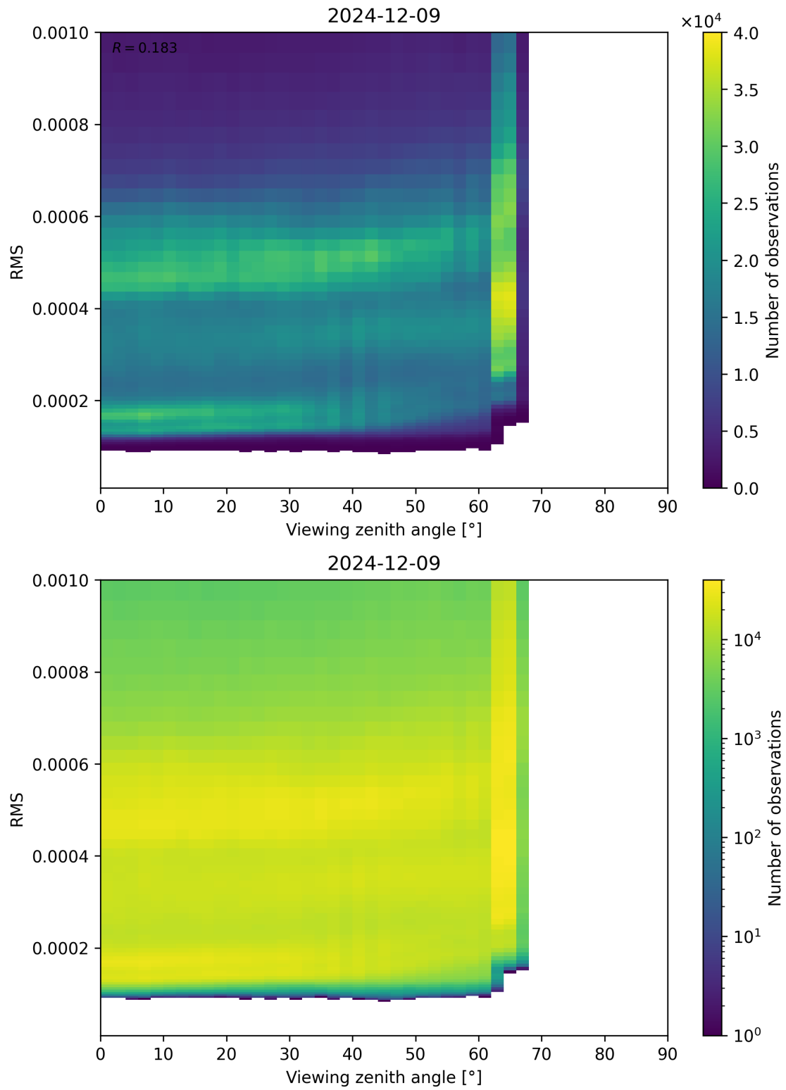
Figure 171: Scatter density plot of “Viewing zenith angle” against “RMS” for 2024-12-08 to 2024-12-10.
