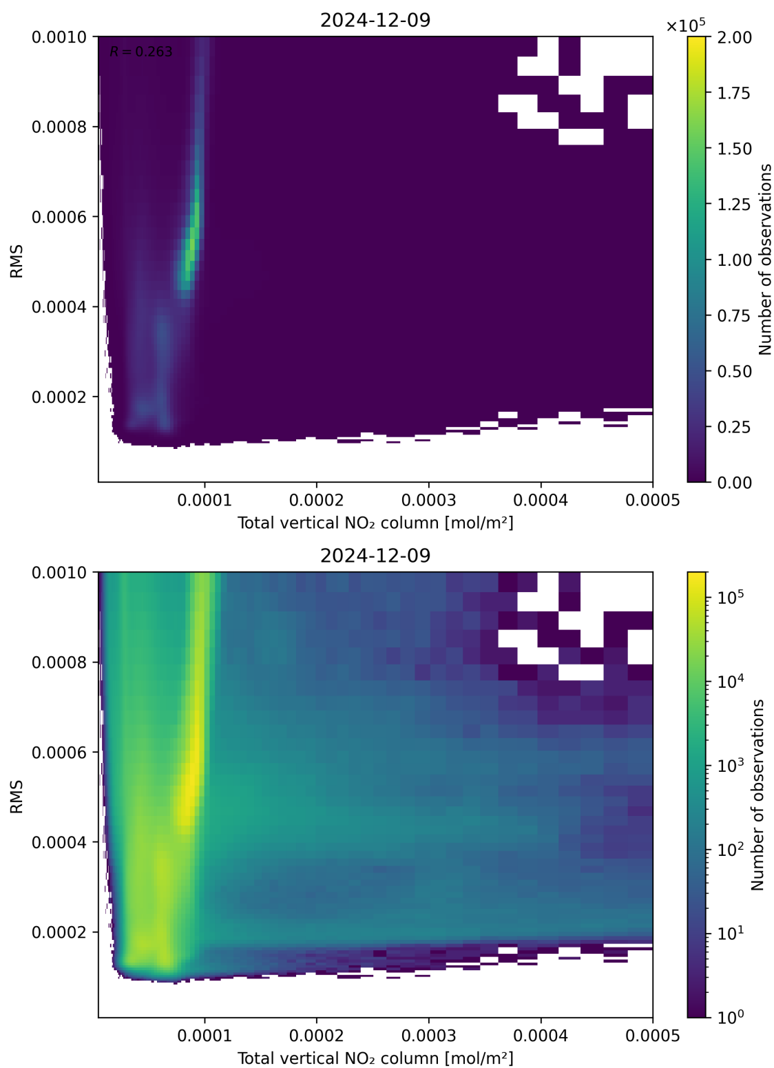
Figure 120: Scatter density plot of “Total vertical NO 2 column” against “RMS” for 2024-12-08 to 2024-12-10.
