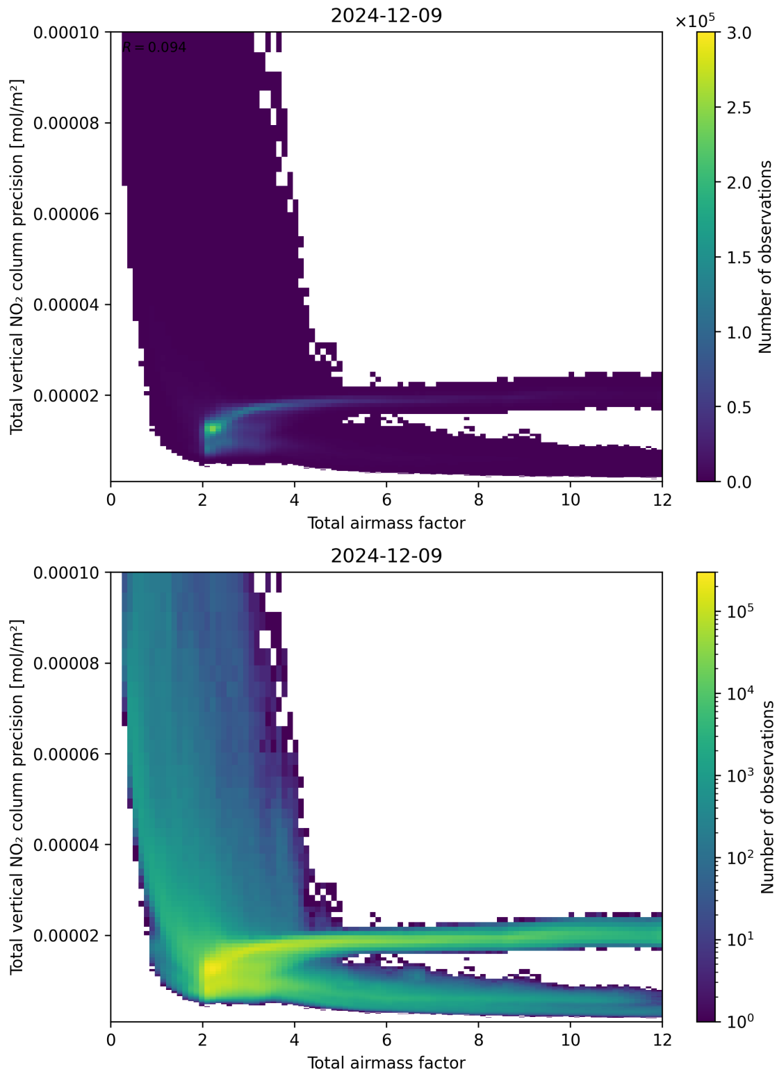
Figure 68: Scatter density plot of “Total airmass factor” against “Total vertical NO 2 column precision” for 2024-12-08 to 2024-12-10.
