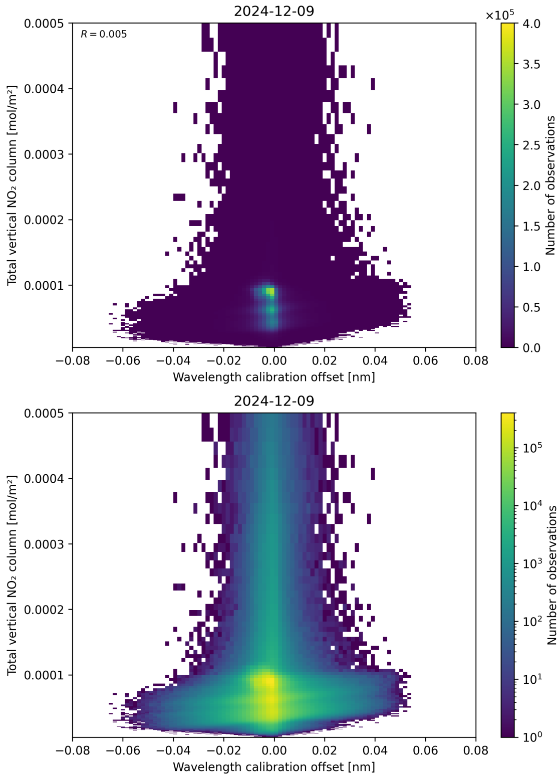
Figure 179: Scatter density plot of “Wavelength calibration offset” against “Total vertical NO 2 column” for 2024-12-08 to 2024-12-10.
