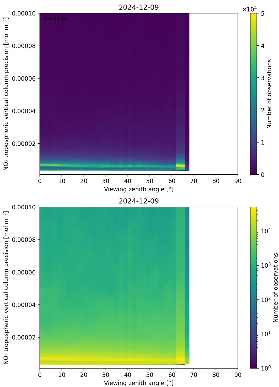
Figure 170: Scatter density plot of “Viewing zenith angle” against “NO 2 tropospheric vertical column precision” for 2024-12-08 to 2024-12-10.
