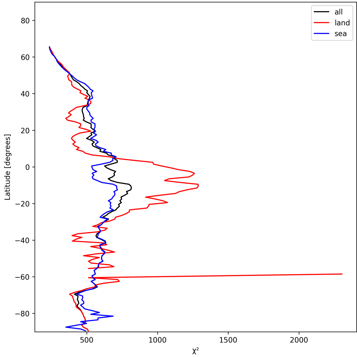
Figure 25: Zonal average of “ \chi^2 ” for 2024-12-08 to 2024-12-10.
