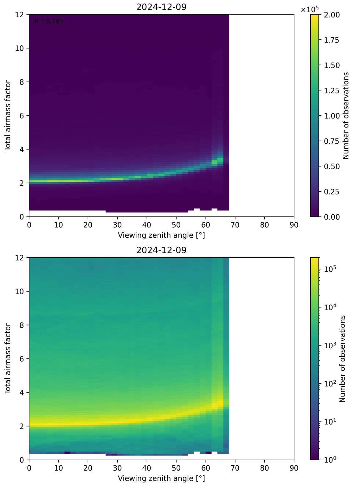
Figure 160: Scatter density plot of “Viewing zenith angle” against “Total airmass factor” for 2024-12-08 to 2024-12-10.
