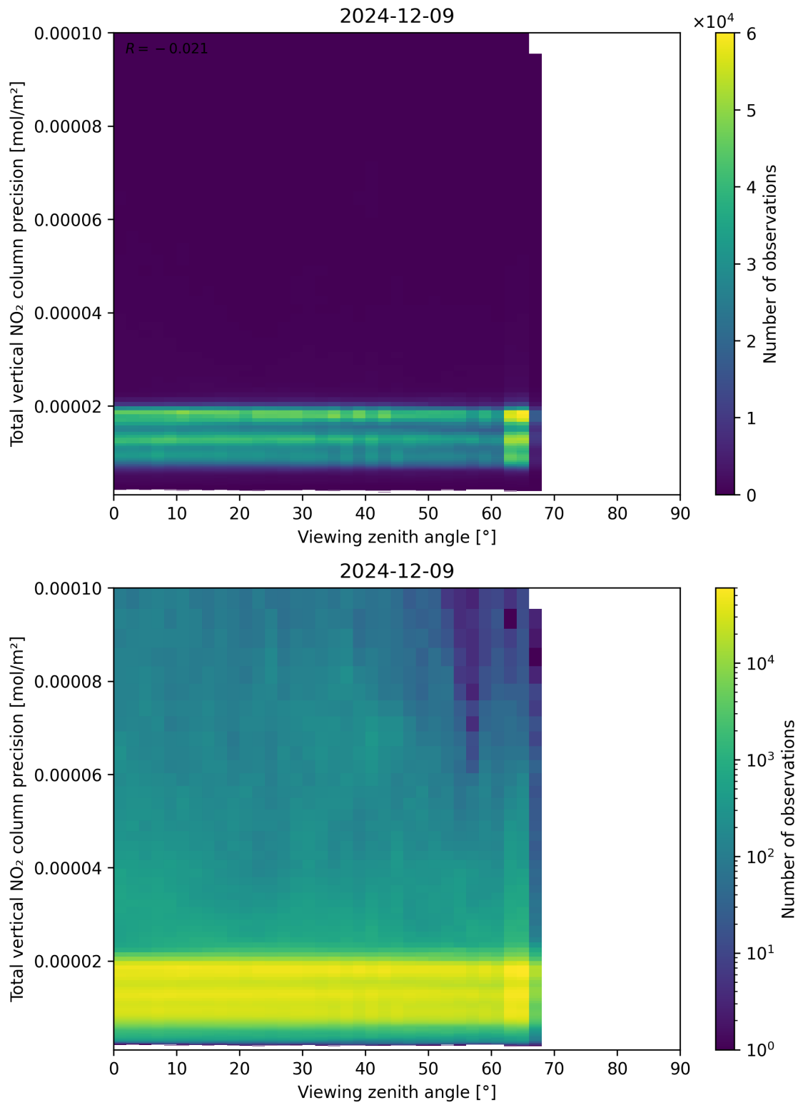
Figure 168: Scatter density plot of “Viewing zenith angle” against “Total vertical NO 2 column precision” for 2024-12-08 to 2024-12-10.
