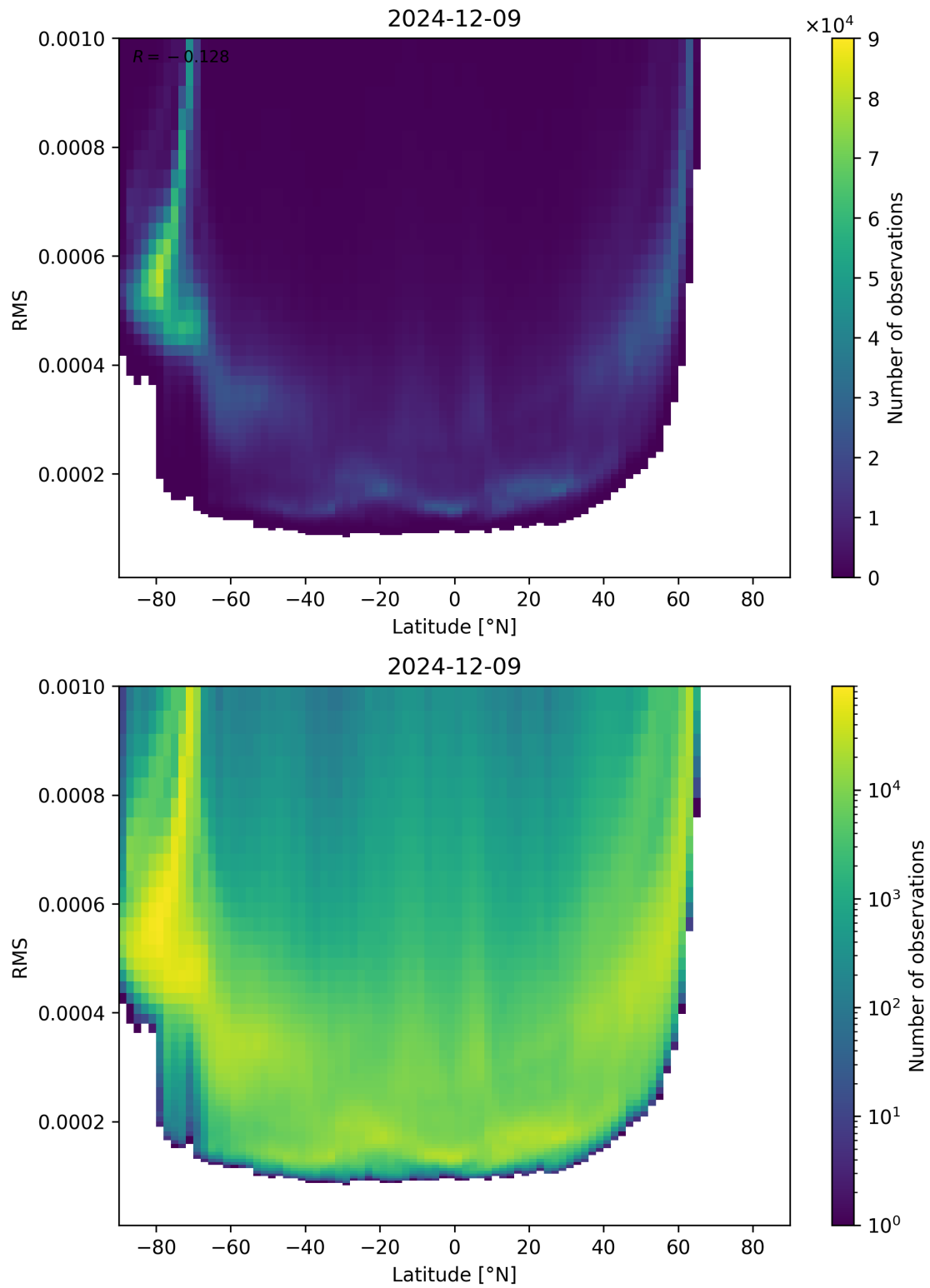
Figure 94: Scatter density plot of “Latitude” against “RMS” for 2024-12-08 to 2024-12-10.
