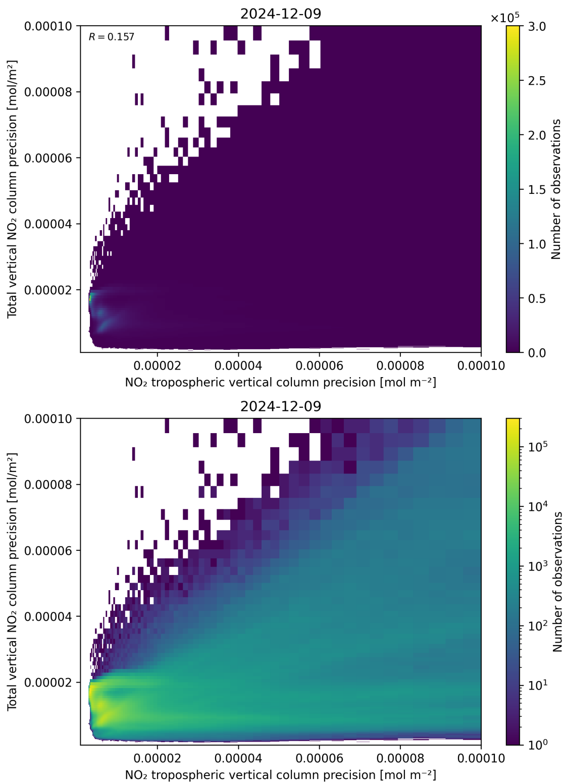
Figure 139: Scatter density plot of “NO 2 tropospheric vertical column precision” against “Total vertical NO 2 column precision” for 2024-12-08 to 2024-12-10.
