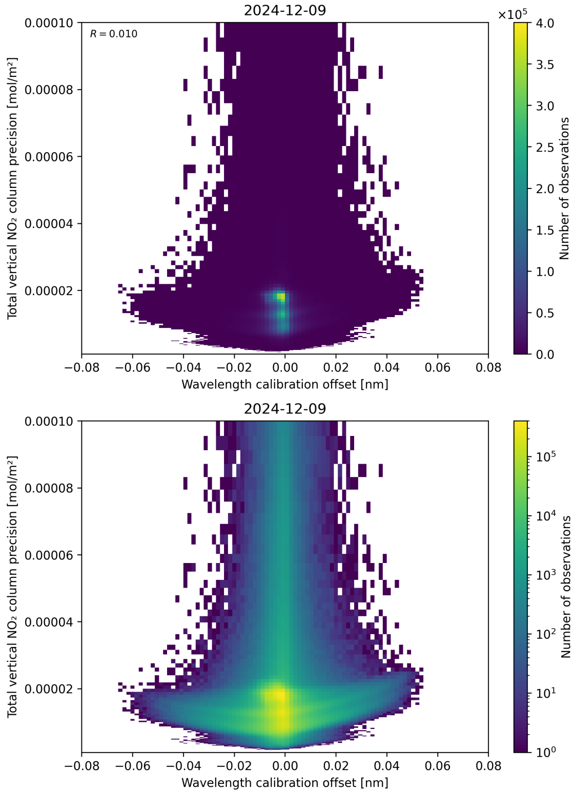
Figure 180: Scatter density plot of “Wavelength calibration offset” against “Total vertical NO 2 column precision” for 2024-12-08 to 2024-12-10.
