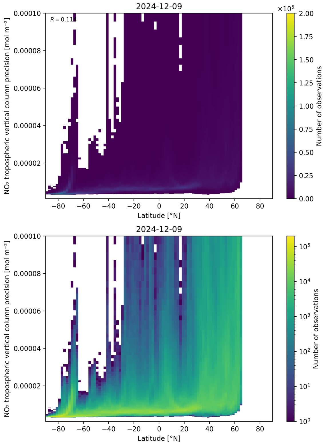
Figure 93: Scatter density plot of “Latitude” against “NO 2 tropospheric vertical column precision” for 2024-12-08 to 2024-12-10.
