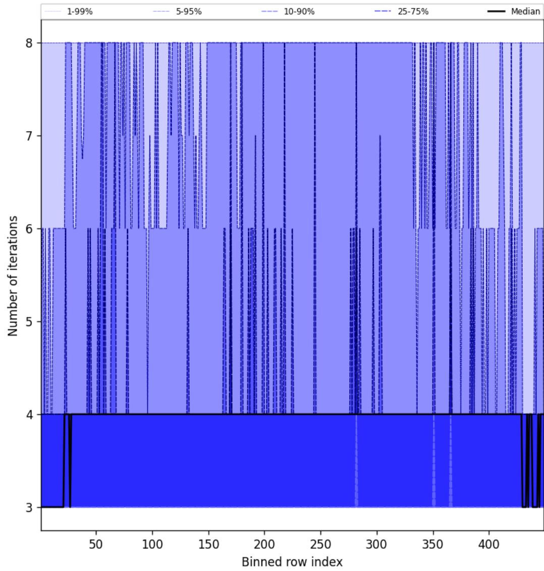
Figure 51: Along track statistics of “Number of iterations” for 2024-12-08 to 2024-12-10
