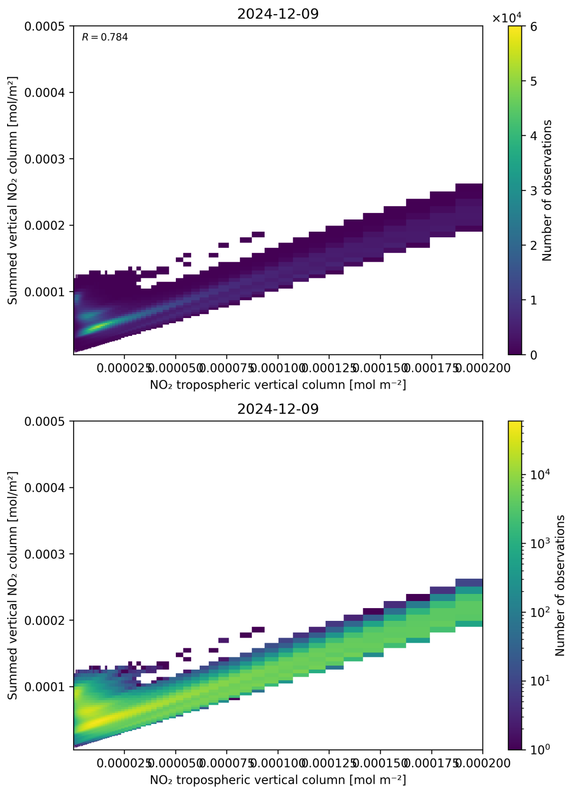
Figure 126: Scatter density plot of “NO 2 tropospheric vertical column” against “Summed vertical NO 2 column” for 2024-12-08 to 2024-12-10.
