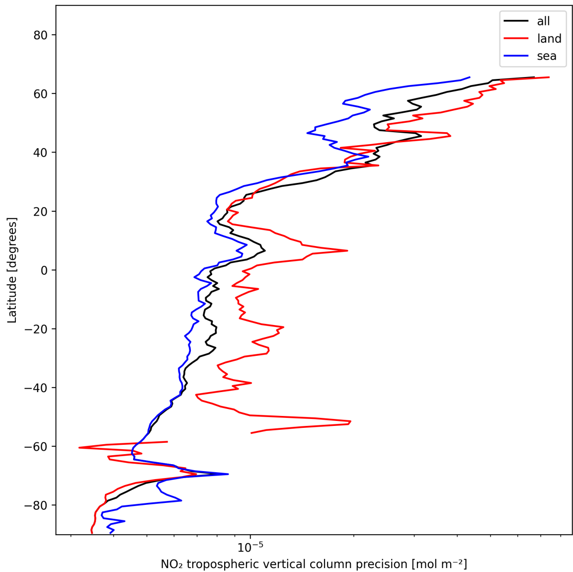
Figure 13: Zonal average of “NO 2 tropospheric vertical column precision” for 2024-12-08 to 2024-12-10.
