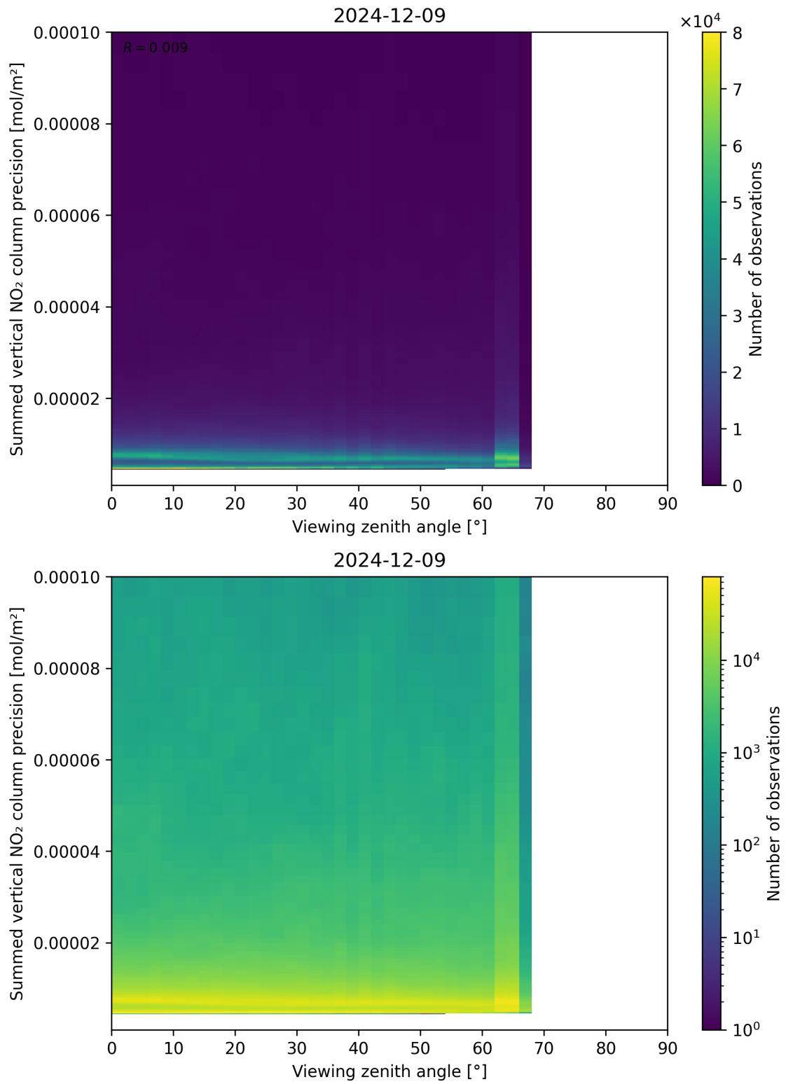
Figure 166: Scatter density plot of “Viewing zenith angle” against “Summed vertical NO 2 column precision” for 2024-12-08 to 2024-12-10.
