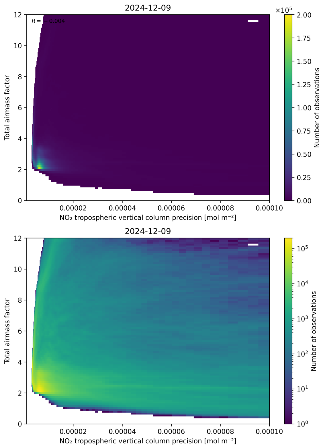
Figure 132: Scatter density plot of “NO 2 tropospheric vertical column precision” against “Total air mass factor” for 2024-12-08 to 2024-12-10.
