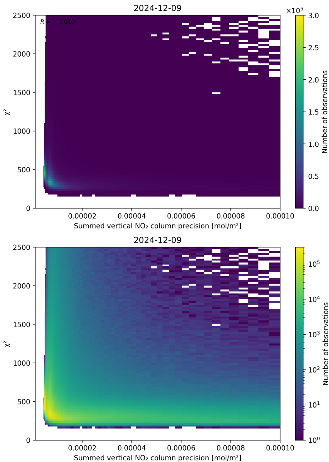
Figure 107: Scatter density plot of “Summed vertical NO 2 column precision” against “ \chi^2 ” for 2024-12-08 to 2024-12-10.
