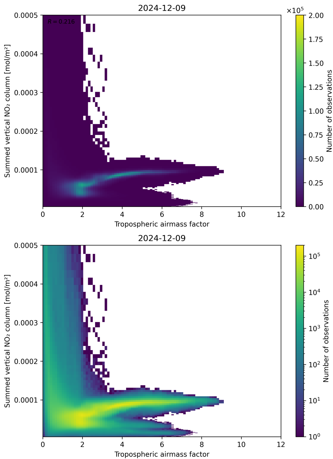
Figure 75: Scatter density plot of “Tropospheric air mass factor” against “Summed vertical NO 2 column” for 2024-12-08 to 2024-12-10.
