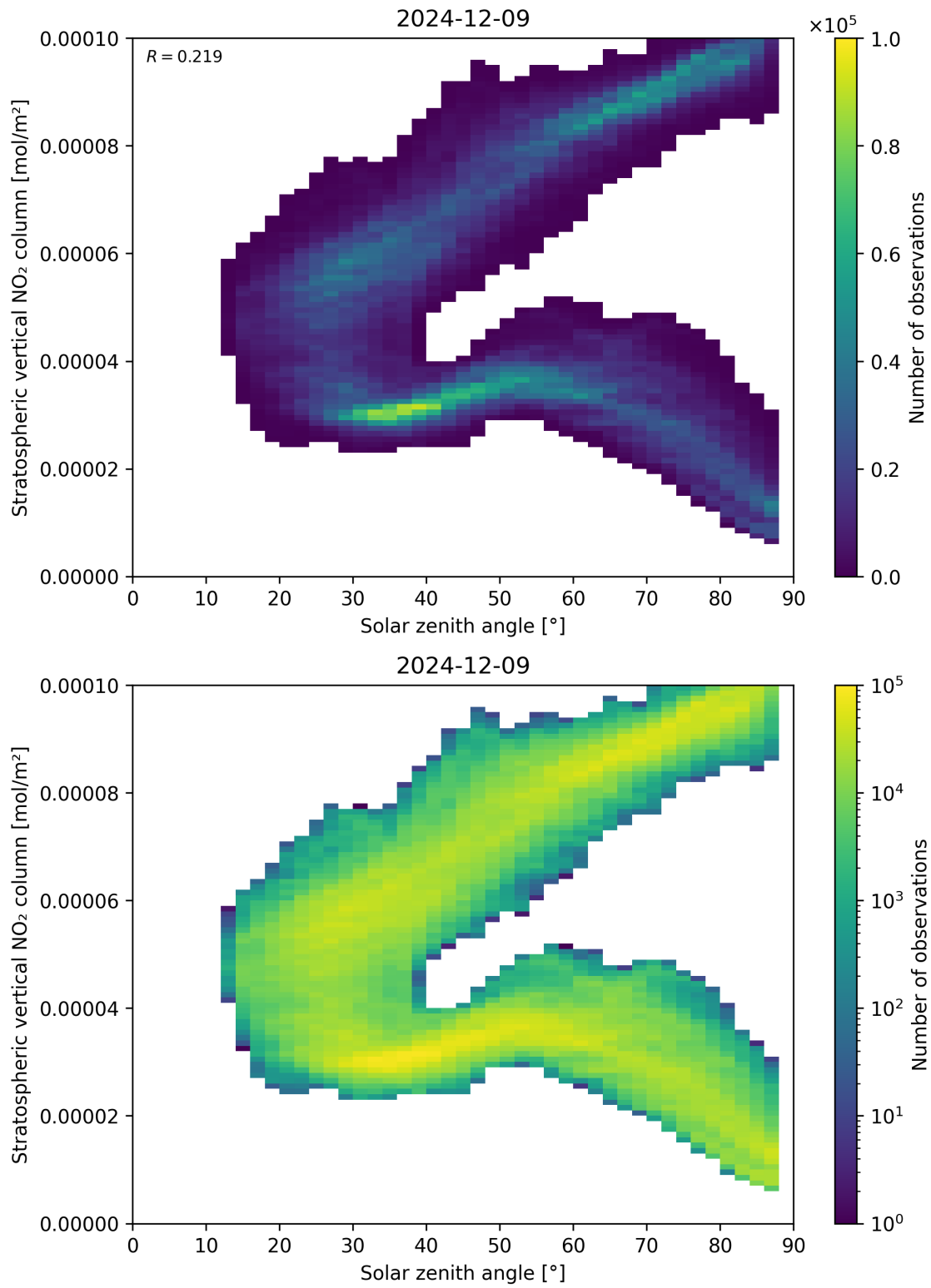
Figure 150: Scatter density plot of “Solar zenith angle” against “Stratospheric vertical NO 2 column” for 2024-12-08 to 2024-12-10.
