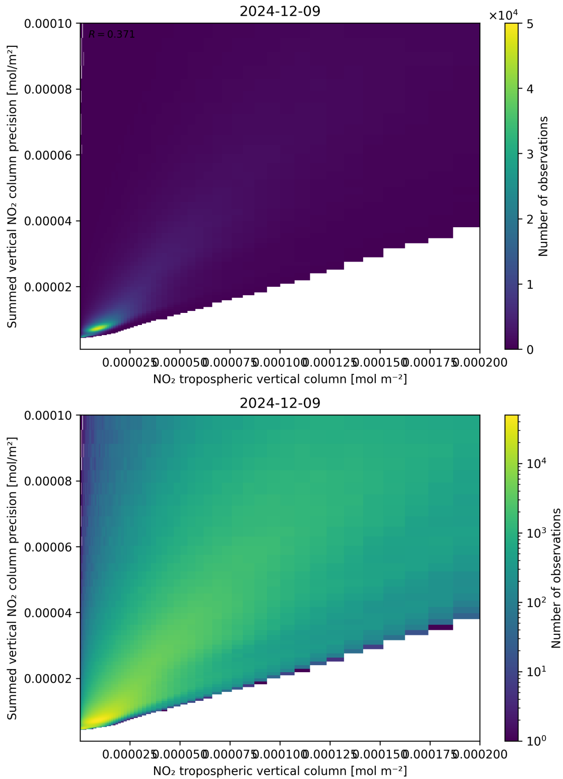
Figure 127: Scatter density plot of “NO 2 tropospheric vertical column” against “Summed vertical NO 2 column precision” for 2024-12-08 to 2024-12-10.
