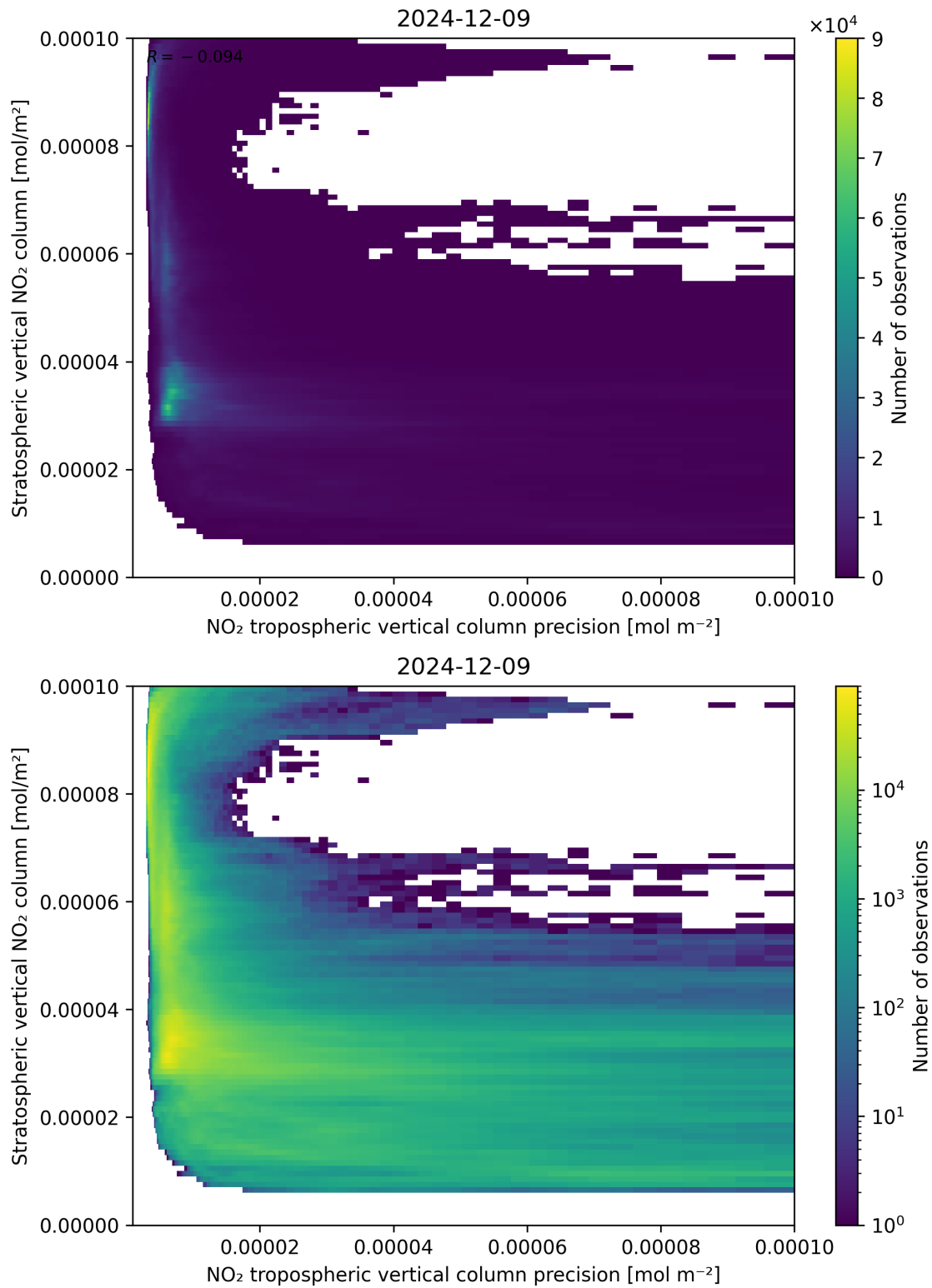
Figure 135: Scatter density plot of “NO 2 tropospheric vertical column precision” against “Stratospheric vertical NO 2 column” for 2024-12-08 to 2024-12-10.
