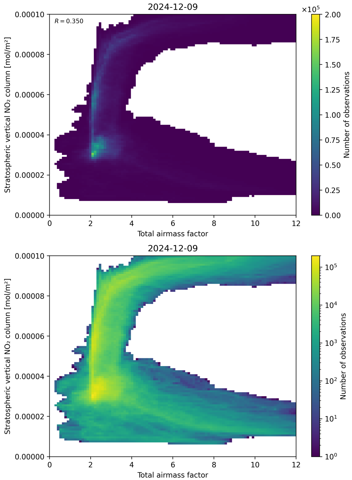
Figure 64: Scatter density plot of “Total airmass factor” against “Stratospheric vertical NO 2 column” for 2024-12-08 to 2024-12-10.
