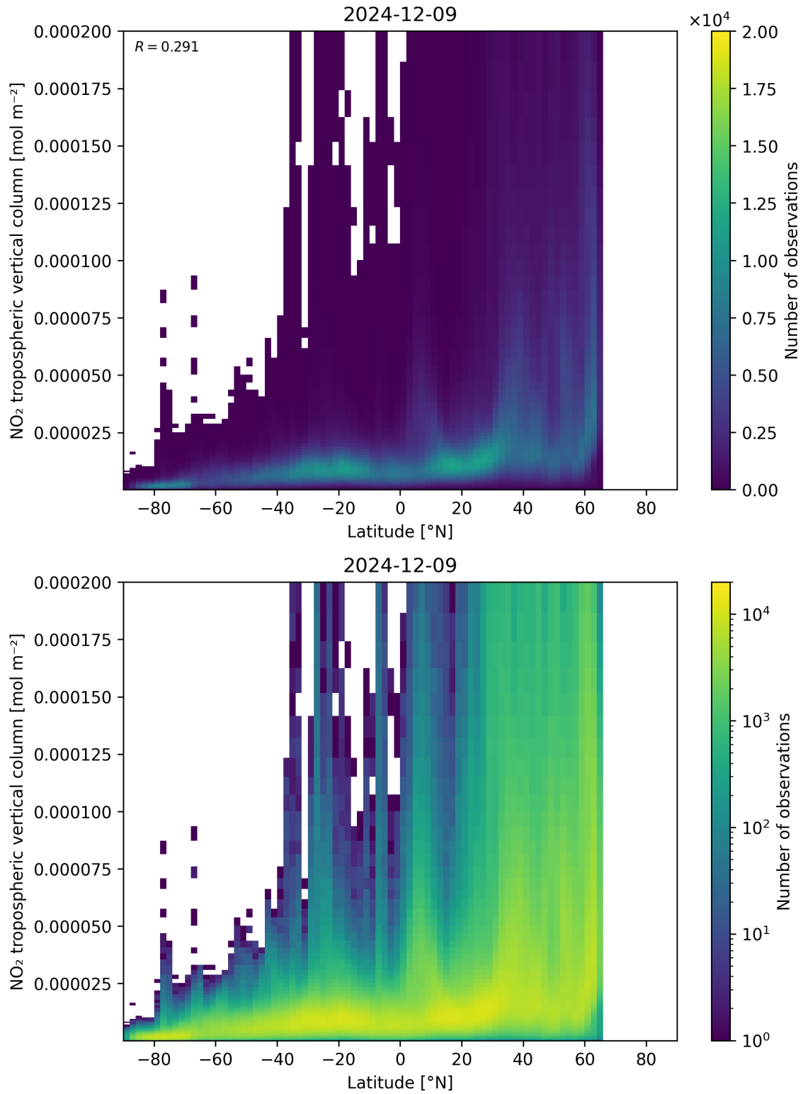
Figure 92: Scatter density plot of “Latitude” against “NO 2 tropospheric vertical column” for 2024-12-08 to 2024-12-10.
