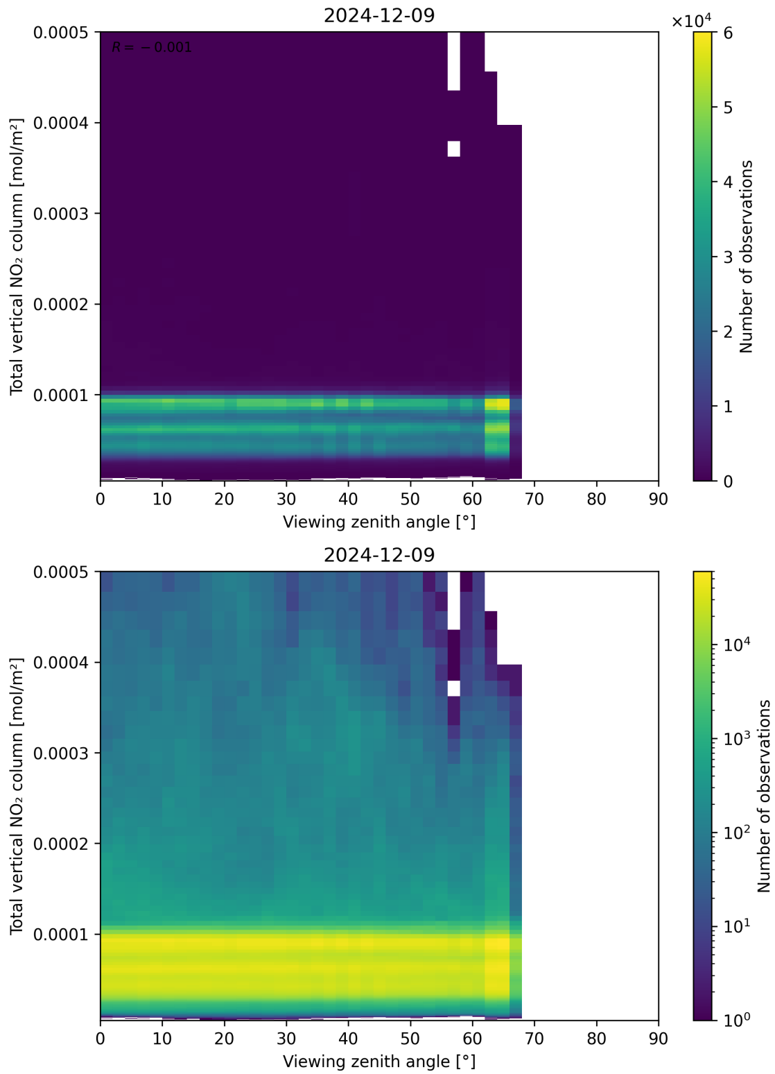
Figure 167: Scatter density plot of “Viewing zenith angle” against “Total vertical NO 2 column” for 2024-12-08 to 2024-12-10.
