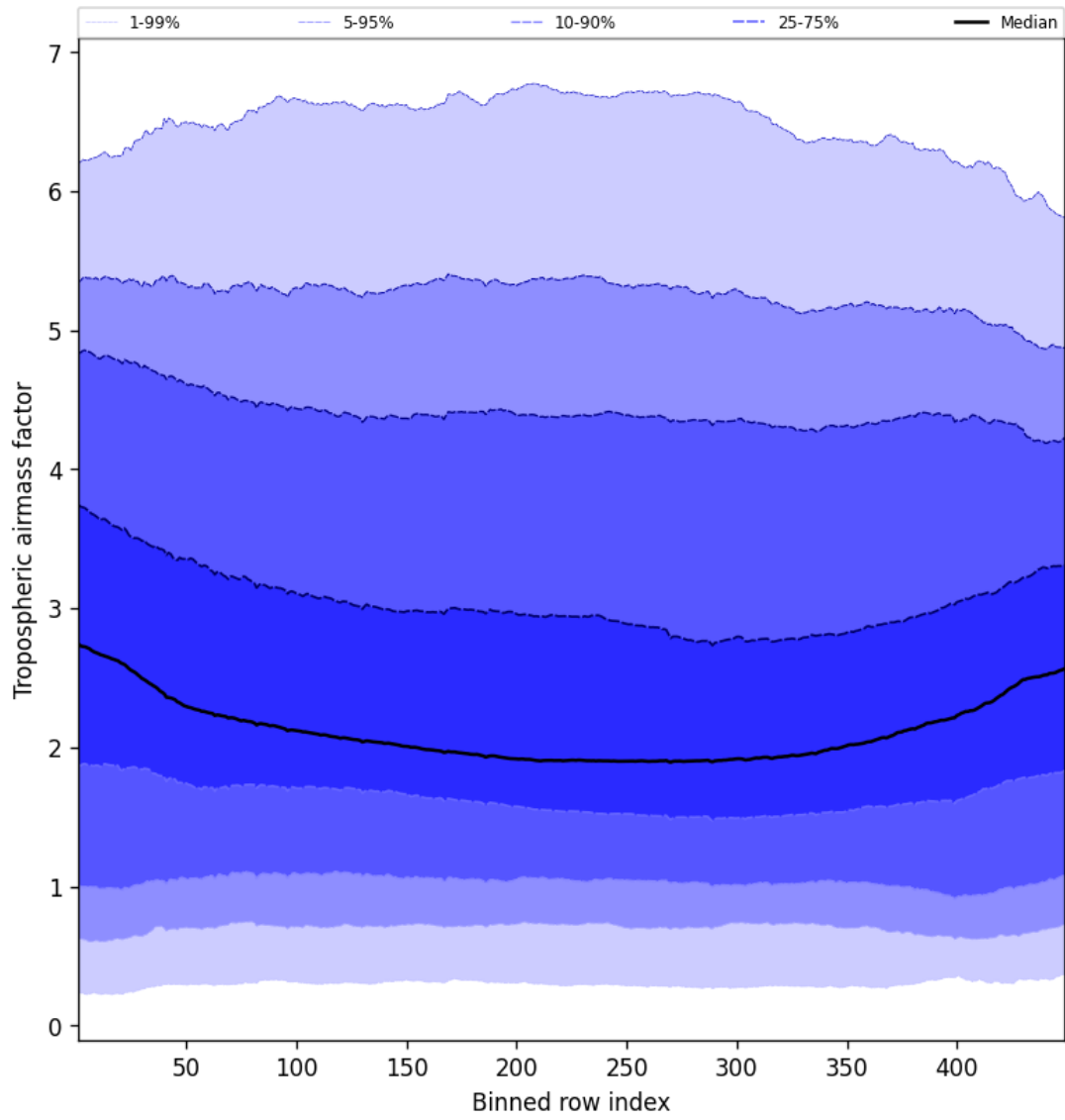
Figure 48: Along track statistics of “Tropospheric airmass factor” for 2024-12-08 to 2024-12-10
