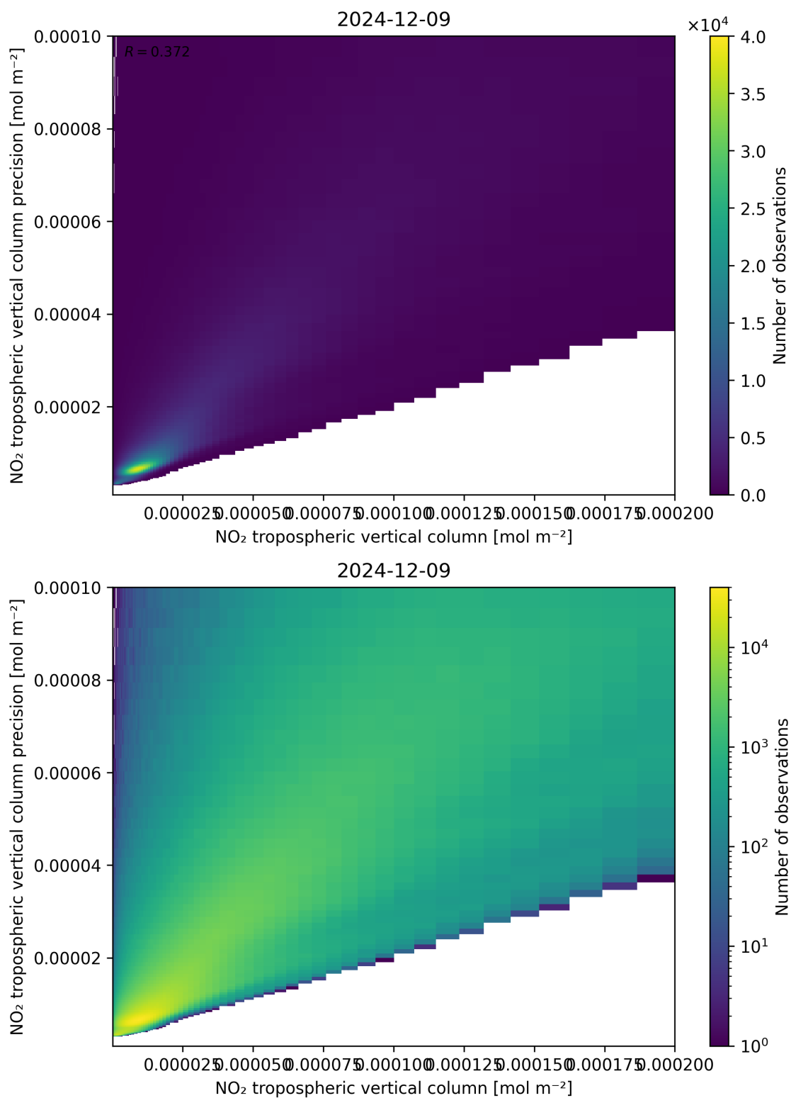
Figure 130: Scatter density plot of “NO 2 tropospheric vertical column” against “NO 2 tropospheric vertical column precision” for 2024-12-08 to 2024-12-10.
