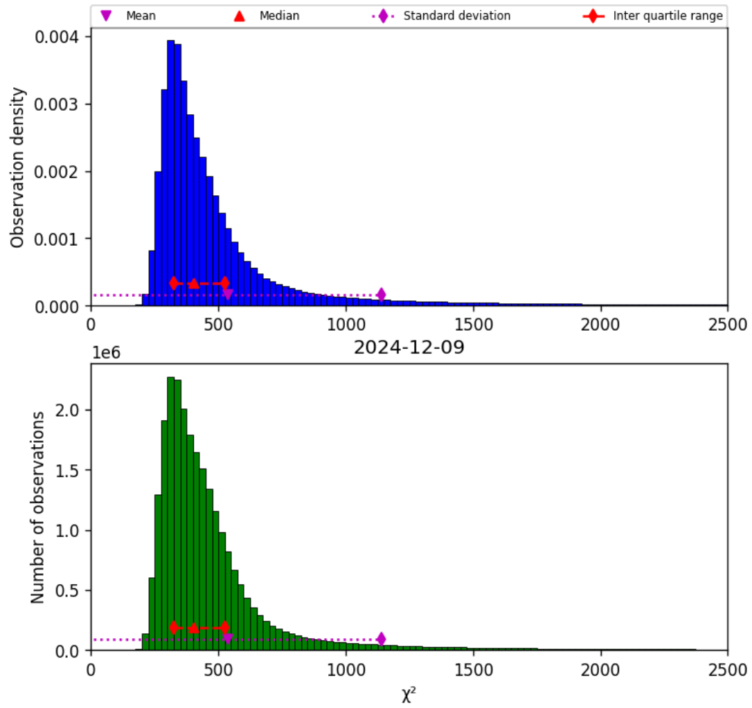
Figure 42: Histogram of “ \chi^2 ” for 2024-12-08 to 2024-12-10
