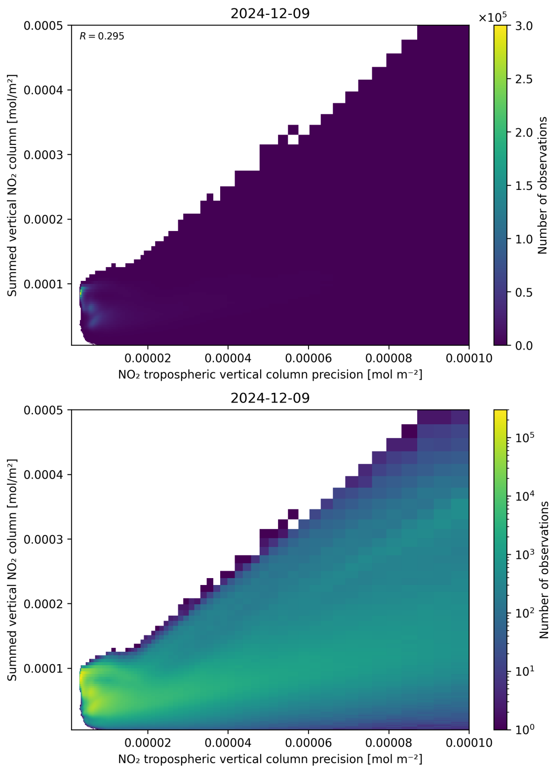
Figure 136: Scatter density plot of “NO 2 tropospheric vertical column precision” against “Summed vertical NO 2 column” for 2024-12-08 to 2024-12-10.
