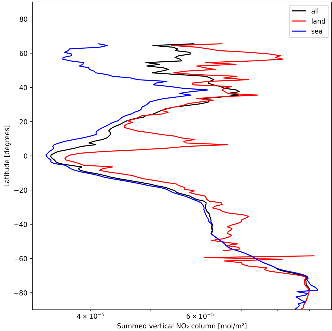
Figure 23: Zonal average of “Summed vertical NO 2 column” for 2024-12-08 to 2024-12-10.
