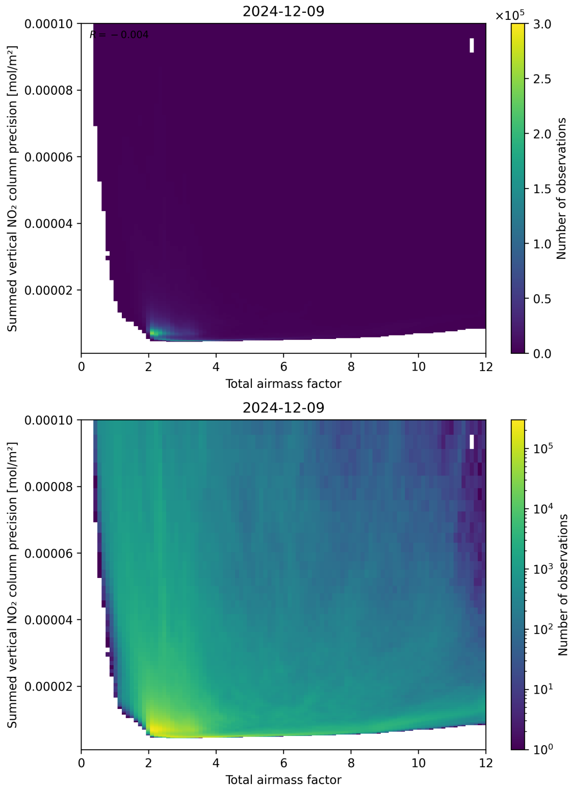
Figure 66: Scatter density plot of “Total airmass factor” against “Summed vertical NO 2 column precision” for 2024-12-08 to 2024-12-10.
