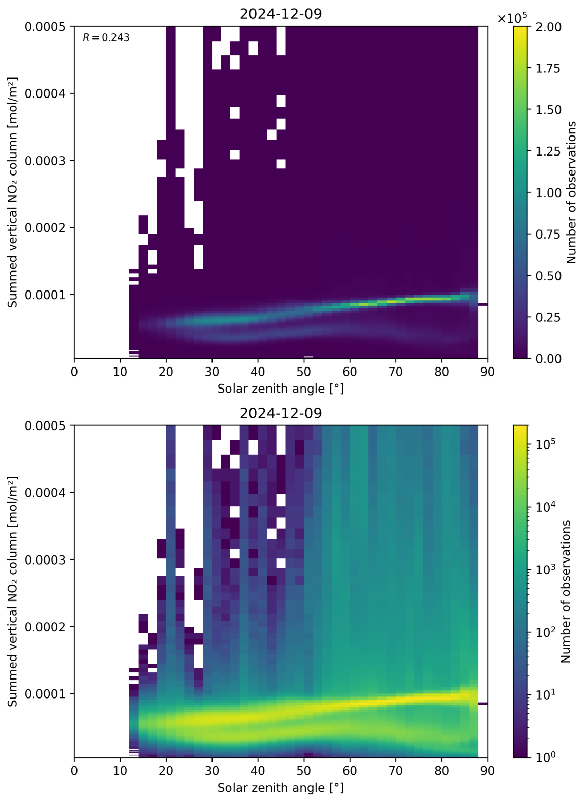
Figure 151: Scatter density plot of “Solar zenith angle” against “Summed vertical NO 2 column” for 2024-12-08 to 2024-12-10.
