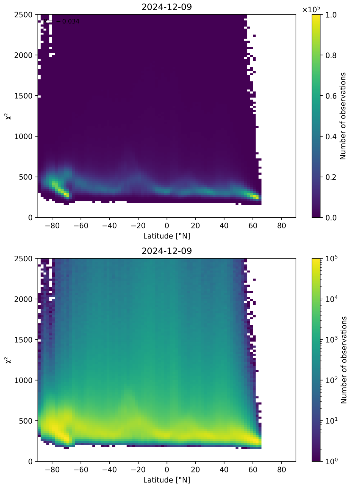
Figure 86: Scatter density plot of “Latitude” against “ \chi^2 ” for 2024-12-08 to 2024-12-10.
