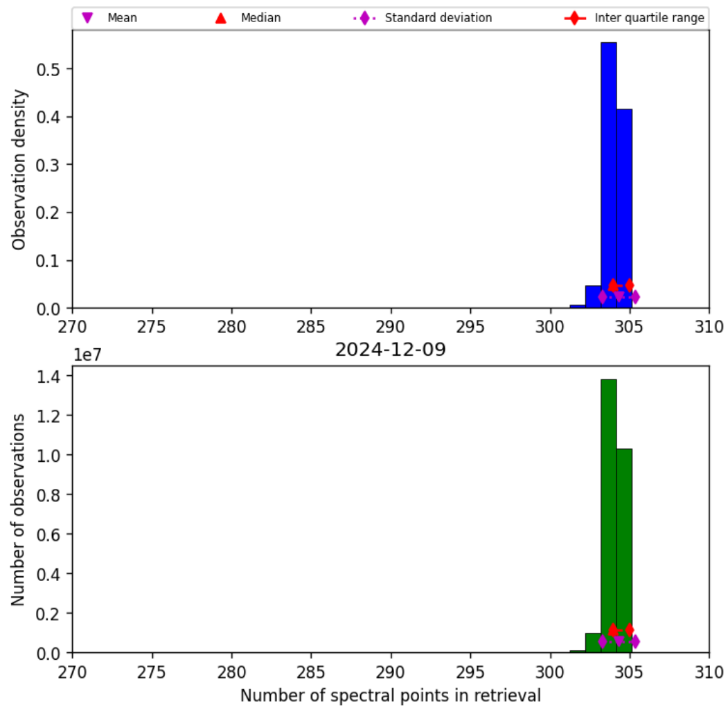
Figure 33: Histogram of “Number of spectral points in retrieval” for 2024-12-08 to 2024-12-10
