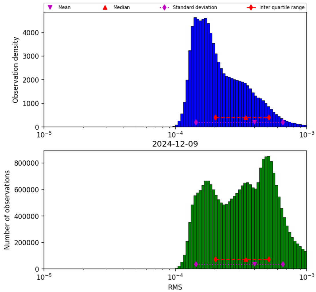
Figure 43: Histogram of “RMS” for 2024-12-08 to 2024-12-10
