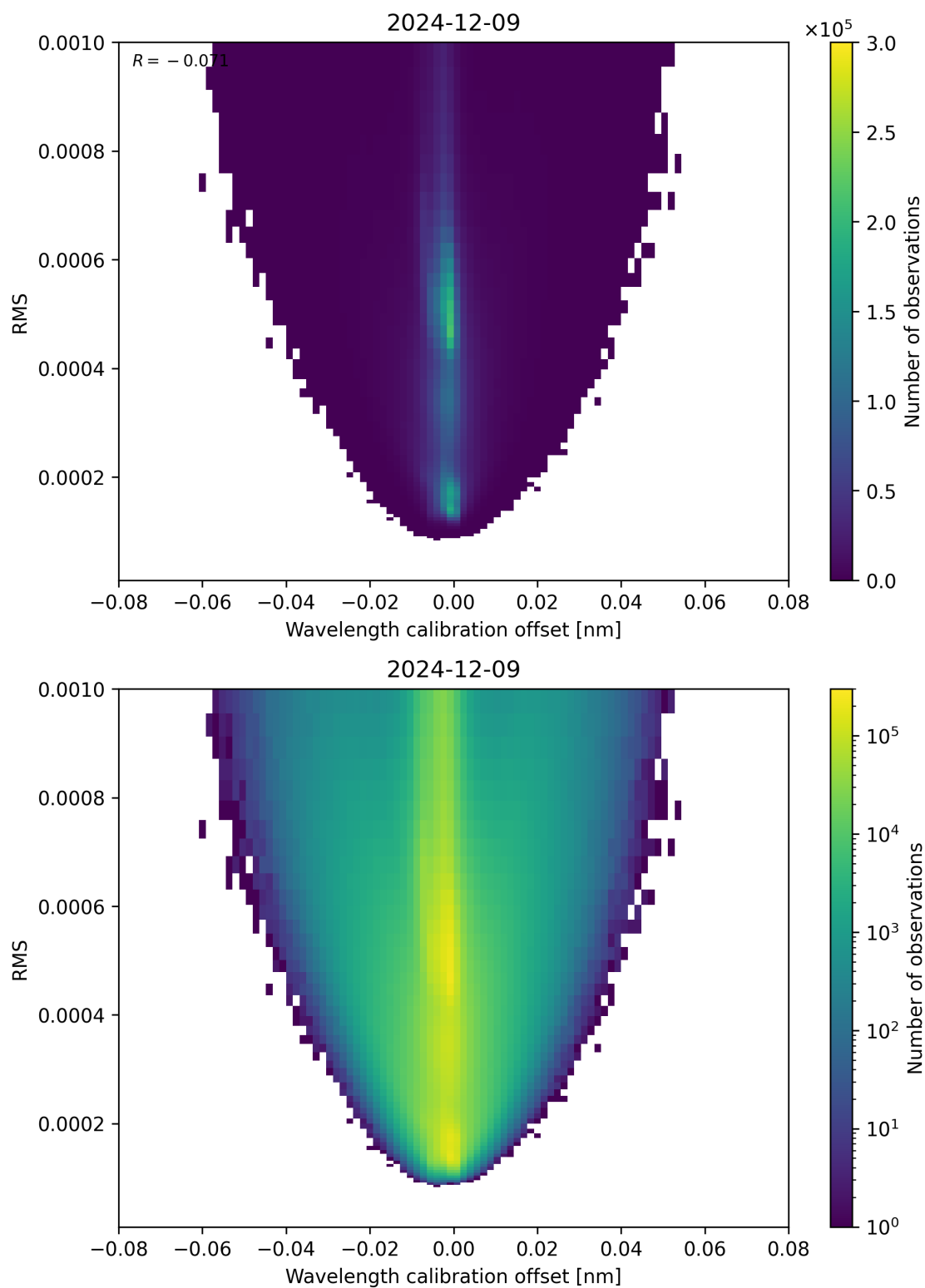
Figure 181: Scatter density plot of “Wavelength calibration offset” against “RMS” for 2024-12-08 to 2024-12-10.
