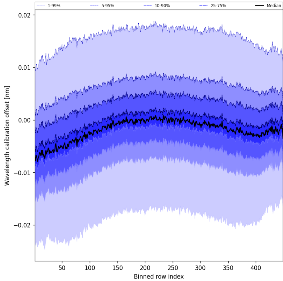
Figure 52: Along track statistics of “Wavelength calibration offset” for 2024-12-08 to 2024-12-10
