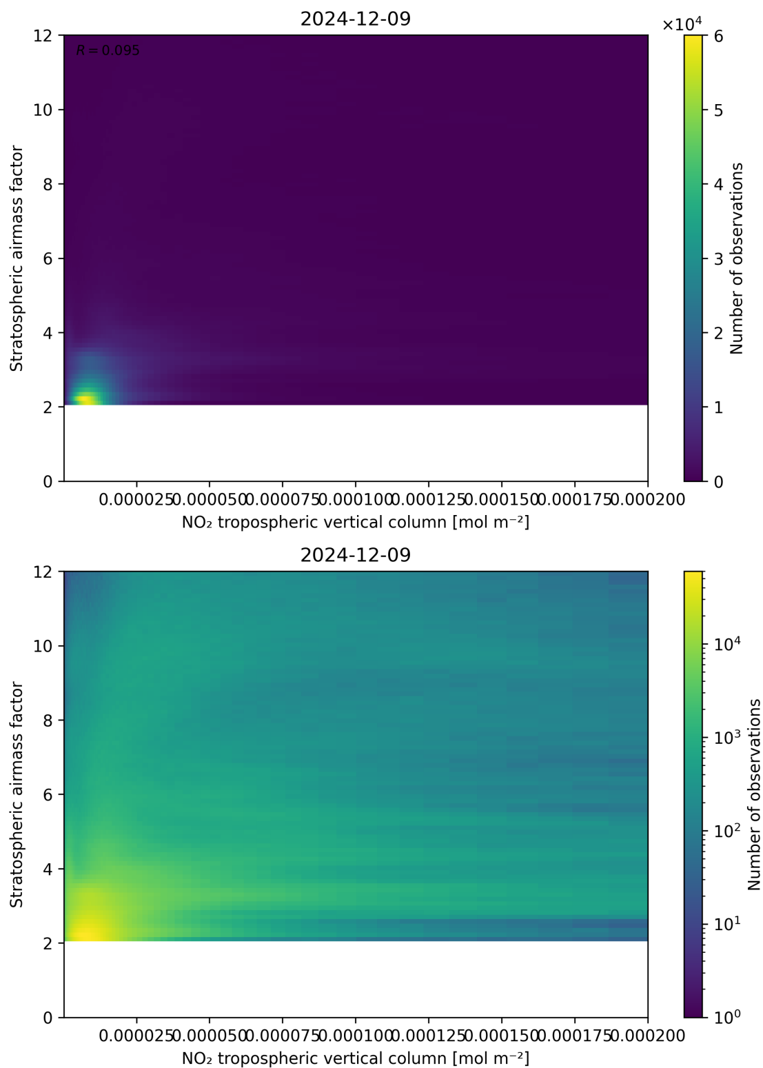
Figure 121: Scatter density plot of “NO 2 tropospheric vertical column” against “Stratospheric airmass factor” for 2024-12-08 to 2024-12-10.
