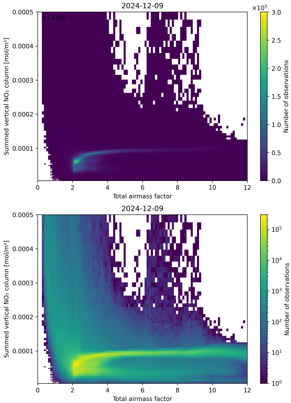
Figure 65: Scatter density plot of “Total airmass factor” against “Summed vertical NO 2 column” for 2024-12-08 to 2024-12-10.
