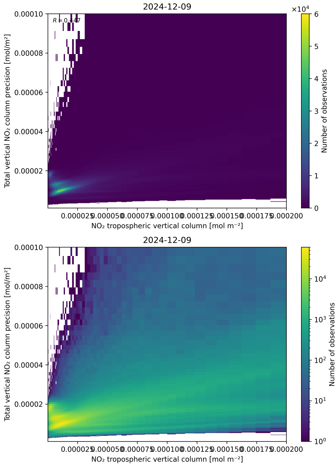
Figure 129: Scatter density plot of “NO 2 tropospheric vertical column” against “Total vertical NO 2 column precision” for 2024-12-08 to 2024-12-10.
