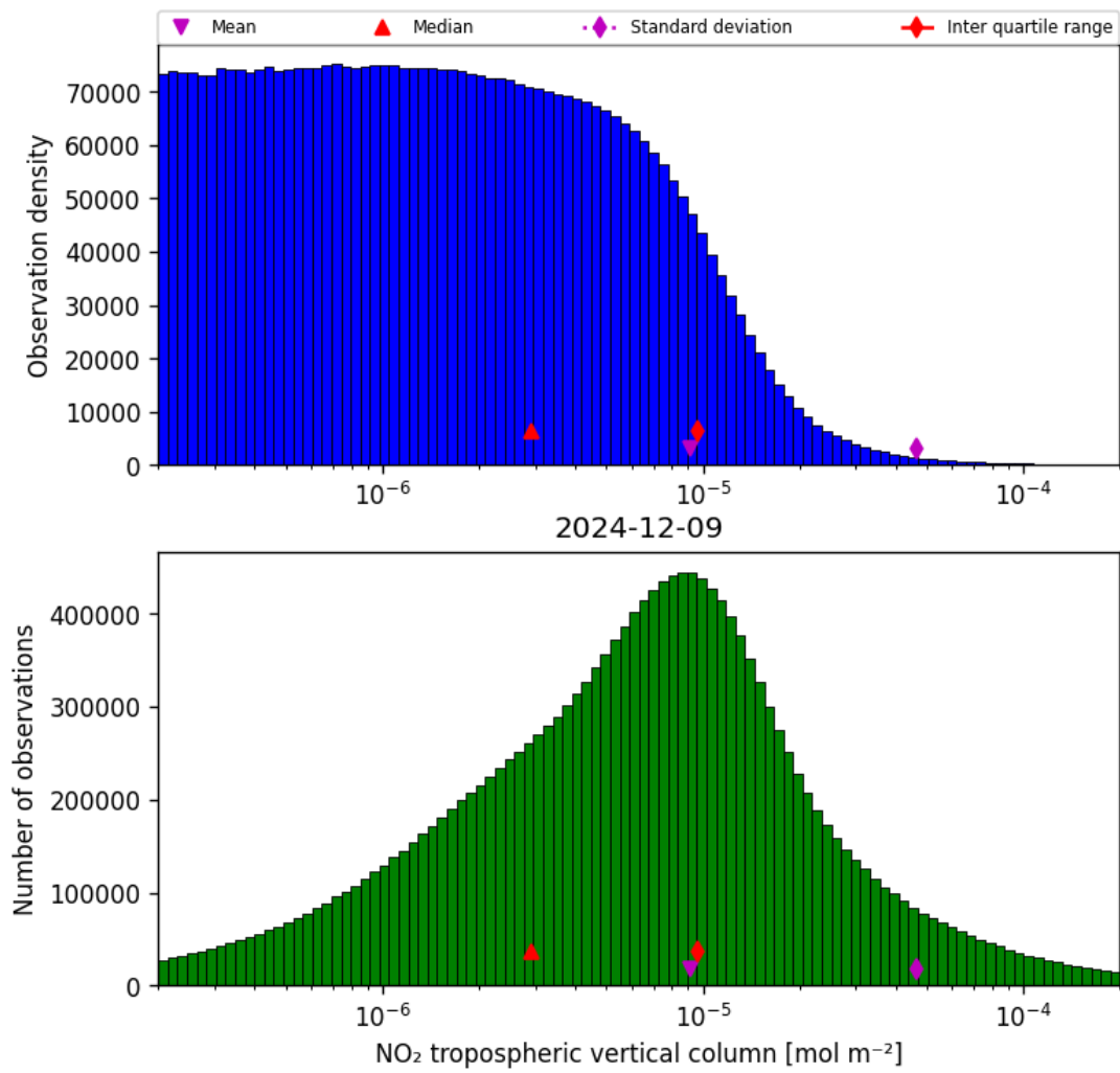
Figure 29: Histogram of “NO 2 tropospheric vertical column” for 2024-12-08 to 2024-12-10
