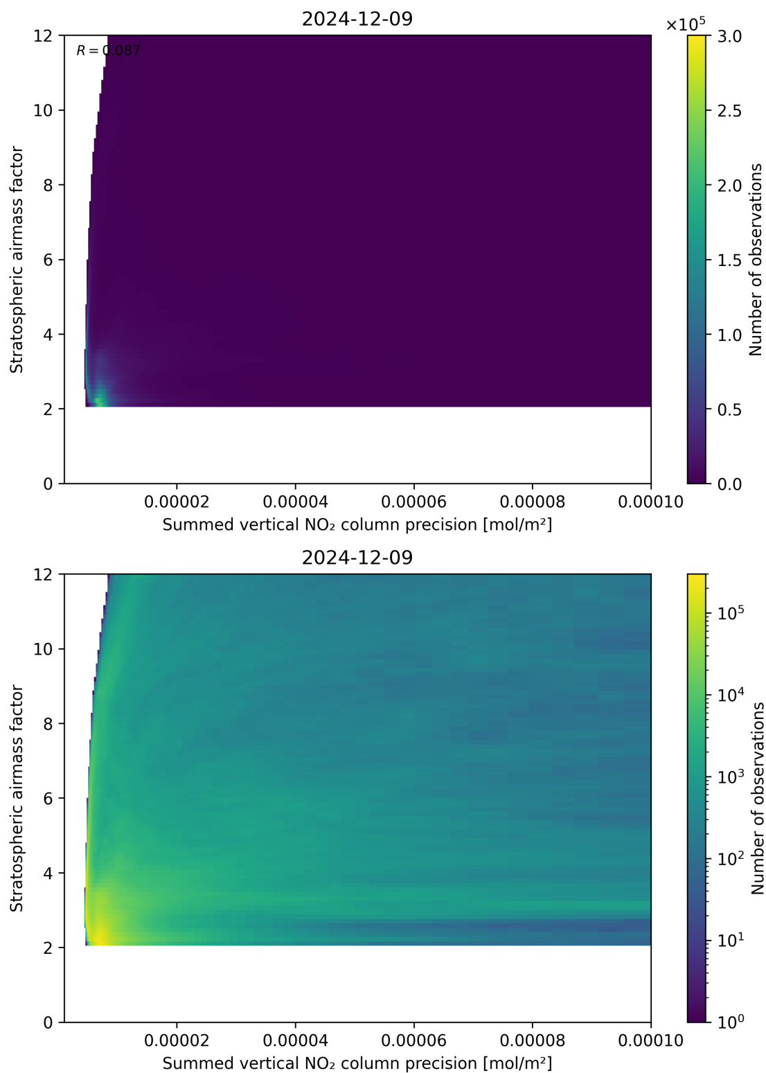
Figure 106: Scatter density plot of “Summed vertical NO 2 column precision” against “Stratospheric airmass factor” for 2024-12-08 to 2024-12-10.
