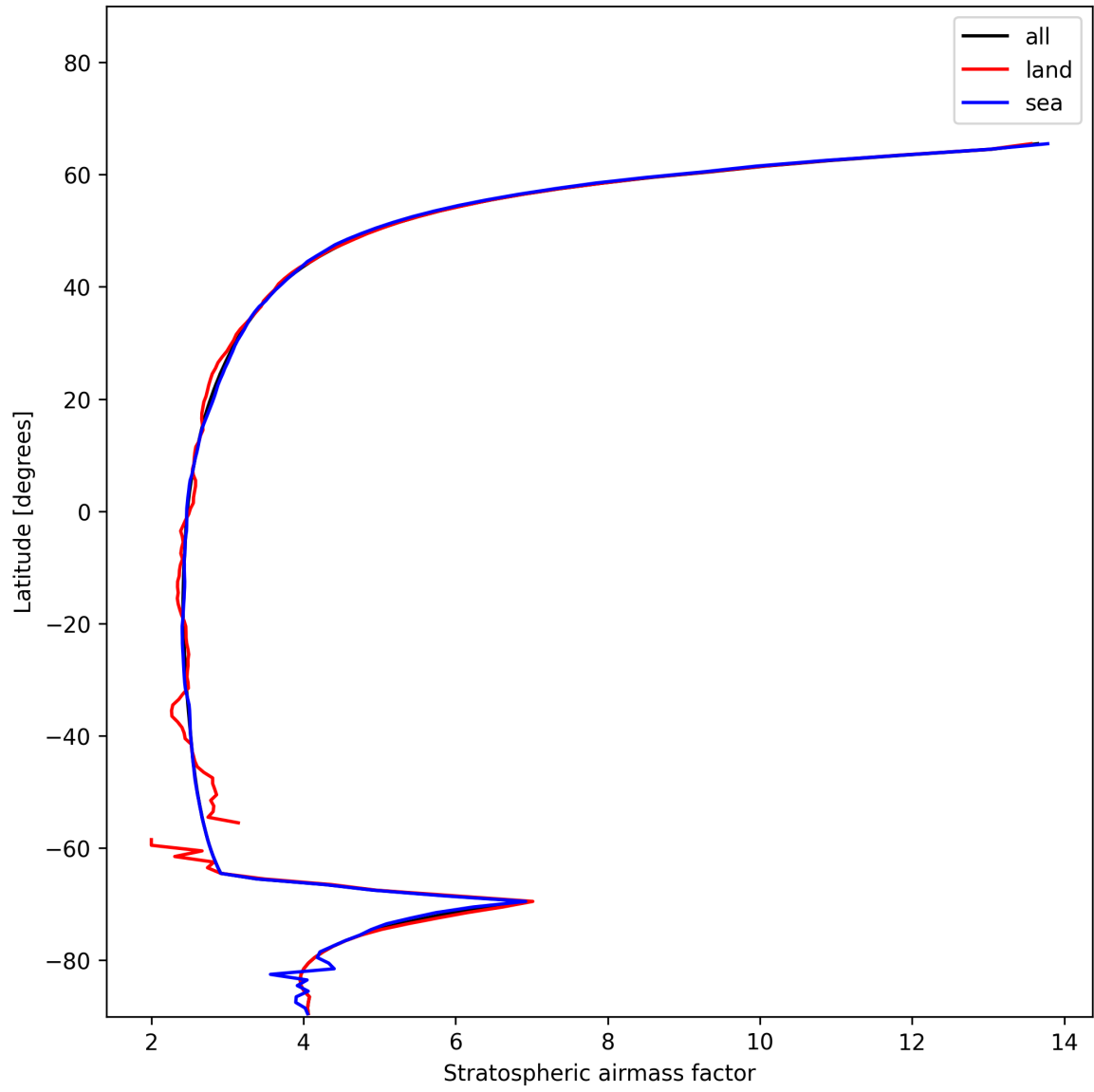
Figure 27: Zonal average of “Stratospheric air mass factor” for 2024-12-08 to 2024-12-10.
