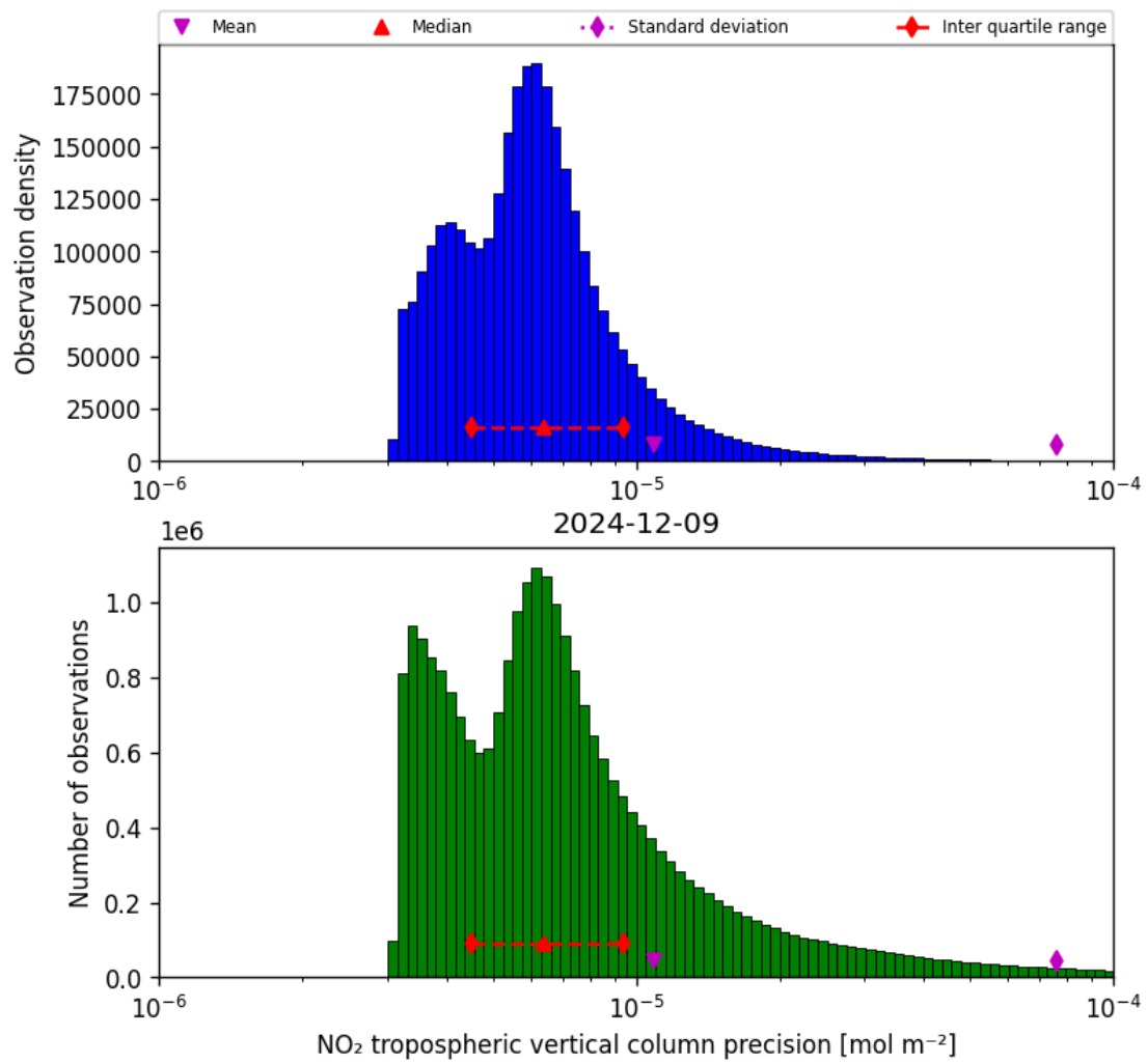
Figure 30: Histogram of “NO 2 tropospheric vertical column precision” for 2024-12-08 to 2024-12-10
