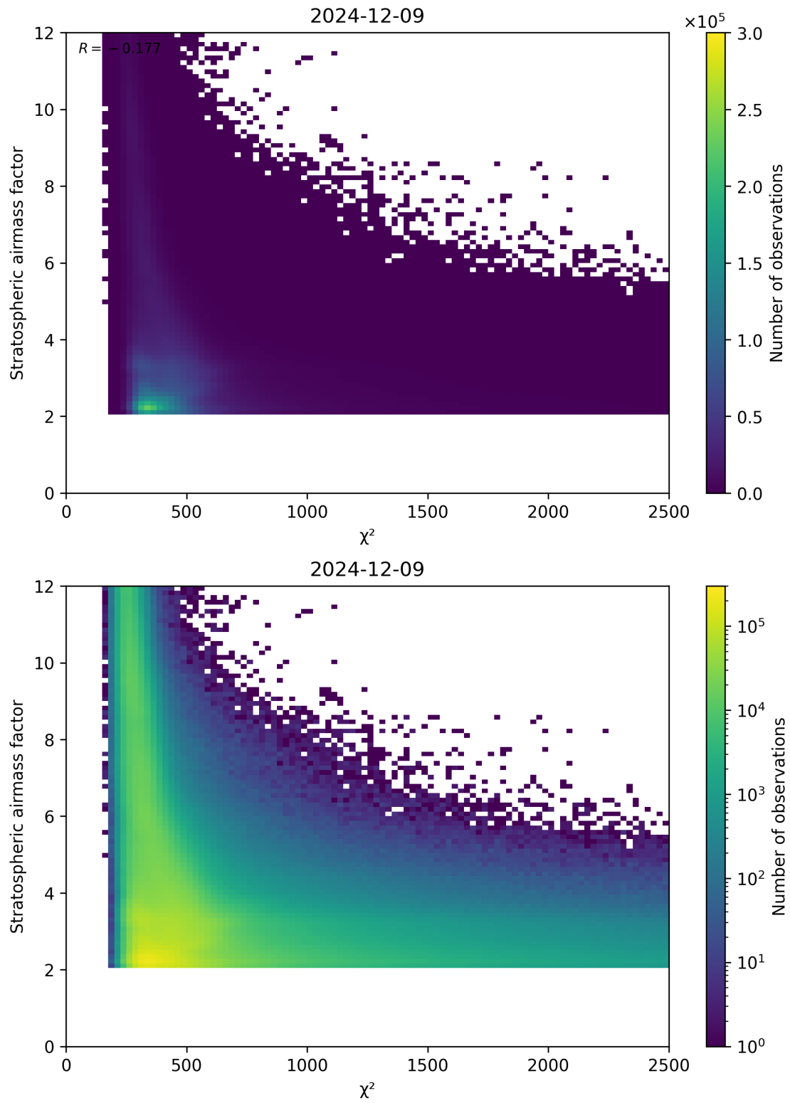
Figure 81: Scatter density plot of “ \chi^2 ” against “Stratospheric airmass factor” for 2024-12-08 to 2024-12-10.
