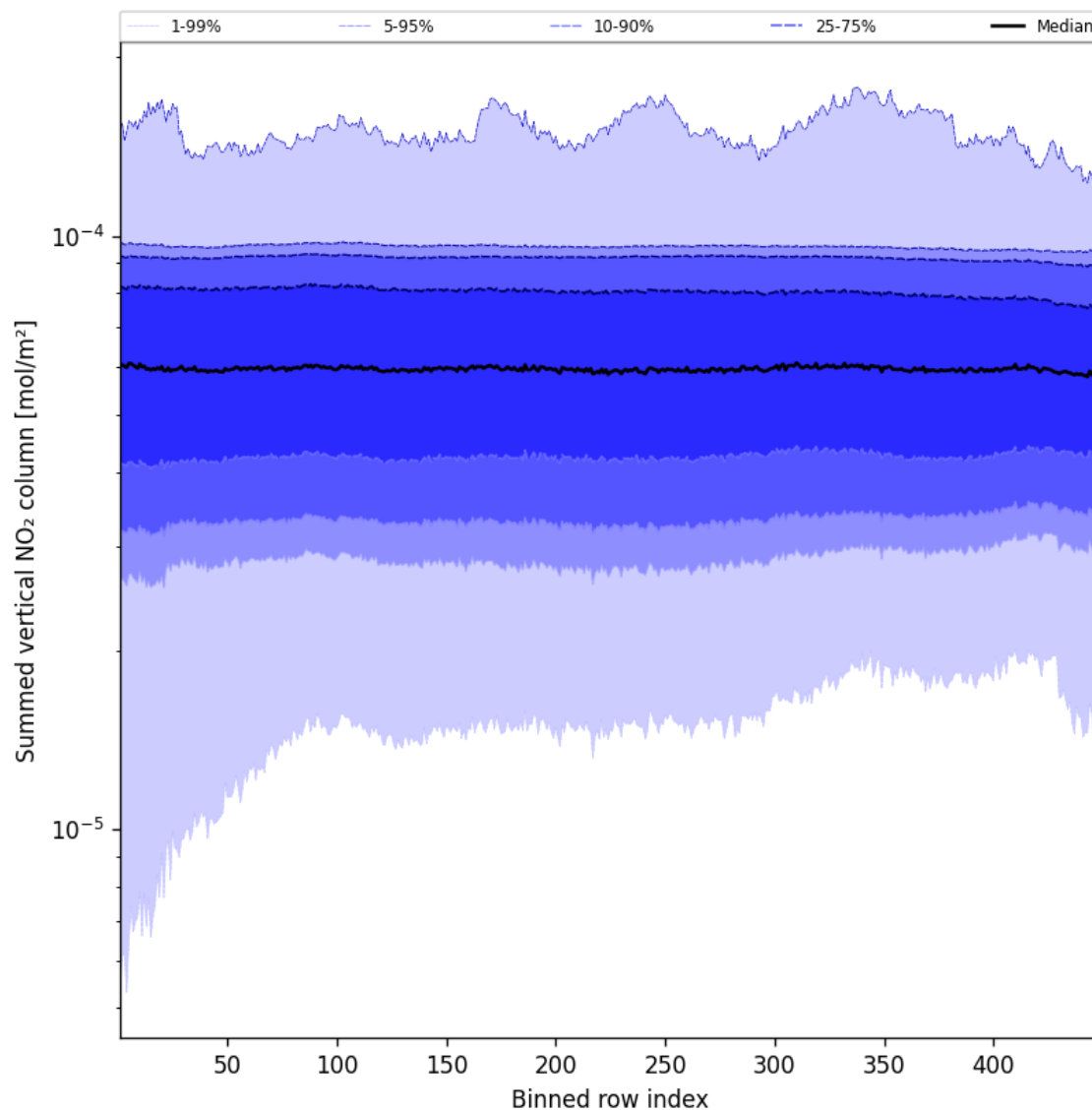
Figure 57: Along track statistics of “Summed vertical NO 2 column” for 2024-12-08 to 2024-12-10
