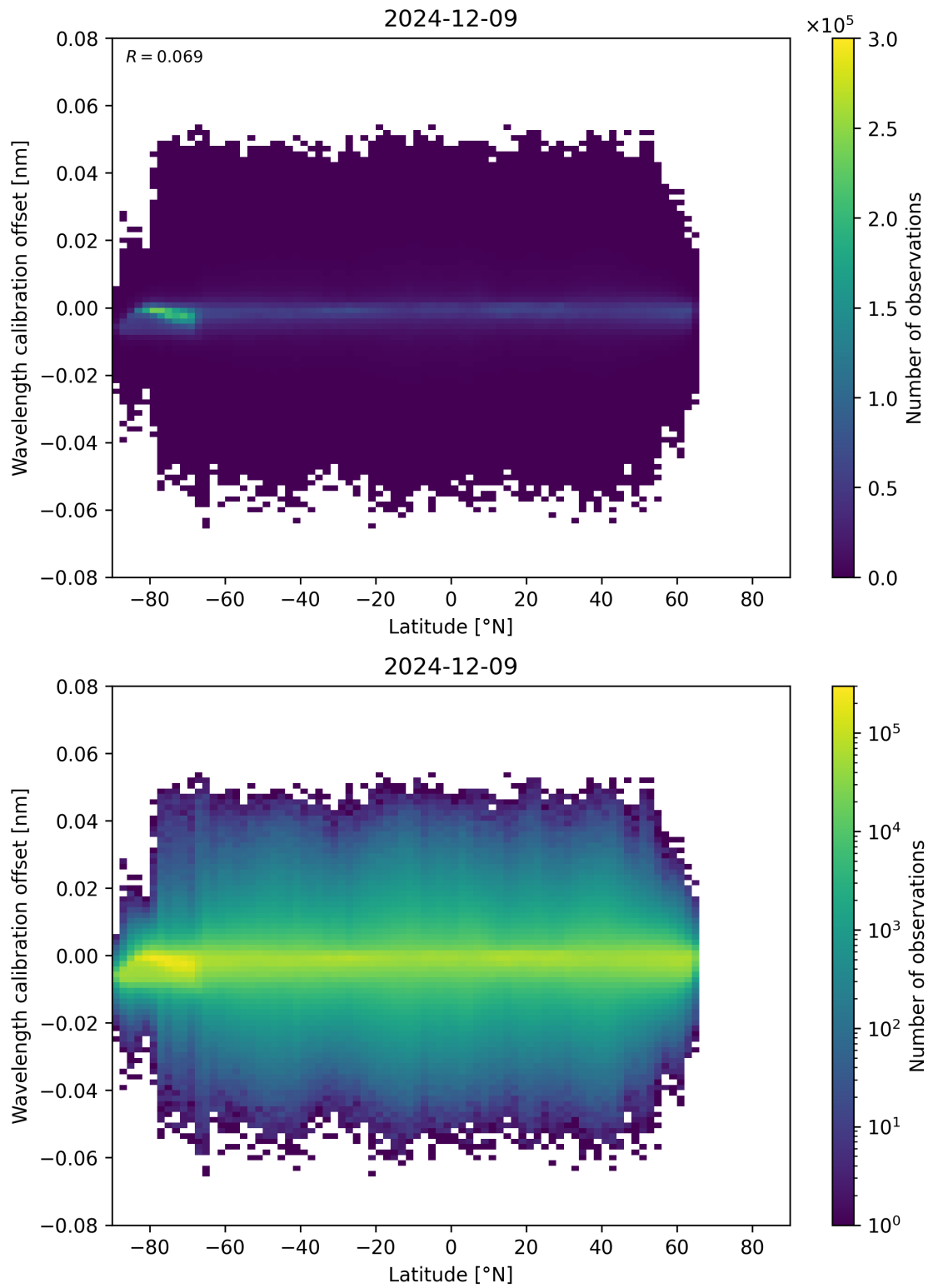
Figure 95: Scatter density plot of “Latitude” against “Wavelength calibration offset” for 2024-12-08 to 2024-12-10.
