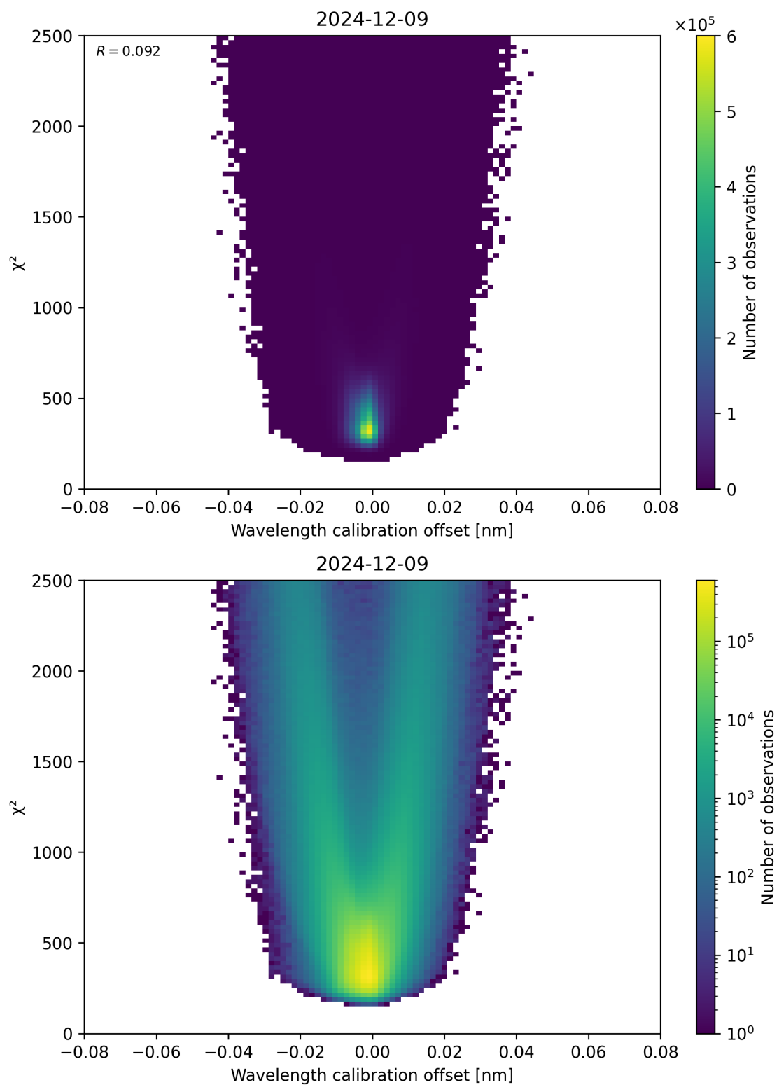
Figure 175: Scatter density plot of “Wavelength calibration offset” against “ \chi^2 ” for 2024-12-08 to 2024-12-10.
