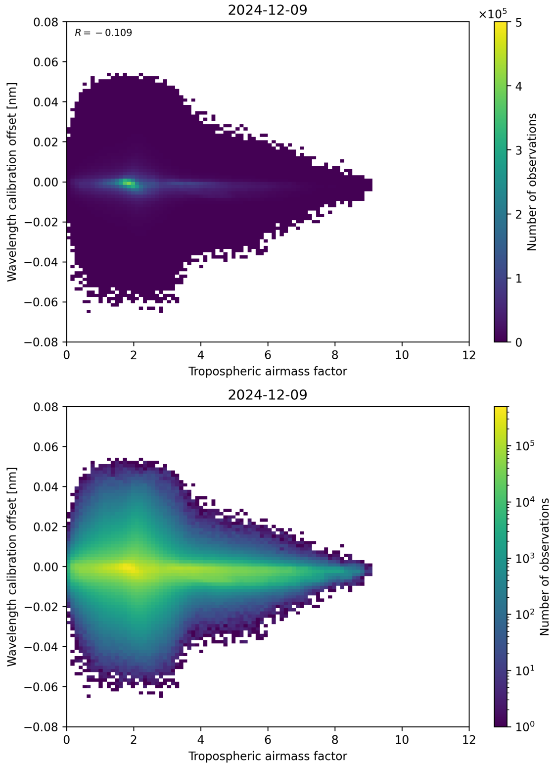
Figure 80: Scatter density plot of “Tropospheric air mass factor” against “Wavelength calibration offset” for 2024-12-08 to 2024-12-10.
