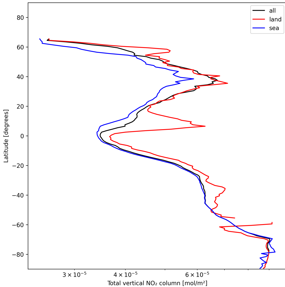
Figure 21: Zonal average of “Total vertical NO 2 column” for 2024-12-08 to 2024-12-10.
