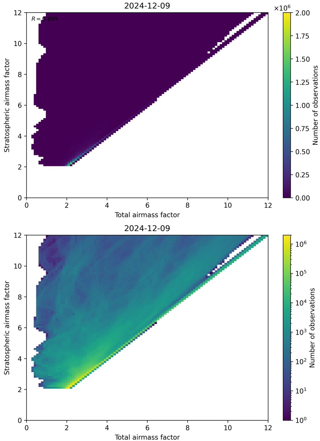
Figure 62: Scatter density plot of “Total airmass factor” against “Stratospheric airmass factor” for 2024-12-08 to 2024-12-10.
