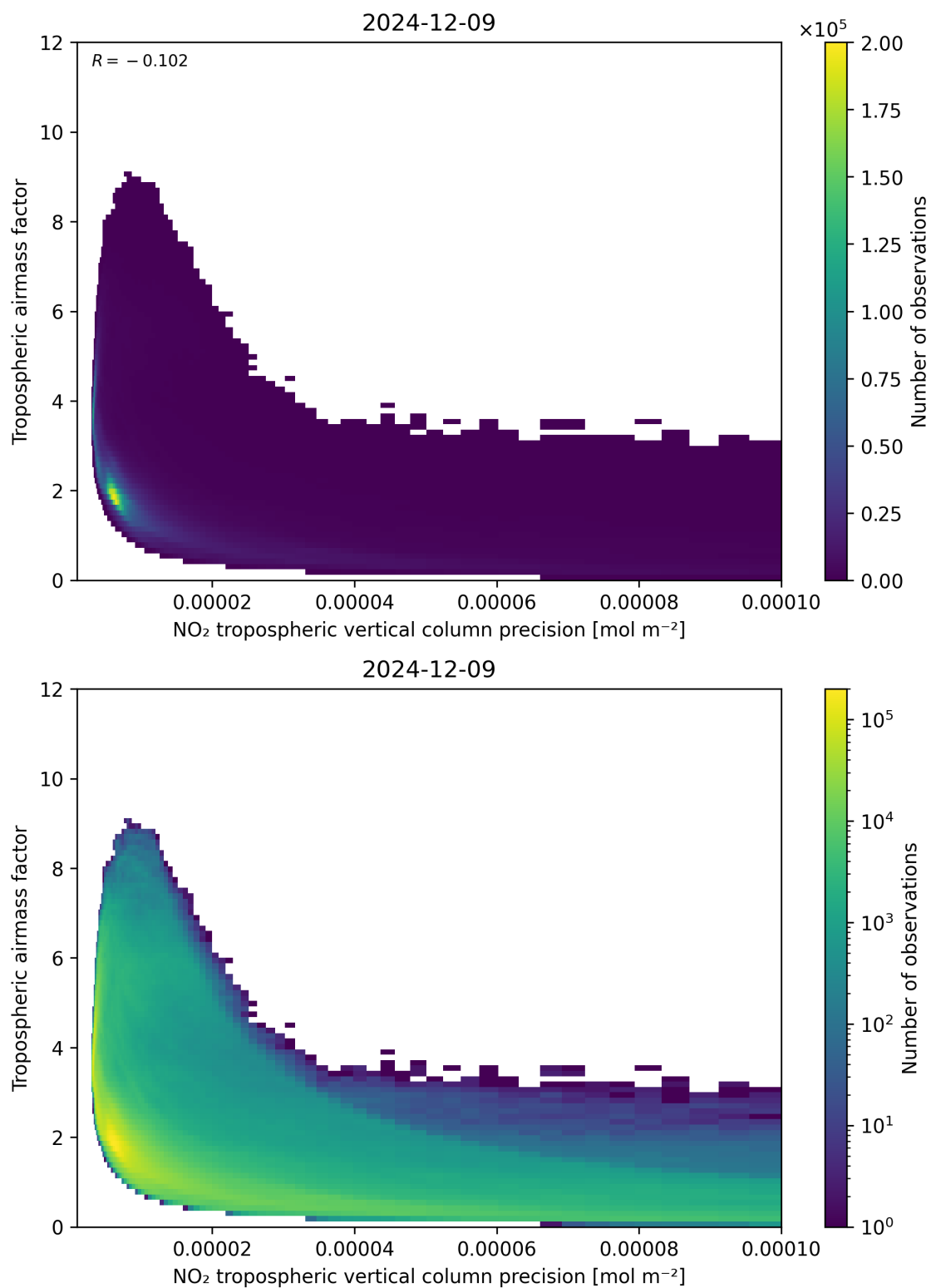
Figure 133: Scatter density plot of “NO 2 tropospheric vertical column precision” against “Tropospheric airmass factor” for 2024-12-08 to 2024-12-10.
