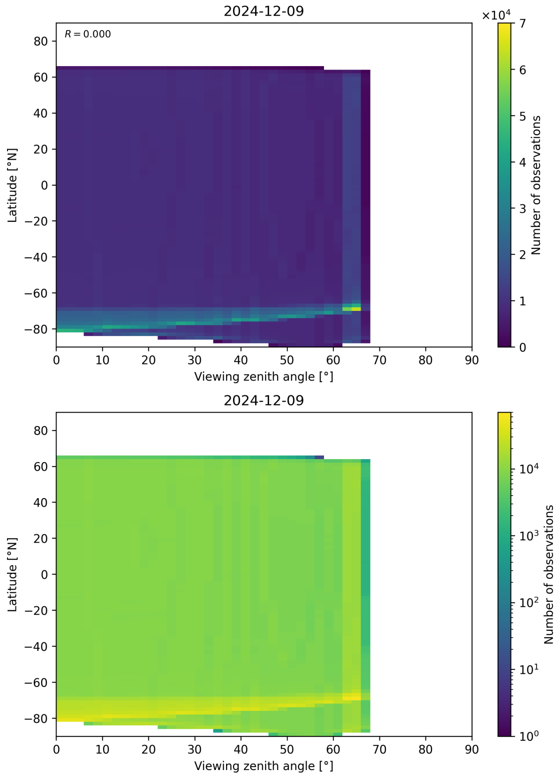
Figure 163: Scatter density plot of “Viewing zenith angle” against “Latitude” for 2024-12-08 to 2024-12-10.
