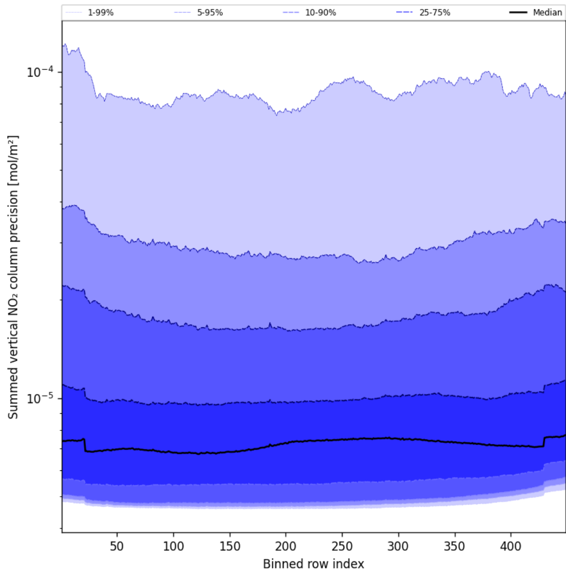
Figure 58: Along track statistics of “Summed vertical NO 2 column precision” for 2024-12-08 to 2024-12-10
