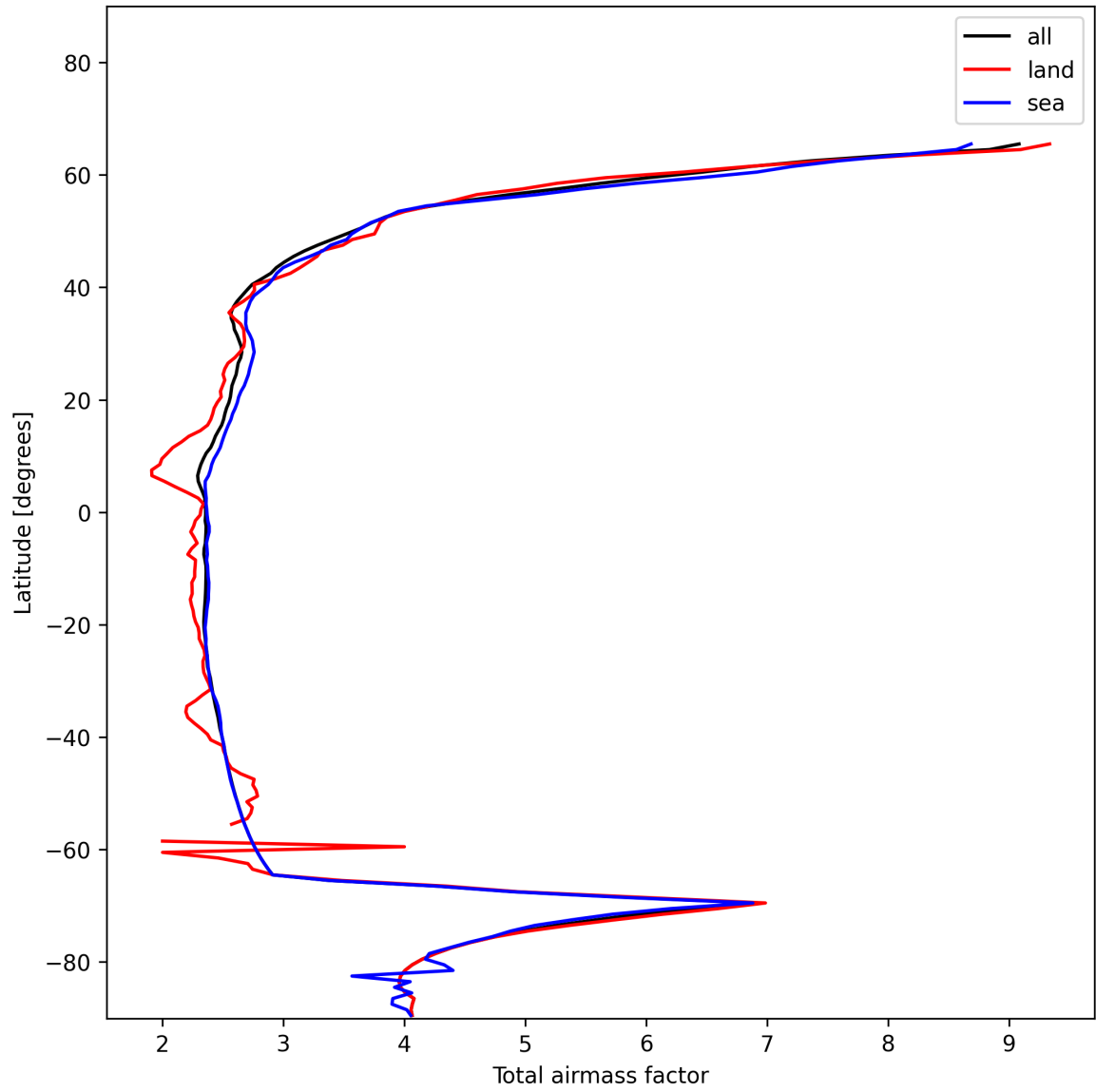
Figure 15: Zonal average of “Total airmass factor” for 2024-12-08 to 2024-12-10.
