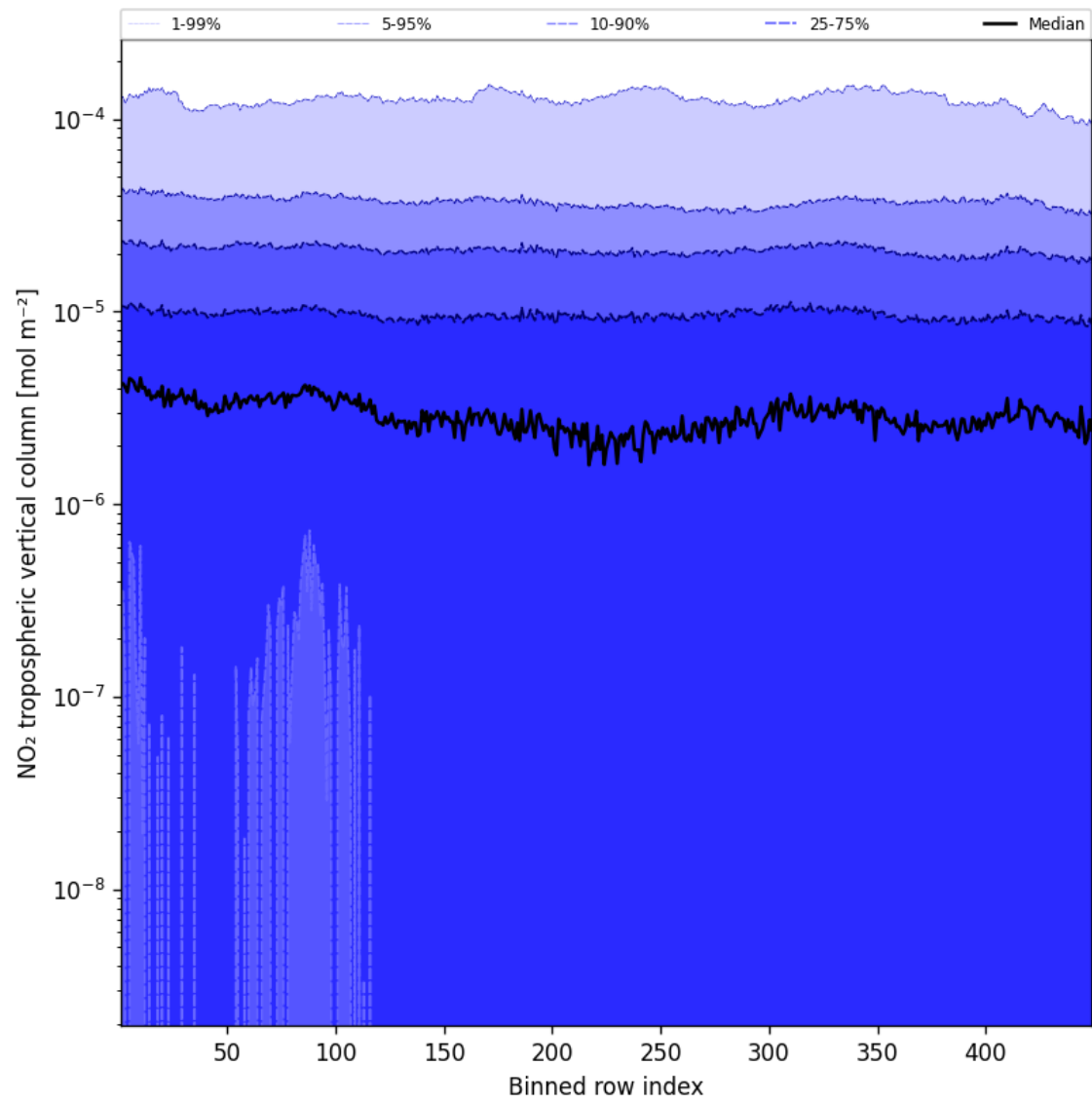
Figure 46: Along track statistics of “NO 2 tropospheric vertical column” for 2024-12-08 to 2024-12-10
