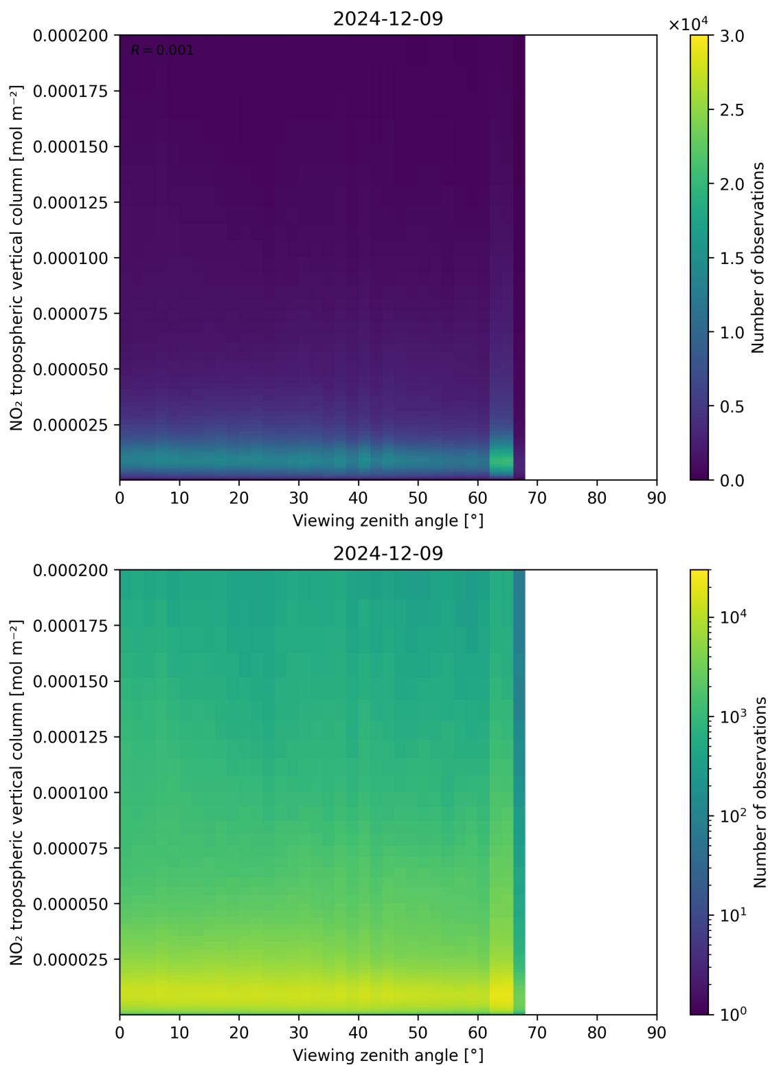
Figure 169: Scatter density plot of “Viewing zenith angle” against “NO 2 tropospheric vertical column” for 2024-12-08 to 2024-12-10.
