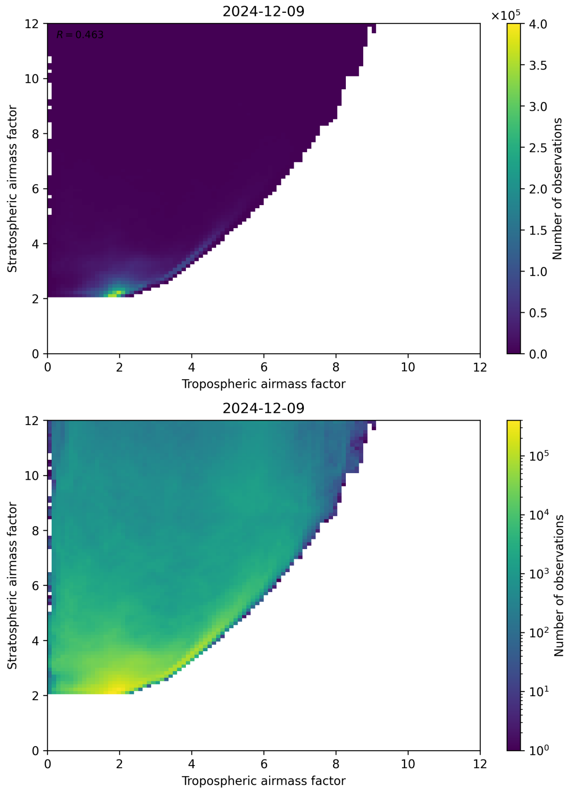
Figure 71: Scatter density plot of “Tropospheric airmass factor” against “Stratospheric airmass factor” for 2024-12-08 to 2024-12-10.
