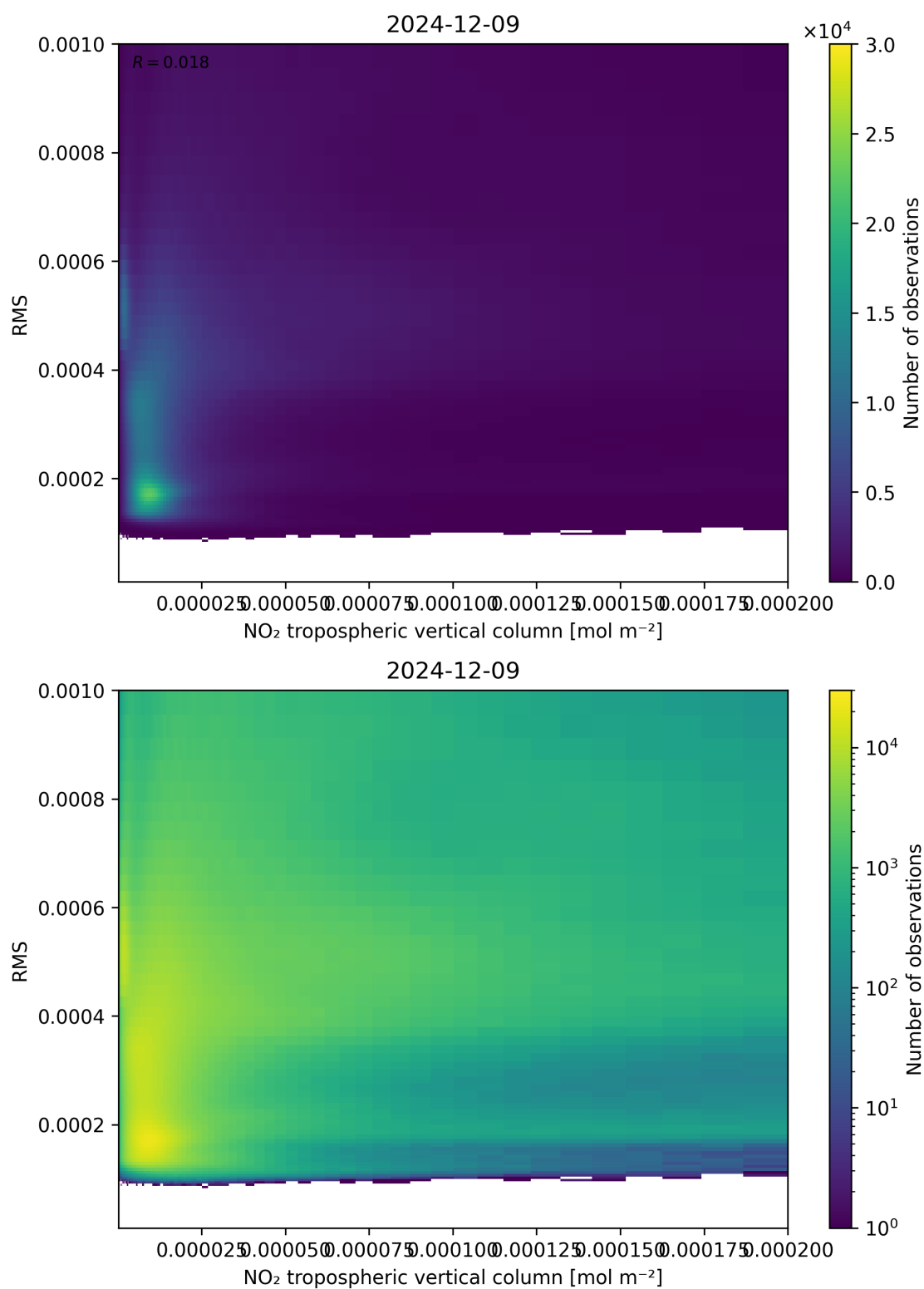
Figure 142: Scatter density plot of “NO 2 tropospheric vertical column” against “RMS” for 2024-12-08 to 2024-12-10.
