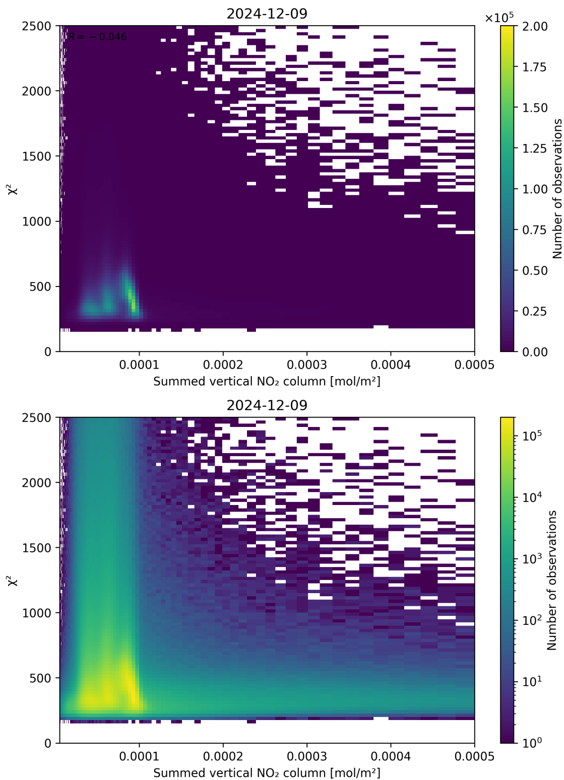
Figure 104: Scatter density plot of “Summed vertical NO 2 column” against “ \chi^2 ” for 2024-12-08 to 2024-12-10.
