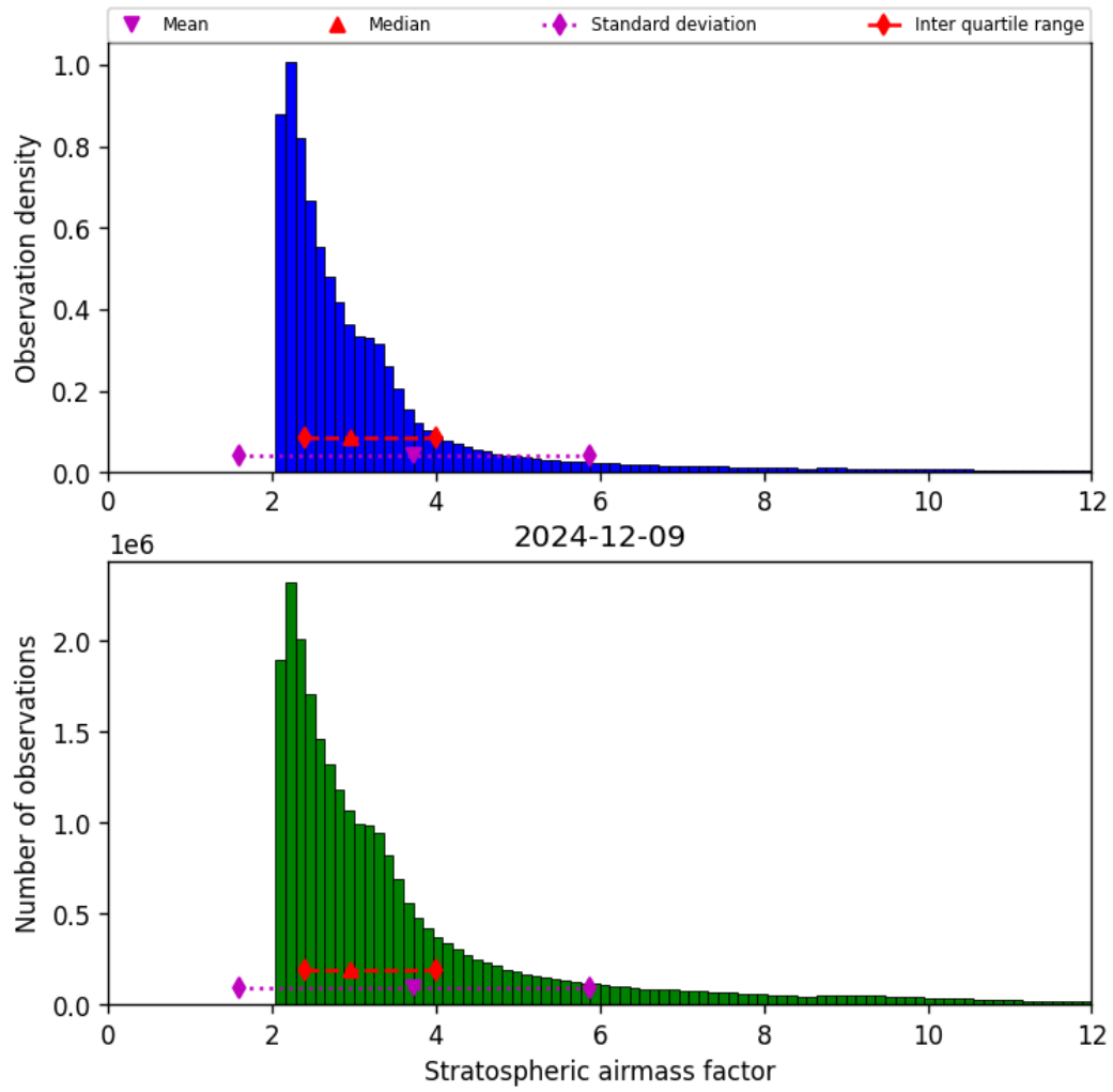
Figure 44: Histogram of “Stratospheric airmass factor” for 2024-12-08 to 2024-12-10
