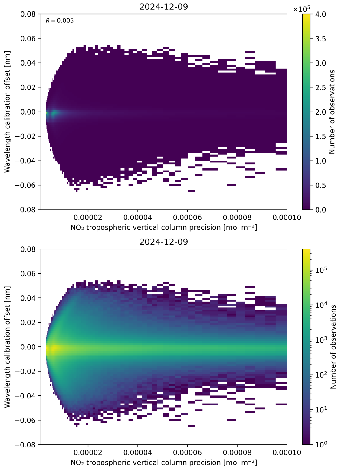
Figure 141: Scatter density plot of “NO 2 tropospheric vertical column precision” against “Wavelength calibration offset” for 2024-12-08 to 2024-12-10.
