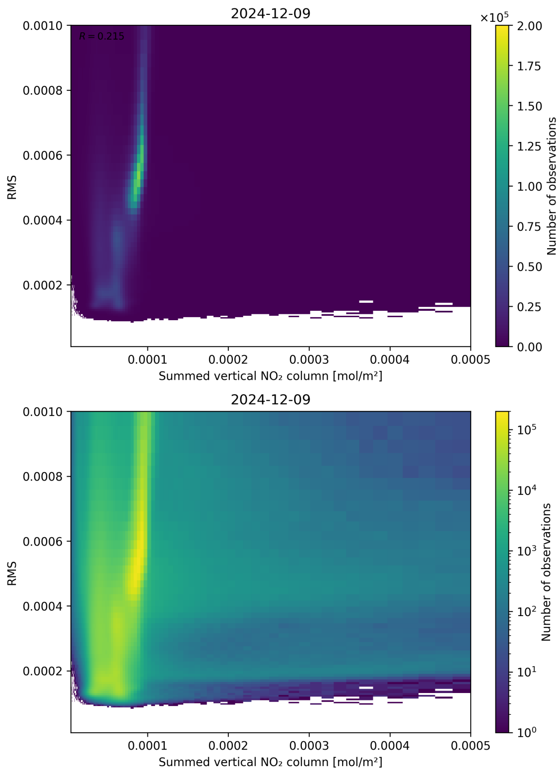
Figure 109: Scatter density plot of “Summed vertical NO 2 column” against “RMS” for 2024-12-08 to 2024-12-10.
