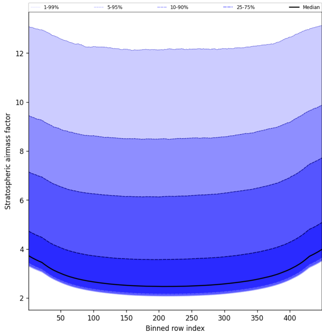
Figure 61: Along track statistics of “Stratospheric airmass factor” for 2024-12-08 to 2024-12-10
