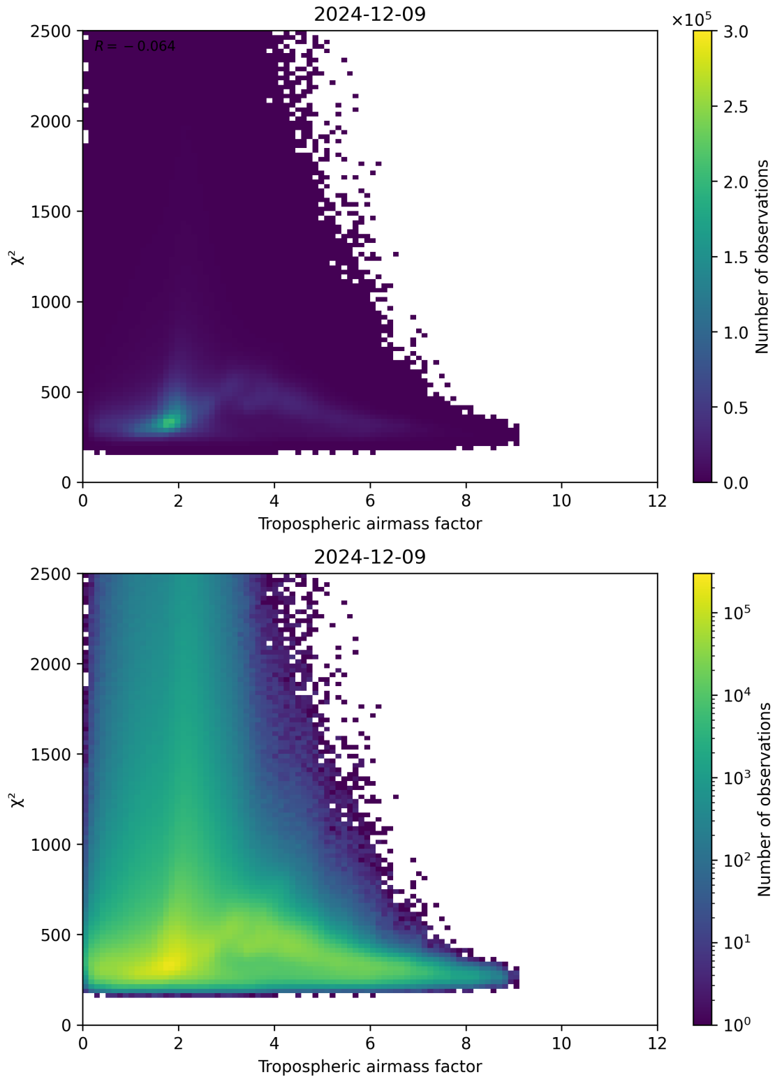
Figure 73: Scatter density plot of “Tropospheric airmass factor” against “ \chi^2 ” for 2024-12-08 to 2024-12-10.
