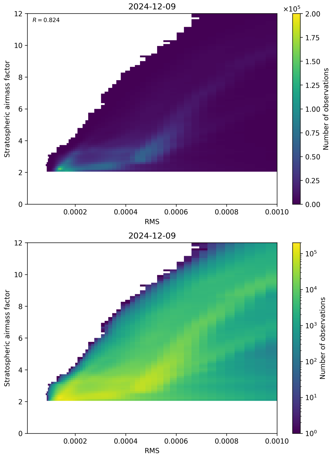
Figure 144: Scatter density plot of “RMS” against “Stratospheric airmass factor” for 2024-12-08 to 2024-12-10.
