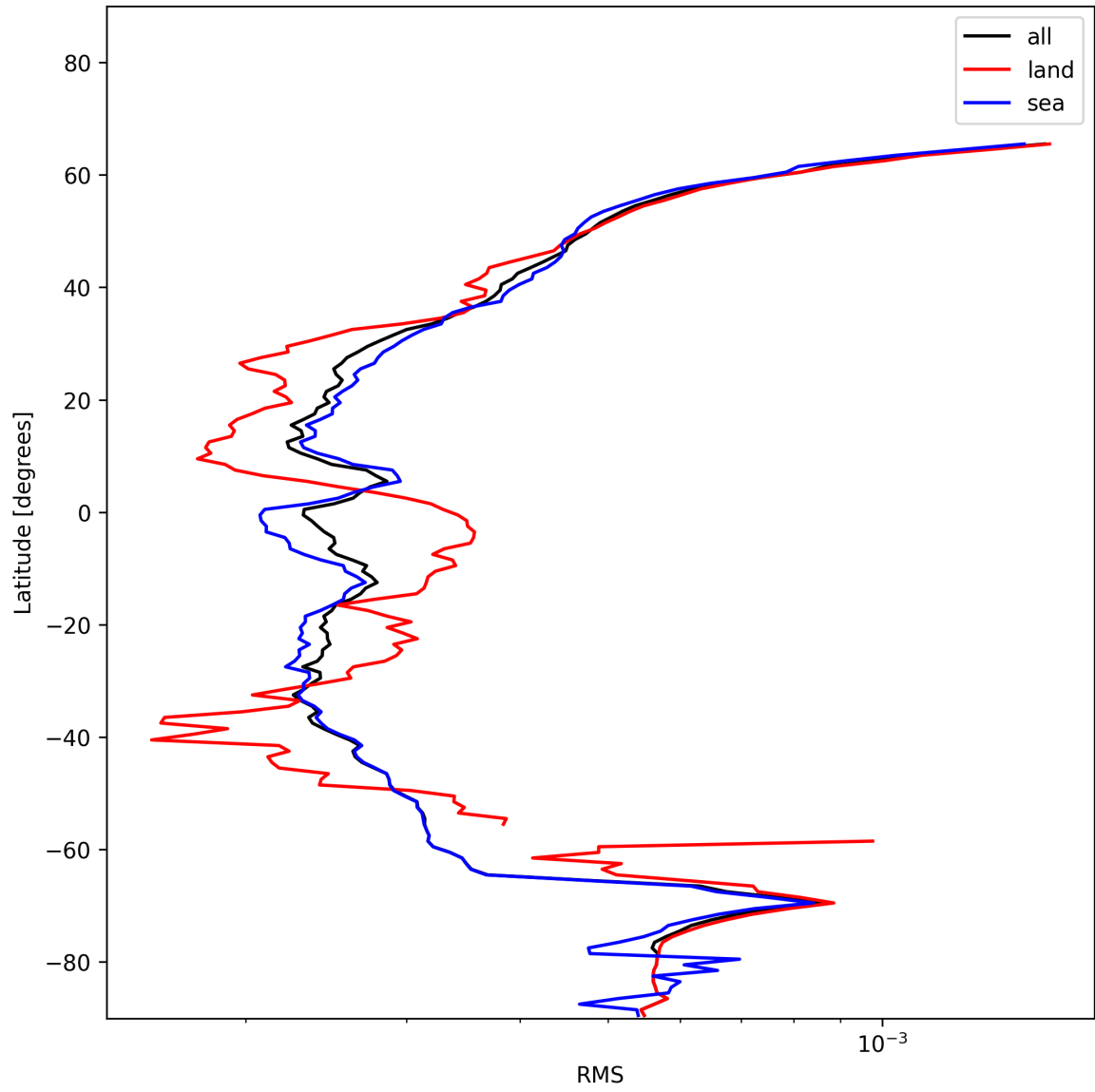
Figure 26: Zonal average of “RMS” for 2024-12-08 to 2024-12-10.
