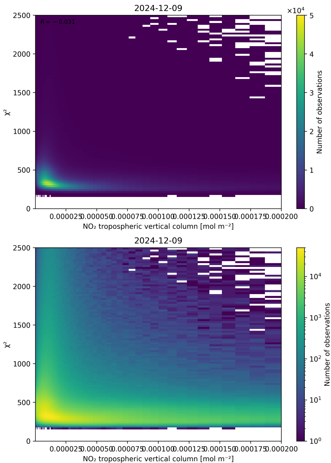
Figure 124: Scatter density plot of “NO 2 tropospheric vertical column” against “ \chi^2 ” for 2024-12-08 to 2024-12-10.
