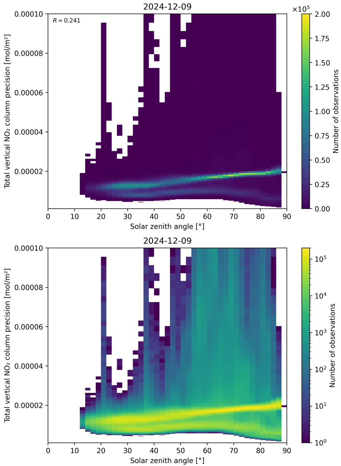
Figure 154: Scatter density plot of “Solar zenith angle” against “Total vertical NO 2 column precision” for 2024-12-08 to 2024-12-10.
