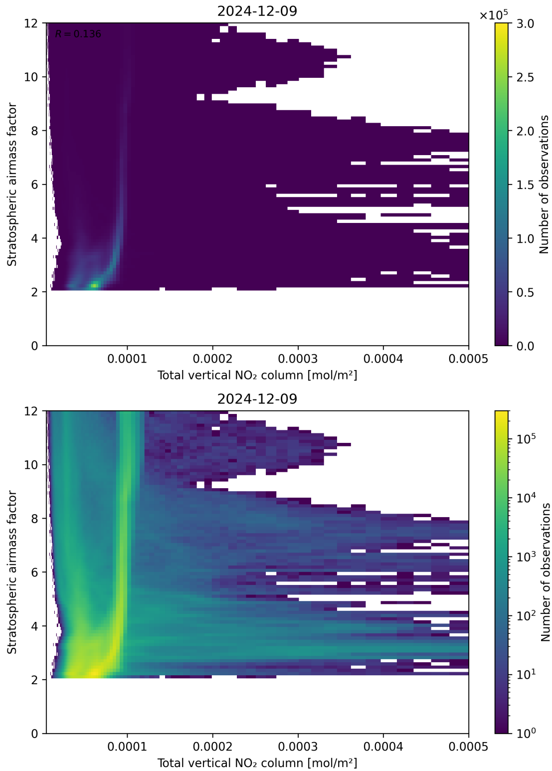
Figure 110: Scatter density plot of “Total vertical NO 2 column” against “Stratospheric airmass factor” for 2024-12-08 to 2024-12-10.
