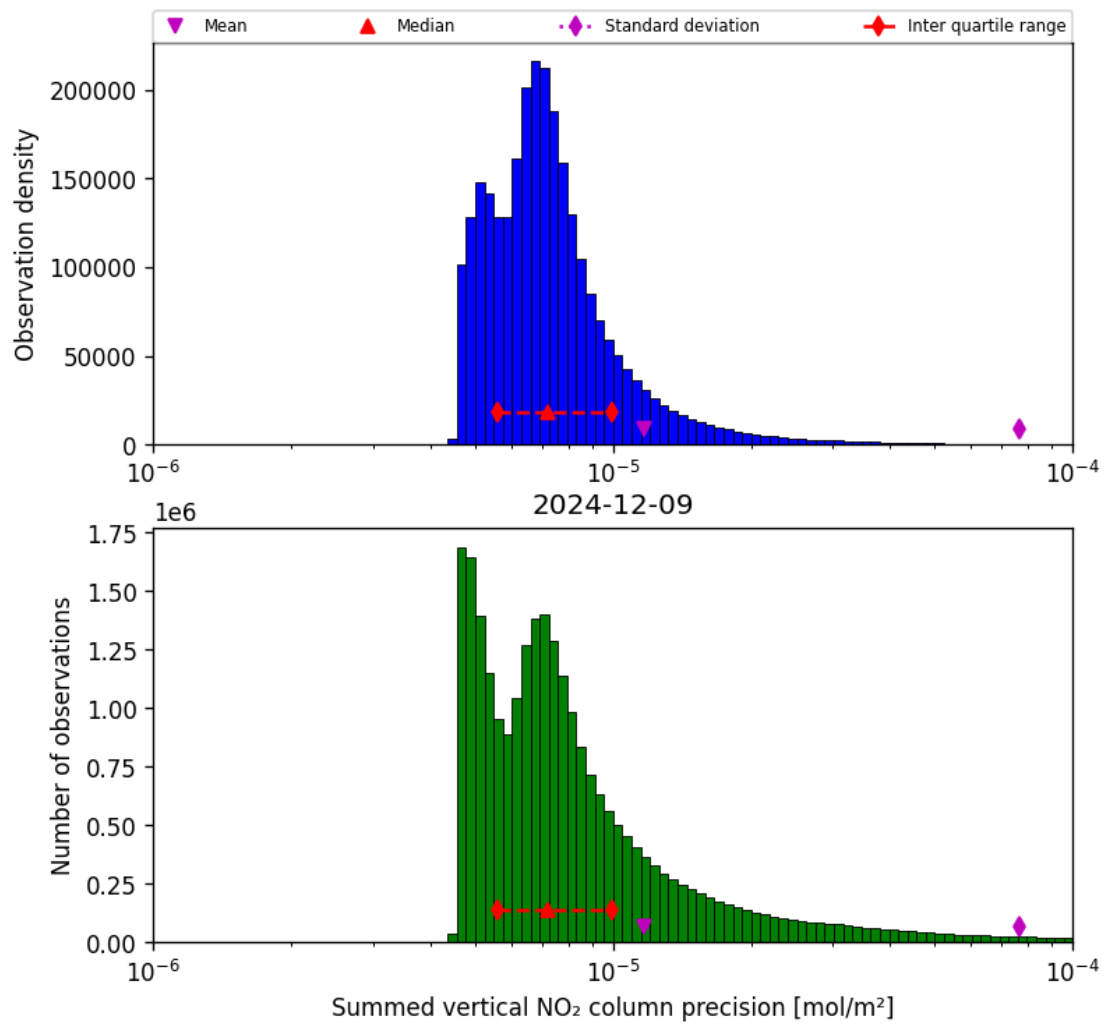
Figure 41: Histogram of “Summed vertical NO 2 column precision” for 2024-12-08 to 2024-12-10
