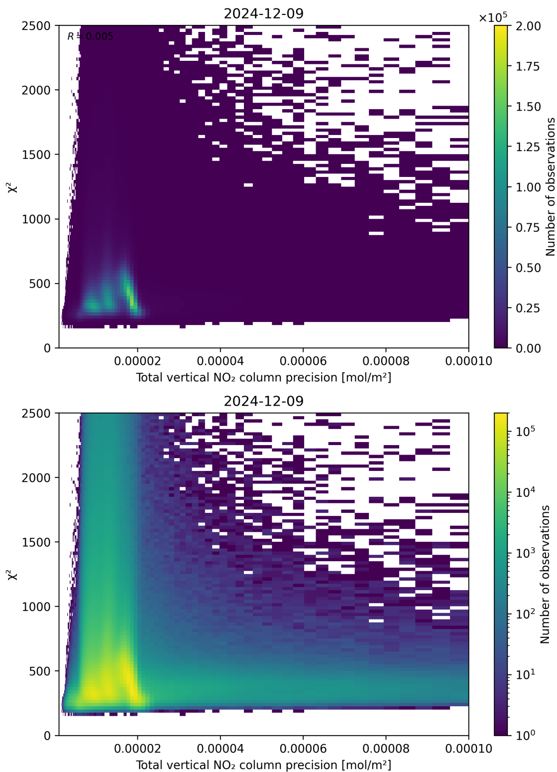
Figure 116: Scatter density plot of “Total vertical NO 2 column precision” against “ \chi^2 ” for 2024-12-08 to 2024-12-10.
