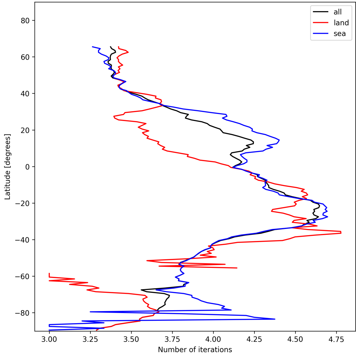
Figure 17: Zonal average of “Number of iterations” for 2024-12-08 to 2024-12-10.
