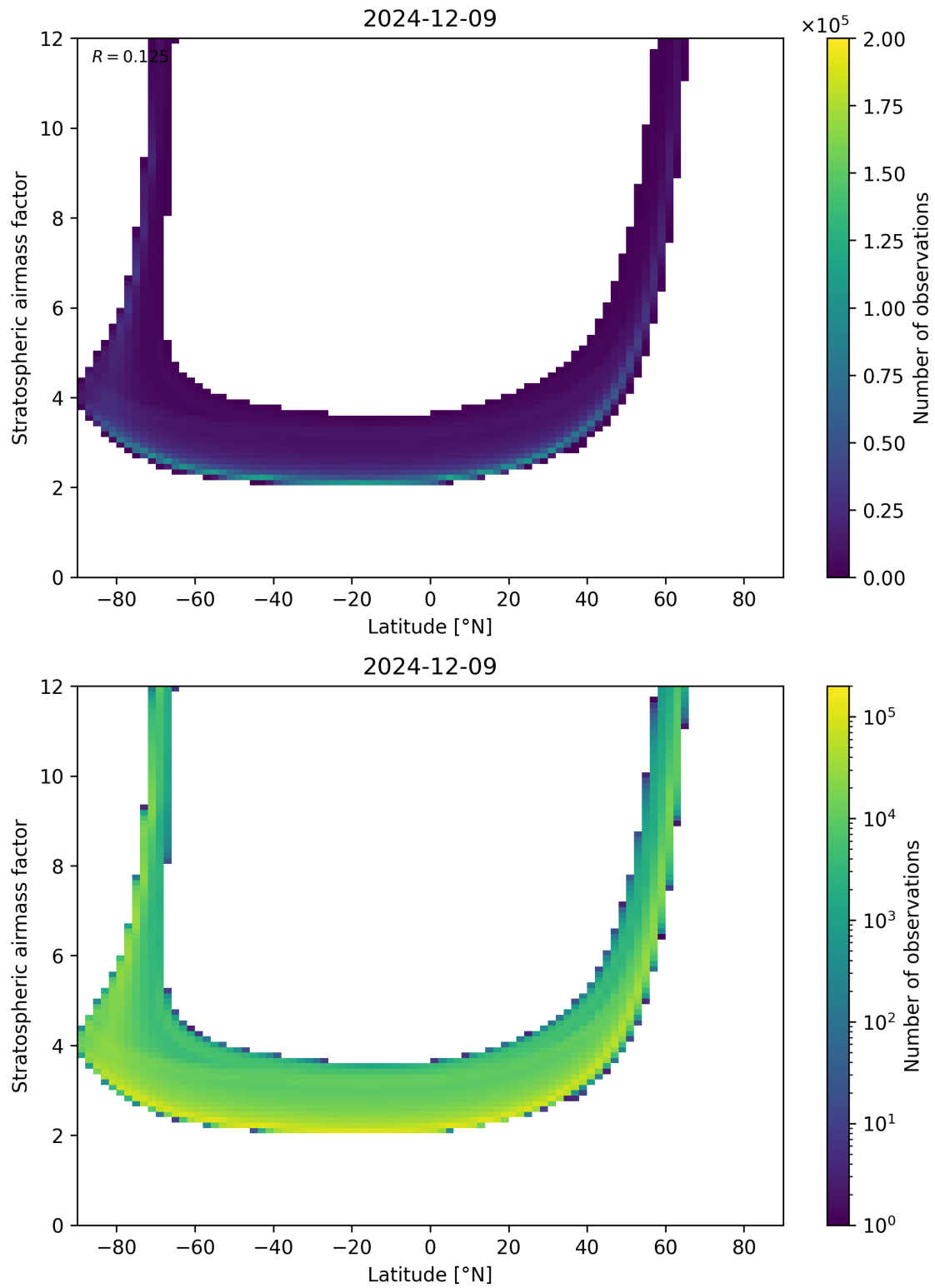
Figure 83: Scatter density plot of “Latitude” against “Stratospheric air mass factor” for 2024-12-08 to 2024-12-10.
