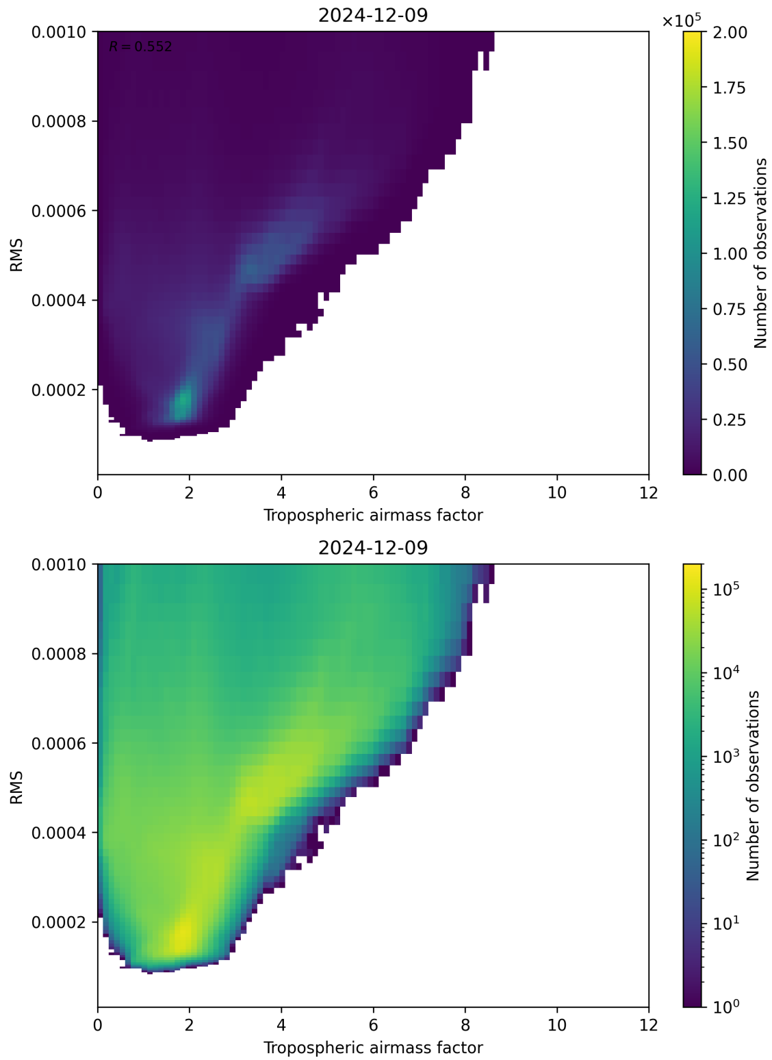
Figure 79: Scatter density plot of “Tropospheric airmass factor” against “RMS” for 2024-12-08 to 2024-12-10.
