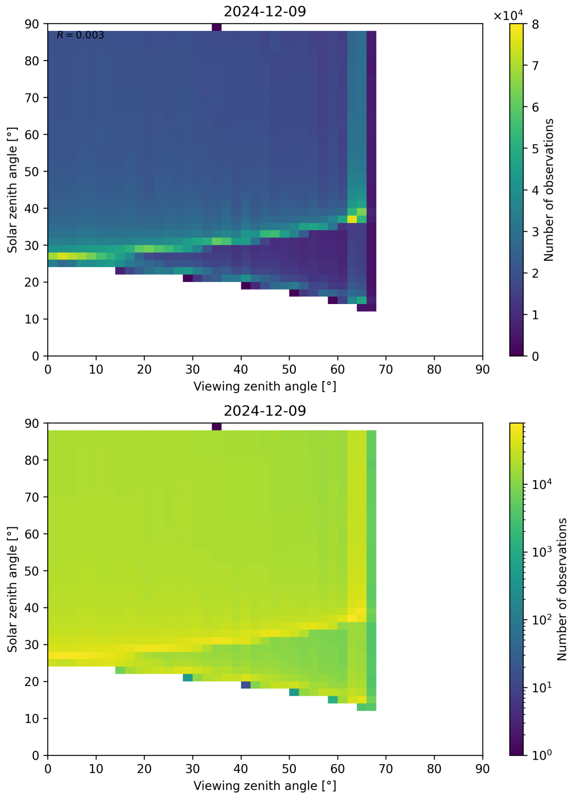
Figure 172: Scatter density plot of “Viewing zenith angle” against “Solar zenith angle” for 2024-12-08 to 2024-12-10.
