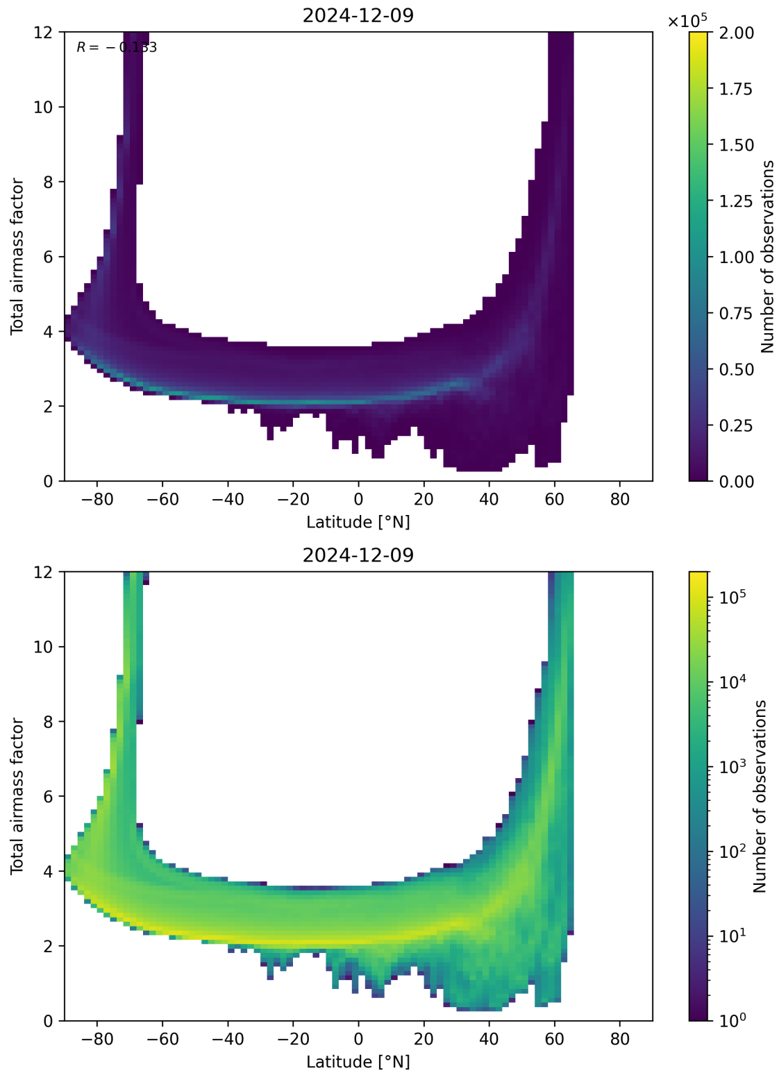
Figure 84: Scatter density plot of “Latitude” against “Total airmass factor” for 2024-12-08 to 2024-12-10.
