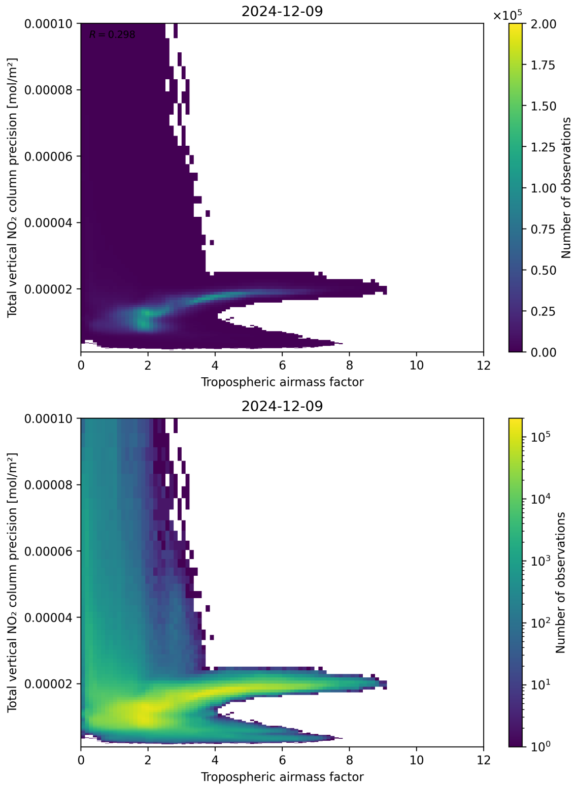
Figure 78: Scatter density plot of “Tropospheric air mass factor” against “Total vertical NO 2 column precision” for 2024-12-08 to 2024-12-10.
