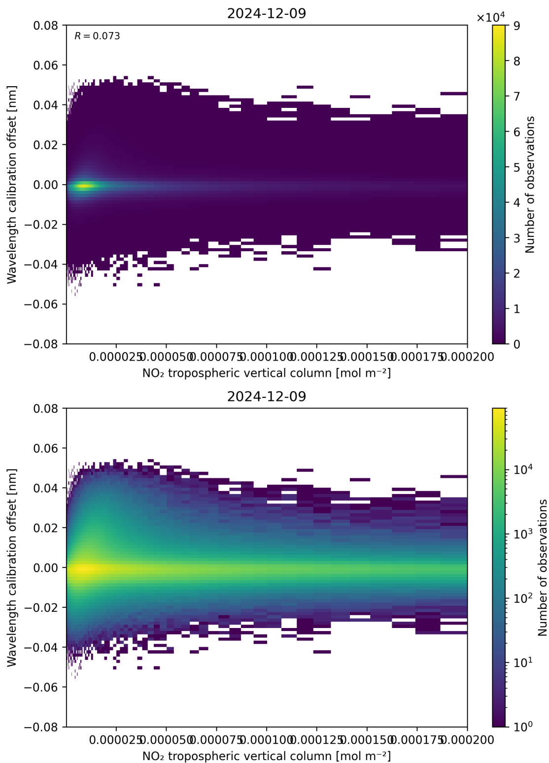
Figure 143: Scatter density plot of “NO 2 tropospheric vertical column” against “Wavelength calibration offset” for 2024-12-08 to 2024-12-10.
