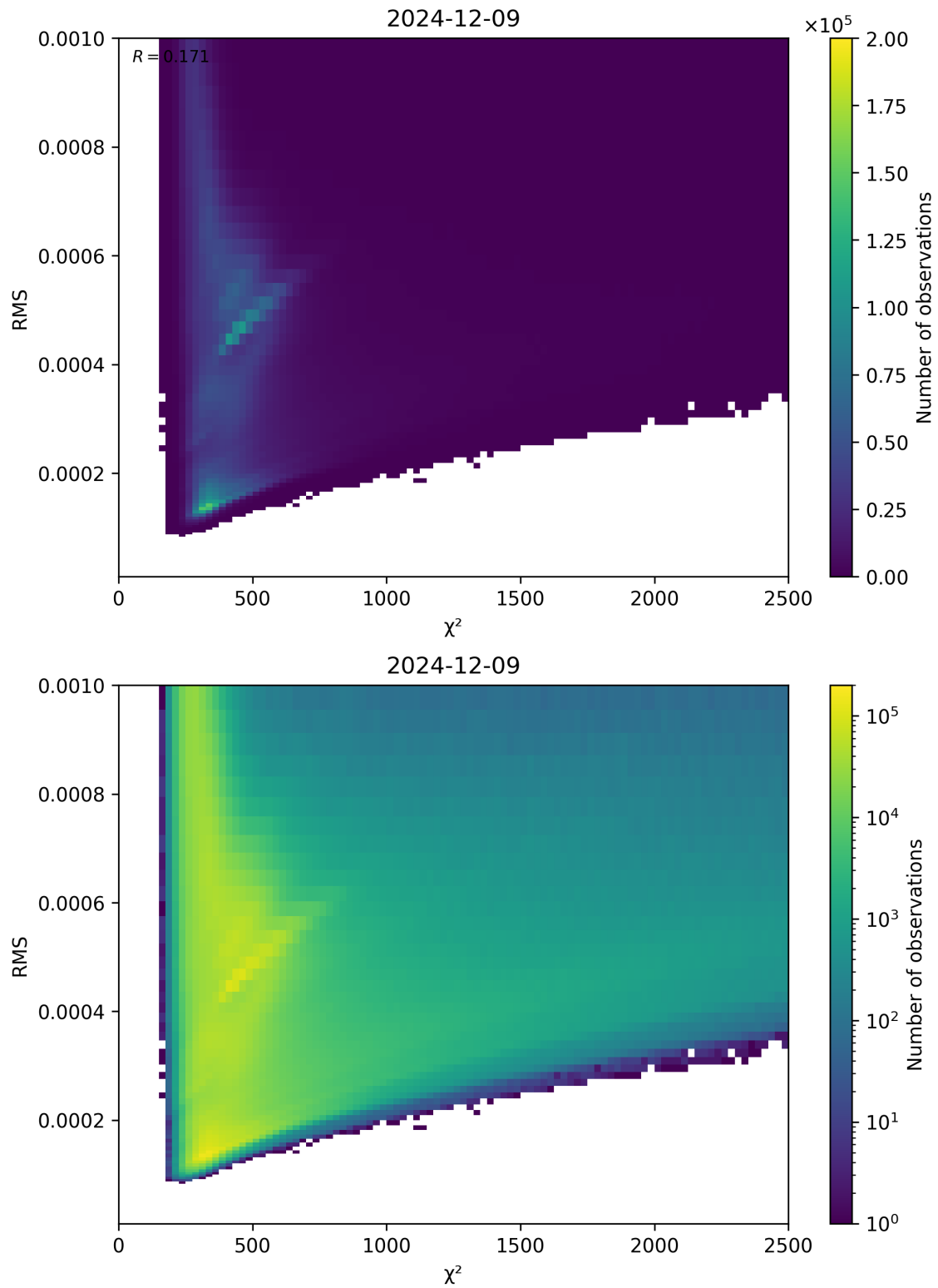
Figure 82: Scatter density plot of “ \chi^2 ” against “RMS” for 2024-12-08 to 2024-12-10.
