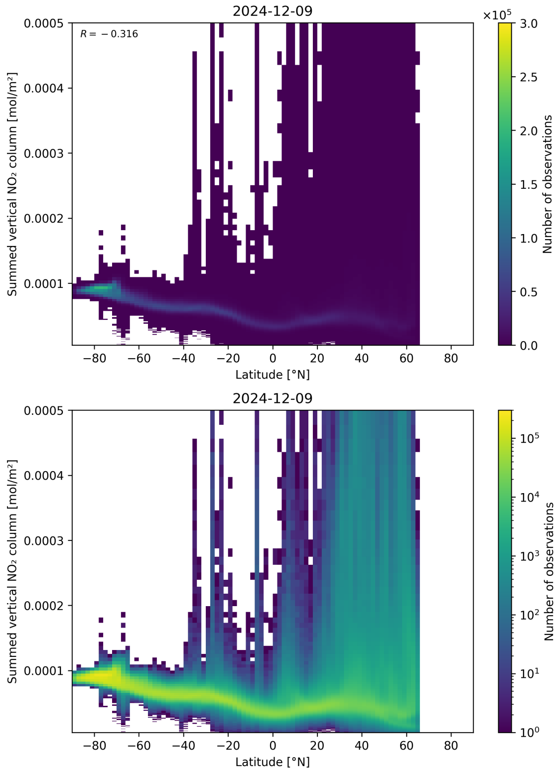
Figure 88: Scatter density plot of “Latitude” against “Summed vertical NO 2 column” for 2024-12-08 to 2024-12-10.
