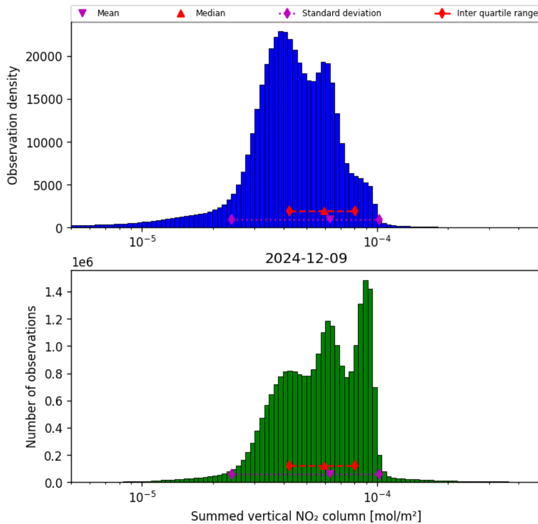
Figure 40: Histogram of “Summed vertical NO 2 column” for 2024-12-08 to 2024-12-10
