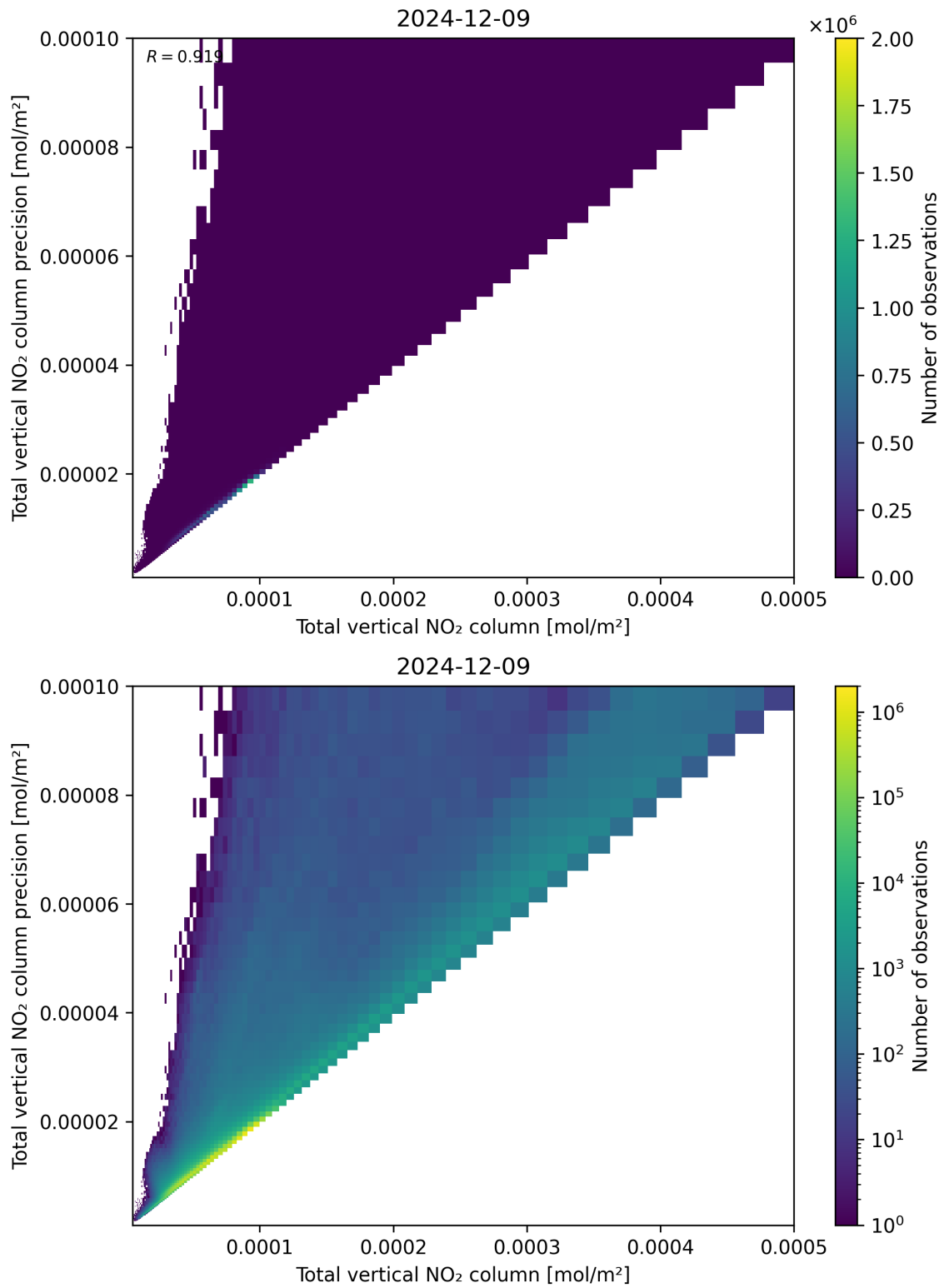
Figure 114: Scatter density plot of “Total vertical NO 2 column” against “Total vertical NO 2 column precision” for 2024-12-08 to 2024-12-10.
