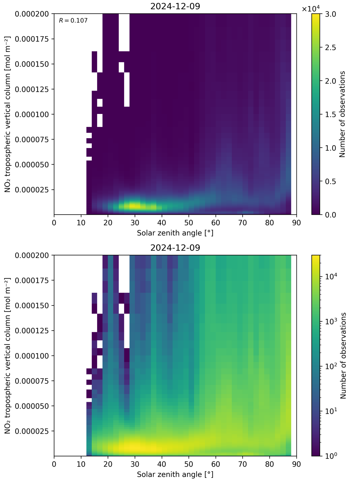
Figure 155: Scatter density plot of “Solar zenith angle” against “NO 2 tropospheric vertical column” for 2024-12-08 to 2024-12-10.
