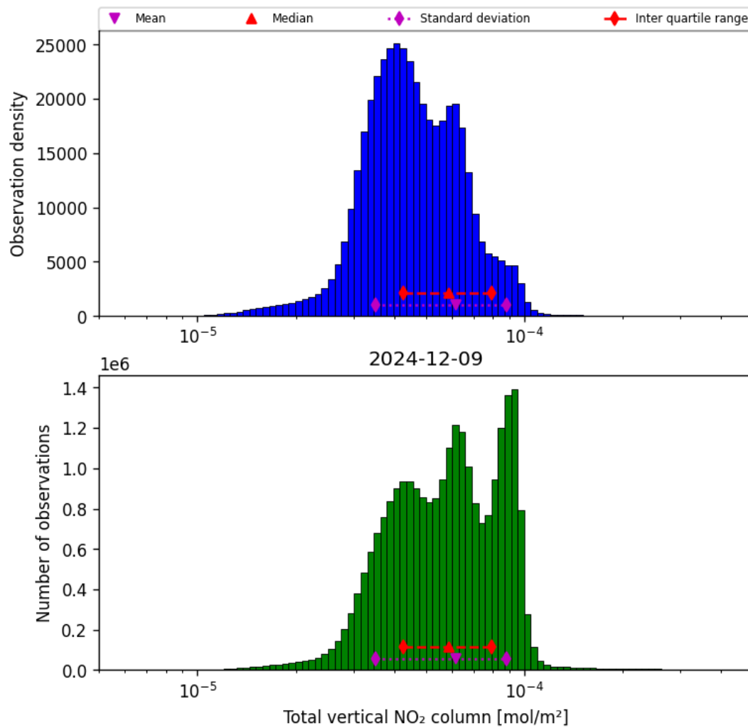
Figure 38: Histogram of “Total vertical NO 2 column” for 2024-12-08 to 2024-12-10
