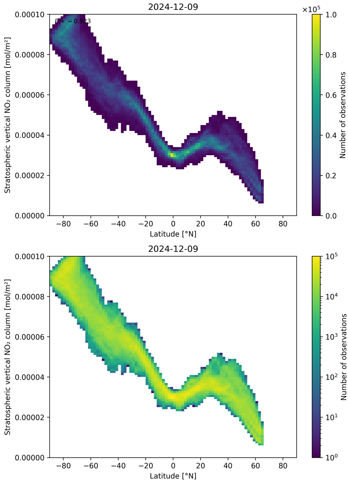
Figure 87: Scatter density plot of “Latitude” against “Stratospheric vertical NO 2 column” for 2024-12-08 to 2024-12-10.
