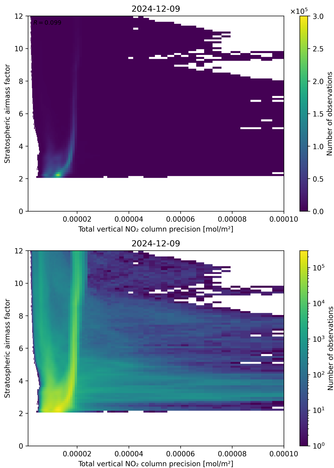
Figure 115: Scatter density plot of “Total vertical NO 2 column precision” against “Stratospheric air mass factor” for 2024-12-08 to 2024-12-10.
