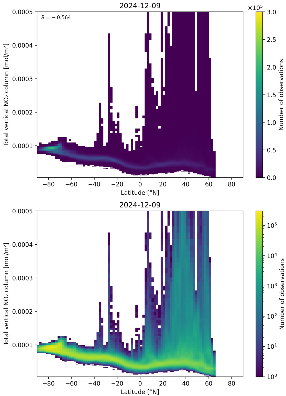
Figure 90: Scatter density plot of “Latitude” against “Total vertical NO 2 column” for 2024-12-08 to 2024-12-10.
