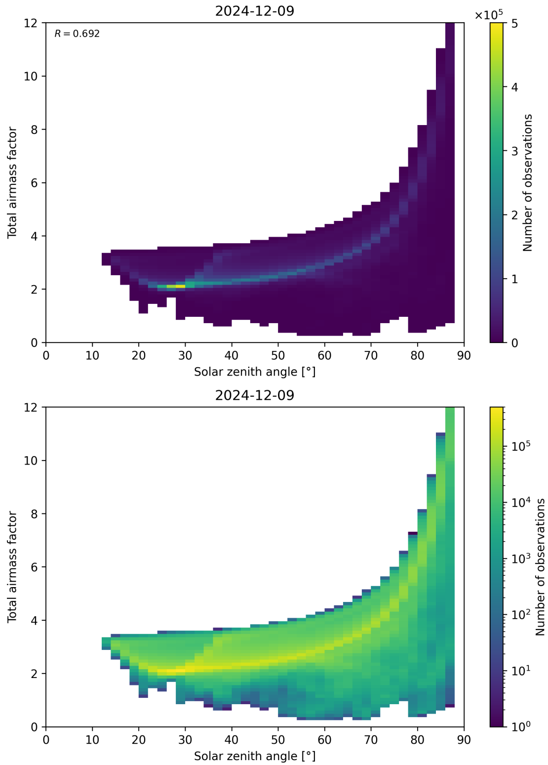
Figure 146: Scatter density plot of “Solar zenith angle” against “Total air mass factor” for 2024-12-08 to 2024-12-10.
