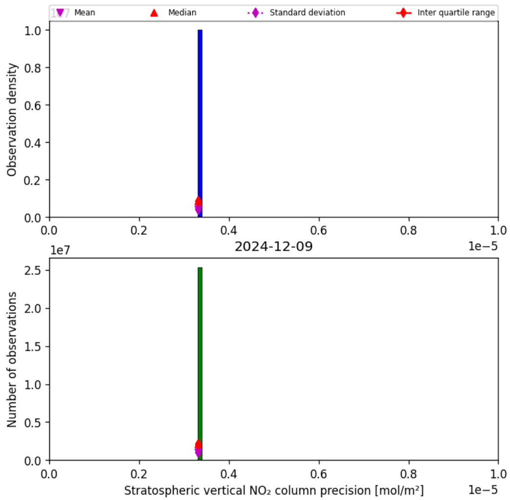
Figure 37: Histogram of “Stratospheric vertical NO 2 column precision” for 2024-12-08 to 2024-12-10
