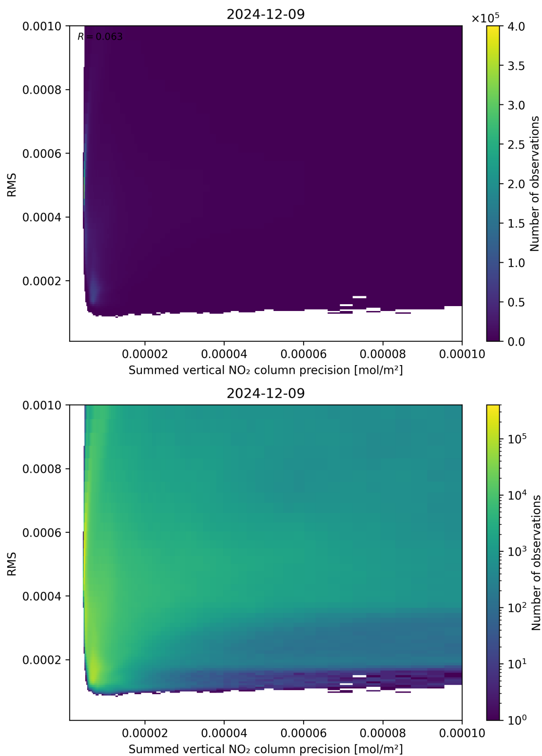
Figure 108: Scatter density plot of “Summed vertical NO 2 column precision” against “RMS” for 2024-12-08 to 2024-12-10.
