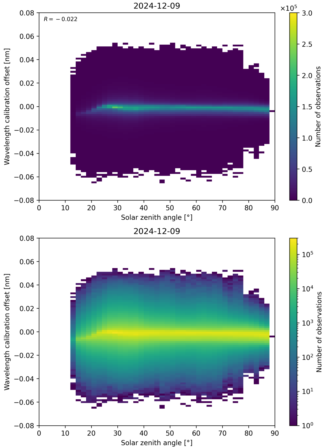
Figure 158: Scatter density plot of “Solar zenith angle” against “Wavelength calibration offset” for 2024-12-08 to 2024-12-10.
