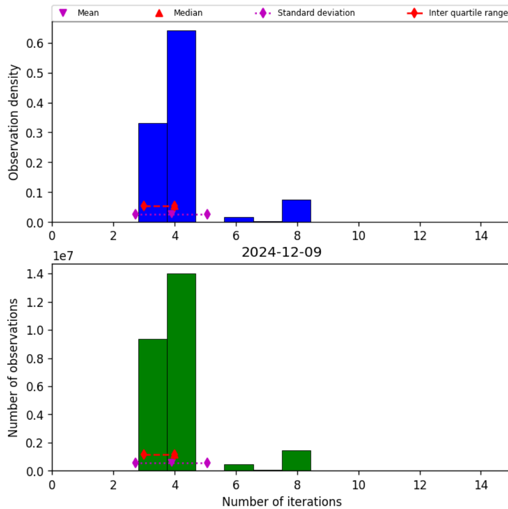
Figure 34: Histogram of “Number of iterations” for 2024-12-08 to 2024-12-10
