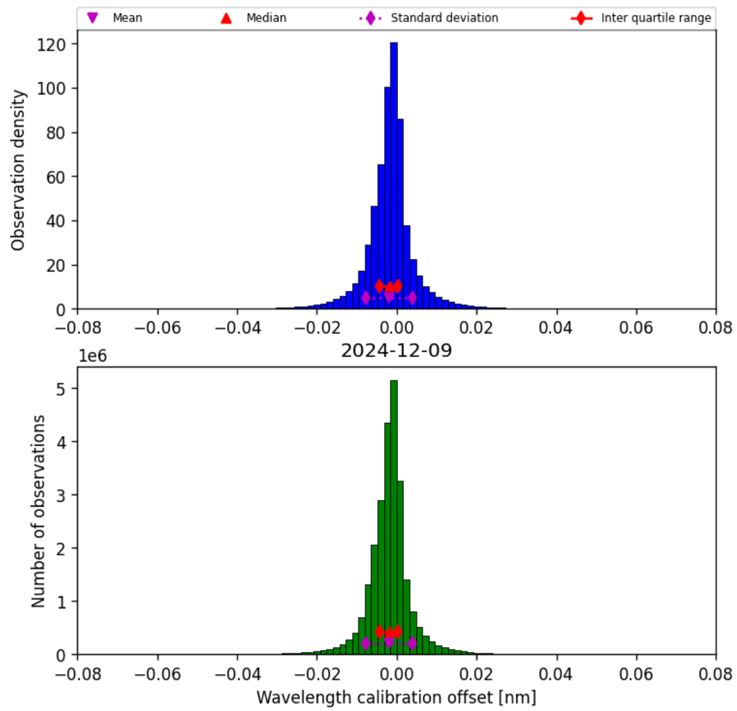
Figure 35: Histogram of “Wavelength calibration offset” for 2024-12-08 to 2024-12-10
