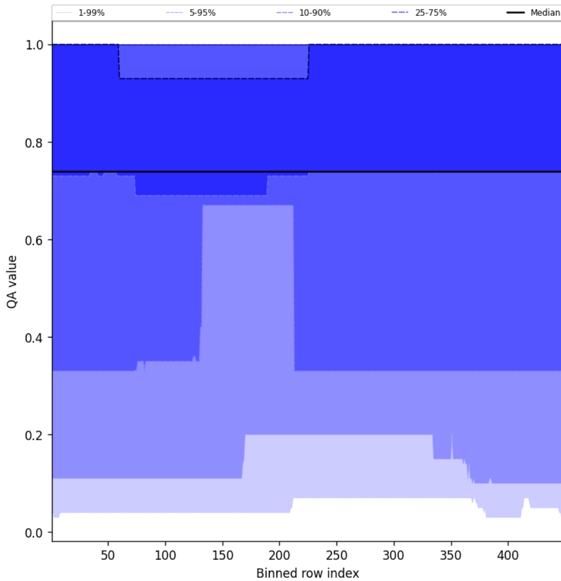
Figure 45: Along track statistics of “QA value” for 2024-12-08 to 2024-12-10
