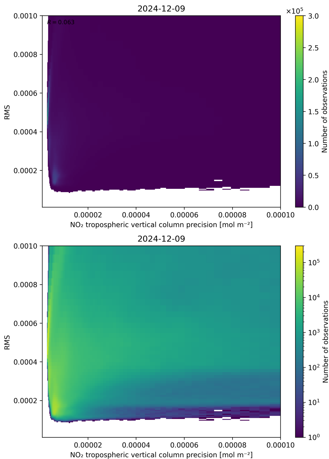
Figure 140: Scatter density plot of “NO 2 tropospheric vertical column precision” against “RMS” for 2024-12-08 to 2024-12-10.
