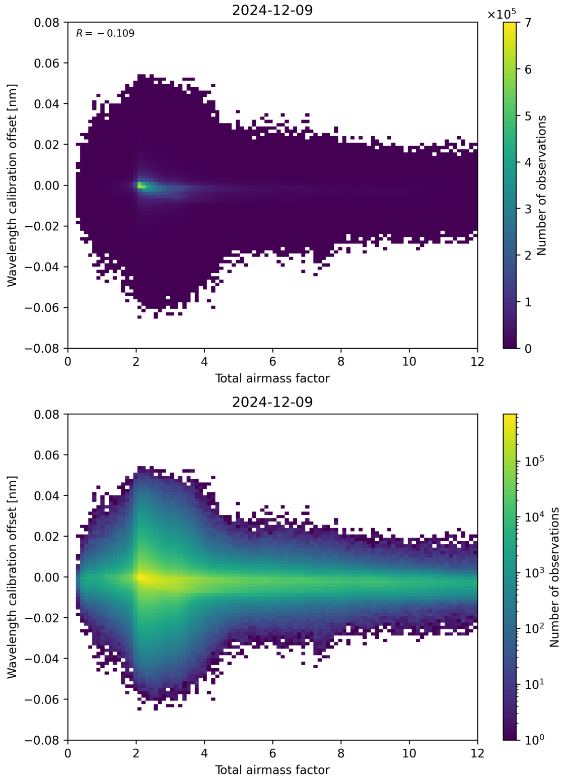
Figure 70: Scatter density plot of “Total airmass factor” against “Wavelength calibration offset” for 2024-12-08 to 2024-12-10.
