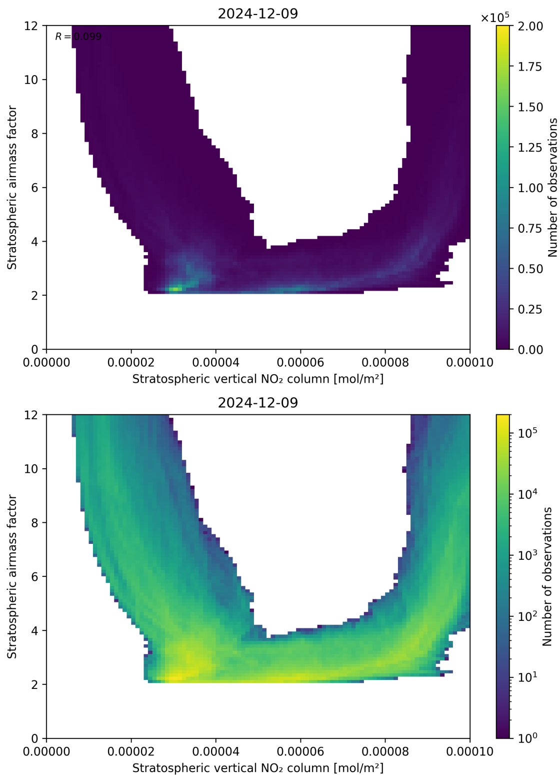
Figure 96: Scatter density plot of “Stratospheric vertical NO 2 column” against “Stratospheric airmass factor” for 2024-12-08 to 2024-12-10.
