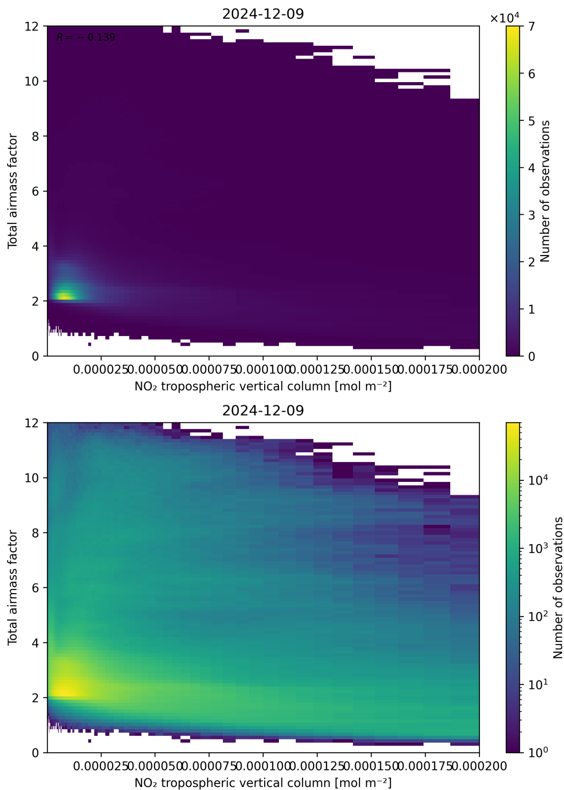
Figure 122: Scatter density plot of “NO 2 tropospheric vertical column” against “Total air mass factor” for 2024-12-08 to 2024-12-10.
