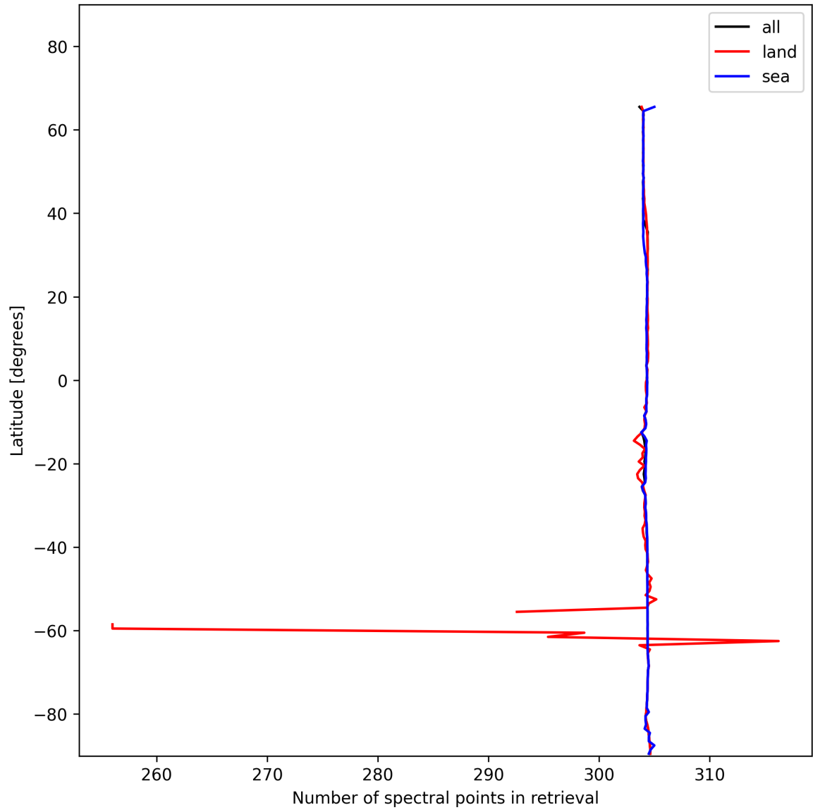
Figure 16: Zonal average of “Number of spectral points in retrieval” for 2024-12-08 to 2024-12-10.
