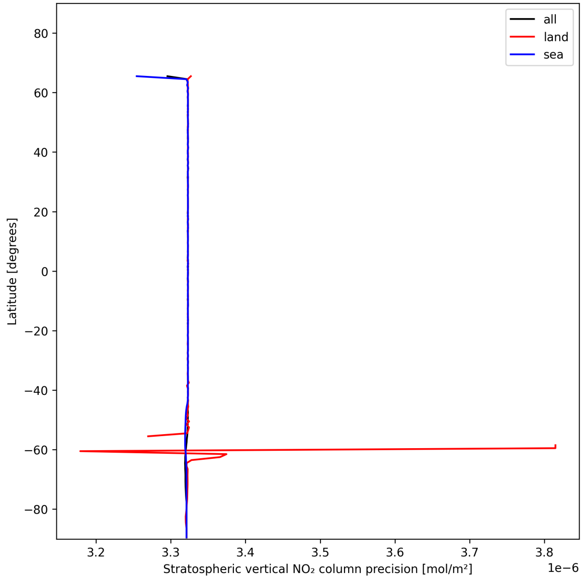
Figure 20: Zonal average of “Stratospheric vertical NO 2 column precision” for 2024-12-08 to 2024-12-10.
