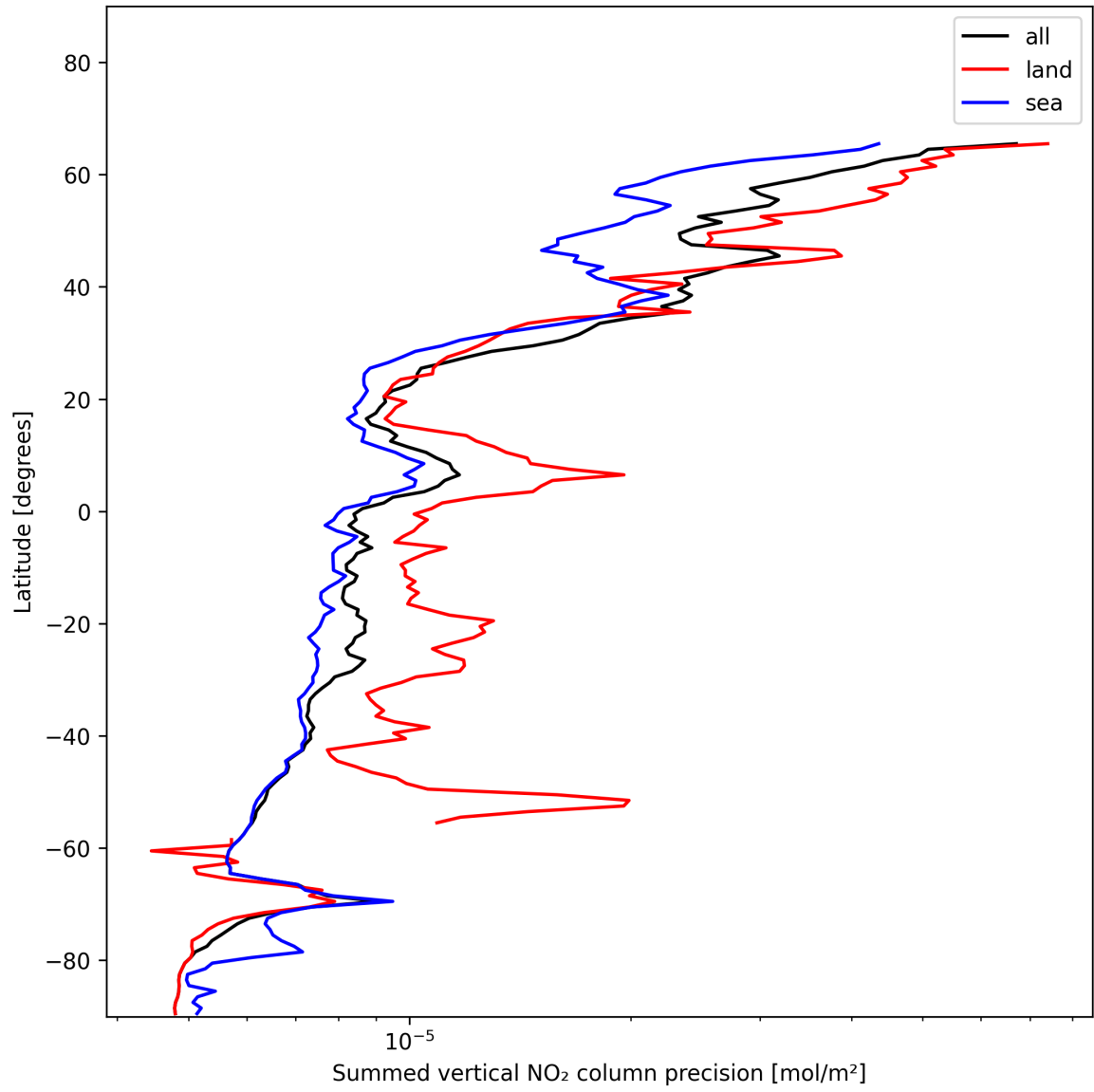
Figure 24: Zonal average of “Summed vertical NO 2 column precision” for 2024-12-08 to 2024-12-10.
