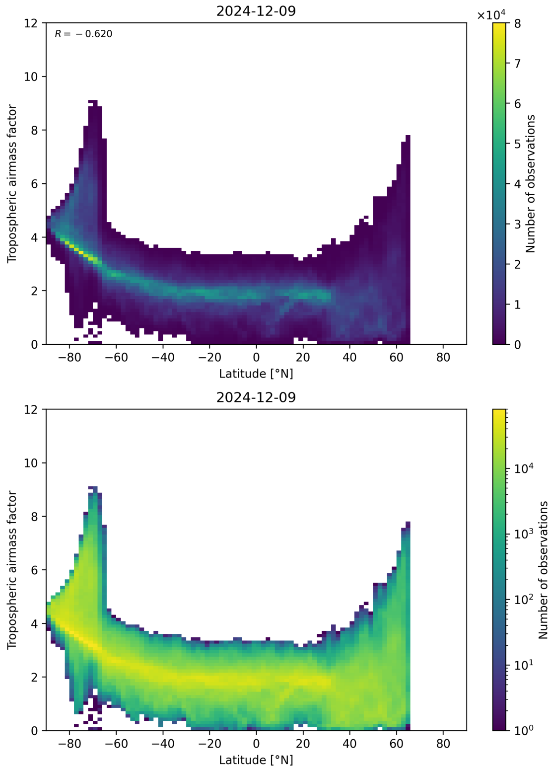
Figure 85: Scatter density plot of “Latitude” against “Tropospheric airmass factor” for 2024-12-08 to 2024-12-10.
