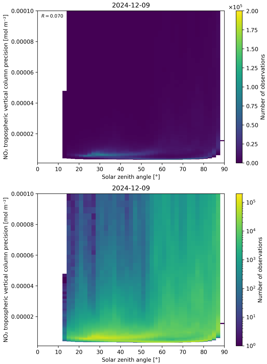
Figure 156: Scatter density plot of “Solar zenith angle” against “NO 2 tropospheric vertical column precision” for 2024-12-08 to 2024-12-10.
