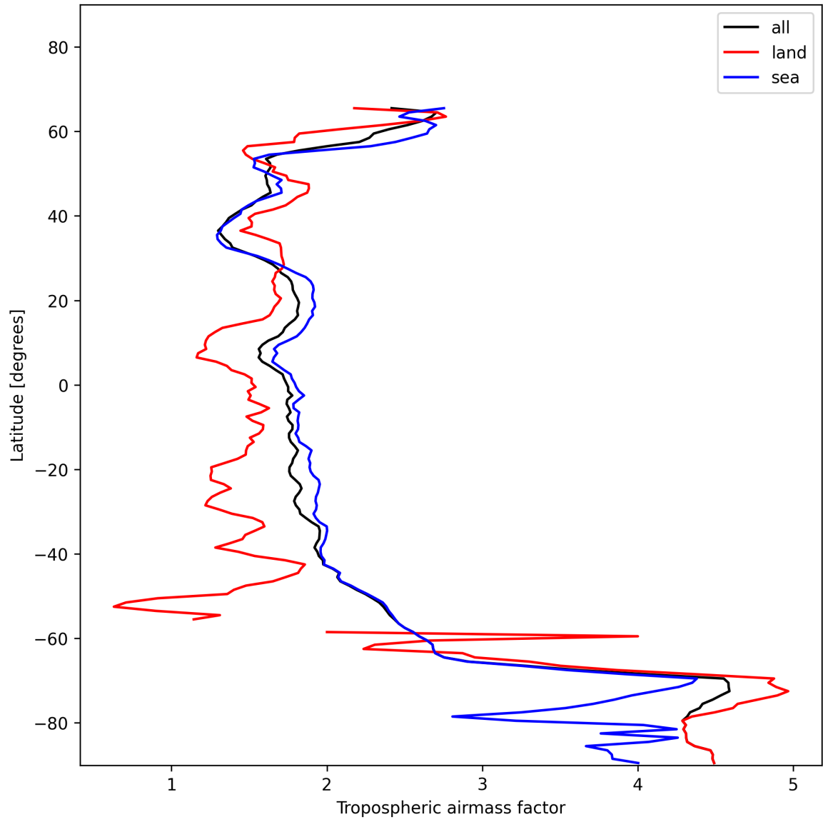
Figure 14: Zonal average of “Tropospheric airmass factor” for 2024-12-08 to 2024-12-10.
