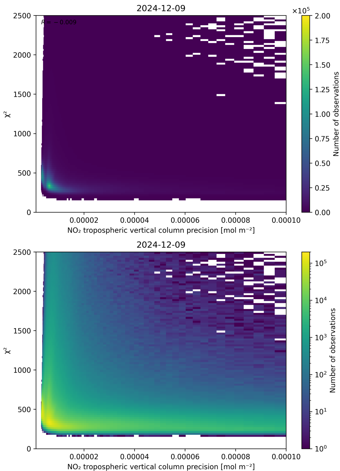
Figure 134: Scatter density plot of “NO 2 tropospheric vertical column precision” against “ \chi^2 ” for 2024-12-08 to 2024-12-10.
