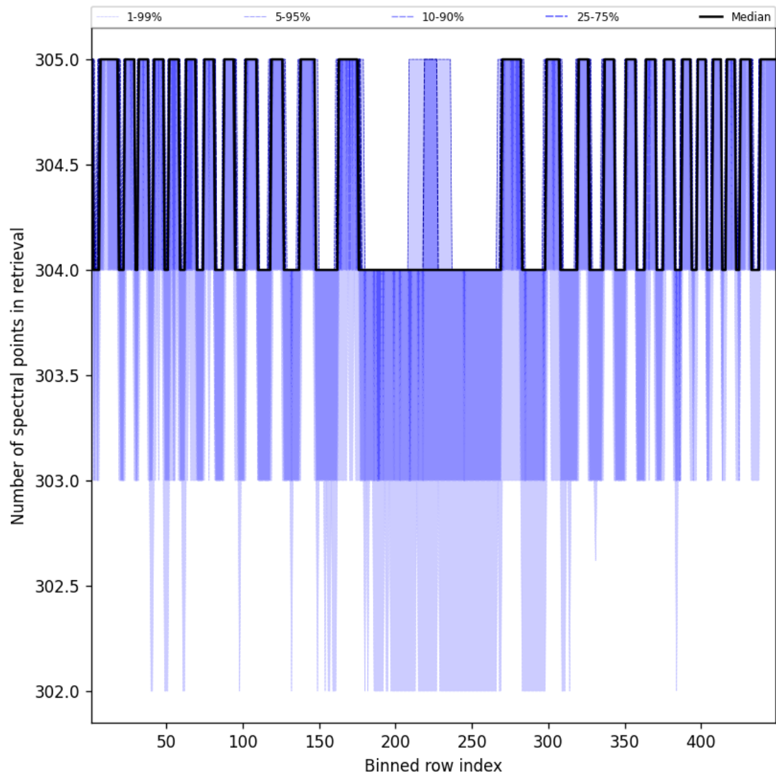
Figure 50: Along track statistics of “Number of spectral points in retrieval” for 2024-12-08 to 2024-12-10
