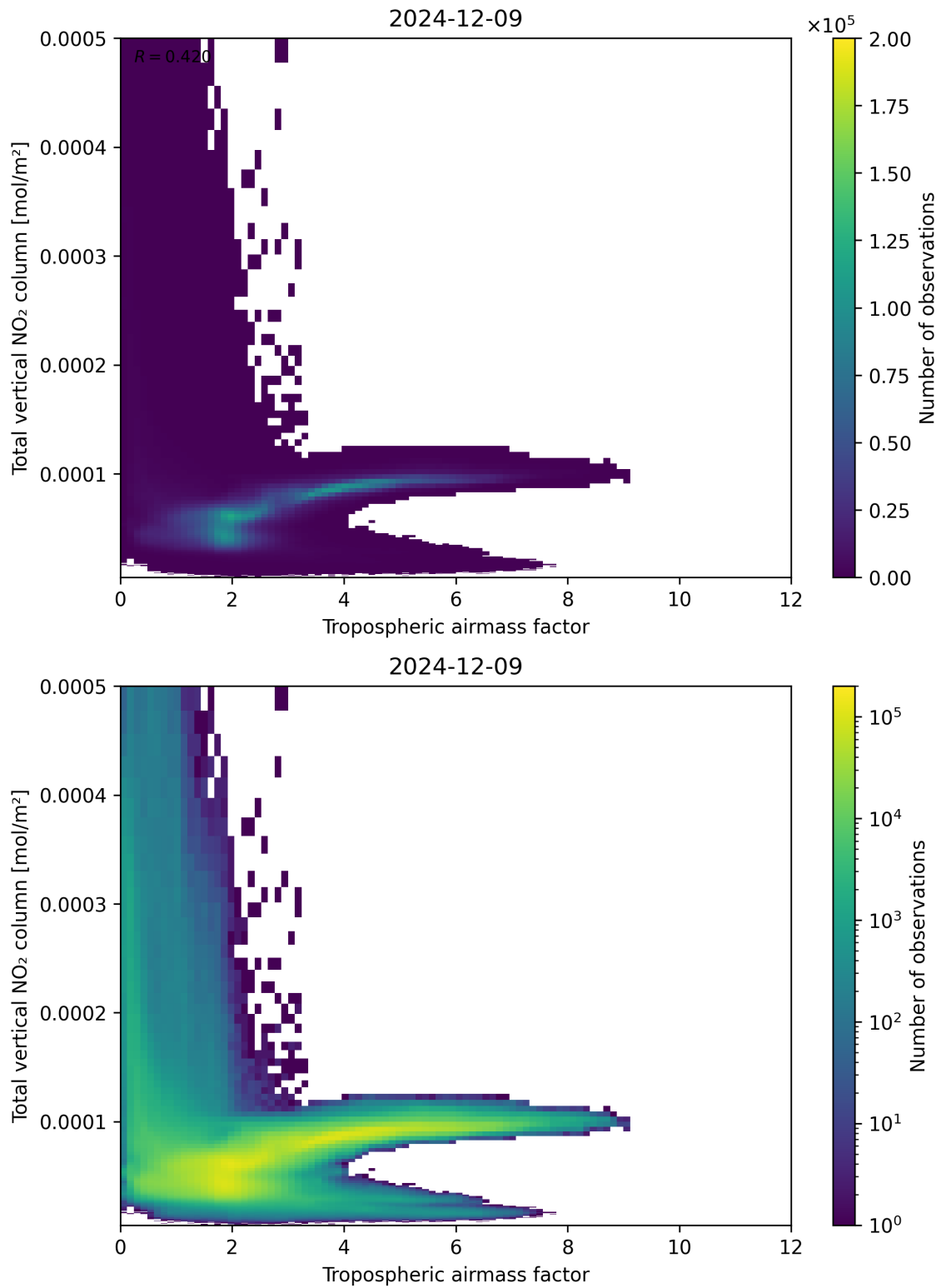
Figure 77: Scatter density plot of “Tropospheric airmass factor” against “Total vertical NO 2 column” for 2024-12-08 to 2024-12-10.
