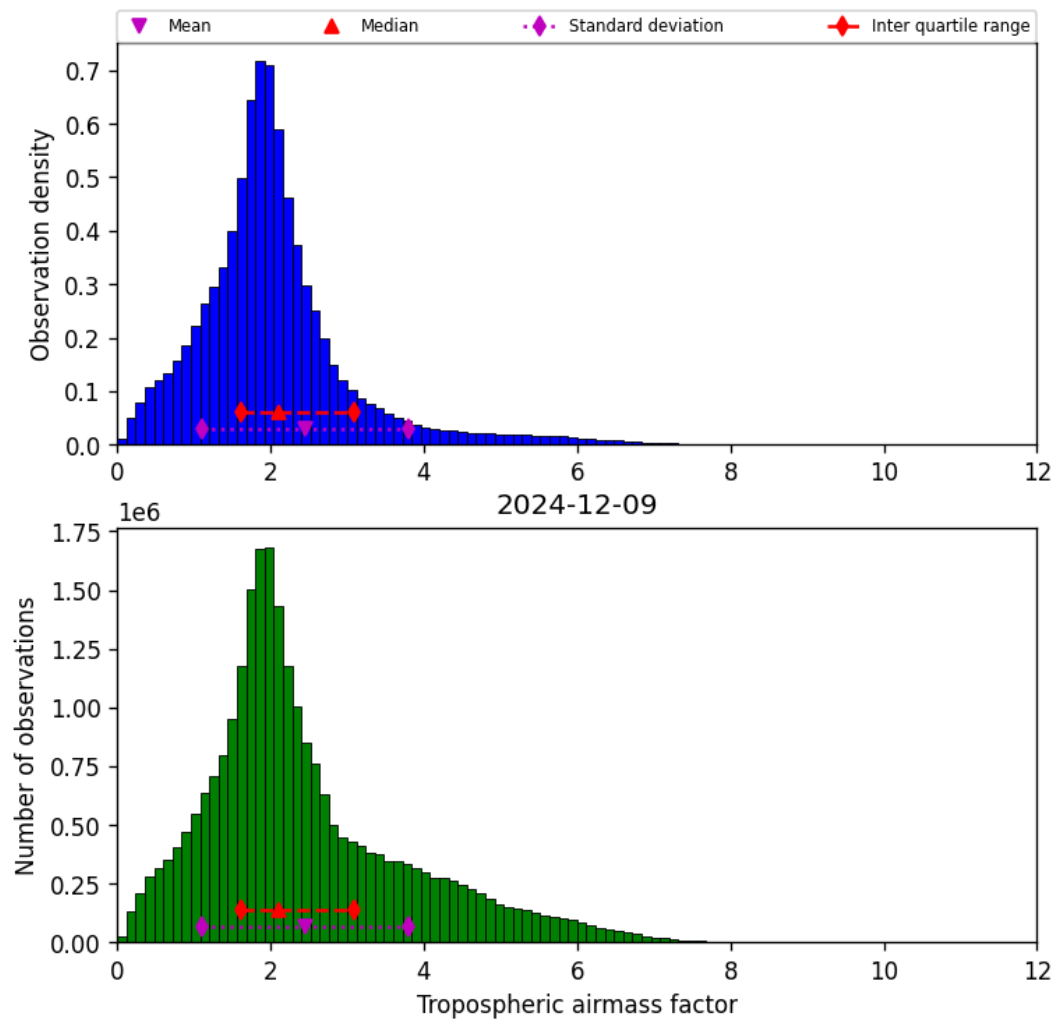
Figure 31: Histogram of “Tropospheric airmass factor” for 2024-12-08 to 2024-12-10
