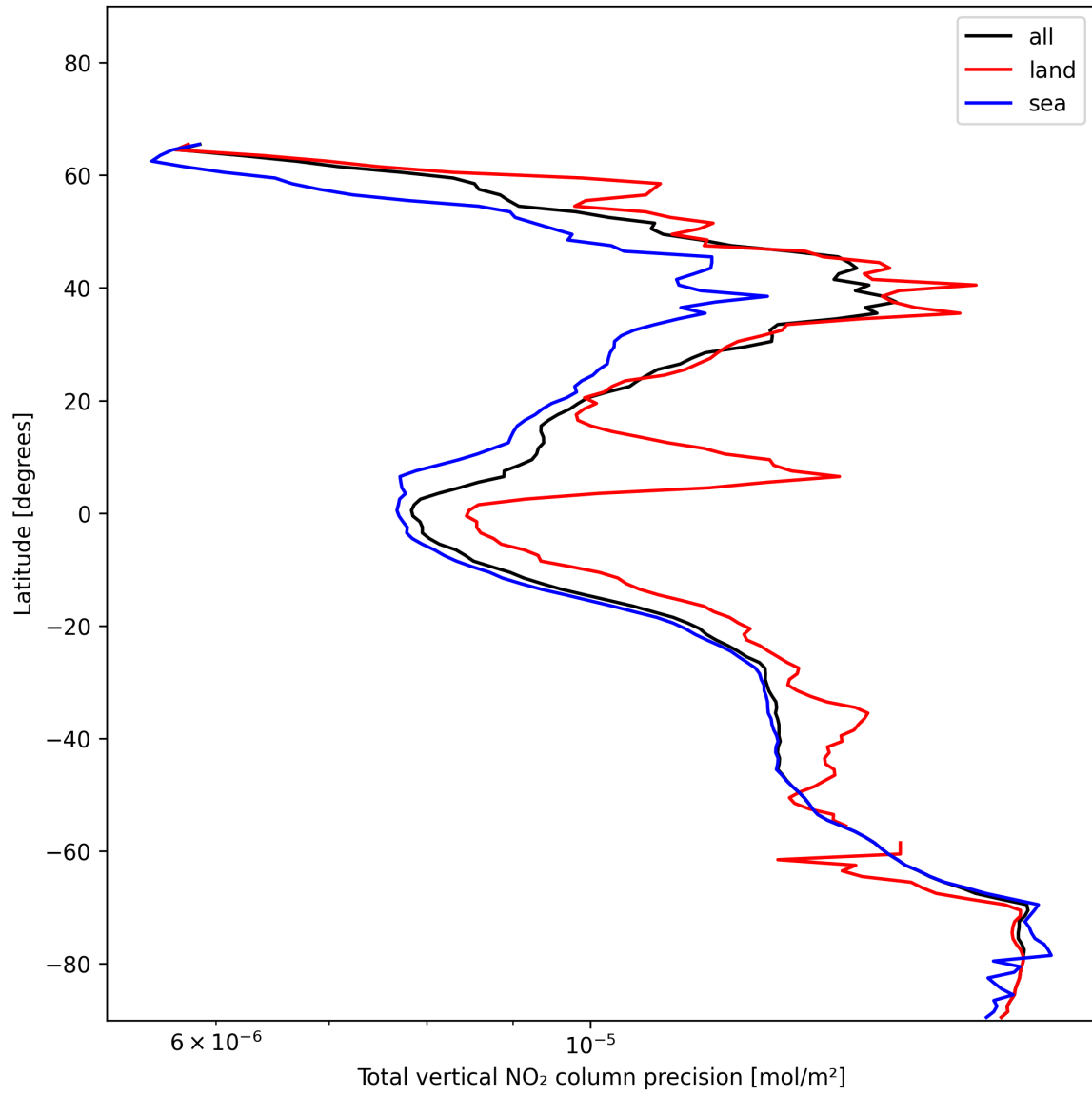
Figure 22: Zonal average of “Total vertical NO 2 column precision” for 2024-12-08 to 2024-12-10.
