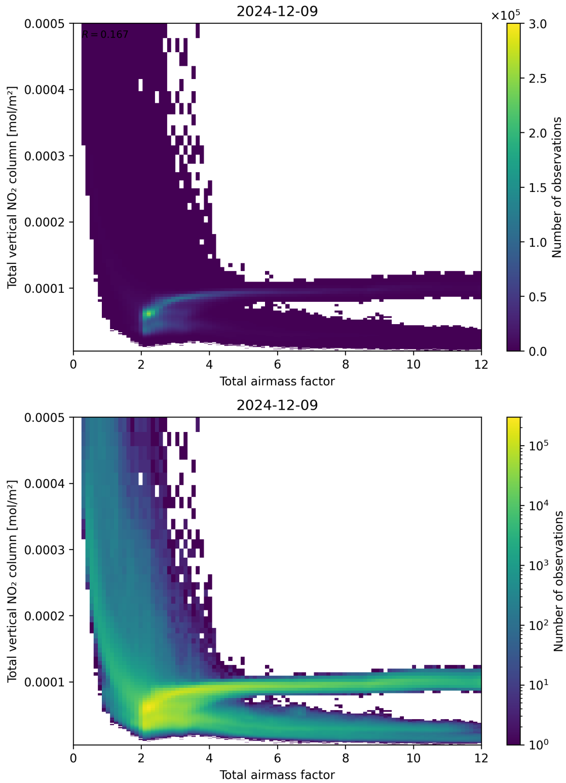
Figure 67: Scatter density plot of “Total airmass factor” against “Total vertical NO 2 column” for 2024-12-08 to 2024-12-10.
