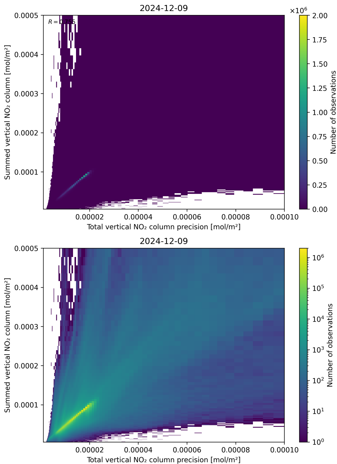
Figure 117: Scatter density plot of “Total vertical NO 2 column precision” against “Summed vertical NO 2 column” for 2024-12-08 to 2024-12-10.
