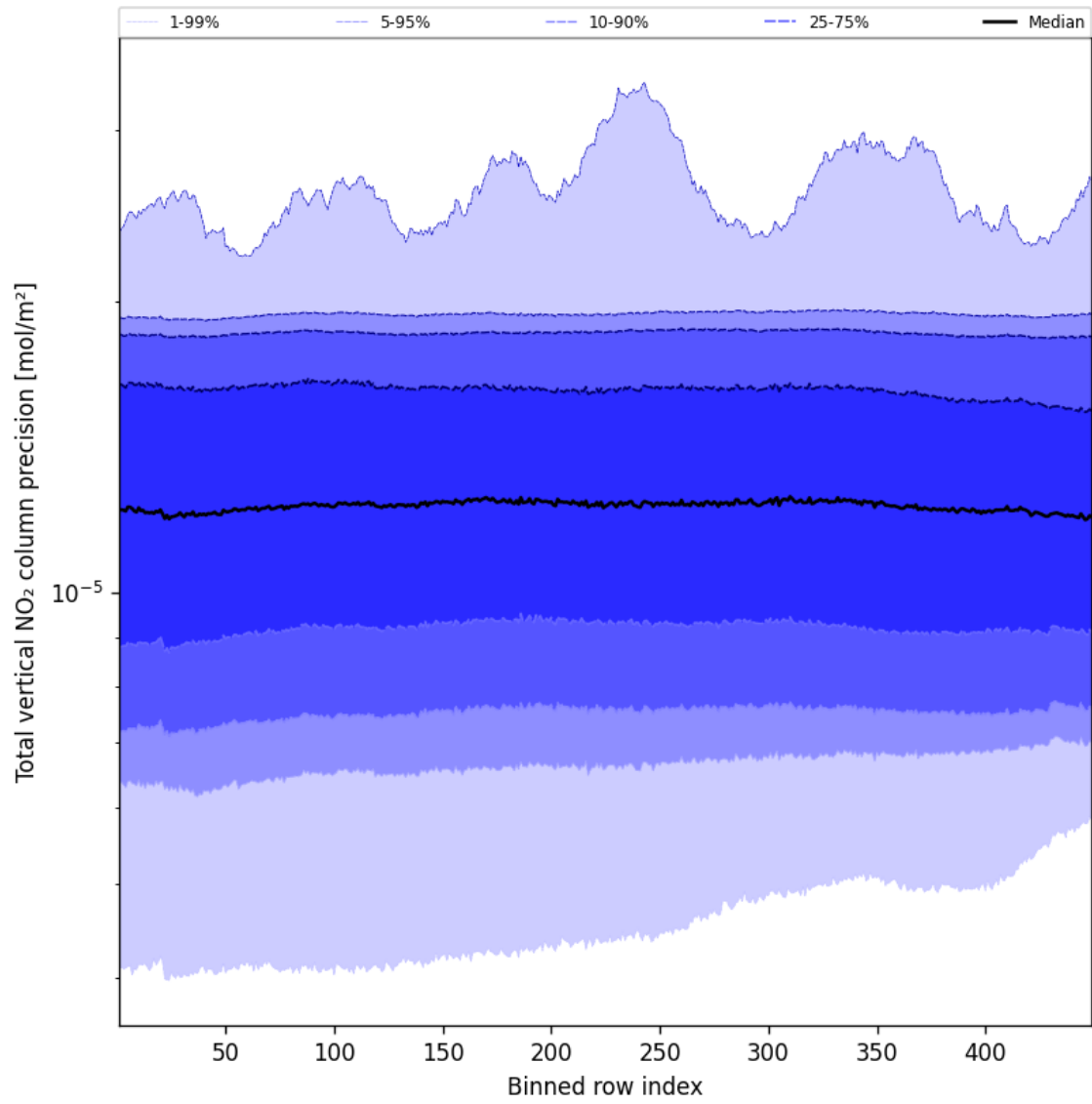
Figure 56: Along track statistics of “Total vertical NO 2 column precision” for 2024-12-08 to 2024-12-10
