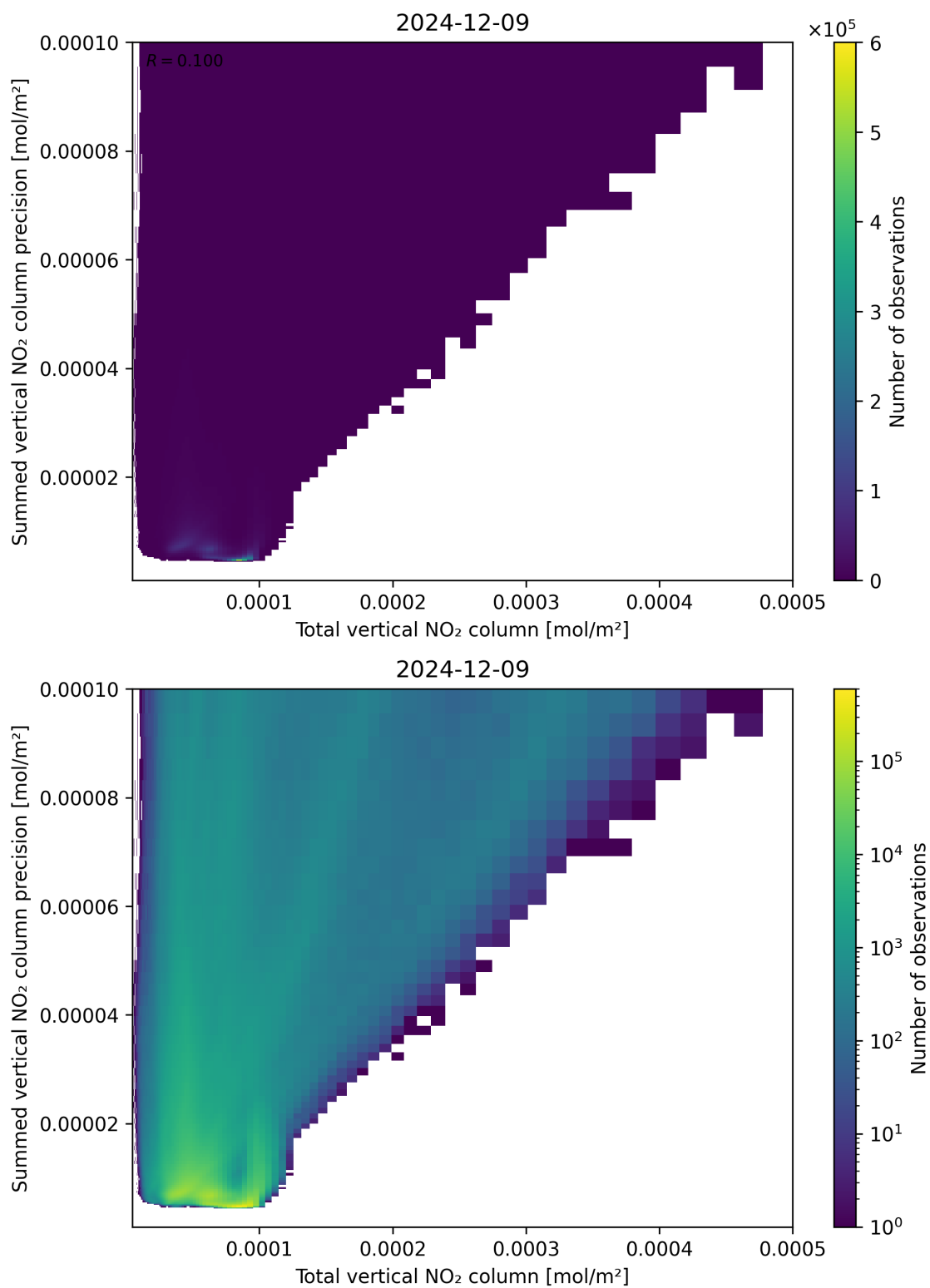
Figure 113: Scatter density plot of “Total vertical NO 2 column” against “Summed vertical NO 2 column precision” for 2024-12-08 to 2024-12-10.
