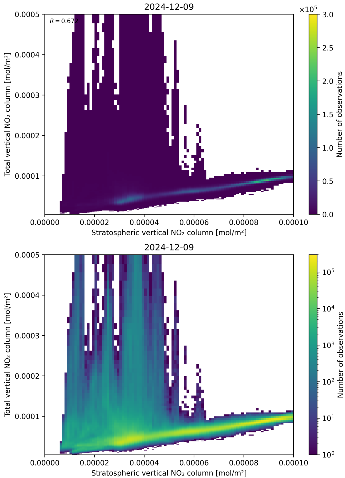
Figure 100: Scatter density plot of “Stratospheric vertical NO 2 column” against “Total vertical NO 2 column” for 2024-12-08 to 2024-12-10.
