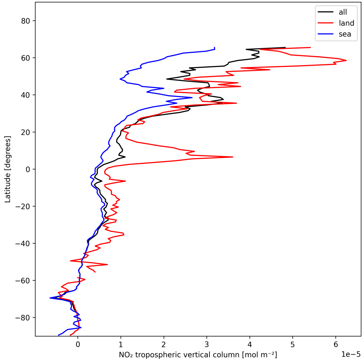
Figure 12: Zonal average of “NO 2 tropospheric vertical column” for 2024-12-08 to 2024-12-10.
