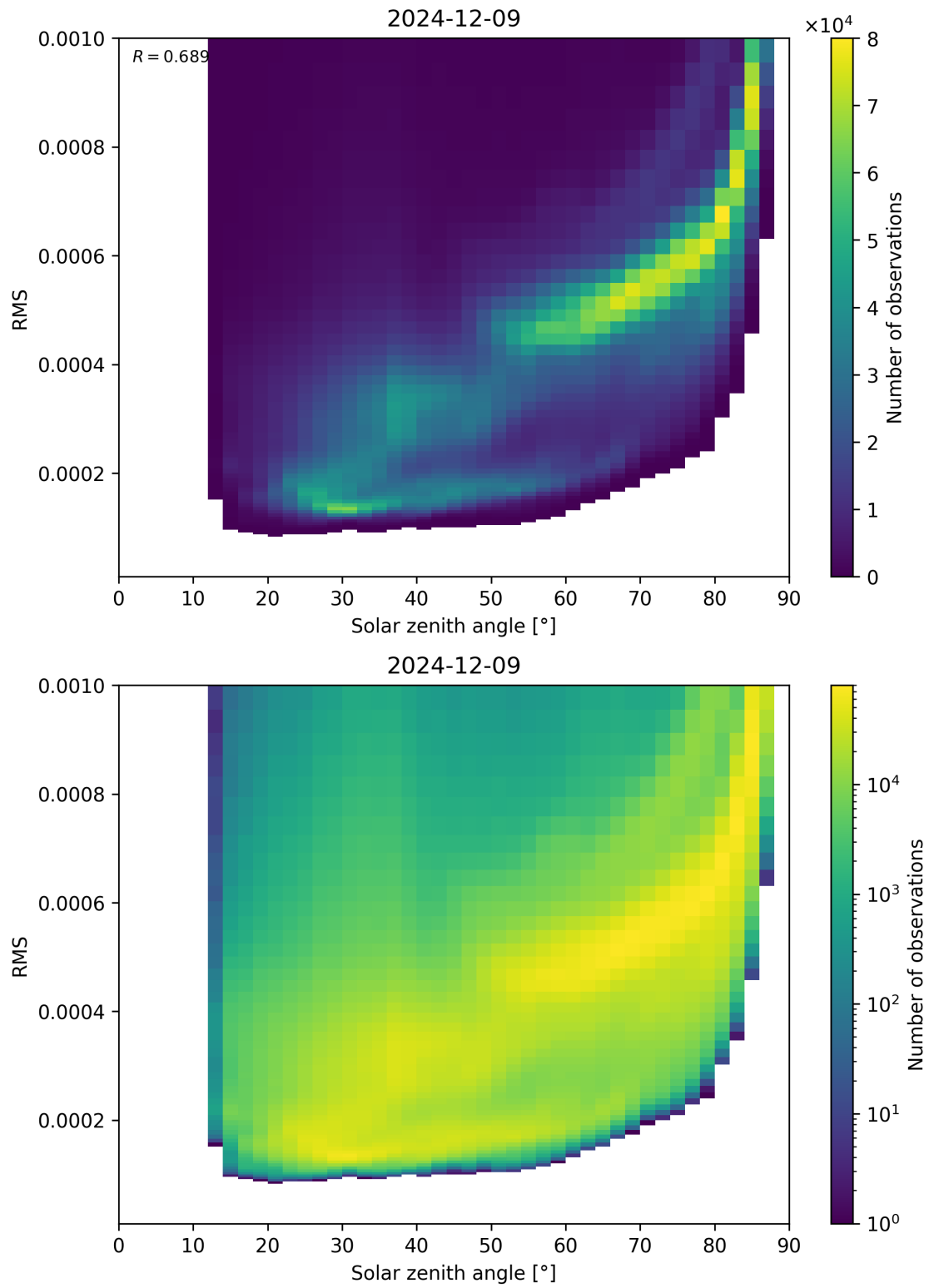
Figure 157: Scatter density plot of “Solar zenith angle” against “RMS” for 2024-12-08 to 2024-12-10.
