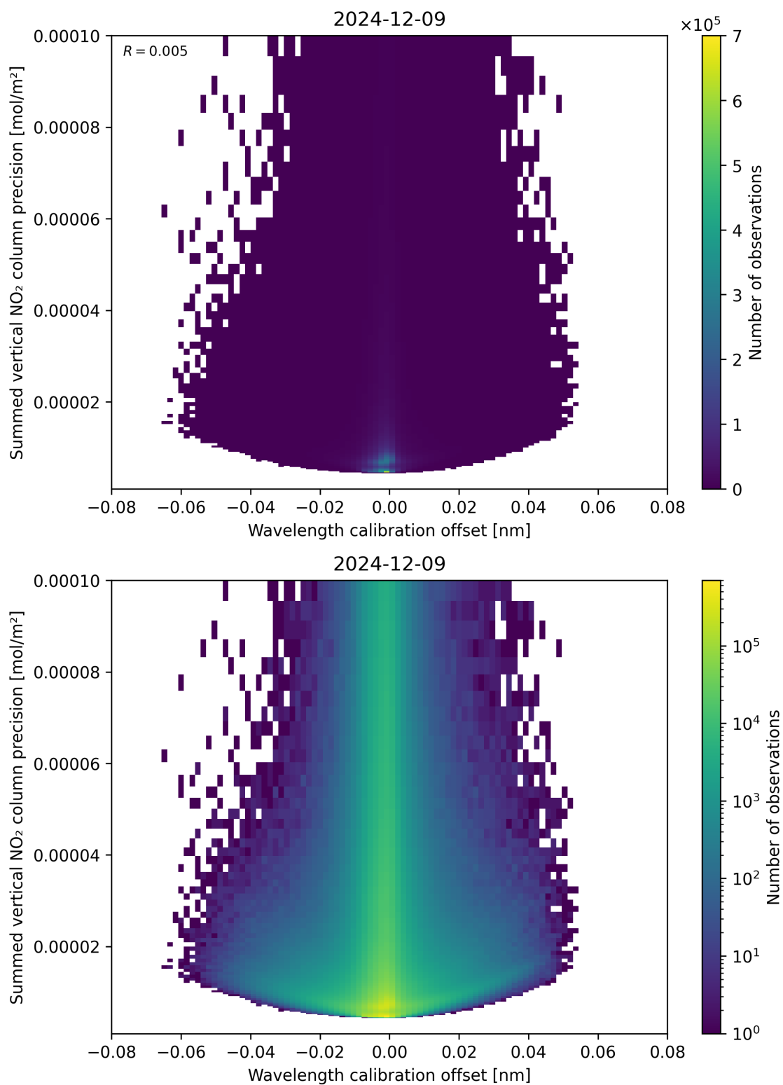
Figure 178: Scatter density plot of “Wavelength calibration offset” against “Summed vertical NO 2 column precision” for 2024-12-08 to 2024-12-10.
