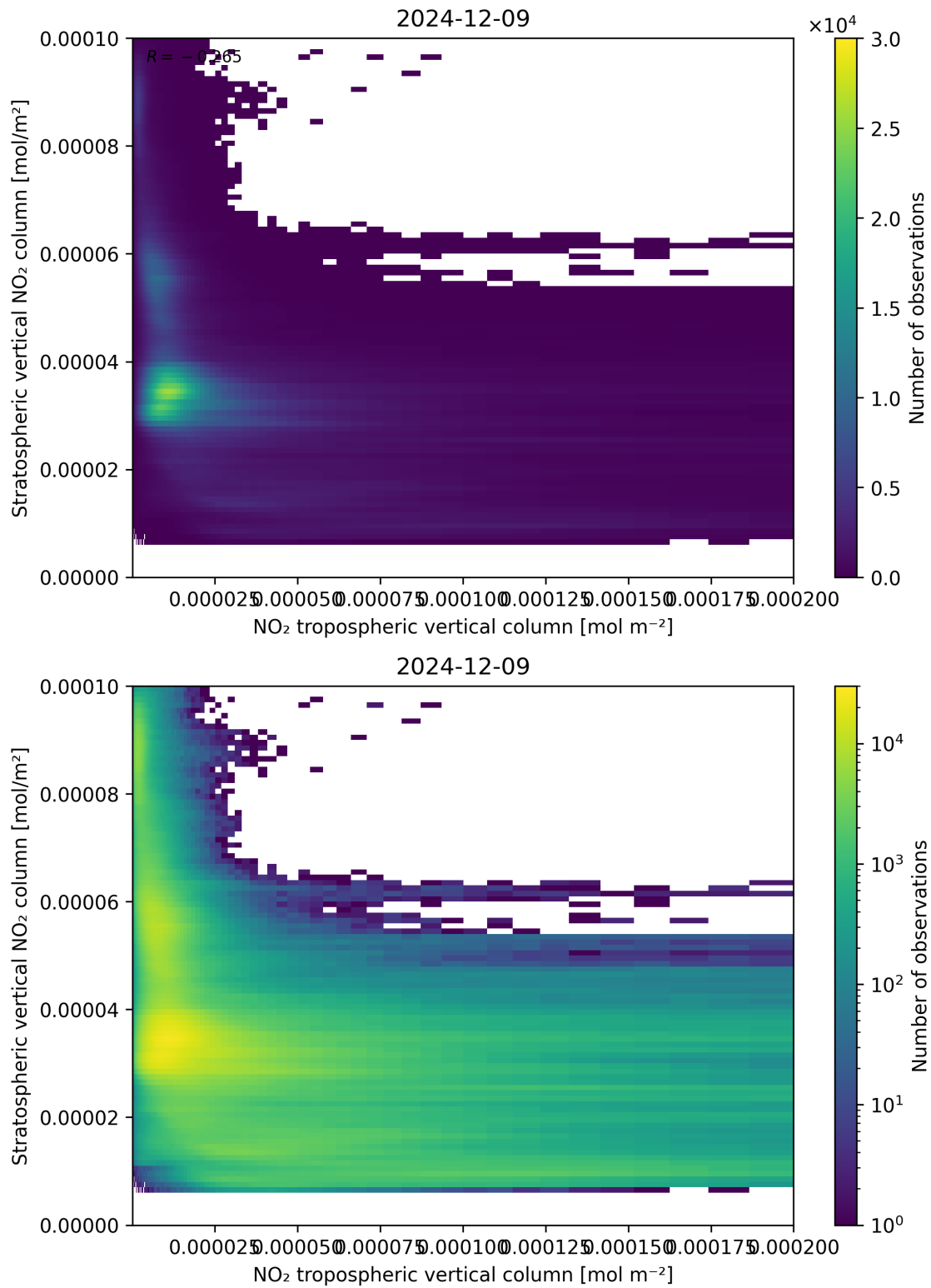
Figure 125: Scatter density plot of “NO 2 tropospheric vertical column” against “Stratospheric vertical NO 2 column” for 2024-12-08 to 2024-12-10.
