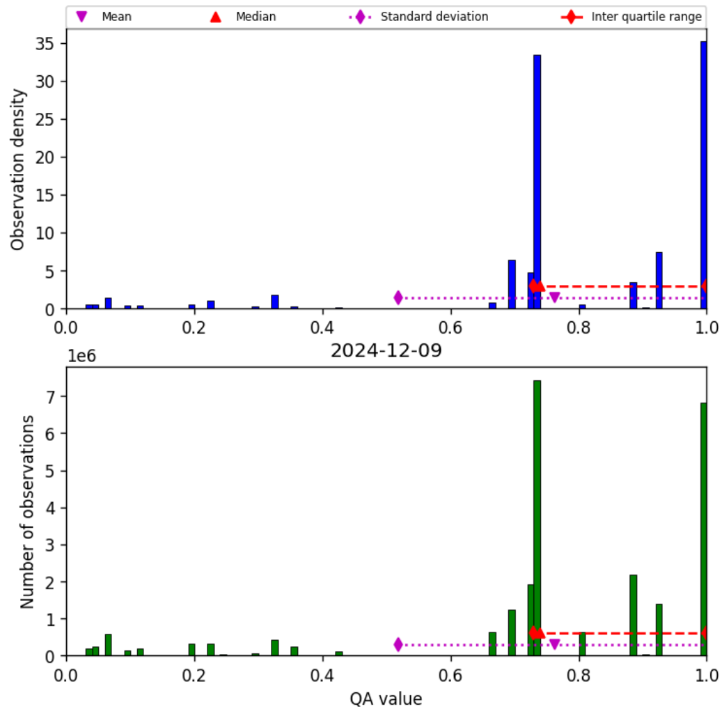
Figure 28: Histogram of “QA value” for 2024-12-08 to 2024-12-10
