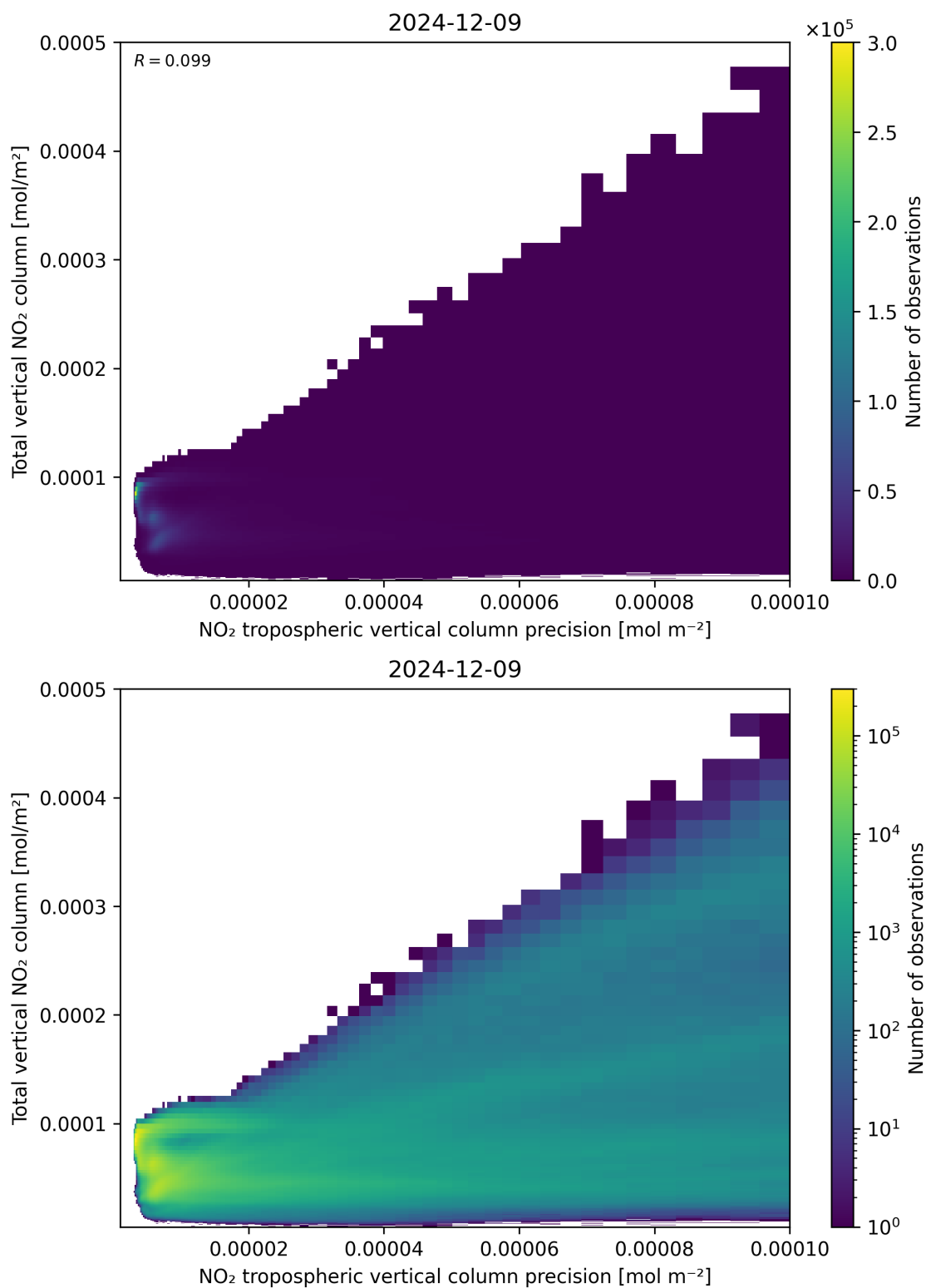
Figure 138: Scatter density plot of “NO 2 tropospheric vertical column precision” against “Total vertical NO 2 column” for 2024-12-08 to 2024-12-10.
