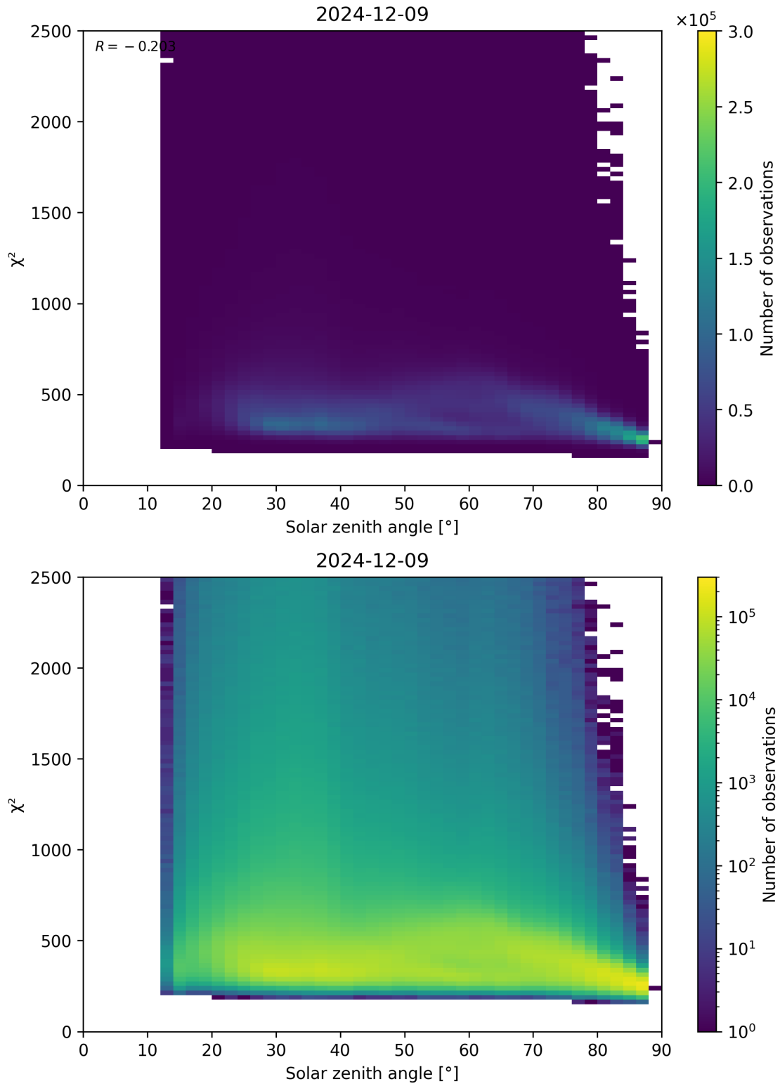
Figure 148: Scatter density plot of “Solar zenith angle” against “ \chi^2 ” for 2024-12-08 to 2024-12-10.
