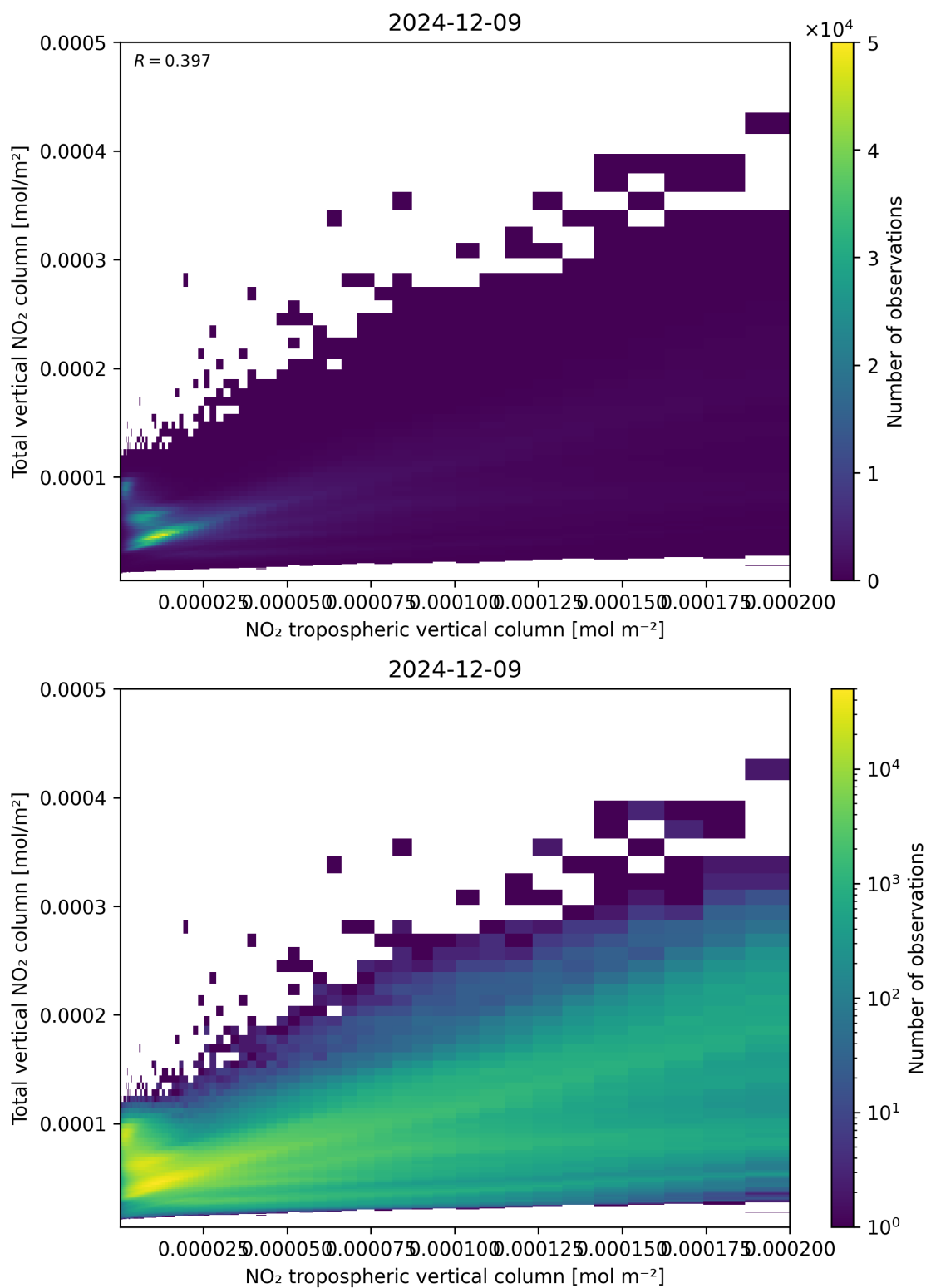
Figure 128: Scatter density plot of “NO 2 tropospheric vertical column” against “Total vertical NO 2 column” for 2024-12-08 to 2024-12-10.
