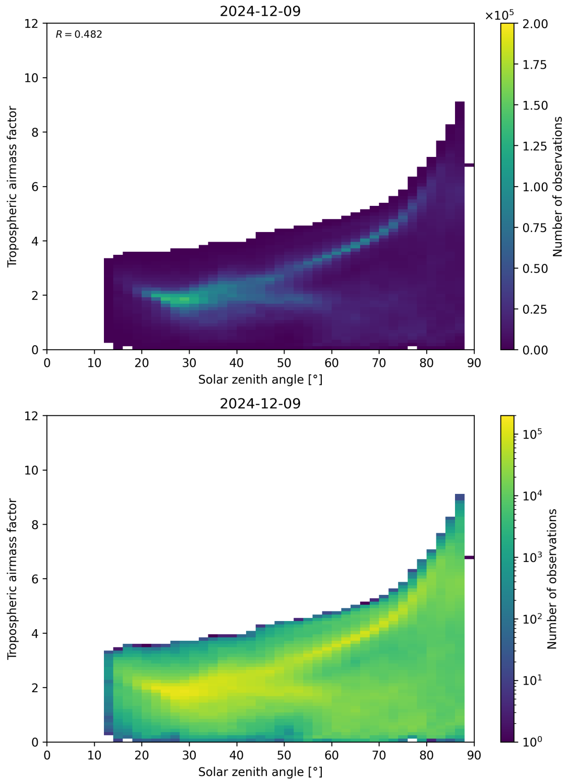
Figure 147: Scatter density plot of “Solar zenith angle” against “Tropospheric airmass factor” for 2024-12-08 to 2024-12-10.
