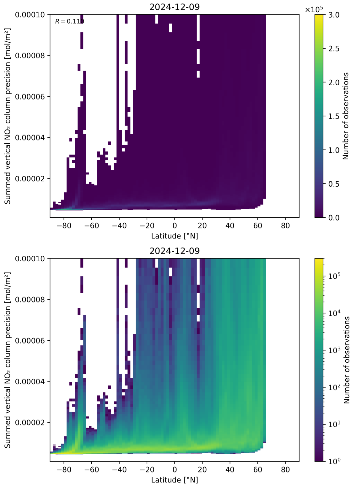
Figure 89: Scatter density plot of “Latitude” against “Summed vertical NO 2 column precision” for 2024-12-08 to 2024-12-10.
