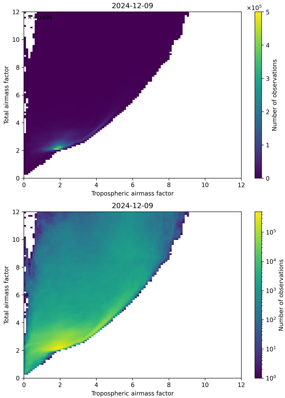
Figure 72: Scatter density plot of “Tropospheric airmass factor” against “Total airmass factor” for 2024-12-08 to 2024-12-10.
