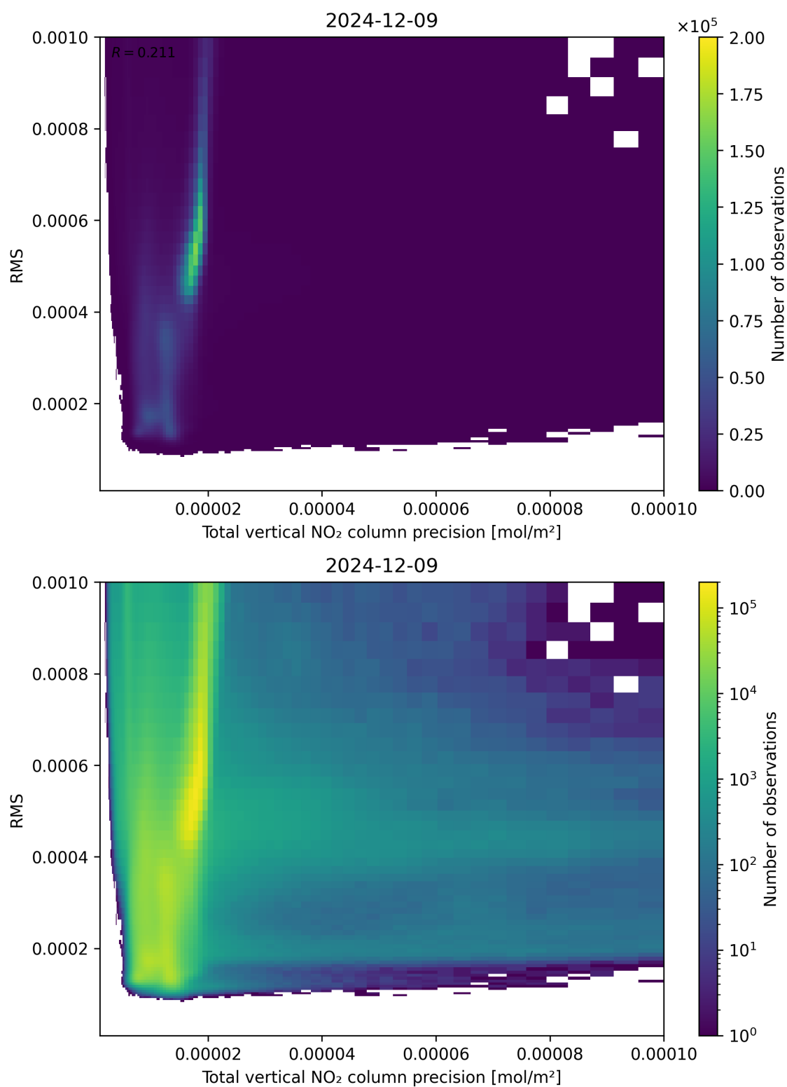
Figure 119: Scatter density plot of “Total vertical NO 2 column precision” against “RMS” for 2024-12-08 to 2024-12-10.
