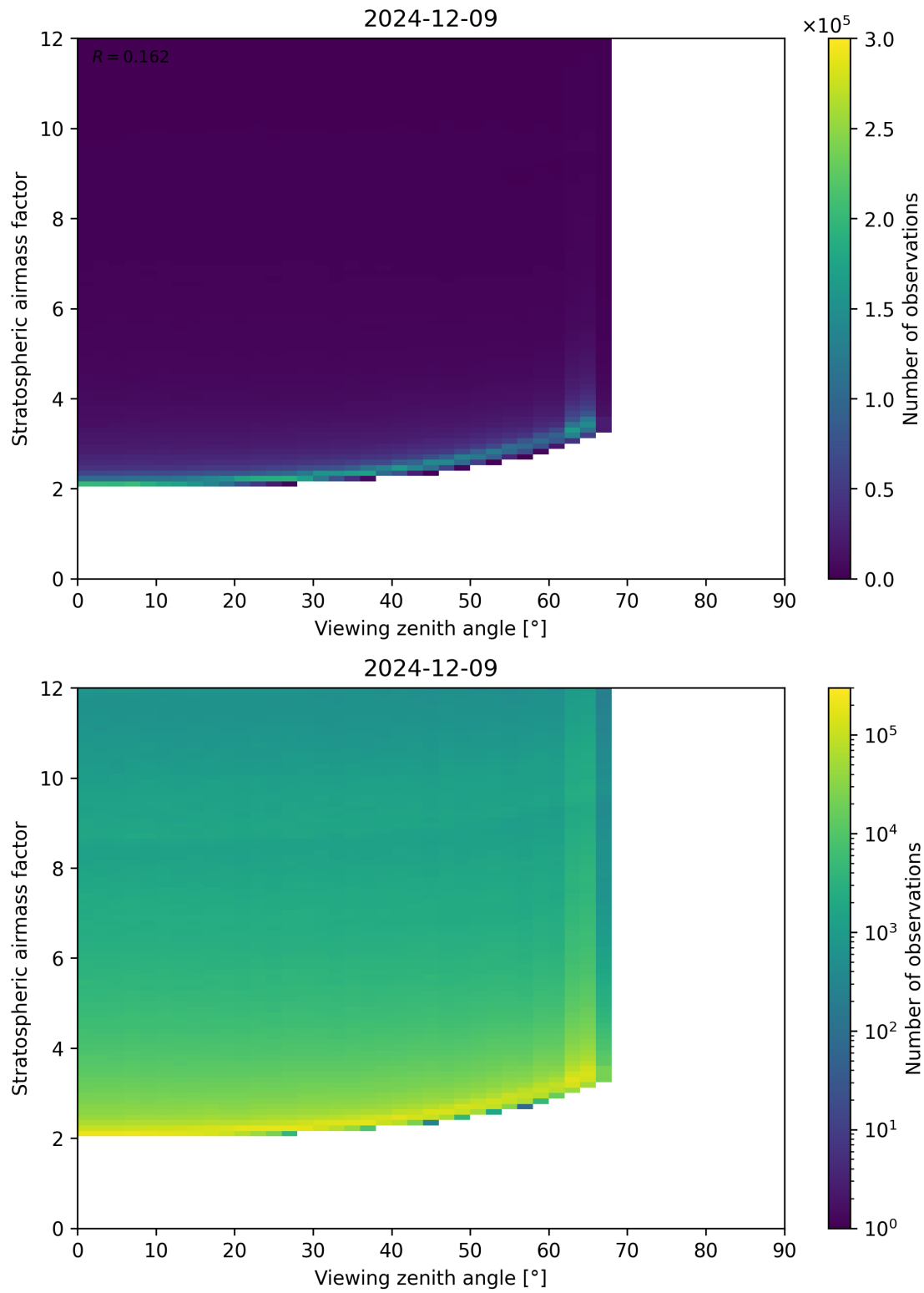
Figure 159: Scatter density plot of “Viewing zenith angle” against “Stratospheric airmass factor” for 2024-12-08 to 2024-12-10.
