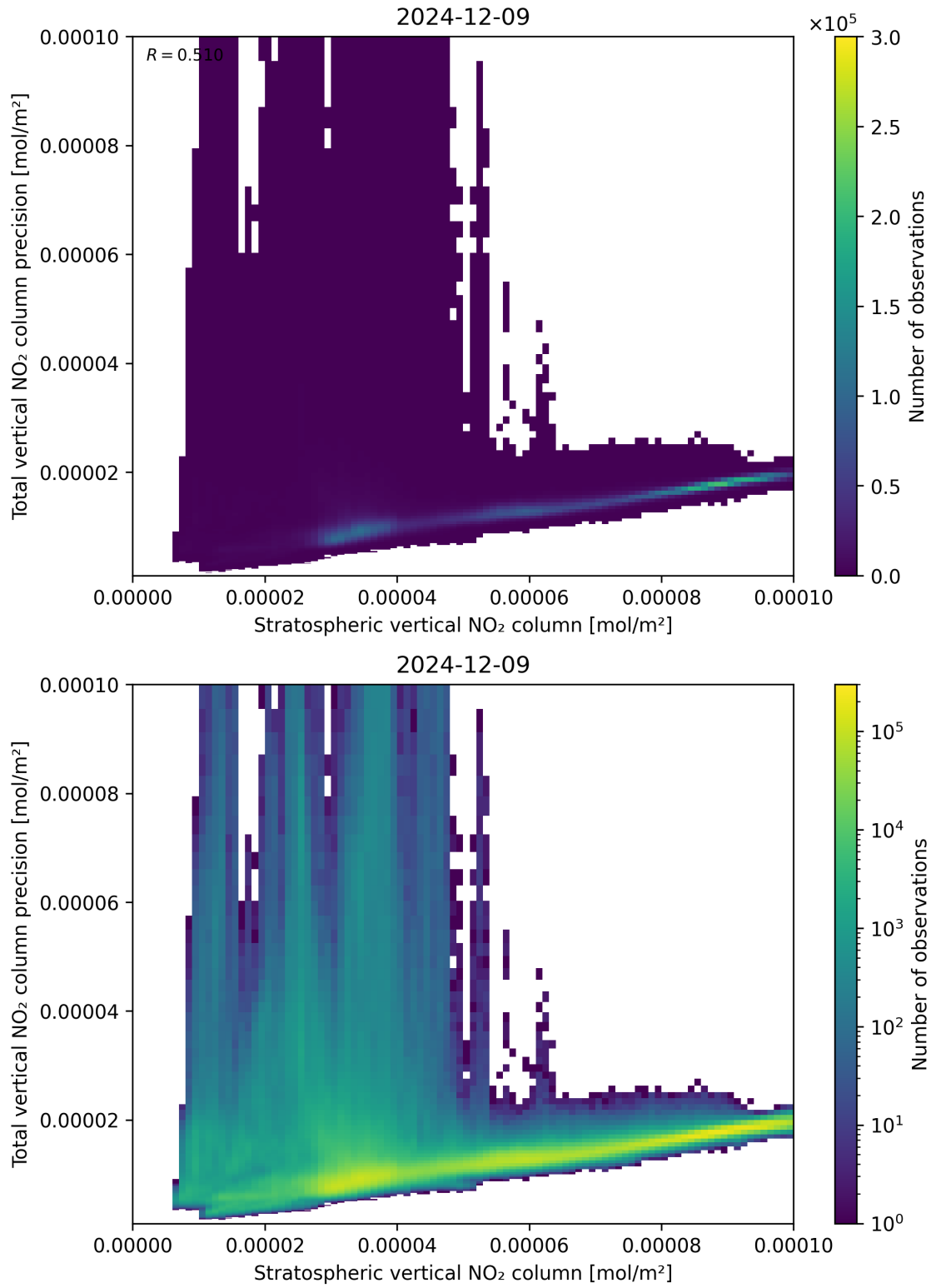
Figure 101: Scatter density plot of “Stratospheric vertical NO 2 column” against “Total vertical NO 2 column precision” for 2024-12-08 to 2024-12-10.
