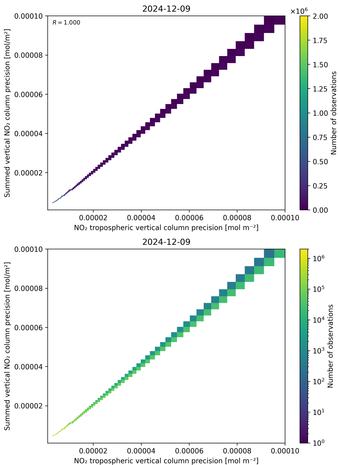
Figure 137: Scatter density plot of “NO 2 tropospheric vertical column precision” against “Summed vertical NO 2 column precision” for 2024-12-08 to 2024-12-10.
