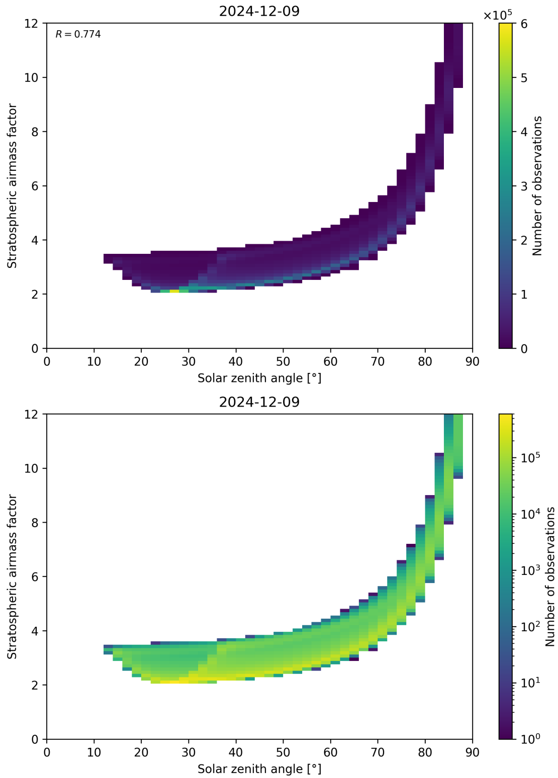
Figure 145: Scatter density plot of “Solar zenith angle” against “Stratospheric airmass factor” for 2024-12-08 to 2024-12-10.
