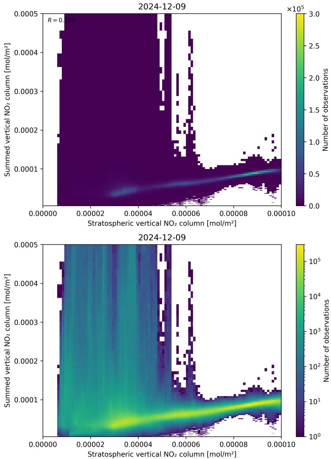
Figure 98: Scatter density plot of “Stratospheric vertical NO 2 column” against “Summed vertical NO 2 column” for 2024-12-08 to 2024-12-10.
