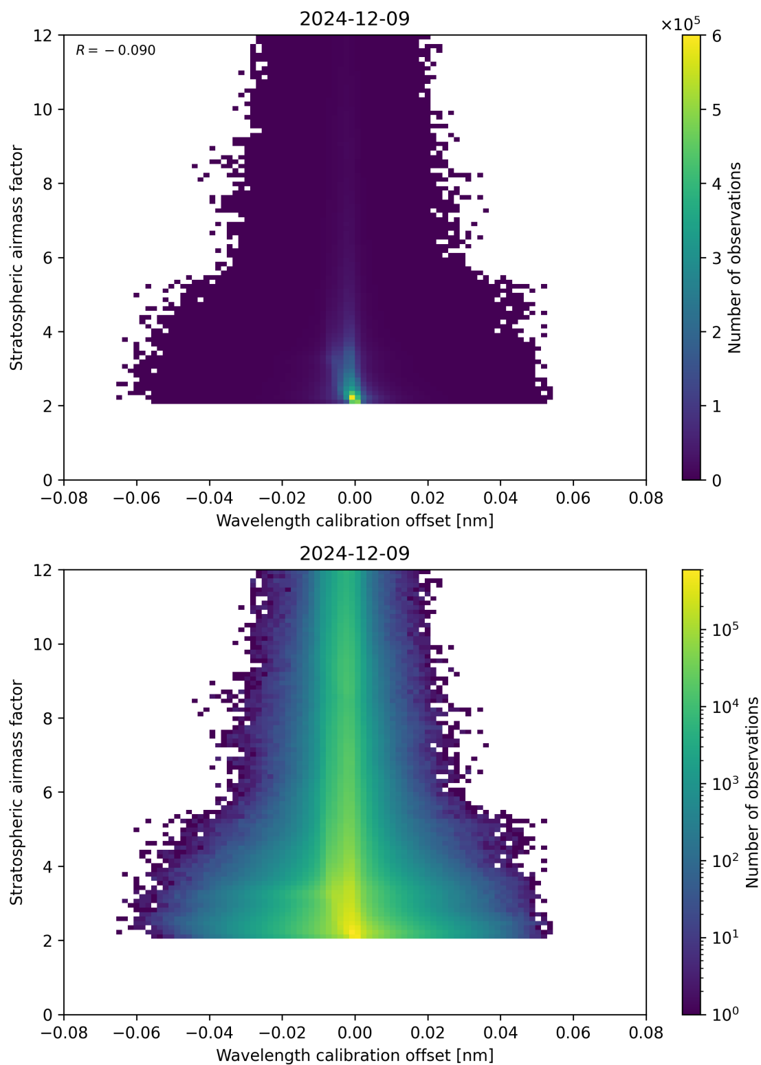
Figure 174: Scatter density plot of “Wavelength calibration offset” against “Stratospheric airmass factor” for 2024-12-08 to 2024-12-10.
