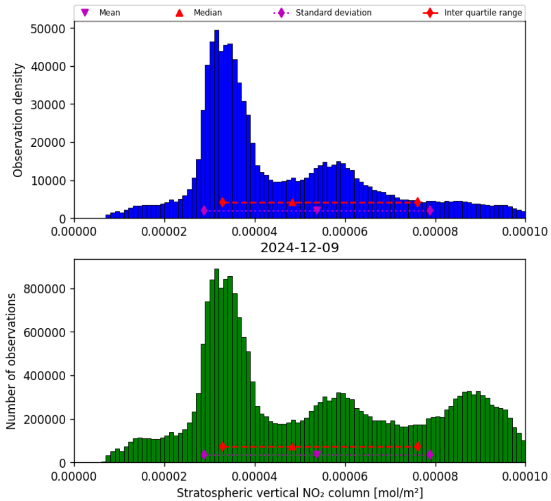
Figure 36: Histogram of “Stratospheric vertical NO 2 column” for 2024-12-08 to 2024-12-10
