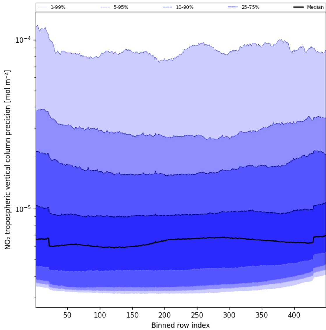
Figure 47: Along track statistics of “NO 2 tropospheric vertical column precision” for 2024-12-08 to 2024-12-10
