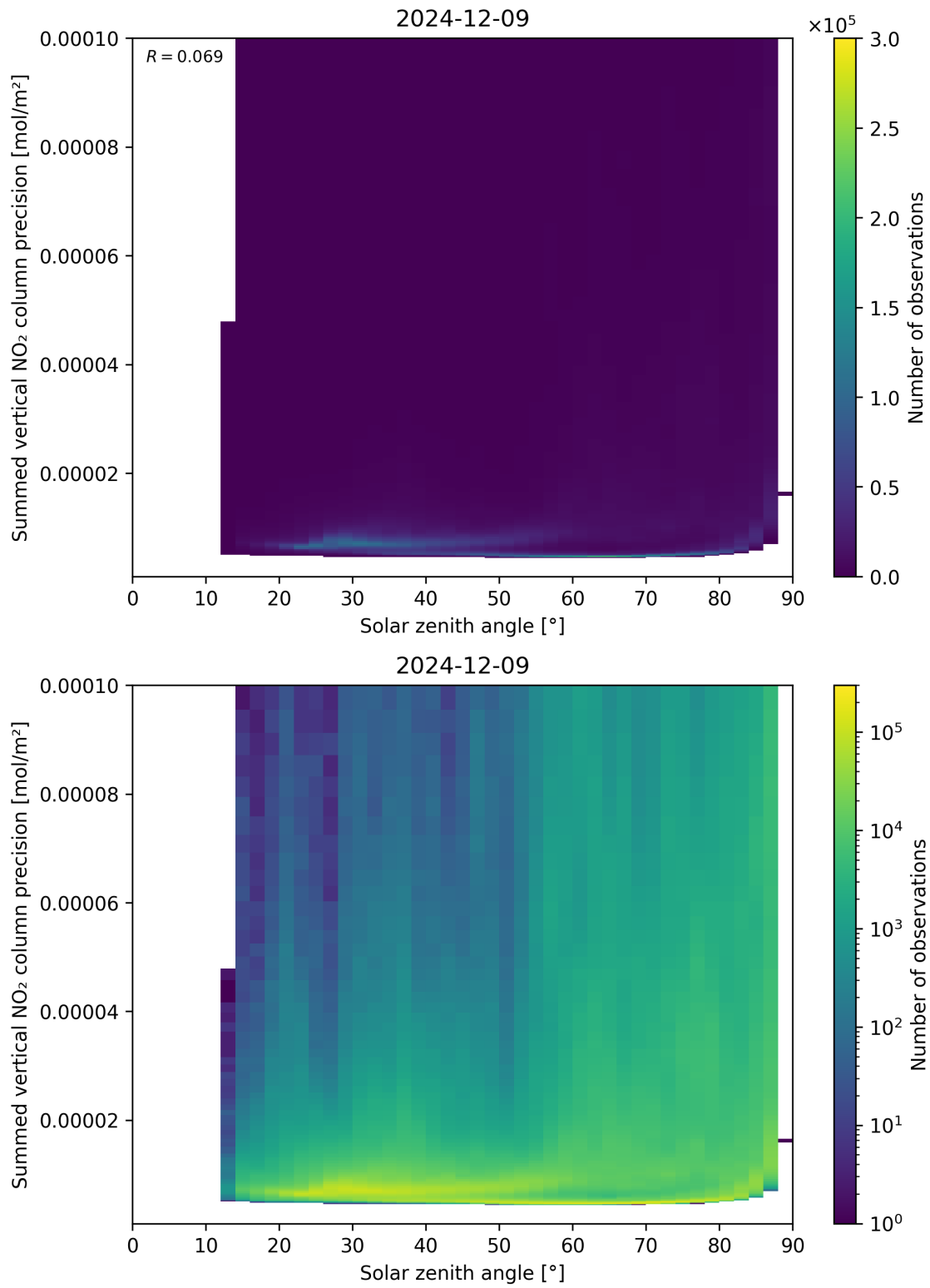
Figure 152: Scatter density plot of “Solar zenith angle” against “Summed vertical NO 2 column precision” for 2024-12-08 to 2024-12-10.
