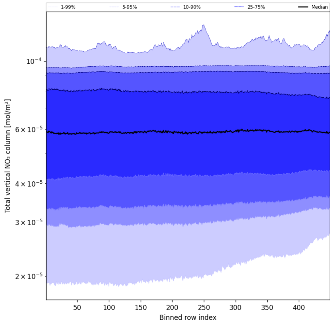
Figure 55: Along track statistics of “Total vertical NO 2 column” for 2024-12-08 to 2024-12-10
