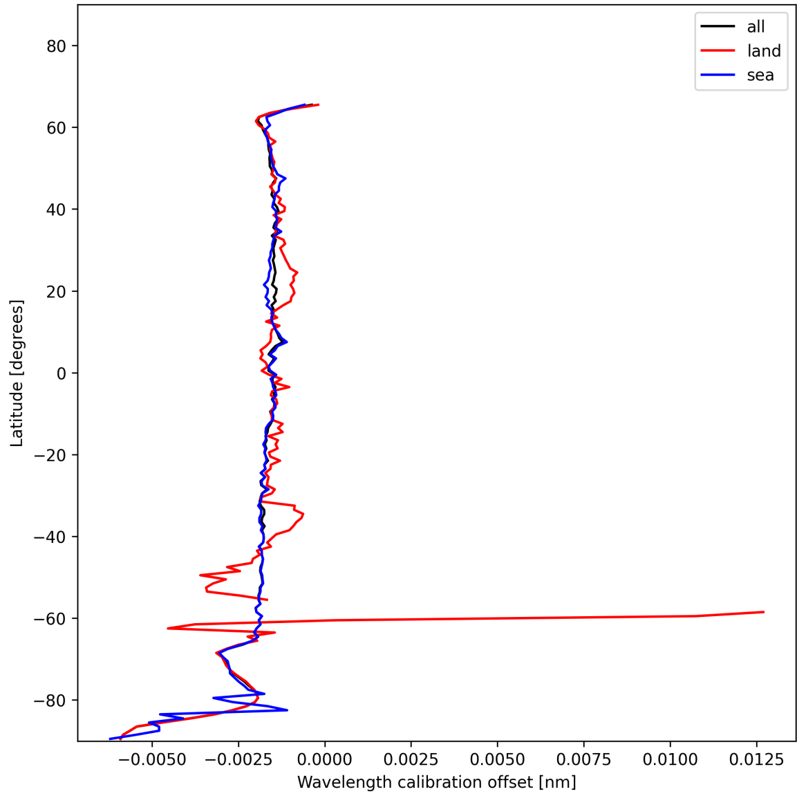
Figure 18: Zonal average of “Wavelength calibration offset” for 2024-12-08 to 2024-12-10.
