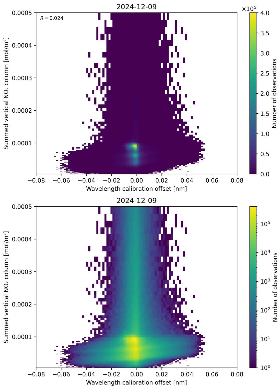
Figure 177: Scatter density plot of “Wavelength calibration offset” against “Summed vertical NO 2 column” for 2024-12-08 to 2024-12-10.
