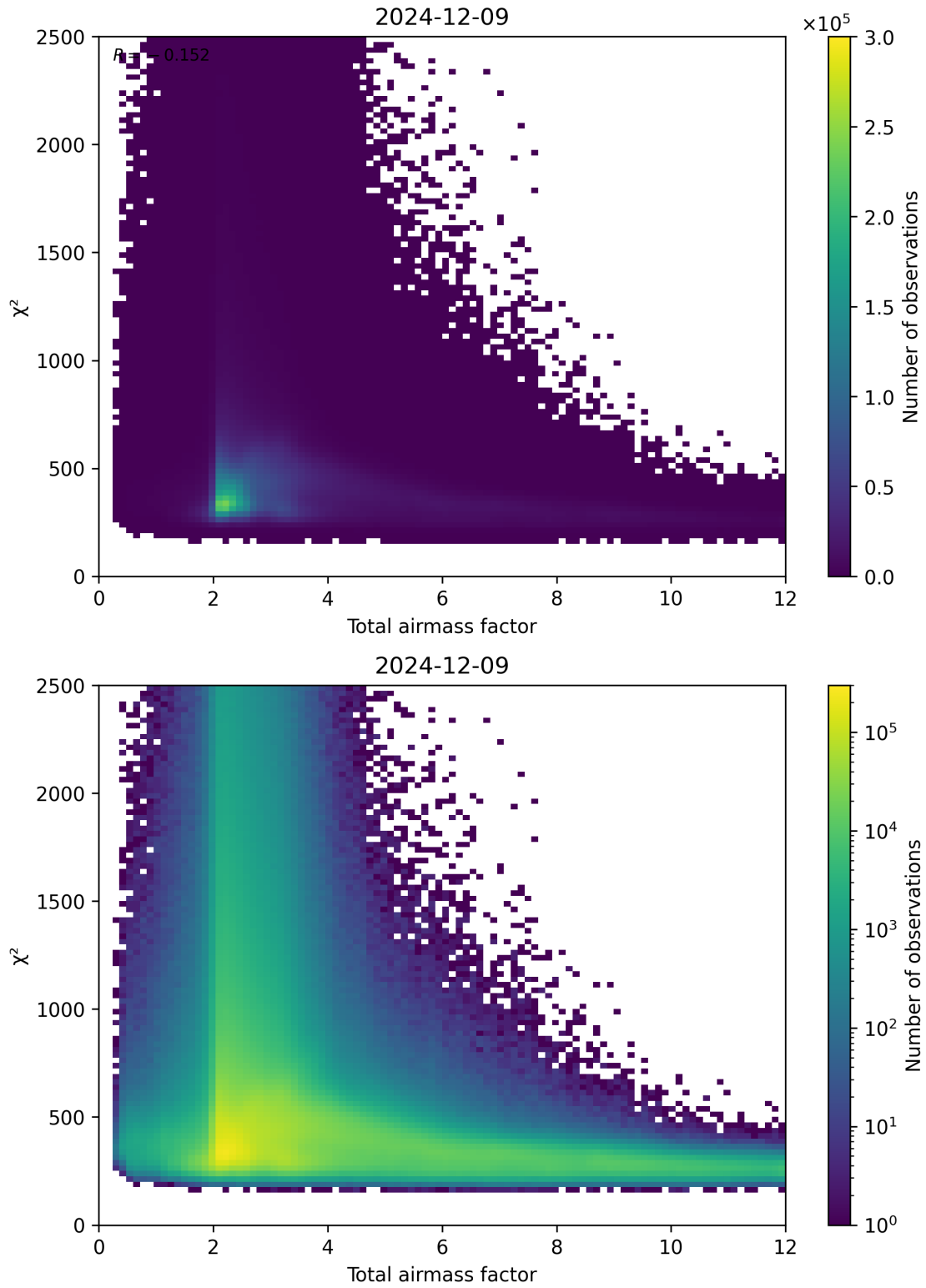
Figure 63: Scatter density plot of “Total airmass factor” against “ \chi^2 ” for 2024-12-08 to 2024-12-10.
