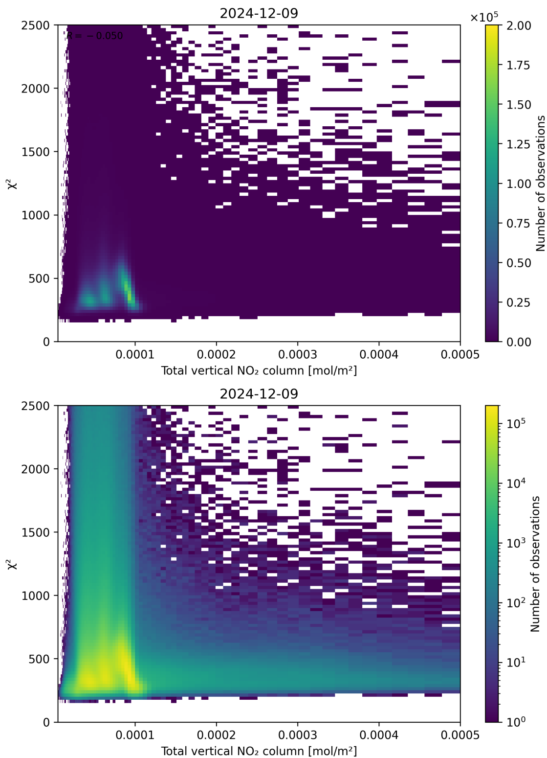
Figure 111: Scatter density plot of “Total vertical NO 2 column” against “ \chi^2 ” for 2024-12-08 to 2024-12-10.
