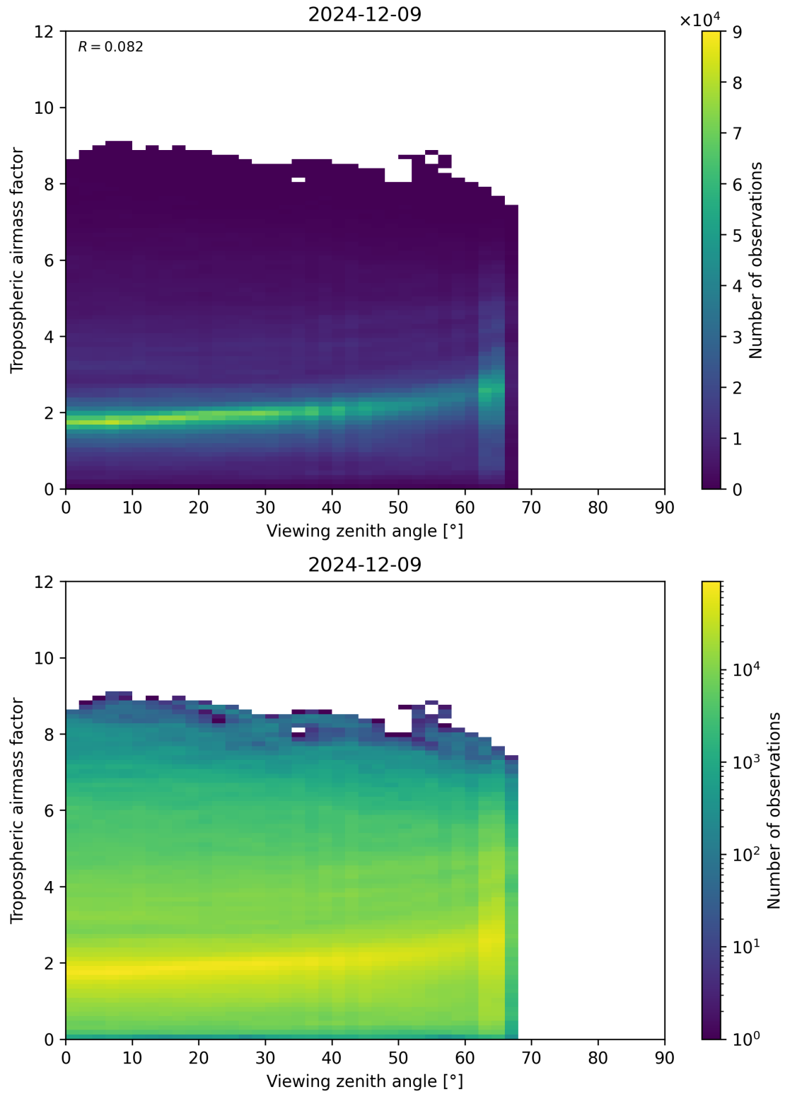
Figure 161: Scatter density plot of “Viewing zenith angle” against “Tropospheric airmass factor” for 2024-12-08 to 2024-12-10.
