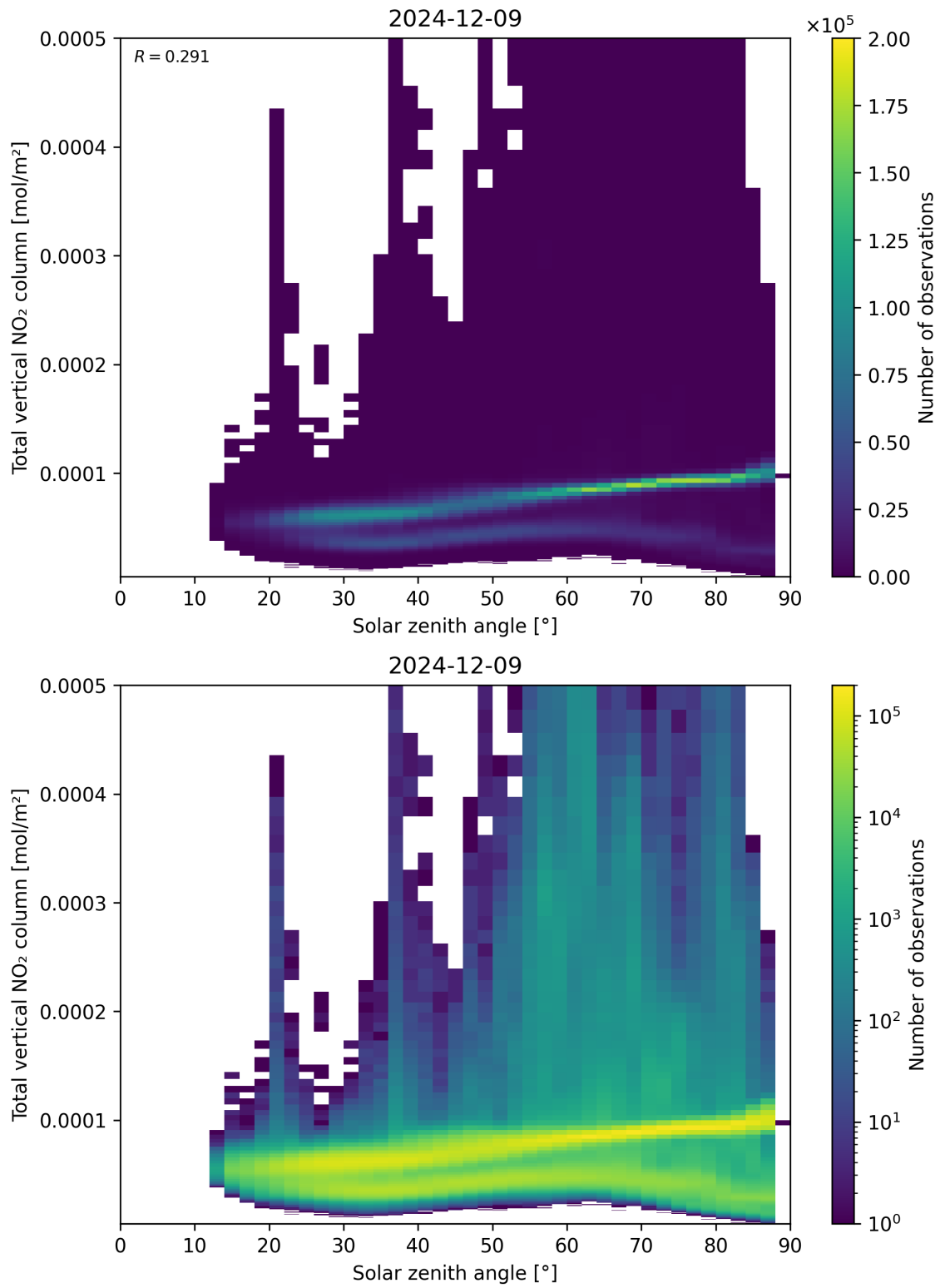
Figure 153: Scatter density plot of “Solar zenith angle” against “Total vertical NO 2 column” for 2024-12-08 to 2024-12-10.
