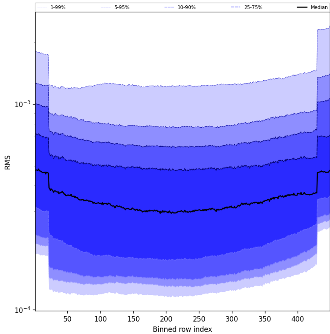
Figure 60: Along track statistics of “RMS” for 2024-12-08 to 2024-12-10
