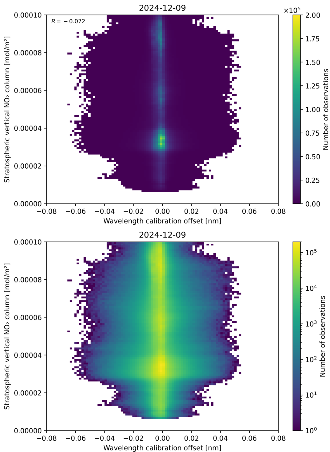
Figure 176: Scatter density plot of “Wavelength calibration offset” against “Stratospheric vertical NO 2 column” for 2024-12-08 to 2024-12-10.
