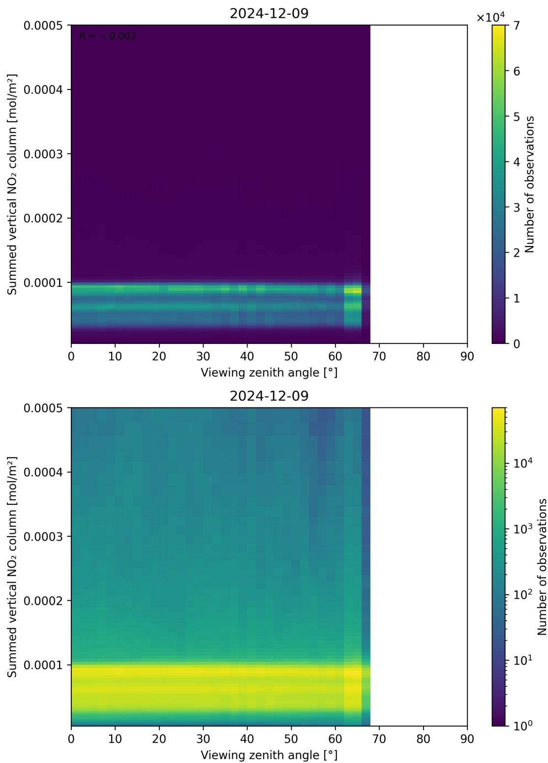
Figure 165: Scatter density plot of “Viewing zenith angle” against “Summed vertical NO 2 column” for 2024-12-08 to 2024-12-10.
