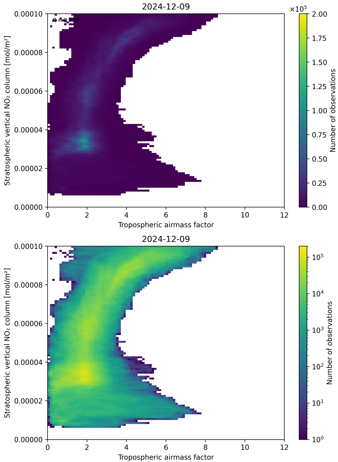
Figure 74: Scatter density plot of “Tropospheric airmass factor” against “Stratospheric vertical NO 2 column” for 2024-12-08 to 2024-12-10.
