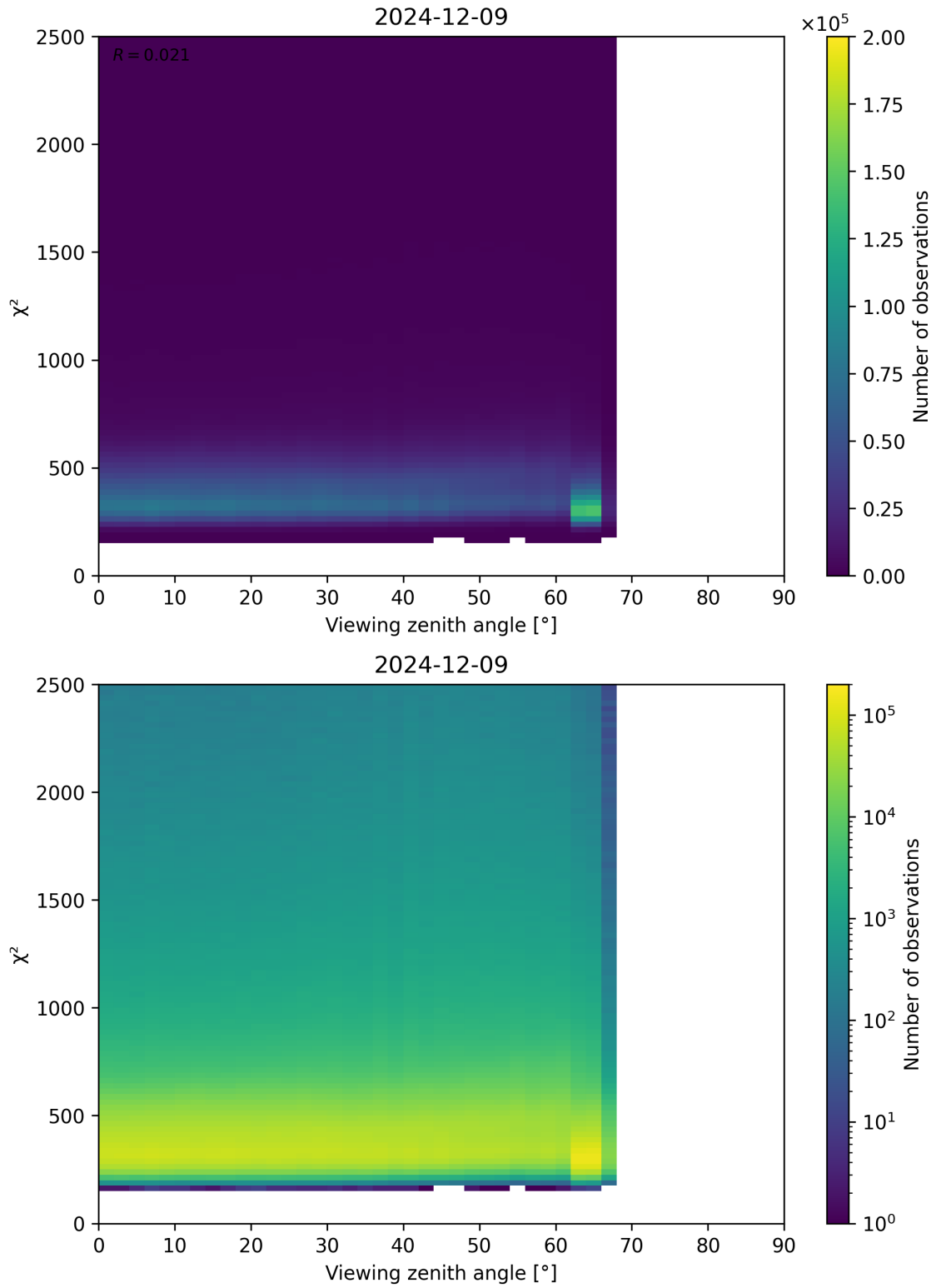
Figure 162: Scatter density plot of “Viewing zenith angle” against “ \chi^2 ” for 2024-12-08 to 2024-12-10.
