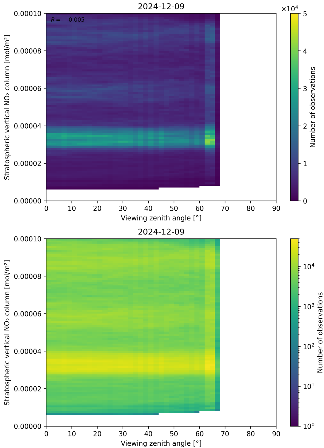
Figure 164: Scatter density plot of “Viewing zenith angle” against “Stratospheric vertical NO 2 column” for 2024-12-08 to 2024-12-10.
