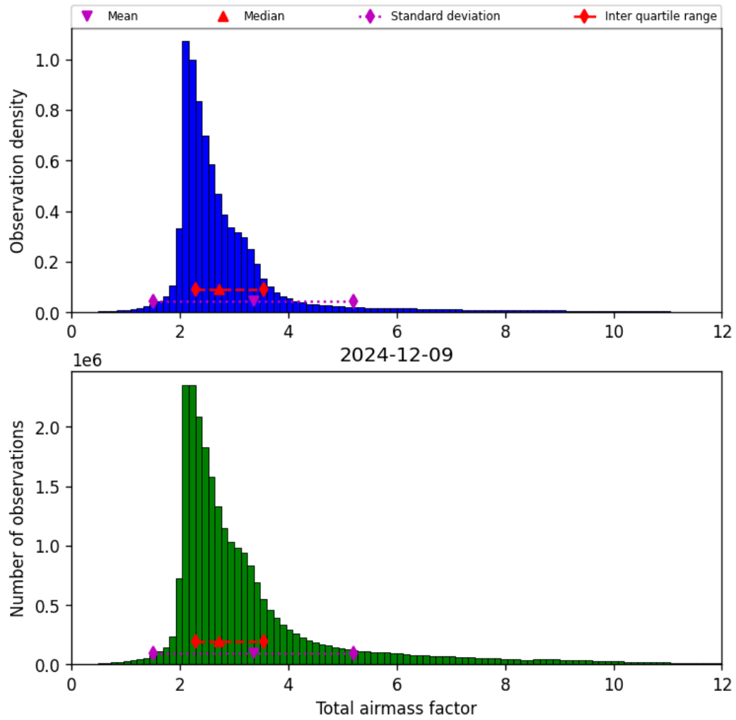
Figure 32: Histogram of “Total airmass factor” for 2024-12-08 to 2024-12-10
