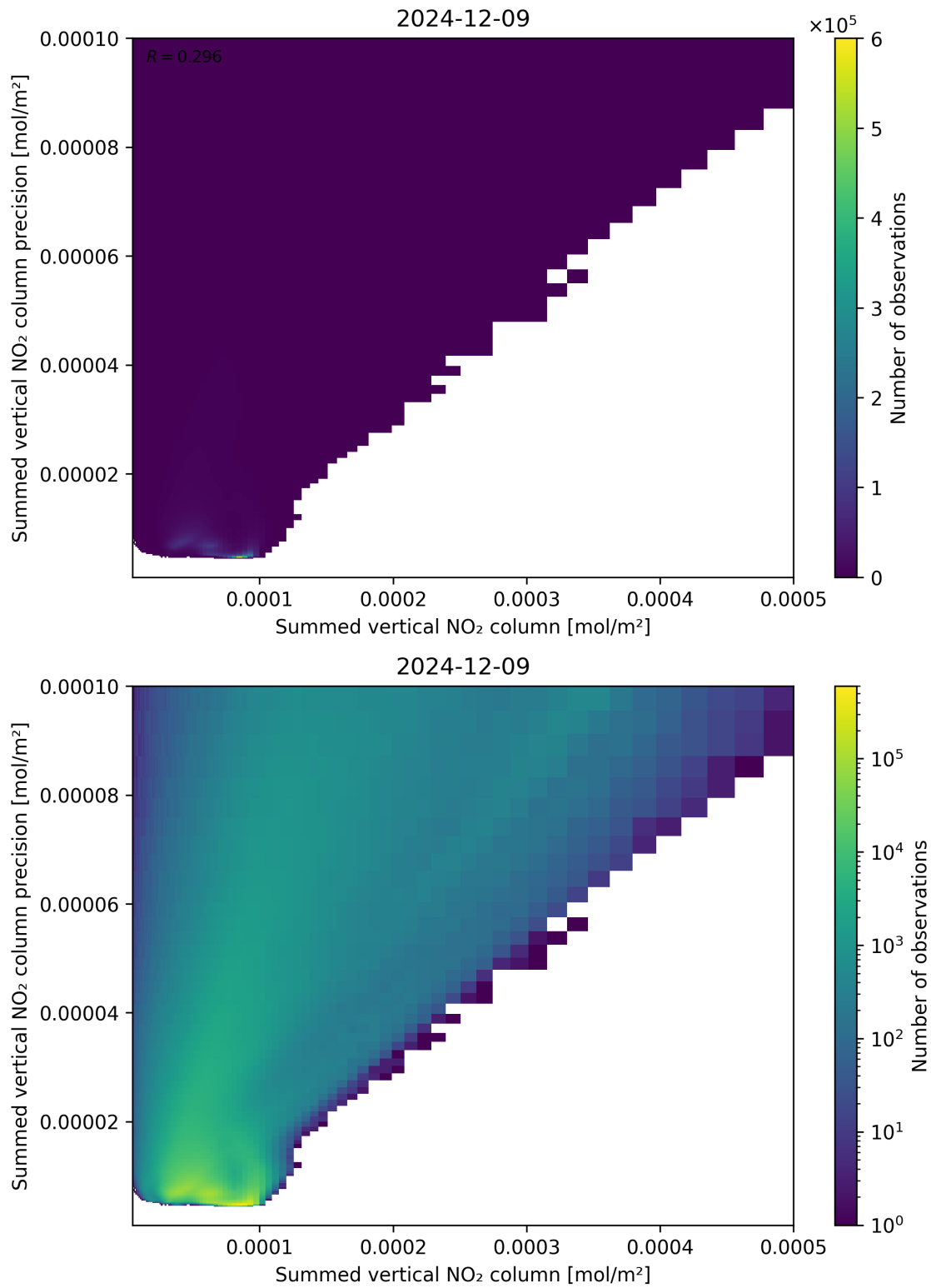
Figure 105: Scatter density plot of “Summed vertical NO 2 column” against “Summed vertical NO 2 column precision” for 2024-12-08 to 2024-12-10.
