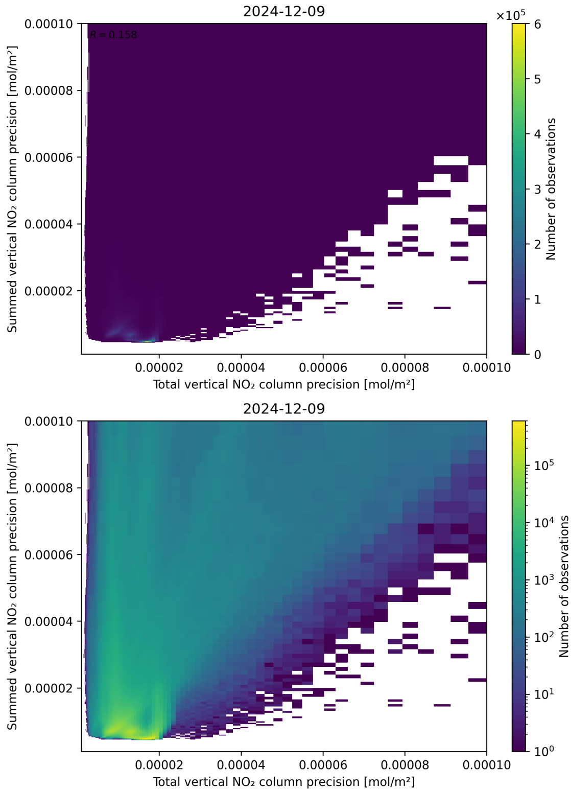
Figure 118: Scatter density plot of “Total vertical NO 2 column precision” against “Summed vertical NO 2 column precision” for 2024-12-08 to 2024-12-10.
