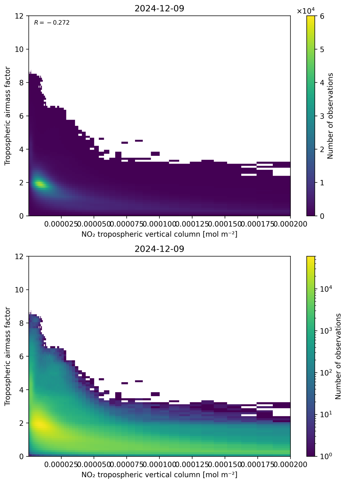
Figure 123: Scatter density plot of “NO 2 tropospheric vertical column” against “Tropospheric air mass factor” for 2024-12-08 to 2024-12-10.
