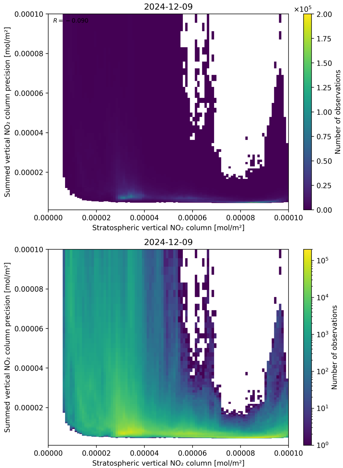
Figure 99: Scatter density plot of “Stratospheric vertical NO 2 column” against “Summed vertical NO 2 column precision” for 2024-12-08 to 2024-12-10.
