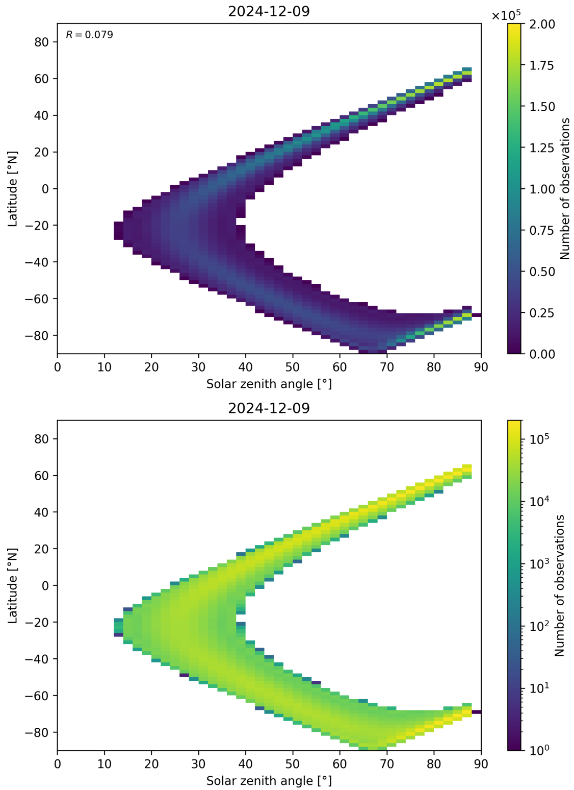
Figure 149: Scatter density plot of “Solar zenith angle” against “Latitude” for 2024-12-08 to 2024-12-10.
