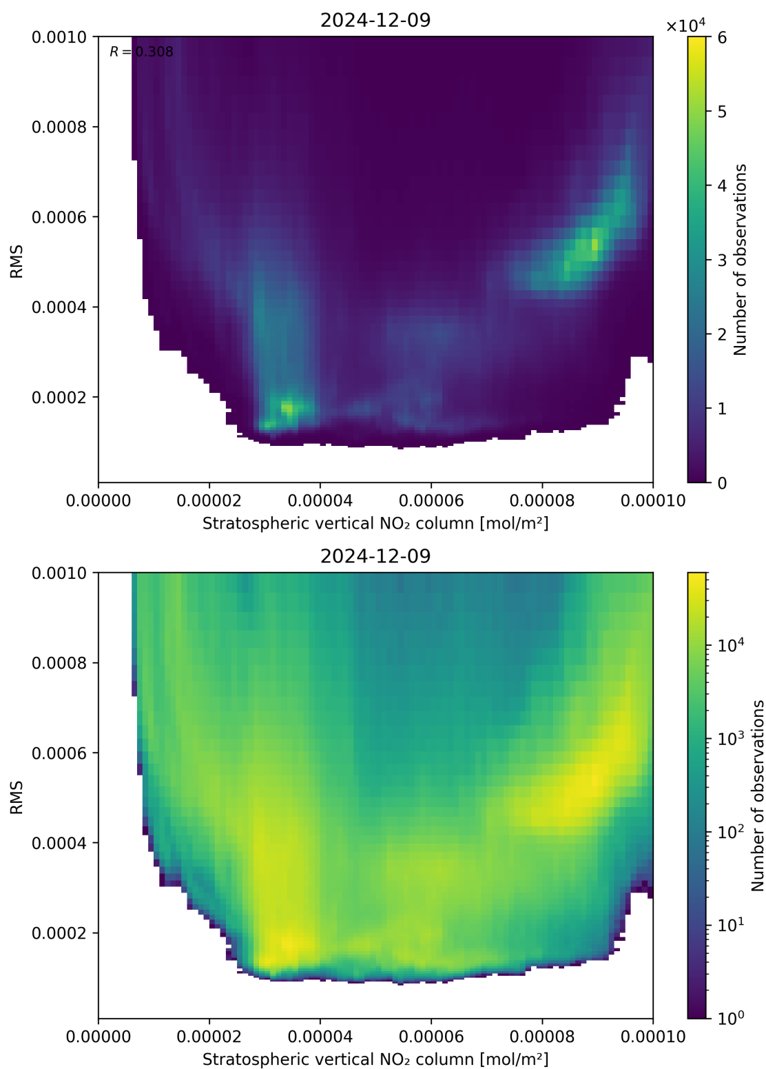
Figure 102: Scatter density plot of “Stratospheric vertical NO 2 column” against “RMS” for 2024-12-08 to 2024-12-10.
