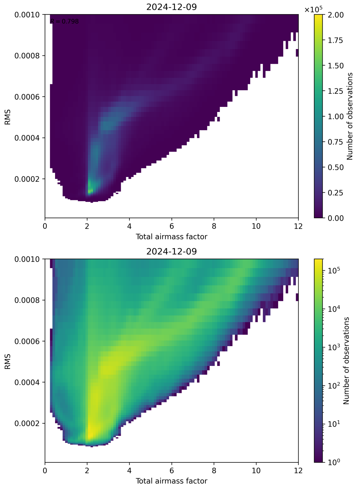
Figure 69: Scatter density plot of “Total airmass factor” against “RMS” for 2024-12-08 to 2024-12-10.
