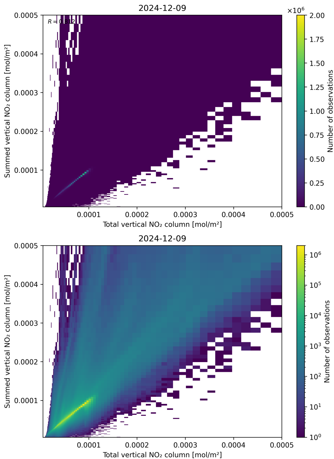
Figure 112: Scatter density plot of “Total vertical NO 2 column” against “Summed vertical NO 2 column” for 2024-12-08 to 2024-12-10.
