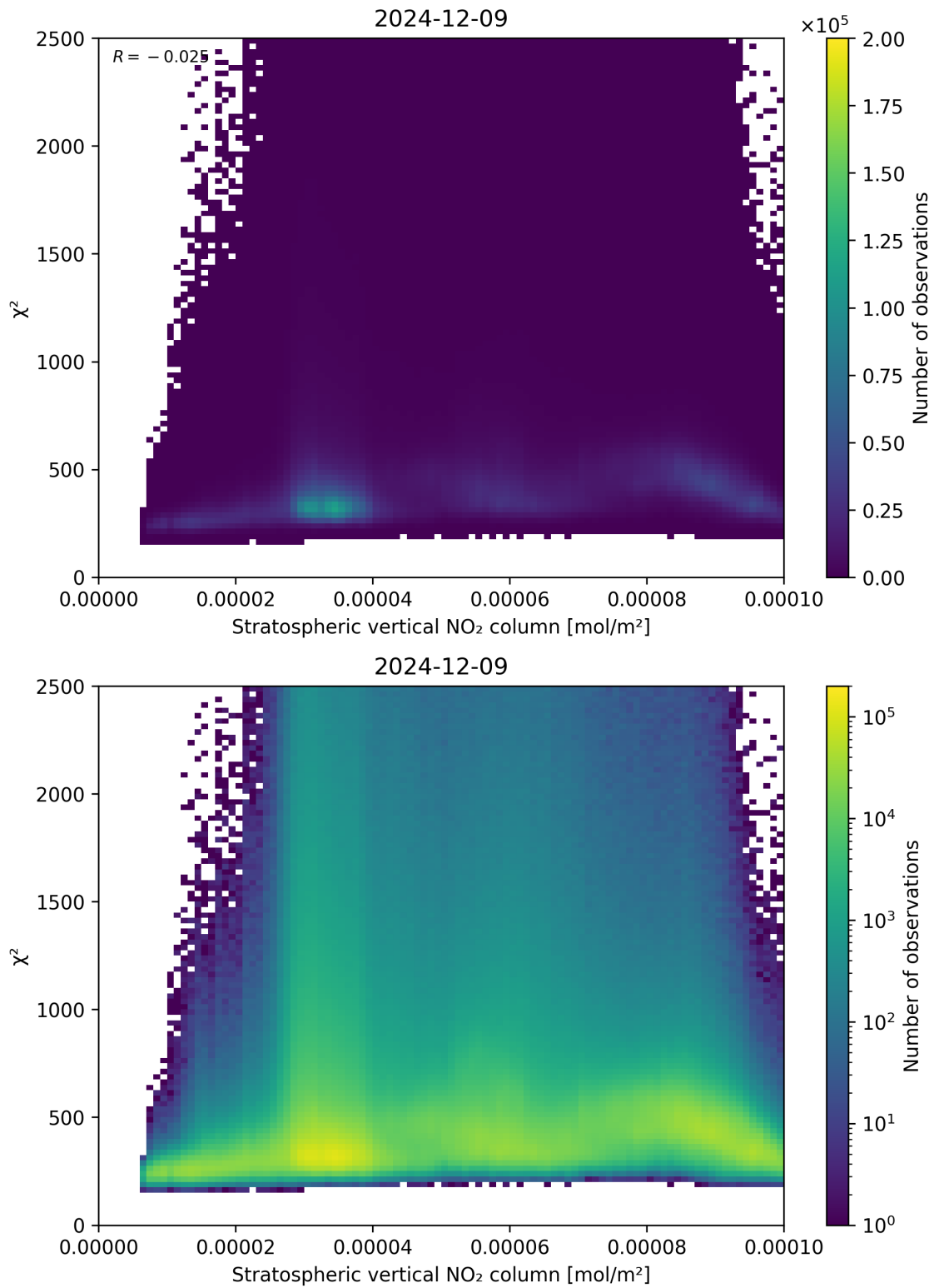
Figure 97: Scatter density plot of “Stratospheric vertical NO 2 column” against “ \chi^2 ” for 2024-12-08 to 2024-12-10.
