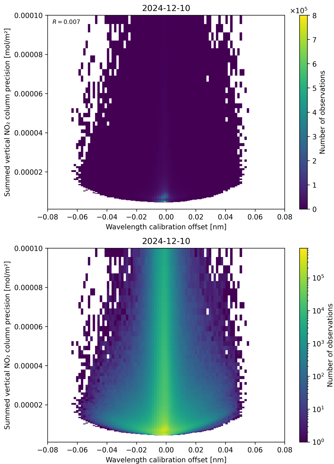
Figure 178: Scatter density plot of “Wavelength calibration offset” against “Summed vertical NO 2 column precision” for 2024-12-09 to 2024-12-11.
