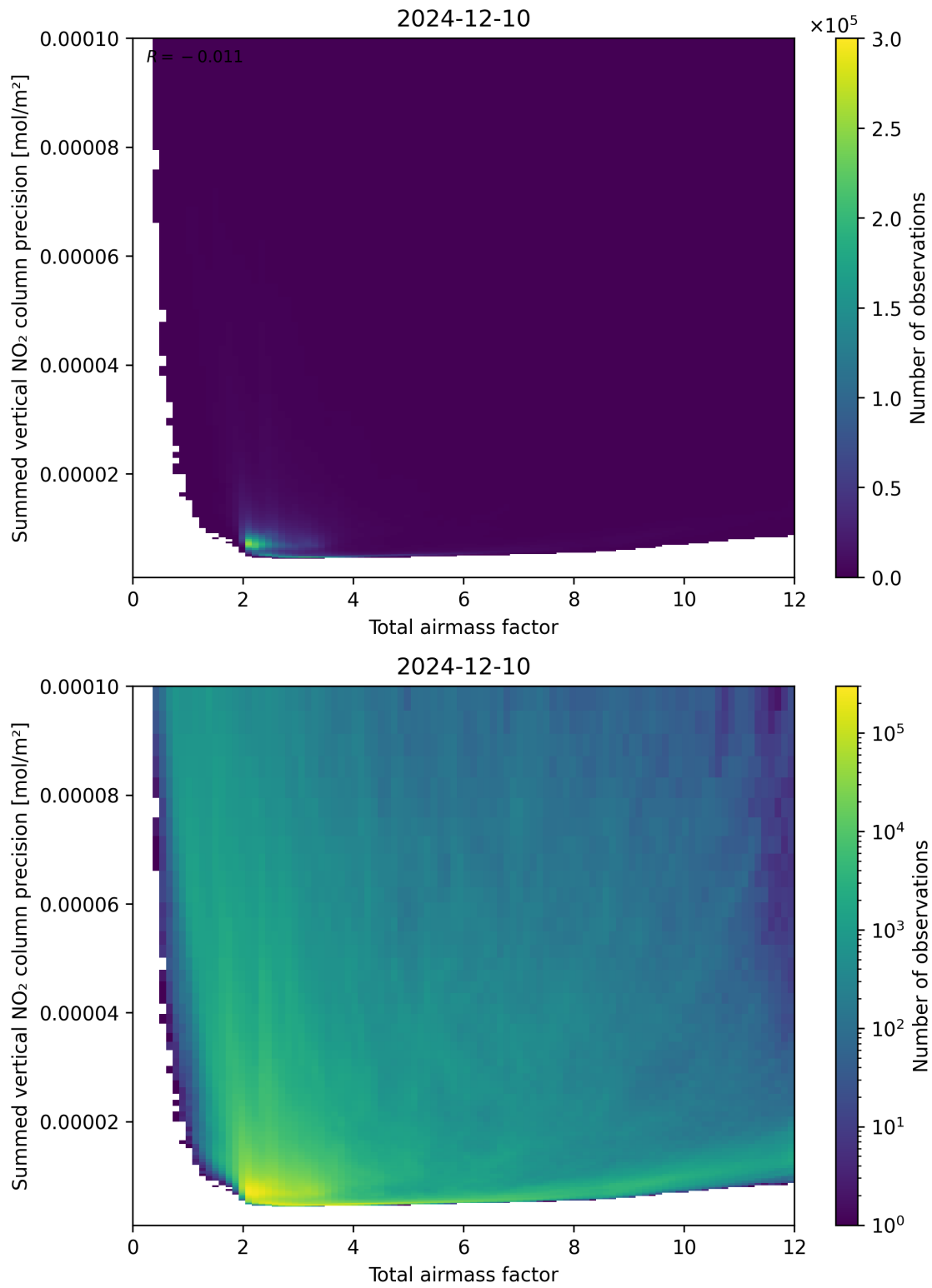
Figure 66: Scatter density plot of “Total airmass factor” against “Summed vertical NO 2 column precision” for 2024-12-09 to 2024-12-11.
