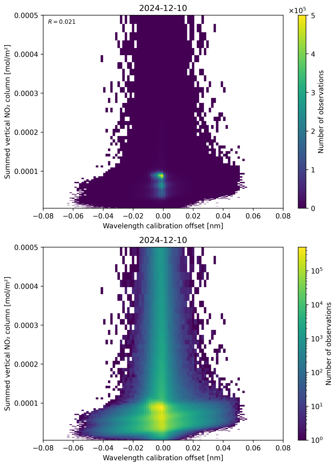
Figure 177: Scatter density plot of “Wavelength calibration offset” against “Summed vertical NO 2 column” for 2024-12-09 to 2024-12-11.
