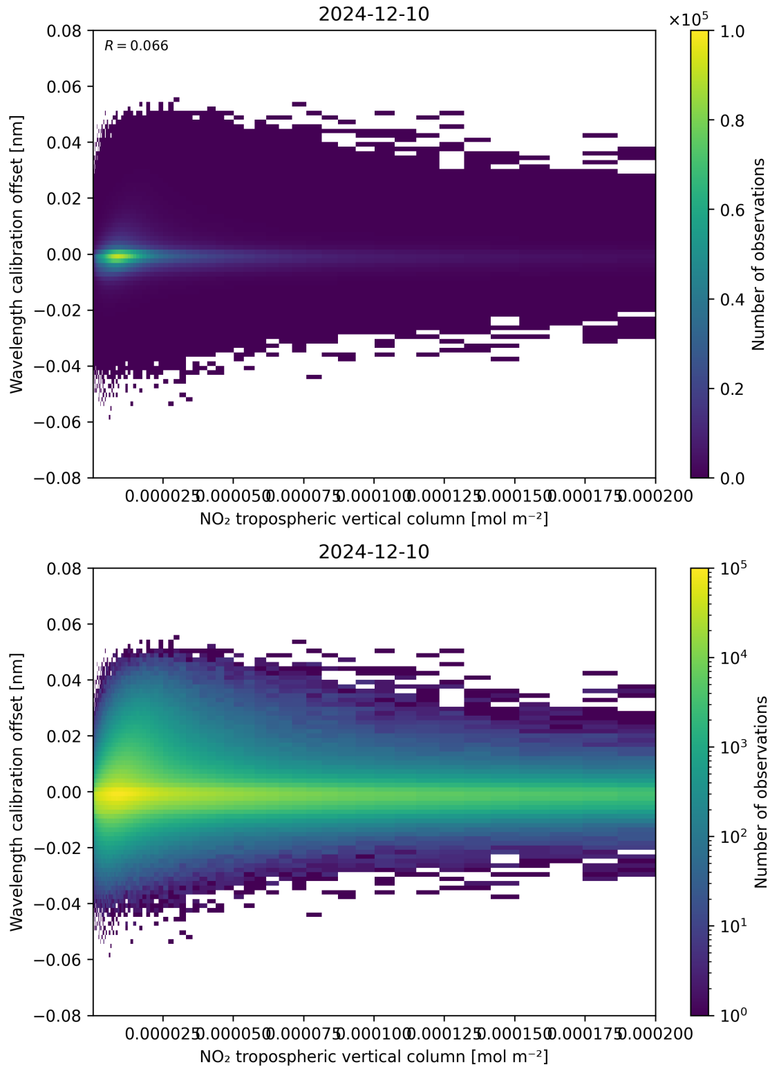
Figure 143: Scatter density plot of “NO 2 tropospheric vertical column” against “Wavelength calibration offset” for 2024-12-09 to 2024-12-11.
