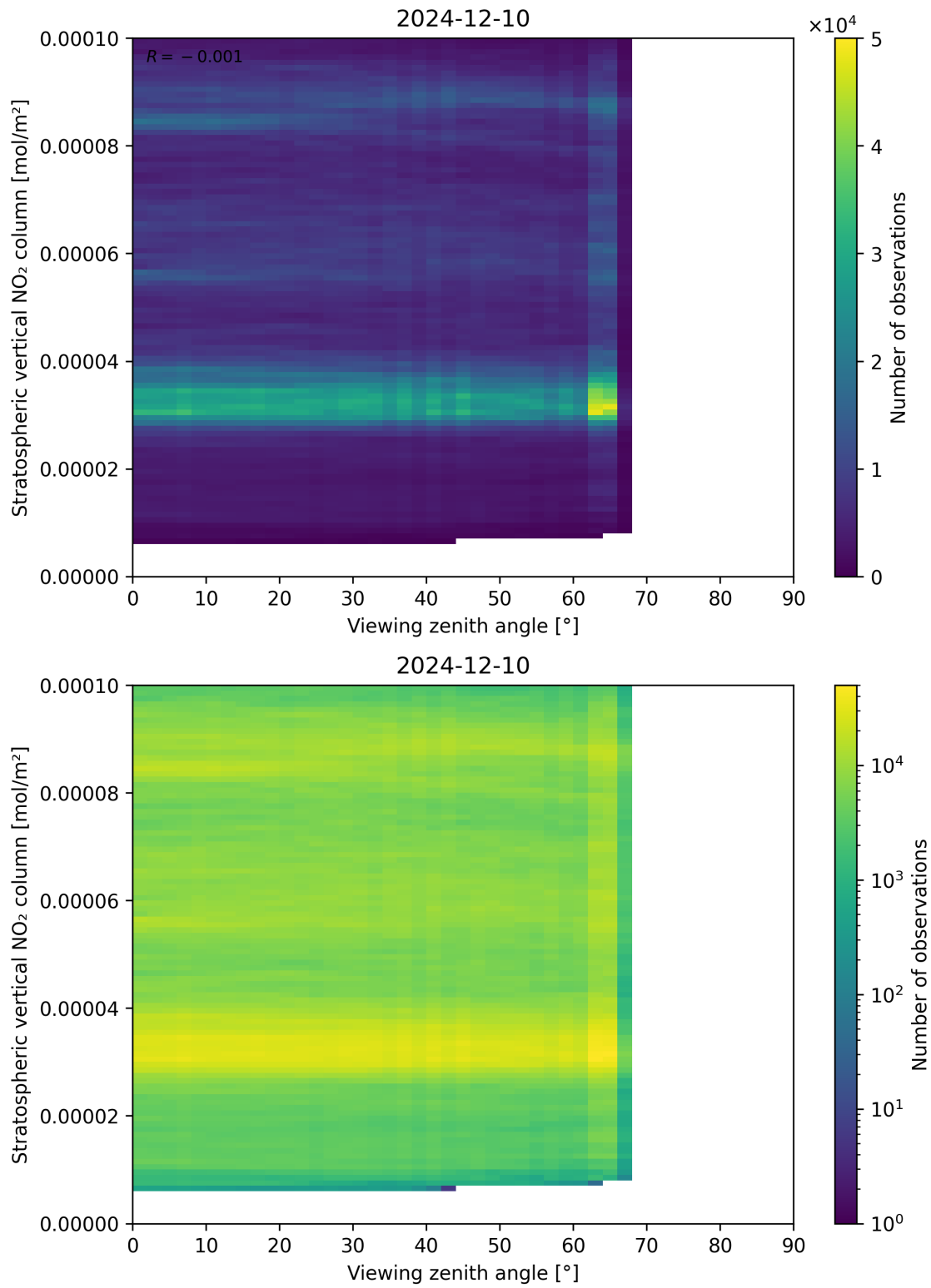
Figure 164: Scatter density plot of “Viewing zenith angle” against “Stratospheric vertical NO 2 column” for 2024-12-09 to 2024-12-11.
