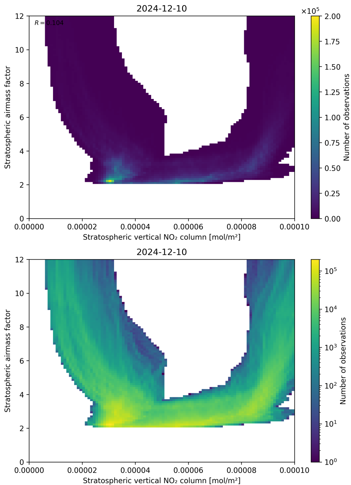
Figure 96: Scatter density plot of “Stratospheric vertical NO 2 column” against “Stratospheric airmass factor” for 2024-12-09 to 2024-12-11.
