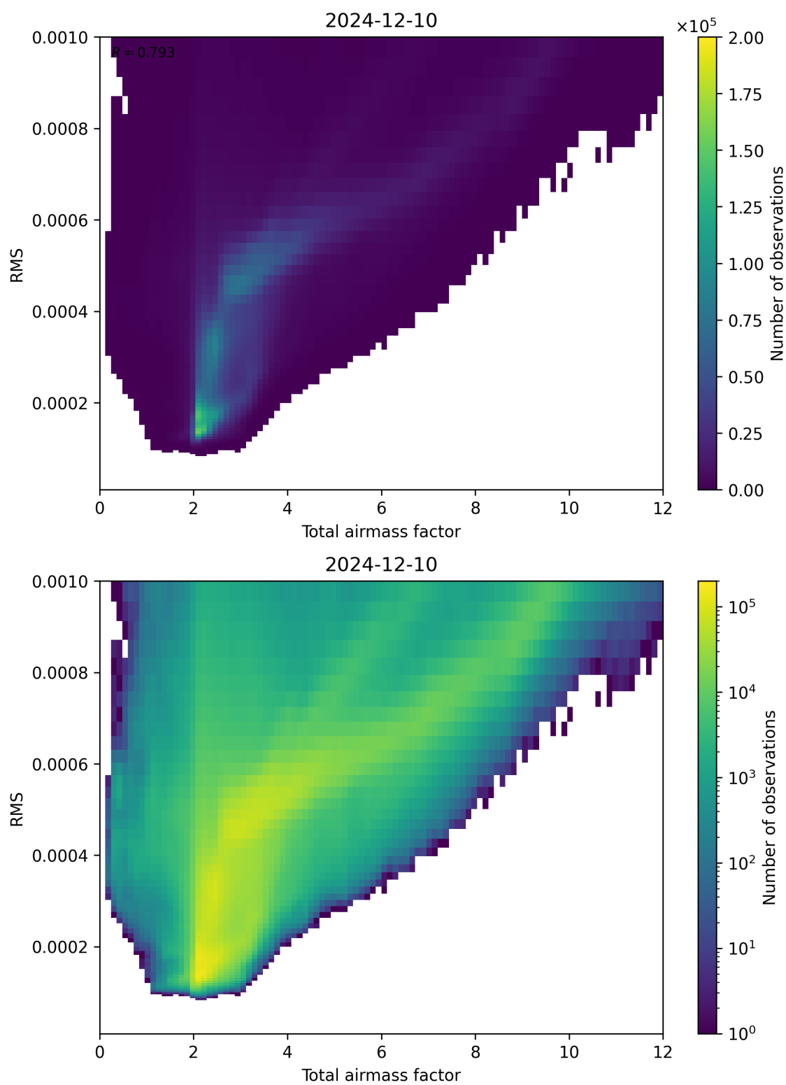
Figure 69: Scatter density plot of “Total airmass factor” against “RMS” for 2024-12-09 to 2024-12-11.
