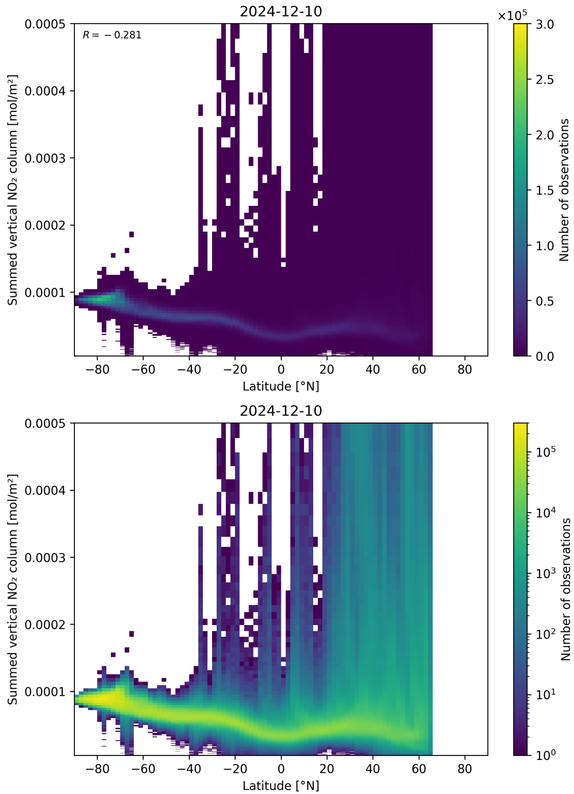
Figure 88: Scatter density plot of “Latitude” against “Summed vertical NO 2 column” for 2024-12-09 to 2024-12-11.
