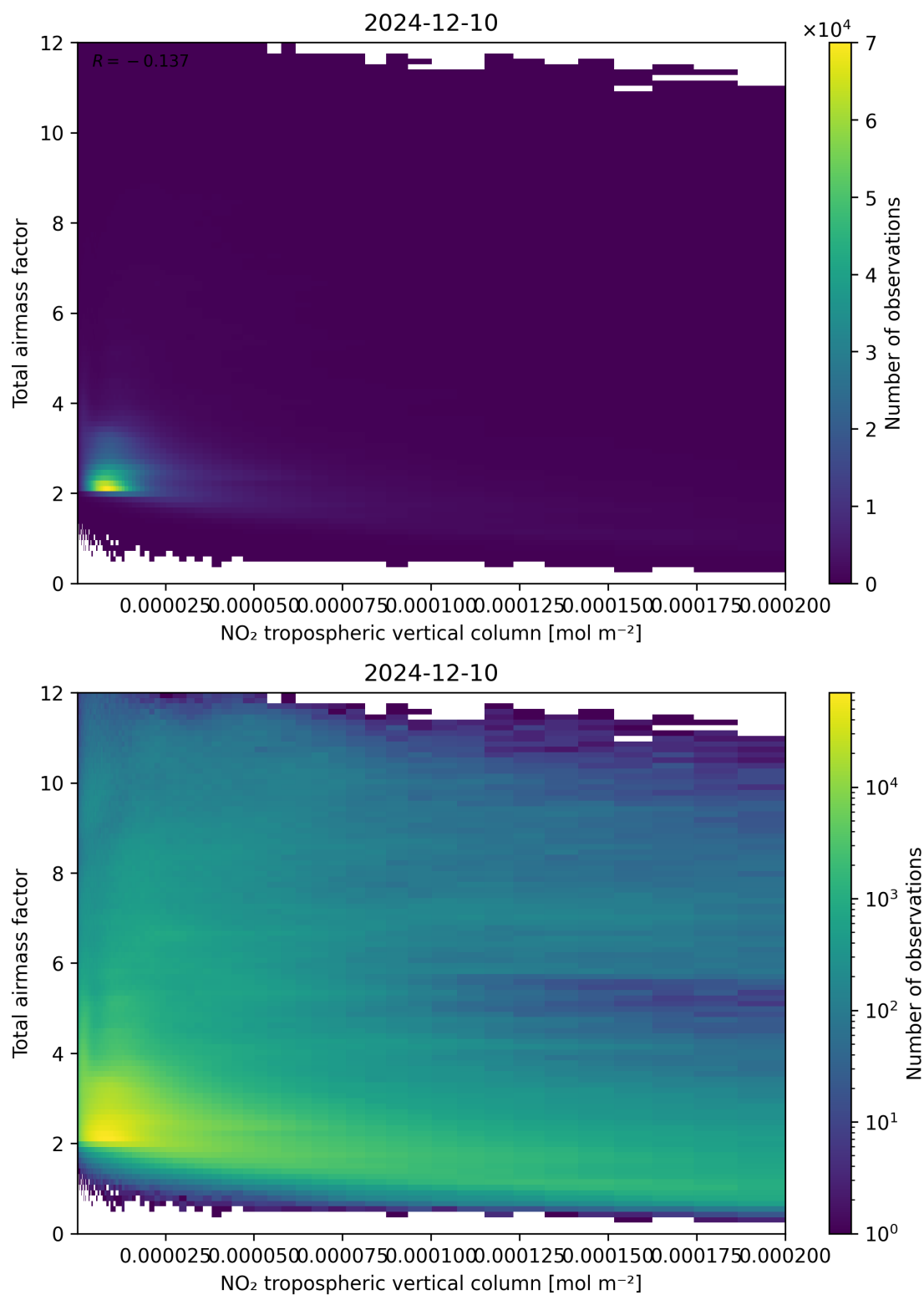
Figure 122: Scatter density plot of “NO 2 tropospheric vertical column” against “Total air mass factor” for 2024-12-09 to 2024-12-11.
