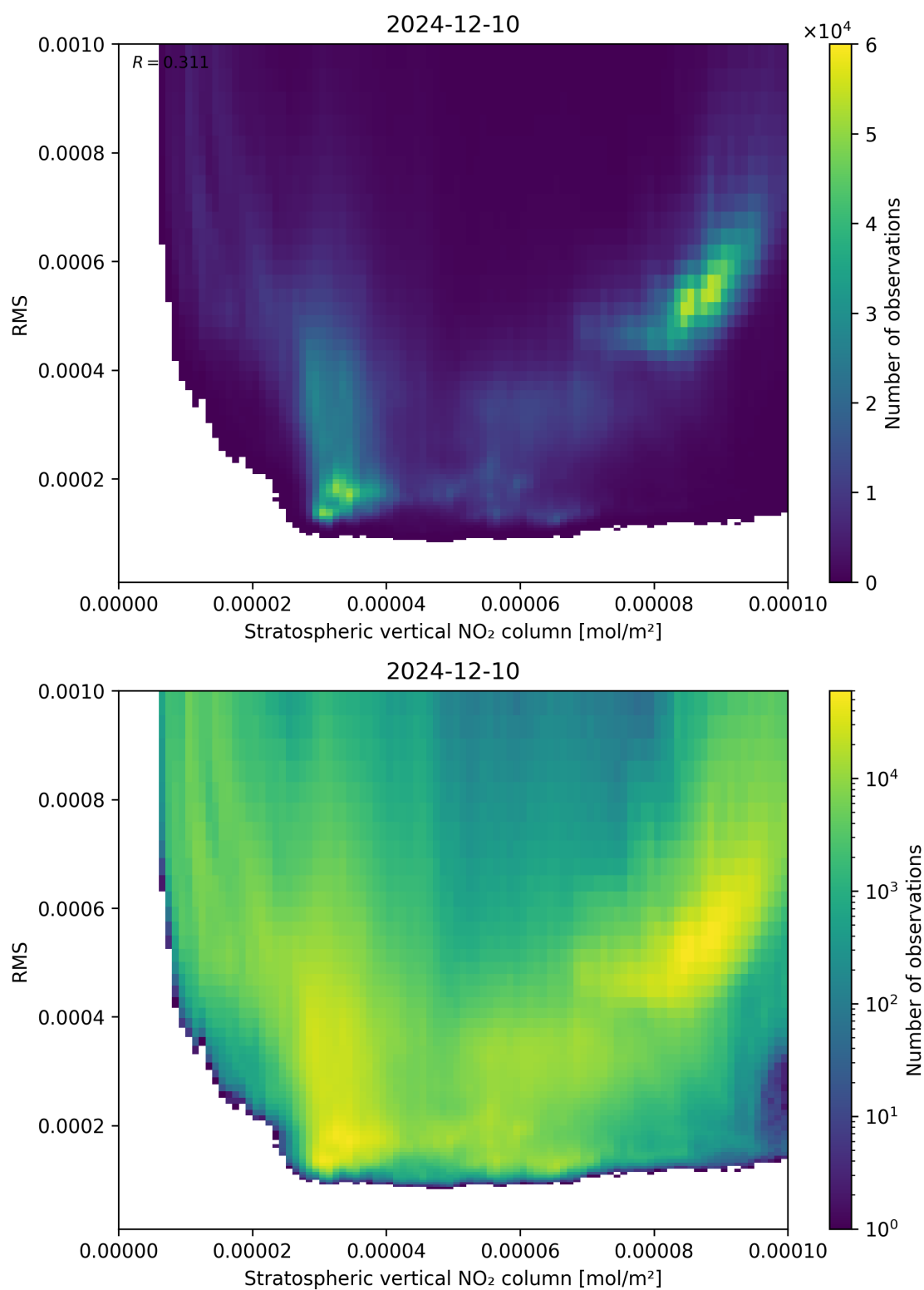
Figure 102: Scatter density plot of “Stratospheric vertical NO 2 column” against “RMS” for 2024-12-09 to 2024-12-11.
