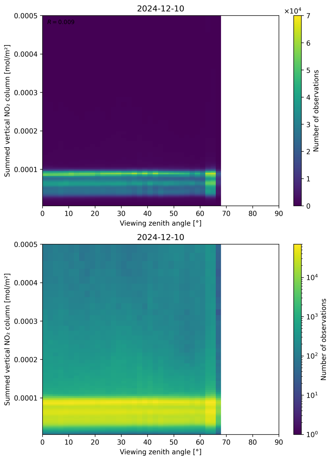
Figure 165: Scatter density plot of “Viewing zenith angle” against “Summed vertical NO 2 column” for 2024-12-09 to 2024-12-11.
