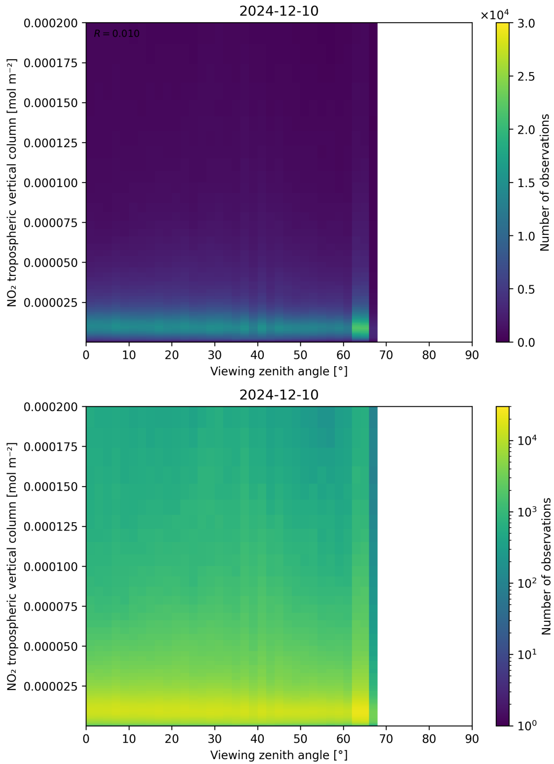
Figure 169: Scatter density plot of “Viewing zenith angle” against “NO 2 tropospheric vertical column” for 2024-12-09 to 2024-12-11.
