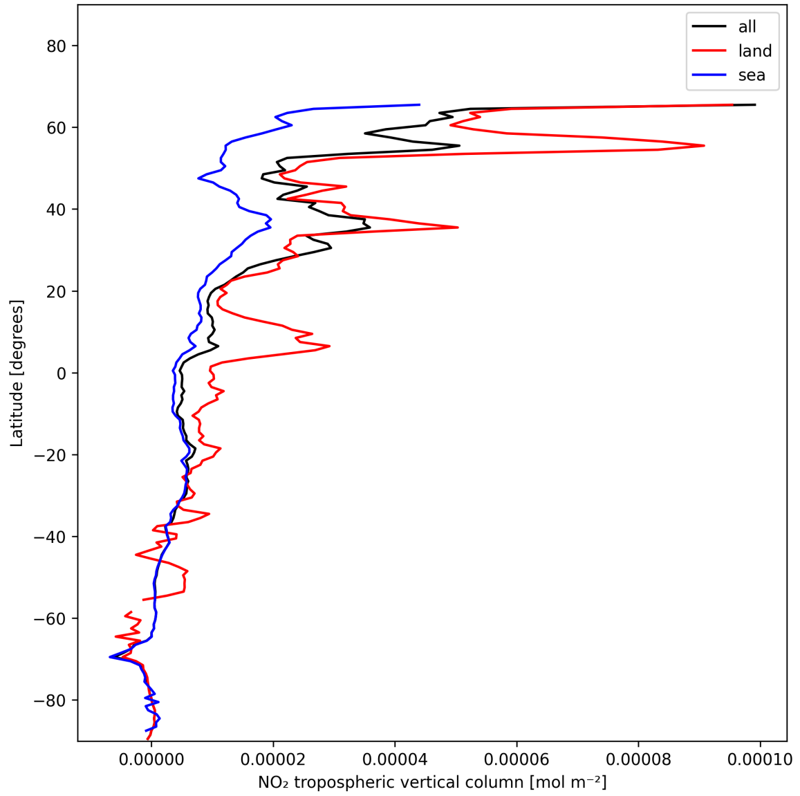
Figure 12: Zonal average of “NO 2 tropospheric vertical column” for 2024-12-09 to 2024-12-11.
