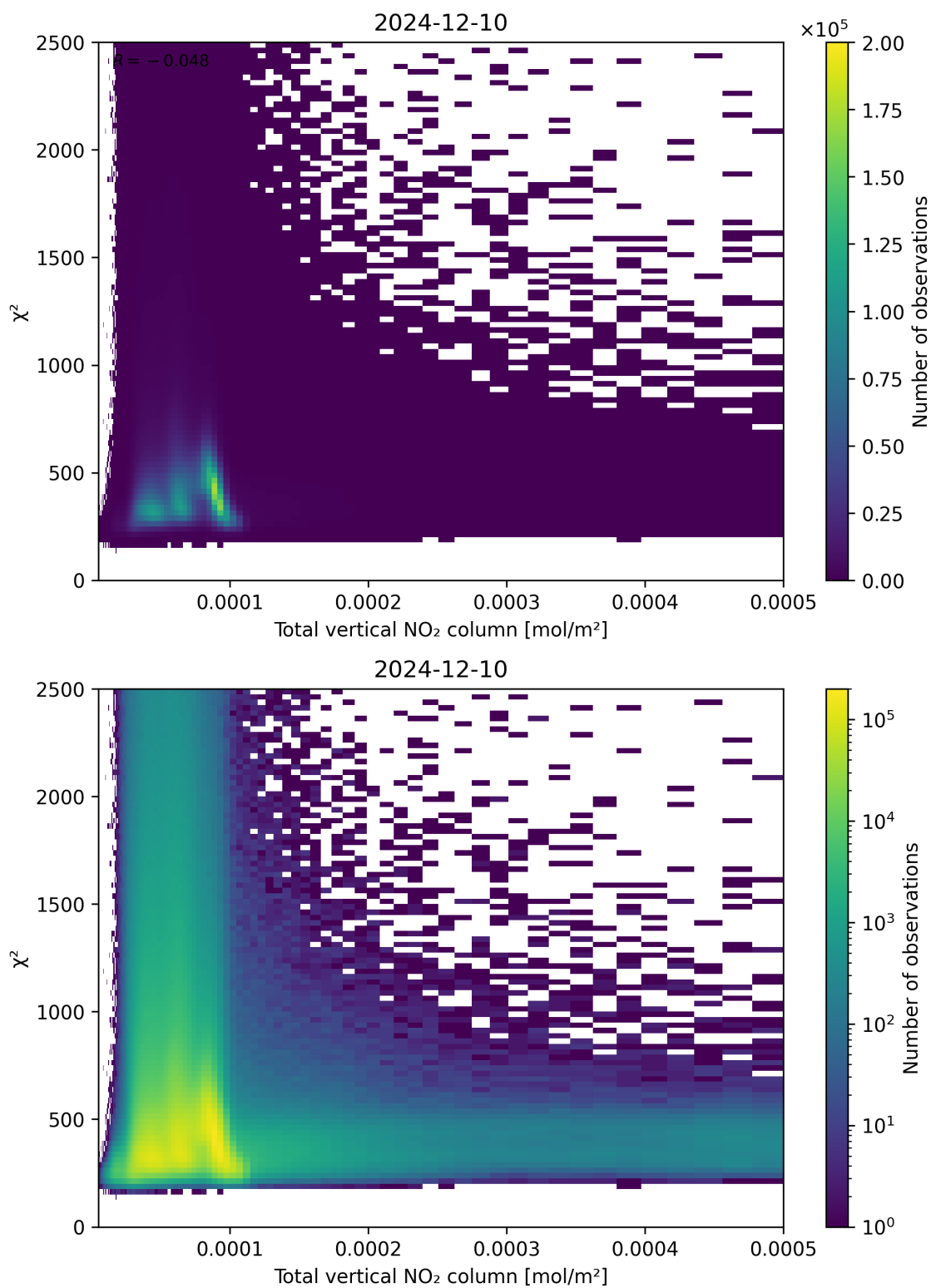
Figure 111: Scatter density plot of “Total vertical NO 2 column” against “ \chi^2 ” for 2024-12-09 to 2024-12-11.
