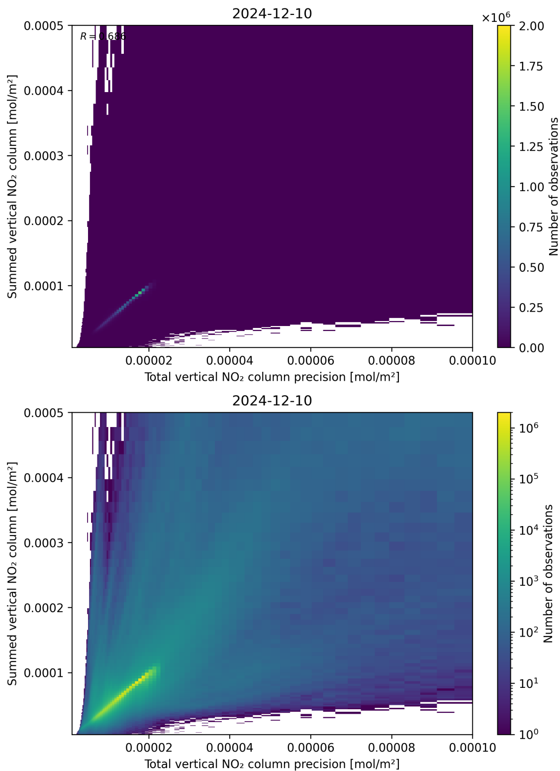
Figure 117: Scatter density plot of “Total vertical NO 2 column precision” against “Summed vertical NO 2 column” for 2024-12-09 to 2024-12-11.
