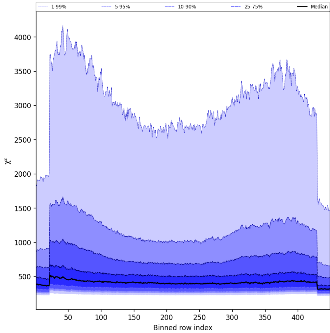
Figure 59: Along track statistics of “ \chi^2 ” for 2024-12-09 to 2024-12-11
