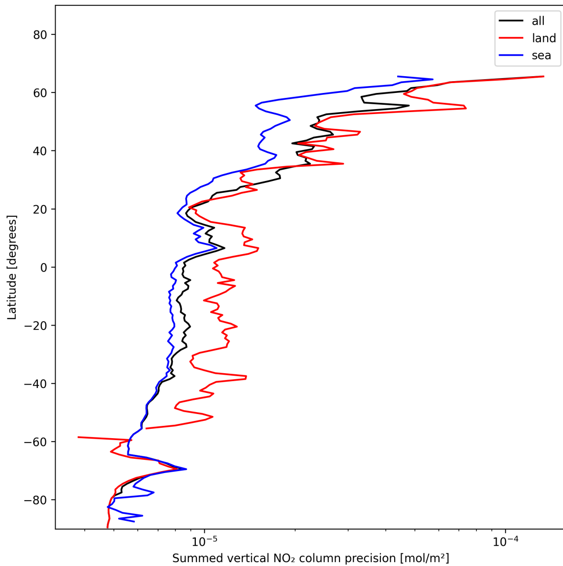
Figure 24: Zonal average of “Summed vertical NO 2 column precision” for 2024-12-09 to 2024-12-11.
