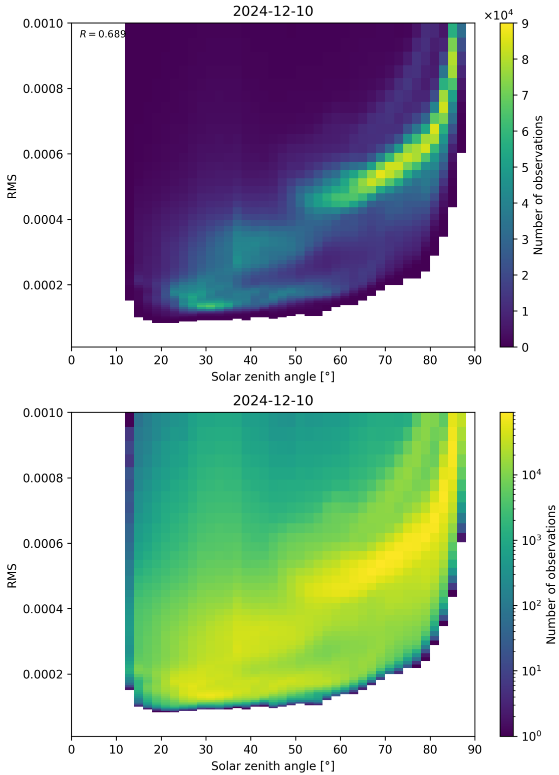
Figure 157: Scatter density plot of “Solar zenith angle” against “RMS” for 2024-12-09 to 2024-12-11.
