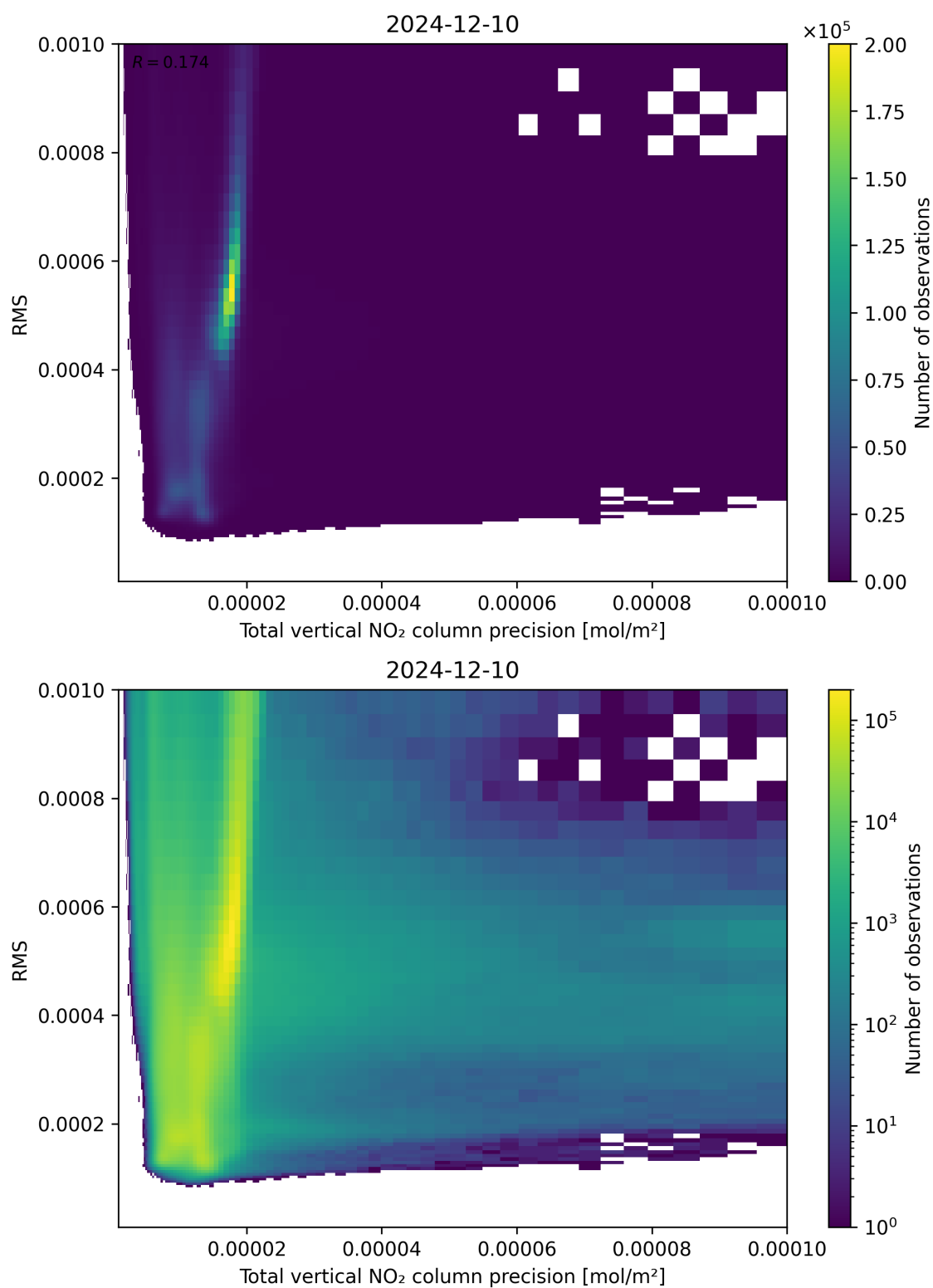
Figure 119: Scatter density plot of “Total vertical NO 2 column precision” against “RMS” for 2024-12-09 to 2024-12-11.
