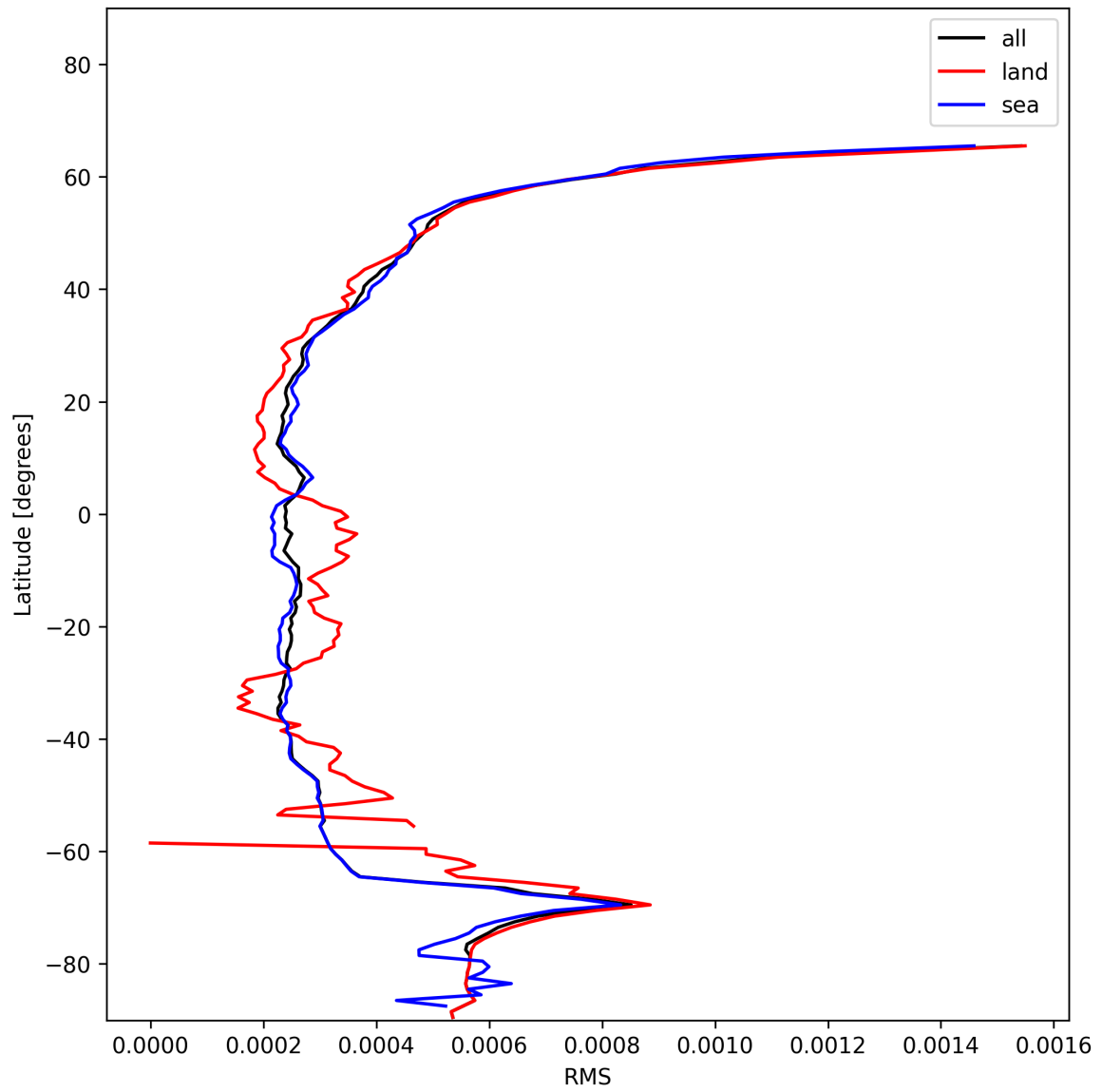
Figure 26: Zonal average of “RMS” for 2024-12-09 to 2024-12-11.
