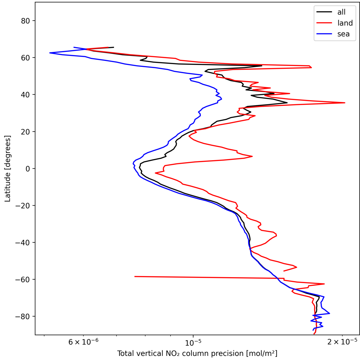
Figure 22: Zonal average of “Total vertical NO 2 column precision” for 2024-12-09 to 2024-12-11.
