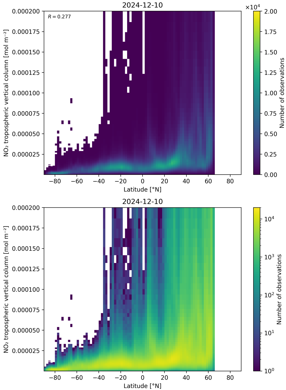
Figure 92: Scatter density plot of “Latitude” against “NO 2 tropospheric vertical column” for 2024-12-09 to 2024-12-11.
