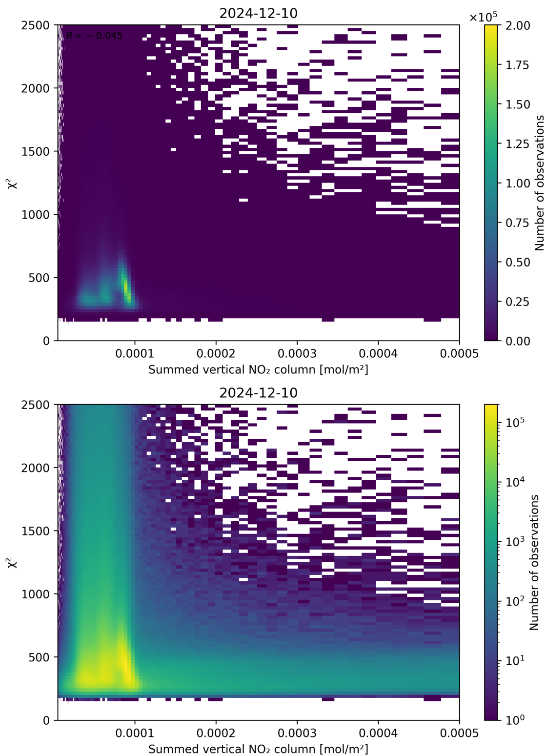
Figure 104: Scatter density plot of “Summed vertical NO 2 column” against “ \chi^2 ” for 2024-12-09 to 2024-12-11.
