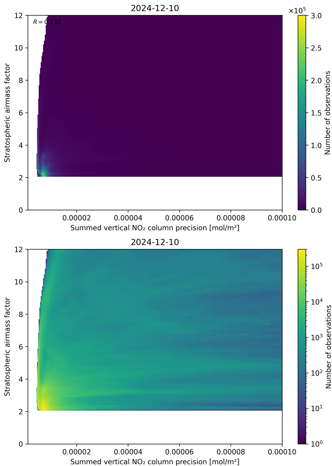
Figure 106: Scatter density plot of “Summed vertical NO 2 column precision” against “Stratospheric airmass factor” for 2024-12-09 to 2024-12-11.
