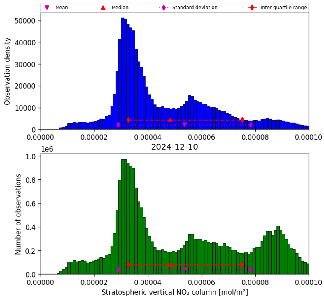
Figure 36: Histogram of “Stratospheric vertical NO 2 column” for 2024-12-09 to 2024-12-11
