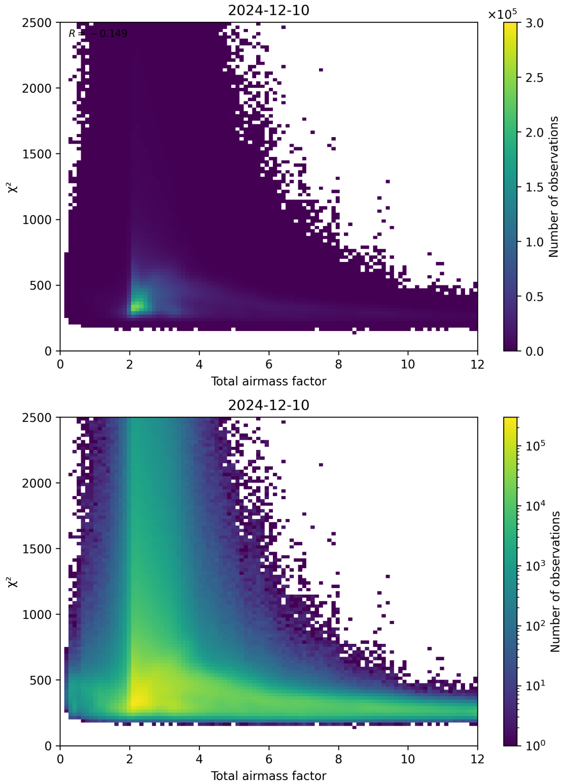
Figure 63: Scatter density plot of “Total airmass factor” against “ \chi^2 ” for 2024-12-09 to 2024-12-11.
