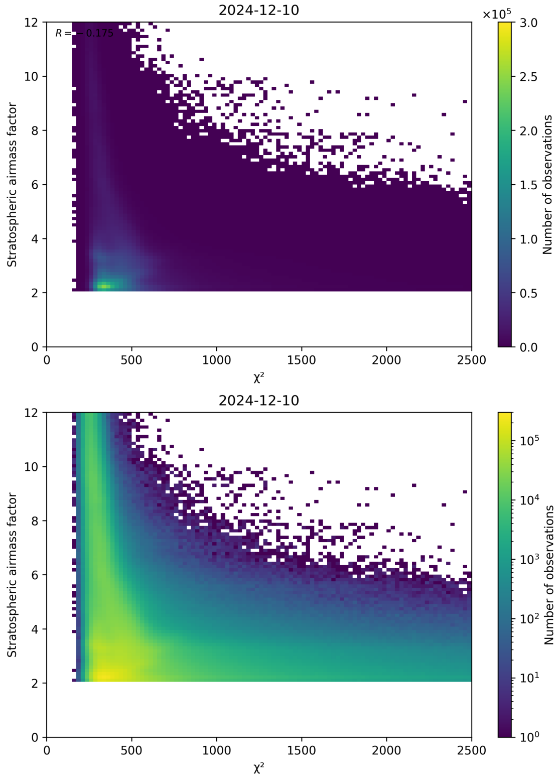
Figure 81: Scatter density plot of “ \chi^2 ” against “Stratospheric airmass factor” for 2024-12-09 to 2024-12-11.
