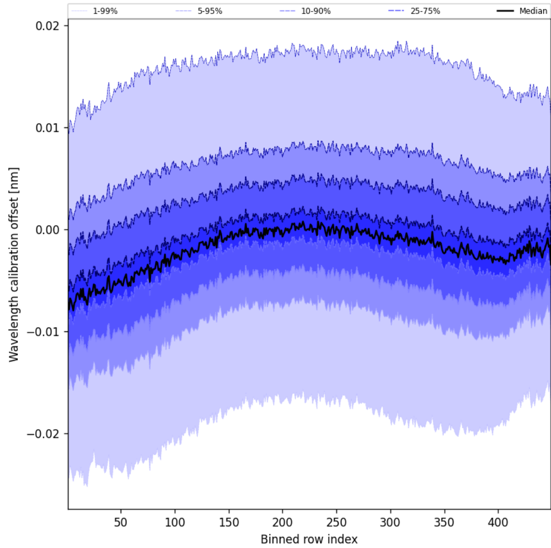
Figure 52: Along track statistics of “Wavelength calibration offset” for 2024-12-09 to 2024-12-11
