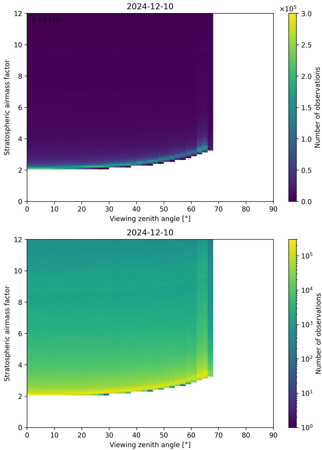
Figure 159: Scatter density plot of “Viewing zenith angle” against “Stratospheric airmass factor” for 2024-12-09 to 2024-12-11.
