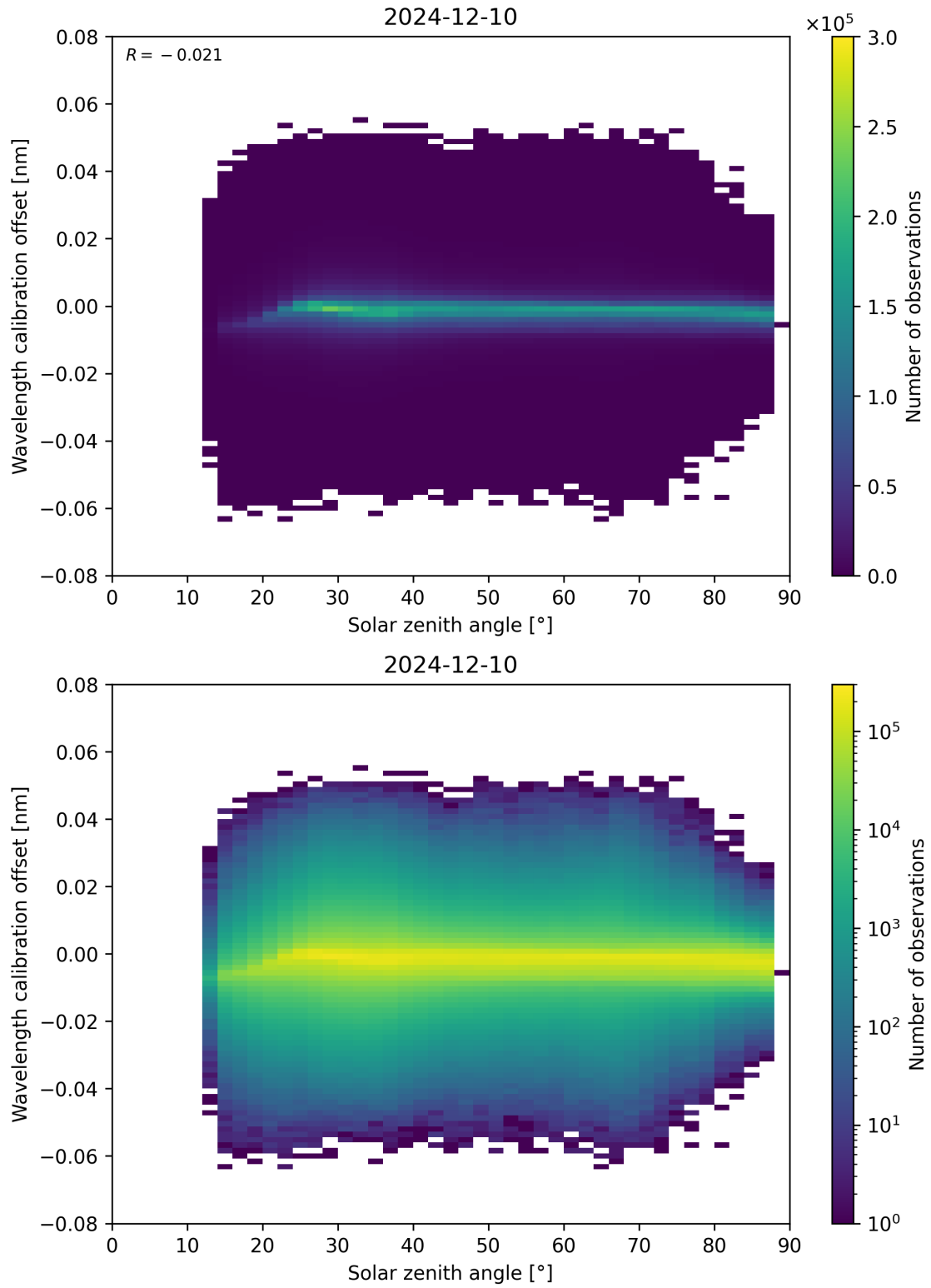
Figure 158: Scatter density plot of “Solar zenith angle” against “Wavelength calibration offset” for 2024-12-09 to 2024-12-11.
