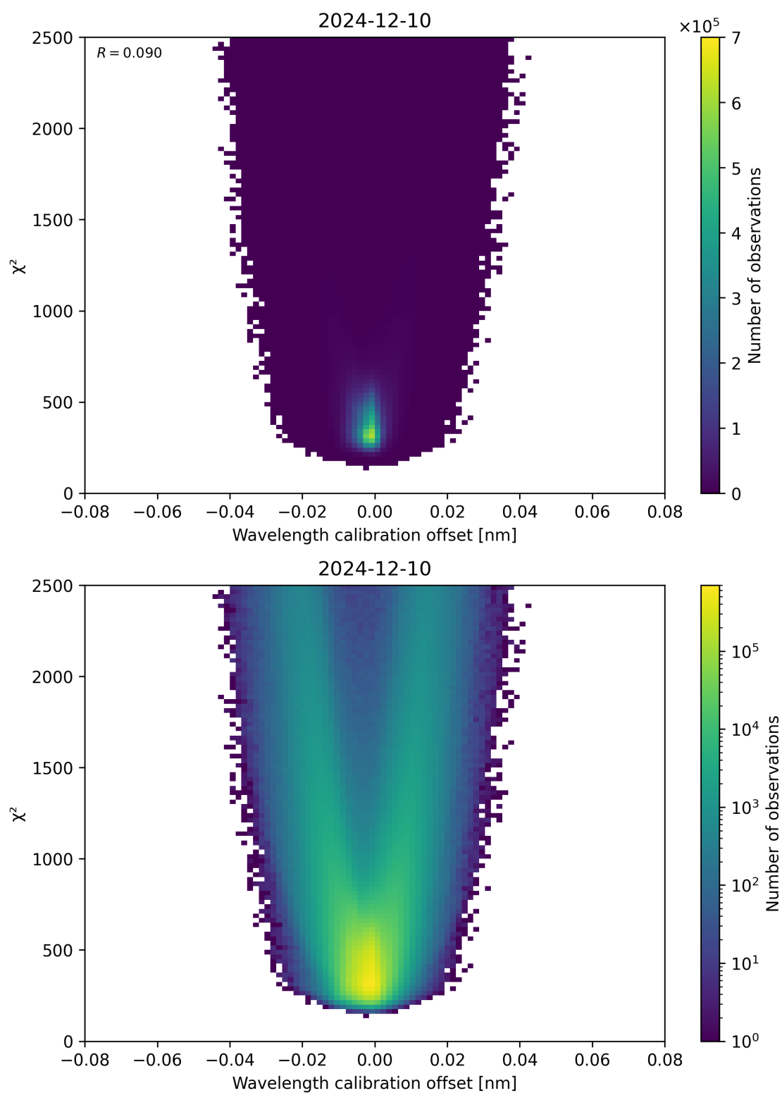
Figure 175: Scatter density plot of “Wavelength calibration offset” against “ \chi^2 ” for 2024-12-09 to 2024-12-11.
