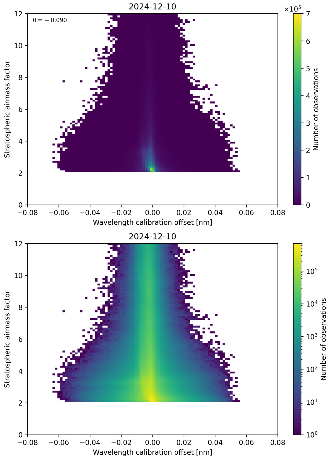
Figure 174: Scatter density plot of “Wavelength calibration offset” against “Stratospheric air mass factor” for 2024-12-09 to 2024-12-11.
