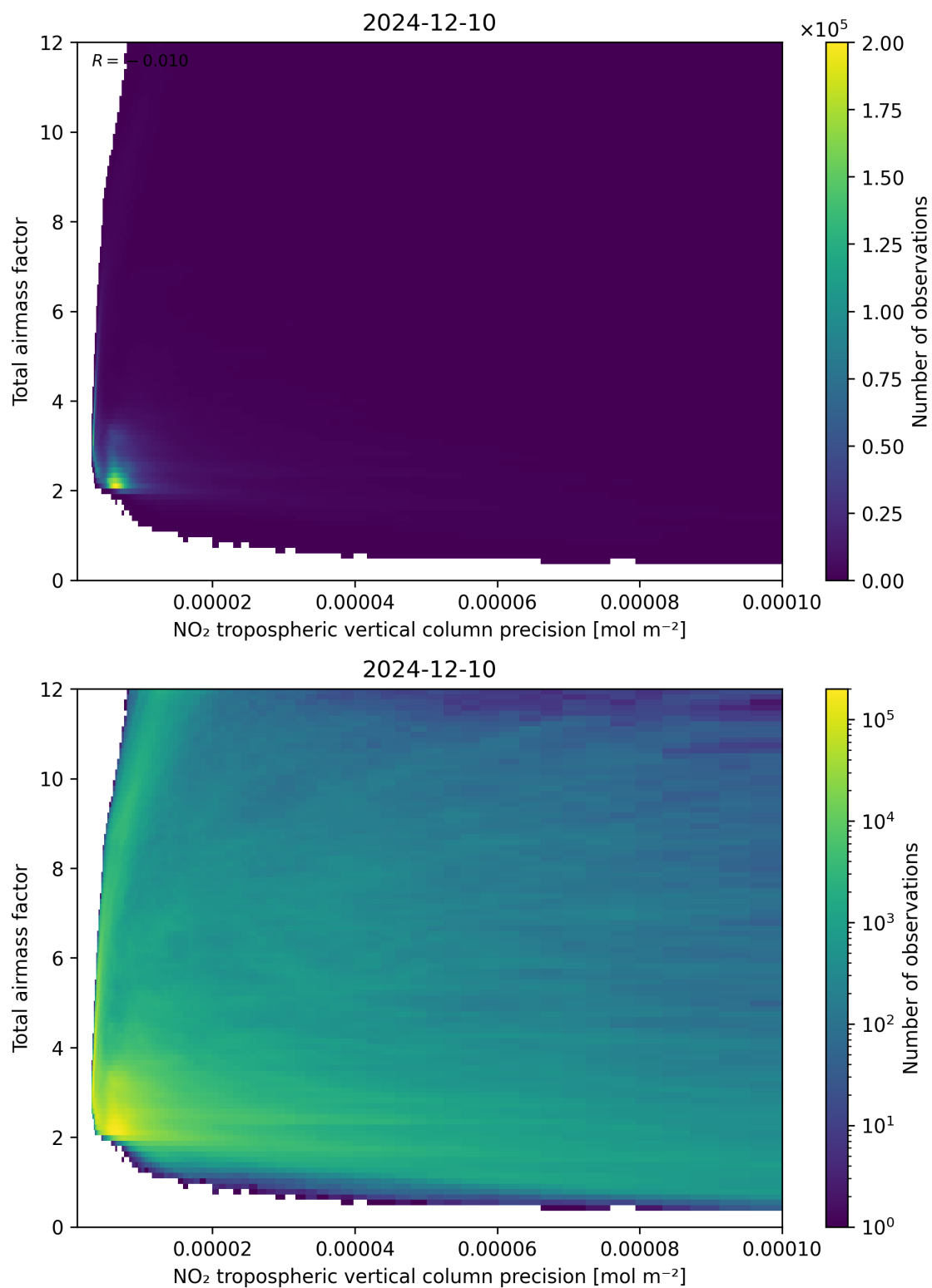
Figure 132: Scatter density plot of “NO 2 tropospheric vertical column precision” against “Total air mass factor” for 2024-12-09 to 2024-12-11.
