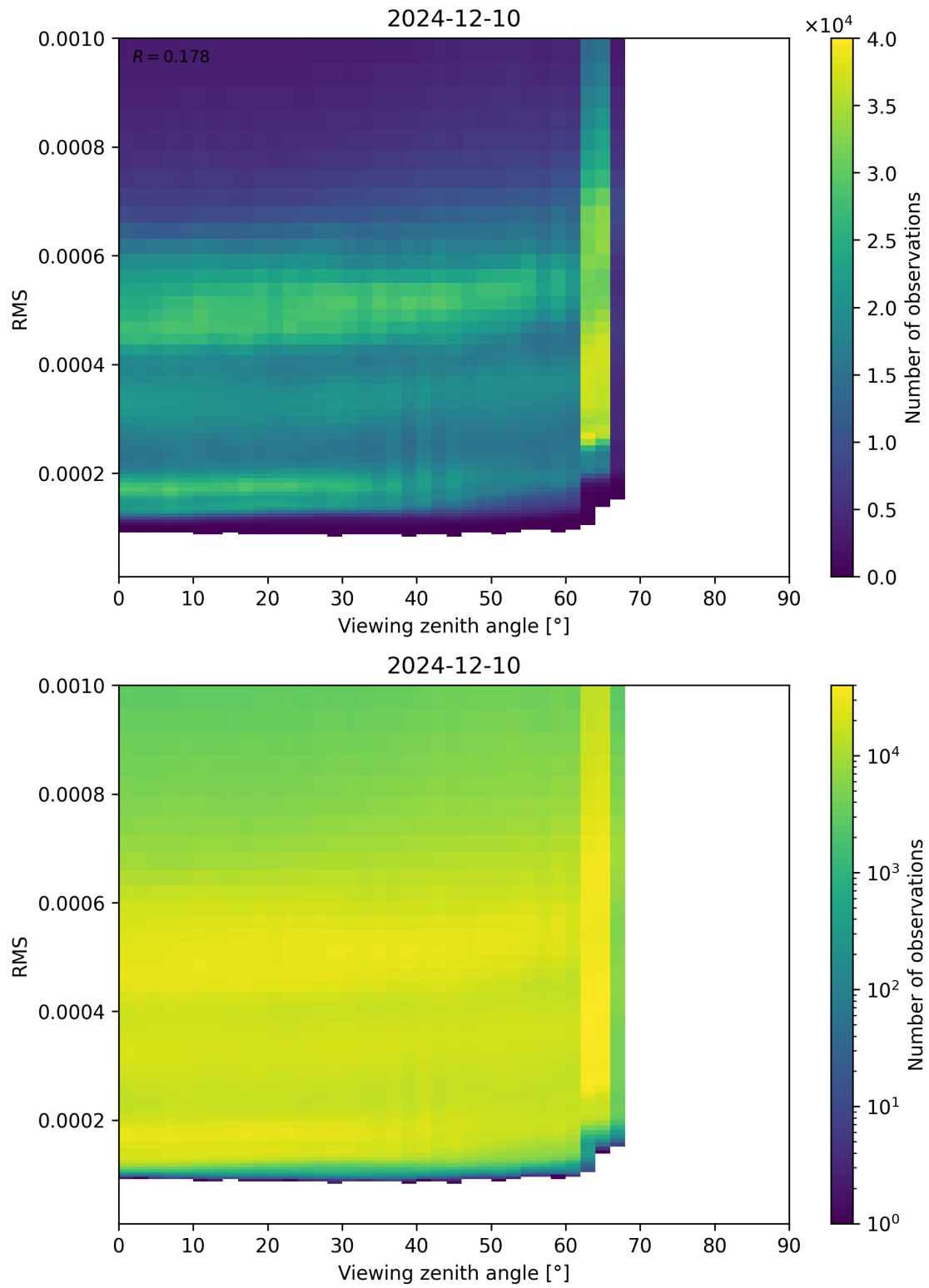
Figure 171: Scatter density plot of “Viewing zenith angle” against “RMS” for 2024-12-09 to 2024-12-11.
