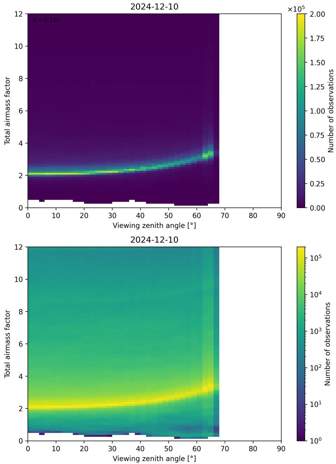
Figure 160: Scatter density plot of “Viewing zenith angle” against “Total airmass factor” for 2024-12-09 to 2024-12-11.
