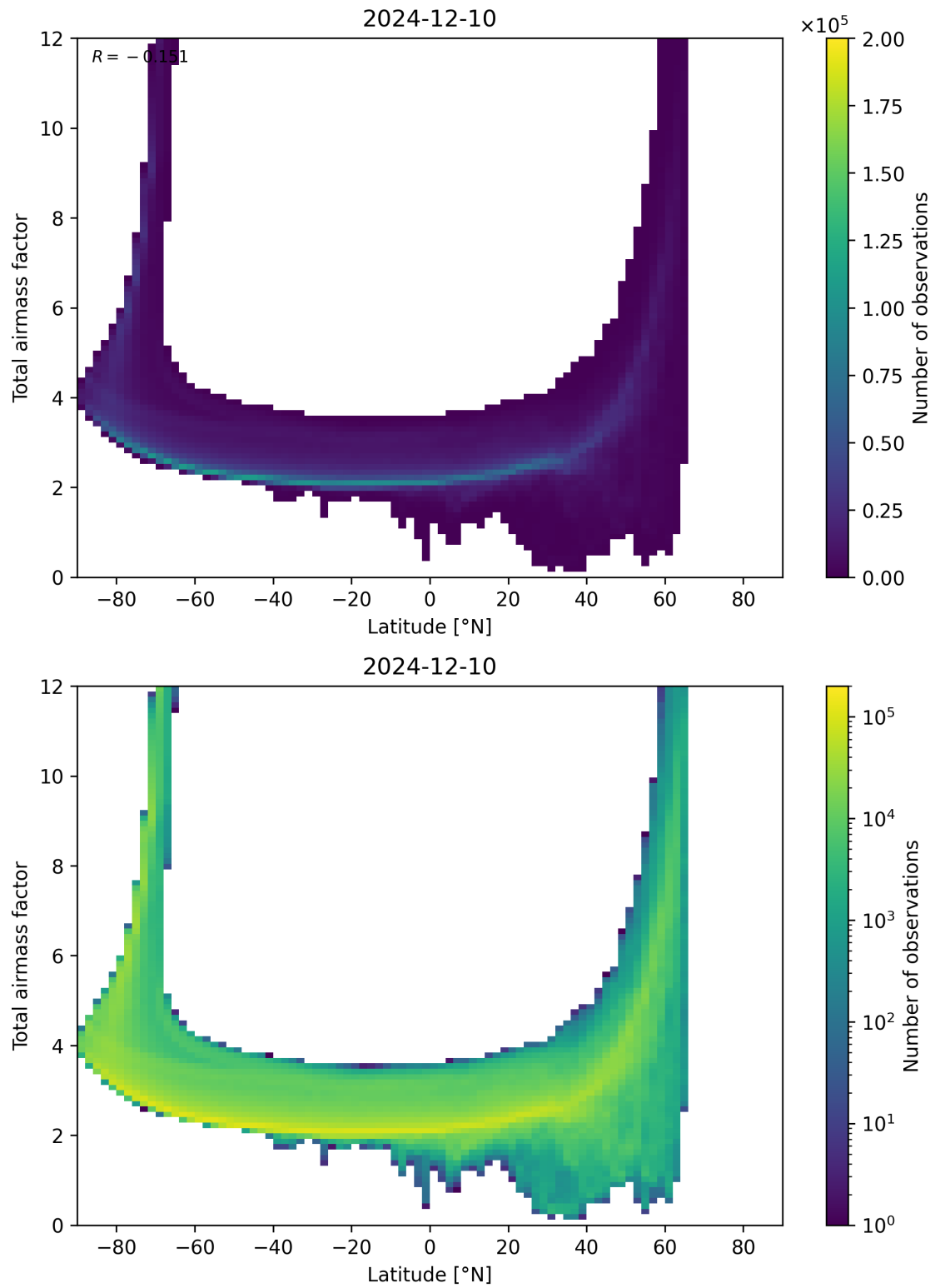
Figure 84: Scatter density plot of “Latitude” against “Total airmass factor” for 2024-12-09 to 2024-12-11.
