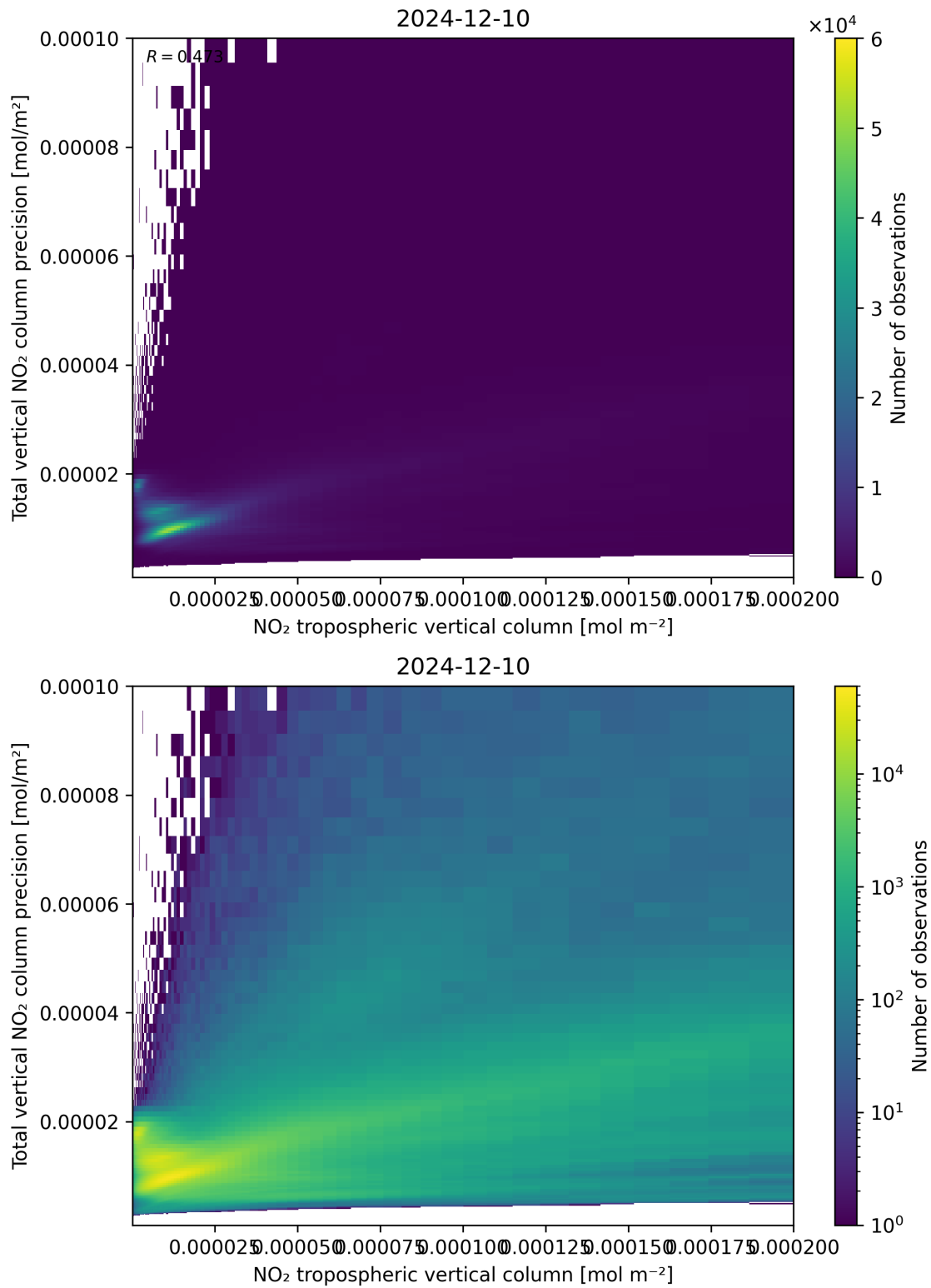
Figure 129: Scatter density plot of “NO 2 tropospheric vertical column” against “Total vertical NO 2 column precision” for 2024-12-09 to 2024-12-11.
