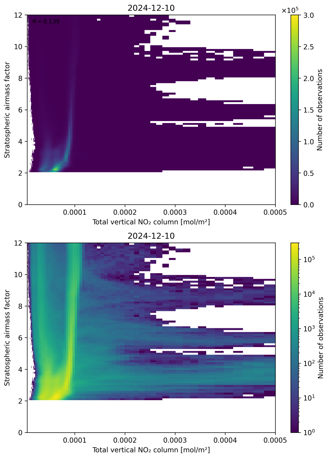
Figure 110: Scatter density plot of “Total vertical NO 2 column” against “Stratospheric air mass factor” for 2024-12-09 to 2024-12-11.
