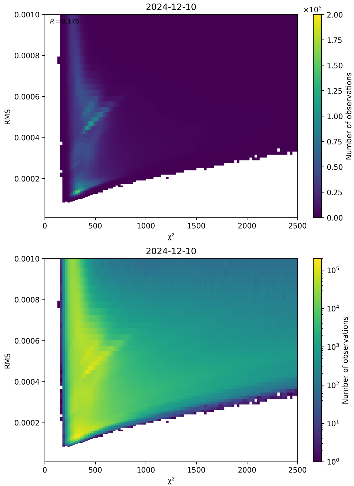
Figure 82: Scatter density plot of “ \chi^2 ” against “RMS” for 2024-12-09 to 2024-12-11.
