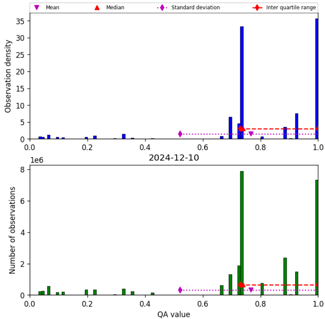
Figure 28: Histogram of “QA value” for 2024-12-09 to 2024-12-11
