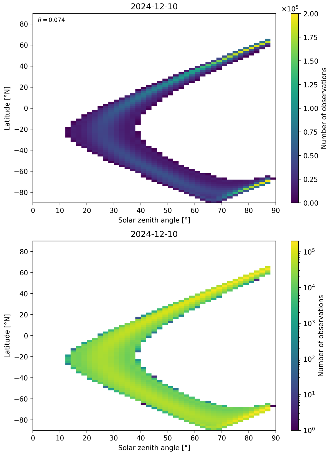
Figure 149: Scatter density plot of “Solar zenith angle” against “Latitude” for 2024-12-09 to 2024-12-11.
