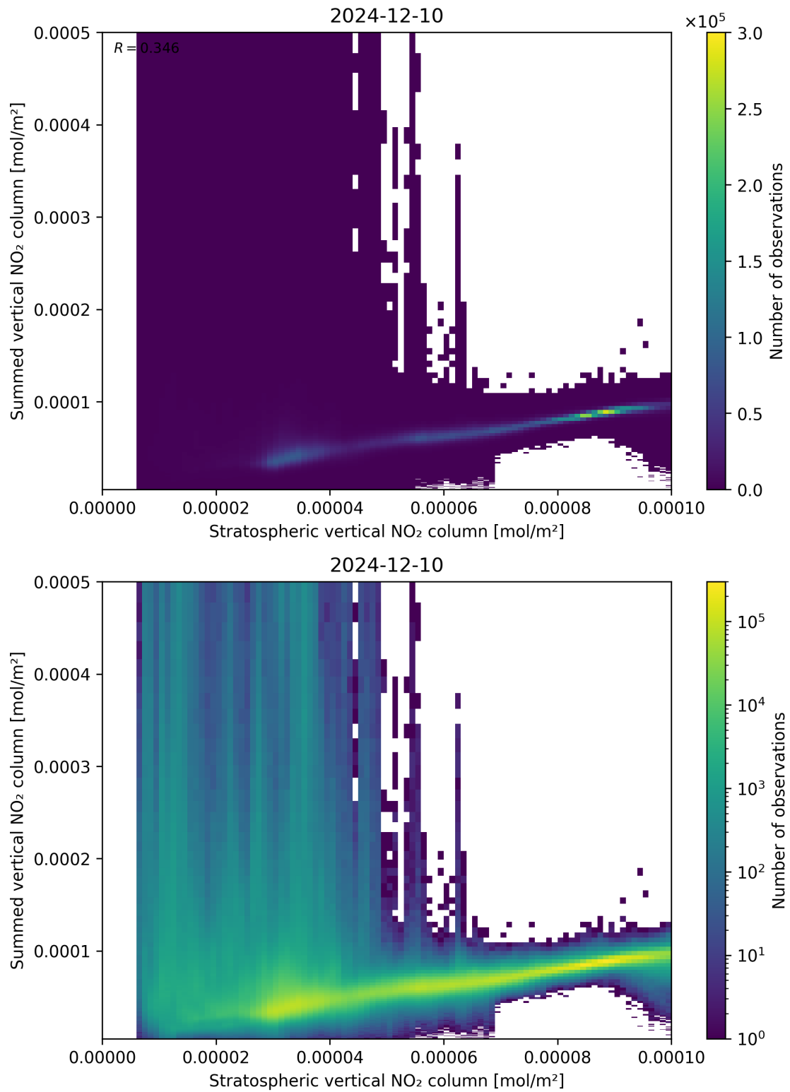
Figure 98: Scatter density plot of “Stratospheric vertical NO 2 column” against “Summed vertical NO 2 column” for 2024-12-09 to 2024-12-11.
