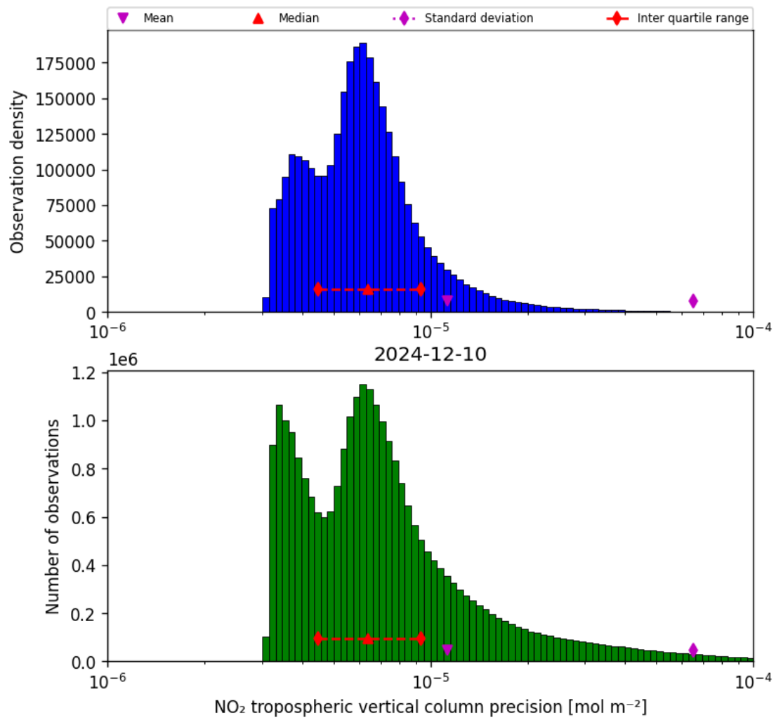
Figure 30: Histogram of “NO 2 tropospheric vertical column precision” for 2024-12-09 to 2024-12-11
