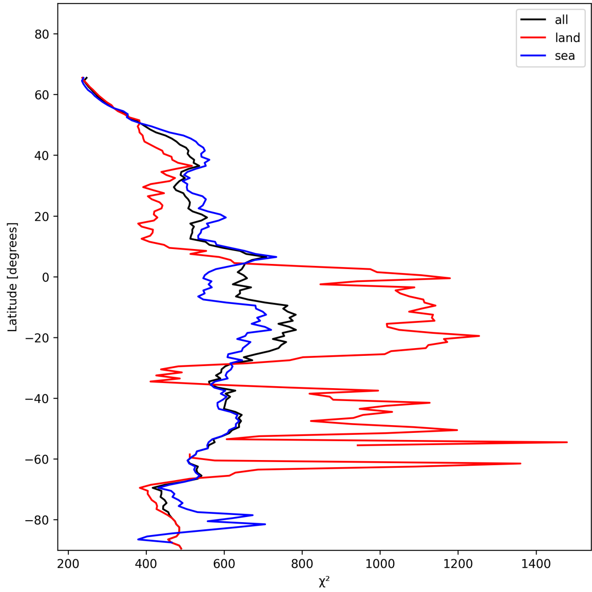
Figure 25: Zonal average of “ \chi^2 ” for 2024-12-09 to 2024-12-11.
