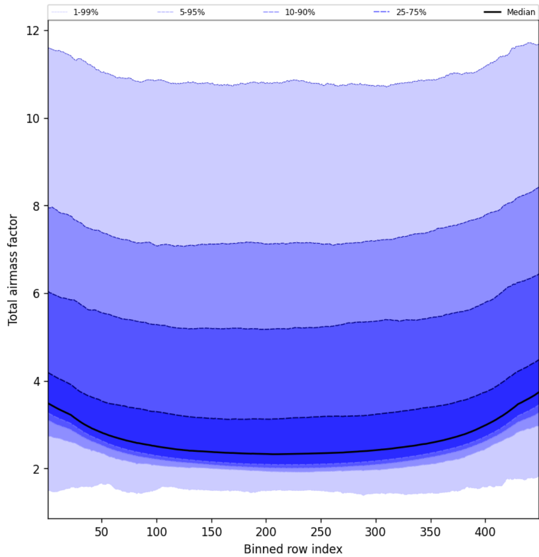
Figure 49: Along track statistics of “Total airmass factor” for 2024-12-09 to 2024-12-11
