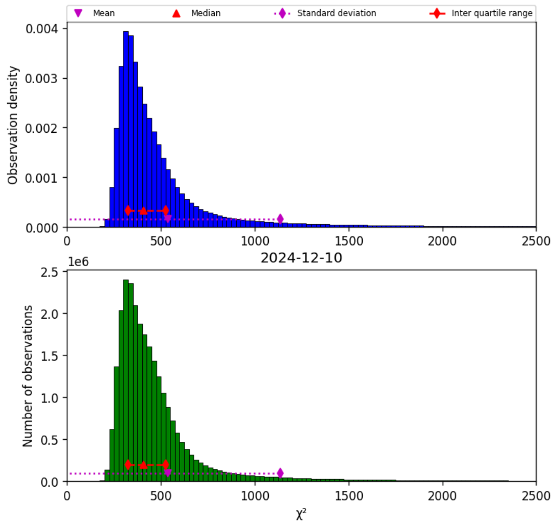
Figure 42: Histogram of “ \chi^2 ” for 2024-12-09 to 2024-12-11
