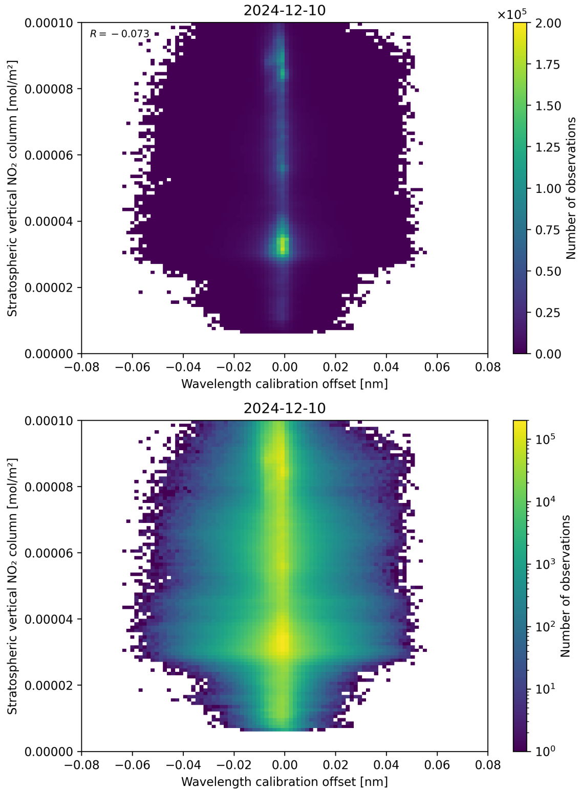
Figure 176: Scatter density plot of “Wavelength calibration offset” against “Stratospheric vertical NO 2 column” for 2024-12-09 to 2024-12-11.
