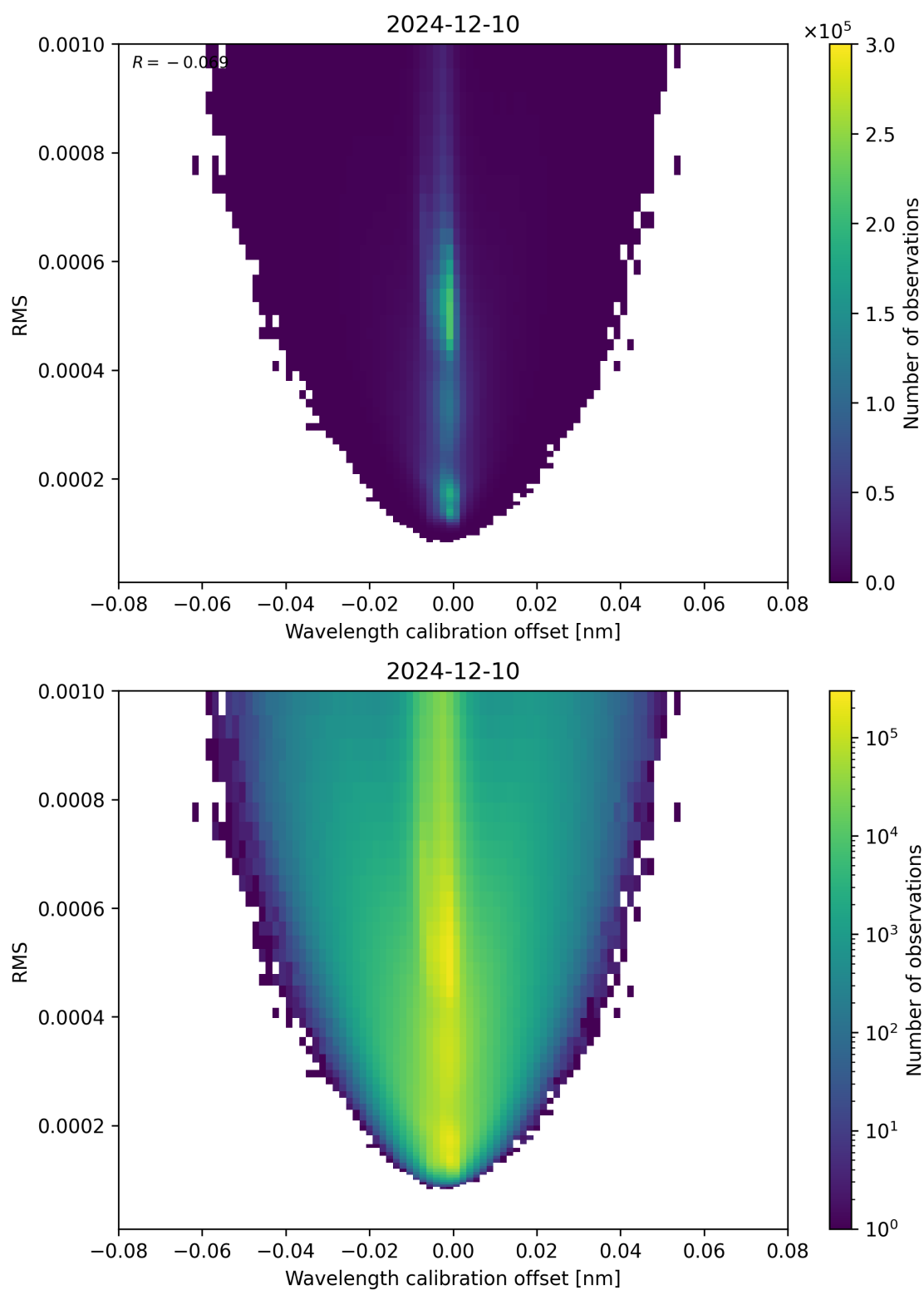
Figure 181: Scatter density plot of “Wavelength calibration offset” against “RMS” for 2024-12-09 to 2024-12-11.
