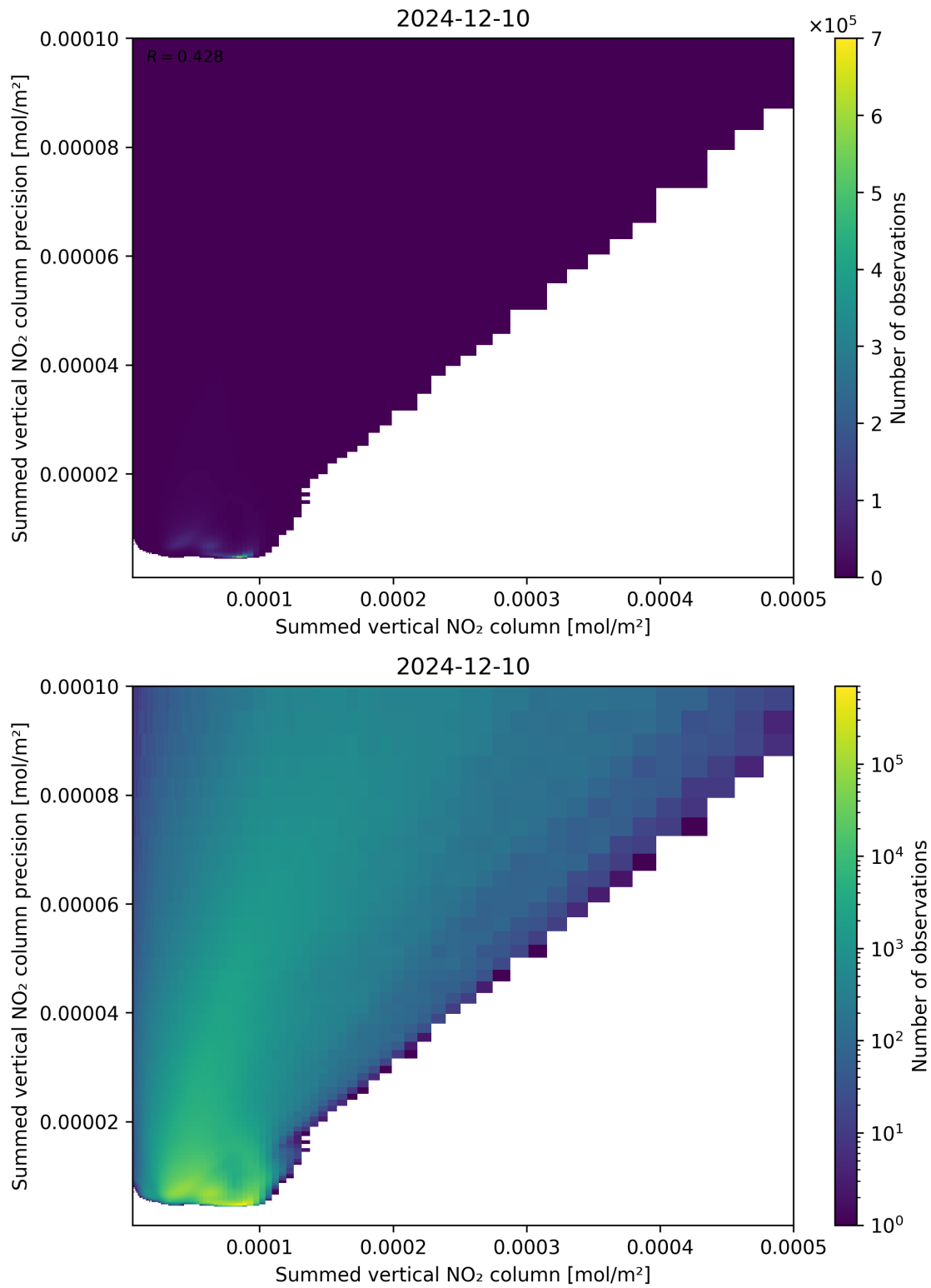
Figure 105: Scatter density plot of “Summed vertical NO 2 column” against “Summed vertical NO 2 column precision” for 2024-12-09 to 2024-12-11.
