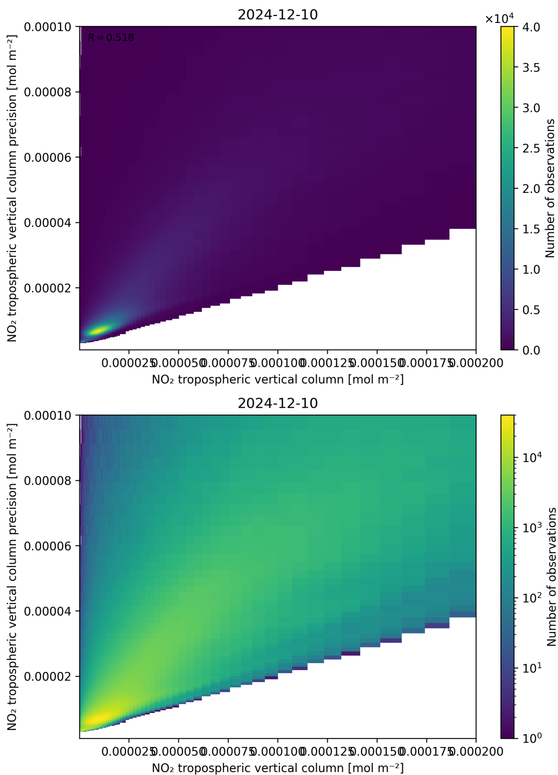
Figure 130: Scatter density plot of “NO 2 tropospheric vertical column” against “NO 2 tropospheric vertical column precision” for 2024-12-09 to 2024-12-11.
