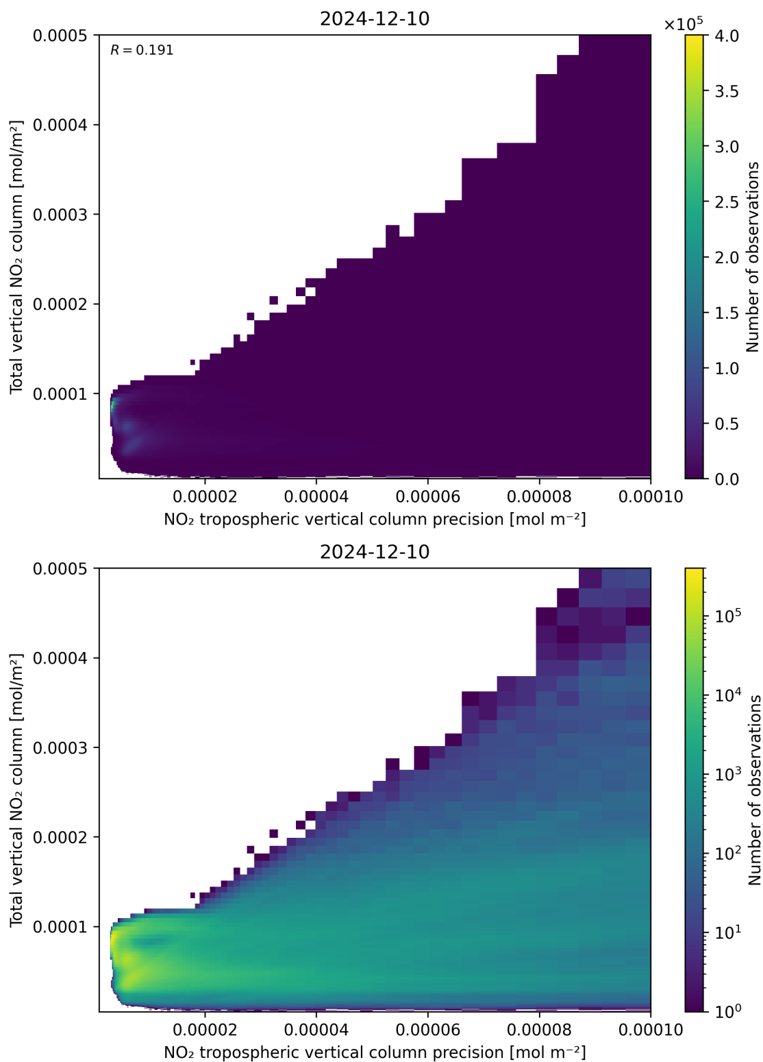
Figure 138: Scatter density plot of “NO 2 tropospheric vertical column precision” against “Total vertical NO 2 column” for 2024-12-09 to 2024-12-11.
