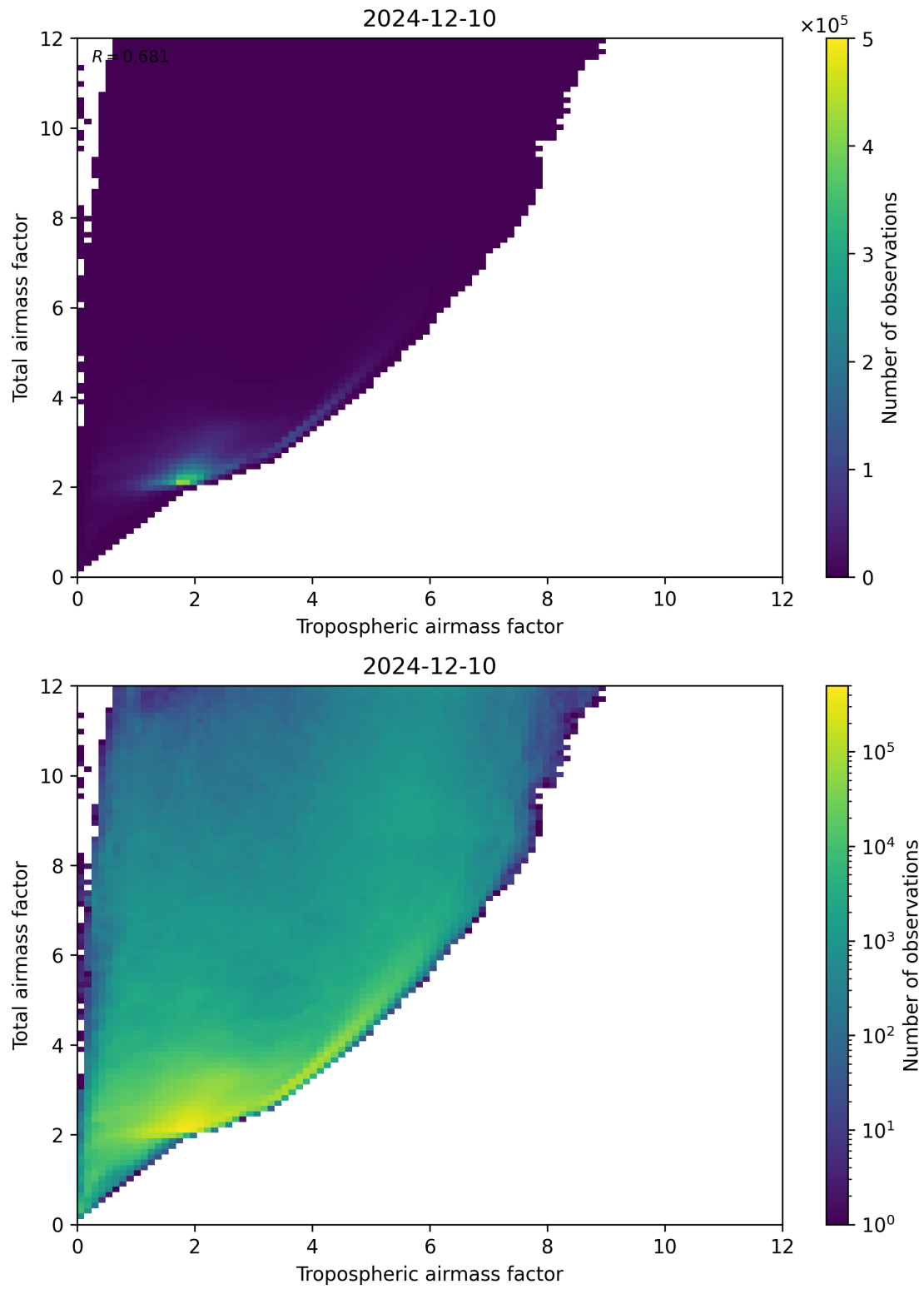
Figure 72: Scatter density plot of “Tropospheric airmass factor” against “Total airmass factor” for 2024-12-09 to 2024-12-11.
