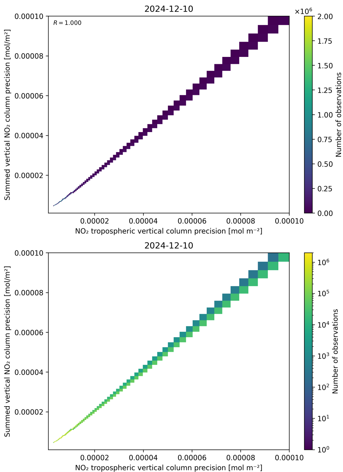
Figure 137: Scatter density plot of “NO 2 tropospheric vertical column precision” against “Summed vertical NO 2 column precision” for 2024-12-09 to 2024-12-11.
