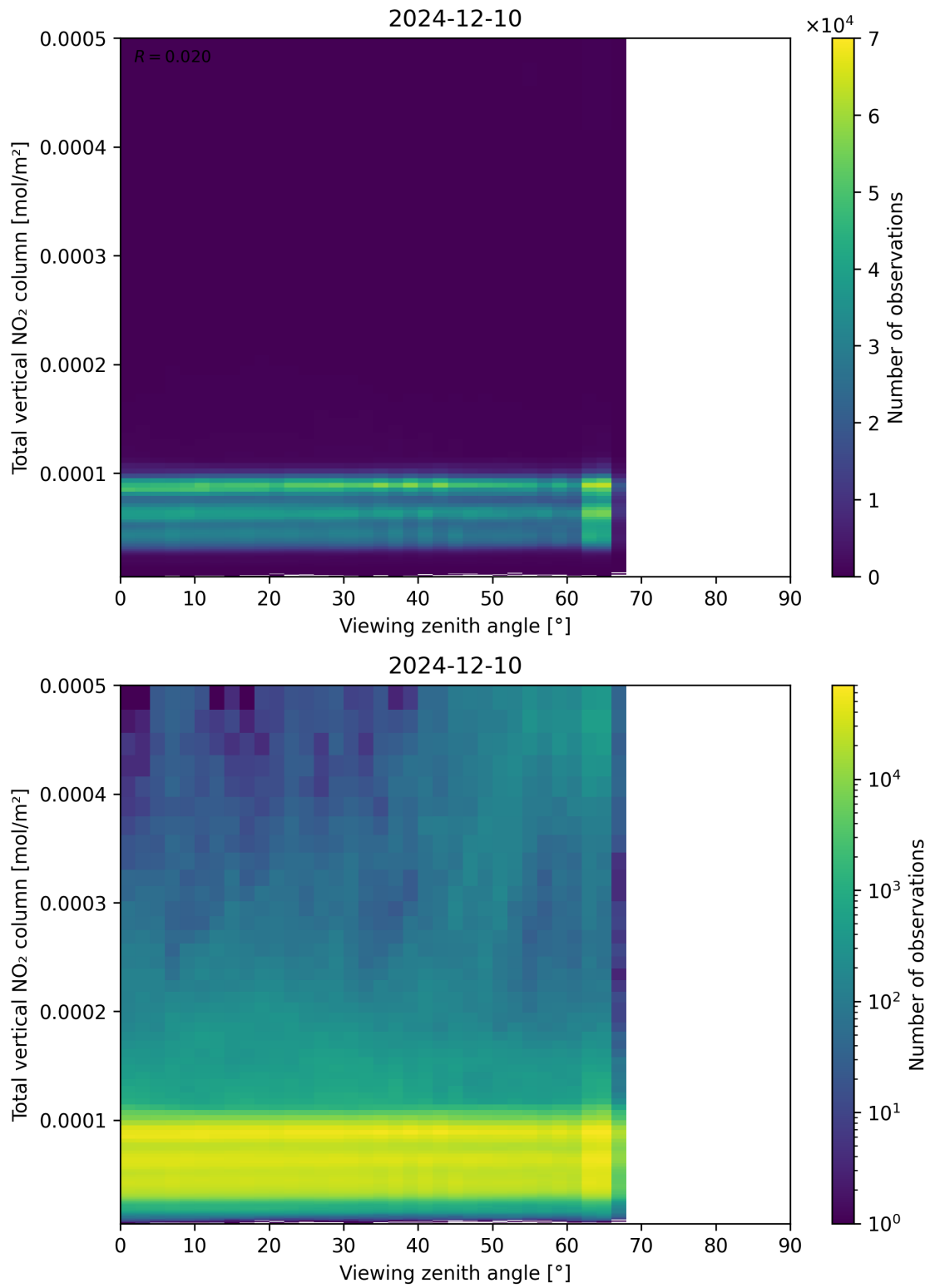
Figure 167: Scatter density plot of “Viewing zenith angle” against “Total vertical NO 2 column” for 2024-12-09 to 2024-12-11.
