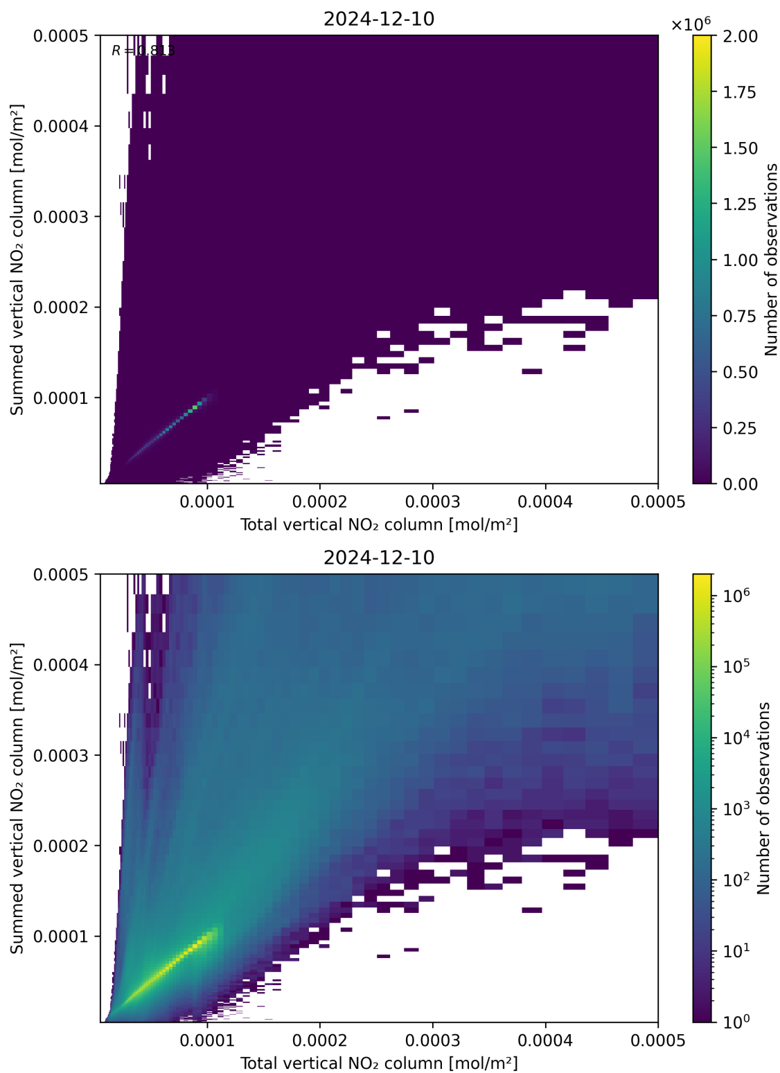
Figure 112: Scatter density plot of “Total vertical NO 2 column” against “Summed vertical NO 2 column” for 2024-12-09 to 2024-12-11.
