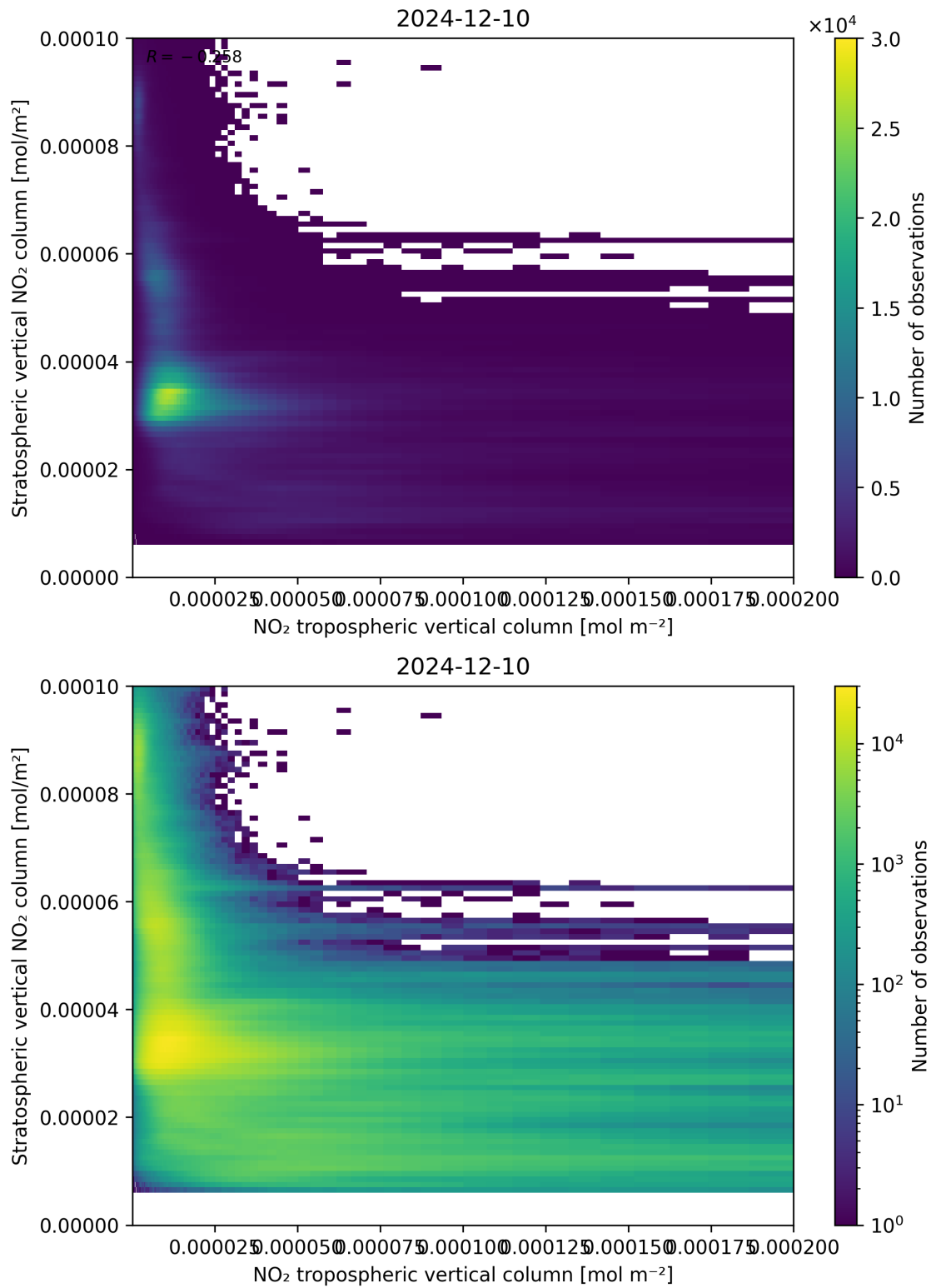
Figure 125: Scatter density plot of “NO 2 tropospheric vertical column” against “Stratospheric vertical NO 2 column” for 2024-12-09 to 2024-12-11.
