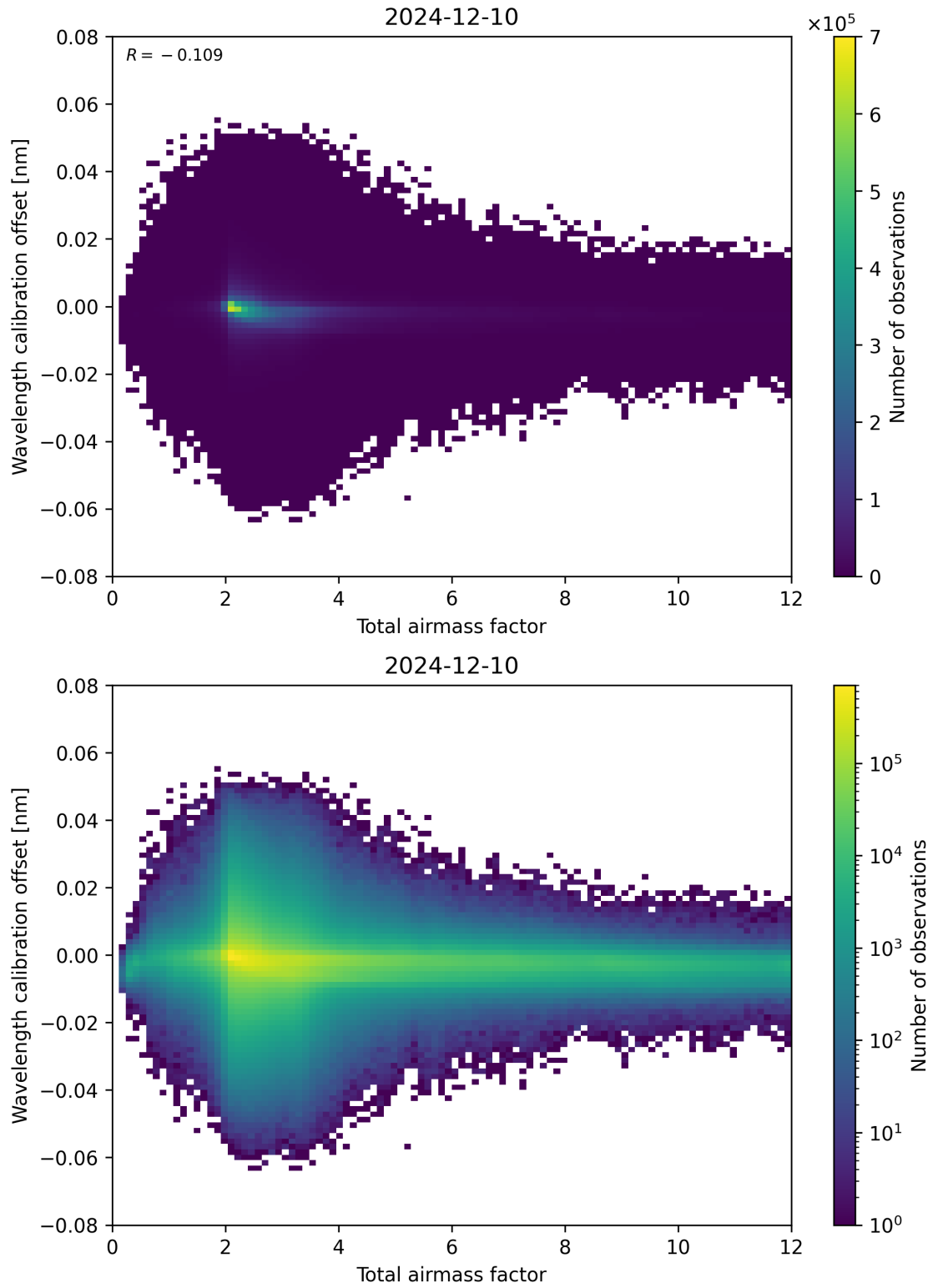
Figure 70: Scatter density plot of “Total airmass factor” against “Wavelength calibration offset” for 2024-12-09 to 2024-12-11.
