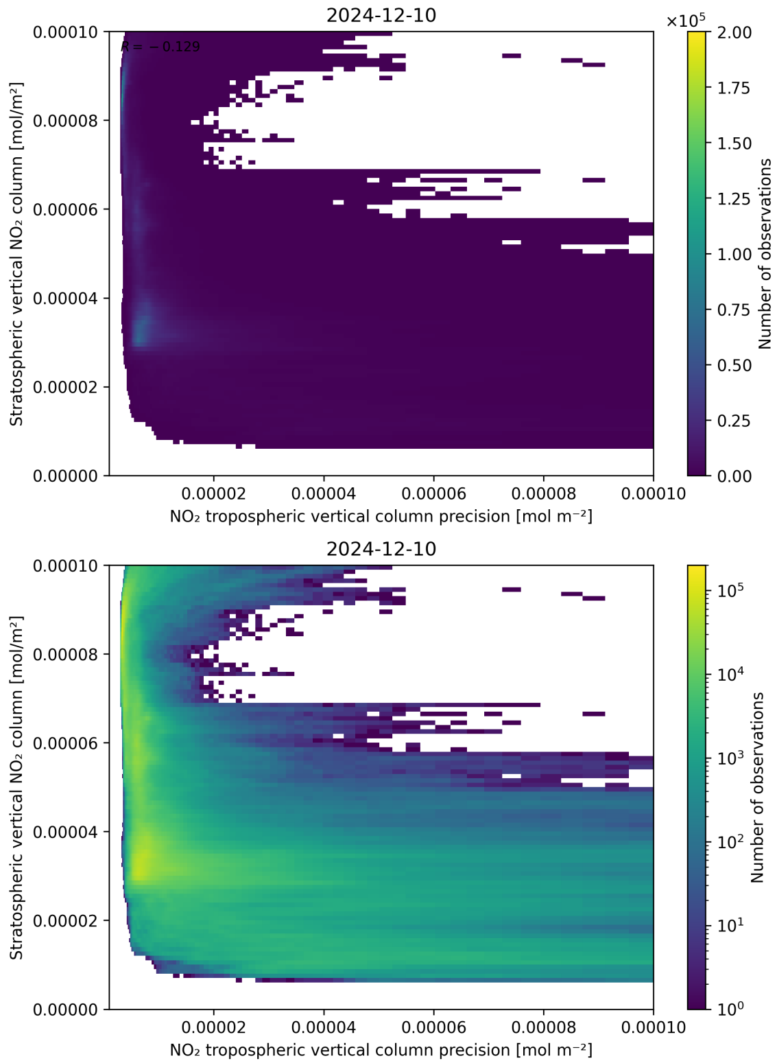
Figure 135: Scatter density plot of “NO 2 tropospheric vertical column precision” against “Stratospheric vertical NO 2 column” for 2024-12-09 to 2024-12-11.
