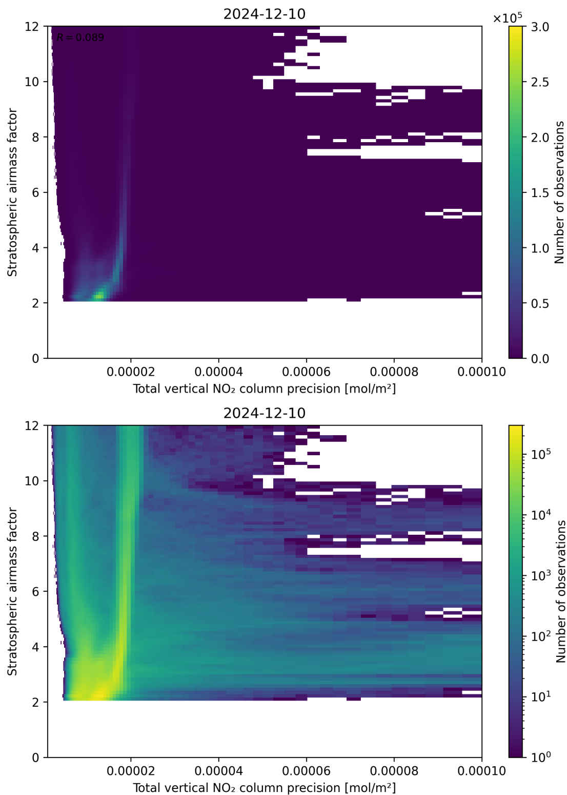
Figure 115: Scatter density plot of “Total vertical NO 2 column precision” against “Stratospheric air mass factor” for 2024-12-09 to 2024-12-11.
