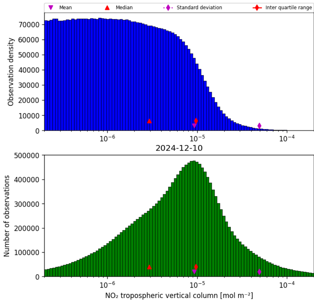
Figure 29: Histogram of “NO 2 tropospheric vertical column” for 2024-12-09 to 2024-12-11
