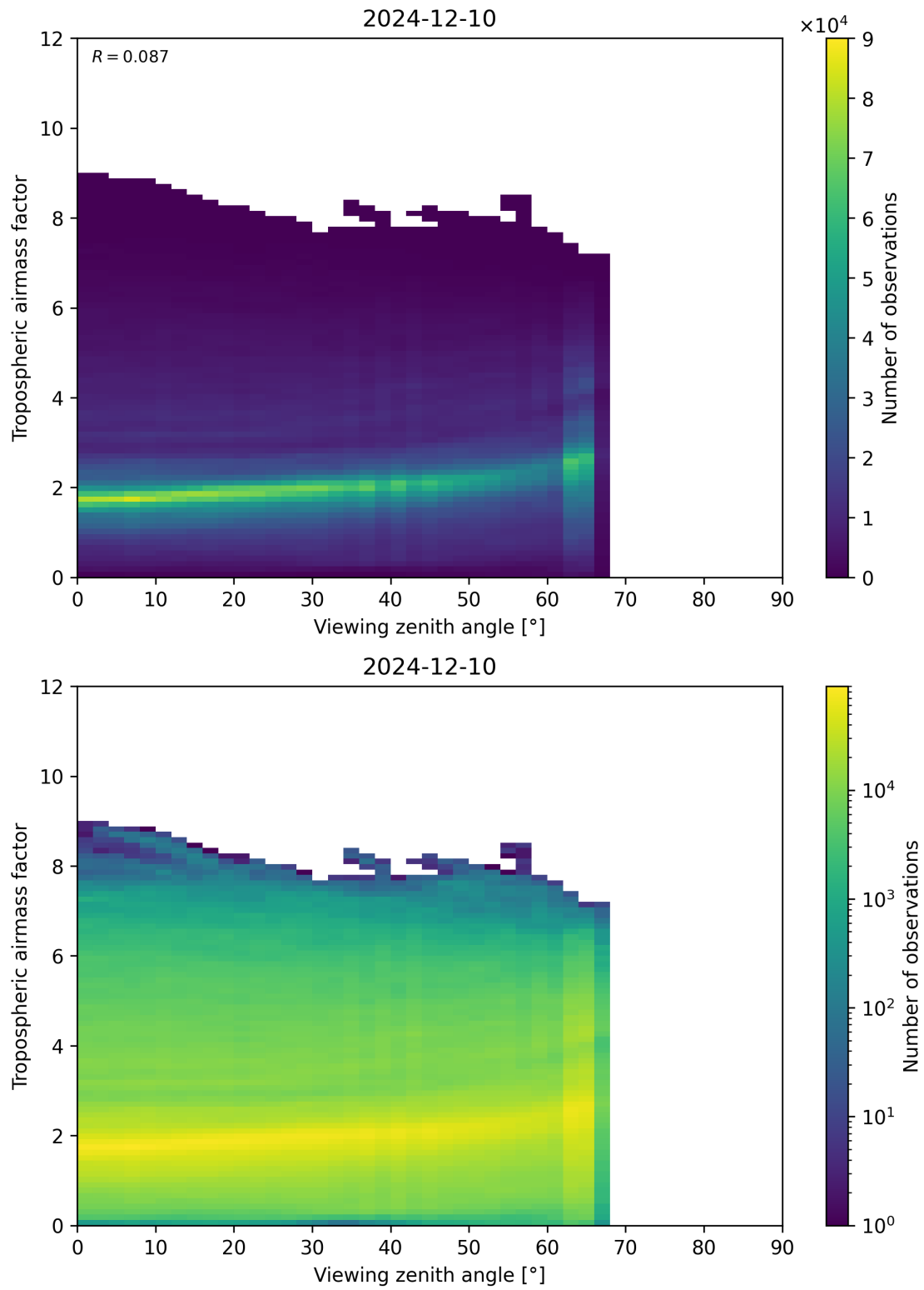
Figure 161: Scatter density plot of “Viewing zenith angle” against “Tropospheric airmass factor” for 2024-12-09 to 2024-12-11.
