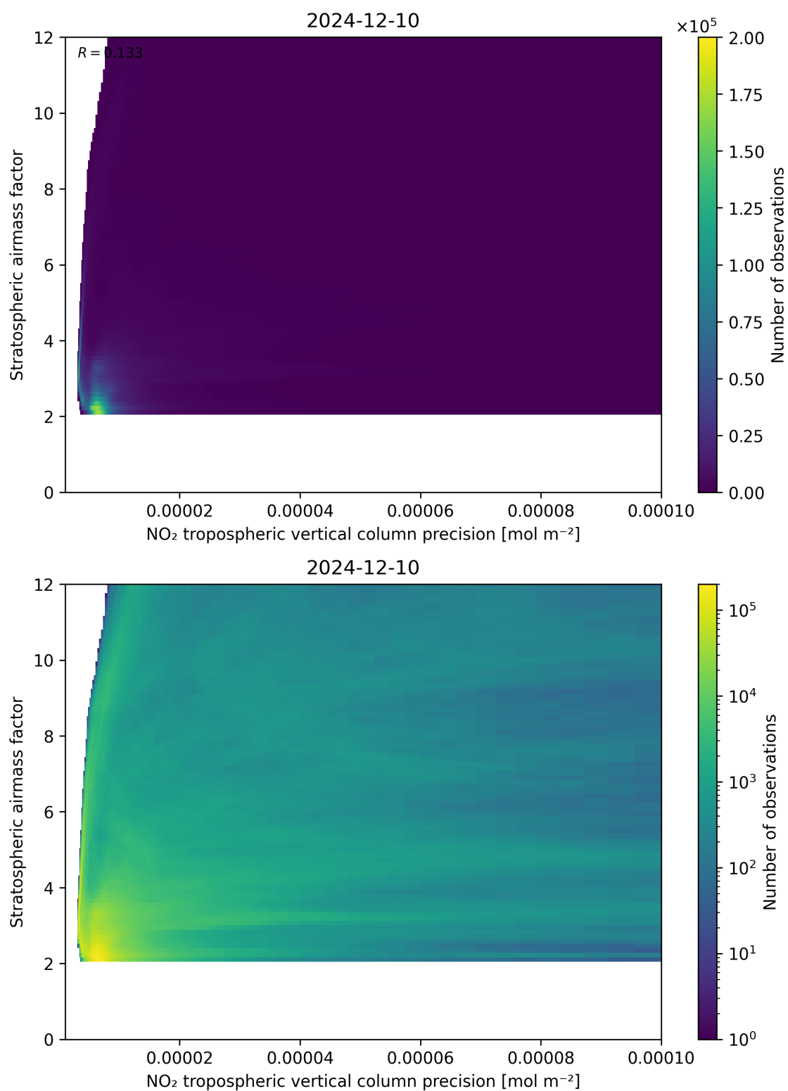
Figure 131: Scatter density plot of “NO 2 tropospheric vertical column precision” against “Stratospheric airmass factor” for 2024-12-09 to 2024-12-11.
