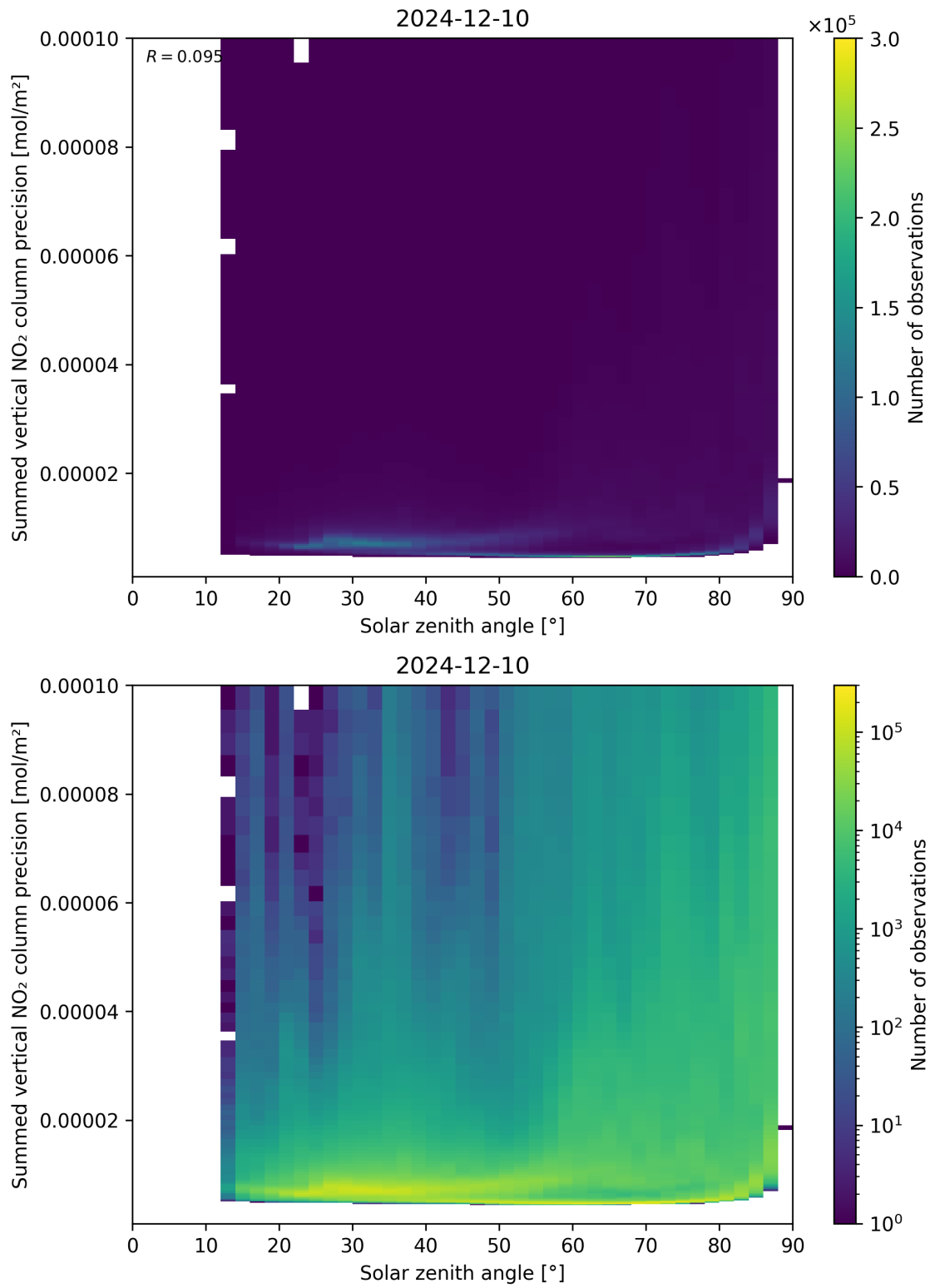
Figure 152: Scatter density plot of “Solar zenith angle” against “Summed vertical NO 2 column precision” for 2024-12-09 to 2024-12-11.
