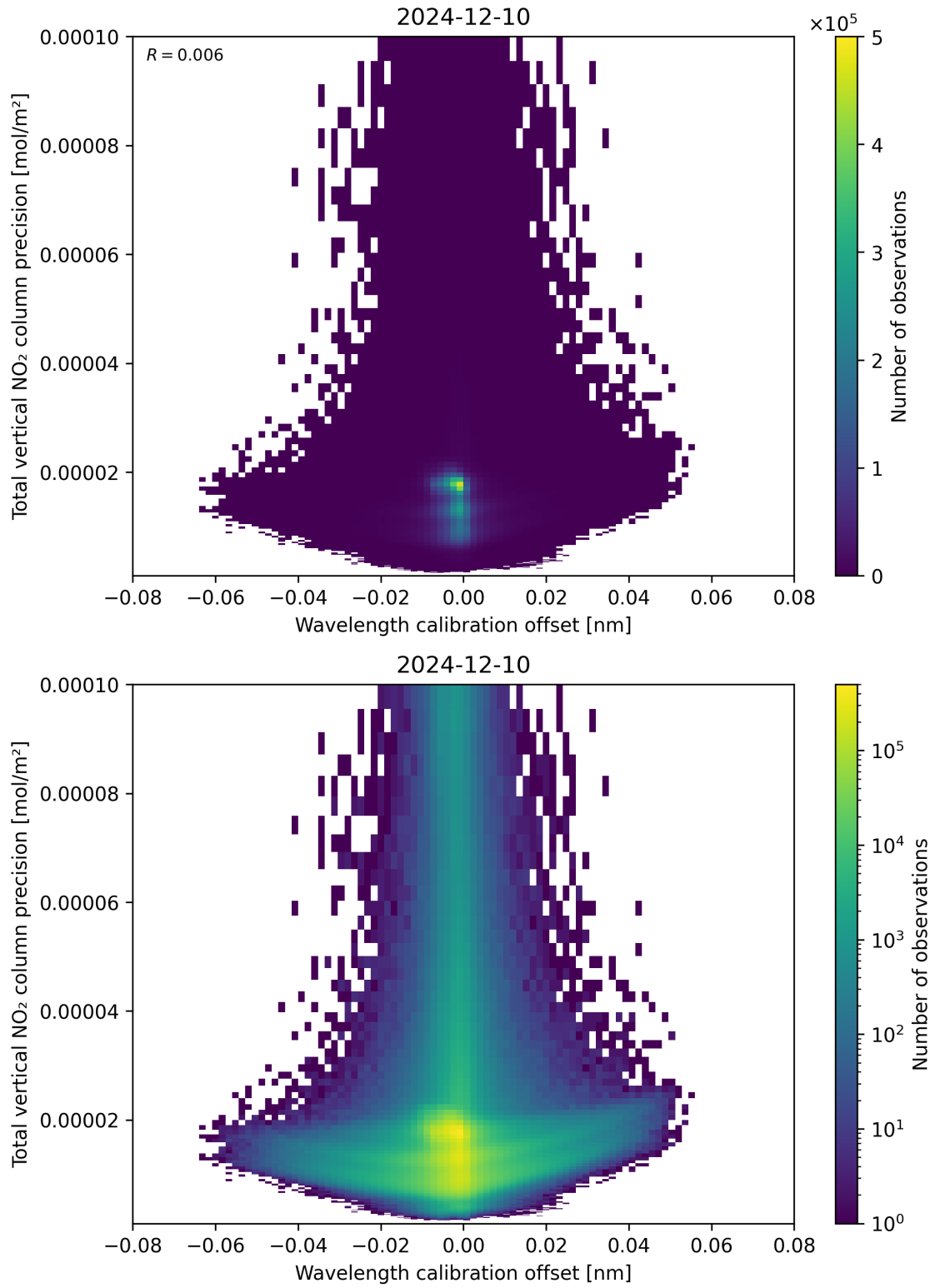
Figure 180: Scatter density plot of “Wavelength calibration offset” against “Total vertical NO 2 column precision” for 2024-12-09 to 2024-12-11.
