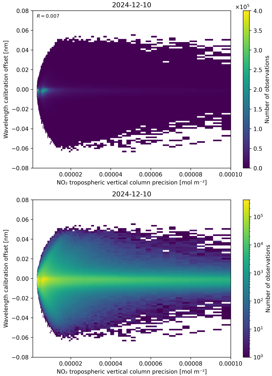
Figure 141: Scatter density plot of “NO 2 tropospheric vertical column precision” against “Wavelength calibration offset” for 2024-12-09 to 2024-12-11.
