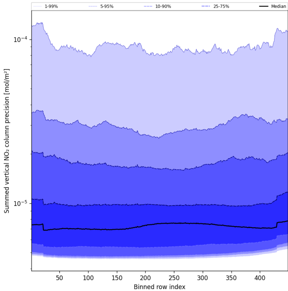
Figure 58: Along track statistics of “Summed vertical NO 2 column precision” for 2024-12-09 to 2024-12-11
