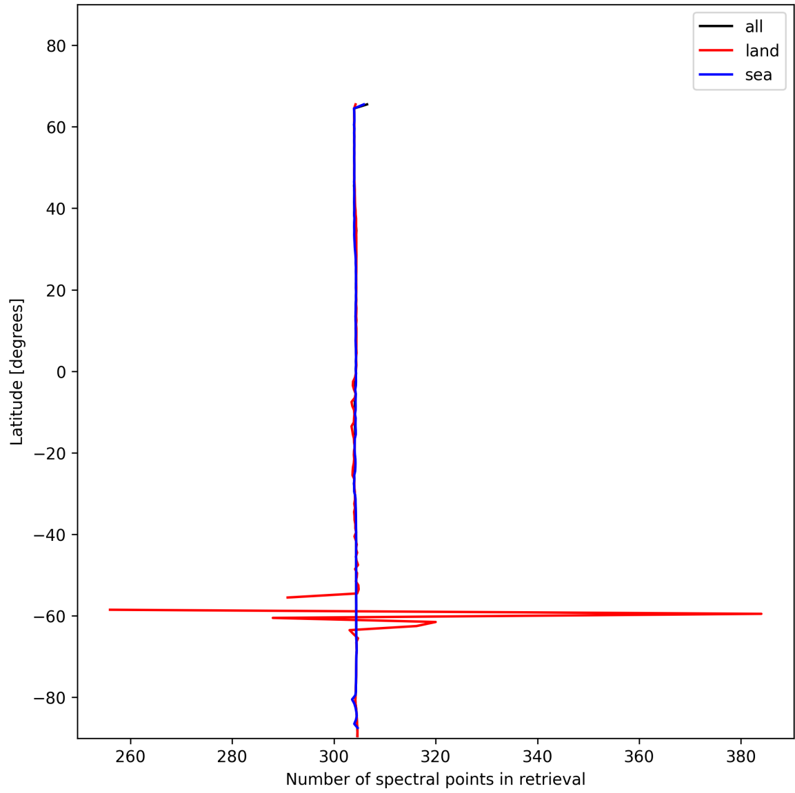
Figure 16: Zonal average of “Number of spectral points in retrieval” for 2024-12-09 to 2024-12-11.
