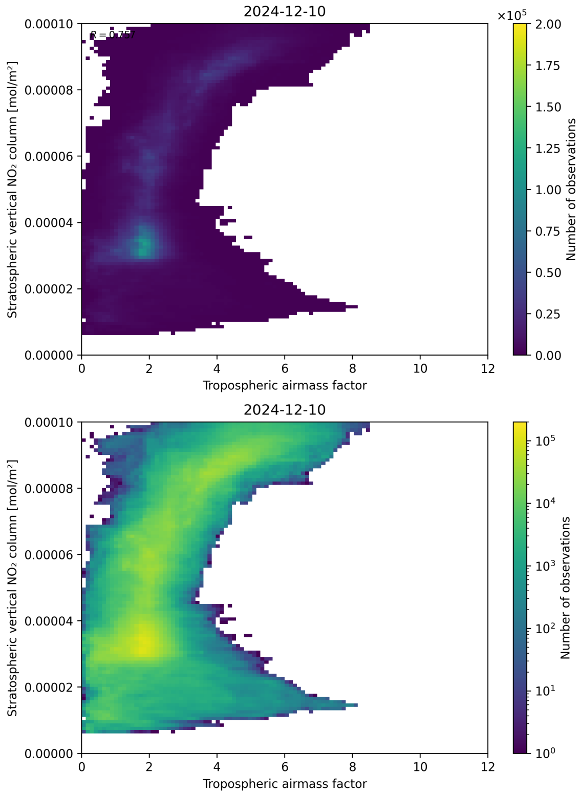
Figure 74: Scatter density plot of “Tropospheric air mass factor” against “Stratospheric vertical NO 2 column” for 2024-12-09 to 2024-12-11.
