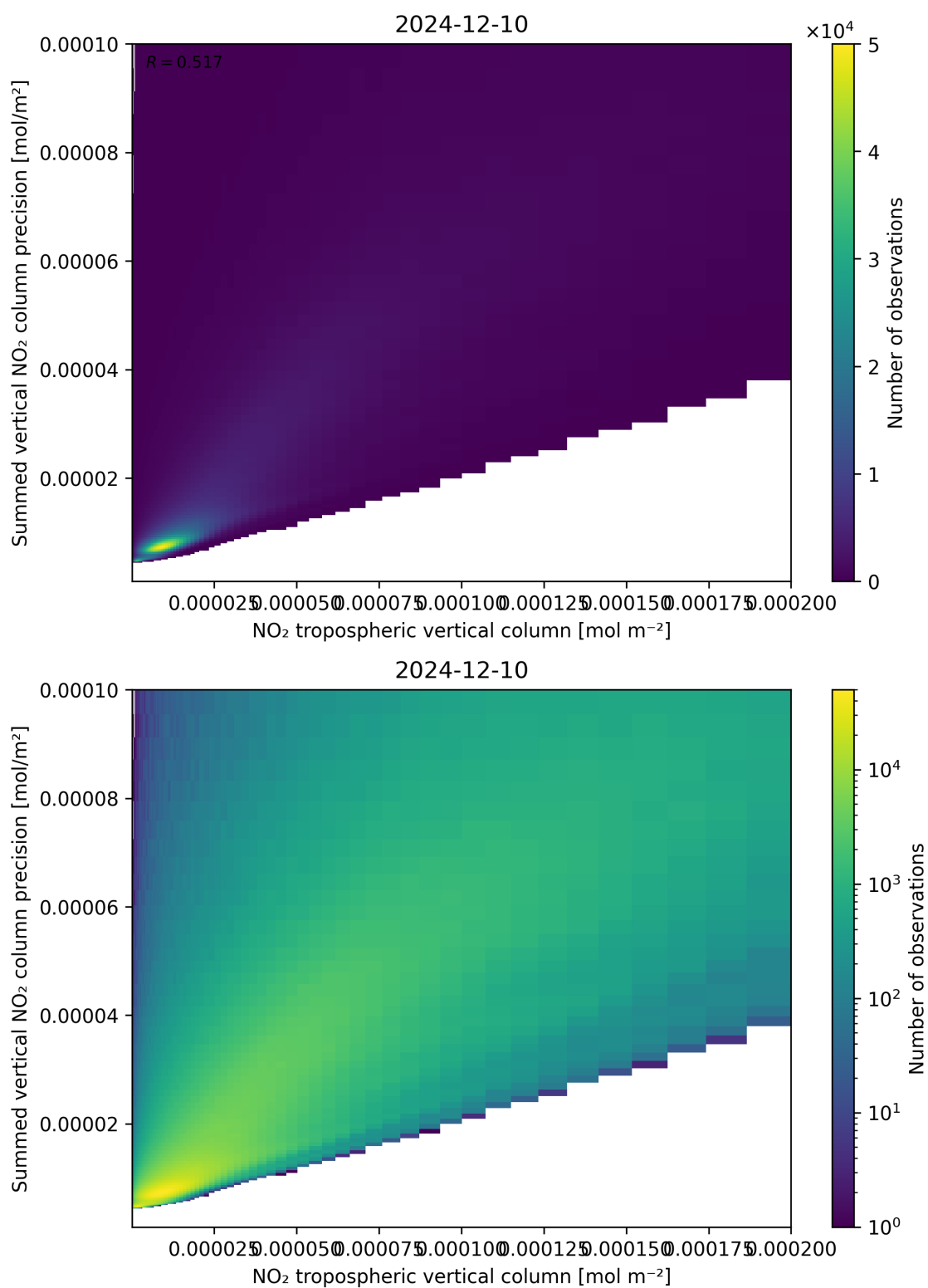
Figure 127: Scatter density plot of “NO 2 tropospheric vertical column” against “Summed vertical NO 2 column precision” for 2024-12-09 to 2024-12-11.
