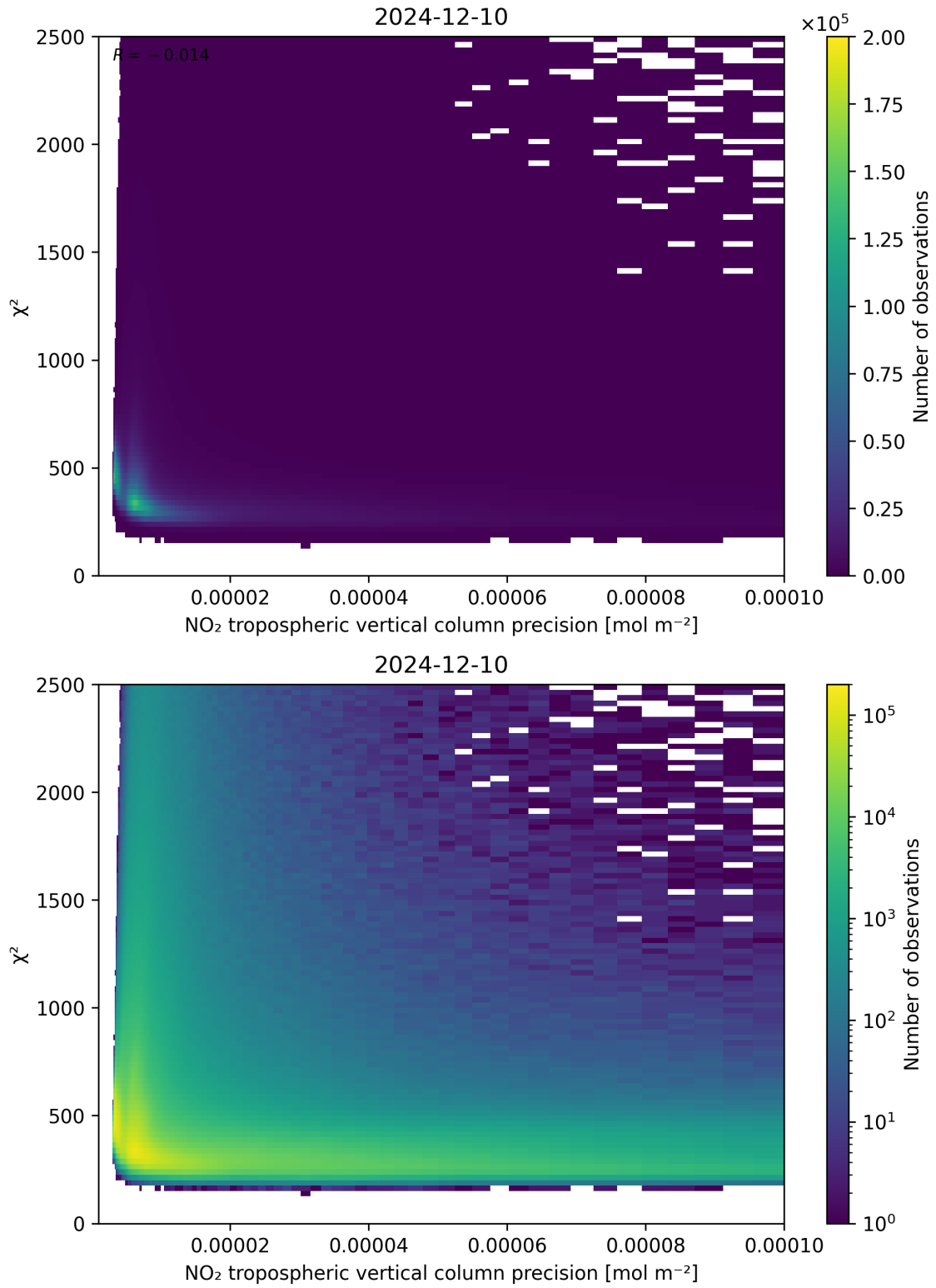
Figure 134: Scatter density plot of “NO 2 tropospheric vertical column precision” against “ \chi^2 ” for 2024-12-09 to 2024-12-11.
