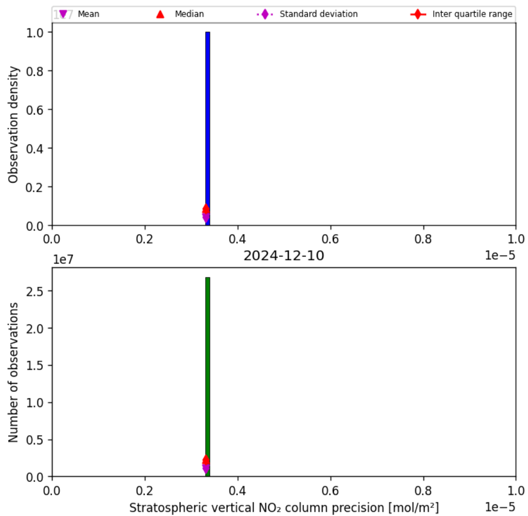
Figure 37: Histogram of “Stratospheric vertical NO 2 column precision” for 2024-12-09 to 2024-12-11
