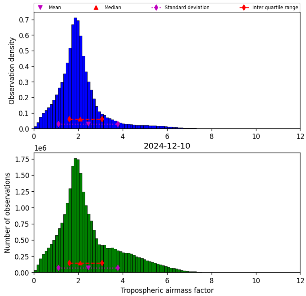
Figure 31: Histogram of “Tropospheric airmass factor” for 2024-12-09 to 2024-12-11
