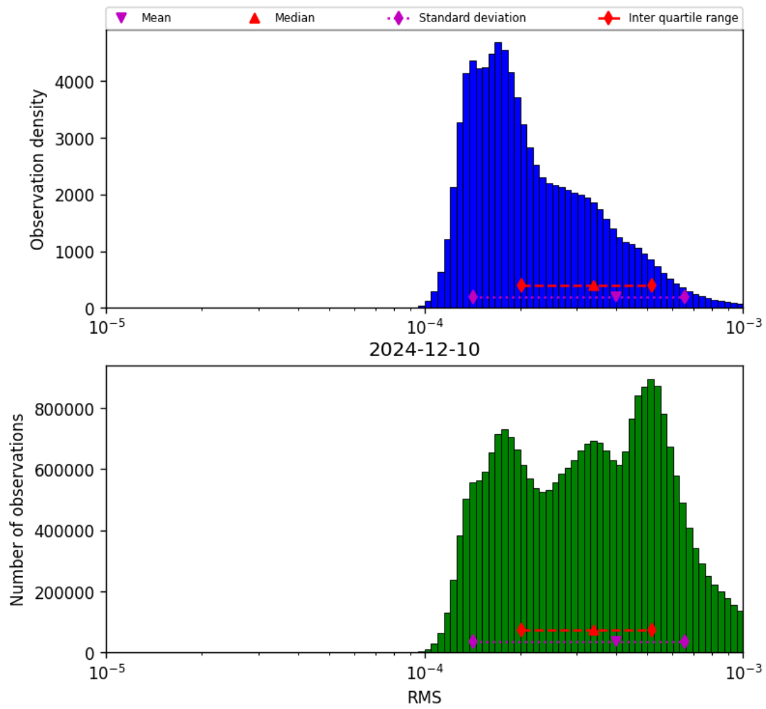
Figure 43: Histogram of “RMS” for 2024-12-09 to 2024-12-11
