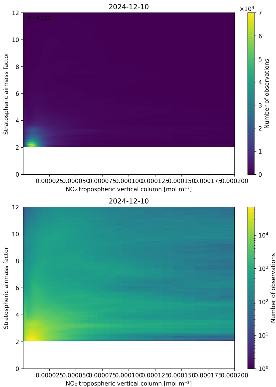
Figure 121: Scatter density plot of “NO 2 tropospheric vertical column” against “Stratospheric airmass factor” for 2024-12-09 to 2024-12-11.
