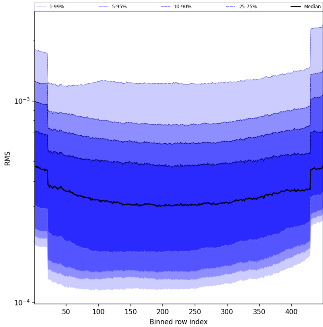
Figure 60: Along track statistics of “RMS” for 2024-12-09 to 2024-12-11
