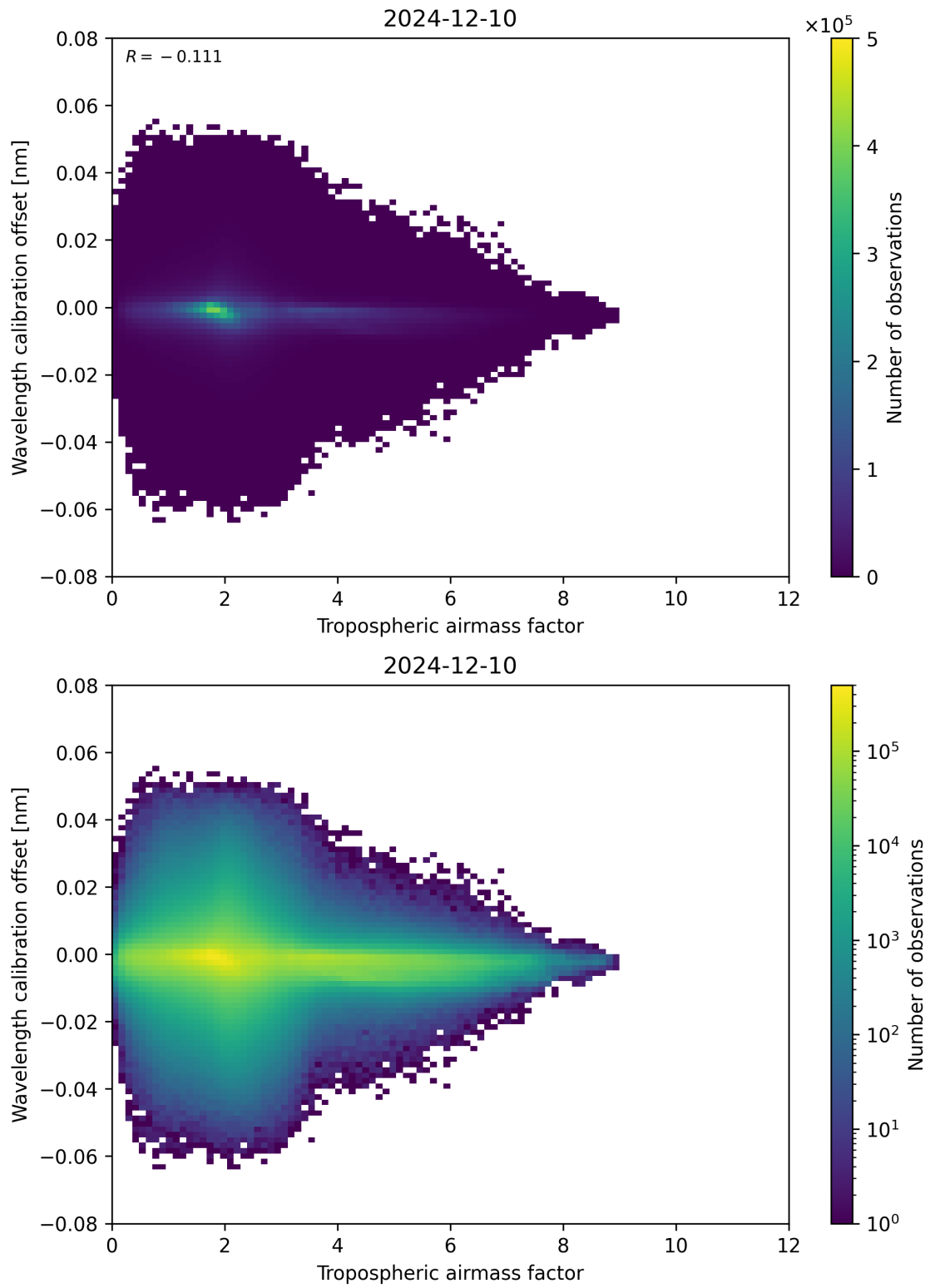
Figure 80: Scatter density plot of “Tropospheric airmass factor” against “Wavelength calibration offset” for 2024-12-09 to 2024-12-11.
