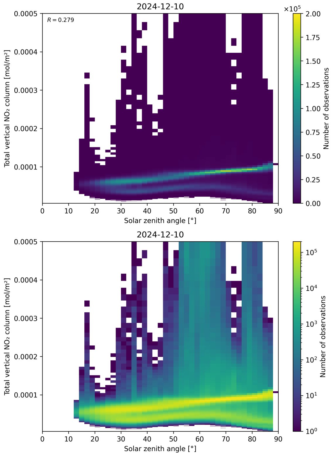
Figure 153: Scatter density plot of “Solar zenith angle” against “Total vertical NO 2 column” for 2024-12-09 to 2024-12-11.
