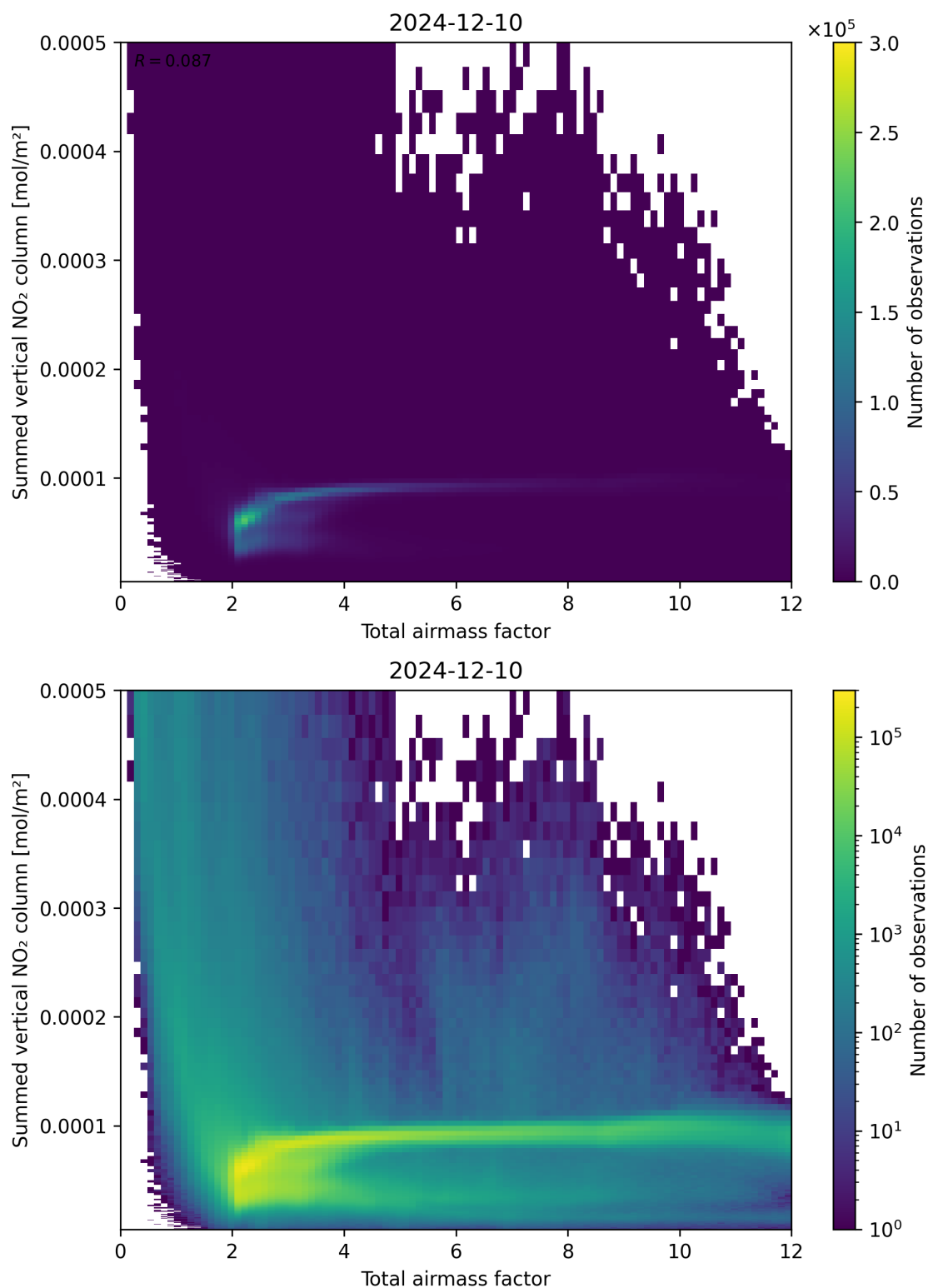
Figure 65: Scatter density plot of “Total airmass factor” against “Summed vertical NO 2 column” for 2024-12-09 to 2024-12-11.
