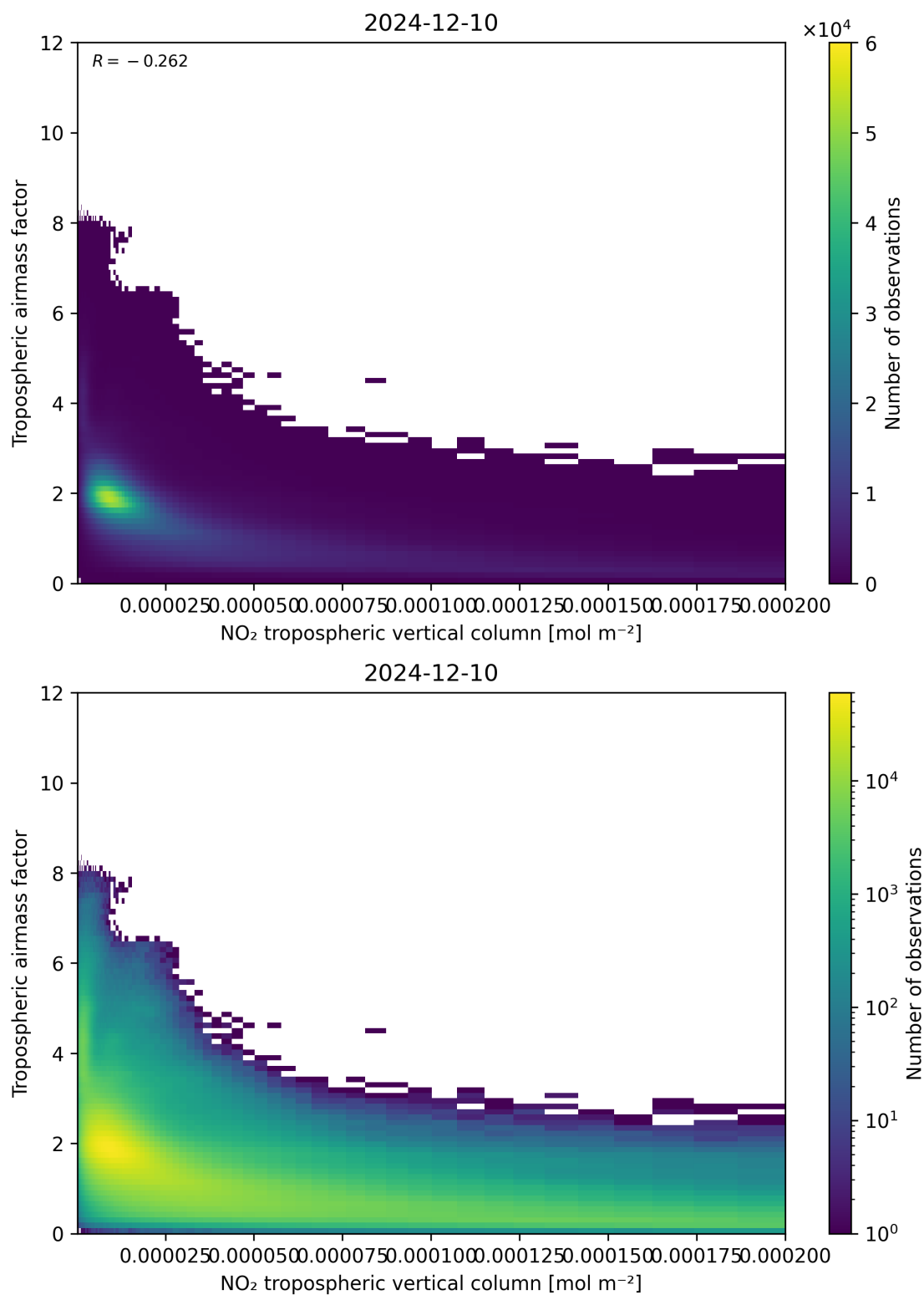
Figure 123: Scatter density plot of “NO 2 tropospheric vertical column” against “Tropospheric airmass factor” for 2024-12-09 to 2024-12-11.
