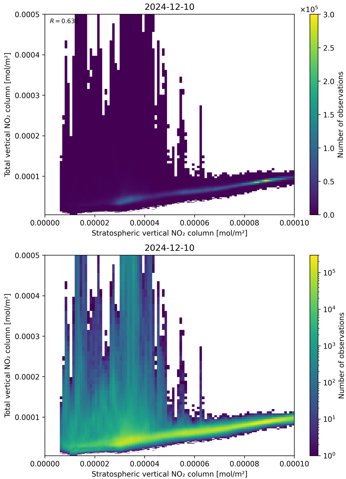
Figure 100: Scatter density plot of “Stratospheric vertical NO 2 column” against “Total vertical NO 2 column” for 2024-12-09 to 2024-12-11.
