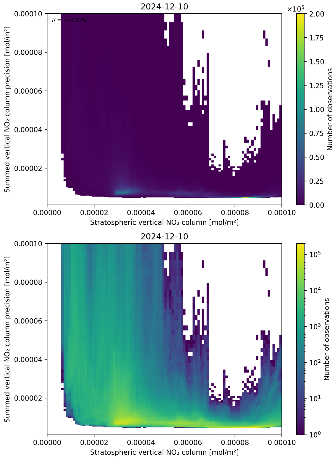
Figure 99: Scatter density plot of “Stratospheric vertical NO 2 column” against “Summed vertical NO 2 column precision” for 2024-12-09 to 2024-12-11.
