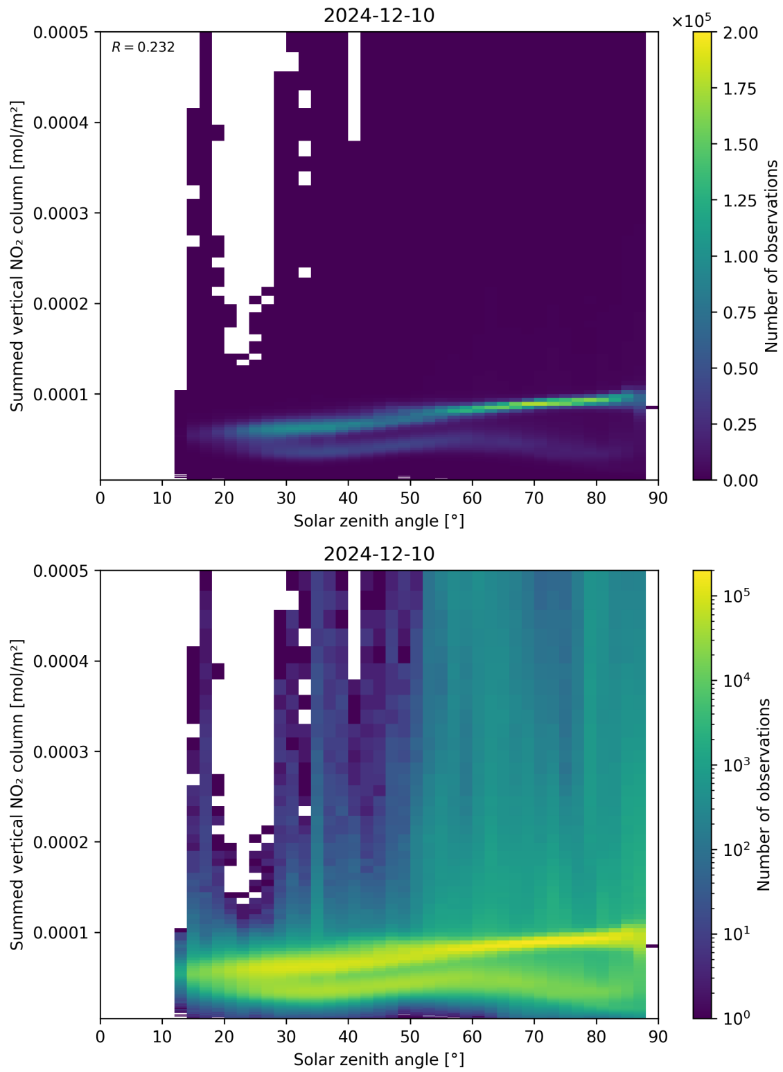
Figure 151: Scatter density plot of “Solar zenith angle” against “Summed vertical NO 2 column” for 2024-12-09 to 2024-12-11.
