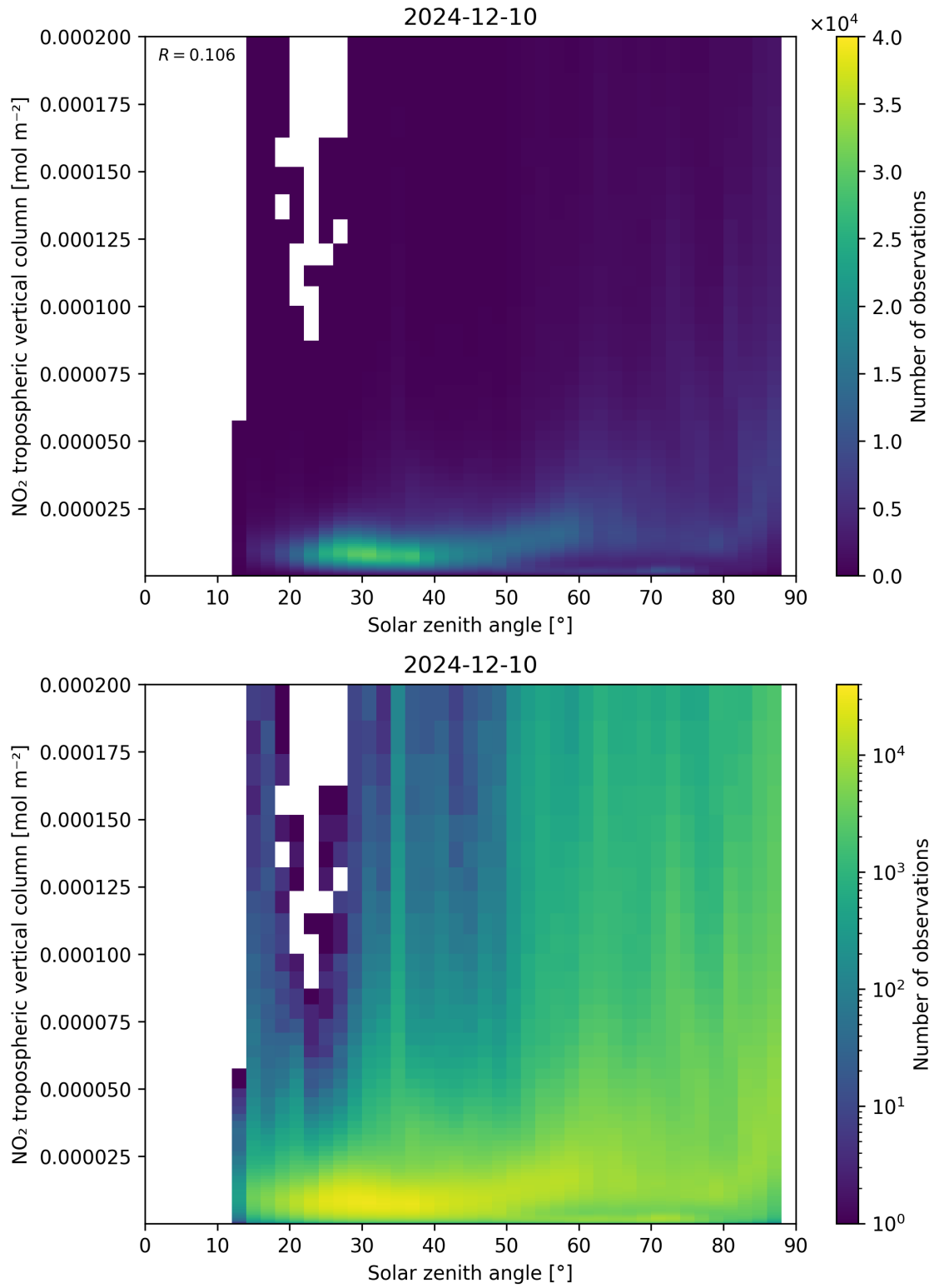
Figure 155: Scatter density plot of “Solar zenith angle” against “NO 2 tropospheric vertical column” for 2024-12-09 to 2024-12-11.
