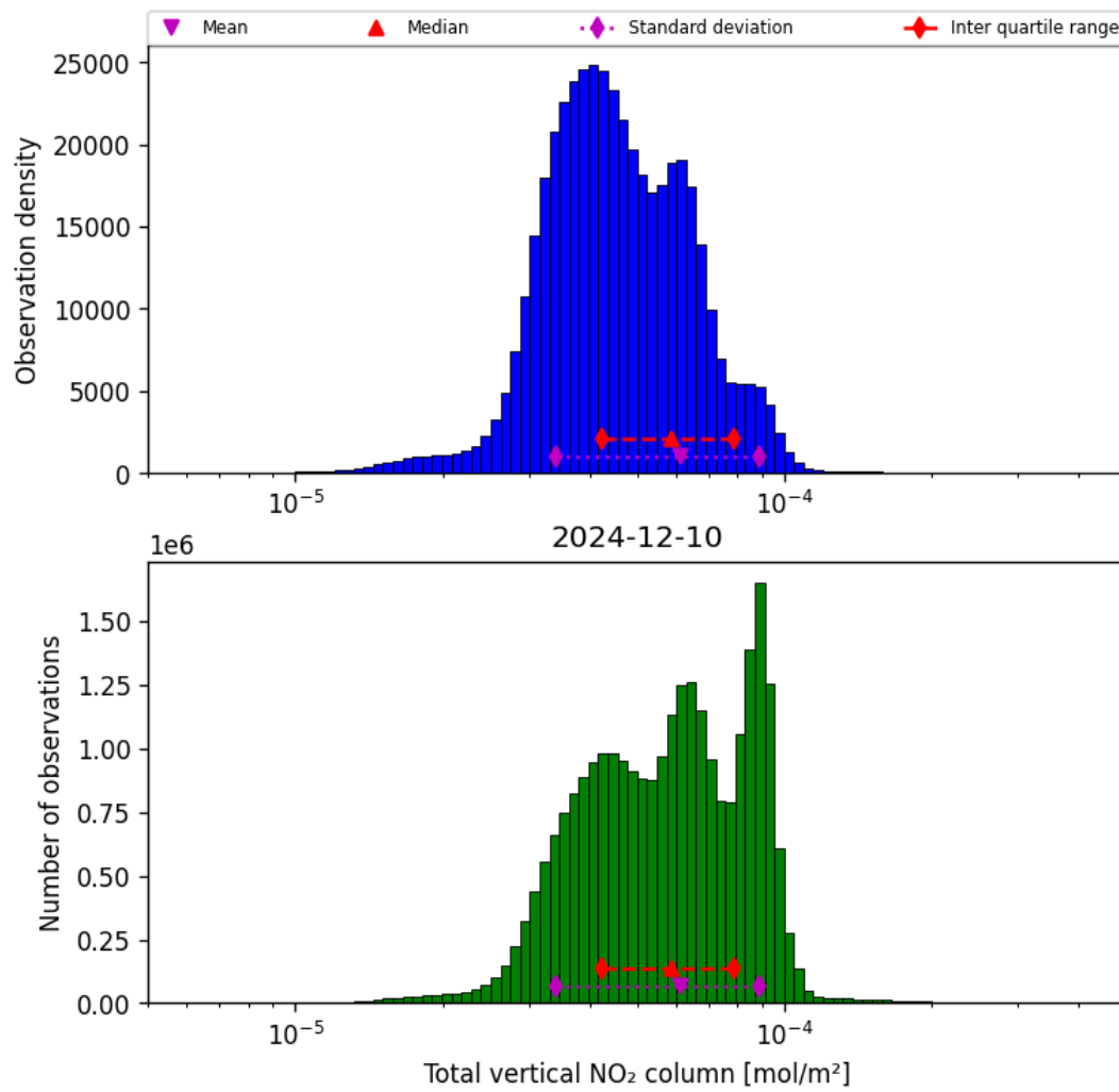
Figure 38: Histogram of “Total vertical NO 2 column” for 2024-12-09 to 2024-12-11
