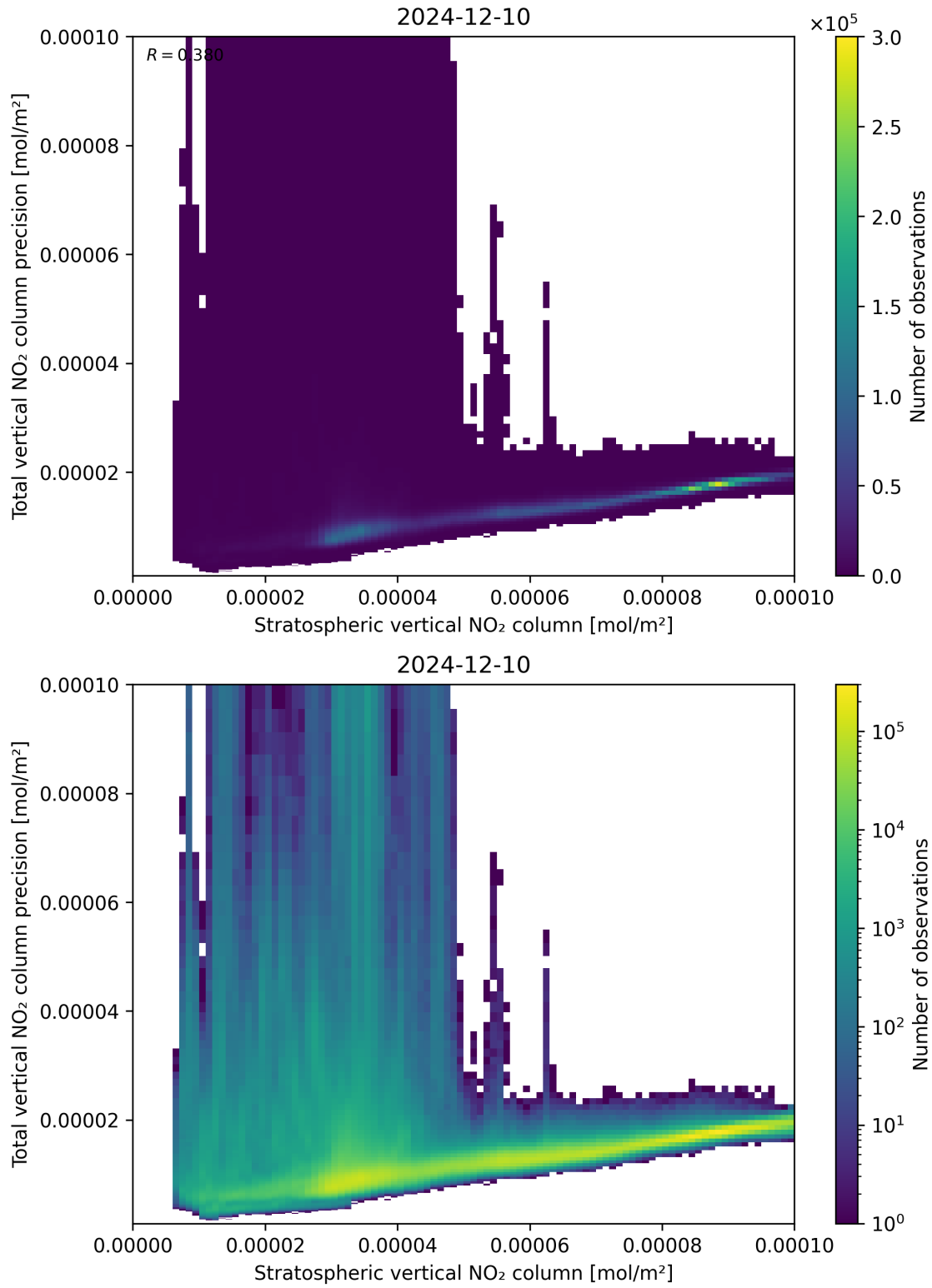
Figure 101: Scatter density plot of “Stratospheric vertical NO 2 column” against “Total vertical NO 2 column precision” for 2024-12-09 to 2024-12-11.
