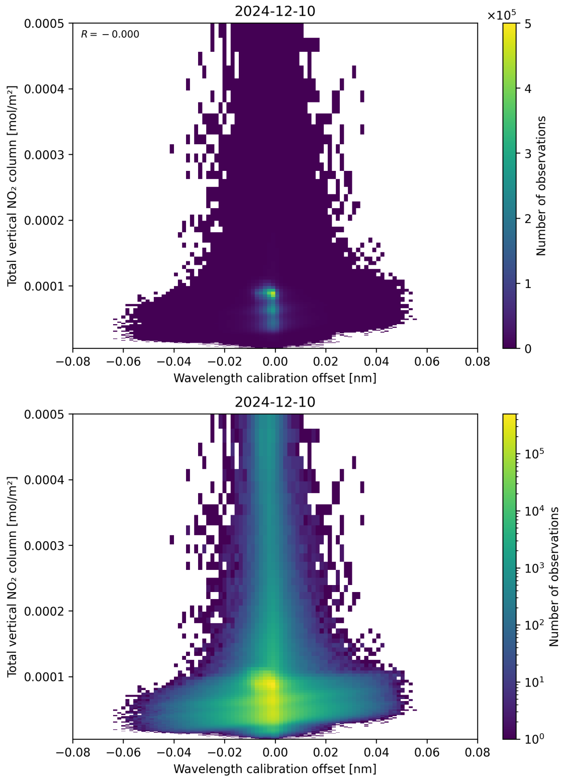
Figure 179: Scatter density plot of “Wavelength calibration offset” against “Total vertical NO 2 column” for 2024-12-09 to 2024-12-11.
