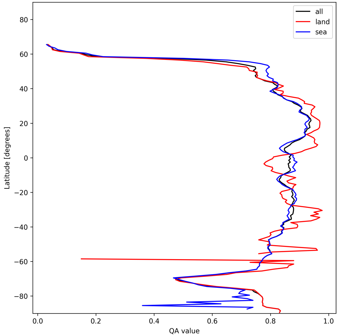
Figure 11: Zonal average of “QA value” for 2024-12-09 to 2024-12-11.
