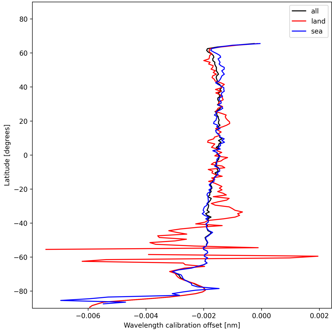
Figure 18: Zonal average of “Wavelength calibration offset” for 2024-12-09 to 2024-12-11.
