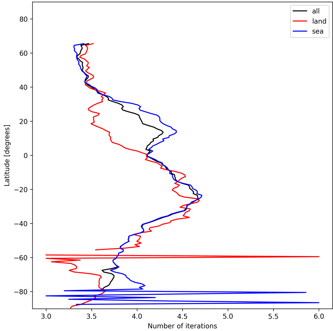
Figure 17: Zonal average of “Number of iterations” for 2024-12-09 to 2024-12-11.
