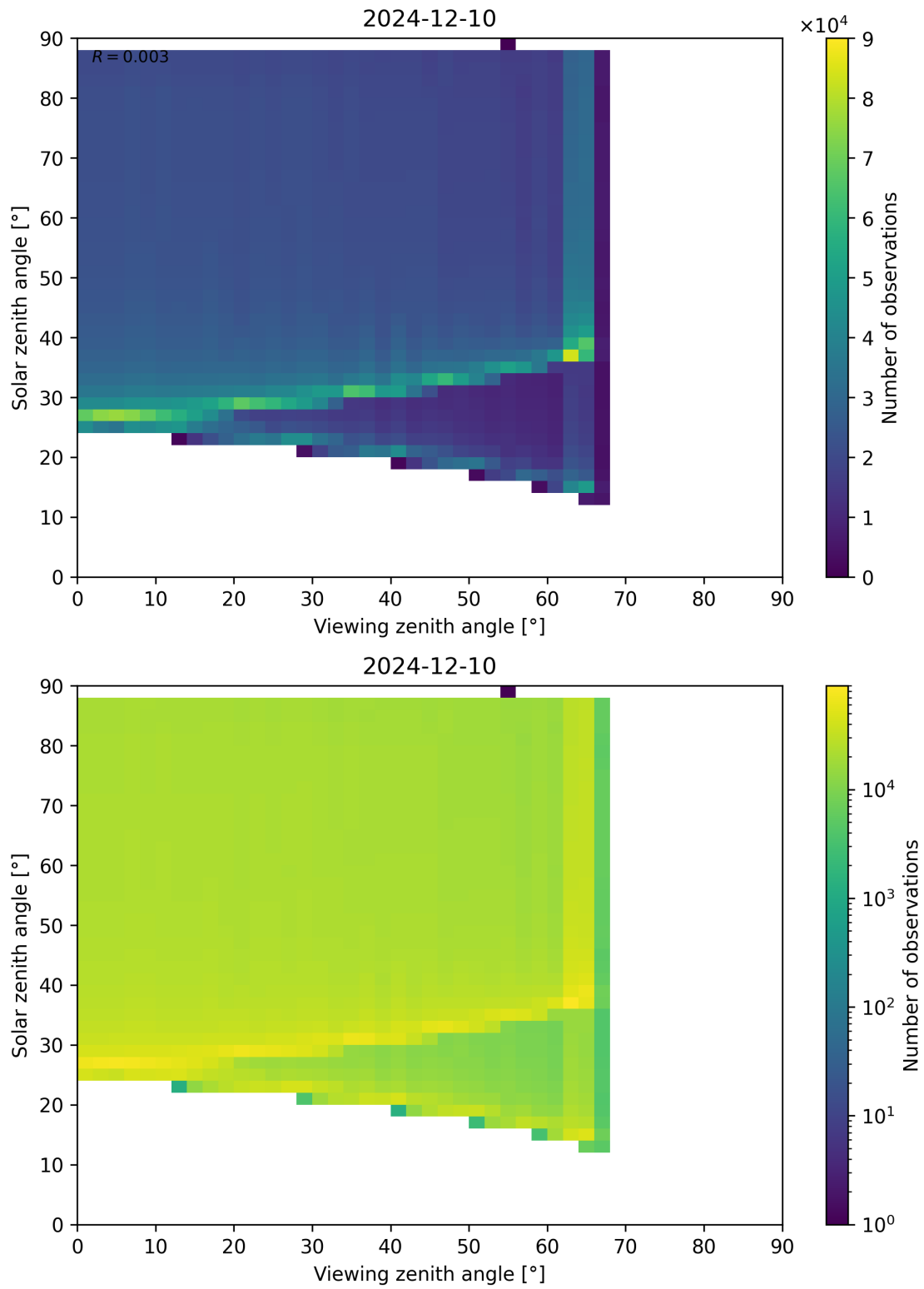
Figure 172: Scatter density plot of “Viewing zenith angle” against “Solar zenith angle” for 2024-12-09 to 2024-12-11.
