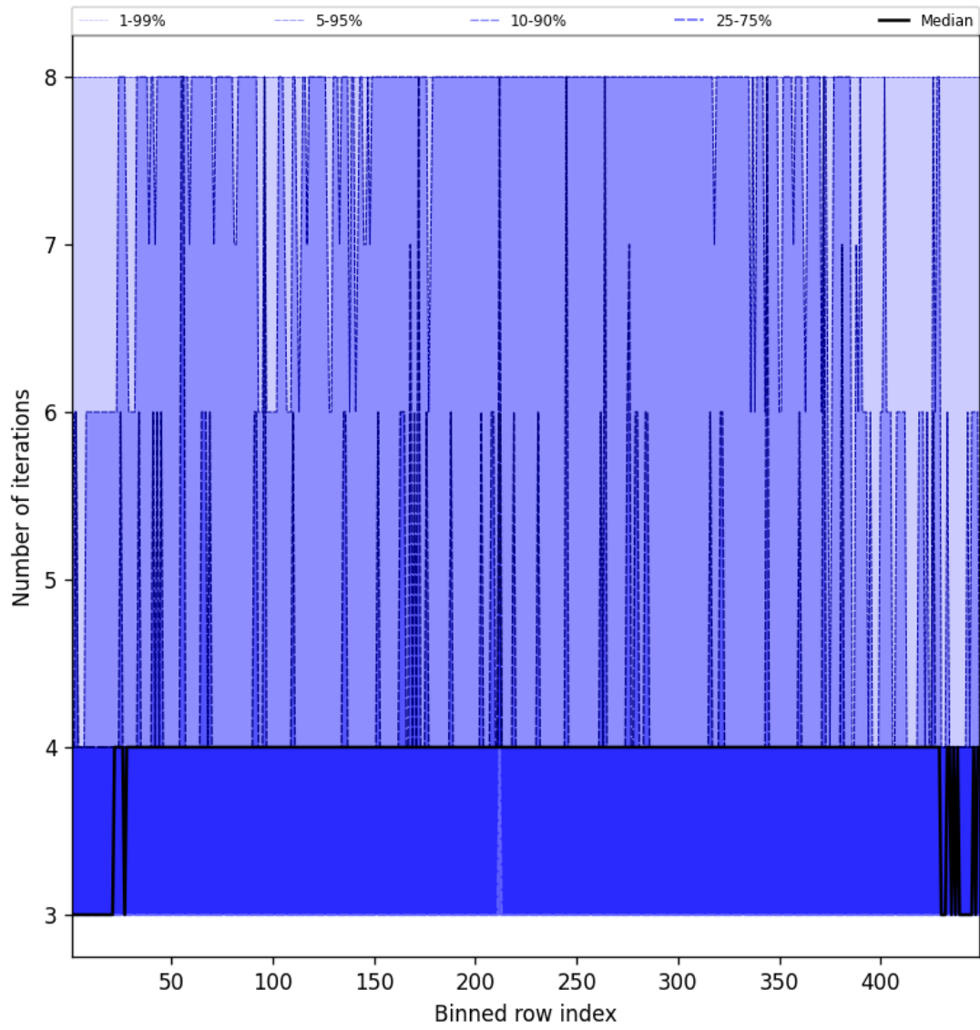
Figure 51: Along track statistics of “Number of iterations” for 2024-12-09 to 2024-12-11
