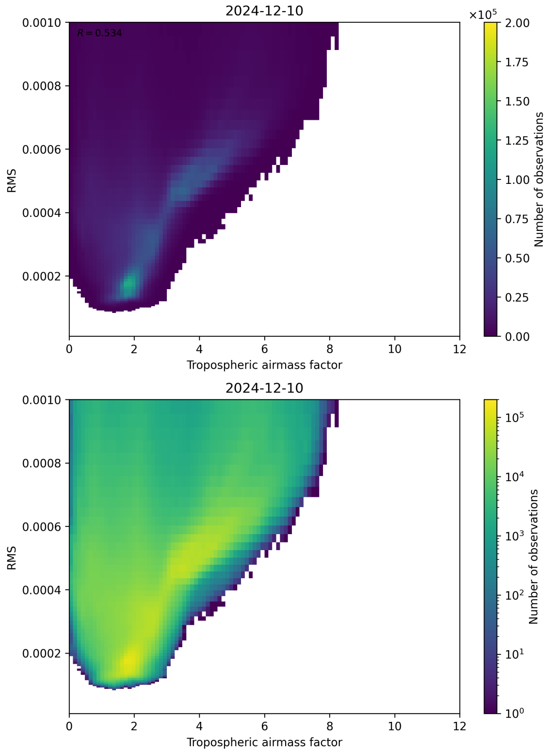
Figure 79: Scatter density plot of “Tropospheric airmass factor” against “RMS” for 2024-12-09 to 2024-12-11.
