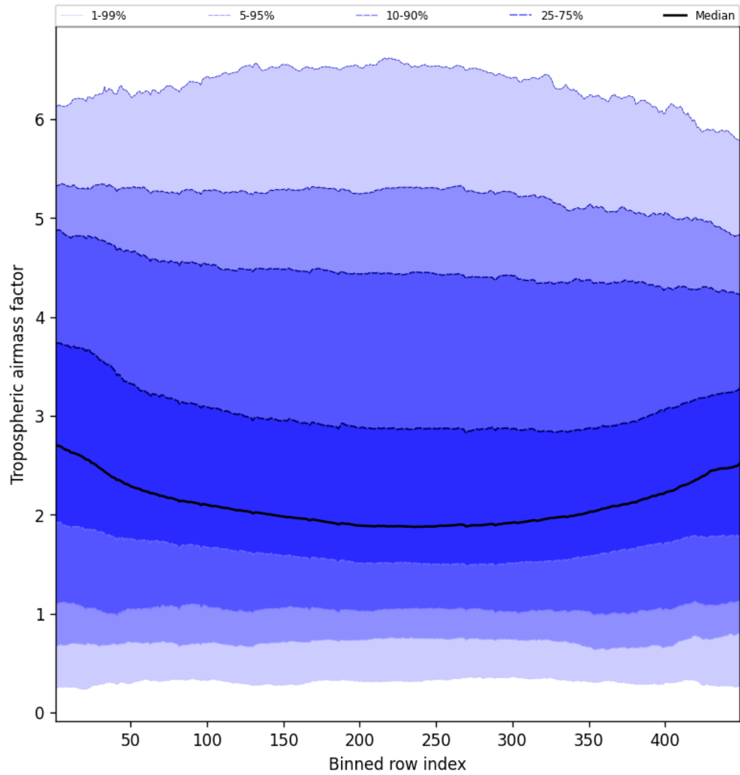
Figure 48: Along track statistics of “Tropospheric air mass factor” for 2024-12-09 to 2024-12-11
