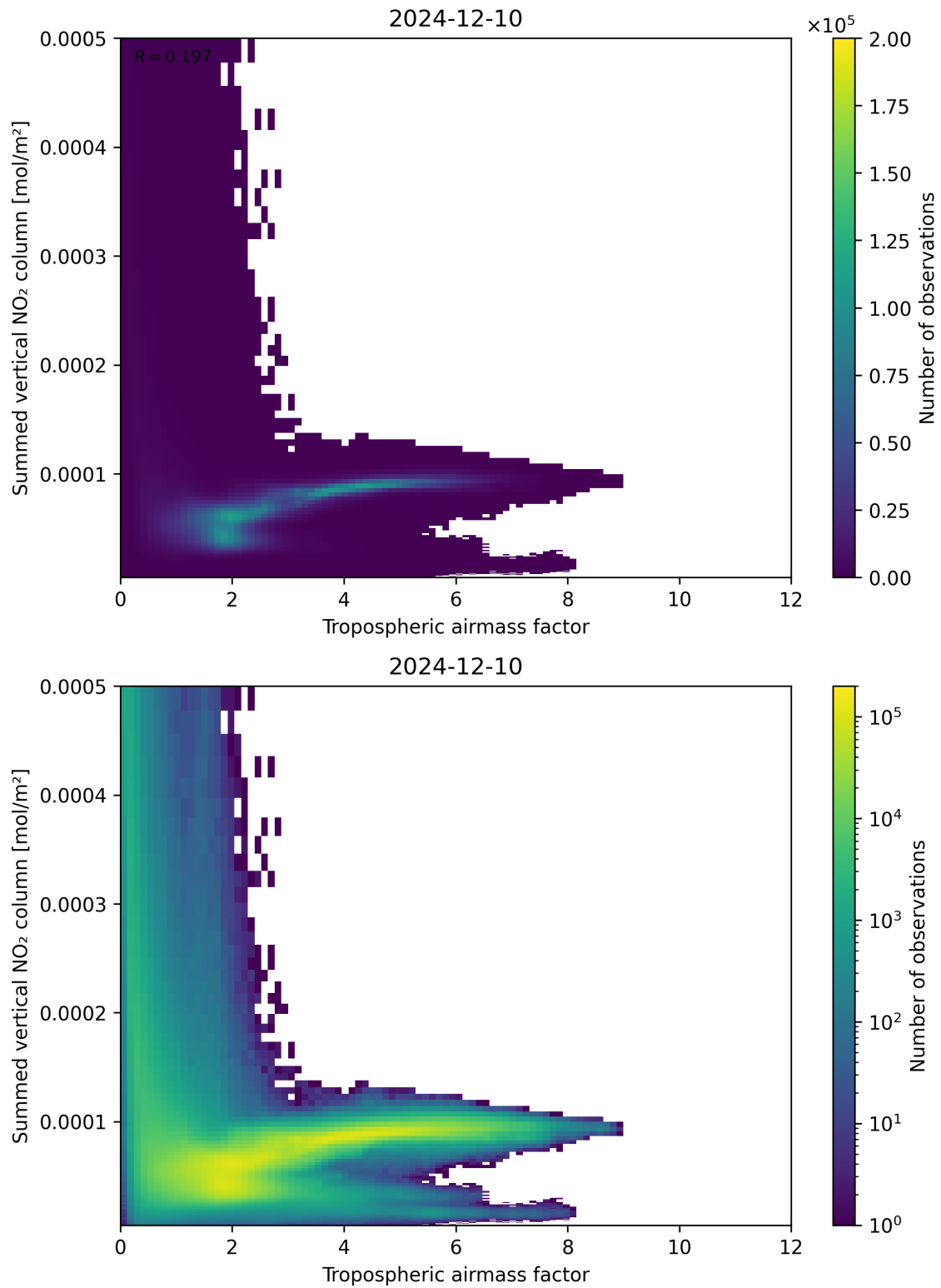
Figure 75: Scatter density plot of “Tropospheric air mass factor” against “Summed vertical NO 2 column” for 2024-12-09 to 2024-12-11.
