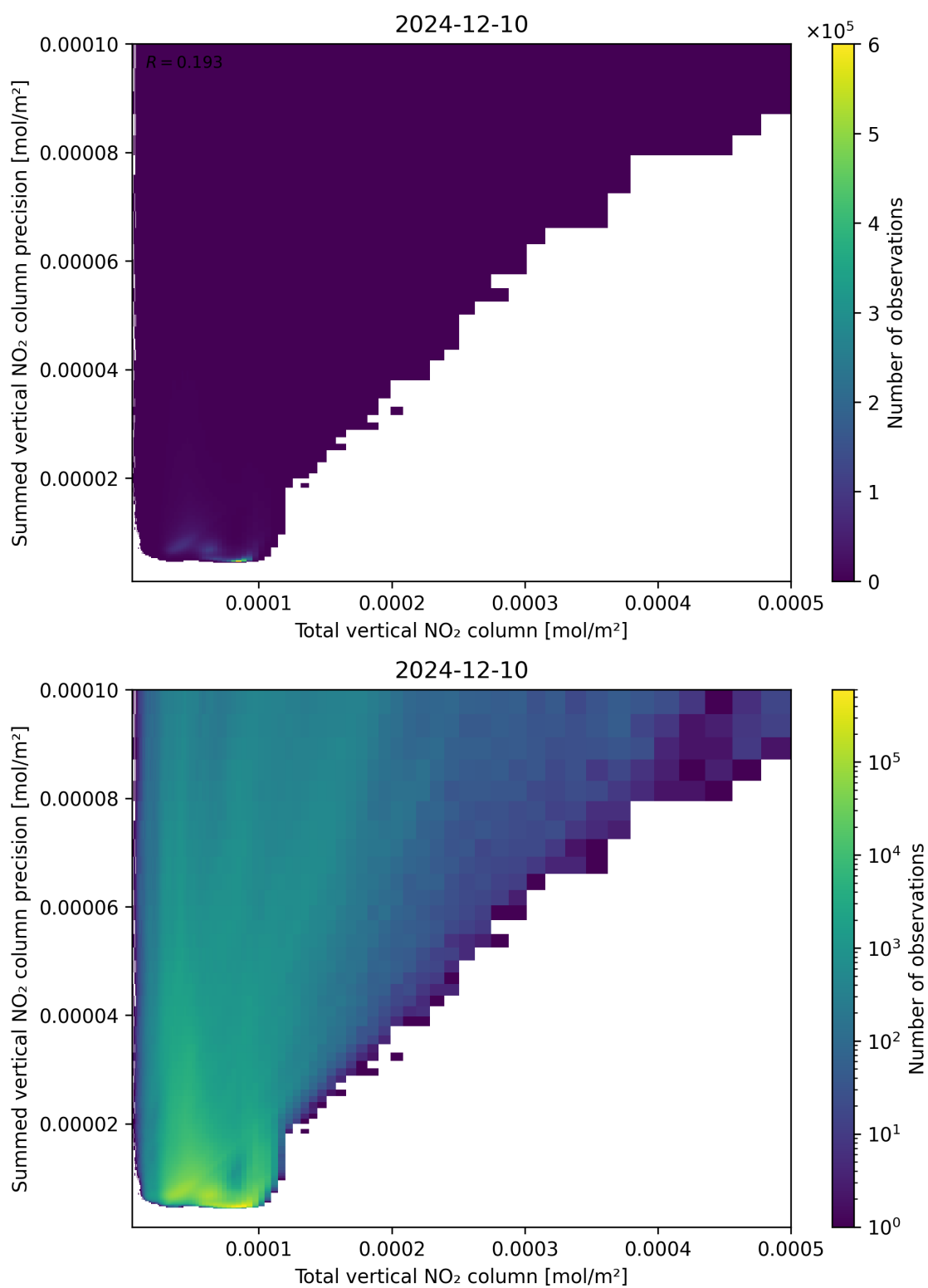
Figure 113: Scatter density plot of “Total vertical NO 2 column” against “Summed vertical NO 2 column precision” for 2024-12-09 to 2024-12-11.
