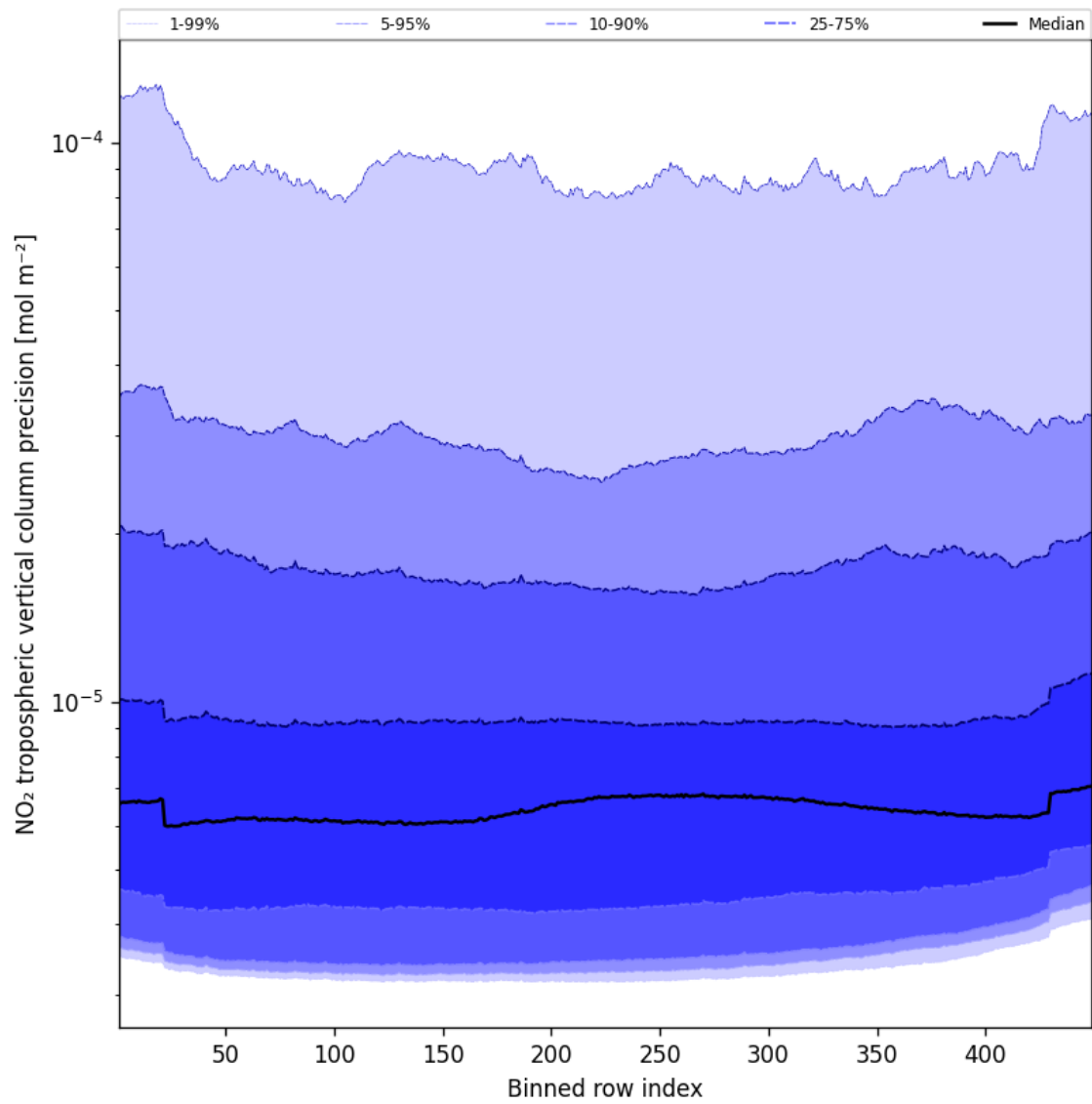
Figure 47: Along track statistics of “NO 2 tropospheric vertical column precision” for 2024-12-09 to 2024-12-11
