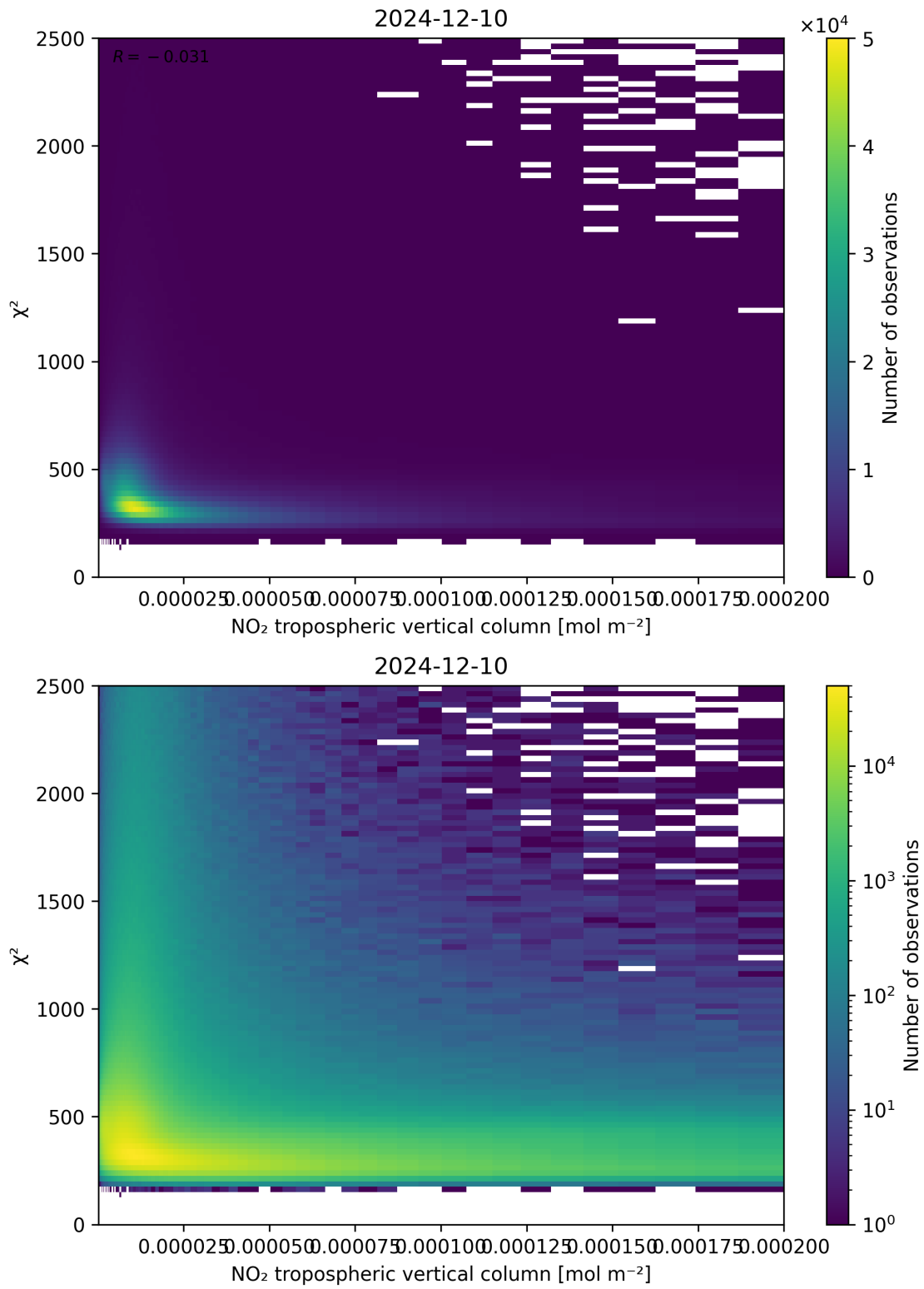
Figure 124: Scatter density plot of “NO 2 tropospheric vertical column” against “ \chi^2 ” for 2024-12-09 to 2024-12-11.
