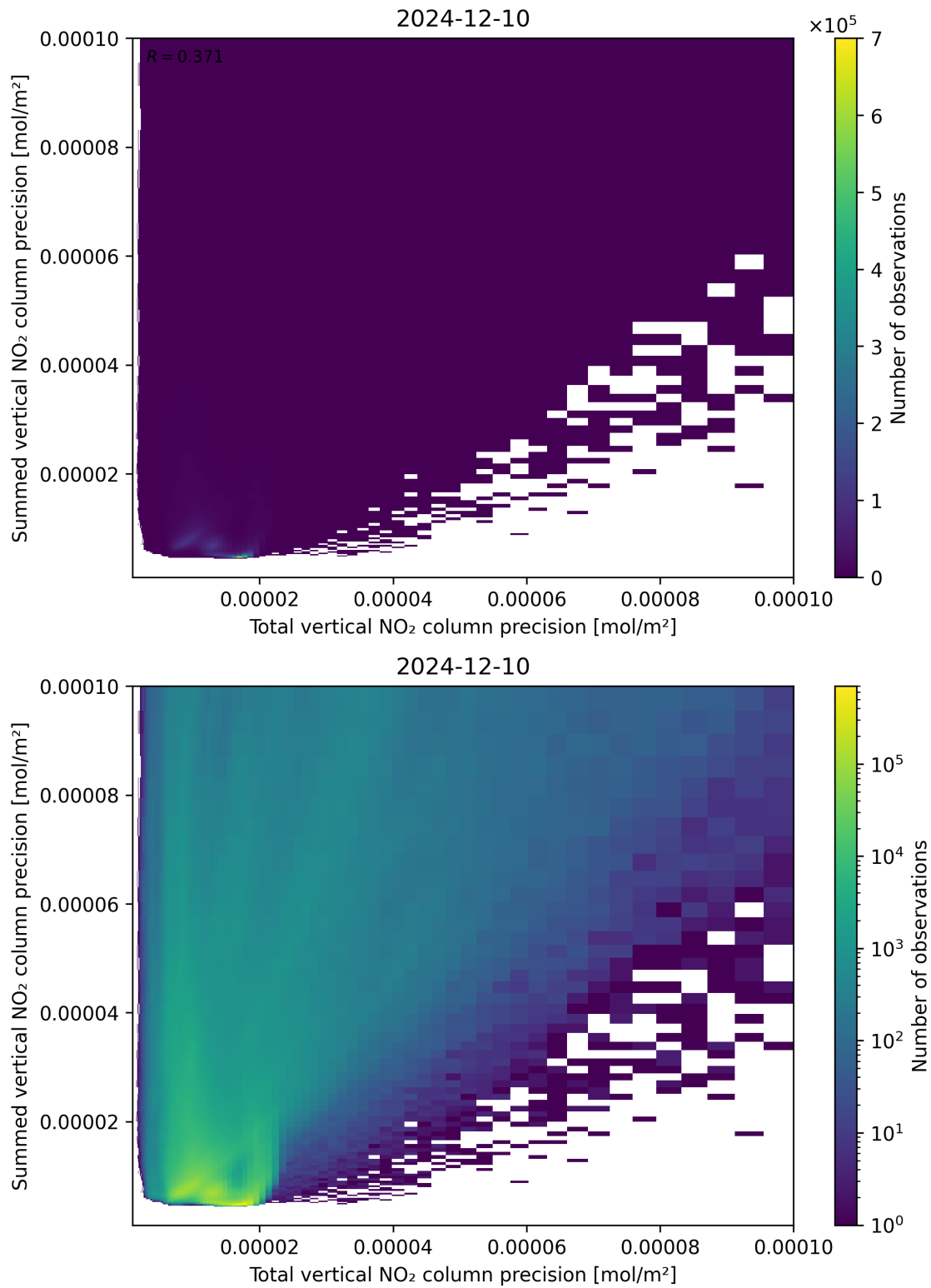
Figure 118: Scatter density plot of “Total vertical NO 2 column precision” against “Summed vertical NO 2 column precision” for 2024-12-09 to 2024-12-11.
