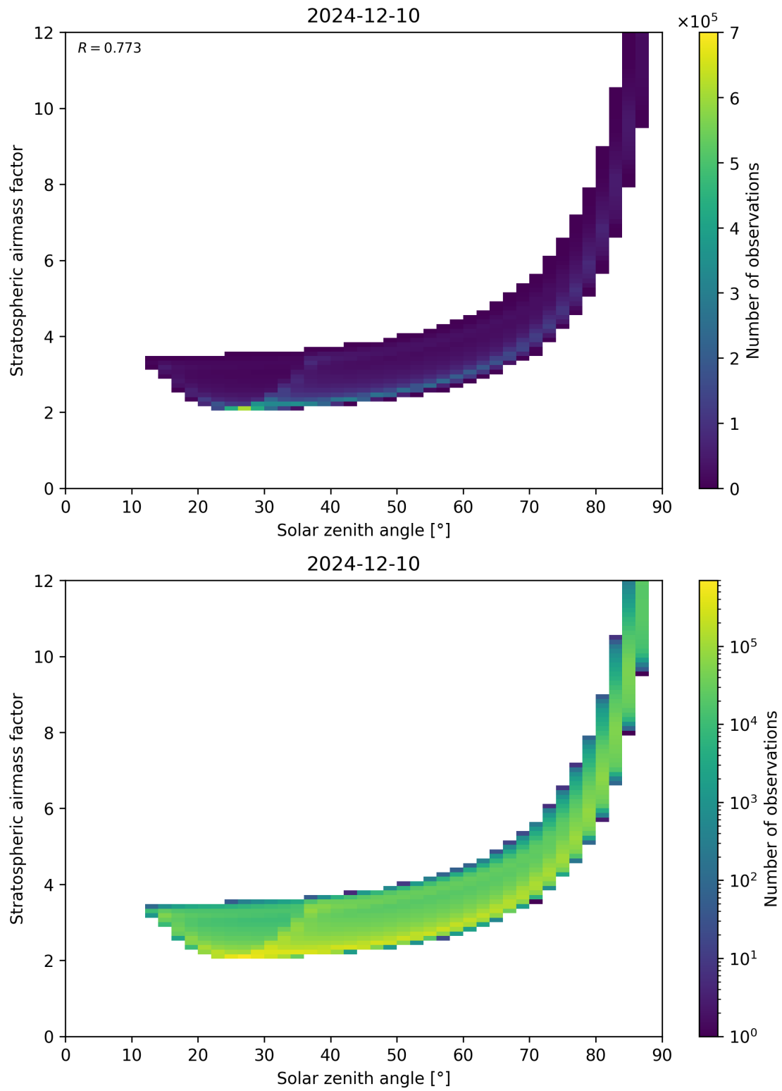
Figure 145: Scatter density plot of “Solar zenith angle” against “Stratospheric airmass factor” for 2024-12-09 to 2024-12-11.
