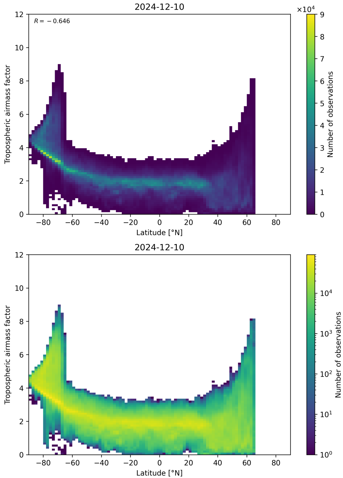
Figure 85: Scatter density plot of “Latitude” against “Tropospheric airmass factor” for 2024-12-09 to 2024-12-11.
