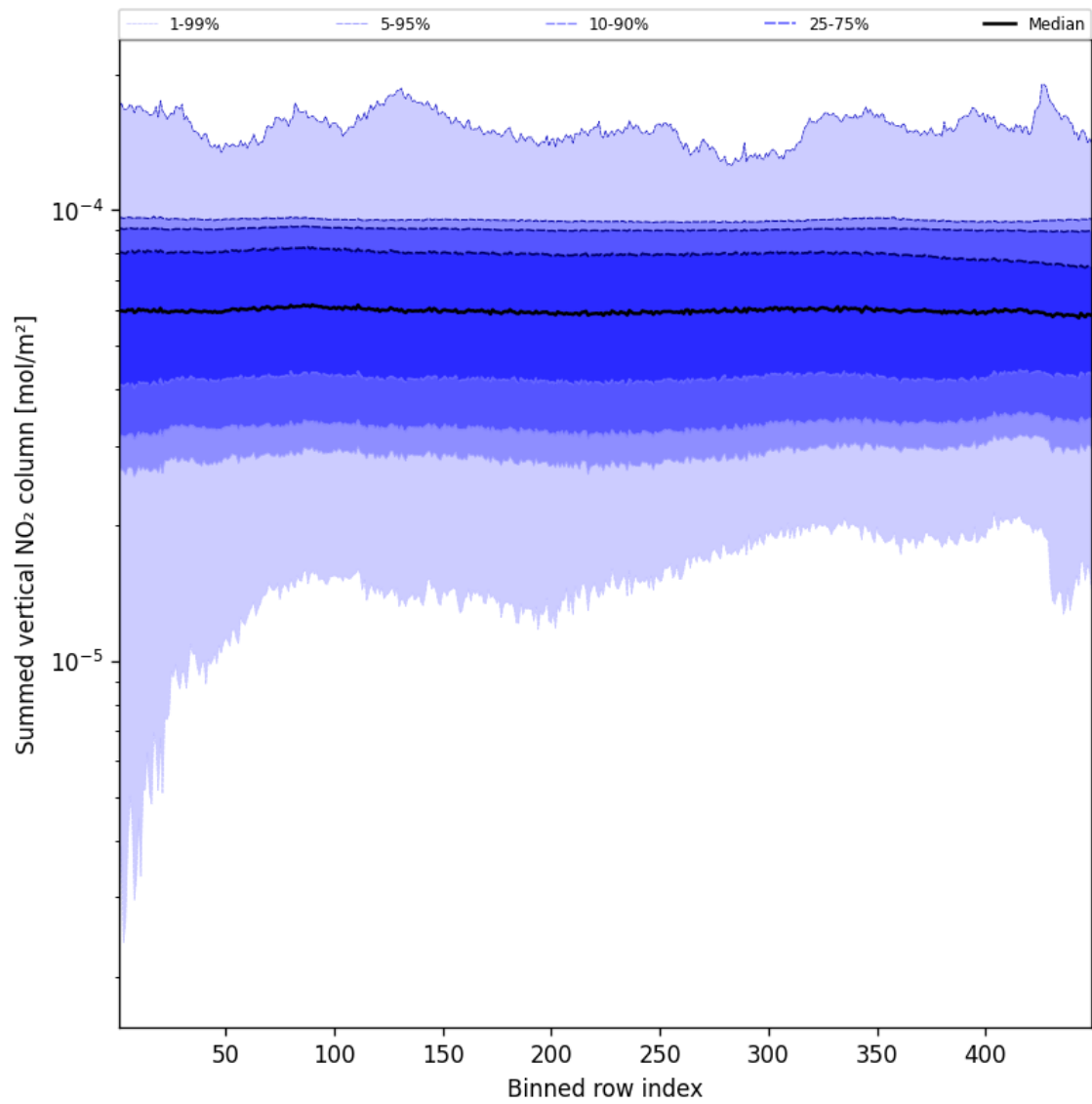
Figure 57: Along track statistics of “Summed vertical NO 2 column” for 2024-12-09 to 2024-12-11
