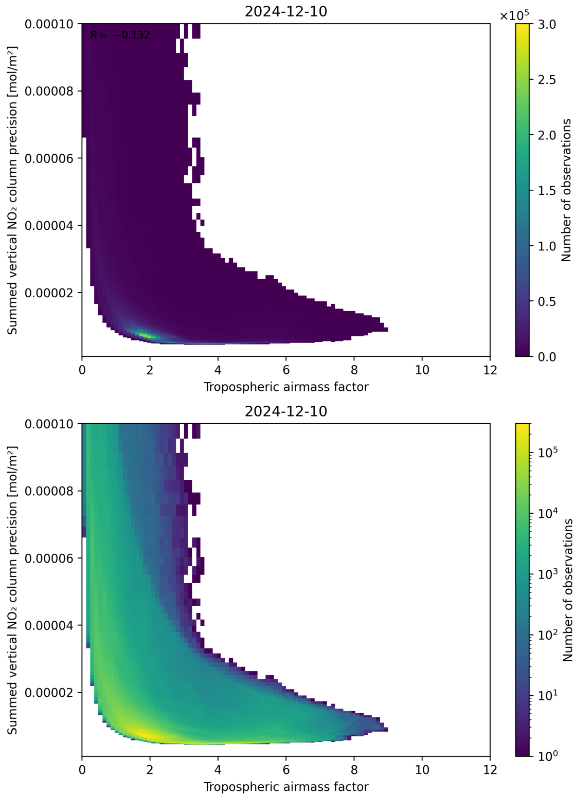
Figure 76: Scatter density plot of “Tropospheric air mass factor” against “Summed vertical NO 2 column precision” for 2024-12-09 to 2024-12-11.
