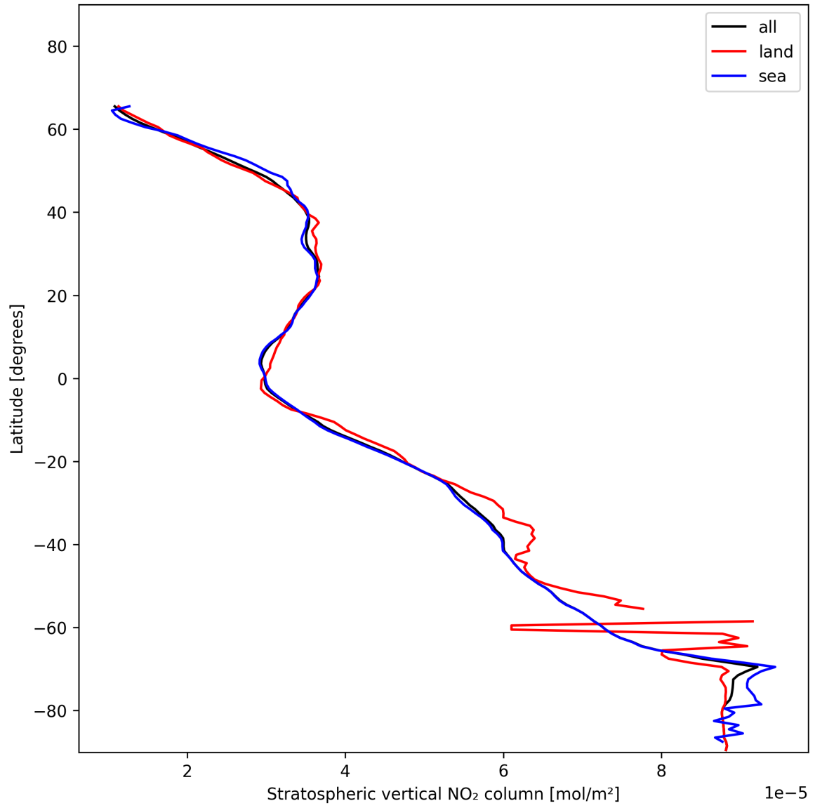
Figure 19: Zonal average of “Stratospheric vertical NO 2 column” for 2024-12-09 to 2024-12-11.
