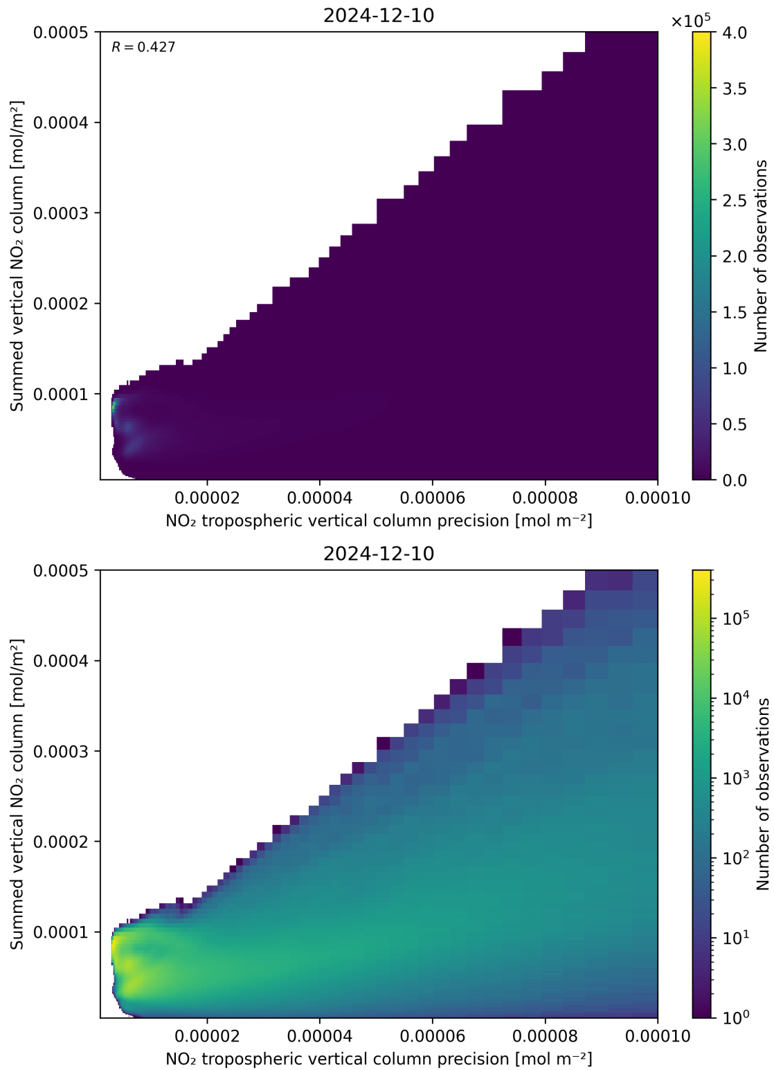
Figure 136: Scatter density plot of “NO 2 tropospheric vertical column precision” against “Summed vertical NO 2 column” for 2024-12-09 to 2024-12-11.
