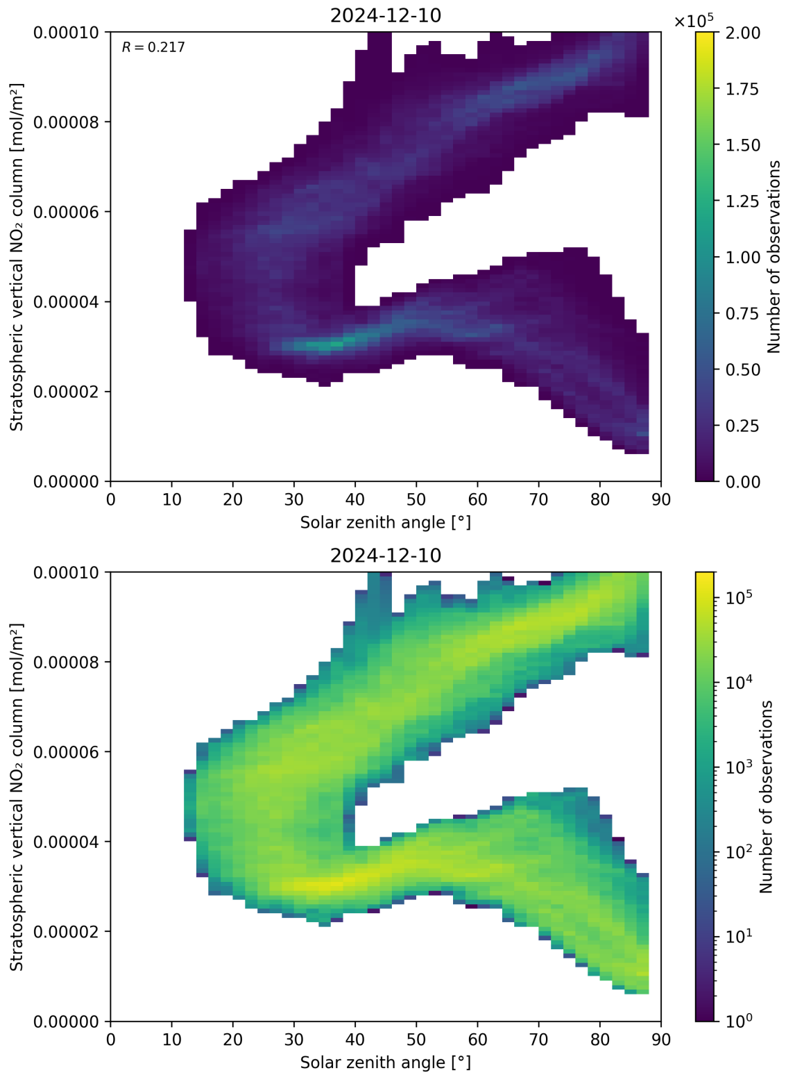
Figure 150: Scatter density plot of “Solar zenith angle” against “Stratospheric vertical NO 2 column” for 2024-12-09 to 2024-12-11.
