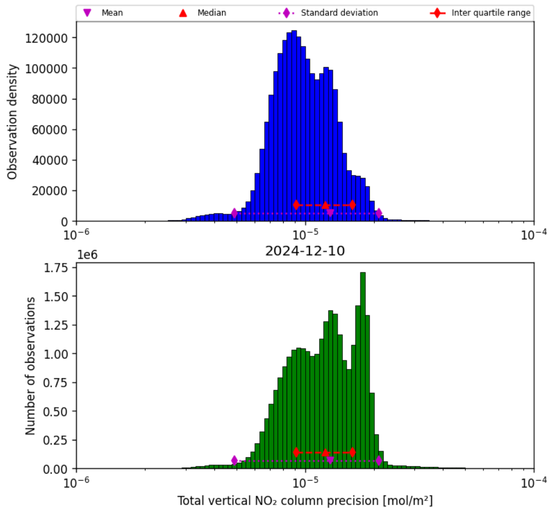
Figure 39: Histogram of “Total vertical NO 2 column precision” for 2024-12-09 to 2024-12-11
