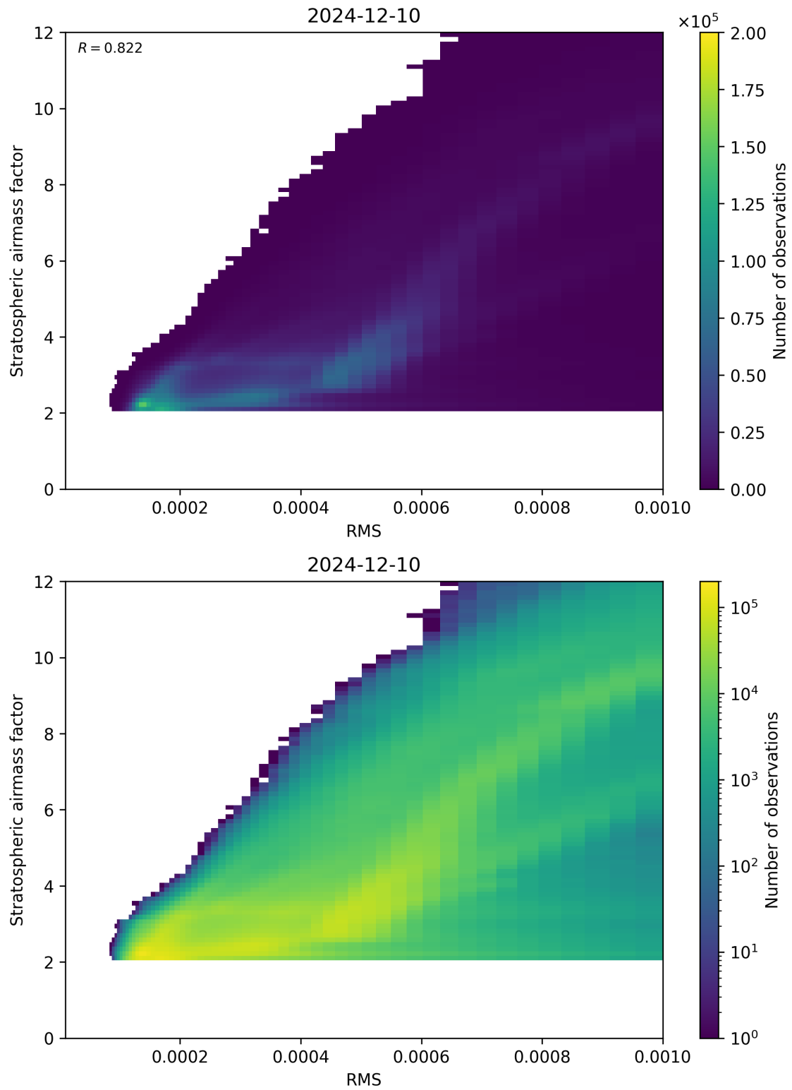
Figure 144: Scatter density plot of “RMS” against “Stratospheric airmass factor” for 2024-12-09 to 2024-12-11.
