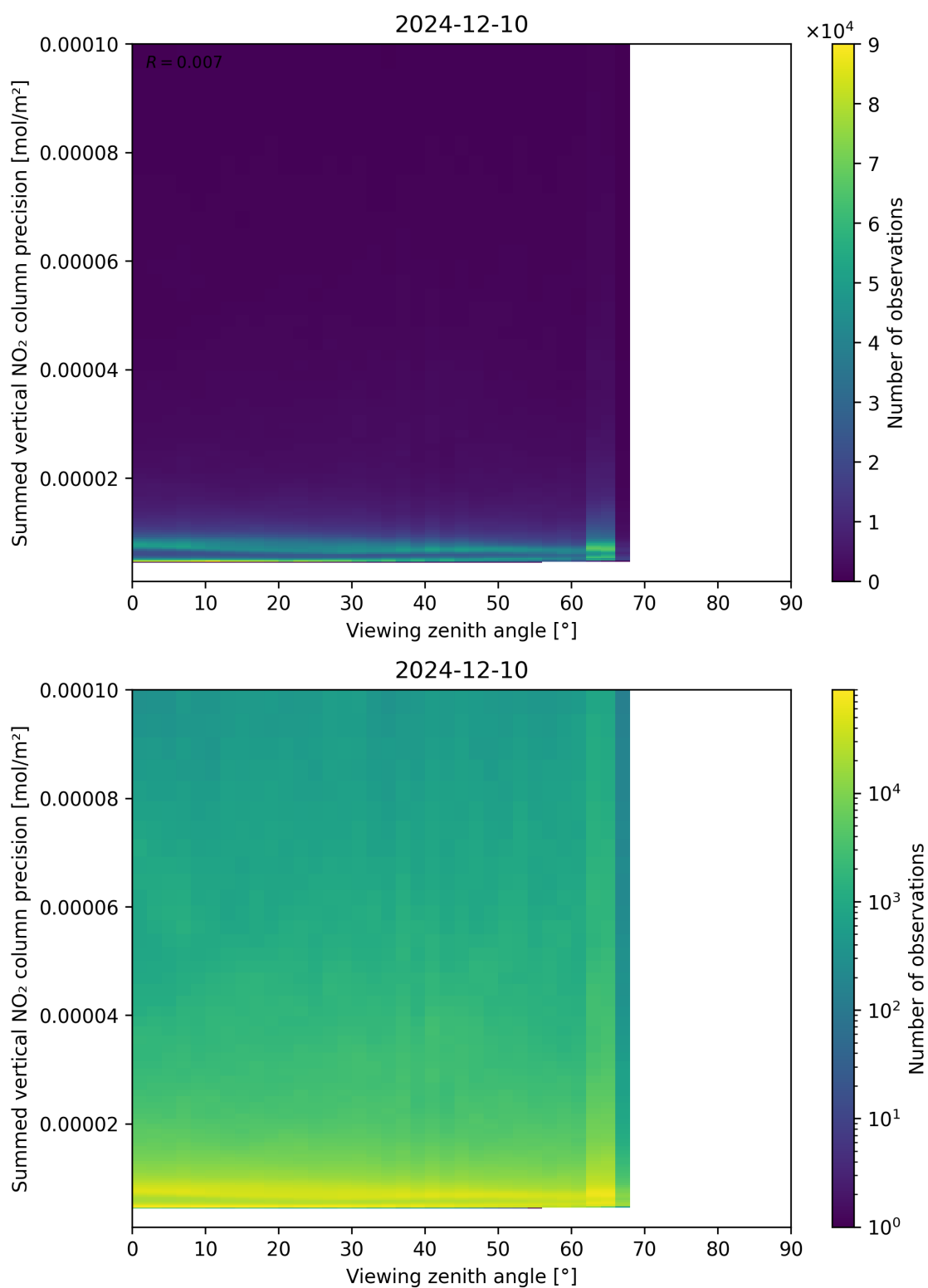
Figure 166: Scatter density plot of “Viewing zenith angle” against “Summed vertical NO 2 column precision” for 2024-12-09 to 2024-12-11.
