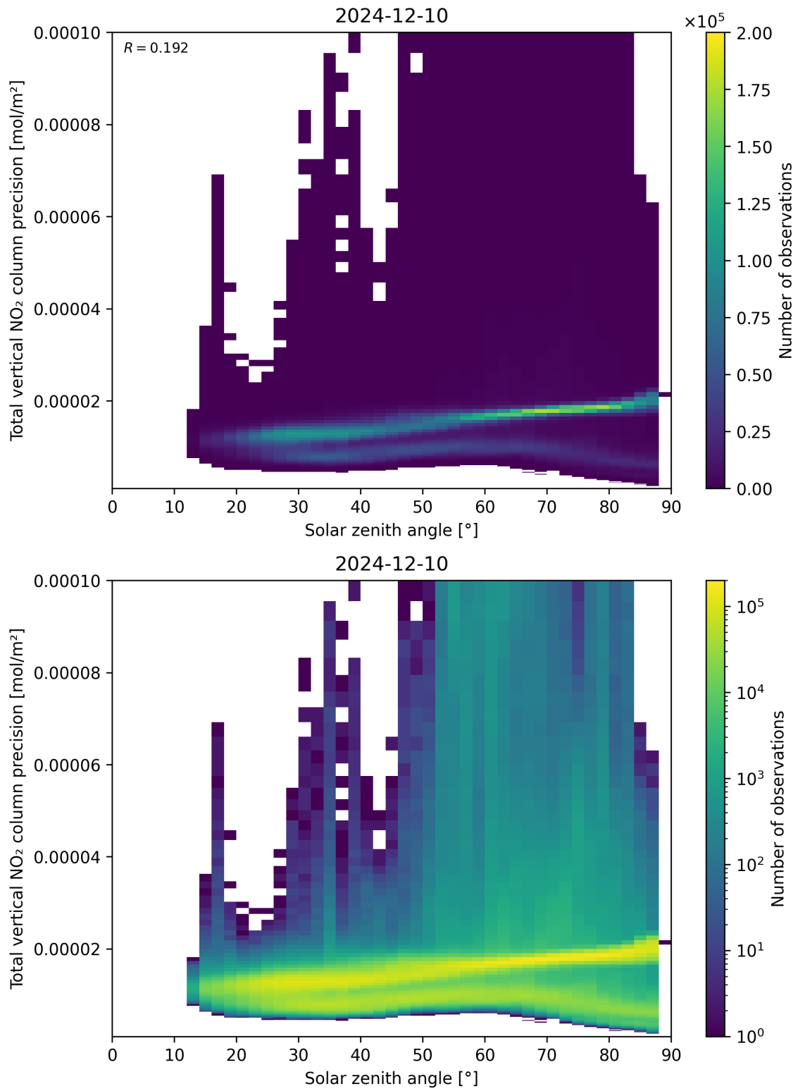
Figure 154: Scatter density plot of “Solar zenith angle” against “Total vertical NO 2 column precision” for 2024-12-09 to 2024-12-11.
