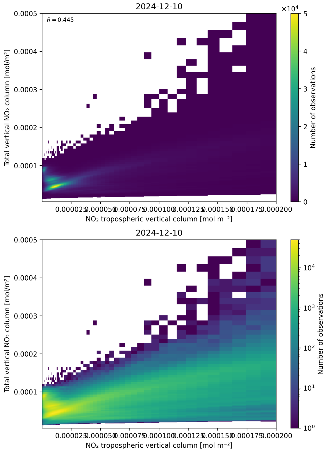
Figure 128: Scatter density plot of “NO 2 tropospheric vertical column” against “Total vertical NO 2 column” for 2024-12-09 to 2024-12-11.
