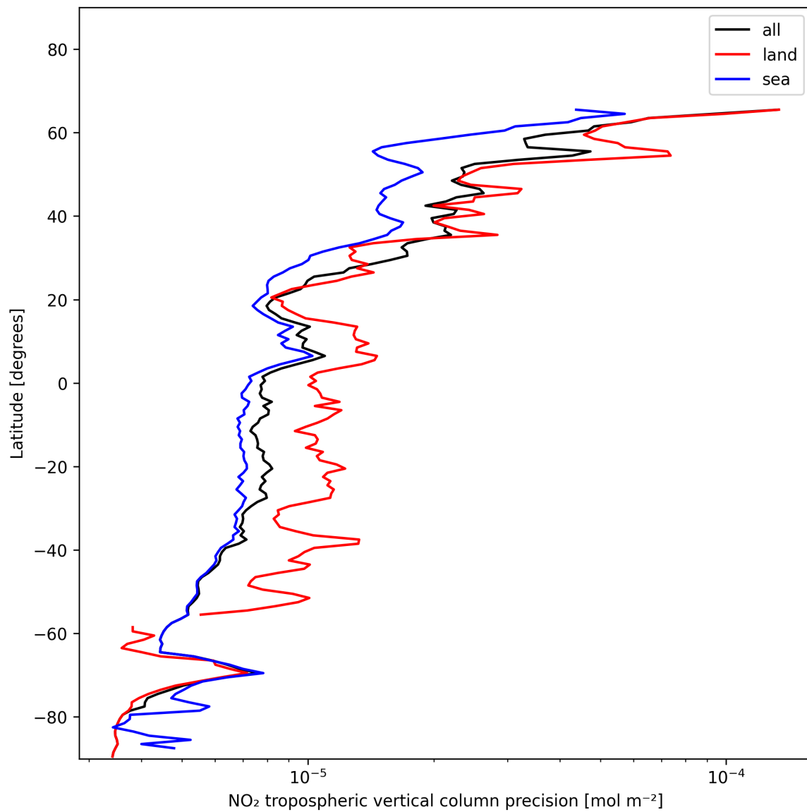
Figure 13: Zonal average of “NO 2 tropospheric vertical column precision” for 2024-12-09 to 2024-12-11.
