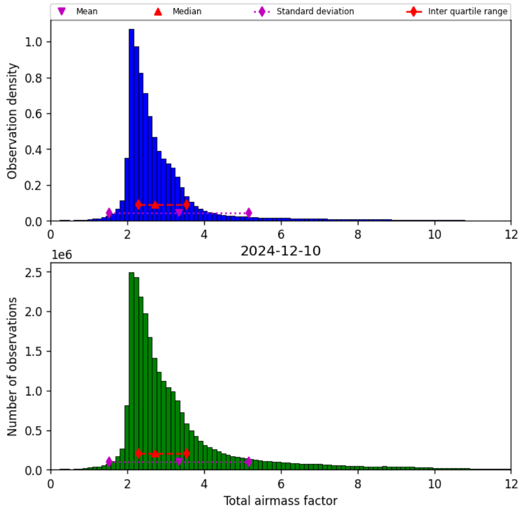
Figure 32: Histogram of “Total airmass factor” for 2024-12-09 to 2024-12-11
