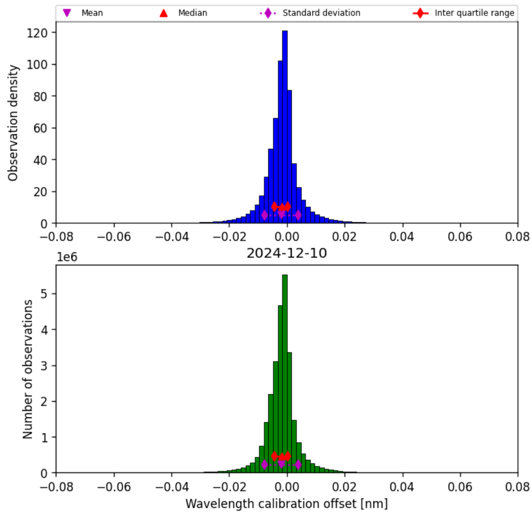
Figure 35: Histogram of "Wavelength calibration offset" for 2024-12-09 to 2024-12-11
