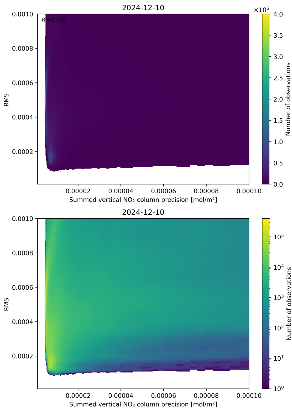
Figure 108: Scatter density plot of “Summed vertical NO 2 column precision” against “RMS” for 2024-12-09 to 2024-12-11.
