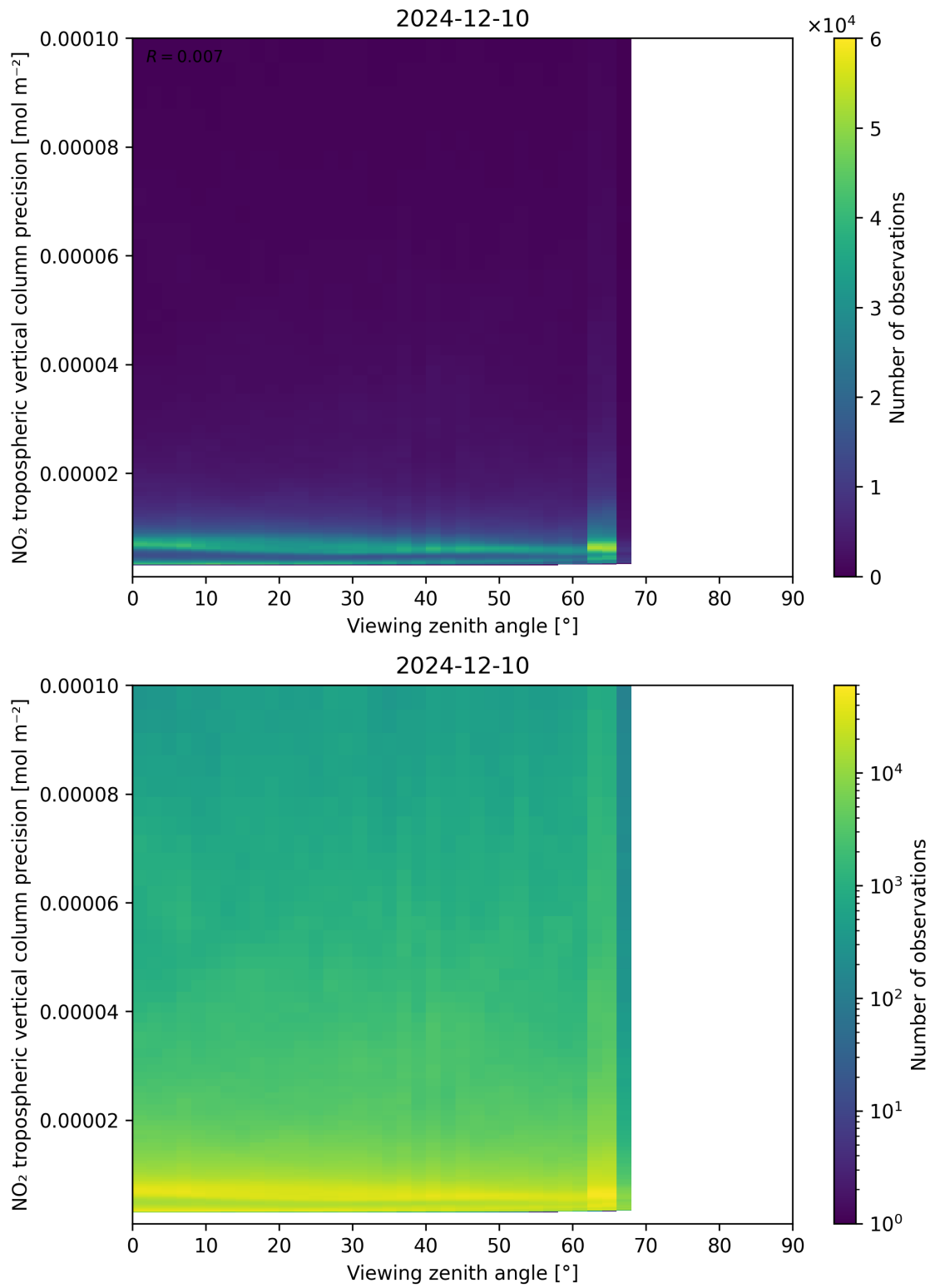
Figure 170: Scatter density plot of “Viewing zenith angle” against “NO 2 tropospheric vertical column precision” for 2024-12-09 to 2024-12-11.
