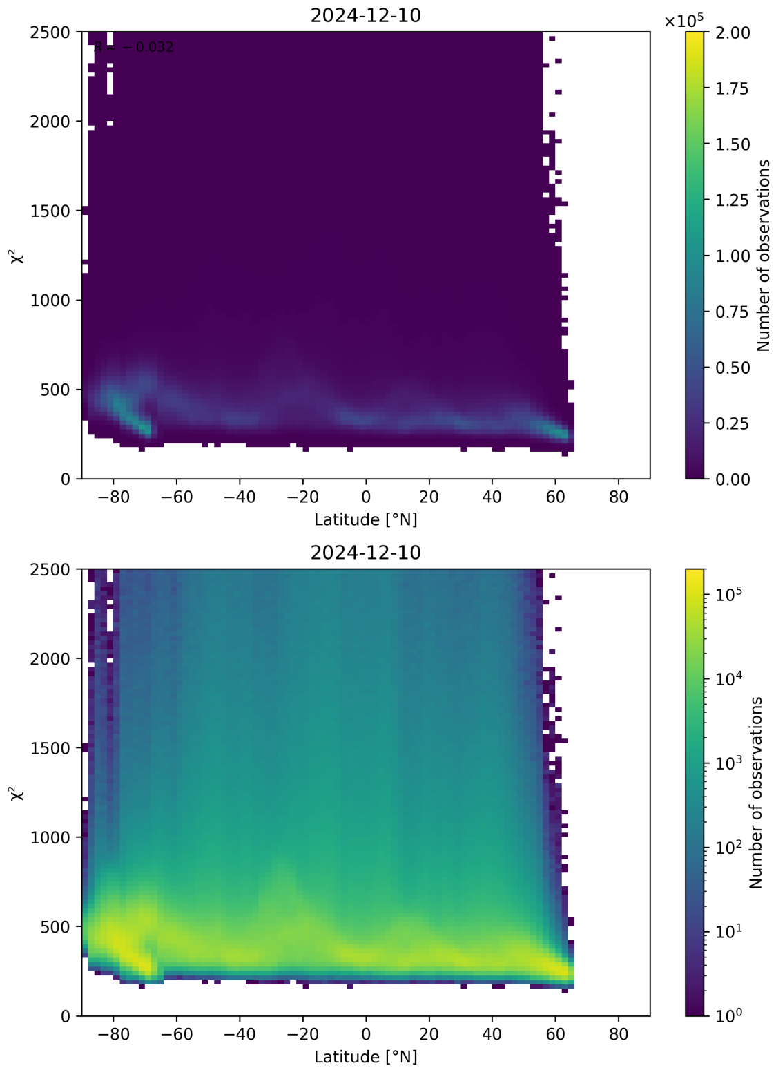
Figure 86: Scatter density plot of “Latitude” against “ \chi^2 ” for 2024-12-09 to 2024-12-11.
