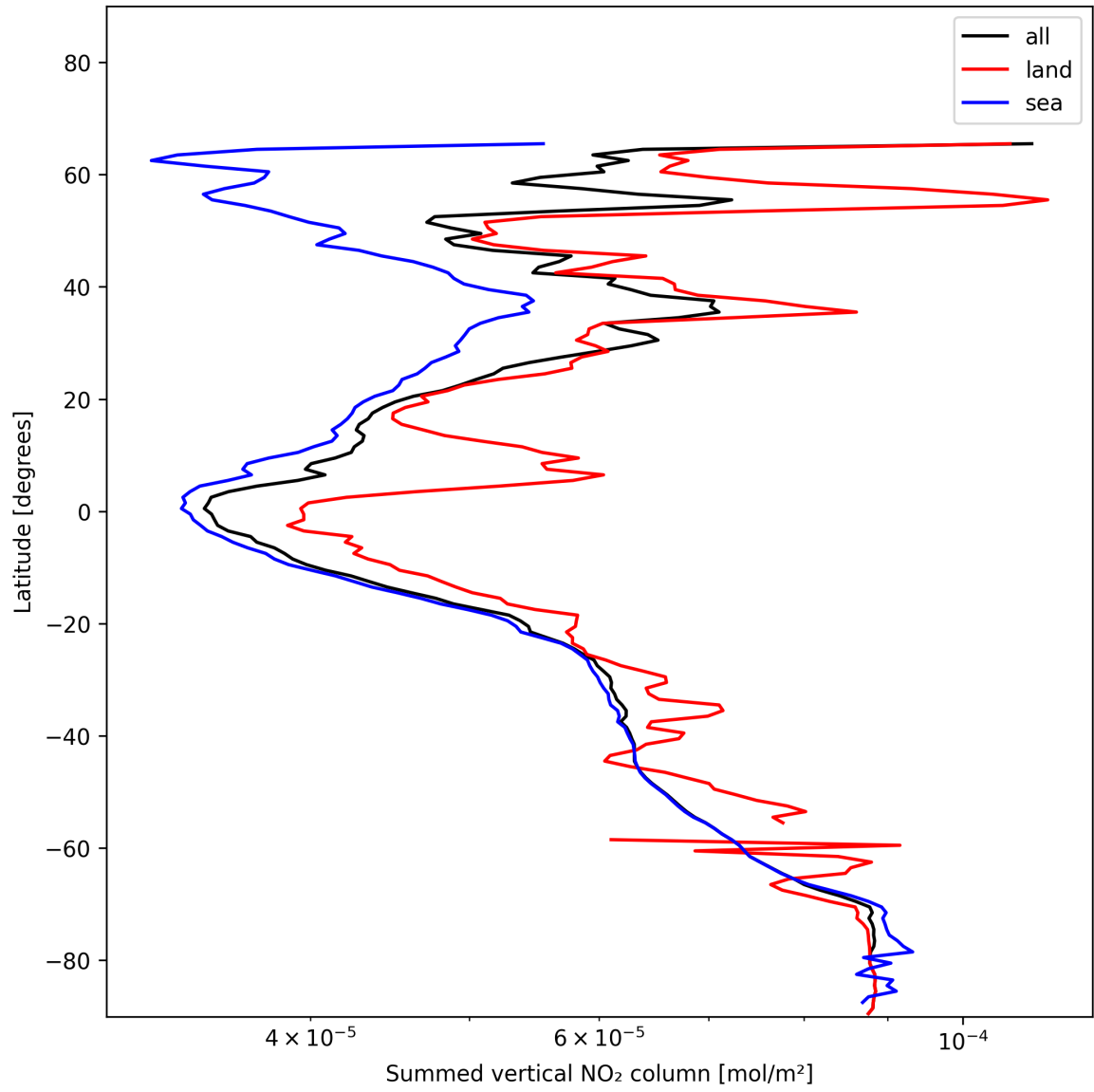
Figure 23: Zonal average of “Summed vertical NO 2 column” for 2024-12-09 to 2024-12-11.
