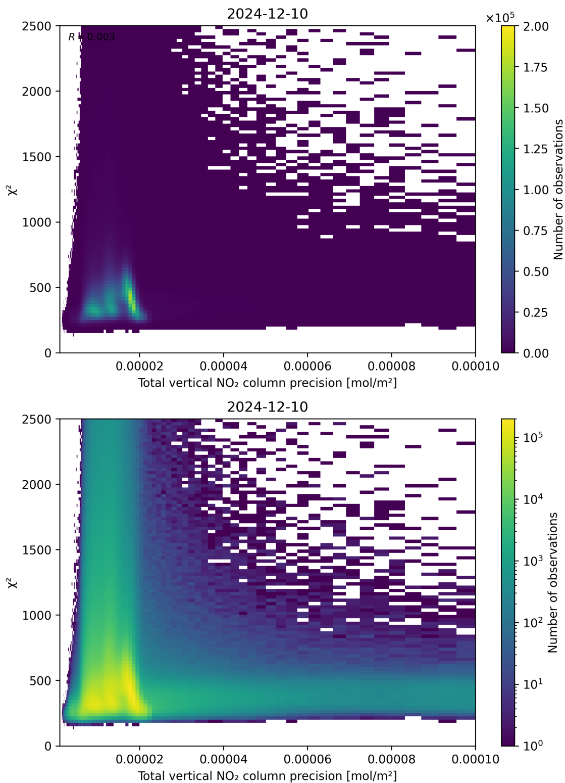
Figure 116: Scatter density plot of “Total vertical NO 2 column precision” against “ \chi^2 ” for 2024-12-09 to 2024-12-11.
