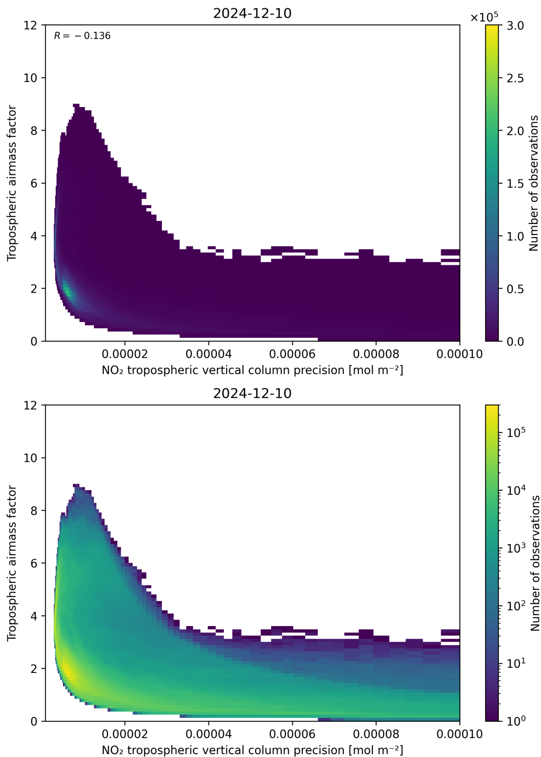
Figure 133: Scatter density plot of “NO 2 tropospheric vertical column precision” against “Tropospheric airmass factor” for 2024-12-09 to 2024-12-11.
