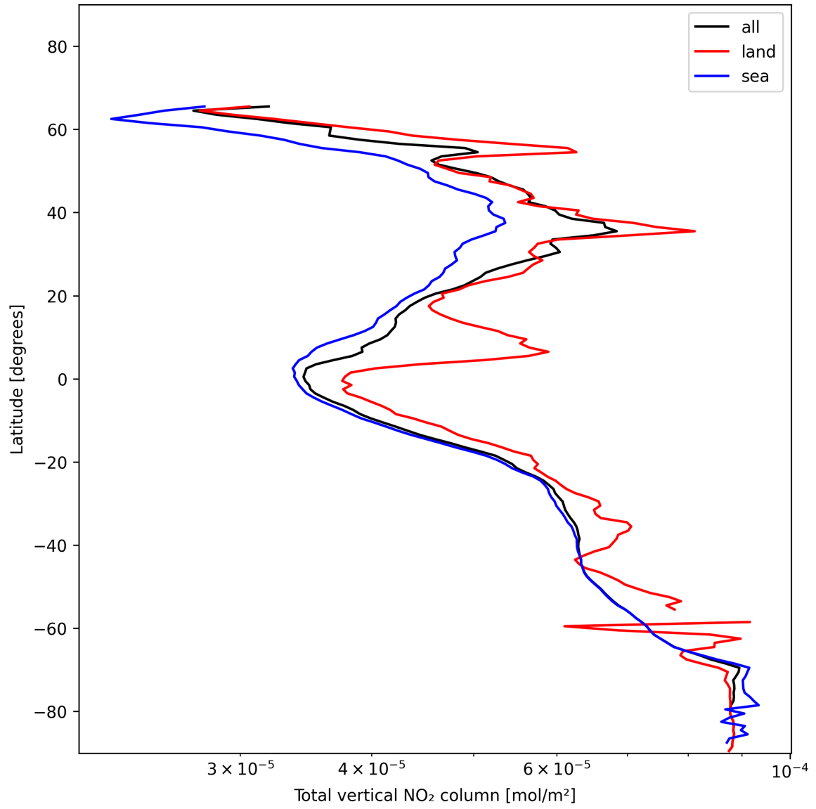
Figure 21: Zonal average of “Total vertical NO 2 column” for 2024-12-09 to 2024-12-11.
