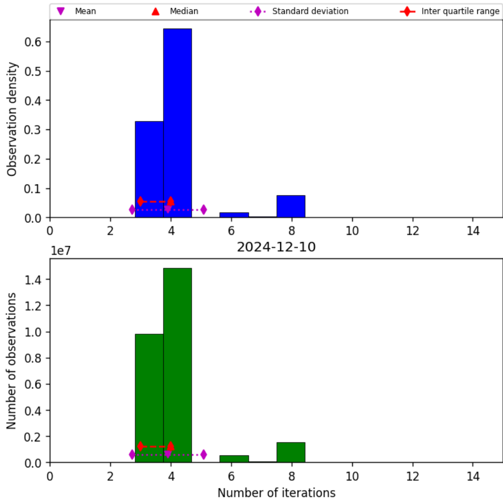
Figure 34: Histogram of “Number of iterations” for 2024-12-09 to 2024-12-11
