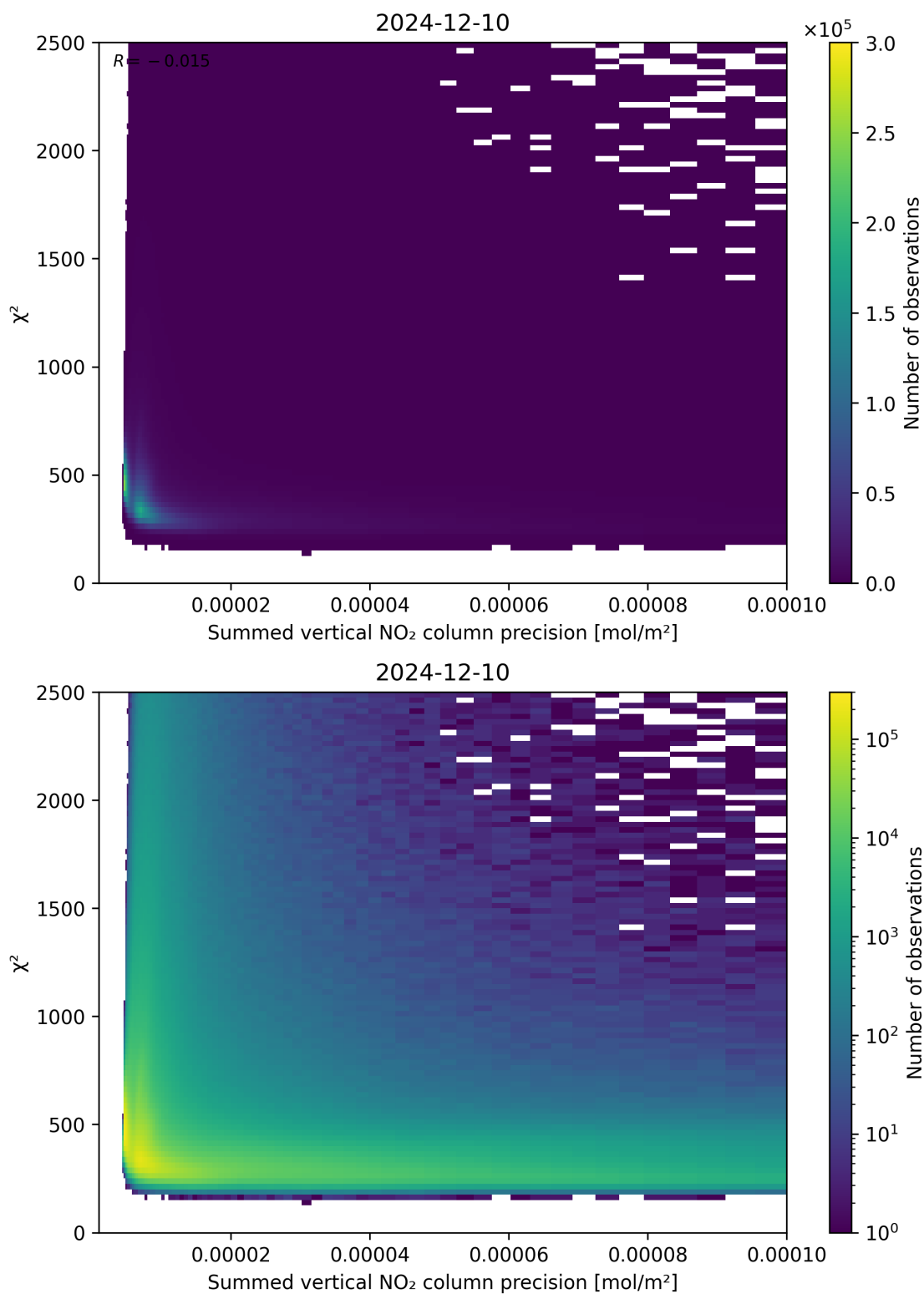
Figure 107: Scatter density plot of “Summed vertical NO 2 column precision” against “ \chi^2 ” for 2024-12-09 to 2024-12-11.
