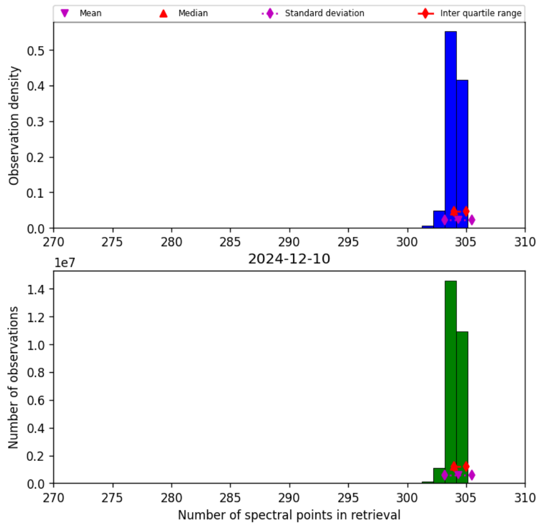
Figure 33: Histogram of “Number of spectral points in retrieval” for 2024-12-09 to 2024-12-11
