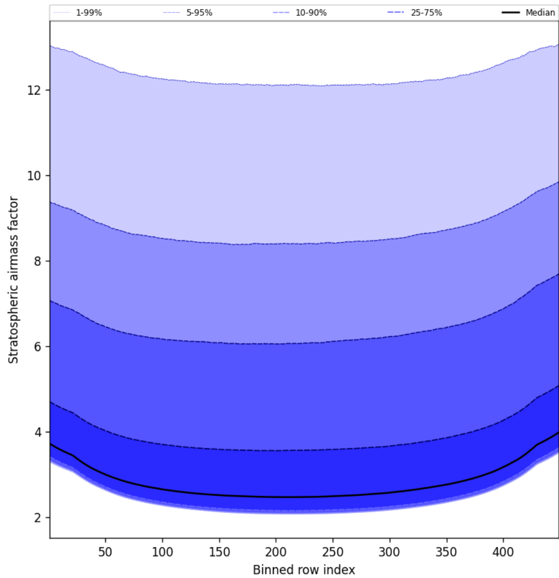
Figure 61: Along track statistics of “Stratospheric airmass factor” for 2024-12-09 to 2024-12-11
