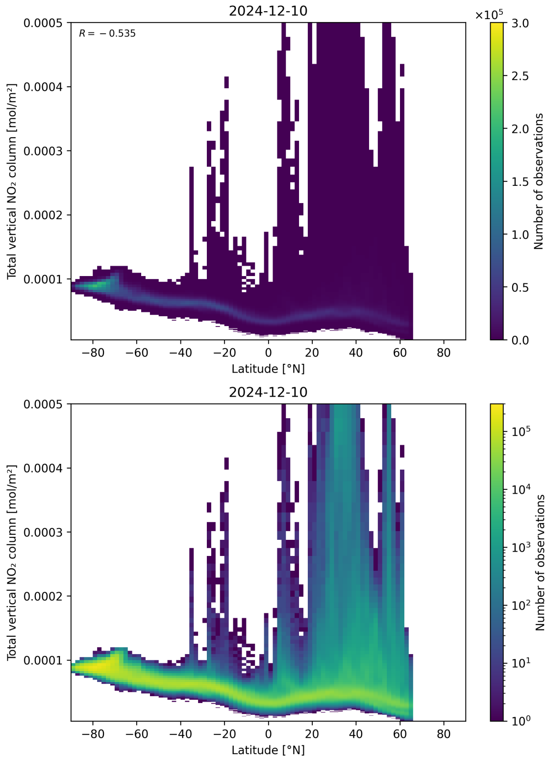
Figure 90: Scatter density plot of “Latitude” against “Total vertical NO 2 column” for 2024-12-09 to 2024-12-11.
