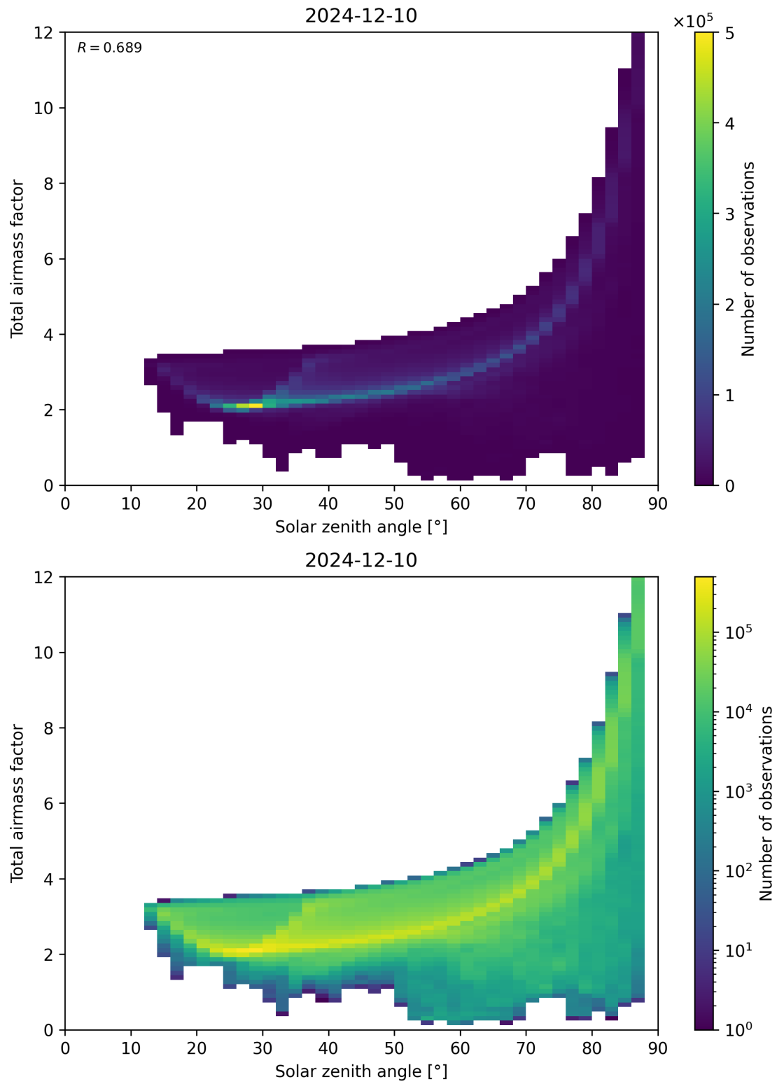
Figure 146: Scatter density plot of “Solar zenith angle” against “Total air mass factor” for 2024-12-09 to 2024-12-11.
