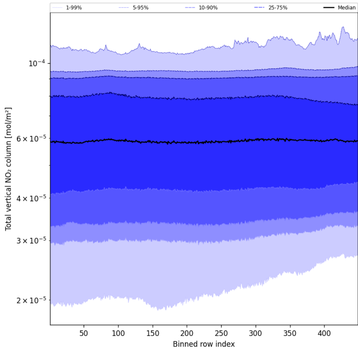
Figure 55: Along track statistics of “Total vertical NO 2 column” for 2024-12-09 to 2024-12-11
