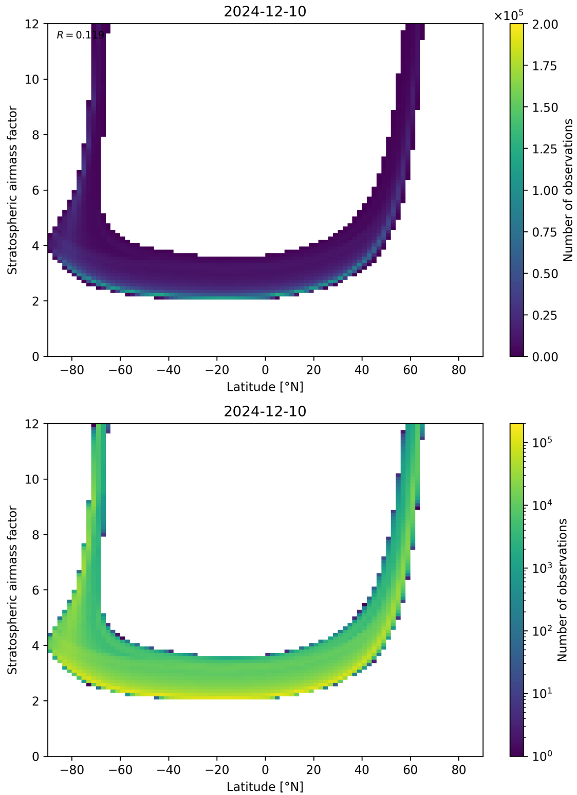
Figure 83: Scatter density plot of “Latitude” against “Stratospheric air mass factor” for 2024-12-09 to 2024-12-11.
