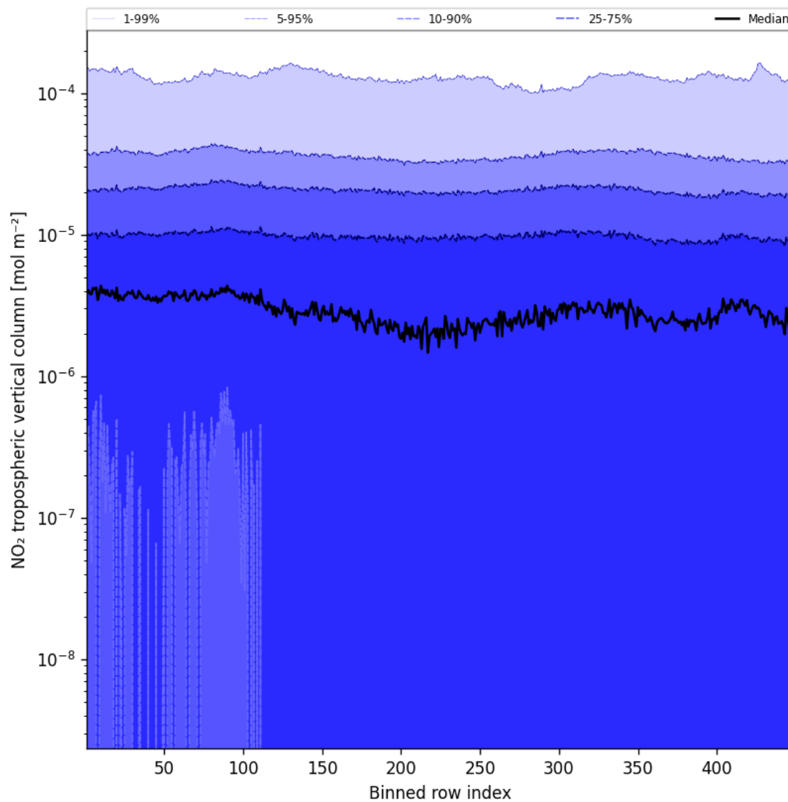
Figure 46: Along track statistics of “NO 2 tropospheric vertical column” for 2024-12-09 to 2024-12-11
