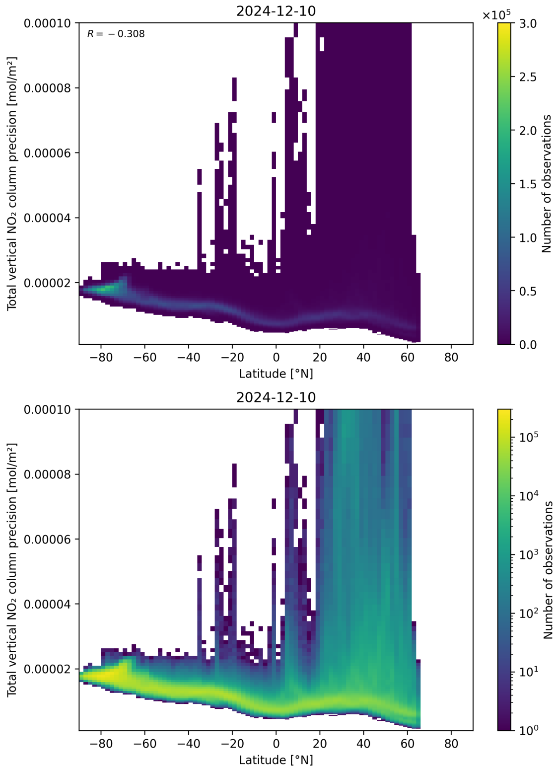
Figure 91: Scatter density plot of “Latitude” against “Total vertical NO 2 column precision” for 2024-12-09 to 2024-12-11.
