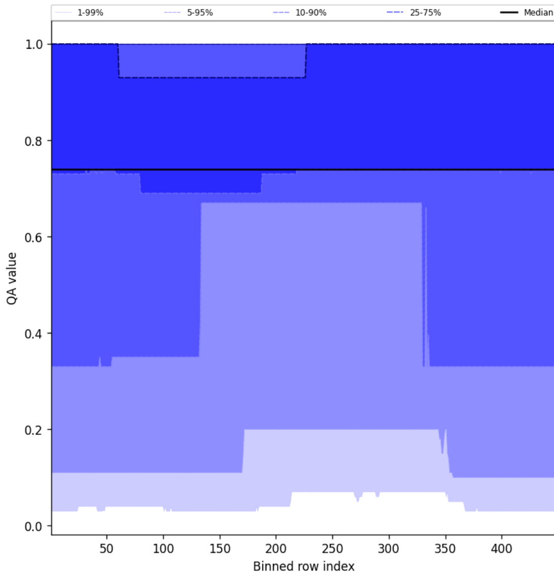
Figure 45: Along track statistics of “QA value” for 2024-12-09 to 2024-12-11
