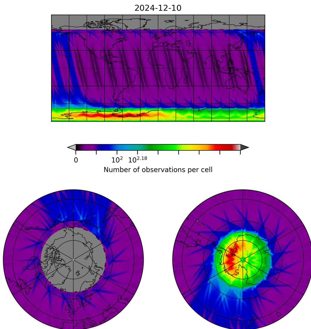
Figure 10: Map of the number of observations for 2024-12-09 to 2024-12-11
