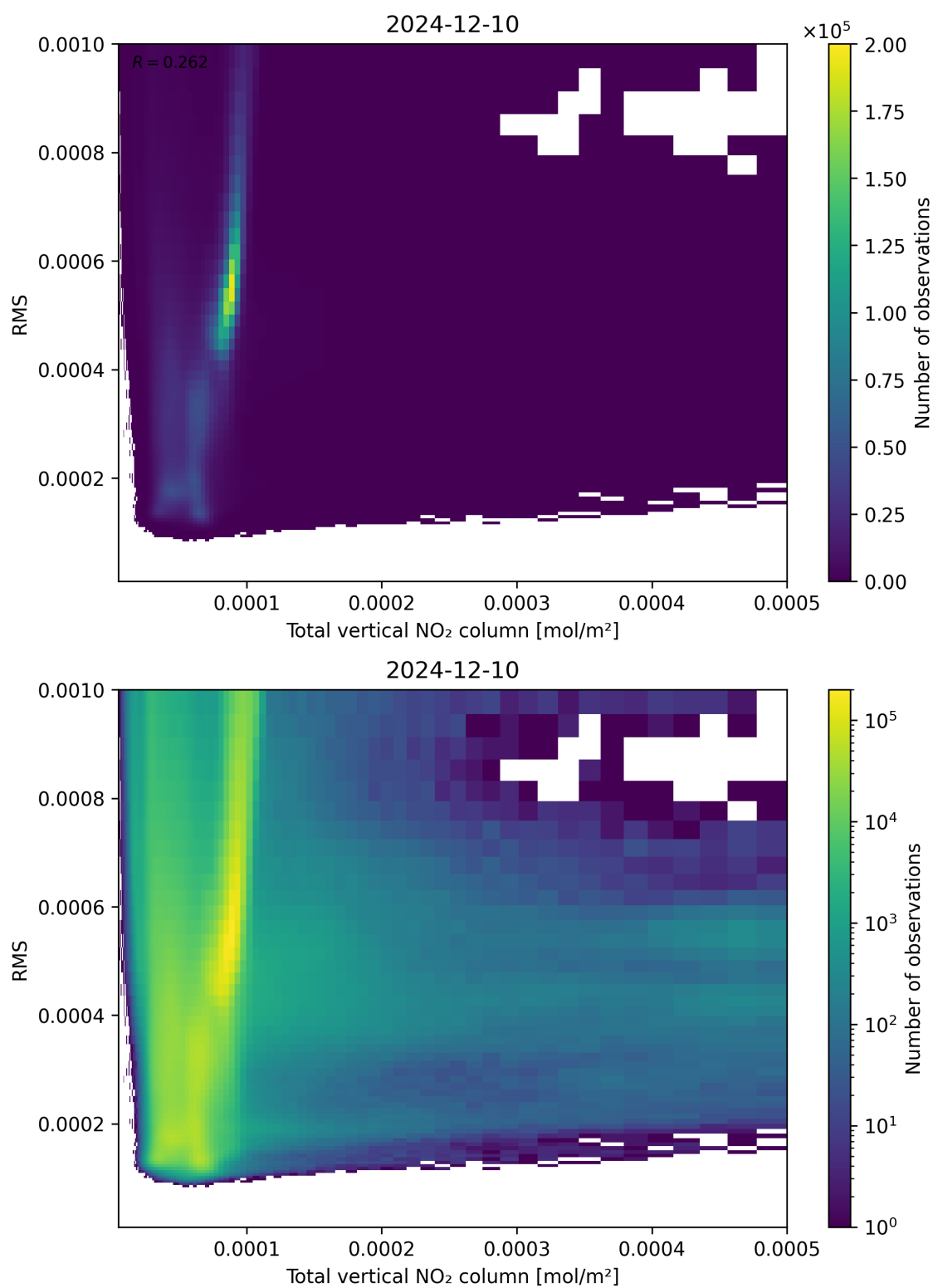
Figure 120: Scatter density plot of “Total vertical NO 2 column” against “RMS” for 2024-12-09 to 2024-12-11.
