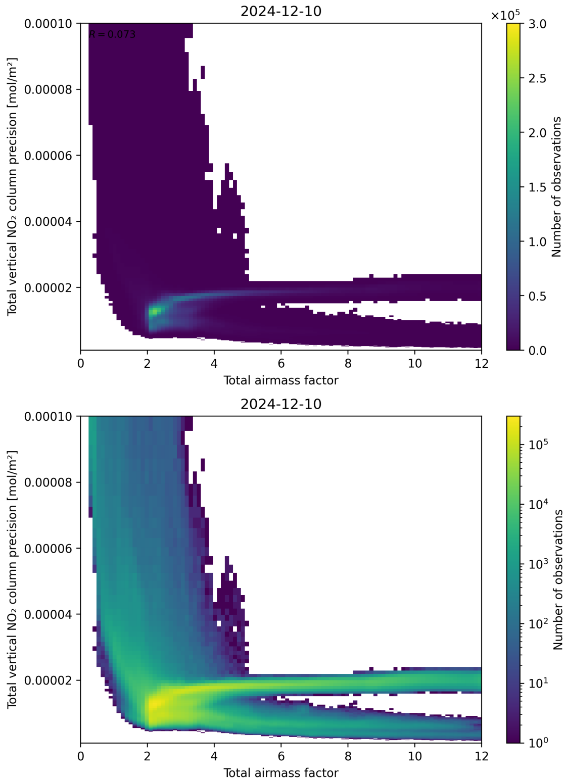
Figure 68: Scatter density plot of “Total airmass factor” against “Total vertical NO 2 column precision” for 2024-12-09 to 2024-12-11.
