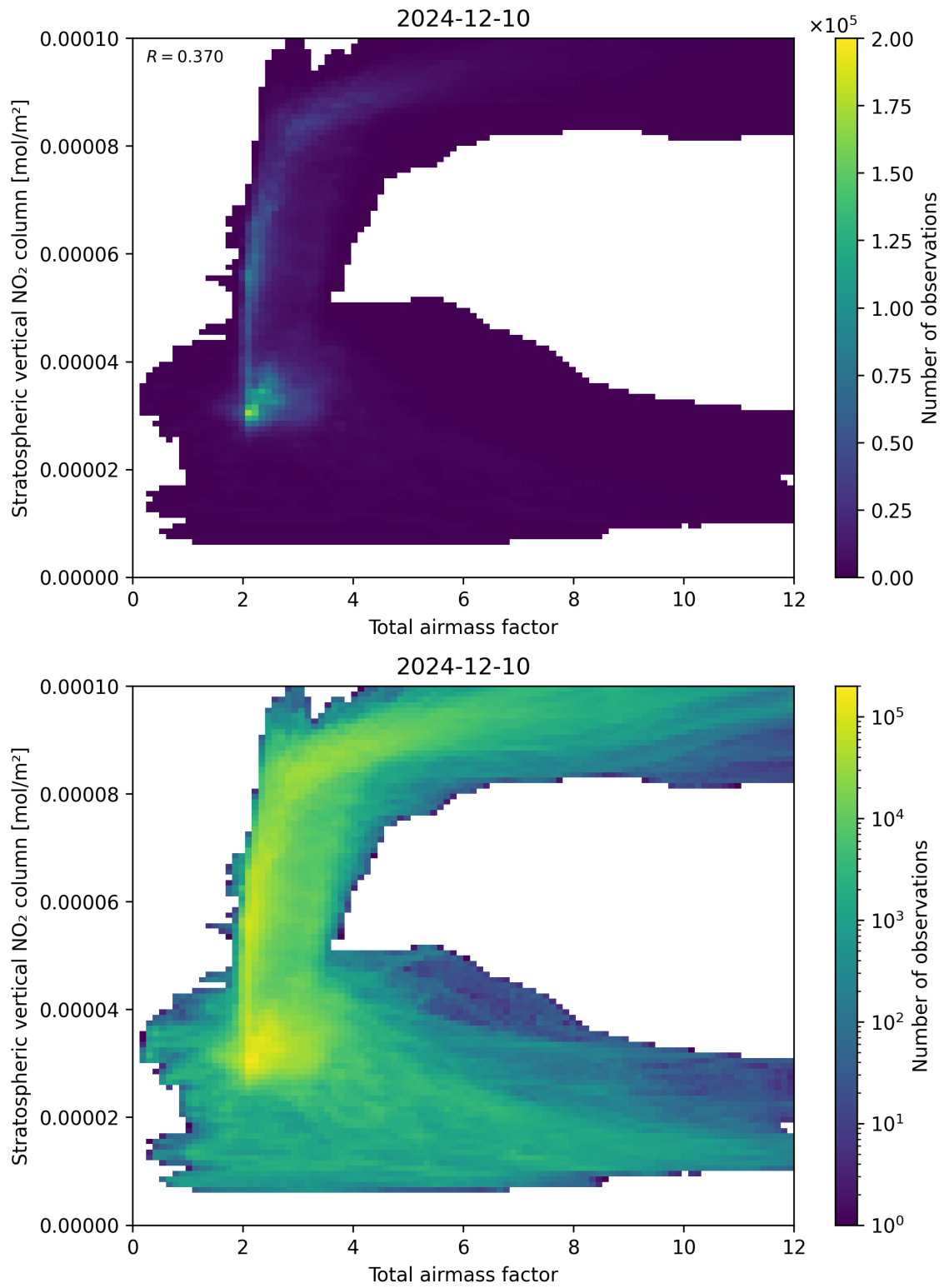
Figure 64: Scatter density plot of “Total airmass factor” against “Stratospheric vertical \text{NO}_2 column” for 2024-12-09 to 2024-12-11.
