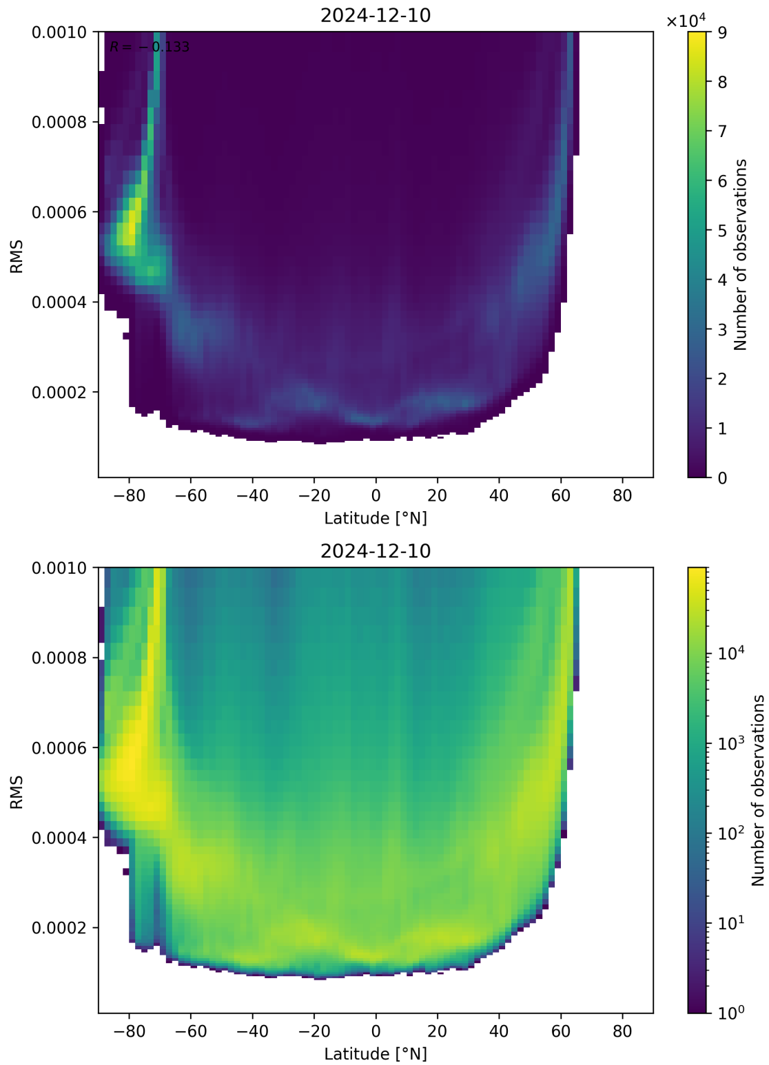
Figure 94: Scatter density plot of “Latitude” against “RMS” for 2024-12-09 to 2024-12-11.
