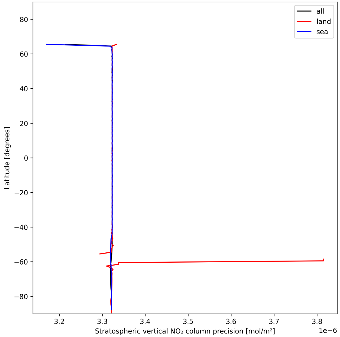
Figure 20: Zonal average of “Stratospheric vertical NO 2 column precision” for 2024-12-09 to 2024-12-11.
