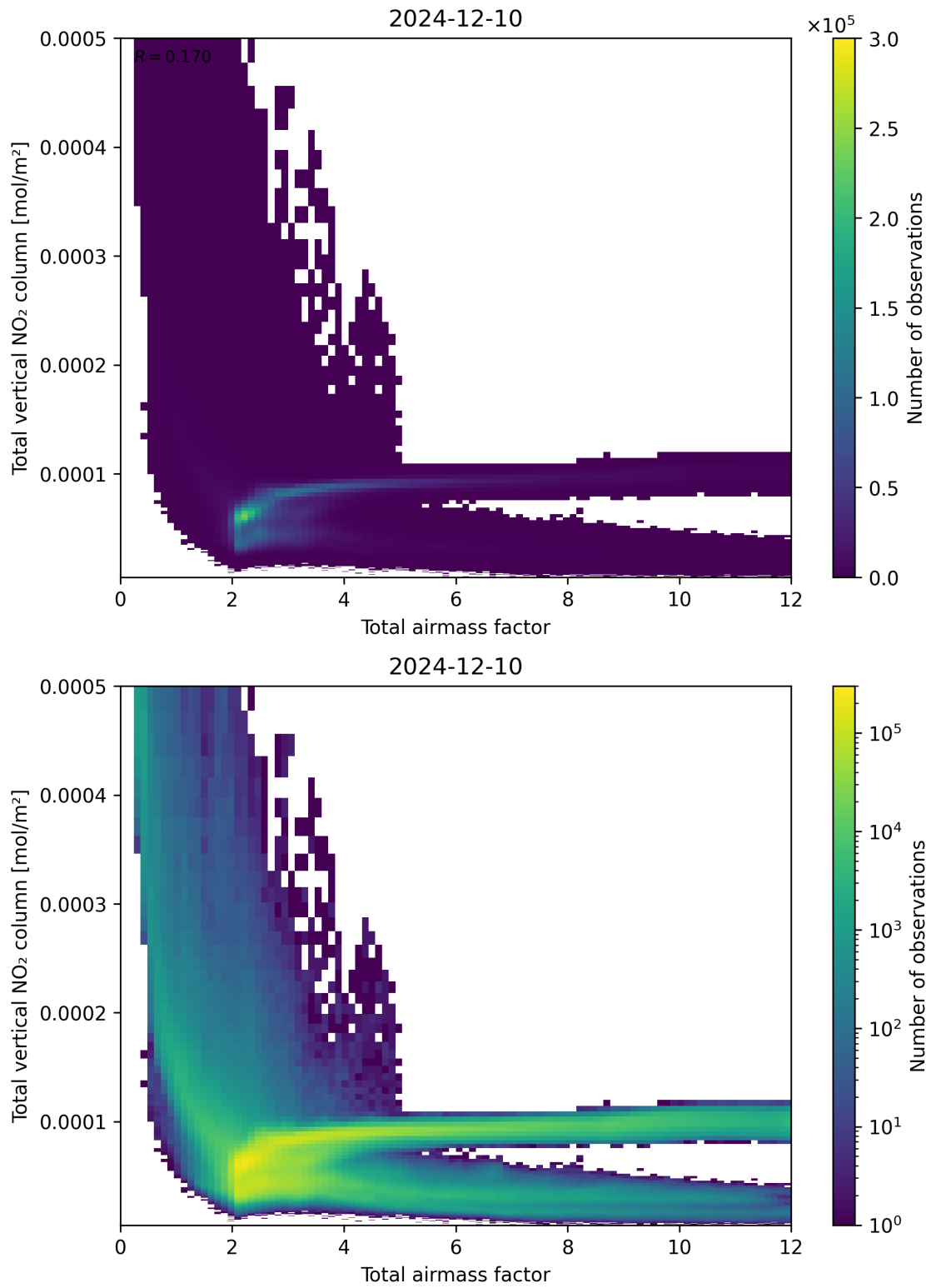
Figure 67: Scatter density plot of “Total air mass factor” against “Total vertical NO 2 column” for 2024-12-09 to 2024-12-11.
