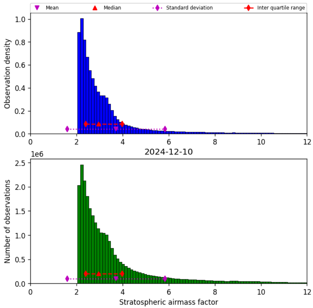
Figure 44: Histogram of “Stratospheric airmass factor” for 2024-12-09 to 2024-12-11
