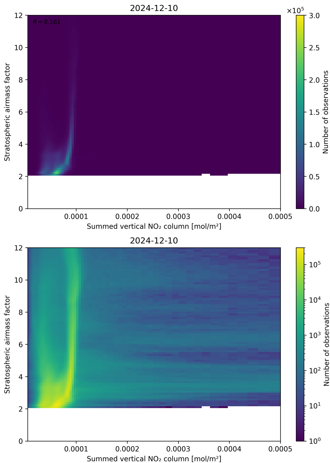
Figure 103: Scatter density plot of “Summed vertical NO 2 column” against “Stratospheric airmass factor” for 2024-12-09 to 2024-12-11.
