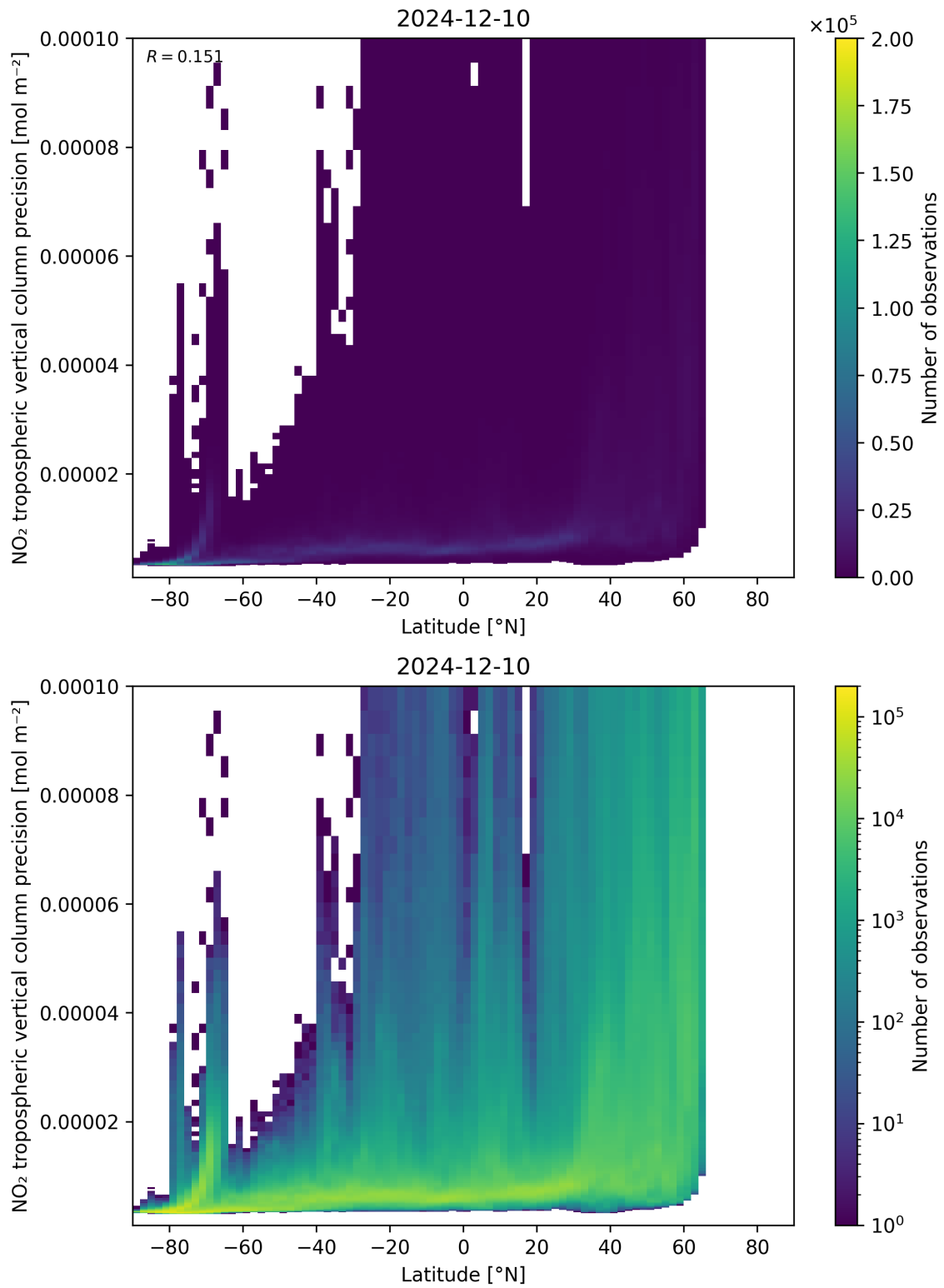
Figure 93: Scatter density plot of “Latitude” against “NO 2 tropospheric vertical column precision” for 2024-12-09 to 2024-12-11.
