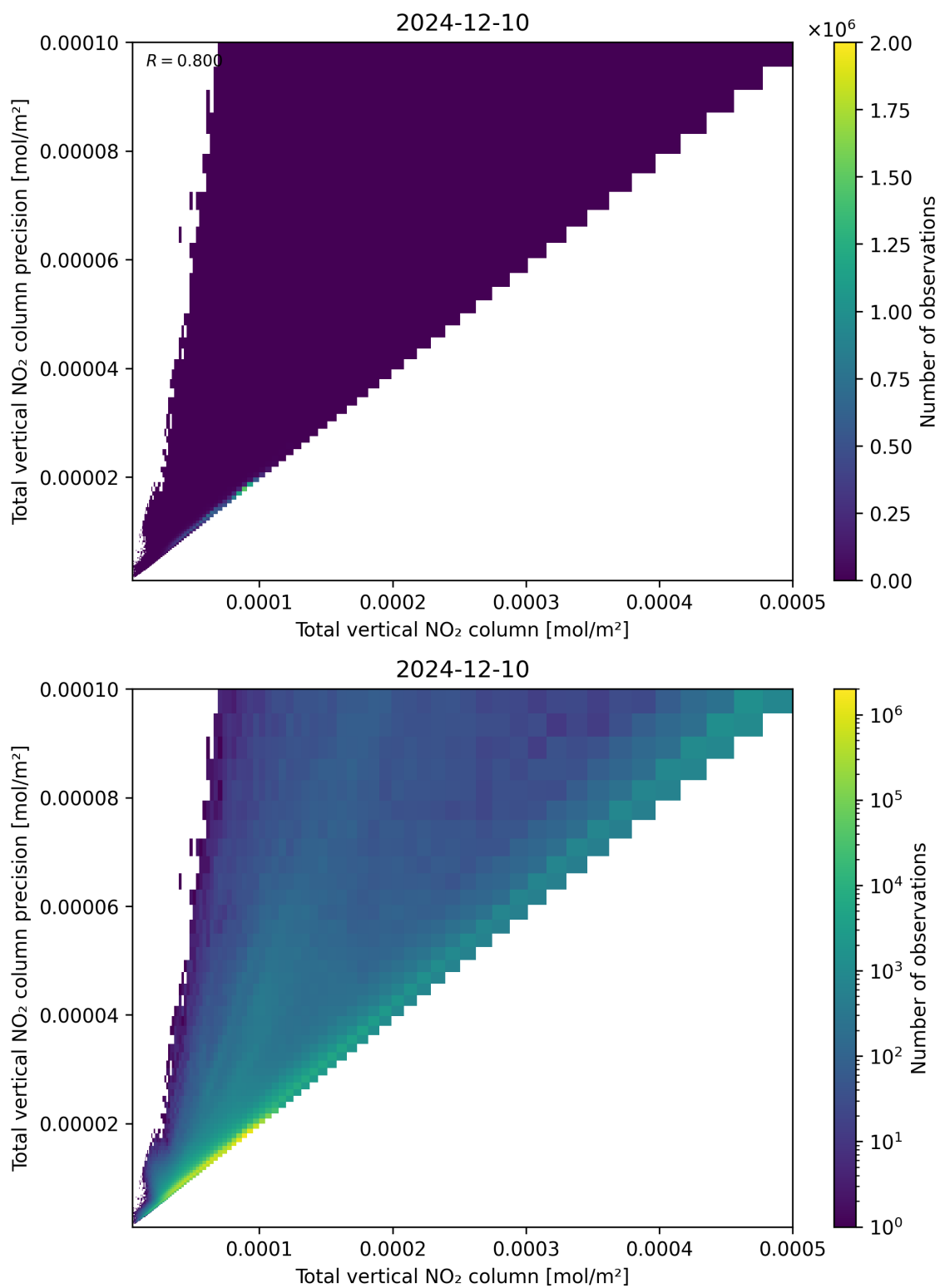
Figure 114: Scatter density plot of “Total vertical NO 2 column” against “Total vertical NO 2 column precision” for 2024-12-09 to 2024-12-11.
