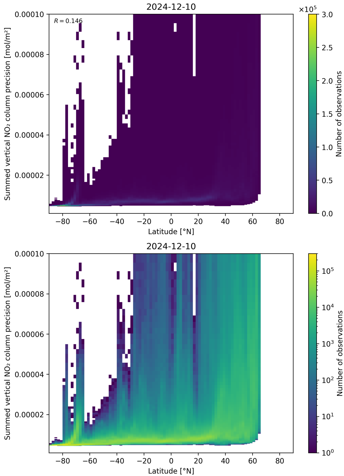
Figure 89: Scatter density plot of “Latitude” against “Summed vertical NO 2 column precision” for 2024-12-09 to 2024-12-11.
