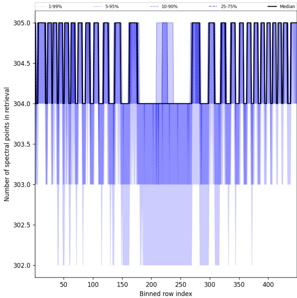
Figure 50: Along track statistics of “Number of spectral points in retrieval” for 2024-12-09 to 2024-12-11
