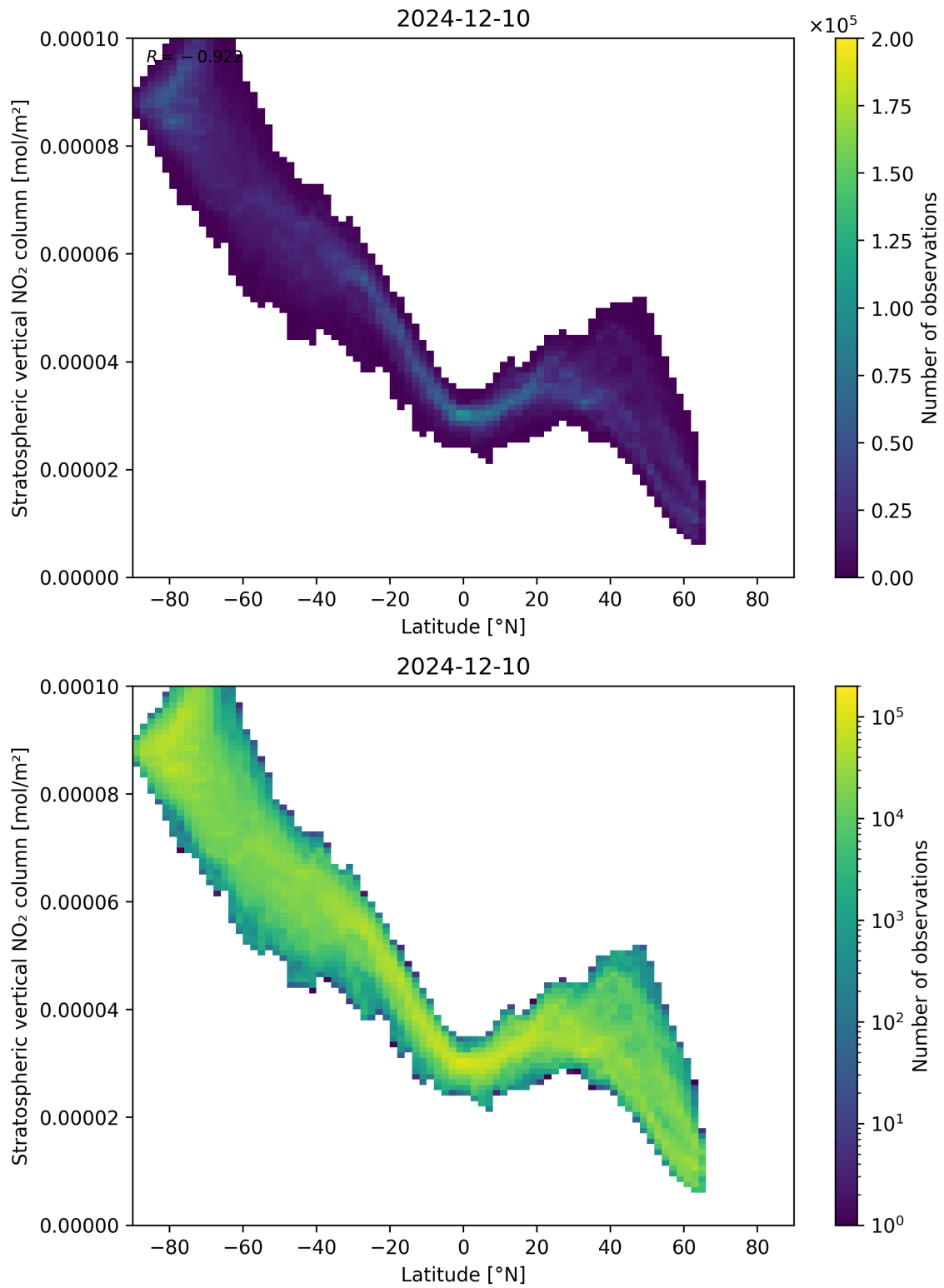
Figure 87: Scatter density plot of “Latitude” against “Stratospheric vertical NO 2 column” for 2024-12-09 to 2024-12-11.
