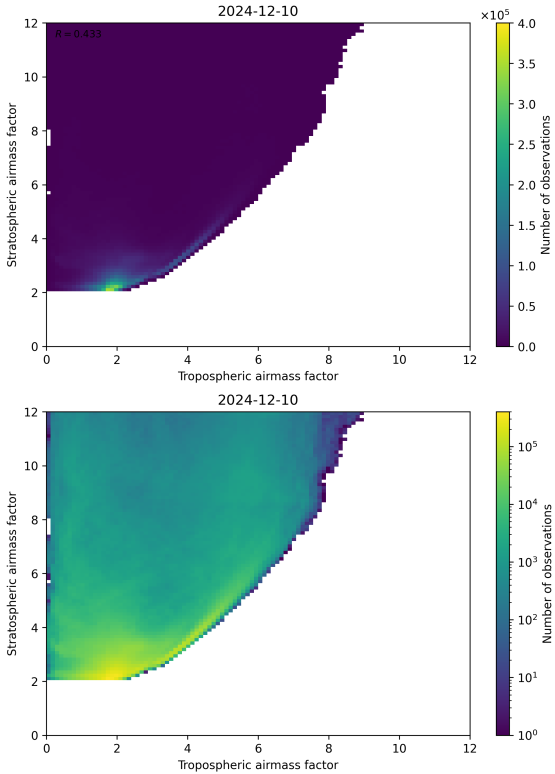
Figure 71: Scatter density plot of “Tropospheric airmass factor” against “Stratospheric airmass factor” for 2024-12-09 to 2024-12-11.
