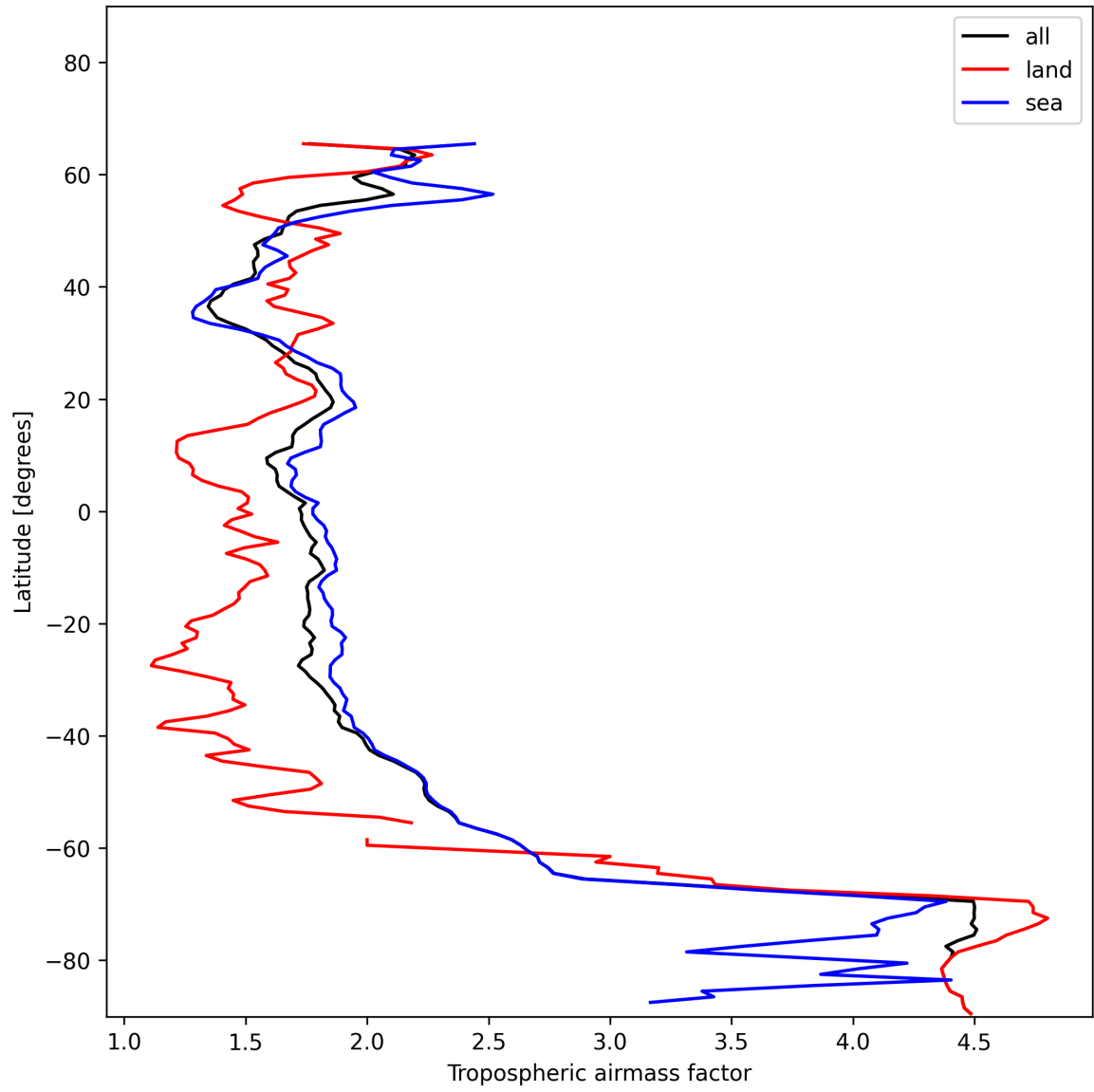
Figure 14: Zonal average of “Tropospheric airmass factor” for 2024-12-09 to 2024-12-11.
