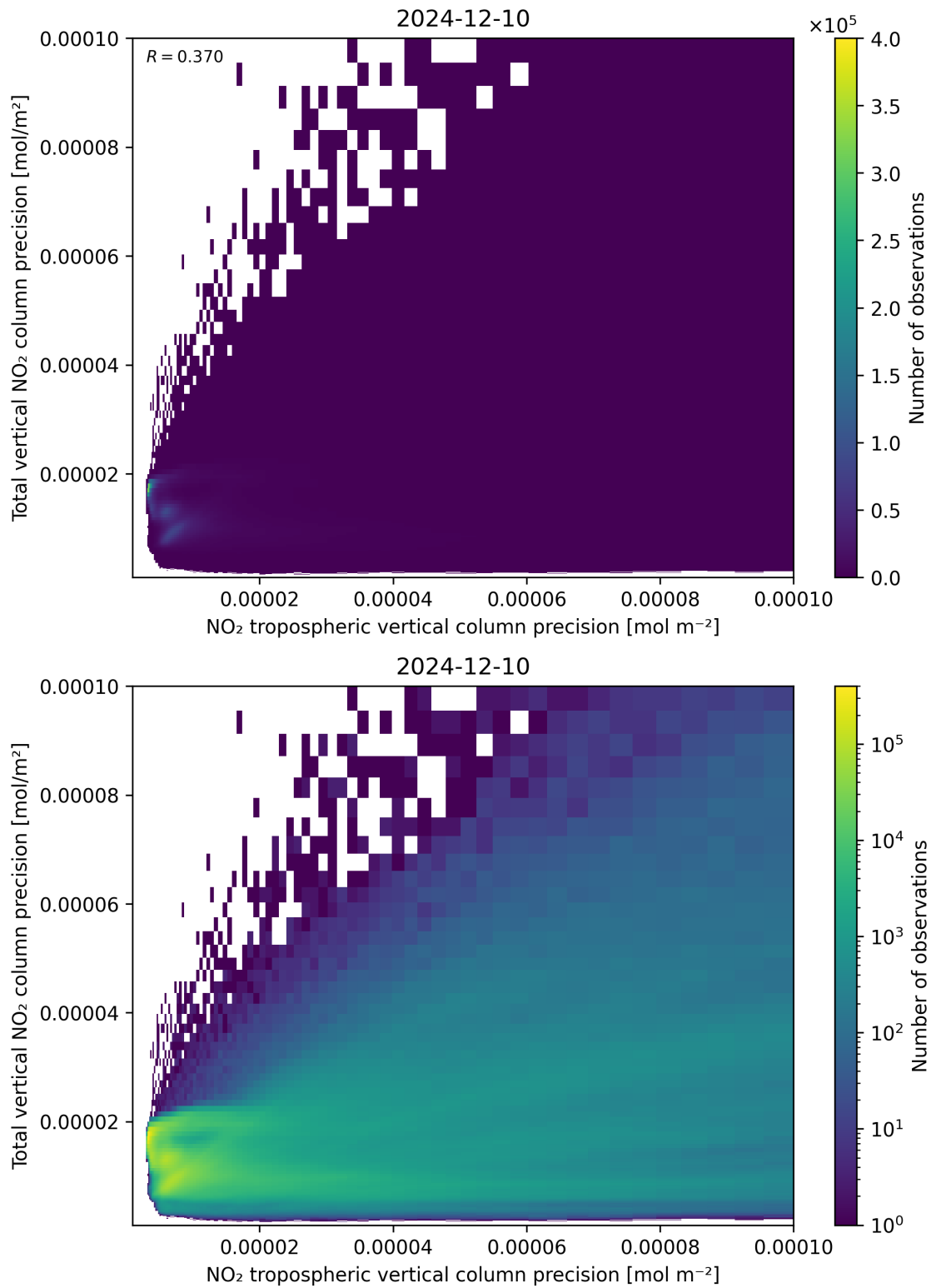
Figure 139: Scatter density plot of “NO 2 tropospheric vertical column precision” against “Total vertical NO 2 column precision” for 2024-12-09 to 2024-12-11.
