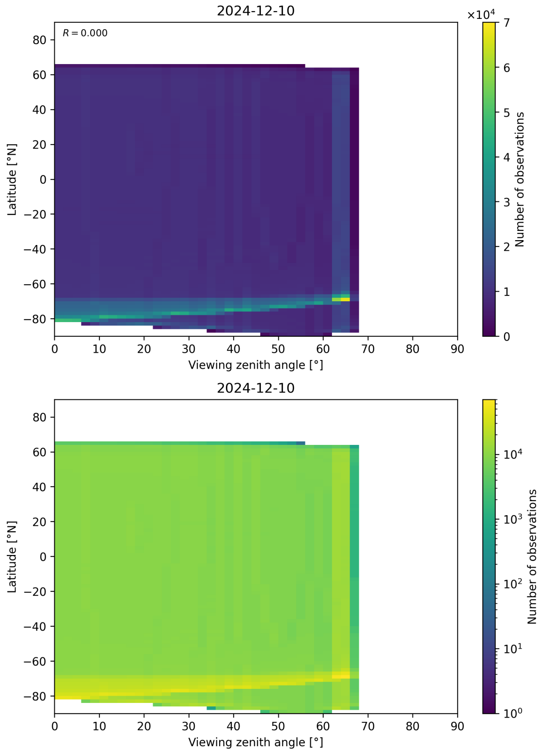
Figure 163: Scatter density plot of “Viewing zenith angle” against “Latitude” for 2024-12-09 to 2024-12-11.
