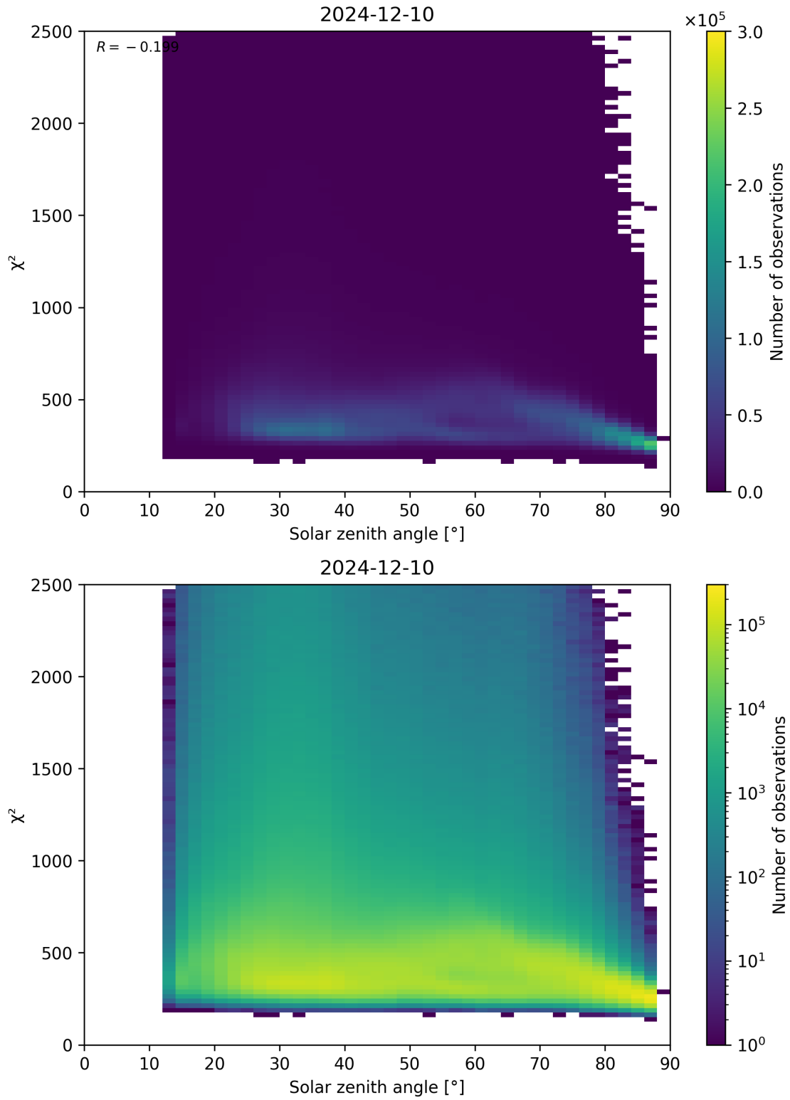
Figure 148: Scatter density plot of “Solar zenith angle” against “ \chi^2 ” for 2024-12-09 to 2024-12-11.
