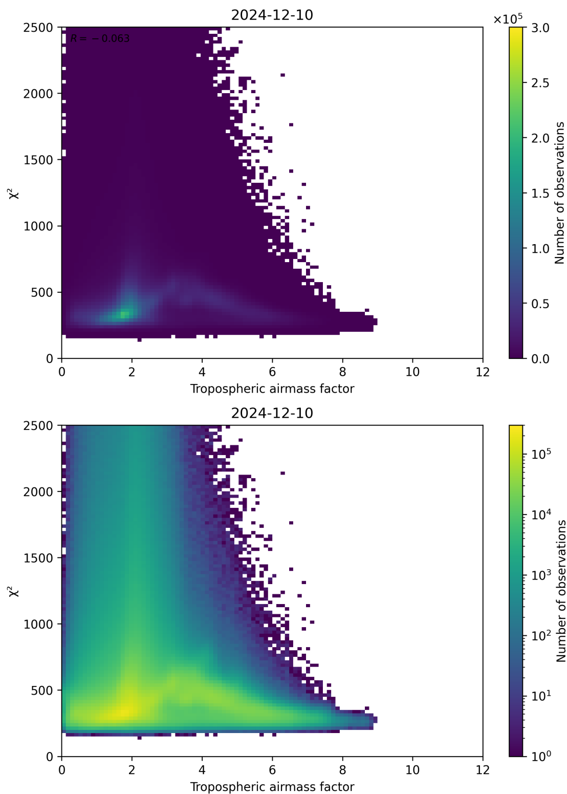
Figure 73: Scatter density plot of “Tropospheric airmass factor” against “ \chi^2 ” for 2024-12-09 to 2024-12-11.
