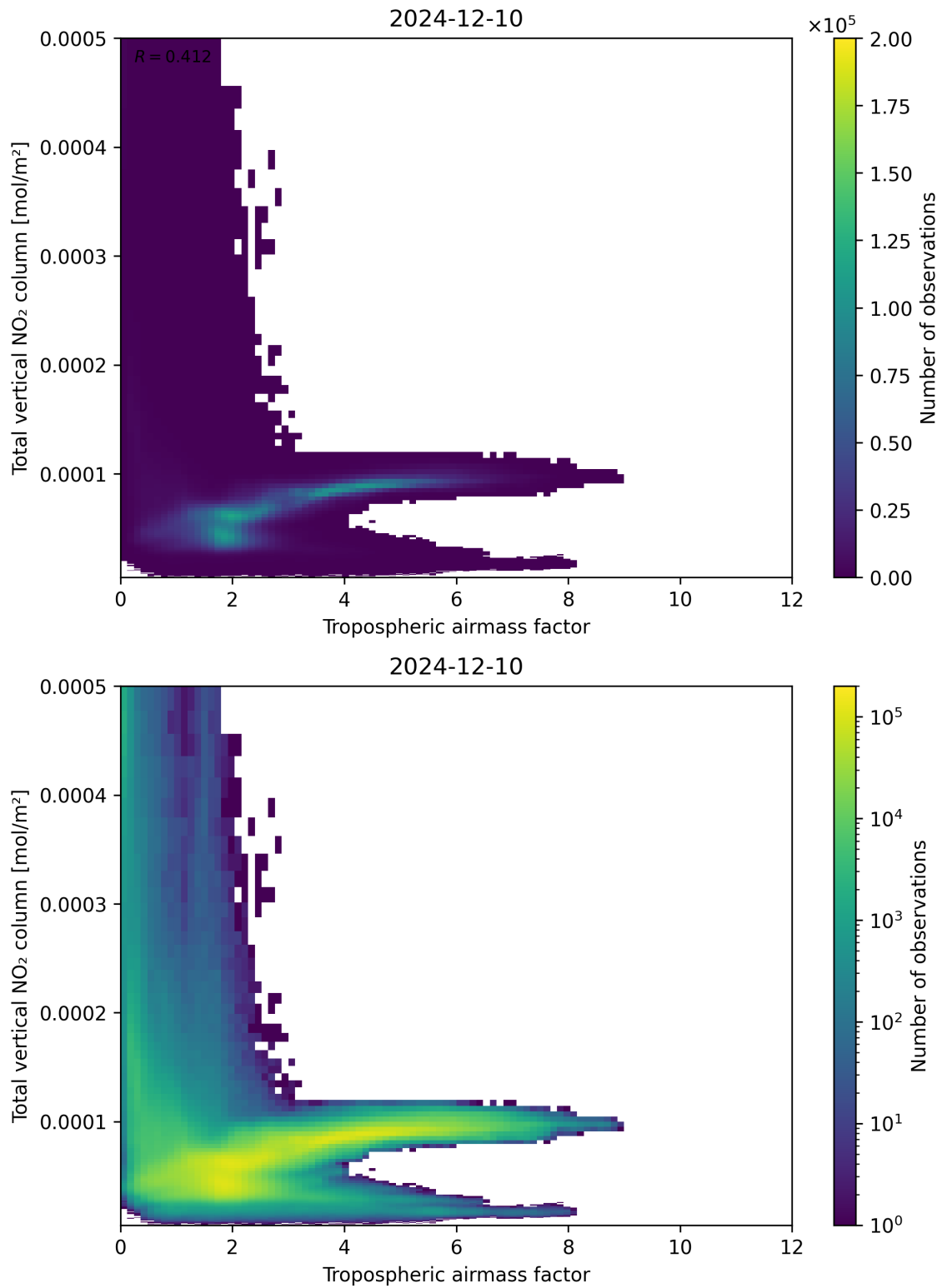
Figure 77: Scatter density plot of “Tropospheric airmass factor” against “Total vertical NO 2 column” for 2024-12-09 to 2024-12-11.
