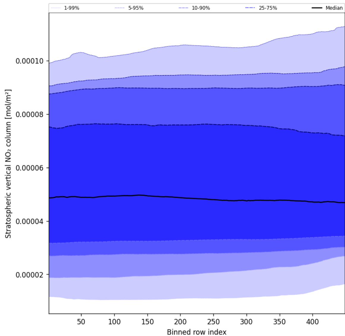
Figure 53: Along track statistics of “Stratospheric vertical NO 2 column” for 2024-12-09 to 2024-12-11
