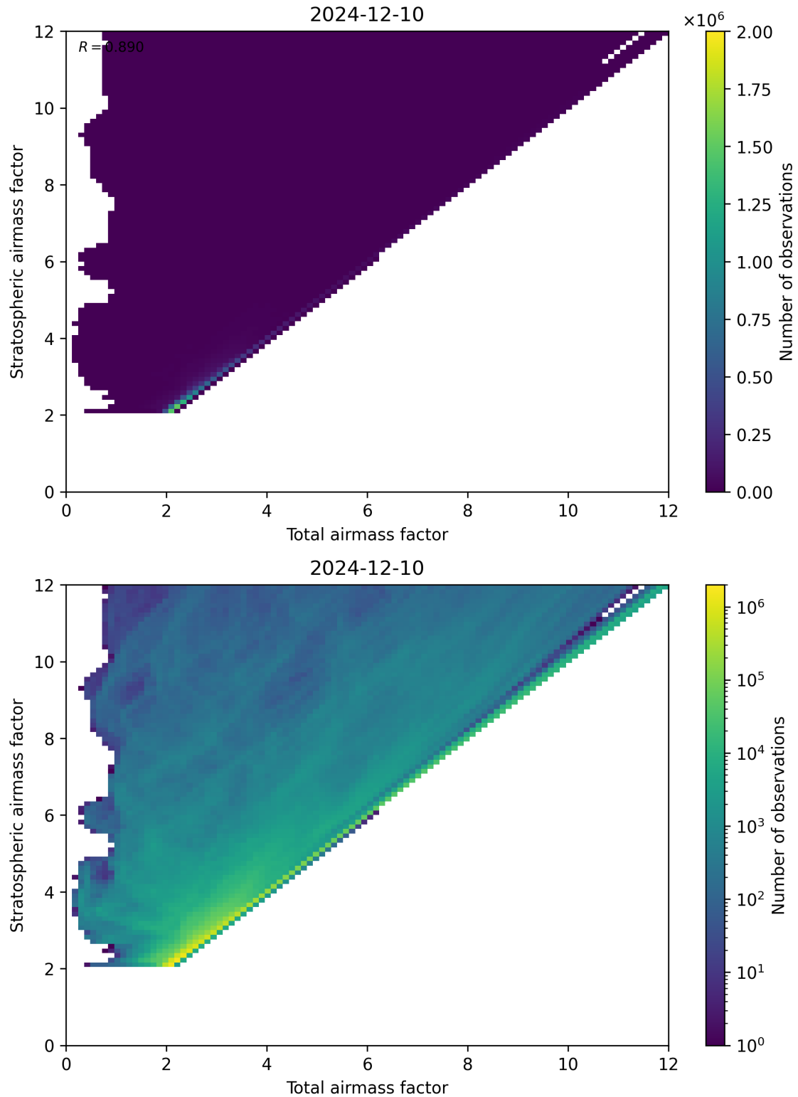
Figure 62: Scatter density plot of “Total airmass factor” against “Stratospheric airmass factor” for 2024-12-09 to 2024-12-11.
