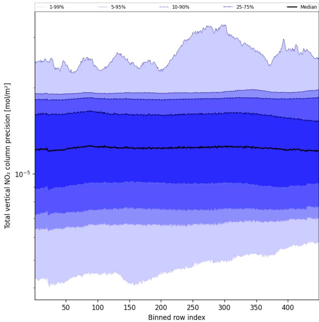
Figure 56: Along track statistics of “Total vertical NO 2 column precision” for 2024-12-09 to 2024-12-11
