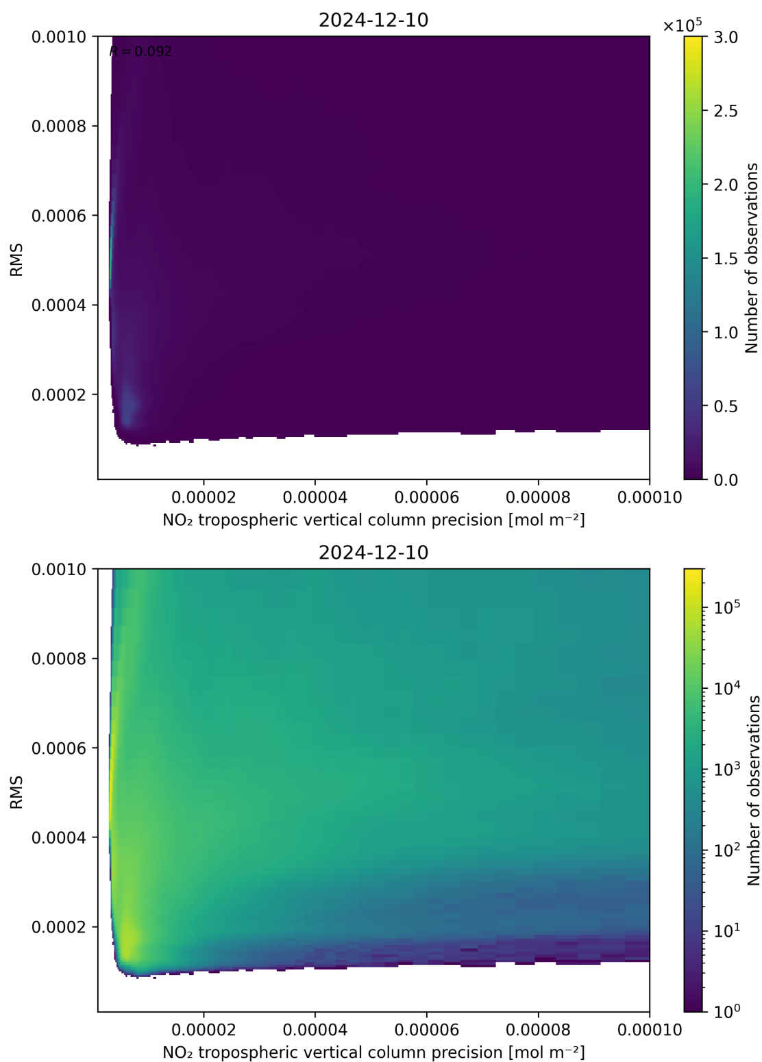
Figure 140: Scatter density plot of “NO 2 tropospheric vertical column precision” against “RMS” for 2024-12-09 to 2024-12-11.
