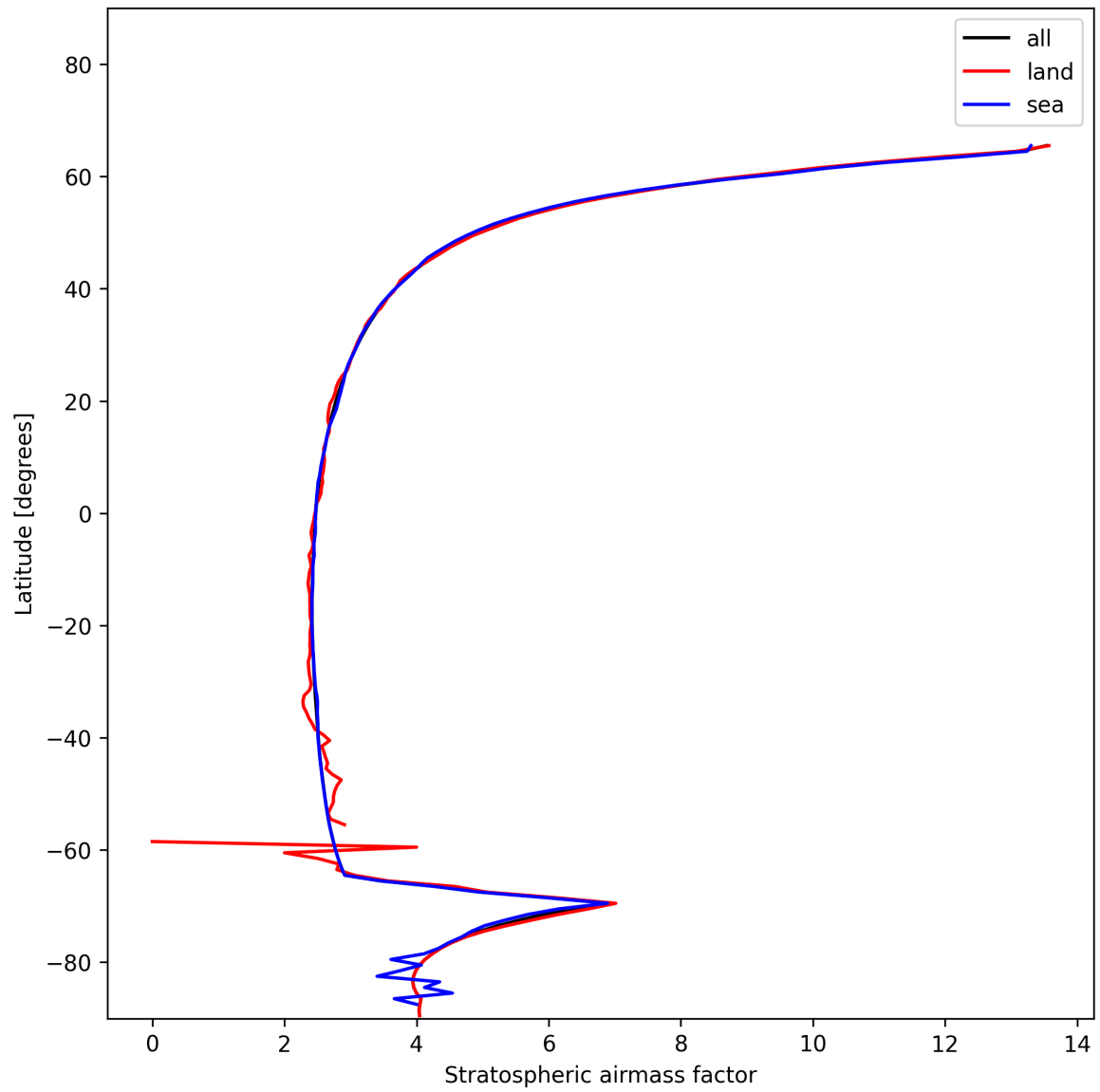
Figure 27: Zonal average of “Stratospheric air mass factor” for 2024-12-09 to 2024-12-11.
