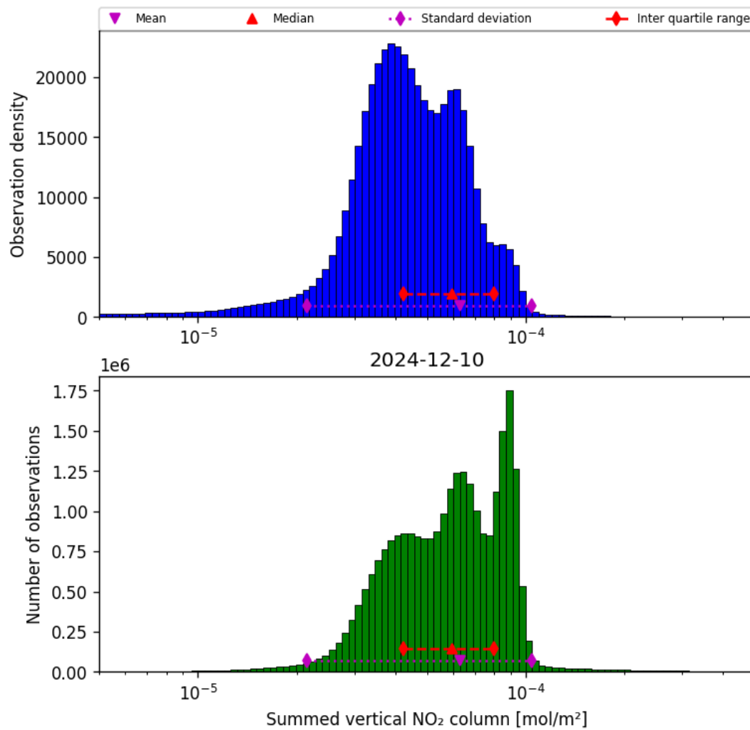
Figure 40: Histogram of “Summed vertical NO 2 column” for 2024-12-09 to 2024-12-11
