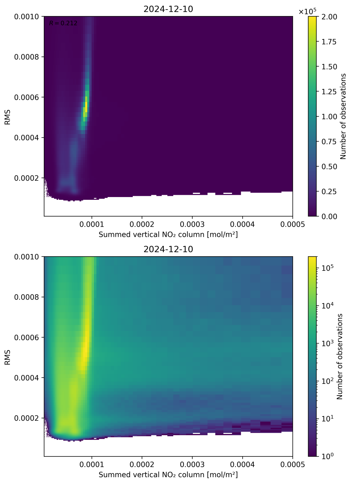
Figure 109: Scatter density plot of “Summed vertical NO 2 column” against “RMS” for 2024-12-09 to 2024-12-11.
