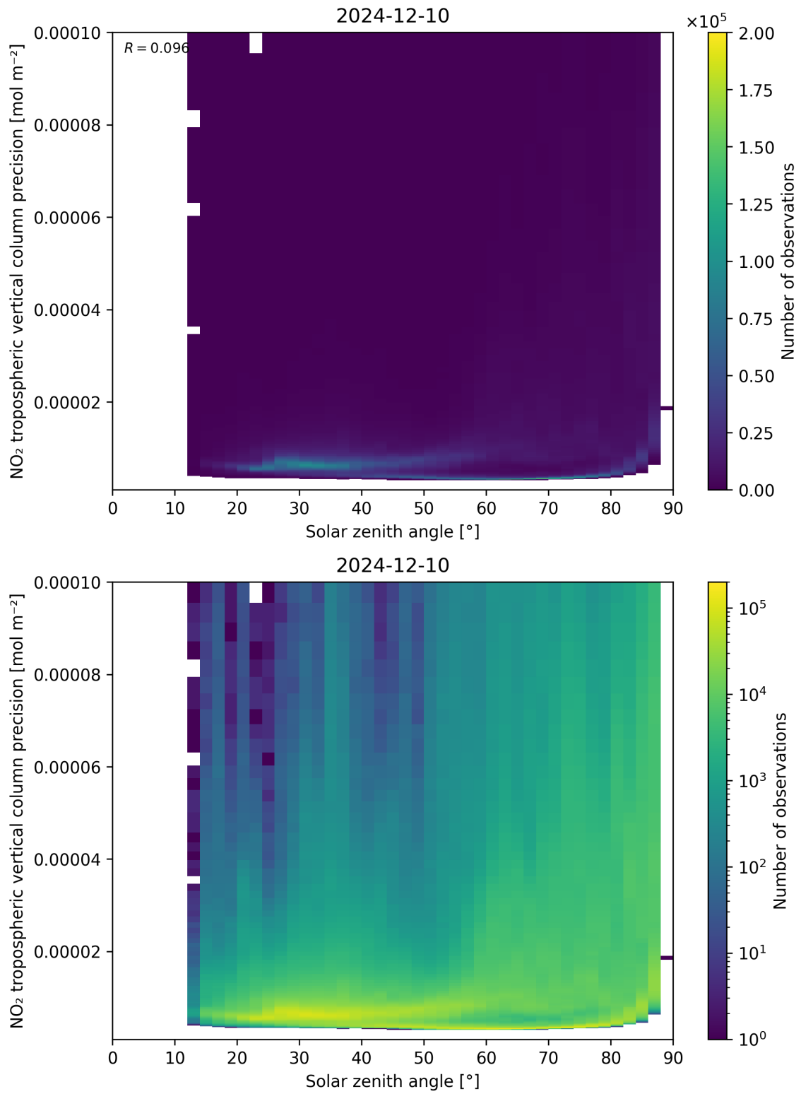
Figure 156: Scatter density plot of “Solar zenith angle” against “NO 2 tropospheric vertical column precision” for 2024-12-09 to 2024-12-11.
