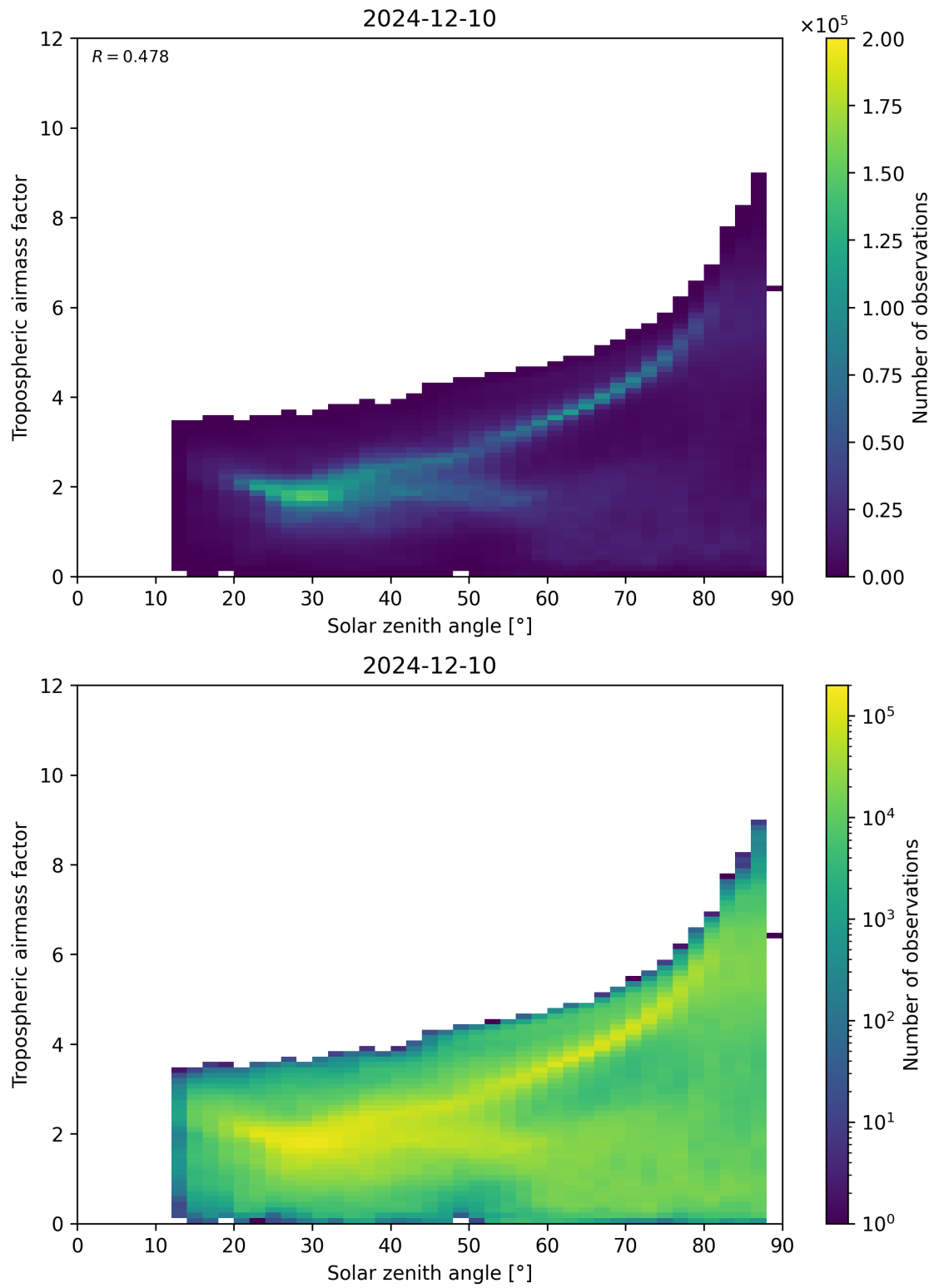
Figure 147: Scatter density plot of “Solar zenith angle” against “Tropospheric airmass factor” for 2024-12-09 to 2024-12-11.
