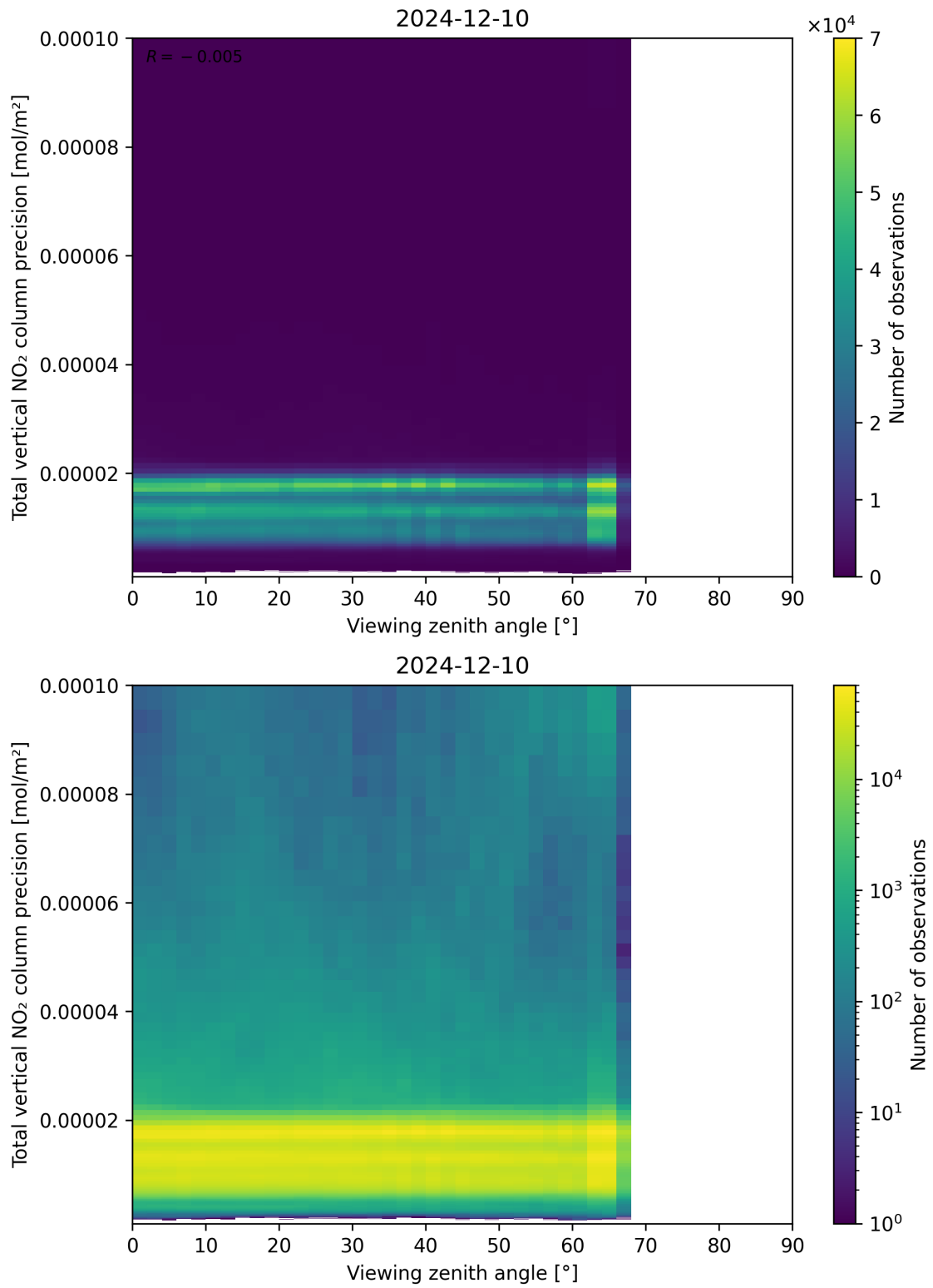
Figure 168: Scatter density plot of “Viewing zenith angle” against “Total vertical NO 2 column precision” for 2024-12-09 to 2024-12-11.
