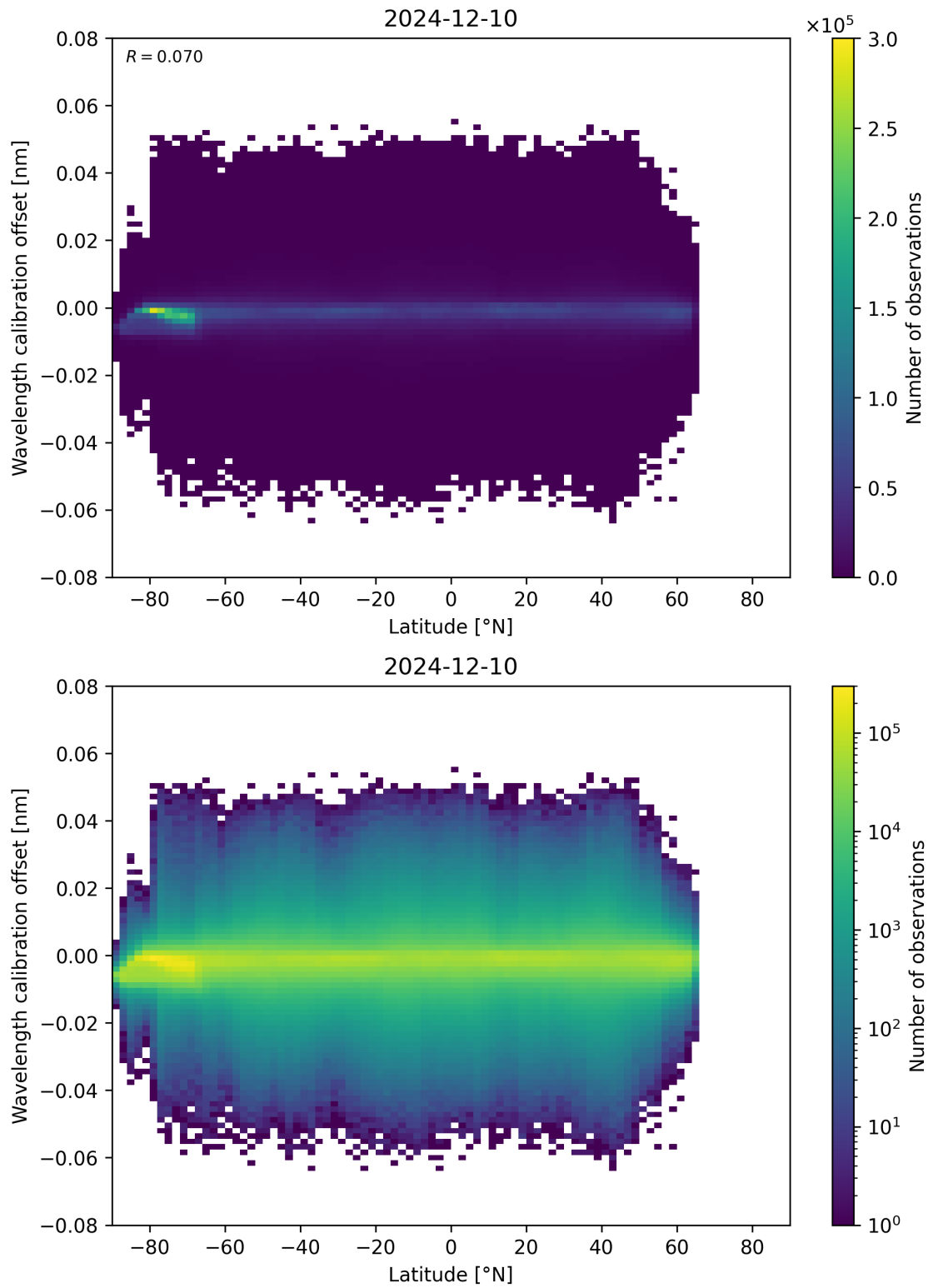
Figure 95: Scatter density plot of “Latitude” against “Wavelength calibration offset” for 2024-12-09 to 2024-12-11.
