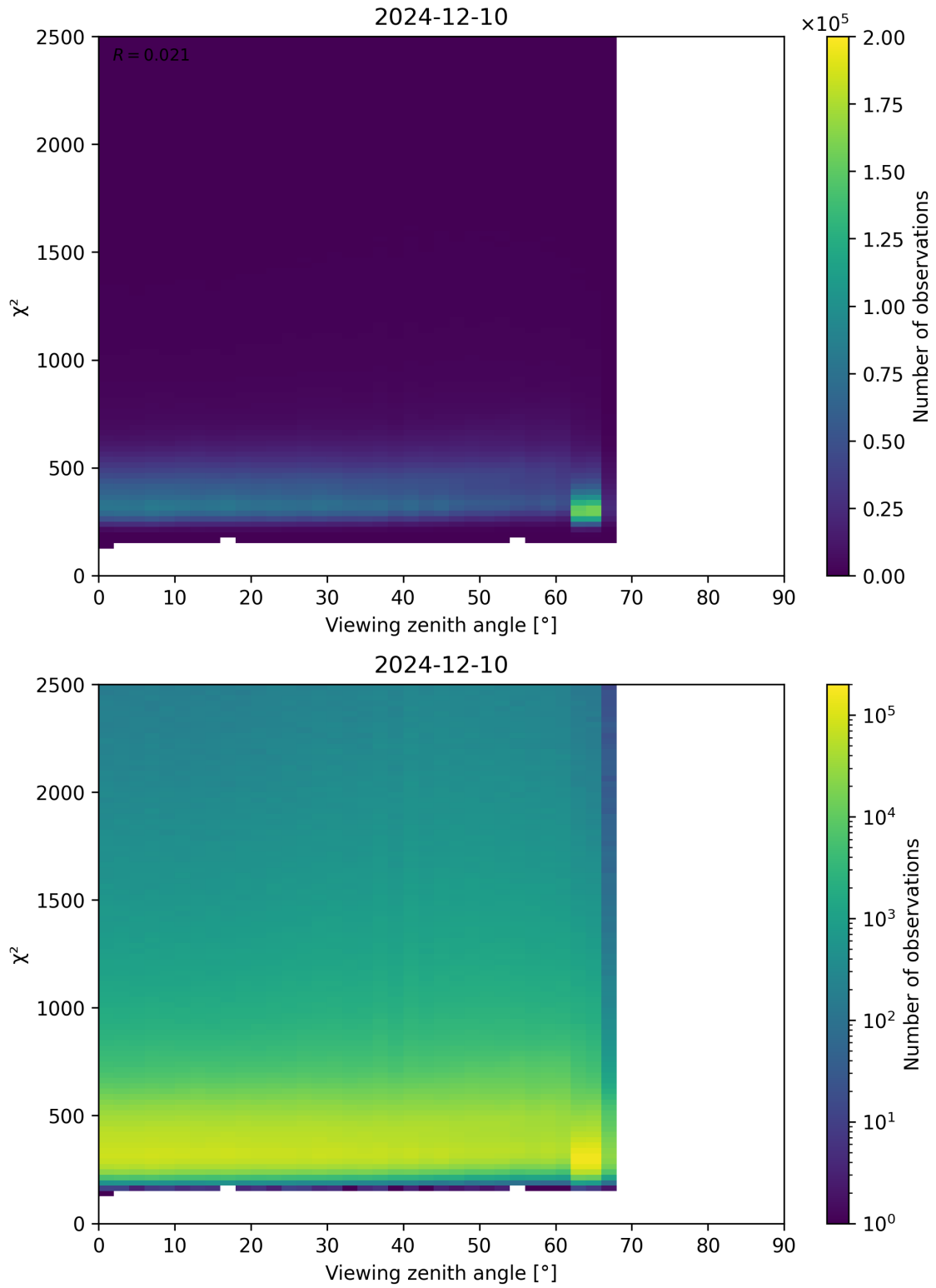
Figure 162: Scatter density plot of “Viewing zenith angle” against “ \chi^2 ” for 2024-12-09 to 2024-12-11.
