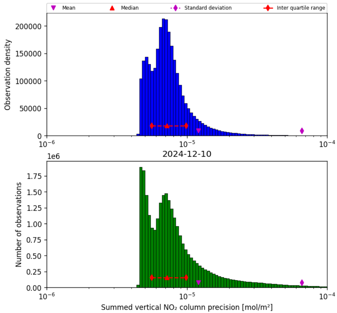
Figure 41: Histogram of “Summed vertical NO 2 column precision” for 2024-12-09 to 2024-12-11
