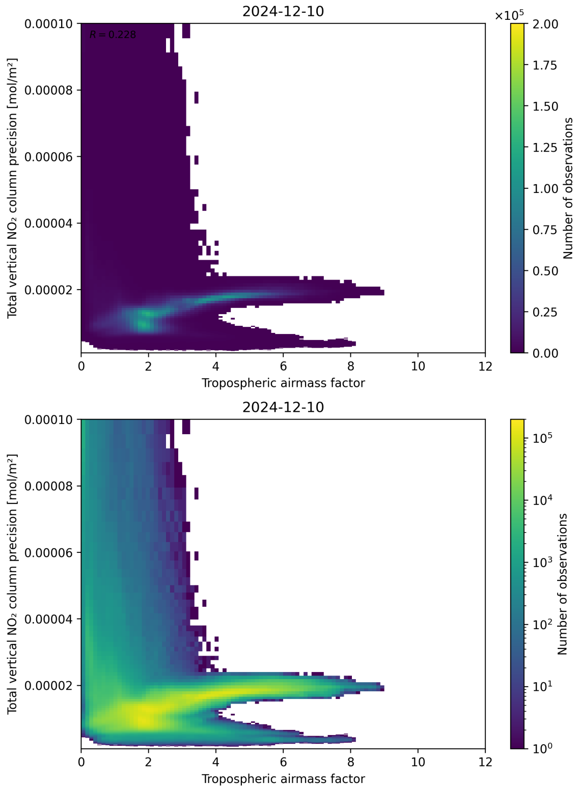
Figure 78: Scatter density plot of “Tropospheric air mass factor” against “Total vertical NO 2 column precision” for 2024-12-09 to 2024-12-11.
