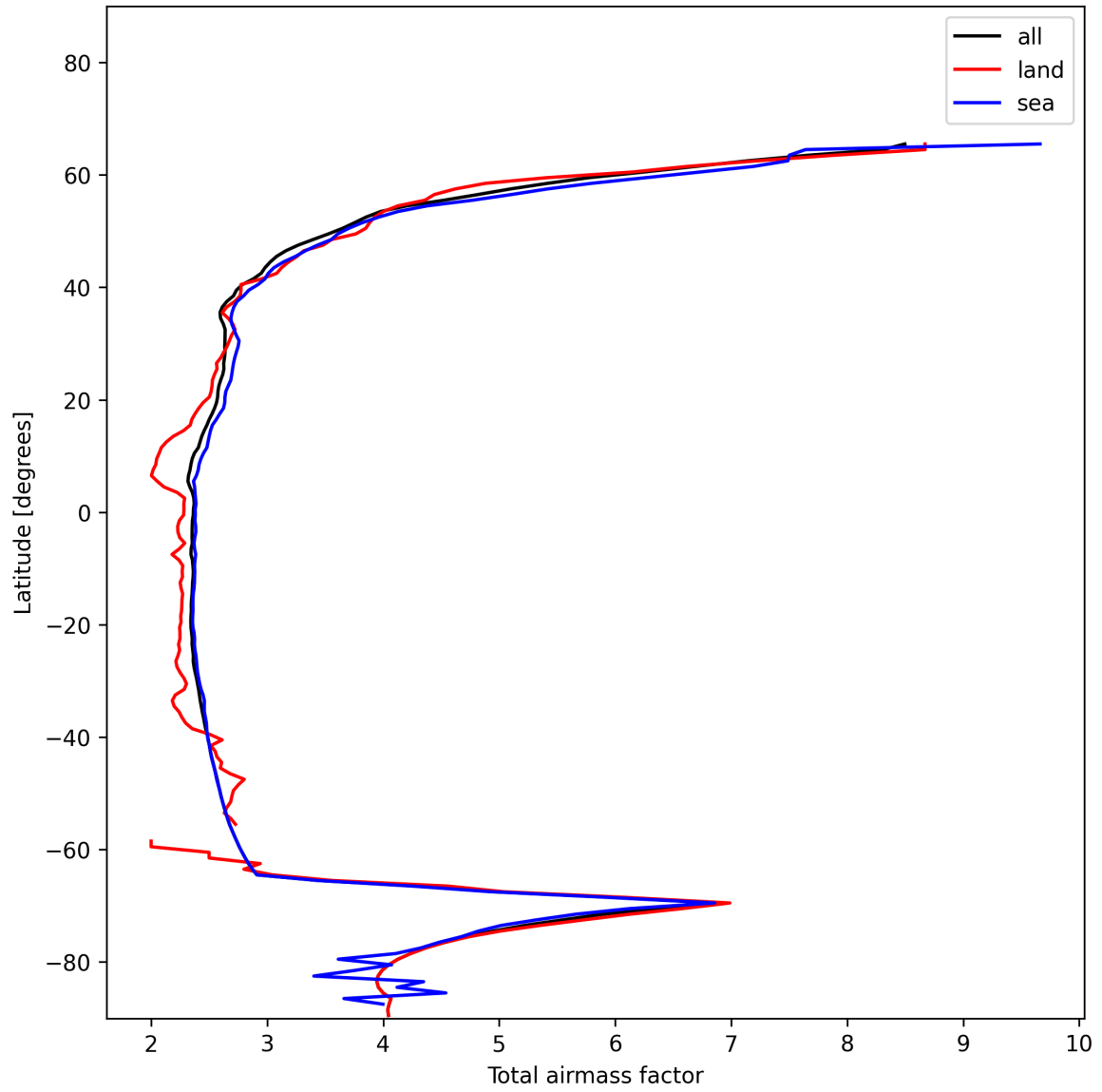
Figure 15: Zonal average of “Total airmass factor” for 2024-12-09 to 2024-12-11.
