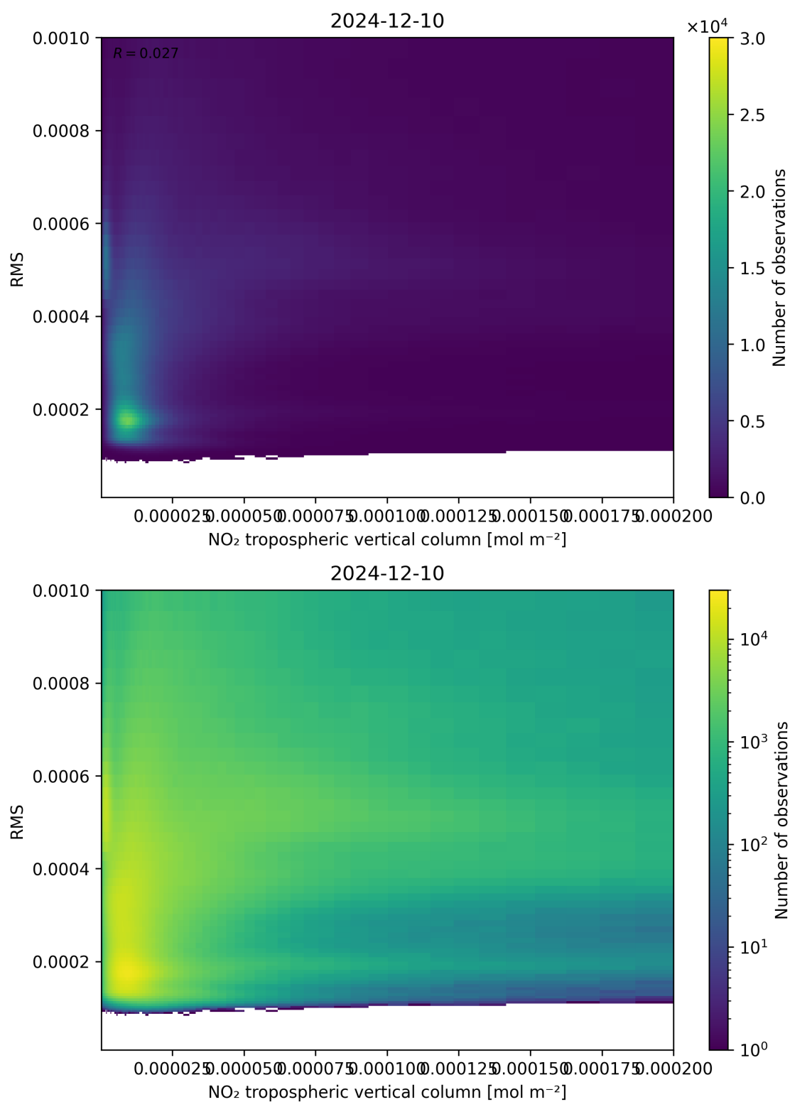
Figure 142: Scatter density plot of “NO 2 tropospheric vertical column” against “RMS” for 2024-12-09 to 2024-12-11.
