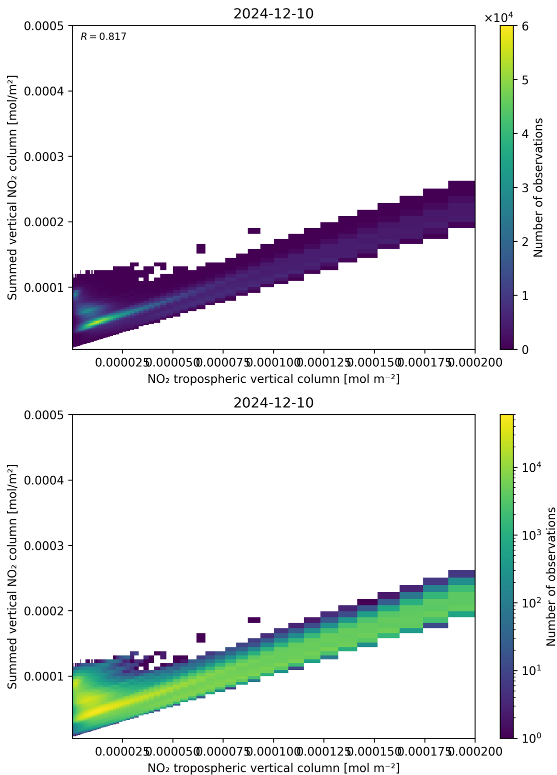
Figure 126: Scatter density plot of “NO 2 tropospheric vertical column” against “Summed vertical NO 2 column” for 2024-12-09 to 2024-12-11.
