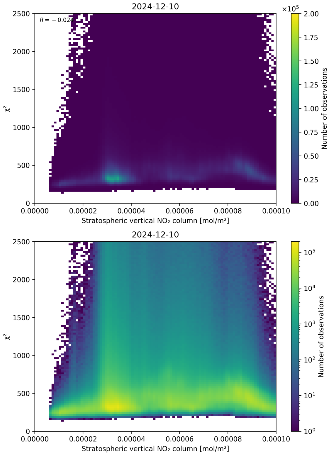
Figure 97: Scatter density plot of “Stratospheric vertical NO 2 column” against “ \chi^2 ” for 2024-12-09 to 2024-12-11.
