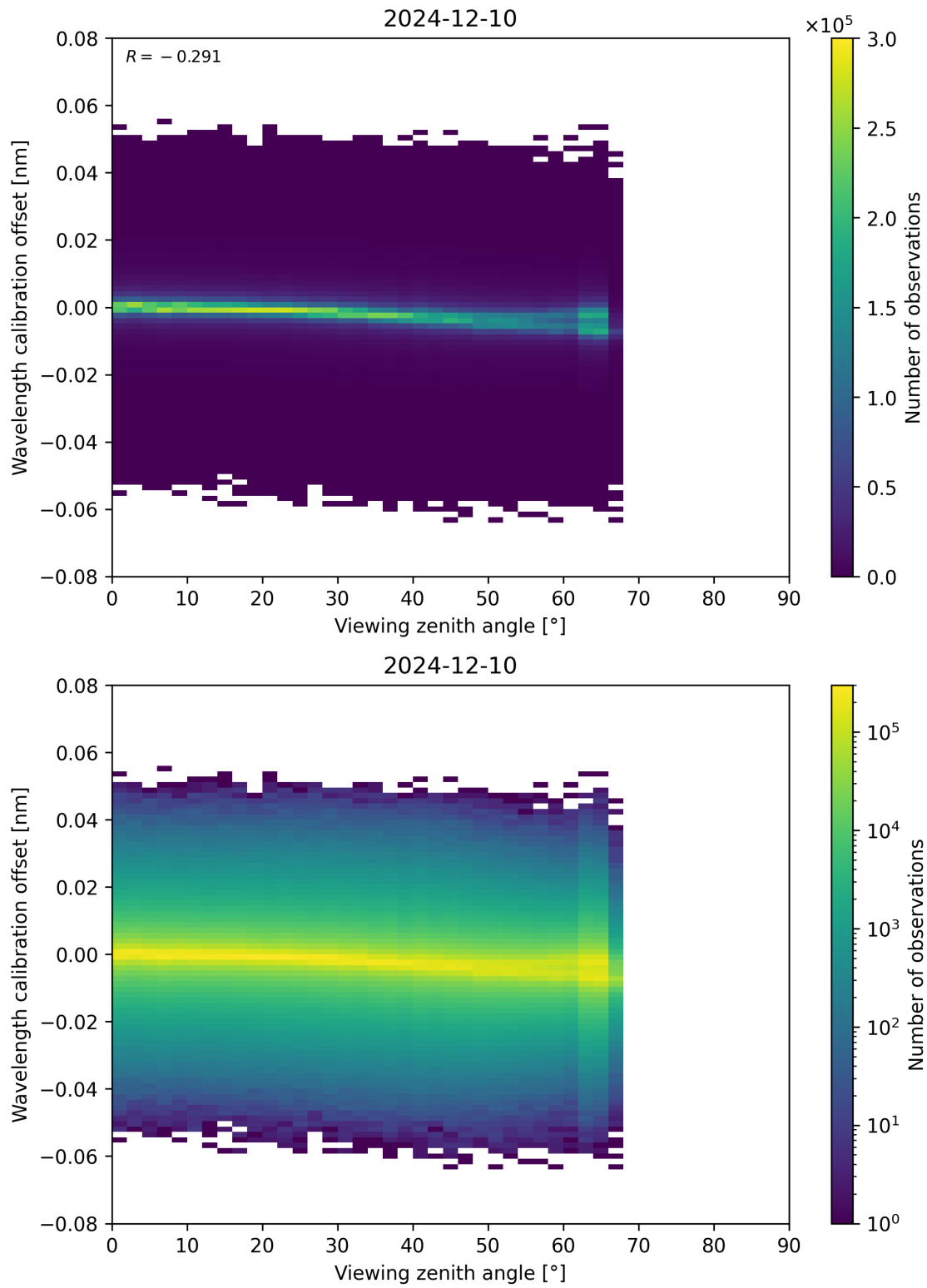
Figure 173: Scatter density plot of “Viewing zenith angle” against “Wavelength calibration offset” for 2024-12-09 to 2024-12-11.
