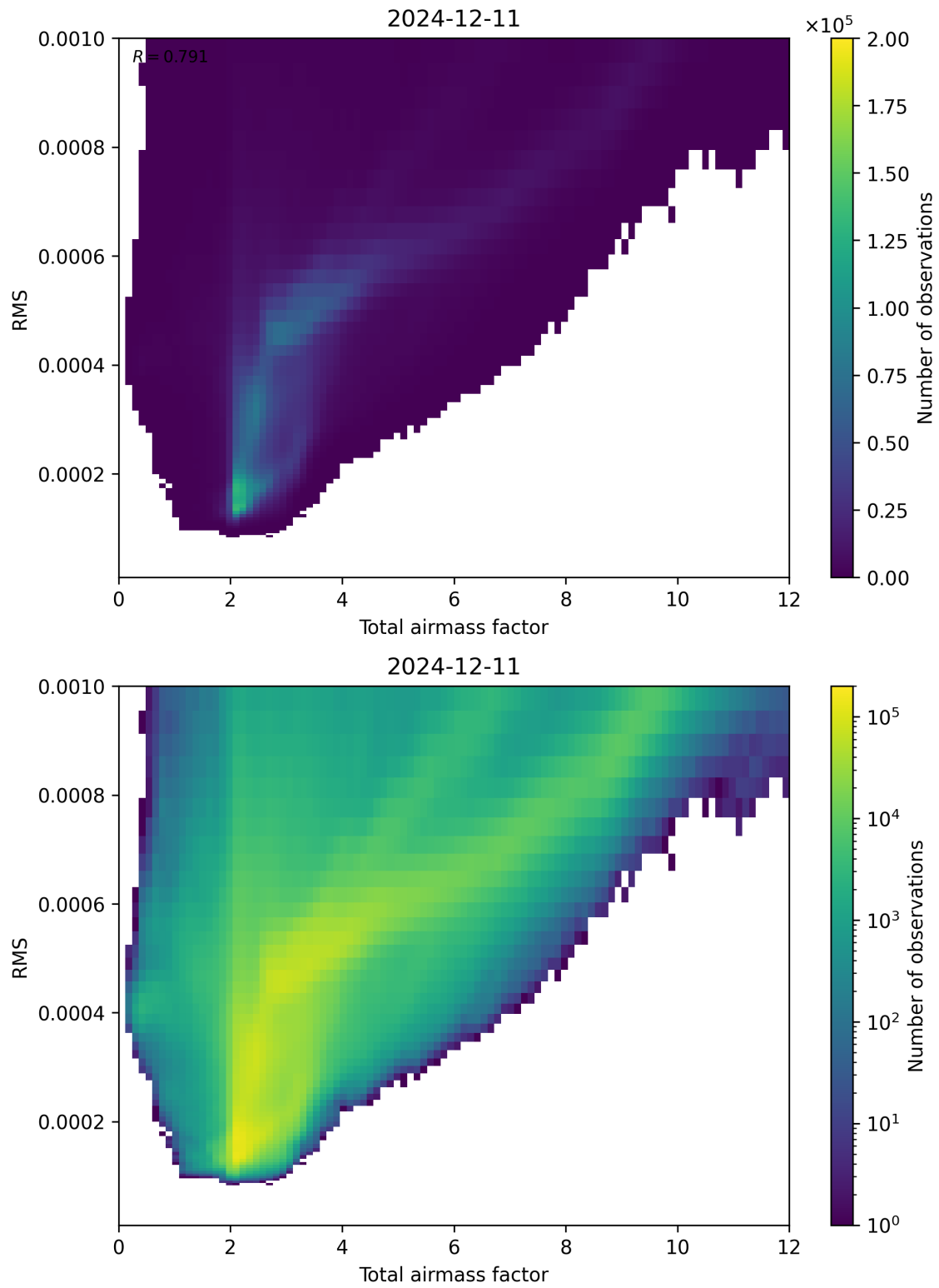
Figure 69: Scatter density plot of “Total airmass factor” against “RMS” for 2024-12-11 to 2024-12-12.
