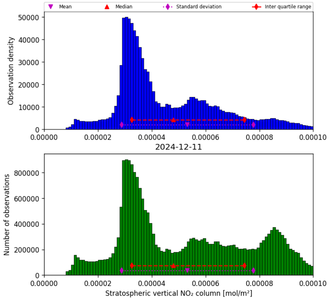
Figure 36: Histogram of “Stratospheric vertical NO 2 column” for 2024-12-11 to 2024-12-12
