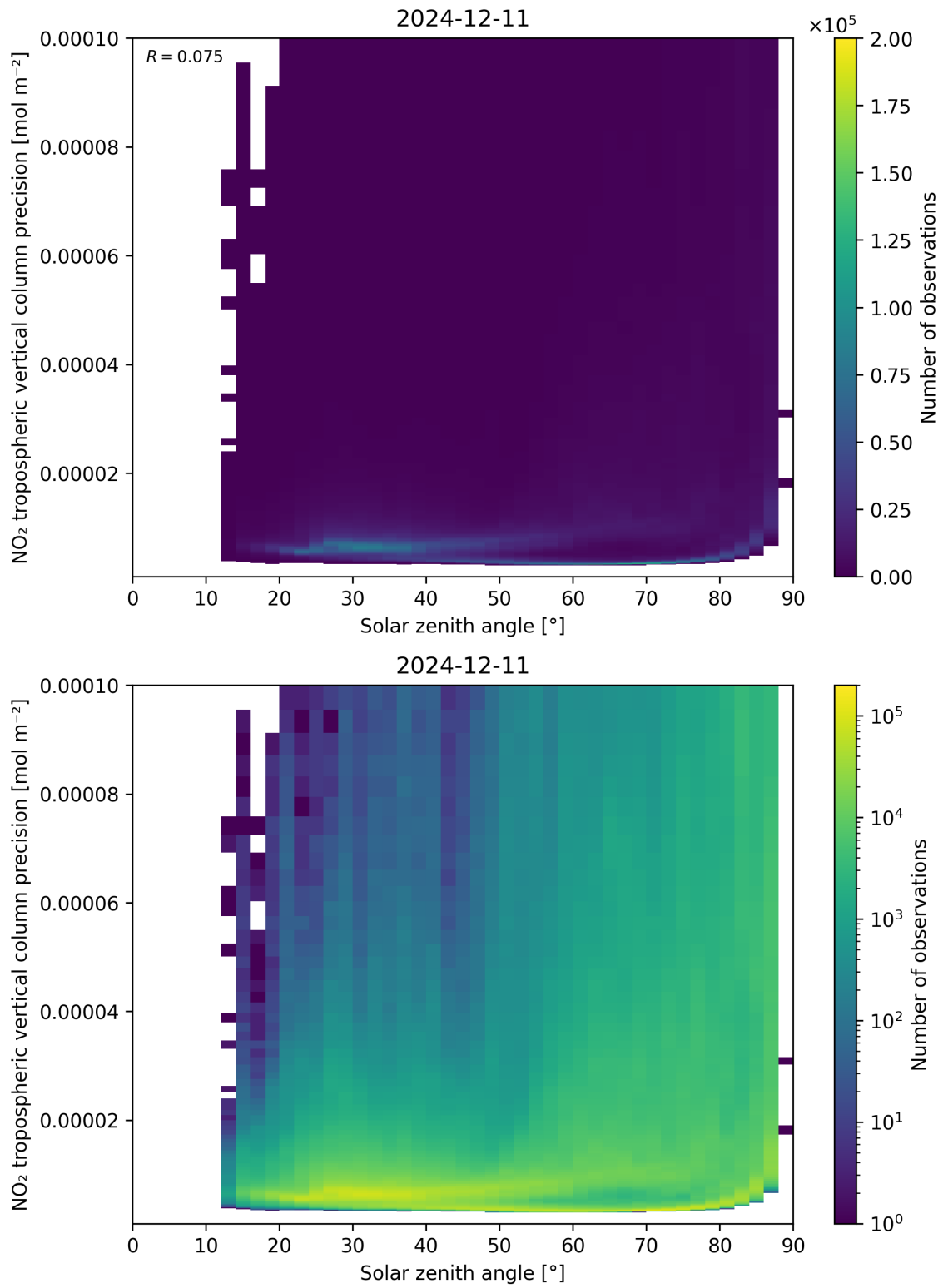
Figure 156: Scatter density plot of “Solar zenith angle” against “NO 2 tropospheric vertical column precision” for 2024-12-11 to 2024-12-12.
