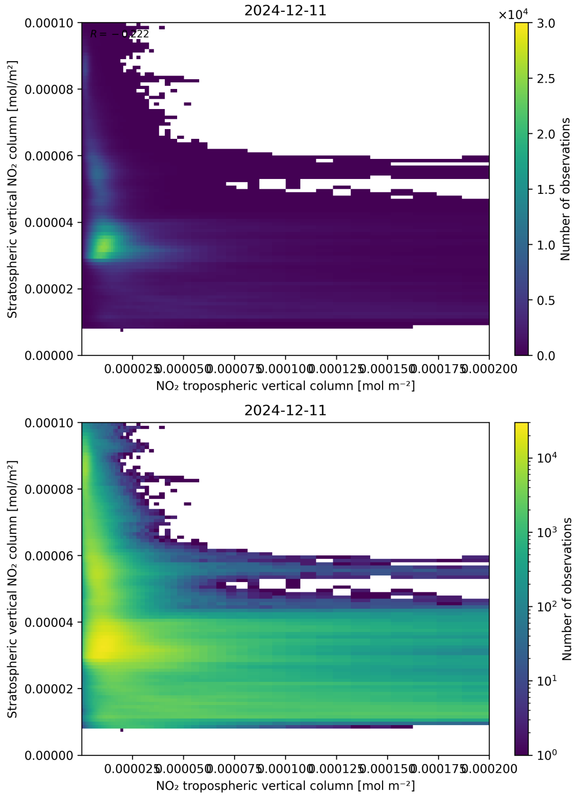
Figure 125: Scatter density plot of “NO 2 tropospheric vertical column” against “Stratospheric vertical NO 2 column” for 2024-12-11 to 2024-12-12.
