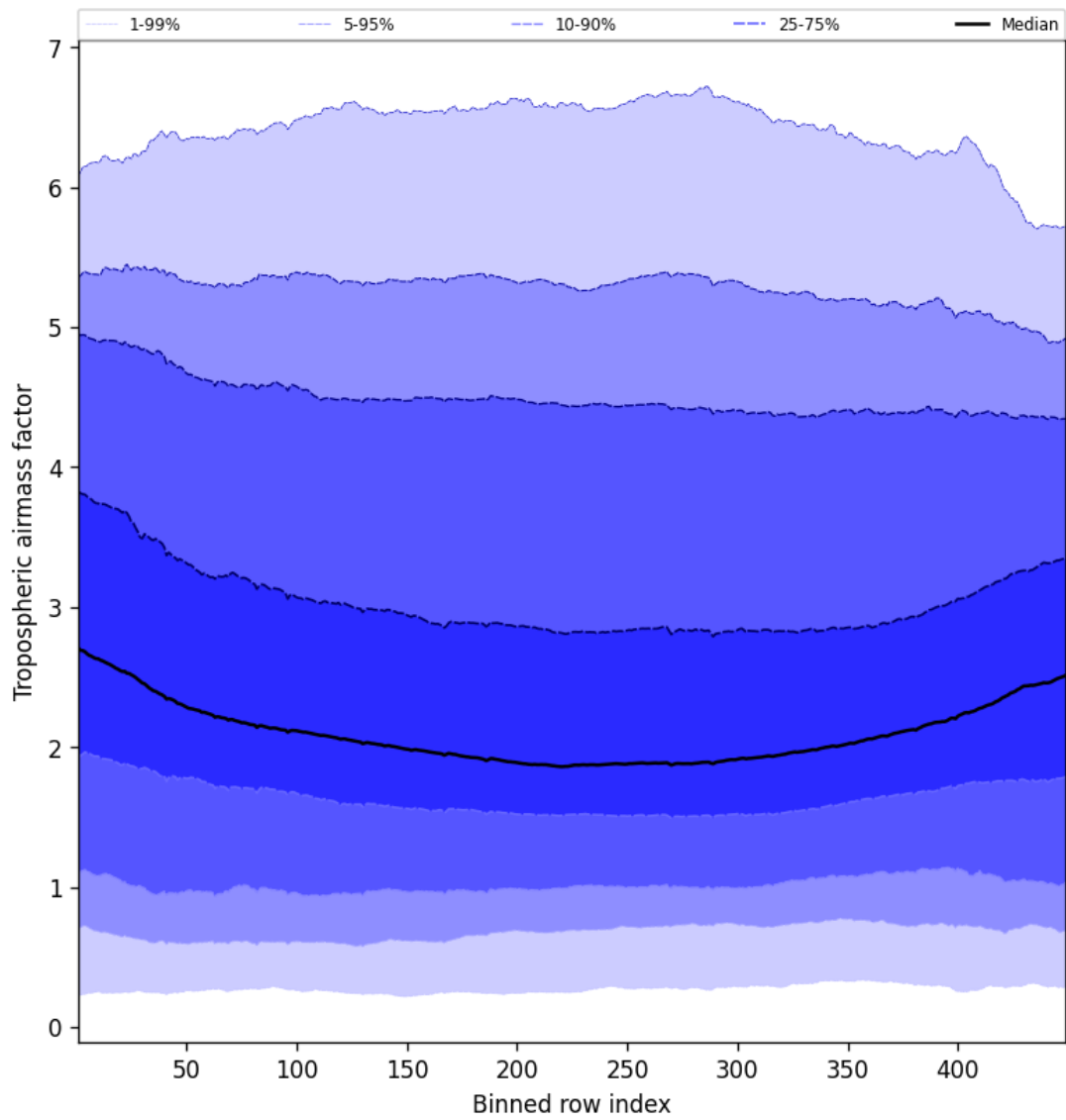
Figure 48: Along track statistics of “Tropospheric airmass factor” for 2024-12-11 to 2024-12-12
