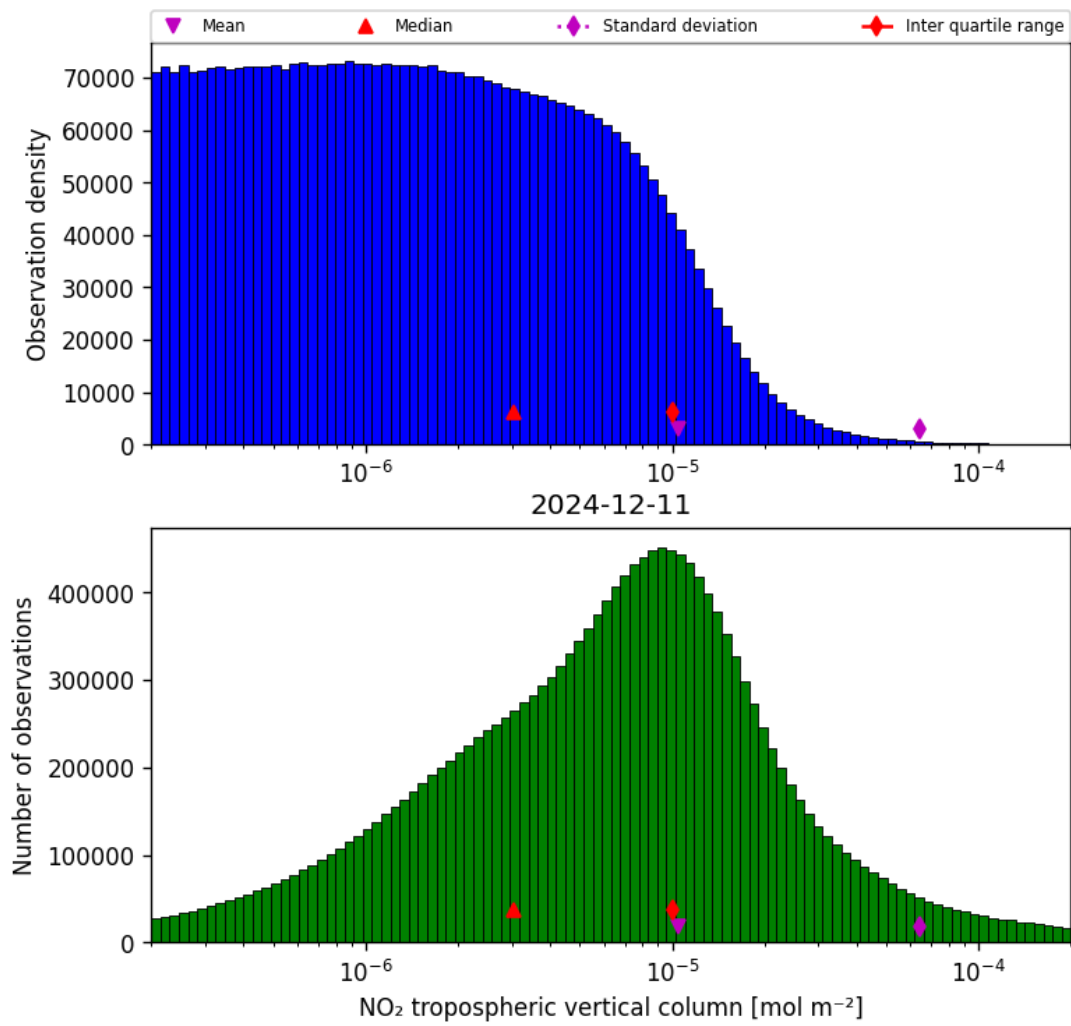
Figure 29: Histogram of “NO 2 tropospheric vertical column” for 2024-12-11 to 2024-12-12
