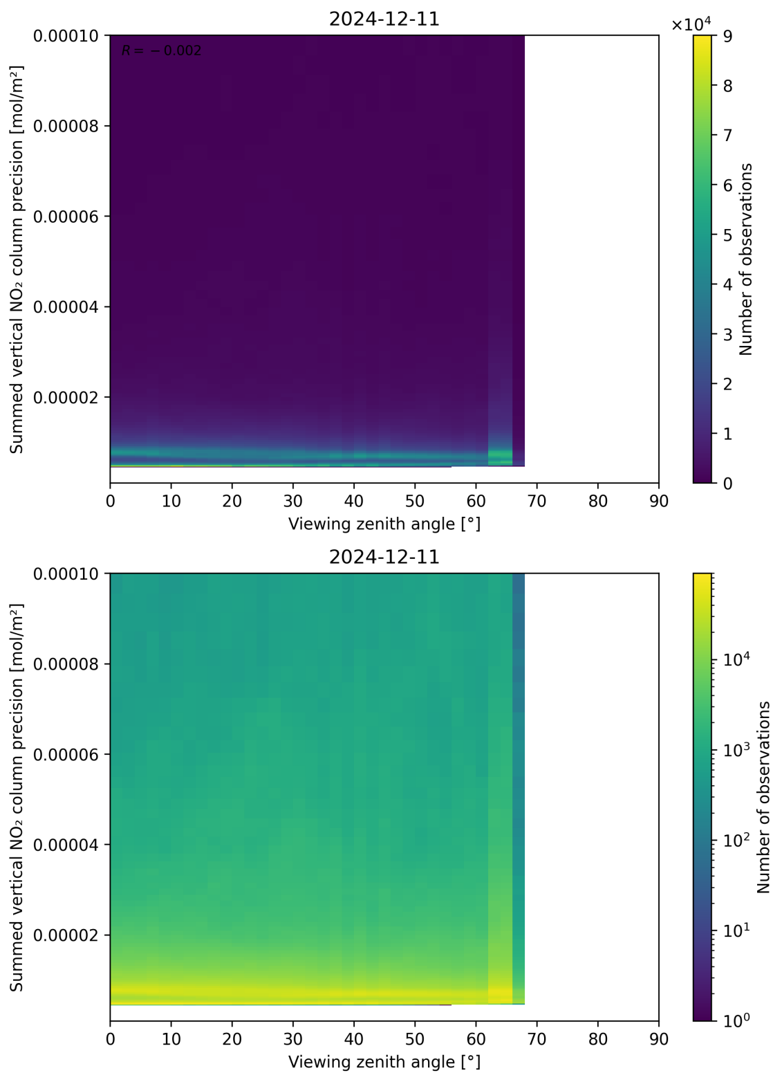
Figure 166: Scatter density plot of “Viewing zenith angle” against “Summed vertical NO 2 column precision” for 2024-12-11 to 2024-12-12.
