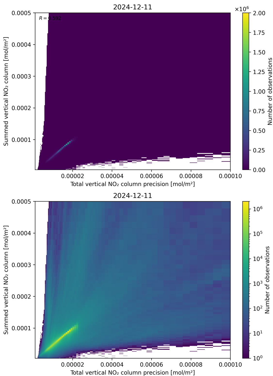
Figure 117: Scatter density plot of “Total vertical NO 2 column precision” against “Summed vertical NO 2 column” for 2024-12-11 to 2024-12-12.
