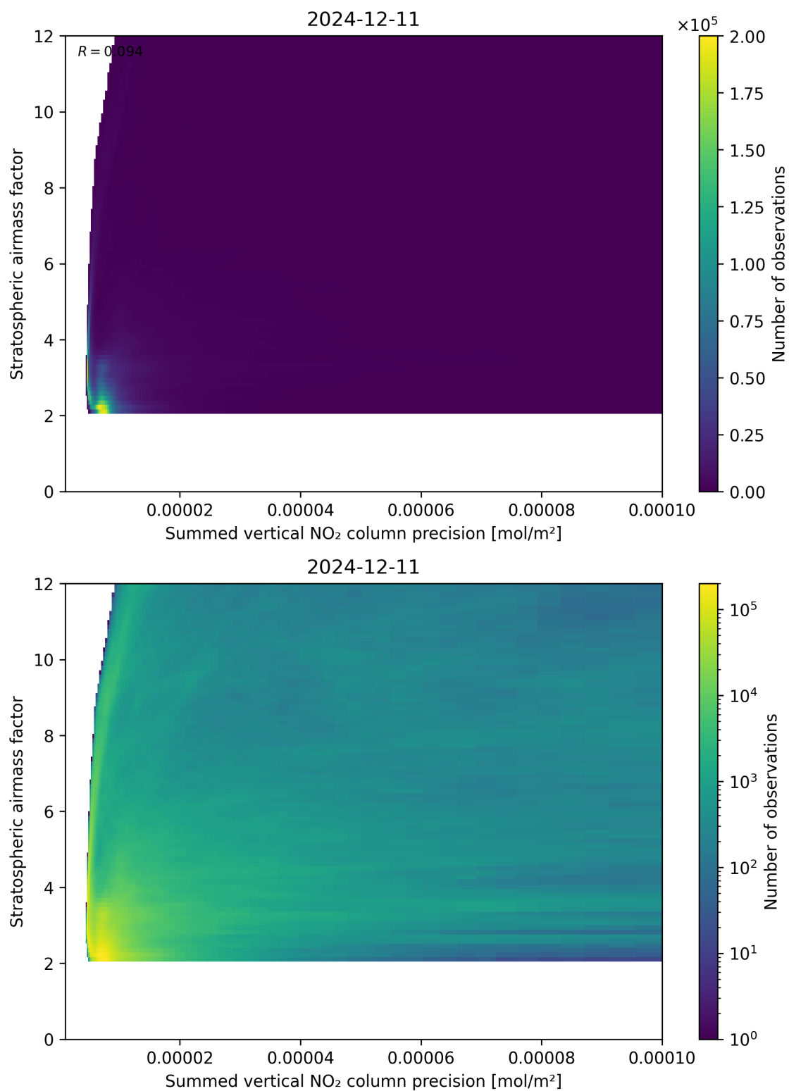
Figure 106: Scatter density plot of “Summed vertical NO 2 column precision” against “Stratospheric airmass factor” for 2024-12-11 to 2024-12-12.
