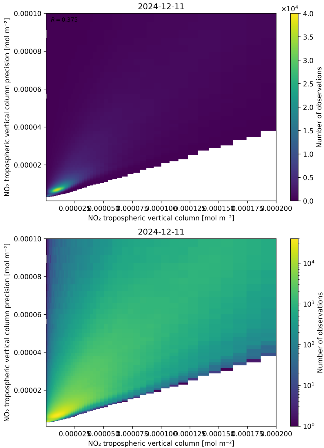
Figure 130: Scatter density plot of “NO 2 tropospheric vertical column” against “NO 2 tropospheric vertical column precision” for 2024-12-11 to 2024-12-12.
