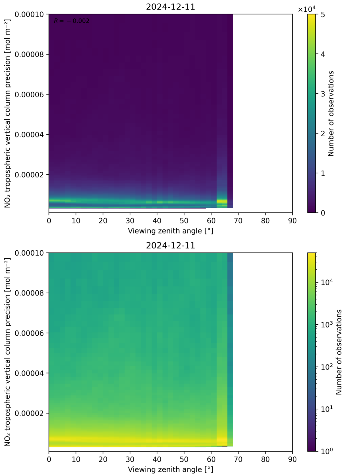
Figure 170: Scatter density plot of “Viewing zenith angle” against “NO 2 tropospheric vertical column precision” for 2024-12-11 to 2024-12-12.
