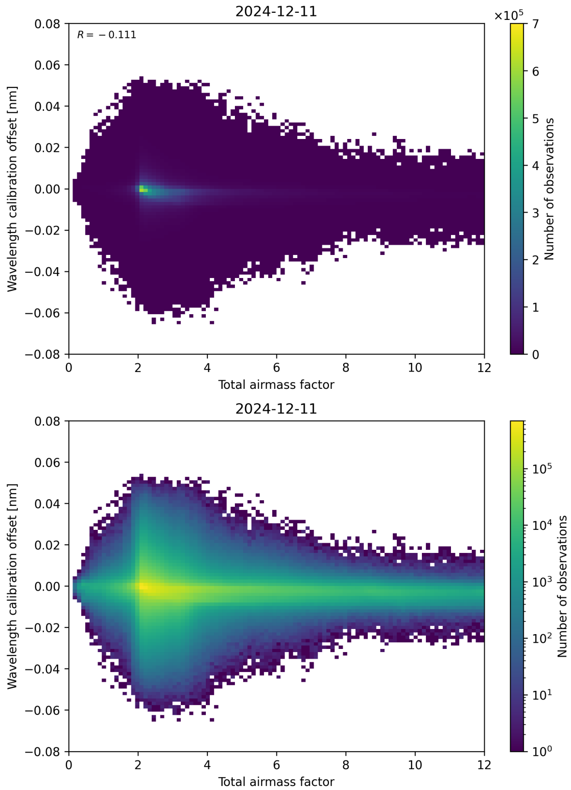
Figure 70: Scatter density plot of “Total airmass factor” against “Wavelength calibration offset” for 2024-12-11 to 2024-12-12.
