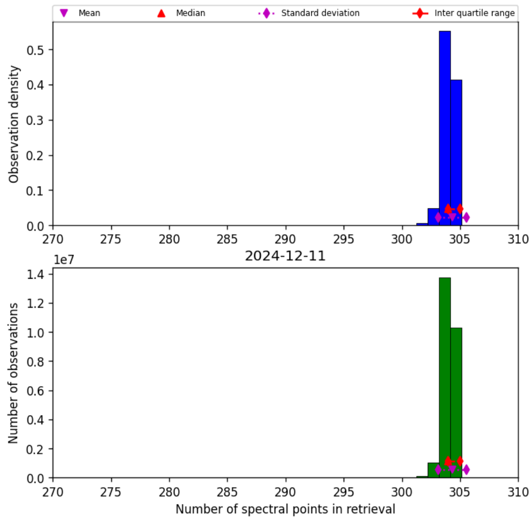
Figure 33: Histogram of “Number of spectral points in retrieval” for 2024-12-11 to 2024-12-12
