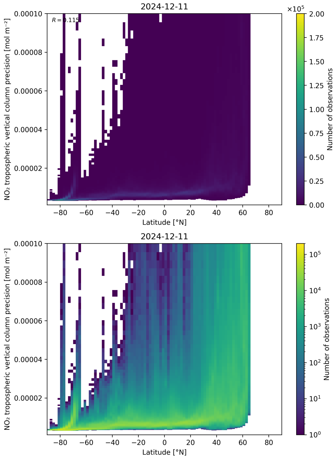
Figure 93: Scatter density plot of “Latitude” against “NO 2 tropospheric vertical column precision” for 2024-12-11 to 2024-12-12.
