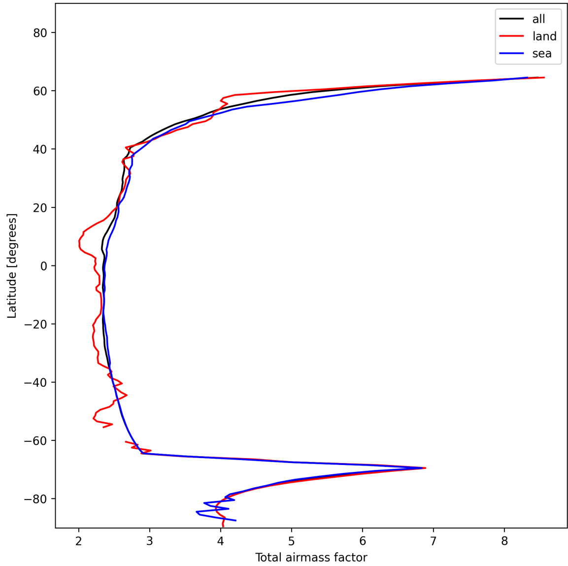
Figure 15: Zonal average of “Total airmass factor” for 2024-12-11 to 2024-12-12.
