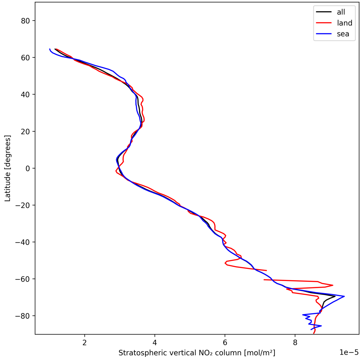
Figure 19: Zonal average of “Stratospheric vertical NO 2 column” for 2024-12-11 to 2024-12-12.
