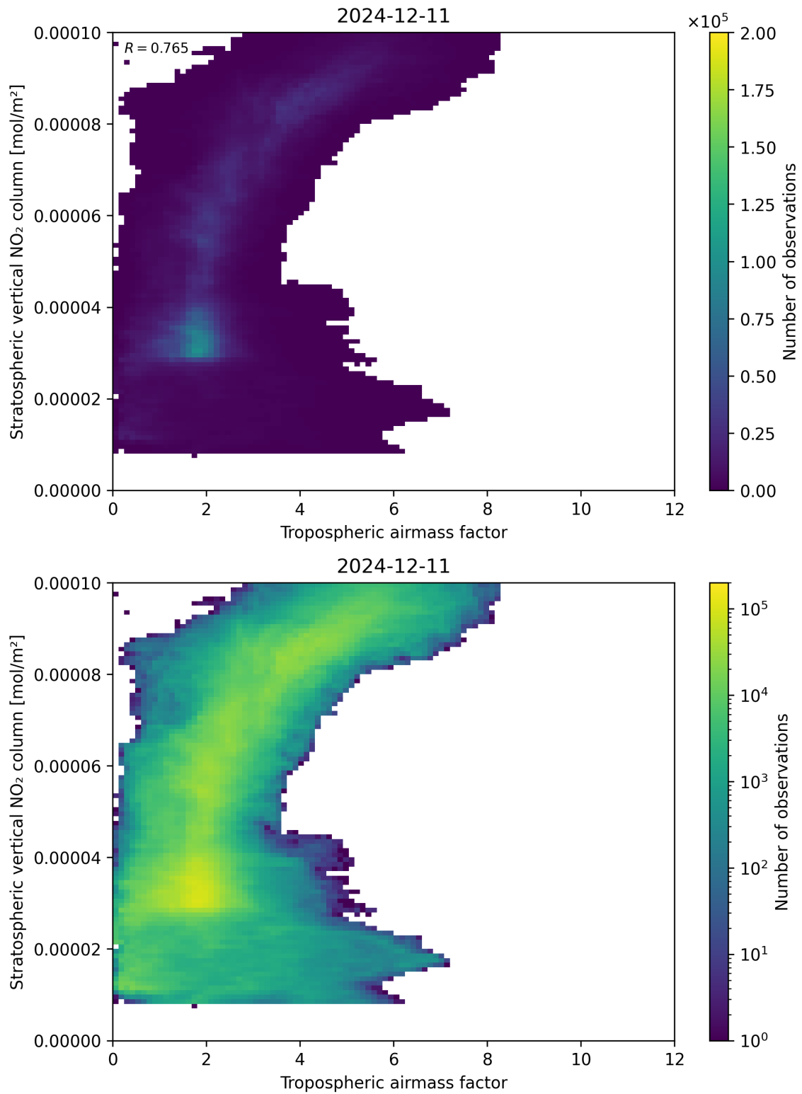
Figure 74: Scatter density plot of “Tropospheric airmass factor” against “Stratospheric vertical NO 2 column” for 2024-12-11 to 2024-12-12.
