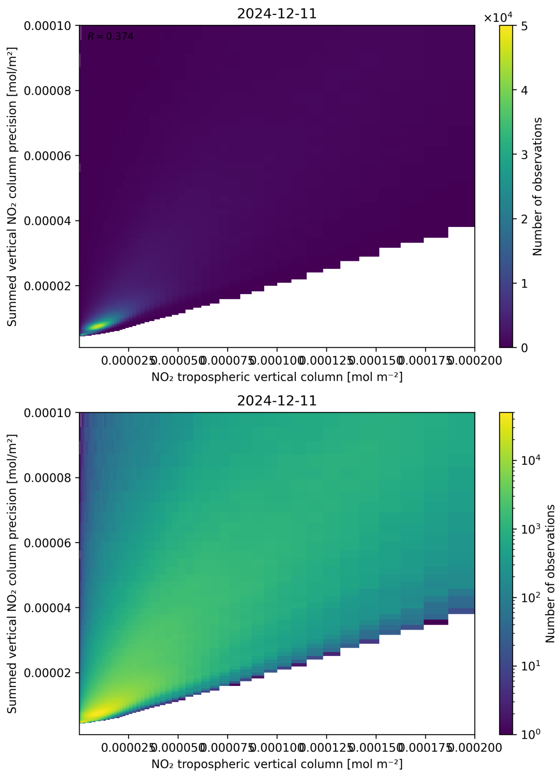
Figure 127: Scatter density plot of “NO 2 tropospheric vertical column” against “Summed vertical NO 2 column precision” for 2024-12-11 to 2024-12-12.
