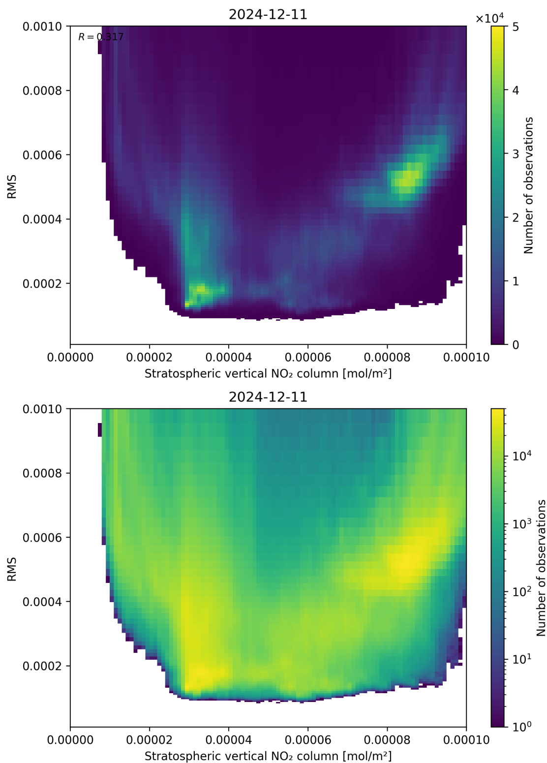
Figure 102: Scatter density plot of “Stratospheric vertical NO 2 column” against “RMS” for 2024-12-11 to 2024-12-12.
