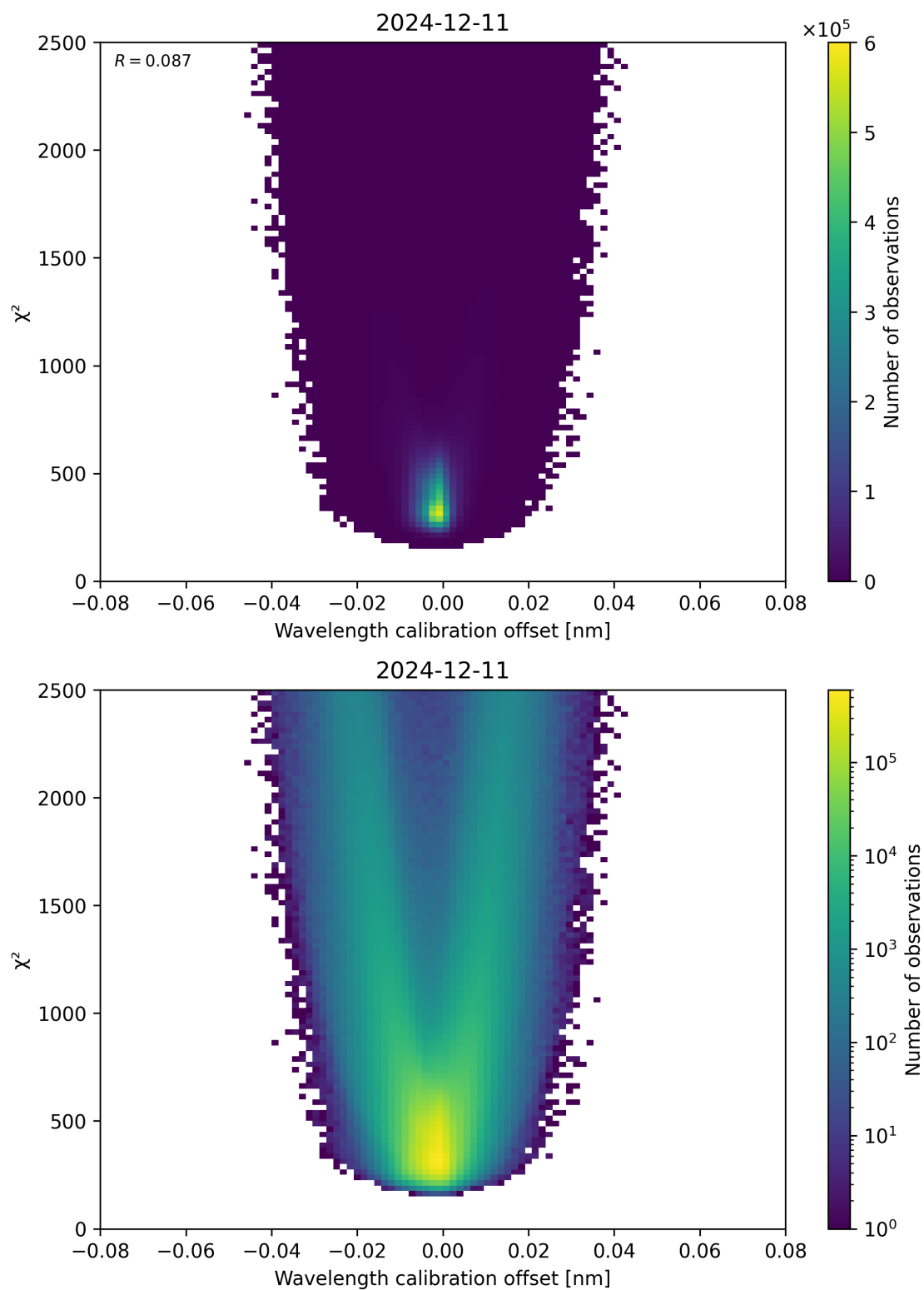
Figure 175: Scatter density plot of “Wavelength calibration offset” against “ \chi^2 ” for 2024-12-11 to 2024-12-12.
