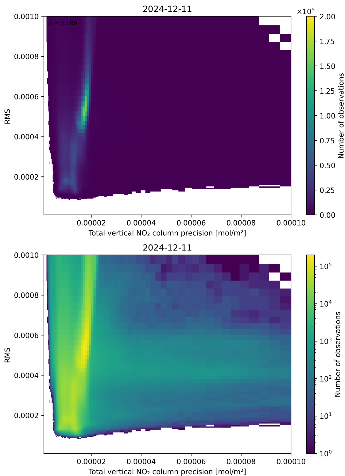
Figure 119: Scatter density plot of “Total vertical NO 2 column precision” against “RMS” for 2024-12-11 to 2024-12-12.
