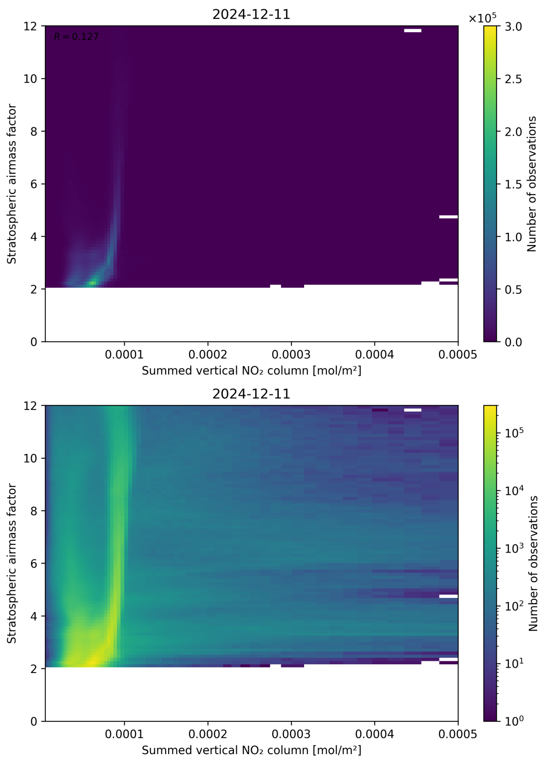
Figure 103: Scatter density plot of “Summed vertical NO 2 column” against “Stratospheric airmass factor” for 2024-12-11 to 2024-12-12.
