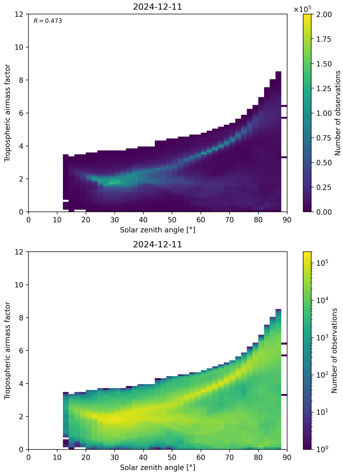
Figure 147: Scatter density plot of “Solar zenith angle” against “Tropospheric airmass factor” for 2024-12-11 to 2024-12-12.
