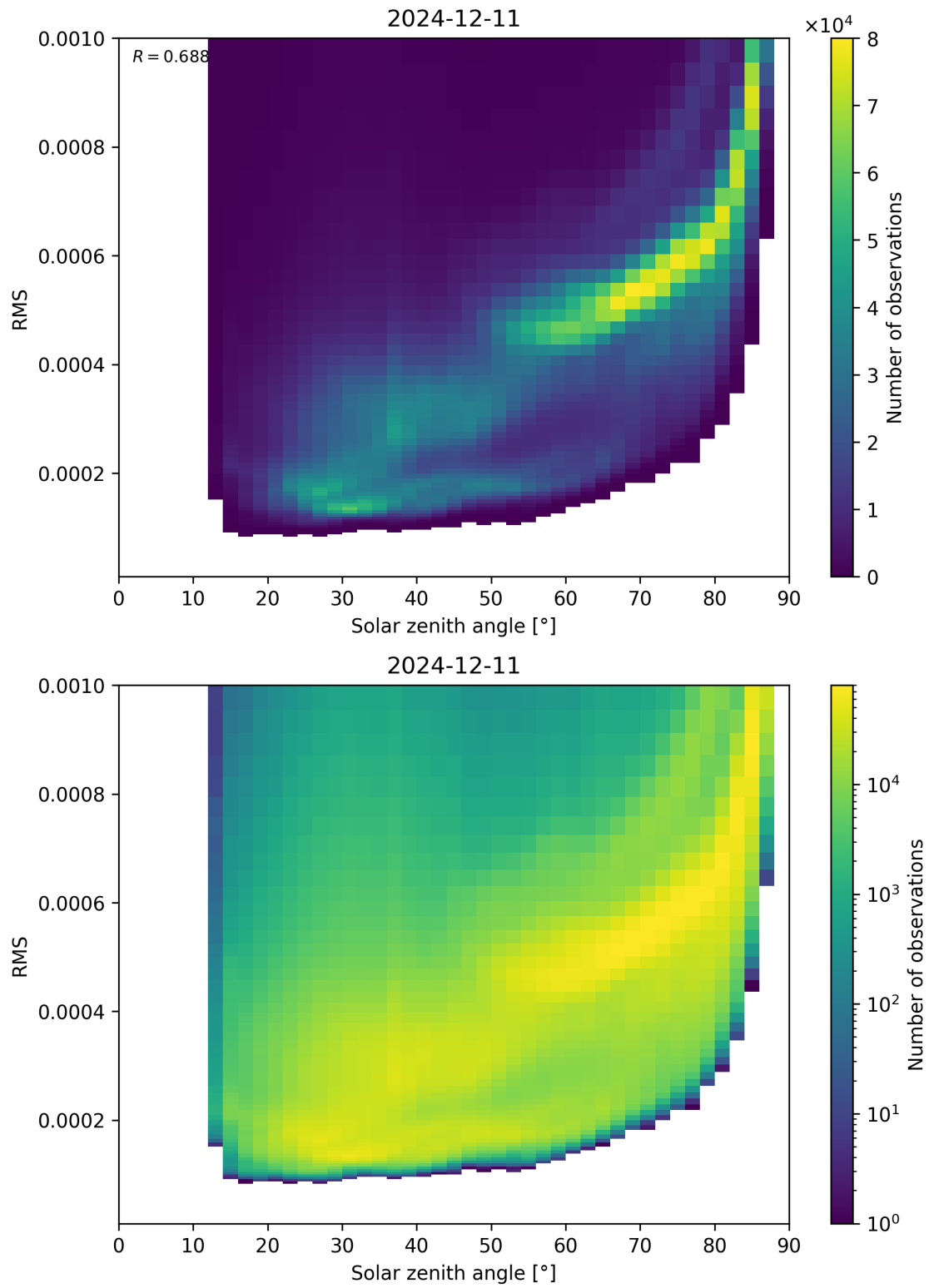
Figure 157: Scatter density plot of “Solar zenith angle” against “RMS” for 2024-12-11 to 2024-12-12.
