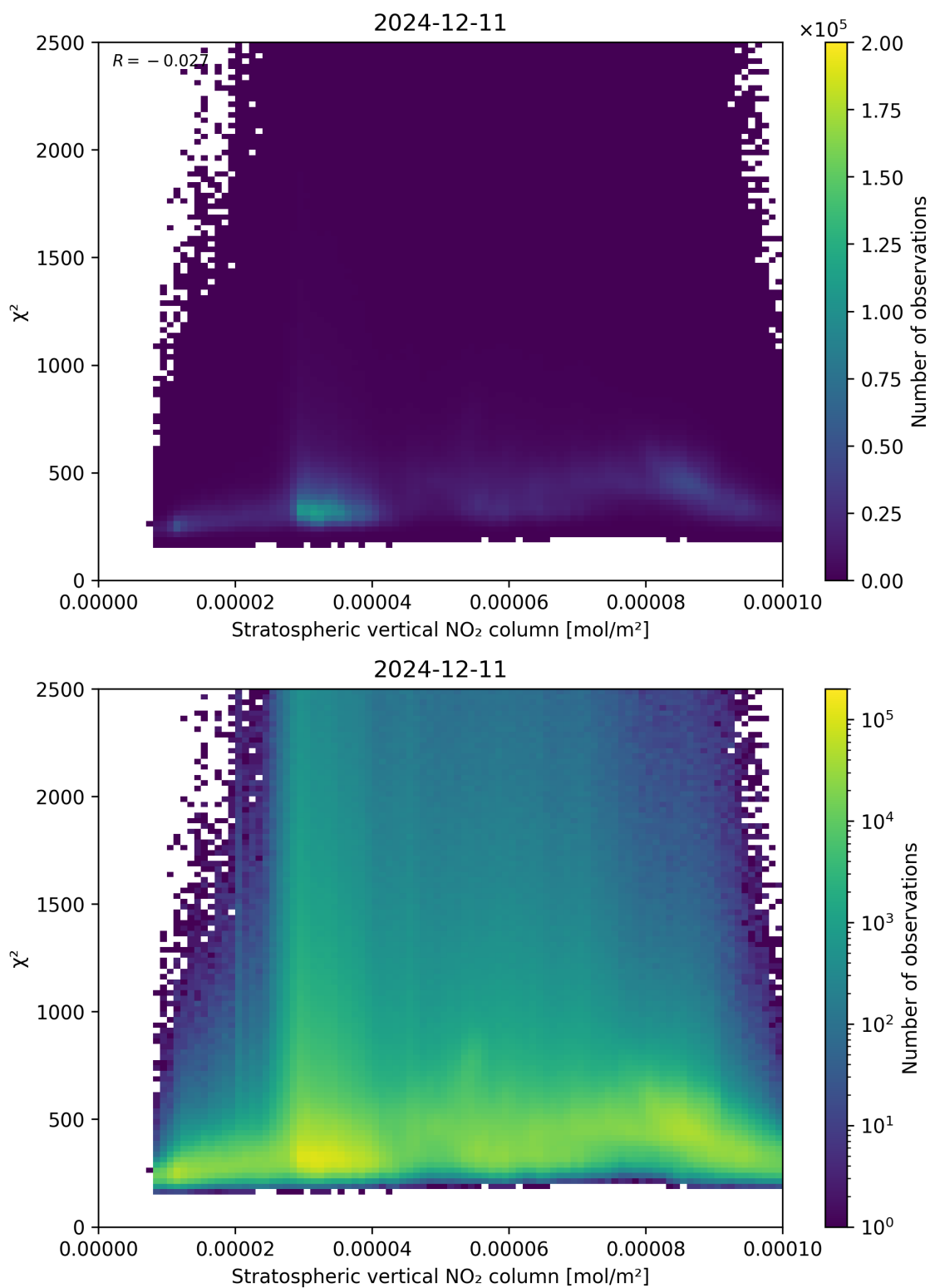
Figure 97: Scatter density plot of “Stratospheric vertical NO 2 column” against “ \chi^2 ” for 2024-12-11 to 2024-12-12.
