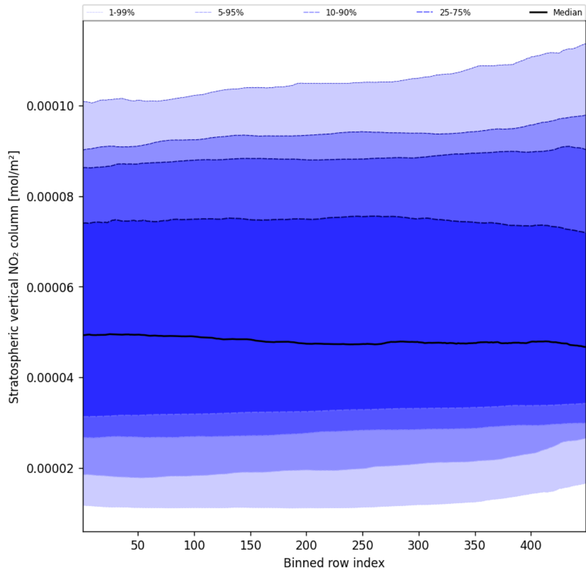
Figure 53: Along track statistics of “Stratospheric vertical NO 2 column” for 2024-12-11 to 2024-12-12
