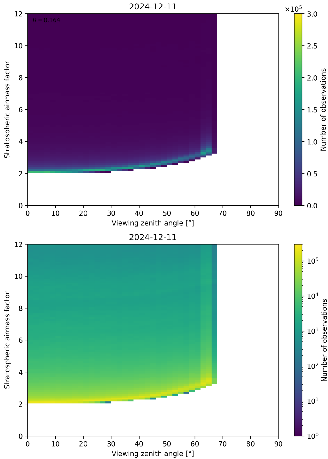
Figure 159: Scatter density plot of “Viewing zenith angle” against “Stratospheric airmass factor” for 2024-12-11 to 2024-12-12.
