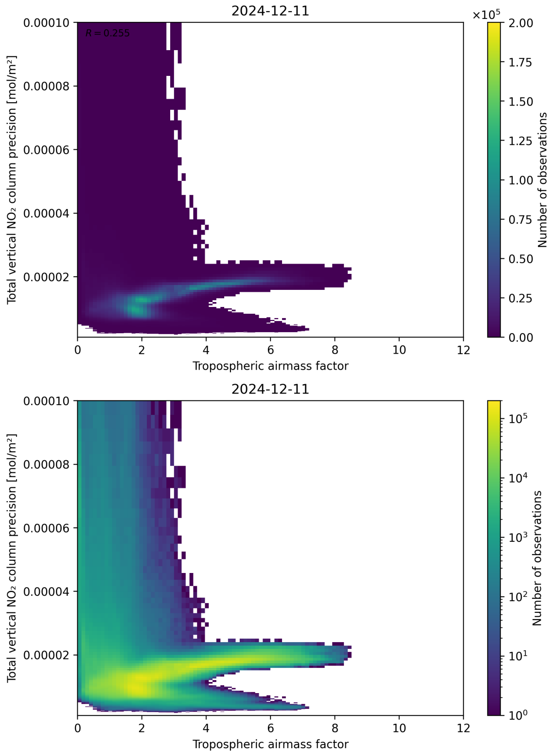
Figure 78: Scatter density plot of “Tropospheric air mass factor” against “Total vertical NO 2 column precision” for 2024-12-11 to 2024-12-12.
