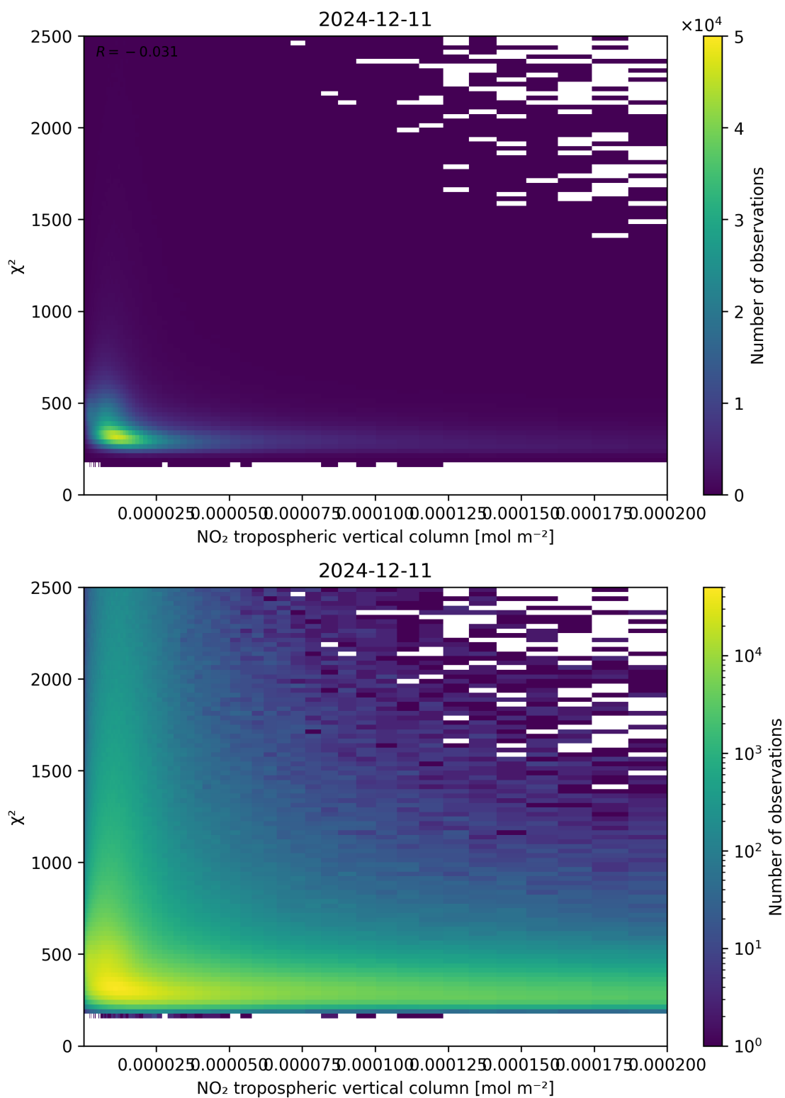
Figure 124: Scatter density plot of “NO 2 tropospheric vertical column” against “ \chi^2 ” for 2024-12-11 to 2024-12-12.
