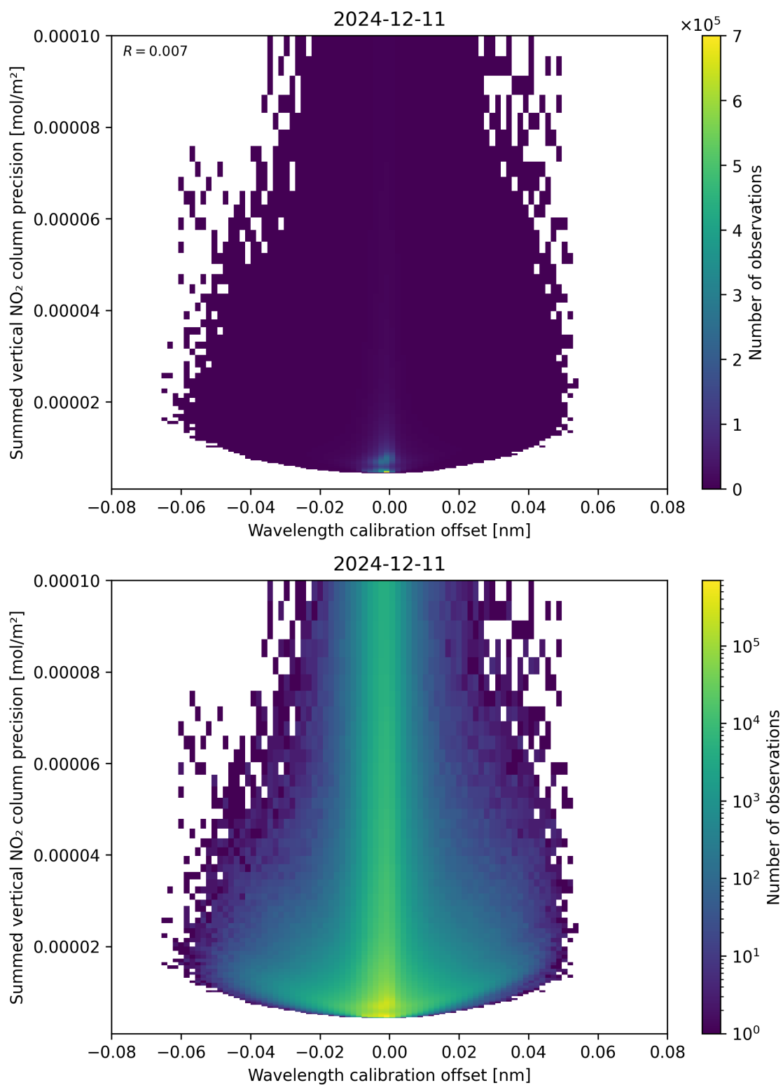
Figure 178: Scatter density plot of “Wavelength calibration offset” against “Summed vertical NO 2 column precision” for 2024-12-11 to 2024-12-12.
