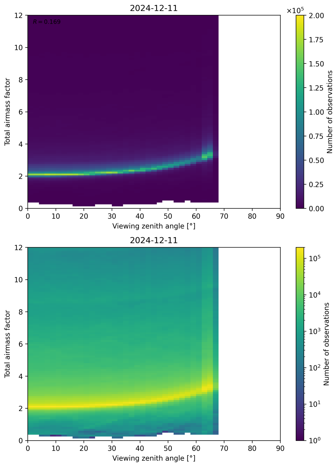
Figure 160: Scatter density plot of “Viewing zenith angle” against “Total airmass factor” for 2024-12-11 to 2024-12-12.
