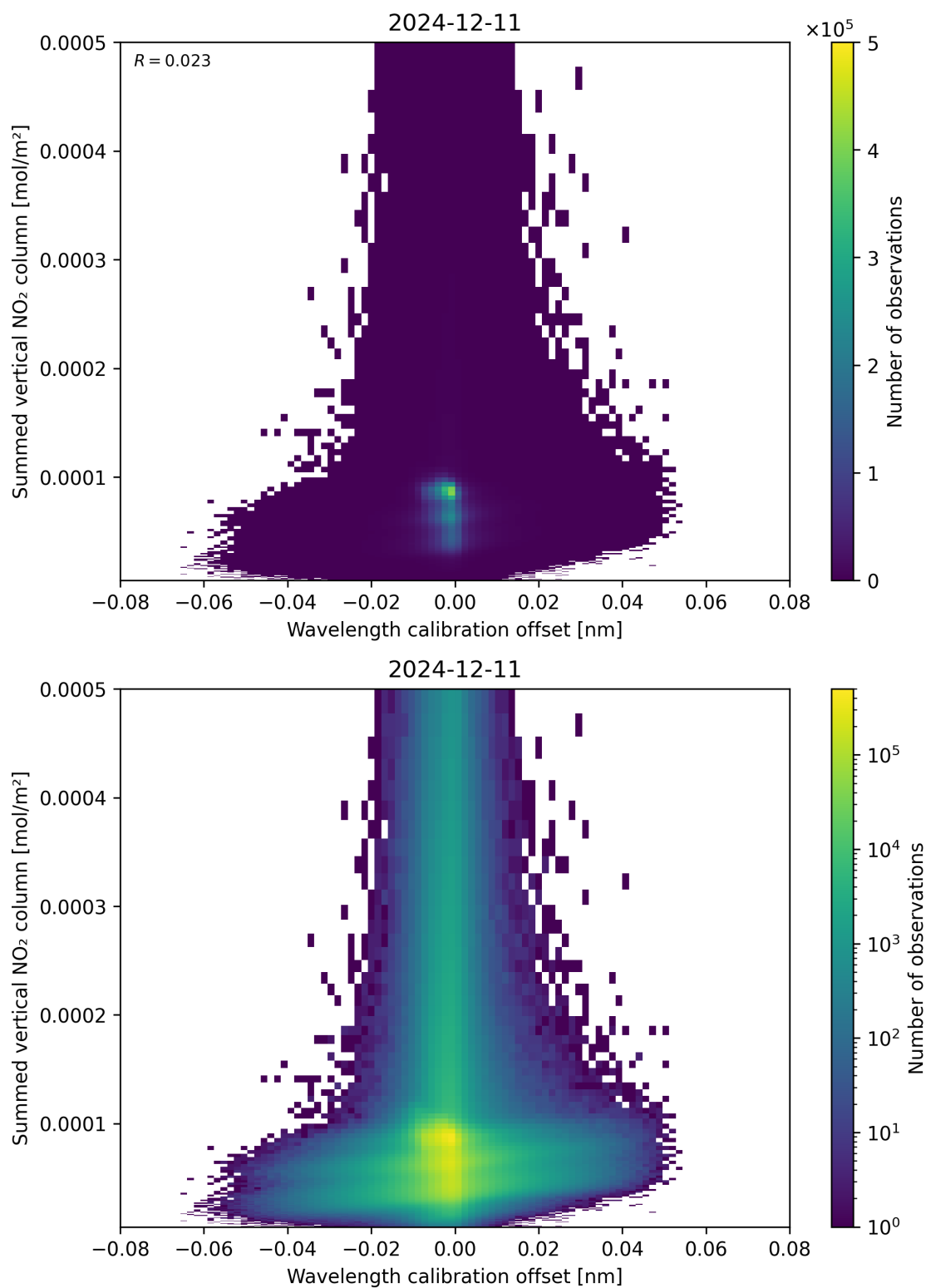
Figure 177: Scatter density plot of “Wavelength calibration offset” against “Summed vertical NO 2 column” for 2024-12-11 to 2024-12-12.
