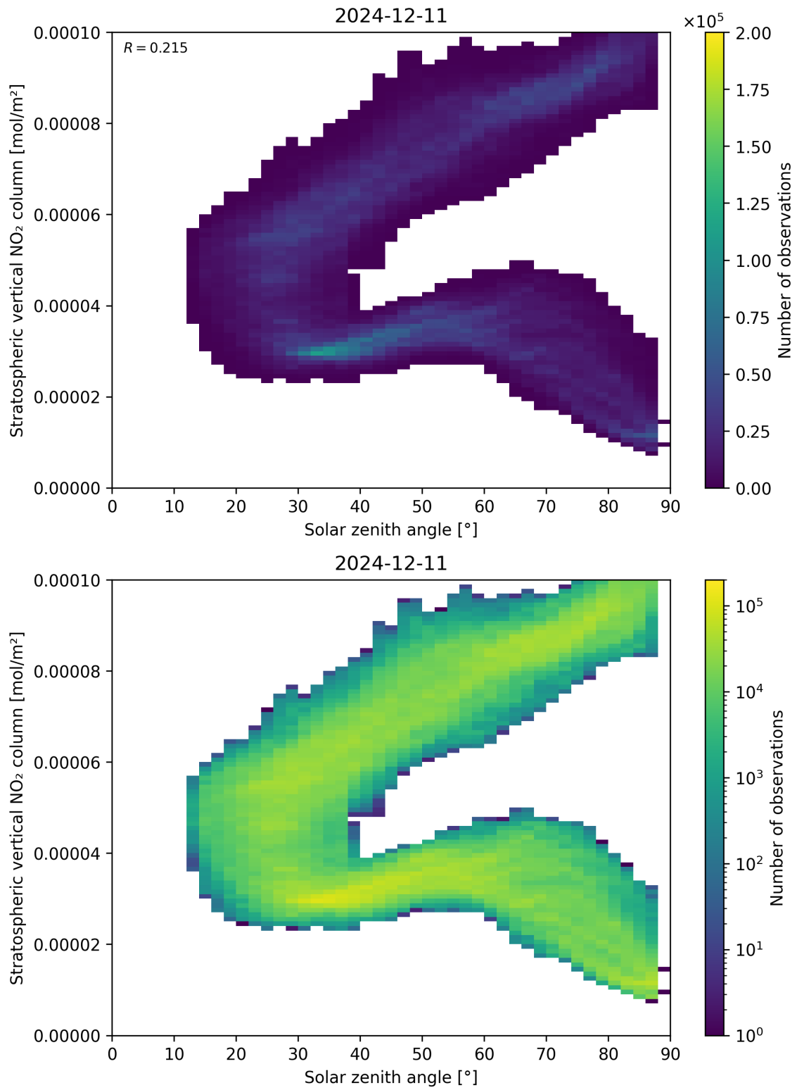
Figure 150: Scatter density plot of “Solar zenith angle” against “Stratospheric vertical NO 2 column” for 2024-12-11 to 2024-12-12.
