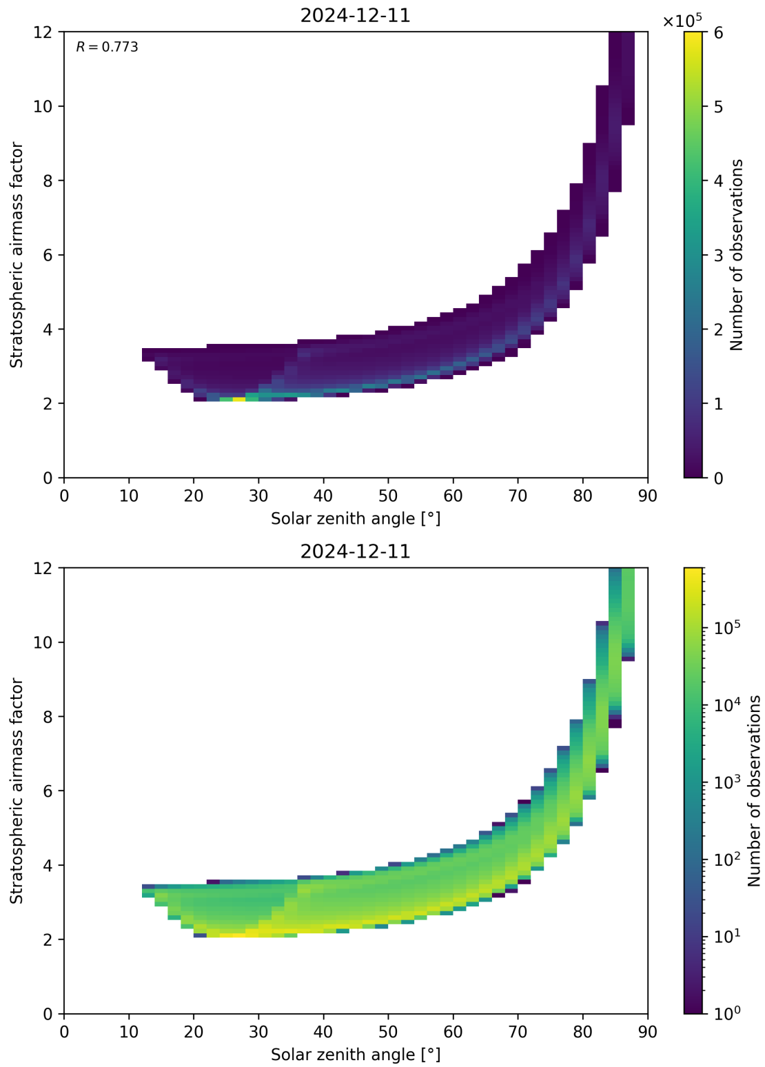
Figure 145: Scatter density plot of “Solar zenith angle” against “Stratospheric airmass factor” for 2024-12-11 to 2024-12-12.
