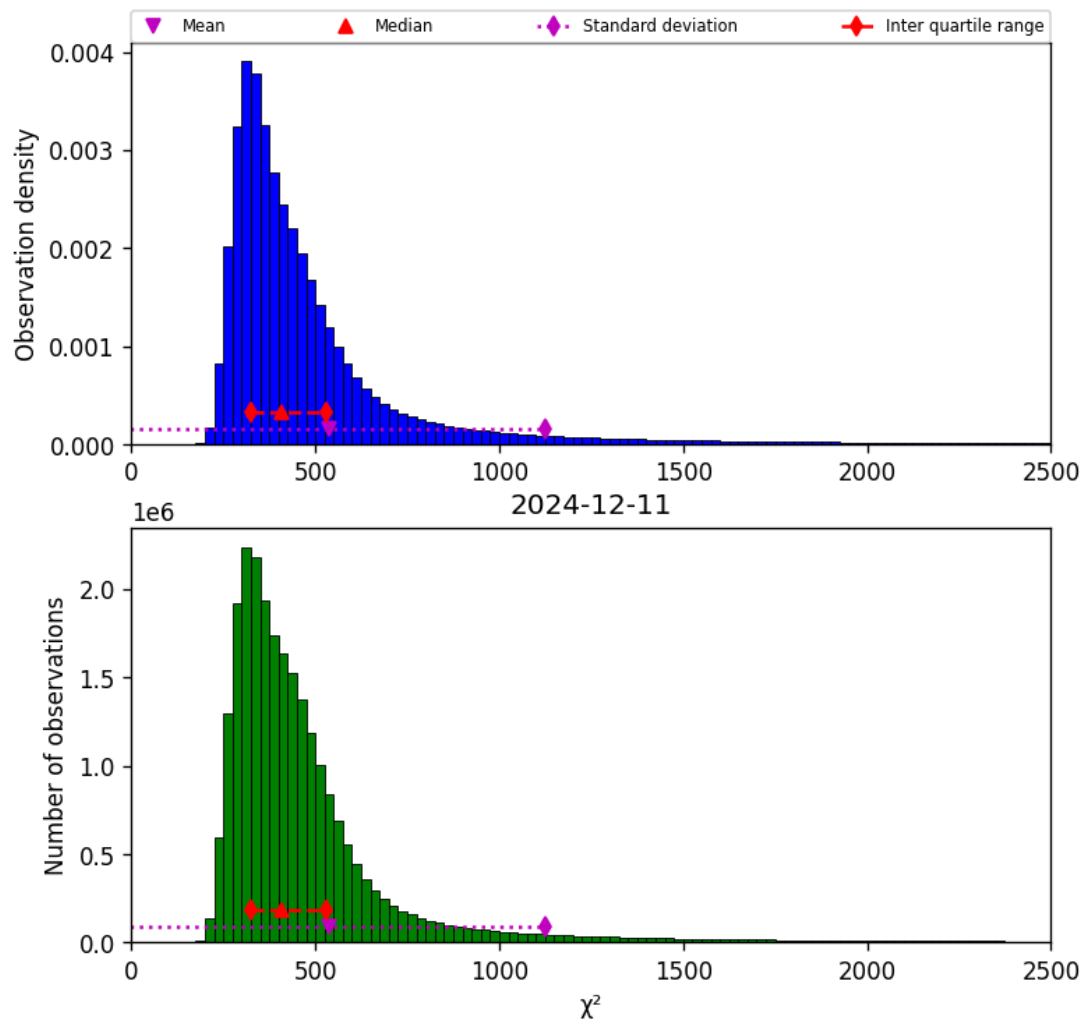
Figure 42: Histogram of “ \chi^2 ” for 2024-12-11 to 2024-12-12
