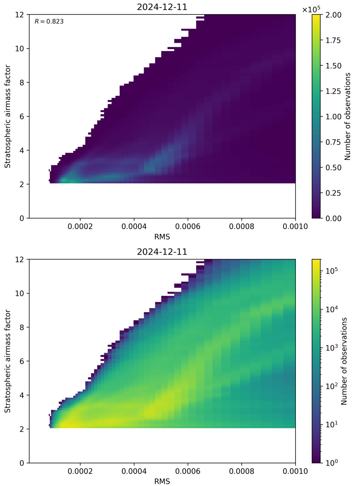
Figure 144: Scatter density plot of “RMS” against “Stratospheric airmass factor” for 2024-12-11 to 2024-12-12.
