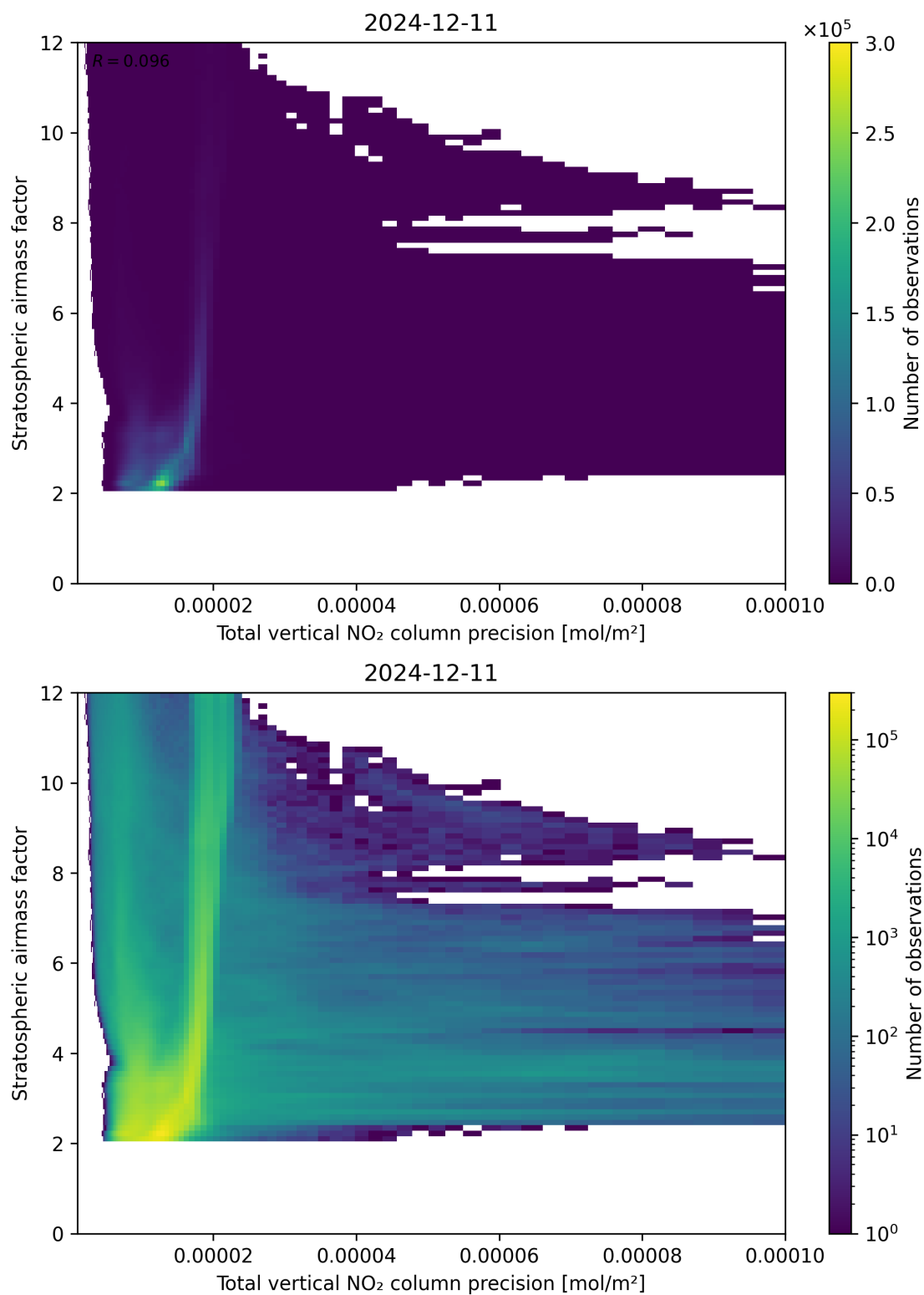
Figure 115: Scatter density plot of “Total vertical NO 2 column precision” against “Stratospheric air mass factor” for 2024-12-11 to 2024-12-12.
