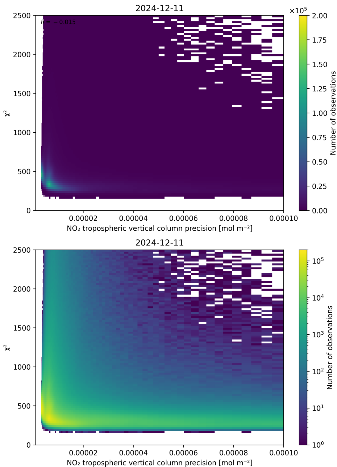
Figure 134: Scatter density plot of “NO 2 tropospheric vertical column precision” against “ \chi^2 ” for 2024-12-11 to 2024-12-12.
