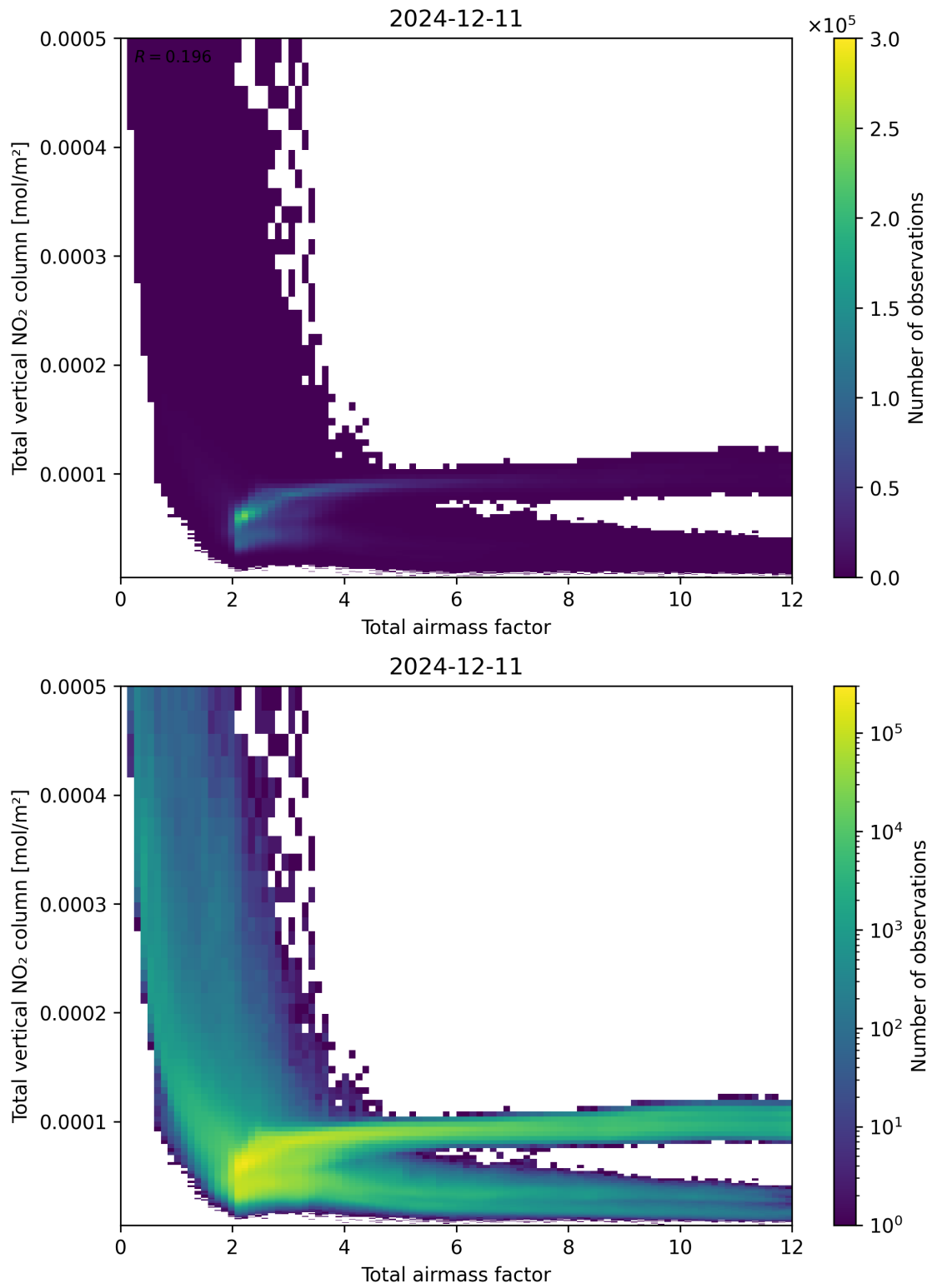
Figure 67: Scatter density plot of “Total airmass factor” against “Total vertical NO 2 column” for 2024-12-11 to 2024-12-12.
