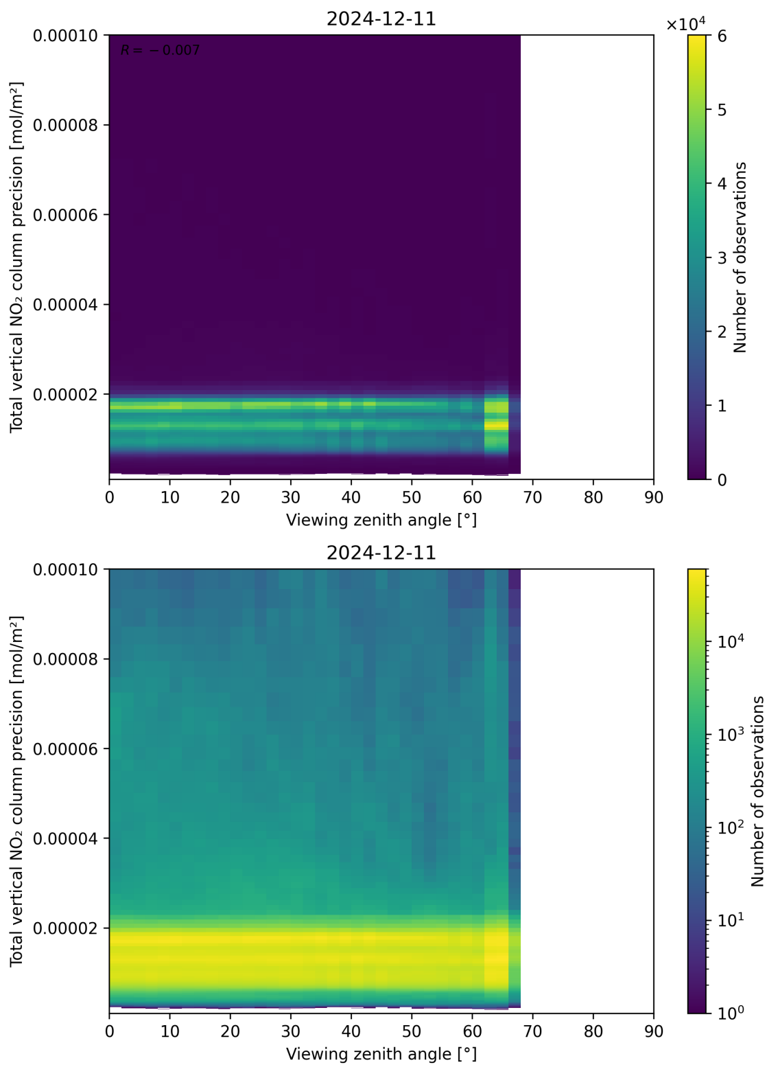
Figure 168: Scatter density plot of “Viewing zenith angle” against “Total vertical NO 2 column precision” for 2024-12-11 to 2024-12-12.
