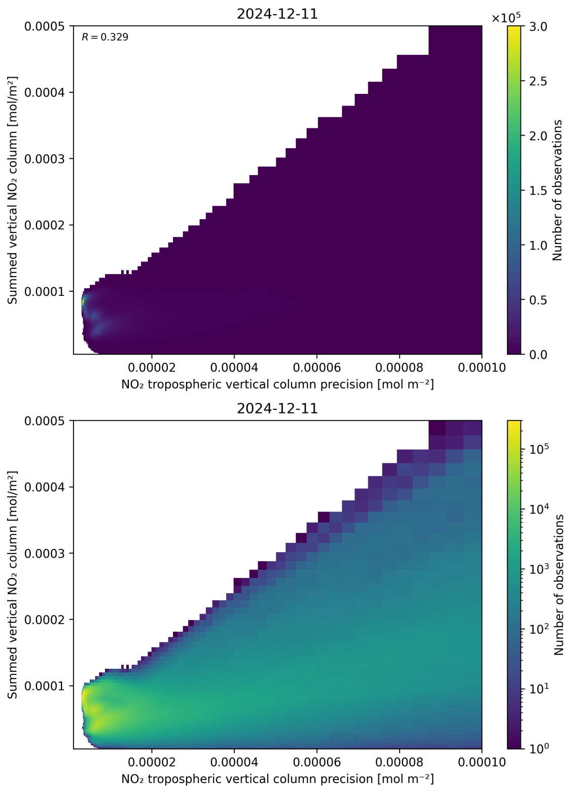
Figure 136: Scatter density plot of “NO 2 tropospheric vertical column precision” against “Summed vertical NO 2 column” for 2024-12-11 to 2024-12-12.
