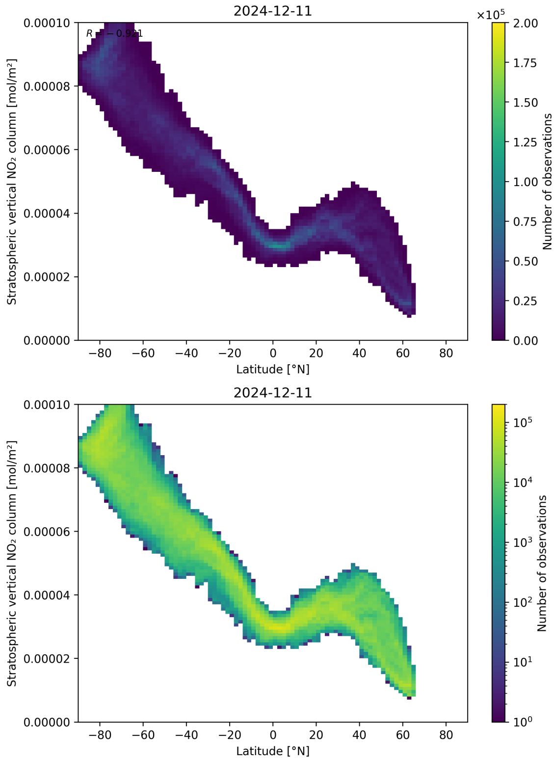
Figure 87: Scatter density plot of “Latitude” against “Stratospheric vertical NO 2 column” for 2024-12-11 to 2024-12-12.
