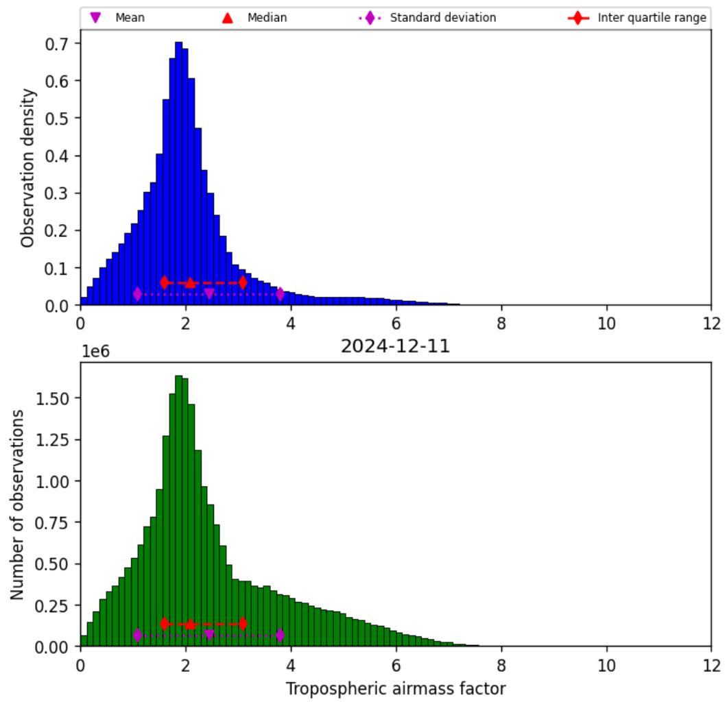
Figure 31: Histogram of “Tropospheric airmass factor” for 2024-12-11 to 2024-12-12
