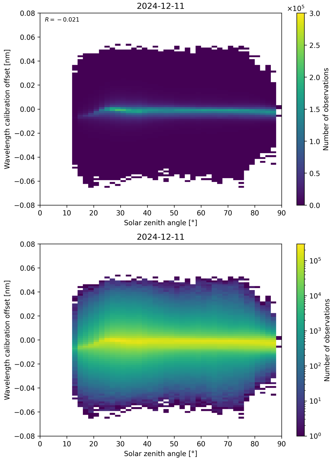
Figure 158: Scatter density plot of “Solar zenith angle” against “Wavelength calibration offset” for 2024-12-11 to 2024-12-12.
