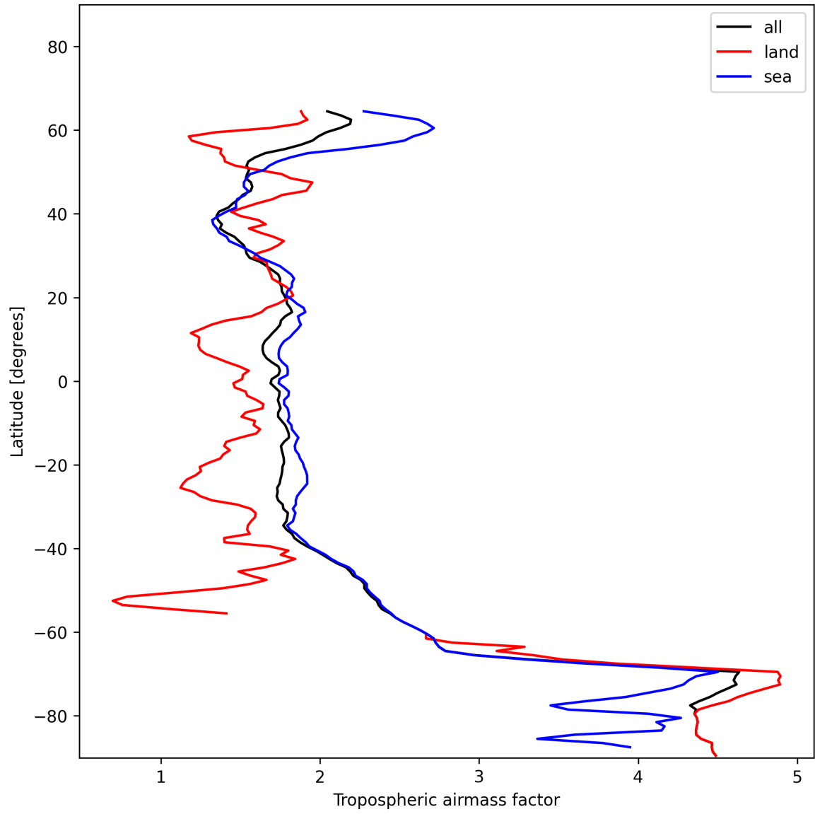
Figure 14: Zonal average of “Tropospheric airmass factor” for 2024-12-11 to 2024-12-12.
