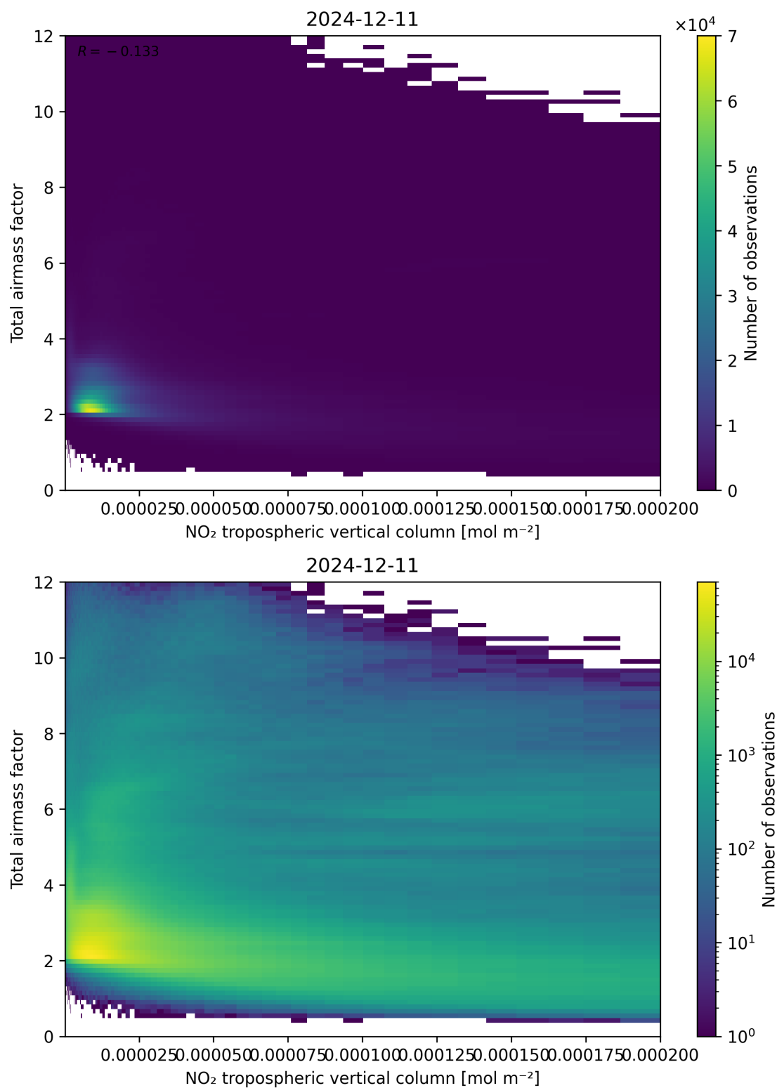
Figure 122: Scatter density plot of “NO 2 tropospheric vertical column” against “Total air mass factor” for 2024-12-11 to 2024-12-12.
