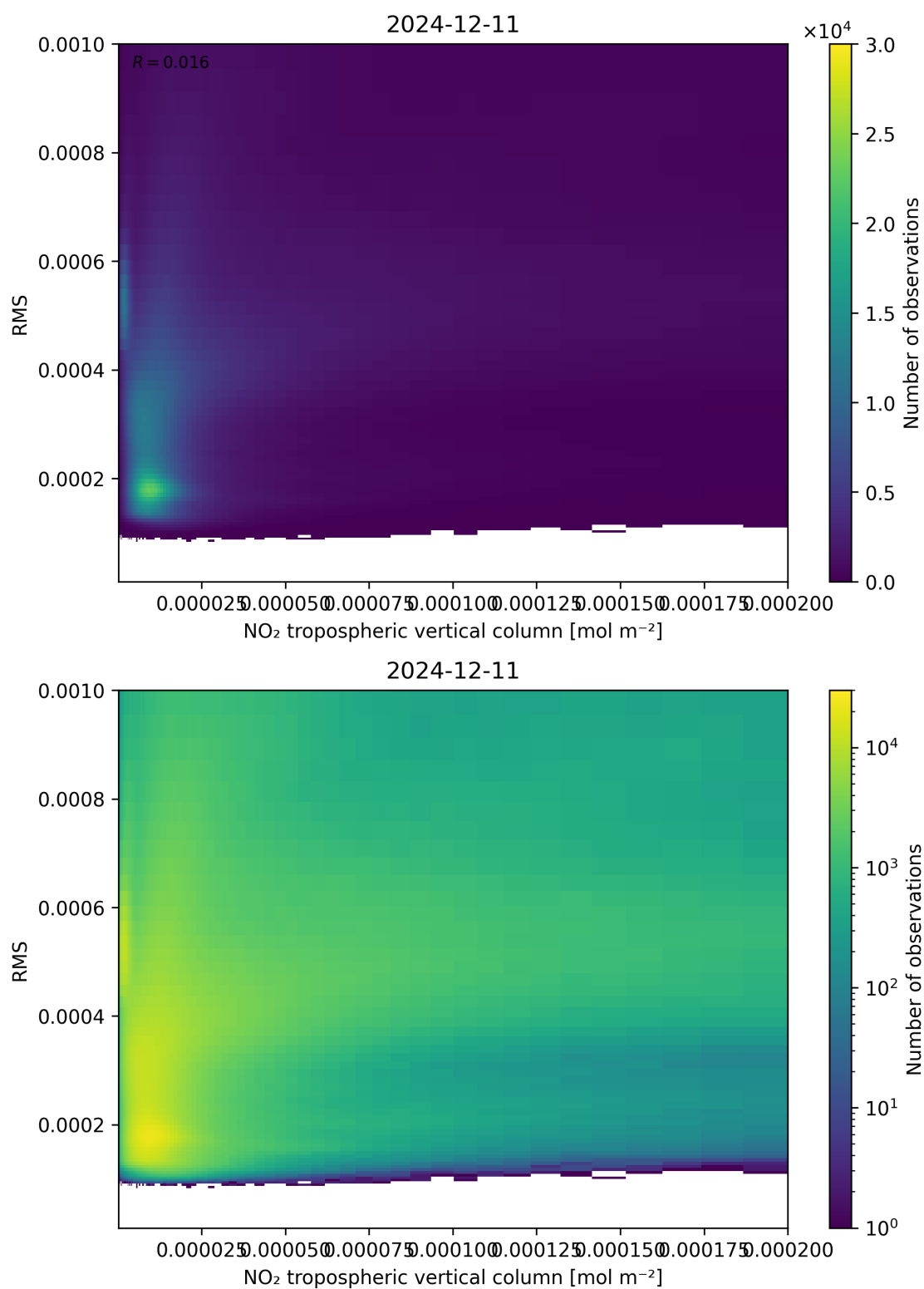
Figure 142: Scatter density plot of “NO 2 tropospheric vertical column” against “RMS” for 2024-12-11 to 2024-12-12.
