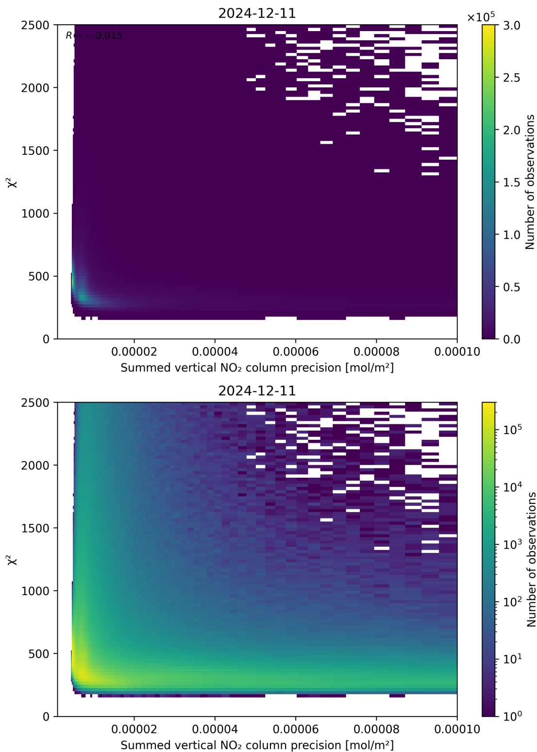
Figure 107: Scatter density plot of “Summed vertical NO 2 column precision” against “ \chi^2 ” for 2024-12-11 to 2024-12-12.
