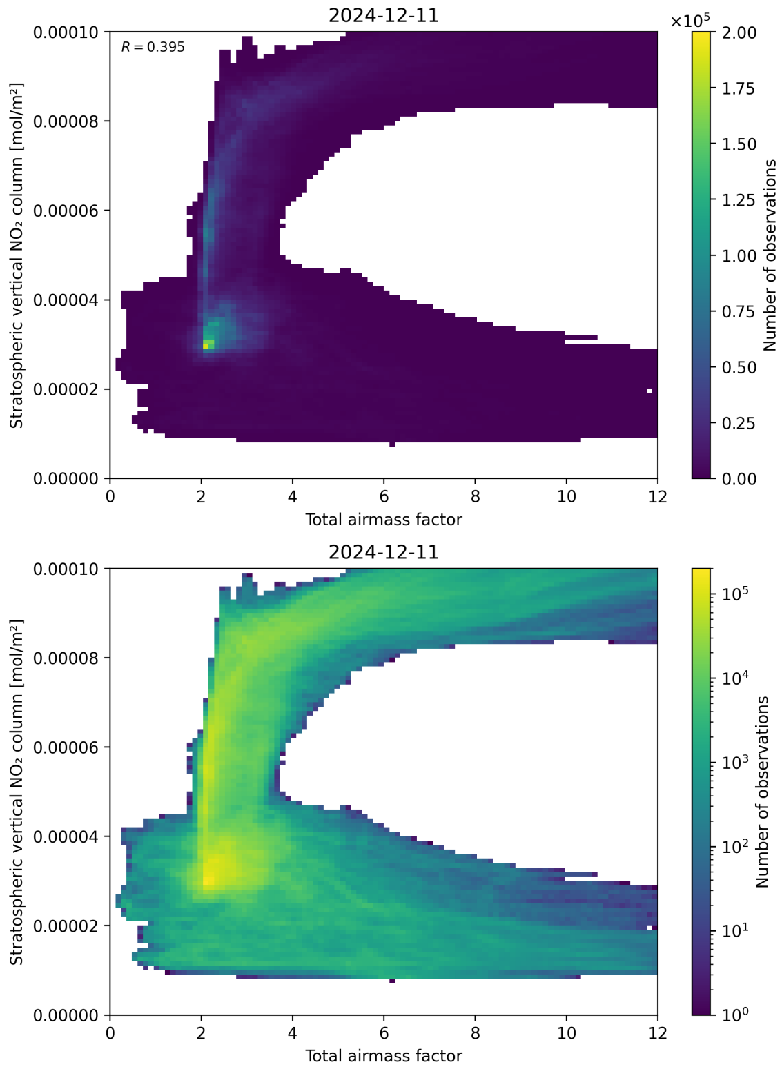
Figure 64: Scatter density plot of “Total airmass factor” against “Stratospheric vertical \text{NO}_2 column” for 2024-12-11 to 2024-12-12.
