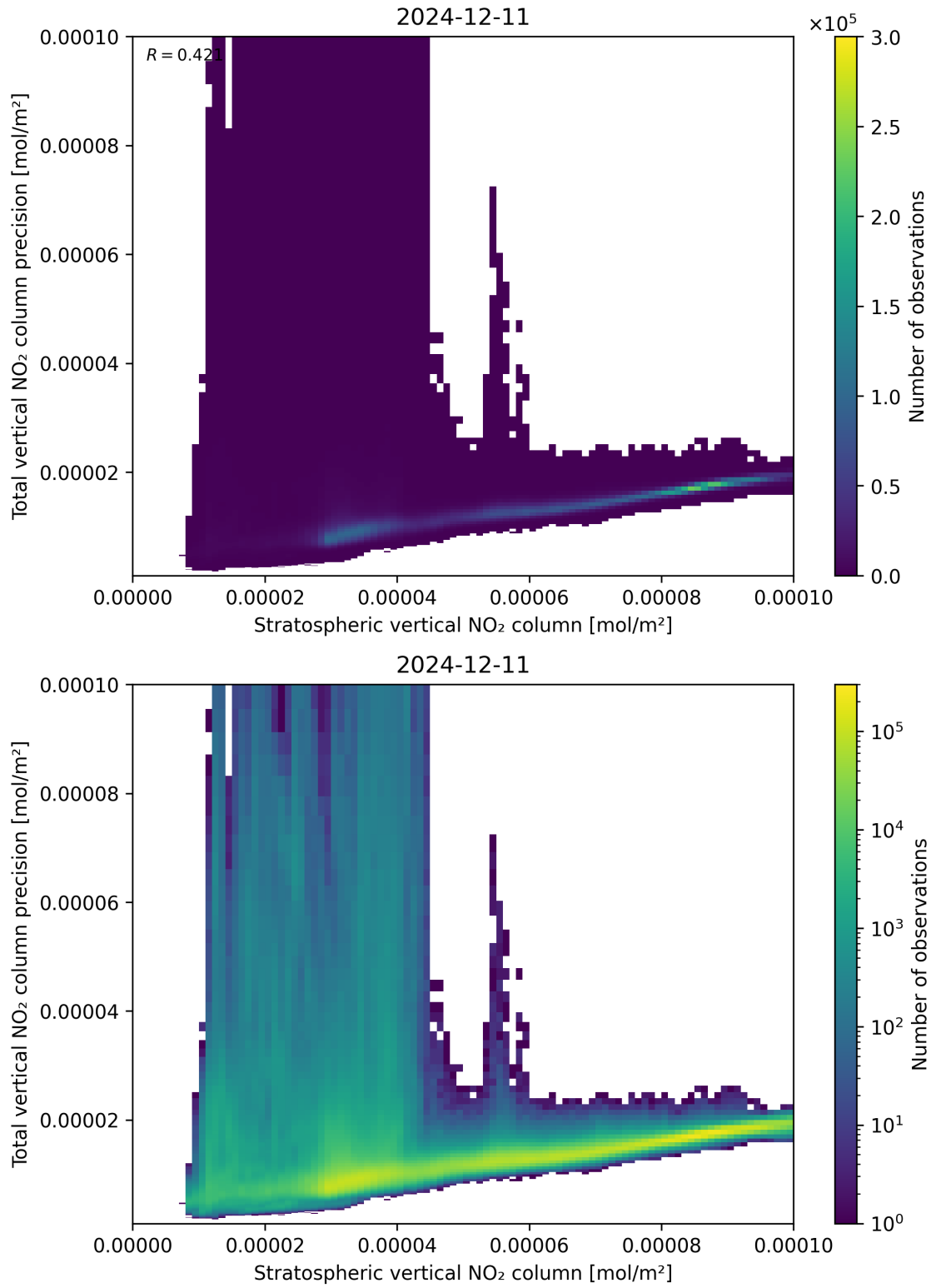
Figure 101: Scatter density plot of “Stratospheric vertical NO 2 column” against “Total vertical NO 2 column precision” for 2024-12-11 to 2024-12-12.
