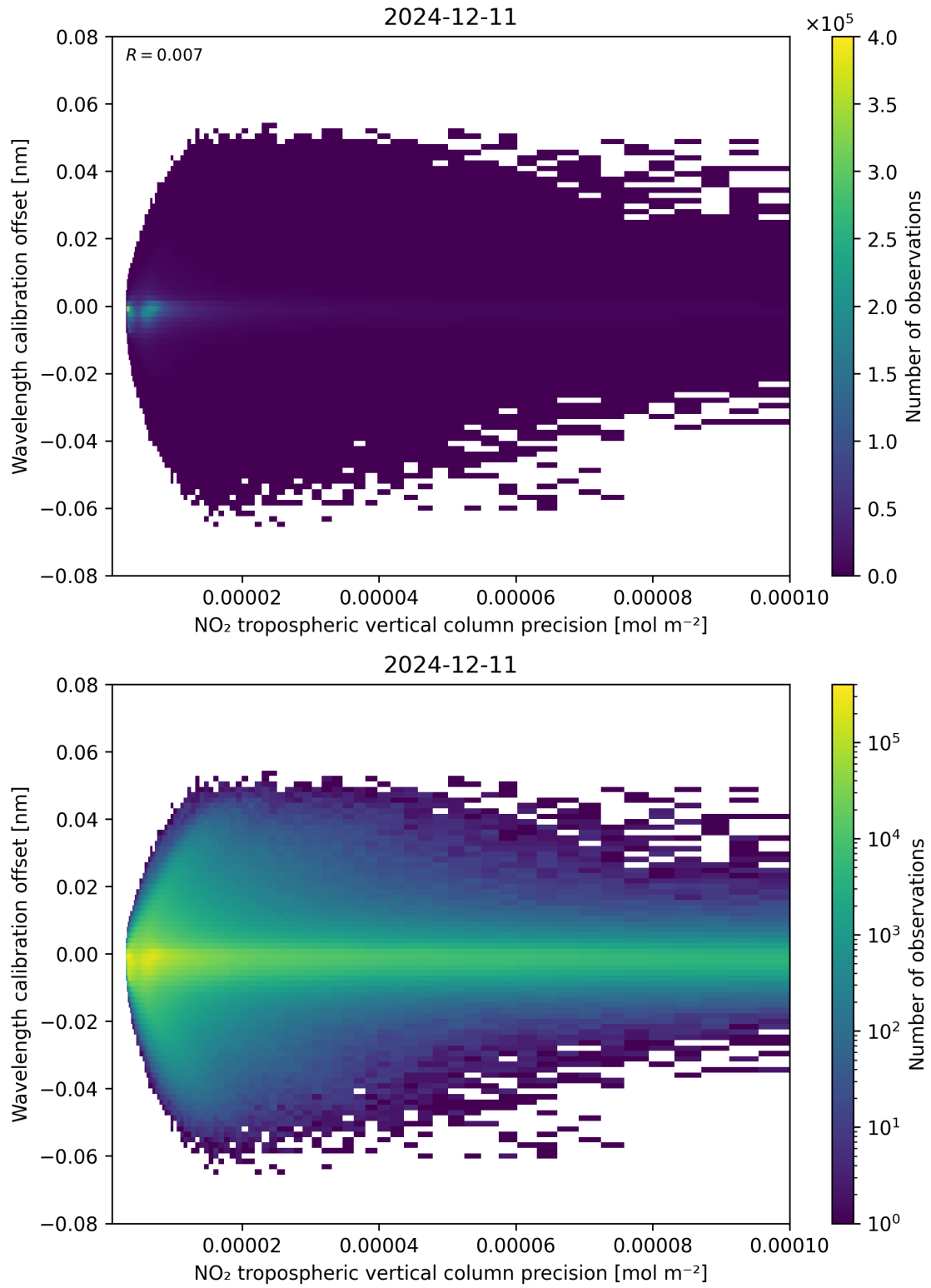
Figure 141: Scatter density plot of “NO 2 tropospheric vertical column precision” against “Wavelength calibration offset” for 2024-12-11 to 2024-12-12.
