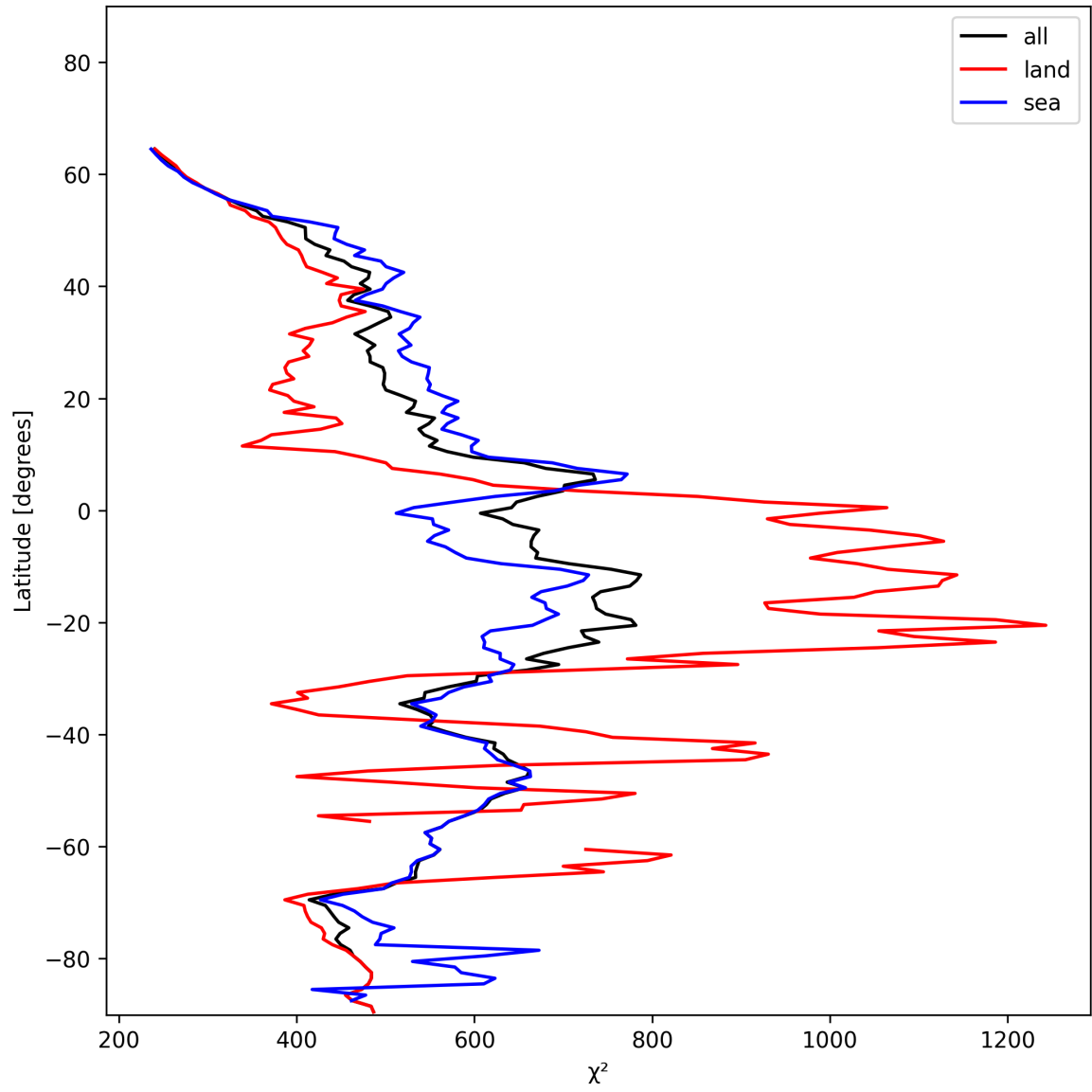
Figure 25: Zonal average of “ \chi^2 ” for 2024-12-11 to 2024-12-12.
