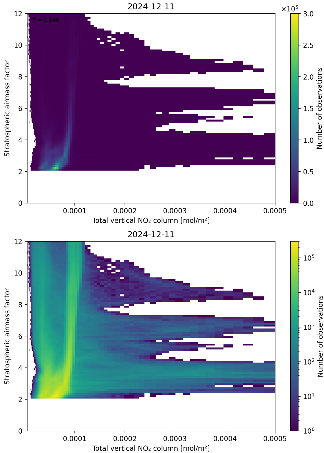
Figure 110: Scatter density plot of “Total vertical NO 2 column” against “Stratospheric airmass factor” for 2024-12-11 to 2024-12-12.
