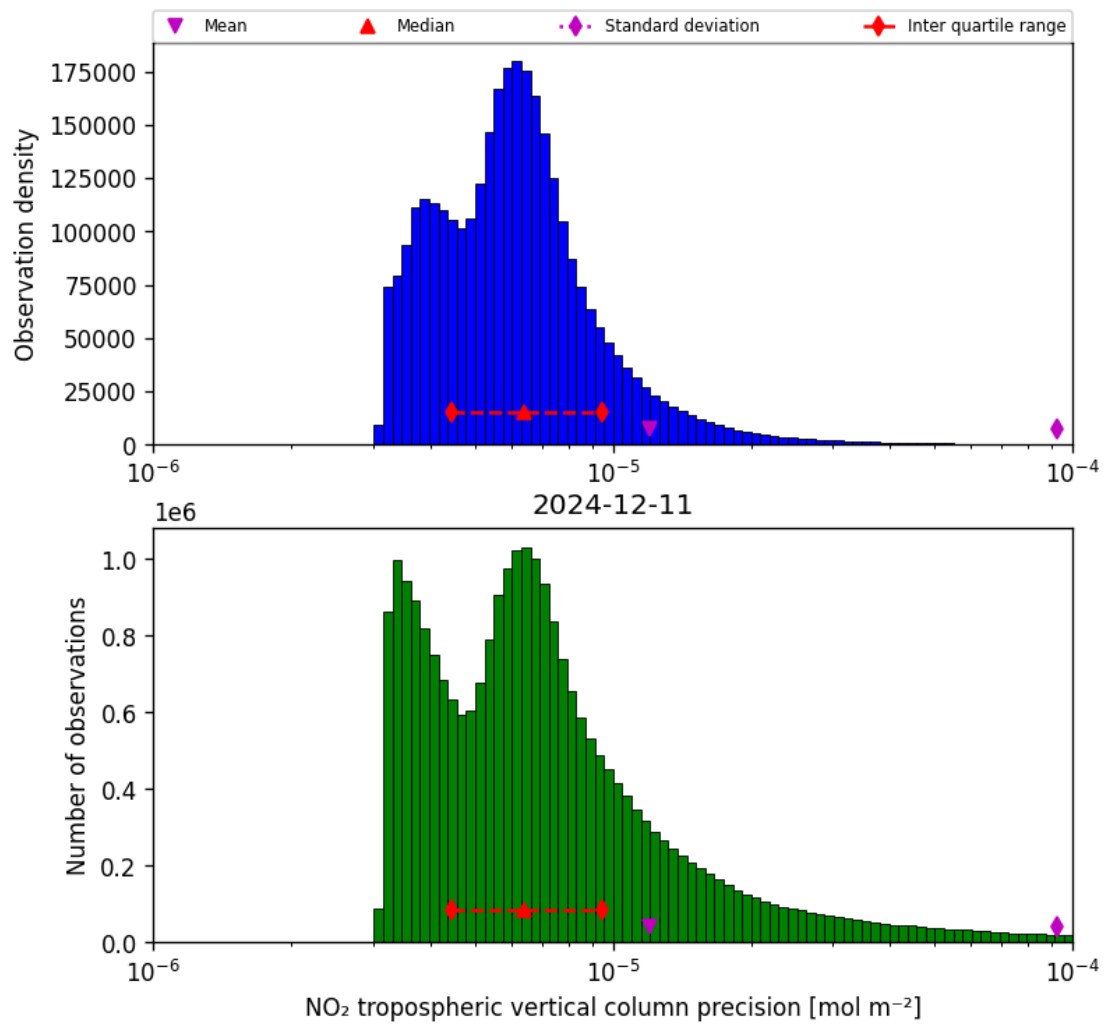
Figure 30: Histogram of “NO 2 tropospheric vertical column precision” for 2024-12-11 to 2024-12-12
