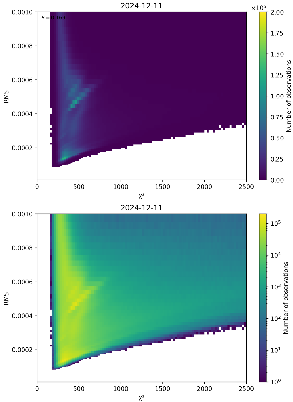
Figure 82: Scatter density plot of “ \chi^2 ” against “RMS” for 2024-12-11 to 2024-12-12.
