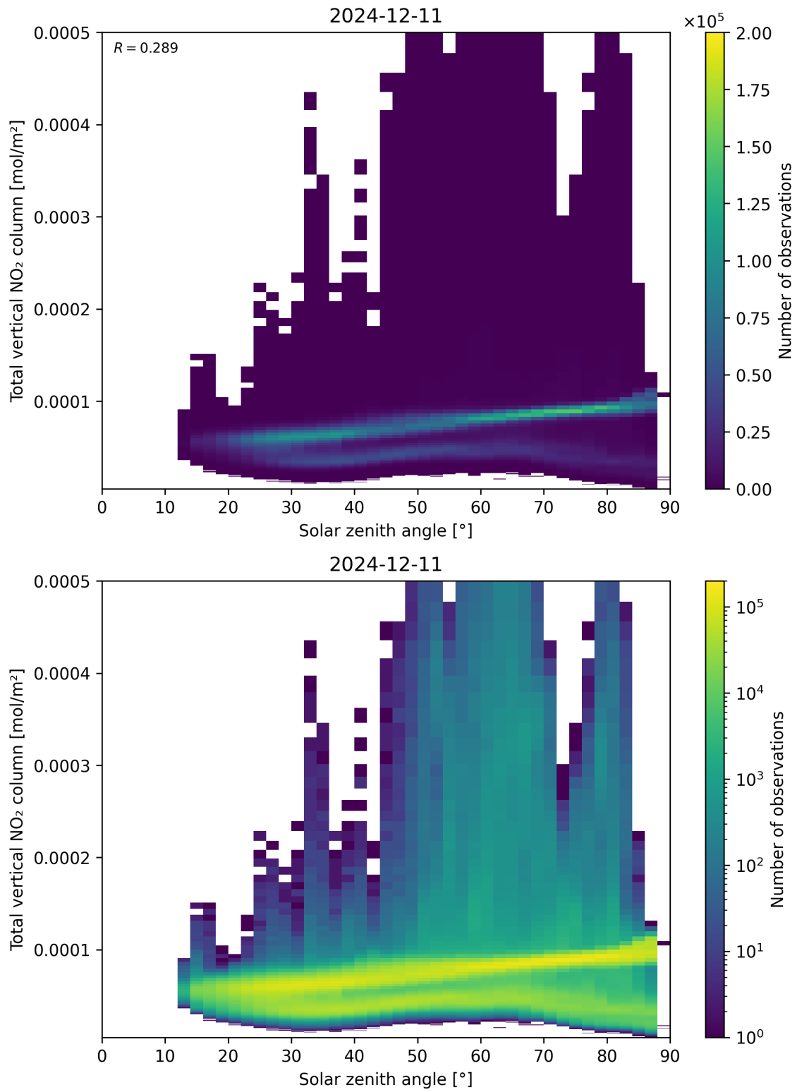
Figure 153: Scatter density plot of “Solar zenith angle” against “Total vertical NO 2 column” for 2024-12-11 to 2024-12-12.
