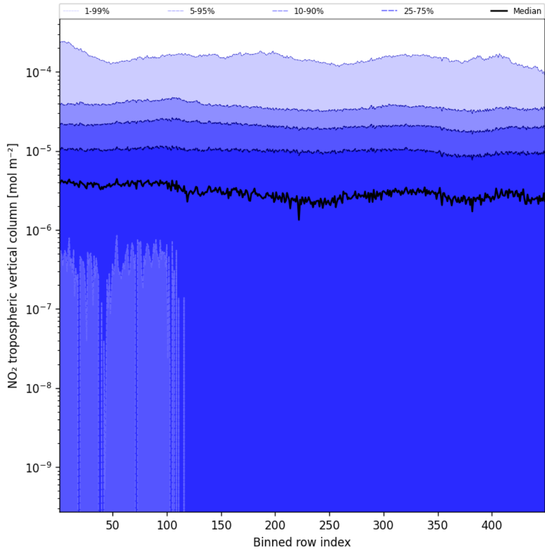
Figure 46: Along track statistics of “NO 2 tropospheric vertical column” for 2024-12-11 to 2024-12-12
