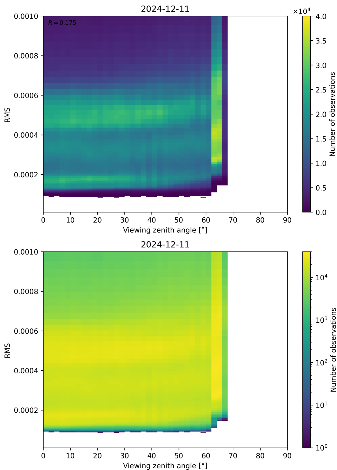
Figure 171: Scatter density plot of “Viewing zenith angle” against “RMS” for 2024-12-11 to 2024-12-12.
