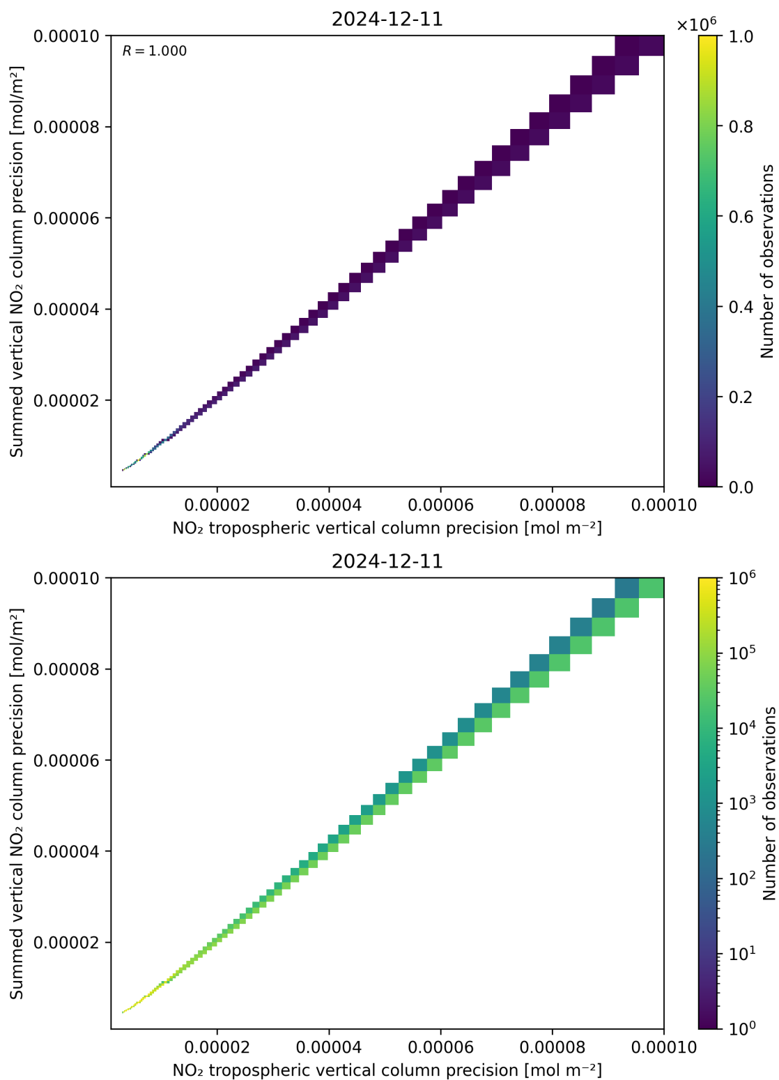
Figure 137: Scatter density plot of “NO 2 tropospheric vertical column precision” against “Summed vertical NO 2 column precision” for 2024-12-11 to 2024-12-12.
