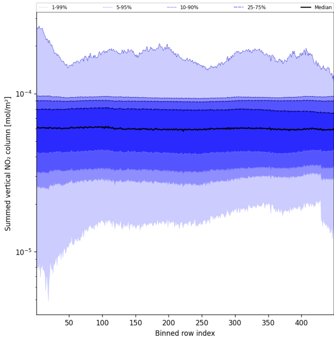
Figure 57: Along track statistics of “Summed vertical NO 2 column” for 2024-12-11 to 2024-12-12
