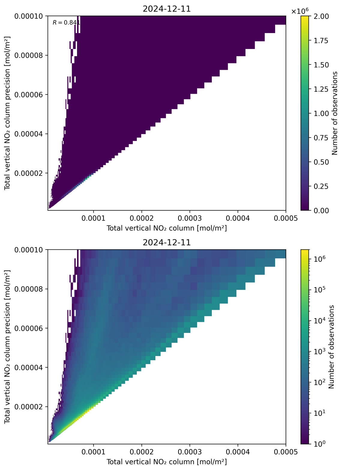
Figure 114: Scatter density plot of “Total vertical NO 2 column” against “Total vertical NO 2 column precision” for 2024-12-11 to 2024-12-12.
