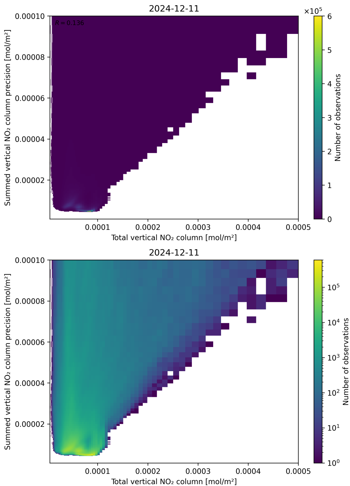
Figure 113: Scatter density plot of “Total vertical NO 2 column” against “Summed vertical NO 2 column precision” for 2024-12-11 to 2024-12-12.
