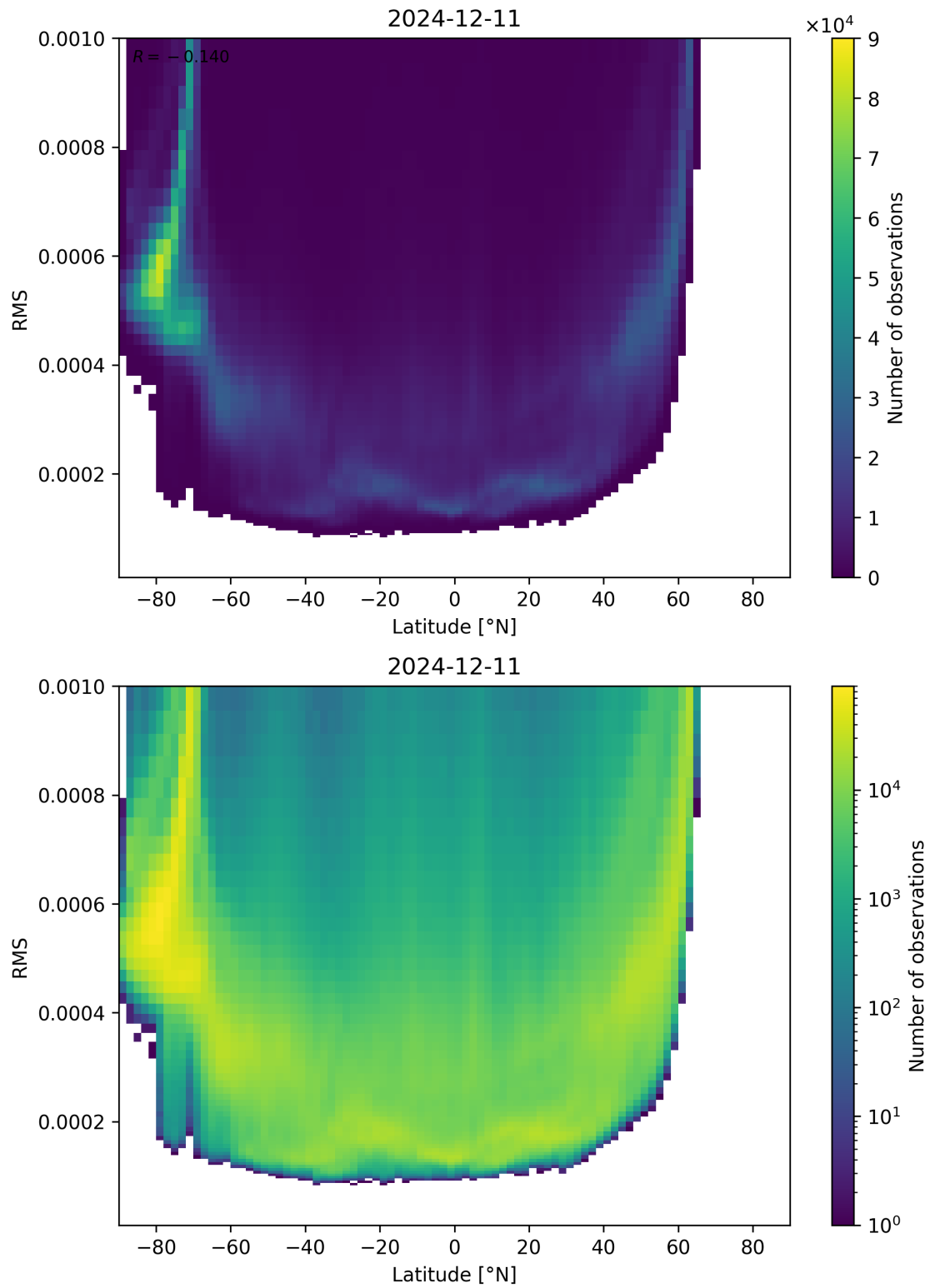
Figure 94: Scatter density plot of “Latitude” against “RMS” for 2024-12-11 to 2024-12-12.
