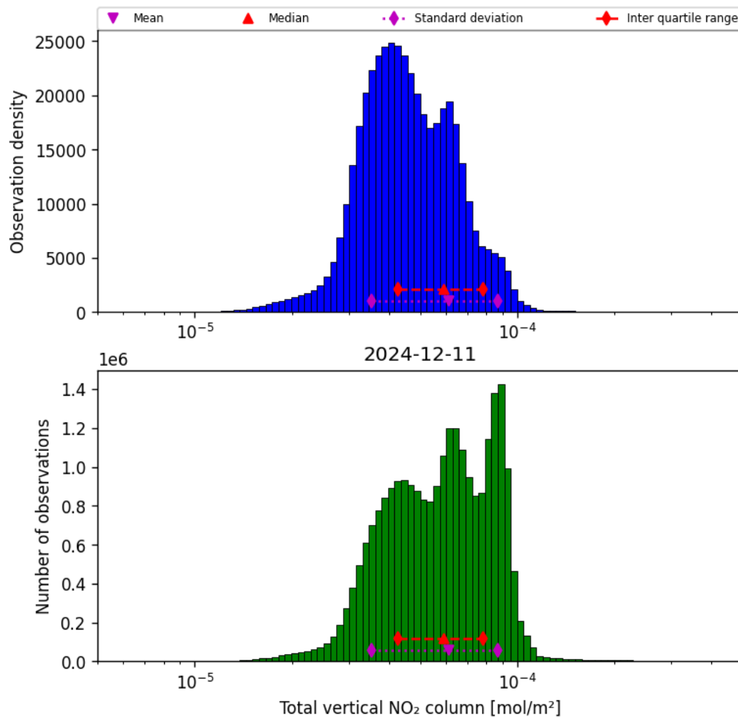
Figure 38: Histogram of “Total vertical NO 2 column” for 2024-12-11 to 2024-12-12
