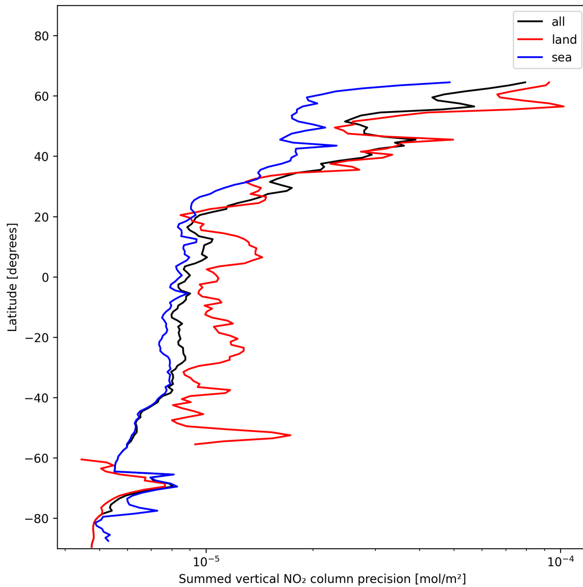
Figure 24: Zonal average of “Summed vertical NO 2 column precision” for 2024-12-11 to 2024-12-12.
