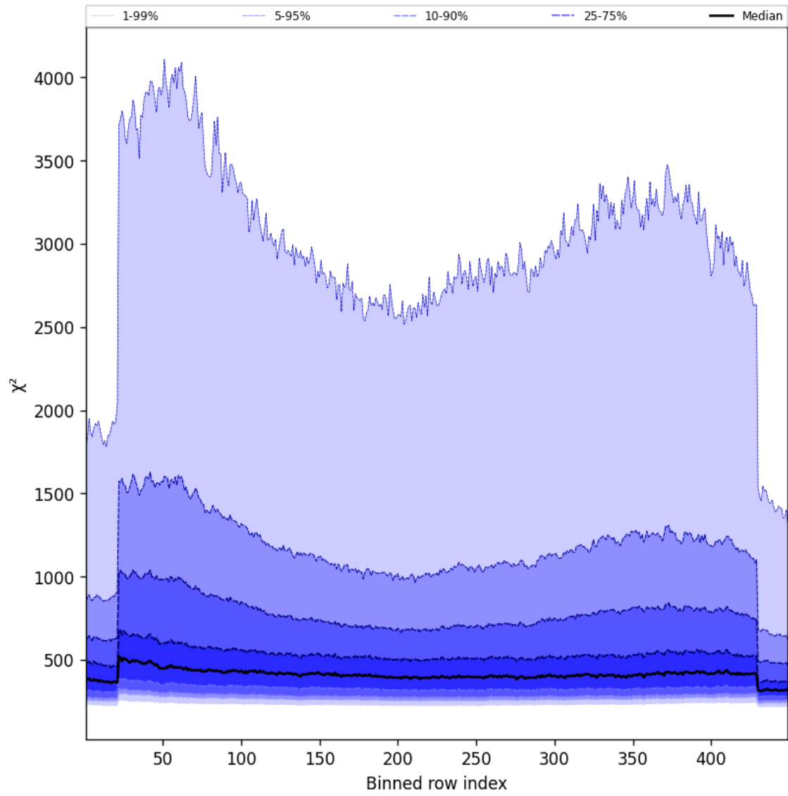
Figure 59: Along track statistics of “ \chi^2 ” for 2024-12-11 to 2024-12-12
