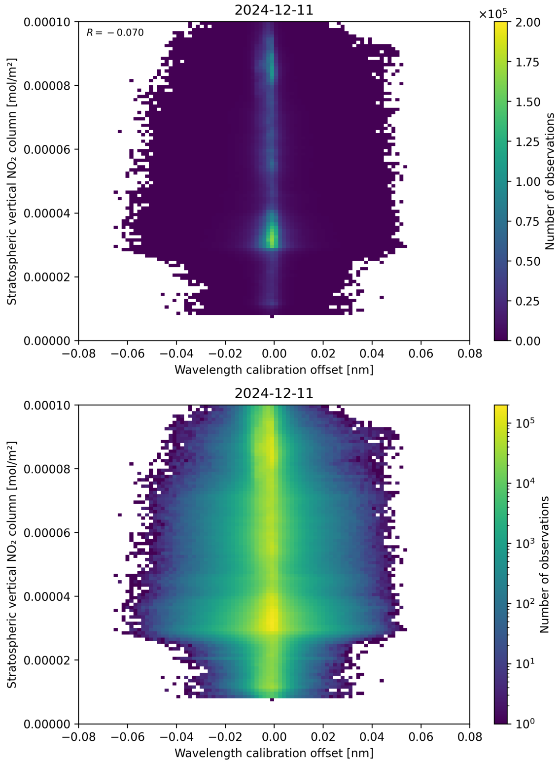
Figure 176: Scatter density plot of “Wavelength calibration offset” against “Stratospheric vertical NO 2 column” for 2024-12-11 to 2024-12-12.
