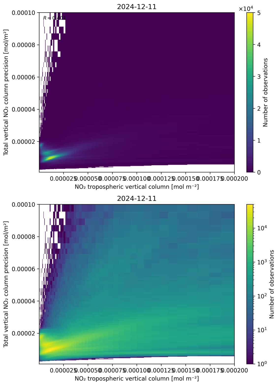
Figure 129: Scatter density plot of “NO 2 tropospheric vertical column” against “Total vertical NO 2 column precision” for 2024-12-11 to 2024-12-12.
