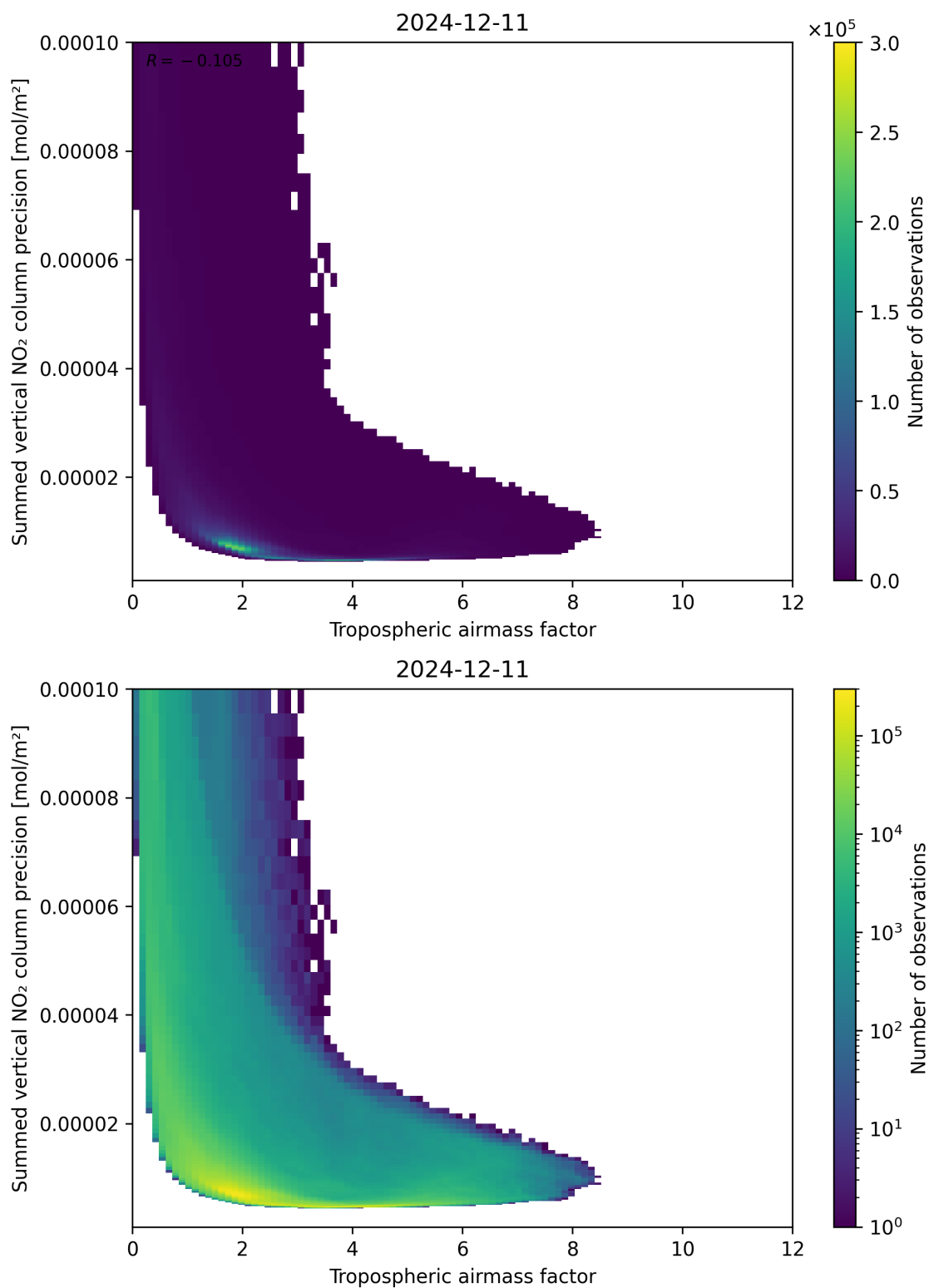
Figure 76: Scatter density plot of “Tropospheric air mass factor” against “Summed vertical NO 2 column precision” for 2024-12-11 to 2024-12-12.
