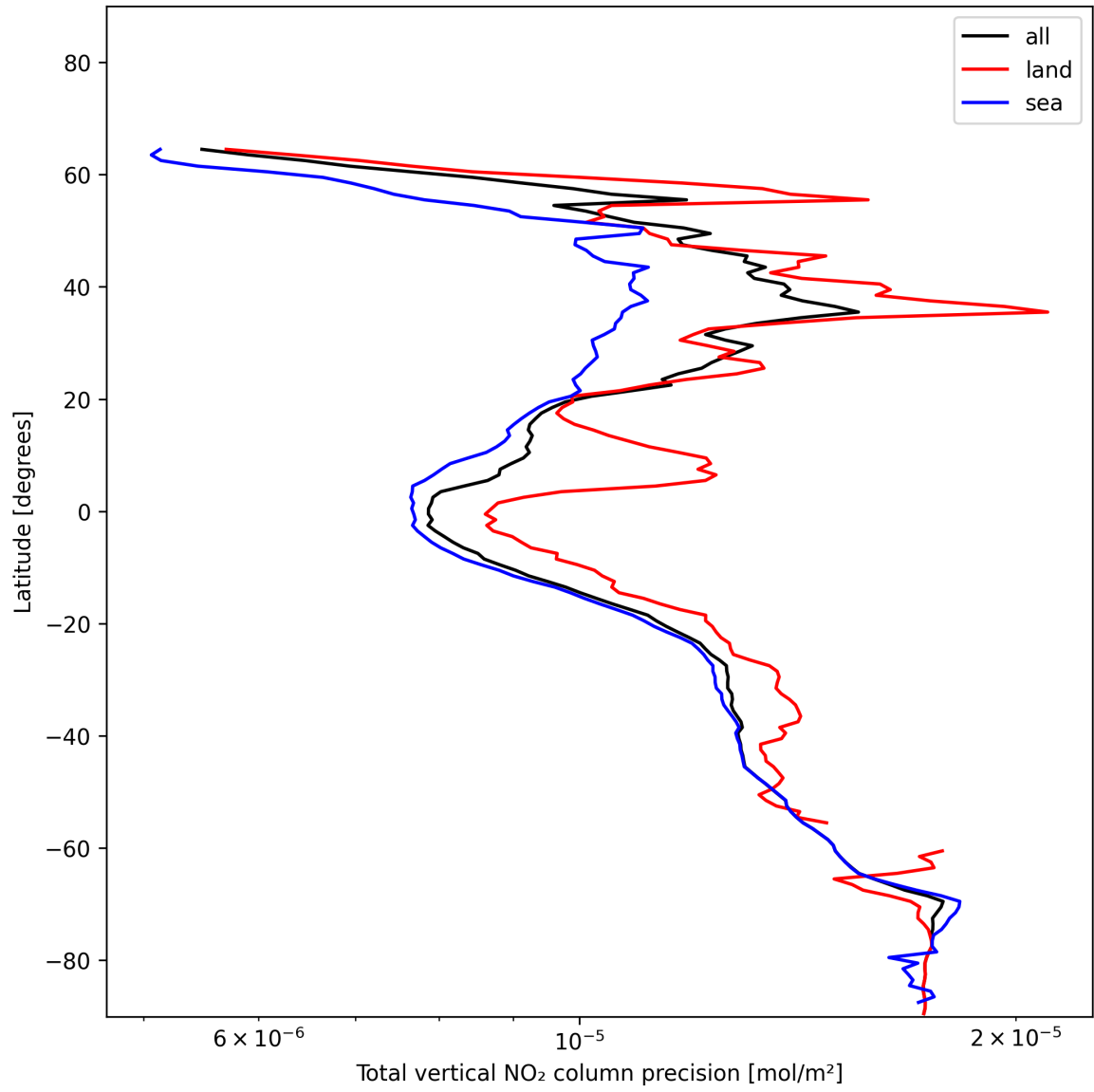
Figure 22: Zonal average of “Total vertical NO 2 column precision” for 2024-12-11 to 2024-12-12.
