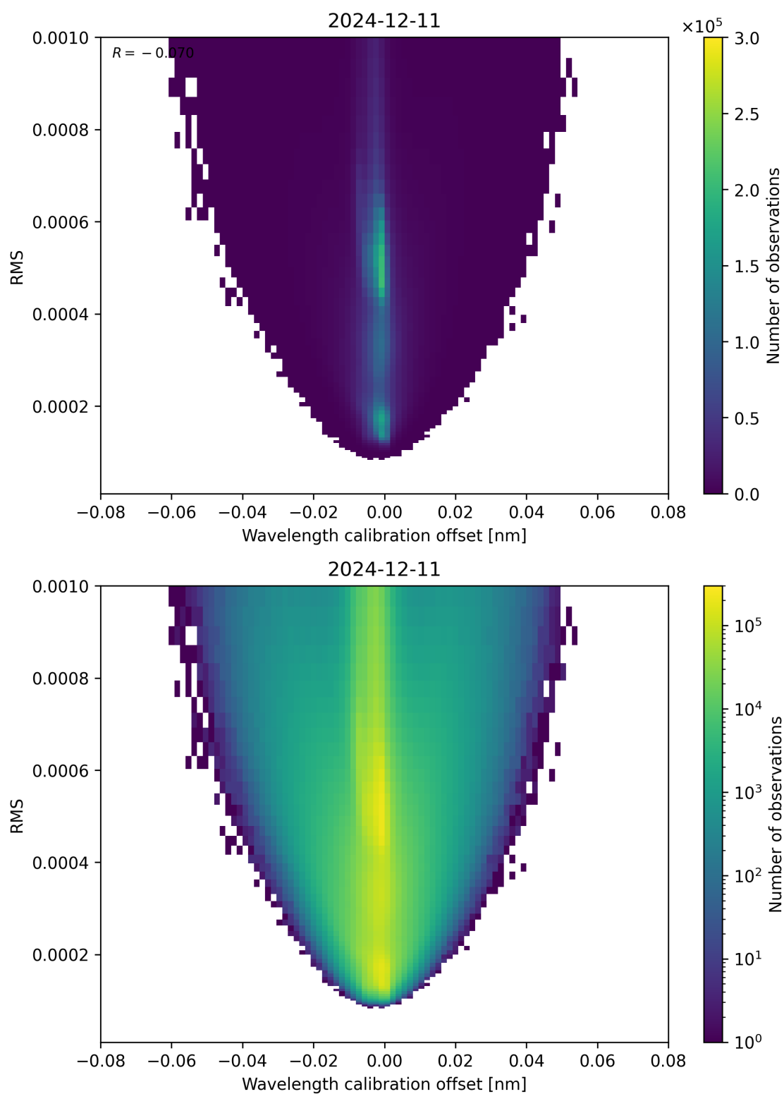
Figure 181: Scatter density plot of “Wavelength calibration offset” against “RMS” for 2024-12-11 to 2024-12-12.
