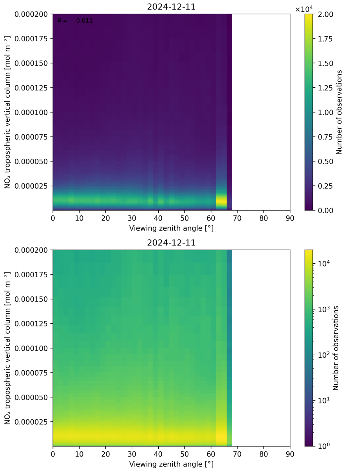
Figure 169: Scatter density plot of “Viewing zenith angle” against “NO 2 tropospheric vertical column” for 2024-12-11 to 2024-12-12.
