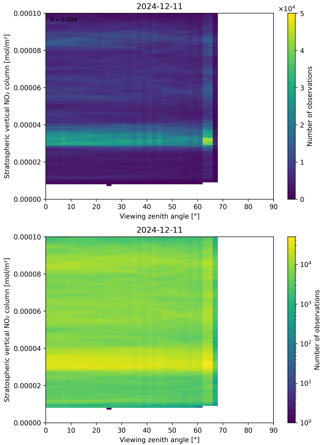
Figure 164: Scatter density plot of “Viewing zenith angle” against “Stratospheric vertical NO 2 column” for 2024-12-11 to 2024-12-12.
