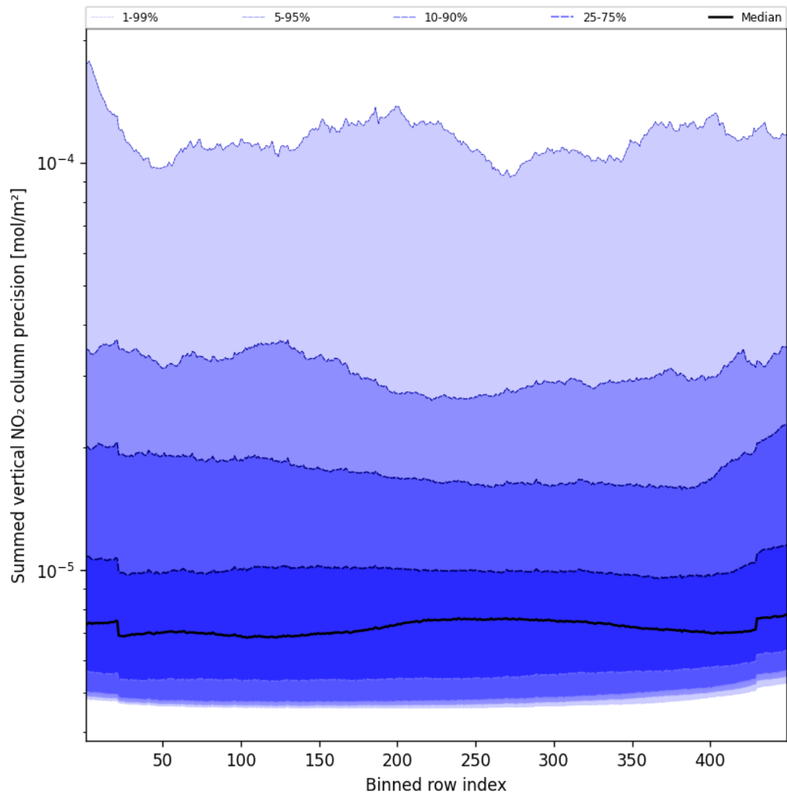
Figure 58: Along track statistics of “Summed vertical NO 2 column precision” for 2024-12-11 to 2024-12-12
