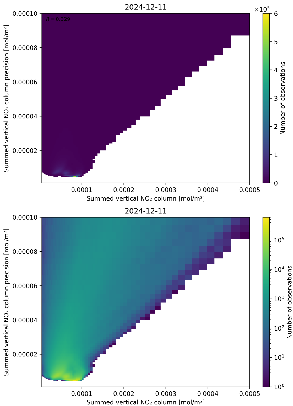
Figure 105: Scatter density plot of “Summed vertical NO 2 column” against “Summed vertical NO 2 column precision” for 2024-12-11 to 2024-12-12.
