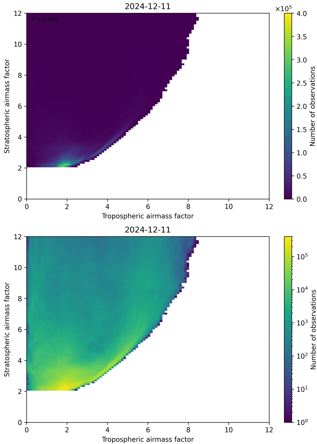
Figure 71: Scatter density plot of “Tropospheric airmass factor” against “Stratospheric airmass factor” for 2024-12-11 to 2024-12-12.
