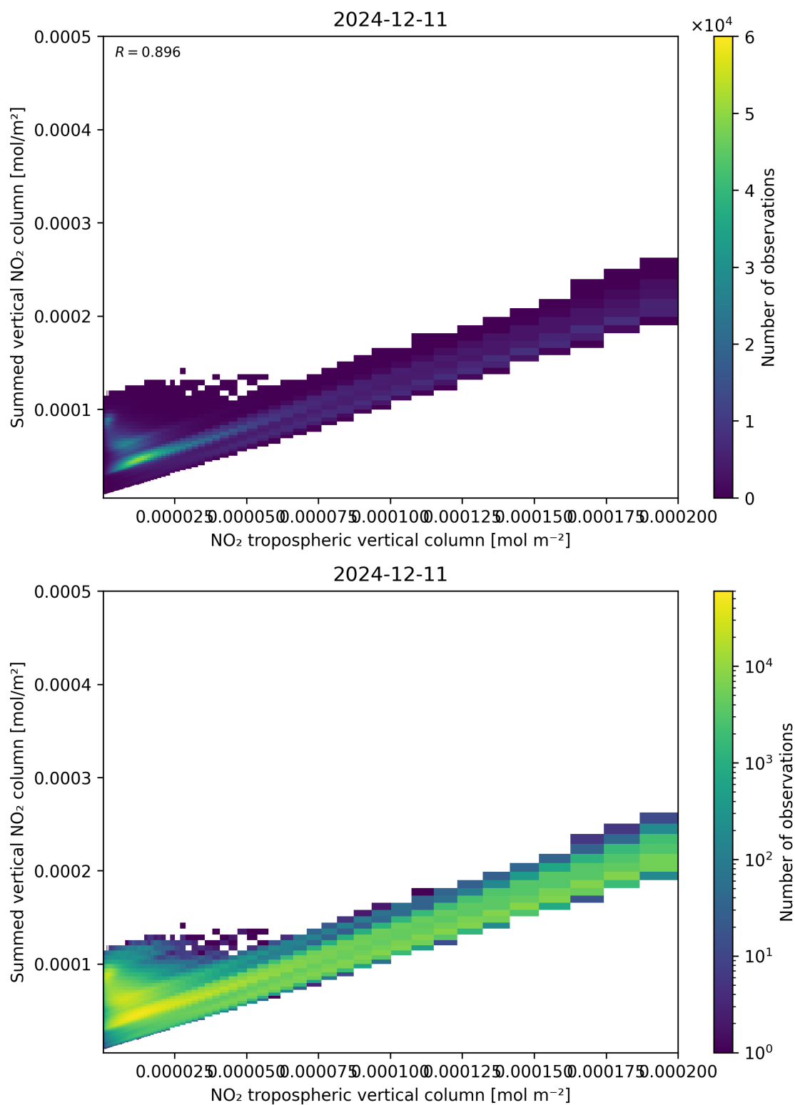
Figure 126: Scatter density plot of “NO 2 tropospheric vertical column” against “Summed vertical NO 2 column” for 2024-12-11 to 2024-12-12.
