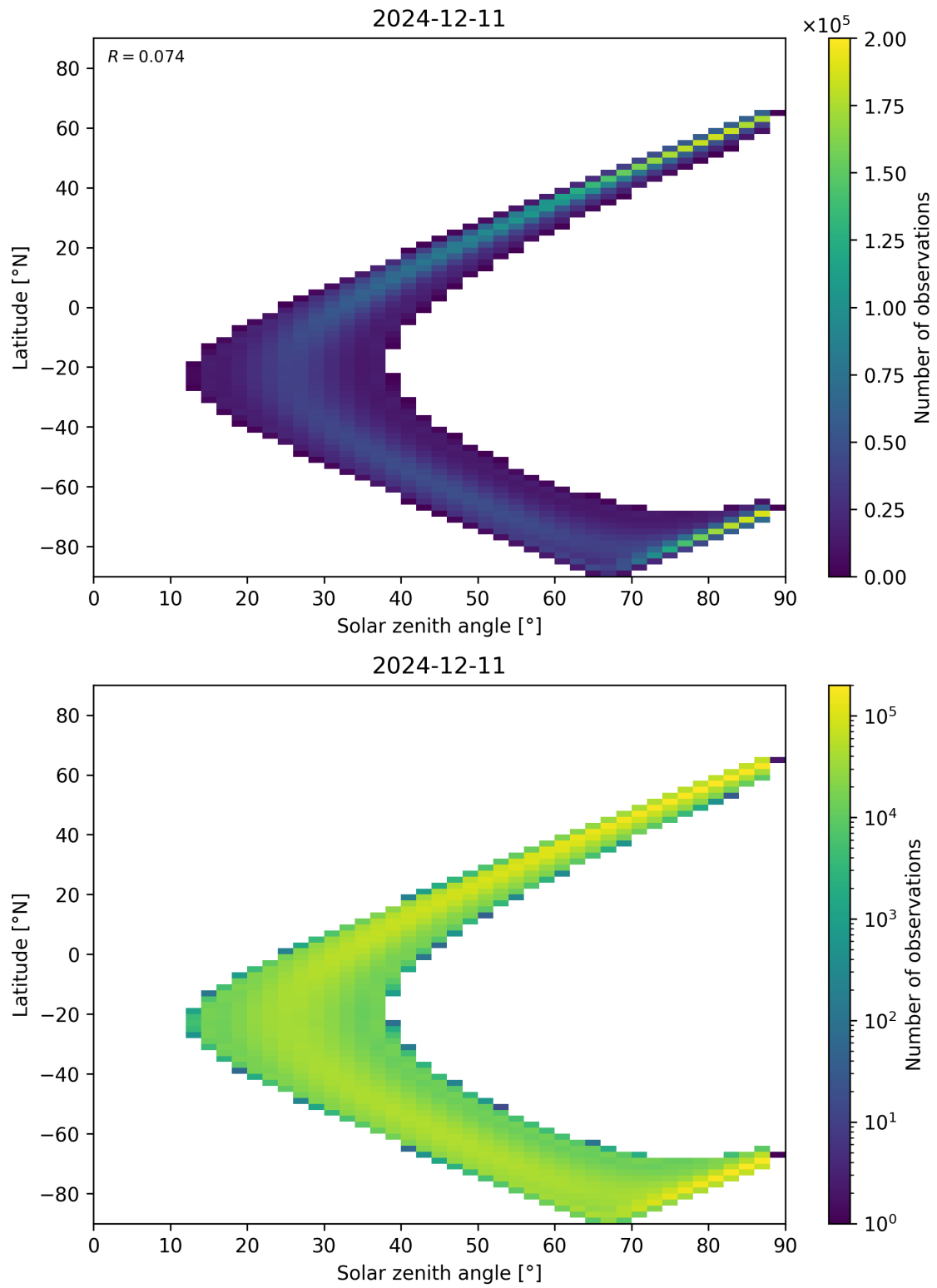
Figure 149: Scatter density plot of “Solar zenith angle” against “Latitude” for 2024-12-11 to 2024-12-12.
