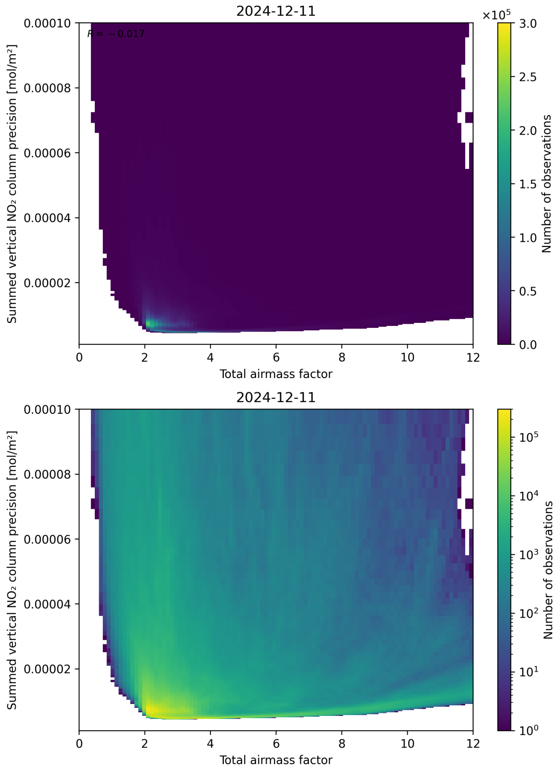
Figure 66: Scatter density plot of “Total airmass factor” against “Summed vertical NO 2 column precision” for 2024-12-11 to 2024-12-12.
