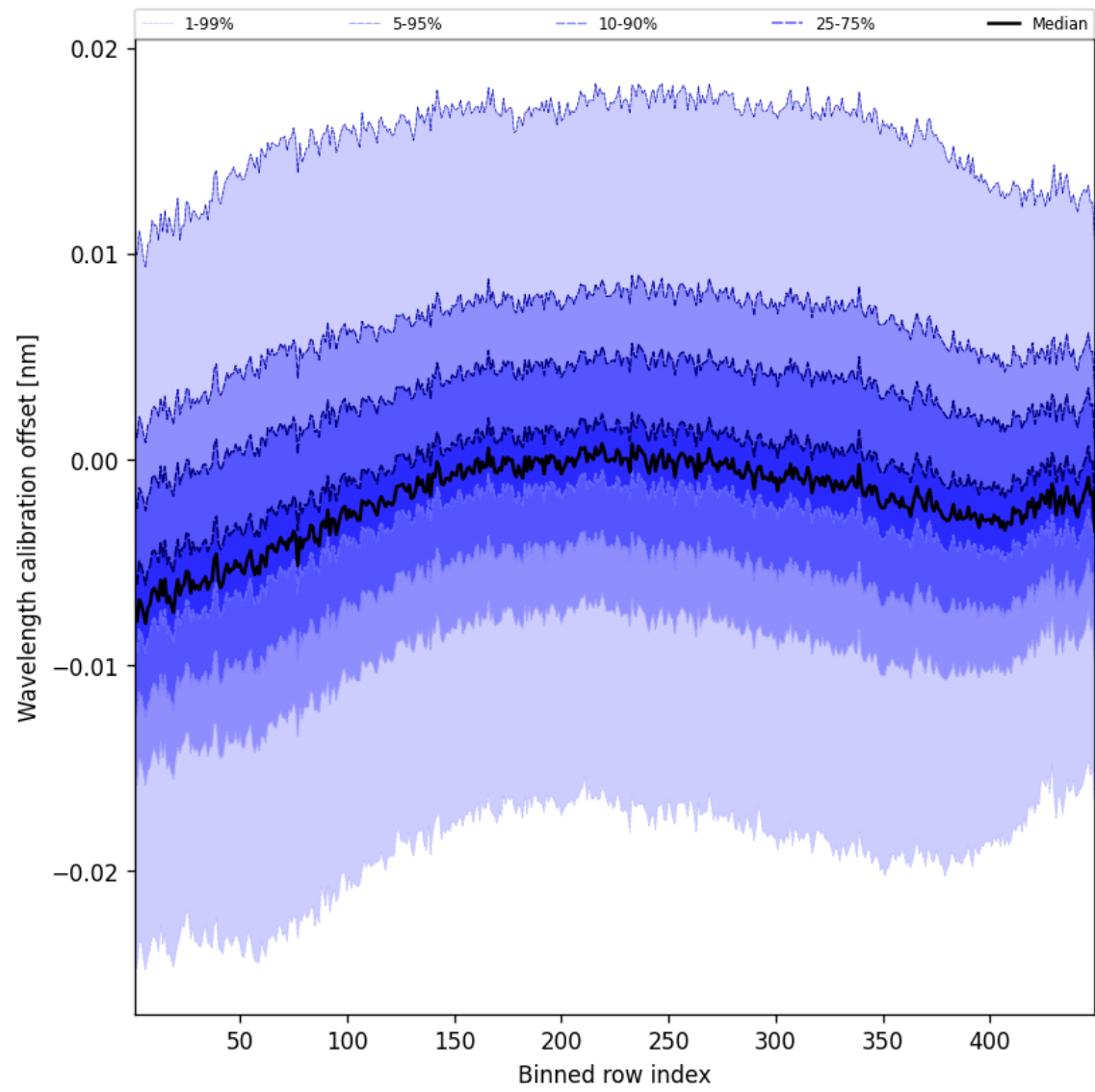
Figure 52: Along track statistics of “Wavelength calibration offset” for 2024-12-11 to 2024-12-12
