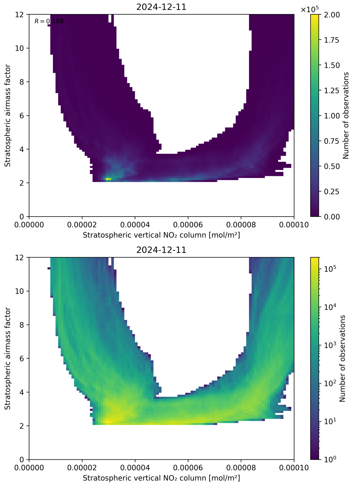
Figure 96: Scatter density plot of “Stratospheric vertical NO 2 column” against “Stratospheric airmass factor” for 2024-12-11 to 2024-12-12.
