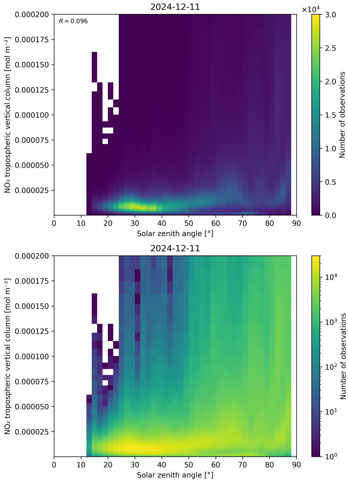
Figure 155: Scatter density plot of “Solar zenith angle” against “NO 2 tropospheric vertical column” for 2024-12-11 to 2024-12-12.
