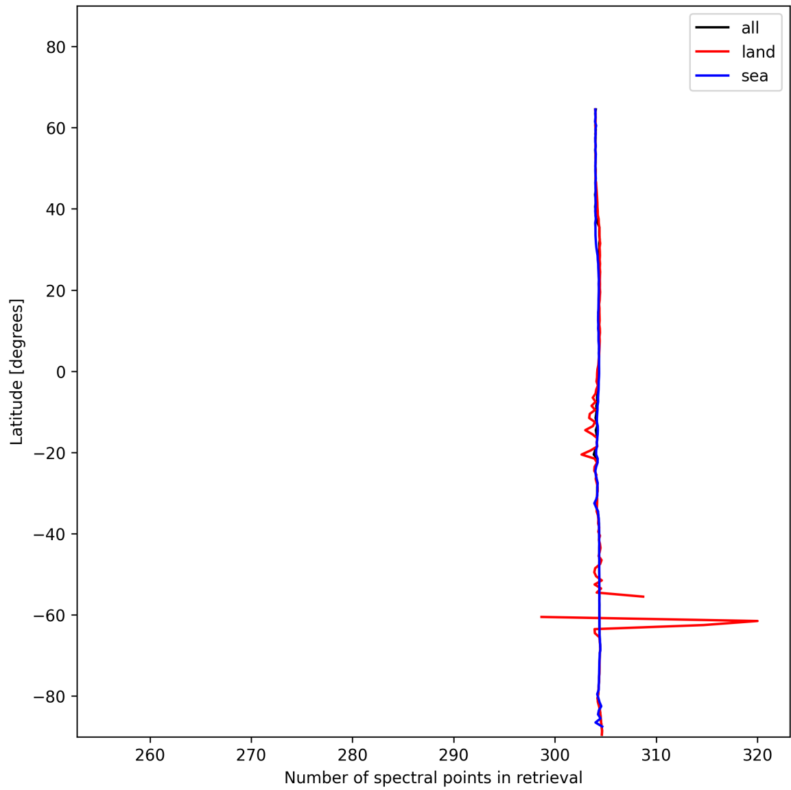
Figure 16: Zonal average of “Number of spectral points in retrieval” for 2024-12-11 to 2024-12-12.
