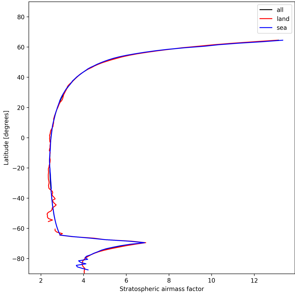
Figure 27: Zonal average of “Stratospheric airmass factor” for 2024-12-11 to 2024-12-12.
