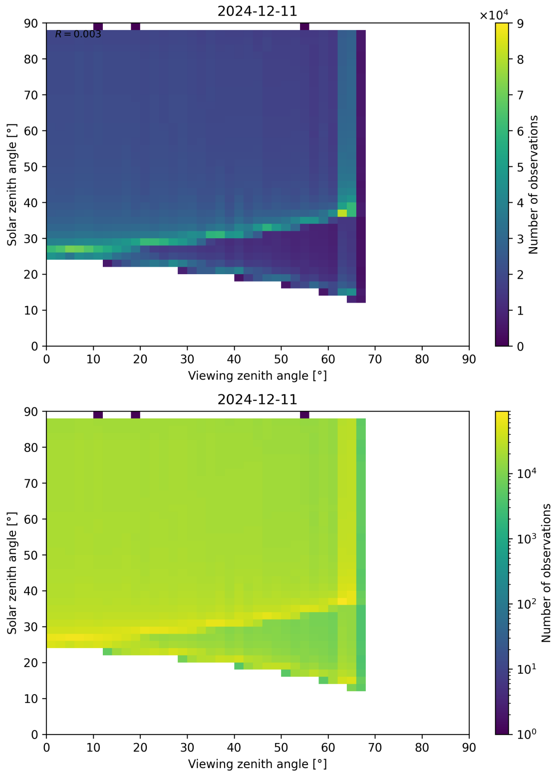
Figure 172: Scatter density plot of “Viewing zenith angle” against “Solar zenith angle” for 2024-12-11 to 2024-12-12.
