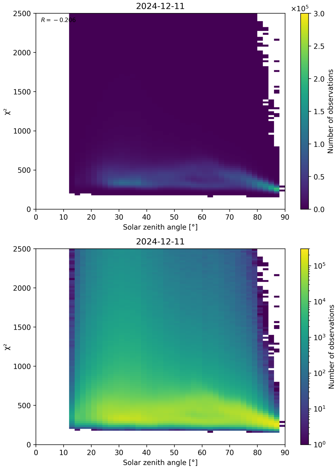
Figure 148: Scatter density plot of “Solar zenith angle” against “ \chi^2 ” for 2024-12-11 to 2024-12-12.
