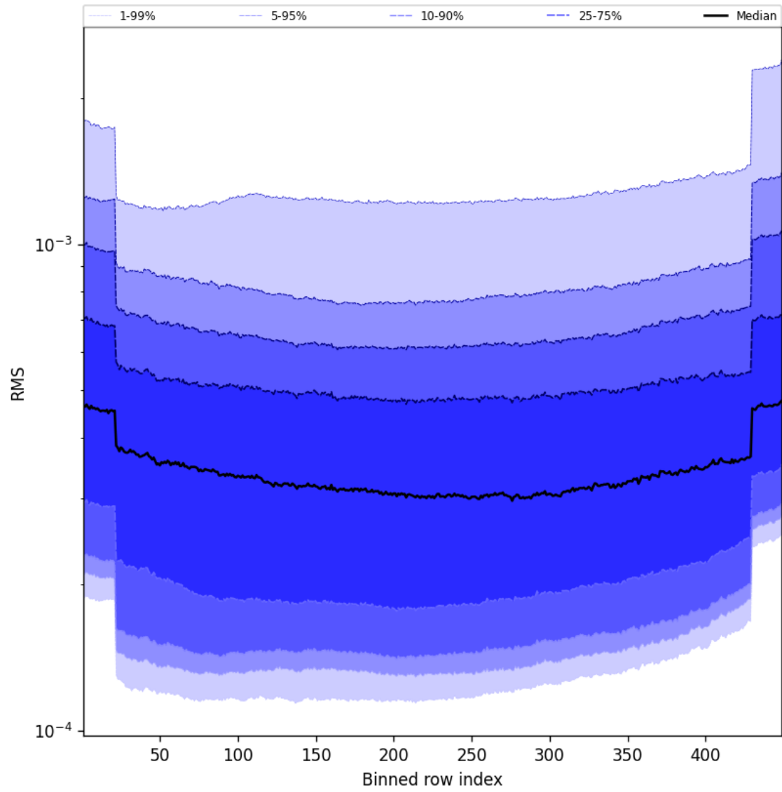
Figure 60: Along track statistics of “RMS” for 2024-12-11 to 2024-12-12
