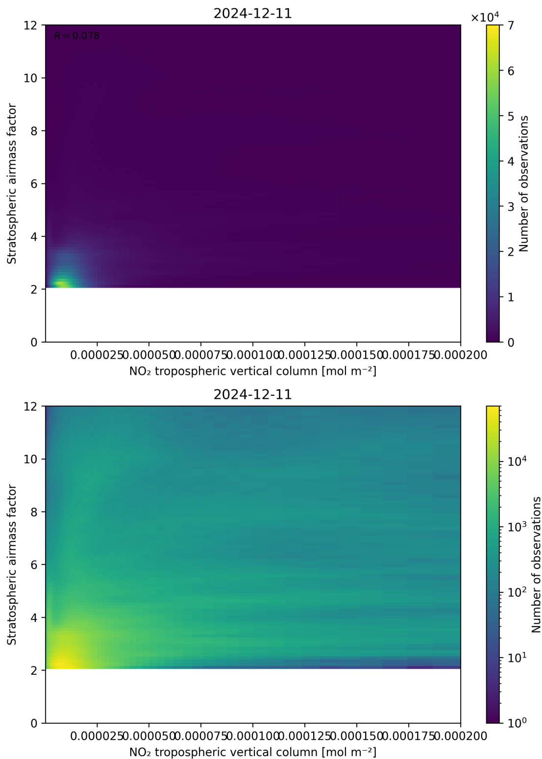
Figure 121: Scatter density plot of “NO 2 tropospheric vertical column” against “Stratospheric airmass factor” for 2024-12-11 to 2024-12-12.
