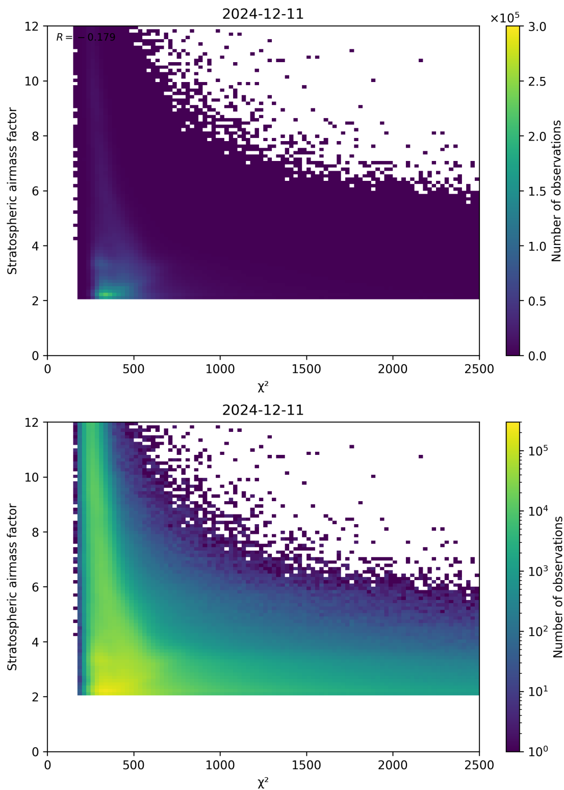
Figure 81: Scatter density plot of “ \chi^2 ” against “Stratospheric airmass factor” for 2024-12-11 to 2024-12-12.
