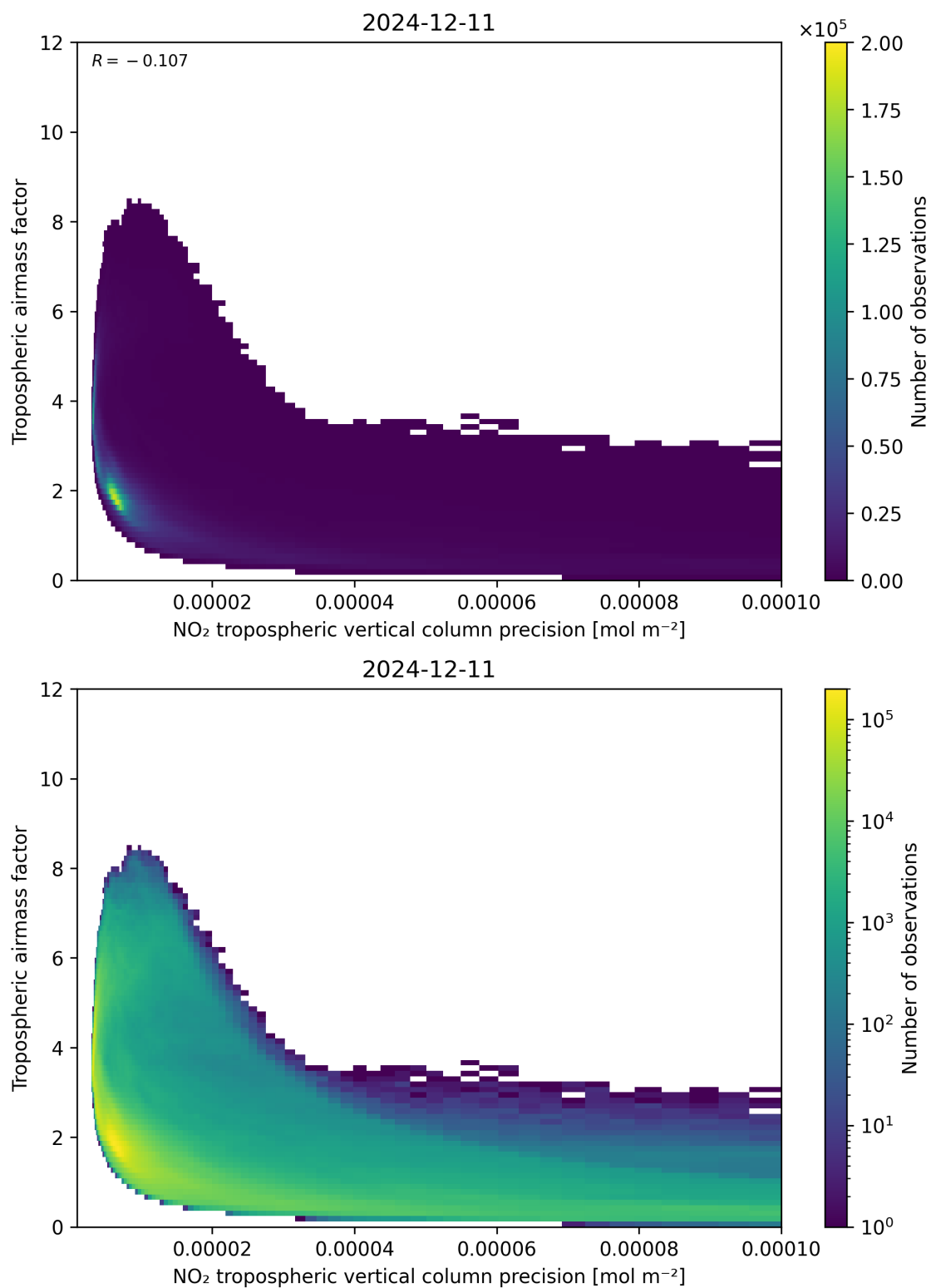
Figure 133: Scatter density plot of “NO 2 tropospheric vertical column precision” against “Tropospheric air mass factor” for 2024-12-11 to 2024-12-12.
