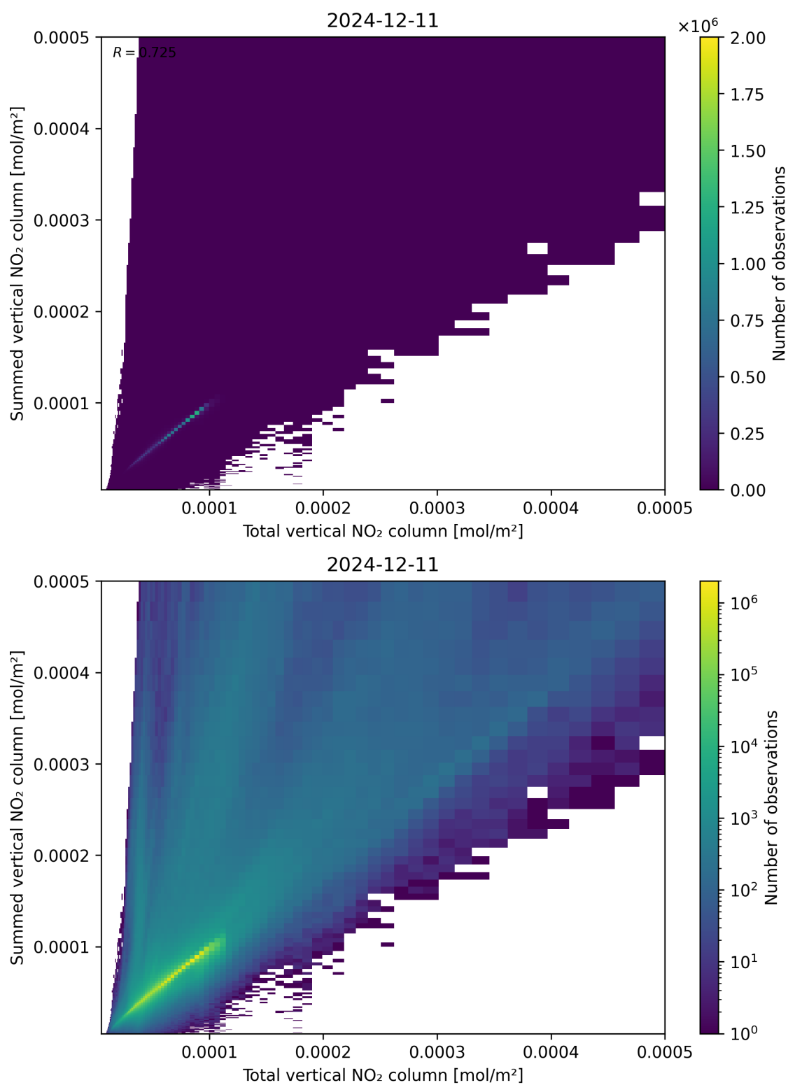
Figure 112: Scatter density plot of “Total vertical NO 2 column” against “Summed vertical NO 2 column” for 2024-12-11 to 2024-12-12.
