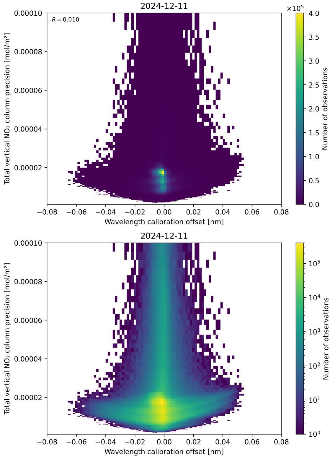
Figure 180: Scatter density plot of “Wavelength calibration offset” against “Total vertical NO 2 column precision” for 2024-12-11 to 2024-12-12.
