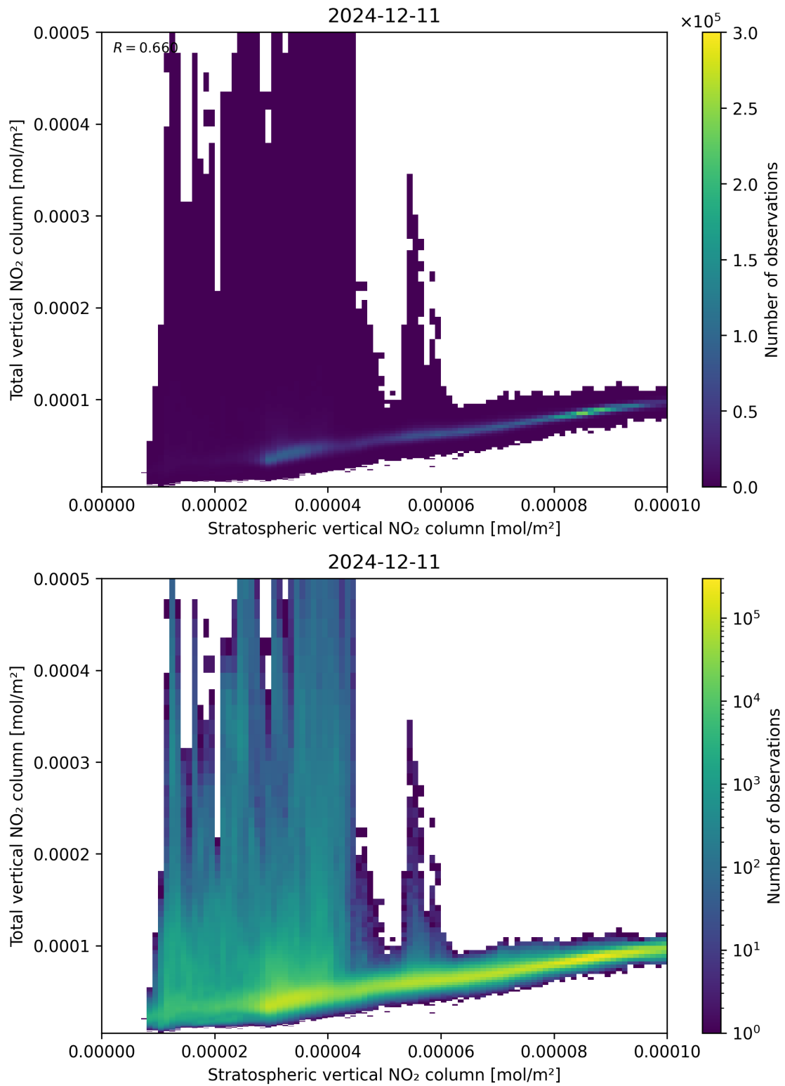
Figure 100: Scatter density plot of “Stratospheric vertical NO 2 column” against “Total vertical NO 2 column” for 2024-12-11 to 2024-12-12.
