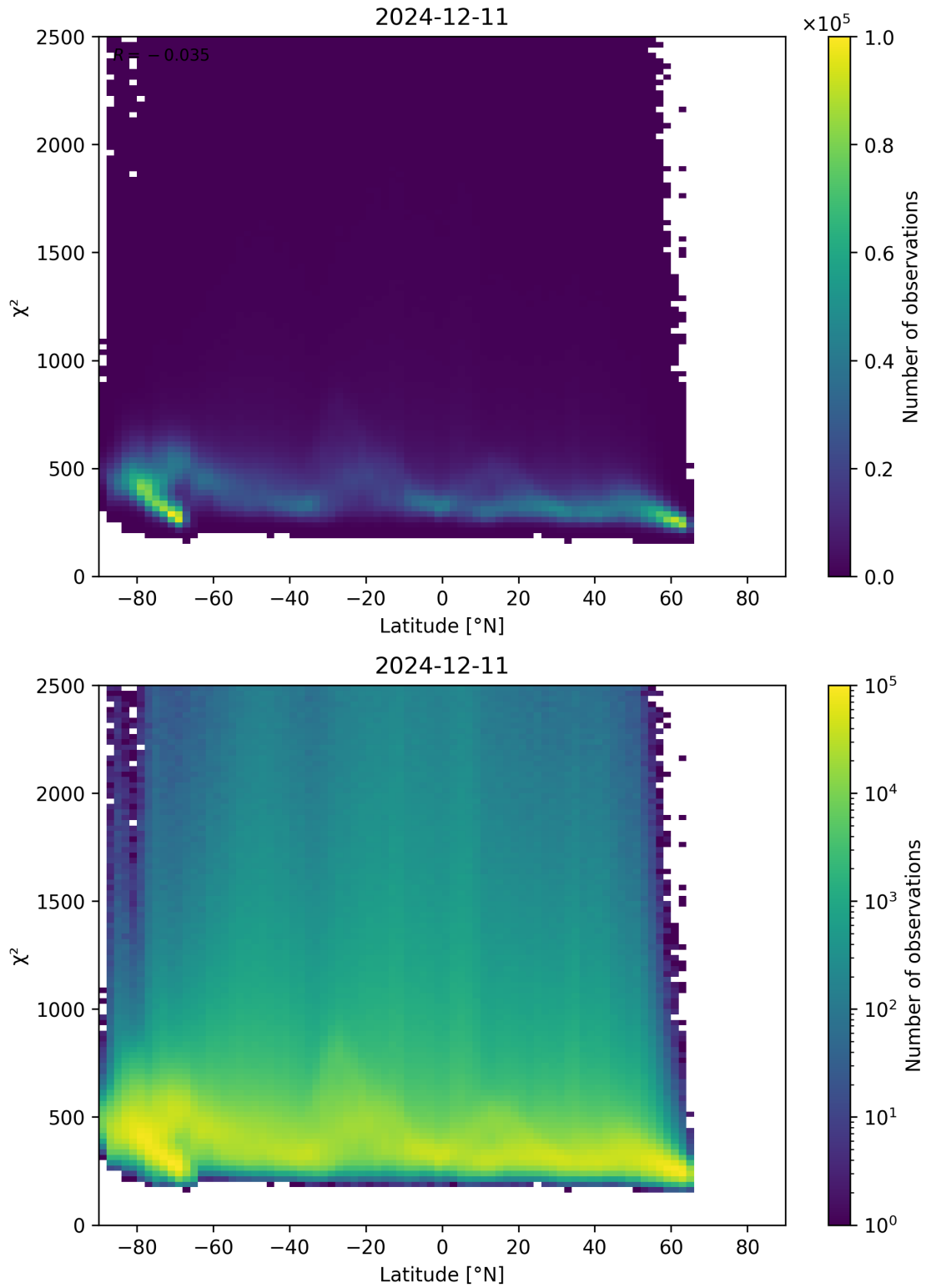
Figure 86: Scatter density plot of “Latitude” against “ \chi^2 ” for 2024-12-11 to 2024-12-12.
