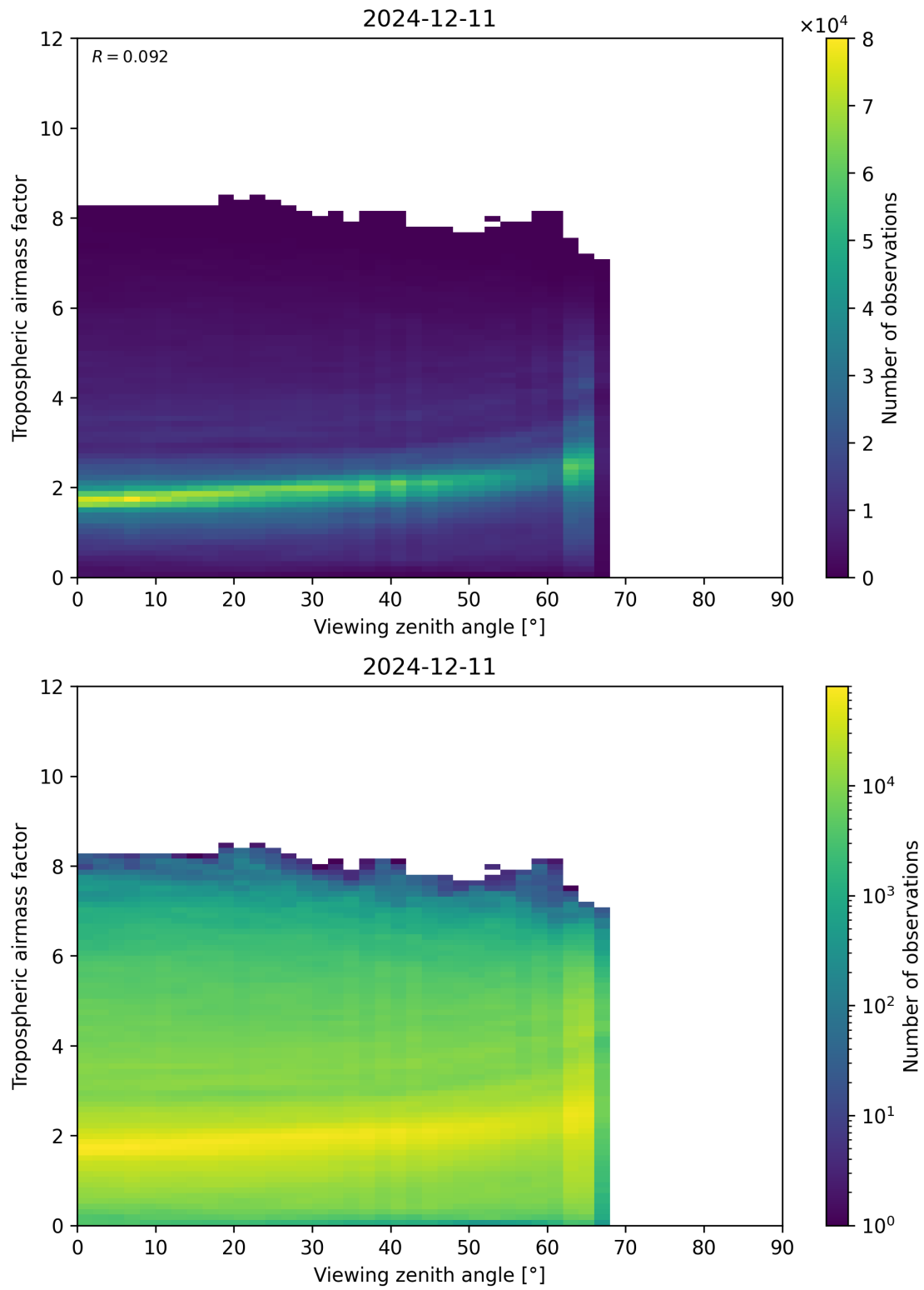
Figure 161: Scatter density plot of “Viewing zenith angle” against “Tropospheric airmass factor” for 2024-12-11 to 2024-12-12.
