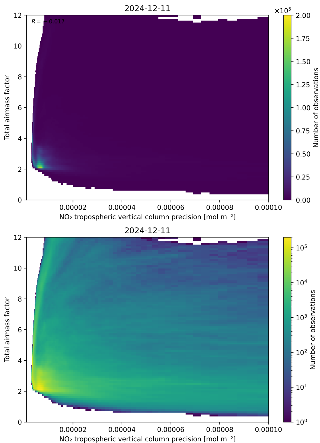
Figure 132: Scatter density plot of “NO 2 tropospheric vertical column precision” against “Total air mass factor” for 2024-12-11 to 2024-12-12.
