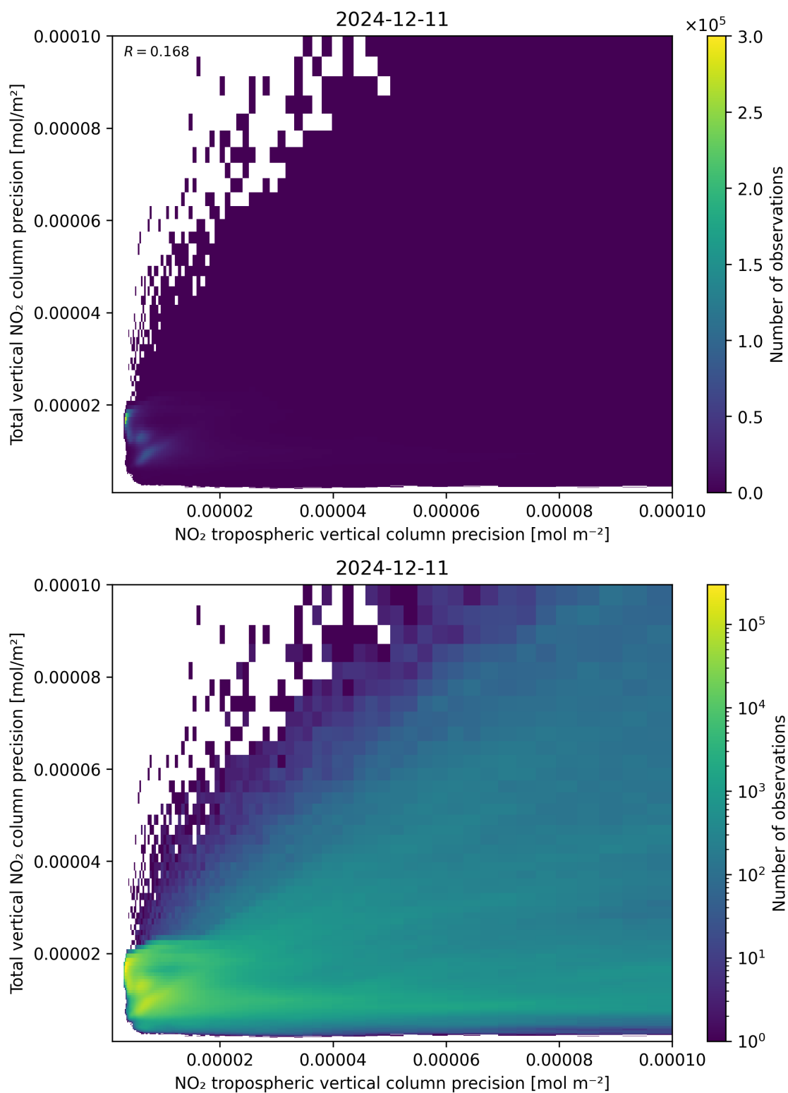
Figure 139: Scatter density plot of “NO 2 tropospheric vertical column precision” against “Total vertical NO 2 column precision” for 2024-12-11 to 2024-12-12.
