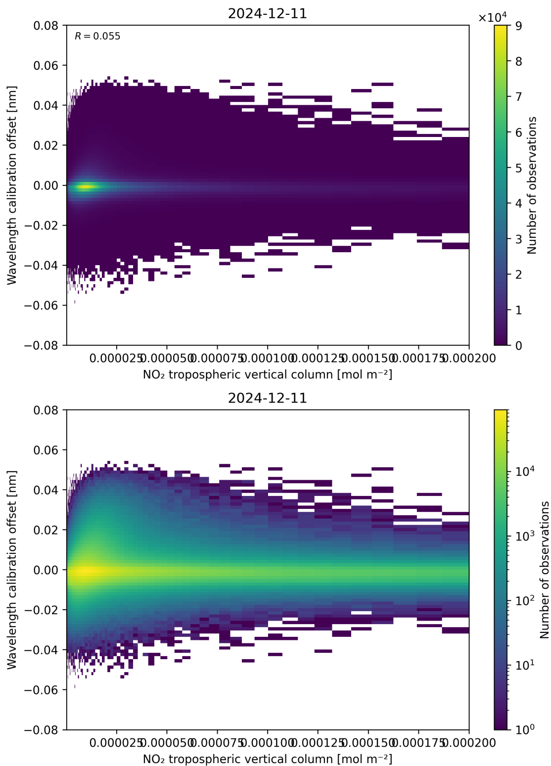
Figure 143: Scatter density plot of “NO 2 tropospheric vertical column” against “Wavelength calibration offset” for 2024-12-11 to 2024-12-12.
