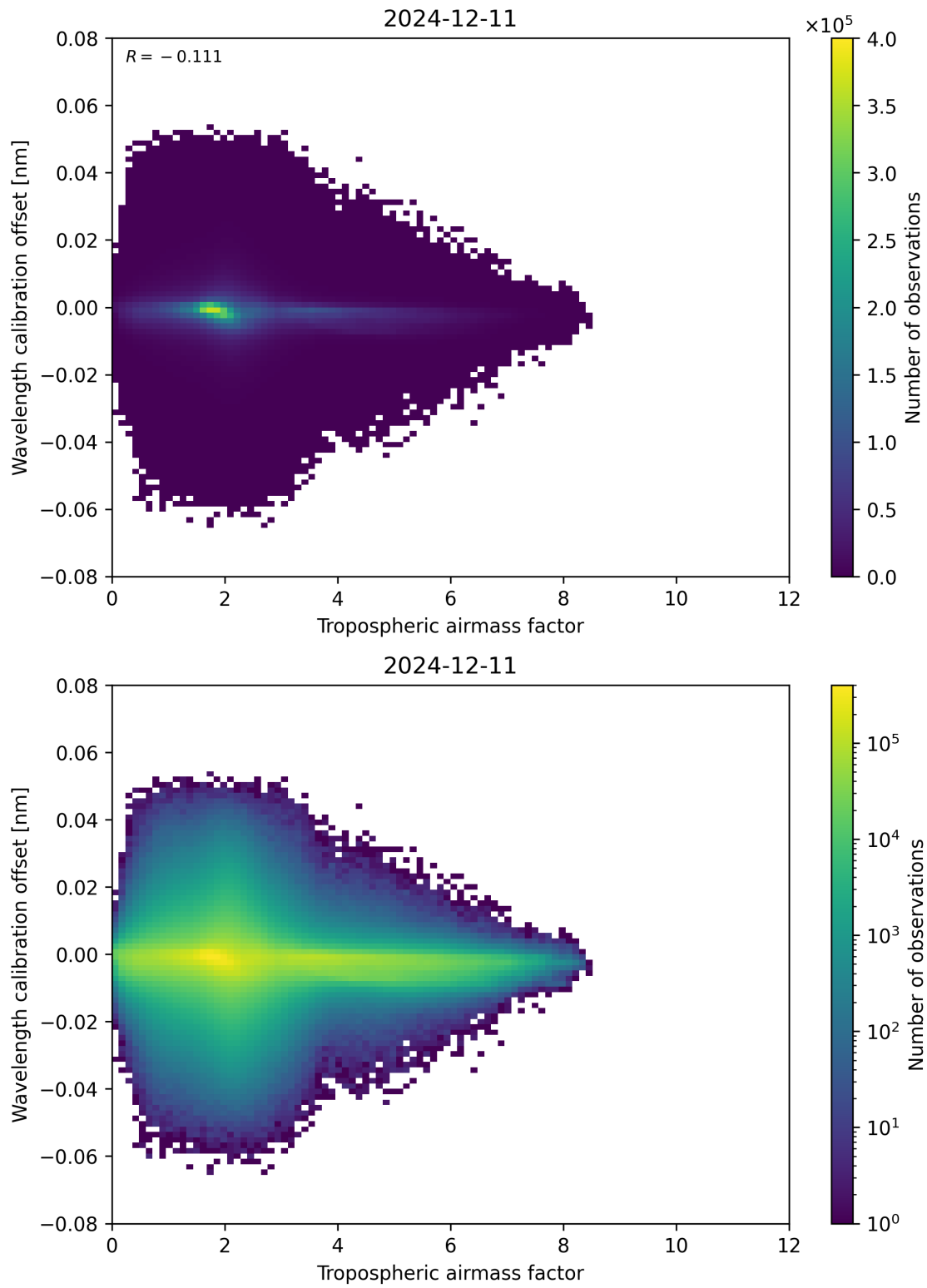
Figure 80: Scatter density plot of “Tropospheric airmass factor” against “Wavelength calibration offset” for 2024-12-11 to 2024-12-12.
