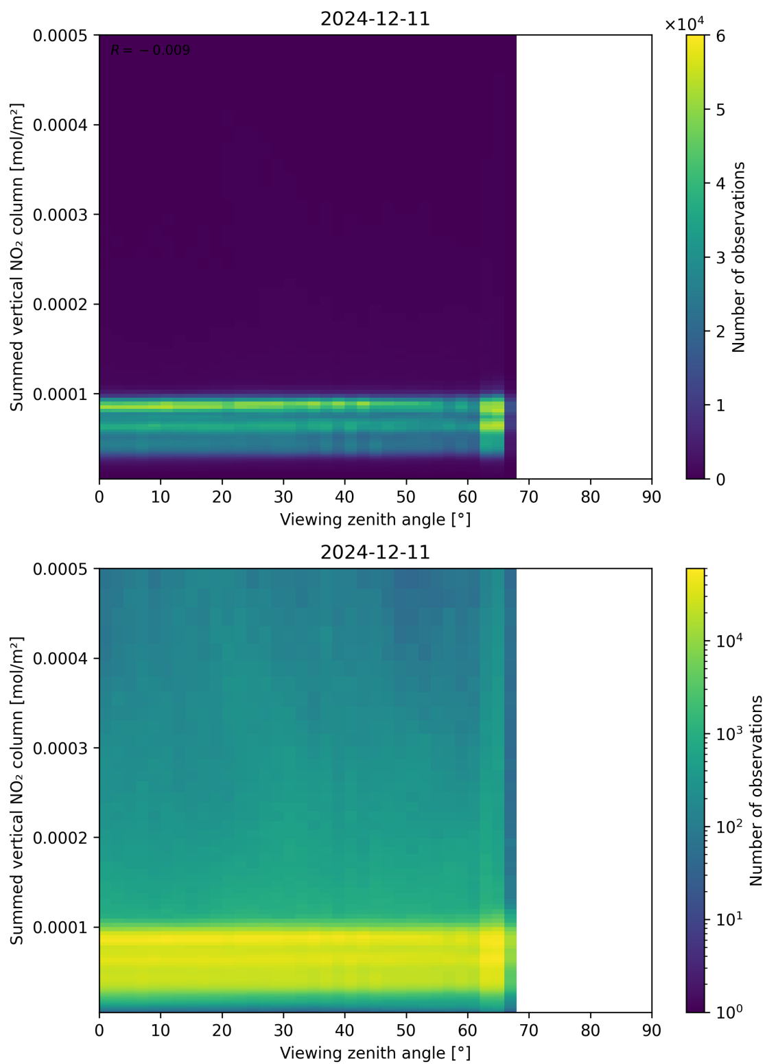
Figure 165: Scatter density plot of “Viewing zenith angle” against “Summed vertical NO 2 column” for 2024-12-11 to 2024-12-12.
