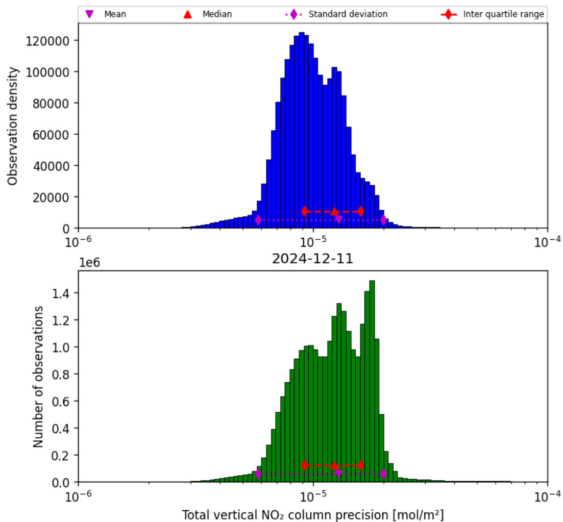
Figure 39: Histogram of “Total vertical NO 2 column precision” for 2024-12-11 to 2024-12-12
