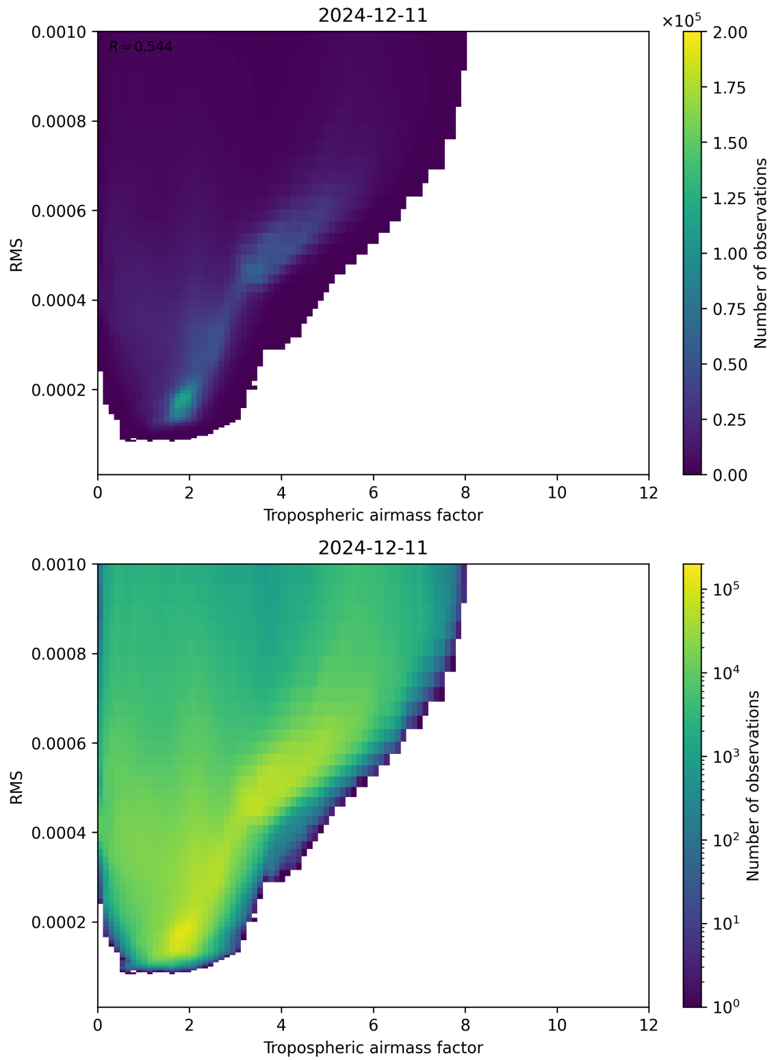
Figure 79: Scatter density plot of “Tropospheric airmass factor” against “RMS” for 2024-12-11 to 2024-12-12.
