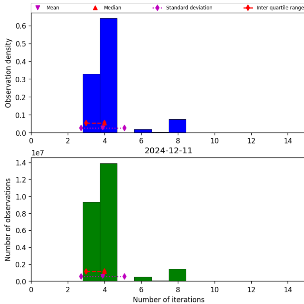
Figure 34: Histogram of “Number of iterations” for 2024-12-11 to 2024-12-12
