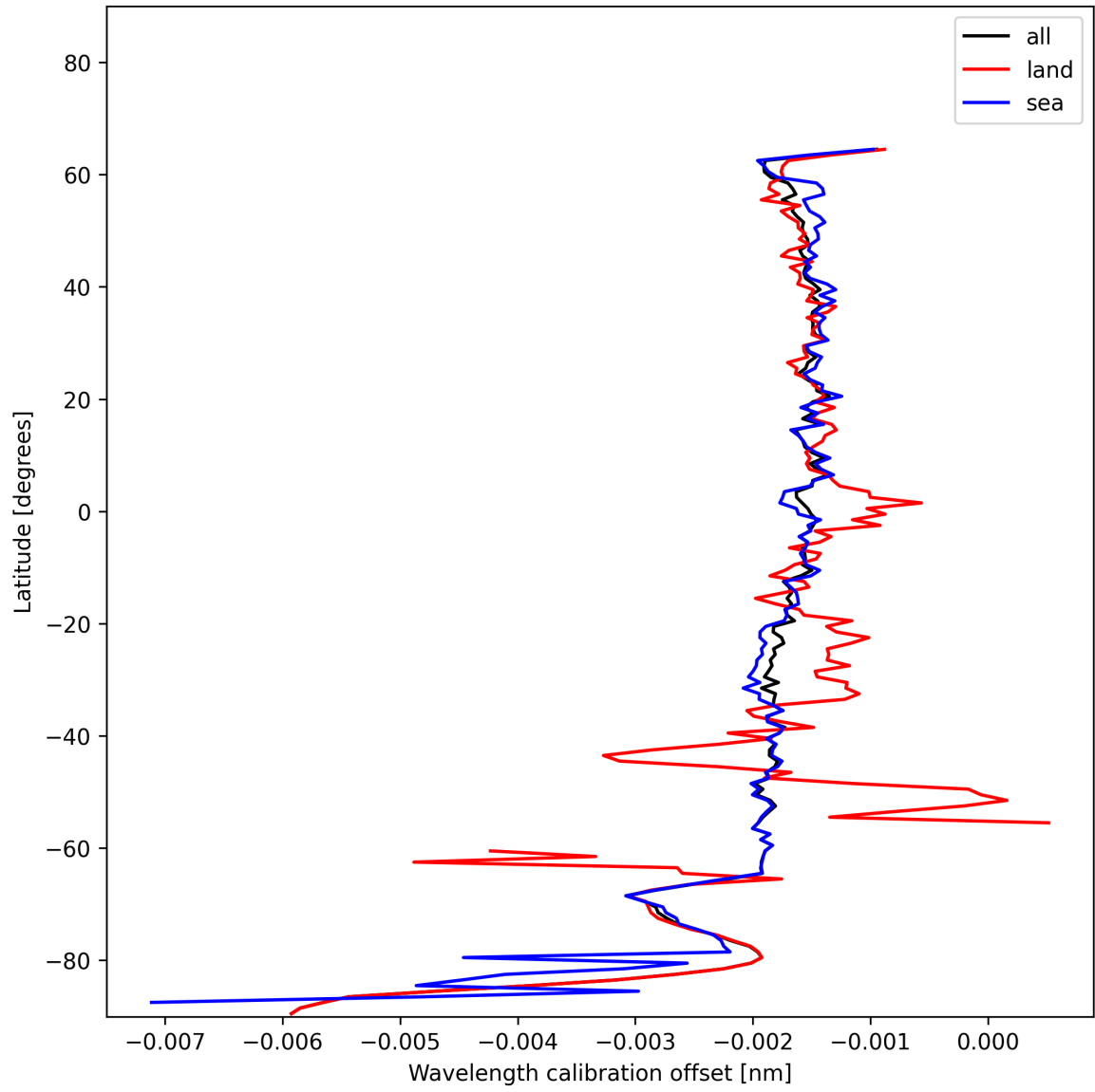
Figure 18: Zonal average of “Wavelength calibration offset” for 2024-12-11 to 2024-12-12.
