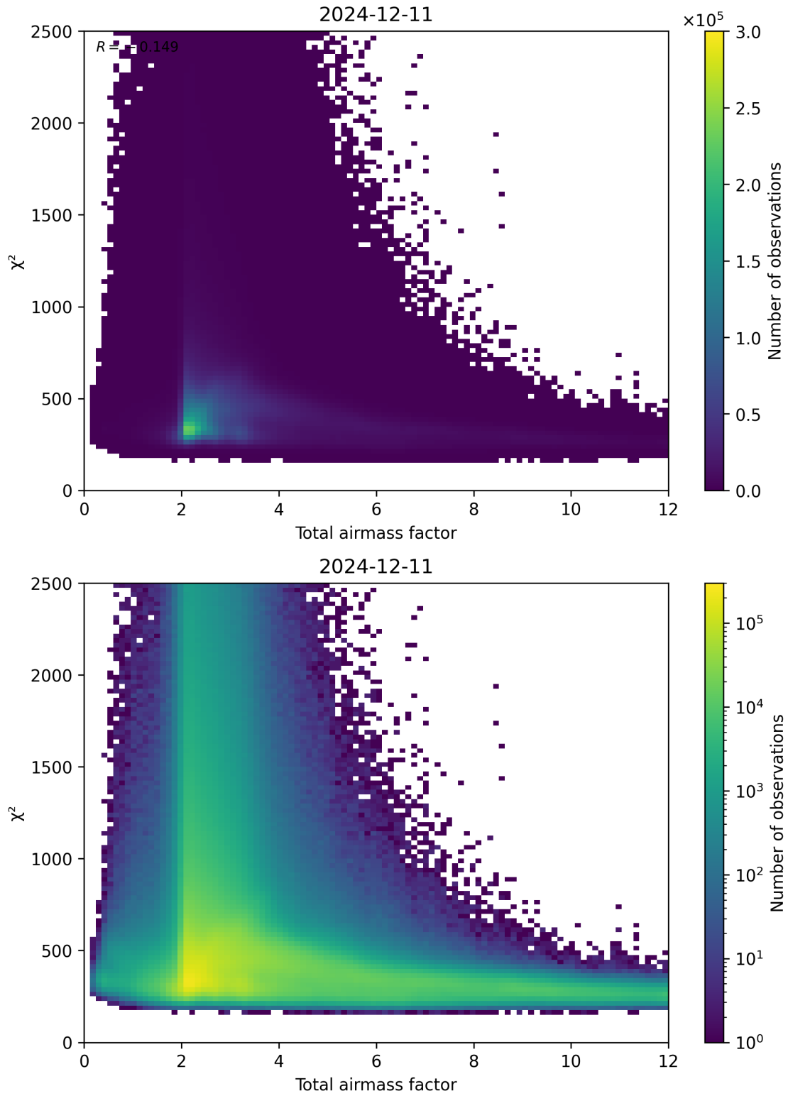
Figure 63: Scatter density plot of “Total airmass factor” against “ \chi^2 ” for 2024-12-11 to 2024-12-12.
