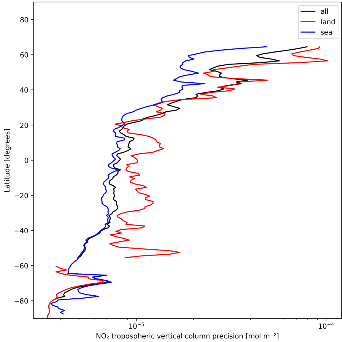
Figure 13: Zonal average of “NO 2 tropospheric vertical column precision” for 2024-12-11 to 2024-12-12.
