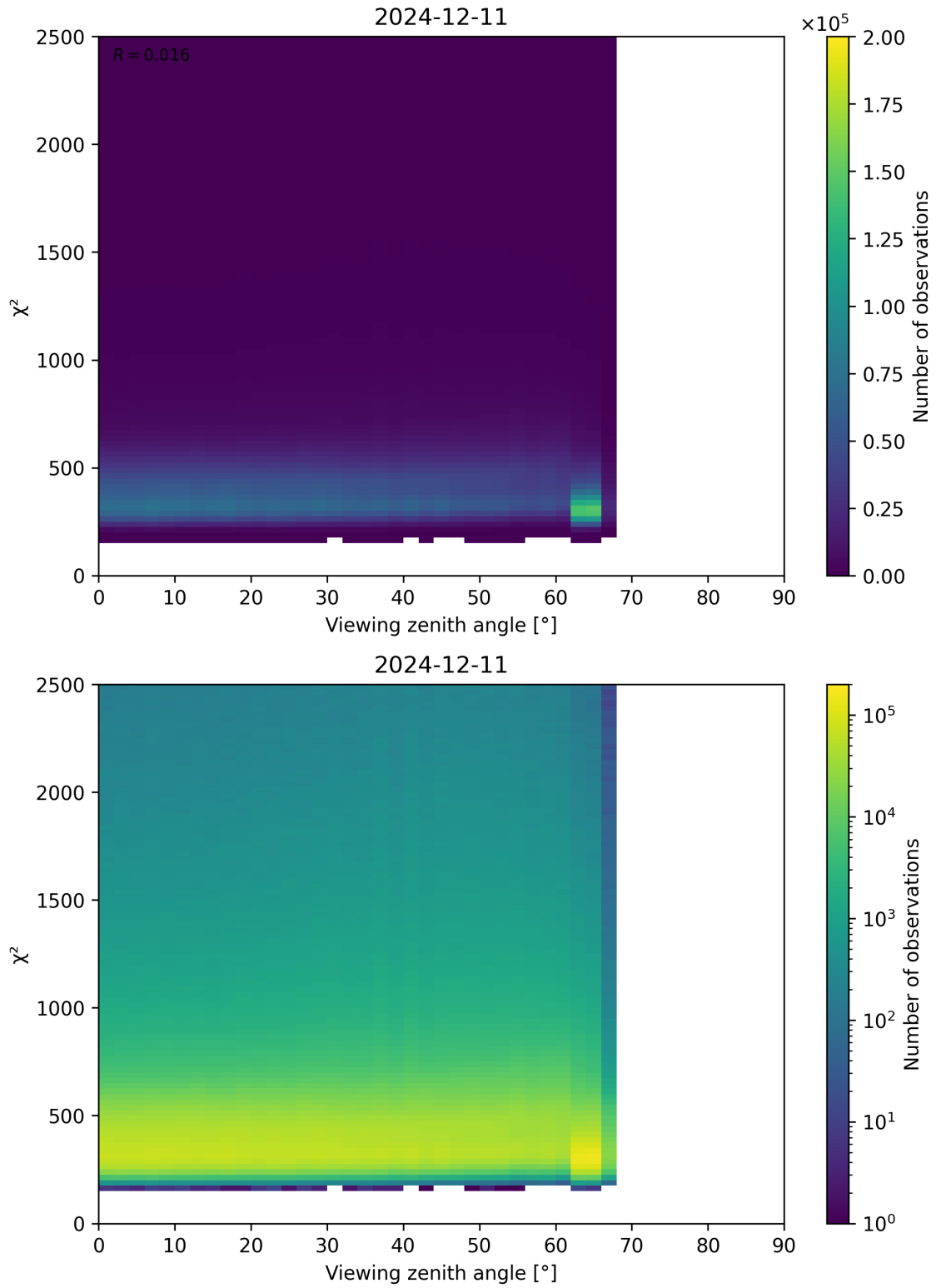
Figure 162: Scatter density plot of “Viewing zenith angle” against “ \chi^2 ” for 2024-12-11 to 2024-12-12.
