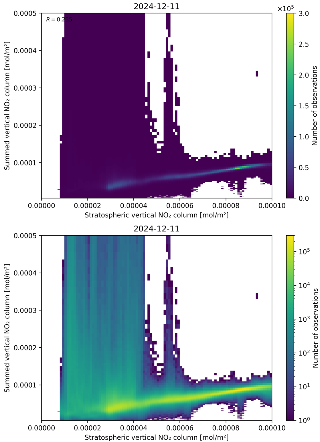
Figure 98: Scatter density plot of “Stratospheric vertical NO 2 column” against “Summed vertical NO 2 column” for 2024-12-11 to 2024-12-12.
