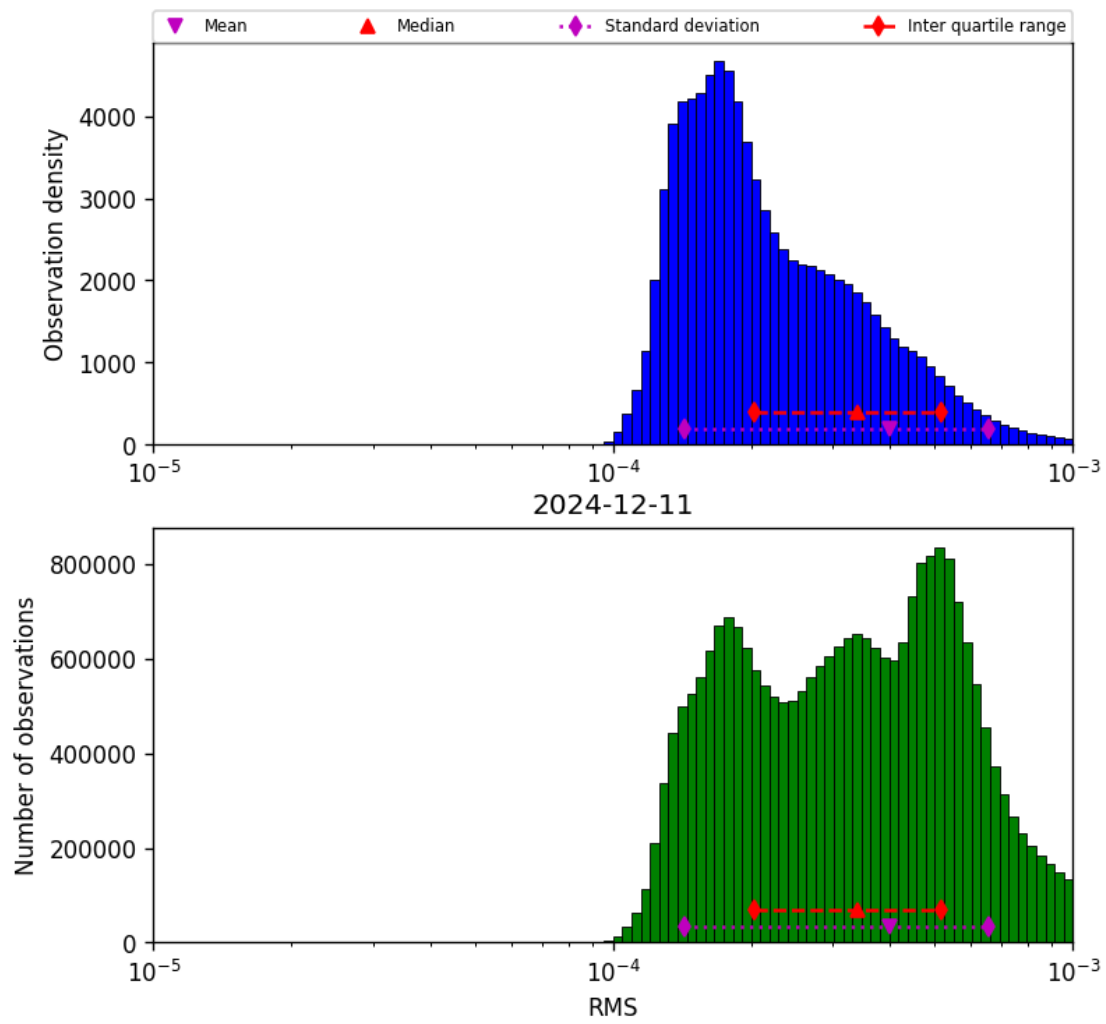
Figure 43: Histogram of “RMS” for 2024-12-11 to 2024-12-12
