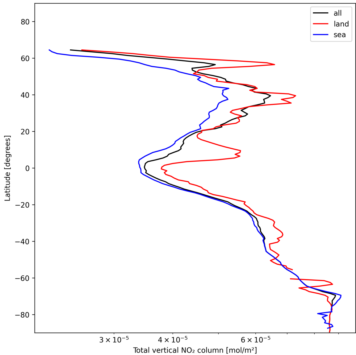
Figure 21: Zonal average of “Total vertical NO 2 column” for 2024-12-11 to 2024-12-12.
