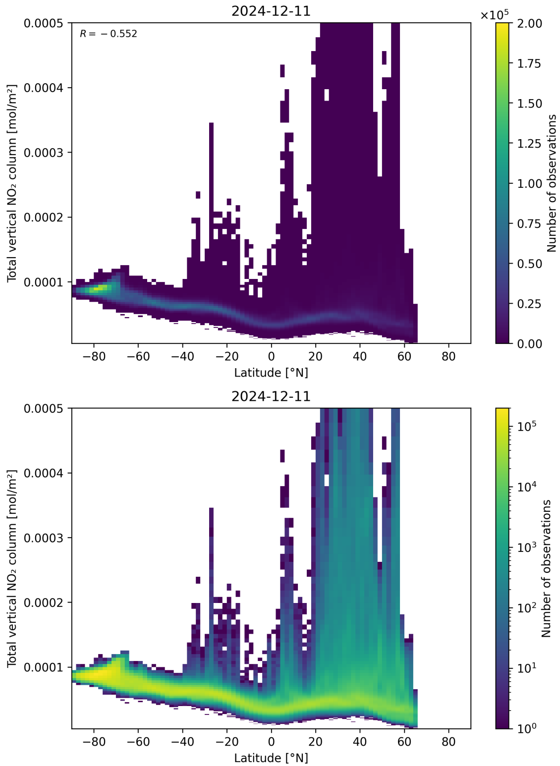
Figure 90: Scatter density plot of “Latitude” against “Total vertical NO 2 column” for 2024-12-11 to 2024-12-12.
