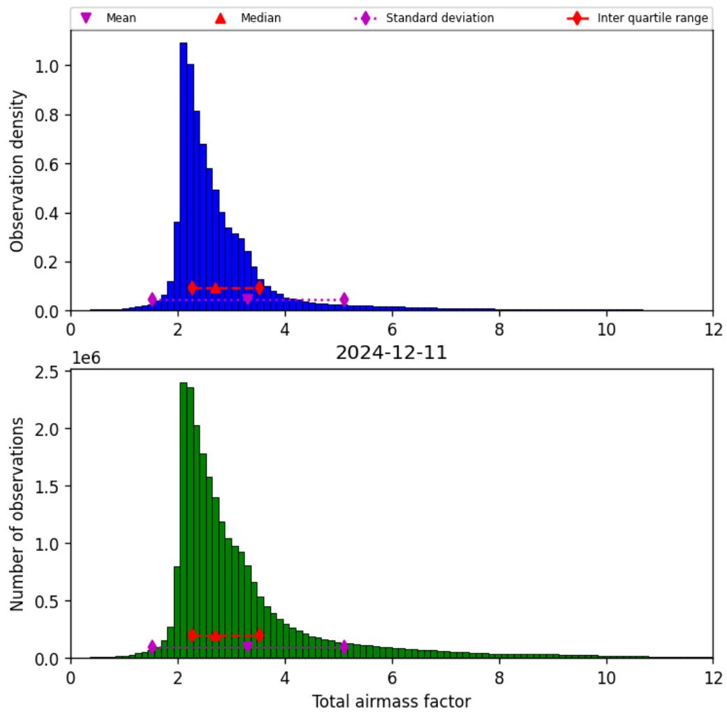
Figure 32: Histogram of “Total airmass factor” for 2024-12-11 to 2024-12-12
