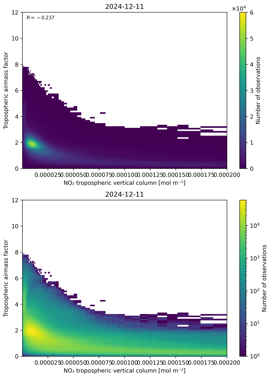
Figure 123: Scatter density plot of “NO 2 tropospheric vertical column” against “Tropospheric air mass factor” for 2024-12-11 to 2024-12-12.
