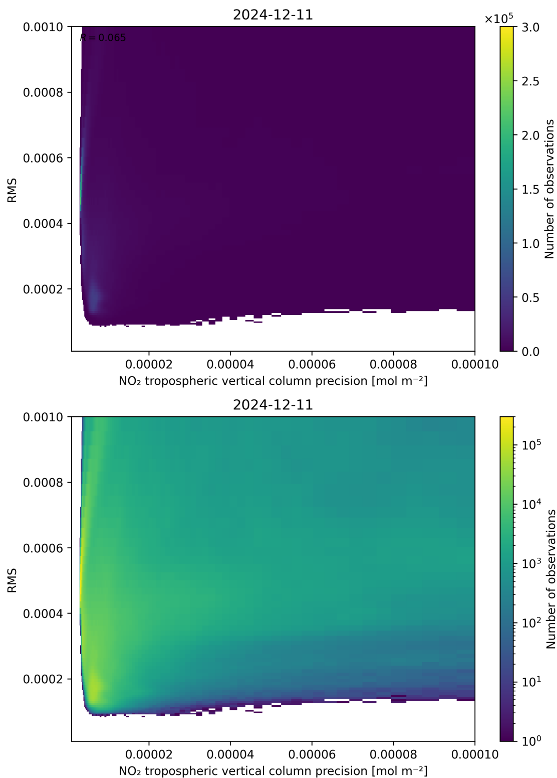
Figure 140: Scatter density plot of “NO 2 tropospheric vertical column precision” against “RMS” for 2024-12-11 to 2024-12-12.
