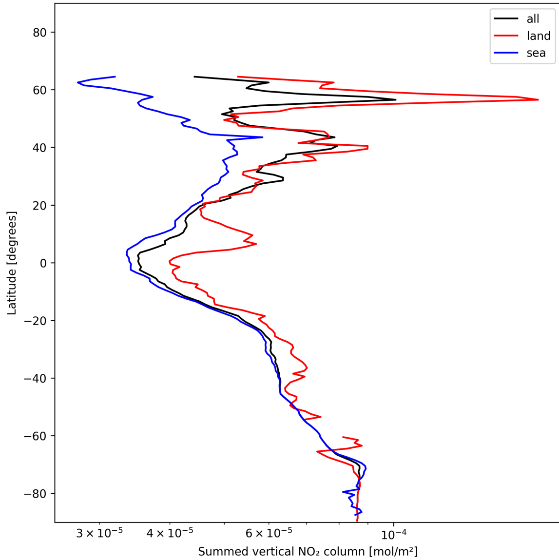
Figure 23: Zonal average of “Summed vertical NO 2 column” for 2024-12-11 to 2024-12-12.
