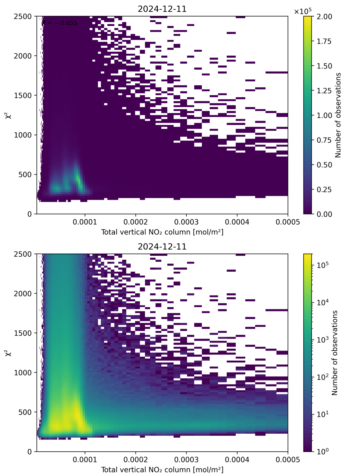
Figure 111: Scatter density plot of “Total vertical NO 2 column” against “ \chi^2 ” for 2024-12-11 to 2024-12-12.
