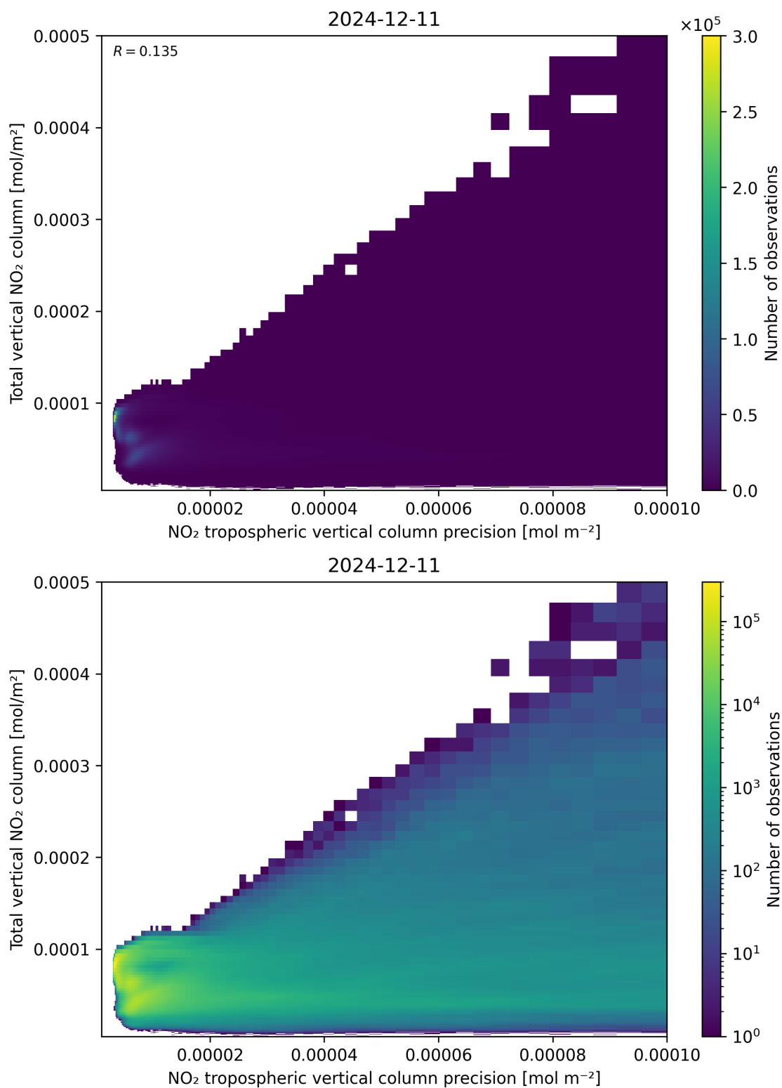
Figure 138: Scatter density plot of “NO 2 tropospheric vertical column precision” against “Total vertical NO 2 column” for 2024-12-11 to 2024-12-12.
