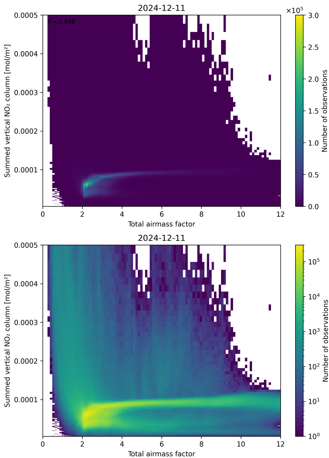
Figure 65: Scatter density plot of “Total airmass factor” against “Summed vertical NO 2 column” for 2024-12-11 to 2024-12-12.
