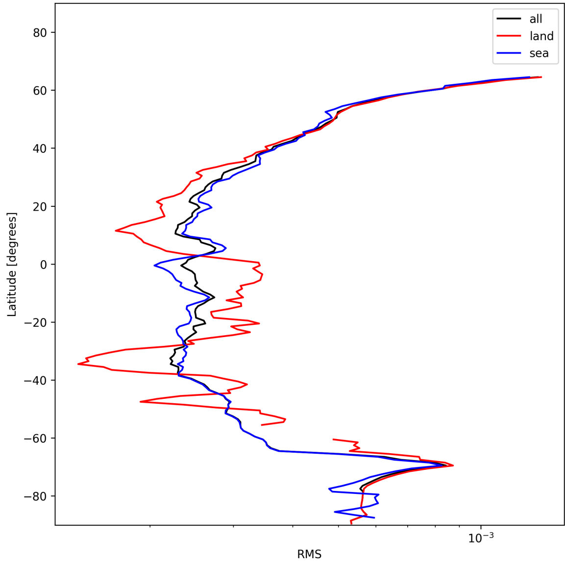
Figure 26: Zonal average of “RMS” for 2024-12-11 to 2024-12-12.
