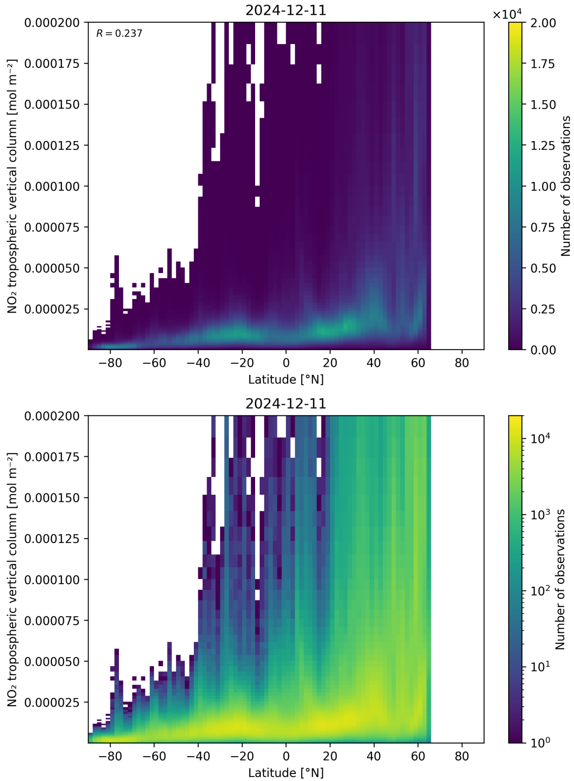
Figure 92: Scatter density plot of “Latitude” against “NO 2 tropospheric vertical column” for 2024-12-11 to 2024-12-12.
