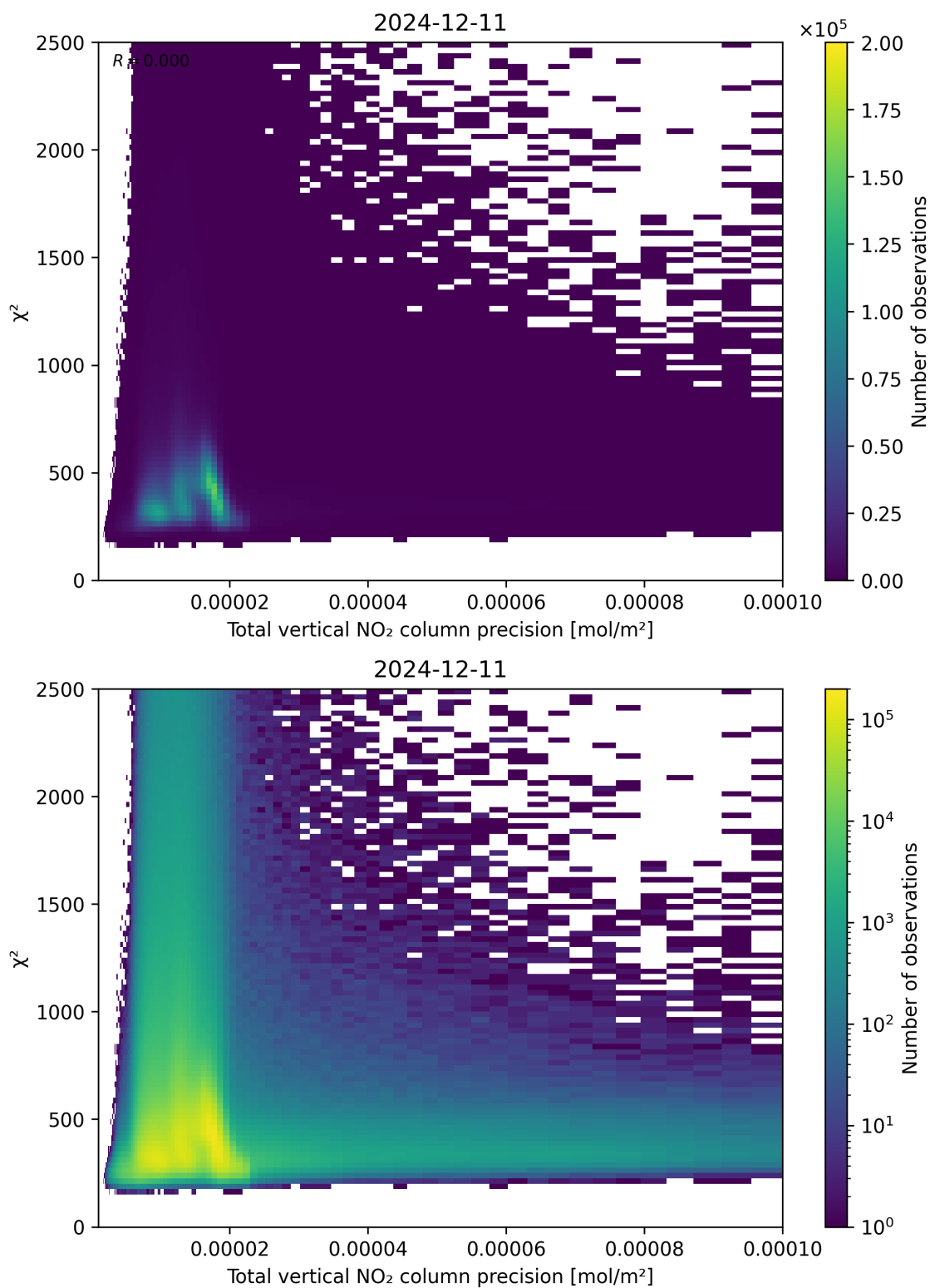
Figure 116: Scatter density plot of “Total vertical NO 2 column precision” against “ \chi^2 ” for 2024-12-11 to 2024-12-12.
