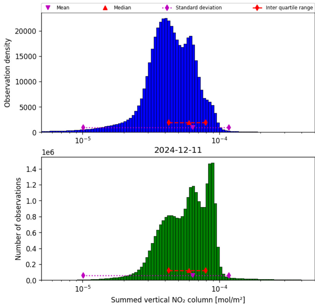
Figure 40: Histogram of “Summed vertical NO 2 column” for 2024-12-11 to 2024-12-12
