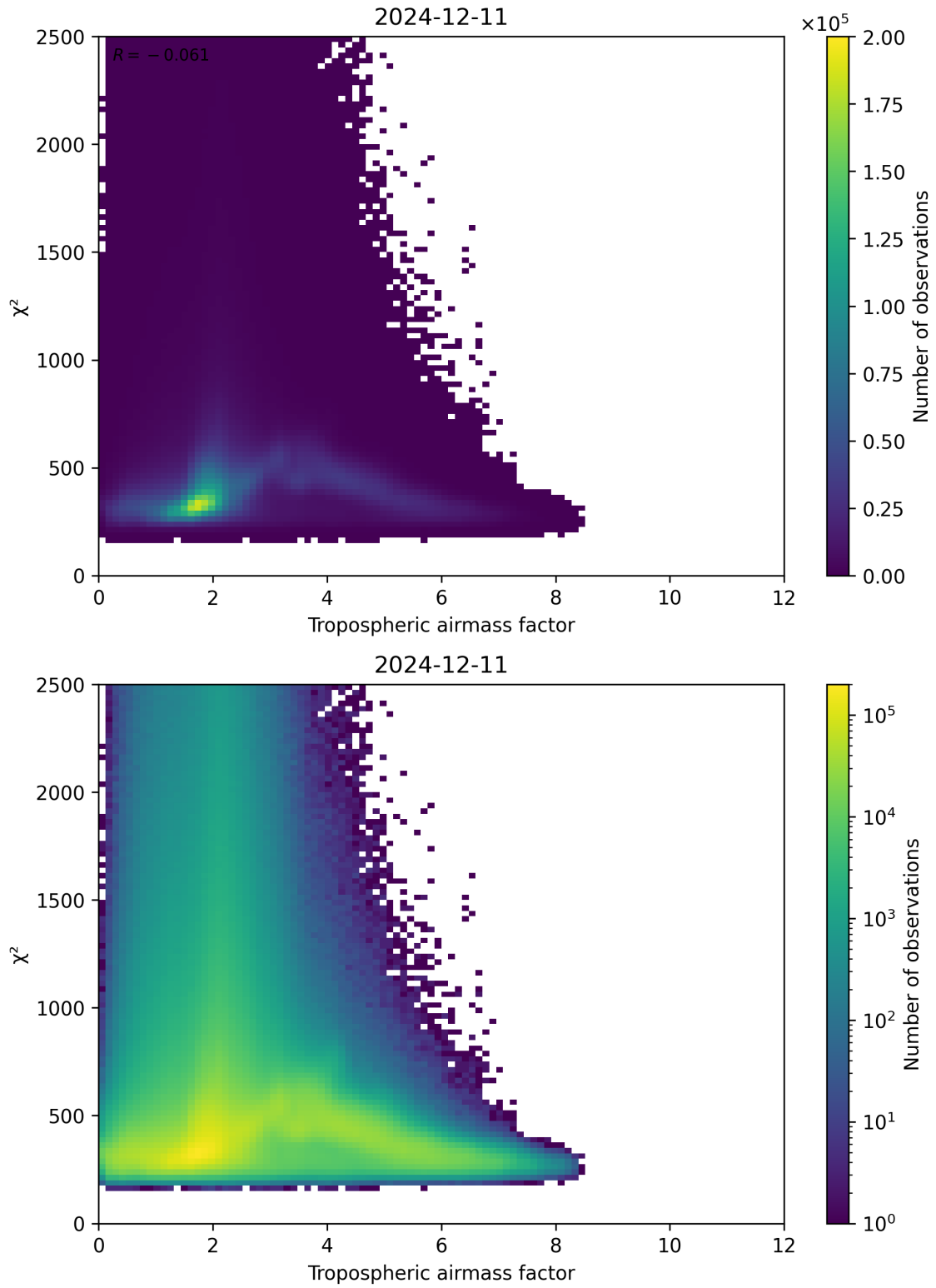
Figure 73: Scatter density plot of “Tropospheric airmass factor” against “ \chi^2 ” for 2024-12-11 to 2024-12-12.
