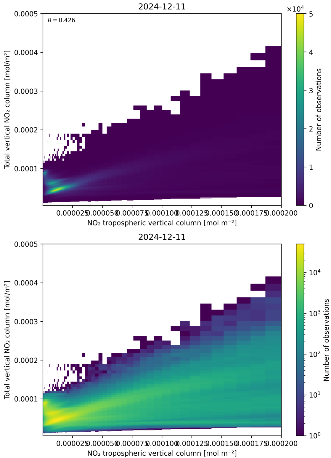
Figure 128: Scatter density plot of “NO 2 tropospheric vertical column” against “Total vertical NO 2 column” for 2024-12-11 to 2024-12-12.
