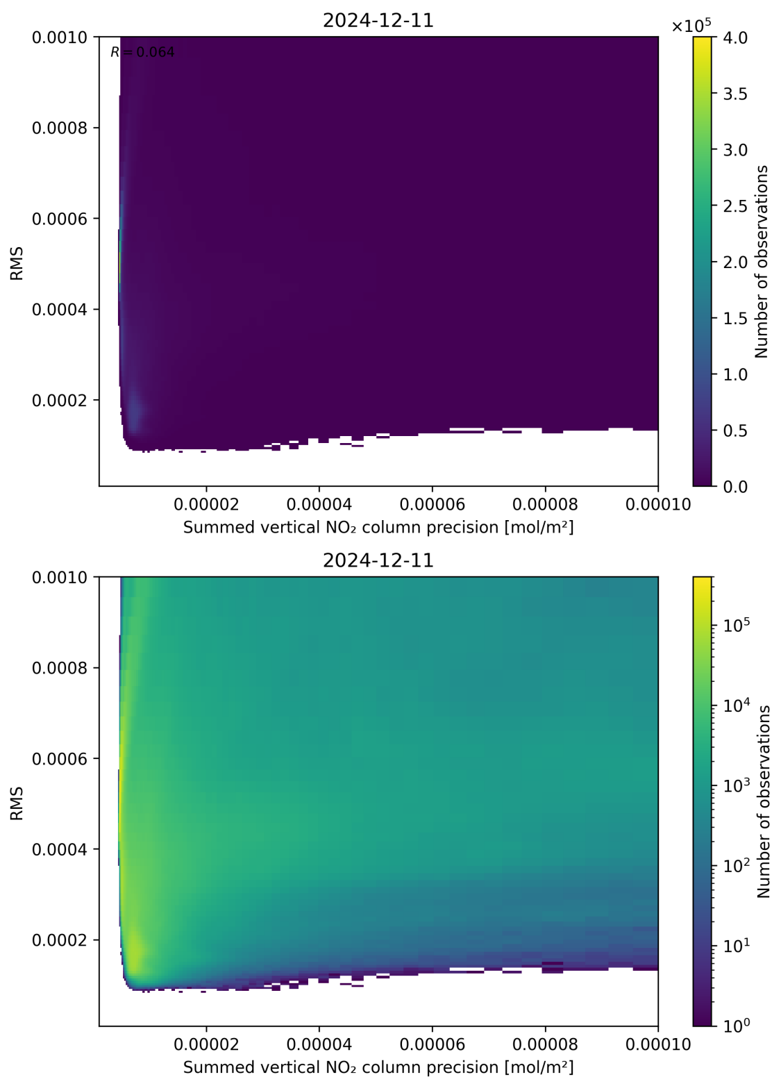
Figure 108: Scatter density plot of “Summed vertical NO 2 column precision” against “RMS” for 2024-12-11 to 2024-12-12.
