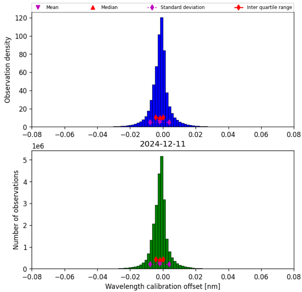
Figure 35: Histogram of “Wavelength calibration offset” for 2024-12-11 to 2024-12-12
