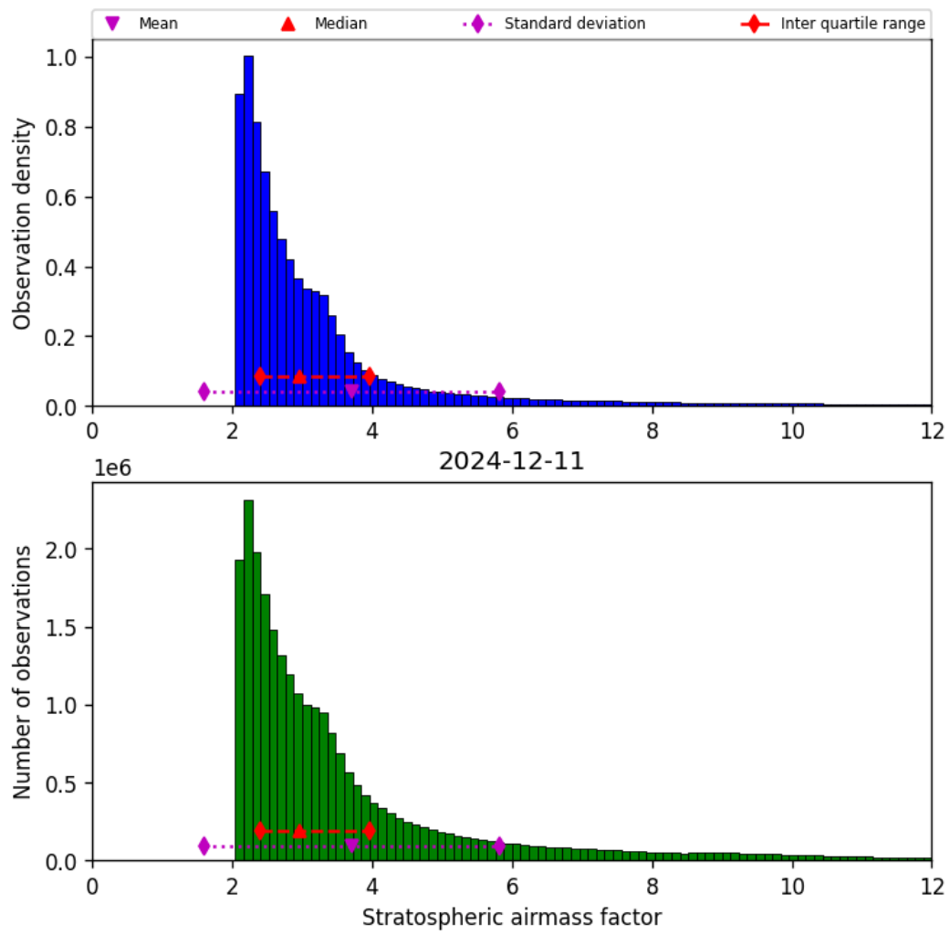
Figure 44: Histogram of “Stratospheric airmass factor” for 2024-12-11 to 2024-12-12
