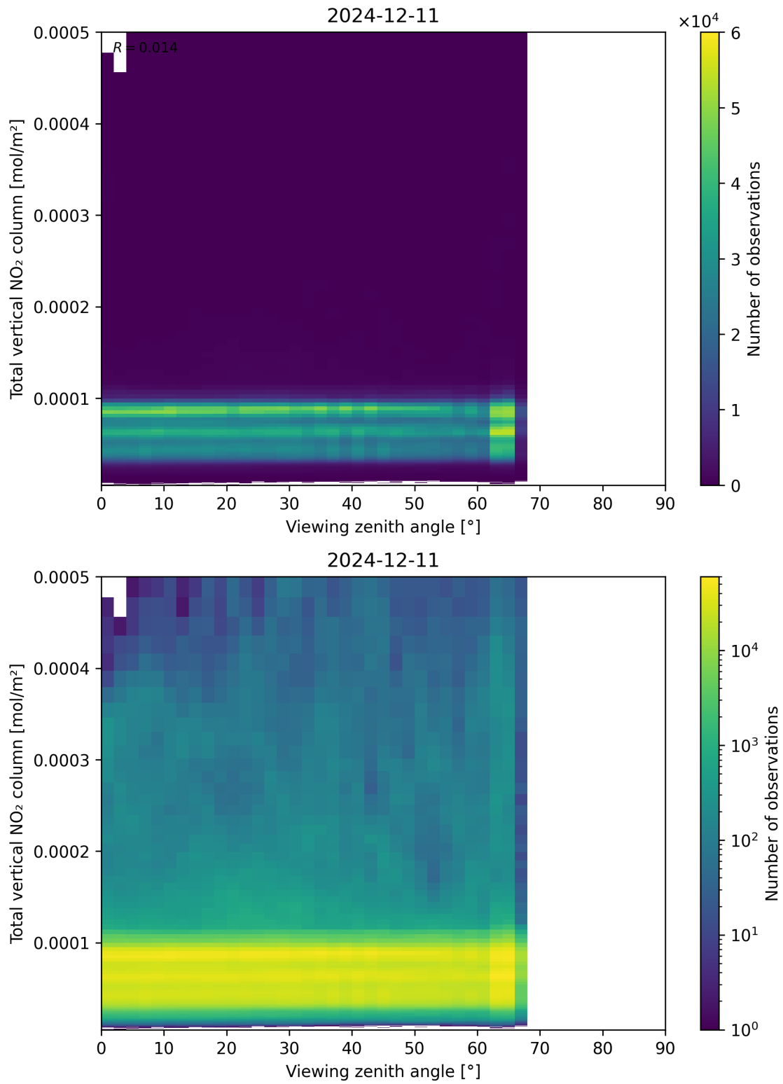
Figure 167: Scatter density plot of “Viewing zenith angle” against “Total vertical NO 2 column” for 2024-12-11 to 2024-12-12.
