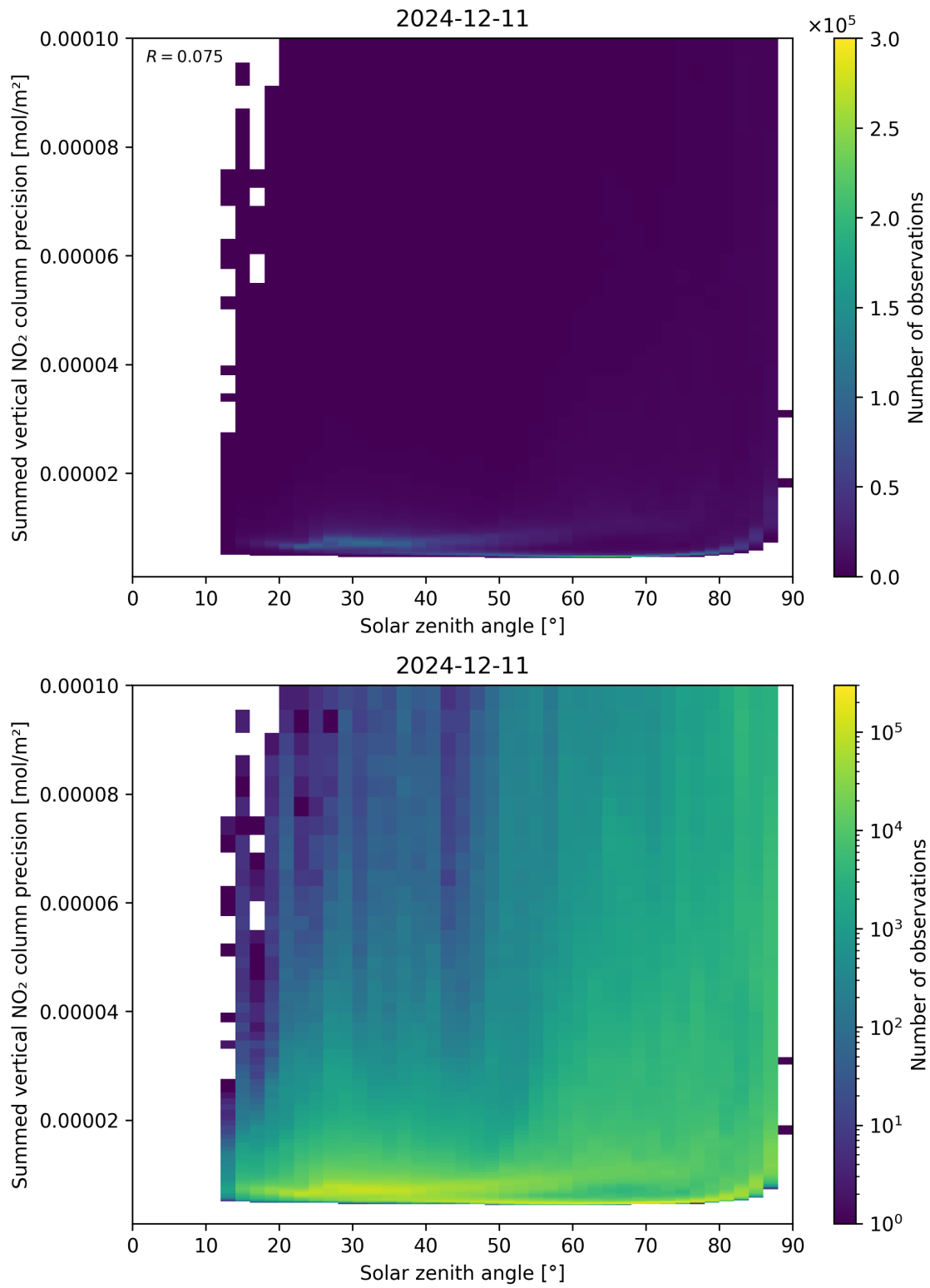
Figure 152: Scatter density plot of “Solar zenith angle” against “Summed vertical NO 2 column precision” for 2024-12-11 to 2024-12-12.
