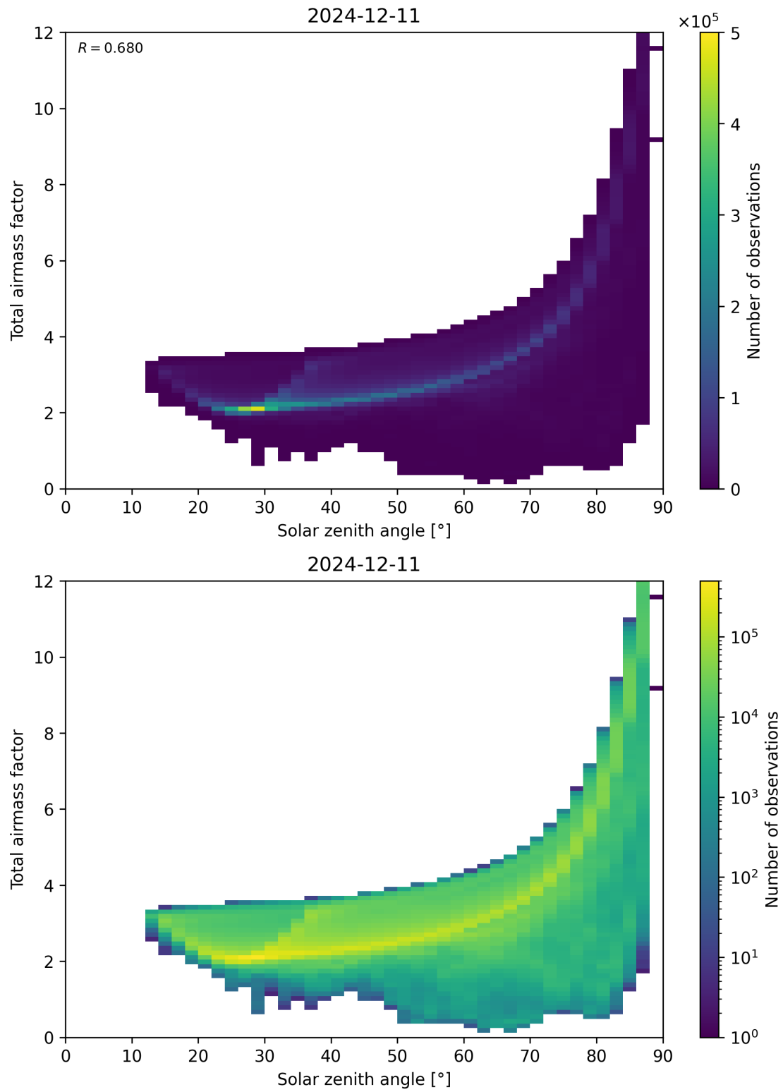
Figure 146: Scatter density plot of “Solar zenith angle” against “Total air mass factor” for 2024-12-11 to 2024-12-12.
