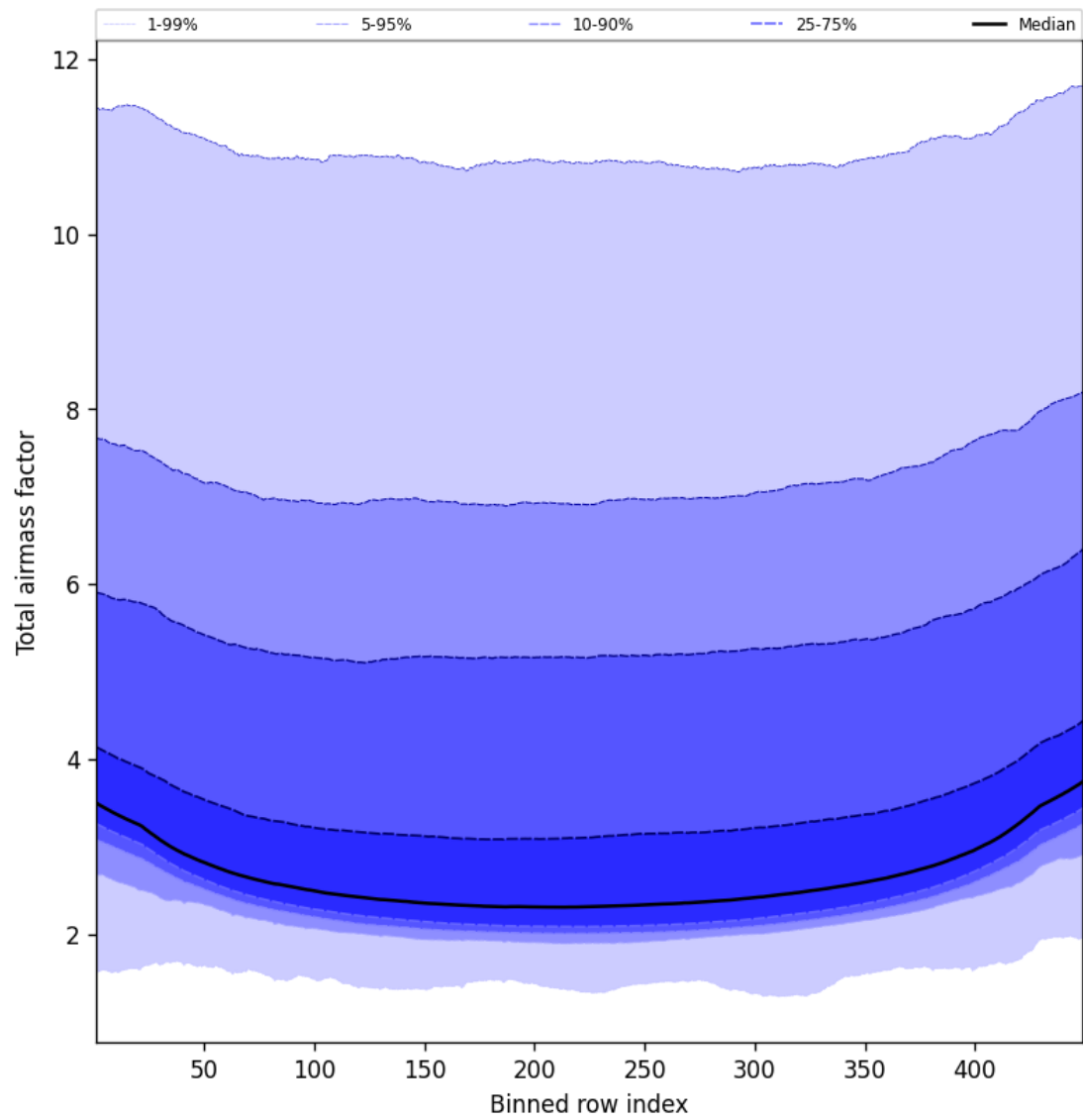
Figure 49: Along track statistics of “Total airmass factor” for 2024-12-11 to 2024-12-12
