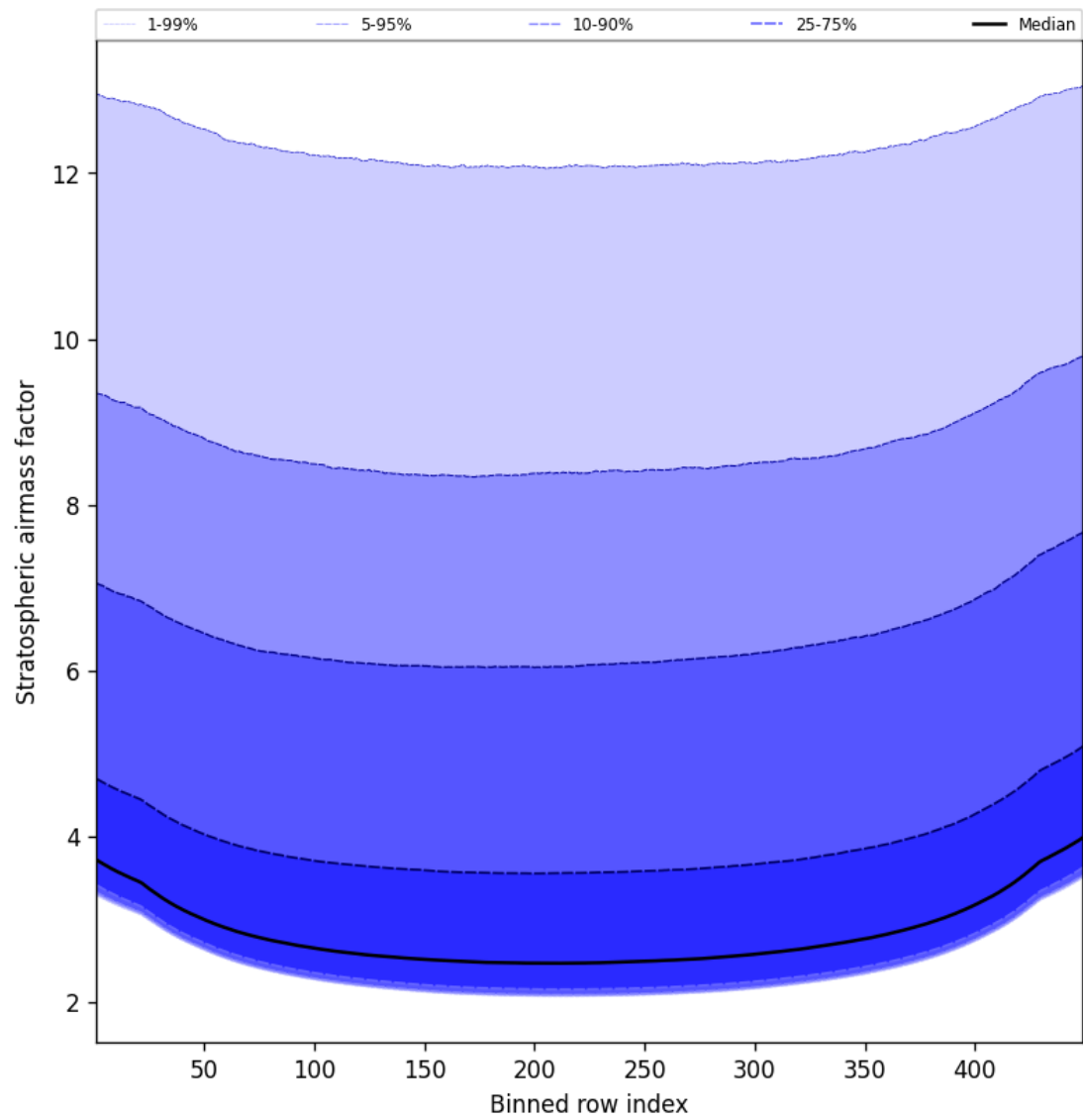
Figure 61: Along track statistics of “Stratospheric airmass factor” for 2024-12-11 to 2024-12-12
