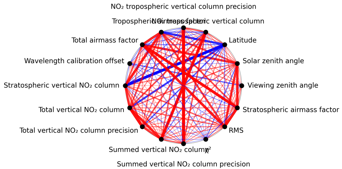
Figure 1: Map of correlation graph for 2024-12-11 to 2024-12-12.
