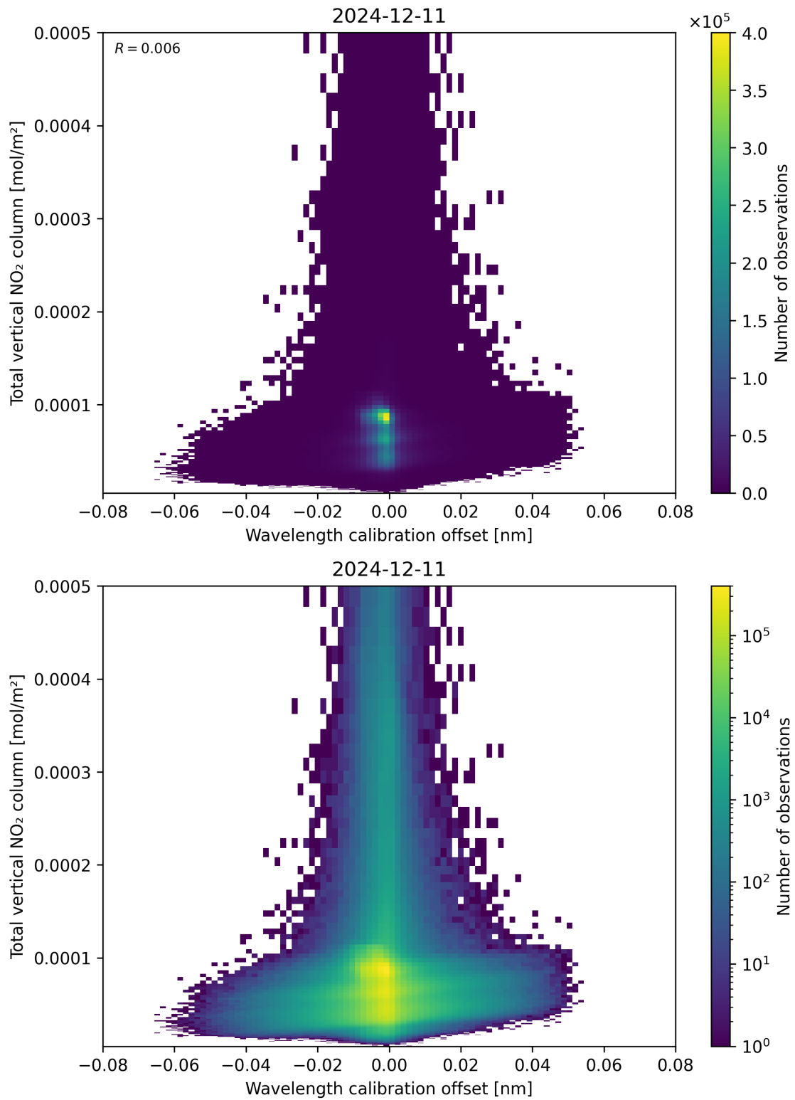
Figure 179: Scatter density plot of “Wavelength calibration offset” against “Total vertical NO 2 column” for 2024-12-11 to 2024-12-12.
