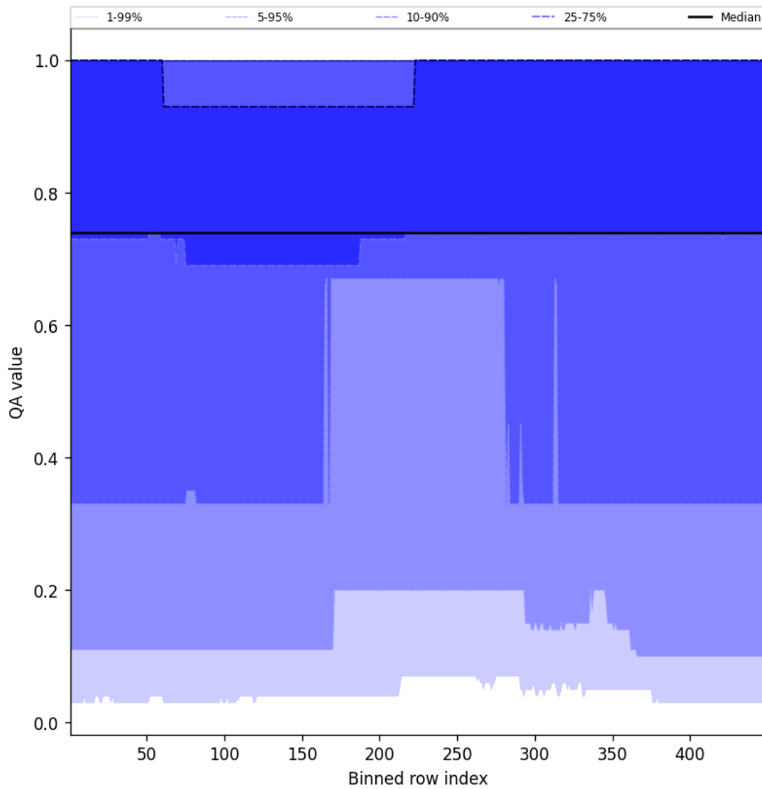
Figure 45: Along track statistics of “QA value” for 2024-12-11 to 2024-12-12
