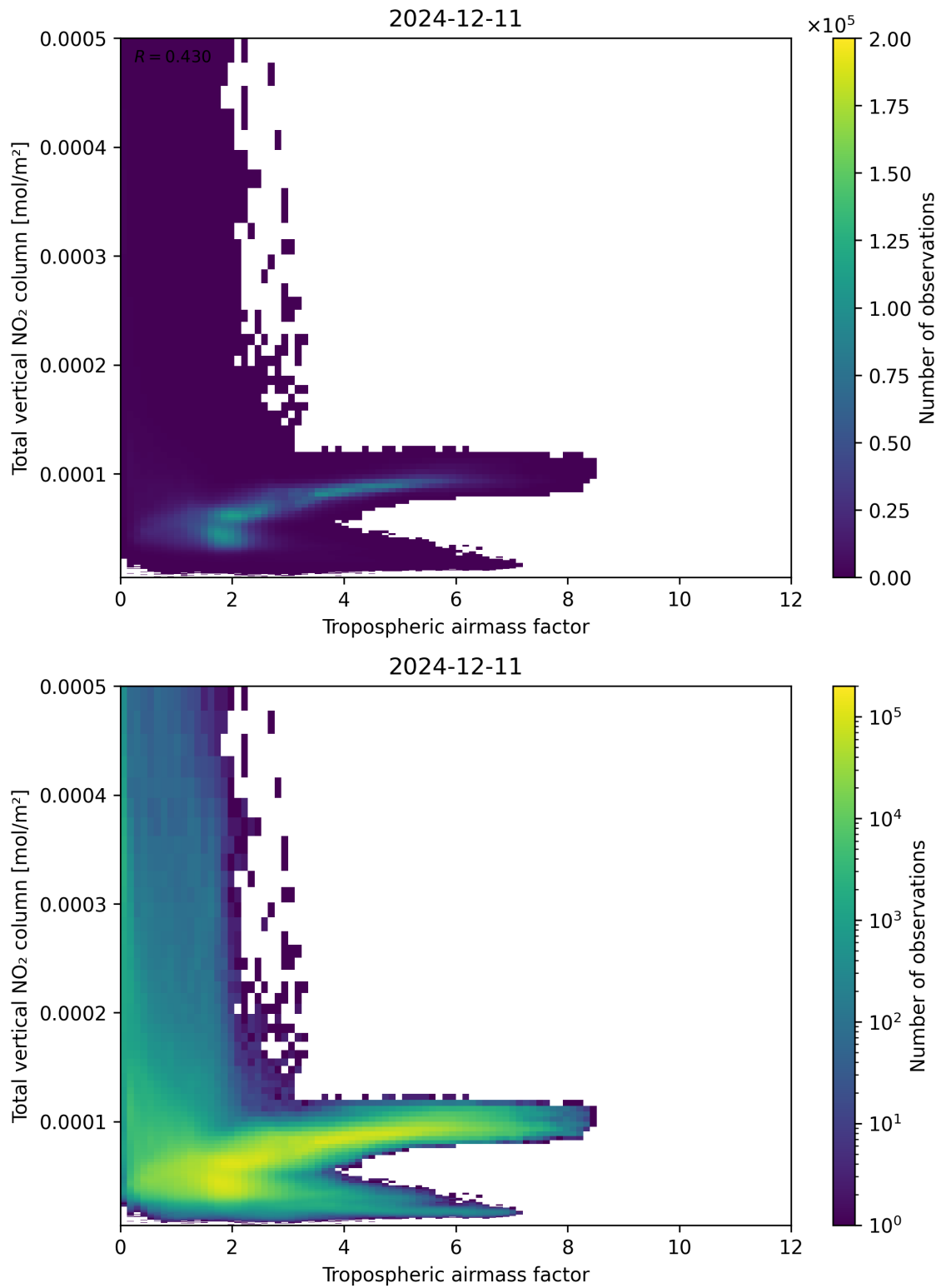
Figure 77: Scatter density plot of “Tropospheric airmass factor” against “Total vertical NO 2 column” for 2024-12-11 to 2024-12-12.
