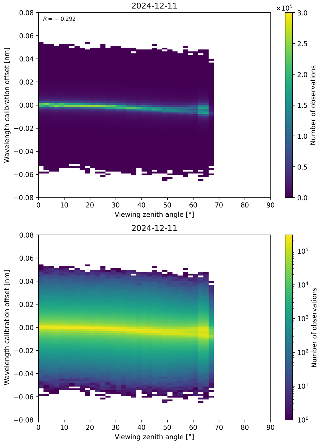
Figure 173: Scatter density plot of “Viewing zenith angle” against “Wavelength calibration offset” for 2024-12-11 to 2024-12-12.
