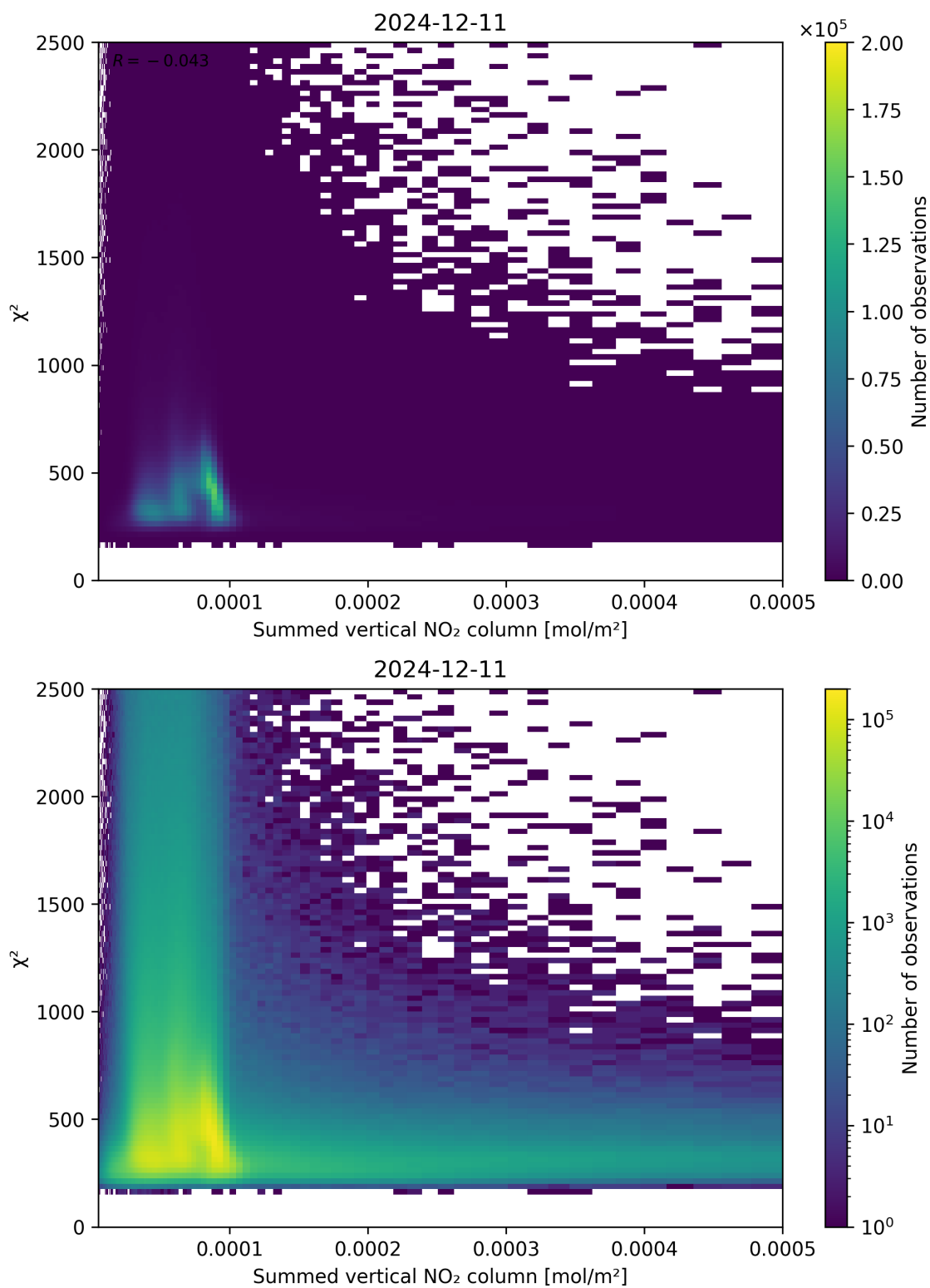
Figure 104: Scatter density plot of “Summed vertical NO 2 column” against “ \chi^2 ” for 2024-12-11 to 2024-12-12.
