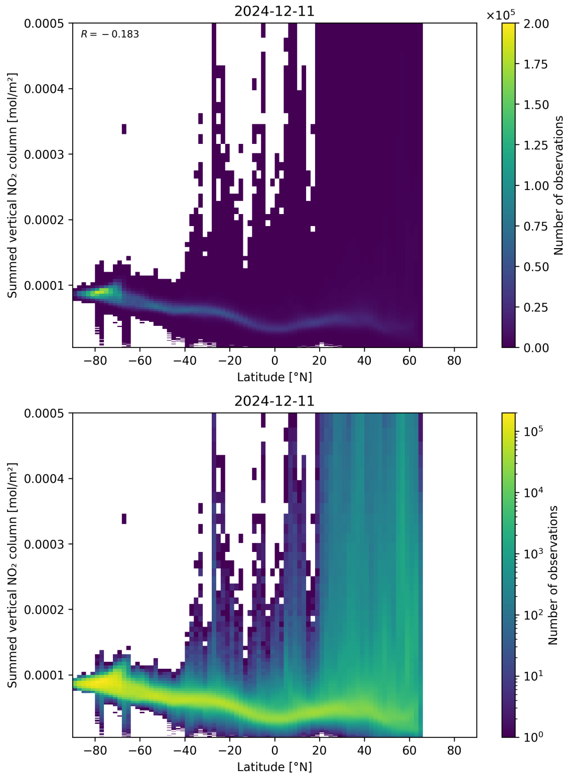
Figure 88: Scatter density plot of “Latitude” against “Summed vertical NO 2 column” for 2024-12-11 to 2024-12-12.
