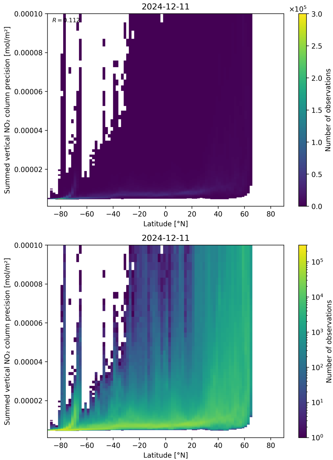
Figure 89: Scatter density plot of “Latitude” against “Summed vertical NO 2 column precision” for 2024-12-11 to 2024-12-12.
