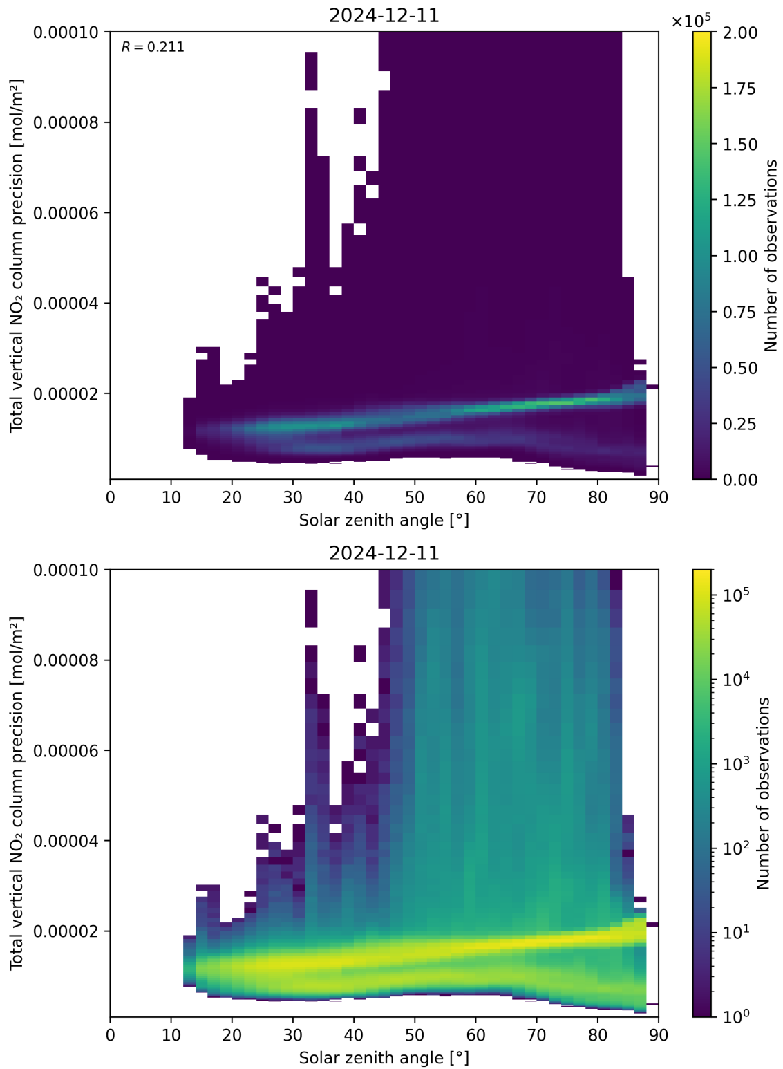
Figure 154: Scatter density plot of “Solar zenith angle” against “Total vertical NO 2 column precision” for 2024-12-11 to 2024-12-12.
