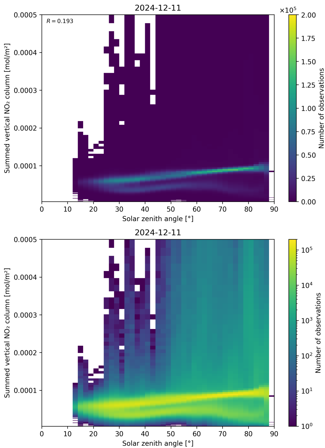
Figure 151: Scatter density plot of “Solar zenith angle” against “Summed vertical NO 2 column” for 2024-12-11 to 2024-12-12.
