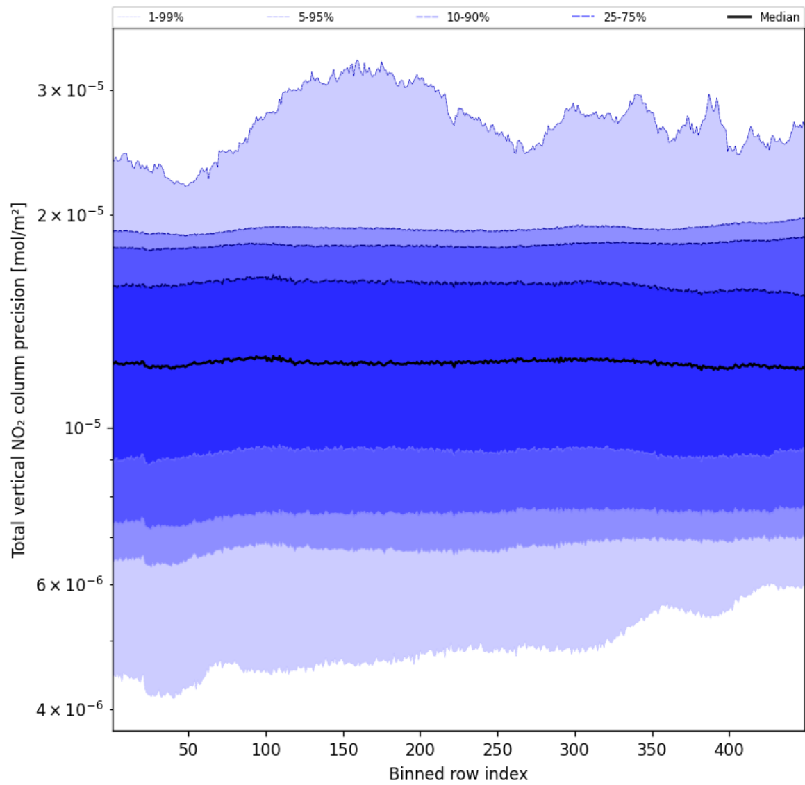
Figure 56: Along track statistics of “Total vertical NO 2 column precision” for 2024-12-11 to 2024-12-12
