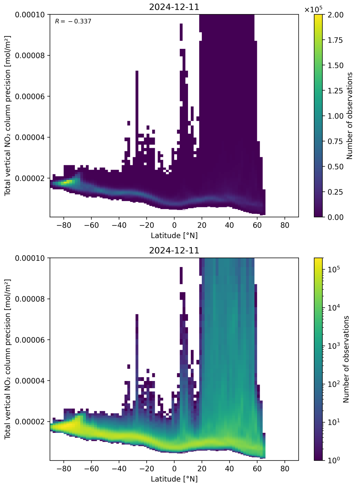
Figure 91: Scatter density plot of “Latitude” against “Total vertical NO 2 column precision” for 2024-12-11 to 2024-12-12.
