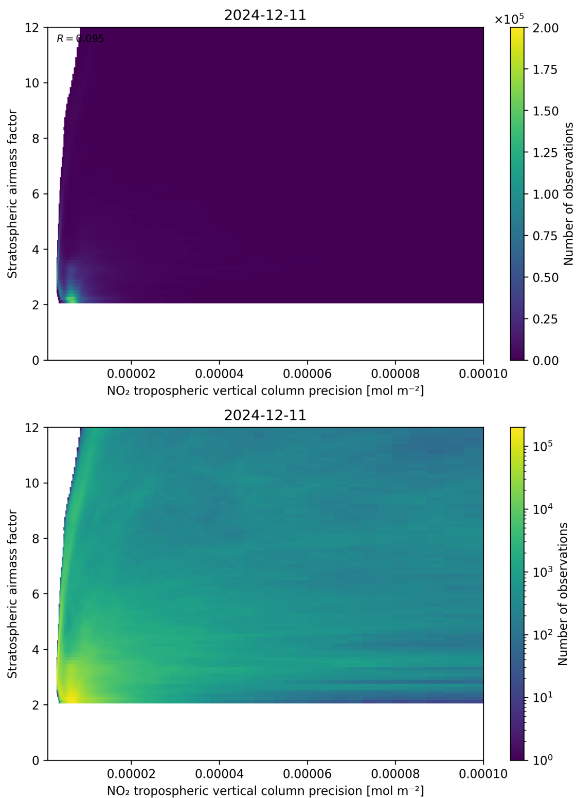
Figure 131: Scatter density plot of “NO 2 tropospheric vertical column precision” against “Stratospheric airmass factor” for 2024-12-11 to 2024-12-12.
