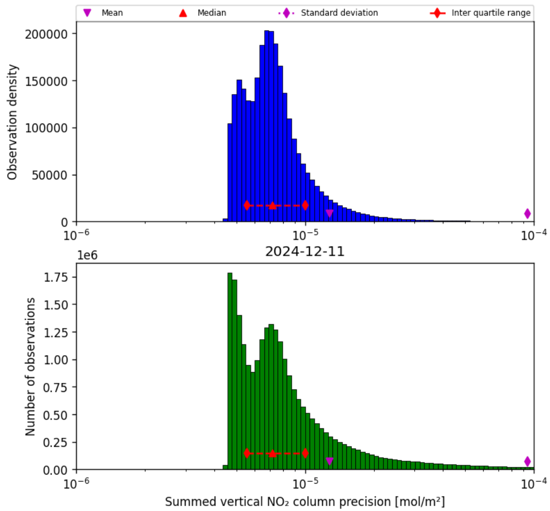
Figure 41: Histogram of “Summed vertical NO 2 column precision” for 2024-12-11 to 2024-12-12
