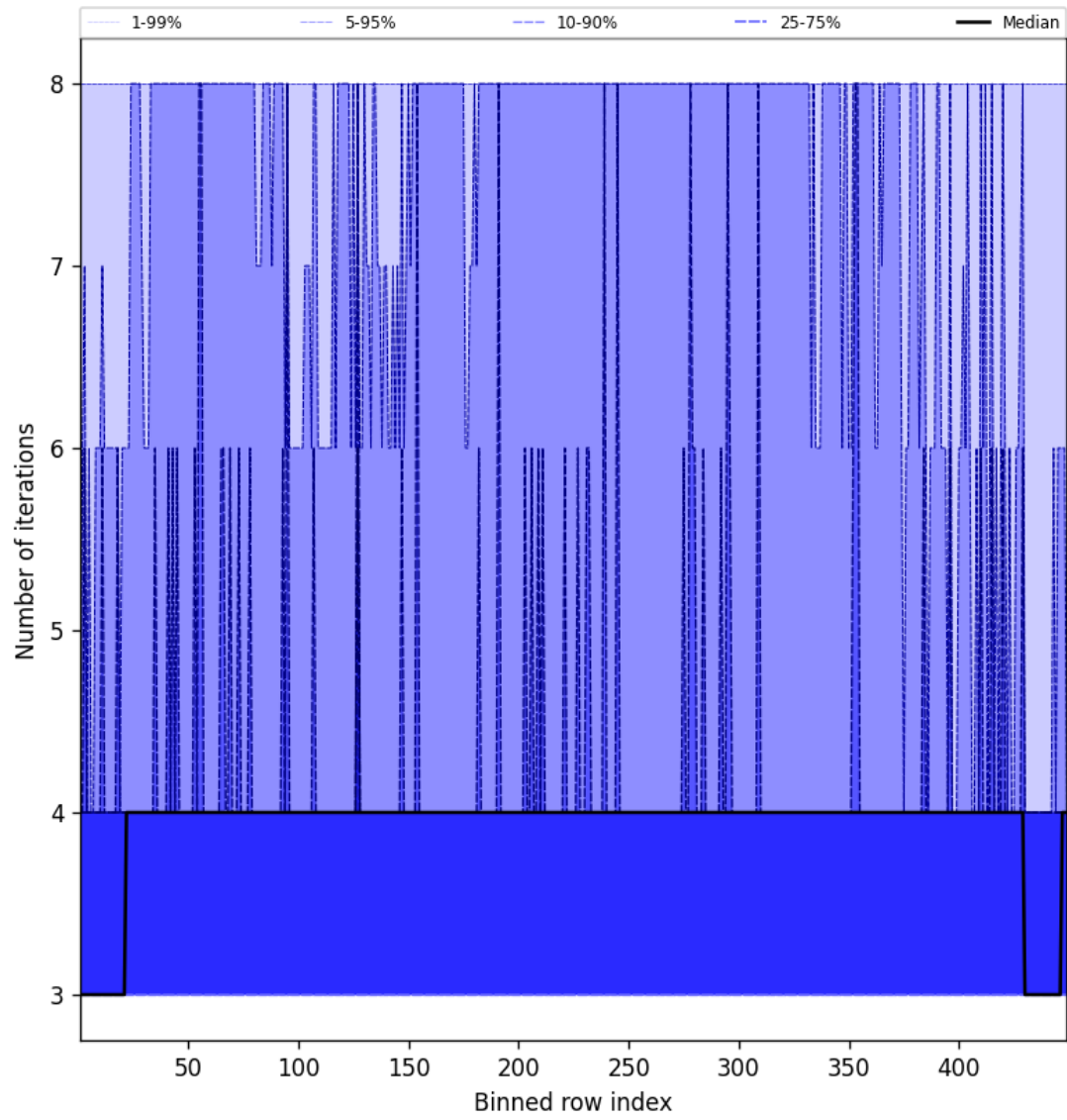
Figure 51: Along track statistics of “Number of iterations” for 2024-12-11 to 2024-12-12
