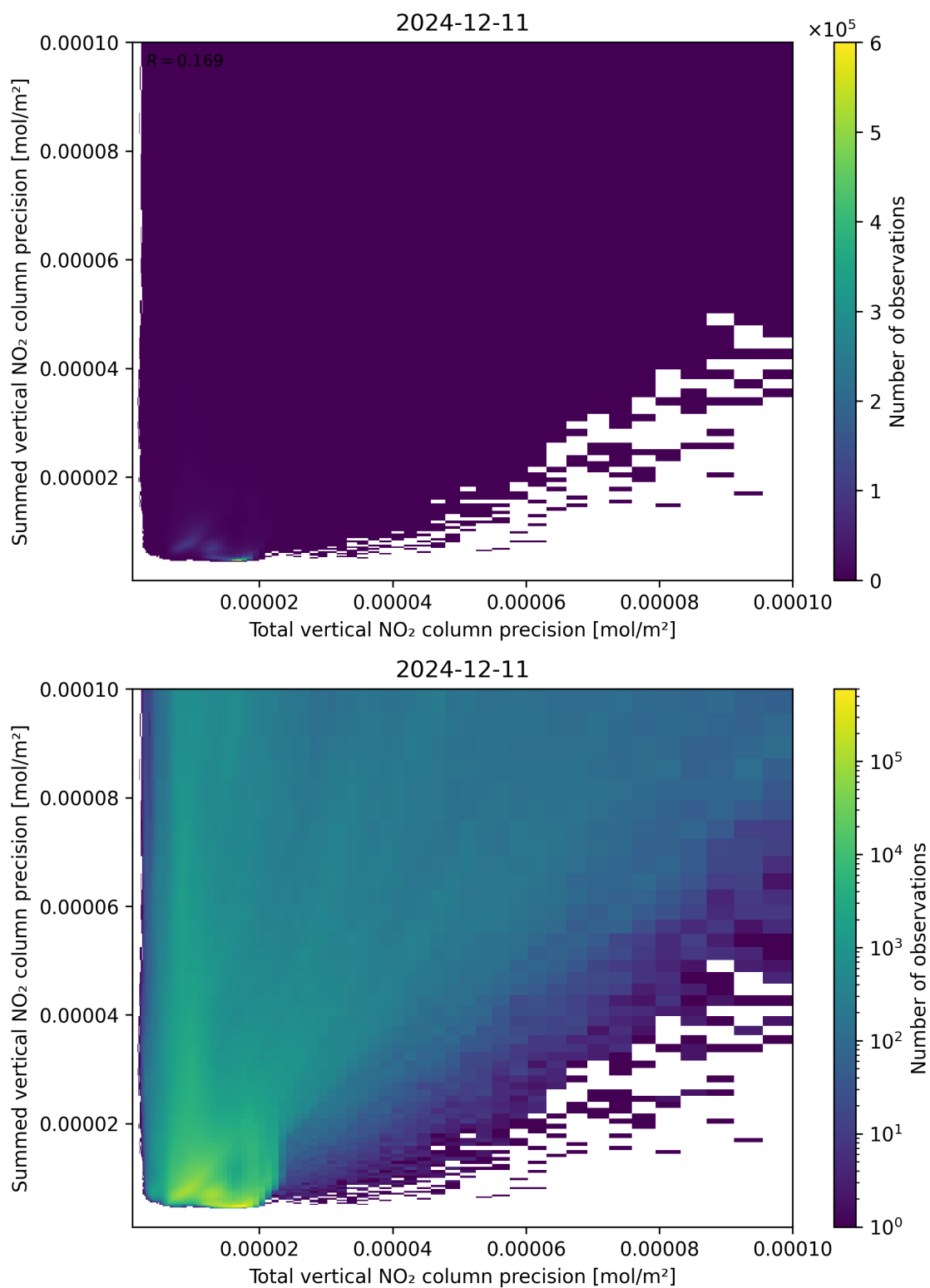
Figure 118: Scatter density plot of “Total vertical NO 2 column precision” against “Summed vertical NO 2 column precision” for 2024-12-11 to 2024-12-12.
