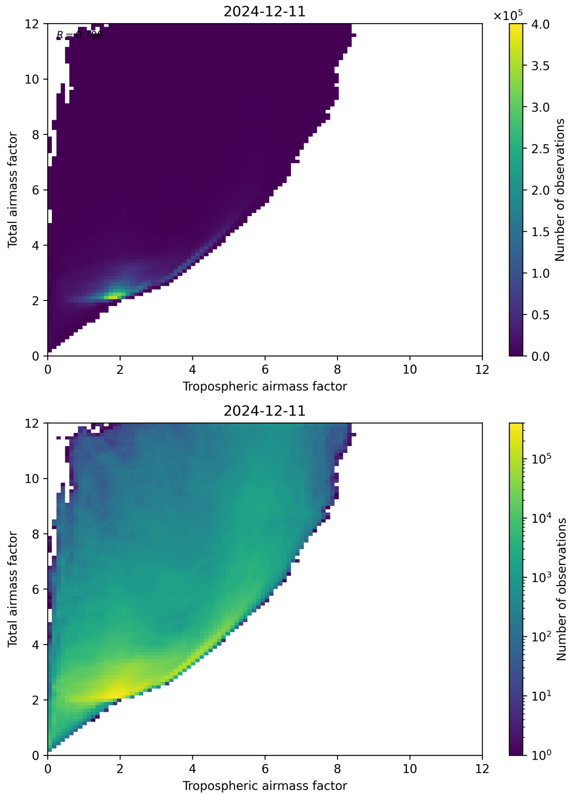
Figure 72: Scatter density plot of “Tropospheric airmass factor” against “Total airmass factor” for 2024-12-11 to 2024-12-12.
