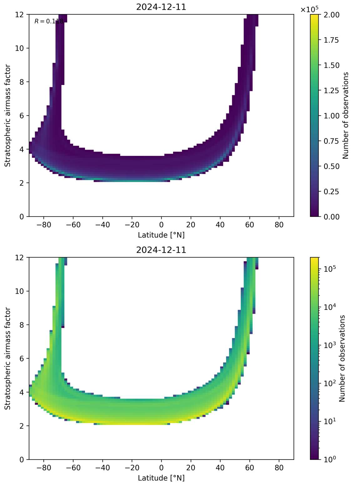
Figure 83: Scatter density plot of “Latitude” against “Stratospheric air mass factor” for 2024-12-11 to 2024-12-12.
