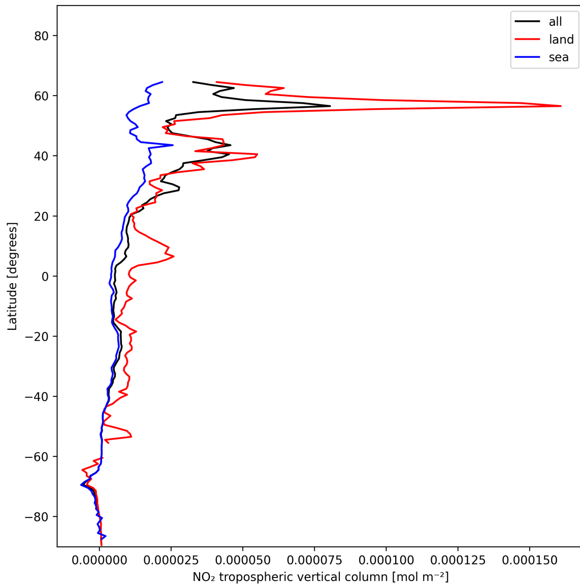
Figure 12: Zonal average of “NO 2 tropospheric vertical column” for 2024-12-11 to 2024-12-12.
