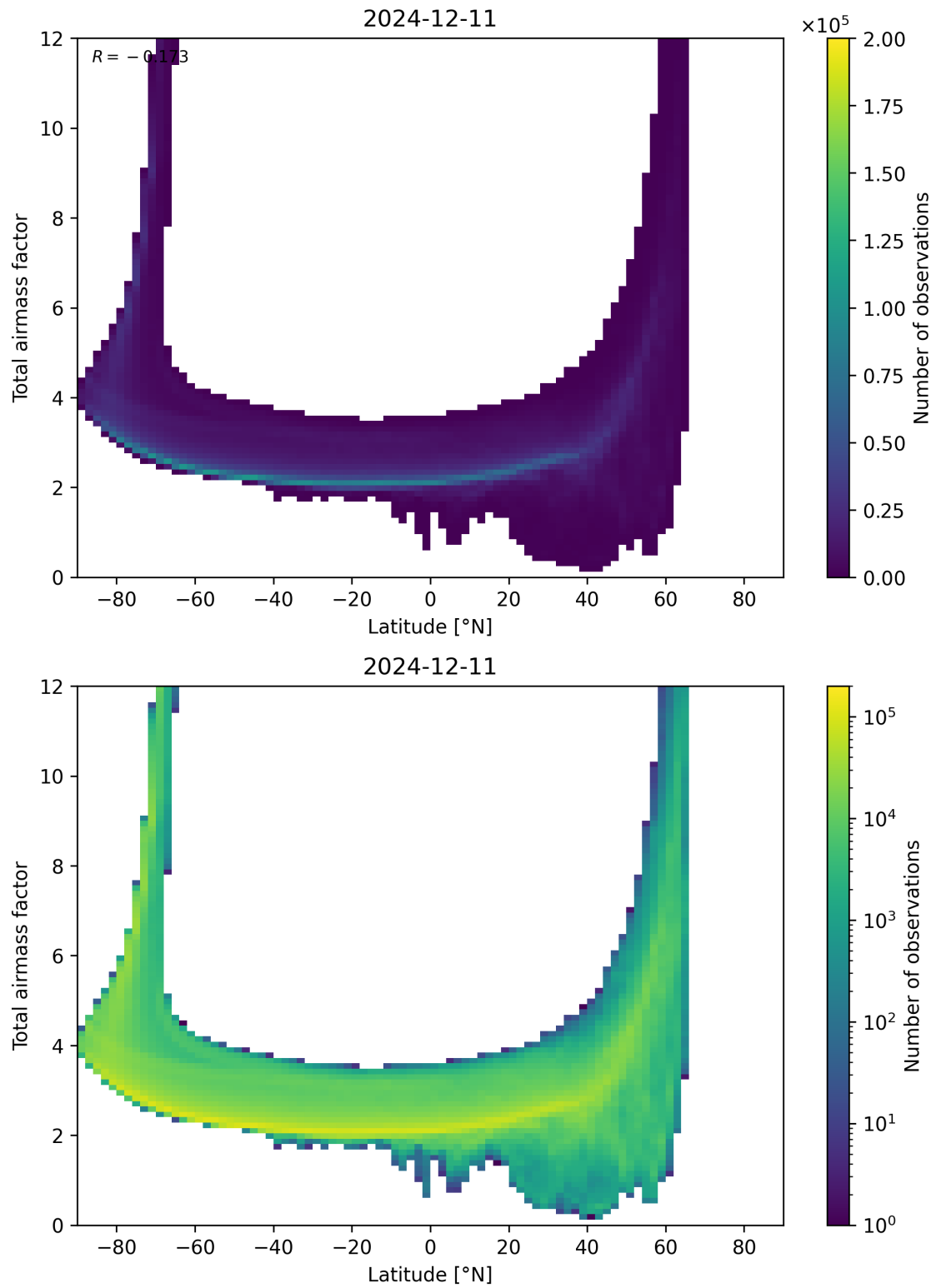
Figure 84: Scatter density plot of “Latitude” against “Total airmass factor” for 2024-12-11 to 2024-12-12.
