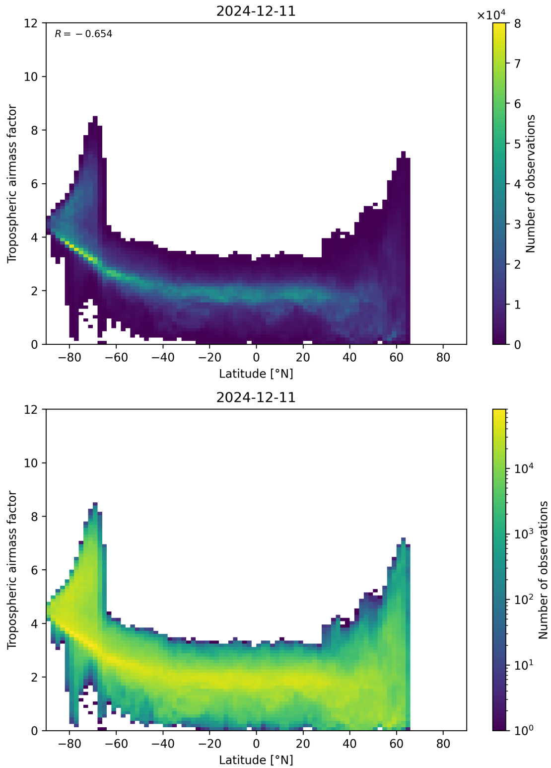
Figure 85: Scatter density plot of “Latitude” against “Tropospheric airmass factor” for 2024-12-11 to 2024-12-12.
