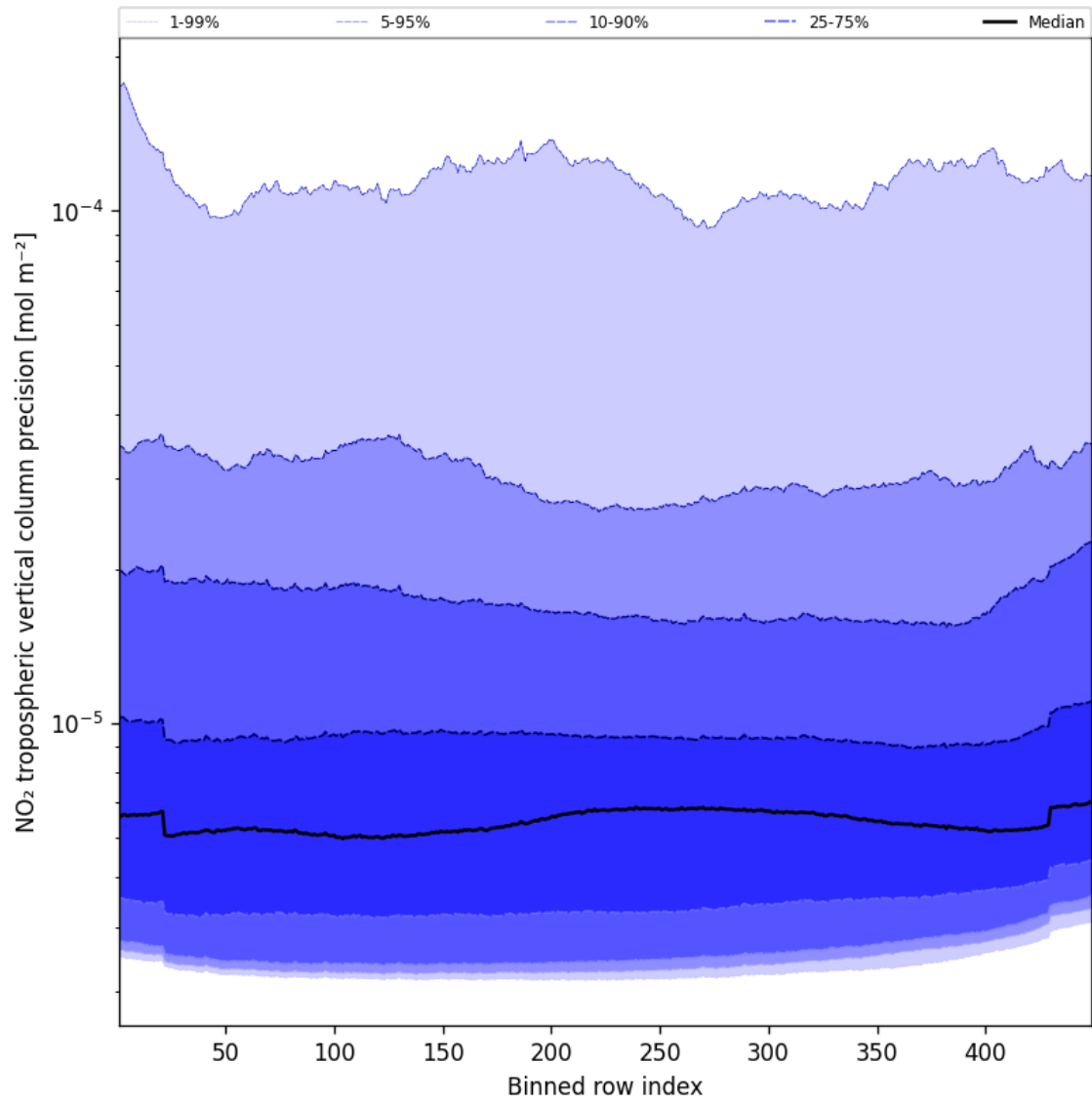
Figure 47: Along track statistics of “NO 2 tropospheric vertical column precision” for 2024-12-11 to 2024-12-12
