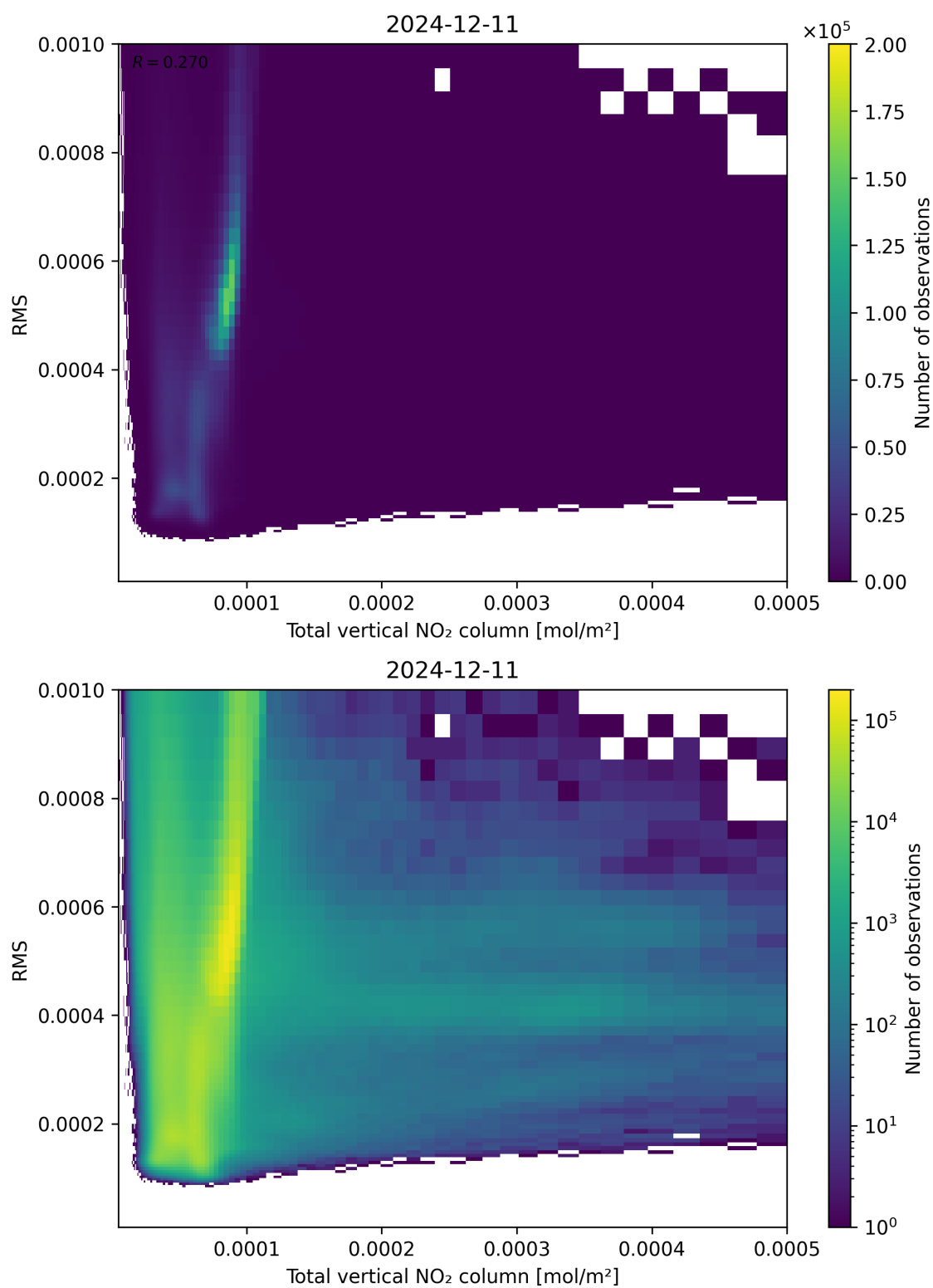
Figure 120: Scatter density plot of “Total vertical NO 2 column” against “RMS” for 2024-12-11 to 2024-12-12.
