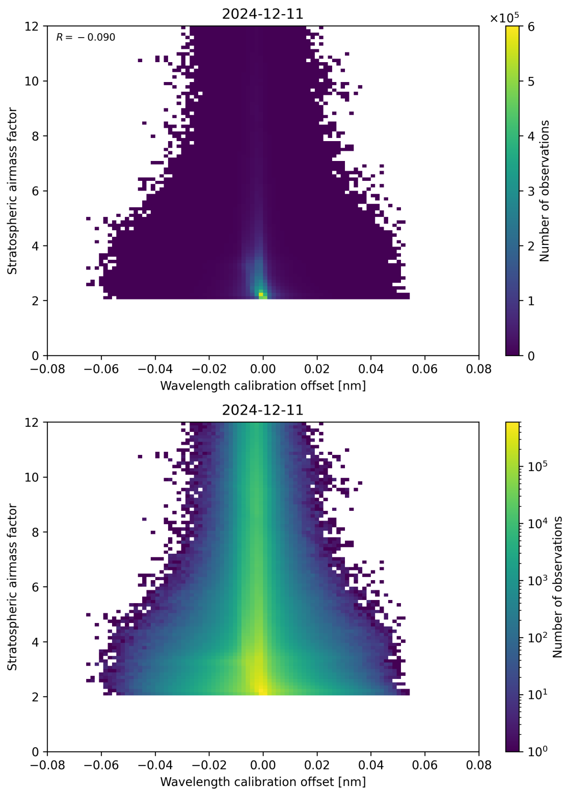
Figure 174: Scatter density plot of “Wavelength calibration offset” against “Stratospheric airmass factor” for 2024-12-11 to 2024-12-12.
