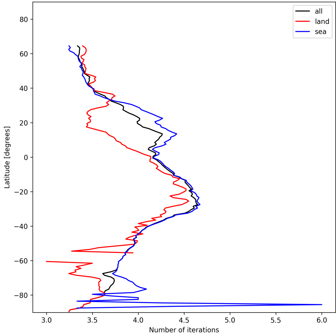
Figure 17: Zonal average of “Number of iterations” for 2024-12-11 to 2024-12-12.
