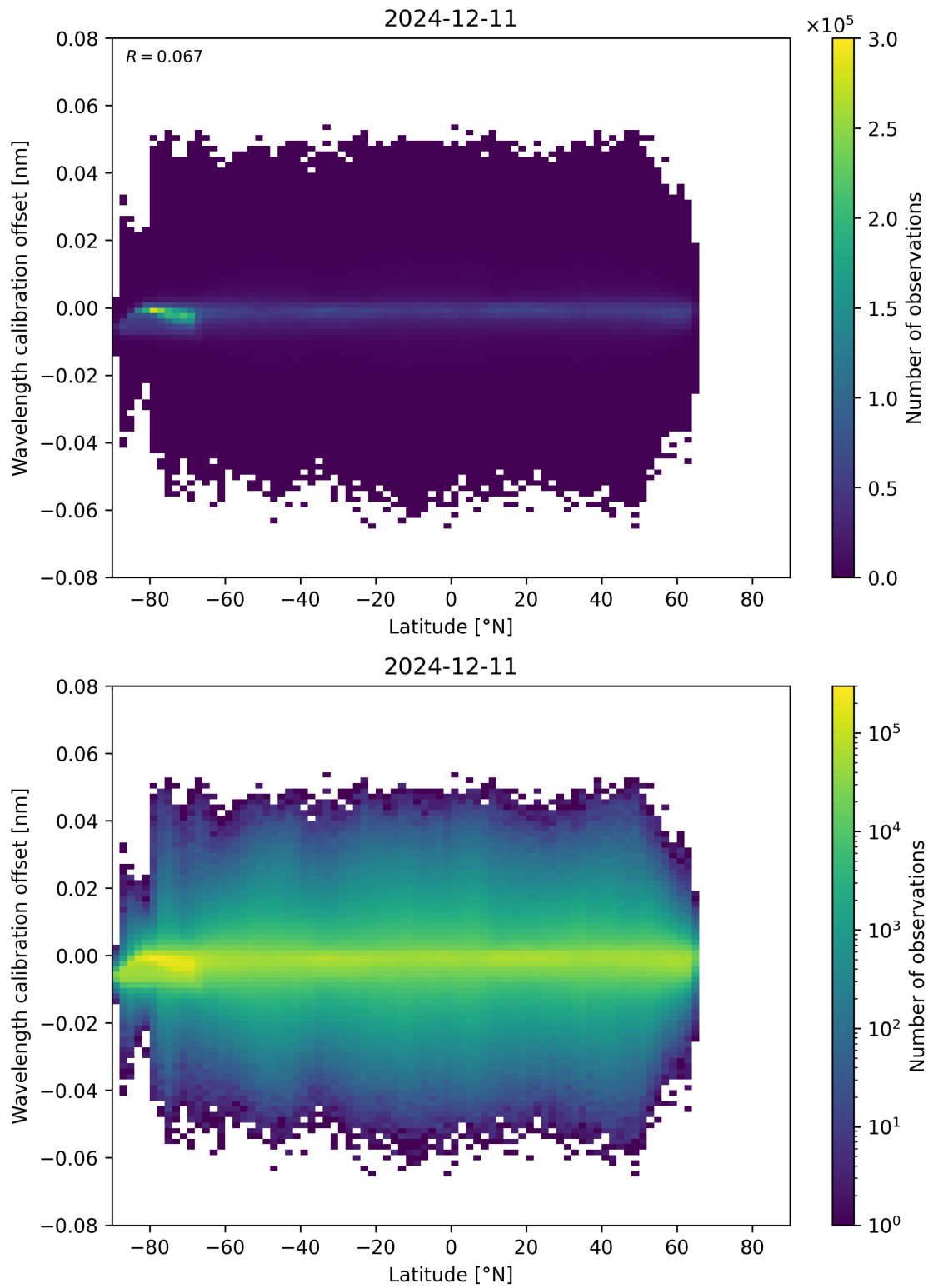
Figure 95: Scatter density plot of “Latitude” against “Wavelength calibration offset” for 2024-12-11 to 2024-12-12.
