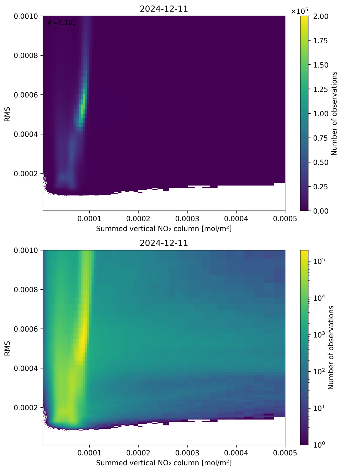
Figure 109: Scatter density plot of “Summed vertical NO 2 column” against “RMS” for 2024-12-11 to 2024-12-12.
