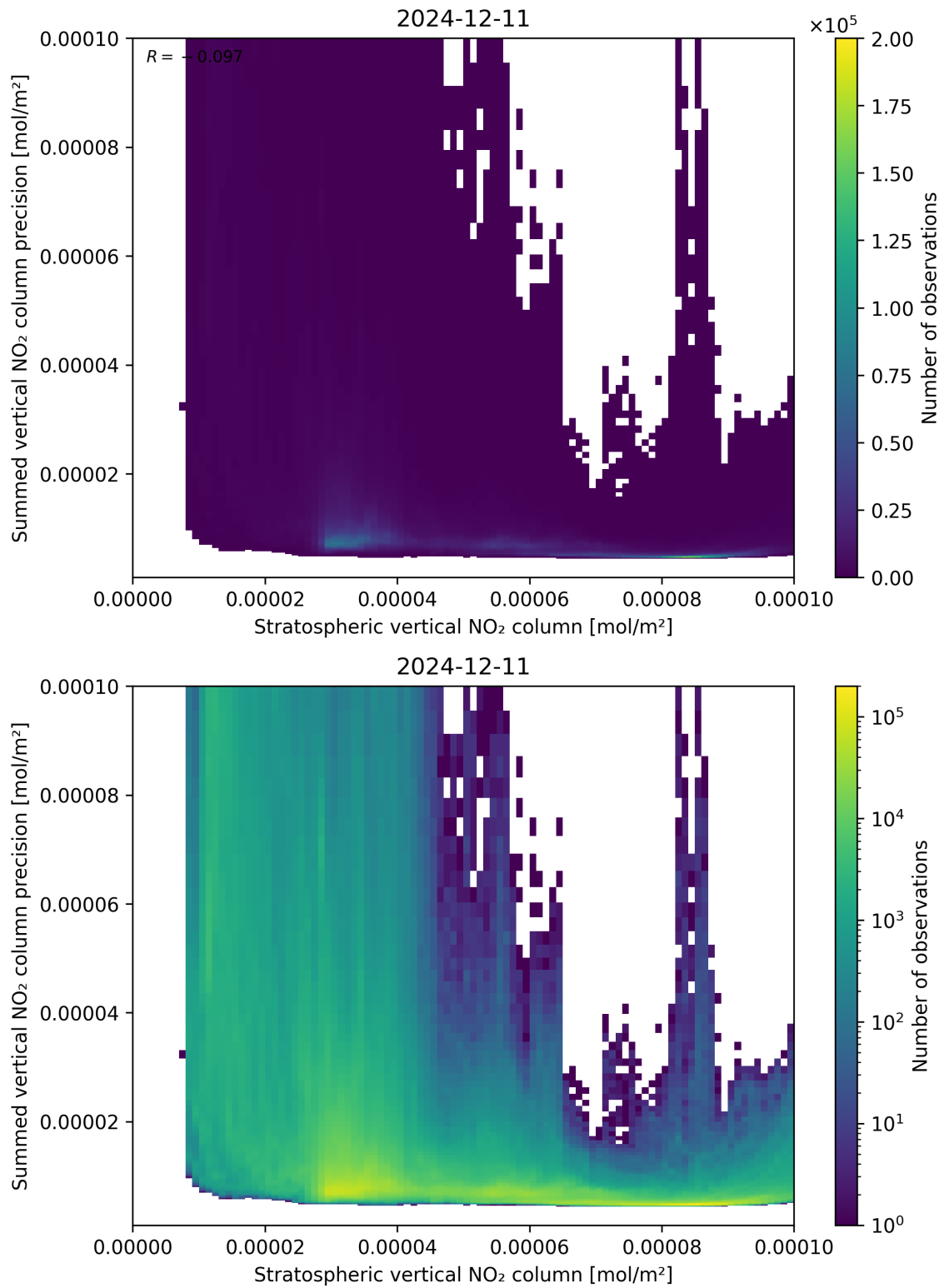
Figure 99: Scatter density plot of “Stratospheric vertical NO 2 column” against “Summed vertical NO 2 column precision” for 2024-12-11 to 2024-12-12.
