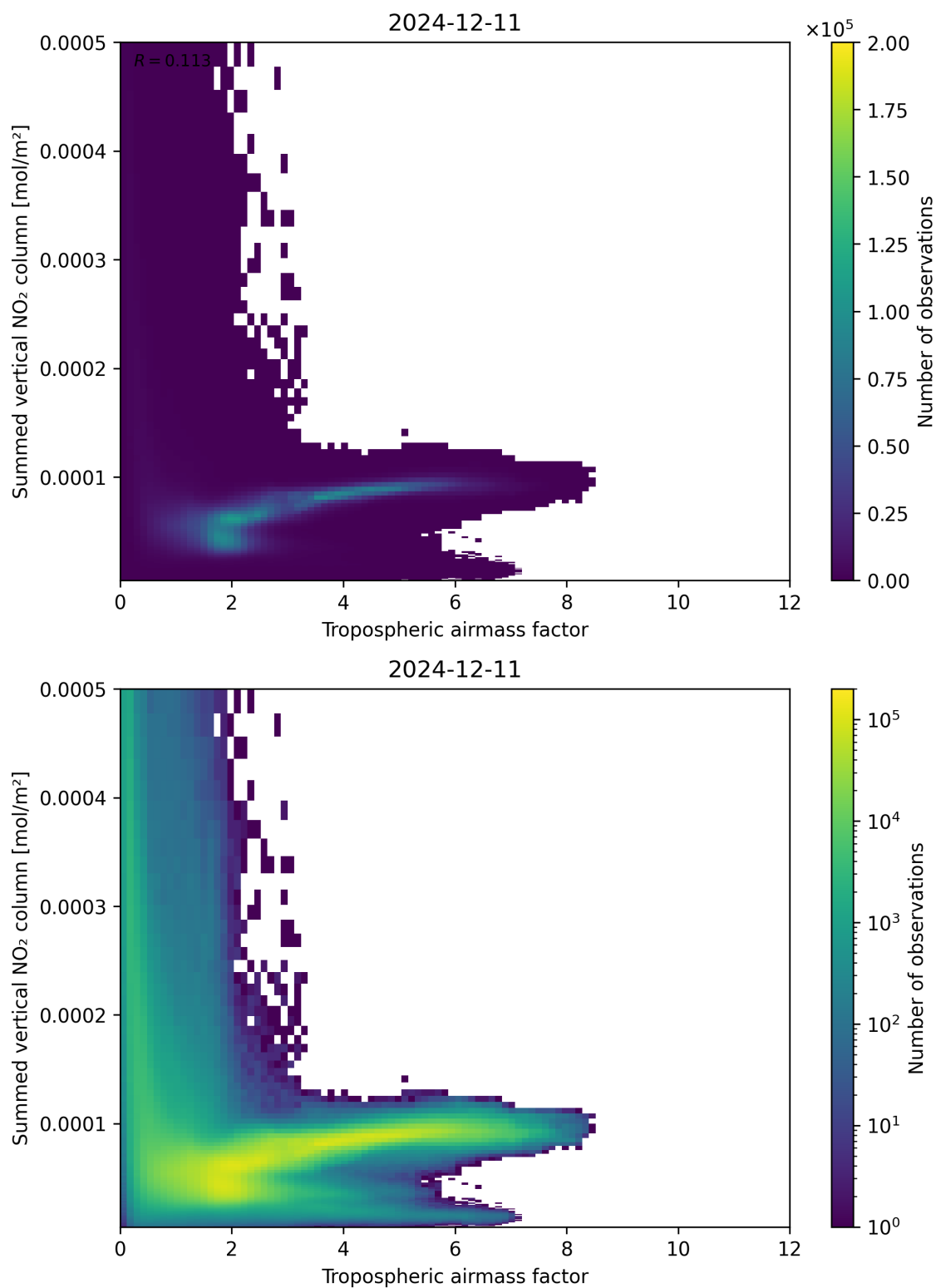
Figure 75: Scatter density plot of “Tropospheric air mass factor” against “Summed vertical NO 2 column” for 2024-12-11 to 2024-12-12.
