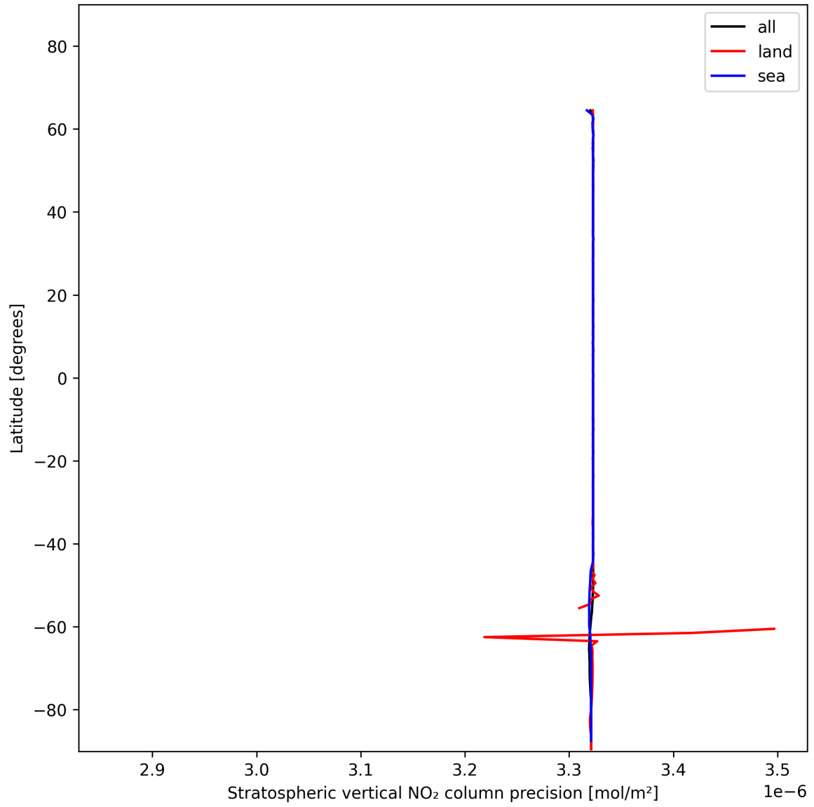
Figure 20: Zonal average of "Stratospheric vertical NO 2 column precision" for 2024-12-11 to 2024-12-12.
