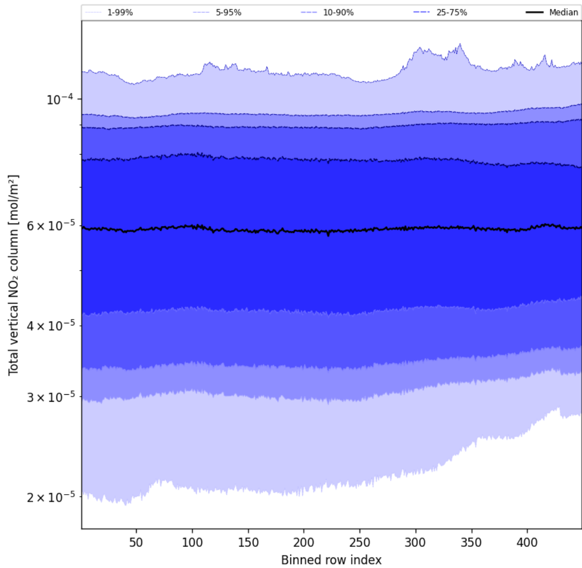
Figure 55: Along track statistics of “Total vertical NO 2 column” for 2024-12-11 to 2024-12-12
