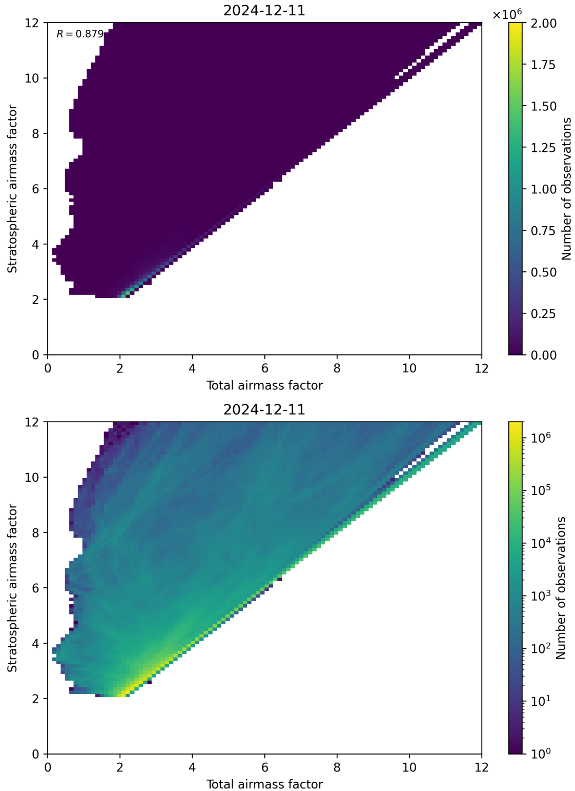
Figure 62: Scatter density plot of “Total airmass factor” against “Stratospheric airmass factor” for 2024-12-11 to 2024-12-12.
