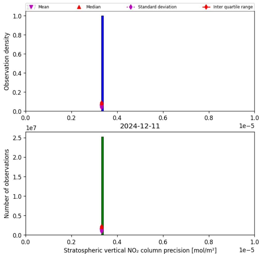
Figure 37: Histogram of “Stratospheric vertical NO 2 column precision” for 2024-12-11 to 2024-12-12
