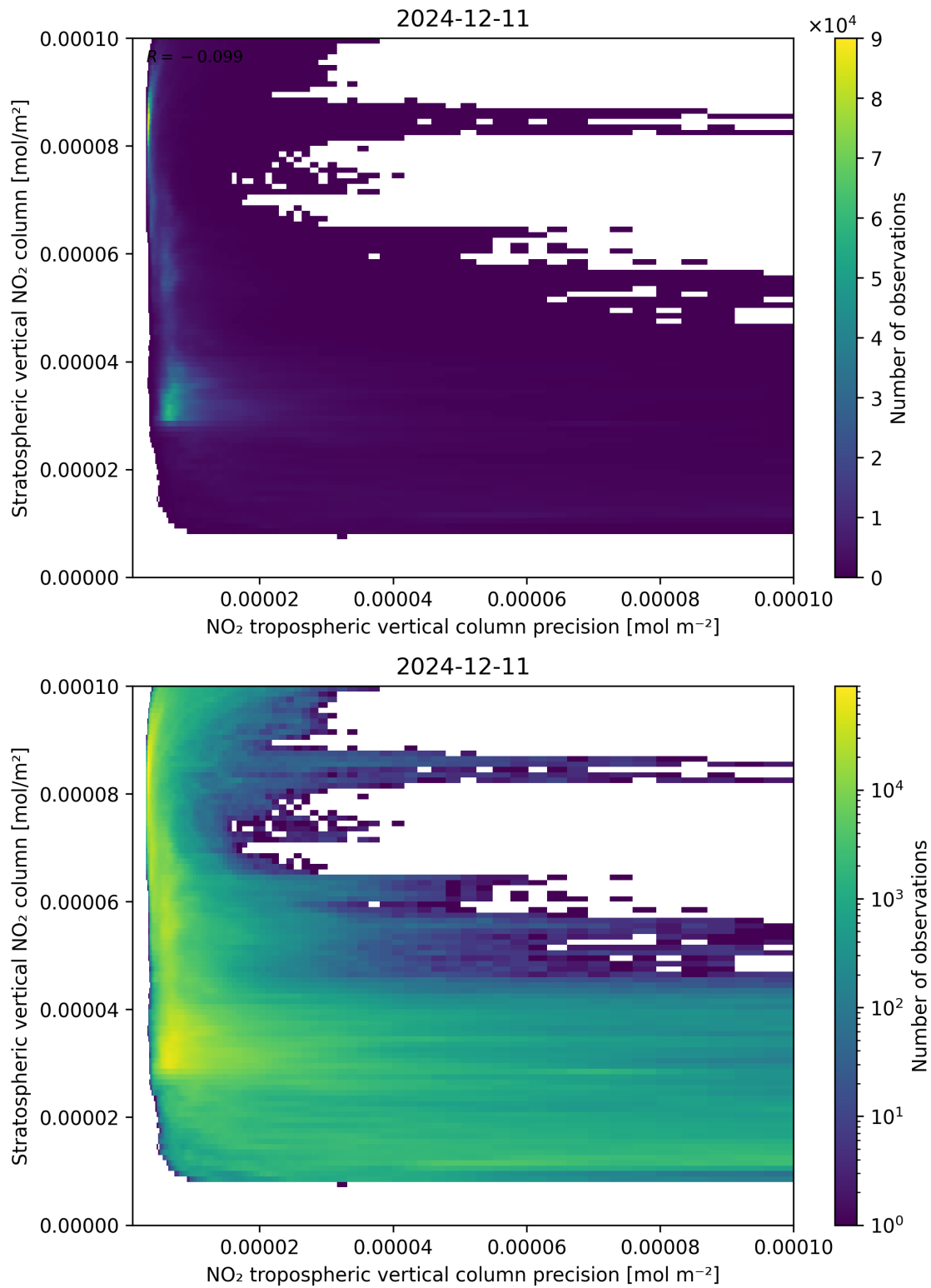
Figure 135: Scatter density plot of “NO 2 tropospheric vertical column precision” against “Stratospheric vertical NO 2 column” for 2024-12-11 to 2024-12-12.
