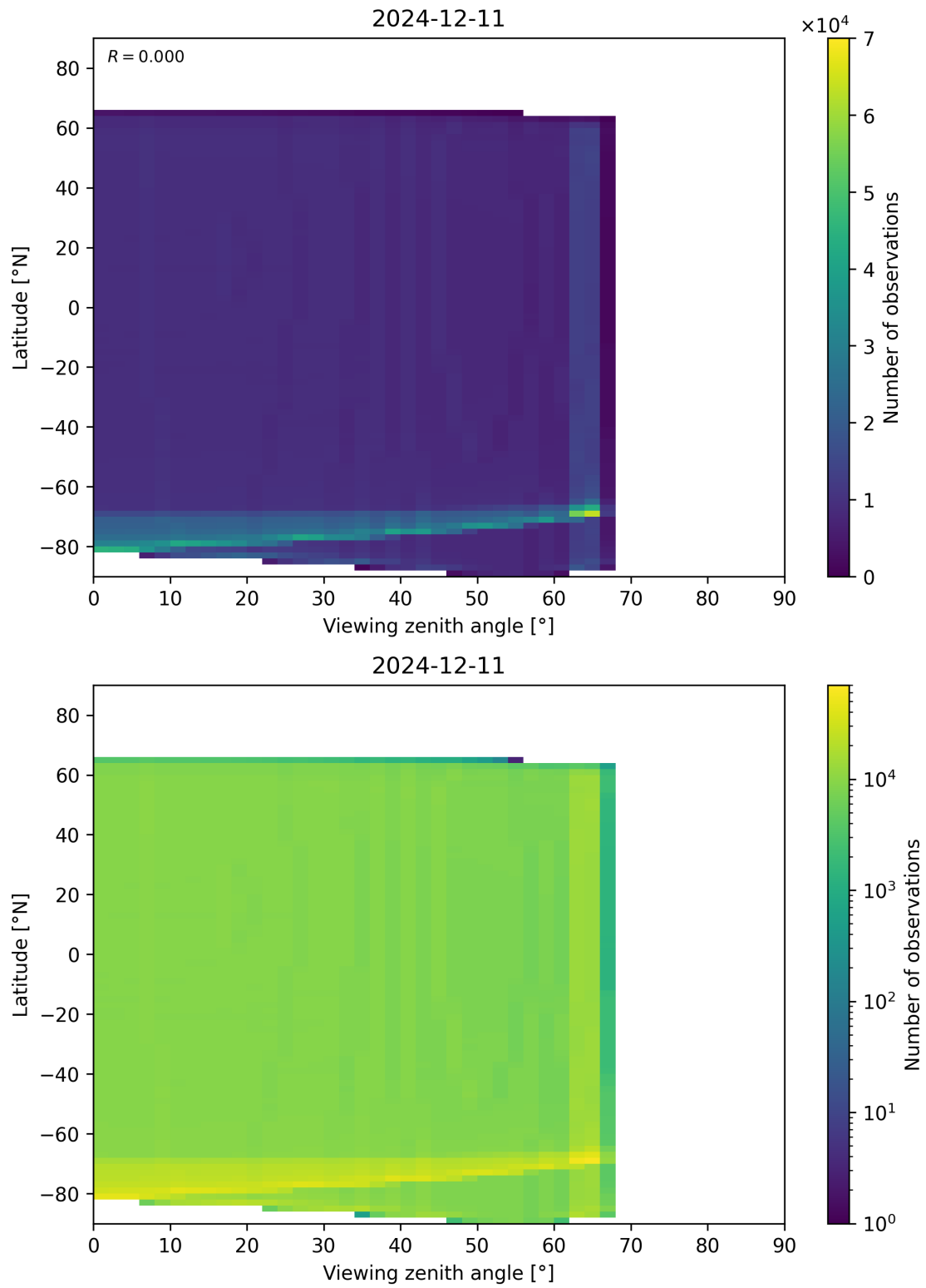
Figure 163: Scatter density plot of “Viewing zenith angle” against “Latitude” for 2024-12-11 to 2024-12-12.
