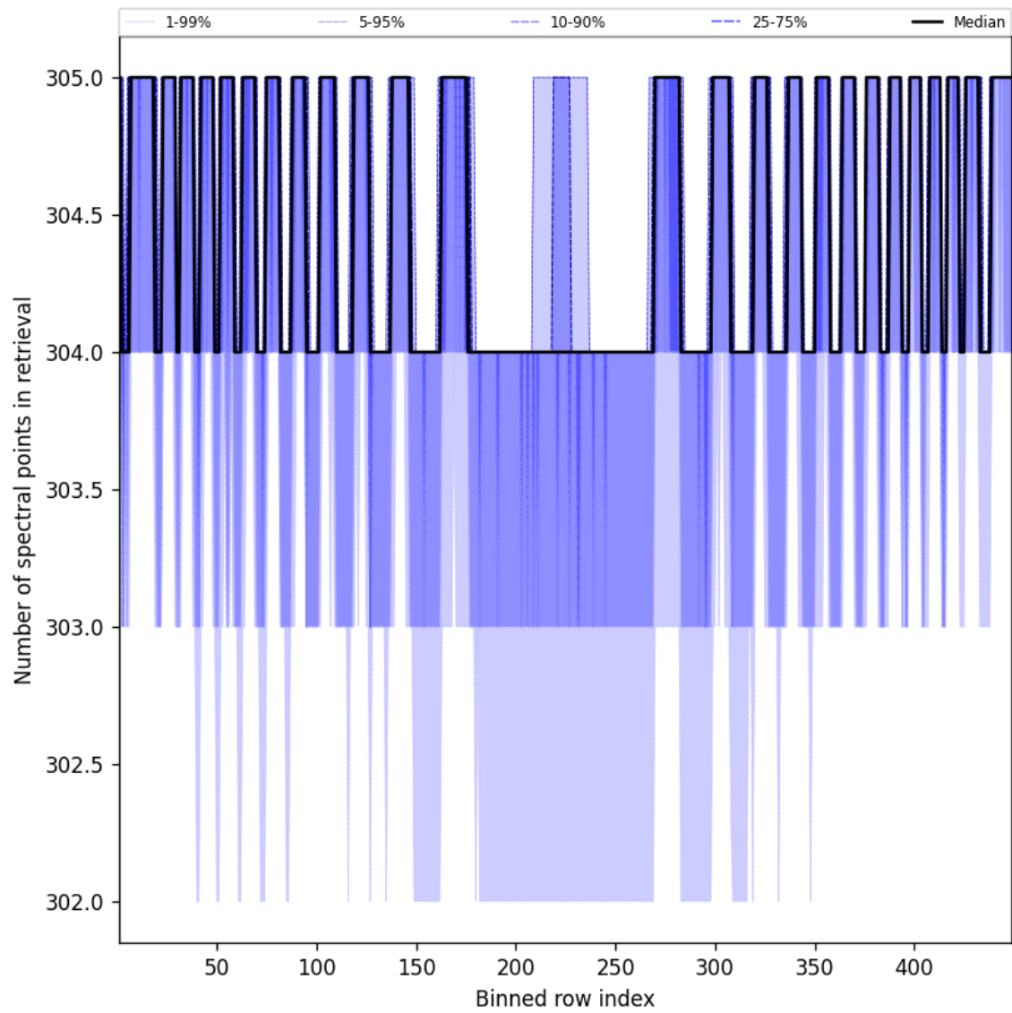
Figure 50: Along track statistics of “Number of spectral points in retrieval” for 2024-12-11 to 2024-12-12
