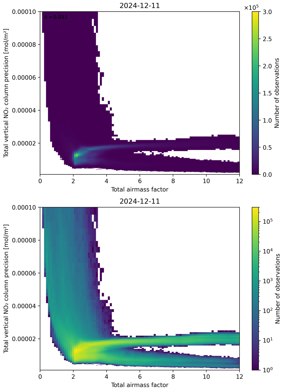
Figure 68: Scatter density plot of “Total airmass factor” against “Total vertical NO 2 column precision” for 2024-12-11 to 2024-12-12.
