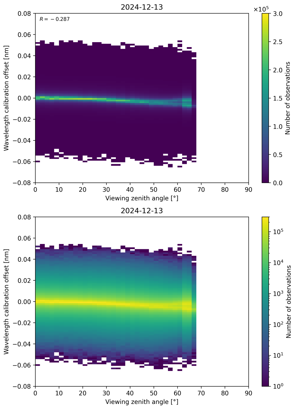
Figure 173: Scatter density plot of “Viewing zenith angle” against “Wavelength calibration offset” for 2024-12-12 to 2024-12-14.
