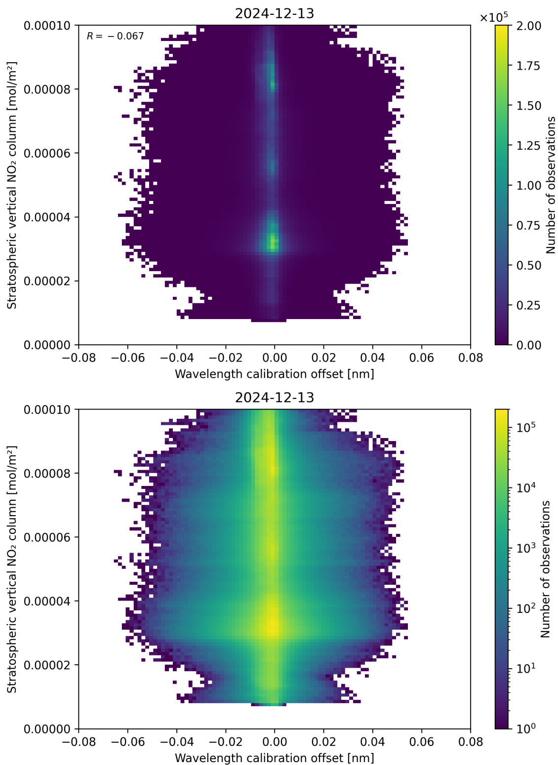
Figure 176: Scatter density plot of “Wavelength calibration offset” against “Stratospheric vertical NO 2 column” for 2024-12-12 to 2024-12-14.
