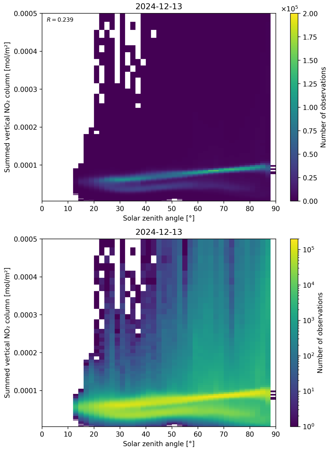
Figure 151: Scatter density plot of “Solar zenith angle” against “Summed vertical NO 2 column” for 2024-12-12 to 2024-12-14.
