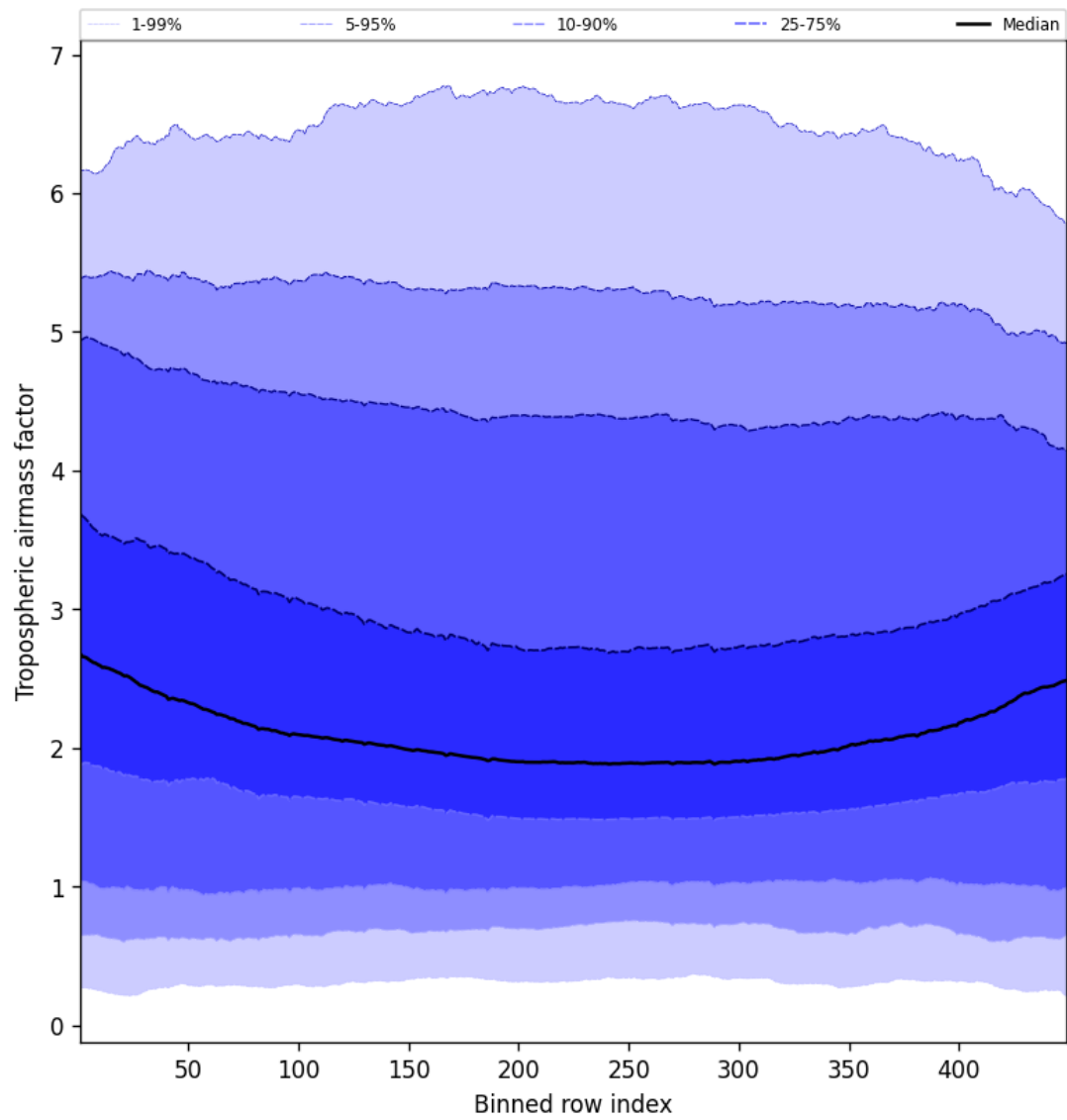
Figure 48: Along track statistics of "Tropospheric airmass factor" for 2024-12-12 to 2024-12-14
