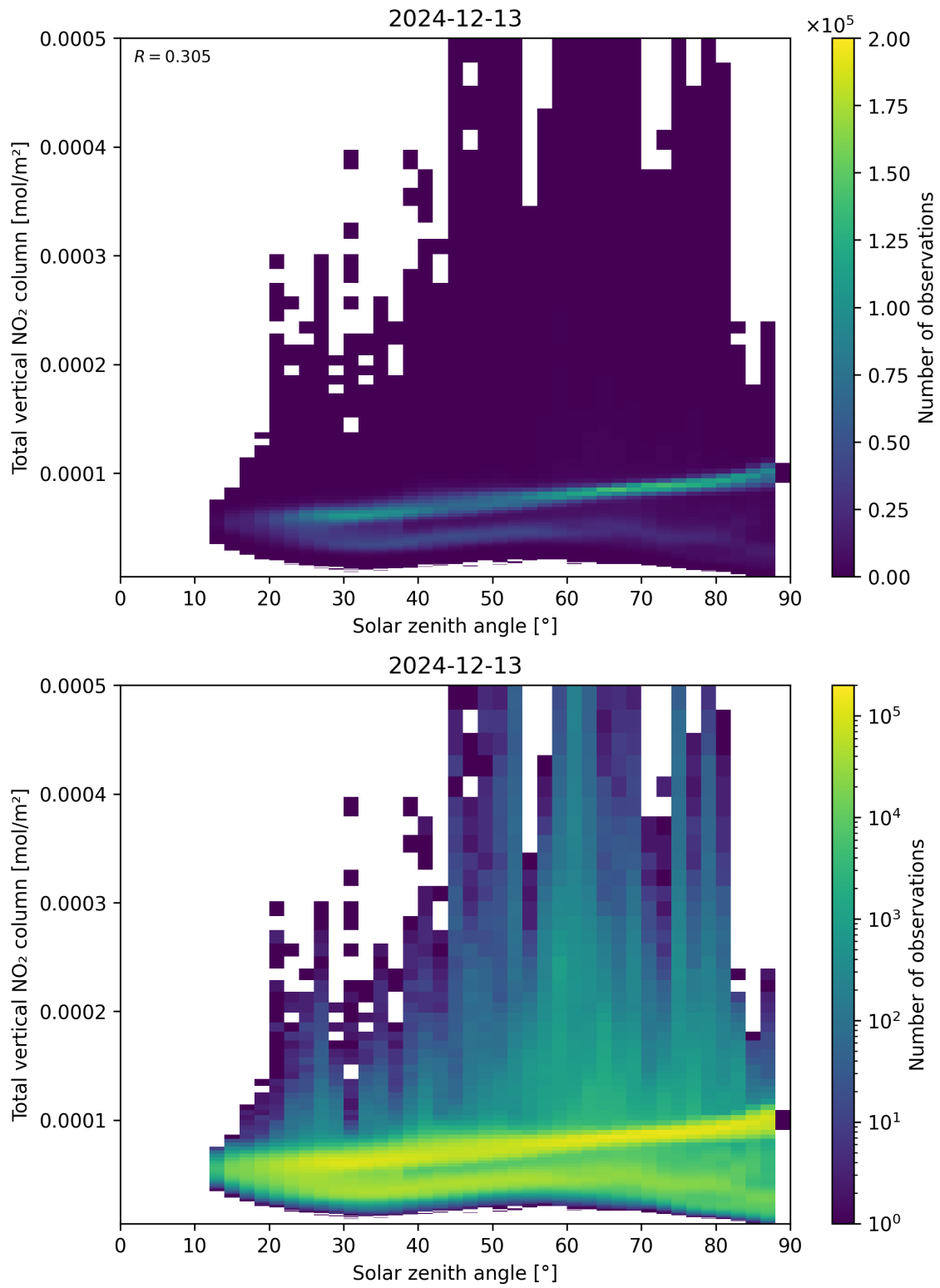
Figure 153: Scatter density plot of “Solar zenith angle” against “Total vertical NO 2 column” for 2024-12-12 to 2024-12-14.
