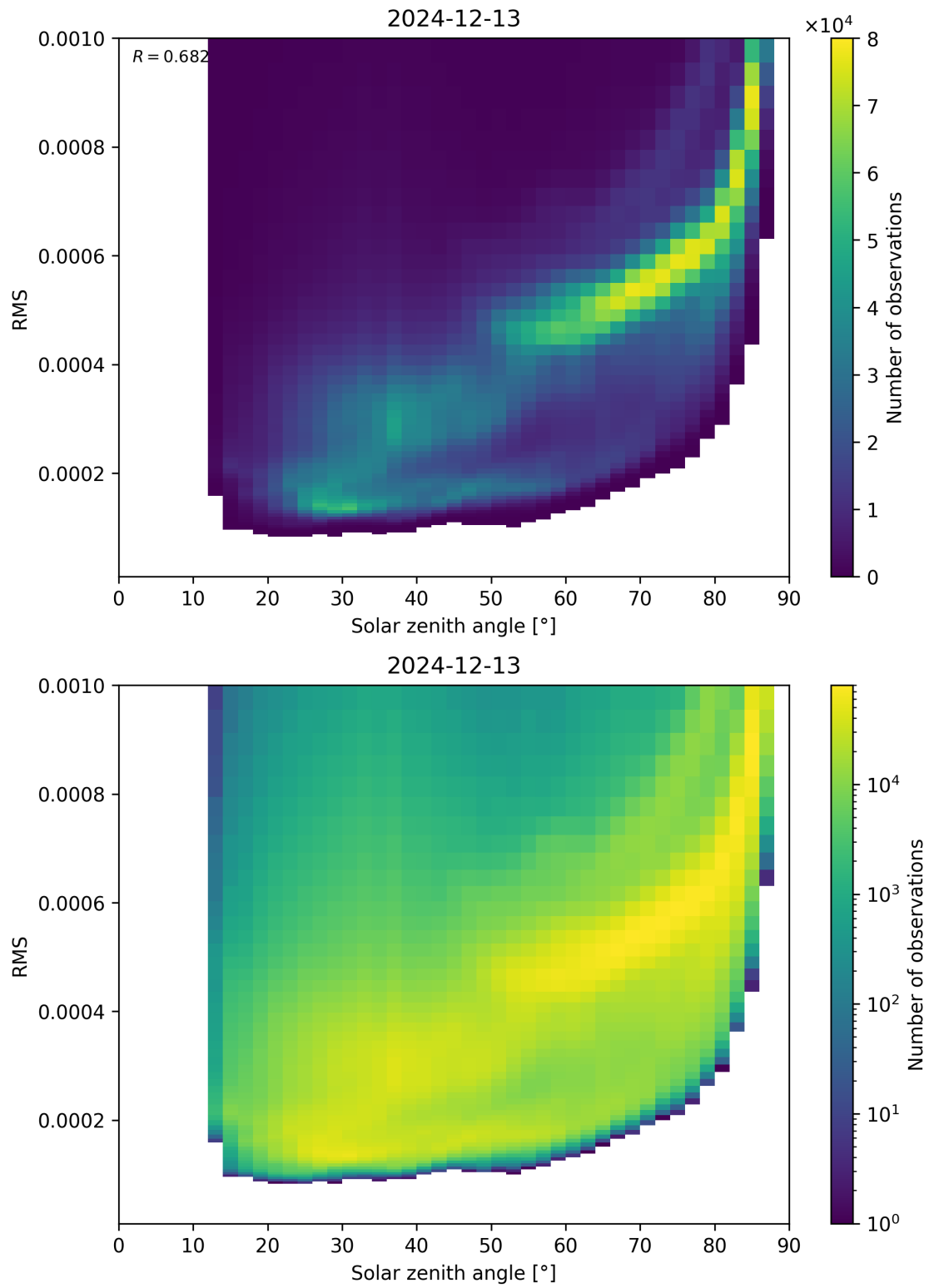
Figure 157: Scatter density plot of “Solar zenith angle” against “RMS” for 2024-12-12 to 2024-12-14.
