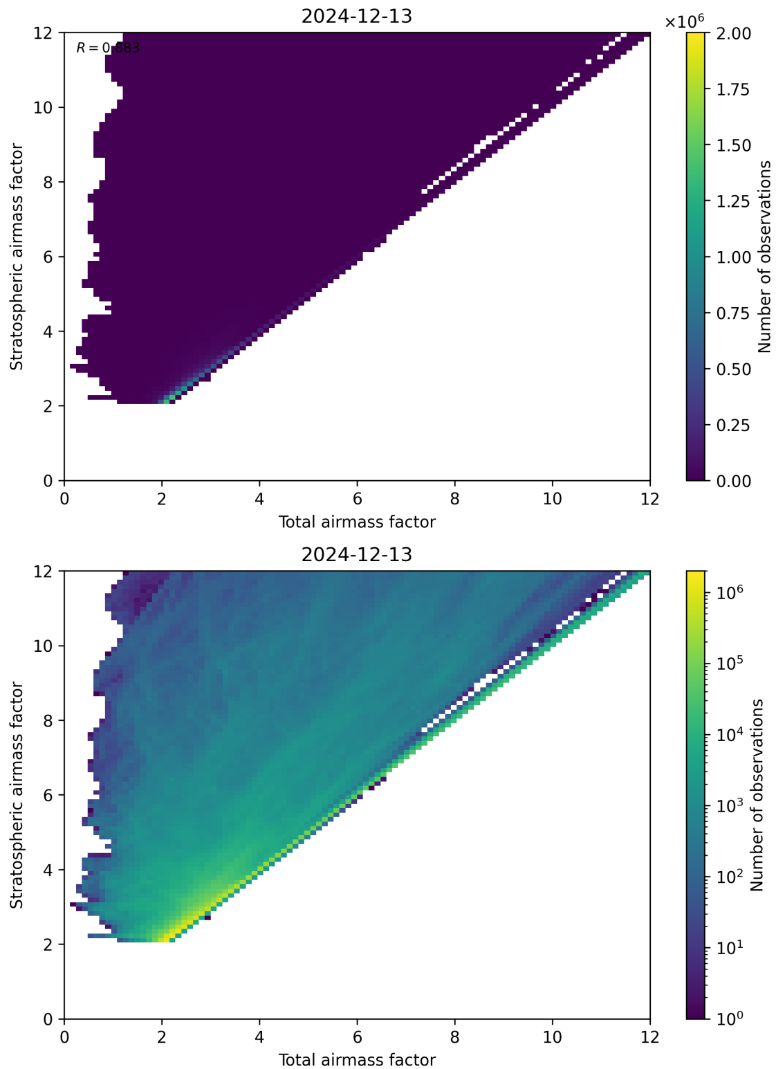
Figure 62: Scatter density plot of “Total airmass factor” against “Stratospheric airmass factor” for 2024-12-12 to 2024-12-14.
