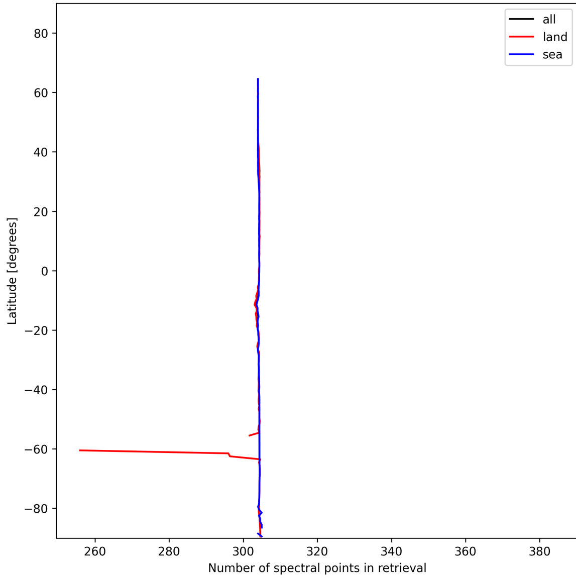
Figure 16: Zonal average of “Number of spectral points in retrieval” for 2024-12-12 to 2024-12-14.
