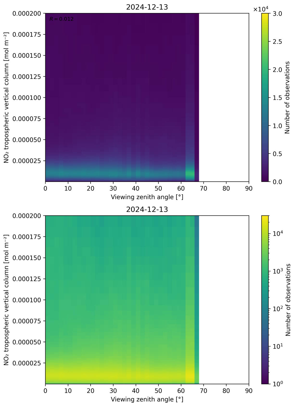
Figure 169: Scatter density plot of “Viewing zenith angle” against “NO 2 tropospheric vertical column” for 2024-12-12 to 2024-12-14.
