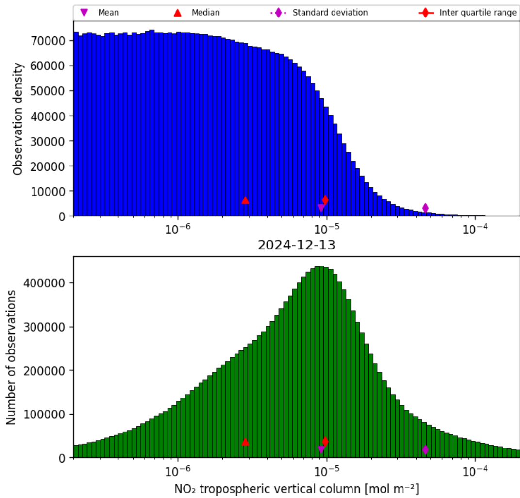
Figure 29: Histogram of “NO 2 tropospheric vertical column” for 2024-12-12 to 2024-12-14
