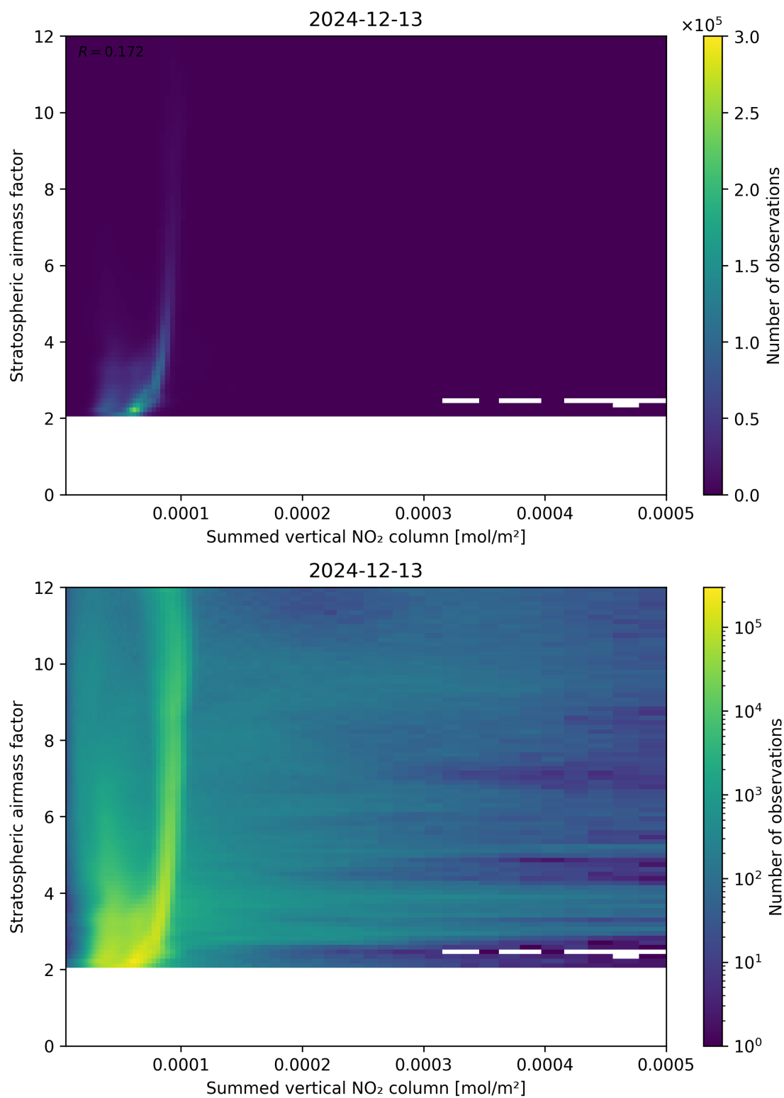
Figure 103: Scatter density plot of “Summed vertical NO 2 column” against “Stratospheric airmass factor” for 2024-12-12 to 2024-12-14.
