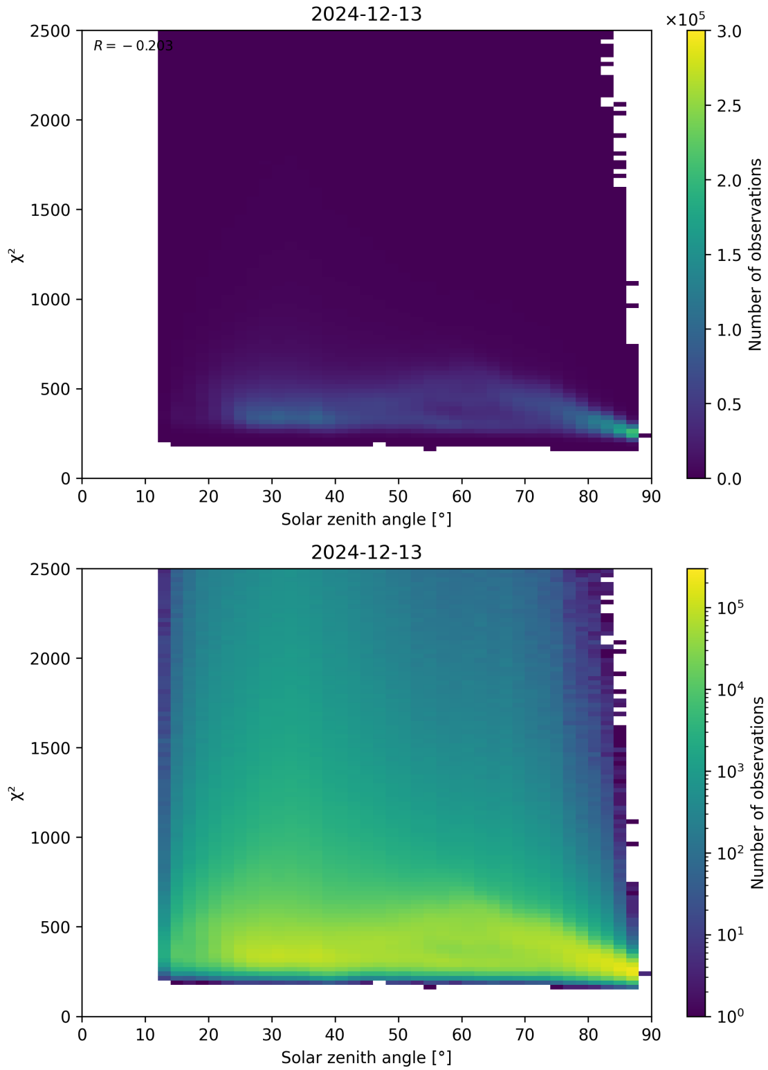
Figure 148: Scatter density plot of “Solar zenith angle” against “ \chi^2 ” for 2024-12-12 to 2024-12-14.
