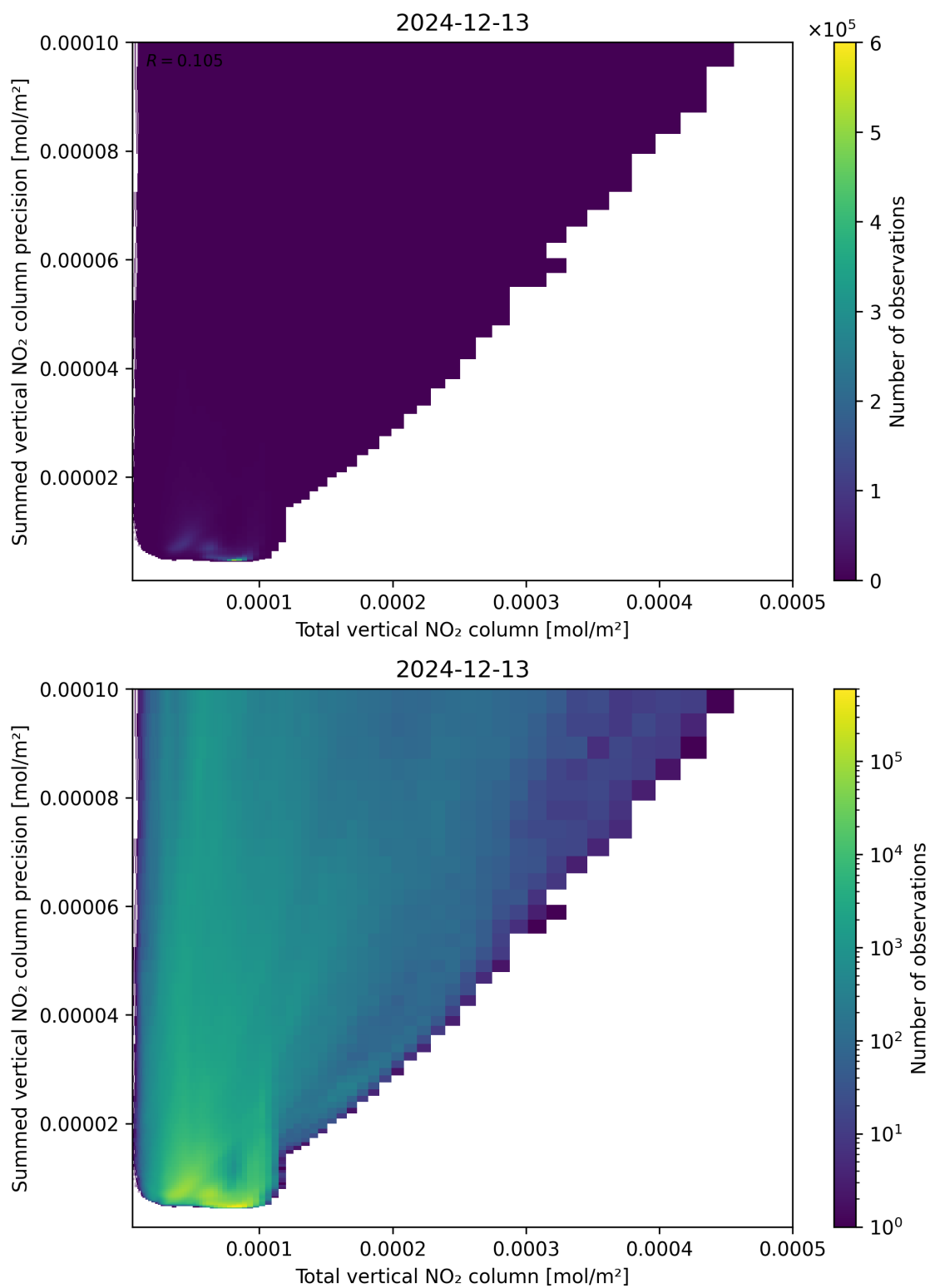
Figure 113: Scatter density plot of “Total vertical NO 2 column” against “Summed vertical NO 2 column precision” for 2024-12-12 to 2024-12-14.
