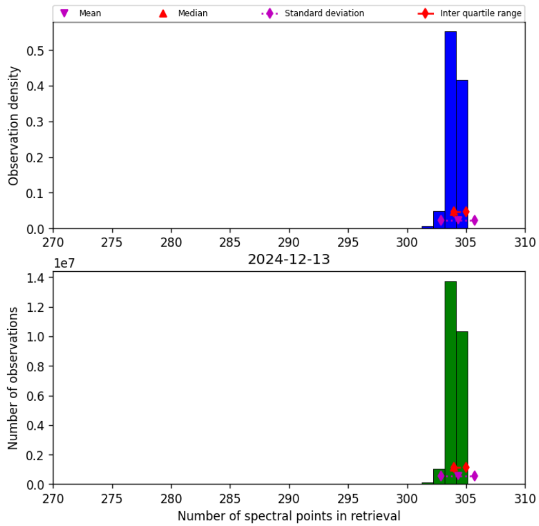
Figure 33: Histogram of “Number of spectral points in retrieval” for 2024-12-12 to 2024-12-14
