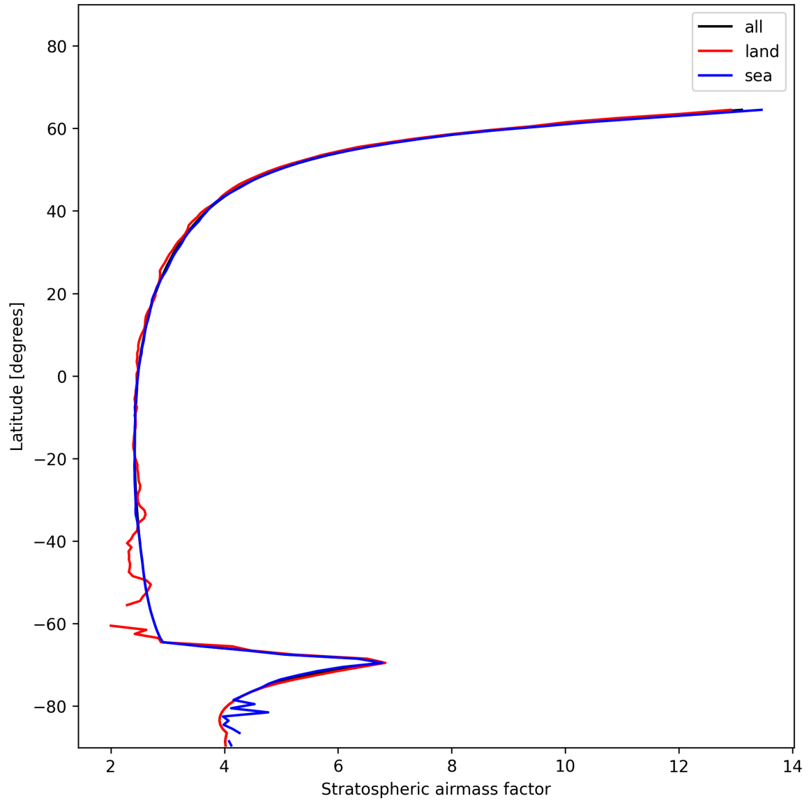
Figure 27: Zonal average of “Stratospheric airmass factor” for 2024-12-12 to 2024-12-14.
