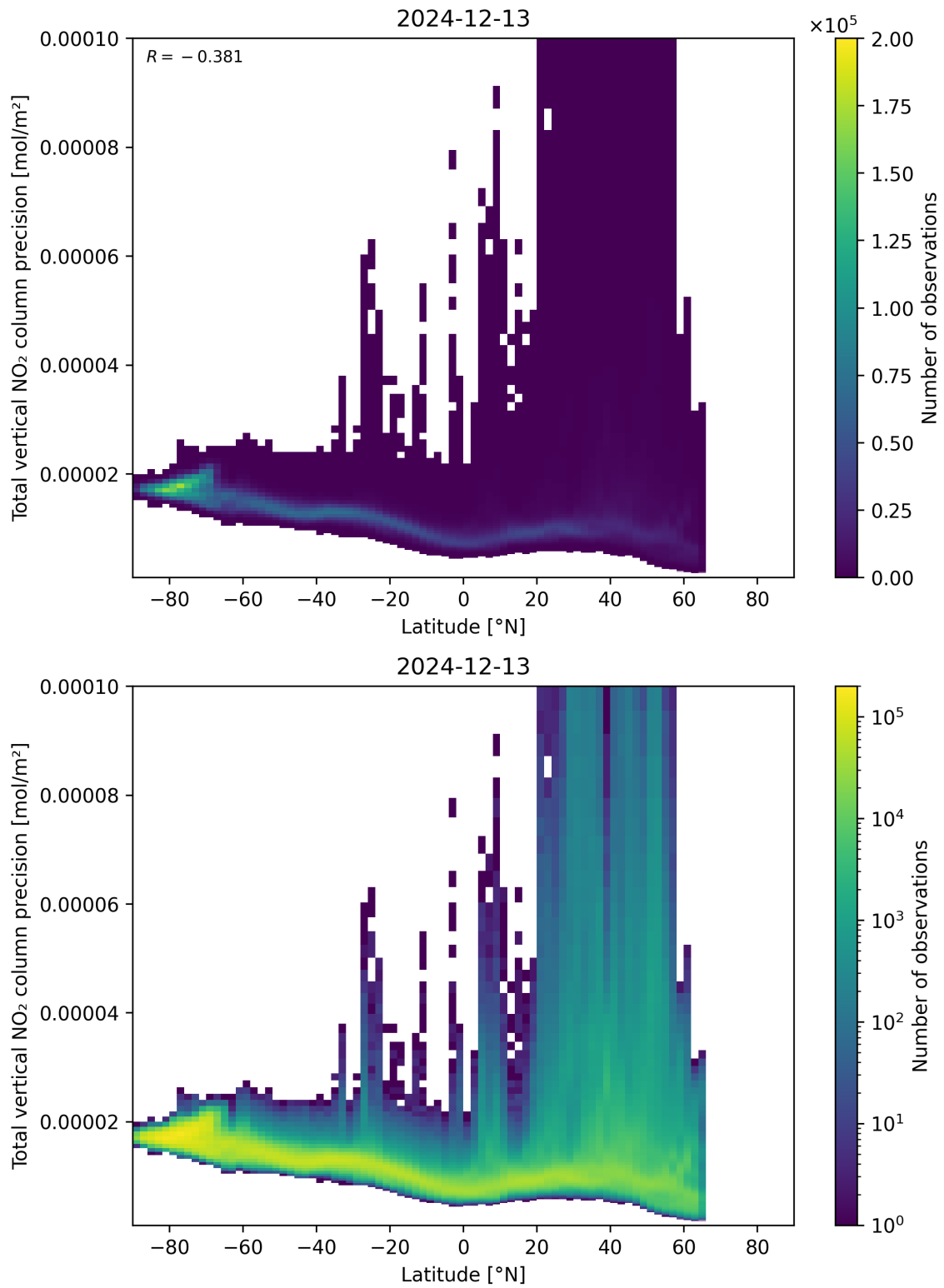
Figure 91: Scatter density plot of “Latitude” against “Total vertical NO 2 column precision” for 2024-12-12 to 2024-12-14.
