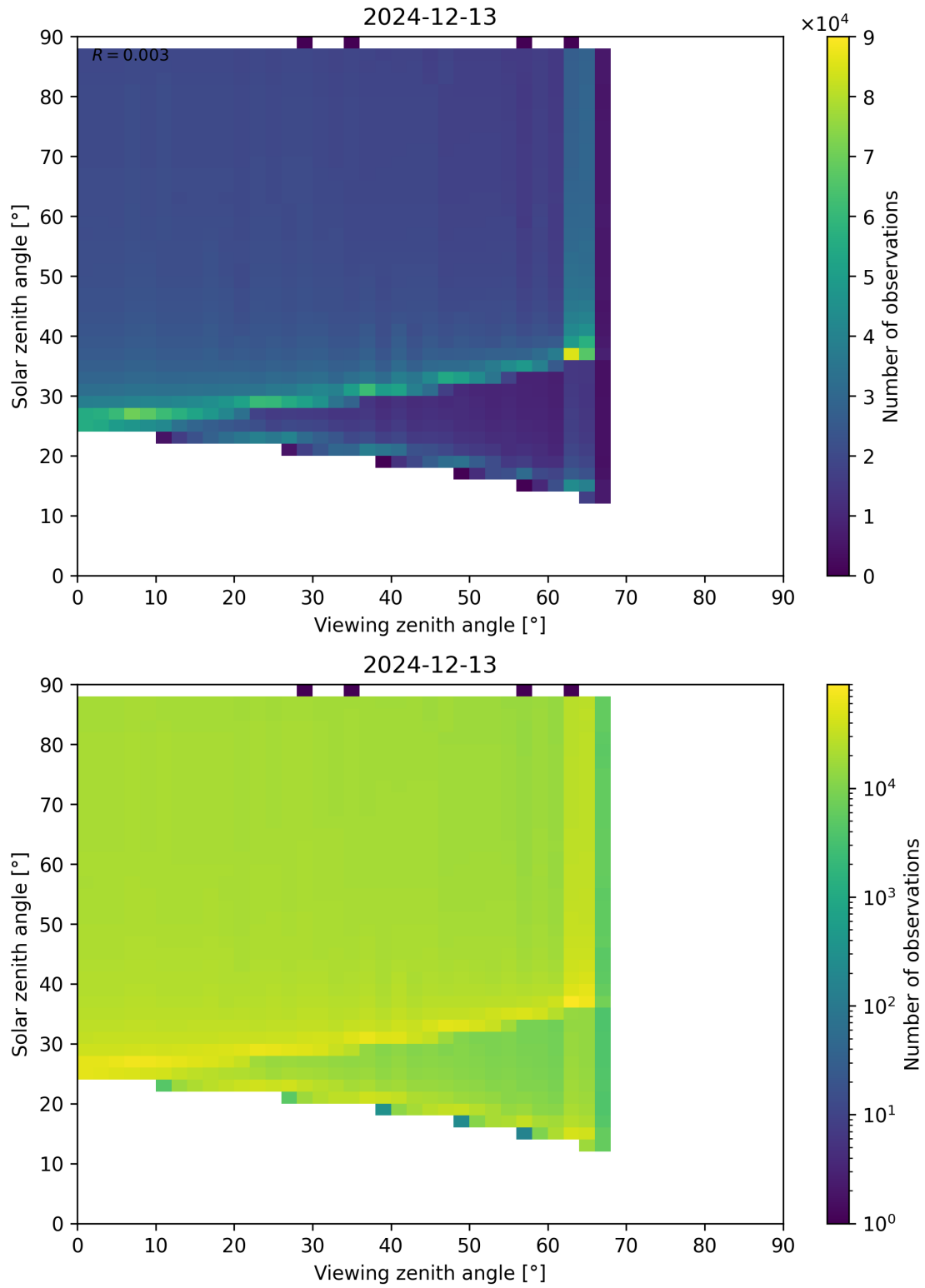
Figure 172: Scatter density plot of “Viewing zenith angle” against “Solar zenith angle” for 2024-12-12 to 2024-12-14.
