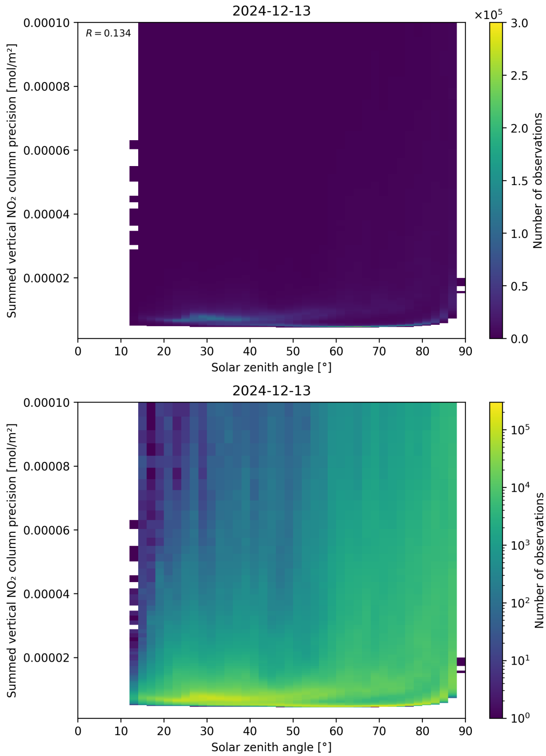
Figure 152: Scatter density plot of “Solar zenith angle” against “Summed vertical NO 2 column precision” for 2024-12-12 to 2024-12-14.
