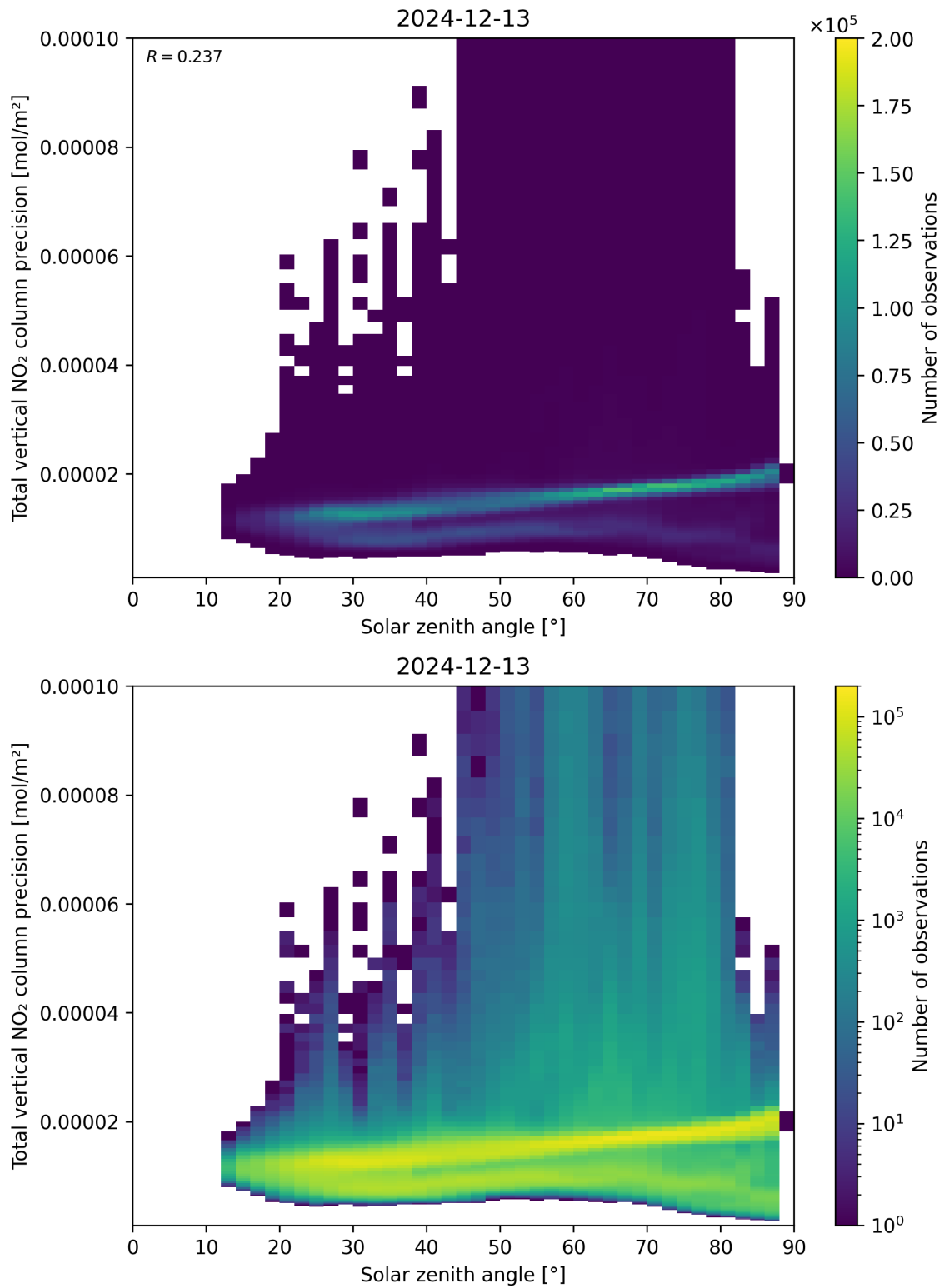
Figure 154: Scatter density plot of “Solar zenith angle” against “Total vertical NO 2 column precision” for 2024-12-12 to 2024-12-14.
