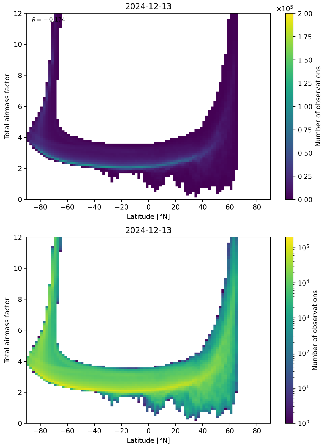
Figure 84: Scatter density plot of “Latitude” against “Total airmass factor” for 2024-12-12 to 2024-12-14.
