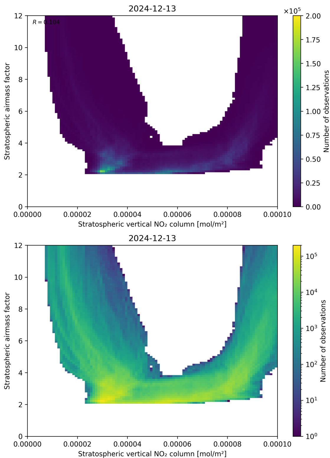
Figure 96: Scatter density plot of “Stratospheric vertical NO 2 column” against “Stratospheric airmass factor” for 2024-12-12 to 2024-12-14.
