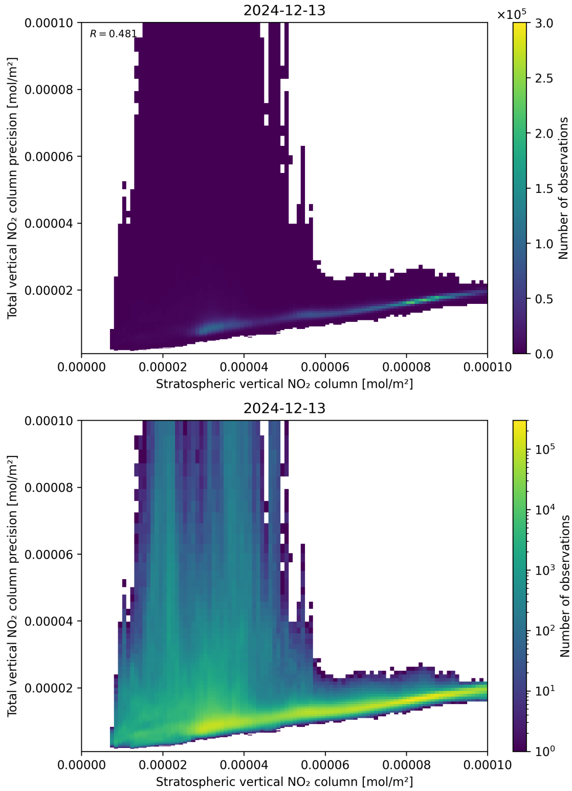
Figure 101: Scatter density plot of “Stratospheric vertical NO 2 column” against “Total vertical NO 2 column precision” for 2024-12-12 to 2024-12-14.
