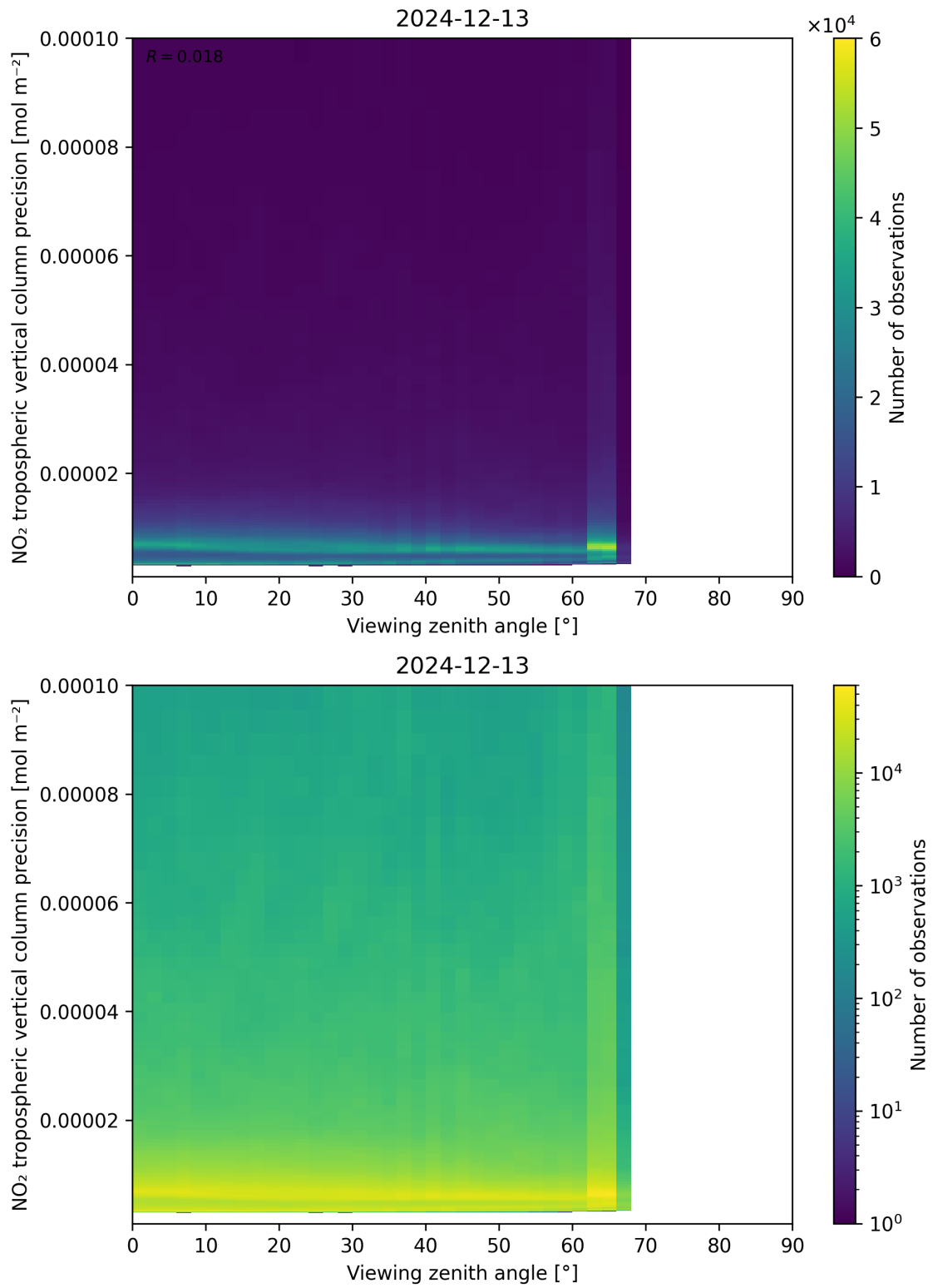
Figure 170: Scatter density plot of “Viewing zenith angle” against “NO 2 tropospheric vertical column precision” for 2024-12-12 to 2024-12-14.
