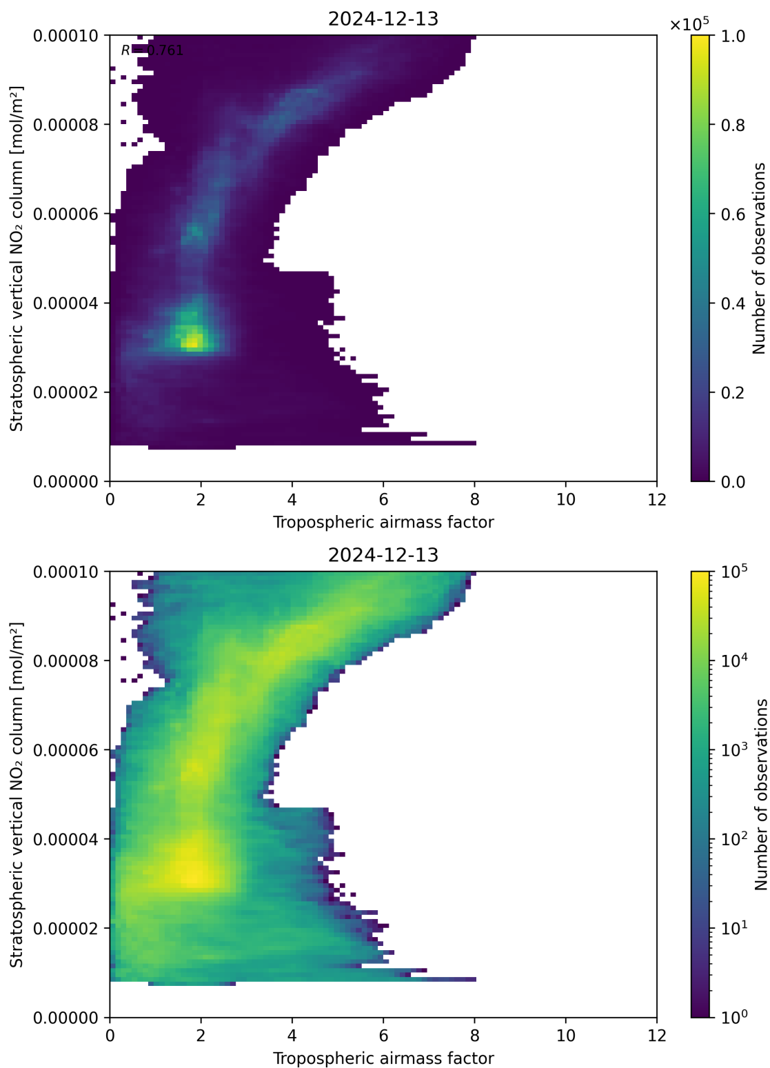
Figure 74: Scatter density plot of “Tropospheric air mass factor” against “Stratospheric vertical NO 2 column” for 2024-12-12 to 2024-12-14.
