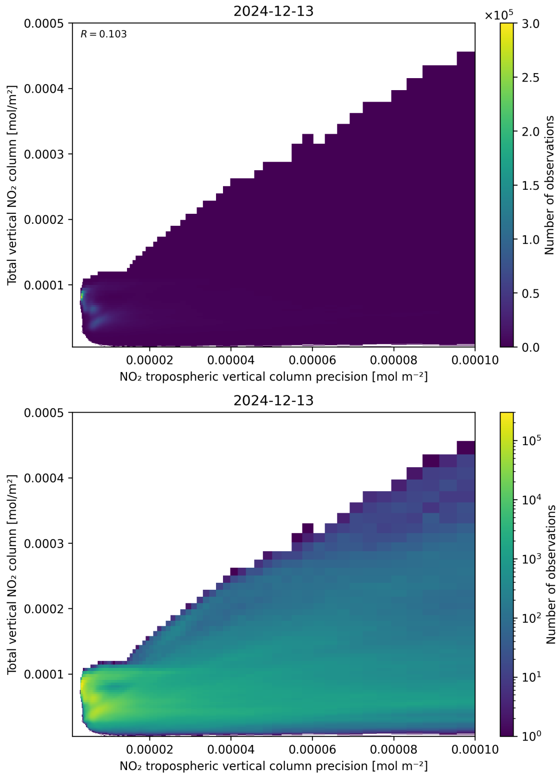
Figure 138: Scatter density plot of “NO 2 tropospheric vertical column precision” against “Total vertical NO 2 column” for 2024-12-12 to 2024-12-14.
