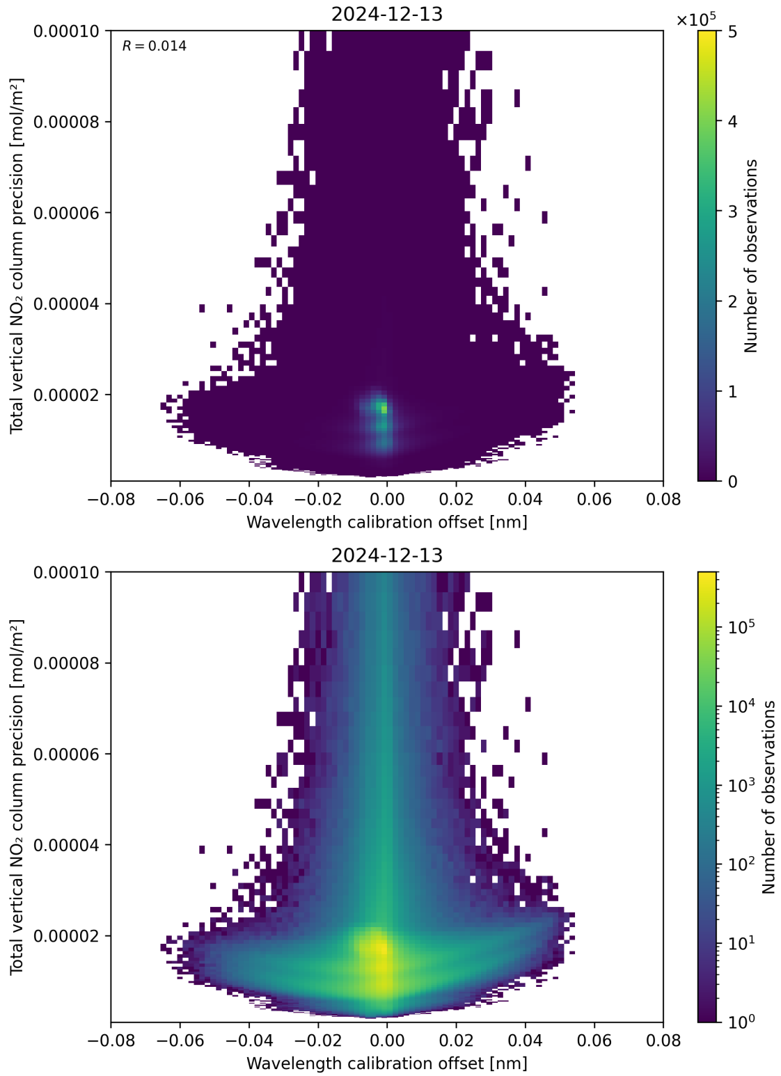
Figure 180: Scatter density plot of “Wavelength calibration offset” against “Total vertical NO 2 column precision” for 2024-12-12 to 2024-12-14.
