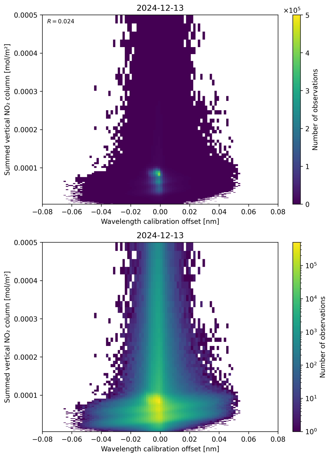
Figure 177: Scatter density plot of “Wavelength calibration offset” against “Summed vertical NO 2 column” for 2024-12-12 to 2024-12-14.
