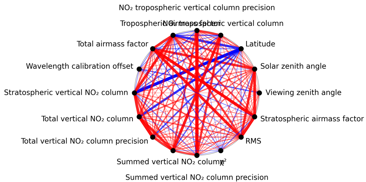
Figure 1: Map of correlation graph for 2024-12-12 to 2024-12-14.
