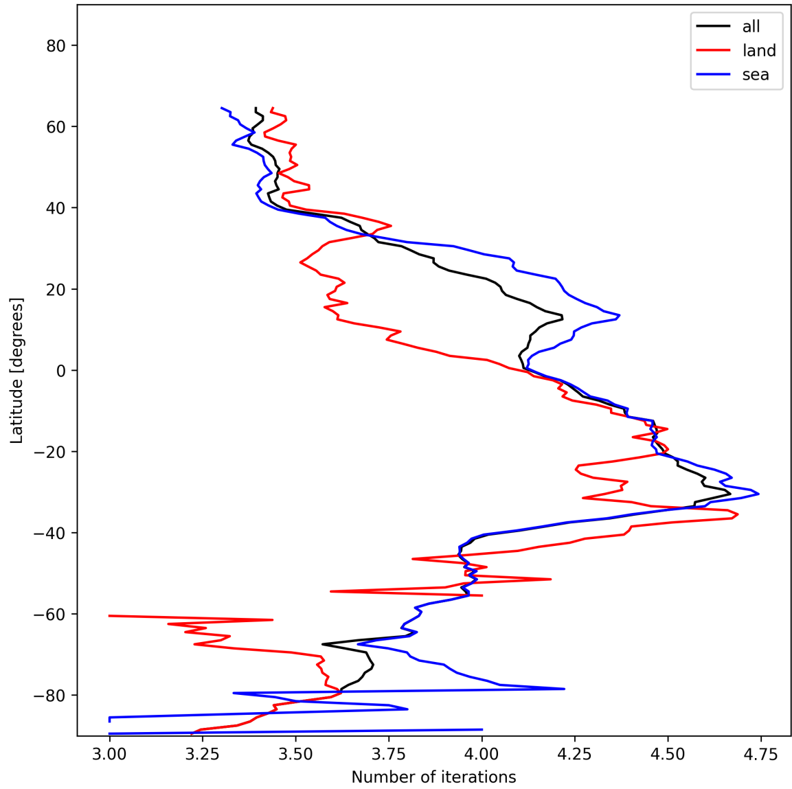
Figure 17: Zonal average of “Number of iterations” for 2024-12-12 to 2024-12-14.
