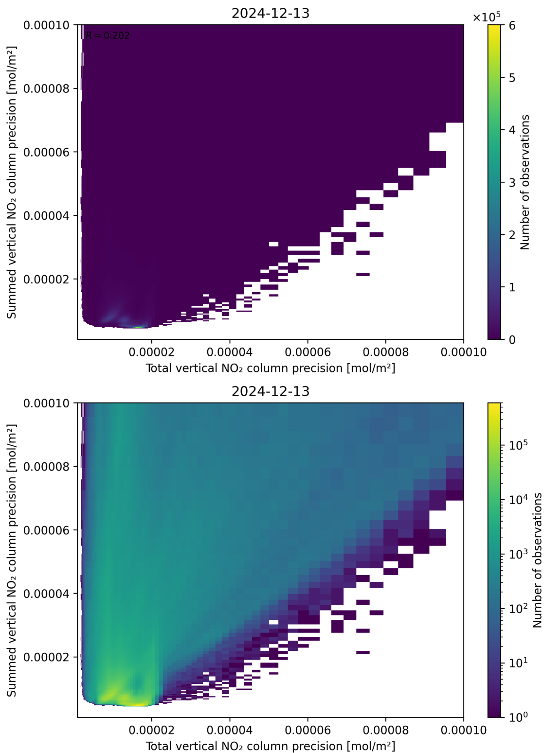
Figure 118: Scatter density plot of “Total vertical NO 2 column precision” against “Summed vertical NO 2 column precision” for 2024-12-12 to 2024-12-14.
