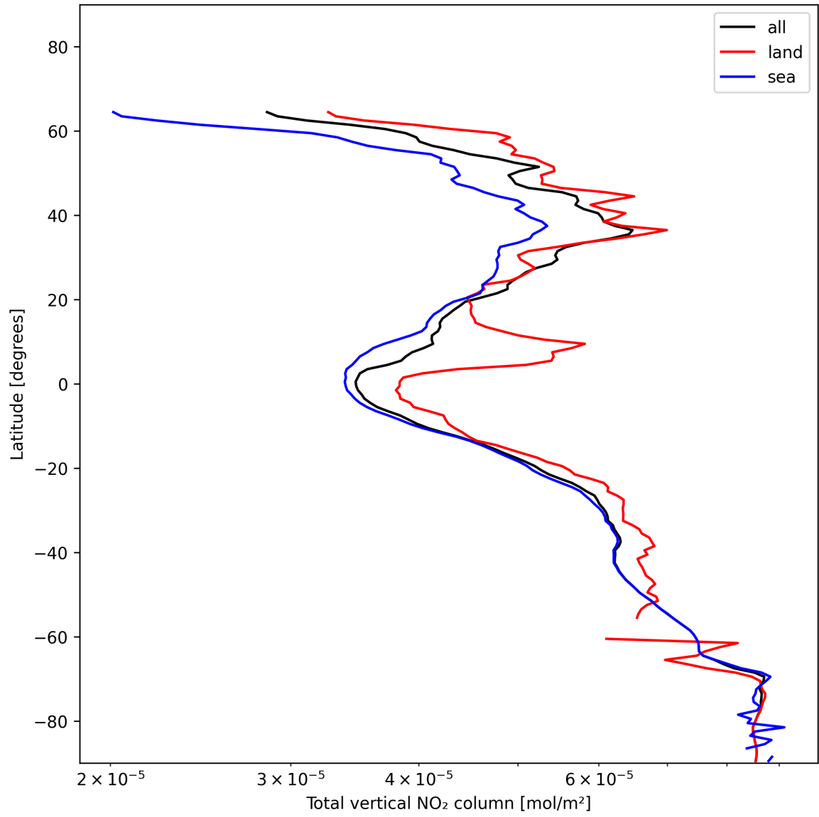
Figure 21: Zonal average of “Total vertical NO 2 column” for 2024-12-12 to 2024-12-14.
