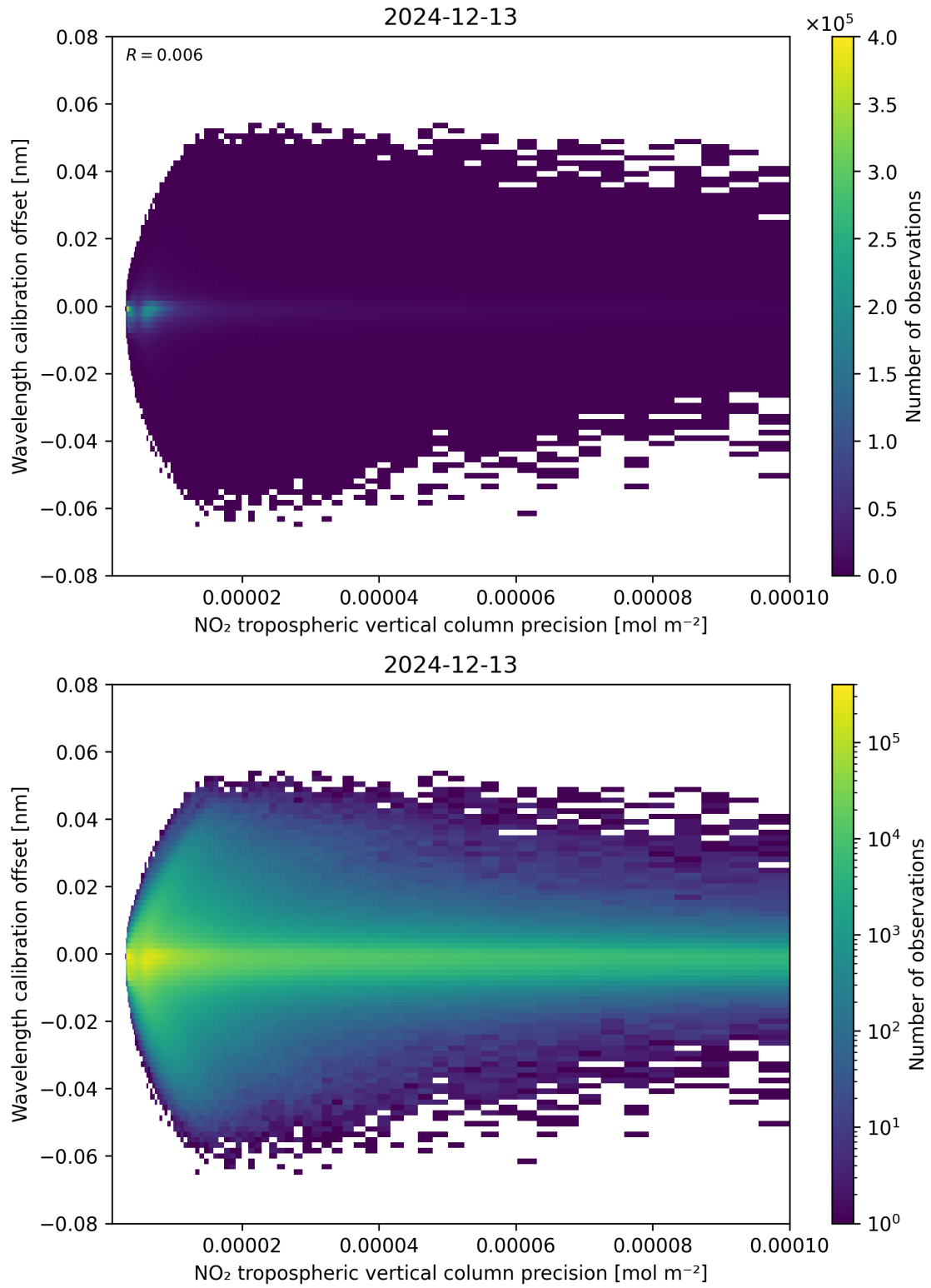
Figure 141: Scatter density plot of “NO 2 tropospheric vertical column precision” against “Wavelength calibration offset” for 2024-12-12 to 2024-12-14.
