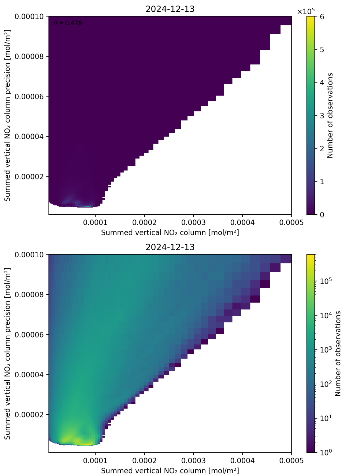
Figure 105: Scatter density plot of “Summed vertical NO 2 column” against “Summed vertical NO 2 column precision” for 2024-12-12 to 2024-12-14.
