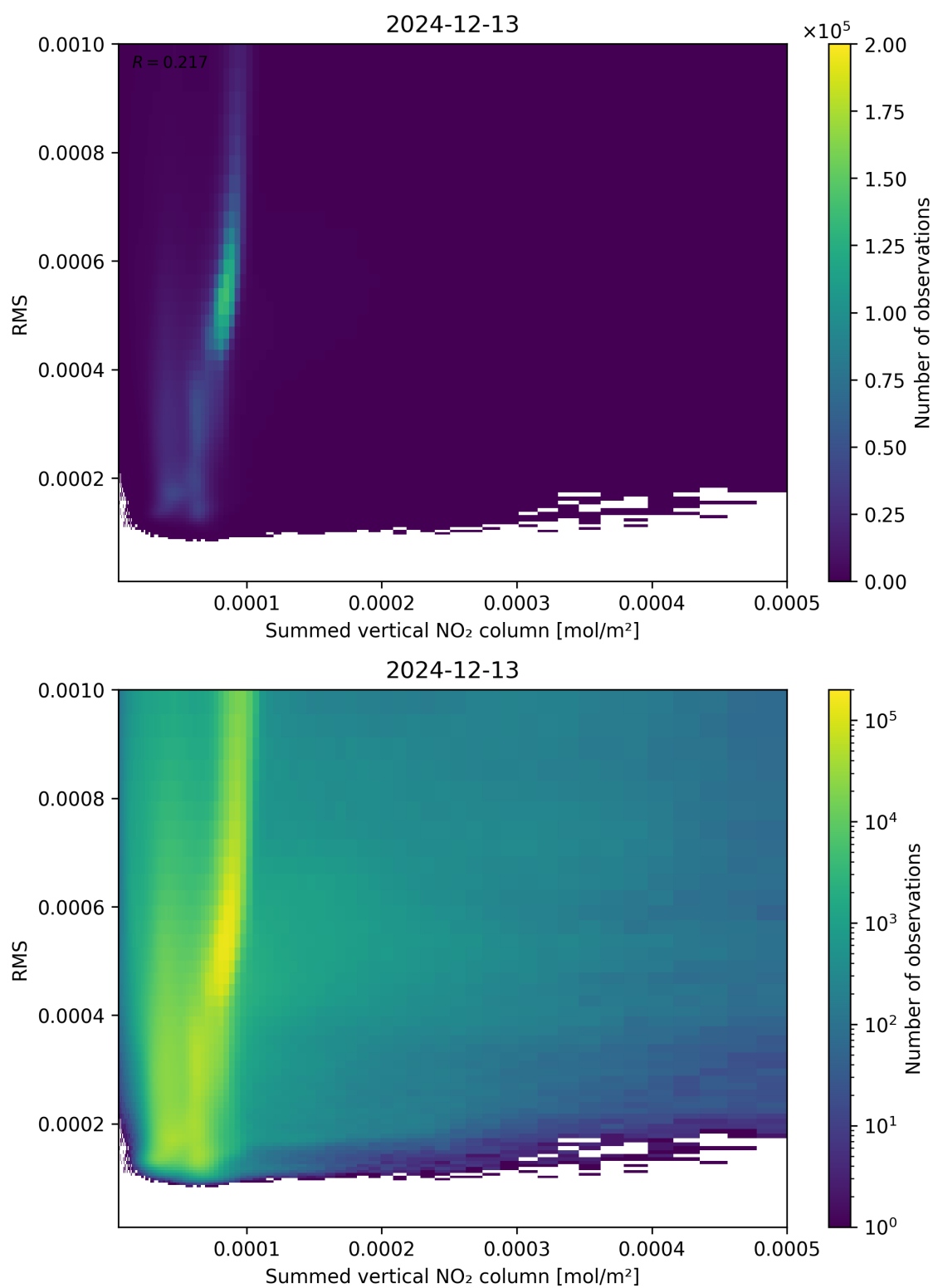
Figure 109: Scatter density plot of “Summed vertical NO 2 column” against “RMS” for 2024-12-12 to 2024-12-14.
