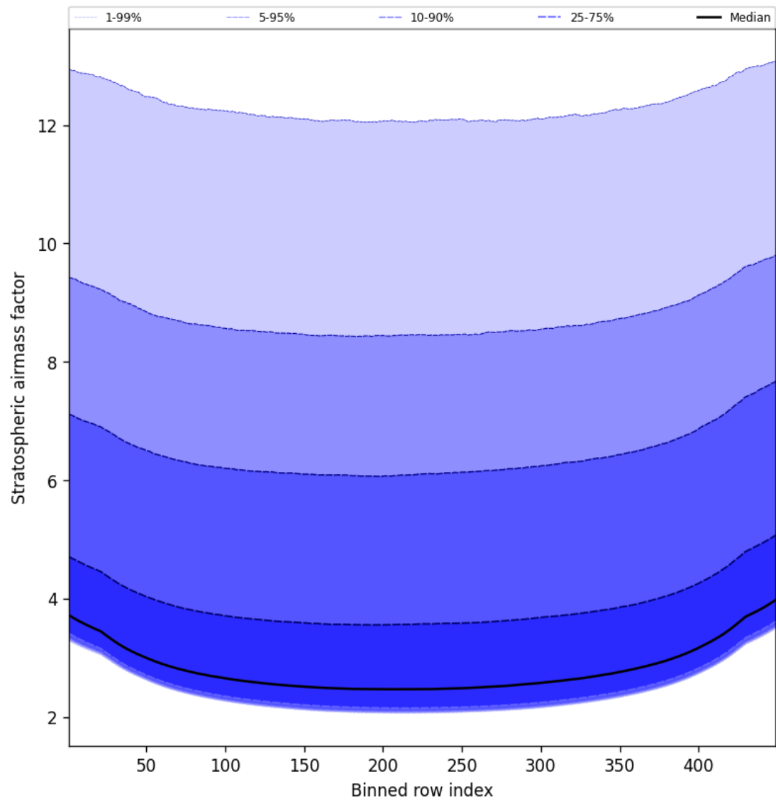
Figure 61: Along track statistics of “Stratospheric airmass factor” for 2024-12-12 to 2024-12-14
