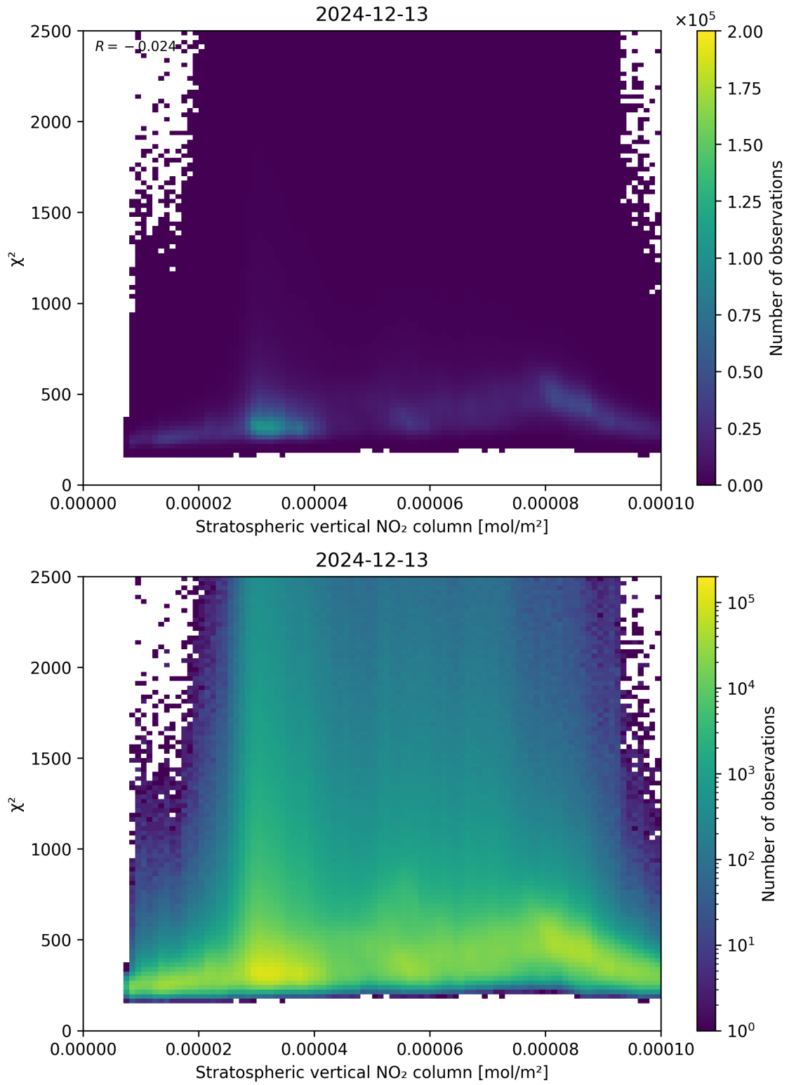
Figure 97: Scatter density plot of “Stratospheric vertical NO 2 column” against “ \chi^2 ” for 2024-12-12 to 2024-12-14.
