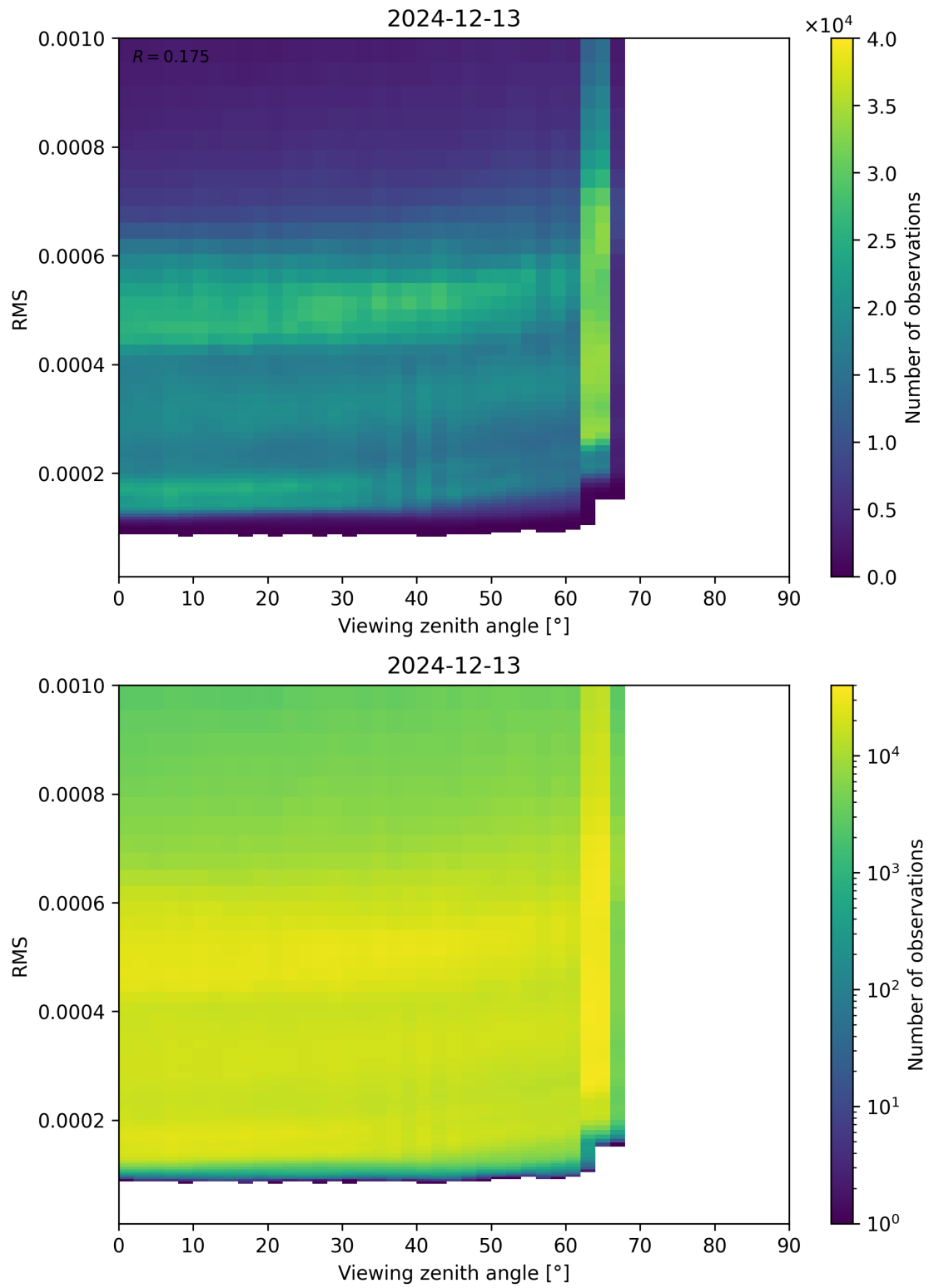
Figure 171: Scatter density plot of “Viewing zenith angle” against “RMS” for 2024-12-12 to 2024-12-14.
