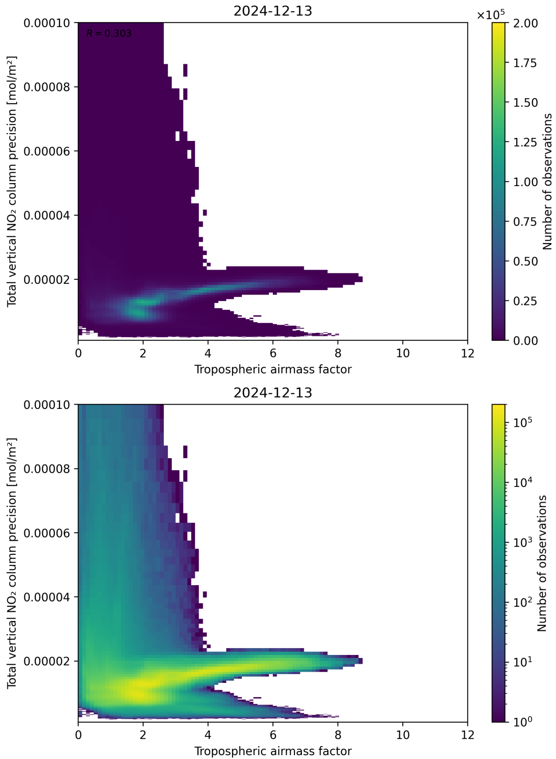
Figure 78: Scatter density plot of “Tropospheric air mass factor” against “Total vertical NO 2 column precision” for 2024-12-12 to 2024-12-14.
