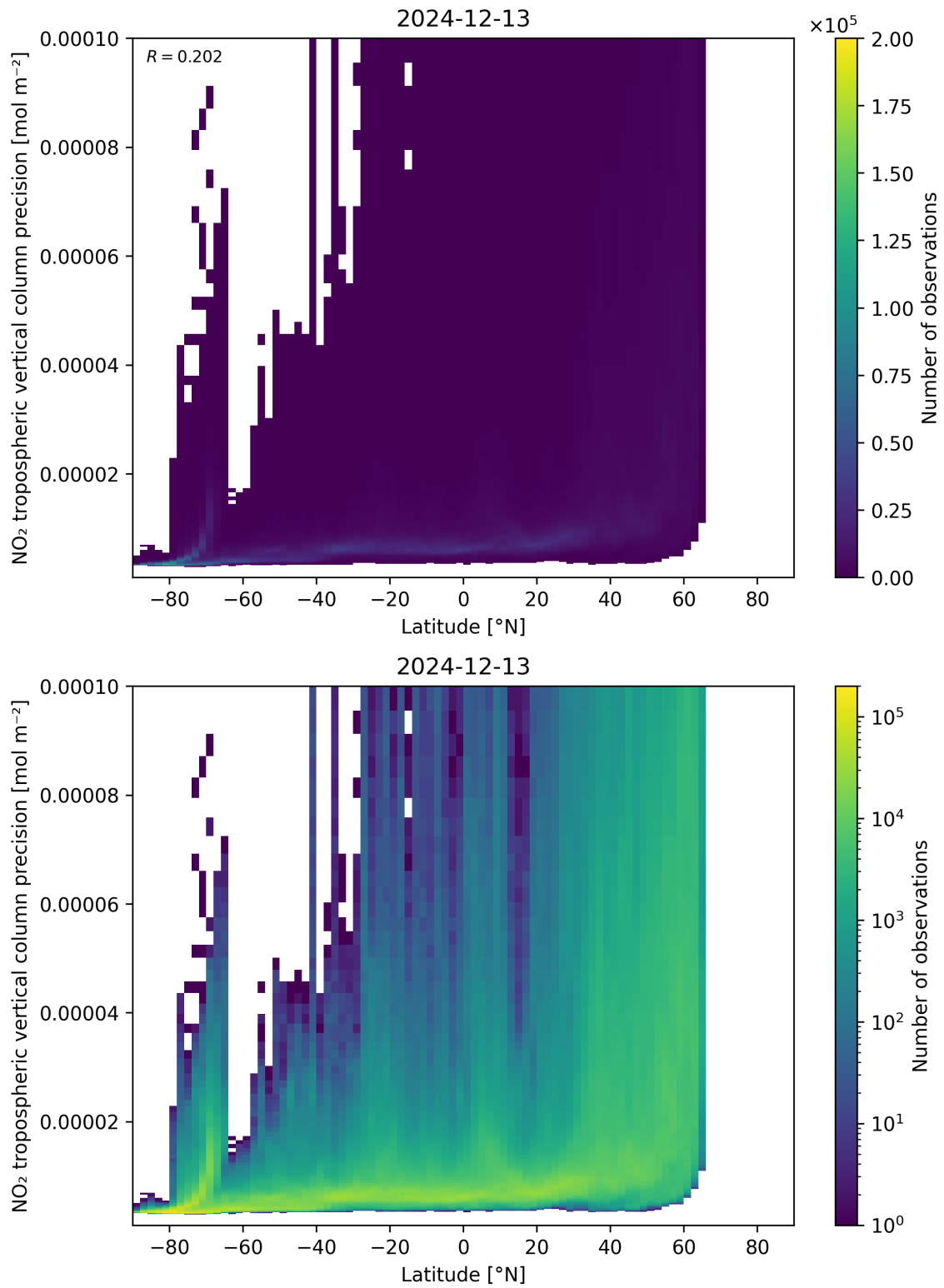
Figure 93: Scatter density plot of “Latitude” against “NO 2 tropospheric vertical column precision” for 2024-12-12 to 2024-12-14.
