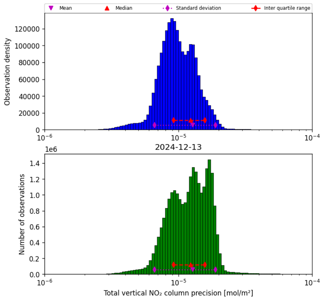
Figure 39: Histogram of “Total vertical NO 2 column precision” for 2024-12-12 to 2024-12-14
