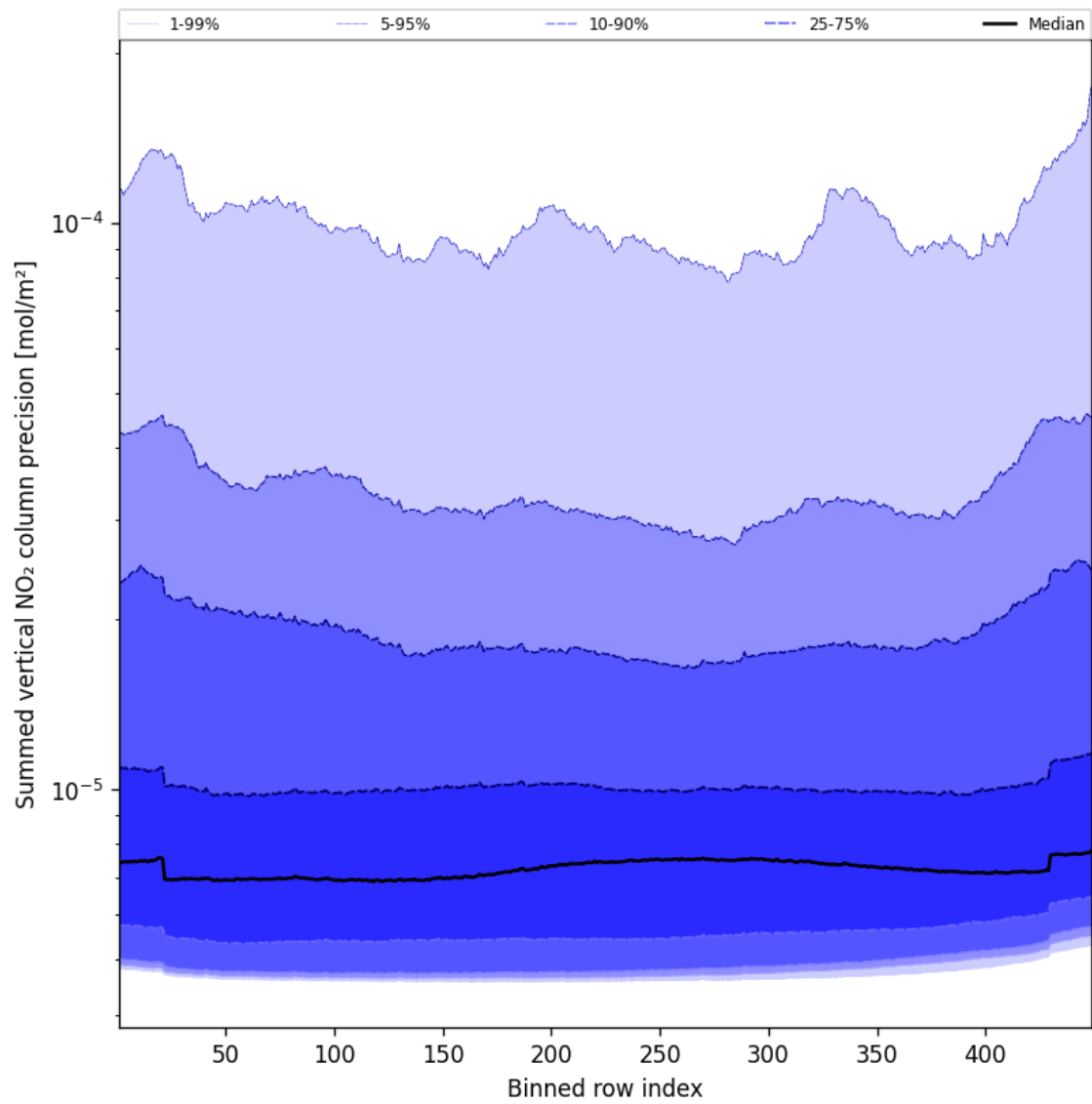
Figure 58: Along track statistics of “Summed vertical NO 2 column precision” for 2024-12-12 to 2024-12-14
