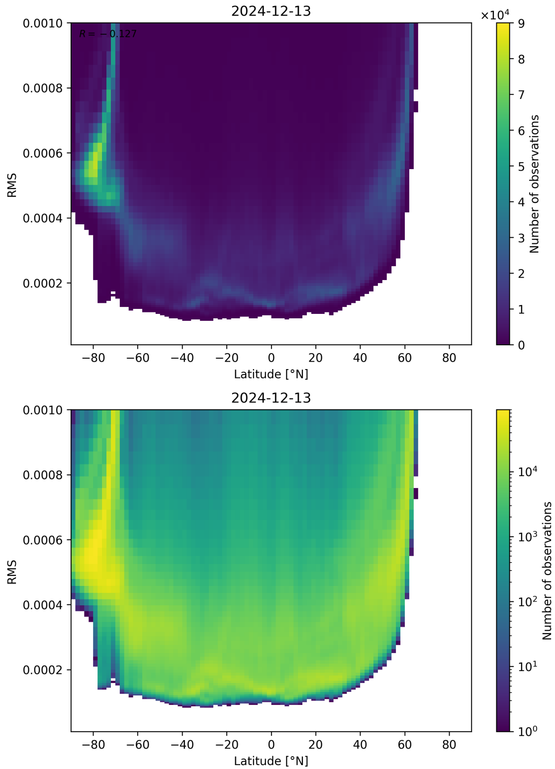
Figure 94: Scatter density plot of “Latitude” against “RMS” for 2024-12-12 to 2024-12-14.
