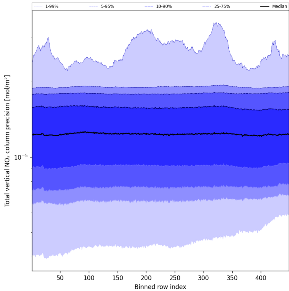
Figure 56: Along track statistics of “Total vertical NO 2 column precision” for 2024-12-12 to 2024-12-14
