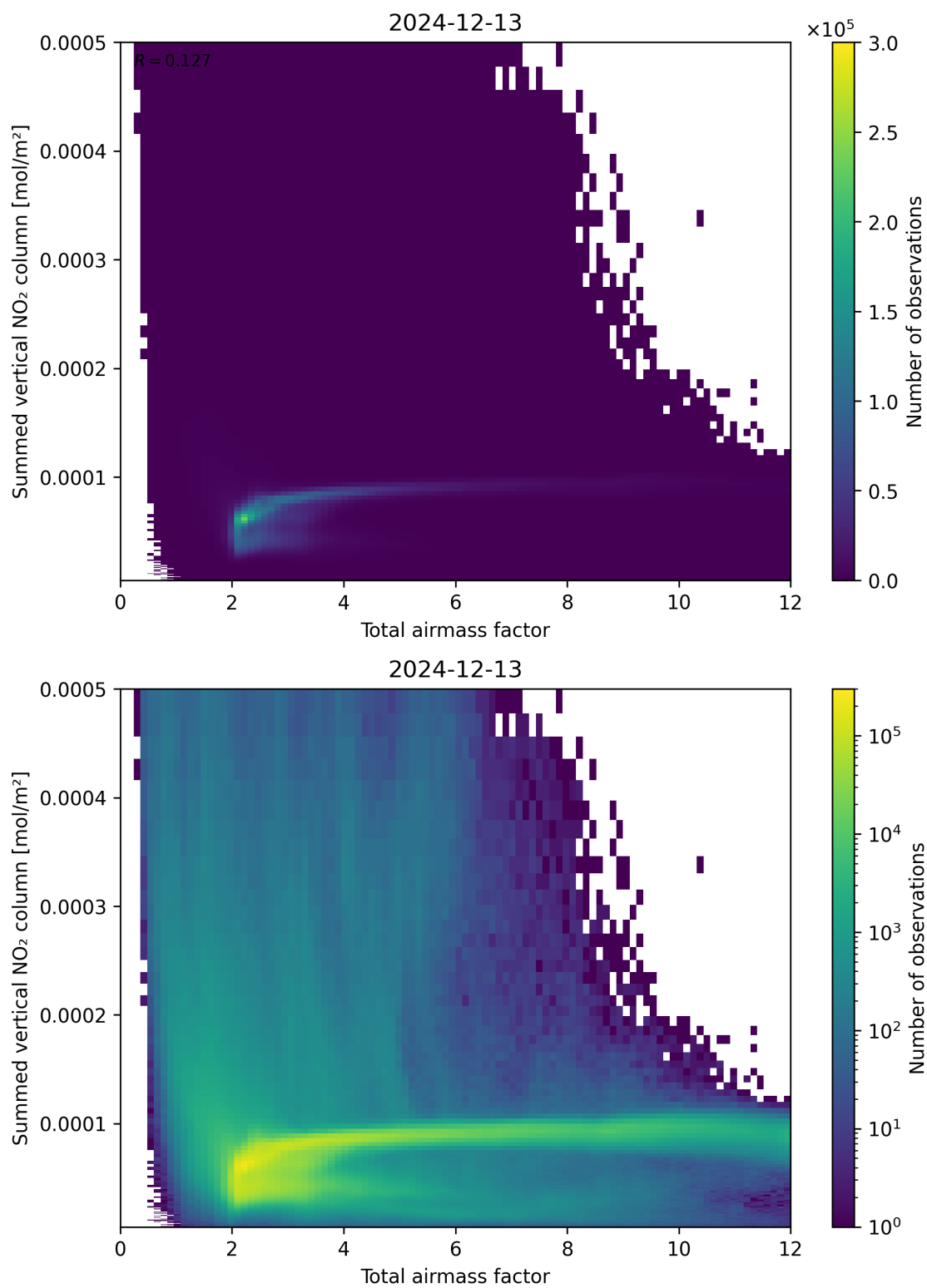
Figure 65: Scatter density plot of “Total airmass factor” against “Summed vertical NO 2 column” for 2024-12-12 to 2024-12-14.
