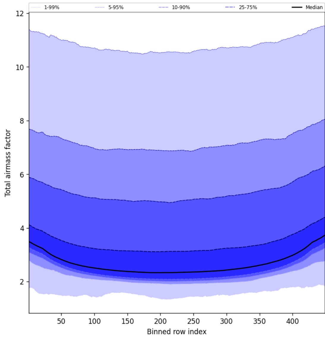
Figure 49: Along track statistics of “Total airmass factor” for 2024-12-12 to 2024-12-14
