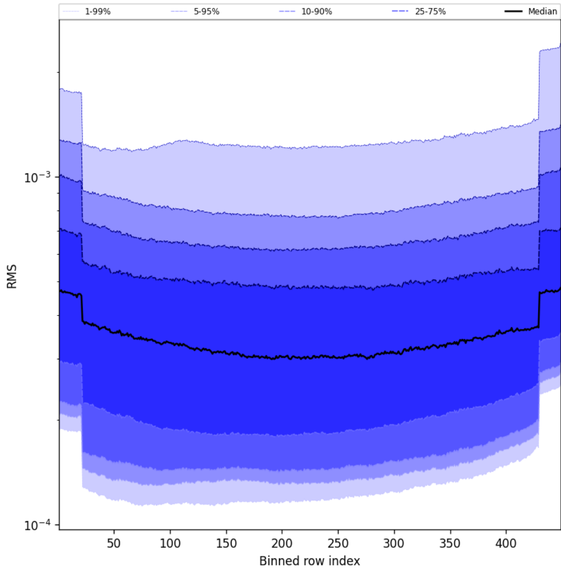
Figure 60: Along track statistics of “RMS” for 2024-12-12 to 2024-12-14
