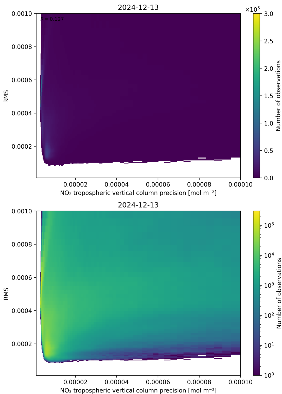
Figure 140: Scatter density plot of “NO 2 tropospheric vertical column precision” against “RMS” for 2024-12-12 to 2024-12-14.
