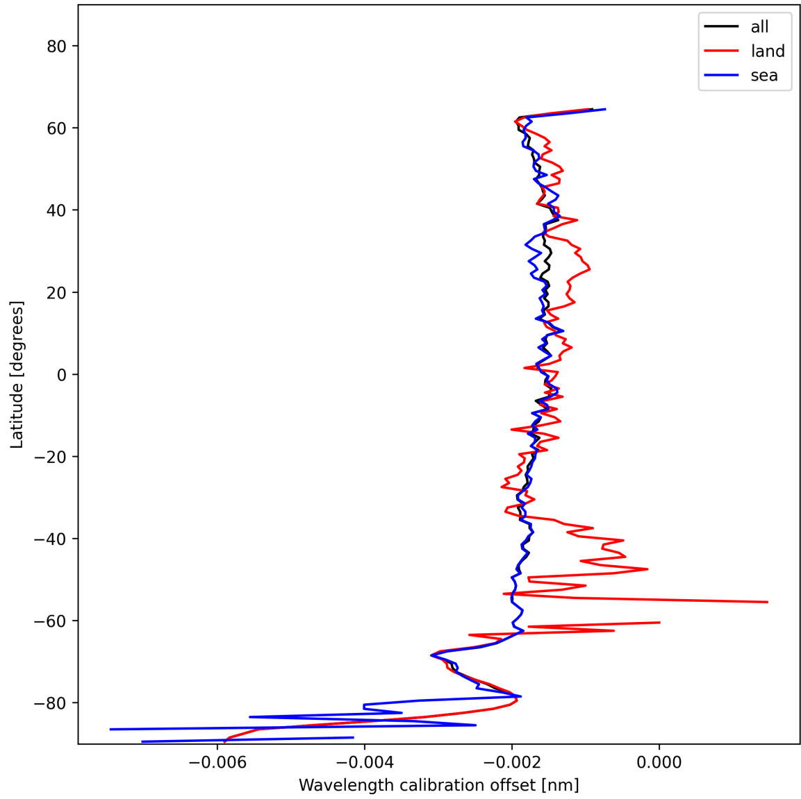
Figure 18: Zonal average of “Wavelength calibration offset” for 2024-12-12 to 2024-12-14.
