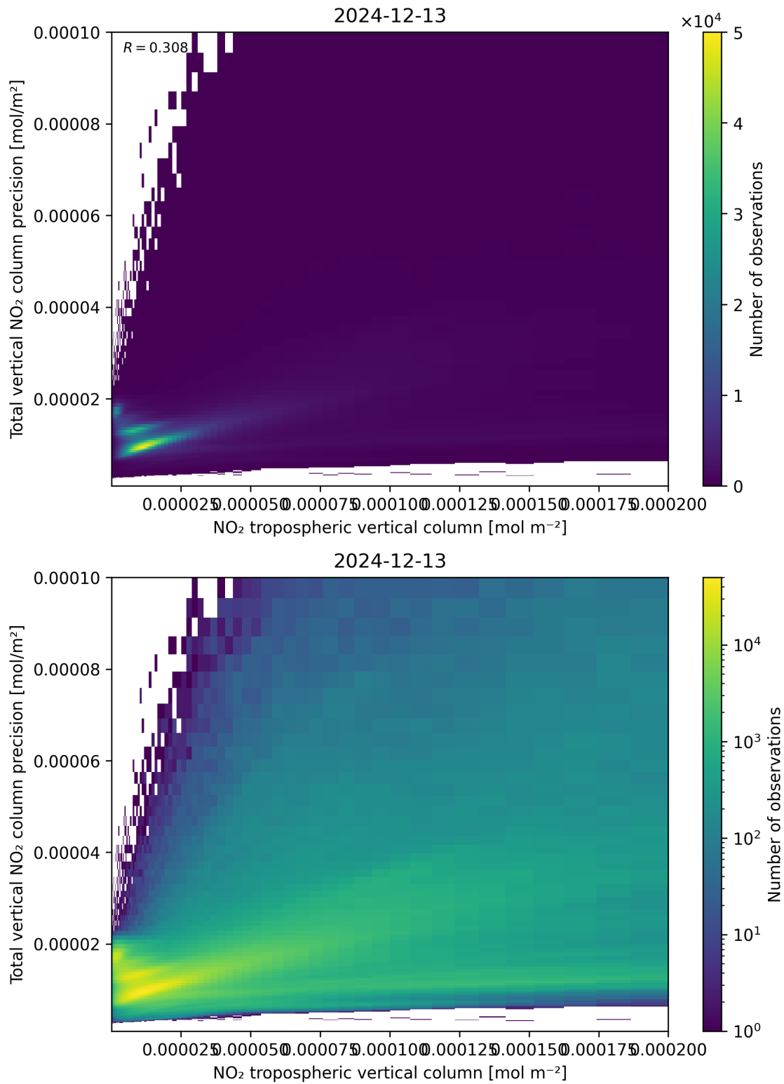
Figure 129: Scatter density plot of “NO 2 tropospheric vertical column” against “Total vertical NO 2 column precision” for 2024-12-12 to 2024-12-14.
