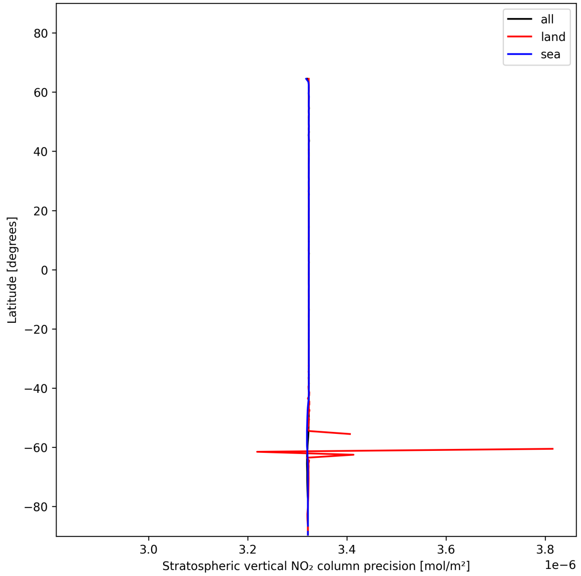
Figure 20: Zonal average of “Stratospheric vertical NO 2 column precision” for 2024-12-12 to 2024-12-14.
