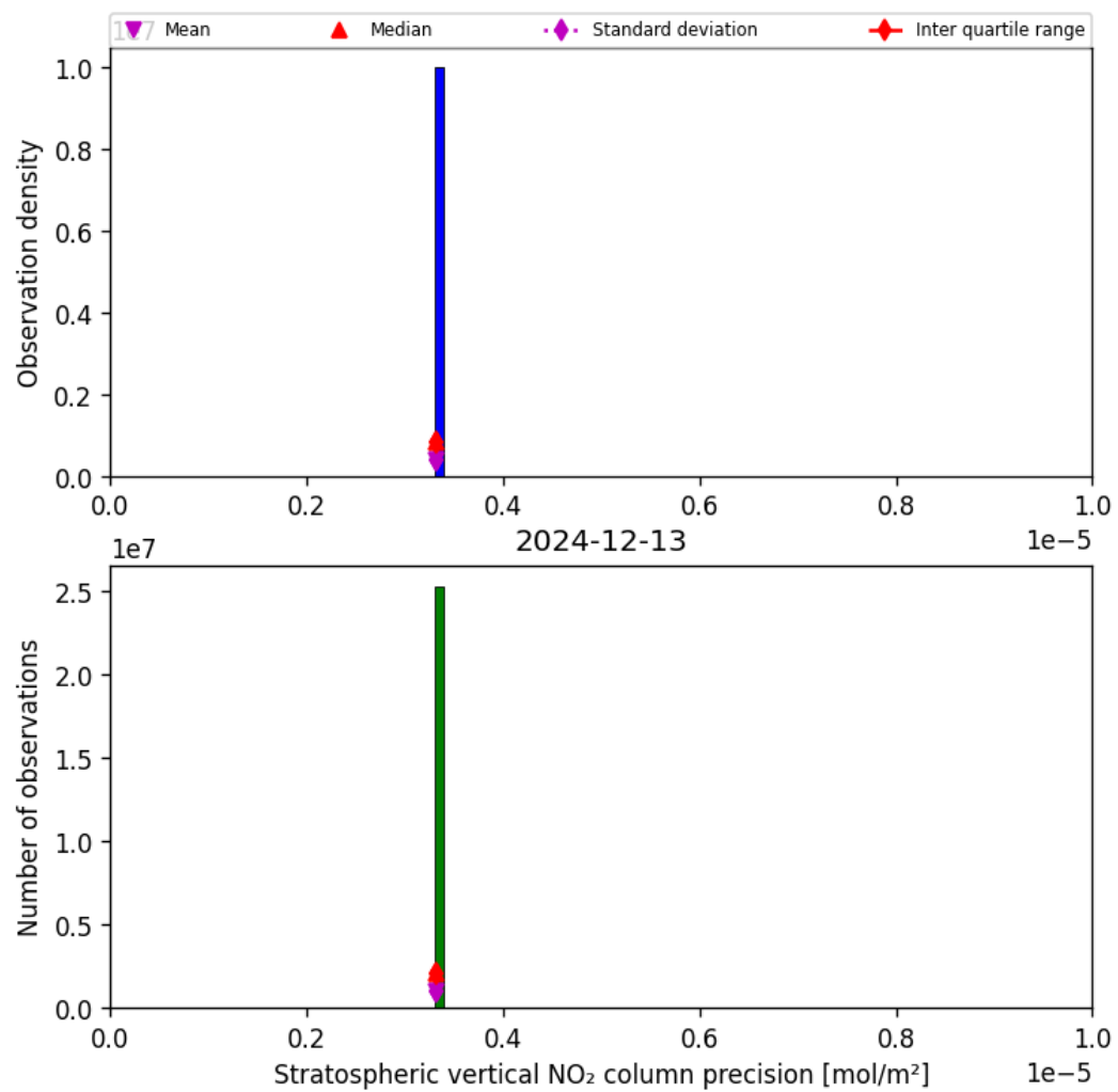
Figure 37: Histogram of “Stratospheric vertical NO 2 column precision” for 2024-12-12 to 2024-12-14
