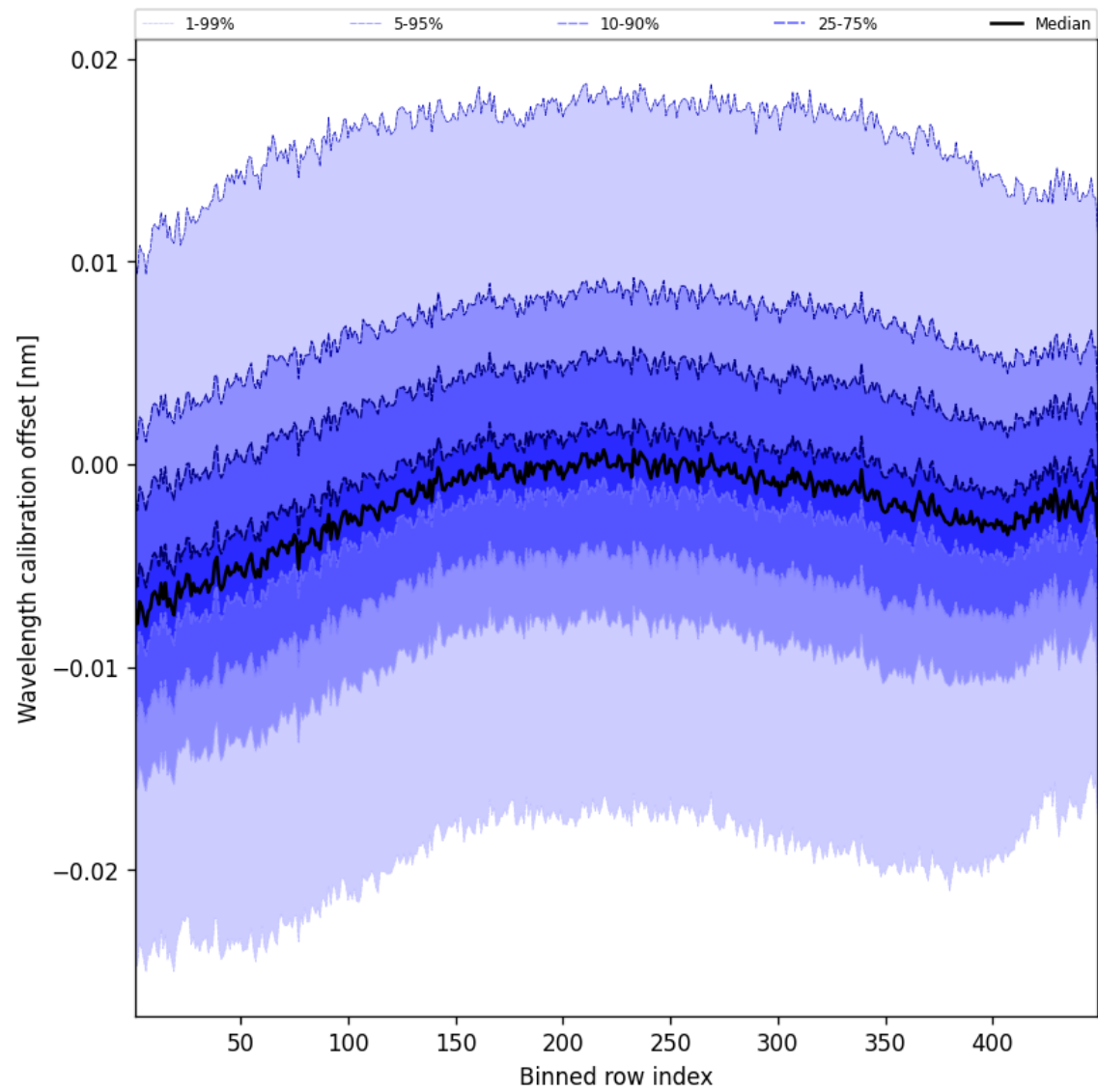
Figure 52: Along track statistics of “Wavelength calibration offset” for 2024-12-12 to 2024-12-14
