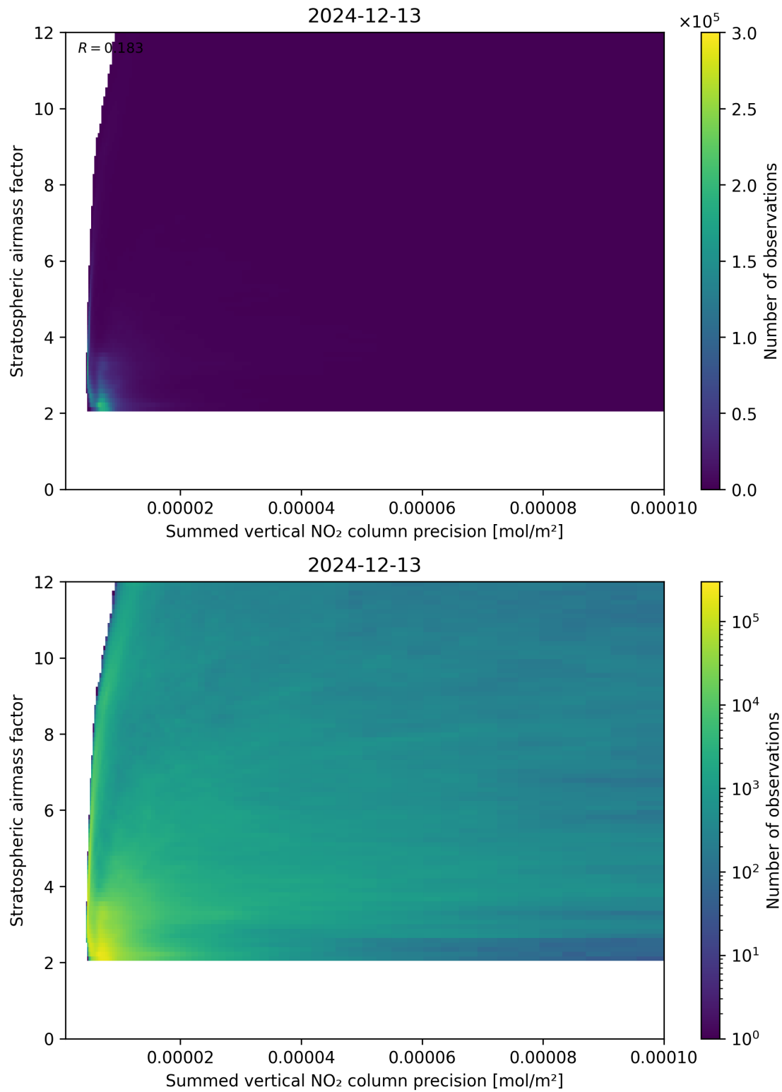
Figure 106: Scatter density plot of “Summed vertical NO 2 column precision” against “Stratospheric airmass factor” for 2024-12-12 to 2024-12-14.
