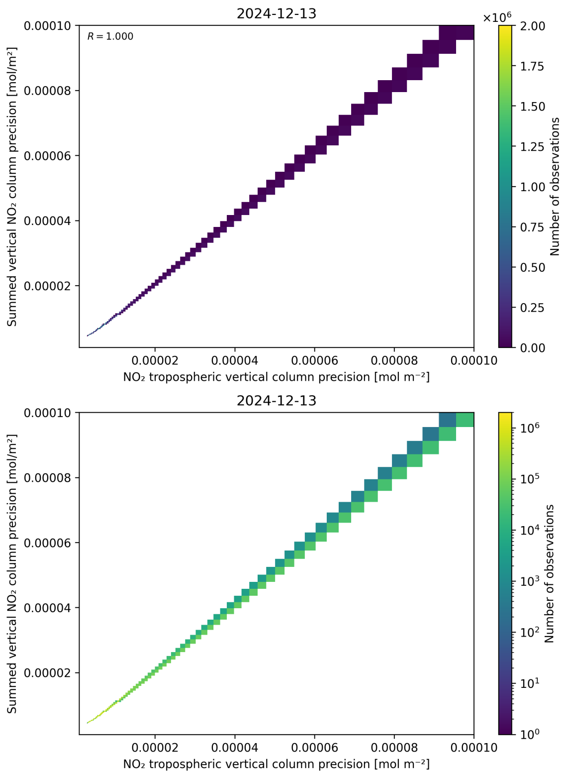
Figure 137: Scatter density plot of “NO 2 tropospheric vertical column precision” against “Summed vertical NO 2 column precision” for 2024-12-12 to 2024-12-14.
