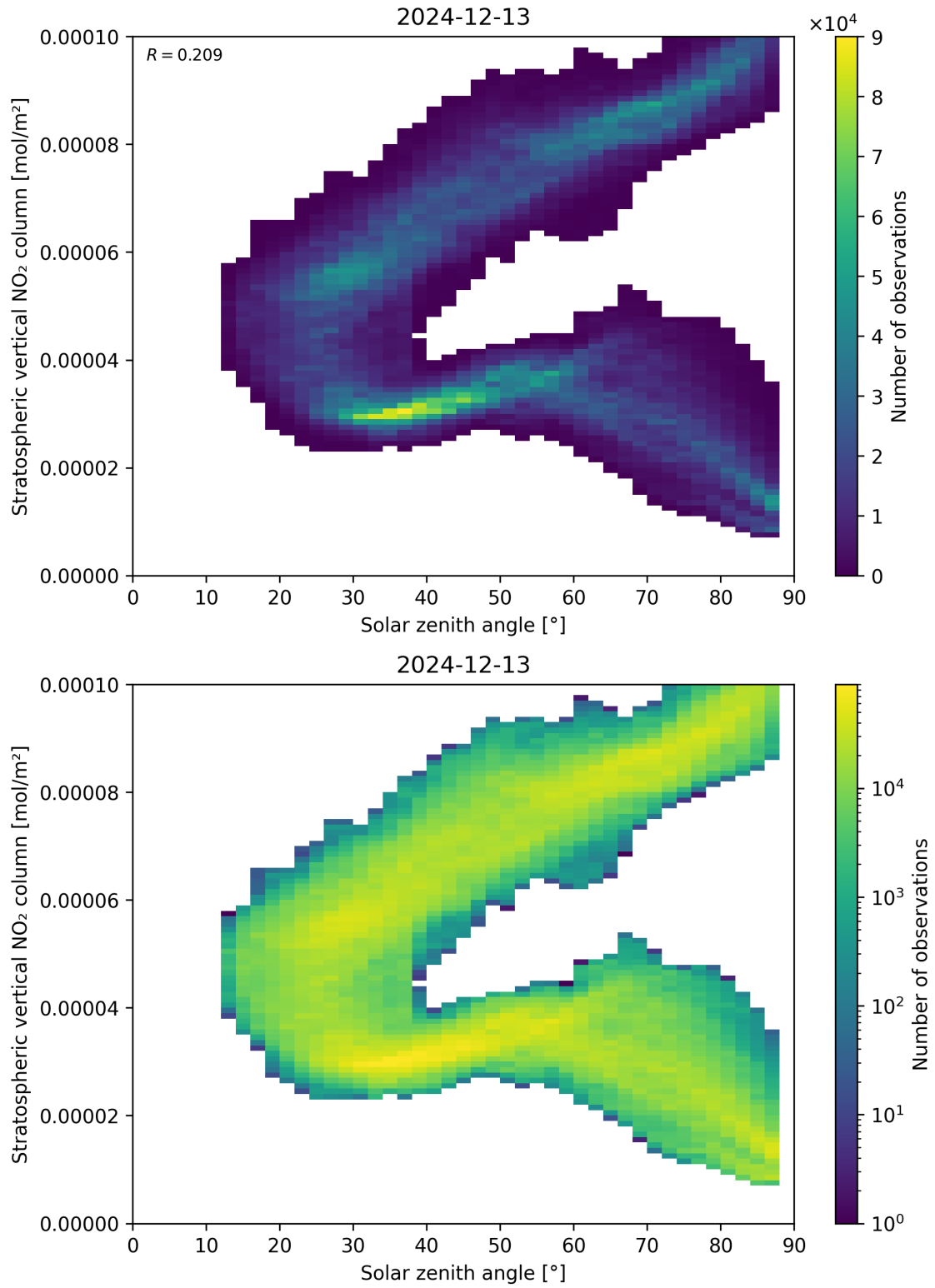
Figure 150: Scatter density plot of “Solar zenith angle” against “Stratospheric vertical NO 2 column” for 2024-12-12 to 2024-12-14.
