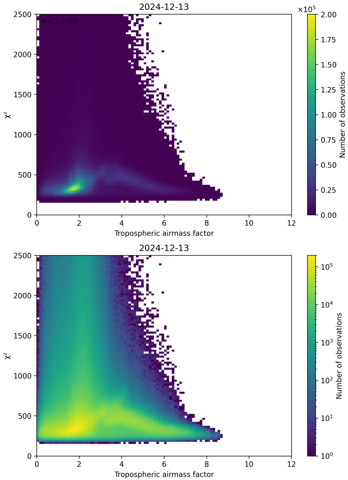
Figure 73: Scatter density plot of “Tropospheric airmass factor” against “ \chi^2 ” for 2024-12-12 to 2024-12-14.
