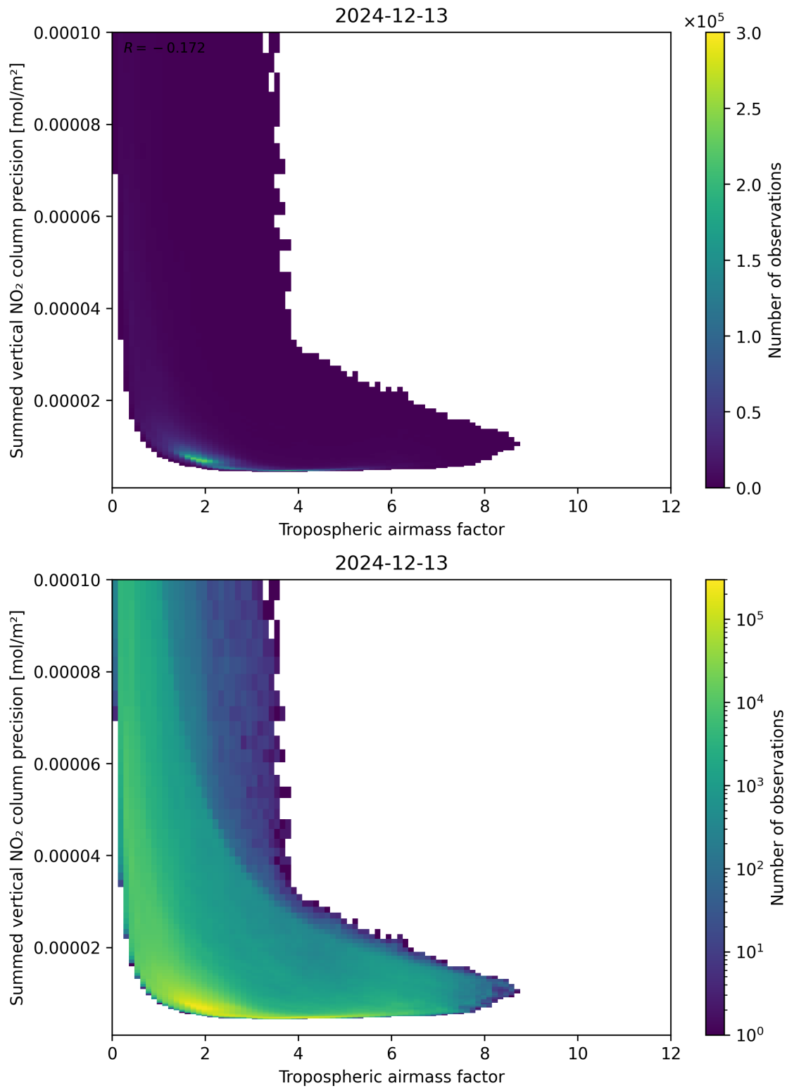
Figure 76: Scatter density plot of “Tropospheric air mass factor” against “Summed vertical NO 2 column precision” for 2024-12-12 to 2024-12-14.
