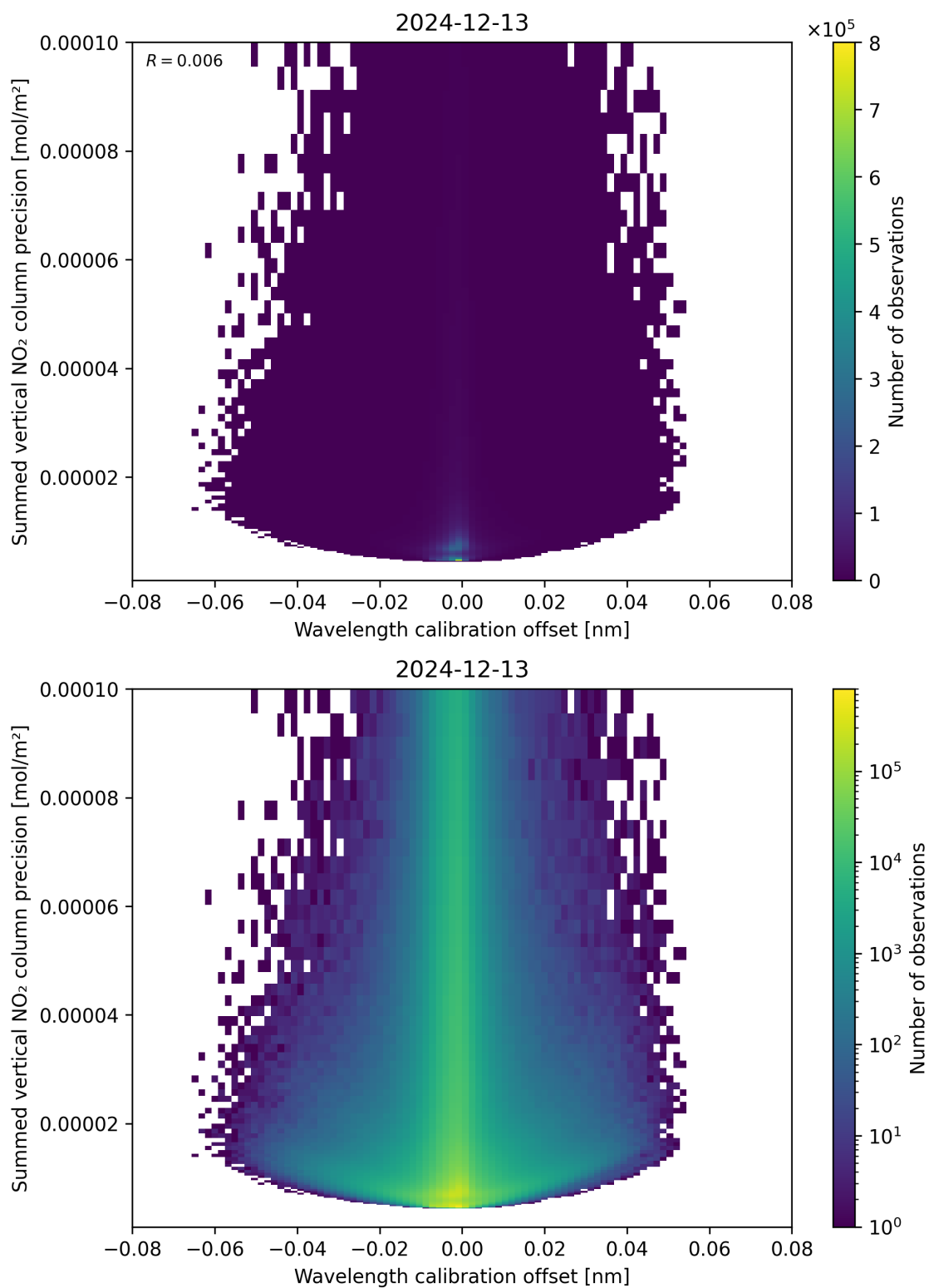
Figure 178: Scatter density plot of “Wavelength calibration offset” against “Summed vertical NO 2 column precision” for 2024-12-12 to 2024-12-14.
