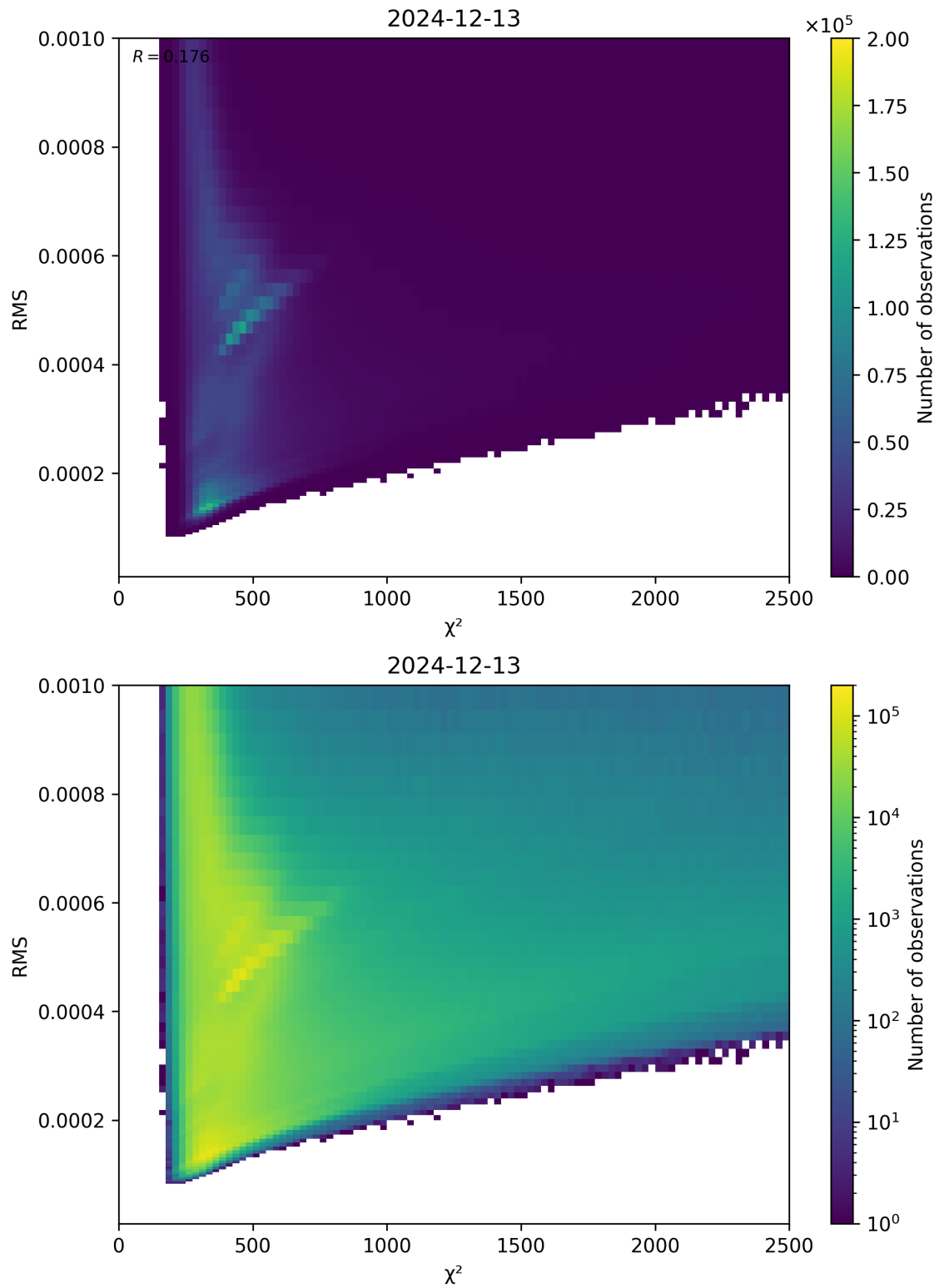
Figure 82: Scatter density plot of “ \chi^2 ” against “RMS” for 2024-12-12 to 2024-12-14.
