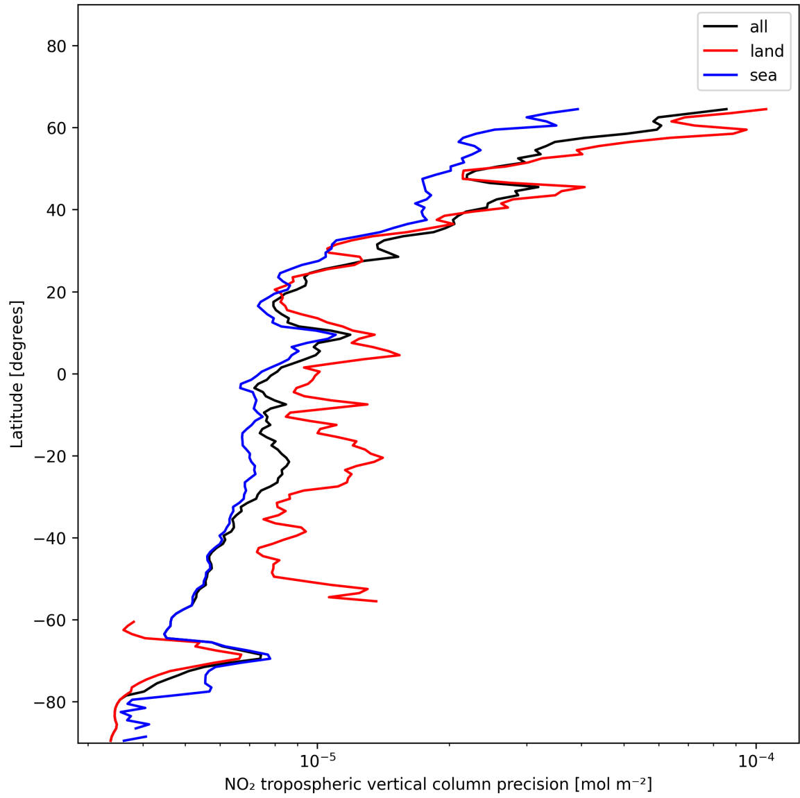
Figure 13: Zonal average of “NO 2 tropospheric vertical column precision” for 2024-12-12 to 2024-12-14.
