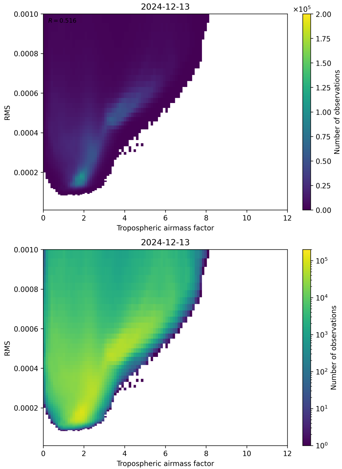
Figure 79: Scatter density plot of “Tropospheric airmass factor” against “RMS” for 2024-12-12 to 2024-12-14.
