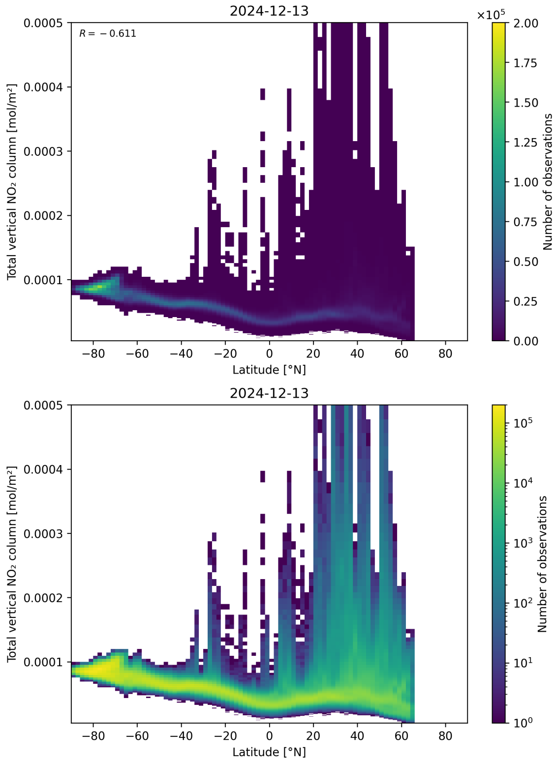
Figure 90: Scatter density plot of “Latitude” against “Total vertical NO 2 column” for 2024-12-12 to 2024-12-14.
