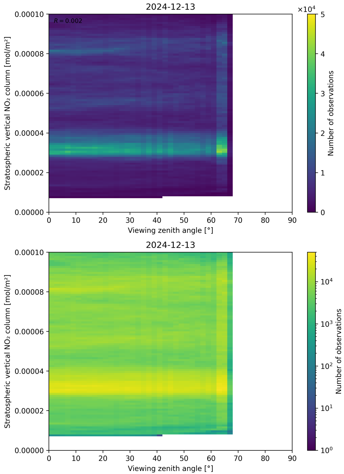
Figure 164: Scatter density plot of “Viewing zenith angle” against “Stratospheric vertical NO 2 column” for 2024-12-12 to 2024-12-14.
