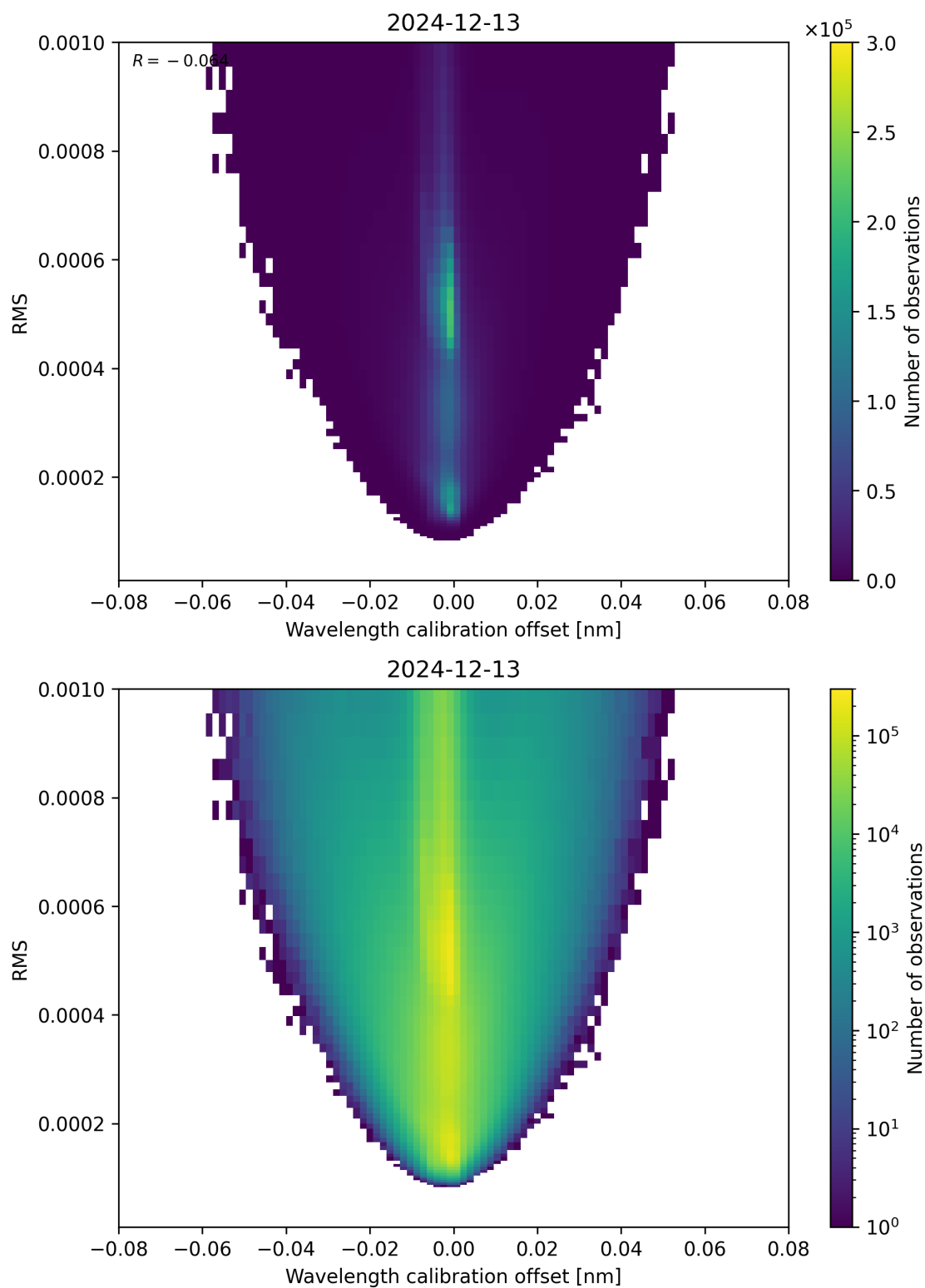
Figure 181: Scatter density plot of “Wavelength calibration offset” against “RMS” for 2024-12-12 to 2024-12-14.
