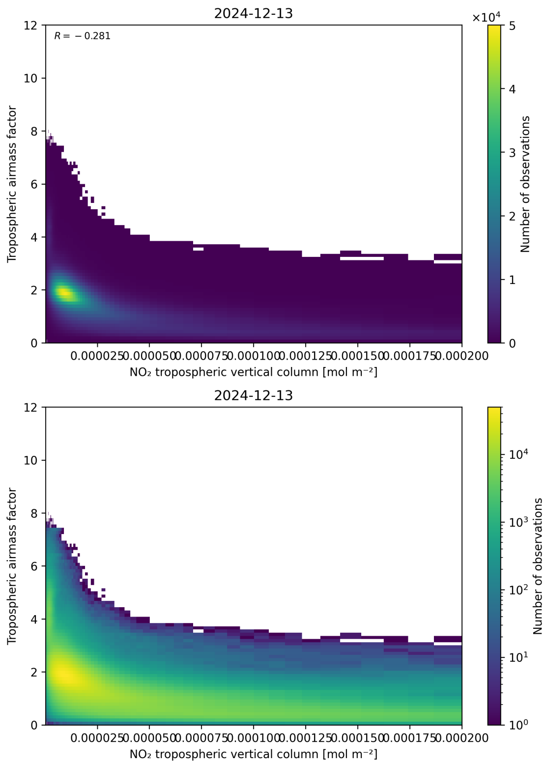
Figure 123: Scatter density plot of “NO 2 tropospheric vertical column” against “Tropospheric air mass factor” for 2024-12-12 to 2024-12-14.
