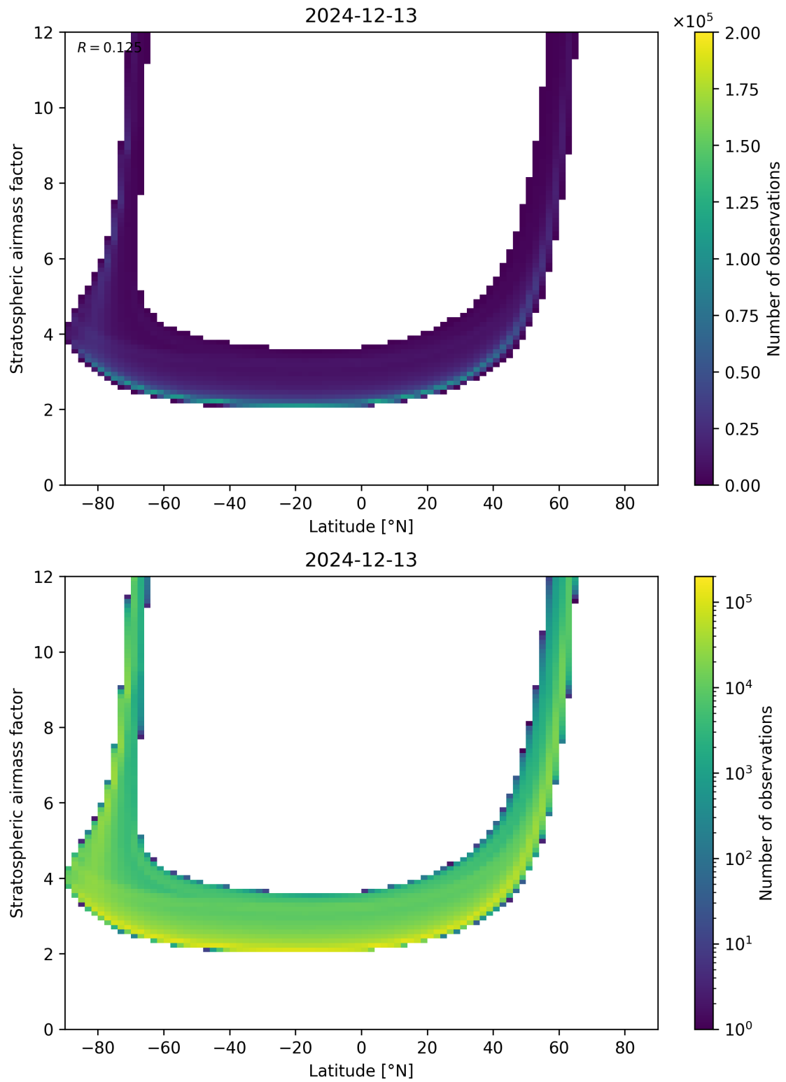
Figure 83: Scatter density plot of “Latitude” against “Stratospheric air mass factor” for 2024-12-12 to 2024-12-14.
