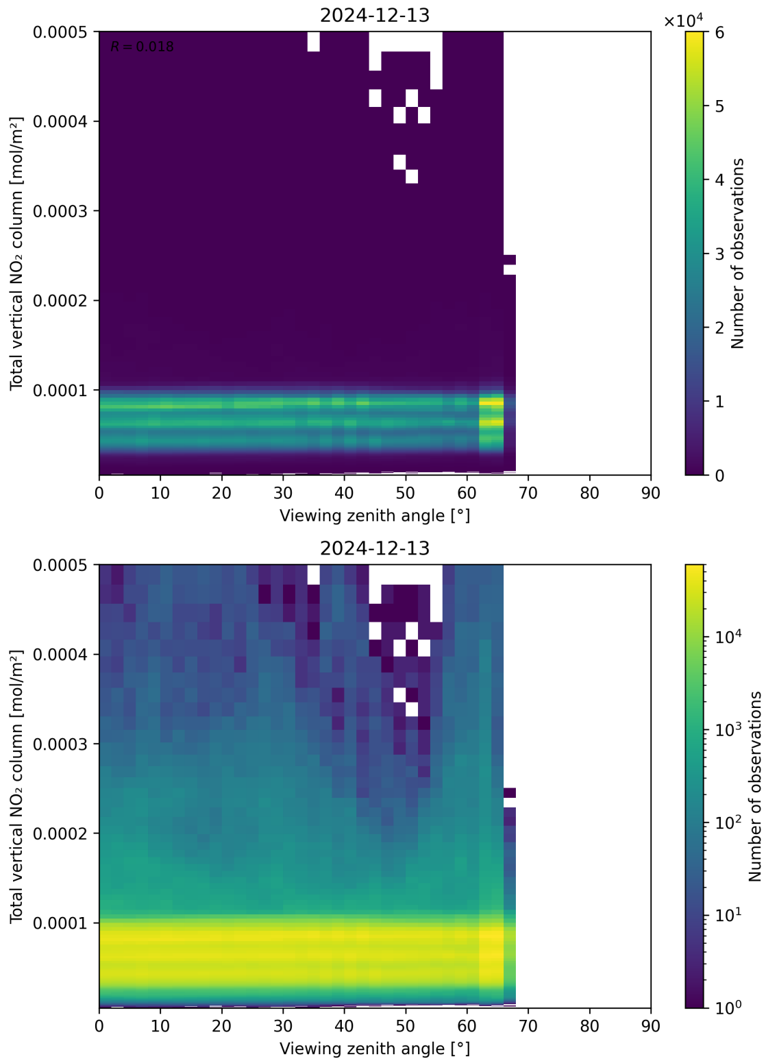
Figure 167: Scatter density plot of “Viewing zenith angle” against “Total vertical NO 2 column” for 2024-12-12 to 2024-12-14.
