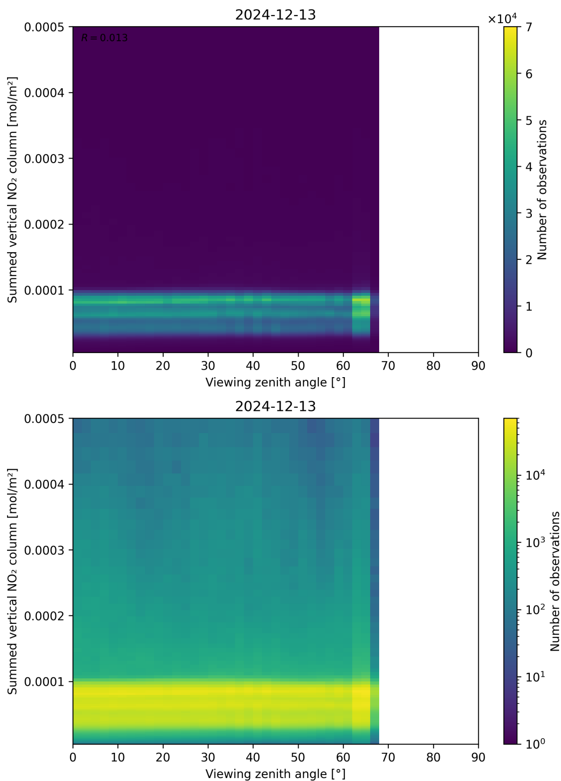
Figure 165: Scatter density plot of “Viewing zenith angle” against “Summed vertical NO 2 column” for 2024-12-12 to 2024-12-14.
