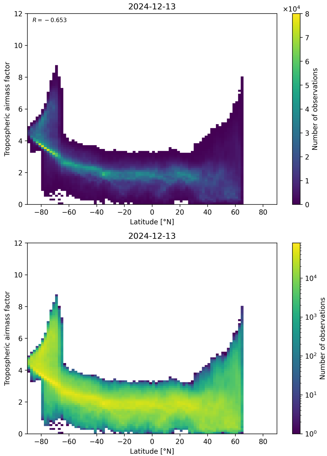
Figure 85: Scatter density plot of “Latitude” against “Tropospheric airmass factor” for 2024-12-12 to 2024-12-14.
