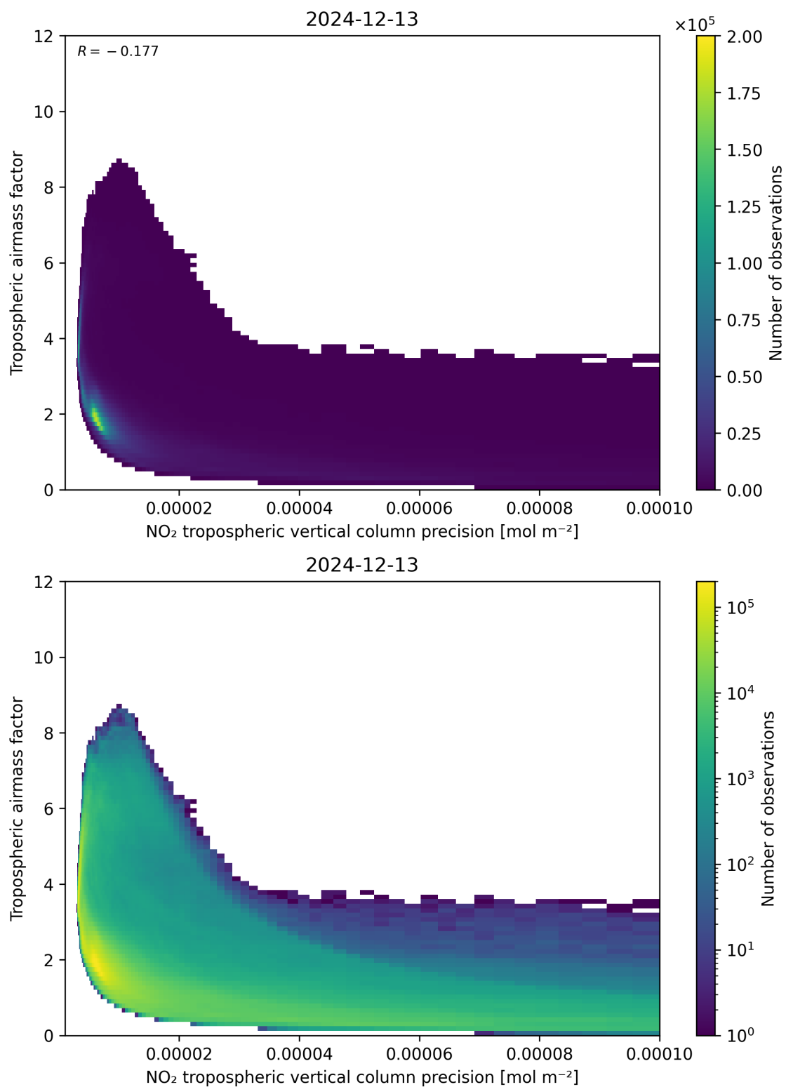
Figure 133: Scatter density plot of “NO 2 tropospheric vertical column precision” against “Tropospheric air mass factor” for 2024-12-12 to 2024-12-14.
