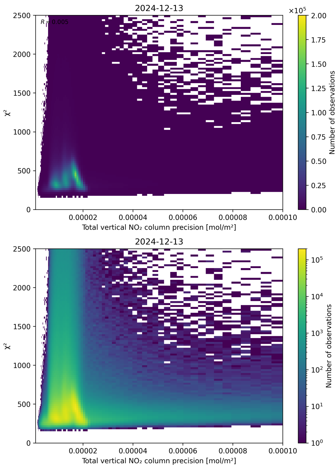
Figure 116: Scatter density plot of “Total vertical NO 2 column precision” against “ \chi^2 ” for 2024-12-12 to 2024-12-14.
