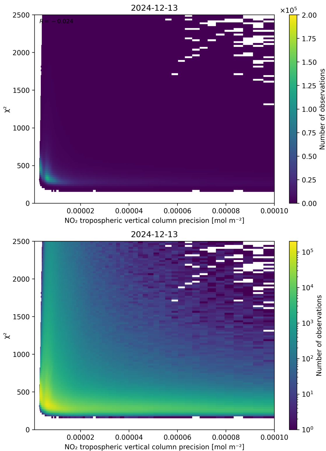
Figure 134: Scatter density plot of “NO 2 tropospheric vertical column precision” against “ \chi^2 ” for 2024-12-12 to 2024-12-14.
