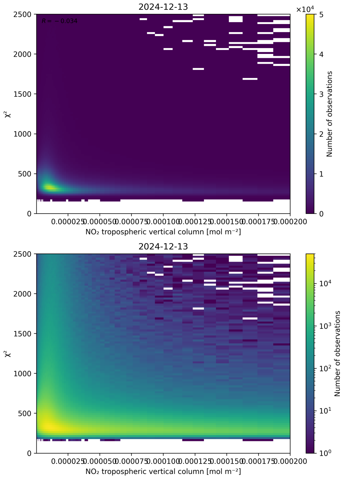
Figure 124: Scatter density plot of “NO 2 tropospheric vertical column” against “ \chi^2 ” for 2024-12-12 to 2024-12-14.
