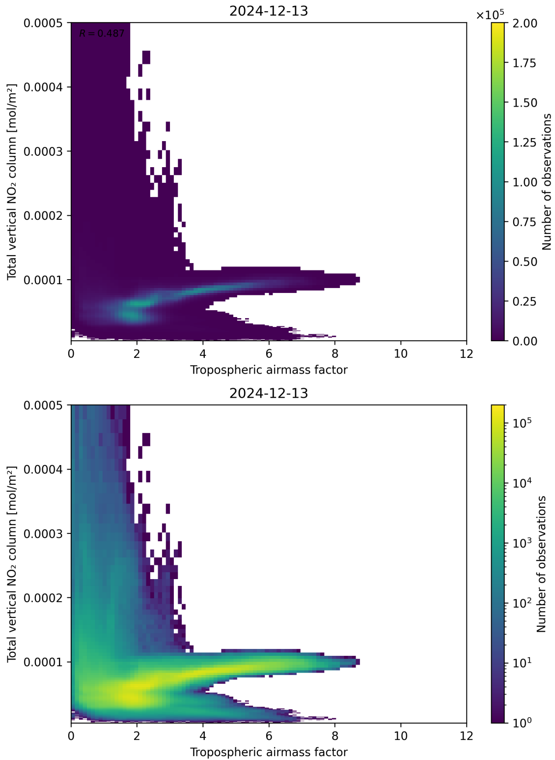
Figure 77: Scatter density plot of “Tropospheric airmass factor” against “Total vertical NO 2 column” for 2024-12-12 to 2024-12-14.
