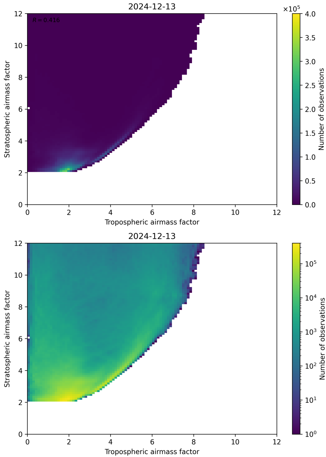
Figure 71: Scatter density plot of “Tropospheric airmass factor” against “Stratospheric airmass factor” for 2024-12-12 to 2024-12-14.
