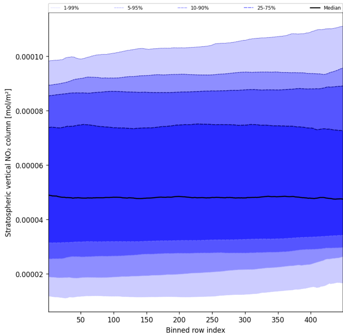
Figure 53: Along track statistics of “Stratospheric vertical NO 2 column” for 2024-12-12 to 2024-12-14
