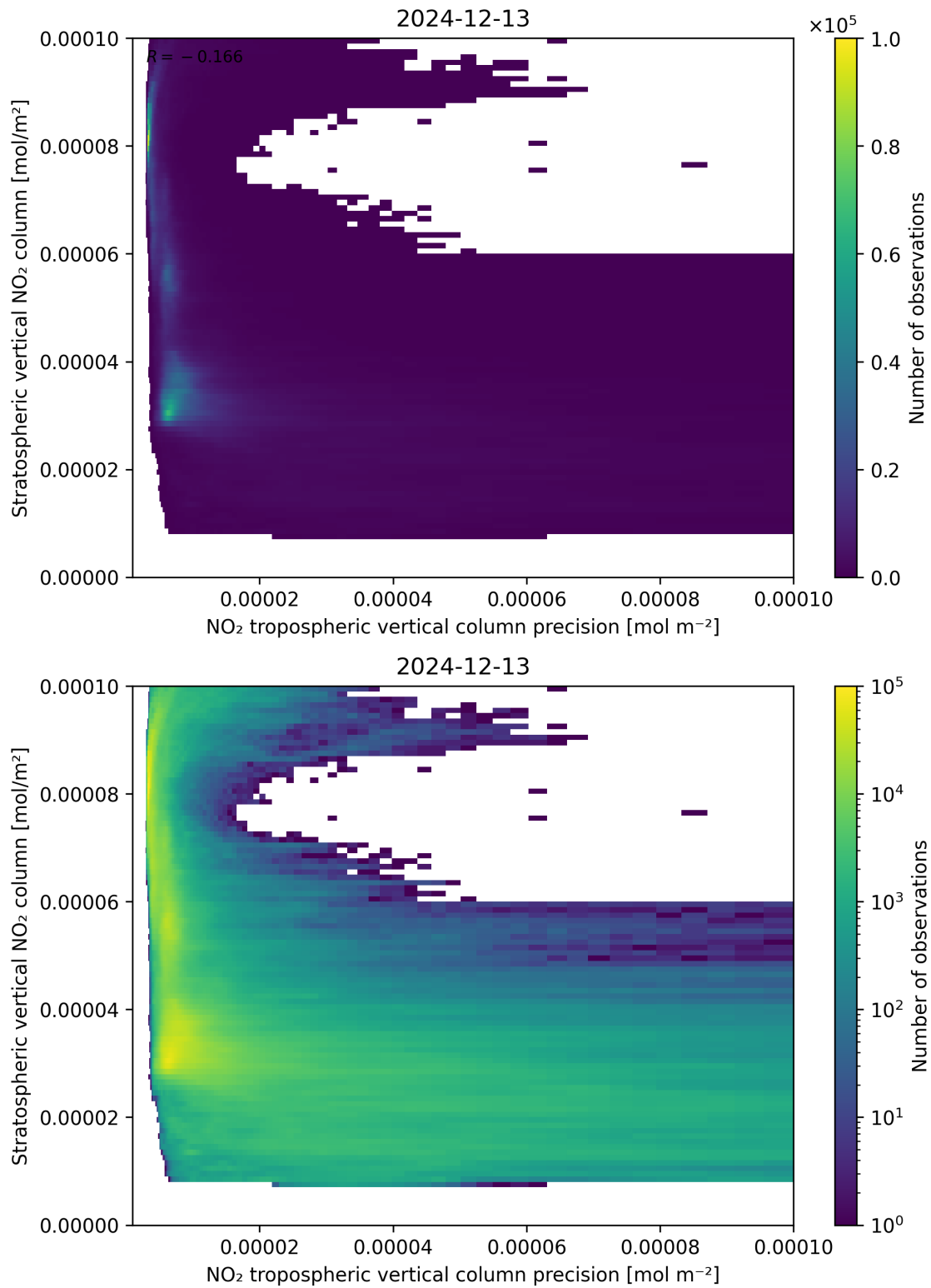
Figure 135: Scatter density plot of “NO 2 tropospheric vertical column precision” against “Stratospheric vertical NO 2 column” for 2024-12-12 to 2024-12-14.
