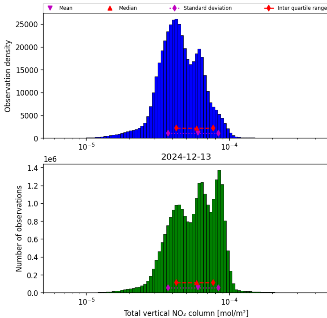
Figure 38: Histogram of “Total vertical NO 2 column” for 2024-12-12 to 2024-12-14
