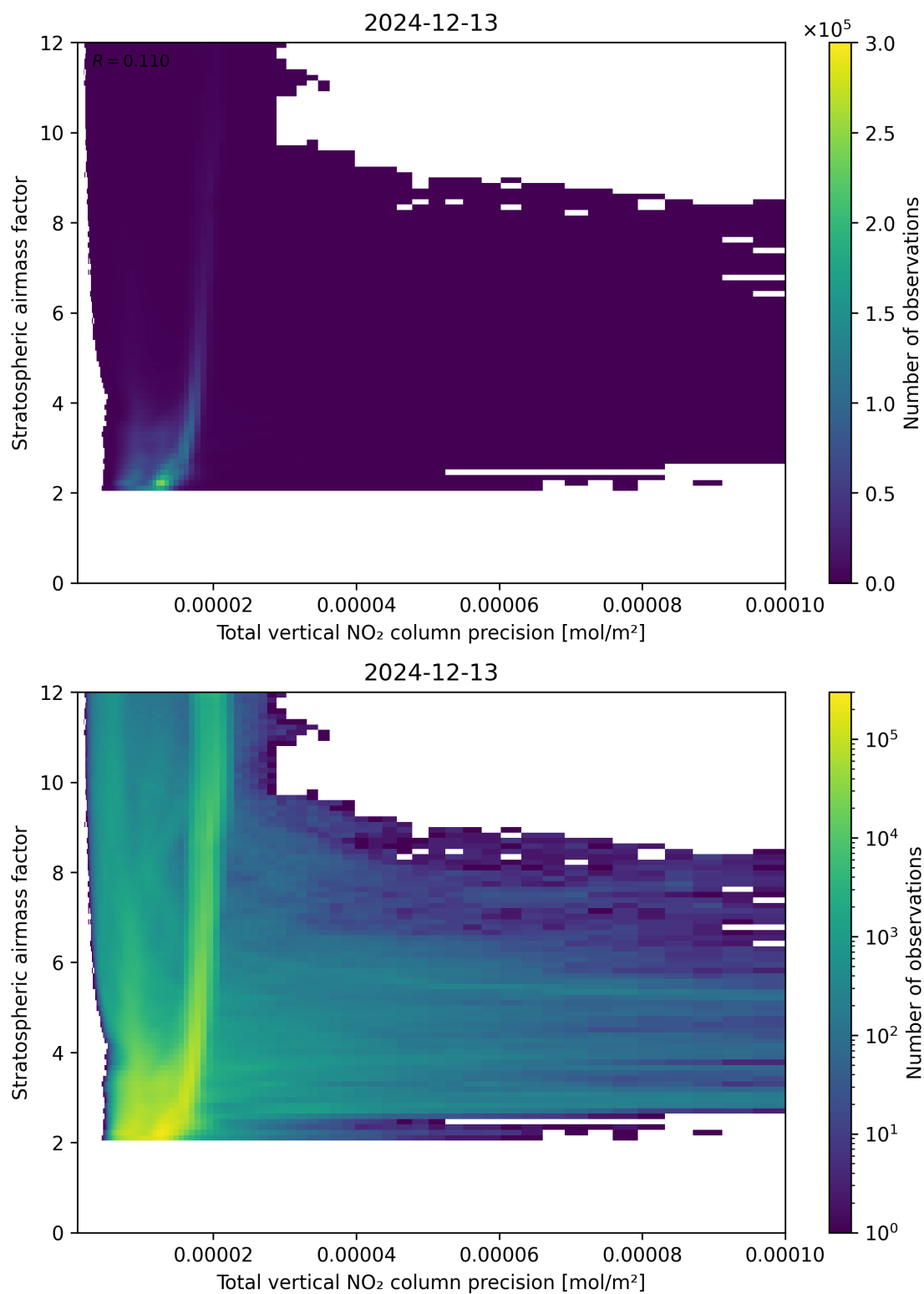
Figure 115: Scatter density plot of “Total vertical NO 2 column precision” against “Stratospheric airmass factor” for 2024-12-12 to 2024-12-14.
