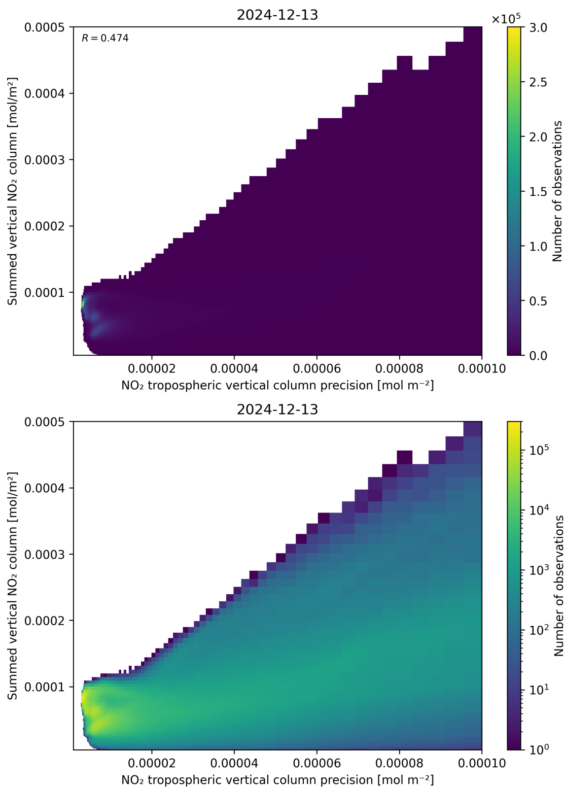
Figure 136: Scatter density plot of “NO 2 tropospheric vertical column precision” against “Summed vertical NO 2 column” for 2024-12-12 to 2024-12-14.
