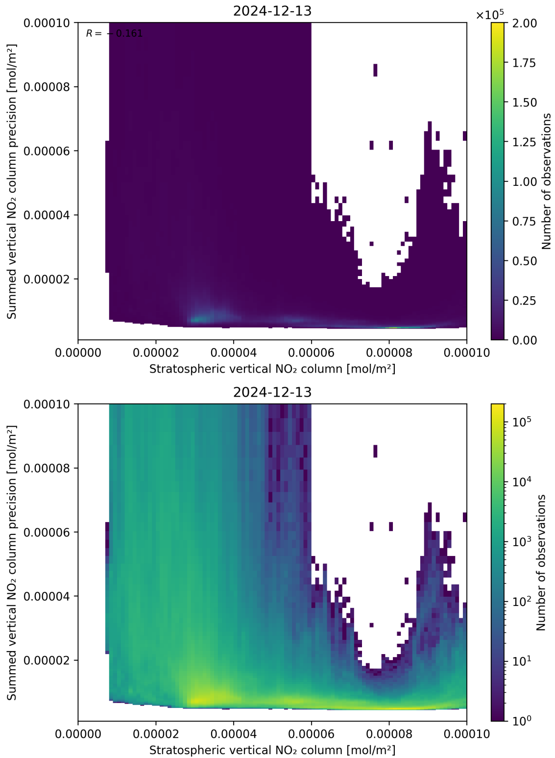
Figure 99: Scatter density plot of “Stratospheric vertical NO 2 column” against “Summed vertical NO 2 column precision” for 2024-12-12 to 2024-12-14.
