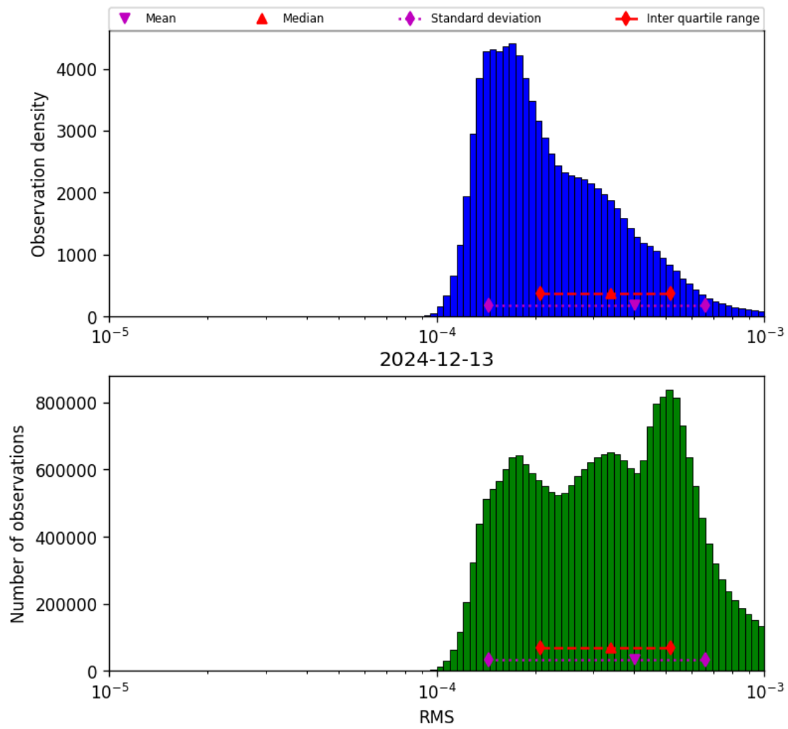
Figure 43: Histogram of “RMS” for 2024-12-12 to 2024-12-14
