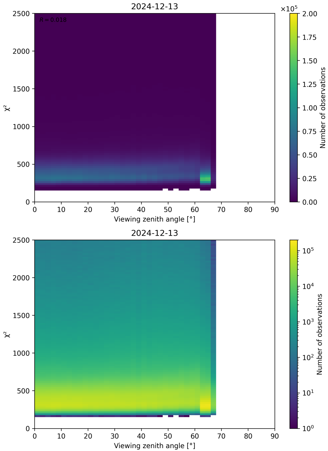
Figure 162: Scatter density plot of “Viewing zenith angle” against “ \chi^2 ” for 2024-12-12 to 2024-12-14.
