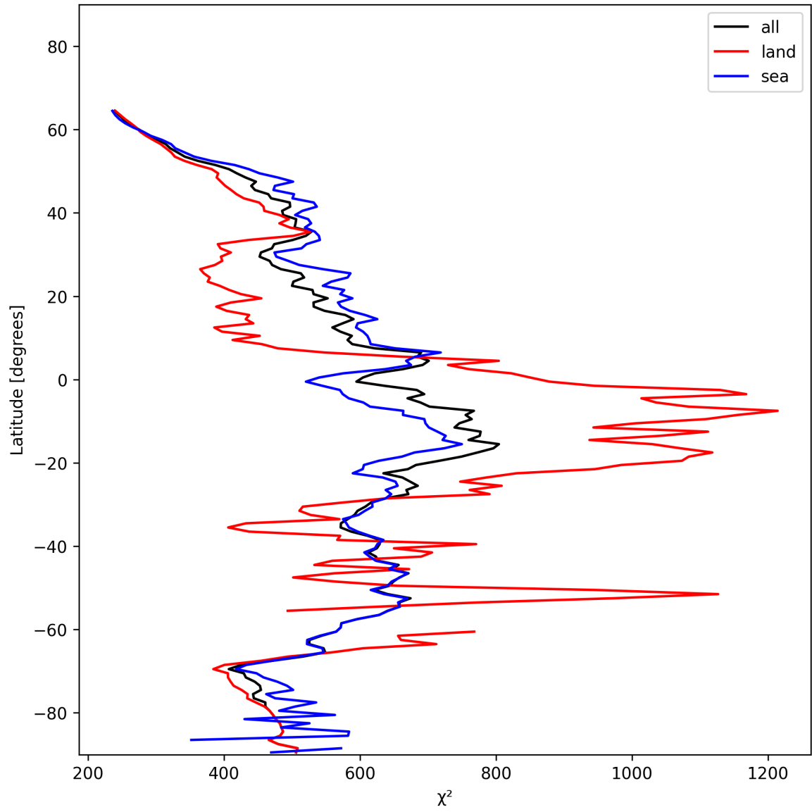
Figure 25: Zonal average of “ \chi^2 ” for 2024-12-12 to 2024-12-14.
