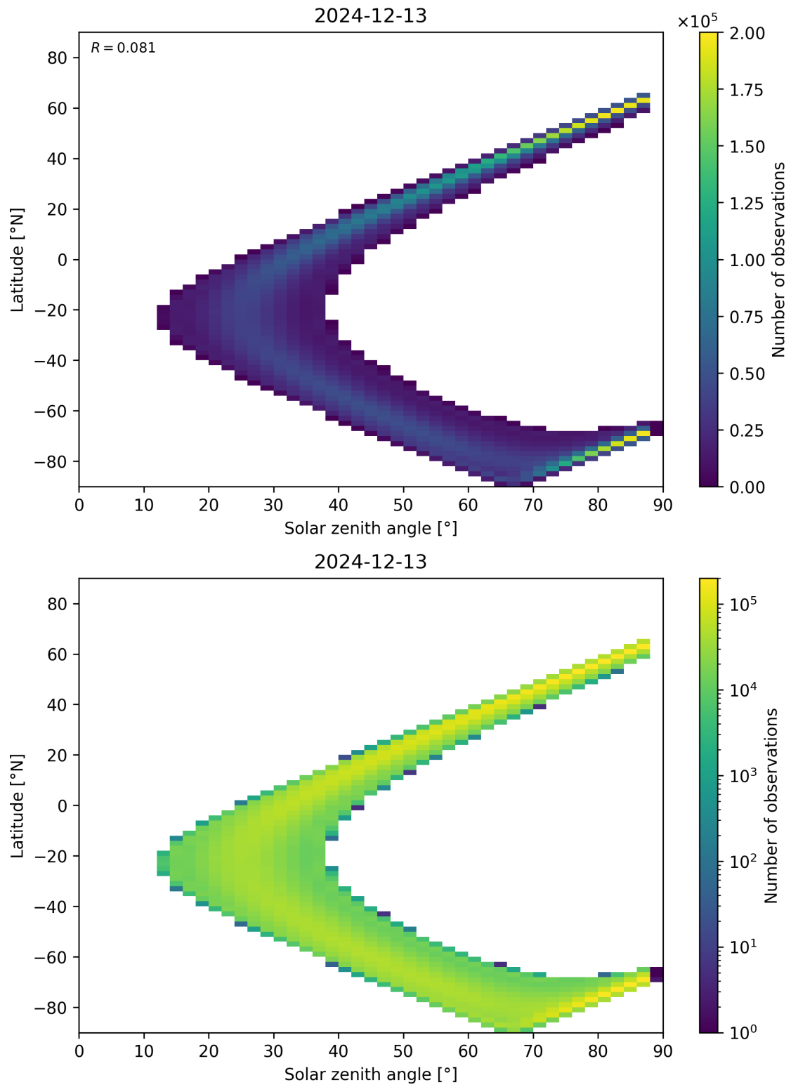
Figure 149: Scatter density plot of “Solar zenith angle” against “Latitude” for 2024-12-12 to 2024-12-14.
