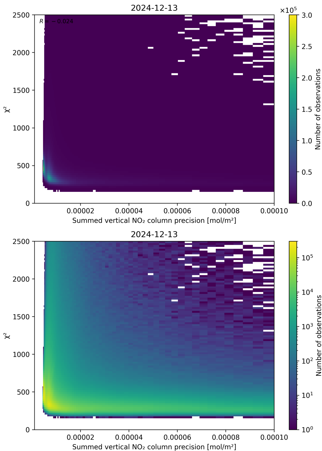
Figure 107: Scatter density plot of “Summed vertical NO 2 column precision” against “ \chi^2 ” for 2024-12-12 to 2024-12-14.
