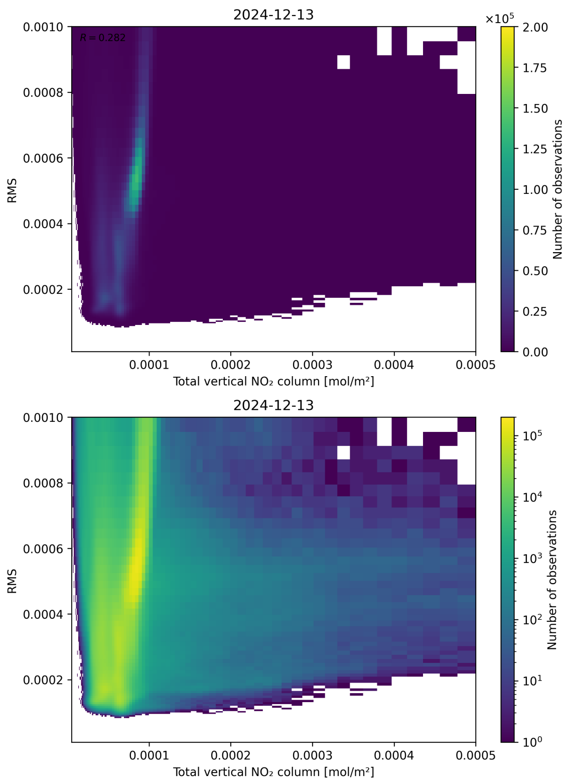
Figure 120: Scatter density plot of “Total vertical NO 2 column” against “RMS” for 2024-12-12 to 2024-12-14.
