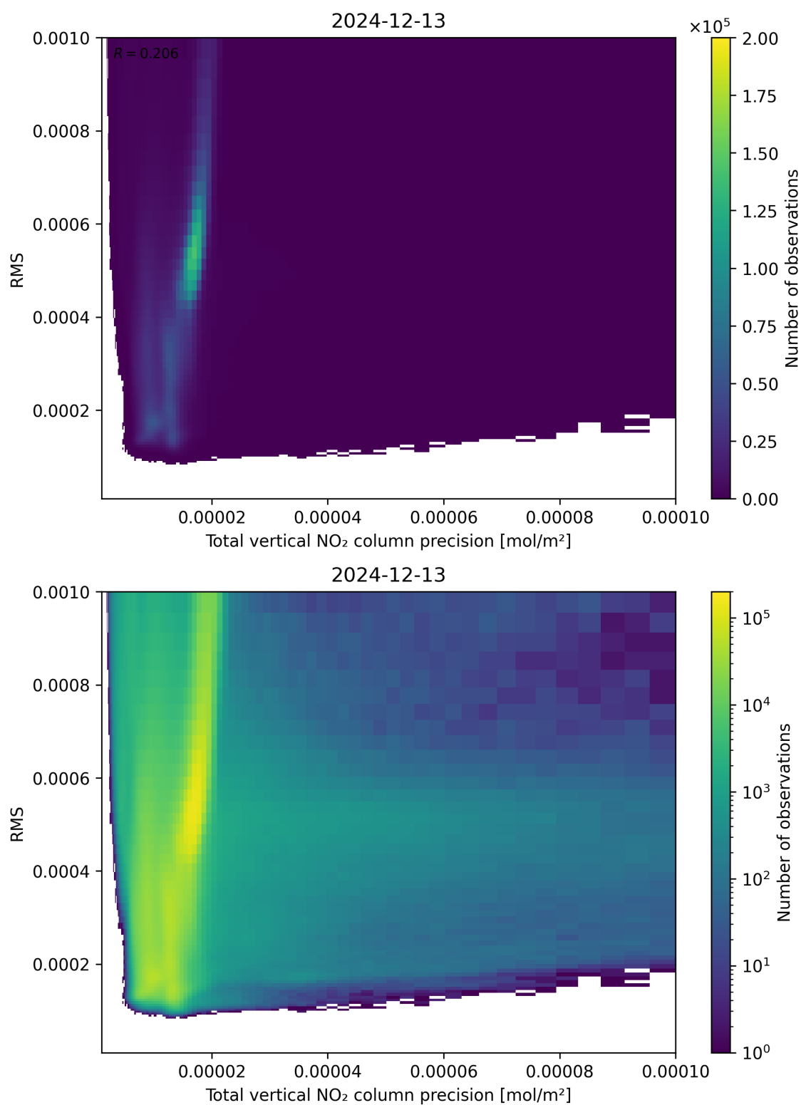
Figure 119: Scatter density plot of “Total vertical NO 2 column precision” against “RMS” for 2024-12-12 to 2024-12-14.
