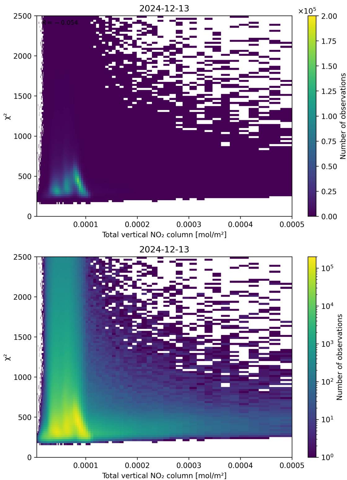
Figure 111: Scatter density plot of “Total vertical NO 2 column” against “ \chi^2 ” for 2024-12-12 to 2024-12-14.
