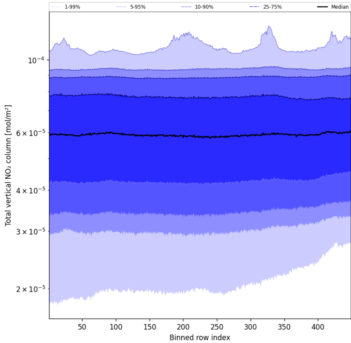
Figure 55: Along track statistics of “Total vertical NO 2 column” for 2024-12-12 to 2024-12-14
