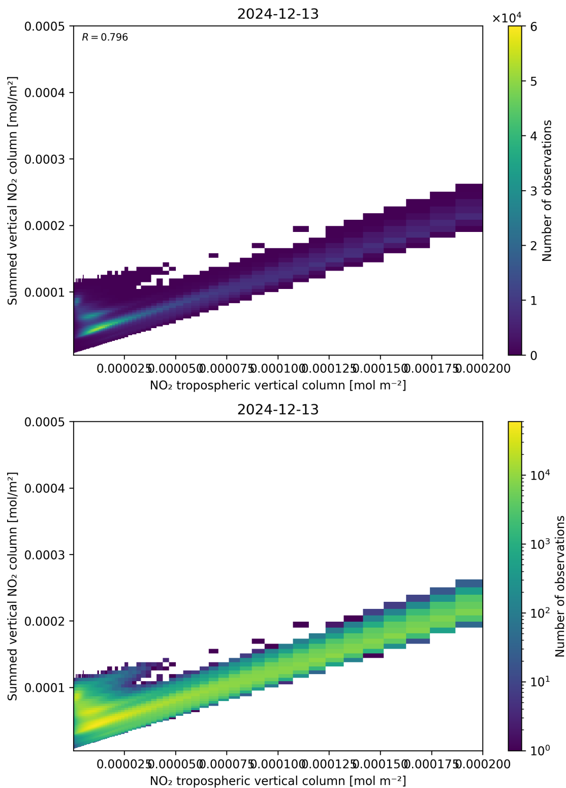
Figure 126: Scatter density plot of “NO 2 tropospheric vertical column” against “Summed vertical NO 2 column” for 2024-12-12 to 2024-12-14.
