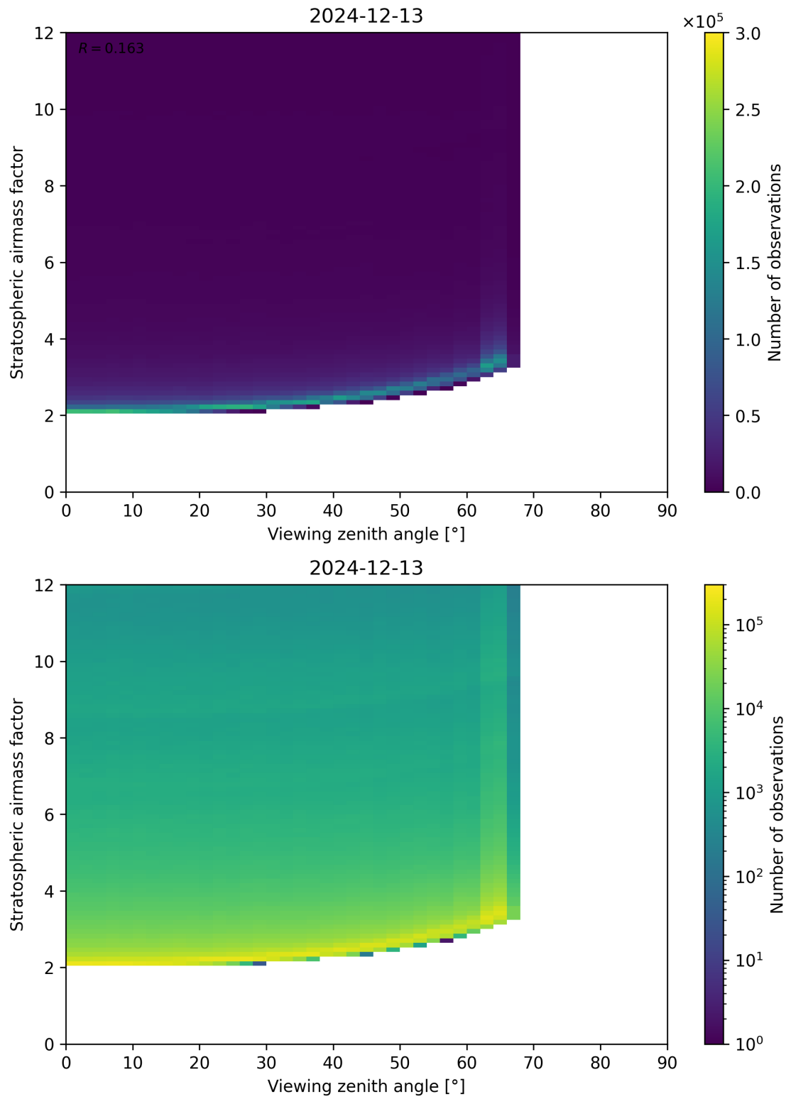
Figure 159: Scatter density plot of “Viewing zenith angle” against “Stratospheric airmass factor” for 2024-12-12 to 2024-12-14.
