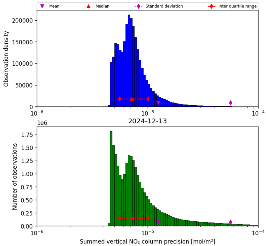
Figure 41: Histogram of "Summed vertical NO 2 column precision" for 2024-12-12 to 2024-12-14
