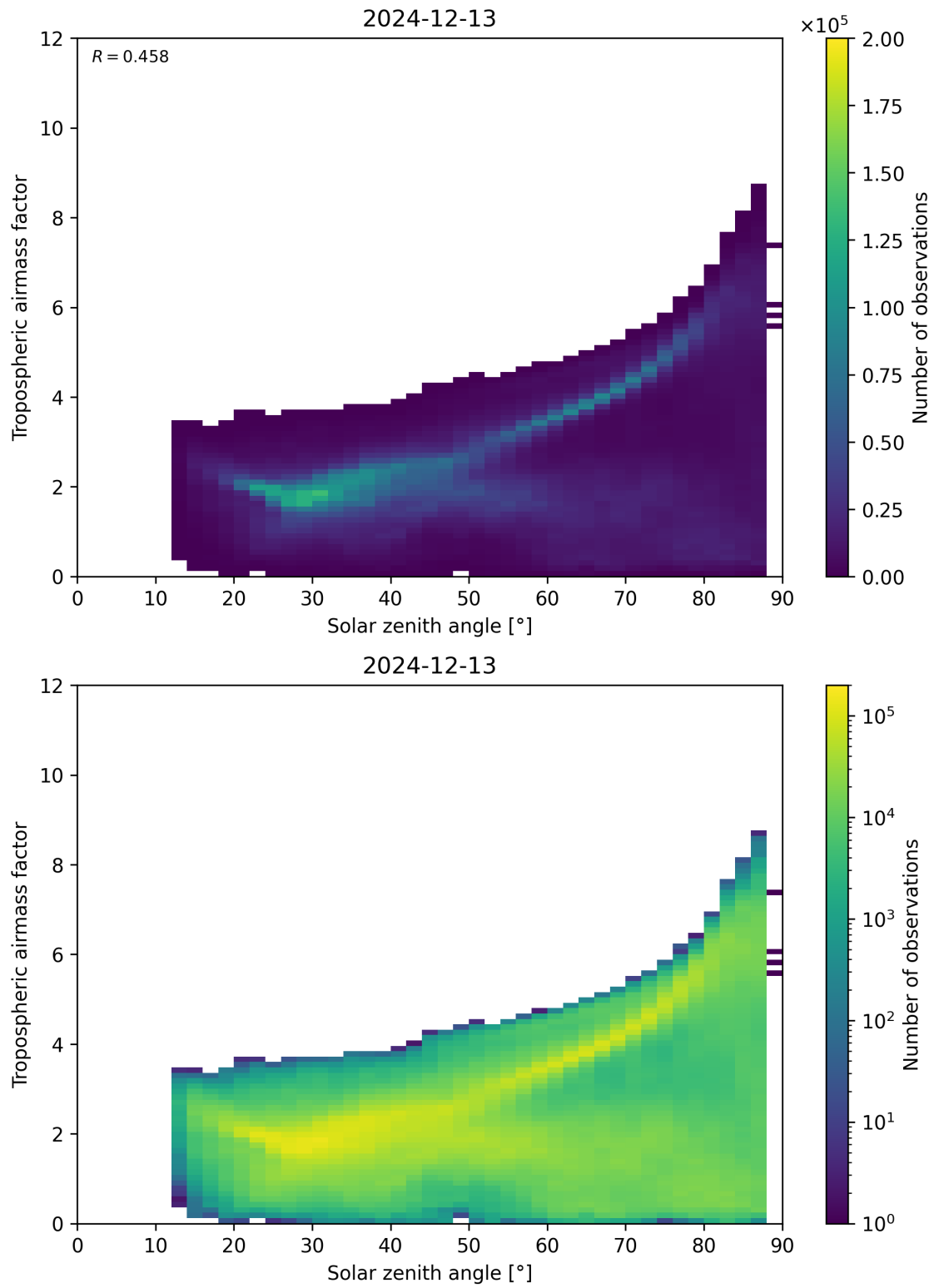
Figure 147: Scatter density plot of “Solar zenith angle” against “Tropospheric airmass factor” for 2024-12-12 to 2024-12-14.
