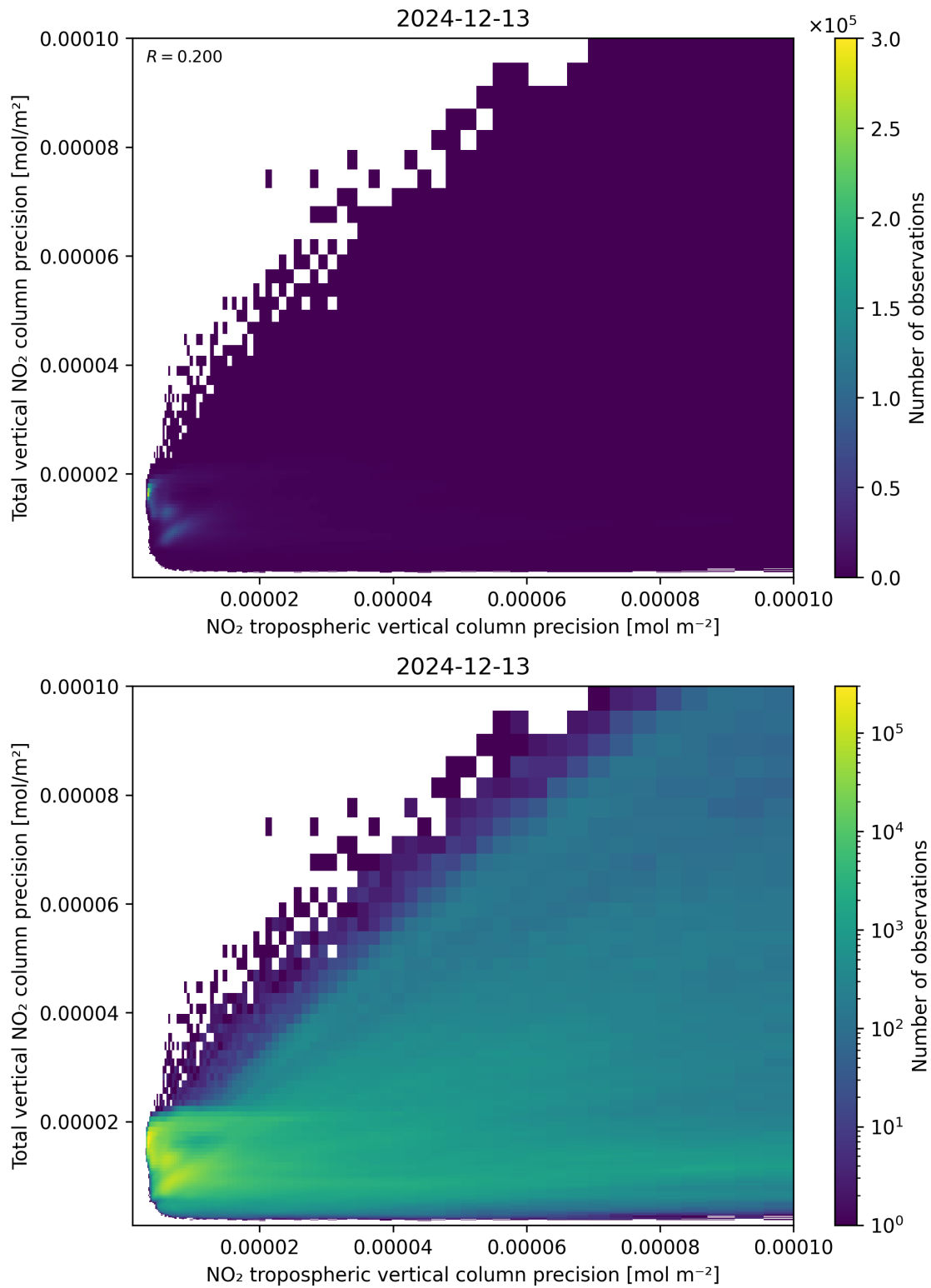
Figure 139: Scatter density plot of “NO 2 tropospheric vertical column precision” against “Total vertical NO 2 column precision” for 2024-12-12 to 2024-12-14.
