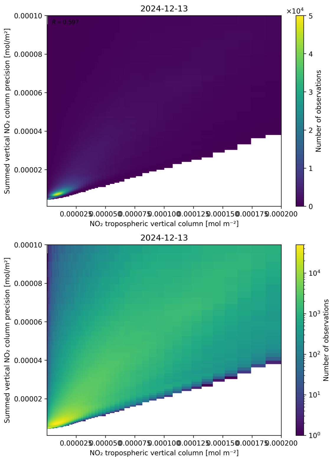
Figure 127: Scatter density plot of “NO 2 tropospheric vertical column” against “Summed vertical NO 2 column precision” for 2024-12-12 to 2024-12-14.
