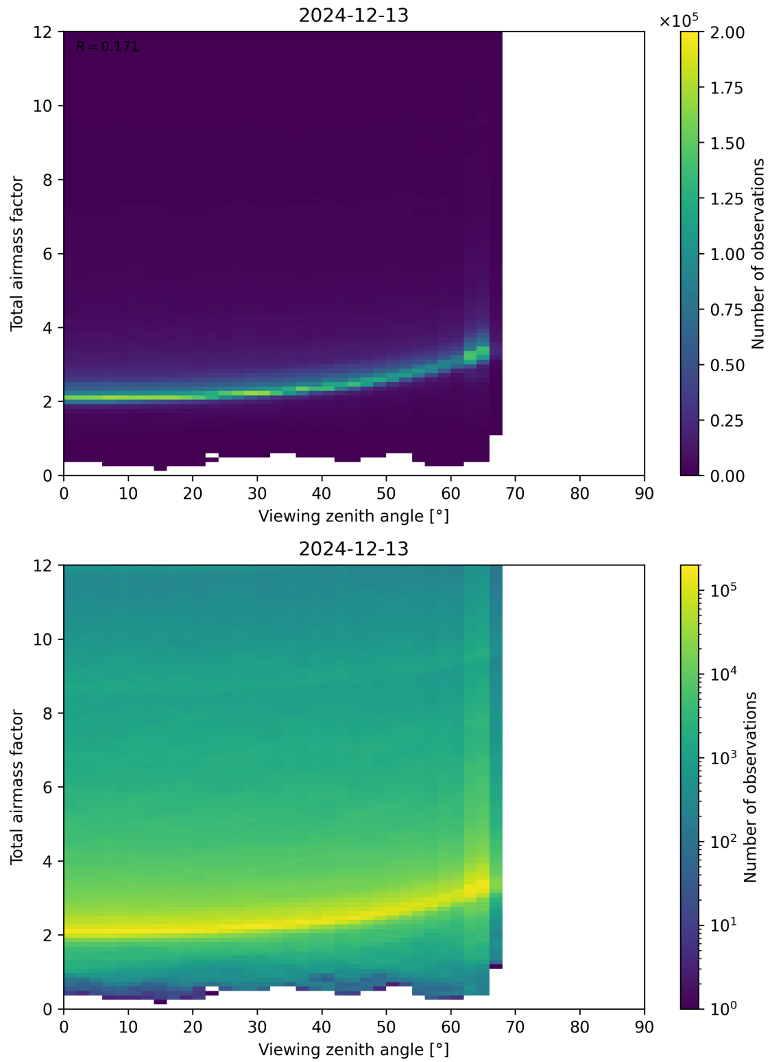
Figure 160: Scatter density plot of “Viewing zenith angle” against “Total airmass factor” for 2024-12-12 to 2024-12-14.
