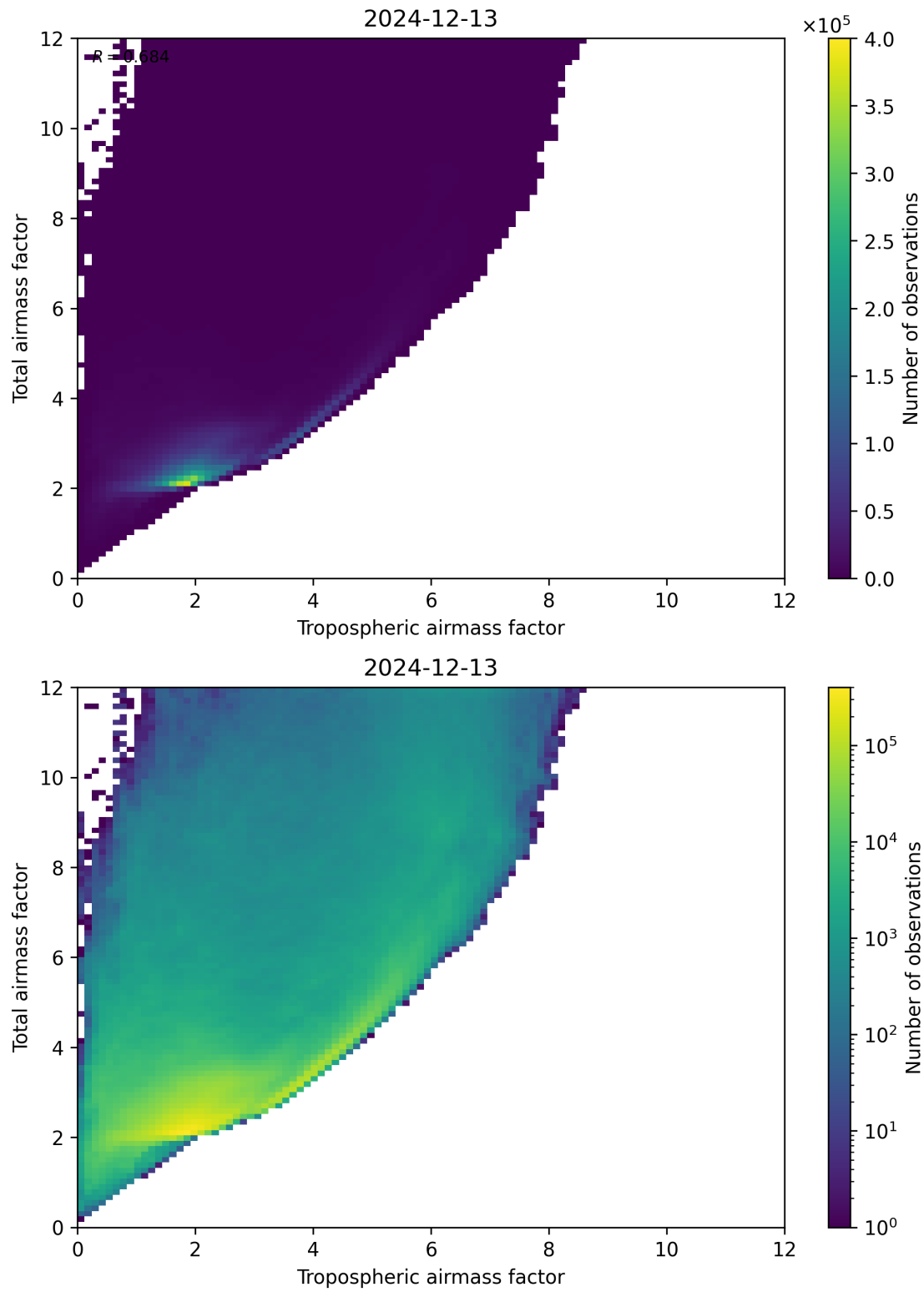
Figure 72: Scatter density plot of “Tropospheric airmass factor” against “Total airmass factor” for 2024-12-12 to 2024-12-14.
