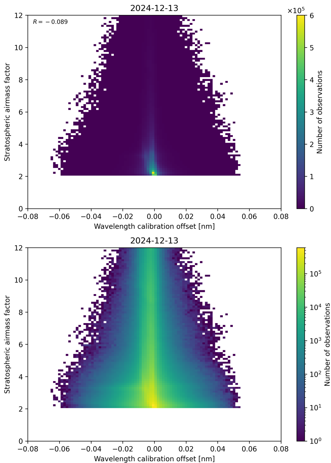
Figure 174: Scatter density plot of “Wavelength calibration offset” against “Stratospheric airmass factor” for 2024-12-12 to 2024-12-14.
