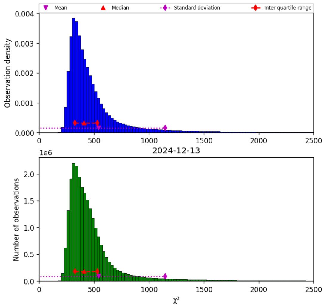
Figure 42: Histogram of " \chi^2 " for 2024-12-12 to 2024-12-14
