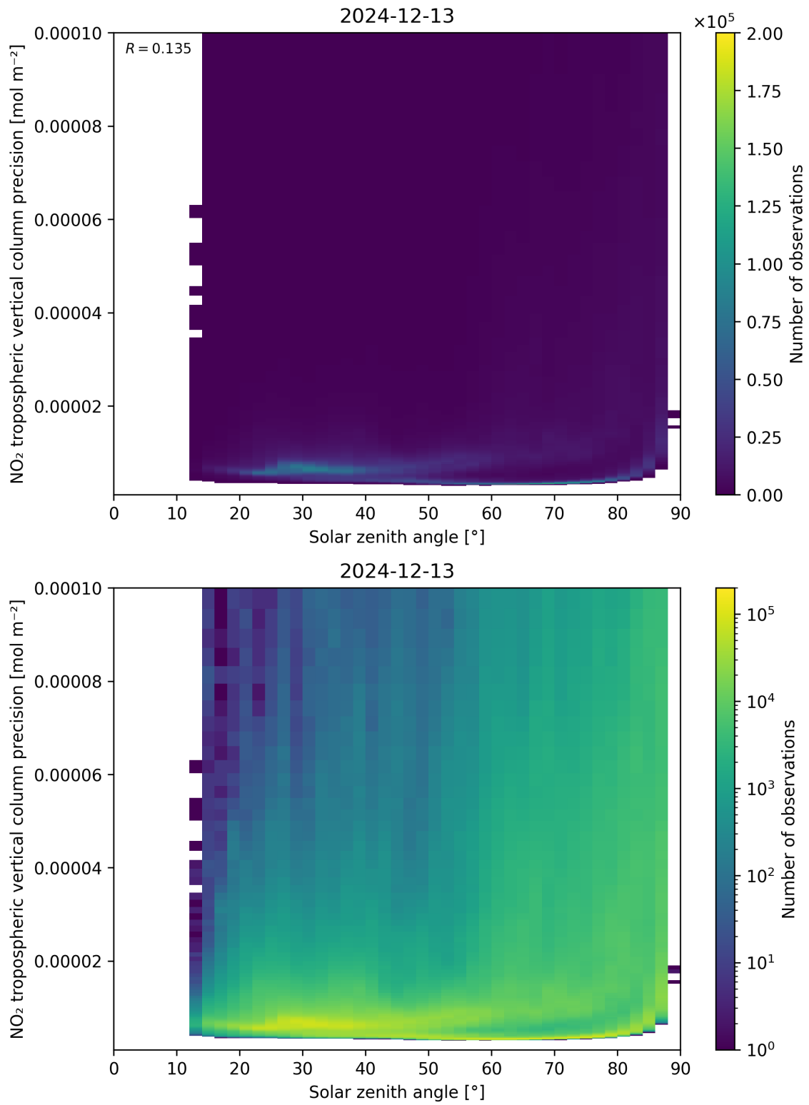
Figure 156: Scatter density plot of “Solar zenith angle” against “NO 2 tropospheric vertical column precision” for 2024-12-12 to 2024-12-14.
