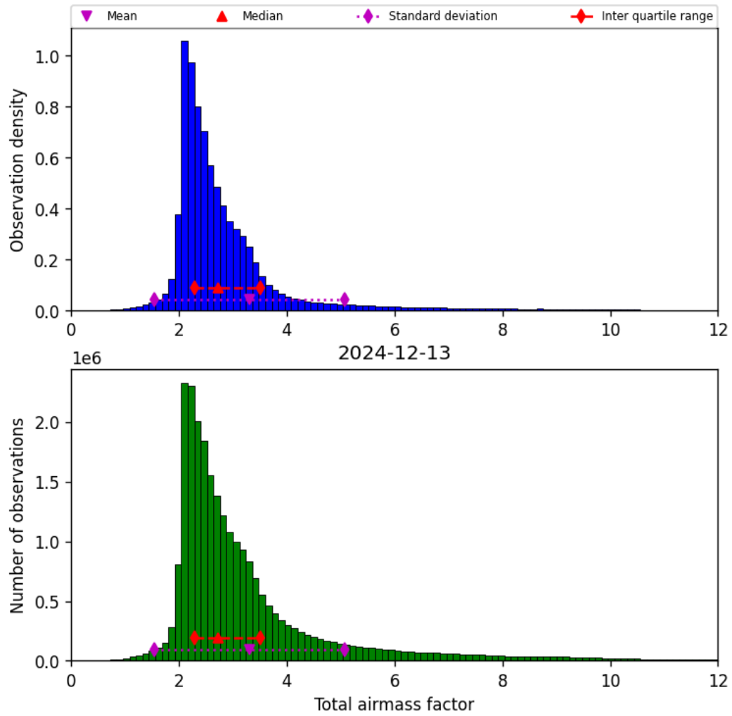
Figure 32: Histogram of “Total airmass factor” for 2024-12-12 to 2024-12-14
