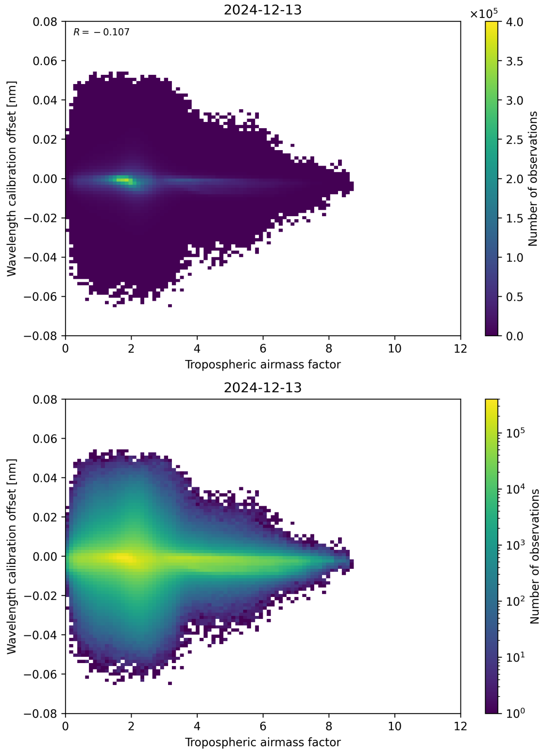
Figure 80: Scatter density plot of “Tropospheric airmass factor” against “Wavelength calibration offset” for 2024-12-12 to 2024-12-14.
