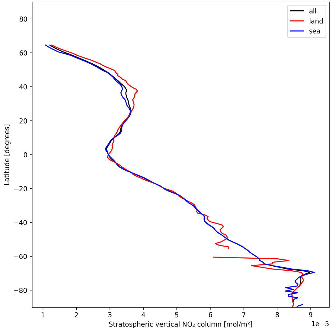
Figure 19: Zonal average of “Stratospheric vertical NO 2 column” for 2024-12-12 to 2024-12-14.
