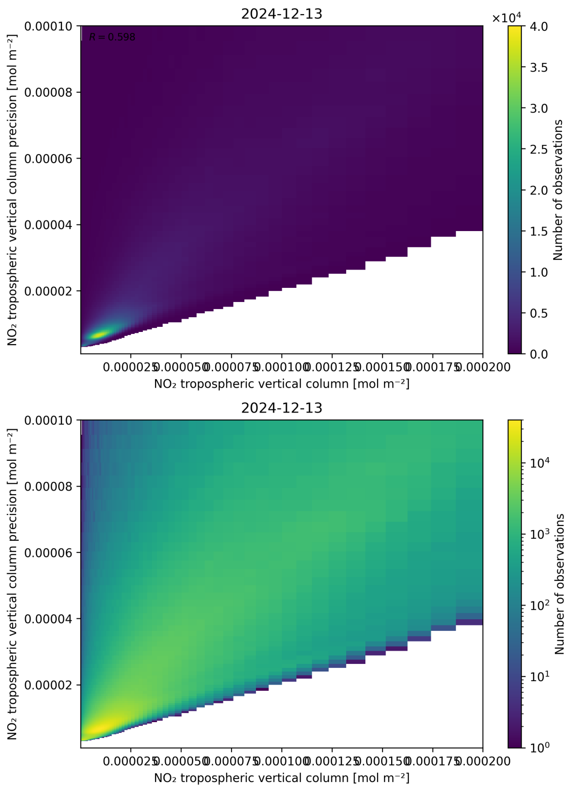
Figure 130: Scatter density plot of “NO 2 tropospheric vertical column” against “NO 2 tropospheric vertical column precision” for 2024-12-12 to 2024-12-14.
