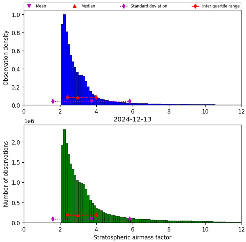
Figure 44: Histogram of “Stratospheric airmass factor” for 2024-12-12 to 2024-12-14
