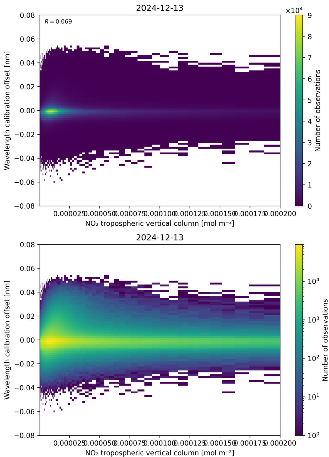
Figure 143: Scatter density plot of “NO 2 tropospheric vertical column” against “Wavelength calibration offset” for 2024-12-12 to 2024-12-14.
