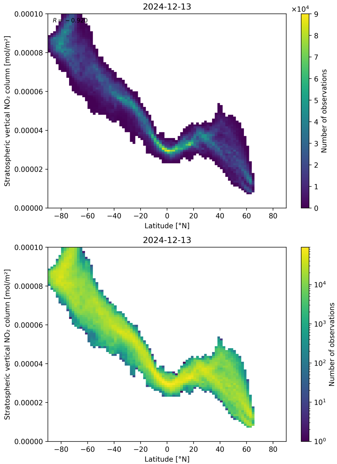
Figure 87: Scatter density plot of “Latitude” against “Stratospheric vertical NO 2 column” for 2024-12-12 to 2024-12-14.
