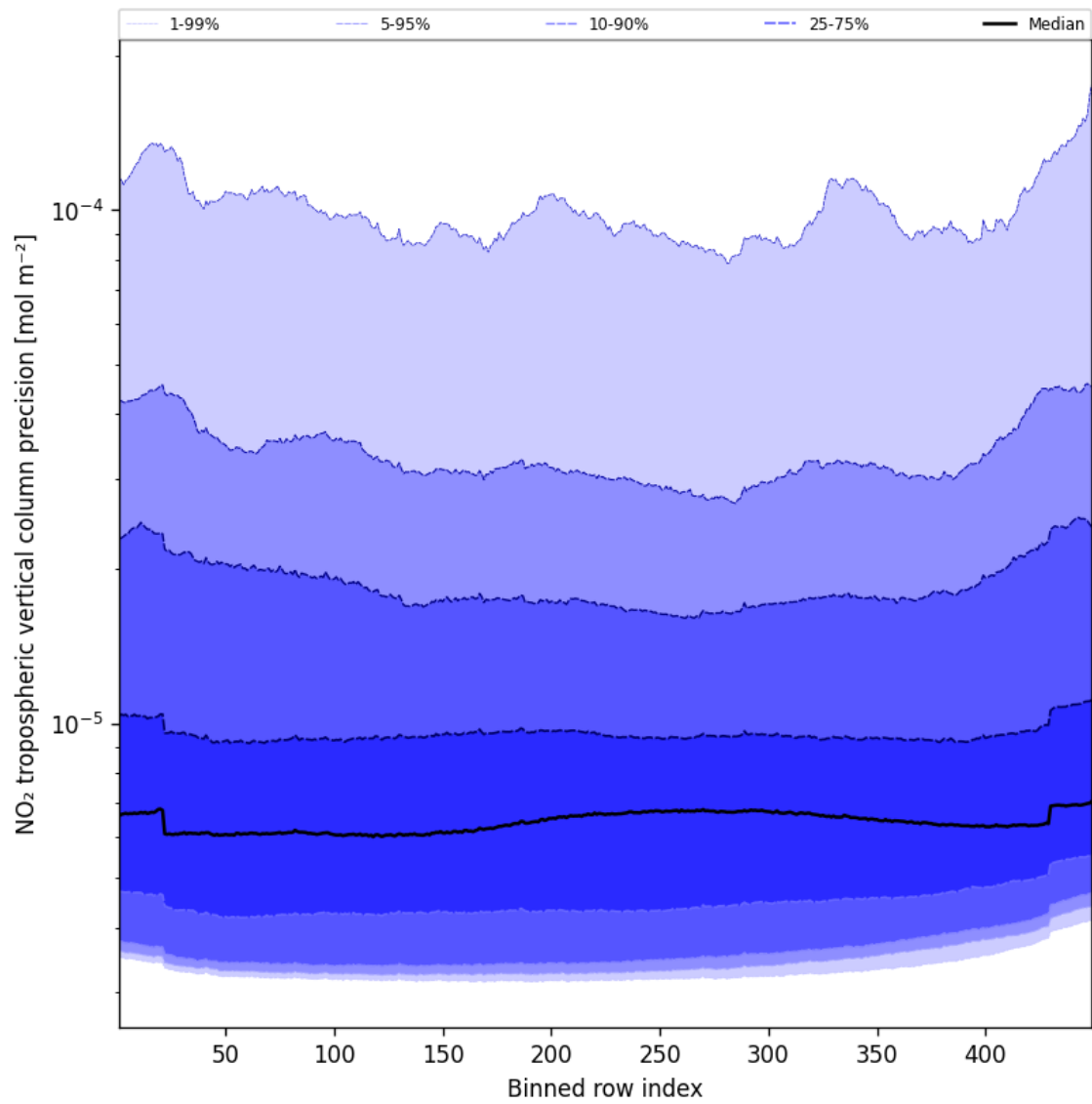
Figure 47: Along track statistics of “NO 2 tropospheric vertical column precision” for 2024-12-12 to 2024-12-14
