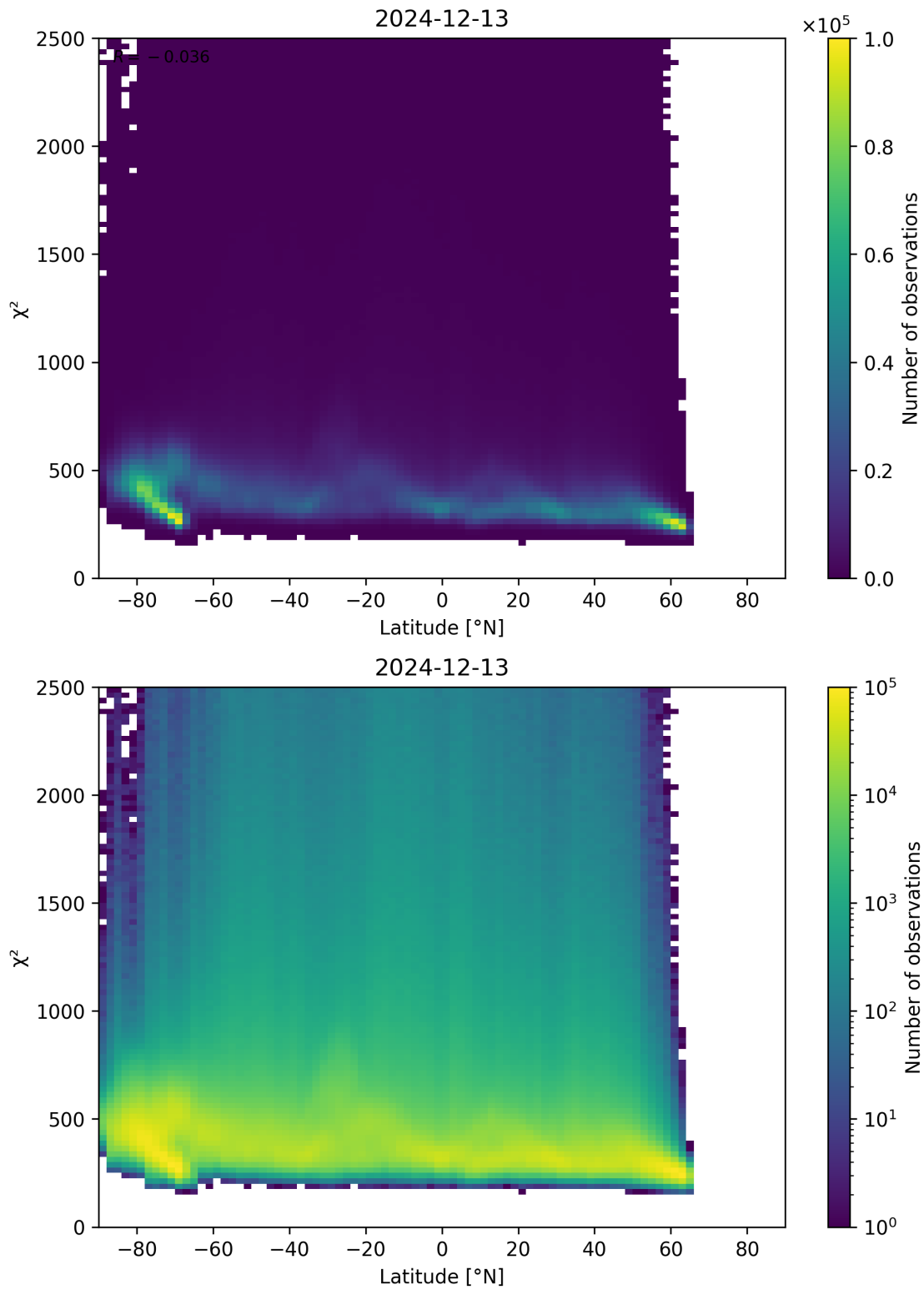
Figure 86: Scatter density plot of “Latitude” against “ \chi^2 ” for 2024-12-12 to 2024-12-14.
