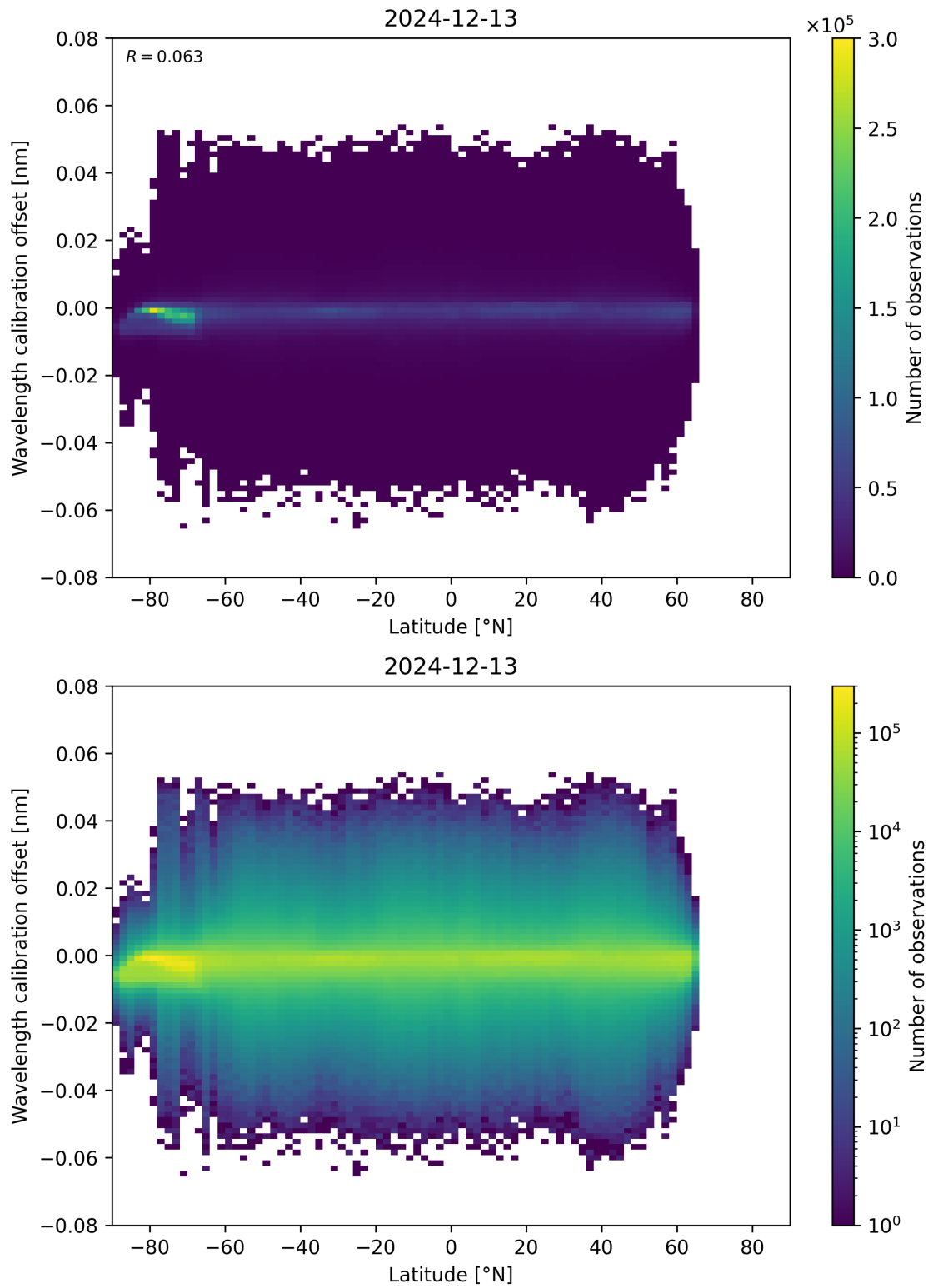
Figure 95: Scatter density plot of “Latitude” against “Wavelength calibration offset” for 2024-12-12 to 2024-12-14.
