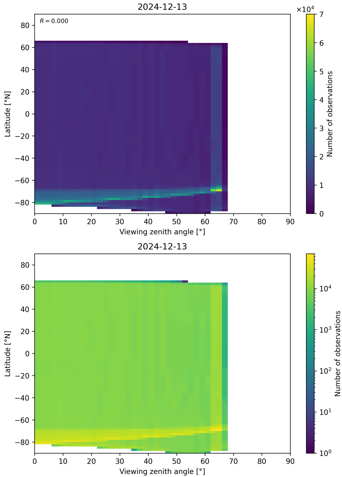
Figure 163: Scatter density plot of “Viewing zenith angle” against “Latitude” for 2024-12-12 to 2024-12-14.
