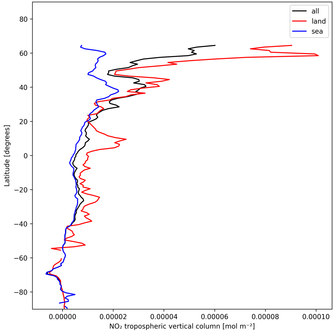
Figure 12: Zonal average of “NO 2 tropospheric vertical column” for 2024-12-12 to 2024-12-14.
