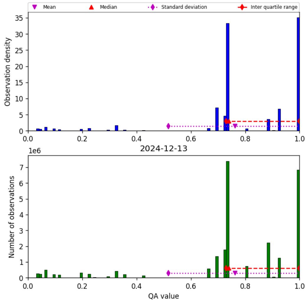
Figure 28: Histogram of “QA value” for 2024-12-12 to 2024-12-14
