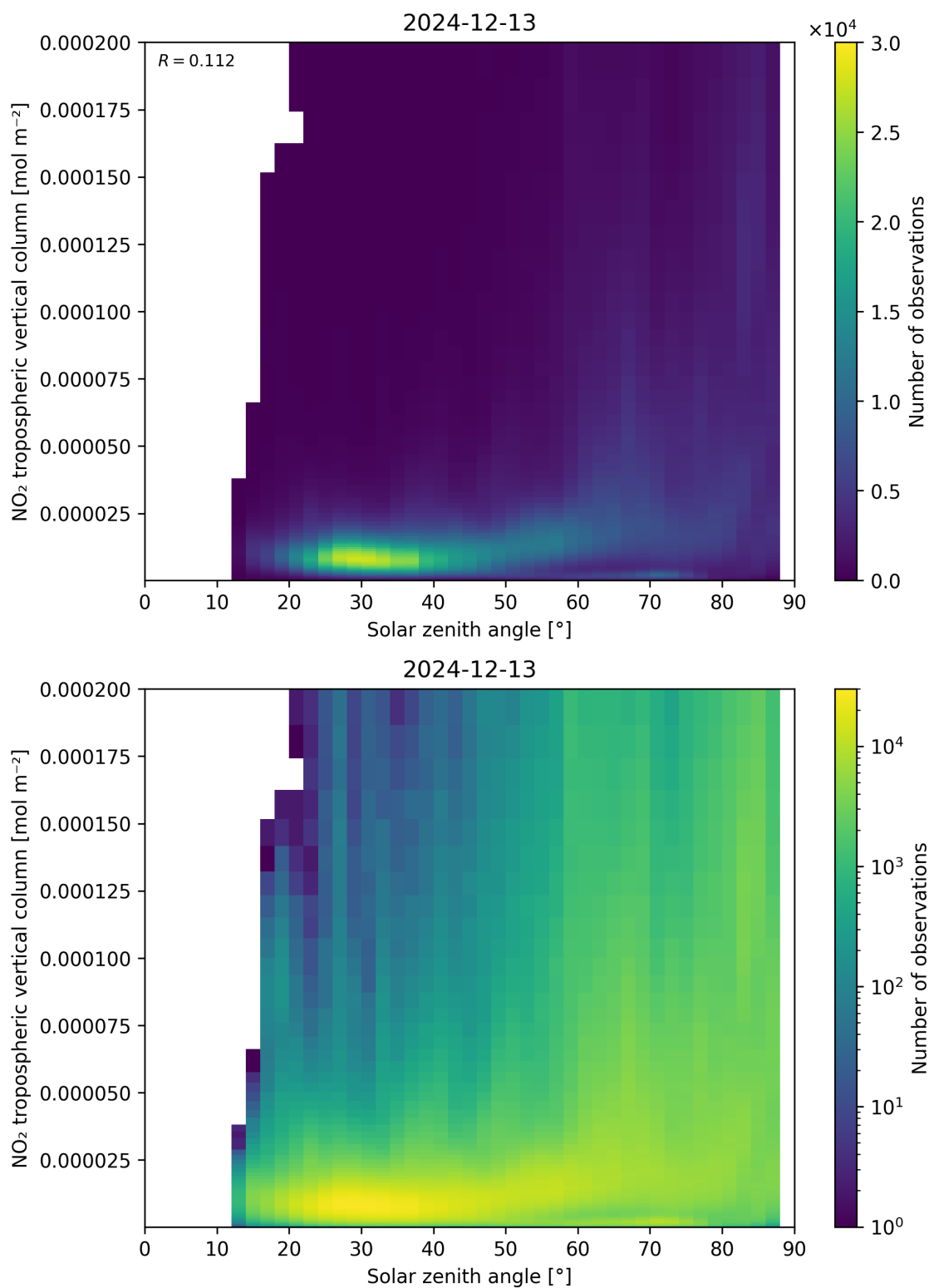
Figure 155: Scatter density plot of “Solar zenith angle” against “NO 2 tropospheric vertical column” for 2024-12-12 to 2024-12-14.
