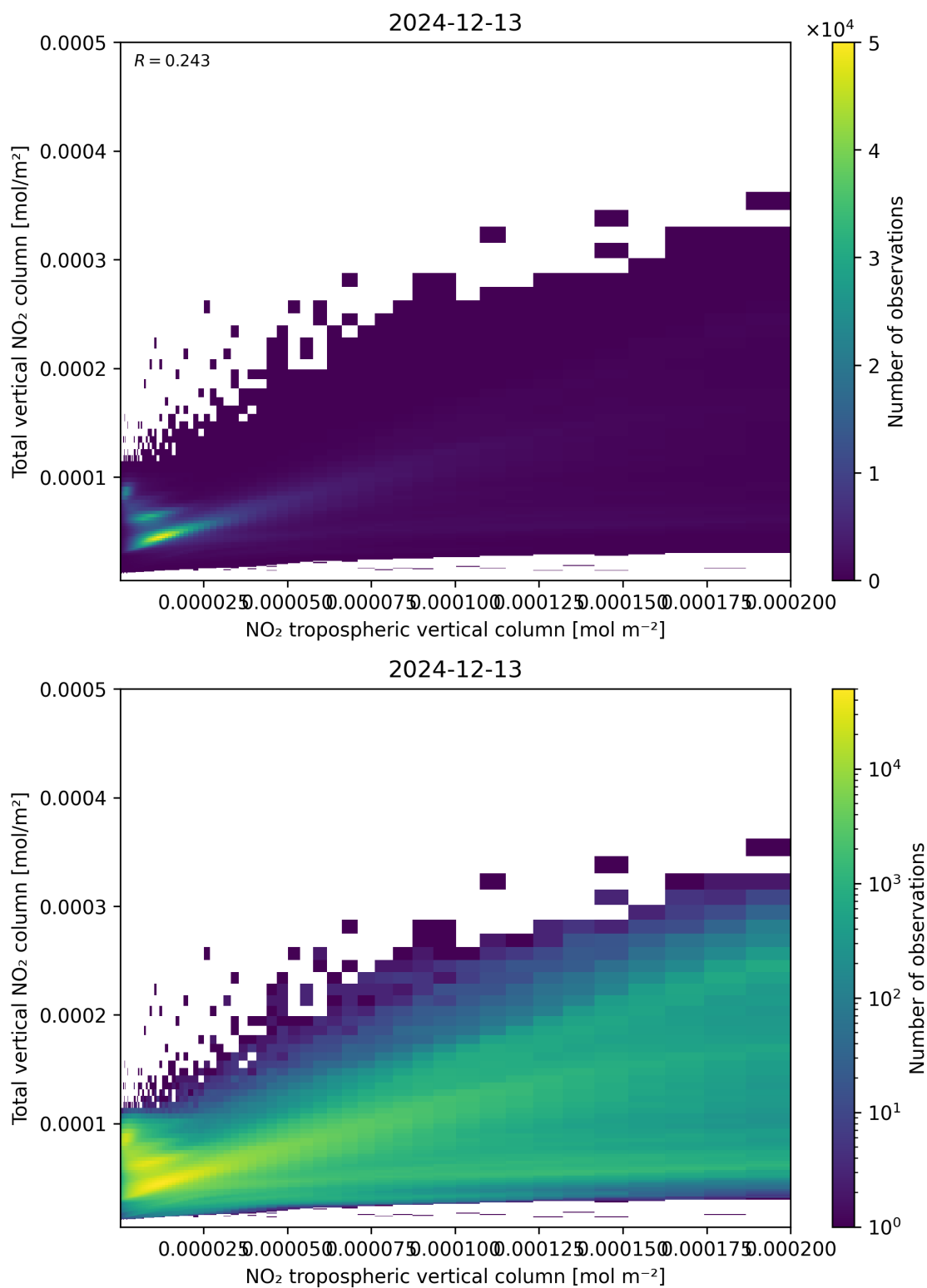
Figure 128: Scatter density plot of “NO 2 tropospheric vertical column” against “Total vertical NO 2 column” for 2024-12-12 to 2024-12-14.
