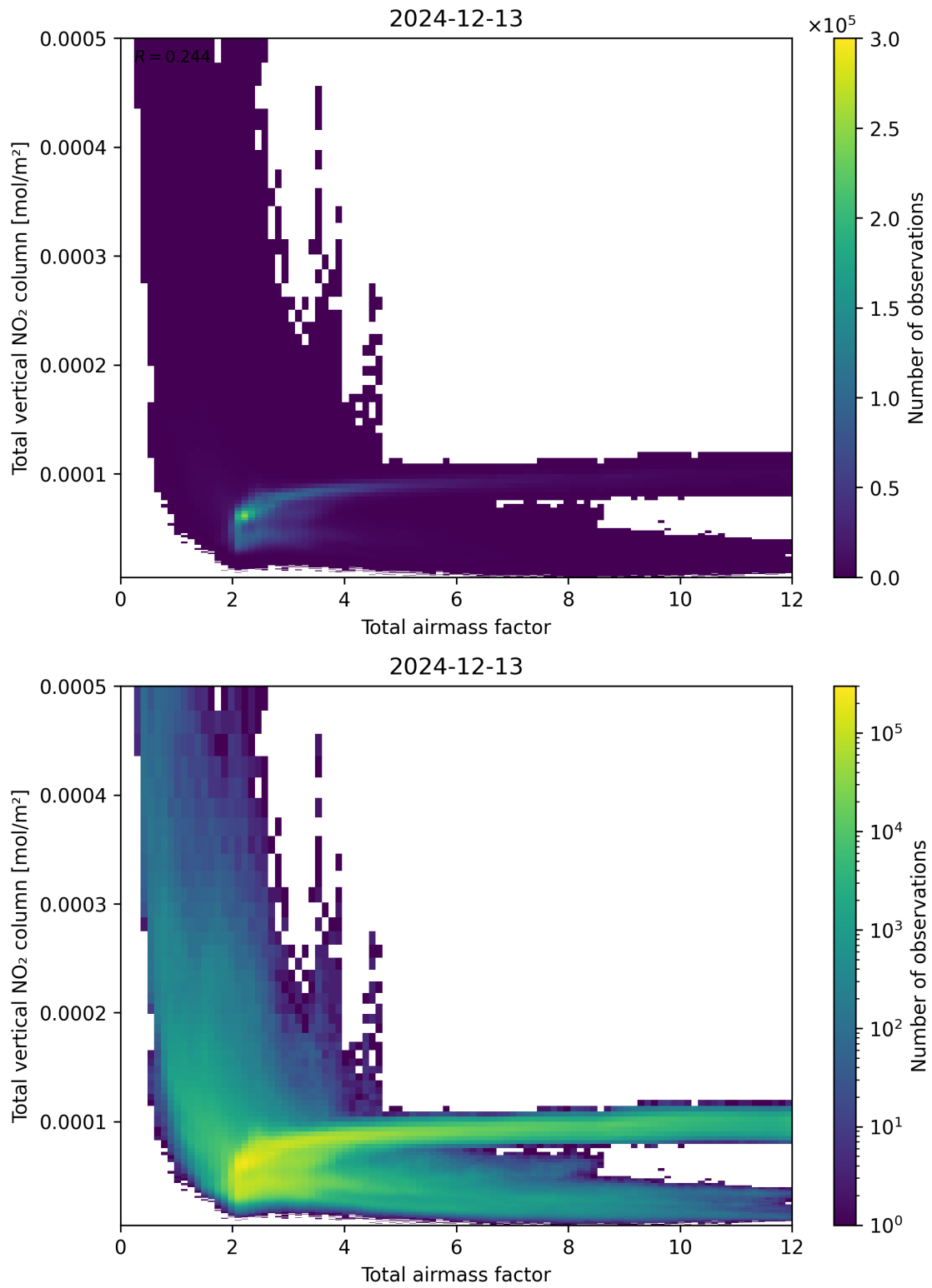
Figure 67: Scatter density plot of “Total airmass factor” against “Total vertical NO 2 column” for 2024-12-12 to 2024-12-14.
