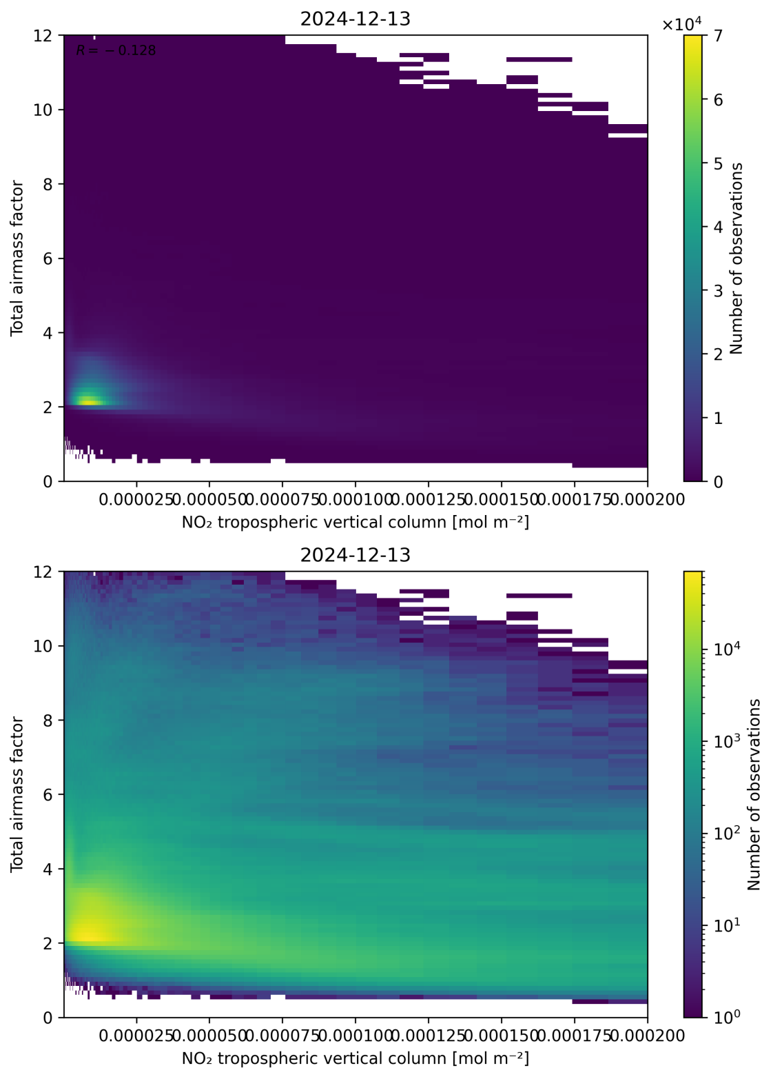
Figure 122: Scatter density plot of “NO 2 tropospheric vertical column” against “Total air mass factor” for 2024-12-12 to 2024-12-14.
