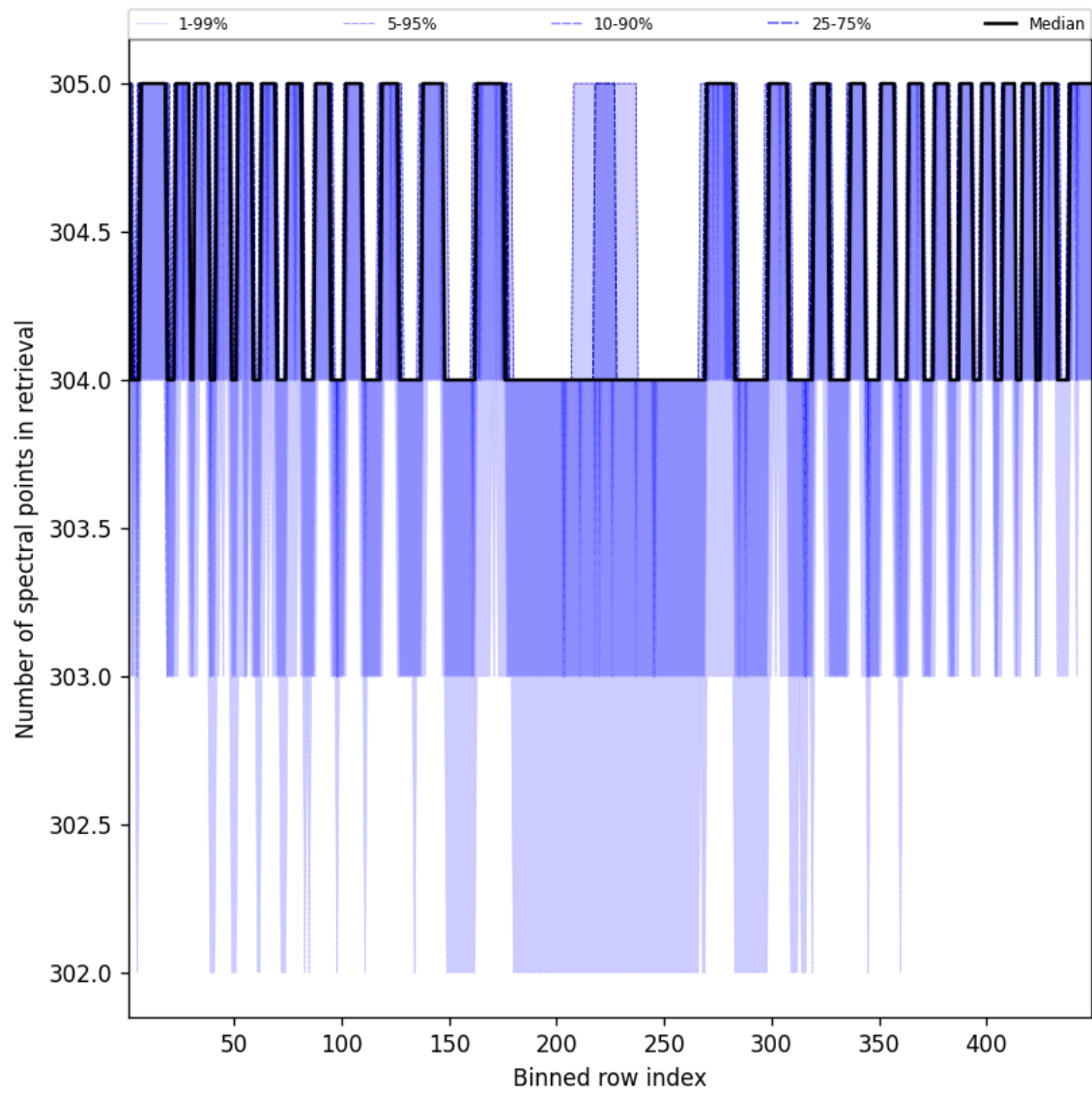
Figure 50: Along track statistics of “Number of spectral points in retrieval” for 2024-12-12 to 2024-12-14
