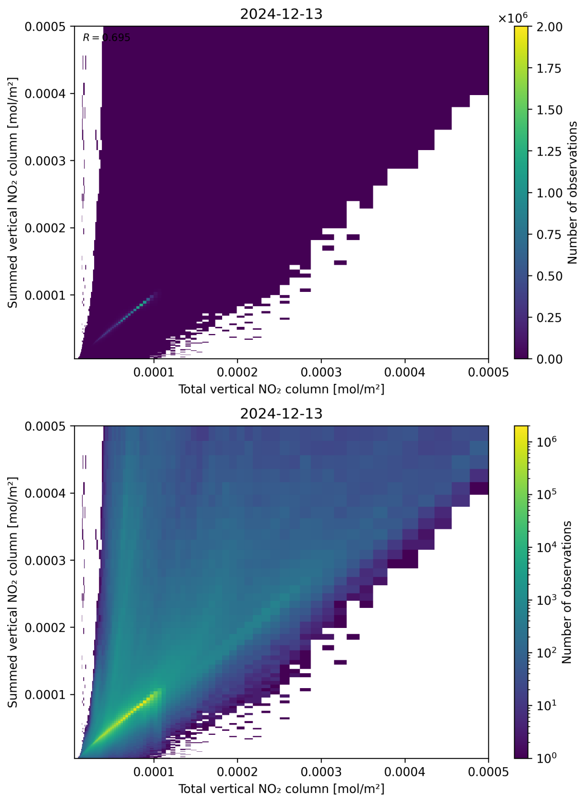
Figure 112: Scatter density plot of “Total vertical NO 2 column” against “Summed vertical NO 2 column” for 2024-12-12 to 2024-12-14.
