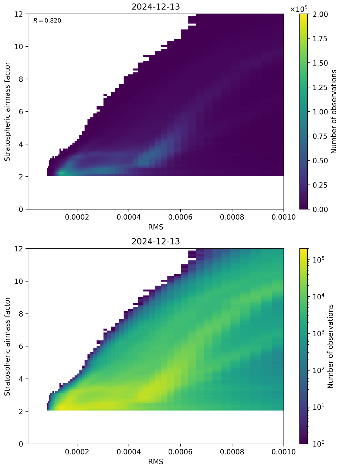
Figure 144: Scatter density plot of “RMS” against “Stratospheric airmass factor” for 2024-12-12 to 2024-12-14.
