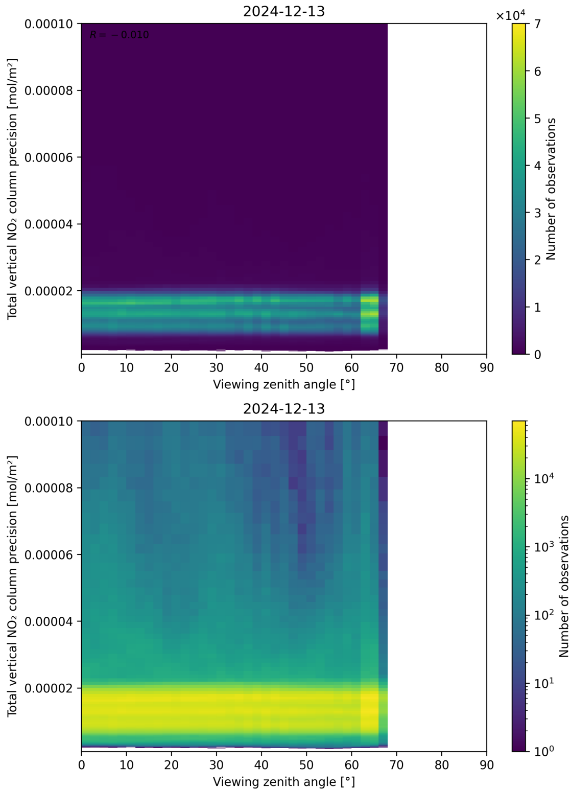
Figure 168: Scatter density plot of “Viewing zenith angle” against “Total vertical NO 2 column precision” for 2024-12-12 to 2024-12-14.
