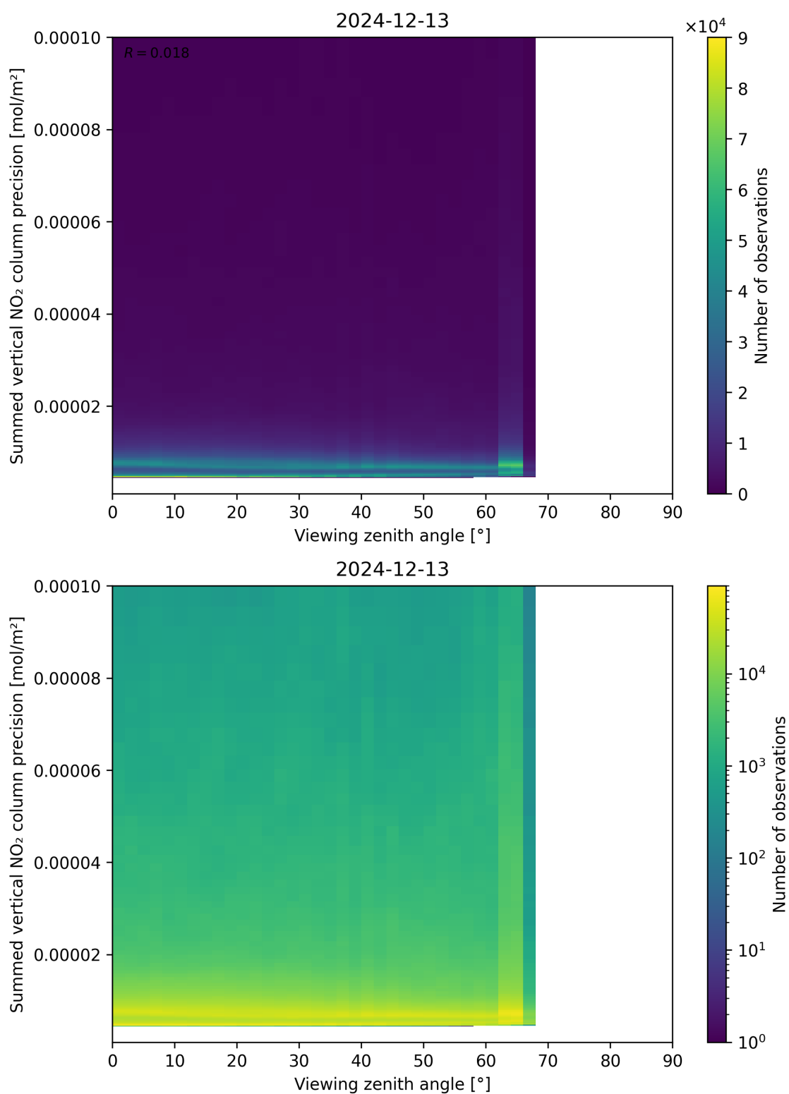
Figure 166: Scatter density plot of “Viewing zenith angle” against “Summed vertical NO 2 column precision” for 2024-12-12 to 2024-12-14.
