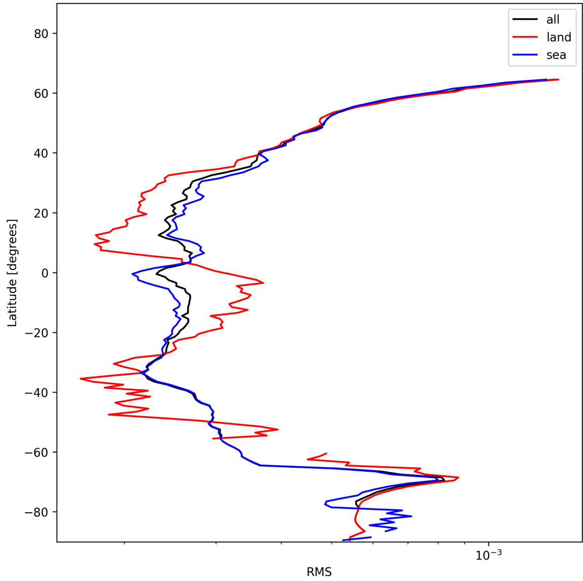
Figure 26: Zonal average of “RMS” for 2024-12-12 to 2024-12-14.
