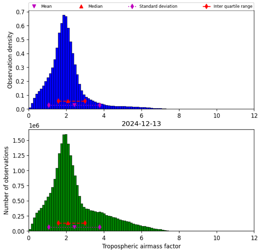
Figure 31: Histogram of “Tropospheric airmass factor” for 2024-12-12 to 2024-12-14
