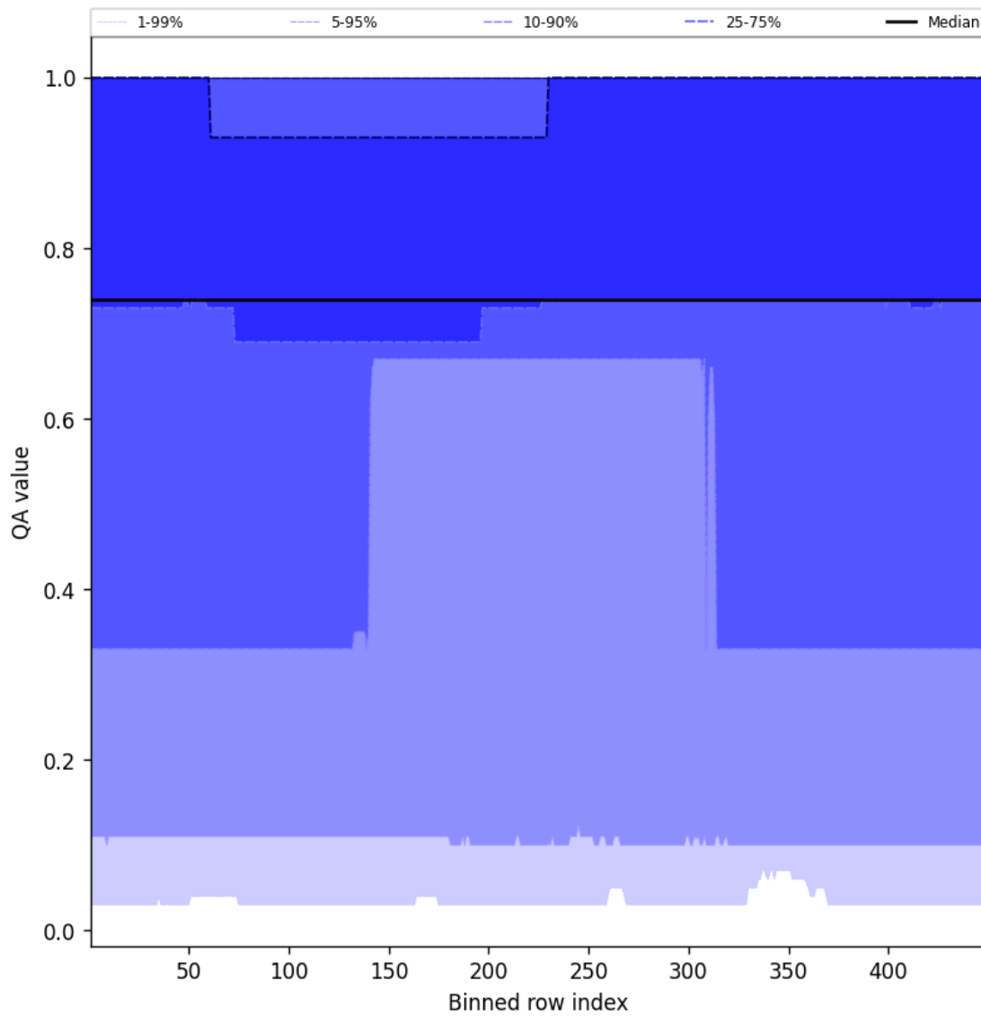
Figure 45: Along track statistics of “QA value” for 2024-12-12 to 2024-12-14
