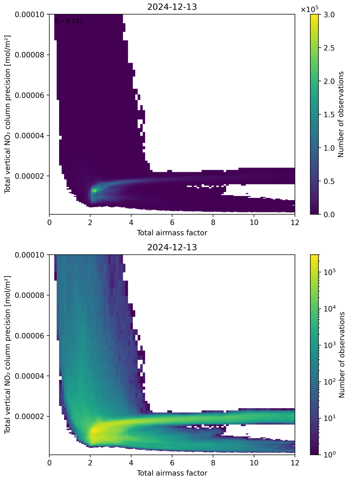
Figure 68: Scatter density plot of “Total airmass factor” against “Total vertical NO 2 column precision” for 2024-12-12 to 2024-12-14.
