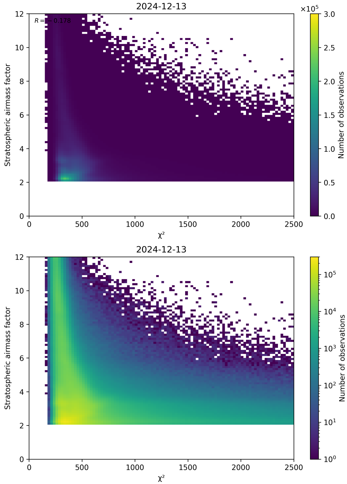
Figure 81: Scatter density plot of “ \chi^2 ” against “Stratospheric air mass factor” for 2024-12-12 to 2024-12-14.
