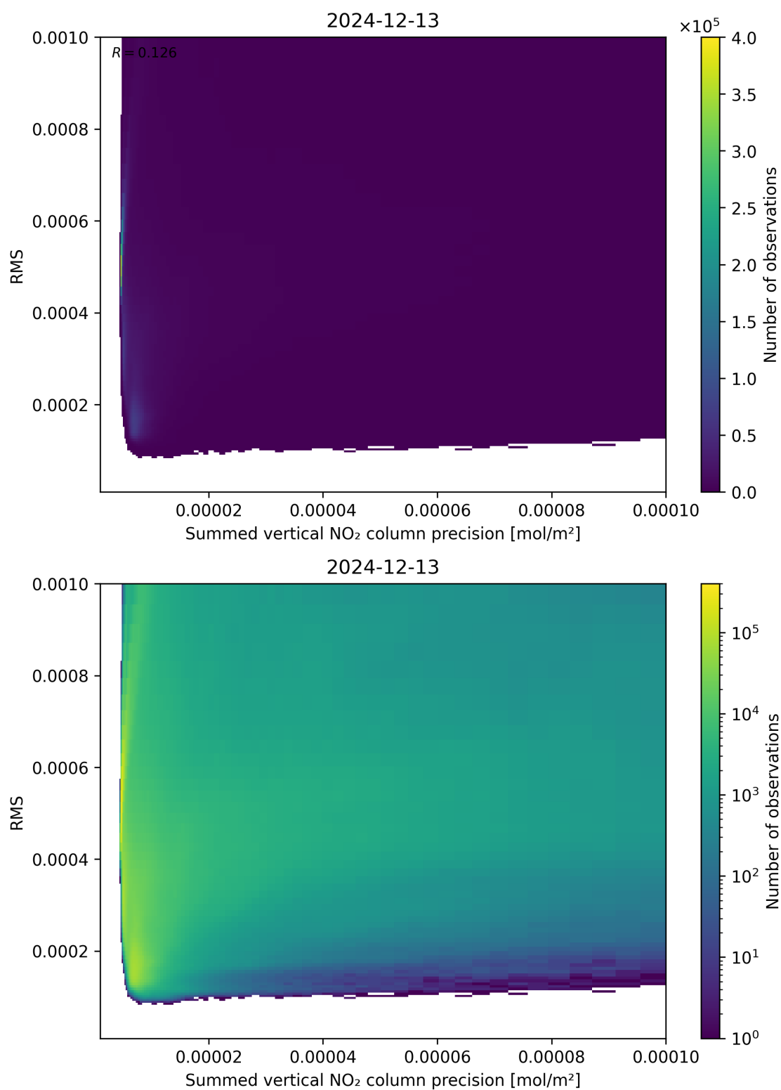
Figure 108: Scatter density plot of “Summed vertical NO 2 column precision” against “RMS” for 2024-12-12 to 2024-12-14.
