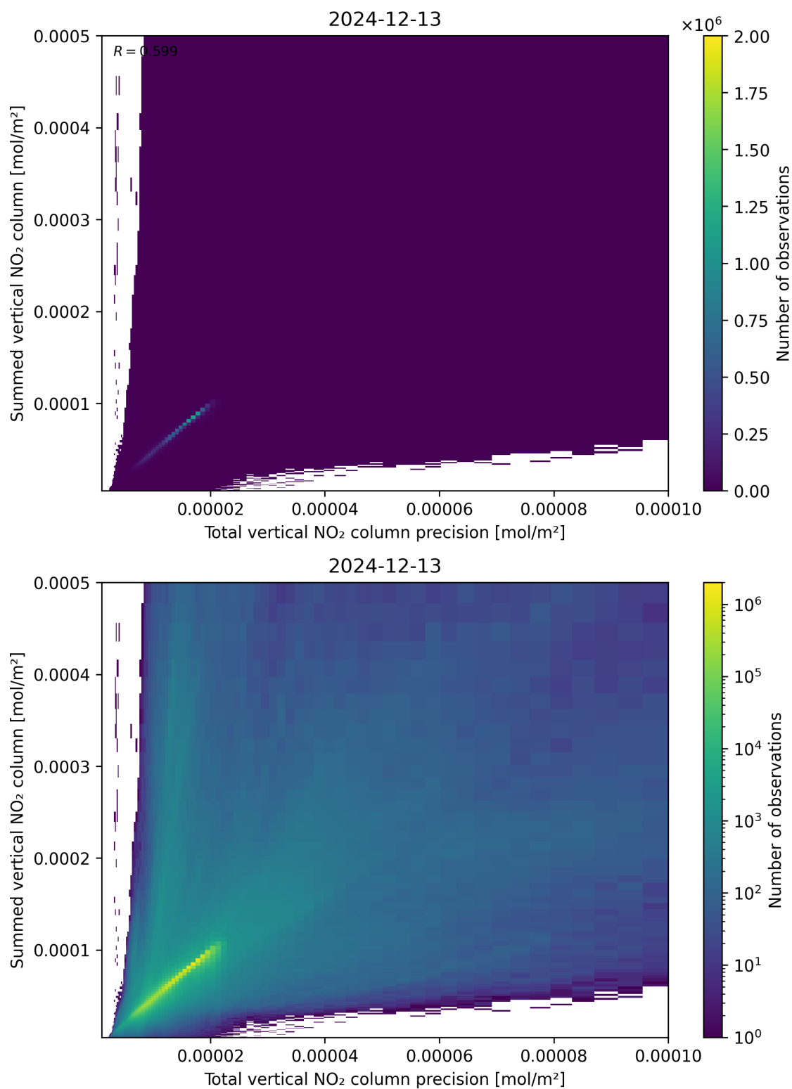
Figure 117: Scatter density plot of “Total vertical NO 2 column precision” against “Summed vertical NO 2 column” for 2024-12-12 to 2024-12-14.
