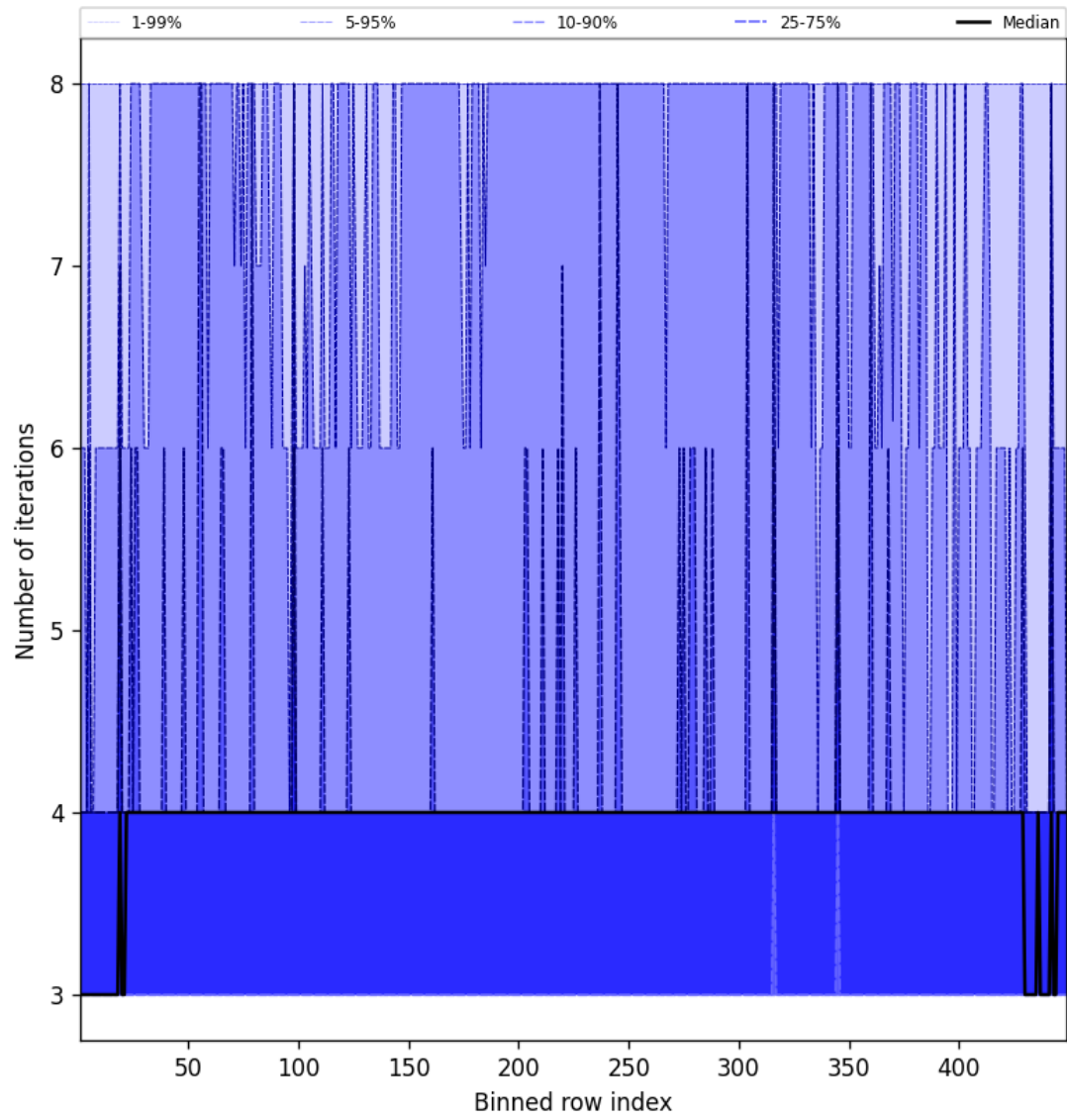
Figure 51: Along track statistics of “Number of iterations” for 2024-12-12 to 2024-12-14
