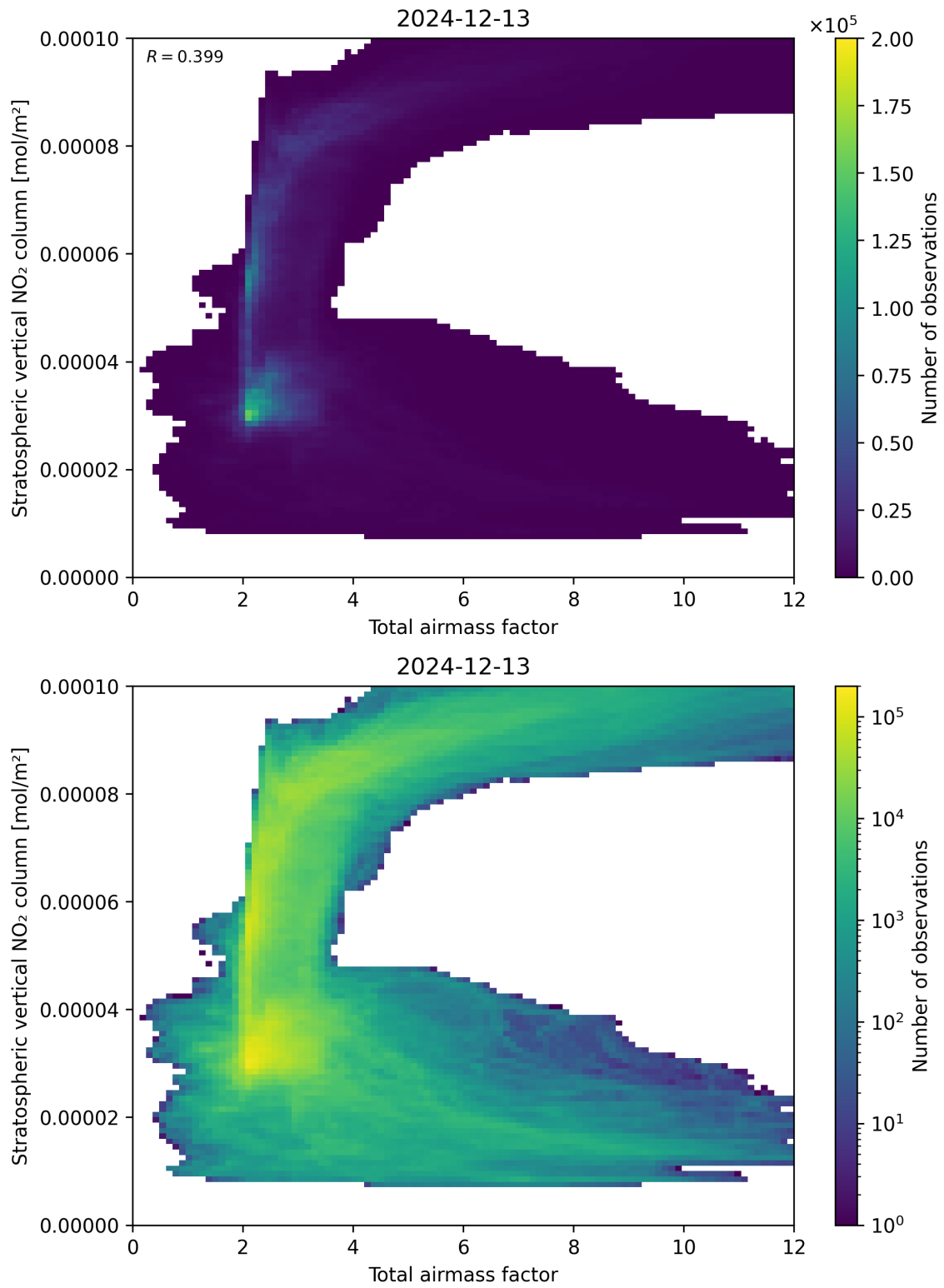
Figure 64: Scatter density plot of “Total airmass factor” against “Stratospheric vertical NO 2 column” for 2024-12-12 to 2024-12-14.
