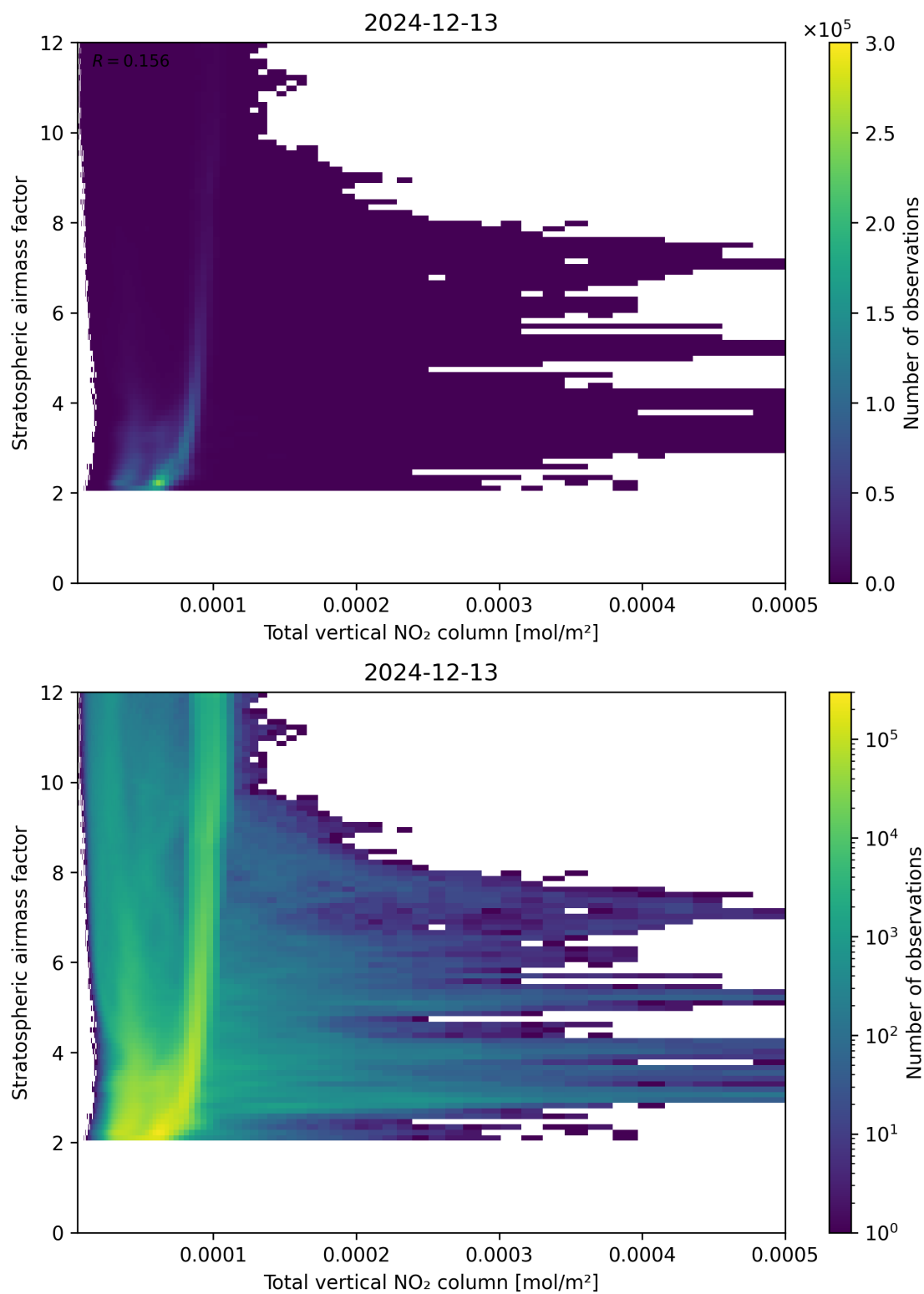
Figure 110: Scatter density plot of “Total vertical NO 2 column” against “Stratospheric airmass factor” for 2024-12-12 to 2024-12-14.
