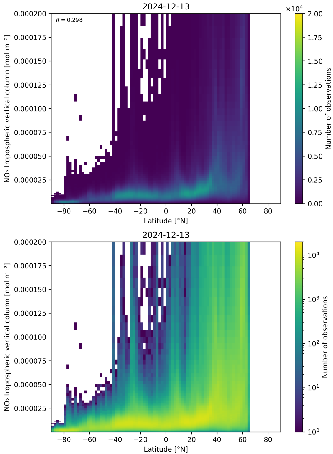
Figure 92: Scatter density plot of “Latitude” against “NO 2 tropospheric vertical column” for 2024-12-12 to 2024-12-14.
