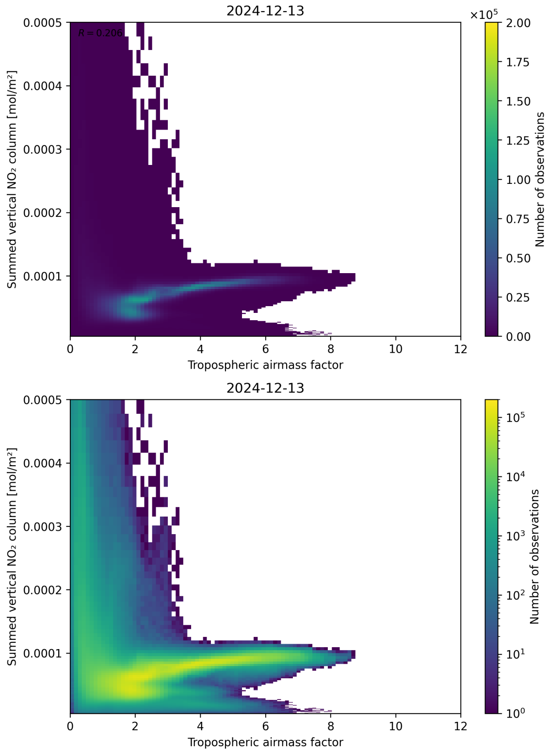
Figure 75: Scatter density plot of “Tropospheric airmass factor” against “Summed vertical NO 2 column” for 2024-12-12 to 2024-12-14.
