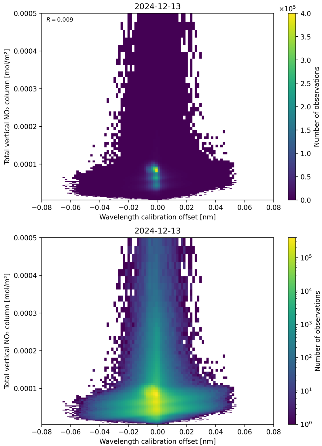
Figure 179: Scatter density plot of “Wavelength calibration offset” against “Total vertical NO 2 column” for 2024-12-12 to 2024-12-14.
