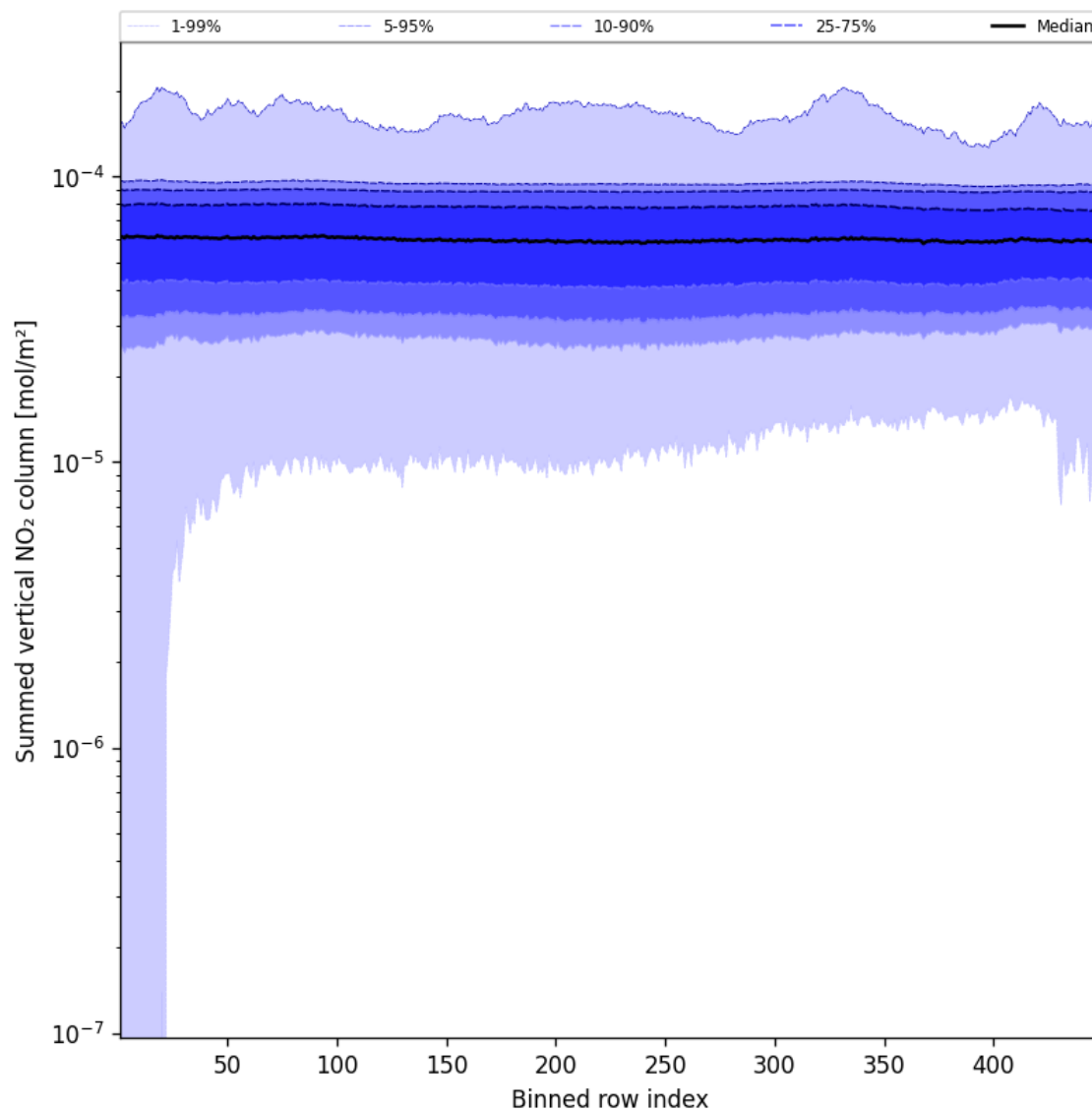
Figure 57: Along track statistics of “Summed vertical NO 2 column” for 2024-12-12 to 2024-12-14
