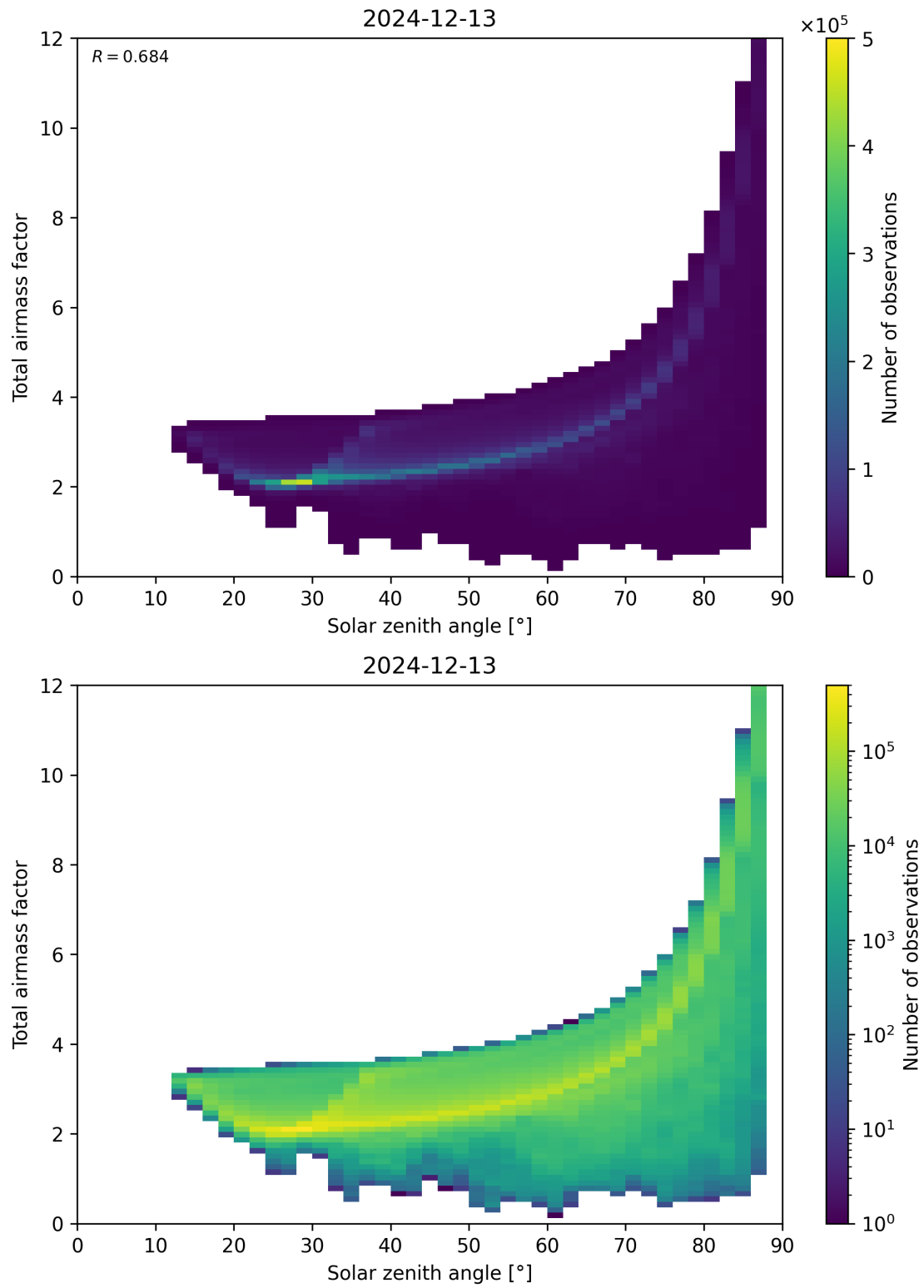
Figure 146: Scatter density plot of “Solar zenith angle” against “Total airmass factor” for 2024-12-12 to 2024-12-14.
