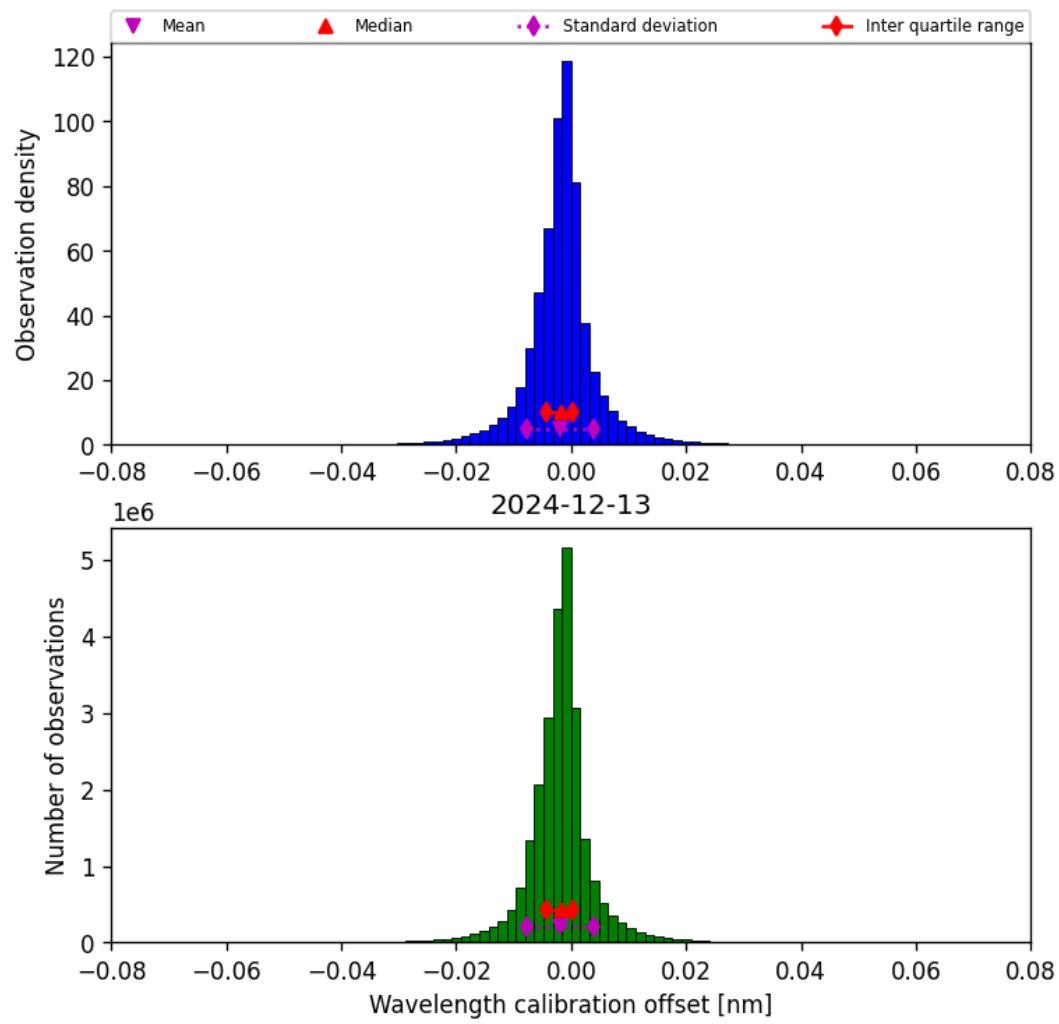
Figure 35: Histogram of “Wavelength calibration offset” for 2024-12-12 to 2024-12-14
