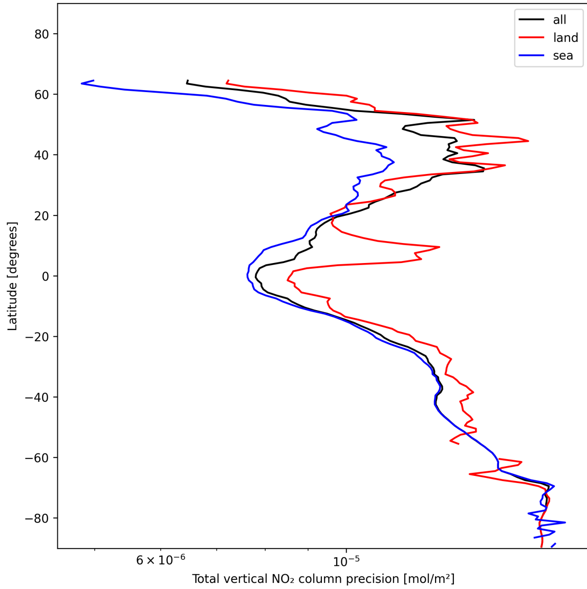
Figure 22: Zonal average of “Total vertical NO 2 column precision” for 2024-12-12 to 2024-12-14.
