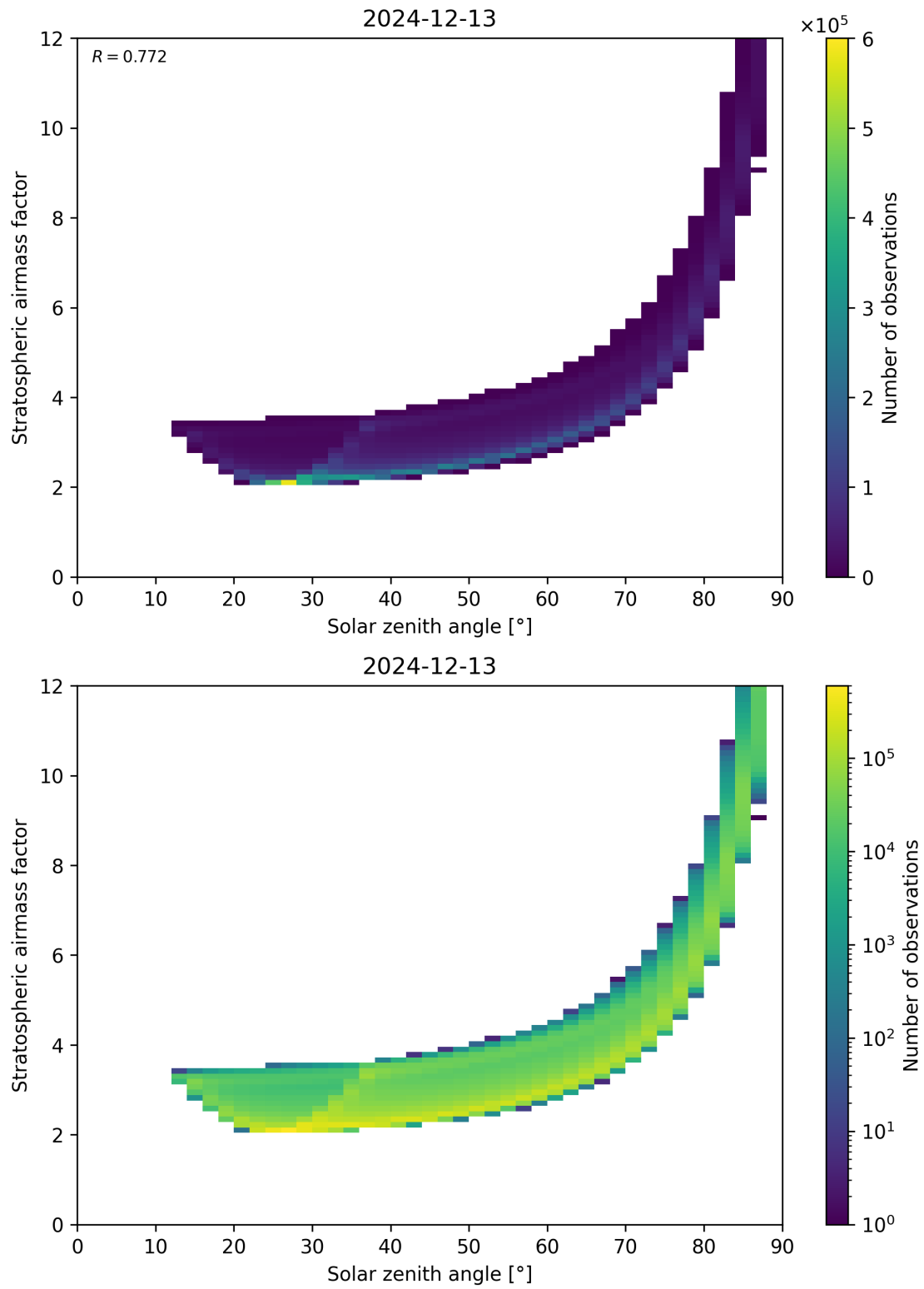
Figure 145: Scatter density plot of “Solar zenith angle” against “Stratospheric airmass factor” for 2024-12-12 to 2024-12-14.
