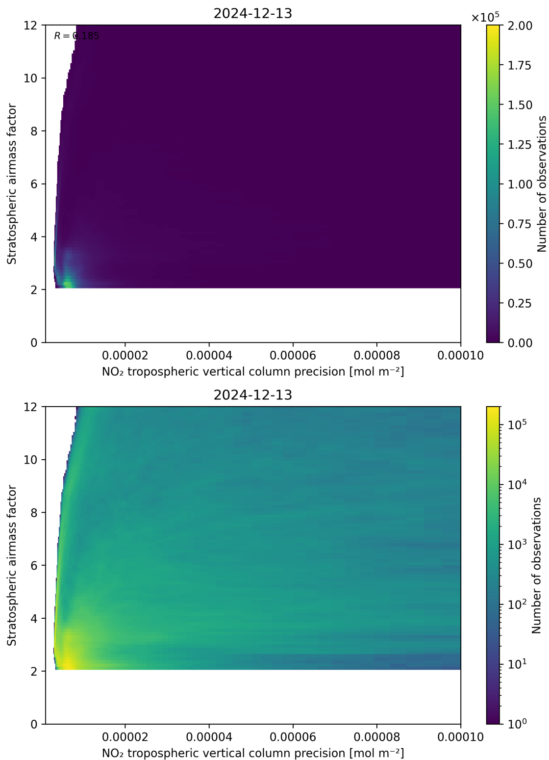
Figure 131: Scatter density plot of “NO 2 tropospheric vertical column precision” against “Stratospheric airmass factor” for 2024-12-12 to 2024-12-14.
