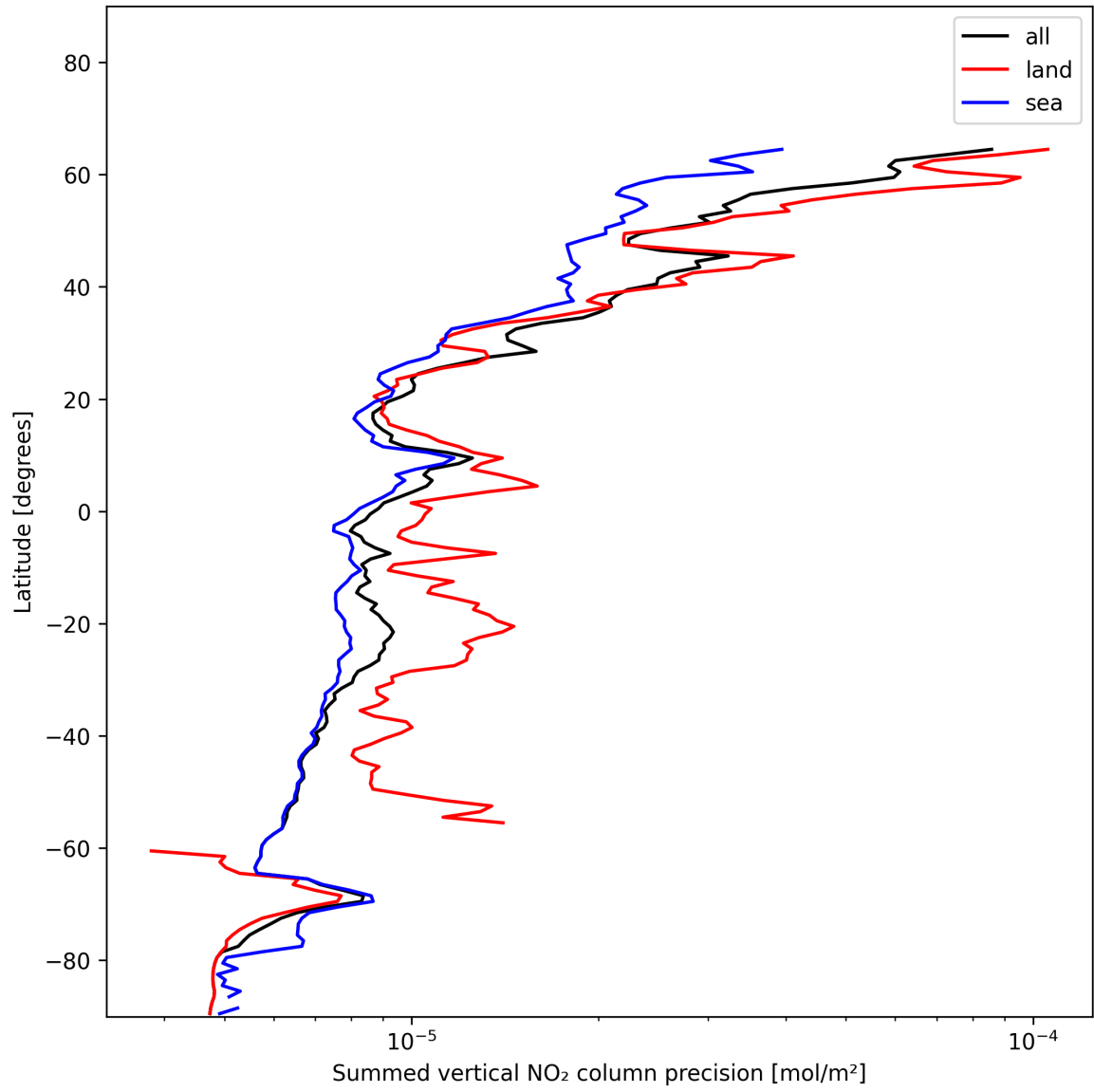
Figure 24: Zonal average of “Summed vertical NO 2 column precision” for 2024-12-12 to 2024-12-14.
