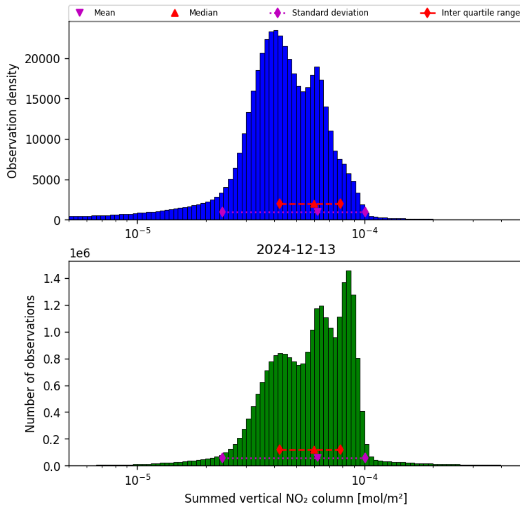
Figure 40: Histogram of “Summed vertical NO 2 column” for 2024-12-12 to 2024-12-14
