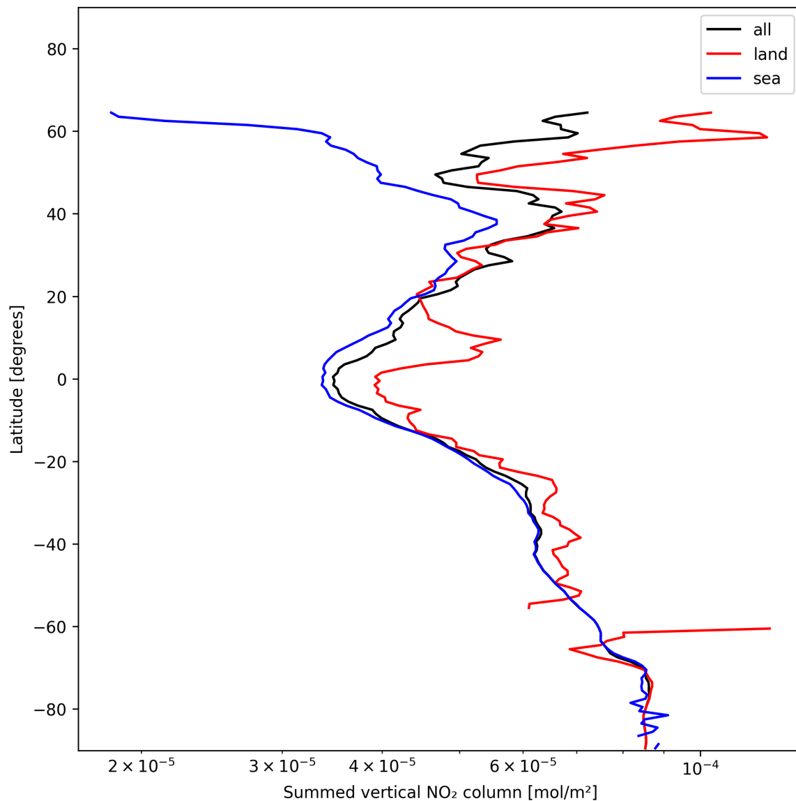
Figure 23: Zonal average of “Summed vertical NO 2 column” for 2024-12-12 to 2024-12-14.
