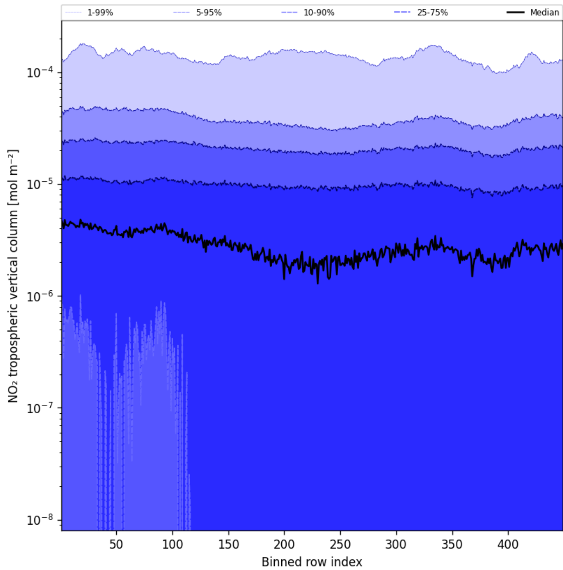
Figure 46: Along track statistics of “NO 2 tropospheric vertical column” for 2024-12-12 to 2024-12-14
