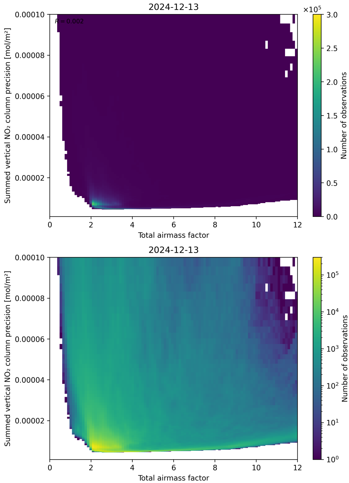
Figure 66: Scatter density plot of “Total airmass factor” against “Summed vertical NO 2 column precision” for 2024-12-12 to 2024-12-14.
