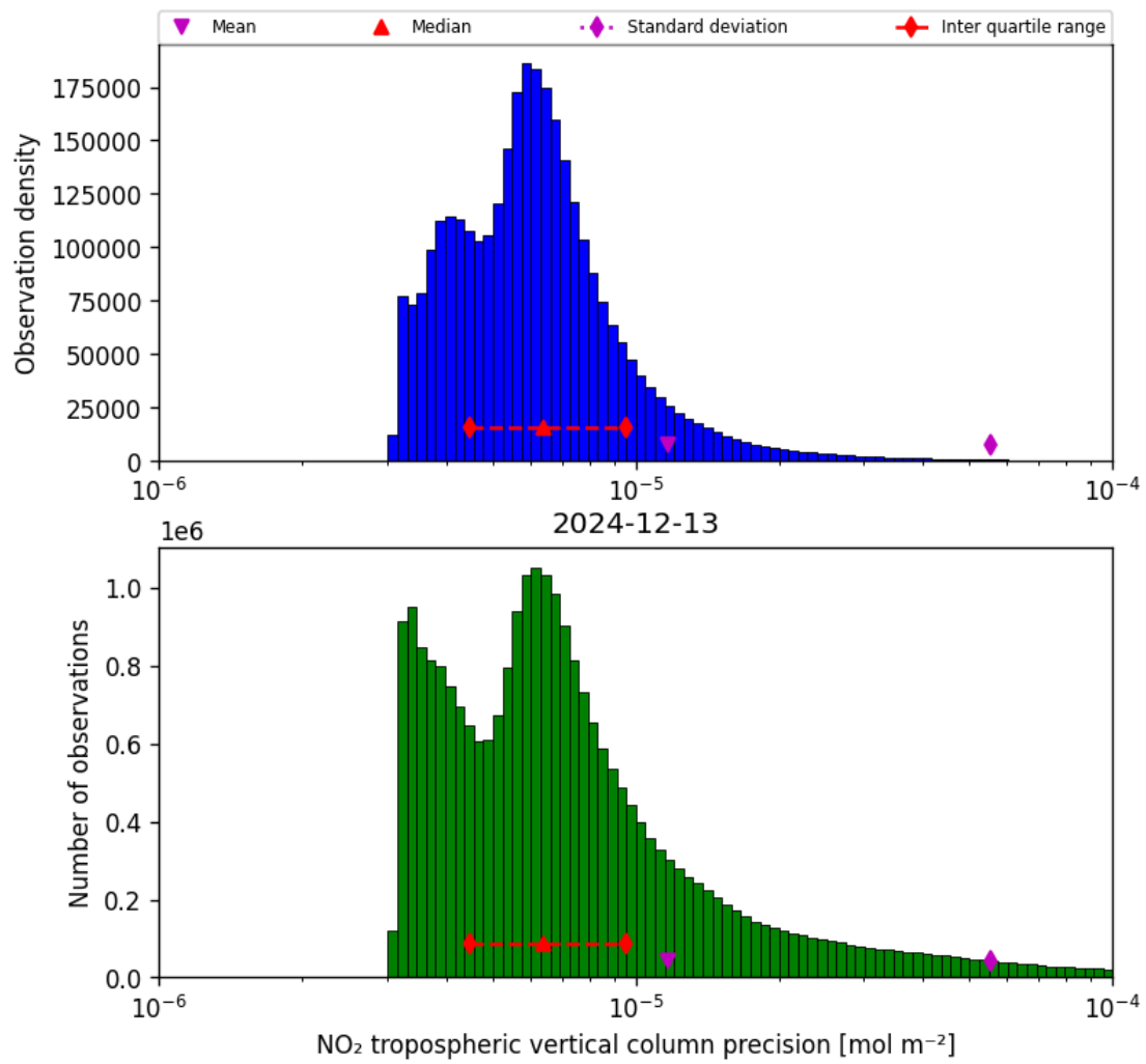
Figure 30: Histogram of “NO 2 tropospheric vertical column precision” for 2024-12-12 to 2024-12-14
