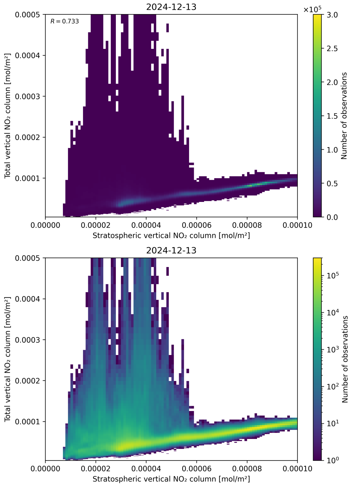
Figure 100: Scatter density plot of “Stratospheric vertical NO 2 column” against “Total vertical NO 2 column” for 2024-12-12 to 2024-12-14.
