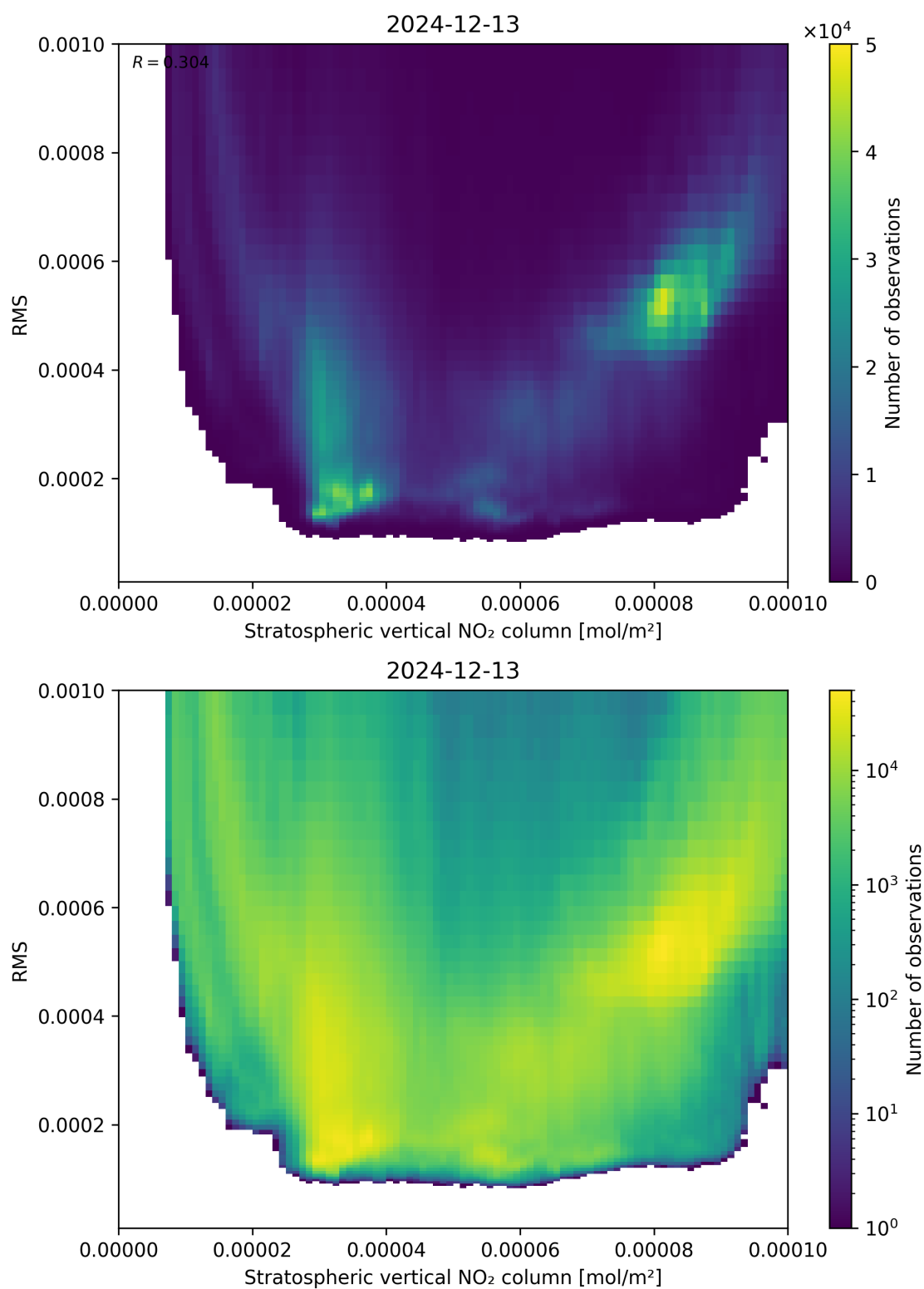
Figure 102: Scatter density plot of “Stratospheric vertical NO 2 column” against “RMS” for 2024-12-12 to 2024-12-14.
