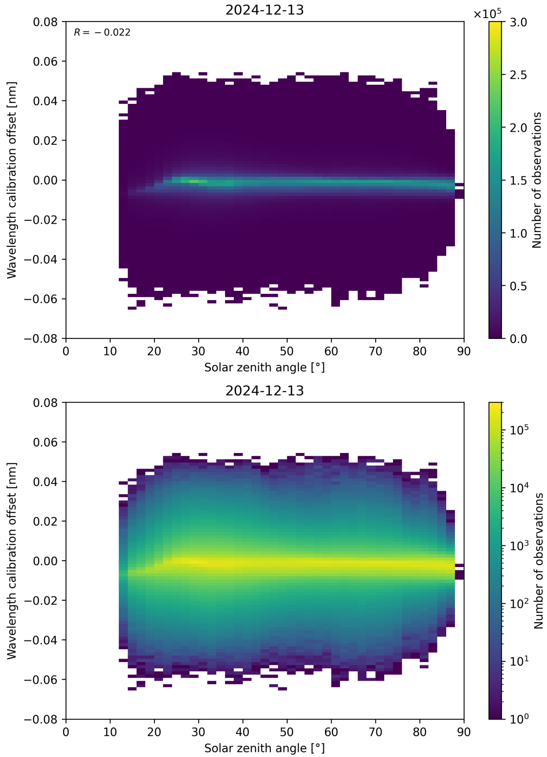
Figure 158: Scatter density plot of “Solar zenith angle” against “Wavelength calibration offset” for 2024-12-12 to 2024-12-14.
