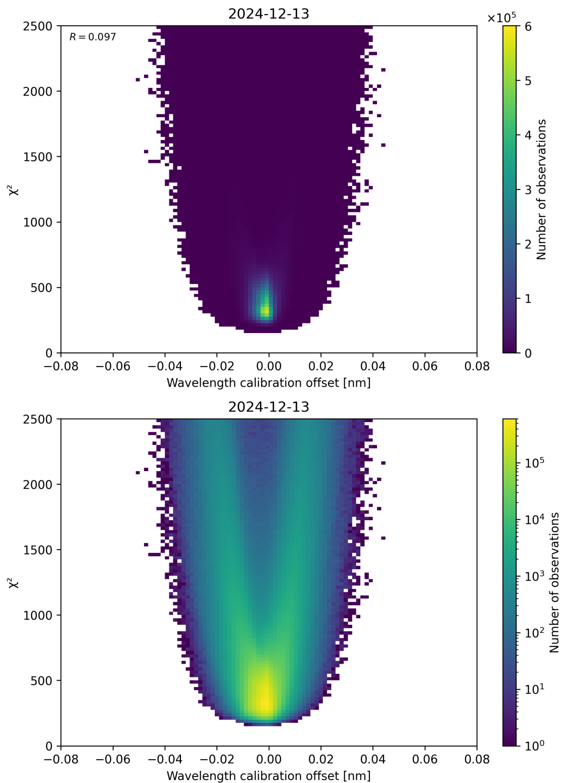
Figure 175: Scatter density plot of “Wavelength calibration offset” against “ \chi^2 ” for 2024-12-12 to 2024-12-14.
