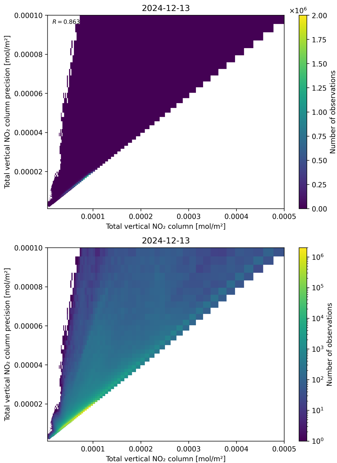
Figure 114: Scatter density plot of “Total vertical NO 2 column” against “Total vertical NO 2 column precision” for 2024-12-12 to 2024-12-14.
