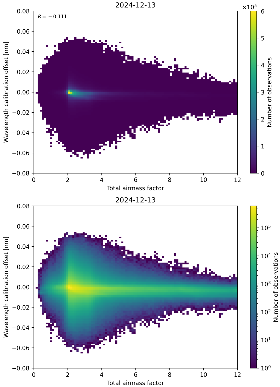
Figure 70: Scatter density plot of “Total airmass factor” against “Wavelength calibration offset” for 2024-12-12 to 2024-12-14.
