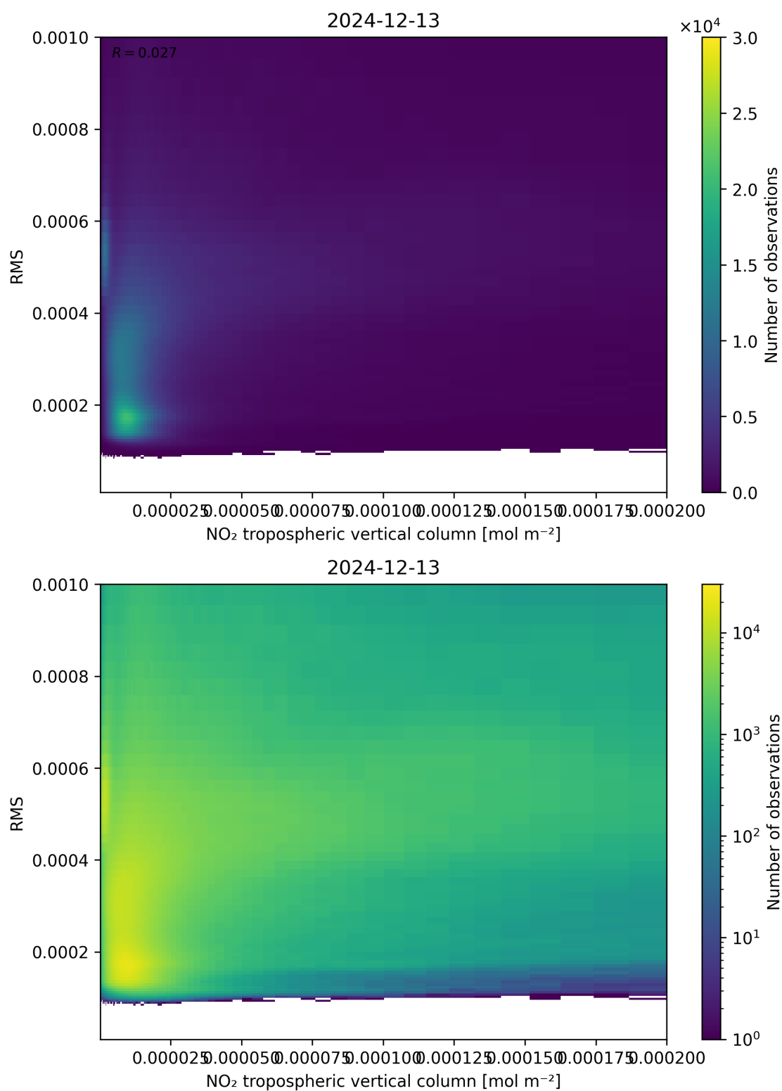
Figure 142: Scatter density plot of “NO 2 tropospheric vertical column” against “RMS” for 2024-12-12 to 2024-12-14.
