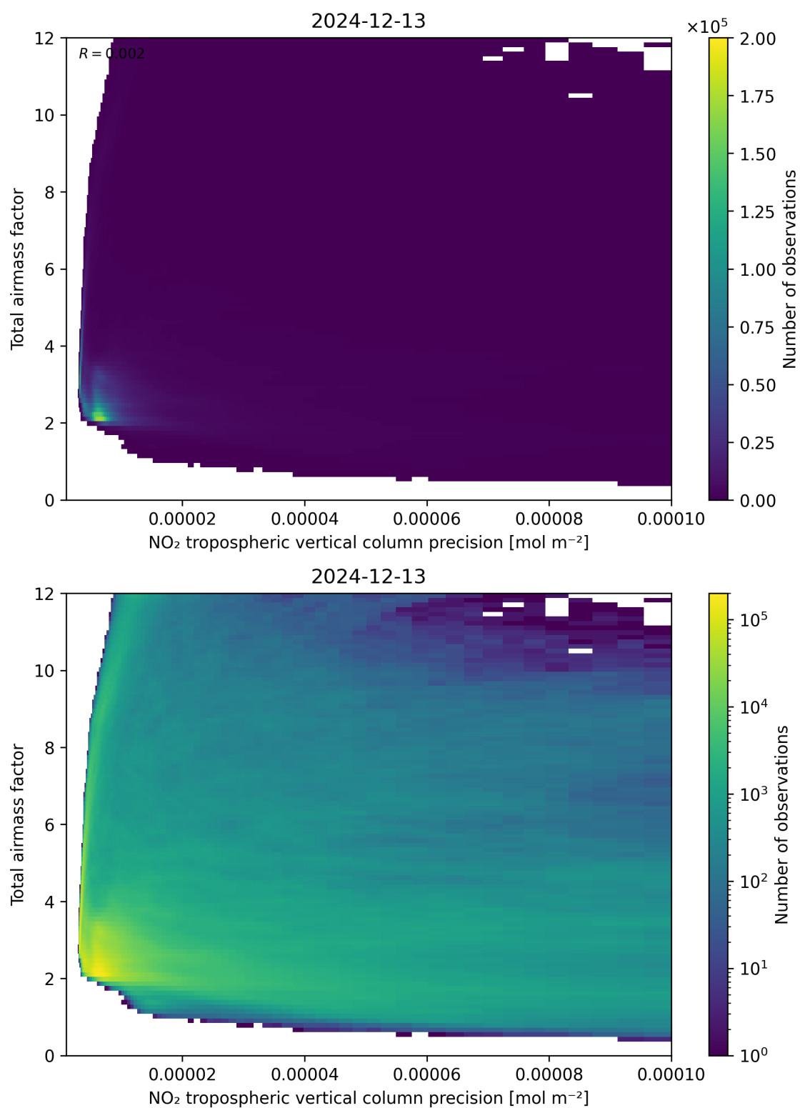
Figure 132: Scatter density plot of “NO 2 tropospheric vertical column precision” against “Total airmass factor” for 2024-12-12 to 2024-12-14.
