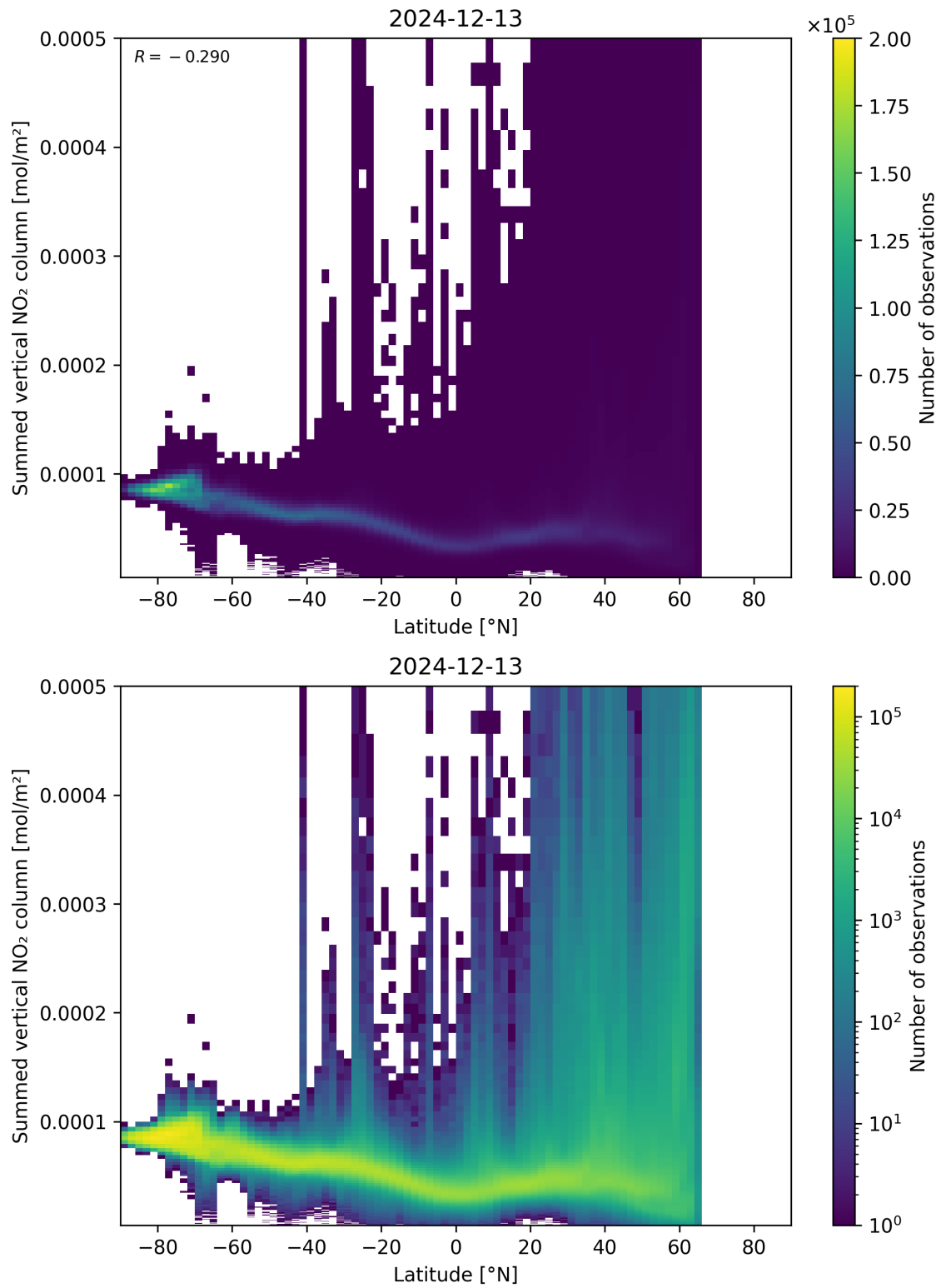
Figure 88: Scatter density plot of “Latitude” against “Summed vertical NO 2 column” for 2024-12-12 to 2024-12-14.
