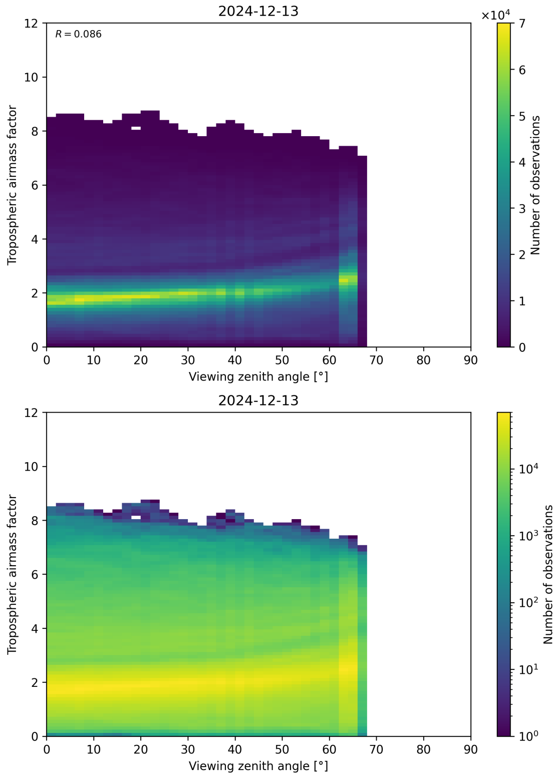
Figure 161: Scatter density plot of “Viewing zenith angle” against “Tropospheric airmass factor” for 2024-12-12 to 2024-12-14.
