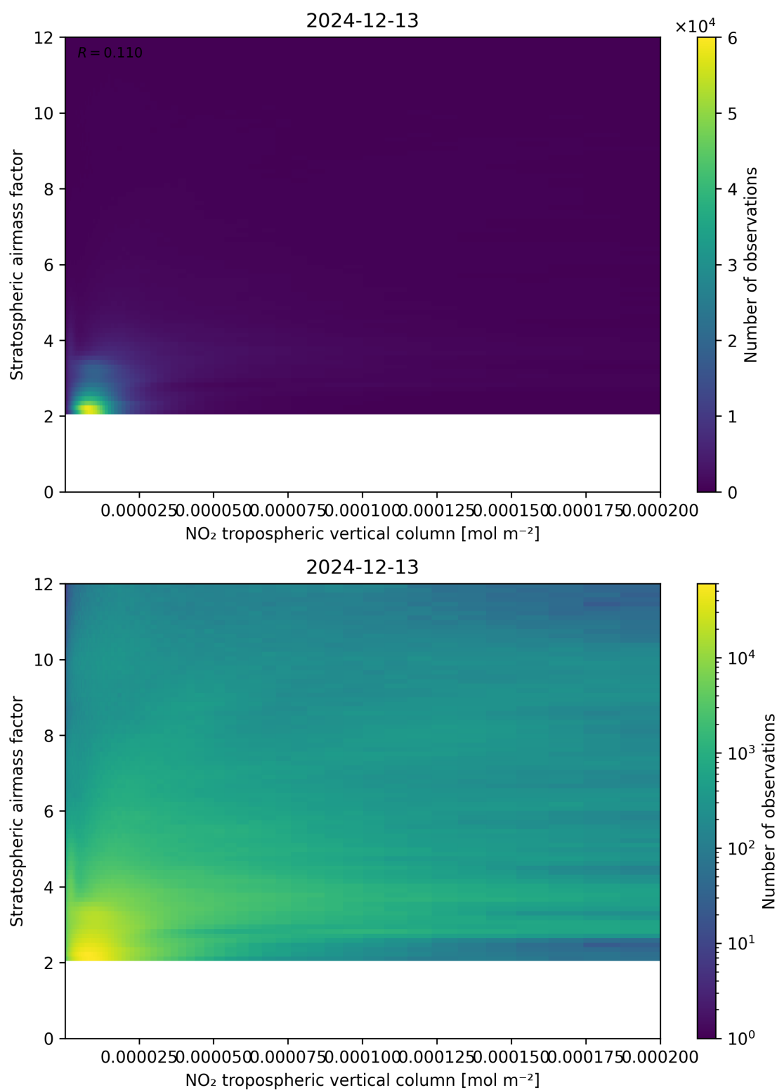
Figure 121: Scatter density plot of “NO 2 tropospheric vertical column” against “Stratospheric airmass factor” for 2024-12-12 to 2024-12-14.
