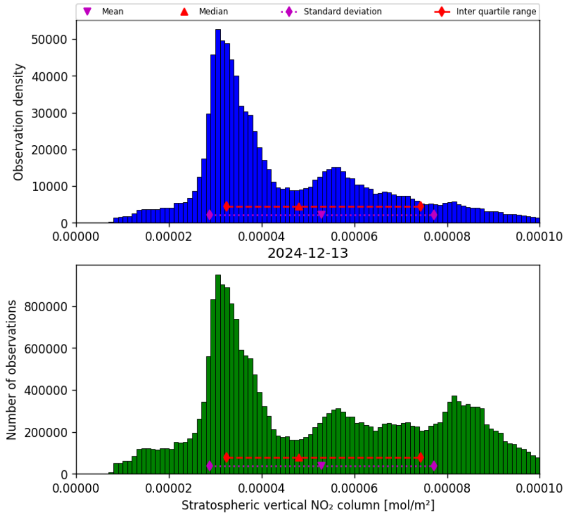
Figure 36: Histogram of “Stratospheric vertical NO 2 column” for 2024-12-12 to 2024-12-14
