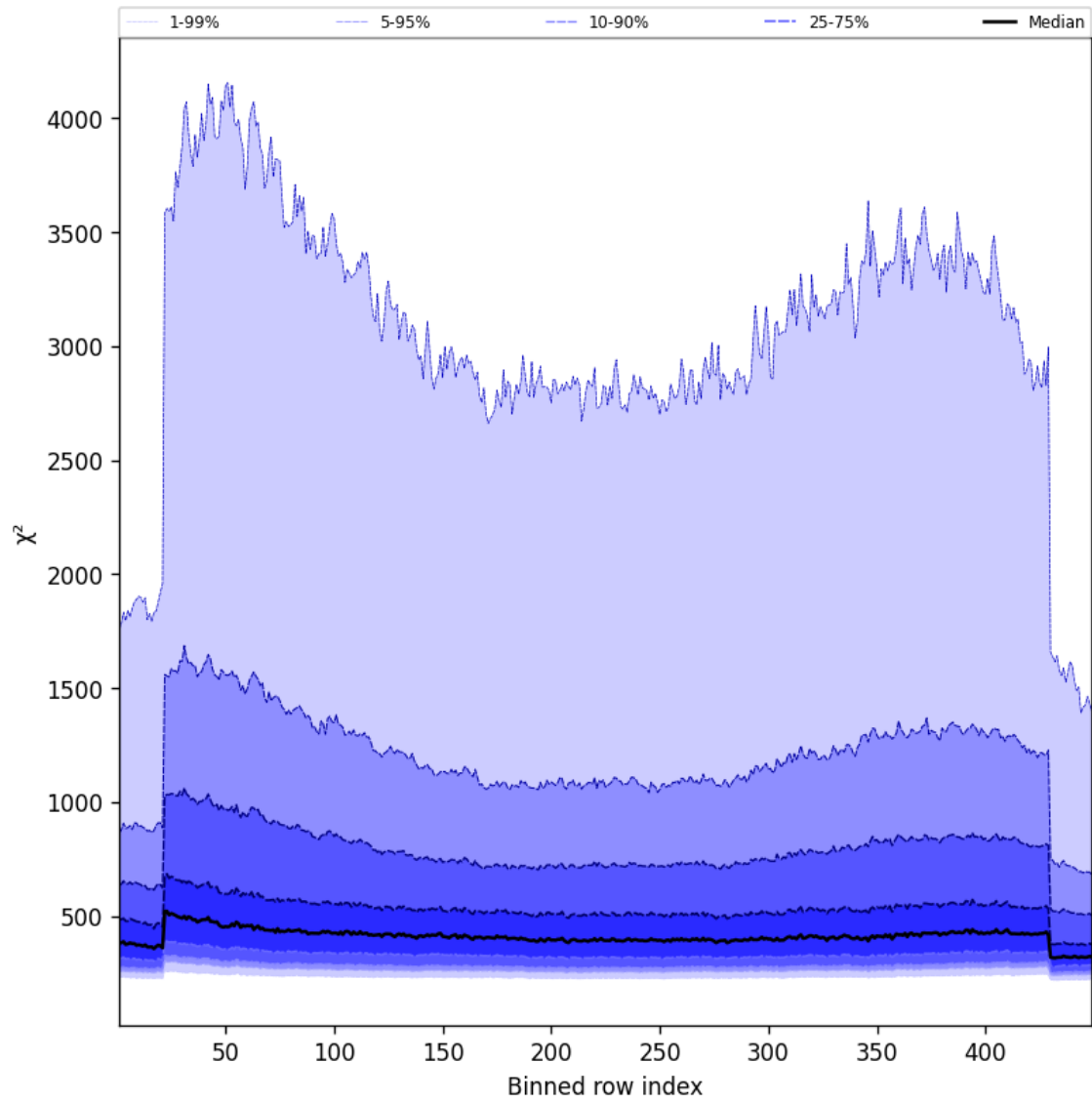
Figure 59: Along track statistics of “ \chi^2 ” for 2024-12-12 to 2024-12-14
