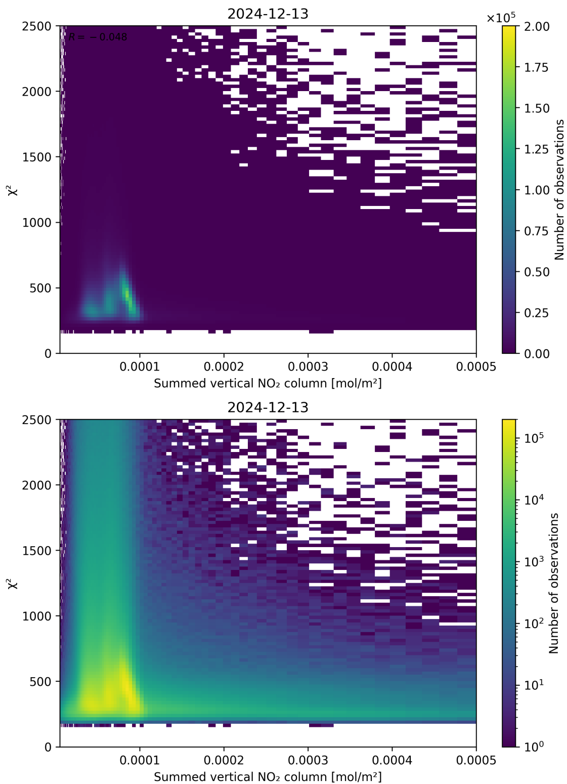
Figure 104: Scatter density plot of “Summed vertical NO 2 column” against “ \chi^2 ” for 2024-12-12 to 2024-12-14.
