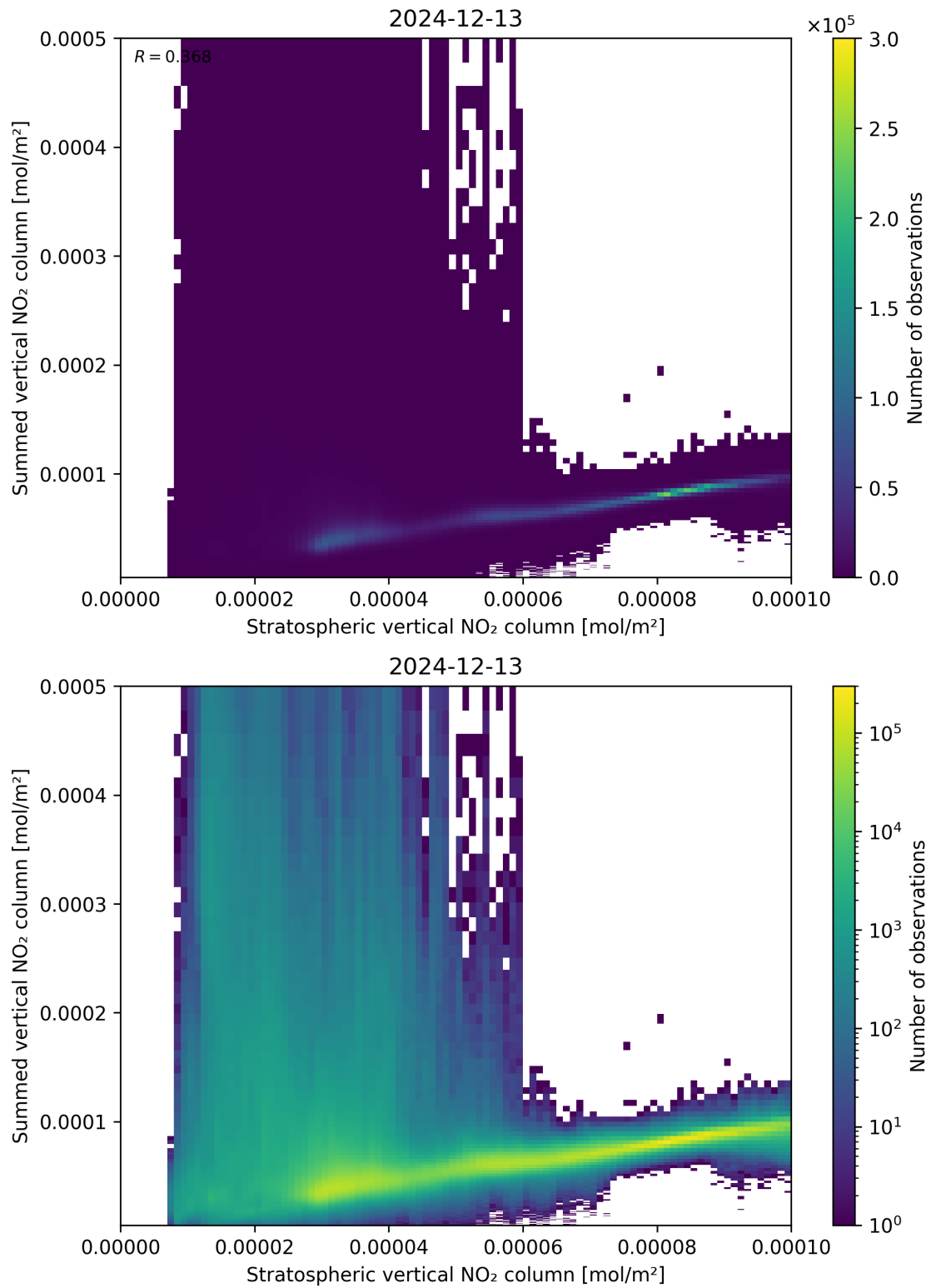
Figure 98: Scatter density plot of “Stratospheric vertical NO 2 column” against “Summed vertical NO 2 column” for 2024-12-12 to 2024-12-14.
