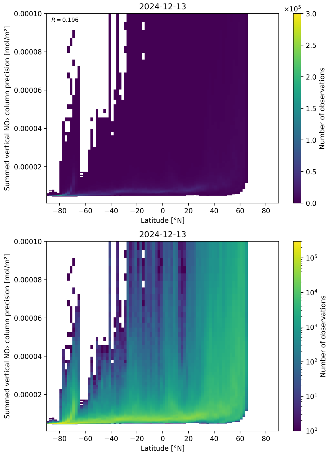
Figure 89: Scatter density plot of “Latitude” against “Summed vertical NO 2 column precision” for 2024-12-12 to 2024-12-14.
