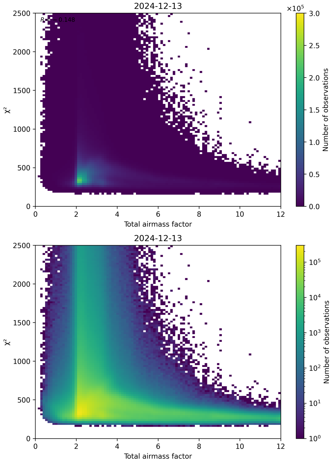
Figure 63: Scatter density plot of “Total airmass factor” against “ \chi^2 ” for 2024-12-12 to 2024-12-14.
