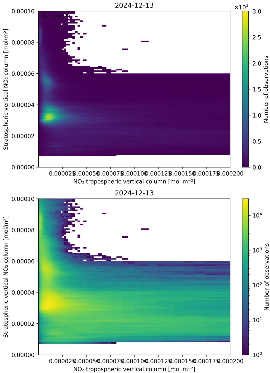
Figure 125: Scatter density plot of “NO 2 tropospheric vertical column” against “Stratospheric vertical NO 2 column” for 2024-12-12 to 2024-12-14.
