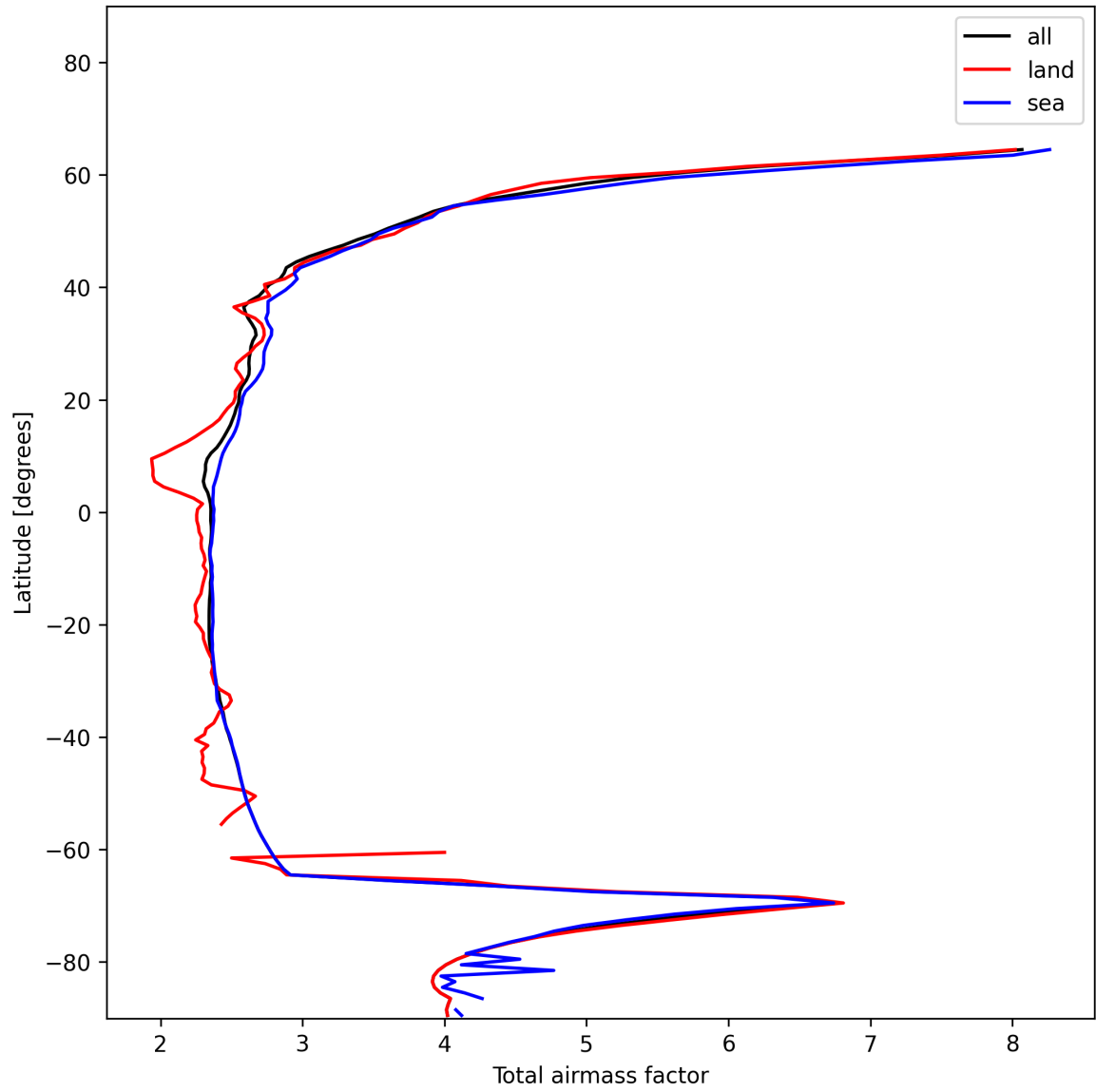
Figure 15: Zonal average of “Total airmass factor” for 2024-12-12 to 2024-12-14.
