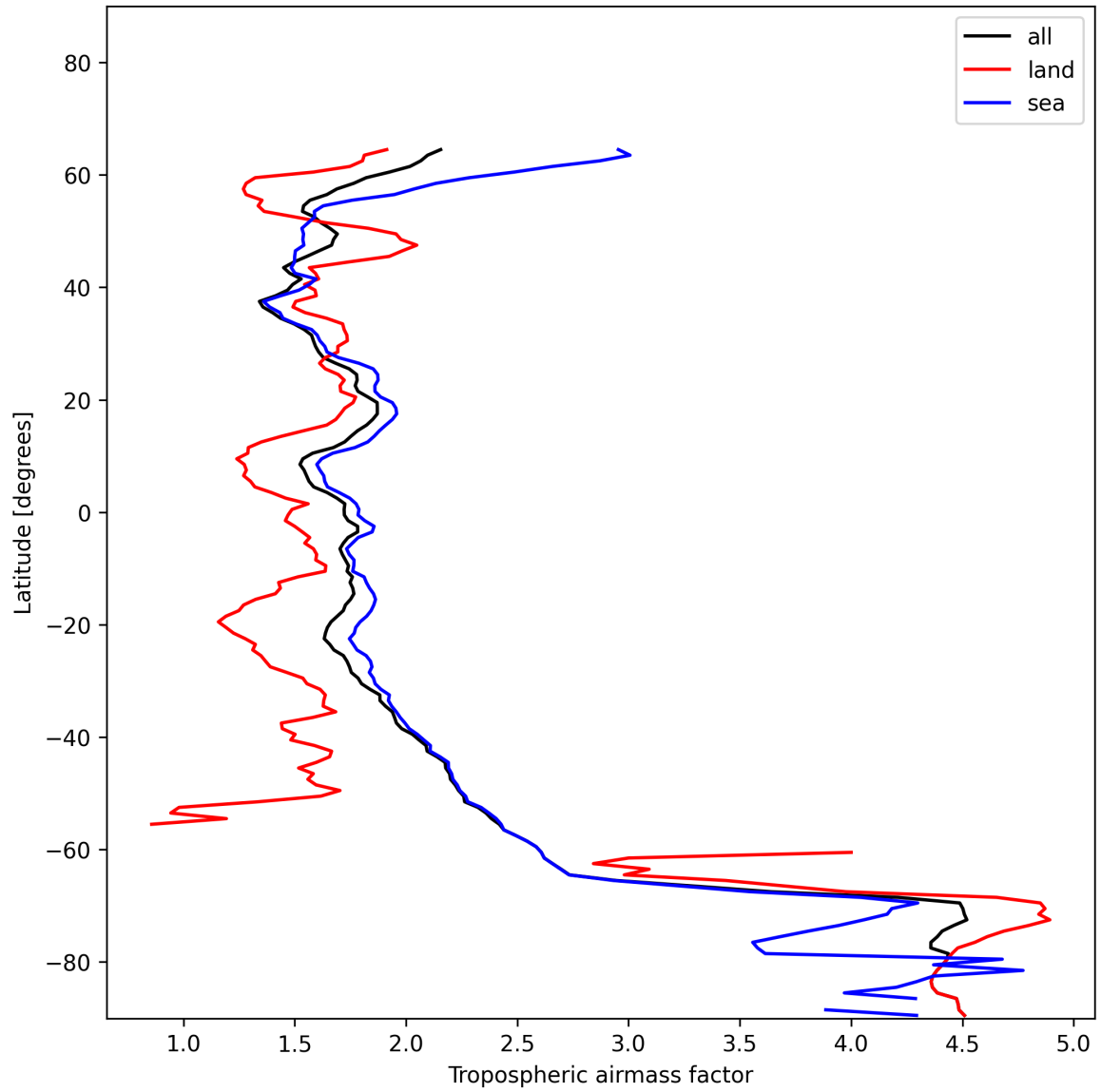
Figure 14: Zonal average of “Tropospheric airmass factor” for 2024-12-12 to 2024-12-14.
