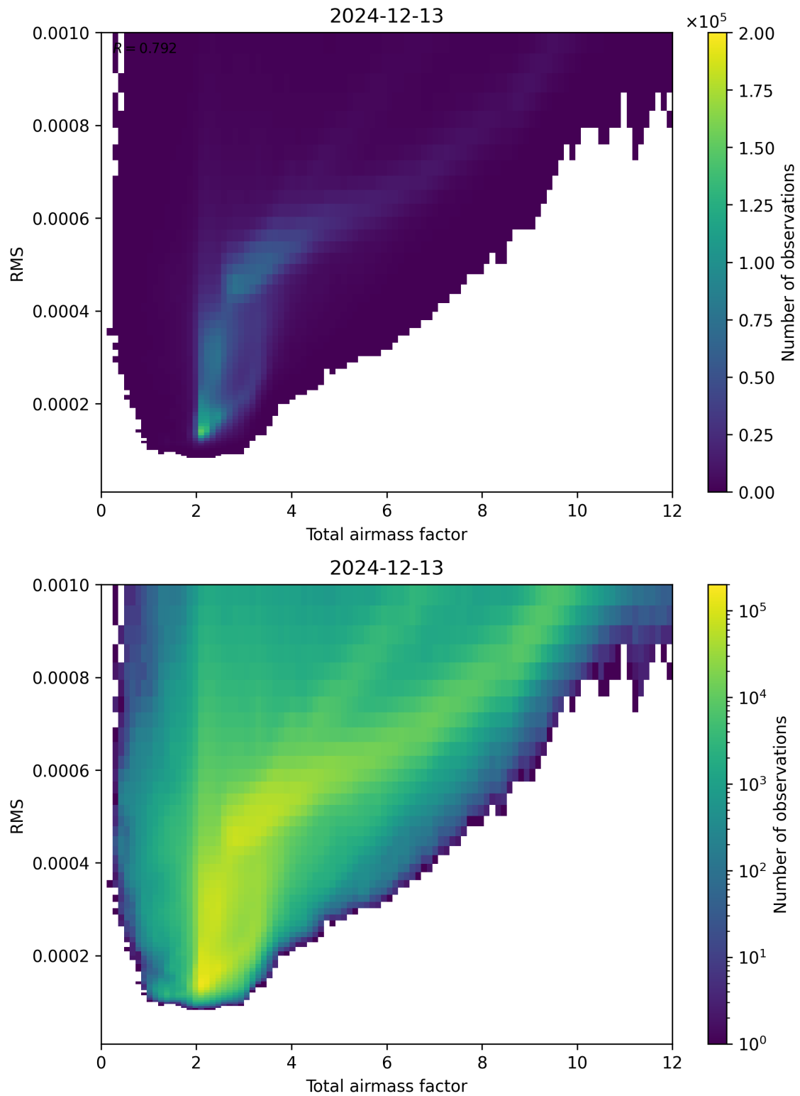
Figure 69: Scatter density plot of “Total airmass factor” against “RMS” for 2024-12-12 to 2024-12-14.
