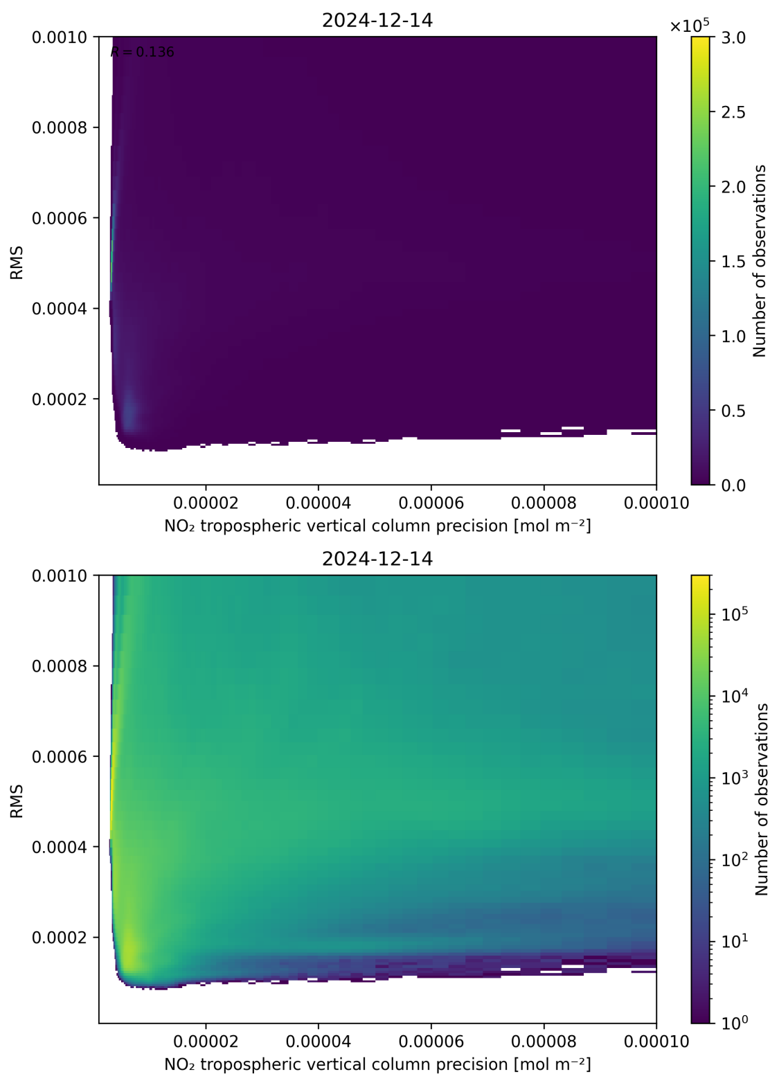
Figure 140: Scatter density plot of “NO 2 tropospheric vertical column precision” against “RMS” for 2024-12-13 to 2024-12-15.
