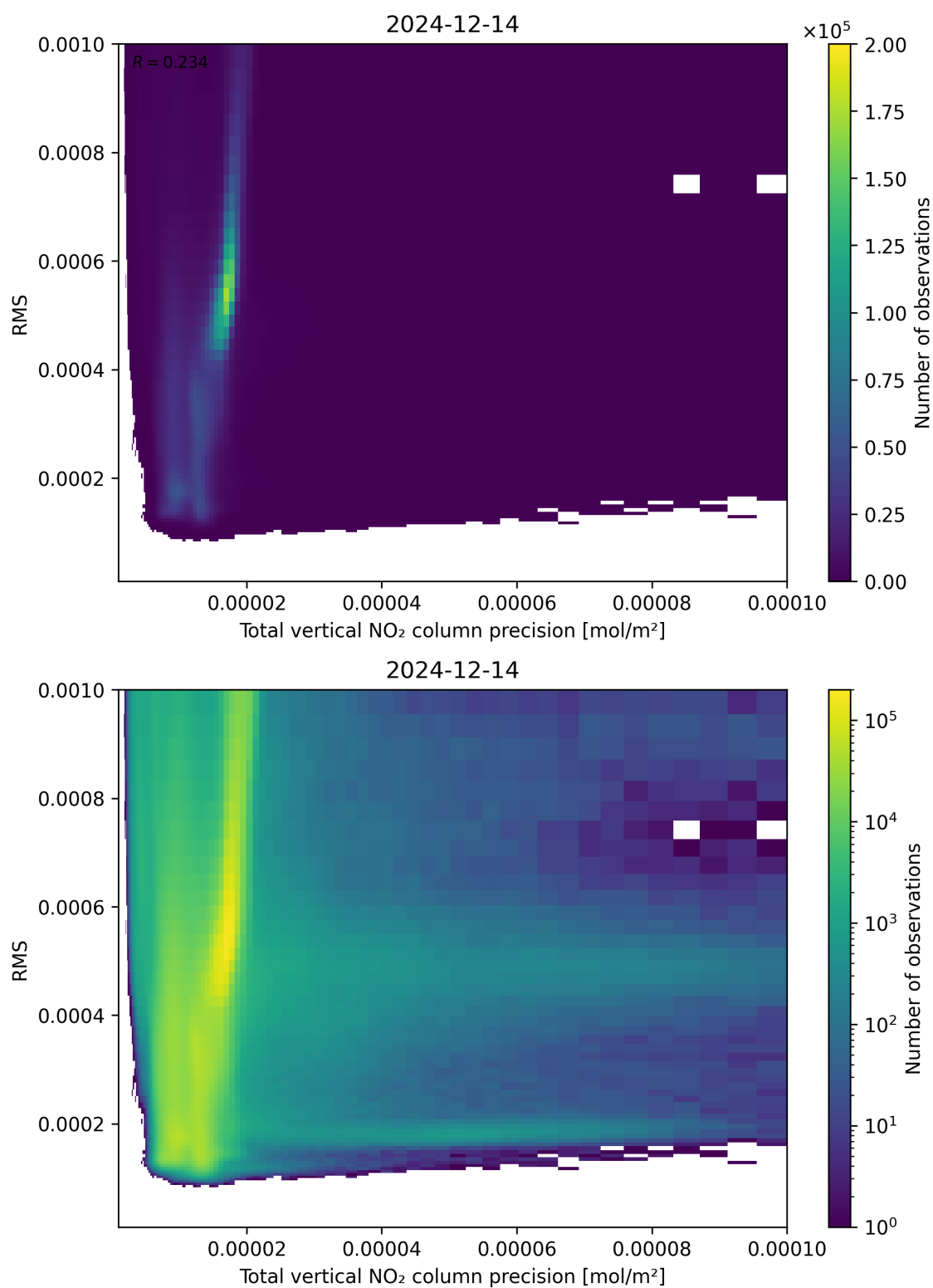
Figure 119: Scatter density plot of “Total vertical NO 2 column precision” against “RMS” for 2024-12-13 to 2024-12-15.
