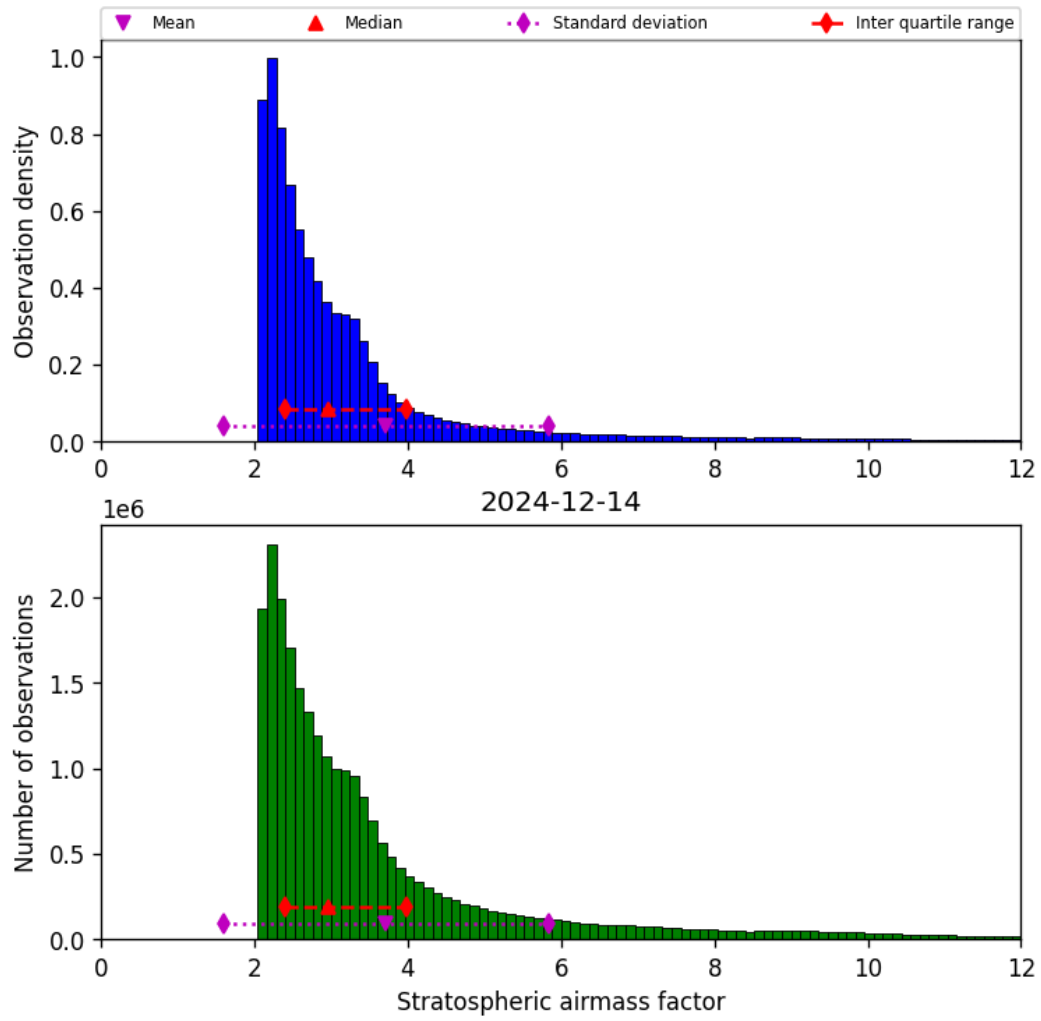
Figure 44: Histogram of “Stratospheric airmass factor” for 2024-12-13 to 2024-12-15
