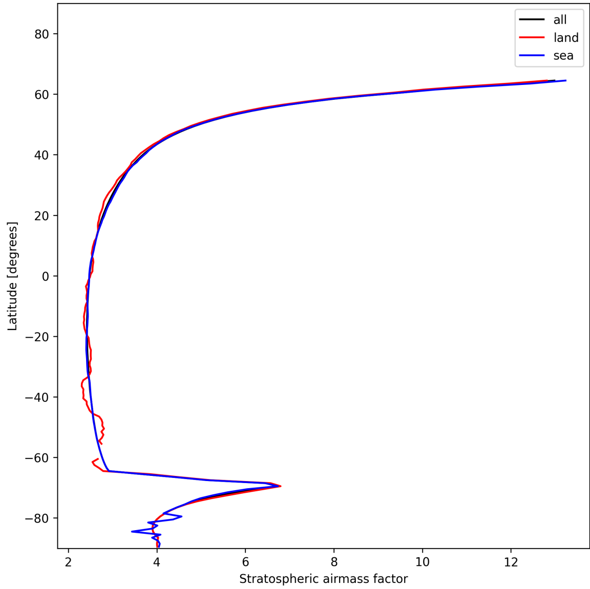
Figure 27: Zonal average of “Stratospheric airmass factor” for 2024-12-13 to 2024-12-15.
