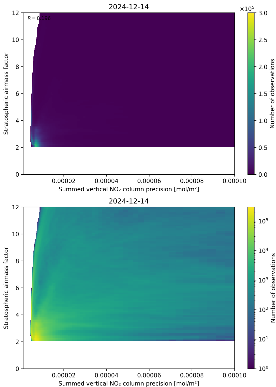
Figure 106: Scatter density plot of “Summed vertical NO 2 column precision” against “Stratospheric airmass factor” for 2024-12-13 to 2024-12-15.
