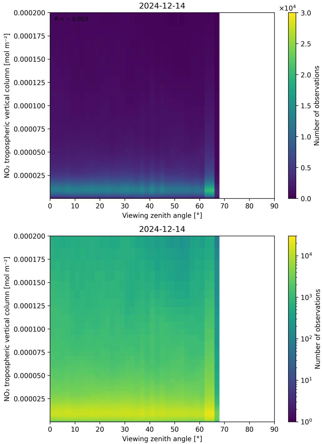
Figure 169: Scatter density plot of “Viewing zenith angle” against “NO 2 tropospheric vertical column” for 2024-12-13 to 2024-12-15.
