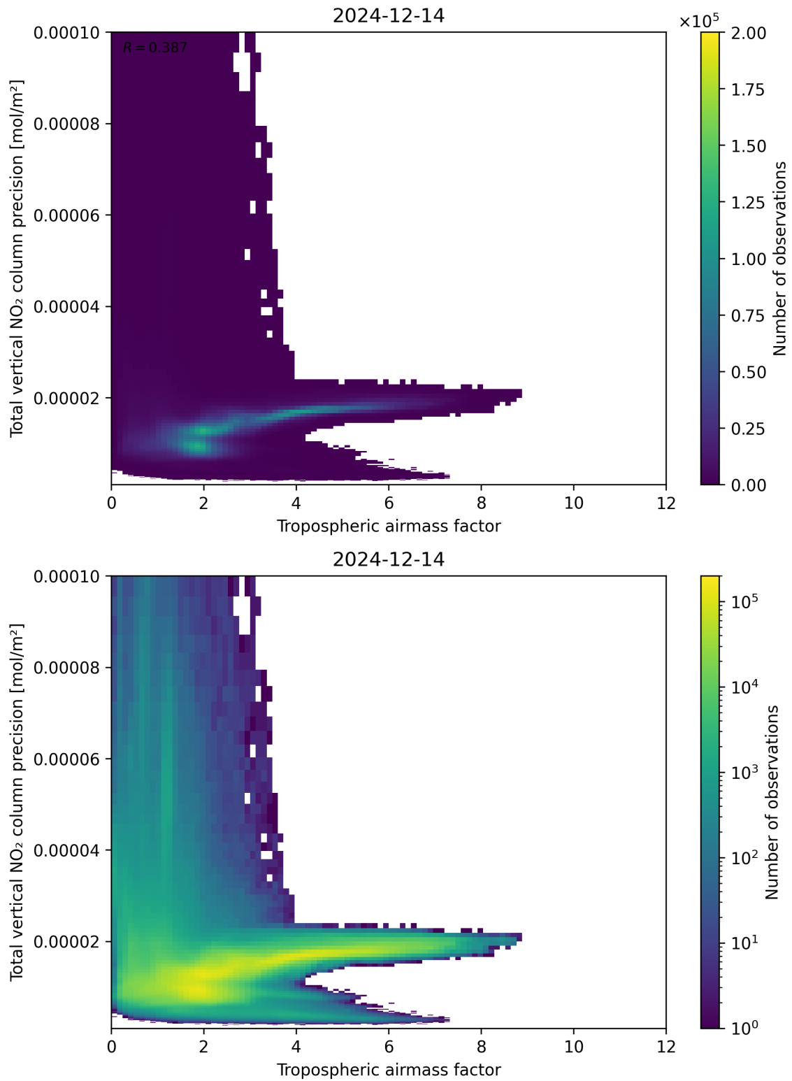
Figure 78: Scatter density plot of “Tropospheric air mass factor” against “Total vertical NO 2 column precision” for 2024-12-13 to 2024-12-15.
