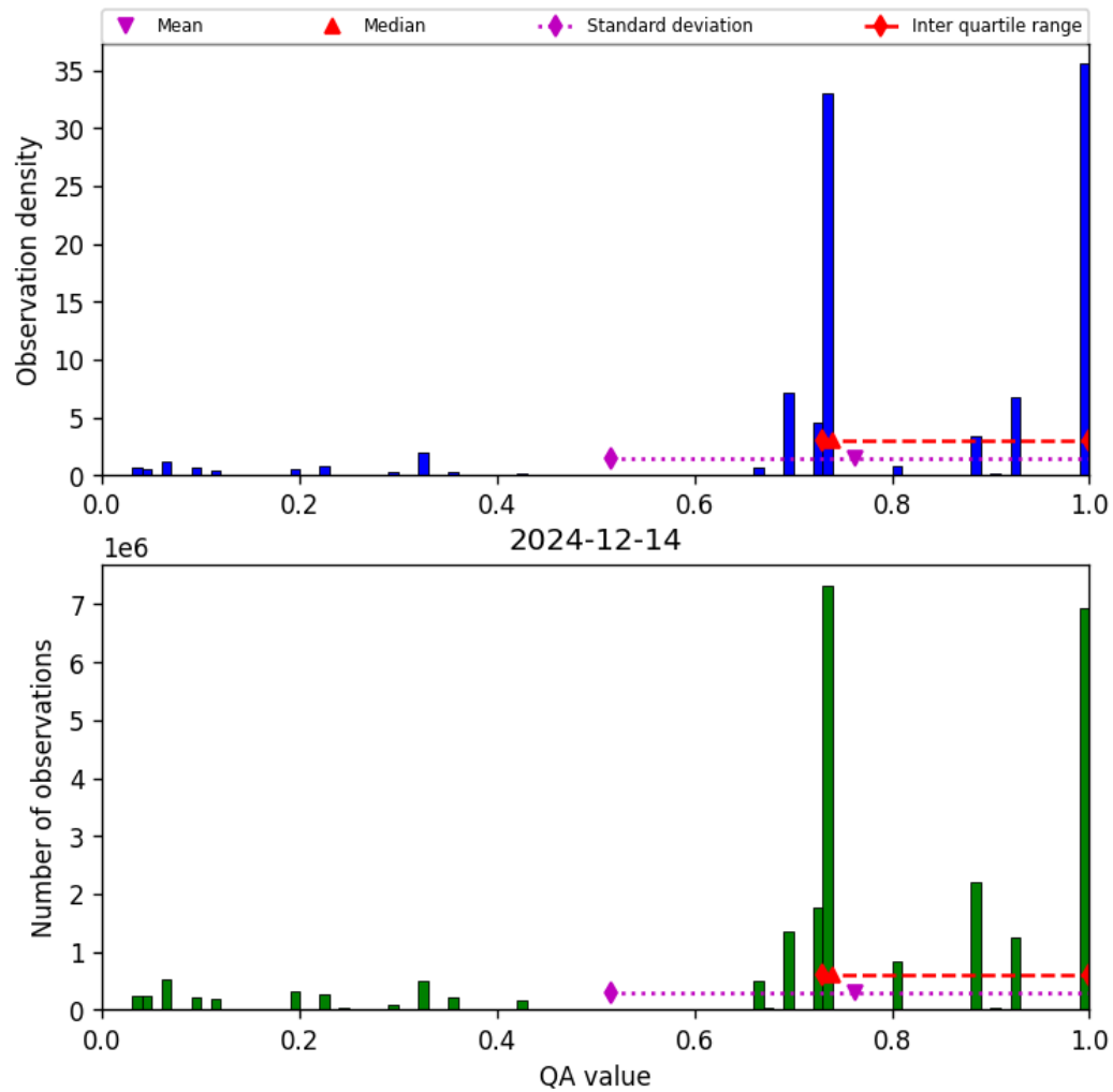
Figure 28: Histogram of “QA value” for 2024-12-13 to 2024-12-15
