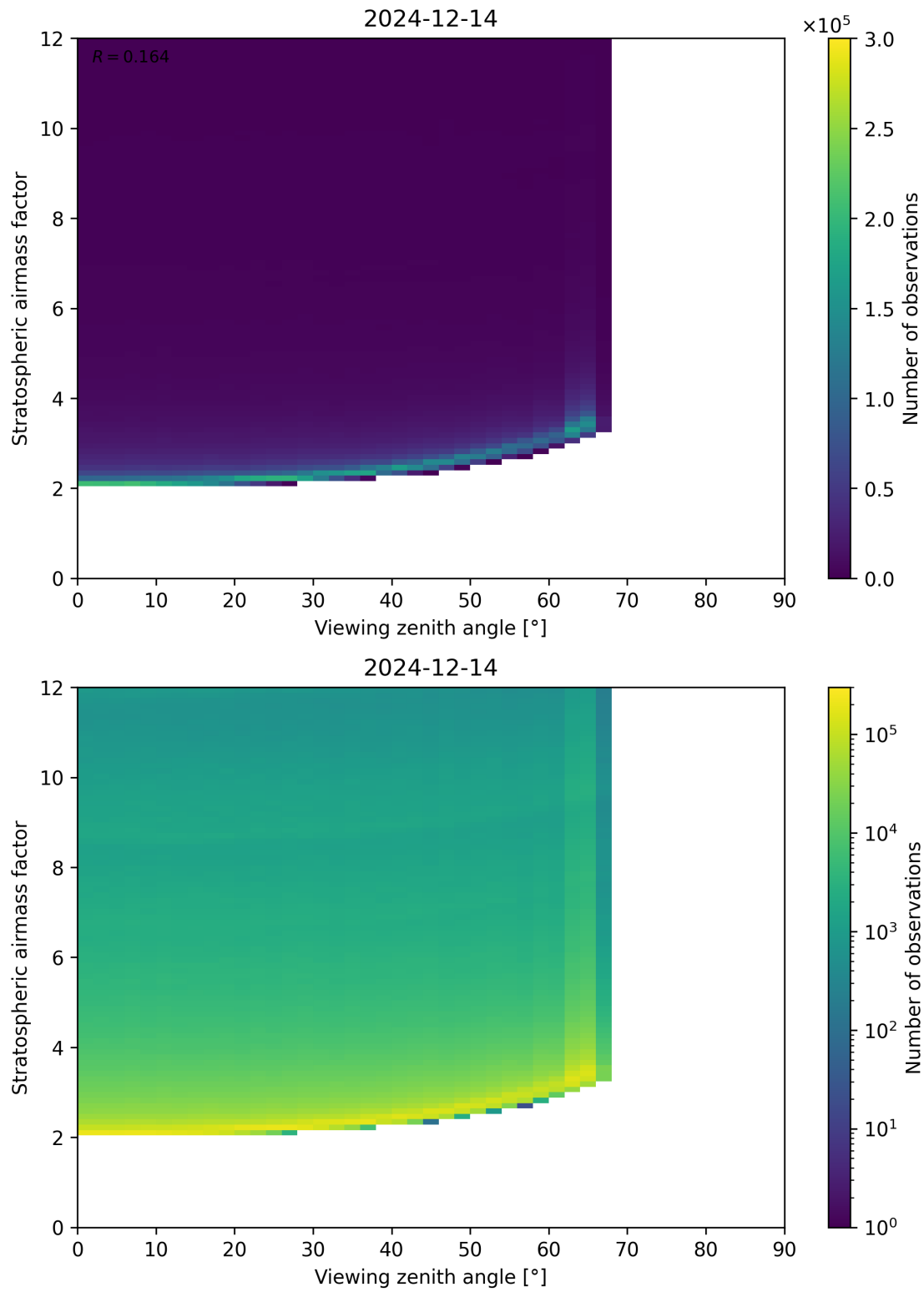
Figure 159: Scatter density plot of “Viewing zenith angle” against “Stratospheric airmass factor” for 2024-12-13 to 2024-12-15.
