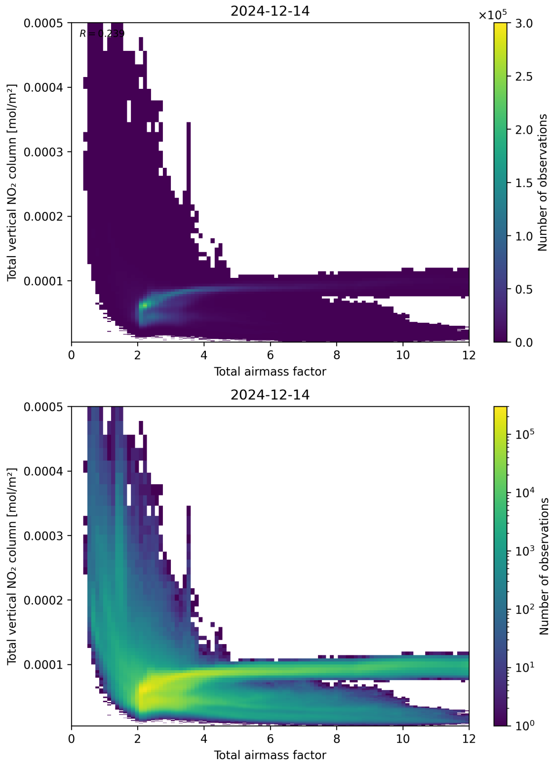
Figure 67: Scatter density plot of “Total air mass factor” against “Total vertical NO 2 column” for 2024-12-13 to 2024-12-15.
