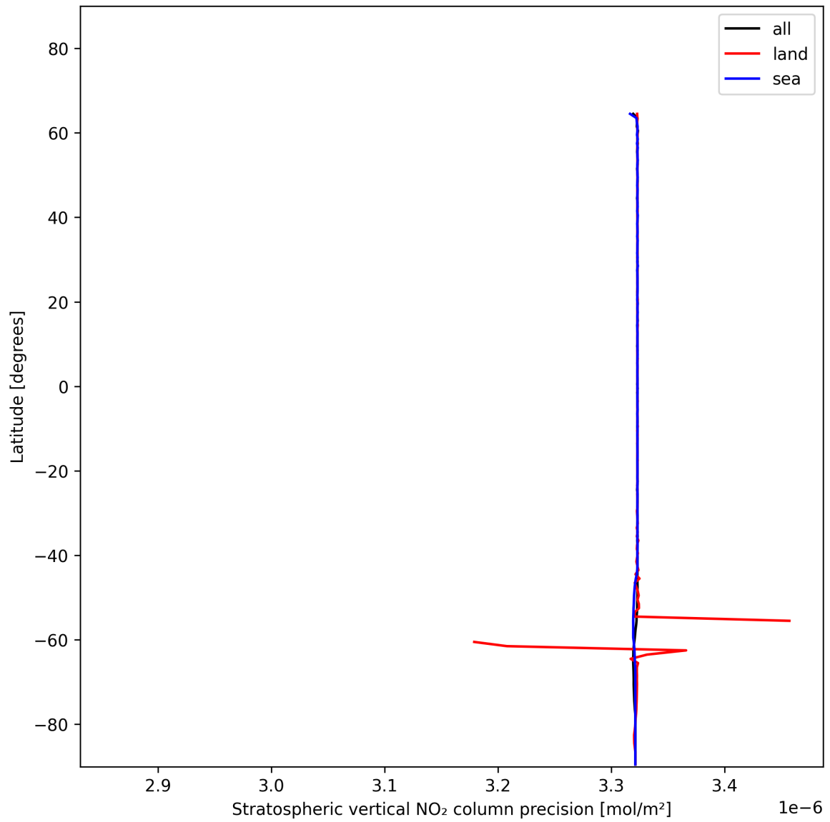
Figure 20: Zonal average of “Stratospheric vertical NO 2 column precision” for 2024-12-13 to 2024-12-15.
