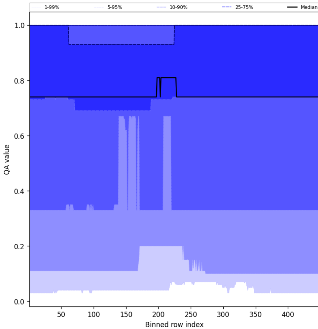
Figure 45: Along track statistics of “QA value” for 2024-12-13 to 2024-12-15
