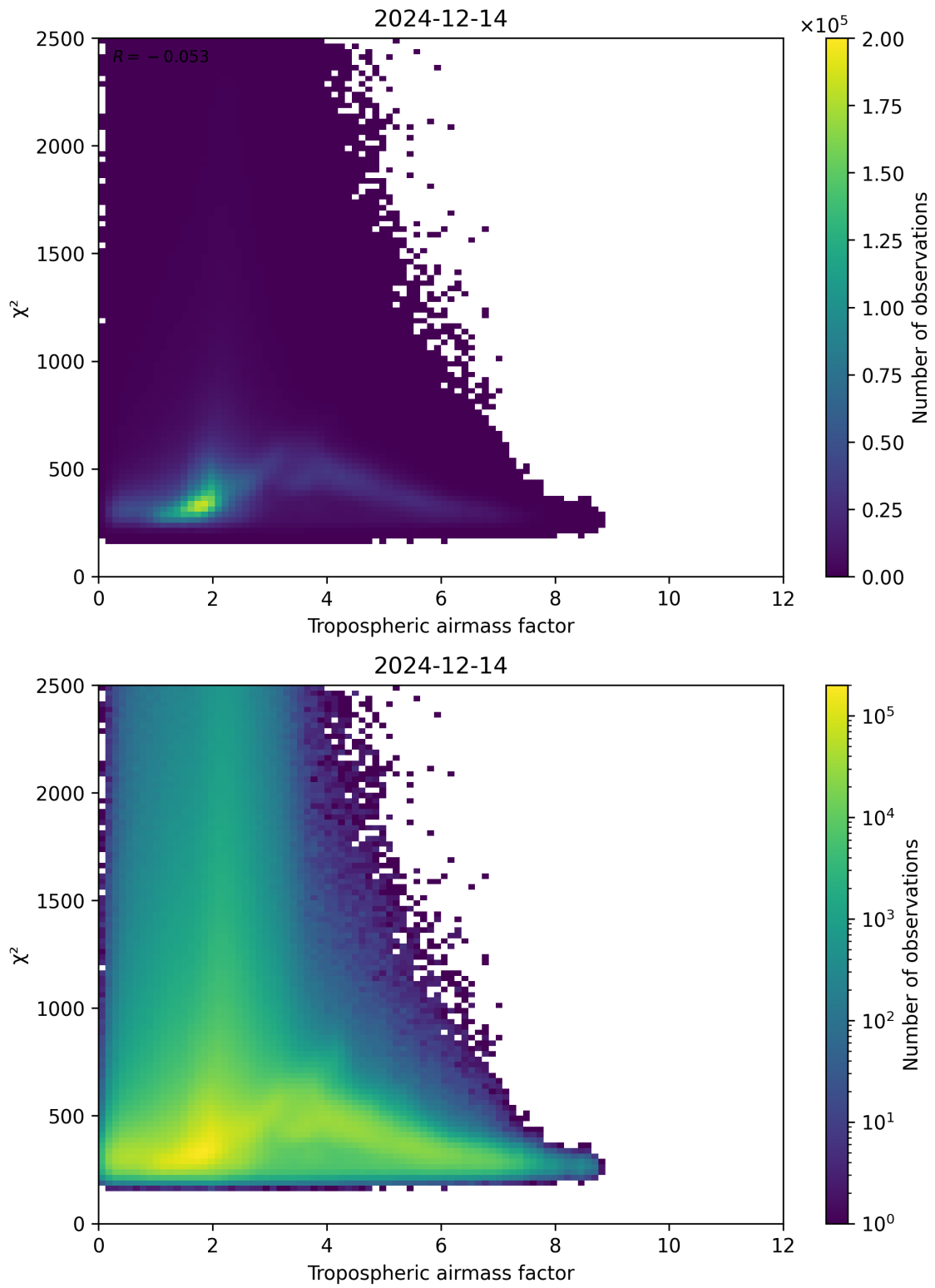
Figure 73: Scatter density plot of “Tropospheric airmass factor” against “ \chi^2 ” for 2024-12-13 to 2024-12-15.
