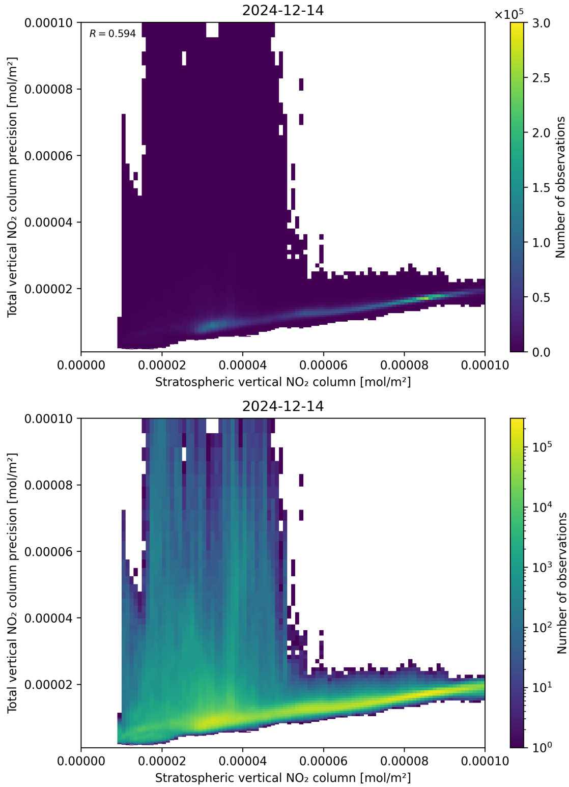
Figure 101: Scatter density plot of “Stratospheric vertical NO 2 column” against “Total vertical NO 2 column precision” for 2024-12-13 to 2024-12-15.
