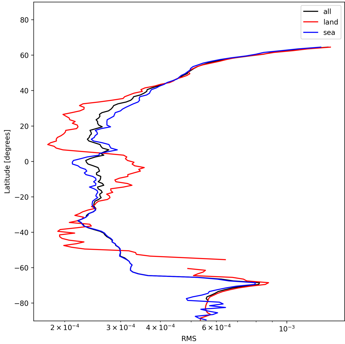
Figure 26: Zonal average of “RMS” for 2024-12-13 to 2024-12-15.
