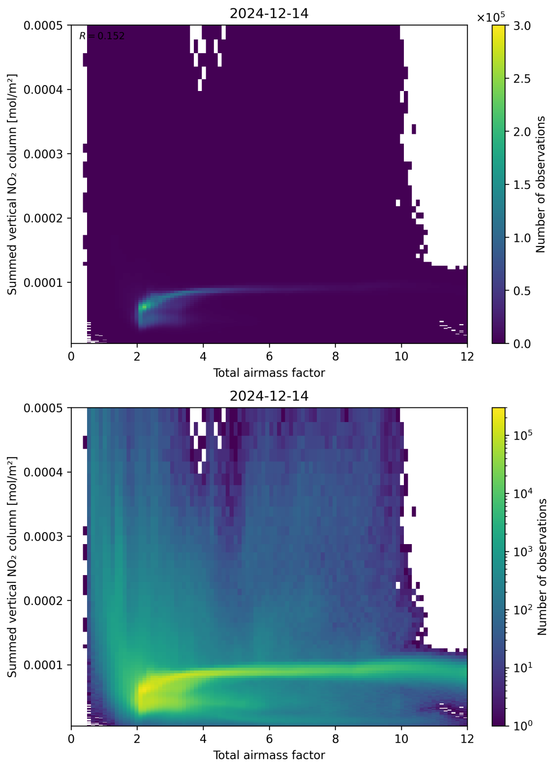
Figure 65: Scatter density plot of “Total airmass factor” against “Summed vertical NO 2 column” for 2024-12-13 to 2024-12-15.
