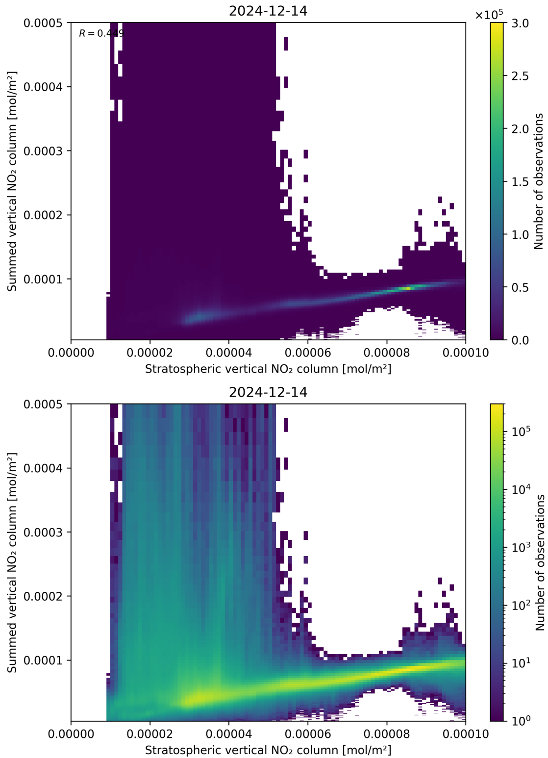
Figure 98: Scatter density plot of “Stratospheric vertical NO 2 column” against “Summed vertical NO 2 column” for 2024-12-13 to 2024-12-15.
