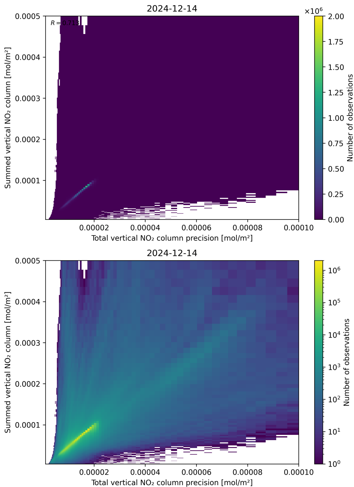
Figure 117: Scatter density plot of “Total vertical NO 2 column precision” against “Summed vertical NO 2 column” for 2024-12-13 to 2024-12-15.
