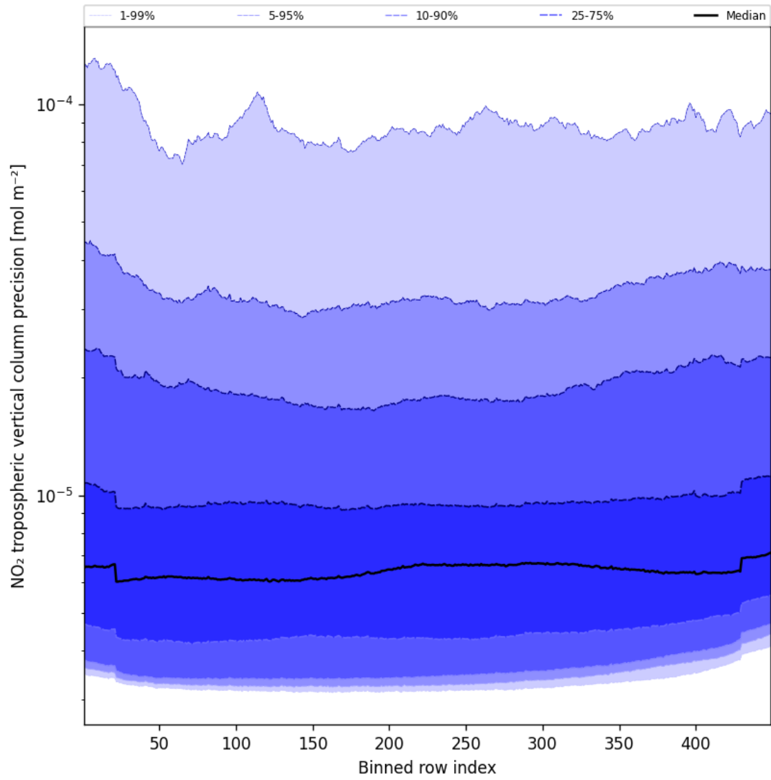
Figure 47: Along track statistics of “NO 2 tropospheric vertical column precision” for 2024-12-13 to 2024-12-15
