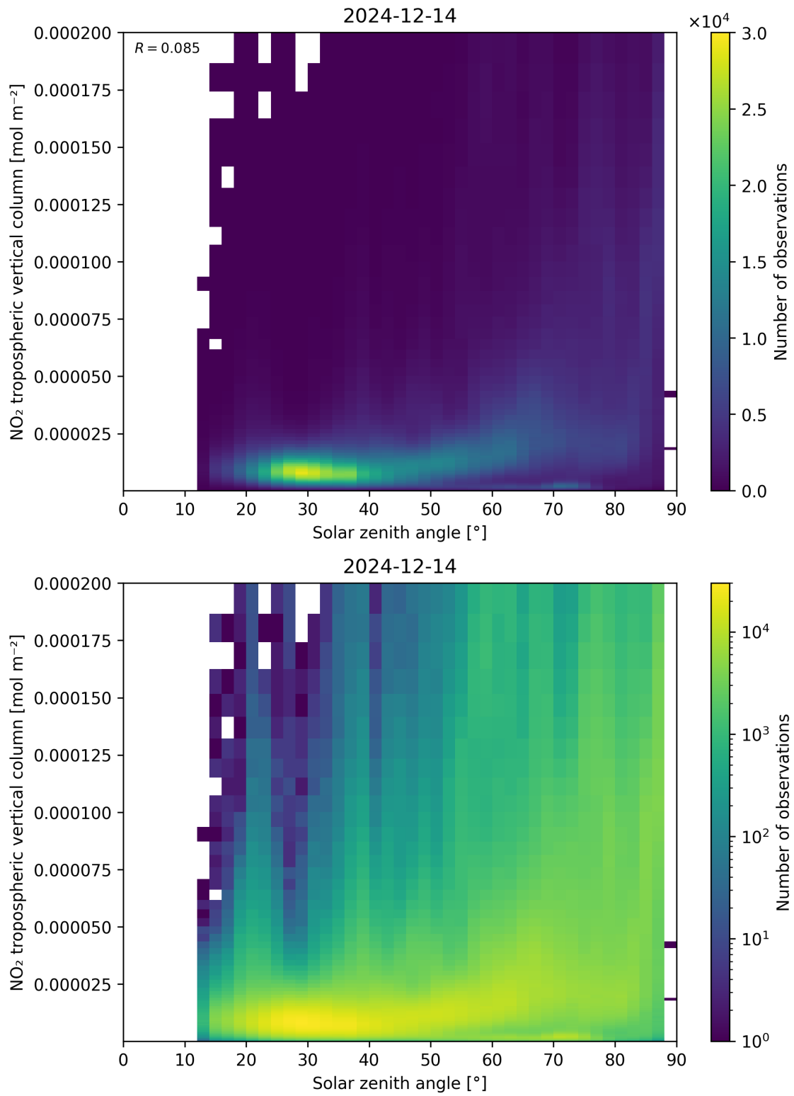
Figure 155: Scatter density plot of “Solar zenith angle” against “NO 2 tropospheric vertical column” for 2024-12-13 to 2024-12-15.
