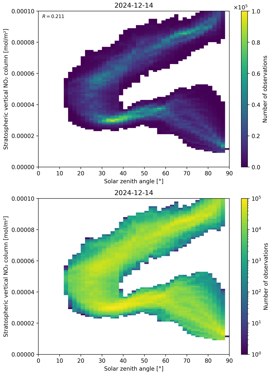
Figure 150: Scatter density plot of “Solar zenith angle” against “Stratospheric vertical NO 2 column” for 2024-12-13 to 2024-12-15.
