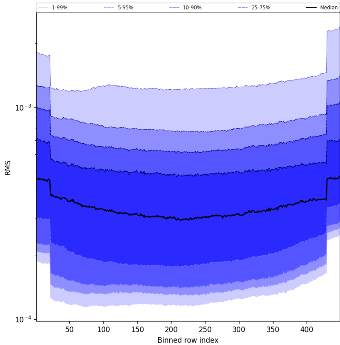
Figure 60: Along track statistics of “RMS” for 2024-12-13 to 2024-12-15
