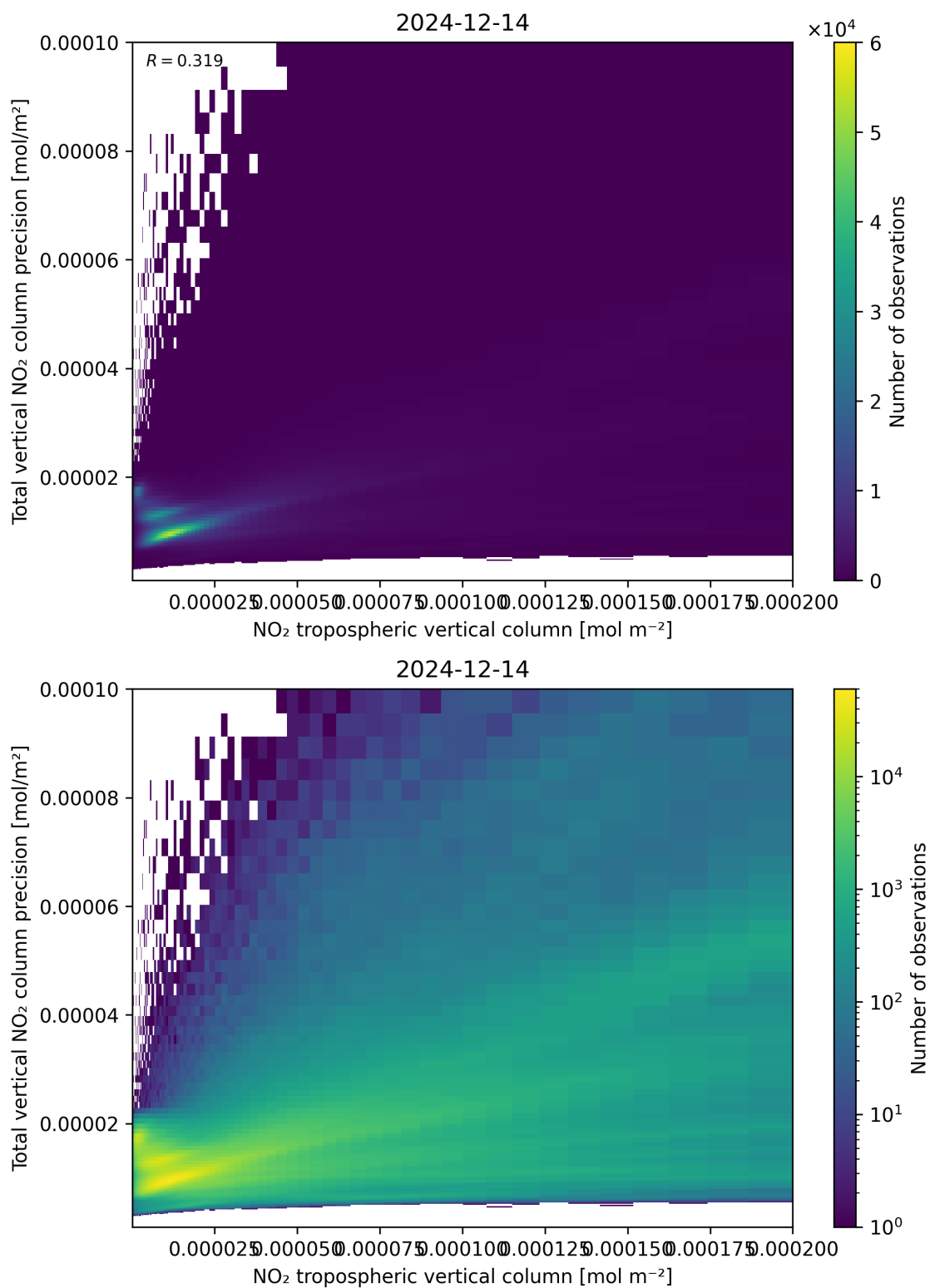
Figure 129: Scatter density plot of “NO 2 tropospheric vertical column” against “Total vertical NO 2 column precision” for 2024-12-13 to 2024-12-15.
