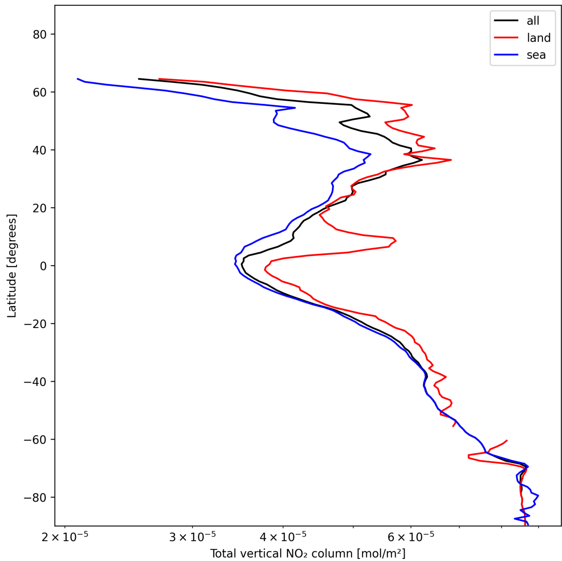
Figure 21: Zonal average of “Total vertical NO 2 column” for 2024-12-13 to 2024-12-15.
