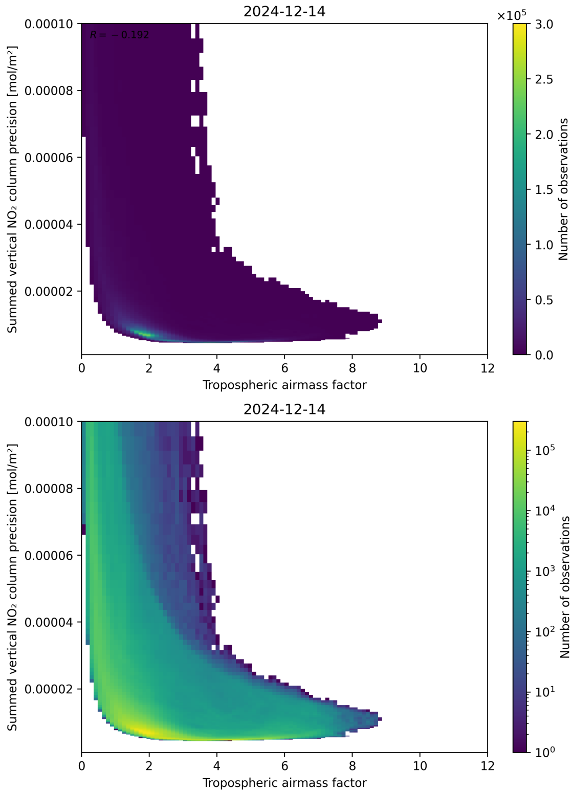
Figure 76: Scatter density plot of “Tropospheric air mass factor” against “Summed vertical NO 2 column precision” for 2024-12-13 to 2024-12-15.
