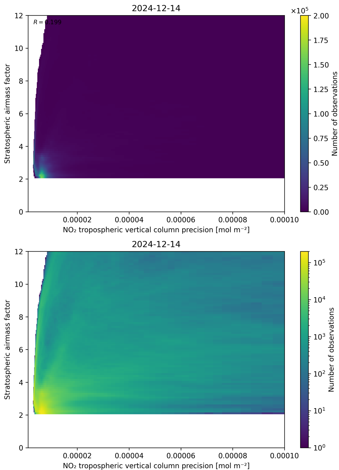
Figure 131: Scatter density plot of “NO 2 tropospheric vertical column precision” against “Stratospheric airmass factor” for 2024-12-13 to 2024-12-15.
