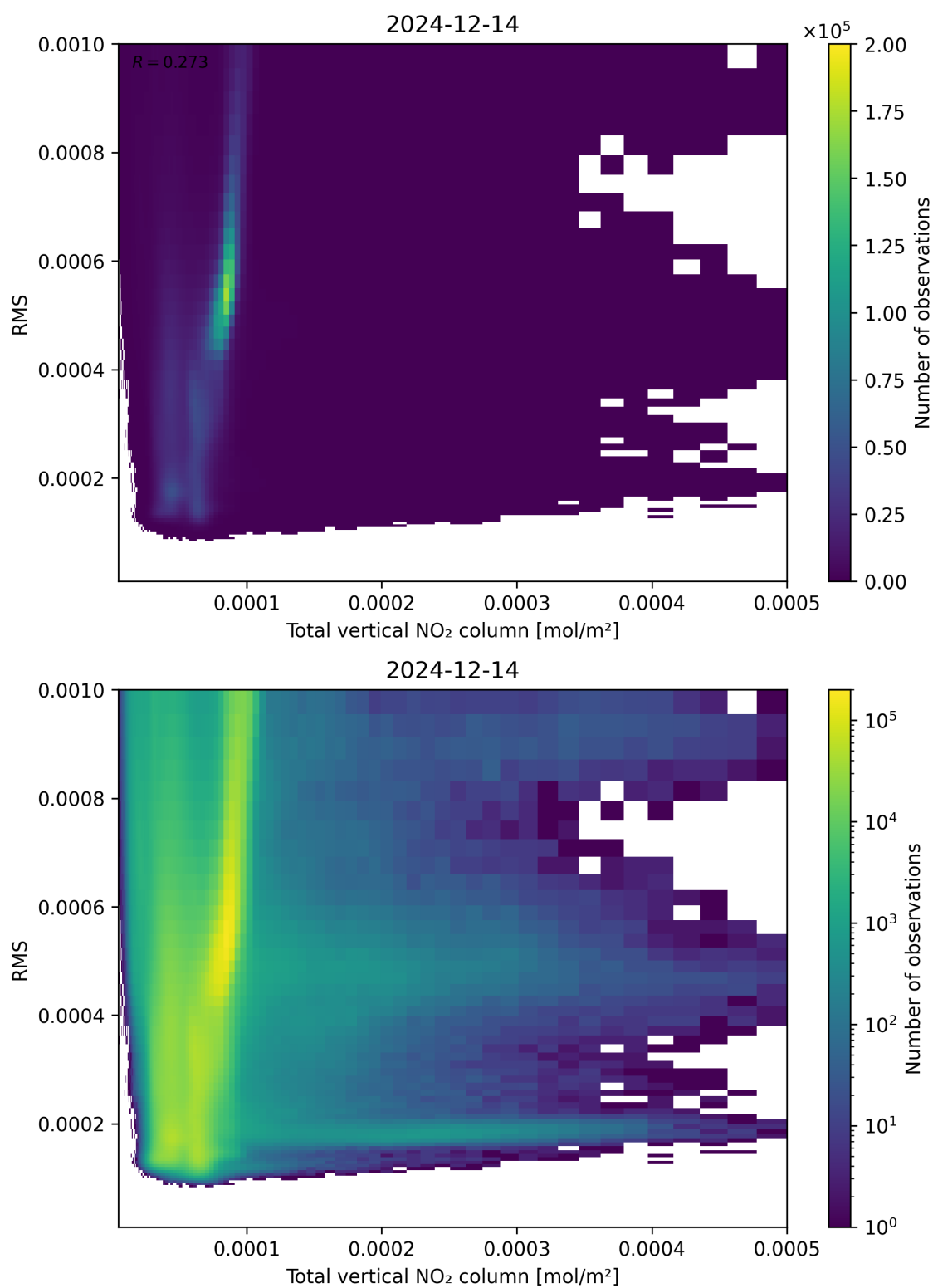
Figure 120: Scatter density plot of “Total vertical NO 2 column” against “RMS” for 2024-12-13 to 2024-12-15.
