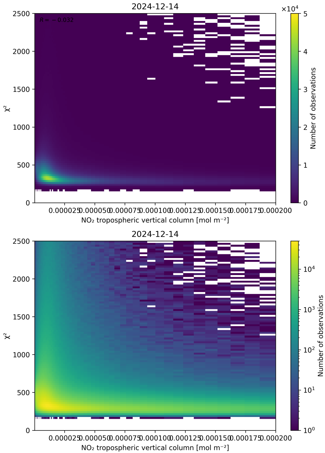
Figure 124: Scatter density plot of “NO 2 tropospheric vertical column” against “ \chi^2 ” for 2024-12-13 to 2024-12-15.
