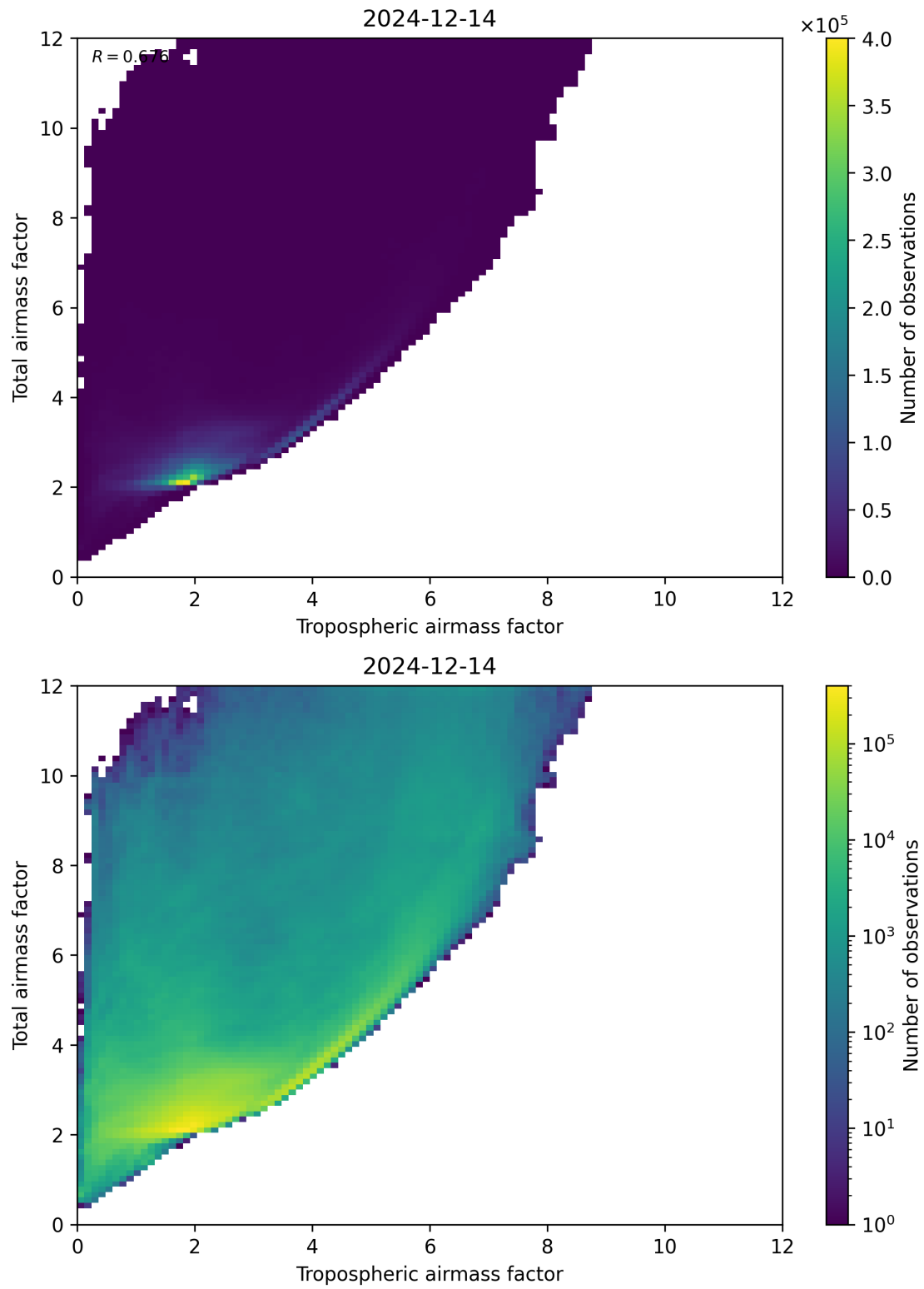
Figure 72: Scatter density plot of “Tropospheric airmass factor” against “Total airmass factor” for 2024-12-13 to 2024-12-15.
