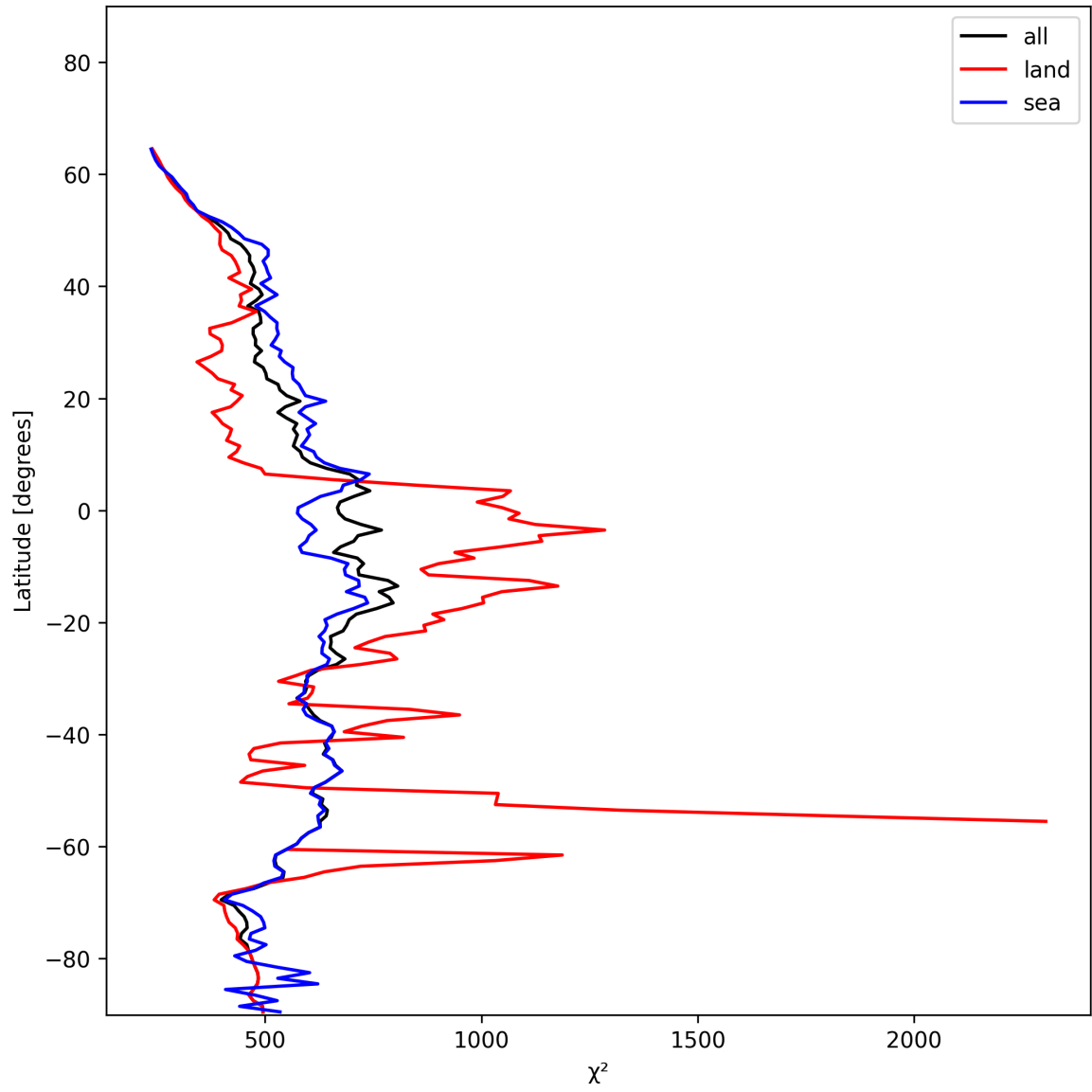
Figure 25: Zonal average of “ \chi^2 ” for 2024-12-13 to 2024-12-15.
