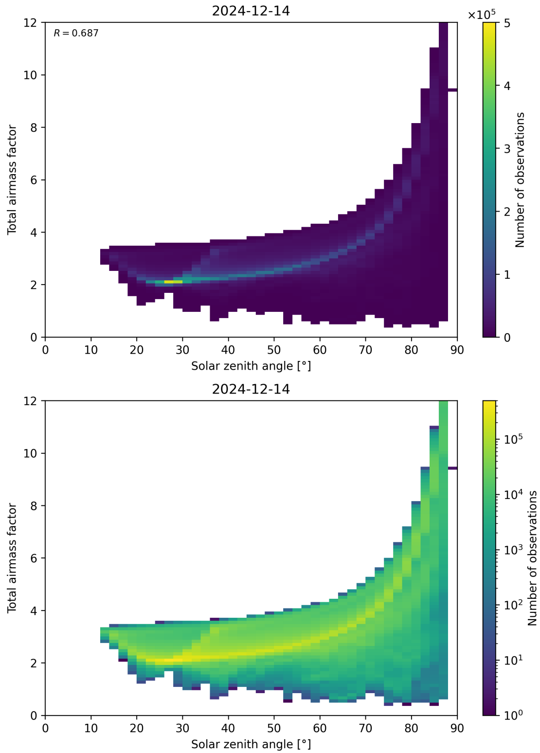
Figure 146: Scatter density plot of “Solar zenith angle” against “Total air mass factor” for 2024-12-13 to 2024-12-15.
