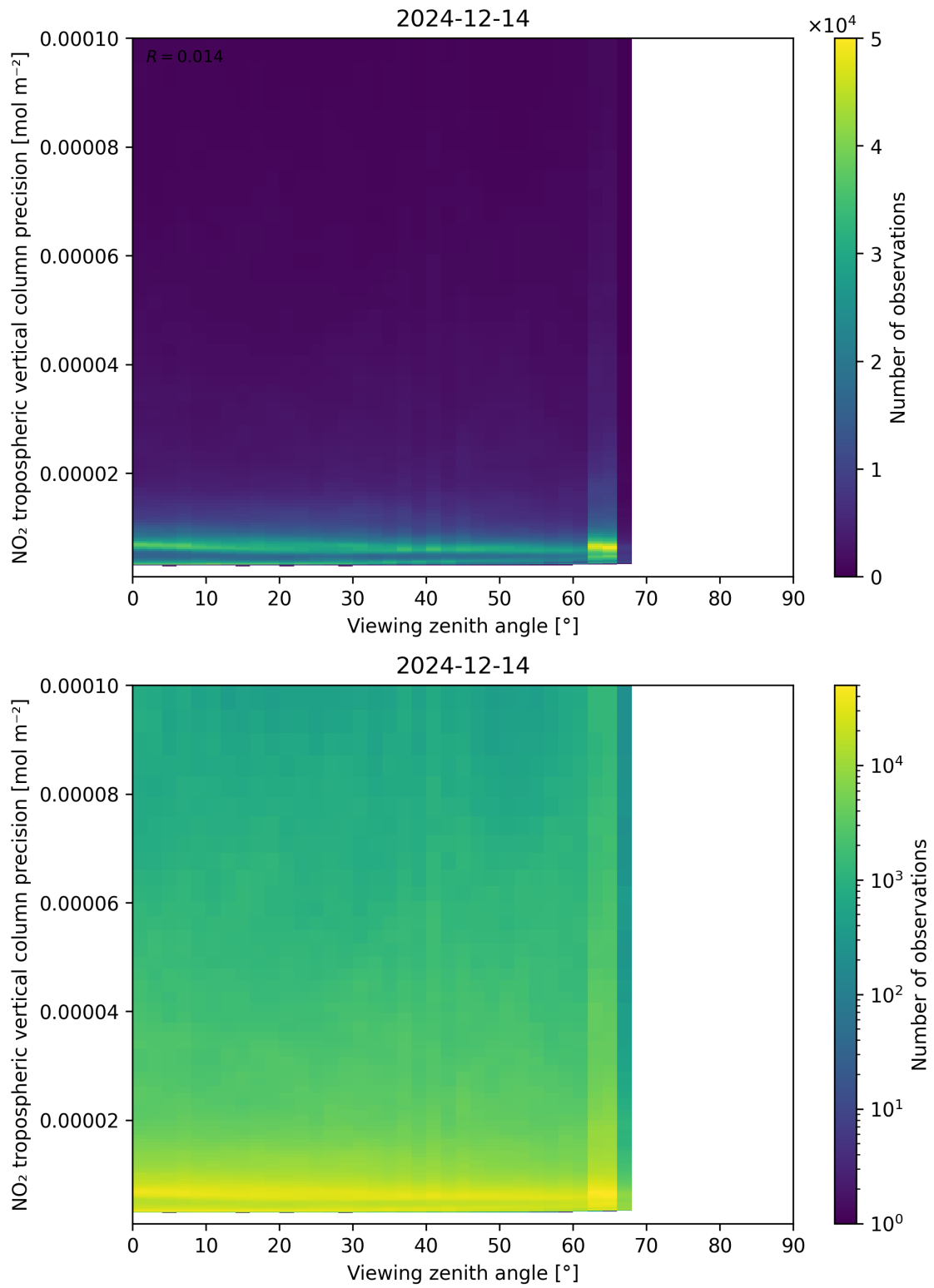
Figure 170: Scatter density plot of “Viewing zenith angle” against “NO 2 tropospheric vertical column precision” for 2024-12-13 to 2024-12-15.
