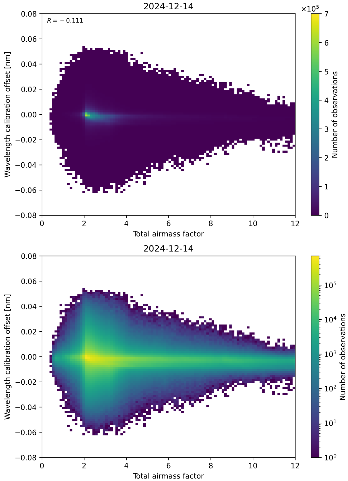
Figure 70: Scatter density plot of “Total airmass factor” against “Wavelength calibration offset” for 2024-12-13 to 2024-12-15.
