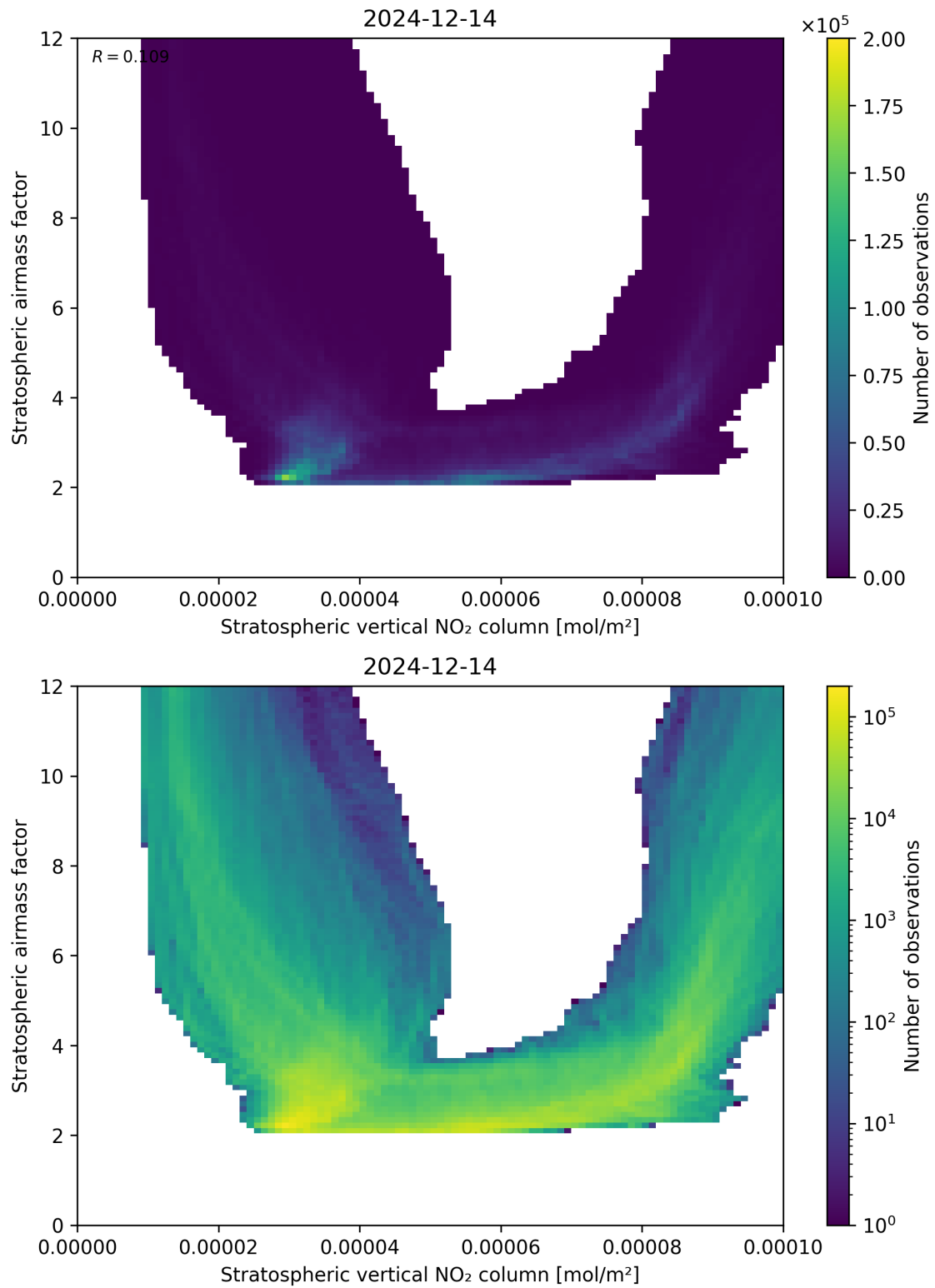
Figure 96: Scatter density plot of “Stratospheric vertical NO 2 column” against “Stratospheric airmass factor” for 2024-12-13 to 2024-12-15.
