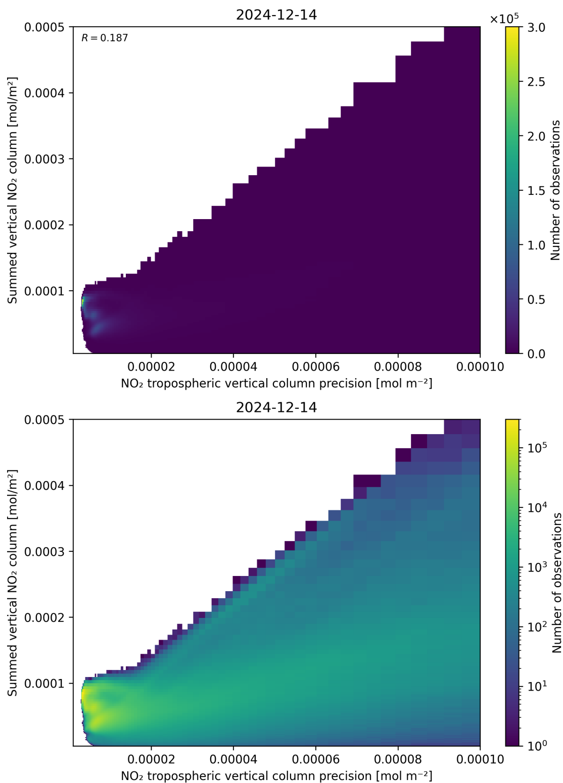
Figure 136: Scatter density plot of “NO 2 tropospheric vertical column precision” against “Summed vertical NO 2 column” for 2024-12-13 to 2024-12-15.
