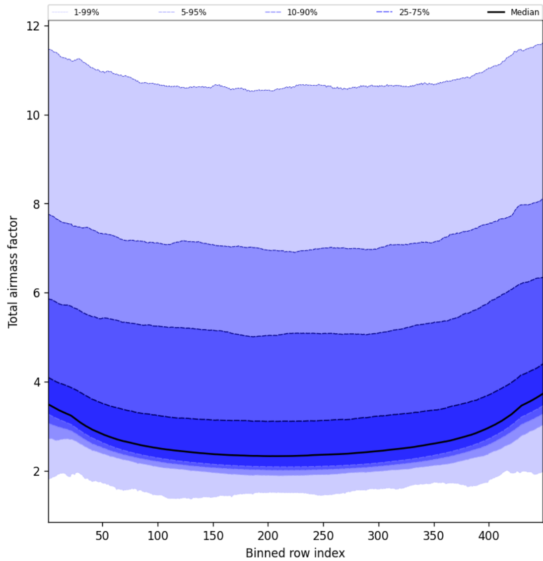
Figure 49: Along track statistics of “Total airmass factor” for 2024-12-13 to 2024-12-15
