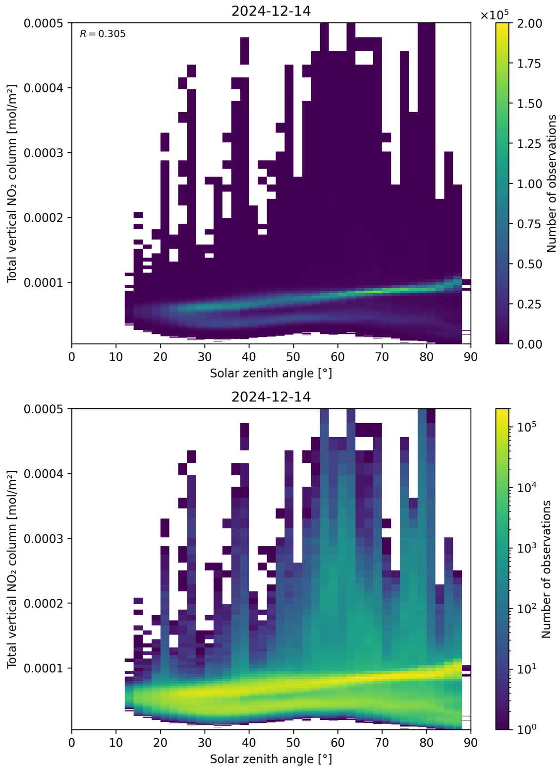
Figure 153: Scatter density plot of “Solar zenith angle” against “Total vertical NO 2 column” for 2024-12-13 to 2024-12-15.
