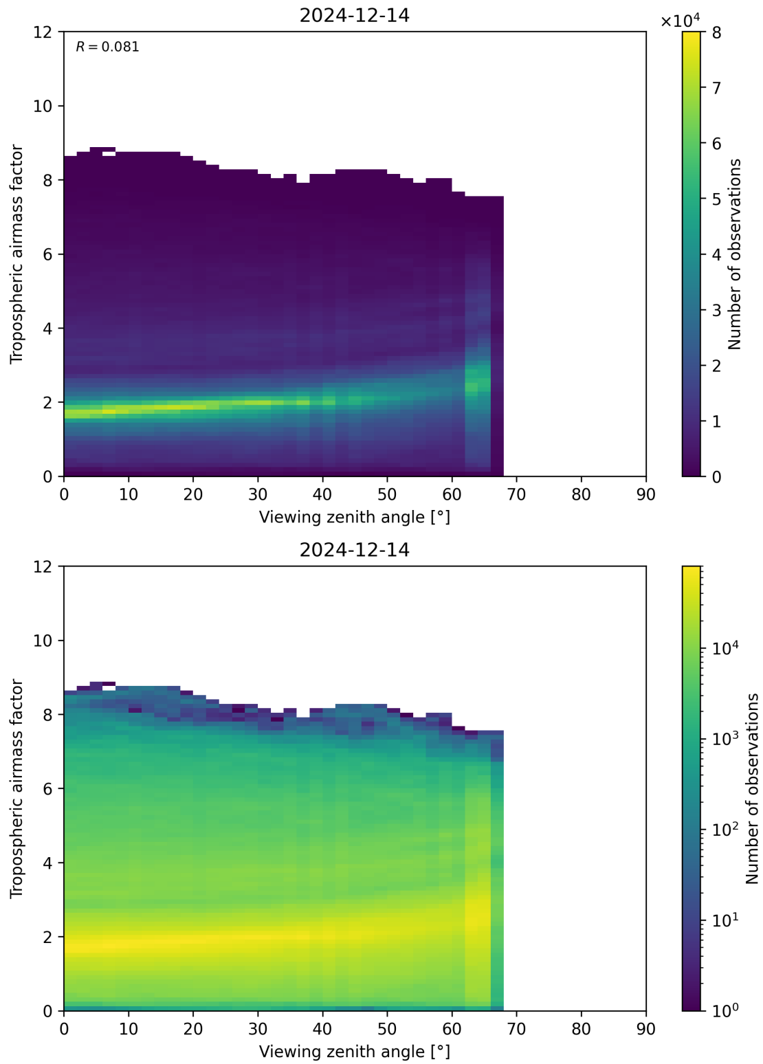
Figure 161: Scatter density plot of “Viewing zenith angle” against “Tropospheric airmass factor” for 2024-12-13 to 2024-12-15.
