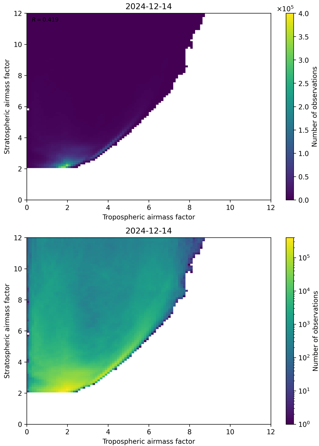
Figure 71: Scatter density plot of “Tropospheric airmass factor” against “Stratospheric airmass factor” for 2024-12-13 to 2024-12-15.
