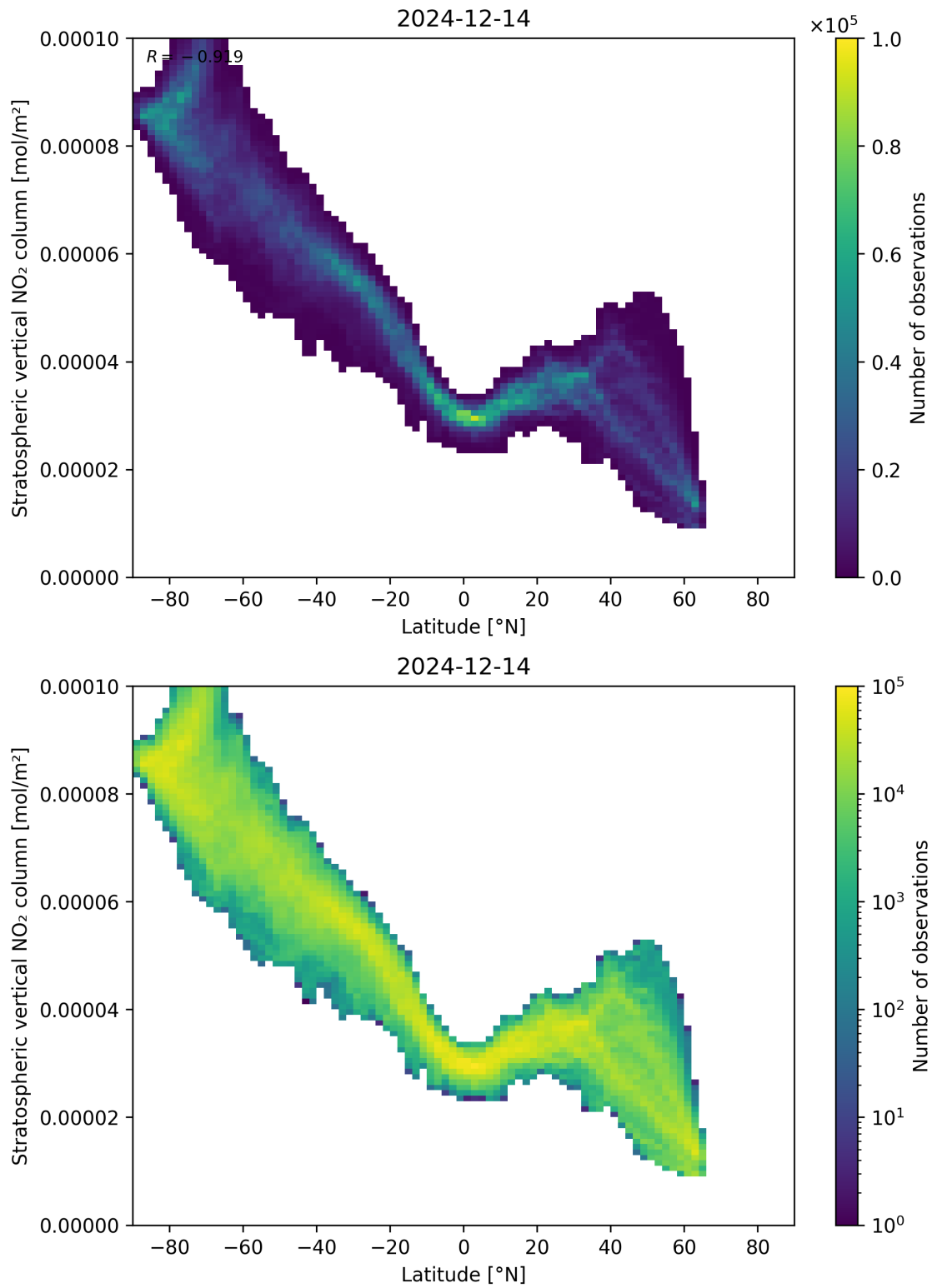
Figure 87: Scatter density plot of “Latitude” against “Stratospheric vertical NO 2 column” for 2024-12-13 to 2024-12-15.
