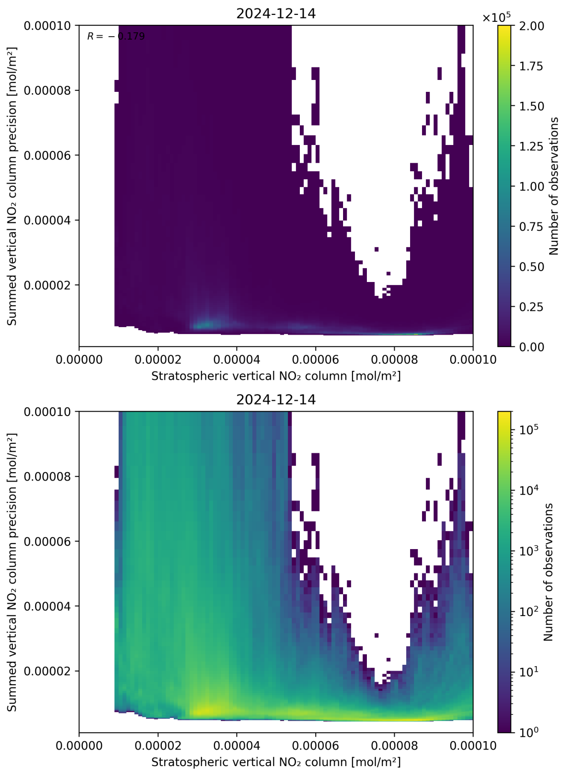
Figure 99: Scatter density plot of “Stratospheric vertical NO 2 column” against “Summed vertical NO 2 column precision” for 2024-12-13 to 2024-12-15.
