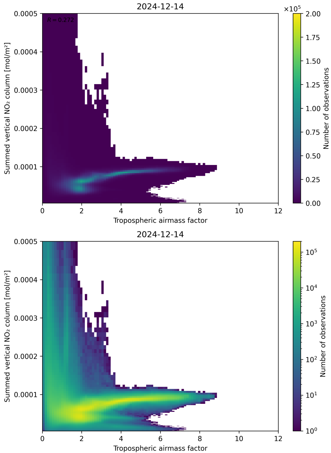
Figure 75: Scatter density plot of “Tropospheric airmass factor” against “Summed vertical NO 2 column” for 2024-12-13 to 2024-12-15.
