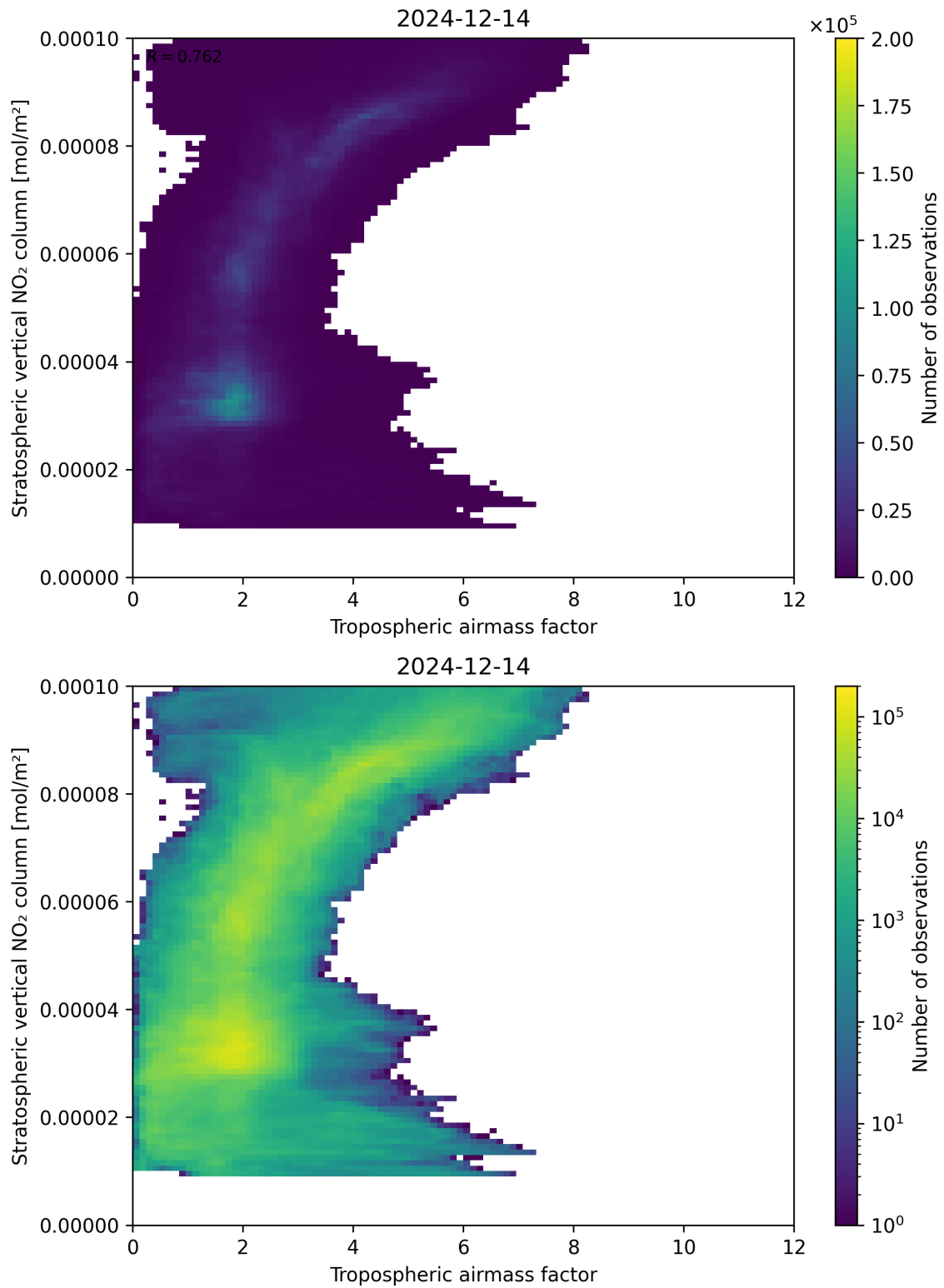
Figure 74: Scatter density plot of “Tropospheric air mass factor” against “Stratospheric vertical NO 2 column” for 2024-12-13 to 2024-12-15.
