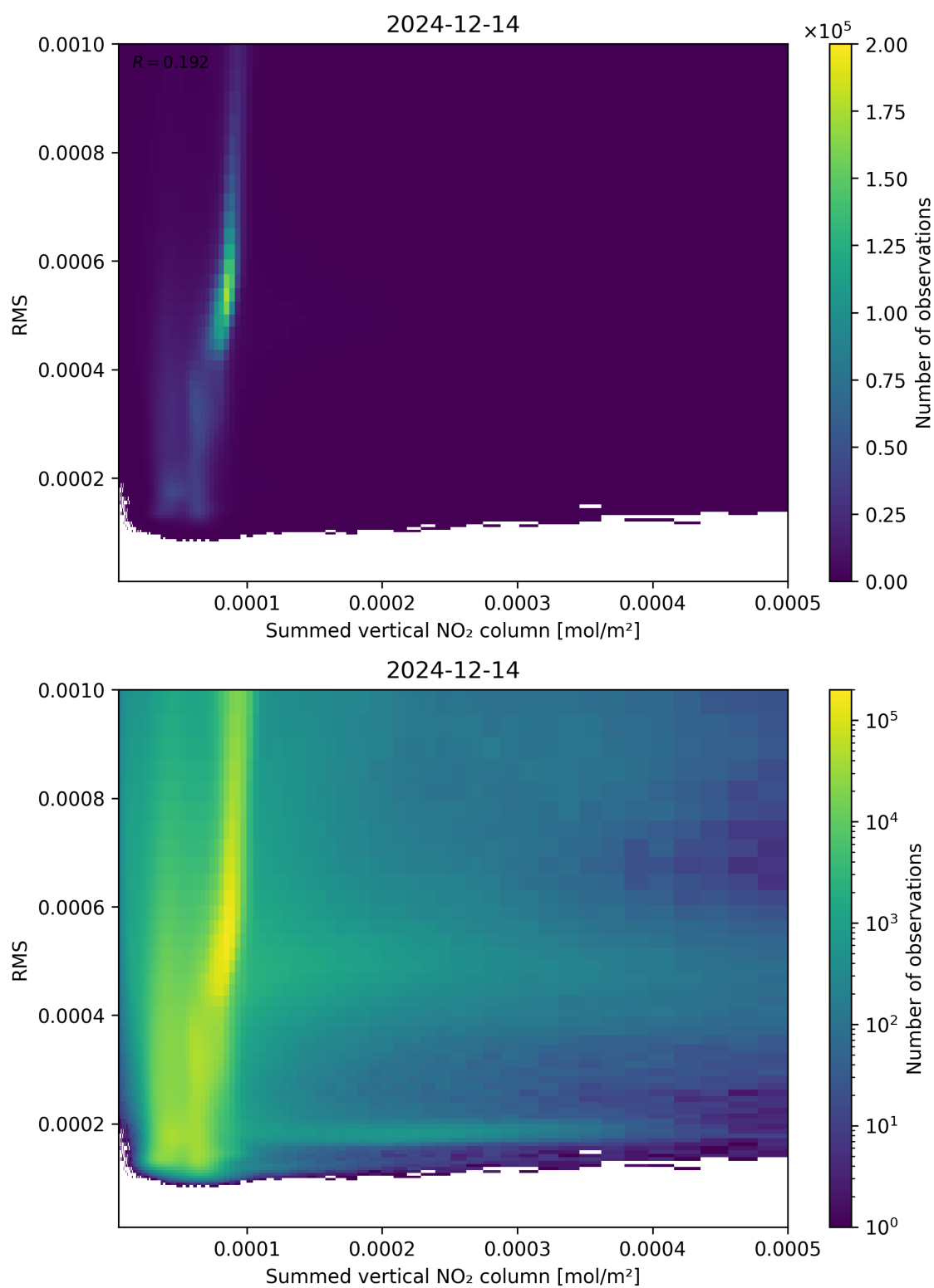
Figure 109: Scatter density plot of “Summed vertical NO 2 column” against “RMS” for 2024-12-13 to 2024-12-15.
