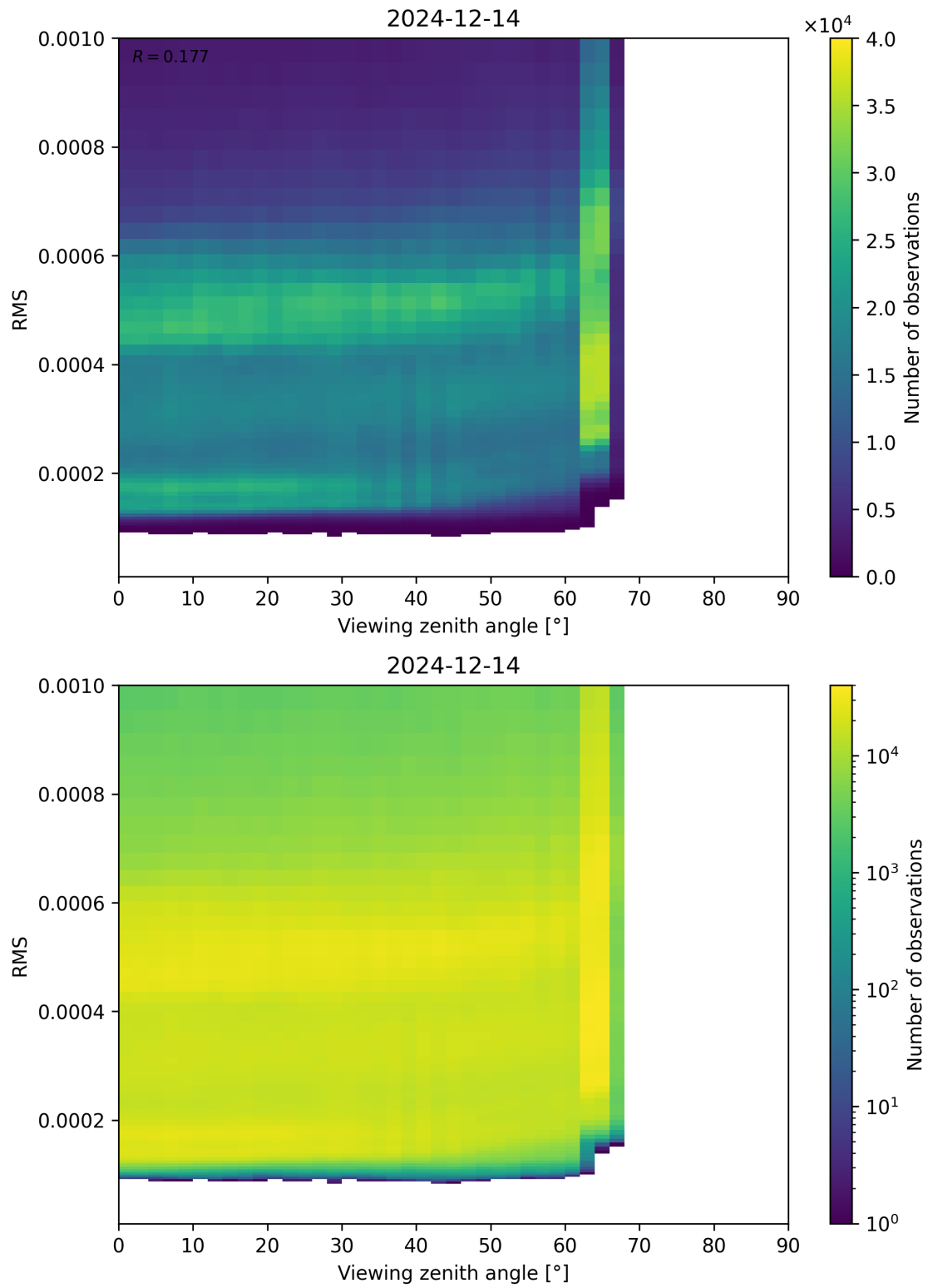
Figure 171: Scatter density plot of “Viewing zenith angle” against “RMS” for 2024-12-13 to 2024-12-15.
