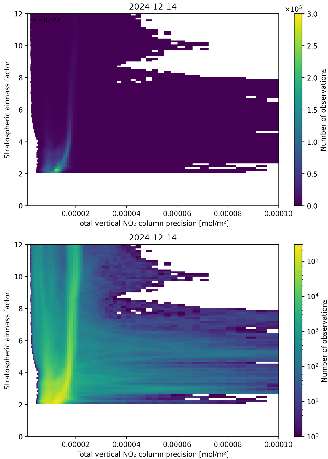
Figure 115: Scatter density plot of “Total vertical NO 2 column precision” against “Stratospheric air mass factor” for 2024-12-13 to 2024-12-15.
