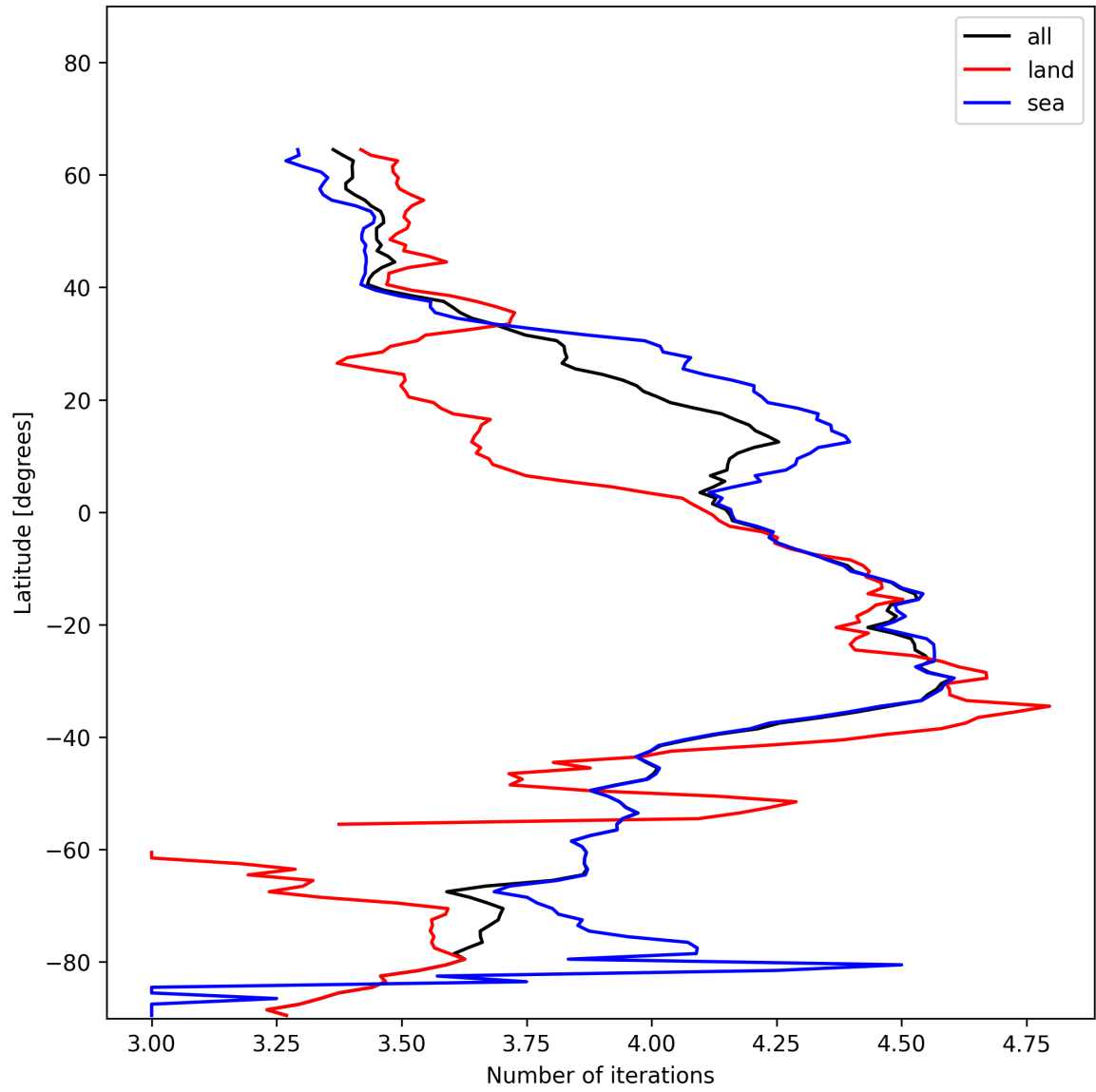
Figure 17: Zonal average of “Number of iterations” for 2024-12-13 to 2024-12-15.
