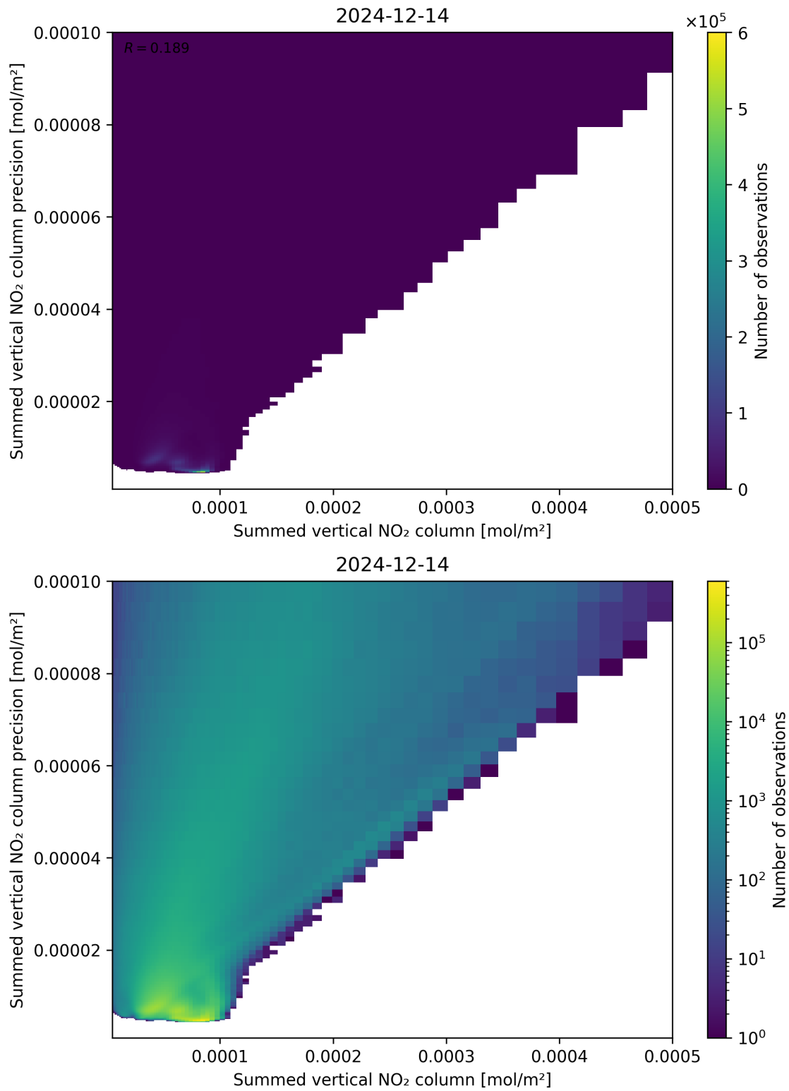
Figure 105: Scatter density plot of “Summed vertical NO 2 column” against “Summed vertical NO 2 column precision” for 2024-12-13 to 2024-12-15.
