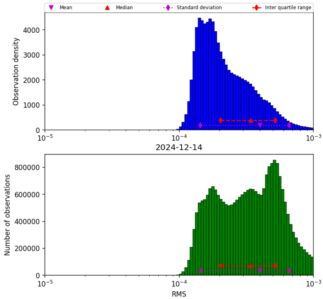
Figure 43: Histogram of “RMS” for 2024-12-13 to 2024-12-15
