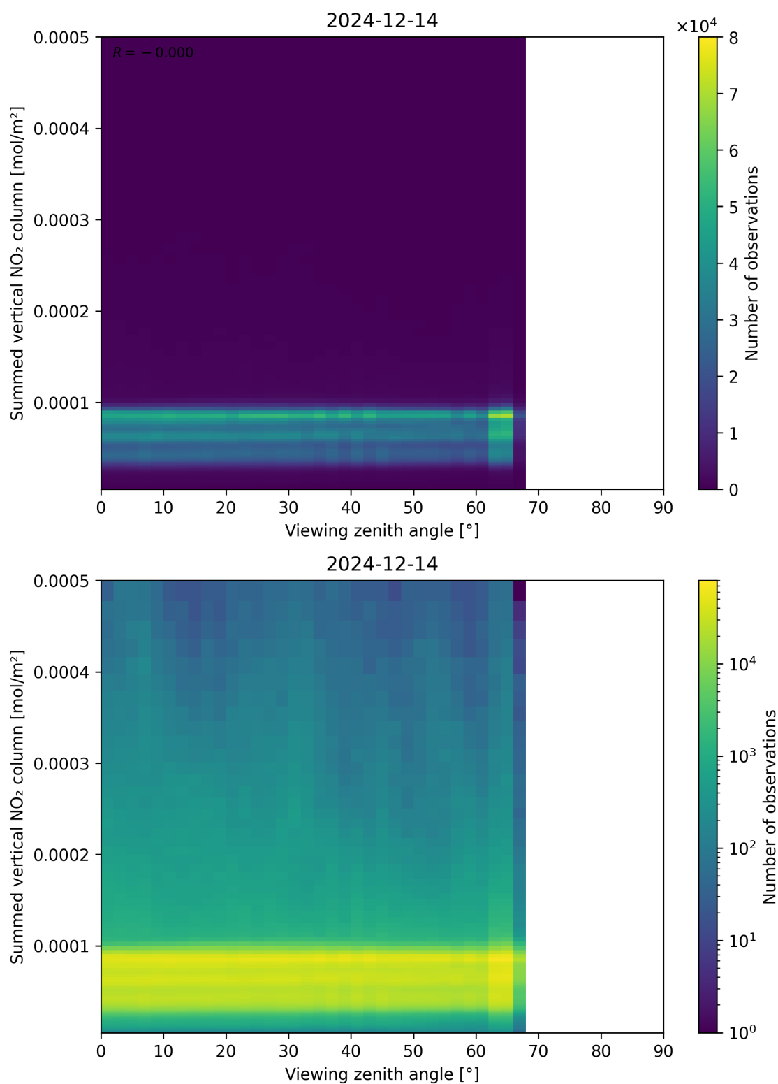
Figure 165: Scatter density plot of “Viewing zenith angle” against “Summed vertical NO 2 column” for 2024-12-13 to 2024-12-15.
