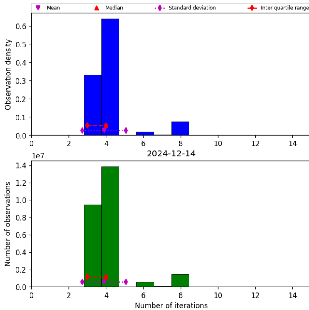
Figure 34: Histogram of “Number of iterations” for 2024-12-13 to 2024-12-15
