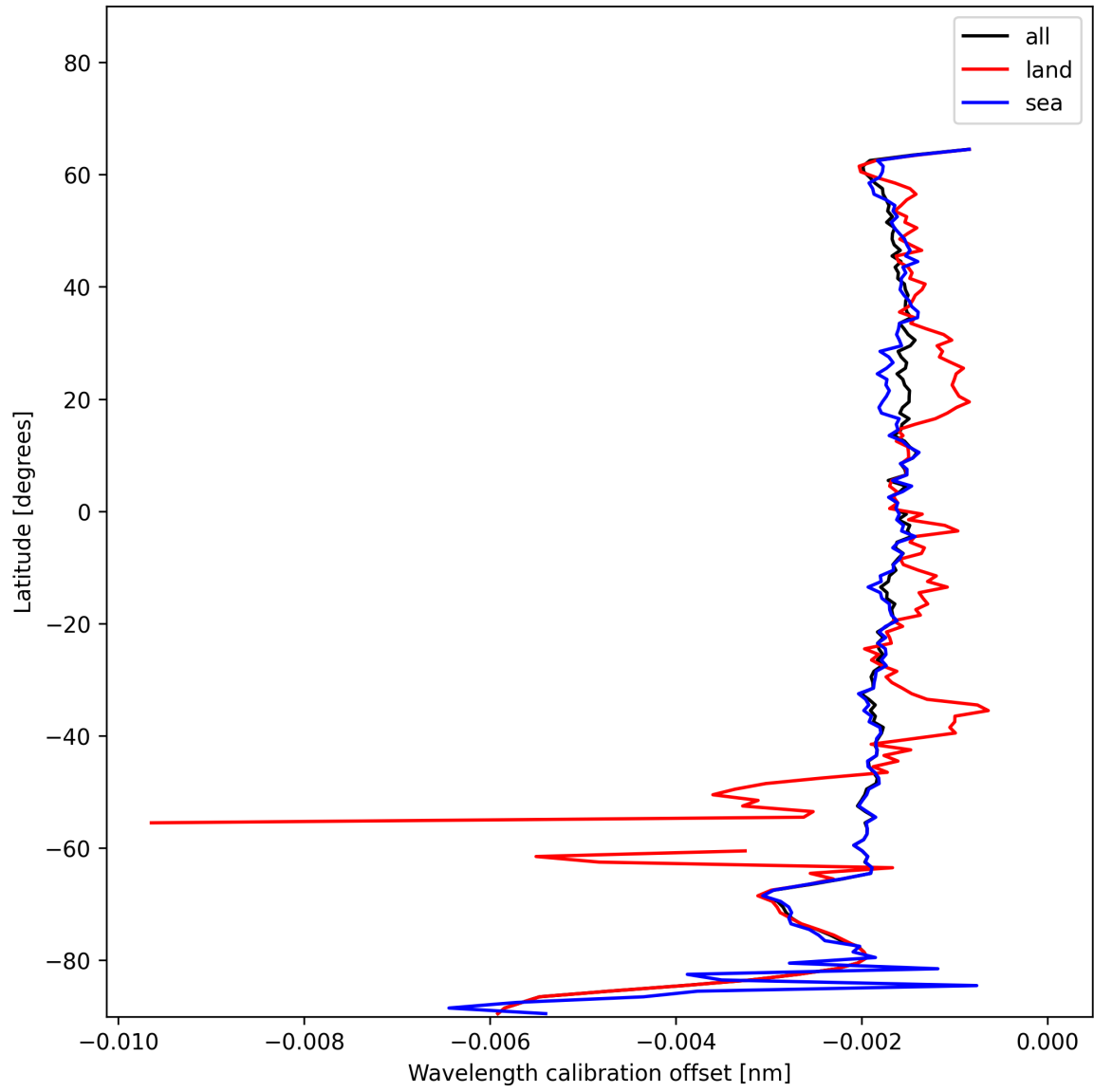
Figure 18: Zonal average of “Wavelength calibration offset” for 2024-12-13 to 2024-12-15.
