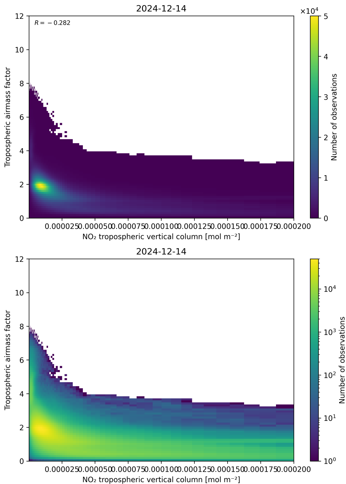
Figure 123: Scatter density plot of “NO 2 tropospheric vertical column” against “Tropospheric air mass factor” for 2024-12-13 to 2024-12-15.
