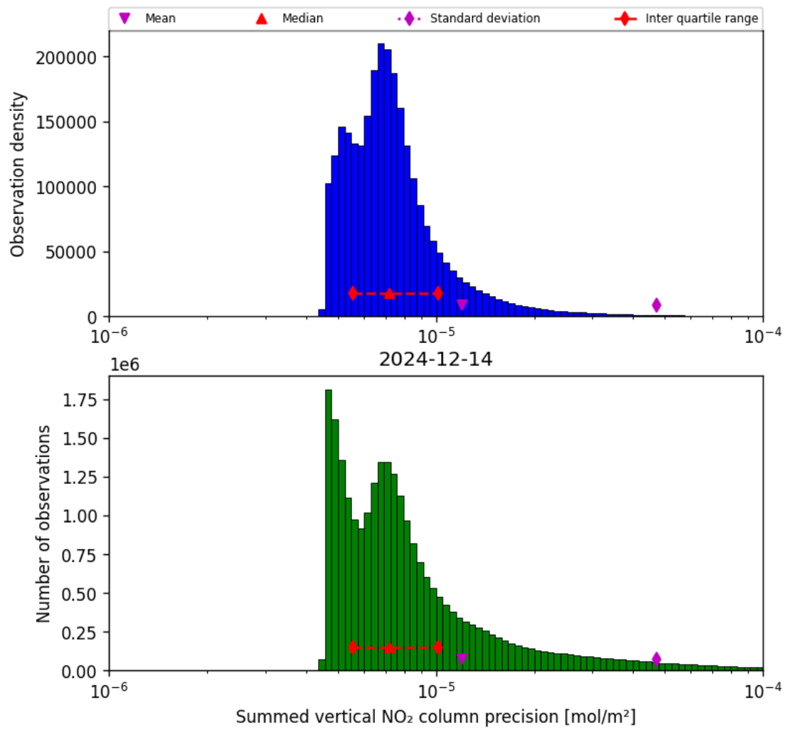
Figure 41: Histogram of "Summed vertical NO 2 column precision" for 2024-12-13 to 2024-12-15
