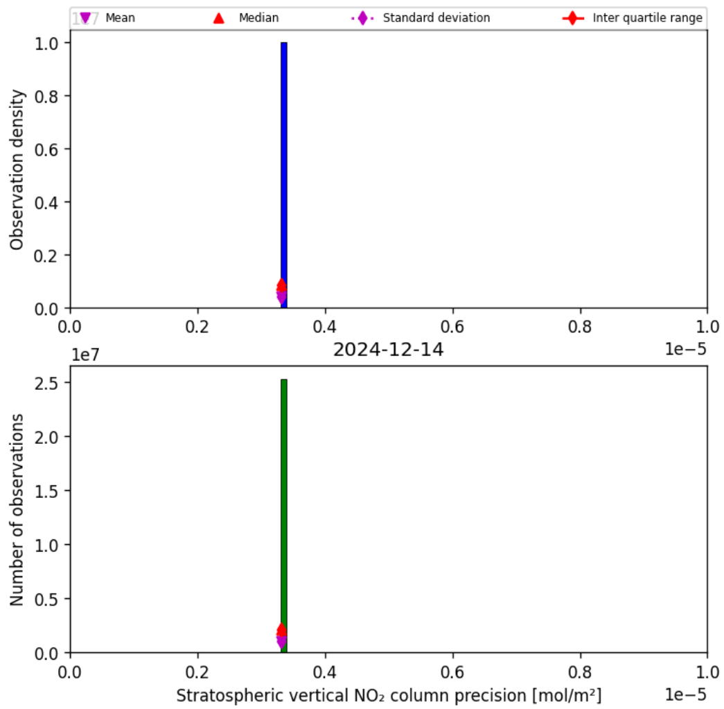
Figure 37: Histogram of “Stratospheric vertical NO 2 column precision” for 2024-12-13 to 2024-12-15
