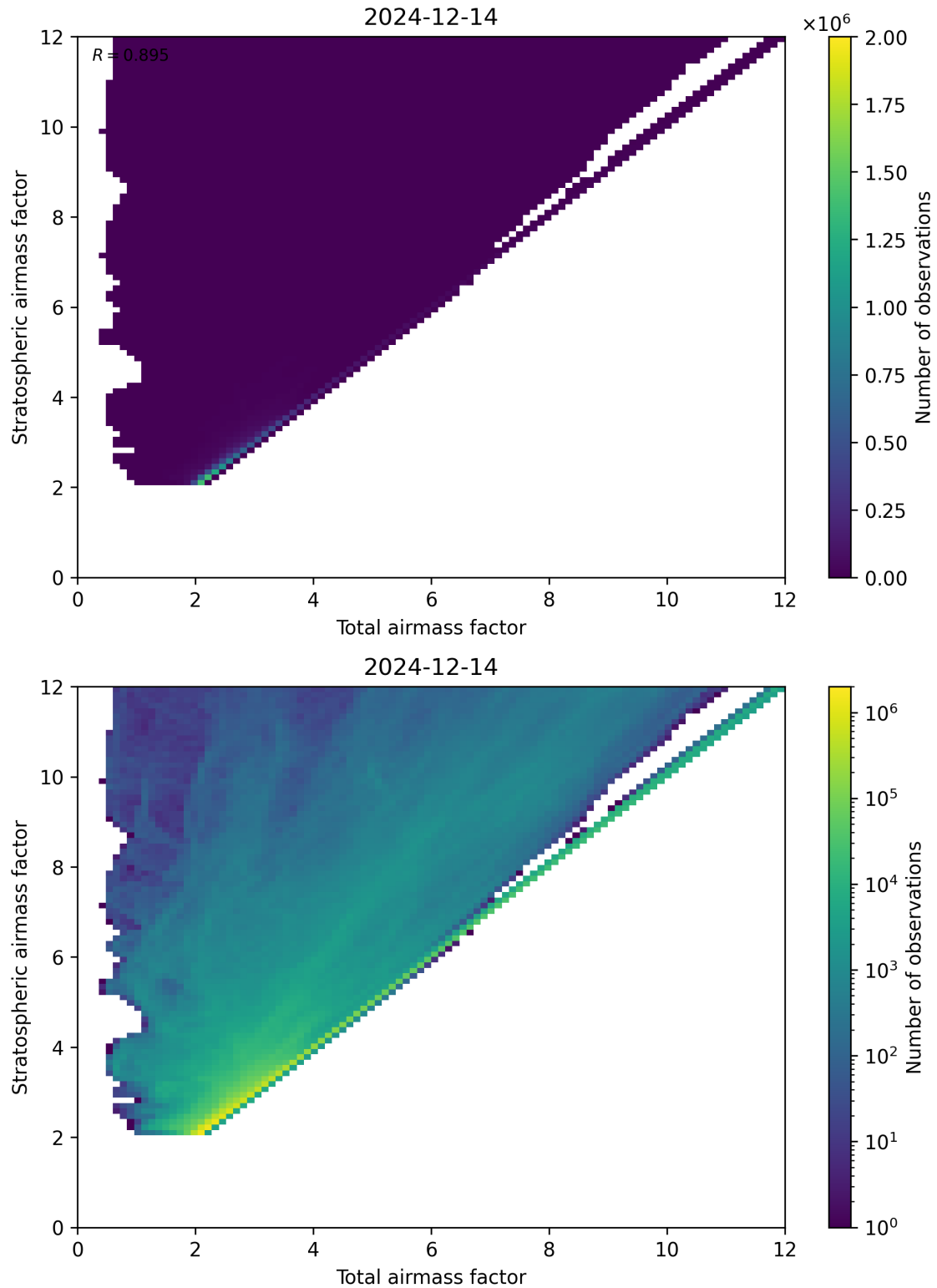
Figure 62: Scatter density plot of “Total airmass factor” against “Stratospheric airmass factor” for 2024-12-13 to 2024-12-15.
