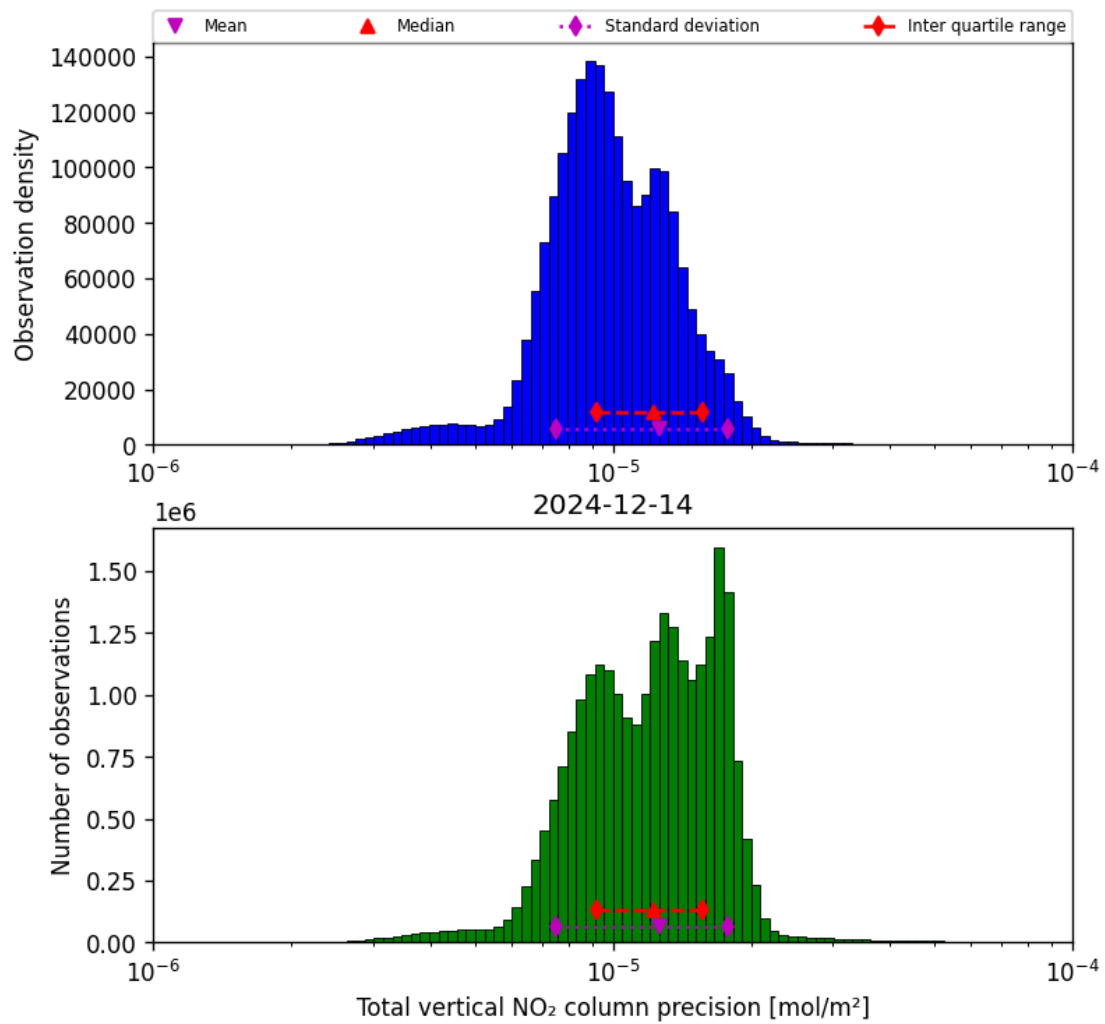
Figure 39: Histogram of “Total vertical NO 2 column precision” for 2024-12-13 to 2024-12-15
