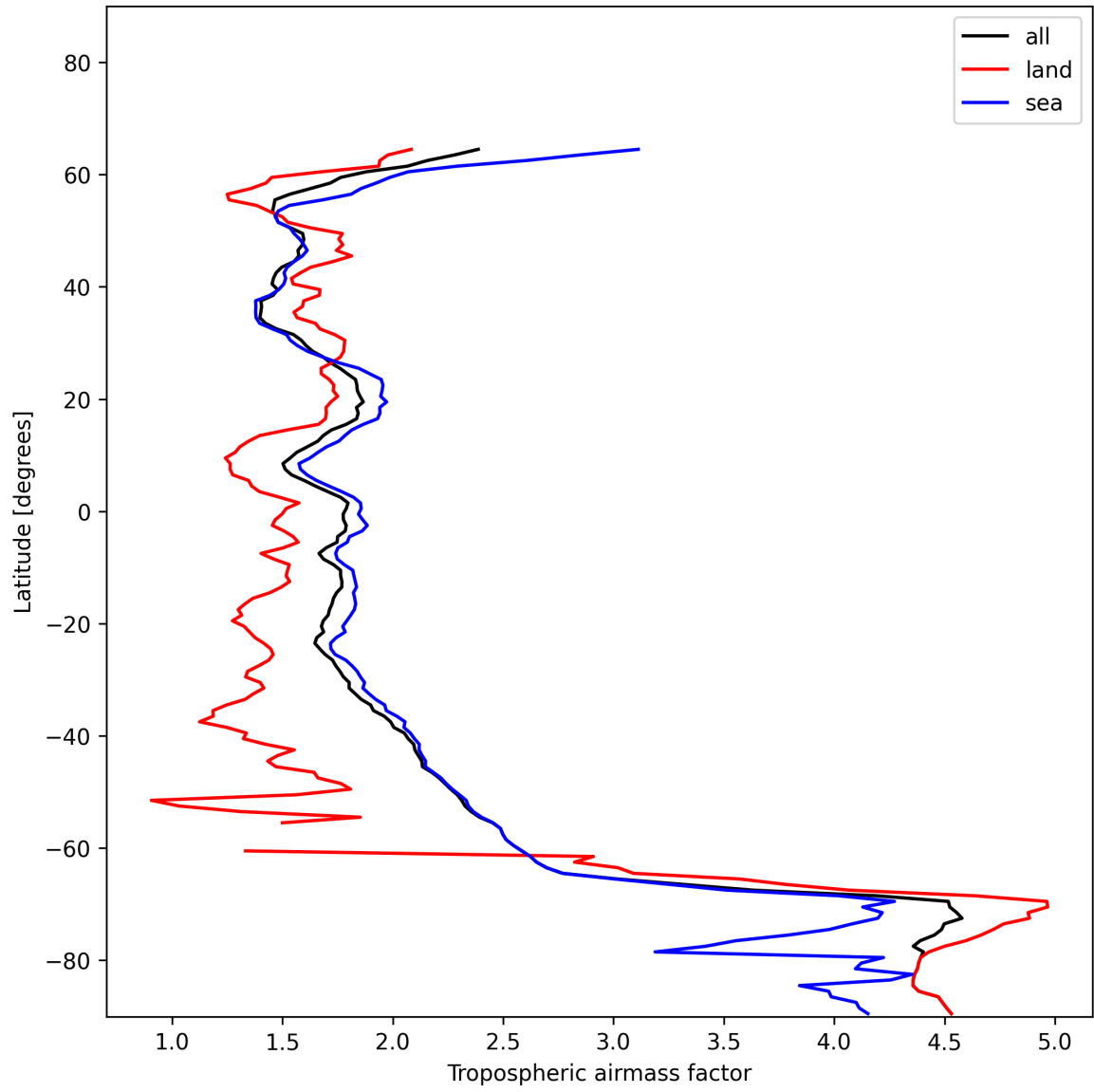
Figure 14: Zonal average of “Tropospheric airmass factor” for 2024-12-13 to 2024-12-15.
