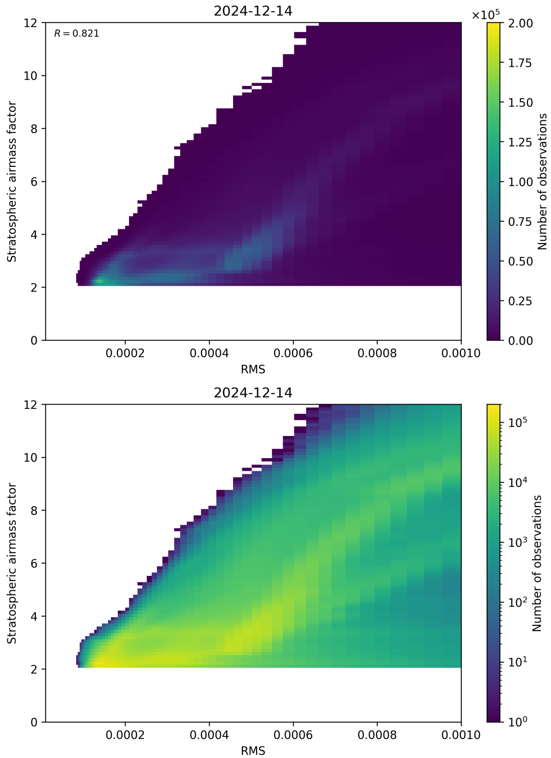
Figure 144: Scatter density plot of “RMS” against “Stratospheric airmass factor” for 2024-12-13 to 2024-12-15.
