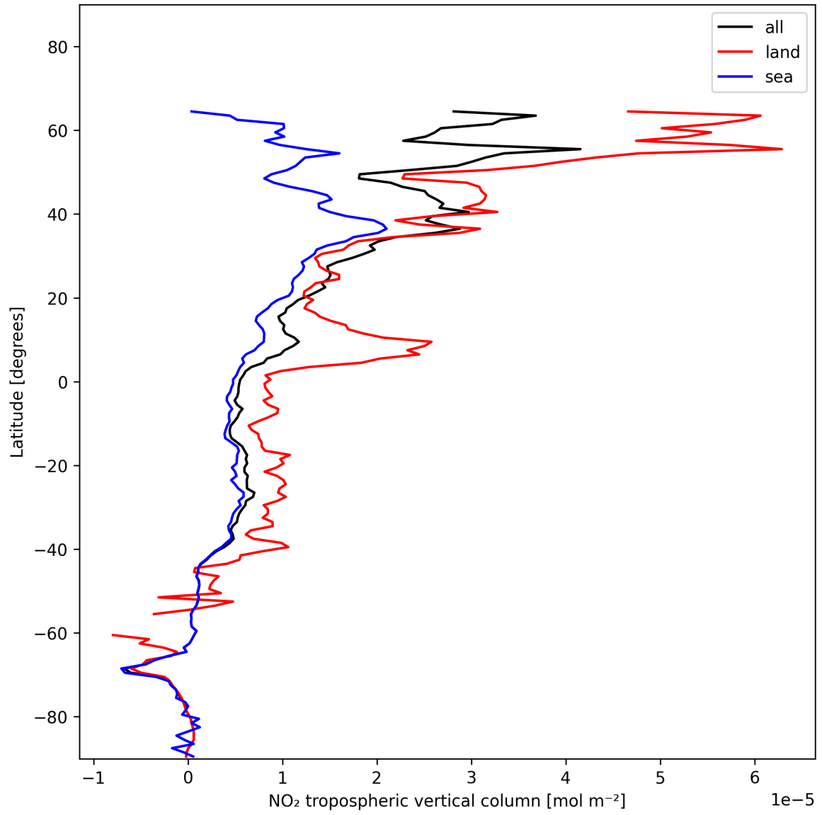
Figure 12: Zonal average of “NO 2 tropospheric vertical column” for 2024-12-13 to 2024-12-15.
