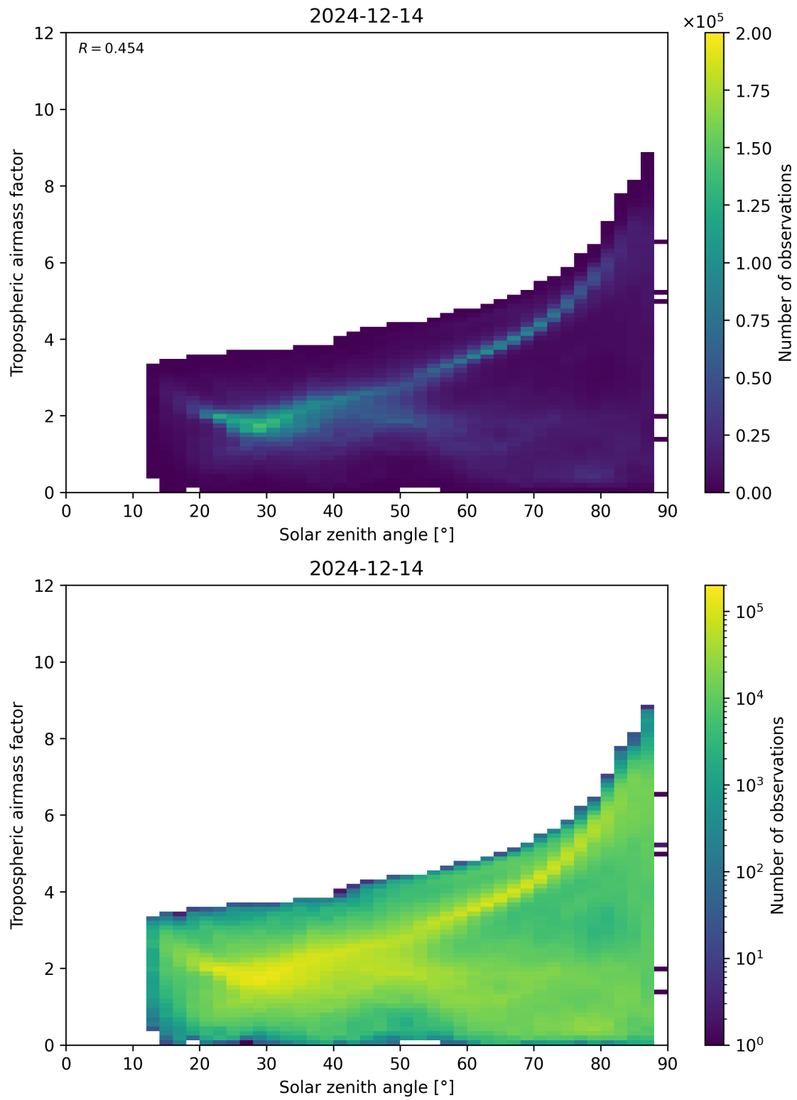
Figure 147: Scatter density plot of “Solar zenith angle” against “Tropospheric airmass factor” for 2024-12-13 to 2024-12-15.
