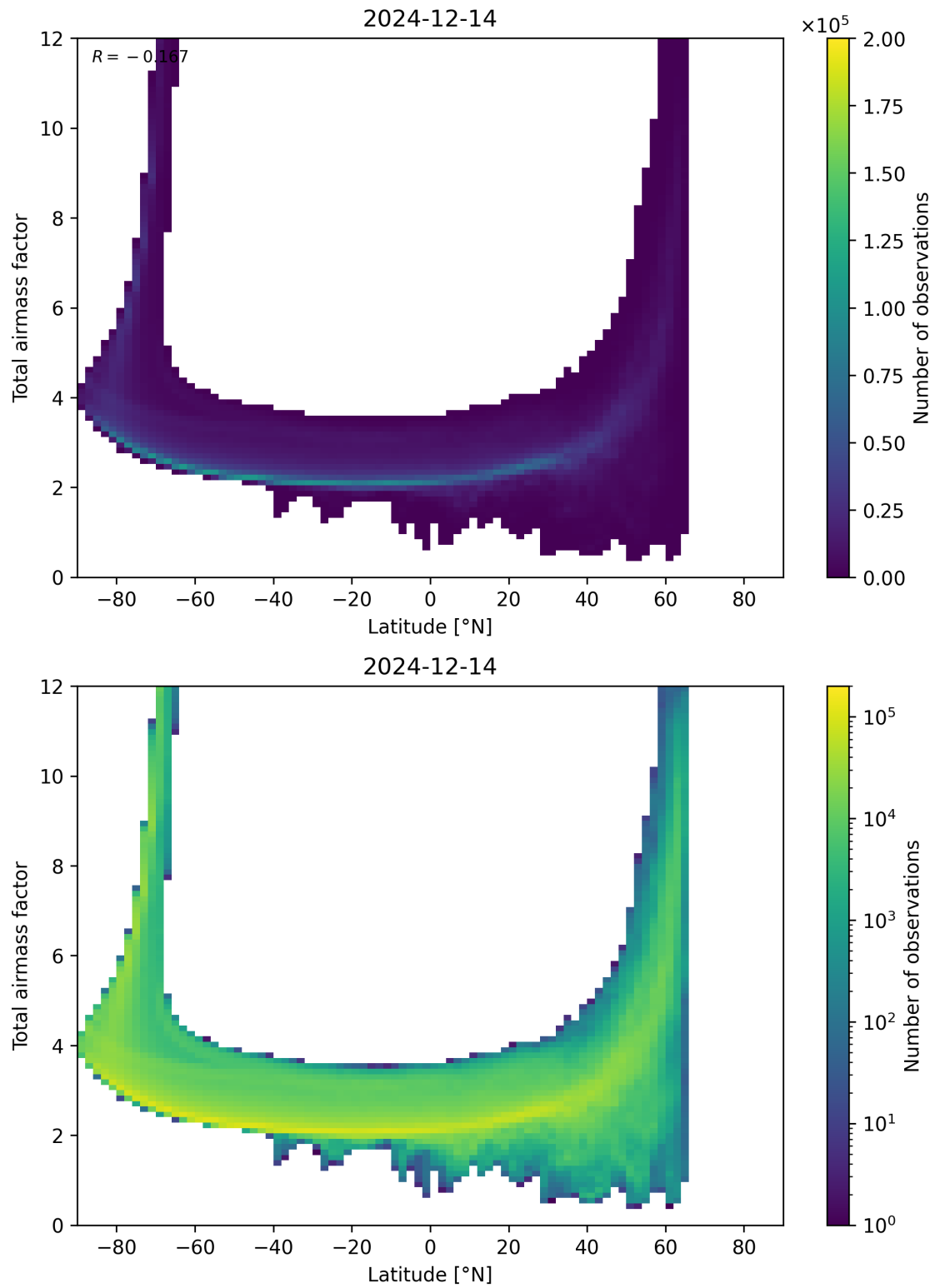
Figure 84: Scatter density plot of “Latitude” against “Total airmass factor” for 2024-12-13 to 2024-12-15.
