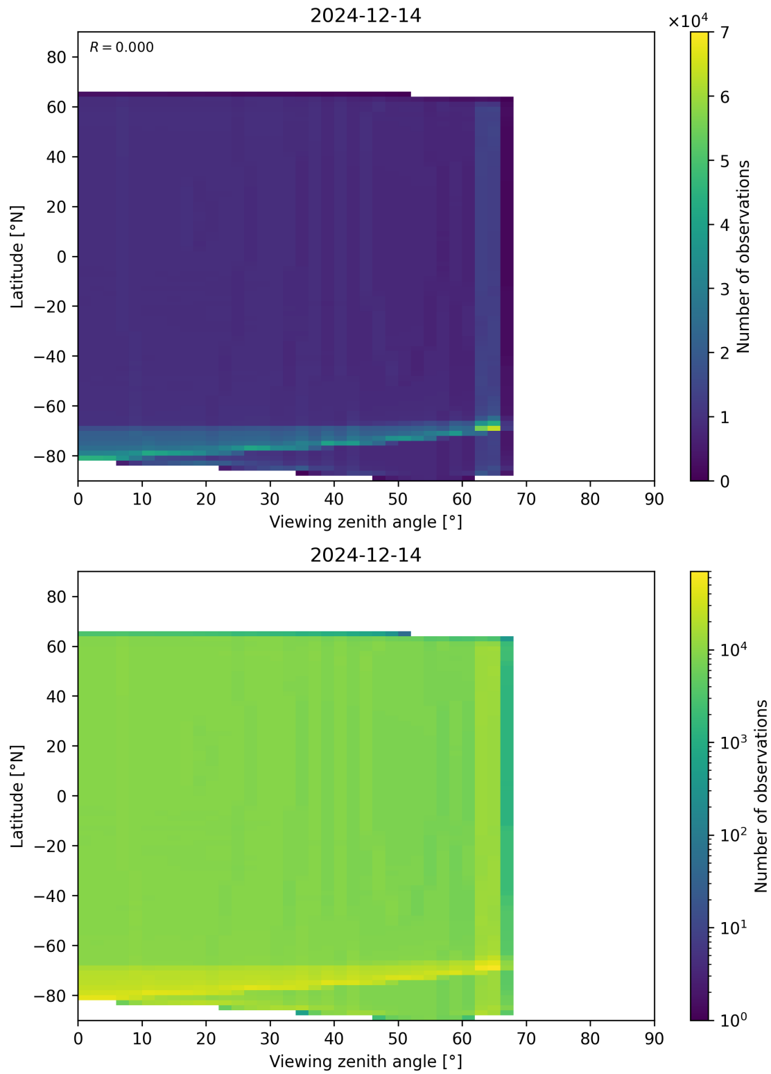
Figure 163: Scatter density plot of “Viewing zenith angle” against “Latitude” for 2024-12-13 to 2024-12-15.
