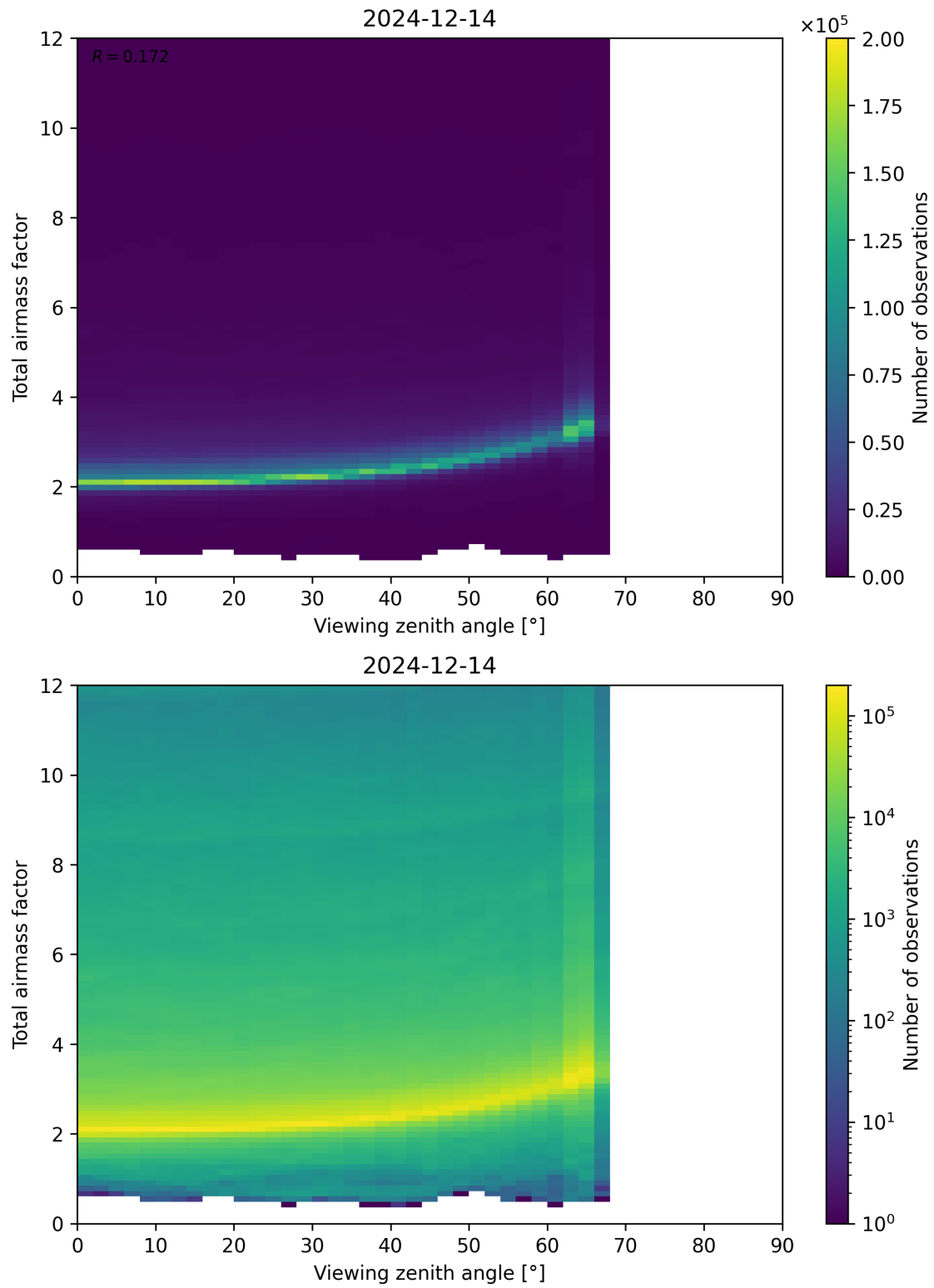
Figure 160: Scatter density plot of “Viewing zenith angle” against “Total airmass factor” for 2024-12-13 to 2024-12-15.
