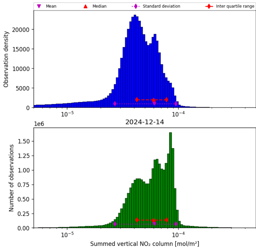
Figure 40: Histogram of “Summed vertical NO 2 column” for 2024-12-13 to 2024-12-15
