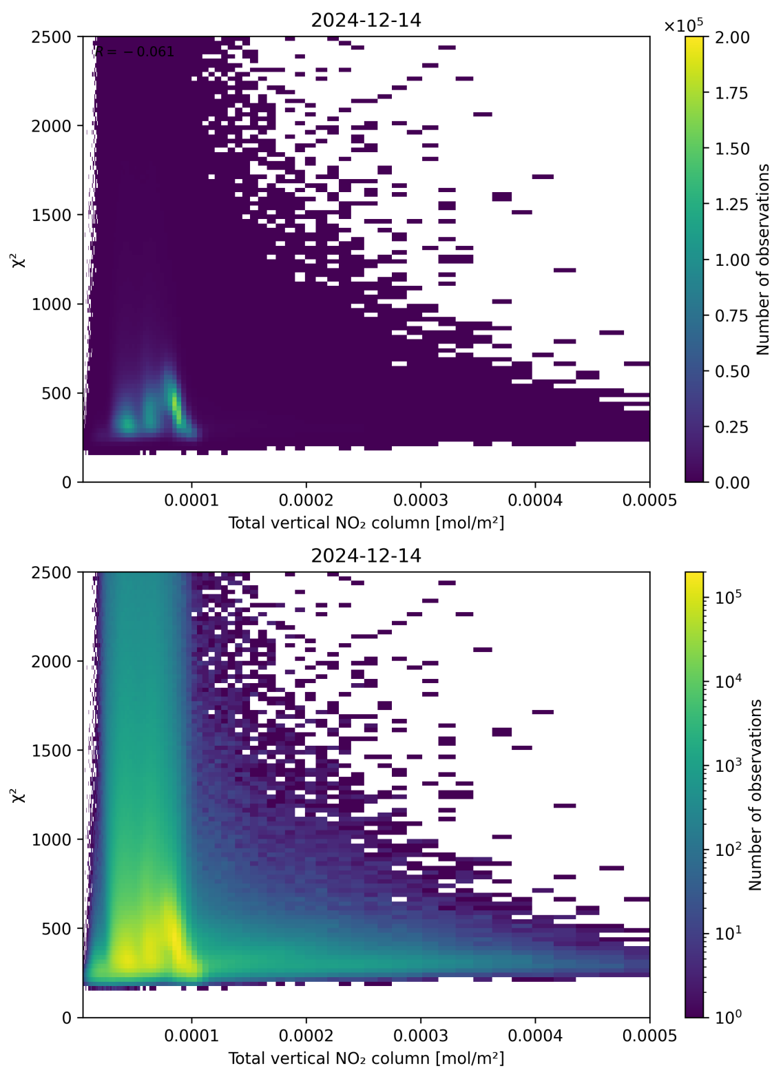
Figure 111: Scatter density plot of “Total vertical NO 2 column” against “ \chi^2 ” for 2024-12-13 to 2024-12-15.
