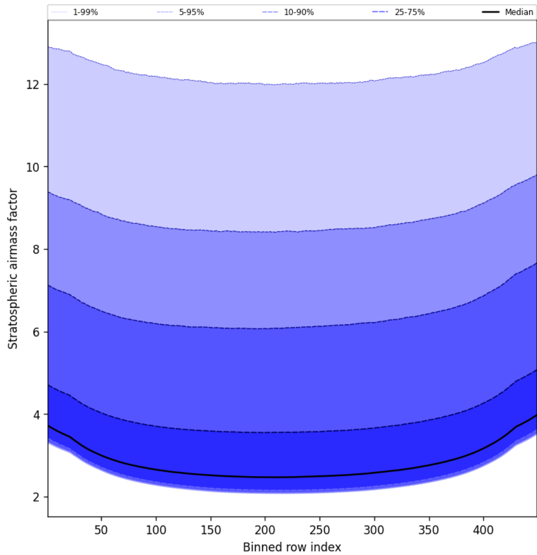
Figure 61: Along track statistics of “Stratospheric airmass factor” for 2024-12-13 to 2024-12-15
