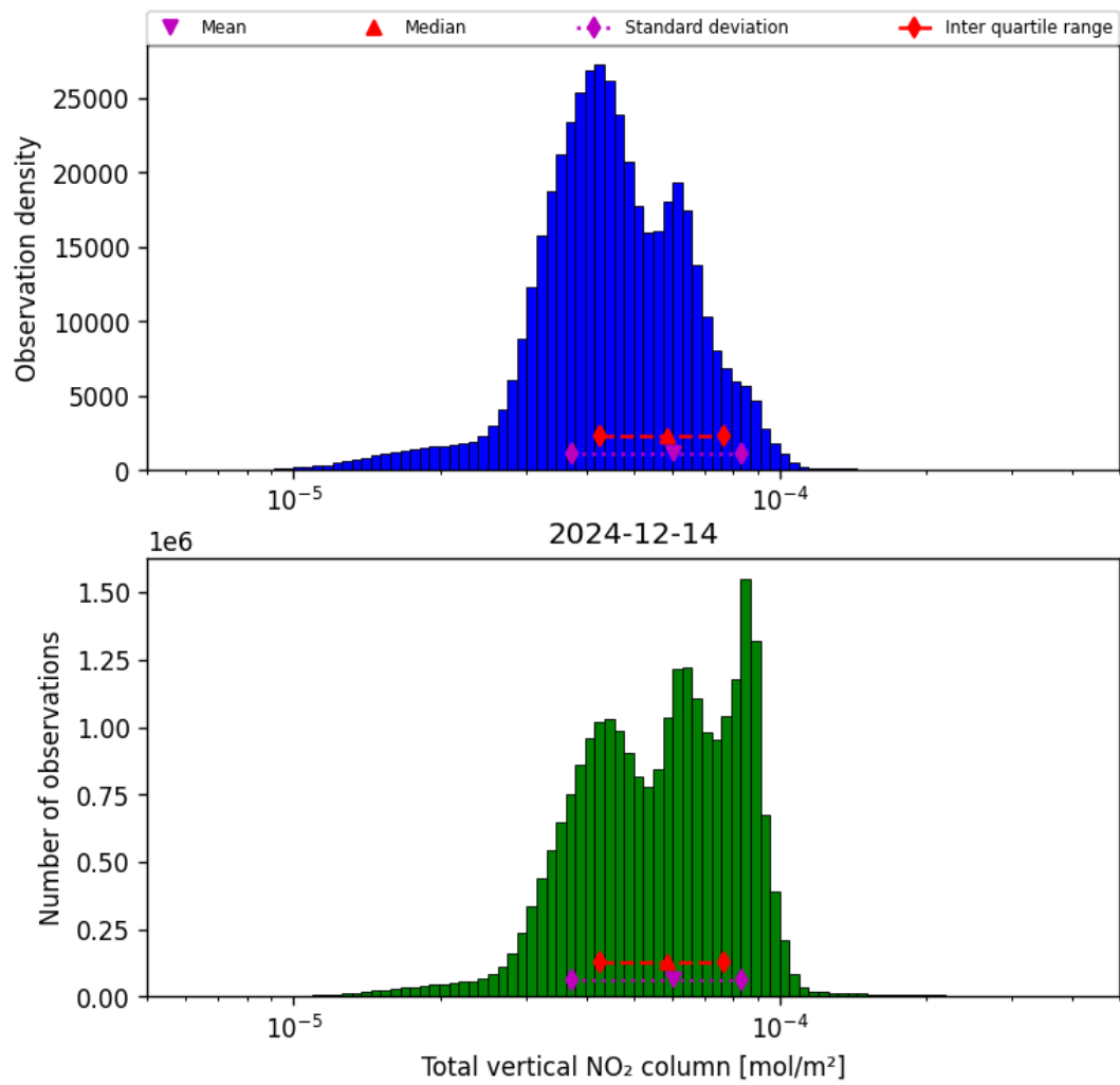
Figure 38: Histogram of “Total vertical NO 2 column” for 2024-12-13 to 2024-12-15
