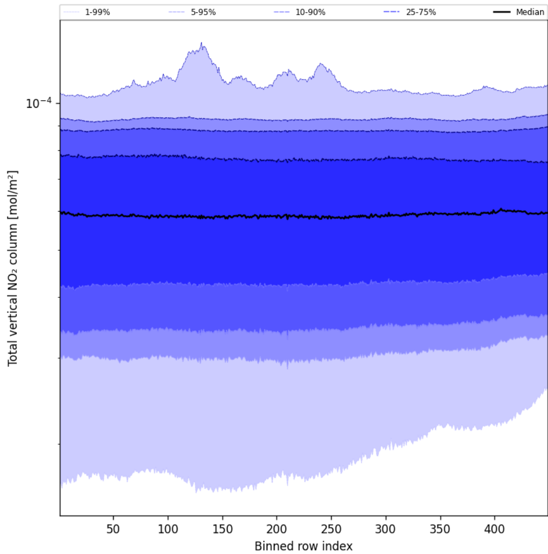
Figure 55: Along track statistics of “Total vertical NO 2 column” for 2024-12-13 to 2024-12-15
