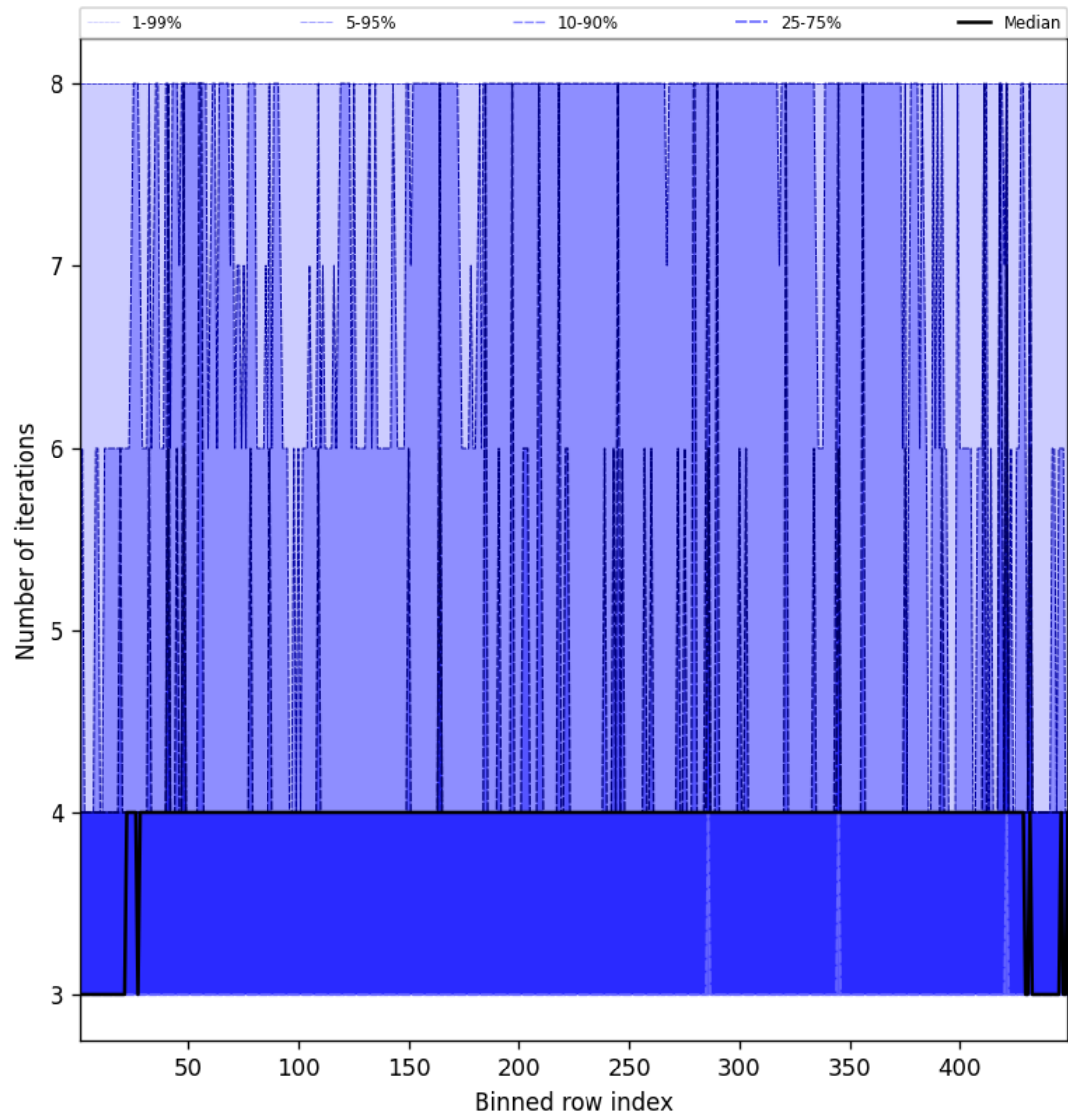
Figure 51: Along track statistics of “Number of iterations” for 2024-12-13 to 2024-12-15
