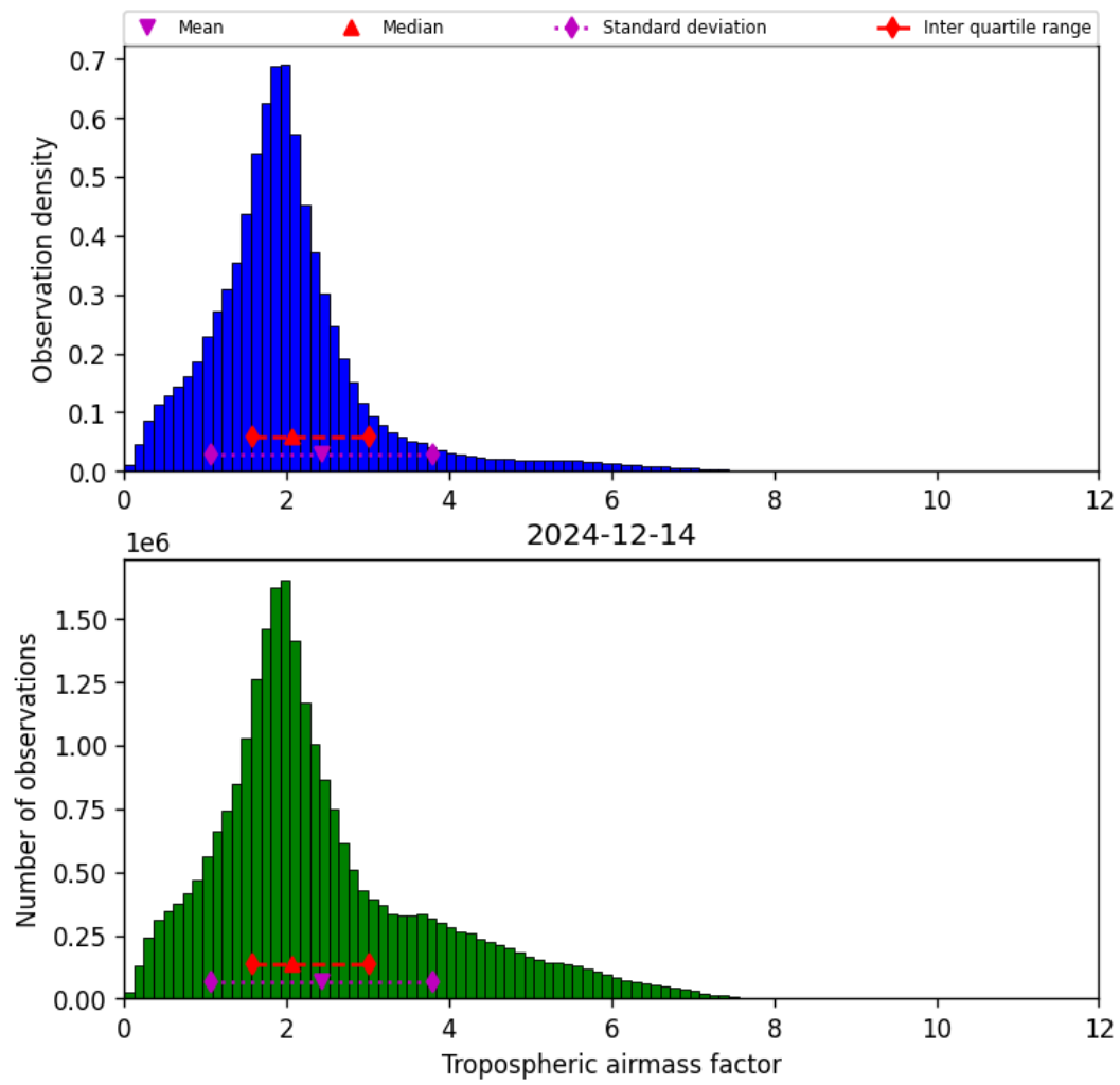
Figure 31: Histogram of “Tropospheric air mass factor” for 2024-12-13 to 2024-12-15
