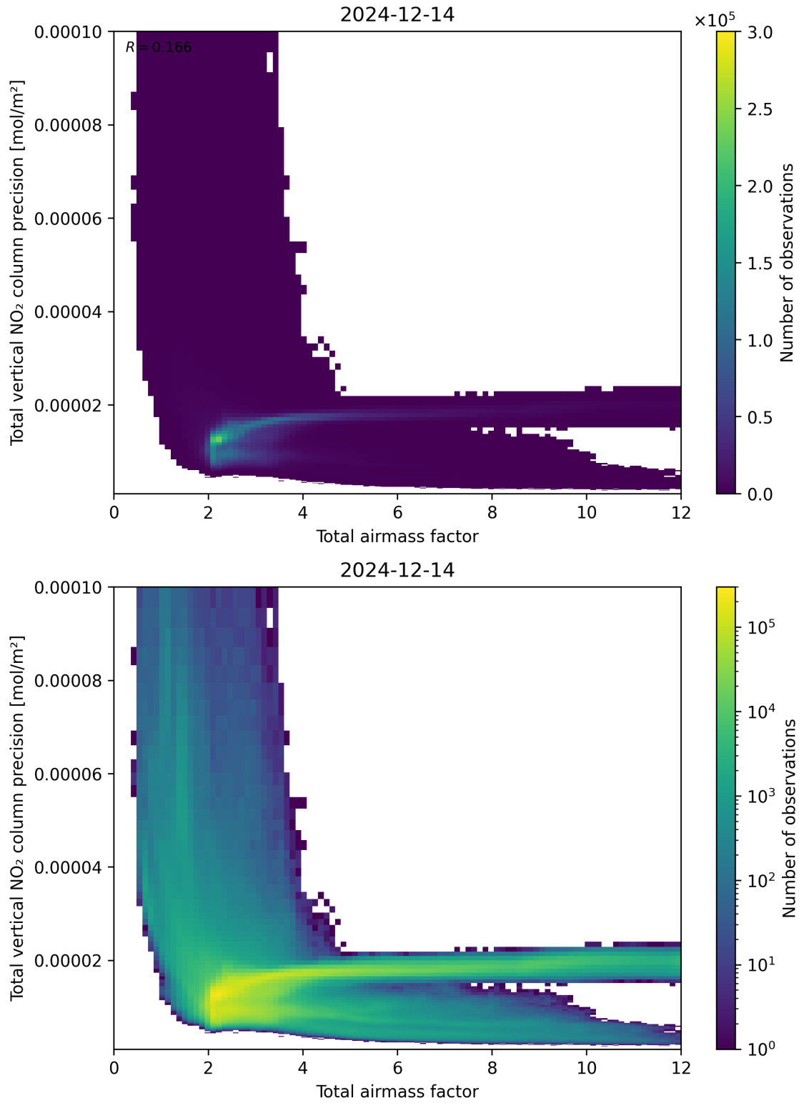
Figure 68: Scatter density plot of “Total airmass factor” against “Total vertical NO 2 column precision” for 2024-12-13 to 2024-12-15.
