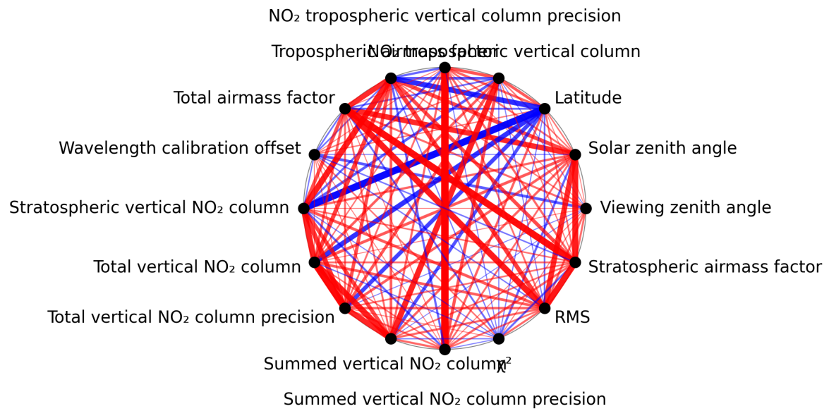
Figure 1: Map of correlation graph for 2024-12-13 to 2024-12-15.
