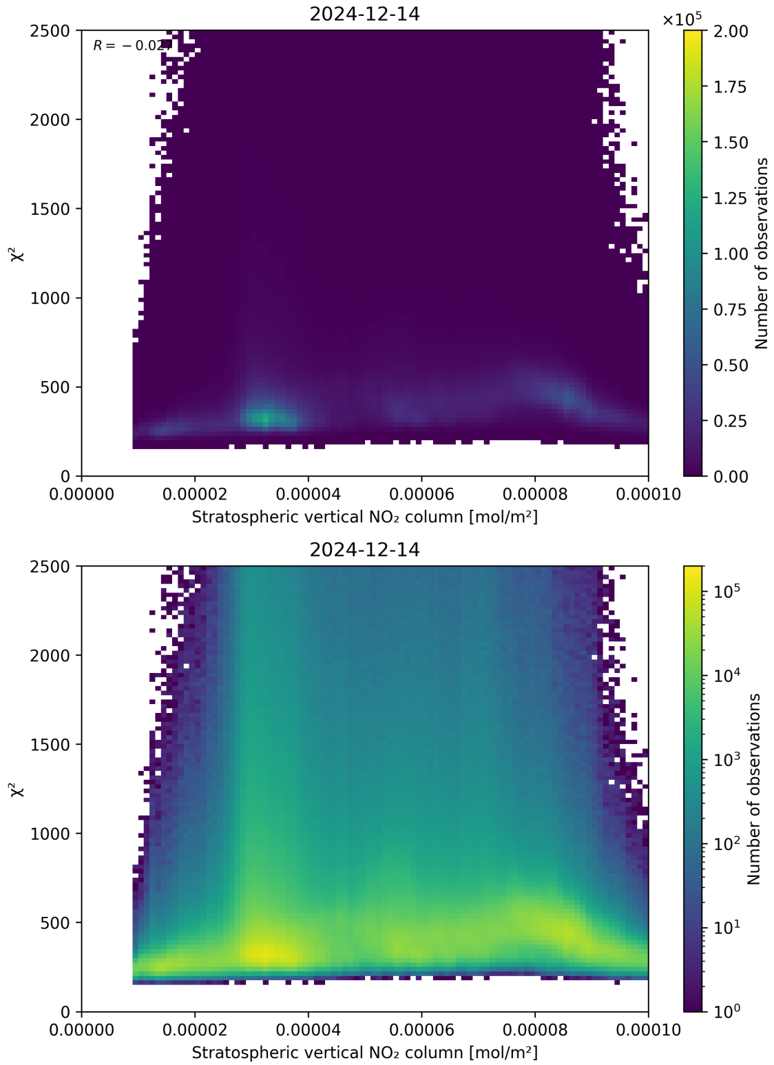
Figure 97: Scatter density plot of “Stratospheric vertical NO 2 column” against “ \chi^2 ” for 2024-12-13 to 2024-12-15.
