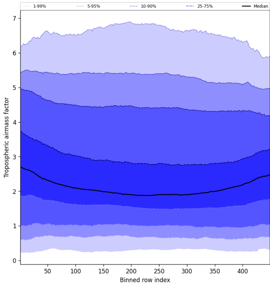
Figure 48: Along track statistics of “Tropospheric airmass factor” for 2024-12-13 to 2024-12-15
