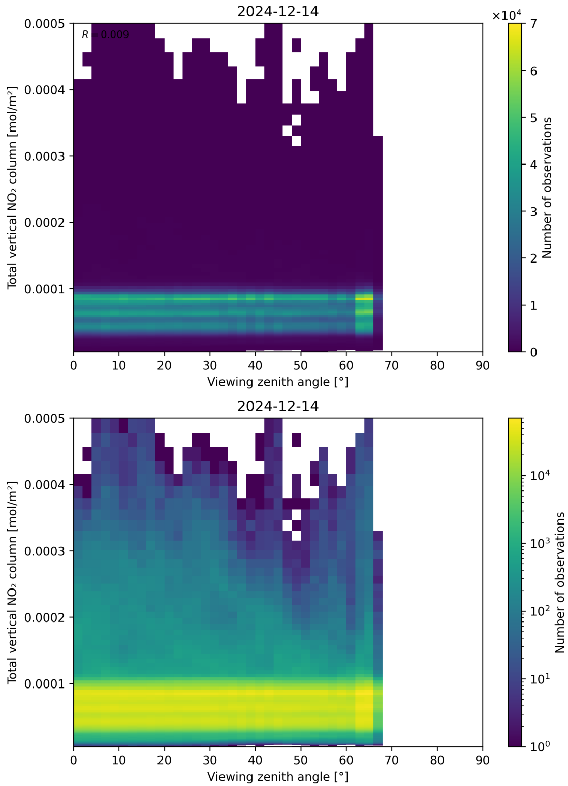
Figure 167: Scatter density plot of “Viewing zenith angle” against “Total vertical NO 2 column” for 2024-12-13 to 2024-12-15.
