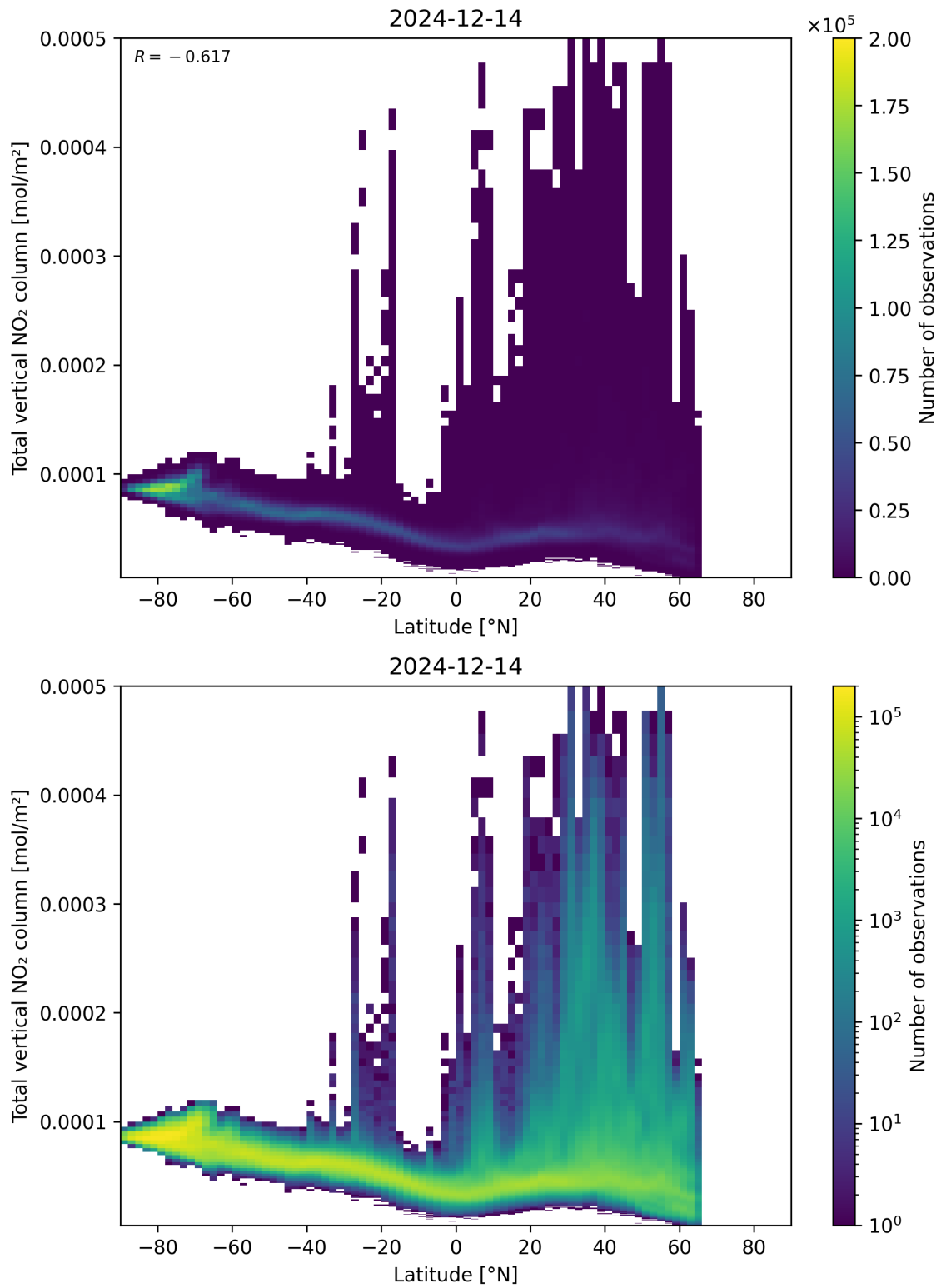
Figure 90: Scatter density plot of “Latitude” against “Total vertical NO 2 column” for 2024-12-13 to 2024-12-15.
