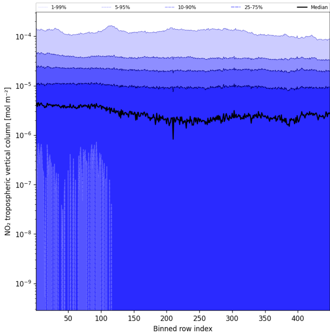
Figure 46: Along track statistics of “NO 2 tropospheric vertical column” for 2024-12-13 to 2024-12-15
