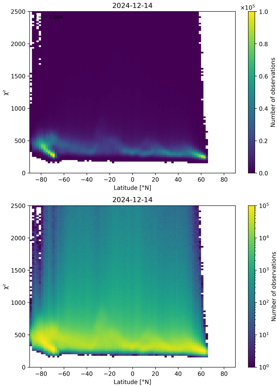
Figure 86: Scatter density plot of “Latitude” against “ \chi^2 ” for 2024-12-13 to 2024-12-15.
