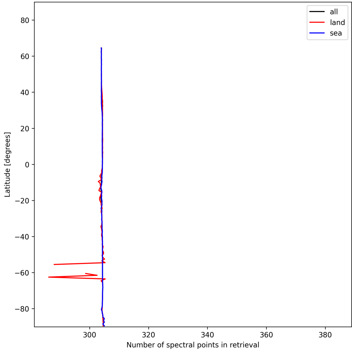
Figure 16: Zonal average of “Number of spectral points in retrieval” for 2024-12-13 to 2024-12-15.
