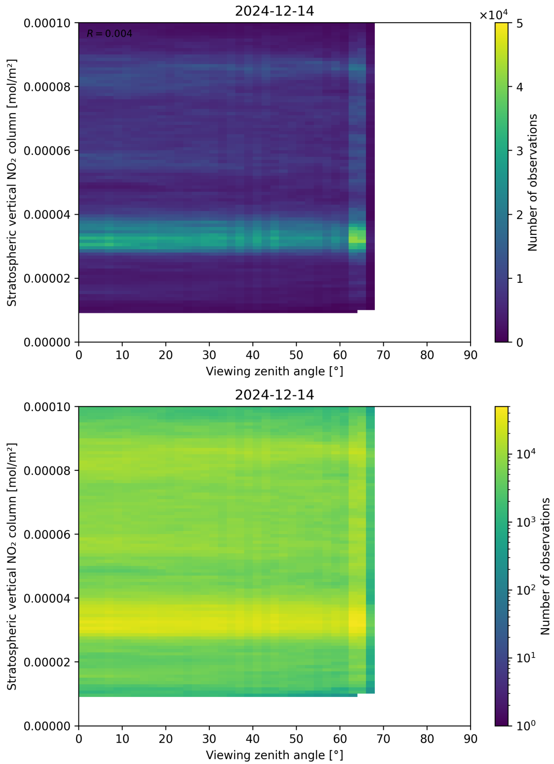
Figure 164: Scatter density plot of “Viewing zenith angle” against “Stratospheric vertical NO 2 column” for 2024-12-13 to 2024-12-15.
