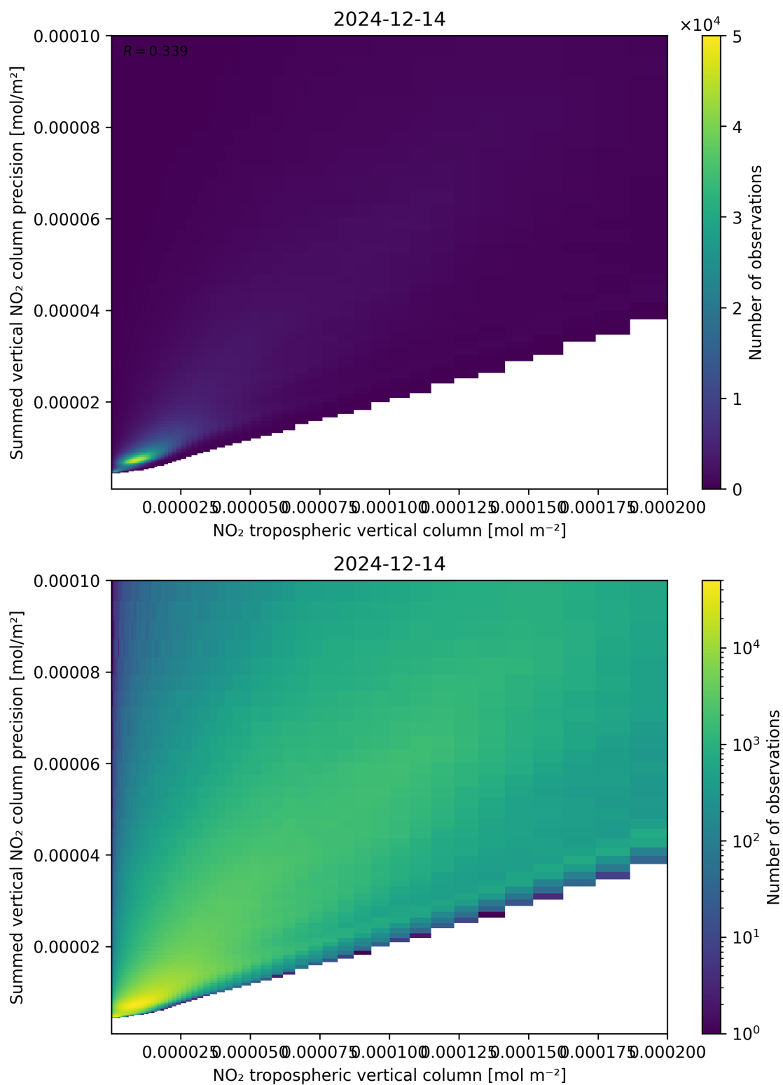
Figure 127: Scatter density plot of “NO 2 tropospheric vertical column” against “Summed vertical NO 2 column precision” for 2024-12-13 to 2024-12-15.
