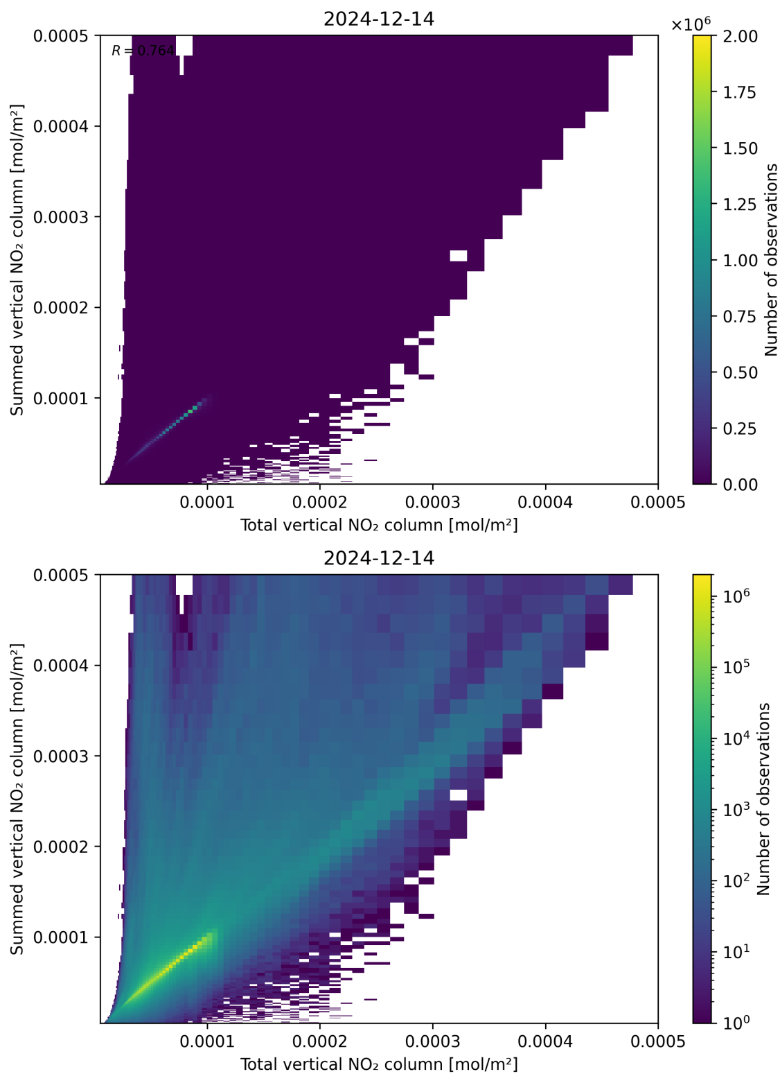
Figure 112: Scatter density plot of “Total vertical NO 2 column” against “Summed vertical NO 2 column” for 2024-12-13 to 2024-12-15.
