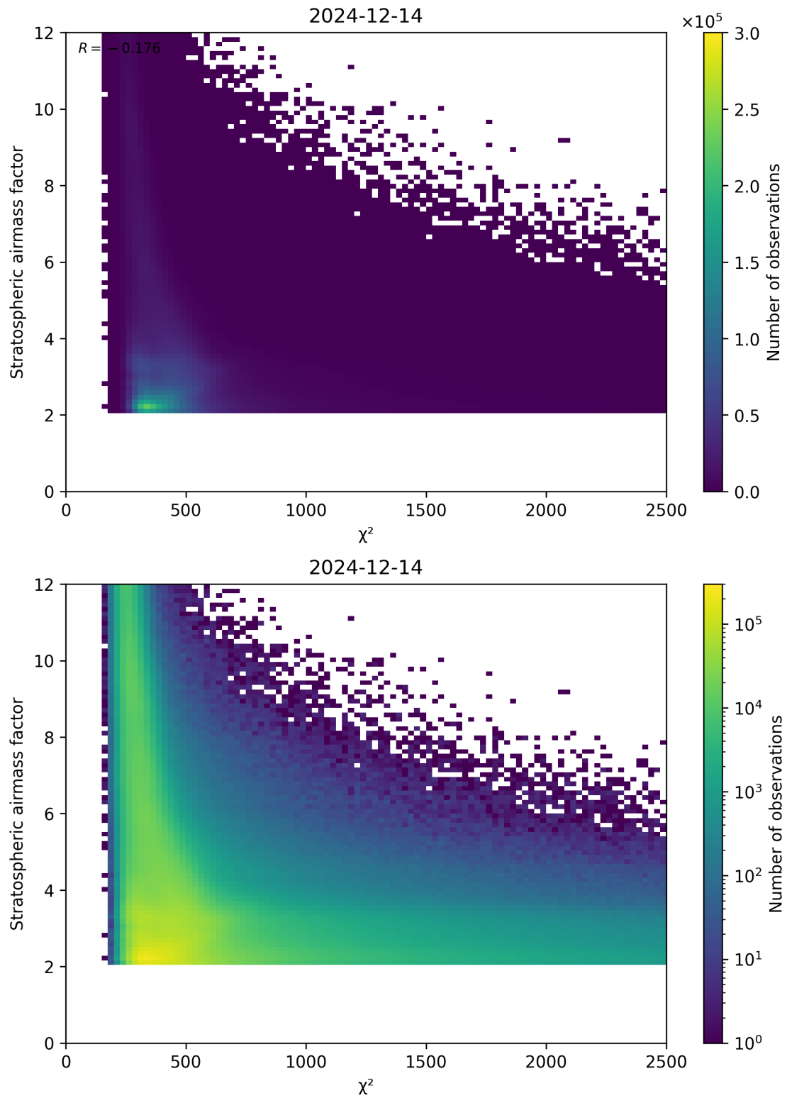
Figure 81: Scatter density plot of “ \chi^2 ” against “Stratospheric airmass factor” for 2024-12-13 to 2024-12-15.
