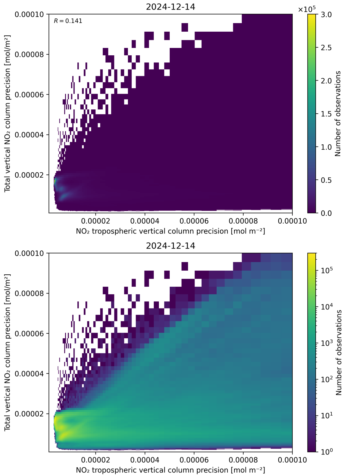
Figure 139: Scatter density plot of “NO 2 tropospheric vertical column precision” against “Total vertical NO 2 column precision” for 2024-12-13 to 2024-12-15.
