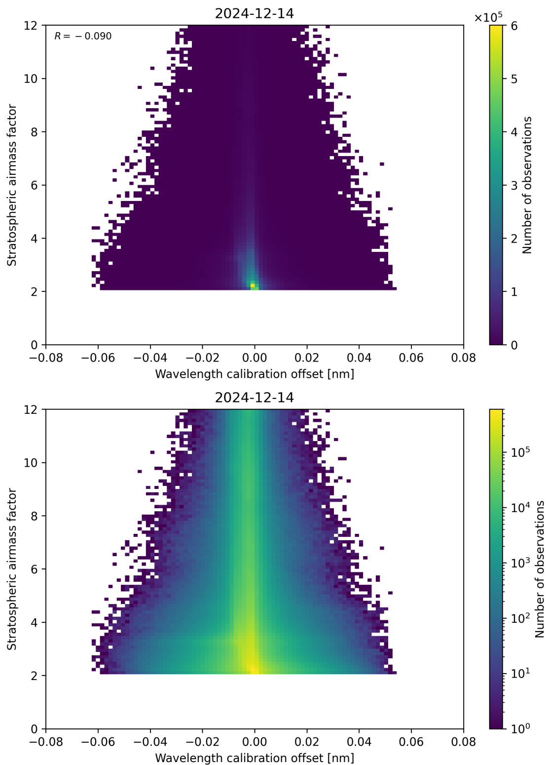
Figure 174: Scatter density plot of “Wavelength calibration offset” against “Stratospheric airmass factor” for 2024-12-13 to 2024-12-15.
