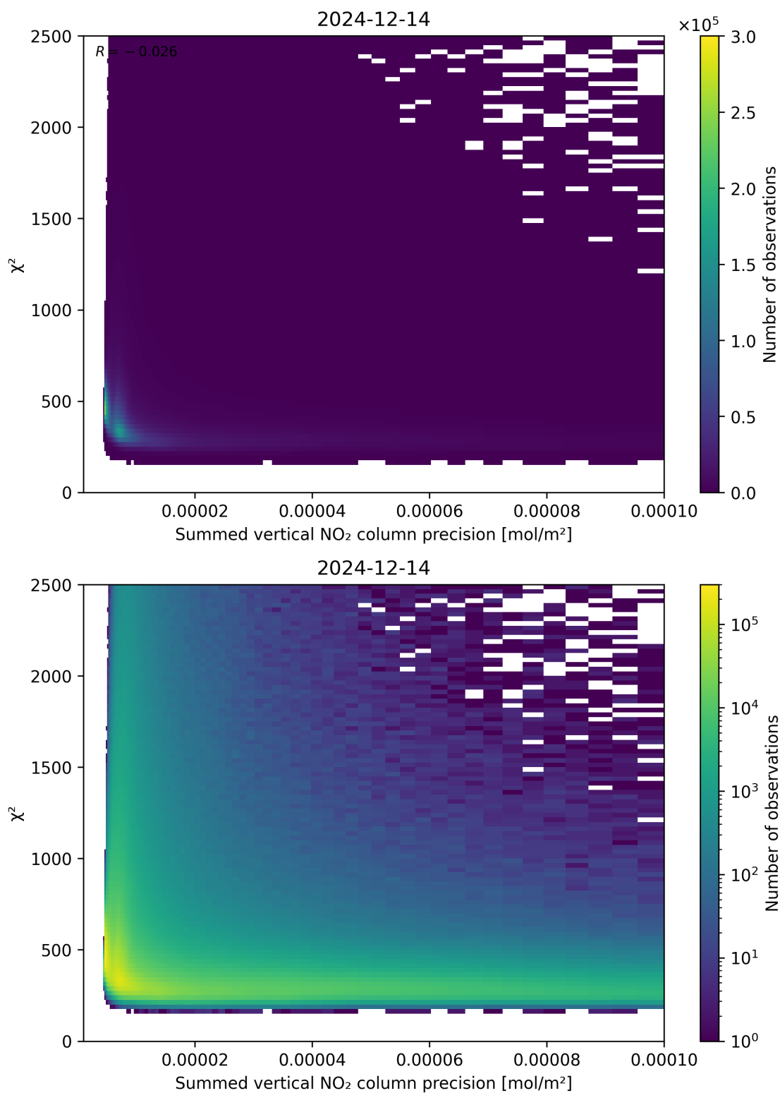
Figure 107: Scatter density plot of “Summed vertical NO 2 column precision” against “ \chi^2 ” for 2024-12-13 to 2024-12-15.
