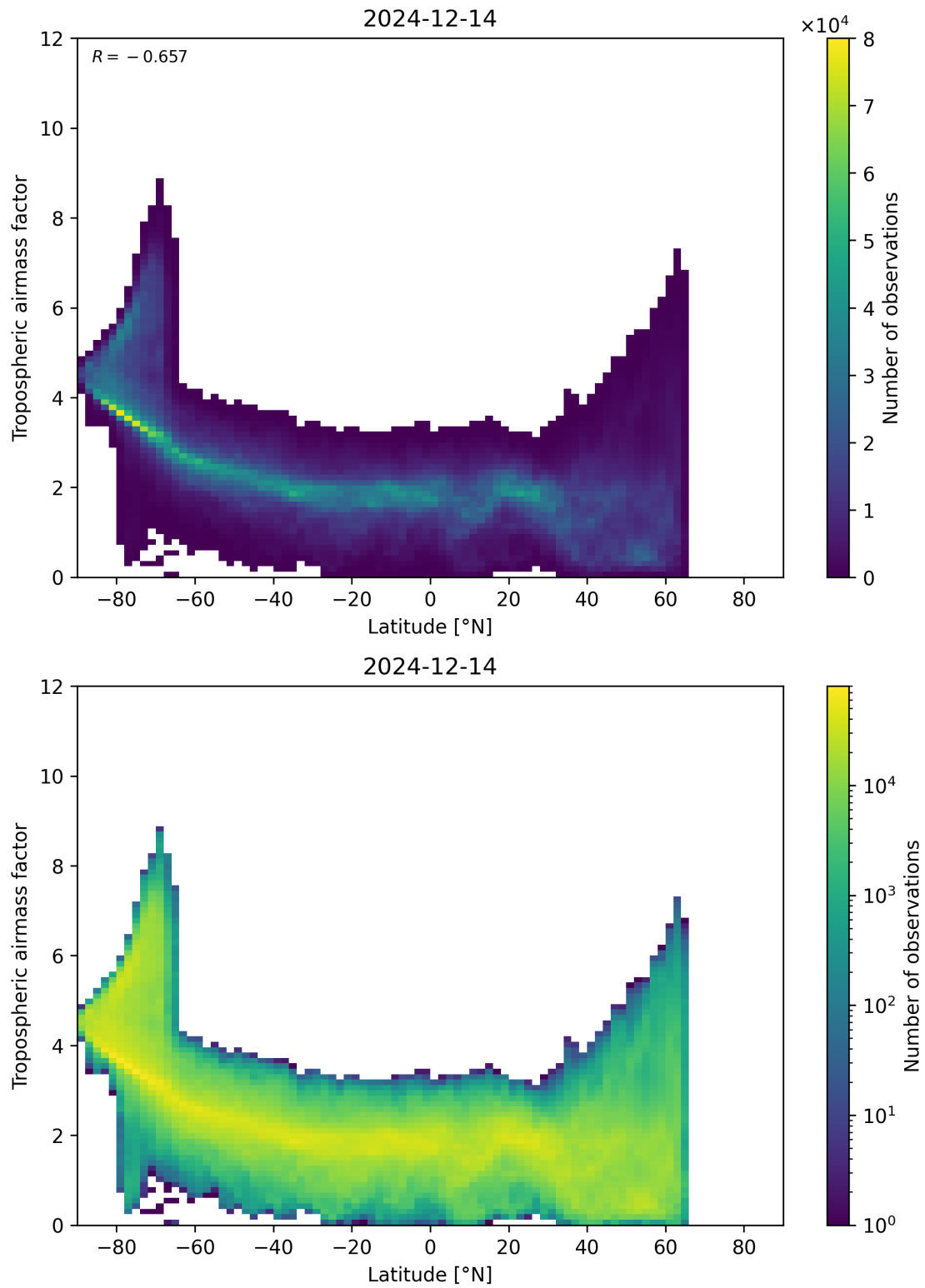
Figure 85: Scatter density plot of “Latitude” against “Tropospheric air mass factor” for 2024-12-13 to 2024-12-15.
