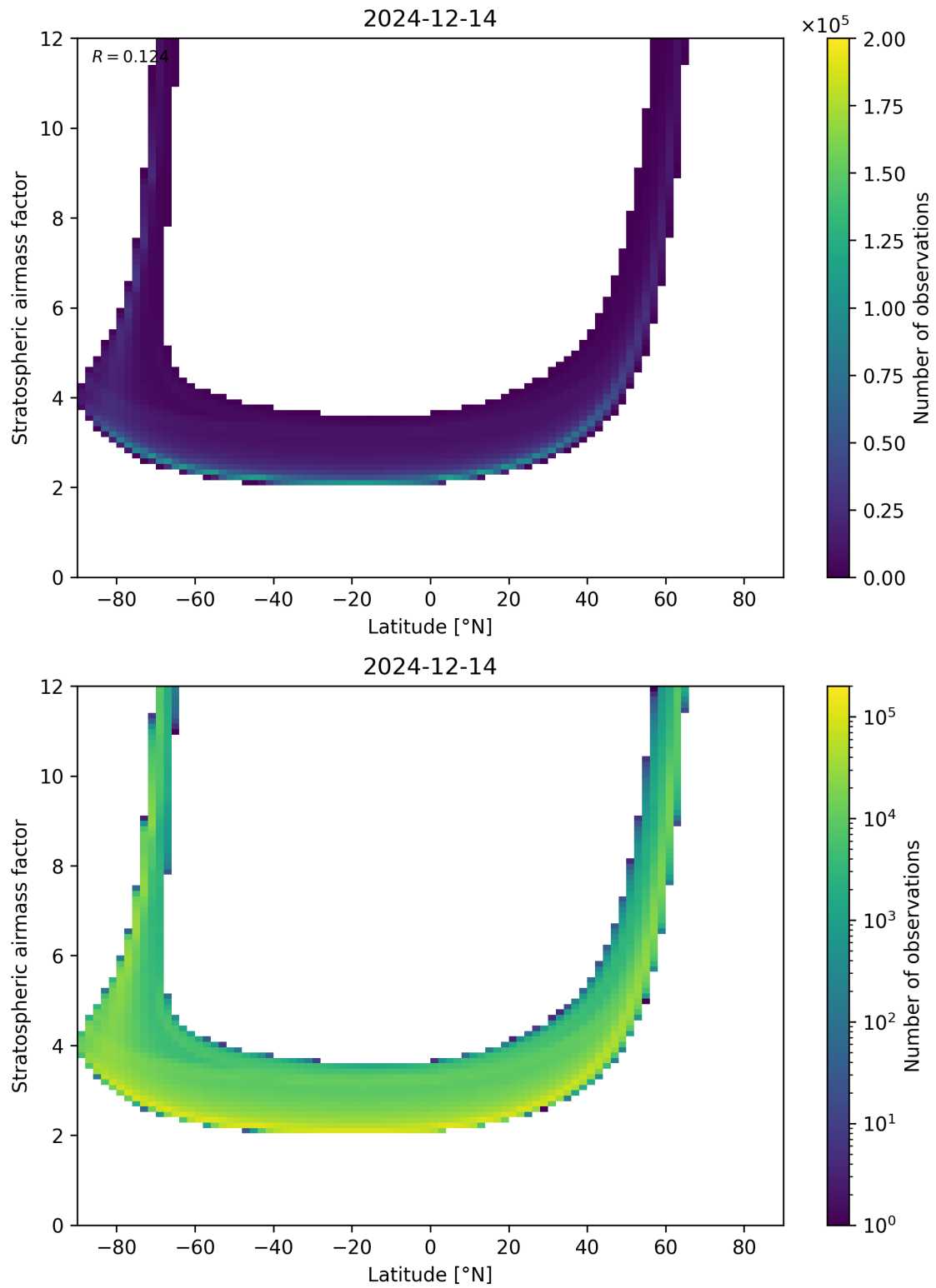
Figure 83: Scatter density plot of “Latitude” against “Stratospheric airmass factor” for 2024-12-13 to 2024-12-15.
