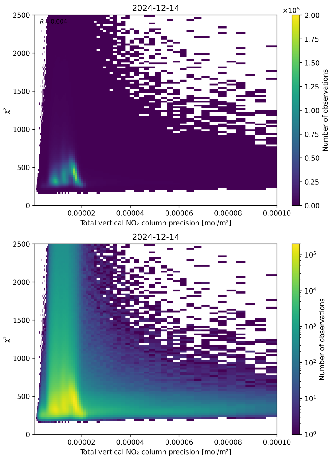
Figure 116: Scatter density plot of “Total vertical NO 2 column precision” against “ \chi^2 ” for 2024-12-13 to 2024-12-15.
