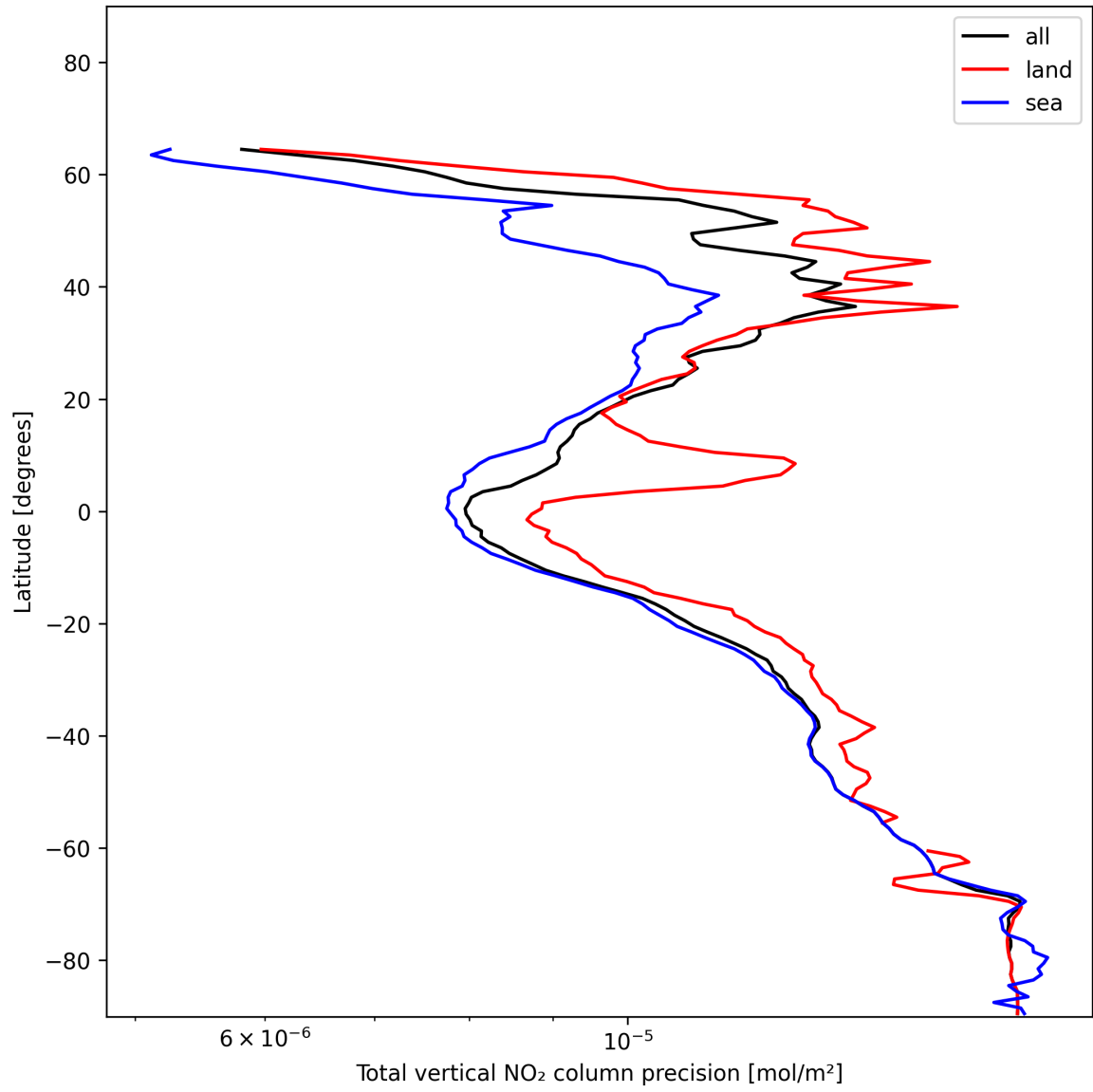
Figure 22: Zonal average of “Total vertical NO 2 column precision” for 2024-12-13 to 2024-12-15.
