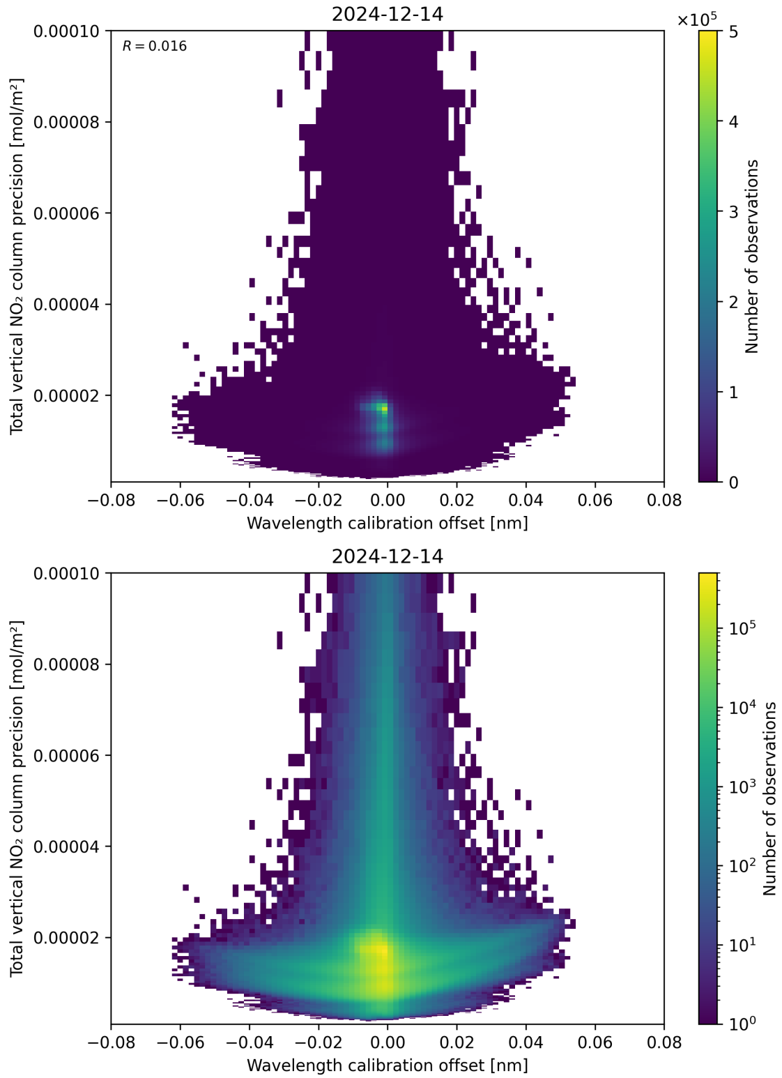
Figure 180: Scatter density plot of “Wavelength calibration offset” against “Total vertical NO 2 column precision” for 2024-12-13 to 2024-12-15.
