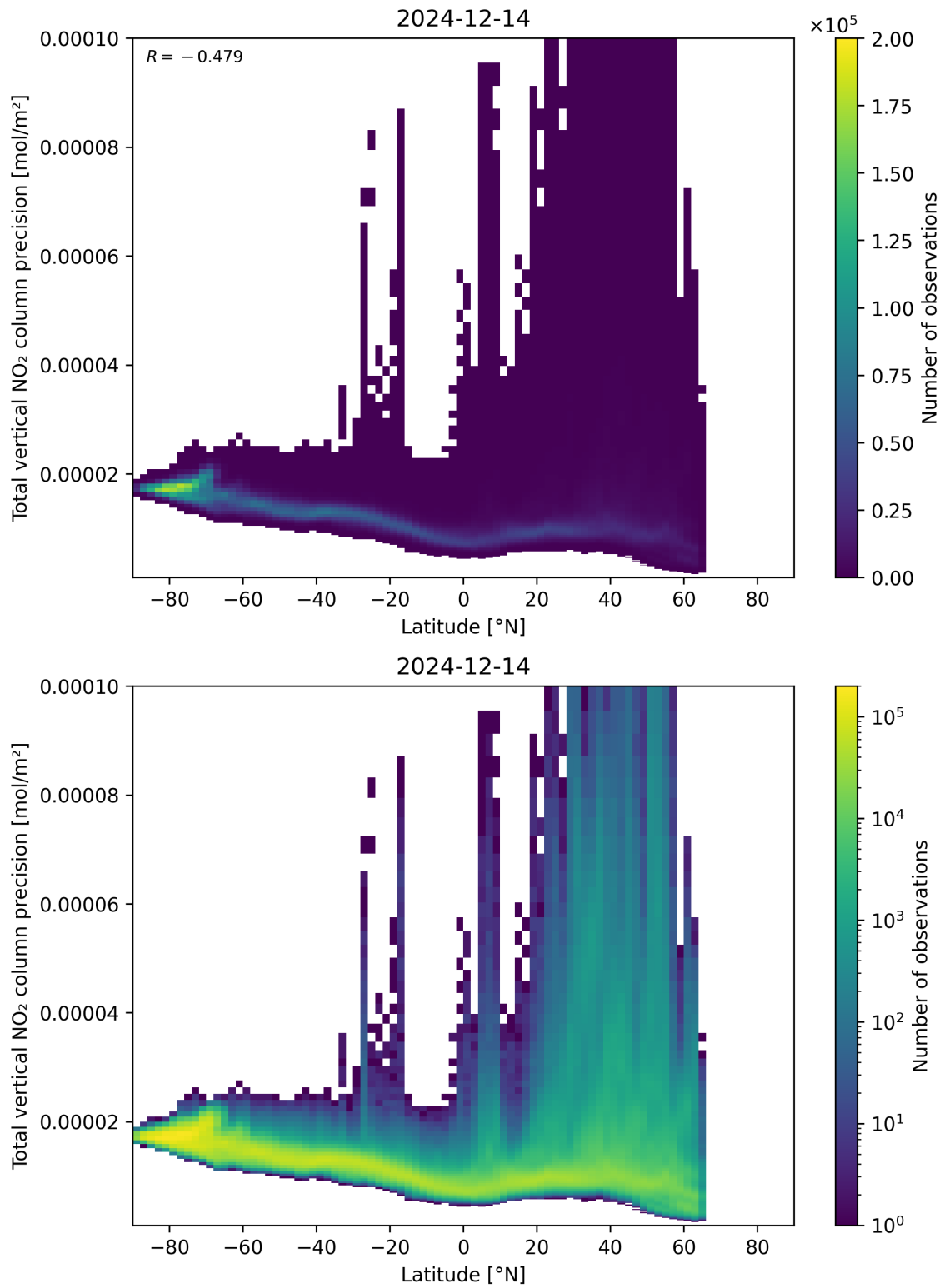
Figure 91: Scatter density plot of “Latitude” against “Total vertical NO 2 column precision” for 2024-12-13 to 2024-12-15.
