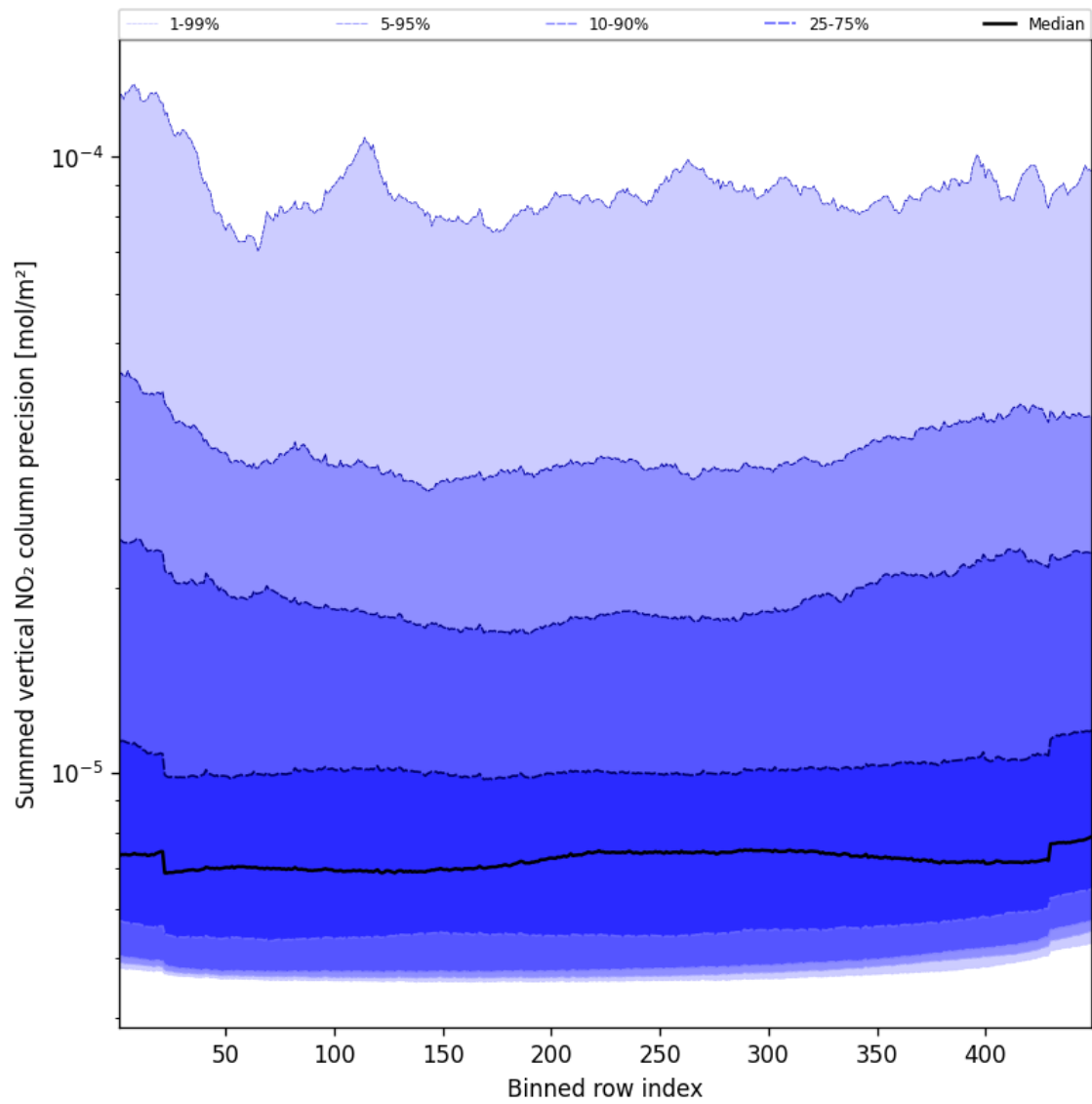
Figure 58: Along track statistics of “Summed vertical NO 2 column precision” for 2024-12-13 to 2024-12-15
