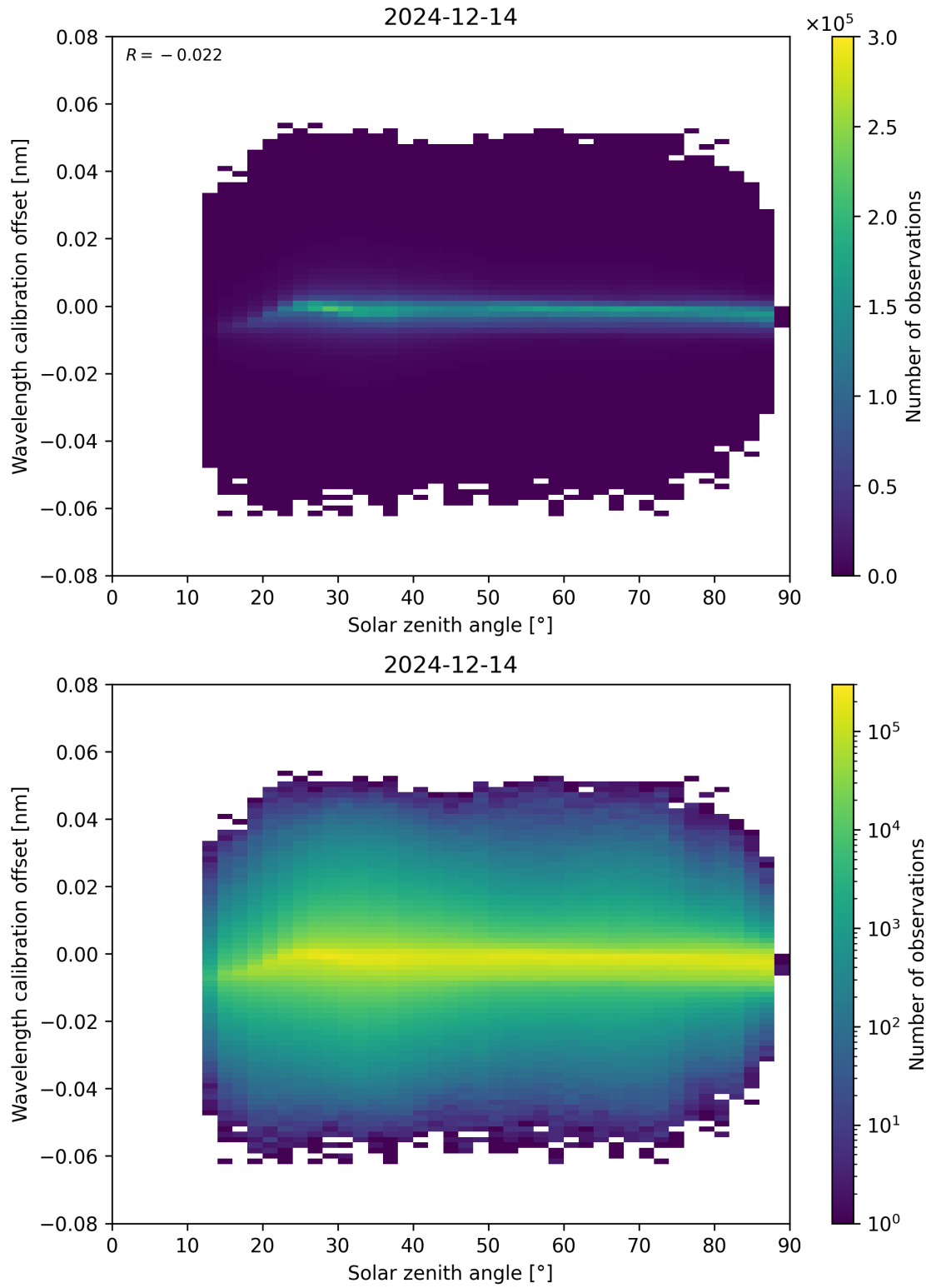
Figure 158: Scatter density plot of “Solar zenith angle” against “Wavelength calibration offset” for 2024-12-13 to 2024-12-15.
