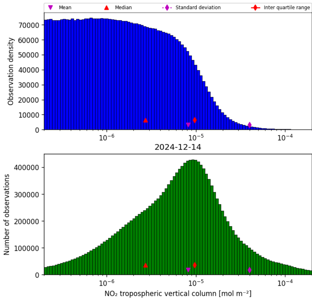
Figure 29: Histogram of “NO 2 tropospheric vertical column” for 2024-12-13 to 2024-12-15
