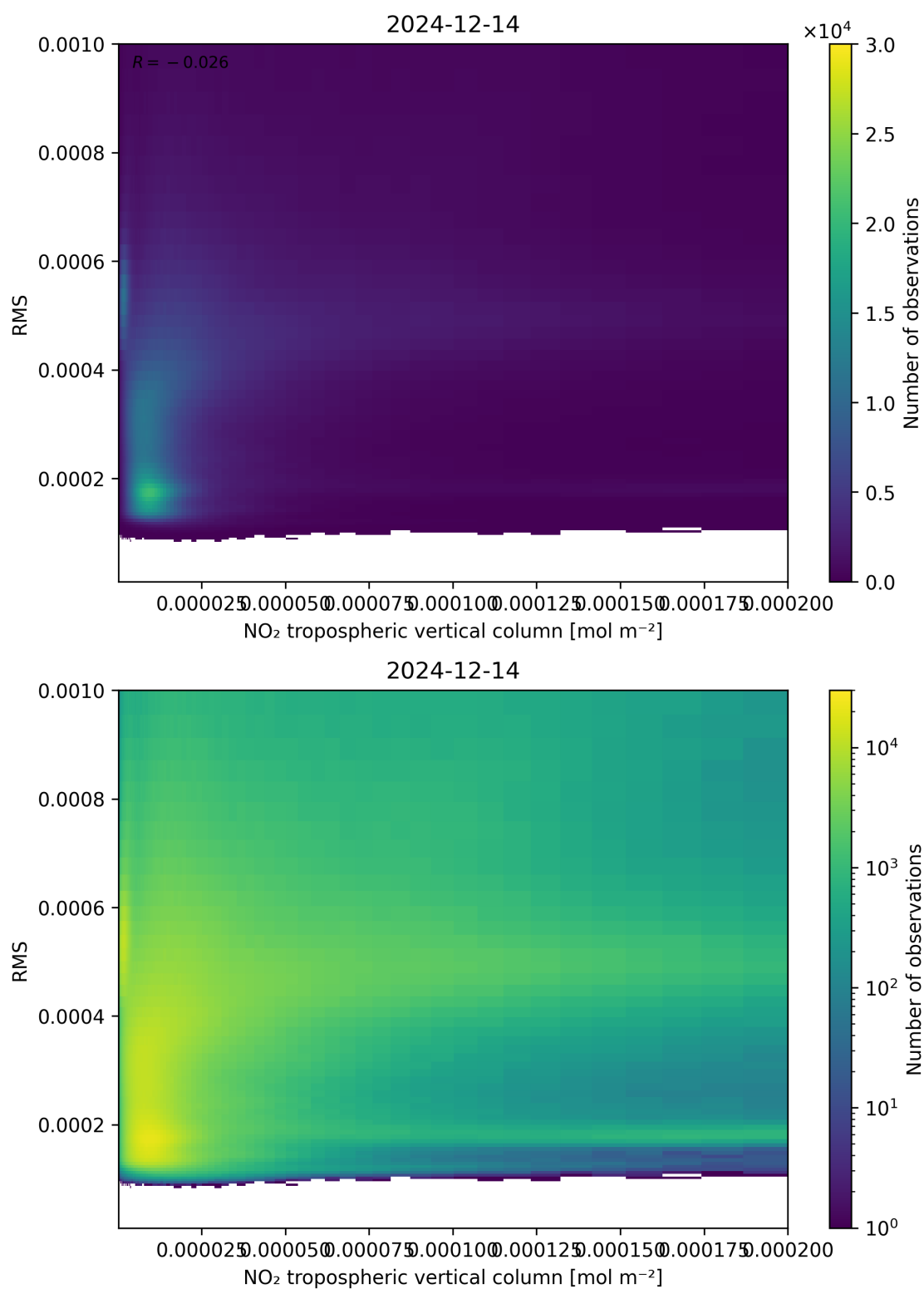
Figure 142: Scatter density plot of “NO 2 tropospheric vertical column” against “RMS” for 2024-12-13 to 2024-12-15.
