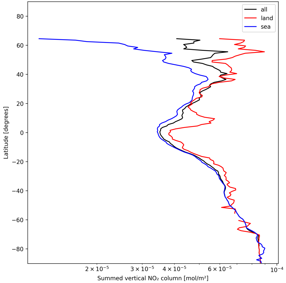
Figure 23: Zonal average of “Summed vertical NO 2 column” for 2024-12-13 to 2024-12-15.
