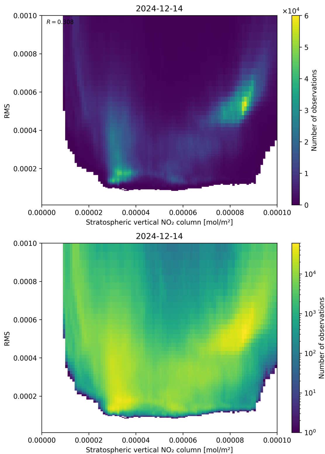
Figure 102: Scatter density plot of “Stratospheric vertical NO 2 column” against “RMS” for 2024-12-13 to 2024-12-15.
