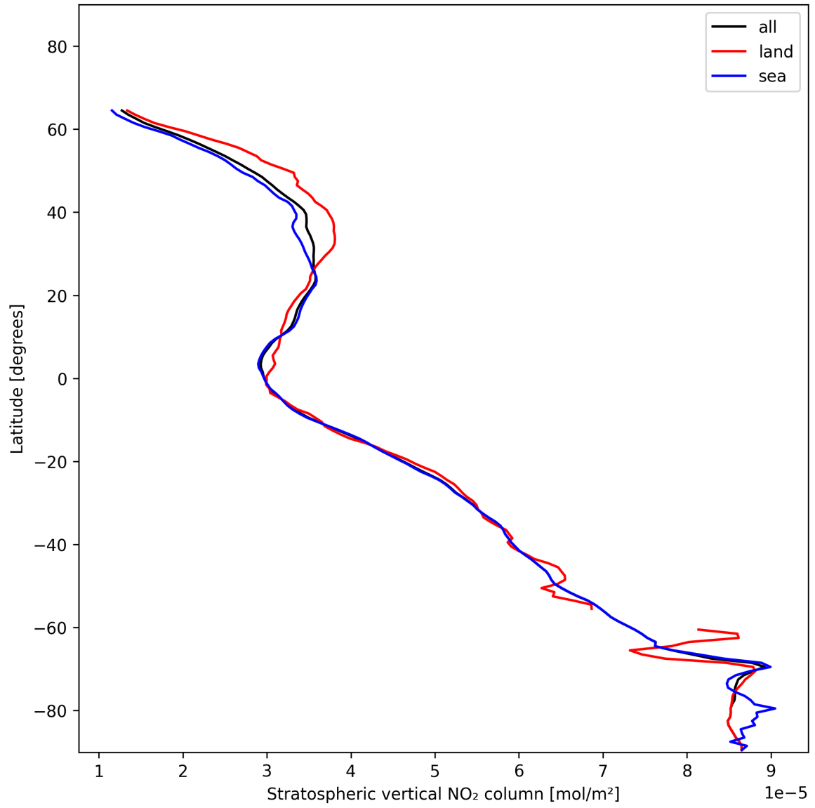
Figure 19: Zonal average of “Stratospheric vertical NO 2 column” for 2024-12-13 to 2024-12-15.
