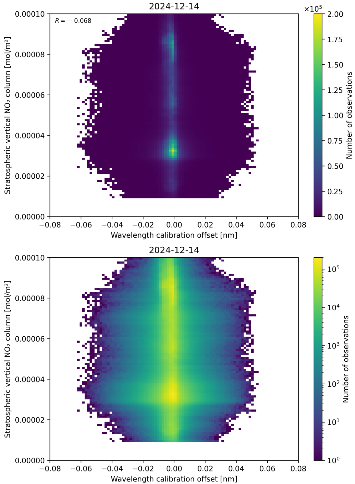
Figure 176: Scatter density plot of “Wavelength calibration offset” against “Stratospheric vertical NO 2 column” for 2024-12-13 to 2024-12-15.
