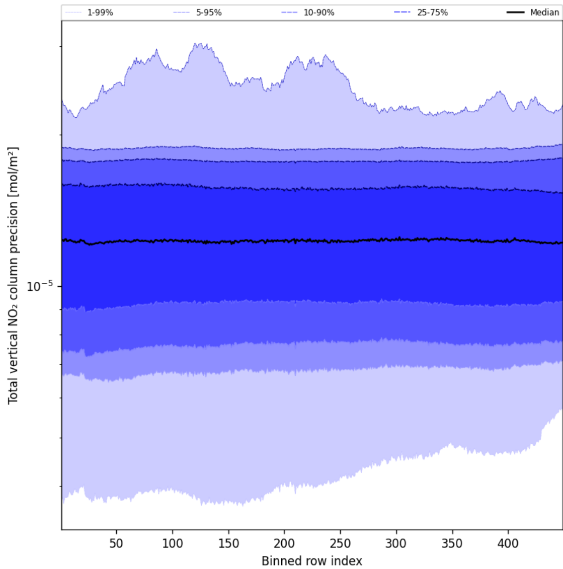
Figure 56: Along track statistics of “Total vertical NO 2 column precision” for 2024-12-13 to 2024-12-15
