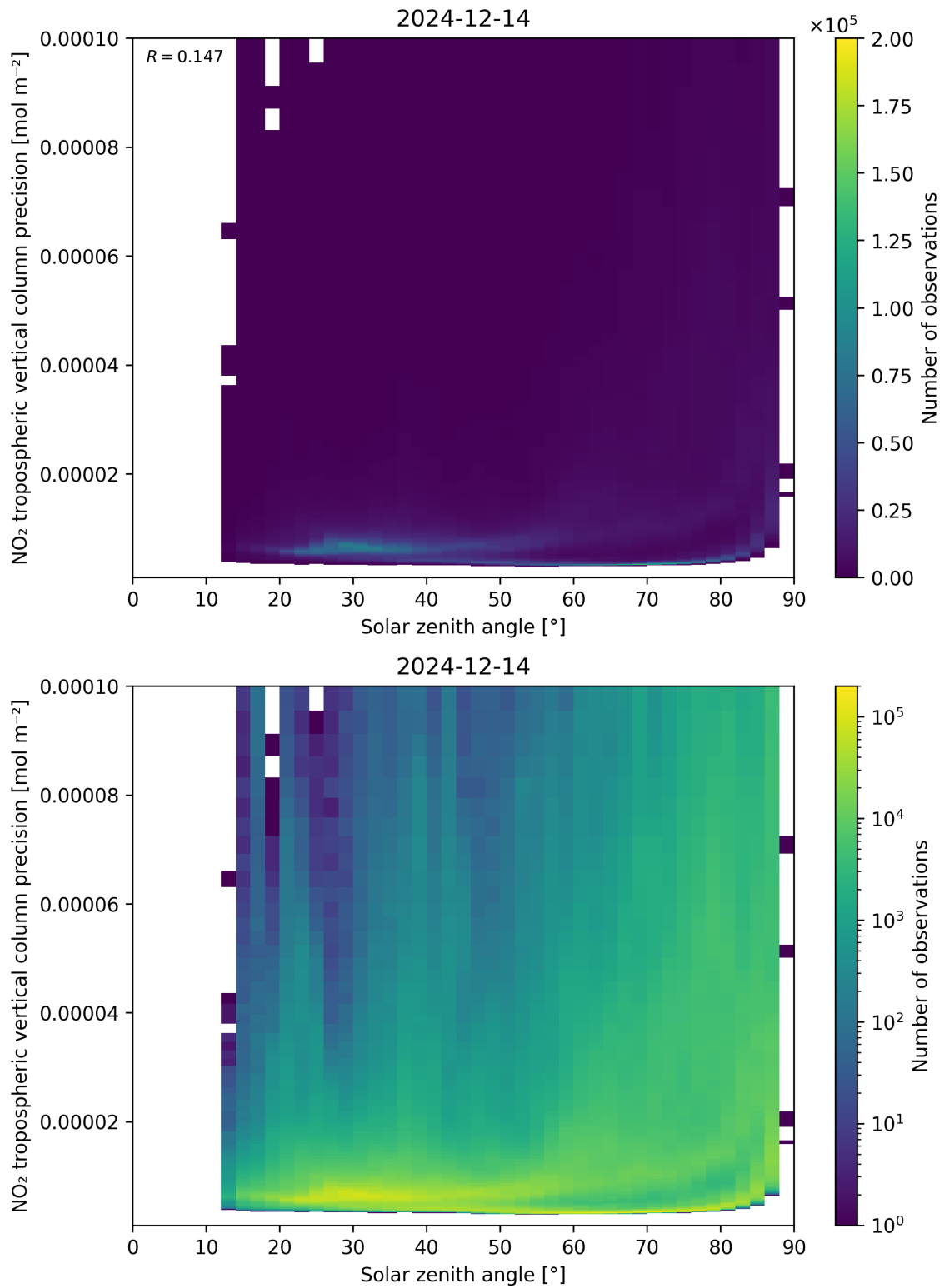
Figure 156: Scatter density plot of “Solar zenith angle” against “NO 2 tropospheric vertical column precision” for 2024-12-13 to 2024-12-15.
