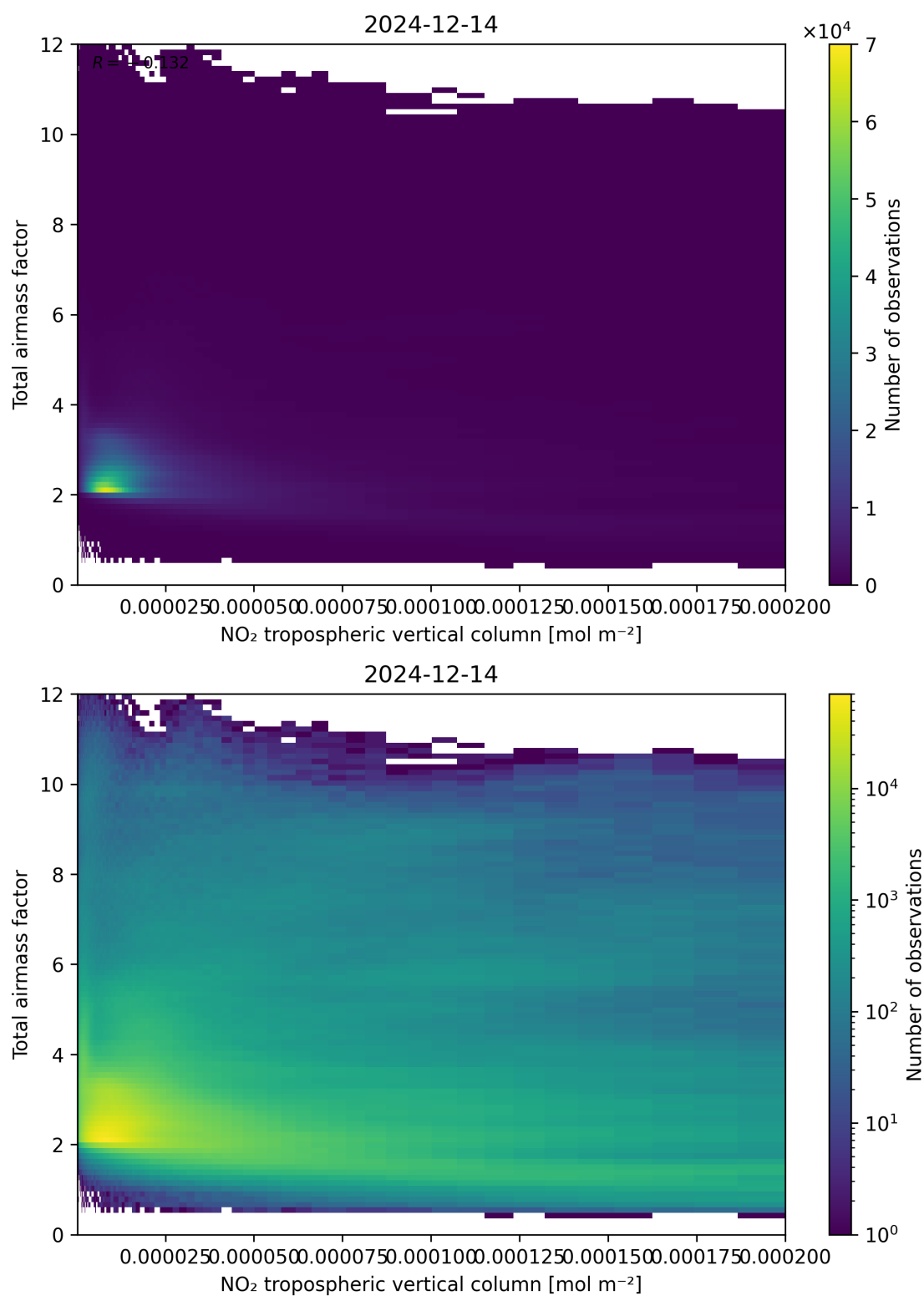
Figure 122: Scatter density plot of “NO 2 tropospheric vertical column” against “Total air mass factor” for 2024-12-13 to 2024-12-15.
