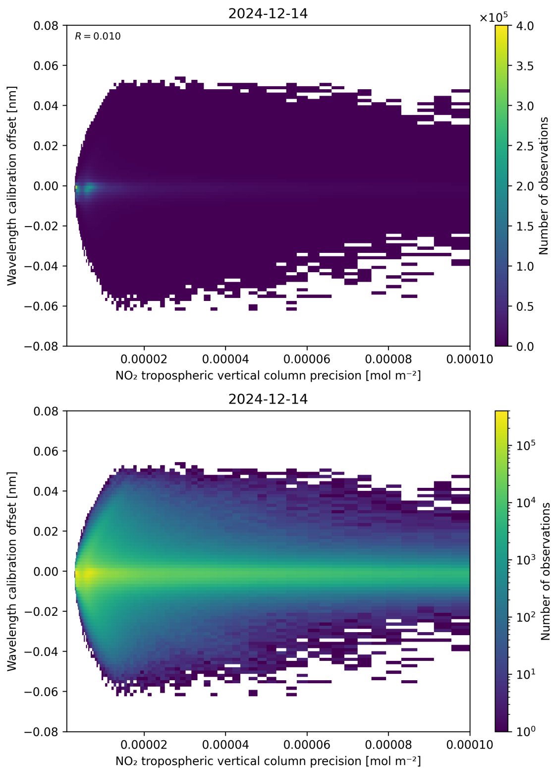
Figure 141: Scatter density plot of “NO 2 tropospheric vertical column precision” against “Wavelength calibration offset” for 2024-12-13 to 2024-12-15.
