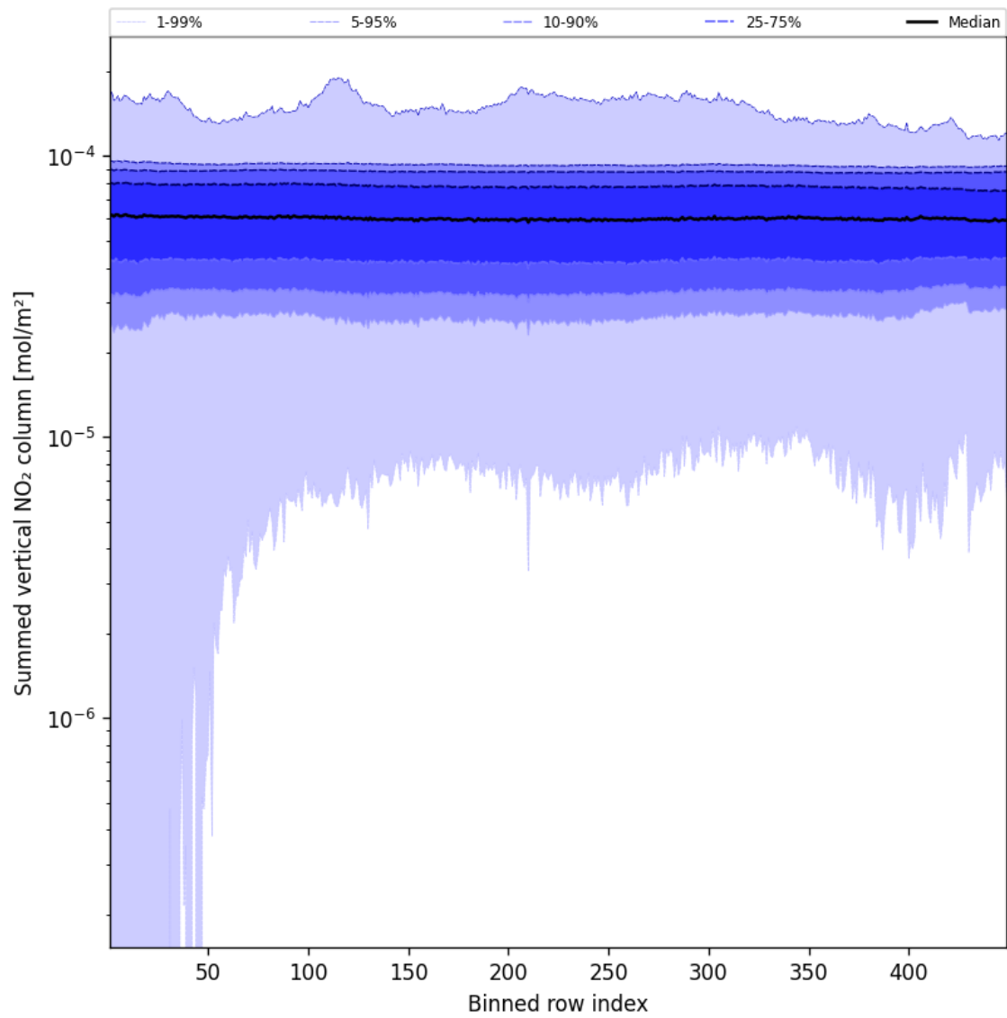
Figure 57: Along track statistics of “Summed vertical NO 2 column” for 2024-12-13 to 2024-12-15
