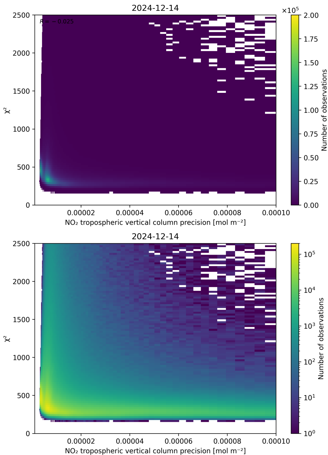
Figure 134: Scatter density plot of “NO 2 tropospheric vertical column precision” against “ \chi^2 ” for 2024-12-13 to 2024-12-15.
