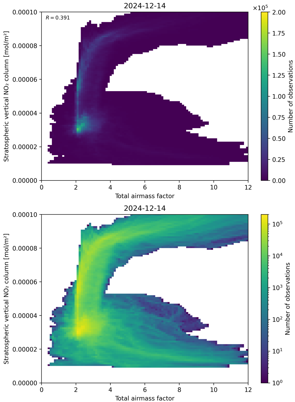
Figure 64: Scatter density plot of “Total airmass factor” against “Stratospheric vertical NO 2 column” for 2024-12-13 to 2024-12-15.
