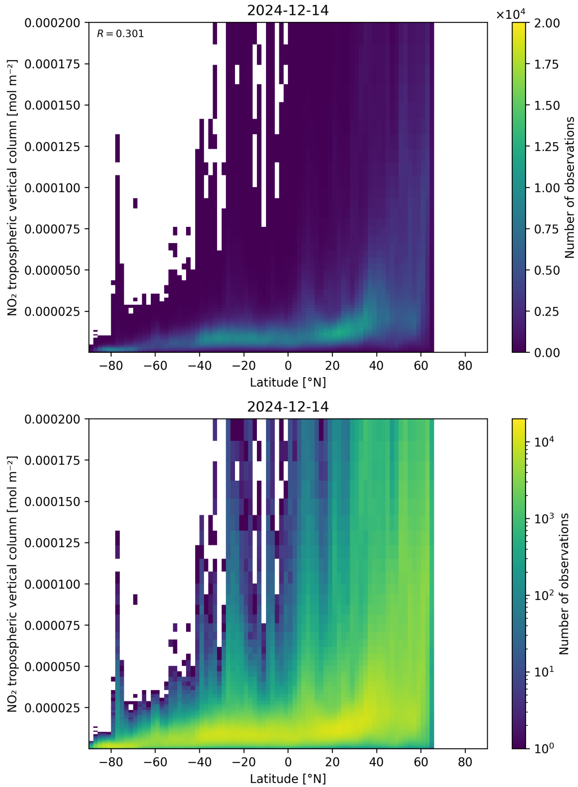
Figure 92: Scatter density plot of “Latitude” against “NO 2 tropospheric vertical column” for 2024-12-13 to 2024-12-15.
