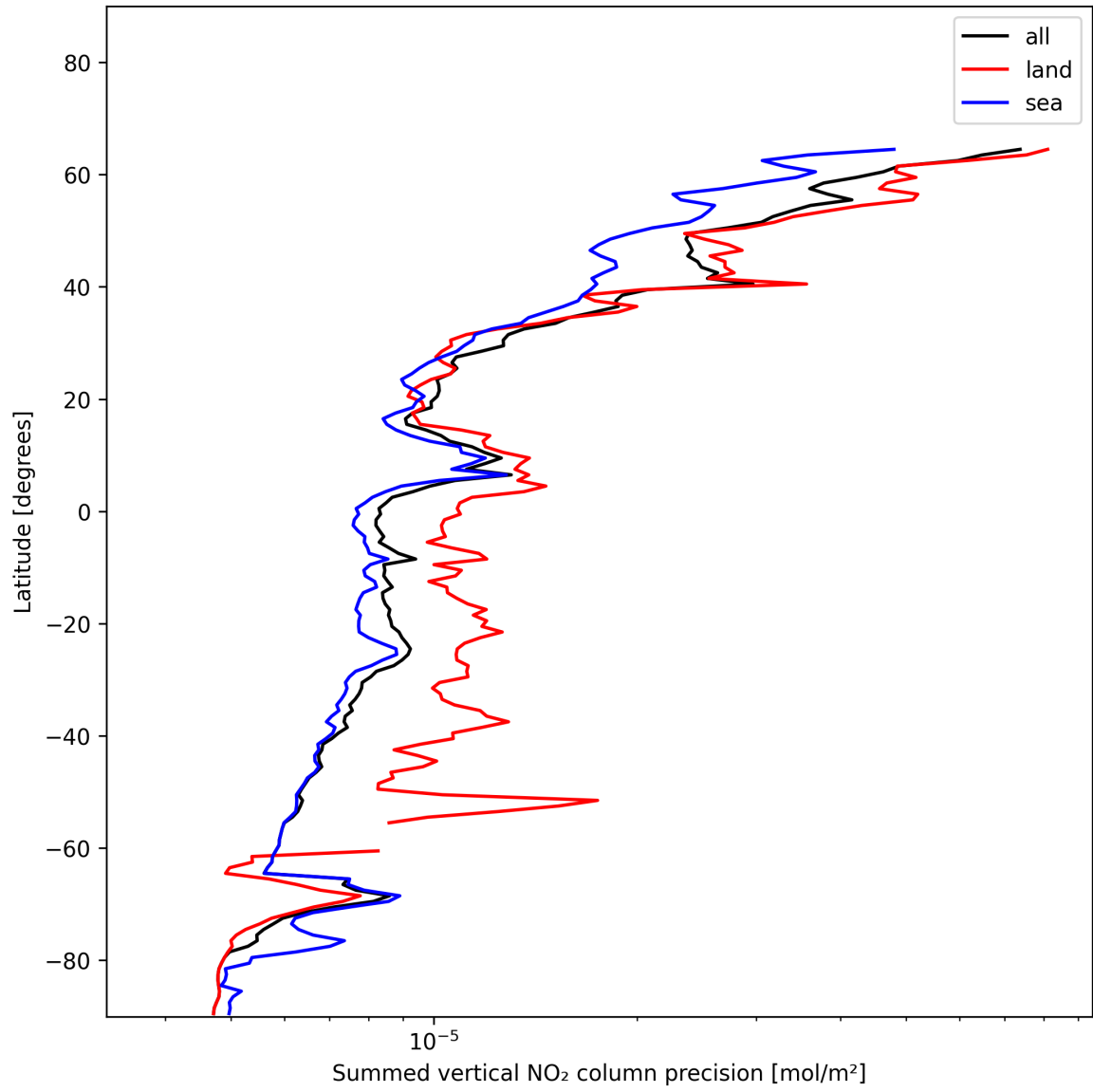
Figure 24: Zonal average of “Summed vertical NO 2 column precision” for 2024-12-13 to 2024-12-15.
