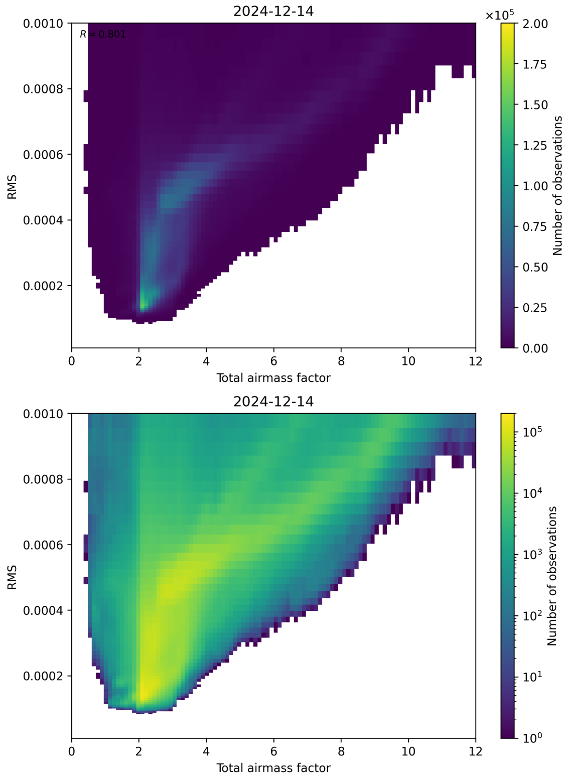
Figure 69: Scatter density plot of “Total airmass factor” against “RMS” for 2024-12-13 to 2024-12-15.
