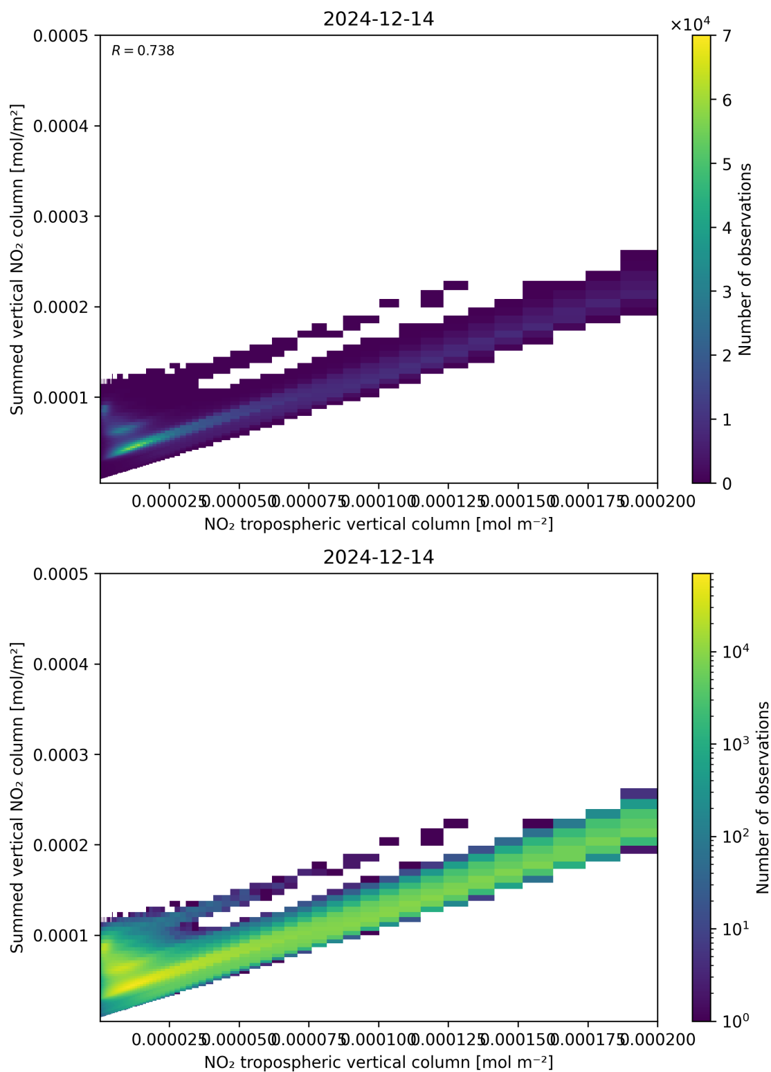
Figure 126: Scatter density plot of “NO 2 tropospheric vertical column” against “Summed vertical NO 2 column” for 2024-12-13 to 2024-12-15.
