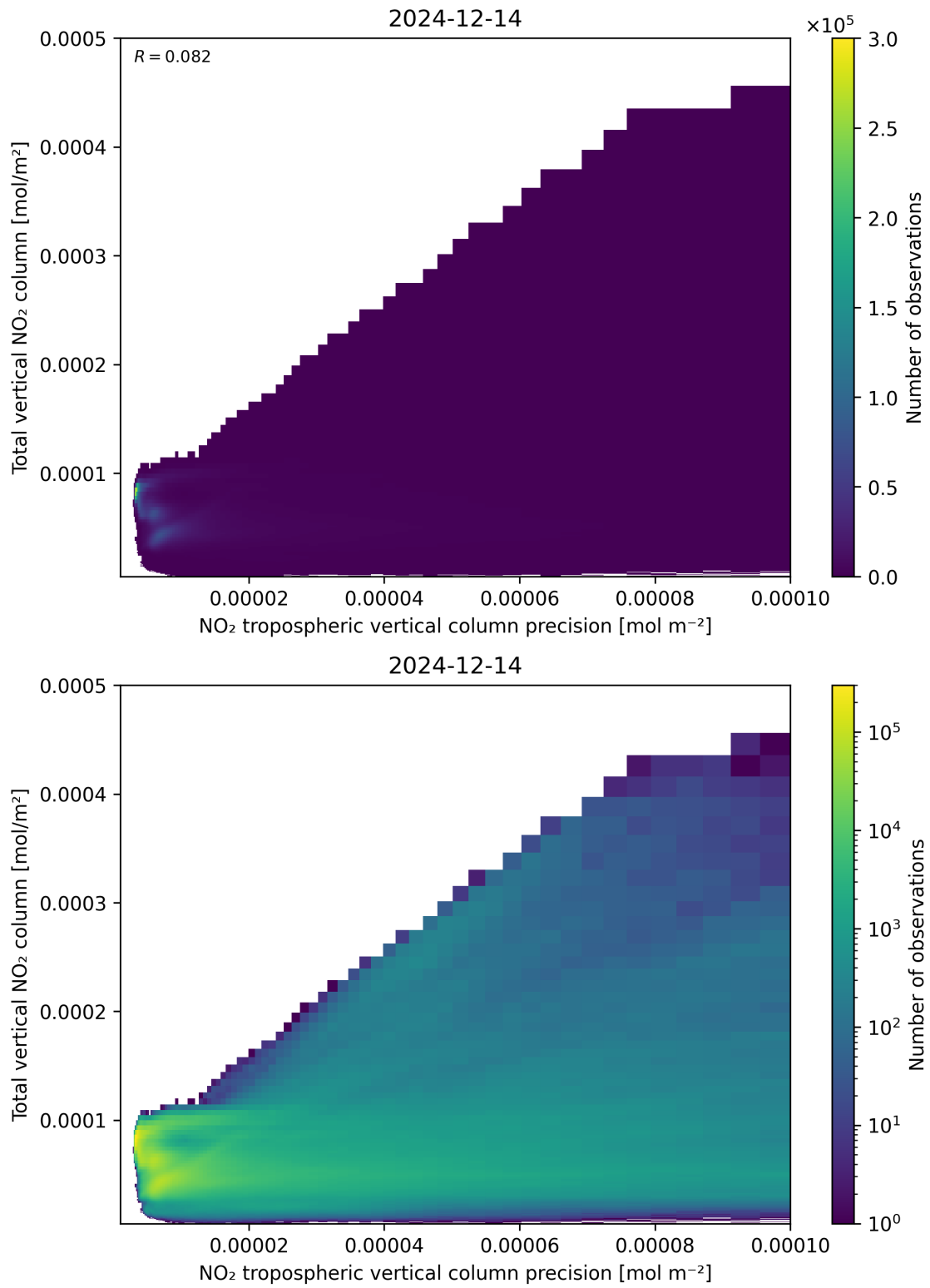
Figure 138: Scatter density plot of “NO 2 tropospheric vertical column precision” against “Total vertical NO 2 column” for 2024-12-13 to 2024-12-15.
