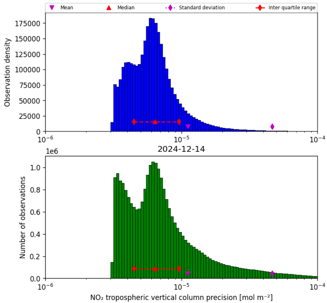
Figure 30: Histogram of “NO 2 tropospheric vertical column precision” for 2024-12-13 to 2024-12-15
