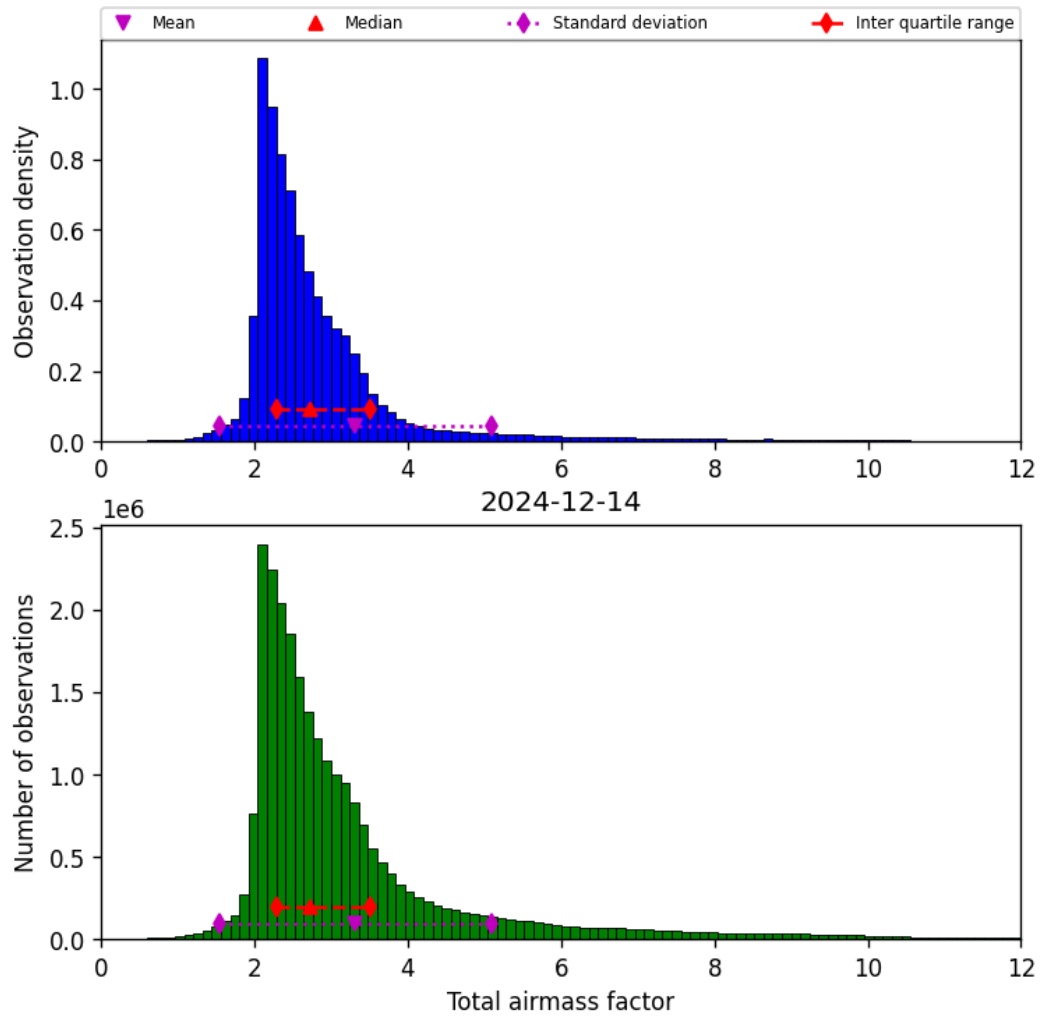
Figure 32: Histogram of “Total airmass factor” for 2024-12-13 to 2024-12-15
