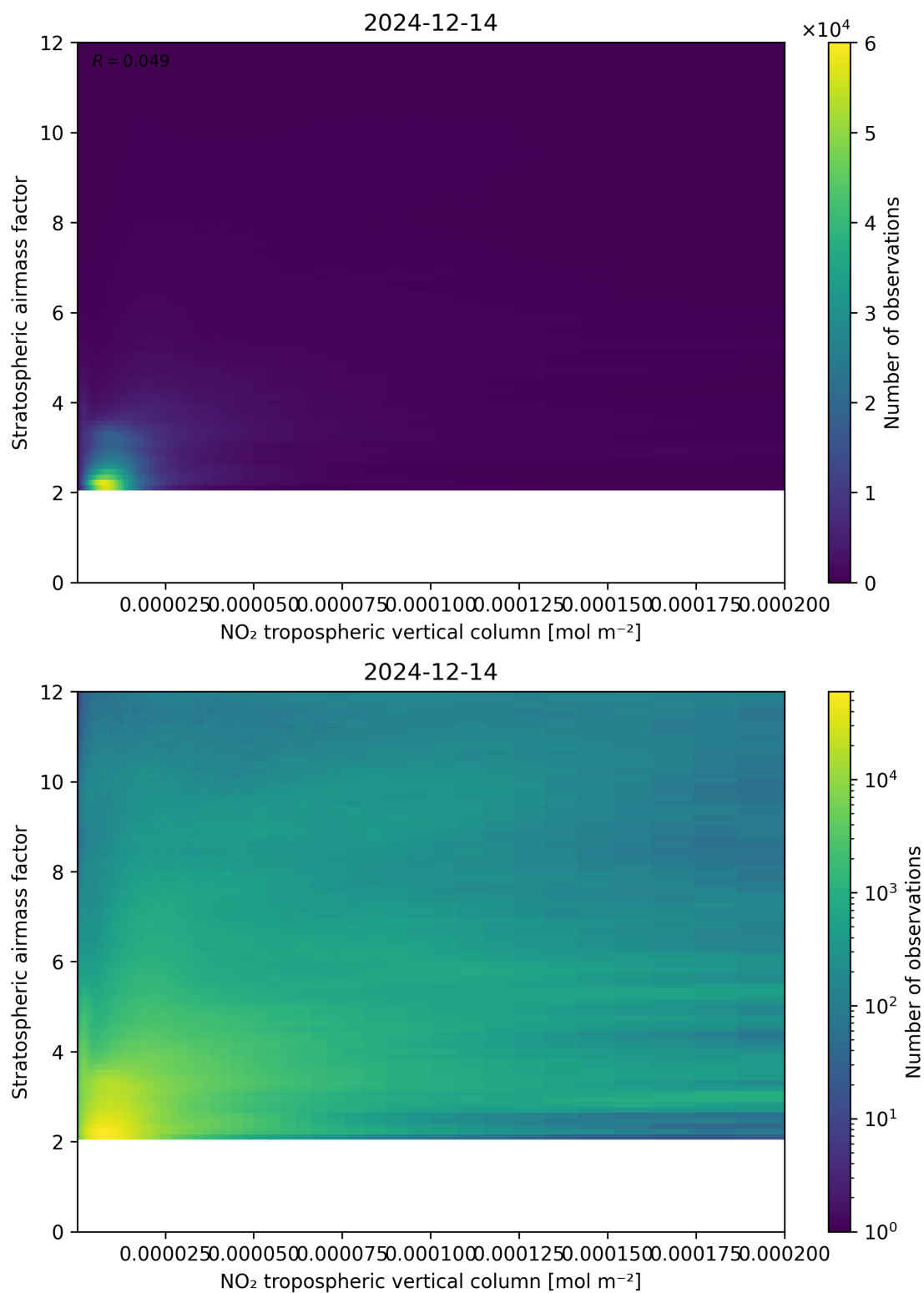
Figure 121: Scatter density plot of “NO 2 tropospheric vertical column” against “Stratospheric airmass factor” for 2024-12-13 to 2024-12-15.
