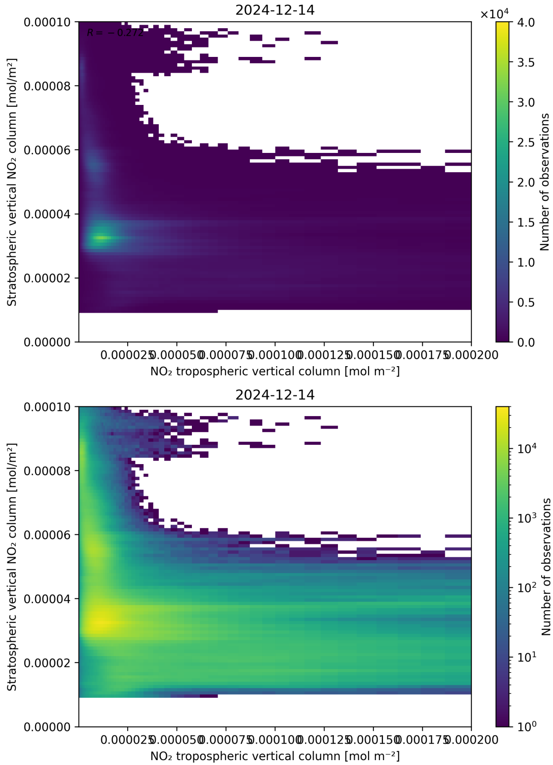
Figure 125: Scatter density plot of “NO 2 tropospheric vertical column” against “Stratospheric vertical NO 2 column” for 2024-12-13 to 2024-12-15.
