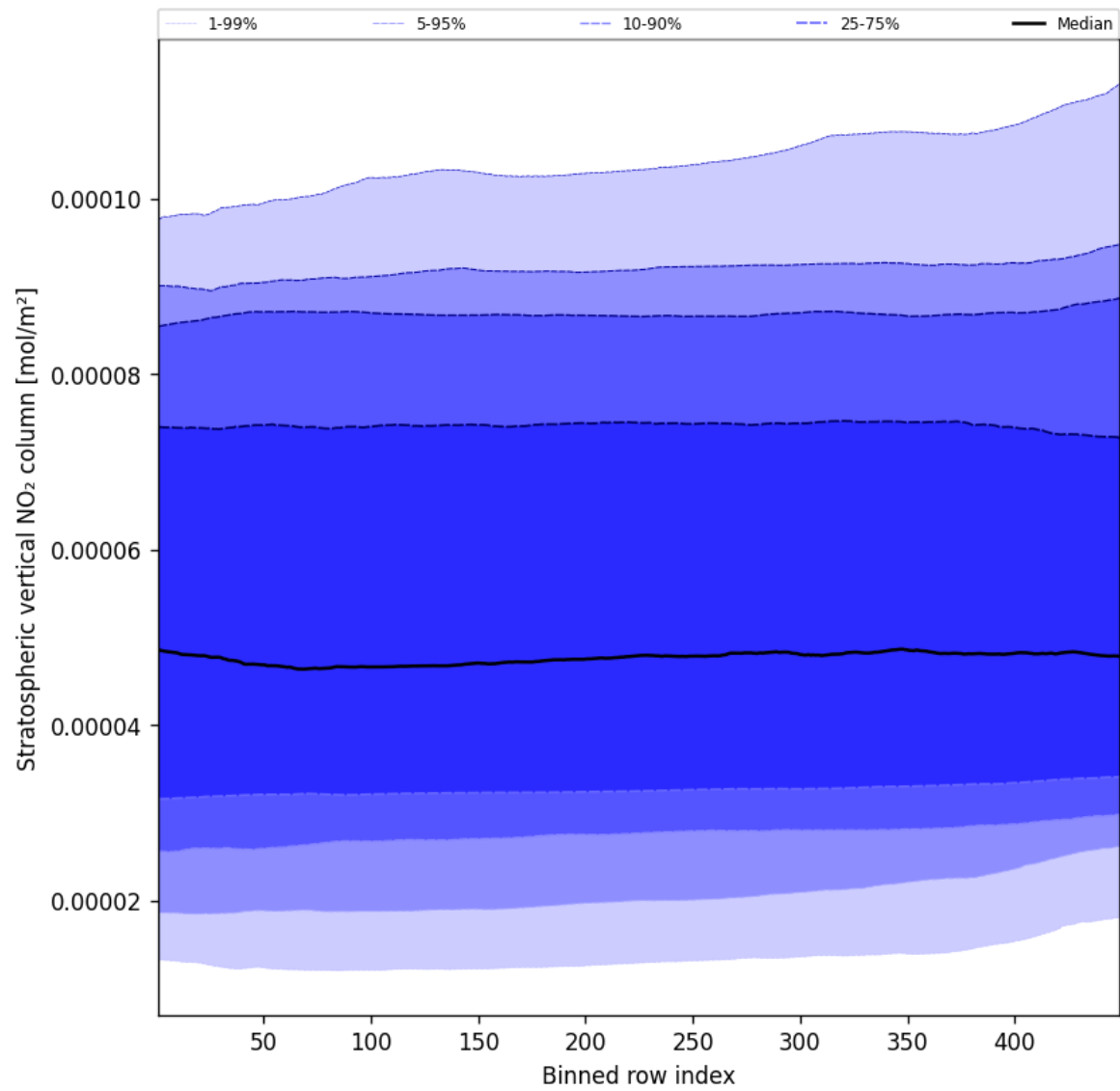
Figure 53: Along track statistics of “Stratospheric vertical NO 2 column” for 2024-12-13 to 2024-12-15
