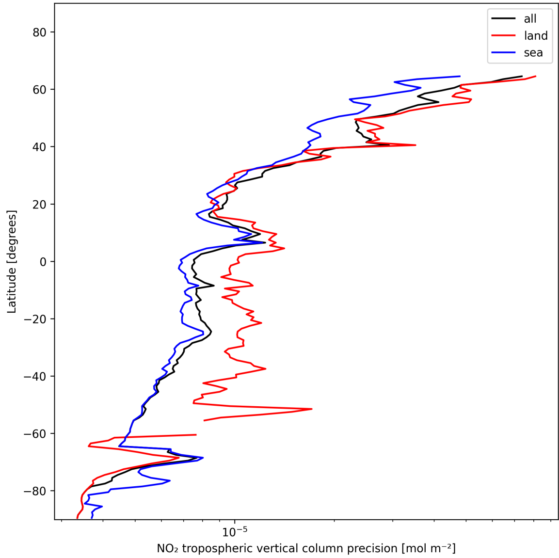
Figure 13: Zonal average of “NO 2 tropospheric vertical column precision” for 2024-12-13 to 2024-12-15.
