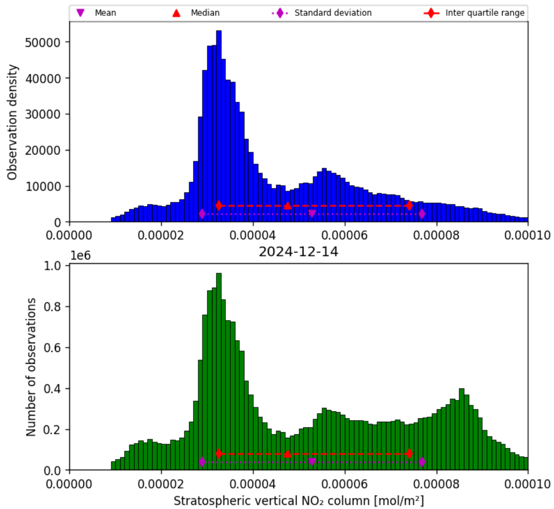
Figure 36: Histogram of “Stratospheric vertical NO 2 column” for 2024-12-13 to 2024-12-15
