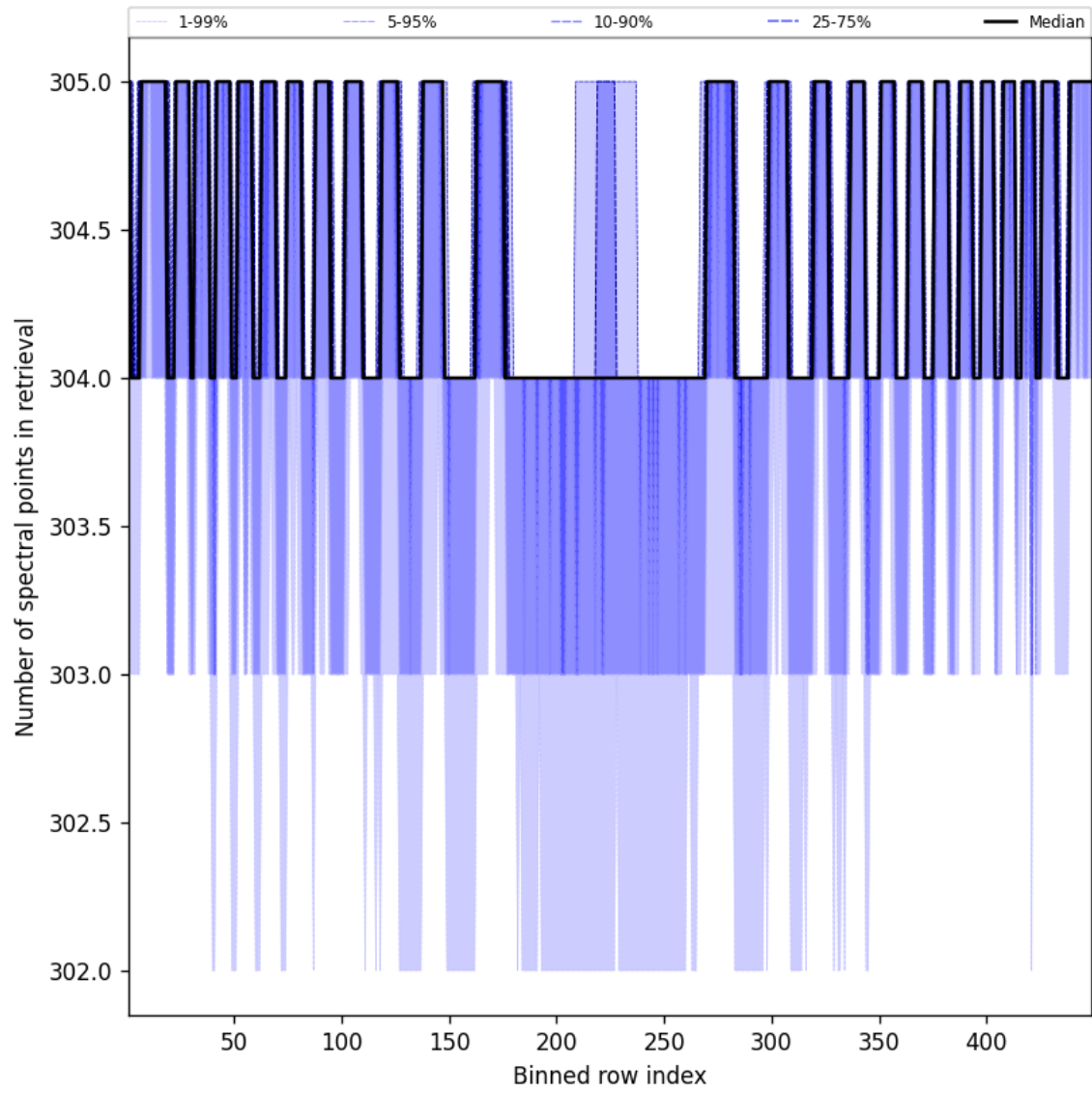
Figure 50: Along track statistics of “Number of spectral points in retrieval” for 2024-12-13 to 2024-12-15
