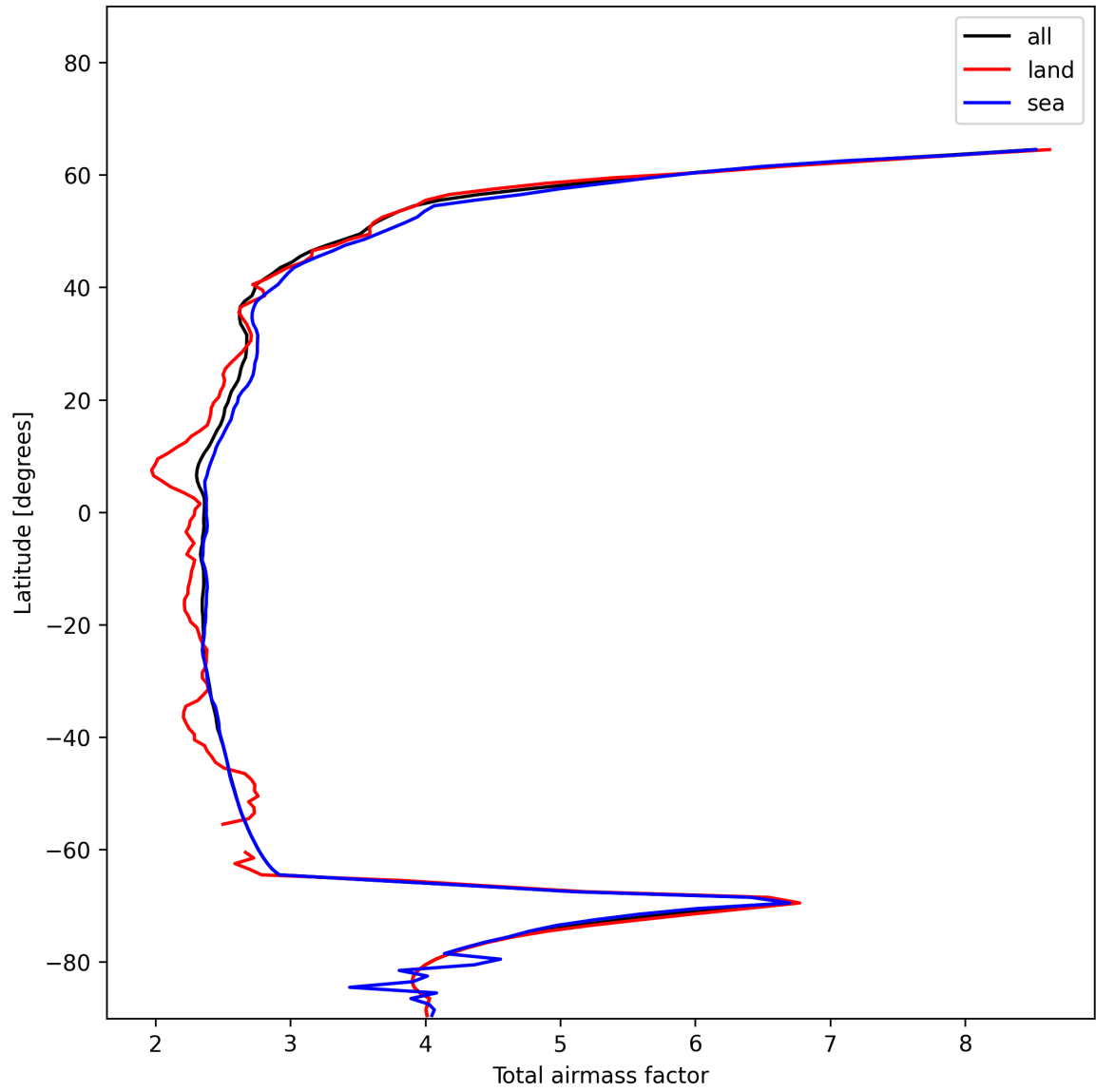
Figure 15: Zonal average of “Total airmass factor” for 2024-12-13 to 2024-12-15.
