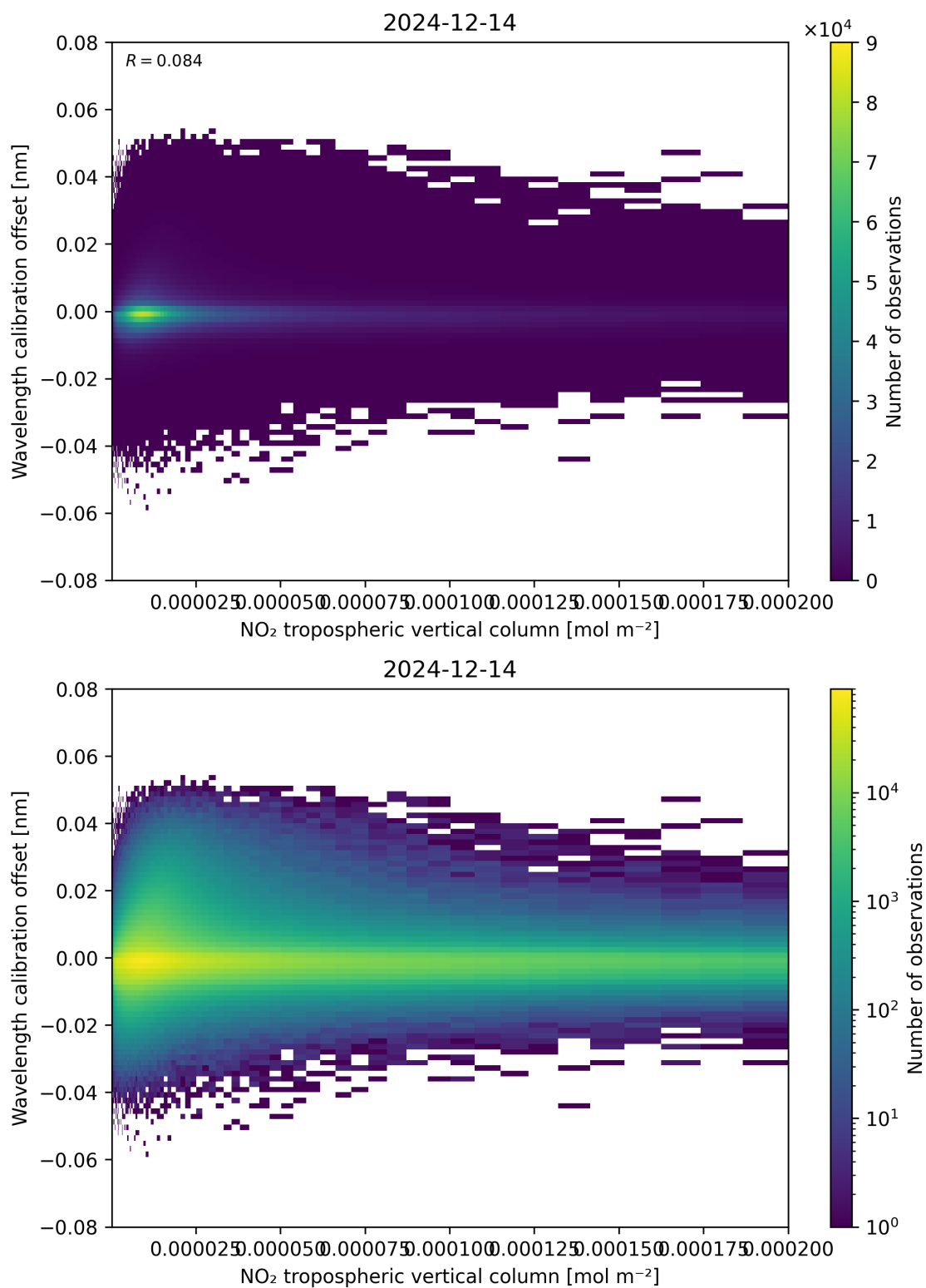
Figure 143: Scatter density plot of “NO 2 tropospheric vertical column” against “Wavelength calibration offset” for 2024-12-13 to 2024-12-15.
