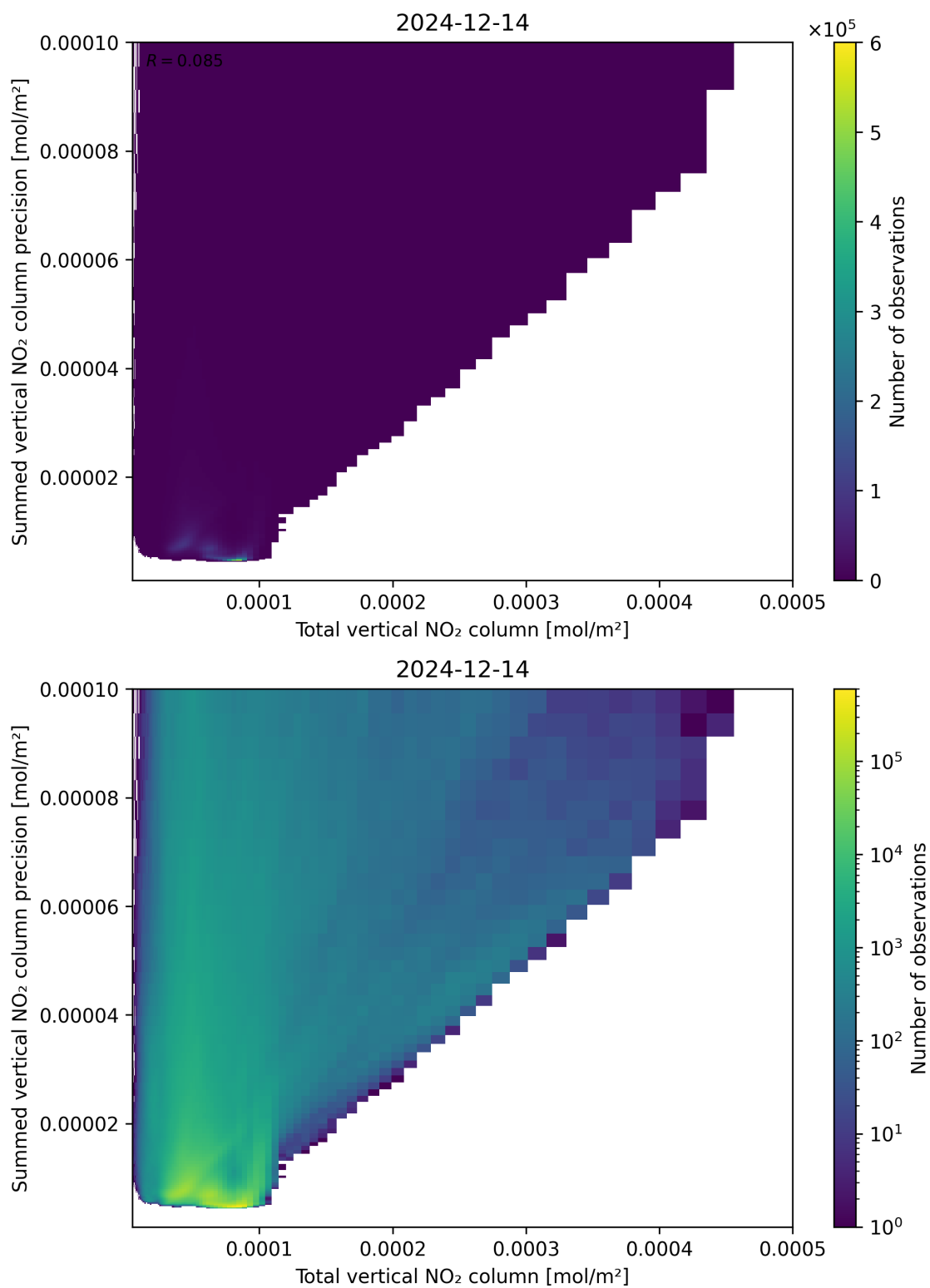
Figure 113: Scatter density plot of “Total vertical NO 2 column” against “Summed vertical NO 2 column precision” for 2024-12-13 to 2024-12-15.
