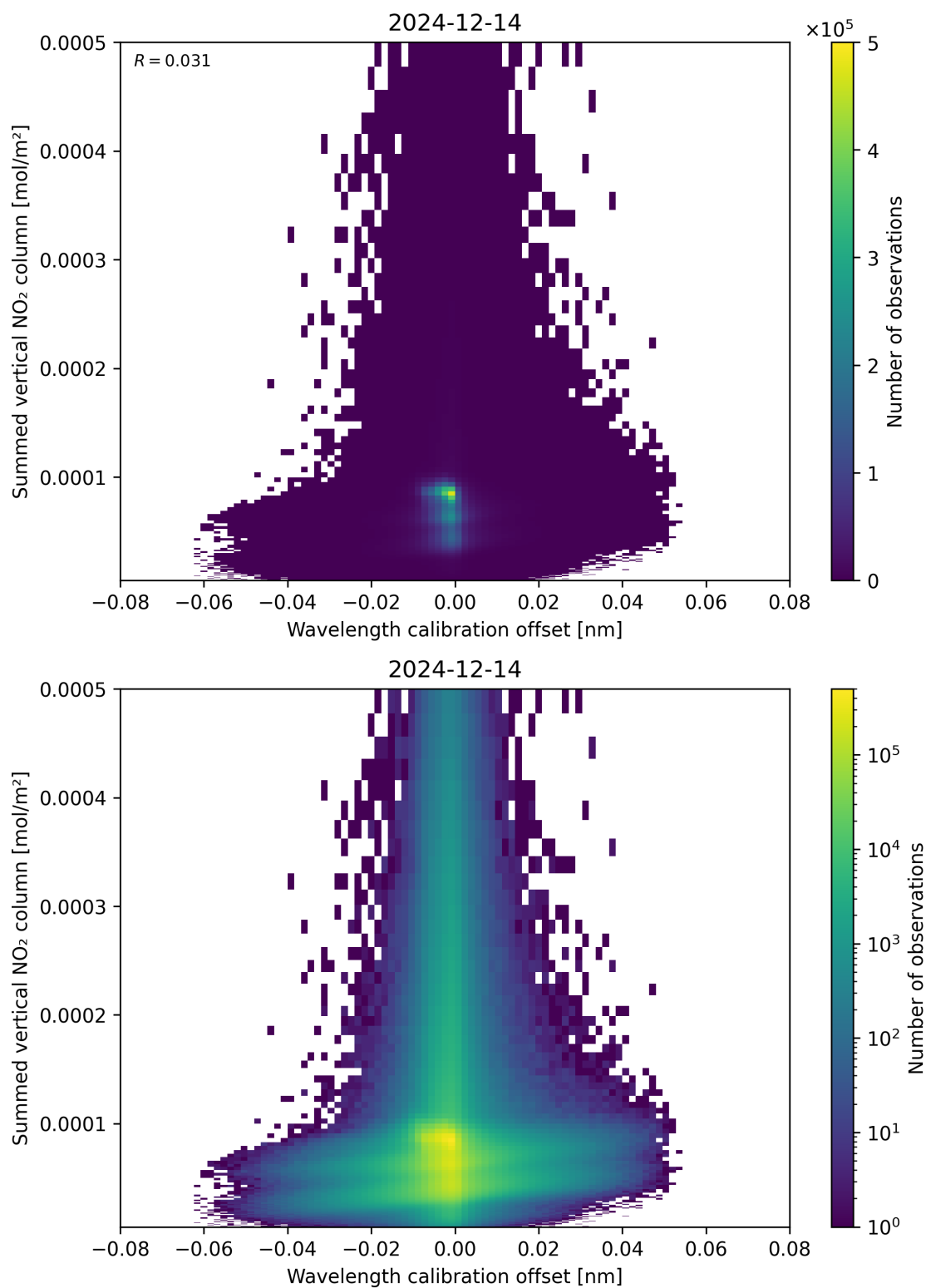
Figure 177: Scatter density plot of “Wavelength calibration offset” against “Summed vertical NO 2 column” for 2024-12-13 to 2024-12-15.
