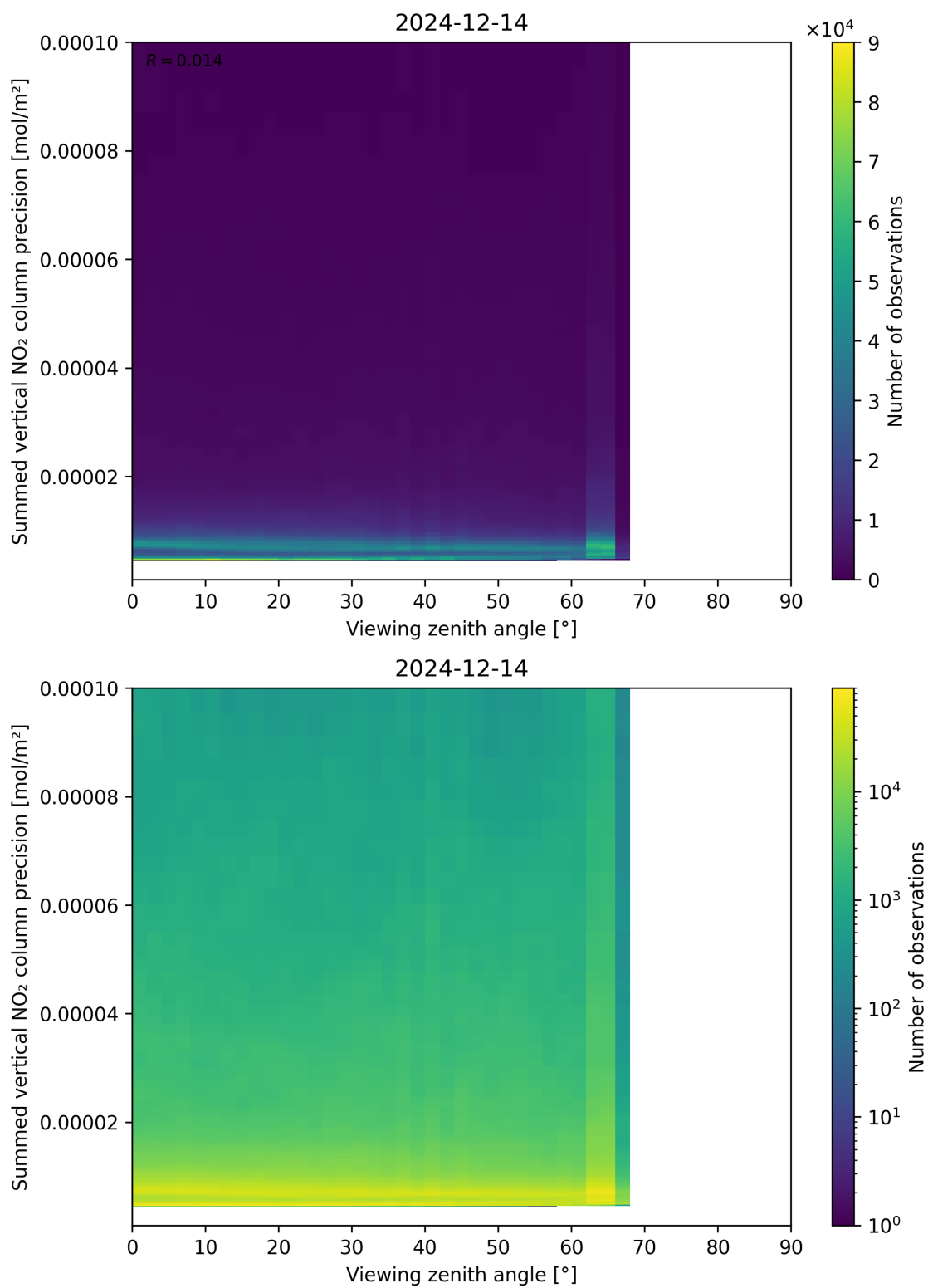
Figure 166: Scatter density plot of “Viewing zenith angle” against “Summed vertical NO 2 column precision” for 2024-12-13 to 2024-12-15.
