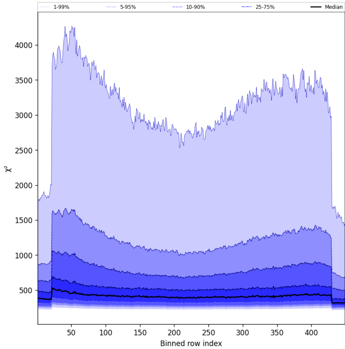
Figure 59: Along track statistics of “ \chi^2 ” for 2024-12-13 to 2024-12-15
