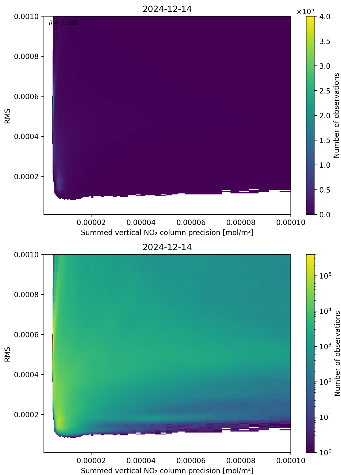
Figure 108: Scatter density plot of “Summed vertical NO 2 column precision” against “RMS” for 2024-12-13 to 2024-12-15.
