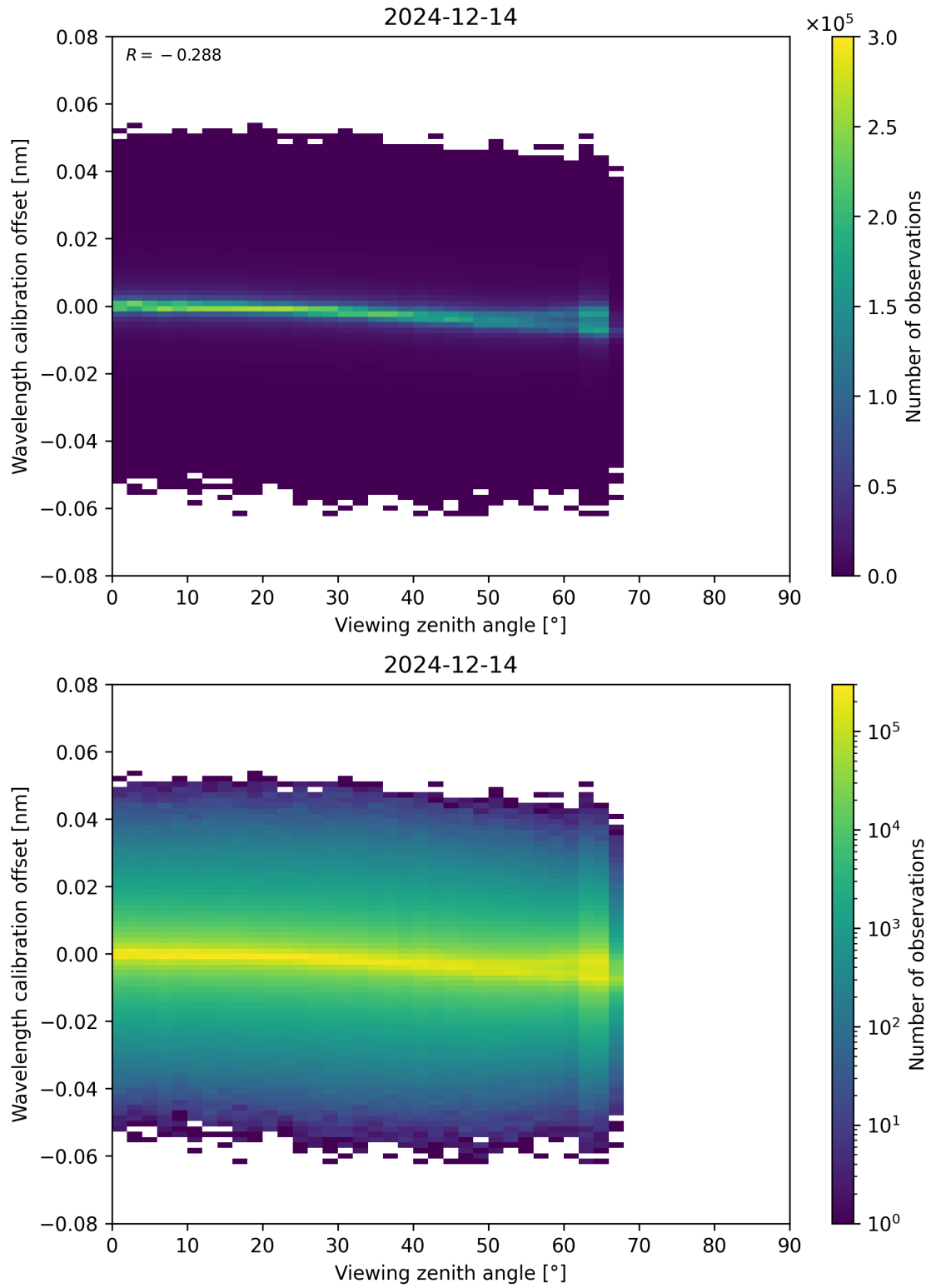
Figure 173: Scatter density plot of “Viewing zenith angle” against “Wavelength calibration offset” for 2024-12-13 to 2024-12-15.
