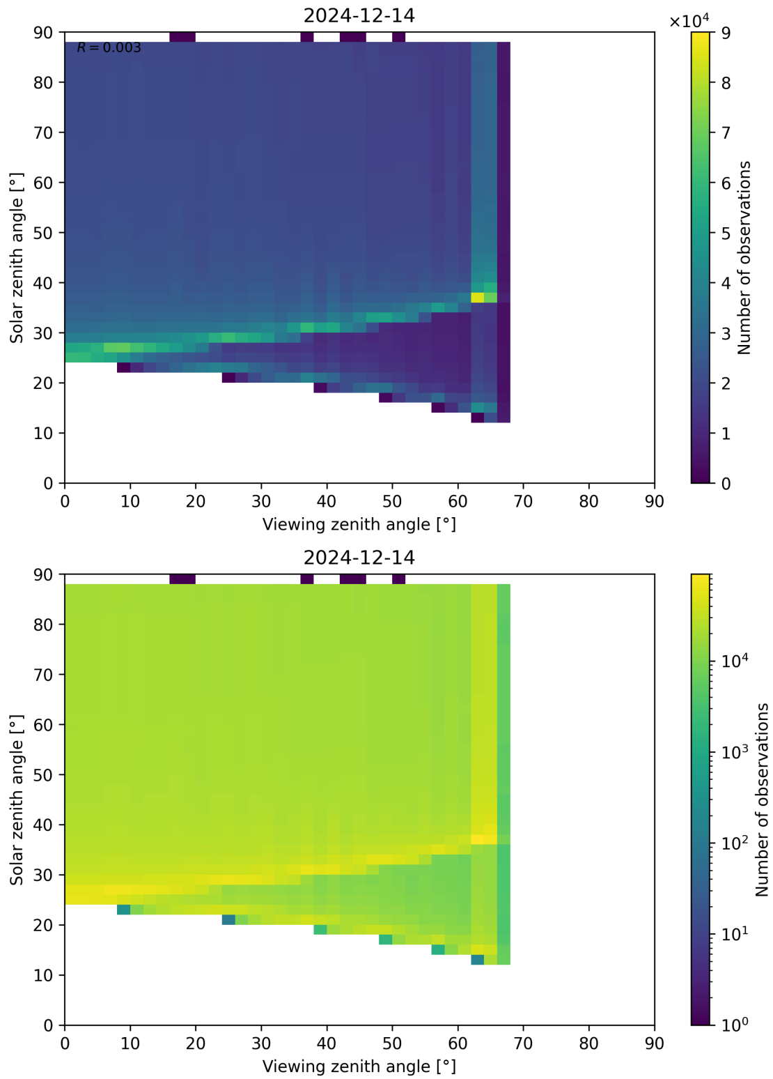
Figure 172: Scatter density plot of “Viewing zenith angle” against “Solar zenith angle” for 2024-12-13 to 2024-12-15.
