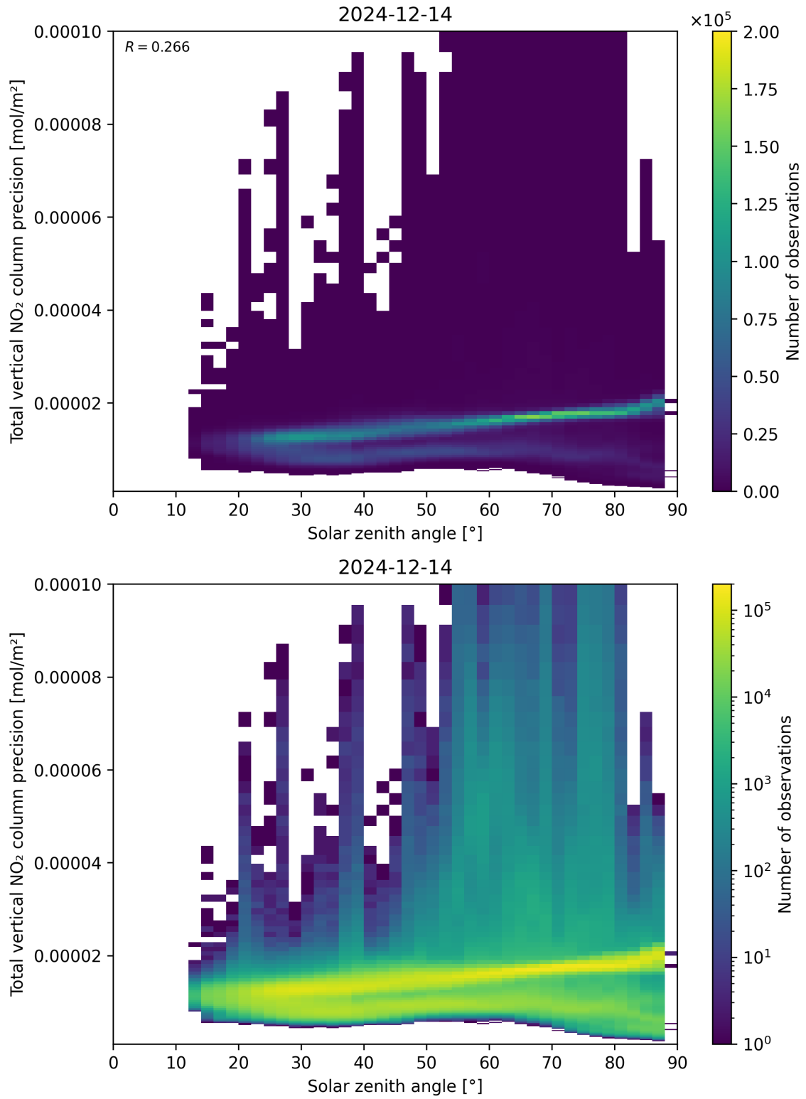
Figure 154: Scatter density plot of “Solar zenith angle” against “Total vertical NO 2 column precision” for 2024-12-13 to 2024-12-15.
