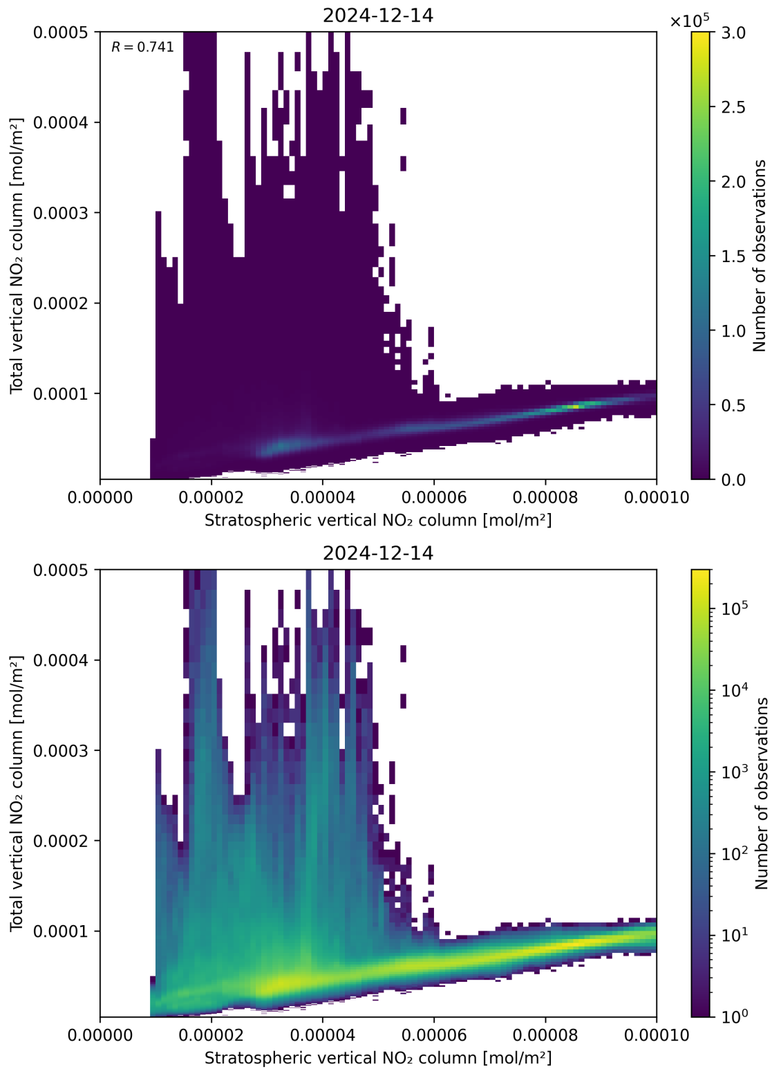
Figure 100: Scatter density plot of “Stratospheric vertical NO 2 column” against “Total vertical NO 2 column” for 2024-12-13 to 2024-12-15.
