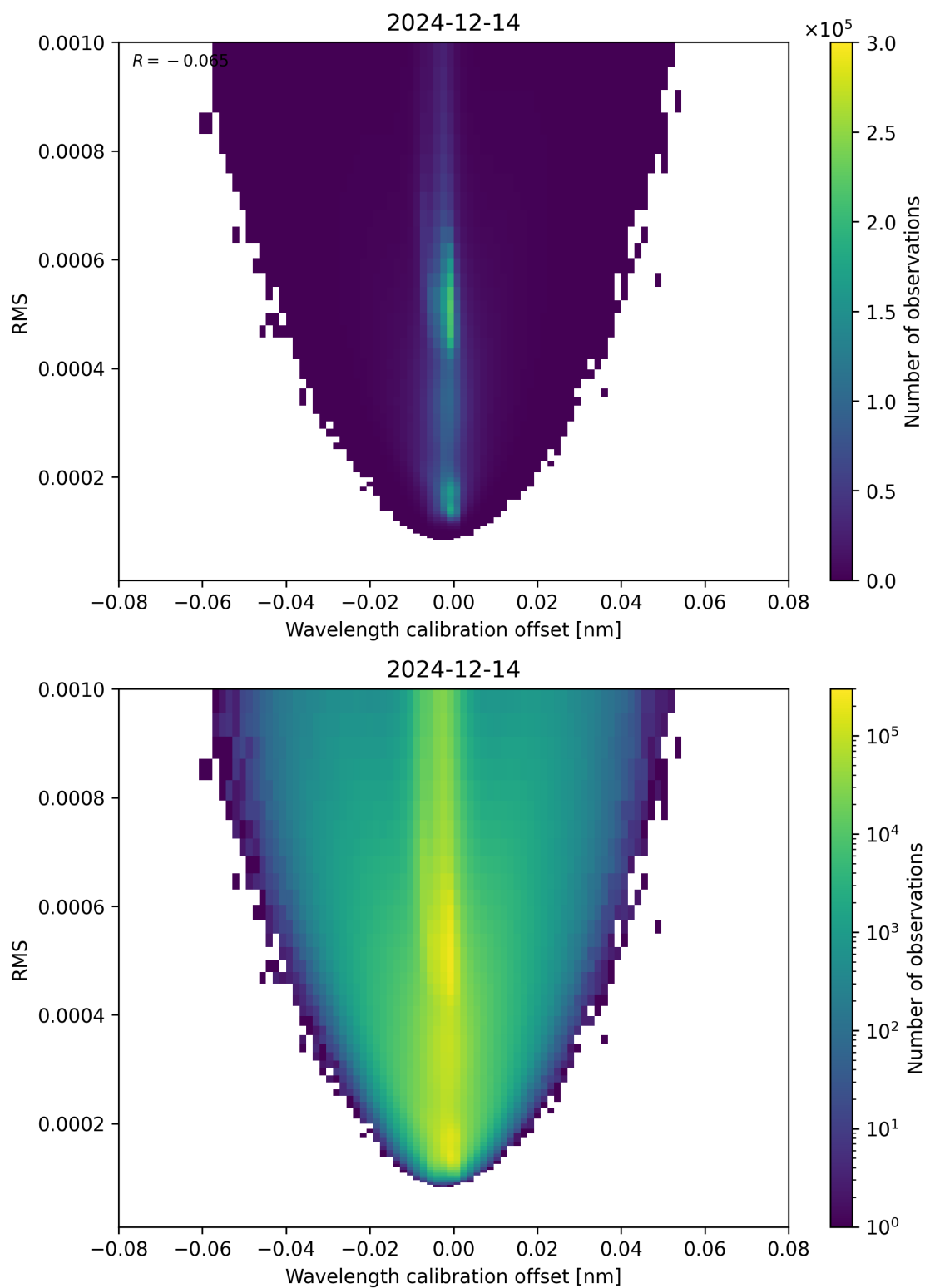
Figure 181: Scatter density plot of “Wavelength calibration offset” against “RMS” for 2024-12-13 to 2024-12-15.
