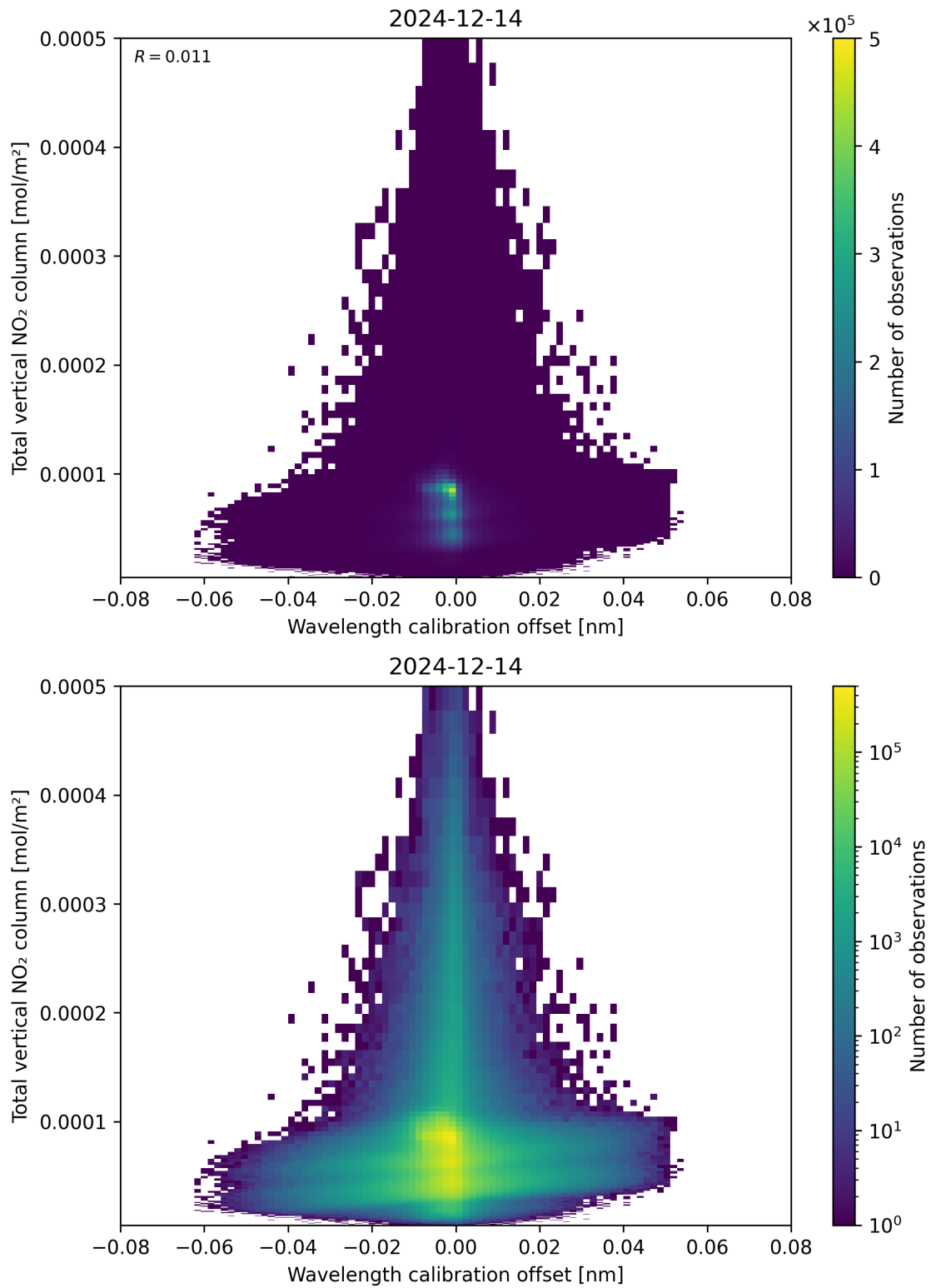
Figure 179: Scatter density plot of “Wavelength calibration offset” against “Total vertical NO 2 column” for 2024-12-13 to 2024-12-15.
