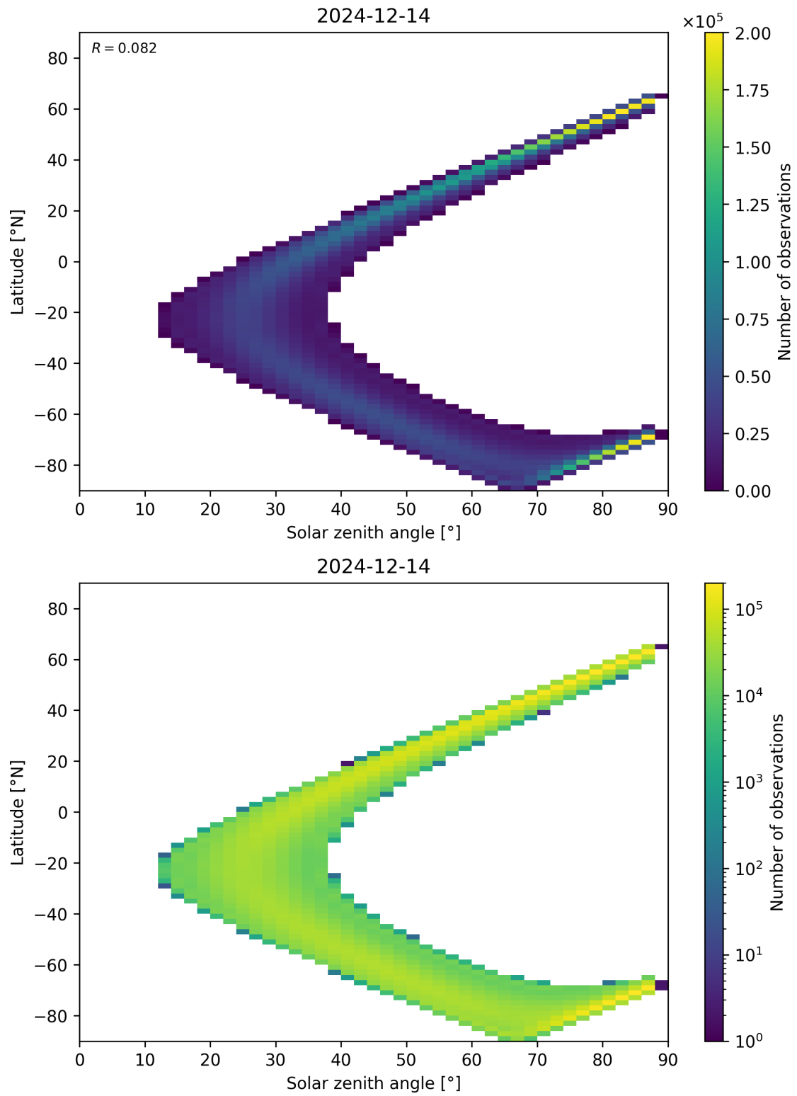
Figure 149: Scatter density plot of “Solar zenith angle” against “Latitude” for 2024-12-13 to 2024-12-15.
