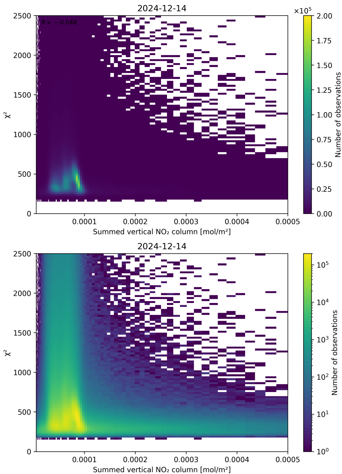
Figure 104: Scatter density plot of “Summed vertical NO 2 column” against “ \chi^2 ” for 2024-12-13 to 2024-12-15.
