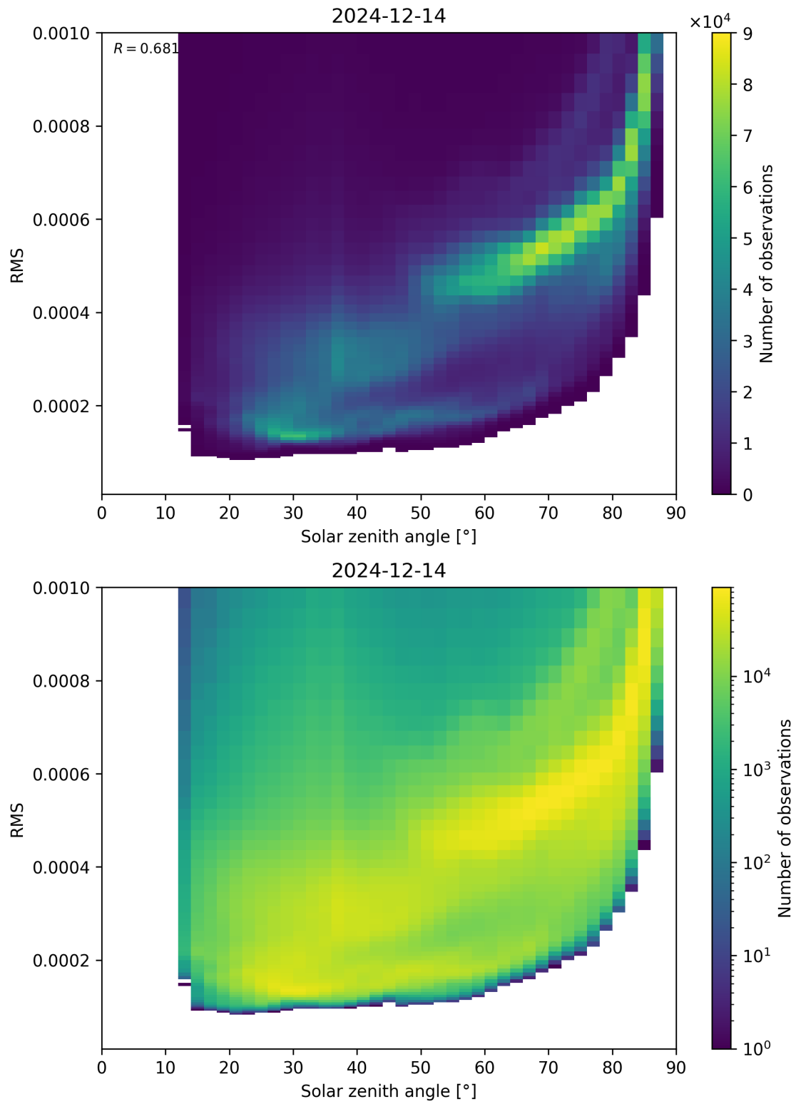
Figure 157: Scatter density plot of “Solar zenith angle” against “RMS” for 2024-12-13 to 2024-12-15.
