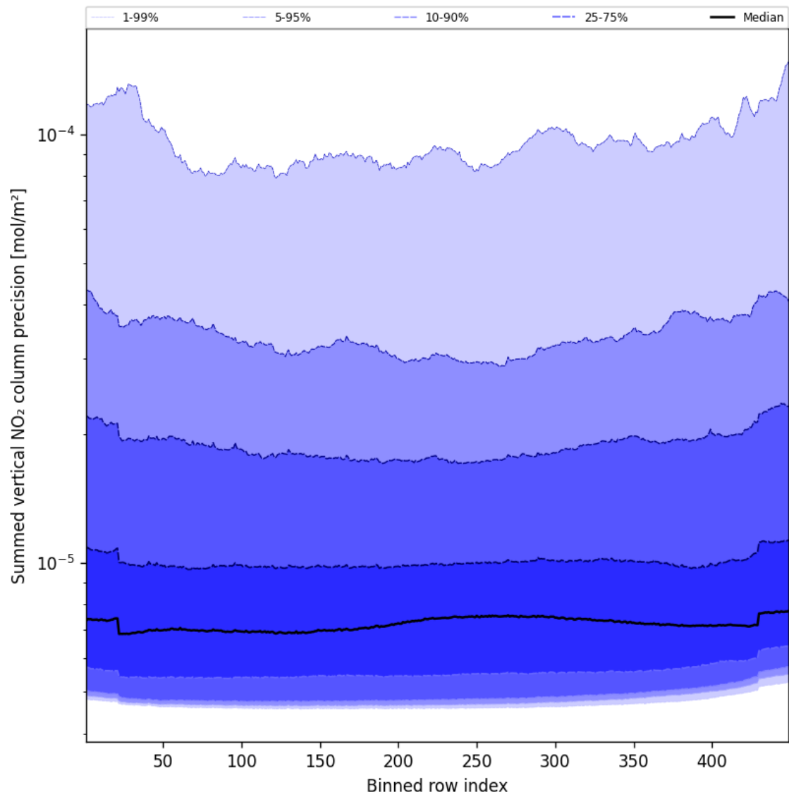
Figure 58: Along track statistics of “Summed vertical NO 2 column precision” for 2024-12-14 to 2024-12-16
