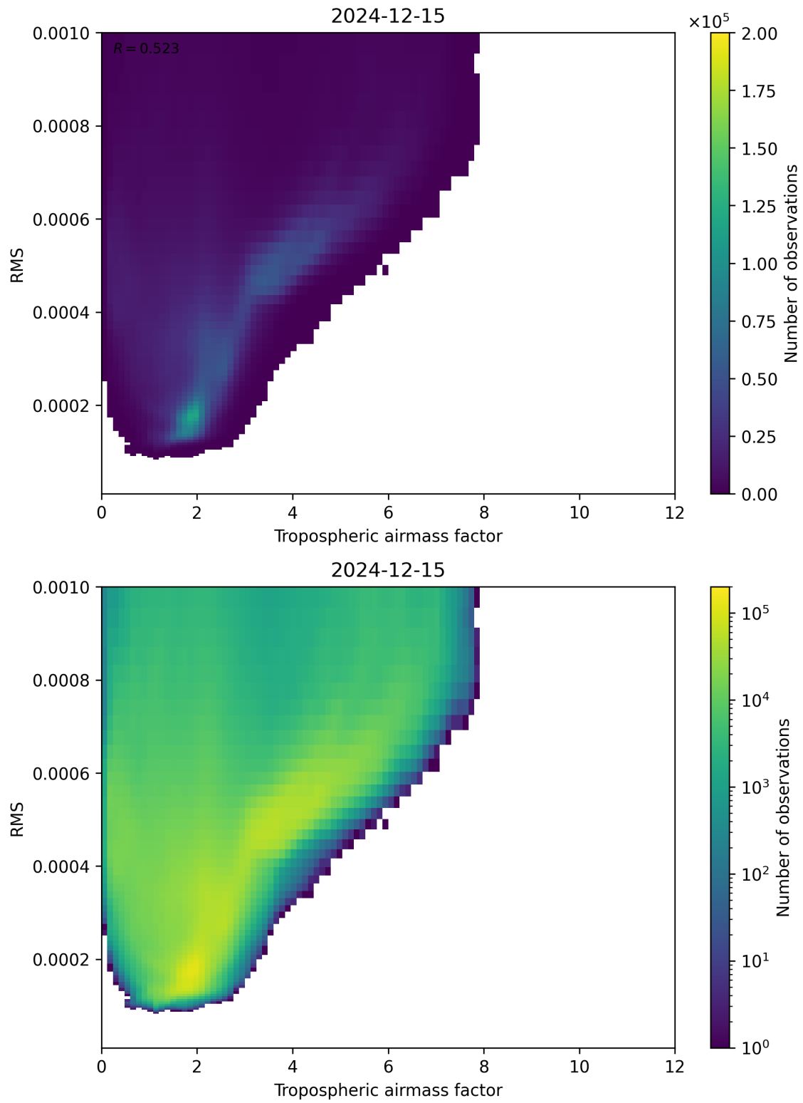
Figure 79: Scatter density plot of “Tropospheric airmass factor” against “RMS” for 2024-12-14 to 2024-12-16.
