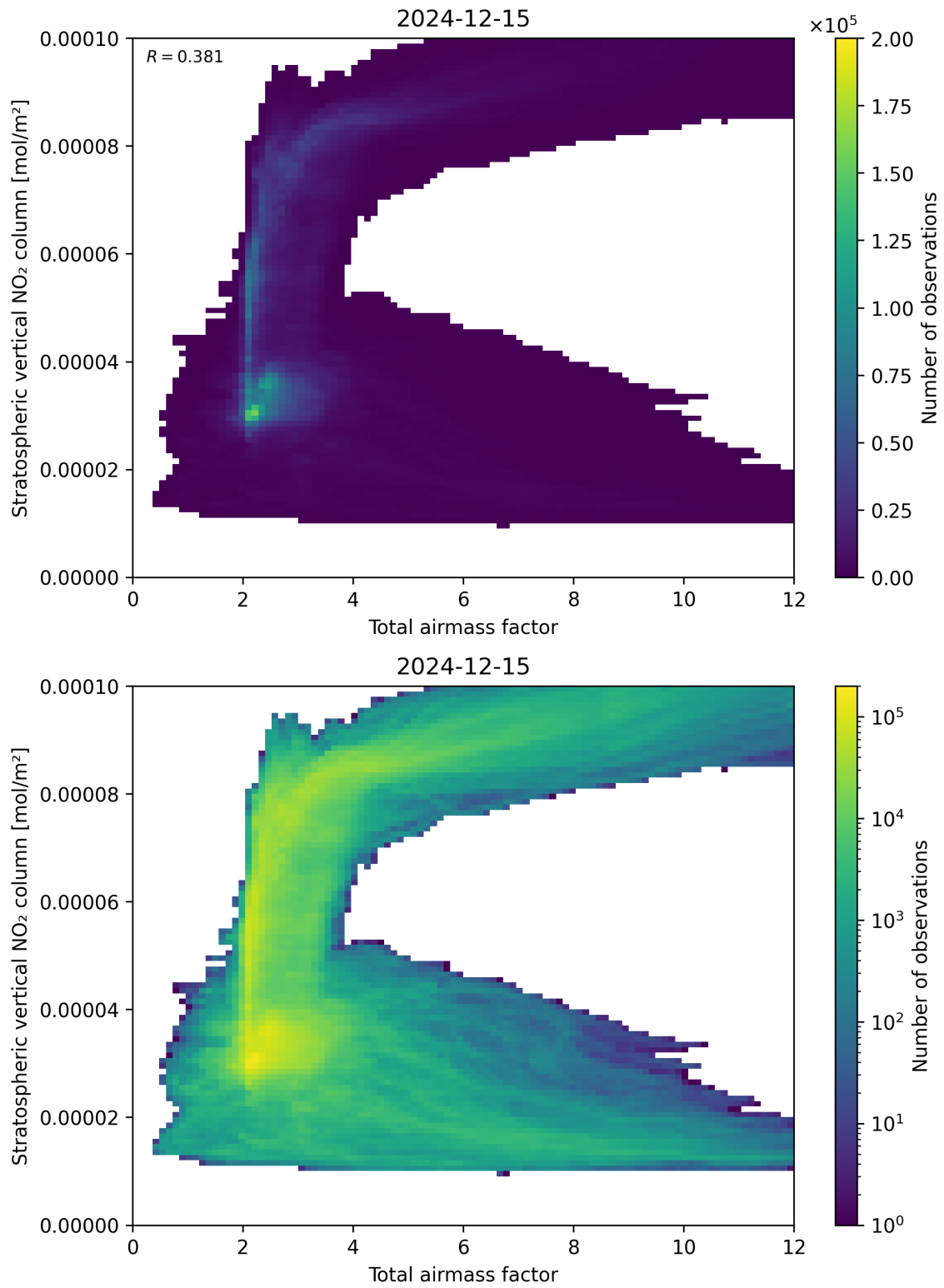
Figure 64: Scatter density plot of “Total airmass factor” against “Stratospheric vertical NO 2 column” for 2024-12-14 to 2024-12-16.
