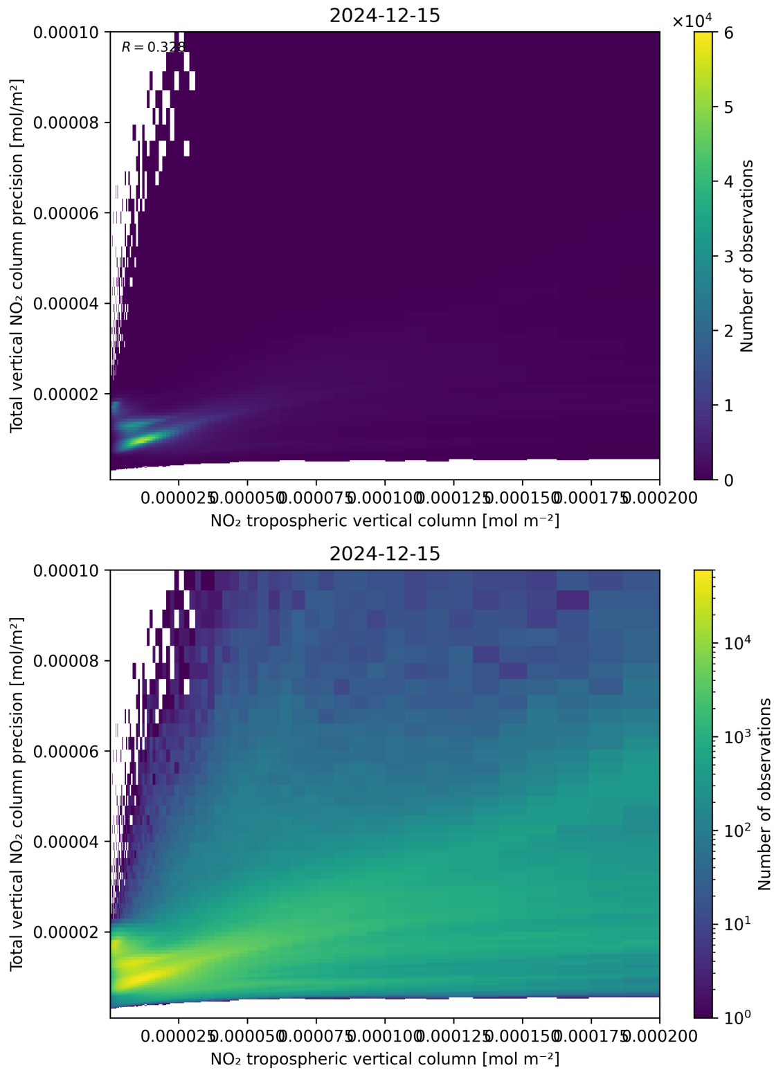
Figure 129: Scatter density plot of “NO 2 tropospheric vertical column” against “Total vertical NO 2 column precision” for 2024-12-14 to 2024-12-16.
