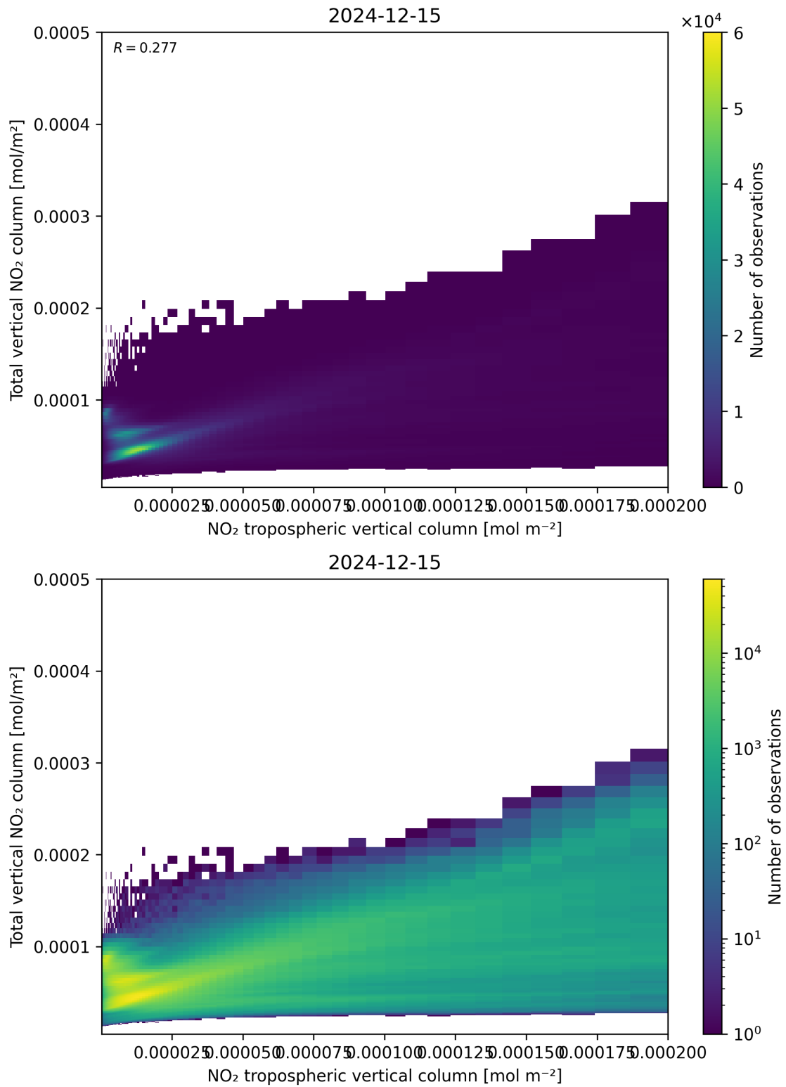
Figure 128: Scatter density plot of “NO 2 tropospheric vertical column” against “Total vertical NO 2 column” for 2024-12-14 to 2024-12-16.
