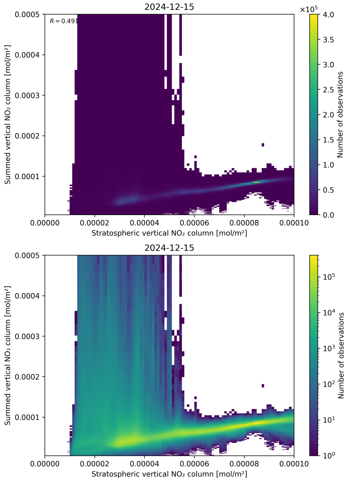
Figure 98: Scatter density plot of “Stratospheric vertical NO 2 column” against “Summed vertical NO 2 column” for 2024-12-14 to 2024-12-16.
