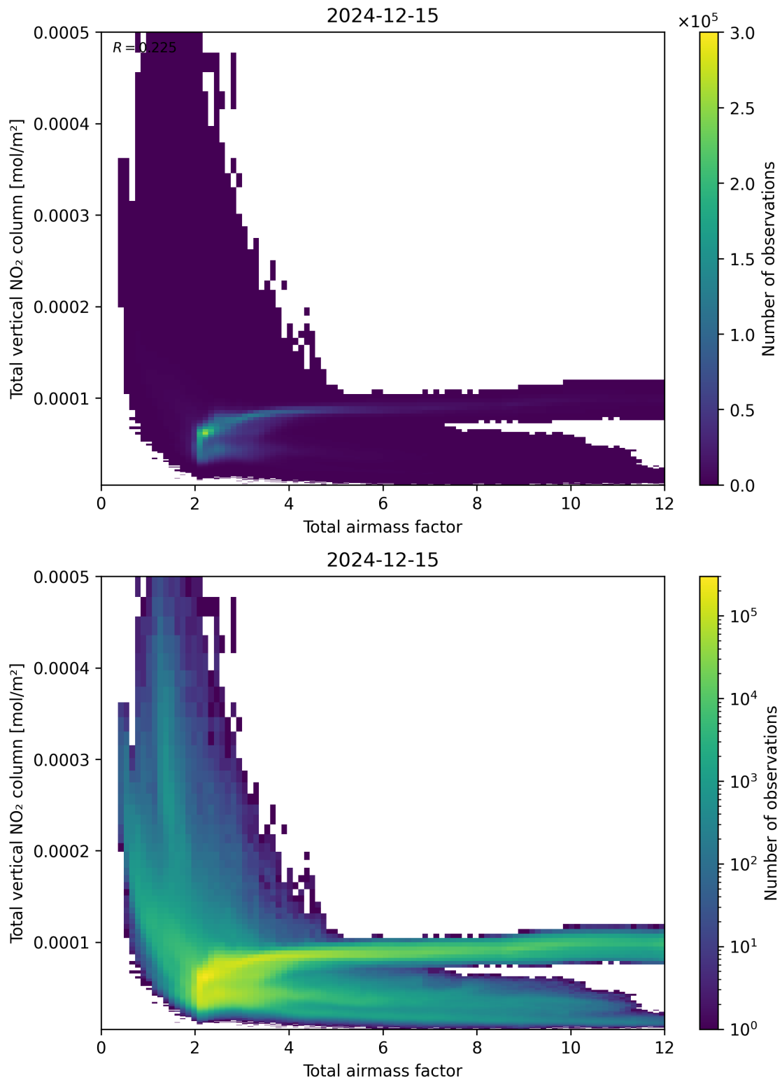
Figure 67: Scatter density plot of “Total airmass factor” against “Total vertical NO 2 column” for 2024-12-14 to 2024-12-16.
