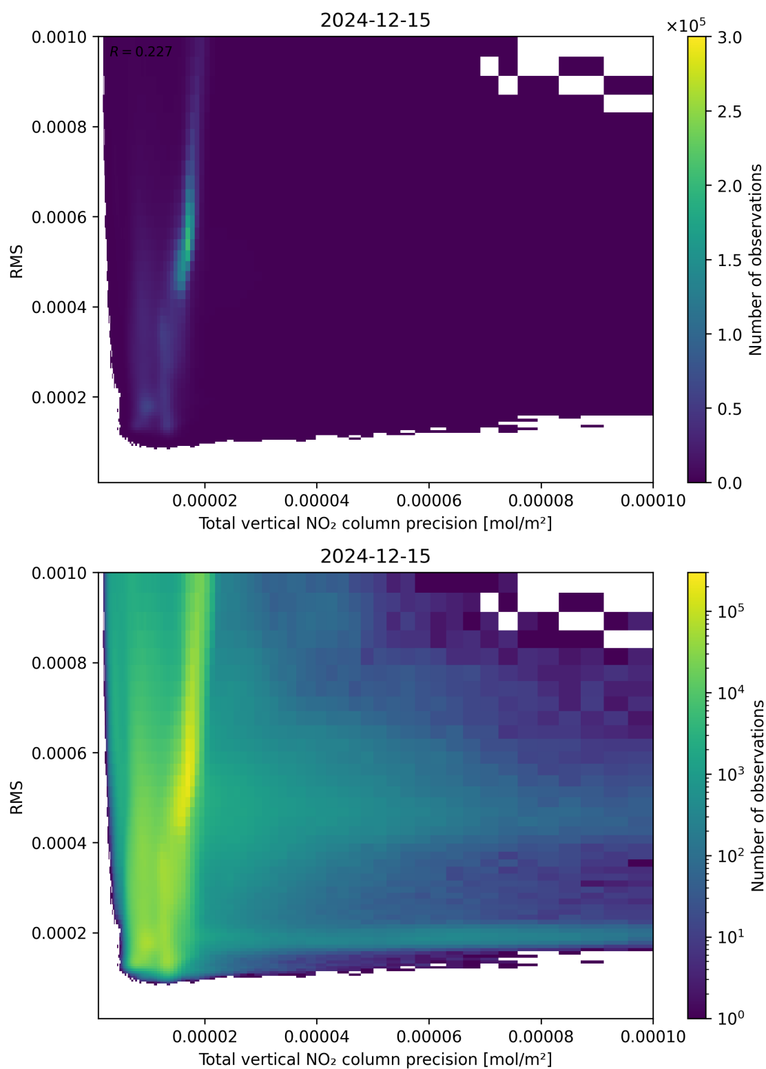
Figure 119: Scatter density plot of “Total vertical NO 2 column precision” against “RMS” for 2024-12-14 to 2024-12-16.
