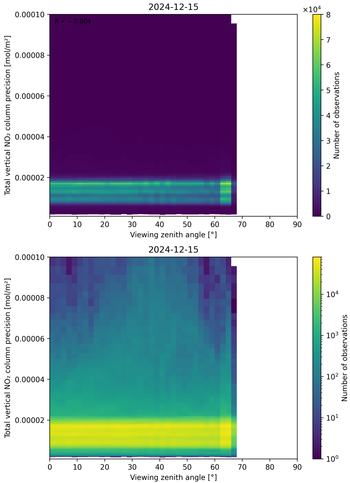
Figure 168: Scatter density plot of “Viewing zenith angle” against “Total vertical NO 2 column precision” for 2024-12-14 to 2024-12-16.
