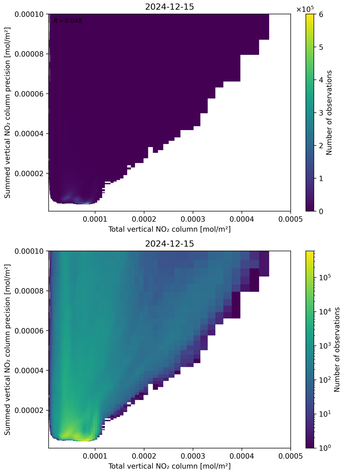
Figure 113: Scatter density plot of “Total vertical NO 2 column” against “Summed vertical NO 2 column precision” for 2024-12-14 to 2024-12-16.
