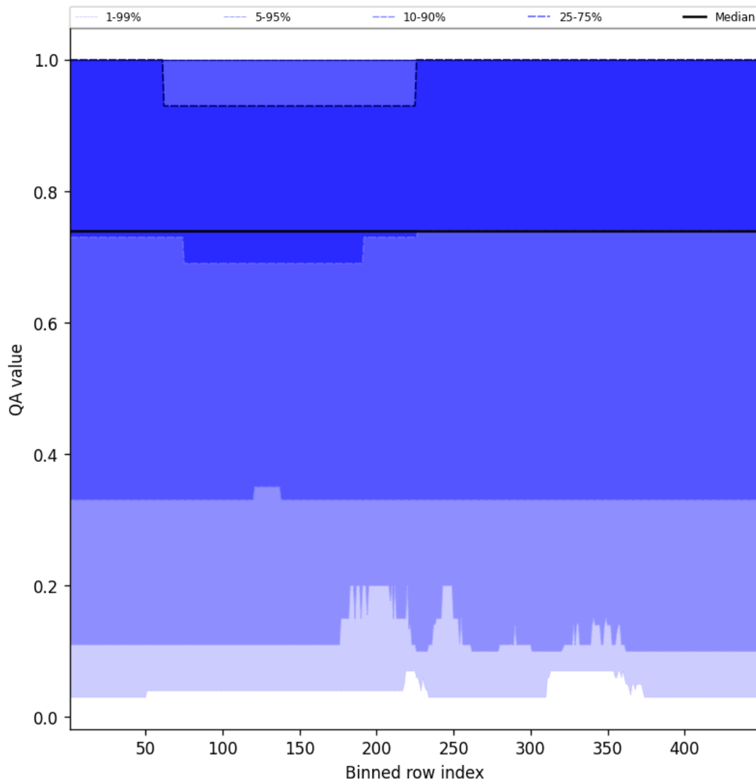
Figure 45: Along track statistics of “QA value” for 2024-12-14 to 2024-12-16
