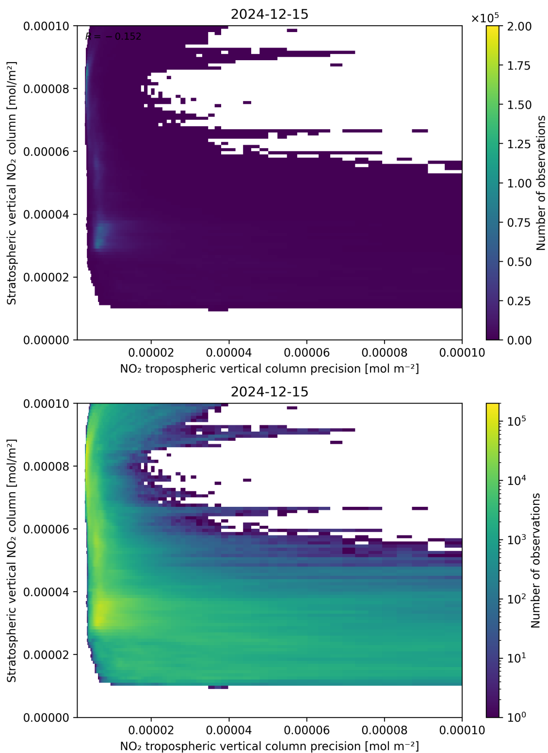
Figure 135: Scatter density plot of “NO 2 tropospheric vertical column precision” against “Stratospheric vertical NO 2 column” for 2024-12-14 to 2024-12-16.
