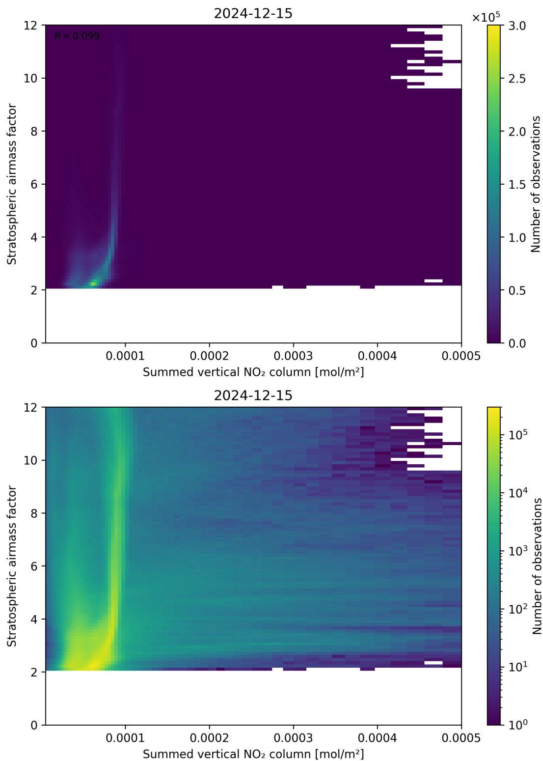
Figure 103: Scatter density plot of “Summed vertical NO 2 column” against “Stratospheric airmass factor” for 2024-12-14 to 2024-12-16.
