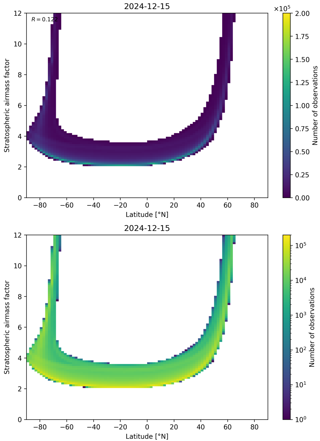
Figure 83: Scatter density plot of “Latitude” against “Stratospheric air mass factor” for 2024-12-14 to 2024-12-16.
