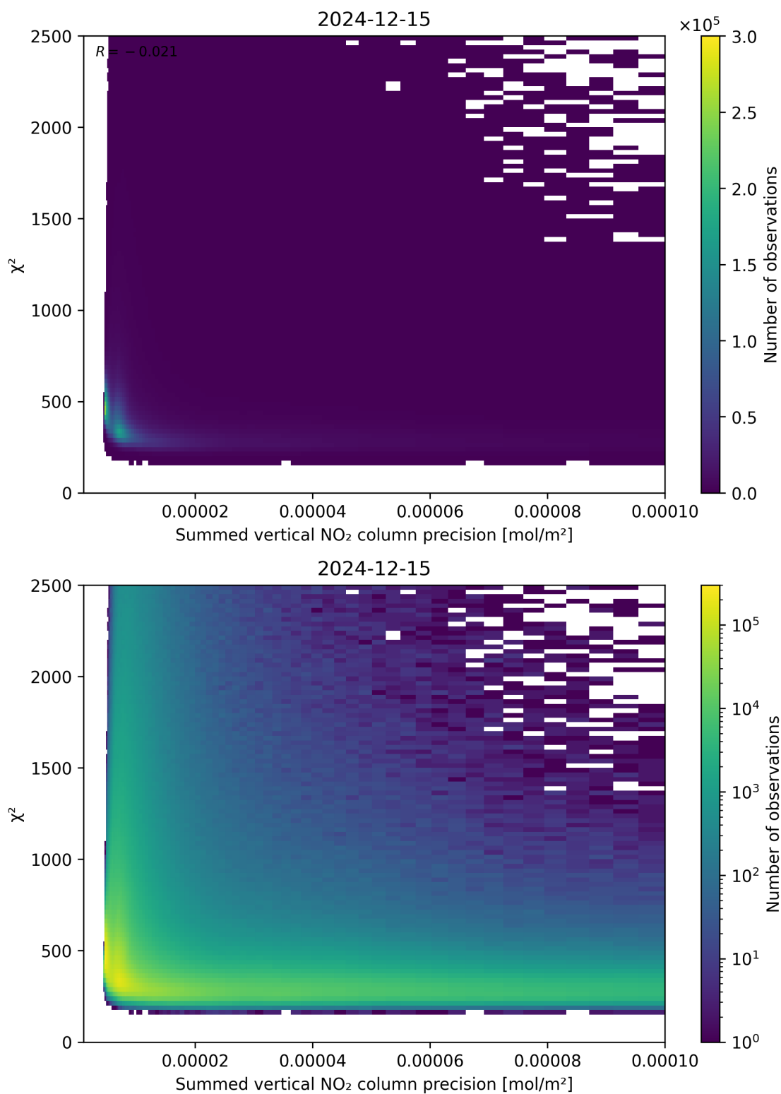
Figure 107: Scatter density plot of “Summed vertical NO 2 column precision” against “ \chi^2 ” for 2024-12-14 to 2024-12-16.
