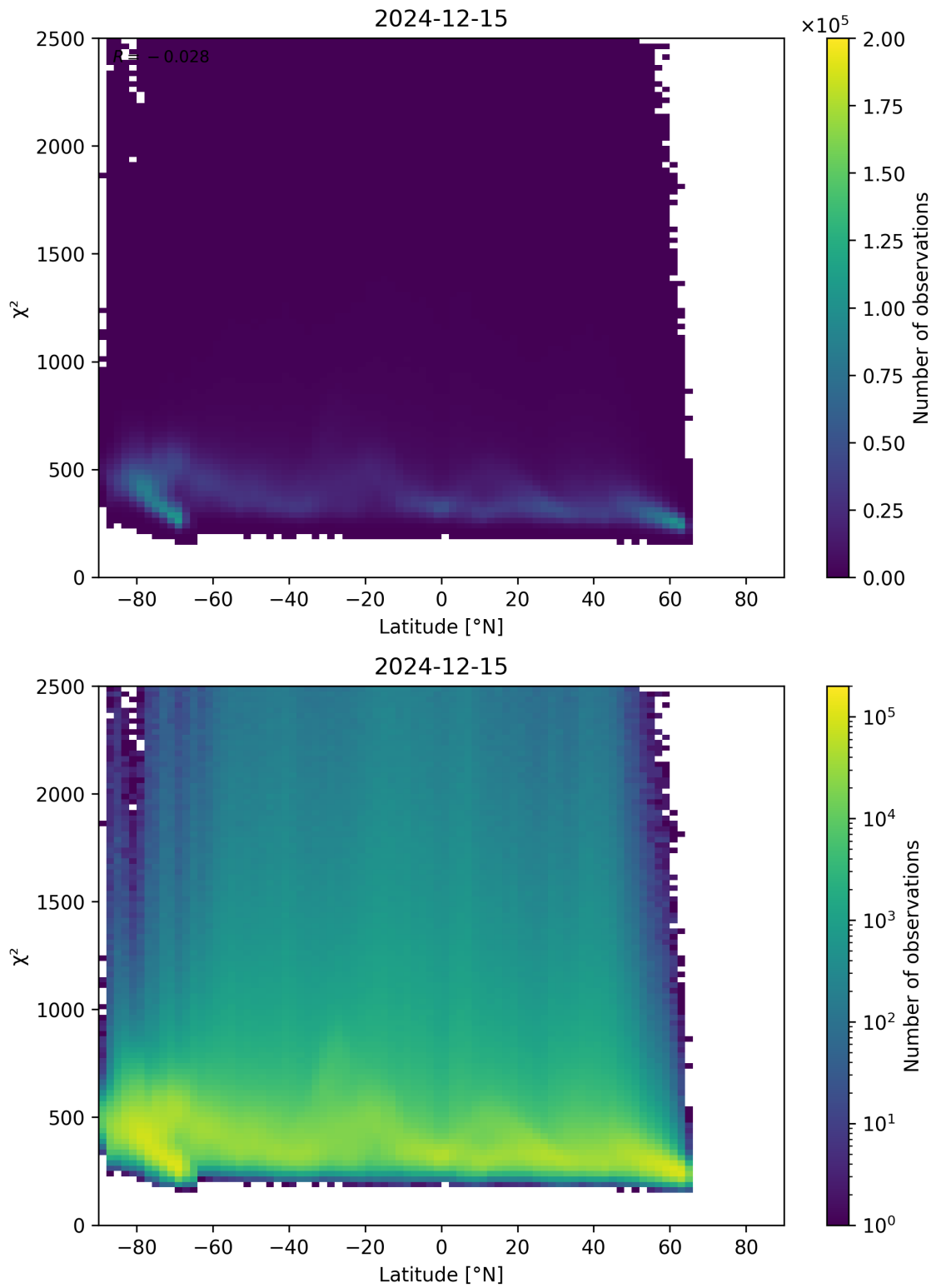
Figure 86: Scatter density plot of “Latitude” against “ \chi^2 ” for 2024-12-14 to 2024-12-16.
