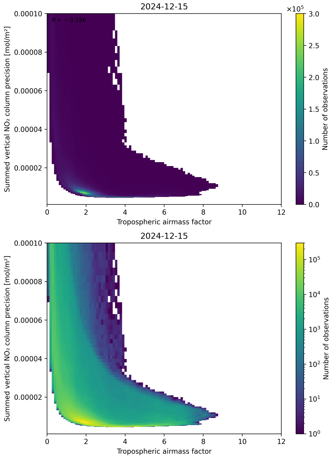
Figure 76: Scatter density plot of “Tropospheric air mass factor” against “Summed vertical NO 2 column precision” for 2024-12-14 to 2024-12-16.
