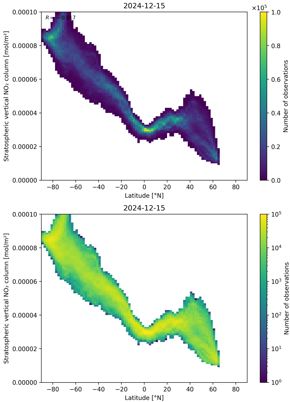
Figure 87: Scatter density plot of “Latitude” against “Stratospheric vertical NO 2 column” for 2024-12-14 to 2024-12-16.
