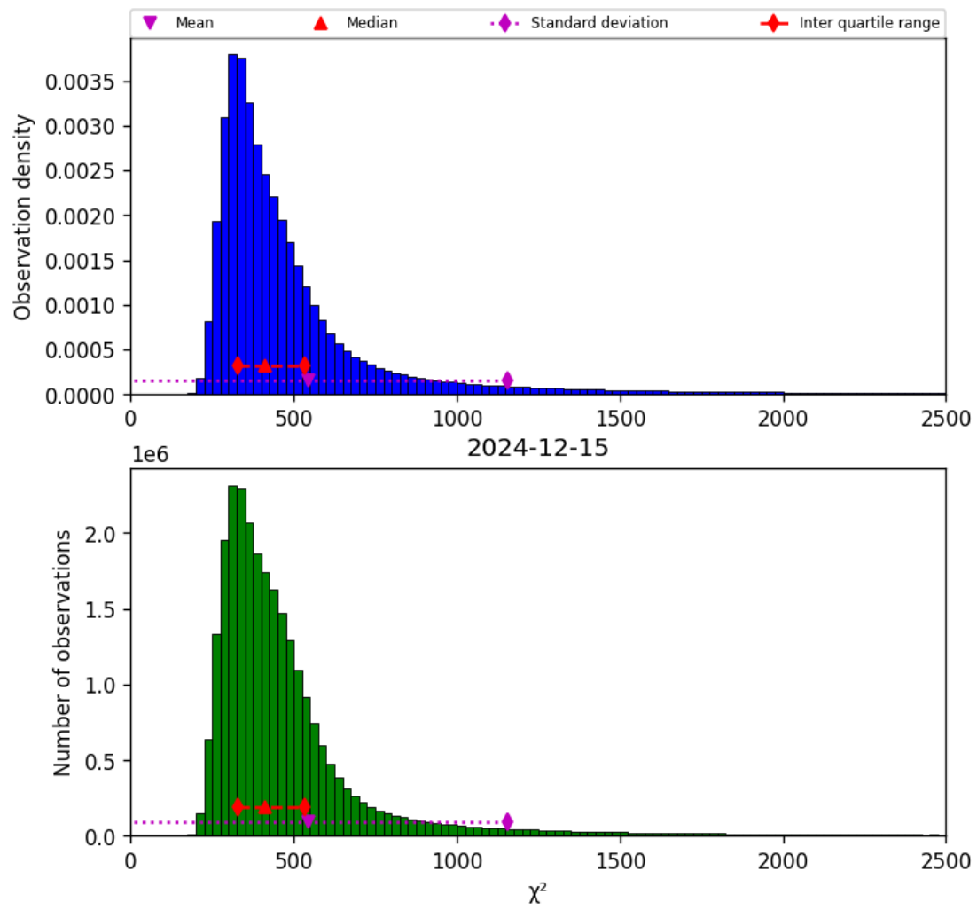
Figure 42: Histogram of “ \chi^2 ” for 2024-12-14 to 2024-12-16
