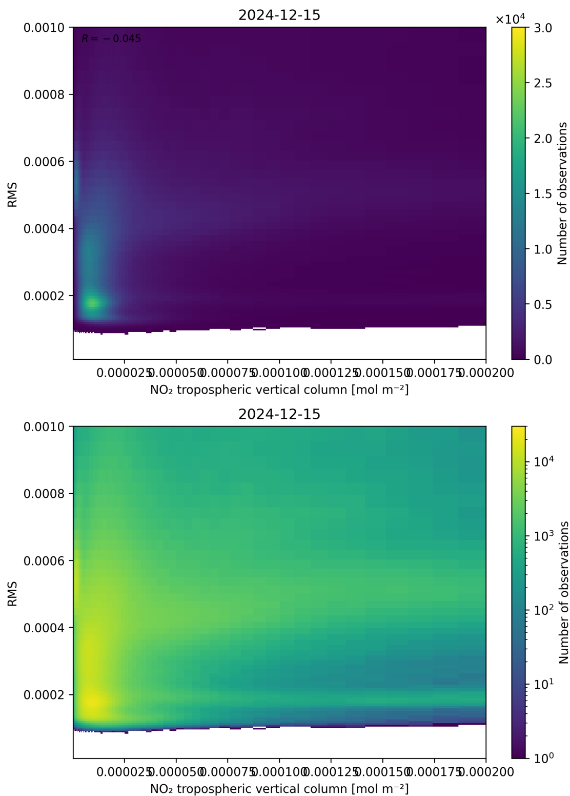
Figure 142: Scatter density plot of “NO 2 tropospheric vertical column” against “RMS” for 2024-12-14 to 2024-12-16.
