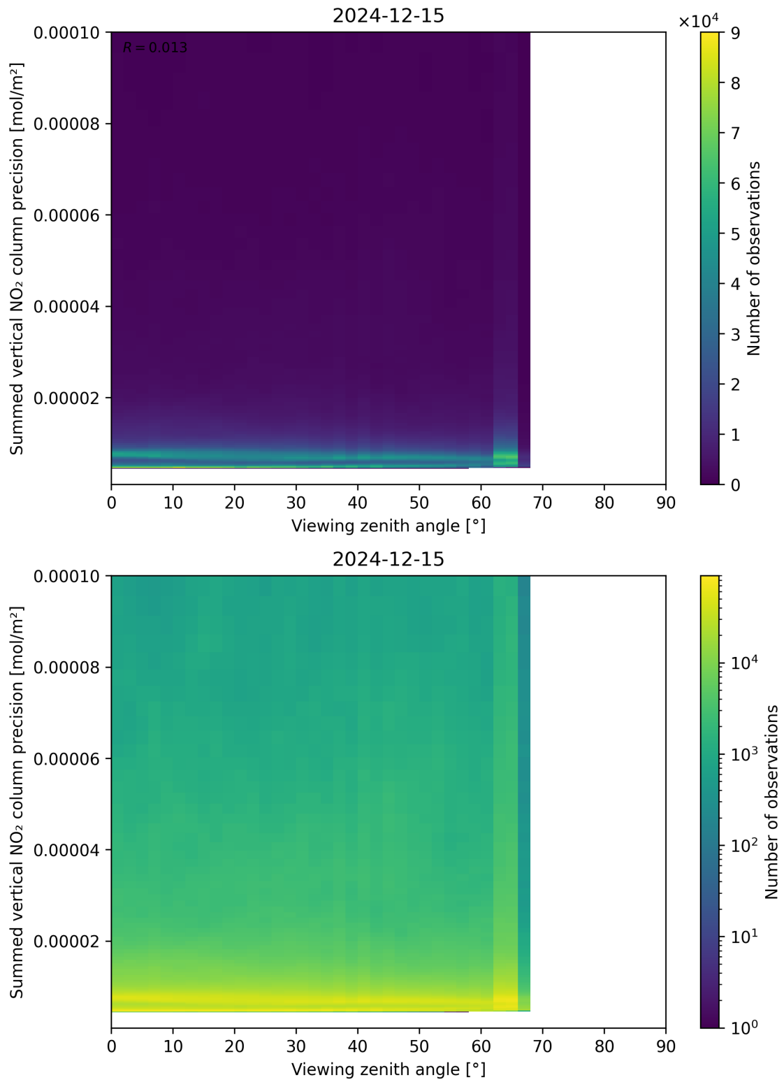
Figure 166: Scatter density plot of “Viewing zenith angle” against “Summed vertical NO 2 column precision” for 2024-12-14 to 2024-12-16.
