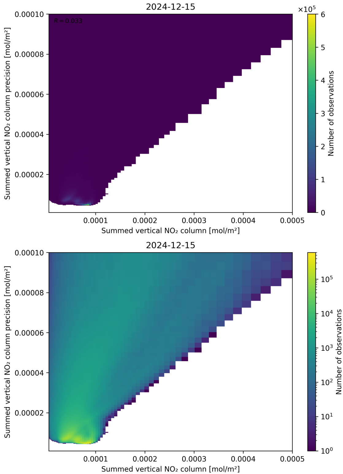
Figure 105: Scatter density plot of “Summed vertical NO 2 column” against “Summed vertical NO 2 column precision” for 2024-12-14 to 2024-12-16.
