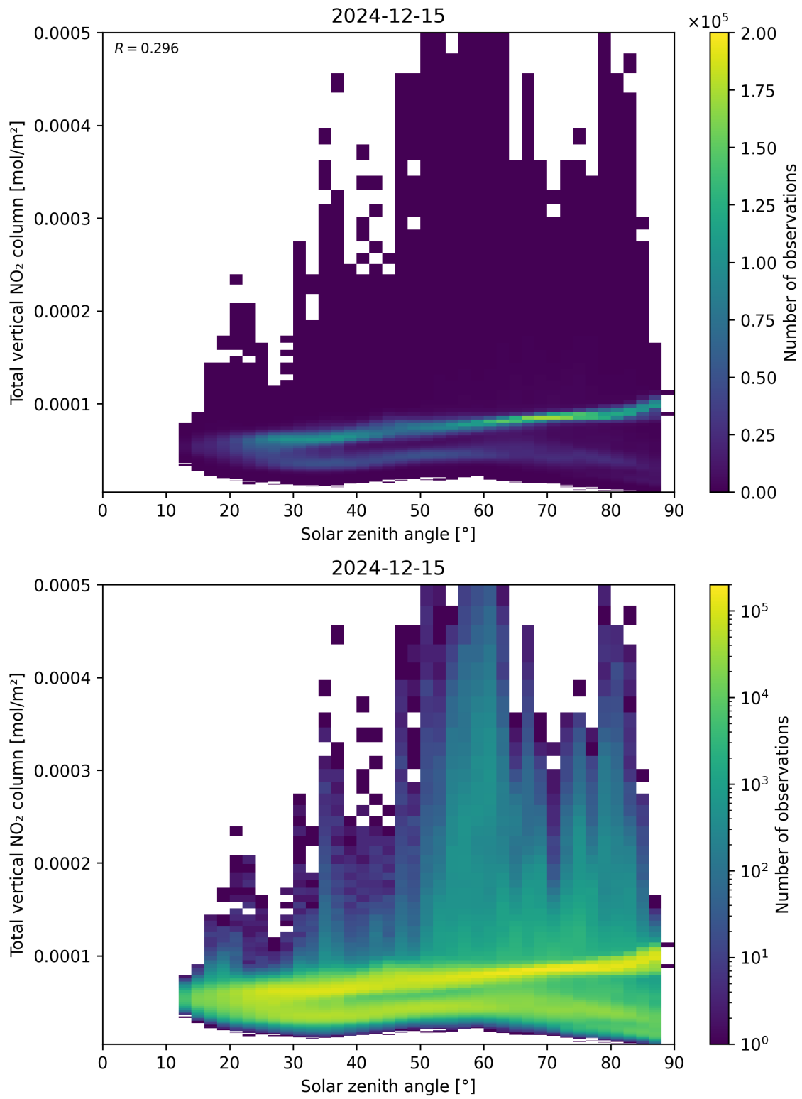
Figure 153: Scatter density plot of “Solar zenith angle” against “Total vertical NO 2 column” for 2024-12-14 to 2024-12-16.
