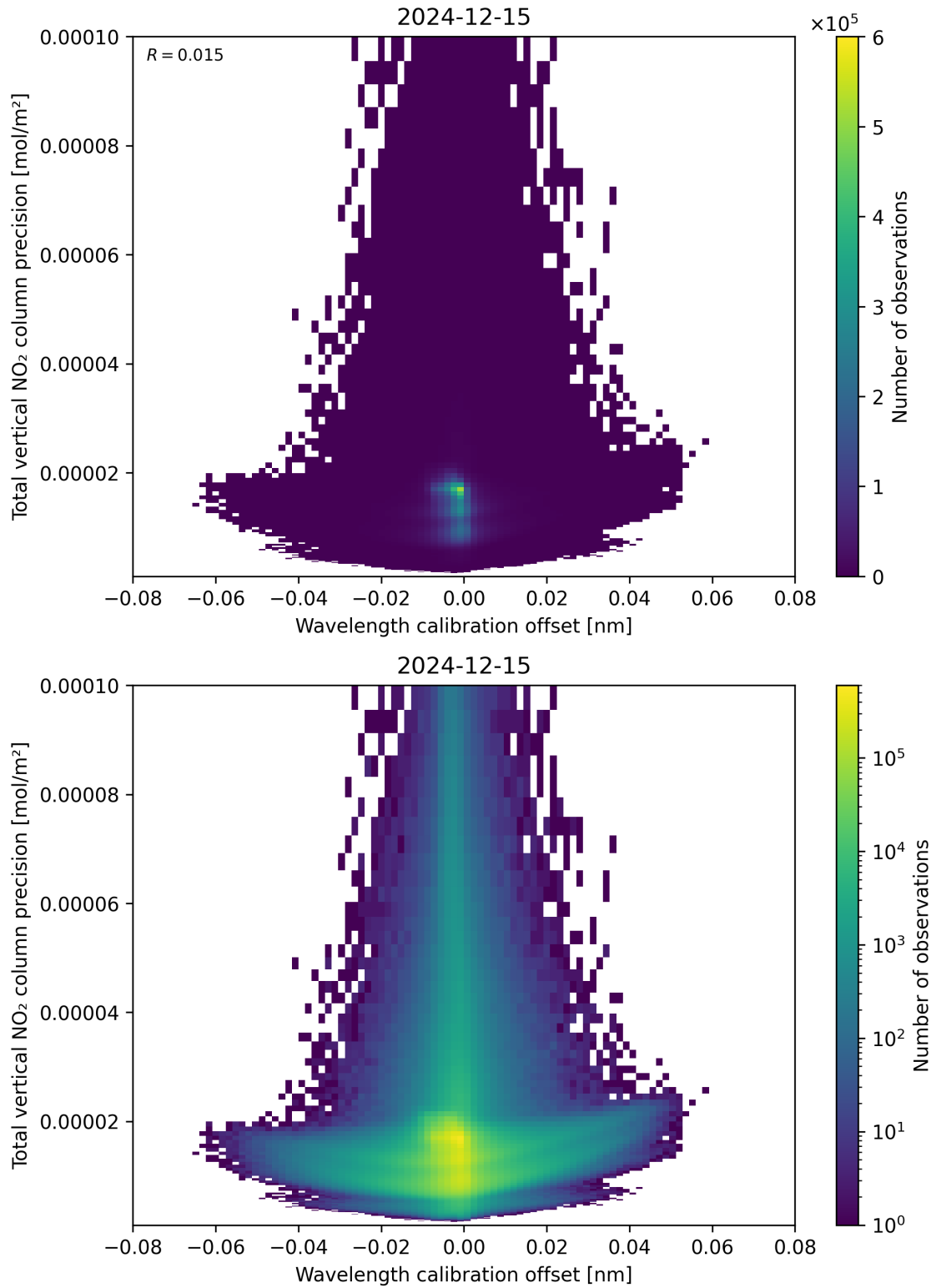
Figure 180: Scatter density plot of “Wavelength calibration offset” against “Total vertical NO 2 column precision” for 2024-12-14 to 2024-12-16.
