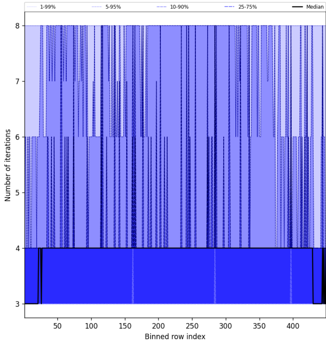
Figure 51: Along track statistics of “Number of iterations” for 2024-12-14 to 2024-12-16
