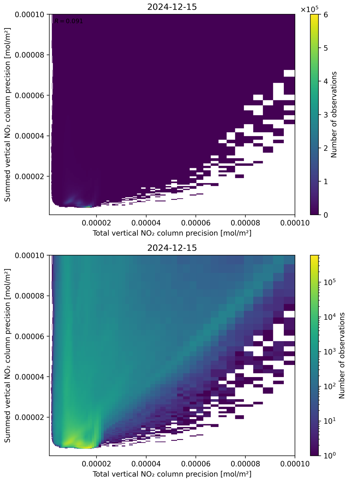
Figure 118: Scatter density plot of “Total vertical NO 2 column precision” against “Summed vertical NO 2 column precision” for 2024-12-14 to 2024-12-16.
