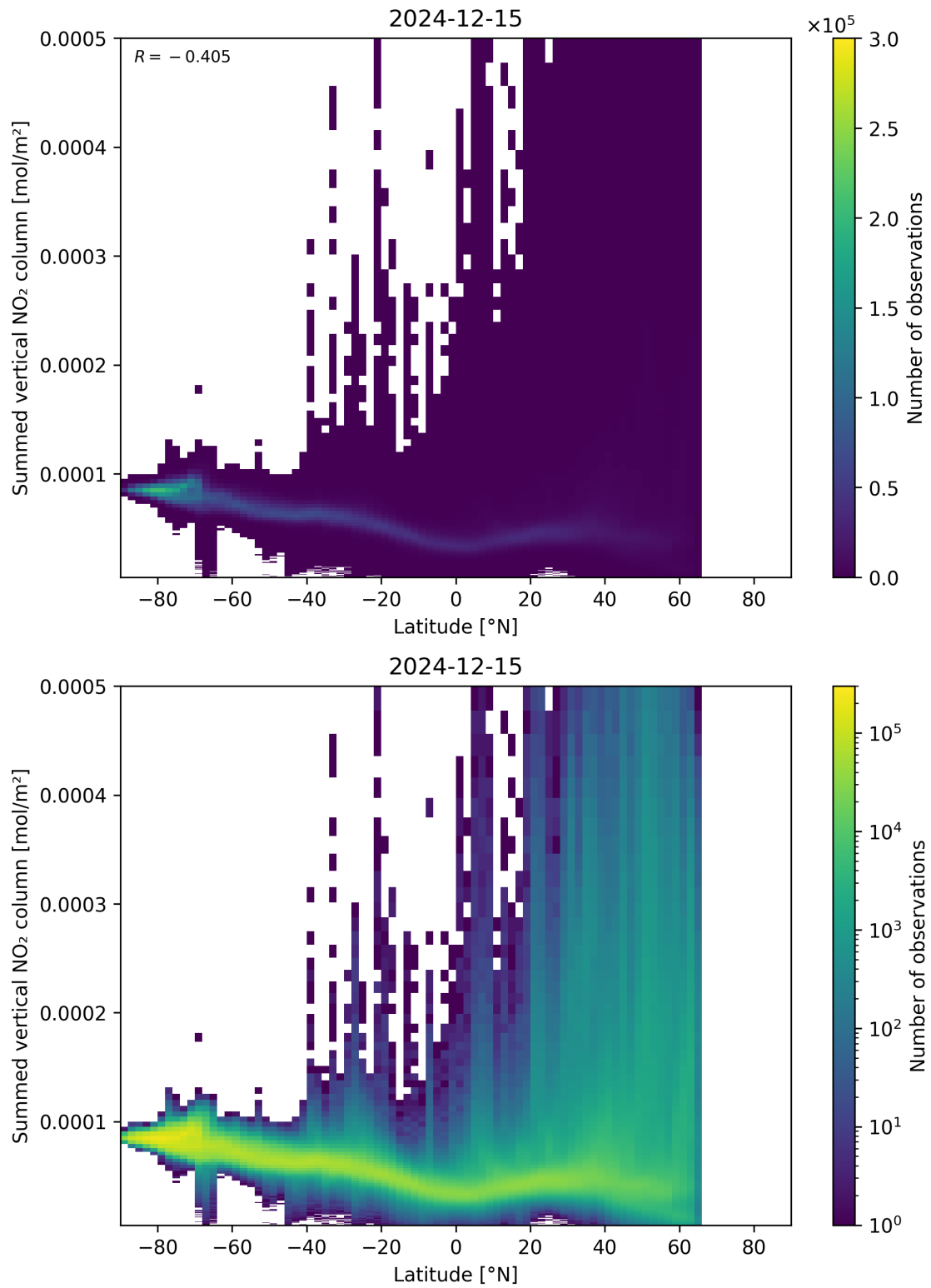
Figure 88: Scatter density plot of “Latitude” against “Summed vertical NO 2 column” for 2024-12-14 to 2024-12-16.
