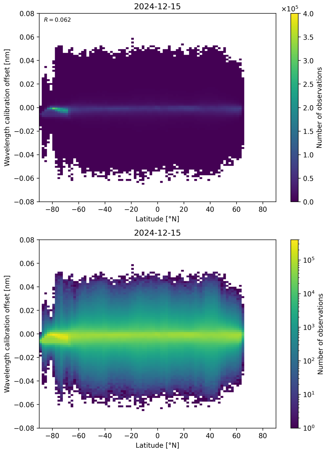
Figure 95: Scatter density plot of “Latitude” against “Wavelength calibration offset” for 2024-12-14 to 2024-12-16.
