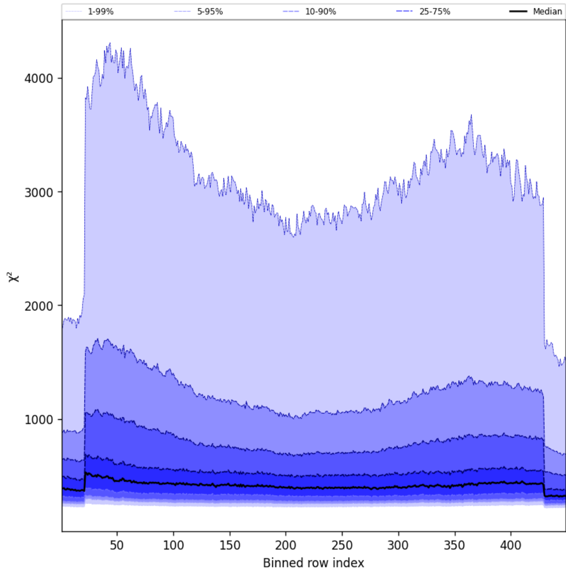
Figure 59: Along track statistics of “ \chi^2 ” for 2024-12-14 to 2024-12-16
