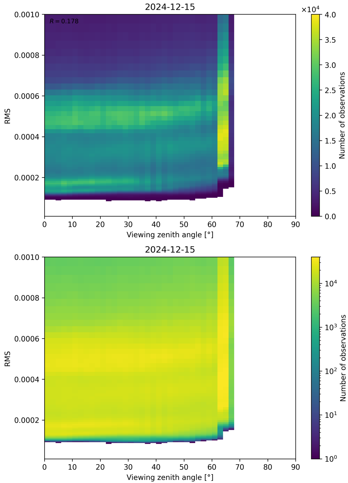
Figure 171: Scatter density plot of “Viewing zenith angle” against “RMS” for 2024-12-14 to 2024-12-16.
