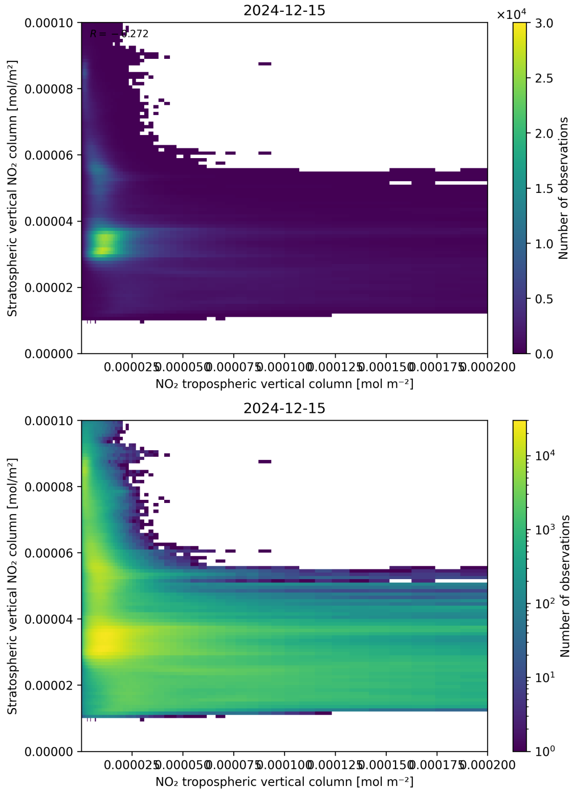
Figure 125: Scatter density plot of “NO 2 tropospheric vertical column” against “Stratospheric vertical NO 2 column” for 2024-12-14 to 2024-12-16.
