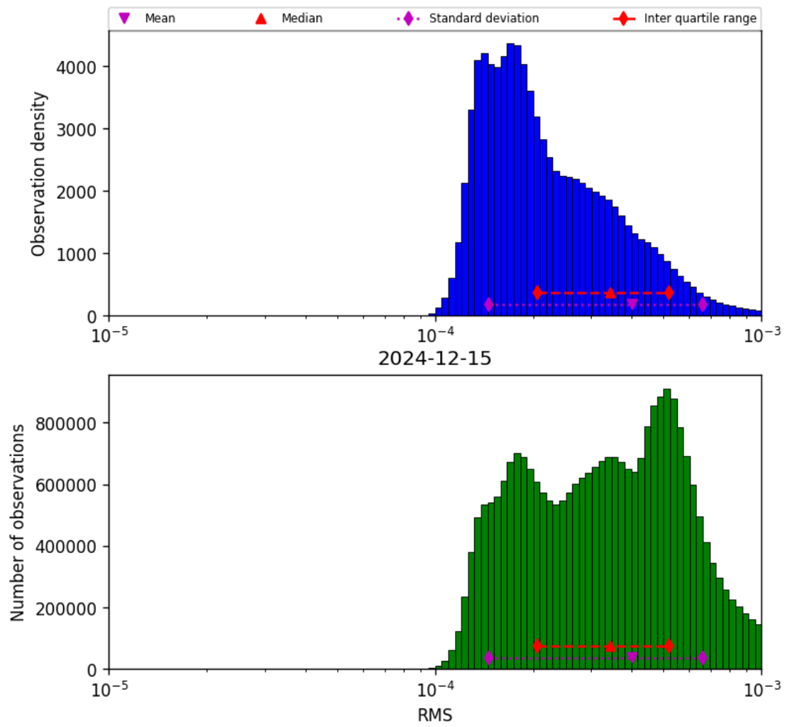
Figure 43: Histogram of “RMS” for 2024-12-14 to 2024-12-16
