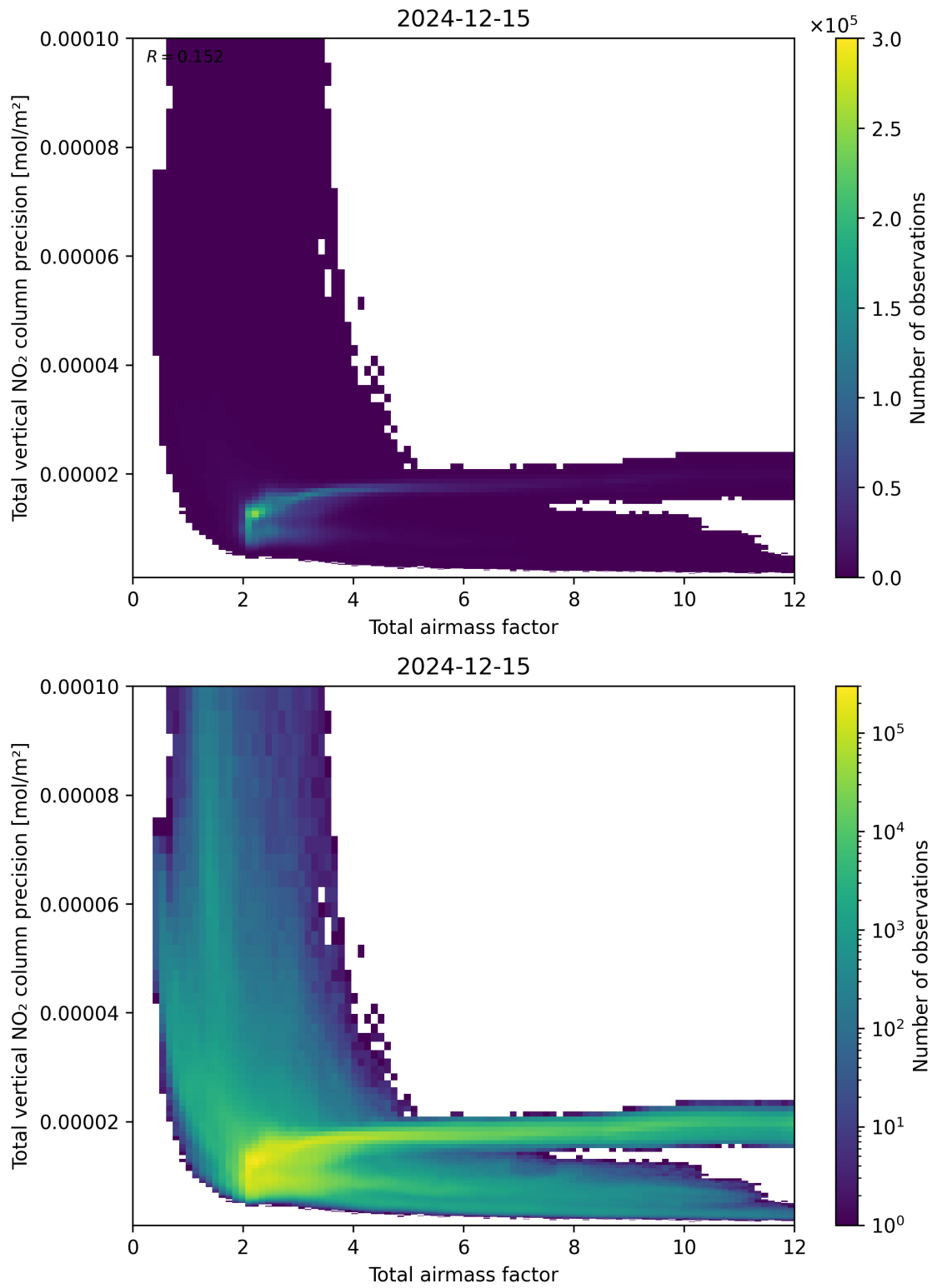
Figure 68: Scatter density plot of “Total airmass factor” against “Total vertical NO 2 column precision” for 2024-12-14 to 2024-12-16.
