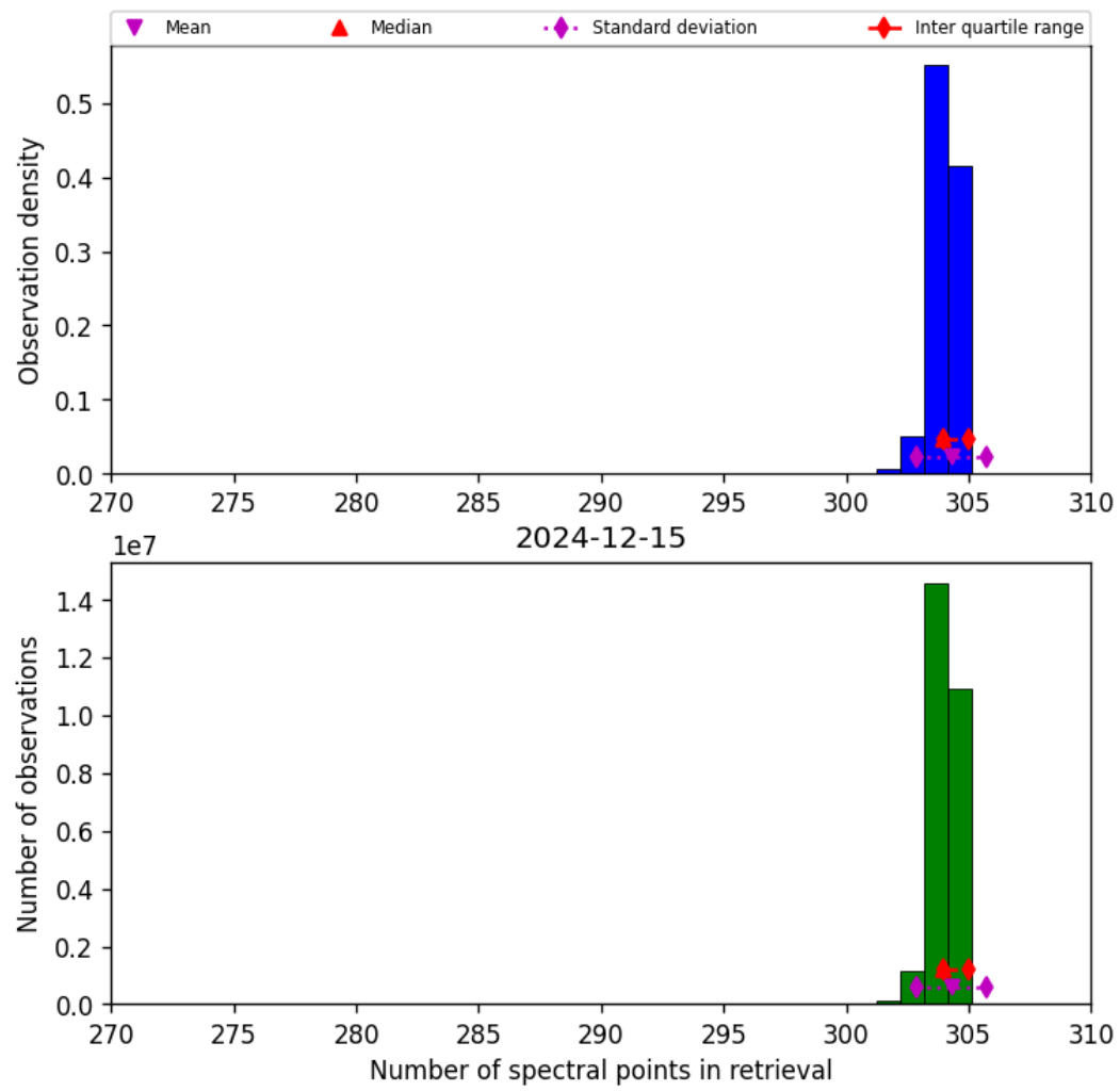
Figure 33: Histogram of “Number of spectral points in retrieval” for 2024-12-14 to 2024-12-16
