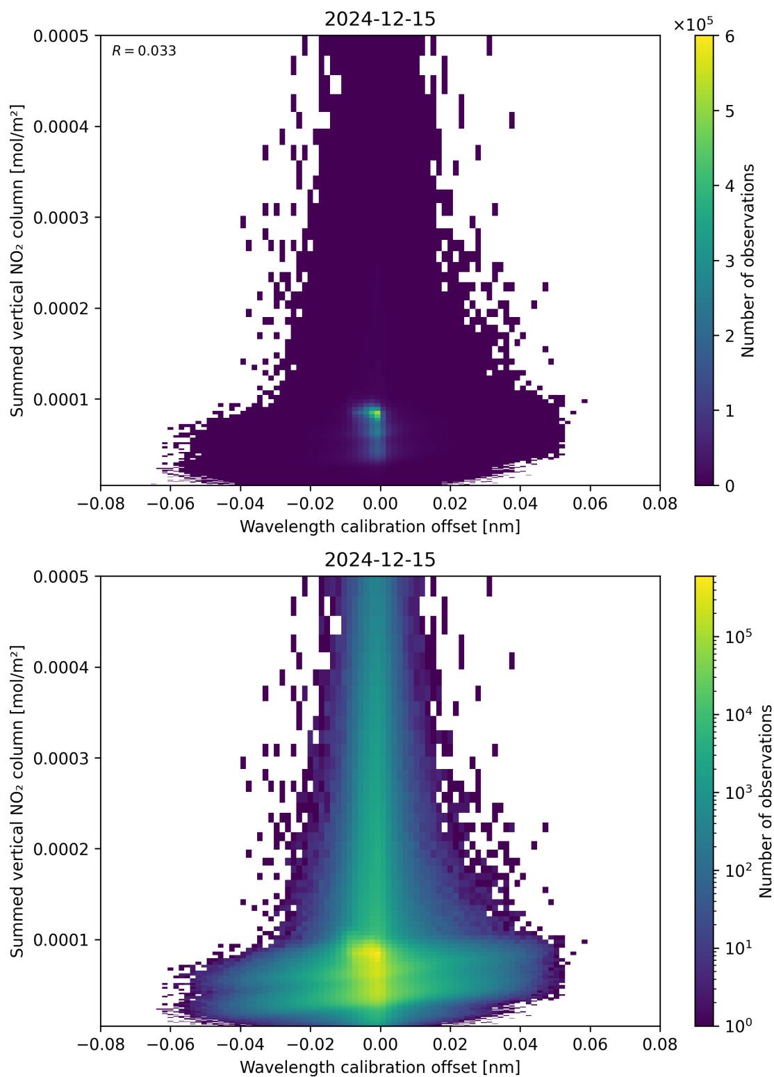
Figure 177: Scatter density plot of “Wavelength calibration offset” against “Summed vertical NO 2 column” for 2024-12-14 to 2024-12-16.
