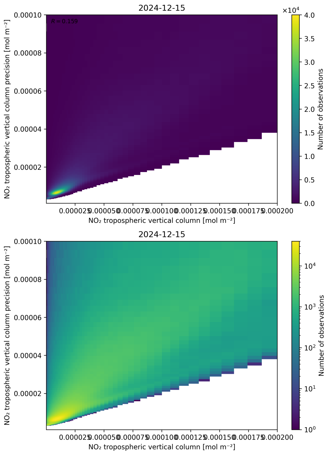
Figure 130: Scatter density plot of “NO 2 tropospheric vertical column” against “NO 2 tropospheric vertical column precision” for 2024-12-14 to 2024-12-16.
