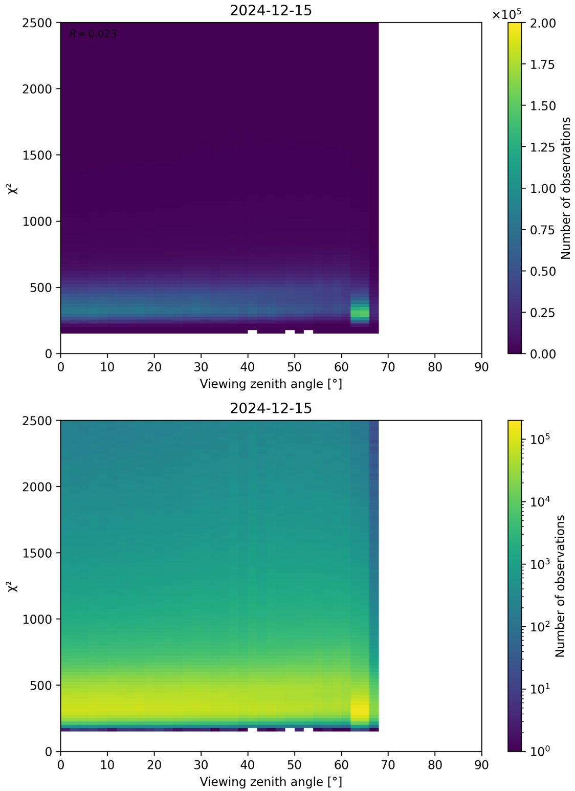
Figure 162: Scatter density plot of “Viewing zenith angle” against “ \chi^2 ” for 2024-12-14 to 2024-12-16.
