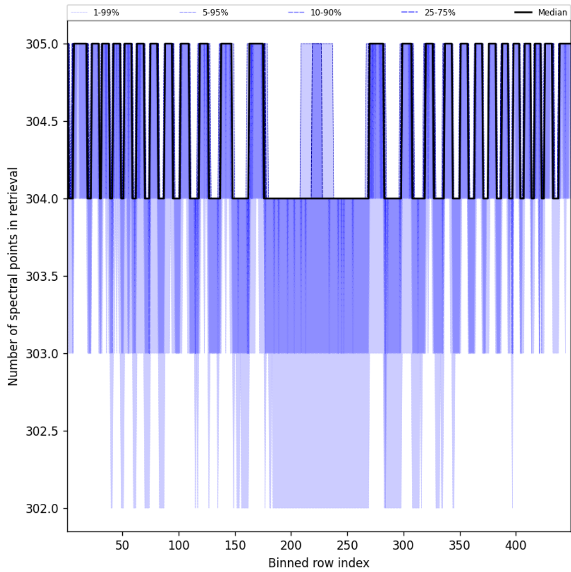
Figure 50: Along track statistics of “Number of spectral points in retrieval” for 2024-12-14 to 2024-12-16
