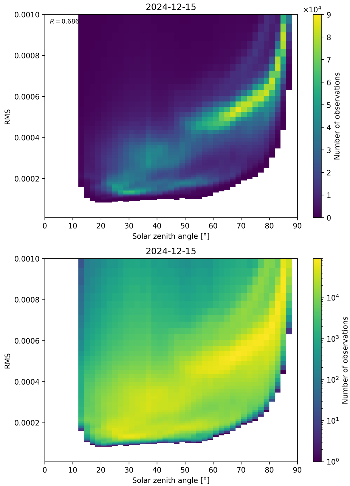
Figure 157: Scatter density plot of “Solar zenith angle” against “RMS” for 2024-12-14 to 2024-12-16.
