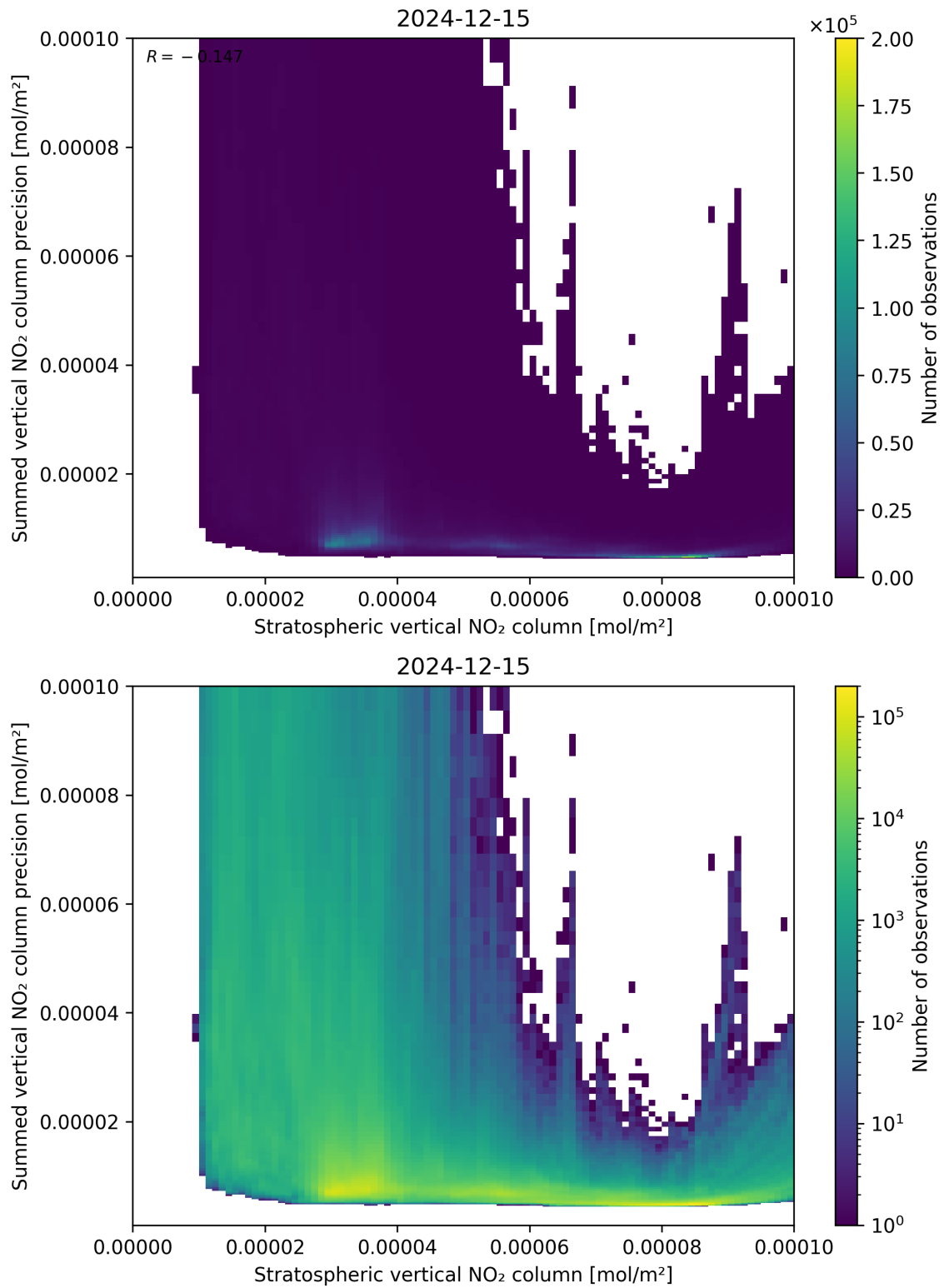
Figure 99: Scatter density plot of “Stratospheric vertical NO 2 column” against “Summed vertical NO 2 column precision” for 2024-12-14 to 2024-12-16.
