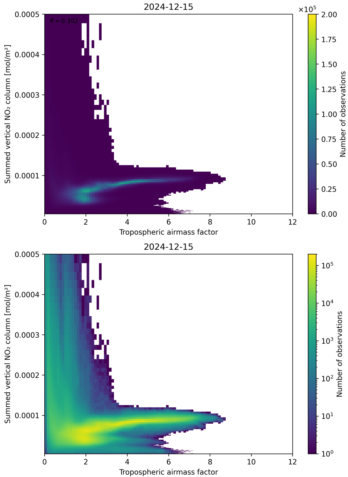
Figure 75: Scatter density plot of “Tropospheric air mass factor” against “Summed vertical NO 2 column” for 2024-12-14 to 2024-12-16.
