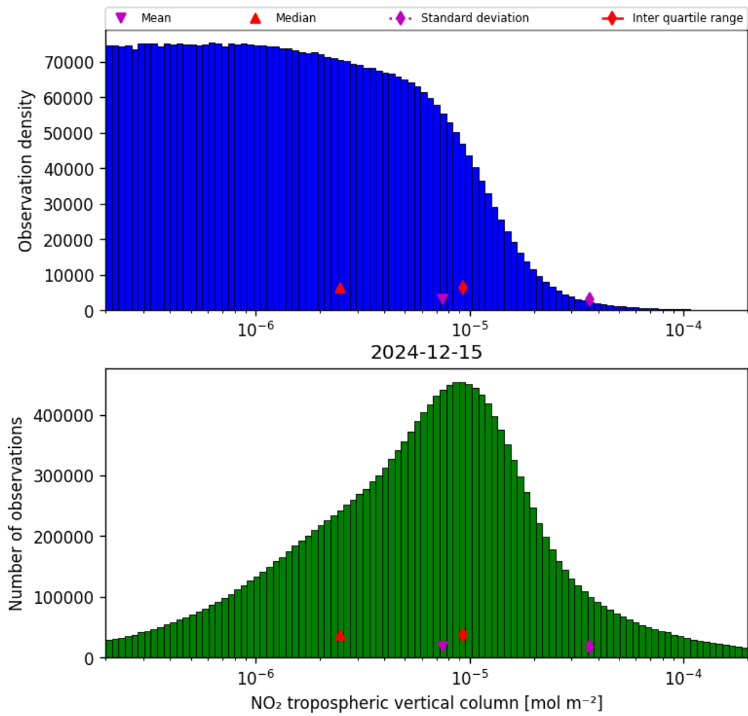
Figure 29: Histogram of “NO 2 tropospheric vertical column” for 2024-12-14 to 2024-12-16
