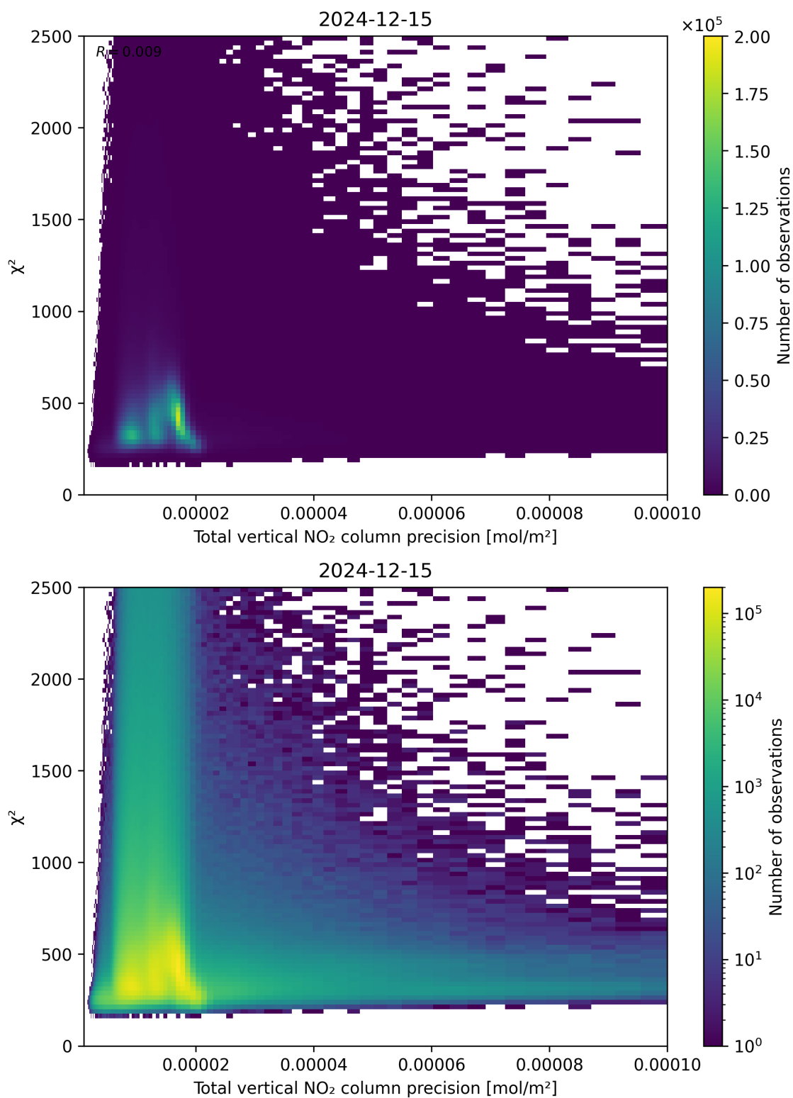
Figure 116: Scatter density plot of “Total vertical NO 2 column precision” against “ \chi^2 ” for 2024-12-14 to 2024-12-16.
