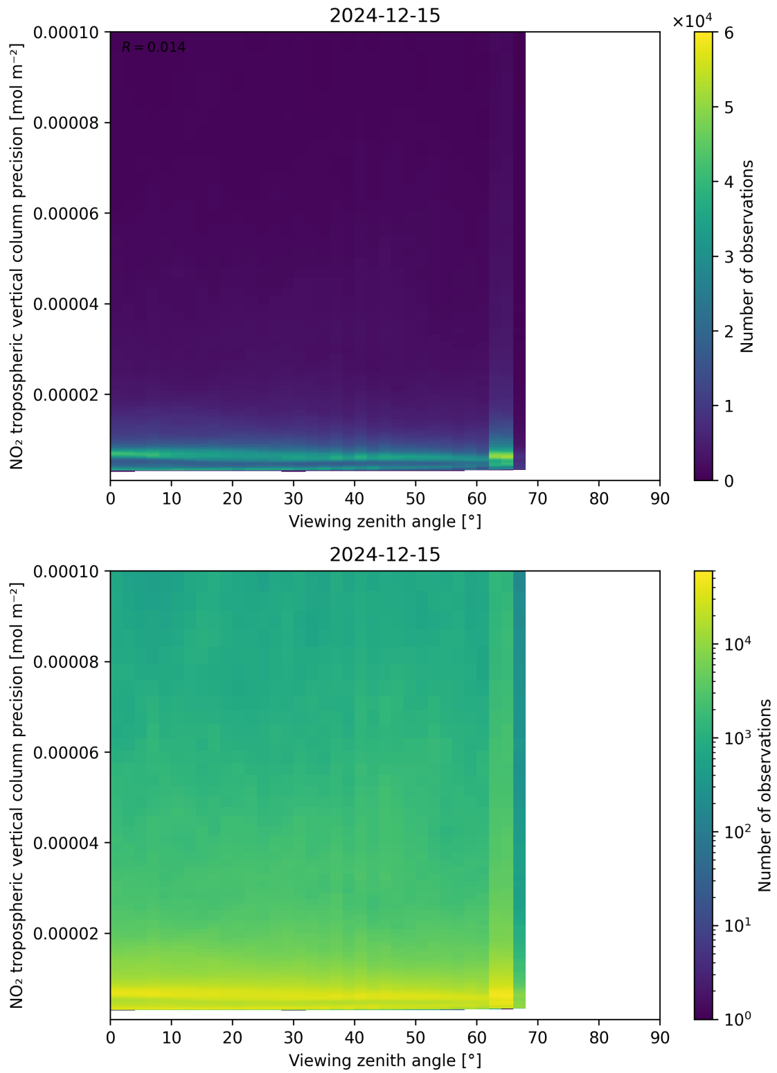
Figure 170: Scatter density plot of “Viewing zenith angle” against “NO 2 tropospheric vertical column precision” for 2024-12-14 to 2024-12-16.
