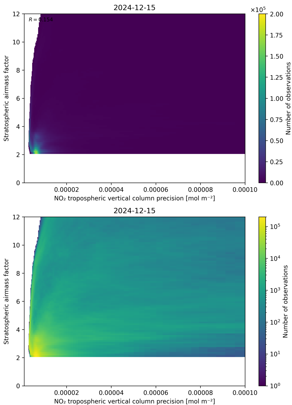
Figure 131: Scatter density plot of “NO 2 tropospheric vertical column precision” against “Stratospheric airmass factor” for 2024-12-14 to 2024-12-16.
