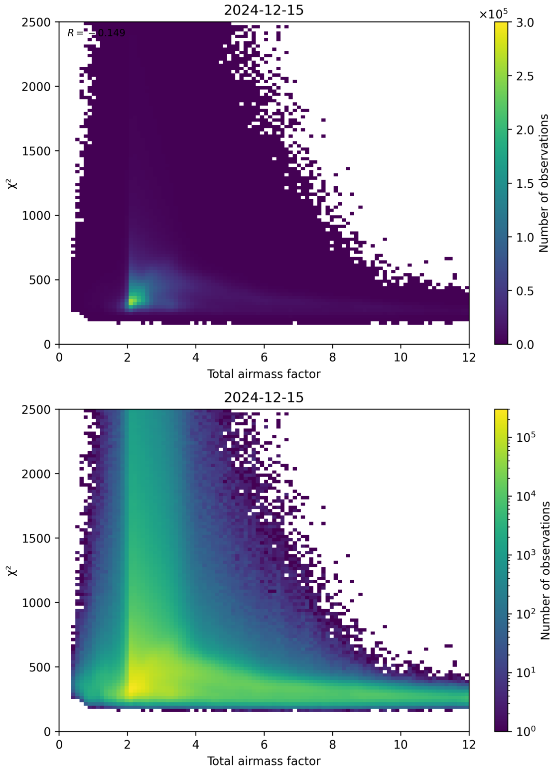
Figure 63: Scatter density plot of “Total airmass factor” against “ \chi^2 ” for 2024-12-14 to 2024-12-16.
