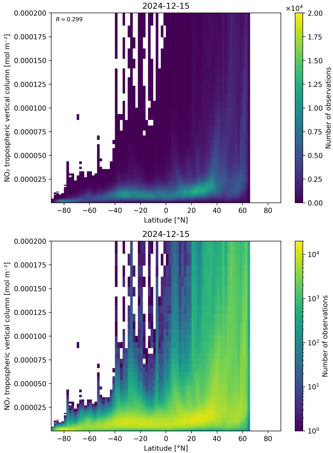
Figure 92: Scatter density plot of “Latitude” against “NO 2 tropospheric vertical column” for 2024-12-14 to 2024-12-16.
