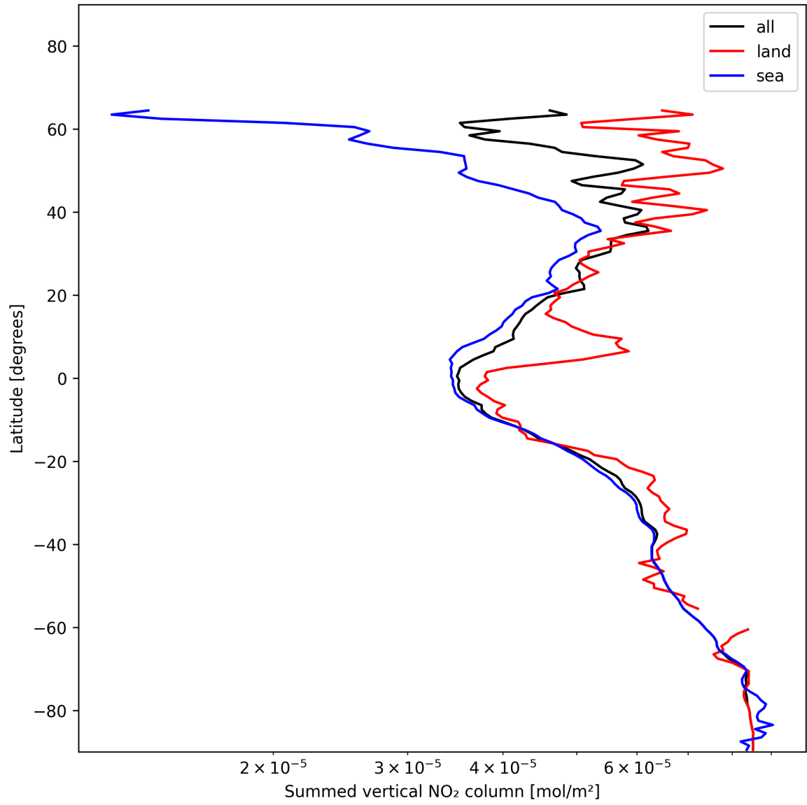
Figure 23: Zonal average of “Summed vertical NO 2 column” for 2024-12-14 to 2024-12-16.
