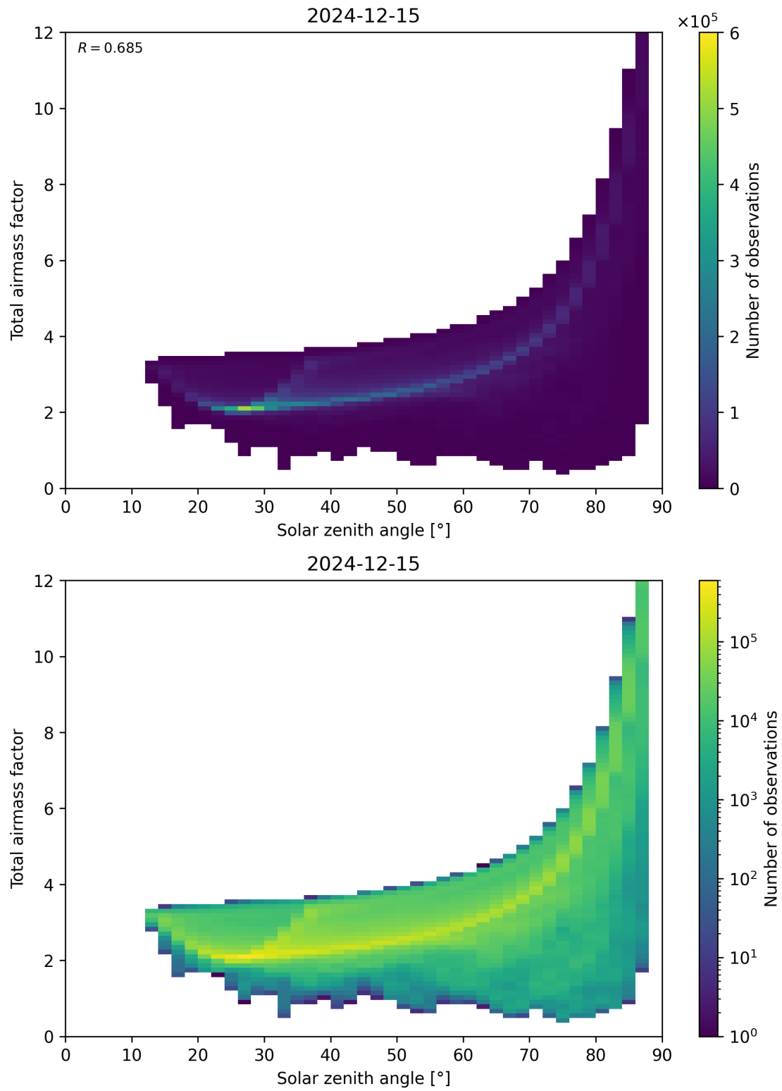
Figure 146: Scatter density plot of “Solar zenith angle” against “Total air mass factor” for 2024-12-14 to 2024-12-16.
