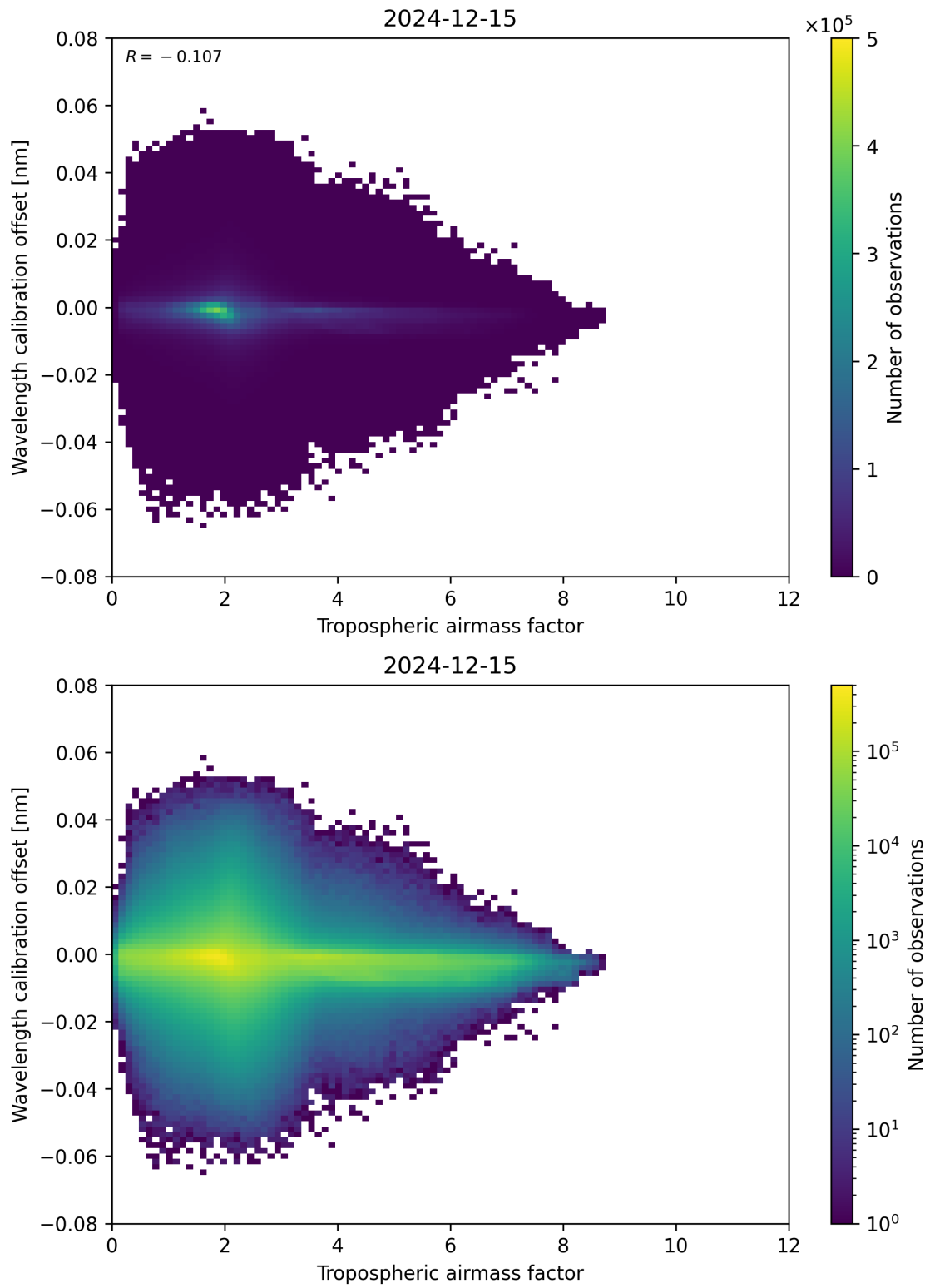
Figure 80: Scatter density plot of “Tropospheric airmass factor” against “Wavelength calibration offset” for 2024-12-14 to 2024-12-16.
