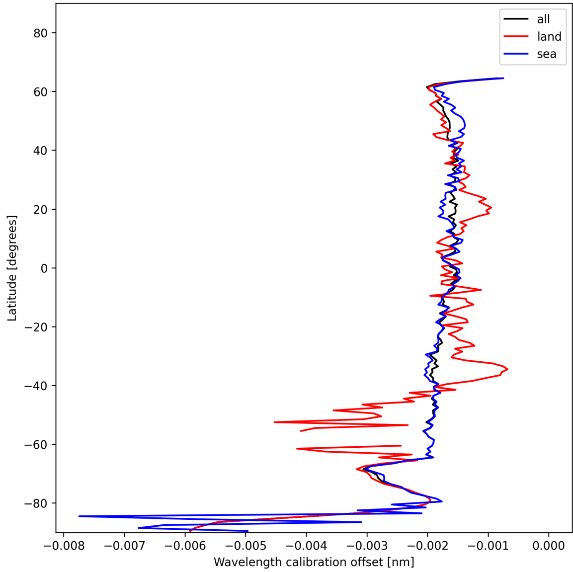
Figure 18: Zonal average of “Wavelength calibration offset” for 2024-12-14 to 2024-12-16.
