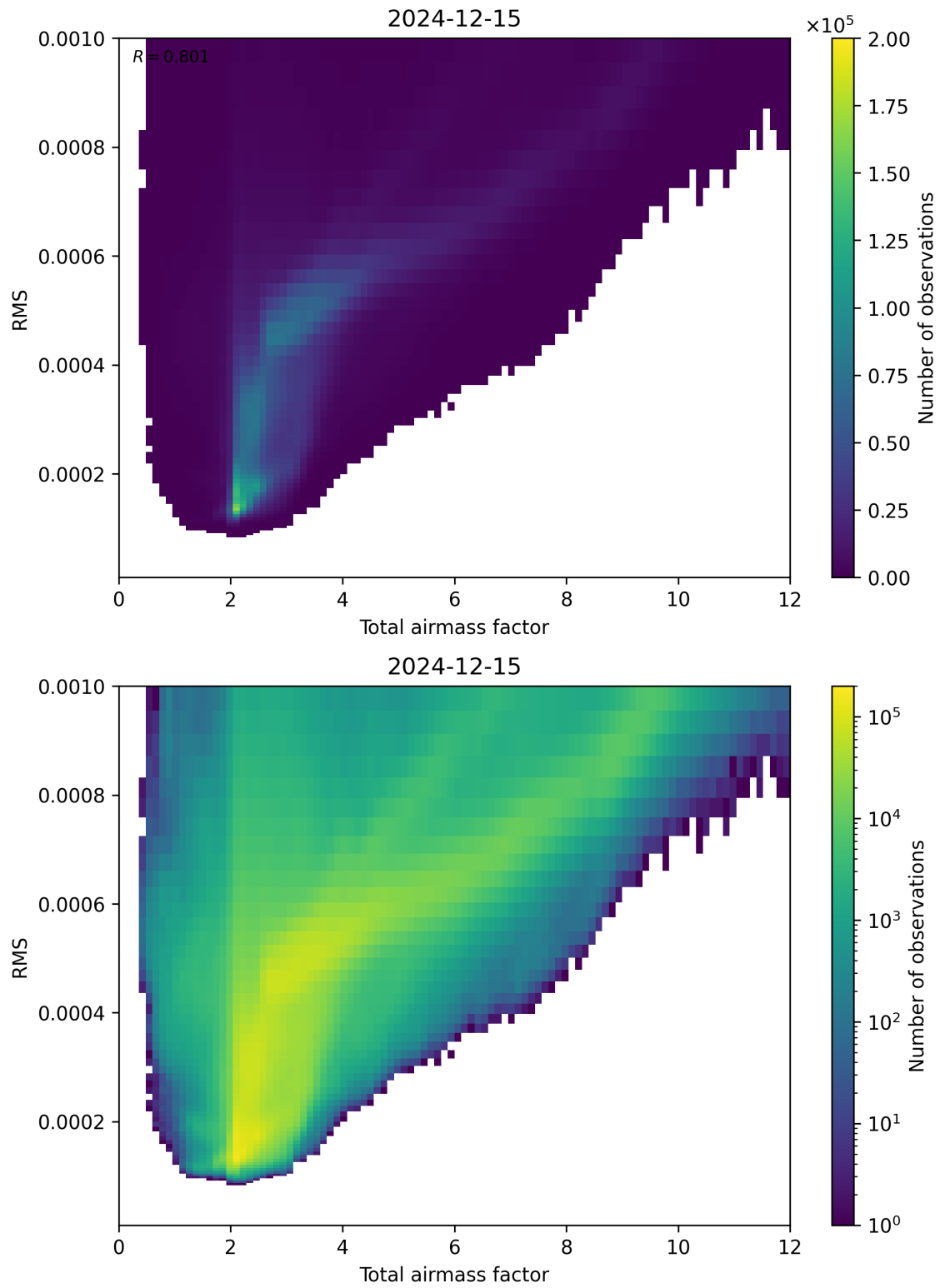
Figure 69: Scatter density plot of “Total airmass factor” against “RMS” for 2024-12-14 to 2024-12-16.
