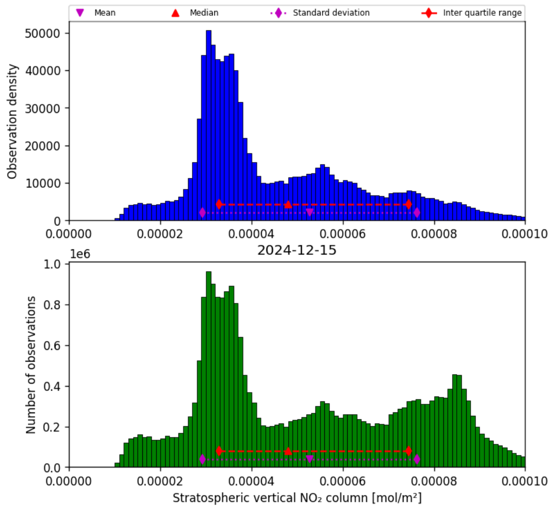
Figure 36: Histogram of “Stratospheric vertical NO 2 column” for 2024-12-14 to 2024-12-16
