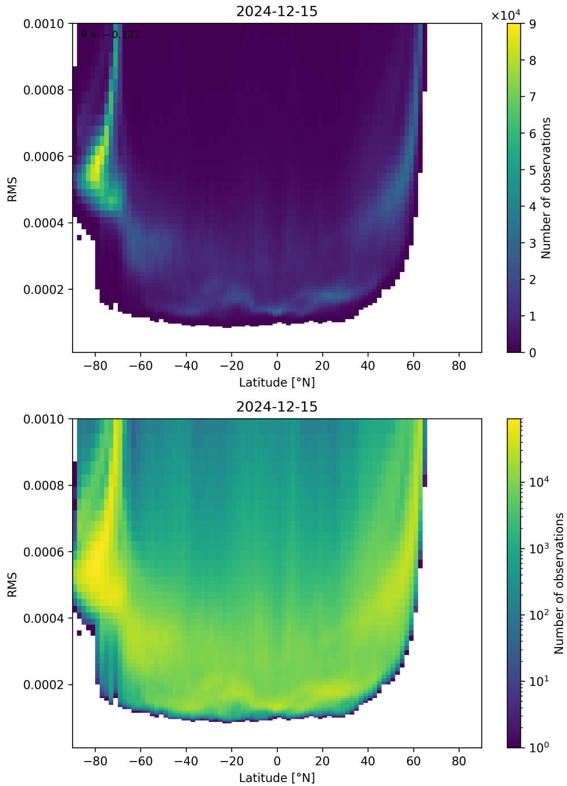
Figure 94: Scatter density plot of “Latitude” against “RMS” for 2024-12-14 to 2024-12-16.
