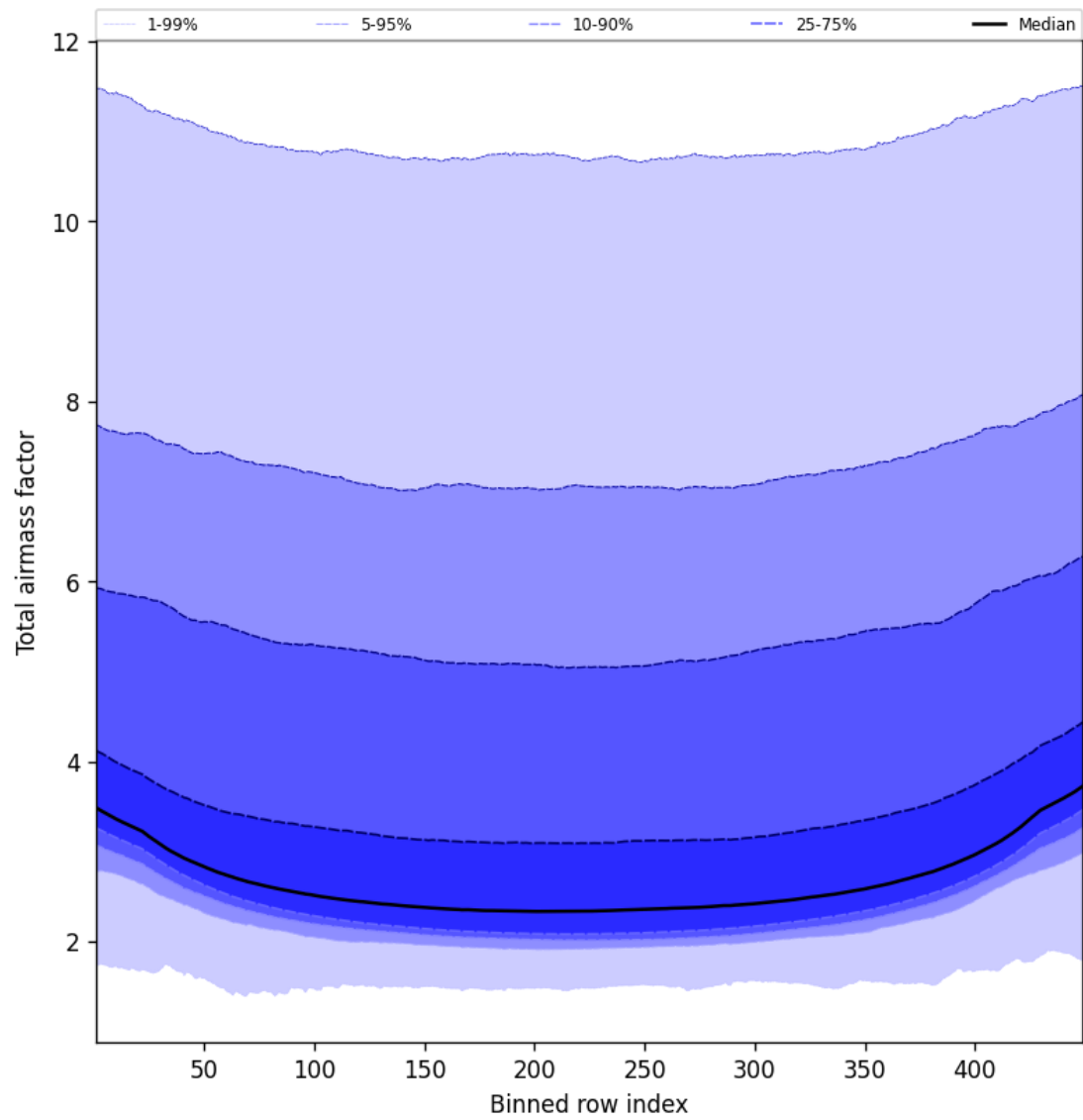
Figure 49: Along track statistics of “Total airmass factor” for 2024-12-14 to 2024-12-16
