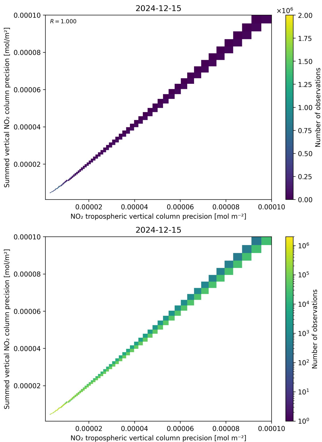
Figure 137: Scatter density plot of “NO 2 tropospheric vertical column precision” against “Summed vertical NO 2 column precision” for 2024-12-14 to 2024-12-16.
