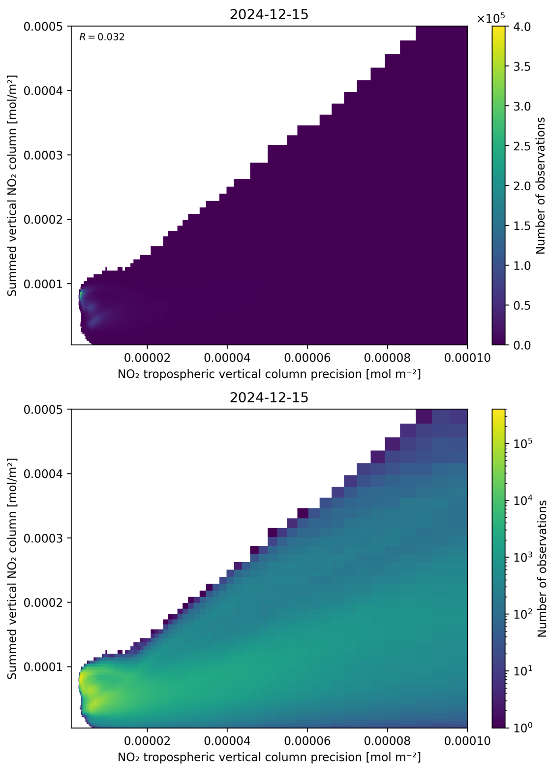
Figure 136: Scatter density plot of “NO 2 tropospheric vertical column precision” against “Summed vertical NO 2 column” for 2024-12-14 to 2024-12-16.
