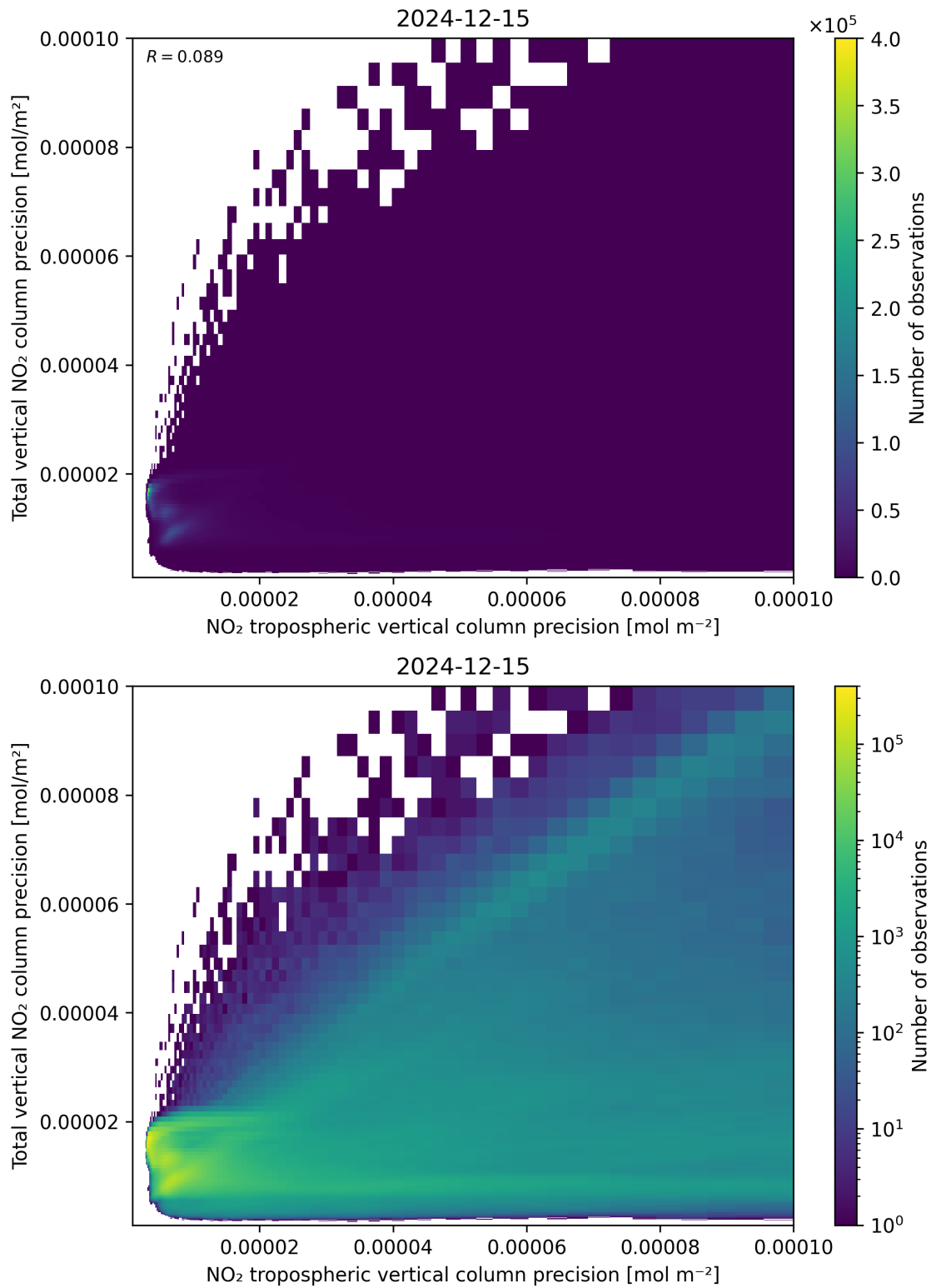
Figure 139: Scatter density plot of “NO 2 tropospheric vertical column precision” against “Total vertical NO 2 column precision” for 2024-12-14 to 2024-12-16.
