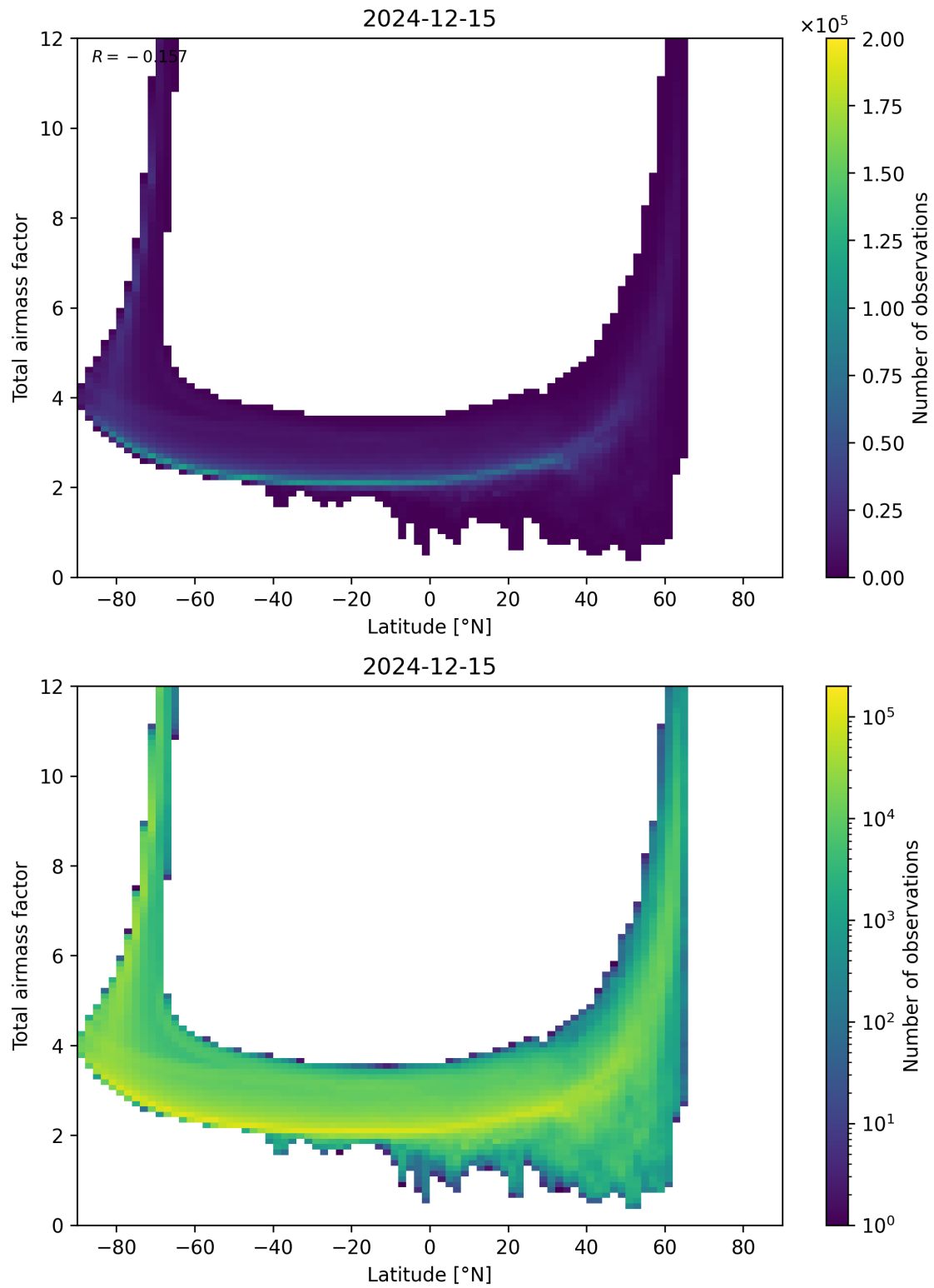
Figure 84: Scatter density plot of “Latitude” against “Total airmass factor” for 2024-12-14 to 2024-12-16.
