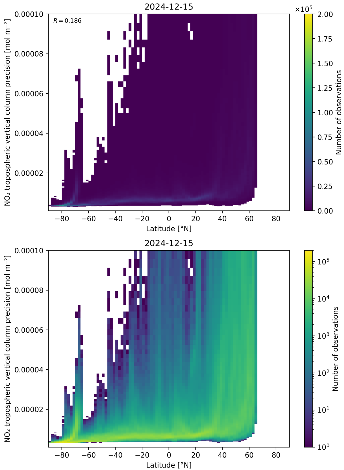
Figure 93: Scatter density plot of “Latitude” against “NO 2 tropospheric vertical column precision” for 2024-12-14 to 2024-12-16.
