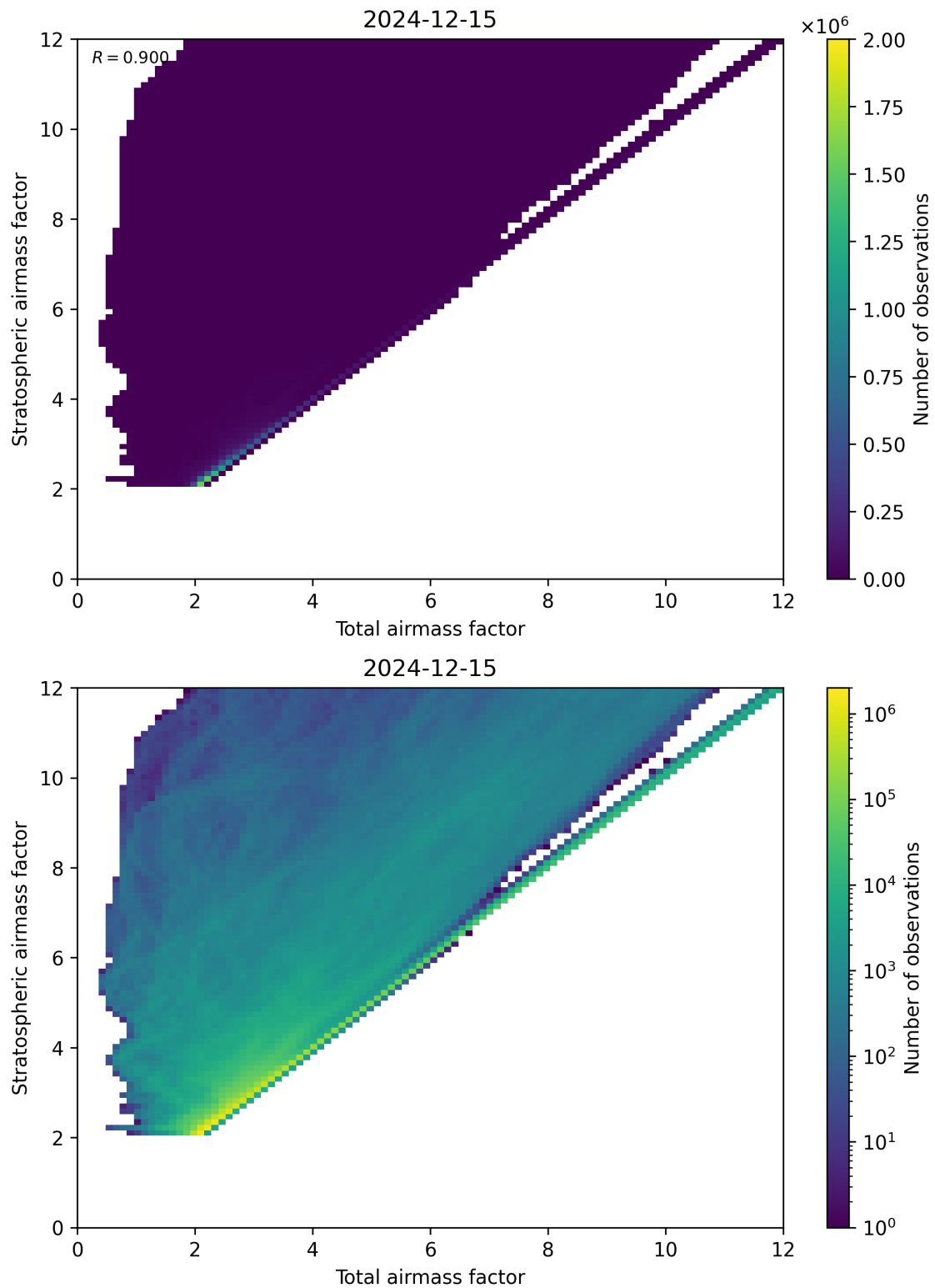
Figure 62: Scatter density plot of “Total airmass factor” against “Stratospheric airmass factor” for 2024-12-14 to 2024-12-16.
