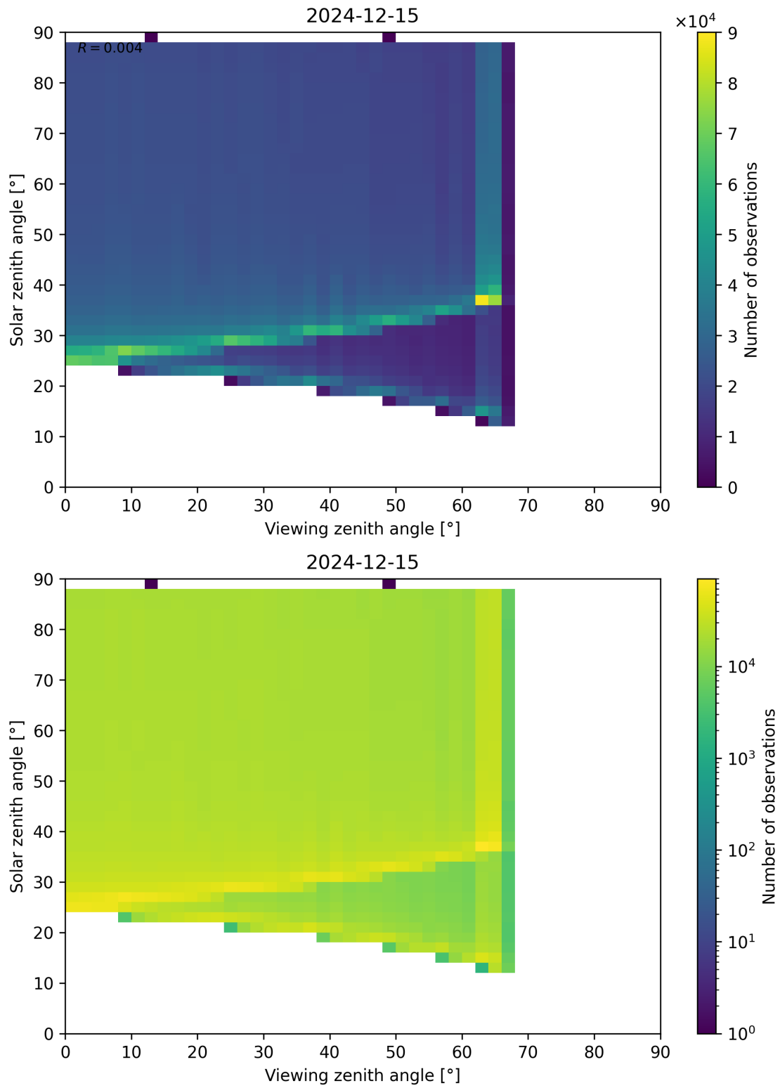
Figure 172: Scatter density plot of “Viewing zenith angle” against “Solar zenith angle” for 2024-12-14 to 2024-12-16.
