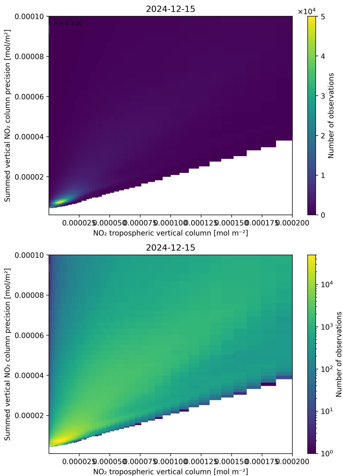
Figure 127: Scatter density plot of “NO 2 tropospheric vertical column” against “Summed vertical NO 2 column precision” for 2024-12-14 to 2024-12-16.
