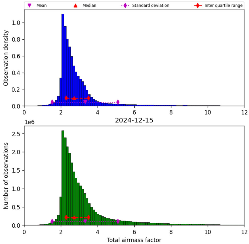
Figure 32: Histogram of “Total airmass factor” for 2024-12-14 to 2024-12-16
