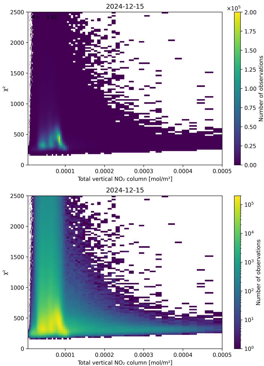
Figure 111: Scatter density plot of “Total vertical NO 2 column” against “ \chi^2 ” for 2024-12-14 to 2024-12-16.
