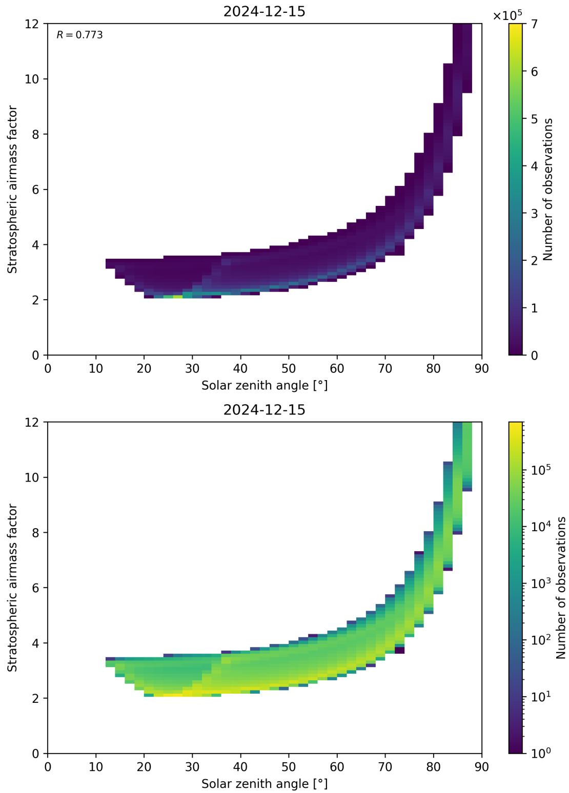
Figure 145: Scatter density plot of “Solar zenith angle” against “Stratospheric airmass factor” for 2024-12-14 to 2024-12-16.
