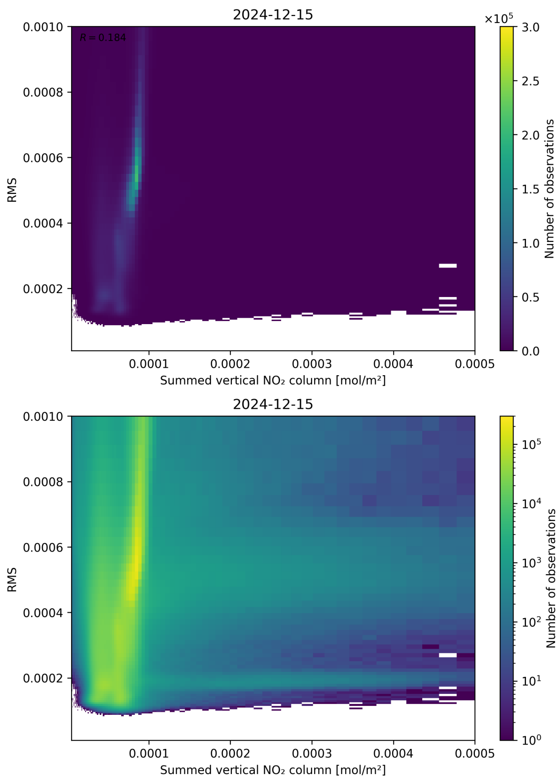
Figure 109: Scatter density plot of “Summed vertical NO 2 column” against “RMS” for 2024-12-14 to 2024-12-16.
