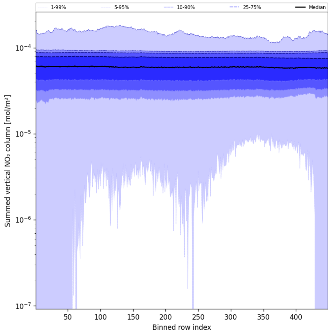
Figure 57: Along track statistics of “Summed vertical NO 2 column” for 2024-12-14 to 2024-12-16
