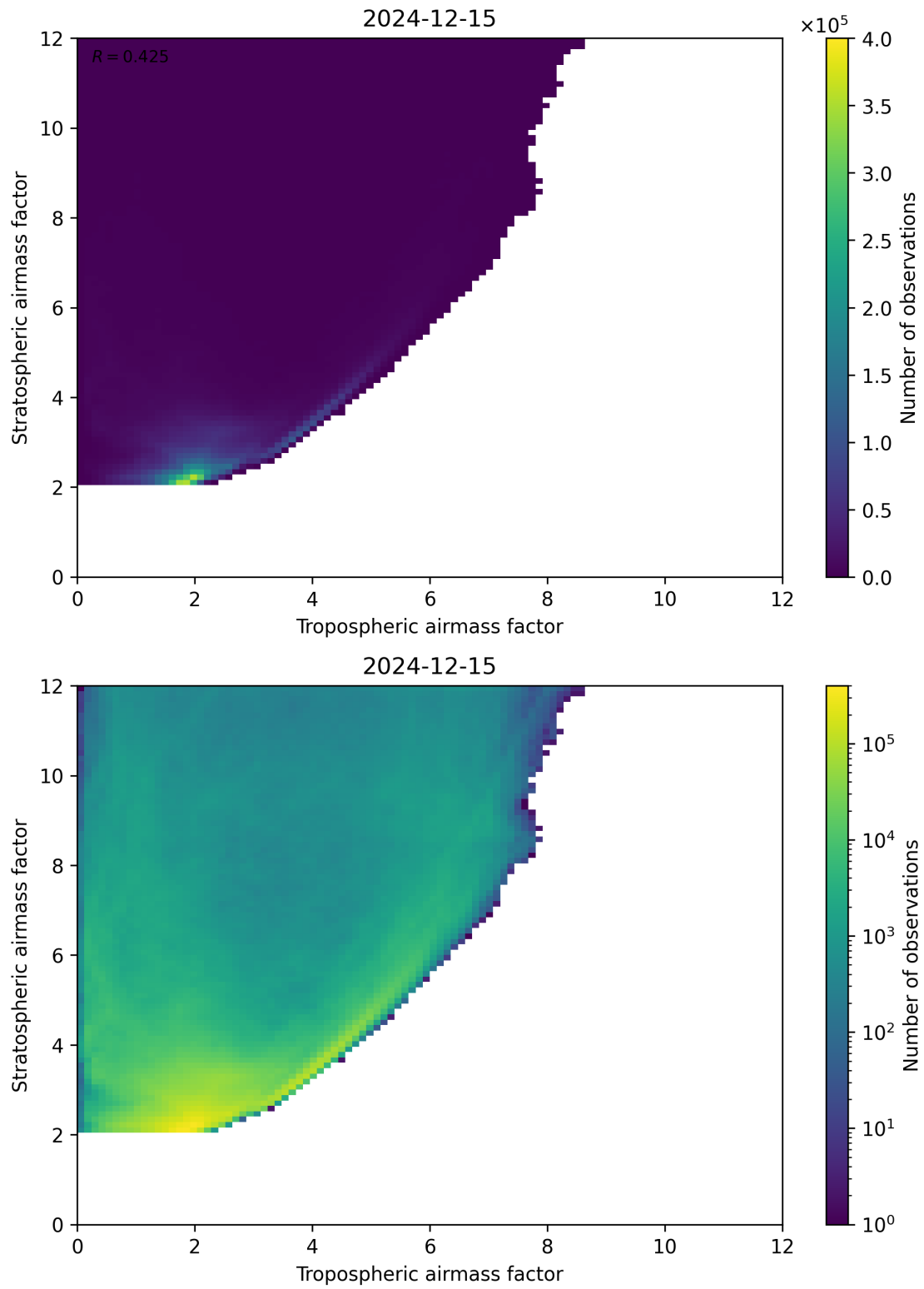
Figure 71: Scatter density plot of “Tropospheric airmass factor” against “Stratospheric airmass factor” for 2024-12-14 to 2024-12-16.
