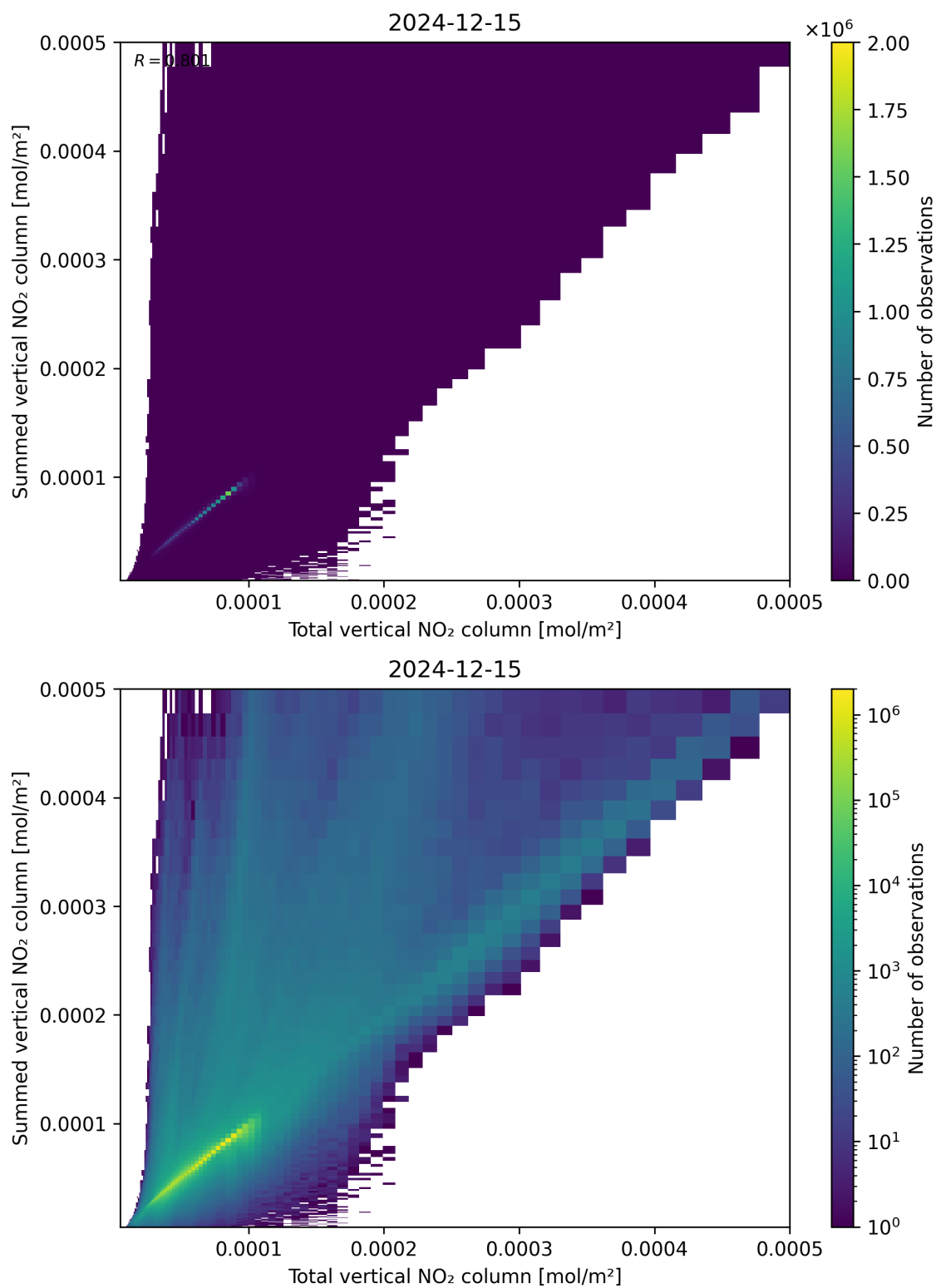
Figure 112: Scatter density plot of “Total vertical NO 2 column” against “Summed vertical NO 2 column” for 2024-12-14 to 2024-12-16.
