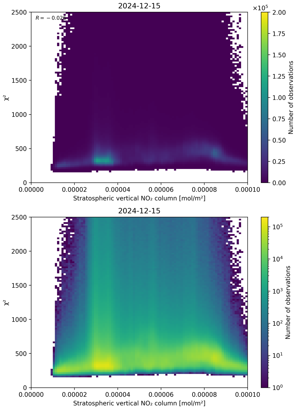
Figure 97: Scatter density plot of “Stratospheric vertical NO 2 column” against “ \chi^2 ” for 2024-12-14 to 2024-12-16.
