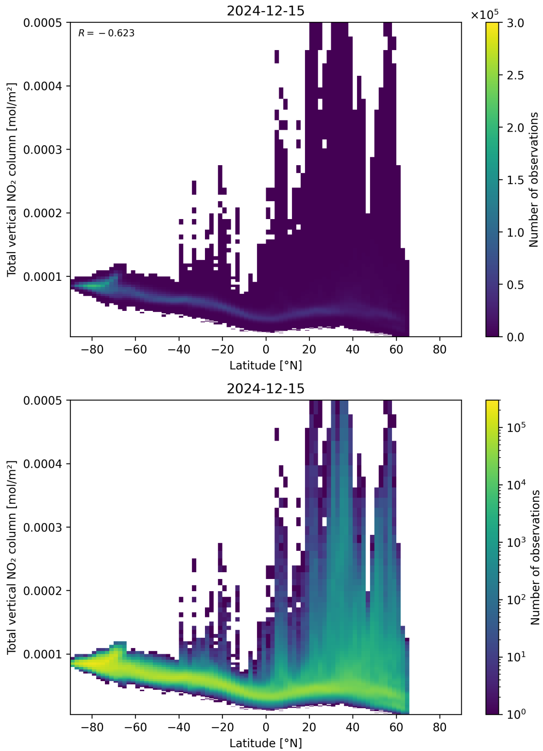
Figure 90: Scatter density plot of “Latitude” against “Total vertical NO 2 column” for 2024-12-14 to 2024-12-16.
