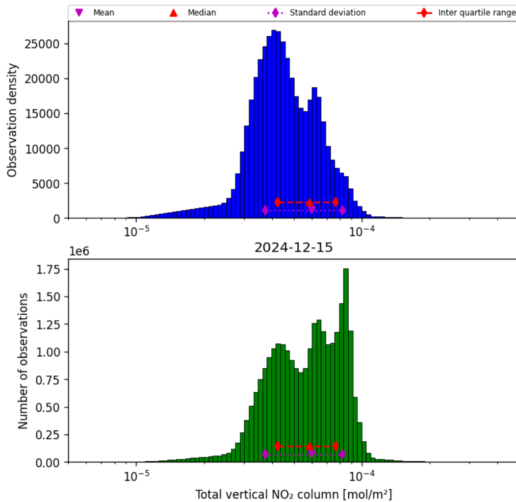
Figure 38: Histogram of “Total vertical NO 2 column” for 2024-12-14 to 2024-12-16
