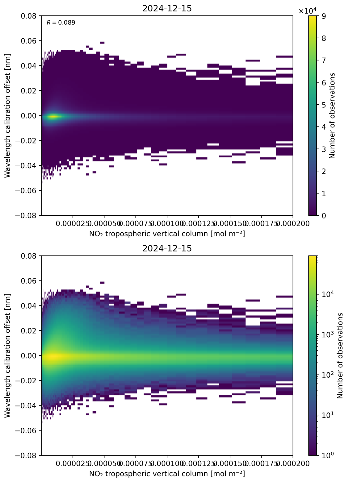
Figure 143: Scatter density plot of “NO 2 tropospheric vertical column” against “Wavelength calibration offset” for 2024-12-14 to 2024-12-16.
