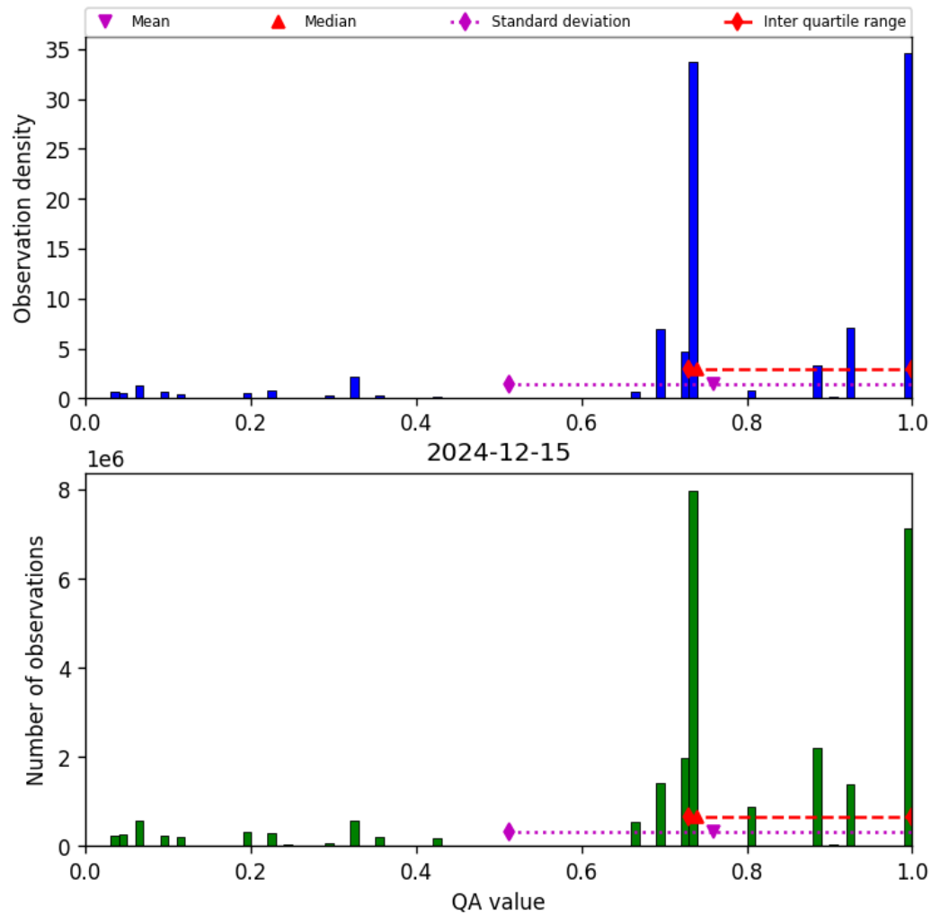
Figure 28: Histogram of “QA value” for 2024-12-14 to 2024-12-16
