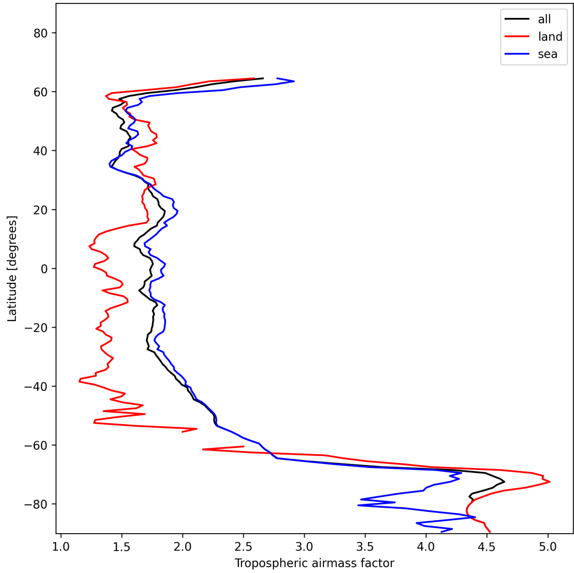
Figure 14: Zonal average of “Tropospheric airmass factor” for 2024-12-14 to 2024-12-16.
