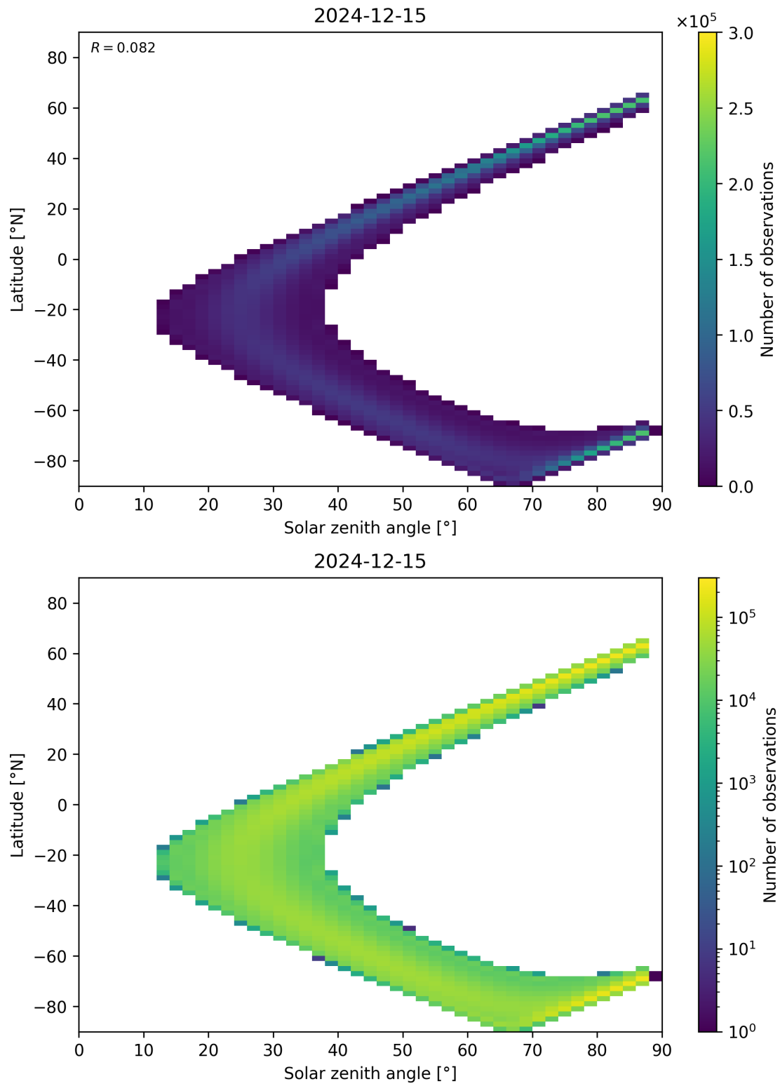
Figure 149: Scatter density plot of “Solar zenith angle” against “Latitude” for 2024-12-14 to 2024-12-16.
