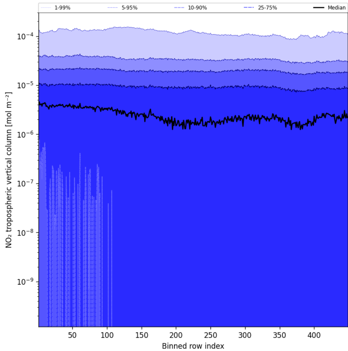
Figure 46: Along track statistics of “NO 2 tropospheric vertical column” for 2024-12-14 to 2024-12-16
