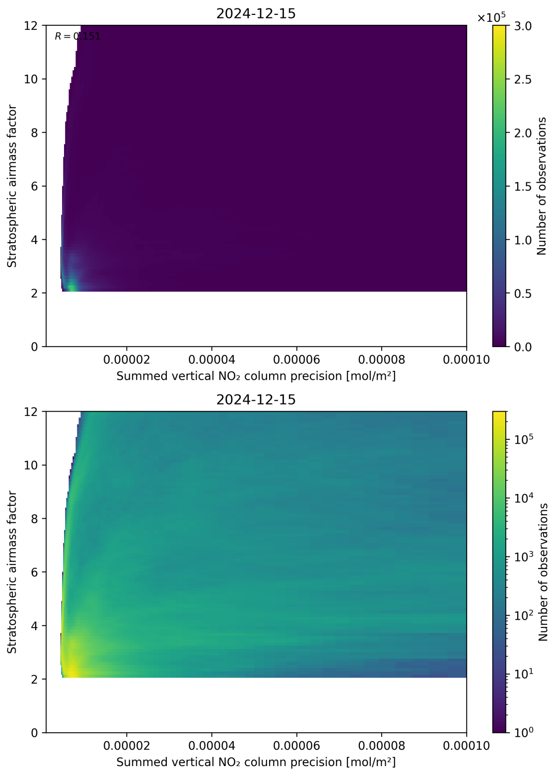
Figure 106: Scatter density plot of “Summed vertical NO 2 column precision” against “Stratospheric airmass factor” for 2024-12-14 to 2024-12-16.
