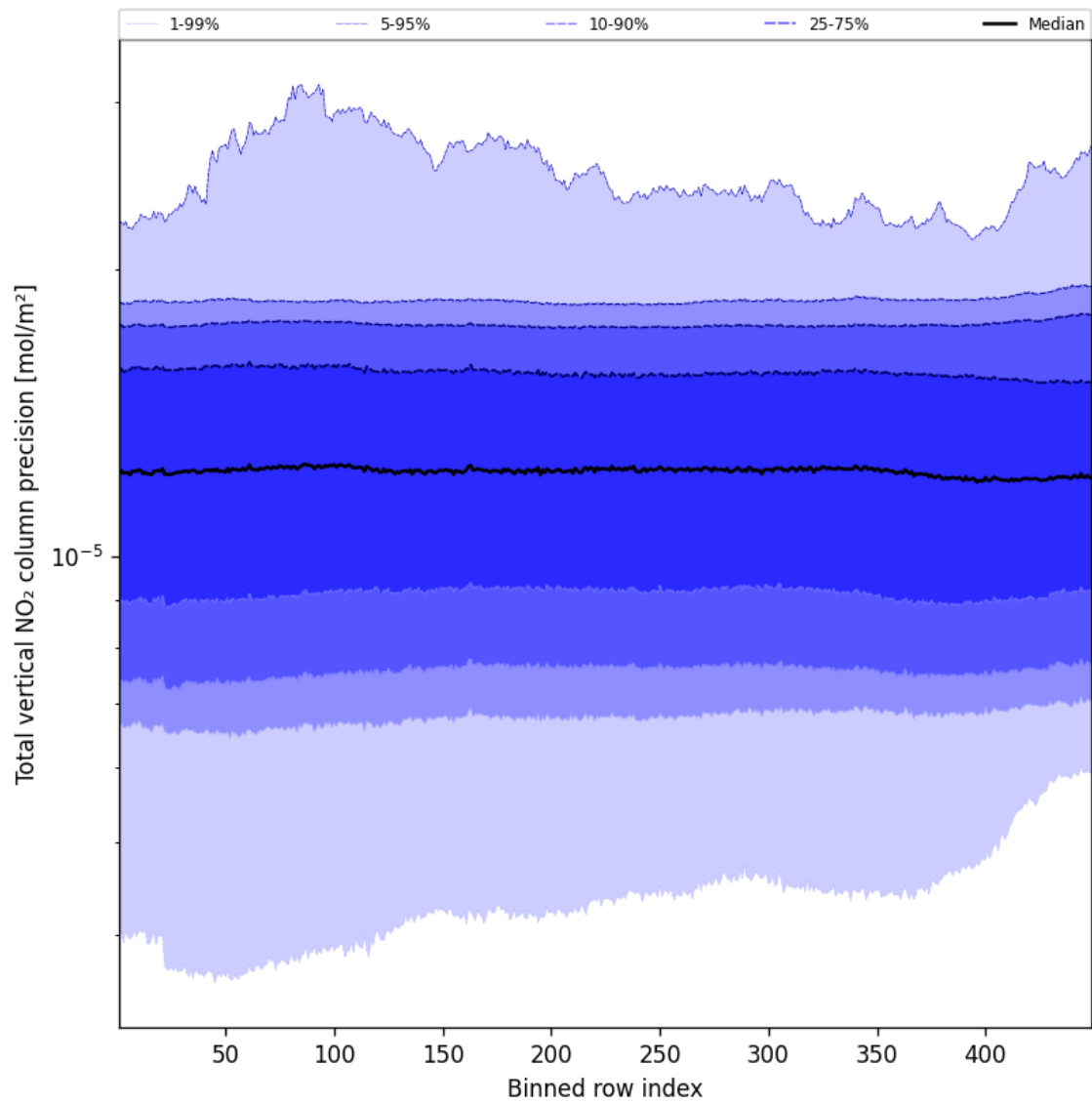
Figure 56: Along track statistics of “Total vertical NO 2 column precision” for 2024-12-14 to 2024-12-16
