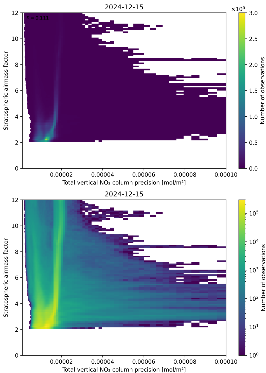
Figure 115: Scatter density plot of “Total vertical NO 2 column precision” against “Stratospheric airmass factor” for 2024-12-14 to 2024-12-16.
