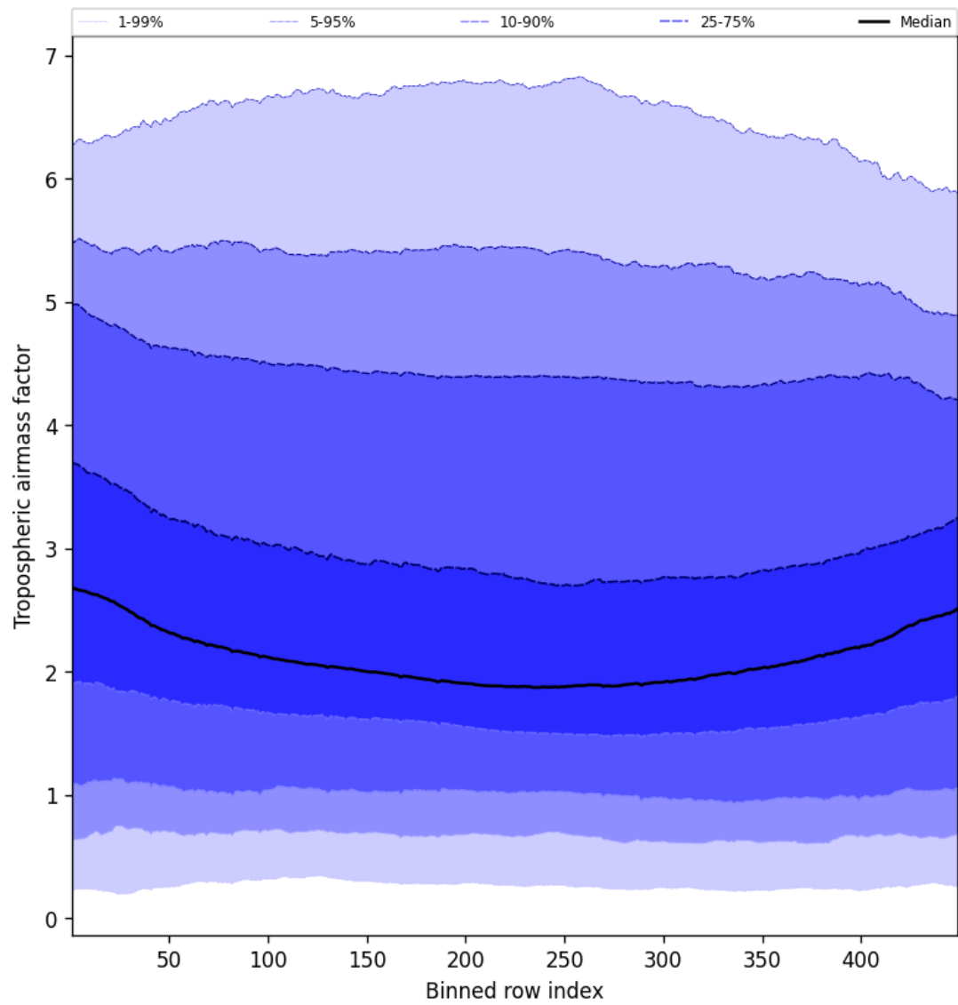
Figure 48: Along track statistics of “Tropospheric airmass factor” for 2024-12-14 to 2024-12-16
