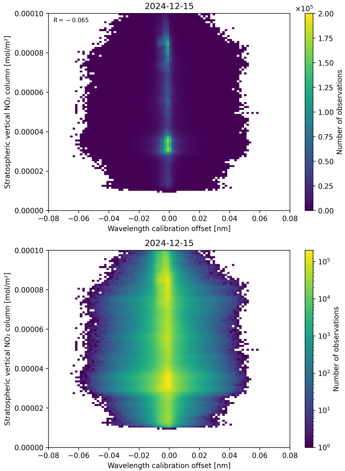
Figure 176: Scatter density plot of “Wavelength calibration offset” against “Stratospheric vertical NO 2 column” for 2024-12-14 to 2024-12-16.
