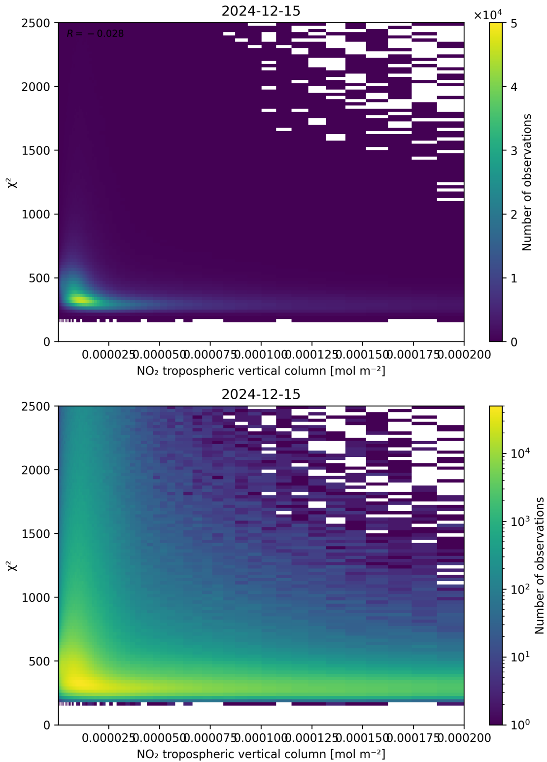
Figure 124: Scatter density plot of “NO 2 tropospheric vertical column” against “ \chi^2 ” for 2024-12-14 to 2024-12-16.
