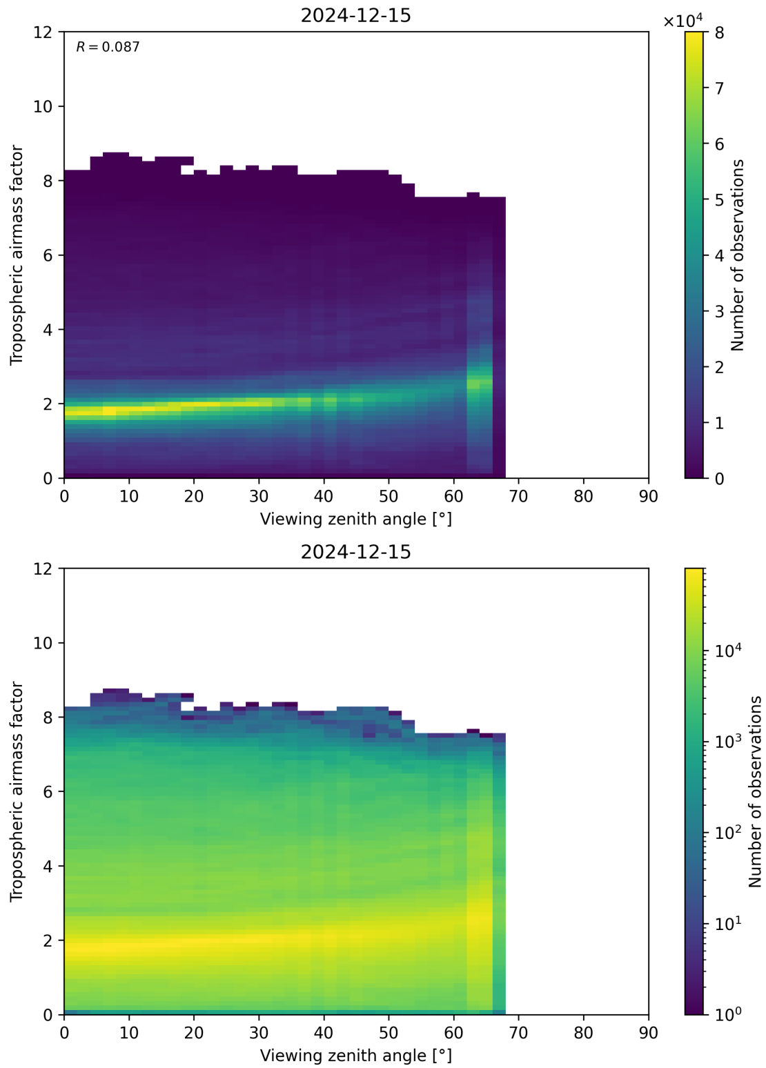
Figure 161: Scatter density plot of “Viewing zenith angle” against “Tropospheric airmass factor” for 2024-12-14 to 2024-12-16.
