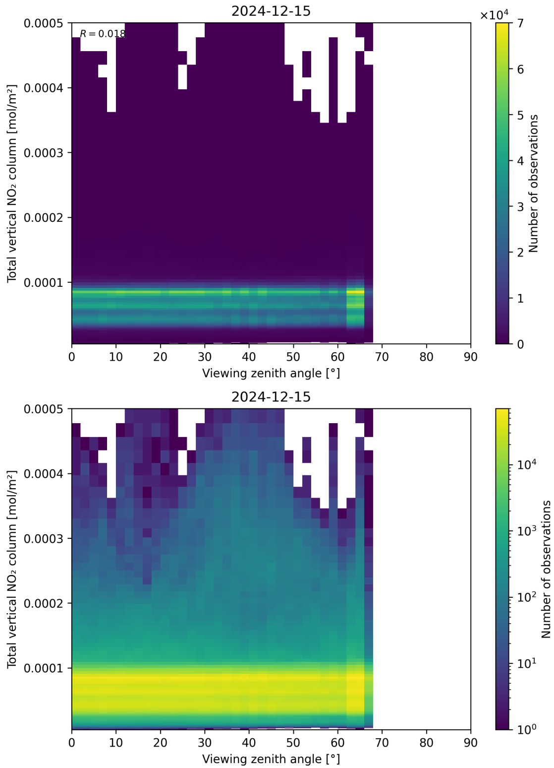
Figure 167: Scatter density plot of “Viewing zenith angle” against “Total vertical NO 2 column” for 2024-12-14 to 2024-12-16.
