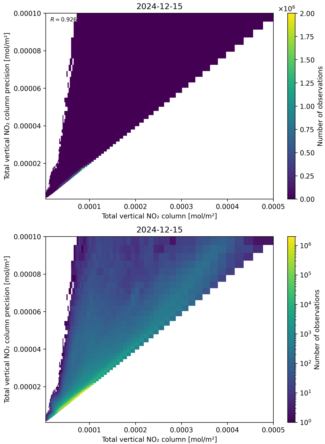
Figure 114: Scatter density plot of “Total vertical NO 2 column” against “Total vertical NO 2 column precision” for 2024-12-14 to 2024-12-16.
