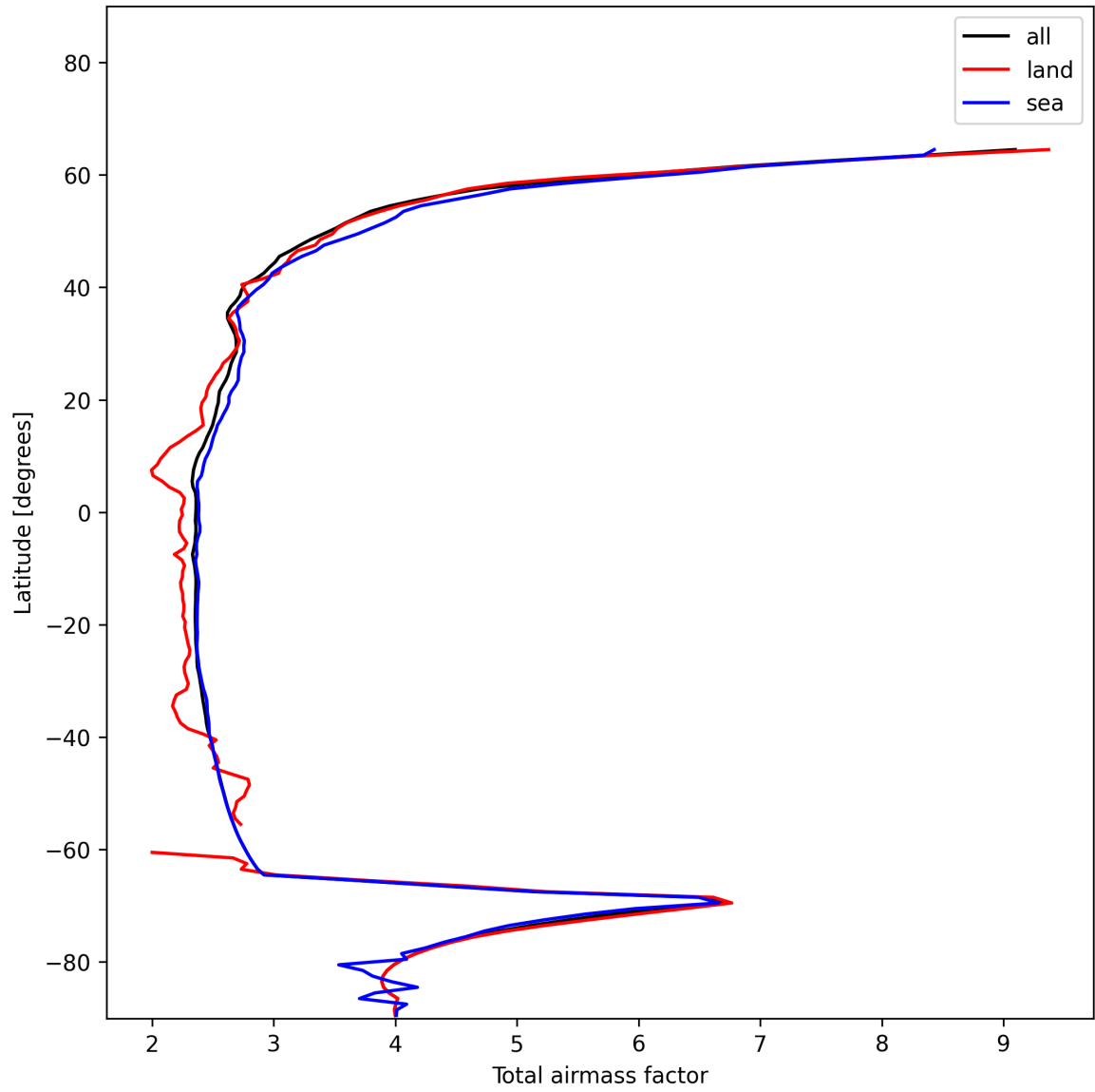
Figure 15: Zonal average of “Total airmass factor” for 2024-12-14 to 2024-12-16.
