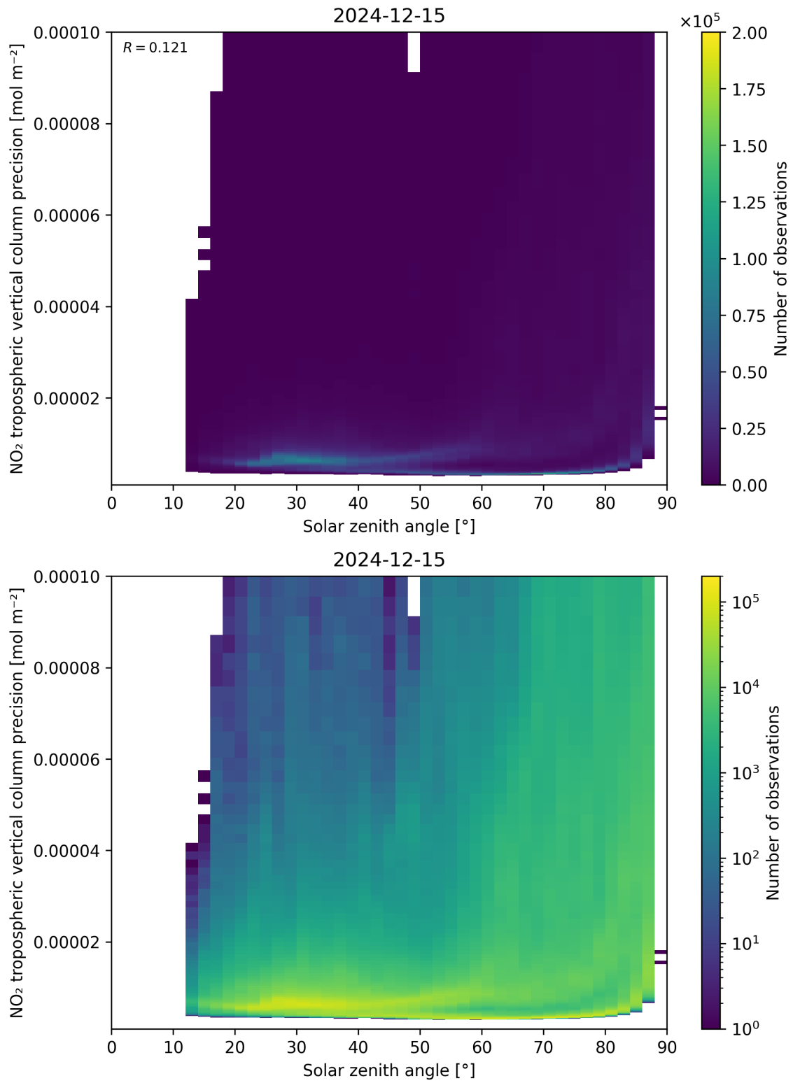
Figure 156: Scatter density plot of “Solar zenith angle” against “NO 2 tropospheric vertical column precision” for 2024-12-14 to 2024-12-16.
