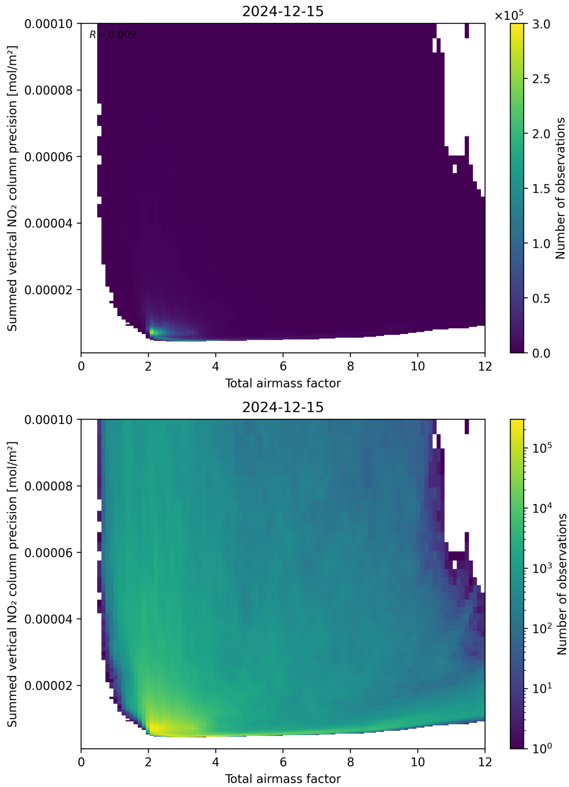
Figure 66: Scatter density plot of “Total airmass factor” against “Summed vertical NO 2 column precision” for 2024-12-14 to 2024-12-16.
