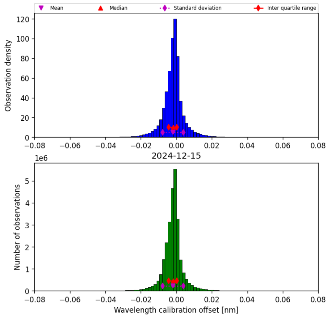
Figure 35: Histogram of “Wavelength calibration offset” for 2024-12-14 to 2024-12-16
