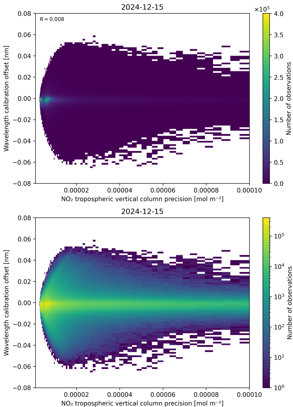
Figure 141: Scatter density plot of “NO 2 tropospheric vertical column precision” against “Wavelength calibration offset” for 2024-12-14 to 2024-12-16.
