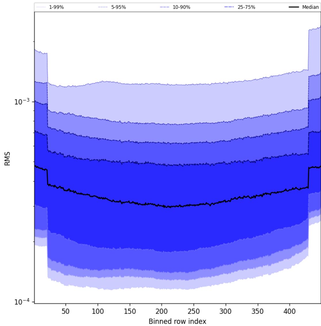
Figure 60: Along track statistics of “RMS” for 2024-12-14 to 2024-12-16
