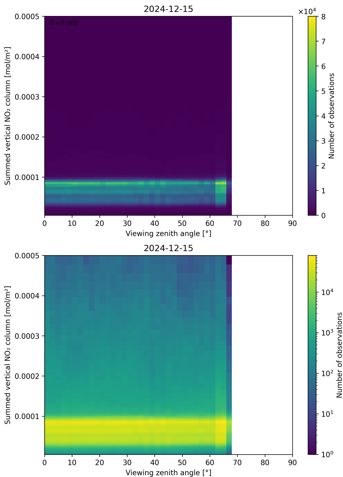
Figure 165: Scatter density plot of “Viewing zenith angle” against “Summed vertical NO 2 column” for 2024-12-14 to 2024-12-16.
