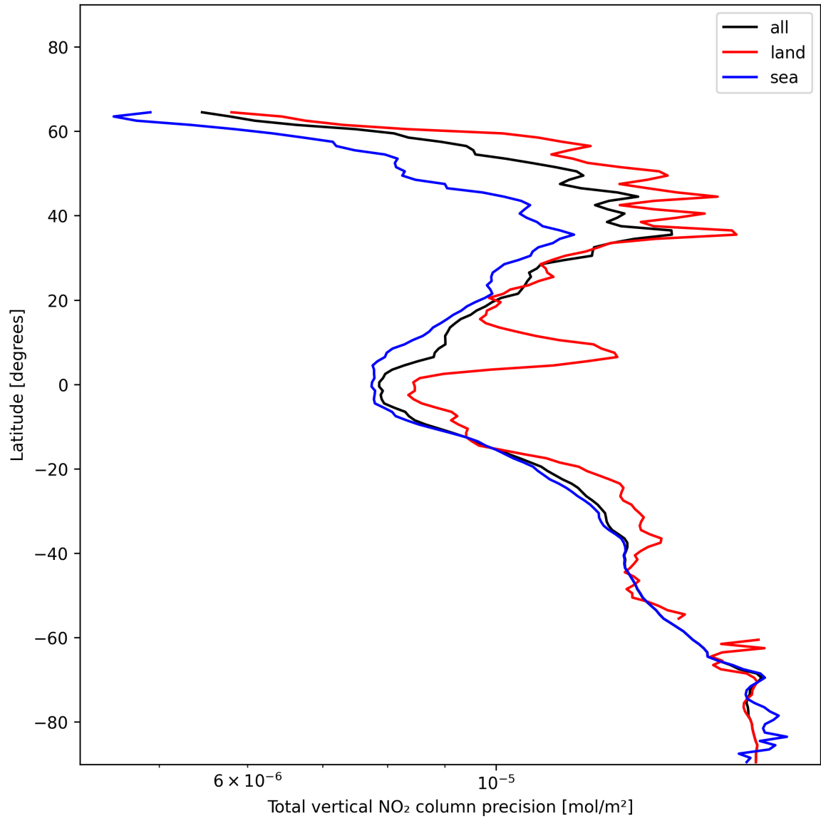
Figure 22: Zonal average of “Total vertical NO 2 column precision” for 2024-12-14 to 2024-12-16.
