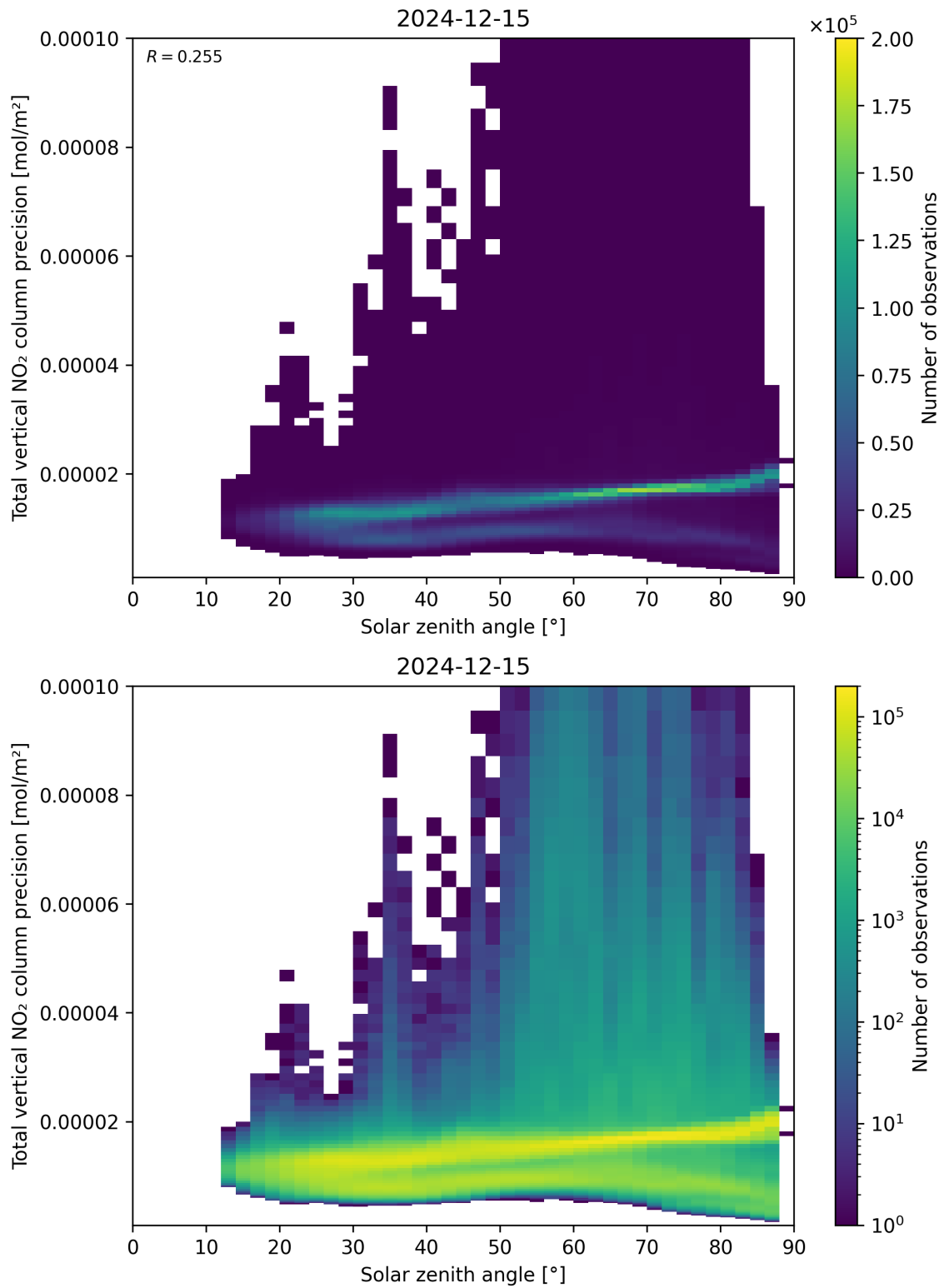
Figure 154: Scatter density plot of “Solar zenith angle” against “Total vertical NO 2 column precision” for 2024-12-14 to 2024-12-16.
