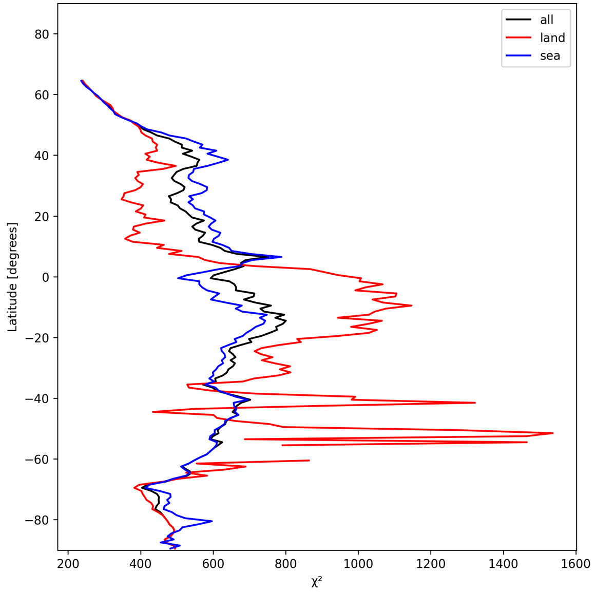
Figure 25: Zonal average of “ \chi^2 ” for 2024-12-14 to 2024-12-16.
