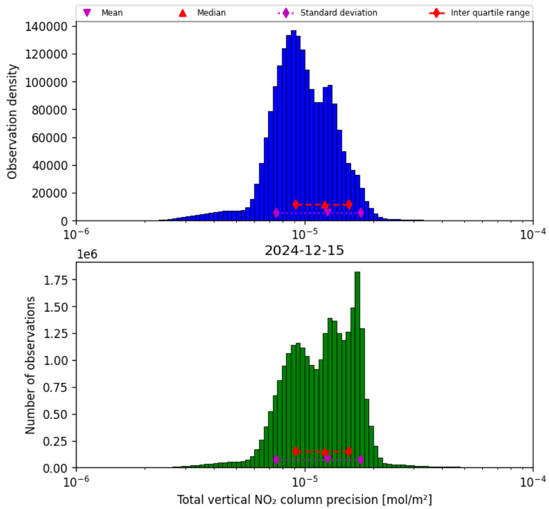
Figure 39: Histogram of “Total vertical NO 2 column precision” for 2024-12-14 to 2024-12-16
