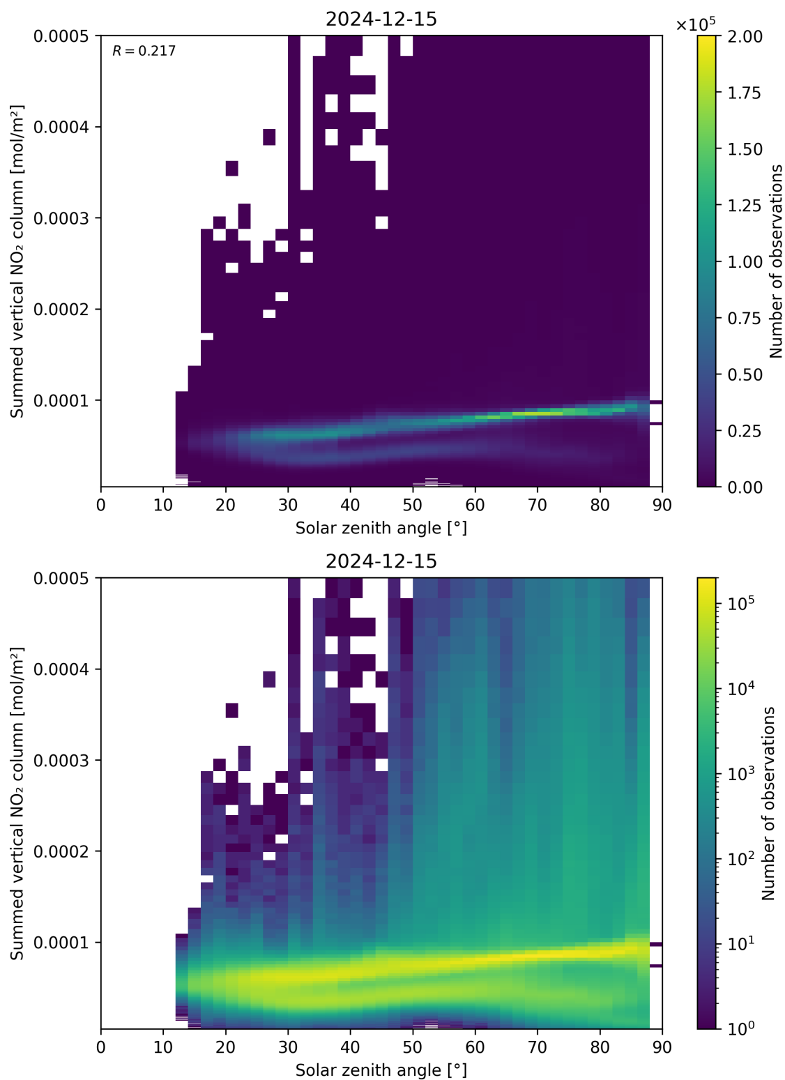
Figure 151: Scatter density plot of “Solar zenith angle” against “Summed vertical NO 2 column” for 2024-12-14 to 2024-12-16.
