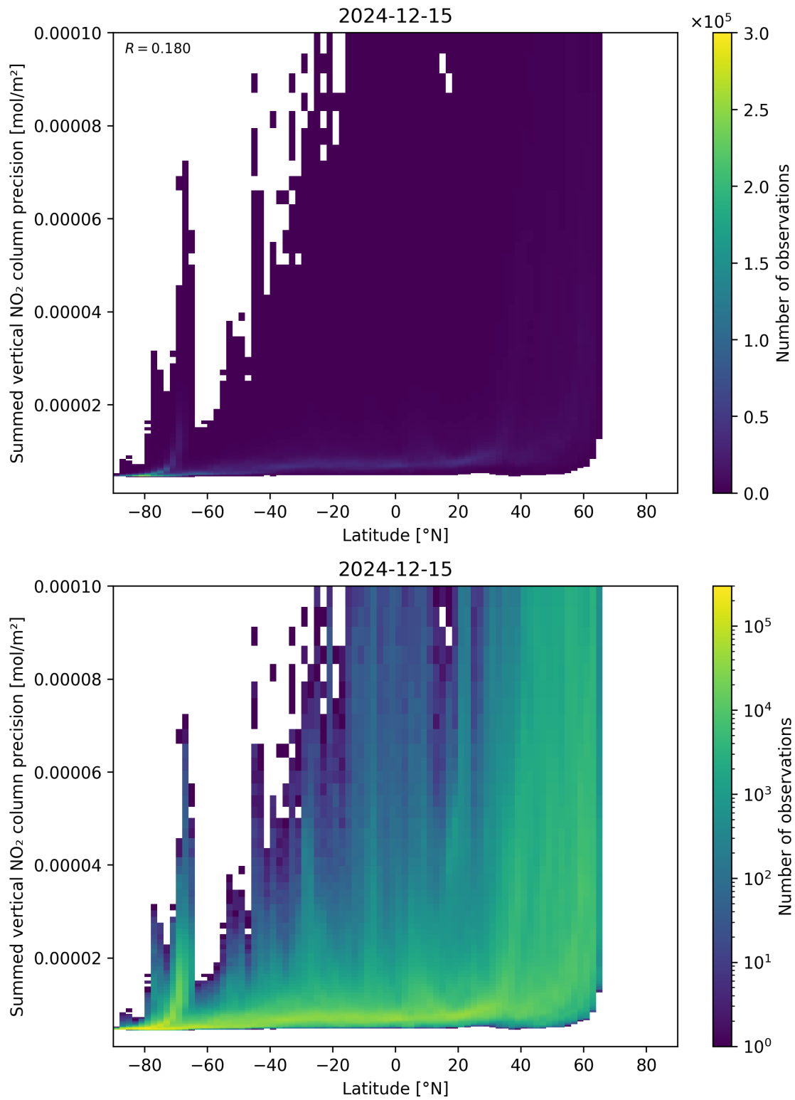
Figure 89: Scatter density plot of “Latitude” against “Summed vertical NO 2 column precision” for 2024-12-14 to 2024-12-16.
