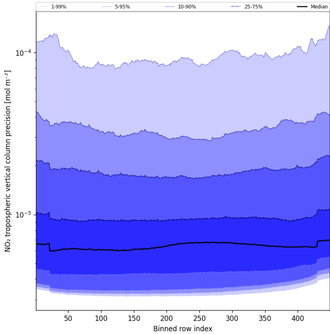
Figure 47: Along track statistics of “NO 2 tropospheric vertical column precision” for 2024-12-14 to 2024-12-16
