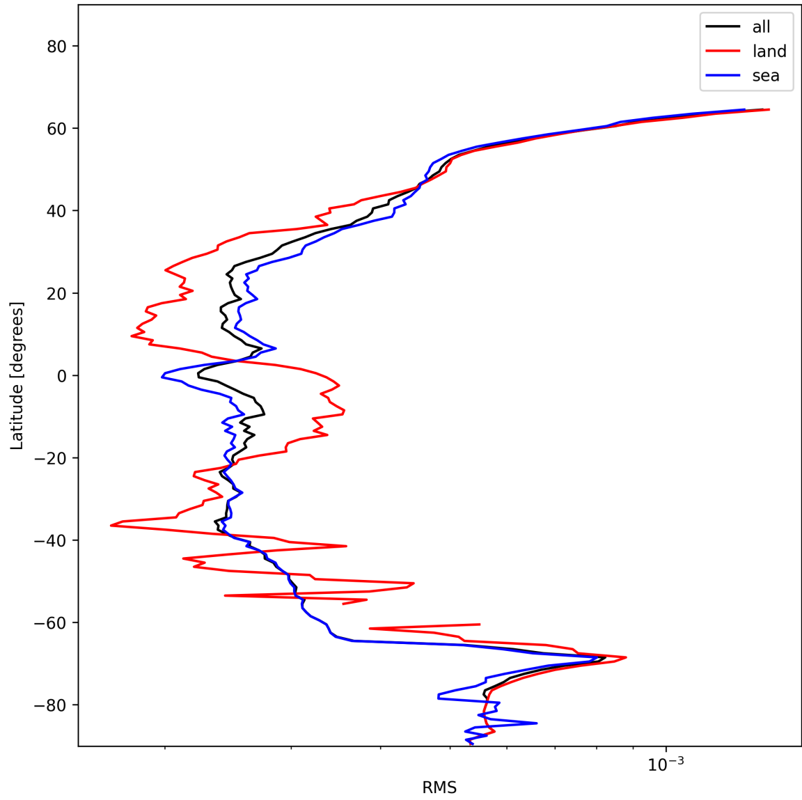
Figure 26: Zonal average of “RMS” for 2024-12-14 to 2024-12-16.
