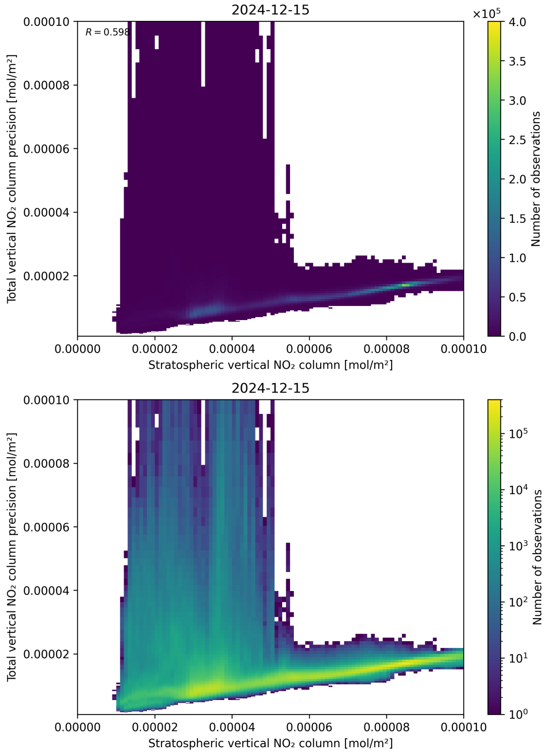
Figure 101: Scatter density plot of “Stratospheric vertical NO 2 column” against “Total vertical NO 2 column precision” for 2024-12-14 to 2024-12-16.
