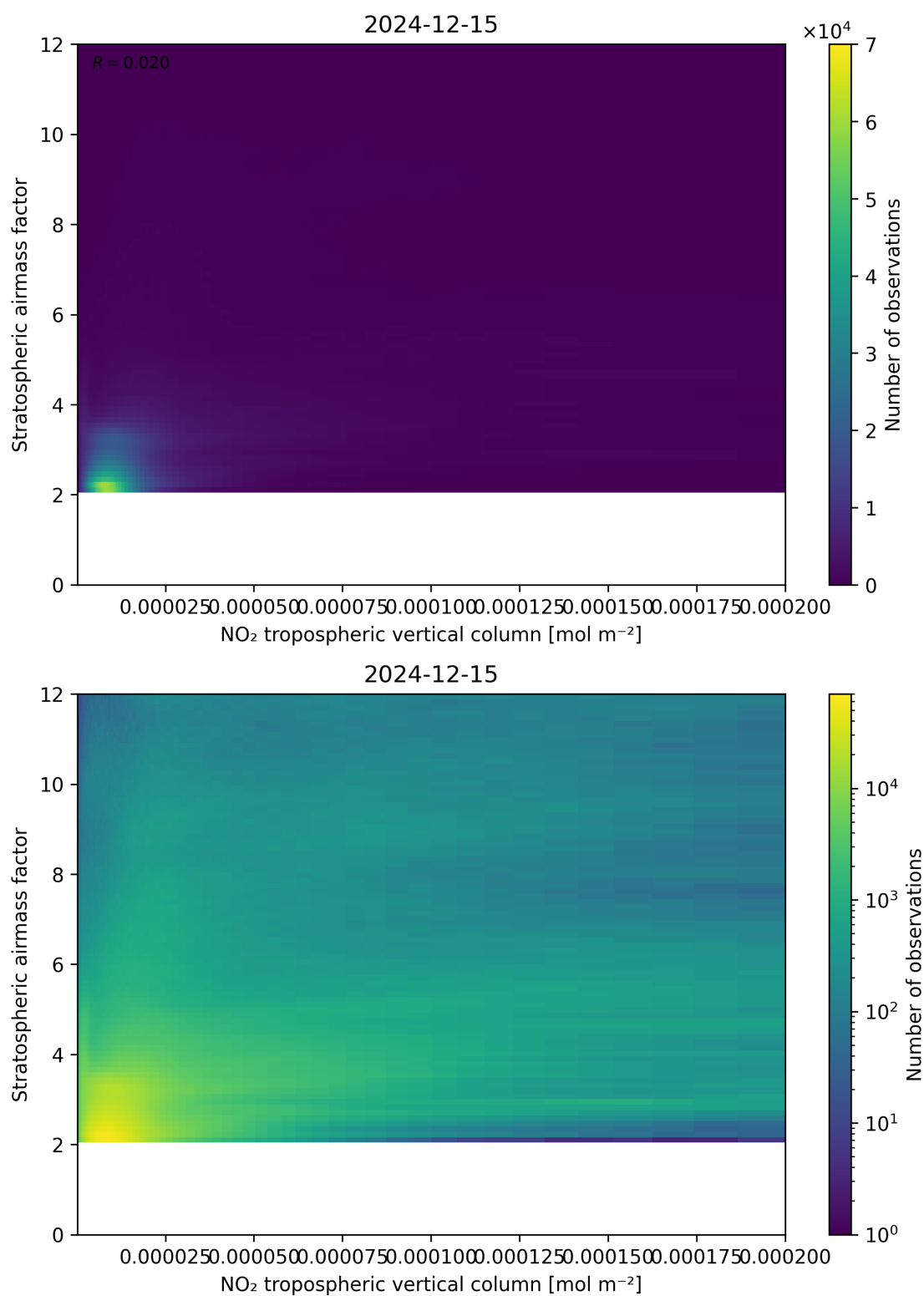
Figure 121: Scatter density plot of “NO 2 tropospheric vertical column” against “Stratospheric airmass factor” for 2024-12-14 to 2024-12-16.
