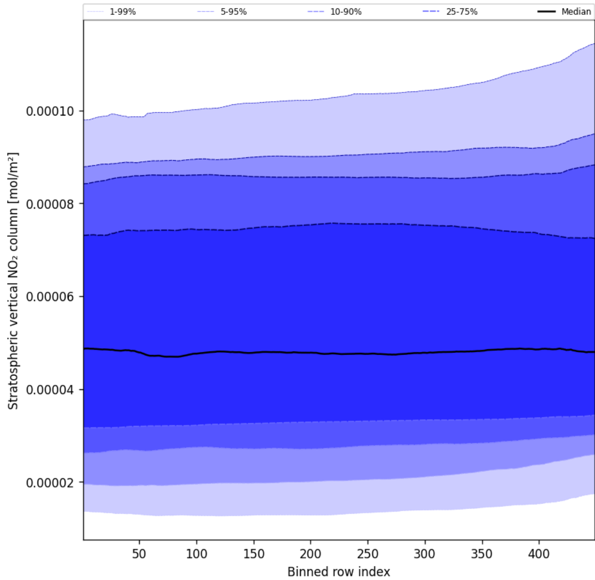
Figure 53: Along track statistics of “Stratospheric vertical NO 2 column” for 2024-12-14 to 2024-12-16
