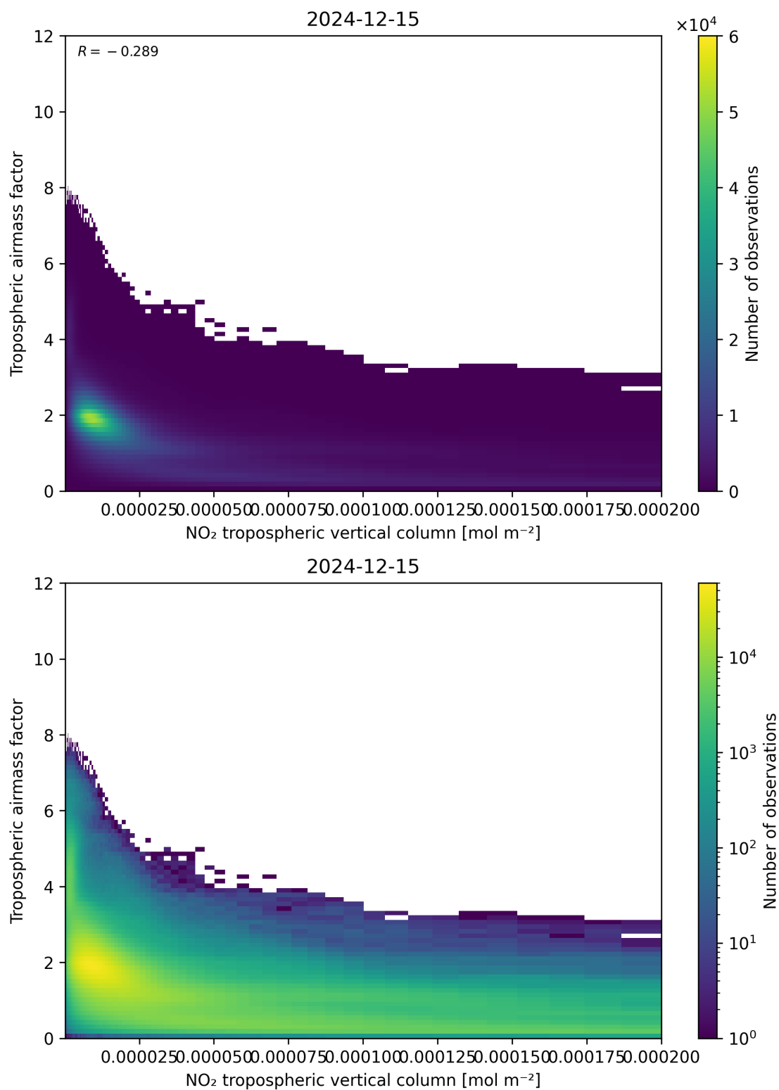
Figure 123: Scatter density plot of “NO 2 tropospheric vertical column” against “Tropospheric air mass factor” for 2024-12-14 to 2024-12-16.
