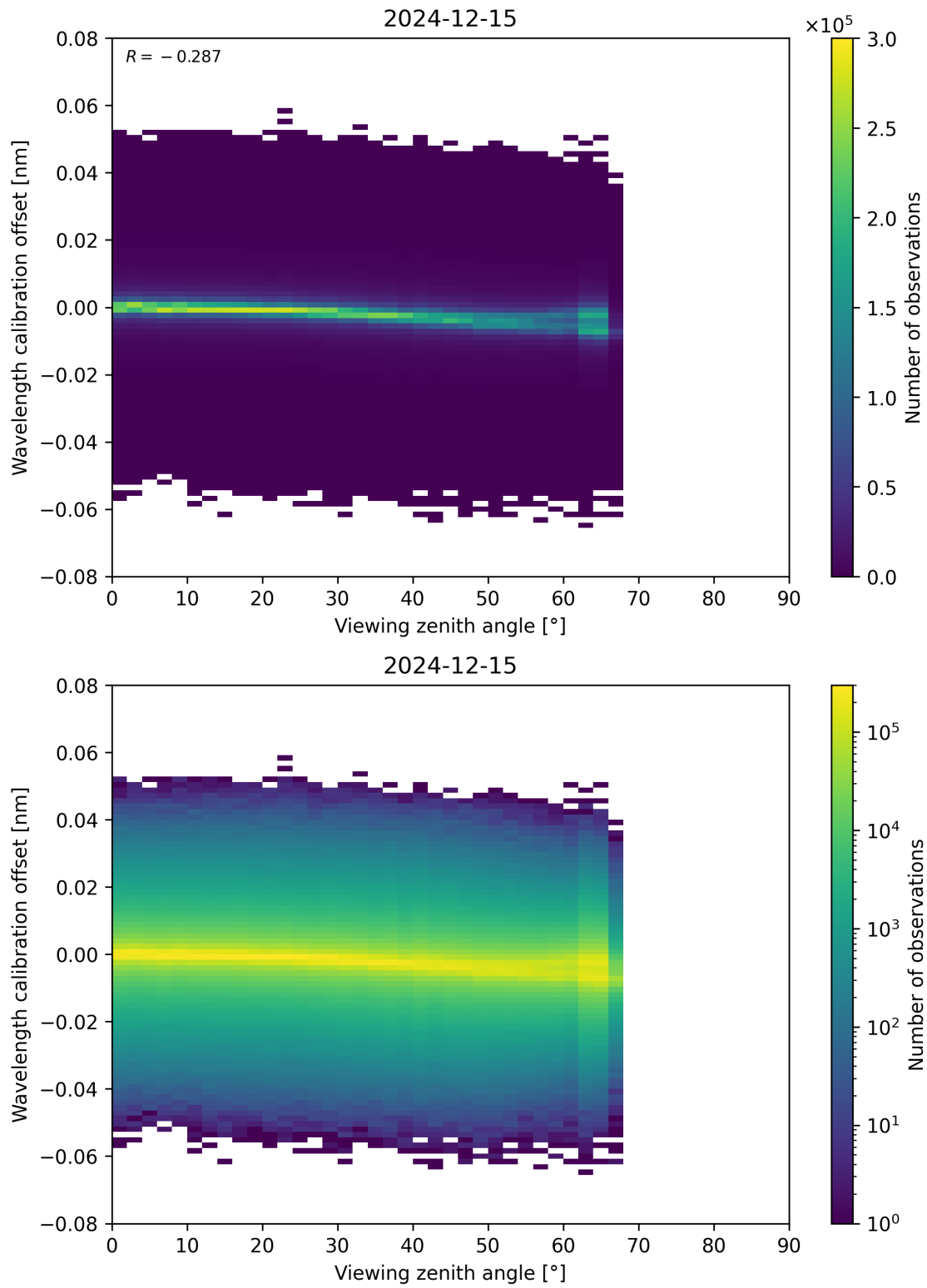
Figure 173: Scatter density plot of “Viewing zenith angle” against “Wavelength calibration offset” for 2024-12-14 to 2024-12-16.
