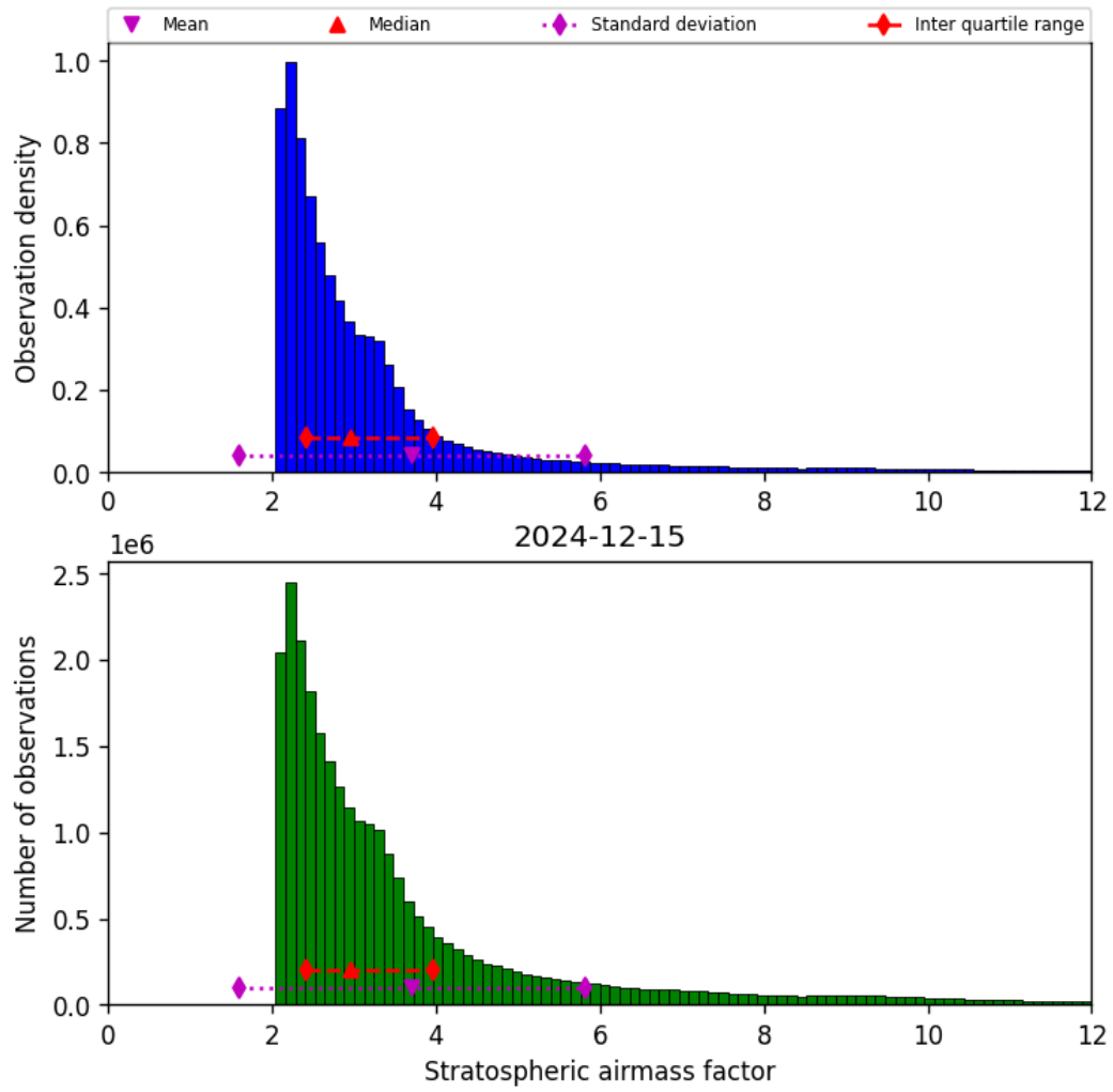
Figure 44: Histogram of “Stratospheric airmass factor” for 2024-12-14 to 2024-12-16
