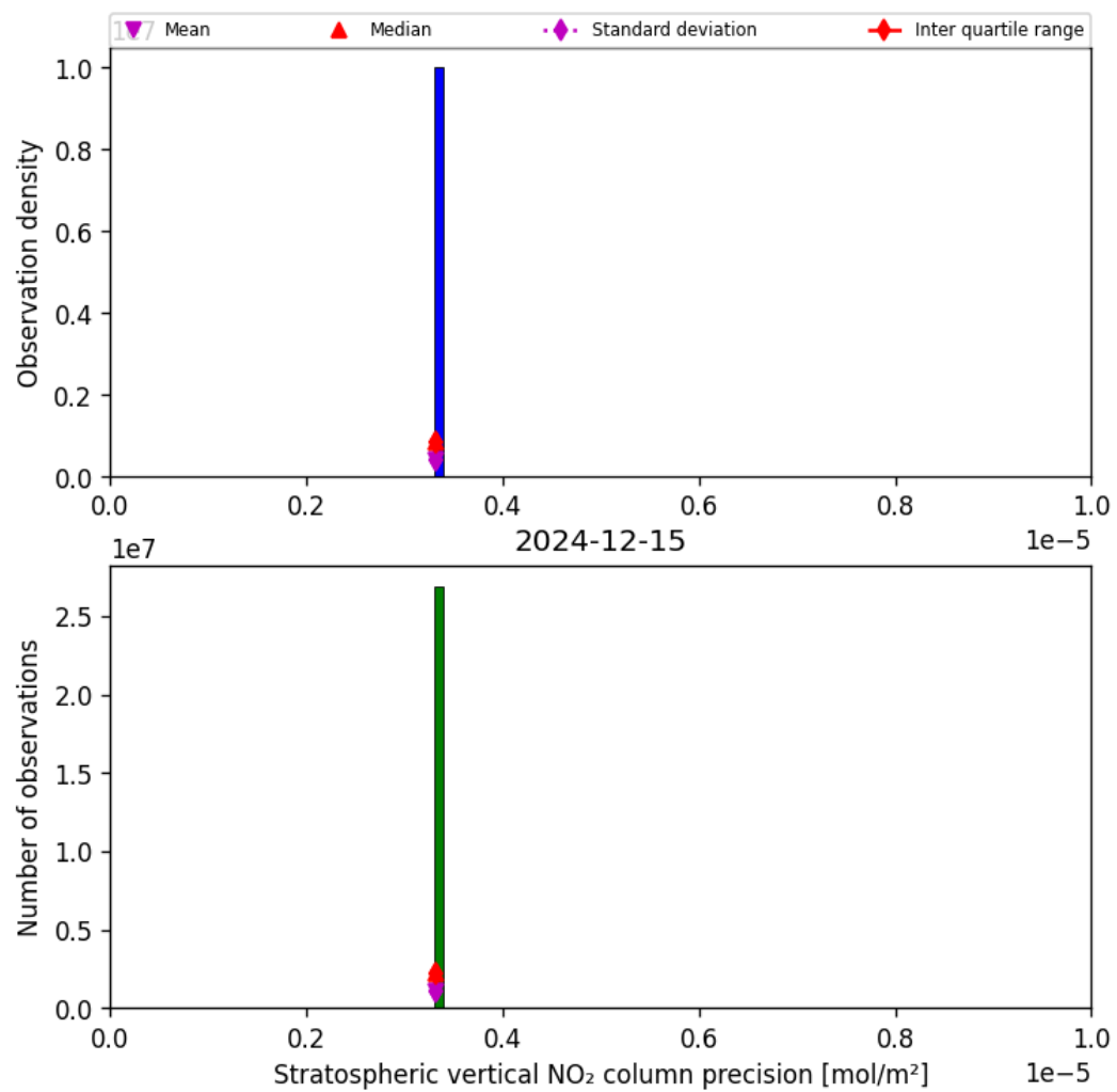
Figure 37: Histogram of “Stratospheric vertical NO 2 column precision” for 2024-12-14 to 2024-12-16
