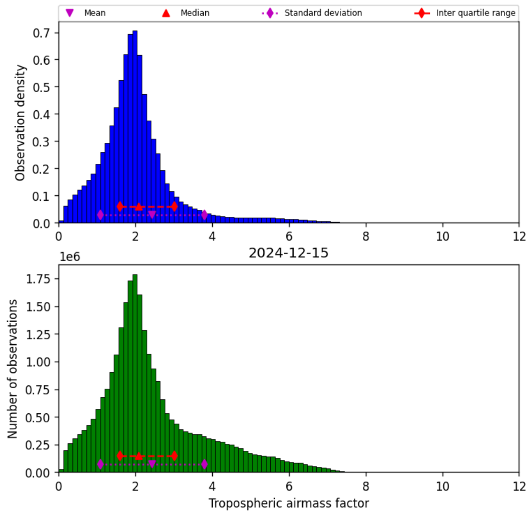
Figure 31: Histogram of “Tropospheric airmass factor” for 2024-12-14 to 2024-12-16
