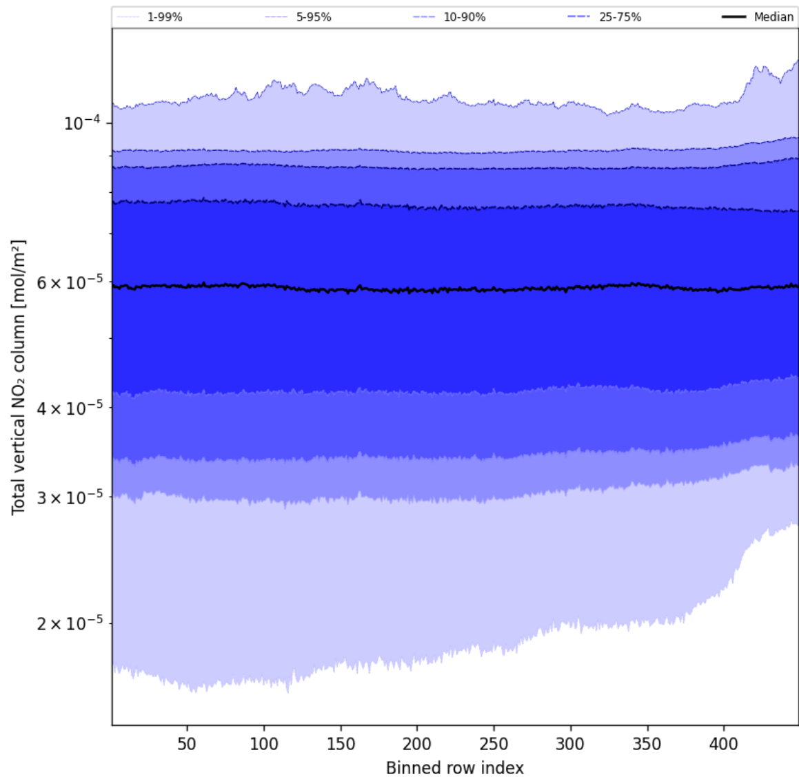
Figure 55: Along track statistics of “Total vertical NO 2 column” for 2024-12-14 to 2024-12-16
