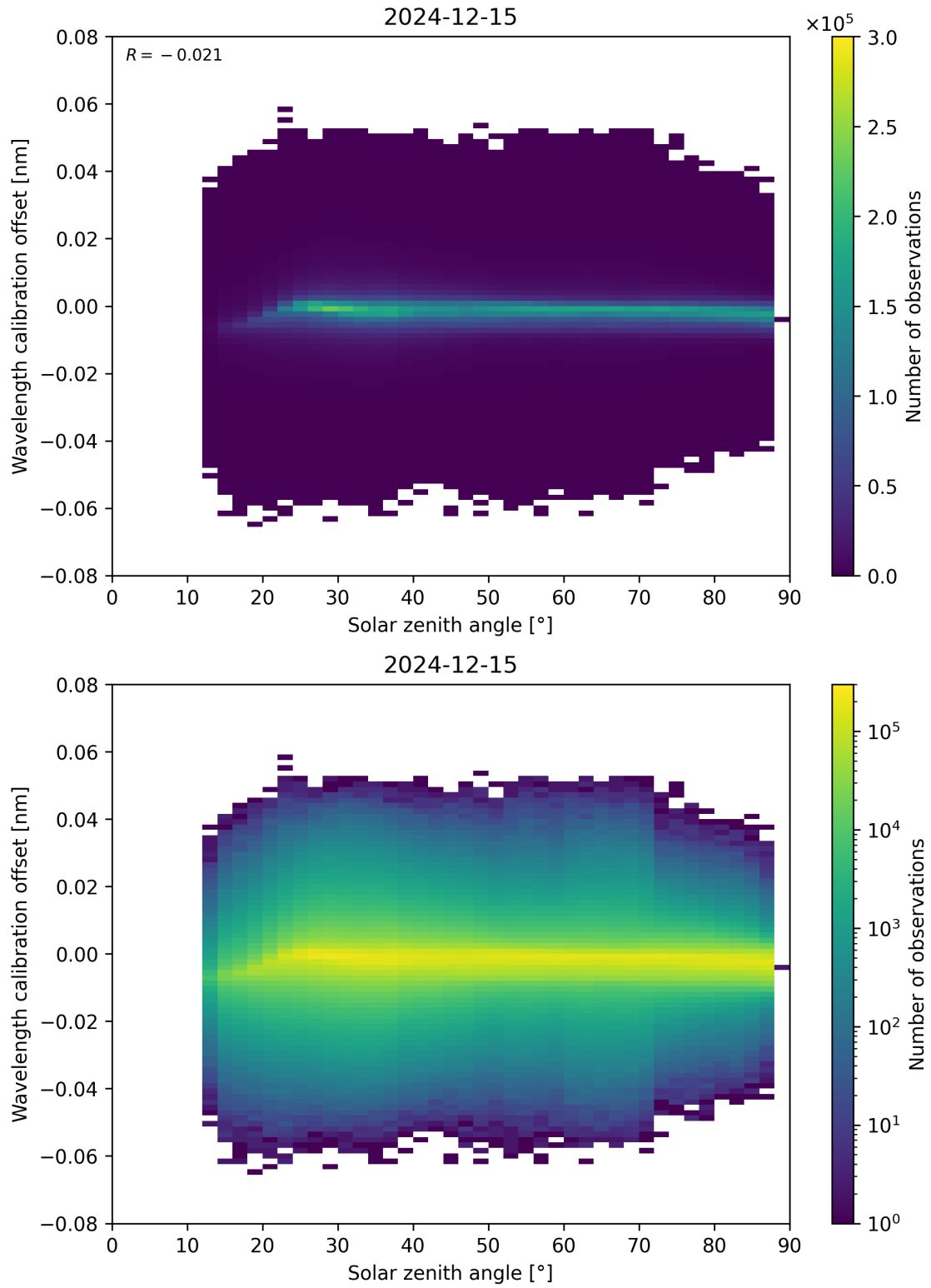
Figure 158: Scatter density plot of “Solar zenith angle” against “Wavelength calibration offset” for 2024-12-14 to 2024-12-16.
