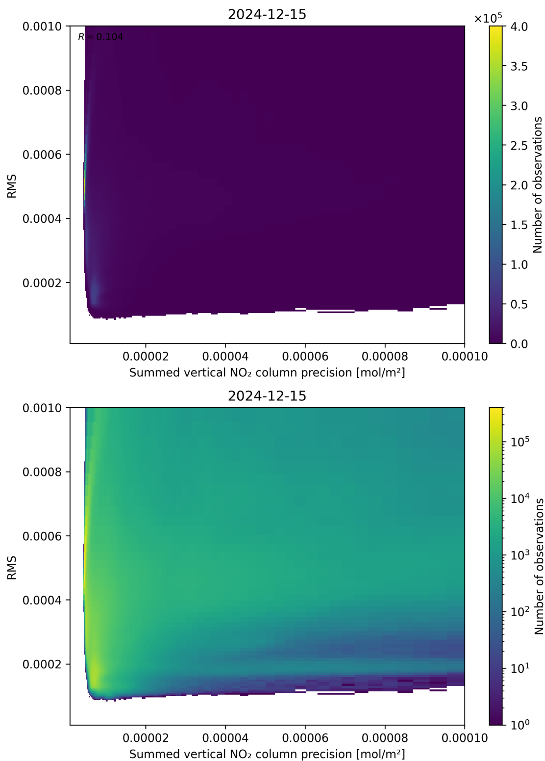
Figure 108: Scatter density plot of “Summed vertical NO 2 column precision” against “RMS” for 2024-12-14 to 2024-12-16.
