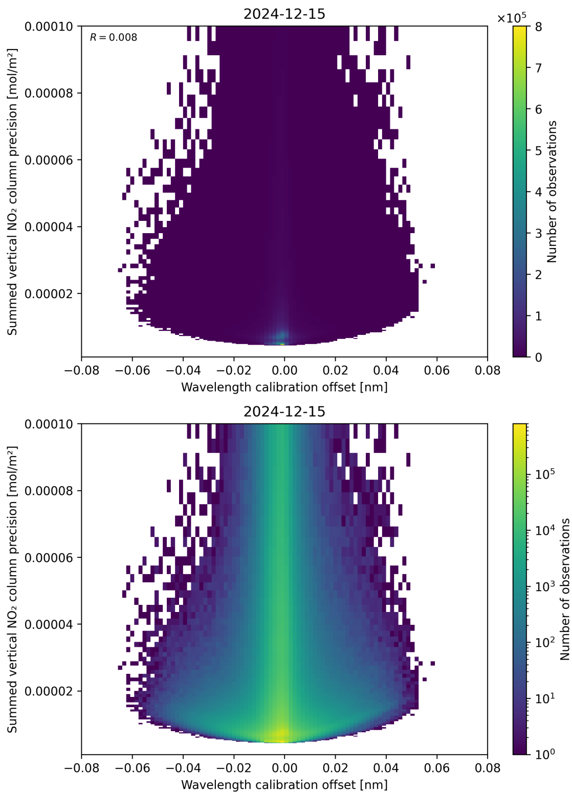
Figure 178: Scatter density plot of “Wavelength calibration offset” against “Summed vertical NO 2 column precision” for 2024-12-14 to 2024-12-16.
