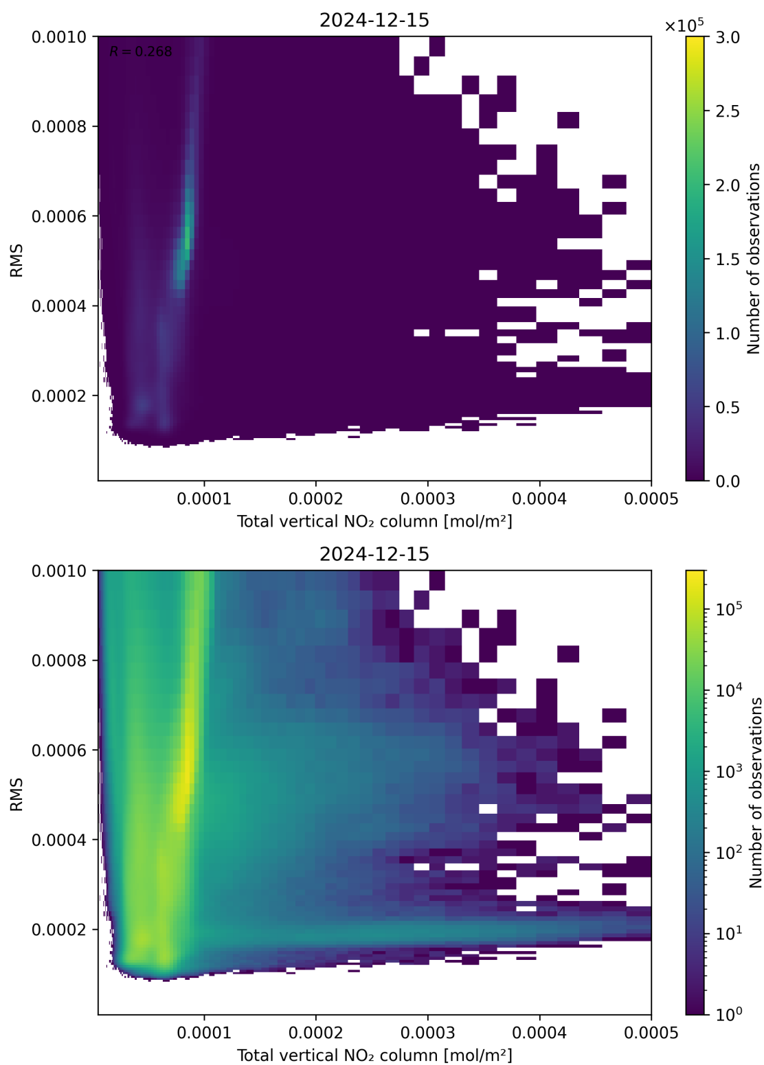
Figure 120: Scatter density plot of “Total vertical NO 2 column” against “RMS” for 2024-12-14 to 2024-12-16.
