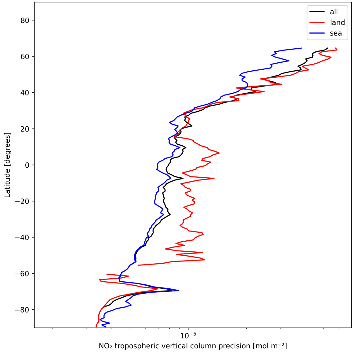
Figure 13: Zonal average of “NO 2 tropospheric vertical column precision” for 2024-12-14 to 2024-12-16.
