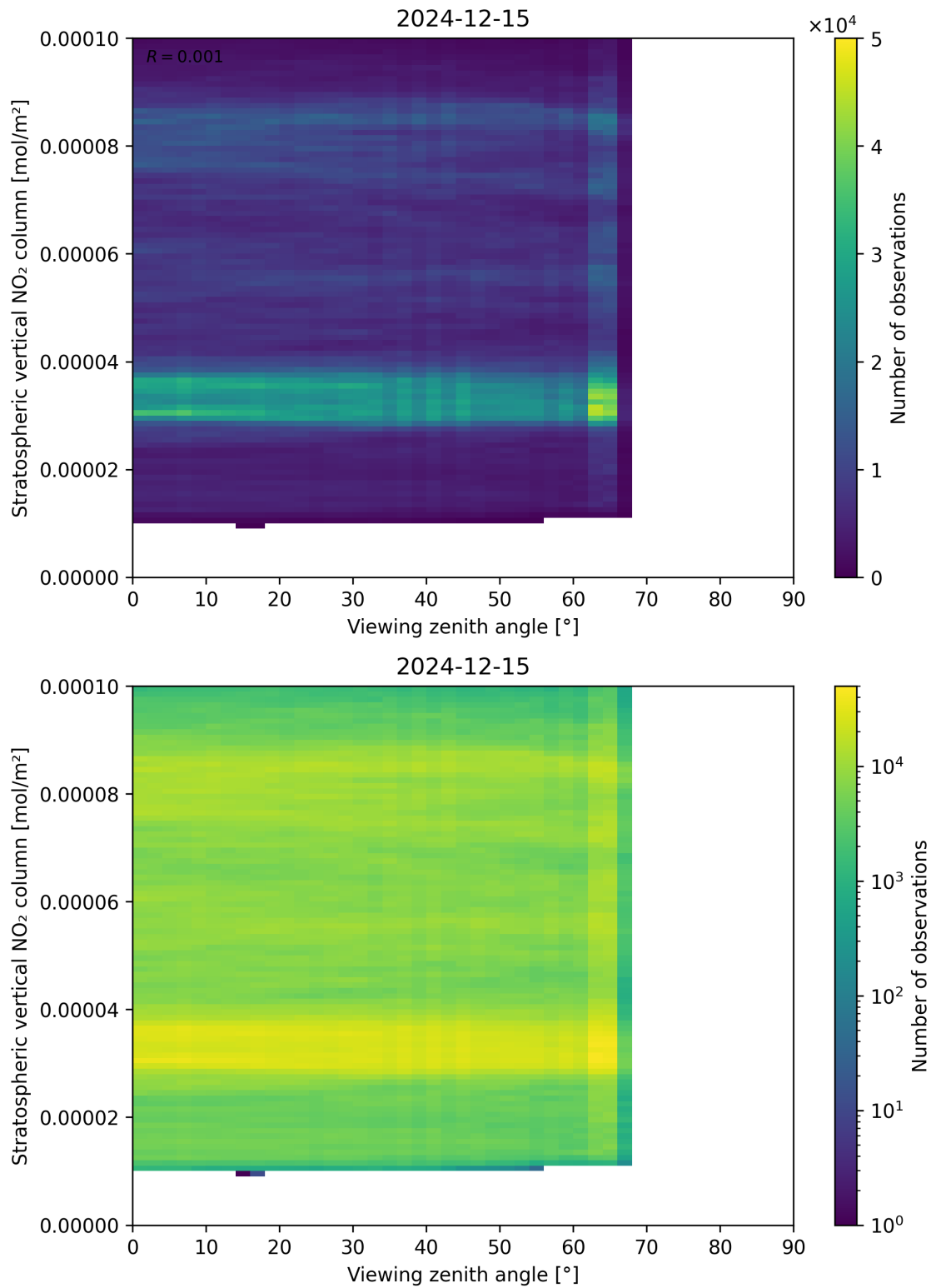
Figure 164: Scatter density plot of “Viewing zenith angle” against “Stratospheric vertical NO 2 column” for 2024-12-14 to 2024-12-16.
