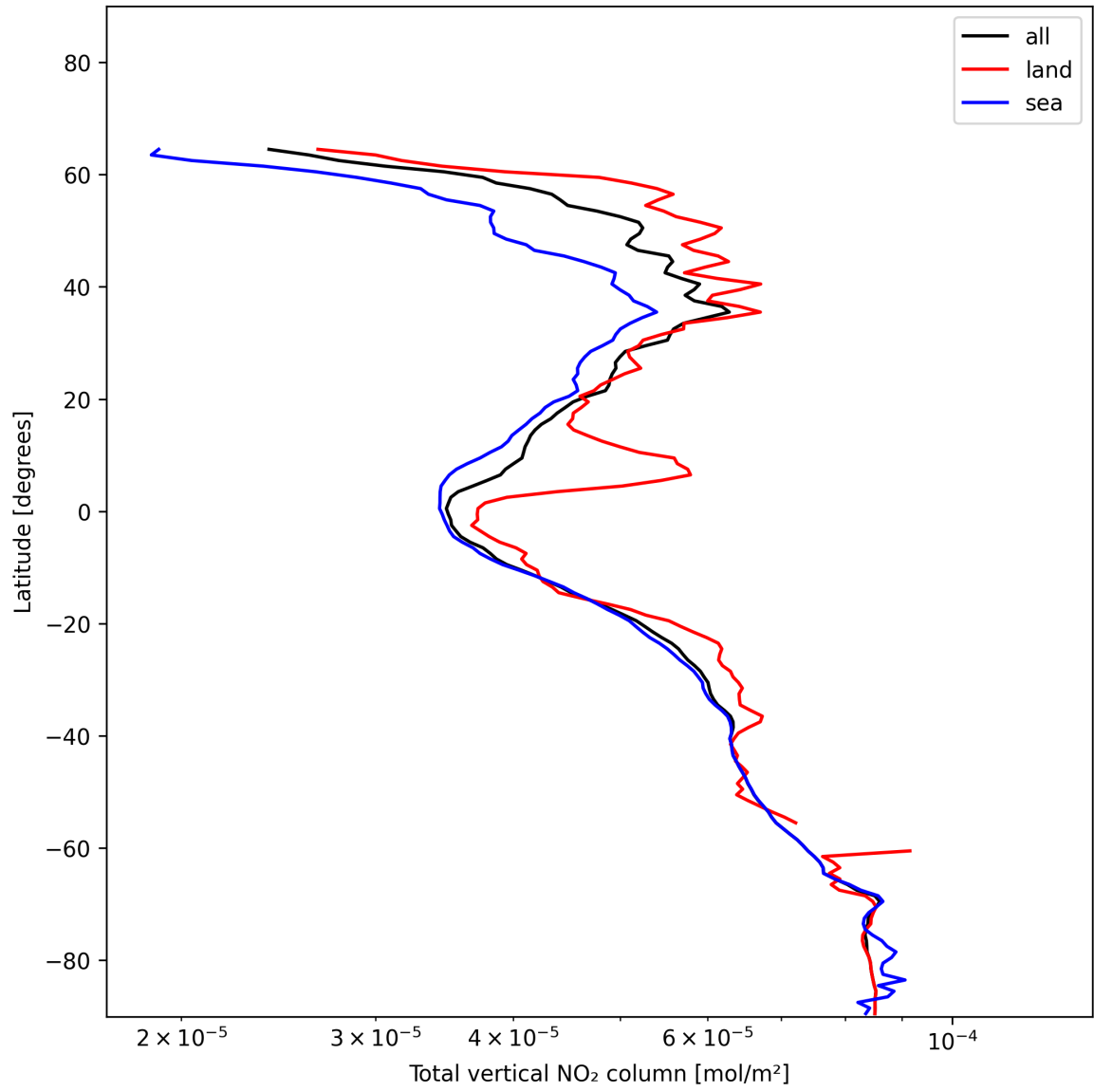
Figure 21: Zonal average of “Total vertical NO 2 column” for 2024-12-14 to 2024-12-16.
