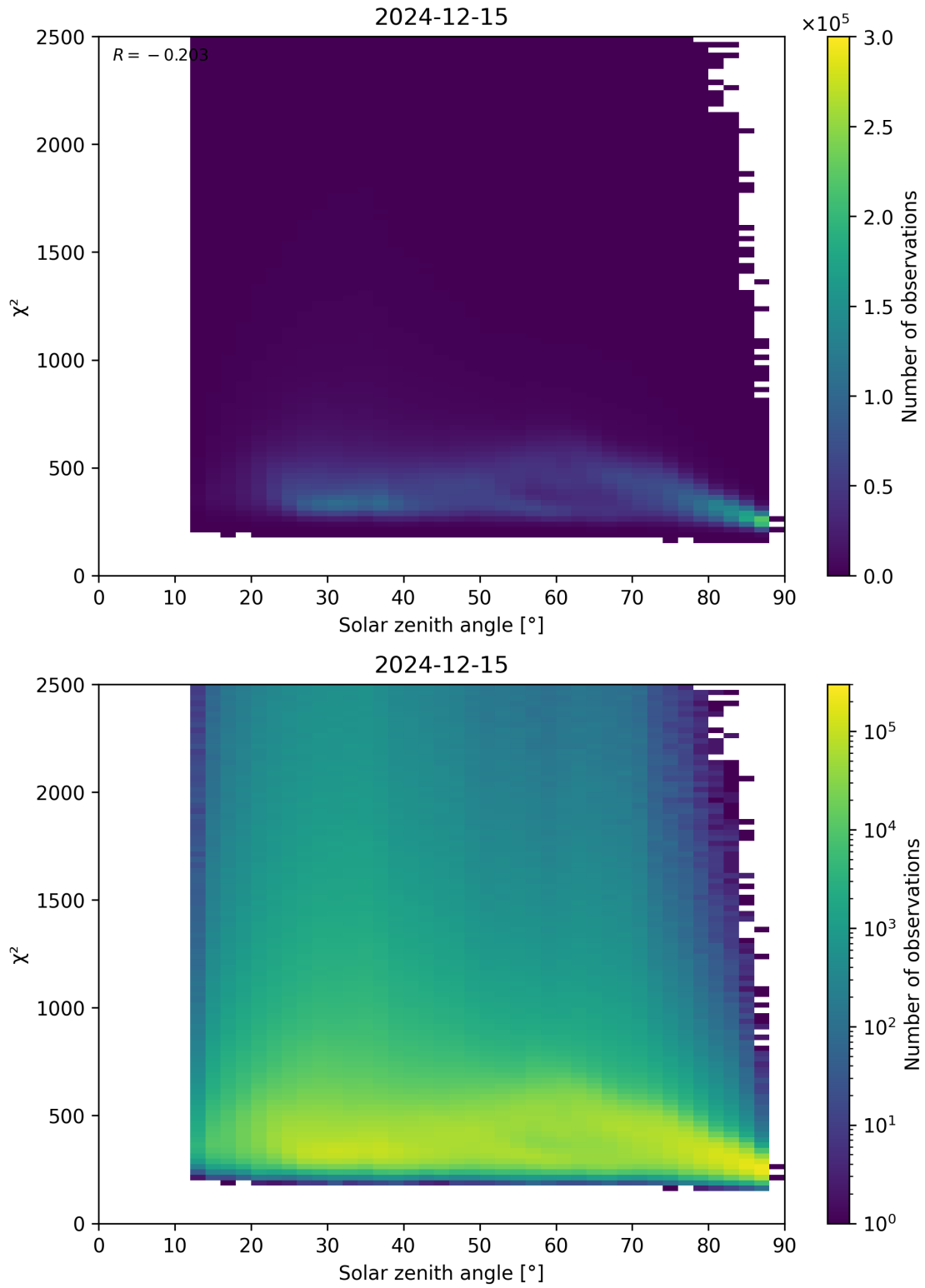
Figure 148: Scatter density plot of “Solar zenith angle” against “ \chi^2 ” for 2024-12-14 to 2024-12-16.
