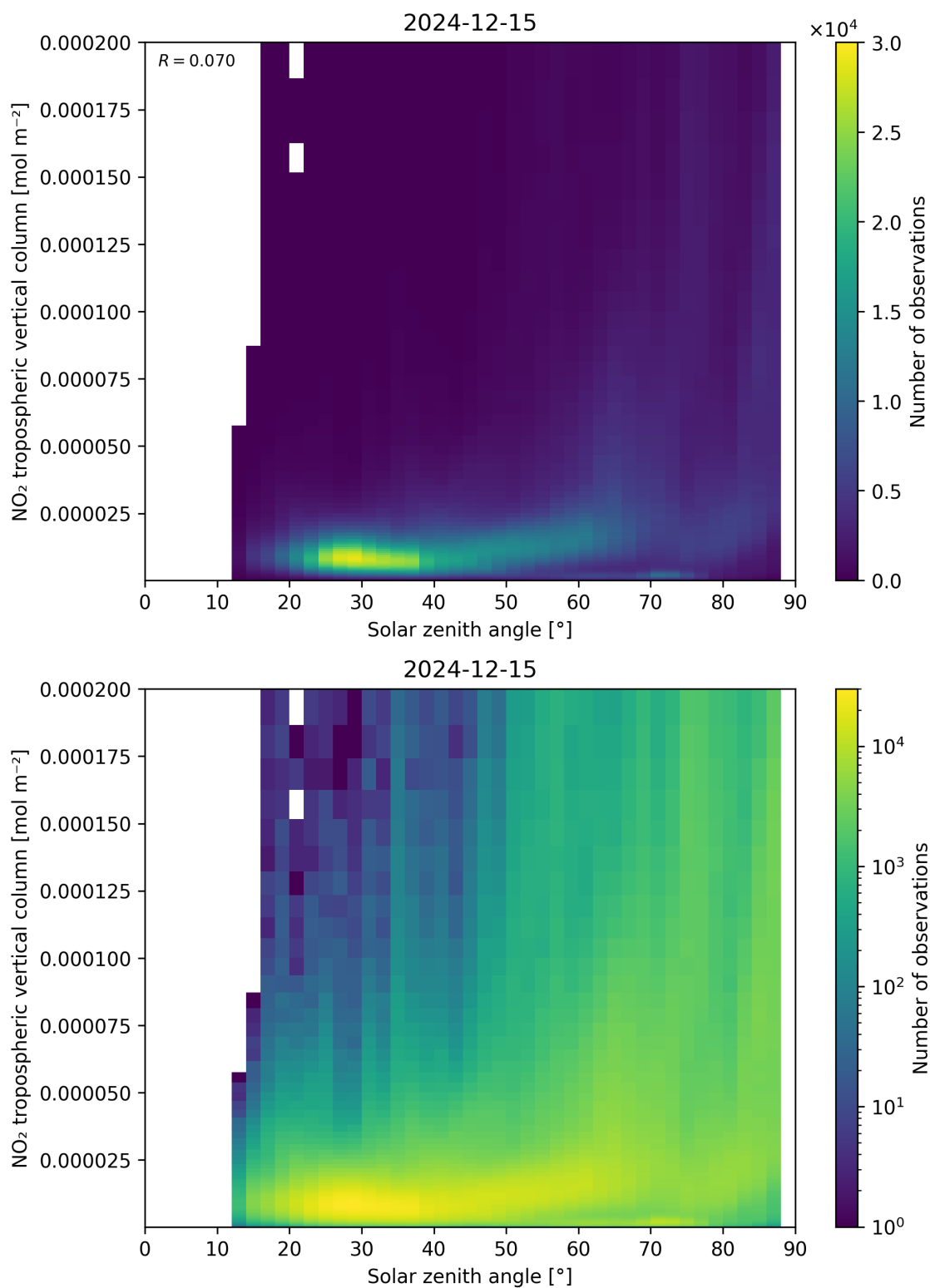
Figure 155: Scatter density plot of “Solar zenith angle” against “NO 2 tropospheric vertical column” for 2024-12-14 to 2024-12-16.
