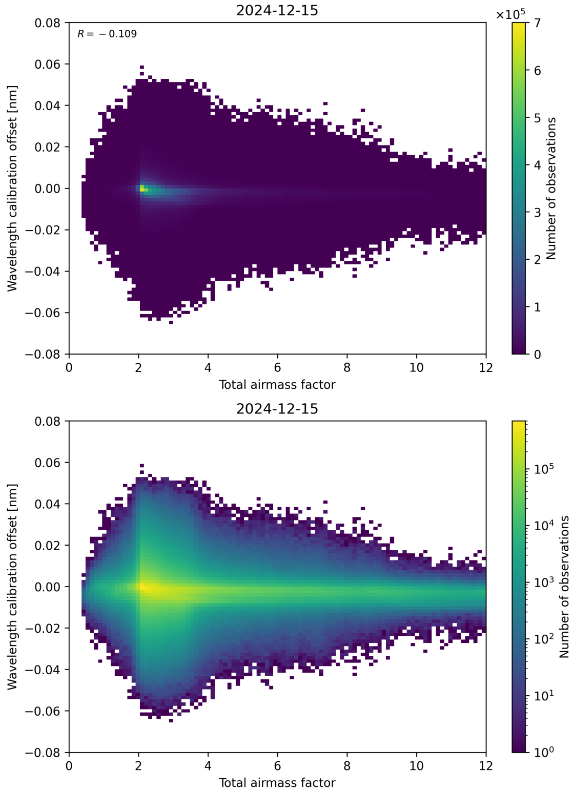
Figure 70: Scatter density plot of “Total airmass factor” against “Wavelength calibration offset” for 2024-12-14 to 2024-12-16.
