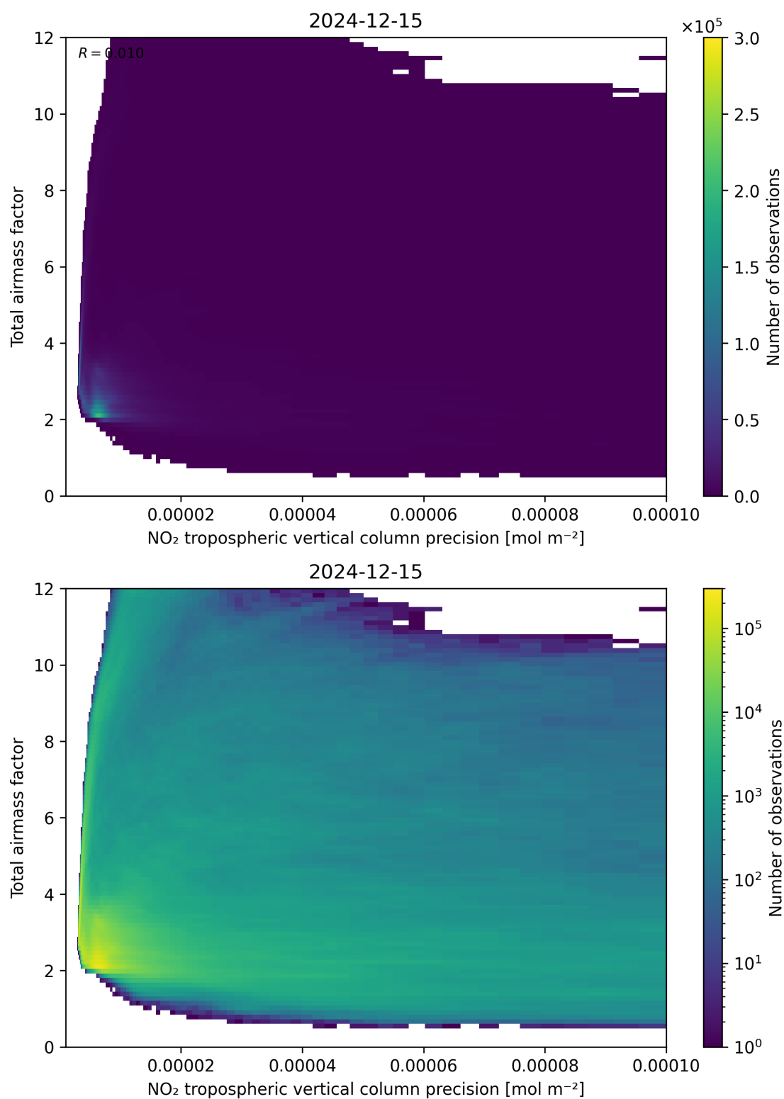
Figure 132: Scatter density plot of “NO 2 tropospheric vertical column precision” against “Total air mass factor” for 2024-12-14 to 2024-12-16.
