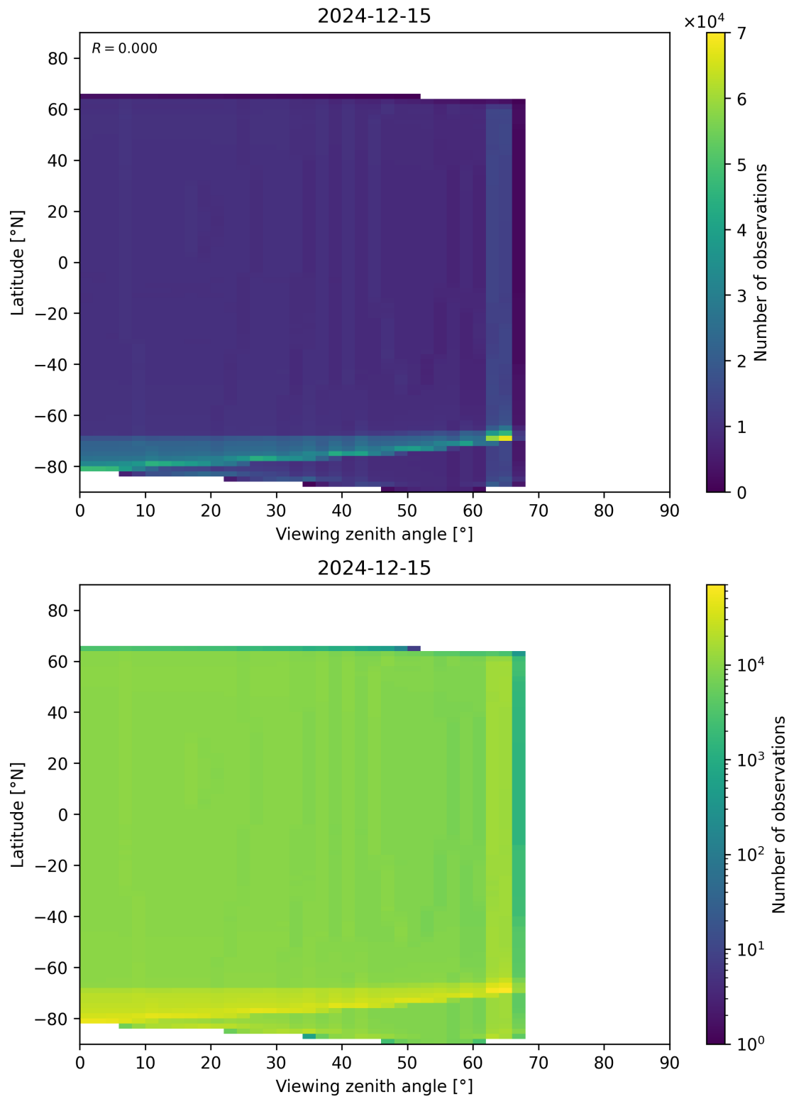
Figure 163: Scatter density plot of “Viewing zenith angle” against “Latitude” for 2024-12-14 to 2024-12-16.
