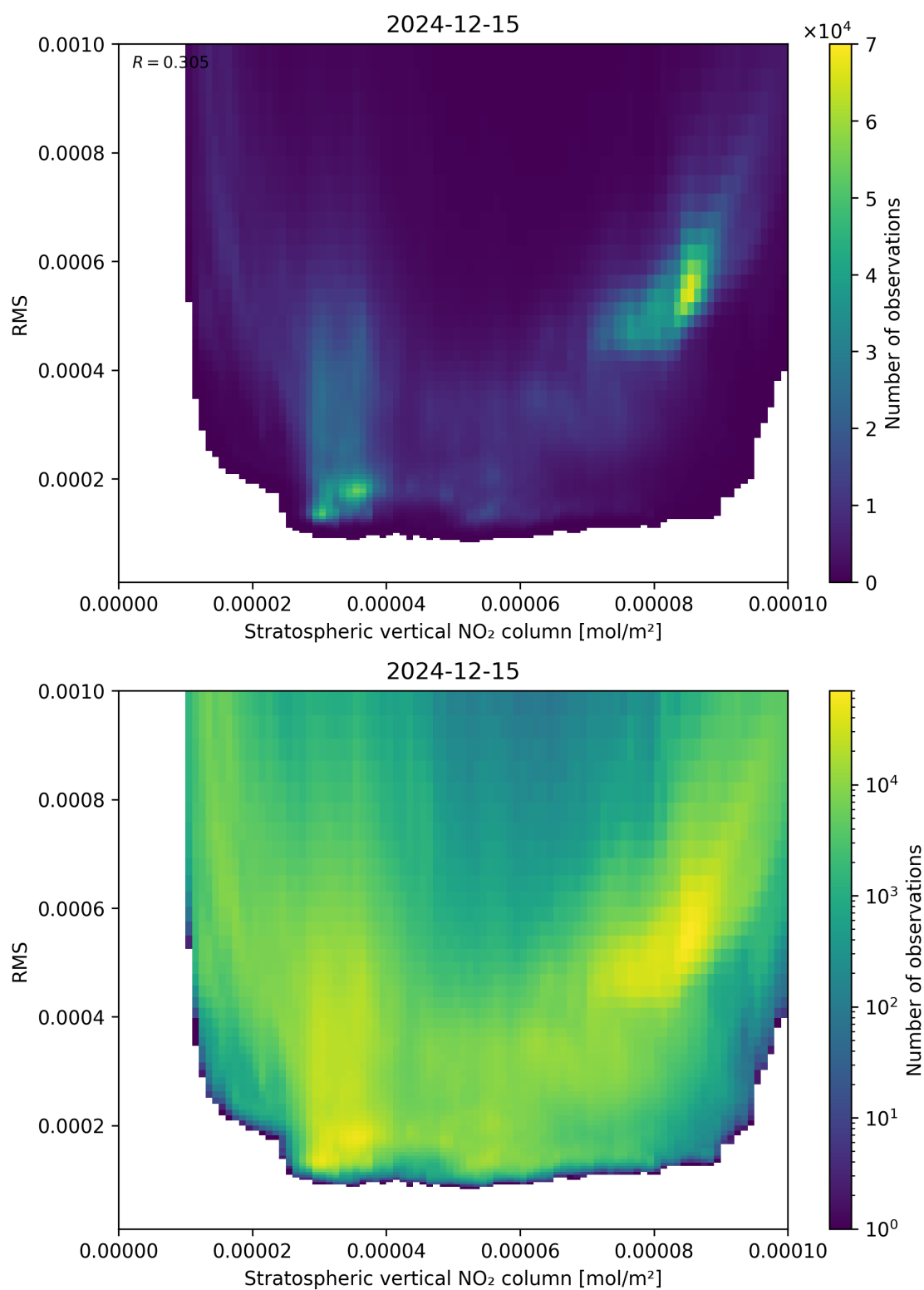
Figure 102: Scatter density plot of “Stratospheric vertical NO 2 column” against “RMS” for 2024-12-14 to 2024-12-16.
