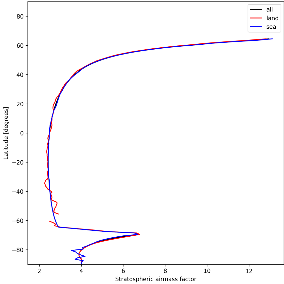
Figure 27: Zonal average of “Stratospheric airmass factor” for 2024-12-14 to 2024-12-16.
