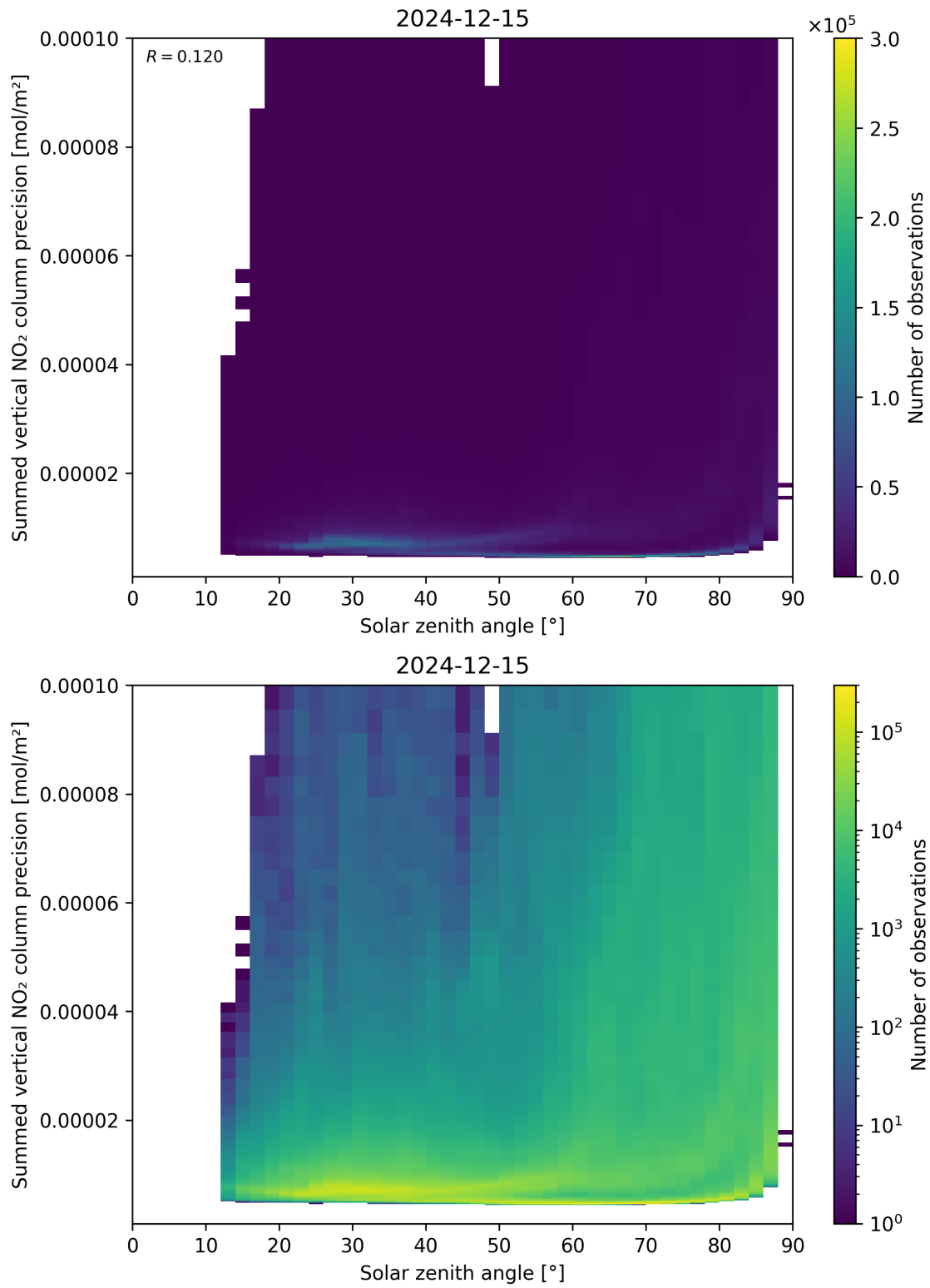
Figure 152: Scatter density plot of “Solar zenith angle” against “Summed vertical NO 2 column precision” for 2024-12-14 to 2024-12-16.
