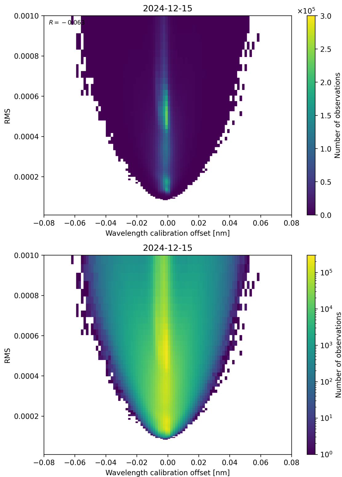
Figure 181: Scatter density plot of “Wavelength calibration offset” against “RMS” for 2024-12-14 to 2024-12-16.
