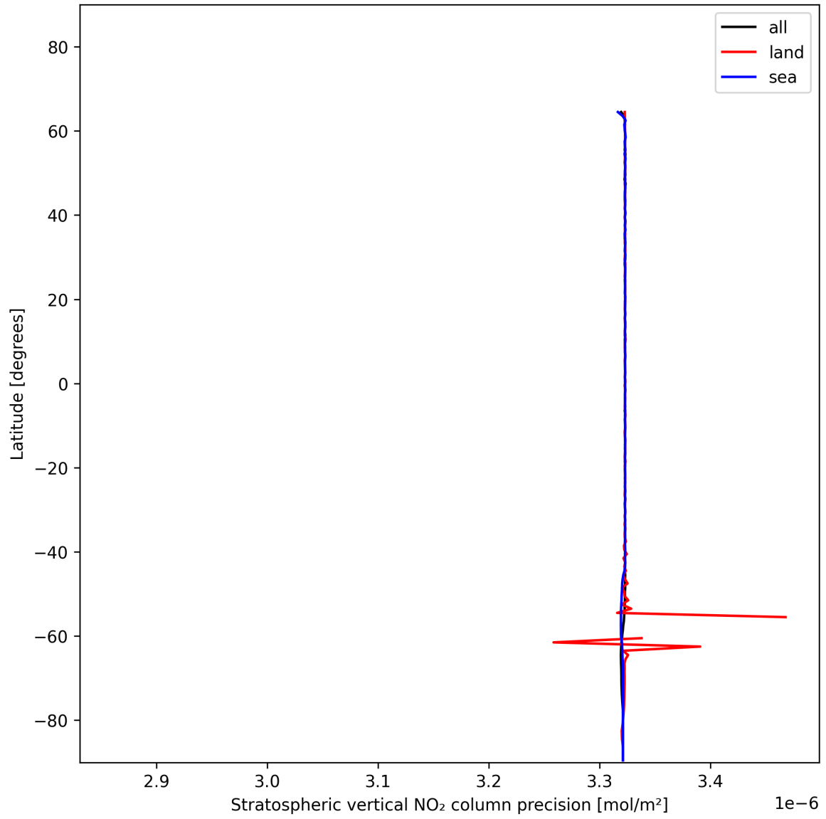
Figure 20: Zonal average of “Stratospheric vertical NO 2 column precision” for 2024-12-14 to 2024-12-16.
