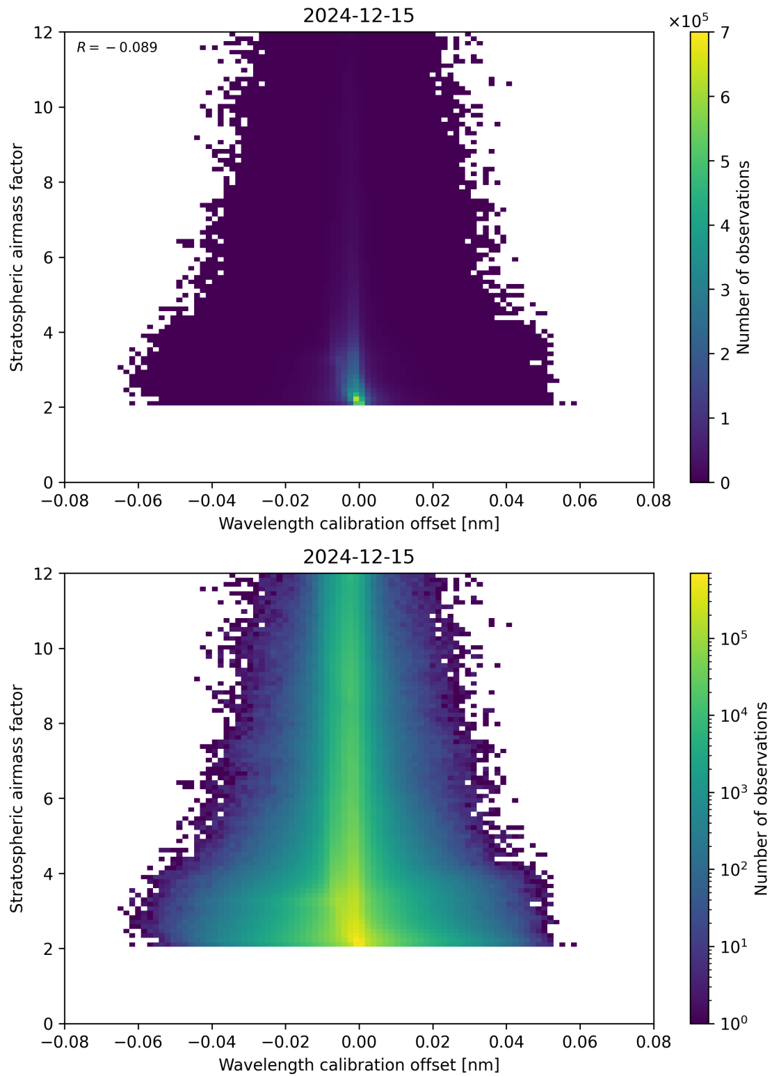
Figure 174: Scatter density plot of “Wavelength calibration offset” against “Stratospheric airmass factor” for 2024-12-14 to 2024-12-16.
