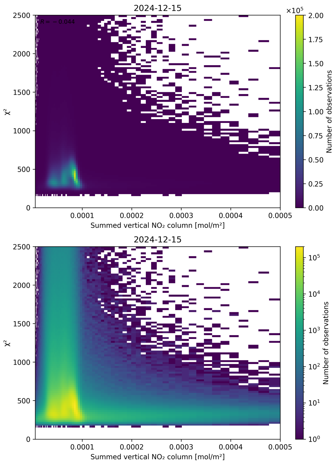
Figure 104: Scatter density plot of “Summed vertical NO 2 column” against “ \chi^2 ” for 2024-12-14 to 2024-12-16.
