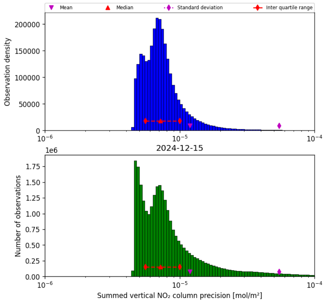
Figure 41: Histogram of “Summed vertical NO 2 column precision” for 2024-12-14 to 2024-12-16
