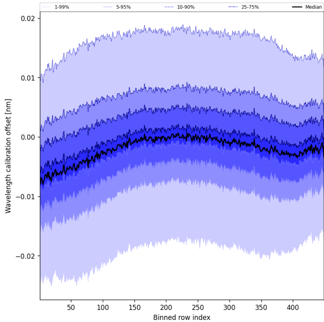
Figure 52: Along track statistics of “Wavelength calibration offset” for 2024-12-14 to 2024-12-16
