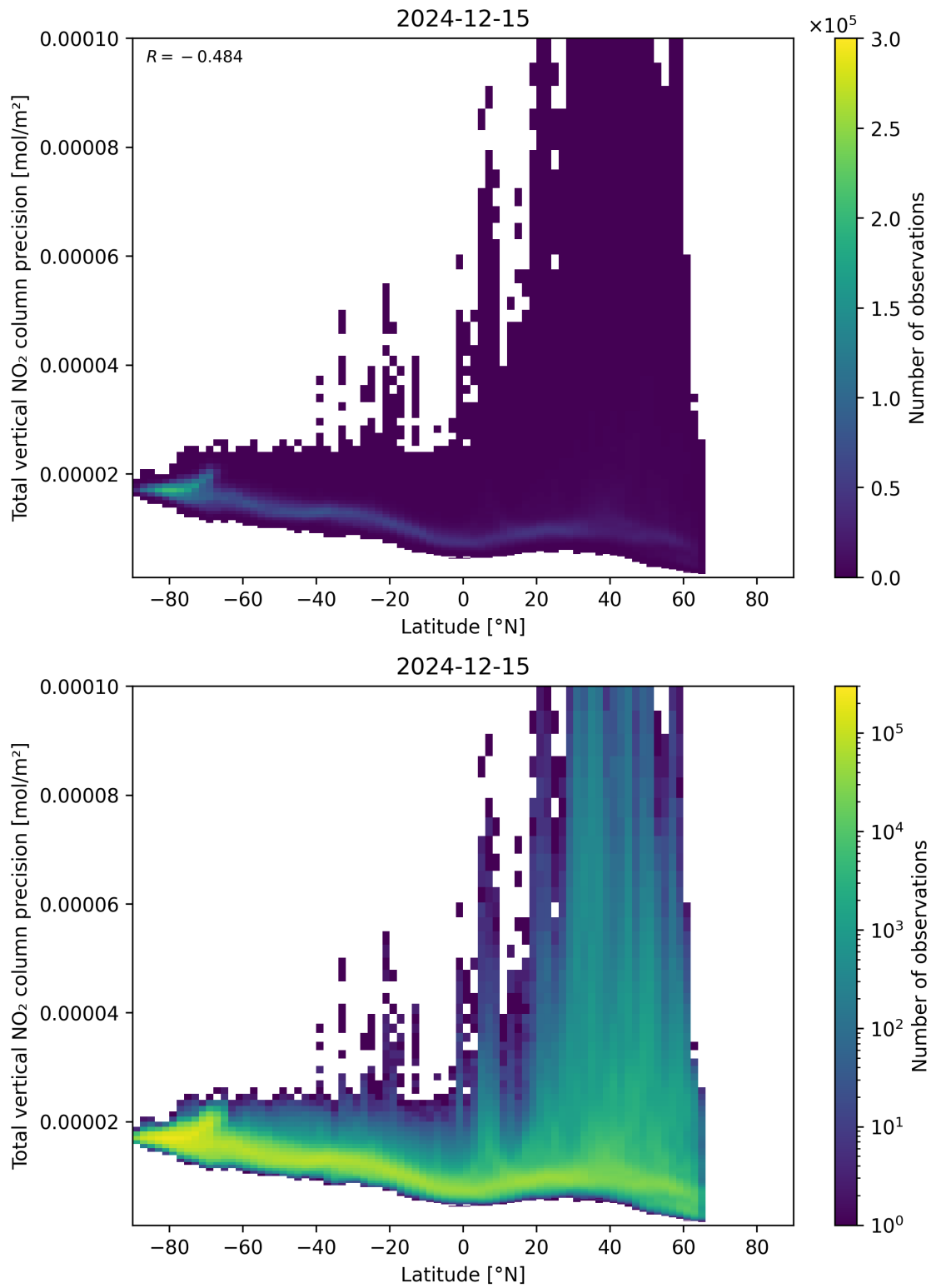
Figure 91: Scatter density plot of “Latitude” against “Total vertical NO 2 column precision” for 2024-12-14 to 2024-12-16.
