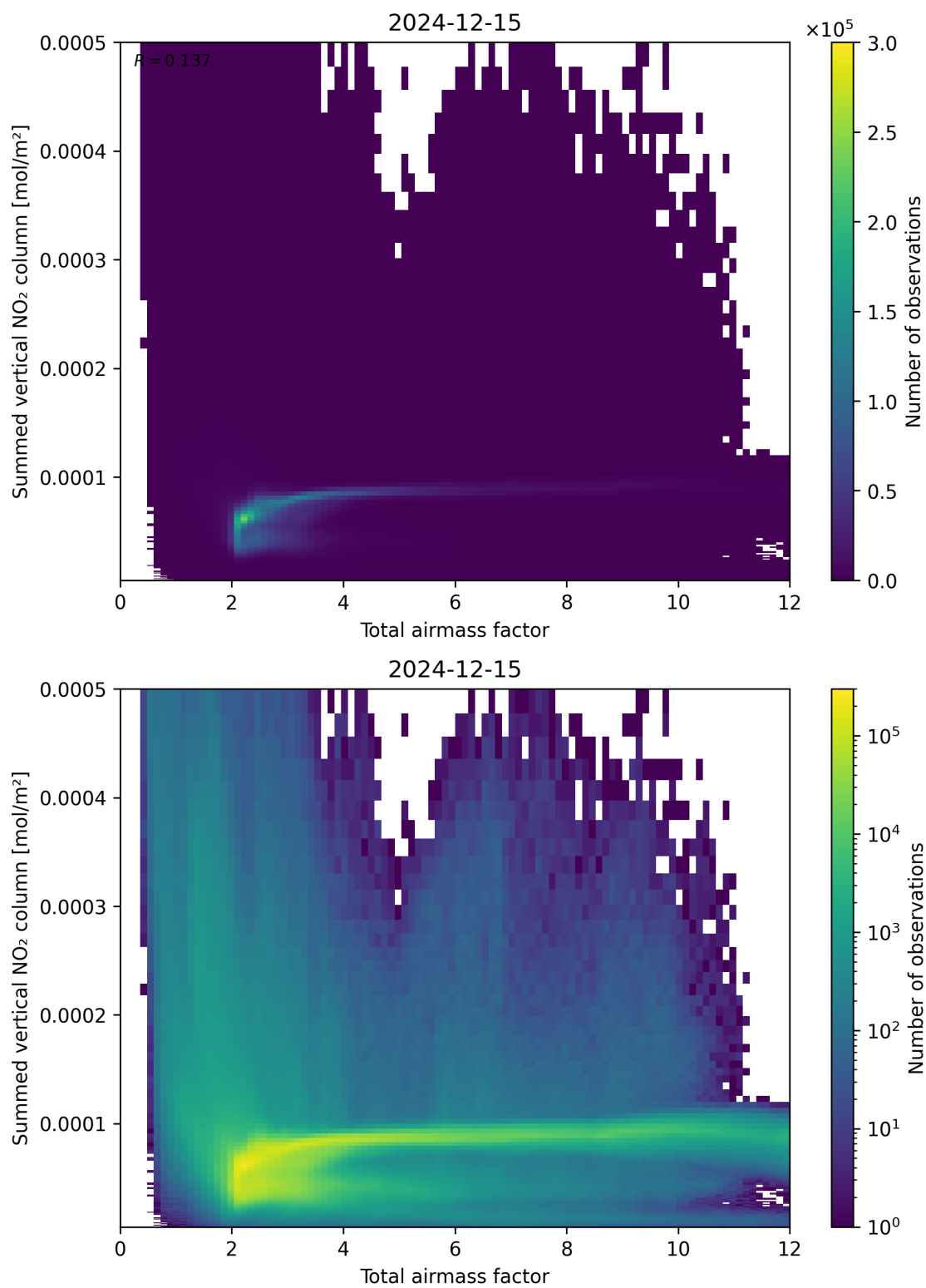
Figure 65: Scatter density plot of “Total airmass factor” against “Summed vertical NO 2 column” for 2024-12-14 to 2024-12-16.
