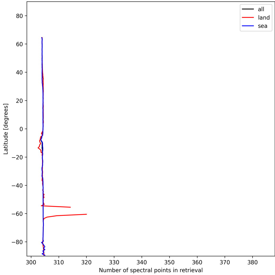
Figure 16: Zonal average of “Number of spectral points in retrieval” for 2024-12-14 to 2024-12-16.
