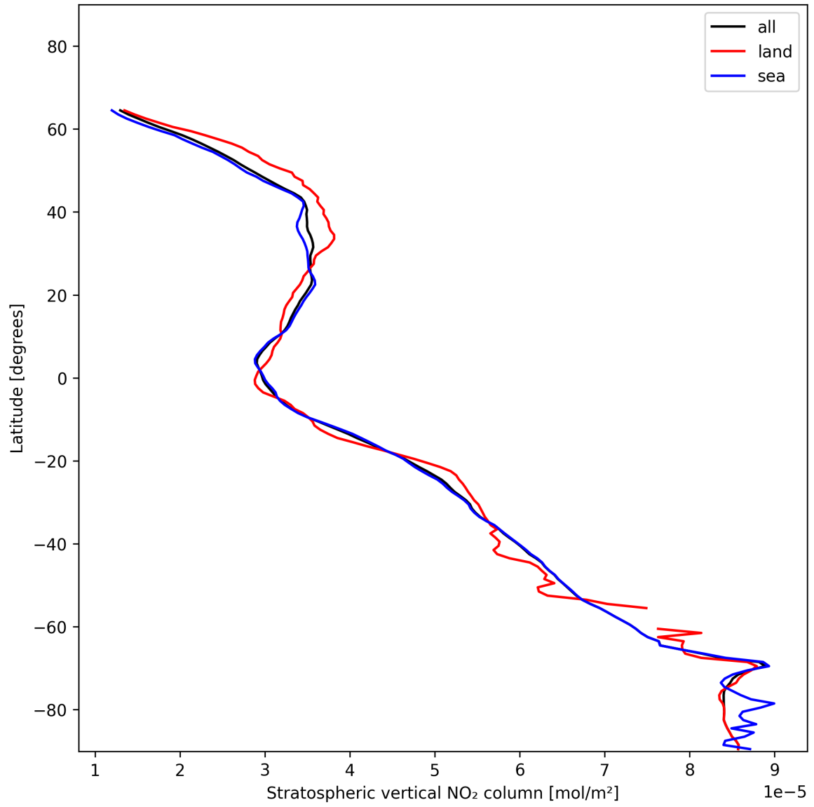
Figure 19: Zonal average of “Stratospheric vertical NO 2 column” for 2024-12-14 to 2024-12-16.
