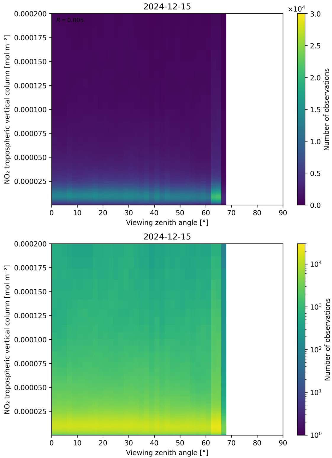
Figure 169: Scatter density plot of “Viewing zenith angle” against “NO 2 tropospheric vertical column” for 2024-12-14 to 2024-12-16.
