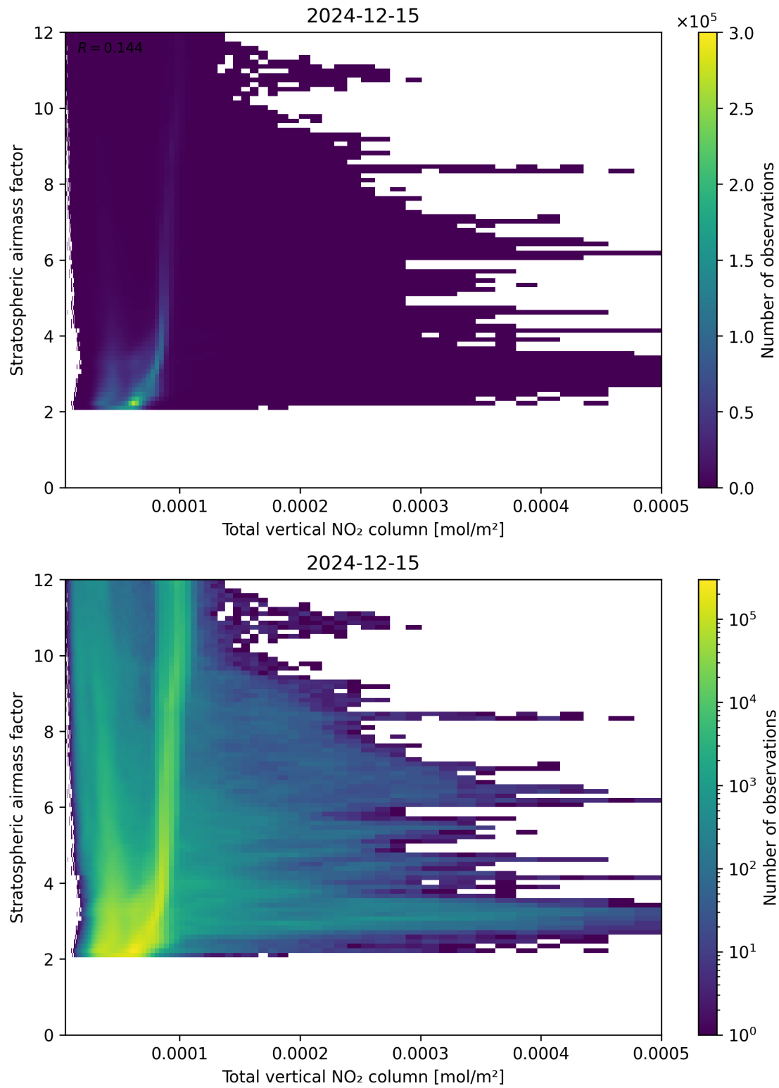
Figure 110: Scatter density plot of “Total vertical NO 2 column” against “Stratospheric airmass factor” for 2024-12-14 to 2024-12-16.
