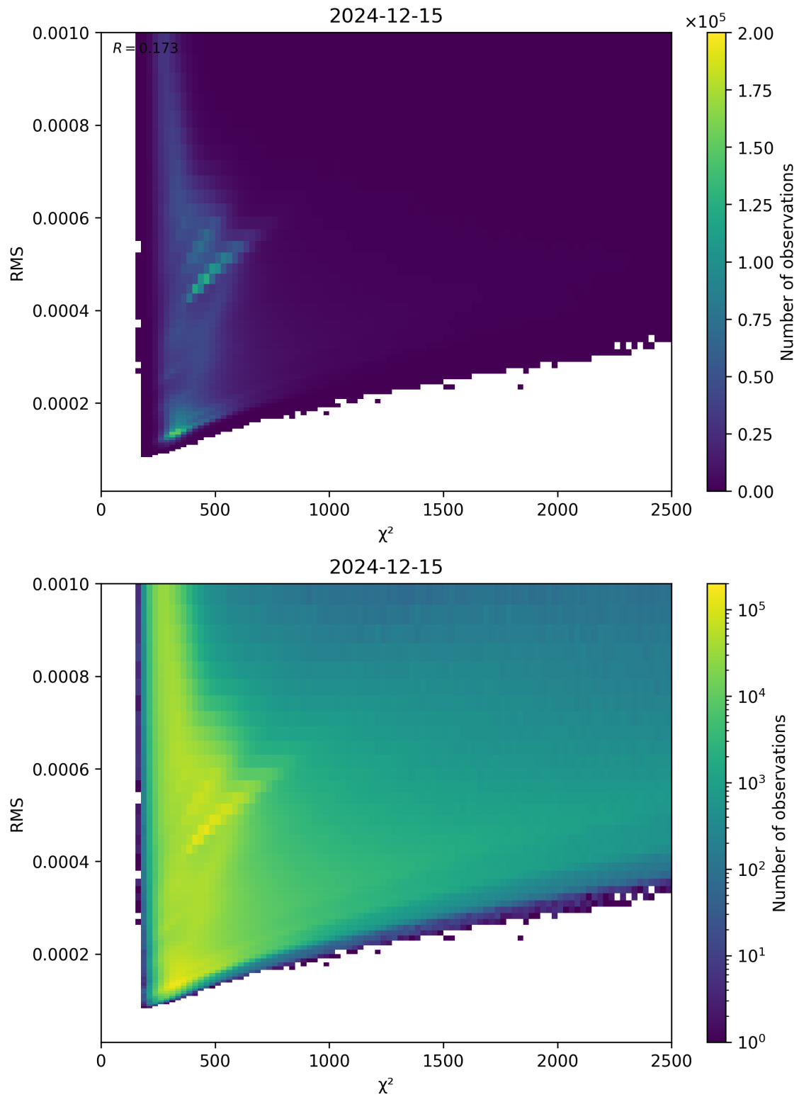
Figure 82: Scatter density plot of “ \chi^2 ” against “RMS” for 2024-12-14 to 2024-12-16.
