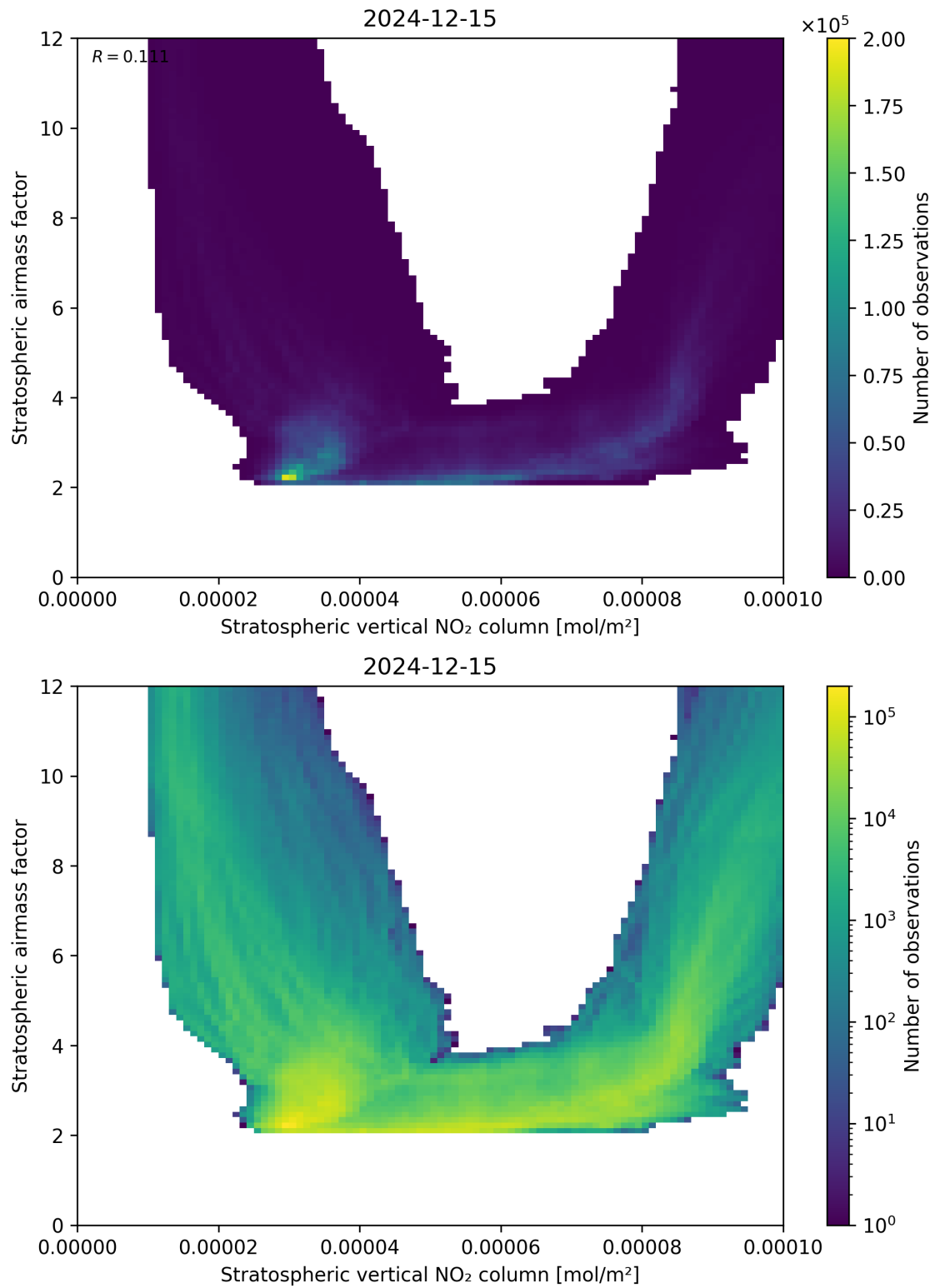
Figure 96: Scatter density plot of “Stratospheric vertical NO 2 column” against “Stratospheric airmass factor” for 2024-12-14 to 2024-12-16.
