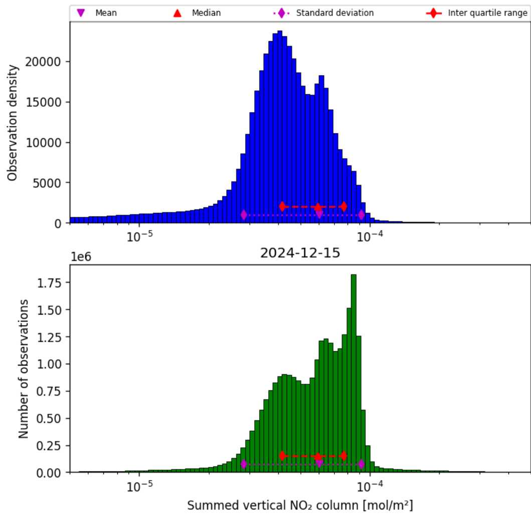
Figure 40: Histogram of “Summed vertical NO 2 column” for 2024-12-14 to 2024-12-16
