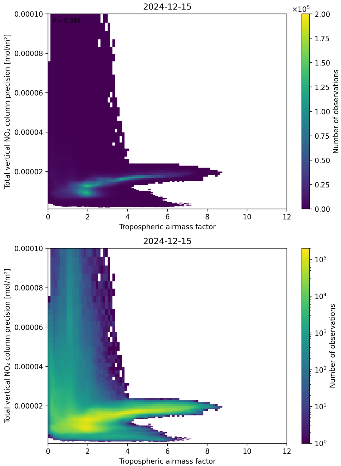
Figure 78: Scatter density plot of “Tropospheric air mass factor” against “Total vertical NO 2 column precision” for 2024-12-14 to 2024-12-16.
