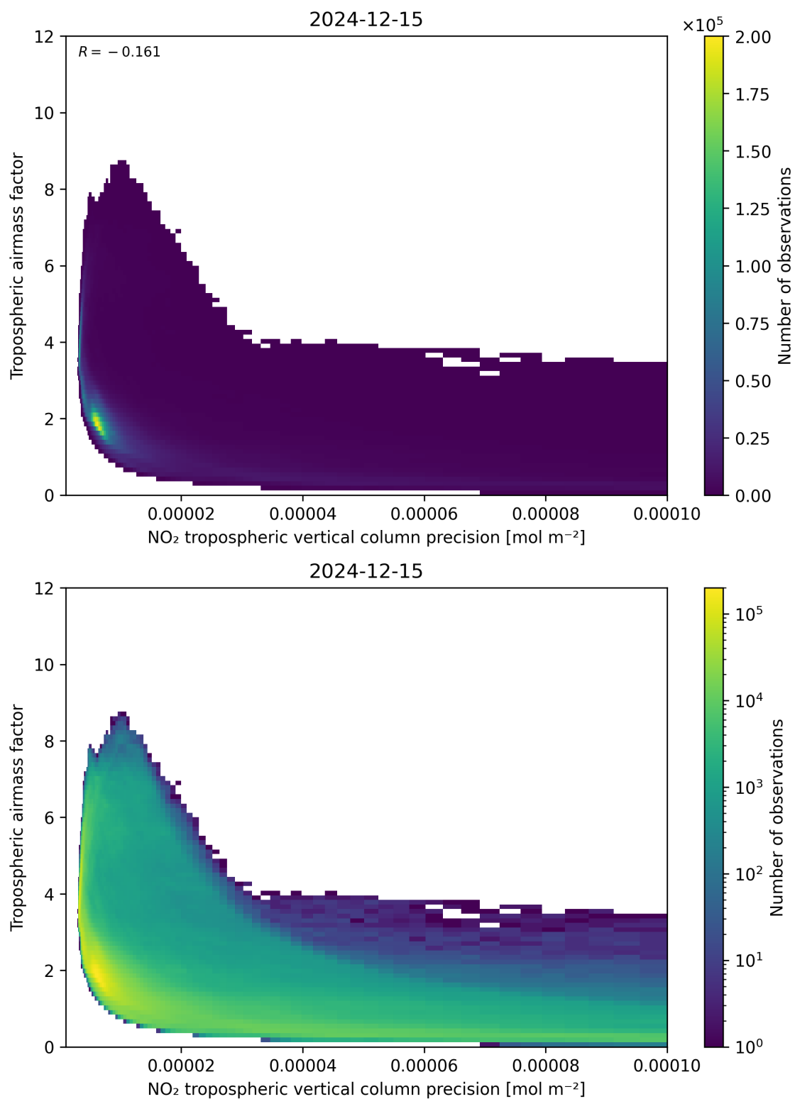
Figure 133: Scatter density plot of “NO 2 tropospheric vertical column precision” against “Tropospheric air mass factor” for 2024-12-14 to 2024-12-16.
