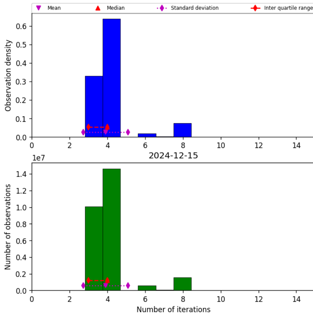
Figure 34: Histogram of “Number of iterations” for 2024-12-14 to 2024-12-16
