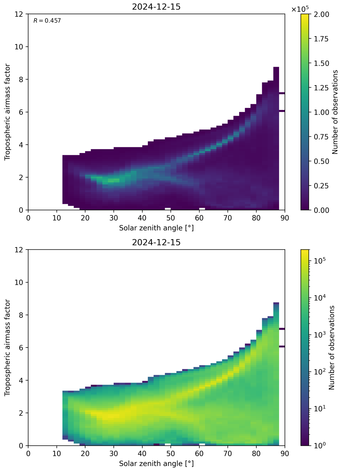
Figure 147: Scatter density plot of “Solar zenith angle” against “Tropospheric airmass factor” for 2024-12-14 to 2024-12-16.
