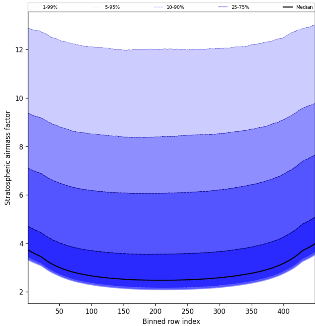
Figure 61: Along track statistics of “Stratospheric airmass factor” for 2024-12-14 to 2024-12-16
