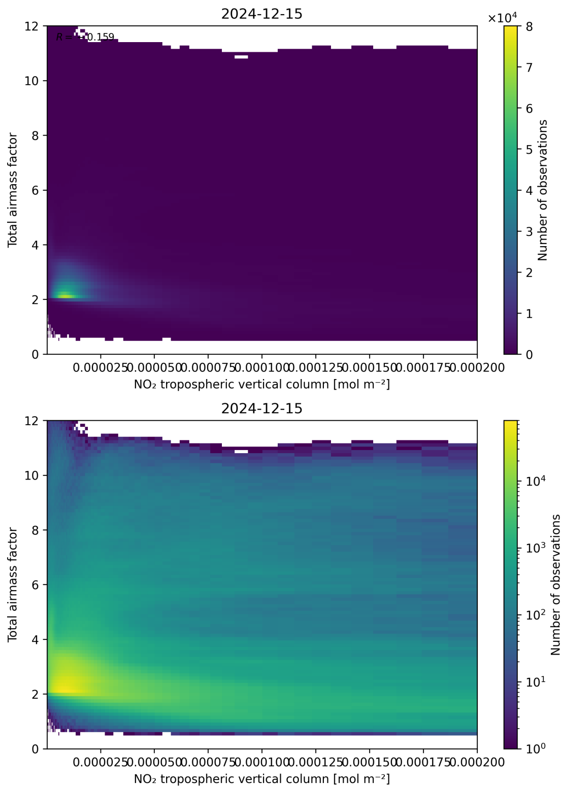
Figure 122: Scatter density plot of “NO 2 tropospheric vertical column” against “Total air mass factor” for 2024-12-14 to 2024-12-16.
