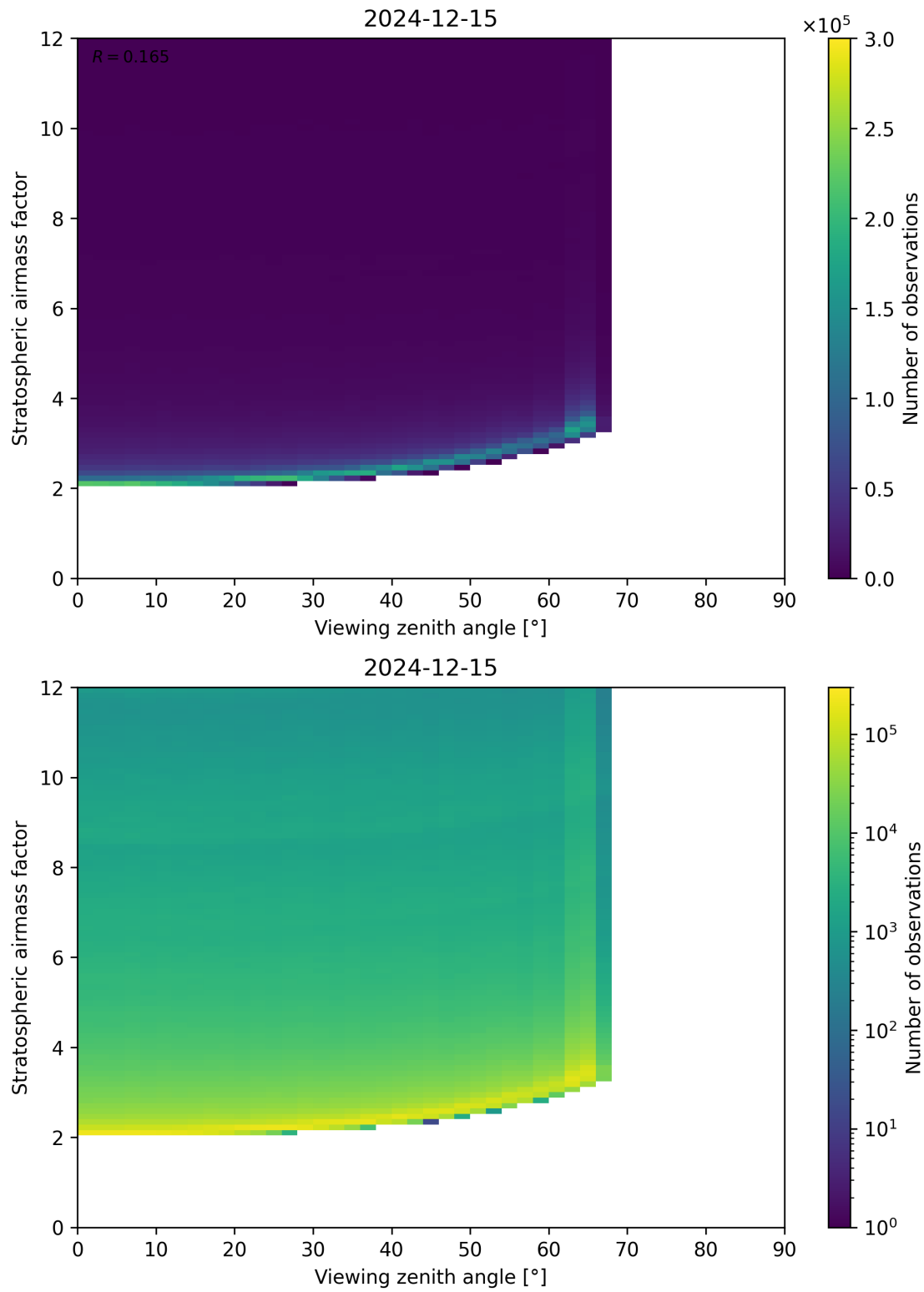
Figure 159: Scatter density plot of “Viewing zenith angle” against “Stratospheric airmass factor” for 2024-12-14 to 2024-12-16.
