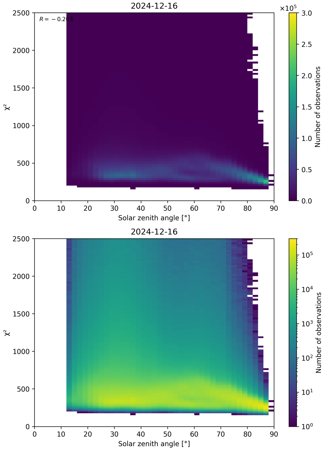
Figure 148: Scatter density plot of “Solar zenith angle” against “ \chi^2 ” for 2024-12-16 to 2024-12-17.
