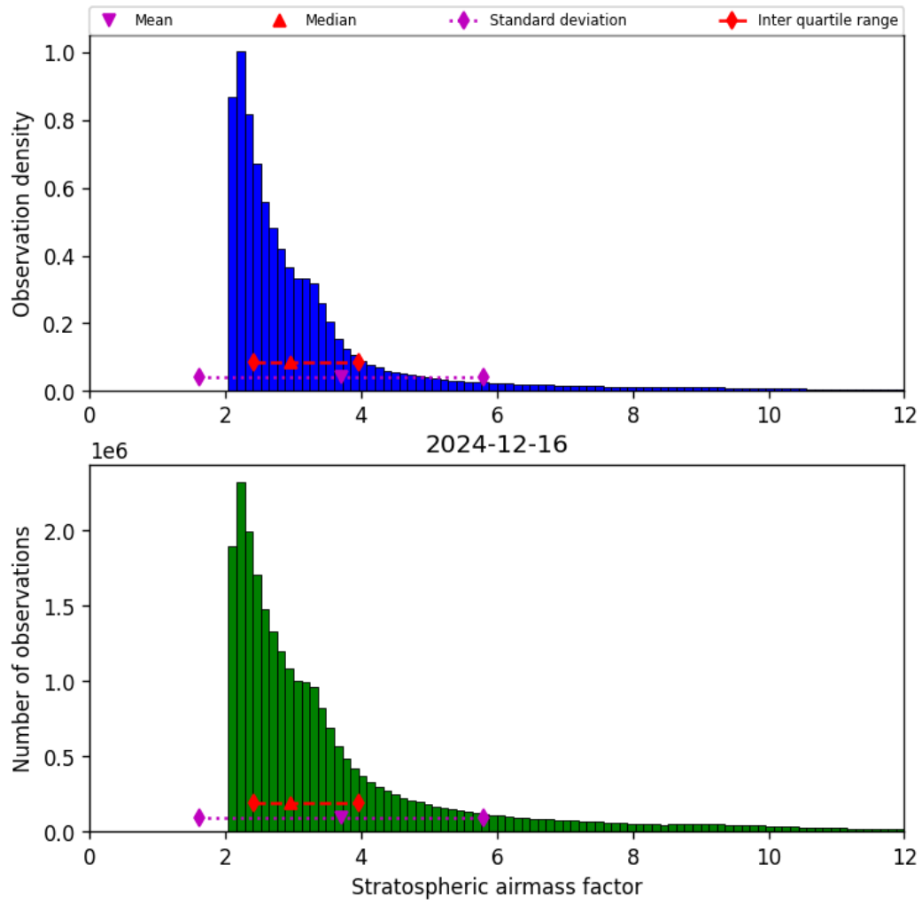
Figure 44: Histogram of “Stratospheric airmass factor” for 2024-12-16 to 2024-12-17
