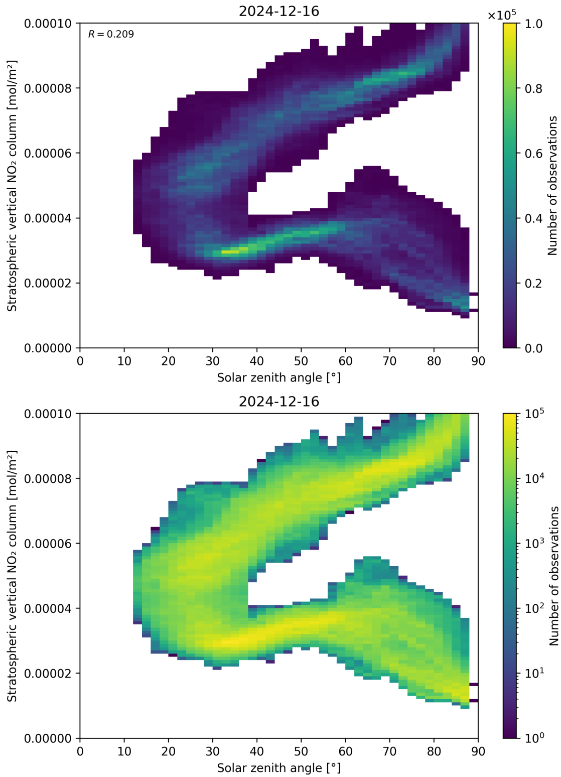
Figure 150: Scatter density plot of “Solar zenith angle” against “Stratospheric vertical NO 2 column” for 2024-12-16 to 2024-12-17.
