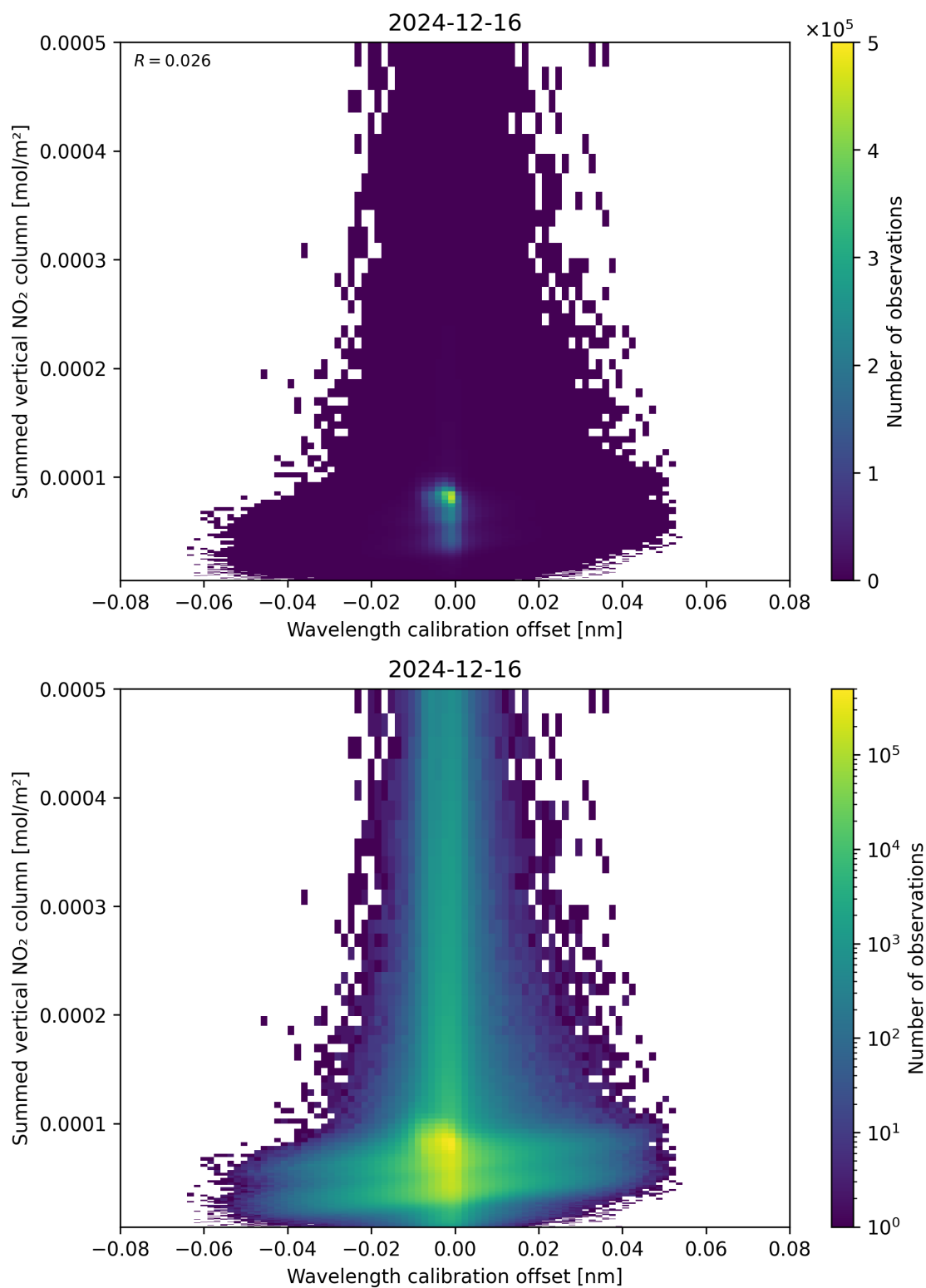
Figure 177: Scatter density plot of “Wavelength calibration offset” against “Summed vertical NO 2 column” for 2024-12-16 to 2024-12-17.
