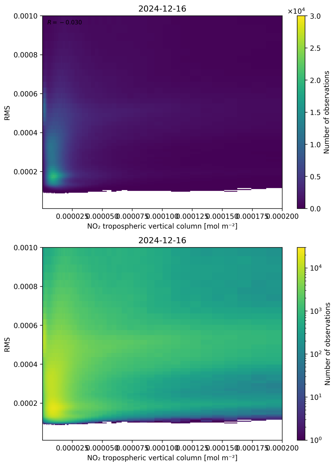
Figure 142: Scatter density plot of “NO 2 tropospheric vertical column” against “RMS” for 2024-12-16 to 2024-12-17.
