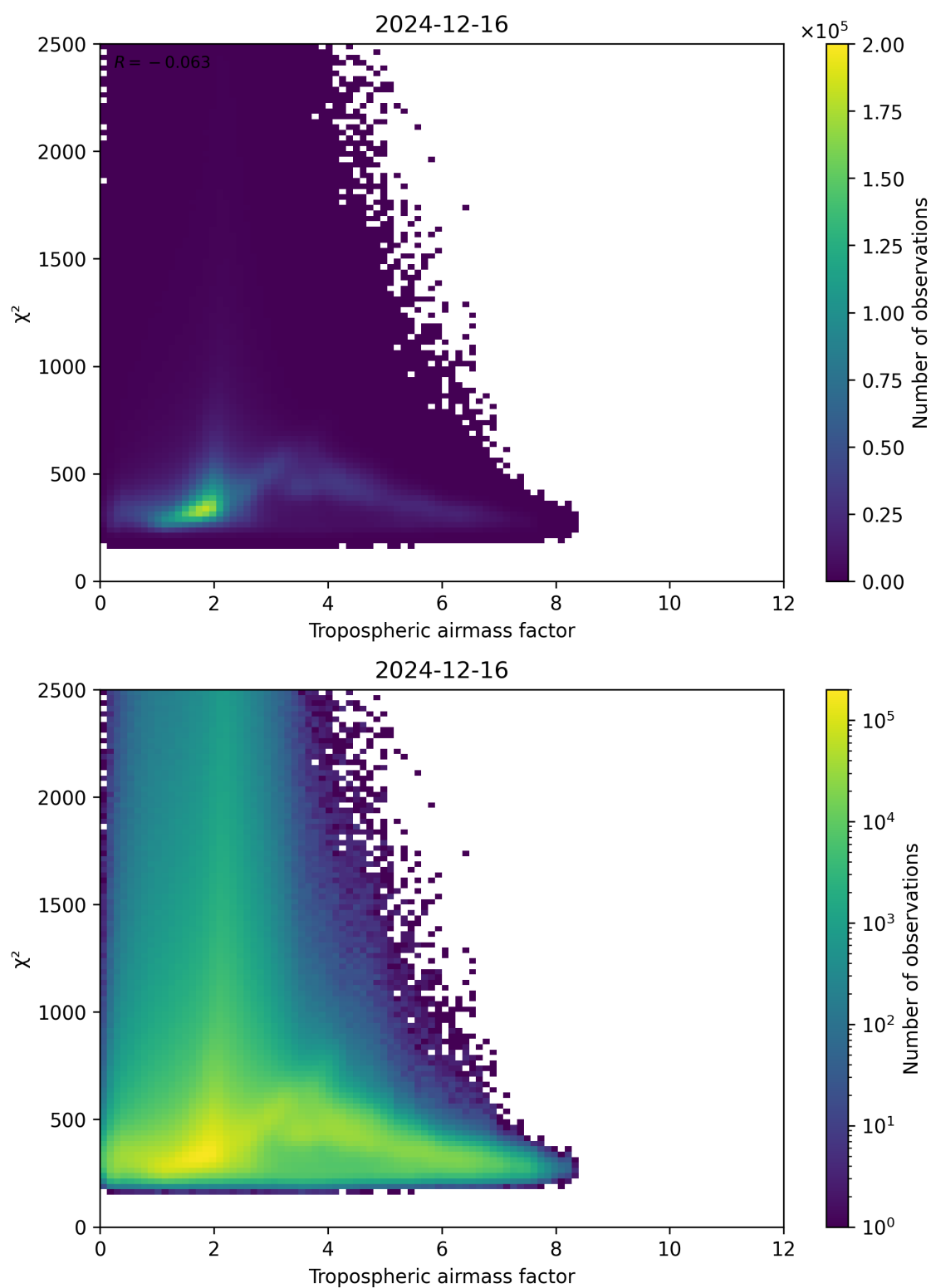
Figure 73: Scatter density plot of “Tropospheric airmass factor” against “ \chi^2 ” for 2024-12-16 to 2024-12-17.
