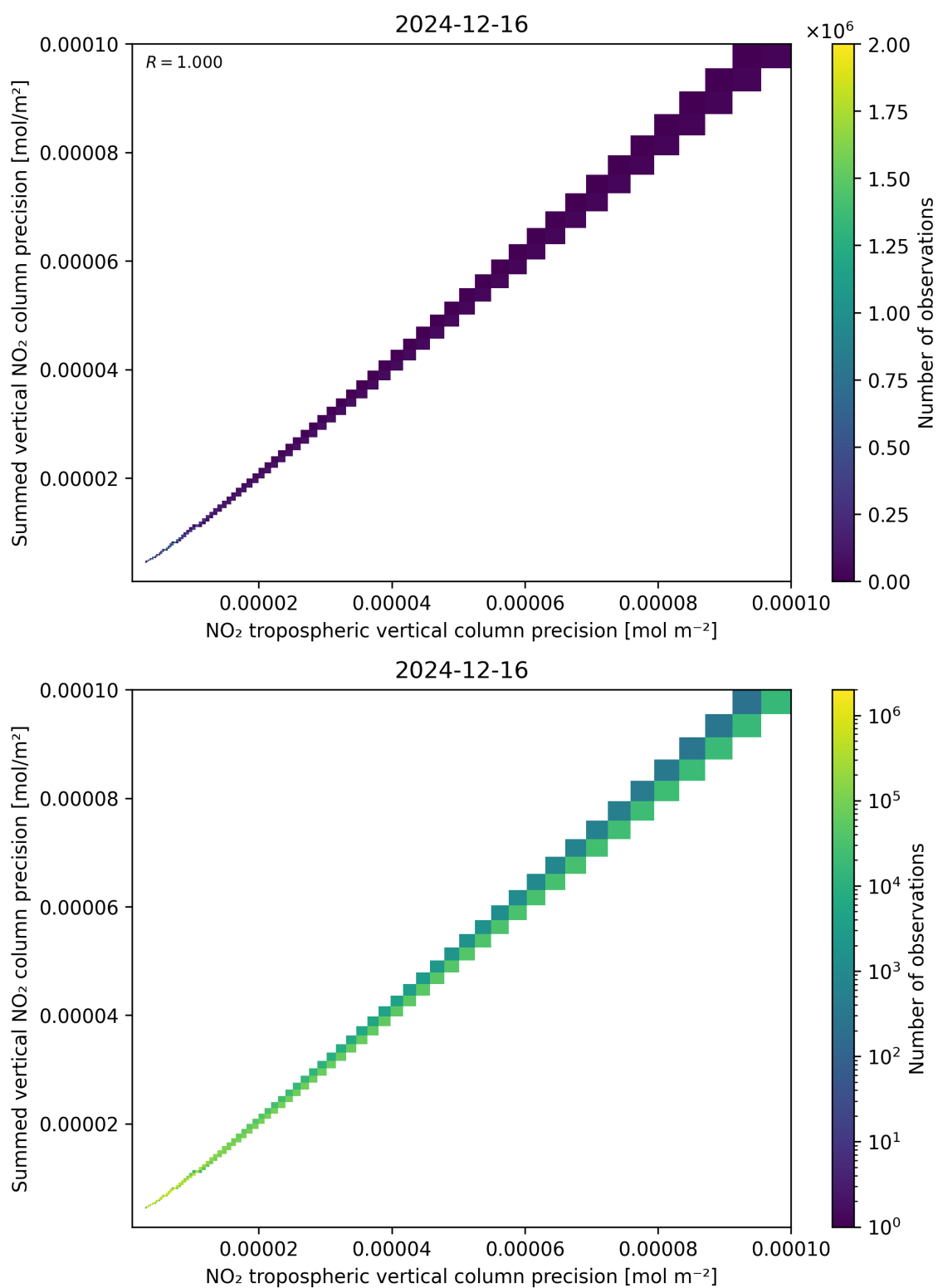
Figure 137: Scatter density plot of “NO 2 tropospheric vertical column precision” against “Summed vertical NO 2 column precision” for 2024-12-16 to 2024-12-17.
