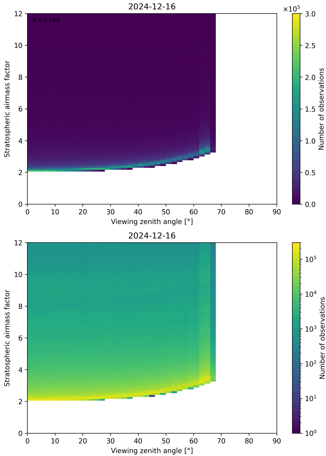
Figure 159: Scatter density plot of “Viewing zenith angle” against “Stratospheric airmass factor” for 2024-12-16 to 2024-12-17.
