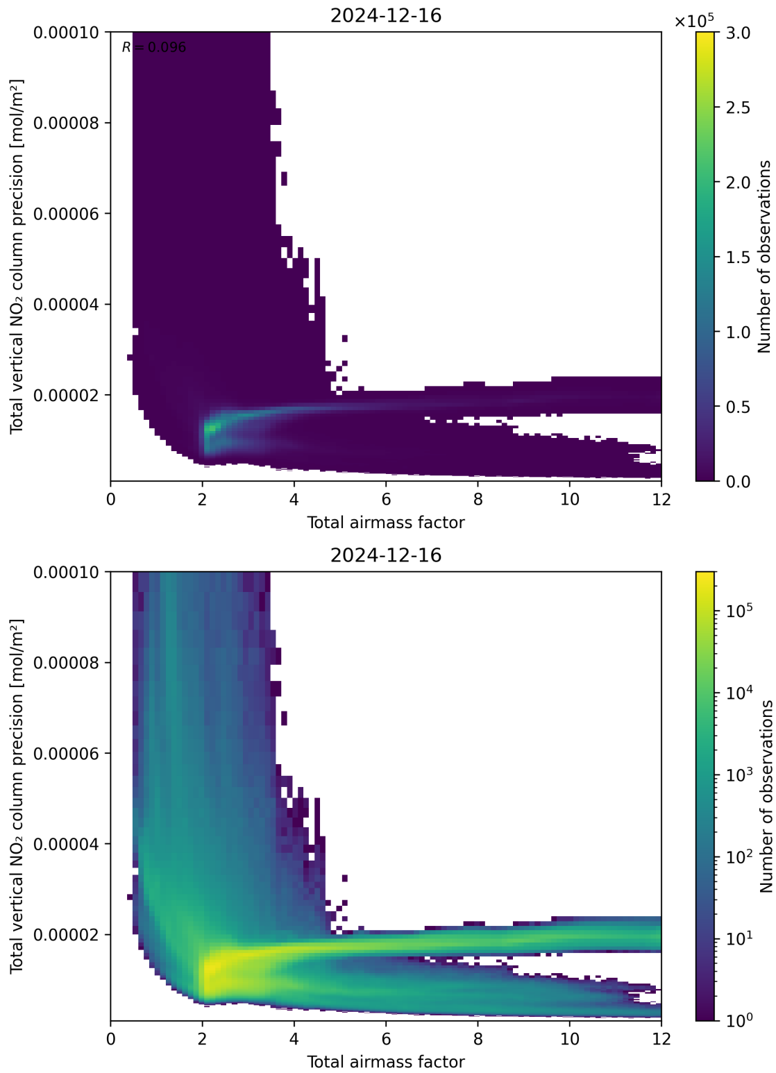
Figure 68: Scatter density plot of “Total airmass factor” against “Total vertical NO 2 column precision” for 2024-12-16 to 2024-12-17.
