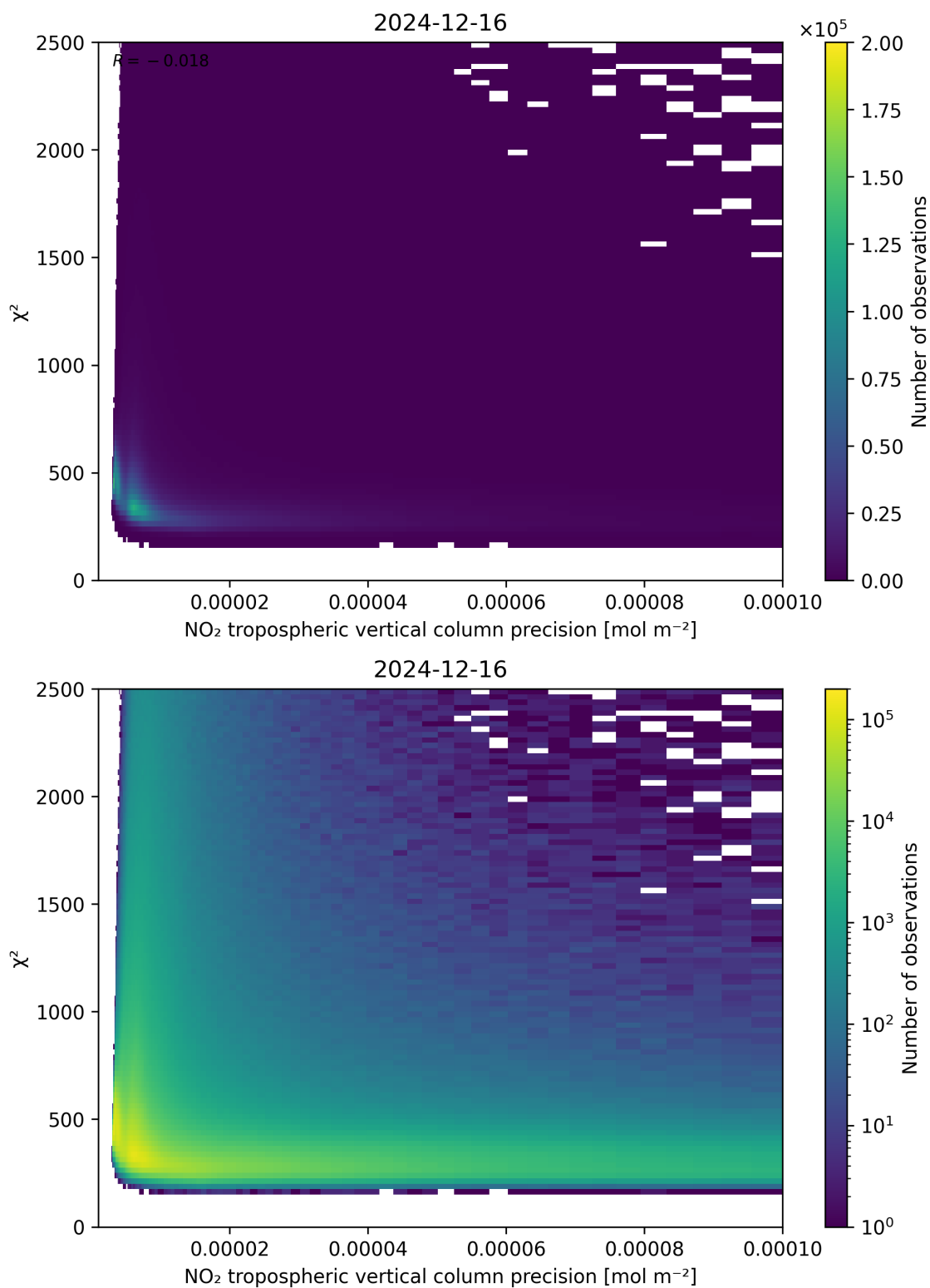
Figure 134: Scatter density plot of “NO 2 tropospheric vertical column precision” against “ \chi^2 ” for 2024-12-16 to 2024-12-17.
