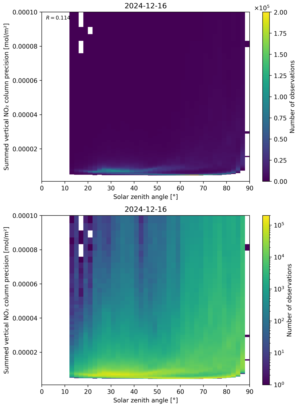
Figure 152: Scatter density plot of “Solar zenith angle” against “Summed vertical NO 2 column precision” for 2024-12-16 to 2024-12-17.
