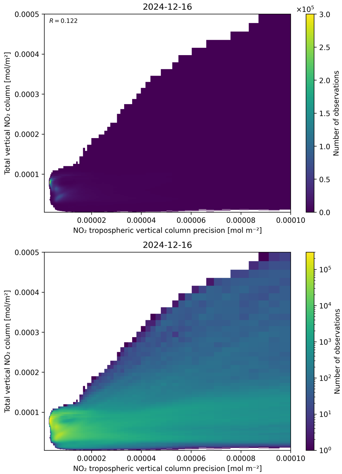
Figure 138: Scatter density plot of “NO 2 tropospheric vertical column precision” against “Total vertical NO 2 column” for 2024-12-16 to 2024-12-17.
