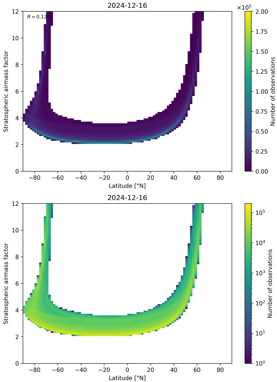
Figure 83: Scatter density plot of “Latitude” against “Stratospheric air mass factor” for 2024-12-16 to 2024-12-17.
