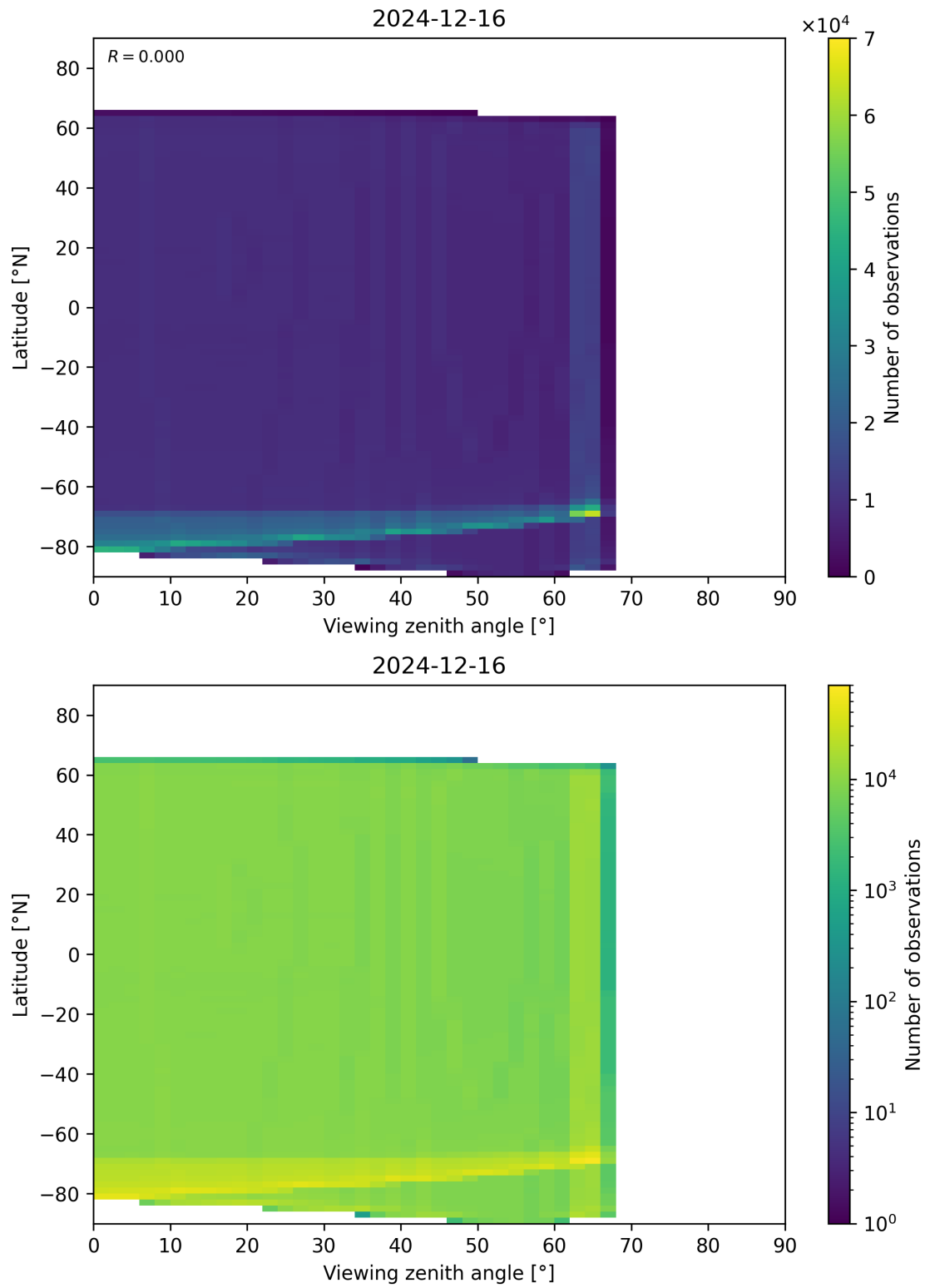
Figure 163: Scatter density plot of “Viewing zenith angle” against “Latitude” for 2024-12-16 to 2024-12-17.
