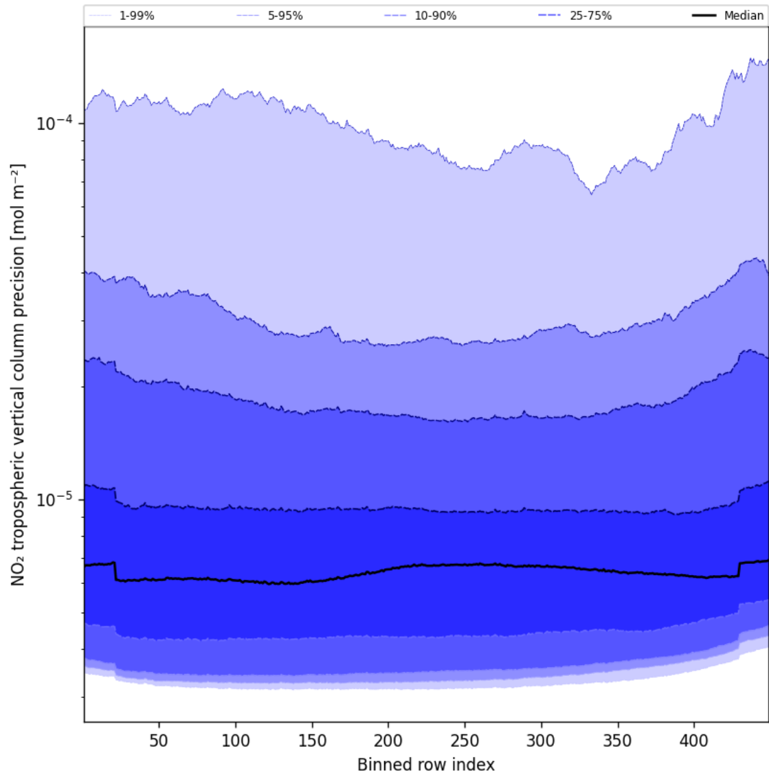
Figure 47: Along track statistics of “NO 2 tropospheric vertical column precision” for 2024-12-16 to 2024-12-17
