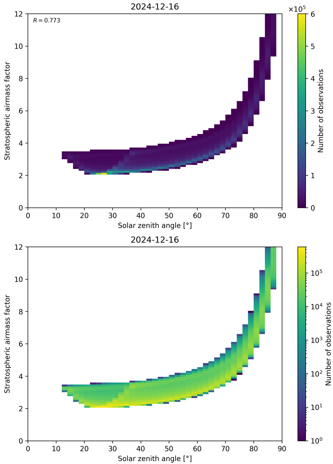
Figure 145: Scatter density plot of “Solar zenith angle” against “Stratospheric airmass factor” for 2024-12-16 to 2024-12-17.
