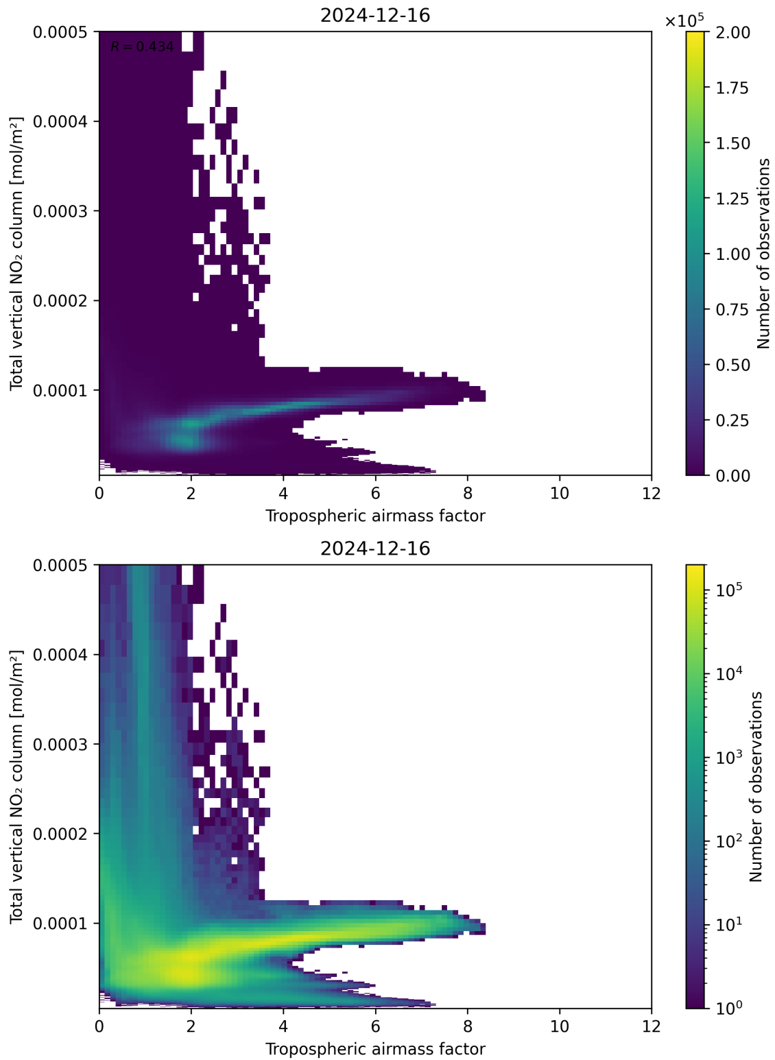
Figure 77: Scatter density plot of “Tropospheric airmass factor” against “Total vertical NO 2 column” for 2024-12-16 to 2024-12-17.
