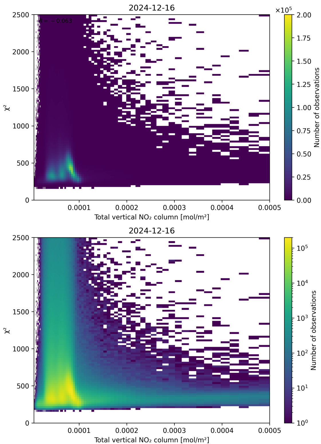
Figure 111: Scatter density plot of “Total vertical NO 2 column” against “ \chi^2 ” for 2024-12-16 to 2024-12-17.
