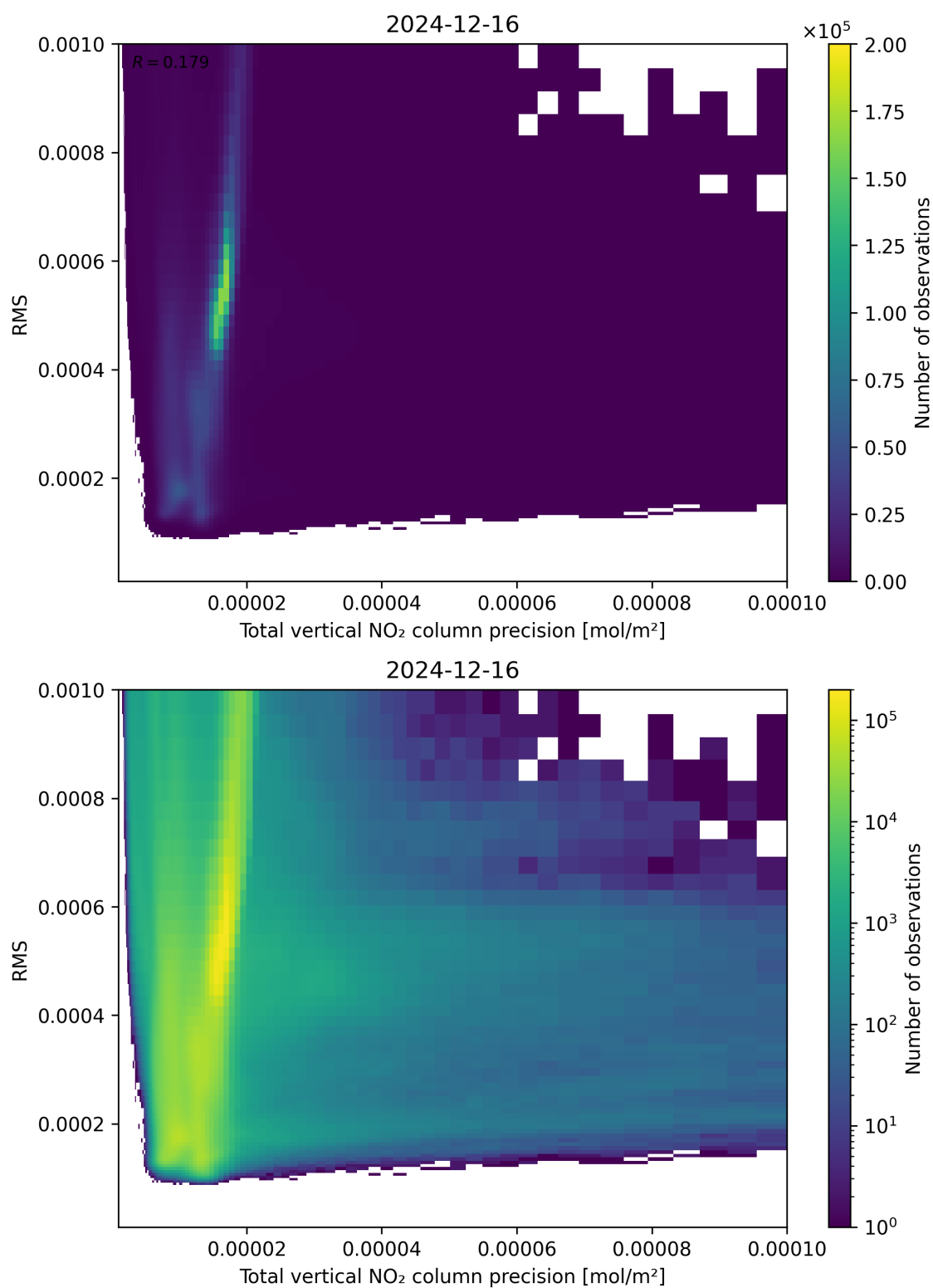
Figure 119: Scatter density plot of “Total vertical NO 2 column precision” against “RMS” for 2024-12-16 to 2024-12-17.
