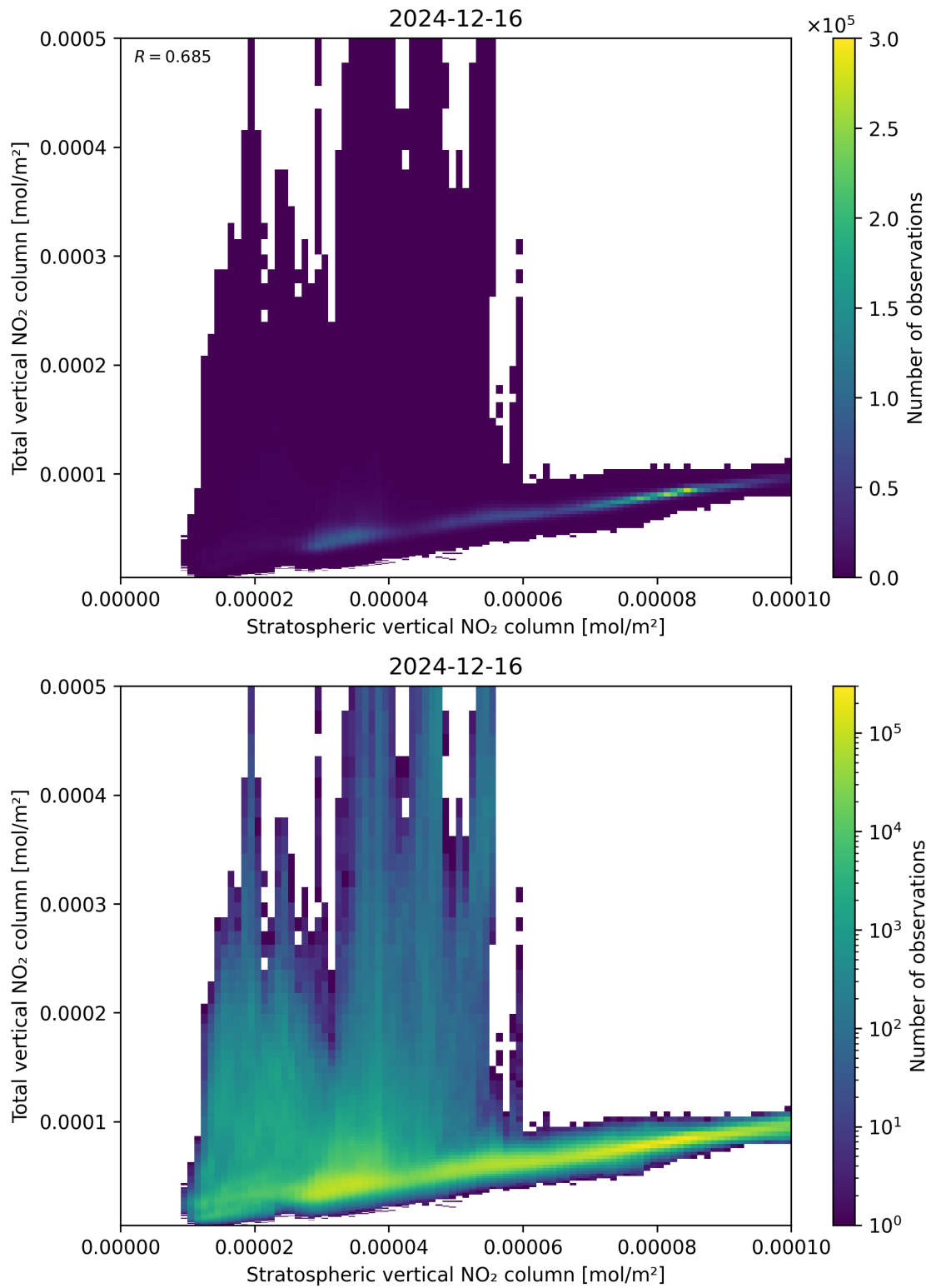
Figure 100: Scatter density plot of “Stratospheric vertical NO 2 column” against “Total vertical NO 2 column” for 2024-12-16 to 2024-12-17.
