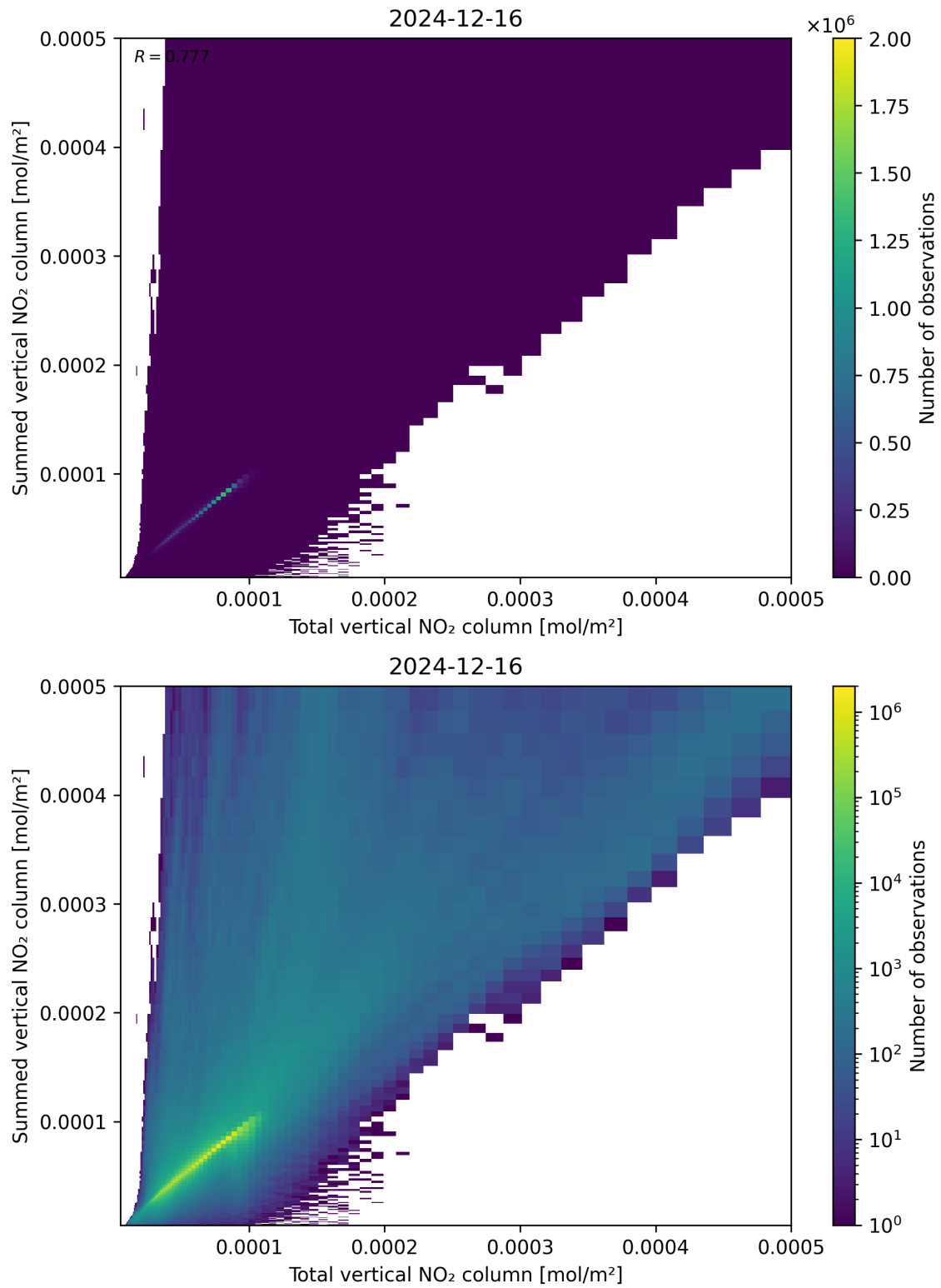
Figure 112: Scatter density plot of “Total vertical NO 2 column” against “Summed vertical NO 2 column” for 2024-12-16 to 2024-12-17.
