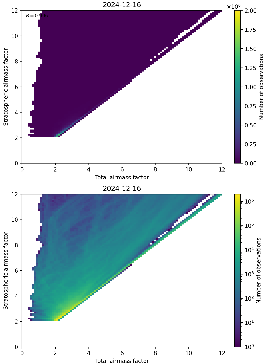
Figure 62: Scatter density plot of “Total airmass factor” against “Stratospheric airmass factor” for 2024-12-16 to 2024-12-17.
