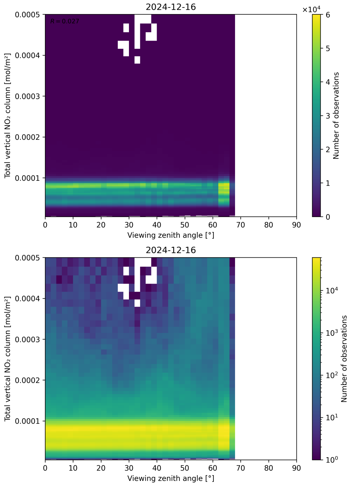
Figure 167: Scatter density plot of “Viewing zenith angle” against “Total vertical NO 2 column” for 2024-12-16 to 2024-12-17.
