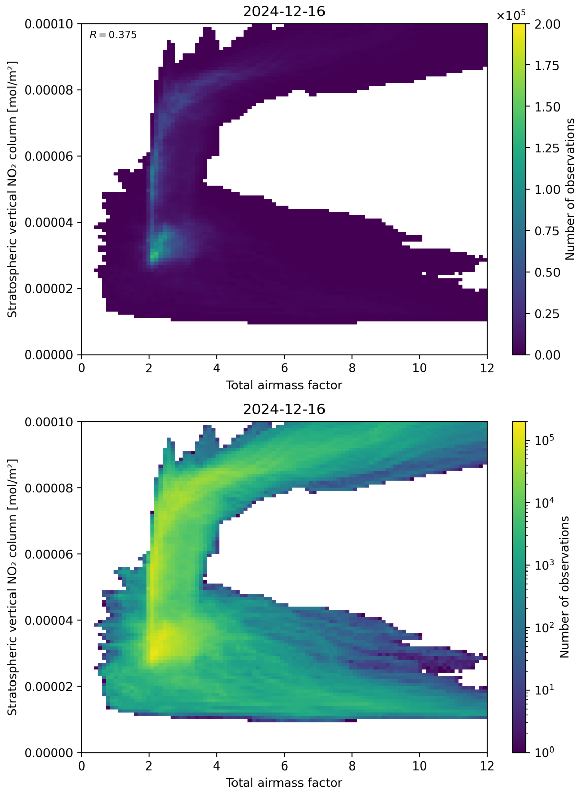
Figure 64: Scatter density plot of “Total airmass factor” against “Stratospheric vertical NO 2 column” for 2024-12-16 to 2024-12-17.
