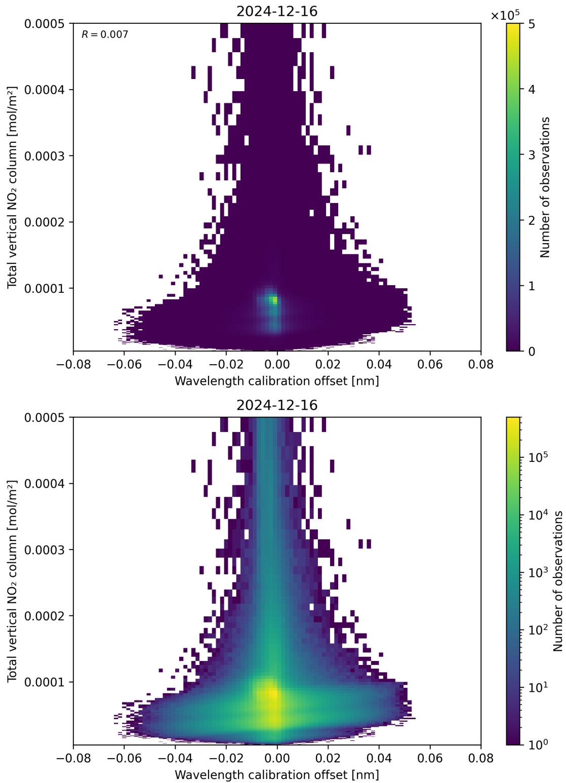
Figure 179: Scatter density plot of “Wavelength calibration offset” against “Total vertical NO 2 column” for 2024-12-16 to 2024-12-17.
