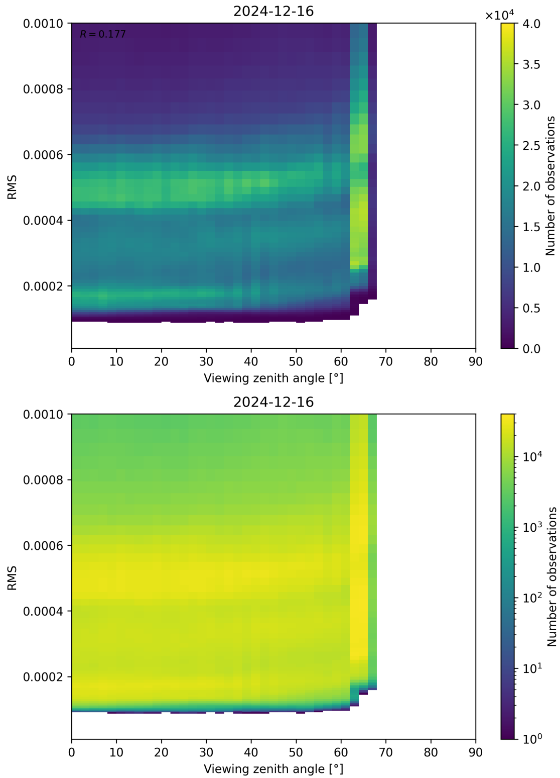
Figure 171: Scatter density plot of “Viewing zenith angle” against “RMS” for 2024-12-16 to 2024-12-17.
