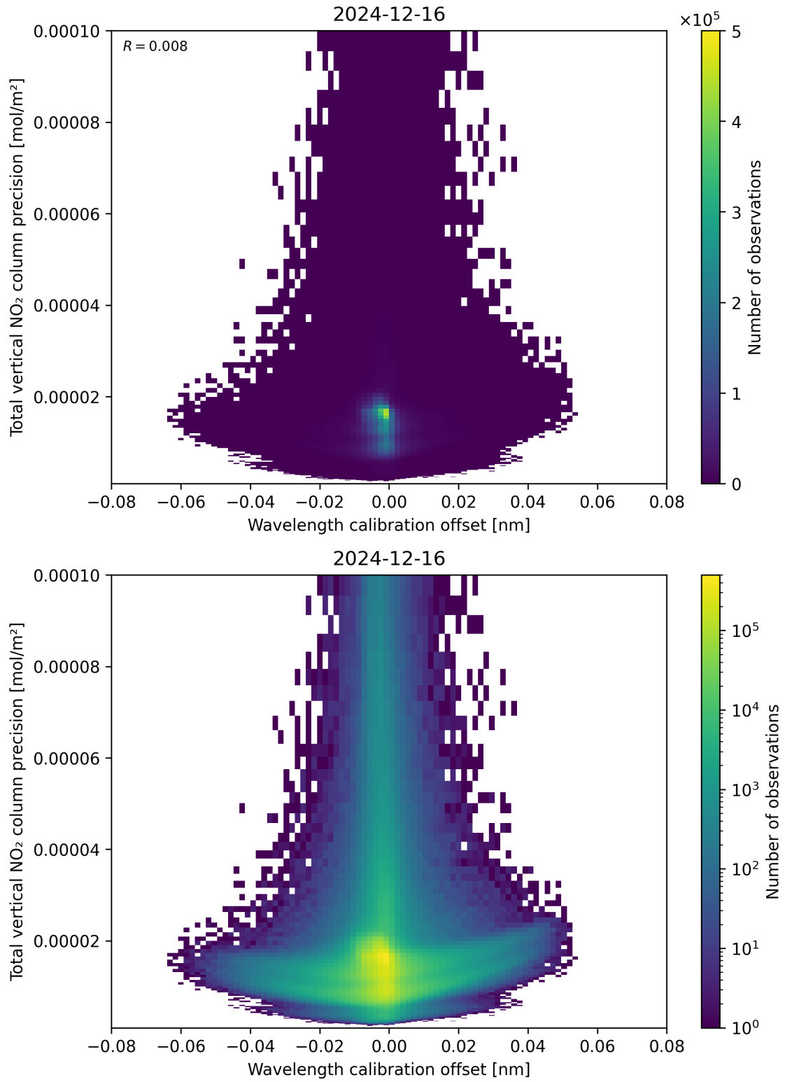
Figure 180: Scatter density plot of “Wavelength calibration offset” against “Total vertical NO 2 column precision” for 2024-12-16 to 2024-12-17.
