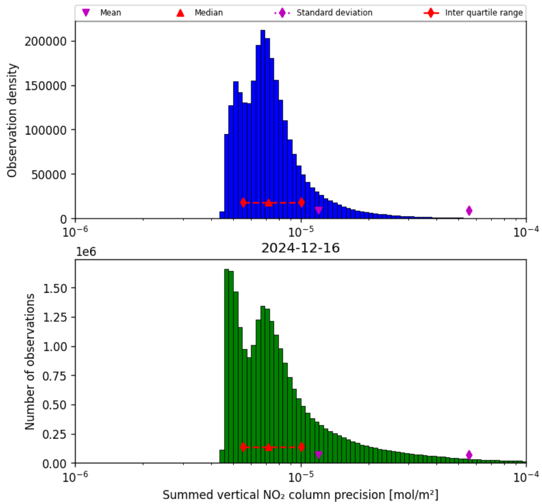
Figure 41: Histogram of “Summed vertical NO 2 column precision” for 2024-12-16 to 2024-12-17
