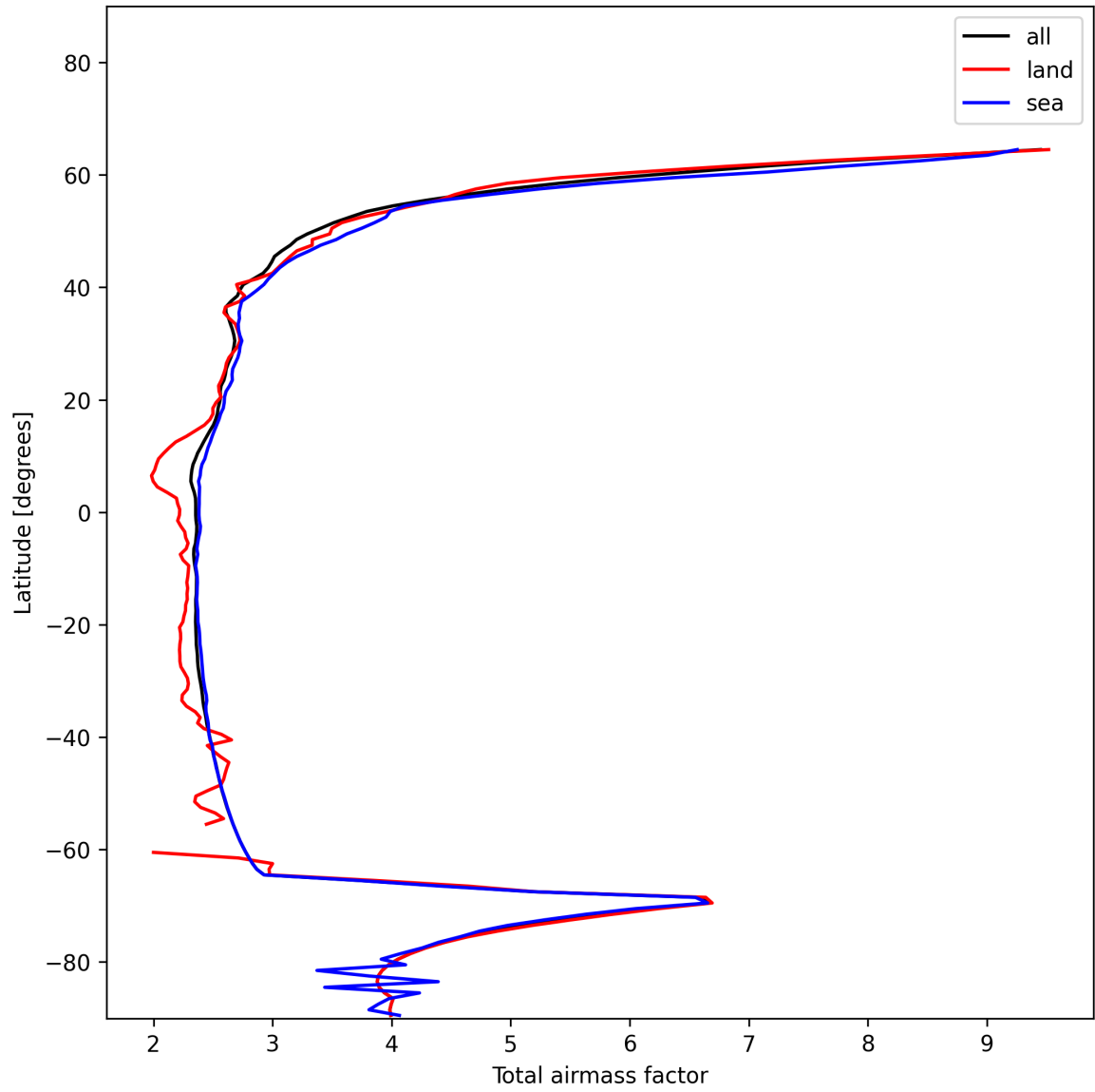
Figure 15: Zonal average of “Total airmass factor” for 2024-12-16 to 2024-12-17.
