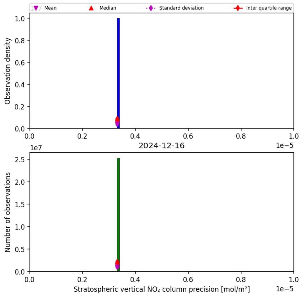
Figure 37: Histogram of “Stratospheric vertical NO 2 column precision” for 2024-12-16 to 2024-12-17
