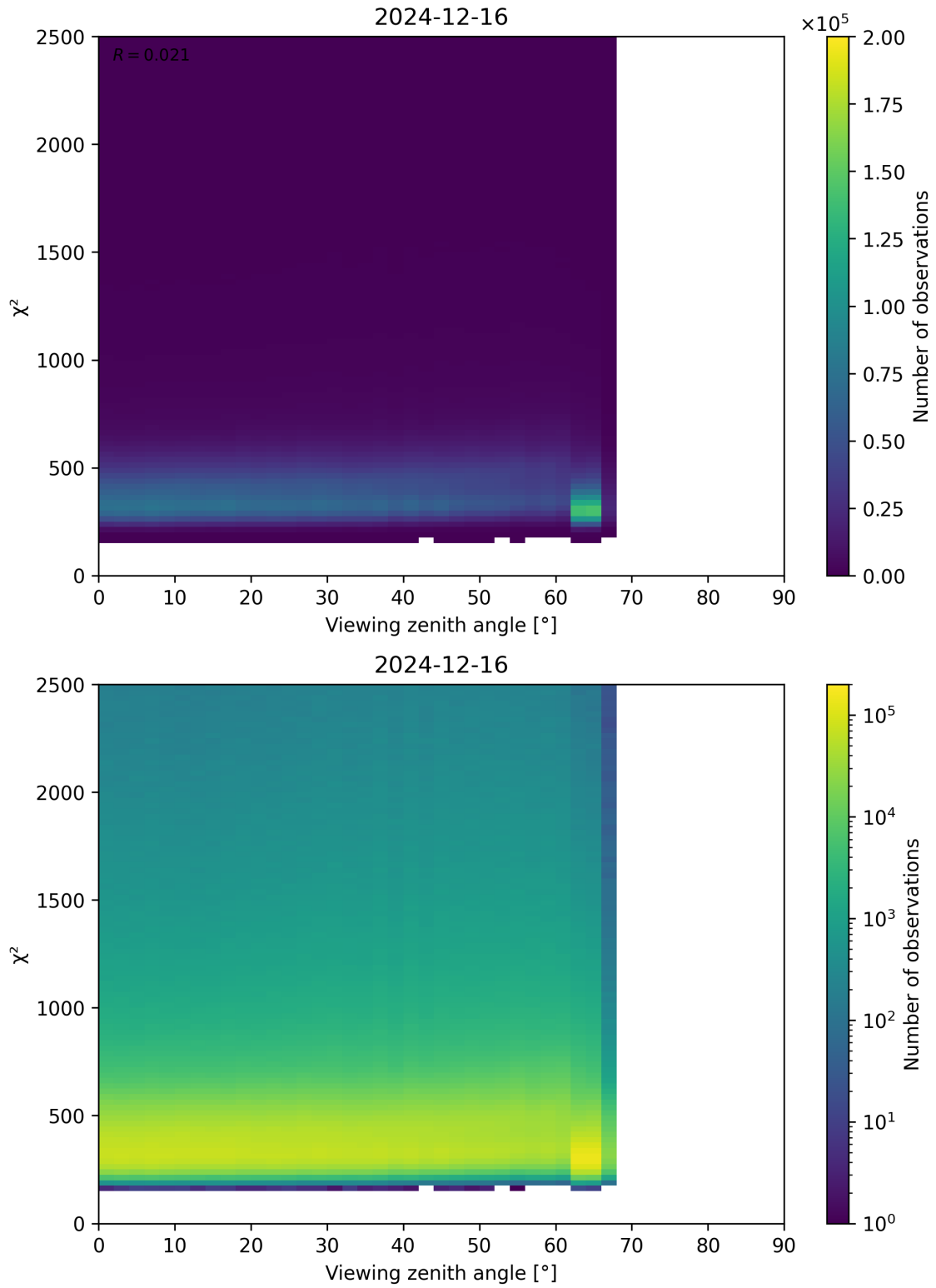
Figure 162: Scatter density plot of “Viewing zenith angle” against “ \chi^2 ” for 2024-12-16 to 2024-12-17.
