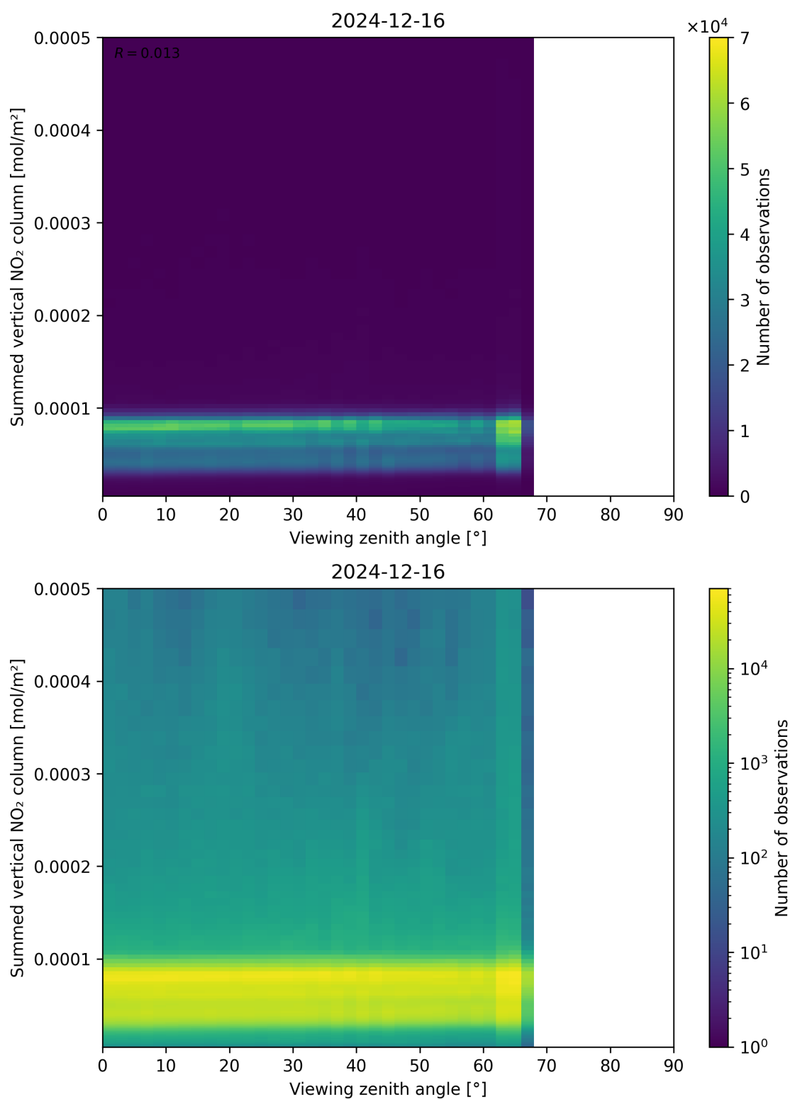
Figure 165: Scatter density plot of “Viewing zenith angle” against “Summed vertical NO 2 column” for 2024-12-16 to 2024-12-17.
