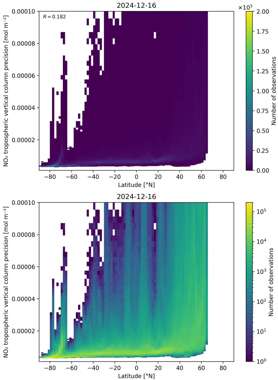
Figure 93: Scatter density plot of “Latitude” against “NO 2 tropospheric vertical column precision” for 2024-12-16 to 2024-12-17.
