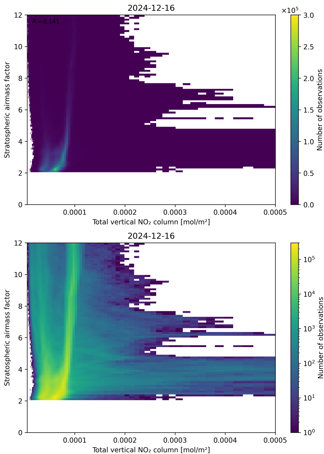
Figure 110: Scatter density plot of “Total vertical NO 2 column” against “Stratospheric airmass factor” for 2024-12-16 to 2024-12-17.
