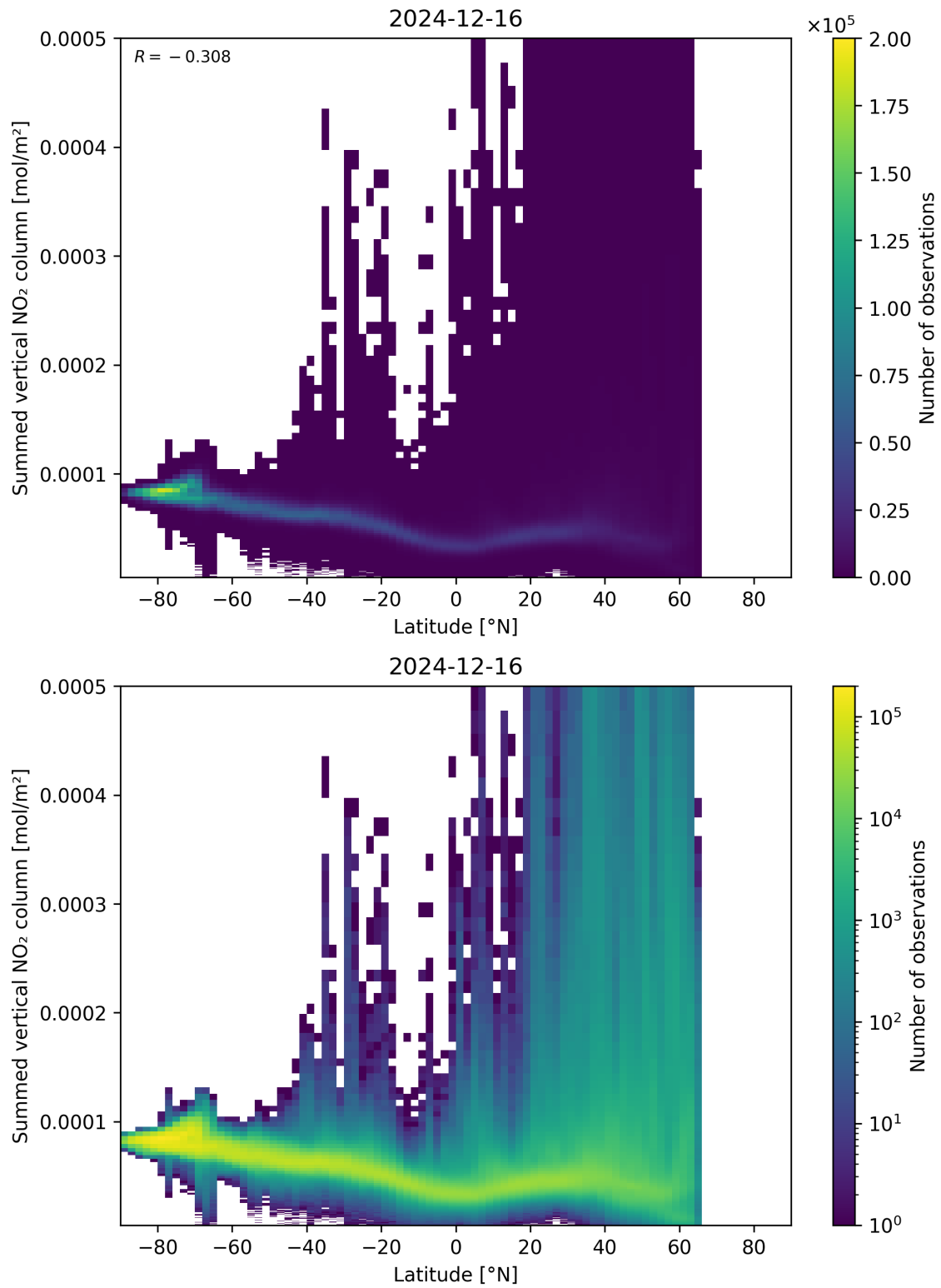
Figure 88: Scatter density plot of “Latitude” against “Summed vertical NO 2 column” for 2024-12-16 to 2024-12-17.
