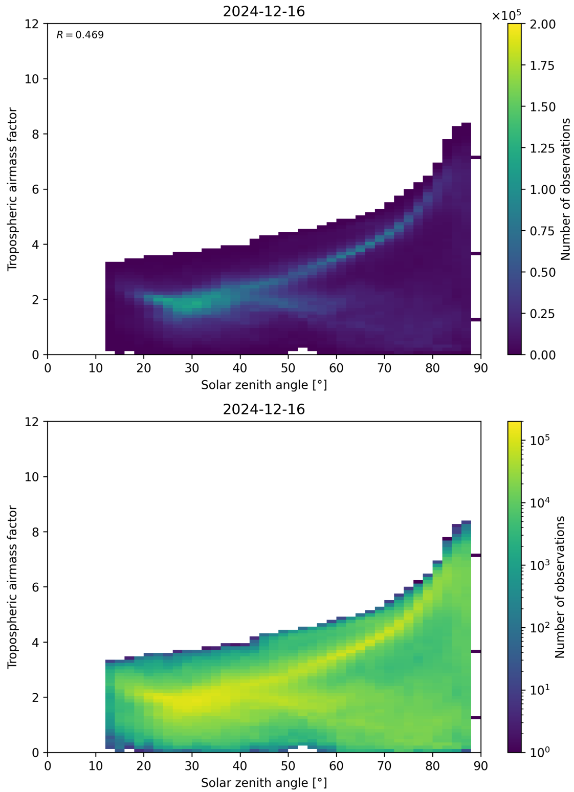
Figure 147: Scatter density plot of “Solar zenith angle” against “Tropospheric airmass factor” for 2024-12-16 to 2024-12-17.
