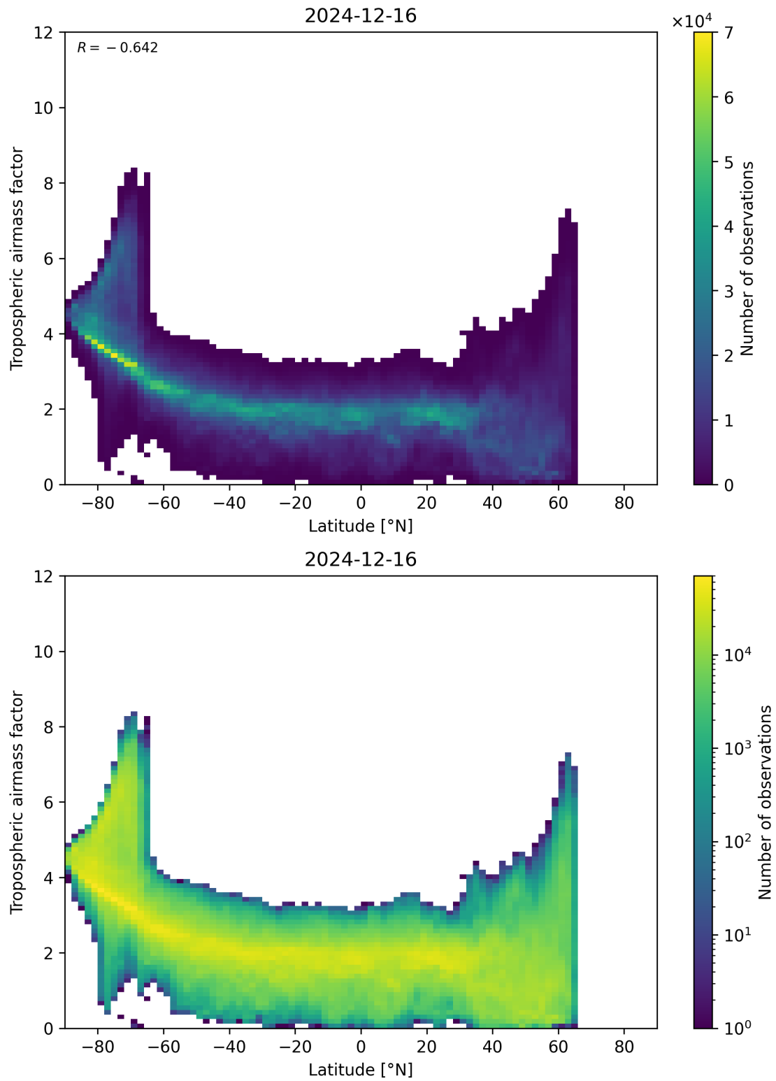
Figure 85: Scatter density plot of “Latitude” against “Tropospheric air mass factor” for 2024-12-16 to 2024-12-17.
