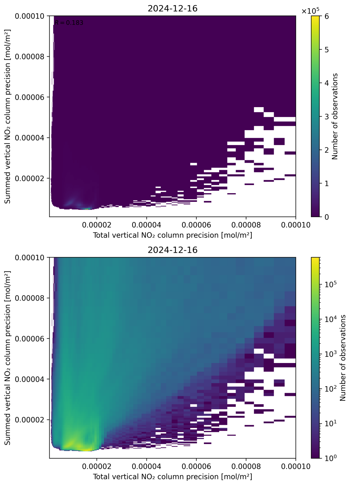
Figure 118: Scatter density plot of “Total vertical NO 2 column precision” against “Summed vertical NO 2 column precision” for 2024-12-16 to 2024-12-17.
