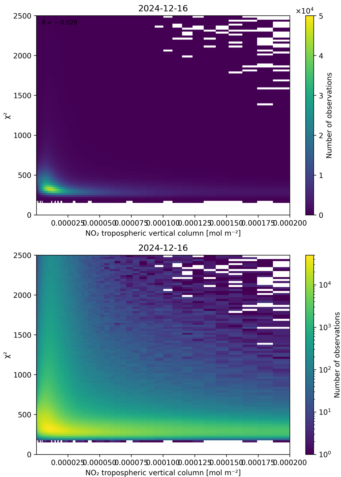
Figure 124: Scatter density plot of “NO 2 tropospheric vertical column” against “ \chi^2 ” for 2024-12-16 to 2024-12-17.
