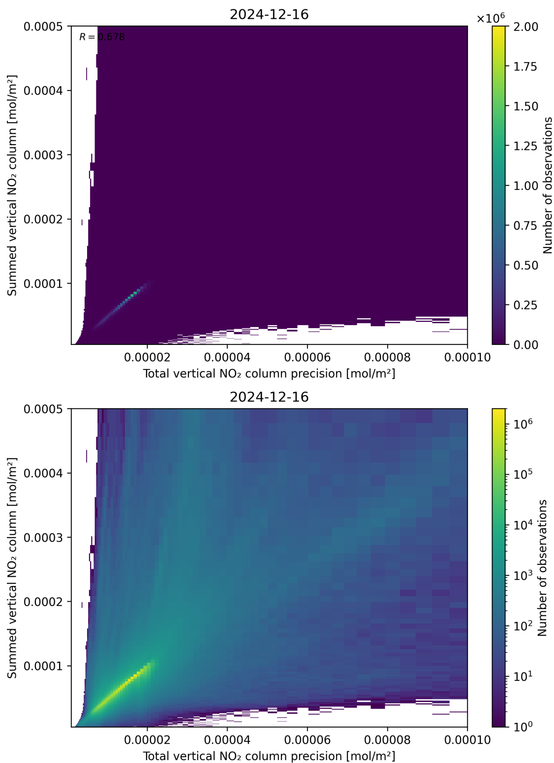
Figure 117: Scatter density plot of “Total vertical NO 2 column precision” against “Summed vertical NO 2 column” for 2024-12-16 to 2024-12-17.
