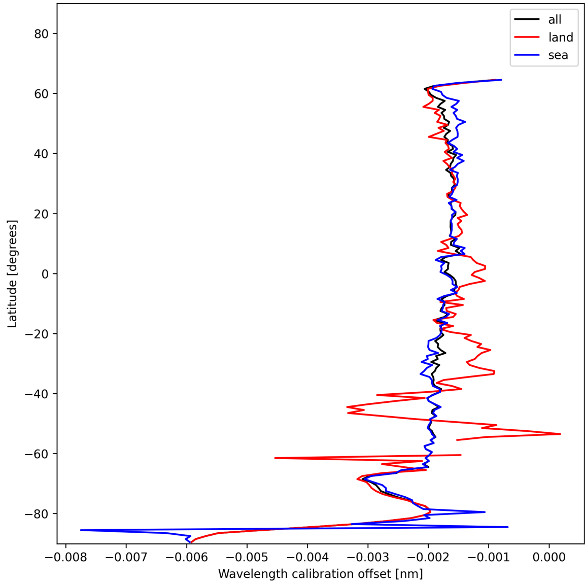
Figure 18: Zonal average of “Wavelength calibration offset” for 2024-12-16 to 2024-12-17.
