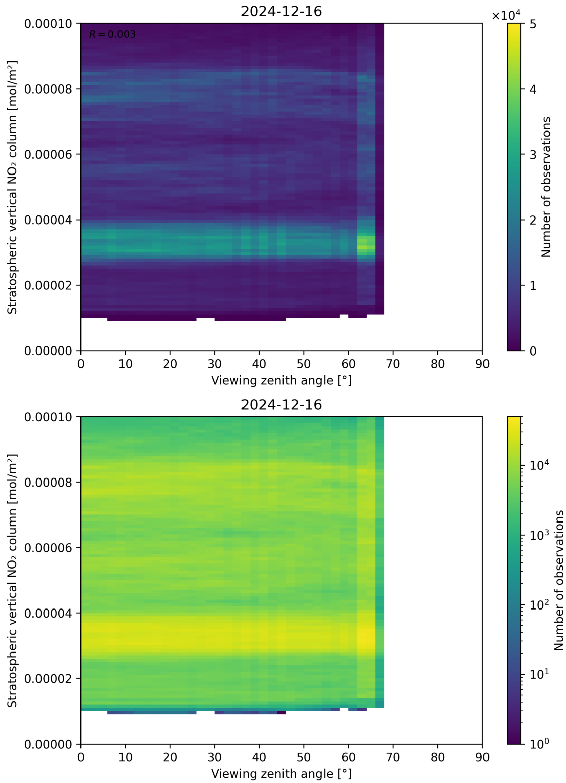
Figure 164: Scatter density plot of “Viewing zenith angle” against “Stratospheric vertical NO 2 column” for 2024-12-16 to 2024-12-17.
