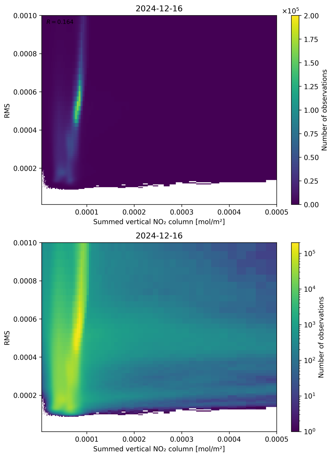
Figure 109: Scatter density plot of “Summed vertical NO 2 column” against “RMS” for 2024-12-16 to 2024-12-17.
