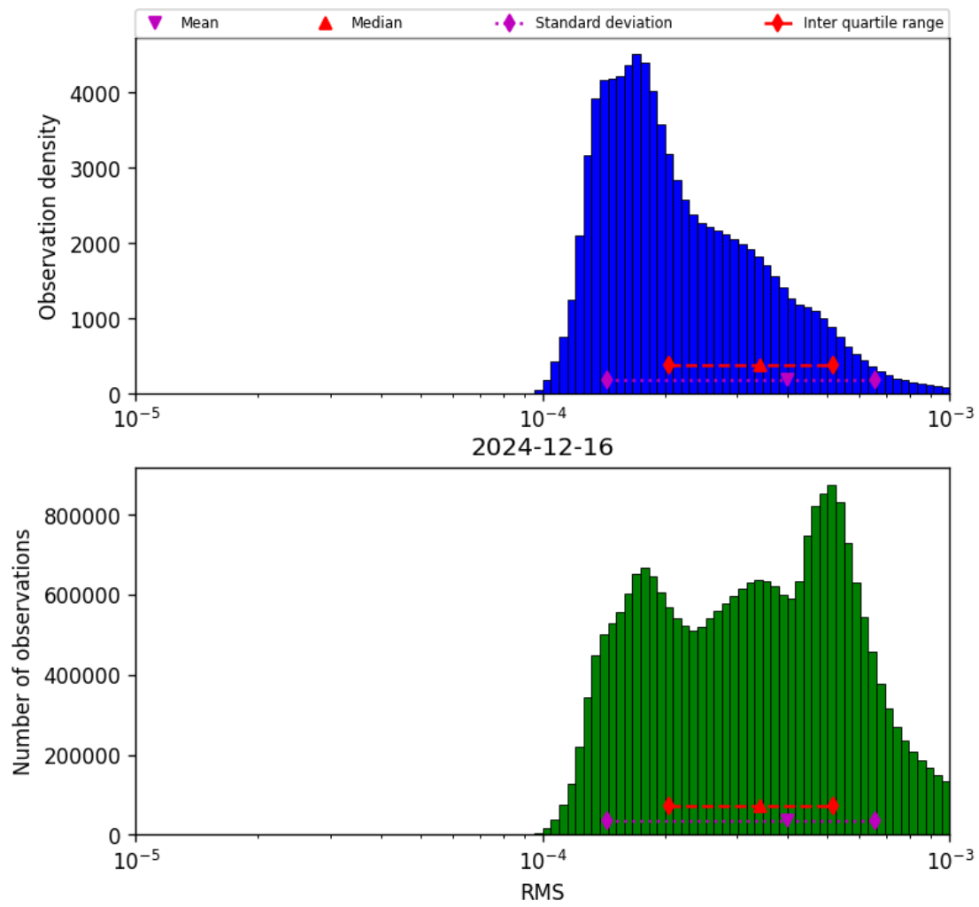
Figure 43: Histogram of “RMS” for 2024-12-16 to 2024-12-17
