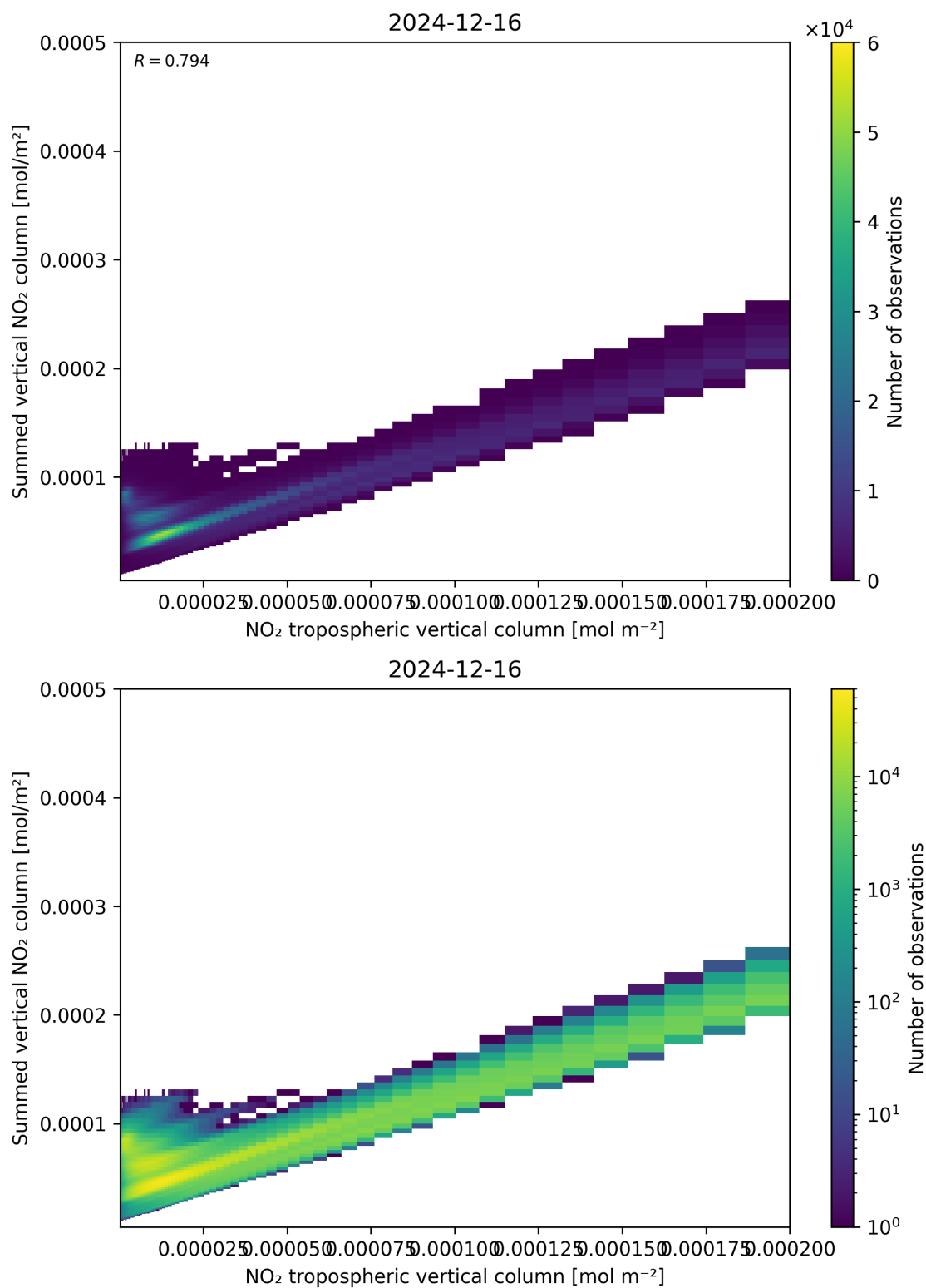
Figure 126: Scatter density plot of “NO 2 tropospheric vertical column” against “Summed vertical NO 2 column” for 2024-12-16 to 2024-12-17.
