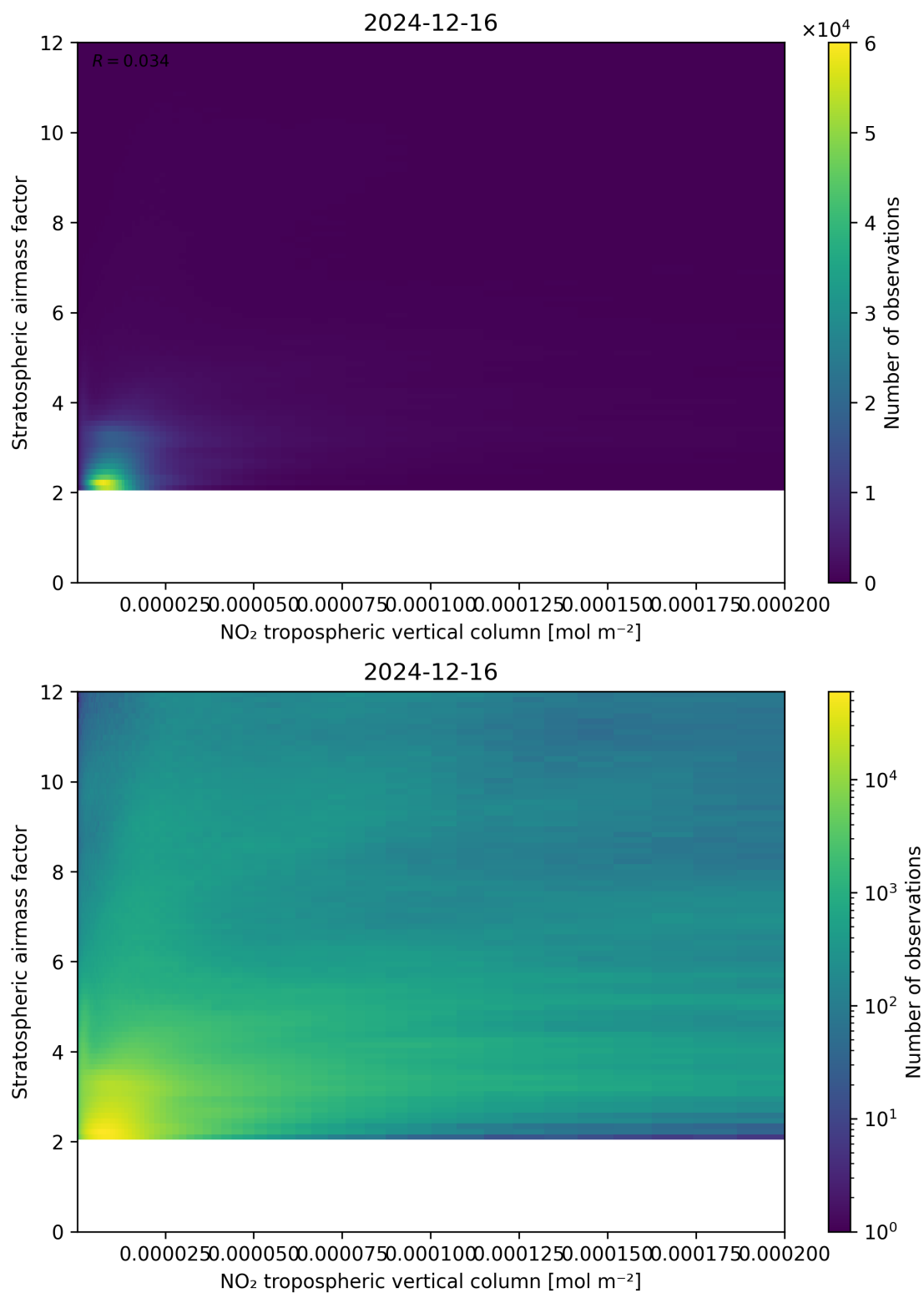
Figure 121: Scatter density plot of “NO 2 tropospheric vertical column” against “Stratospheric airmass factor” for 2024-12-16 to 2024-12-17.
