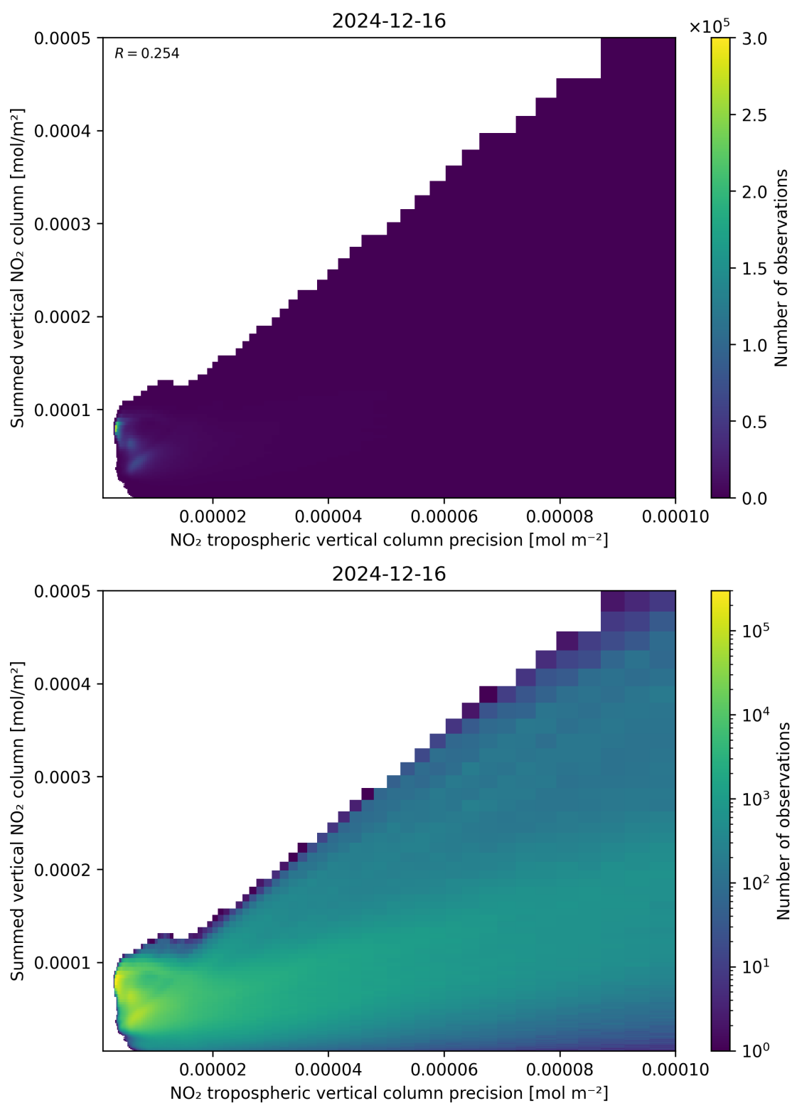
Figure 136: Scatter density plot of “NO 2 tropospheric vertical column precision” against “Summed vertical NO 2 column” for 2024-12-16 to 2024-12-17.
