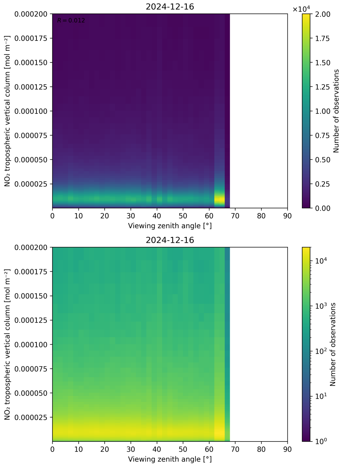
Figure 169: Scatter density plot of “Viewing zenith angle” against “NO 2 tropospheric vertical column” for 2024-12-16 to 2024-12-17.
