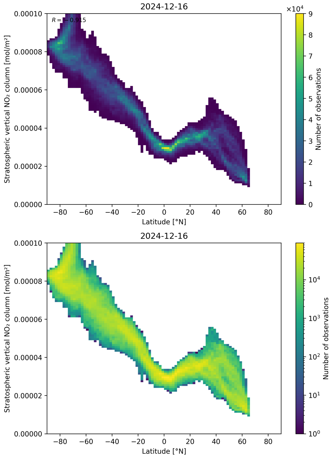
Figure 87: Scatter density plot of “Latitude” against “Stratospheric vertical NO 2 column” for 2024-12-16 to 2024-12-17.
