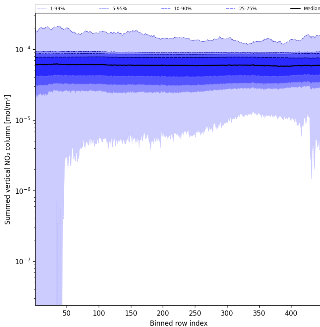
Figure 57: Along track statistics of “Summed vertical NO 2 column” for 2024-12-16 to 2024-12-17
