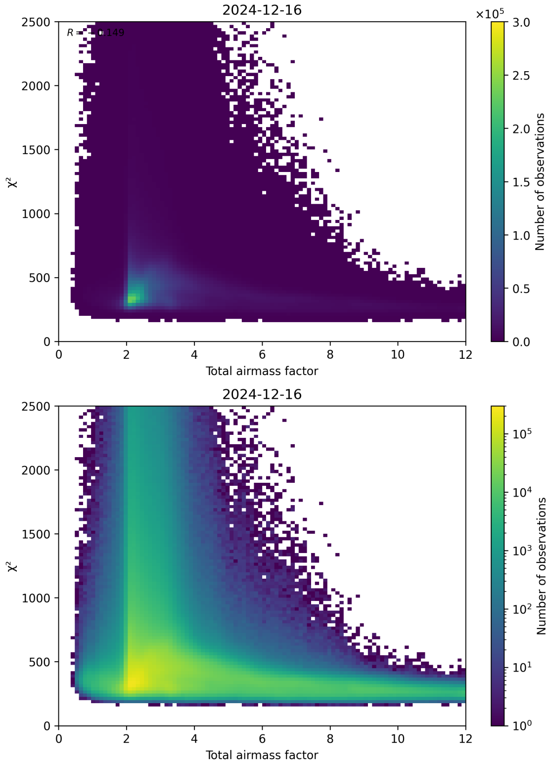
Figure 63: Scatter density plot of “Total airmass factor” against “ \chi^2 ” for 2024-12-16 to 2024-12-17.
