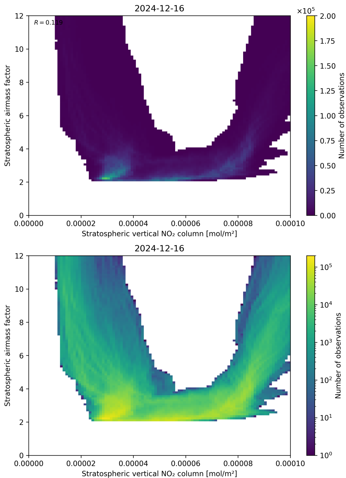
Figure 96: Scatter density plot of “Stratospheric vertical NO 2 column” against “Stratospheric airmass factor” for 2024-12-16 to 2024-12-17.
