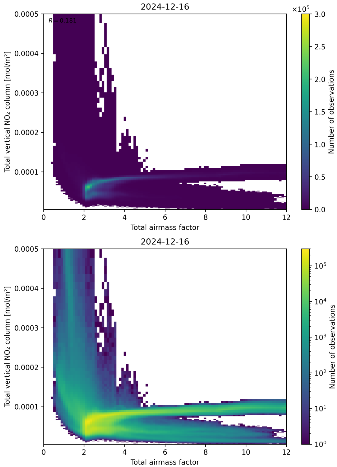
Figure 67: Scatter density plot of “Total airmass factor” against “Total vertical NO 2 column” for 2024-12-16 to 2024-12-17.
