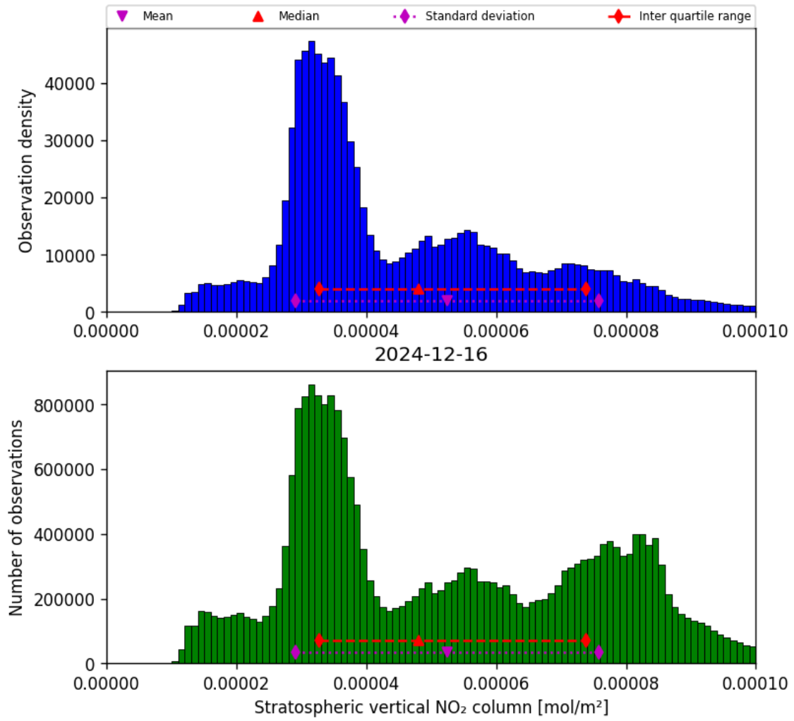
Figure 36: Histogram of “Stratospheric vertical NO 2 column” for 2024-12-16 to 2024-12-17
