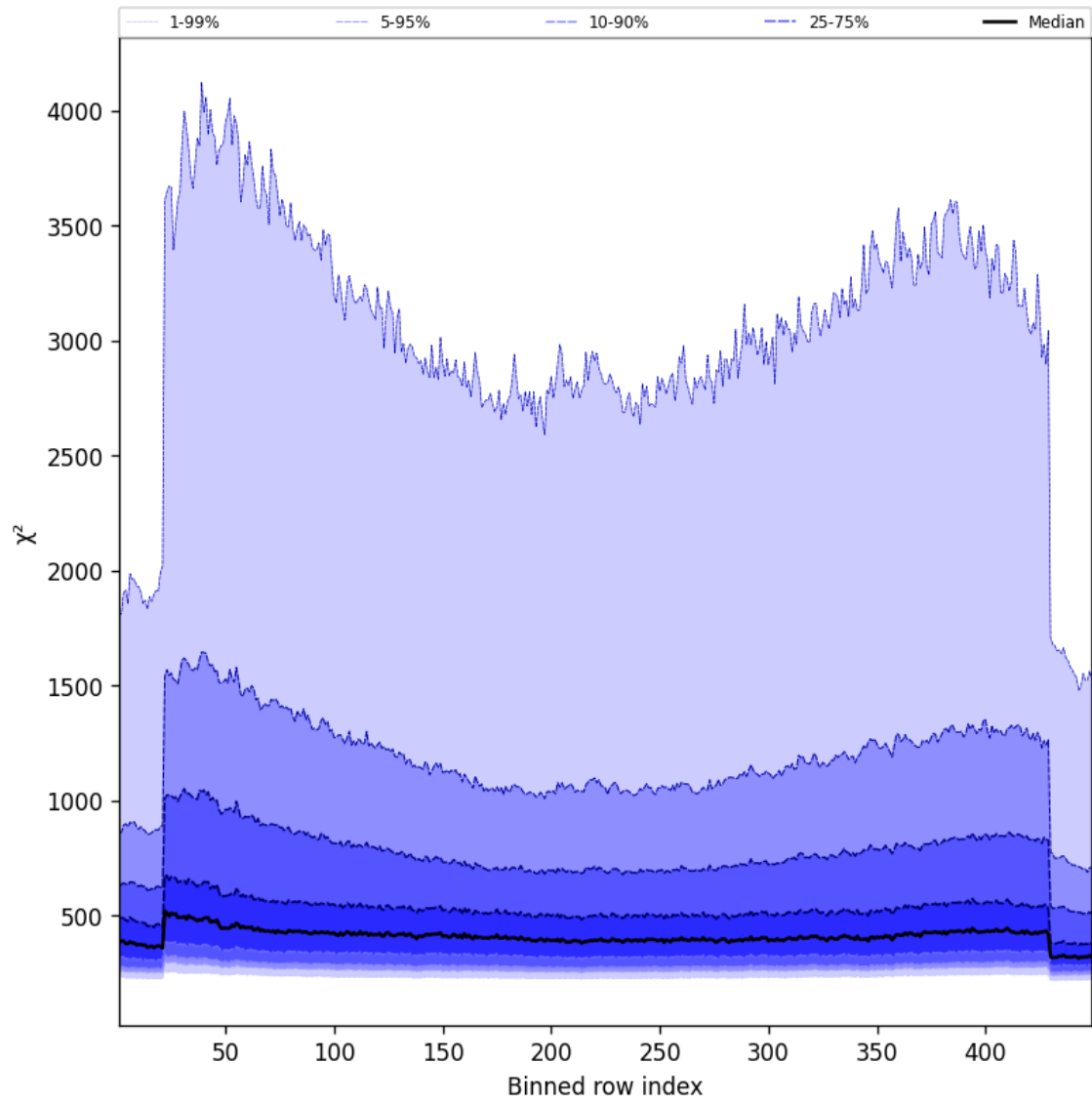
Figure 59: Along track statistics of “ \chi^2 ” for 2024-12-16 to 2024-12-17
