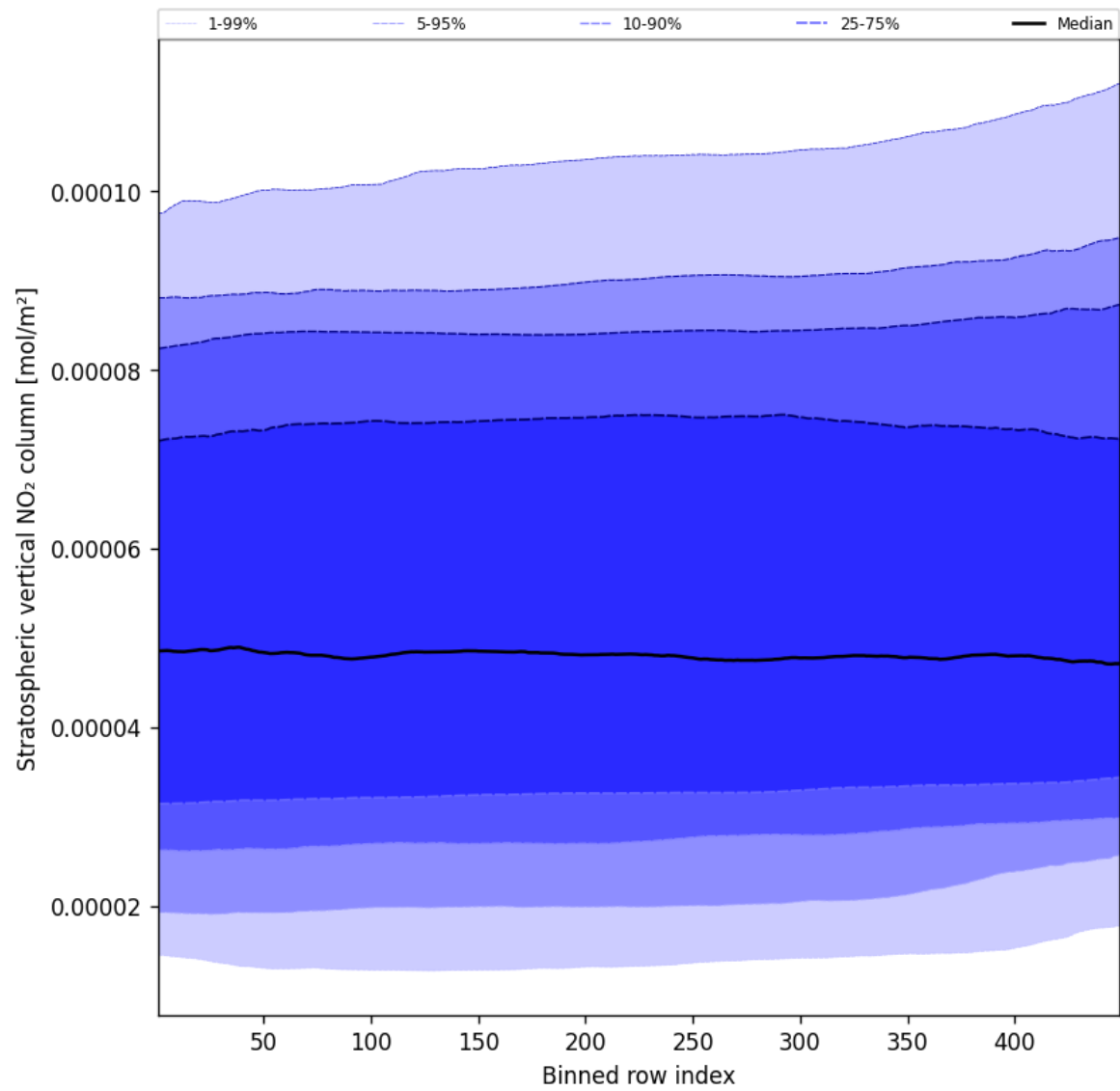
Figure 53: Along track statistics of “Stratospheric vertical NO 2 column” for 2024-12-16 to 2024-12-17
