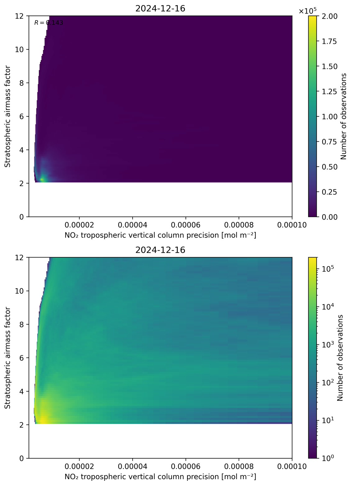
Figure 131: Scatter density plot of “NO 2 tropospheric vertical column precision” against “Stratospheric airmass factor” for 2024-12-16 to 2024-12-17.
