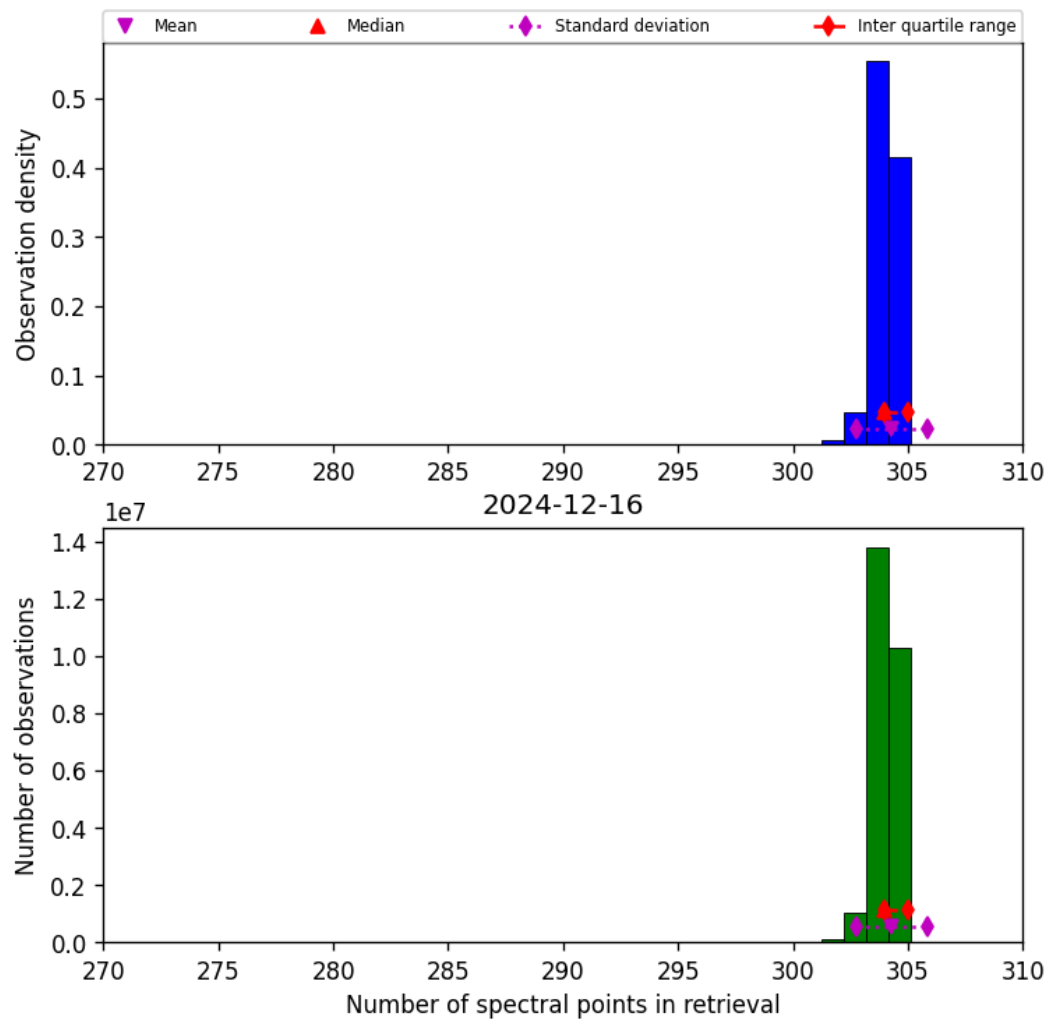
Figure 33: Histogram of “Number of spectral points in retrieval” for 2024-12-16 to 2024-12-17
