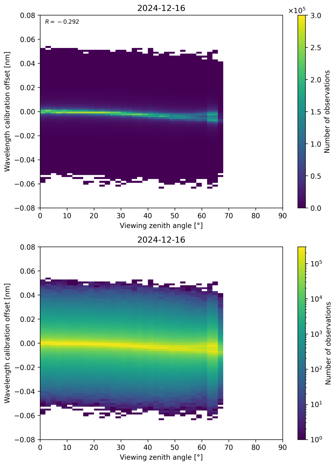
Figure 173: Scatter density plot of “Viewing zenith angle” against “Wavelength calibration offset” for 2024-12-16 to 2024-12-17.
