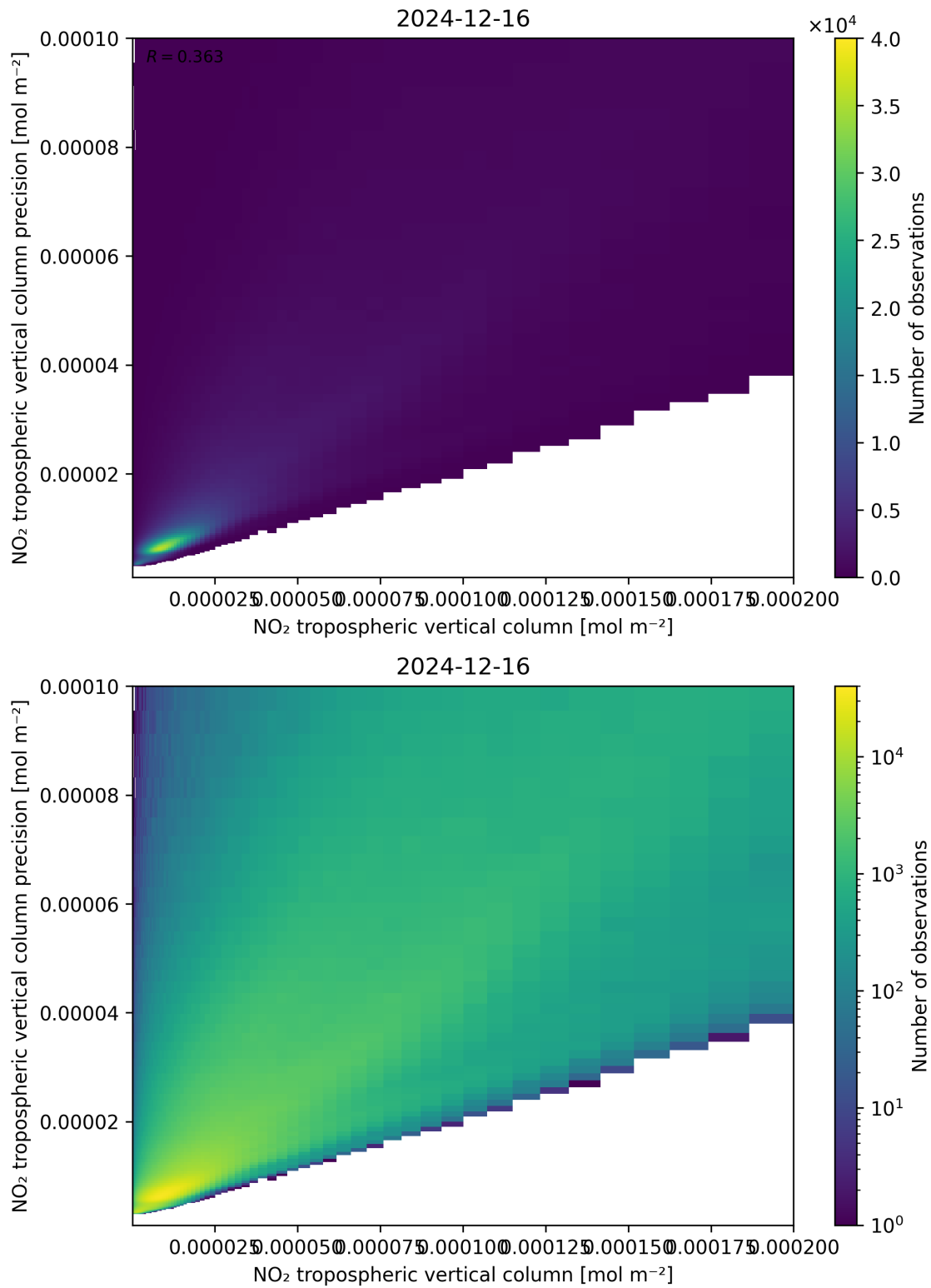
Figure 130: Scatter density plot of “NO 2 tropospheric vertical column” against “NO 2 tropospheric vertical column precision” for 2024-12-16 to 2024-12-17.
