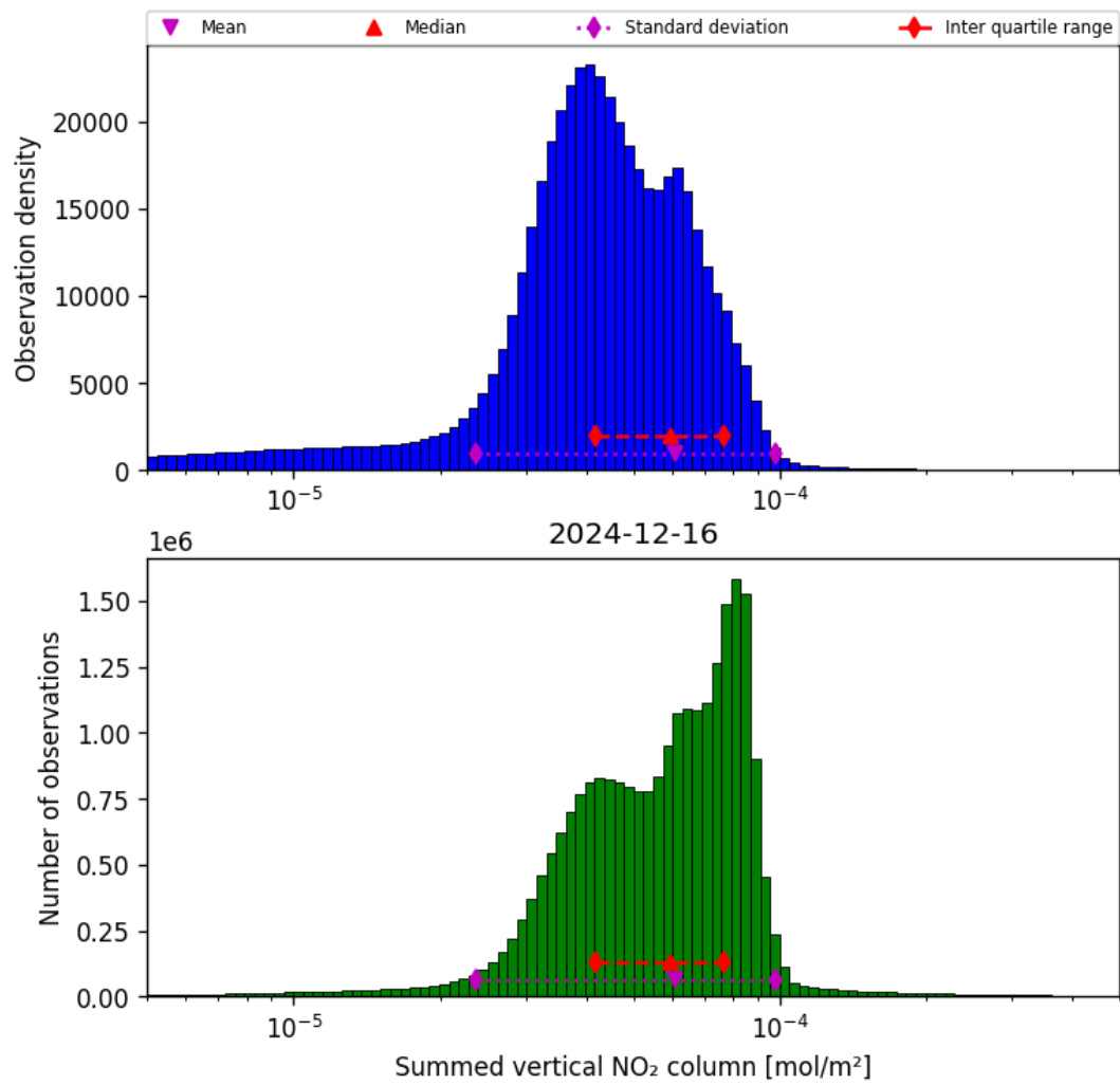
Figure 40: Histogram of “Summed vertical NO 2 column” for 2024-12-16 to 2024-12-17
