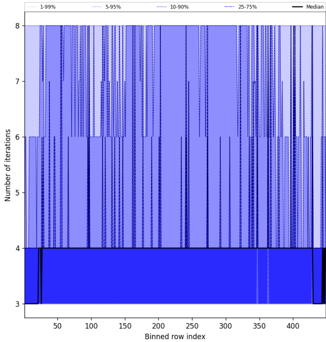
Figure 51: Along track statistics of “Number of iterations” for 2024-12-16 to 2024-12-17
