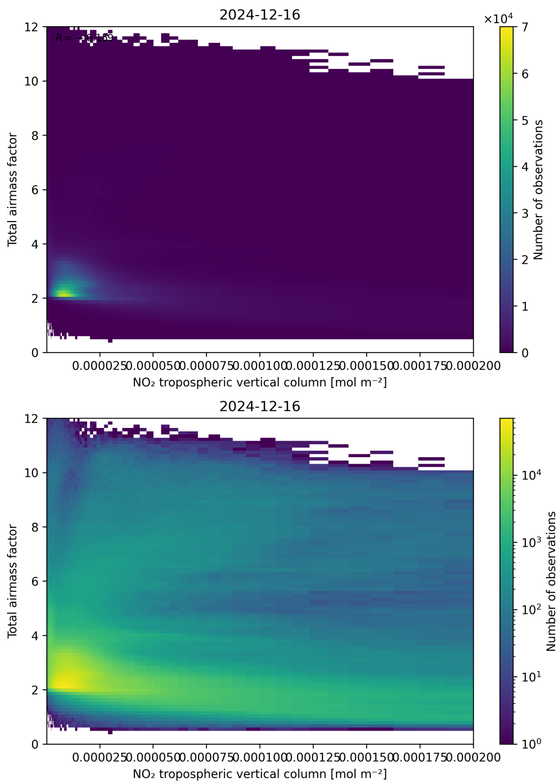
Figure 122: Scatter density plot of “NO 2 tropospheric vertical column” against “Total airmass factor” for 2024-12-16 to 2024-12-17.
