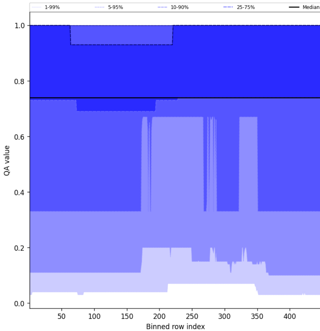
Figure 45: Along track statistics of “QA value” for 2024-12-16 to 2024-12-17
