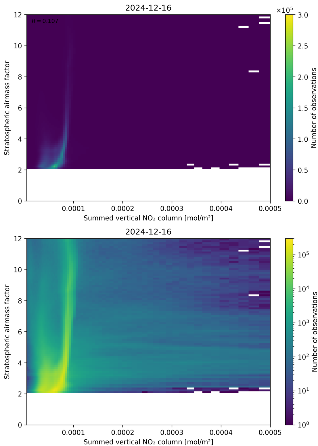
Figure 103: Scatter density plot of “Summed vertical NO 2 column” against “Stratospheric airmass factor” for 2024-12-16 to 2024-12-17.
