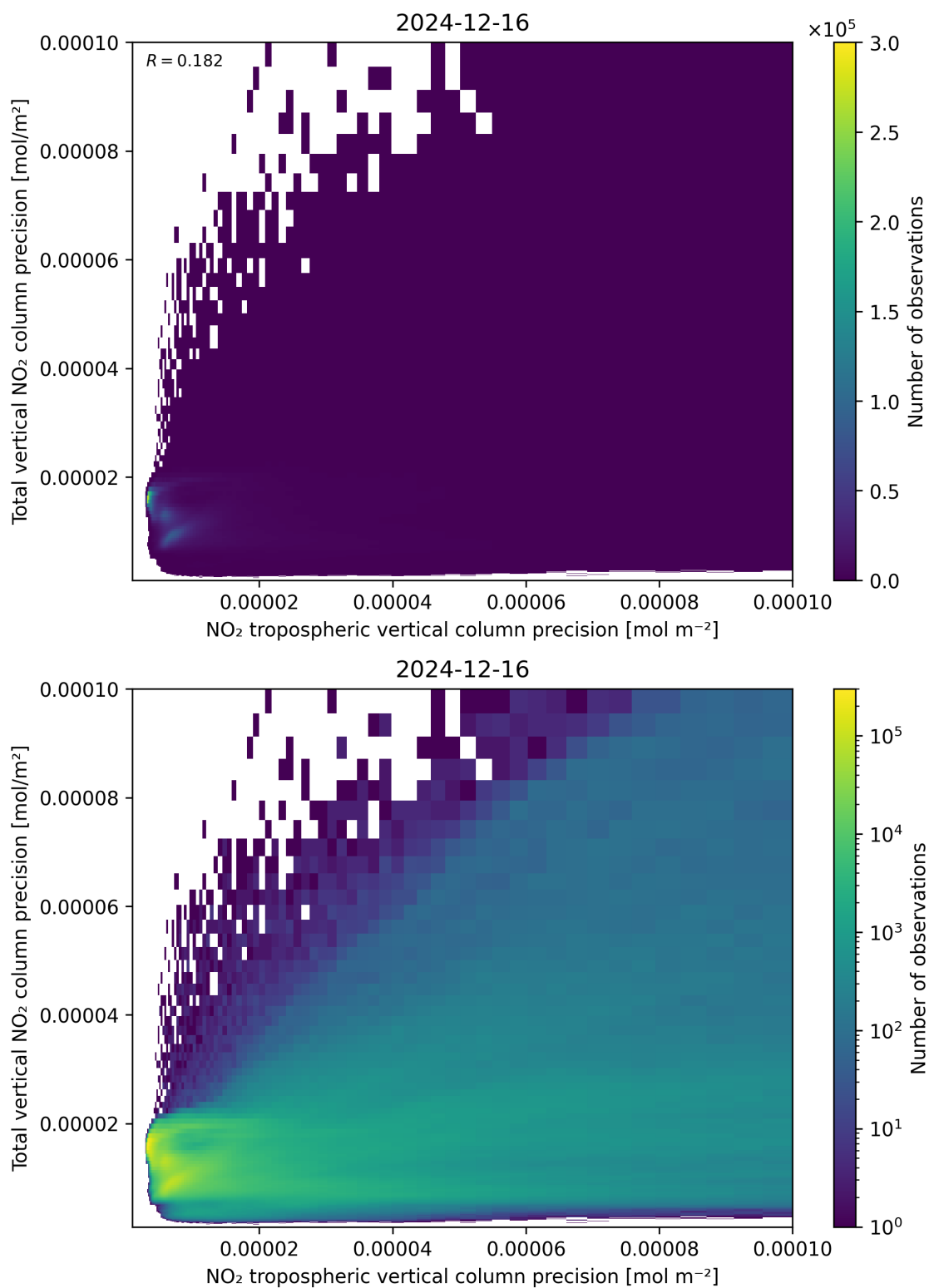
Figure 139: Scatter density plot of “NO 2 tropospheric vertical column precision” against “Total vertical NO 2 column precision” for 2024-12-16 to 2024-12-17.
