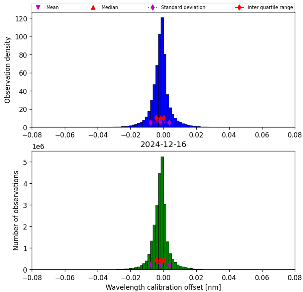
Figure 35: Histogram of “Wavelength calibration offset” for 2024-12-16 to 2024-12-17
