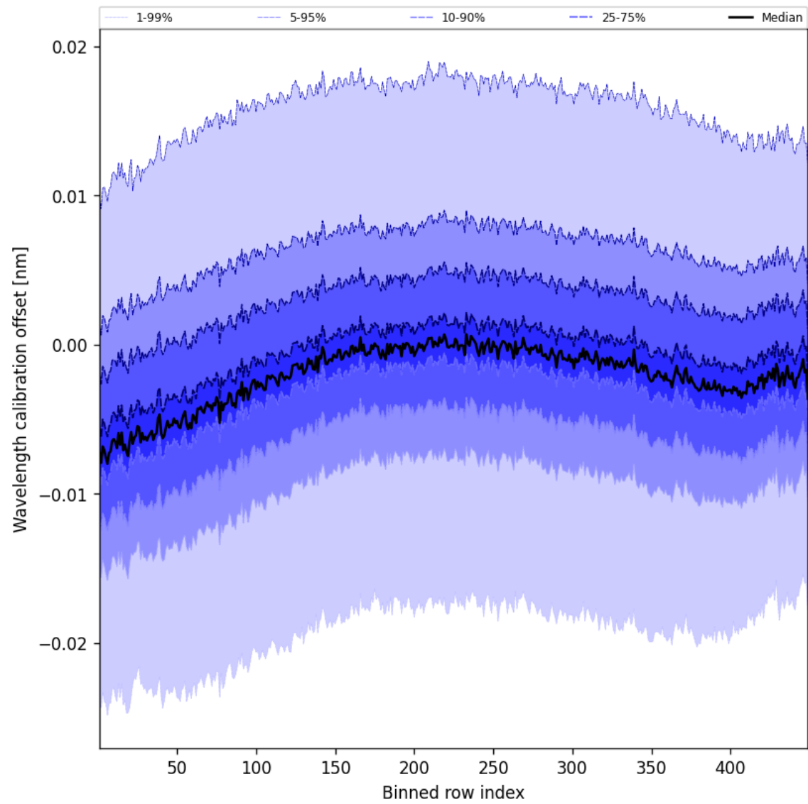
Figure 52: Along track statistics of “Wavelength calibration offset” for 2024-12-16 to 2024-12-17
