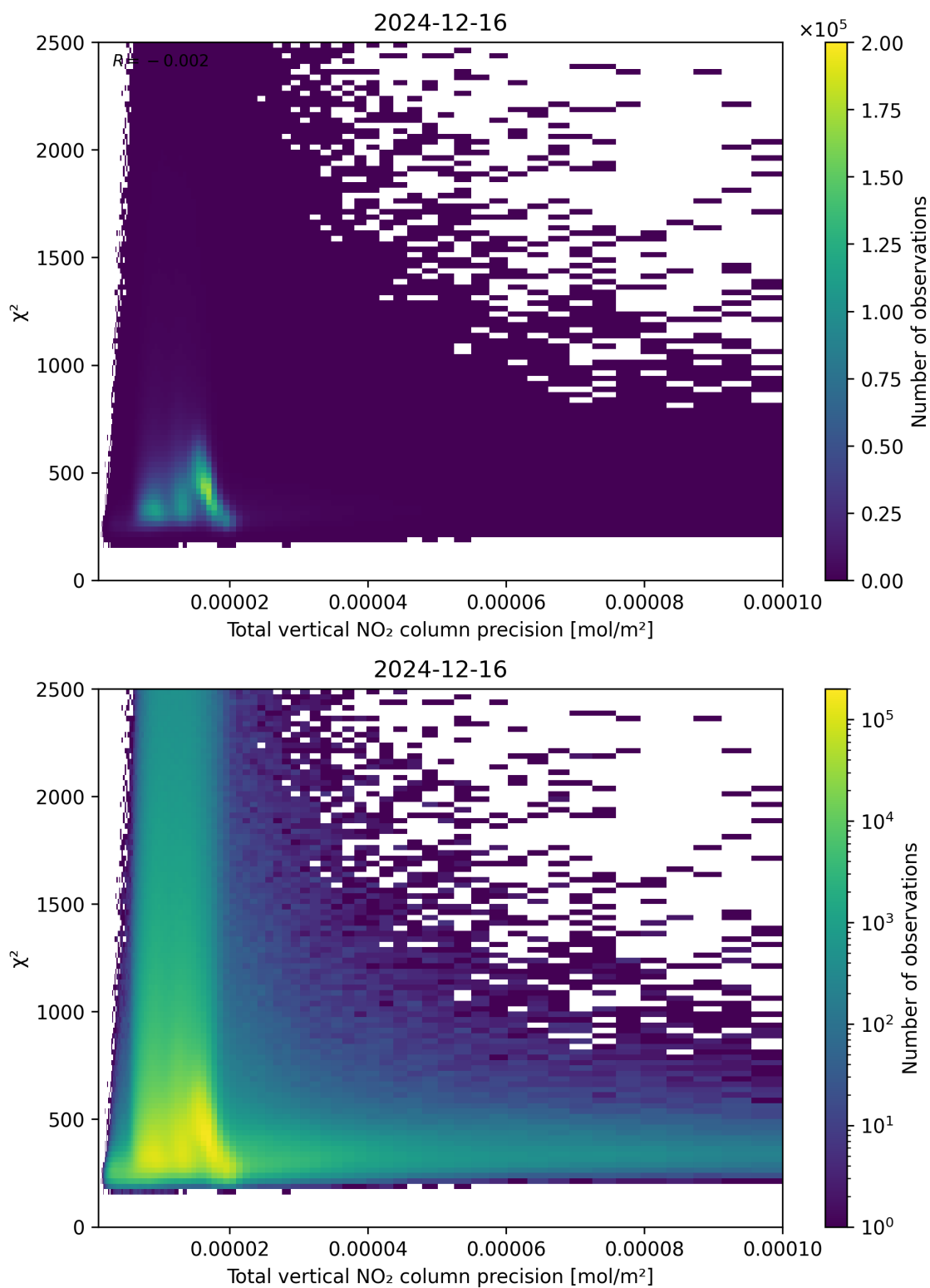
Figure 116: Scatter density plot of “Total vertical NO 2 column precision” against “ \chi^2 ” for 2024-12-16 to 2024-12-17.
