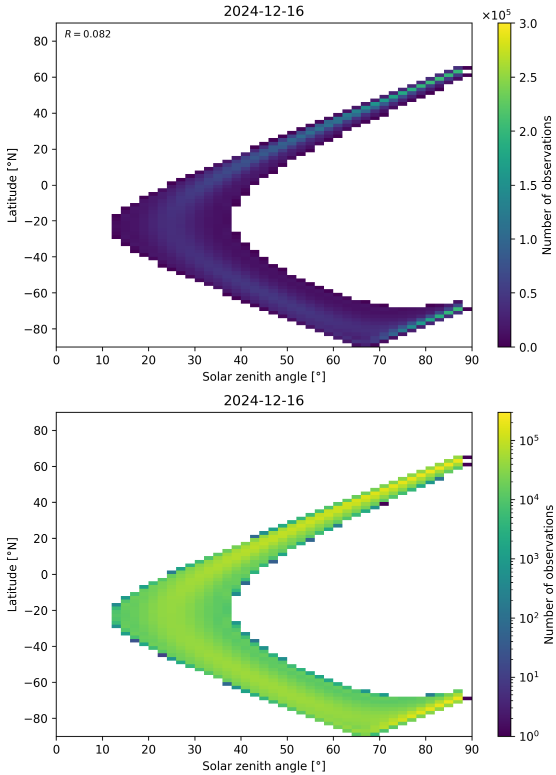
Figure 149: Scatter density plot of “Solar zenith angle” against “Latitude” for 2024-12-16 to 2024-12-17.
