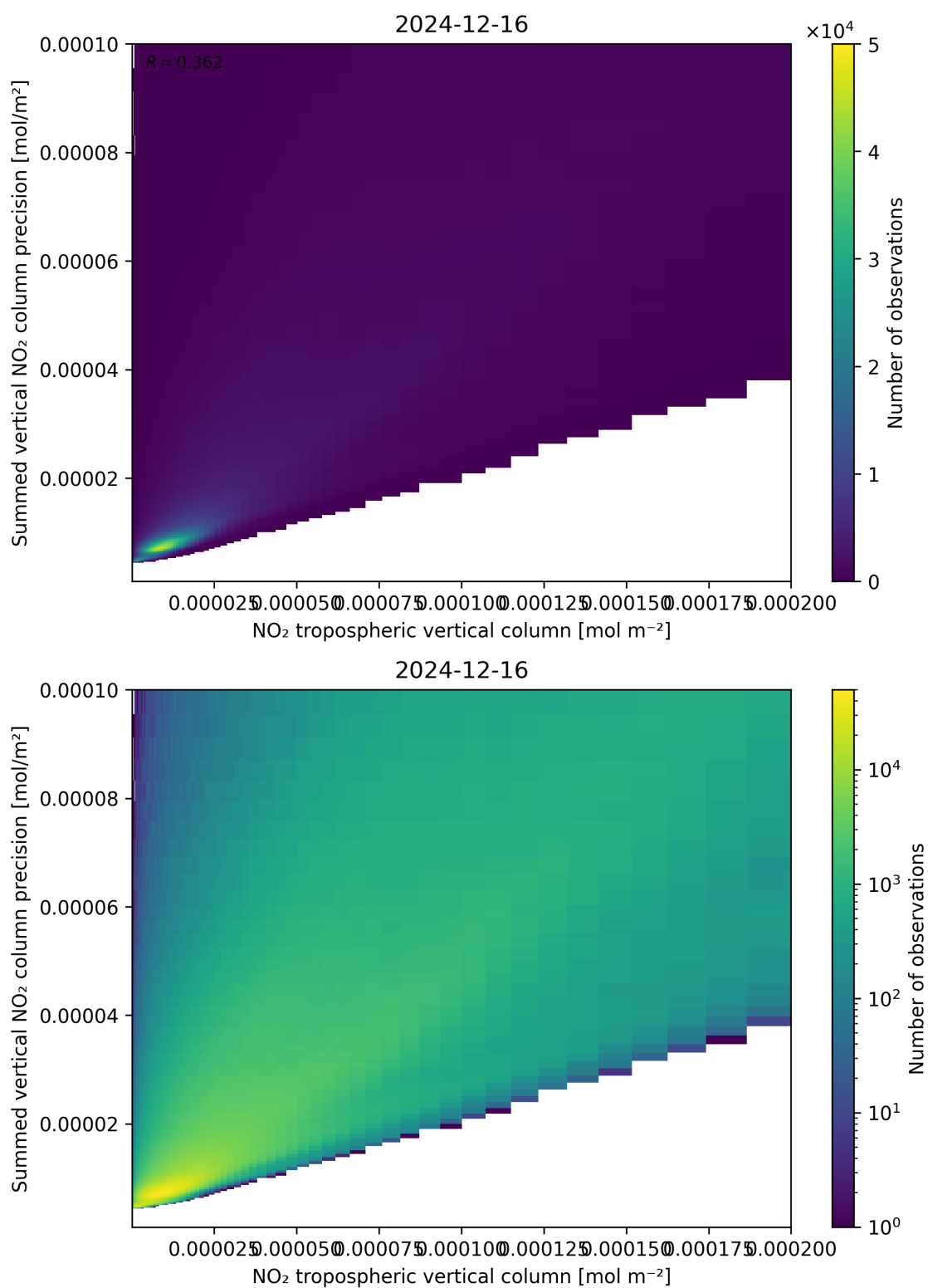
Figure 127: Scatter density plot of “NO 2 tropospheric vertical column” against “Summed vertical NO 2 column precision” for 2024-12-16 to 2024-12-17.
