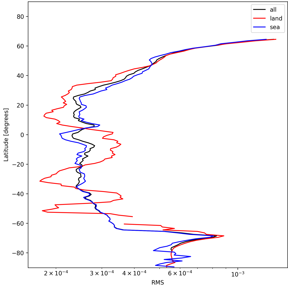
Figure 26: Zonal average of “RMS” for 2024-12-16 to 2024-12-17.
