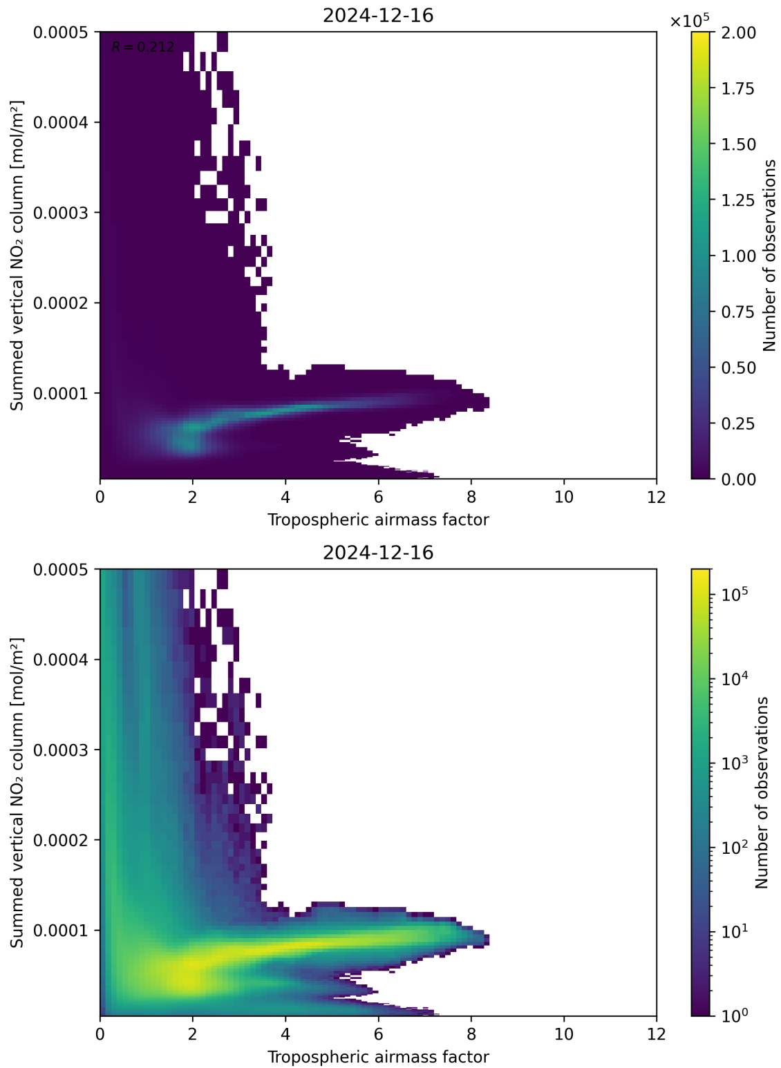
Figure 75: Scatter density plot of “Tropospheric air mass factor” against “Summed vertical NO 2 column” for 2024-12-16 to 2024-12-17.
