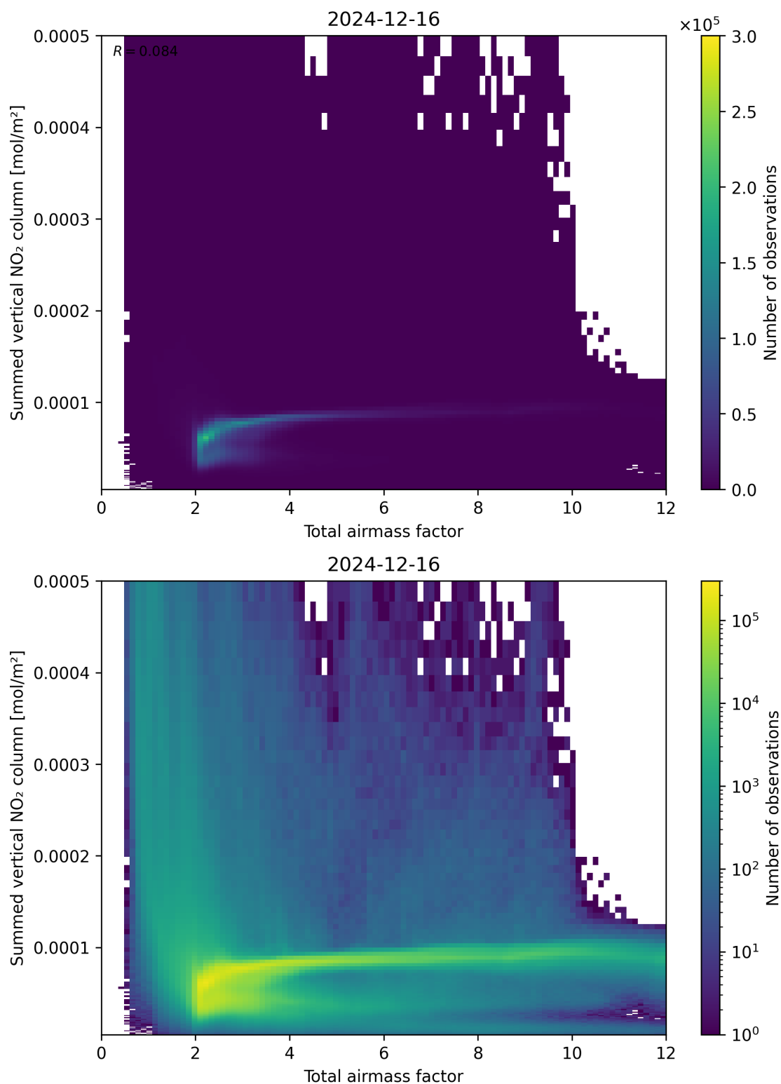
Figure 65: Scatter density plot of “Total airmass factor” against “Summed vertical NO 2 column” for 2024-12-16 to 2024-12-17.
