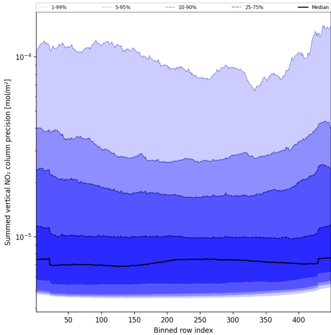
Figure 58: Along track statistics of “Summed vertical NO 2 column precision” for 2024-12-16 to 2024-12-17
