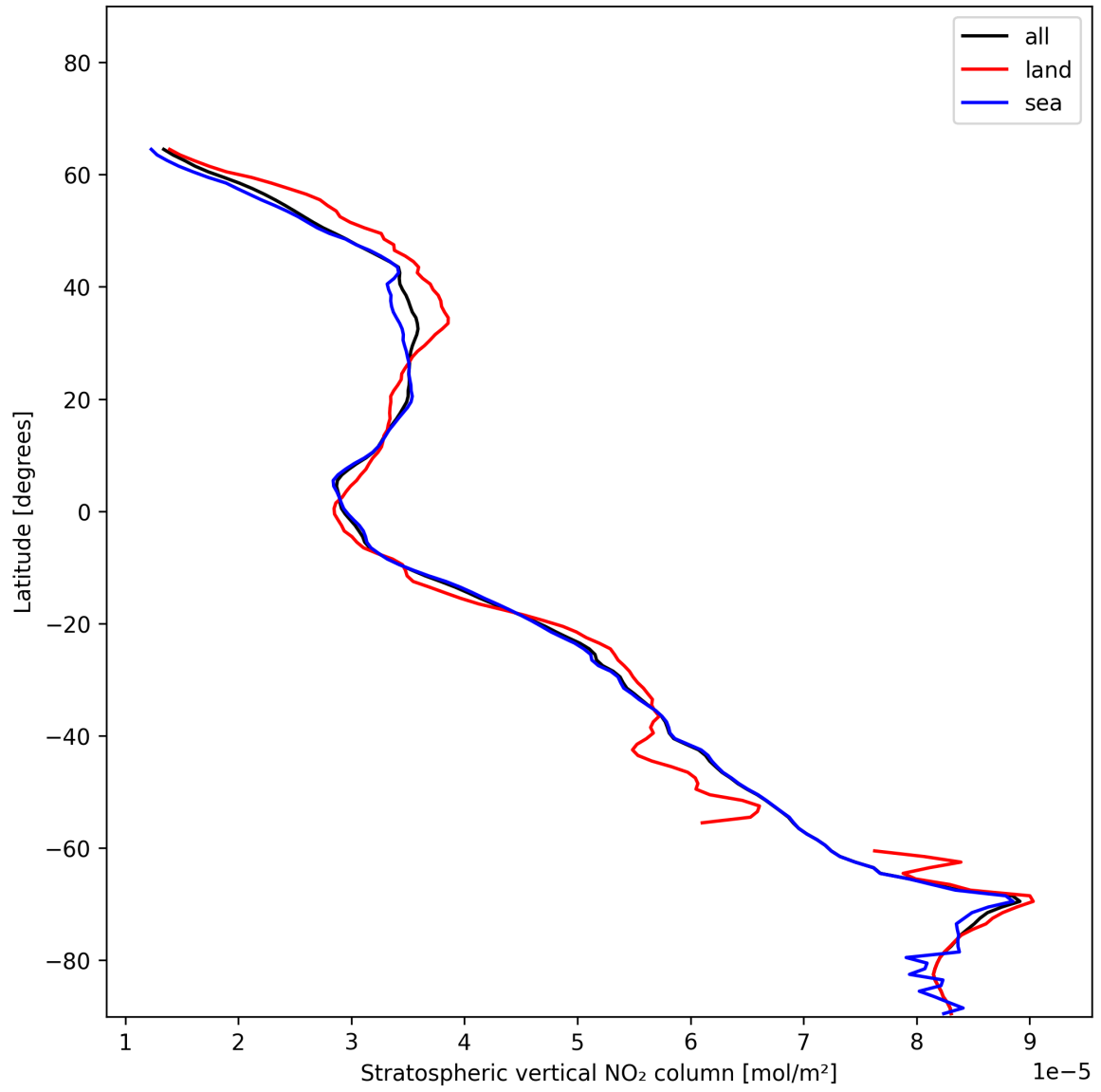
Figure 19: Zonal average of “Stratospheric vertical NO 2 column” for 2024-12-16 to 2024-12-17.
