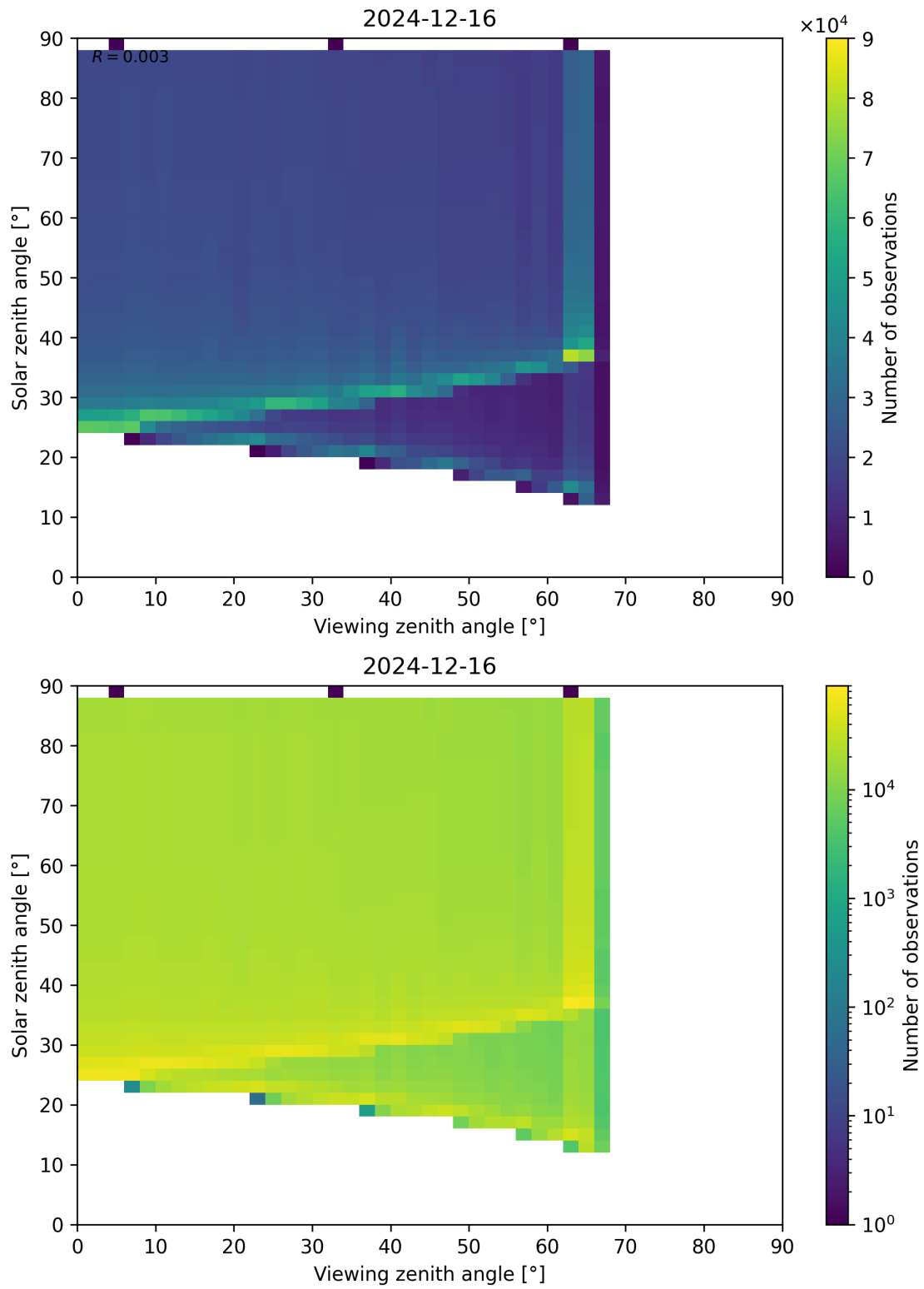
Figure 172: Scatter density plot of “Viewing zenith angle” against “Solar zenith angle” for 2024-12-16 to 2024-12-17.
