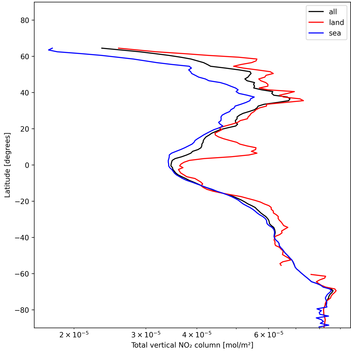
Figure 21: Zonal average of “Total vertical NO 2 column” for 2024-12-16 to 2024-12-17.
