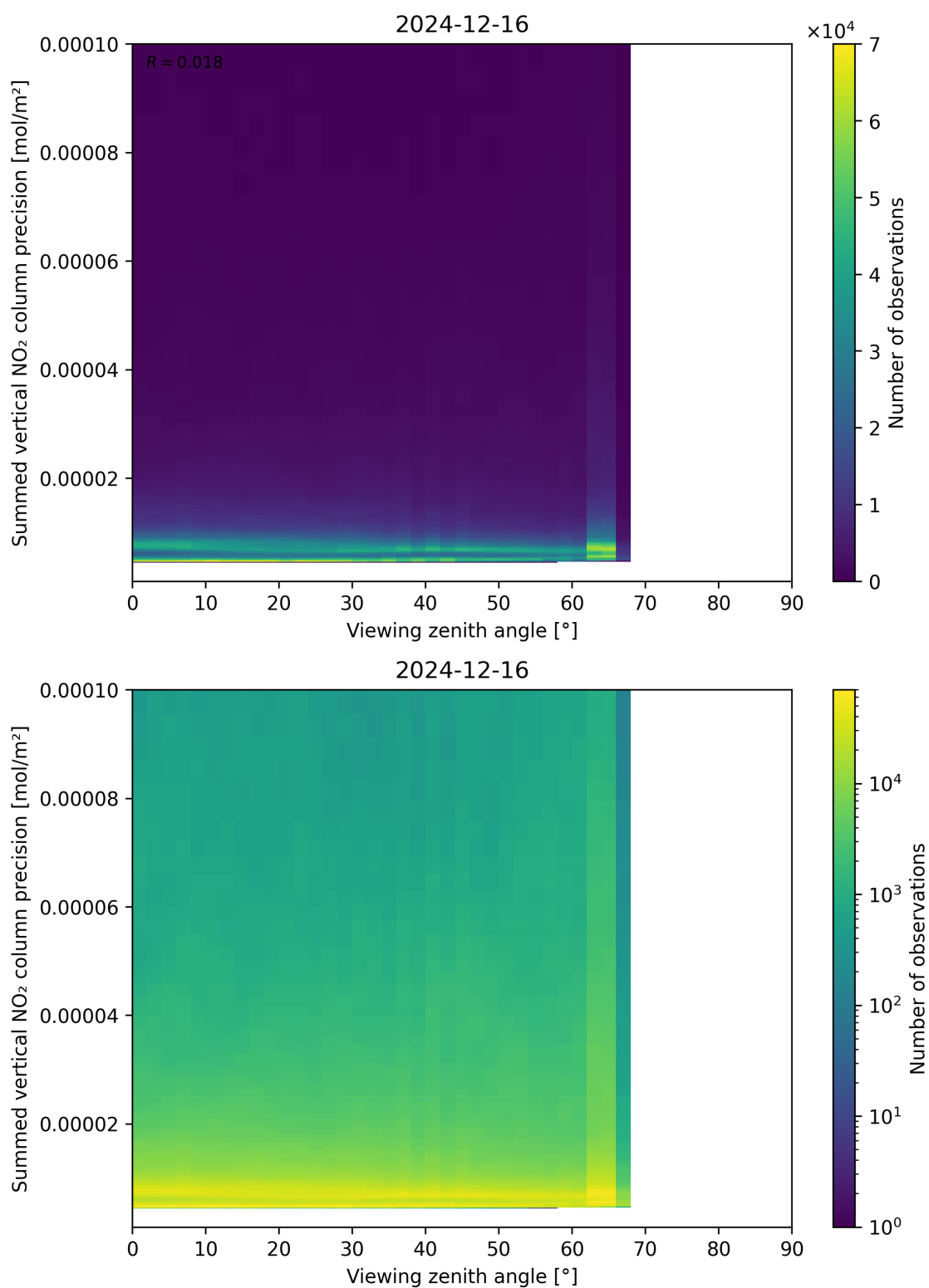
Figure 166: Scatter density plot of “Viewing zenith angle” against “Summed vertical NO 2 column precision” for 2024-12-16 to 2024-12-17.
