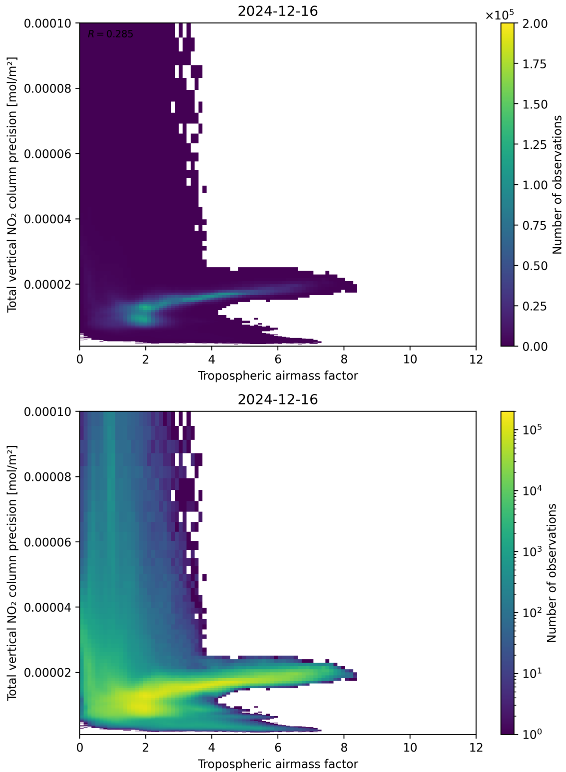
Figure 78: Scatter density plot of “Tropospheric air mass factor” against “Total vertical NO 2 column precision” for 2024-12-16 to 2024-12-17.
