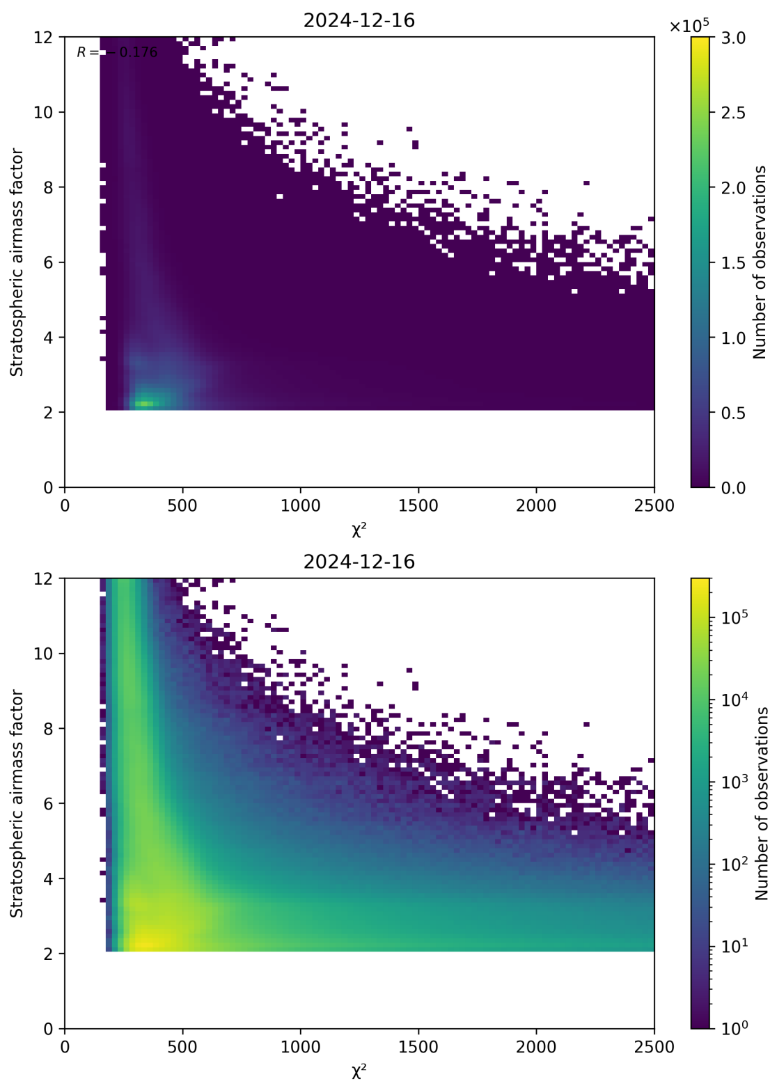
Figure 81: Scatter density plot of “ \chi^2 ” against “Stratospheric airmass factor” for 2024-12-16 to 2024-12-17.
