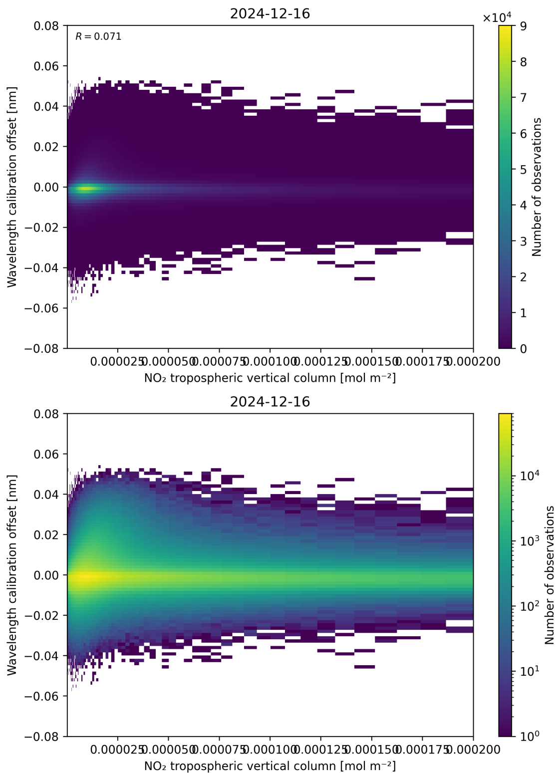
Figure 143: Scatter density plot of “NO 2 tropospheric vertical column” against “Wavelength calibration offset” for 2024-12-16 to 2024-12-17.
