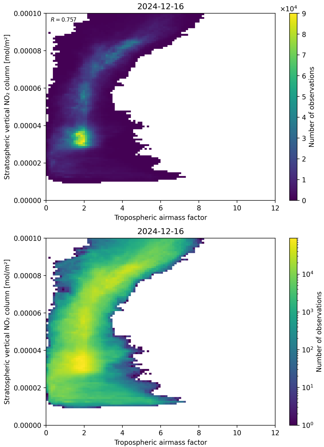
Figure 74: Scatter density plot of “Tropospheric air mass factor” against “Stratospheric vertical NO 2 column” for 2024-12-16 to 2024-12-17.
