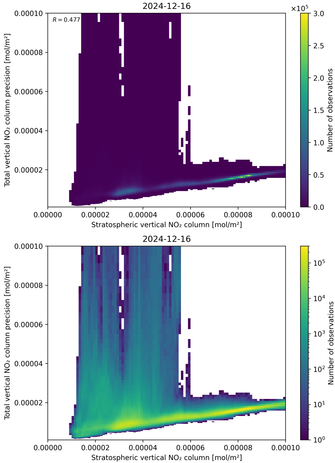
Figure 101: Scatter density plot of “Stratospheric vertical NO 2 column” against “Total vertical NO 2 column precision” for 2024-12-16 to 2024-12-17.
