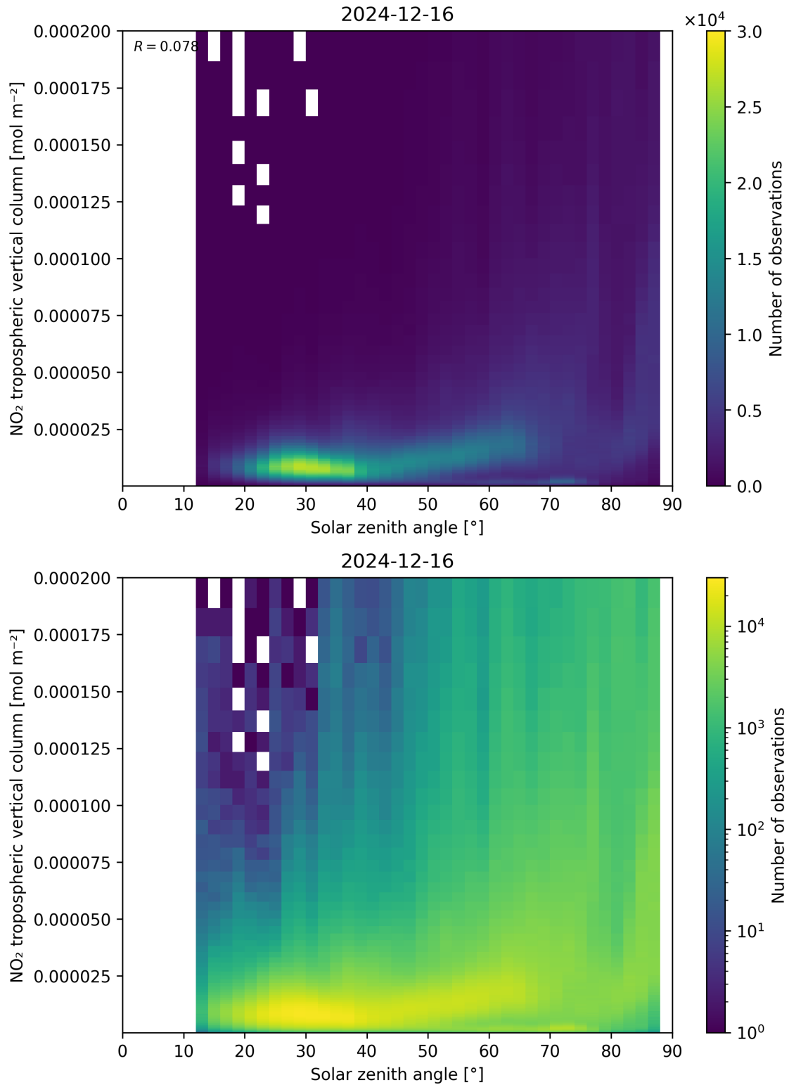
Figure 155: Scatter density plot of “Solar zenith angle” against “NO 2 tropospheric vertical column” for 2024-12-16 to 2024-12-17.
