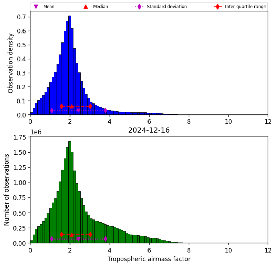
Figure 31: Histogram of “Tropospheric airmass factor” for 2024-12-16 to 2024-12-17
