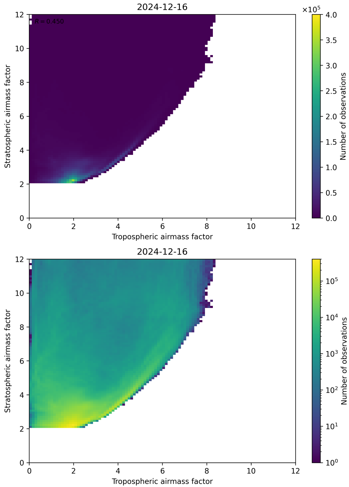
Figure 71: Scatter density plot of “Tropospheric airmass factor” against “Stratospheric airmass factor” for 2024-12-16 to 2024-12-17.
