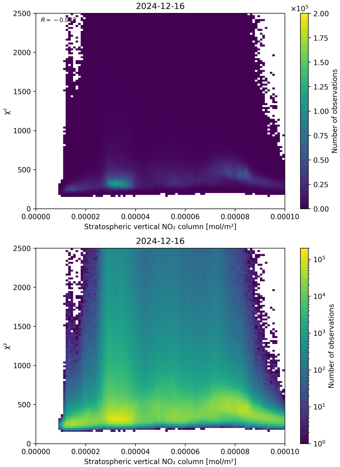
Figure 97: Scatter density plot of “Stratospheric vertical NO 2 column” against “ \chi^2 ” for 2024-12-16 to 2024-12-17.
