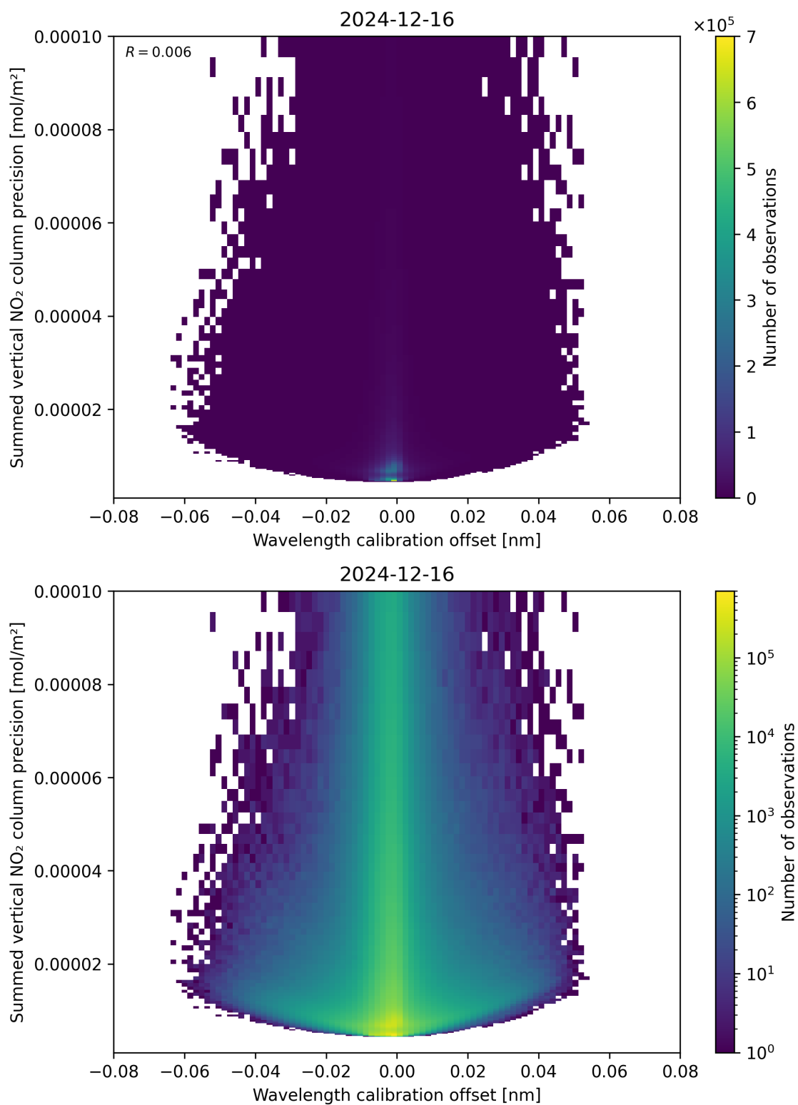
Figure 178: Scatter density plot of “Wavelength calibration offset” against “Summed vertical NO 2 column precision” for 2024-12-16 to 2024-12-17.
