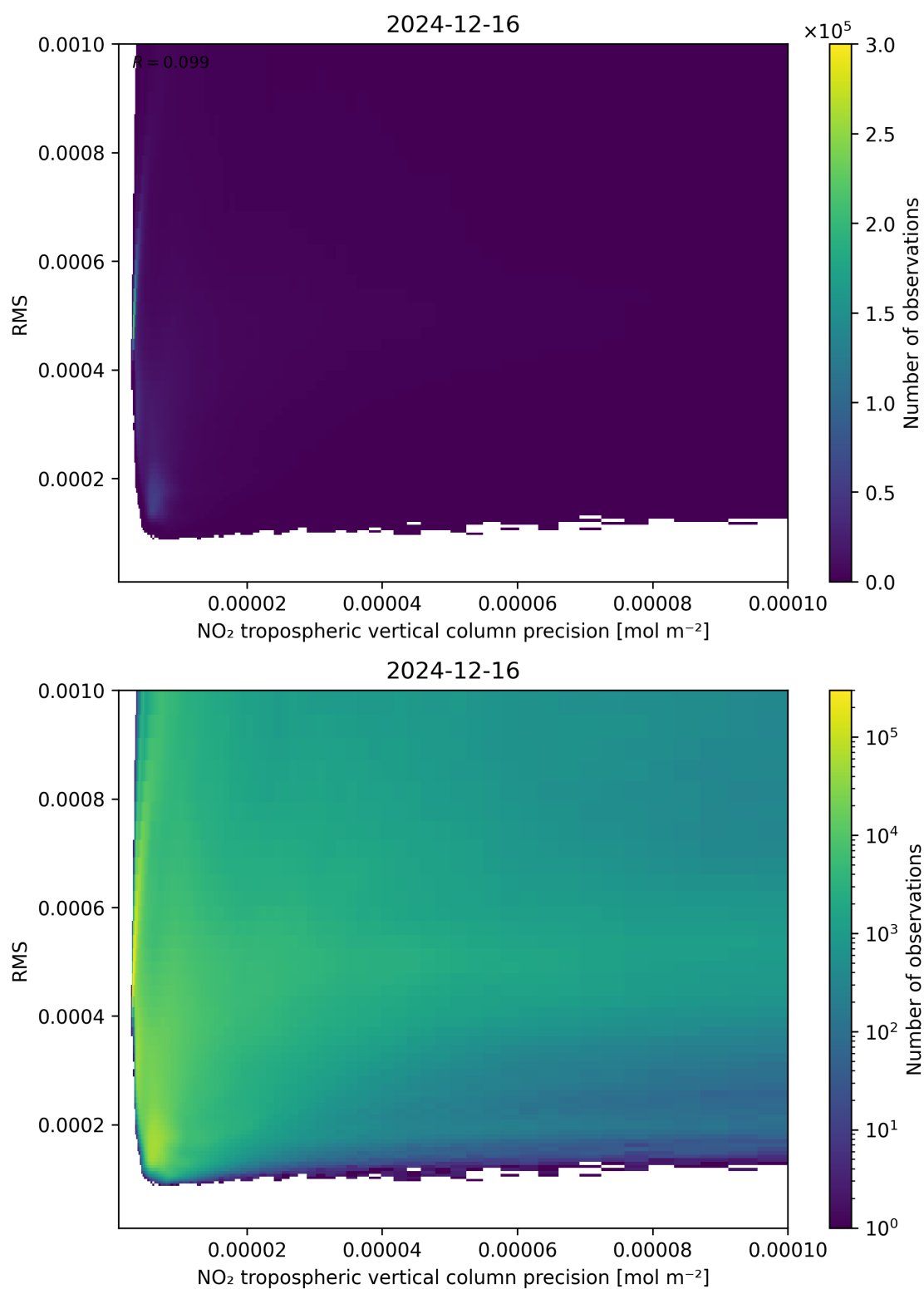
Figure 140: Scatter density plot of “NO 2 tropospheric vertical column precision” against “RMS” for 2024-12-16 to 2024-12-17.
