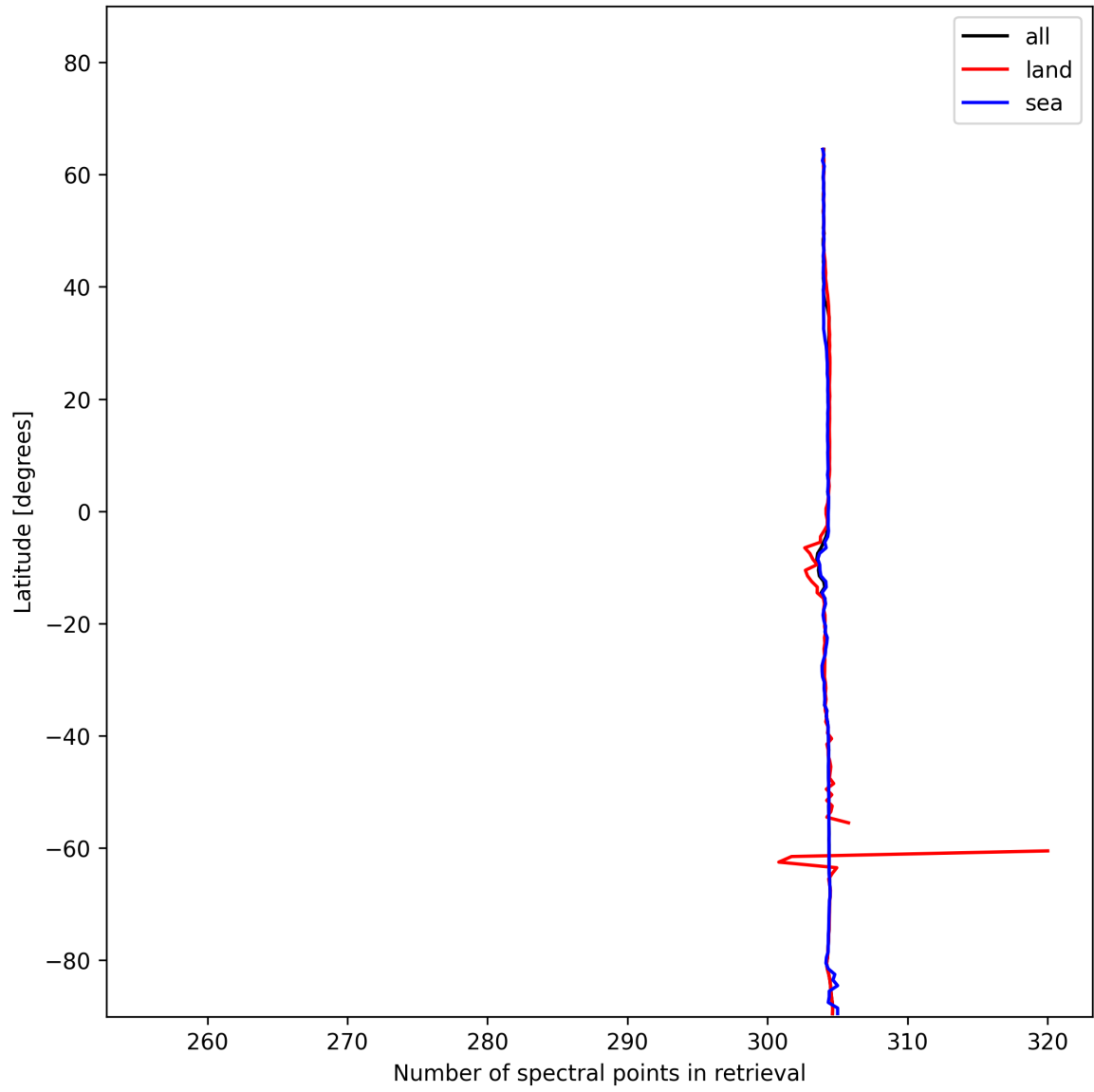
Figure 16: Zonal average of “Number of spectral points in retrieval” for 2024-12-16 to 2024-12-17.
