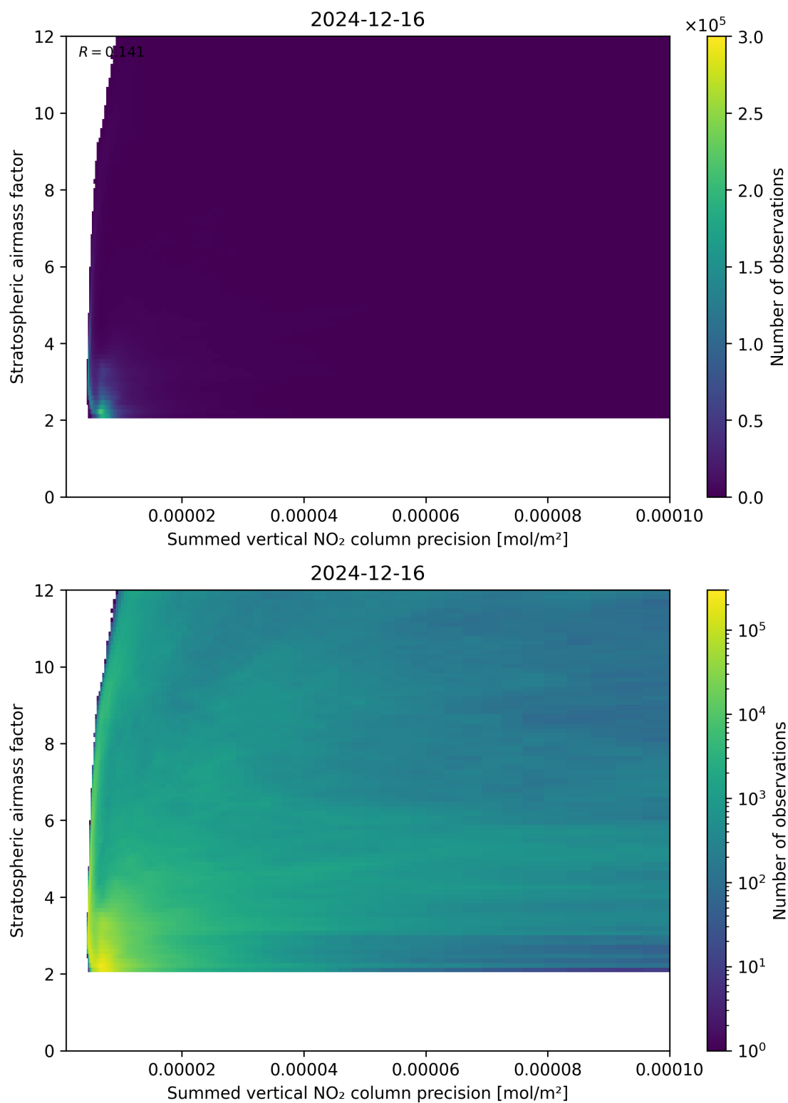
Figure 106: Scatter density plot of “Summed vertical NO 2 column precision” against “Stratospheric airmass factor” for 2024-12-16 to 2024-12-17.
