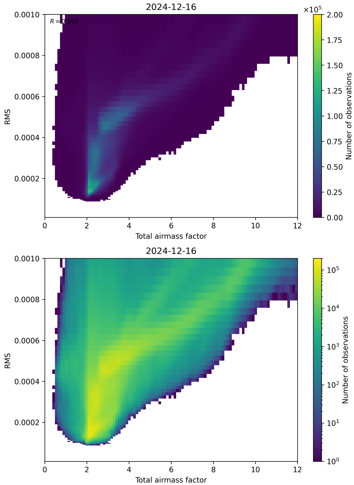
Figure 69: Scatter density plot of “Total airmass factor” against “RMS” for 2024-12-16 to 2024-12-17.
