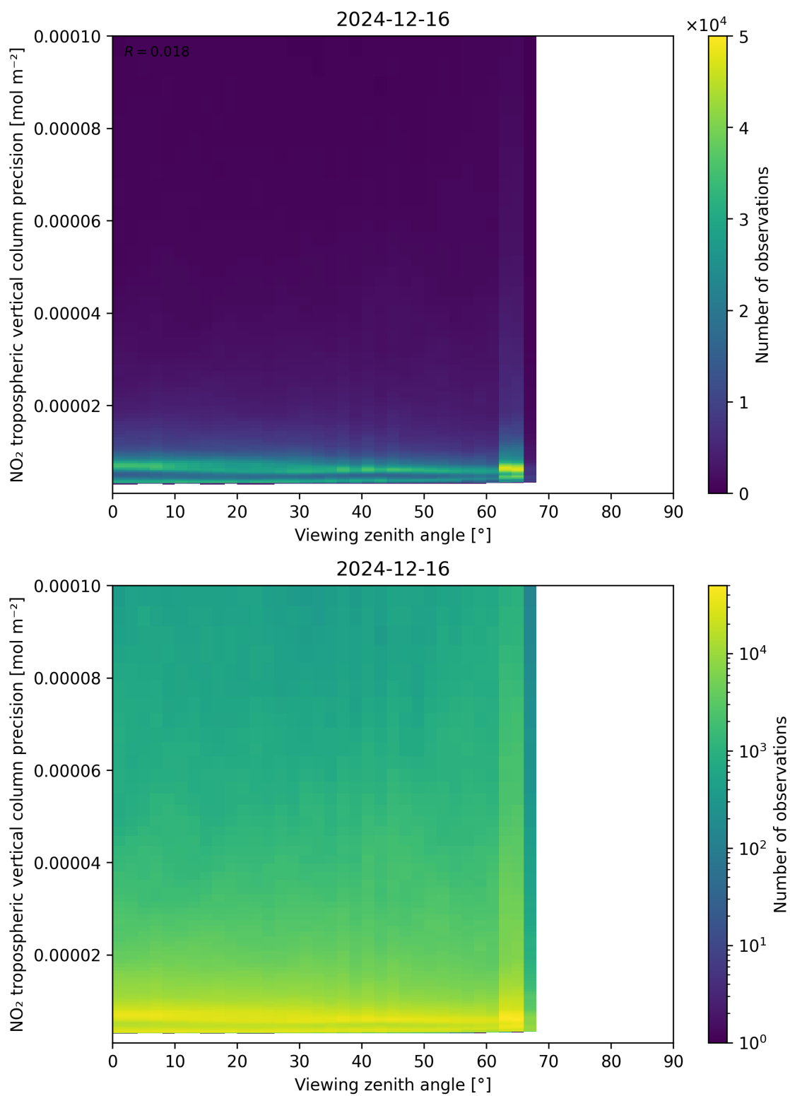
Figure 170: Scatter density plot of “Viewing zenith angle” against “NO 2 tropospheric vertical column precision” for 2024-12-16 to 2024-12-17.
