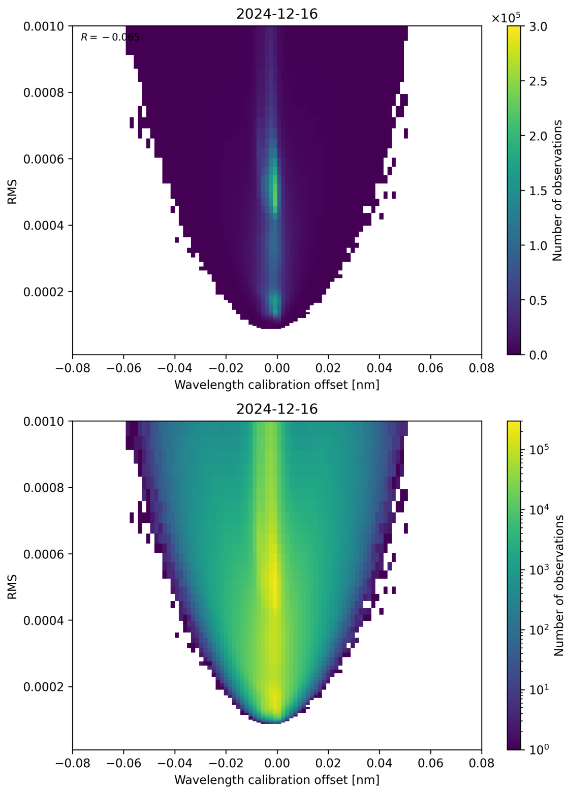
Figure 181: Scatter density plot of “Wavelength calibration offset” against “RMS” for 2024-12-16 to 2024-12-17.
