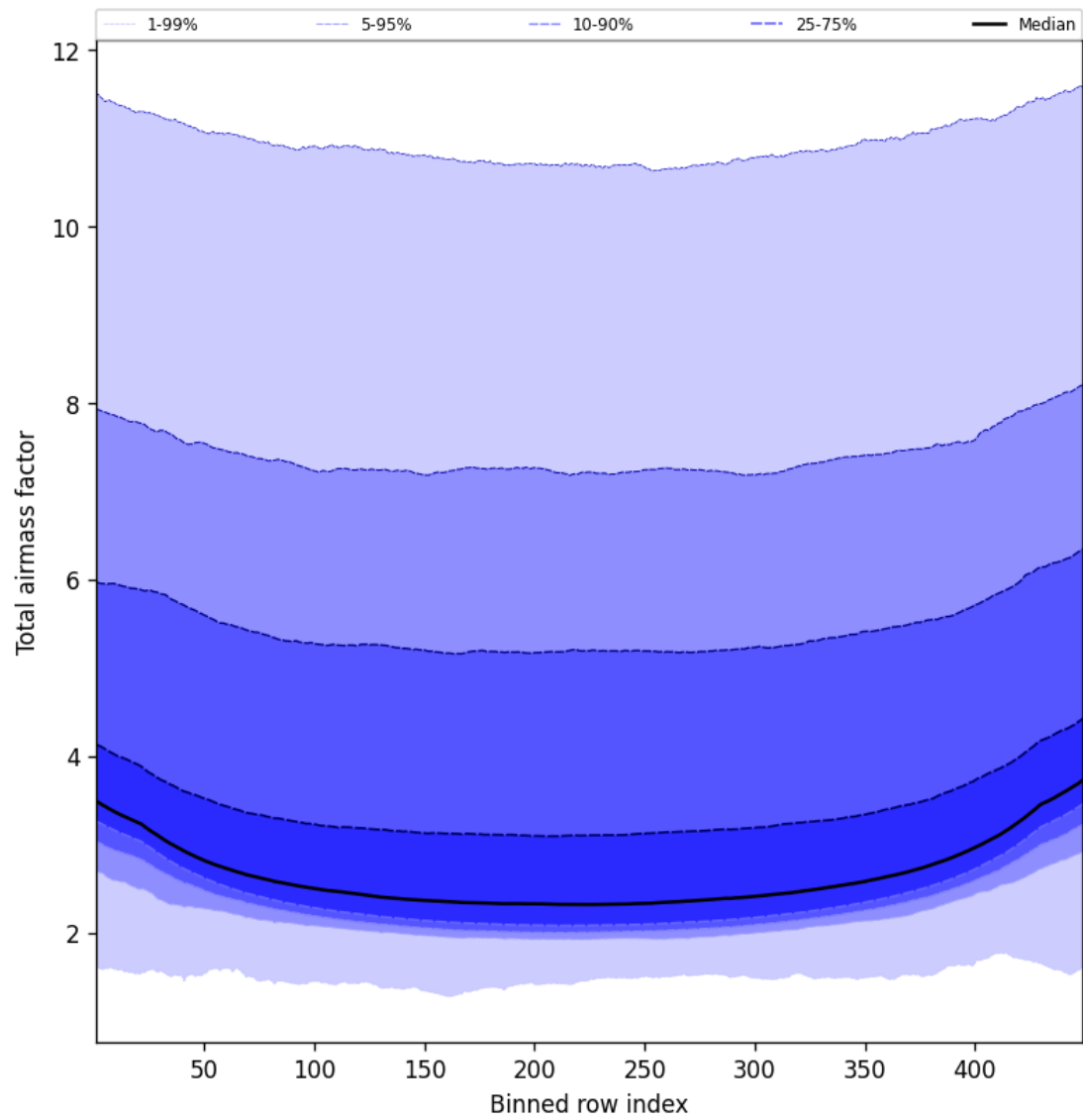
Figure 49: Along track statistics of “Total airmass factor” for 2024-12-16 to 2024-12-17
