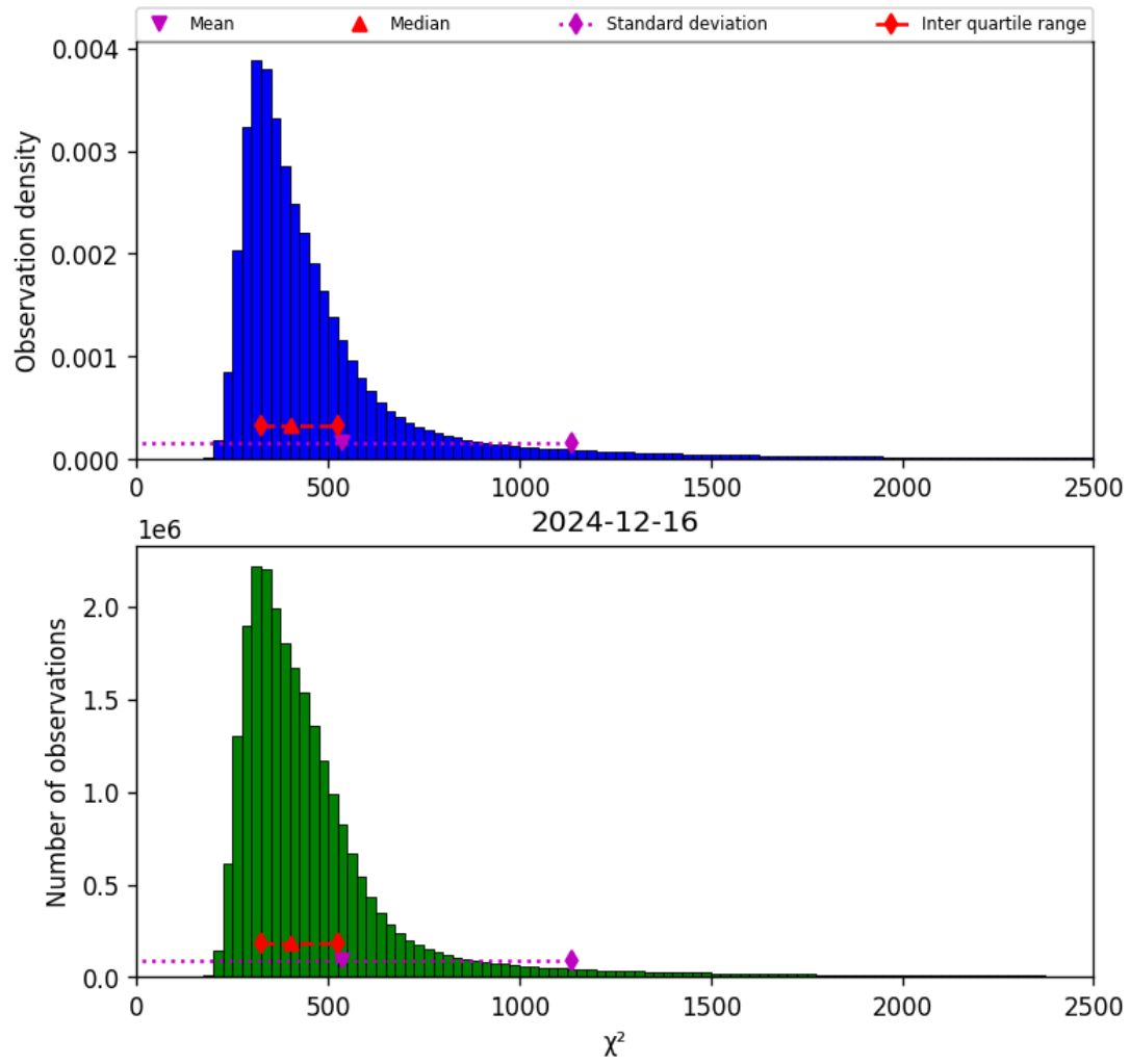
Figure 42: Histogram of “ \chi^2 ” for 2024-12-16 to 2024-12-17
