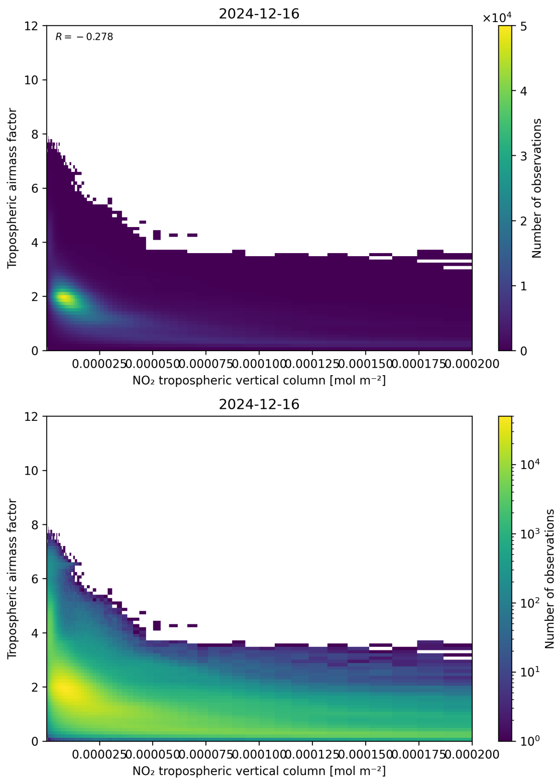
Figure 123: Scatter density plot of “NO 2 tropospheric vertical column” against “Tropospheric air mass factor” for 2024-12-16 to 2024-12-17.
