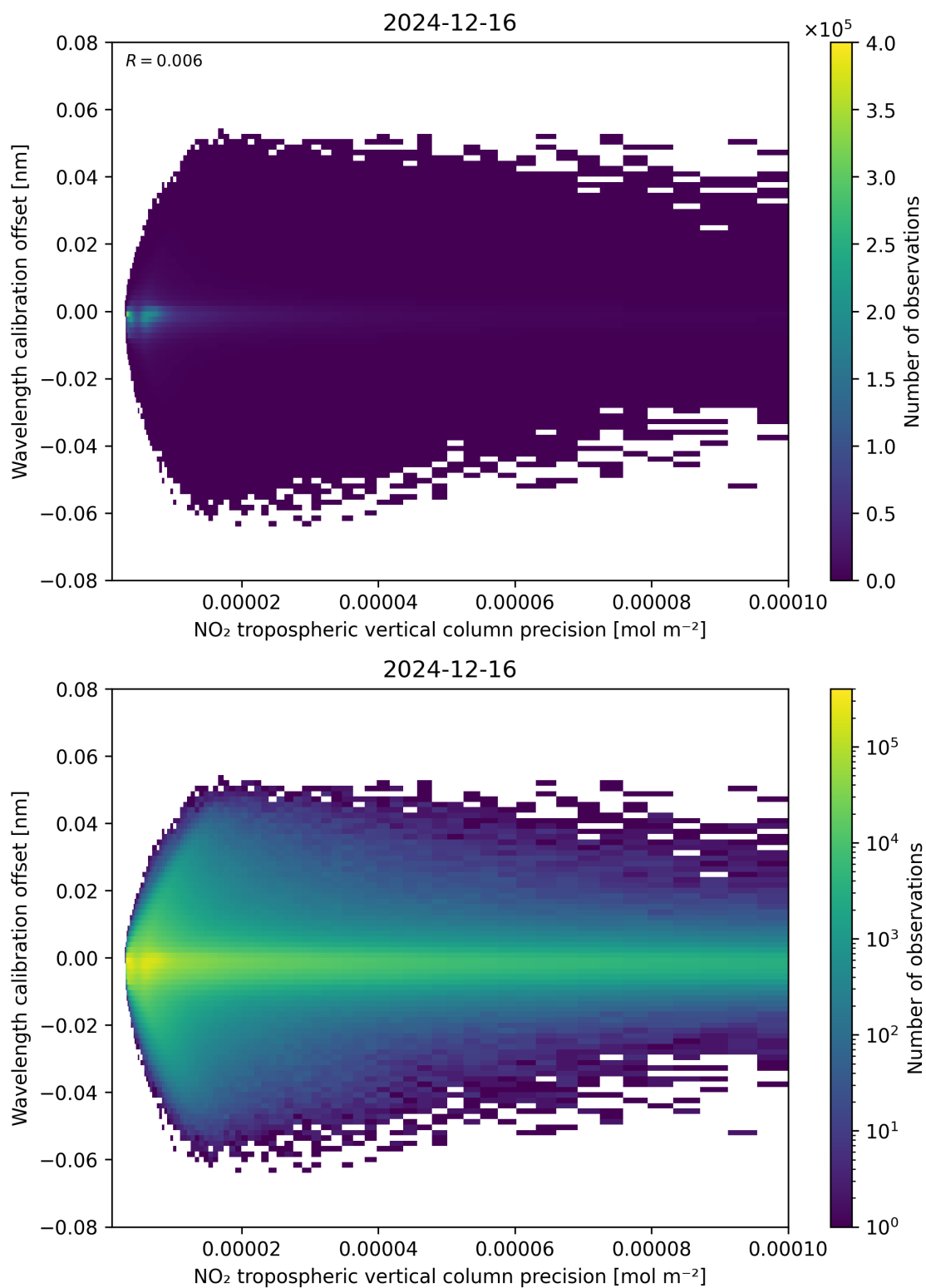
Figure 141: Scatter density plot of “NO 2 tropospheric vertical column precision” against “Wavelength calibration offset” for 2024-12-16 to 2024-12-17.
