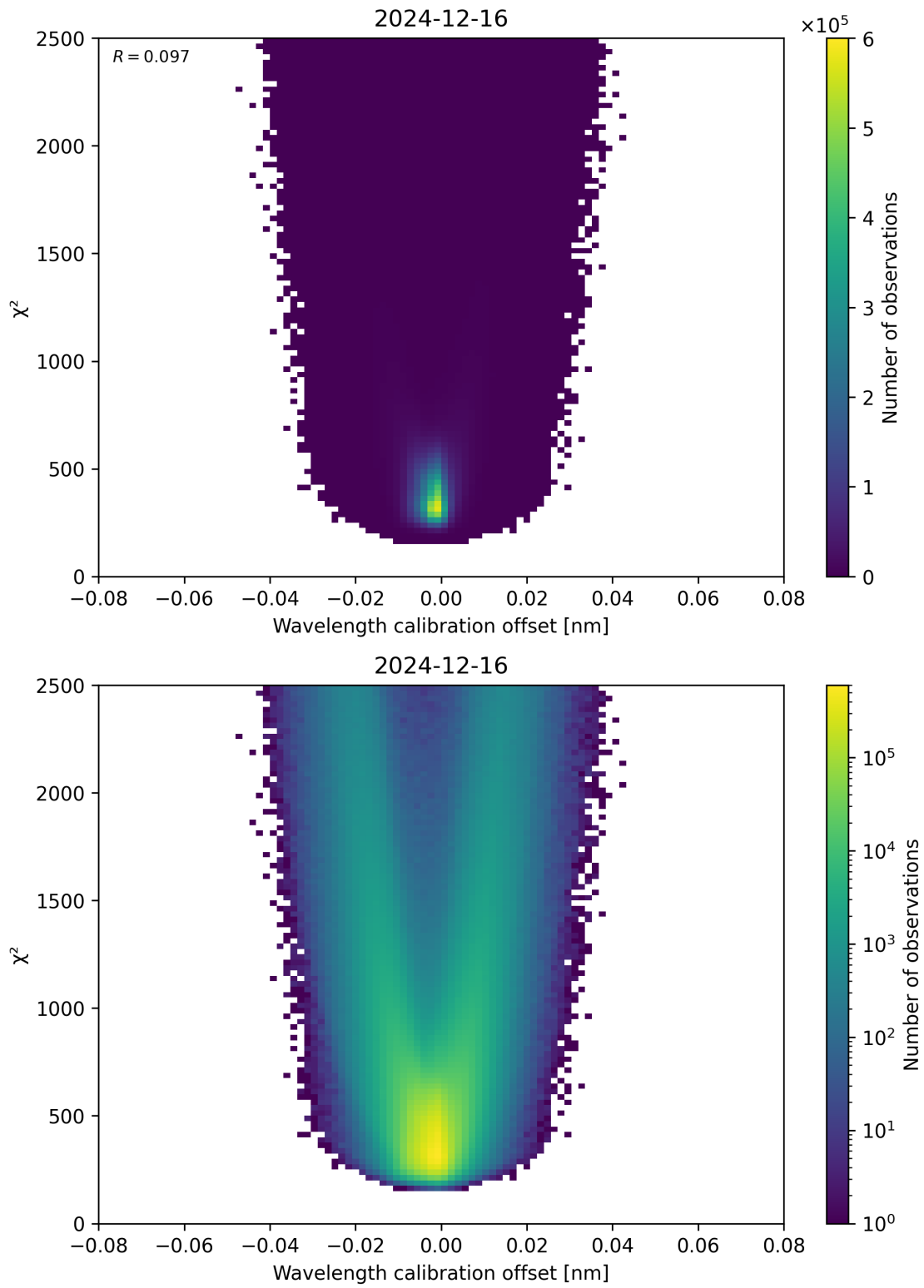
Figure 175: Scatter density plot of “Wavelength calibration offset” against “ \chi^2 ” for 2024-12-16 to 2024-12-17.
