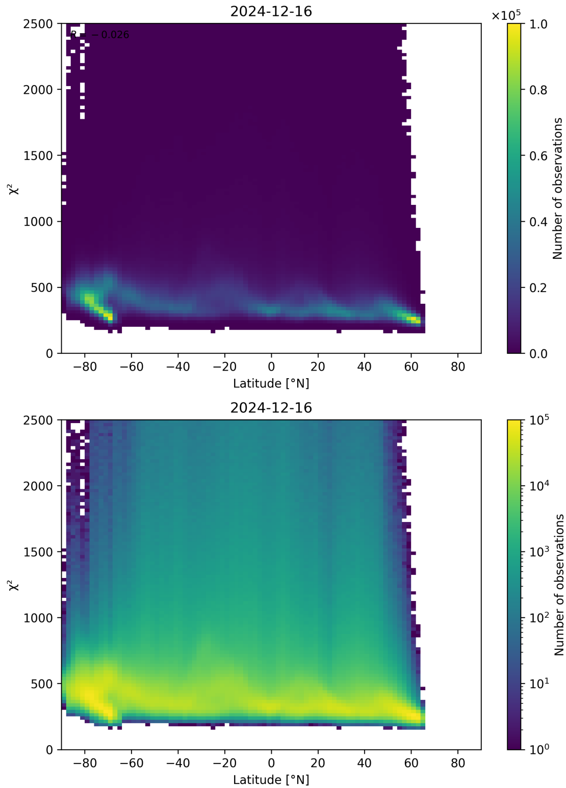
Figure 86: Scatter density plot of “Latitude” against “ \chi^2 ” for 2024-12-16 to 2024-12-17.
