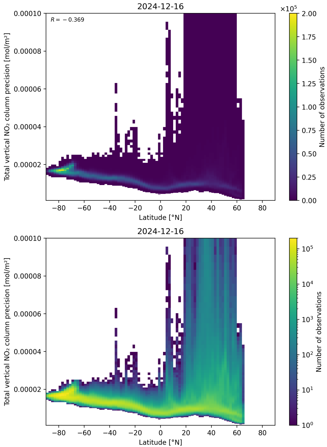
Figure 91: Scatter density plot of “Latitude” against “Total vertical NO 2 column precision” for 2024-12-16 to 2024-12-17.
