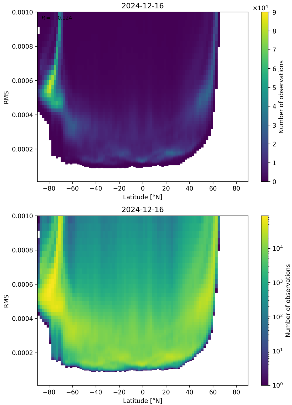
Figure 94: Scatter density plot of “Latitude” against “RMS” for 2024-12-16 to 2024-12-17.
