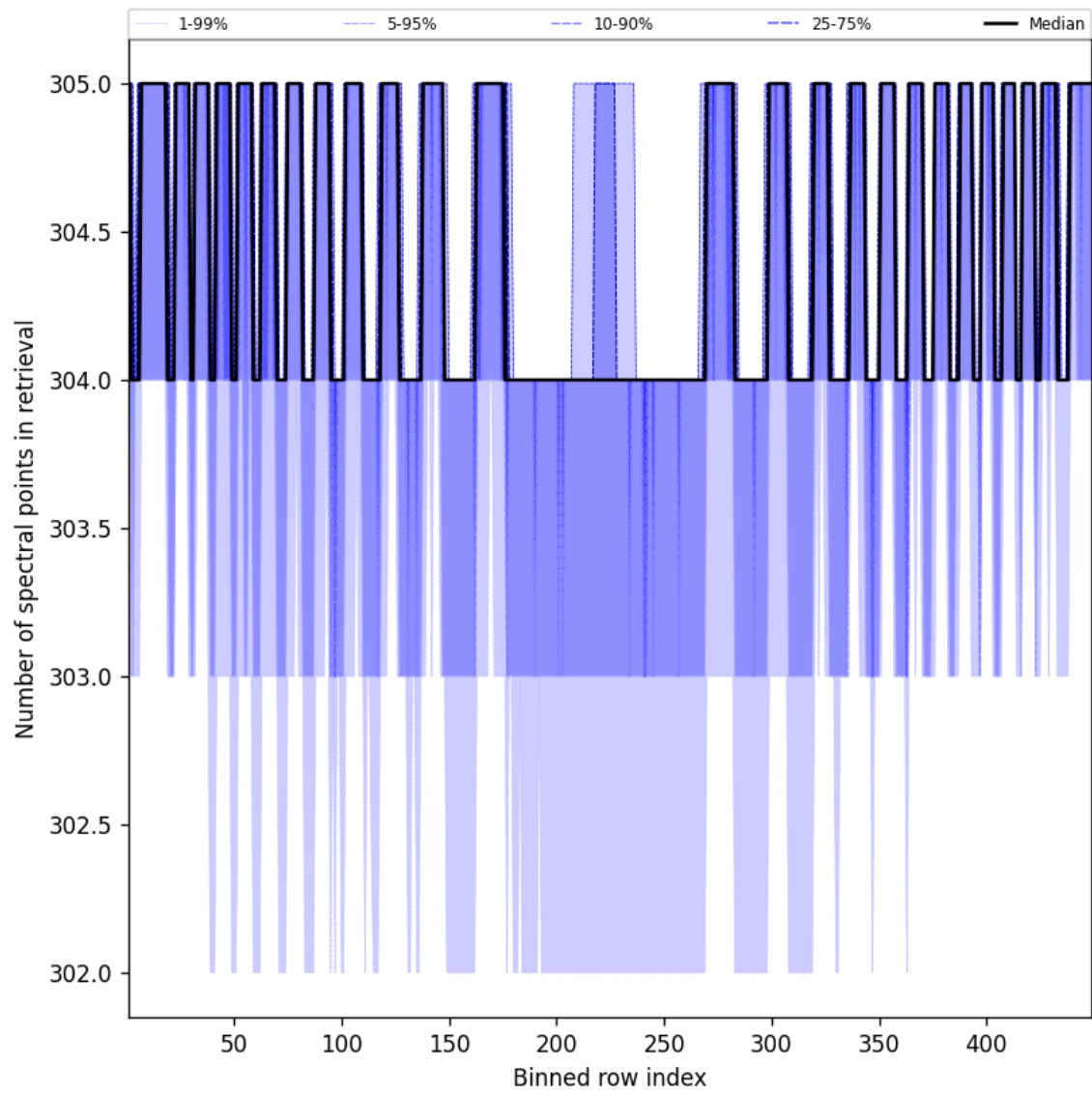
Figure 50: Along track statistics of “Number of spectral points in retrieval” for 2024-12-16 to 2024-12-17
