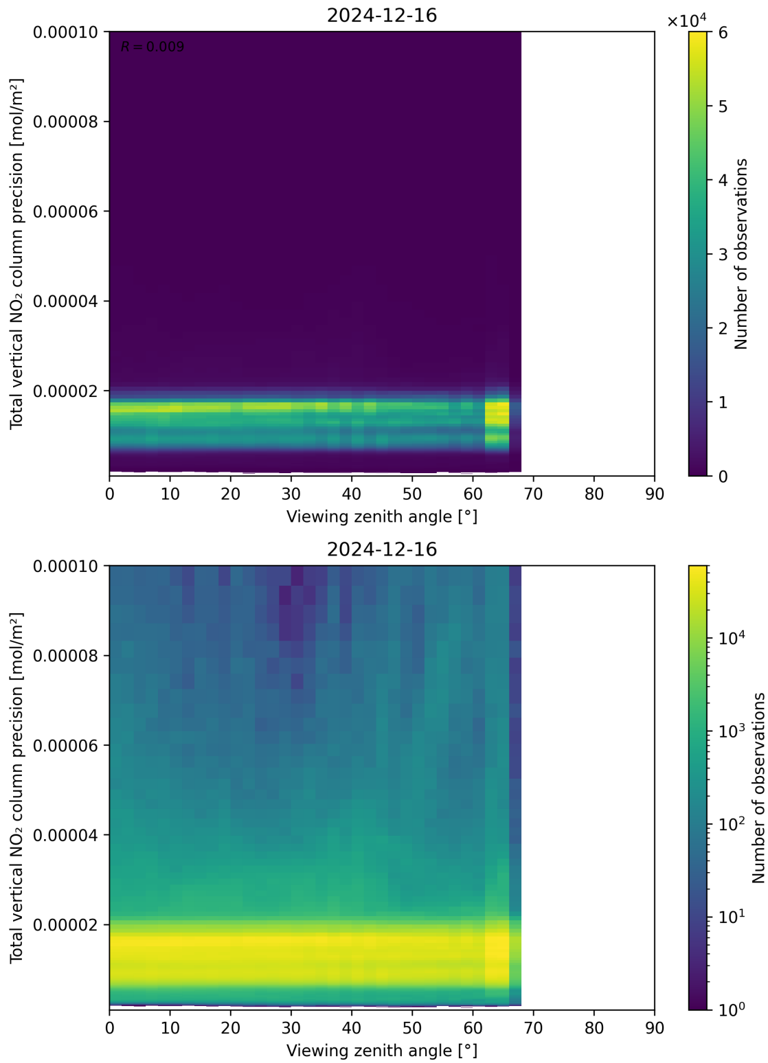
Figure 168: Scatter density plot of “Viewing zenith angle” against “Total vertical NO 2 column precision” for 2024-12-16 to 2024-12-17.
