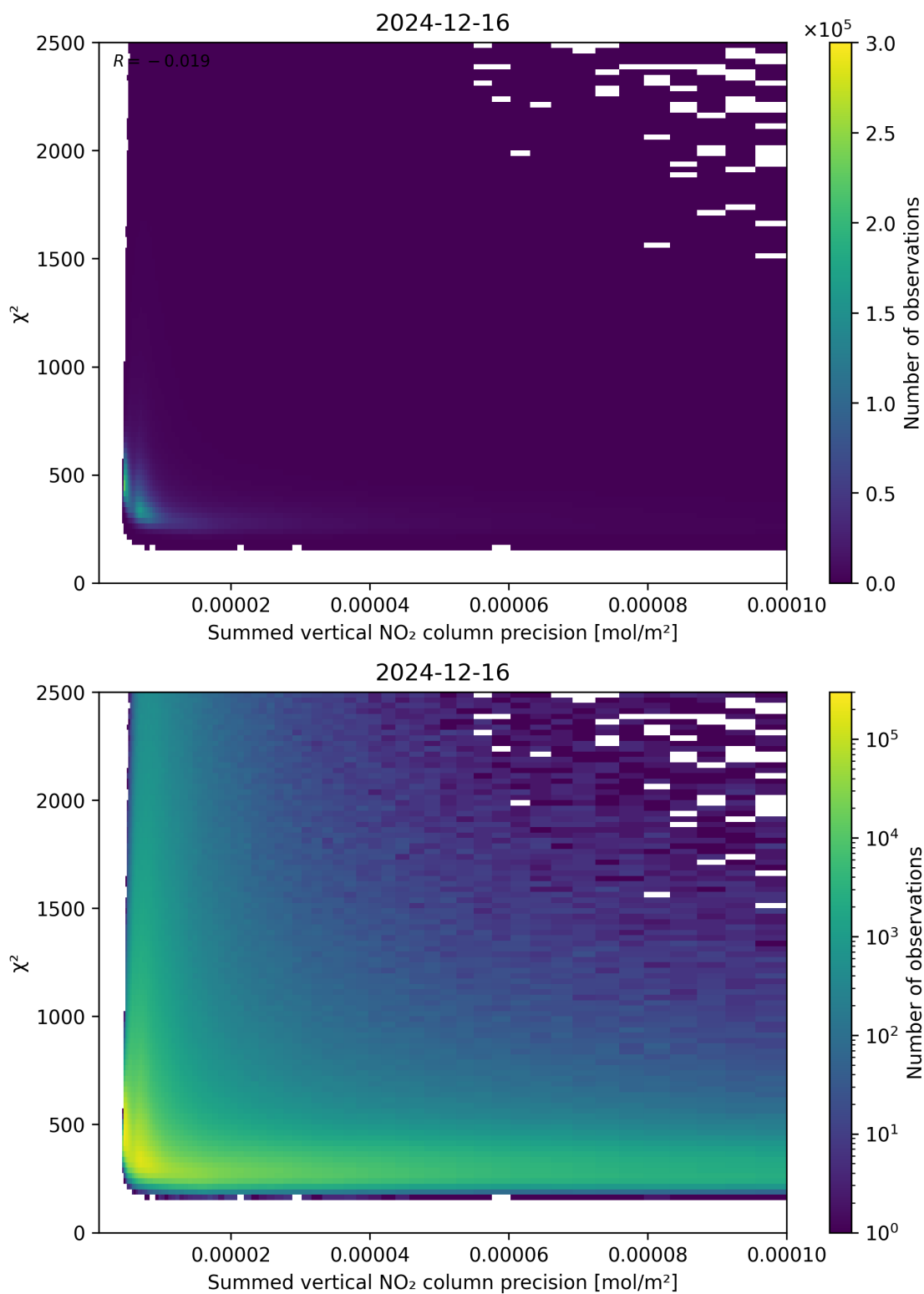
Figure 107: Scatter density plot of “Summed vertical NO 2 column precision” against “ \chi^2 ” for 2024-12-16 to 2024-12-17.
