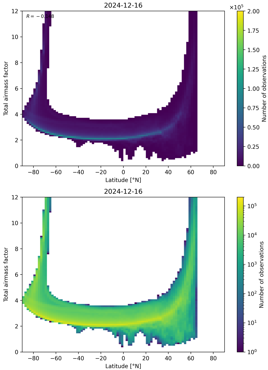
Figure 84: Scatter density plot of “Latitude” against “Total airmass factor” for 2024-12-16 to 2024-12-17.
