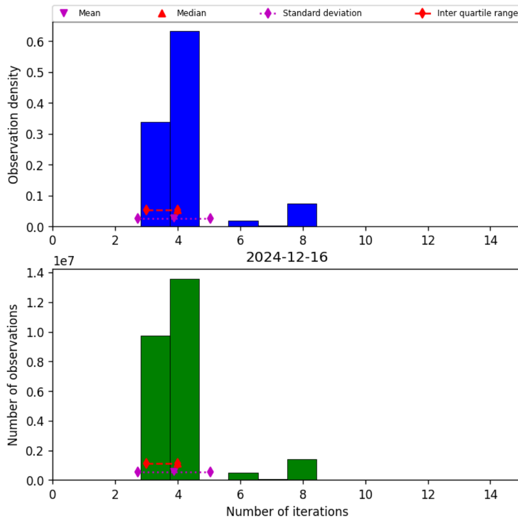
Figure 34: Histogram of “Number of iterations” for 2024-12-16 to 2024-12-17
