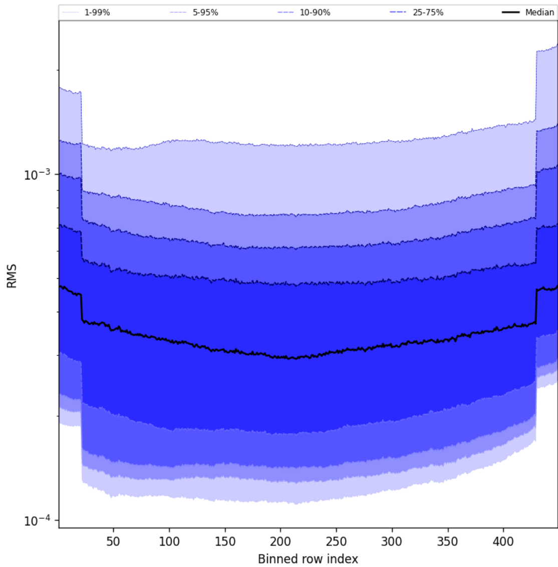
Figure 60: Along track statistics of “RMS” for 2024-12-16 to 2024-12-17
