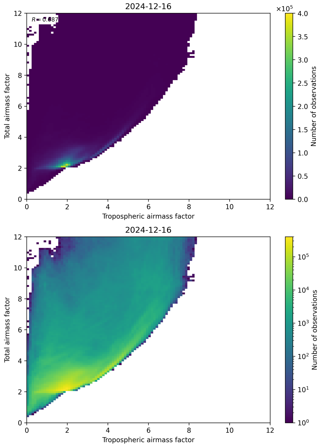
Figure 72: Scatter density plot of “Tropospheric airmass factor” against “Total airmass factor” for 2024-12-16 to 2024-12-17.
