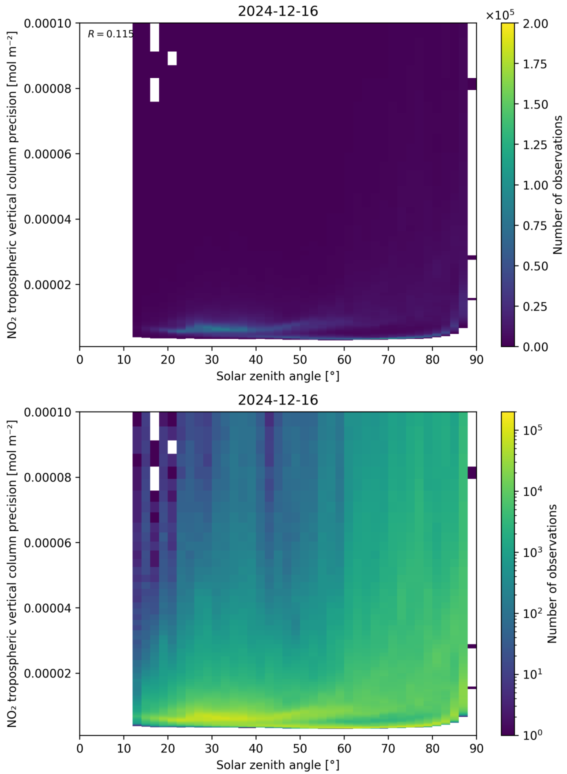
Figure 156: Scatter density plot of “Solar zenith angle” against “NO 2 tropospheric vertical column precision” for 2024-12-16 to 2024-12-17.
