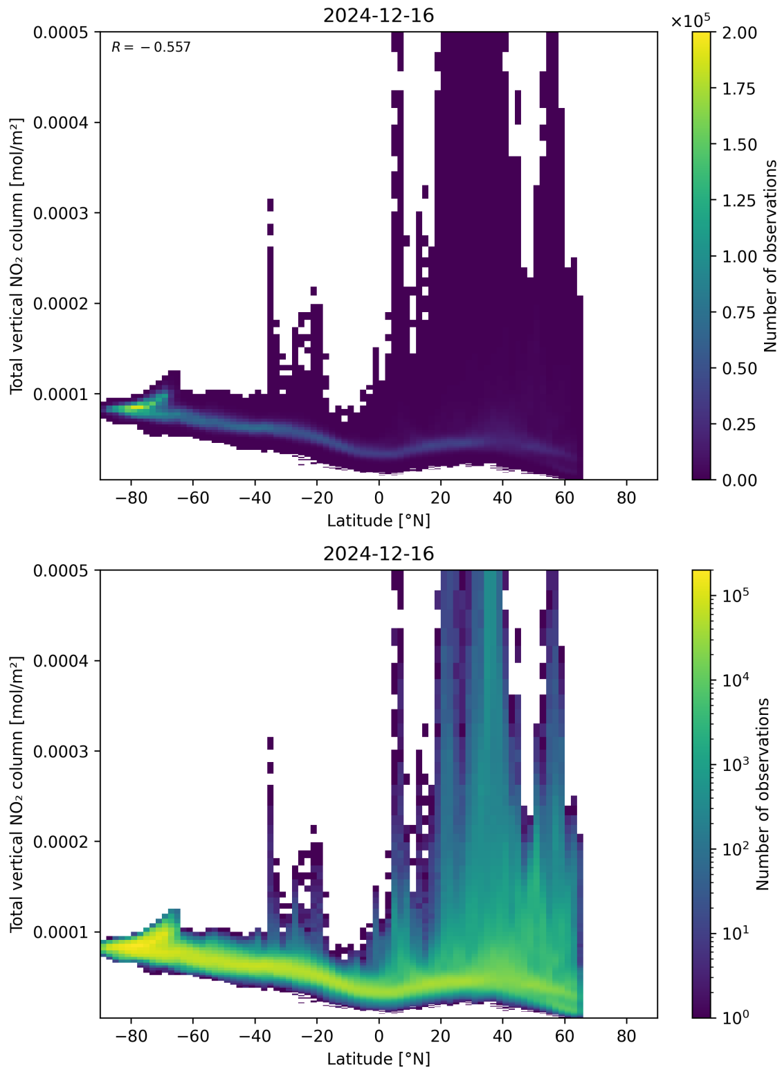
Figure 90: Scatter density plot of “Latitude” against “Total vertical NO 2 column” for 2024-12-16 to 2024-12-17.
