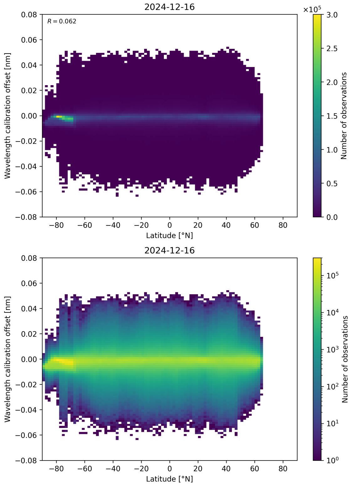
Figure 95: Scatter density plot of “Latitude” against “Wavelength calibration offset” for 2024-12-16 to 2024-12-17.
