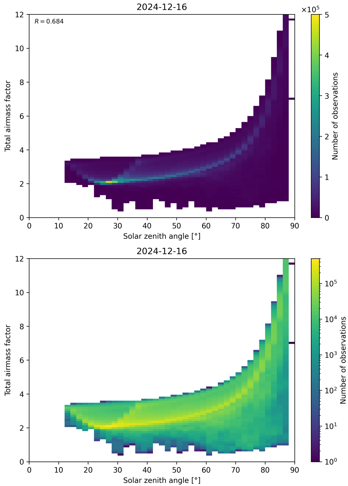
Figure 146: Scatter density plot of “Solar zenith angle” against “Total air mass factor” for 2024-12-16 to 2024-12-17.
