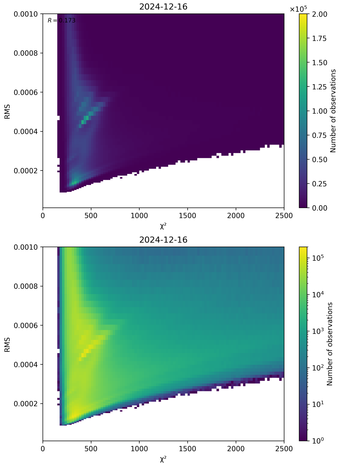
Figure 82: Scatter density plot of “ \chi^2 ” against “RMS” for 2024-12-16 to 2024-12-17.
