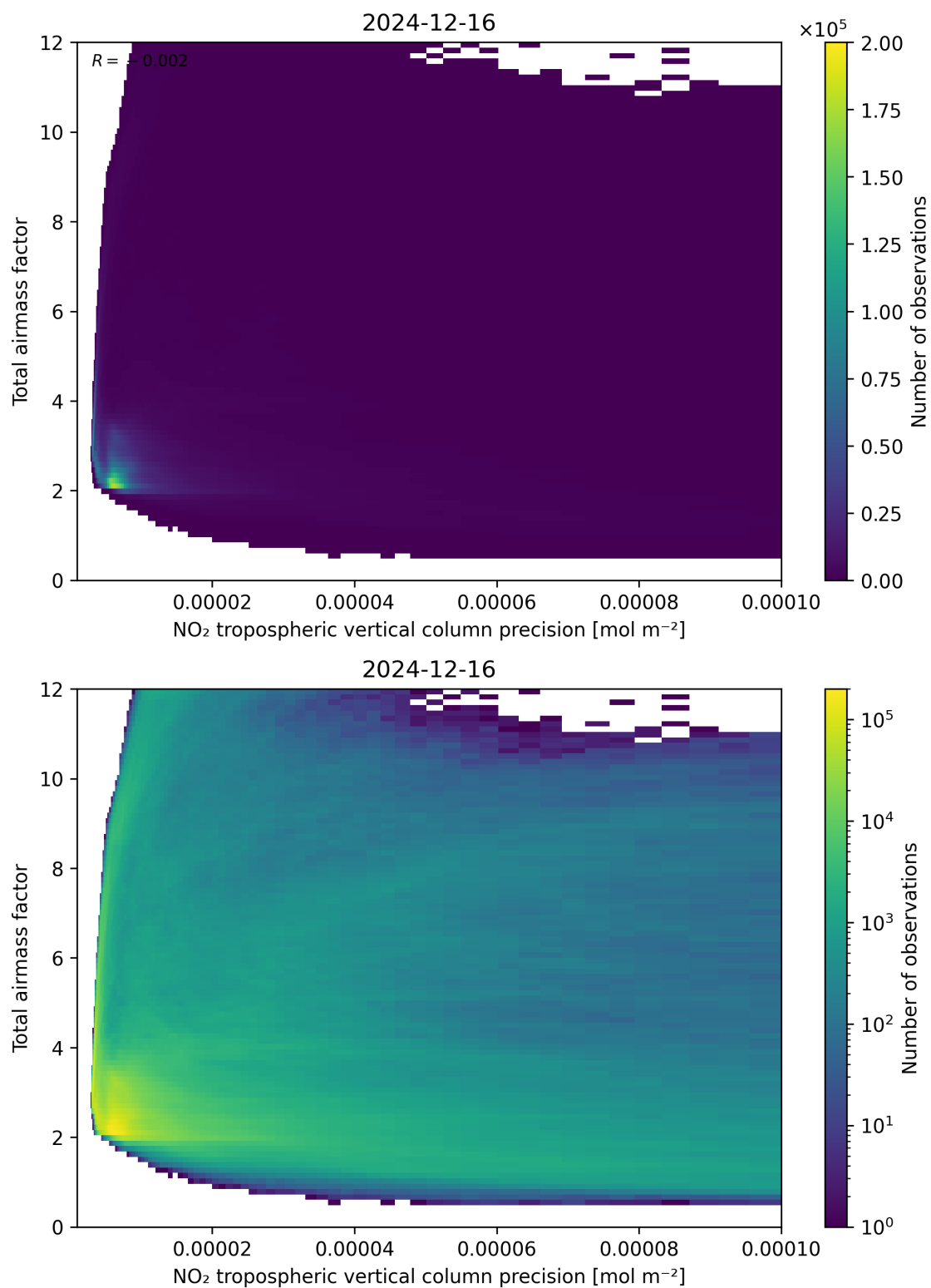
Figure 132: Scatter density plot of “NO 2 tropospheric vertical column precision” against “Total air mass factor” for 2024-12-16 to 2024-12-17.
