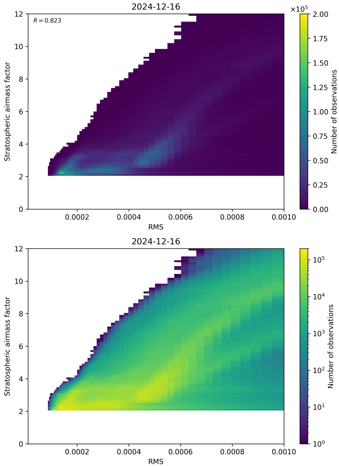
Figure 144: Scatter density plot of “RMS” against “Stratospheric airmass factor” for 2024-12-16 to 2024-12-17.
