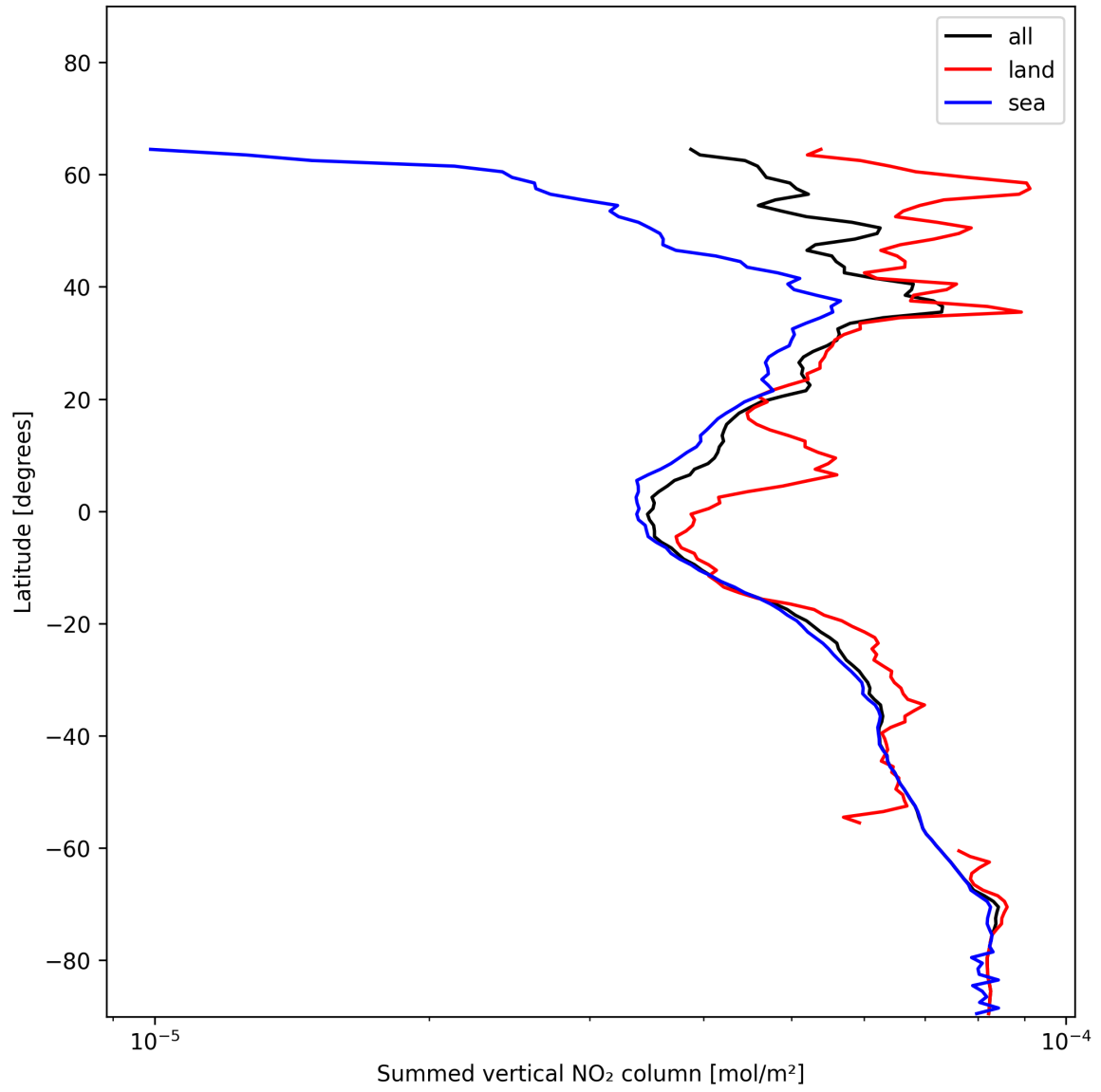
Figure 23: Zonal average of “Summed vertical NO 2 column” for 2024-12-16 to 2024-12-17.
