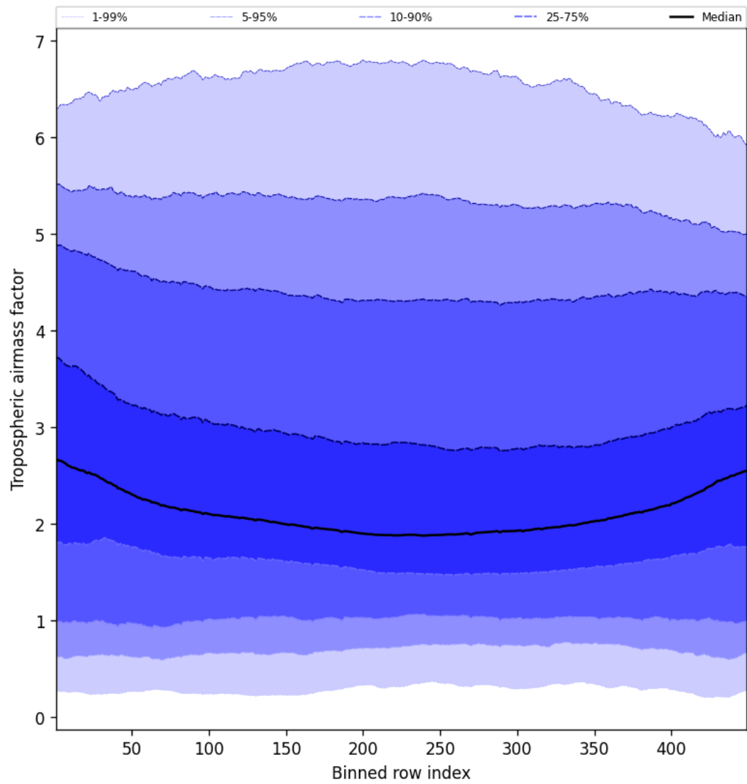
Figure 48: Along track statistics of “Tropospheric airmass factor” for 2024-12-16 to 2024-12-17
