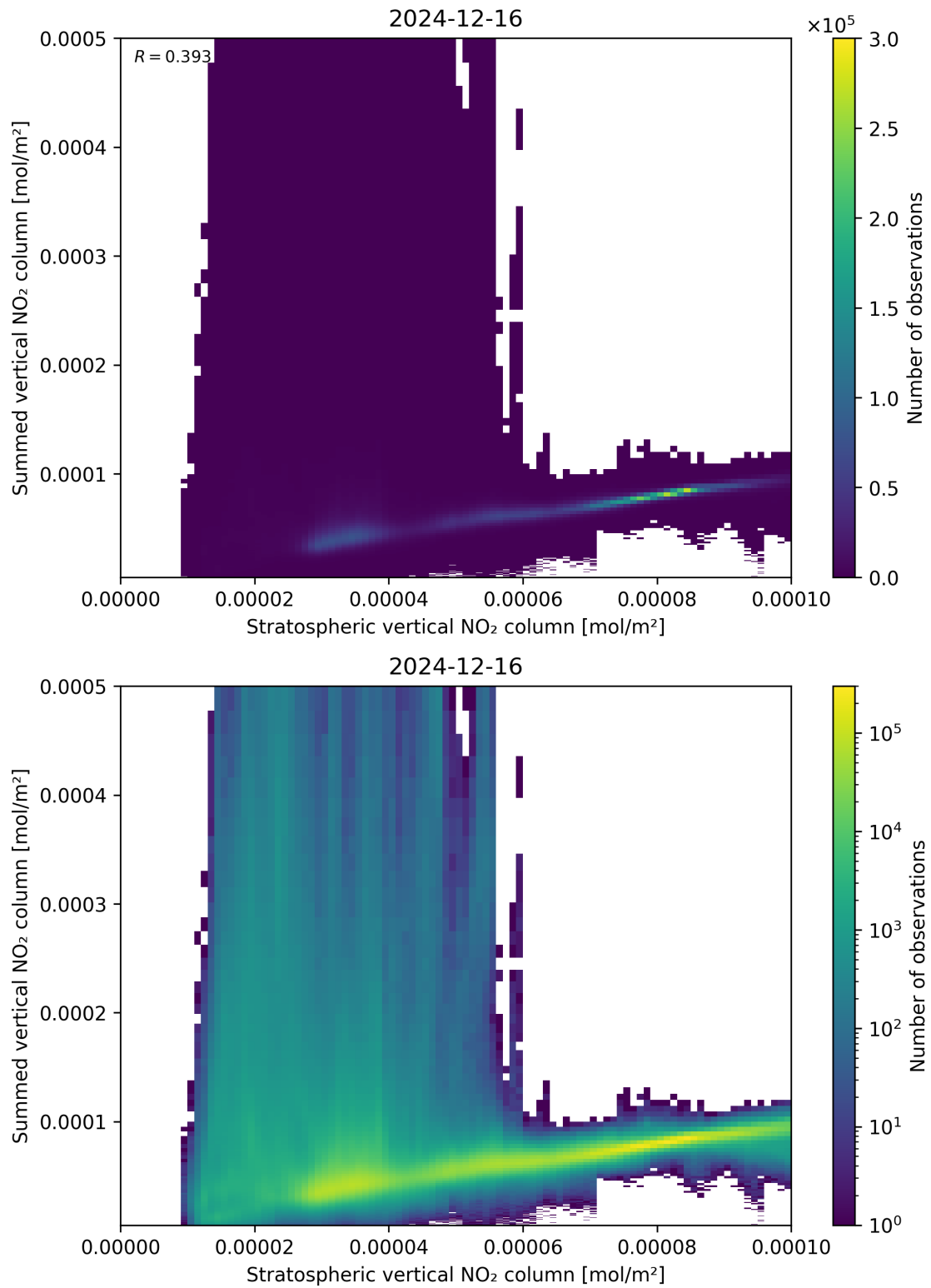
Figure 98: Scatter density plot of “Stratospheric vertical NO 2 column” against “Summed vertical NO 2 column” for 2024-12-16 to 2024-12-17.
