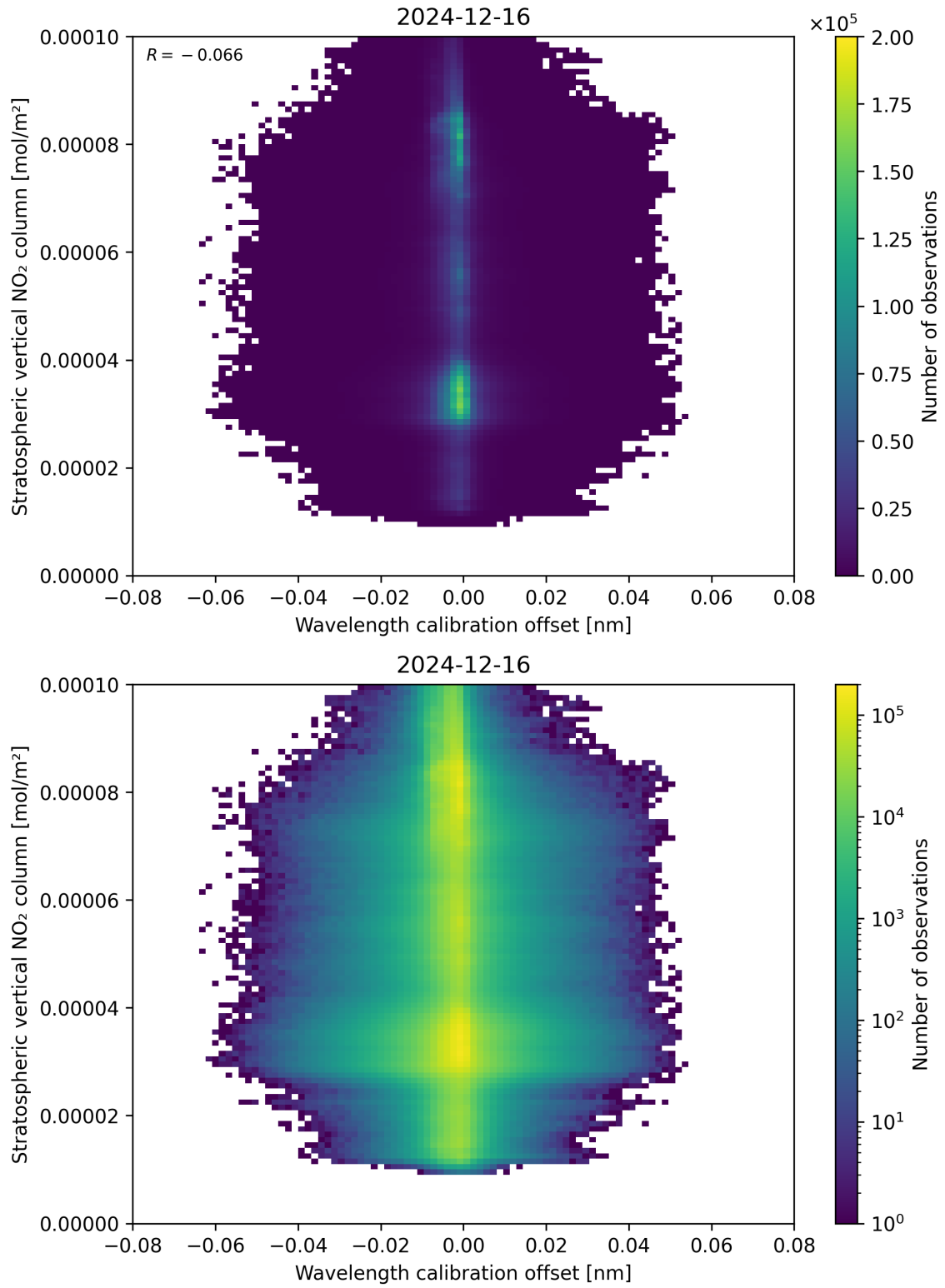
Figure 176: Scatter density plot of “Wavelength calibration offset” against “Stratospheric vertical NO 2 column” for 2024-12-16 to 2024-12-17.
