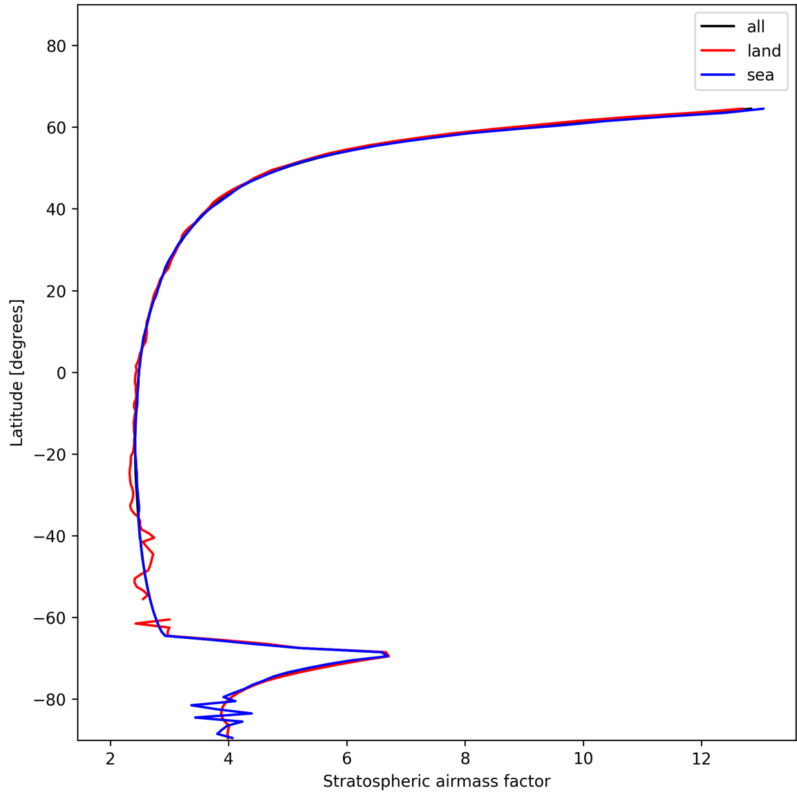
Figure 27: Zonal average of “Stratospheric airmass factor” for 2024-12-16 to 2024-12-17.
