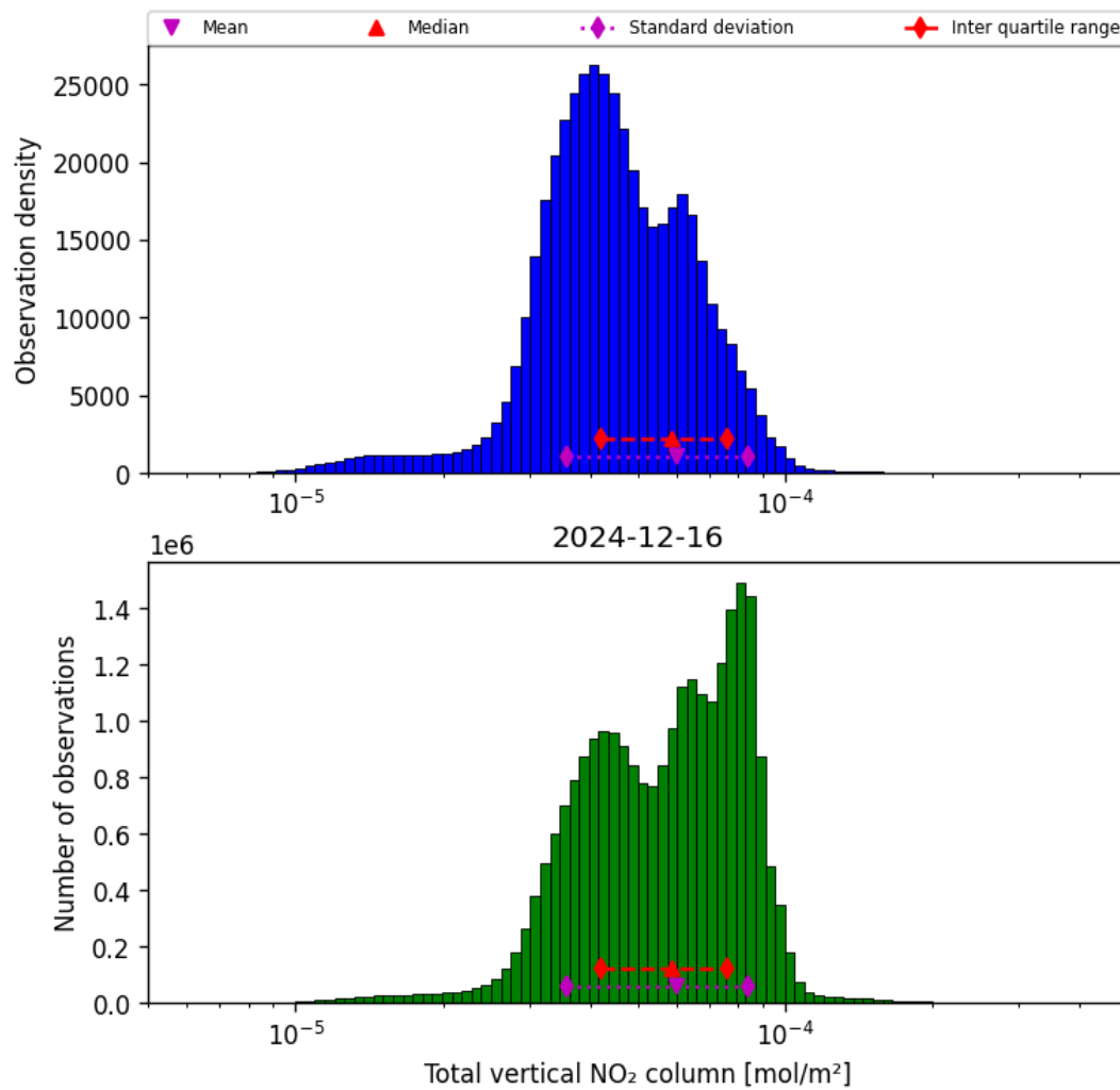
Figure 38: Histogram of “Total vertical NO 2 column” for 2024-12-16 to 2024-12-17
