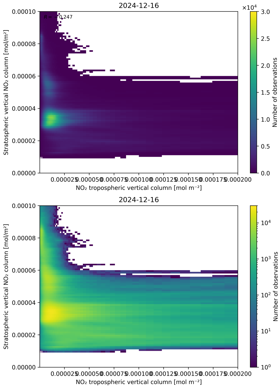
Figure 125: Scatter density plot of “NO 2 tropospheric vertical column” against “Stratospheric vertical NO 2 column” for 2024-12-16 to 2024-12-17.
