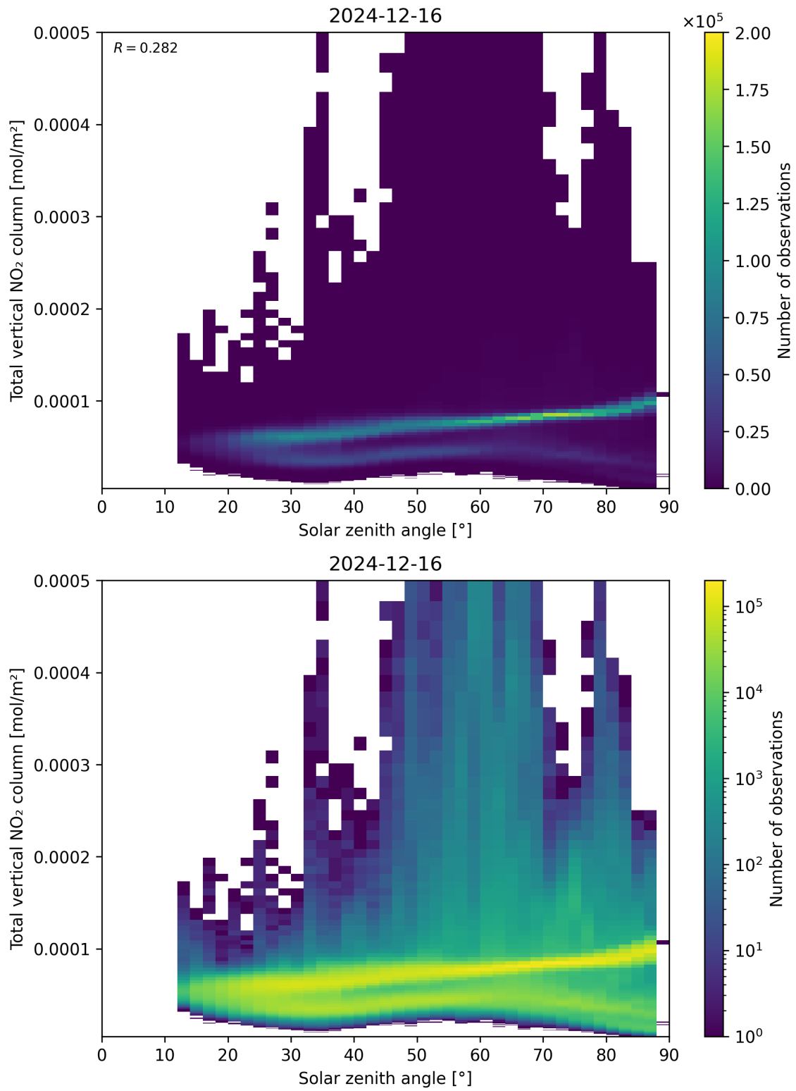
Figure 153: Scatter density plot of “Solar zenith angle” against “Total vertical NO 2 column” for 2024-12-16 to 2024-12-17.
