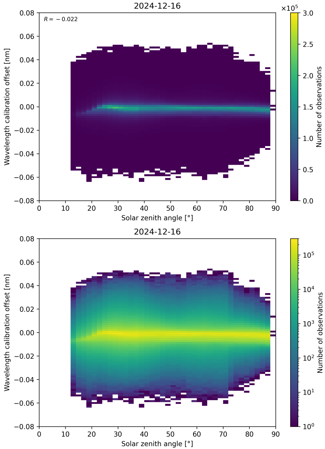
Figure 158: Scatter density plot of “Solar zenith angle” against “Wavelength calibration offset” for 2024-12-16 to 2024-12-17.
