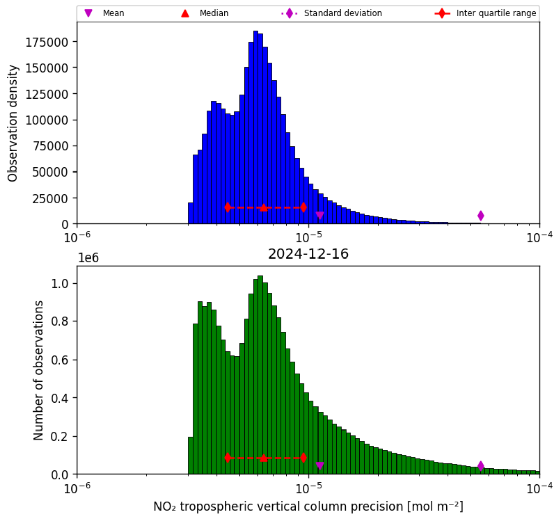
Figure 30: Histogram of “NO 2 tropospheric vertical column precision” for 2024-12-16 to 2024-12-17
