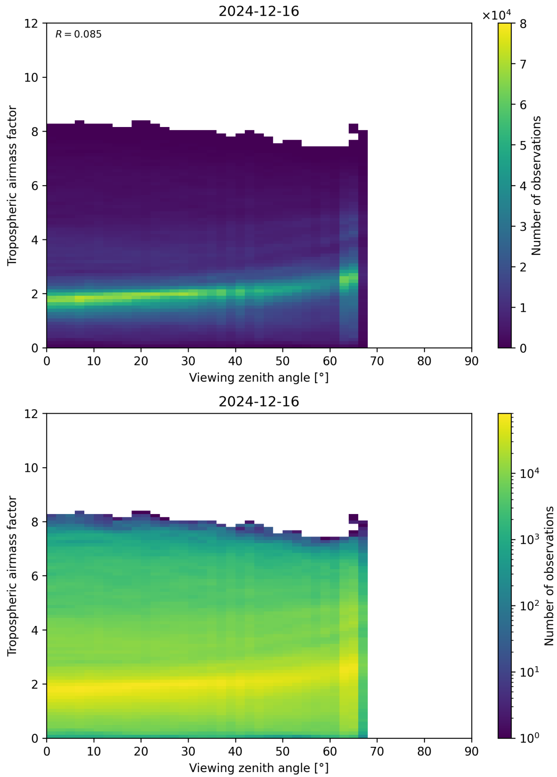
Figure 161: Scatter density plot of “Viewing zenith angle” against “Tropospheric airmass factor” for 2024-12-16 to 2024-12-17.
