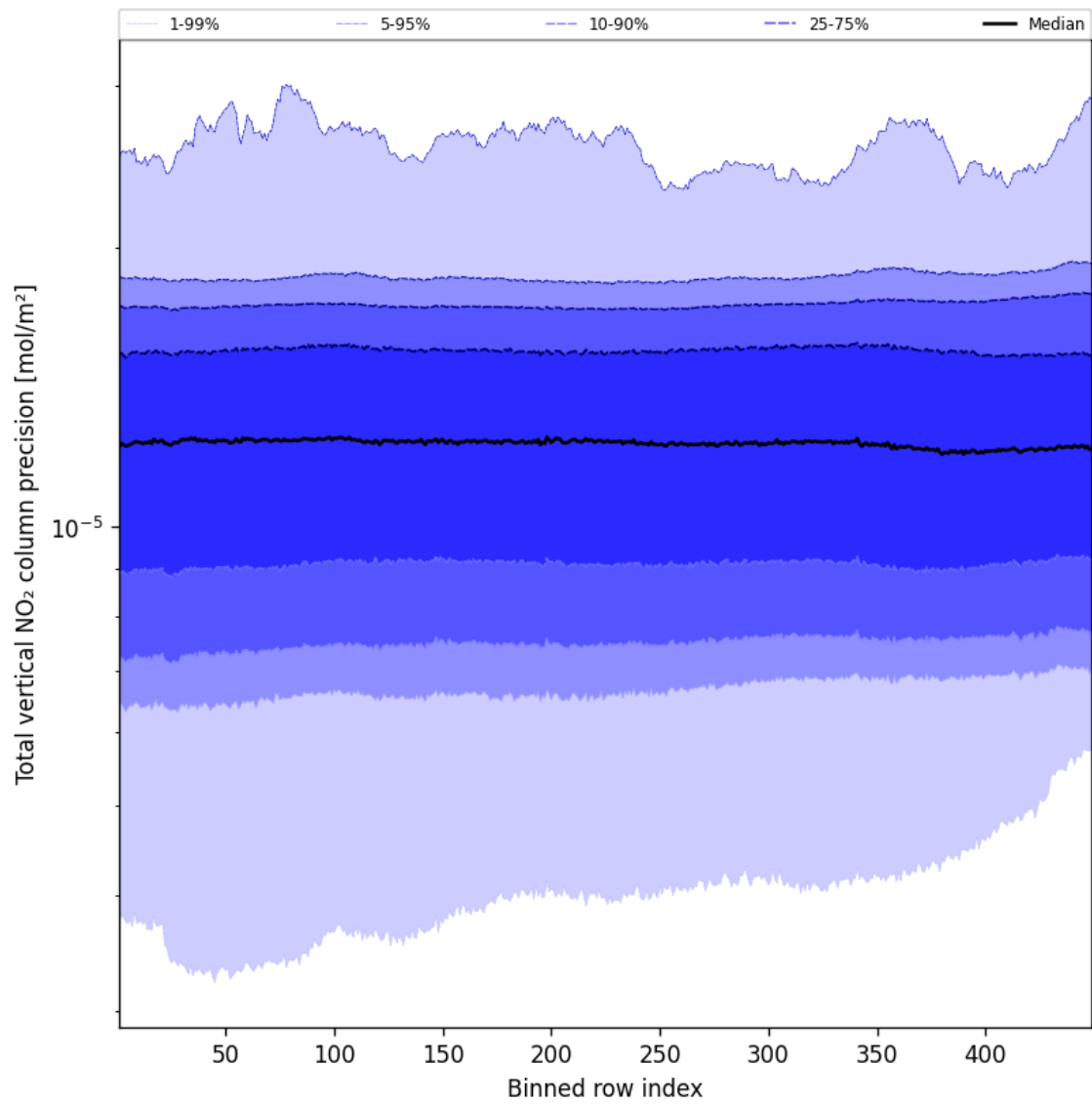
Figure 56: Along track statistics of “Total vertical NO 2 column precision” for 2024-12-16 to 2024-12-17
