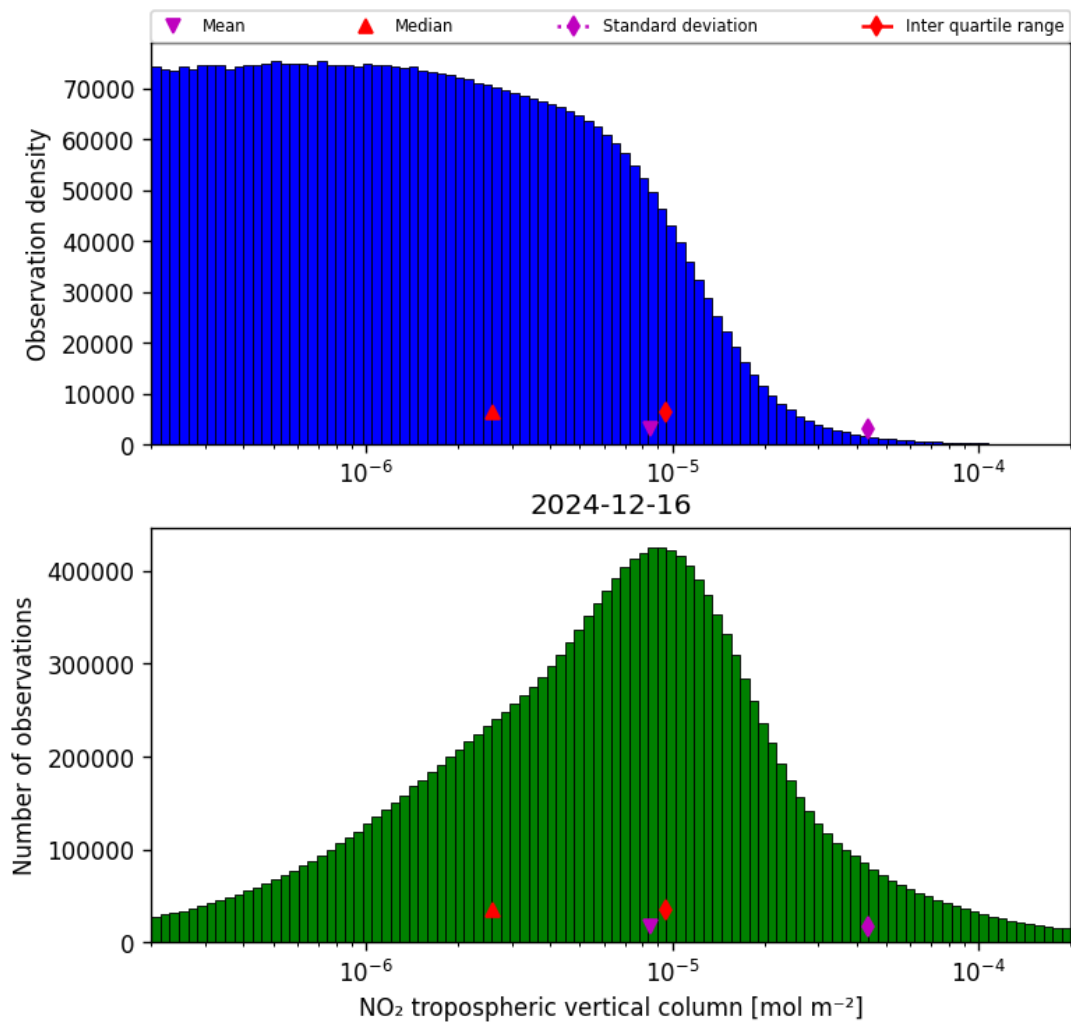
Figure 29: Histogram of “NO 2 tropospheric vertical column” for 2024-12-16 to 2024-12-17
