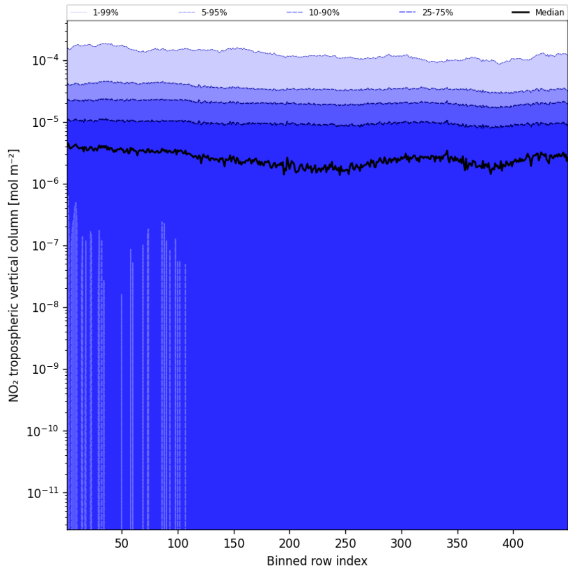
Figure 46: Along track statistics of “NO 2 tropospheric vertical column” for 2024-12-16 to 2024-12-17
