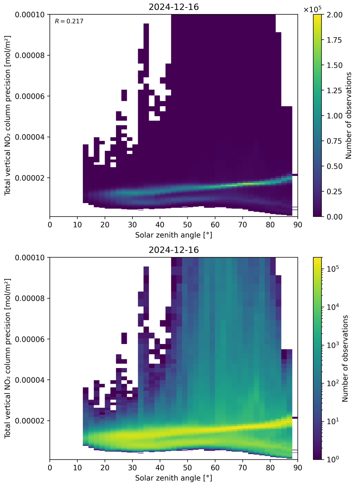
Figure 154: Scatter density plot of “Solar zenith angle” against “Total vertical NO 2 column precision” for 2024-12-16 to 2024-12-17.
