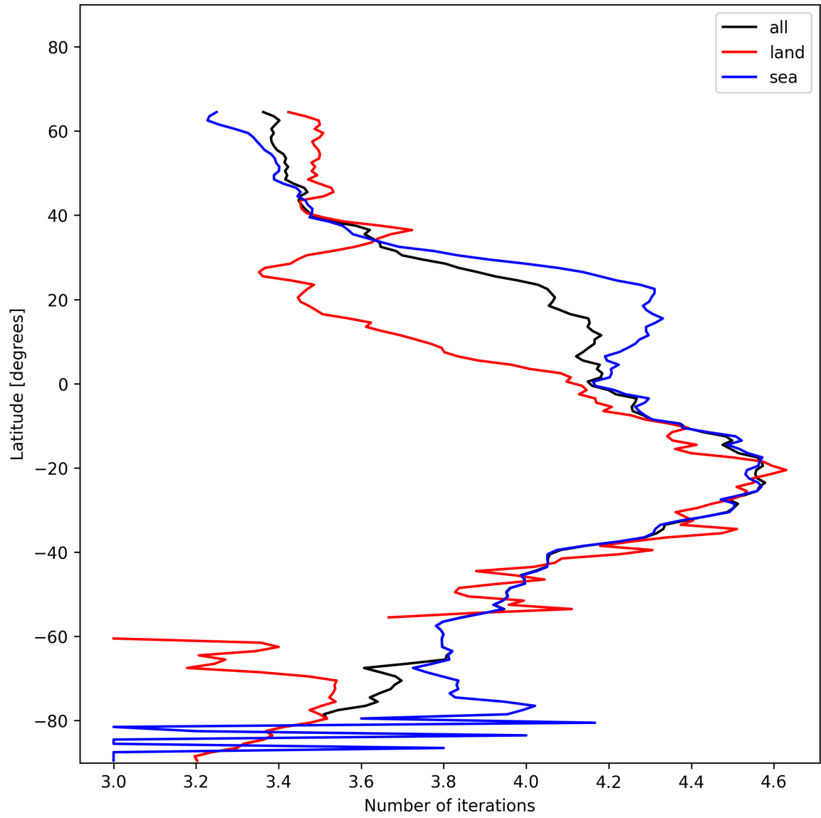
Figure 17: Zonal average of “Number of iterations” for 2024-12-16 to 2024-12-17.
