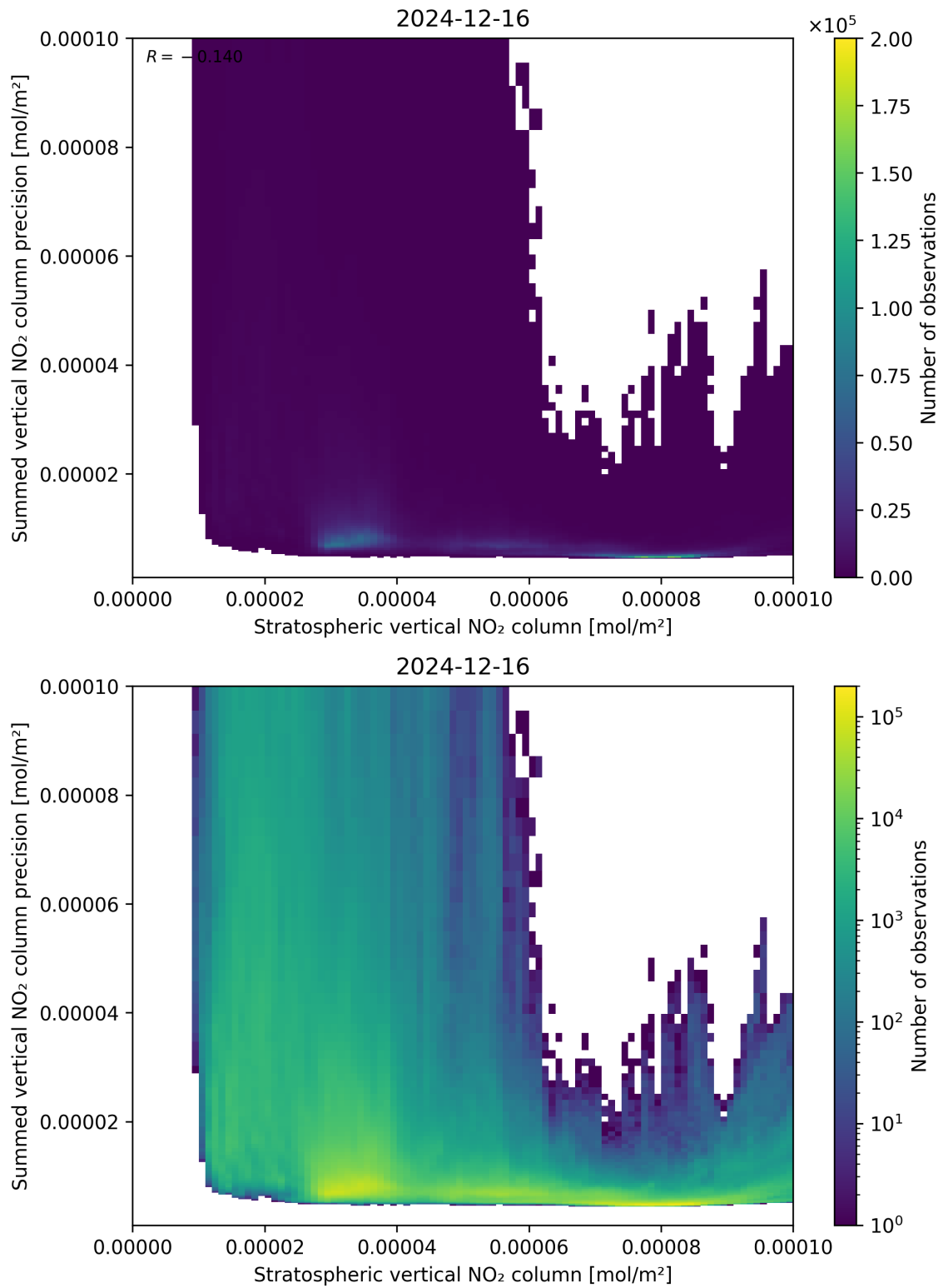
Figure 99: Scatter density plot of “Stratospheric vertical NO 2 column” against “Summed vertical NO 2 column precision” for 2024-12-16 to 2024-12-17.
