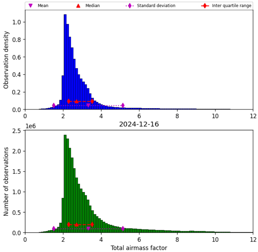
Figure 32: Histogram of “Total airmass factor” for 2024-12-16 to 2024-12-17
