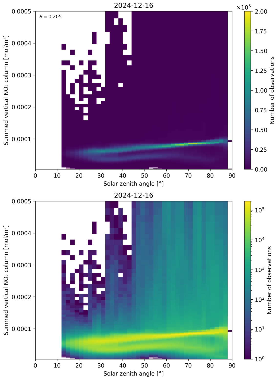
Figure 151: Scatter density plot of “Solar zenith angle” against “Summed vertical NO 2 column” for 2024-12-16 to 2024-12-17.
