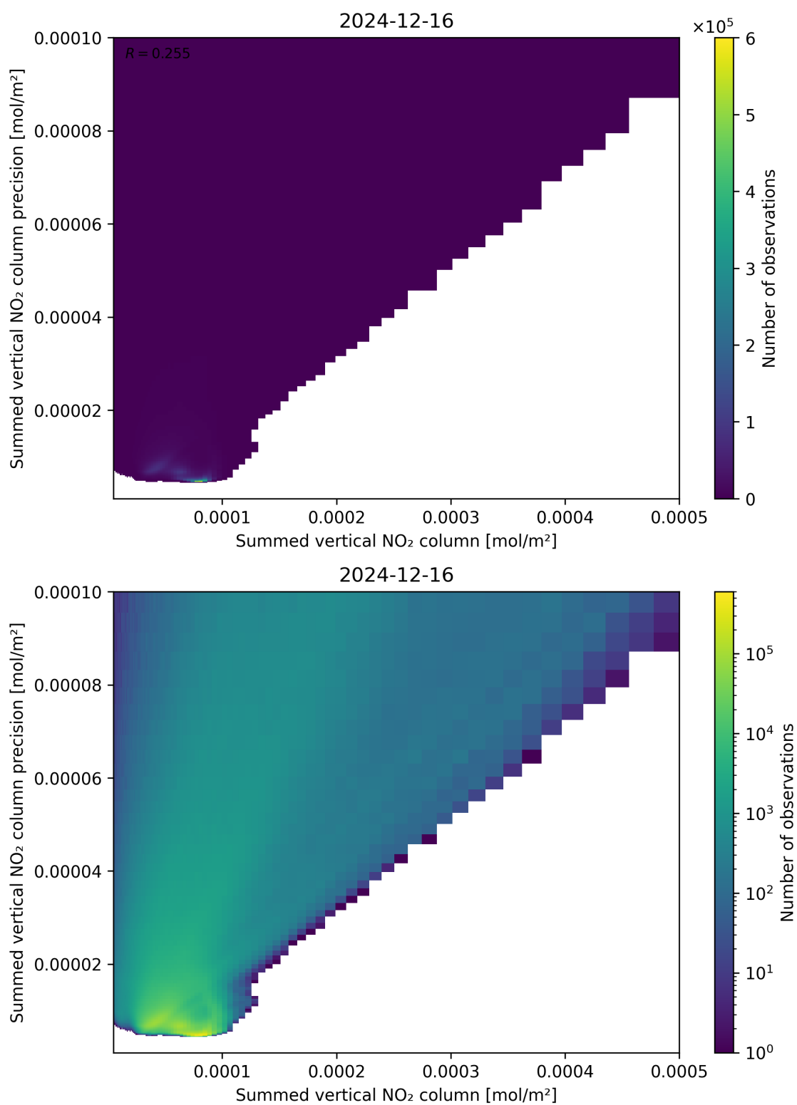
Figure 105: Scatter density plot of “Summed vertical NO 2 column” against “Summed vertical NO 2 column precision” for 2024-12-16 to 2024-12-17.
