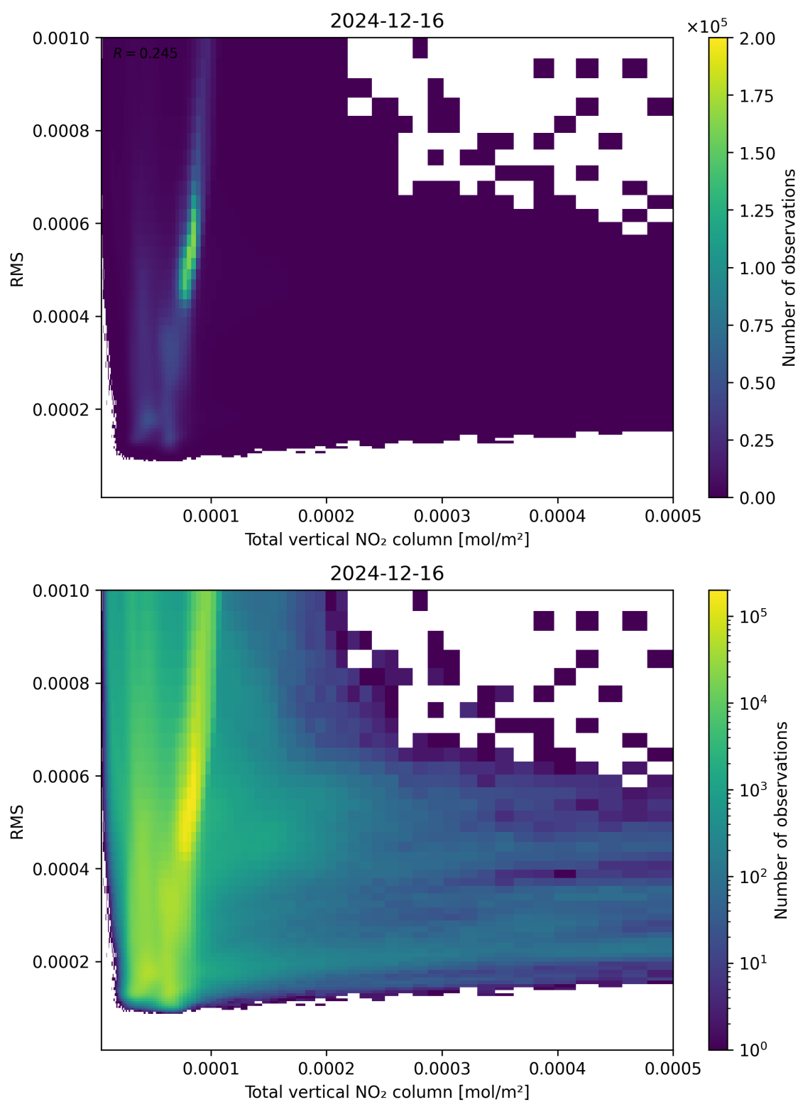
Figure 120: Scatter density plot of “Total vertical NO 2 column” against “RMS” for 2024-12-16 to 2024-12-17.
