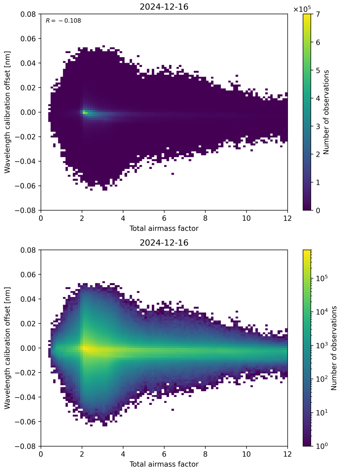
Figure 70: Scatter density plot of “Total airmass factor” against “Wavelength calibration offset” for 2024-12-16 to 2024-12-17.
