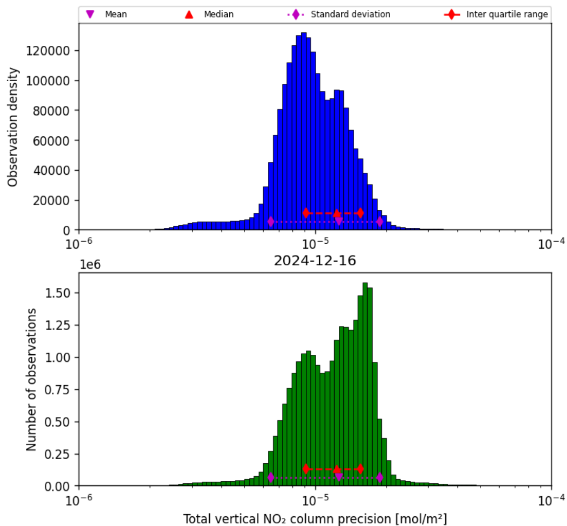
Figure 39: Histogram of “Total vertical NO 2 column precision” for 2024-12-16 to 2024-12-17
