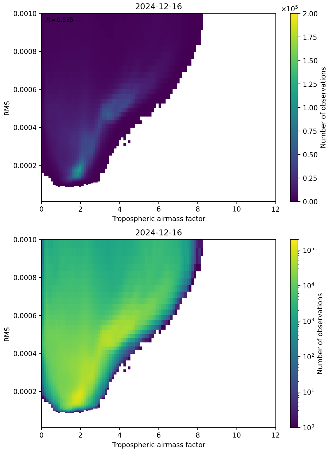
Figure 79: Scatter density plot of “Tropospheric airmass factor” against “RMS” for 2024-12-16 to 2024-12-17.
