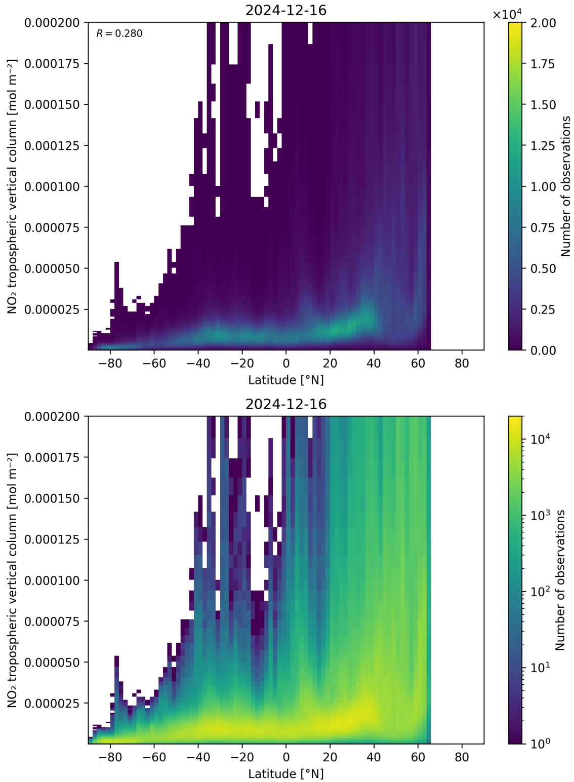
Figure 92: Scatter density plot of “Latitude” against “NO 2 tropospheric vertical column” for 2024-12-16 to 2024-12-17.
