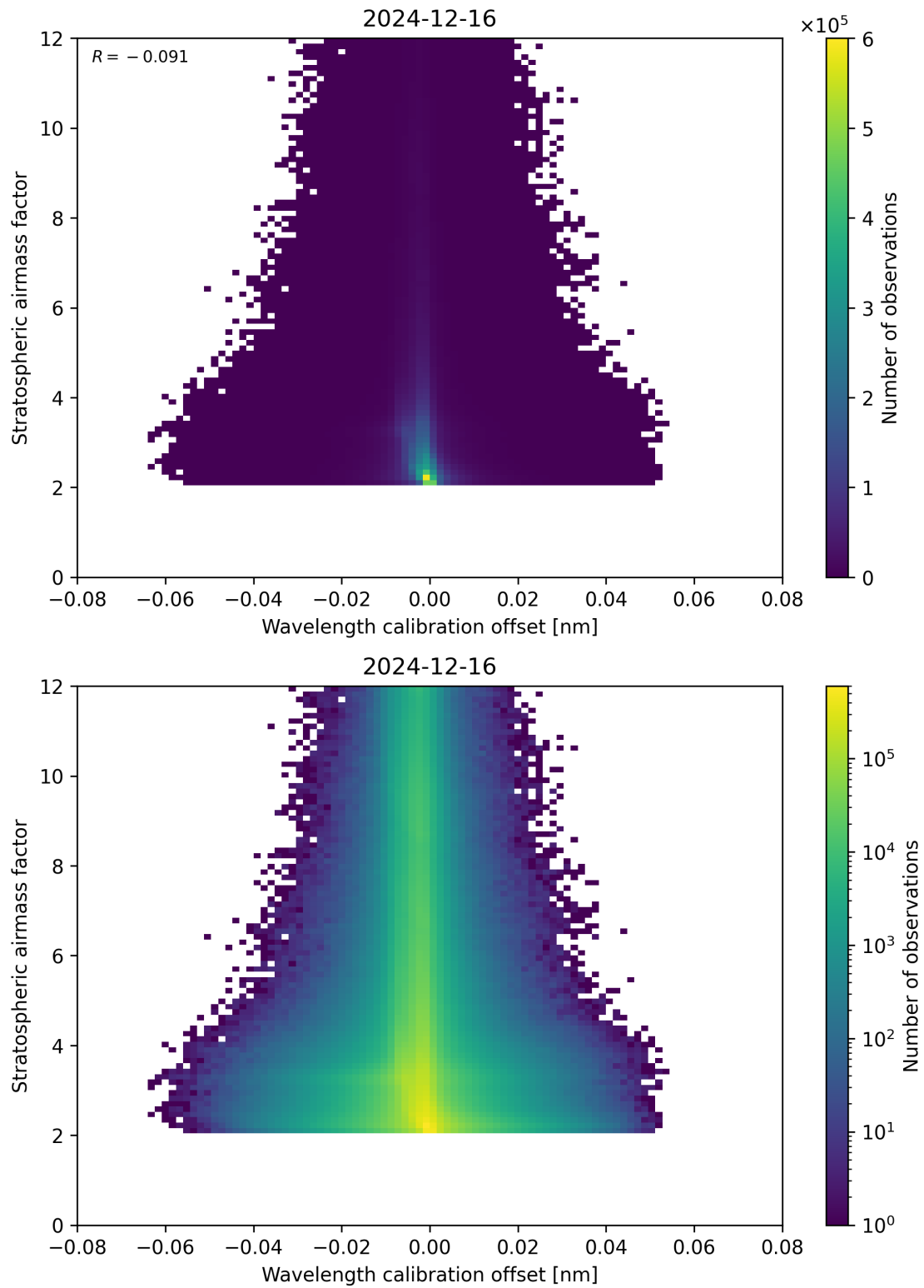
Figure 174: Scatter density plot of “Wavelength calibration offset” against “Stratospheric air mass factor” for 2024-12-16 to 2024-12-17.
