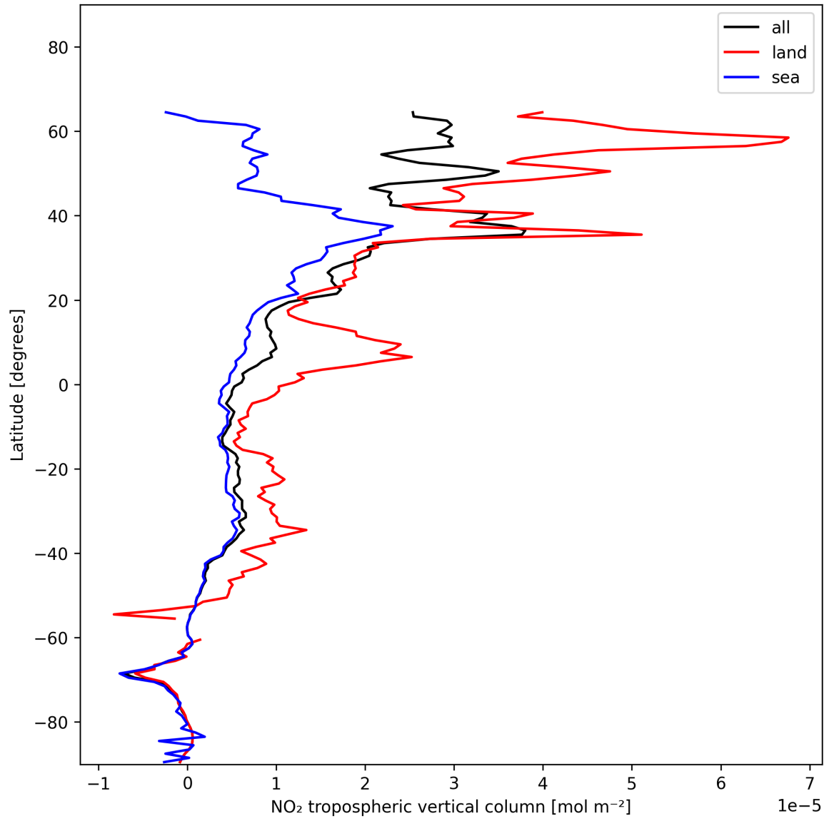
Figure 12: Zonal average of “NO 2 tropospheric vertical column” for 2024-12-16 to 2024-12-17.
