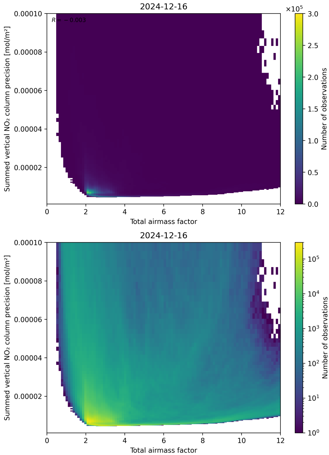
Figure 66: Scatter density plot of “Total airmass factor” against “Summed vertical NO 2 column precision” for 2024-12-16 to 2024-12-17.
