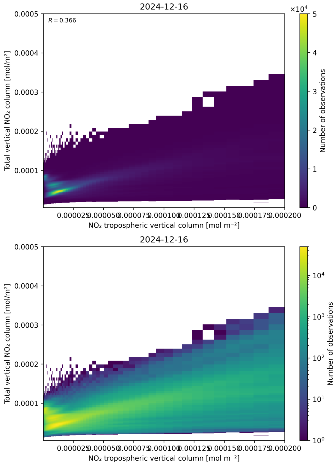
Figure 128: Scatter density plot of “NO 2 tropospheric vertical column” against “Total vertical NO 2 column” for 2024-12-16 to 2024-12-17.
