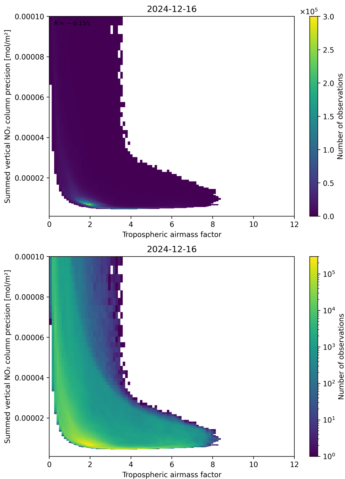
Figure 76: Scatter density plot of “Tropospheric air mass factor” against “Summed vertical NO 2 column precision” for 2024-12-16 to 2024-12-17.
