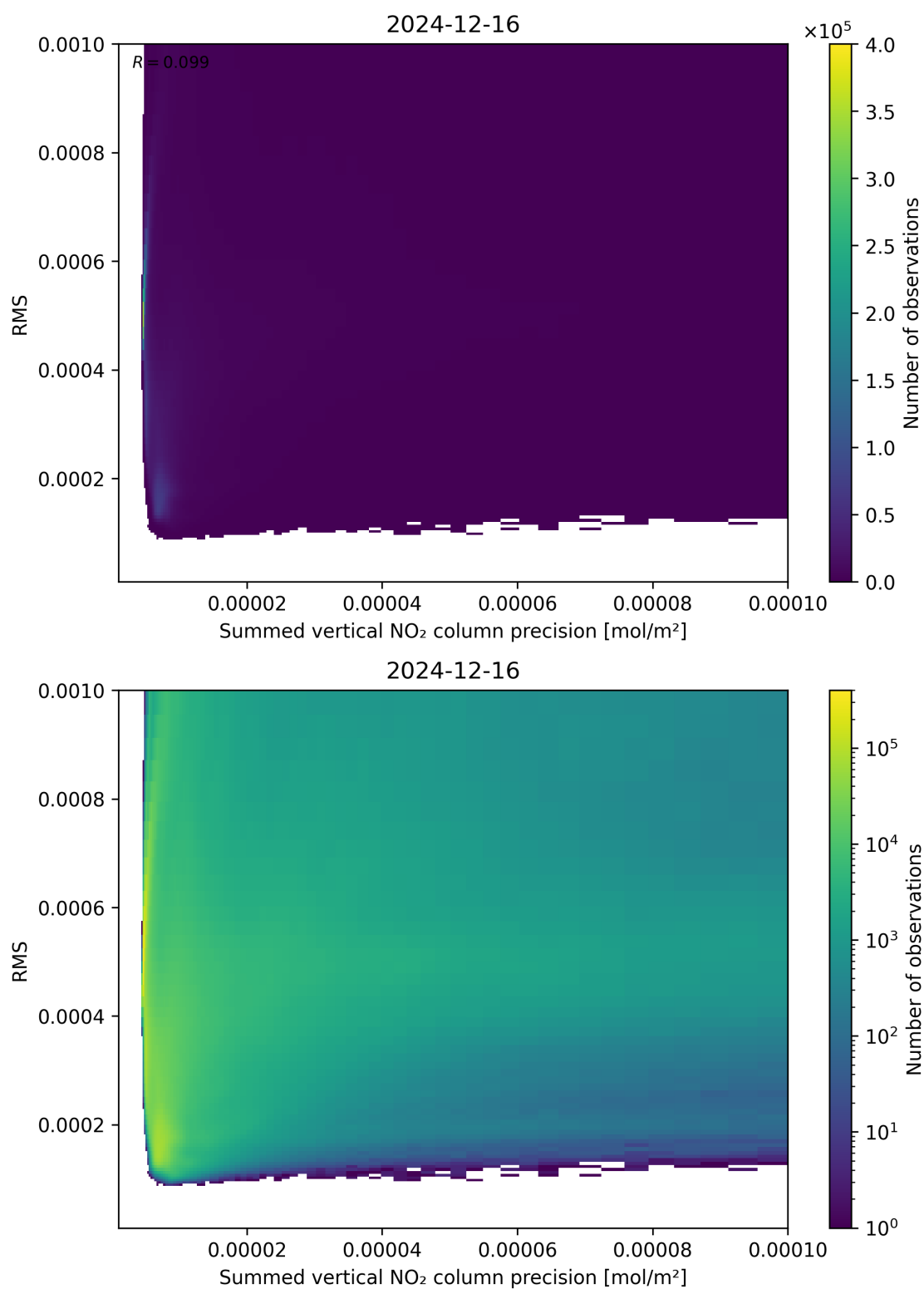
Figure 108: Scatter density plot of “Summed vertical NO 2 column precision” against “RMS” for 2024-12-16 to 2024-12-17.
