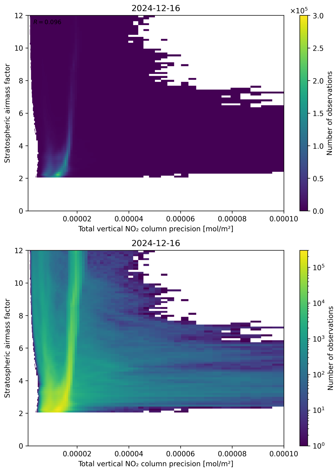
Figure 115: Scatter density plot of “Total vertical NO 2 column precision” against “Stratospheric air mass factor” for 2024-12-16 to 2024-12-17.
