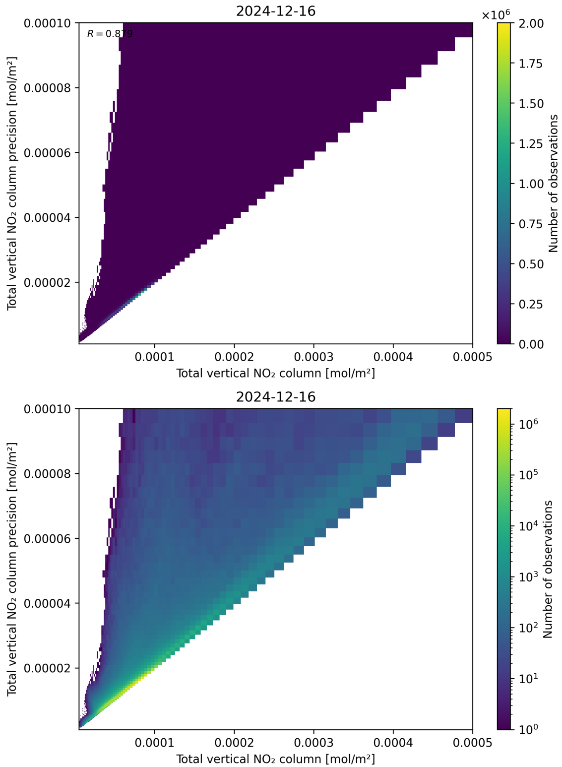
Figure 114: Scatter density plot of “Total vertical NO 2 column” against “Total vertical NO 2 column precision” for 2024-12-16 to 2024-12-17.
