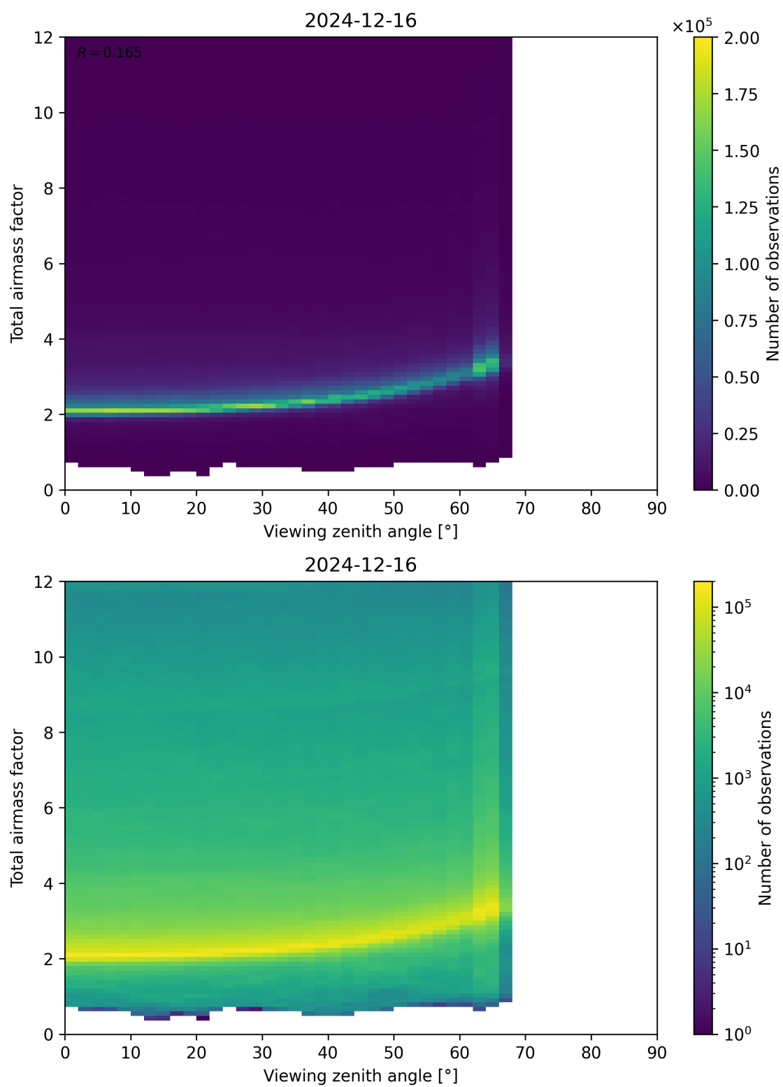
Figure 160: Scatter density plot of “Viewing zenith angle” against “Total airmass factor” for 2024-12-16 to 2024-12-17.
