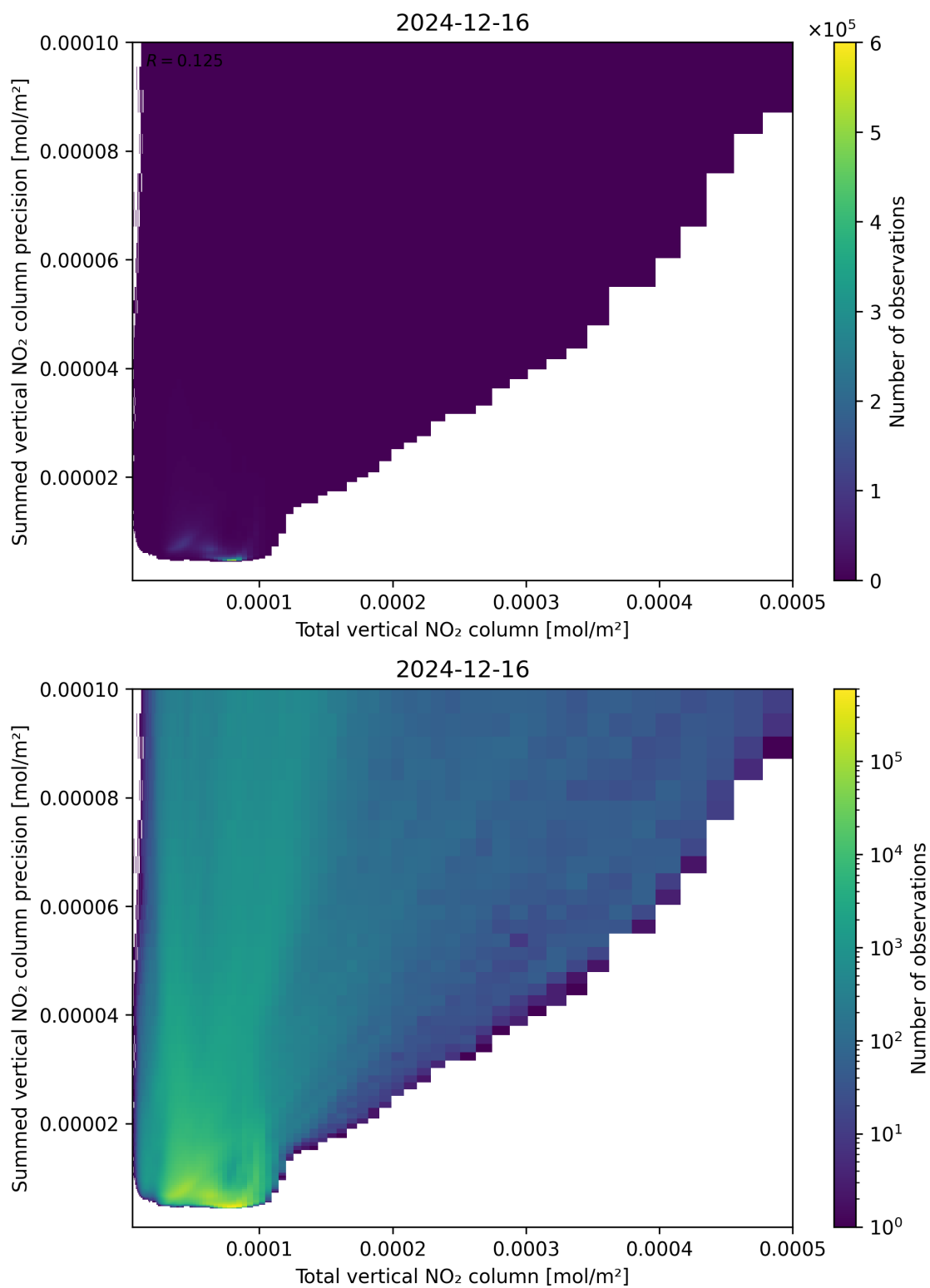
Figure 113: Scatter density plot of “Total vertical NO 2 column” against “Summed vertical NO 2 column precision” for 2024-12-16 to 2024-12-17.
