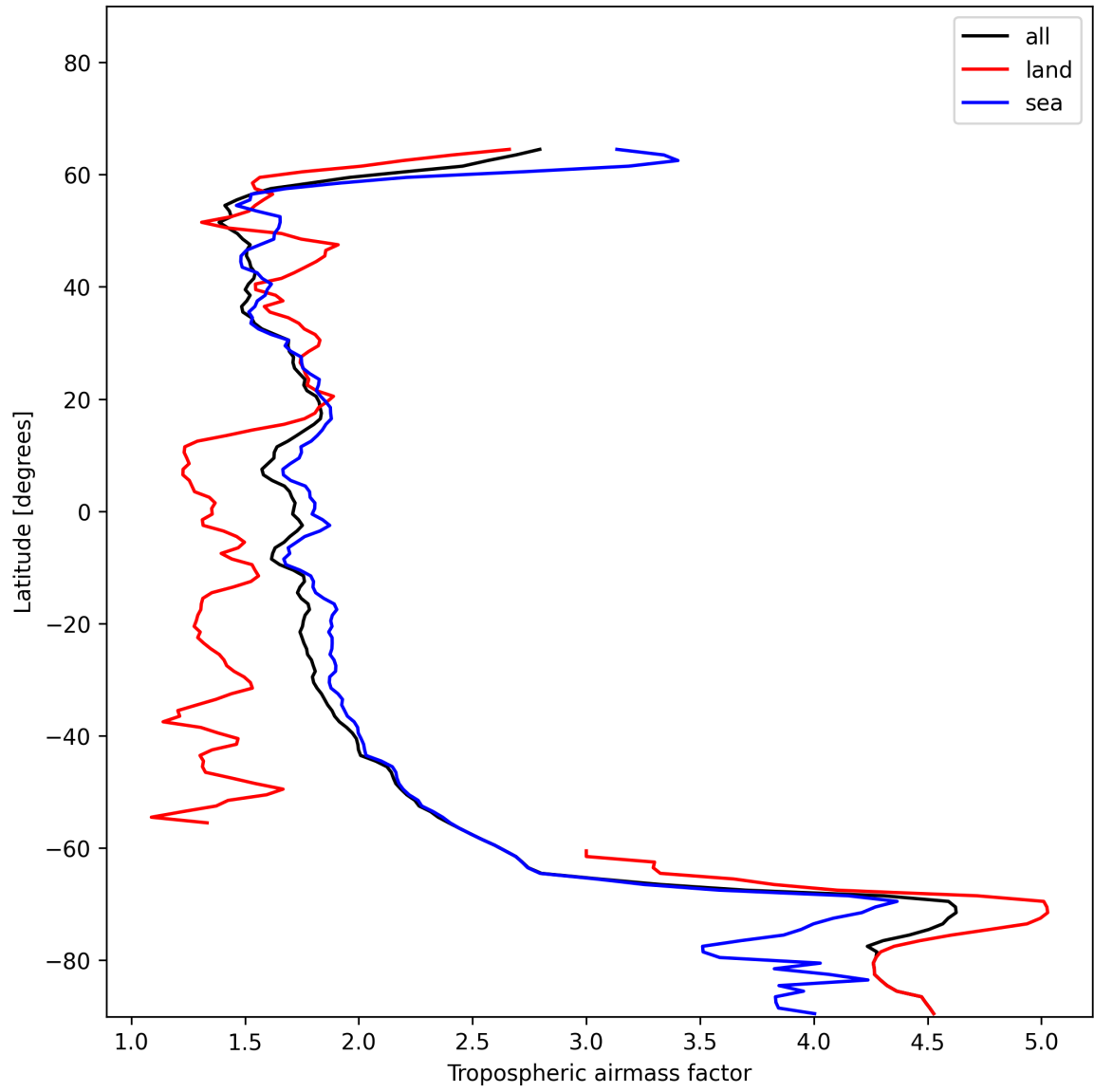
Figure 14: Zonal average of “Tropospheric airmass factor” for 2024-12-16 to 2024-12-17.
