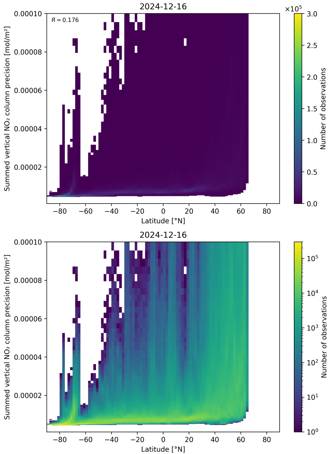
Figure 89: Scatter density plot of “Latitude” against “Summed vertical NO 2 column precision” for 2024-12-16 to 2024-12-17.
