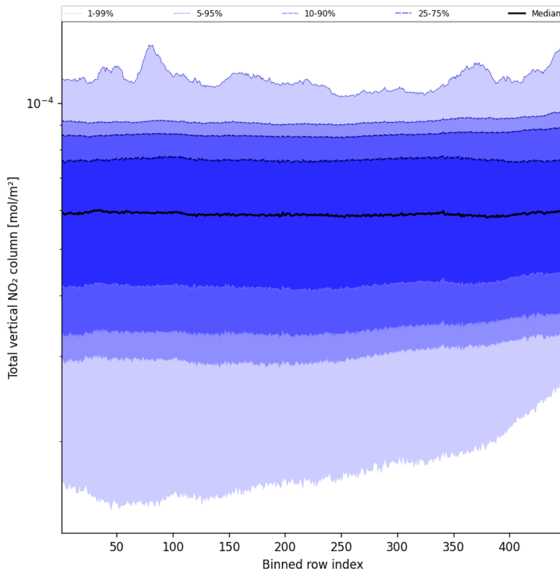
Figure 55: Along track statistics of “Total vertical NO 2 column” for 2024-12-16 to 2024-12-17
