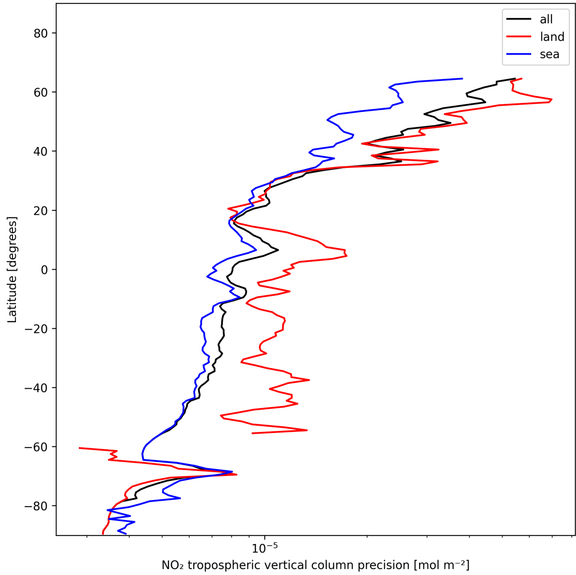
Figure 13: Zonal average of “NO 2 tropospheric vertical column precision” for 2024-12-16 to 2024-12-17.
