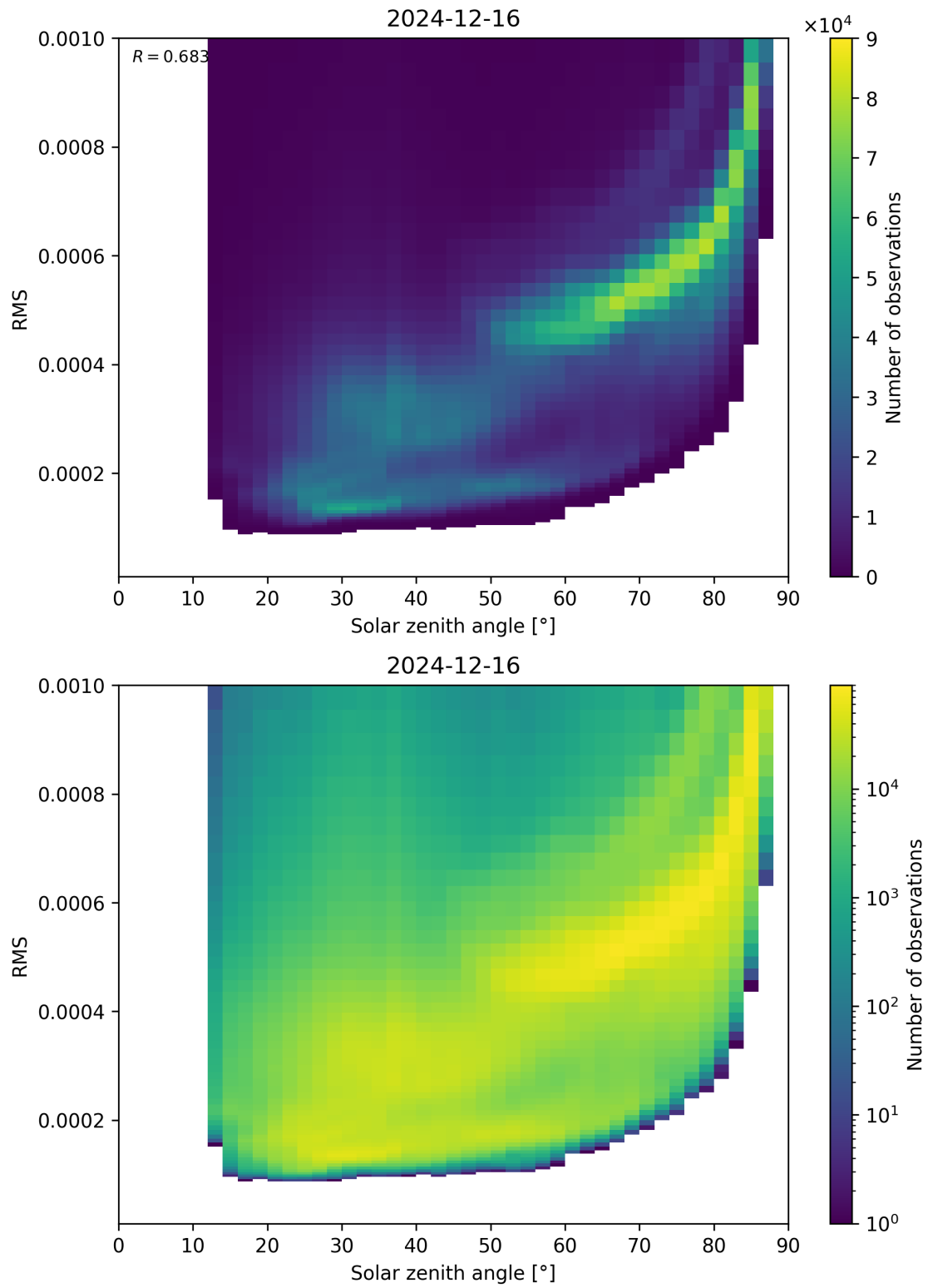
Figure 157: Scatter density plot of “Solar zenith angle” against “RMS” for 2024-12-16 to 2024-12-17.
