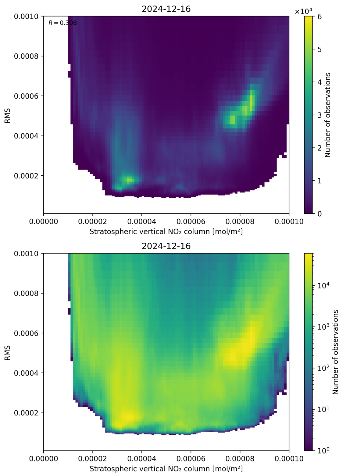
Figure 102: Scatter density plot of “Stratospheric vertical NO 2 column” against “RMS” for 2024-12-16 to 2024-12-17.
