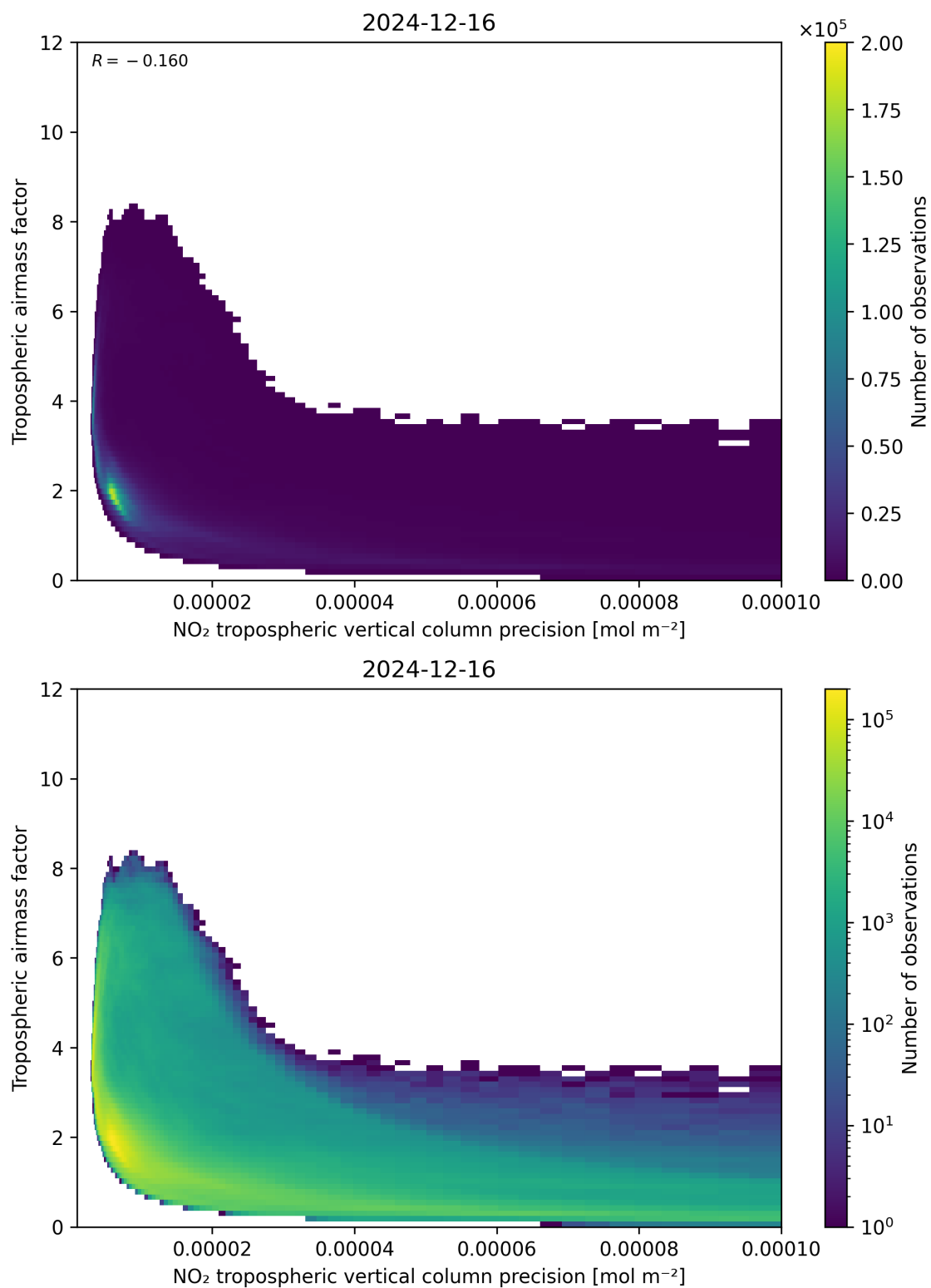
Figure 133: Scatter density plot of “NO 2 tropospheric vertical column precision” against “Tropospheric air mass factor” for 2024-12-16 to 2024-12-17.
