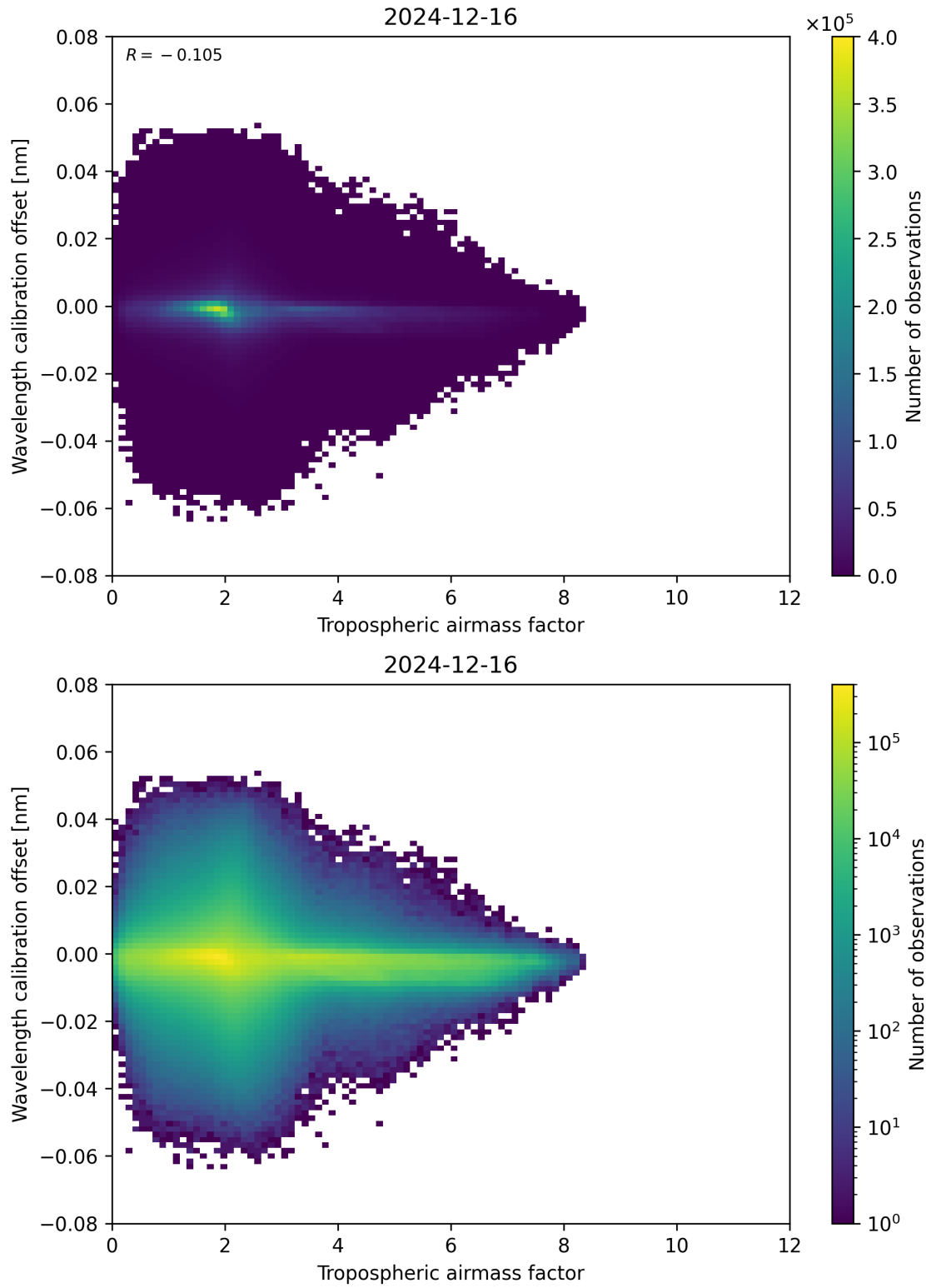
Figure 80: Scatter density plot of “Tropospheric airmass factor” against “Wavelength calibration offset” for 2024-12-16 to 2024-12-17.
