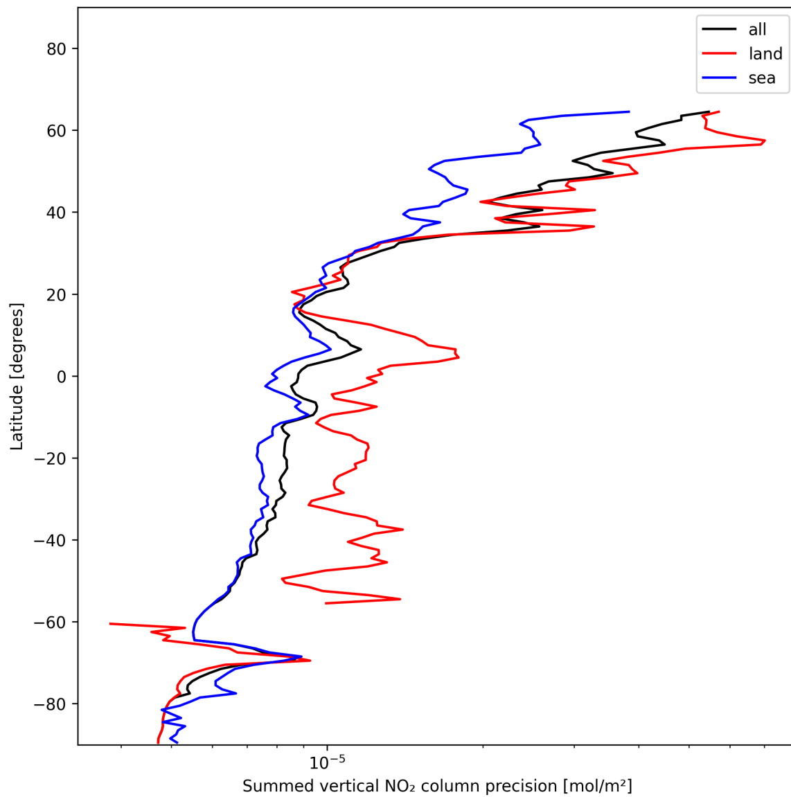
Figure 24: Zonal average of “Summed vertical NO 2 column precision” for 2024-12-16 to 2024-12-17.
