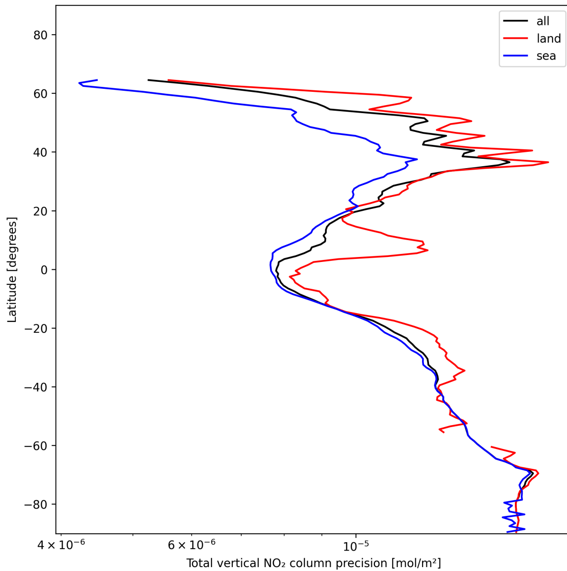
Figure 22: Zonal average of “Total vertical NO 2 column precision” for 2024-12-16 to 2024-12-17.
