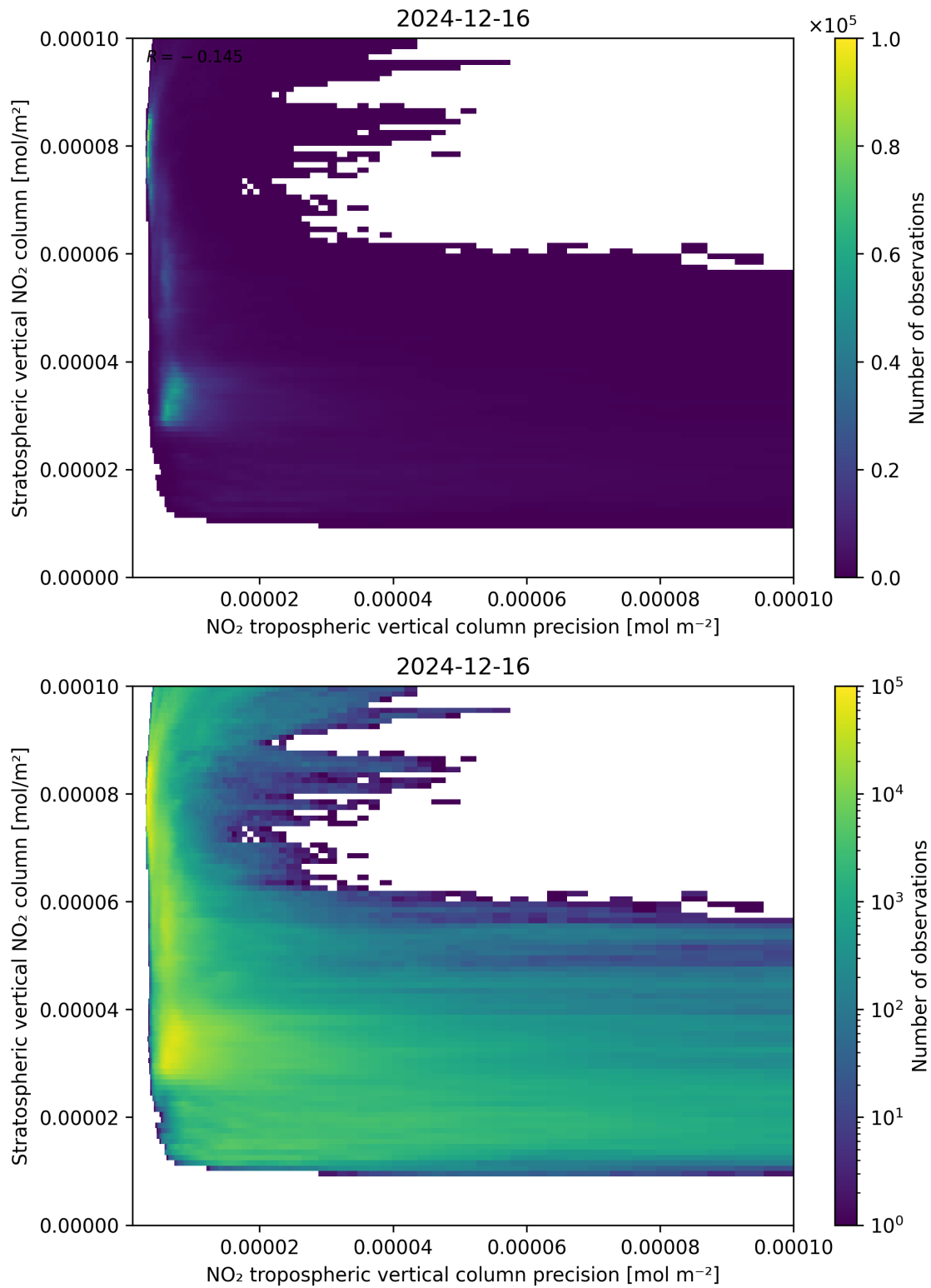
Figure 135: Scatter density plot of “NO 2 tropospheric vertical column precision” against “Stratospheric vertical NO 2 column” for 2024-12-16 to 2024-12-17.
