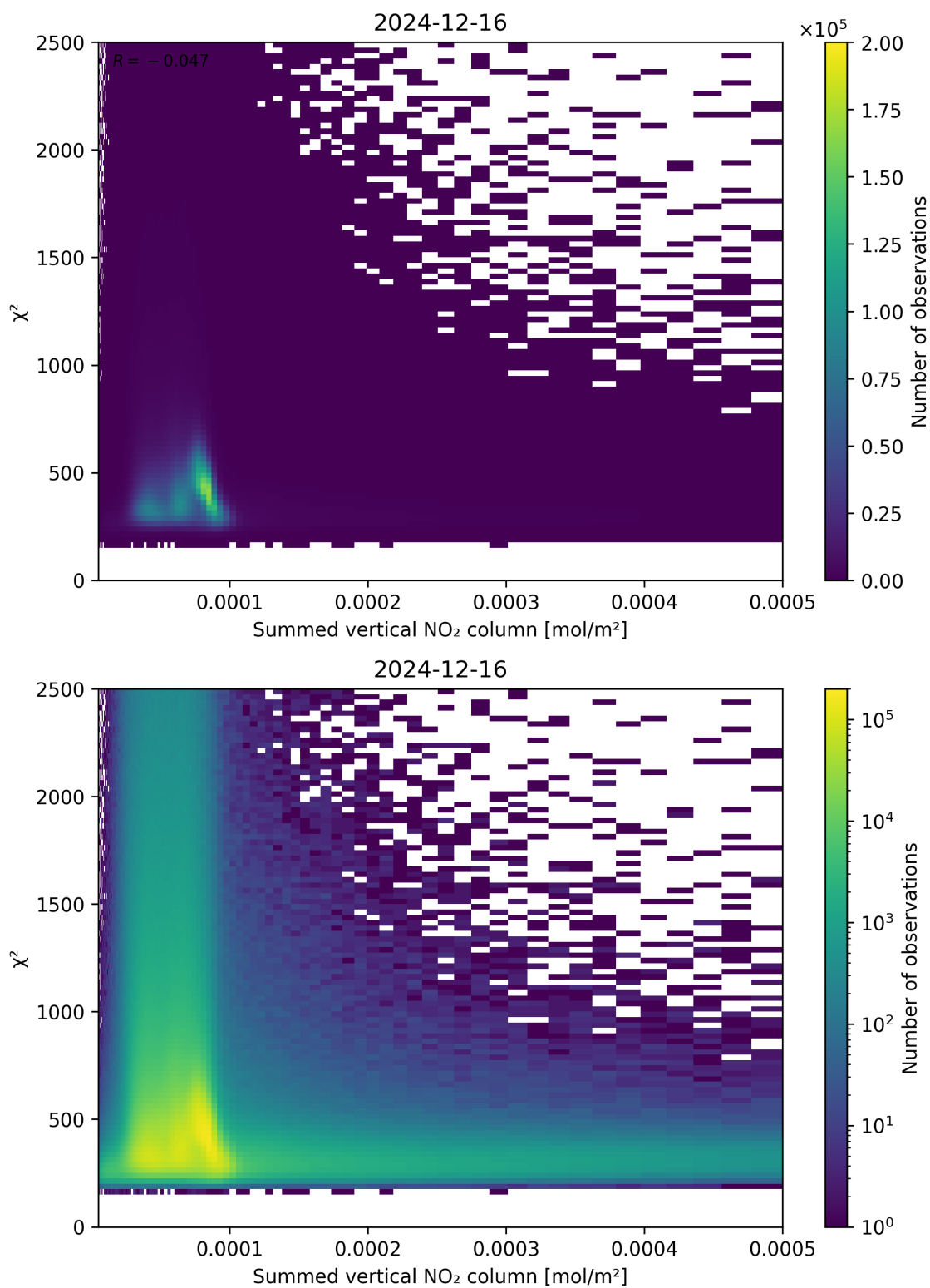
Figure 104: Scatter density plot of “Summed vertical NO 2 column” against “ \chi^2 ” for 2024-12-16 to 2024-12-17.
