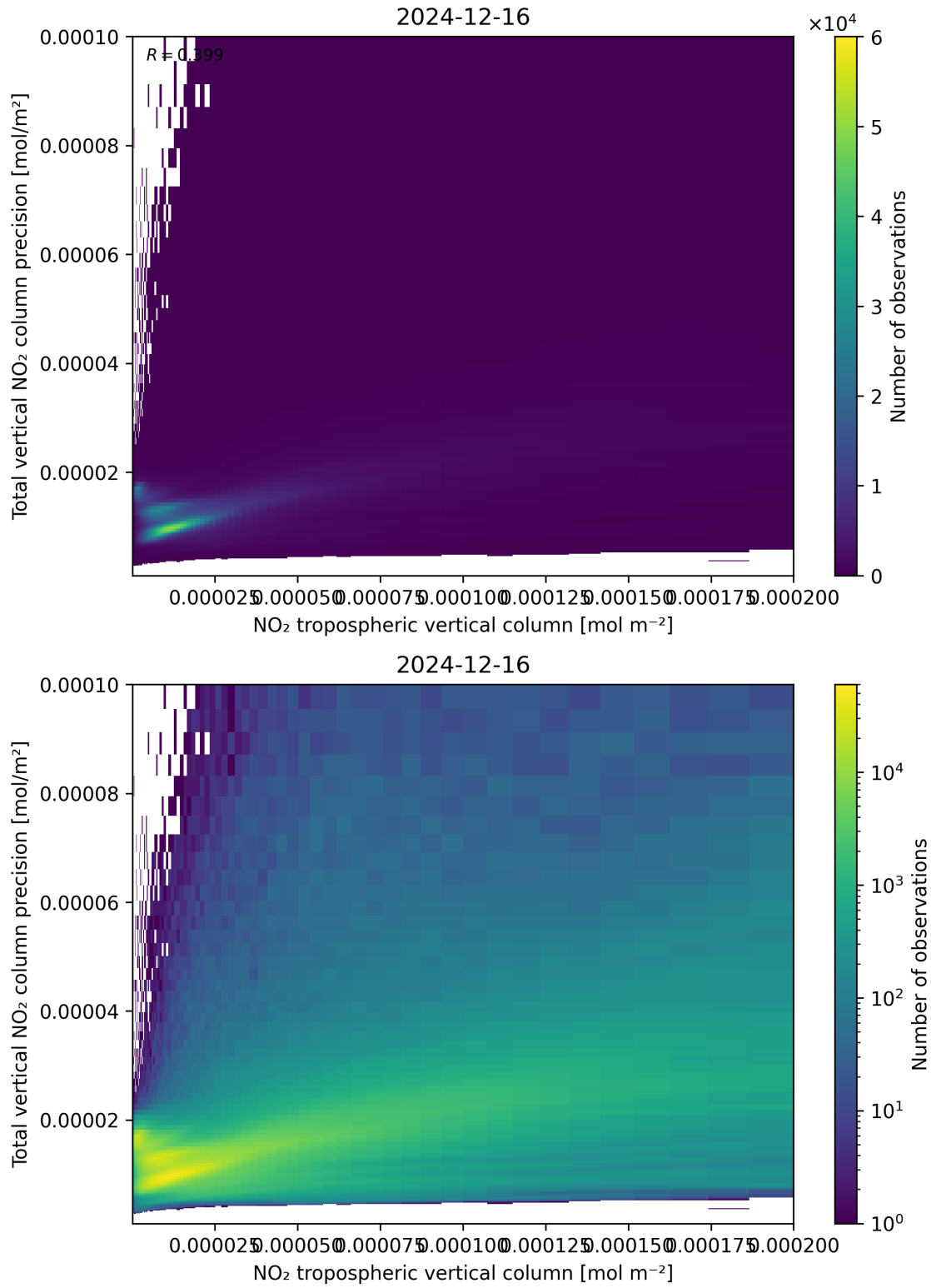
Figure 129: Scatter density plot of “NO 2 tropospheric vertical column” against “Total vertical NO 2 column precision” for 2024-12-16 to 2024-12-17.
