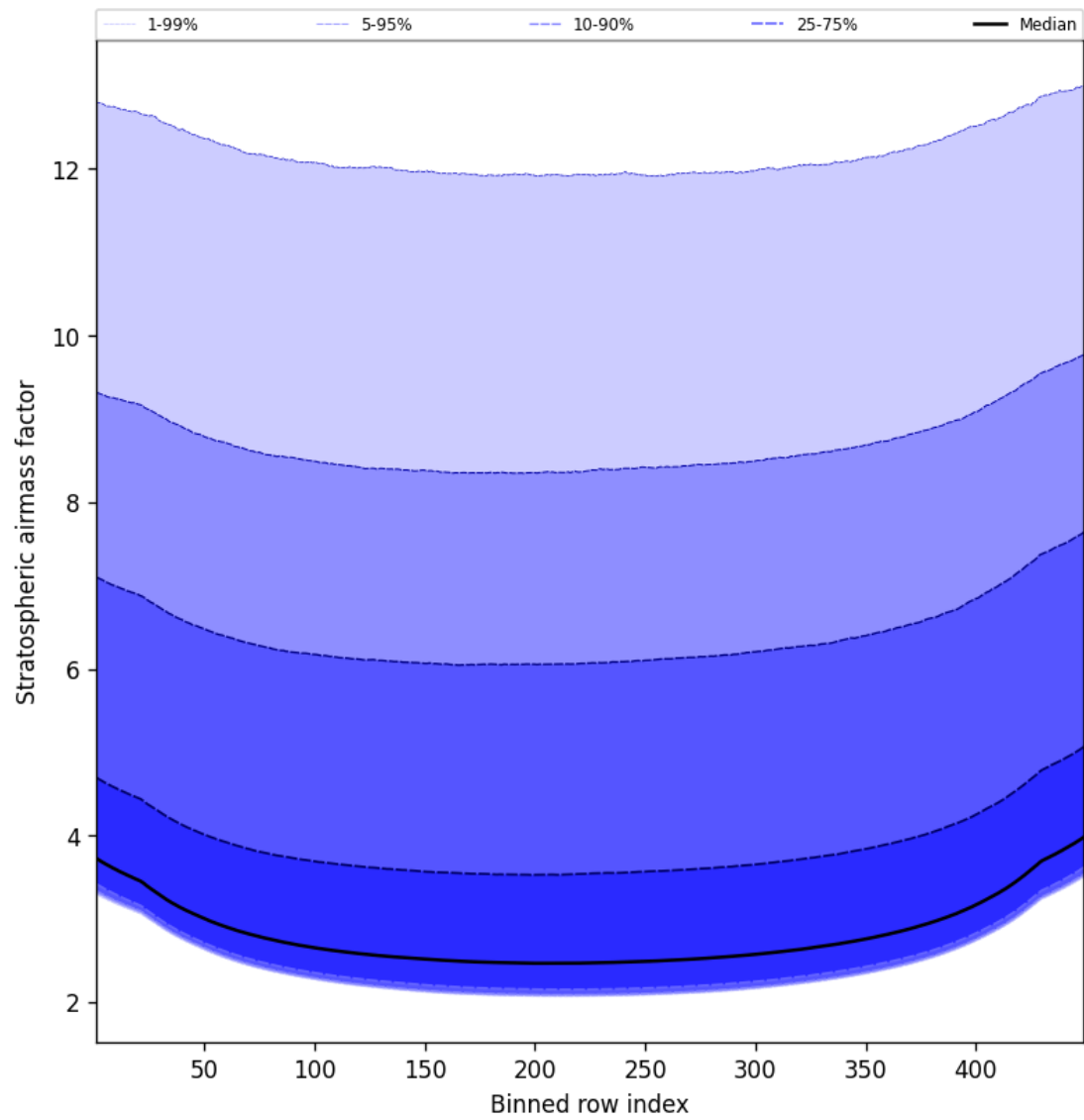
Figure 61: Along track statistics of “Stratospheric airmass factor” for 2024-12-16 to 2024-12-17
