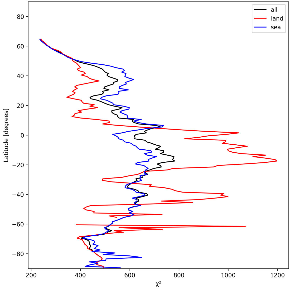
Figure 25: Zonal average of “ \chi^2 ” for 2024-12-16 to 2024-12-17.
