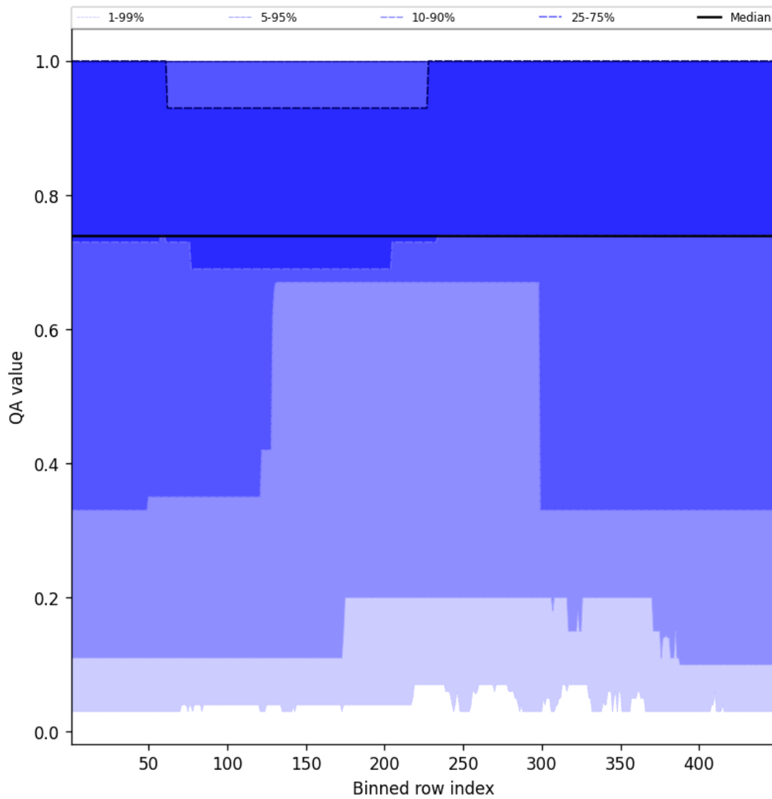
Figure 45: Along track statistics of “QA value” for 2024-12-17 to 2024-12-19
