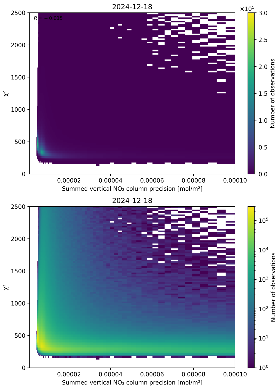
Figure 107: Scatter density plot of “Summed vertical NO 2 column precision” against “ \chi^2 ” for 2024-12-17 to 2024-12-19.
