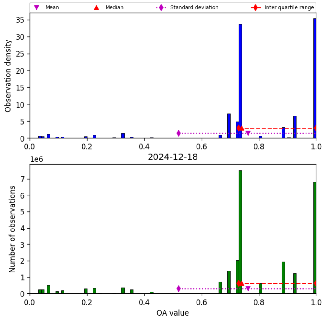
Figure 28: Histogram of “QA value” for 2024-12-17 to 2024-12-19
