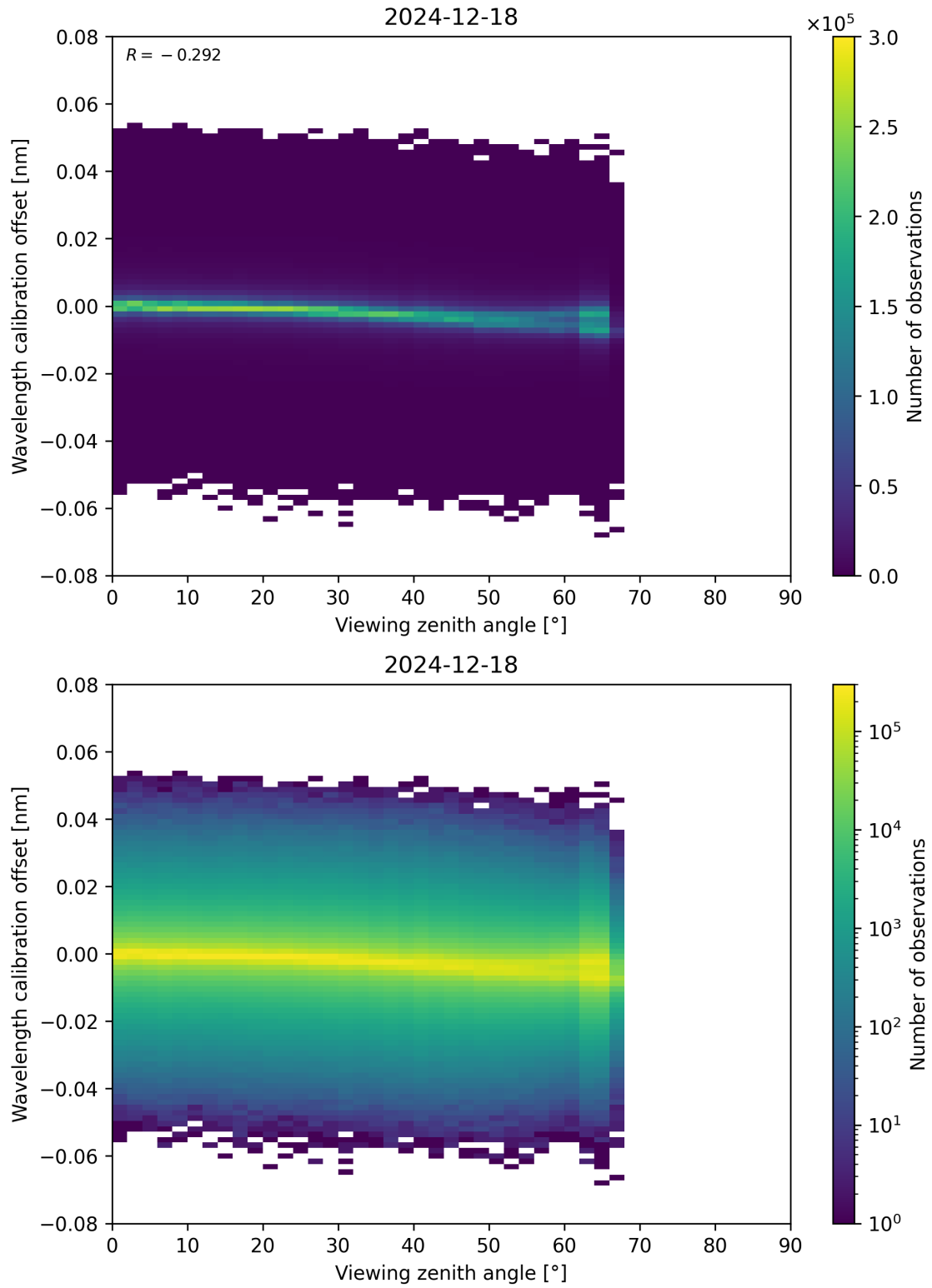
Figure 173: Scatter density plot of “Viewing zenith angle” against “Wavelength calibration offset” for 2024-12-17 to 2024-12-19.
