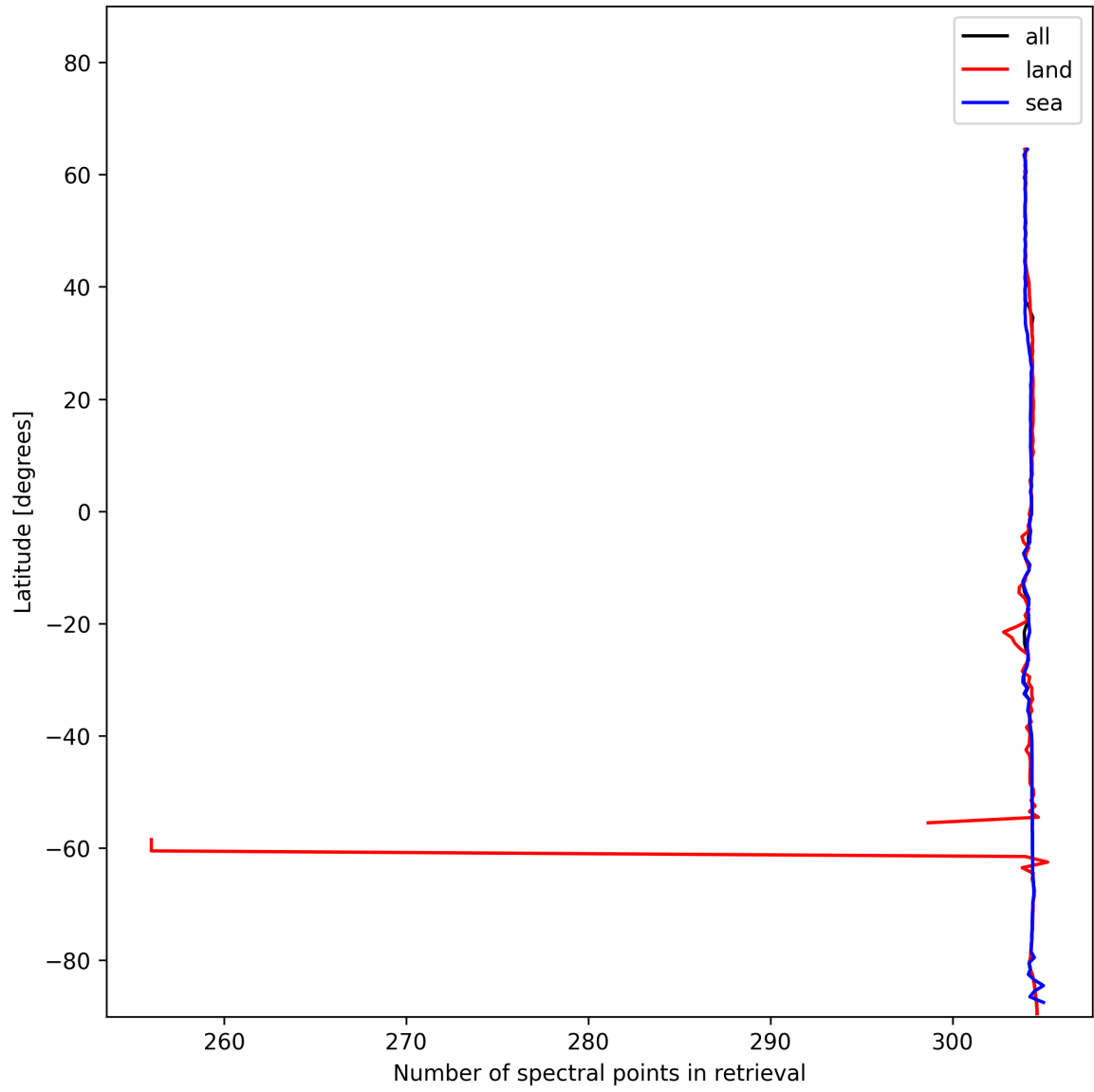
Figure 16: Zonal average of “Number of spectral points in retrieval” for 2024-12-17 to 2024-12-19.
