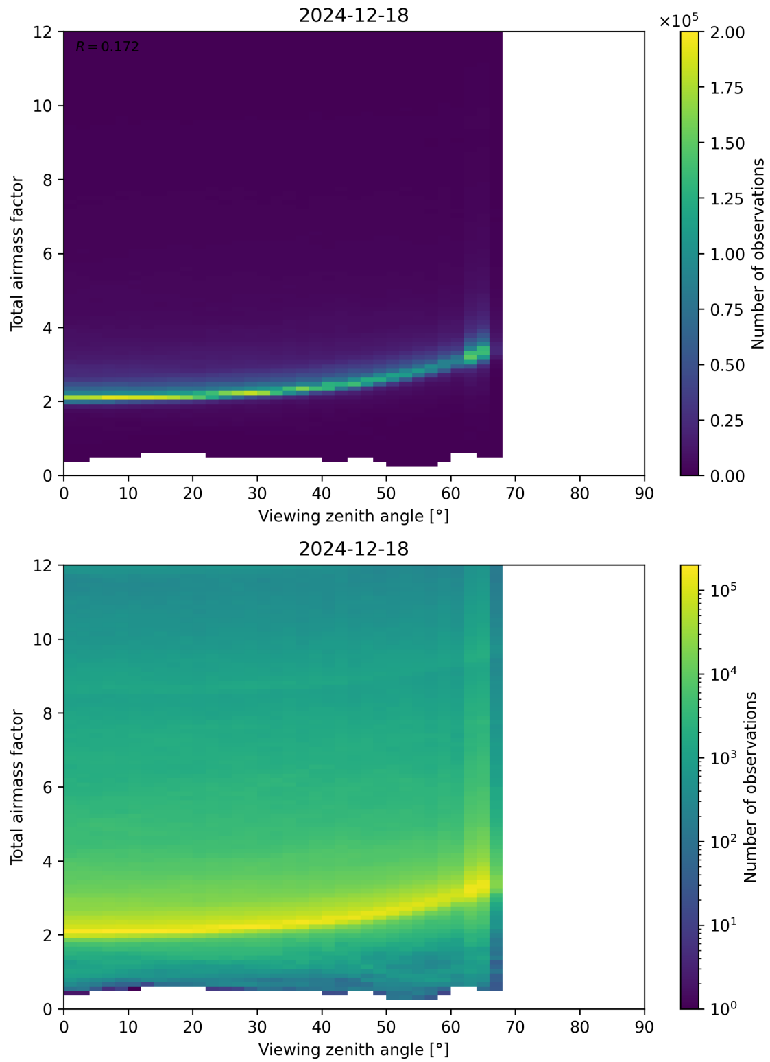
Figure 160: Scatter density plot of “Viewing zenith angle” against “Total airmass factor” for 2024-12-17 to 2024-12-19.
