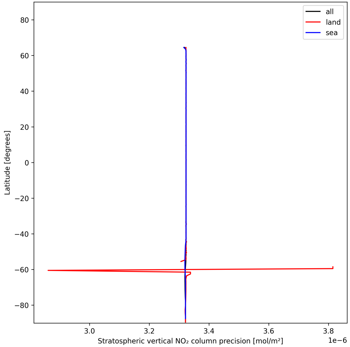
Figure 20: Zonal average of “Stratospheric vertical NO 2 column precision” for 2024-12-17 to 2024-12-19.
