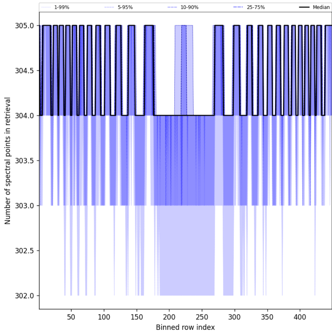
Figure 50: Along track statistics of “Number of spectral points in retrieval” for 2024-12-17 to 2024-12-19
