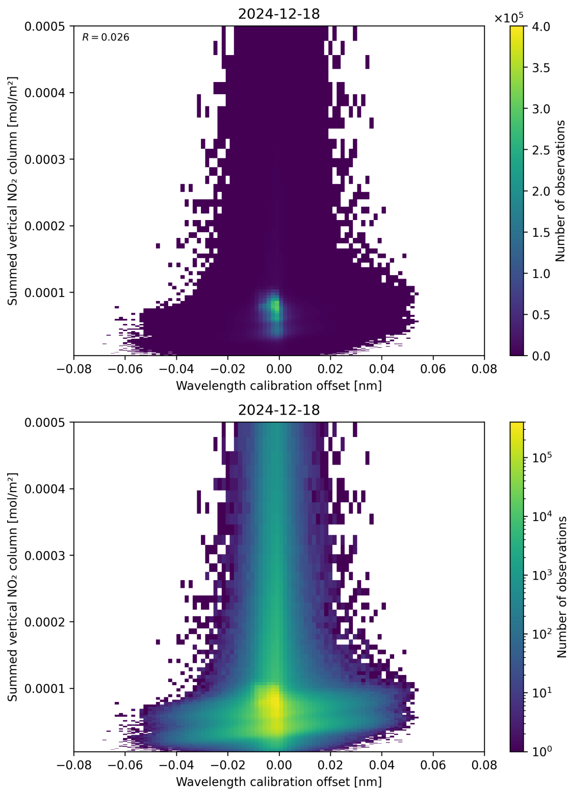
Figure 177: Scatter density plot of “Wavelength calibration offset” against “Summed vertical NO 2 column” for 2024-12-17 to 2024-12-19.
