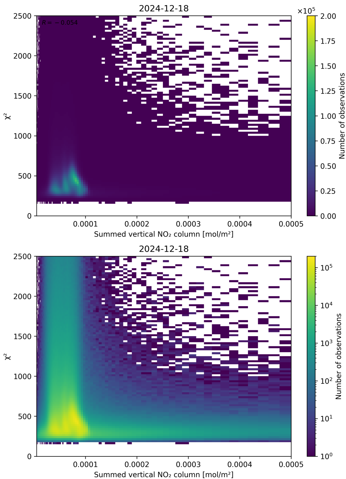
Figure 104: Scatter density plot of “Summed vertical NO 2 column” against “ \chi^2 ” for 2024-12-17 to 2024-12-19.
