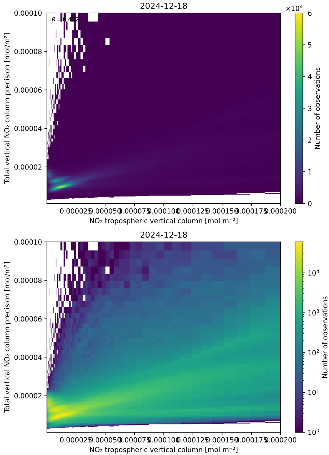
Figure 129: Scatter density plot of “NO 2 tropospheric vertical column” against “Total vertical NO 2 column precision” for 2024-12-17 to 2024-12-19.
