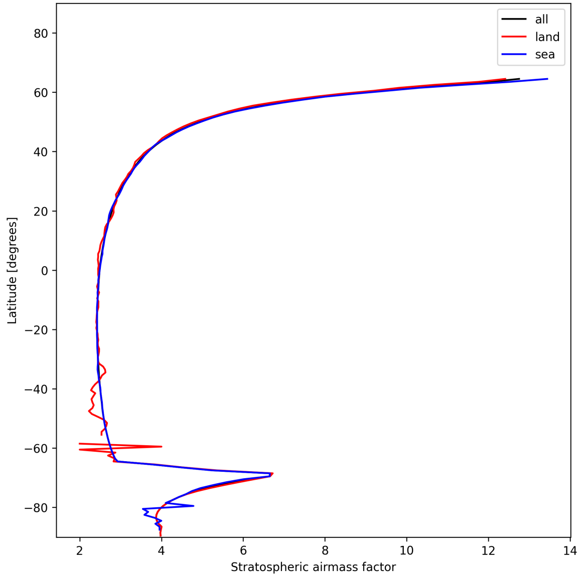
Figure 27: Zonal average of “Stratospheric air mass factor” for 2024-12-17 to 2024-12-19.
