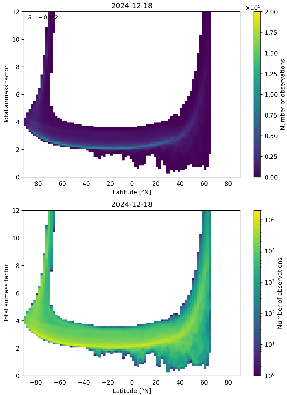
Figure 84: Scatter density plot of “Latitude” against “Total airmass factor” for 2024-12-17 to 2024-12-19.
