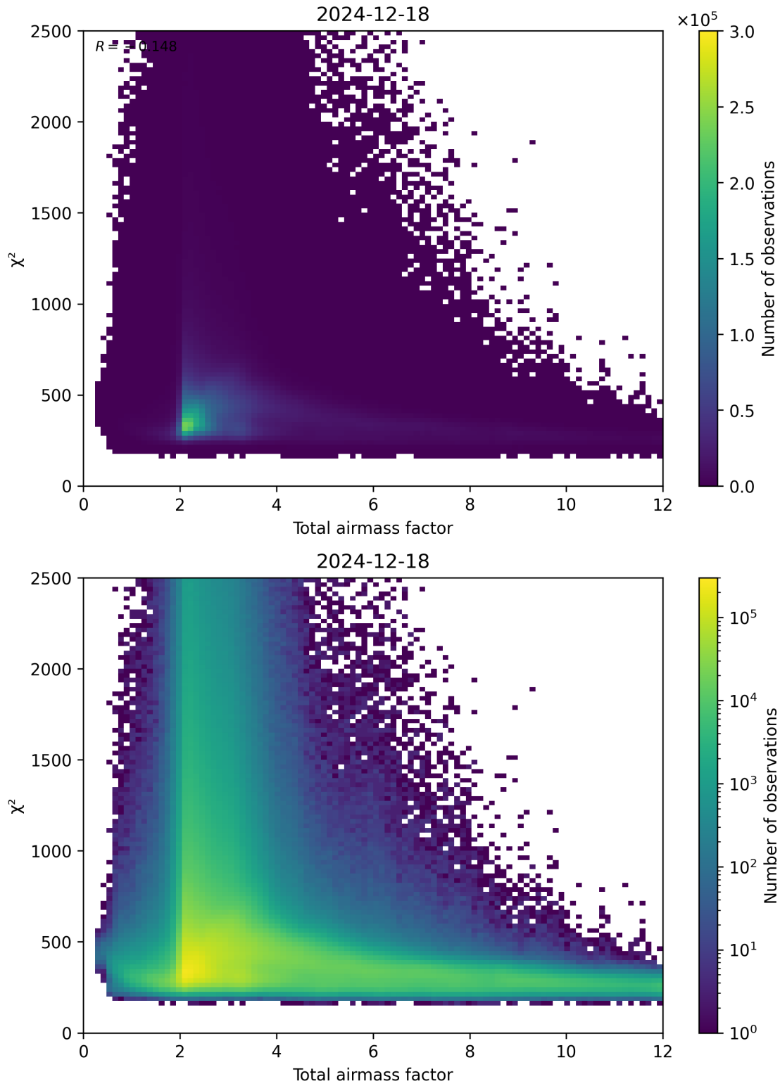
Figure 63: Scatter density plot of “Total airmass factor” against “ \chi^2 ” for 2024-12-17 to 2024-12-19.
