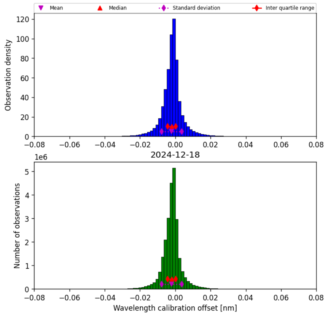
Figure 35: Histogram of “Wavelength calibration offset” for 2024-12-17 to 2024-12-19
