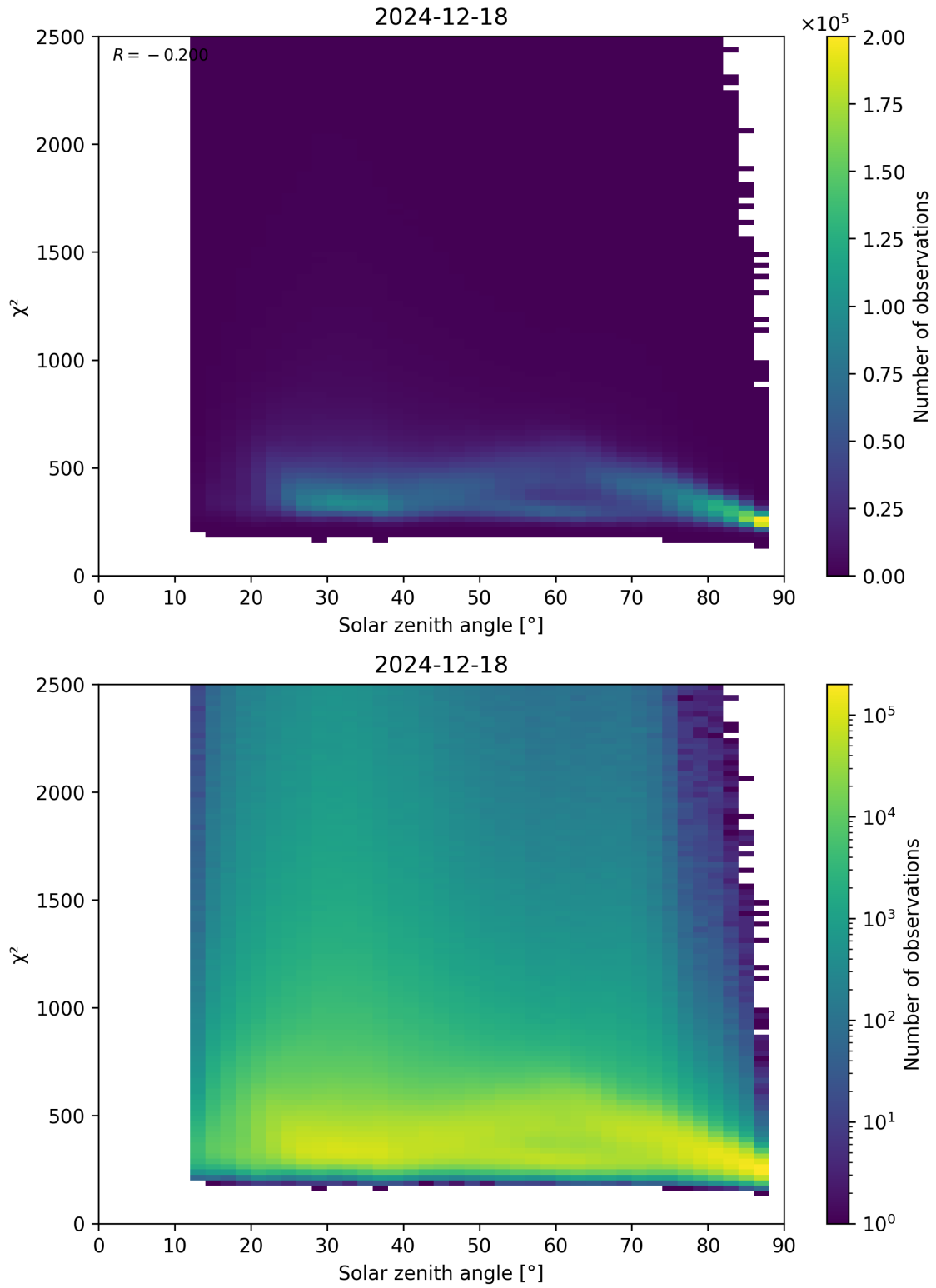
Figure 148: Scatter density plot of “Solar zenith angle” against “ \chi^2 ” for 2024-12-17 to 2024-12-19.
