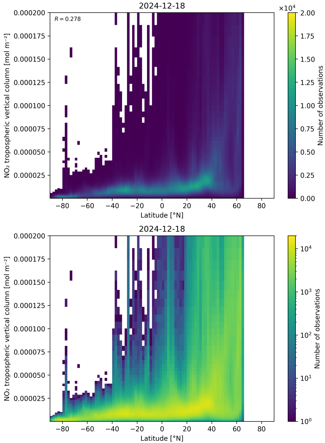
Figure 92: Scatter density plot of “Latitude” against “NO 2 tropospheric vertical column” for 2024-12-17 to 2024-12-19.
