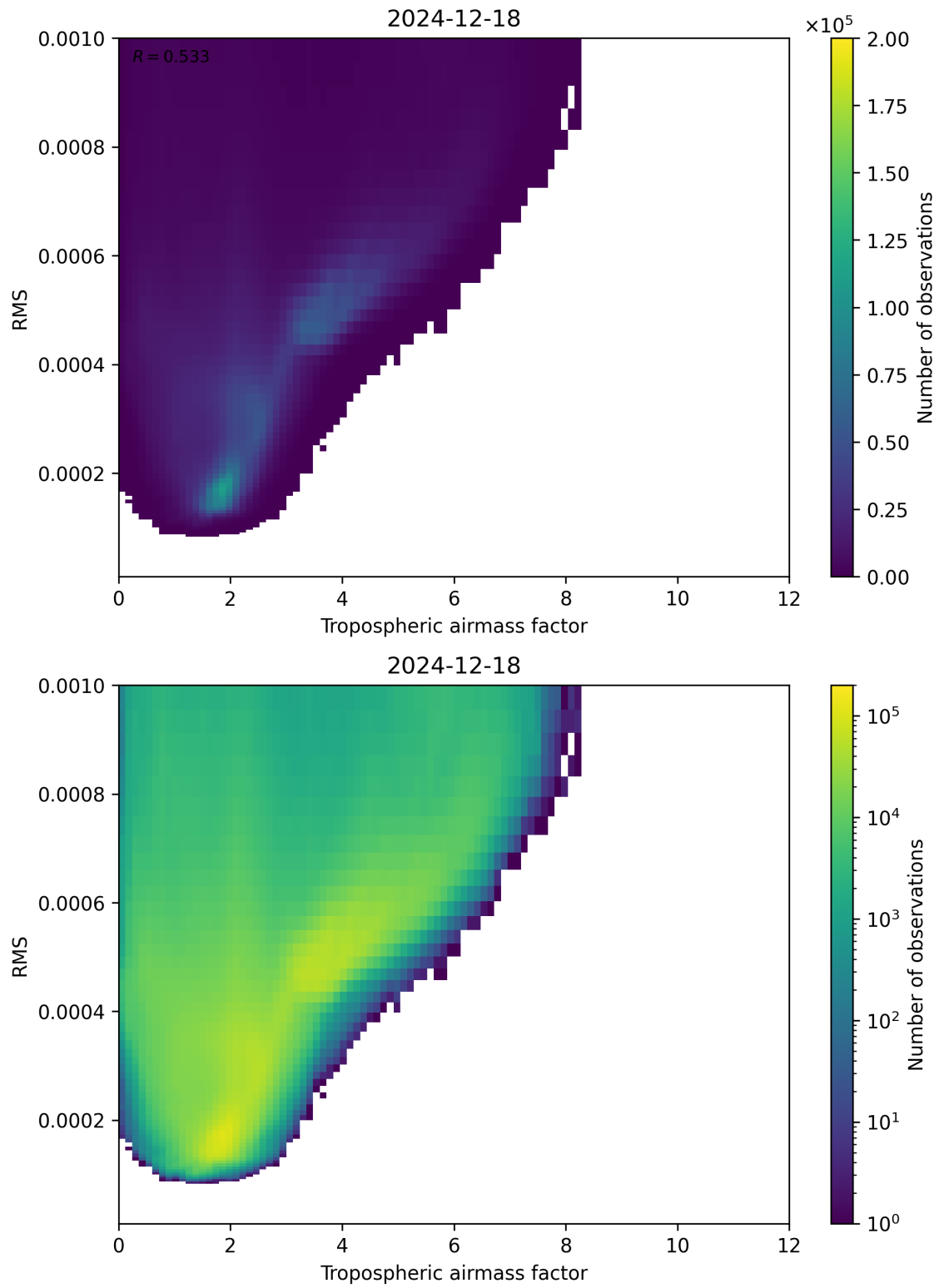
Figure 79: Scatter density plot of “Tropospheric airmass factor” against “RMS” for 2024-12-17 to 2024-12-19.
