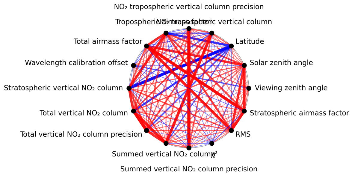
Figure 1: Map of correlation graph for 2024-12-17 to 2024-12-19.
