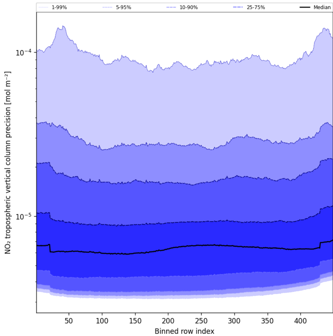
Figure 47: Along track statistics of “NO 2 tropospheric vertical column precision” for 2024-12-17 to 2024-12-19
