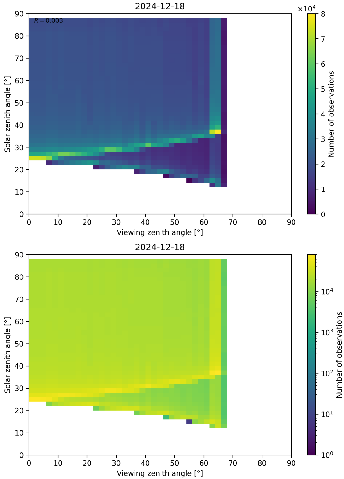
Figure 172: Scatter density plot of “Viewing zenith angle” against “Solar zenith angle” for 2024-12-17 to 2024-12-19.
