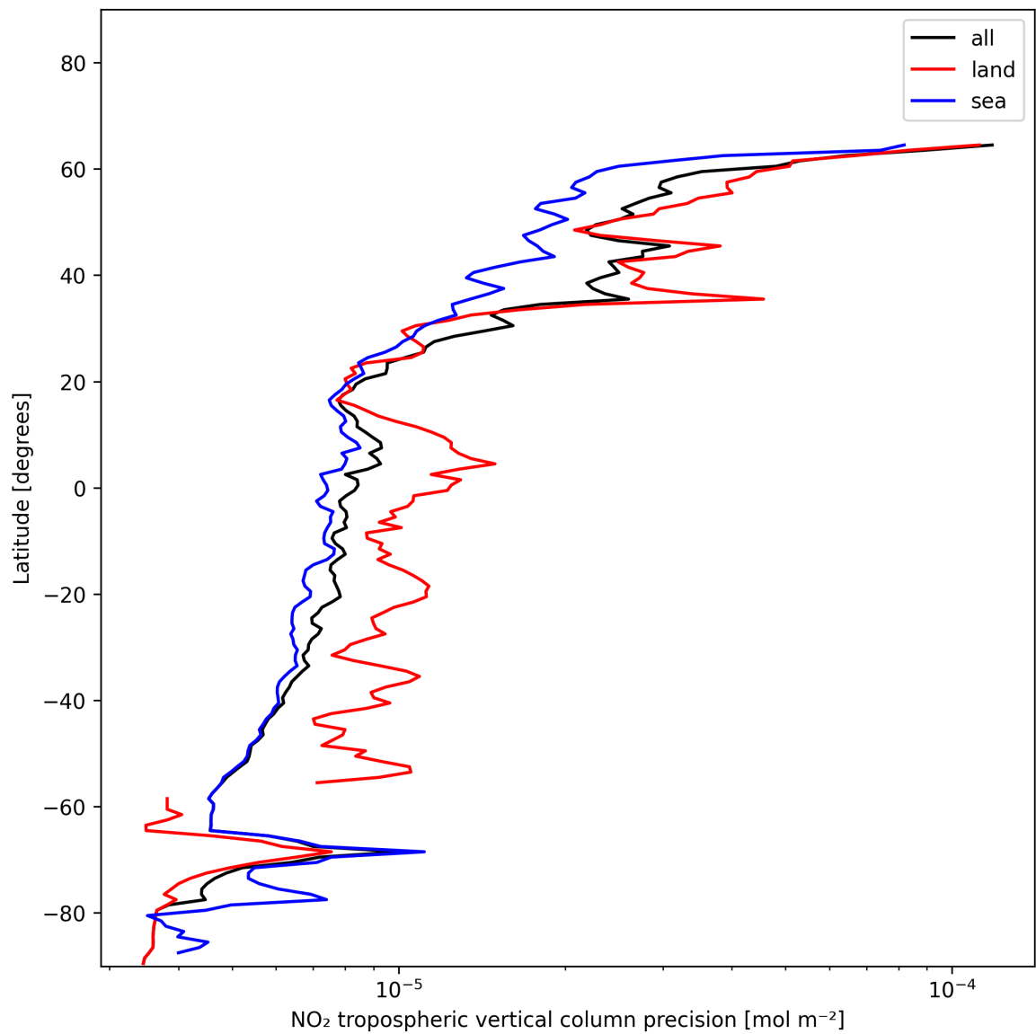
Figure 13: Zonal average of “NO 2 tropospheric vertical column precision” for 2024-12-17 to 2024-12-19.
