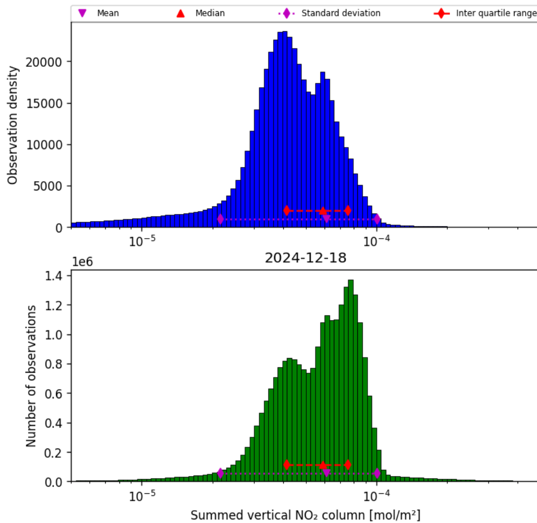
Figure 40: Histogram of “Summed vertical NO 2 column” for 2024-12-17 to 2024-12-19
