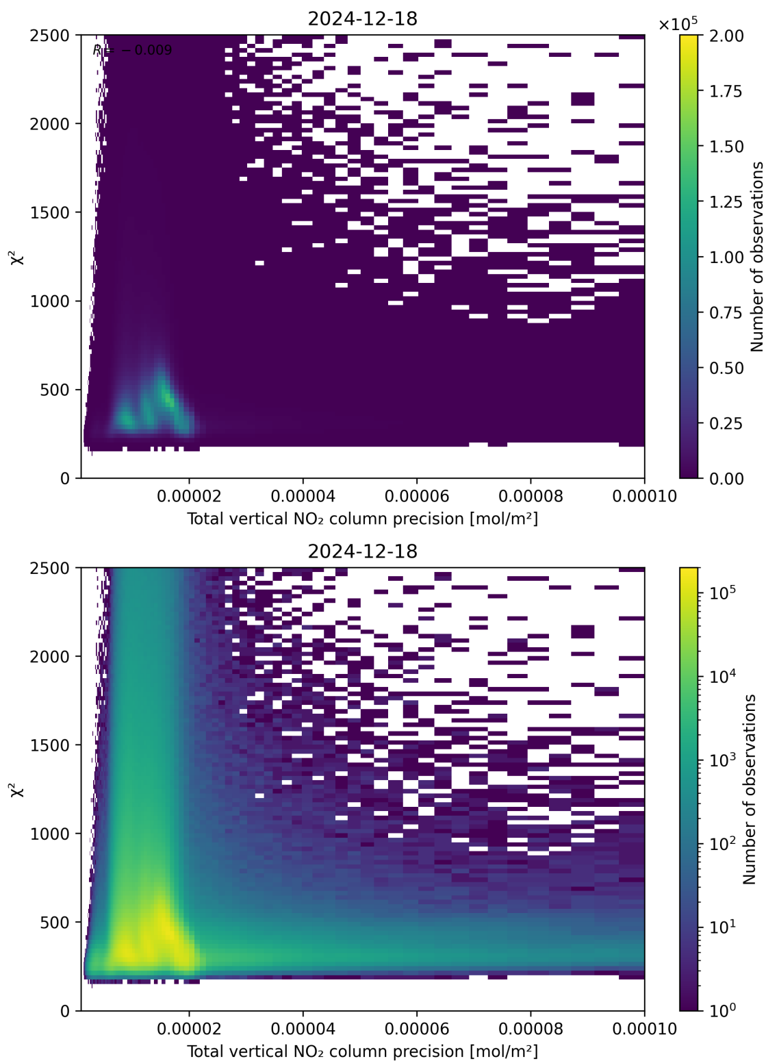
Figure 116: Scatter density plot of “Total vertical NO 2 column precision” against “ \chi^2 ” for 2024-12-17 to 2024-12-19.
