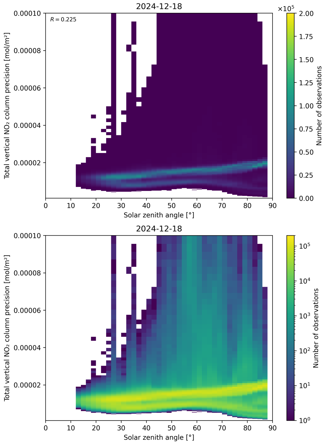
Figure 154: Scatter density plot of “Solar zenith angle” against “Total vertical NO 2 column precision” for 2024-12-17 to 2024-12-19.
