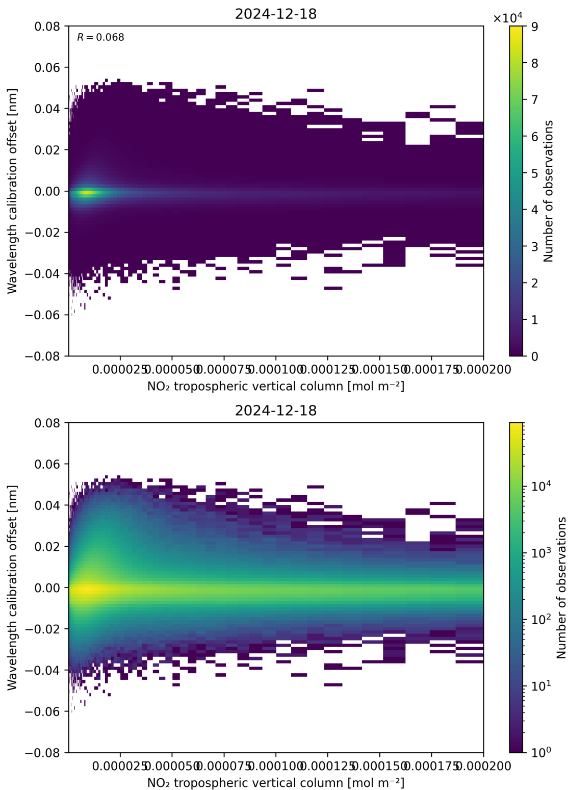
Figure 143: Scatter density plot of “NO 2 tropospheric vertical column” against “Wavelength calibration offset” for 2024-12-17 to 2024-12-19.
