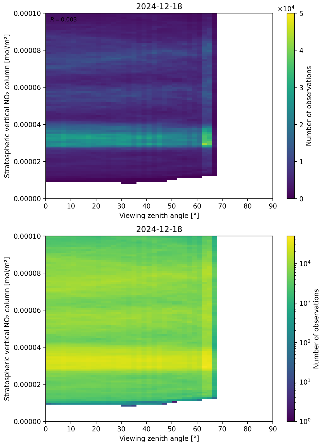
Figure 164: Scatter density plot of “Viewing zenith angle” against “Stratospheric vertical NO 2 column” for 2024-12-17 to 2024-12-19.
