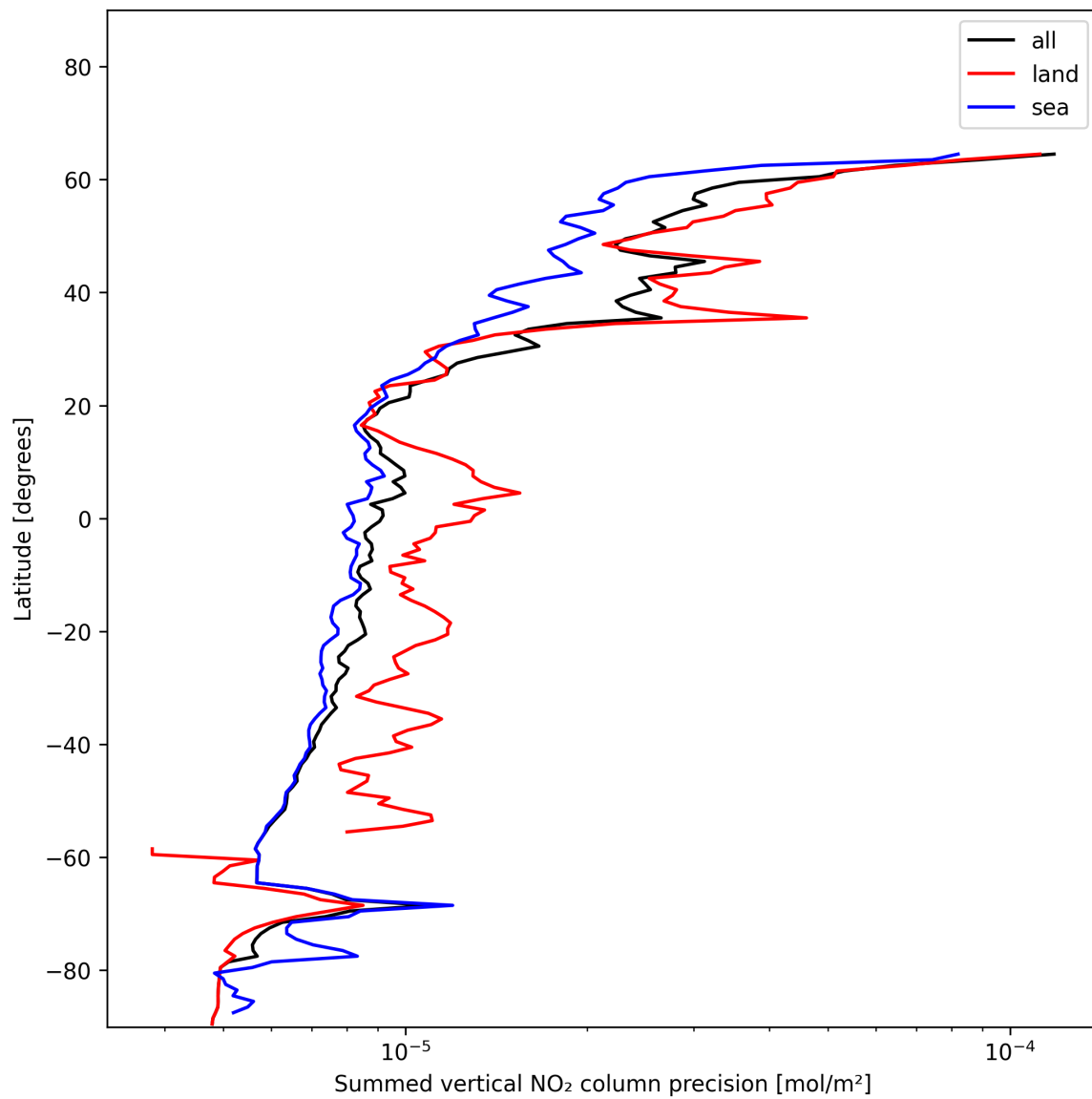
Figure 24: Zonal average of “Summed vertical NO 2 column precision” for 2024-12-17 to 2024-12-19.
