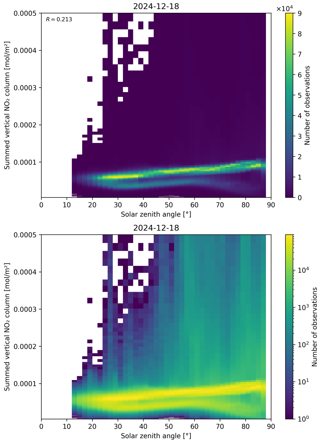
Figure 151: Scatter density plot of “Solar zenith angle” against “Summed vertical NO 2 column” for 2024-12-17 to 2024-12-19.
