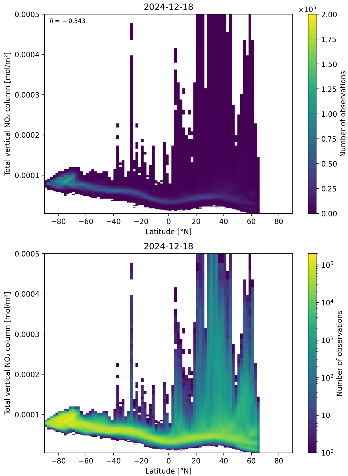
Figure 90: Scatter density plot of “Latitude” against “Total vertical NO 2 column” for 2024-12-17 to 2024-12-19.
