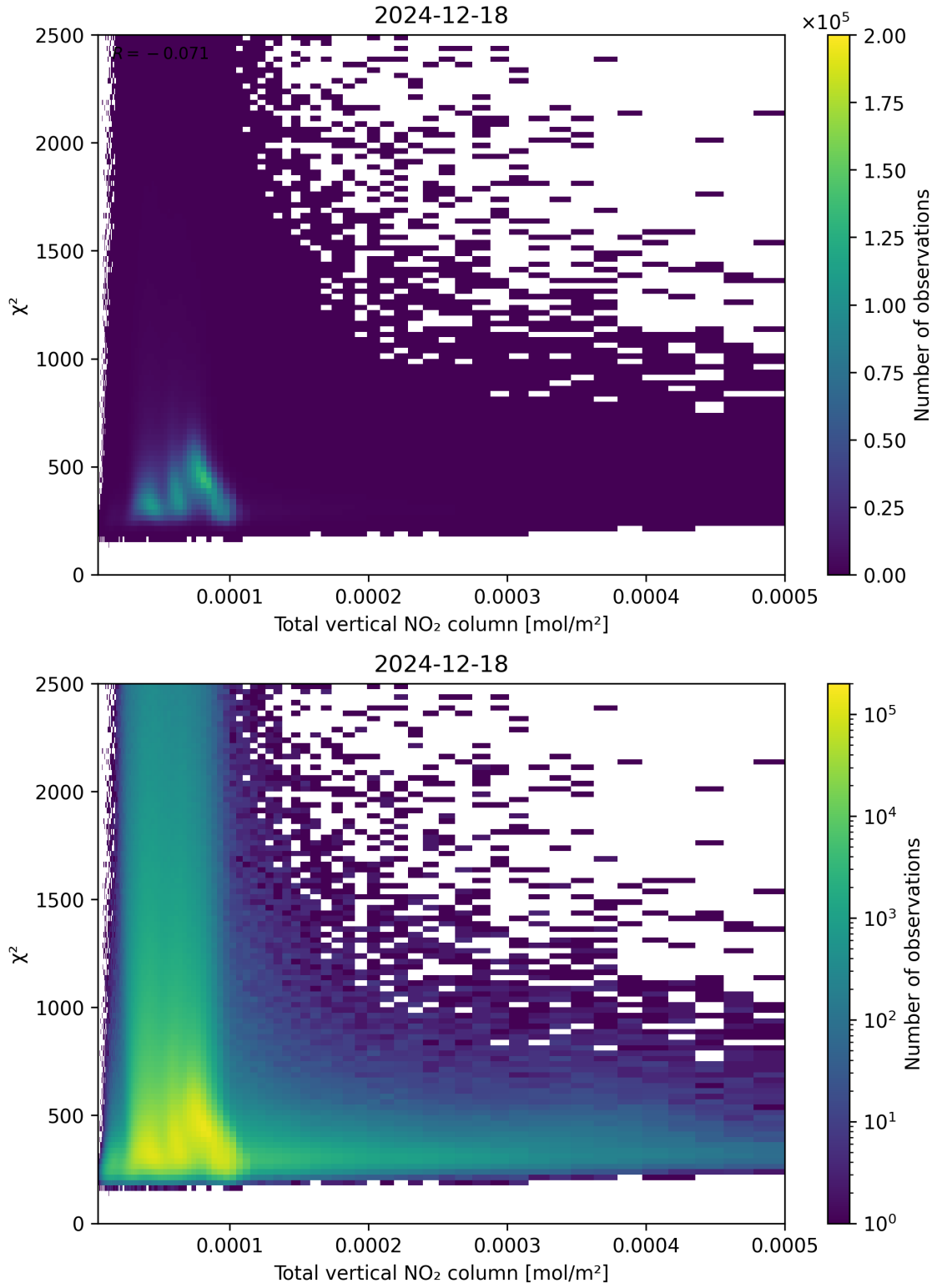
Figure 111: Scatter density plot of “Total vertical NO 2 column” against “ \chi^2 ” for 2024-12-17 to 2024-12-19.
