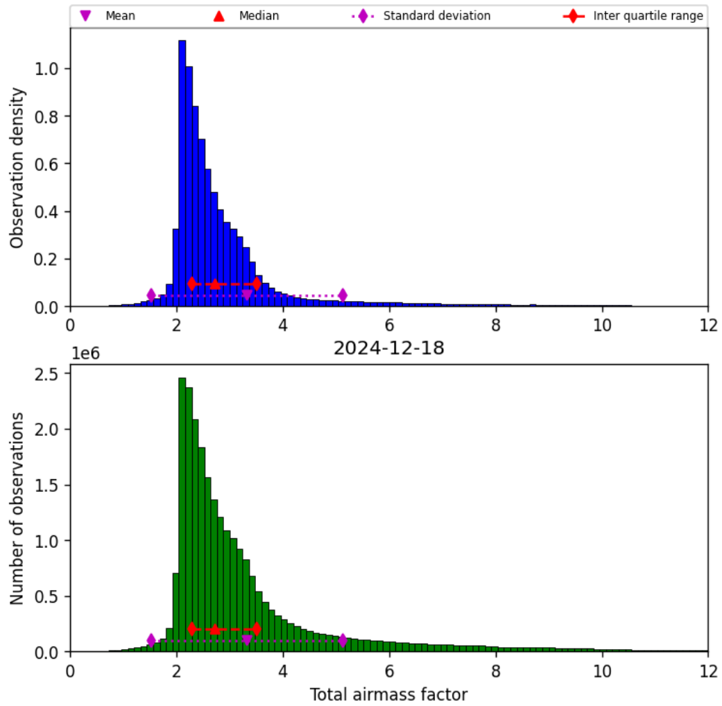
Figure 32: Histogram of “Total airmass factor” for 2024-12-17 to 2024-12-19
