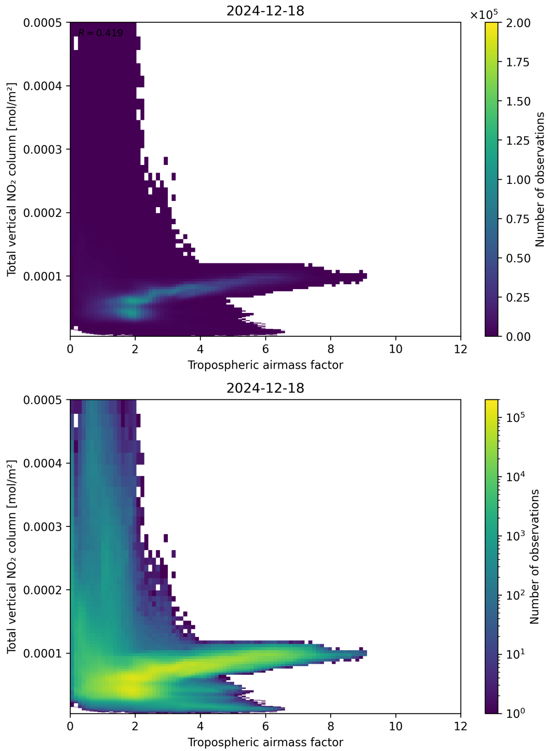
Figure 77: Scatter density plot of “Tropospheric airmass factor” against “Total vertical NO 2 column” for 2024-12-17 to 2024-12-19.
