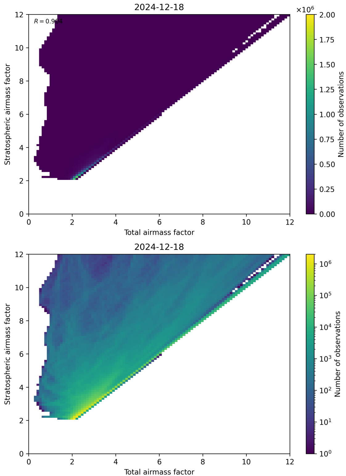
Figure 62: Scatter density plot of “Total airmass factor” against “Stratospheric airmass factor” for 2024-12-17 to 2024-12-19.
