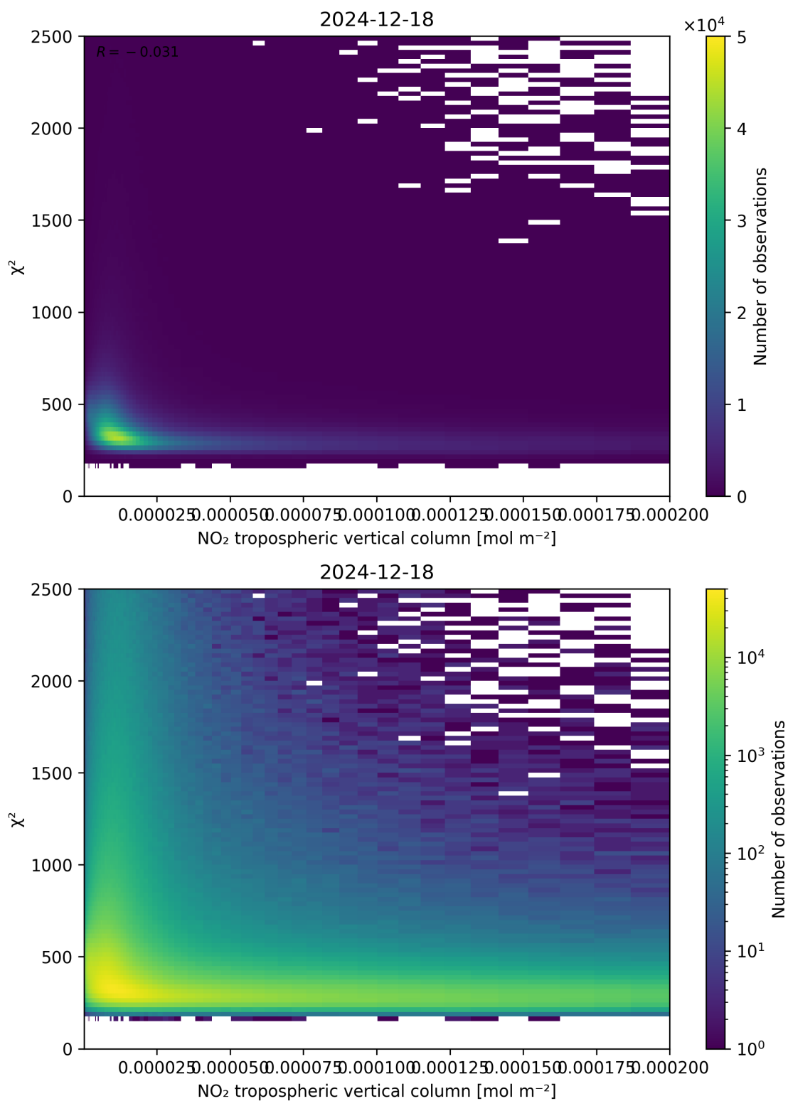
Figure 124: Scatter density plot of “NO 2 tropospheric vertical column” against “ \chi^2 ” for 2024-12-17 to 2024-12-19.
