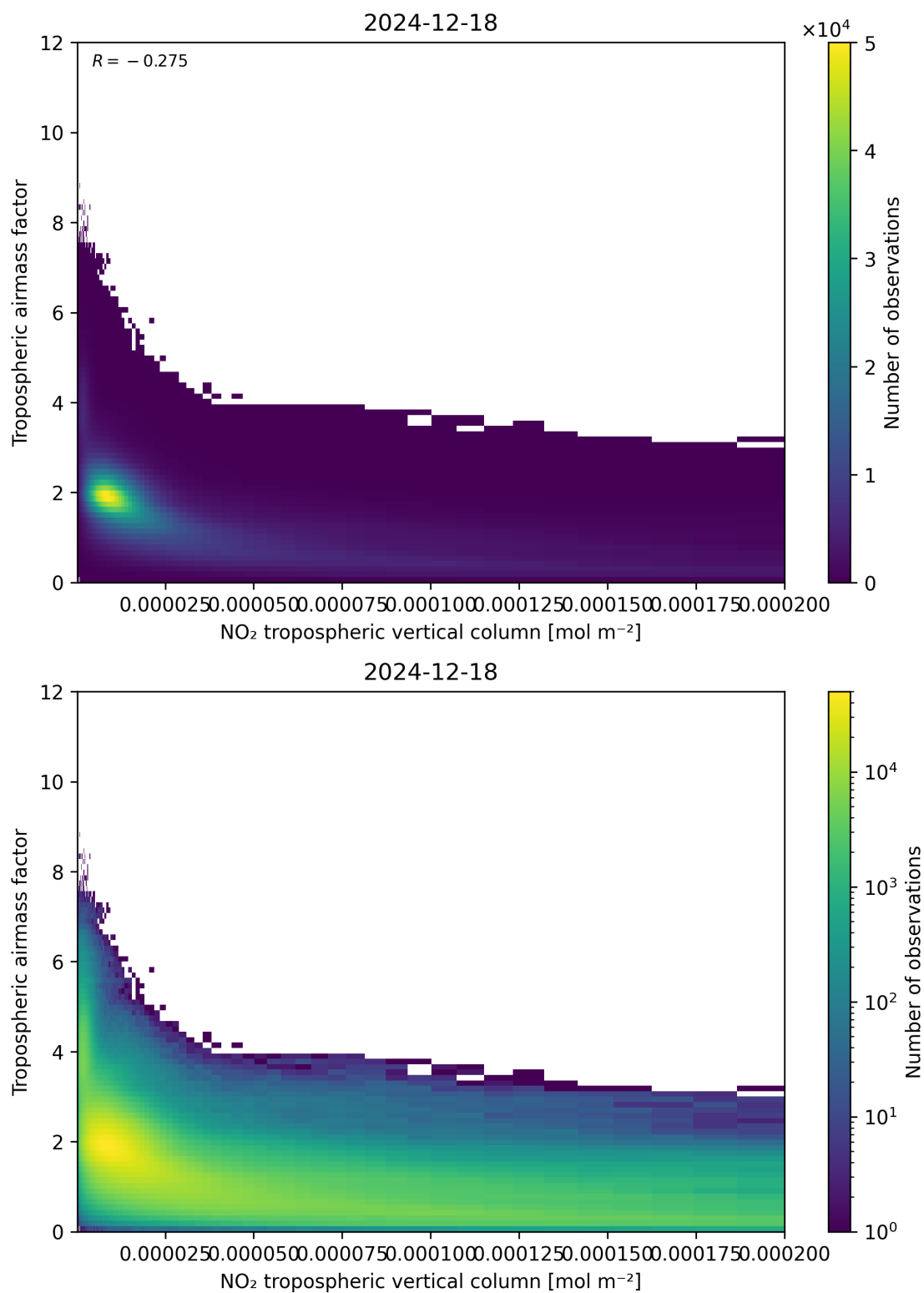
Figure 123: Scatter density plot of “NO 2 tropospheric vertical column” against “Tropospheric air mass factor” for 2024-12-17 to 2024-12-19.
