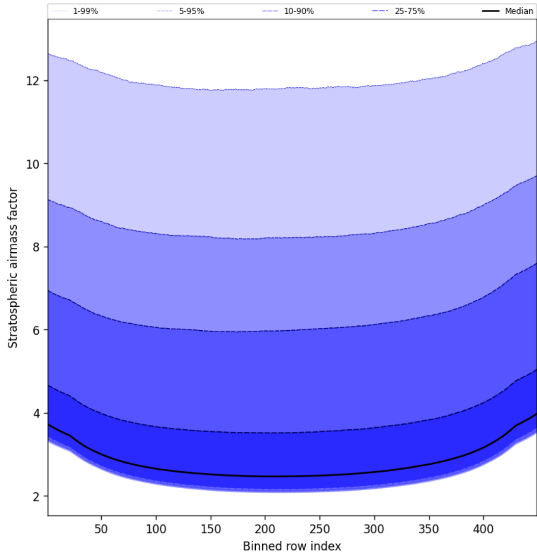
Figure 61: Along track statistics of “Stratospheric airmass factor” for 2024-12-17 to 2024-12-19
