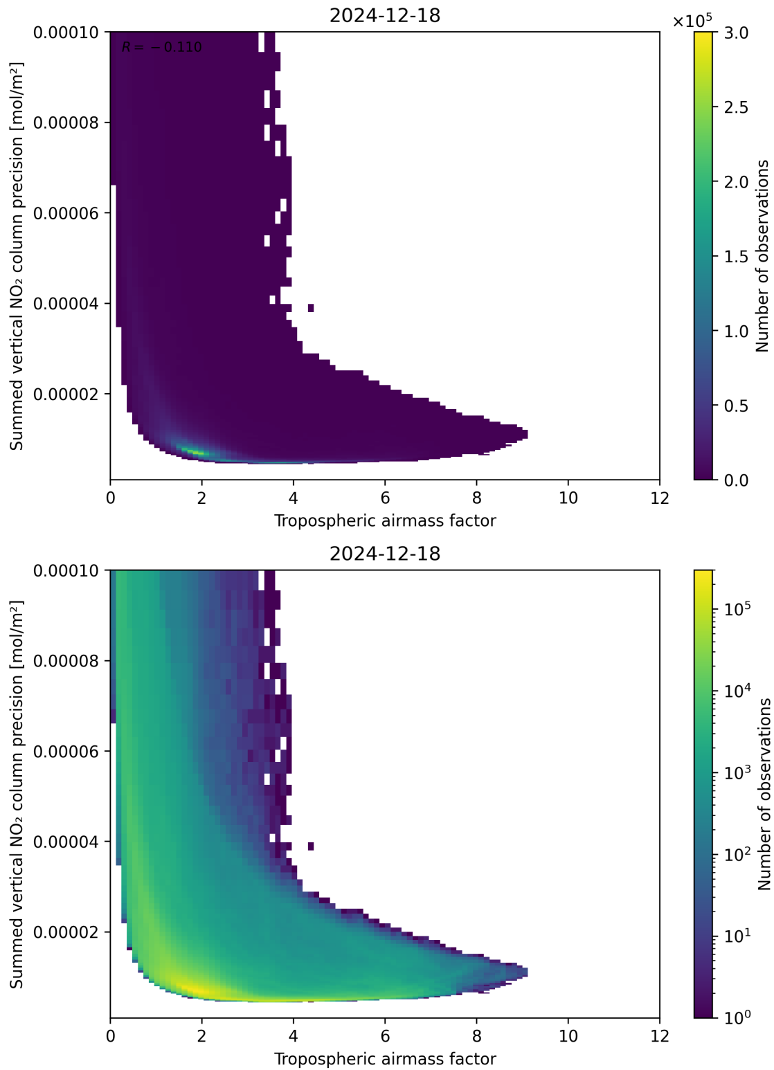
Figure 76: Scatter density plot of “Tropospheric airmass factor” against “Summed vertical NO 2 column precision” for 2024-12-17 to 2024-12-19.
