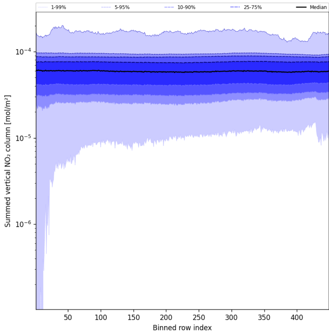
Figure 57: Along track statistics of “Summed vertical NO 2 column” for 2024-12-17 to 2024-12-19
