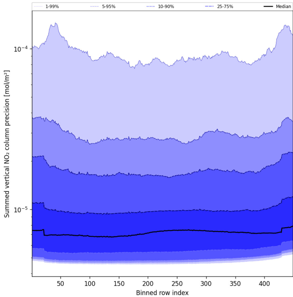
Figure 58: Along track statistics of “Summed vertical NO 2 column precision” for 2024-12-17 to 2024-12-19
