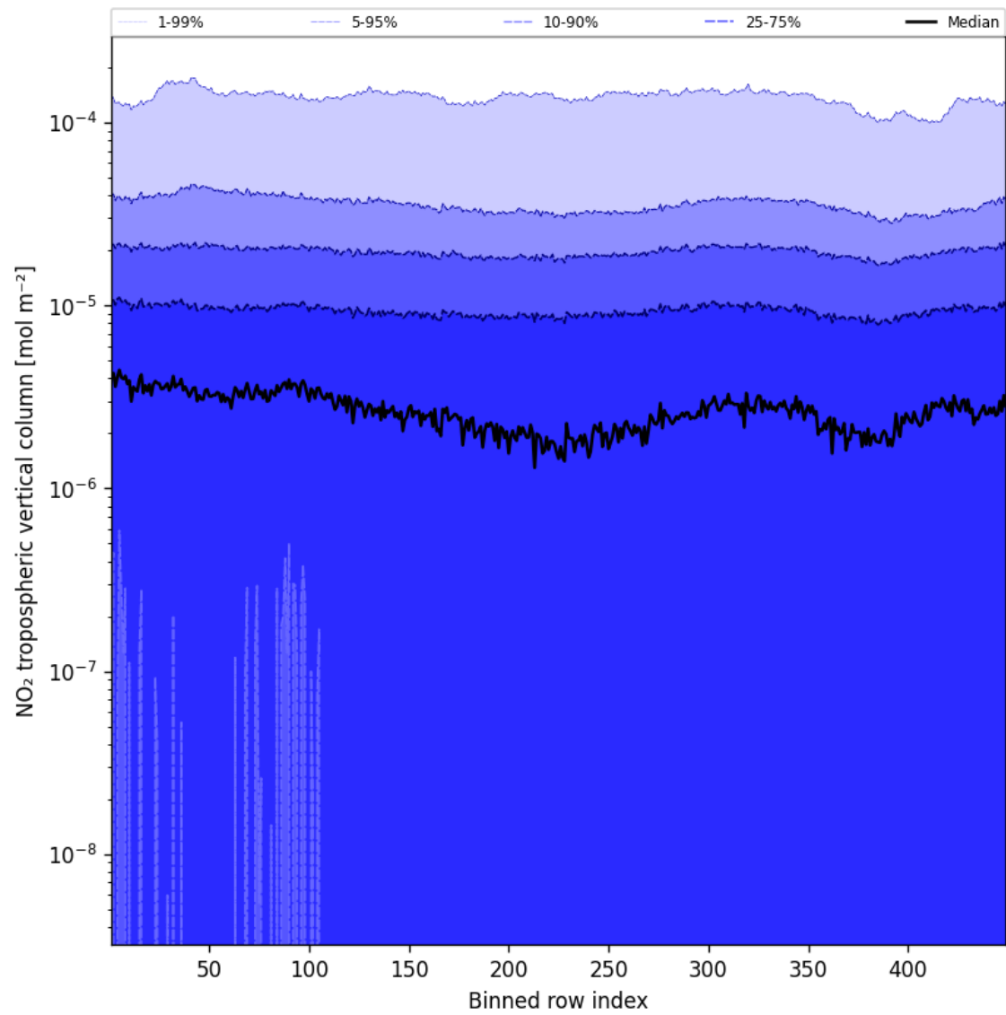
Figure 46: Along track statistics of “NO 2 tropospheric vertical column” for 2024-12-17 to 2024-12-19
