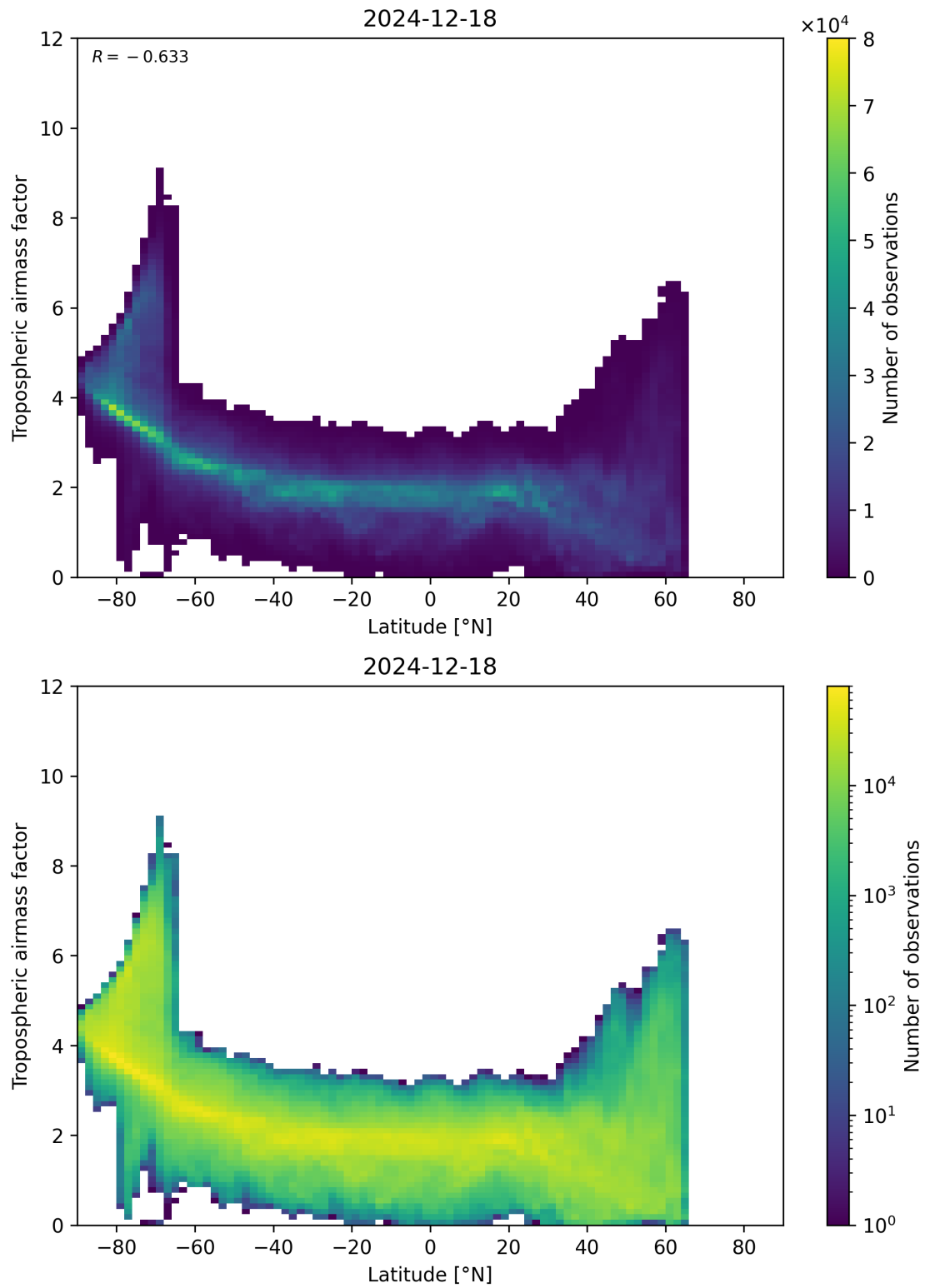
Figure 85: Scatter density plot of “Latitude” against “Tropospheric airmass factor” for 2024-12-17 to 2024-12-19.
