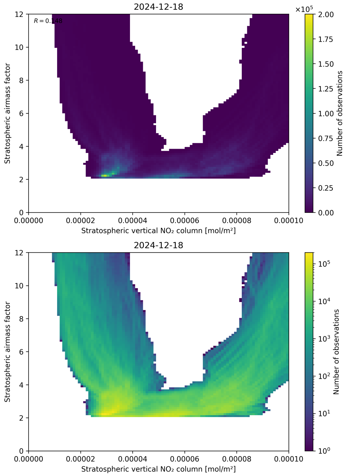
Figure 96: Scatter density plot of “Stratospheric vertical NO 2 column” against “Stratospheric airmass factor” for 2024-12-17 to 2024-12-19.
