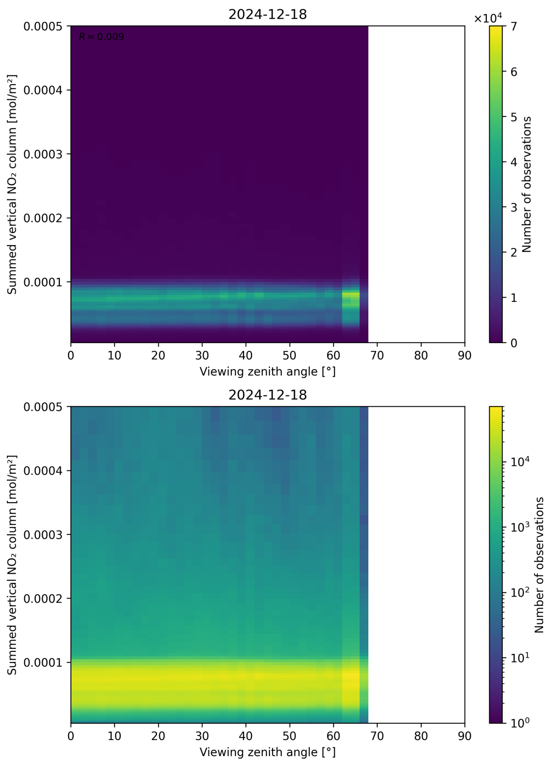
Figure 165: Scatter density plot of “Viewing zenith angle” against “Summed vertical NO 2 column” for 2024-12-17 to 2024-12-19.
