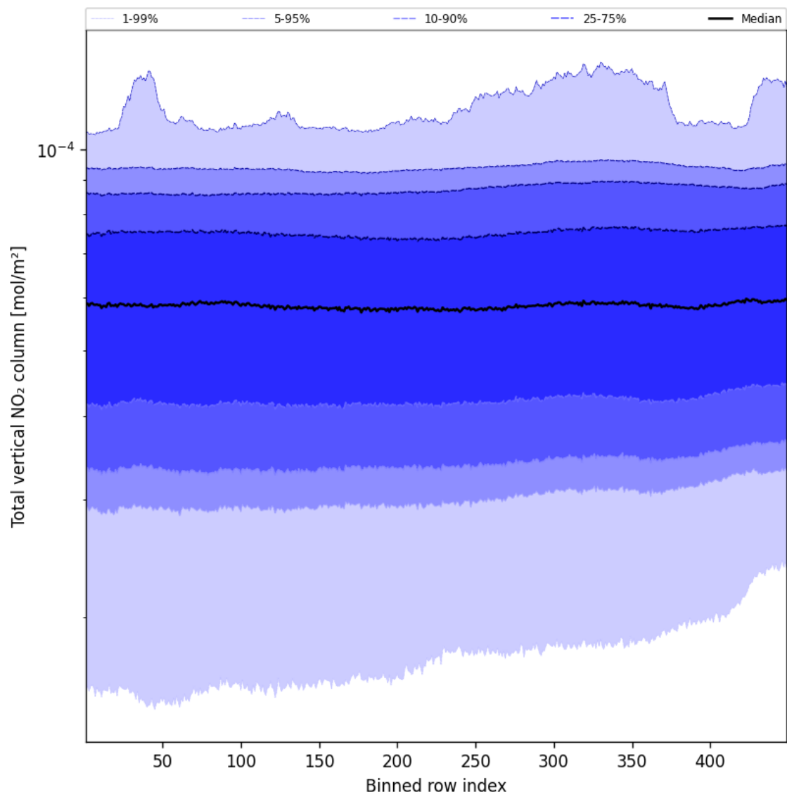
Figure 55: Along track statistics of “Total vertical NO 2 column” for 2024-12-17 to 2024-12-19
