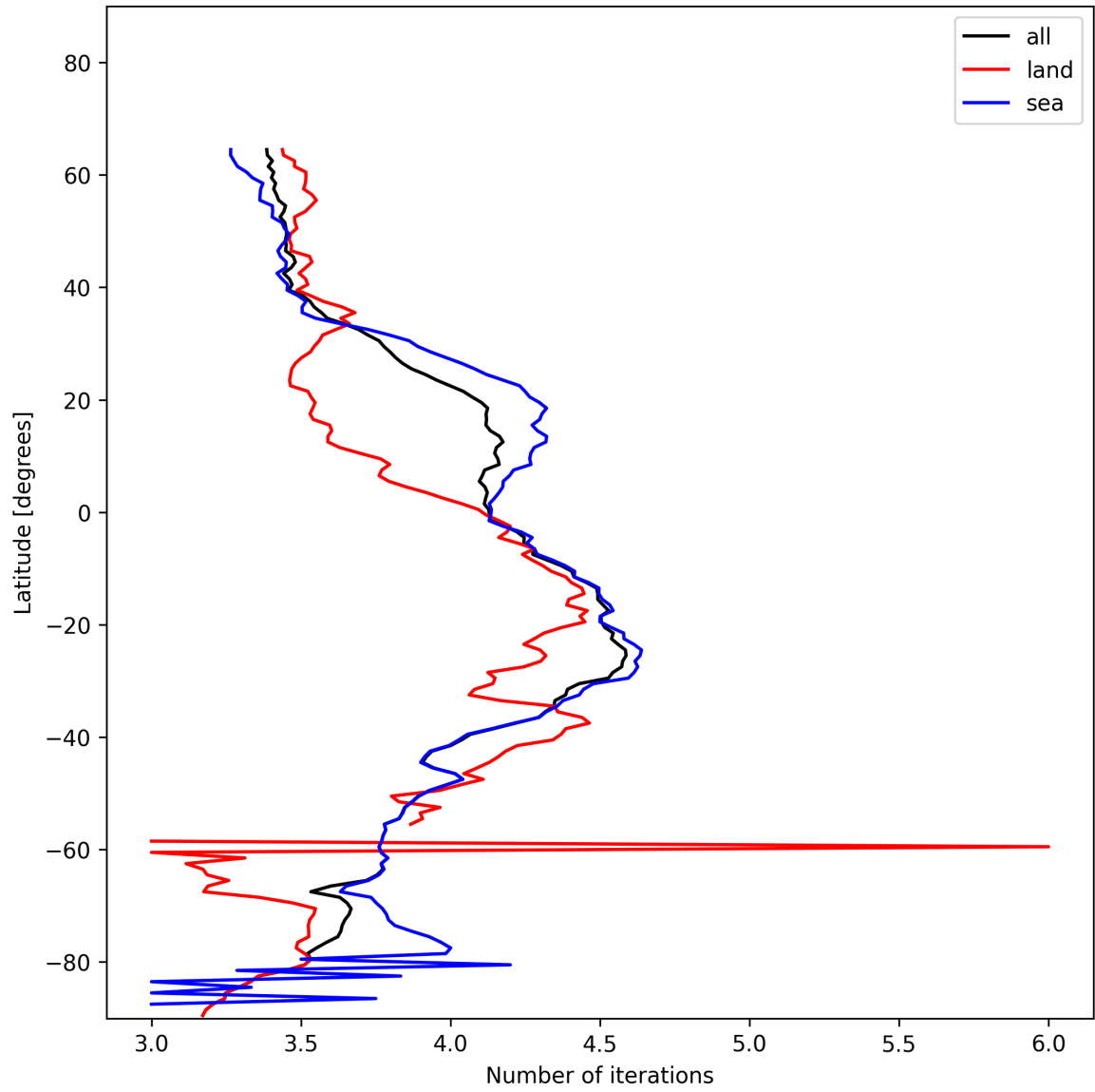
Figure 17: Zonal average of “Number of iterations” for 2024-12-17 to 2024-12-19.
