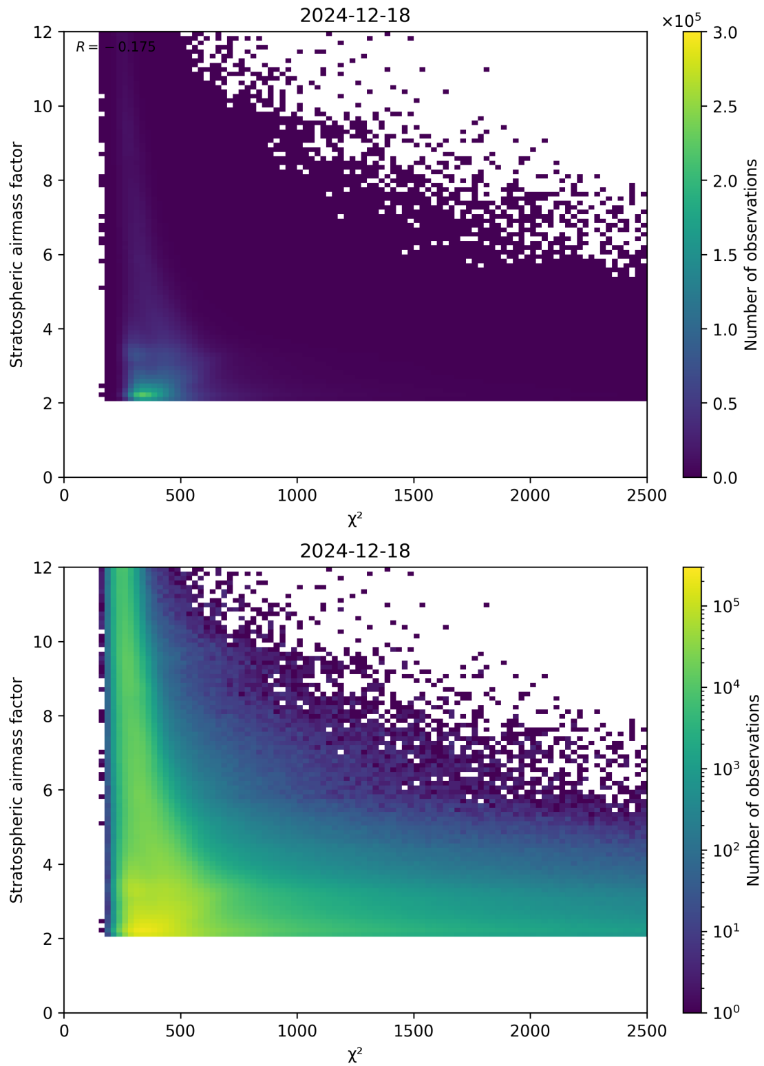
Figure 81: Scatter density plot of “ \chi^2 ” against “Stratospheric airmass factor” for 2024-12-17 to 2024-12-19.
