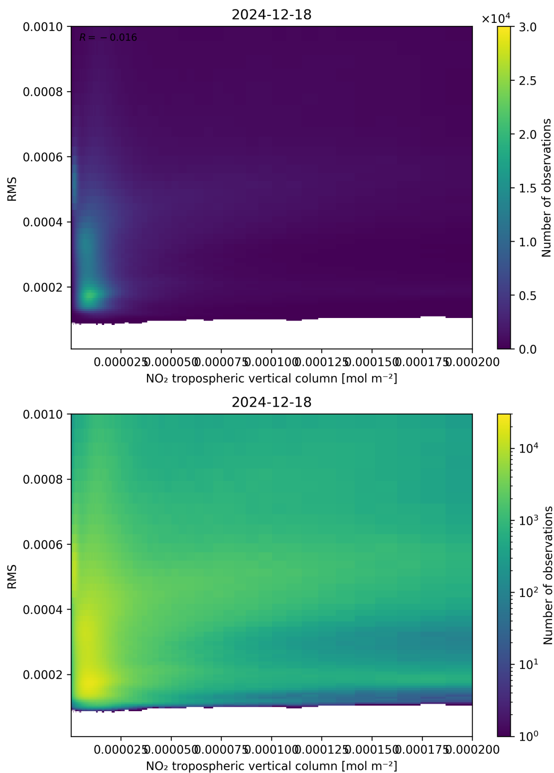
Figure 142: Scatter density plot of “NO 2 tropospheric vertical column” against “RMS” for 2024-12-17 to 2024-12-19.
