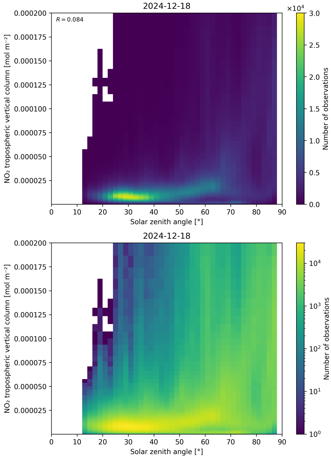
Figure 155: Scatter density plot of “Solar zenith angle” against “NO 2 tropospheric vertical column” for 2024-12-17 to 2024-12-19.
