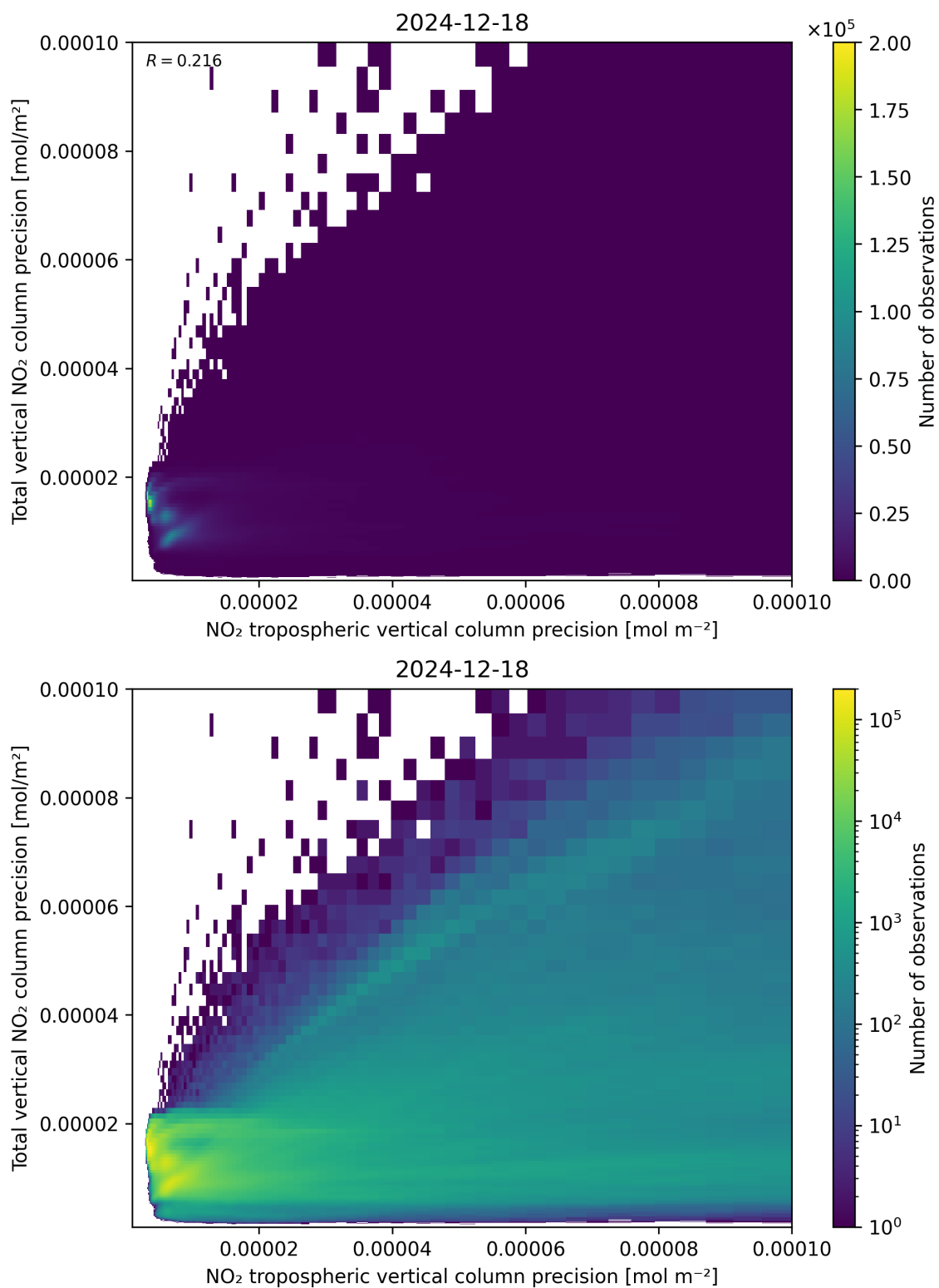
Figure 139: Scatter density plot of “NO 2 tropospheric vertical column precision” against “Total vertical NO 2 column precision” for 2024-12-17 to 2024-12-19.
