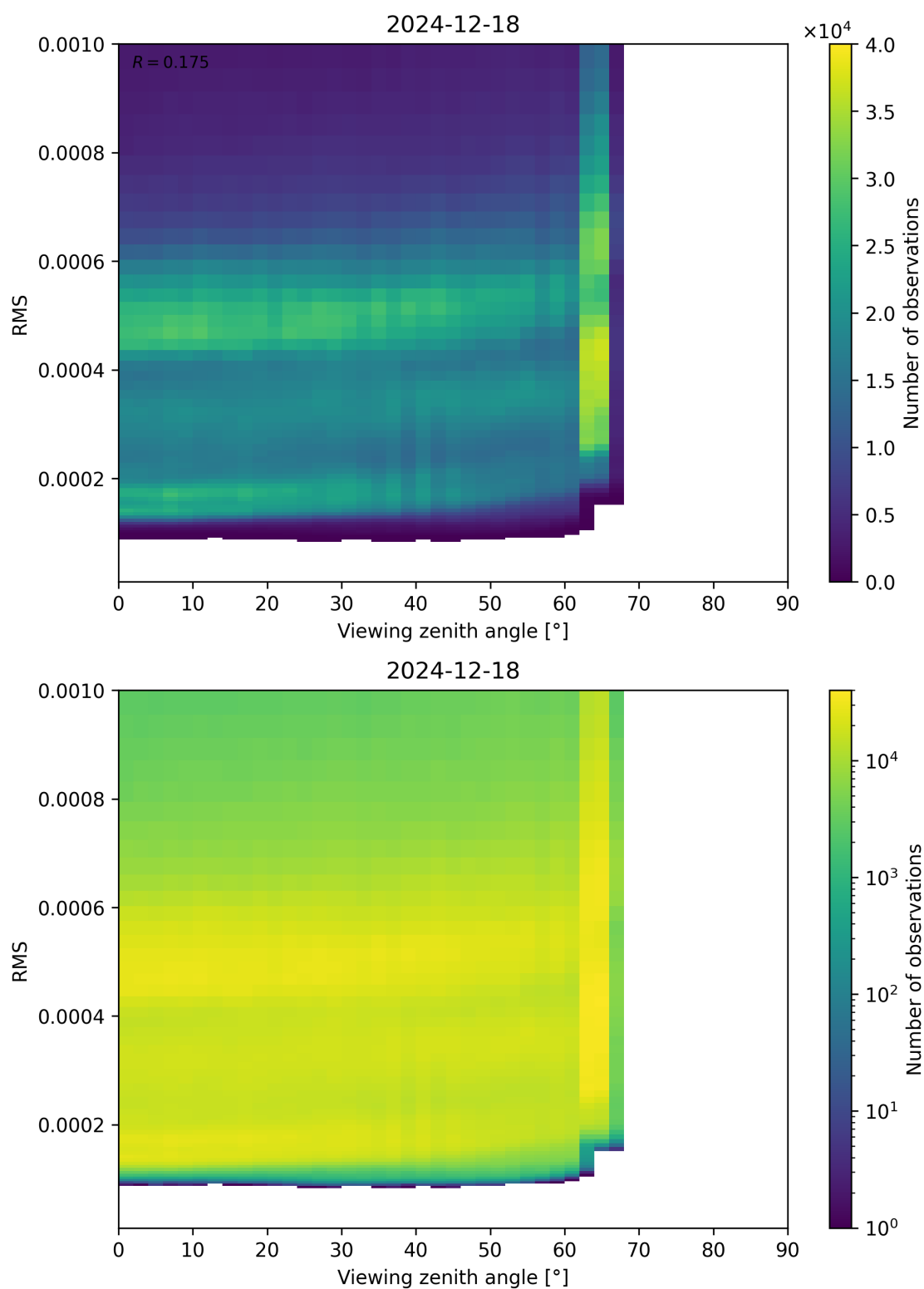
Figure 171: Scatter density plot of “Viewing zenith angle” against “RMS” for 2024-12-17 to 2024-12-19.
