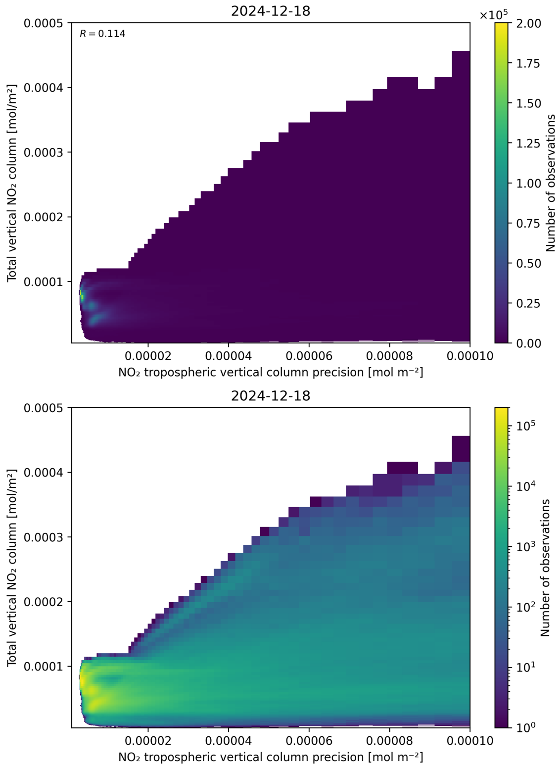
Figure 138: Scatter density plot of “NO 2 tropospheric vertical column precision” against “Total vertical NO 2 column” for 2024-12-17 to 2024-12-19.
