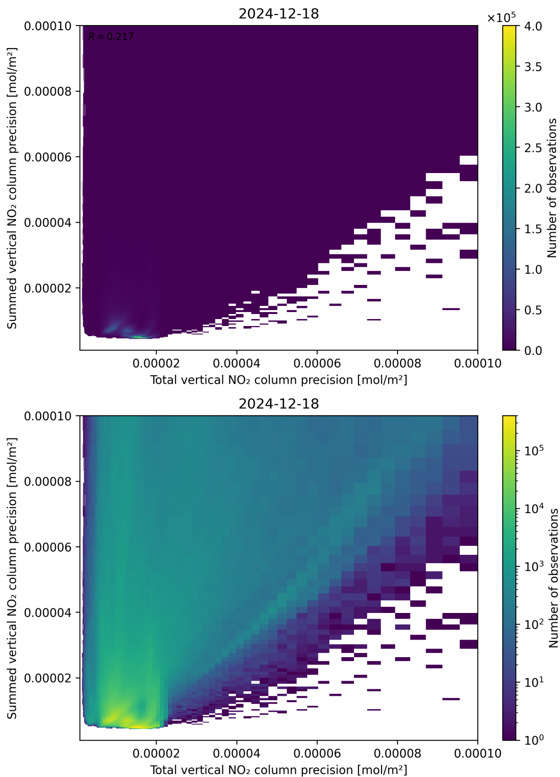
Figure 118: Scatter density plot of “Total vertical NO 2 column precision” against “Summed vertical NO 2 column precision” for 2024-12-17 to 2024-12-19.
