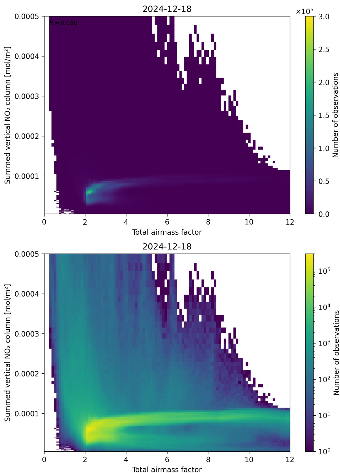
Figure 65: Scatter density plot of “Total airmass factor” against “Summed vertical NO 2 column” for 2024-12-17 to 2024-12-19.
