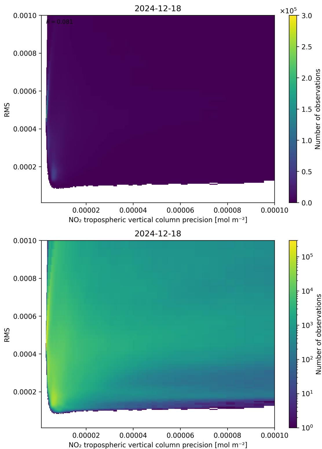
Figure 140: Scatter density plot of “NO 2 tropospheric vertical column precision” against “RMS” for 2024-12-17 to 2024-12-19.
