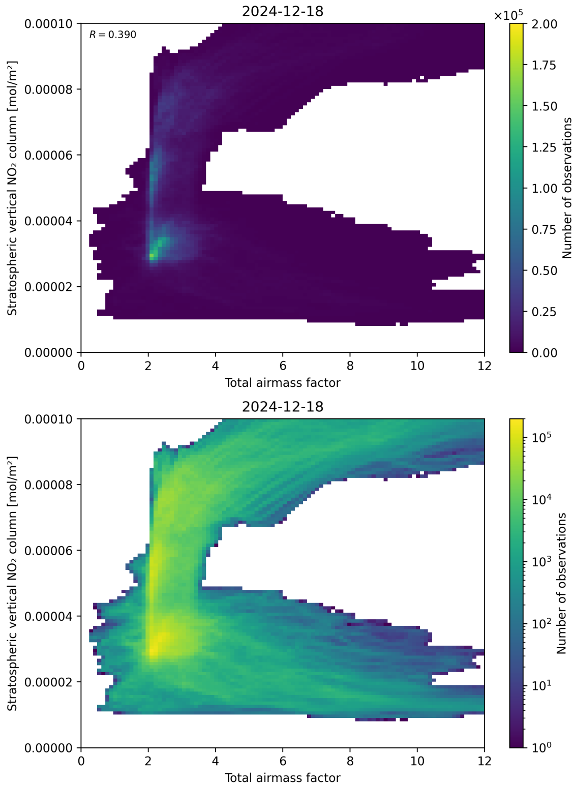
Figure 64: Scatter density plot of “Total airmass factor” against “Stratospheric vertical NO 2 column” for 2024-12-17 to 2024-12-19.
