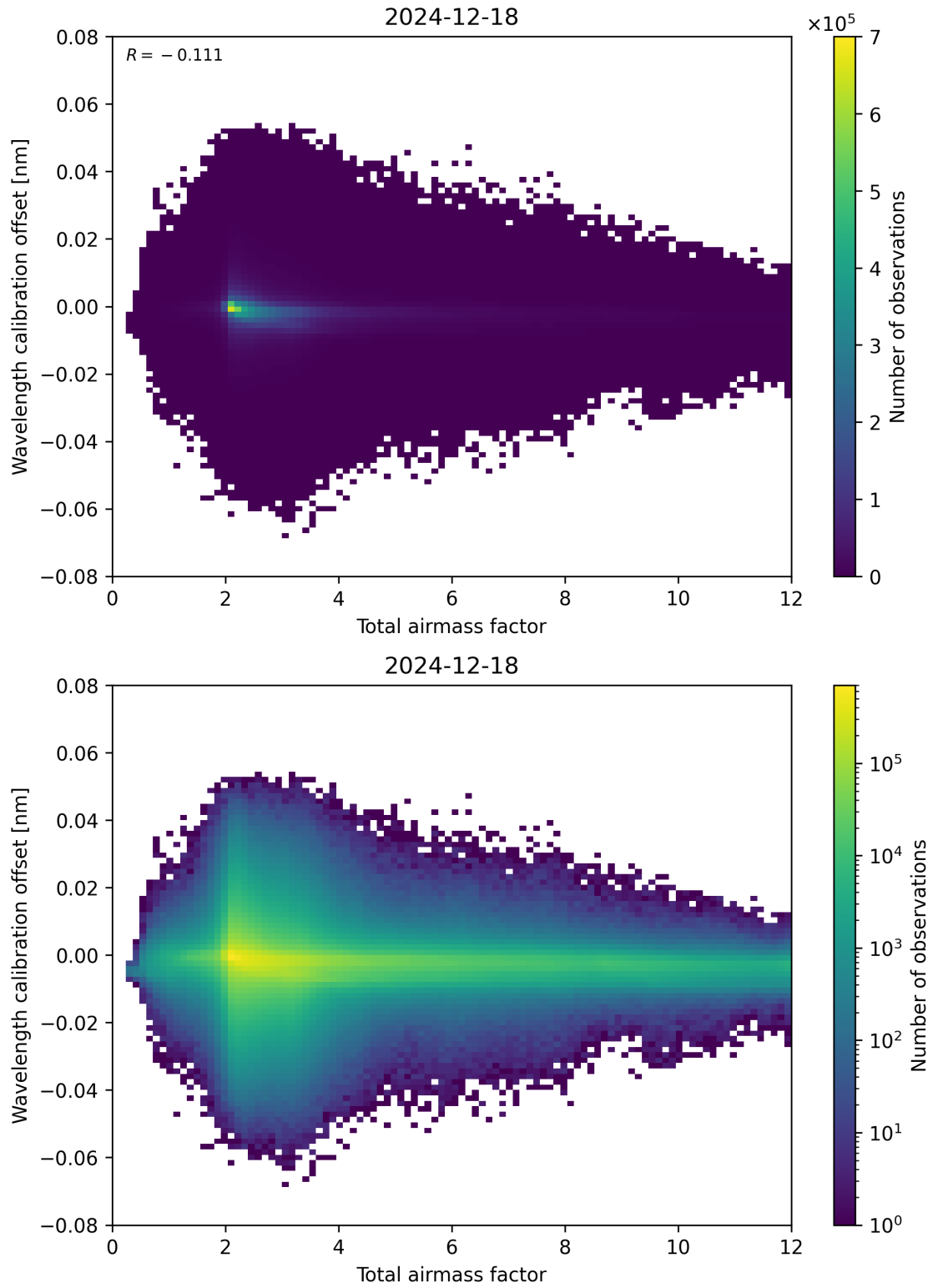
Figure 70: Scatter density plot of “Total airmass factor” against “Wavelength calibration offset” for 2024-12-17 to 2024-12-19.
