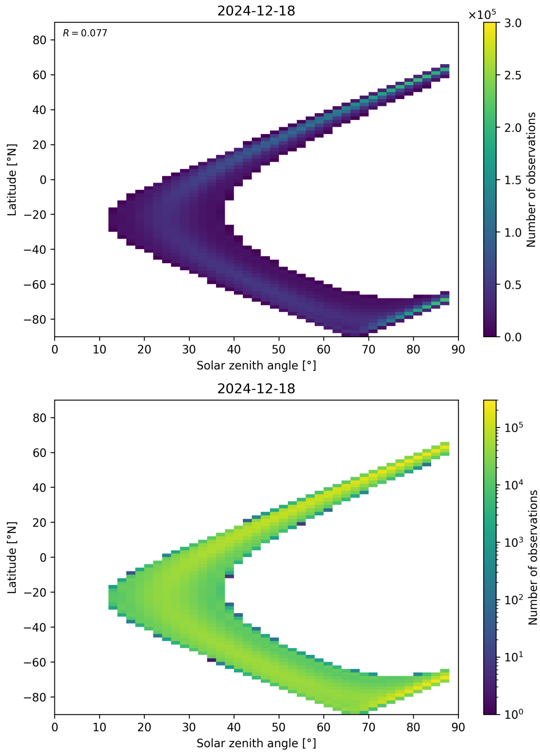
Figure 149: Scatter density plot of “Solar zenith angle” against “Latitude” for 2024-12-17 to 2024-12-19.
