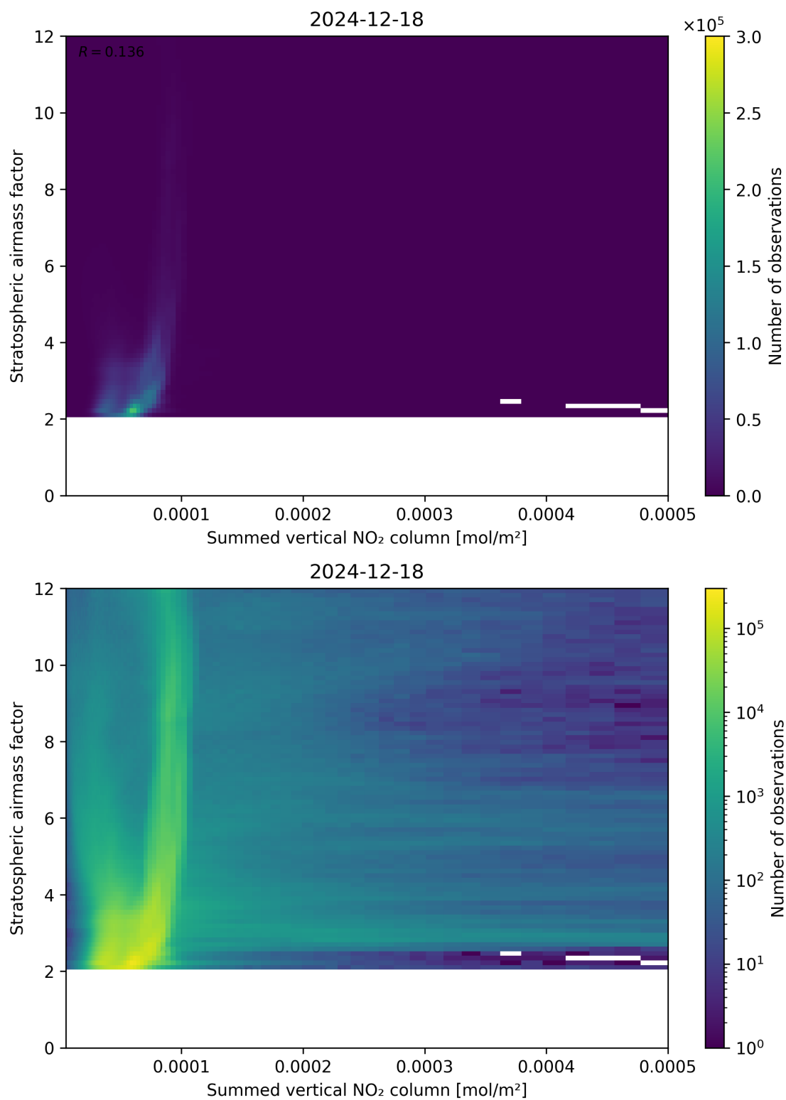
Figure 103: Scatter density plot of “Summed vertical NO 2 column” against “Stratospheric airmass factor” for 2024-12-17 to 2024-12-19.
