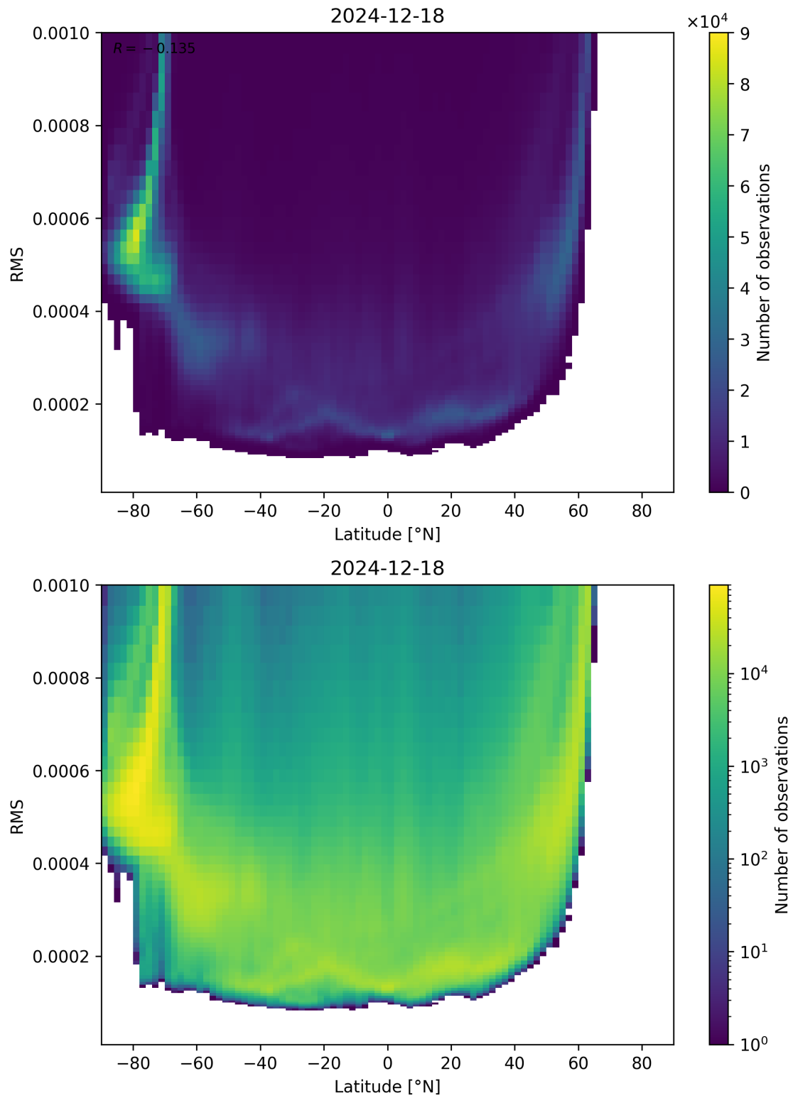
Figure 94: Scatter density plot of “Latitude” against “RMS” for 2024-12-17 to 2024-12-19.
