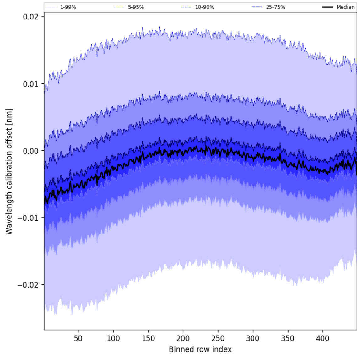
Figure 52: Along track statistics of “Wavelength calibration offset” for 2024-12-17 to 2024-12-19
