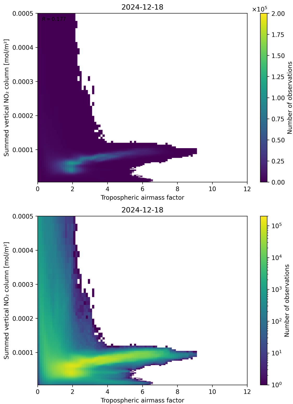
Figure 75: Scatter density plot of “Tropospheric airmass factor” against “Summed vertical NO 2 column” for 2024-12-17 to 2024-12-19.
