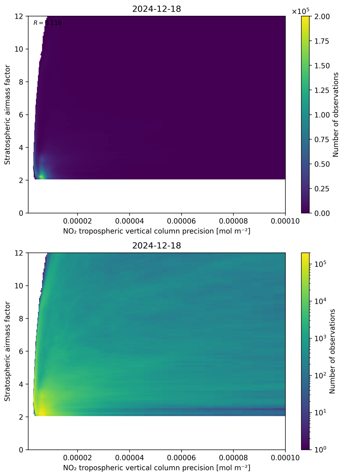
Figure 131: Scatter density plot of “NO 2 tropospheric vertical column precision” against “Stratospheric airmass factor” for 2024-12-17 to 2024-12-19.
