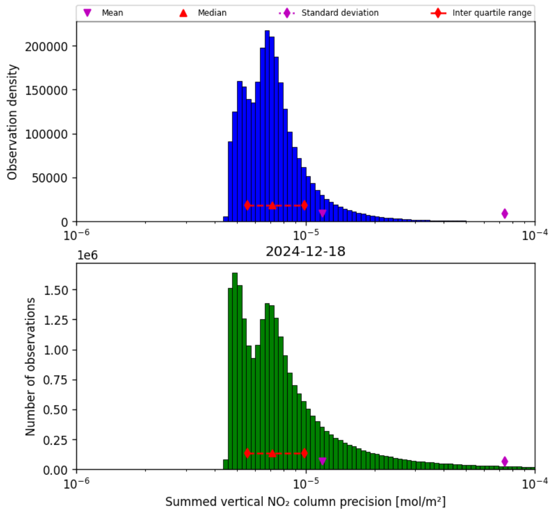
Figure 41: Histogram of “Summed vertical NO 2 column precision” for 2024-12-17 to 2024-12-19
