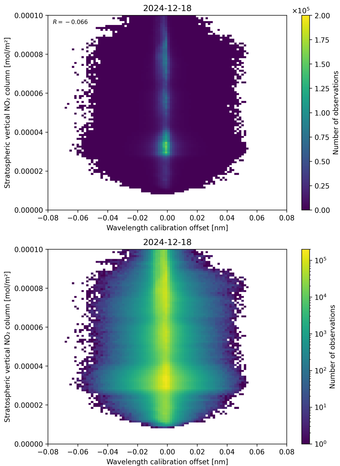
Figure 176: Scatter density plot of “Wavelength calibration offset” against “Stratospheric vertical NO 2 column” for 2024-12-17 to 2024-12-19.
