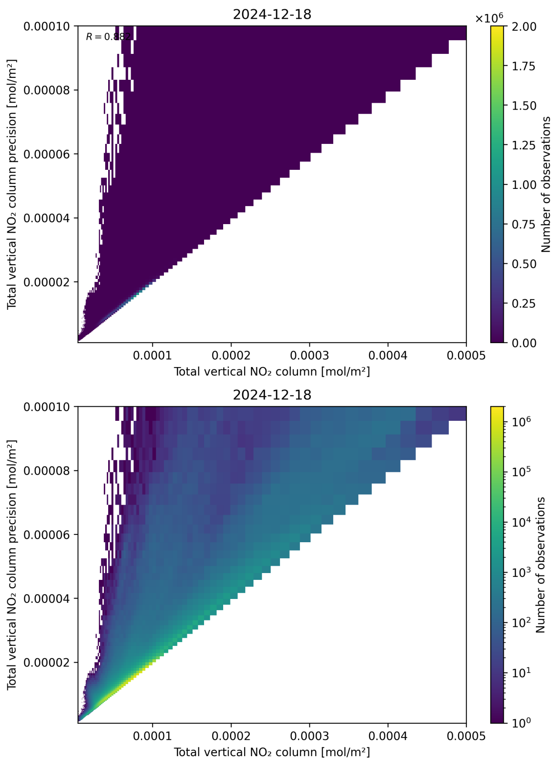
Figure 114: Scatter density plot of “Total vertical NO 2 column” against “Total vertical NO 2 column precision” for 2024-12-17 to 2024-12-19.
