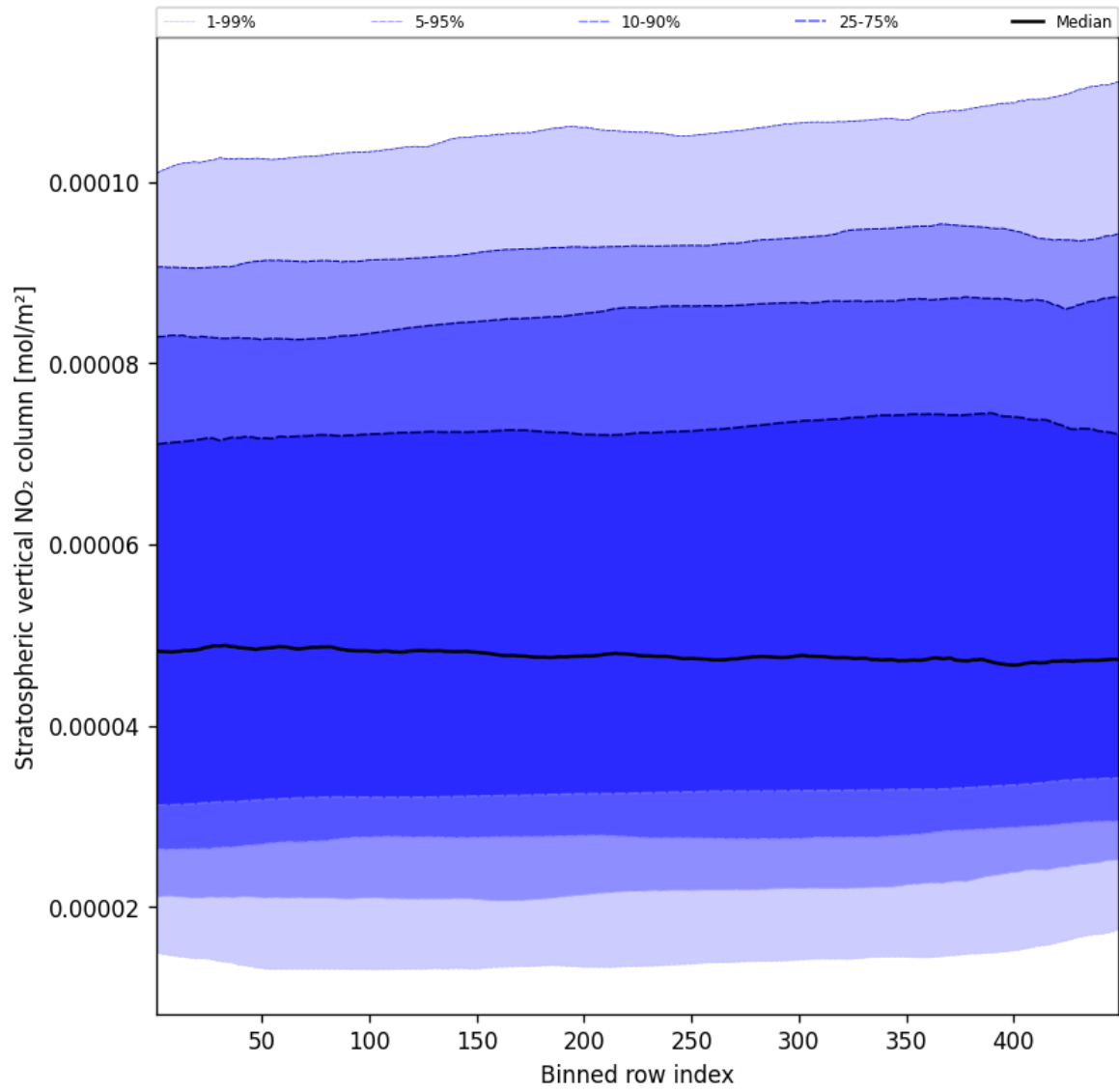
Figure 53: Along track statistics of “Stratospheric vertical NO 2 column” for 2024-12-17 to 2024-12-19
