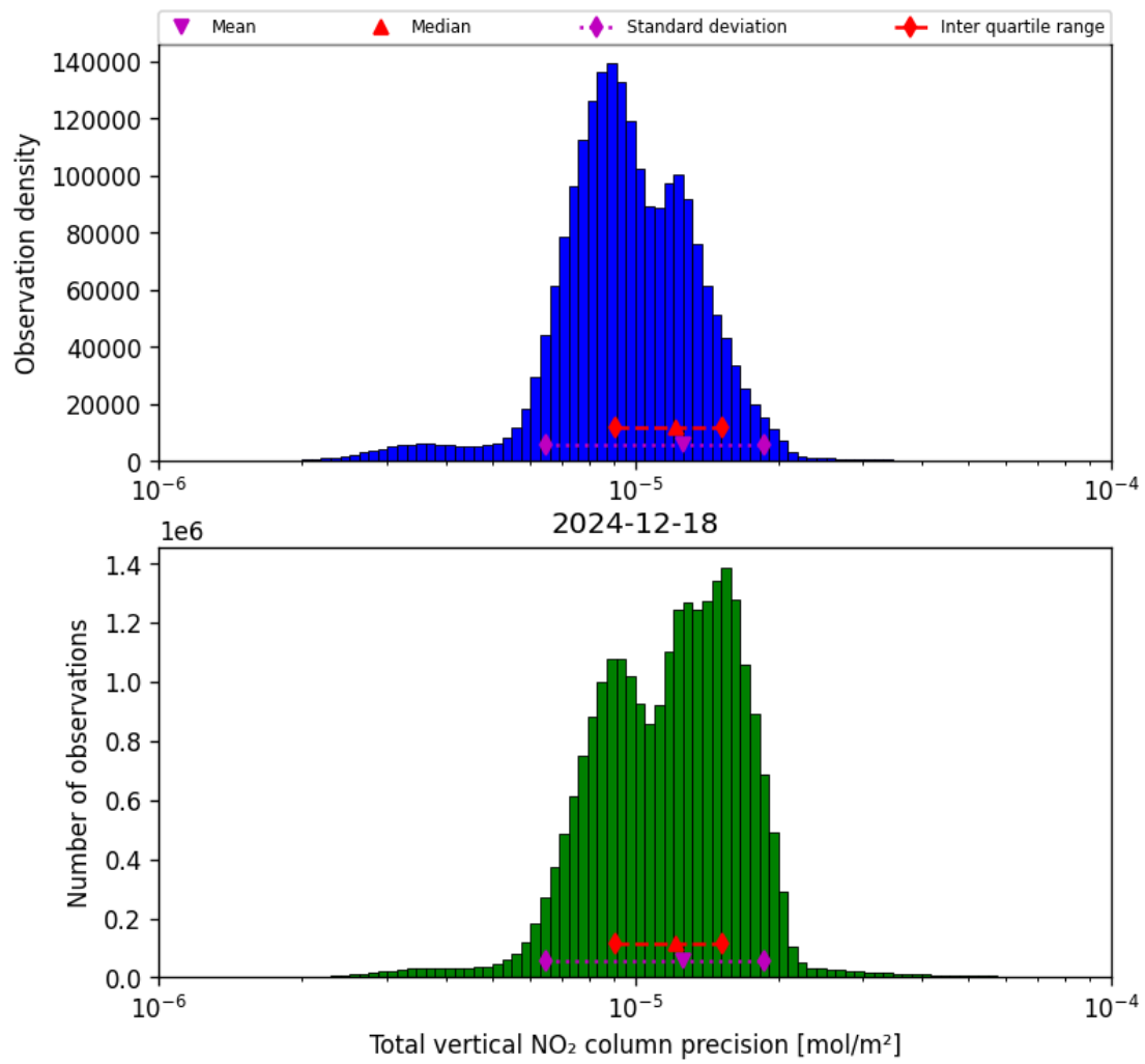
Figure 39: Histogram of “Total vertical NO 2 column precision” for 2024-12-17 to 2024-12-19
