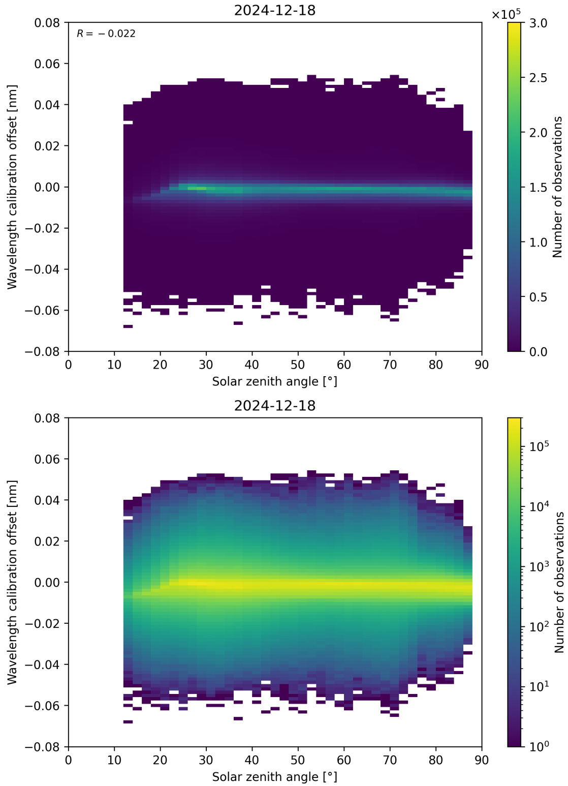
Figure 158: Scatter density plot of “Solar zenith angle” against “Wavelength calibration offset” for 2024-12-17 to 2024-12-19.
