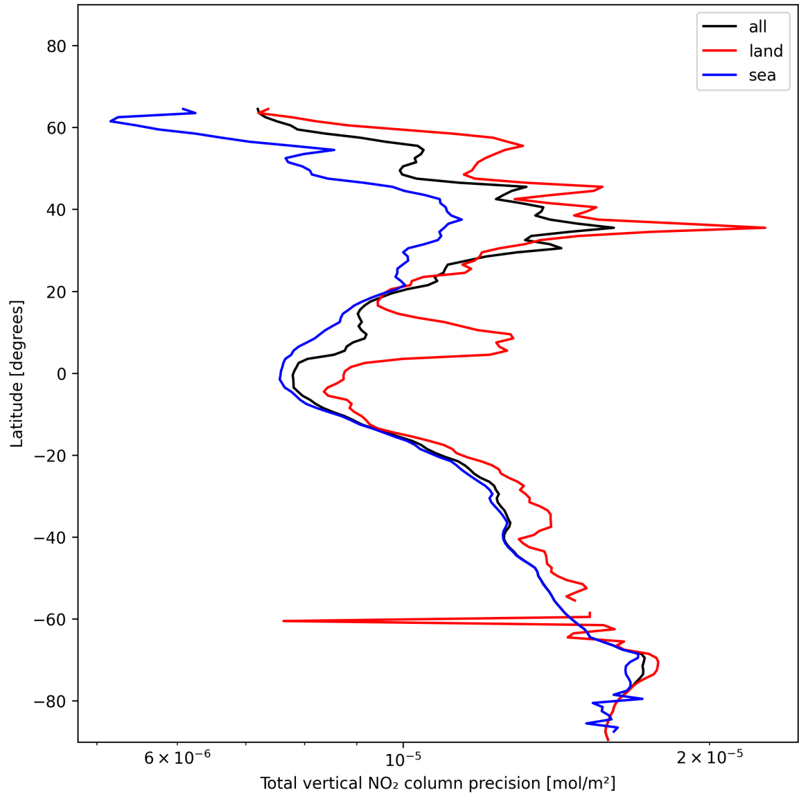
Figure 22: Zonal average of “Total vertical NO 2 column precision” for 2024-12-17 to 2024-12-19.
