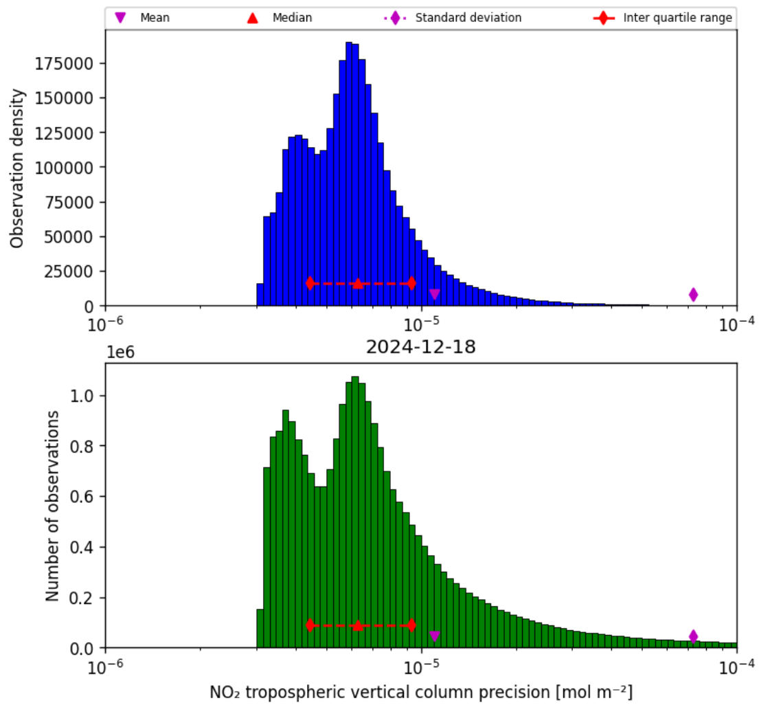
Figure 30: Histogram of “NO 2 tropospheric vertical column precision” for 2024-12-17 to 2024-12-19
