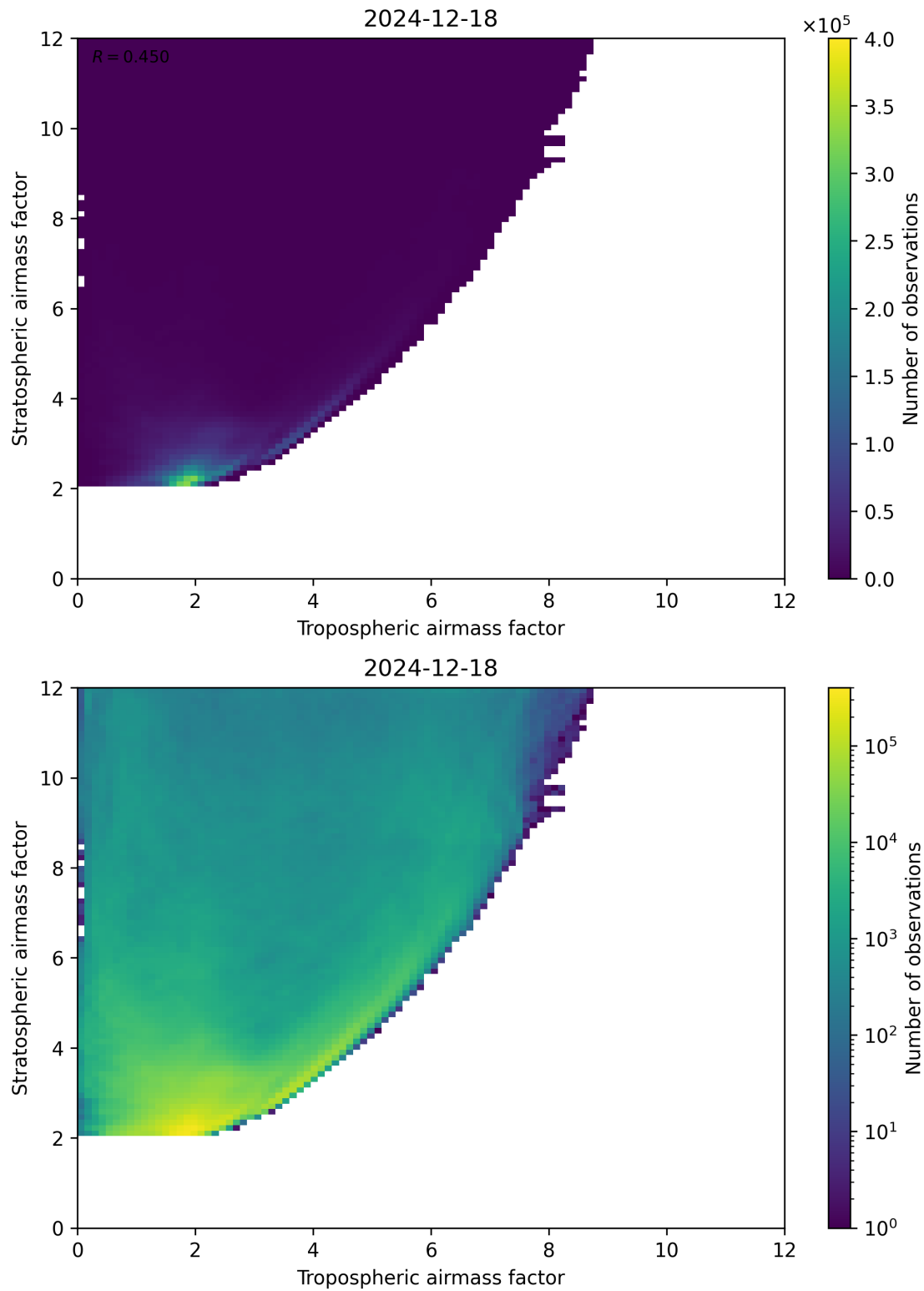
Figure 71: Scatter density plot of “Tropospheric airmass factor” against “Stratospheric airmass factor” for 2024-12-17 to 2024-12-19.
