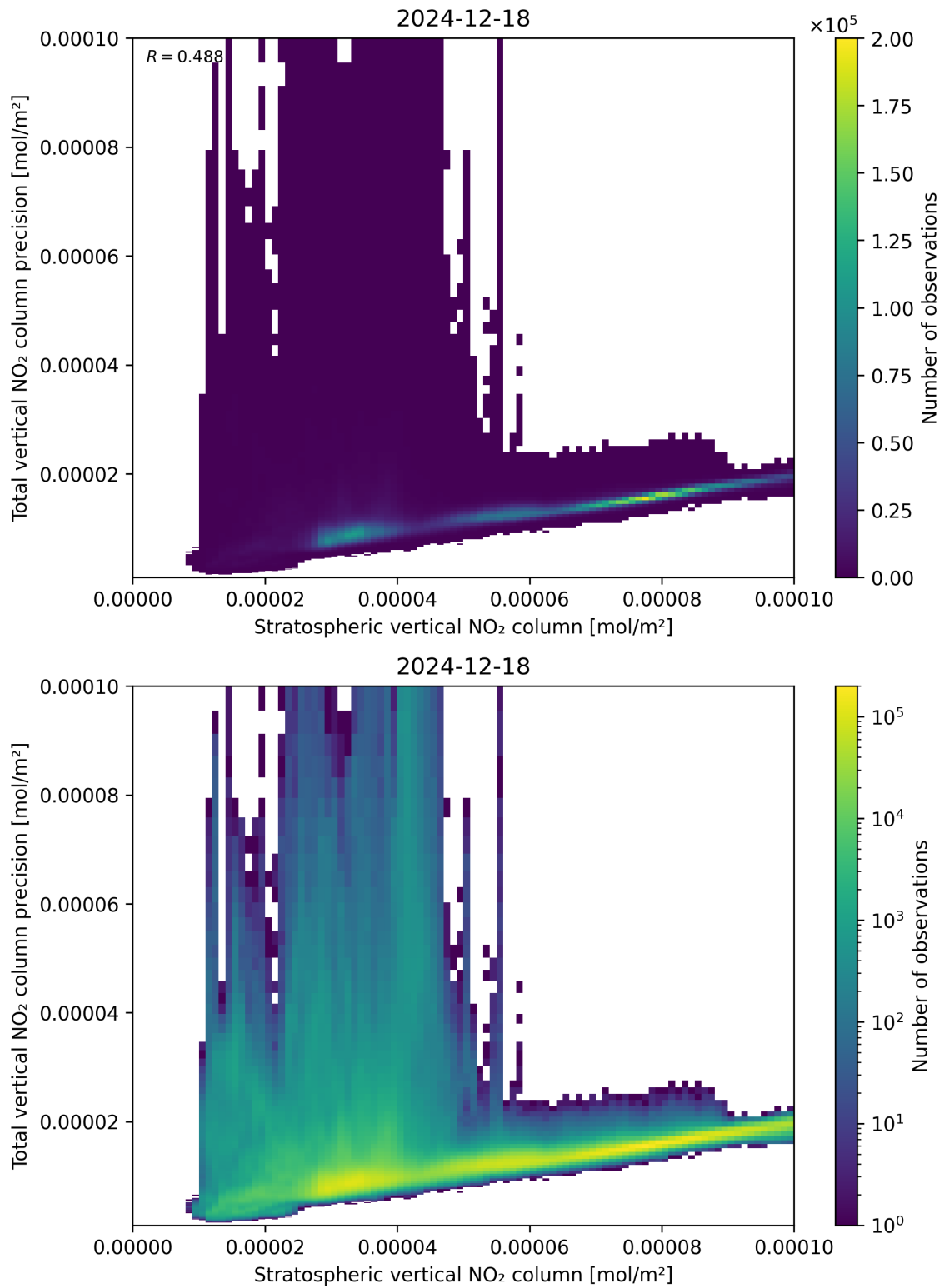
Figure 101: Scatter density plot of “Stratospheric vertical NO 2 column” against “Total vertical NO 2 column precision” for 2024-12-17 to 2024-12-19.
