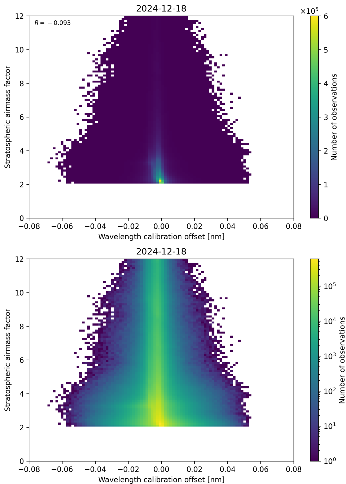
Figure 174: Scatter density plot of “Wavelength calibration offset” against “Stratospheric airmass factor” for 2024-12-17 to 2024-12-19.
