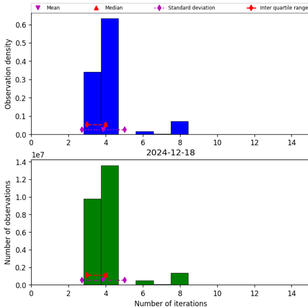
Figure 34: Histogram of “Number of iterations” for 2024-12-17 to 2024-12-19
