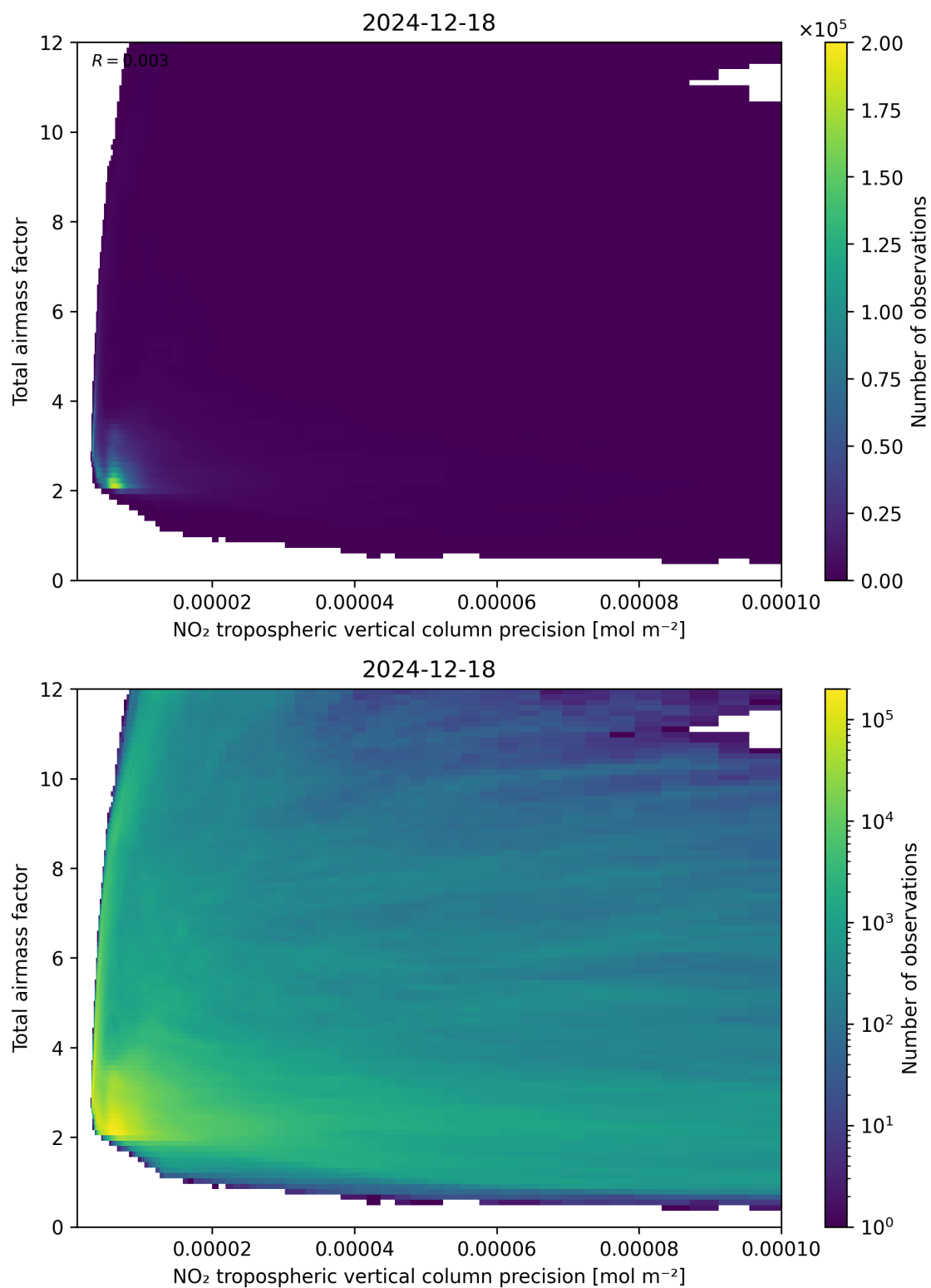
Figure 132: Scatter density plot of “NO 2 tropospheric vertical column precision” against “Total air mass factor” for 2024-12-17 to 2024-12-19.
