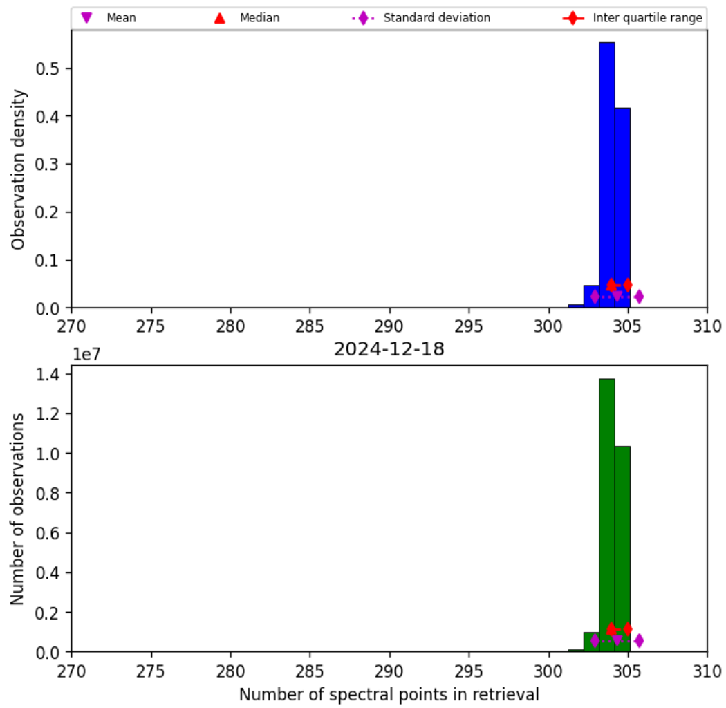
Figure 33: Histogram of “Number of spectral points in retrieval” for 2024-12-17 to 2024-12-19
