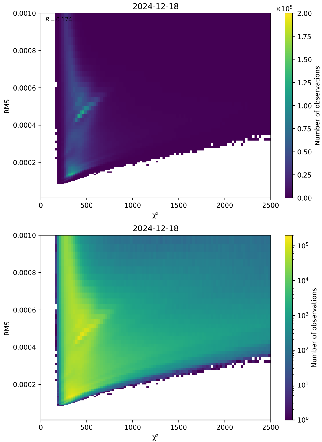
Figure 82: Scatter density plot of “ \chi^2 ” against “RMS” for 2024-12-17 to 2024-12-19.
