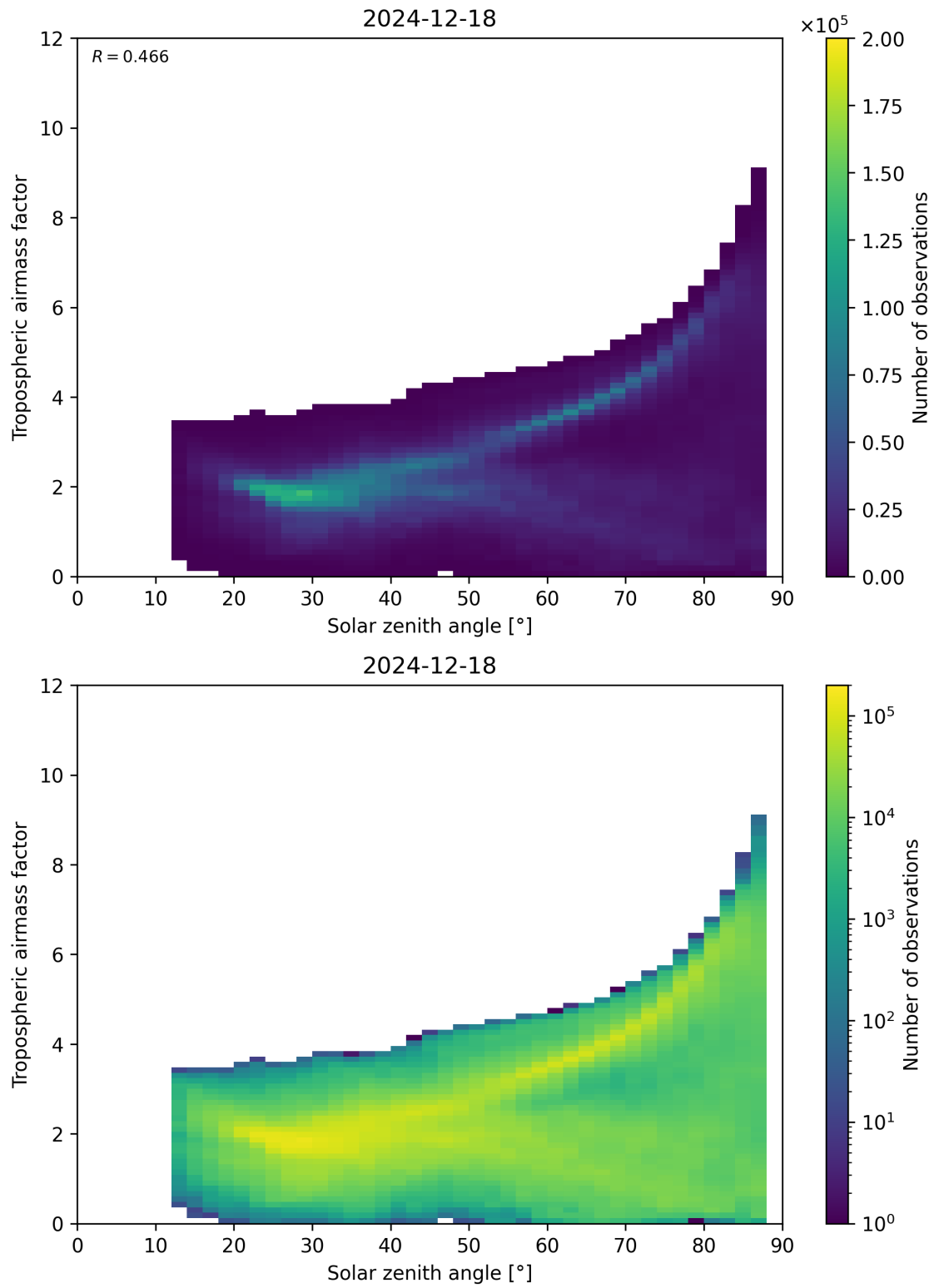
Figure 147: Scatter density plot of “Solar zenith angle” against “Tropospheric airmass factor” for 2024-12-17 to 2024-12-19.
