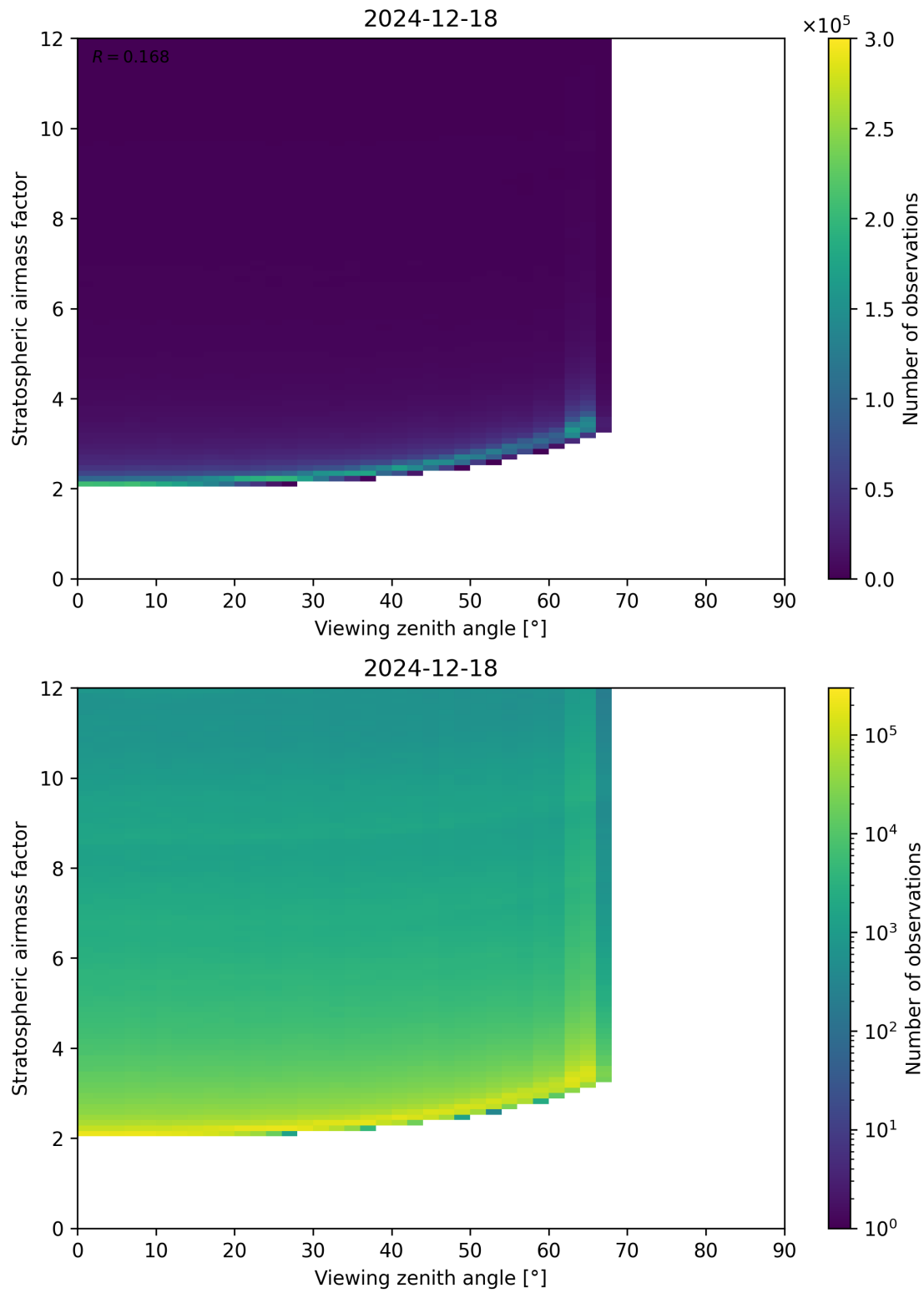
Figure 159: Scatter density plot of “Viewing zenith angle” against “Stratospheric airmass factor” for 2024-12-17 to 2024-12-19.
