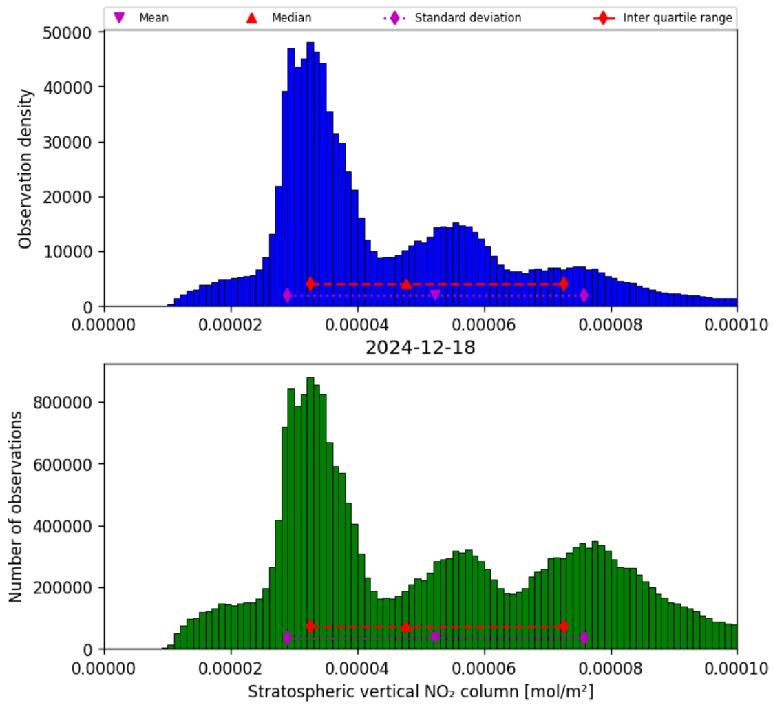
Figure 36: Histogram of “Stratospheric vertical NO 2 column” for 2024-12-17 to 2024-12-19
