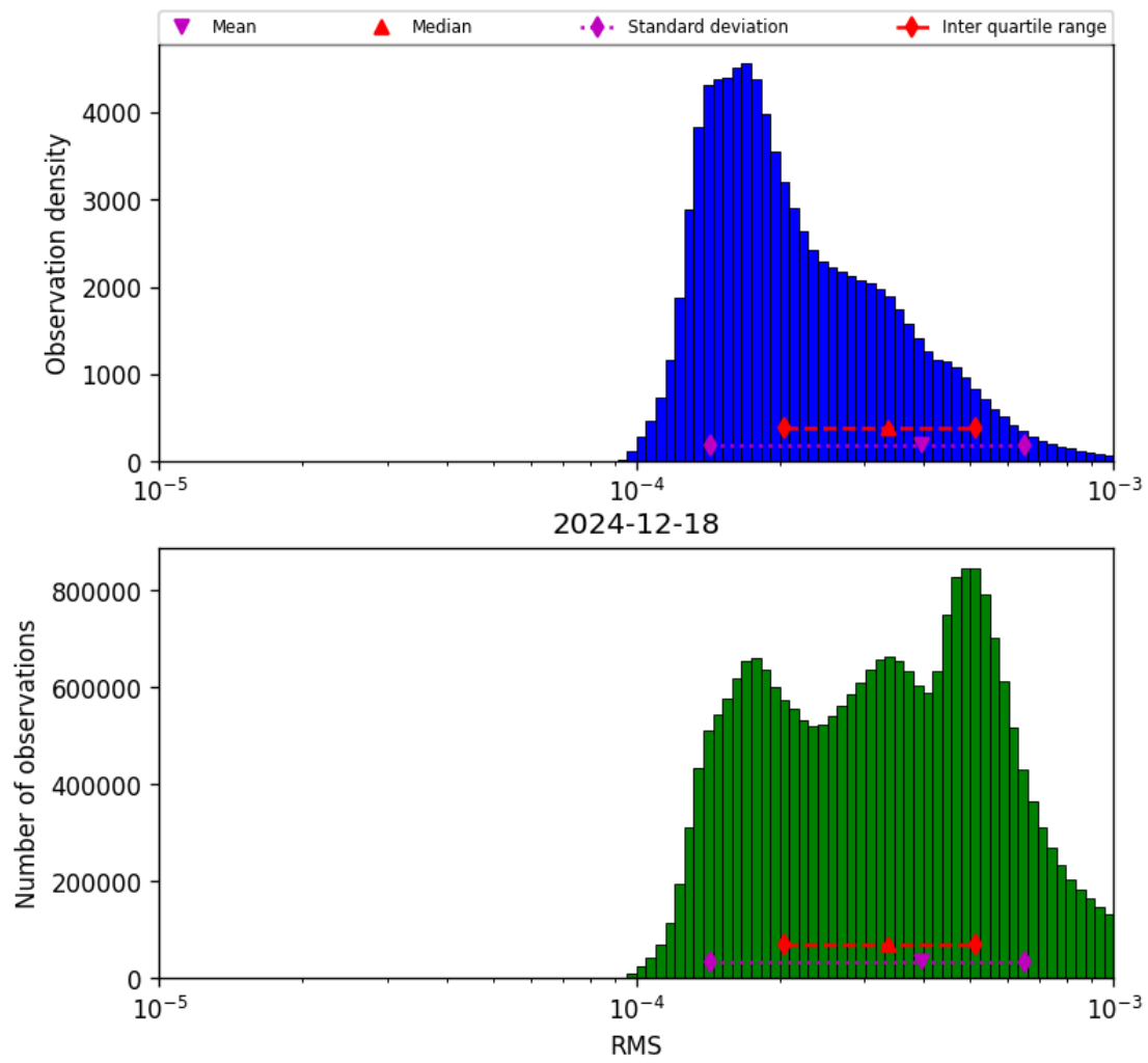
Figure 43: Histogram of “RMS” for 2024-12-17 to 2024-12-19
