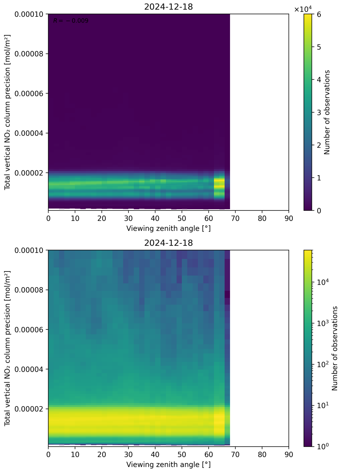
Figure 168: Scatter density plot of “Viewing zenith angle” against “Total vertical NO 2 column precision” for 2024-12-17 to 2024-12-19.
