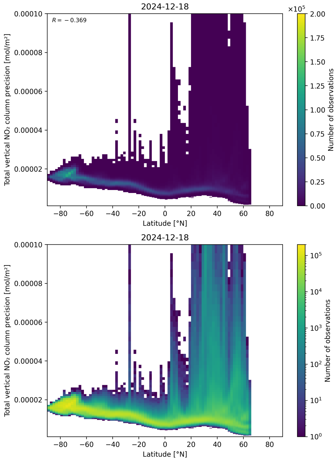
Figure 91: Scatter density plot of “Latitude” against “Total vertical NO 2 column precision” for 2024-12-17 to 2024-12-19.
