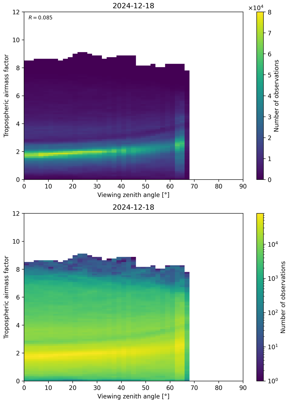
Figure 161: Scatter density plot of “Viewing zenith angle” against “Tropospheric airmass factor” for 2024-12-17 to 2024-12-19.
