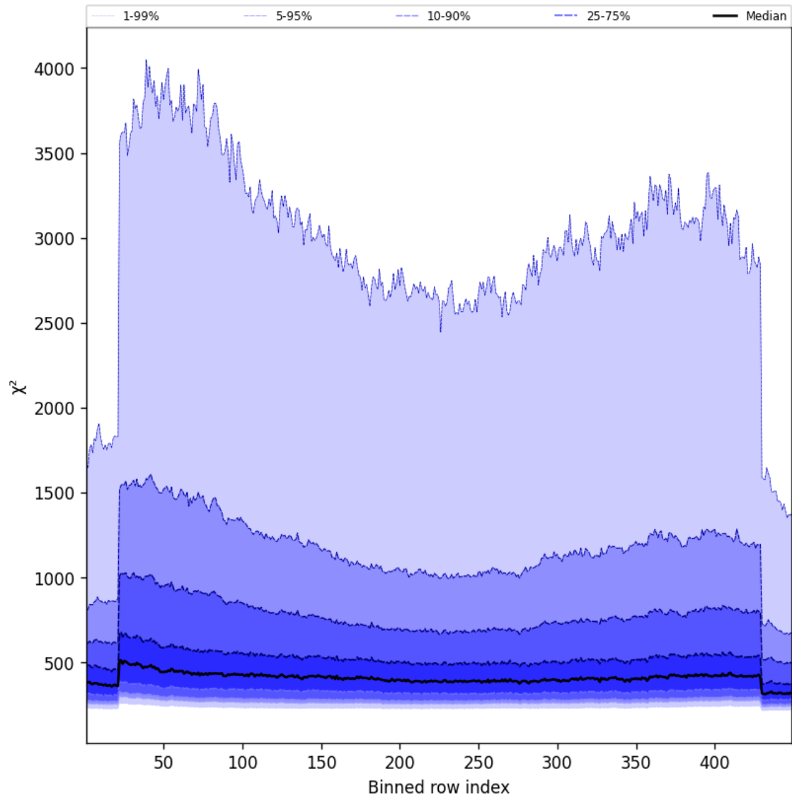
Figure 59: Along track statistics of " \chi^2 " for 2024-12-17 to 2024-12-19
