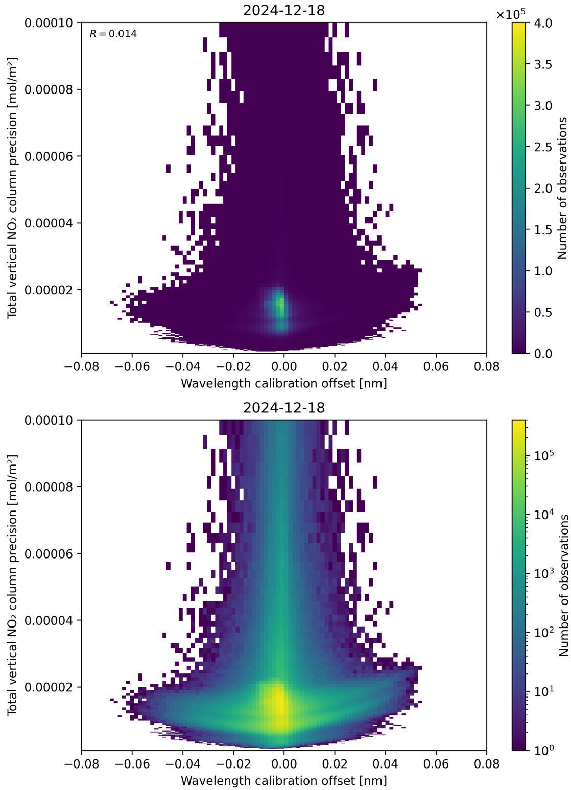
Figure 180: Scatter density plot of “Wavelength calibration offset” against “Total vertical NO 2 column precision” for 2024-12-17 to 2024-12-19.
