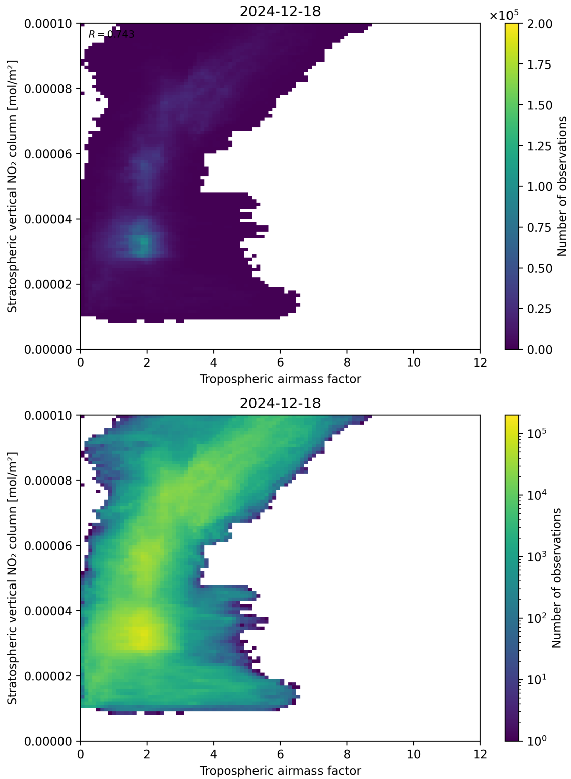
Figure 74: Scatter density plot of “Tropospheric air mass factor” against “Stratospheric vertical NO 2 column” for 2024-12-17 to 2024-12-19.
