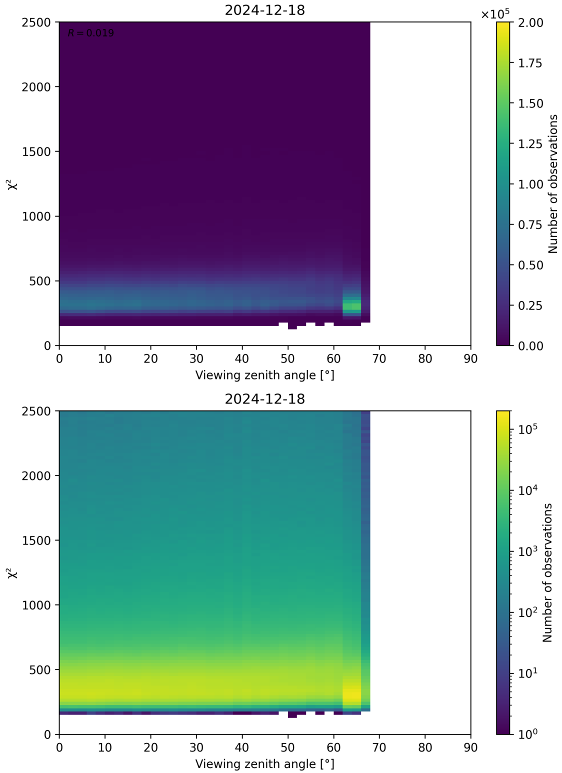
Figure 162: Scatter density plot of “Viewing zenith angle” against “ \chi^2 ” for 2024-12-17 to 2024-12-19.
