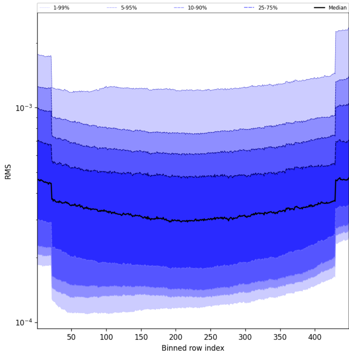
Figure 60: Along track statistics of “RMS” for 2024-12-17 to 2024-12-19
