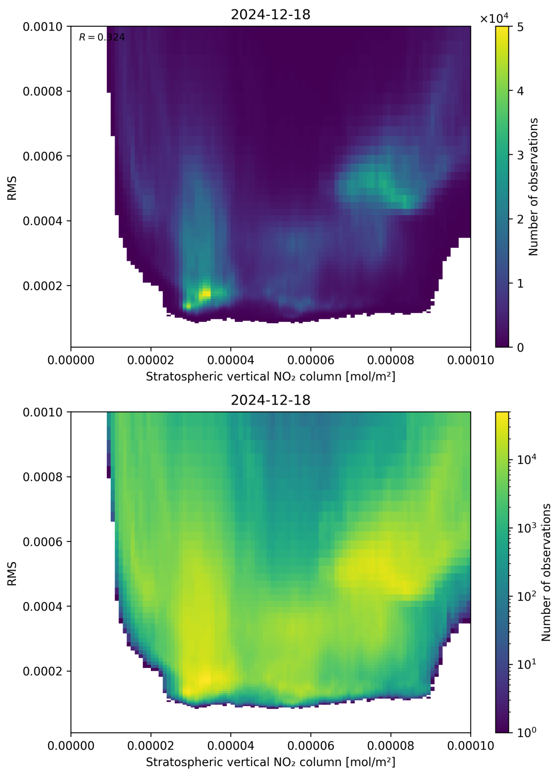
Figure 102: Scatter density plot of “Stratospheric vertical NO 2 column” against “RMS” for 2024-12-17 to 2024-12-19.
