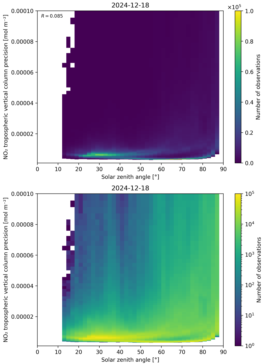
Figure 156: Scatter density plot of “Solar zenith angle” against “NO 2 tropospheric vertical column precision” for 2024-12-17 to 2024-12-19.
