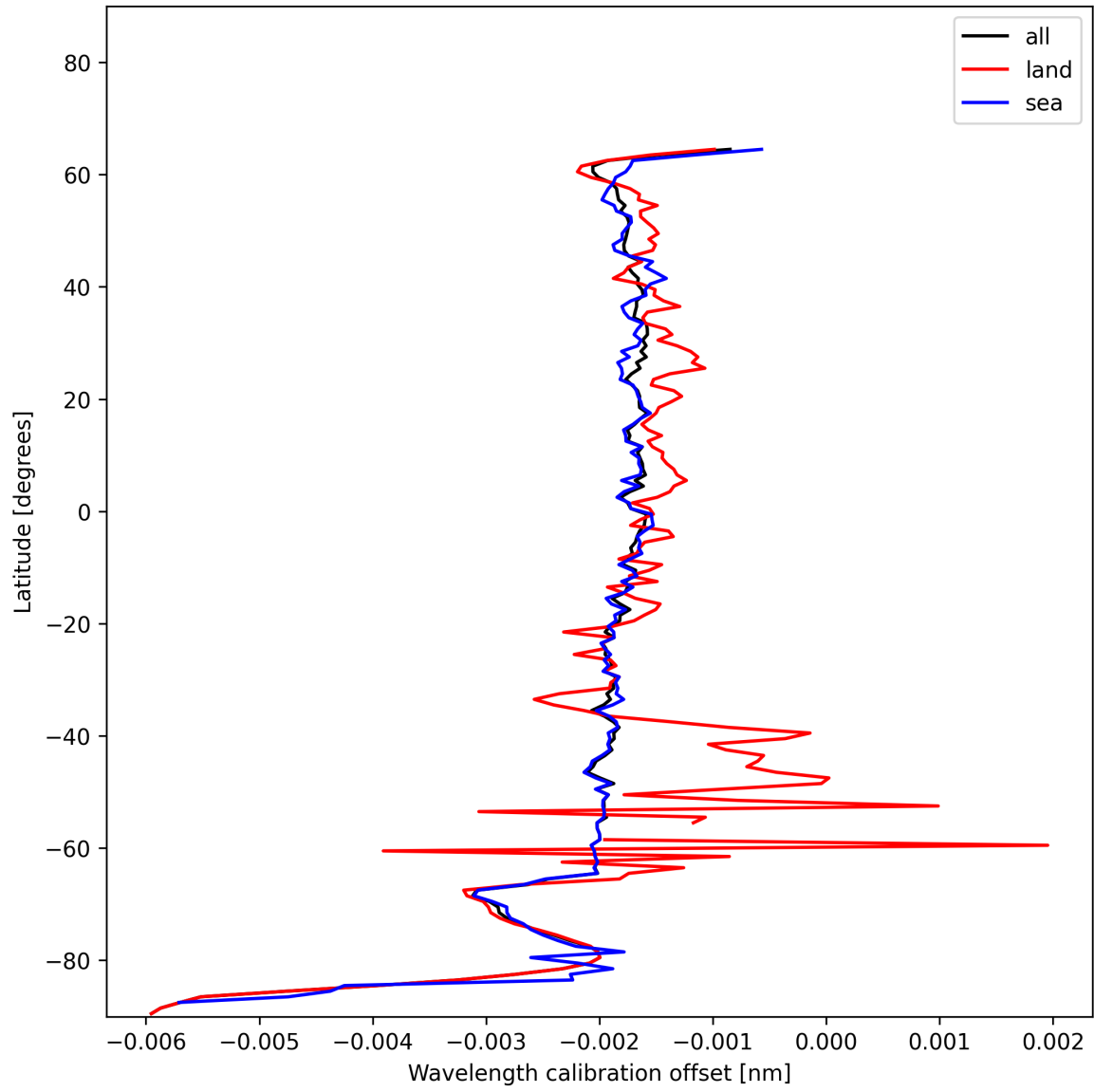
Figure 18: Zonal average of “Wavelength calibration offset” for 2024-12-17 to 2024-12-19.
