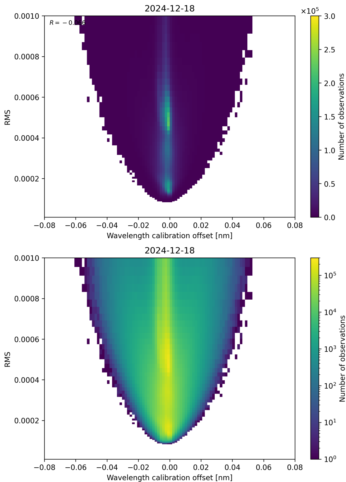
Figure 181: Scatter density plot of “Wavelength calibration offset” against “RMS” for 2024-12-17 to 2024-12-19.
