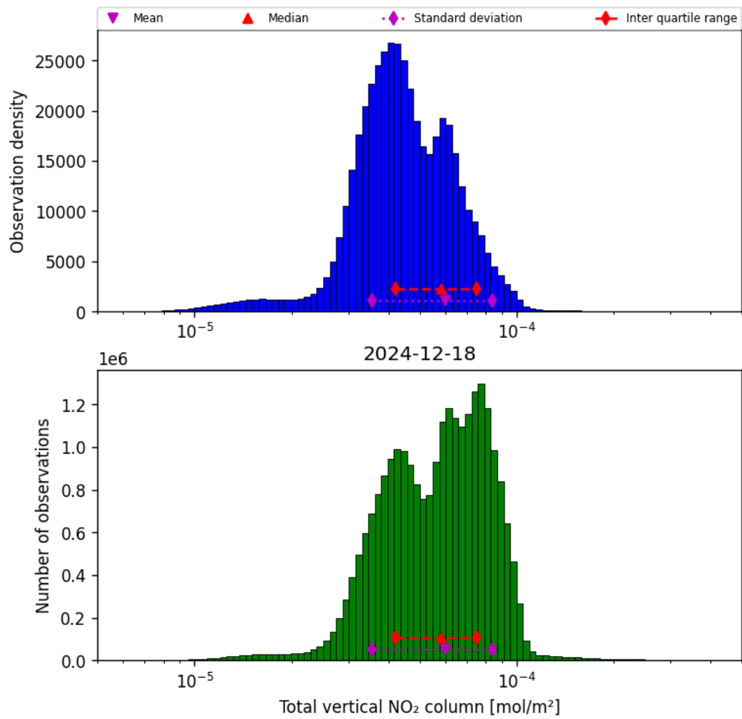
Figure 38: Histogram of “Total vertical NO 2 column” for 2024-12-17 to 2024-12-19
