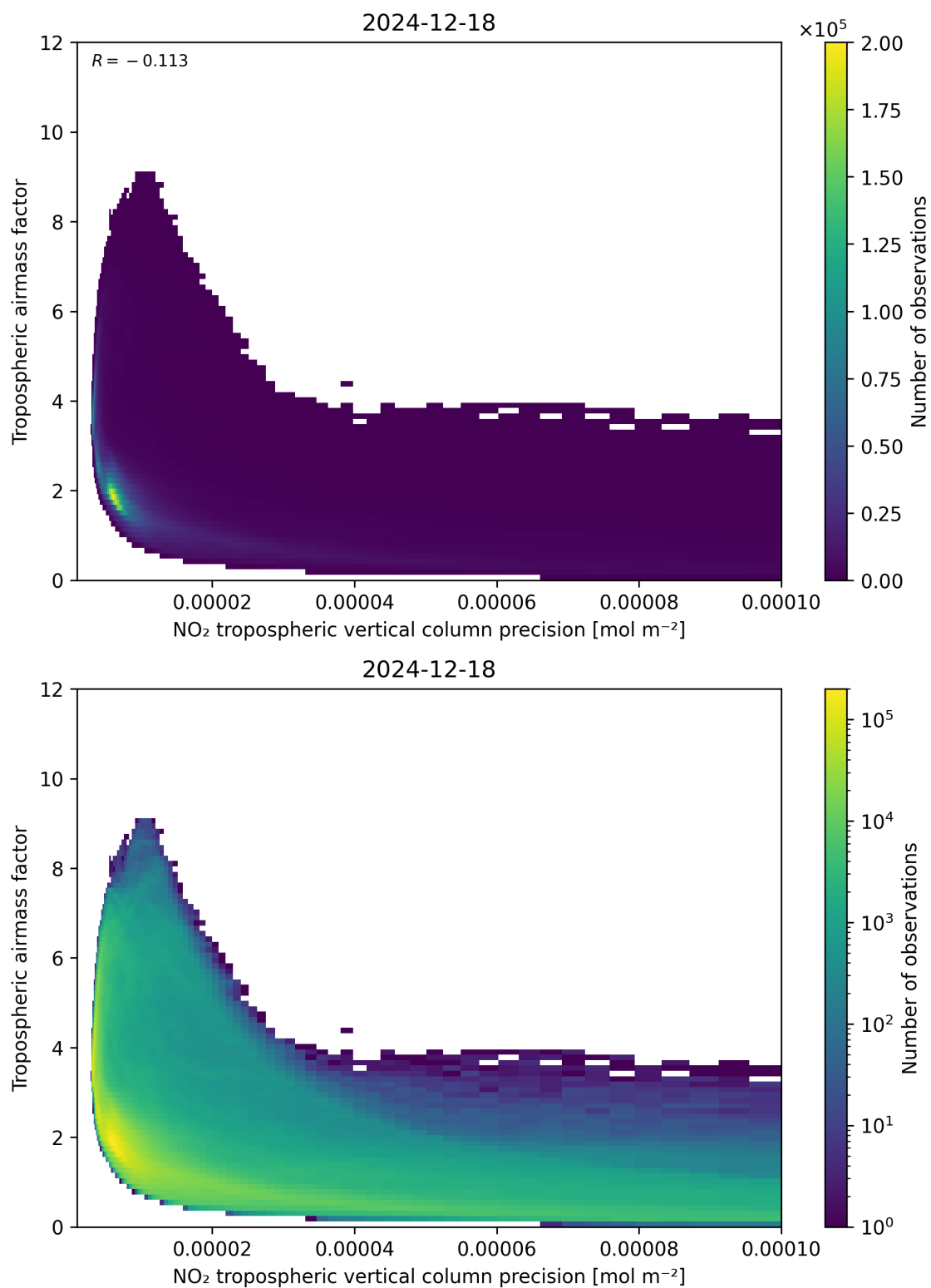
Figure 133: Scatter density plot of “NO 2 tropospheric vertical column precision” against “Tropospheric air mass factor” for 2024-12-17 to 2024-12-19.
