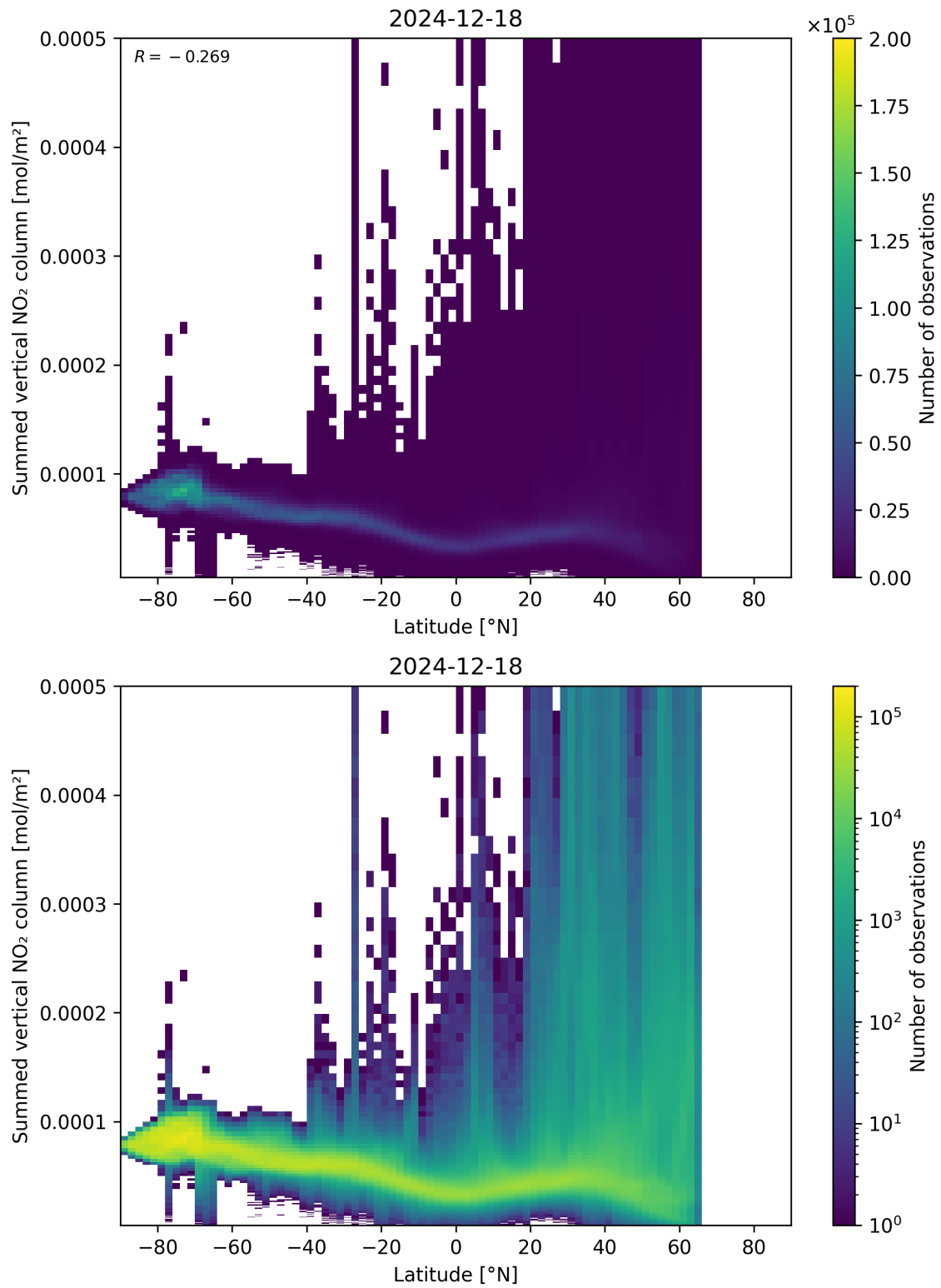
Figure 88: Scatter density plot of “Latitude” against “Summed vertical NO 2 column” for 2024-12-17 to 2024-12-19.
