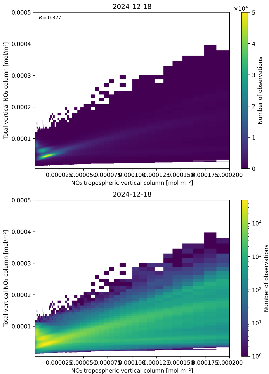
Figure 128: Scatter density plot of “NO 2 tropospheric vertical column” against “Total vertical NO 2 column” for 2024-12-17 to 2024-12-19.
