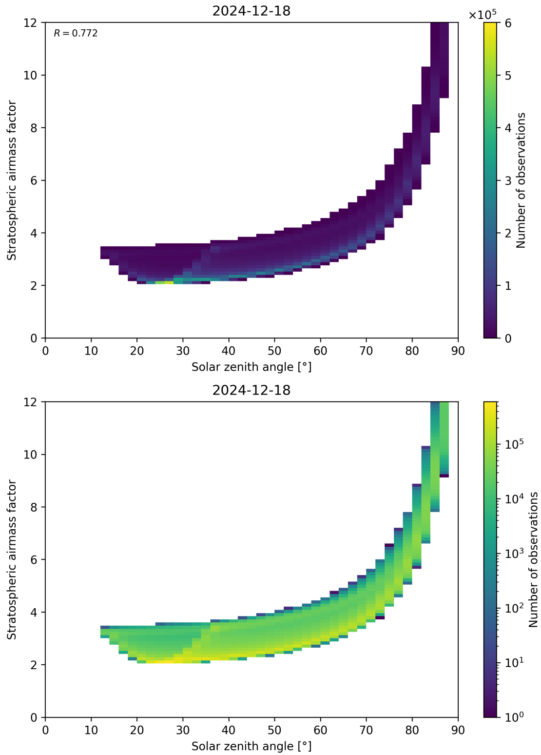
Figure 145: Scatter density plot of “Solar zenith angle” against “Stratospheric airmass factor” for 2024-12-17 to 2024-12-19.
