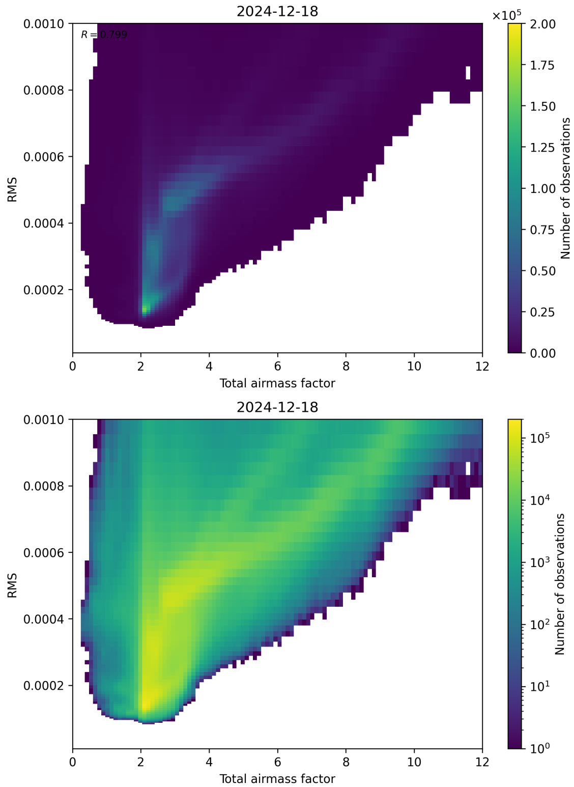
Figure 69: Scatter density plot of “Total airmass factor” against “RMS” for 2024-12-17 to 2024-12-19.
