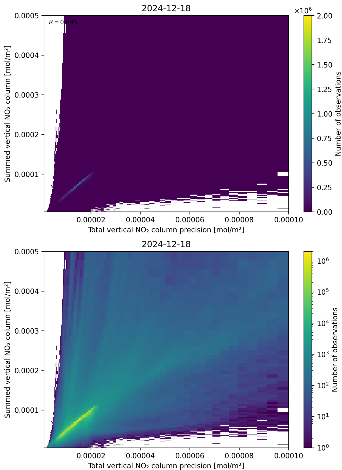
Figure 117: Scatter density plot of “Total vertical NO 2 column precision” against “Summed vertical NO 2 column” for 2024-12-17 to 2024-12-19.
