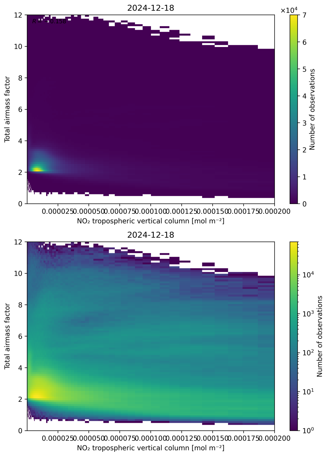
Figure 122: Scatter density plot of “NO 2 tropospheric vertical column” against “Total airmass factor” for 2024-12-17 to 2024-12-19.
