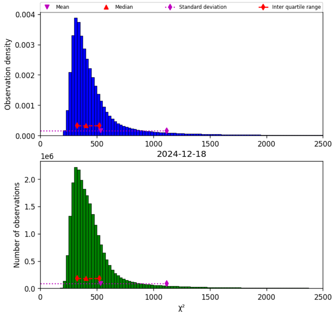
Figure 42: Histogram of “ \chi^2 ” for 2024-12-17 to 2024-12-19
