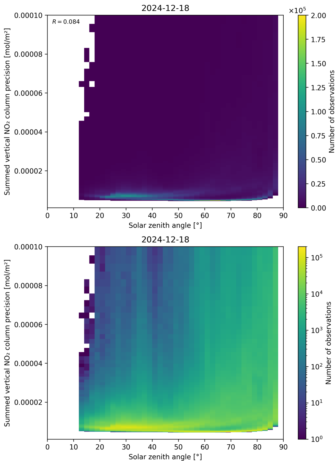
Figure 152: Scatter density plot of “Solar zenith angle” against “Summed vertical NO 2 column precision” for 2024-12-17 to 2024-12-19.
