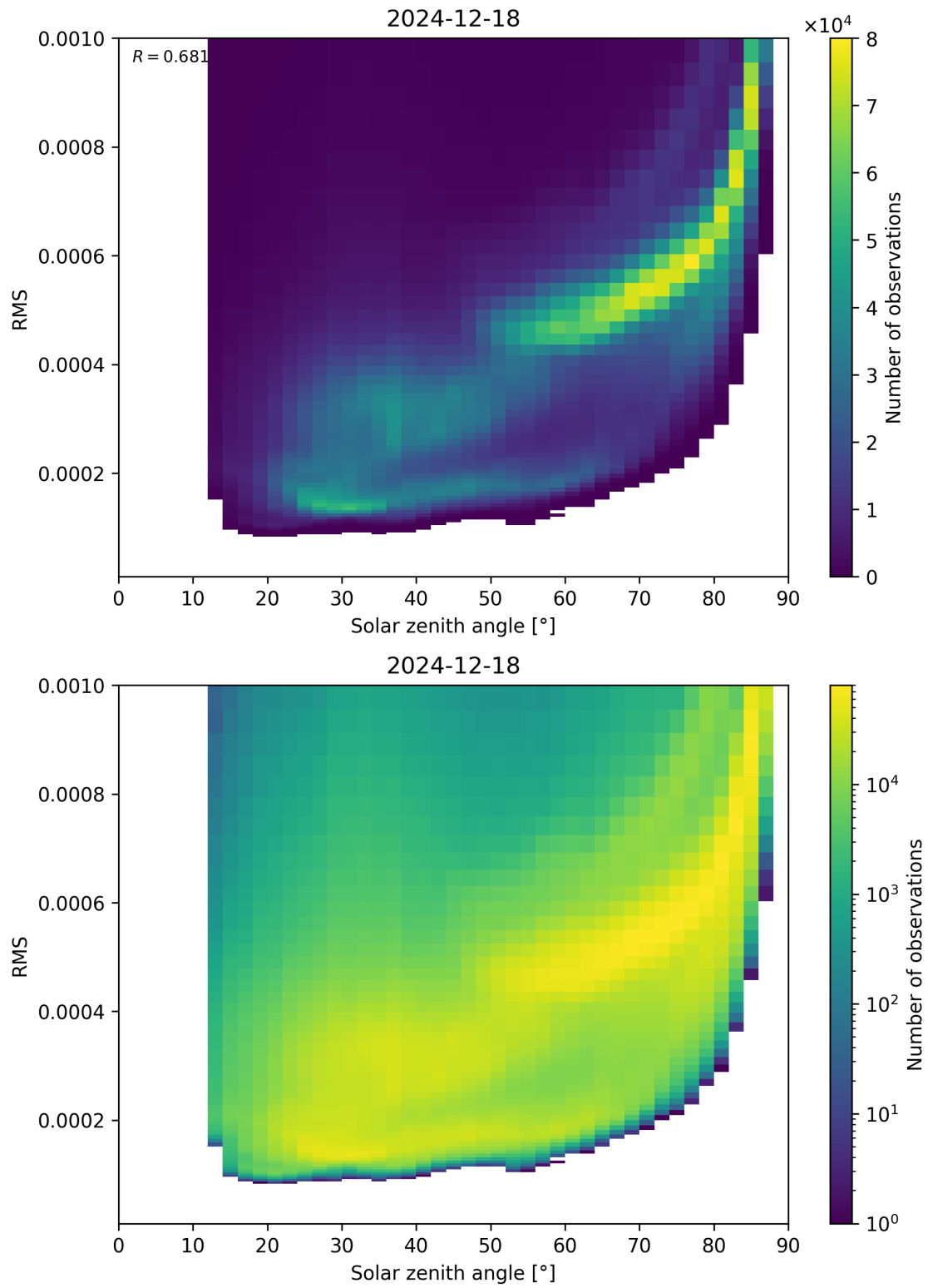
Figure 157: Scatter density plot of “Solar zenith angle” against “RMS” for 2024-12-17 to 2024-12-19.
