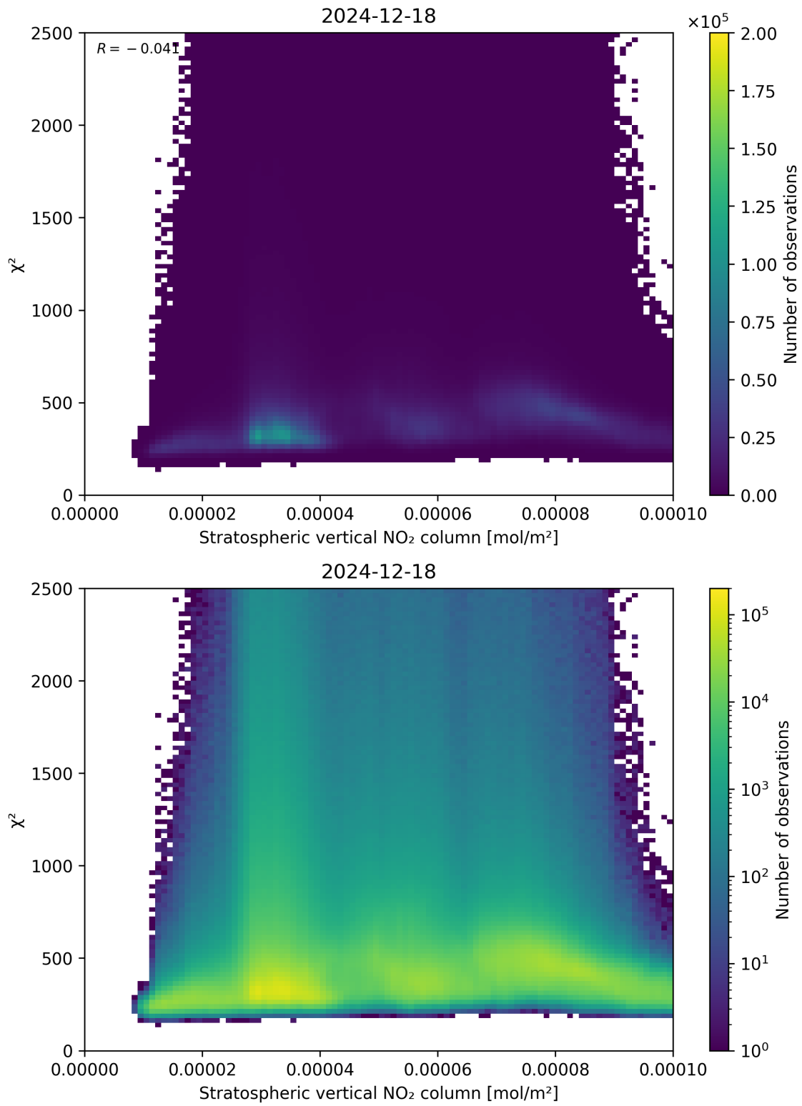
Figure 97: Scatter density plot of “Stratospheric vertical NO 2 column” against “ \chi^2 ” for 2024-12-17 to 2024-12-19.
