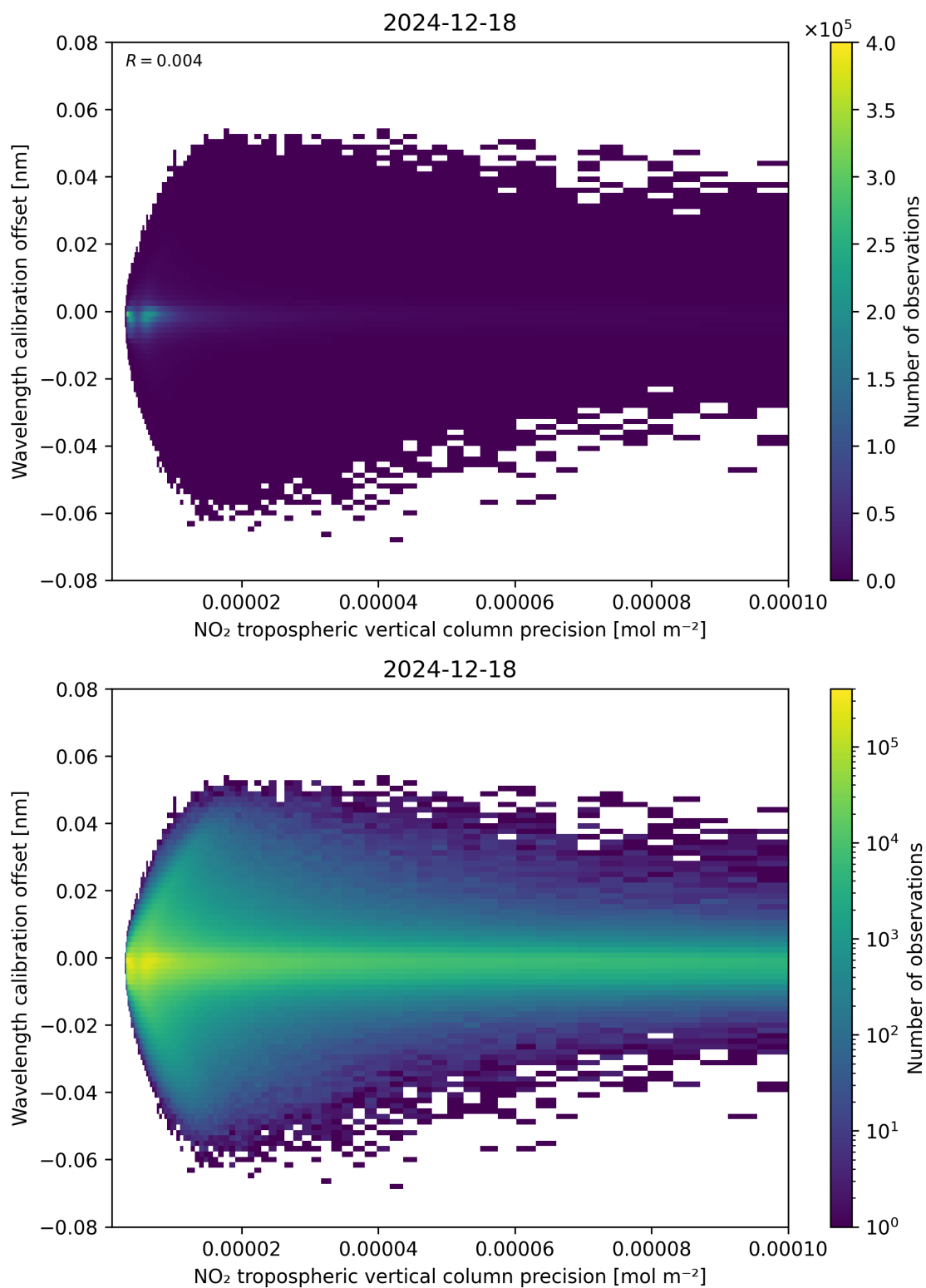
Figure 141: Scatter density plot of “NO 2 tropospheric vertical column precision” against “Wavelength calibration offset” for 2024-12-17 to 2024-12-19.
