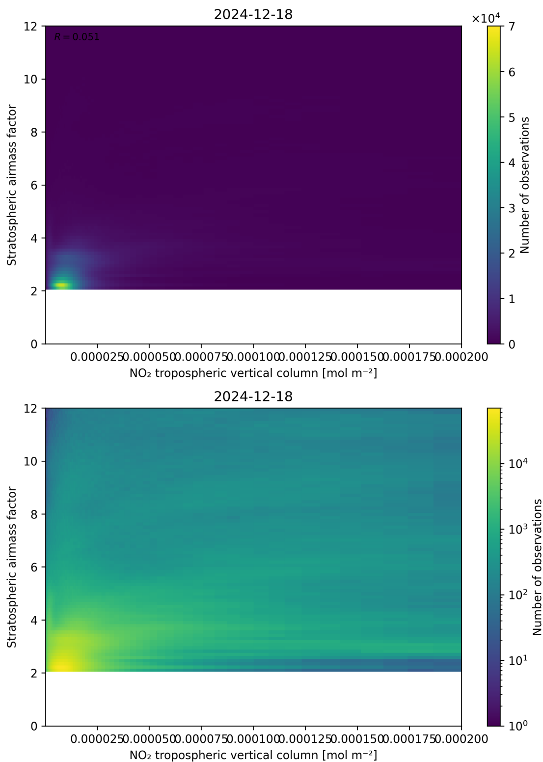
Figure 121: Scatter density plot of “NO 2 tropospheric vertical column” against “Stratospheric airmass factor” for 2024-12-17 to 2024-12-19.
