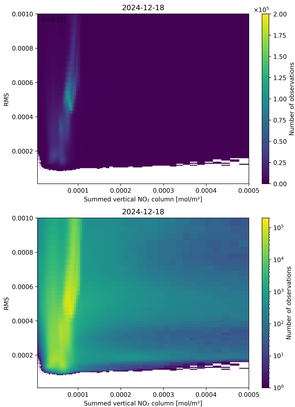
Figure 109: Scatter density plot of “Summed vertical NO 2 column” against “RMS” for 2024-12-17 to 2024-12-19.
