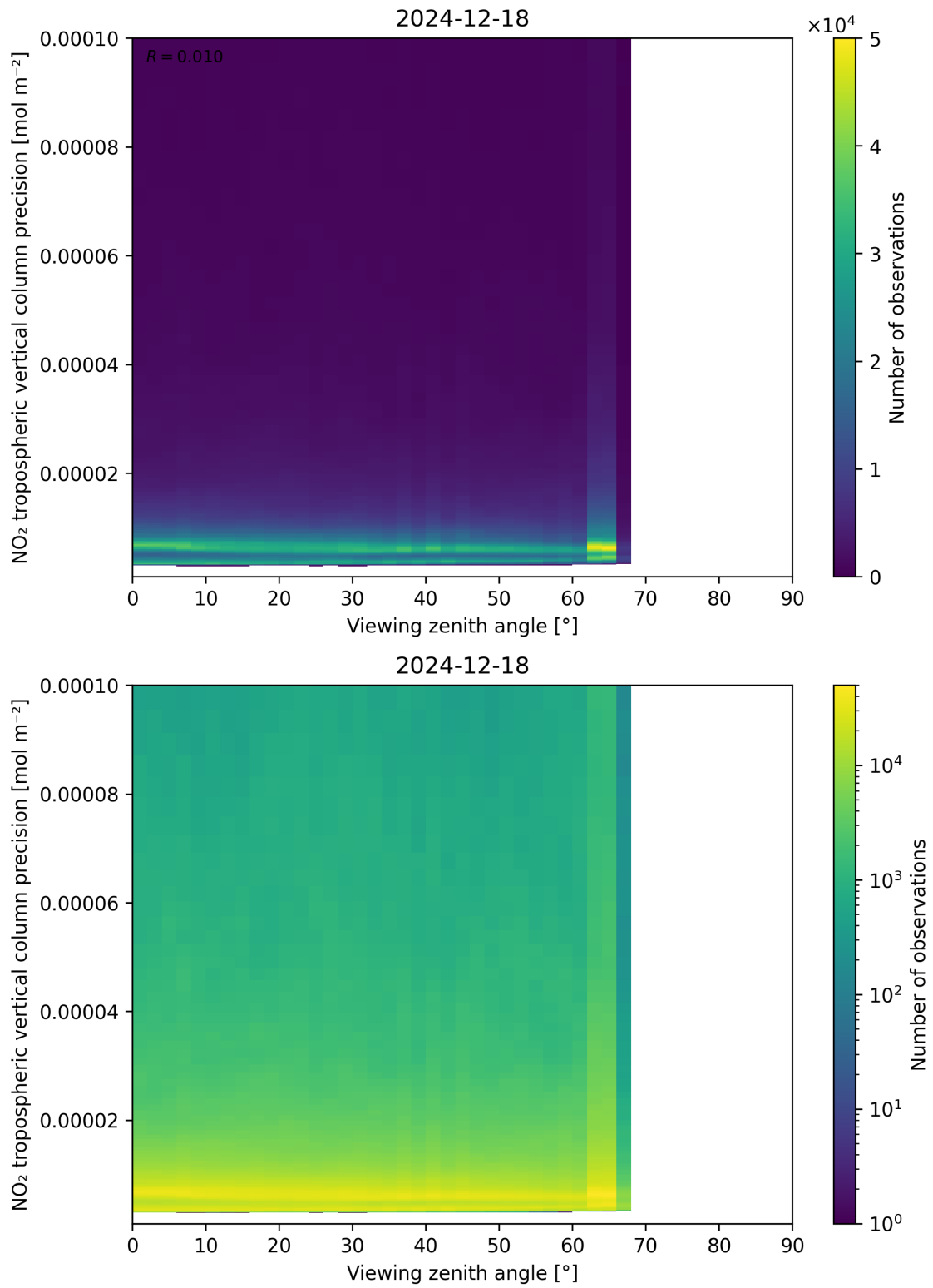
Figure 170: Scatter density plot of “Viewing zenith angle” against “NO 2 tropospheric vertical column precision” for 2024-12-17 to 2024-12-19.
