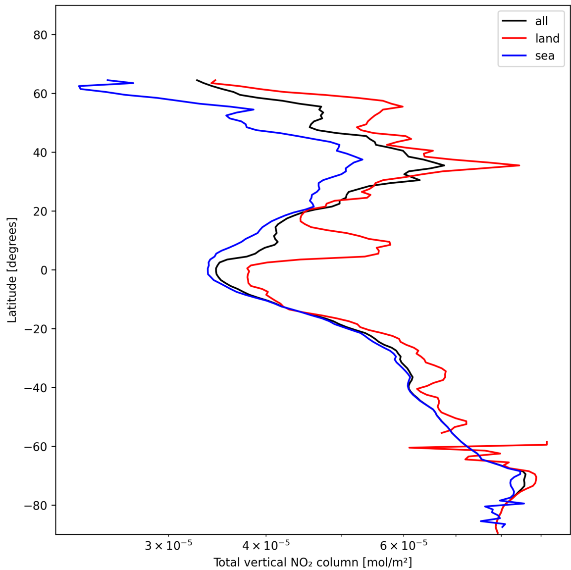
Figure 21: Zonal average of “Total vertical NO 2 column” for 2024-12-17 to 2024-12-19.
