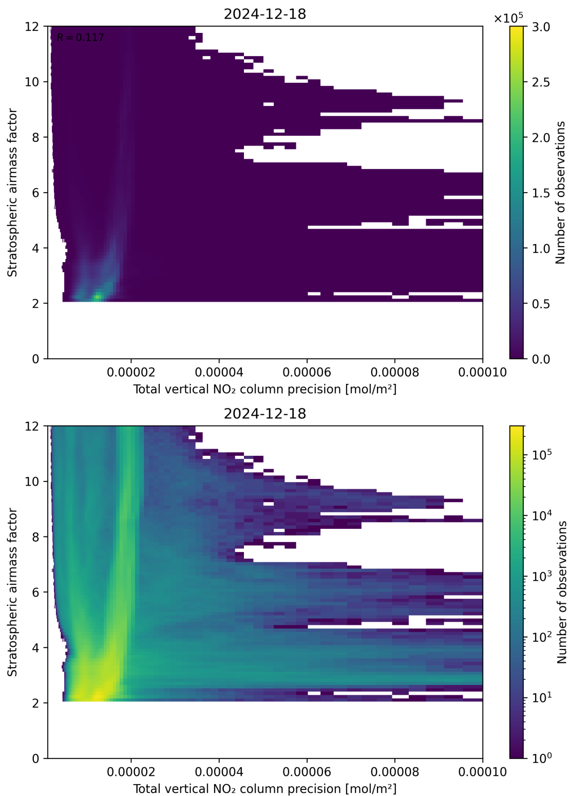
Figure 115: Scatter density plot of “Total vertical NO 2 column precision” against “Stratospheric air mass factor” for 2024-12-17 to 2024-12-19.
