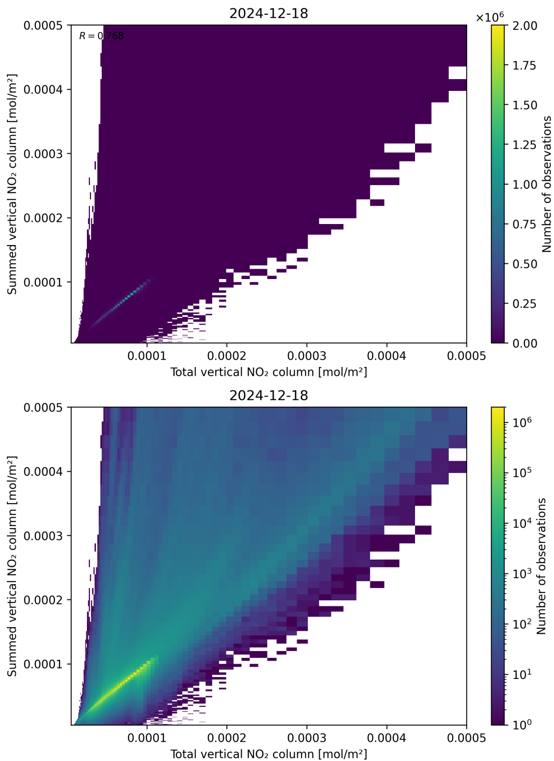
Figure 112: Scatter density plot of “Total vertical NO 2 column” against “Summed vertical NO 2 column” for 2024-12-17 to 2024-12-19.
