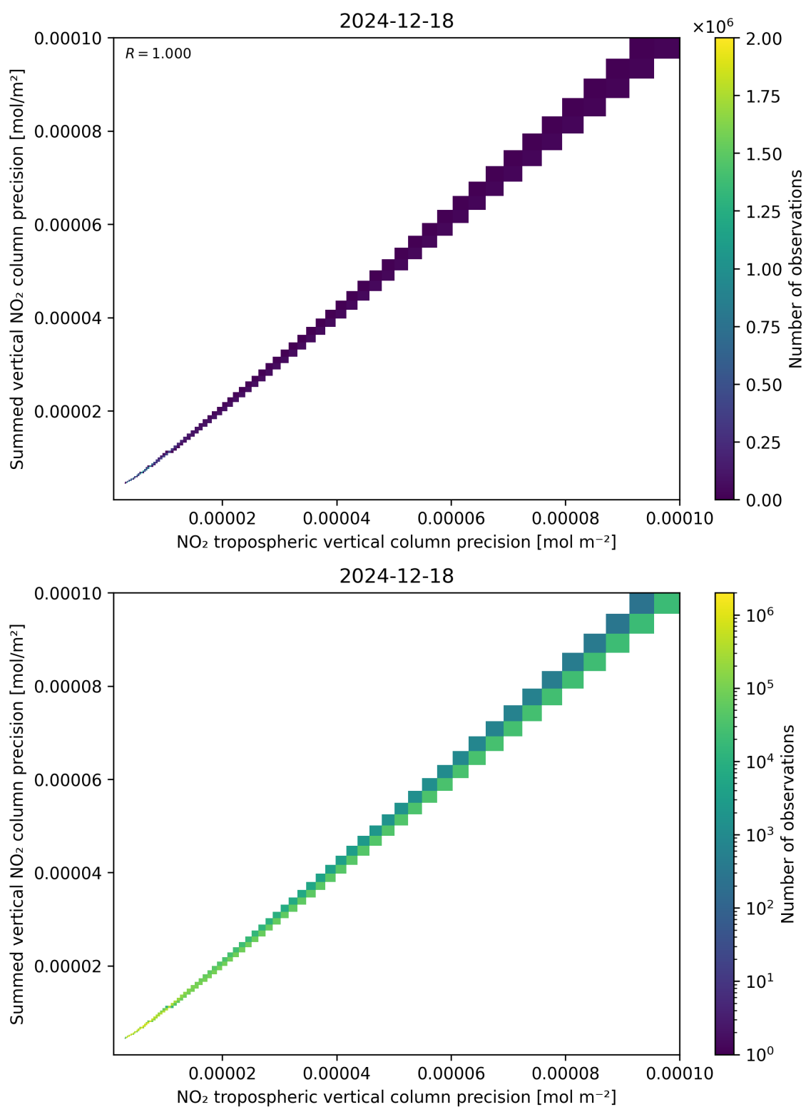
Figure 137: Scatter density plot of “NO 2 tropospheric vertical column precision” against “Summed vertical NO 2 column precision” for 2024-12-17 to 2024-12-19.
