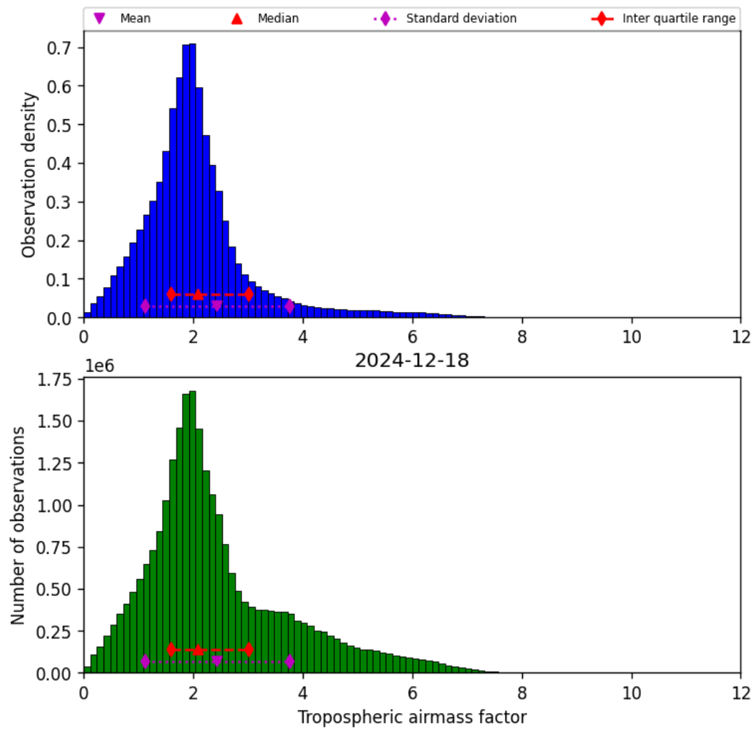
Figure 31: Histogram of “Tropospheric airmass factor” for 2024-12-17 to 2024-12-19
