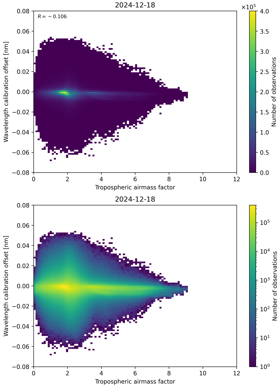
Figure 80: Scatter density plot of “Tropospheric airmass factor” against “Wavelength calibration offset” for 2024-12-17 to 2024-12-19.
