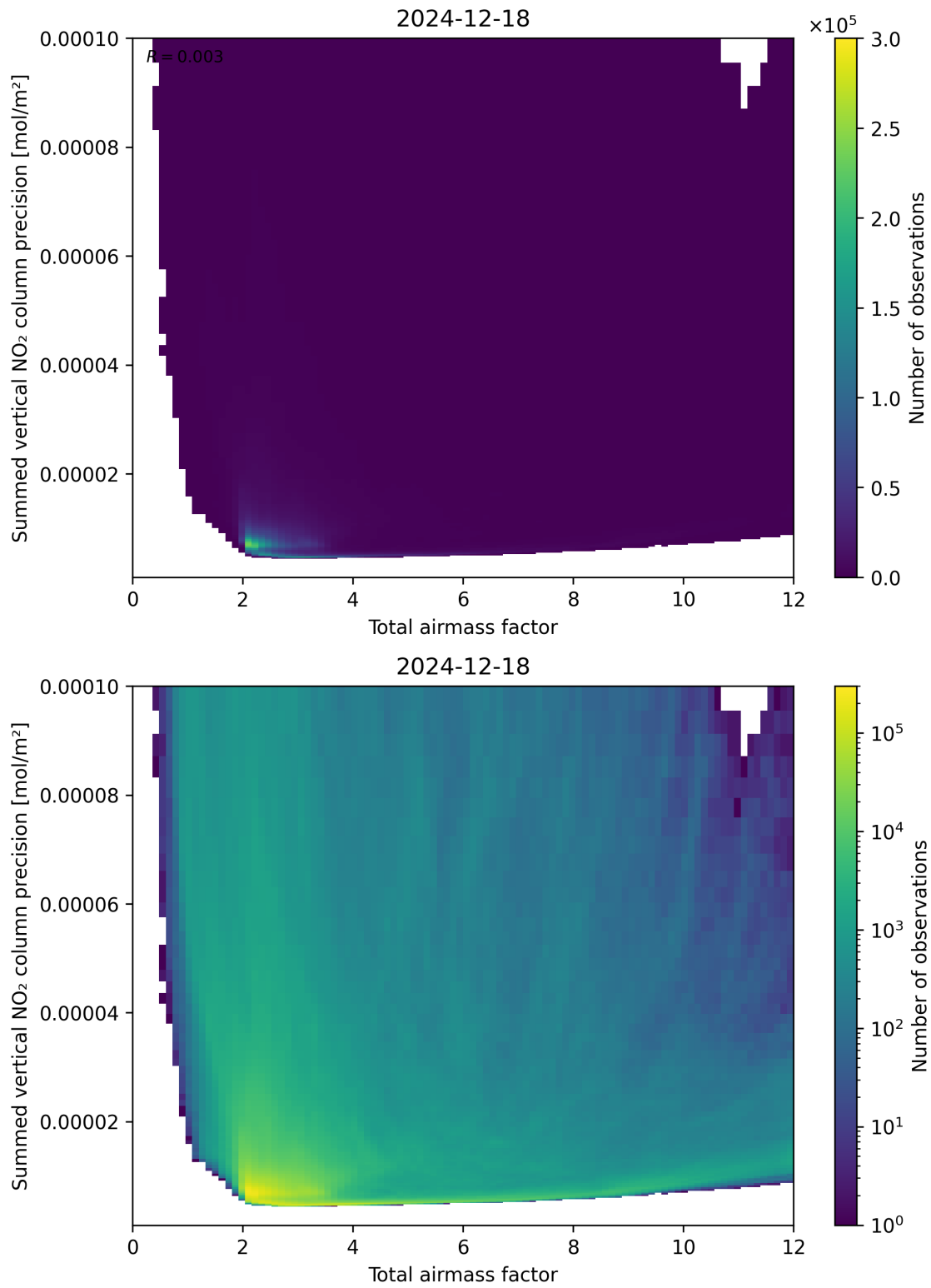
Figure 66: Scatter density plot of “Total airmass factor” against “Summed vertical NO 2 column precision” for 2024-12-17 to 2024-12-19.
