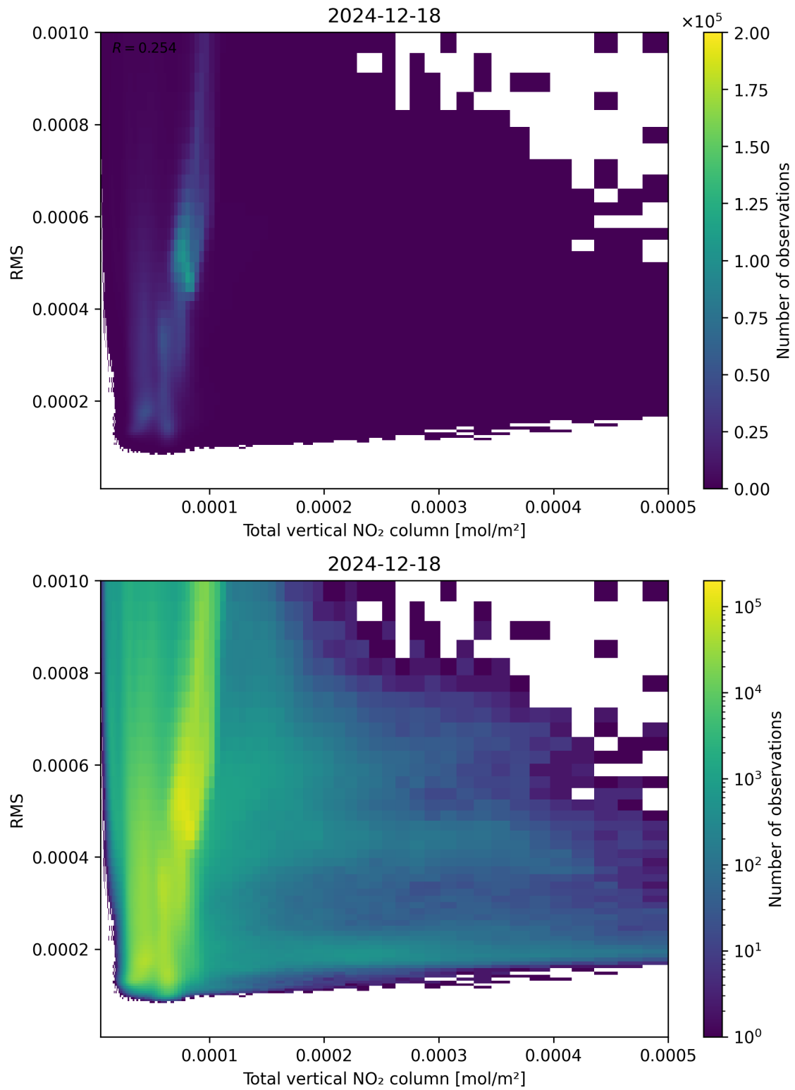
Figure 120: Scatter density plot of “Total vertical NO 2 column” against “RMS” for 2024-12-17 to 2024-12-19.
