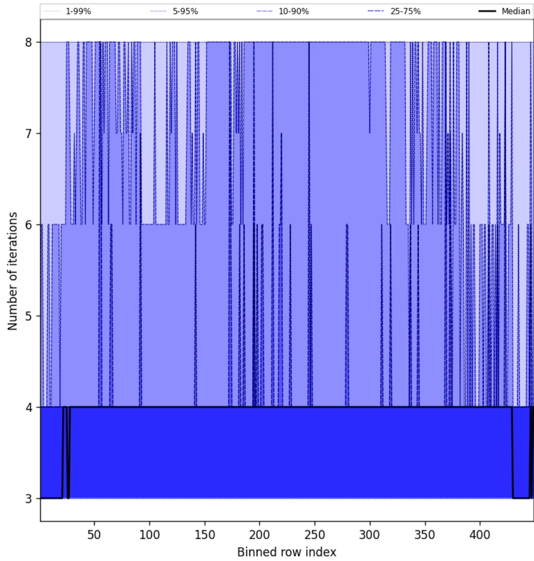
Figure 51: Along track statistics of “Number of iterations” for 2024-12-17 to 2024-12-19
