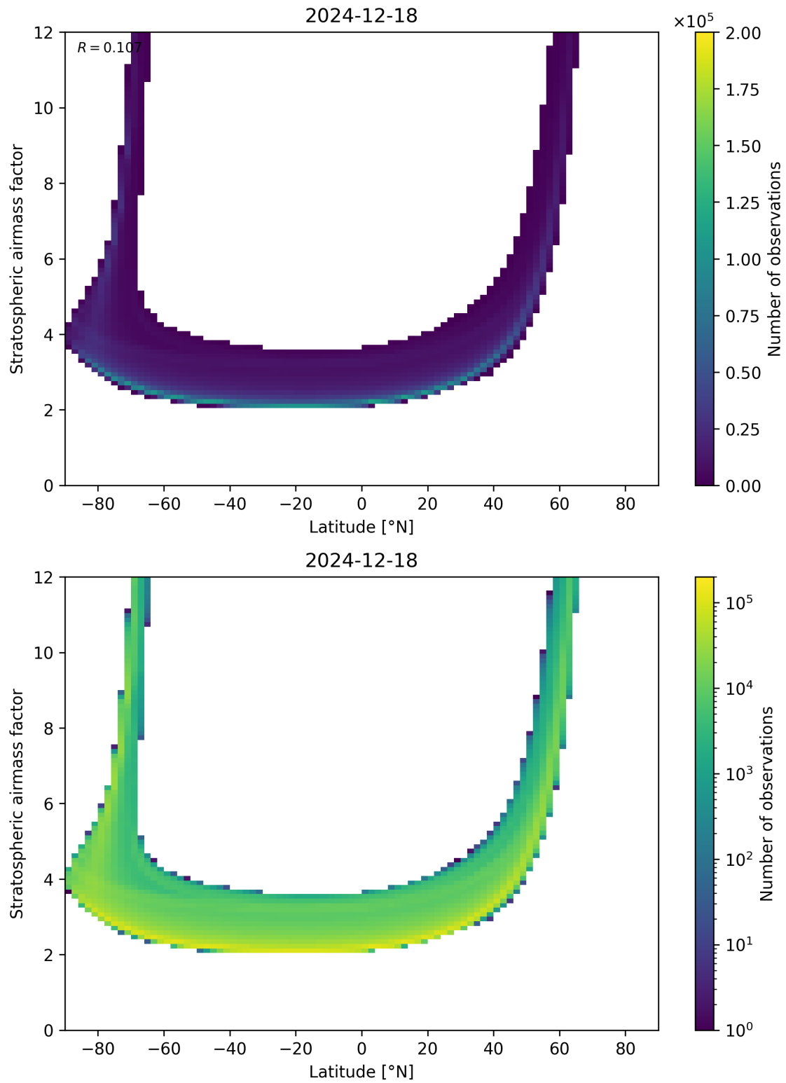
Figure 83: Scatter density plot of “Latitude” against “Stratospheric airmass factor” for 2024-12-17 to 2024-12-19.
