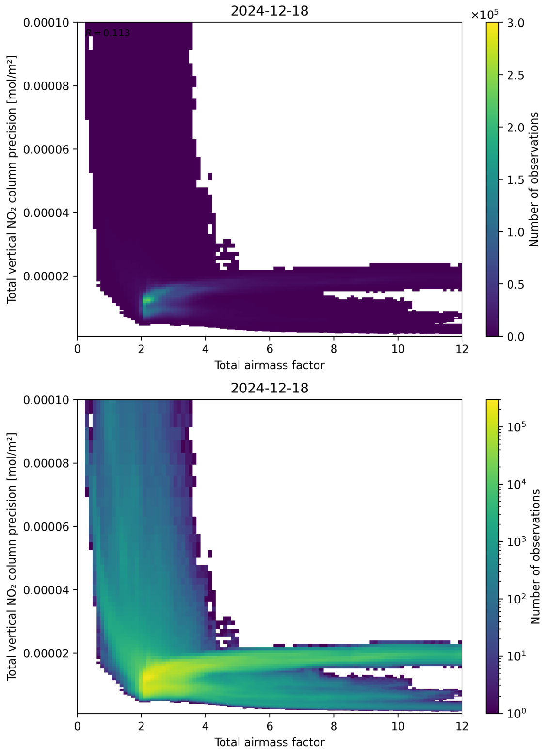
Figure 68: Scatter density plot of “Total airmass factor” against “Total vertical NO 2 column precision” for 2024-12-17 to 2024-12-19.
