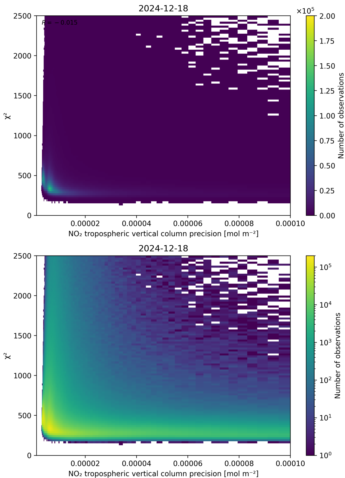
Figure 134: Scatter density plot of “NO 2 tropospheric vertical column precision” against “ \chi^2 ” for 2024-12-17 to 2024-12-19.
