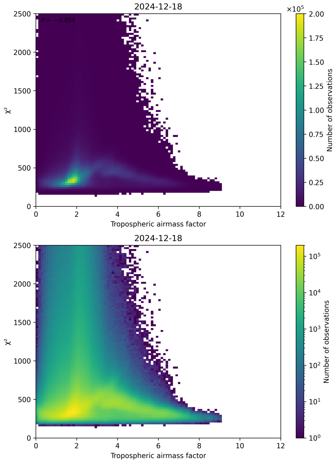
Figure 73: Scatter density plot of “Tropospheric airmass factor” against “ \chi^2 ” for 2024-12-17 to 2024-12-19.
