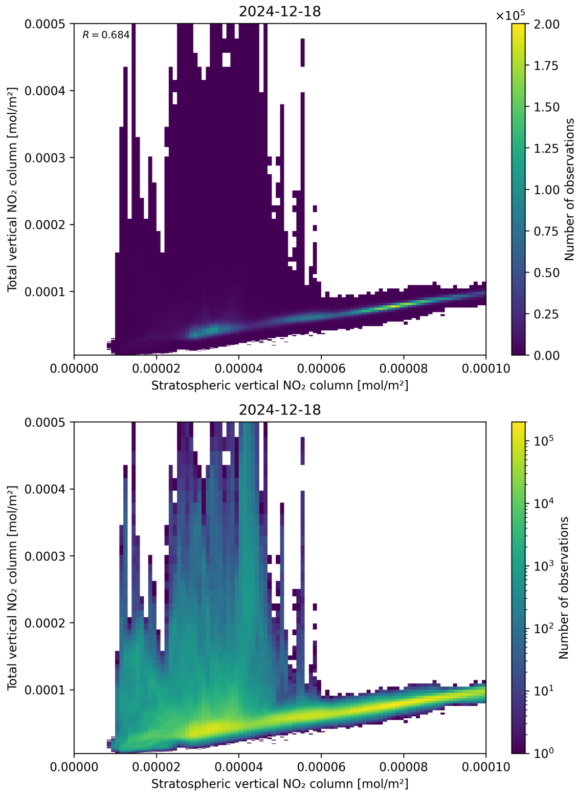
Figure 100: Scatter density plot of “Stratospheric vertical NO 2 column” against “Total vertical NO 2 column” for 2024-12-17 to 2024-12-19.
