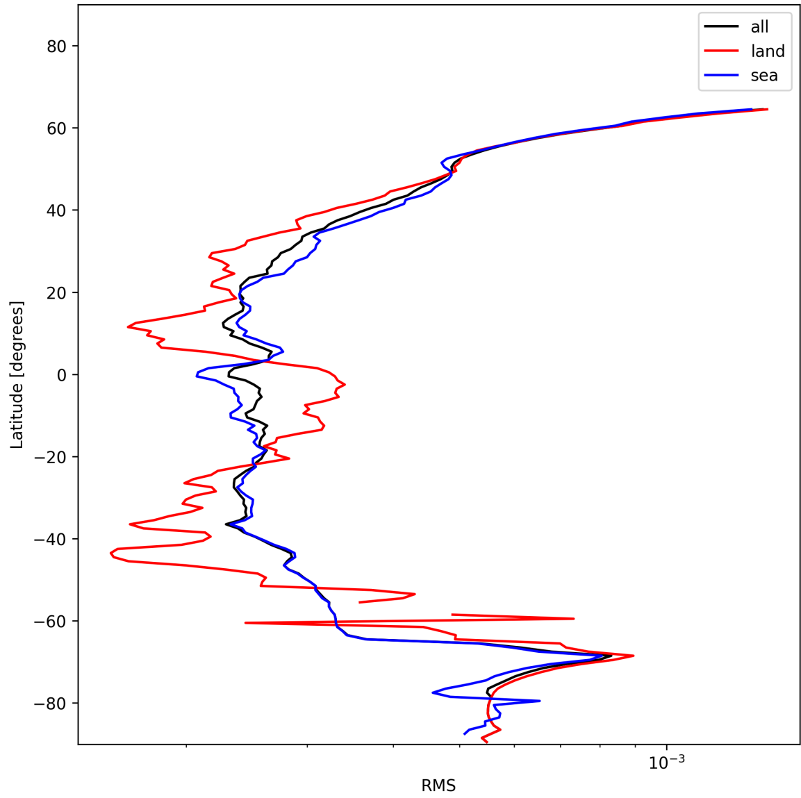
Figure 26: Zonal average of “RMS” for 2024-12-17 to 2024-12-19.
