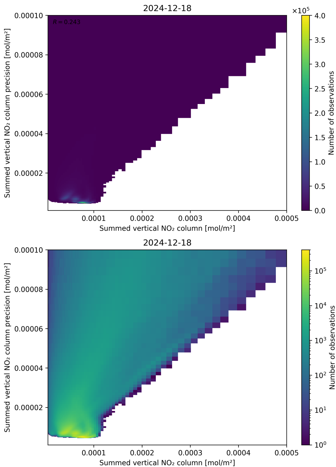
Figure 105: Scatter density plot of “Summed vertical NO 2 column” against “Summed vertical NO 2 column precision” for 2024-12-17 to 2024-12-19.
