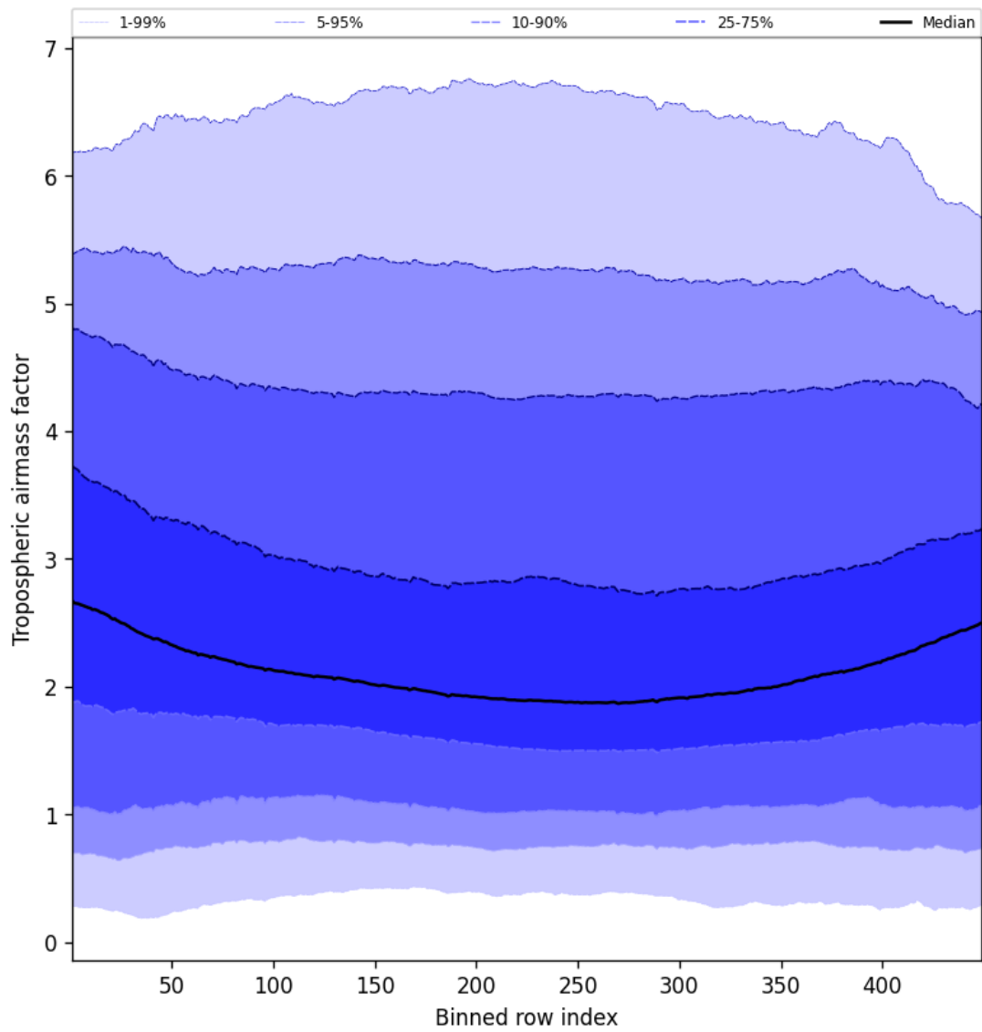
Figure 48: Along track statistics of “Tropospheric airmass factor” for 2024-12-17 to 2024-12-19
