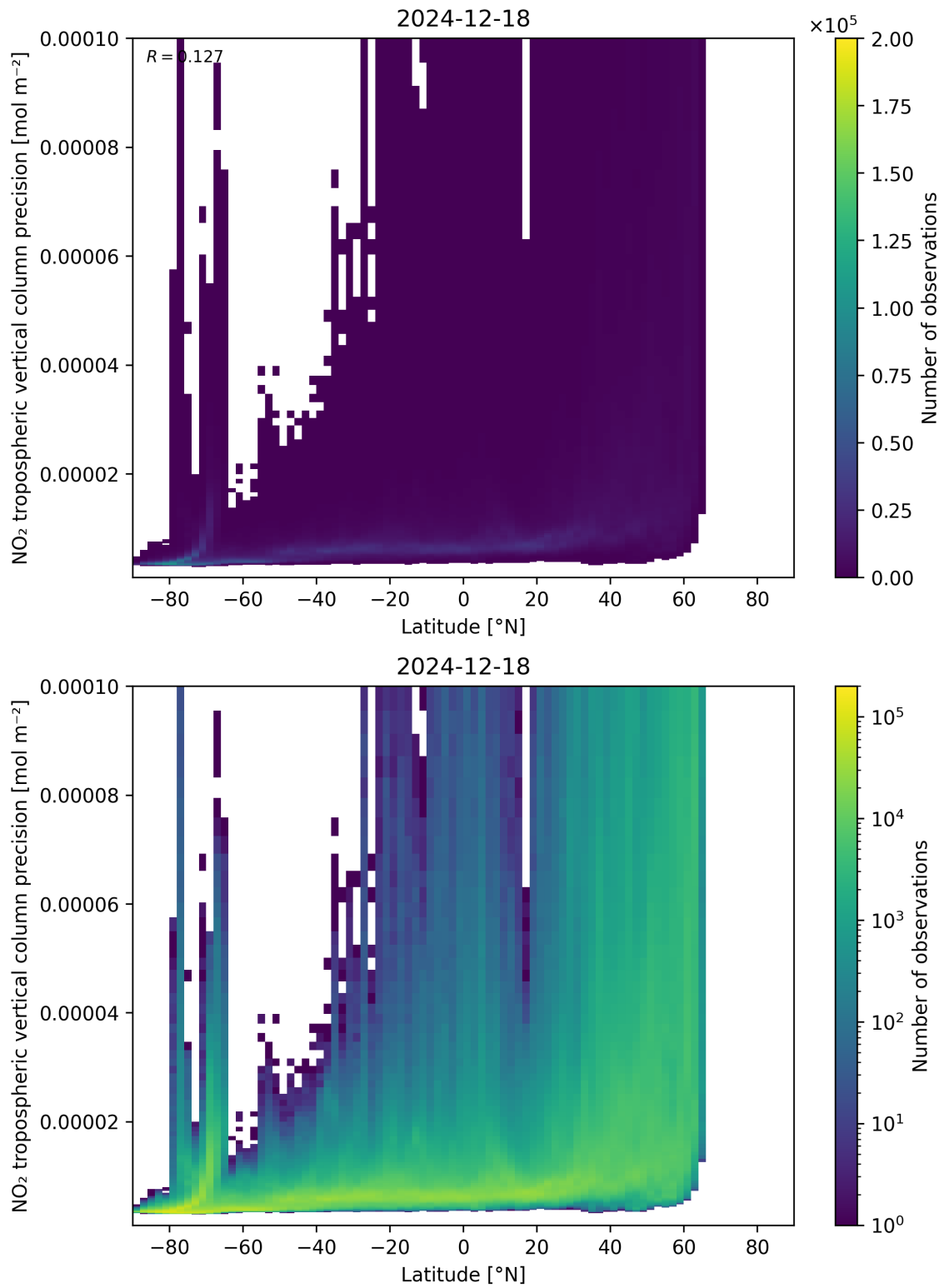
Figure 93: Scatter density plot of “Latitude” against “NO 2 tropospheric vertical column precision” for 2024-12-17 to 2024-12-19.
