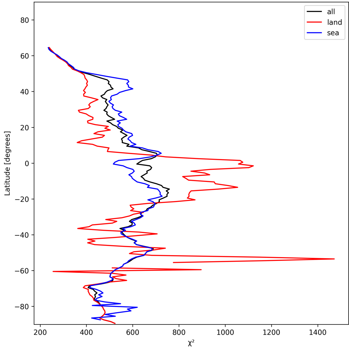
Figure 25: Zonal average of “ \chi^2 ” for 2024-12-17 to 2024-12-19.
