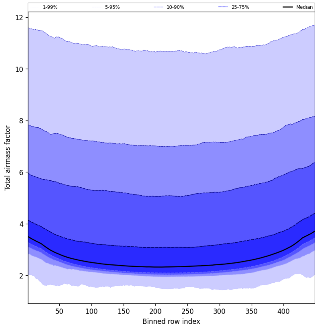
Figure 49: Along track statistics of “Total airmass factor” for 2024-12-17 to 2024-12-19
