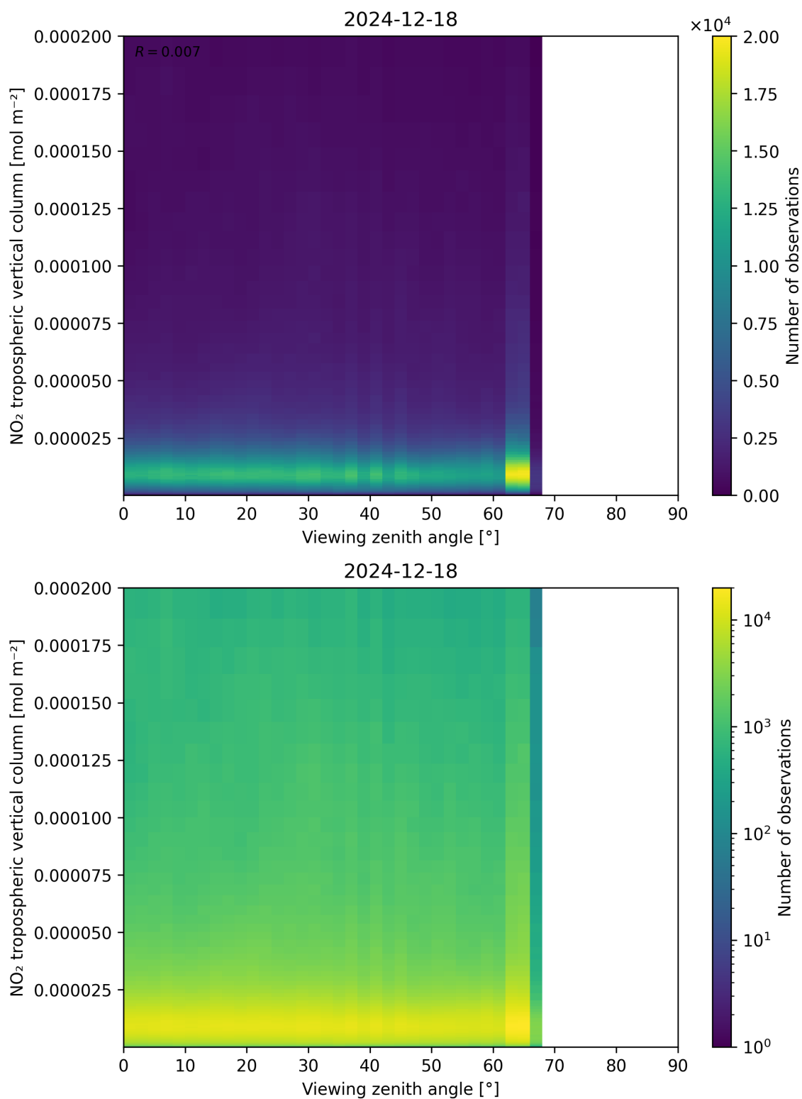
Figure 169: Scatter density plot of “Viewing zenith angle” against “NO 2 tropospheric vertical column” for 2024-12-17 to 2024-12-19.
