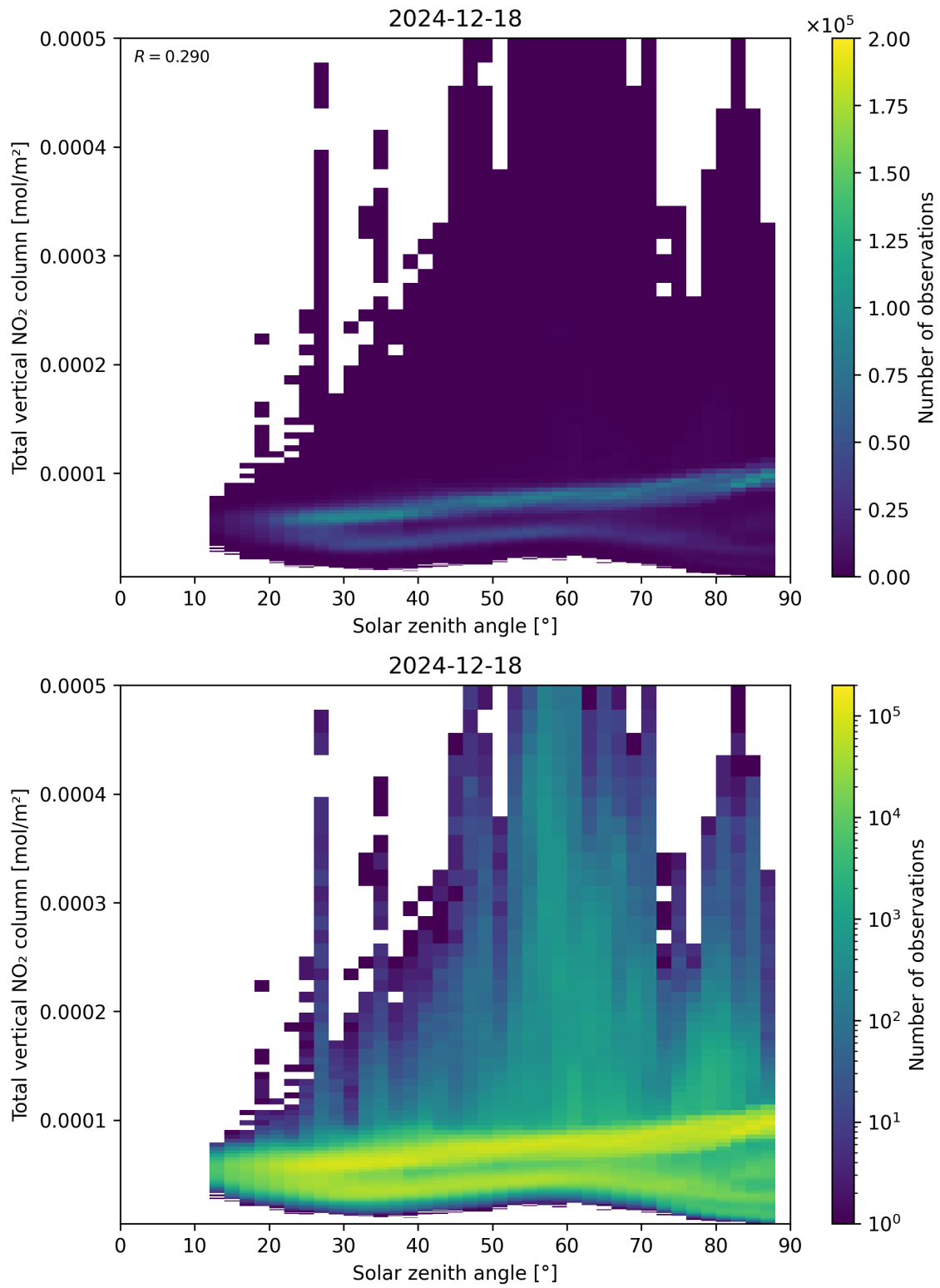
Figure 153: Scatter density plot of “Solar zenith angle” against “Total vertical \text{NO}_2 column” for 2024-12-17 to 2024-12-19.
