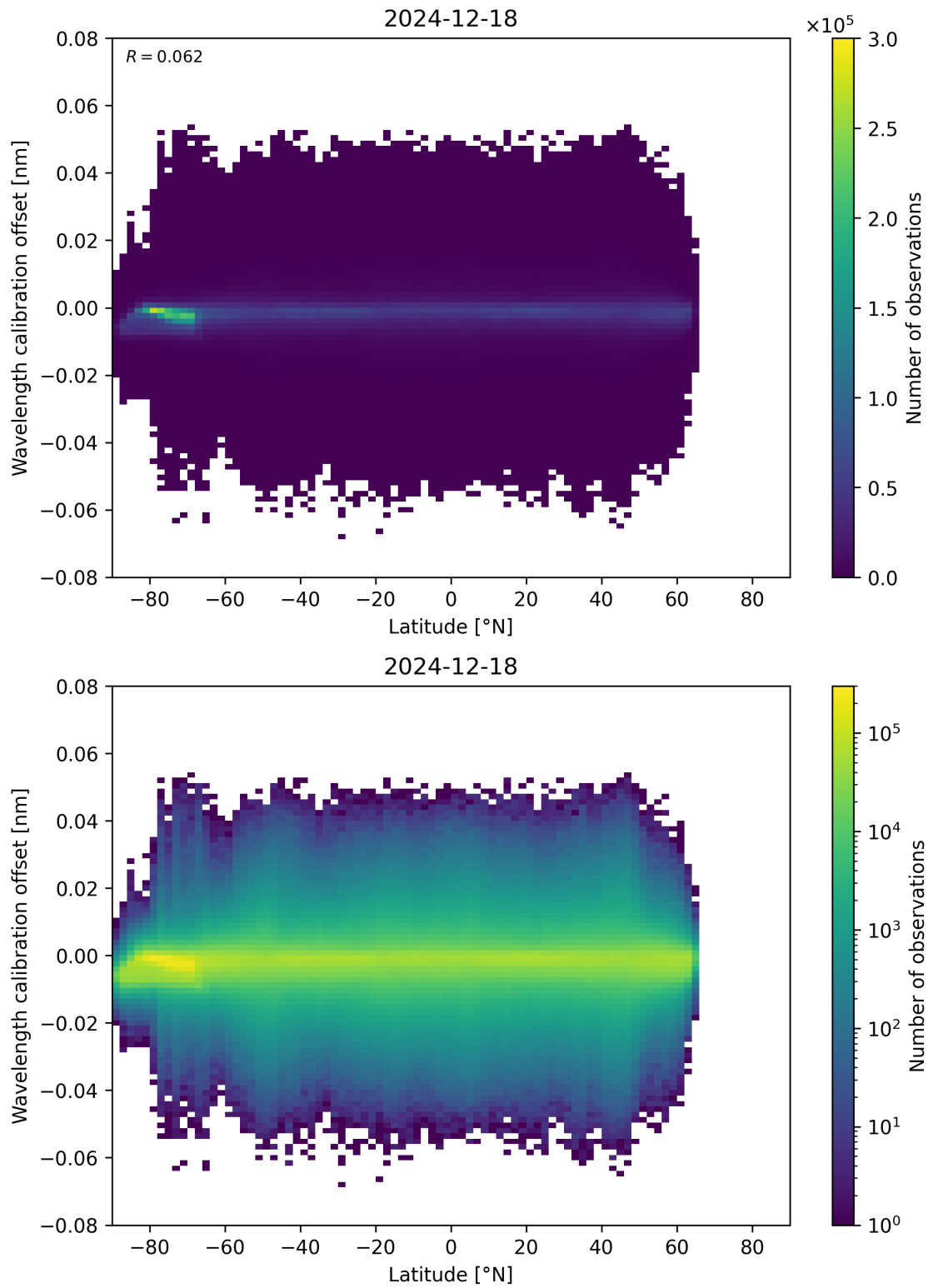
Figure 95: Scatter density plot of “Latitude” against “Wavelength calibration offset” for 2024-12-17 to 2024-12-19.
