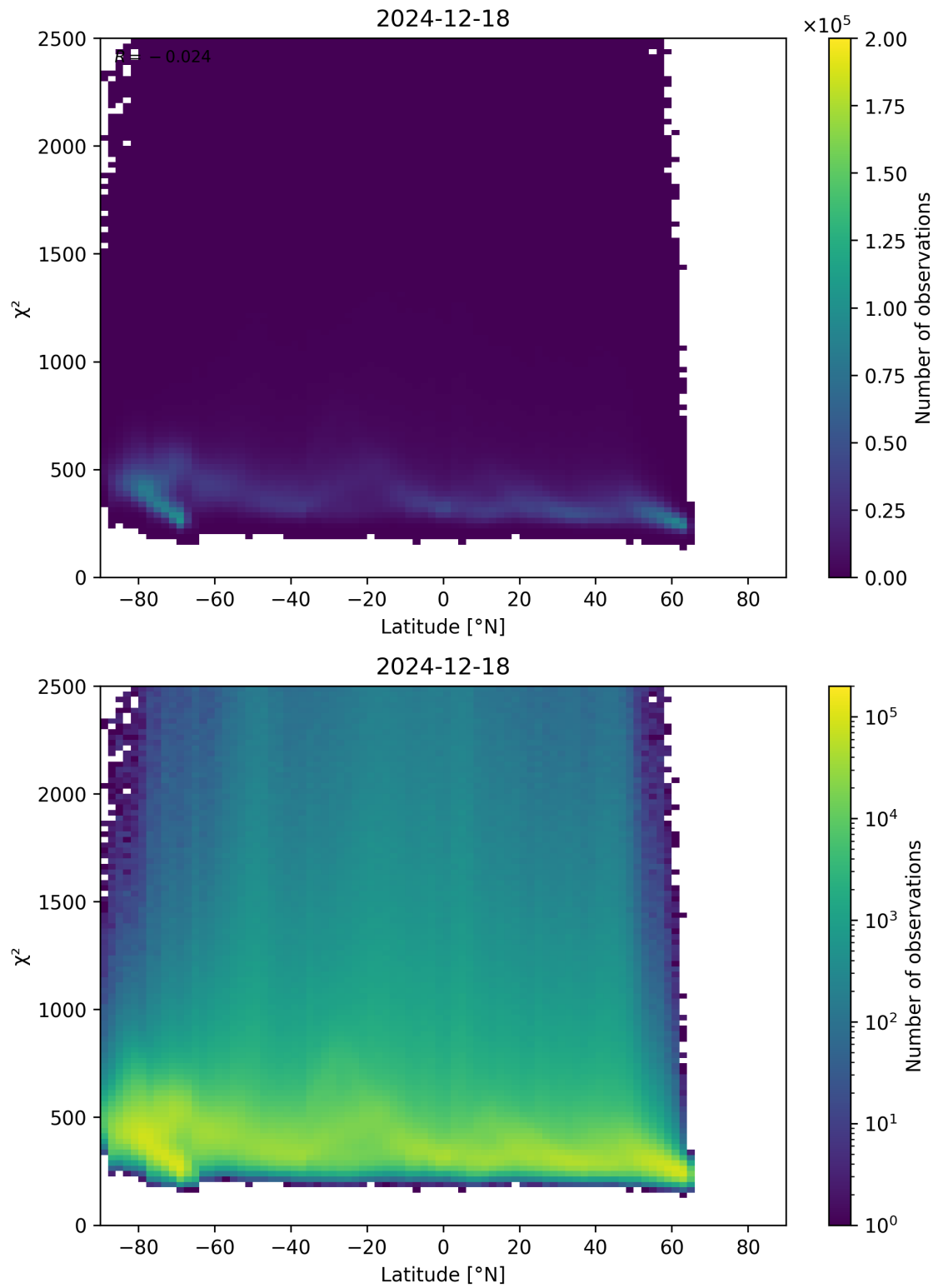
Figure 86: Scatter density plot of “Latitude” against “ \chi^2 ” for 2024-12-17 to 2024-12-19.
