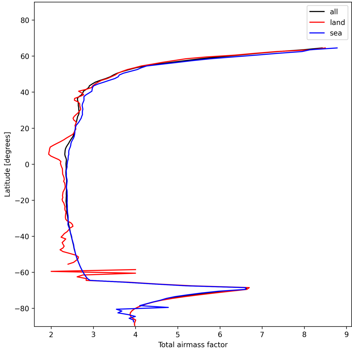
Figure 15: Zonal average of “Total airmass factor” for 2024-12-17 to 2024-12-19.
