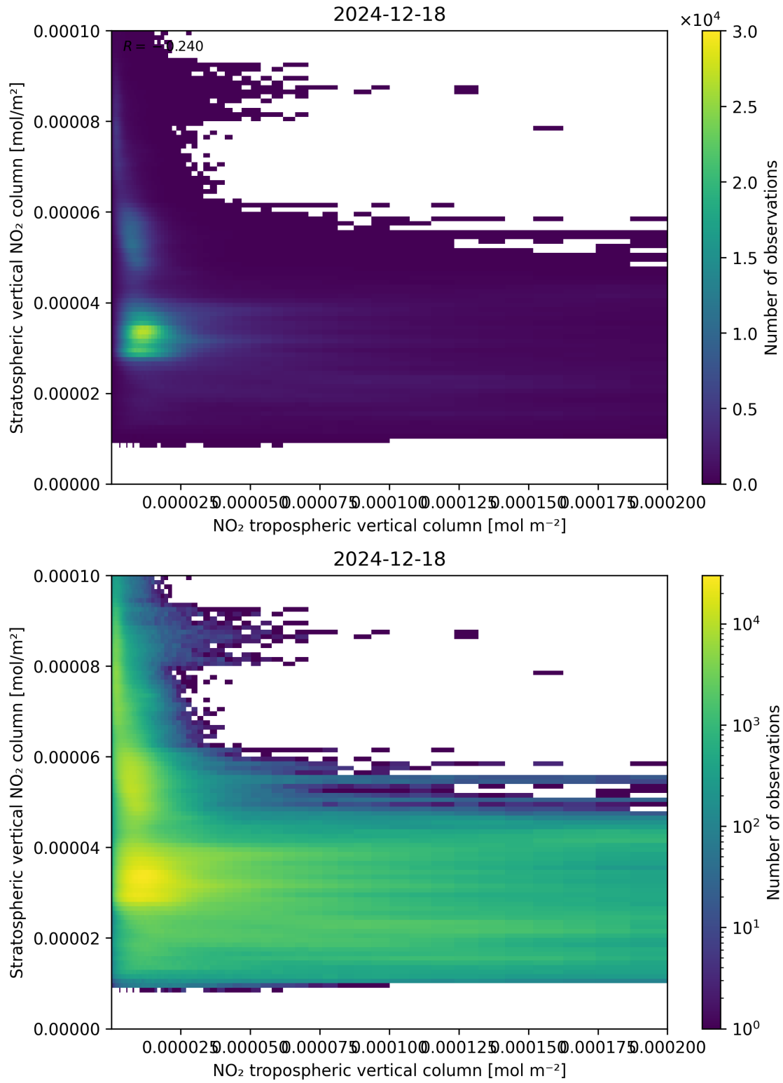
Figure 125: Scatter density plot of “NO 2 tropospheric vertical column” against “Stratospheric vertical NO 2 column” for 2024-12-17 to 2024-12-19.
