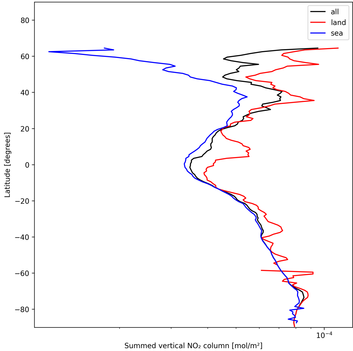
Figure 23: Zonal average of “Summed vertical NO 2 column” for 2024-12-17 to 2024-12-19.
