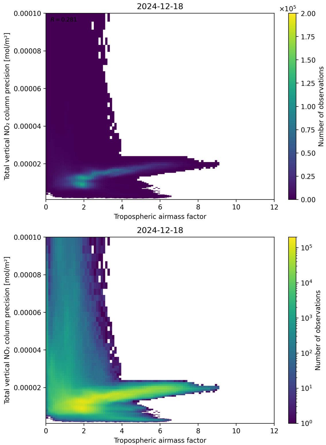
Figure 78: Scatter density plot of “Tropospheric air mass factor” against “Total vertical NO 2 column precision” for 2024-12-17 to 2024-12-19.
