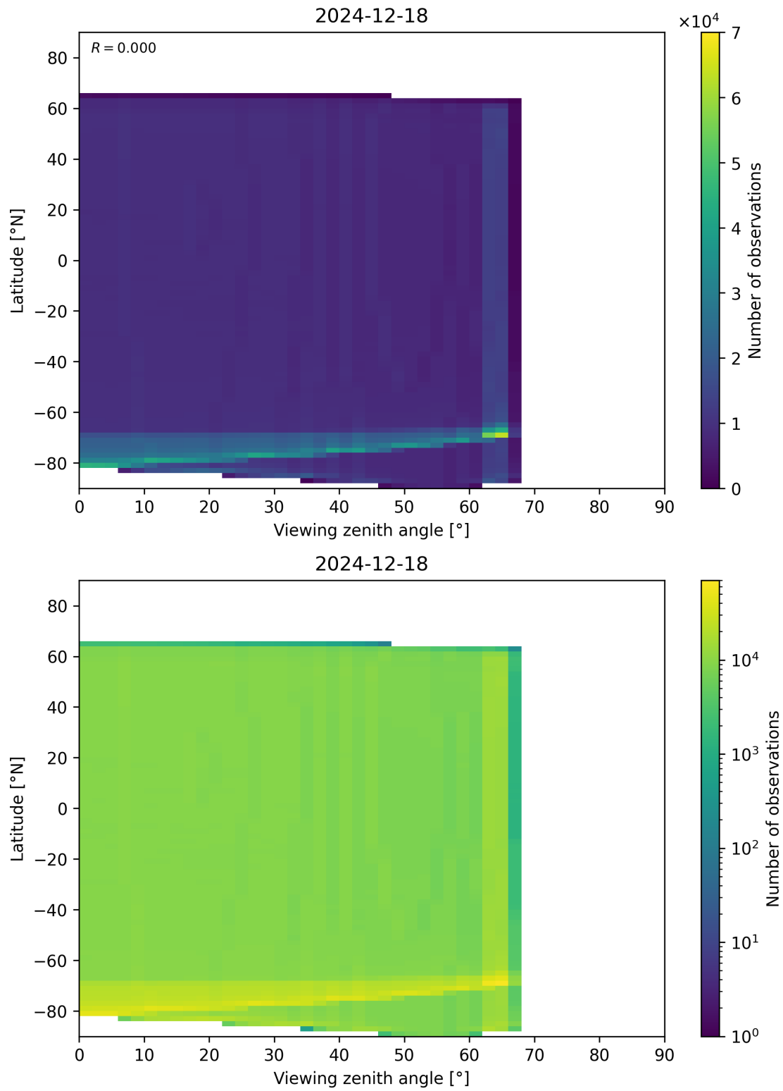
Figure 163: Scatter density plot of “Viewing zenith angle” against “Latitude” for 2024-12-17 to 2024-12-19.
