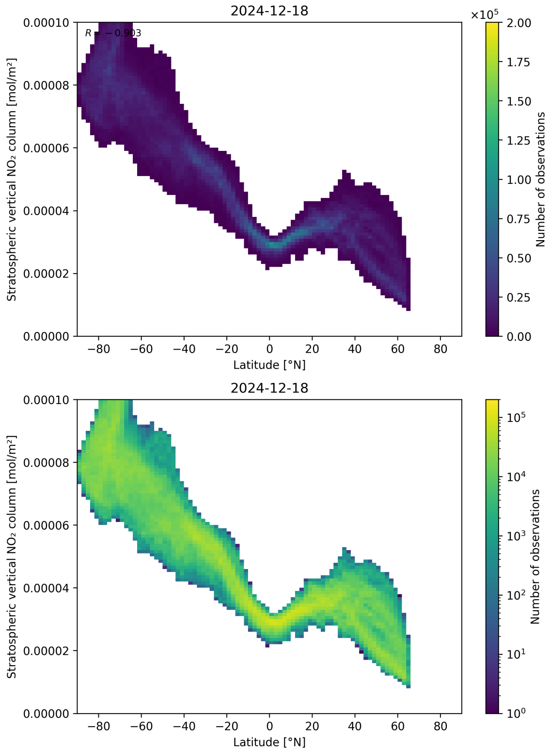
Figure 87: Scatter density plot of “Latitude” against “Stratospheric vertical NO 2 column” for 2024-12-17 to 2024-12-19.
