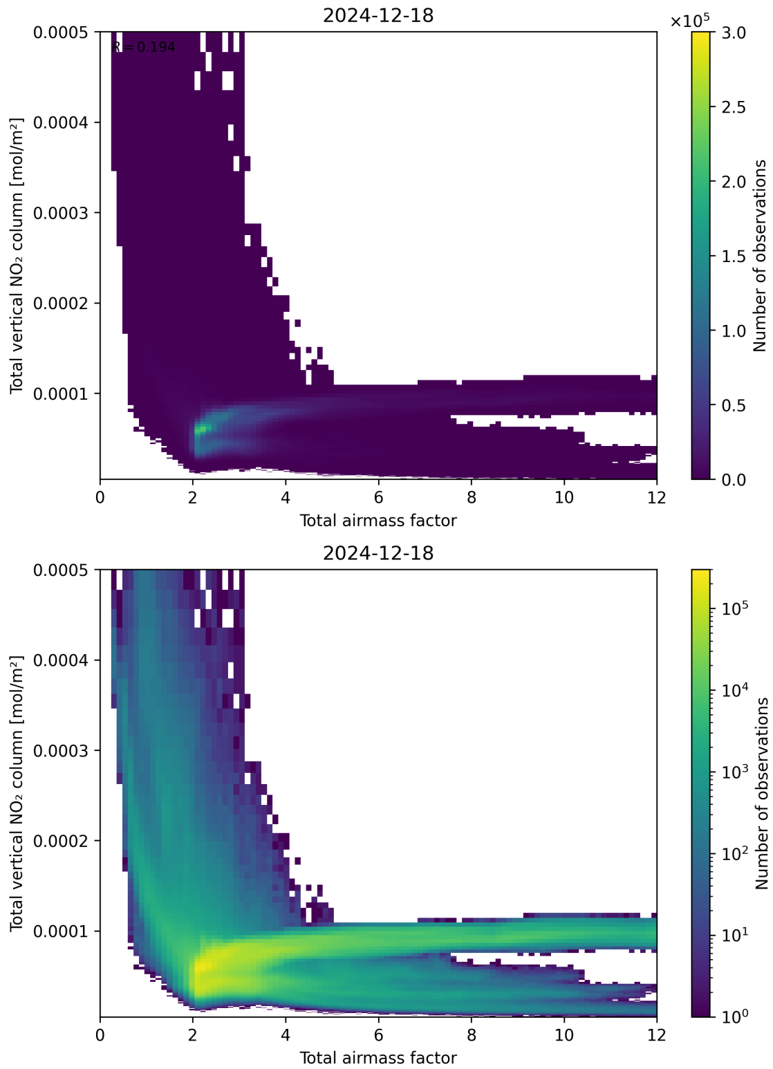
Figure 67: Scatter density plot of “Total airmass factor” against “Total vertical NO 2 column” for 2024-12-17 to 2024-12-19.
