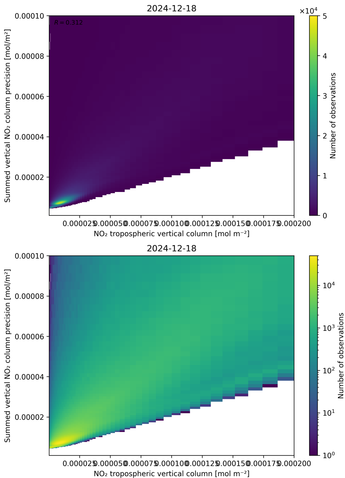
Figure 127: Scatter density plot of “NO 2 tropospheric vertical column” against “Summed vertical NO 2 column precision” for 2024-12-17 to 2024-12-19.
