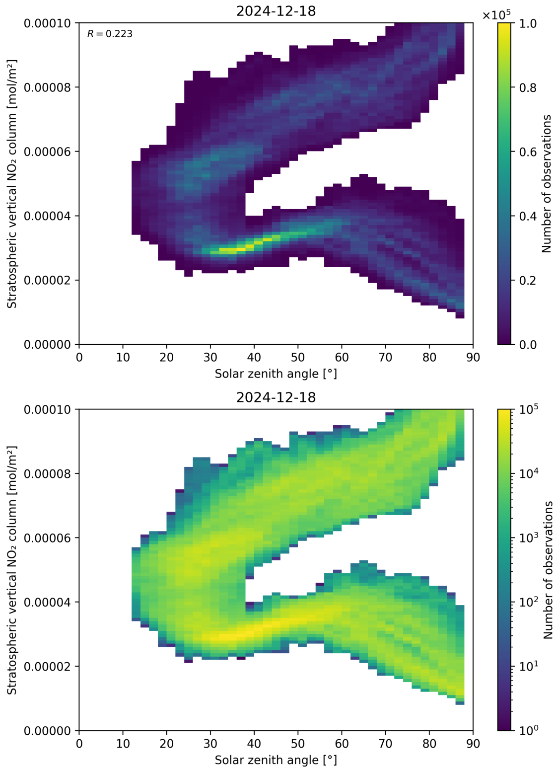
Figure 150: Scatter density plot of “Solar zenith angle” against “Stratospheric vertical NO 2 column” for 2024-12-17 to 2024-12-19.
