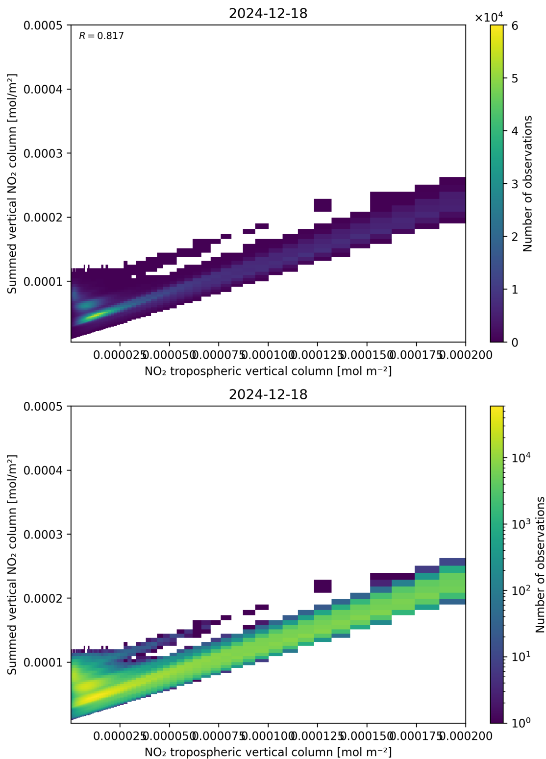
Figure 126: Scatter density plot of “NO 2 tropospheric vertical column” against “Summed vertical NO 2 column” for 2024-12-17 to 2024-12-19.
