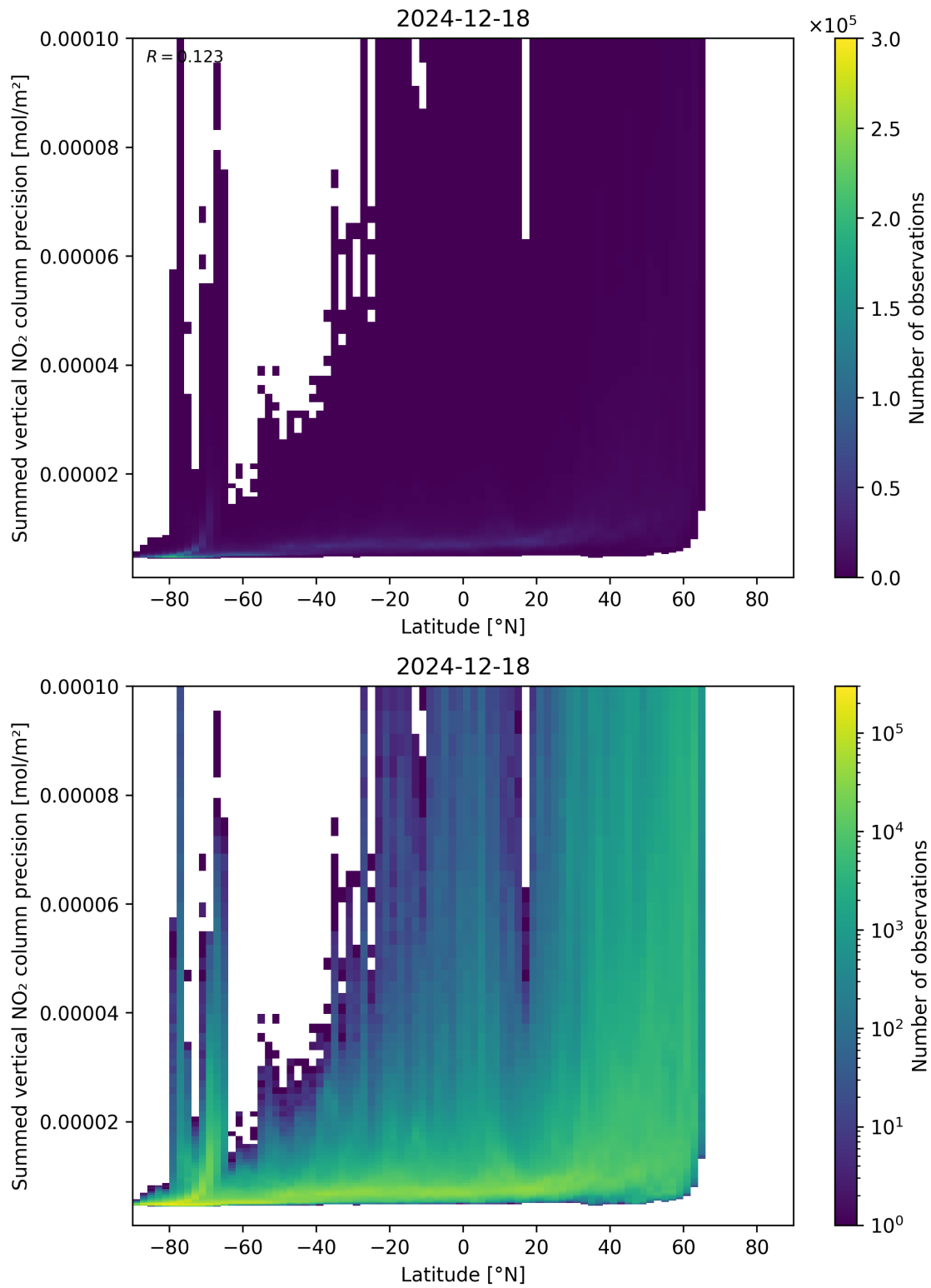
Figure 89: Scatter density plot of “Latitude” against “Summed vertical NO 2 column precision” for 2024-12-17 to 2024-12-19.
