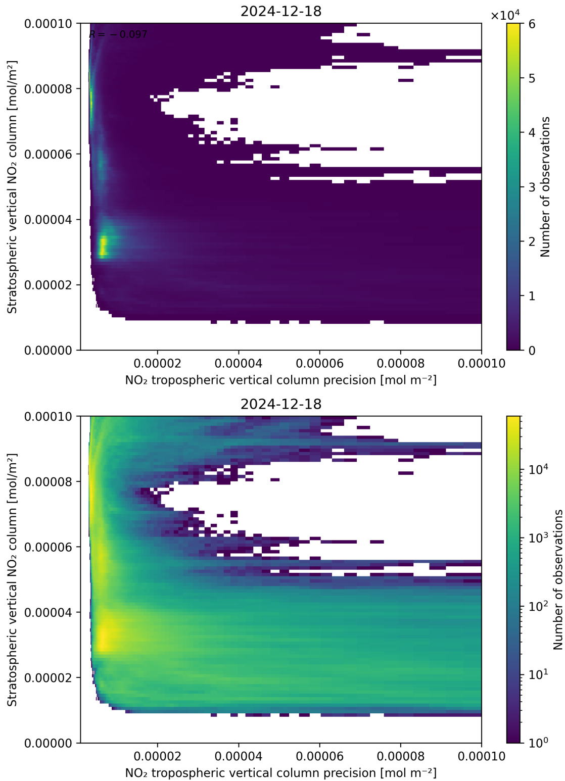
Figure 135: Scatter density plot of “NO 2 tropospheric vertical column precision” against “Stratospheric vertical NO 2 column” for 2024-12-17 to 2024-12-19.
