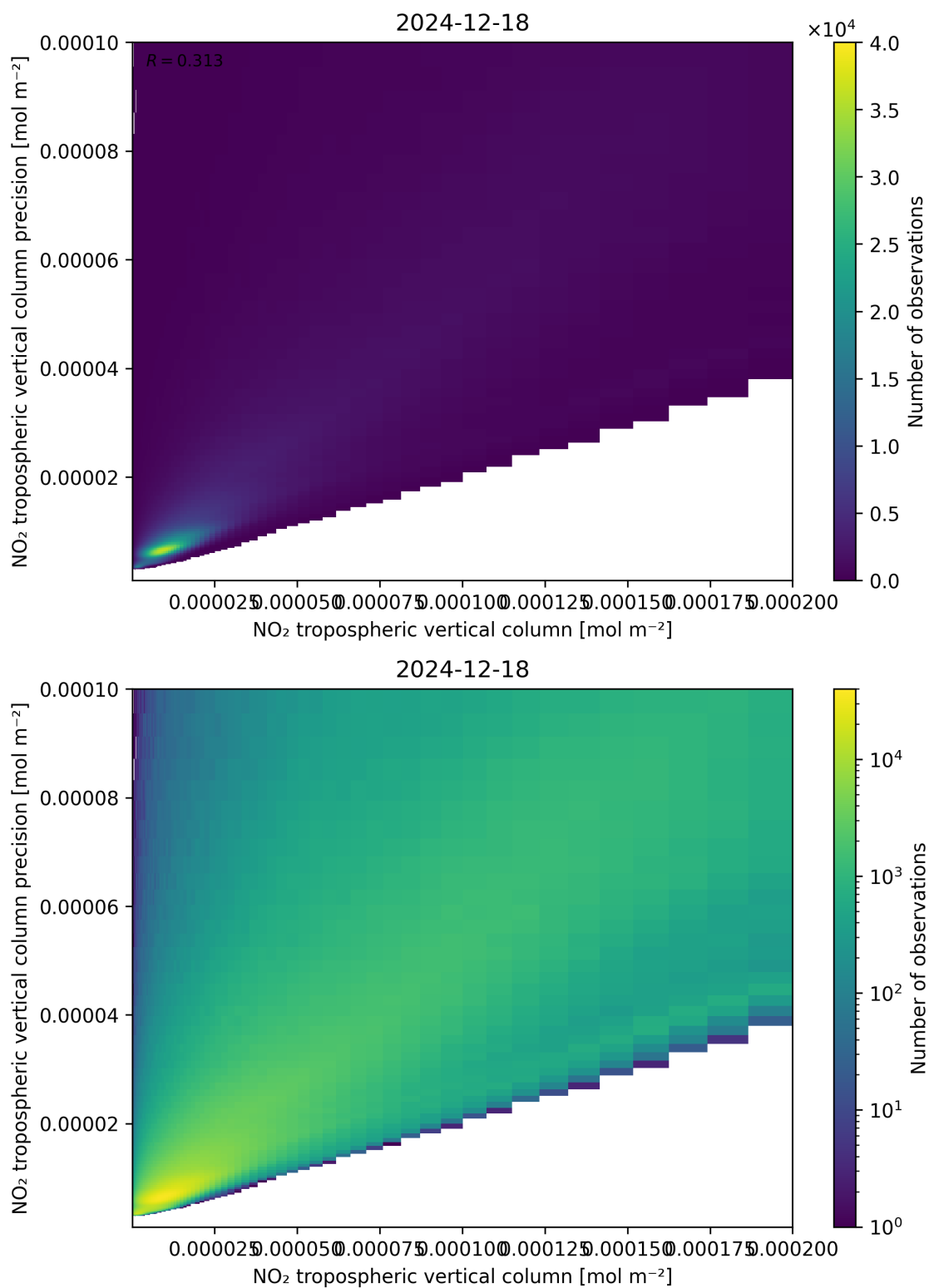
Figure 130: Scatter density plot of “NO 2 tropospheric vertical column” against “NO 2 tropospheric vertical column precision” for 2024-12-17 to 2024-12-19.
