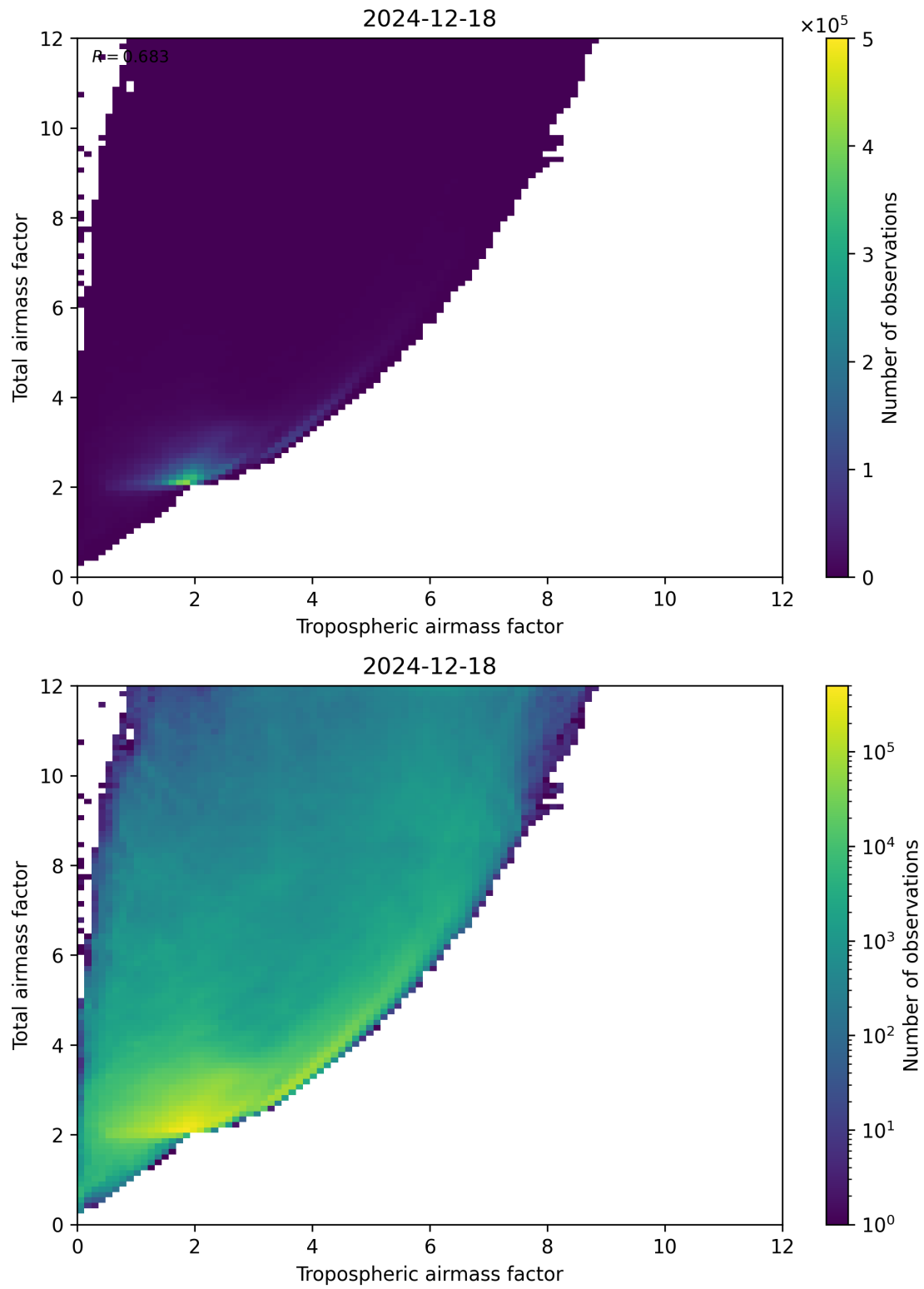
Figure 72: Scatter density plot of “Tropospheric airmass factor” against “Total airmass factor” for 2024-12-17 to 2024-12-19.
