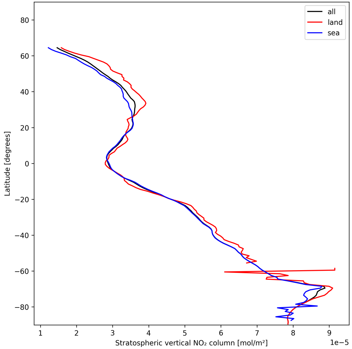
Figure 19: Zonal average of “Stratospheric vertical NO 2 column” for 2024-12-17 to 2024-12-19.
