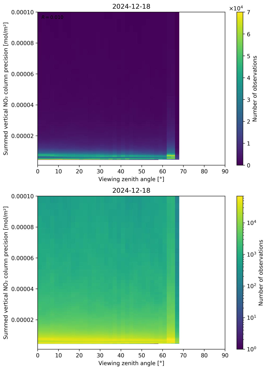
Figure 166: Scatter density plot of “Viewing zenith angle” against “Summed vertical NO 2 column precision” for 2024-12-17 to 2024-12-19.
