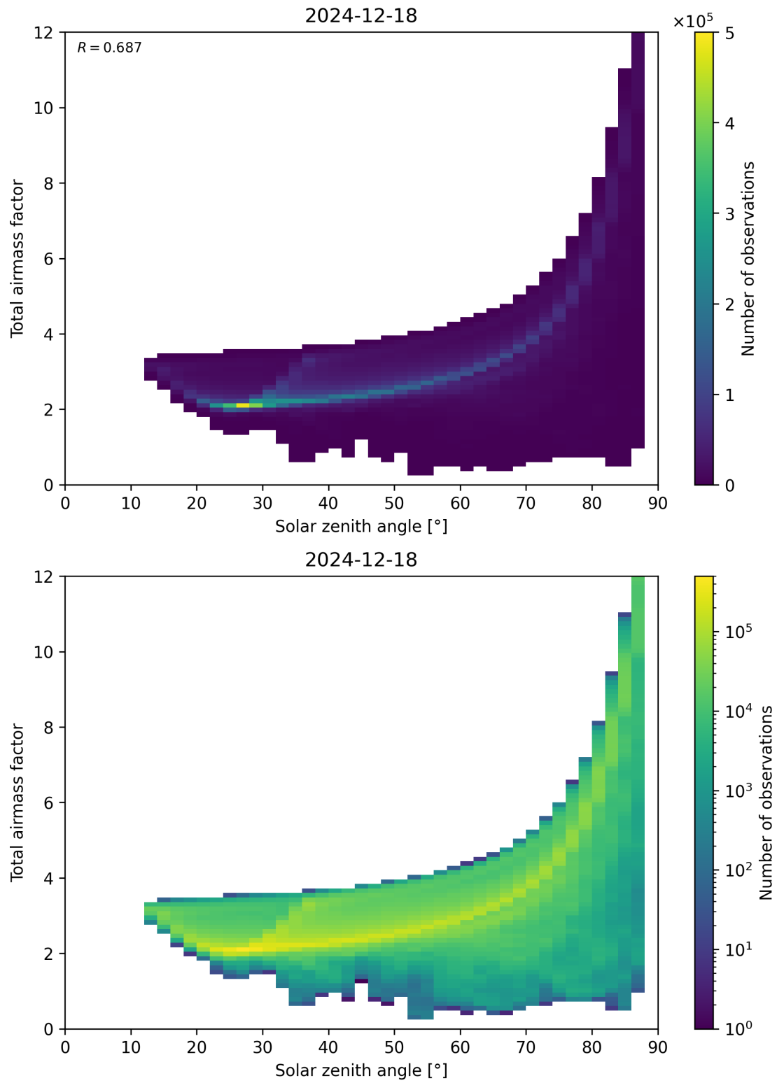
Figure 146: Scatter density plot of “Solar zenith angle” against “Total air mass factor” for 2024-12-17 to 2024-12-19.
