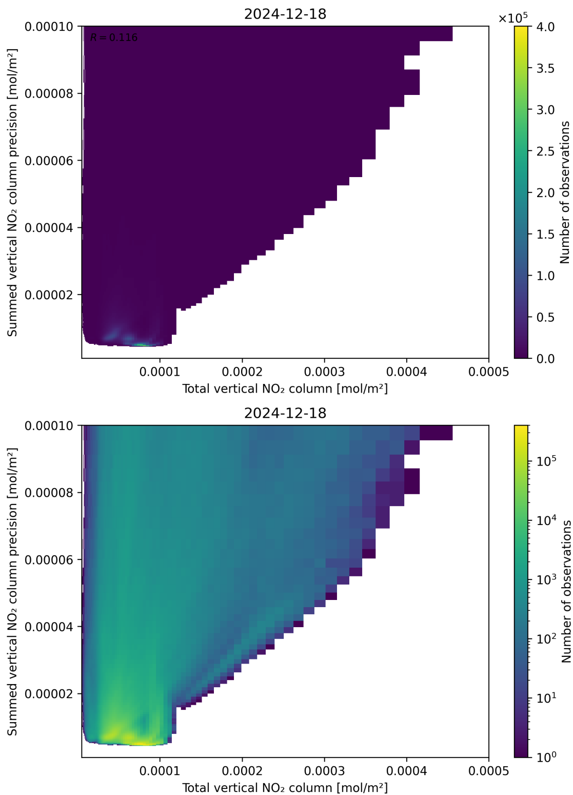
Figure 113: Scatter density plot of “Total vertical NO 2 column” against “Summed vertical NO 2 column precision” for 2024-12-17 to 2024-12-19.
