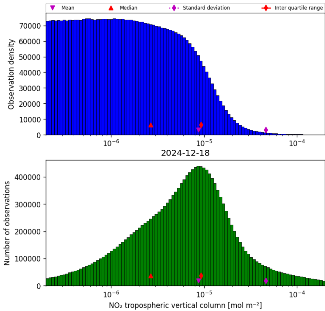
Figure 29: Histogram of “NO 2 tropospheric vertical column” for 2024-12-17 to 2024-12-19
