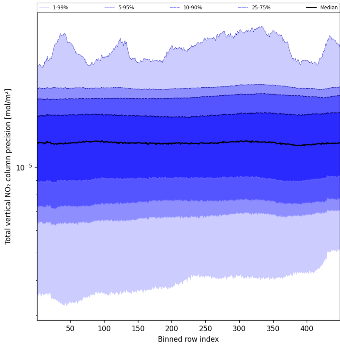
Figure 56: Along track statistics of “Total vertical NO 2 column precision” for 2024-12-17 to 2024-12-19
