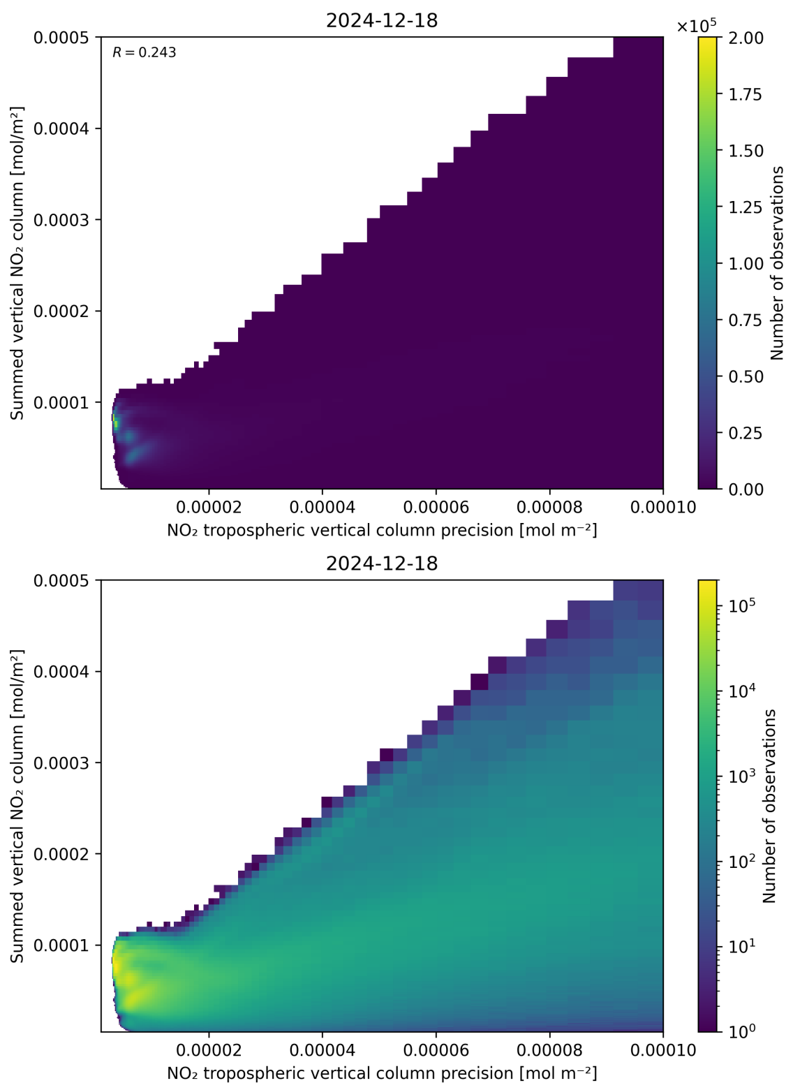
Figure 136: Scatter density plot of “NO 2 tropospheric vertical column precision” against “Summed vertical NO 2 column” for 2024-12-17 to 2024-12-19.
