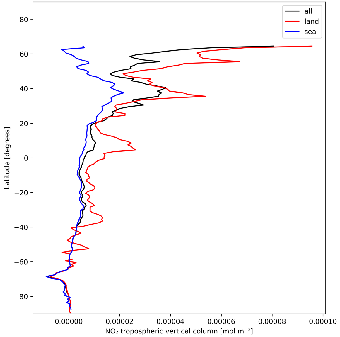
Figure 12: Zonal average of “NO 2 tropospheric vertical column” for 2024-12-17 to 2024-12-19.
