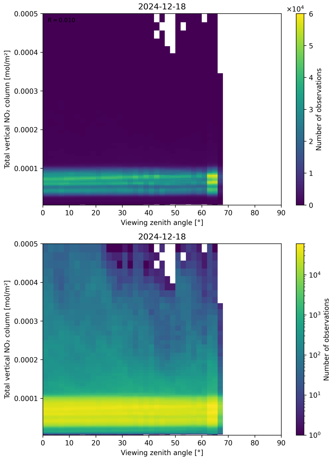
Figure 167: Scatter density plot of “Viewing zenith angle” against “Total vertical NO 2 column” for 2024-12-17 to 2024-12-19.
