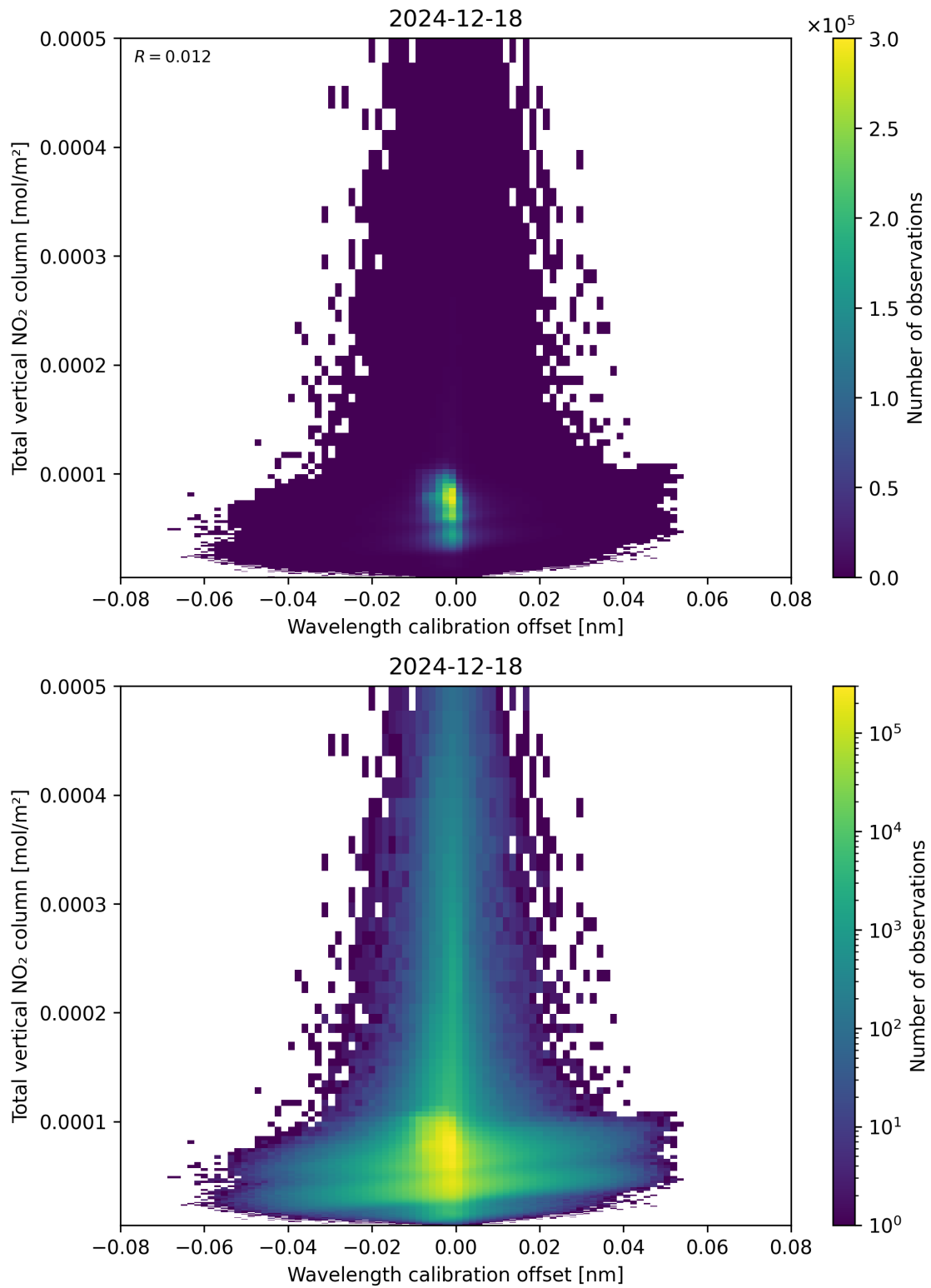
Figure 179: Scatter density plot of “Wavelength calibration offset” against “Total vertical NO 2 column” for 2024-12-17 to 2024-12-19.
