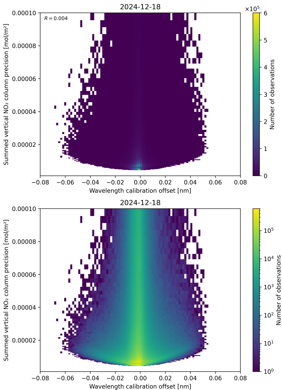
Figure 178: Scatter density plot of “Wavelength calibration offset” against “Summed vertical NO 2 column precision” for 2024-12-17 to 2024-12-19.
