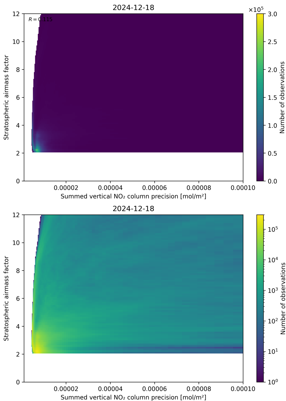
Figure 106: Scatter density plot of “Summed vertical NO 2 column precision” against “Stratospheric airmass factor” for 2024-12-17 to 2024-12-19.
