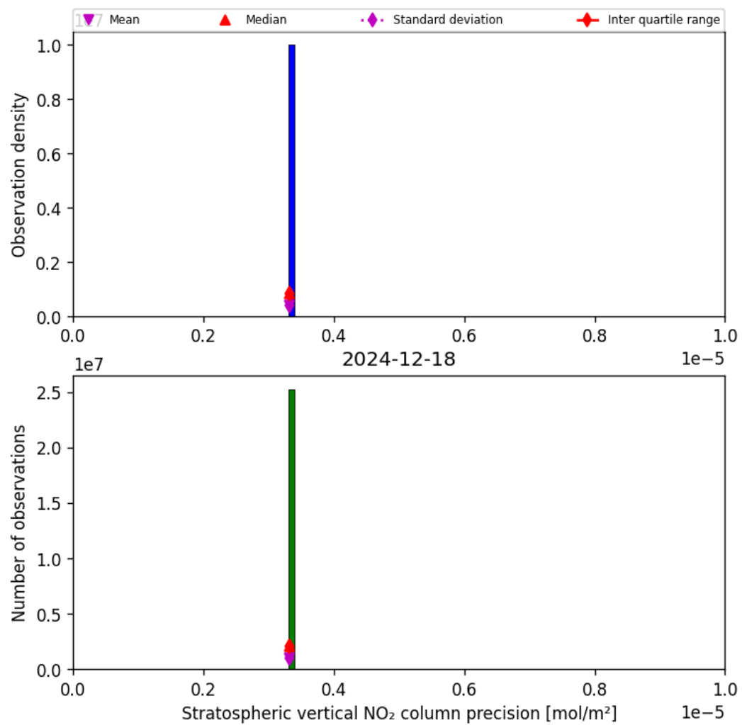
Figure 37: Histogram of “Stratospheric vertical NO 2 column precision” for 2024-12-17 to 2024-12-19
