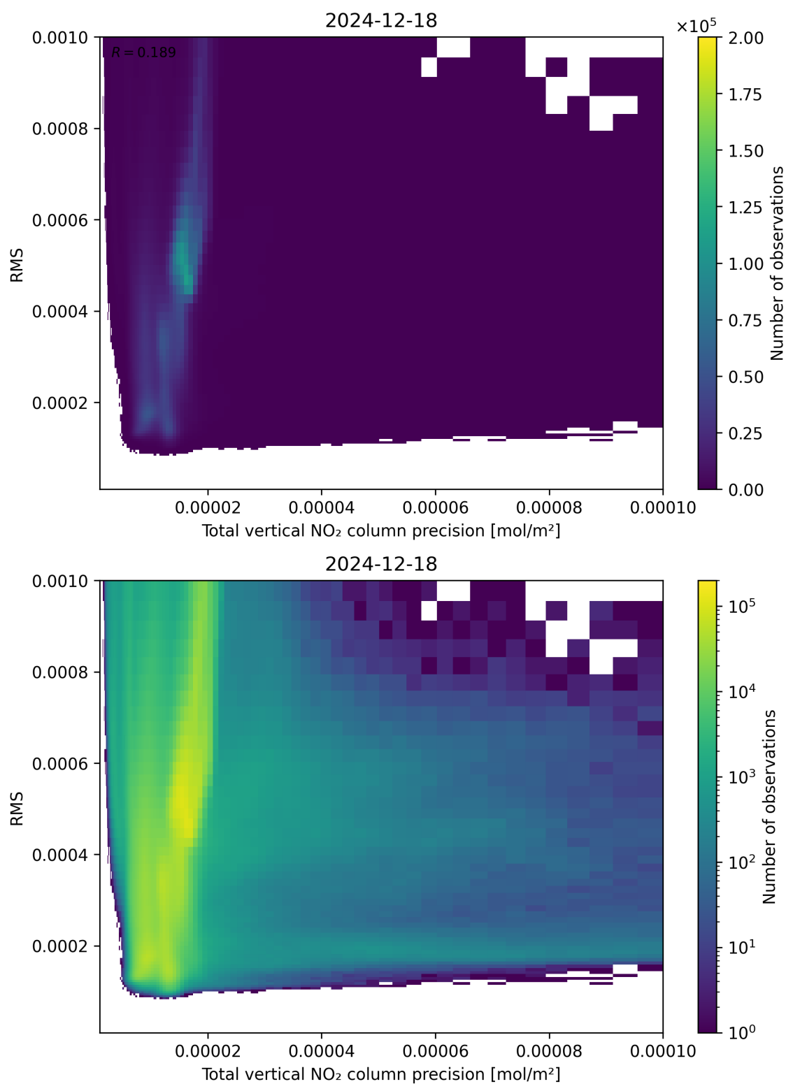
Figure 119: Scatter density plot of “Total vertical NO 2 column precision” against “RMS” for 2024-12-17 to 2024-12-19.
