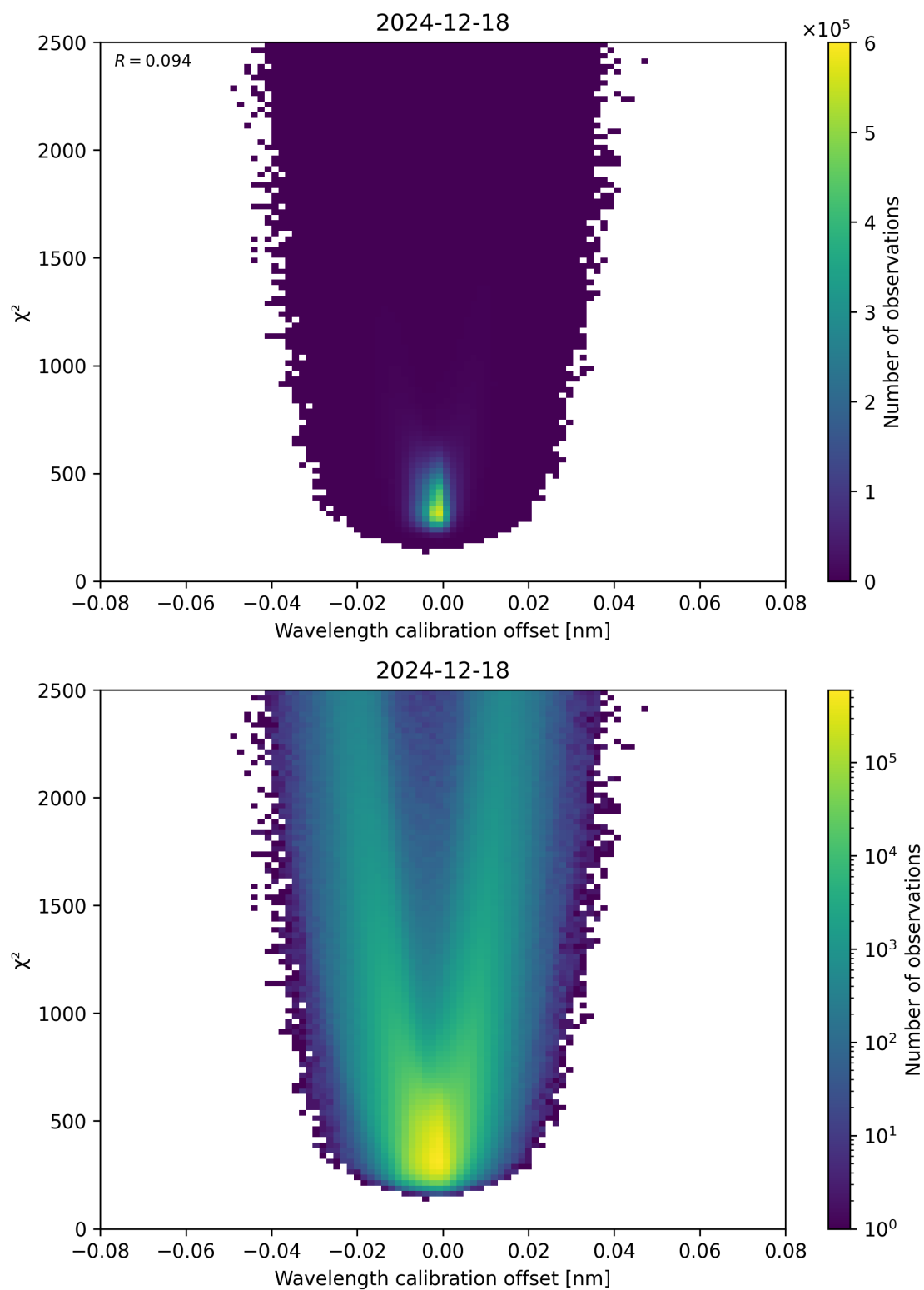
Figure 175: Scatter density plot of “Wavelength calibration offset” against “ \chi^2 ” for 2024-12-17 to 2024-12-19.
