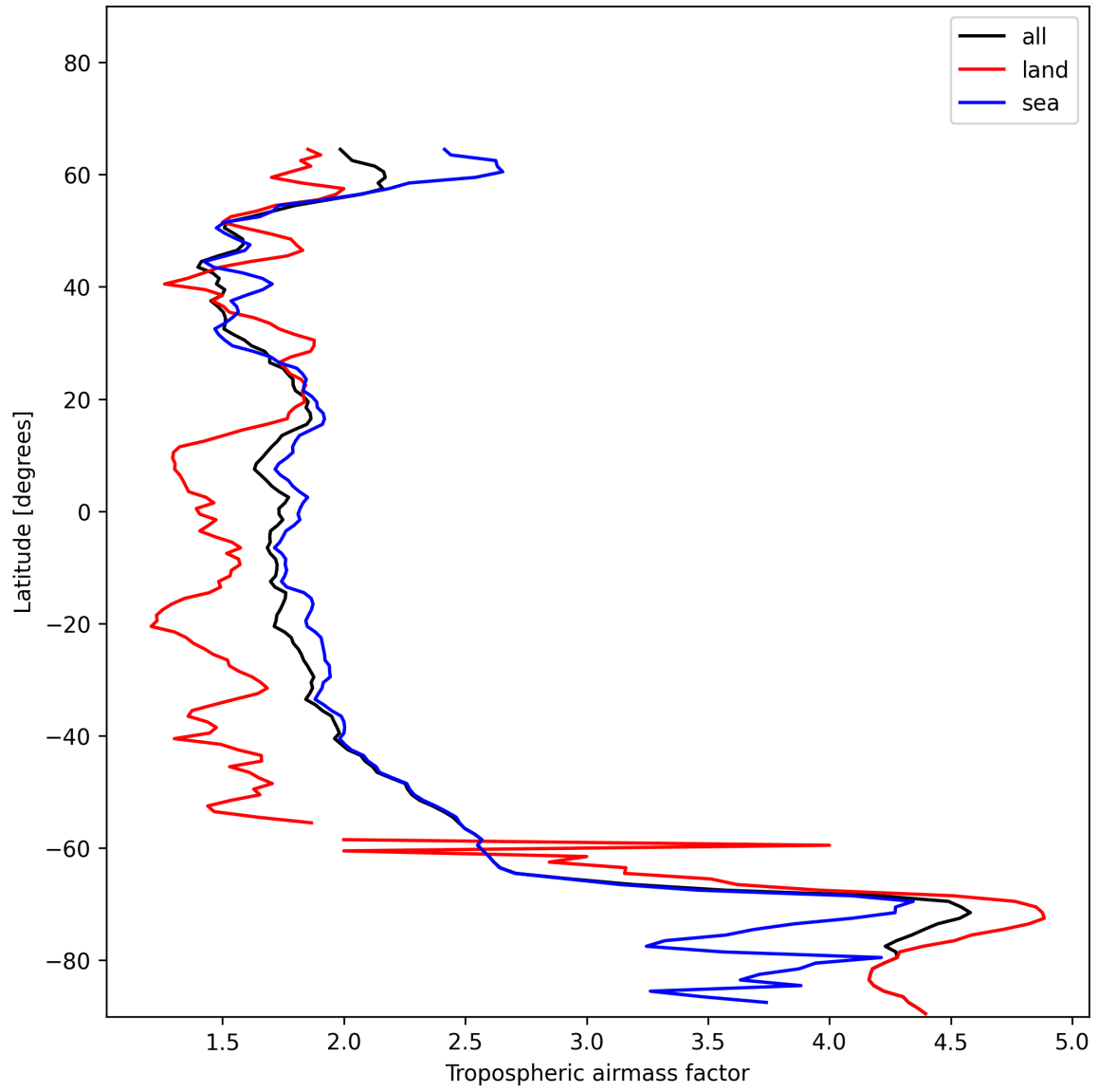
Figure 14: Zonal average of “Tropospheric airmass factor” for 2024-12-17 to 2024-12-19.
