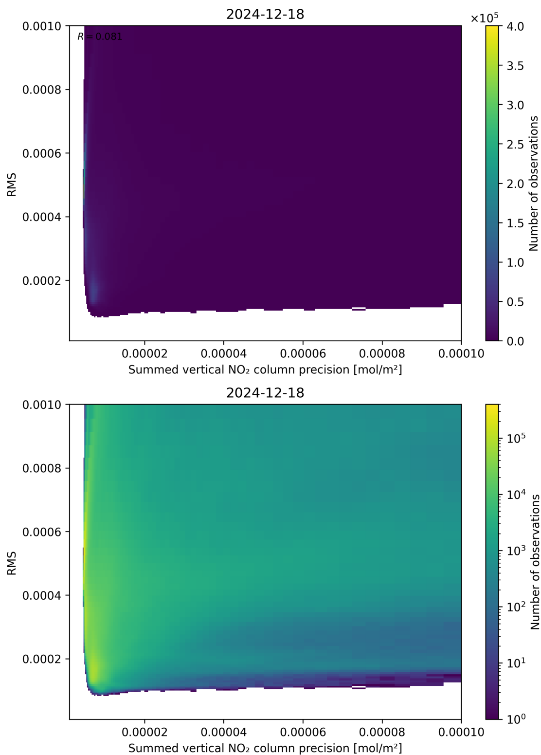
Figure 108: Scatter density plot of “Summed vertical NO 2 column precision” against “RMS” for 2024-12-17 to 2024-12-19.
