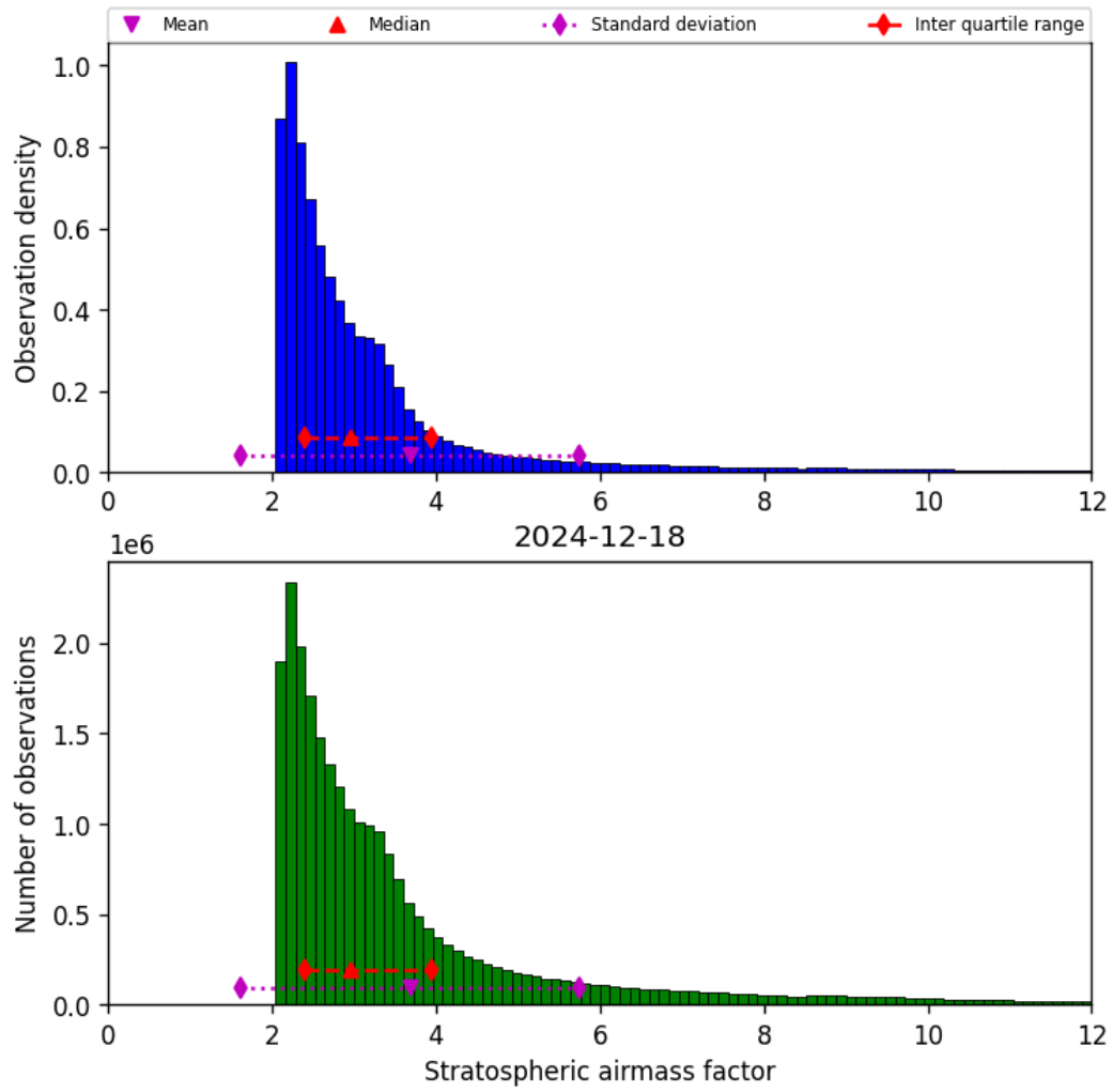
Figure 44: Histogram of “Stratospheric airmass factor” for 2024-12-17 to 2024-12-19
