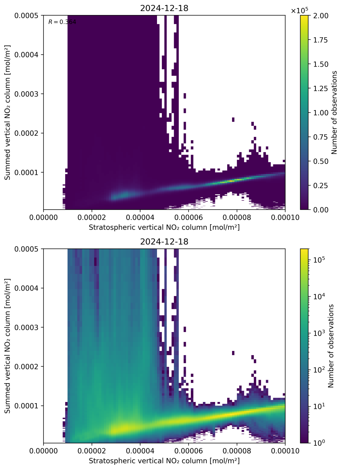
Figure 98: Scatter density plot of “Stratospheric vertical NO 2 column” against “Summed vertical NO 2 column” for 2024-12-17 to 2024-12-19.
