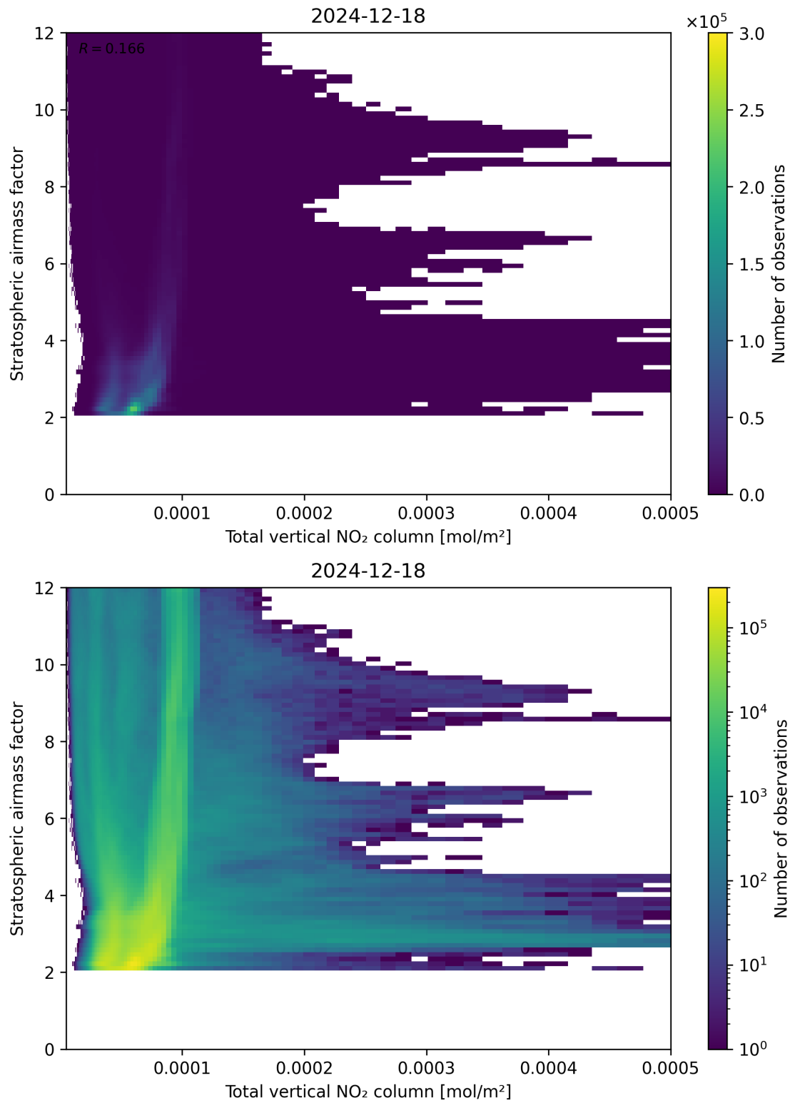
Figure 110: Scatter density plot of “Total vertical NO 2 column” against “Stratospheric air mass factor” for 2024-12-17 to 2024-12-19.
