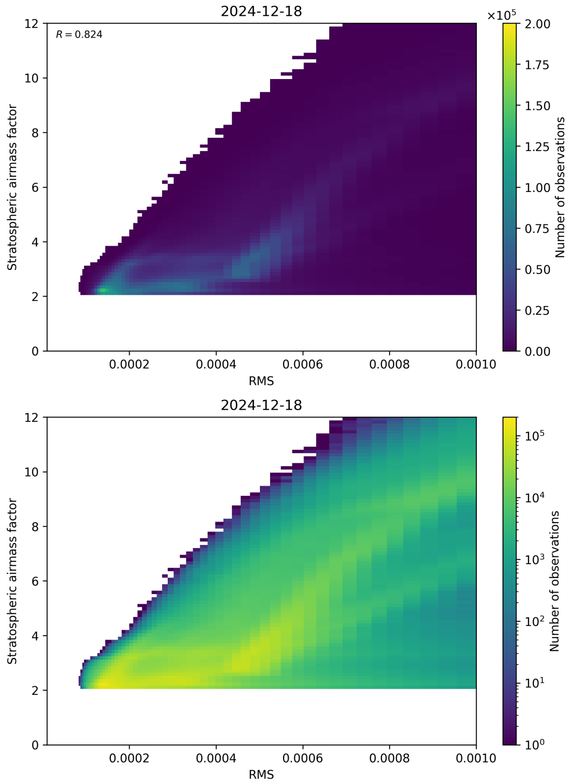
Figure 144: Scatter density plot of “RMS” against “Stratospheric airmass factor” for 2024-12-17 to 2024-12-19.
