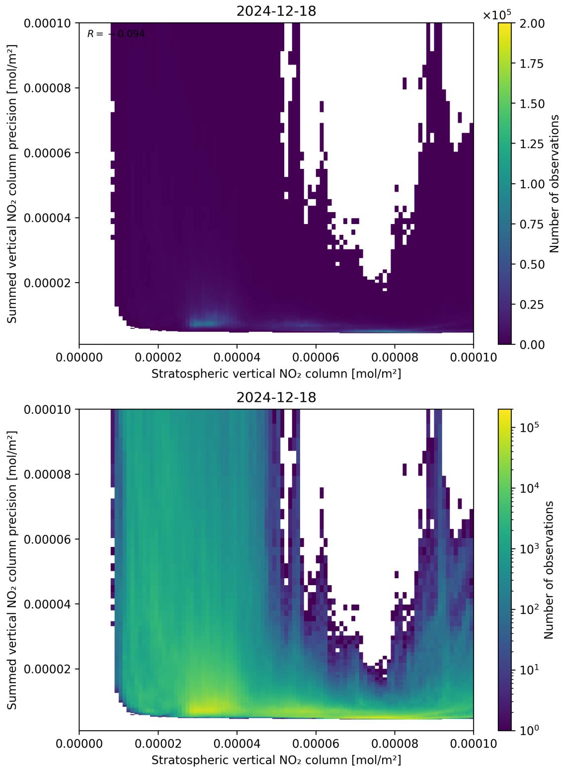
Figure 99: Scatter density plot of “Stratospheric vertical NO 2 column” against “Summed vertical NO 2 column precision” for 2024-12-17 to 2024-12-19.
